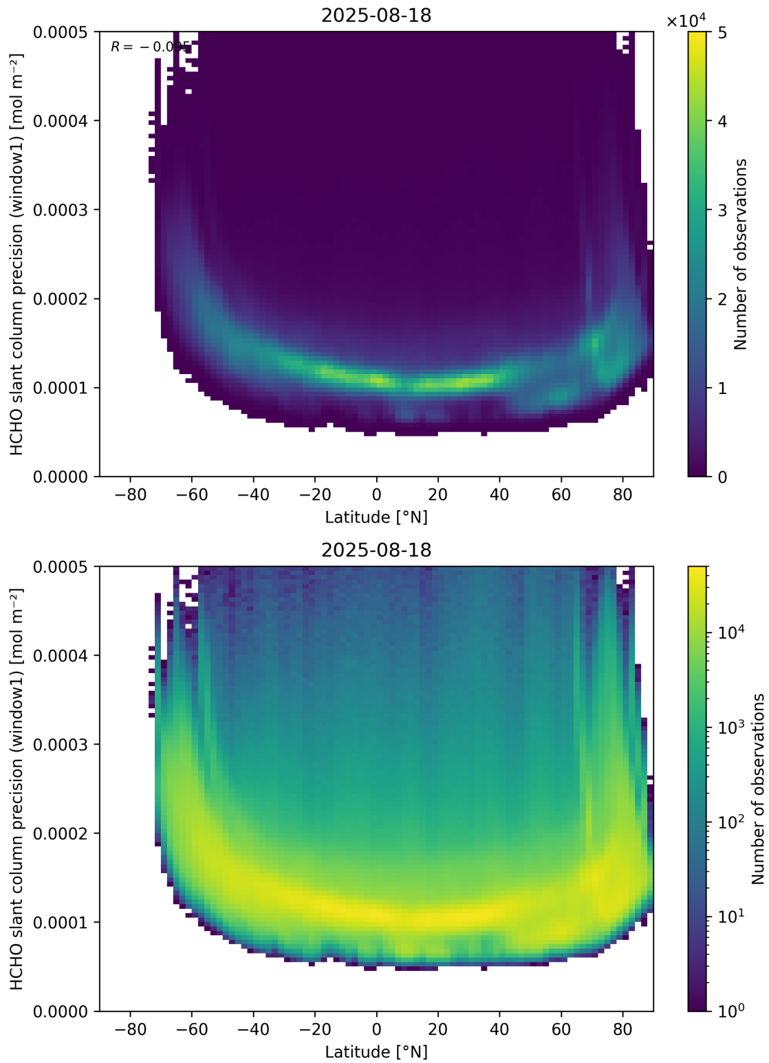
Figure 160: Scatter density plot of “Latitude” against “HCHO slant column precision (window1)” for 2025-08-17 to 2025-08-19.
