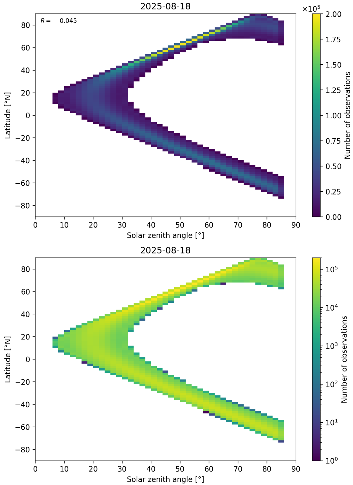
Figure 181: Scatter density plot of “Solar zenith angle” against “Latitude” for 2025-08-17 to 2025-08-19.
