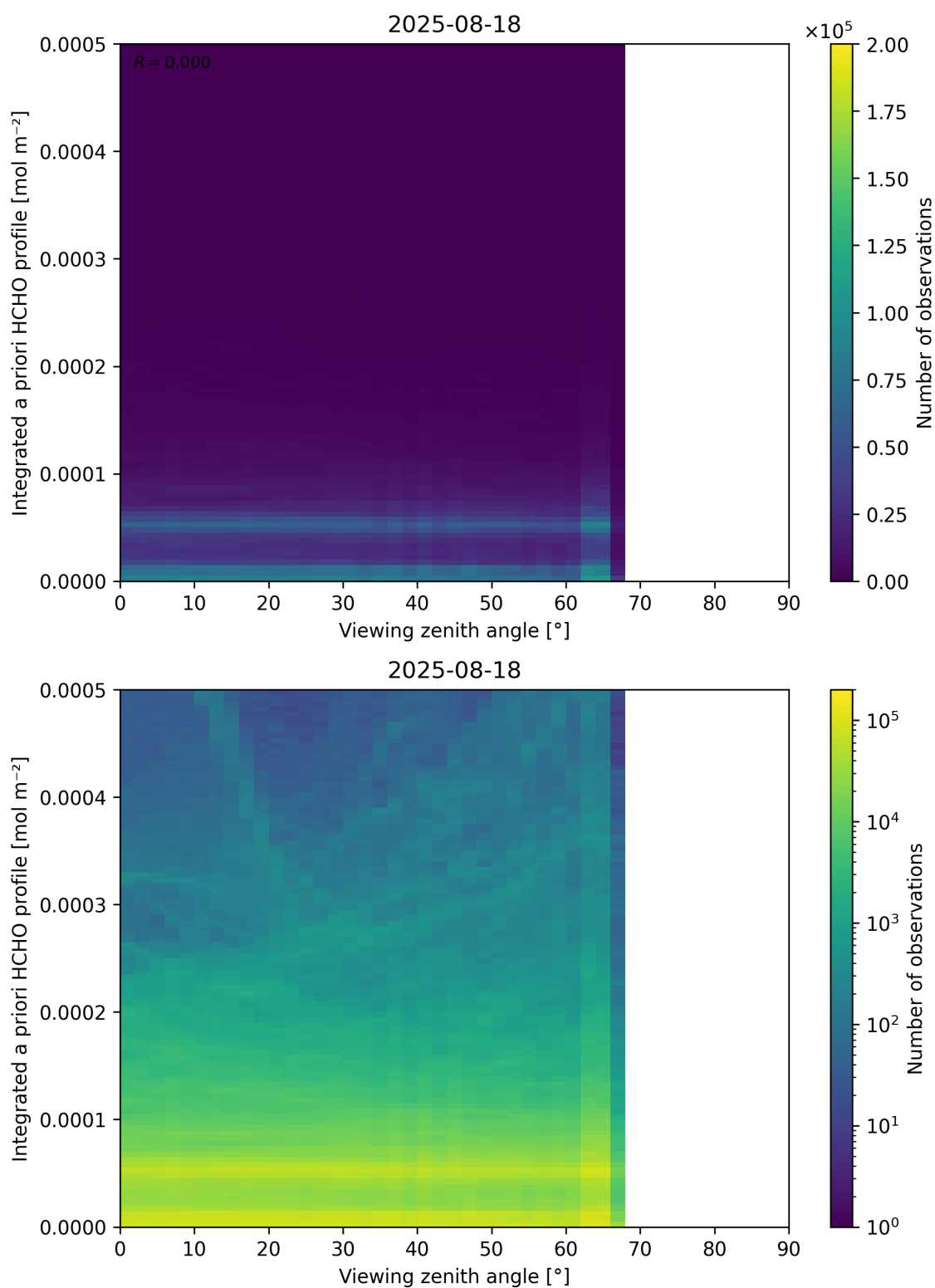
Figure 195: Scatter density plot of “Viewing zenith angle” against “Integrated a priori HCHO profile” for 2025-08-17 to 2025-08-19.
