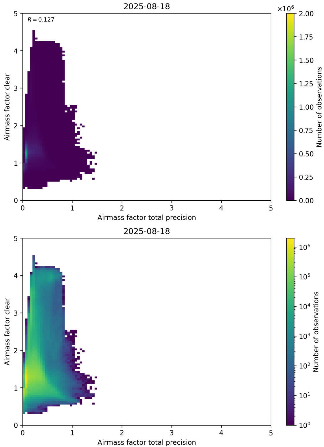
Figure 108: Scatter density plot of “Airmass factor total precision” against “Airmass factor clear” for 2025-08-17 to 2025-08-19.
