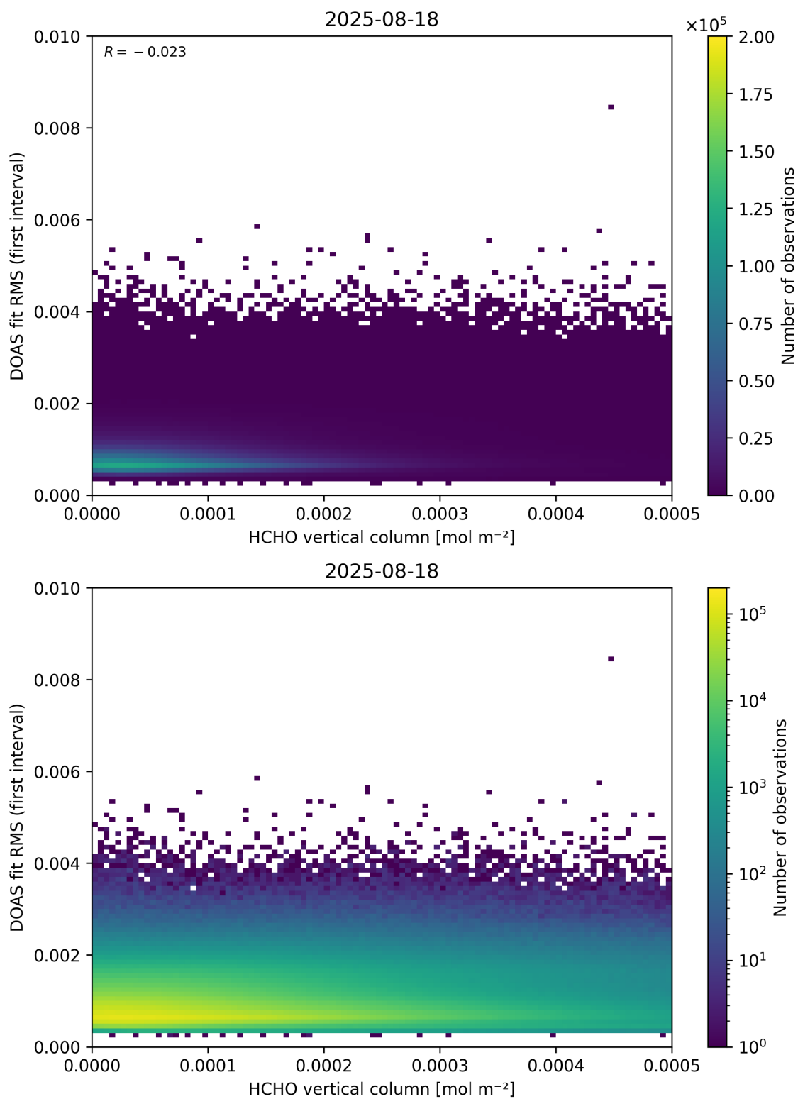
Figure 123: Scatter density plot of “HCHO vertical column” against “DOAS fit RMS (first interval)” for 2025-08-17 to 2025-08-19.
