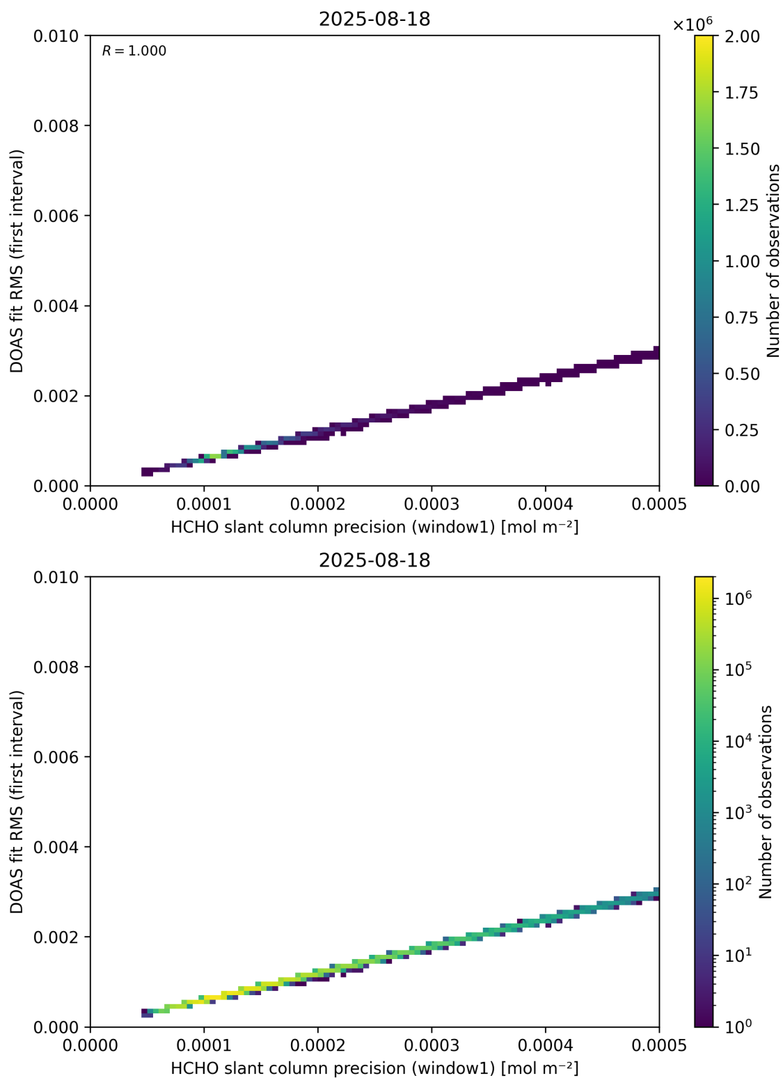
Figure 88: Scatter density plot of “HCHO slant column precision (window1)” against “DOAS fit RMS (first interval)” for 2025-08-17 to 2025-08-19.
