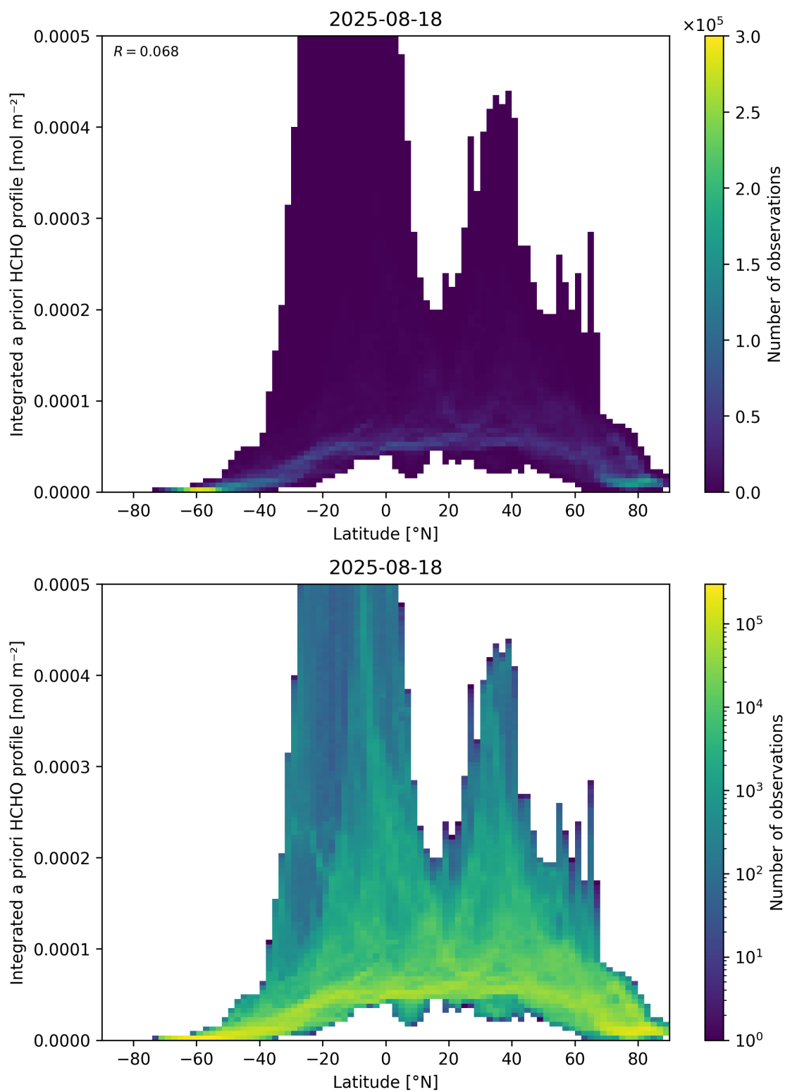
Figure 166: Scatter density plot of “Latitude” against “Integrated a priori HCHO profile” for 2025-08-17 to 2025-08-19.
