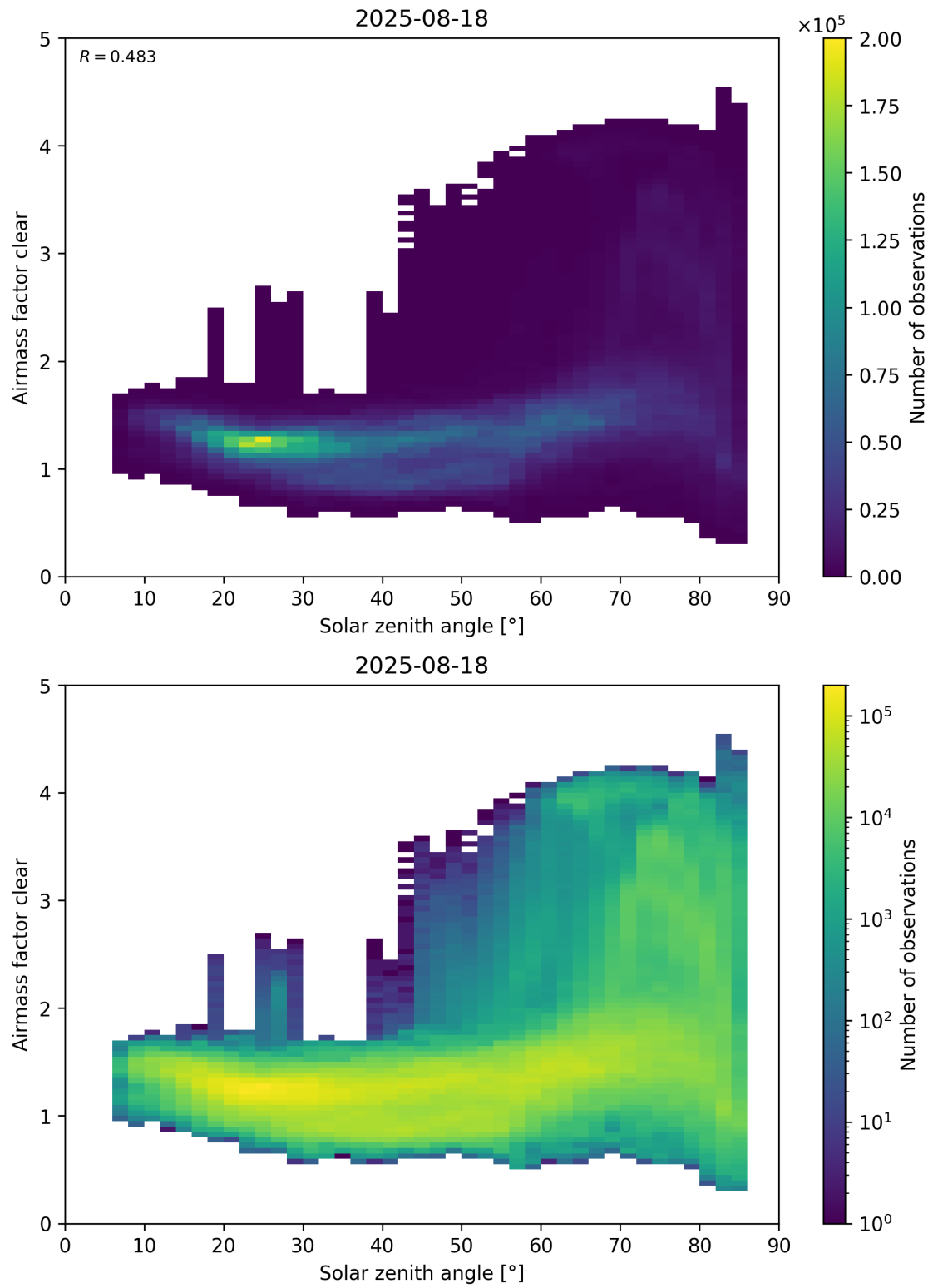
Figure 170: Scatter density plot of “Solar zenith angle” against “Airmass factor clear” for 2025-08-17 to 2025-08-19.
