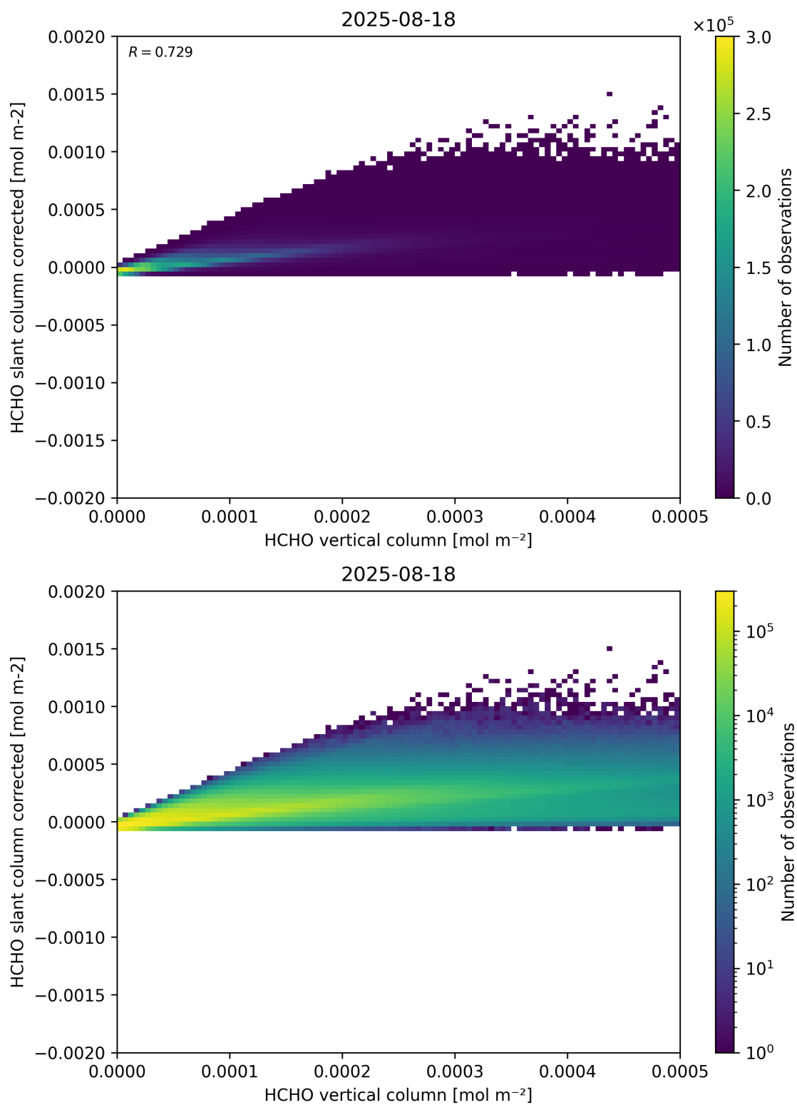
Figure 127: Scatter density plot of “HCHO vertical column” against “HCHO slant column corrected” for 2025-08-17 to 2025-08-19.
