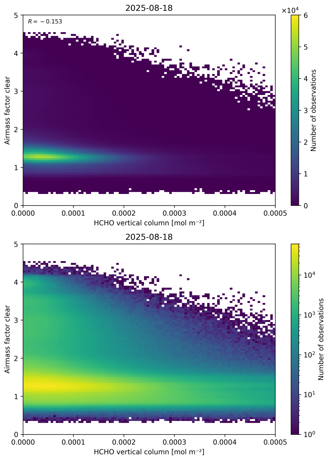
Figure 126: Scatter density plot of “HCHO vertical column” against “Airmass factor clear” for 2025-08-17 to 2025-08-19.
