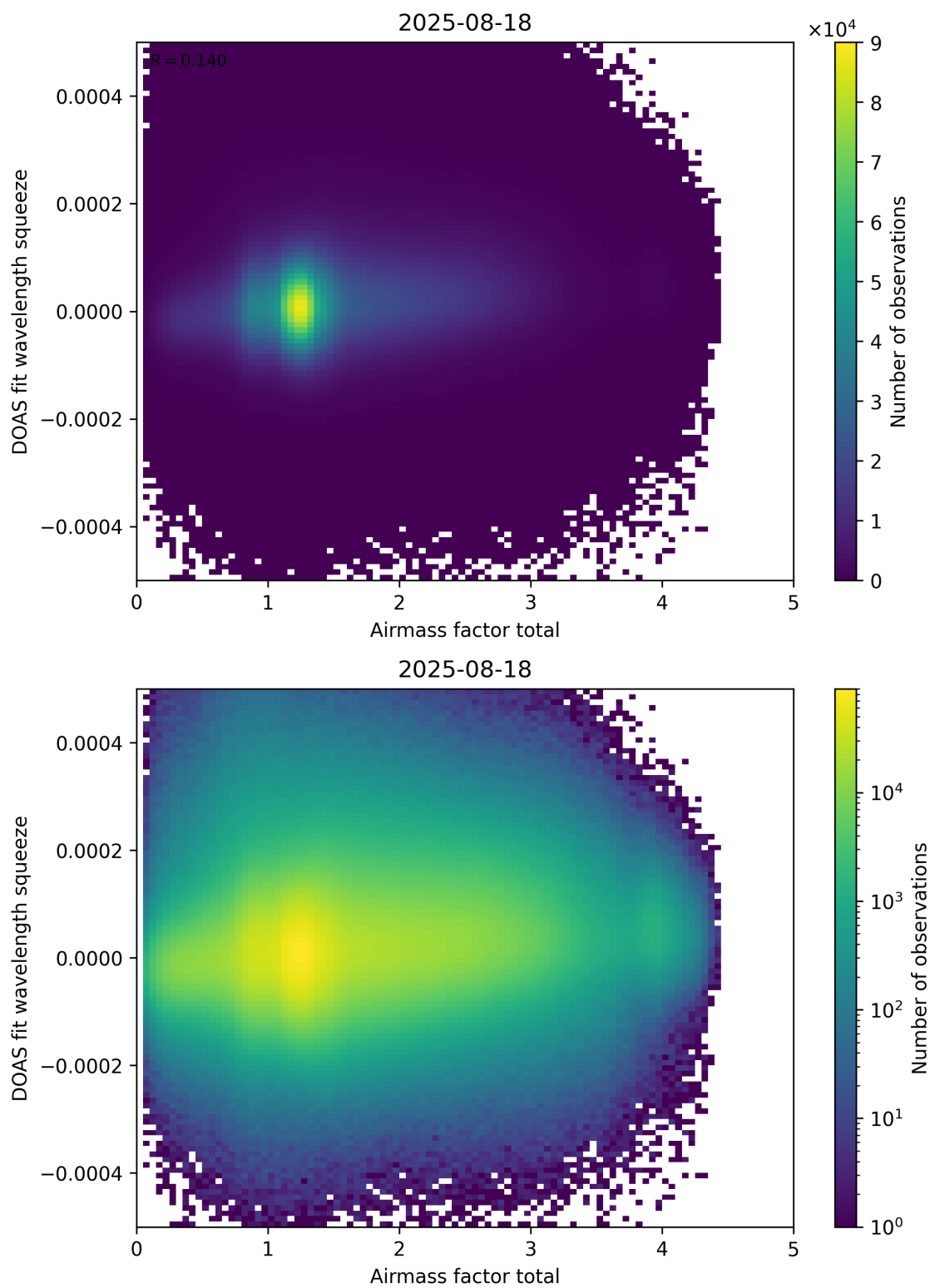
Figure 99: Scatter density plot of “Airmass factor total” against “DOAS fit wavelength squeeze” for 2025-08-17 to 2025-08-19.
