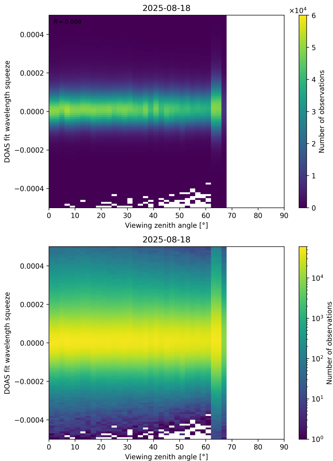
Figure 184: Scatter density plot of “Viewing zenith angle” against “DOAS fit wavelength squeeze” for 2025-08-17 to 2025-08-19.
