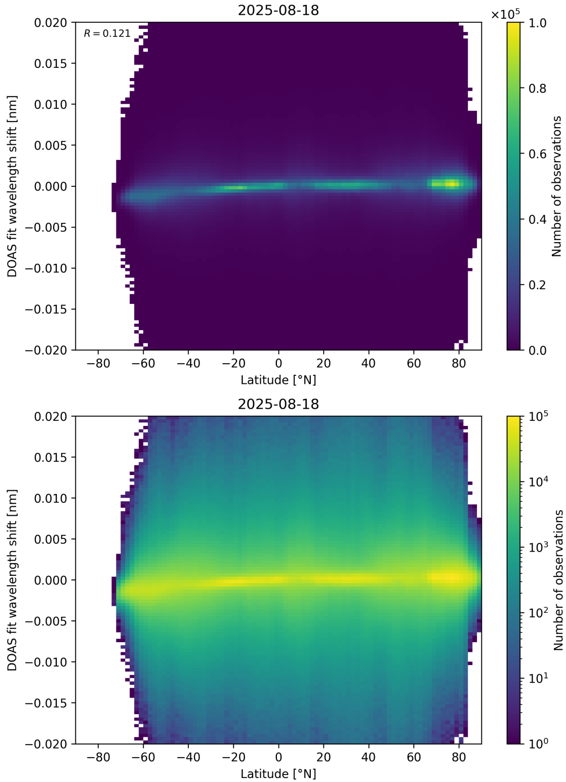
Figure 154: Scatter density plot of “Latitude” against “DOAS fit wavelength shift” for 2025-08-17 to 2025-08-19.
