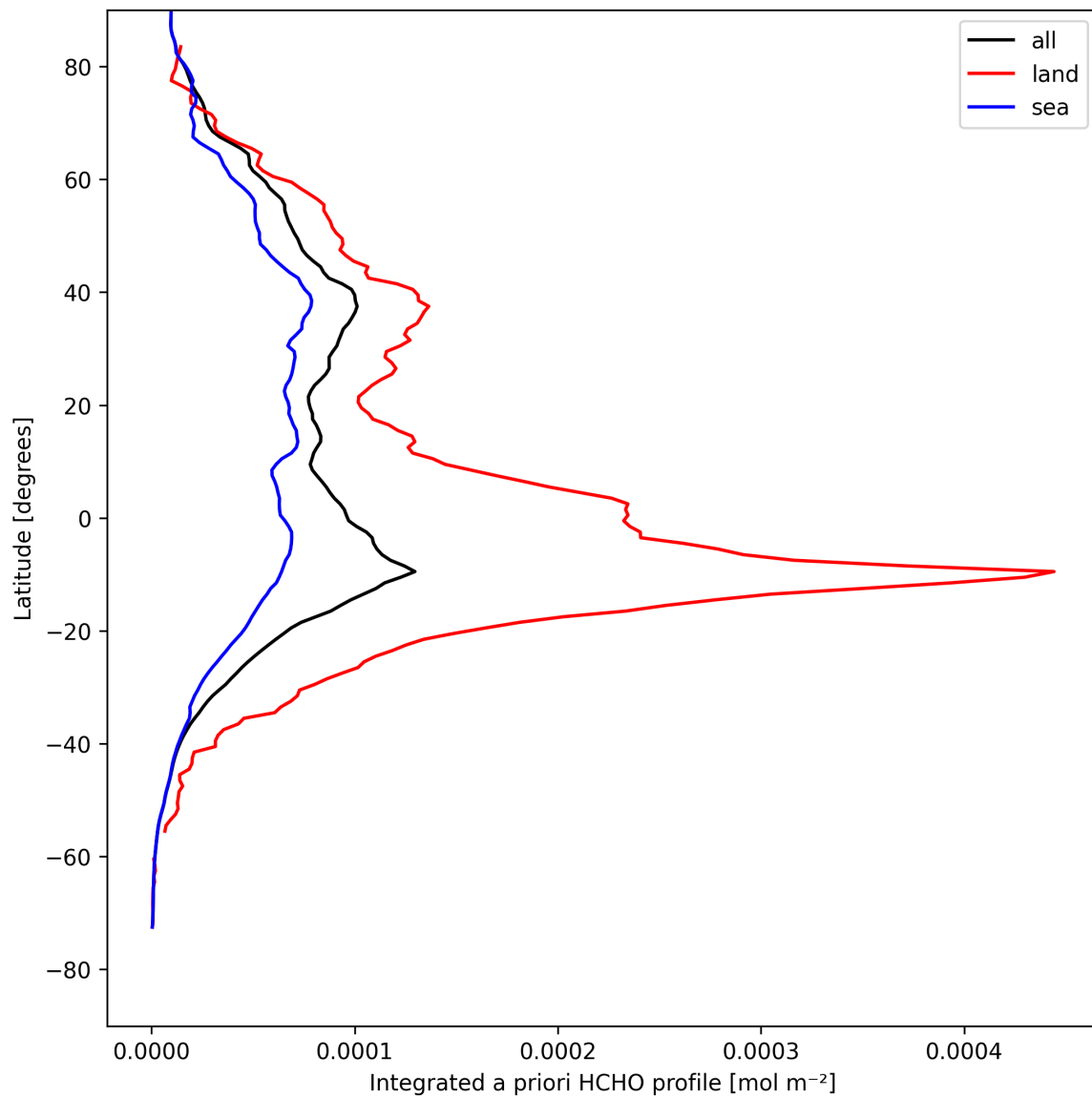
Figure 29: Zonal average of “Integrated a priori HCHO profile” for 2025-08-17 to 2025-08-19.
