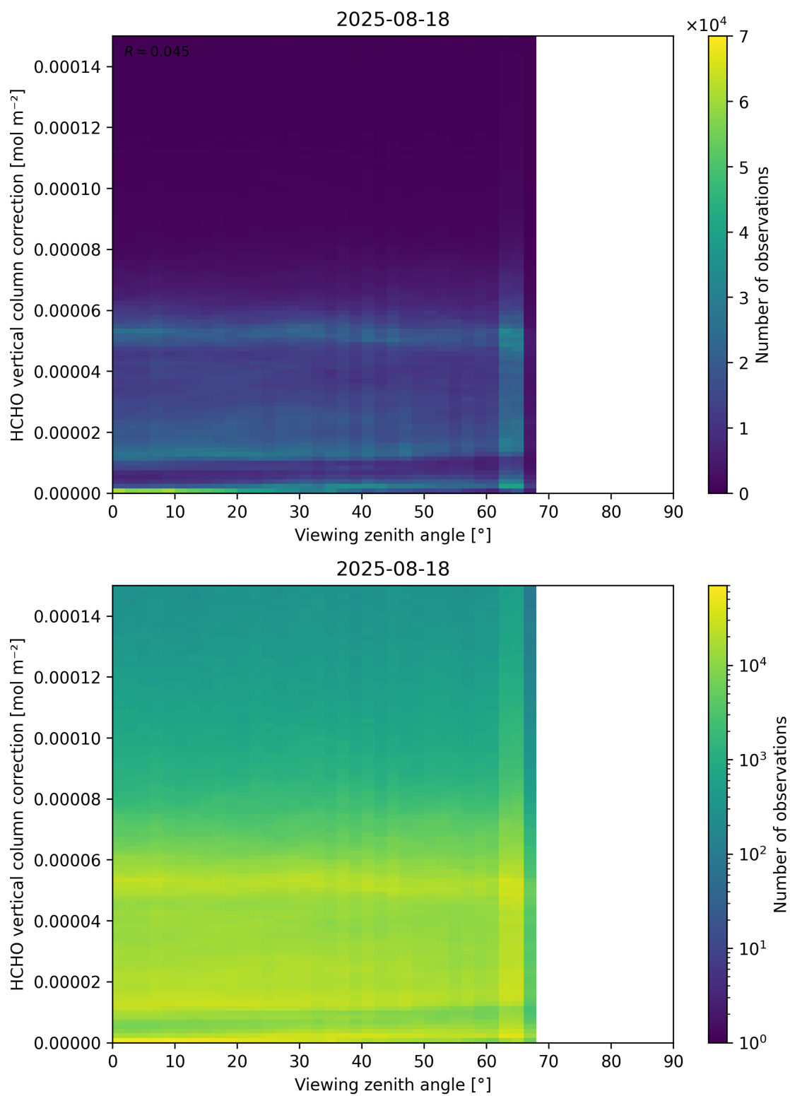
Figure 193: Scatter density plot of “Viewing zenith angle” against “HCHO vertical column correction” for 2025-08-17 to 2025-08-19.
