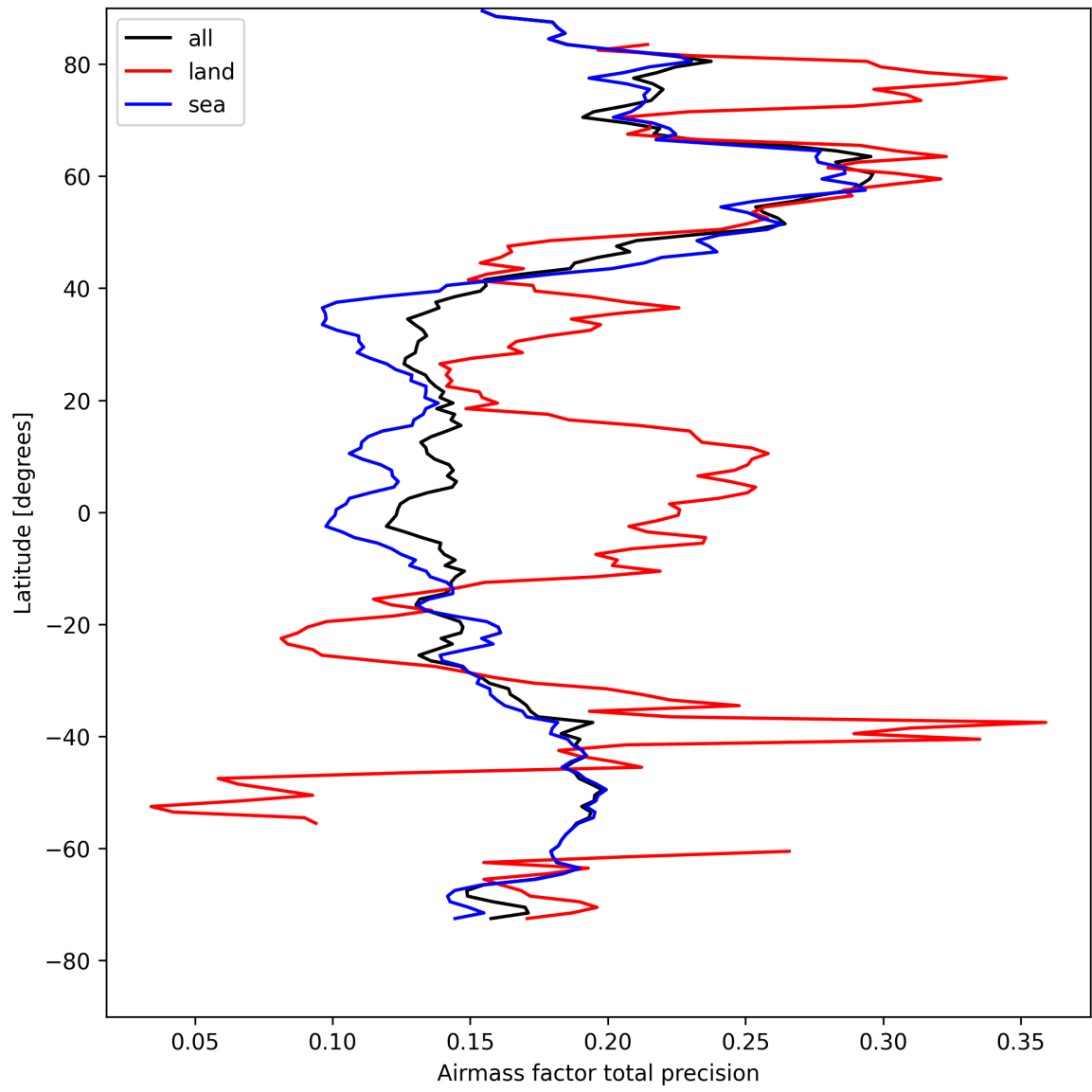
Figure 27: Zonal average of “Airmass factor total precision” for 2025-08-17 to 2025-08-19.
