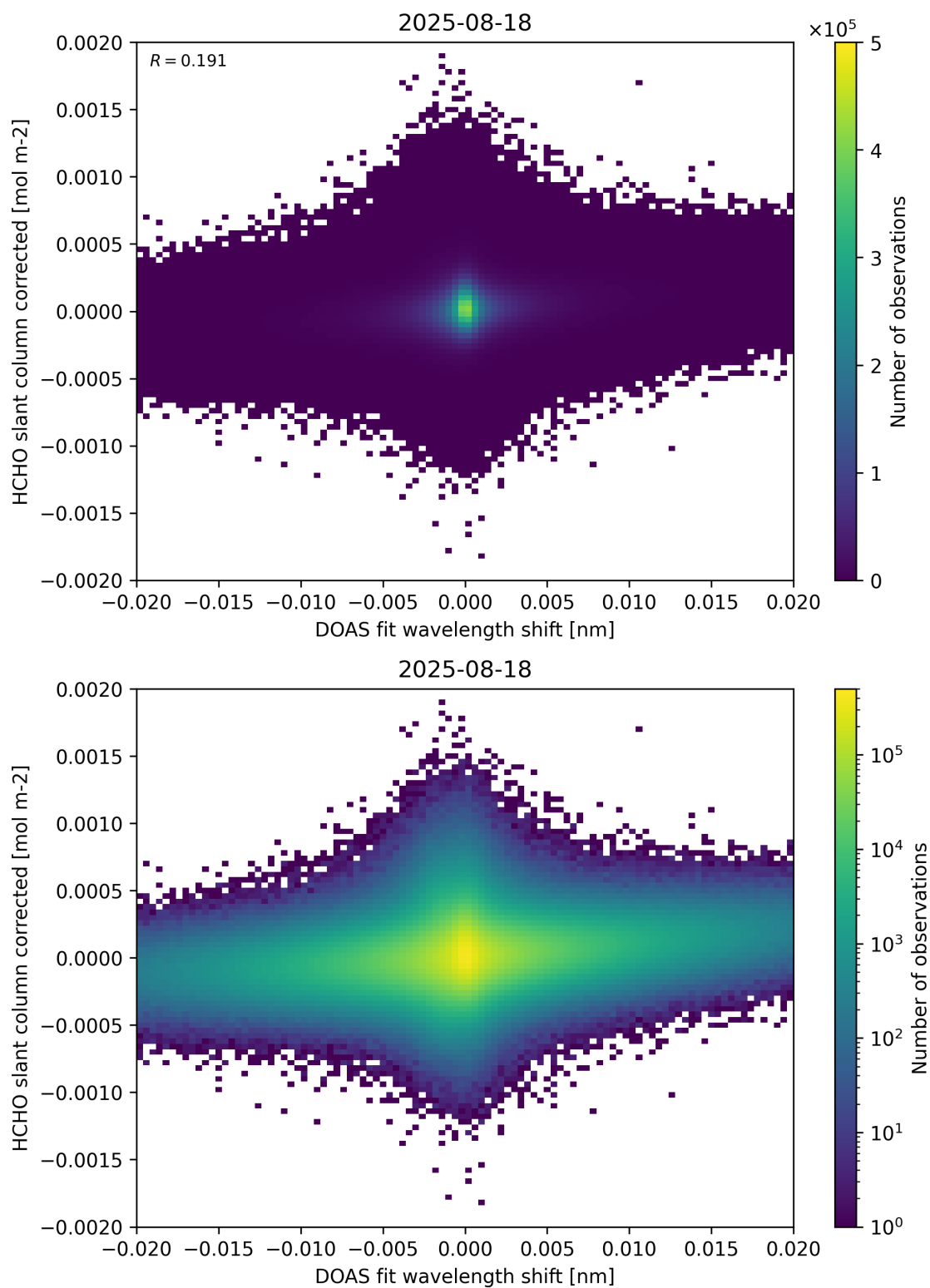
Figure 66: Scatter density plot of “DOAS fit wavelength shift” against “HCHO slant column corrected” for 2025-08-17 to 2025-08-19.
