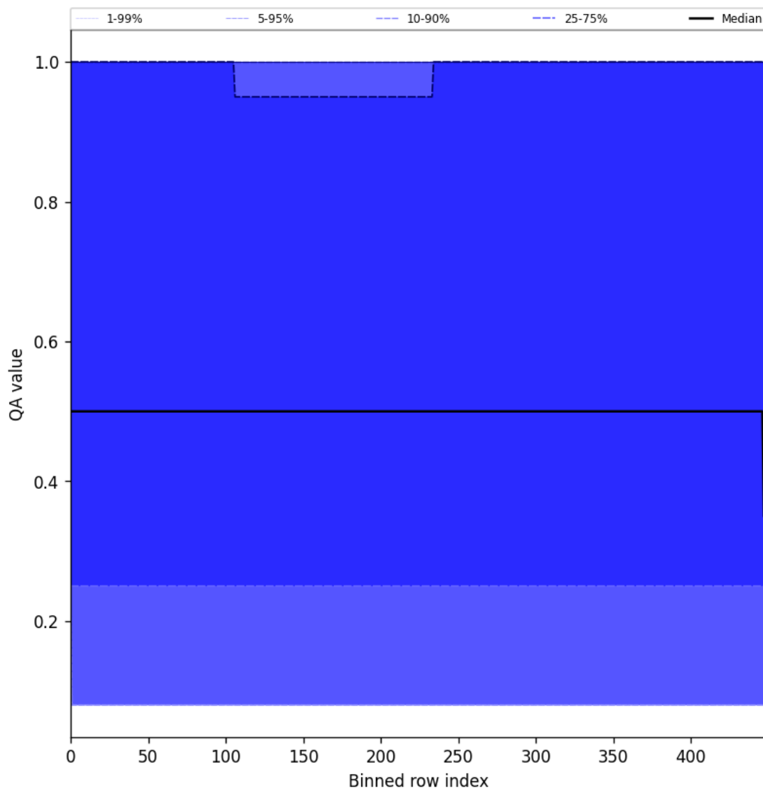
Figure 48: Along track statistics of “QA value” for 2025-08-17 to 2025-08-19
