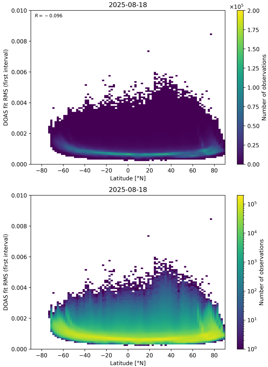
Figure 153: Scatter density plot of “Latitude” against “DOAS fit RMS (first interval)” for 2025-08-17 to 2025-08-19.
