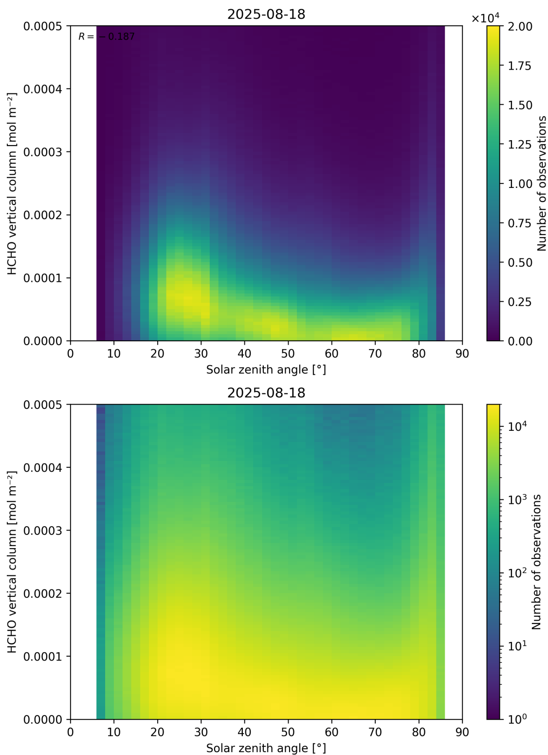
Figure 177: Scatter density plot of “Solar zenith angle” against “HCHO vertical column” for 2025-08-17 to 2025-08-19.
