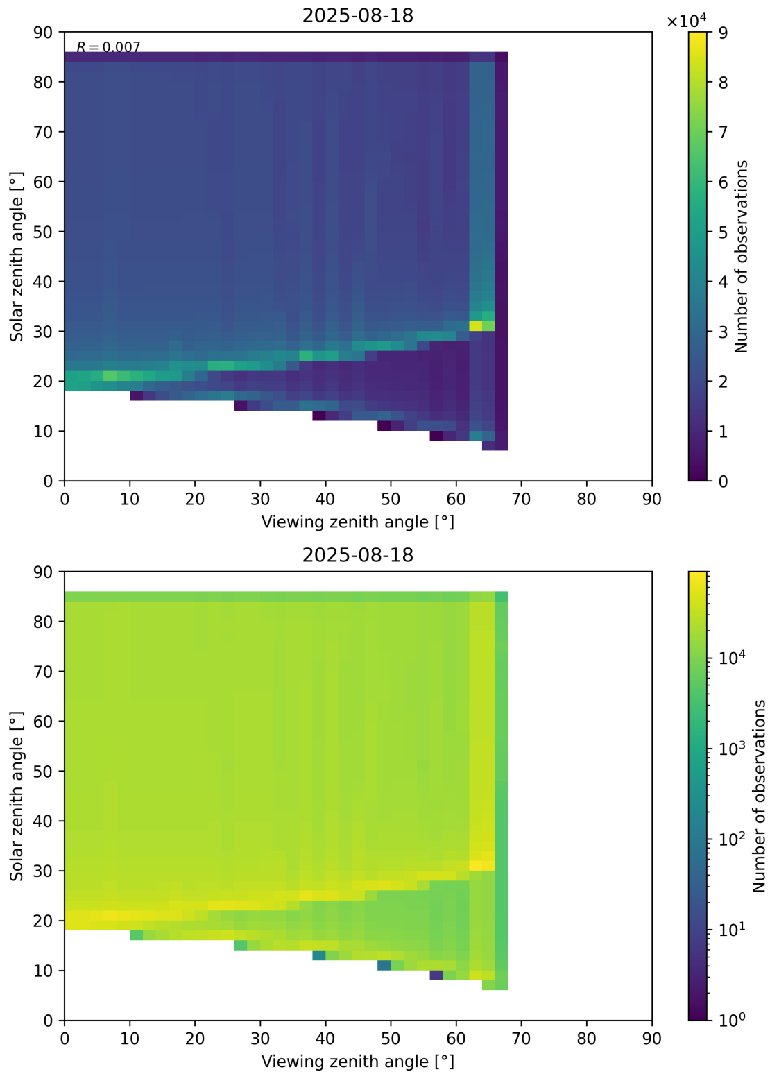
Figure 197: Scatter density plot of “Viewing zenith angle” against “Solar zenith angle” for 2025-08-17 to 2025-08-19.
