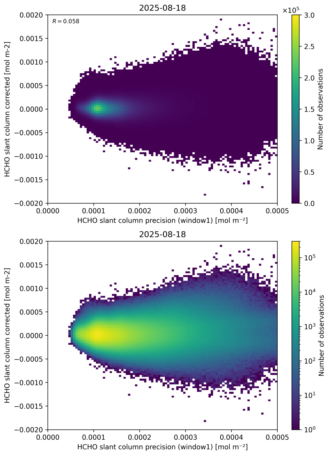
Figure 92: Scatter density plot of “HCHO slant column precision (window1)” against “HCHO slant column corrected” for 2025-08-17 to 2025-08-19.
