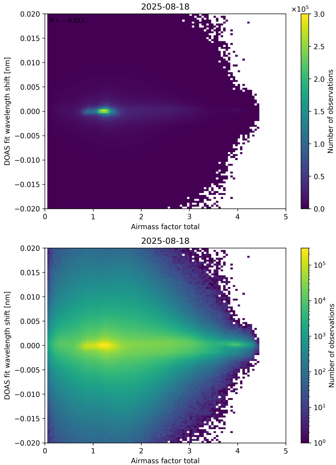
Figure 98: Scatter density plot of “Airmass factor total” against “DOAS fit wavelength shift” for 2025-08-17 to 2025-08-19.
