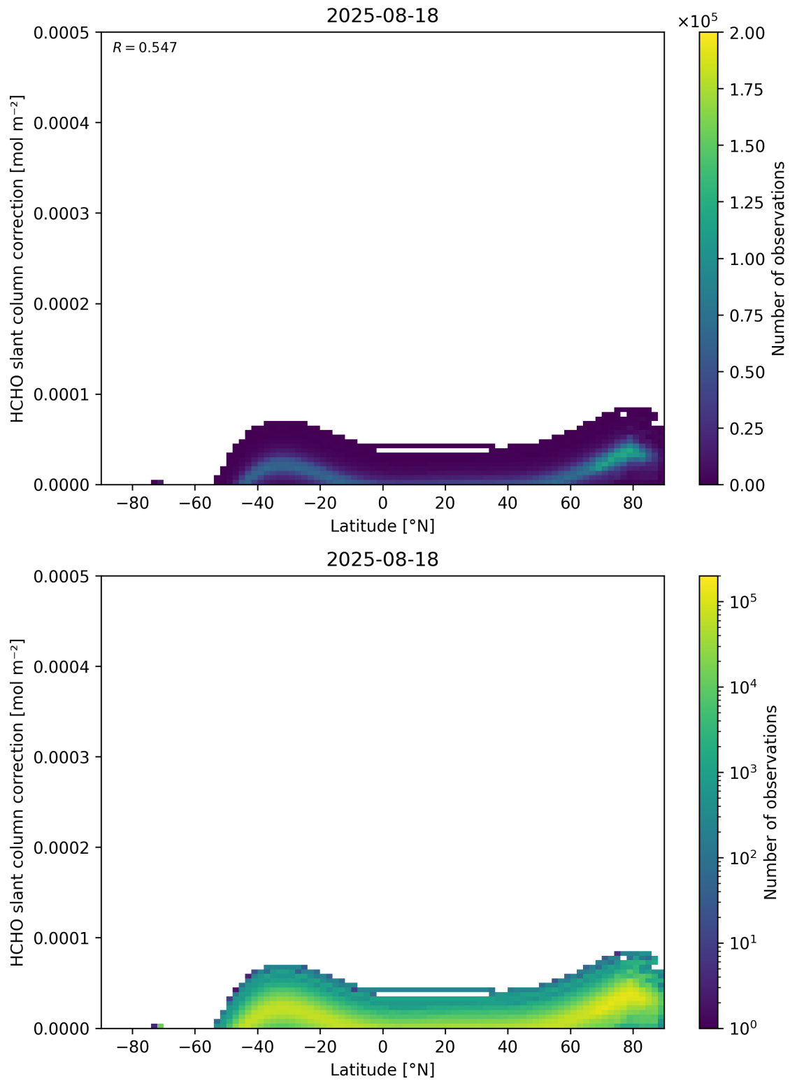
Figure 158: Scatter density plot of “Latitude” against “HCHO slant column correction” for 2025-08-17 to 2025-08-19.
