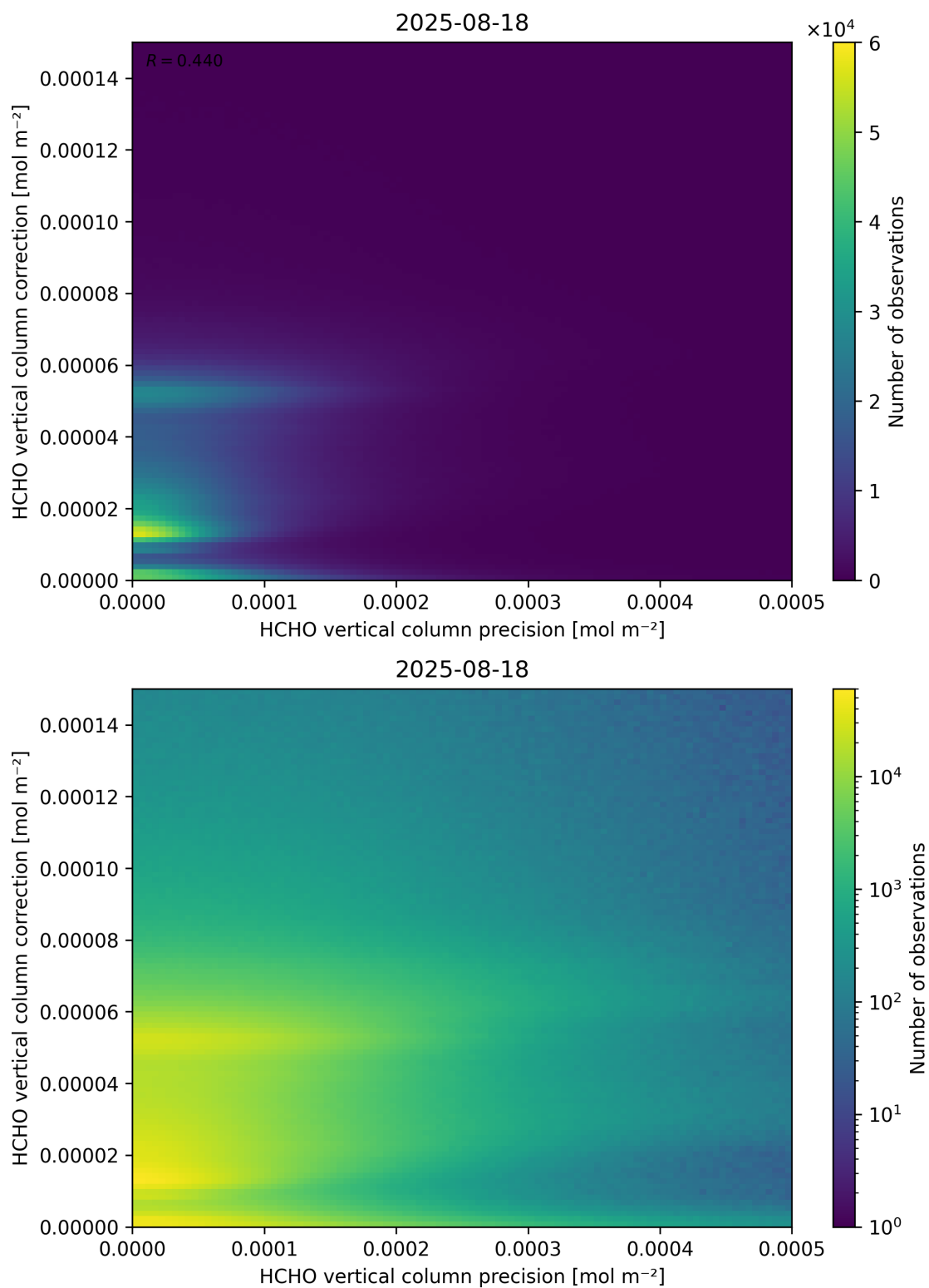
Figure 146: Scatter density plot of “HCHO vertical column precision” against “HCHO vertical column correction” for 2025-08-17 to 2025-08-19.
