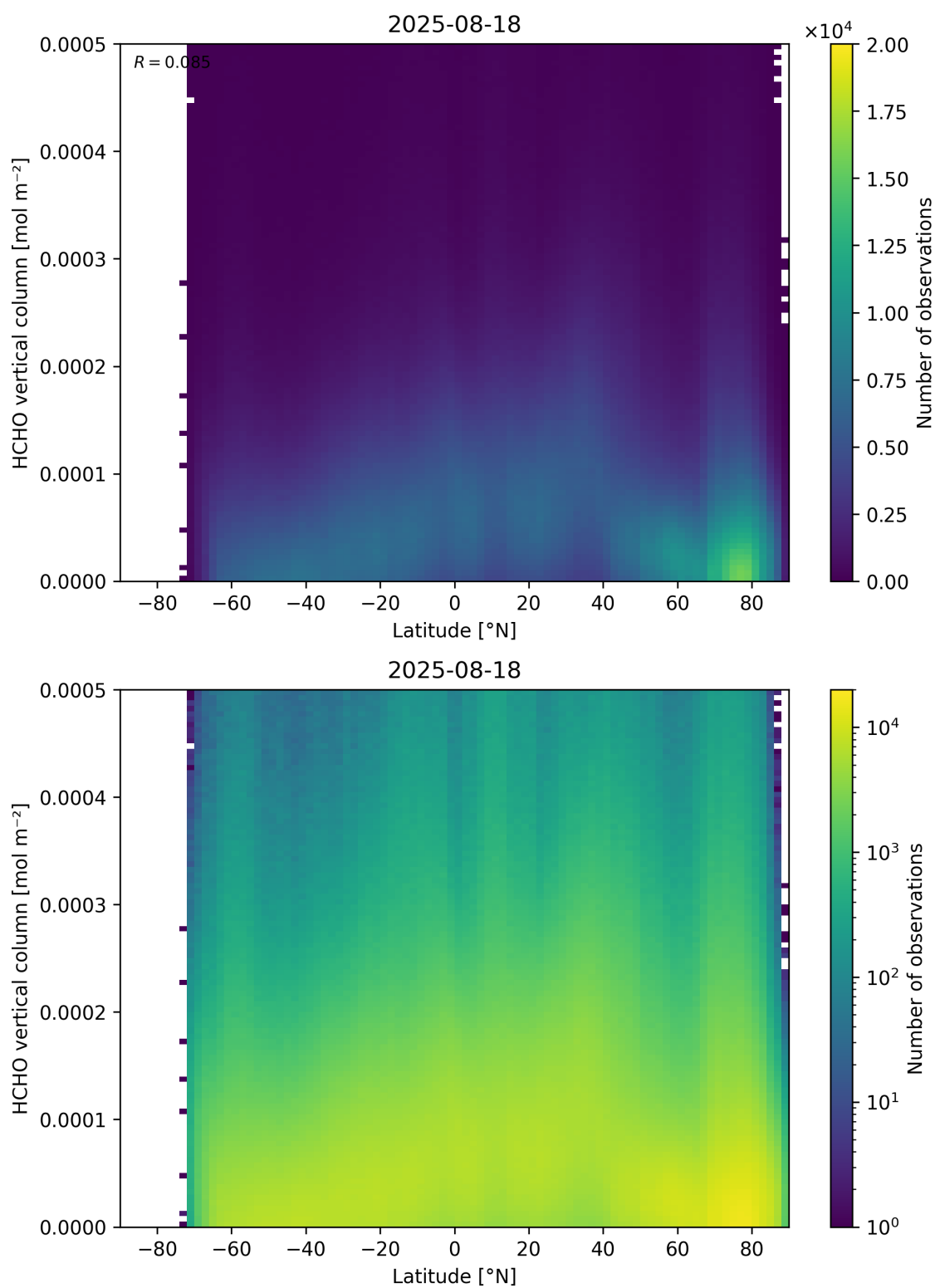
Figure 163: Scatter density plot of “Latitude” against “HCHO vertical column” for 2025-08-17 to 2025-08-19.
