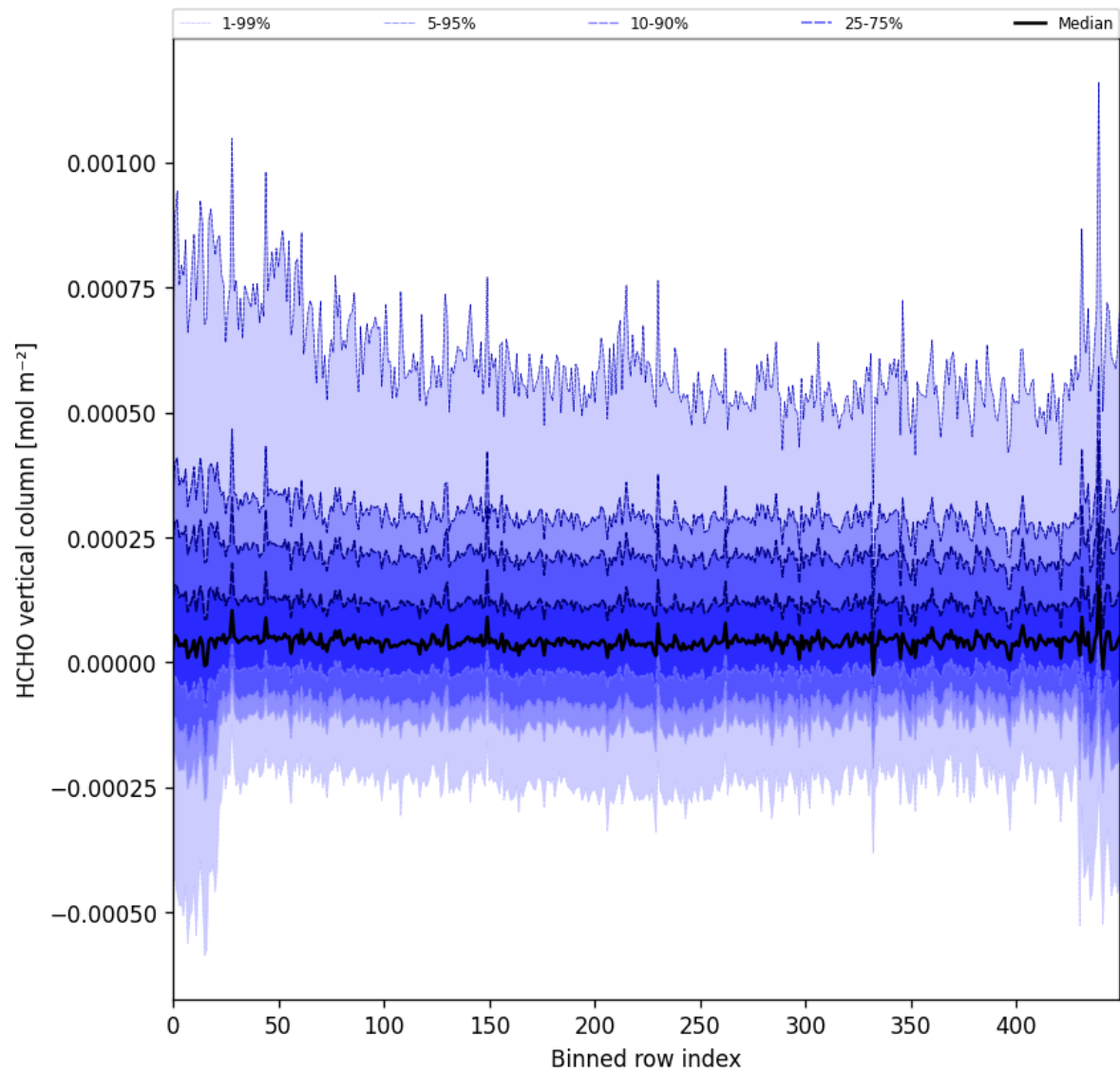
Figure 49: Along track statistics of “HCHO vertical column” for 2025-08-17 to 2025-08-19
