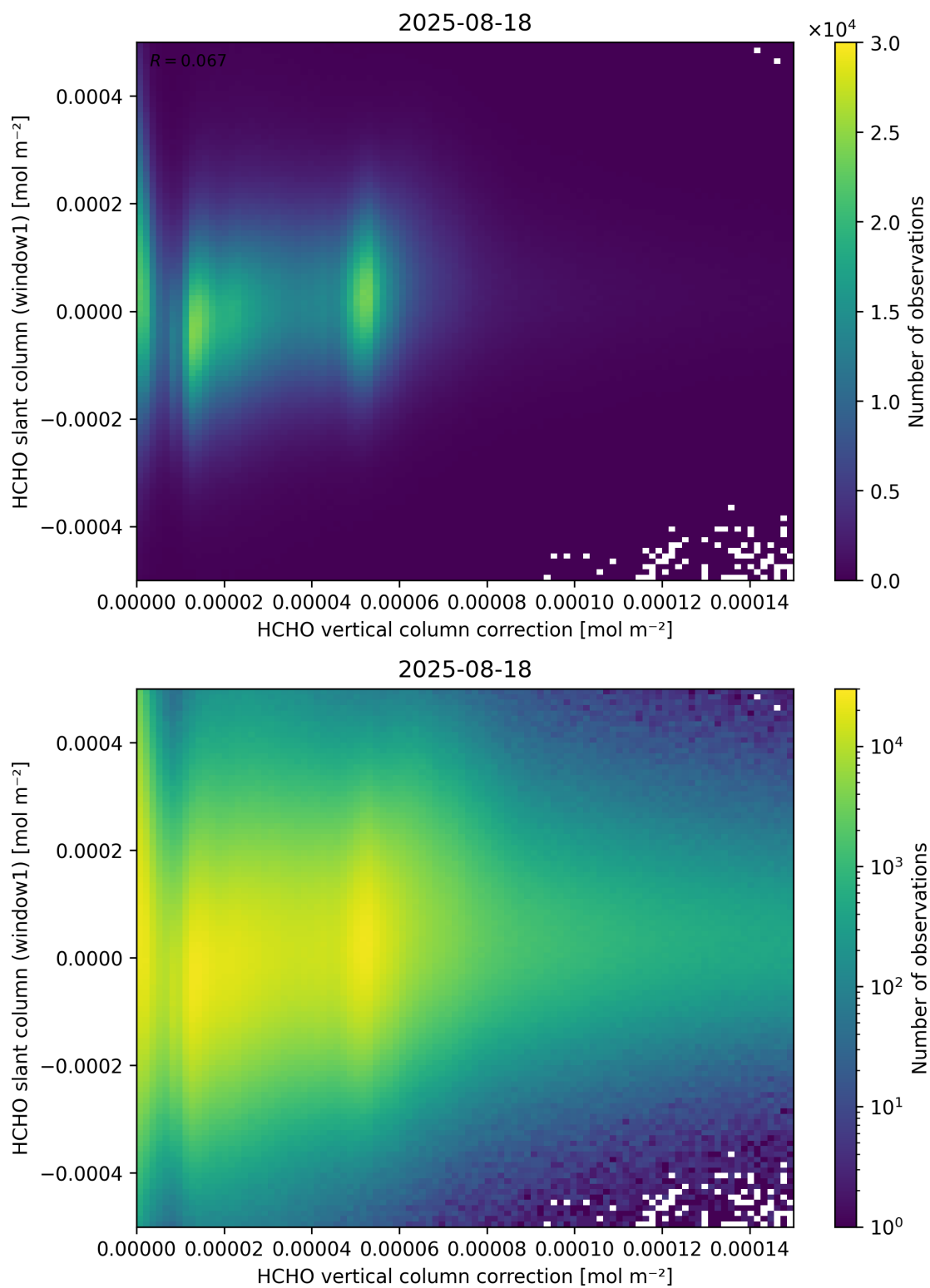
Figure 118: Scatter density plot of “HCHO vertical column correction” against “HCHO slant column (window1)” for 2025-08-17 to 2025-08-19.
