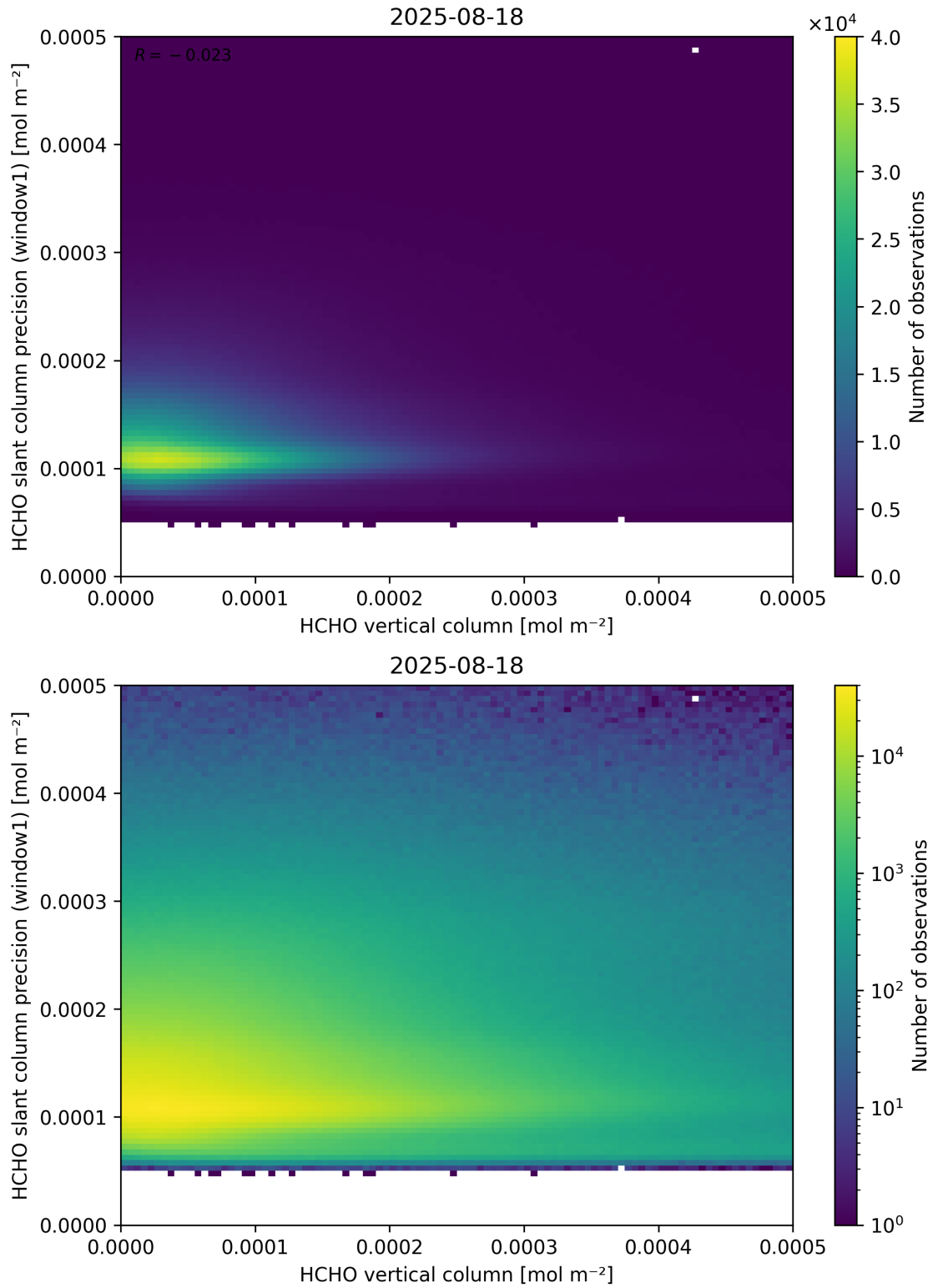
Figure 130: Scatter density plot of “HCHO vertical column” against “HCHO slant column precision (window1)” for 2025-08-17 to 2025-08-19.
