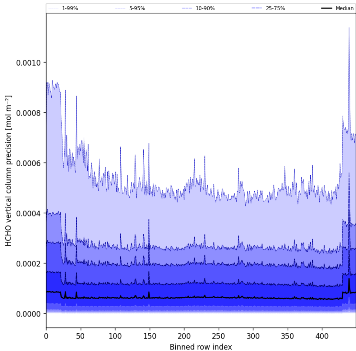
Figure 50: Along track statistics of “HCHO vertical column precision” for 2025-08-17 to 2025-08-19
