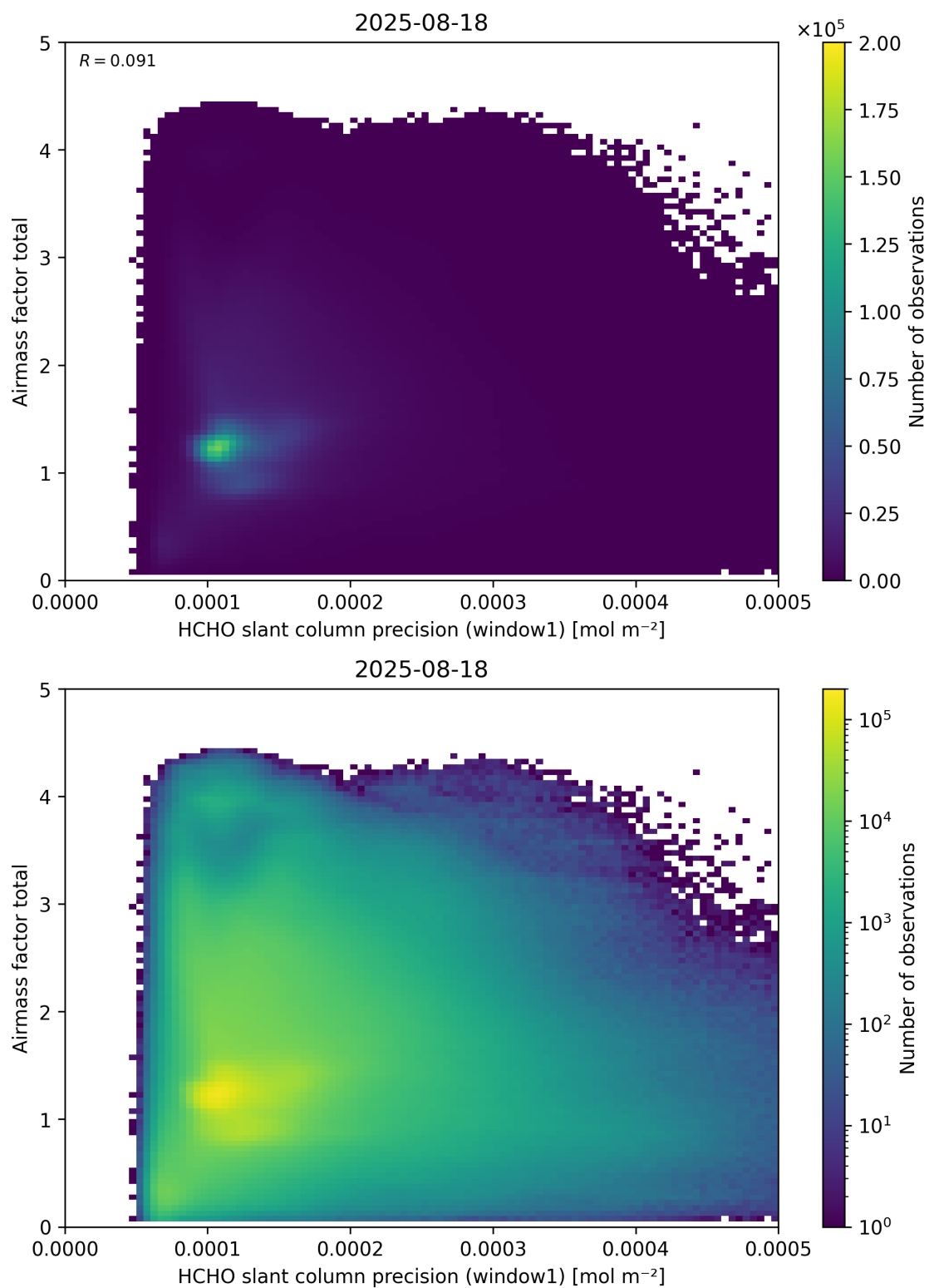
Figure 94: Scatter density plot of “HCHO slant column precision (window1)” against “Airmass factor total” for 2025-08-17 to 2025-08-19.
