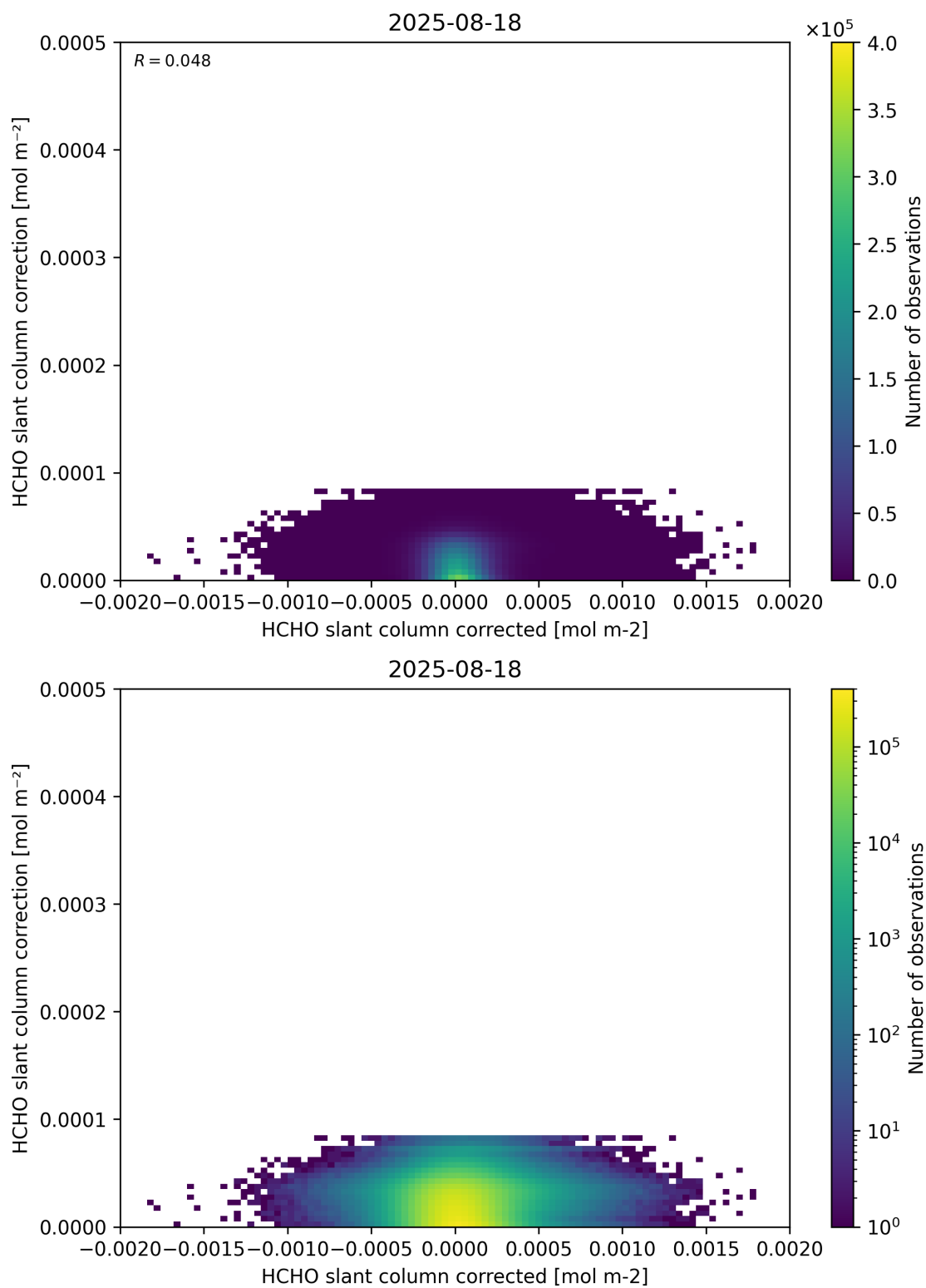
Figure 77: Scatter density plot of “HCHO slant column corrected” against “HCHO slant column correction” for 2025-08-17 to 2025-08-19.
