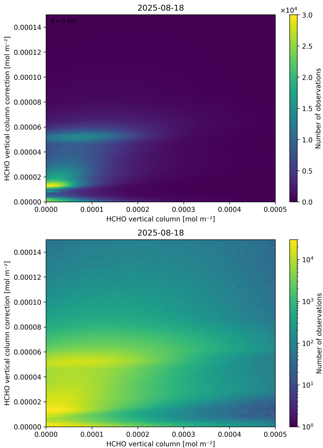
Figure 133: Scatter density plot of “HCHO vertical column” against “HCHO vertical column correction” for 2025-08-17 to 2025-08-19.
