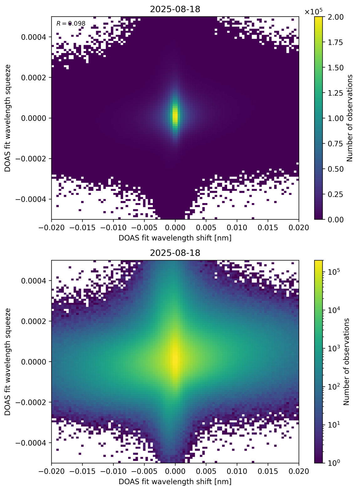
Figure 65: Scatter density plot of “DOAS fit wavelength shift” against “DOAS fit wavelength squeeze” for 2025-08-17 to 2025-08-19.
