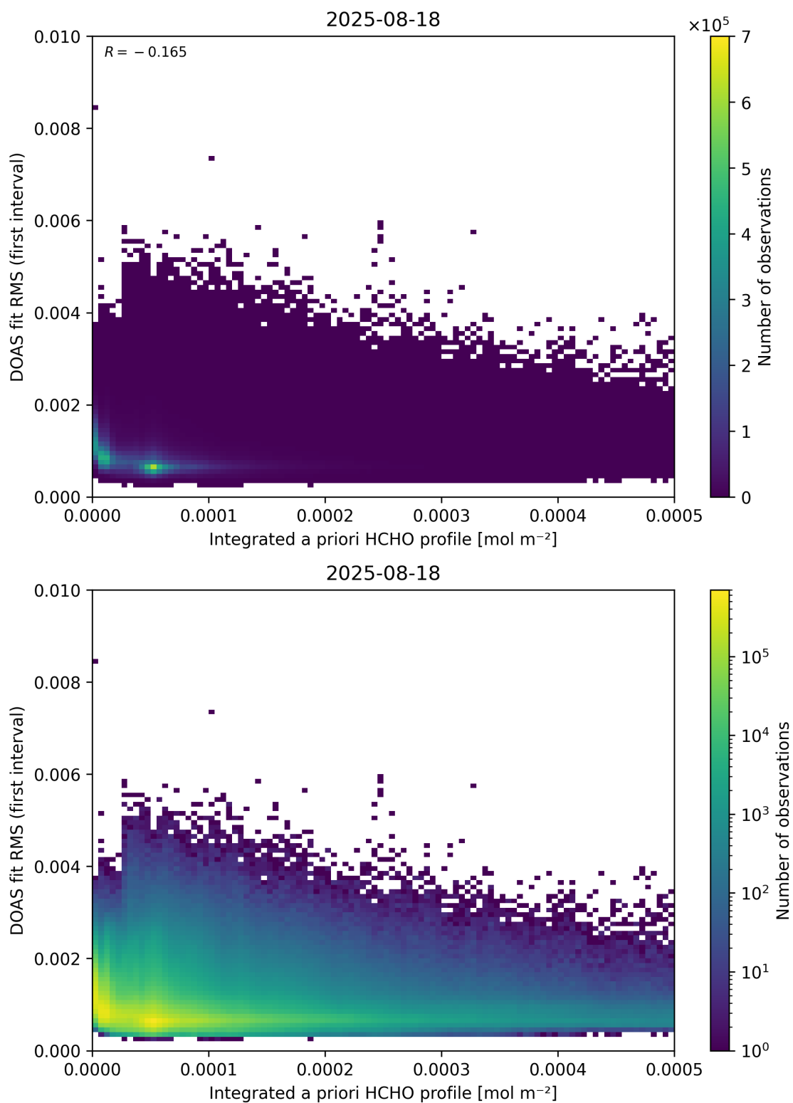
Figure 148: Scatter density plot of “Integrated a priori HCHO profile” against “DOAS fit RMS (first interval)” for 2025-08-17 to 2025-08-19.
