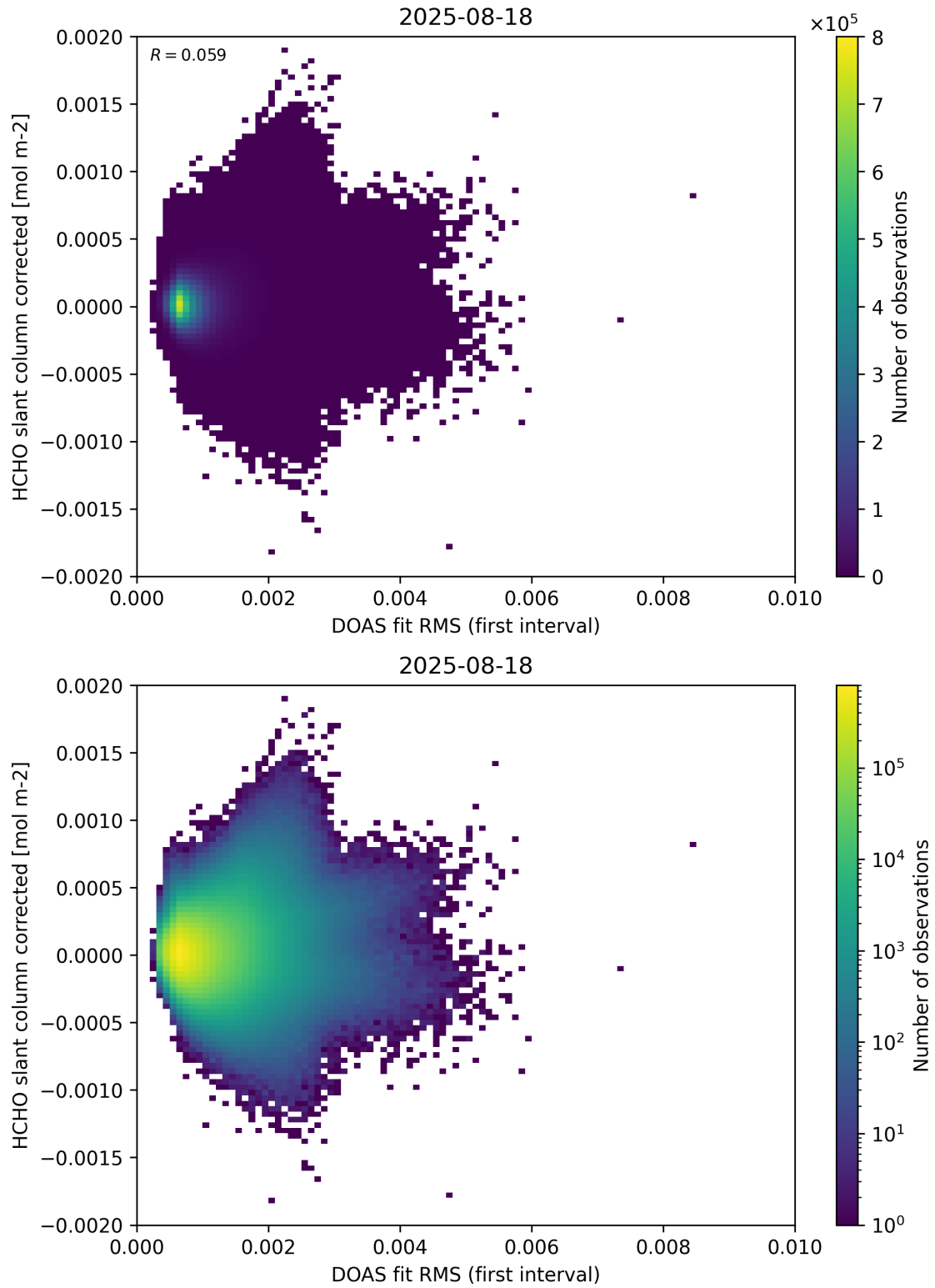
Figure 62: Scatter density plot of “DOAS fit RMS (first interval)” against “HCHO slant column corrected” for 2025-08-17 to 2025-08-19.
