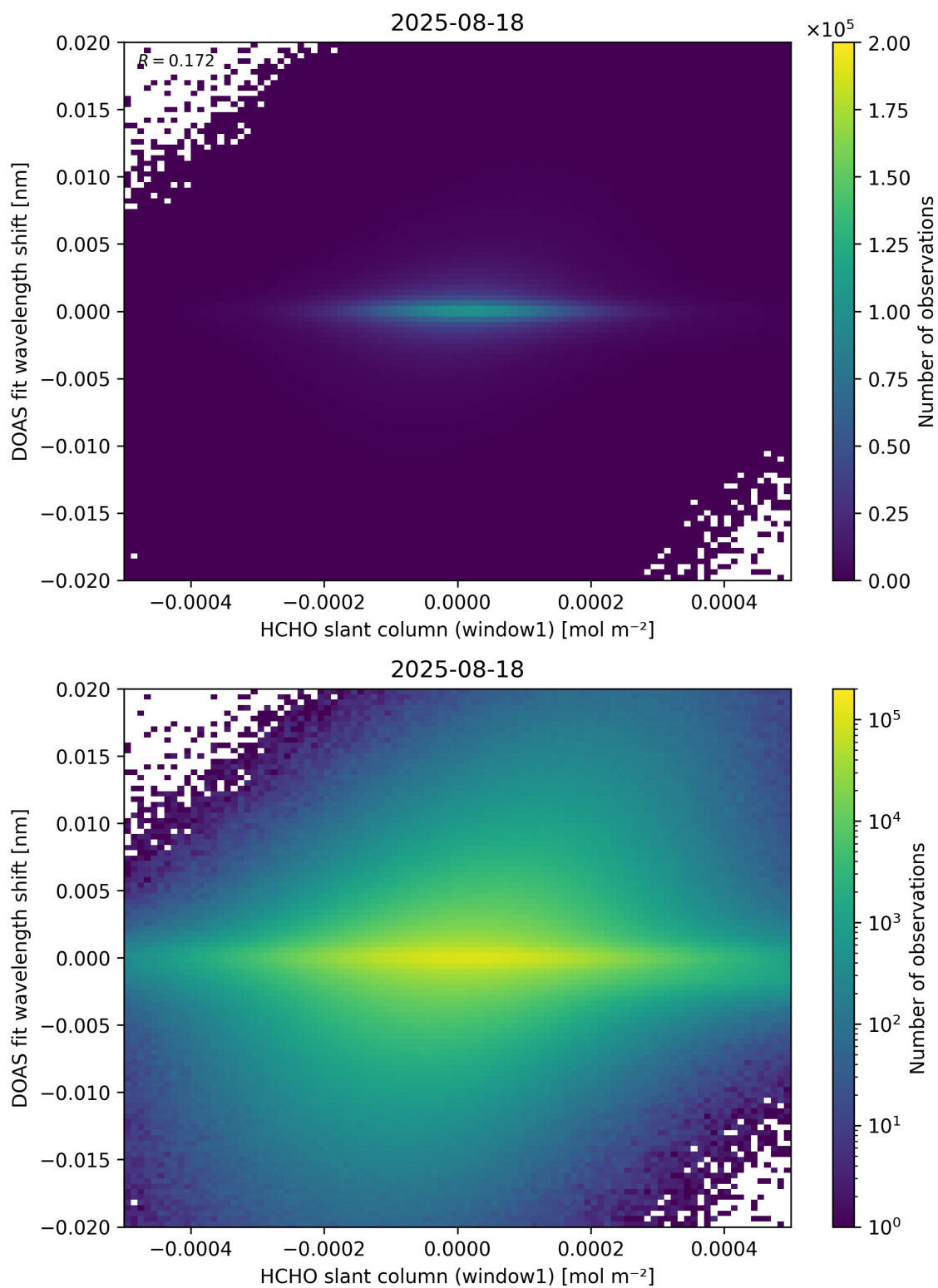
Figure 79: Scatter density plot of “HCHO slant column (window1)” against “DOAS fit wavelength shift” for 2025-08-17 to 2025-08-19.
