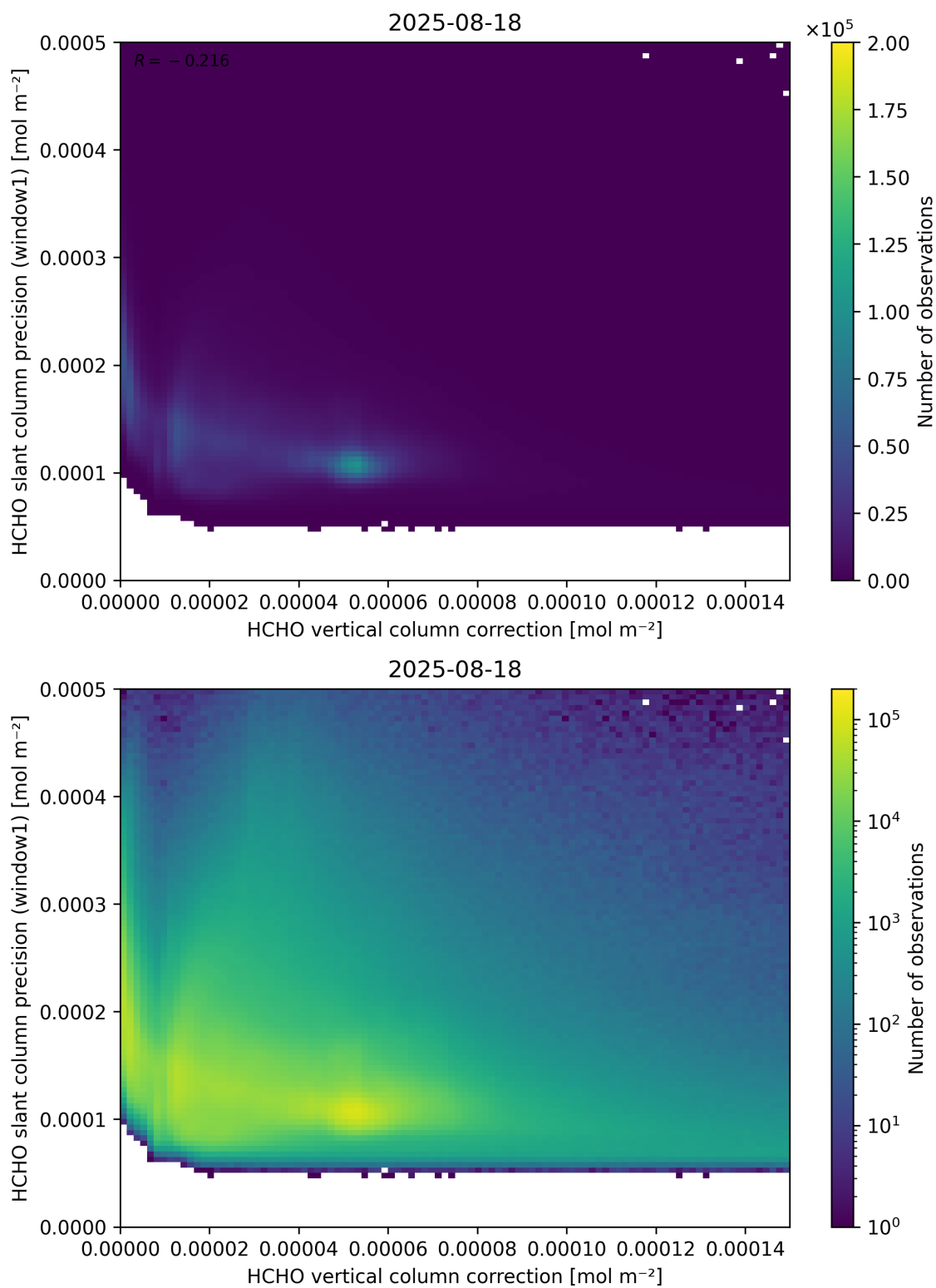
Figure 119: Scatter density plot of “HCHO vertical column correction” against “HCHO slant column precision (window1)” for 2025-08-17 to 2025-08-19.
