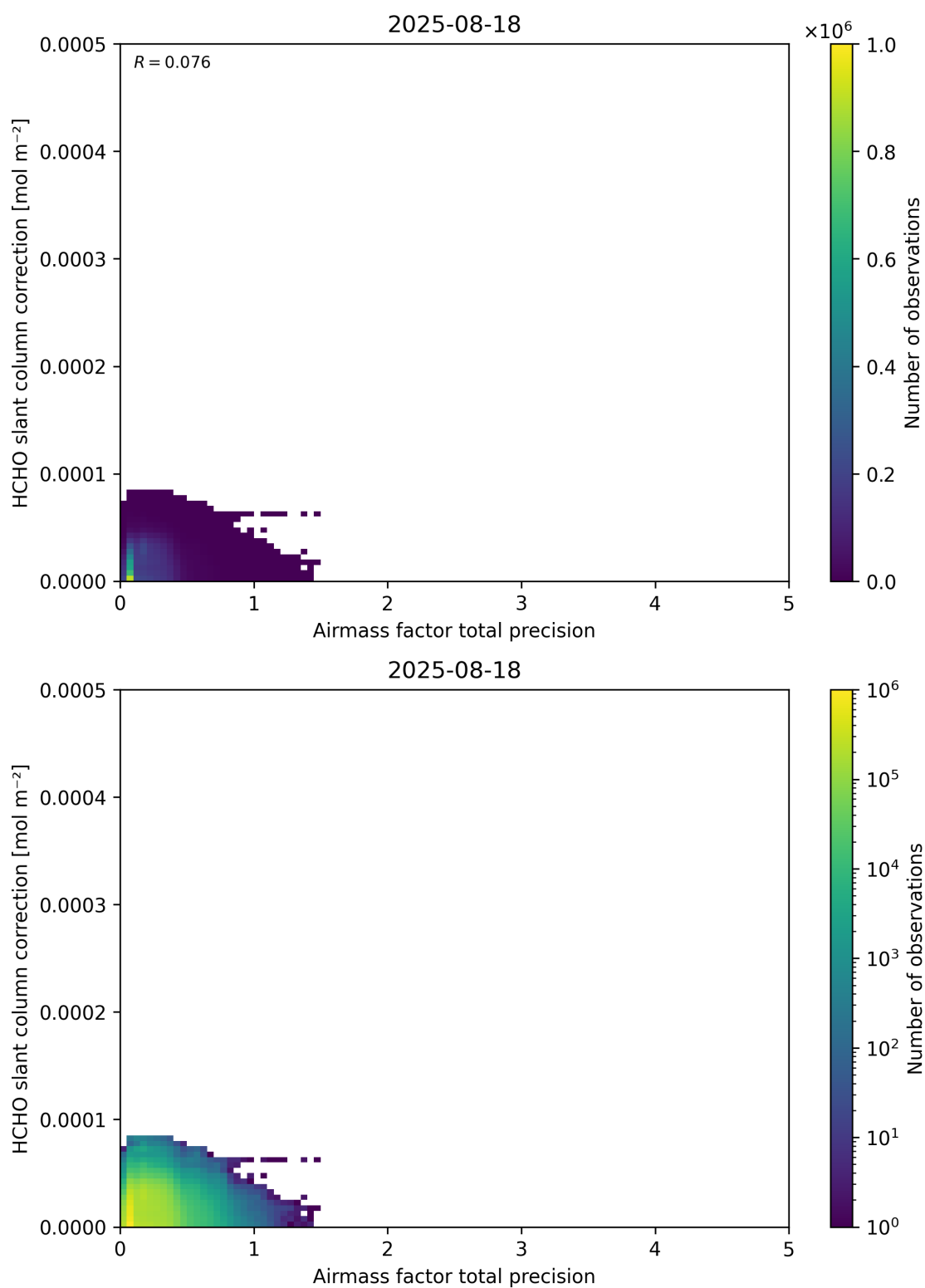
Figure 110: Scatter density plot of “Airmass factor total precision” against “HCHO slant column correction” for 2025-08-17 to 2025-08-19.
