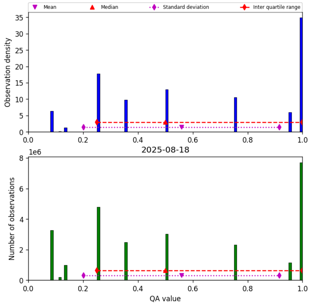
Figure 34: Histogram of “QA value” for 2025-08-17 to 2025-08-19
