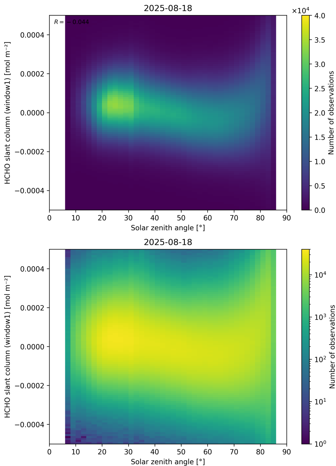
Figure 173: Scatter density plot of “Solar zenith angle” against “HCHO slant column (window1)” for 2025-08-17 to 2025-08-19.
