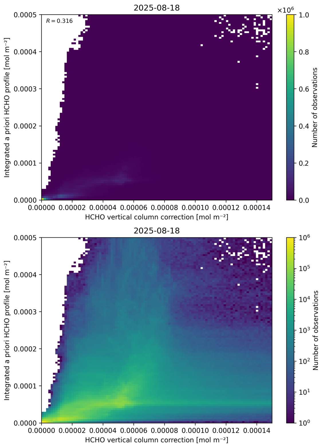
Figure 122: Scatter density plot of “HCHO vertical column correction” against “Integrated a priori HCHO profile” for 2025-08-17 to 2025-08-19.
