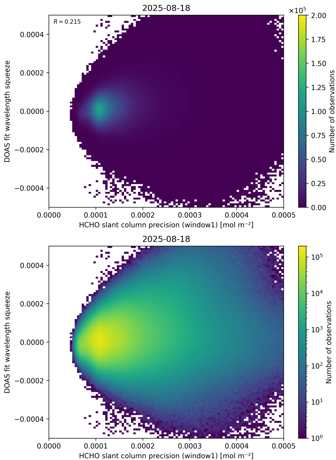
Figure 90: Scatter density plot of “HCHO slant column precision (window1)” against “DOAS fit wavelength squeeze” for 2025-08-17 to 2025-08-19.
