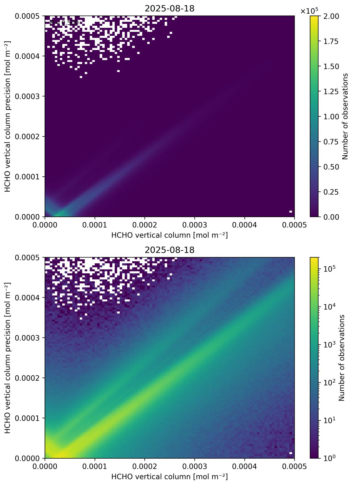
Figure 134: Scatter density plot of “HCHO vertical column” against “HCHO vertical column precision” for 2025-08-17 to 2025-08-19.
