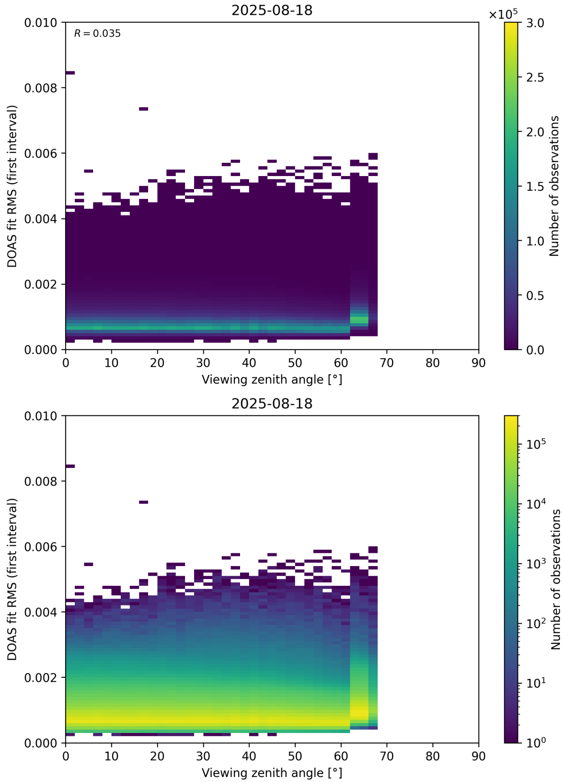
Figure 182: Scatter density plot of “Viewing zenith angle” against “DOAS fit RMS (first interval)” for 2025-08-17 to 2025-08-19.
