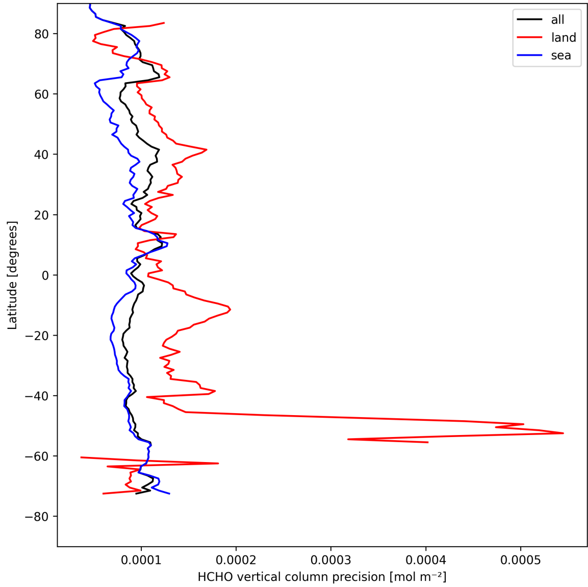
Figure 22: Zonal average of “HCHO vertical column precision” for 2025-08-17 to 2025-08-19.
