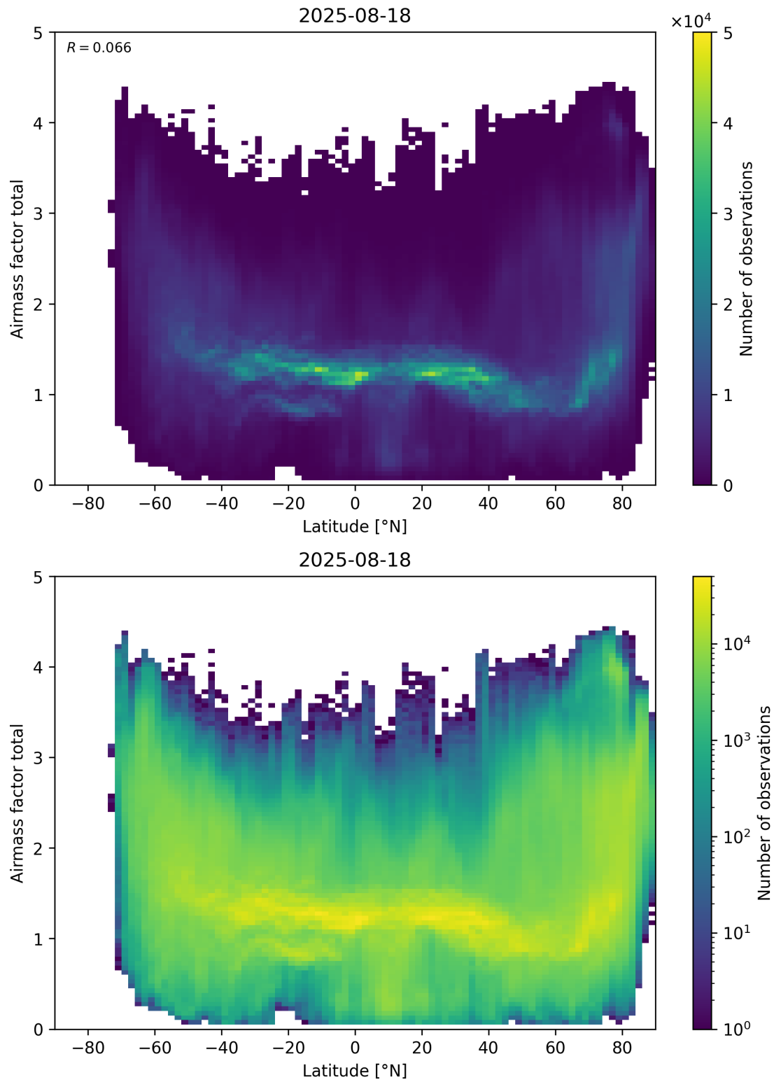
Figure 161: Scatter density plot of “Latitude” against “Airmass factor total” for 2025-08-17 to 2025-08-19.
