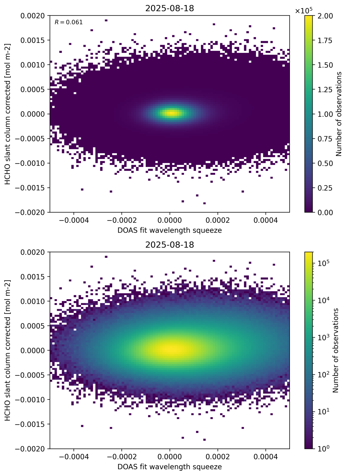
Figure 69: Scatter density plot of “DOAS fit wavelength squeeze” against “HCHO slant column corrected” for 2025-08-17 to 2025-08-19.
