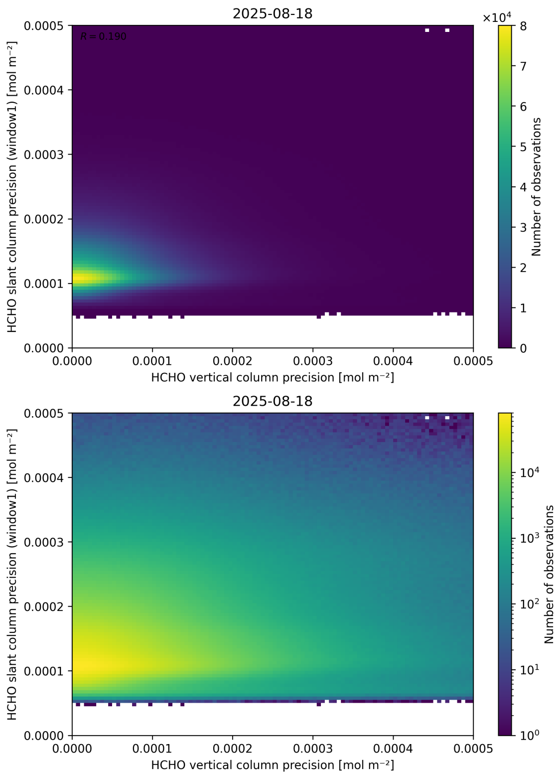
Figure 143: Scatter density plot of “HCHO vertical column precision” against “HCHO slant column precision (window1)” for 2025-08-17 to 2025-08-19.
