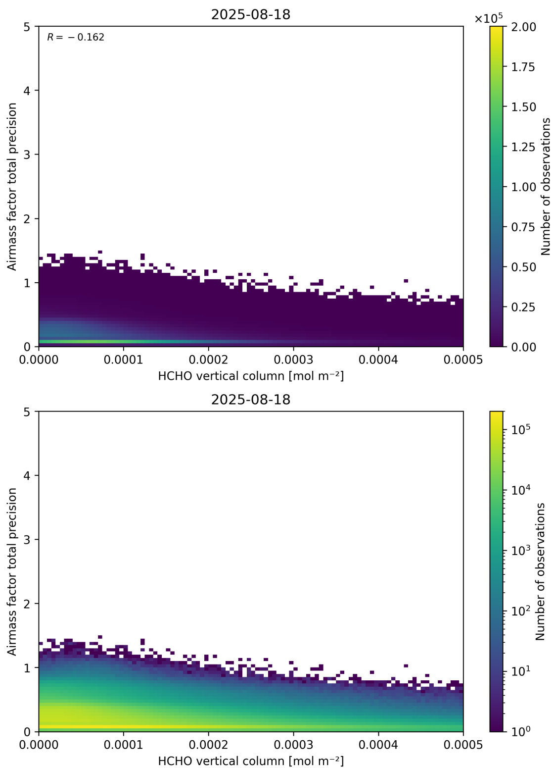
Figure 132: Scatter density plot of “HCHO vertical column” against “Airmass factor total precision” for 2025-08-17 to 2025-08-19.
