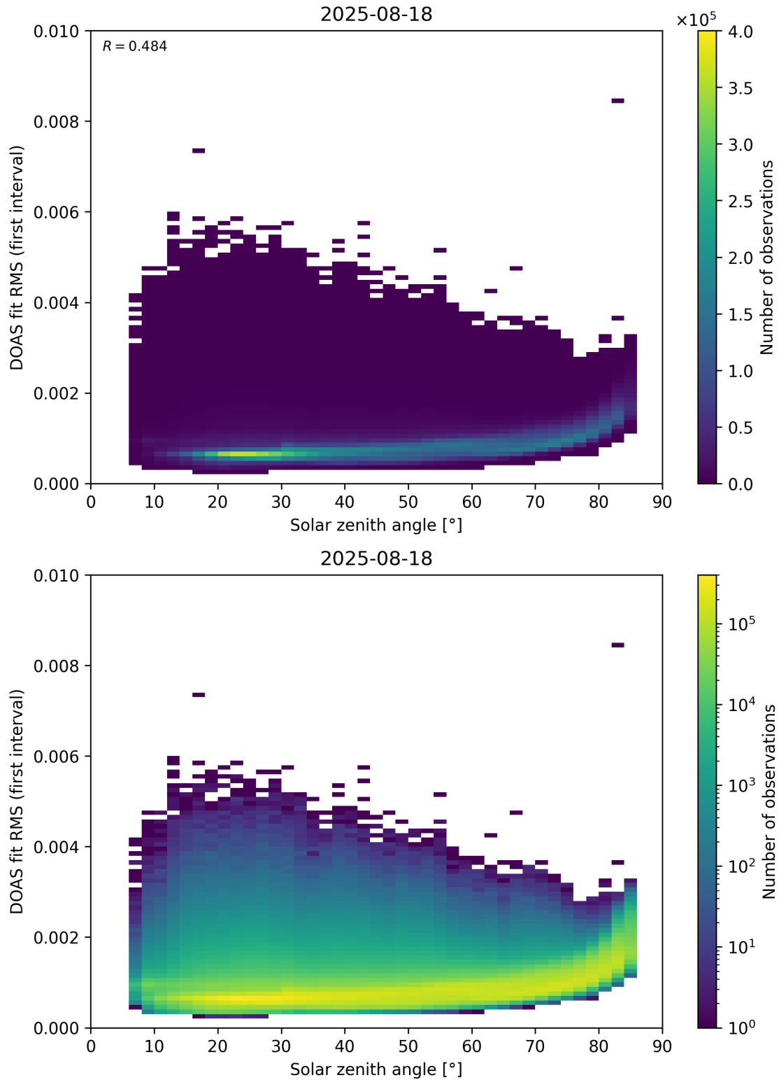
Figure 167: Scatter density plot of “Solar zenith angle” against “DOAS fit RMS (first interval)” for 2025-08-17 to 2025-08-19.
