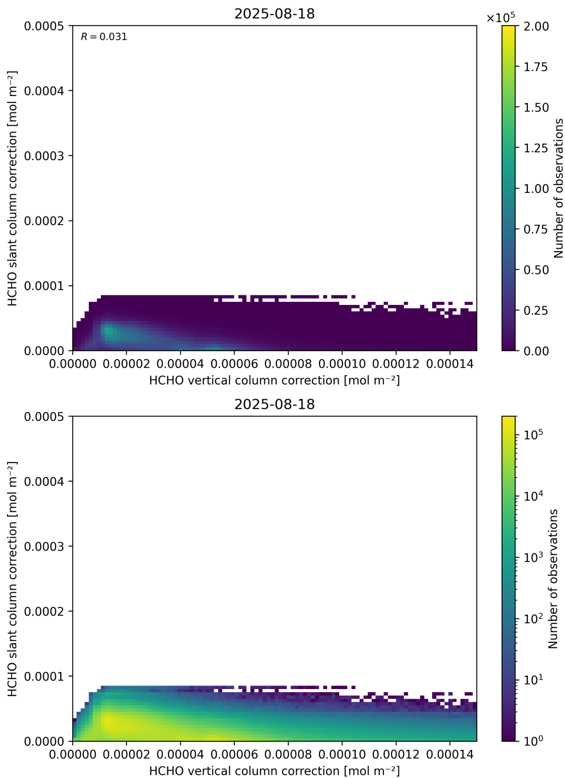
Figure 117: Scatter density plot of “HCHO vertical column correction” against “HCHO slant column correction” for 2025-08-17 to 2025-08-19.
