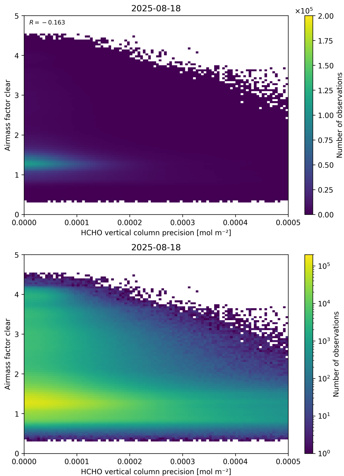
Figure 139: Scatter density plot of “HCHO vertical column precision” against “Airmass factor clear” for 2025-08-17 to 2025-08-19.
