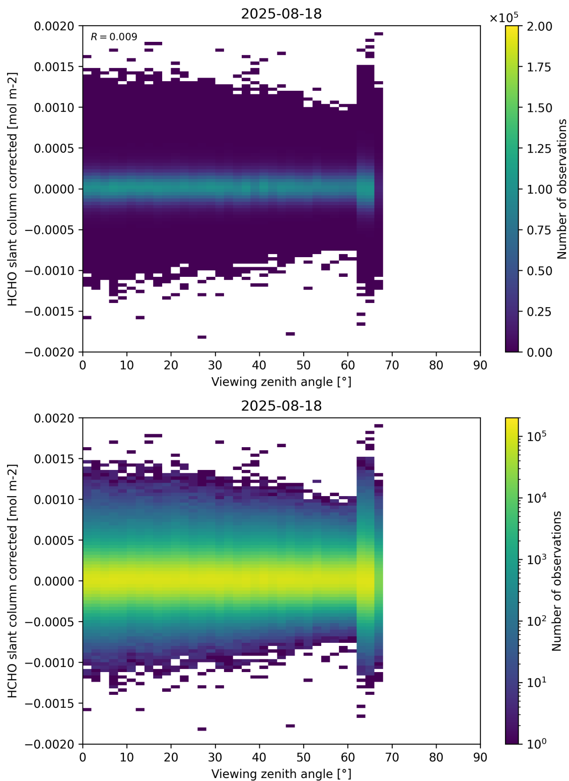
Figure 186: Scatter density plot of “Viewing zenith angle” against “HCHO slant column corrected” for 2025-08-17 to 2025-08-19.
