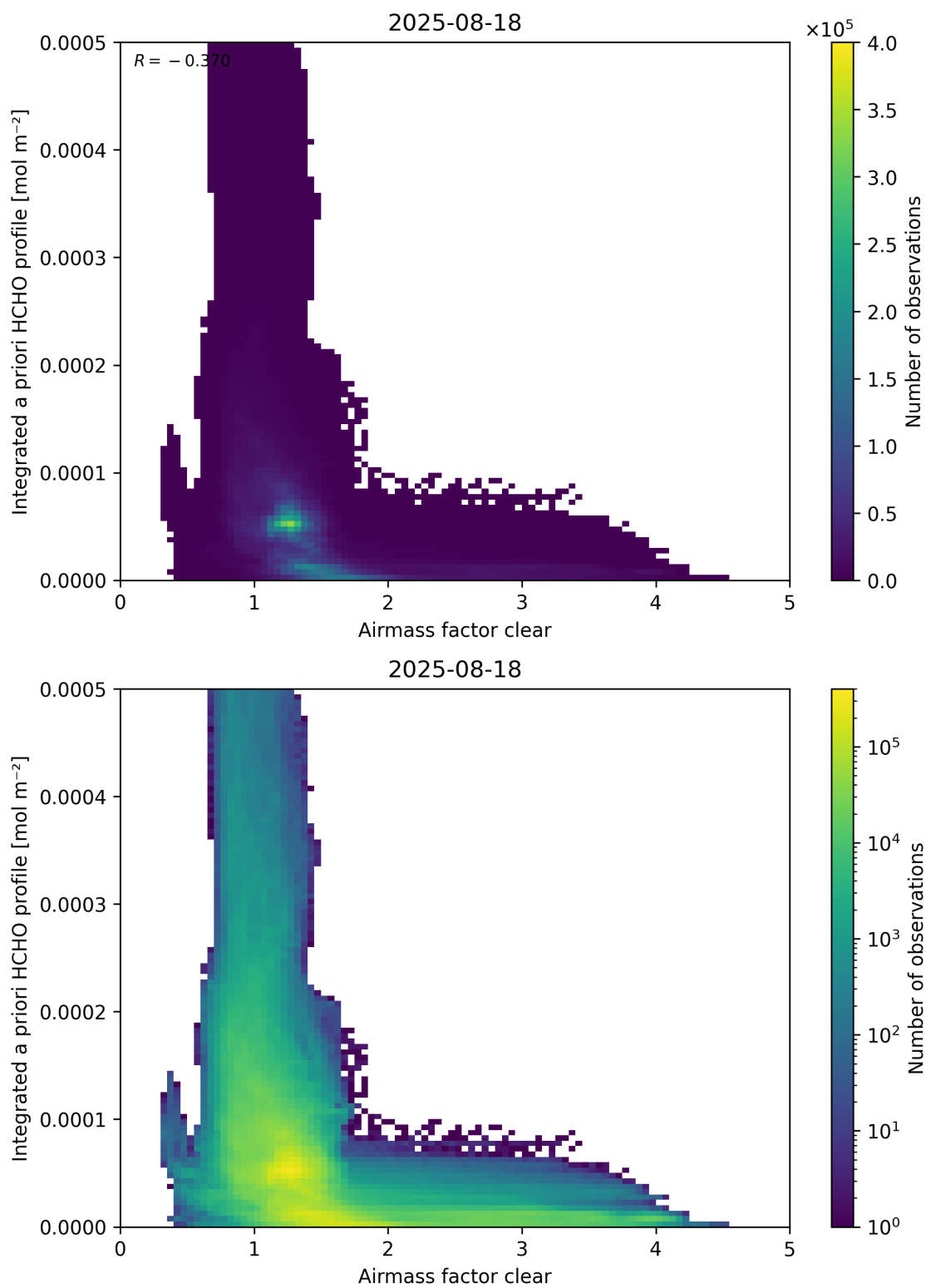
Figure 76: Scatter density plot of “Airmass factor clear” against “Integrated a priori HCHO profile” for 2025-08-17 to 2025-08-19.
