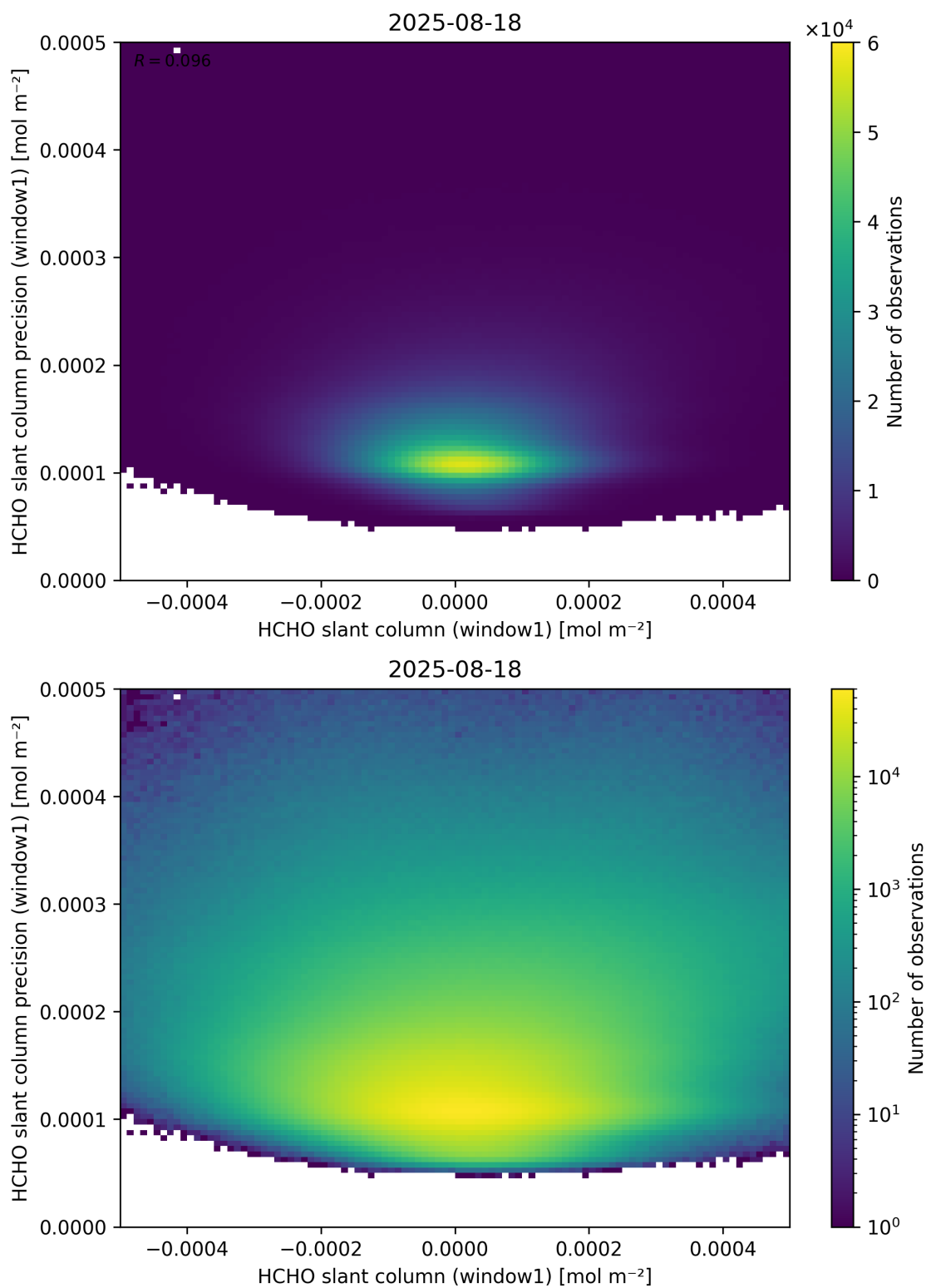
Figure 84: Scatter density plot of “HCHO slant column (window1)” against “HCHO slant column precision (window1)” for 2025-08-17 to 2025-08-19.
