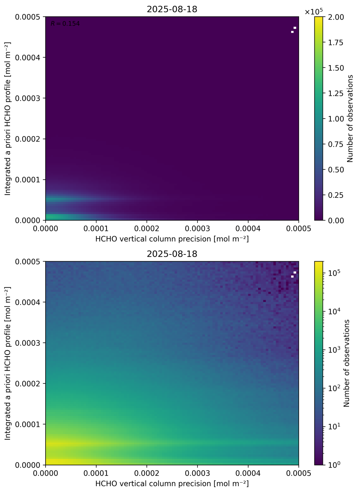
Figure 147: Scatter density plot of “HCHO vertical column precision” against “Integrated a priori HCHO profile” for 2025-08-17 to 2025-08-19.
