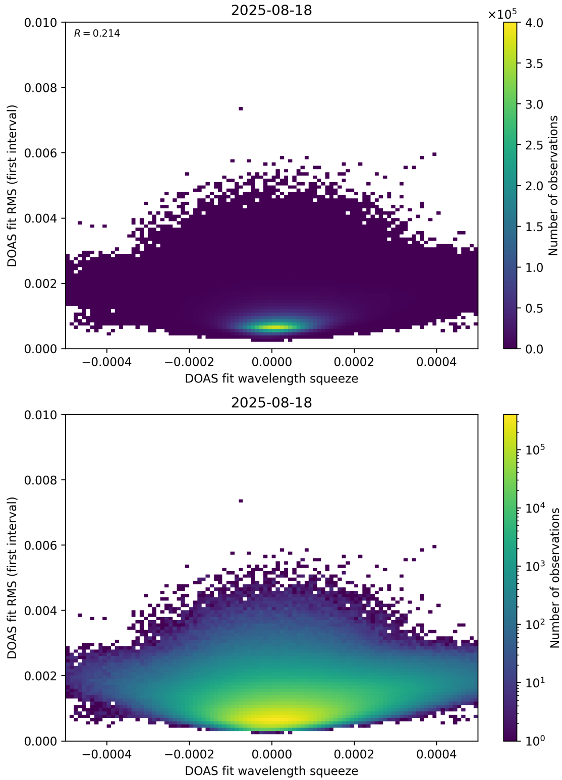
Figure 68: Scatter density plot of “DOAS fit wavelength squeeze” against “DOAS fit RMS (first interval)” for 2025-08-17 to 2025-08-19.
