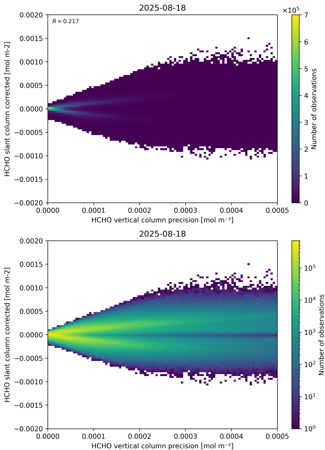
Figure 140: Scatter density plot of “HCHO vertical column precision” against “HCHO slant column corrected” for 2025-08-17 to 2025-08-19.
