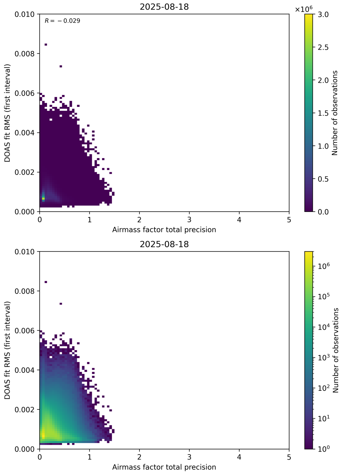
Figure 105: Scatter density plot of “Airmass factor total precision” against “DOAS fit RMS (first interval)” for 2025-08-17 to 2025-08-19.
