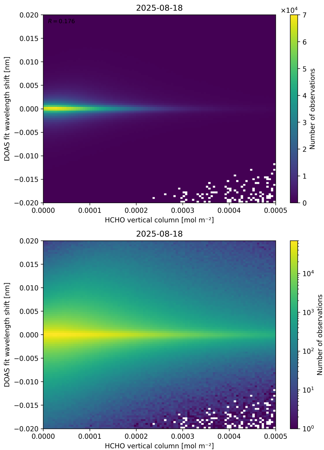
Figure 124: Scatter density plot of “HCHO vertical column” against “DOAS fit wavelength shift” for 2025-08-17 to 2025-08-19.
