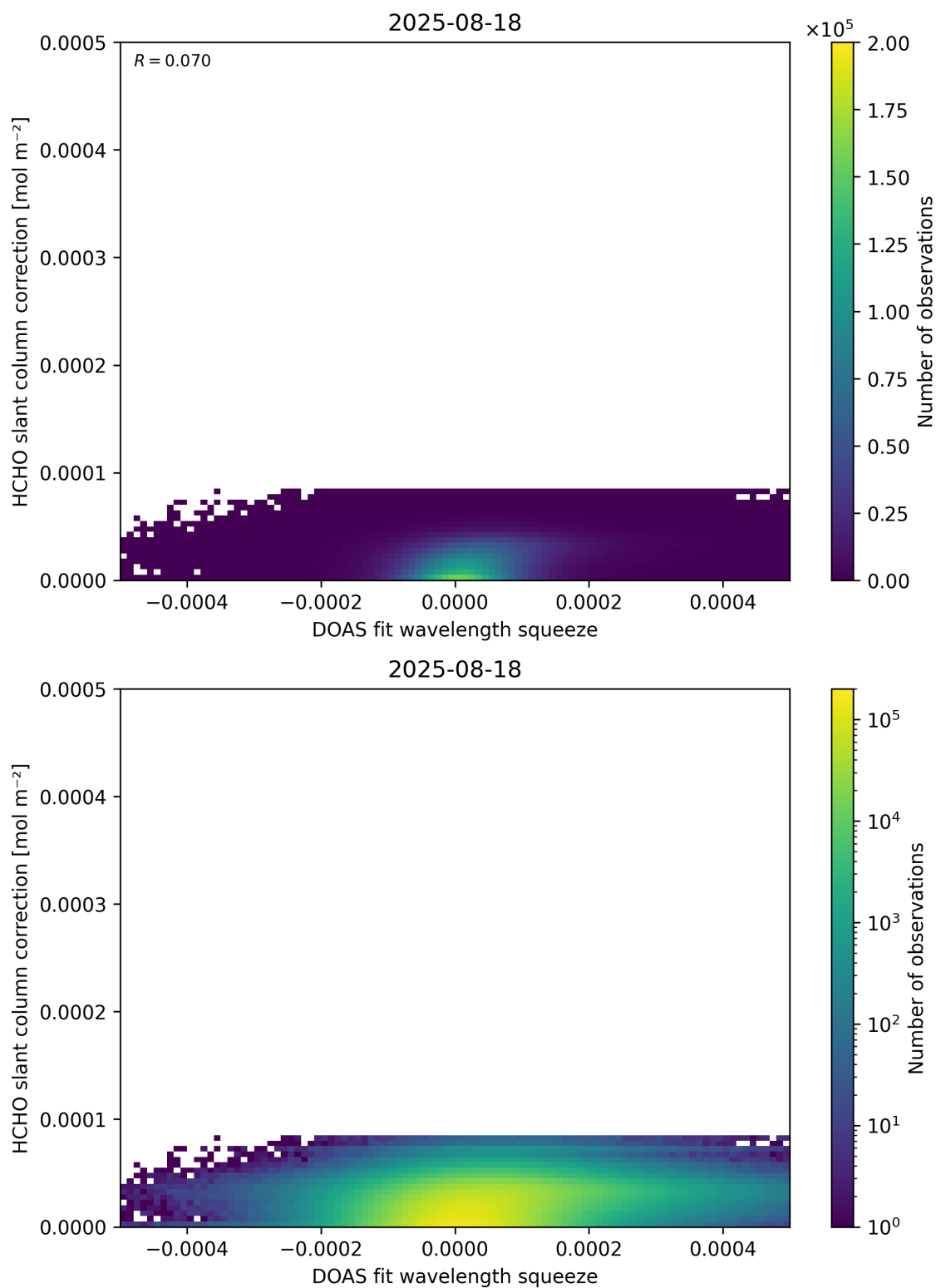
Figure 70: Scatter density plot of “DOAS fit wavelength squeeze” against “HCHO slant column correction” for 2025-08-17 to 2025-08-19.
