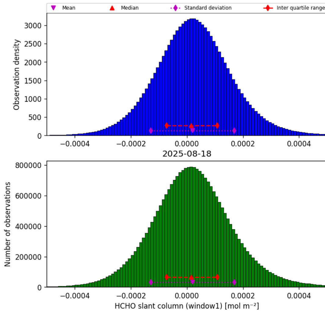
Figure 38: Histogram of “HCHO slant column (window1)” for 2025-08-17 to 2025-08-19
