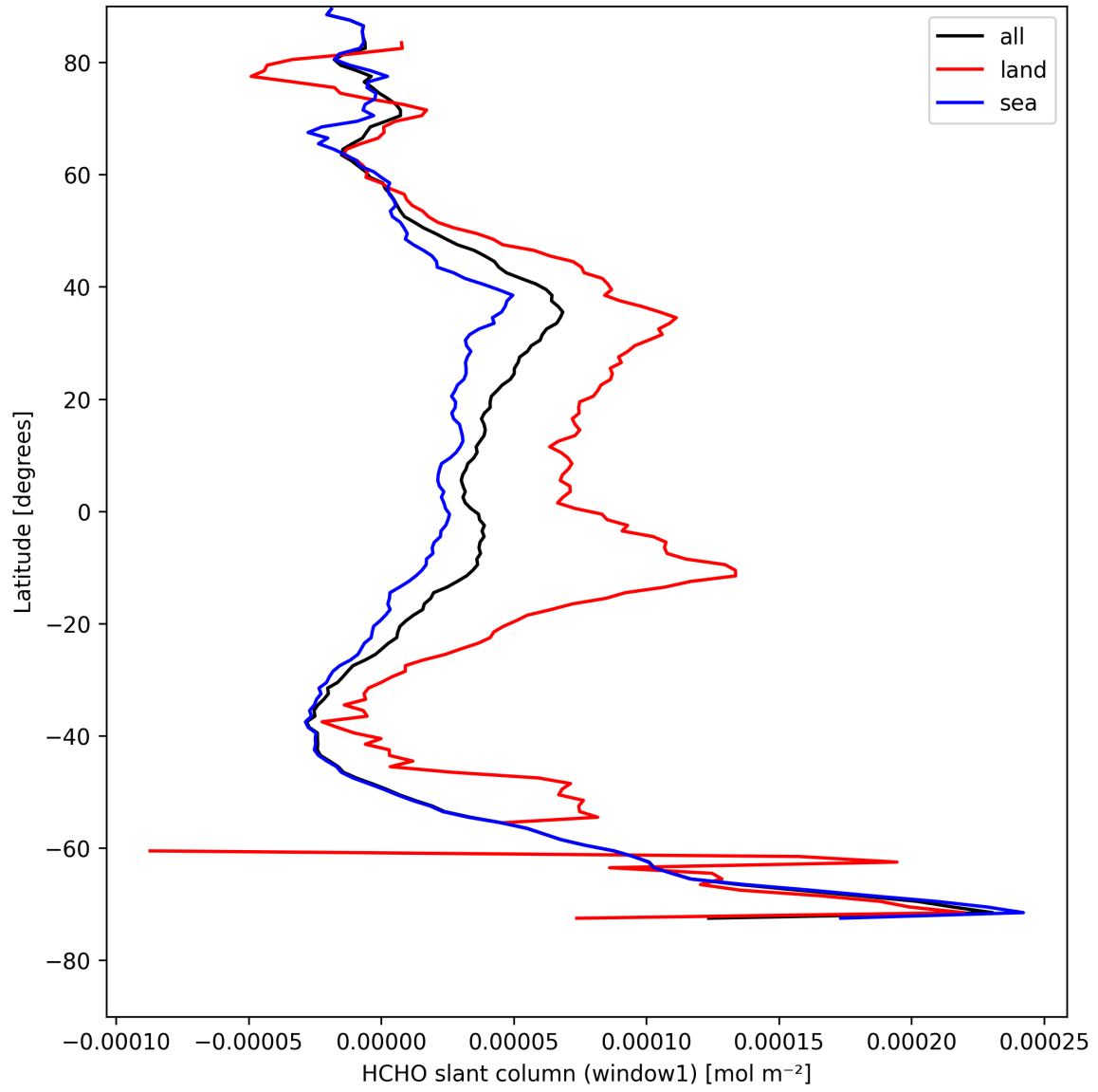
Figure 24: Zonal average of “HCHO slant column (window1)” for 2025-08-17 to 2025-08-19.
