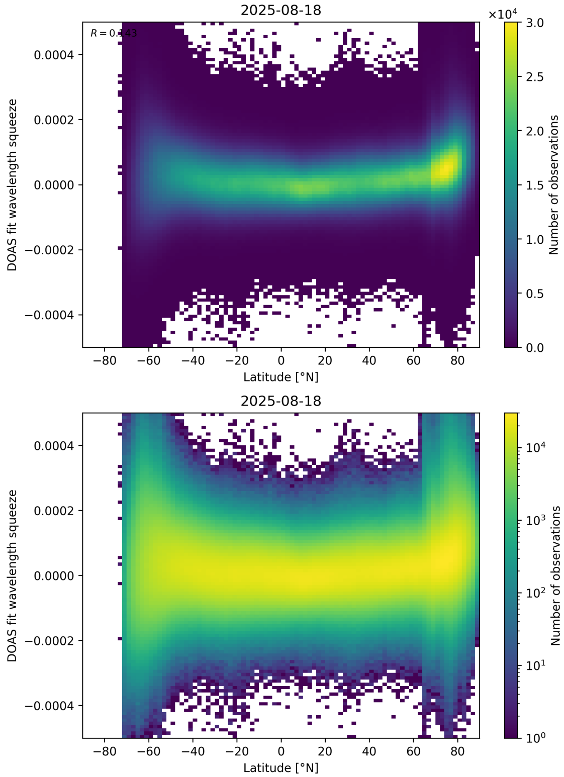
Figure 155: Scatter density plot of “Latitude” against “DOAS fit wavelength squeeze” for 2025-08-17 to 2025-08-19.
