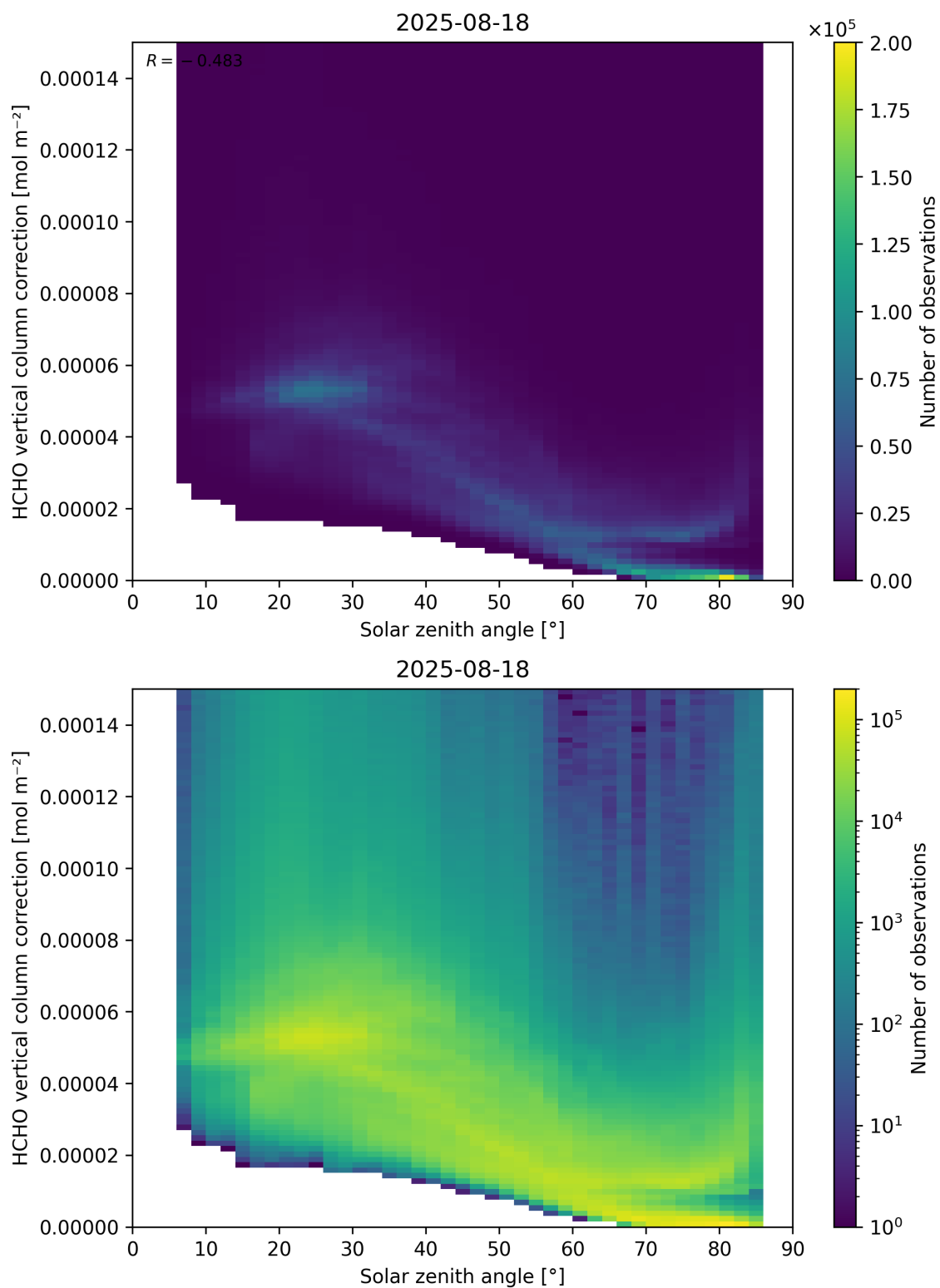
Figure 178: Scatter density plot of “Solar zenith angle” against “HCHO vertical column correction” for 2025-08-17 to 2025-08-19.
