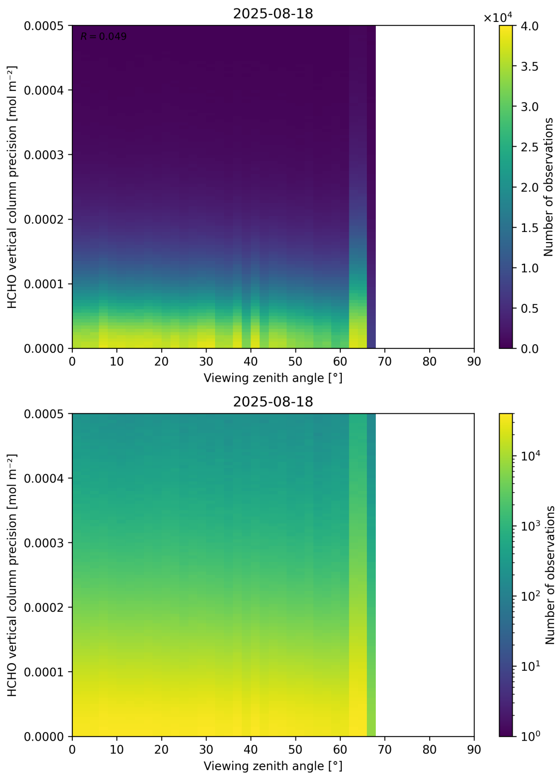
Figure 194: Scatter density plot of “Viewing zenith angle” against “HCHO vertical column precision” for 2025-08-17 to 2025-08-19.
