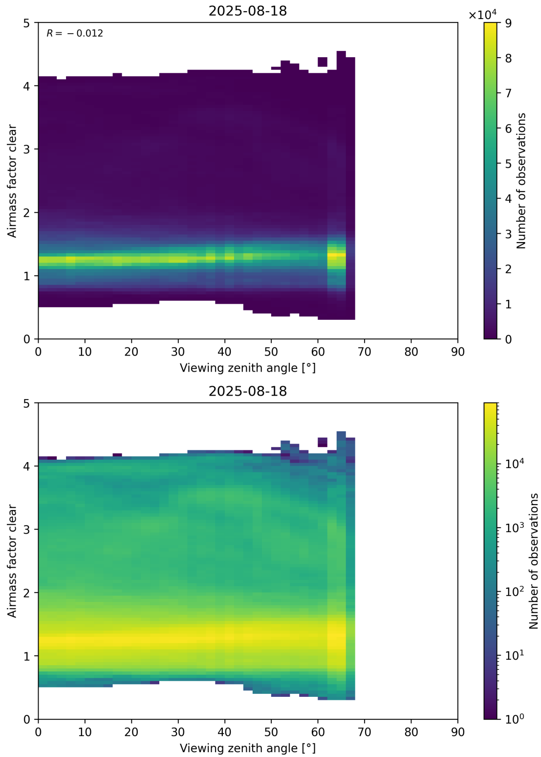
Figure 185: Scatter density plot of “Viewing zenith angle” against “Airmass factor clear” for 2025-08-17 to 2025-08-19.
