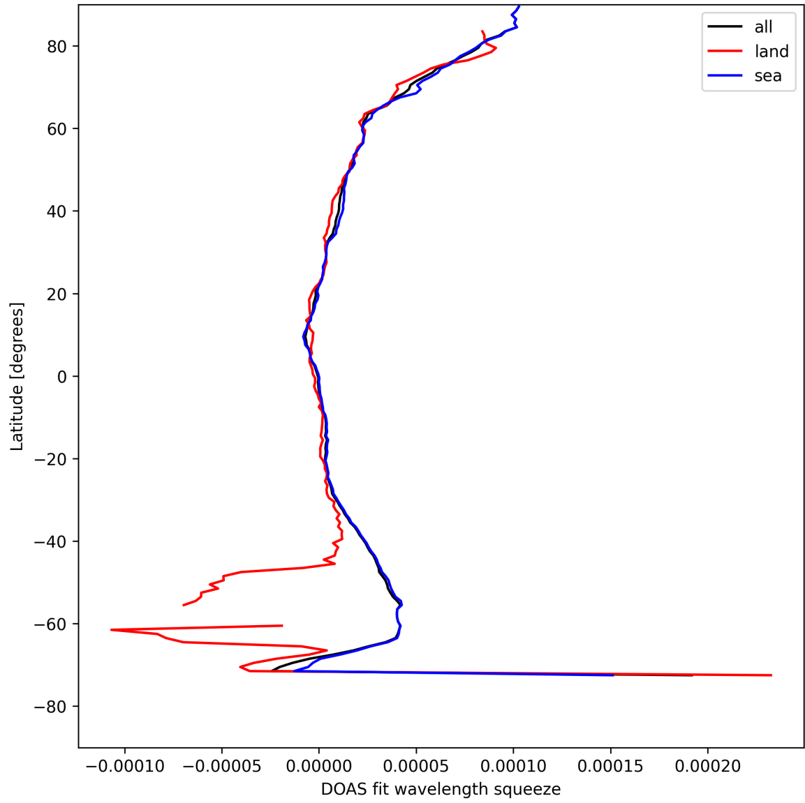
Figure 31: Zonal average of “DOAS fit wavelength squeeze” for 2025-08-17 to 2025-08-19.
