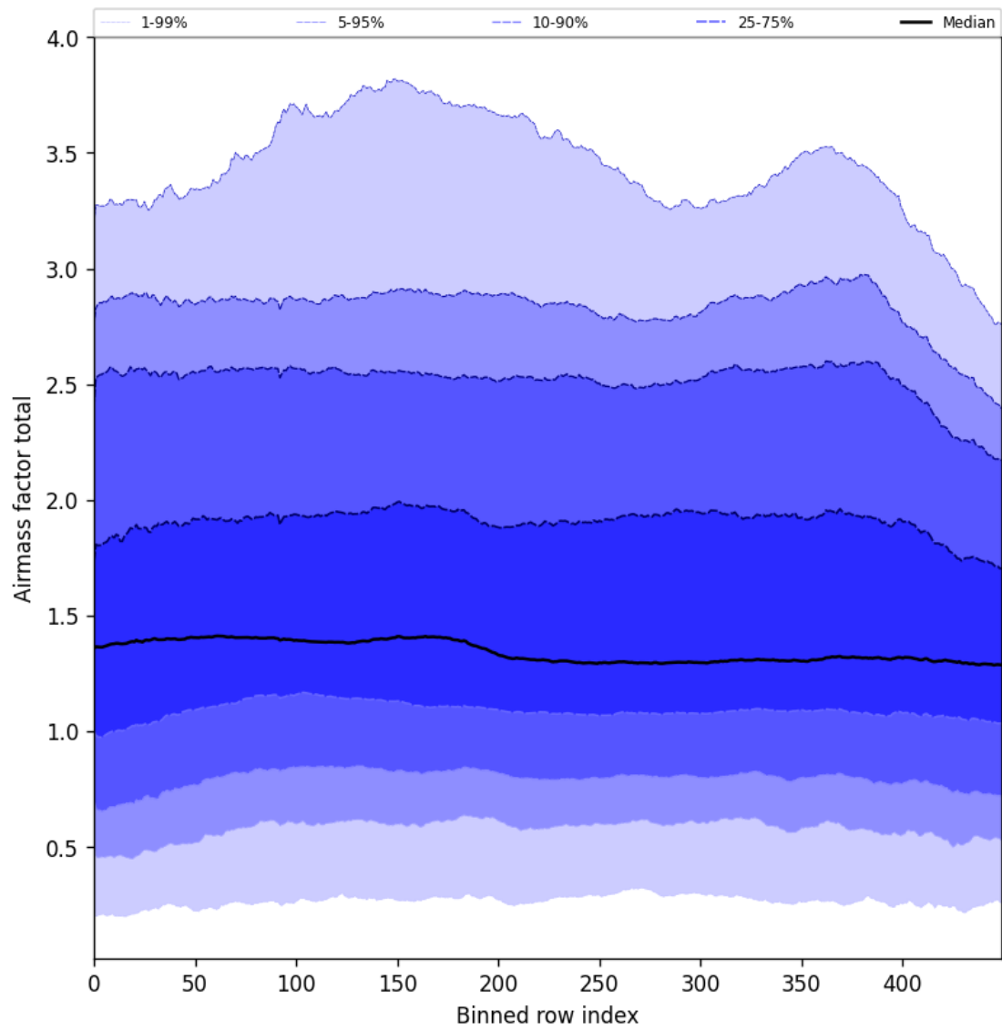
Figure 54: Along track statistics of “Airmass factor total” for 2025-08-17 to 2025-08-19
