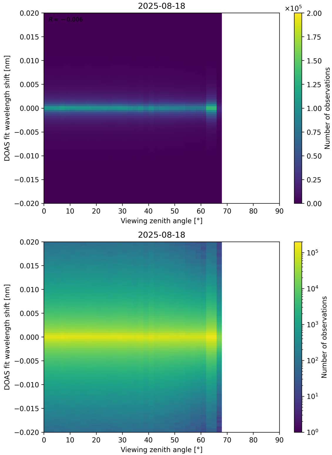
Figure 183: Scatter density plot of “Viewing zenith angle” against “DOAS fit wavelength shift” for 2025-08-17 to 2025-08-19.
