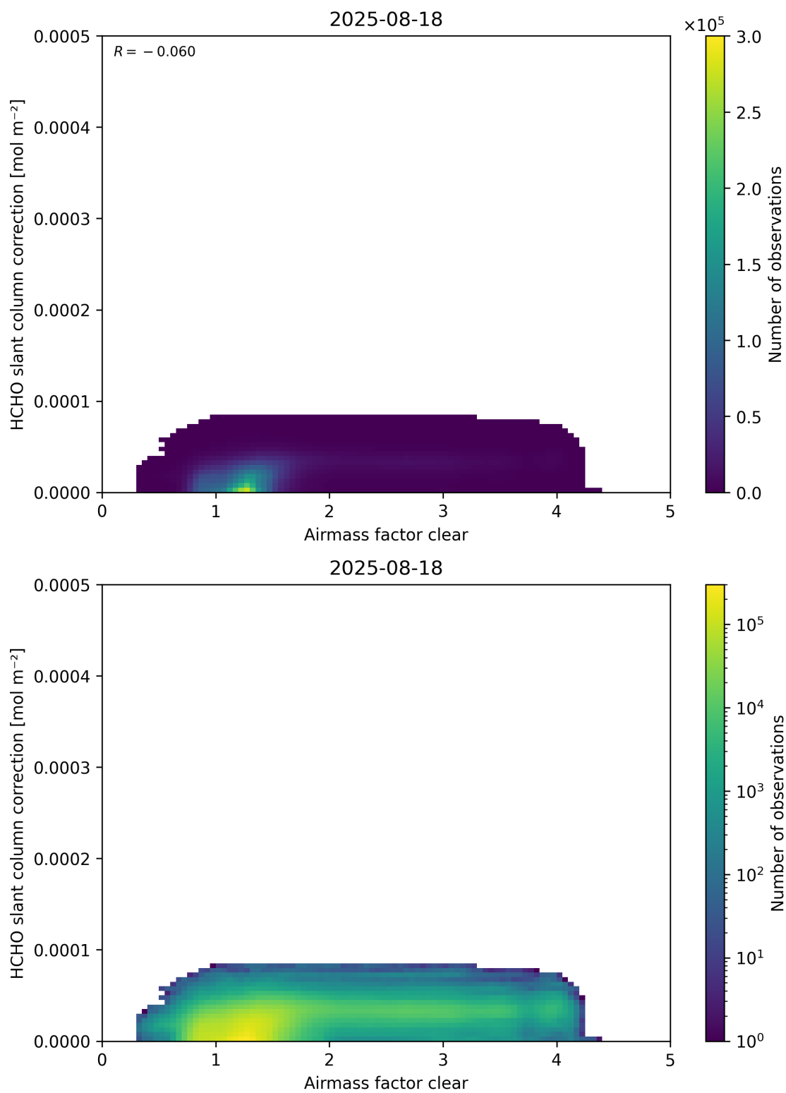
Figure 75: Scatter density plot of “Airmass factor clear” against “HCHO slant column correction” for 2025-08-17 to 2025-08-19.
