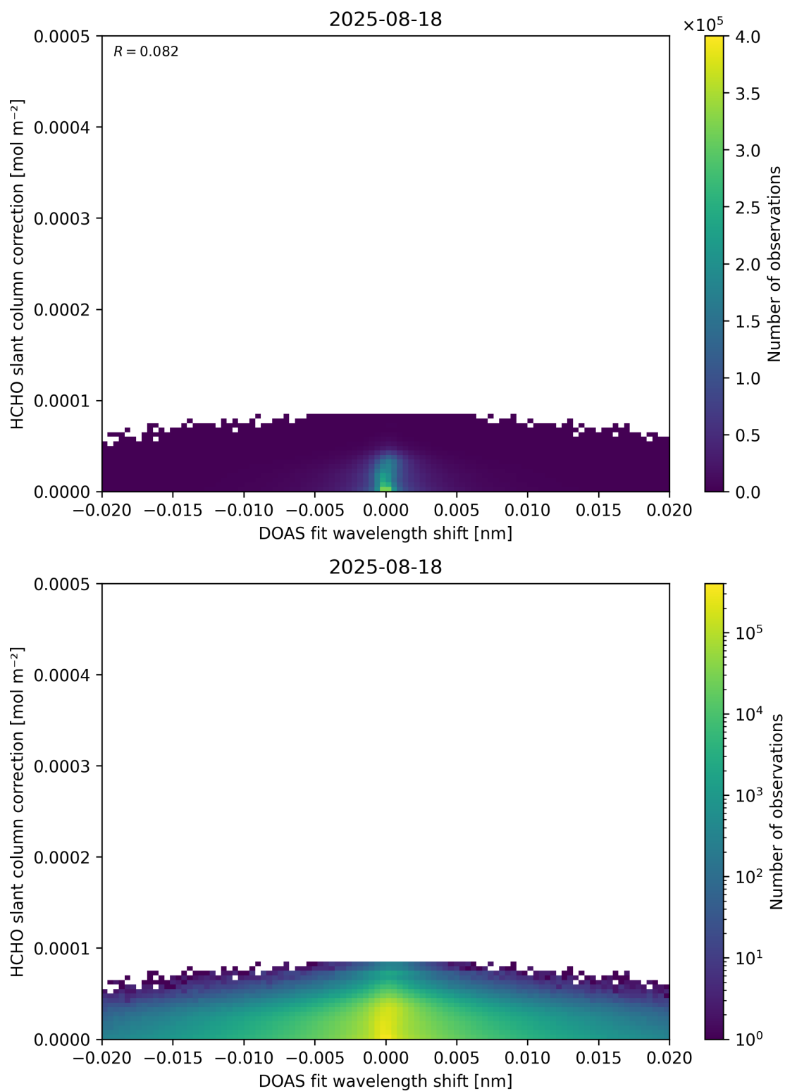
Figure 67: Scatter density plot of “DOAS fit wavelength shift” against “HCHO slant column correction” for 2025-08-17 to 2025-08-19.
