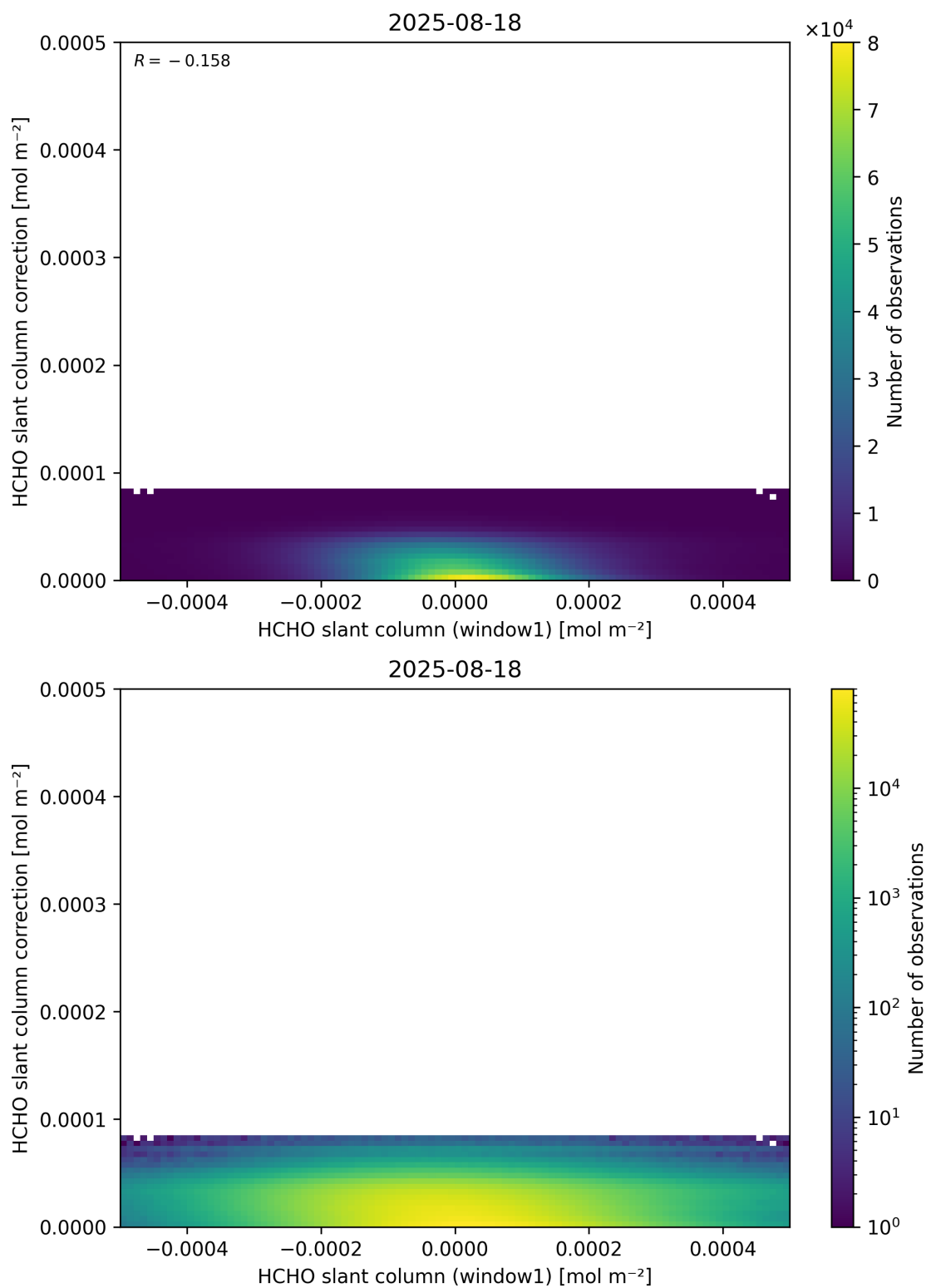
Figure 83: Scatter density plot of “HCHO slant column (window1)” against “HCHO slant column correction” for 2025-08-17 to 2025-08-19.
