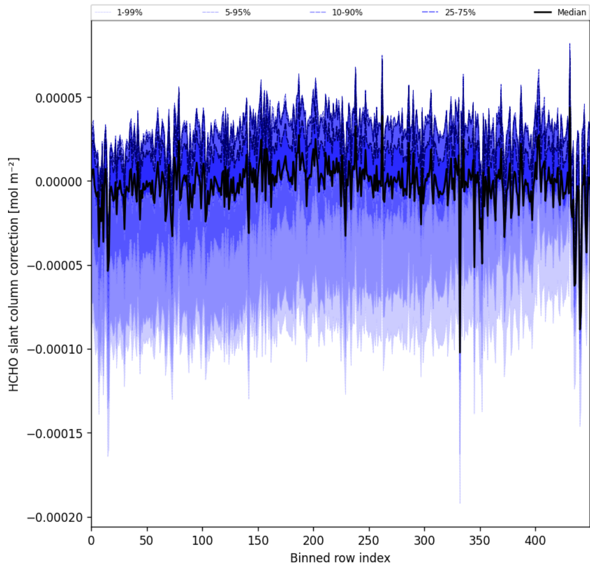
Figure 61: Along track statistics of “HCHO slant column correction” for 2025-08-17 to 2025-08-19
