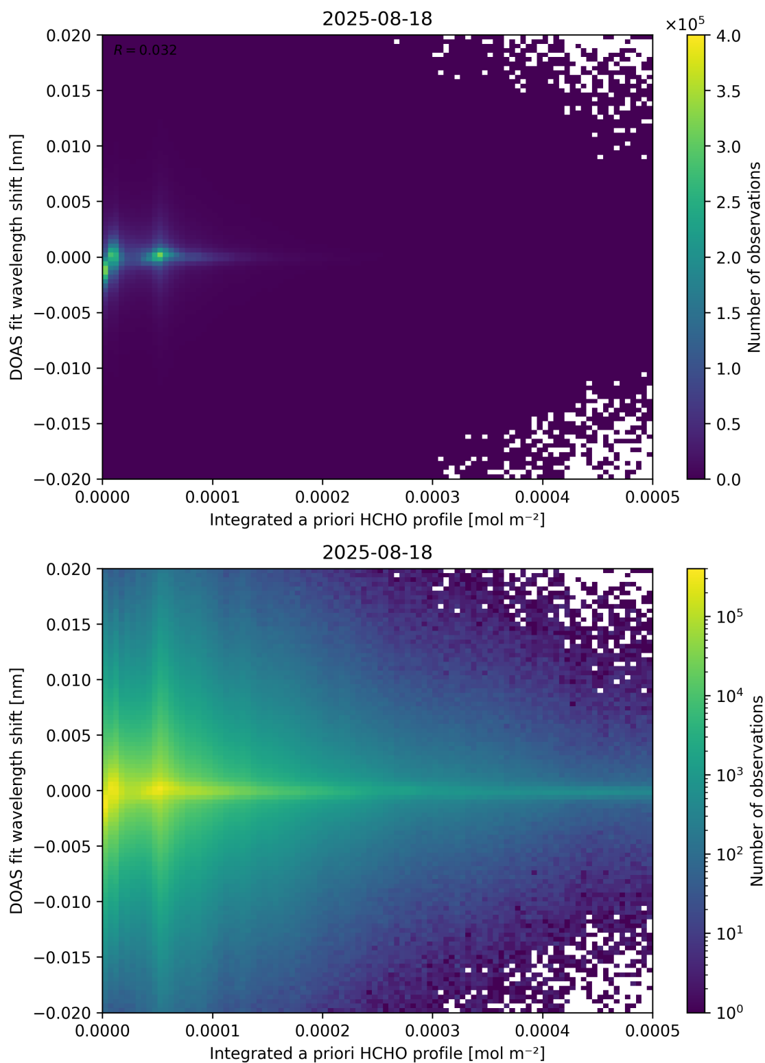
Figure 149: Scatter density plot of “Integrated a priori HCHO profile” against “DOAS fit wavelength shift” for 2025-08-17 to 2025-08-19.
