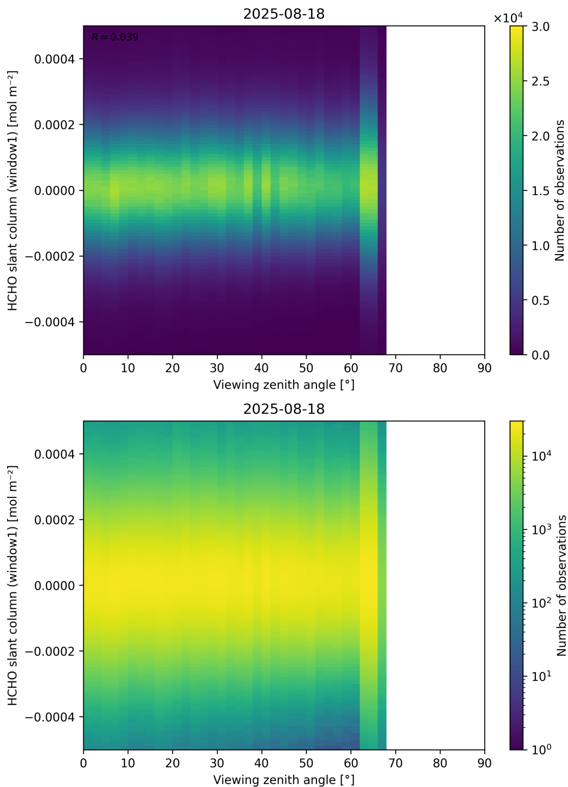
Figure 188: Scatter density plot of “Viewing zenith angle” against “HCHO slant column (window1)” for 2025-08-17 to 2025-08-19.
