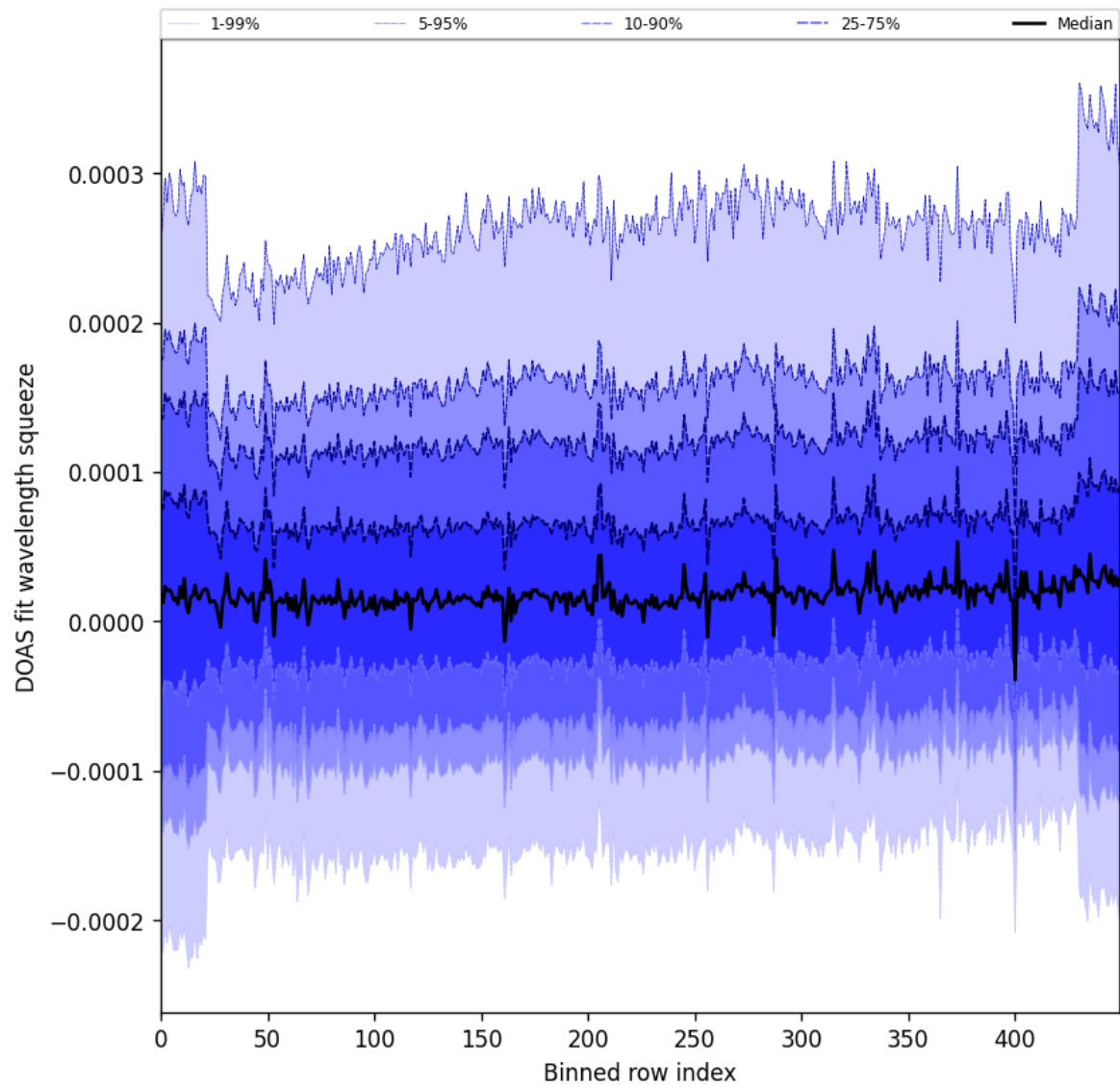
Figure 59: Along track statistics of “DOAS fit wavelength squeeze” for 2025-08-17 to 2025-08-19
