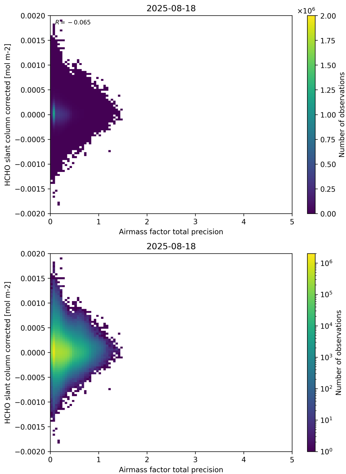
Figure 109: Scatter density plot of “Airmass factor total precision” against “HCHO slant column corrected” for 2025-08-17 to 2025-08-19.
