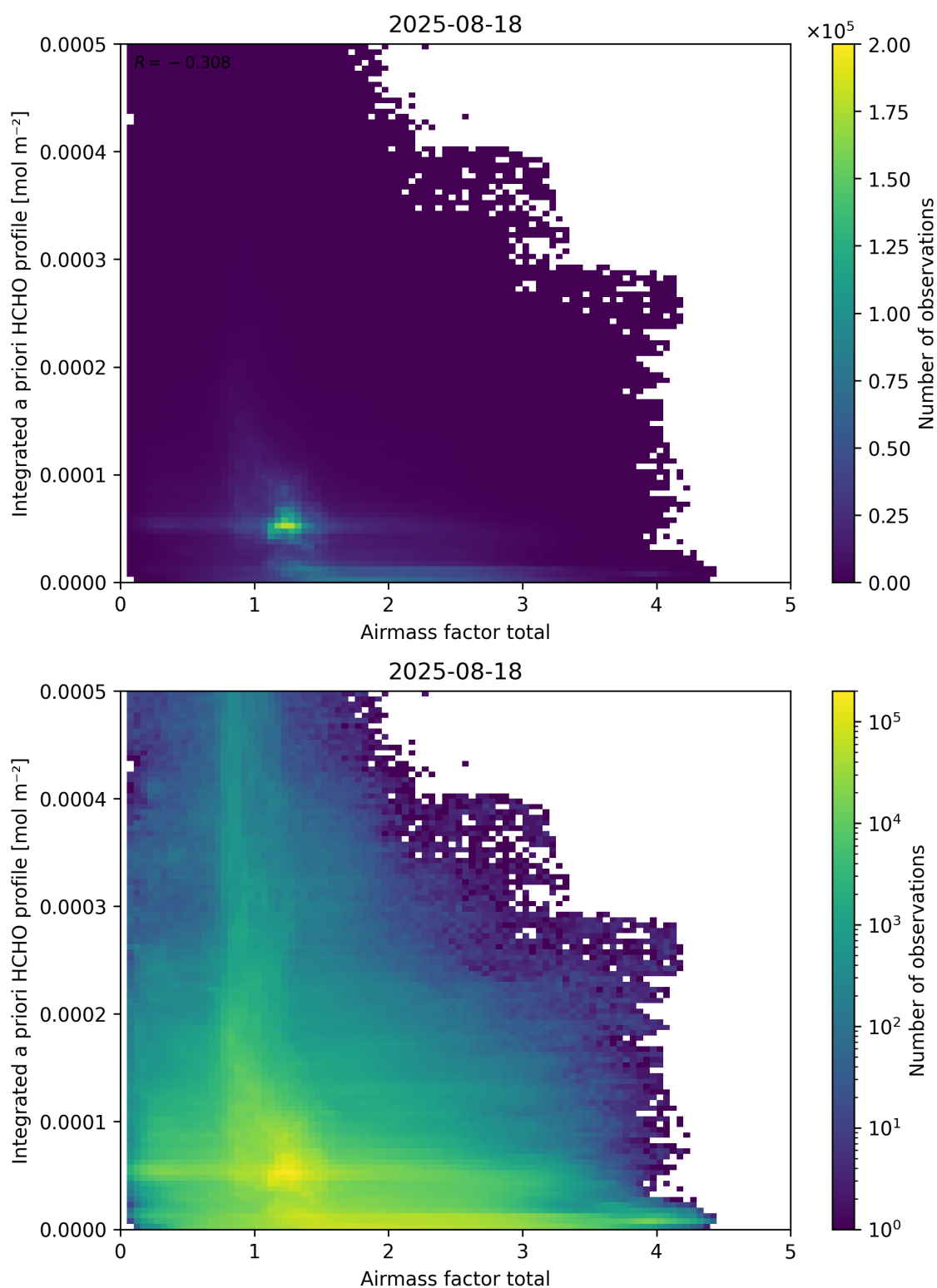
Figure 104: Scatter density plot of “Airmass factor total” against “Integrated a priori HCHO profile” for 2025-08-17 to 2025-08-19.
