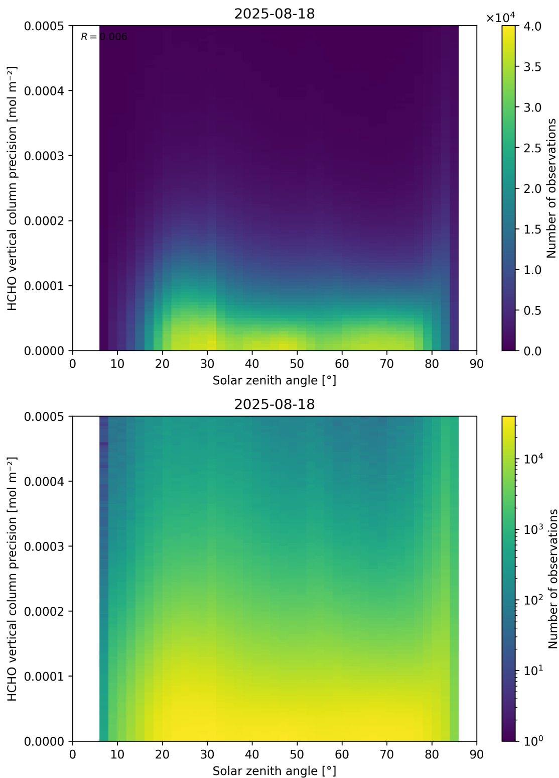
Figure 179: Scatter density plot of “Solar zenith angle” against “HCHO vertical column precision” for 2025-08-17 to 2025-08-19.
