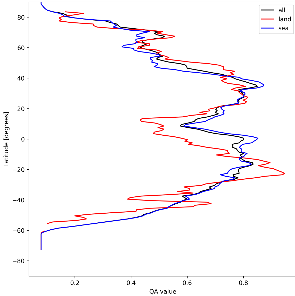
Figure 20: Zonal average of “QA value” for 2025-08-17 to 2025-08-19.
