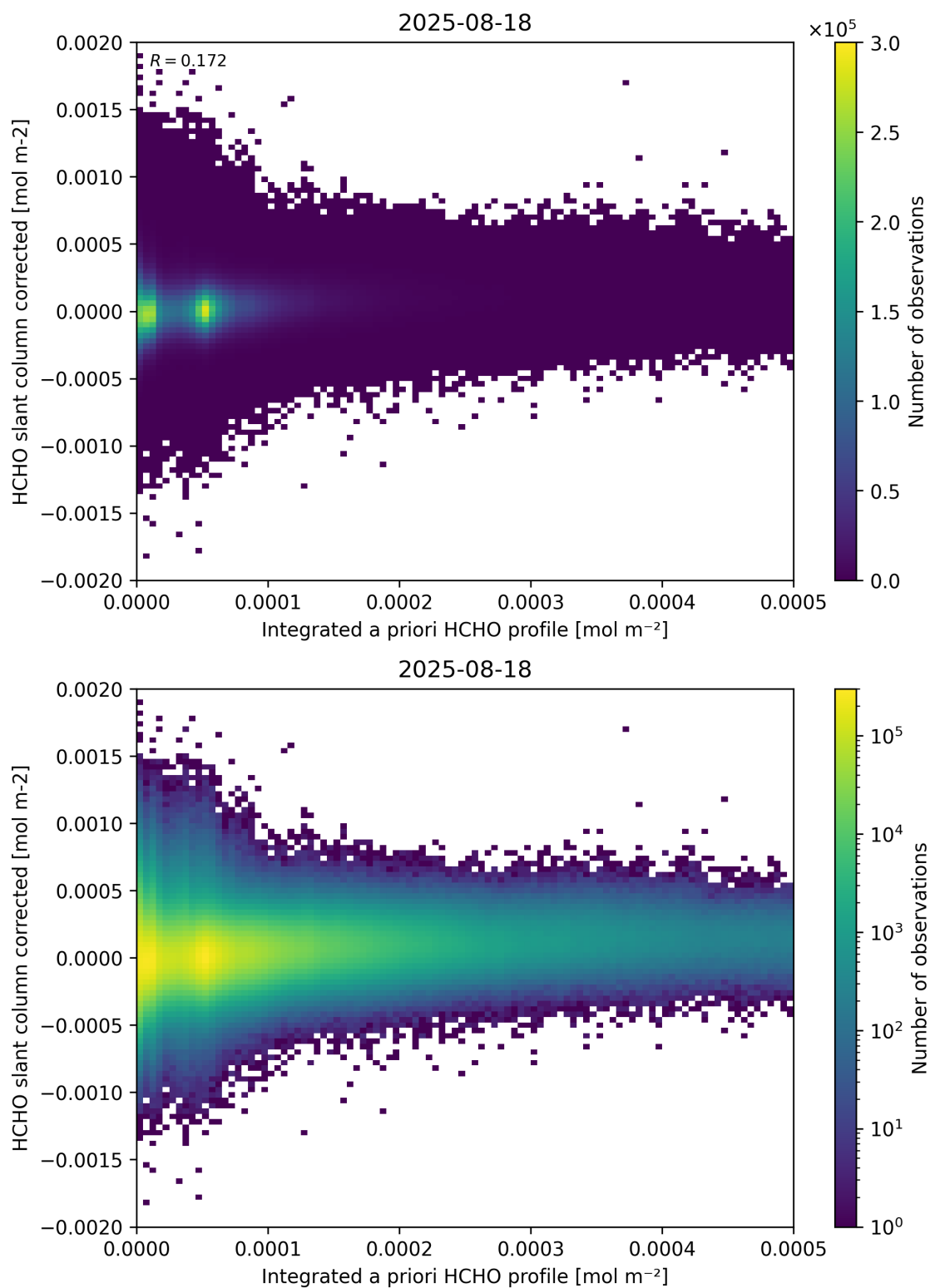
Figure 151: Scatter density plot of “Integrated a priori HCHO profile” against “HCHO slant column corrected” for 2025-08-17 to 2025-08-19.
