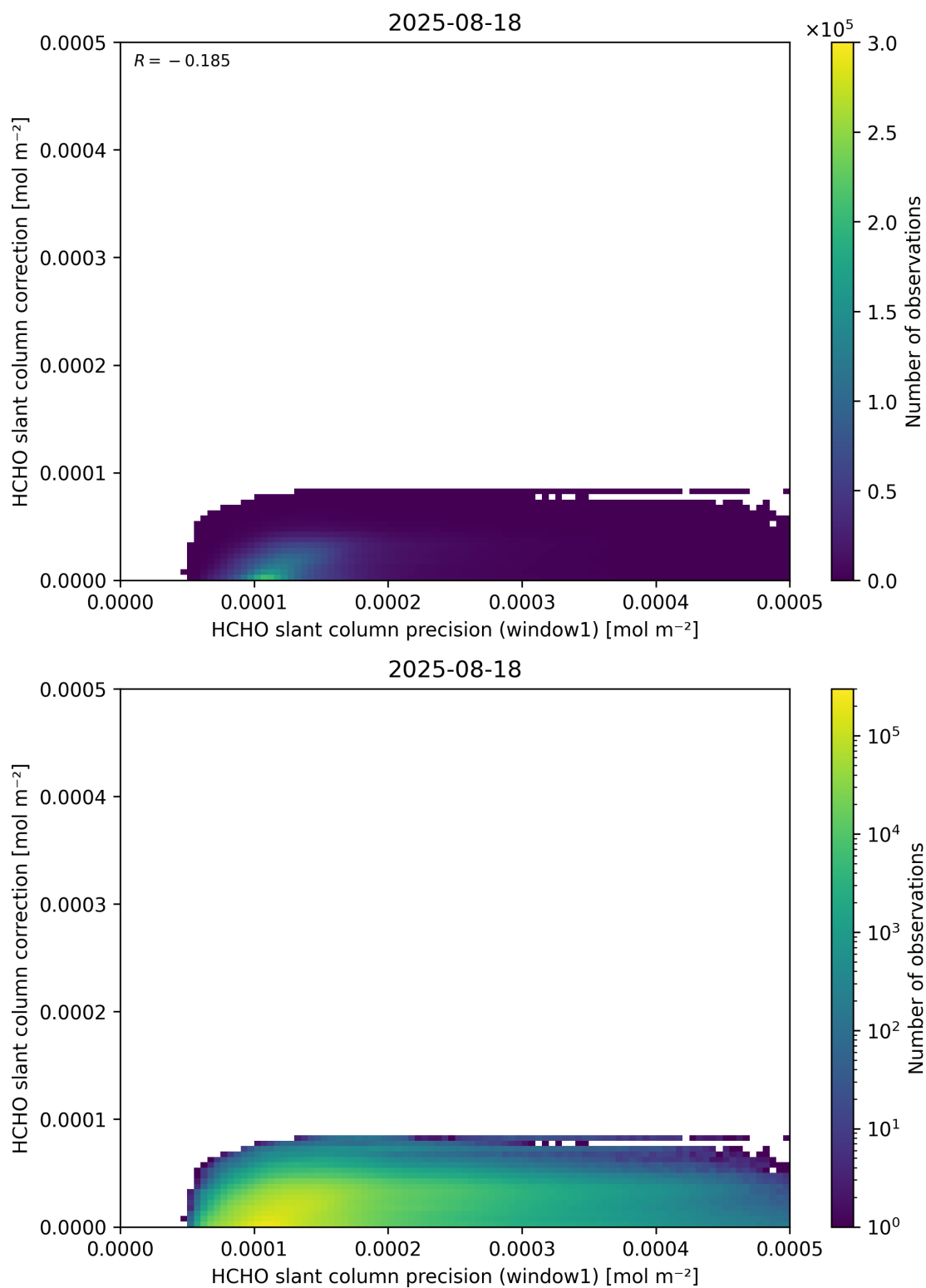
Figure 93: Scatter density plot of “HCHO slant column precision (window1)” against “HCHO slant column correction” for 2025-08-17 to 2025-08-19.
