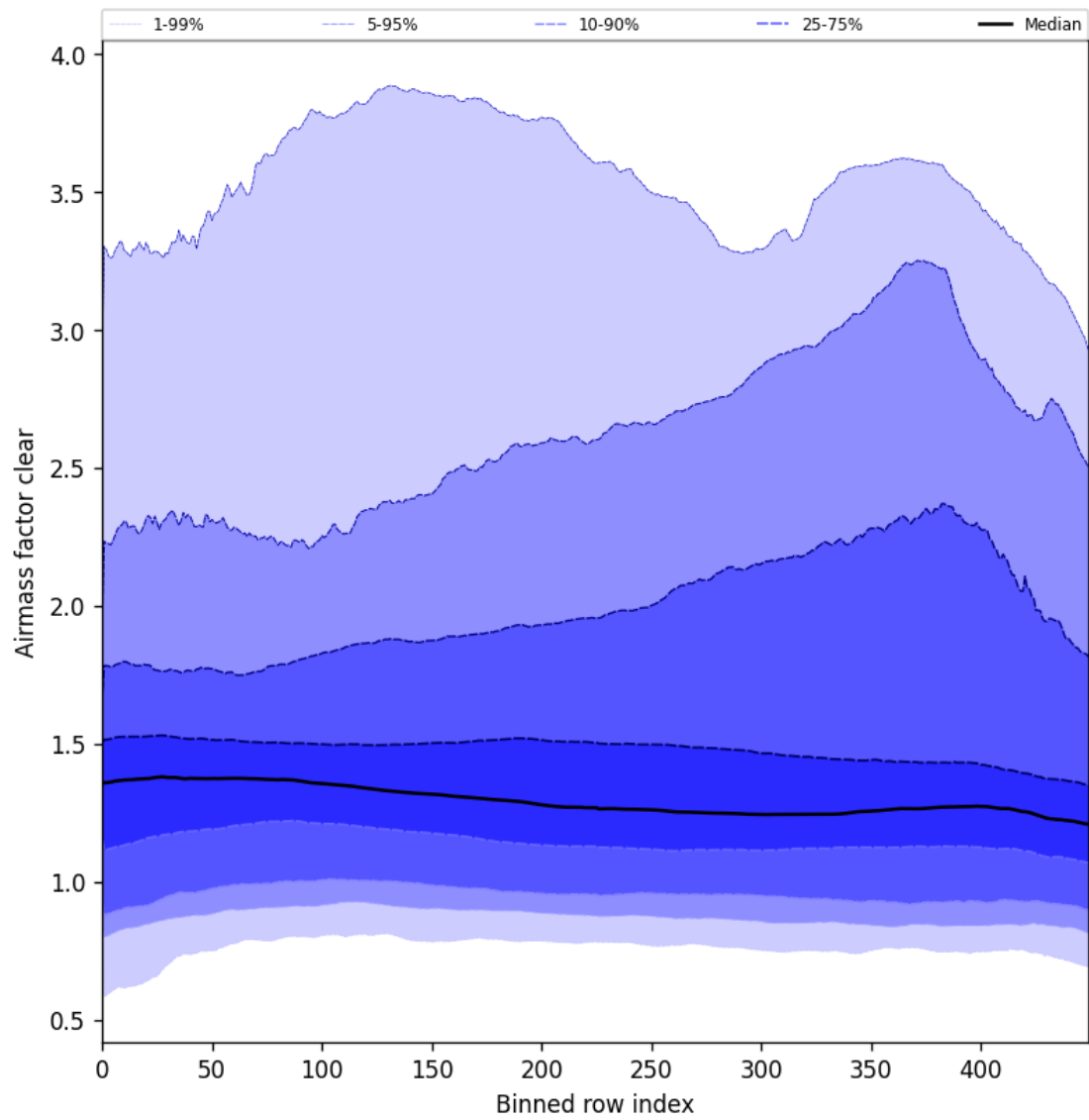
Figure 56: Along track statistics of “Airmass factor clear” for 2025-08-17 to 2025-08-19
