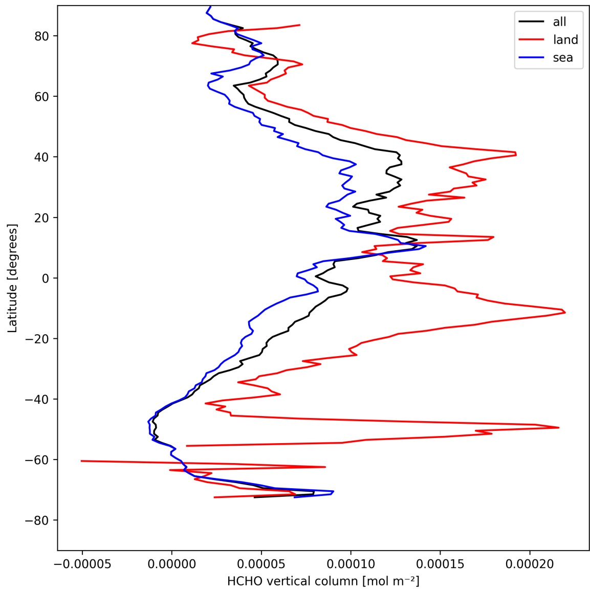
Figure 21: Zonal average of “HCHO vertical column” for 2025-08-17 to 2025-08-19.
