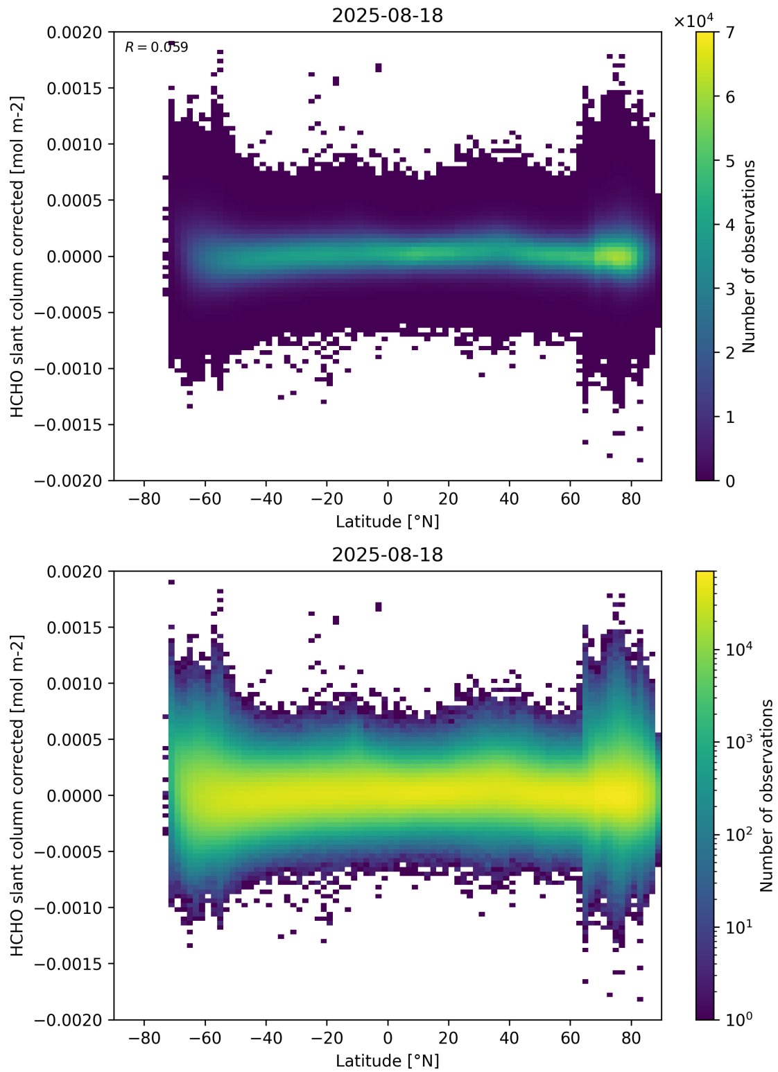
Figure 157: Scatter density plot of “Latitude” against “HCHO slant column corrected” for 2025-08-17 to 2025-08-19.
