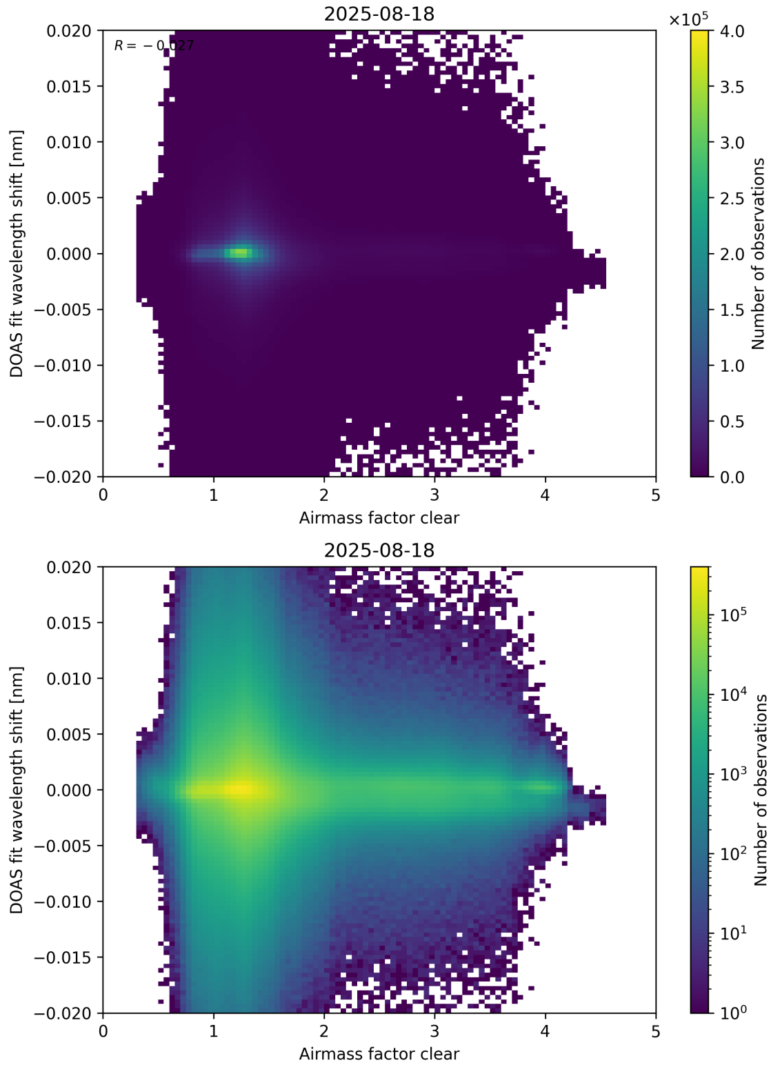
Figure 72: Scatter density plot of “Airmass factor clear” against “DOAS fit wavelength shift” for 2025-08-17 to 2025-08-19.
