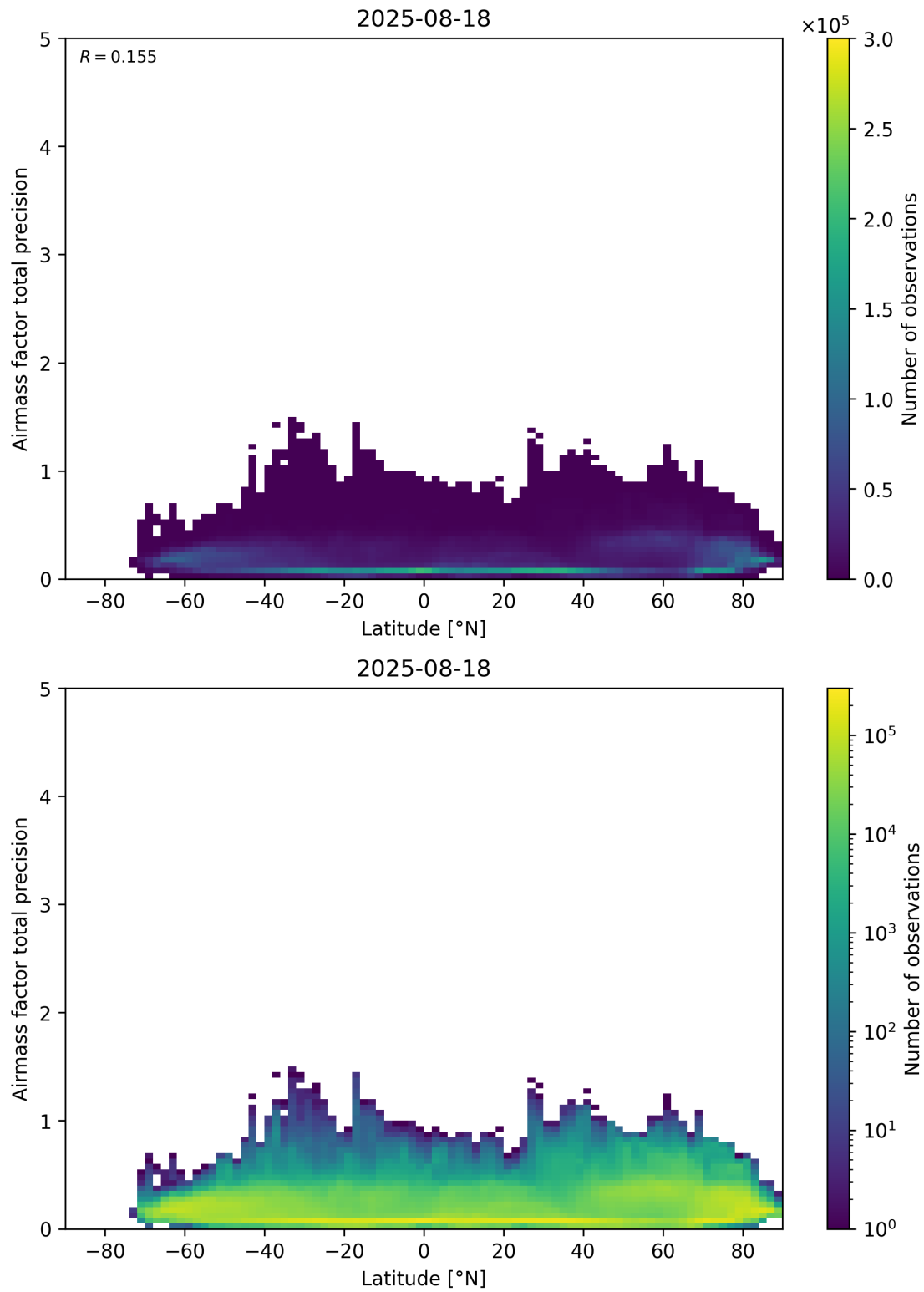
Figure 162: Scatter density plot of “Latitude” against “Airmass factor total precision” for 2025-08-17 to 2025-08-19.
