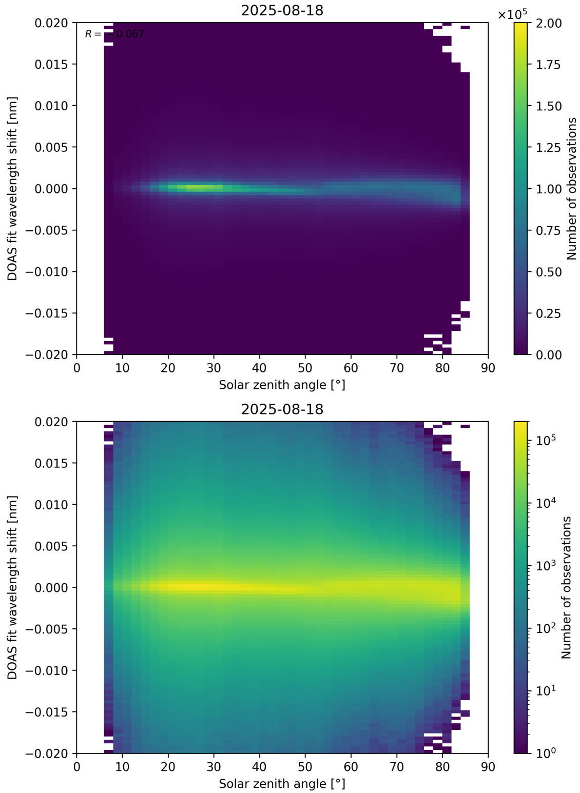
Figure 168: Scatter density plot of “Solar zenith angle” against “DOAS fit wavelength shift” for 2025-08-17 to 2025-08-19.
