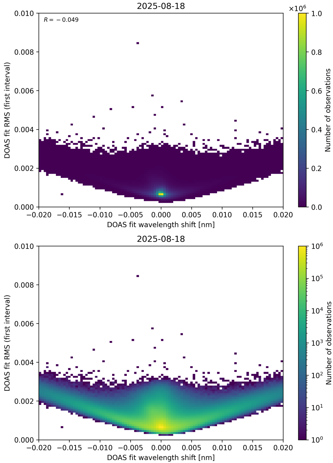
Figure 64: Scatter density plot of “DOAS fit wavelength shift” against “DOAS fit RMS (first interval)” for 2025-08-17 to 2025-08-19.
