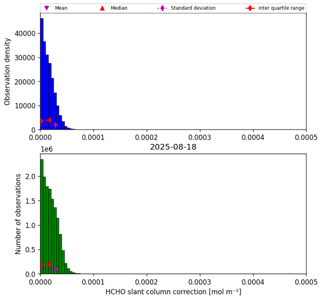
Figure 47: Histogram of “HCHO slant column correction” for 2025-08-17 to 2025-08-19
