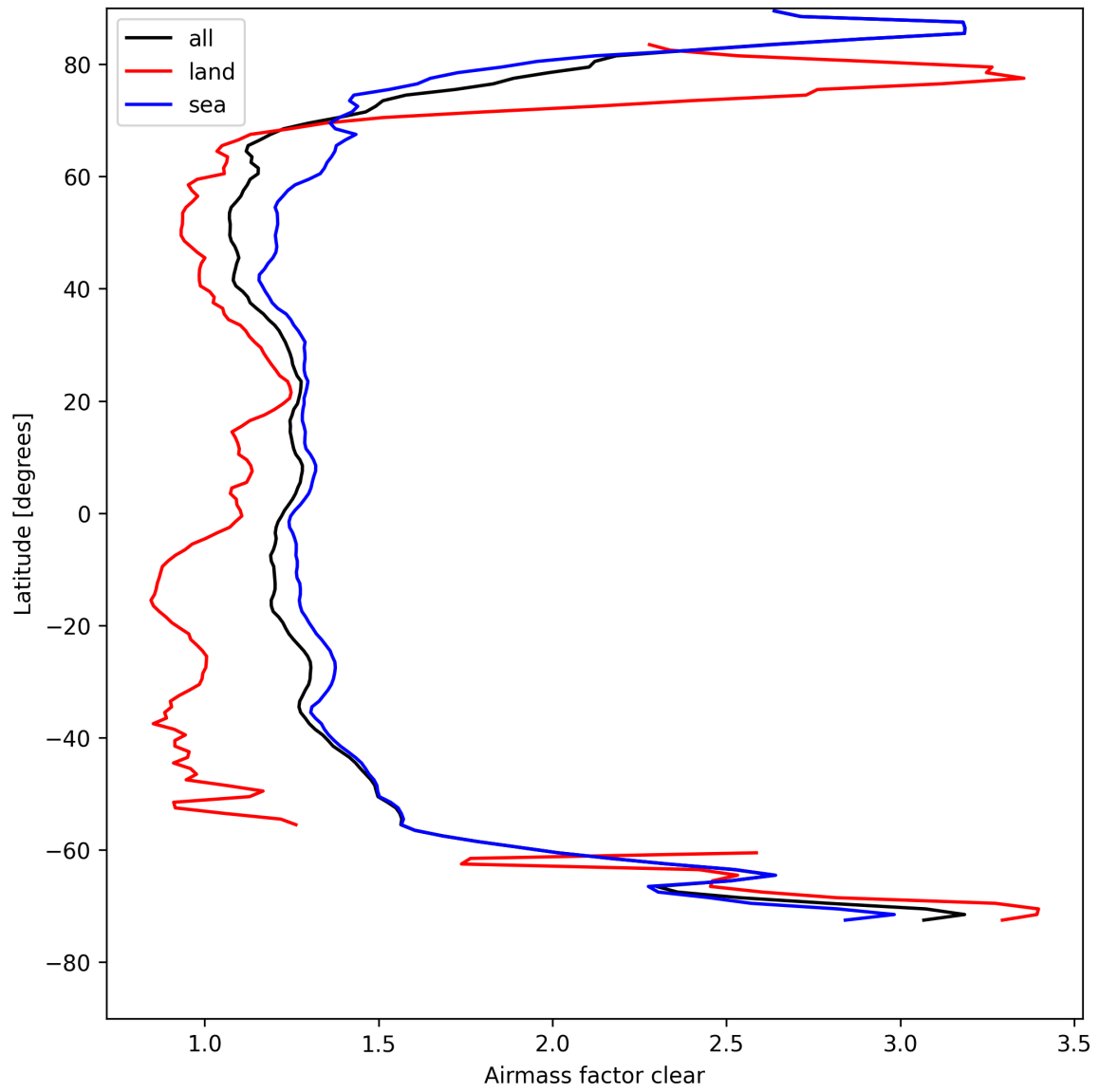
Figure 28: Zonal average of “Airmass factor clear” for 2025-08-17 to 2025-08-19.
