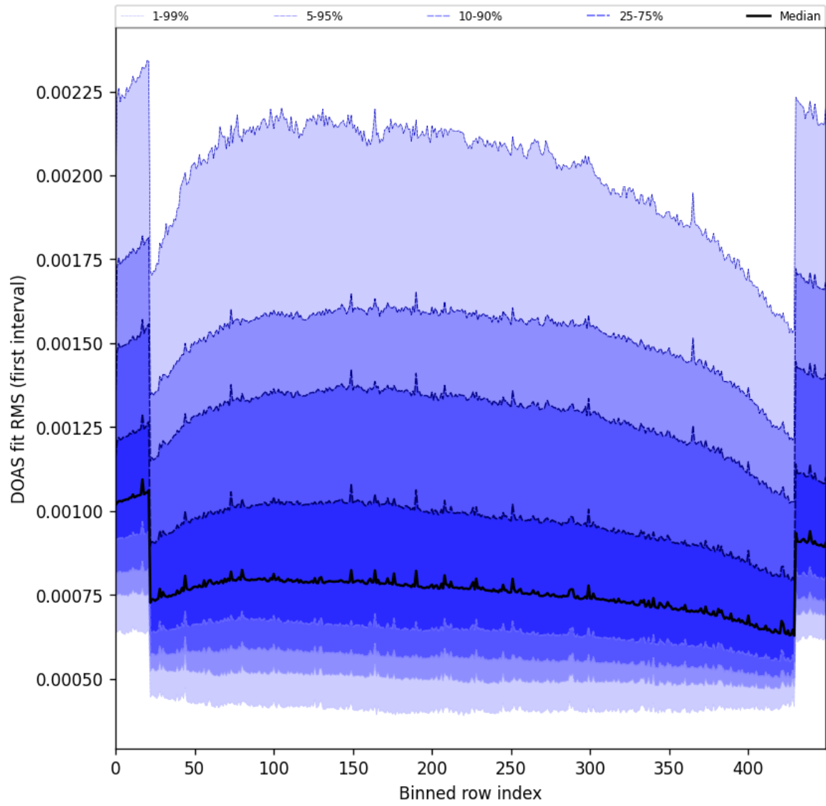
Figure 60: Along track statistics of “DOAS fit RMS (first interval)” for 2025-08-17 to 2025-08-19
