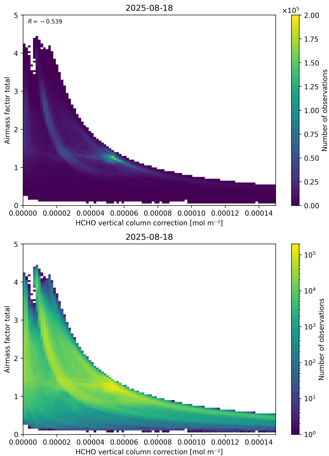
Figure 120: Scatter density plot of “HCHO vertical column correction” against “Airmass factor total” for 2025-08-17 to 2025-08-19.
