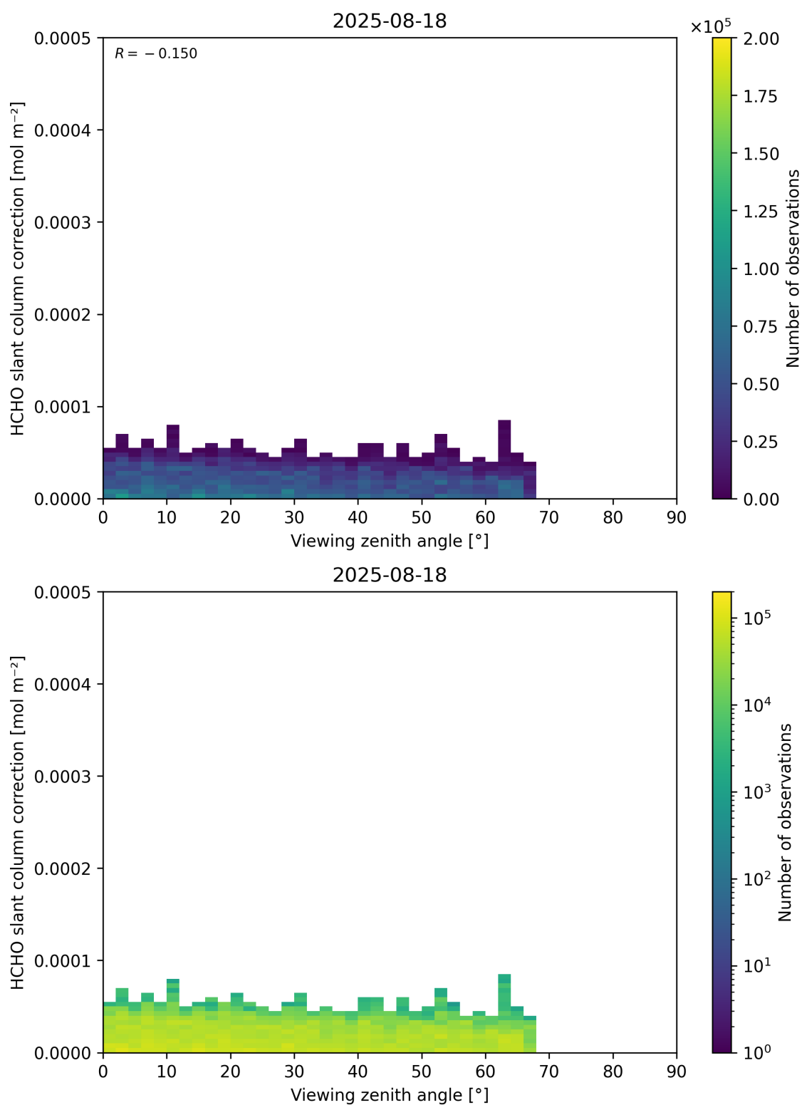
Figure 187: Scatter density plot of “Viewing zenith angle” against “HCHO slant column correction” for 2025-08-17 to 2025-08-19.
