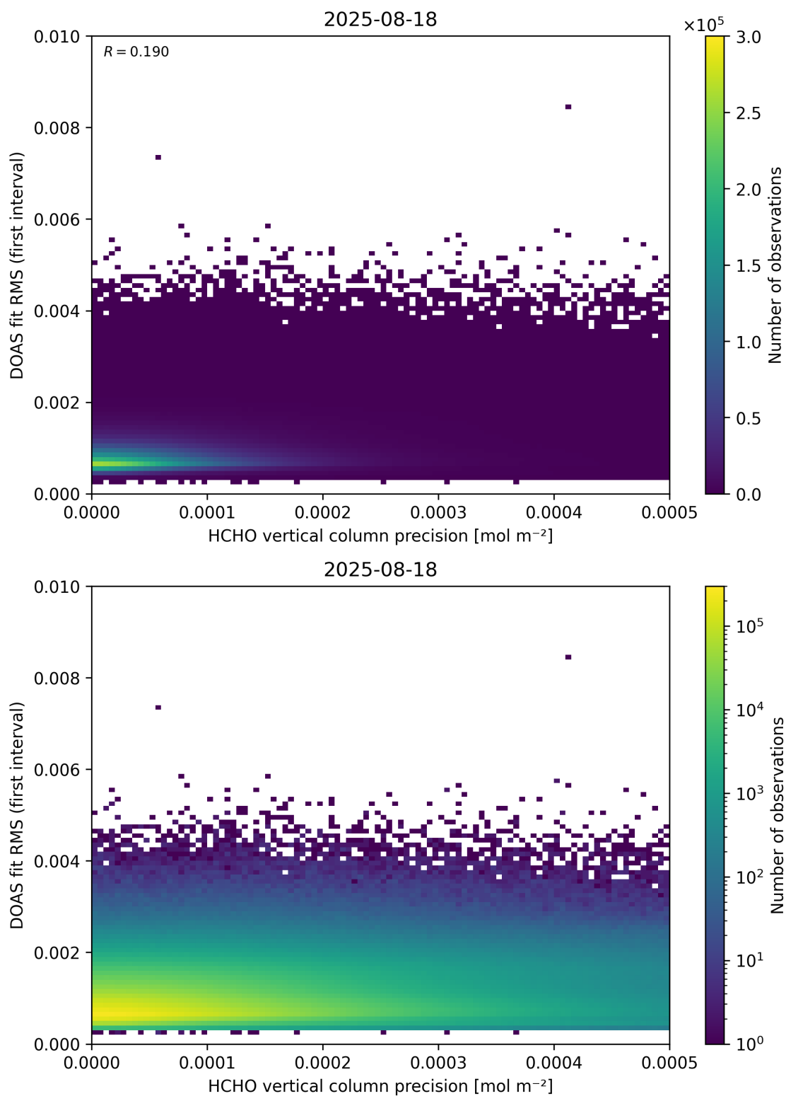
Figure 136: Scatter density plot of “HCHO vertical column precision” against “DOAS fit RMS (first interval)” for 2025-08-17 to 2025-08-19.
