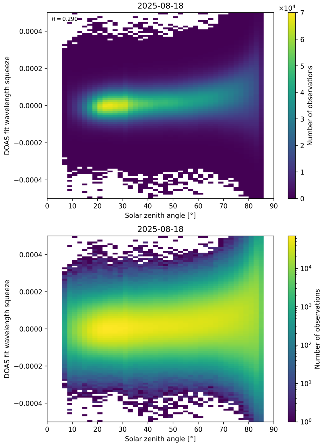
Figure 169: Scatter density plot of “Solar zenith angle” against “DOAS fit wavelength squeeze” for 2025-08-17 to 2025-08-19.
