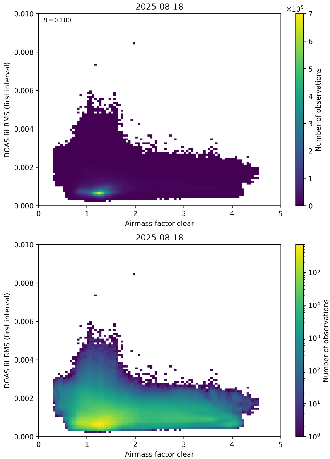
Figure 71: Scatter density plot of “Airmass factor clear” against “DOAS fit RMS (first interval)” for 2025-08-17 to 2025-08-19.
