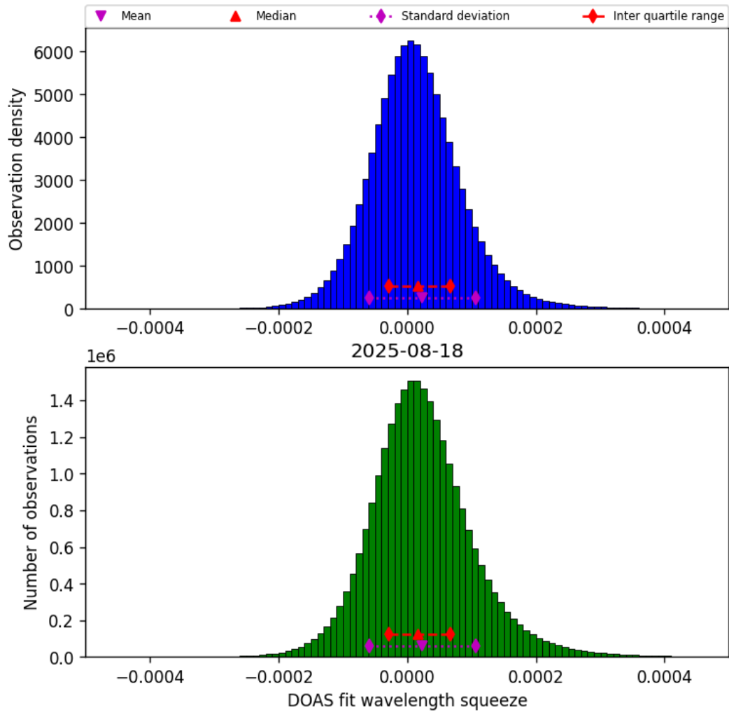
Figure 45: Histogram of “DOAS fit wavelength squeeze” for 2025-08-17 to 2025-08-19
