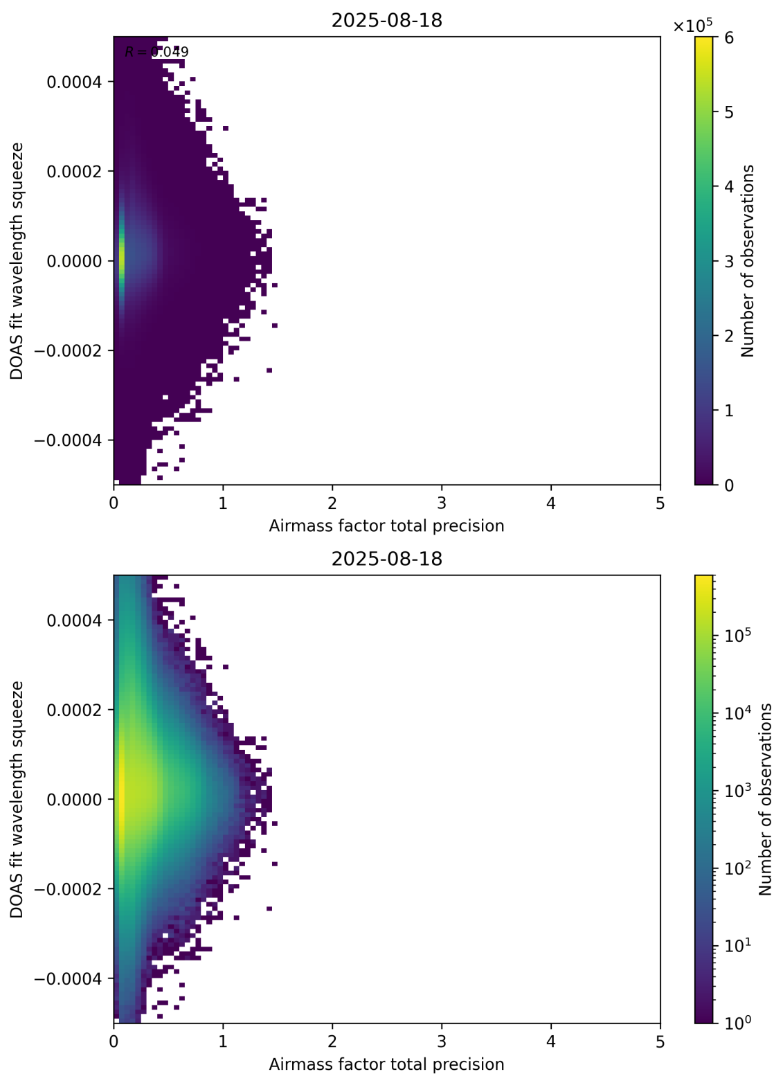
Figure 107: Scatter density plot of “Airmass factor total precision” against “DOAS fit wavelength squeeze” for 2025-08-17 to 2025-08-19.
