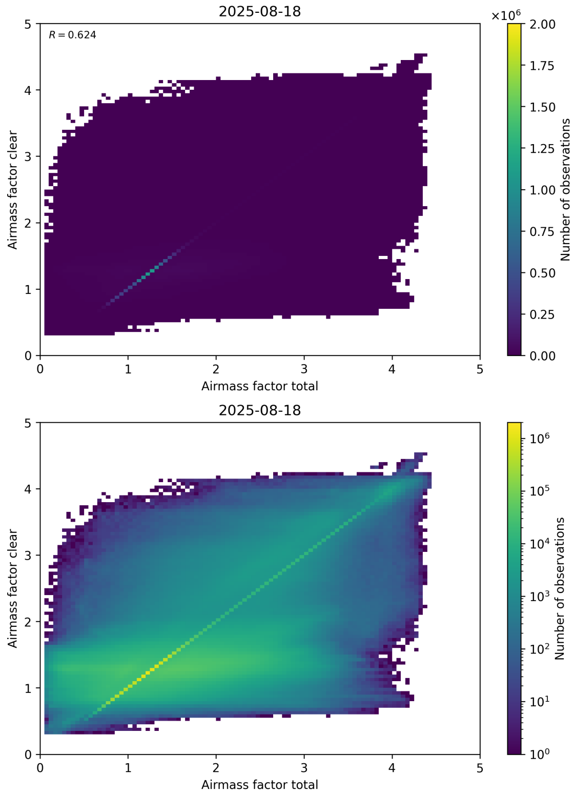
Figure 100: Scatter density plot of “Airmass factor total” against “Airmass factor clear” for 2025-08-17 to 2025-08-19.
