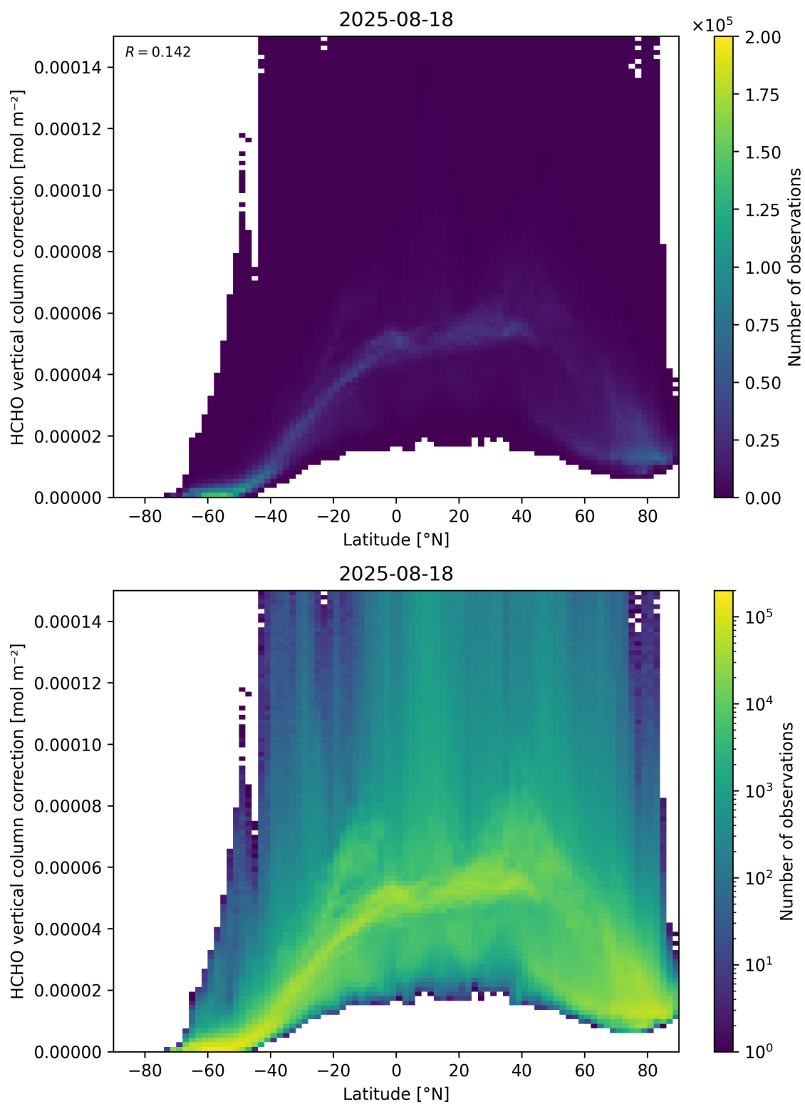
Figure 164: Scatter density plot of “Latitude” against “HCHO vertical column correction” for 2025-08-17 to 2025-08-19.
