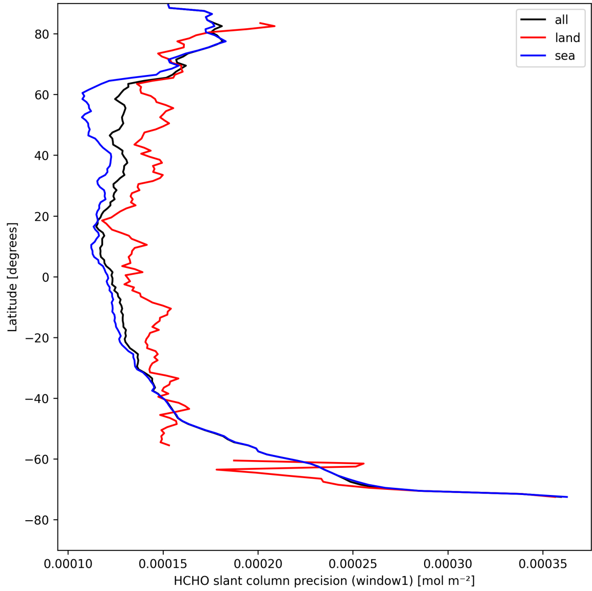
Figure 25: Zonal average of "HCHO slant column precision (window1)" for 2025-08-17 to 2025-08-19.
