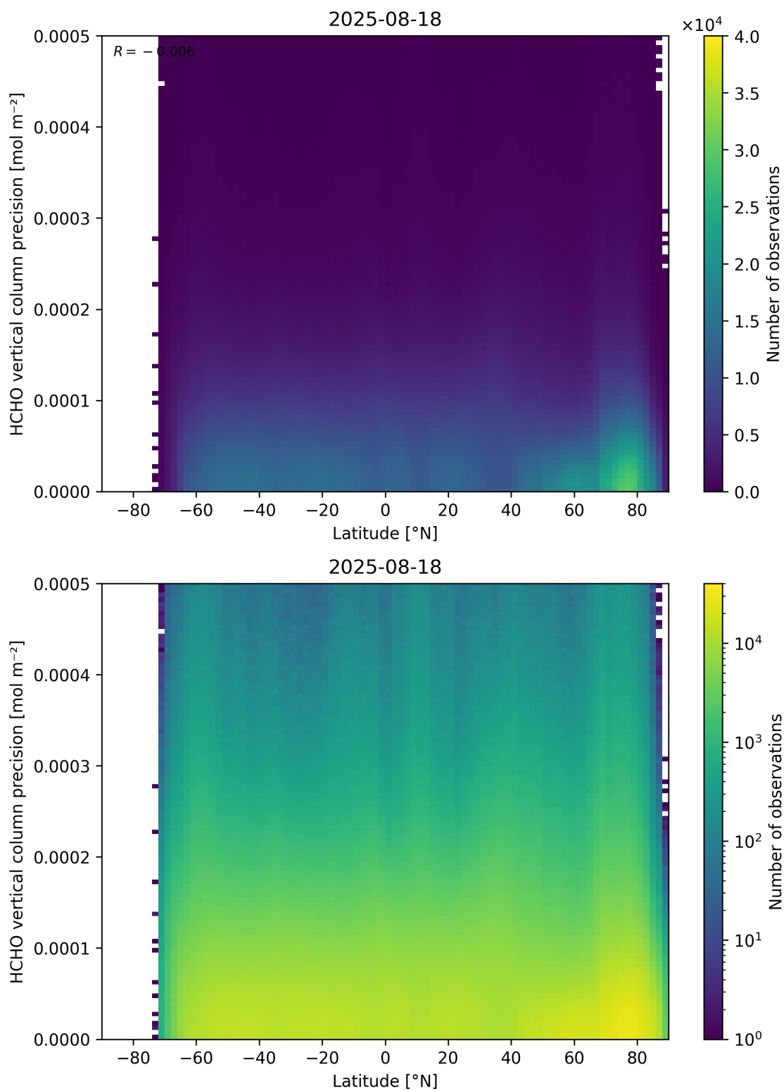
Figure 165: Scatter density plot of “Latitude” against “HCHO vertical column precision” for 2025-08-17 to 2025-08-19.
