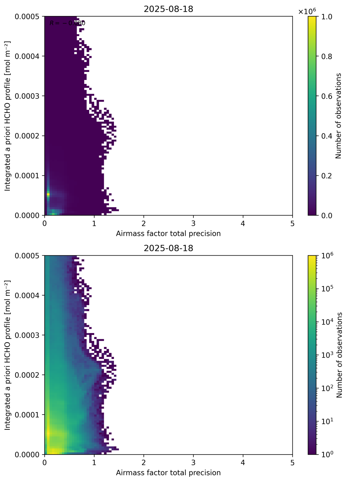
Figure 111: Scatter density plot of “Airmass factor total precision” against “Integrated a priori HCHO profile” for 2025-08-17 to 2025-08-19.
