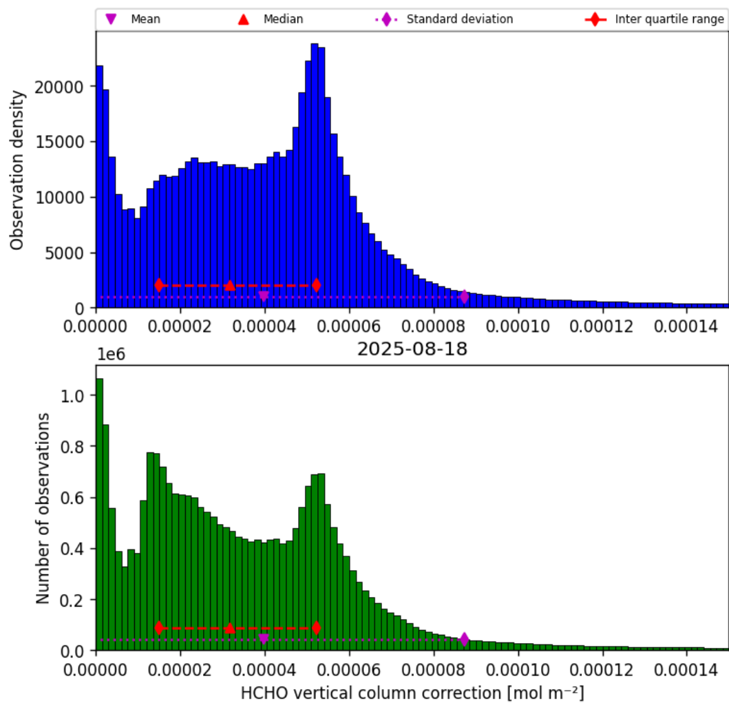
Figure 37: Histogram of “HCHO vertical column correction” for 2025-08-17 to 2025-08-19
