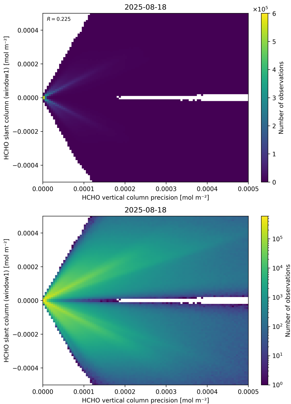
Figure 142: Scatter density plot of “HCHO vertical column precision” against “HCHO slant column (window1)” for 2025-08-17 to 2025-08-19.
