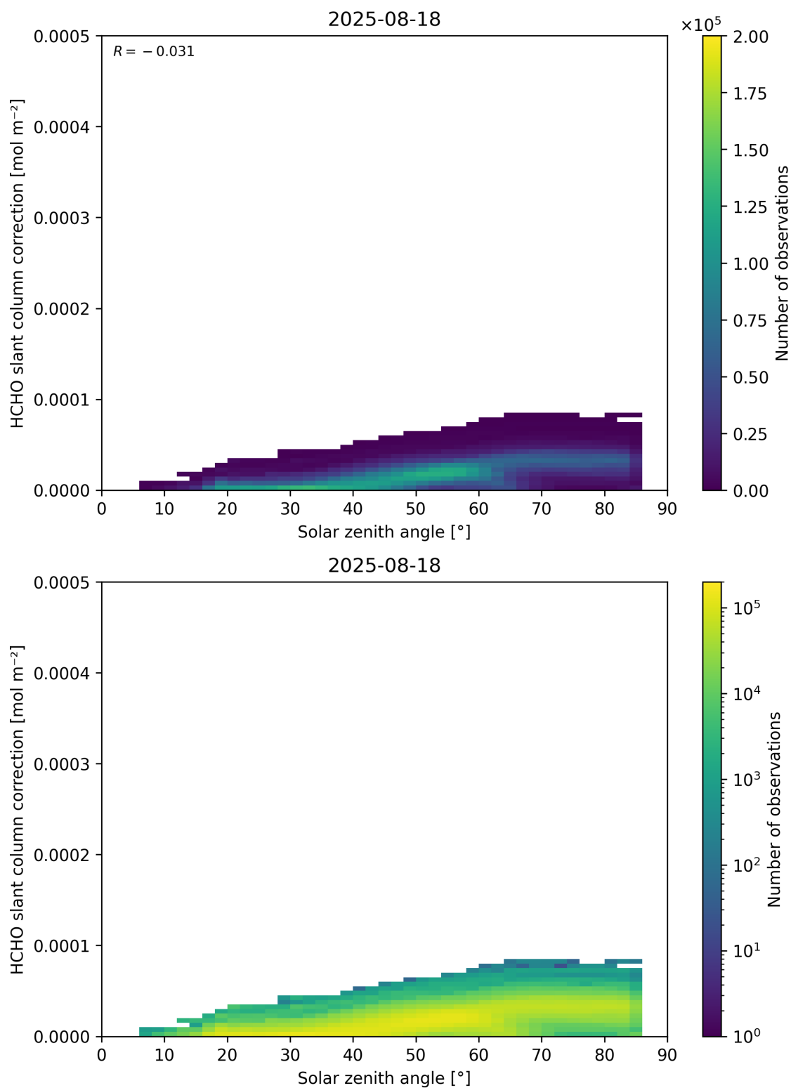
Figure 172: Scatter density plot of “Solar zenith angle” against “HCHO slant column correction” for 2025-08-17 to 2025-08-19.
