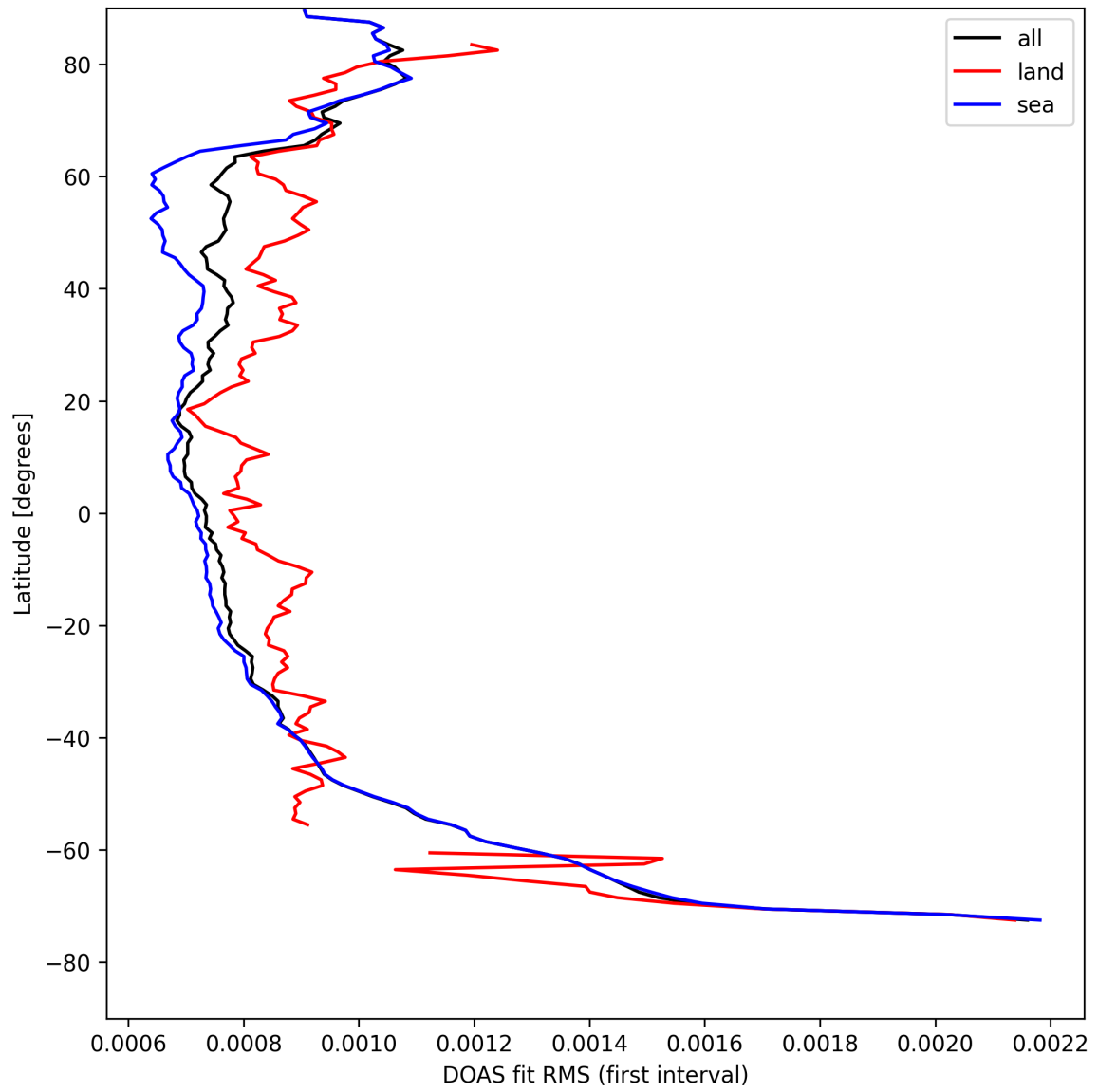
Figure 32: Zonal average of “DOAS fit RMS (first interval)” for 2025-08-17 to 2025-08-19.
