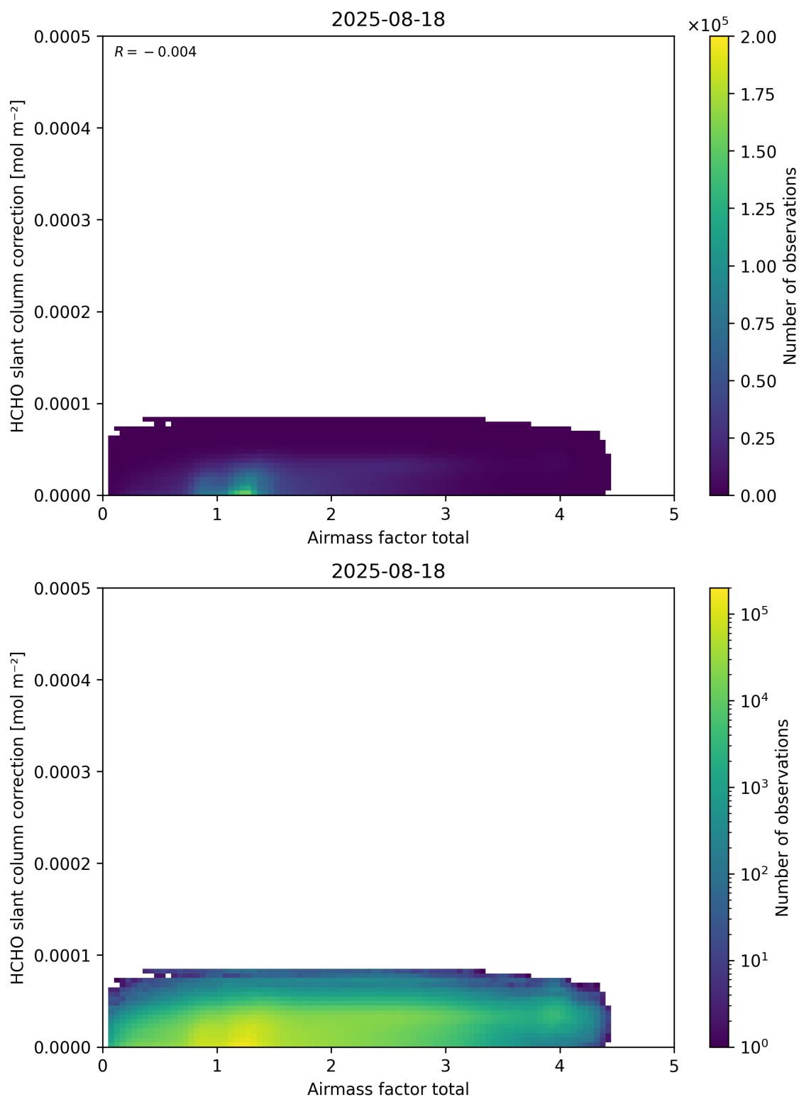
Figure 102: Scatter density plot of “Airmass factor total” against “HCHO slant column correction” for 2025-08-17 to 2025-08-19.
