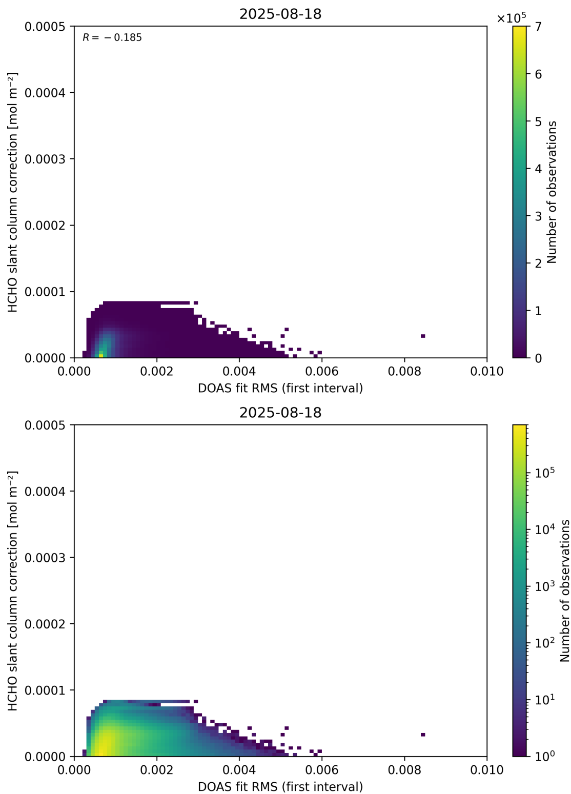
Figure 63: Scatter density plot of “DOAS fit RMS (first interval)” against “HCHO slant column correction” for 2025-08-17 to 2025-08-19.
