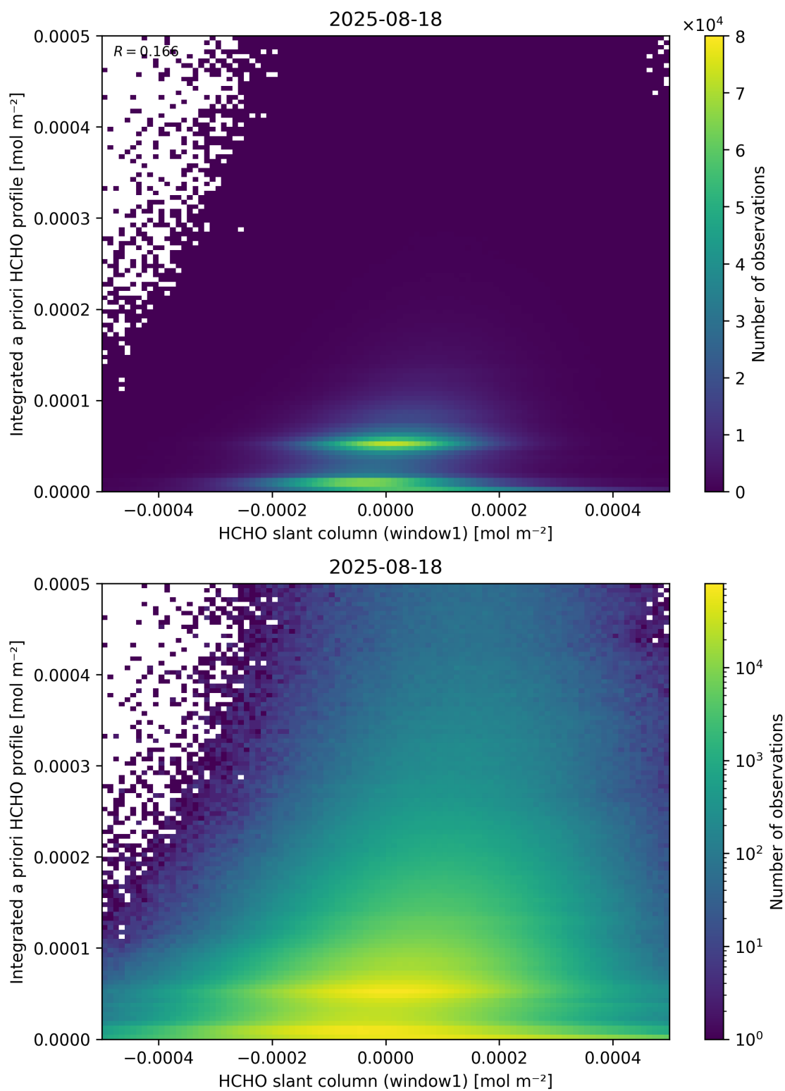
Figure 87: Scatter density plot of “HCHO slant column (window1)” against “Integrated a priori HCHO profile” for 2025-08-17 to 2025-08-19.
