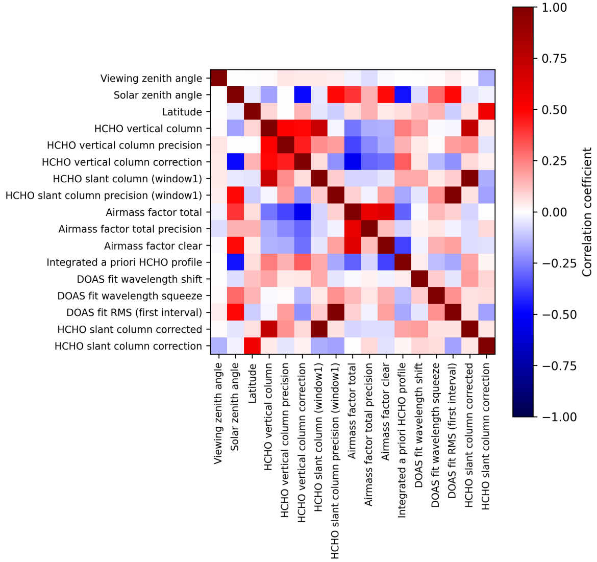
Figure 2: Map of correlation matrix for 2025-08-17 to 2025-08-19.
