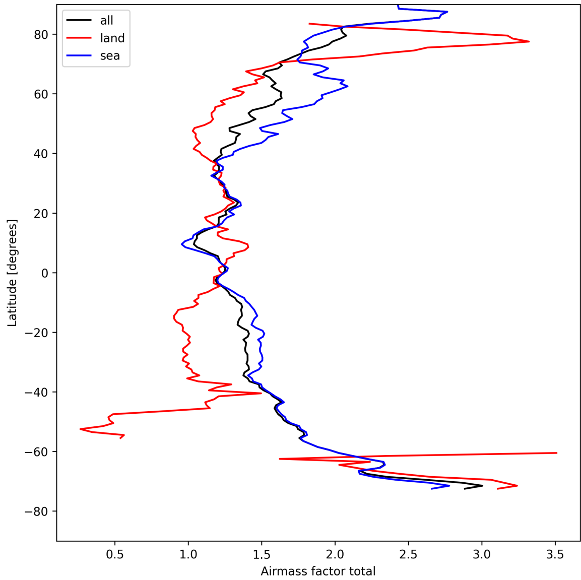
Figure 26: Zonal average of “Airmass factor total” for 2025-08-17 to 2025-08-19.
