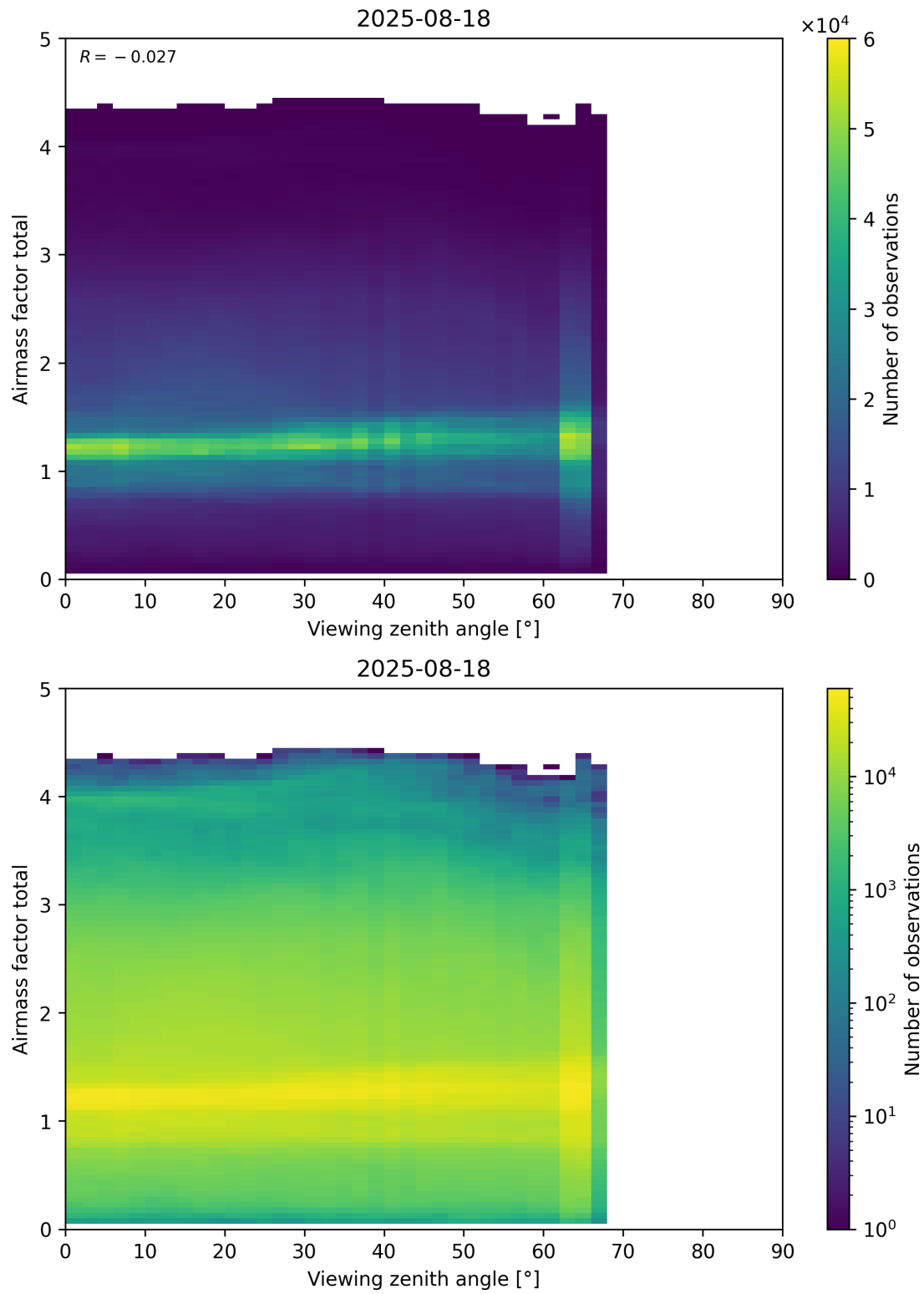
Figure 190: Scatter density plot of “Viewing zenith angle” against “Airmass factor total” for 2025-08-17 to 2025-08-19.
