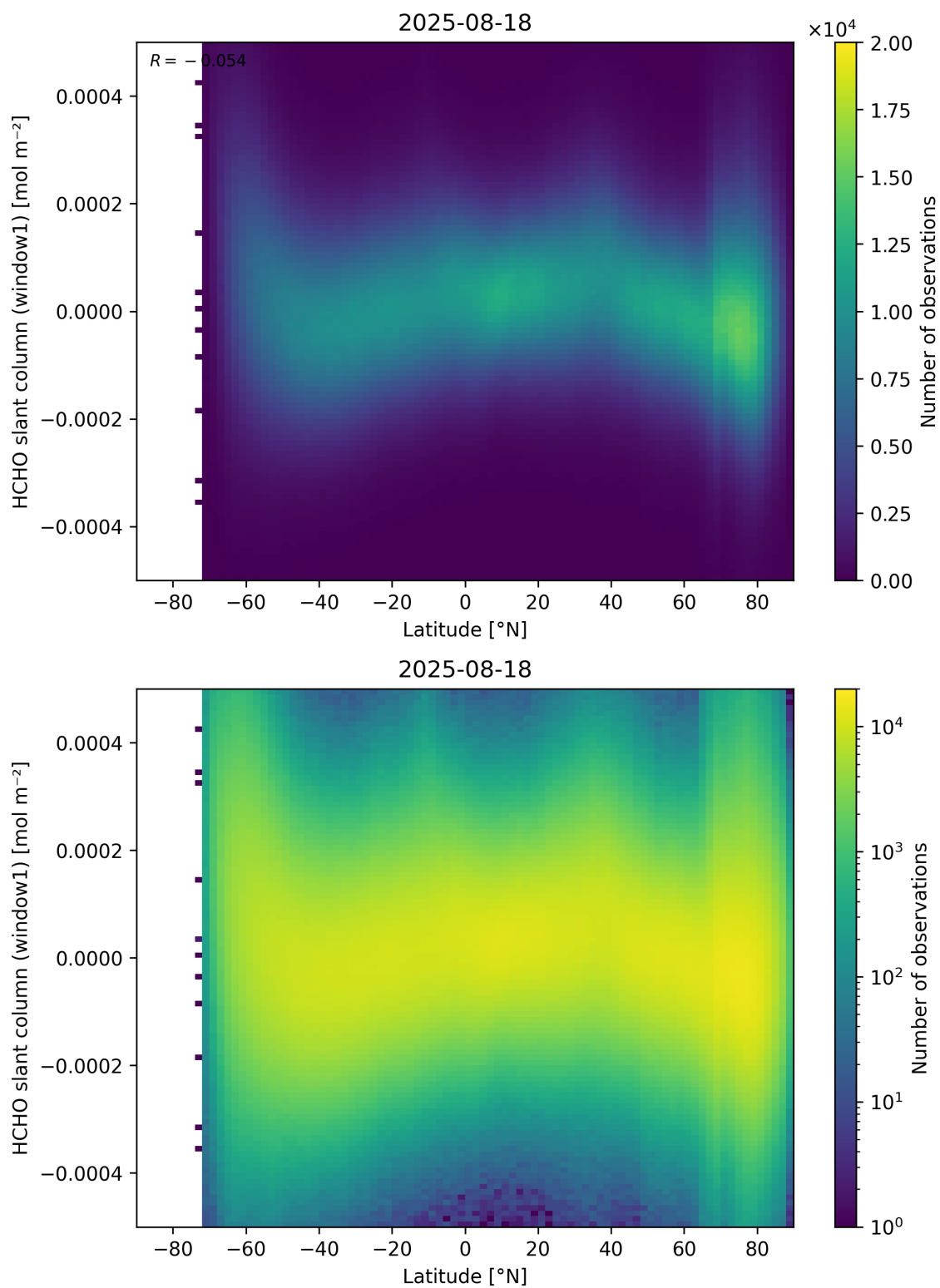
Figure 159: Scatter density plot of “Latitude” against “HCHO slant column (window1)” for 2025-08-17 to 2025-08-19.
