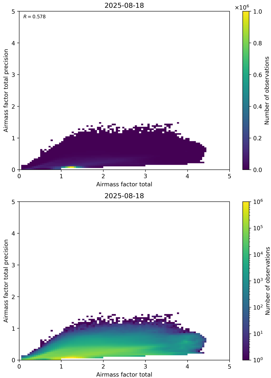
Figure 103: Scatter density plot of “Airmass factor total” against “Airmass factor total precision” for 2025-08-17 to 2025-08-19.
