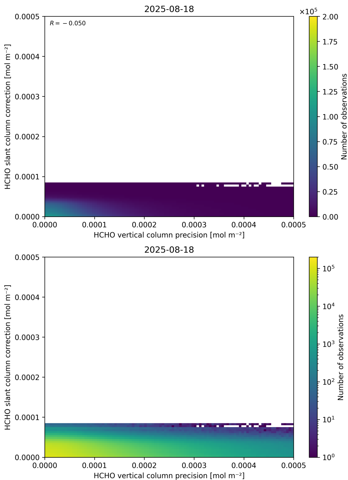
Figure 141: Scatter density plot of “HCHO vertical column precision” against “HCHO slant column correction” for 2025-08-17 to 2025-08-19.
