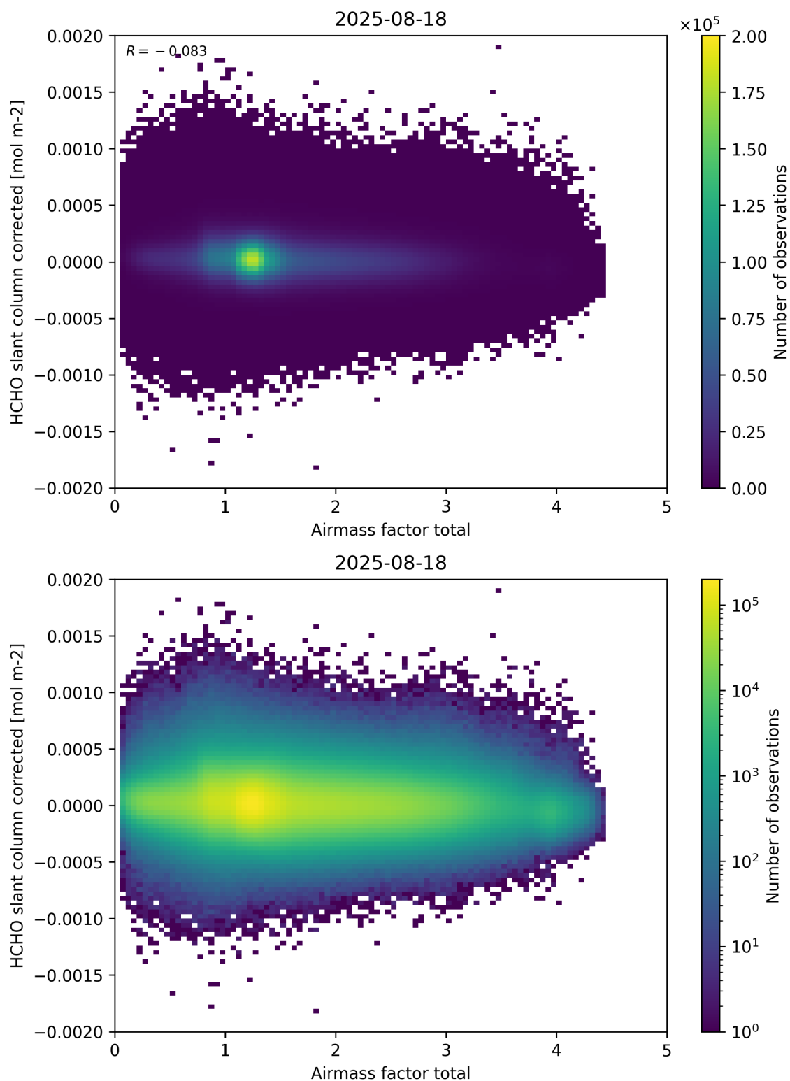
Figure 101: Scatter density plot of “Airmass factor total” against “HCHO slant column corrected” for 2025-08-17 to 2025-08-19.
