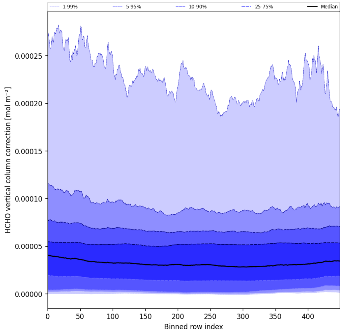
Figure 51: Along track statistics of "HCHO vertical column correction" for 2025-08-17 to 2025-08-19
