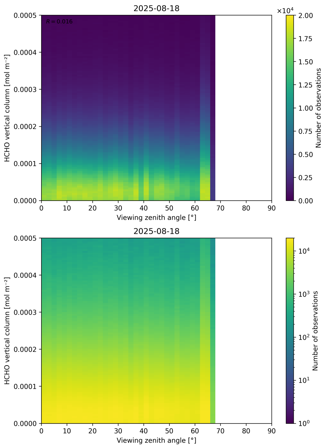
Figure 192: Scatter density plot of “Viewing zenith angle” against “HCHO vertical column” for 2025-08-17 to 2025-08-19.
