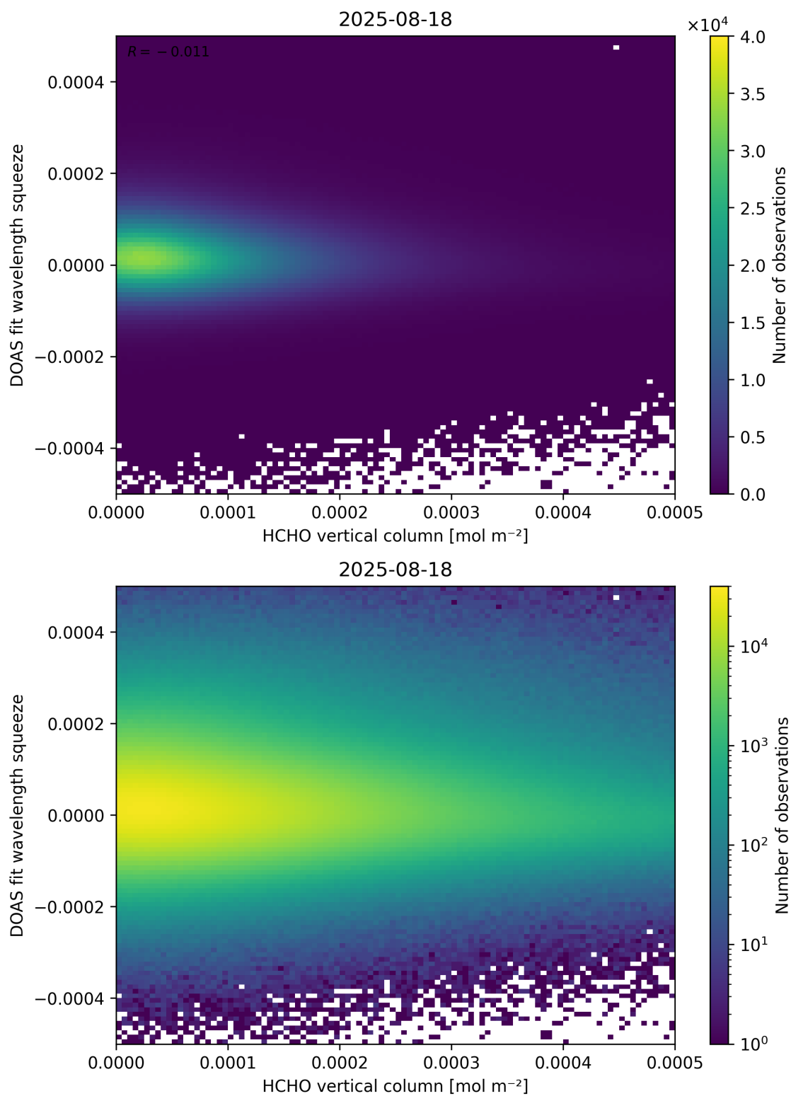
Figure 125: Scatter density plot of “HCHO vertical column” against “DOAS fit wavelength squeeze” for 2025-08-17 to 2025-08-19.
