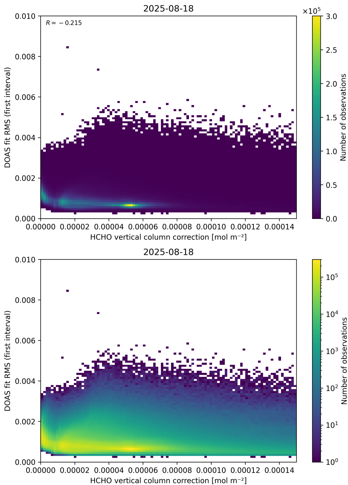
Figure 112: Scatter density plot of “HCHO vertical column correction” against “DOAS fit RMS (first interval)” for 2025-08-17 to 2025-08-19.
