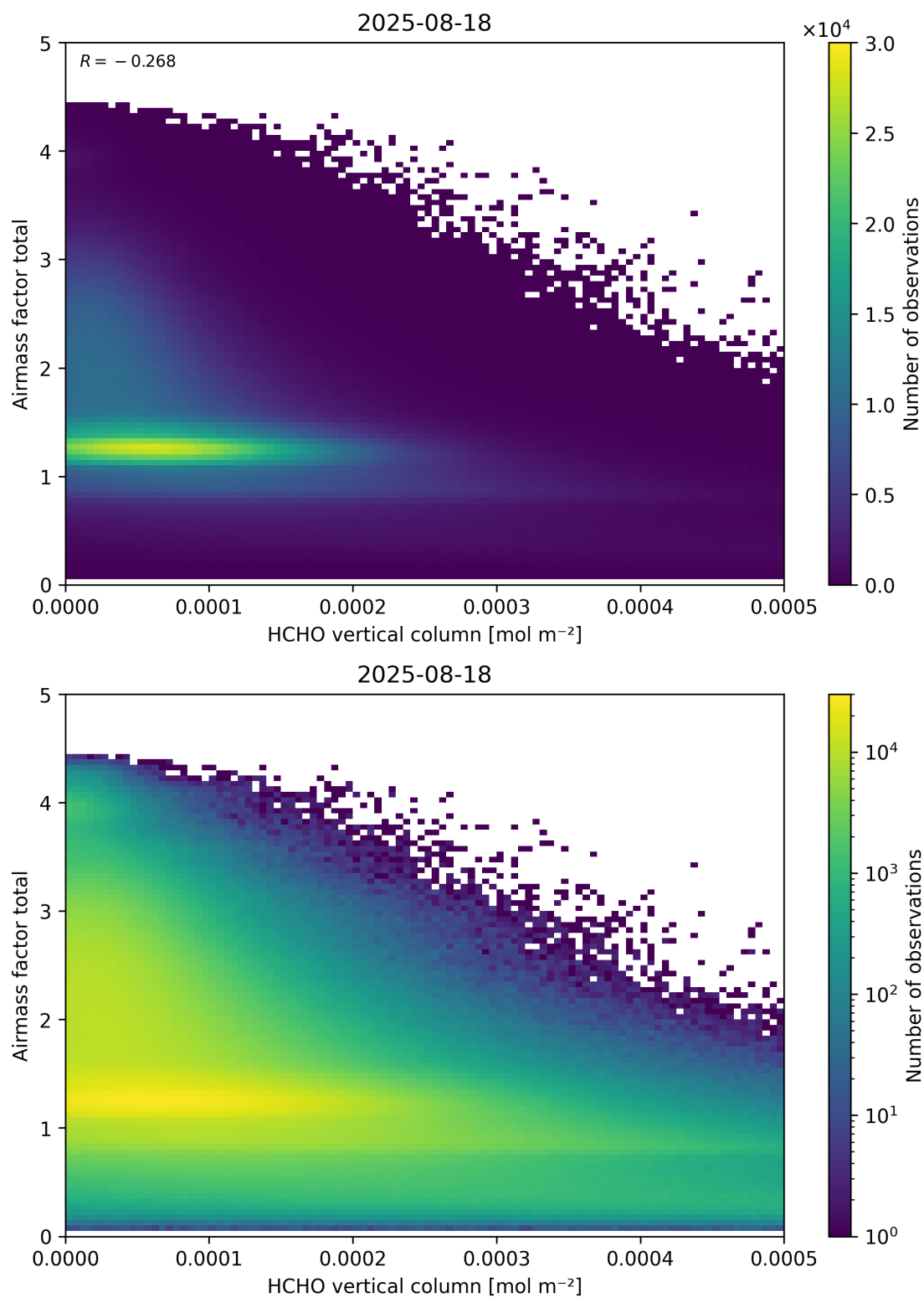
Figure 131: Scatter density plot of “HCHO vertical column” against “Airmass factor total” for 2025-08-17 to 2025-08-19.
