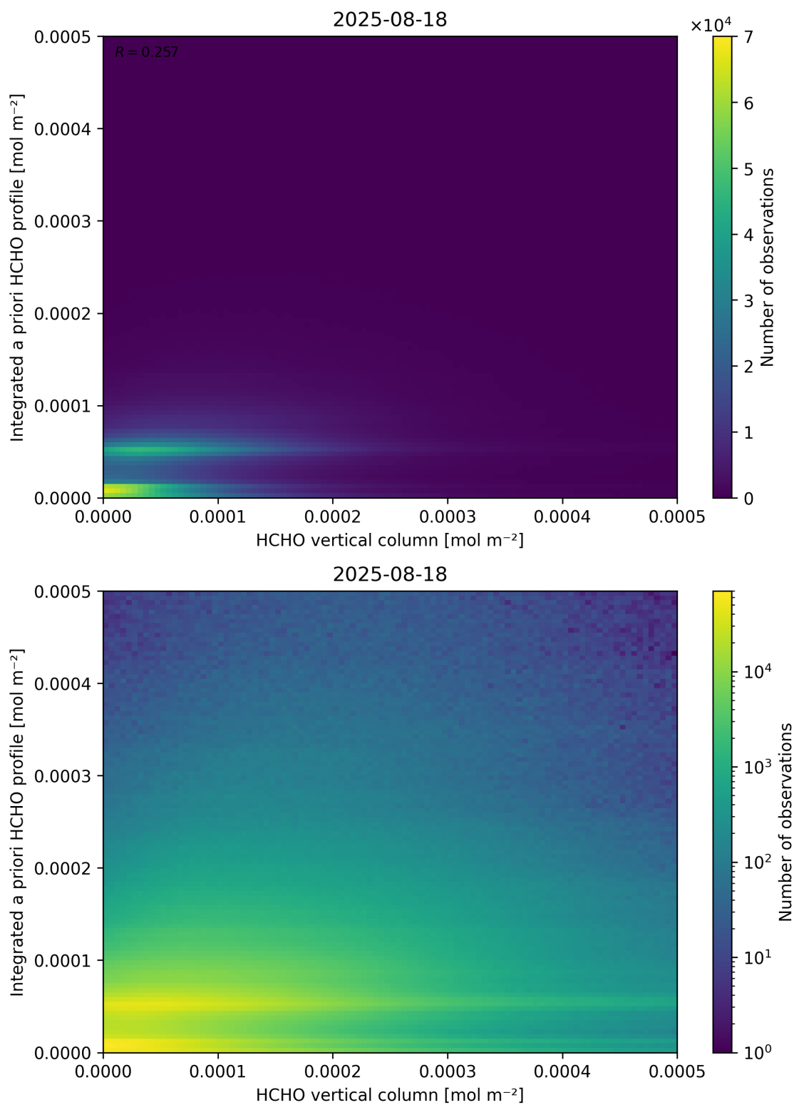
Figure 135: Scatter density plot of “HCHO vertical column” against “Integrated a priori HCHO profile” for 2025-08-17 to 2025-08-19.
