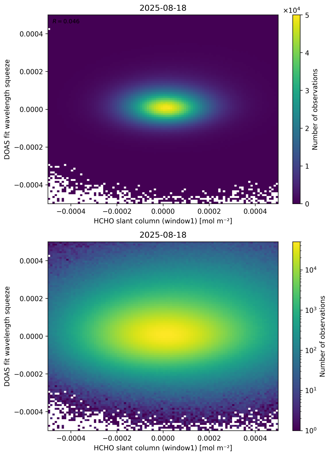
Figure 80: Scatter density plot of “HCHO slant column (window1)” against “DOAS fit wavelength squeeze” for 2025-08-17 to 2025-08-19.
