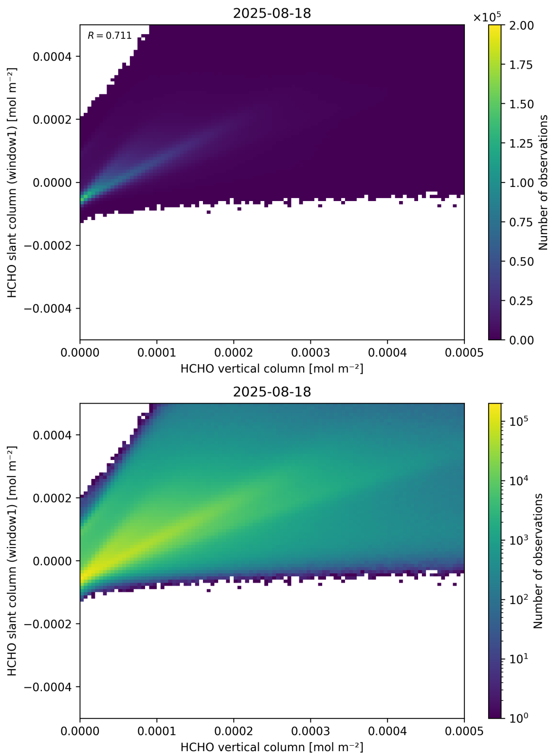
Figure 129: Scatter density plot of “HCHO vertical column” against “HCHO slant column (window1)” for 2025-08-17 to 2025-08-19.
