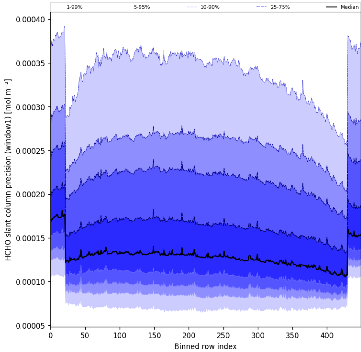
Figure 53: Along track statistics of “HCHO slant column precision (window1)” for 2025-08-17 to 2025-08-19
