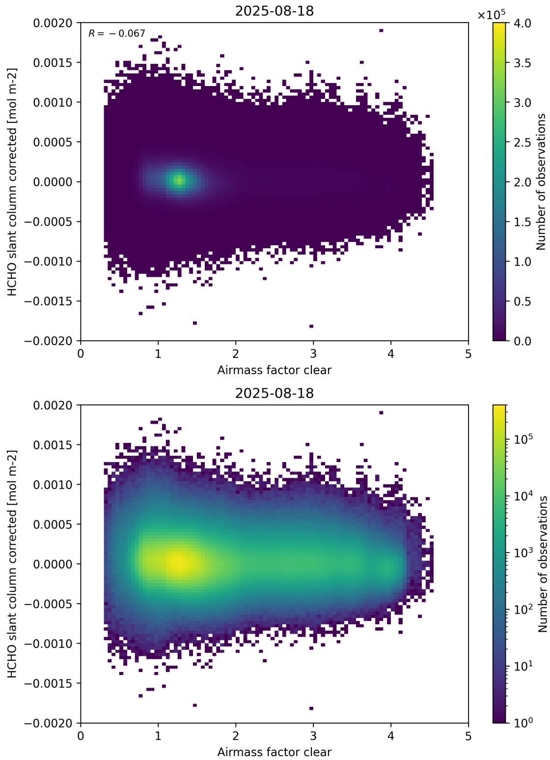
Figure 74: Scatter density plot of “Airmass factor clear” against “HCHO slant column corrected” for 2025-08-17 to 2025-08-19.
