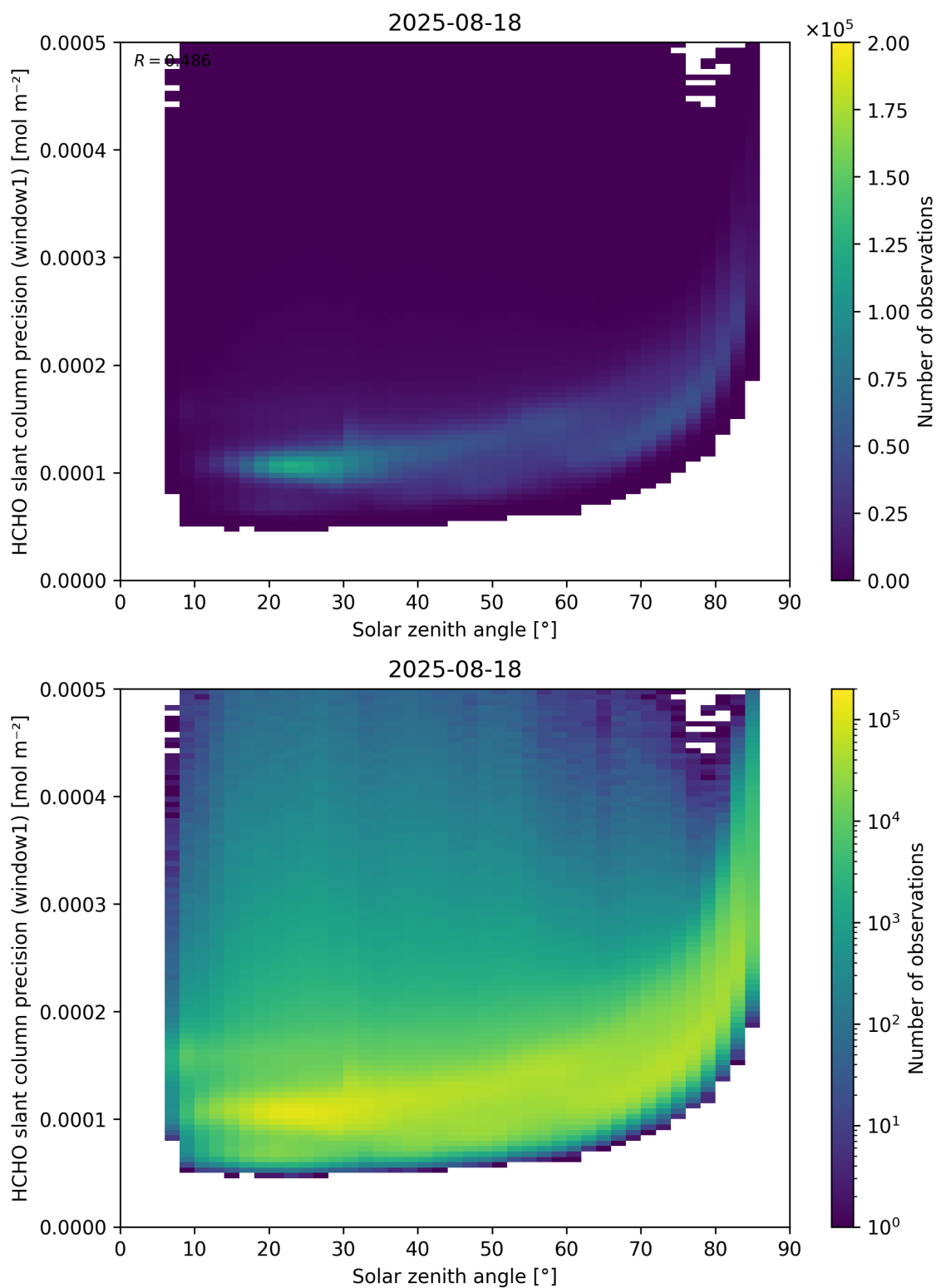
Figure 174: Scatter density plot of “Solar zenith angle” against “HCHO slant column precision (window1)” for 2025-08-17 to 2025-08-19.
