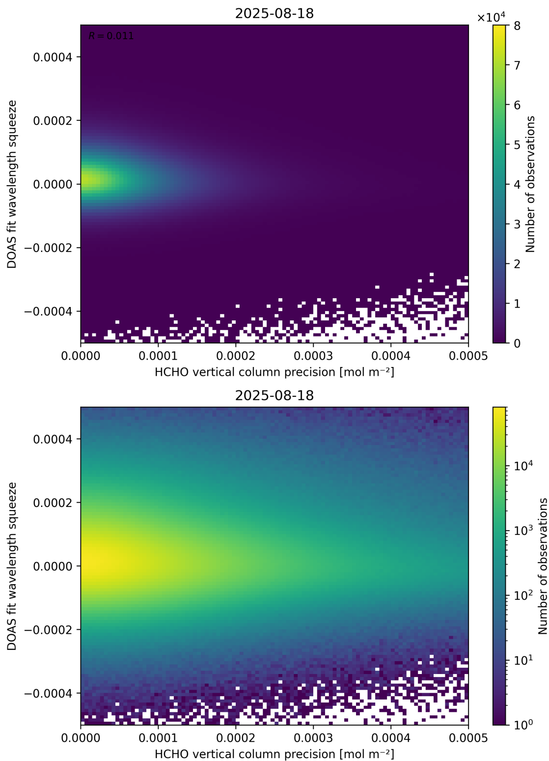
Figure 138: Scatter density plot of “HCHO vertical column precision” against “DOAS fit wavelength squeeze” for 2025-08-17 to 2025-08-19.
