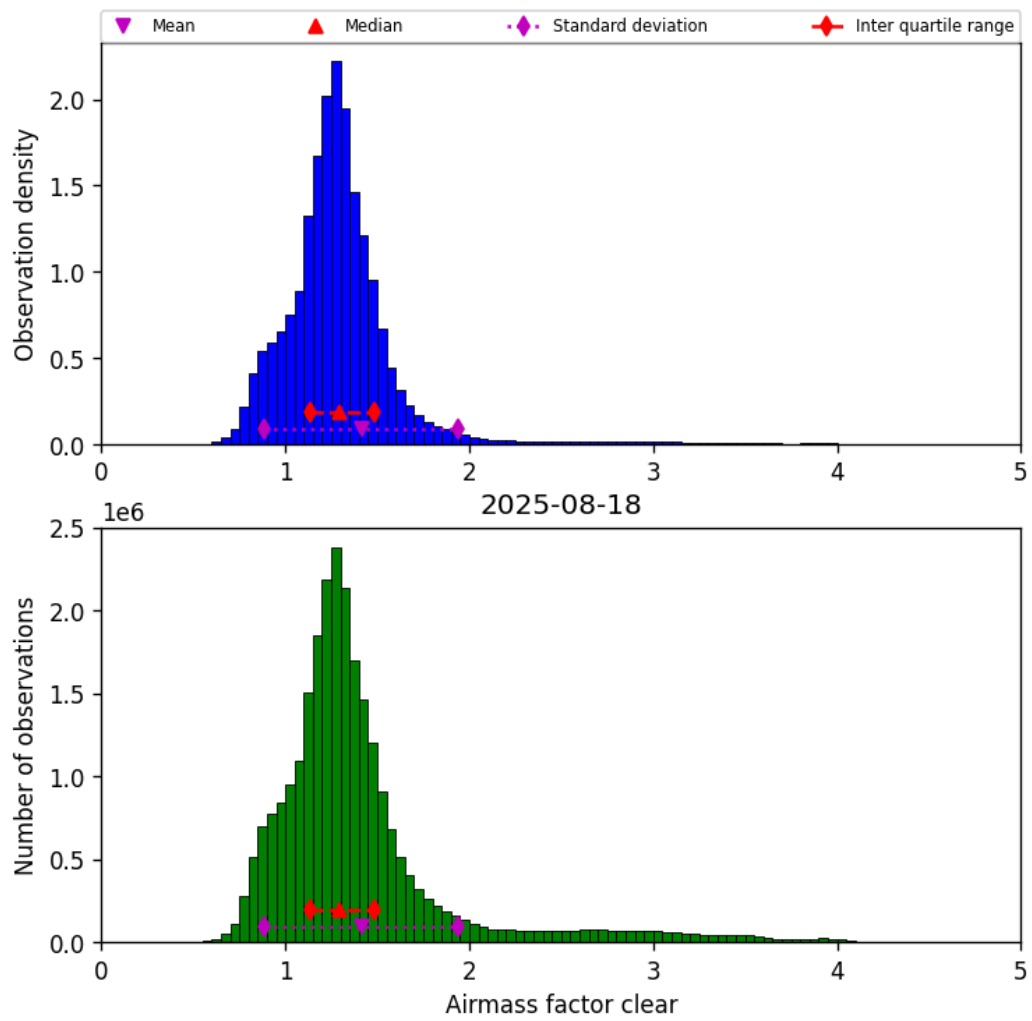
Figure 42: Histogram of “Airmass factor clear” for 2025-08-17 to 2025-08-19
