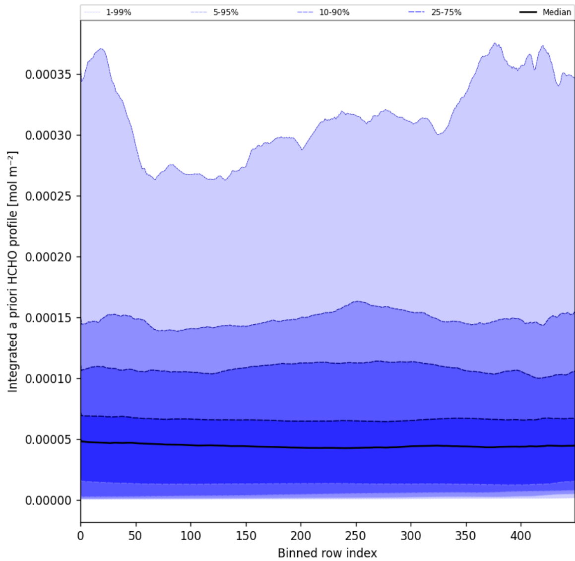
Figure 57: Along track statistics of “Integrated a priori HCHO profile” for 2025-08-17 to 2025-08-19
