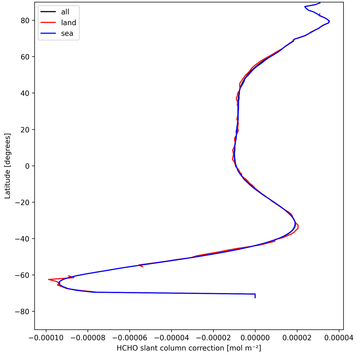
Figure 33: Zonal average of “HCHO slant column correction” for 2025-08-17 to 2025-08-19.
