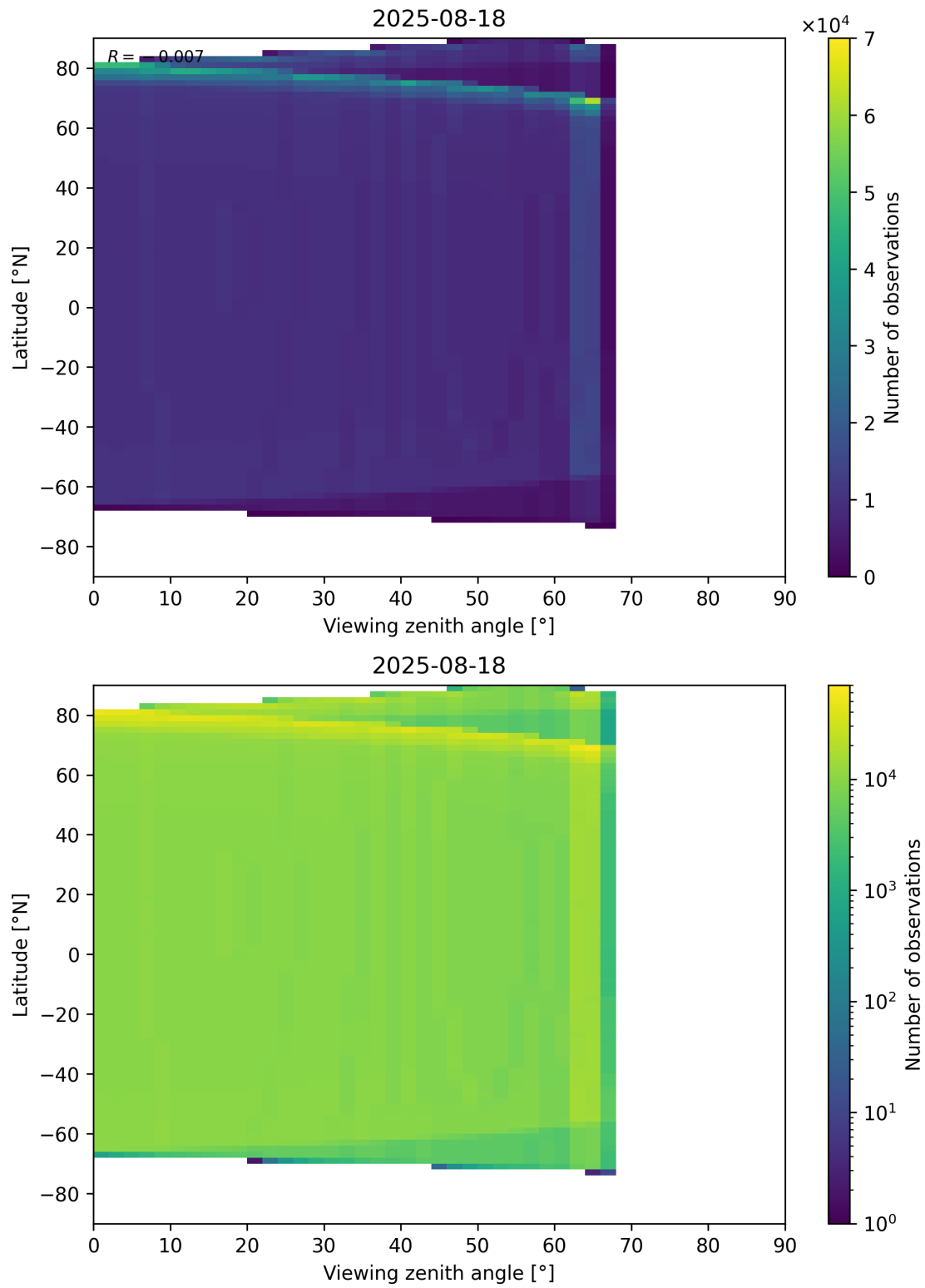
Figure 196: Scatter density plot of “Viewing zenith angle” against “Latitude” for 2025-08-17 to 2025-08-19.
