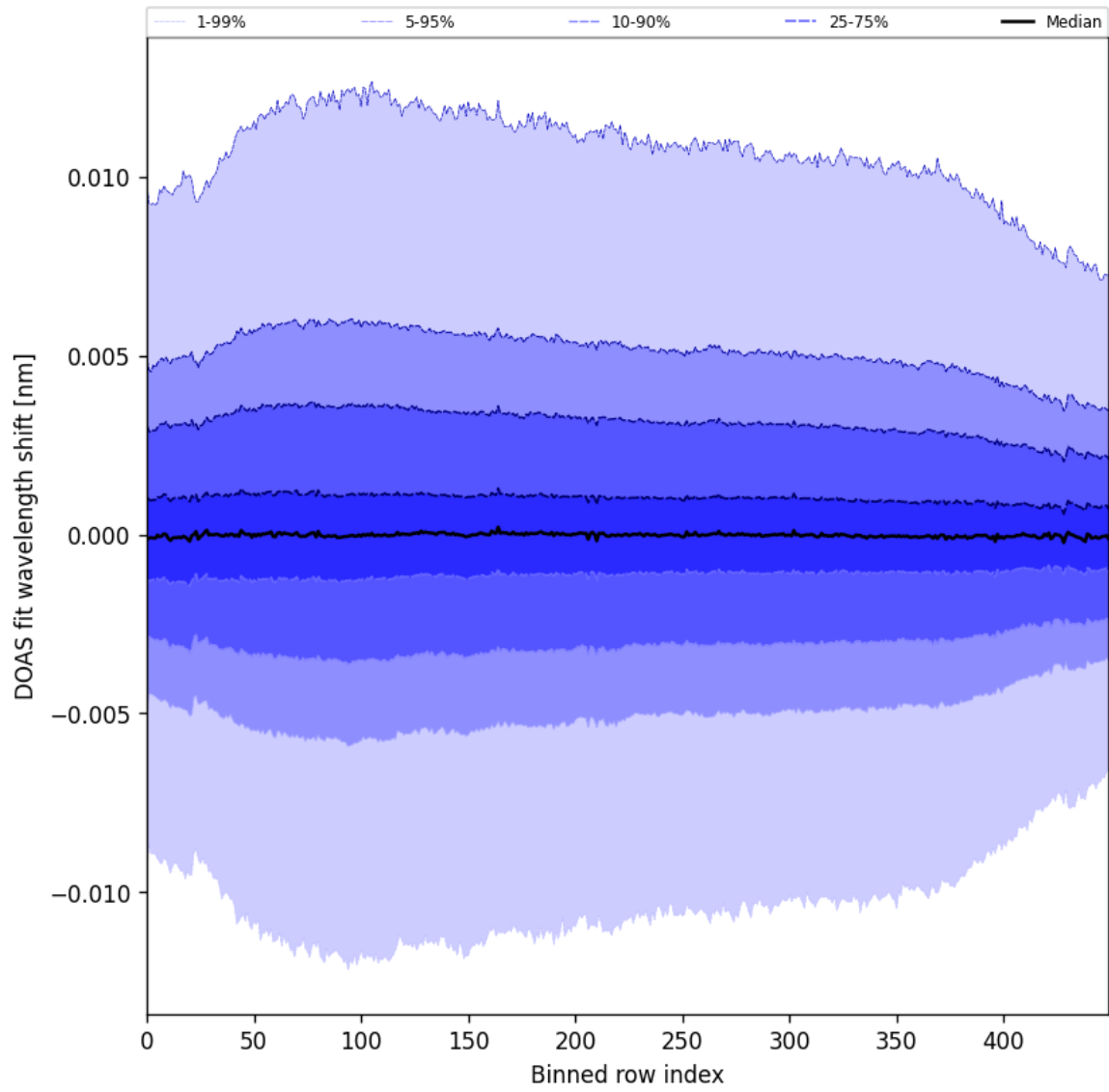
Figure 58: Along track statistics of “DOAS fit wavelength shift” for 2025-08-17 to 2025-08-19
