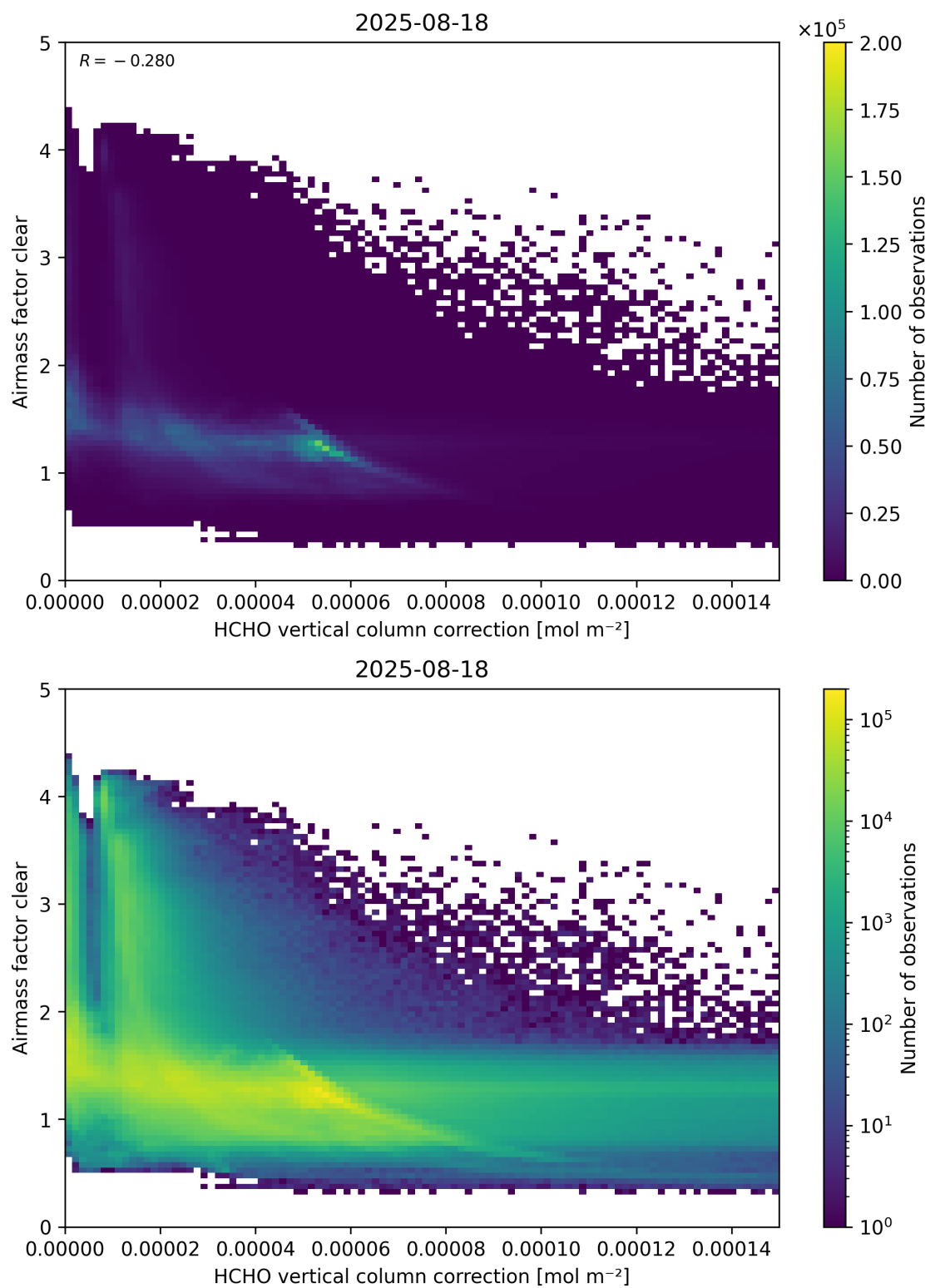
Figure 115: Scatter density plot of “HCHO vertical column correction” against “Airmass factor clear” for 2025-08-17 to 2025-08-19.
