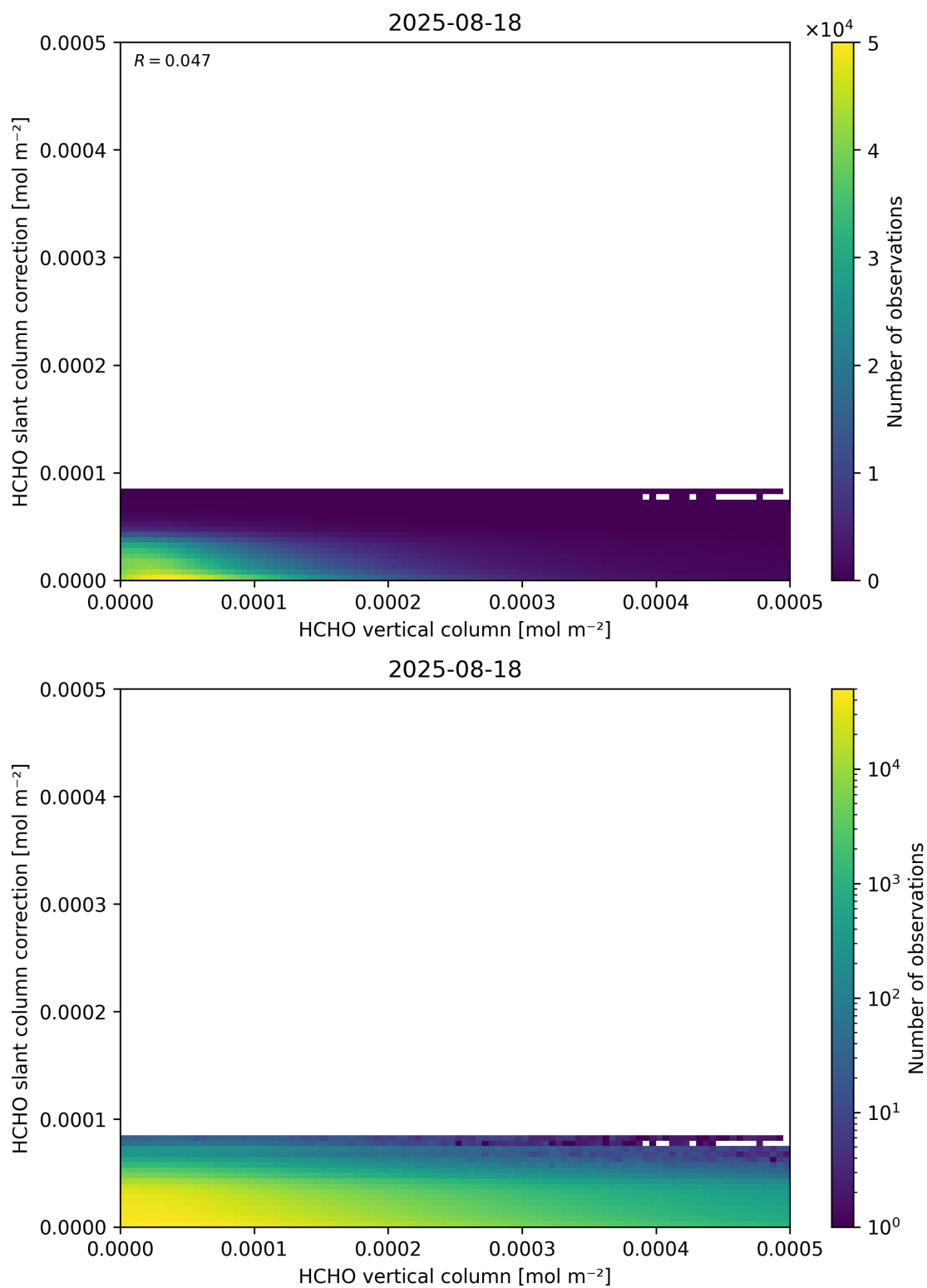
Figure 128: Scatter density plot of “HCHO vertical column” against “HCHO slant column correction” for 2025-08-17 to 2025-08-19.
