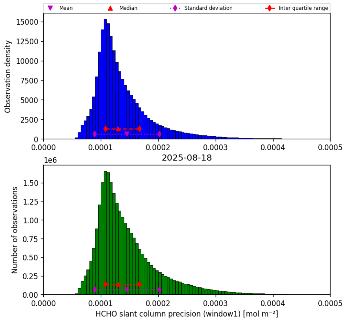
Figure 39: Histogram of “HCHO slant column precision (window1)” for 2025-08-17 to 2025-08-19
