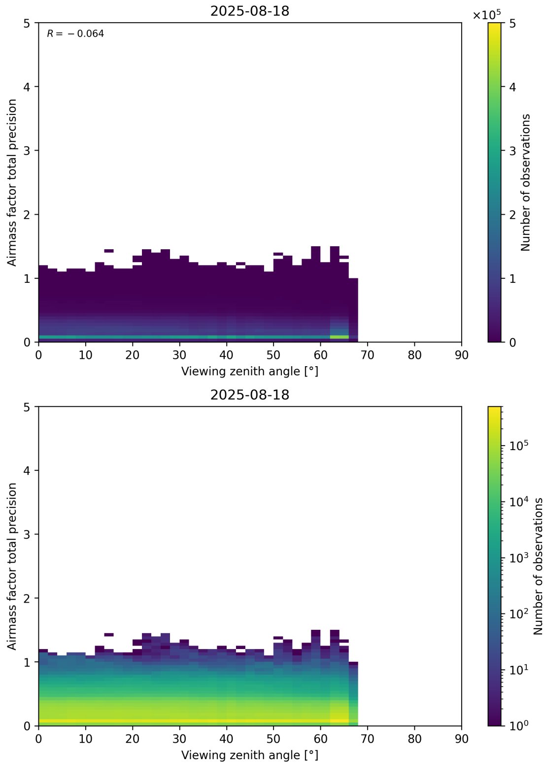
Figure 191: Scatter density plot of “Viewing zenith angle” against “Airmass factor total precision” for 2025-08-17 to 2025-08-19.
