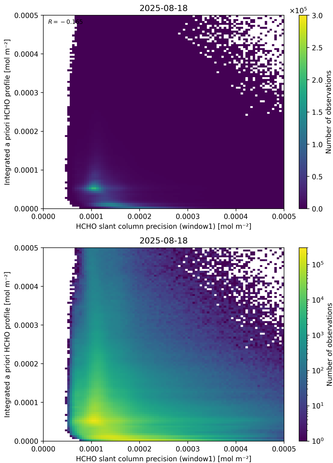
Figure 96: Scatter density plot of “HCHO slant column precision (window1)” against “Integrated a priori HCHO profile” for 2025-08-17 to 2025-08-19.
