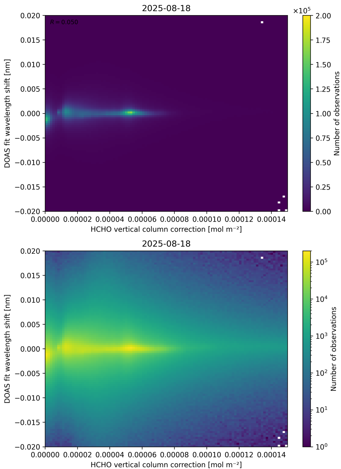
Figure 113: Scatter density plot of “HCHO vertical column correction” against “DOAS fit wavelength shift” for 2025-08-17 to 2025-08-19.
