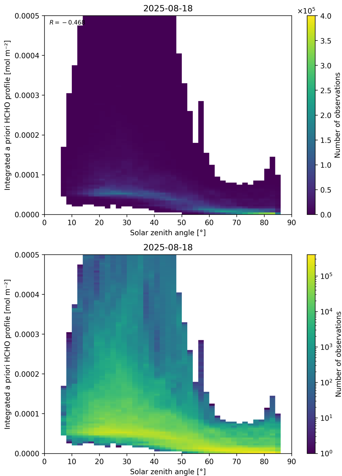
Figure 180: Scatter density plot of “Solar zenith angle” against “Integrated a priori HCHO profile” for 2025-08-17 to 2025-08-19.
