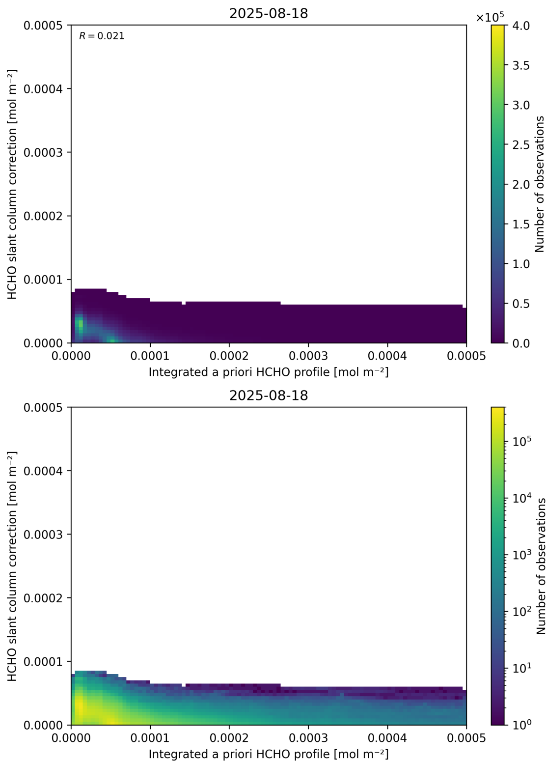
Figure 152: Scatter density plot of “Integrated a priori HCHO profile” against “HCHO slant column correction” for 2025-08-17 to 2025-08-19.
