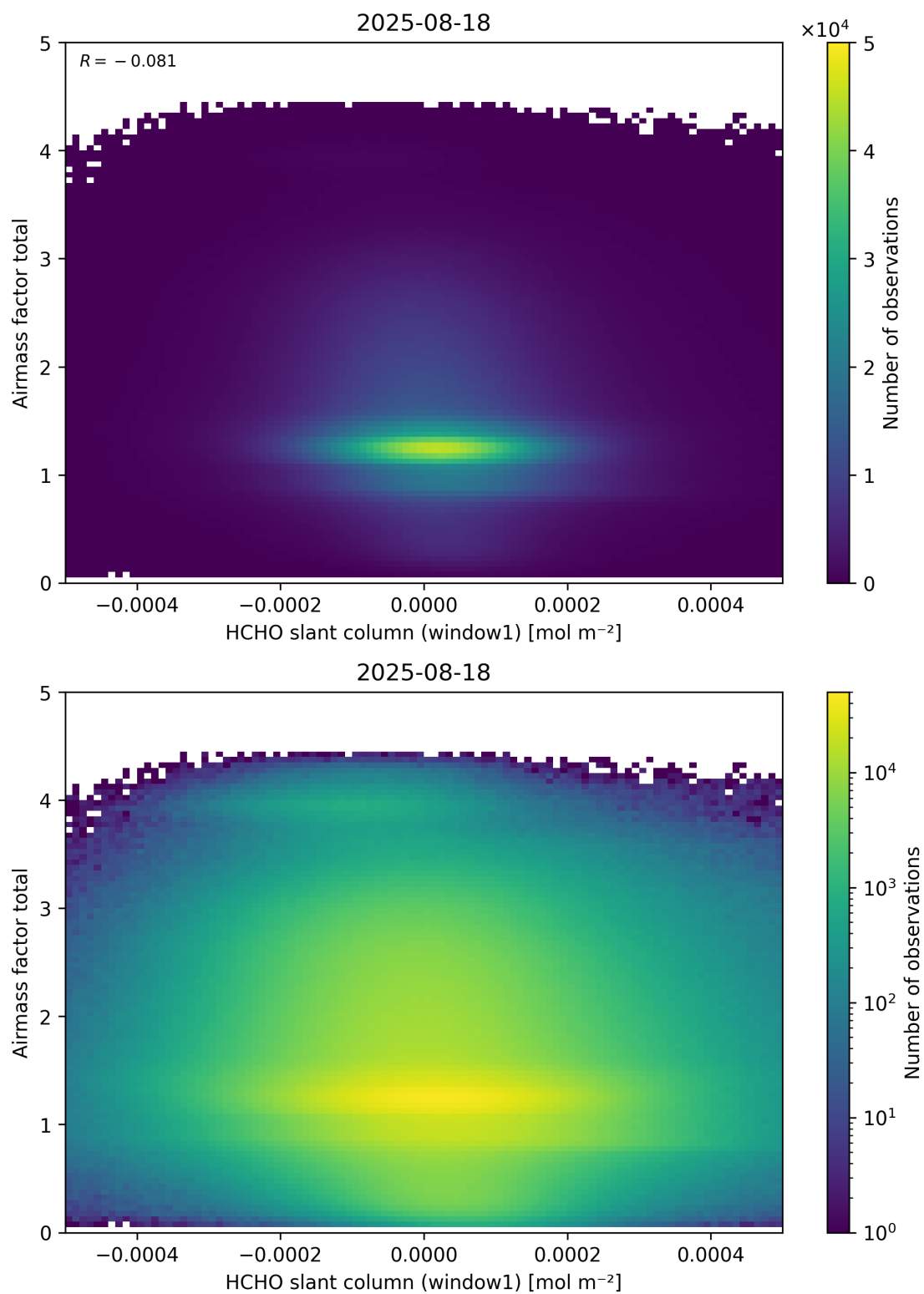
Figure 85: Scatter density plot of “HCHO slant column (window1)” against “Airmass factor total” for 2025-08-17 to 2025-08-19.
