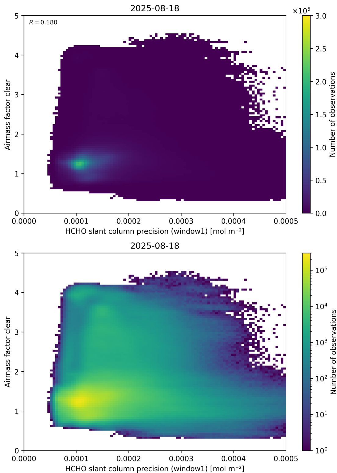
Figure 91: Scatter density plot of “HCHO slant column precision (window1)” against “Airmass factor clear” for 2025-08-17 to 2025-08-19.
