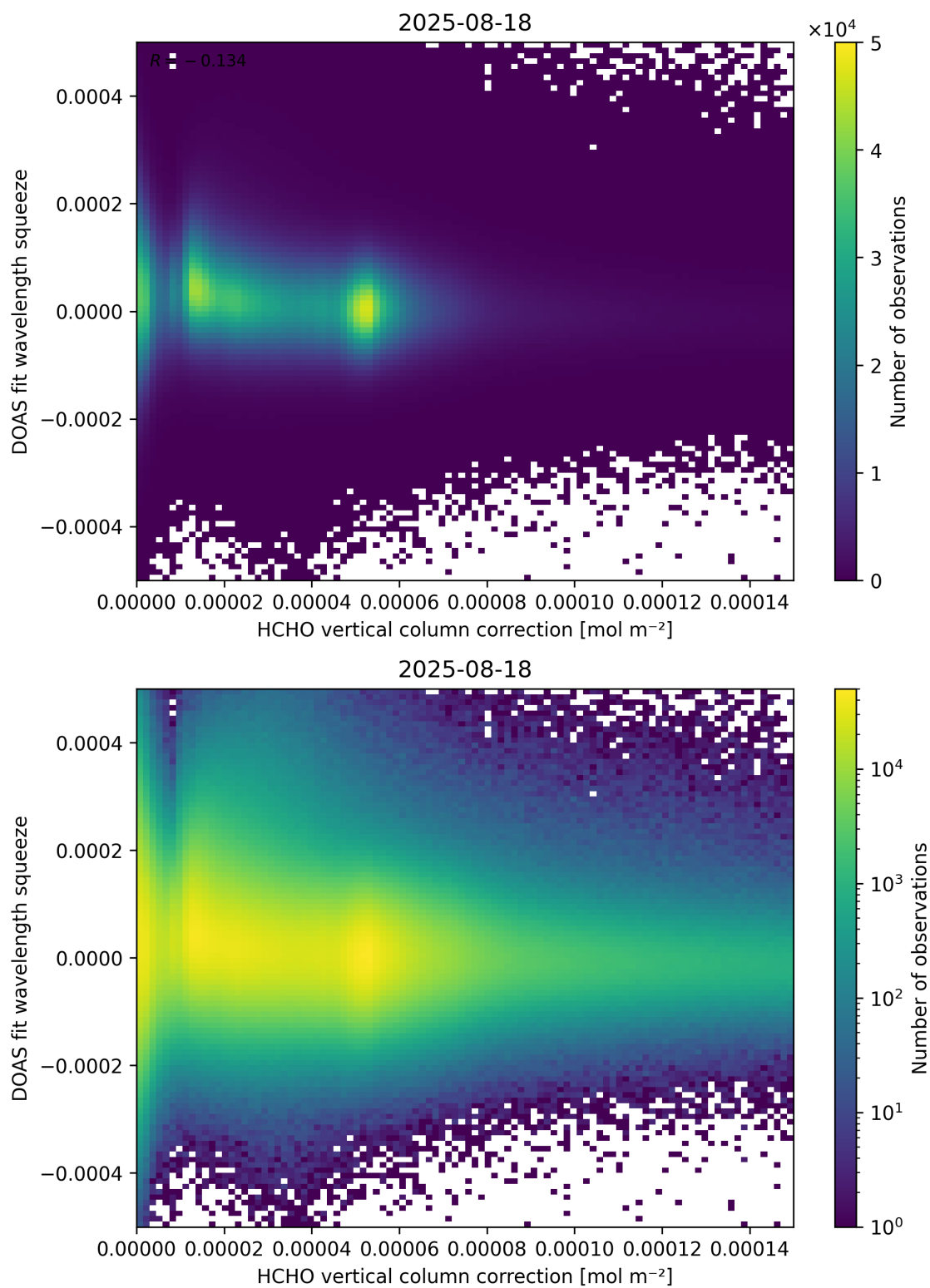
Figure 114: Scatter density plot of “HCHO vertical column correction” against “DOAS fit wavelength squeeze” for 2025-08-17 to 2025-08-19.
