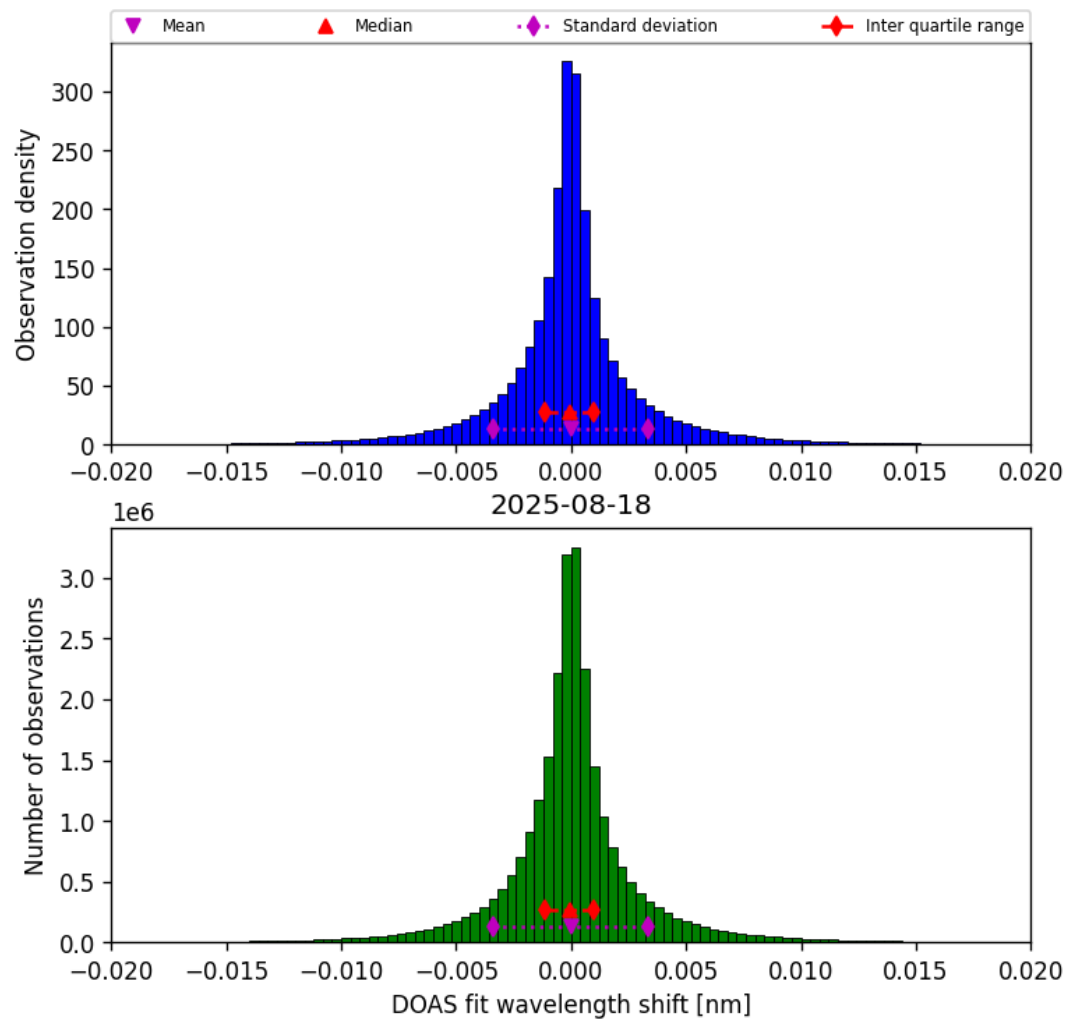
Figure 44: Histogram of “DOAS fit wavelength shift” for 2025-08-17 to 2025-08-19
