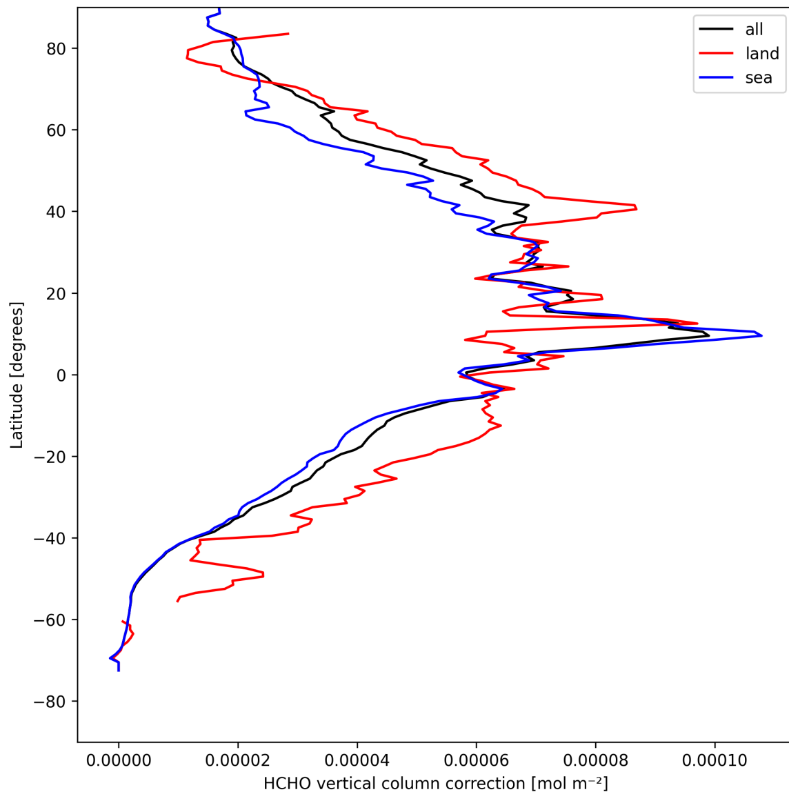
Figure 23: Zonal average of “HCHO vertical column correction” for 2025-08-17 to 2025-08-19.
