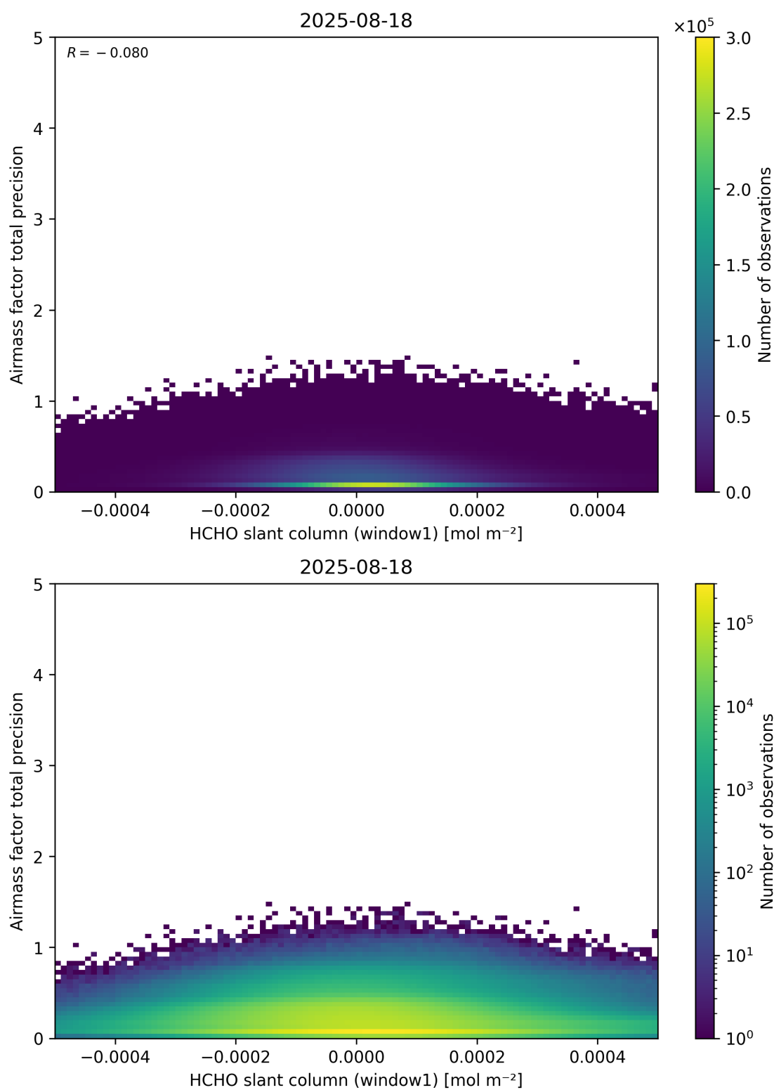
Figure 86: Scatter density plot of “HCHO slant column (window1)” against “Airmass factor total precision” for 2025-08-17 to 2025-08-19.
