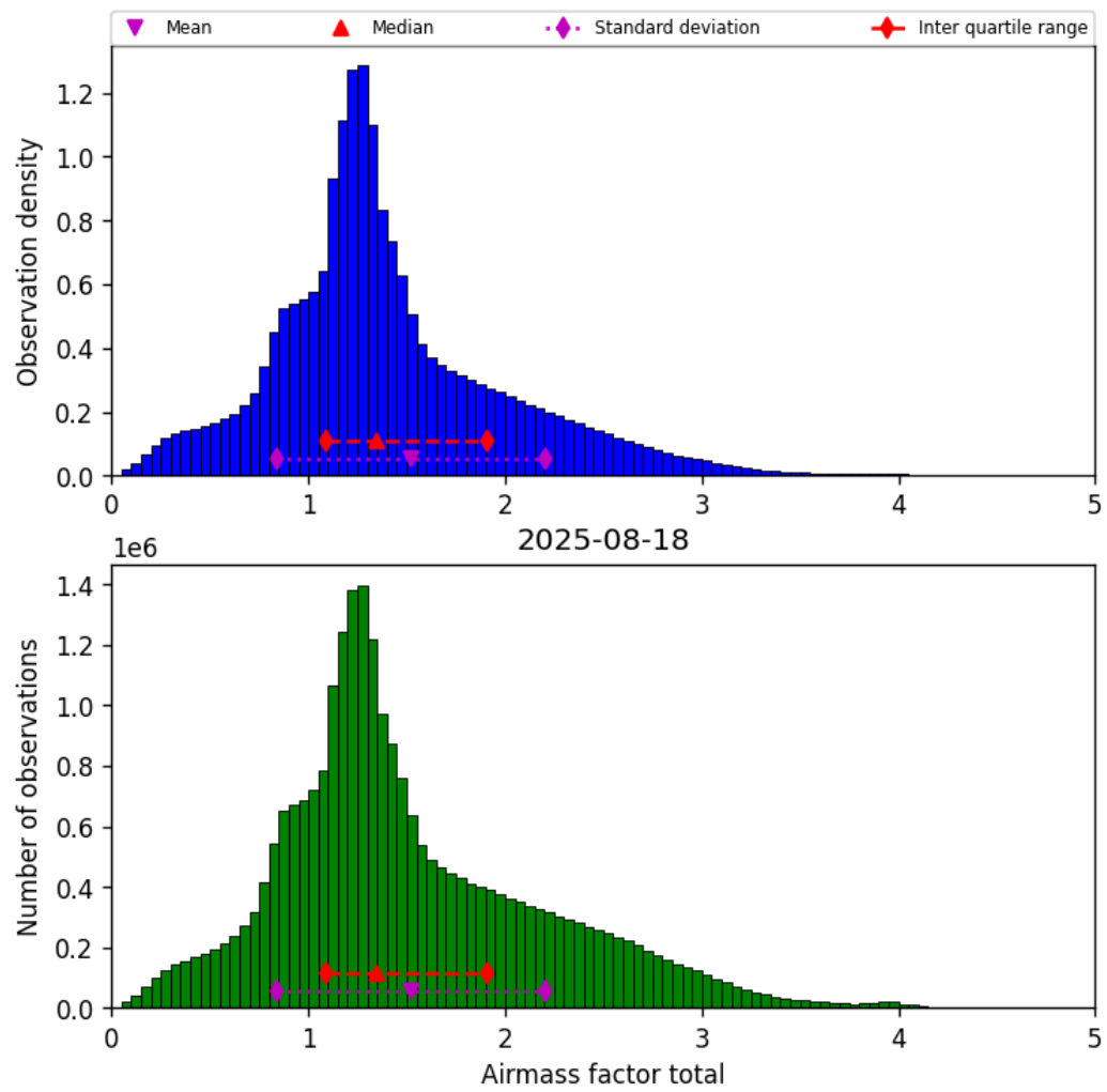
Figure 40: Histogram of “Airmass factor total” for 2025-08-17 to 2025-08-19
