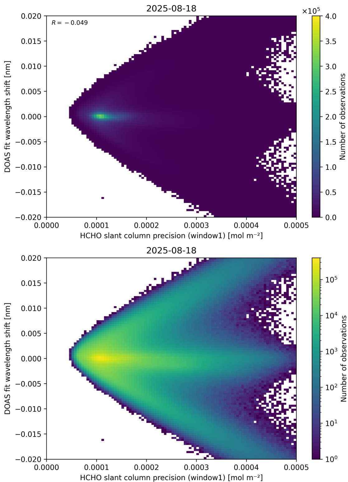
Figure 89: Scatter density plot of “HCHO slant column precision (window1)” against “DOAS fit wavelength shift” for 2025-08-17 to 2025-08-19.
