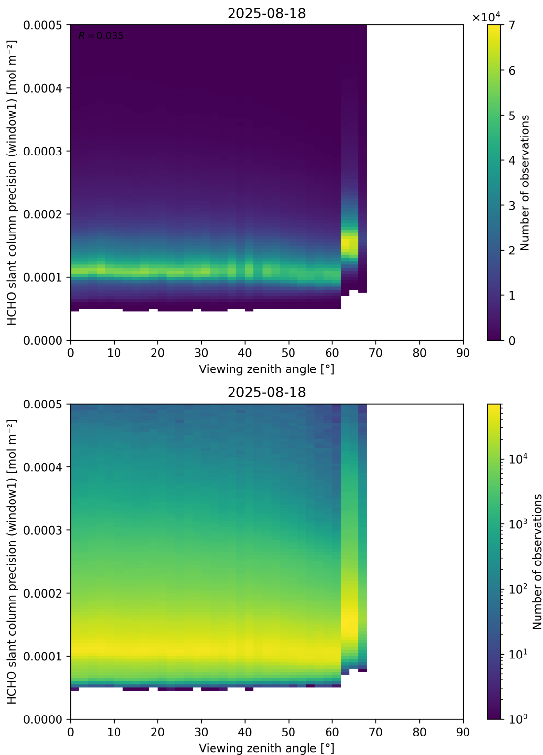
Figure 189: Scatter density plot of “Viewing zenith angle” against “HCHO slant column precision (window1)” for 2025-08-17 to 2025-08-19.
