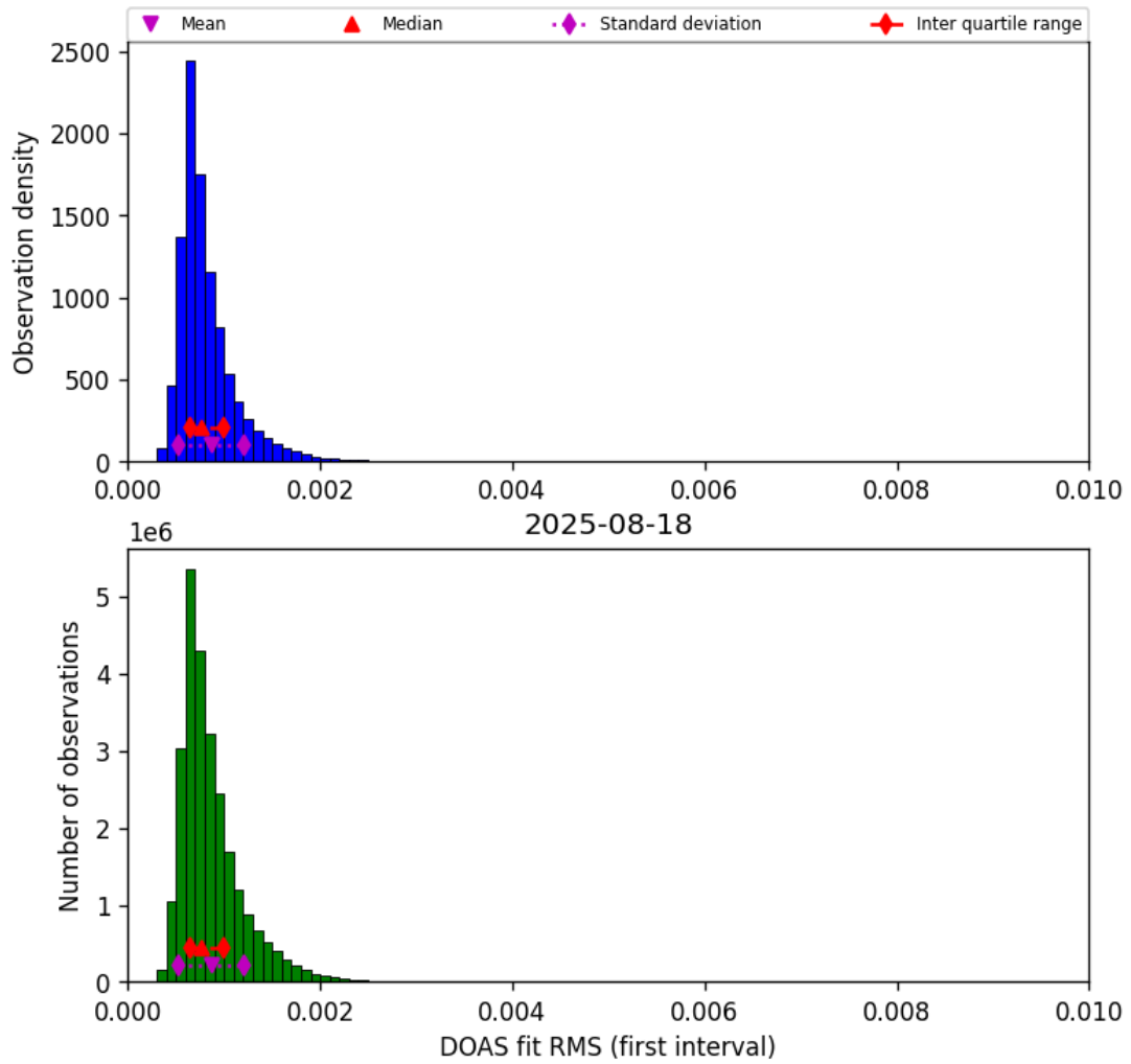
Figure 46: Histogram of “DOAS fit RMS (first interval)” for 2025-08-17 to 2025-08-19
