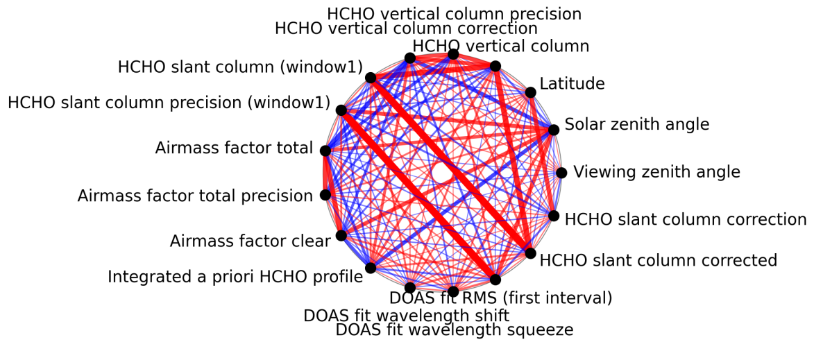
Figure 1: Map of correlation graph for 2025-08-17 to 2025-08-19.
