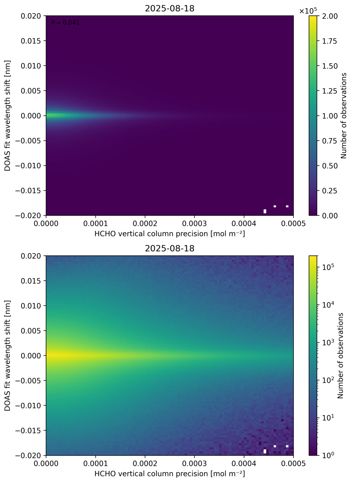
Figure 137: Scatter density plot of “HCHO vertical column precision” against “DOAS fit wavelength shift” for 2025-08-17 to 2025-08-19.
