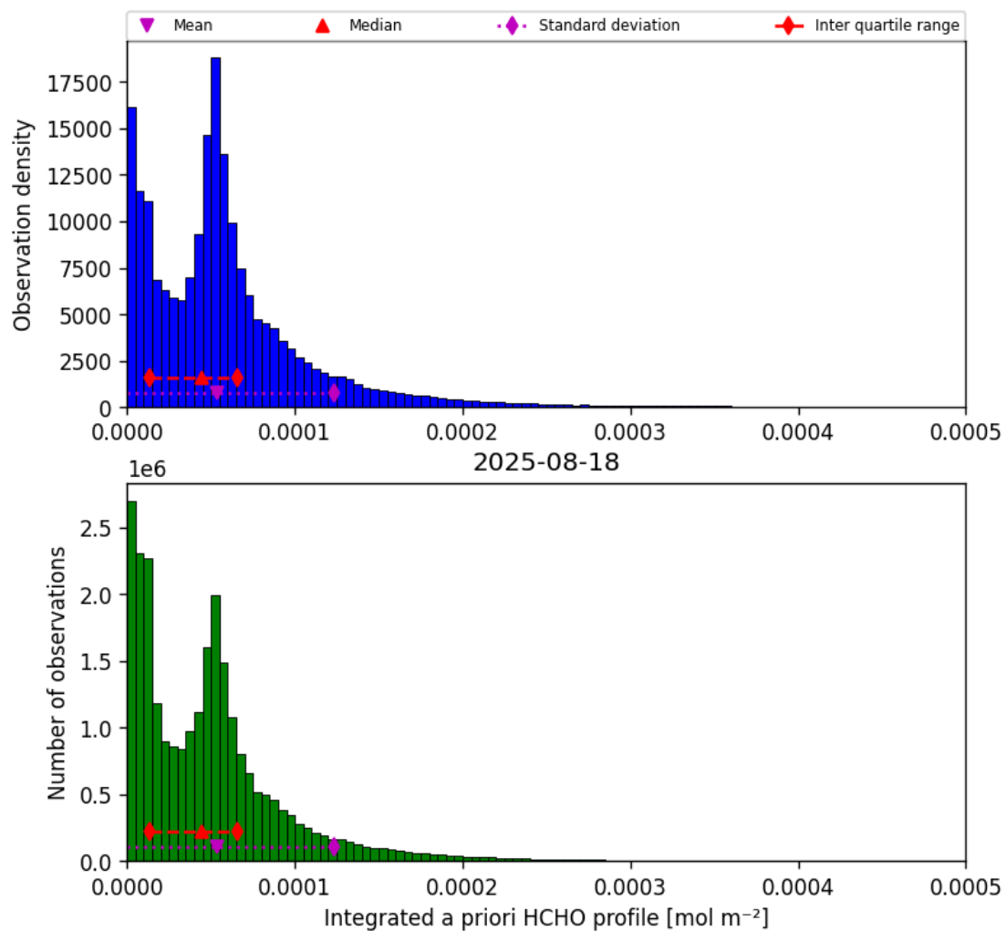
Figure 43: Histogram of “Integrated a priori HCHO profile” for 2025-08-17 to 2025-08-19
