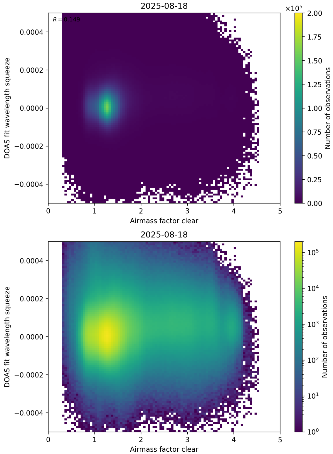
Figure 73: Scatter density plot of “Airmass factor clear” against “DOAS fit wavelength squeeze” for 2025-08-17 to 2025-08-19.
