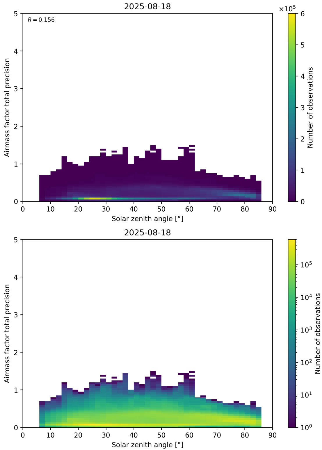
Figure 176: Scatter density plot of “Solar zenith angle” against “Airmass factor total precision” for 2025-08-17 to 2025-08-19.
