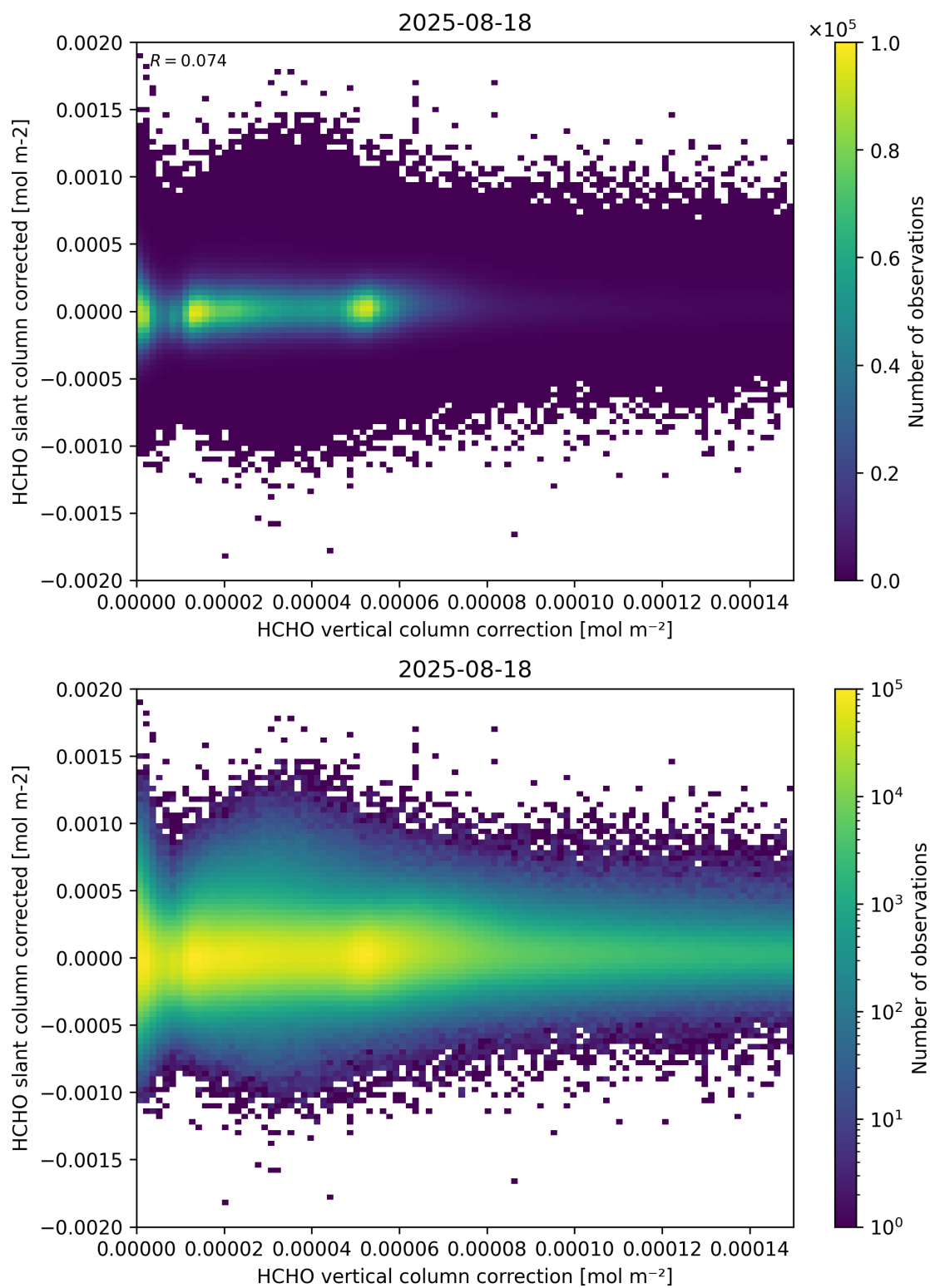
Figure 116: Scatter density plot of “HCHO vertical column correction” against “HCHO slant column corrected” for 2025-08-17 to 2025-08-19.
