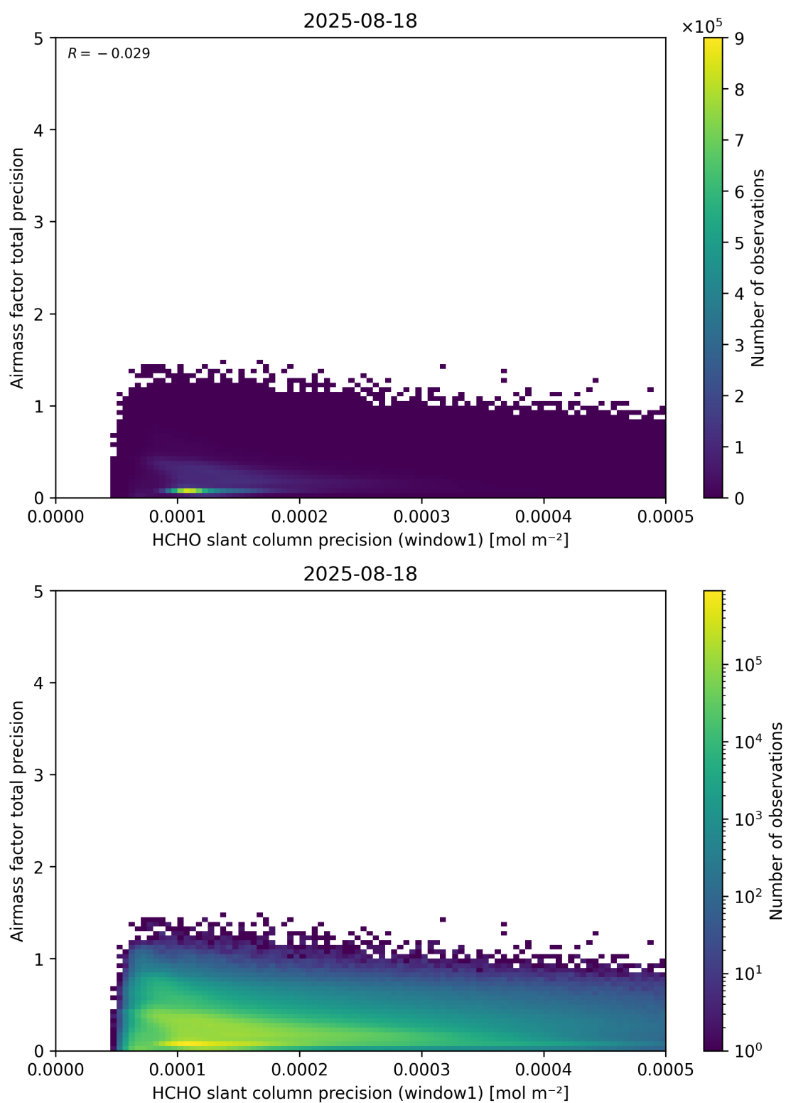
Figure 95: Scatter density plot of “HCHO slant column precision (window1)” against “Airmass factor total precision” for 2025-08-17 to 2025-08-19.
