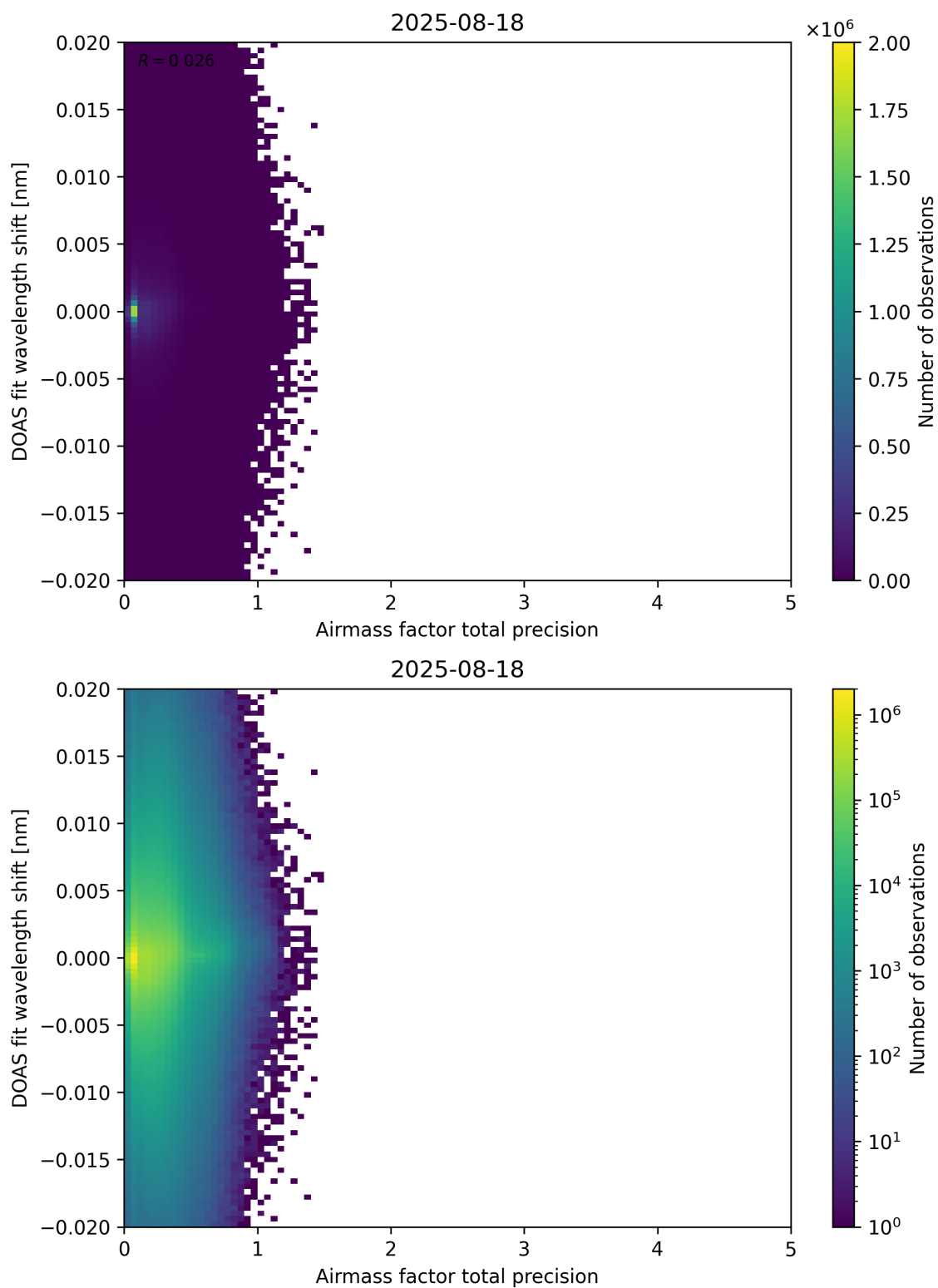
Figure 106: Scatter density plot of “Airmass factor total precision” against “DOAS fit wavelength shift” for 2025-08-17 to 2025-08-19.
