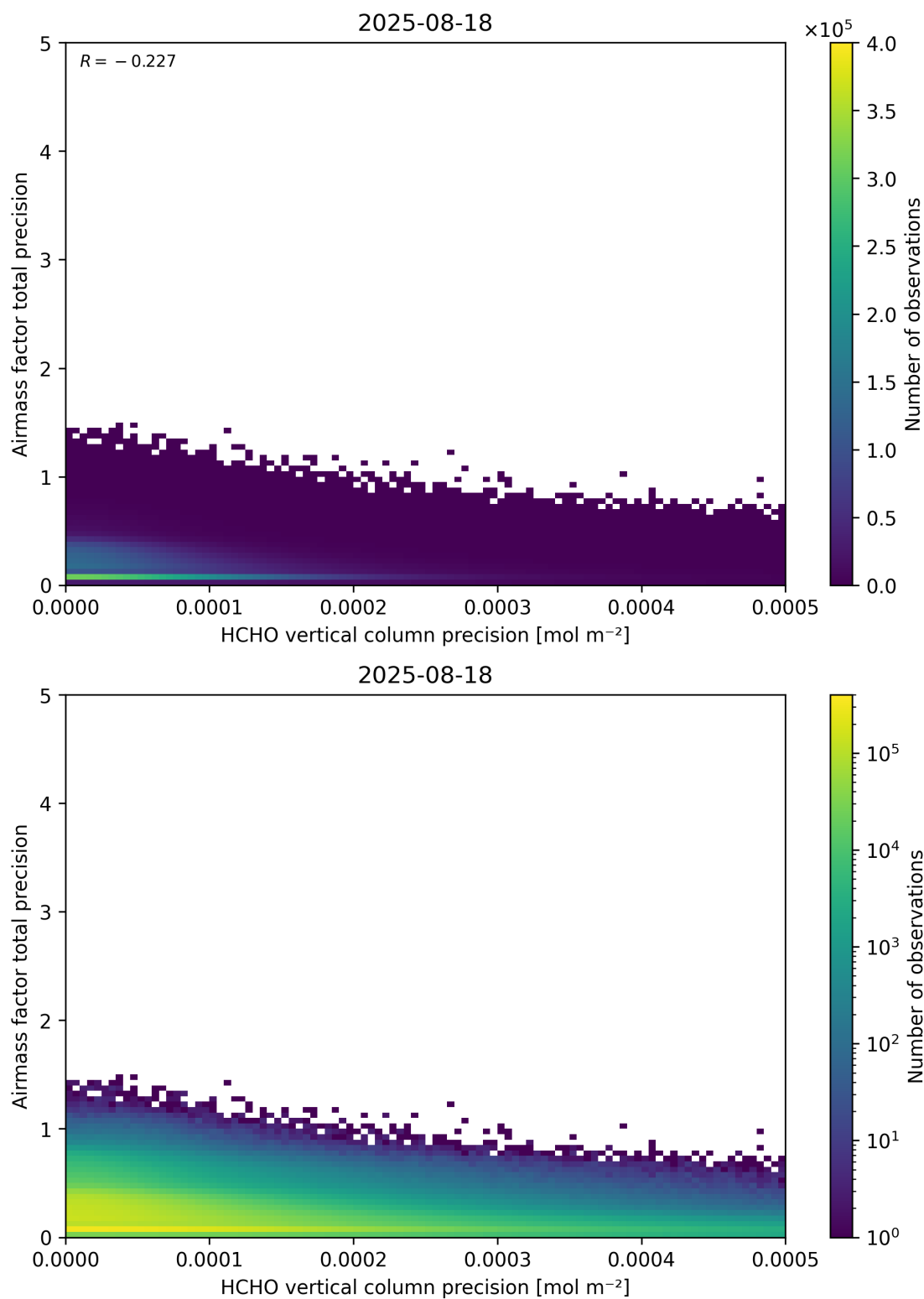
Figure 145: Scatter density plot of “HCHO vertical column precision” against “Airmass factor total precision” for 2025-08-17 to 2025-08-19.
