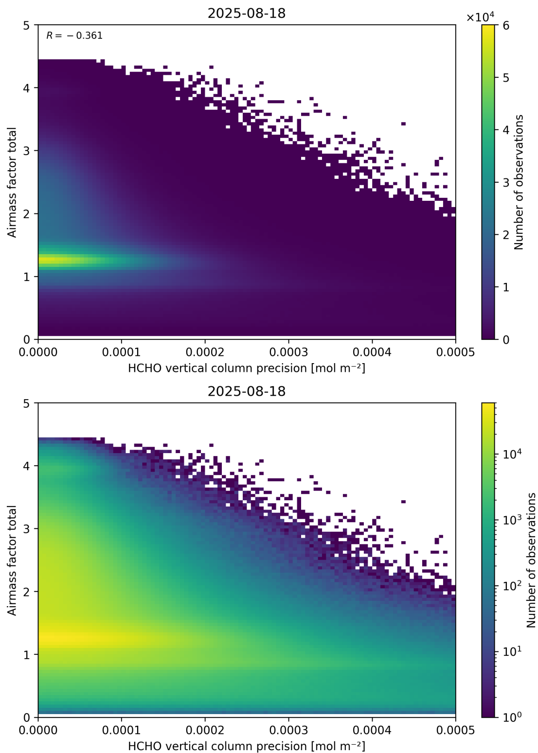
Figure 144: Scatter density plot of “HCHO vertical column precision” against “Airmass factor total” for 2025-08-17 to 2025-08-19.
