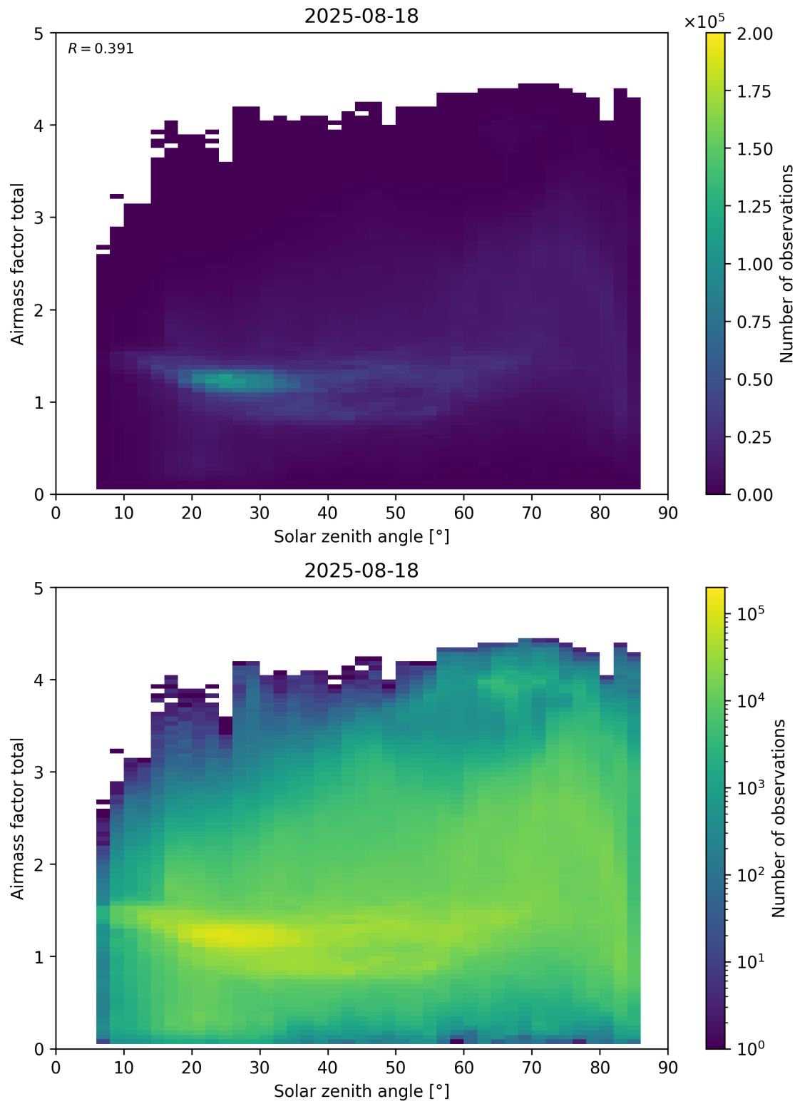
Figure 175: Scatter density plot of “Solar zenith angle” against “Airmass factor total” for 2025-08-17 to 2025-08-19.
