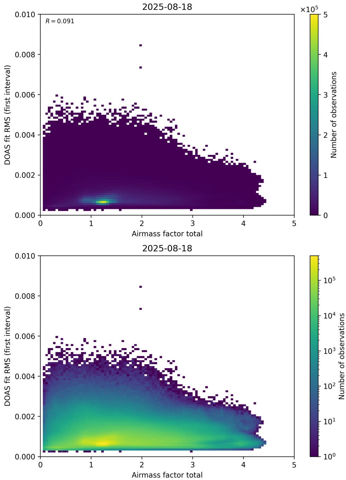
Figure 97: Scatter density plot of “Airmass factor total” against “DOAS fit RMS (first interval)” for 2025-08-17 to 2025-08-19.
