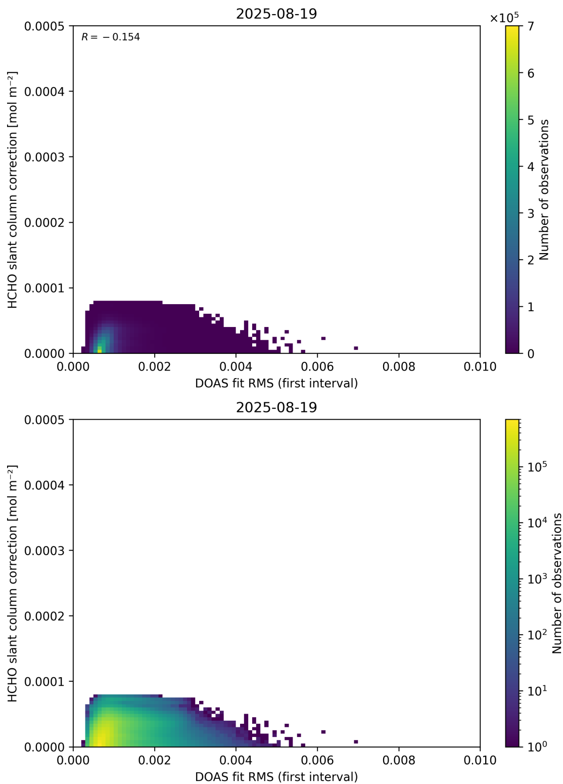
Figure 63: Scatter density plot of “DOAS fit RMS (first interval)” against “HCHO slant column correction” for 2025-08-19 to 2025-08-20.
