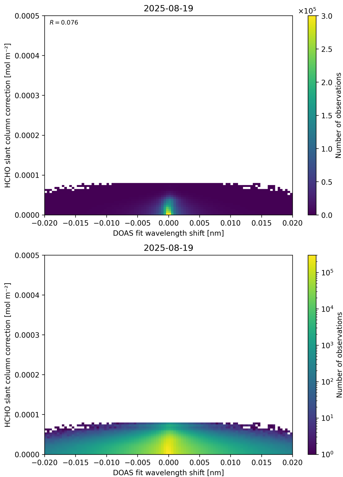
Figure 67: Scatter density plot of “DOAS fit wavelength shift” against “HCHO slant column correction” for 2025-08-19 to 2025-08-20.
