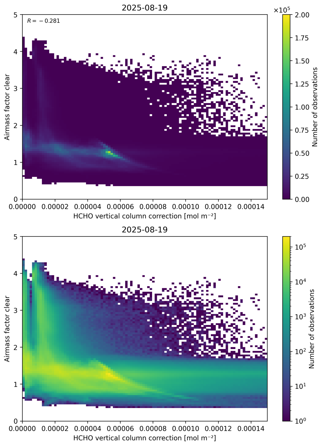
Figure 115: Scatter density plot of “HCHO vertical column correction” against “Airmass factor clear” for 2025-08-19 to 2025-08-20.
