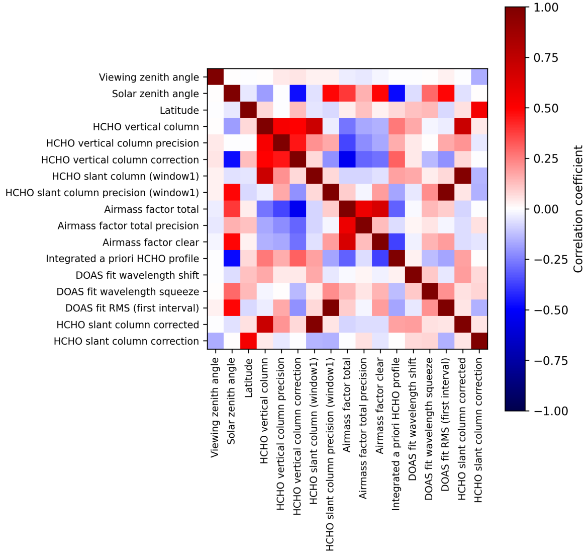
Figure 2: Map of correlation matrix for 2025-08-19 to 2025-08-20.
