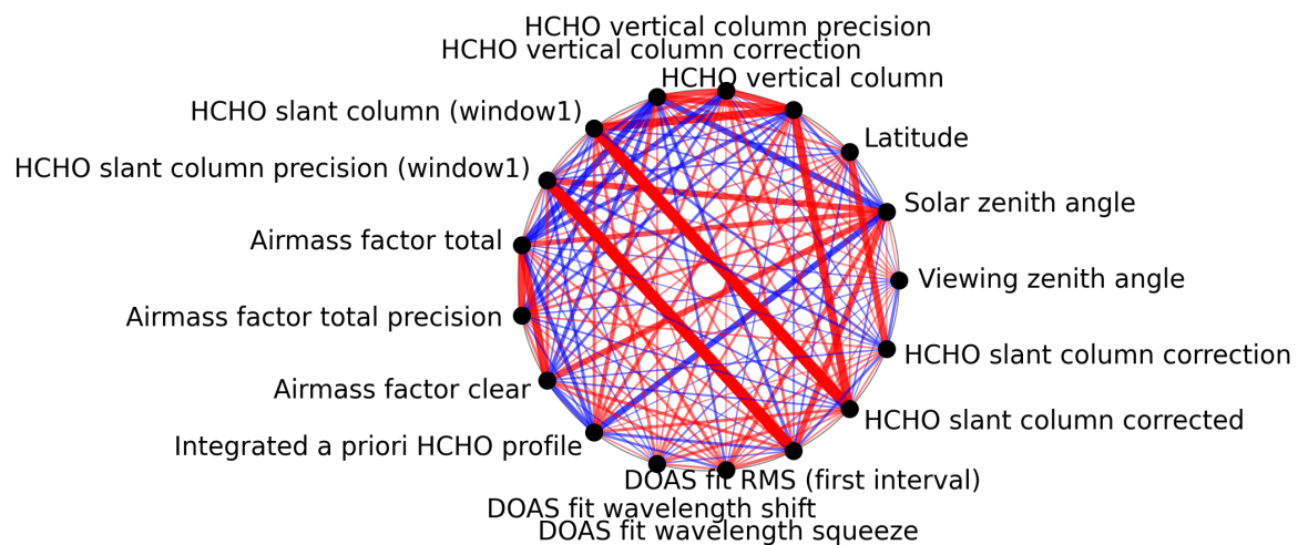
Figure 1: Map of correlation graph for 2025-08-19 to 2025-08-20.
