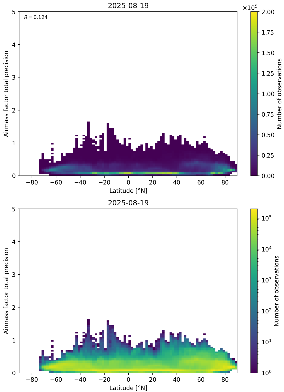
Figure 162: Scatter density plot of “Latitude” against “Airmass factor total precision” for 2025-08-19 to 2025-08-20.
