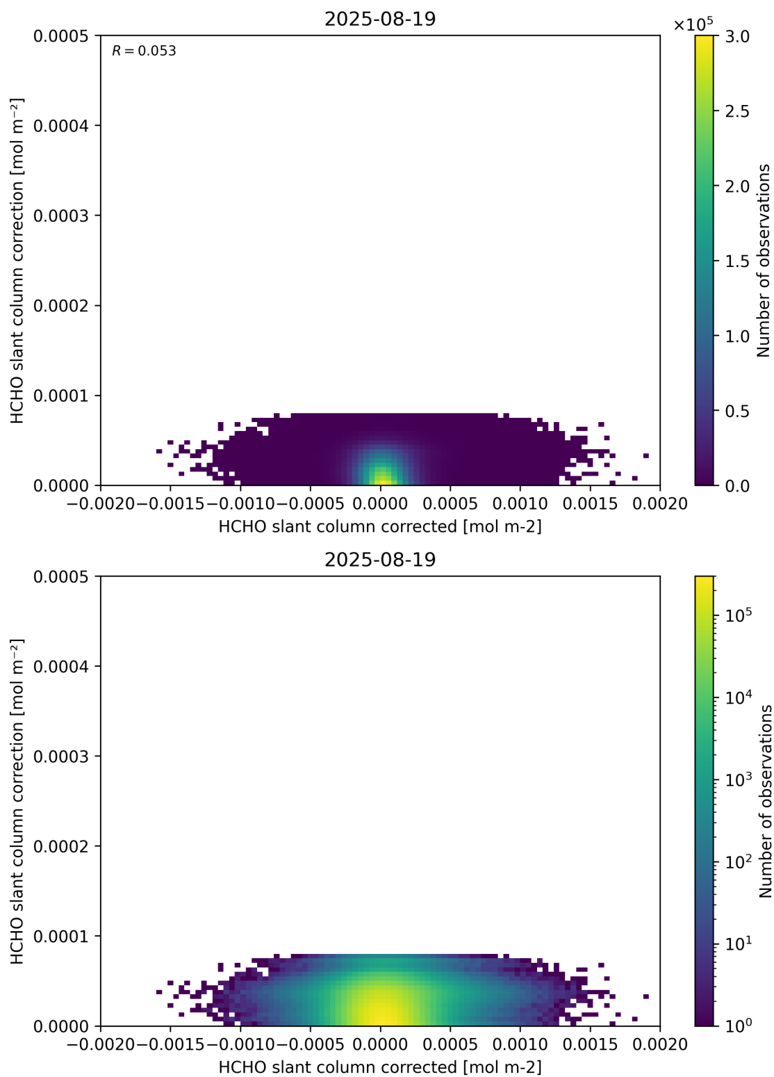
Figure 77: Scatter density plot of “HCHO slant column corrected” against “HCHO slant column correction” for 2025-08-19 to 2025-08-20.
