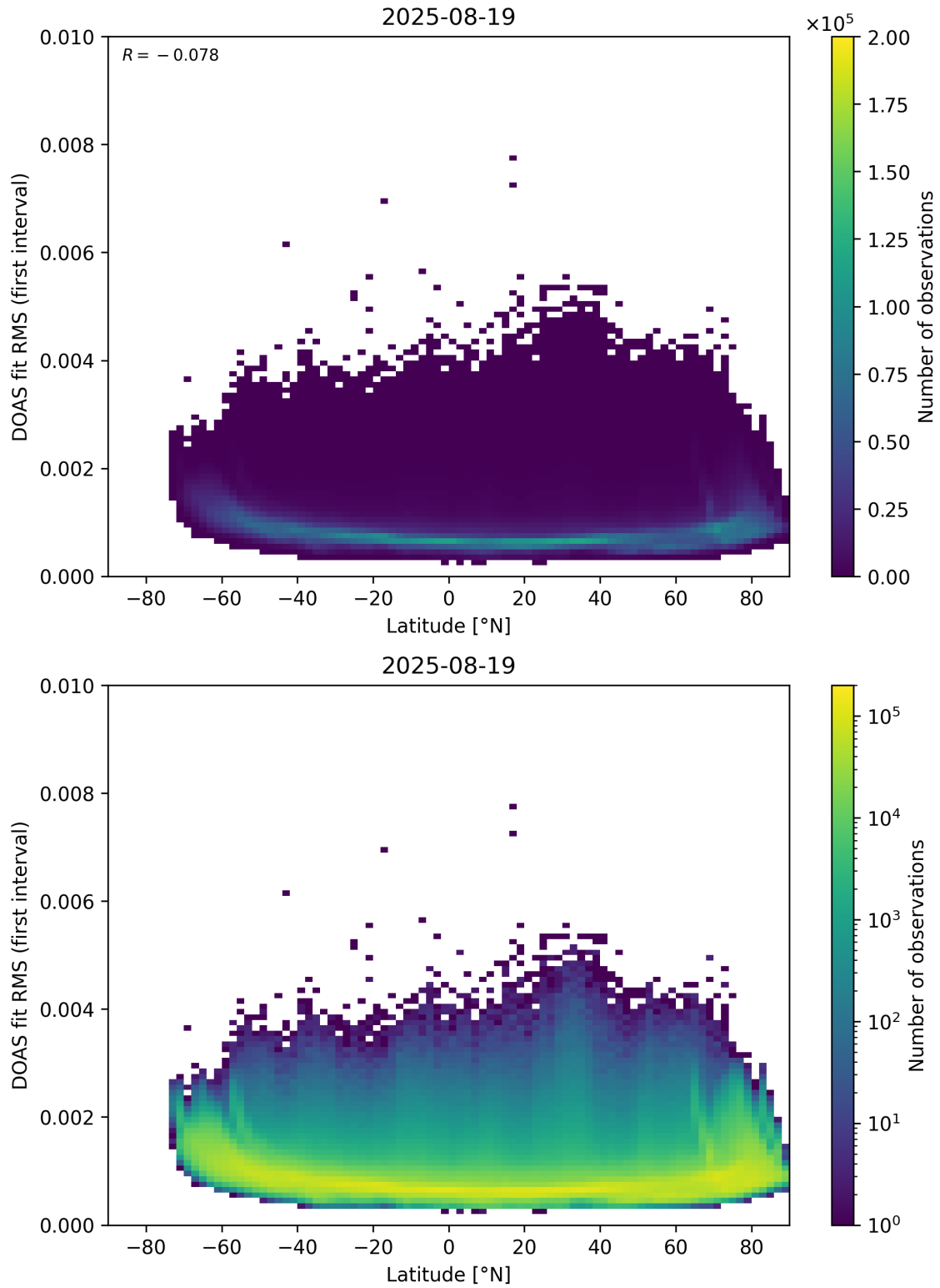
Figure 153: Scatter density plot of “Latitude” against “DOAS fit RMS (first interval)” for 2025-08-19 to 2025-08-20.
