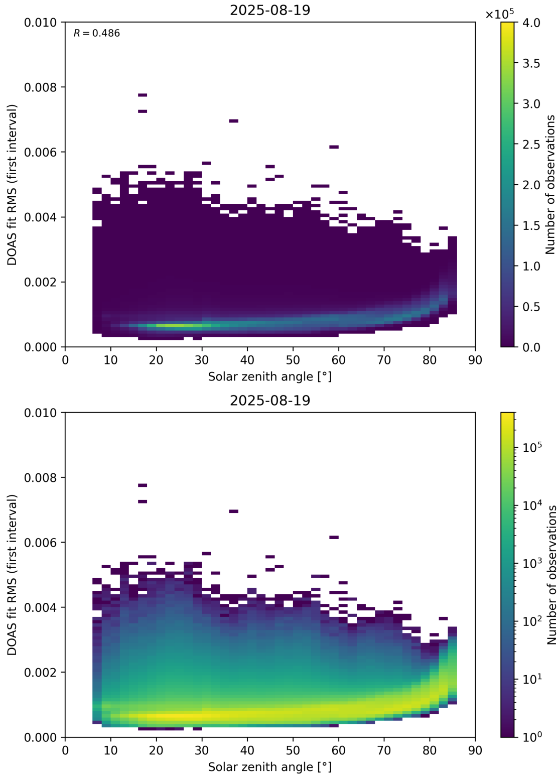
Figure 167: Scatter density plot of “Solar zenith angle” against “DOAS fit RMS (first interval)” for 2025-08-19 to 2025-08-20.
