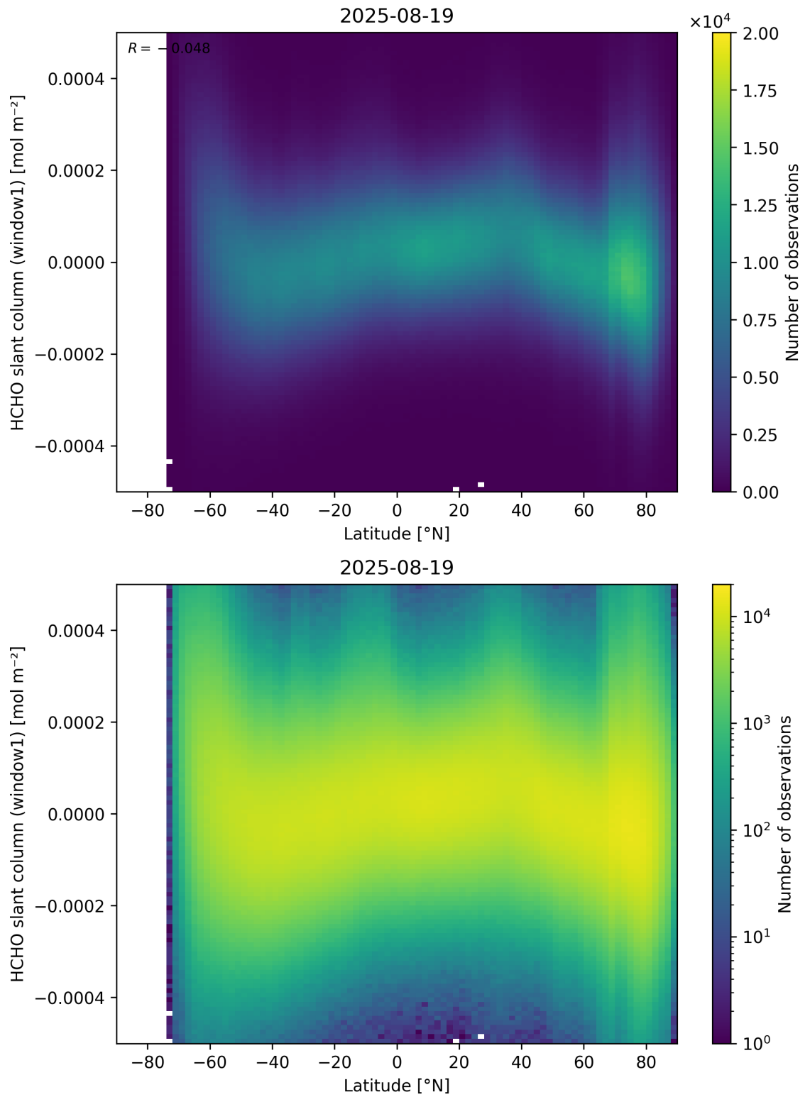
Figure 159: Scatter density plot of “Latitude” against “HCHO slant column (window1)” for 2025-08-19 to 2025-08-20.
