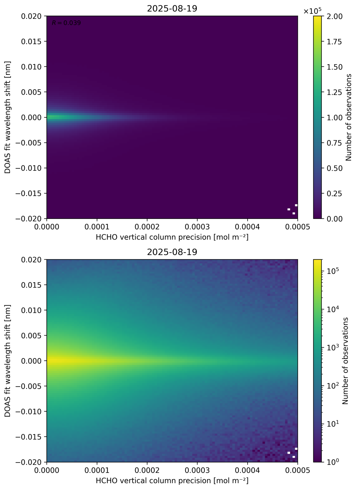
Figure 137: Scatter density plot of “HCHO vertical column precision” against “DOAS fit wavelength shift” for 2025-08-19 to 2025-08-20.
