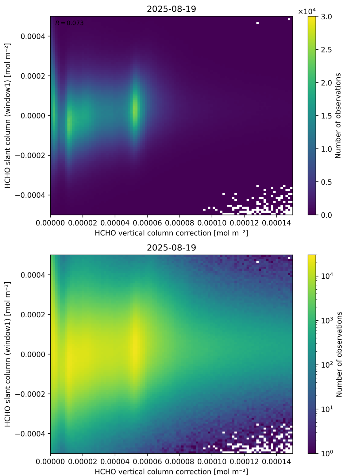
Figure 118: Scatter density plot of “HCHO vertical column correction” against “HCHO slant column (window1)” for 2025-08-19 to 2025-08-20.
