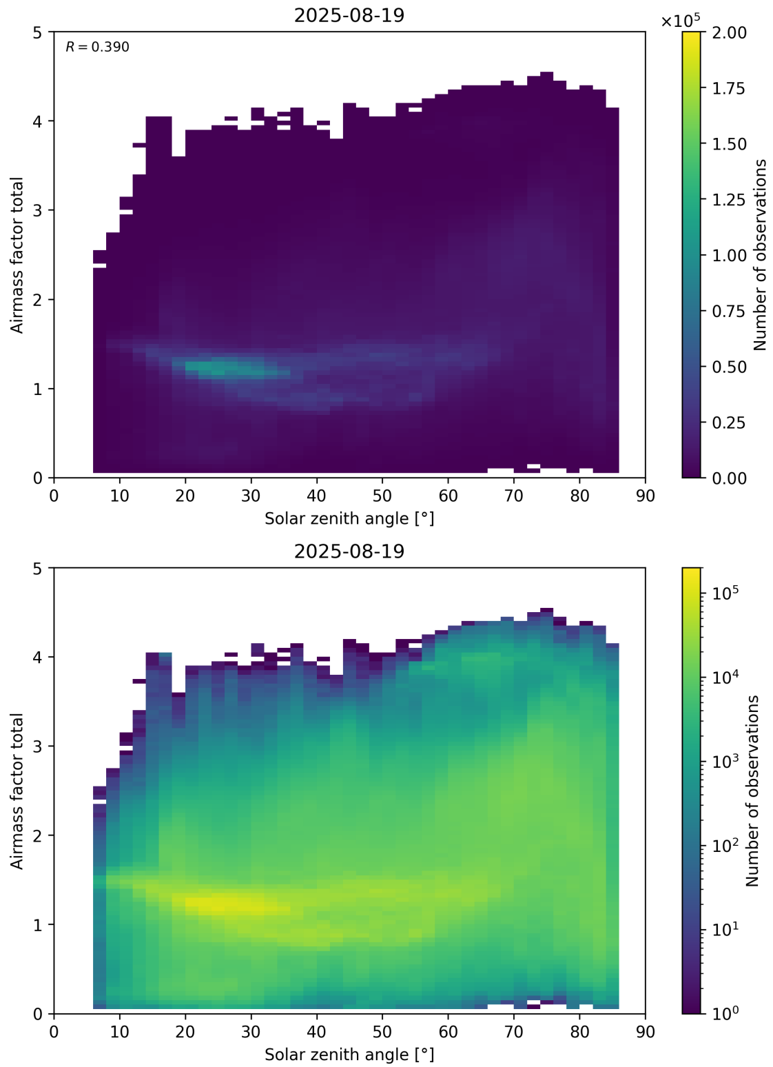
Figure 175: Scatter density plot of “Solar zenith angle” against “Airmass factor total” for 2025-08-19 to 2025-08-20.
