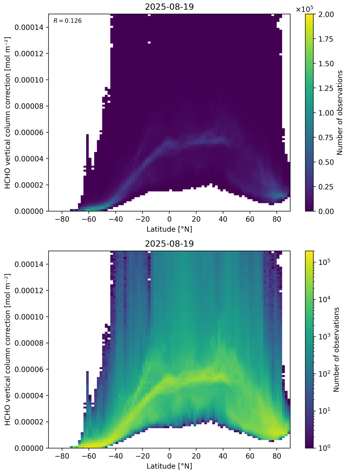
Figure 164: Scatter density plot of “Latitude” against “HCHO vertical column correction” for 2025-08-19 to 2025-08-20.
