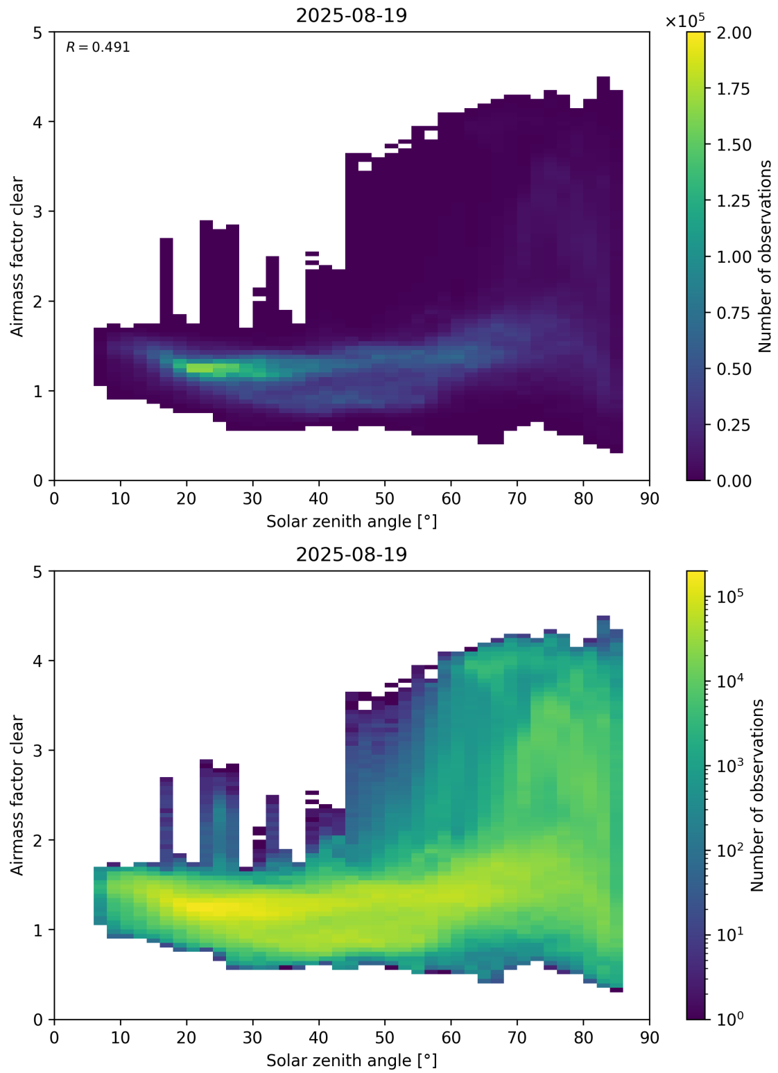
Figure 170: Scatter density plot of “Solar zenith angle” against “Airmass factor clear” for 2025-08-19 to 2025-08-20.
