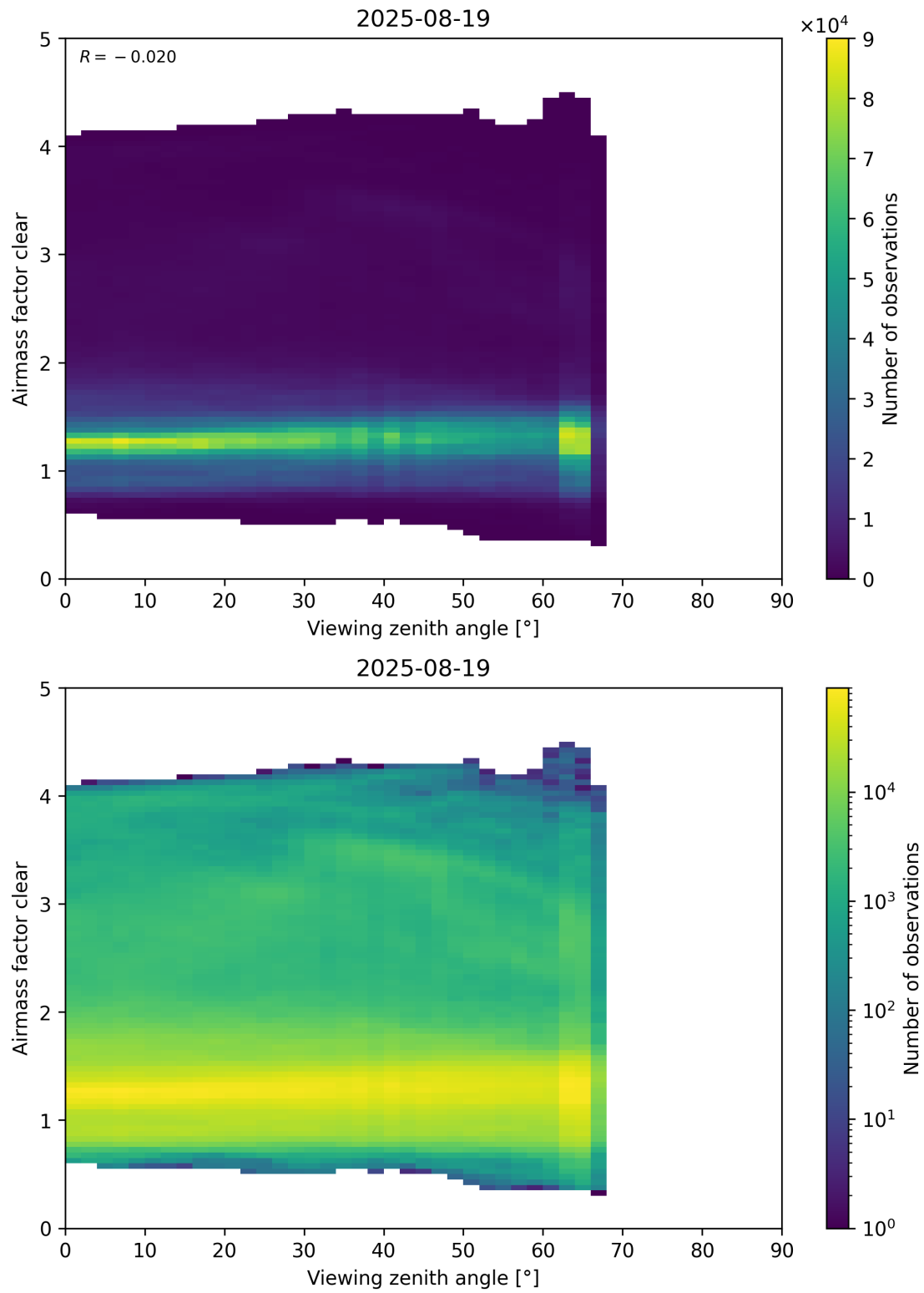
Figure 185: Scatter density plot of “Viewing zenith angle” against “Airmass factor clear” for 2025-08-19 to 2025-08-20.
