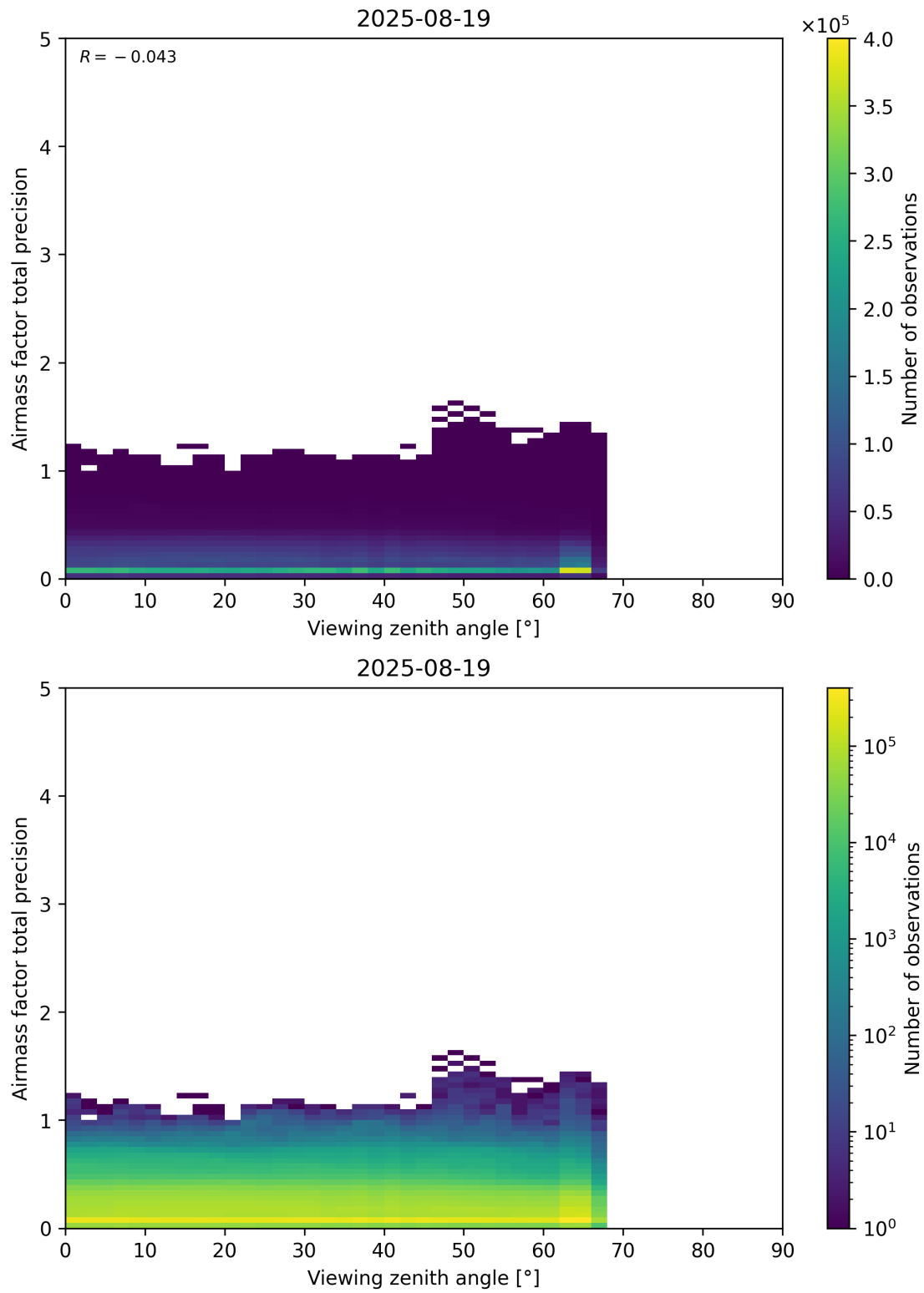
Figure 191: Scatter density plot of “Viewing zenith angle” against “Airmass factor total precision” for 2025-08-19 to 2025-08-20.
