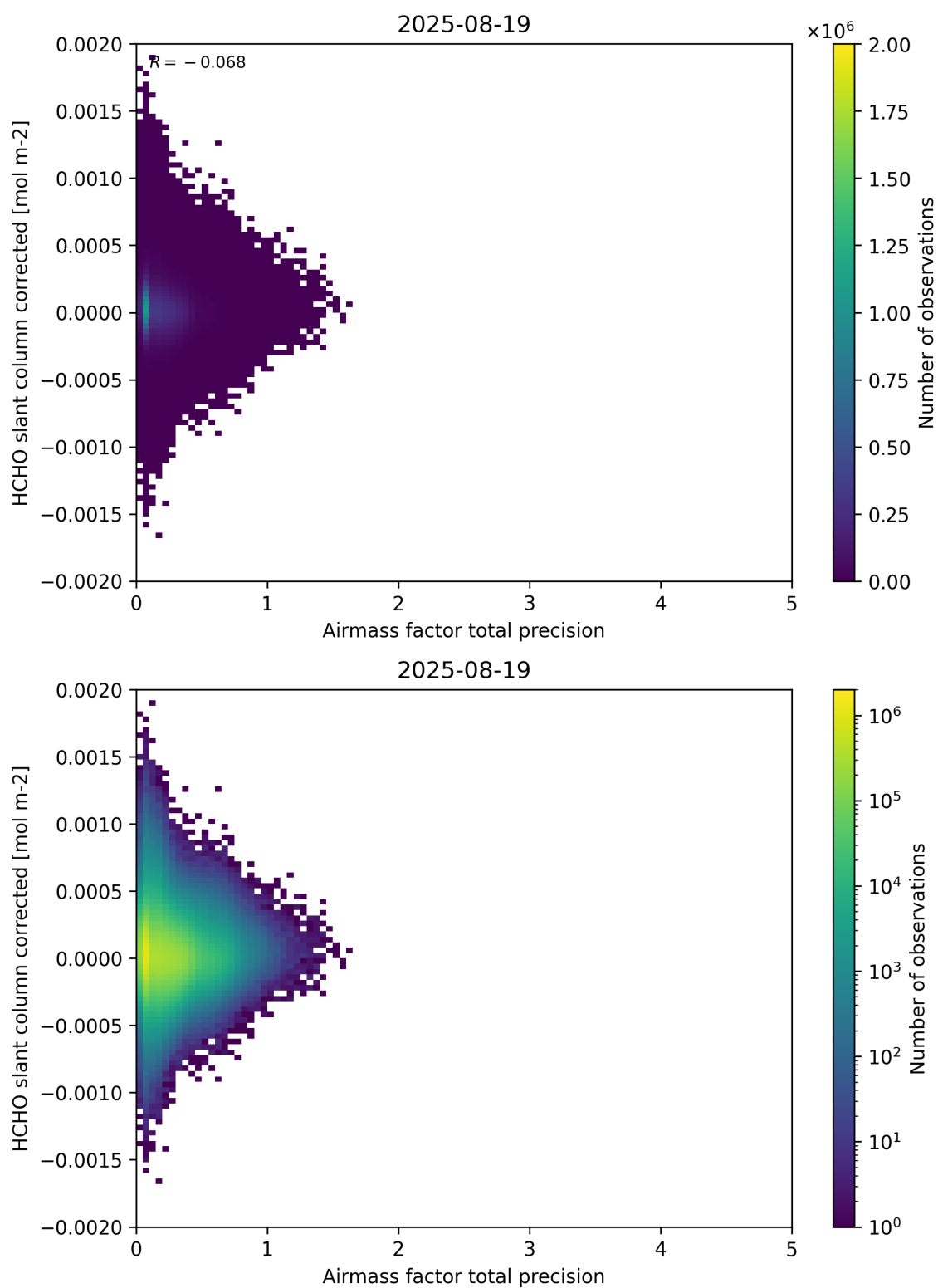
Figure 109: Scatter density plot of “Airmass factor total precision” against “HCHO slant column corrected” for 2025-08-19 to 2025-08-20.
