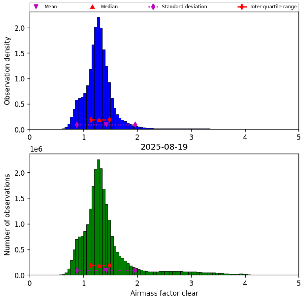
Figure 42: Histogram of “Airmass factor clear” for 2025-08-19 to 2025-08-20
