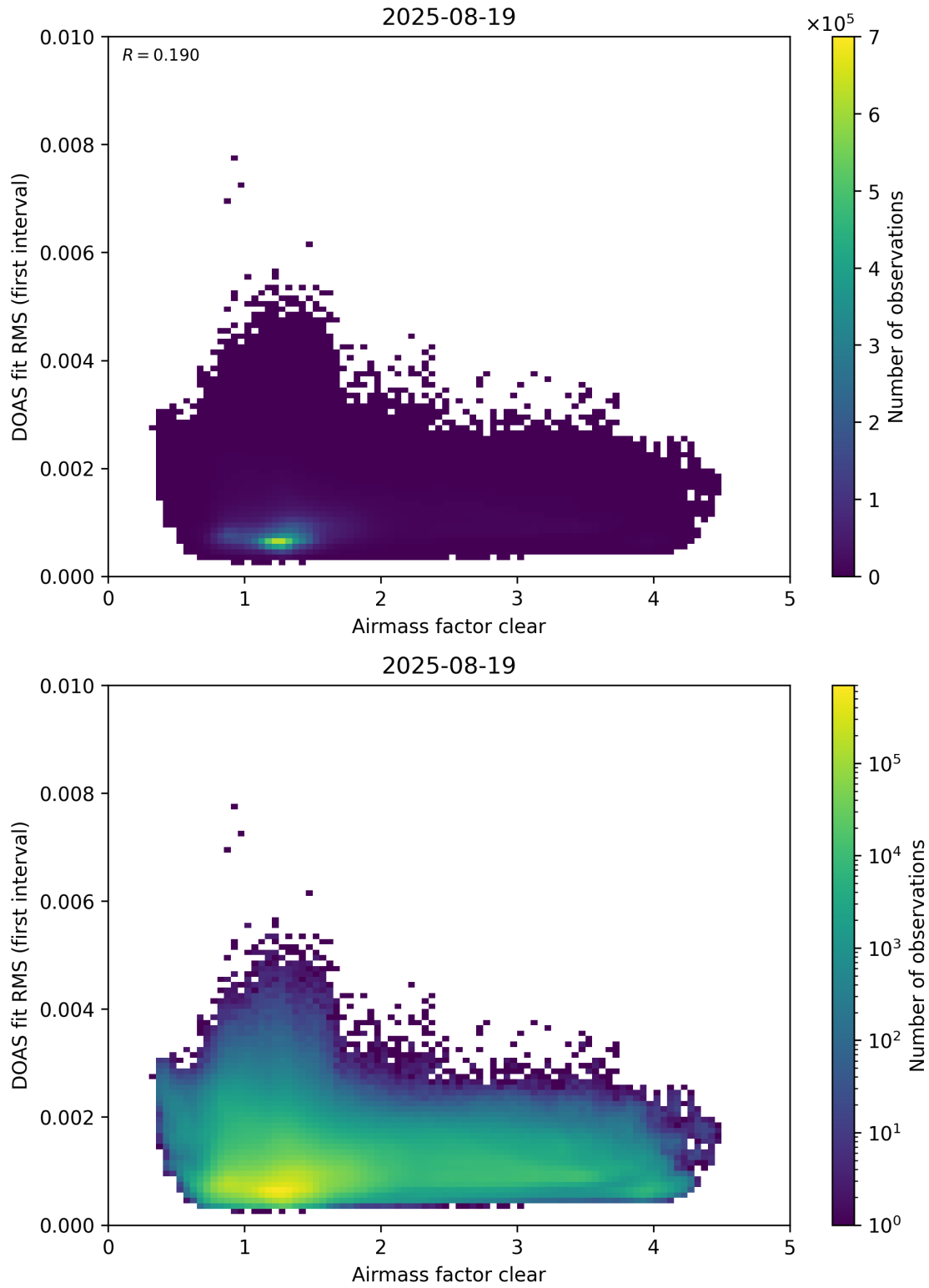
Figure 71: Scatter density plot of “Airmass factor clear” against “DOAS fit RMS (first interval)” for 2025-08-19 to 2025-08-20.
