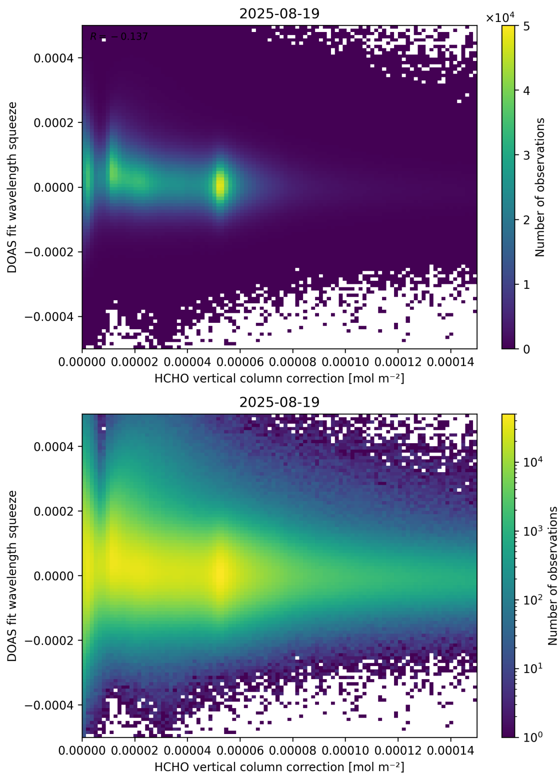
Figure 114: Scatter density plot of “HCHO vertical column correction” against “DOAS fit wavelength squeeze” for 2025-08-19 to 2025-08-20.
