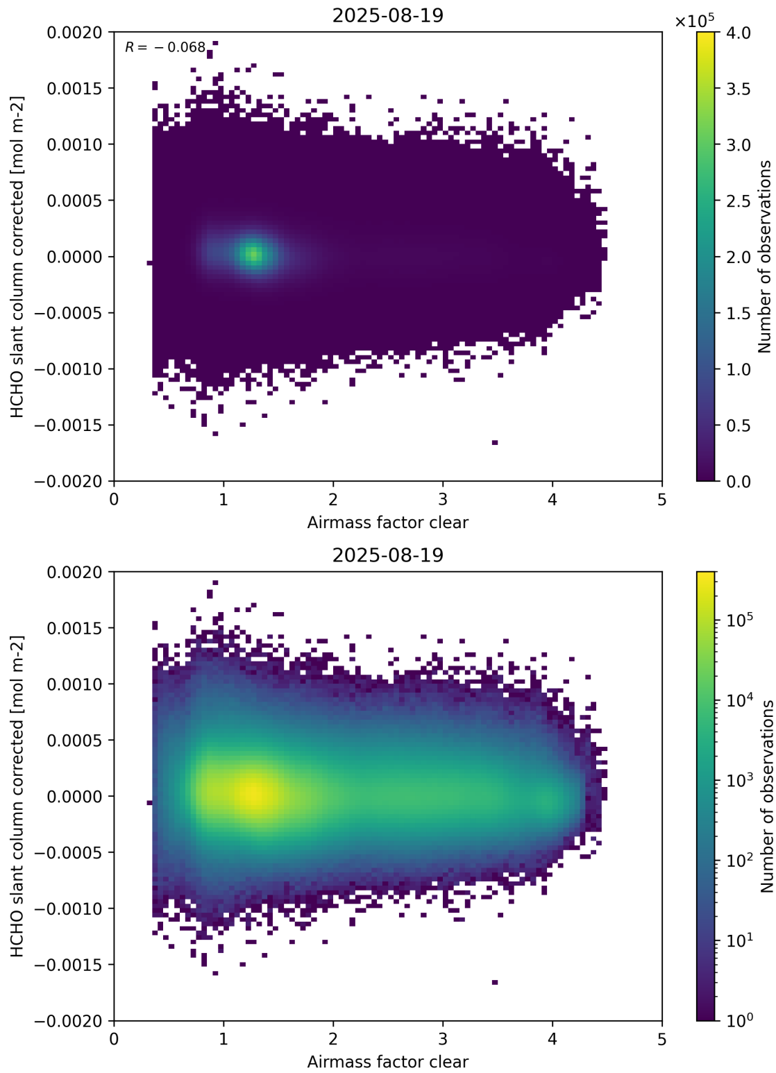
Figure 74: Scatter density plot of “Airmass factor clear” against “HCHO slant column corrected” for 2025-08-19 to 2025-08-20.
