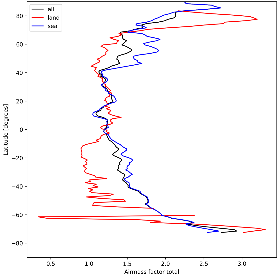
Figure 26: Zonal average of “Airmass factor total” for 2025-08-19 to 2025-08-20.
