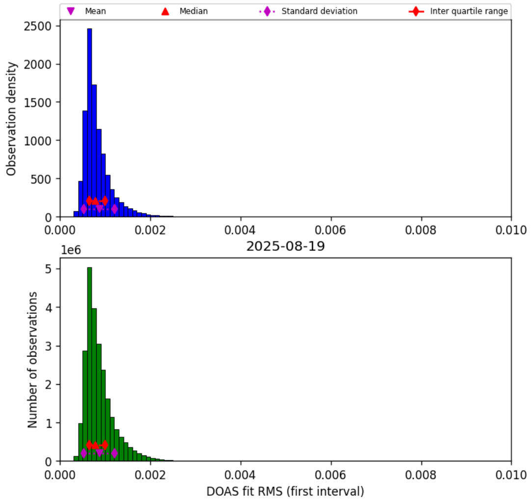
Figure 46: Histogram of “DOAS fit RMS (first interval)” for 2025-08-19 to 2025-08-20
