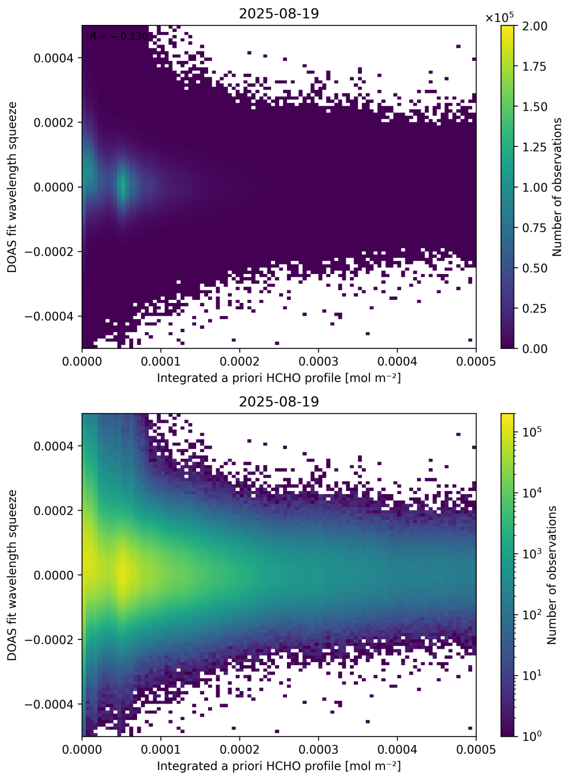
Figure 150: Scatter density plot of “Integrated a priori HCHO profile” against “DOAS fit wavelength squeeze” for 2025-08-19 to 2025-08-20.
