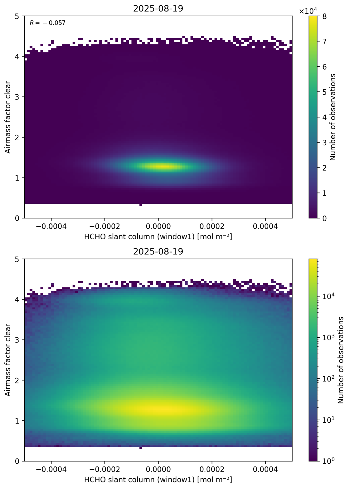
Figure 81: Scatter density plot of “HCHO slant column (window1)” against “Airmass factor clear” for 2025-08-19 to 2025-08-20.
