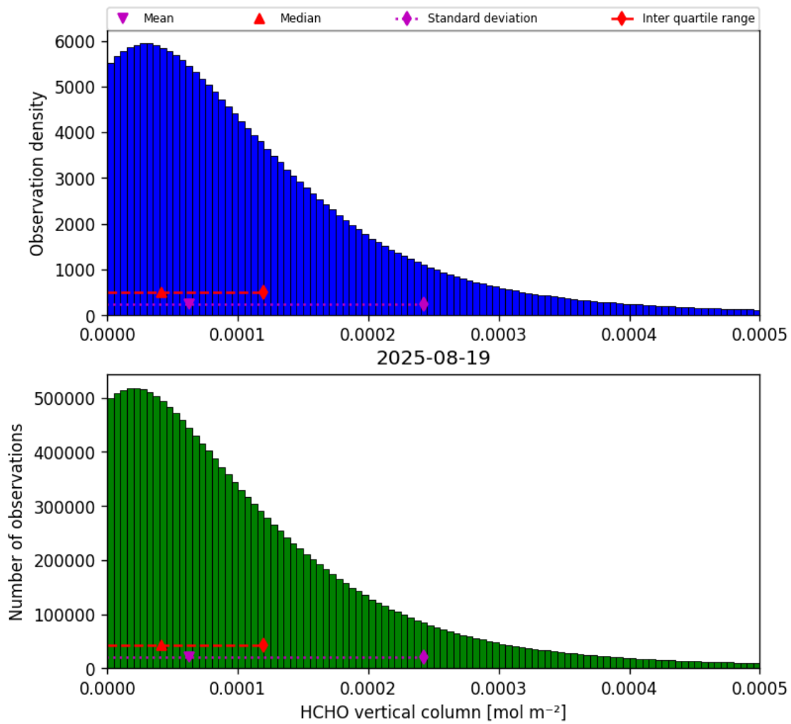
Figure 35: Histogram of “HCHO vertical column” for 2025-08-19 to 2025-08-20
