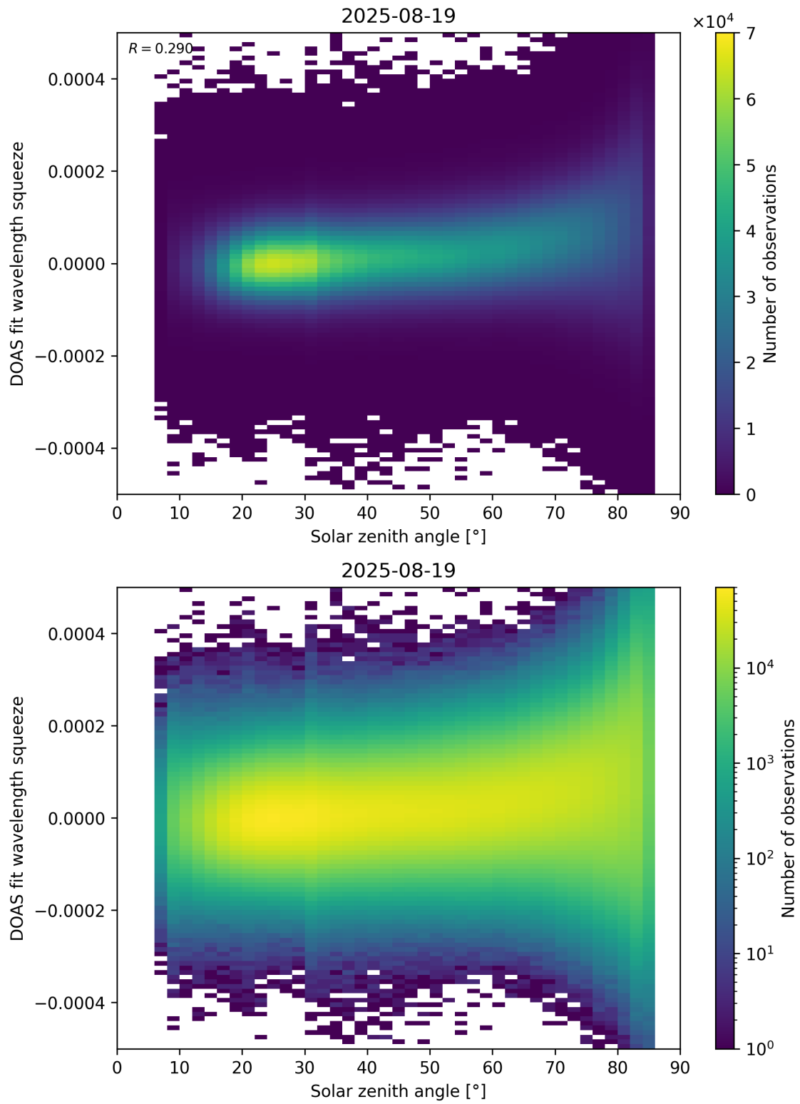
Figure 169: Scatter density plot of “Solar zenith angle” against “DOAS fit wavelength squeeze” for 2025-08-19 to 2025-08-20.
