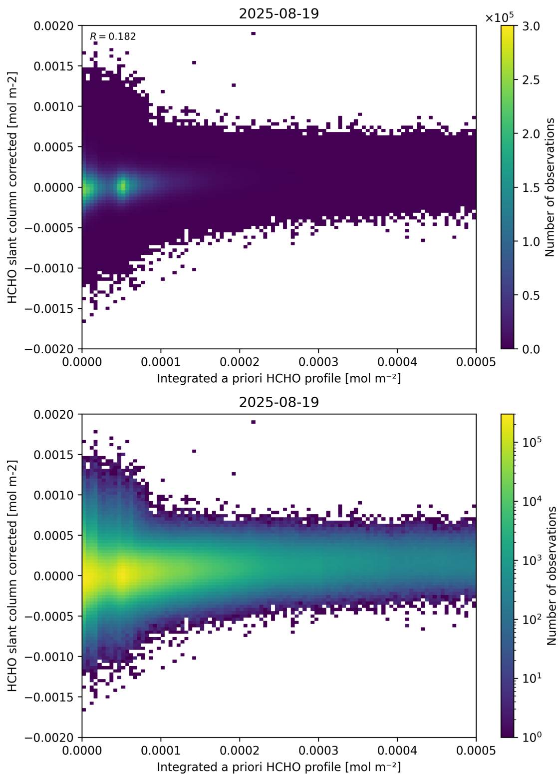
Figure 151: Scatter density plot of “Integrated a priori HCHO profile” against “HCHO slant column corrected” for 2025-08-19 to 2025-08-20.
