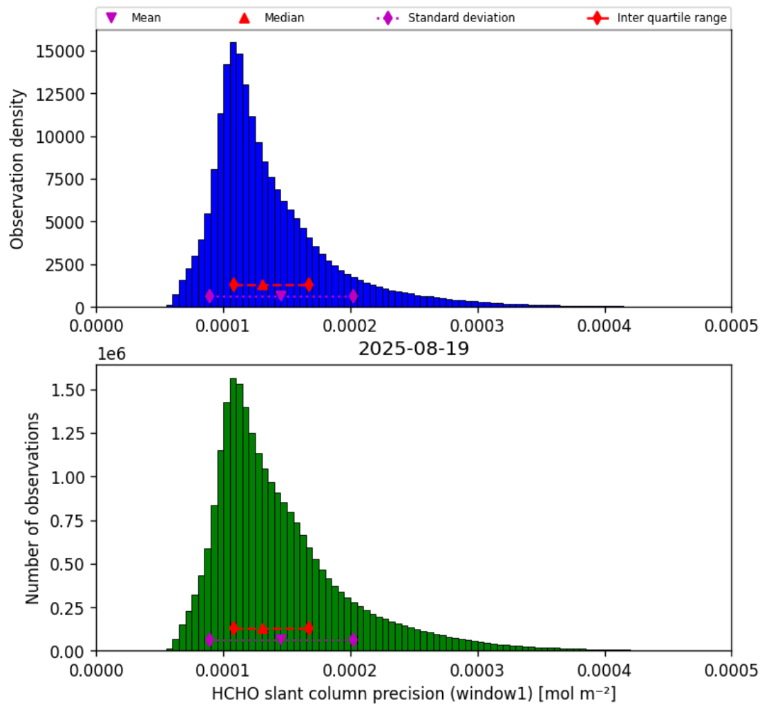
Figure 39: Histogram of “HCHO slant column precision (window1)” for 2025-08-19 to 2025-08-20
