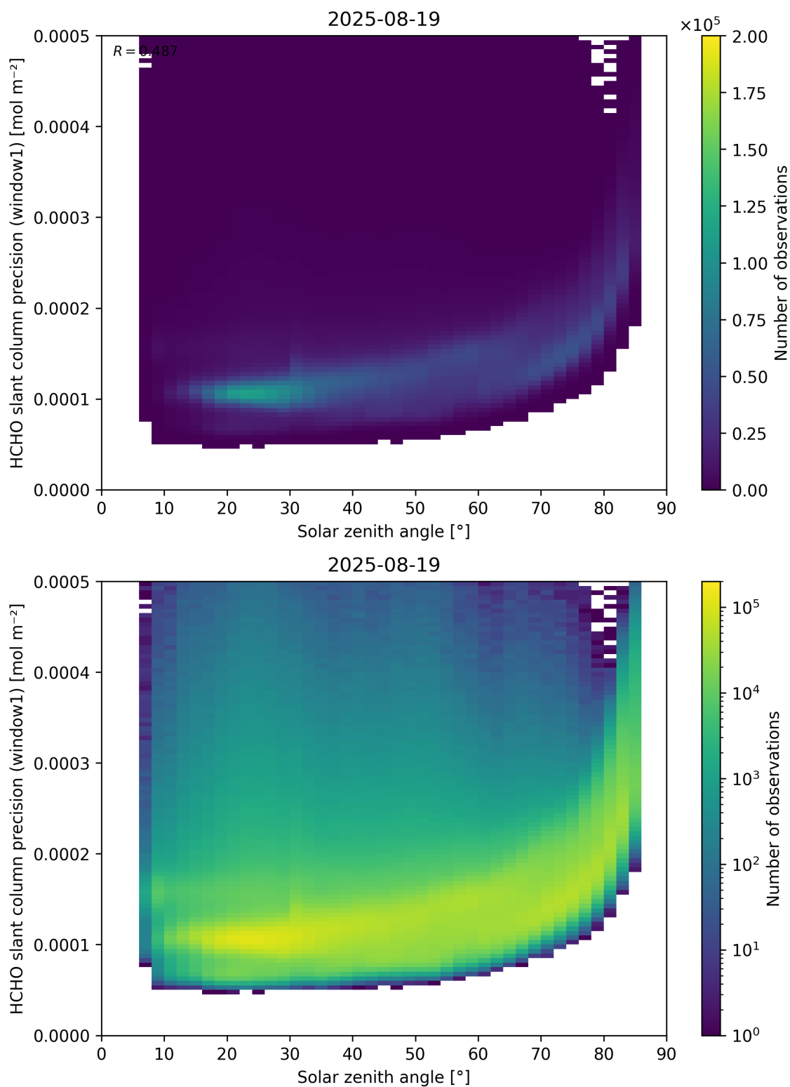
Figure 174: Scatter density plot of “Solar zenith angle” against “HCHO slant column precision (window1)” for 2025-08-19 to 2025-08-20.
