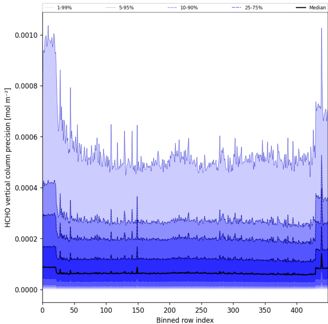
Figure 50: Along track statistics of “HCHO vertical column precision” for 2025-08-19 to 2025-08-20
