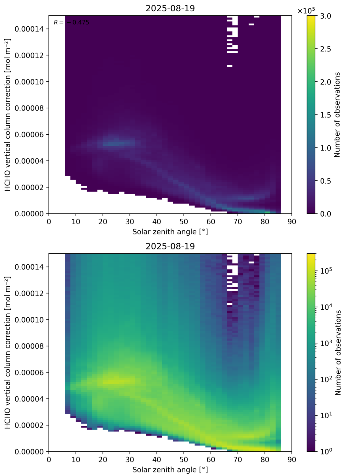
Figure 178: Scatter density plot of “Solar zenith angle” against “HCHO vertical column correction” for 2025-08-19 to 2025-08-20.
