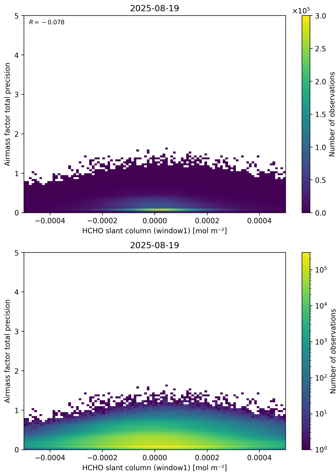
Figure 86: Scatter density plot of “HCHO slant column (window1)” against “Airmass factor total precision” for 2025-08-19 to 2025-08-20.
