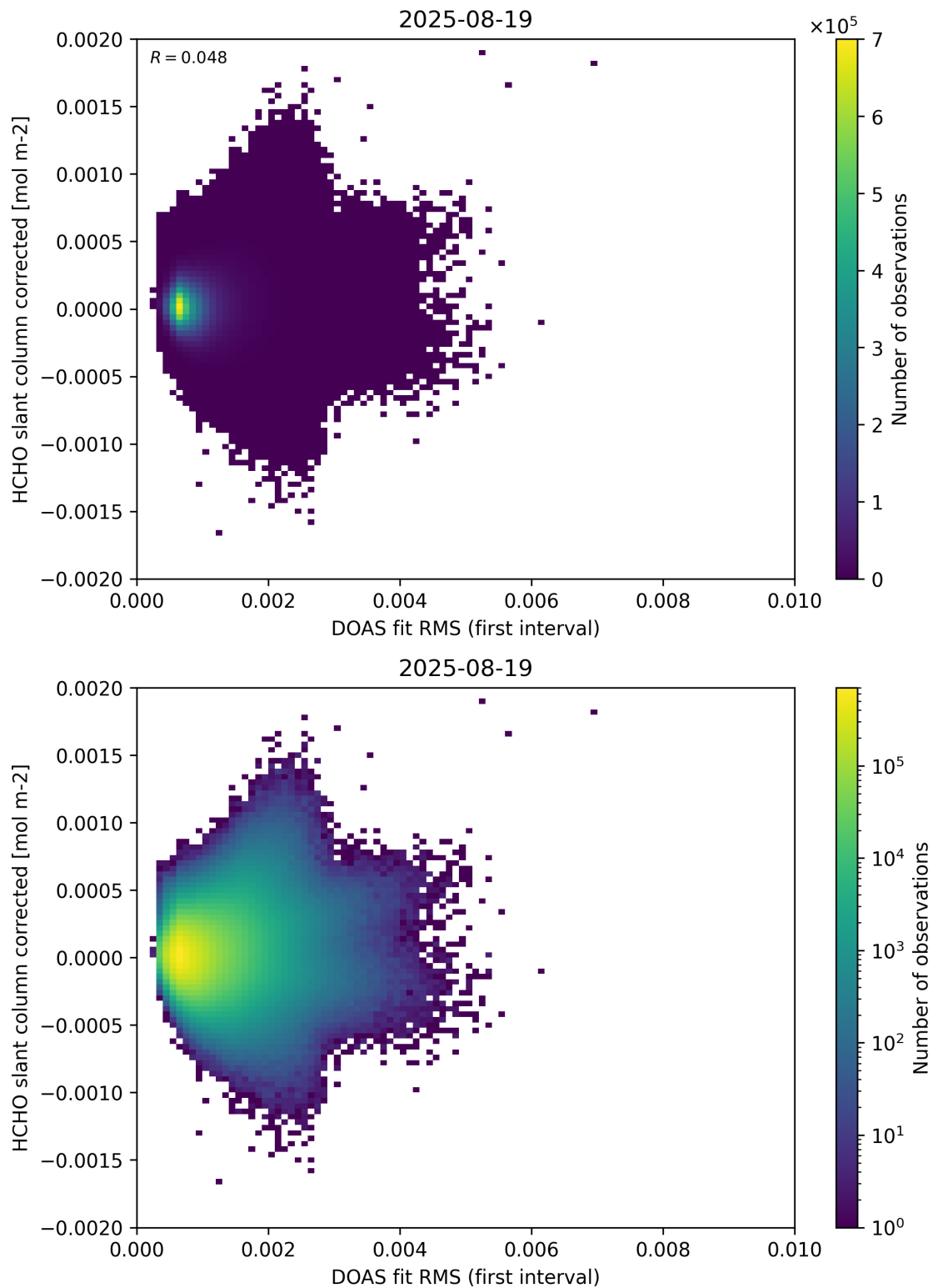
Figure 62: Scatter density plot of “DOAS fit RMS (first interval)” against “HCHO slant column corrected” for 2025-08-19 to 2025-08-20.
