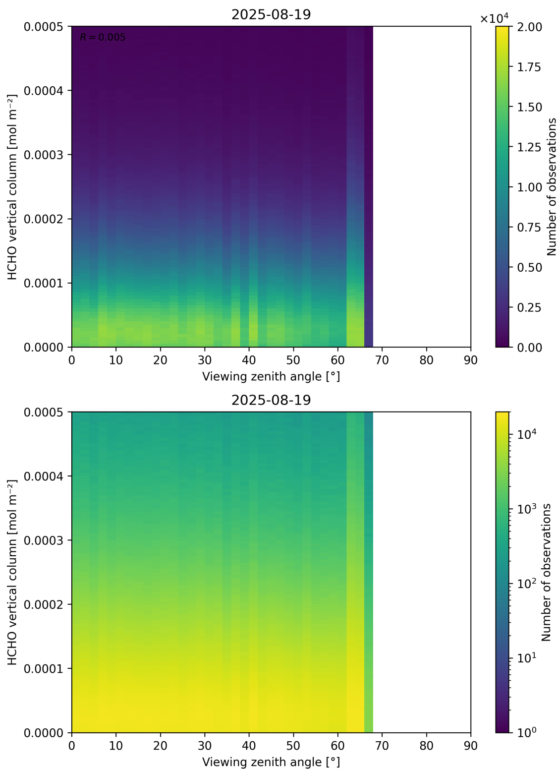
Figure 192: Scatter density plot of “Viewing zenith angle” against “HCHO vertical column” for 2025-08-19 to 2025-08-20.
