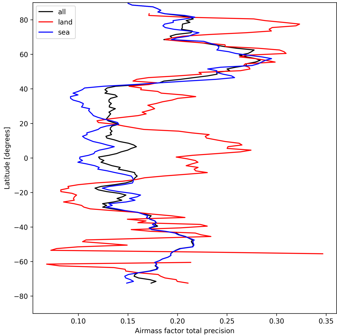
Figure 27: Zonal average of “Airmass factor total precision” for 2025-08-19 to 2025-08-20.
