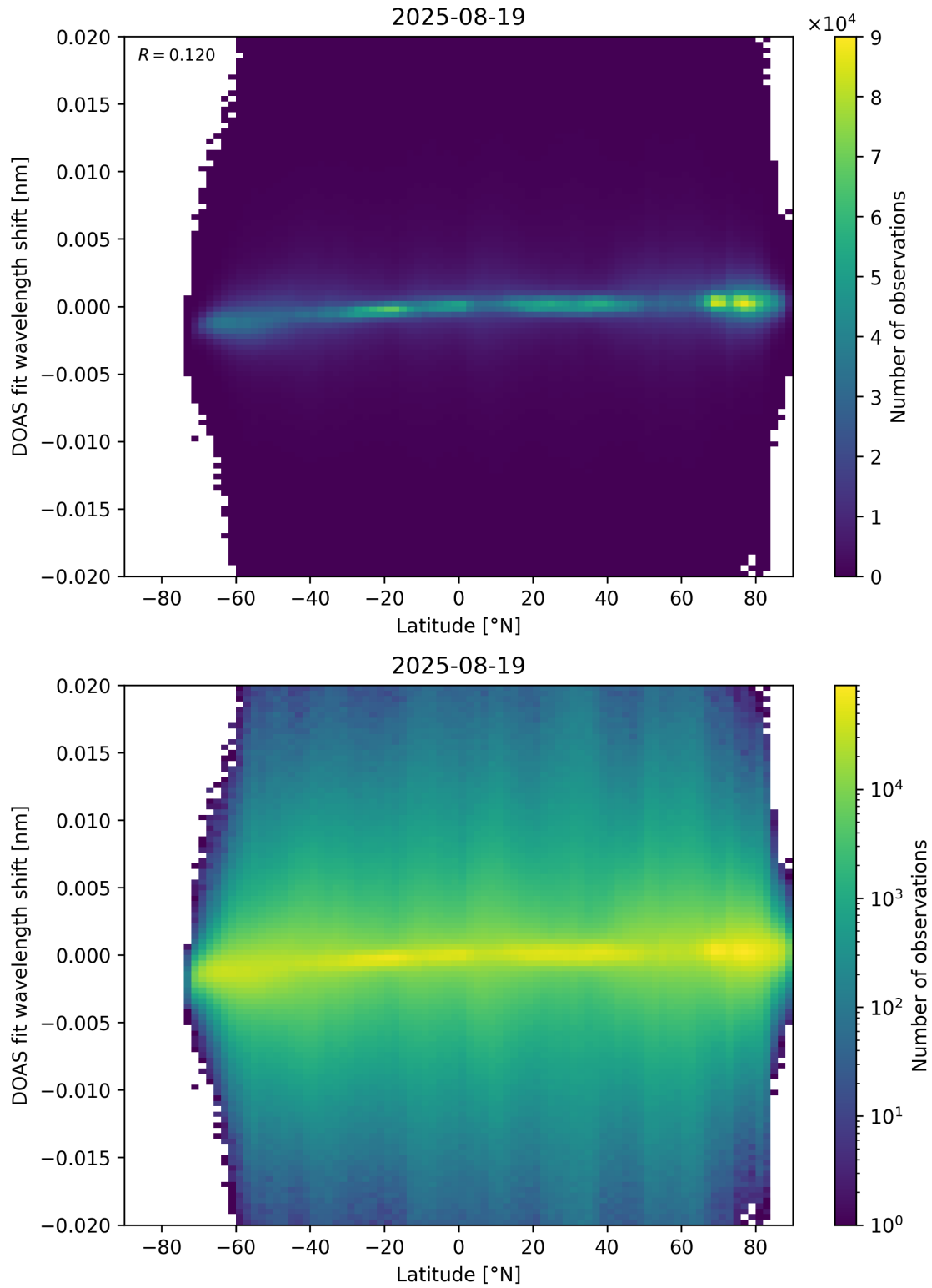
Figure 154: Scatter density plot of “Latitude” against “DOAS fit wavelength shift” for 2025-08-19 to 2025-08-20.
