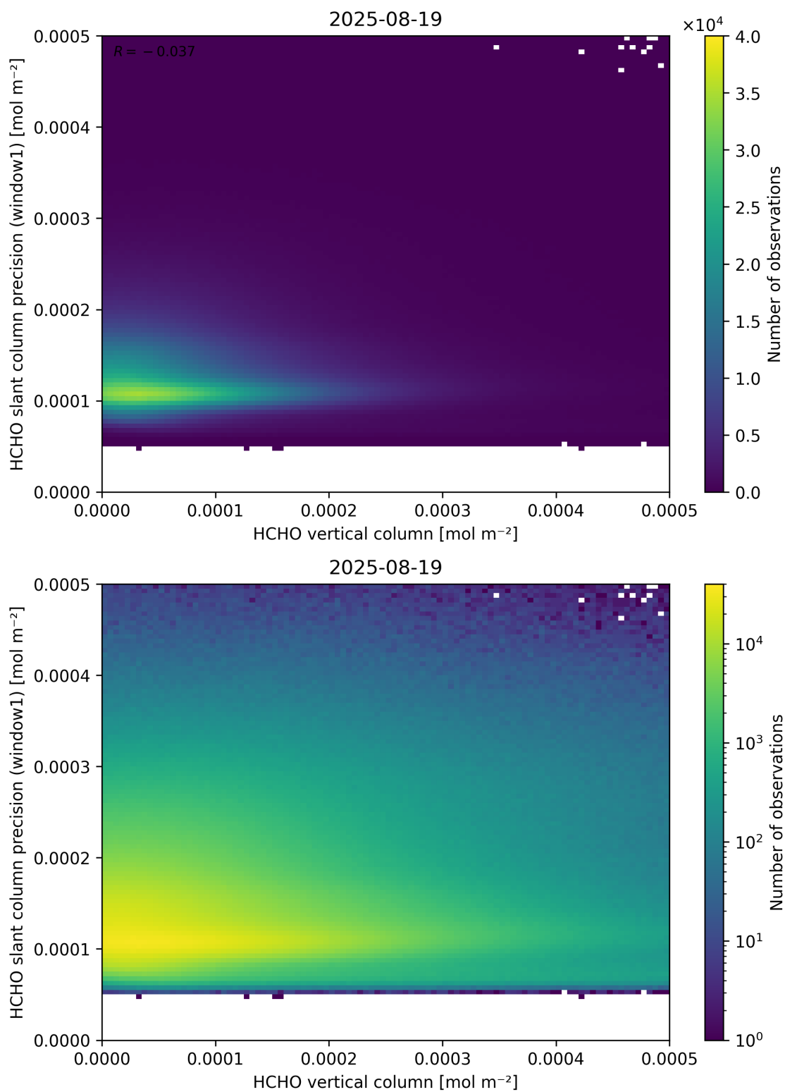
Figure 130: Scatter density plot of “HCHO vertical column” against “HCHO slant column precision (window1)” for 2025-08-19 to 2025-08-20.
