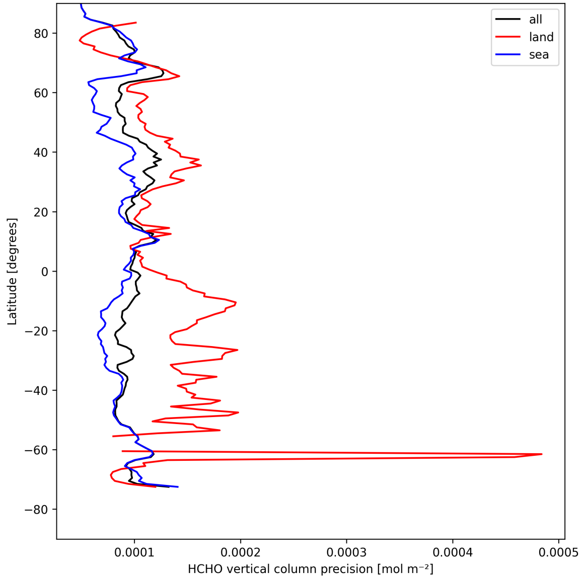
Figure 22: Zonal average of “HCHO vertical column precision” for 2025-08-19 to 2025-08-20.
