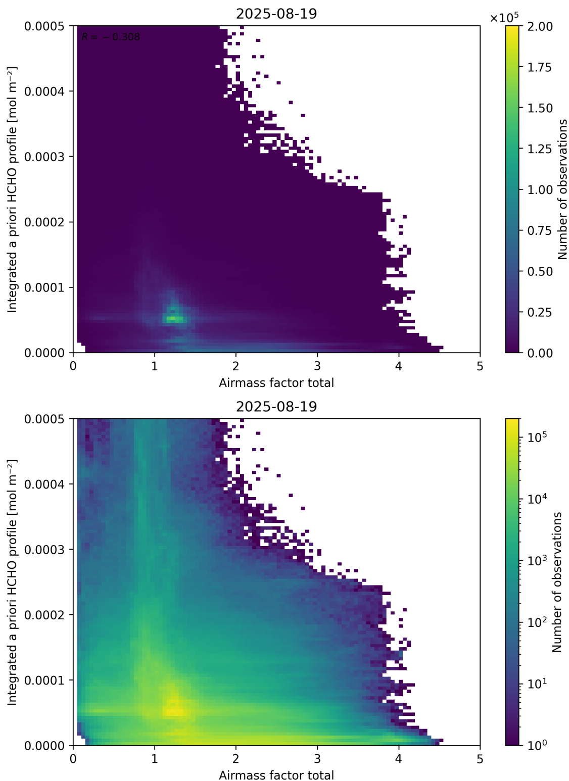
Figure 104: Scatter density plot of “Airmass factor total” against “Integrated a priori HCHO profile” for 2025-08-19 to 2025-08-20.
