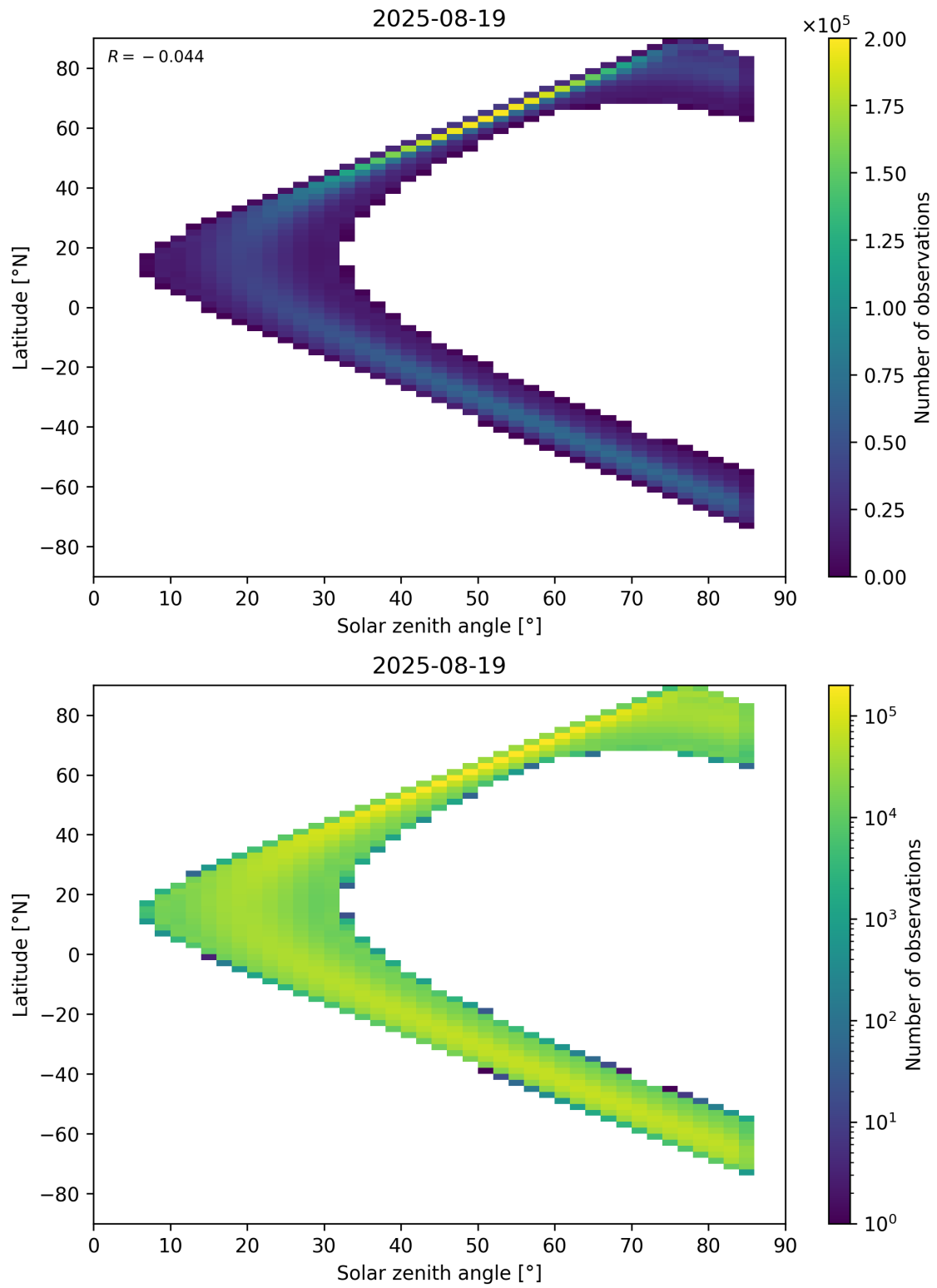
Figure 181: Scatter density plot of “Solar zenith angle” against “Latitude” for 2025-08-19 to 2025-08-20.
