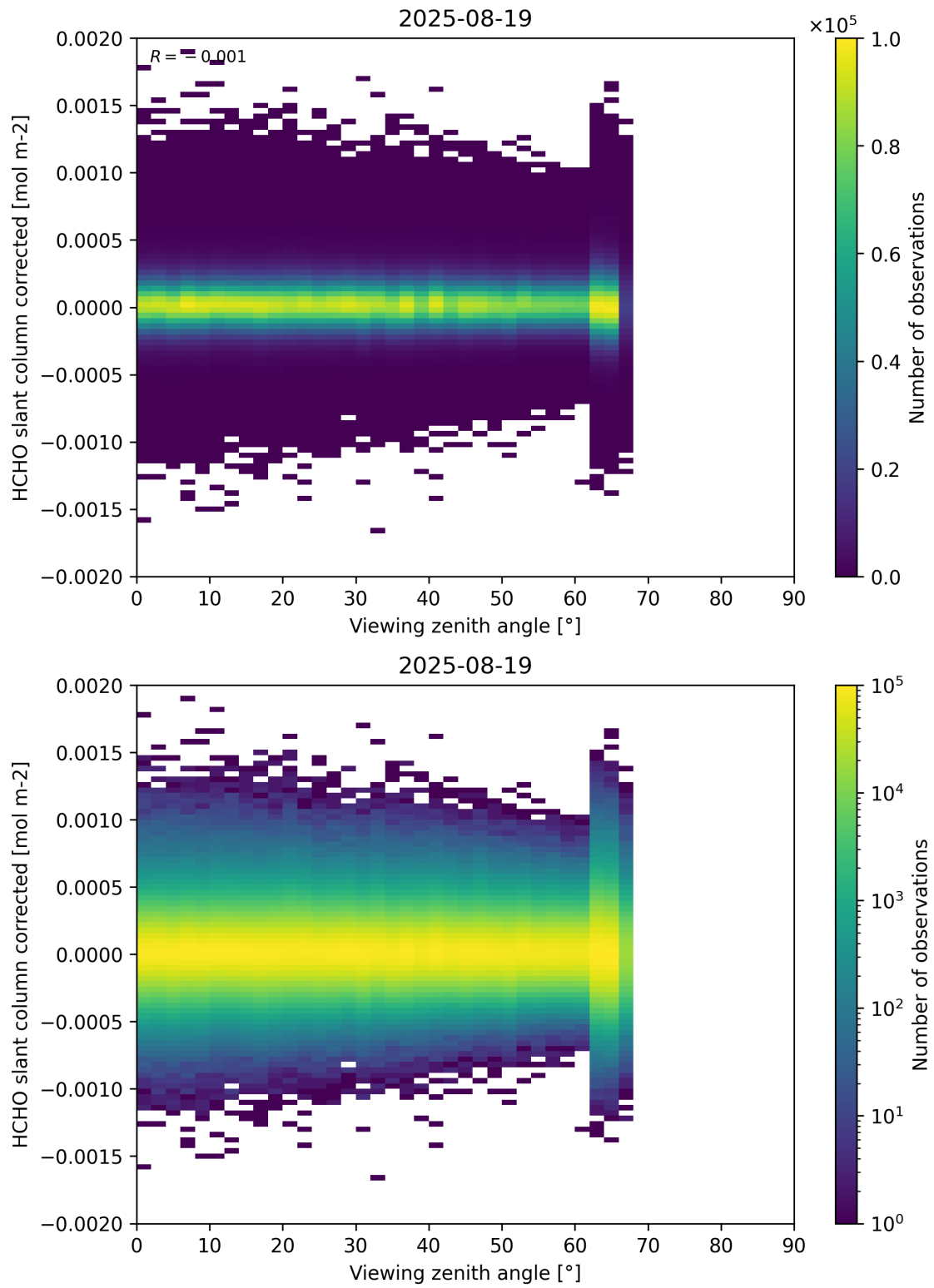
Figure 186: Scatter density plot of “Viewing zenith angle” against “HCHO slant column corrected” for 2025-08-19 to 2025-08-20.
