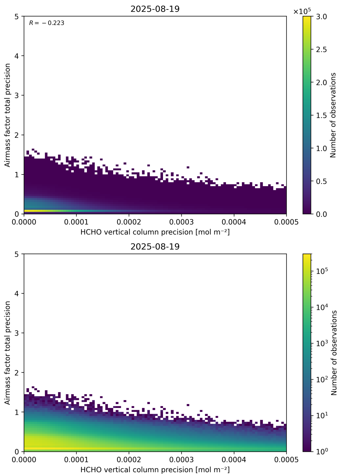
Figure 145: Scatter density plot of “HCHO vertical column precision” against “Airmass factor total precision” for 2025-08-19 to 2025-08-20.
