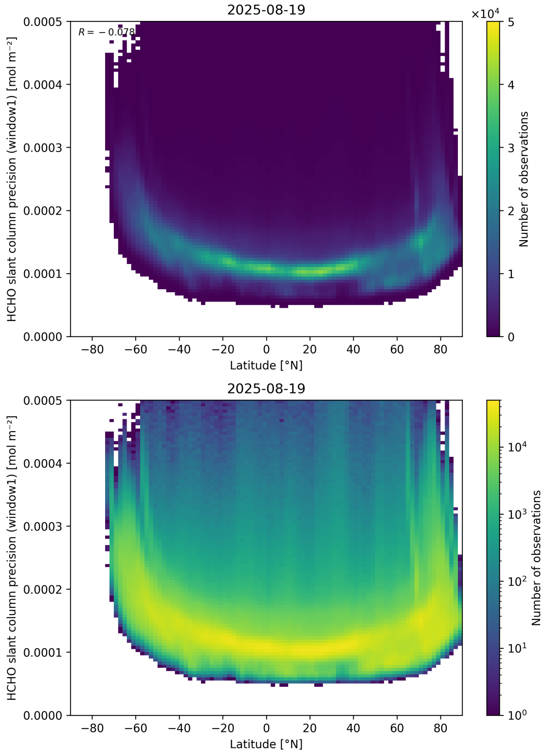
Figure 160: Scatter density plot of “Latitude” against “HCHO slant column precision (window1)” for 2025-08-19 to 2025-08-20.
