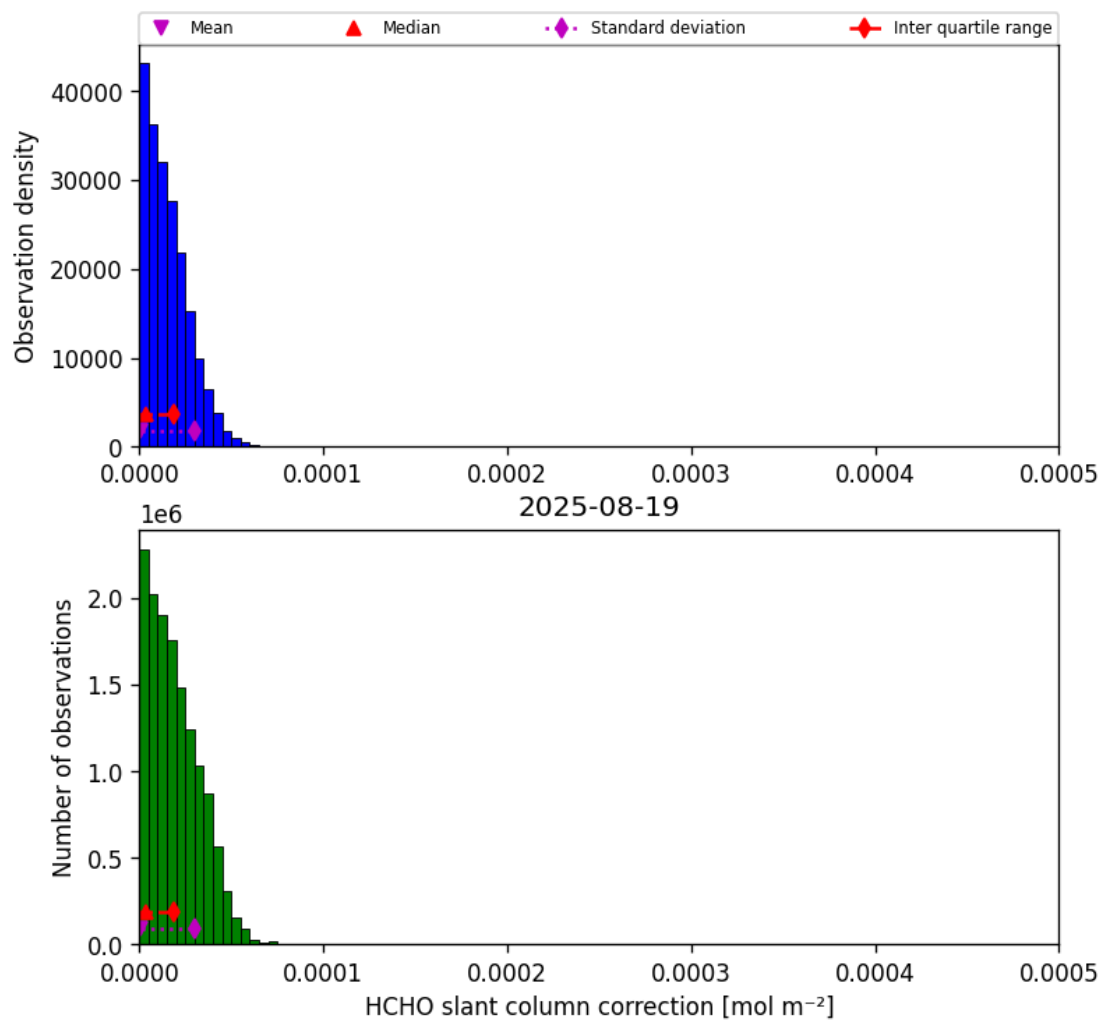
Figure 47: Histogram of “HCHO slant column correction” for 2025-08-19 to 2025-08-20
