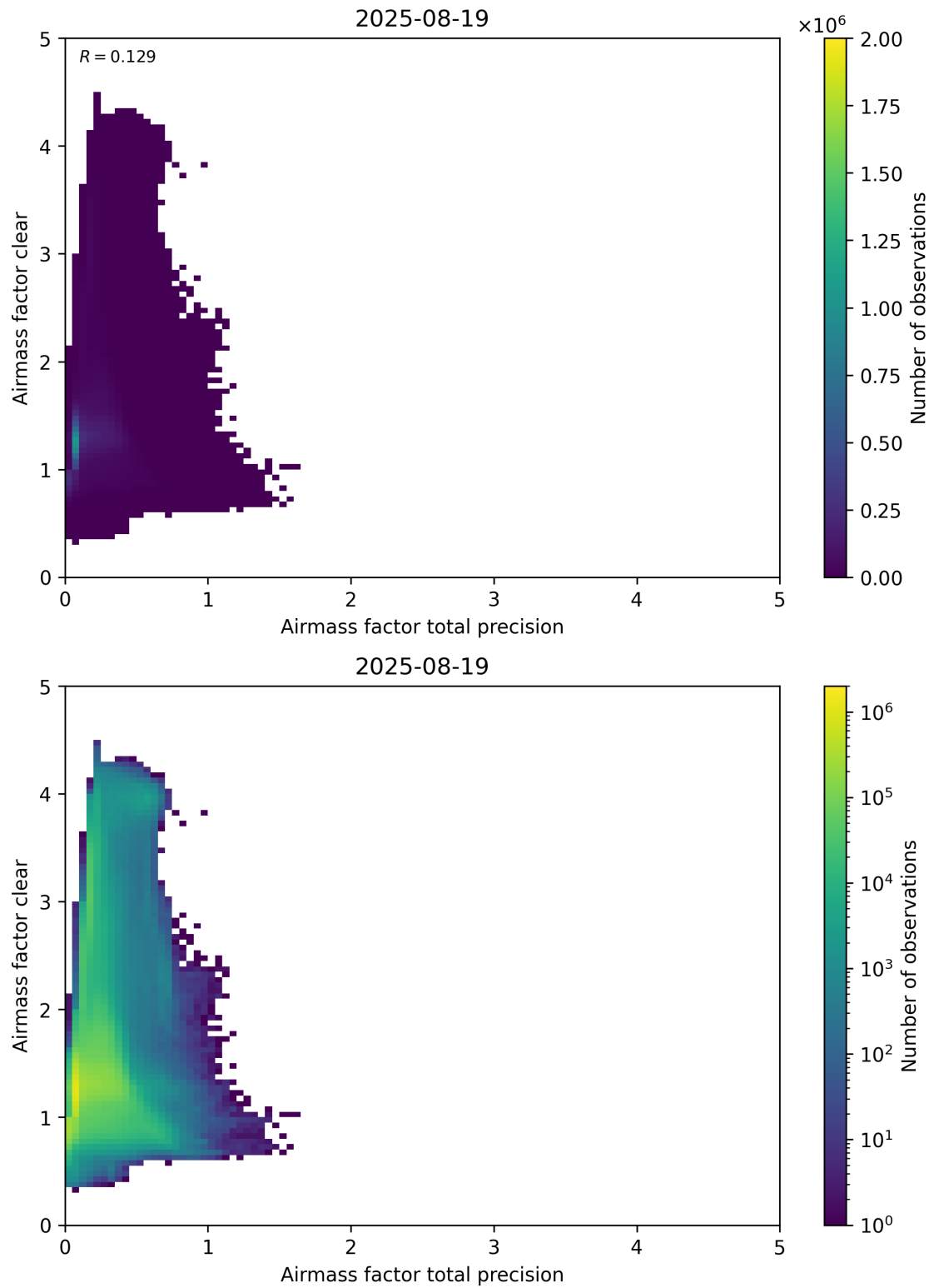
Figure 108: Scatter density plot of “Airmass factor total precision” against “Airmass factor clear” for 2025-08-19 to 2025-08-20.
