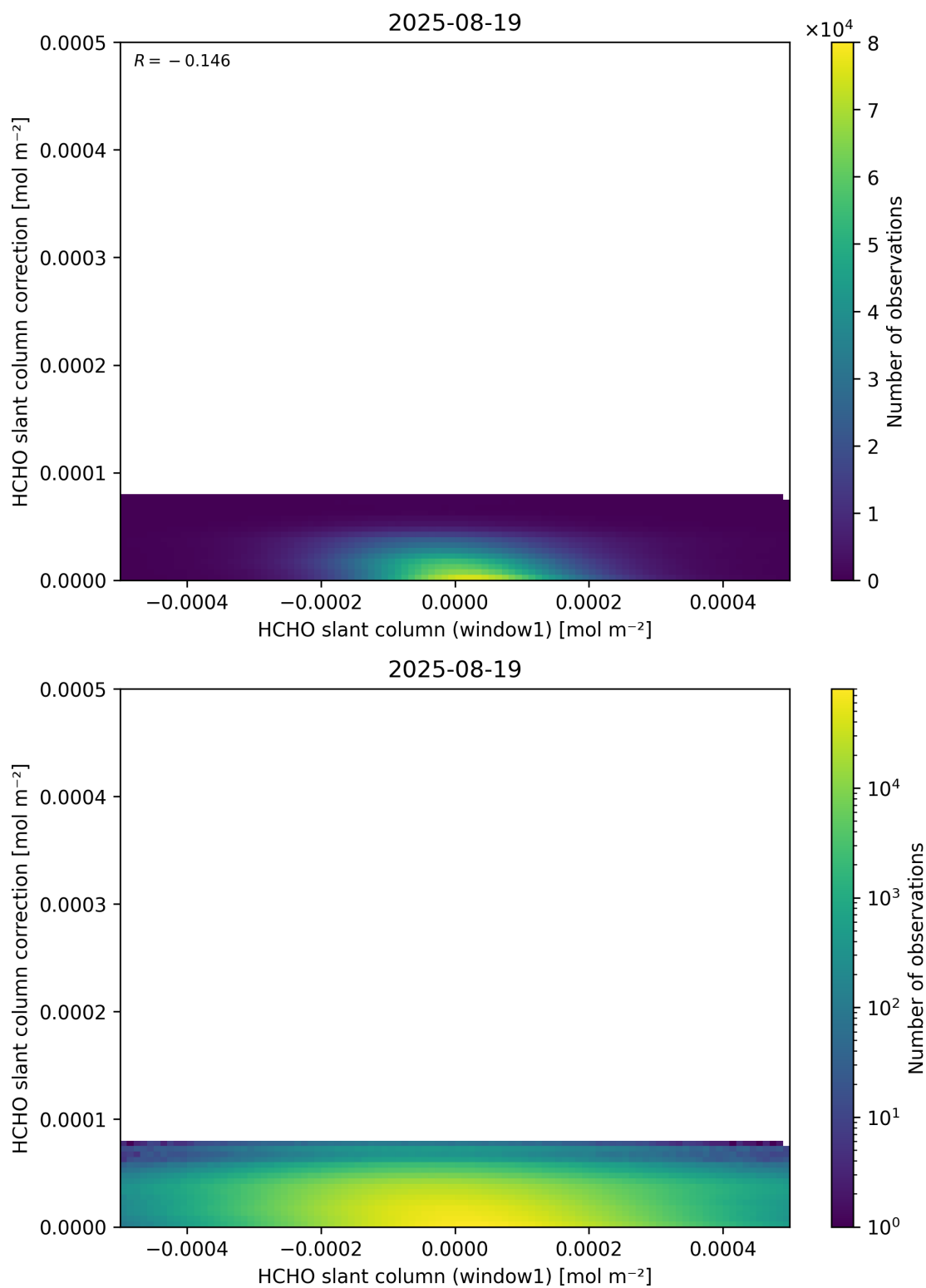
Figure 83: Scatter density plot of “HCHO slant column (window1)” against “HCHO slant column correction” for 2025-08-19 to 2025-08-20.
