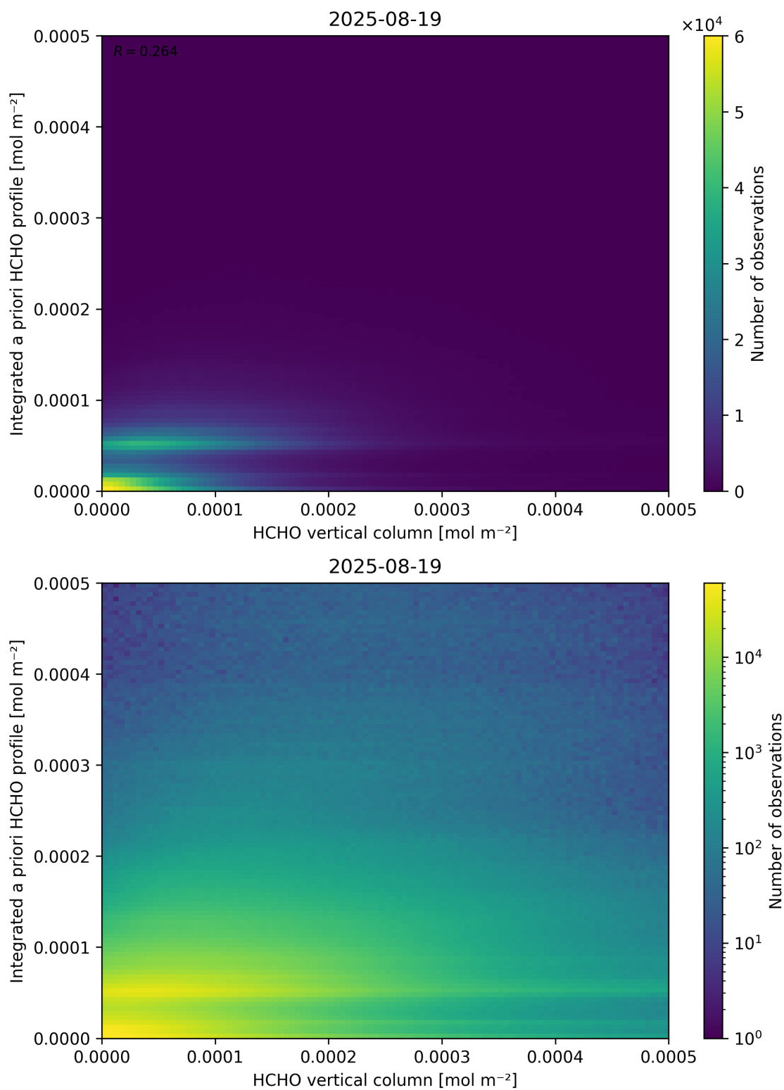
Figure 135: Scatter density plot of “HCHO vertical column” against “Integrated a priori HCHO profile” for 2025-08-19 to 2025-08-20.
