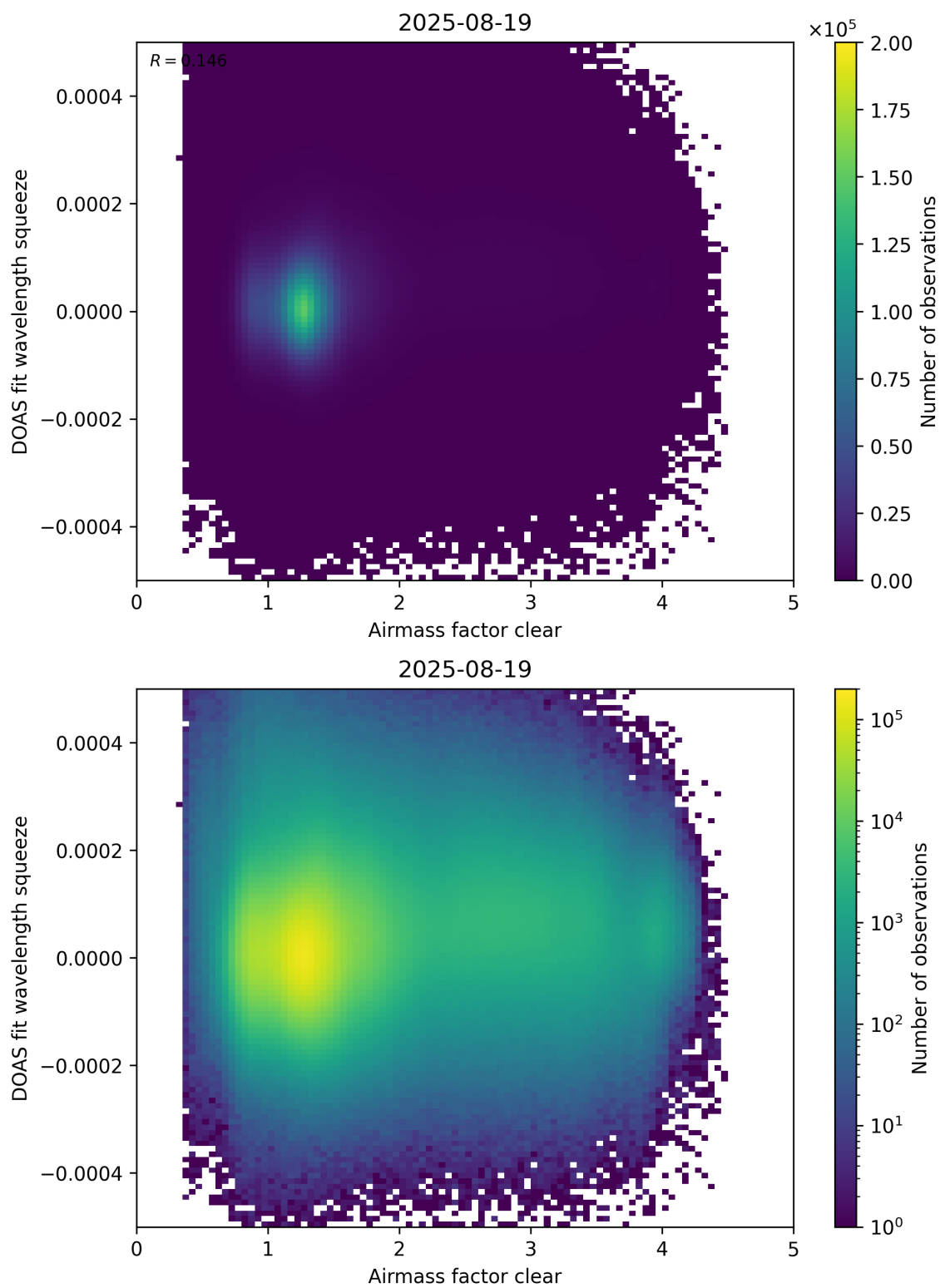
Figure 73: Scatter density plot of “Airmass factor clear” against “DOAS fit wavelength squeeze” for 2025-08-19 to 2025-08-20.
