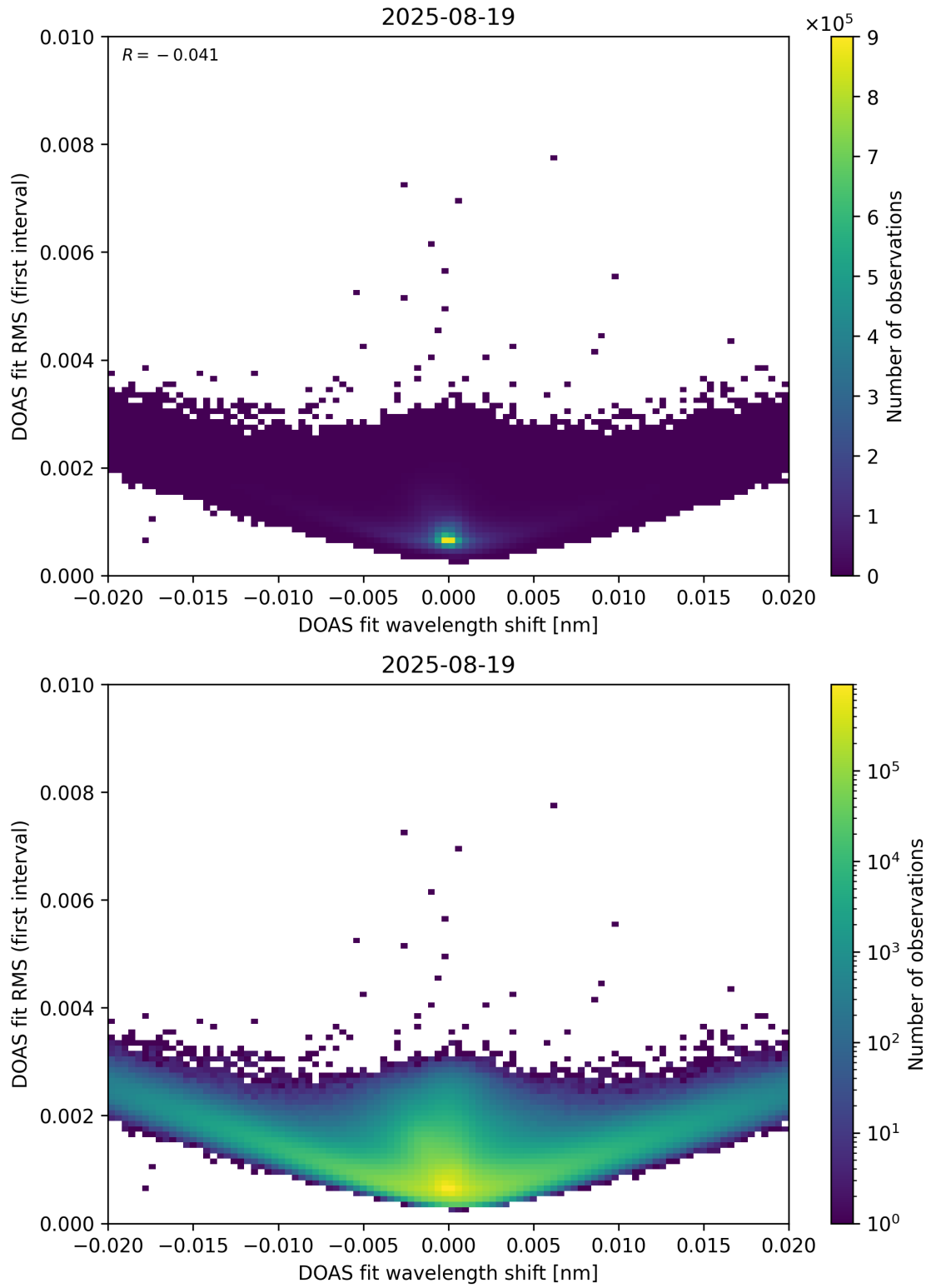
Figure 64: Scatter density plot of “DOAS fit wavelength shift” against “DOAS fit RMS (first interval)” for 2025-08-19 to 2025-08-20.
