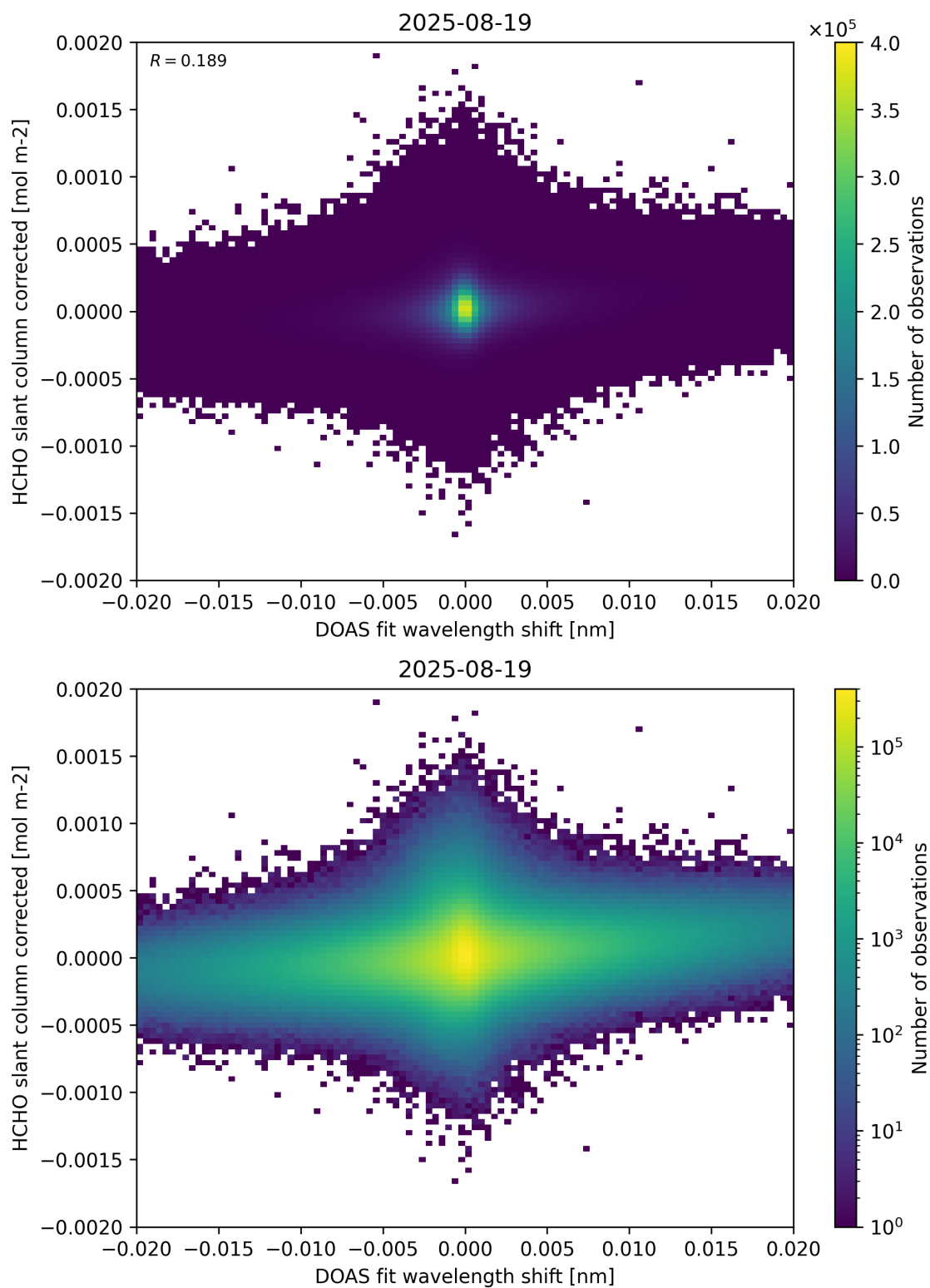
Figure 66: Scatter density plot of “DOAS fit wavelength shift” against “HCHO slant column corrected” for 2025-08-19 to 2025-08-20.
