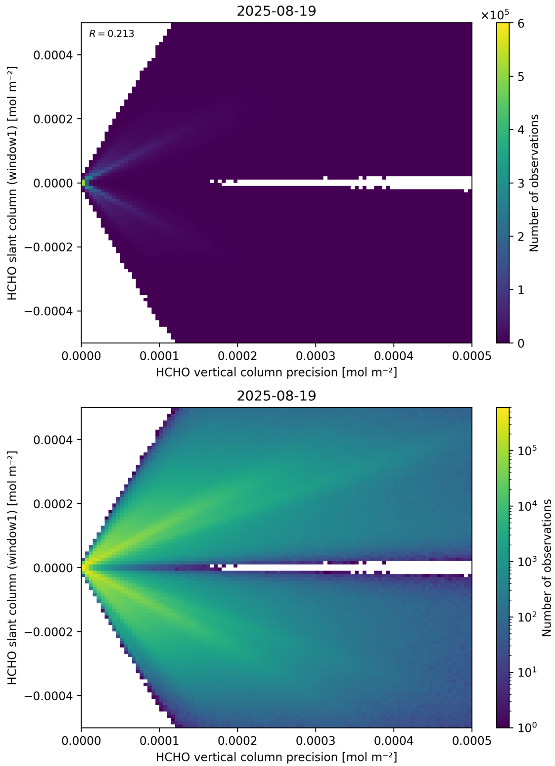
Figure 142: Scatter density plot of “HCHO vertical column precision” against “HCHO slant column (window1)” for 2025-08-19 to 2025-08-20.
