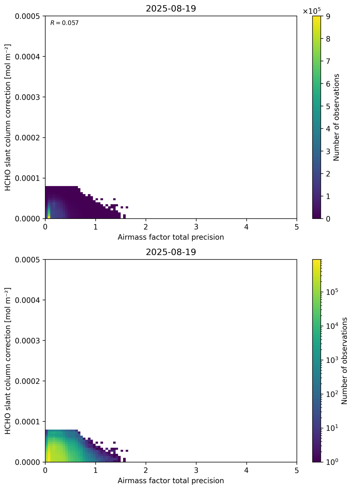
Figure 110: Scatter density plot of “Airmass factor total precision” against “HCHO slant column correction” for 2025-08-19 to 2025-08-20.
