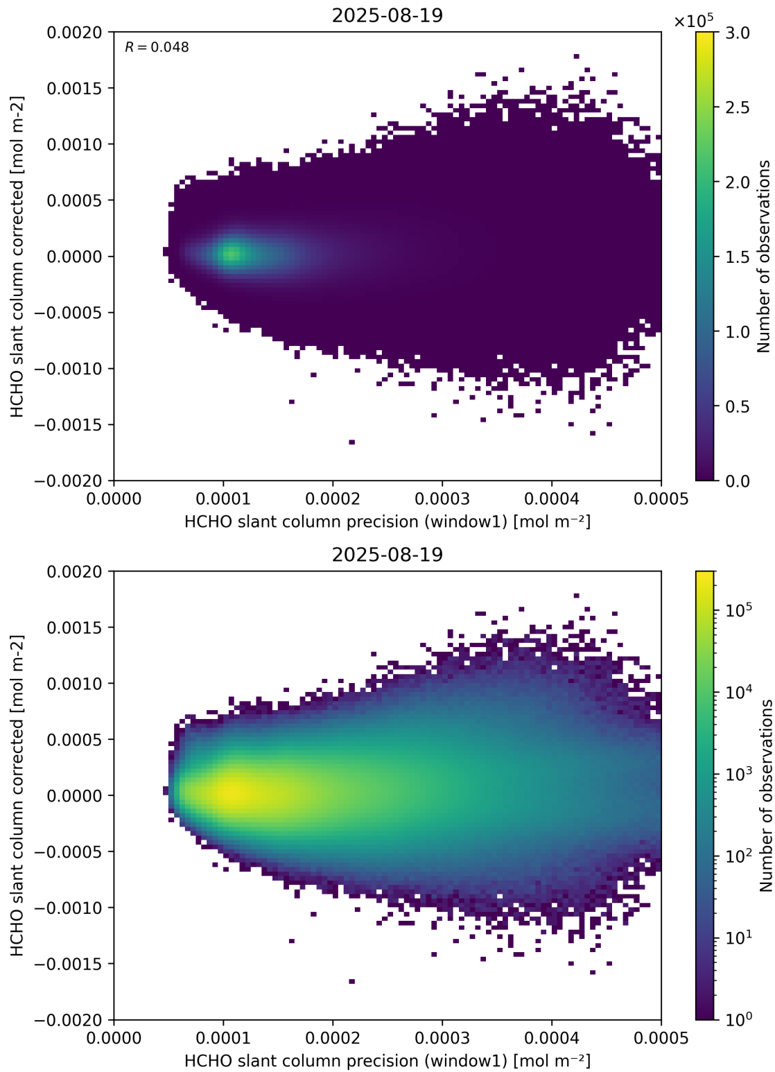
Figure 92: Scatter density plot of “HCHO slant column precision (window1)” against “HCHO slant column corrected” for 2025-08-19 to 2025-08-20.
