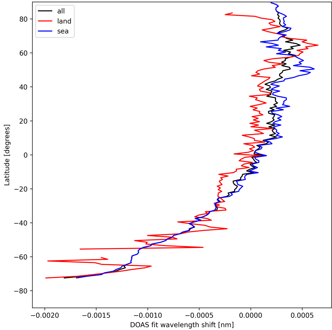
Figure 30: Zonal average of “DOAS fit wavelength shift” for 2025-08-19 to 2025-08-20.
