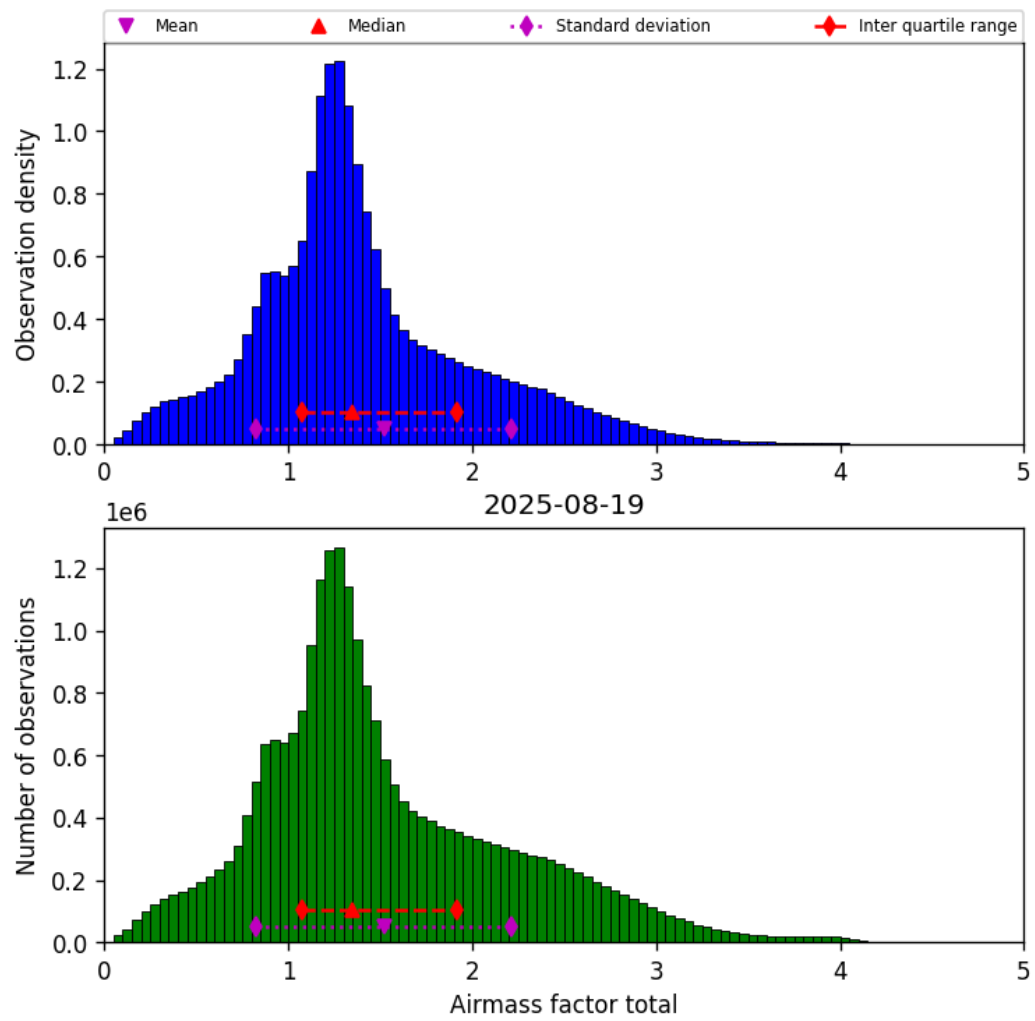
Figure 40: Histogram of “Airmass factor total” for 2025-08-19 to 2025-08-20
