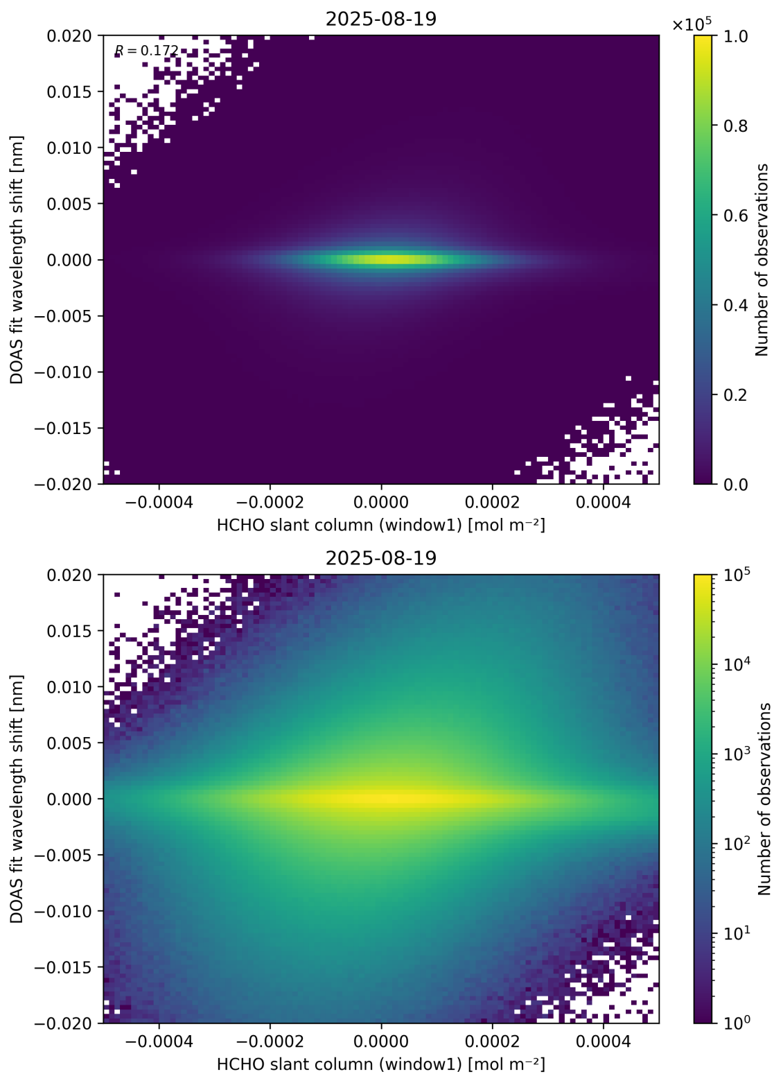
Figure 79: Scatter density plot of “HCHO slant column (window1)” against “DOAS fit wavelength shift” for 2025-08-19 to 2025-08-20.
