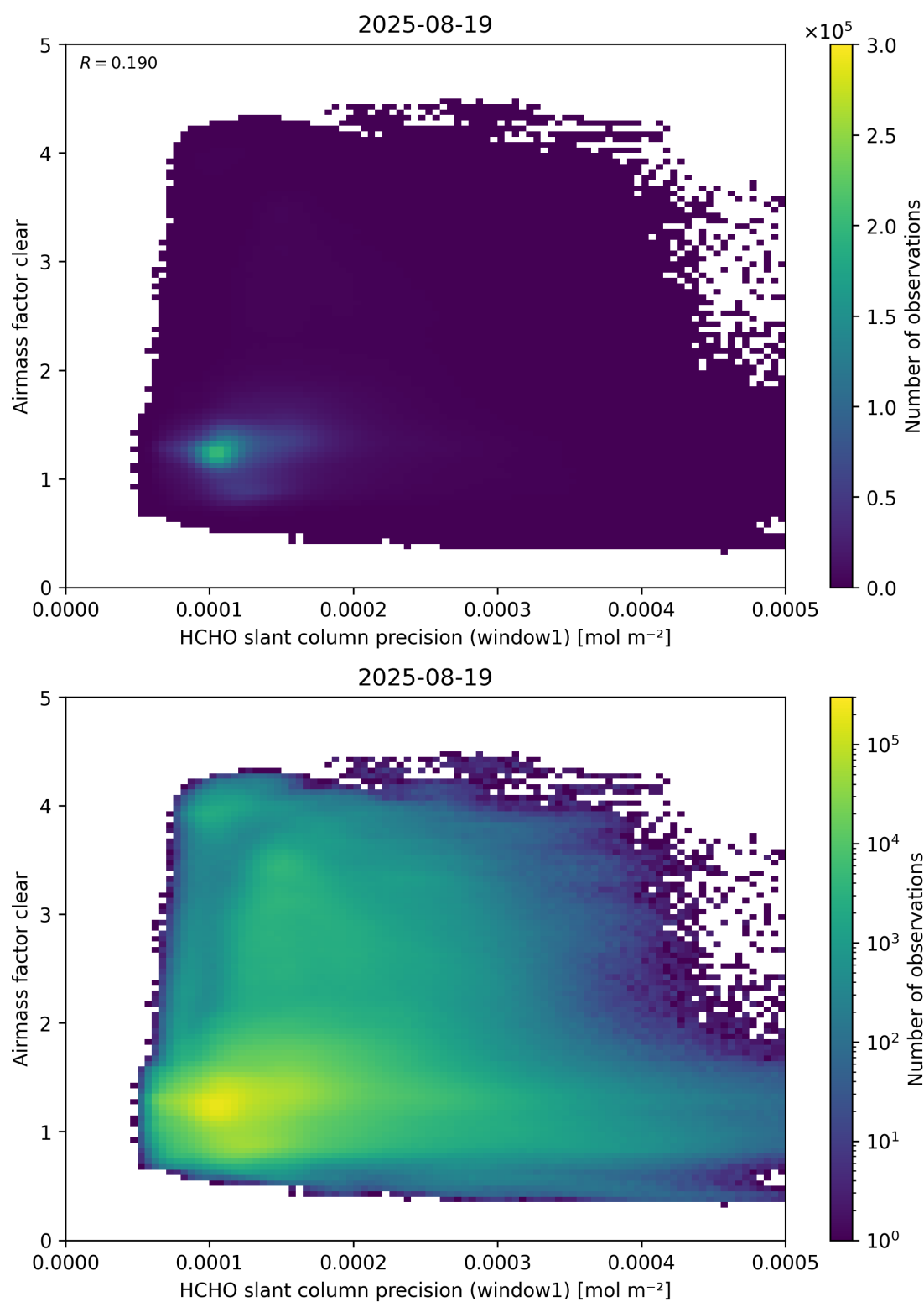
Figure 91: Scatter density plot of “HCHO slant column precision (window1)” against “Airmass factor clear” for 2025-08-19 to 2025-08-20.
