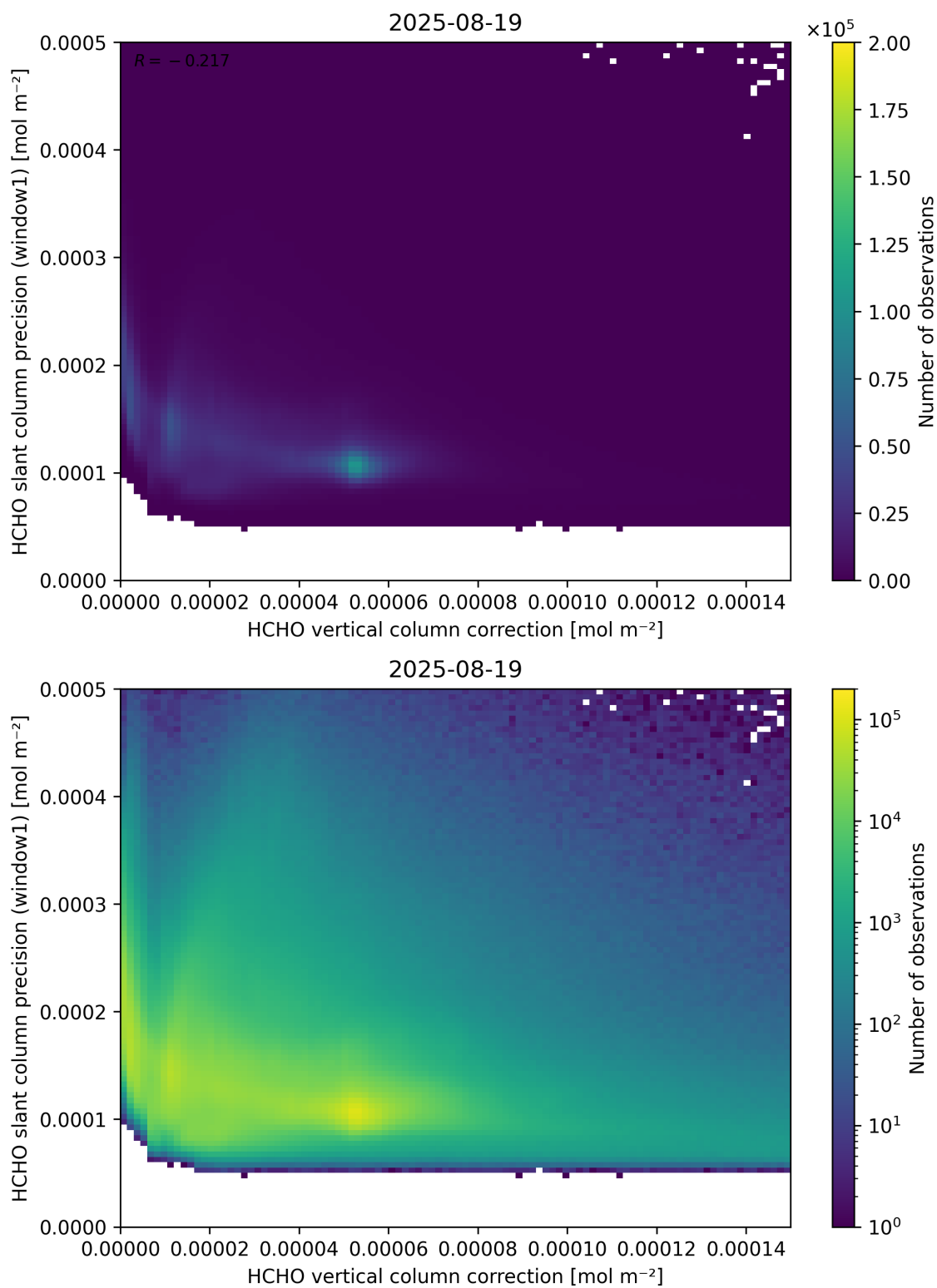
Figure 119: Scatter density plot of “HCHO vertical column correction” against “HCHO slant column precision (window1)” for 2025-08-19 to 2025-08-20.
