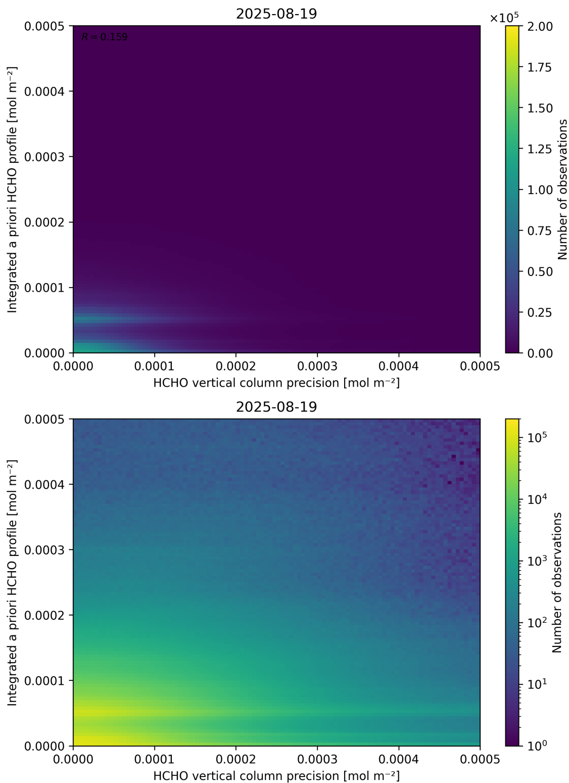
Figure 147: Scatter density plot of “HCHO vertical column precision” against “Integrated a priori HCHO profile” for 2025-08-19 to 2025-08-20.
