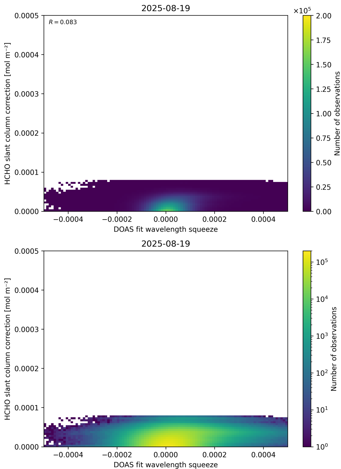
Figure 70: Scatter density plot of “DOAS fit wavelength squeeze” against “HCHO slant column correction” for 2025-08-19 to 2025-08-20.
