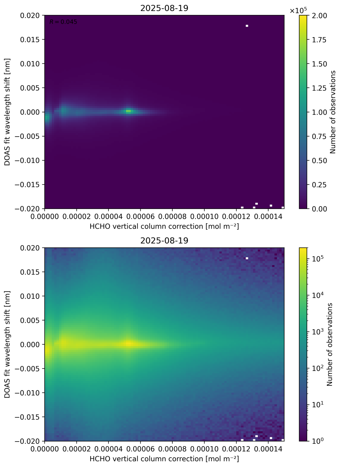
Figure 113: Scatter density plot of “HCHO vertical column correction” against “DOAS fit wavelength shift” for 2025-08-19 to 2025-08-20.
