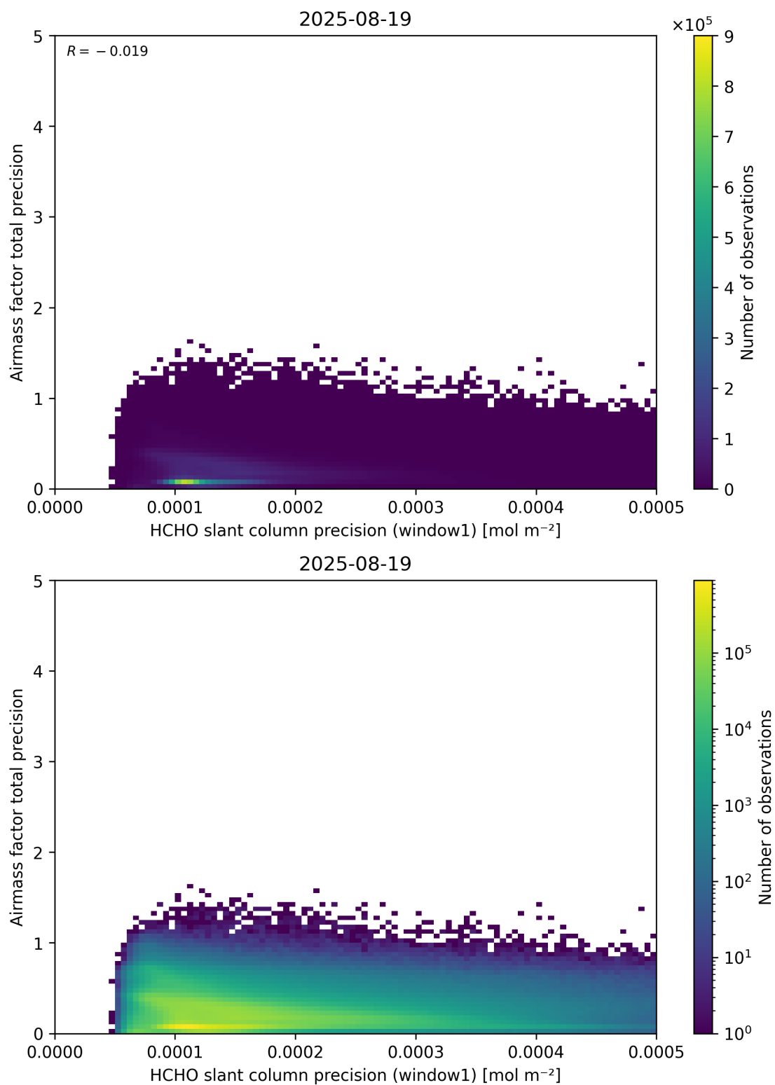
Figure 95: Scatter density plot of “HCHO slant column precision (window1)” against “Airmass factor total precision” for 2025-08-19 to 2025-08-20.
