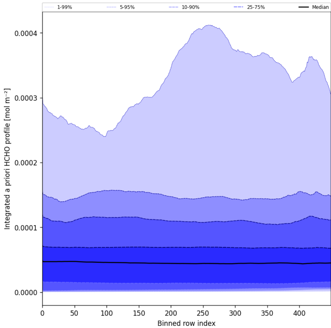
Figure 57: Along track statistics of “Integrated a priori HCHO profile” for 2025-08-19 to 2025-08-20
