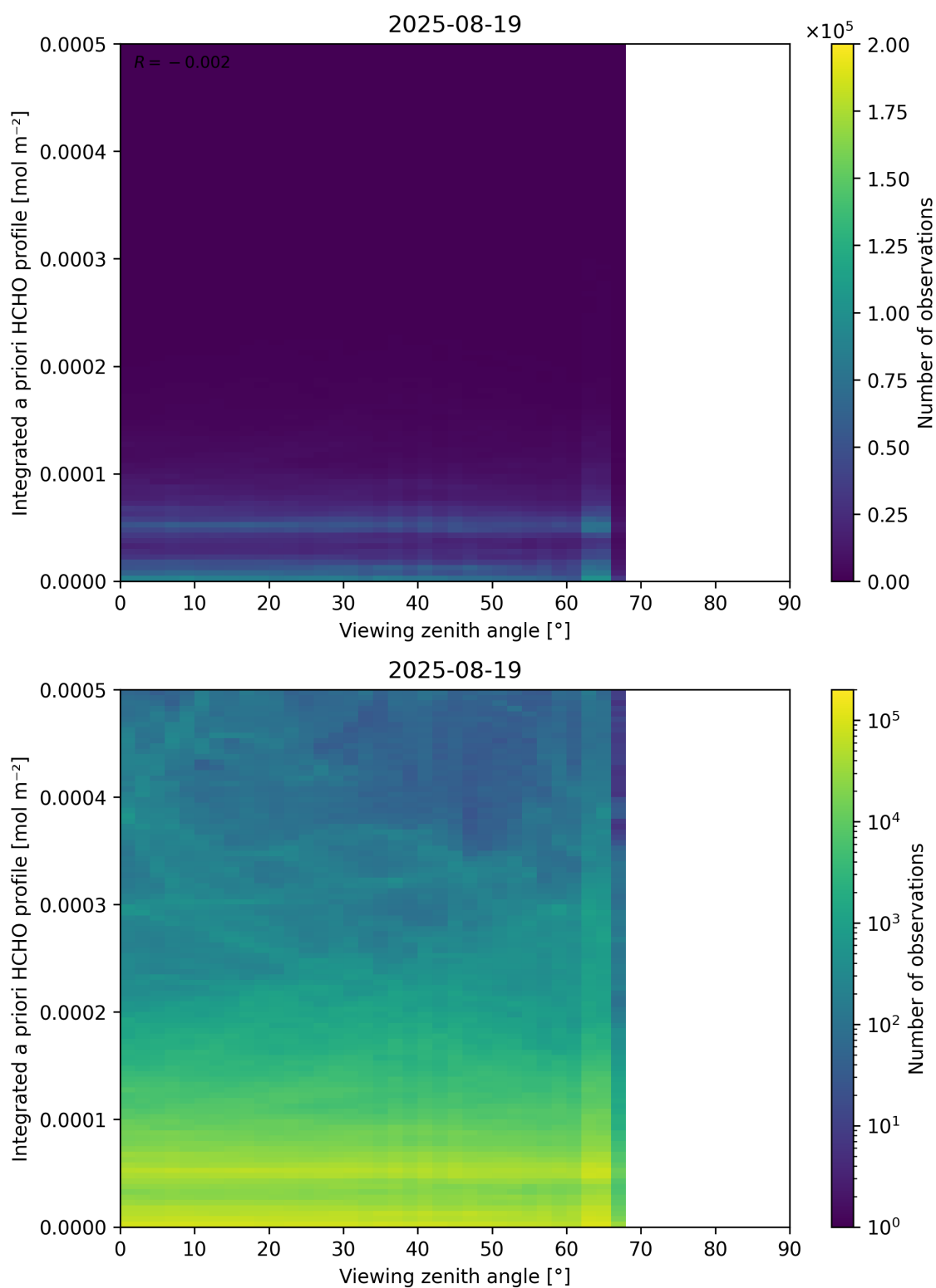
Figure 195: Scatter density plot of “Viewing zenith angle” against “Integrated a priori HCHO profile” for 2025-08-19 to 2025-08-20.
