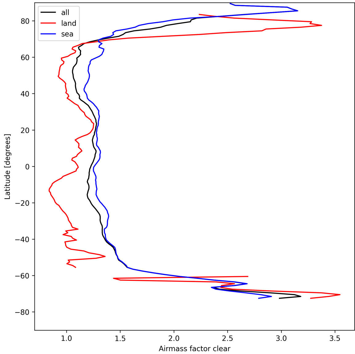
Figure 28: Zonal average of “Airmass factor clear” for 2025-08-19 to 2025-08-20.
