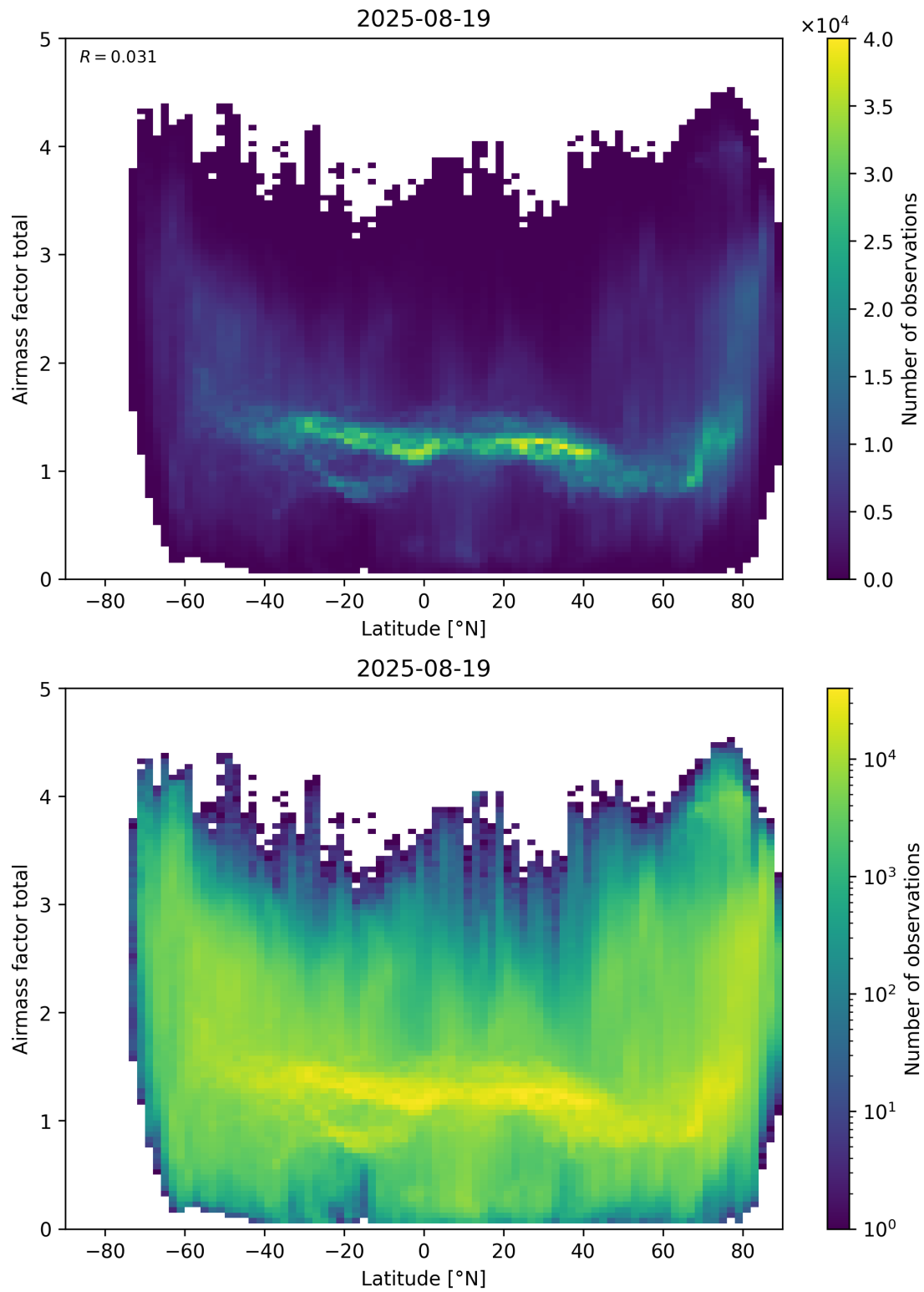
Figure 161: Scatter density plot of “Latitude” against “Airmass factor total” for 2025-08-19 to 2025-08-20.
