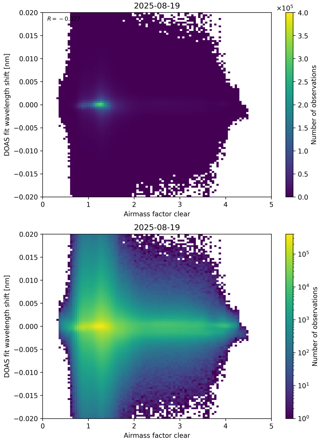
Figure 72: Scatter density plot of “Airmass factor clear” against “DOAS fit wavelength shift” for 2025-08-19 to 2025-08-20.
