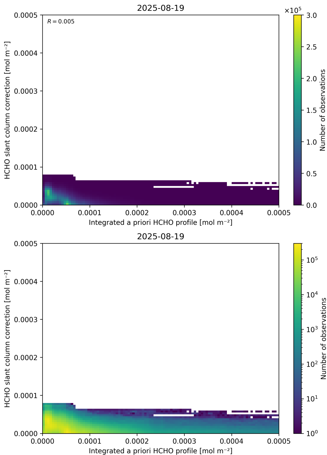
Figure 152: Scatter density plot of “Integrated a priori HCHO profile” against “HCHO slant column correction” for 2025-08-19 to 2025-08-20.
