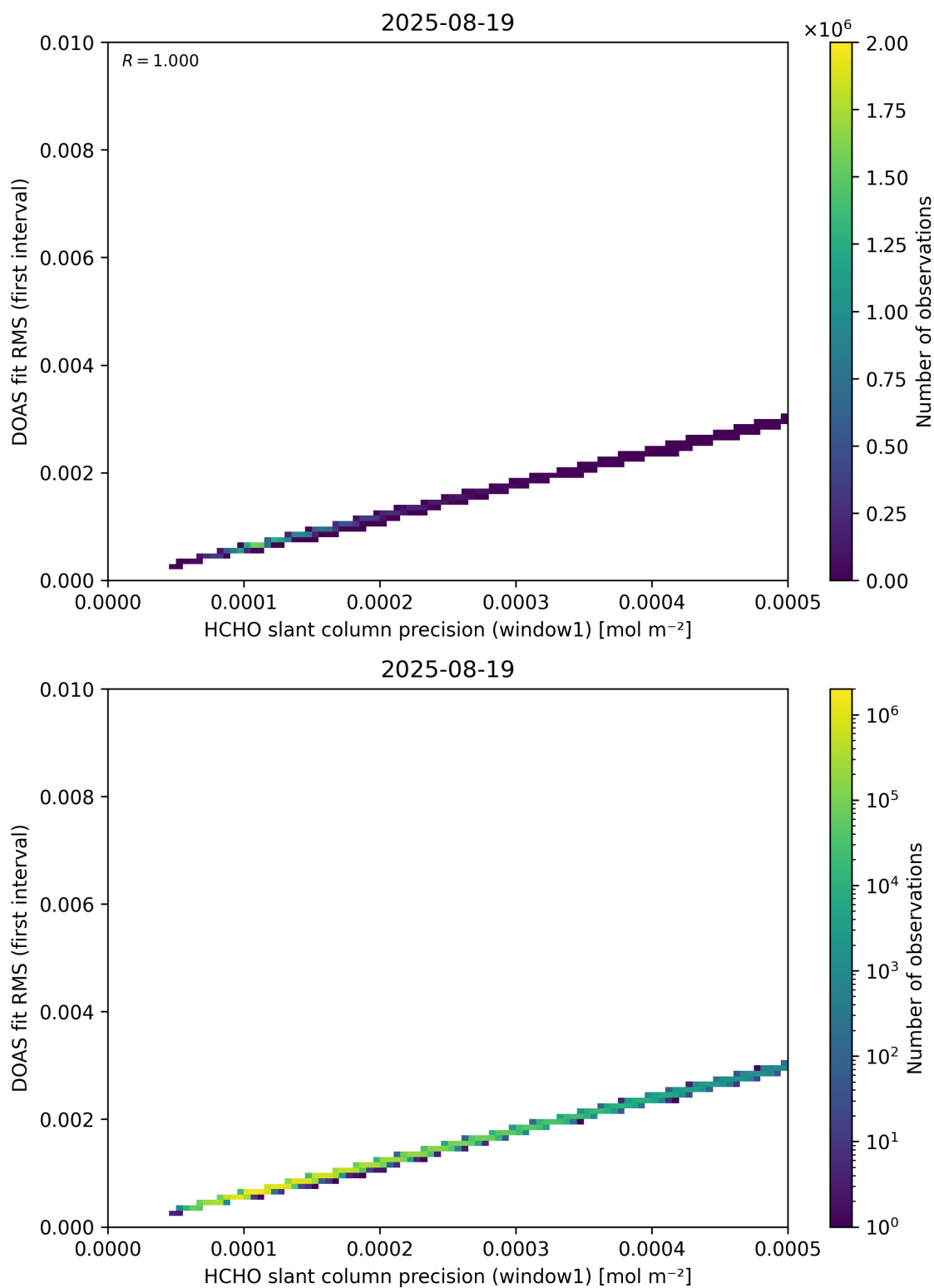
Figure 88: Scatter density plot of “HCHO slant column precision (window1)” against “DOAS fit RMS (first interval)” for 2025-08-19 to 2025-08-20.
