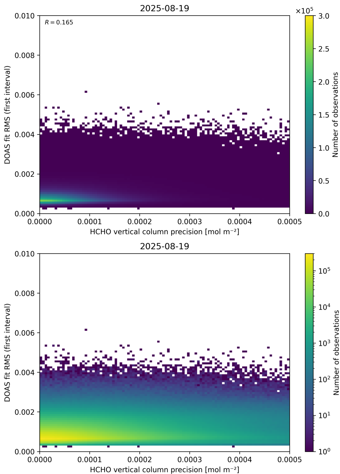
Figure 136: Scatter density plot of “HCHO vertical column precision” against “DOAS fit RMS (first interval)” for 2025-08-19 to 2025-08-20.
