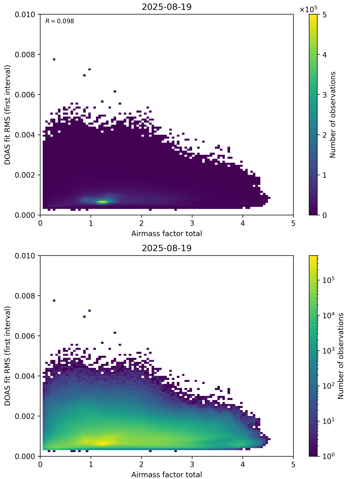
Figure 97: Scatter density plot of “Airmass factor total” against “DOAS fit RMS (first interval)” for 2025-08-19 to 2025-08-20.
