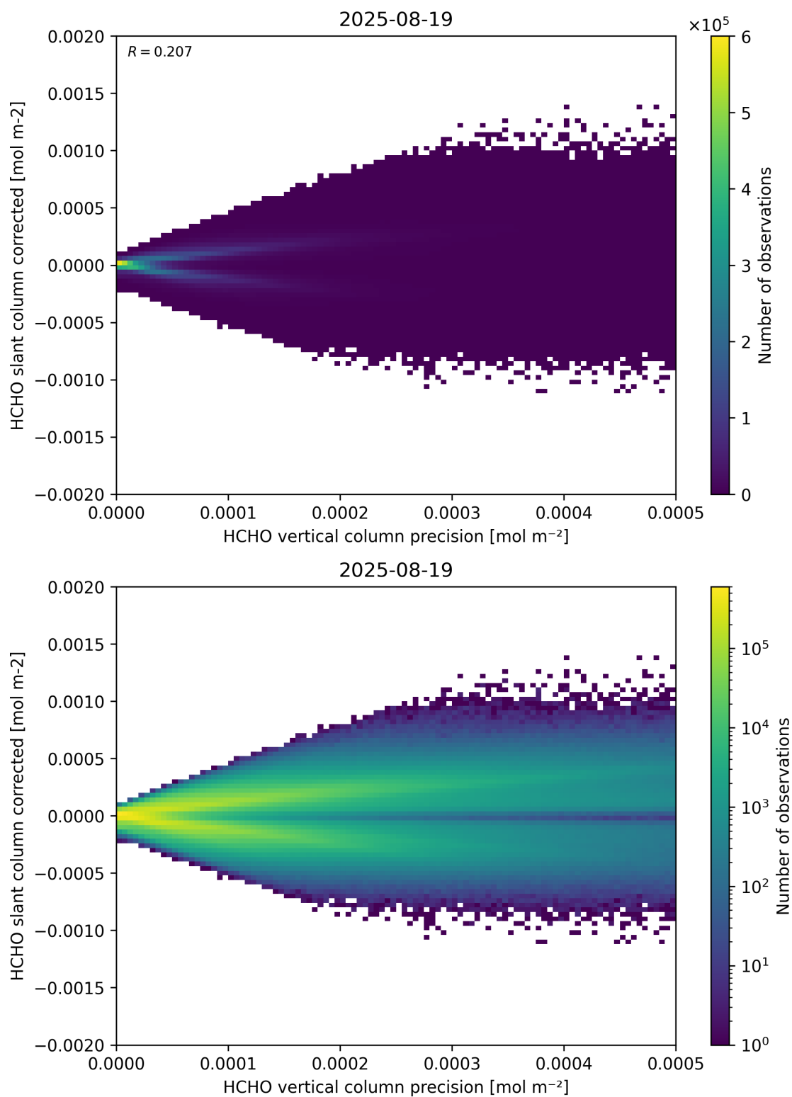
Figure 140: Scatter density plot of “HCHO vertical column precision” against “HCHO slant column corrected” for 2025-08-19 to 2025-08-20.
