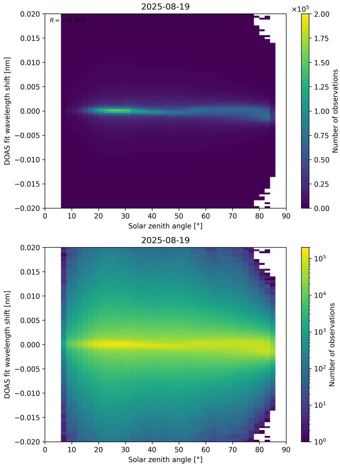
Figure 168: Scatter density plot of “Solar zenith angle” against “DOAS fit wavelength shift” for 2025-08-19 to 2025-08-20.
