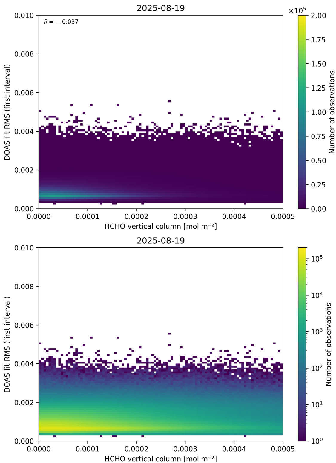
Figure 123: Scatter density plot of “HCHO vertical column” against “DOAS fit RMS (first interval)” for 2025-08-19 to 2025-08-20.
