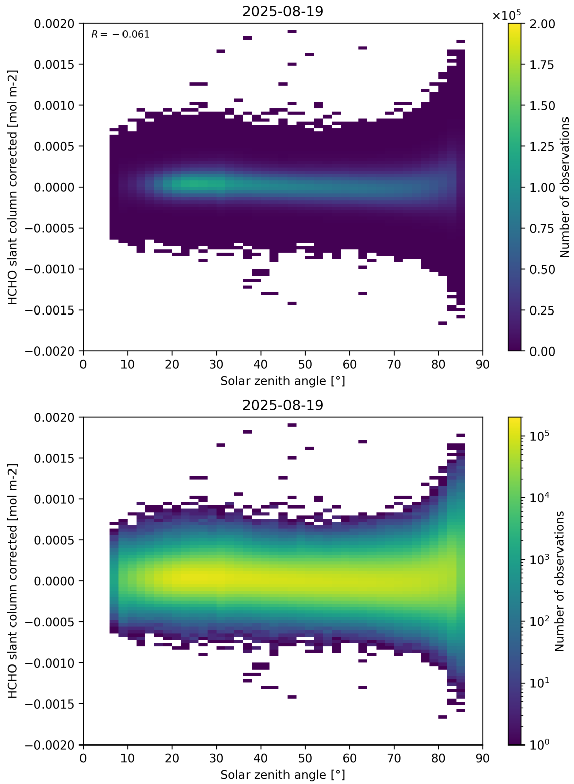
Figure 171: Scatter density plot of “Solar zenith angle” against “HCHO slant column corrected” for 2025-08-19 to 2025-08-20.
