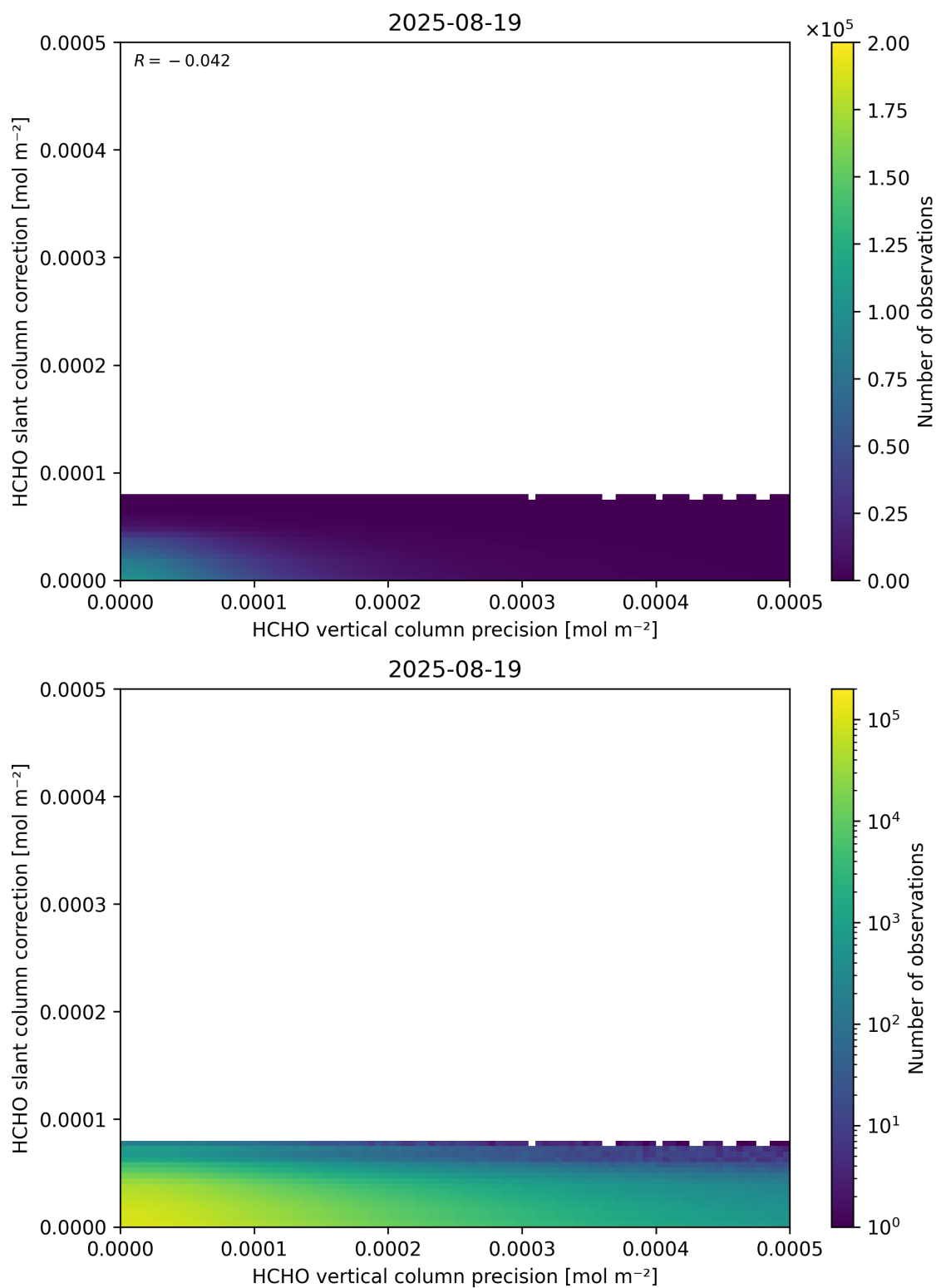
Figure 141: Scatter density plot of “HCHO vertical column precision” against “HCHO slant column correction” for 2025-08-19 to 2025-08-20.
