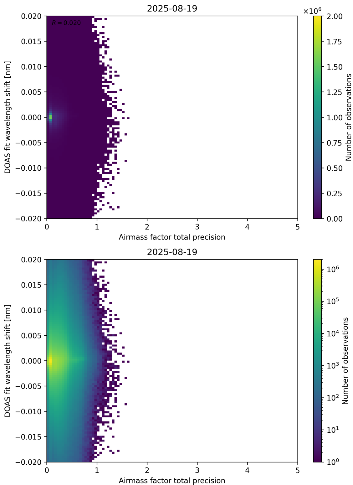
Figure 106: Scatter density plot of “Airmass factor total precision” against “DOAS fit wavelength shift” for 2025-08-19 to 2025-08-20.
