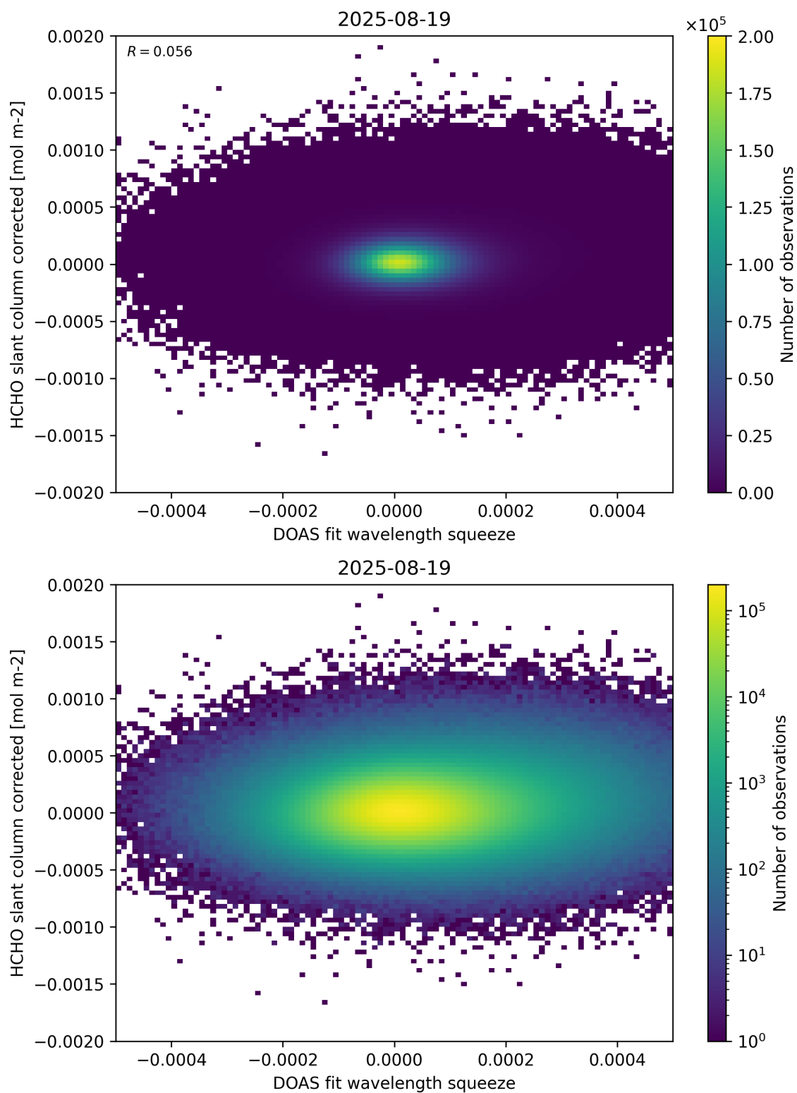
Figure 69: Scatter density plot of “DOAS fit wavelength squeeze” against “HCHO slant column corrected” for 2025-08-19 to 2025-08-20.
