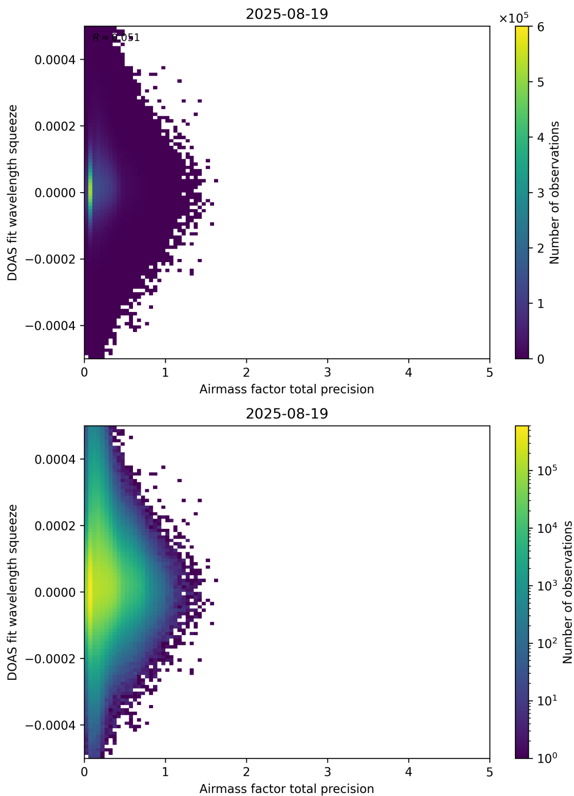
Figure 107: Scatter density plot of “Airmass factor total precision” against “DOAS fit wavelength squeeze” for 2025-08-19 to 2025-08-20.
