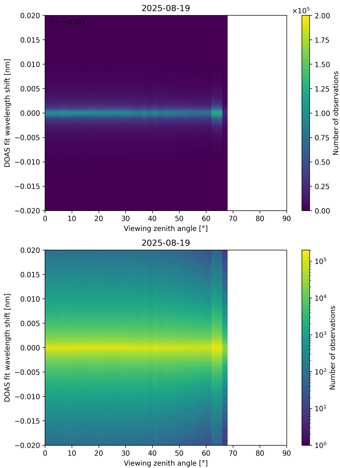
Figure 183: Scatter density plot of “Viewing zenith angle” against “DOAS fit wavelength shift” for 2025-08-19 to 2025-08-20.
