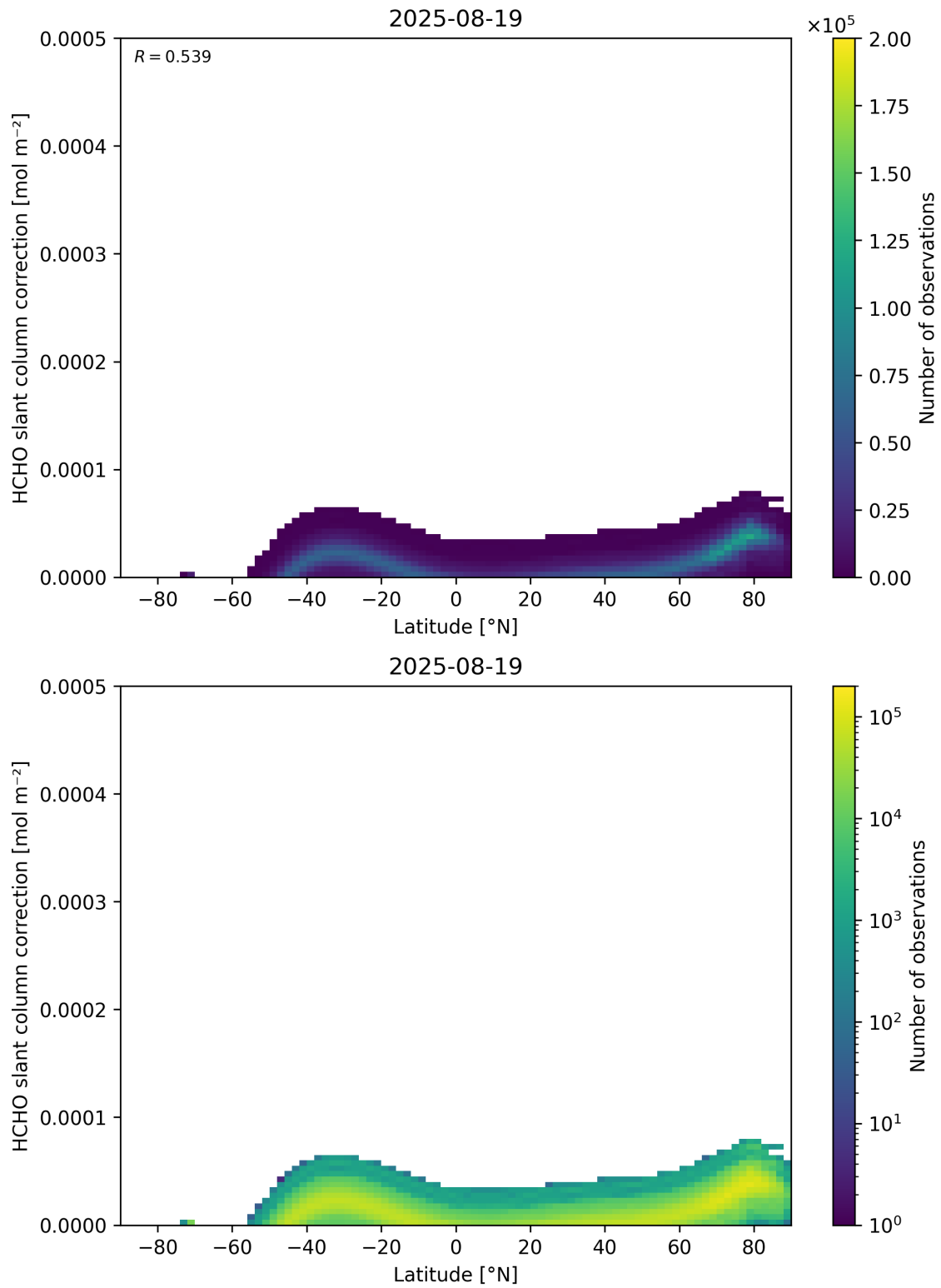
Figure 158: Scatter density plot of “Latitude” against “HCHO slant column correction” for 2025-08-19 to 2025-08-20.
