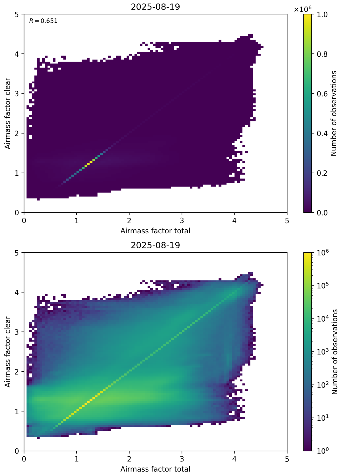
Figure 100: Scatter density plot of “Airmass factor total” against “Airmass factor clear” for 2025-08-19 to 2025-08-20.
