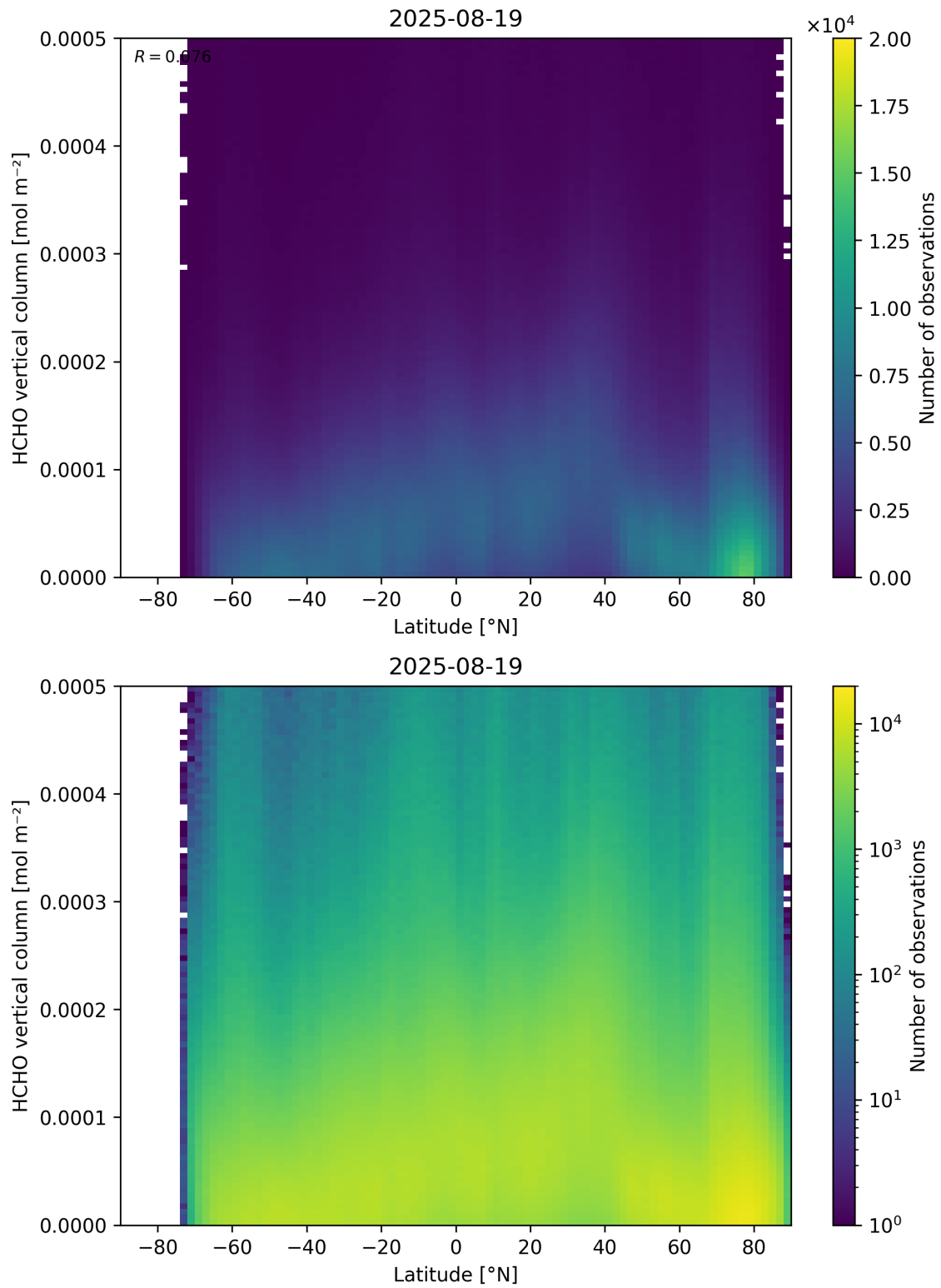
Figure 163: Scatter density plot of “Latitude” against “HCHO vertical column” for 2025-08-19 to 2025-08-20.
