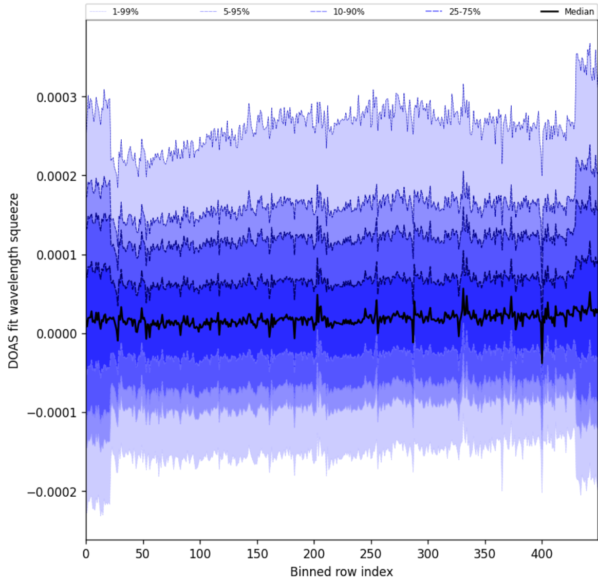
Figure 59: Along track statistics of “DOAS fit wavelength squeeze” for 2025-08-19 to 2025-08-20
