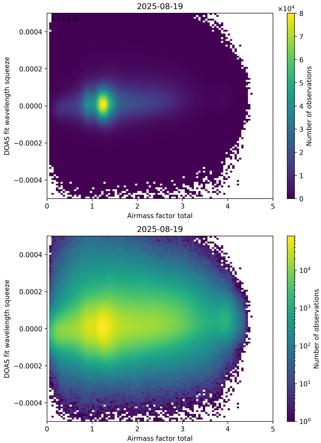
Figure 99: Scatter density plot of “Airmass factor total” against “DOAS fit wavelength squeeze” for 2025-08-19 to 2025-08-20.
