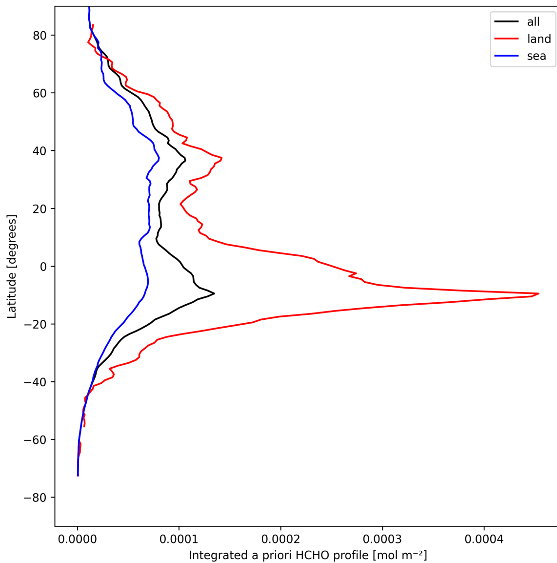
Figure 29: Zonal average of “Integrated a priori HCHO profile” for 2025-08-19 to 2025-08-20.
