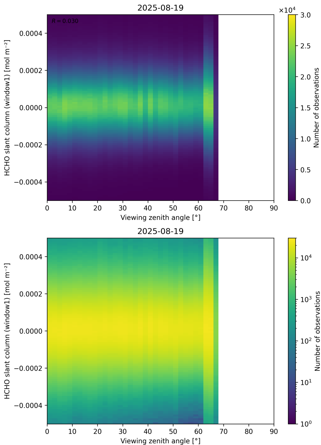
Figure 188: Scatter density plot of “Viewing zenith angle” against “HCHO slant column (window1)” for 2025-08-19 to 2025-08-20.
