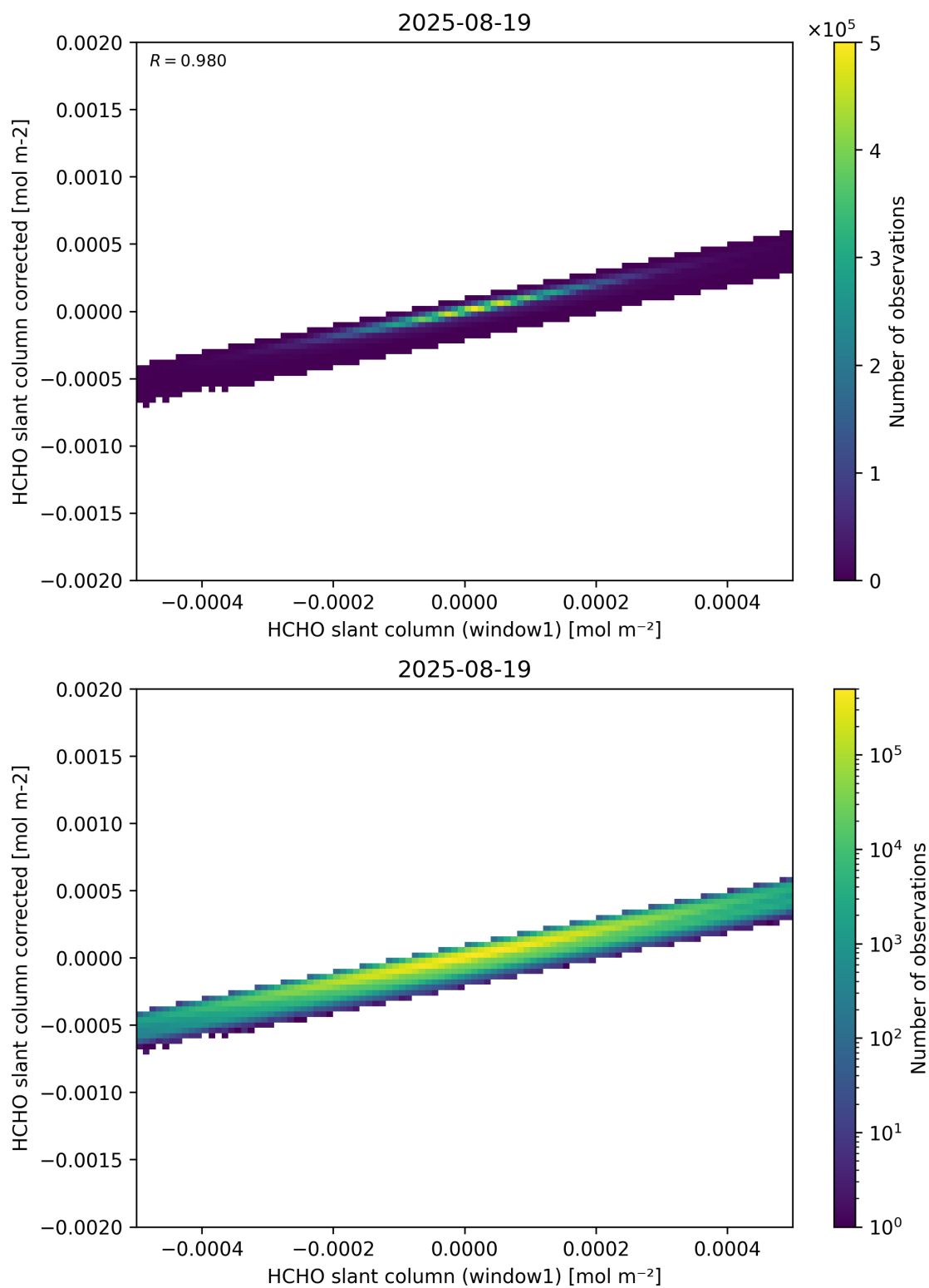
Figure 82: Scatter density plot of “HCHO slant column (window1)” against “HCHO slant column corrected” for 2025-08-19 to 2025-08-20.
