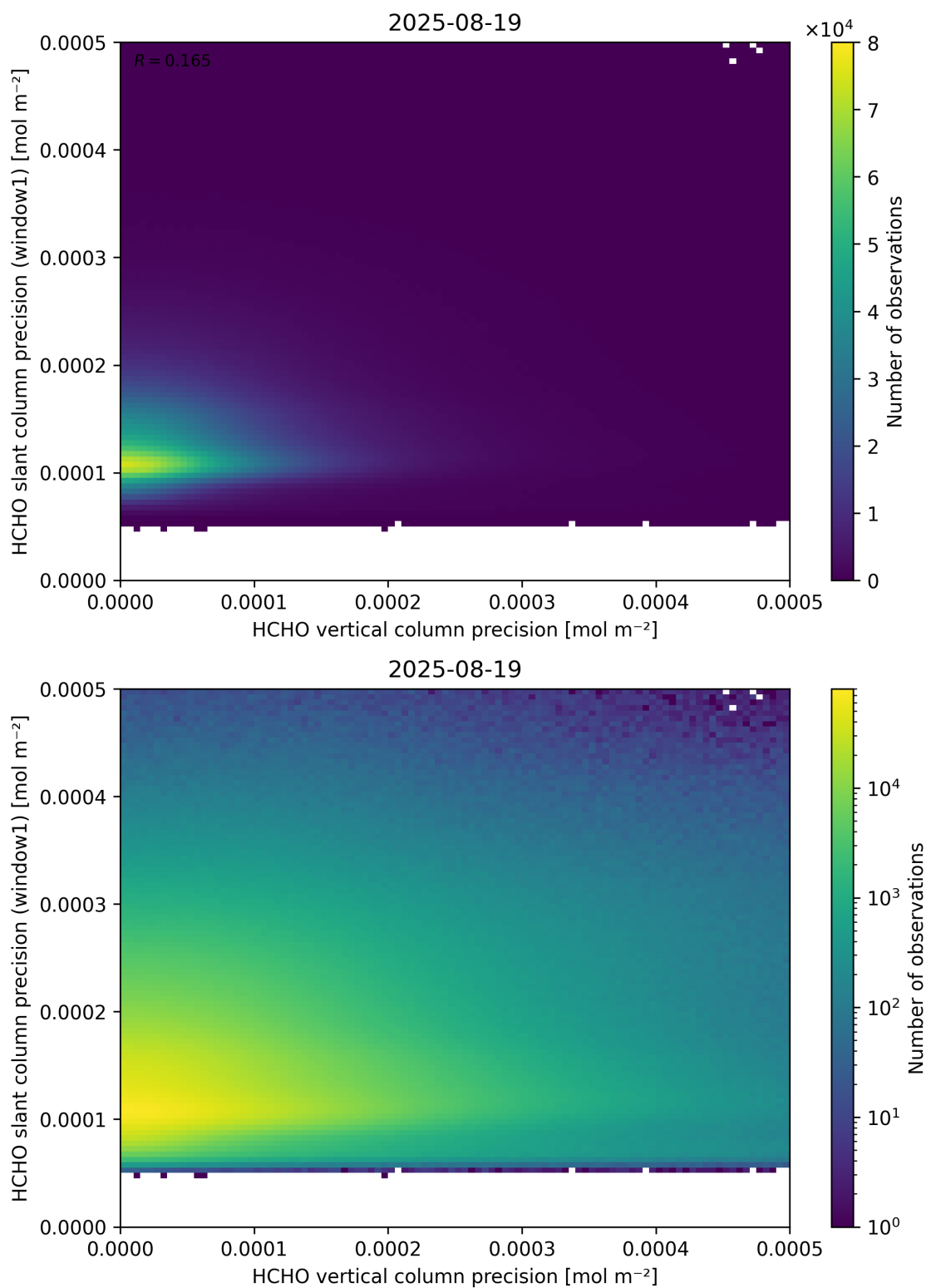
Figure 143: Scatter density plot of “HCHO vertical column precision” against “HCHO slant column precision (window1)” for 2025-08-19 to 2025-08-20.
