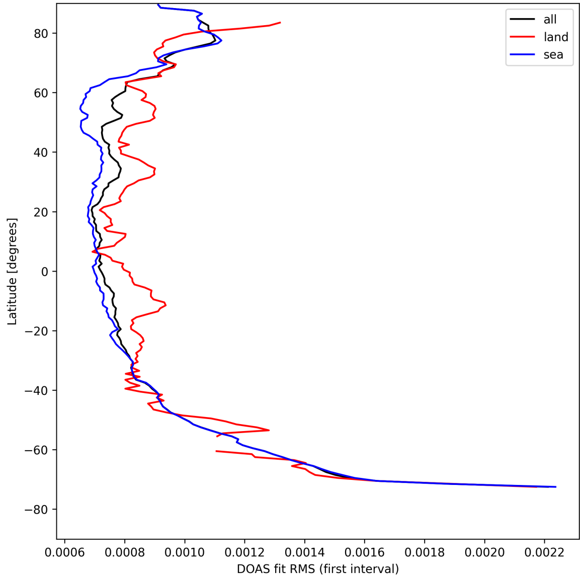
Figure 32: Zonal average of “DOAS fit RMS (first interval)” for 2025-08-19 to 2025-08-20.
