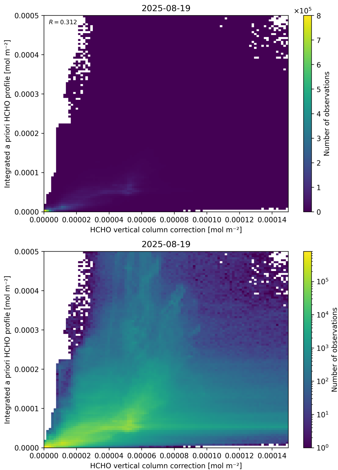
Figure 122: Scatter density plot of “HCHO vertical column correction” against “Integrated a priori HCHO profile” for 2025-08-19 to 2025-08-20.
