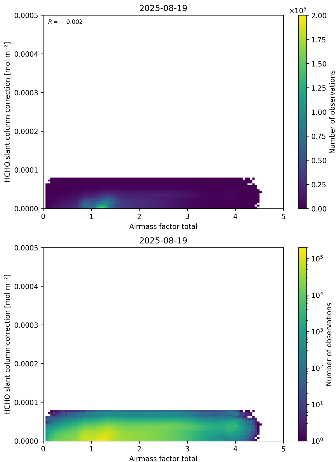
Figure 102: Scatter density plot of “Airmass factor total” against “HCHO slant column correction” for 2025-08-19 to 2025-08-20.
