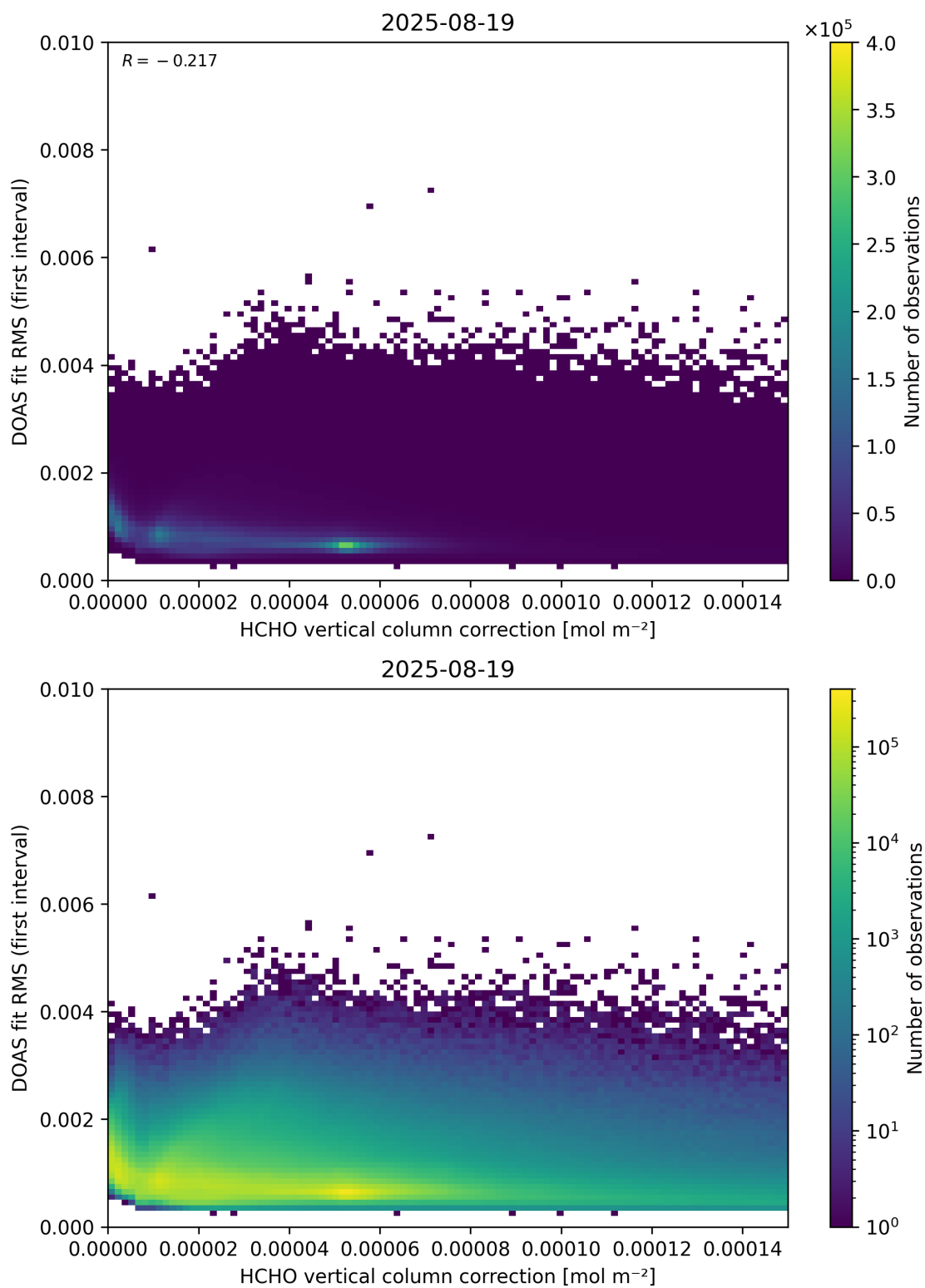
Figure 112: Scatter density plot of “HCHO vertical column correction” against “DOAS fit RMS (first interval)” for 2025-08-19 to 2025-08-20.
