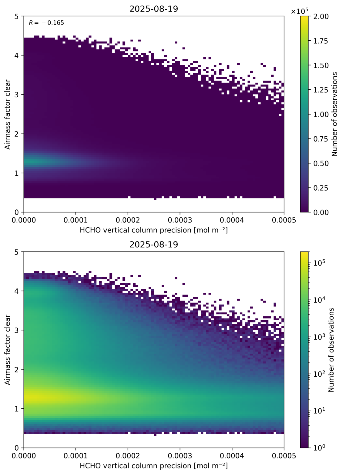
Figure 139: Scatter density plot of “HCHO vertical column precision” against “Airmass factor clear” for 2025-08-19 to 2025-08-20.
