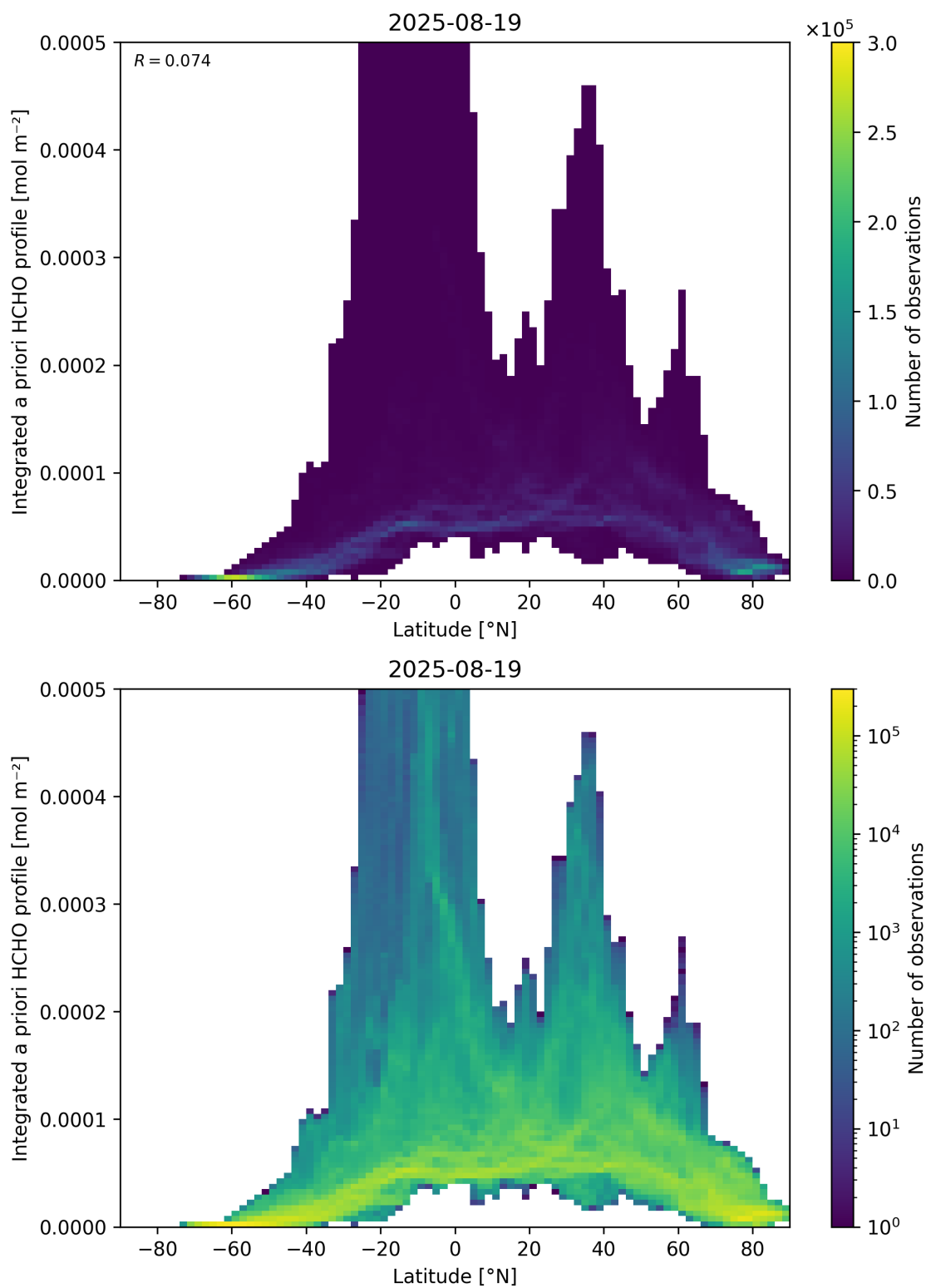
Figure 166: Scatter density plot of “Latitude” against “Integrated a priori HCHO profile” for 2025-08-19 to 2025-08-20.
