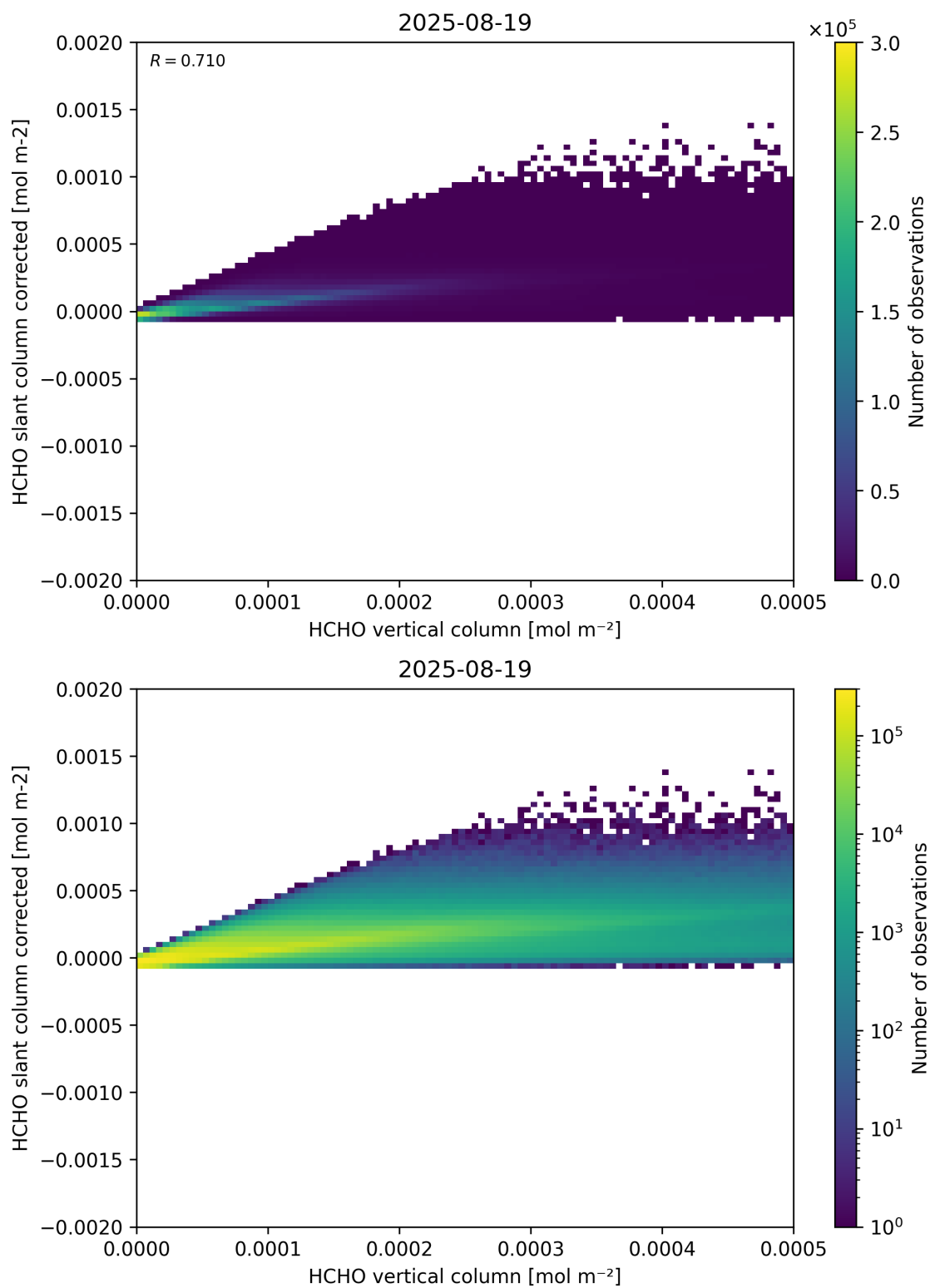
Figure 127: Scatter density plot of “HCHO vertical column” against “HCHO slant column corrected” for 2025-08-19 to 2025-08-20.
