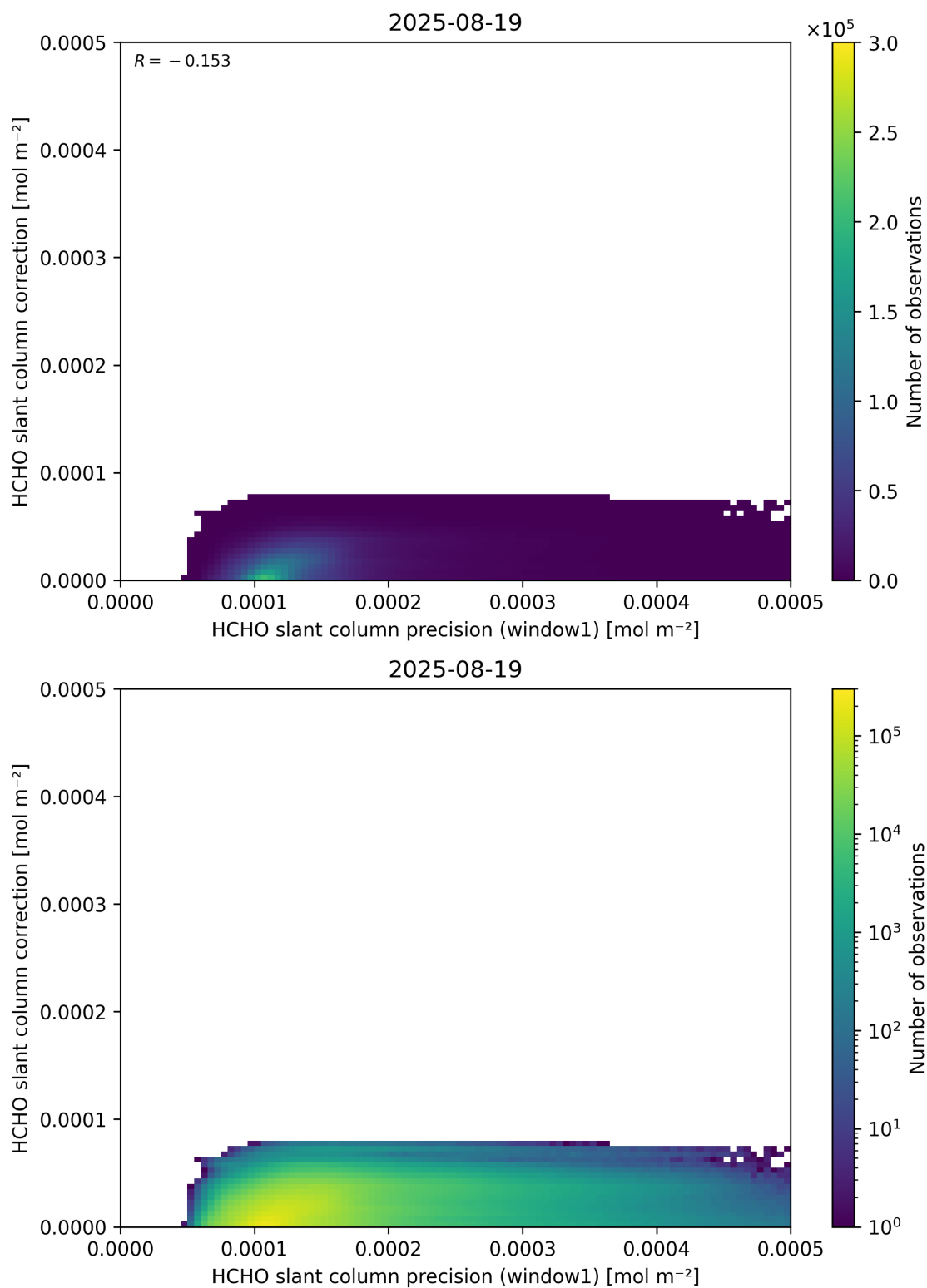
Figure 93: Scatter density plot of “HCHO slant column precision (window1)” against “HCHO slant column correction” for 2025-08-19 to 2025-08-20.
