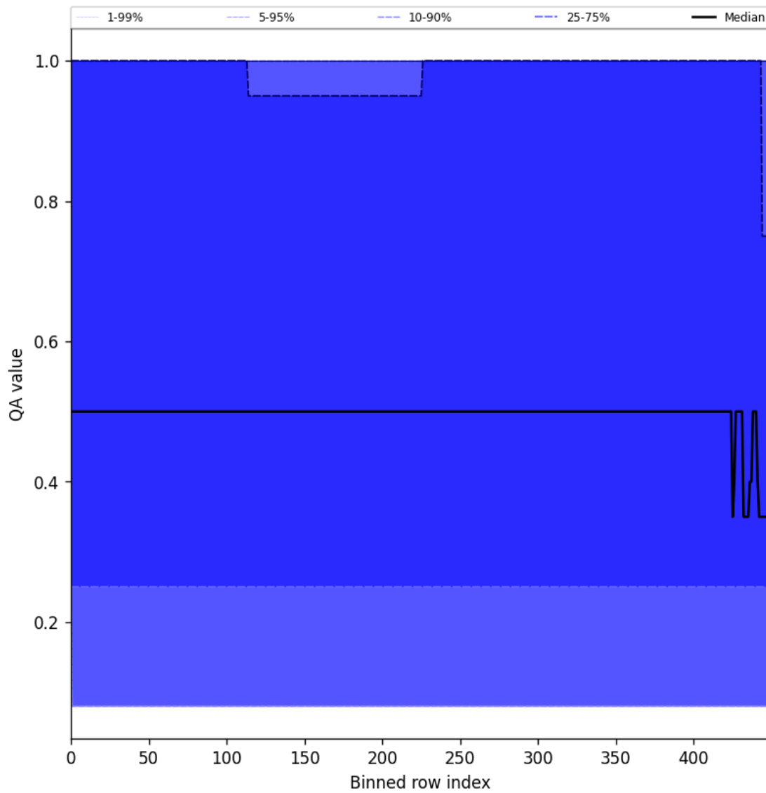
Figure 48: Along track statistics of “QA value” for 2025-08-19 to 2025-08-20
