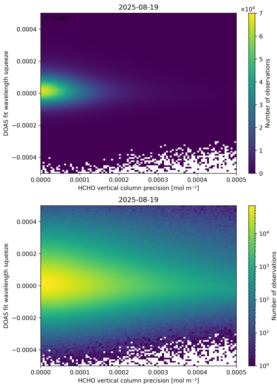
Figure 138: Scatter density plot of “HCHO vertical column precision” against “DOAS fit wavelength squeeze” for 2025-08-19 to 2025-08-20.
