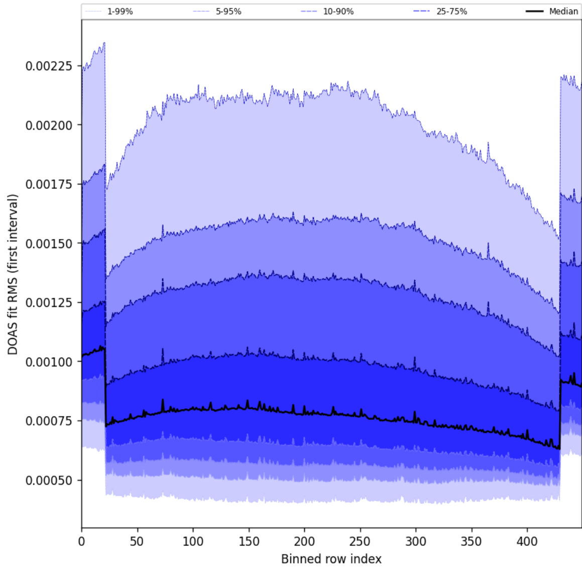
Figure 60: Along track statistics of “DOAS fit RMS (first interval)” for 2025-08-19 to 2025-08-20
