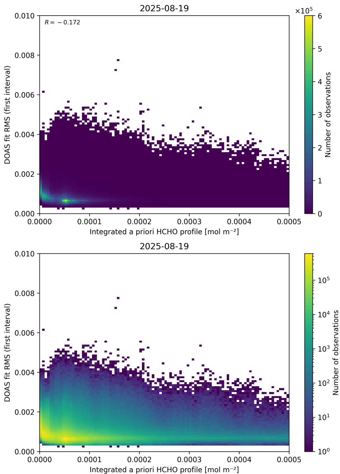
Figure 148: Scatter density plot of “Integrated a priori HCHO profile” against “DOAS fit RMS (first interval)” for 2025-08-19 to 2025-08-20.
