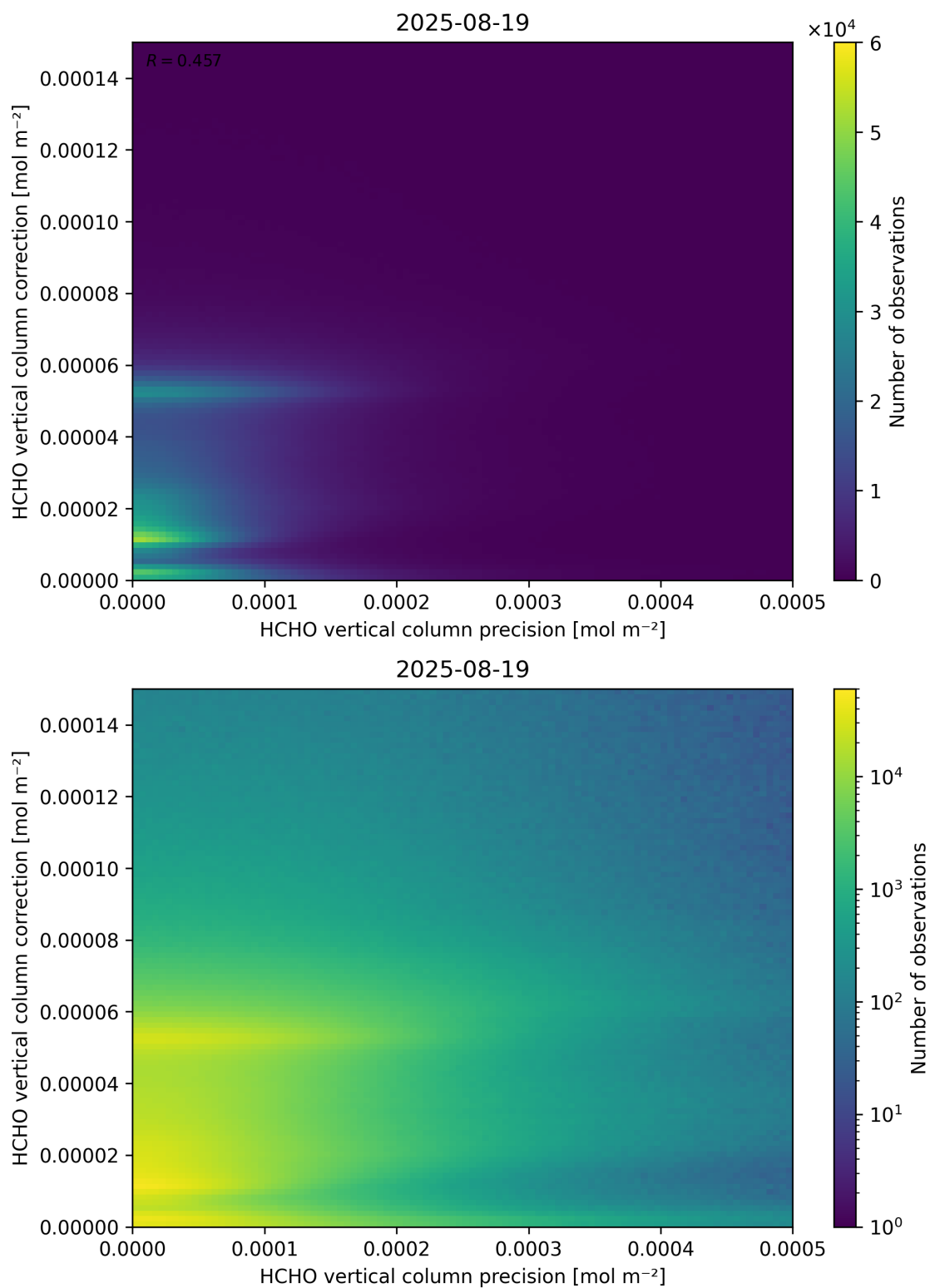
Figure 146: Scatter density plot of “HCHO vertical column precision” against “HCHO vertical column correction” for 2025-08-19 to 2025-08-20.
