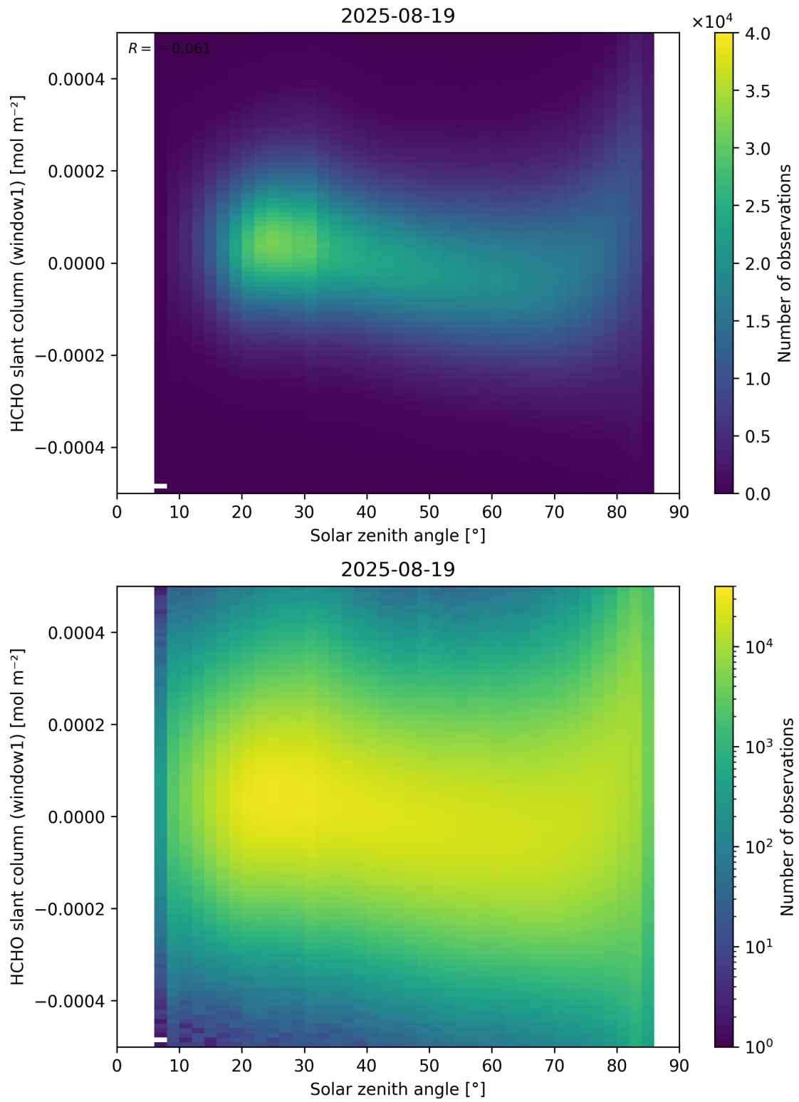
Figure 173: Scatter density plot of “Solar zenith angle” against “HCHO slant column (window1)” for 2025-08-19 to 2025-08-20.
