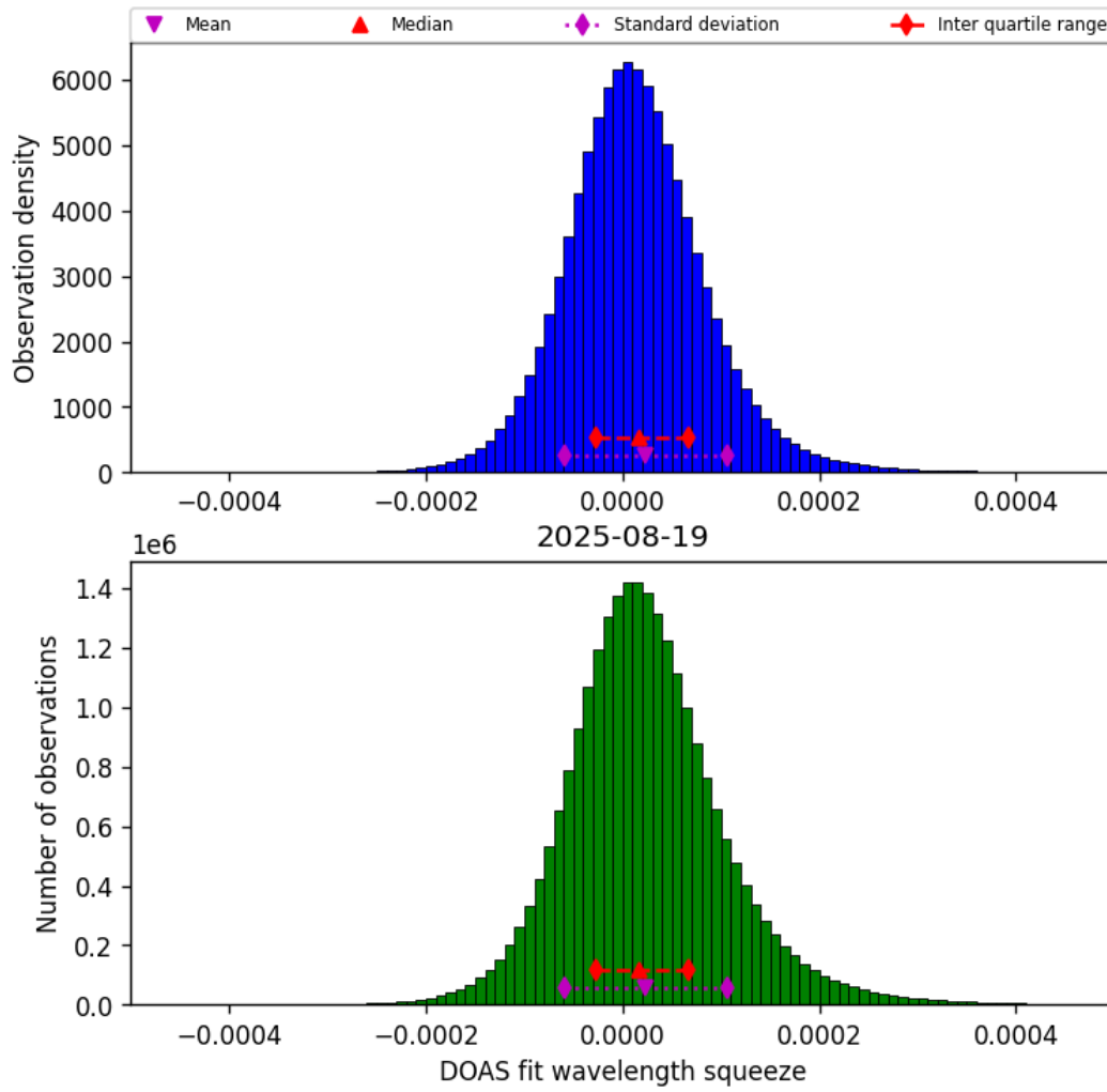
Figure 45: Histogram of “DOAS fit wavelength squeeze” for 2025-08-19 to 2025-08-20
