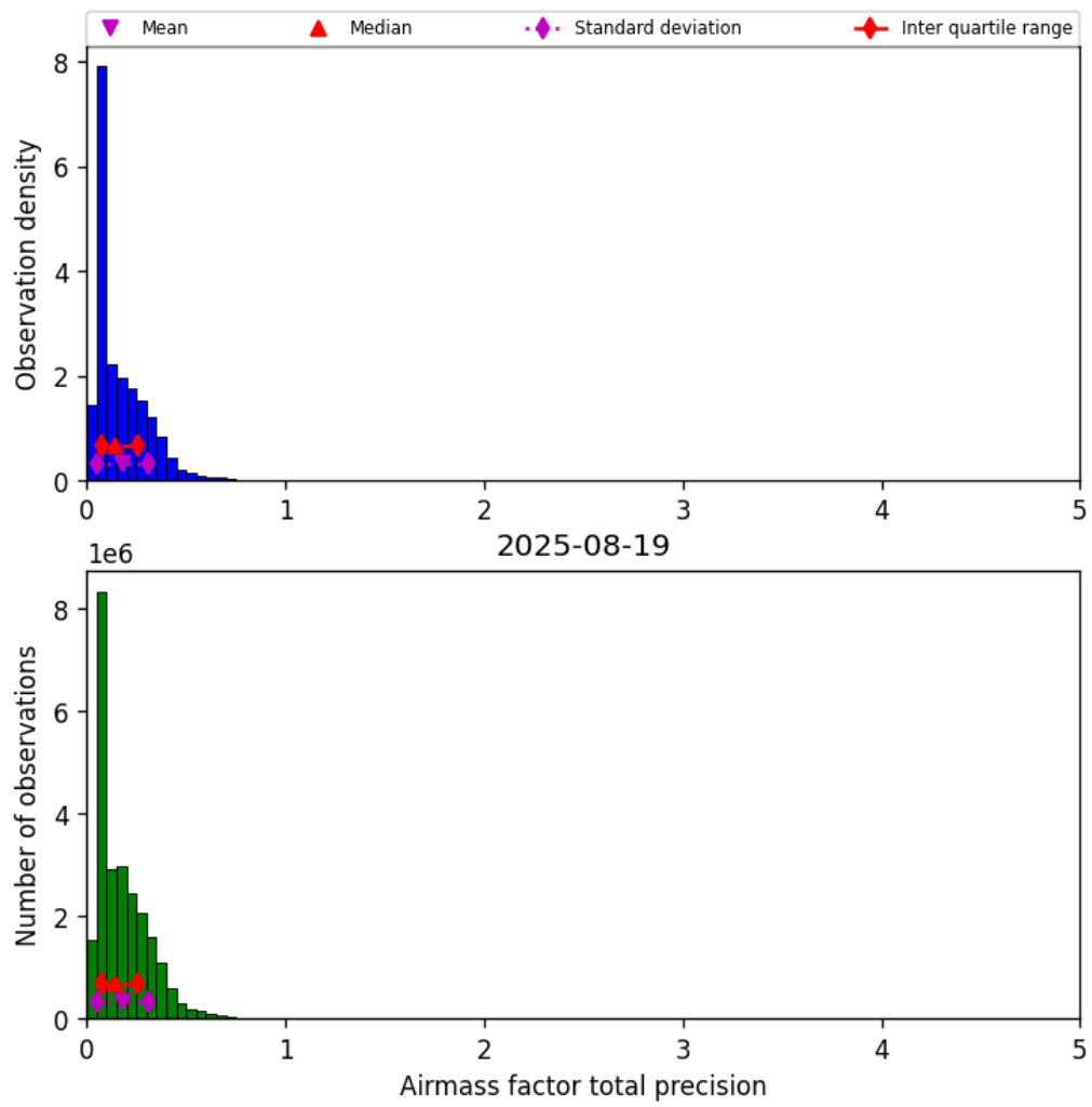
Figure 41: Histogram of “Airmass factor total precision” for 2025-08-19 to 2025-08-20
