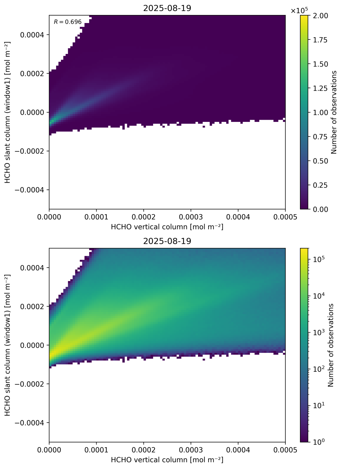
Figure 129: Scatter density plot of “HCHO vertical column” against “HCHO slant column (window1)” for 2025-08-19 to 2025-08-20.
