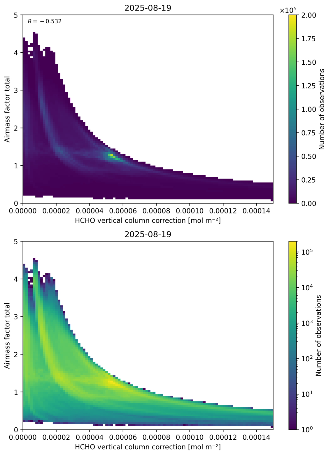
Figure 120: Scatter density plot of “HCHO vertical column correction” against “Airmass factor total” for 2025-08-19 to 2025-08-20.
