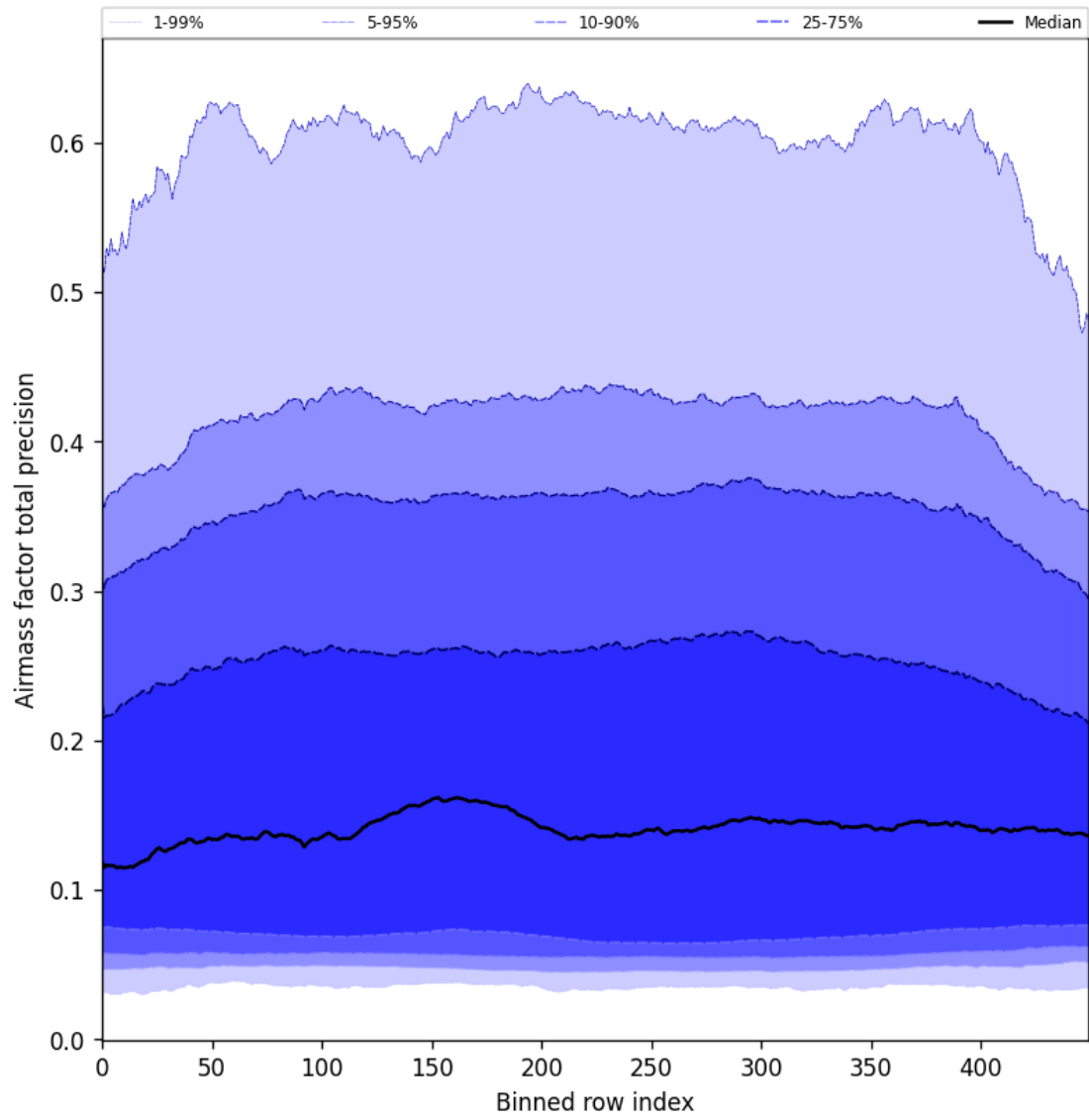
Figure 55: Along track statistics of “Airmass factor total precision” for 2025-08-19 to 2025-08-20
