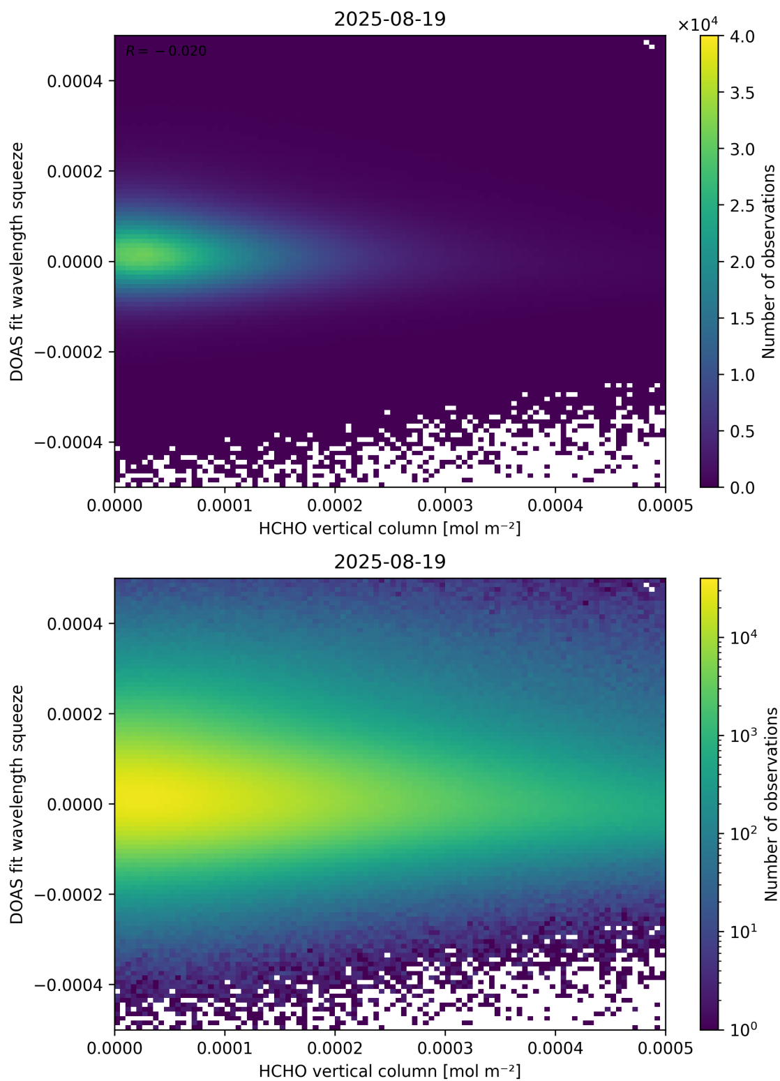
Figure 125: Scatter density plot of “HCHO vertical column” against “DOAS fit wavelength squeeze” for 2025-08-19 to 2025-08-20.
