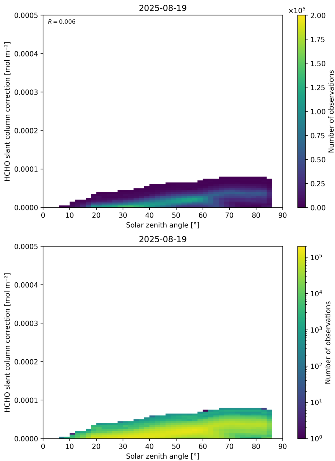
Figure 172: Scatter density plot of “Solar zenith angle” against “HCHO slant column correction” for 2025-08-19 to 2025-08-20.
