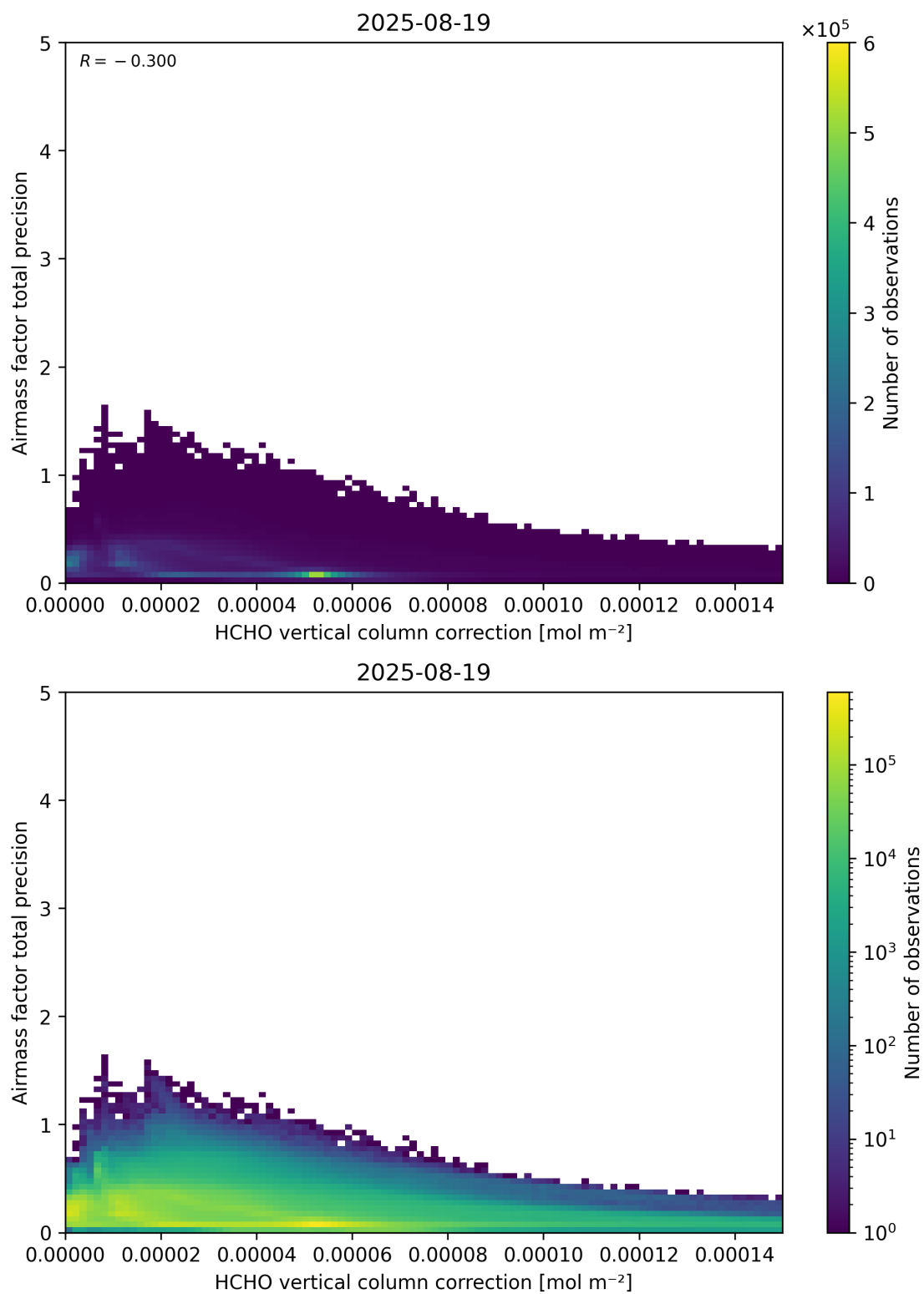
Figure 121: Scatter density plot of “HCHO vertical column correction” against “Airmass factor total precision” for 2025-08-19 to 2025-08-20.
