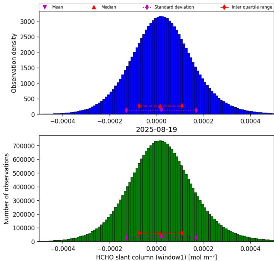
Figure 38: Histogram of "HCHO slant column (window1)" for 2025-08-19 to 2025-08-20
