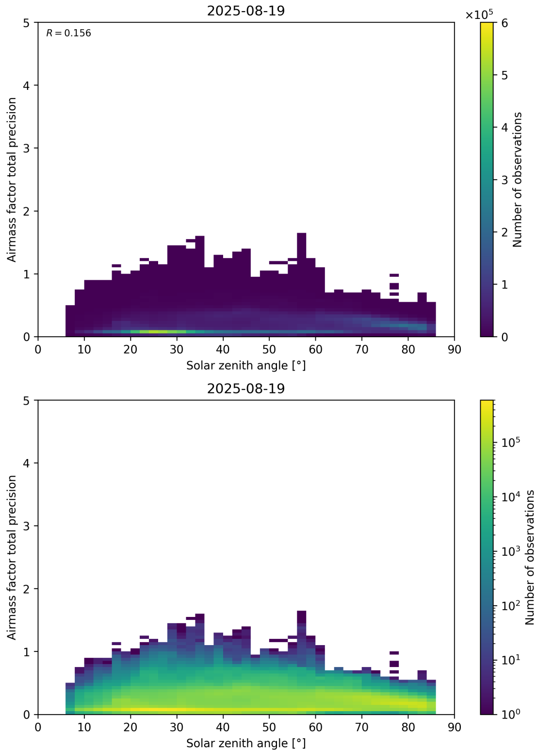
Figure 176: Scatter density plot of “Solar zenith angle” against “Airmass factor total precision” for 2025-08-19 to 2025-08-20.
