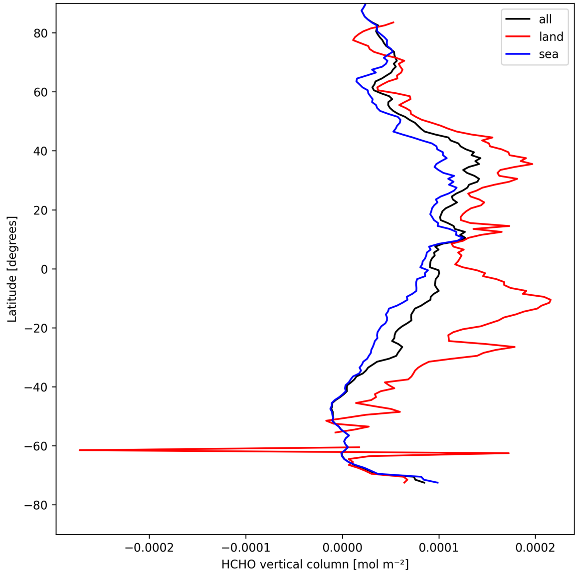
Figure 21: Zonal average of “HCHO vertical column” for 2025-08-19 to 2025-08-20.
