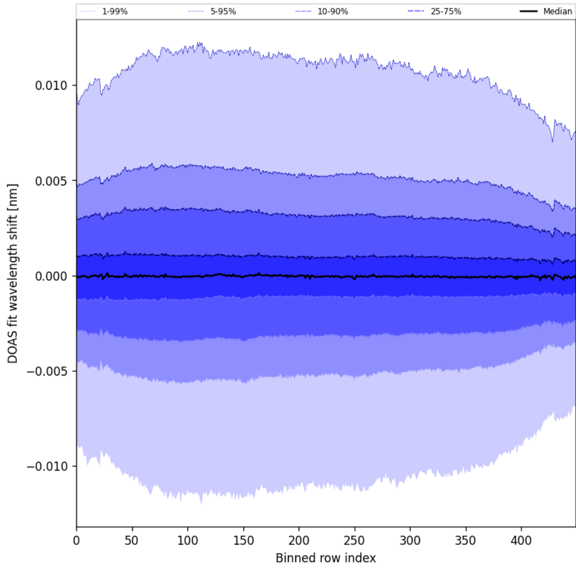
Figure 58: Along track statistics of “DOAS fit wavelength shift” for 2025-08-19 to 2025-08-20
