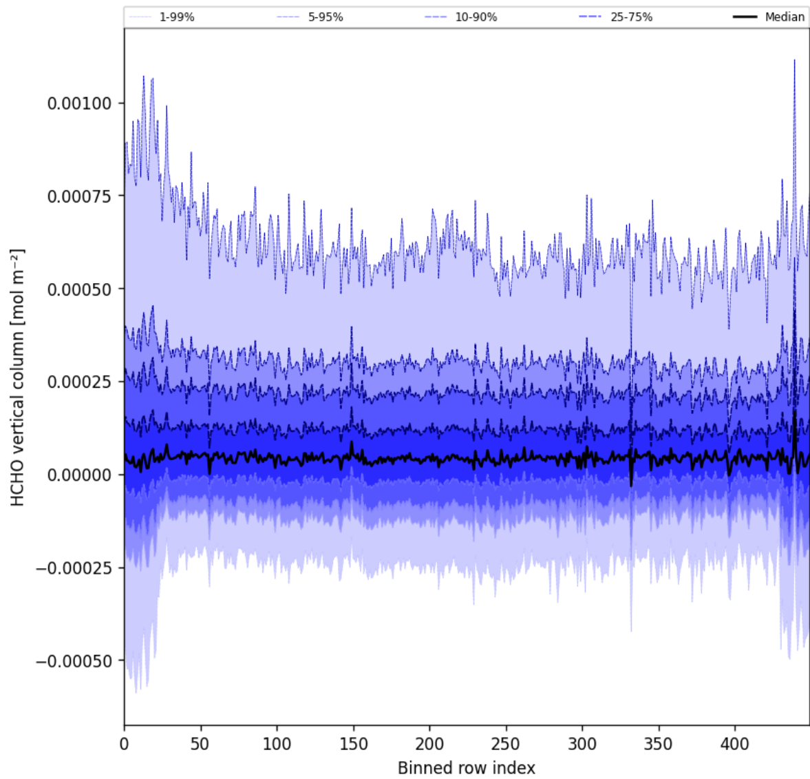
Figure 49: Along track statistics of “HCHO vertical column” for 2025-08-19 to 2025-08-20
