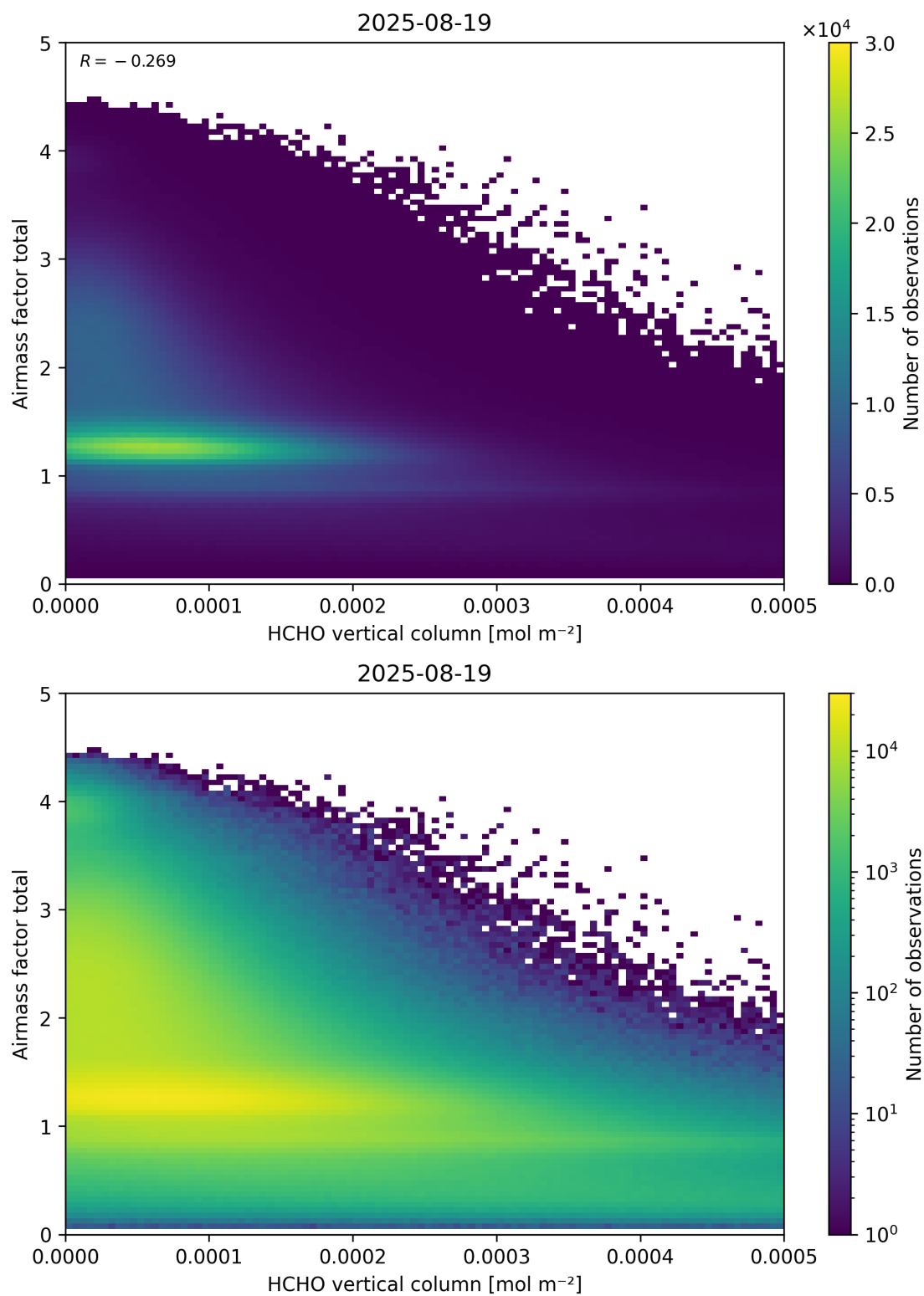
Figure 131: Scatter density plot of “HCHO vertical column” against “Airmass factor total” for 2025-08-19 to 2025-08-20.
