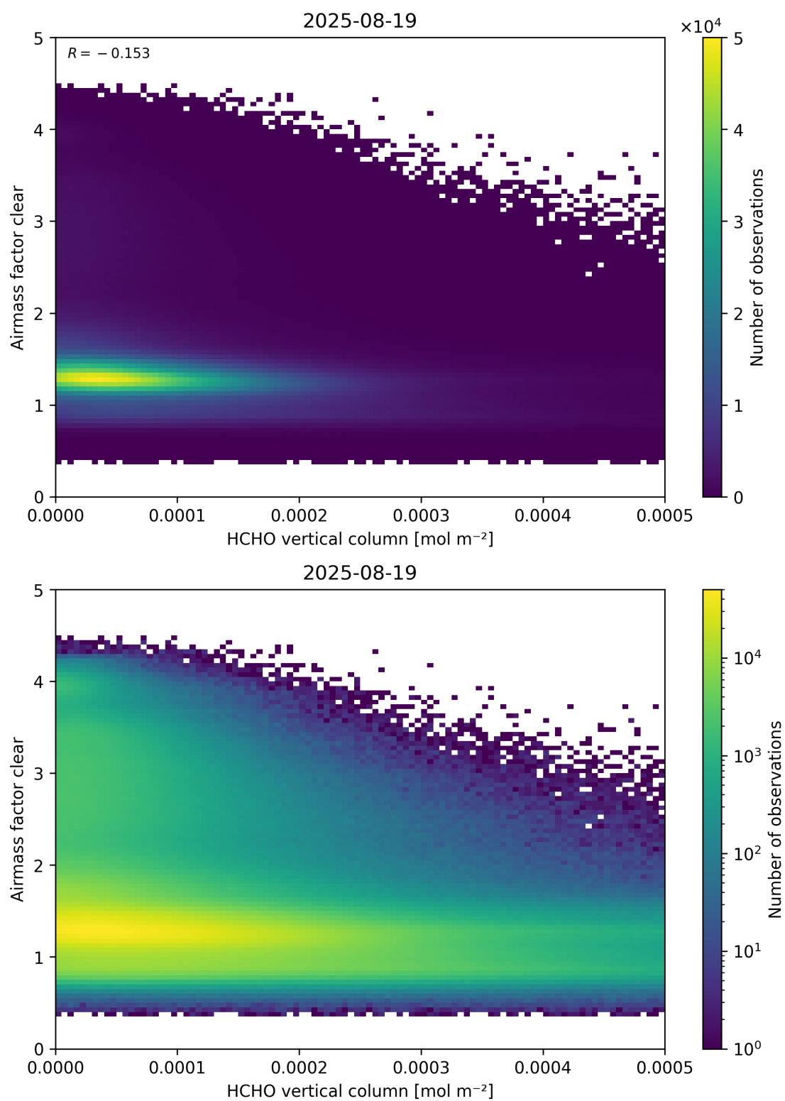
Figure 126: Scatter density plot of “HCHO vertical column” against “Airmass factor clear” for 2025-08-19 to 2025-08-20.
