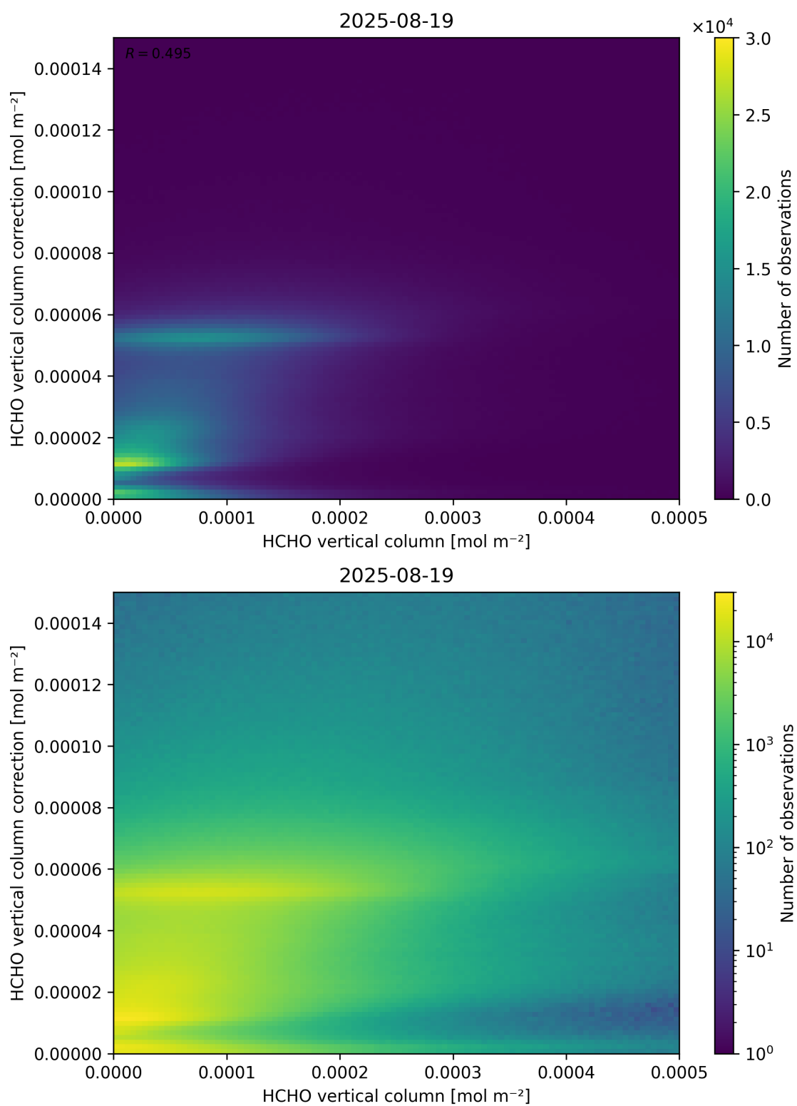
Figure 133: Scatter density plot of “HCHO vertical column” against “HCHO vertical column correction” for 2025-08-19 to 2025-08-20.
