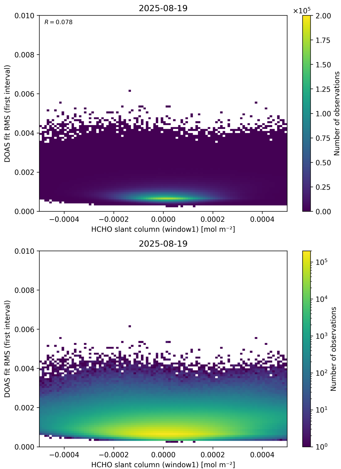
Figure 78: Scatter density plot of “HCHO slant column (window1)” against “DOAS fit RMS (first interval)” for 2025-08-19 to 2025-08-20.
