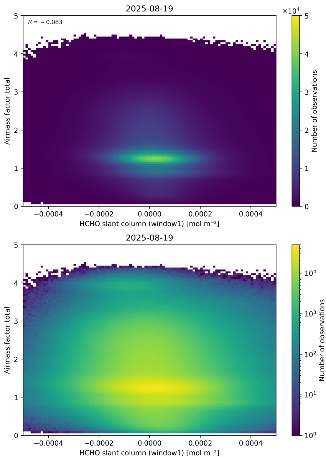
Figure 85: Scatter density plot of “HCHO slant column (window1)” against “Airmass factor total” for 2025-08-19 to 2025-08-20.
