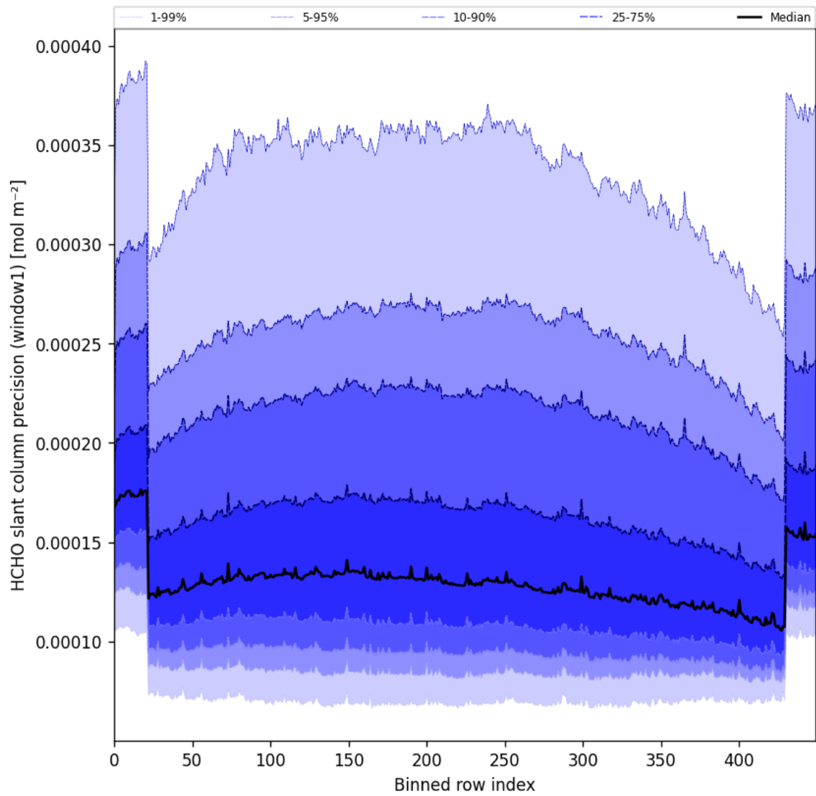
Figure 53: Along track statistics of “HCHO slant column precision (window1)” for 2025-08-19 to 2025-08-20
