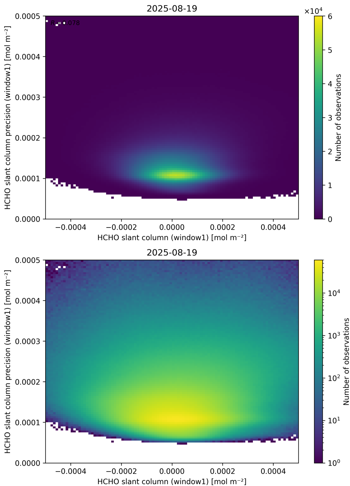
Figure 84: Scatter density plot of “HCHO slant column (window1)” against “HCHO slant column precision (window1)” for 2025-08-19 to 2025-08-20.
