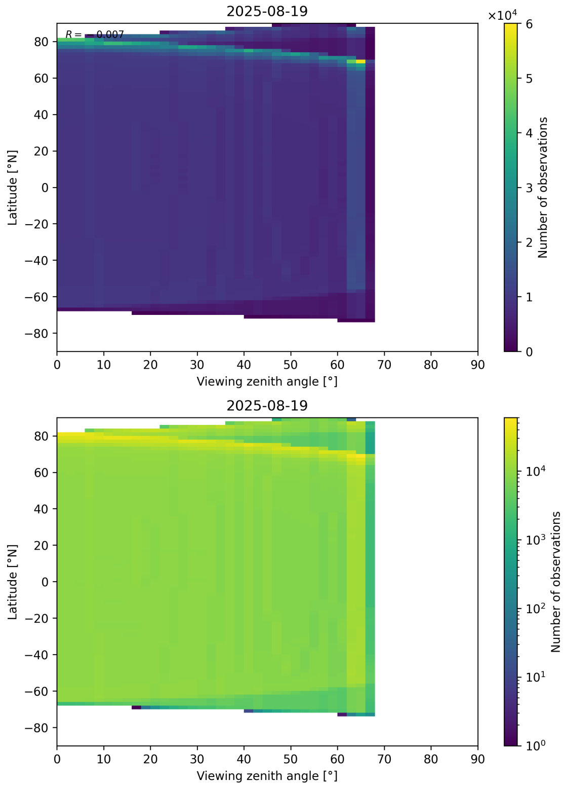
Figure 196: Scatter density plot of “Viewing zenith angle” against “Latitude” for 2025-08-19 to 2025-08-20.
