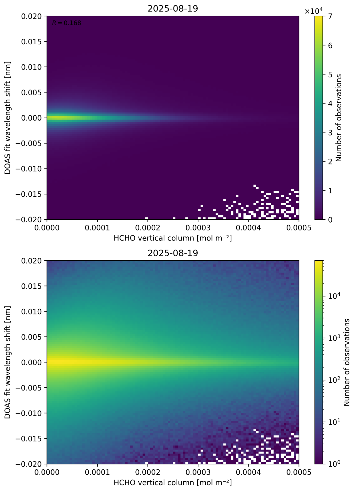
Figure 124: Scatter density plot of “HCHO vertical column” against “DOAS fit wavelength shift” for 2025-08-19 to 2025-08-20.
