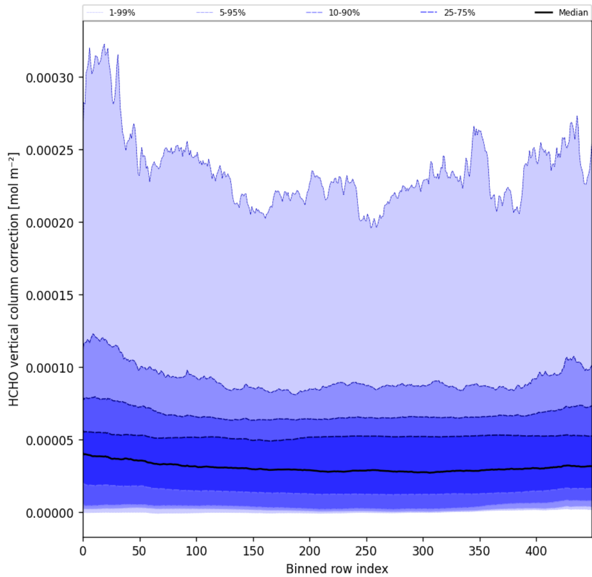
Figure 51: Along track statistics of “HCHO vertical column correction” for 2025-08-19 to 2025-08-20
