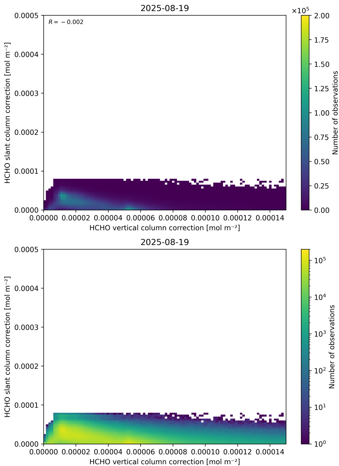
Figure 117: Scatter density plot of “HCHO vertical column correction” against “HCHO slant column correction” for 2025-08-19 to 2025-08-20.
