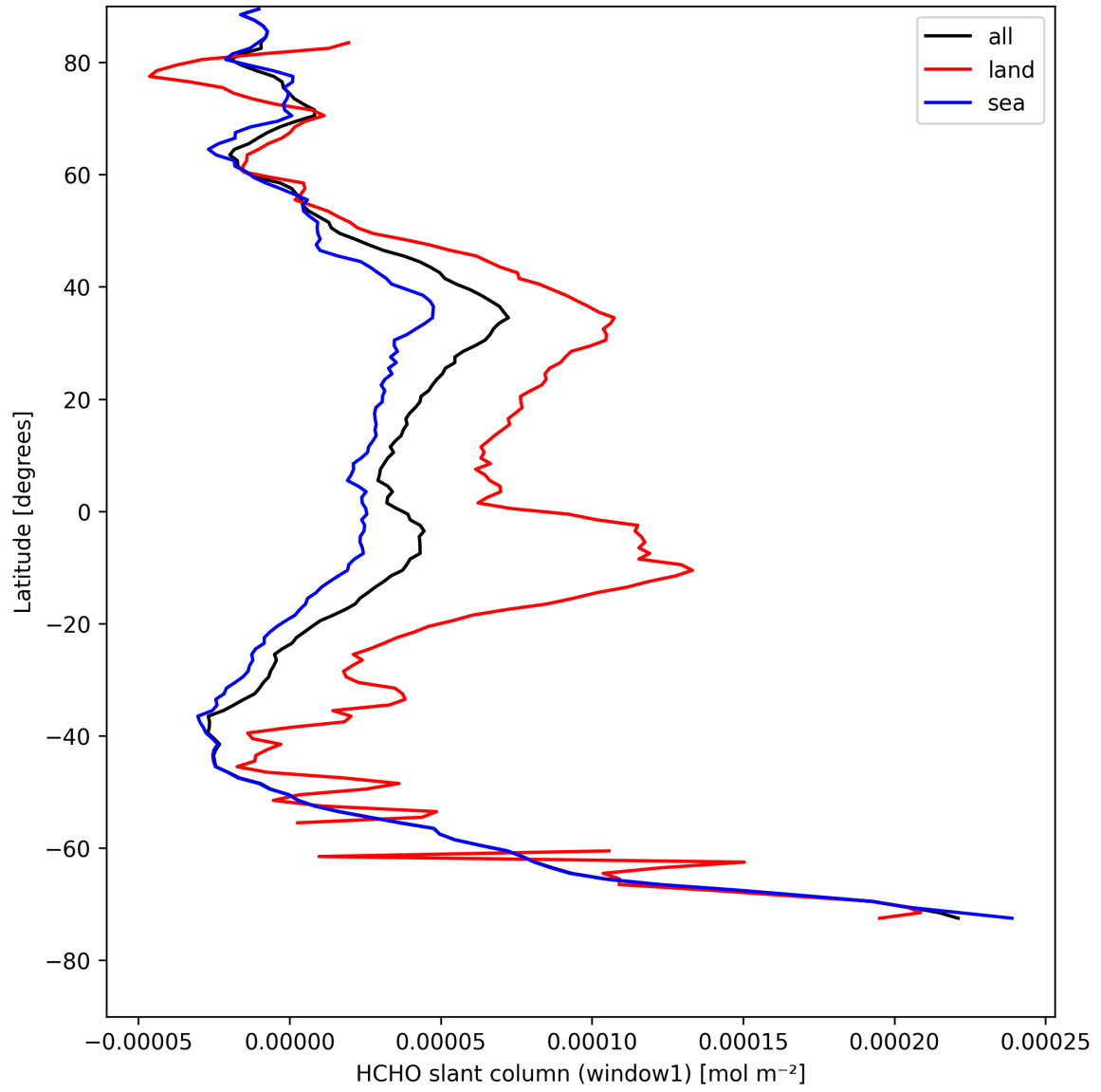
Figure 24: Zonal average of “HCHO slant column (window1)” for 2025-08-19 to 2025-08-20.
