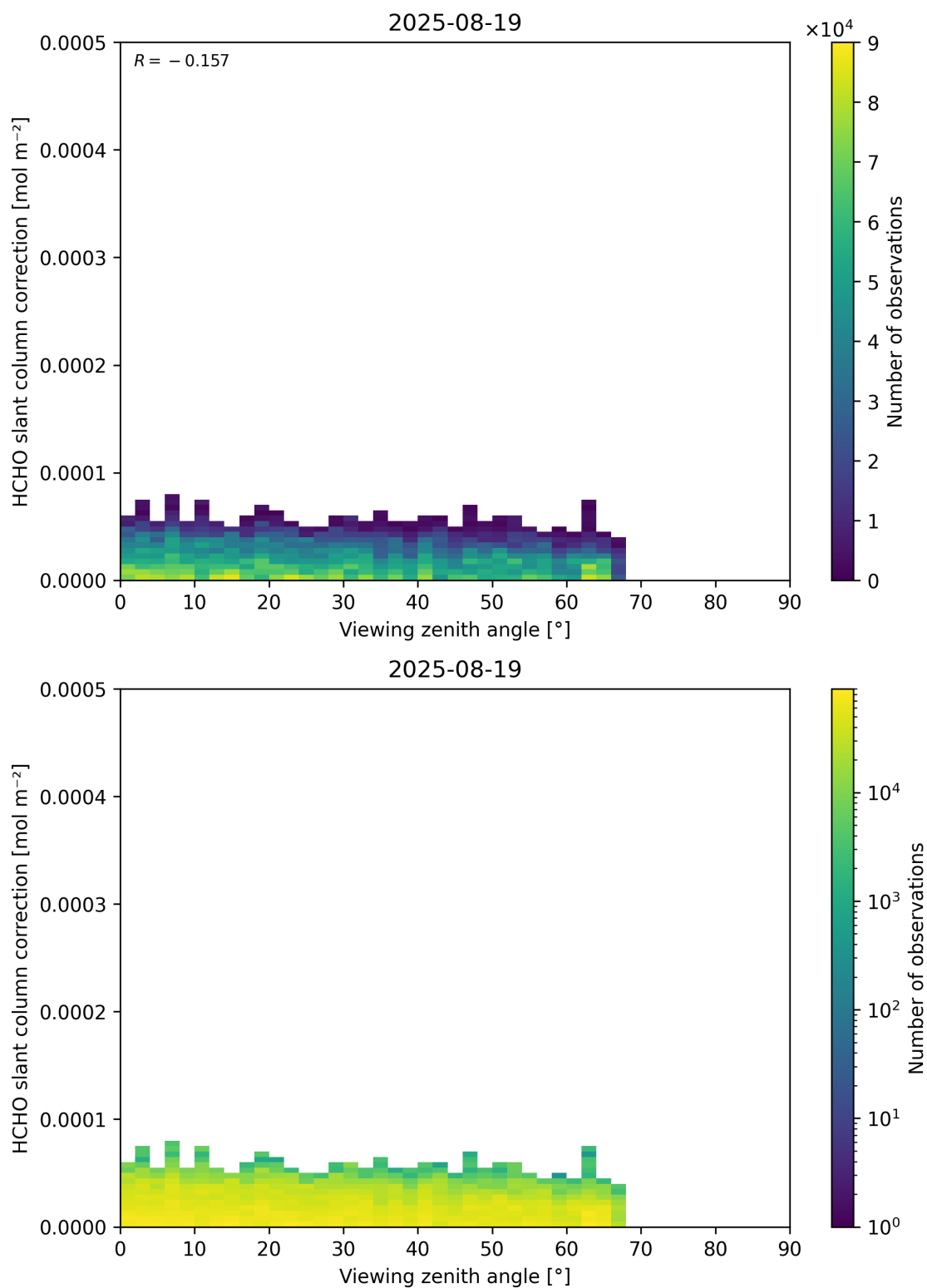
Figure 187: Scatter density plot of “Viewing zenith angle” against “HCHO slant column correction” for 2025-08-19 to 2025-08-20.
