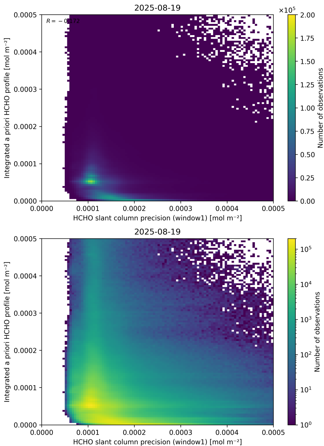
Figure 96: Scatter density plot of “HCHO slant column precision (window1)” against “Integrated a priori HCHO profile” for 2025-08-19 to 2025-08-20.
