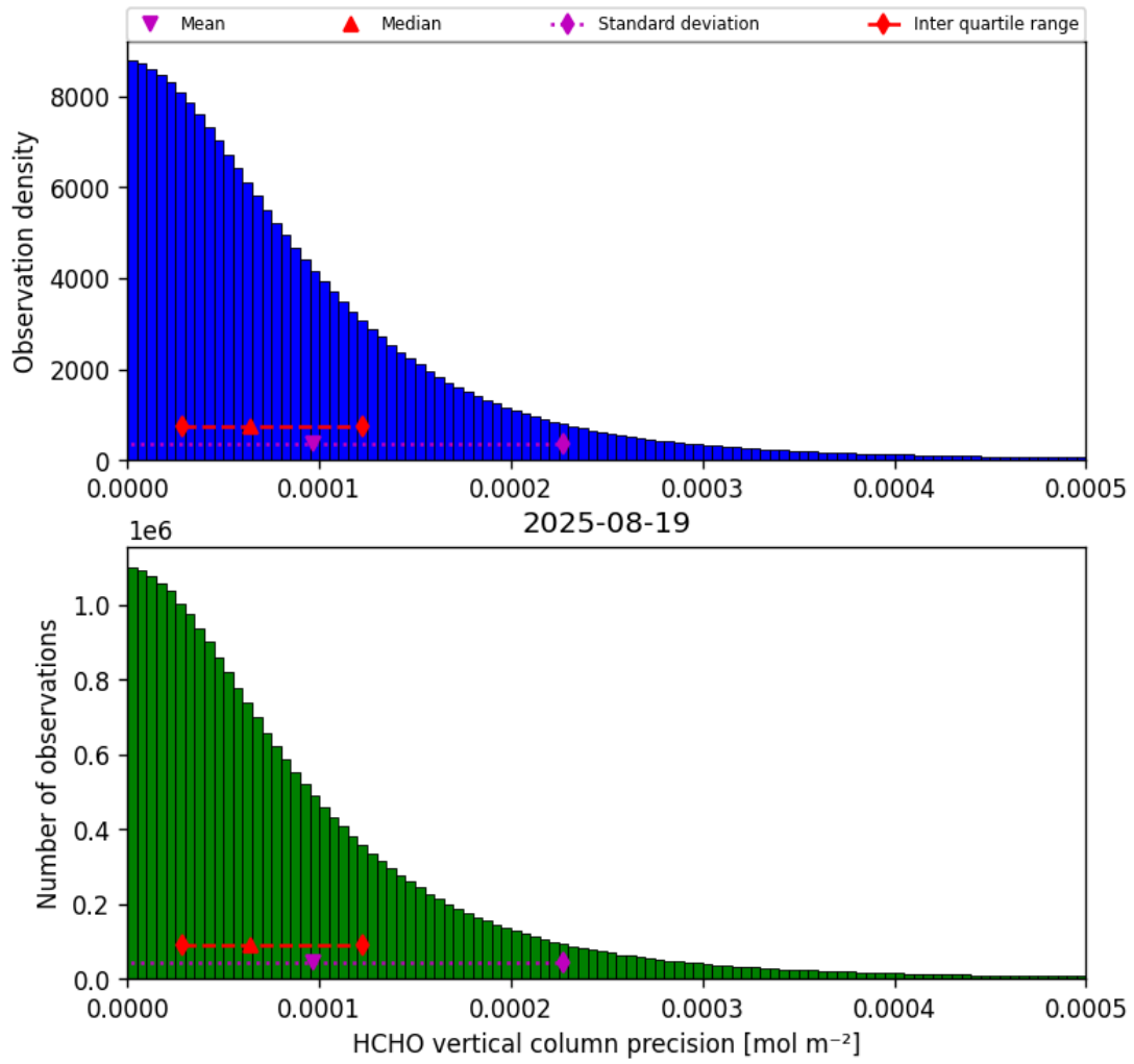
Figure 36: Histogram of “HCHO vertical column precision” for 2025-08-19 to 2025-08-20
