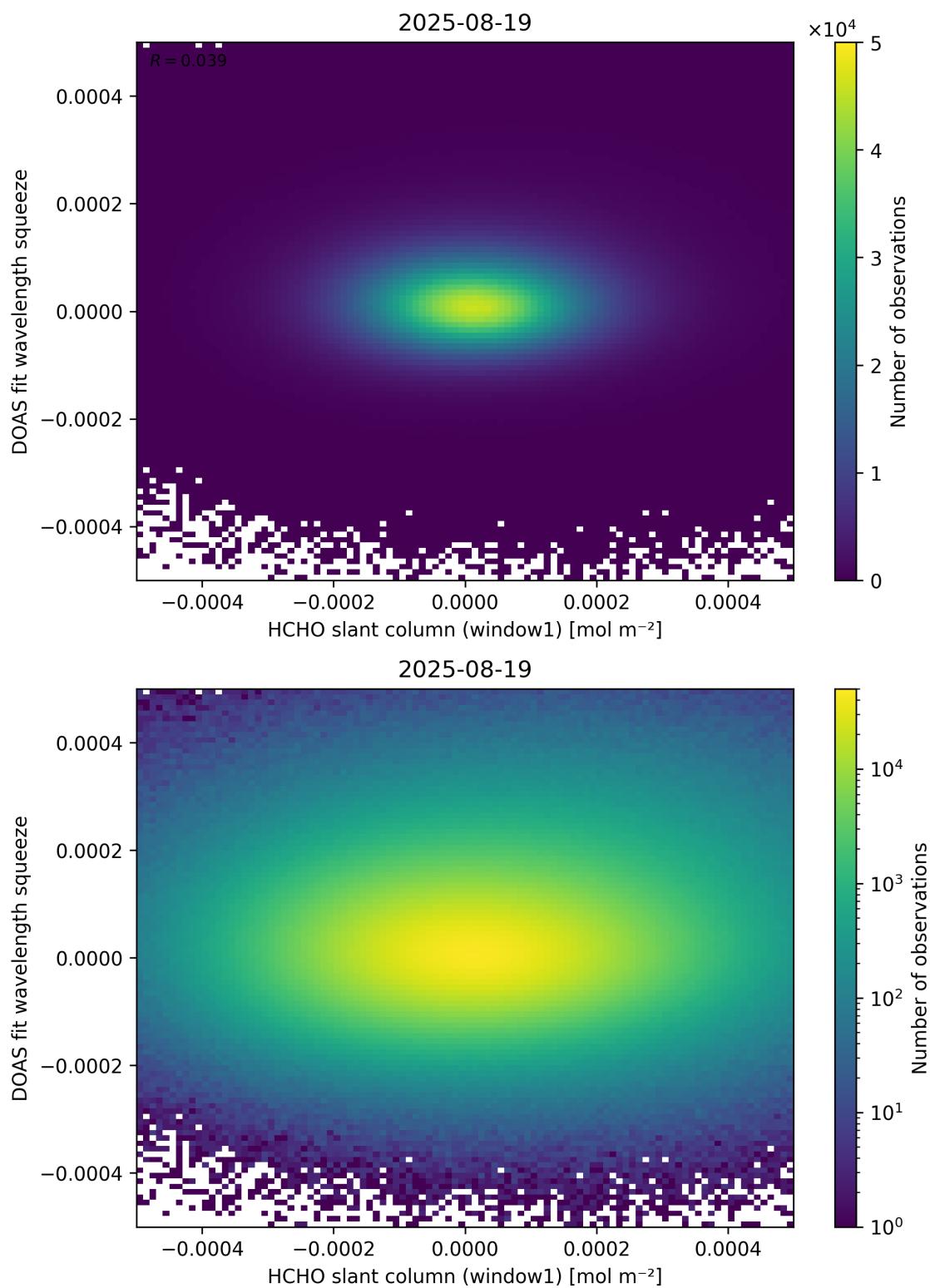
Figure 80: Scatter density plot of “HCHO slant column (window1)” against “DOAS fit wavelength squeeze” for 2025-08-19 to 2025-08-20.
