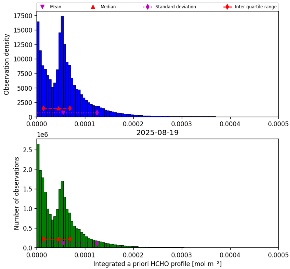
Figure 43: Histogram of “Integrated a priori HCHO profile” for 2025-08-19 to 2025-08-20
