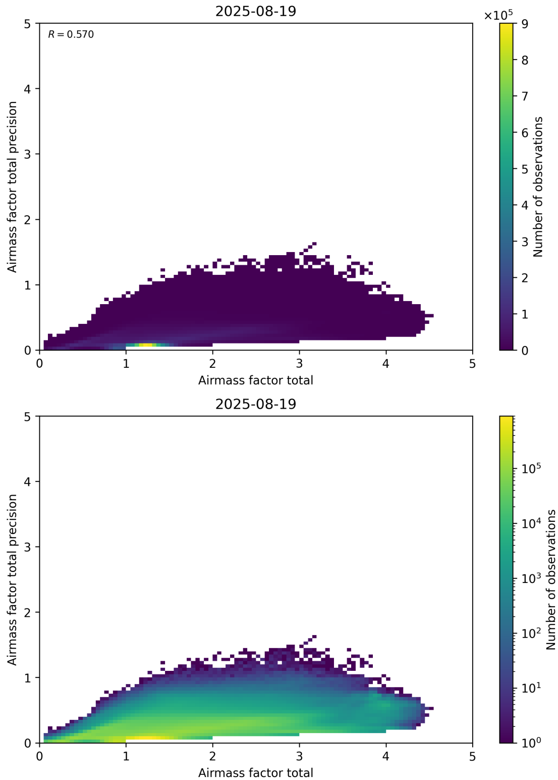
Figure 103: Scatter density plot of “Airmass factor total” against “Airmass factor total precision” for 2025-08-19 to 2025-08-20.
