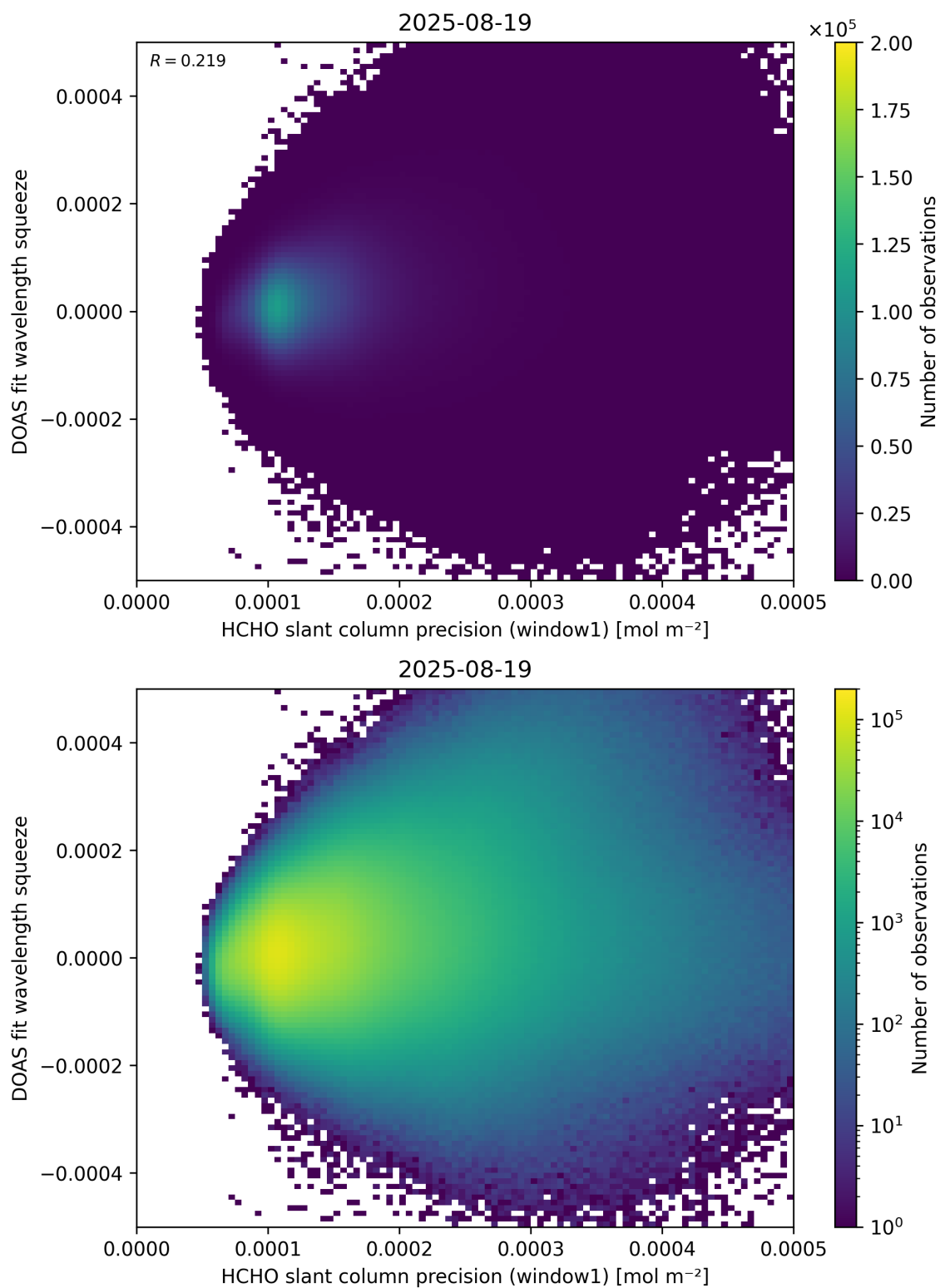
Figure 90: Scatter density plot of “HCHO slant column precision (window1)” against “DOAS fit wavelength squeeze” for 2025-08-19 to 2025-08-20.
