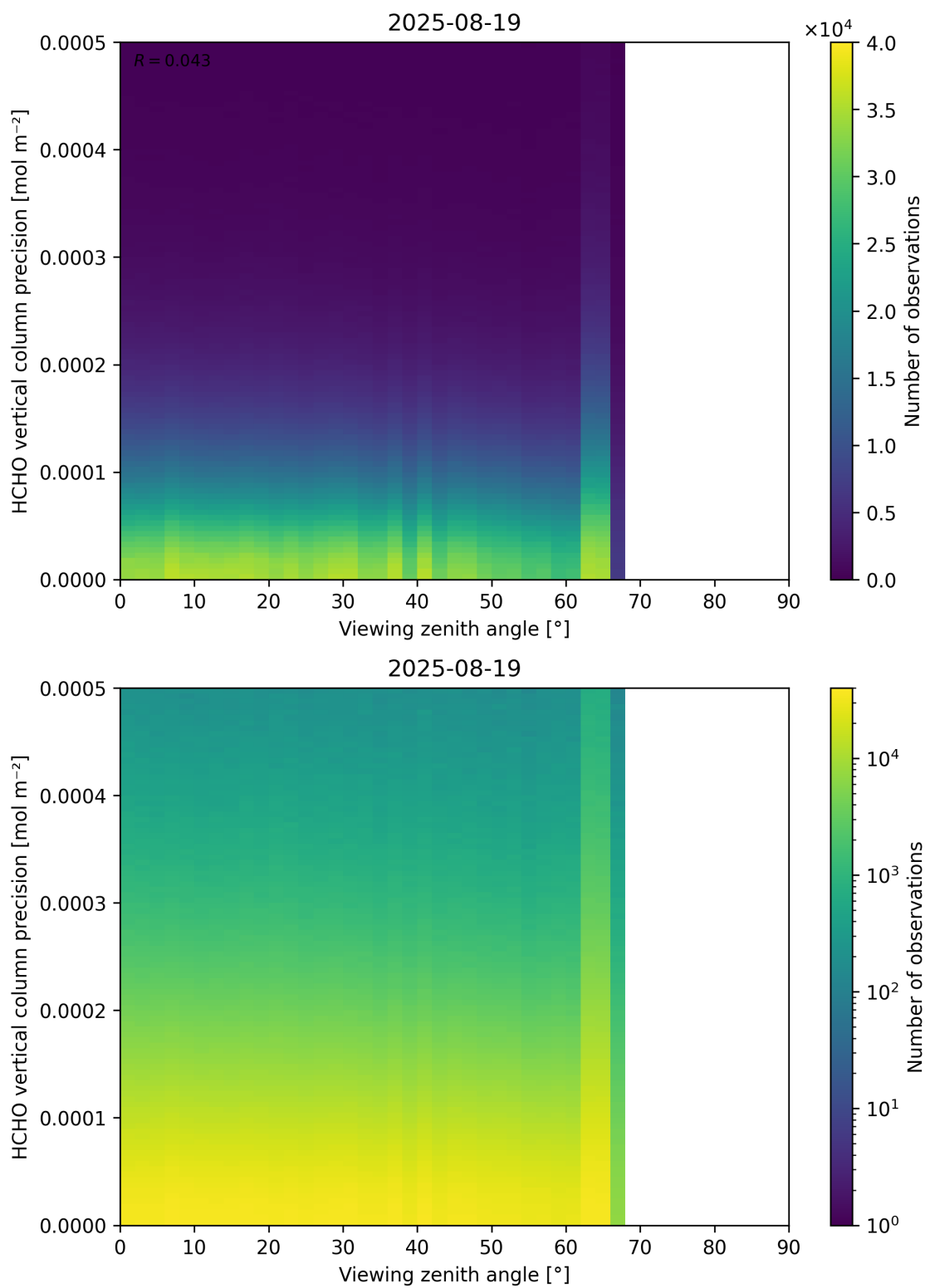
Figure 194: Scatter density plot of “Viewing zenith angle” against “HCHO vertical column precision” for 2025-08-19 to 2025-08-20.
