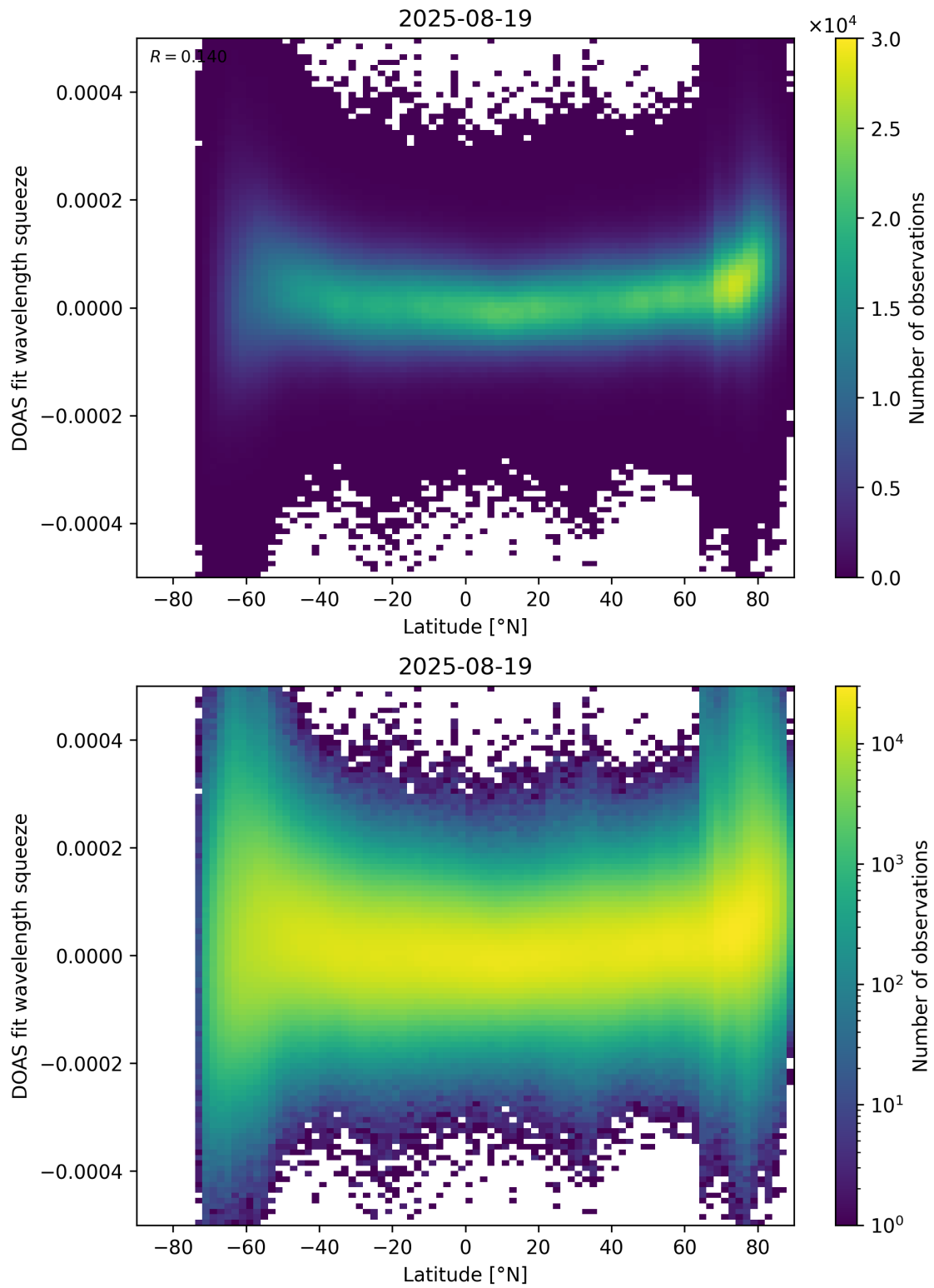
Figure 155: Scatter density plot of “Latitude” against “DOAS fit wavelength squeeze” for 2025-08-19 to 2025-08-20.
