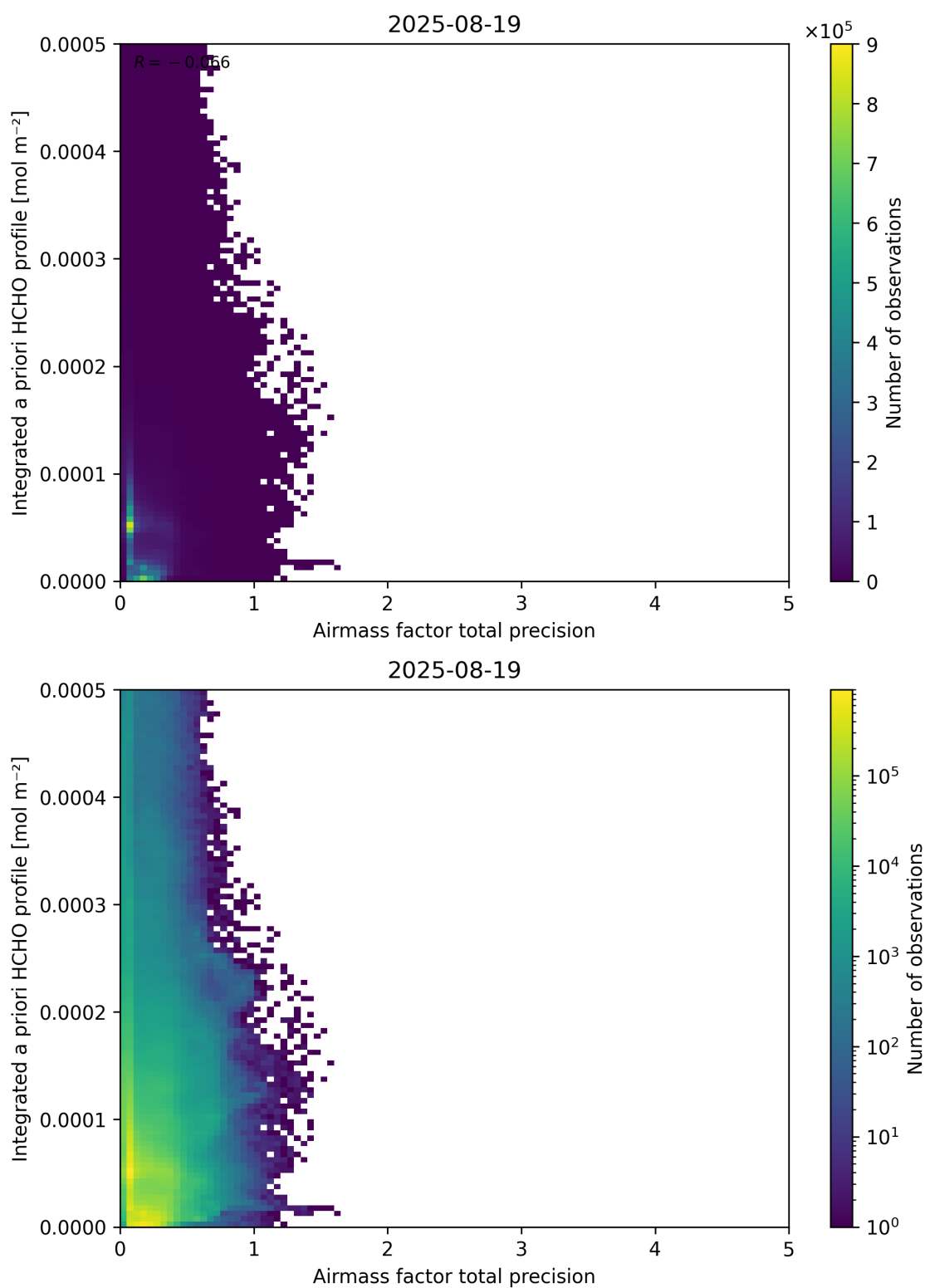
Figure 111: Scatter density plot of “Airmass factor total precision” against “Integrated a priori HCHO profile” for 2025-08-19 to 2025-08-20.
