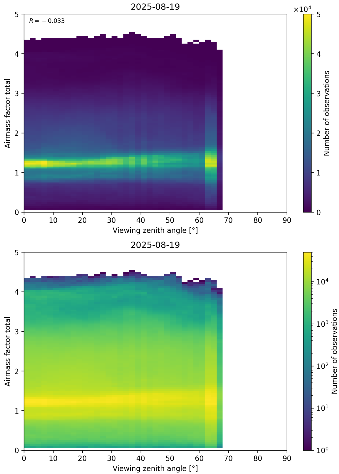
Figure 190: Scatter density plot of “Viewing zenith angle” against “Airmass factor total” for 2025-08-19 to 2025-08-20.
