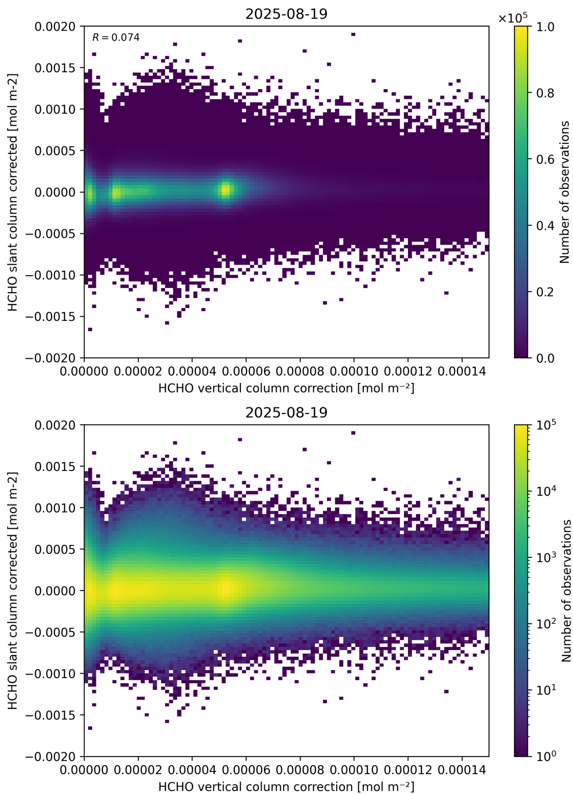
Figure 116: Scatter density plot of “HCHO vertical column correction” against “HCHO slant column corrected” for 2025-08-19 to 2025-08-20.
