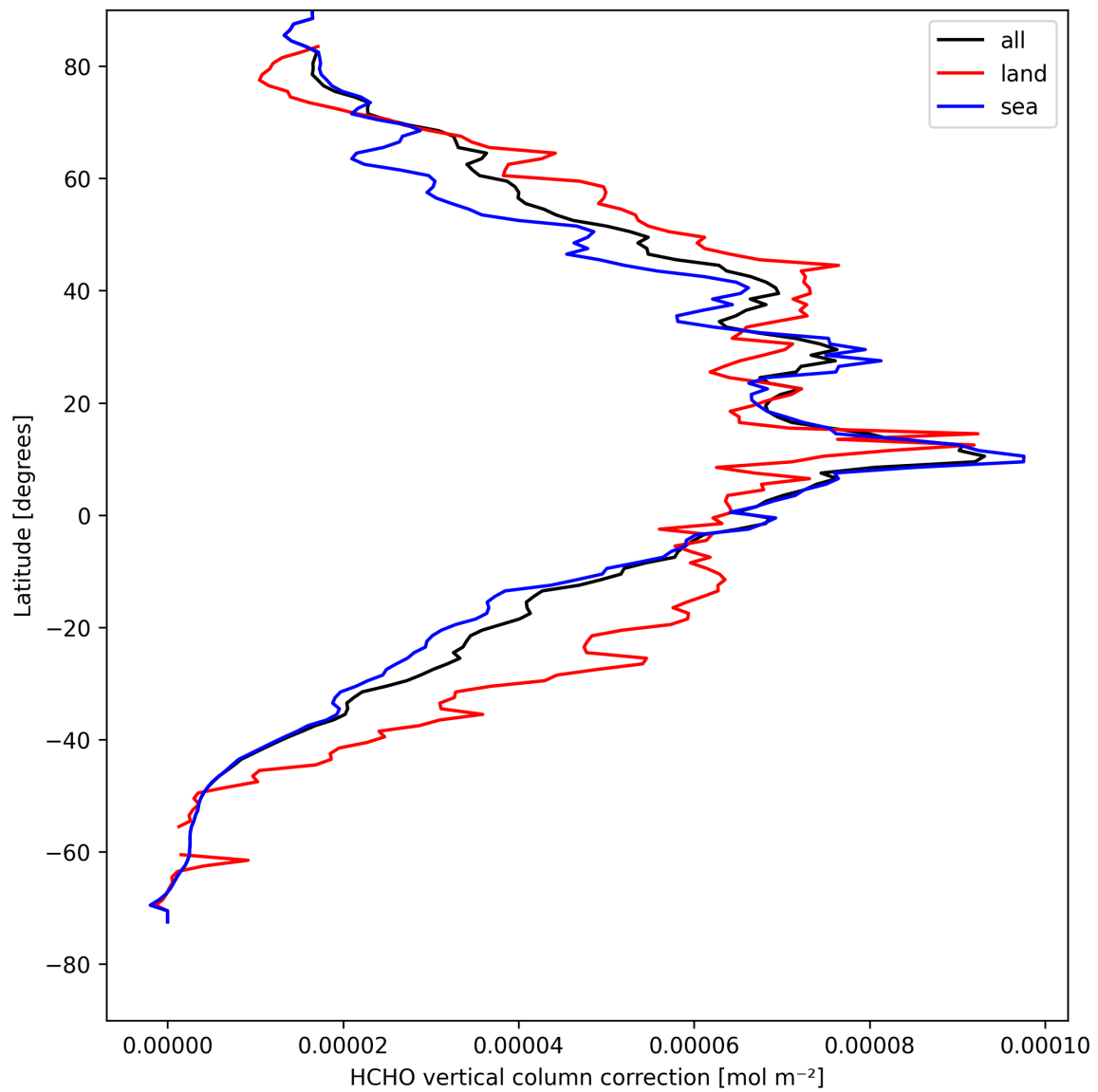
Figure 23: Zonal average of “HCHO vertical column correction” for 2025-08-19 to 2025-08-20.
