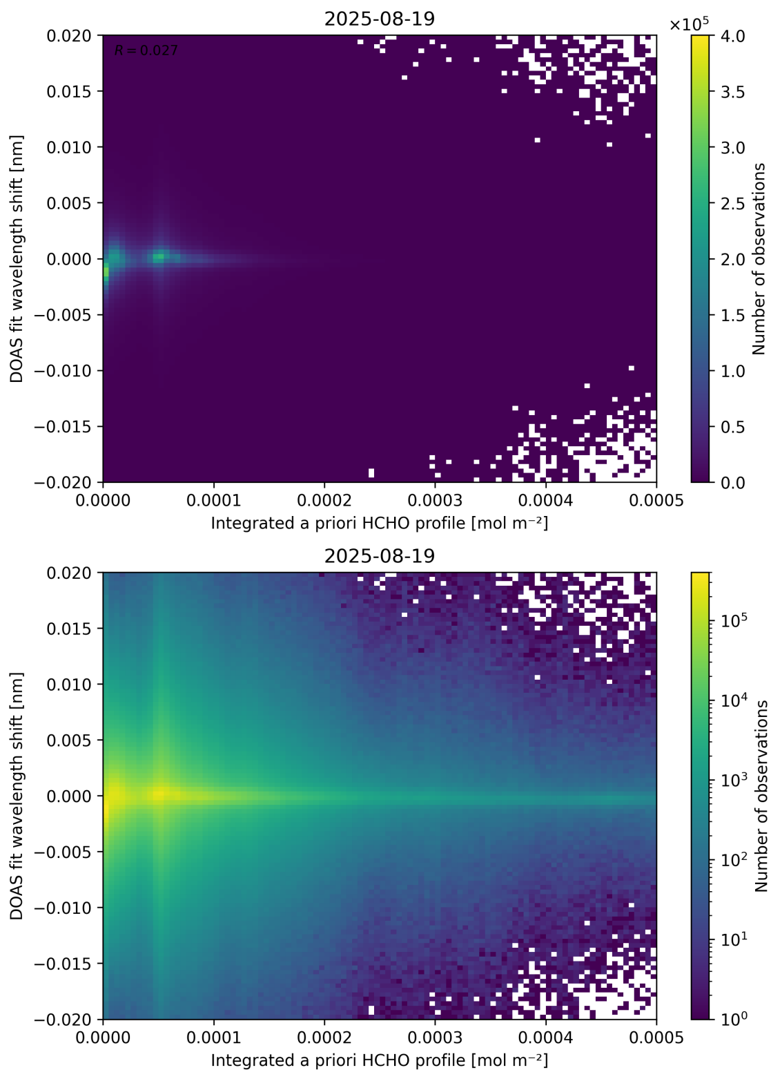
Figure 149: Scatter density plot of “Integrated a priori HCHO profile” against “DOAS fit wavelength shift” for 2025-08-19 to 2025-08-20.
