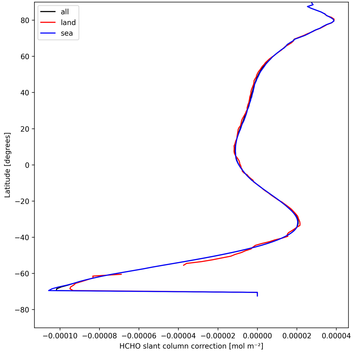
Figure 33: Zonal average of “HCHO slant column correction” for 2025-08-19 to 2025-08-20.
