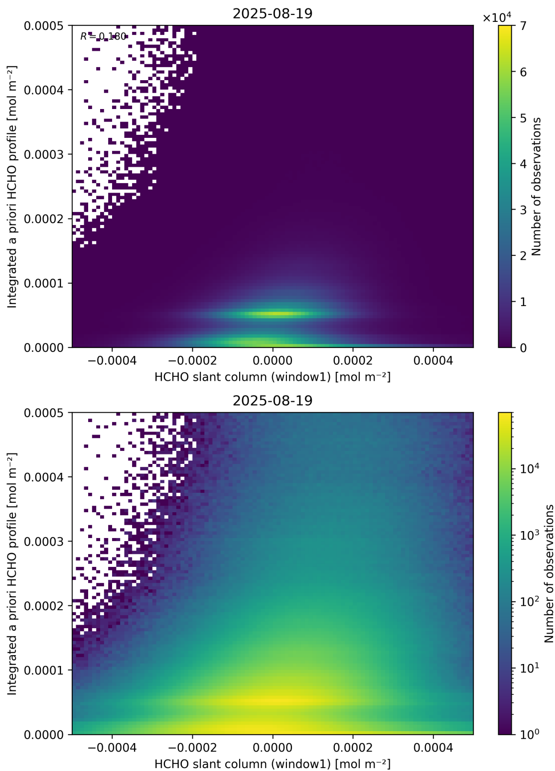
Figure 87: Scatter density plot of “HCHO slant column (window1)” against “Integrated a priori HCHO profile” for 2025-08-19 to 2025-08-20.
