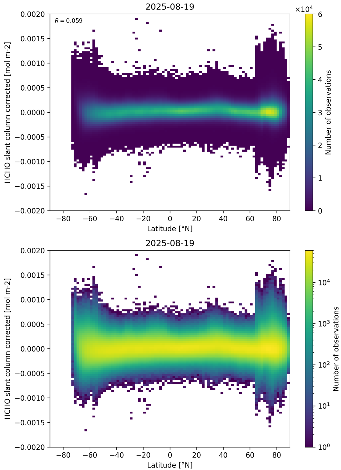
Figure 157: Scatter density plot of “Latitude” against “HCHO slant column corrected” for 2025-08-19 to 2025-08-20.
