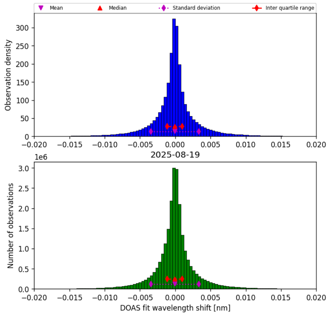
Figure 44: Histogram of “DOAS fit wavelength shift” for 2025-08-19 to 2025-08-20
