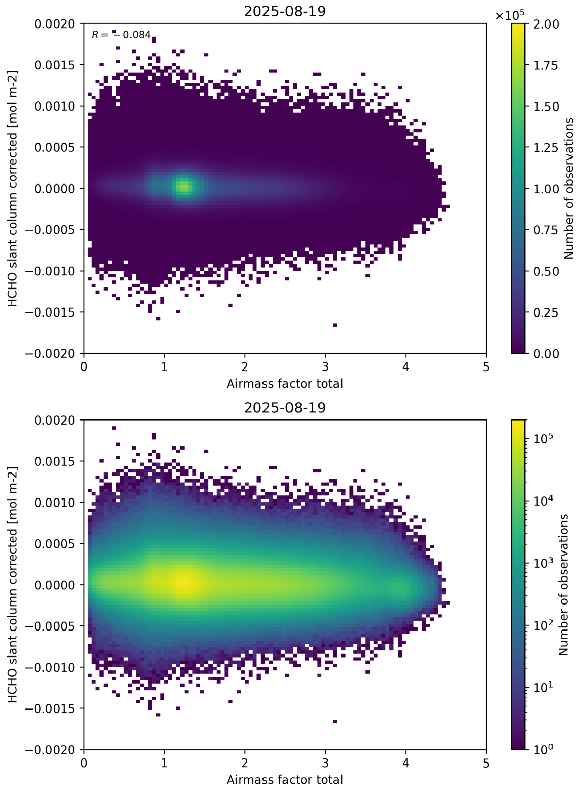
Figure 101: Scatter density plot of “Airmass factor total” against “HCHO slant column corrected” for 2025-08-19 to 2025-08-20.
