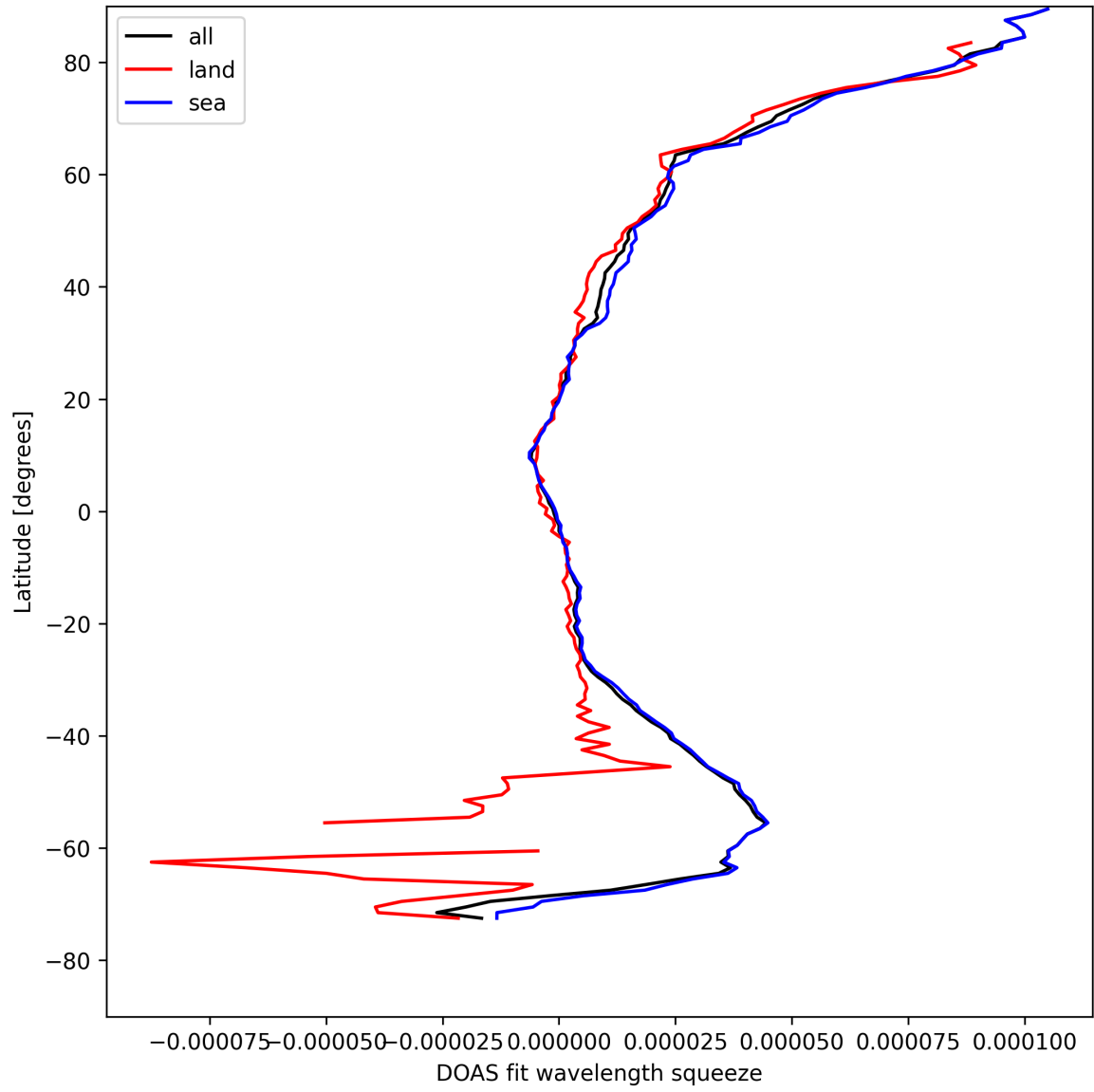
Figure 31: Zonal average of “DOAS fit wavelength squeeze” for 2025-08-19 to 2025-08-20.
