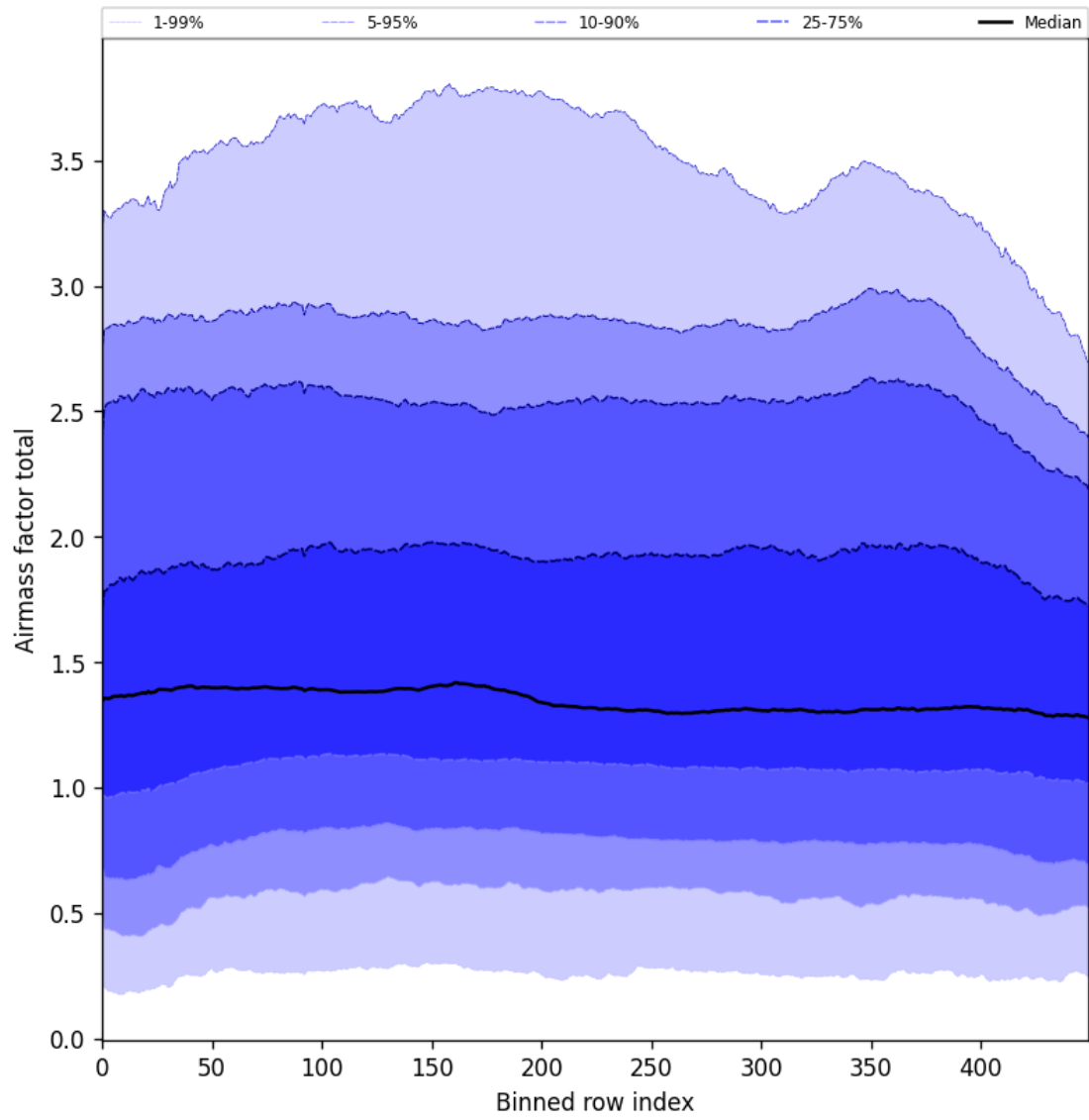
Figure 54: Along track statistics of “Airmass factor total” for 2025-08-19 to 2025-08-20
