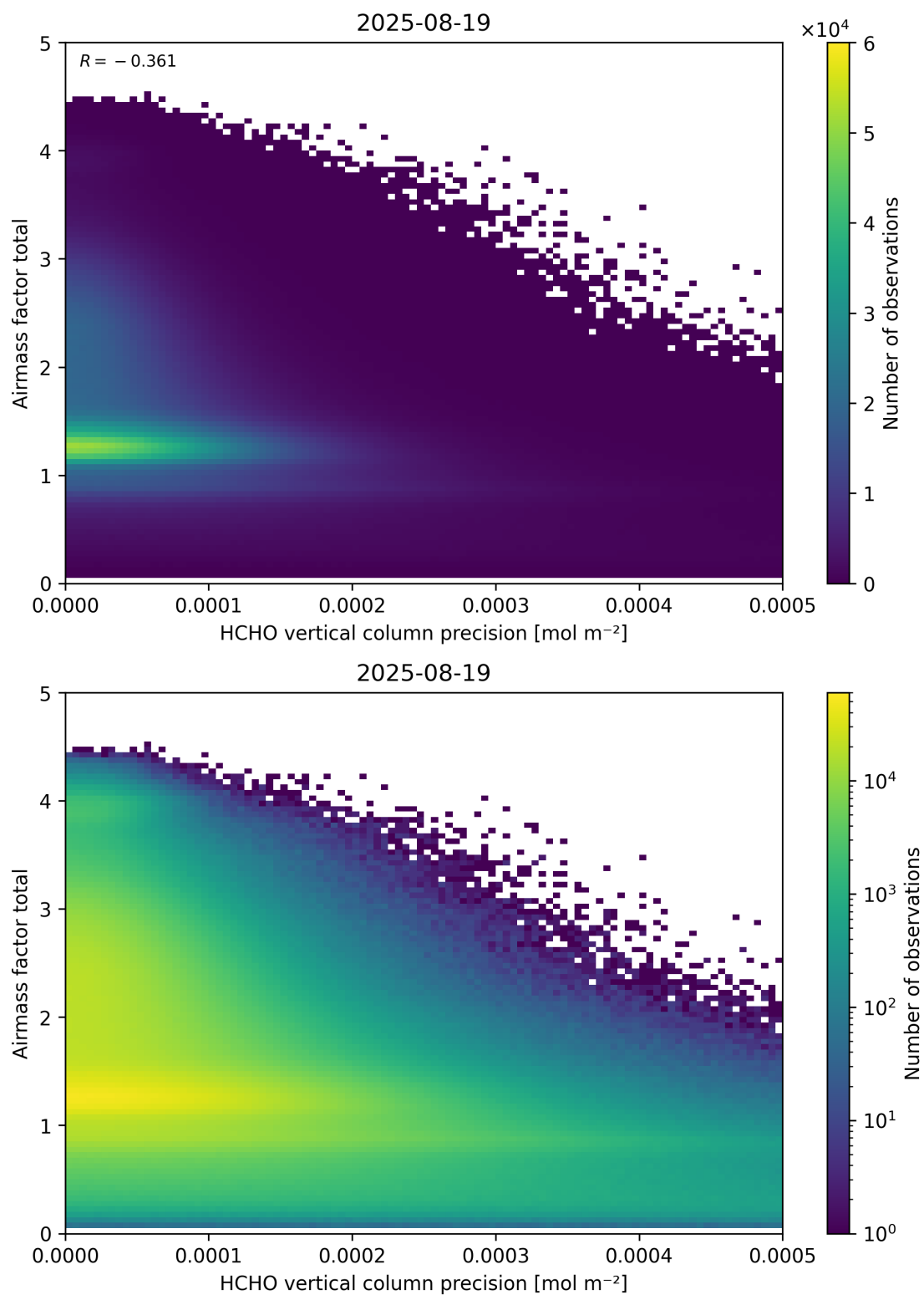
Figure 144: Scatter density plot of “HCHO vertical column precision” against “Airmass factor total” for 2025-08-19 to 2025-08-20.
