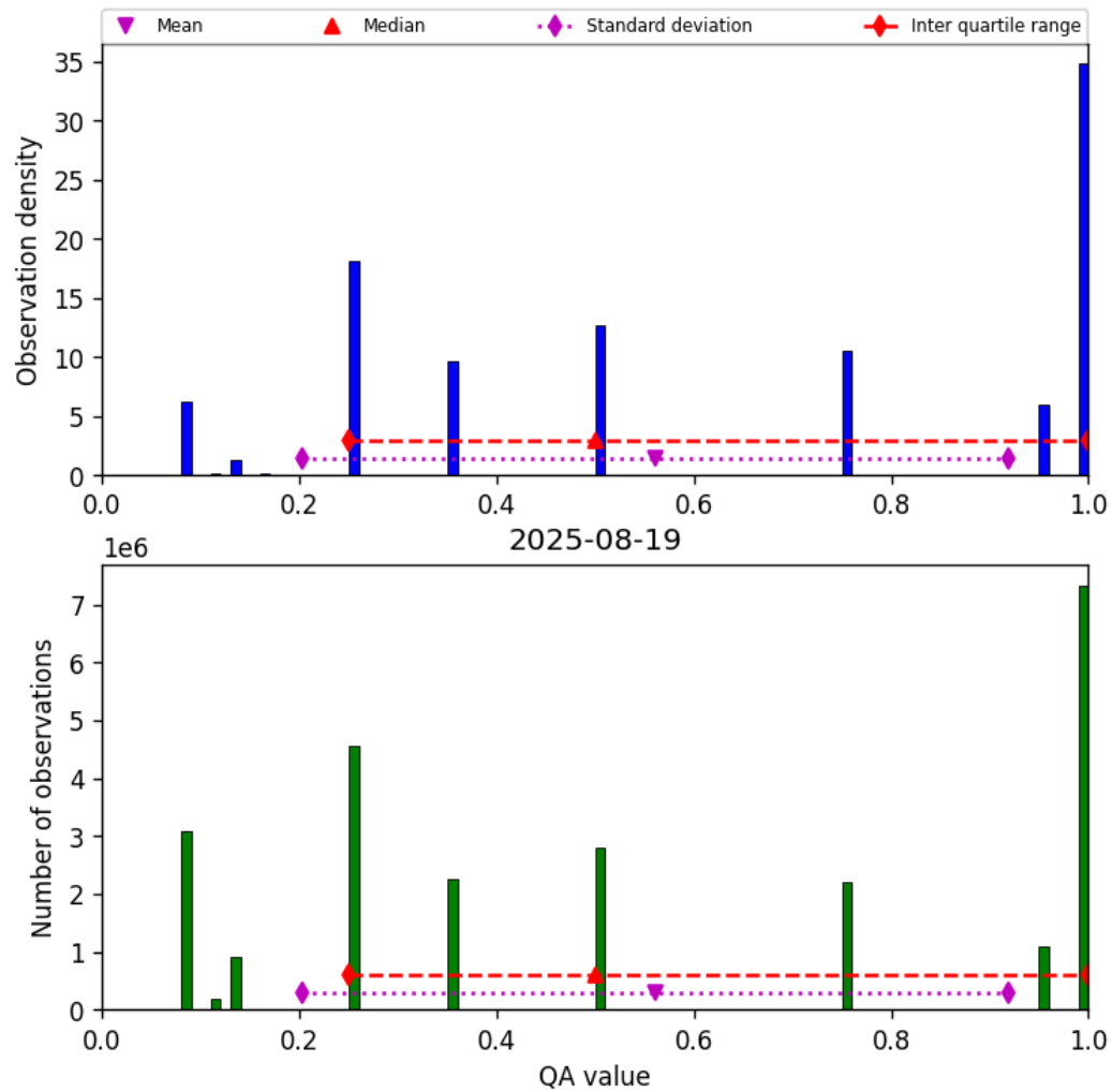
Figure 34: Histogram of “QA value” for 2025-08-19 to 2025-08-20
