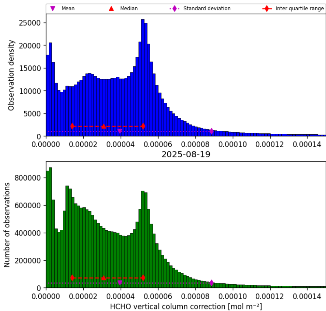
Figure 37: Histogram of “HCHO vertical column correction” for 2025-08-19 to 2025-08-20
