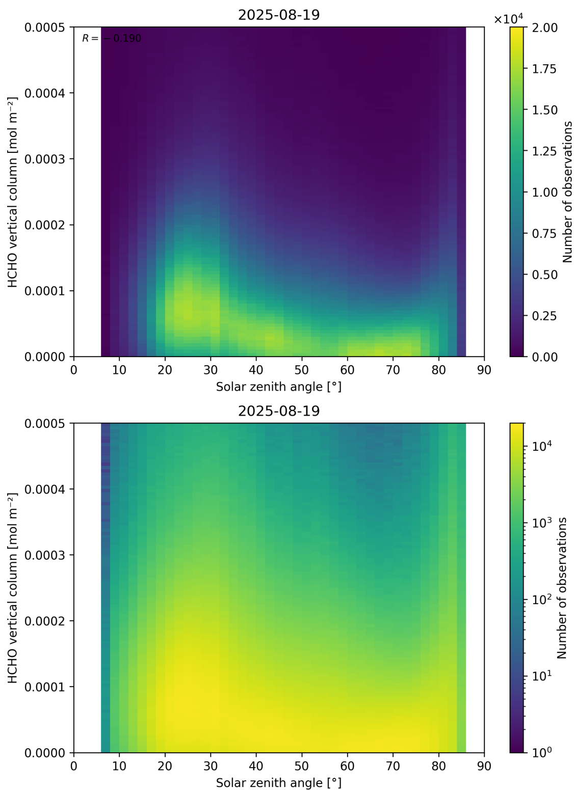
Figure 177: Scatter density plot of “Solar zenith angle” against “HCHO vertical column” for 2025-08-19 to 2025-08-20.
