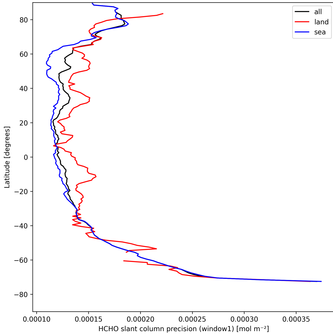
Figure 25: Zonal average of “HCHO slant column precision (window1)” for 2025-08-19 to 2025-08-20.
