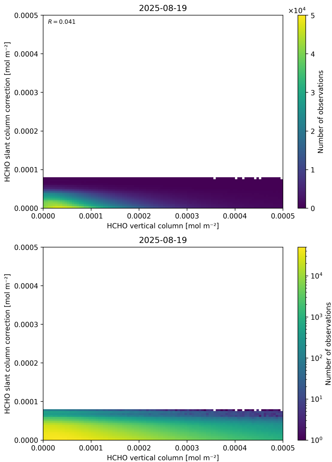
Figure 128: Scatter density plot of “HCHO vertical column” against “HCHO slant column correction” for 2025-08-19 to 2025-08-20.
