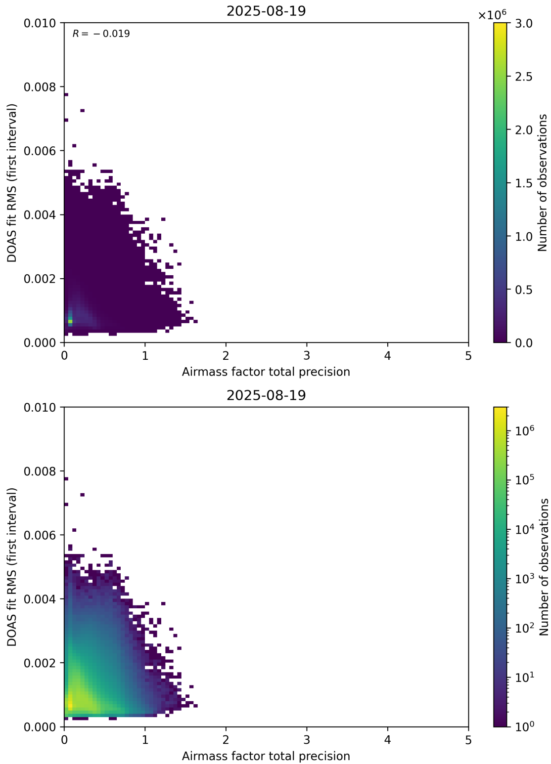
Figure 105: Scatter density plot of “Airmass factor total precision” against “DOAS fit RMS (first interval)” for 2025-08-19 to 2025-08-20.
