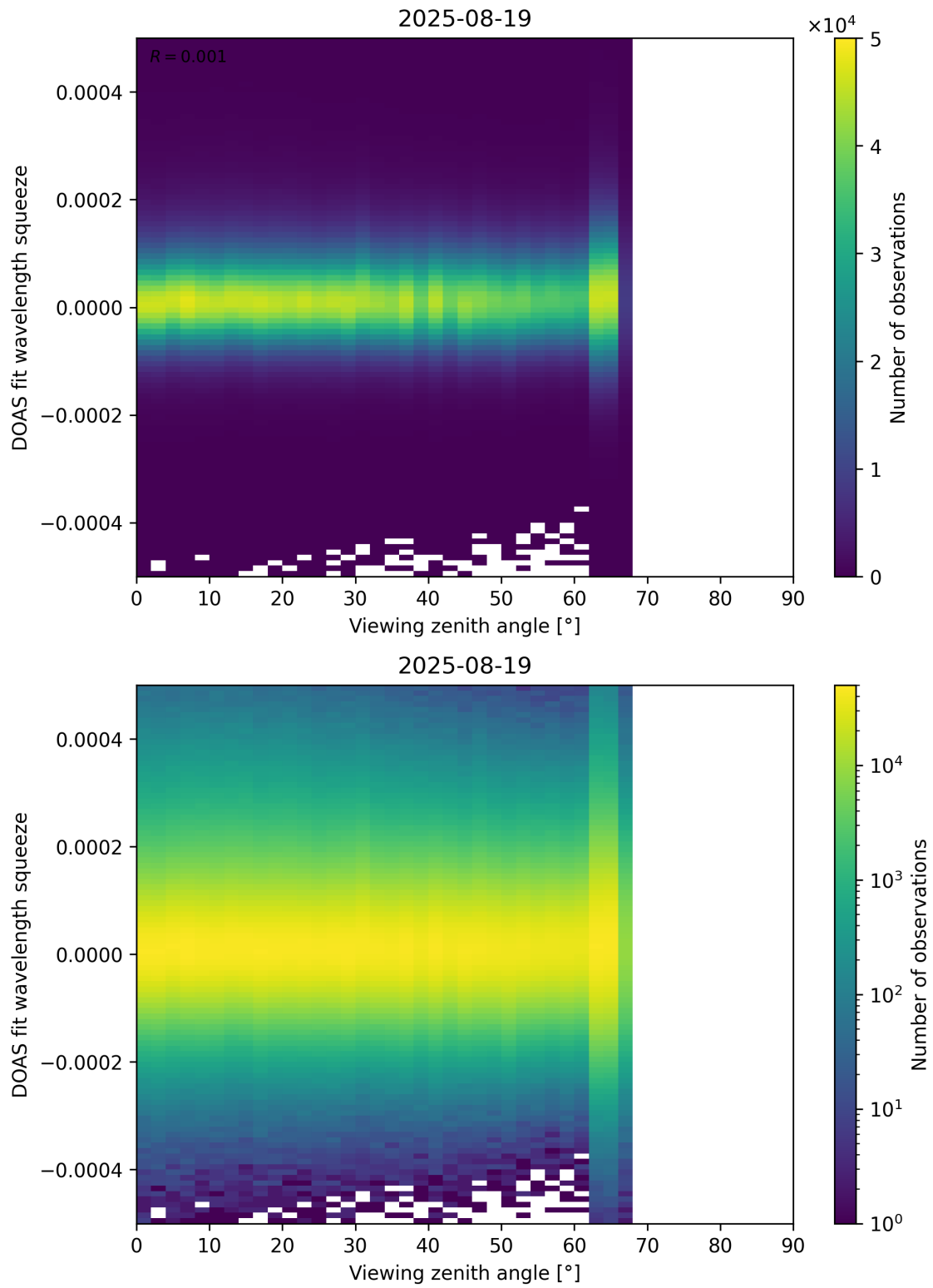
Figure 184: Scatter density plot of “Viewing zenith angle” against “DOAS fit wavelength squeeze” for 2025-08-19 to 2025-08-20.
