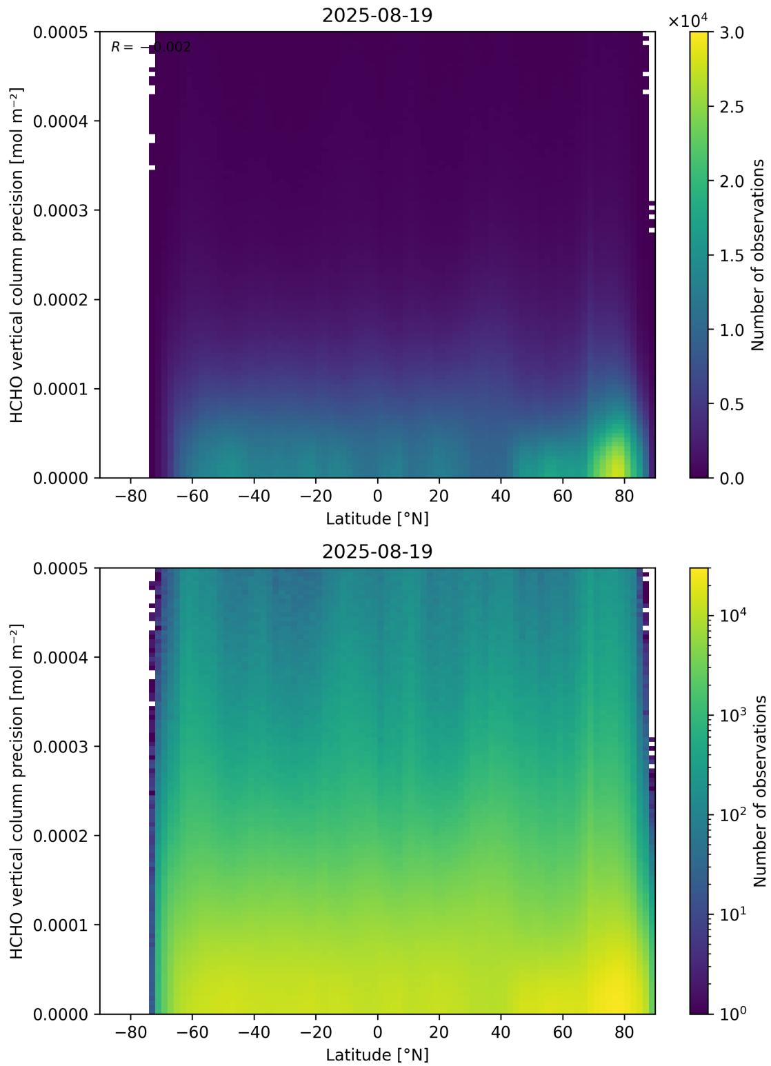
Figure 165: Scatter density plot of “Latitude” against “HCHO vertical column precision” for 2025-08-19 to 2025-08-20.
