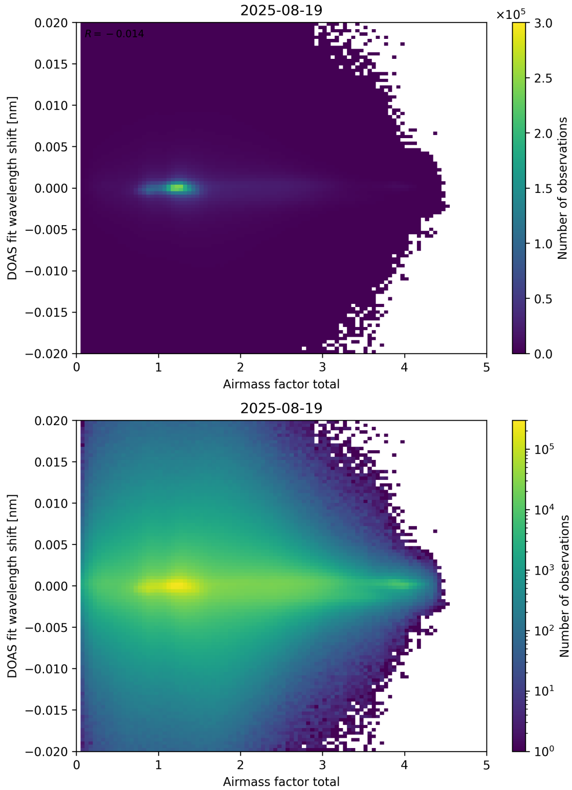
Figure 98: Scatter density plot of “Airmass factor total” against “DOAS fit wavelength shift” for 2025-08-19 to 2025-08-20.
