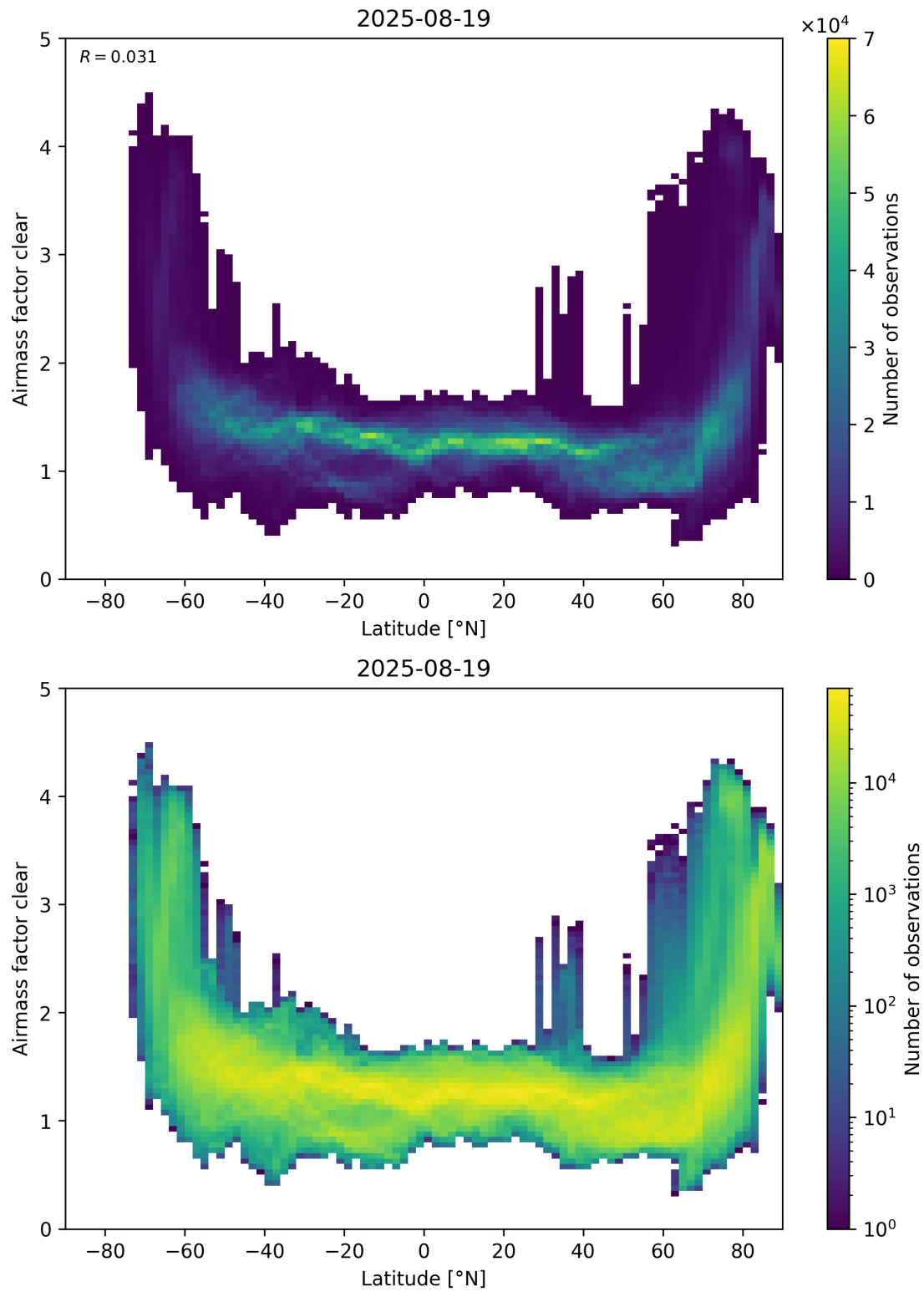
Figure 156: Scatter density plot of “Latitude” against “Airmass factor clear” for 2025-08-19 to 2025-08-20.
