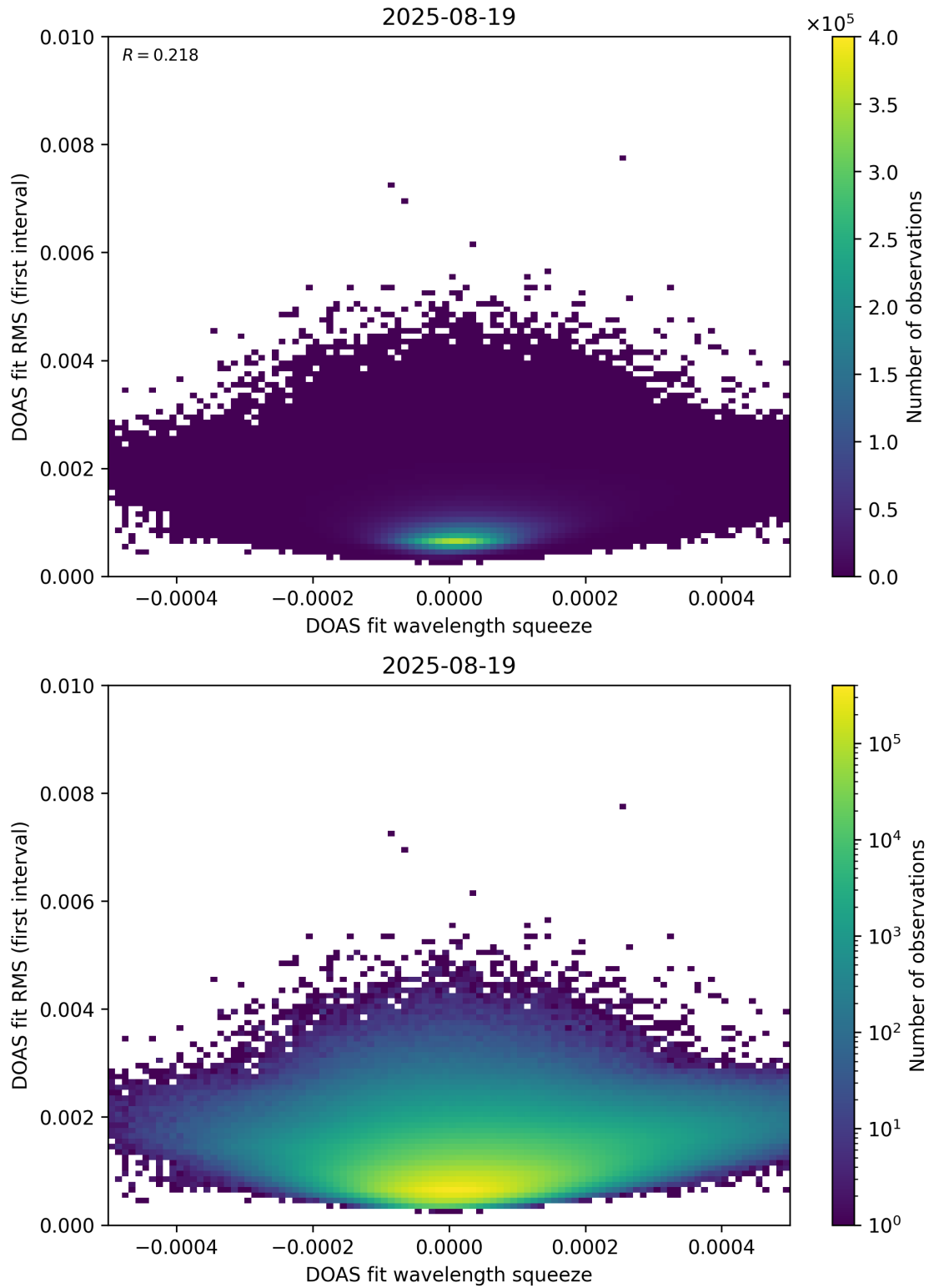
Figure 68: Scatter density plot of “DOAS fit wavelength squeeze” against “DOAS fit RMS (first interval)” for 2025-08-19 to 2025-08-20.
