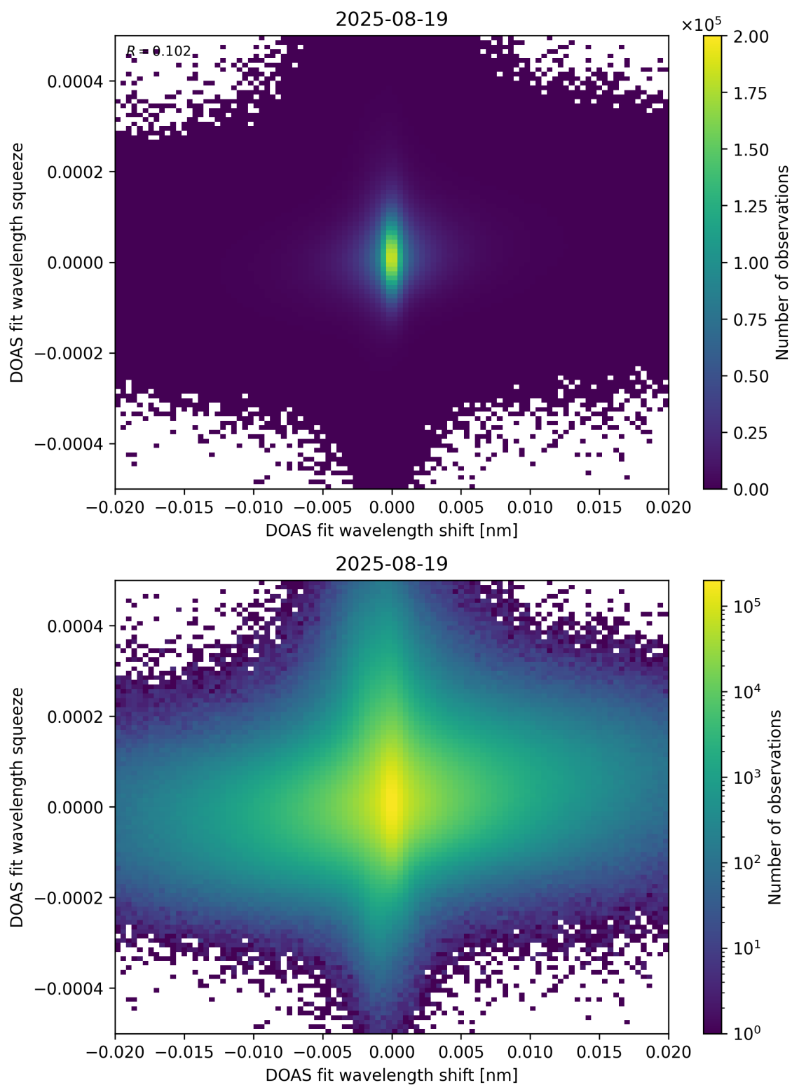
Figure 65: Scatter density plot of “DOAS fit wavelength shift” against “DOAS fit wavelength squeeze” for 2025-08-19 to 2025-08-20.
