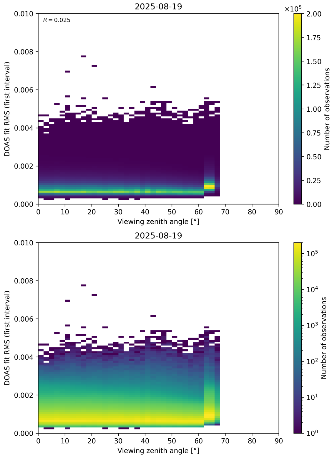
Figure 182: Scatter density plot of “Viewing zenith angle” against “DOAS fit RMS (first interval)” for 2025-08-19 to 2025-08-20.
