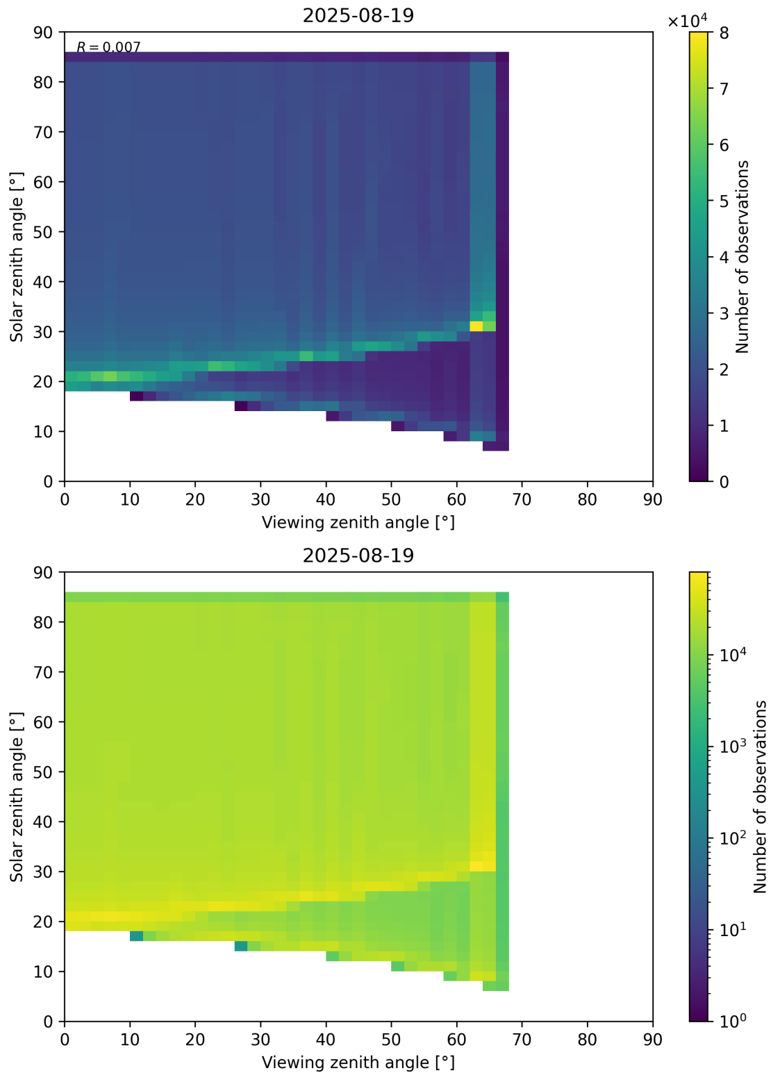
Figure 197: Scatter density plot of “Viewing zenith angle” against “Solar zenith angle” for 2025-08-19 to 2025-08-20.
