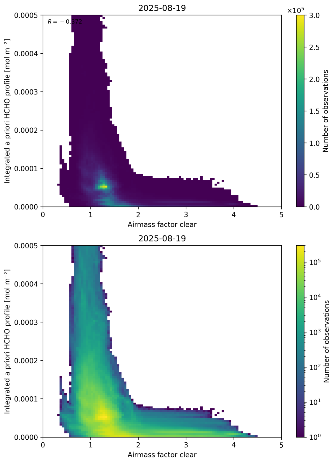
Figure 76: Scatter density plot of “Airmass factor clear” against “Integrated a priori HCHO profile” for 2025-08-19 to 2025-08-20.
