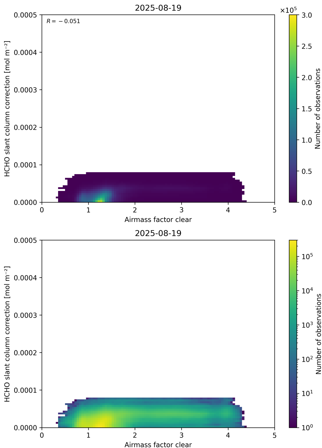
Figure 75: Scatter density plot of “Airmass factor clear” against “HCHO slant column correction” for 2025-08-19 to 2025-08-20.
