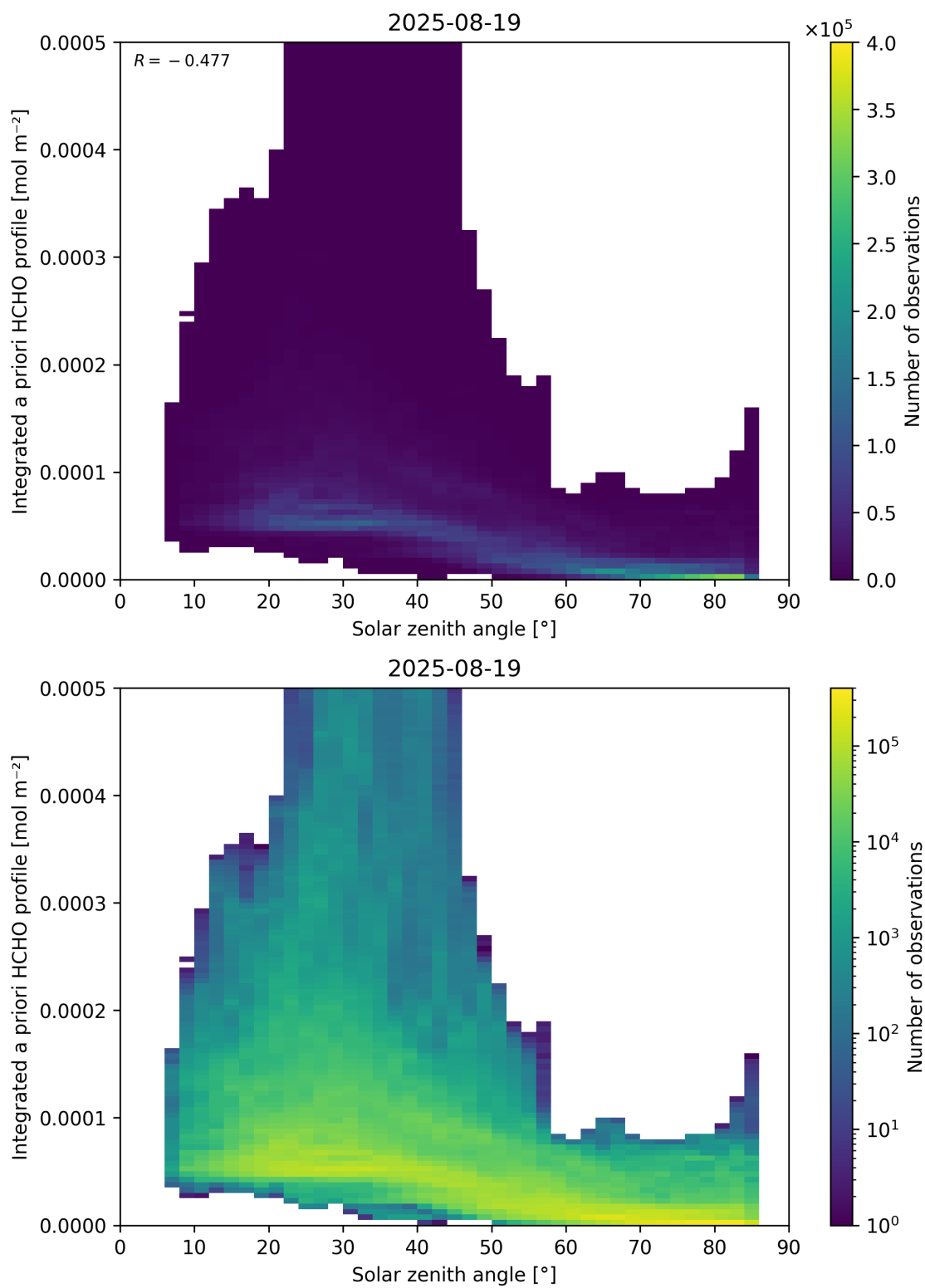
Figure 180: Scatter density plot of “Solar zenith angle” against “Integrated a priori HCHO profile” for 2025-08-19 to 2025-08-20.
