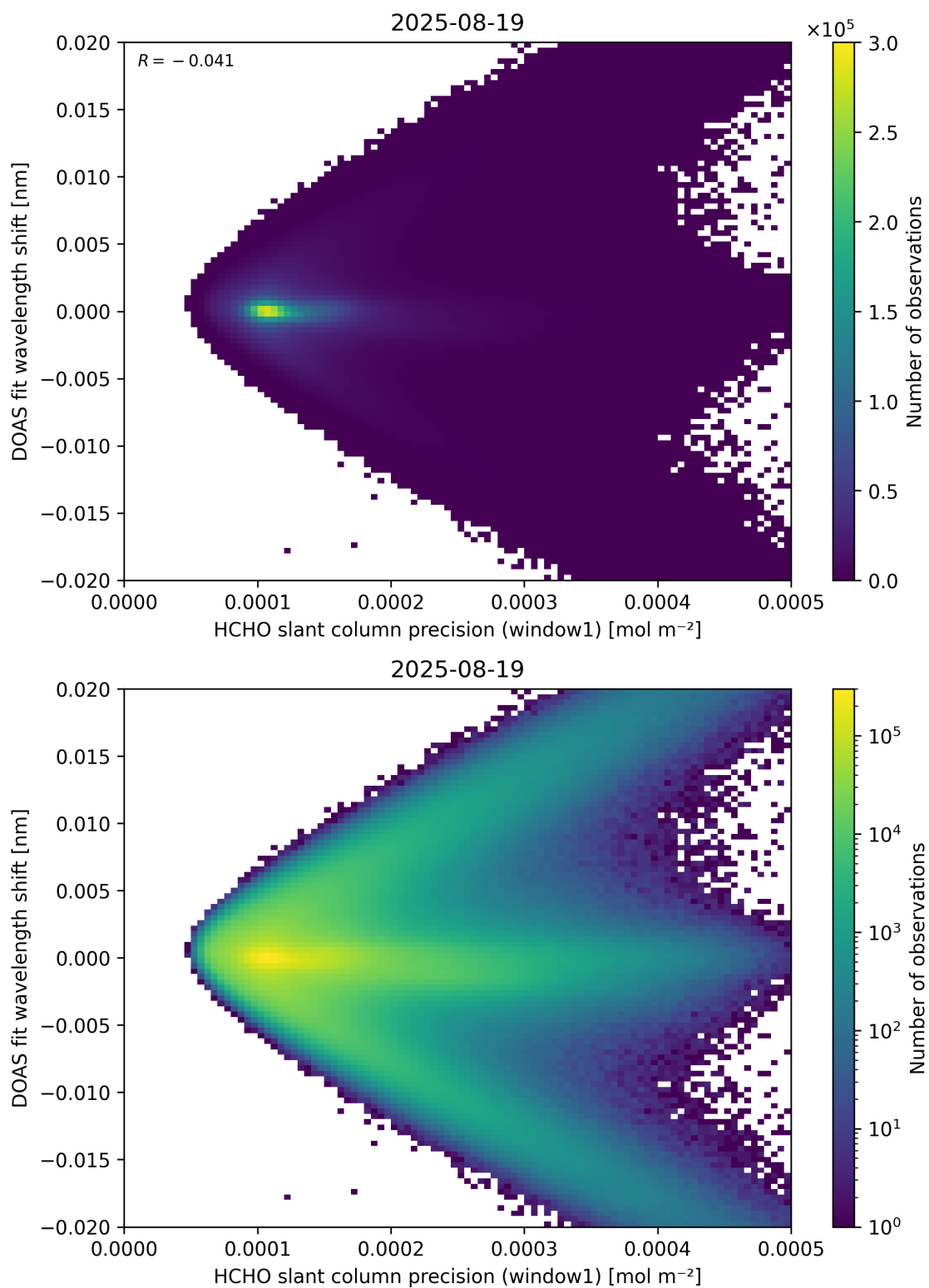
Figure 89: Scatter density plot of “HCHO slant column precision (window1)” against “DOAS fit wavelength shift” for 2025-08-19 to 2025-08-20.
