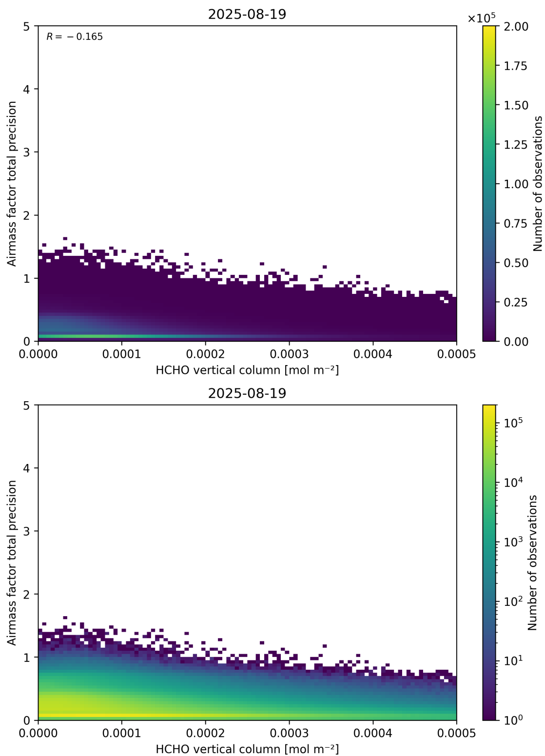
Figure 132: Scatter density plot of “HCHO vertical column” against “Airmass factor total precision” for 2025-08-19 to 2025-08-20.
