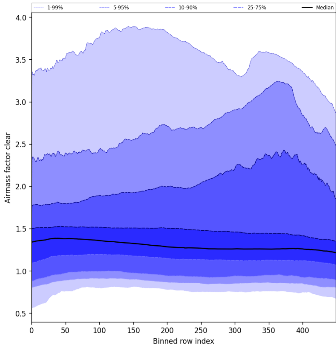
Figure 56: Along track statistics of “Airmass factor clear” for 2025-08-19 to 2025-08-20
