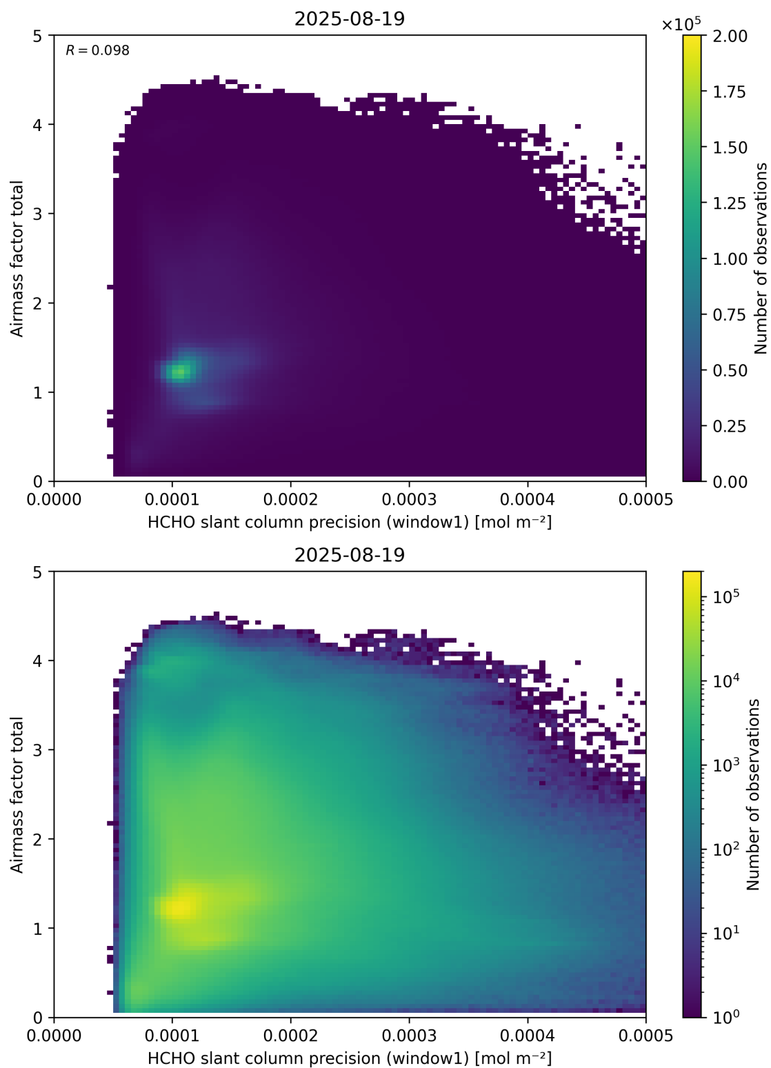
Figure 94: Scatter density plot of “HCHO slant column precision (window1)” against “Airmass factor total” for 2025-08-19 to 2025-08-20.
