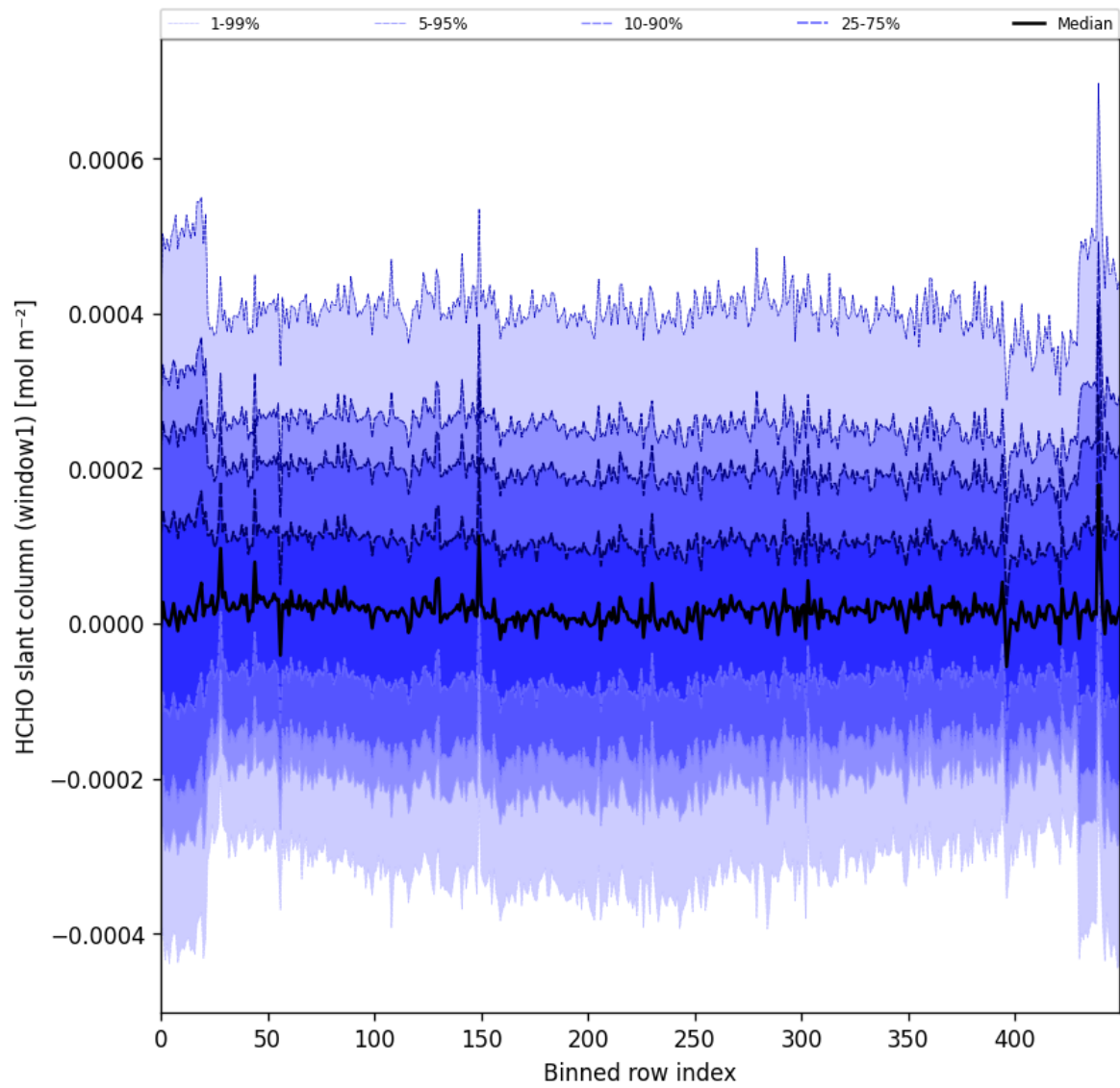
Figure 52: Along track statistics of "HCHO slant column (window1)" for 2025-08-19 to 2025-08-20
