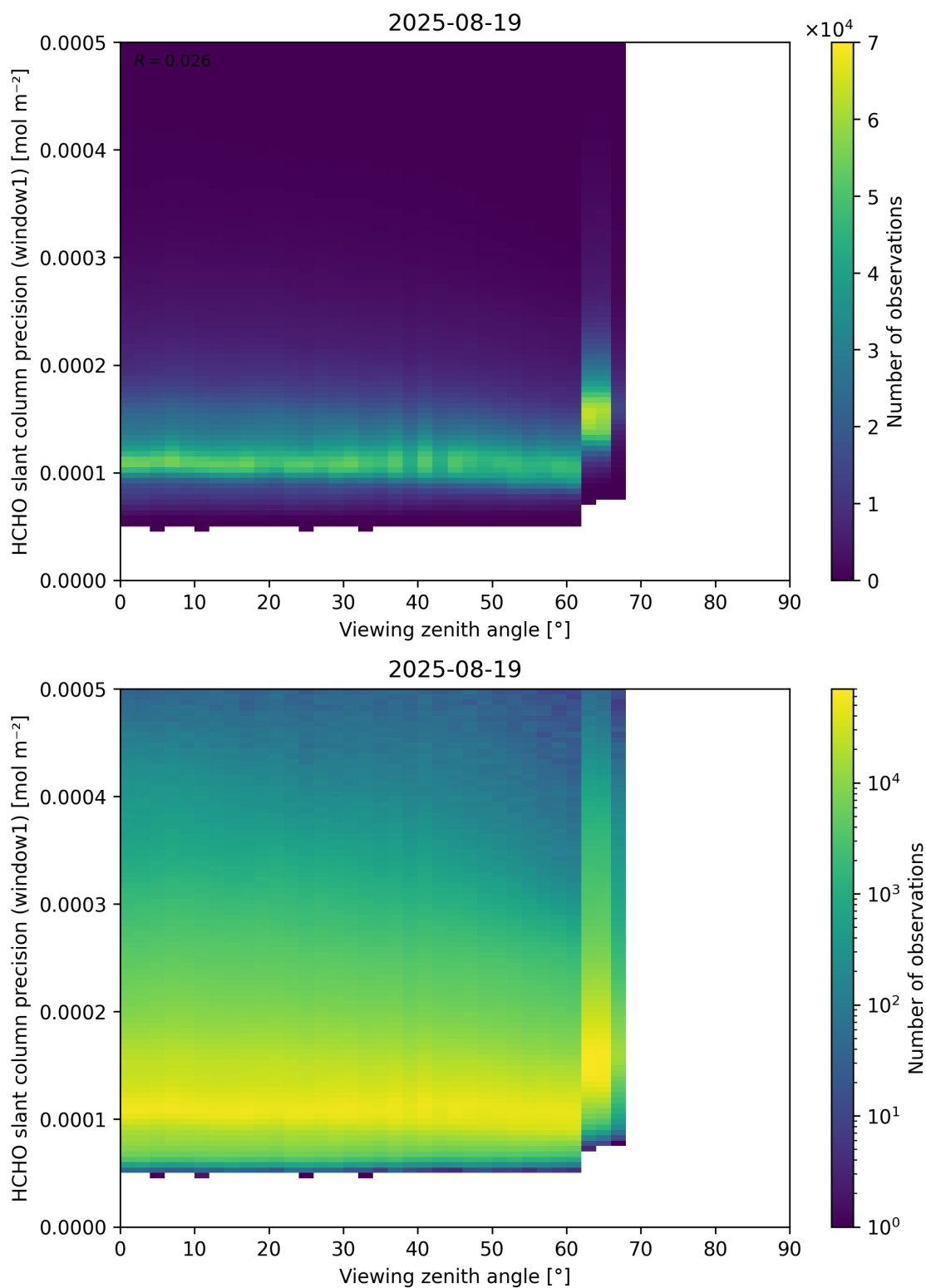
Figure 189: Scatter density plot of “Viewing zenith angle” against “HCHO slant column precision (window1)” for 2025-08-19 to 2025-08-20.
