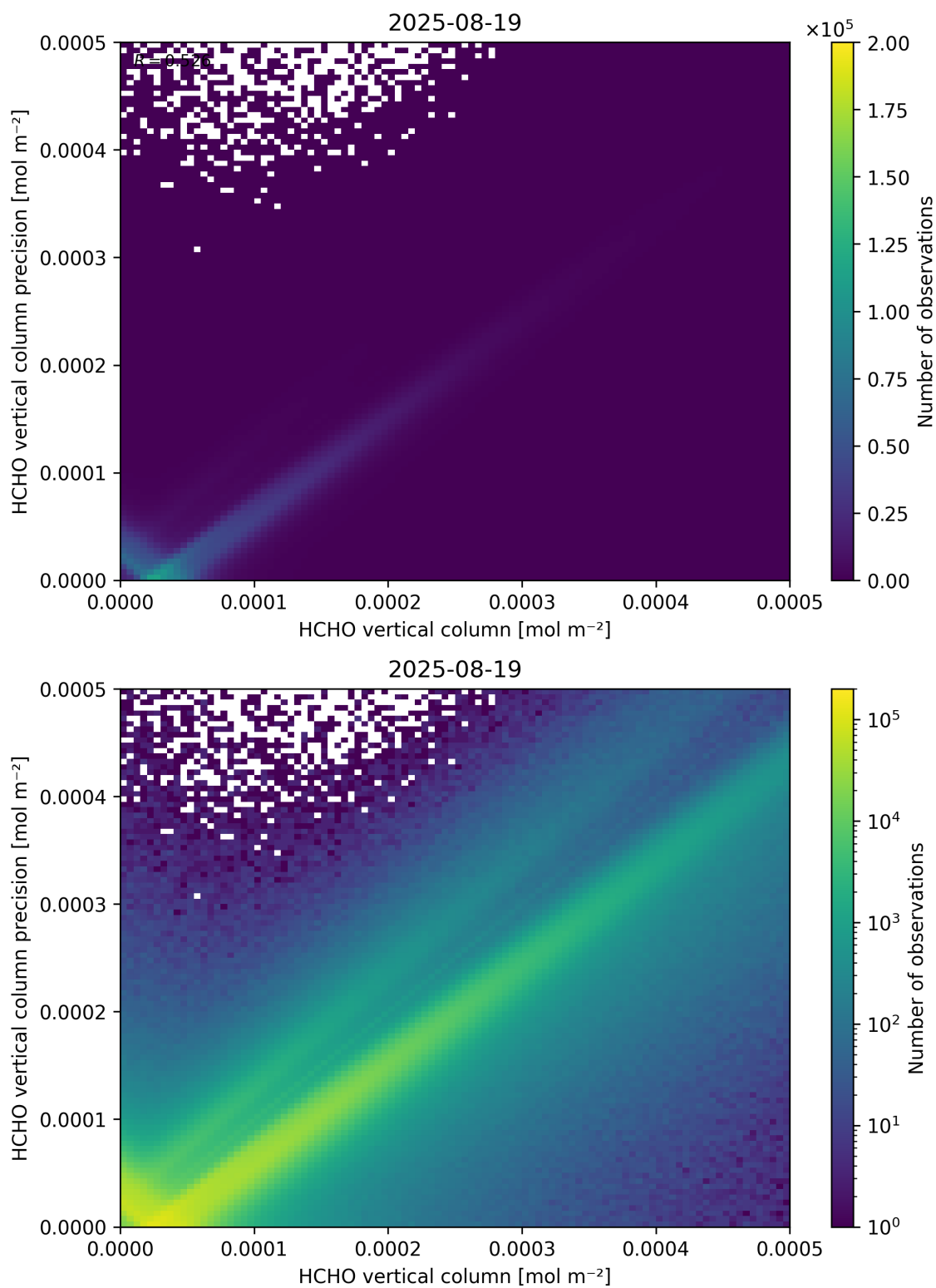
Figure 134: Scatter density plot of “HCHO vertical column” against “HCHO vertical column precision” for 2025-08-19 to 2025-08-20.
