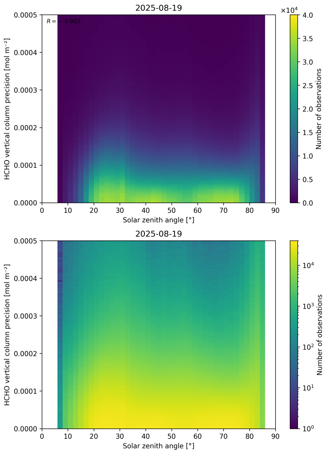
Figure 179: Scatter density plot of “Solar zenith angle” against “HCHO vertical column precision” for 2025-08-19 to 2025-08-20.
