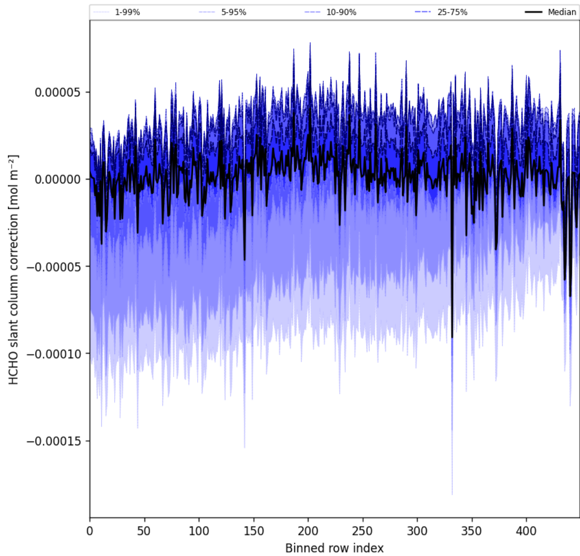
Figure 61: Along track statistics of “HCHO slant column correction” for 2025-08-19 to 2025-08-20
