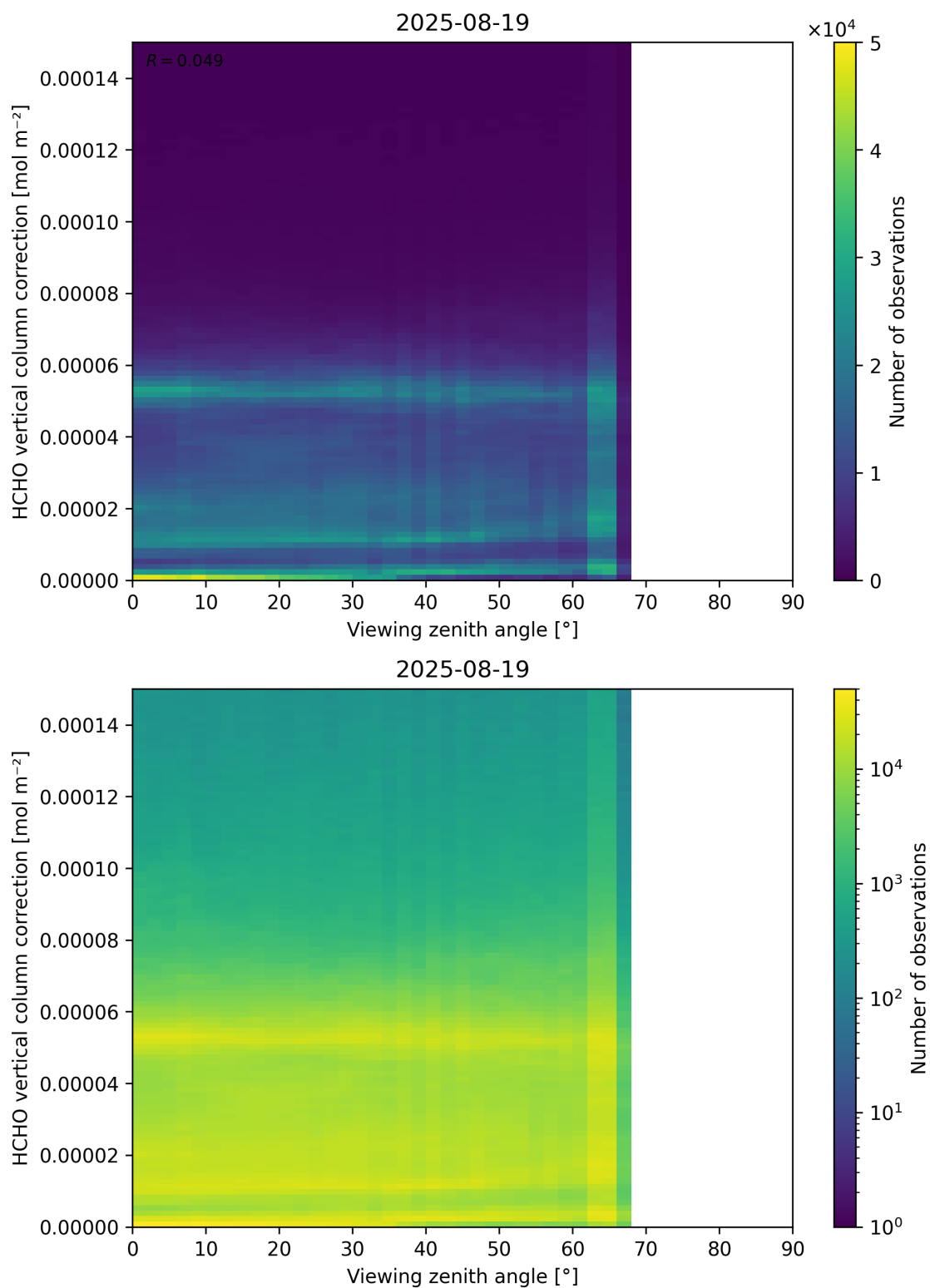
Figure 193: Scatter density plot of “Viewing zenith angle” against “HCHO vertical column correction” for 2025-08-19 to 2025-08-20.
