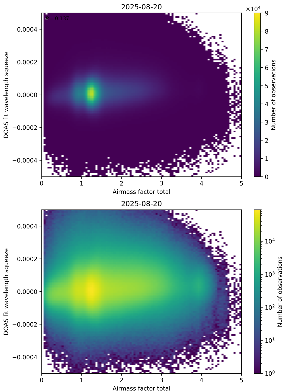
Figure 99: Scatter density plot of “Airmass factor total” against “DOAS fit wavelength squeeze” for 2025-08-19 to 2025-08-21.
