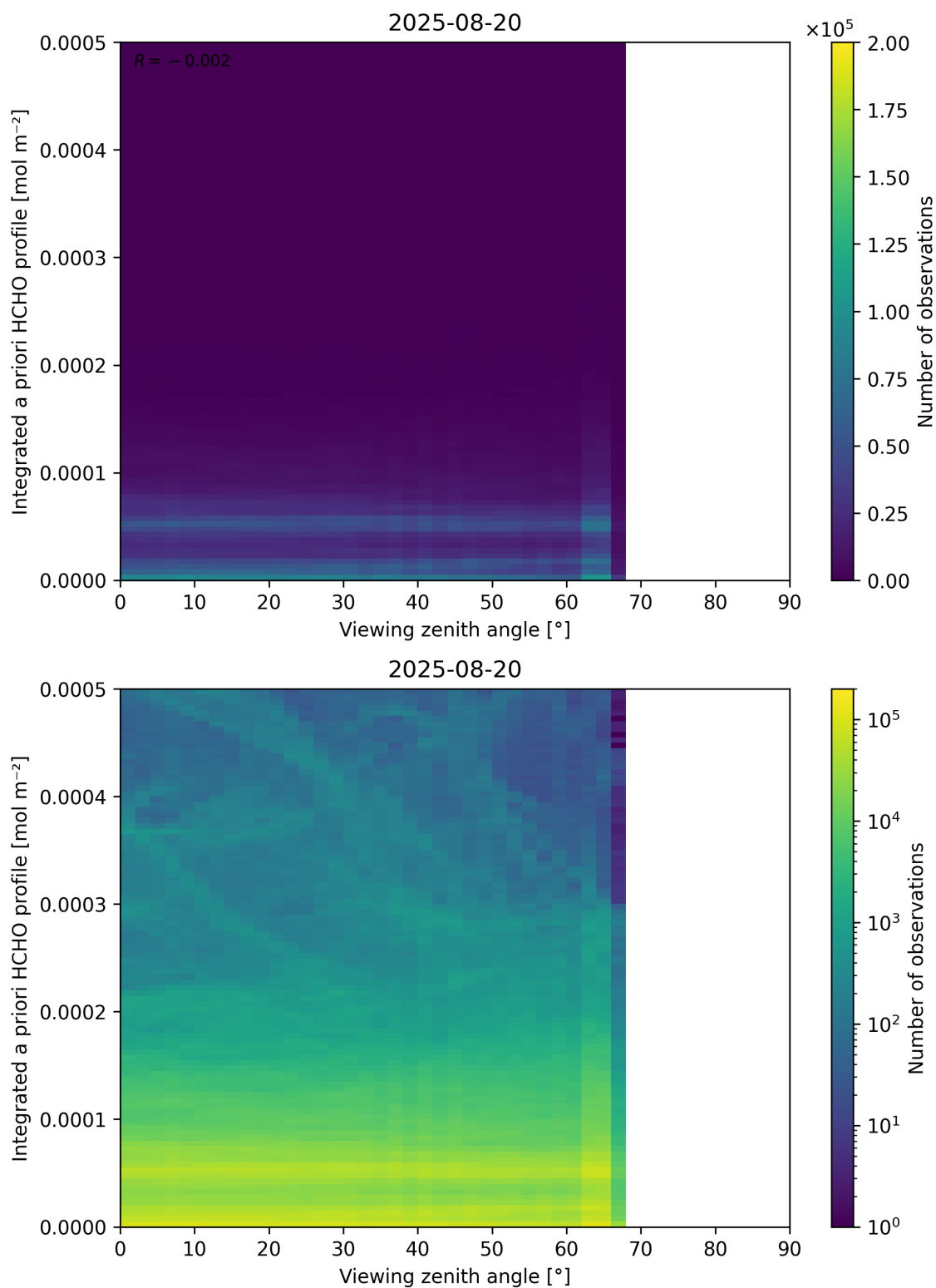
Figure 195: Scatter density plot of “Viewing zenith angle” against “Integrated a priori HCHO profile” for 2025-08-19 to 2025-08-21.
