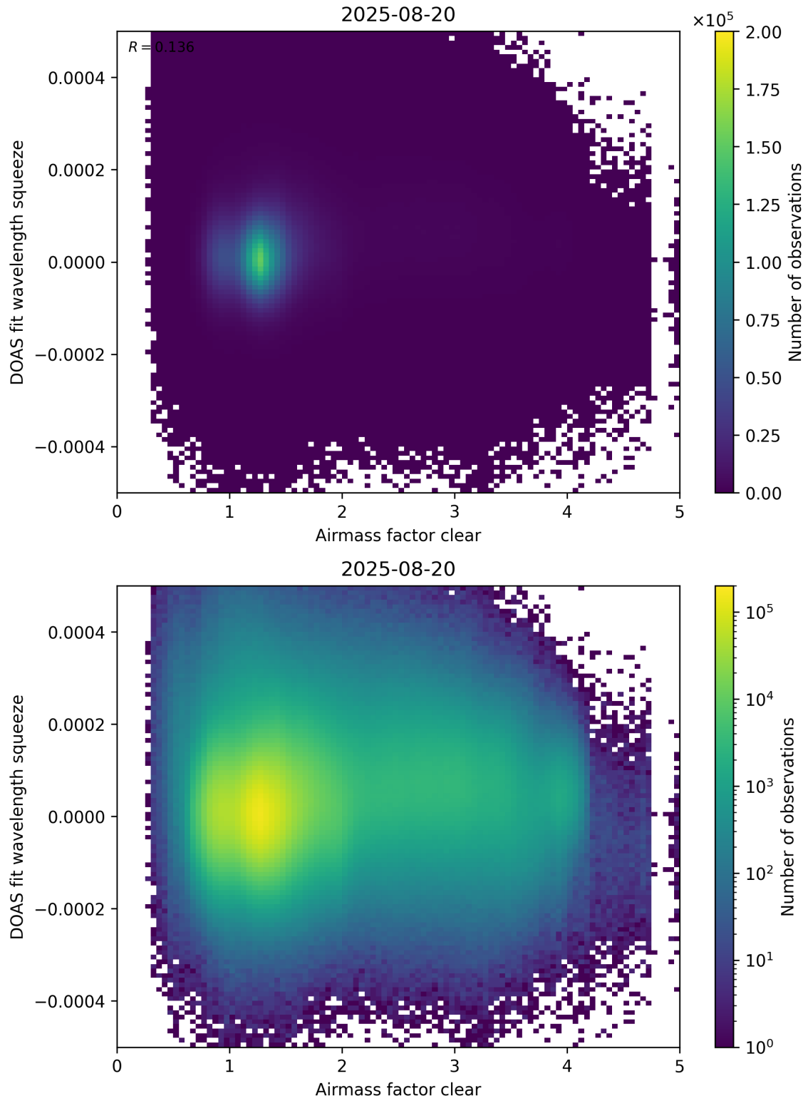
Figure 73: Scatter density plot of “Airmass factor clear” against “DOAS fit wavelength squeeze” for 2025-08-19 to 2025-08-21.
