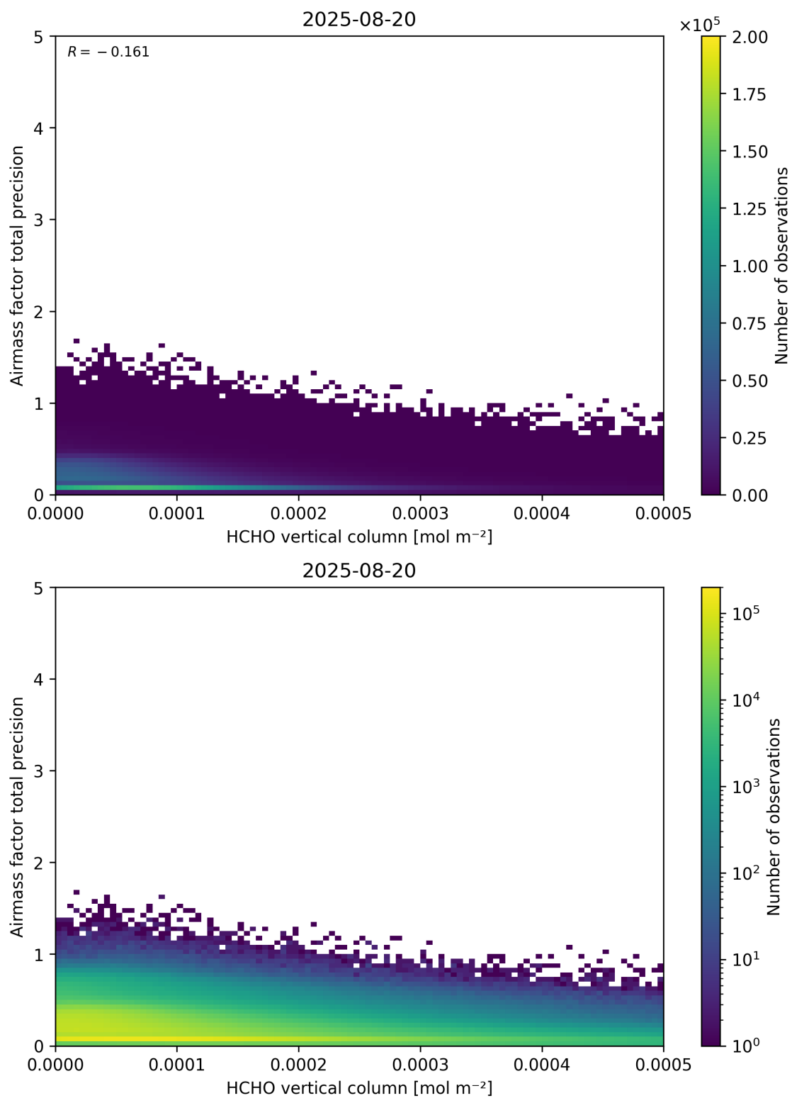
Figure 132: Scatter density plot of “HCHO vertical column” against “Airmass factor total precision” for 2025-08-19 to 2025-08-21.
