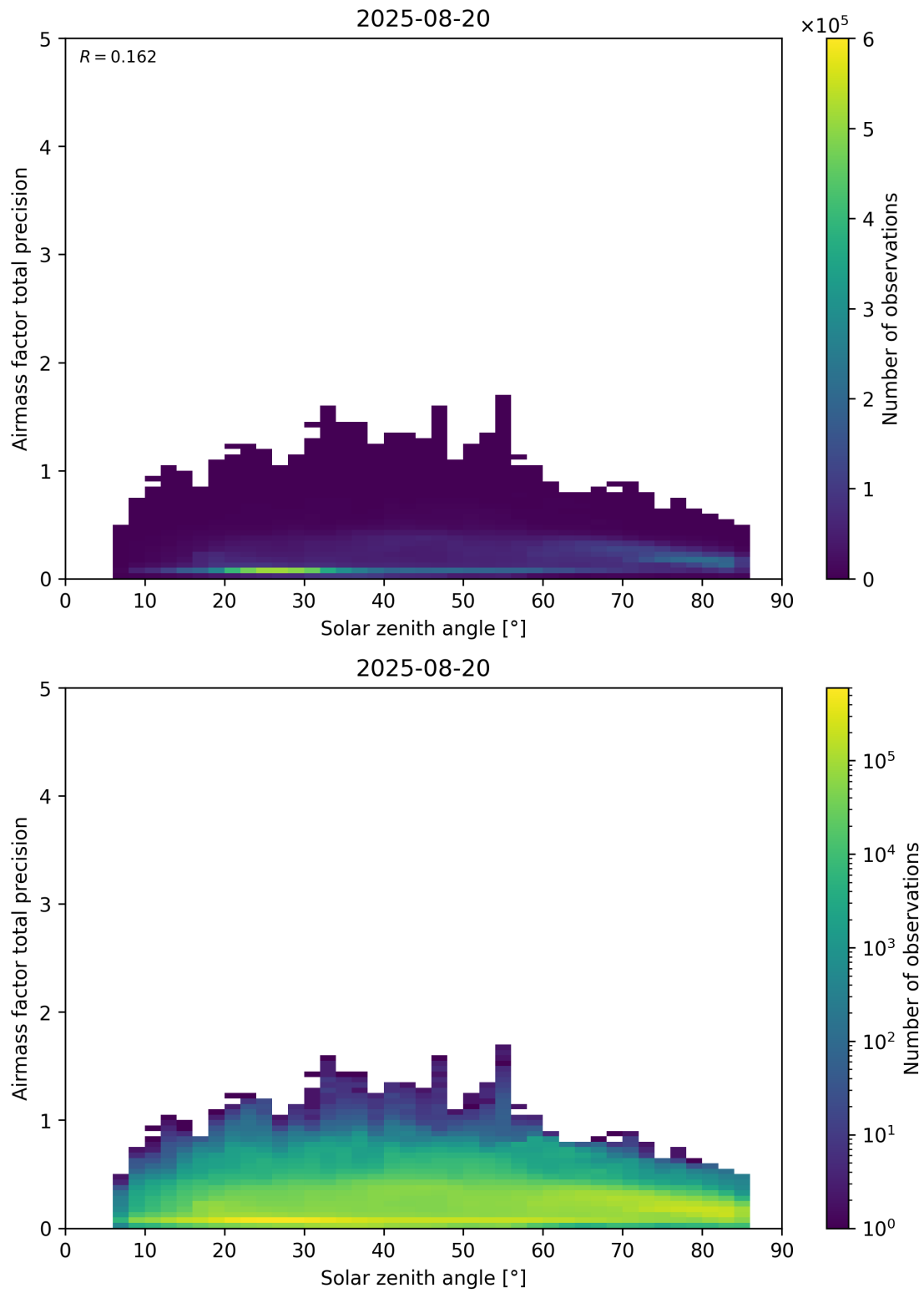
Figure 176: Scatter density plot of “Solar zenith angle” against “Airmass factor total precision” for 2025-08-19 to 2025-08-21.
