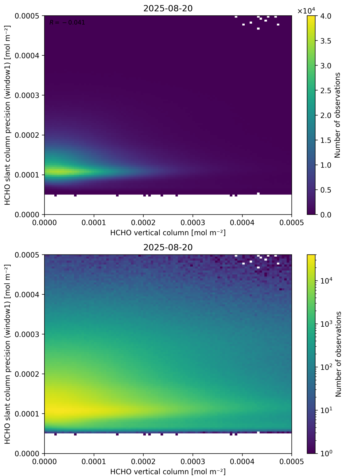
Figure 130: Scatter density plot of “HCHO vertical column” against “HCHO slant column precision (window1)” for 2025-08-19 to 2025-08-21.
