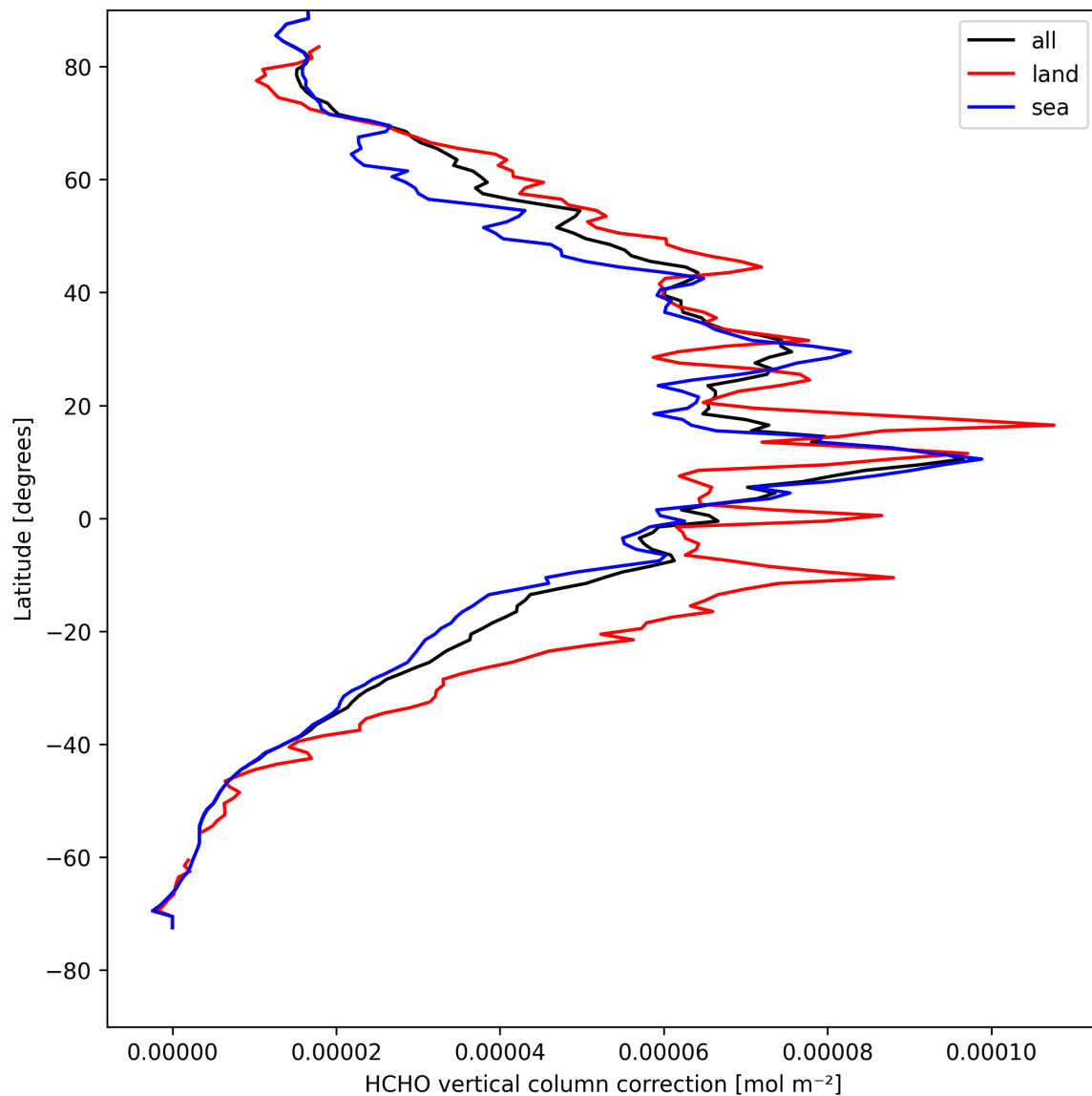
Figure 23: Zonal average of “HCHO vertical column correction” for 2025-08-19 to 2025-08-21.
