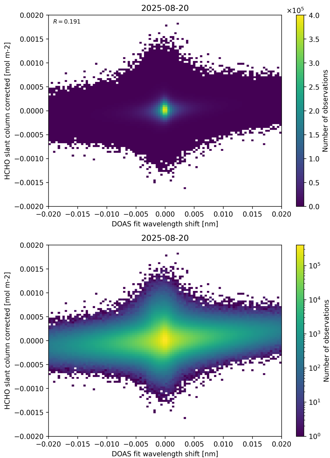
Figure 66: Scatter density plot of “DOAS fit wavelength shift” against “HCHO slant column corrected” for 2025-08-19 to 2025-08-21.
