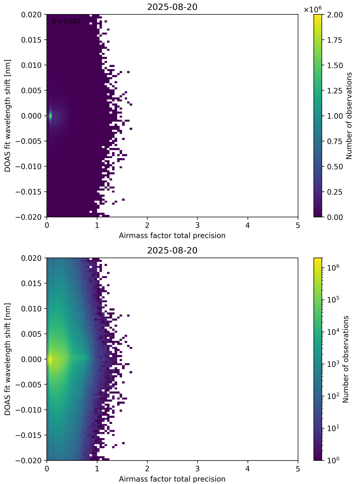
Figure 106: Scatter density plot of “Airmass factor total precision” against “DOAS fit wavelength shift” for 2025-08-19 to 2025-08-21.
