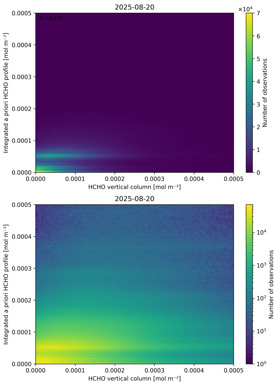
Figure 135: Scatter density plot of “HCHO vertical column” against “Integrated a priori HCHO profile” for 2025-08-19 to 2025-08-21.
