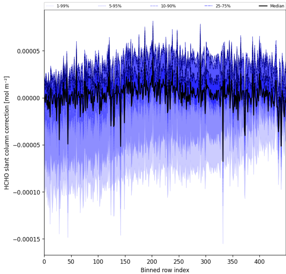
Figure 61: Along track statistics of “HCHO slant column correction” for 2025-08-19 to 2025-08-21
