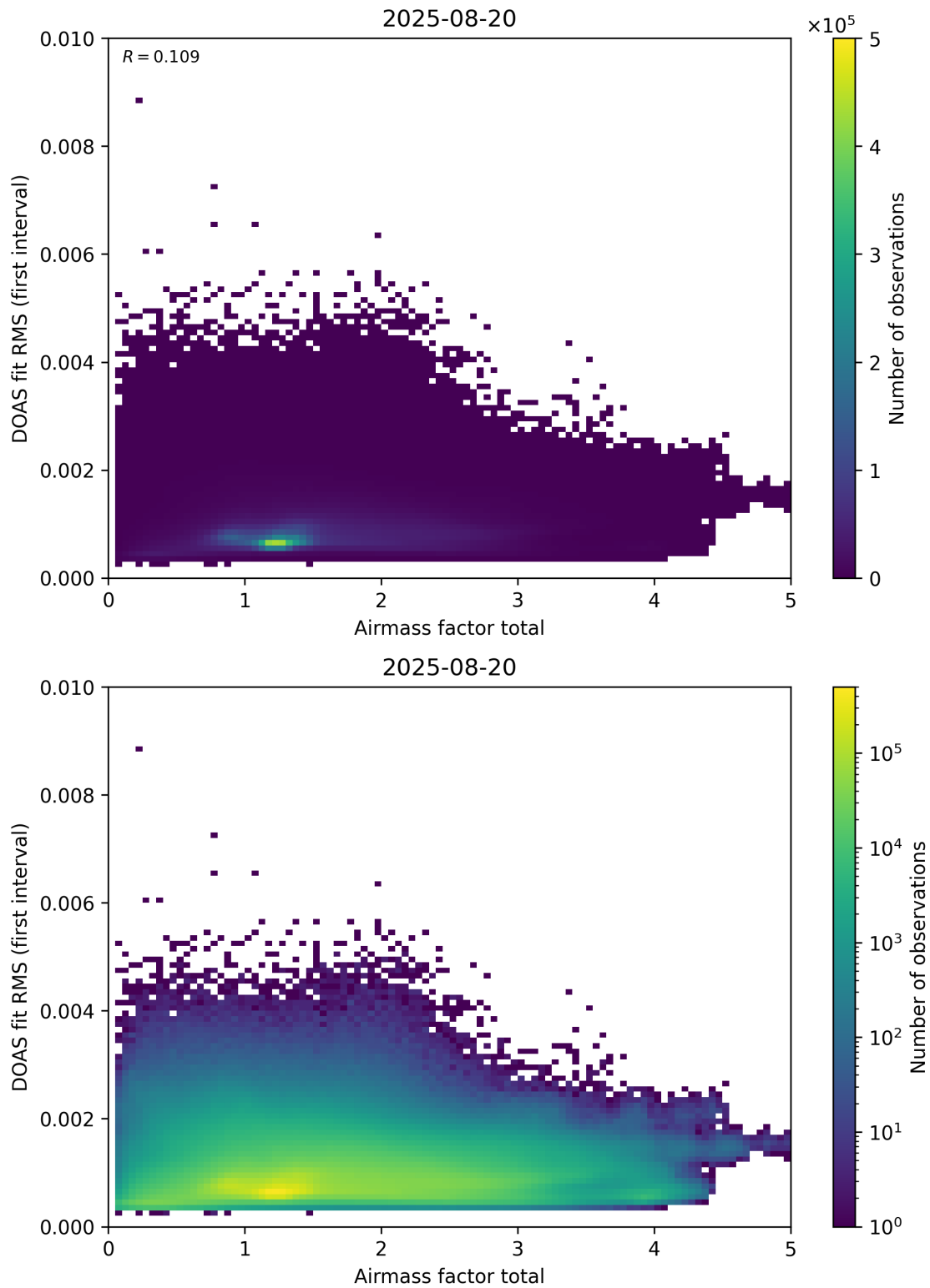
Figure 97: Scatter density plot of “Airmass factor total” against “DOAS fit RMS (first interval)” for 2025-08-19 to 2025-08-21.
