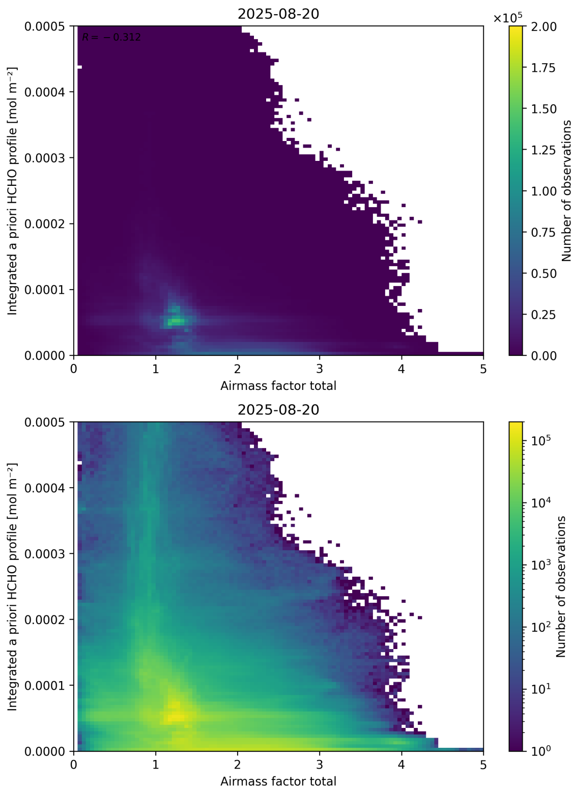
Figure 104: Scatter density plot of “Airmass factor total” against “Integrated a priori HCHO profile” for 2025-08-19 to 2025-08-21.
