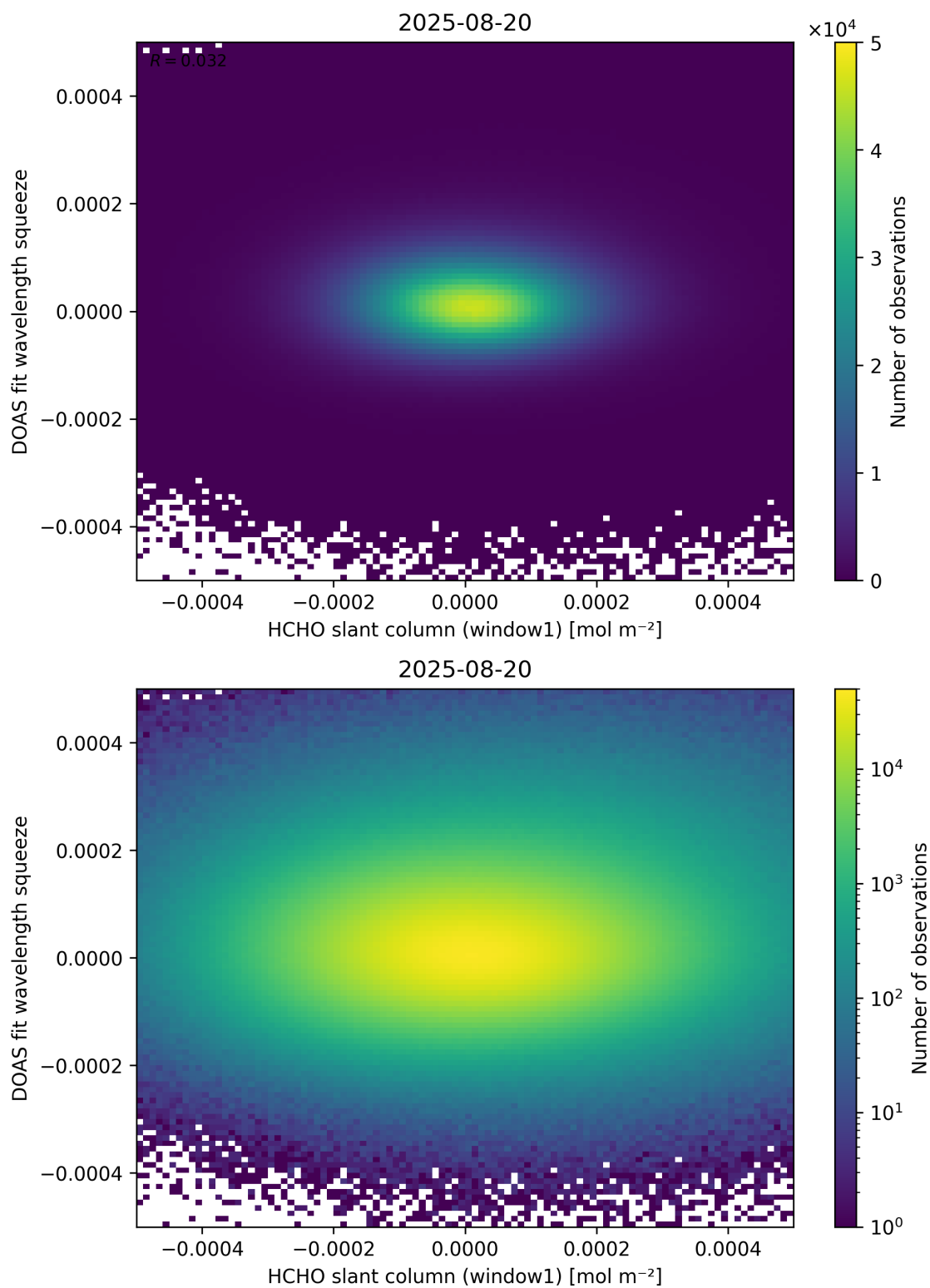
Figure 80: Scatter density plot of “HCHO slant column (window1)” against “DOAS fit wavelength squeeze” for 2025-08-19 to 2025-08-21.
