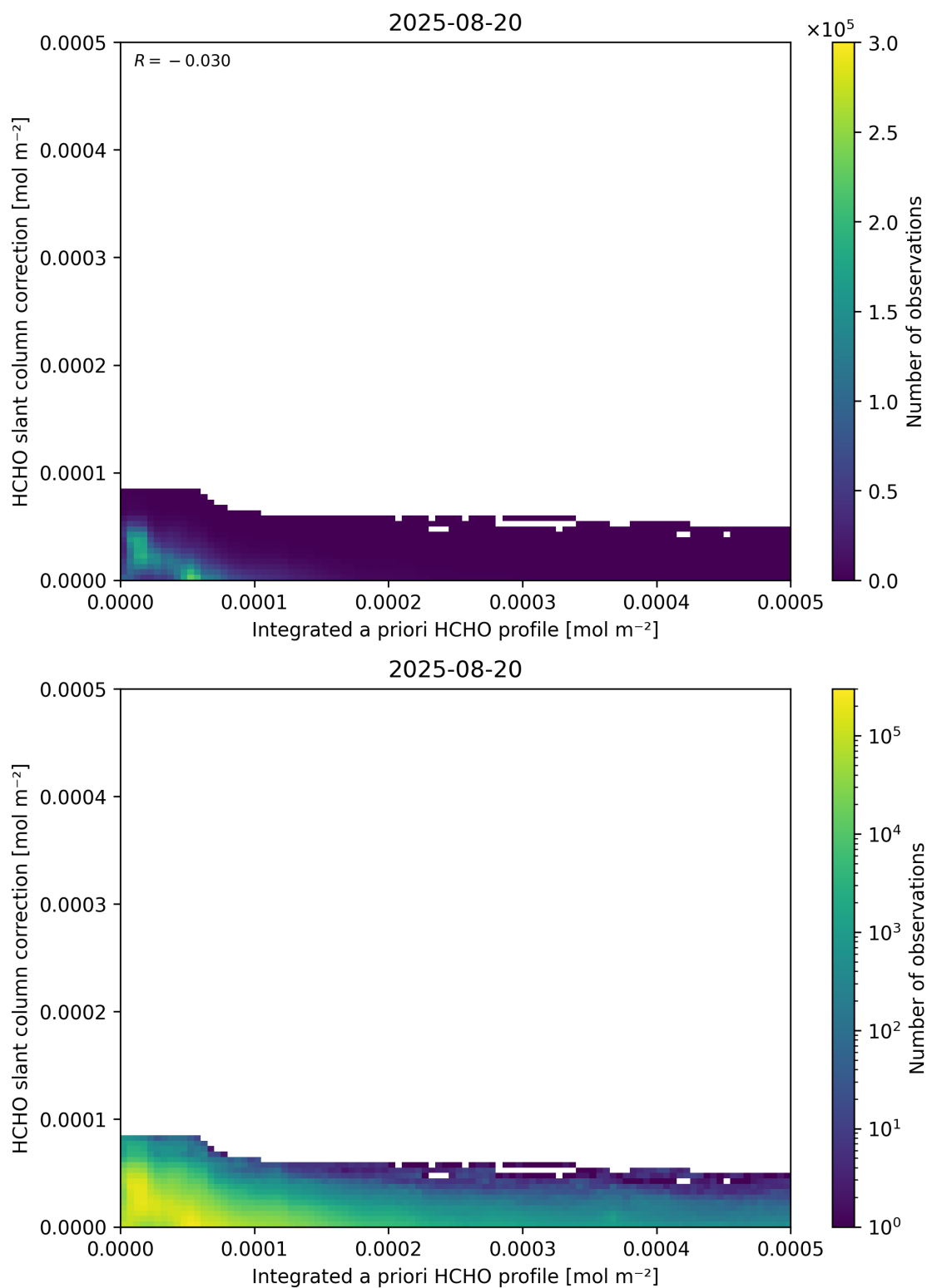
Figure 152: Scatter density plot of “Integrated a priori HCHO profile” against “HCHO slant column correction” for 2025-08-19 to 2025-08-21.
