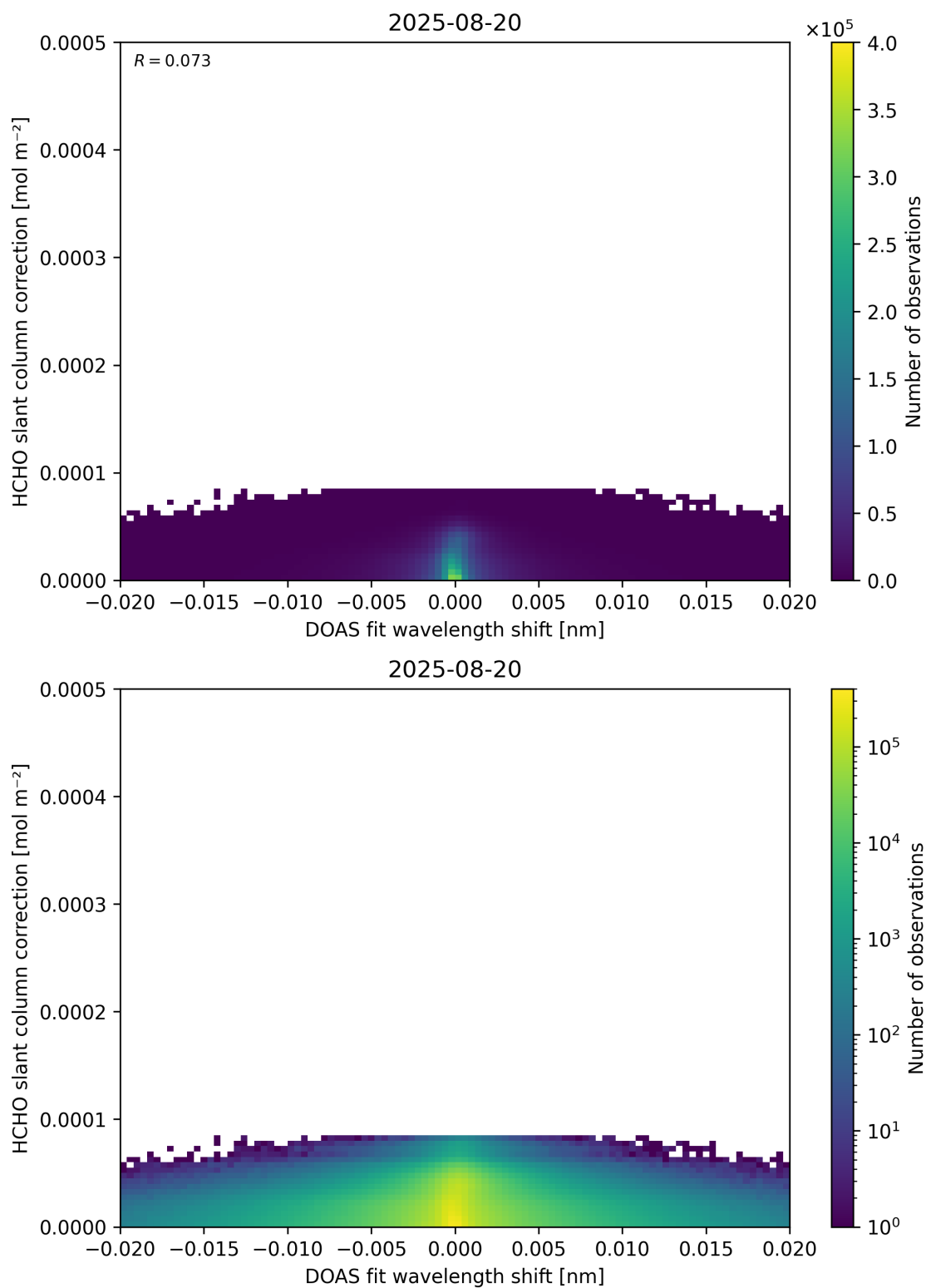
Figure 67: Scatter density plot of “DOAS fit wavelength shift” against “HCHO slant column correction” for 2025-08-19 to 2025-08-21.
