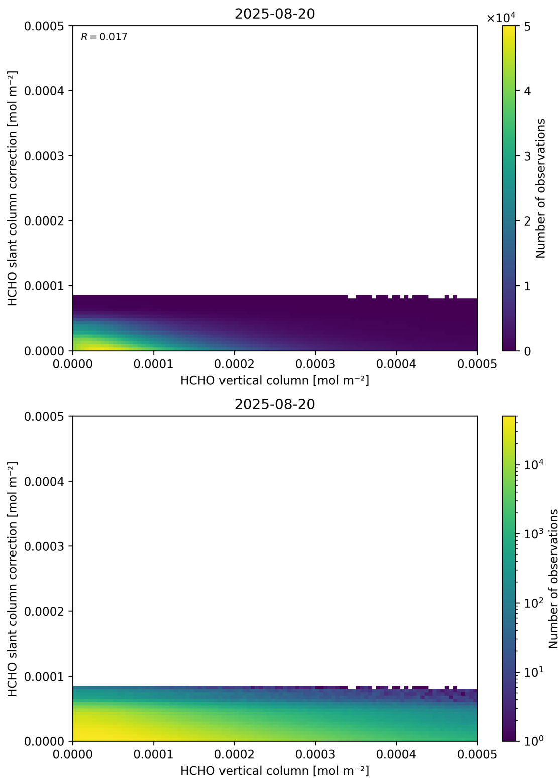
Figure 128: Scatter density plot of “HCHO vertical column” against “HCHO slant column correction” for 2025-08-19 to 2025-08-21.
