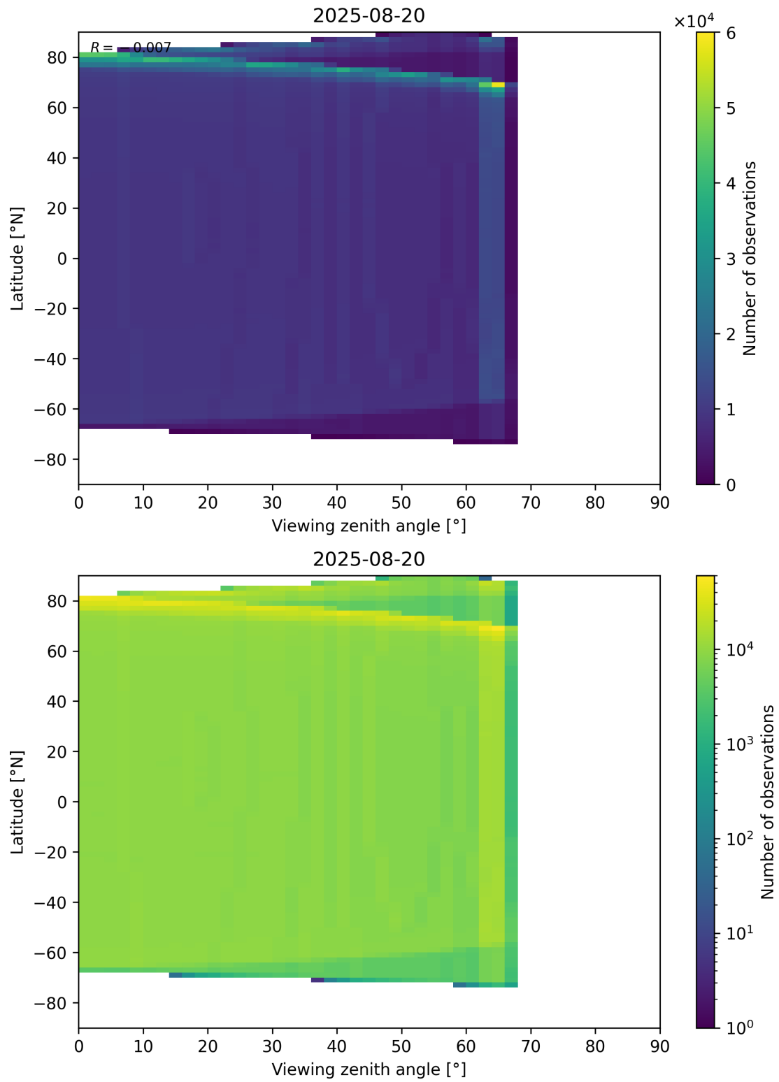
Figure 196: Scatter density plot of “Viewing zenith angle” against “Latitude” for 2025-08-19 to 2025-08-21.
