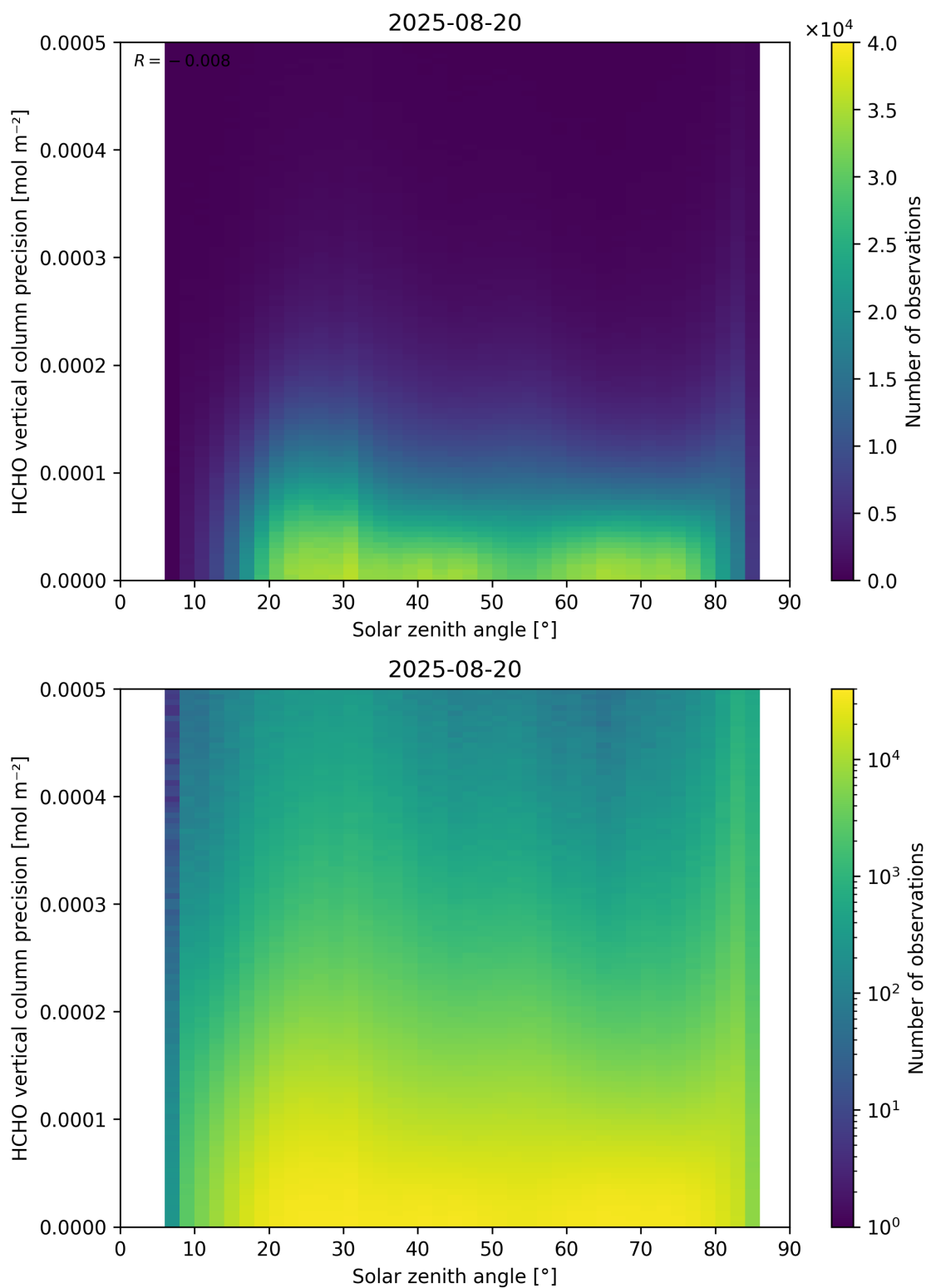
Figure 179: Scatter density plot of “Solar zenith angle” against “HCHO vertical column precision” for 2025-08-19 to 2025-08-21.
