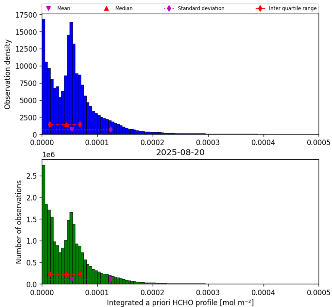
Figure 43: Histogram of “Integrated a priori HCHO profile” for 2025-08-19 to 2025-08-21
