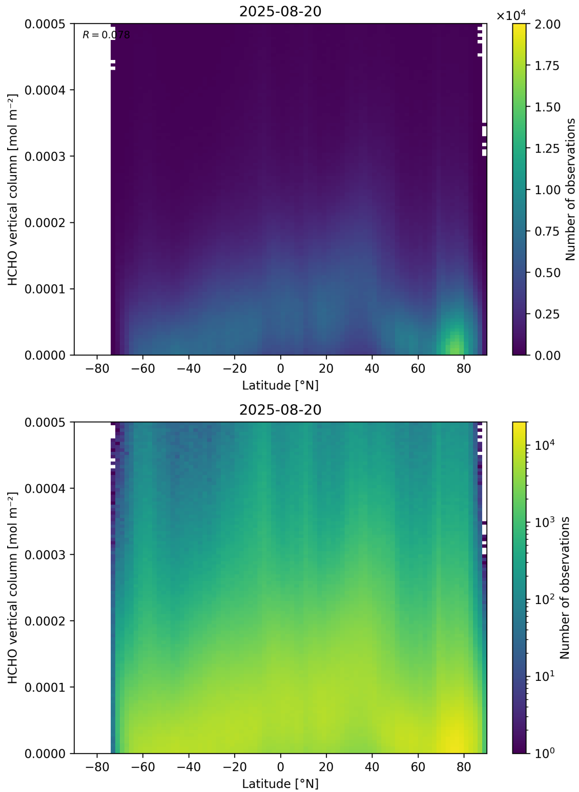
Figure 163: Scatter density plot of “Latitude” against “HCHO vertical column” for 2025-08-19 to 2025-08-21.
