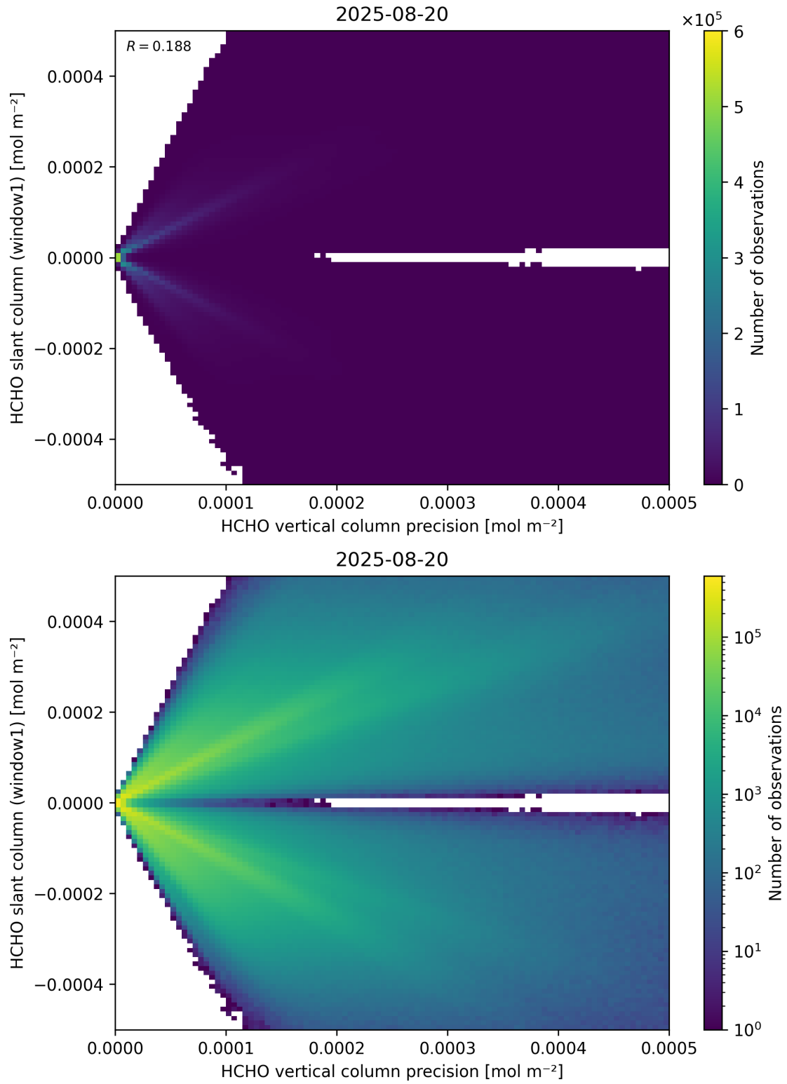
Figure 142: Scatter density plot of “HCHO vertical column precision” against “HCHO slant column (window1)” for 2025-08-19 to 2025-08-21.
