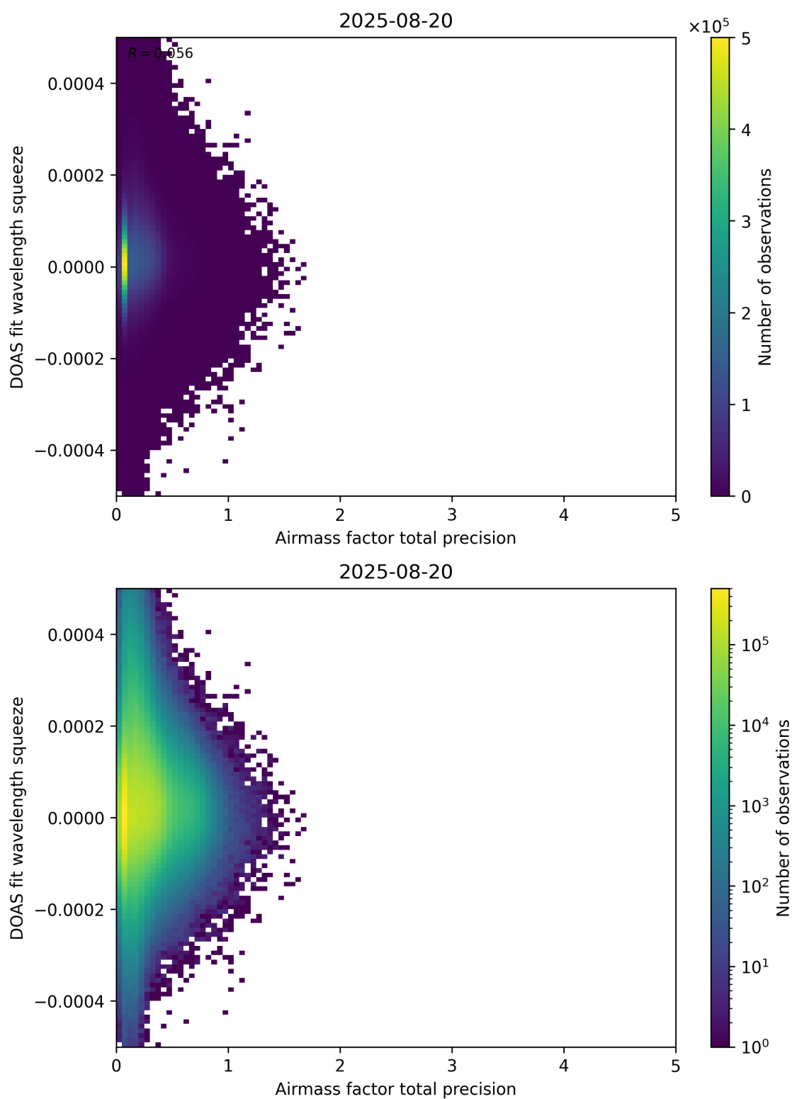
Figure 107: Scatter density plot of “Airmass factor total precision” against “DOAS fit wavelength squeeze” for 2025-08-19 to 2025-08-21.
