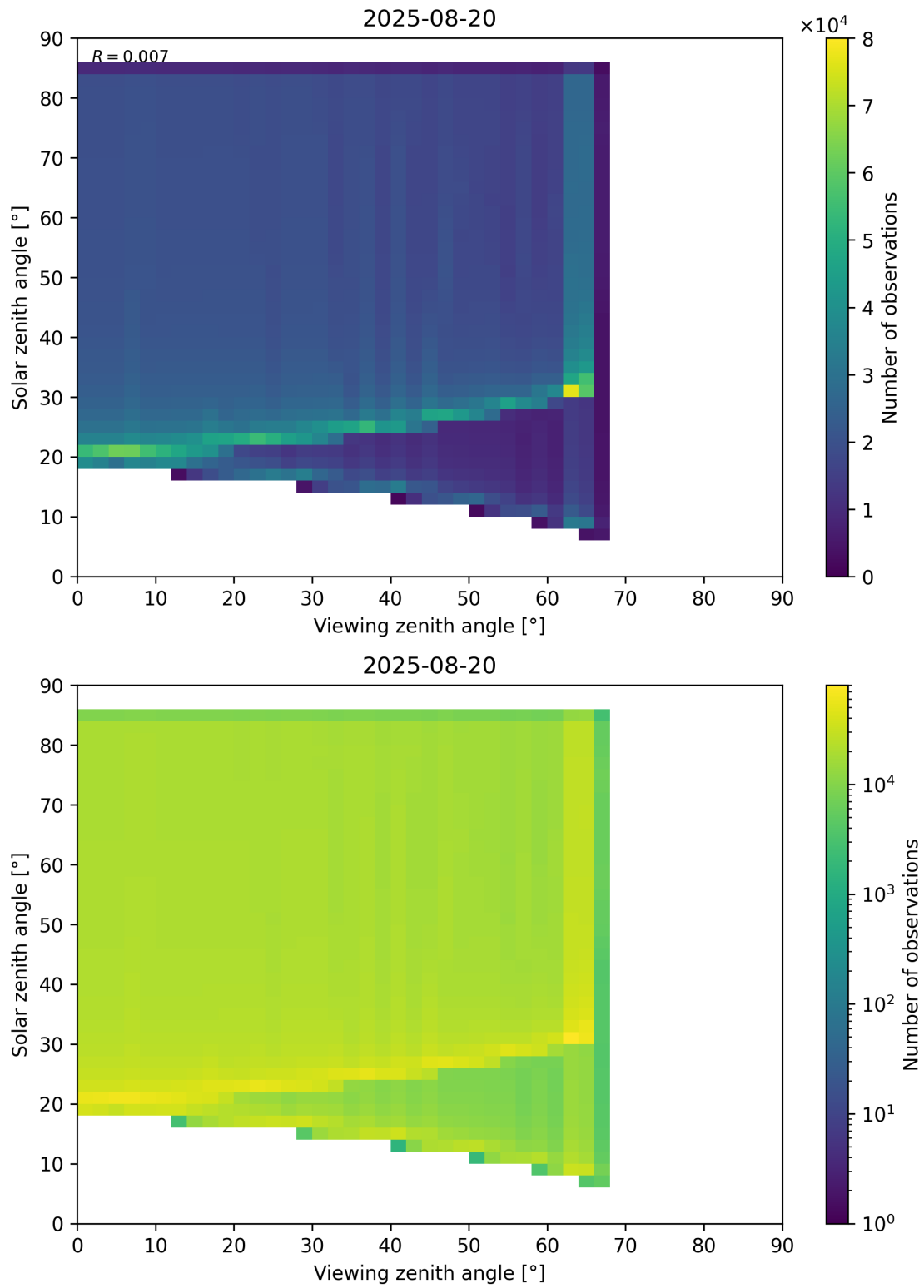
Figure 197: Scatter density plot of “Viewing zenith angle” against “Solar zenith angle” for 2025-08-19 to 2025-08-21.
