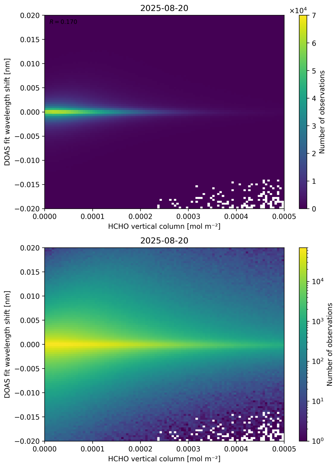
Figure 124: Scatter density plot of “HCHO vertical column” against “DOAS fit wavelength shift” for 2025-08-19 to 2025-08-21.
