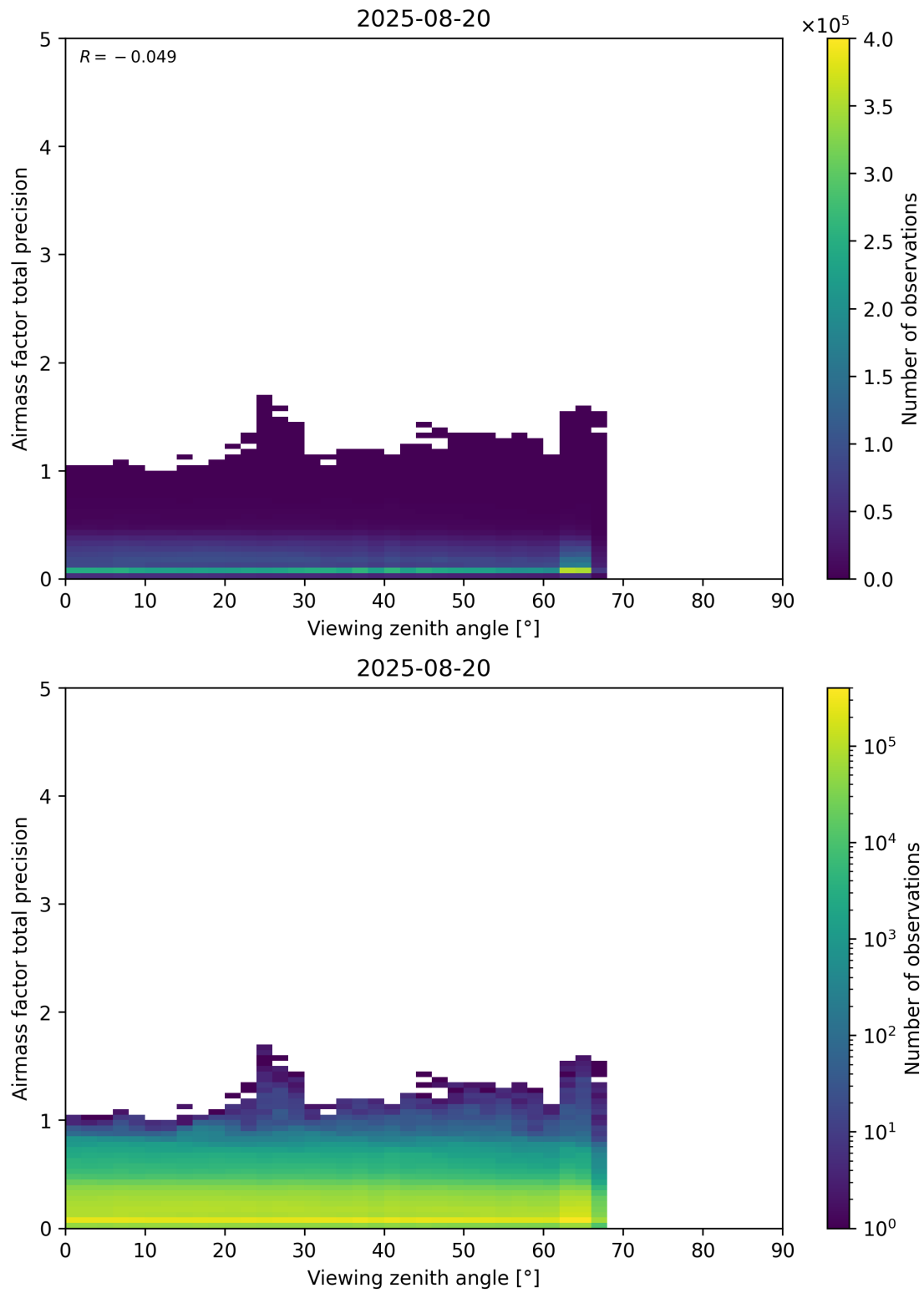
Figure 191: Scatter density plot of “Viewing zenith angle” against “Airmass factor total precision” for 2025-08-19 to 2025-08-21.
