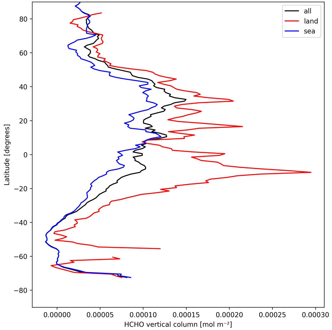
Figure 21: Zonal average of “HCHO vertical column” for 2025-08-19 to 2025-08-21.
