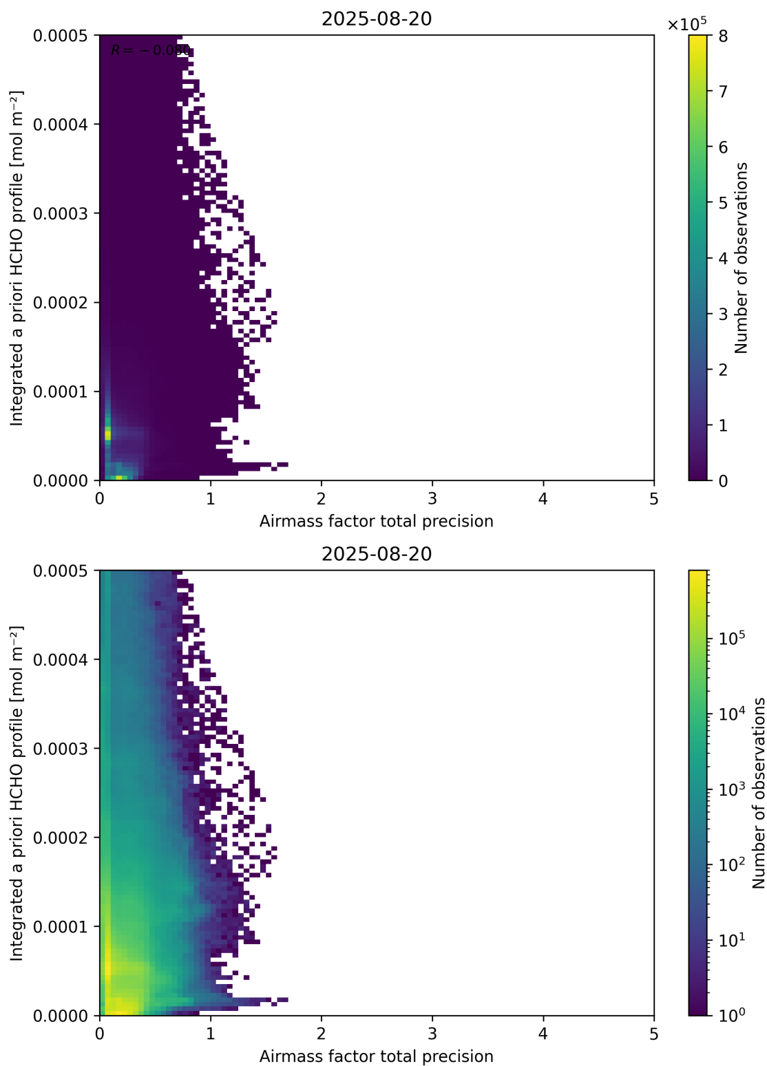
Figure 111: Scatter density plot of “Airmass factor total precision” against “Integrated a priori HCHO profile” for 2025-08-19 to 2025-08-21.
