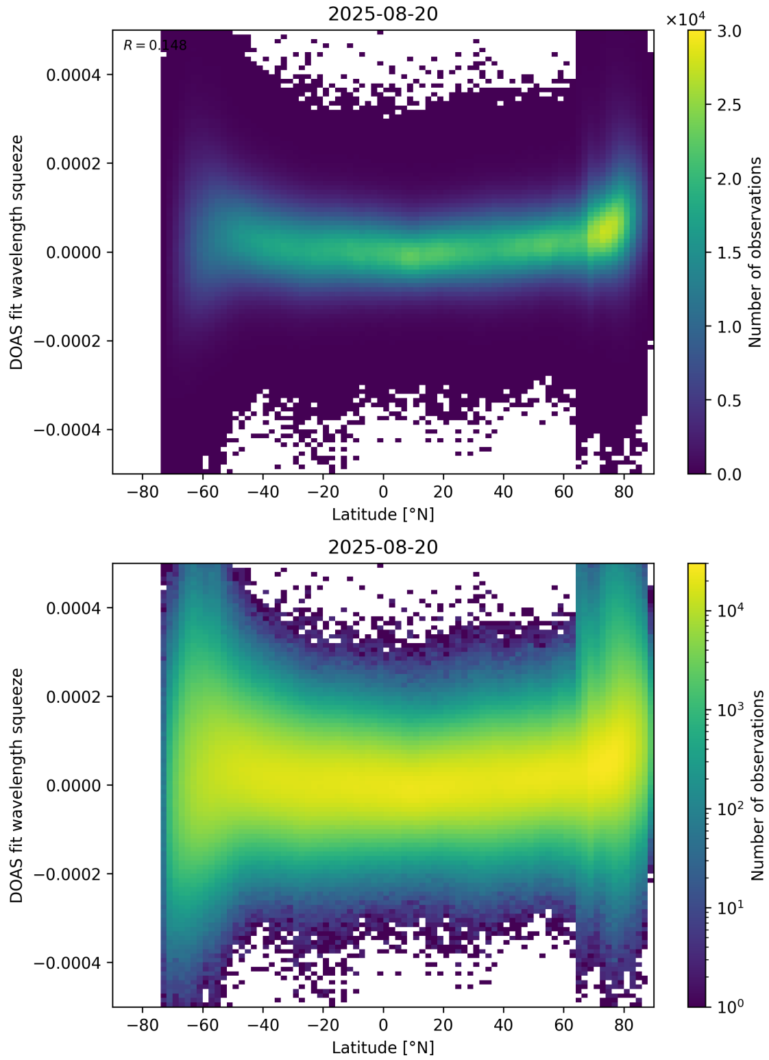
Figure 155: Scatter density plot of “Latitude” against “DOAS fit wavelength squeeze” for 2025-08-19 to 2025-08-21.
