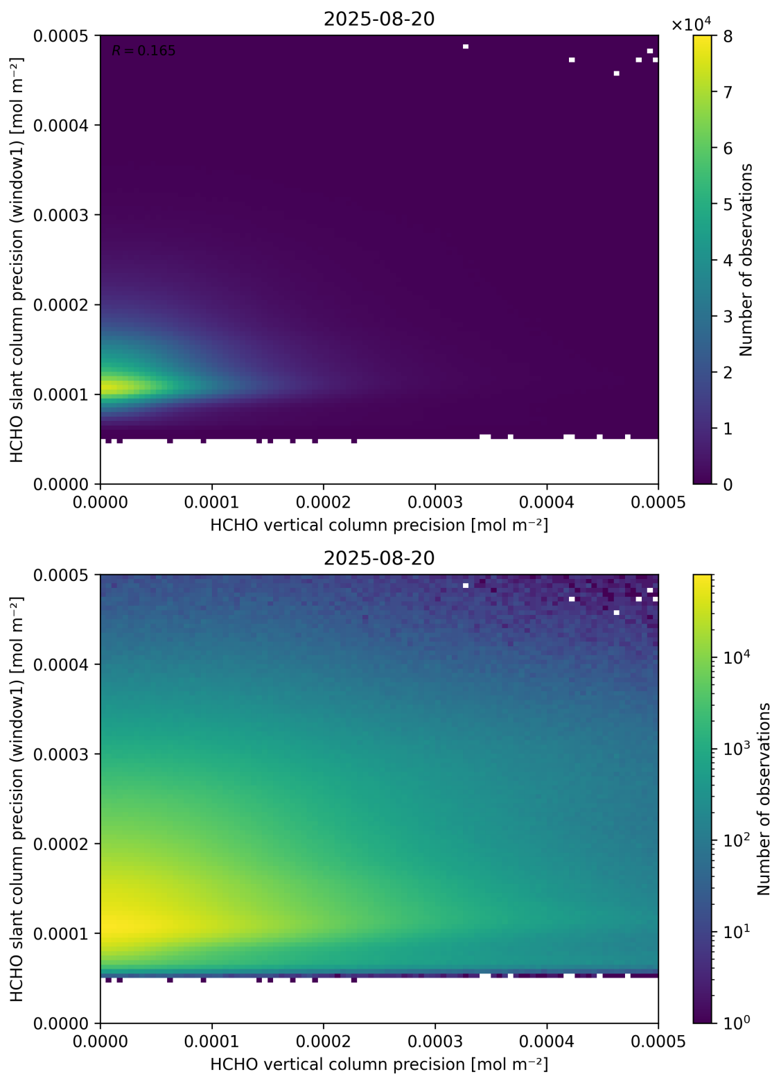
Figure 143: Scatter density plot of “HCHO vertical column precision” against “HCHO slant column precision (window1)” for 2025-08-19 to 2025-08-21.
