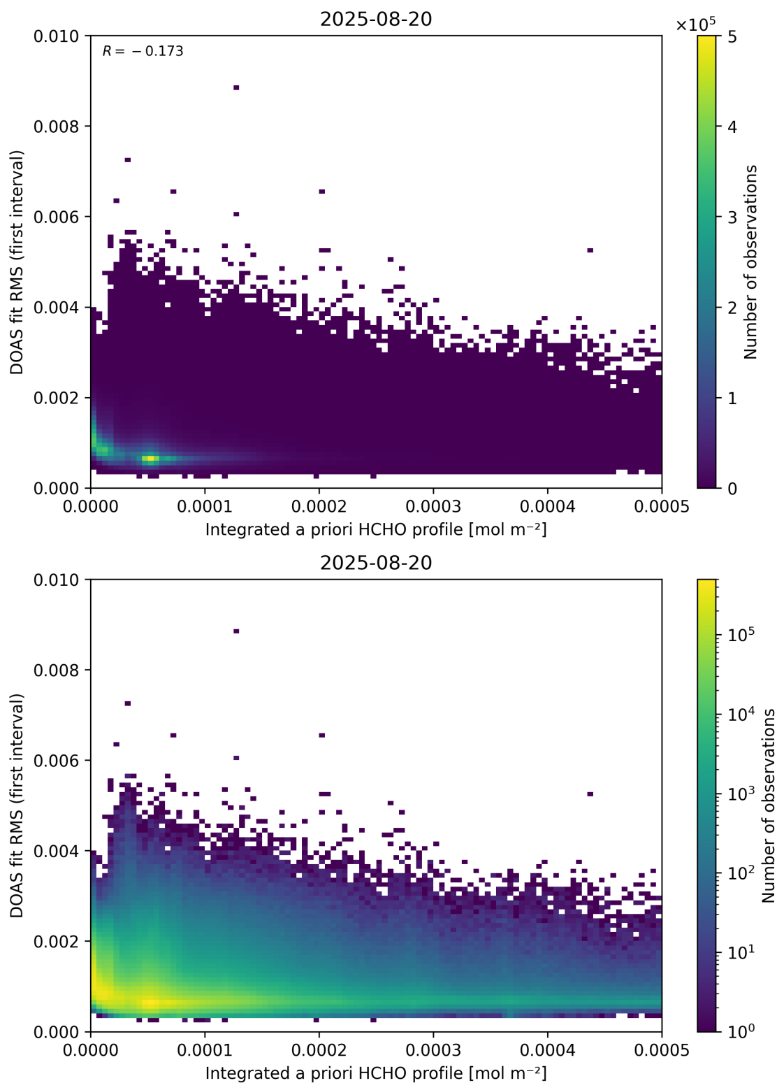
Figure 148: Scatter density plot of “Integrated a priori HCHO profile” against “DOAS fit RMS (first interval)” for 2025-08-19 to 2025-08-21.
