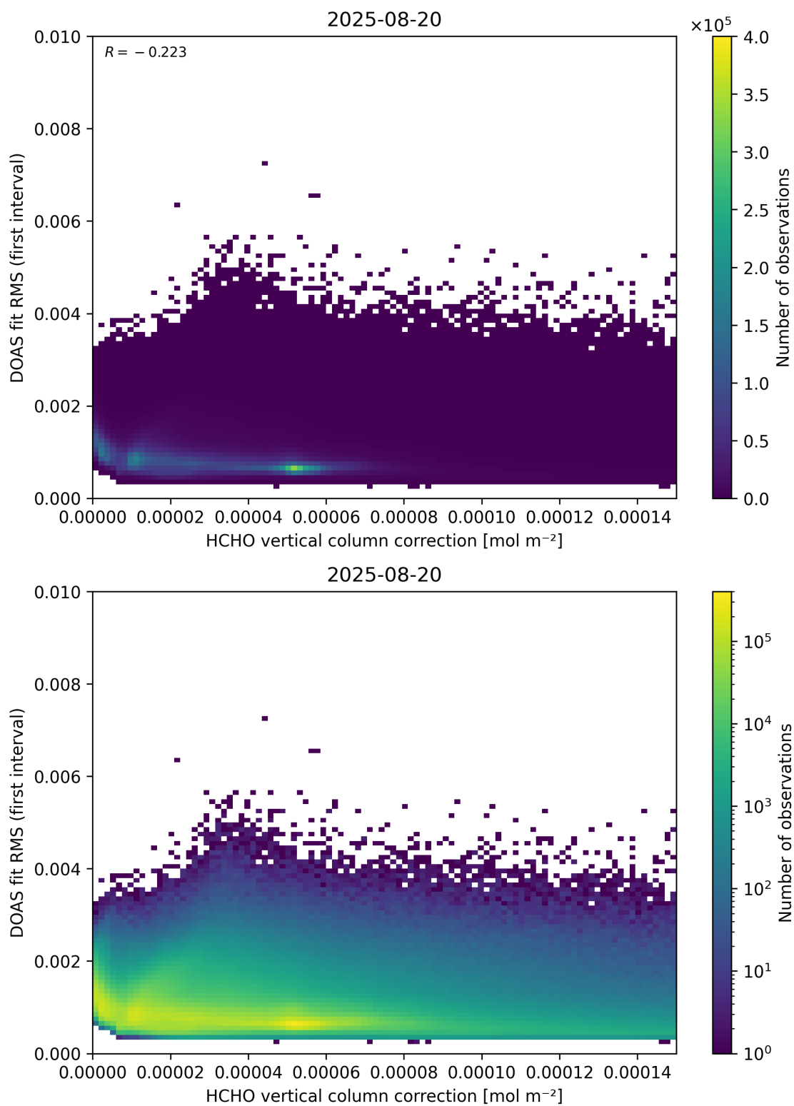
Figure 112: Scatter density plot of “HCHO vertical column correction” against “DOAS fit RMS (first interval)” for 2025-08-19 to 2025-08-21.
