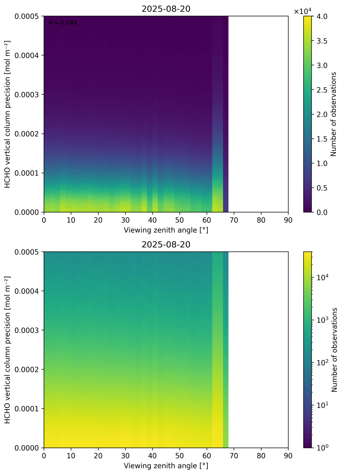
Figure 194: Scatter density plot of “Viewing zenith angle” against “HCHO vertical column precision” for 2025-08-19 to 2025-08-21.
