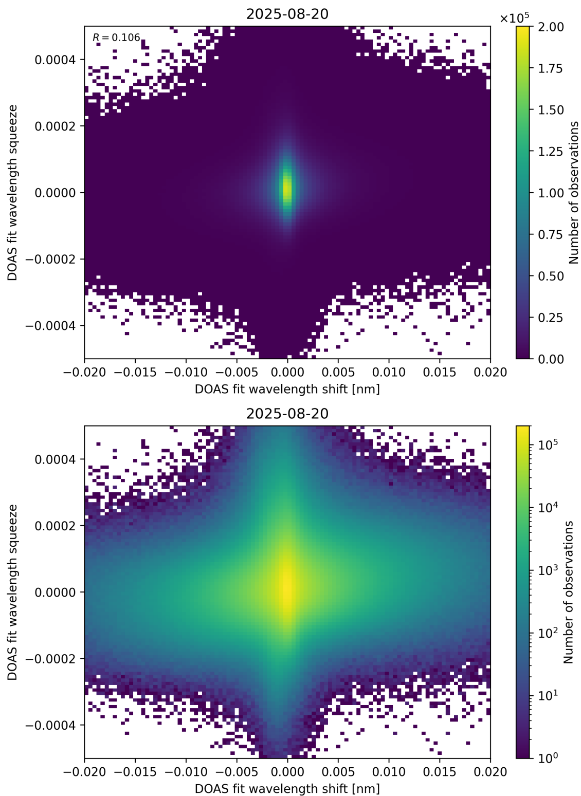
Figure 65: Scatter density plot of “DOAS fit wavelength shift” against “DOAS fit wavelength squeeze” for 2025-08-19 to 2025-08-21.
