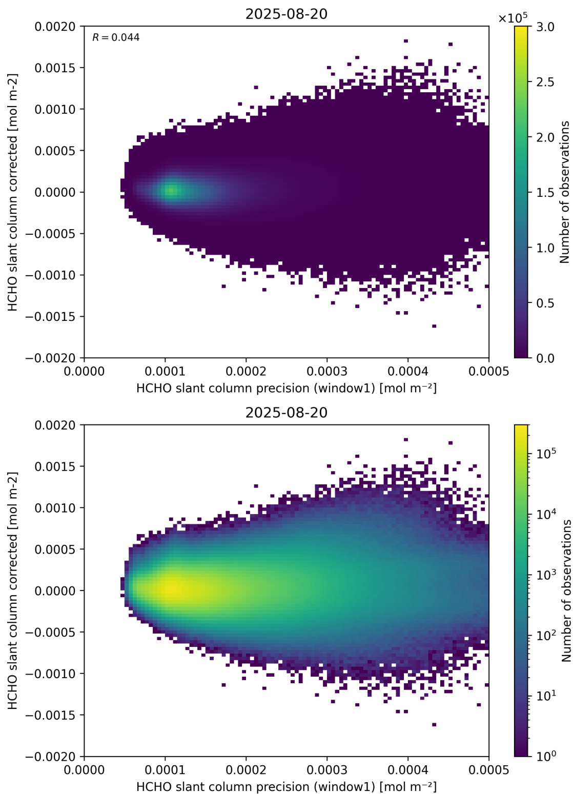
Figure 92: Scatter density plot of “HCHO slant column precision (window1)” against “HCHO slant column corrected” for 2025-08-19 to 2025-08-21.
