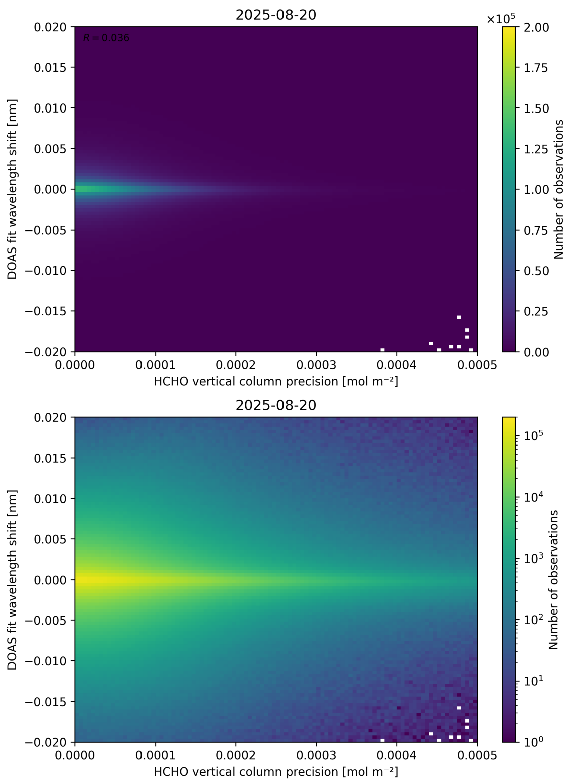
Figure 137: Scatter density plot of “HCHO vertical column precision” against “DOAS fit wavelength shift” for 2025-08-19 to 2025-08-21.
