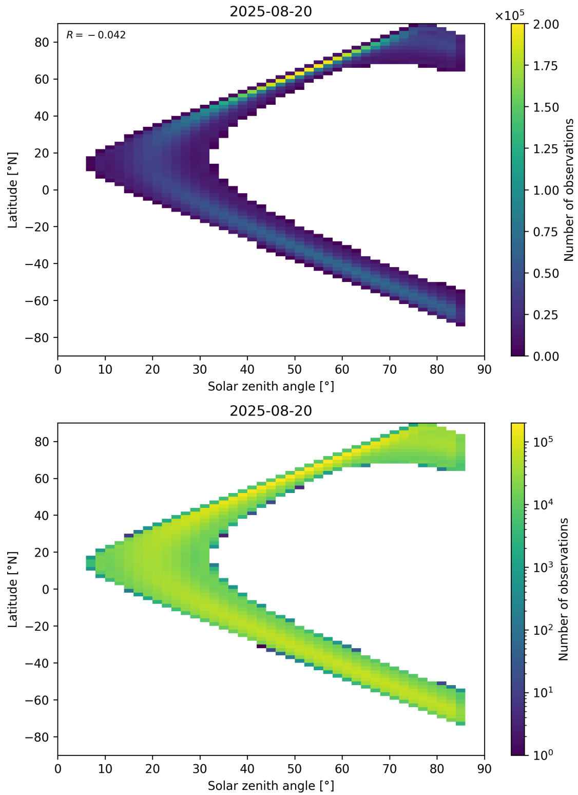
Figure 181: Scatter density plot of “Solar zenith angle” against “Latitude” for 2025-08-19 to 2025-08-21.
