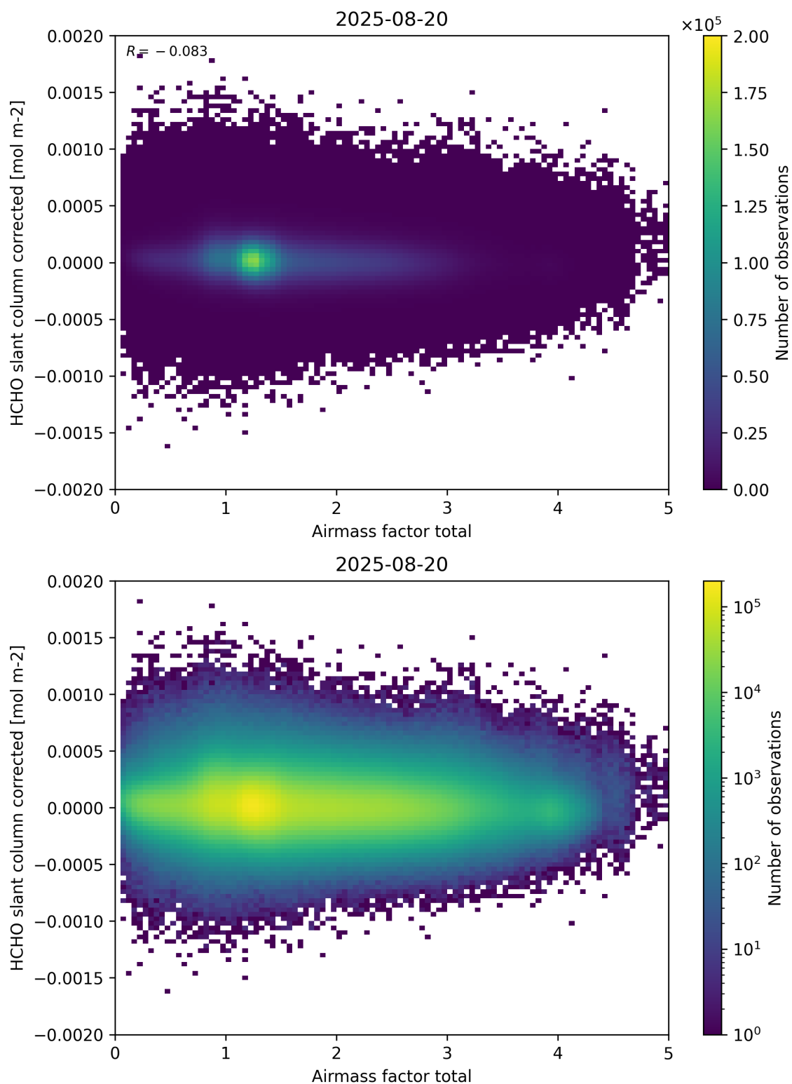
Figure 101: Scatter density plot of “Airmass factor total” against “HCHO slant column corrected” for 2025-08-19 to 2025-08-21.
