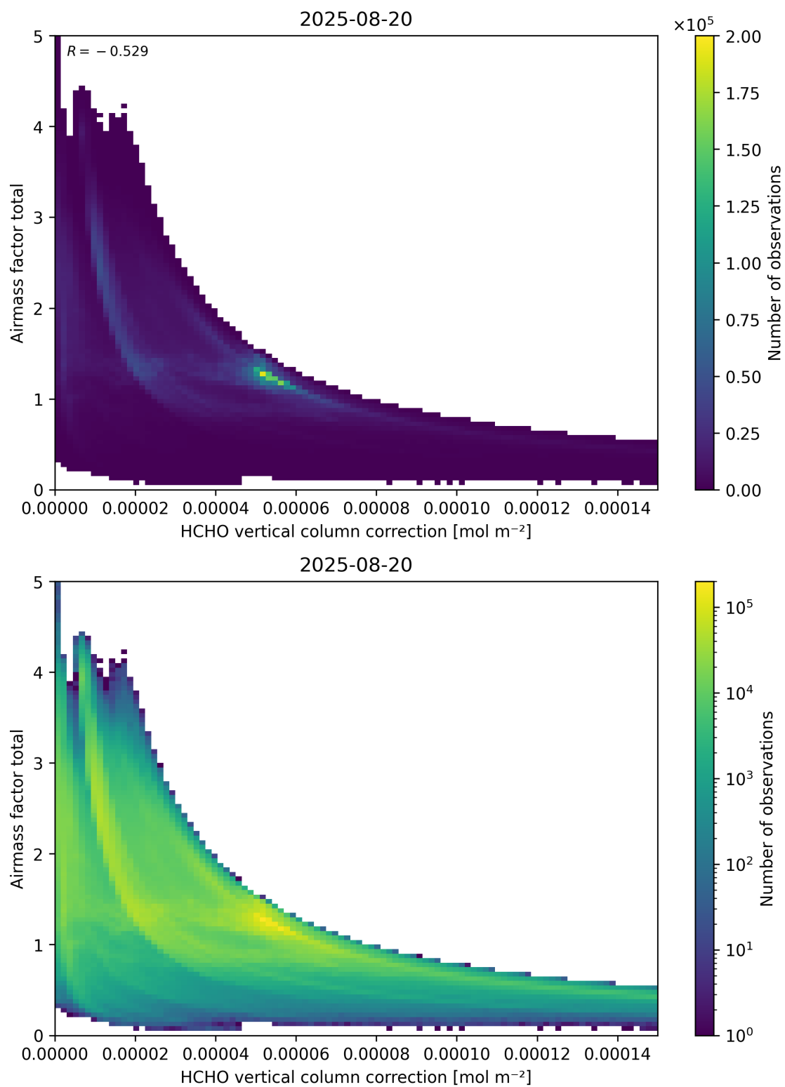
Figure 120: Scatter density plot of “HCHO vertical column correction” against “Airmass factor total” for 2025-08-19 to 2025-08-21.
