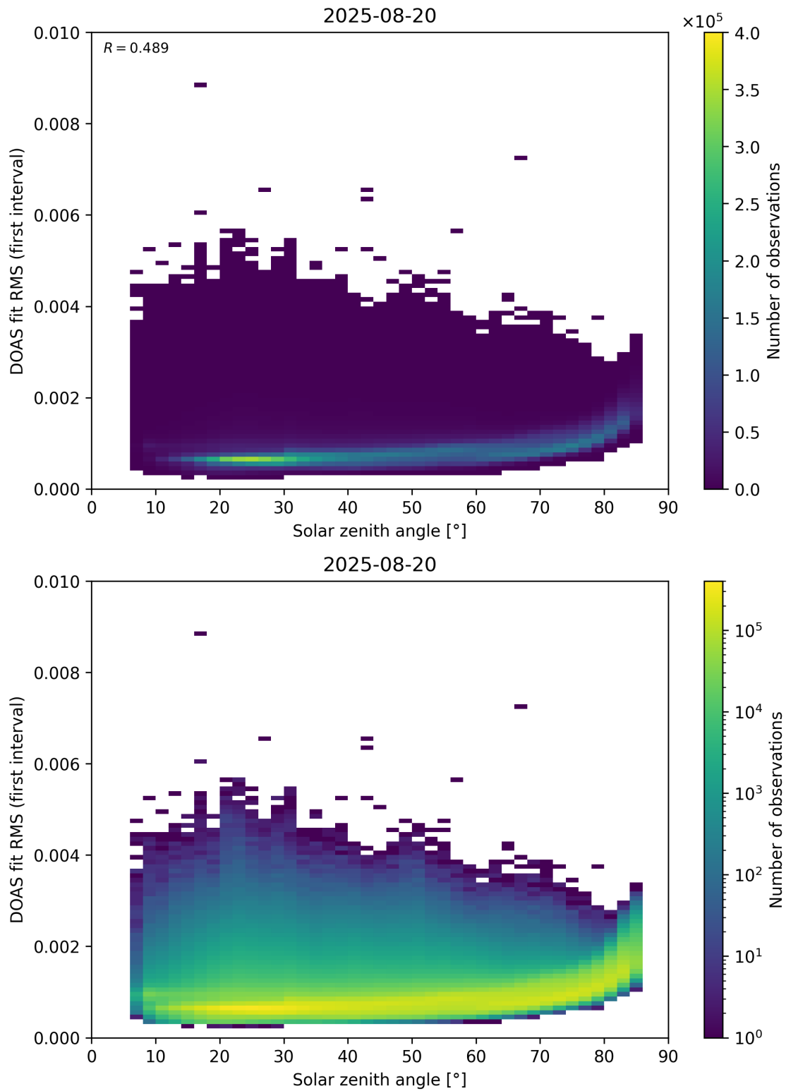
Figure 167: Scatter density plot of “Solar zenith angle” against “DOAS fit RMS (first interval)” for 2025-08-19 to 2025-08-21.
