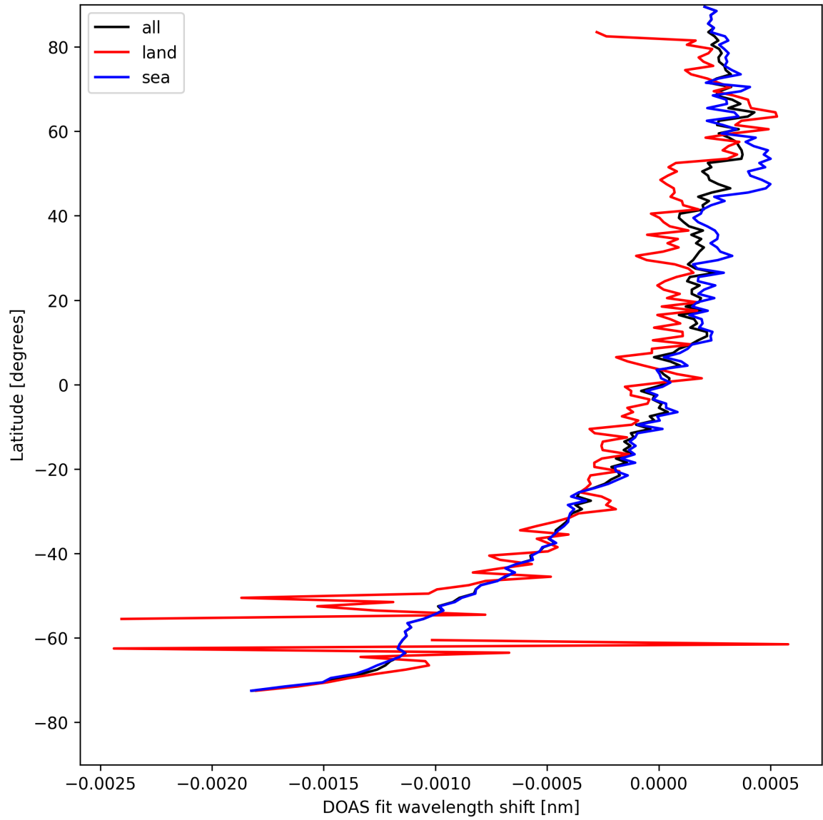
Figure 30: Zonal average of “DOAS fit wavelength shift” for 2025-08-19 to 2025-08-21.
