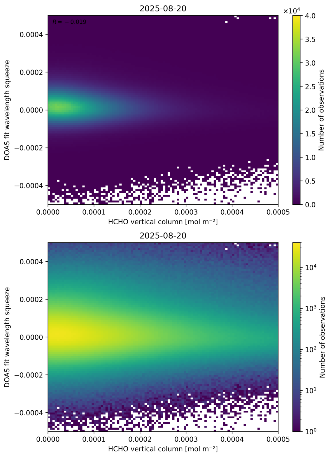
Figure 125: Scatter density plot of “HCHO vertical column” against “DOAS fit wavelength squeeze” for 2025-08-19 to 2025-08-21.
