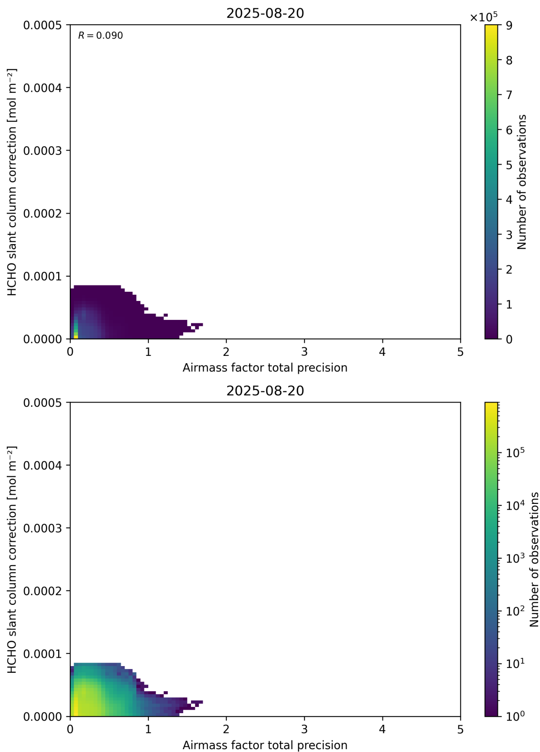
Figure 110: Scatter density plot of “Airmass factor total precision” against “HCHO slant column correction” for 2025-08-19 to 2025-08-21.
