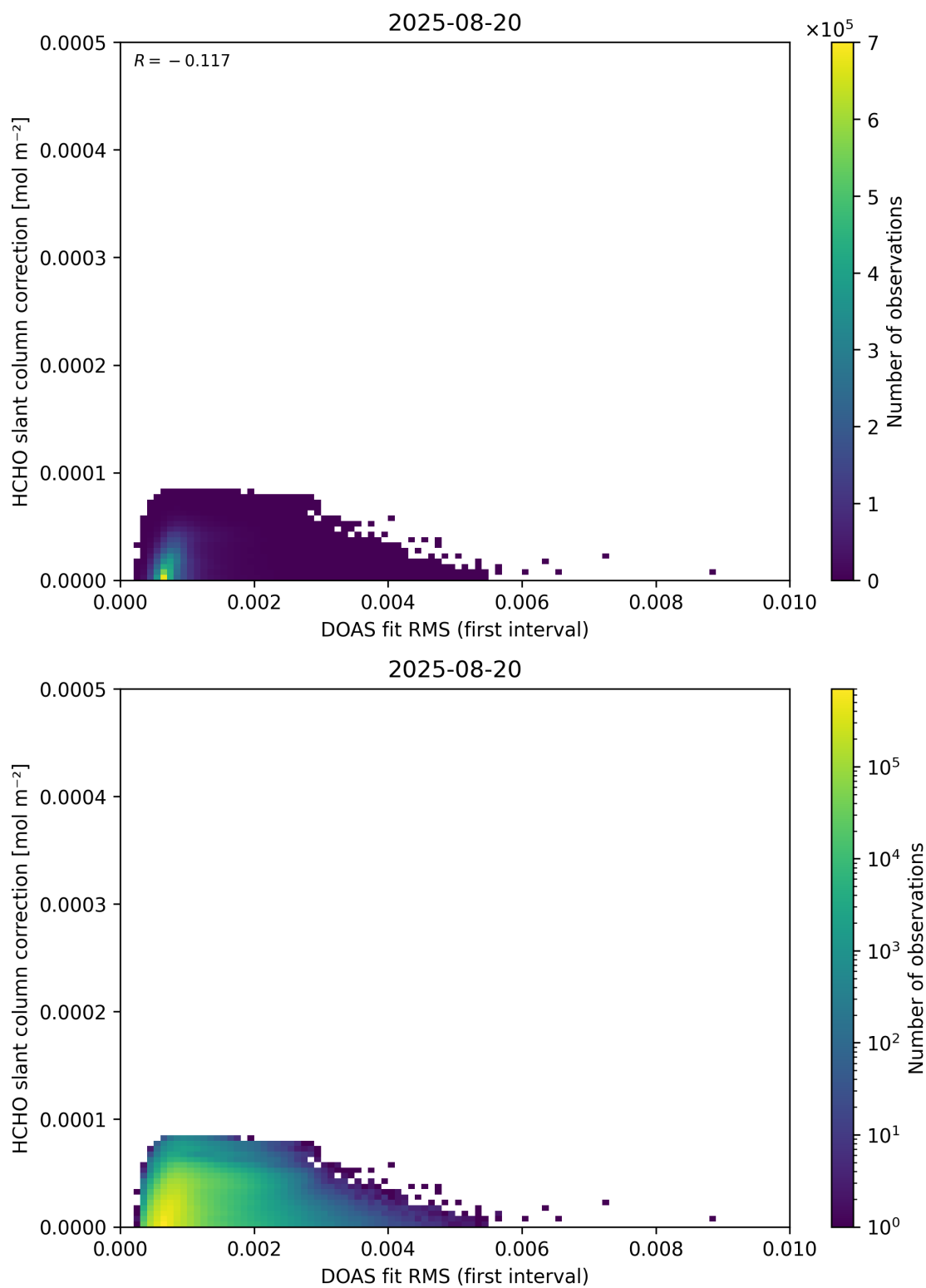
Figure 63: Scatter density plot of “DOAS fit RMS (first interval)” against “HCHO slant column correction” for 2025-08-19 to 2025-08-21.
