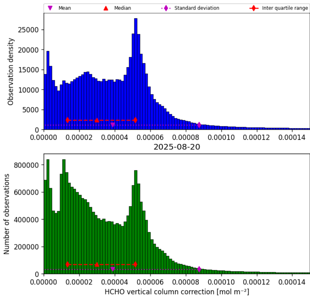
Figure 37: Histogram of “HCHO vertical column correction” for 2025-08-19 to 2025-08-21
