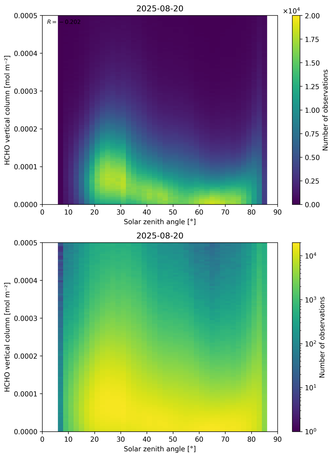
Figure 177: Scatter density plot of “Solar zenith angle” against “HCHO vertical column” for 2025-08-19 to 2025-08-21.
