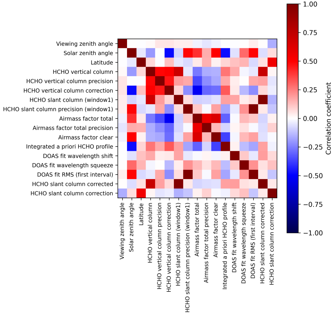
Figure 2: Map of correlation matrix for 2025-08-19 to 2025-08-21.
