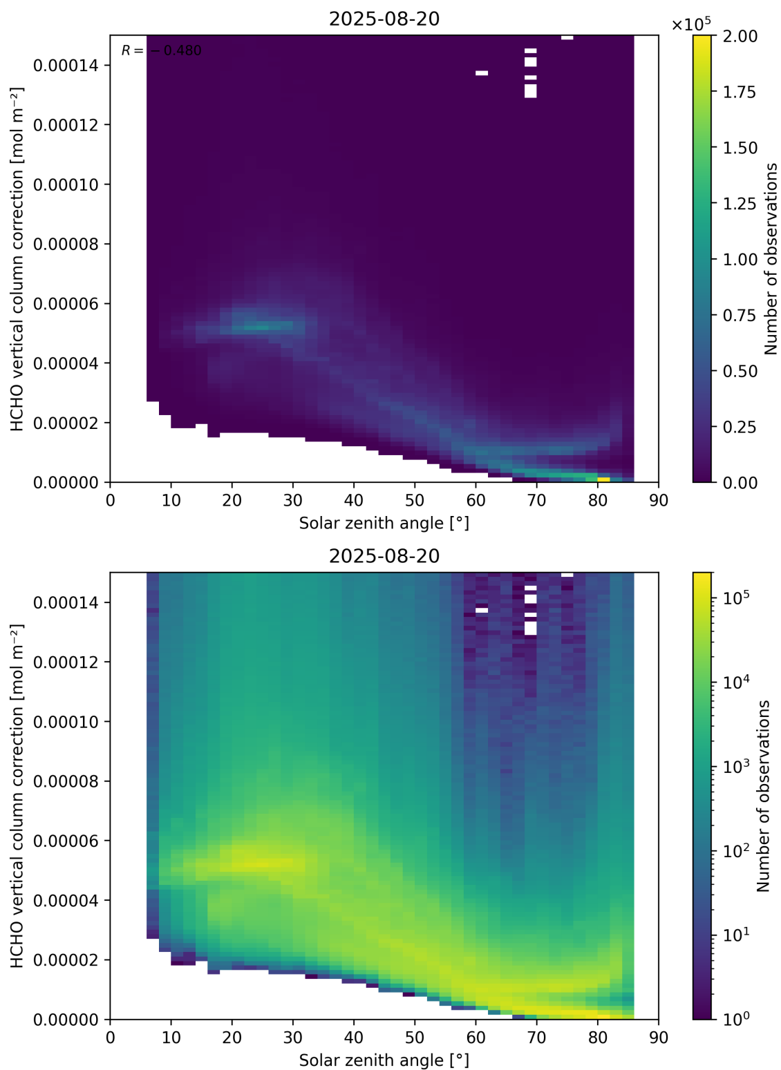
Figure 178: Scatter density plot of “Solar zenith angle” against “HCHO vertical column correction” for 2025-08-19 to 2025-08-21.
