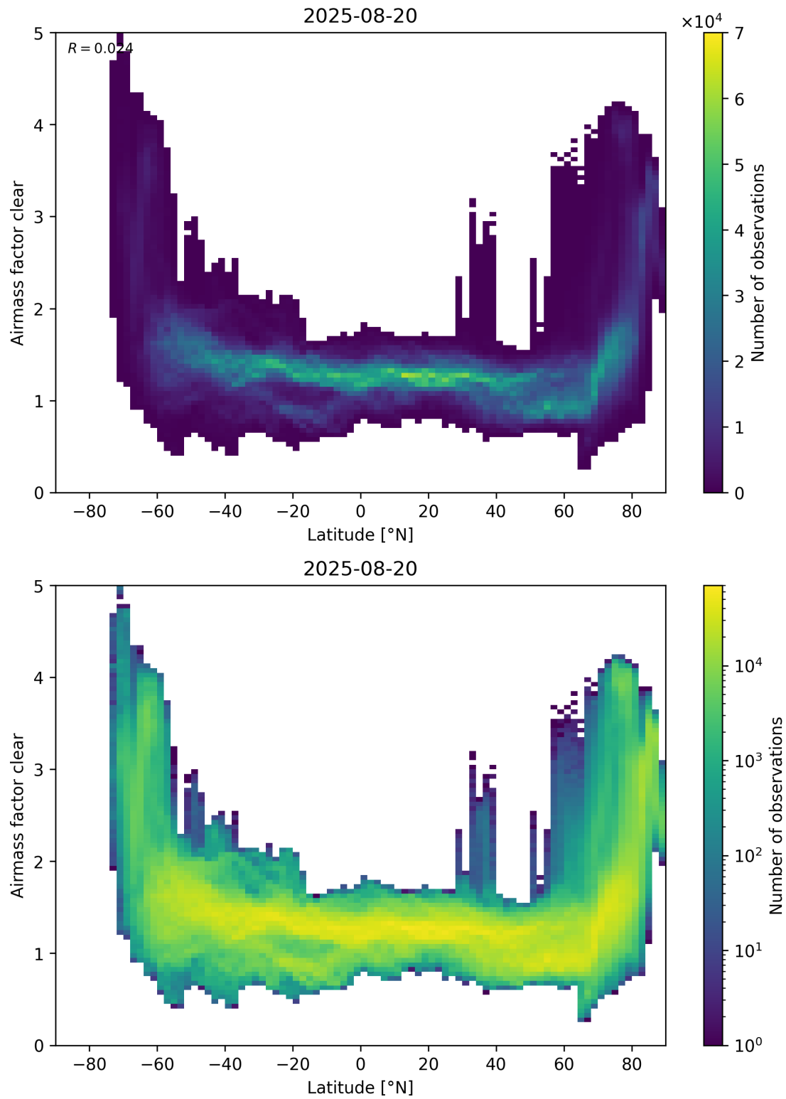
Figure 156: Scatter density plot of “Latitude” against “Airmass factor clear” for 2025-08-19 to 2025-08-21.
