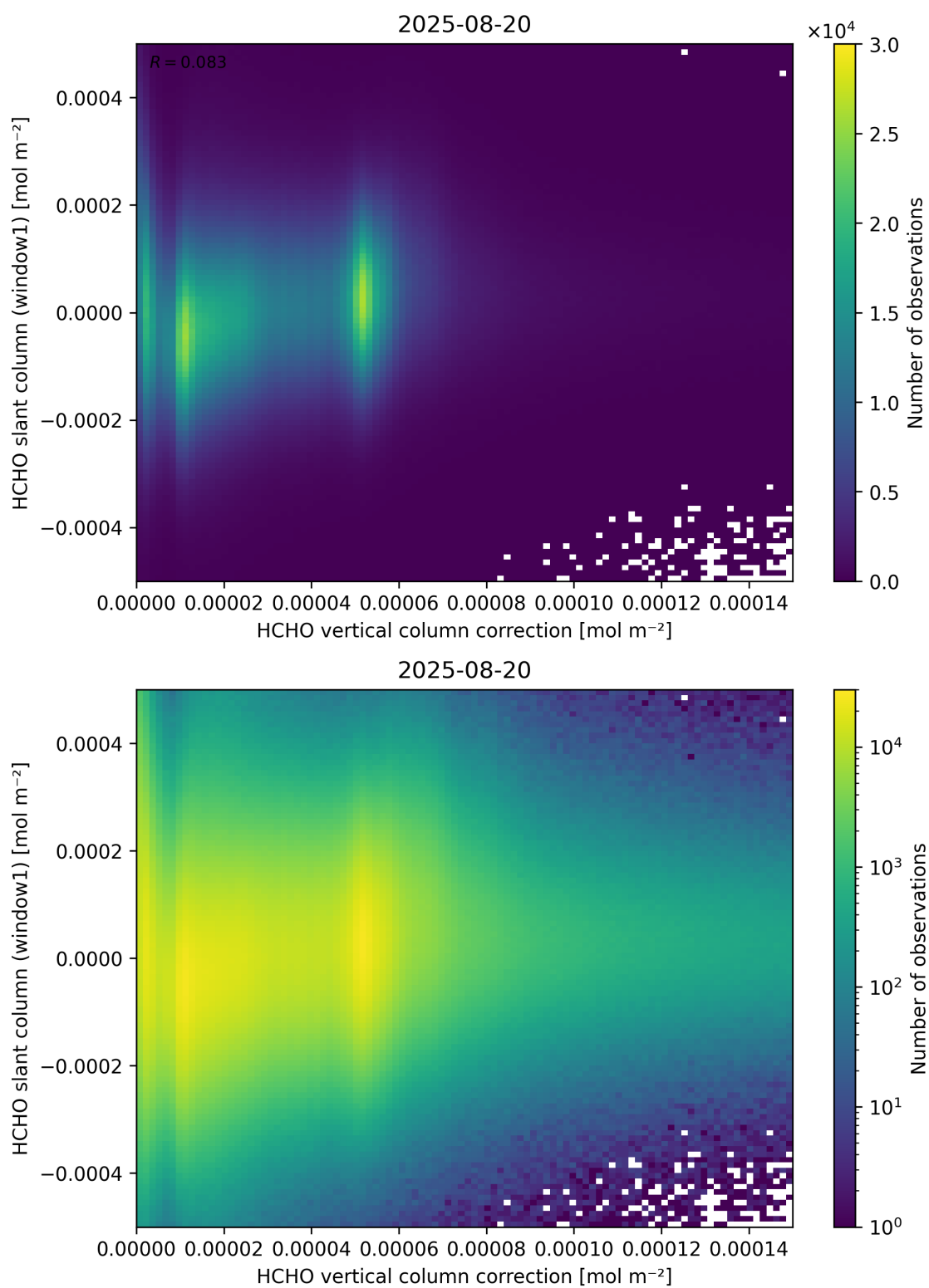
Figure 118: Scatter density plot of “HCHO vertical column correction” against “HCHO slant column (window1)” for 2025-08-19 to 2025-08-21.
