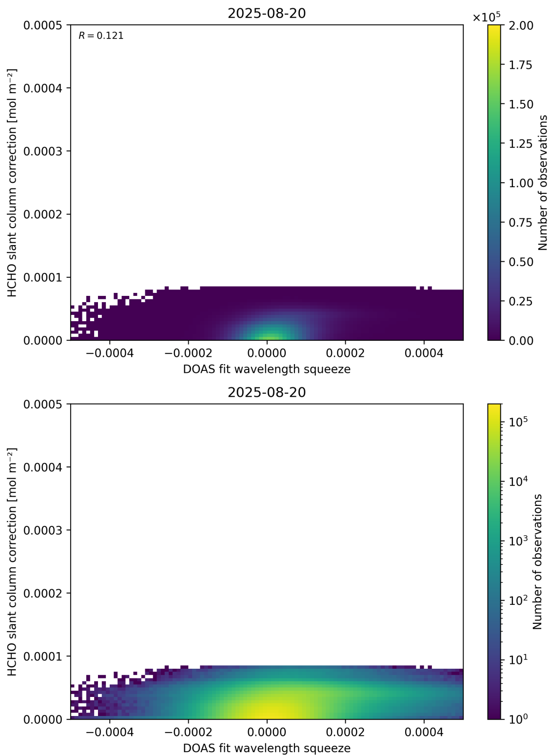
Figure 70: Scatter density plot of “DOAS fit wavelength squeeze” against “HCHO slant column correction” for 2025-08-19 to 2025-08-21.
