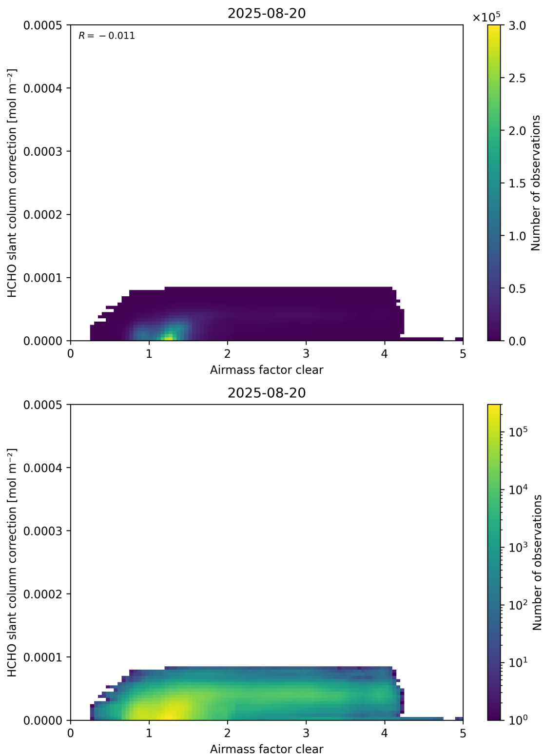
Figure 75: Scatter density plot of “Airmass factor clear” against “HCHO slant column correction” for 2025-08-19 to 2025-08-21.
