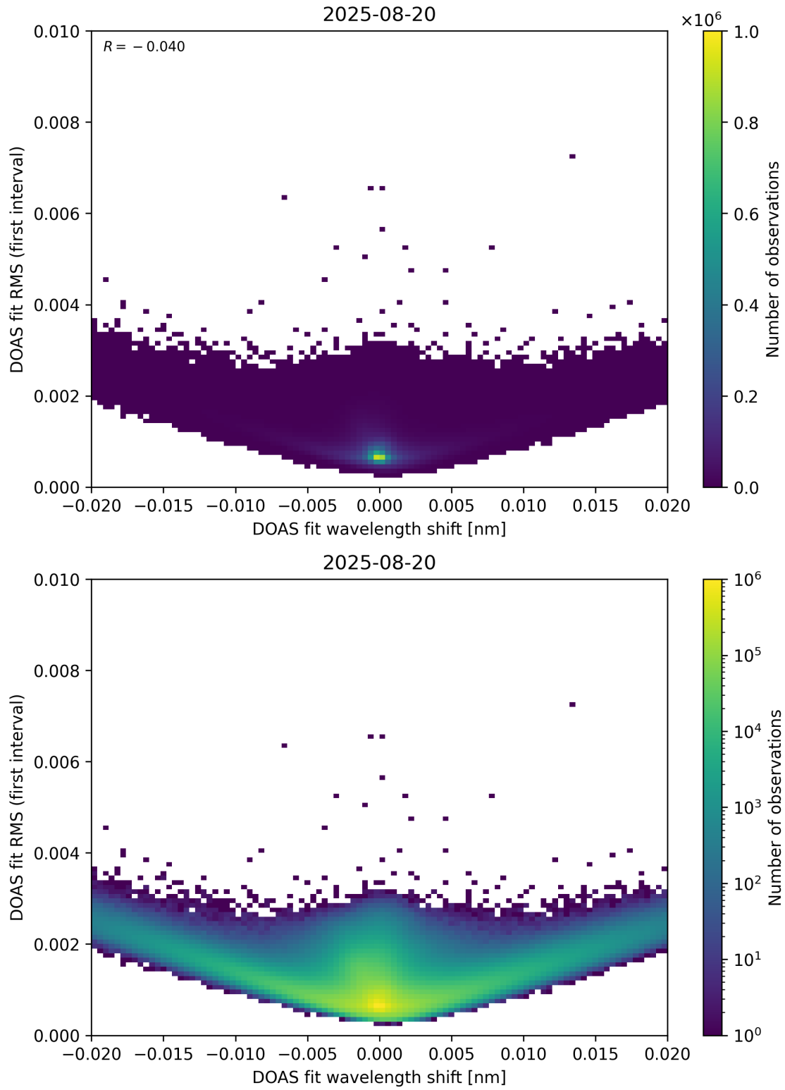
Figure 64: Scatter density plot of “DOAS fit wavelength shift” against “DOAS fit RMS (first interval)” for 2025-08-19 to 2025-08-21.
