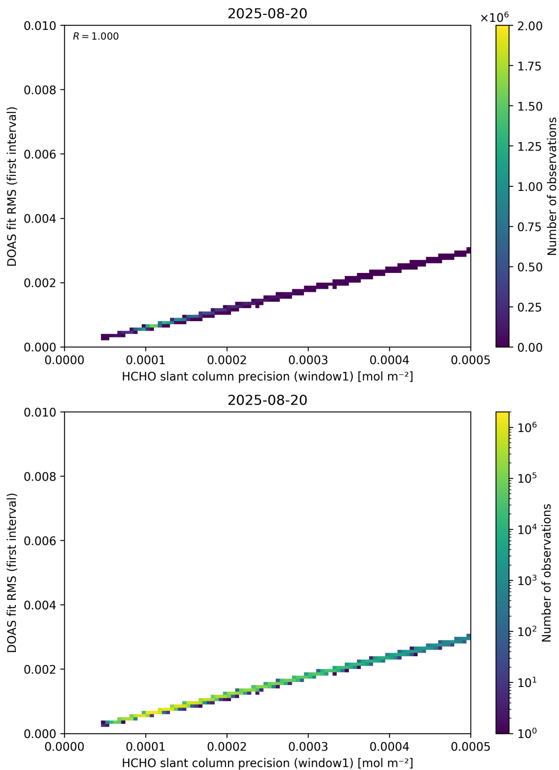
Figure 88: Scatter density plot of “HCHO slant column precision (window1)” against “DOAS fit RMS (first interval)” for 2025-08-19 to 2025-08-21.
