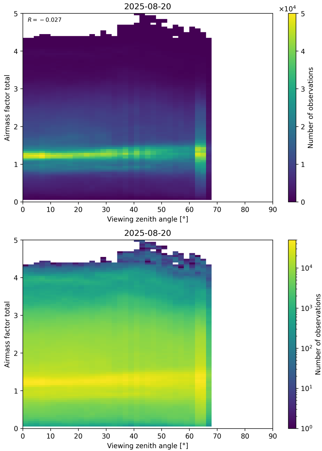
Figure 190: Scatter density plot of “Viewing zenith angle” against “Airmass factor total” for 2025-08-19 to 2025-08-21.
