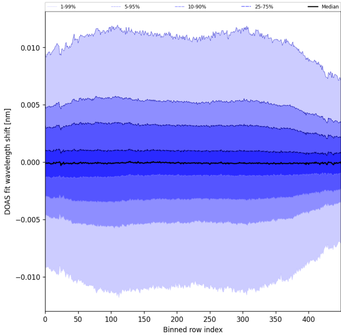
Figure 58: Along track statistics of “DOAS fit wavelength shift” for 2025-08-19 to 2025-08-21
