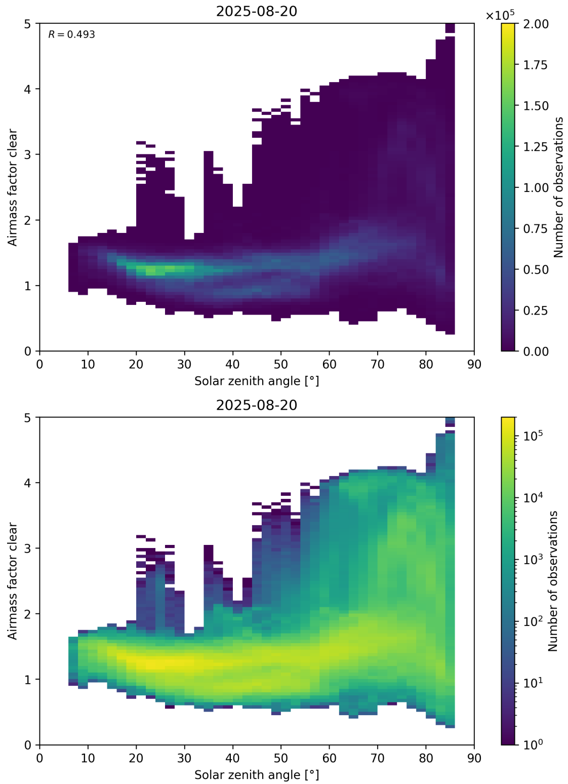
Figure 170: Scatter density plot of “Solar zenith angle” against “Airmass factor clear” for 2025-08-19 to 2025-08-21.
