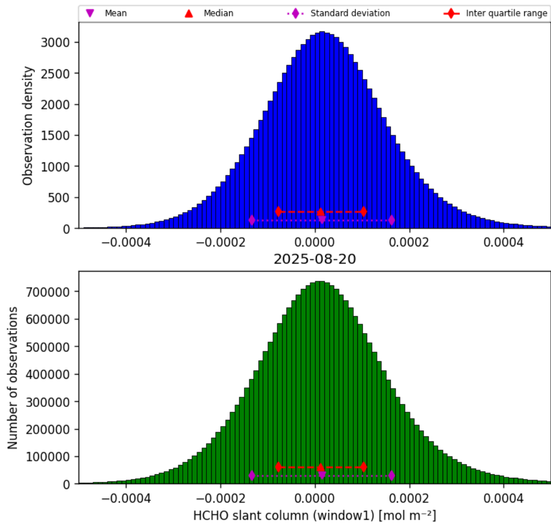
Figure 38: Histogram of “HCHO slant column (window1)” for 2025-08-19 to 2025-08-21
