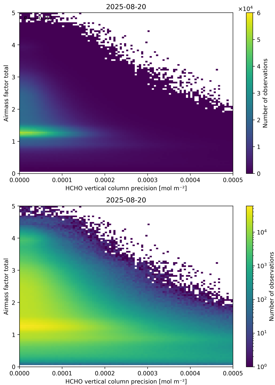
Figure 144: Scatter density plot of “HCHO vertical column precision” against “Airmass factor total” for 2025-08-19 to 2025-08-21.
