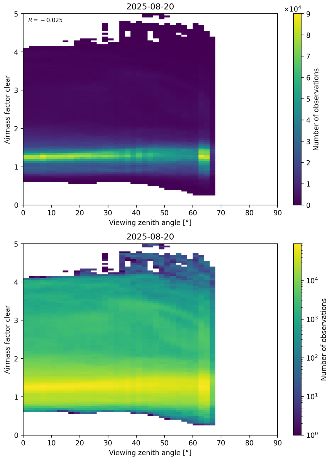
Figure 185: Scatter density plot of “Viewing zenith angle” against “Airmass factor clear” for 2025-08-19 to 2025-08-21.
