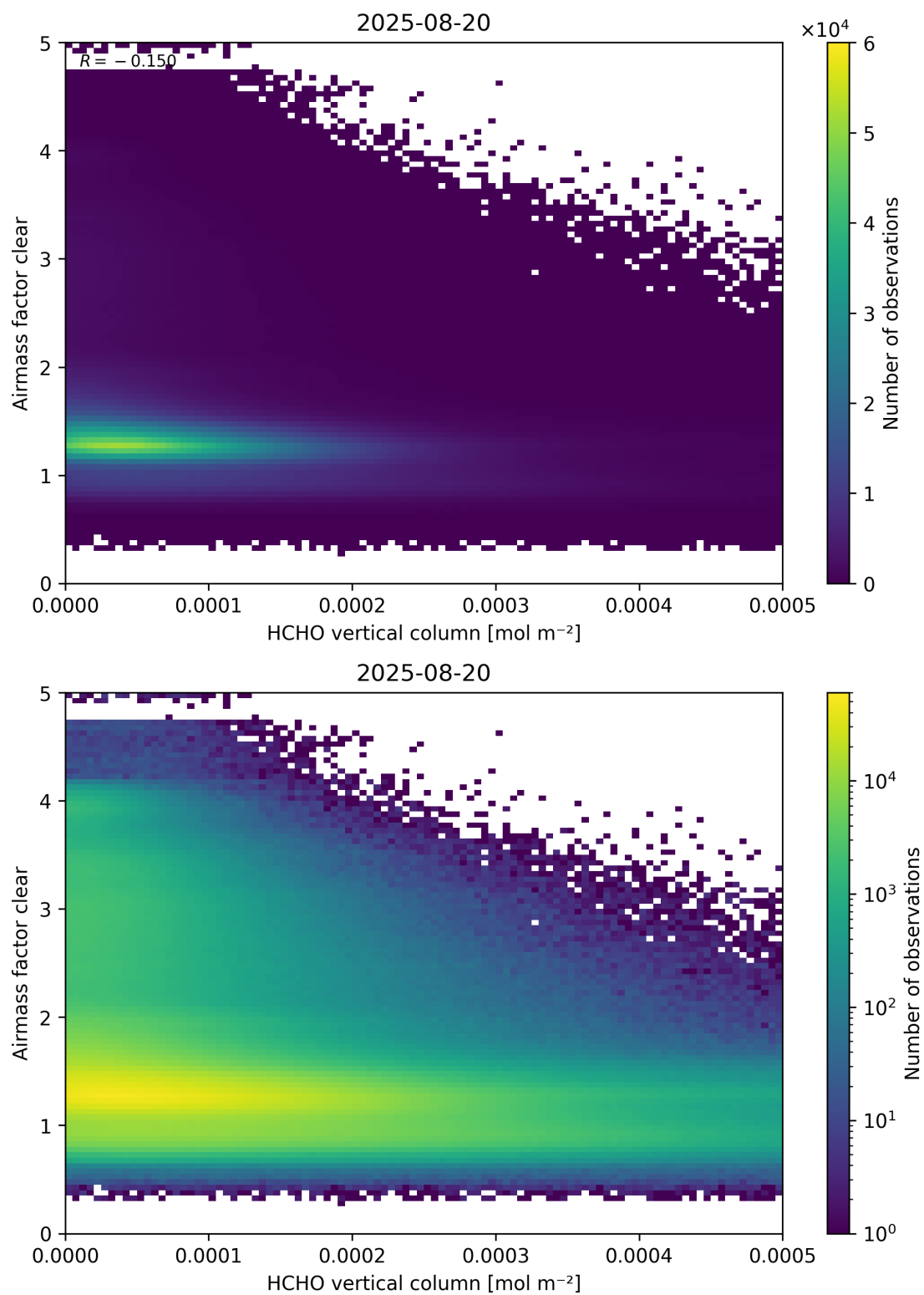
Figure 126: Scatter density plot of “HCHO vertical column” against “Airmass factor clear” for 2025-08-19 to 2025-08-21.
