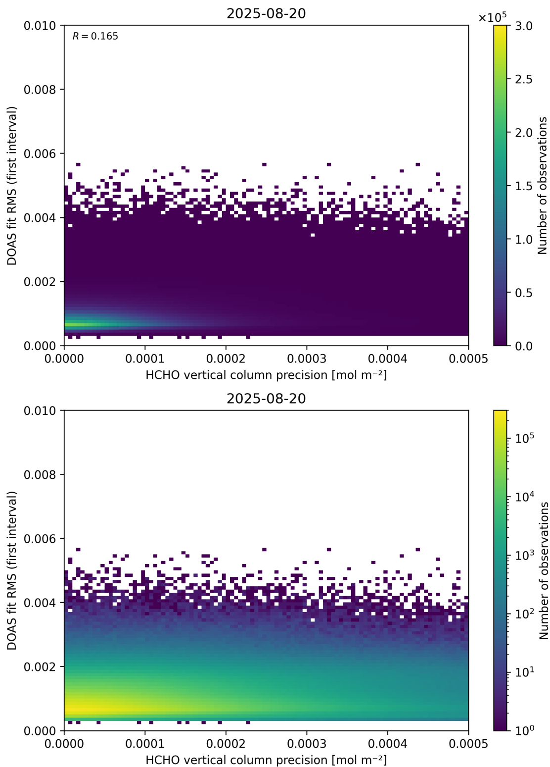
Figure 136: Scatter density plot of “HCHO vertical column precision” against “DOAS fit RMS (first interval)” for 2025-08-19 to 2025-08-21.
