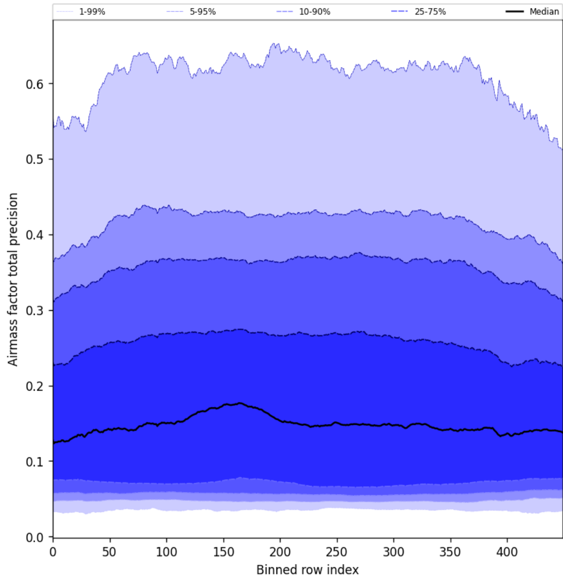
Figure 55: Along track statistics of “Airmass factor total precision” for 2025-08-19 to 2025-08-21
