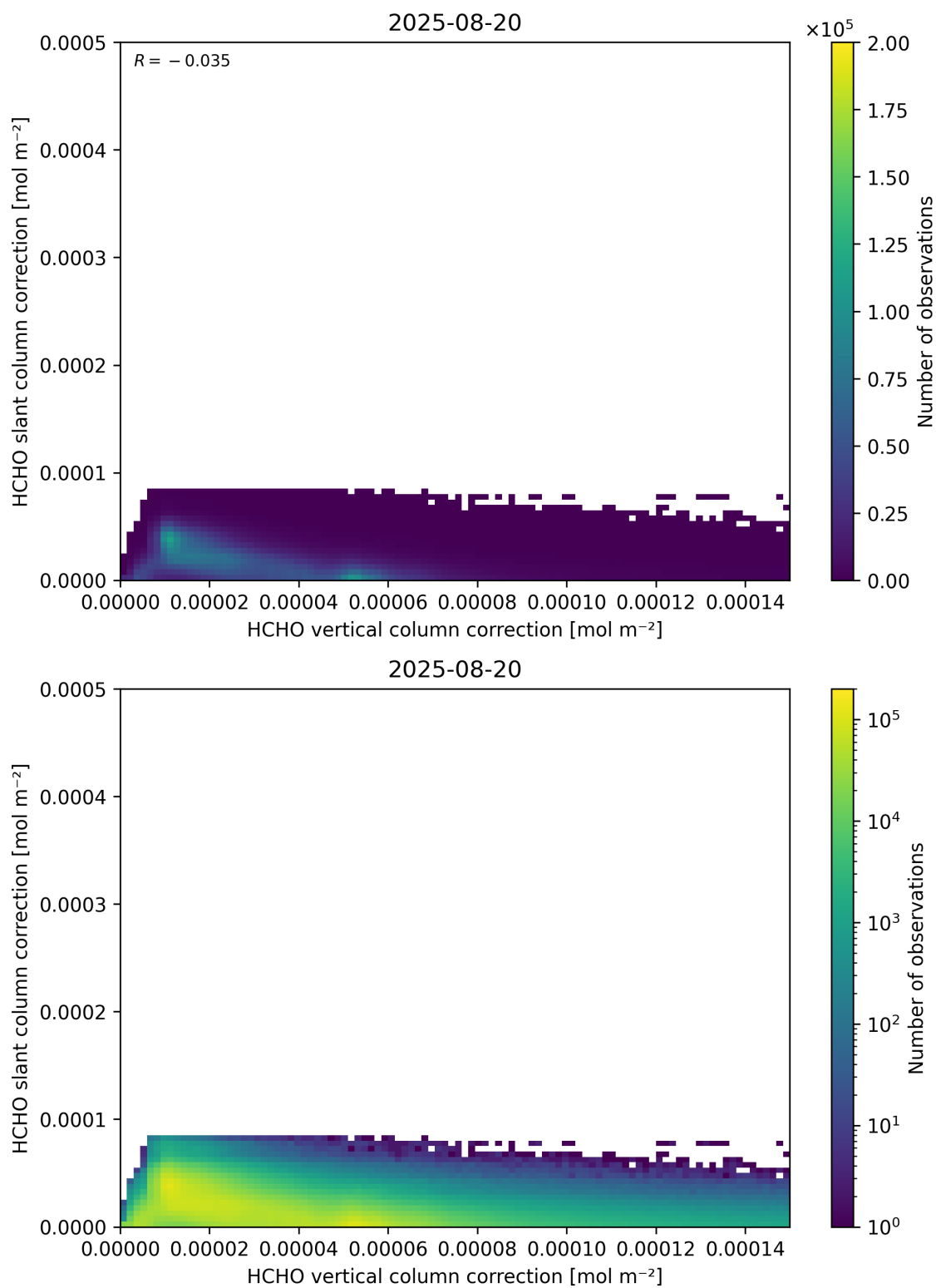
Figure 117: Scatter density plot of “HCHO vertical column correction” against “HCHO slant column correction” for 2025-08-19 to 2025-08-21.
