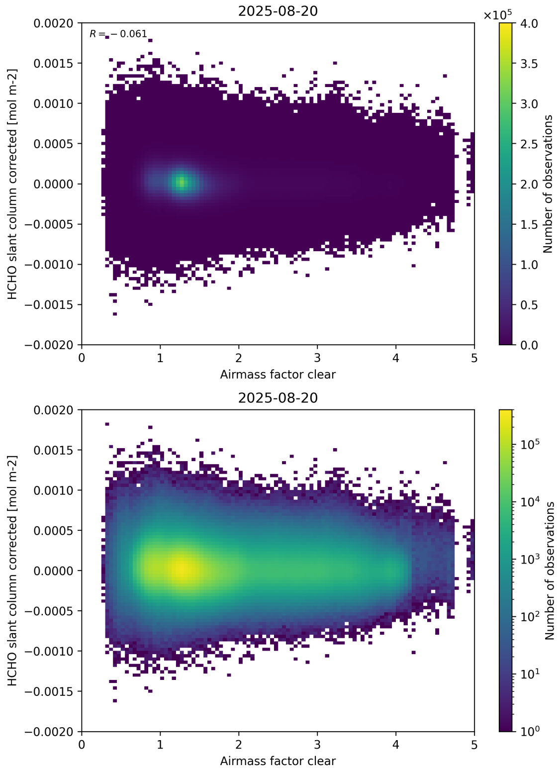
Figure 74: Scatter density plot of “Airmass factor clear” against “HCHO slant column corrected” for 2025-08-19 to 2025-08-21.
