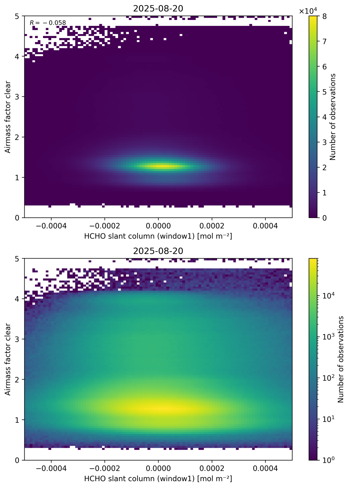
Figure 81: Scatter density plot of “HCHO slant column (window1)” against “Airmass factor clear” for 2025-08-19 to 2025-08-21.
