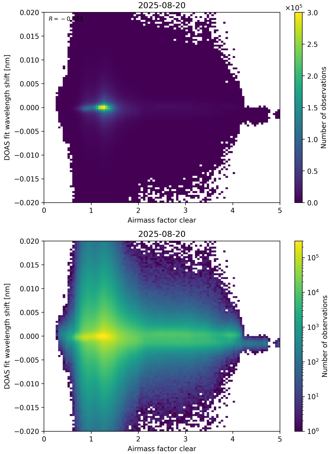
Figure 72: Scatter density plot of “Airmass factor clear” against “DOAS fit wavelength shift” for 2025-08-19 to 2025-08-21.
