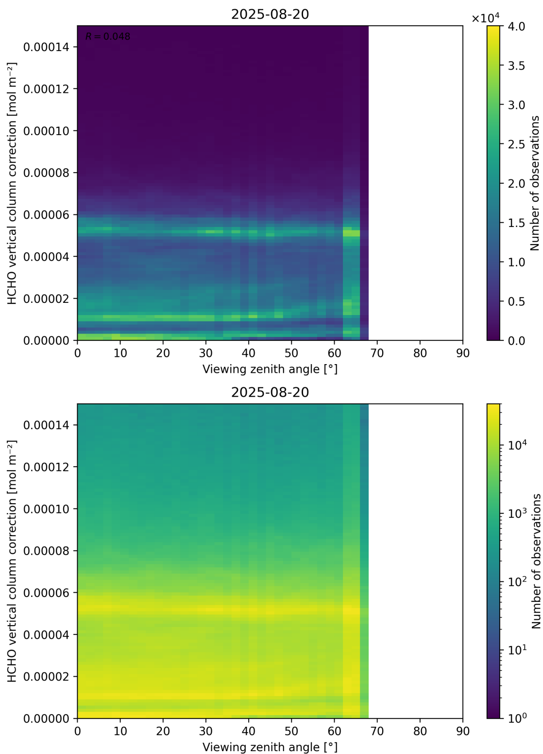
Figure 193: Scatter density plot of “Viewing zenith angle” against “HCHO vertical column correction” for 2025-08-19 to 2025-08-21.
