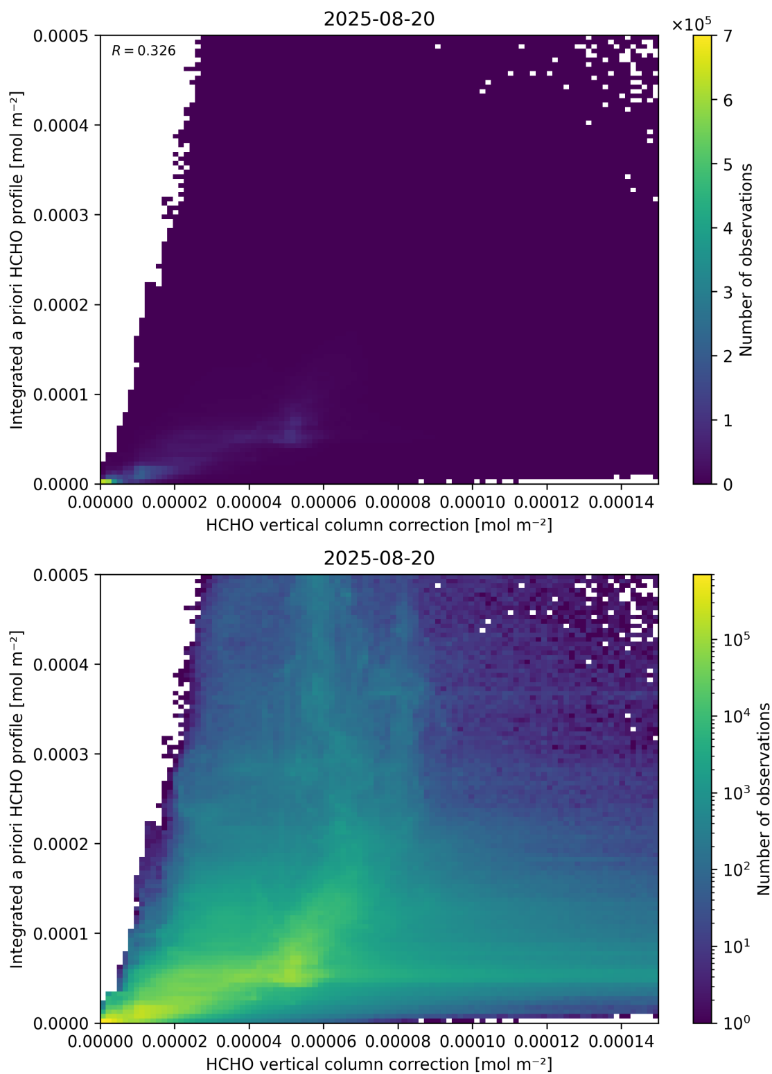
Figure 122: Scatter density plot of “HCHO vertical column correction” against “Integrated a priori HCHO profile” for 2025-08-19 to 2025-08-21.
