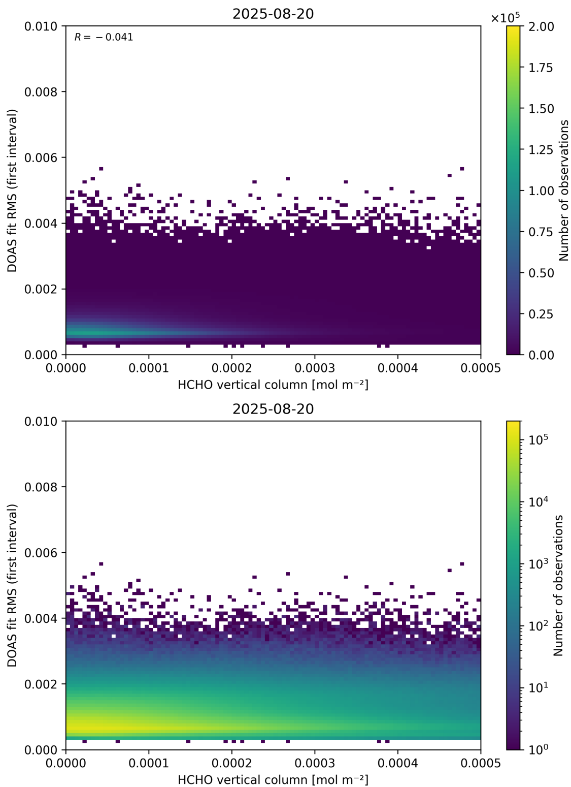
Figure 123: Scatter density plot of “HCHO vertical column” against “DOAS fit RMS (first interval)” for 2025-08-19 to 2025-08-21.
