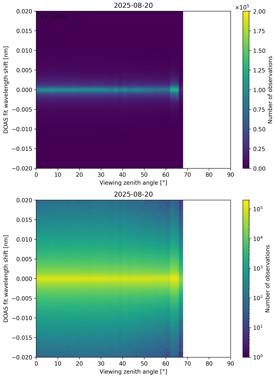
Figure 183: Scatter density plot of “Viewing zenith angle” against “DOAS fit wavelength shift” for 2025-08-19 to 2025-08-21.
