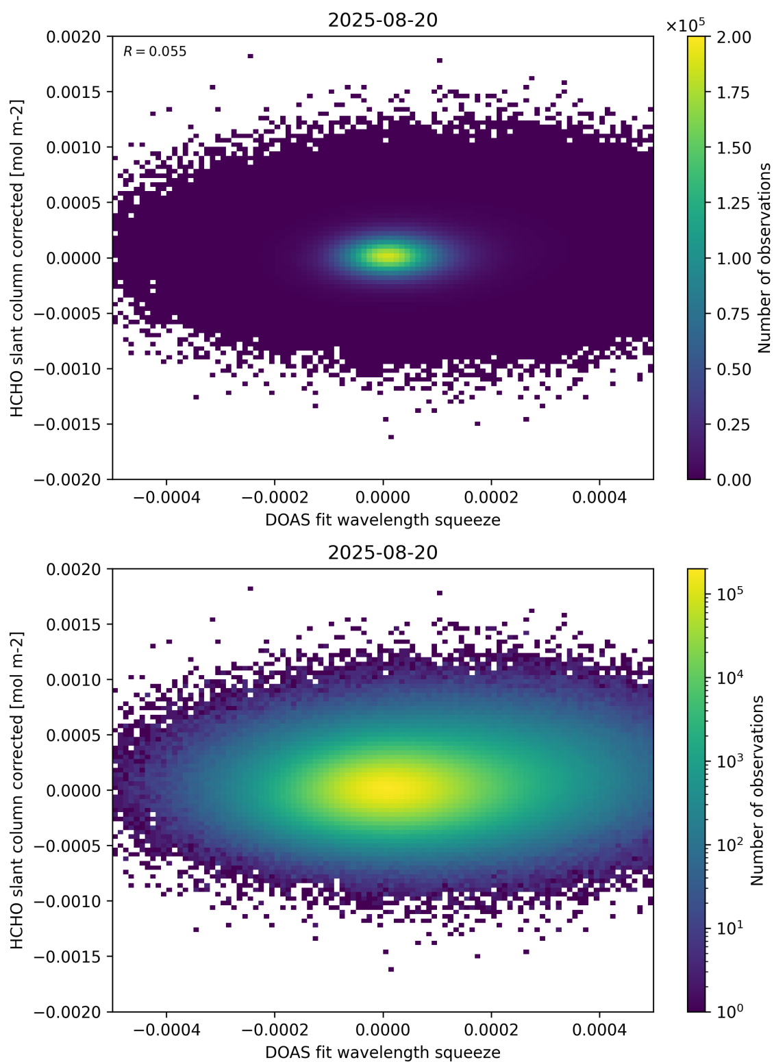
Figure 69: Scatter density plot of “DOAS fit wavelength squeeze” against “HCHO slant column corrected” for 2025-08-19 to 2025-08-21.
