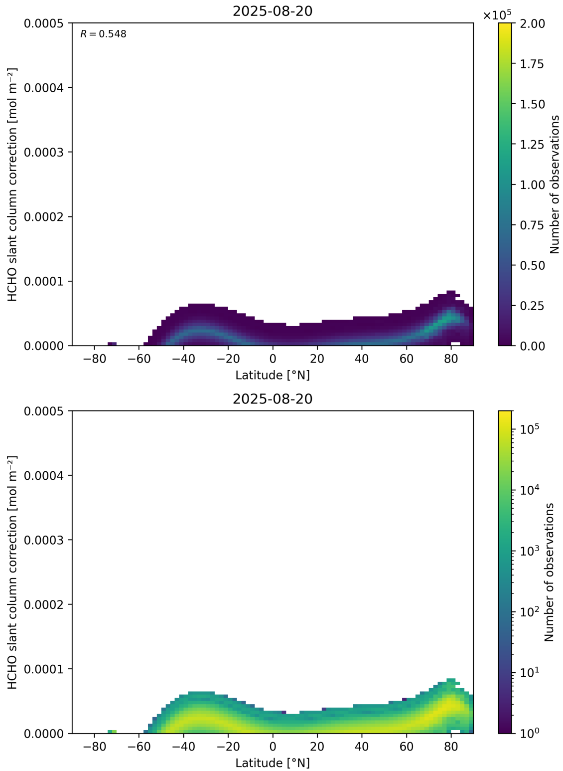
Figure 158: Scatter density plot of “Latitude” against “HCHO slant column correction” for 2025-08-19 to 2025-08-21.
