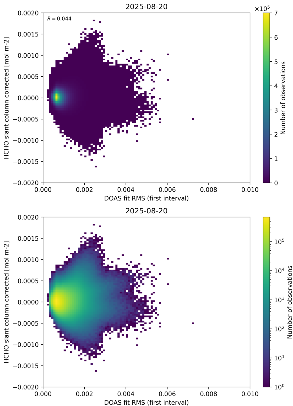
Figure 62: Scatter density plot of “DOAS fit RMS (first interval)” against “HCHO slant column corrected” for 2025-08-19 to 2025-08-21.
