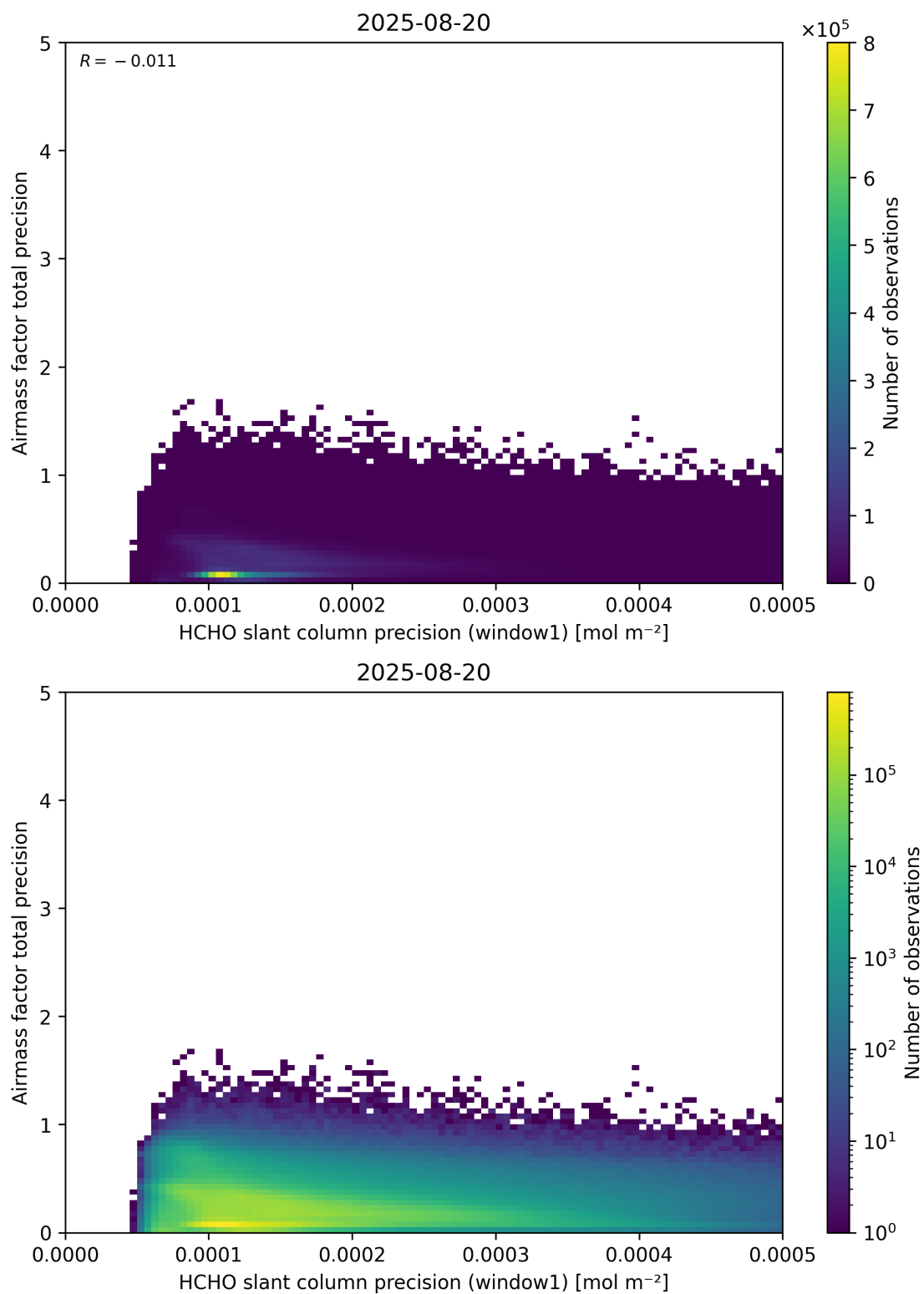
Figure 95: Scatter density plot of “HCHO slant column precision (window1)” against “Airmass factor total precision” for 2025-08-19 to 2025-08-21.
