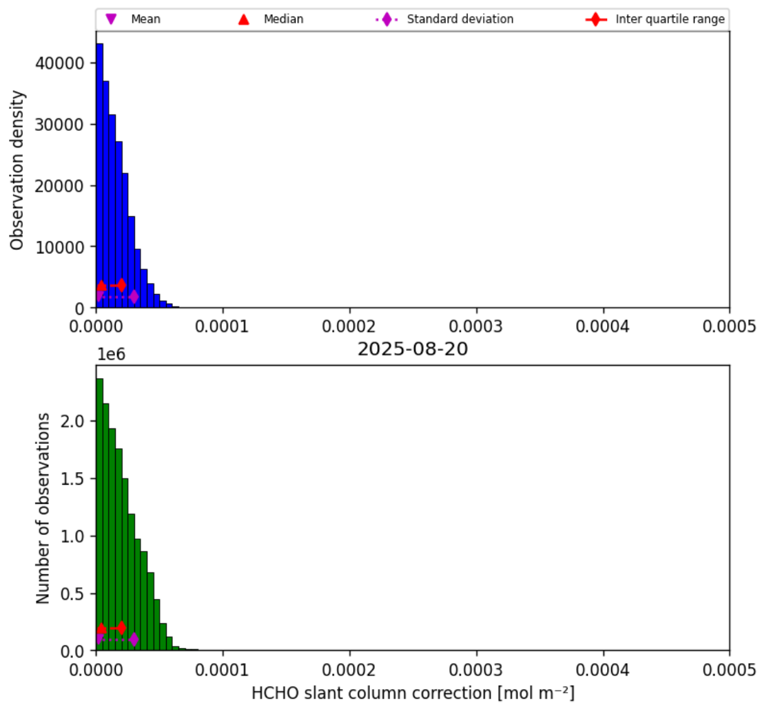
Figure 47: Histogram of “HCHO slant column correction” for 2025-08-19 to 2025-08-21
