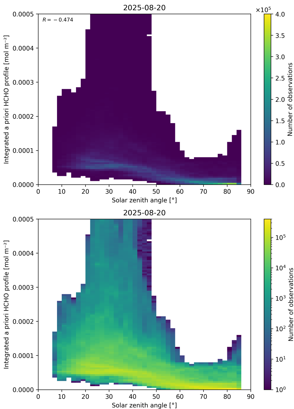
Figure 180: Scatter density plot of “Solar zenith angle” against “Integrated a priori HCHO profile” for 2025-08-19 to 2025-08-21.
