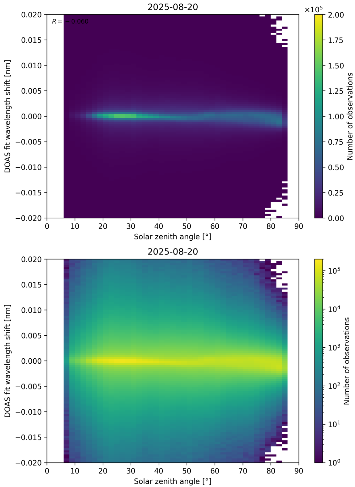
Figure 168: Scatter density plot of “Solar zenith angle” against “DOAS fit wavelength shift” for 2025-08-19 to 2025-08-21.
