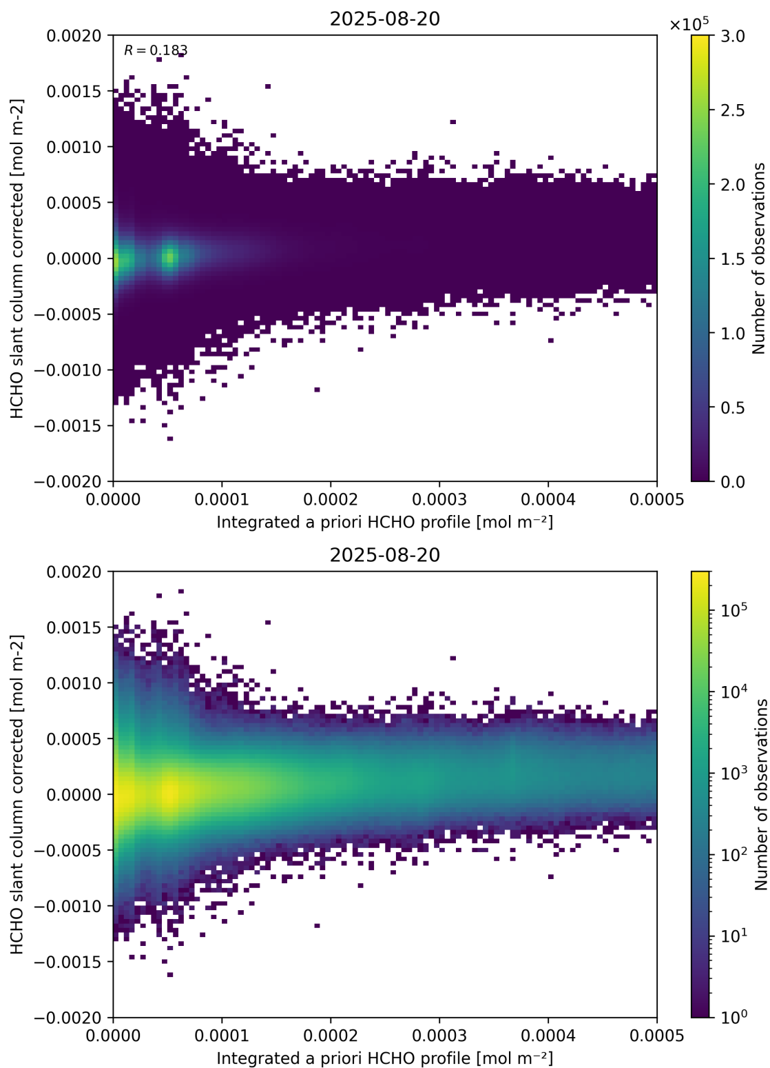
Figure 151: Scatter density plot of “Integrated a priori HCHO profile” against “HCHO slant column corrected” for 2025-08-19 to 2025-08-21.
