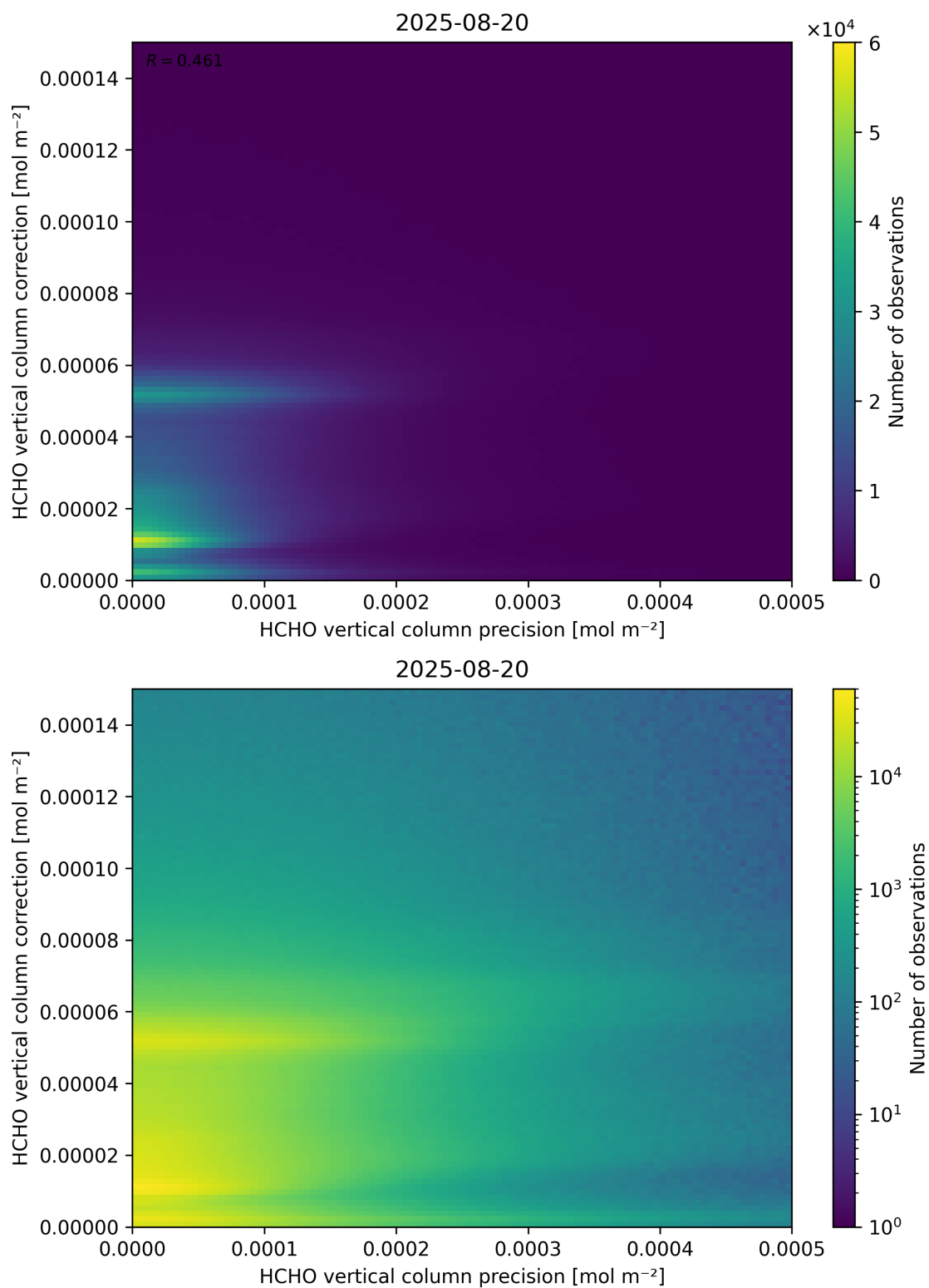
Figure 146: Scatter density plot of “HCHO vertical column precision” against “HCHO vertical column correction” for 2025-08-19 to 2025-08-21.
