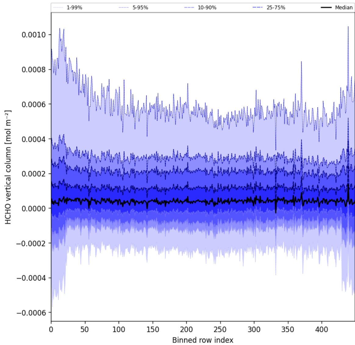
Figure 49: Along track statistics of “HCHO vertical column” for 2025-08-19 to 2025-08-21
