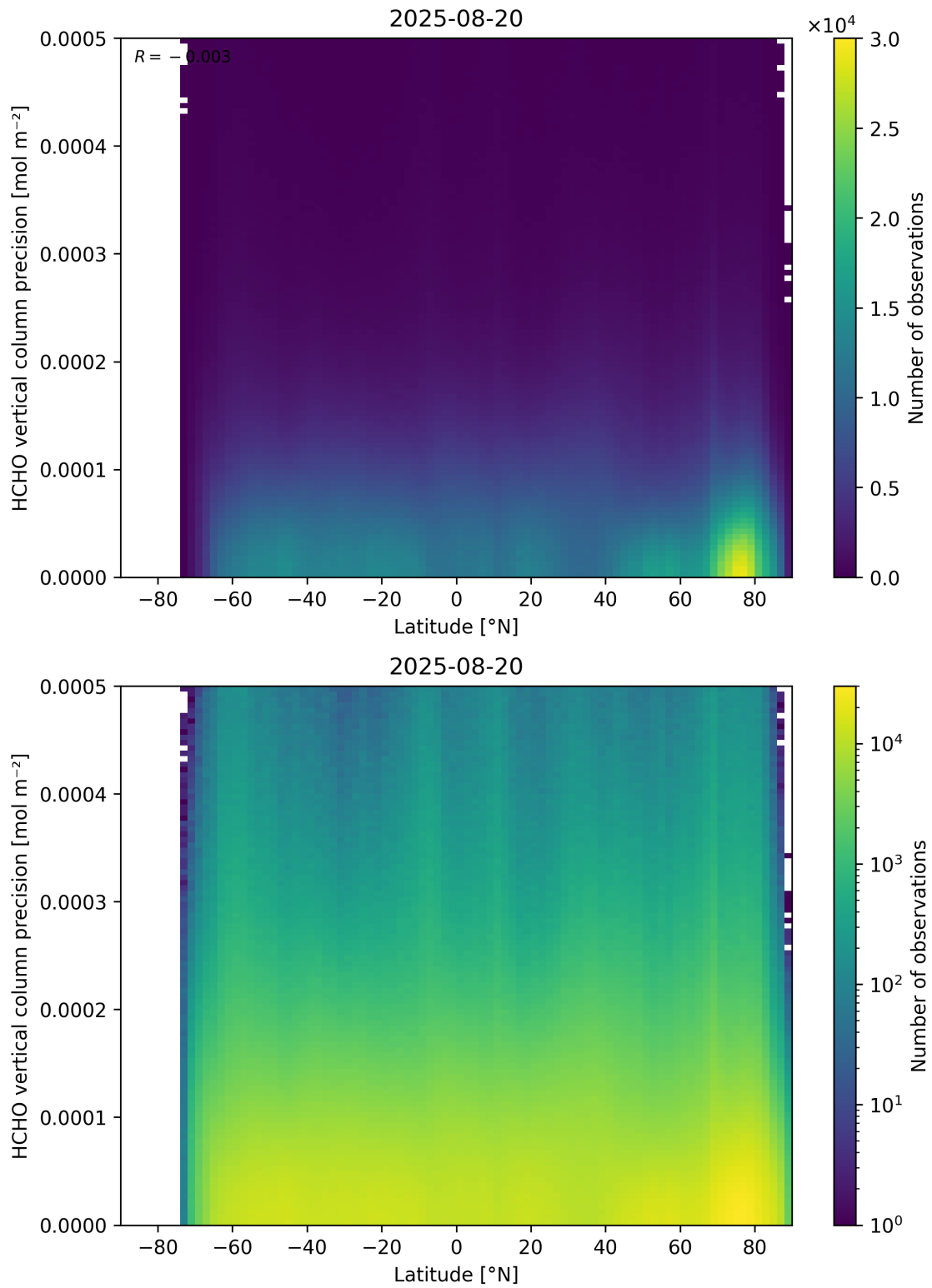
Figure 165: Scatter density plot of “Latitude” against “HCHO vertical column precision” for 2025-08-19 to 2025-08-21.
