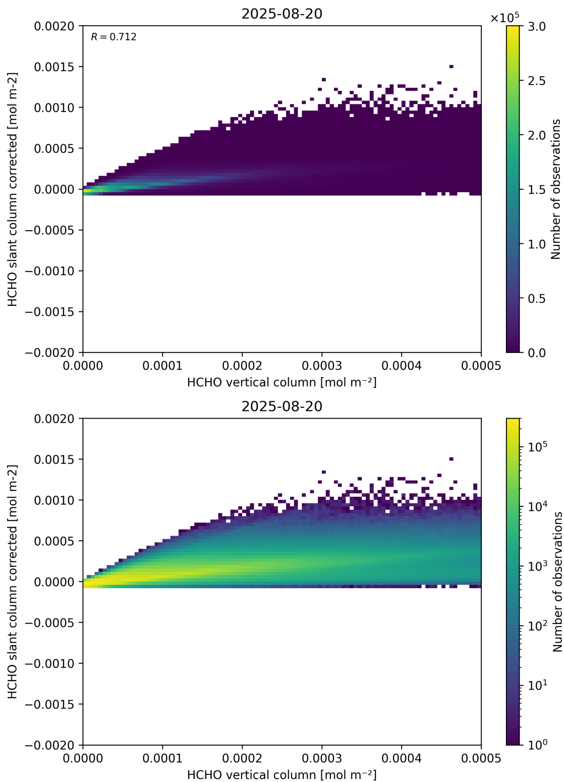
Figure 127: Scatter density plot of “HCHO vertical column” against “HCHO slant column corrected” for 2025-08-19 to 2025-08-21.
