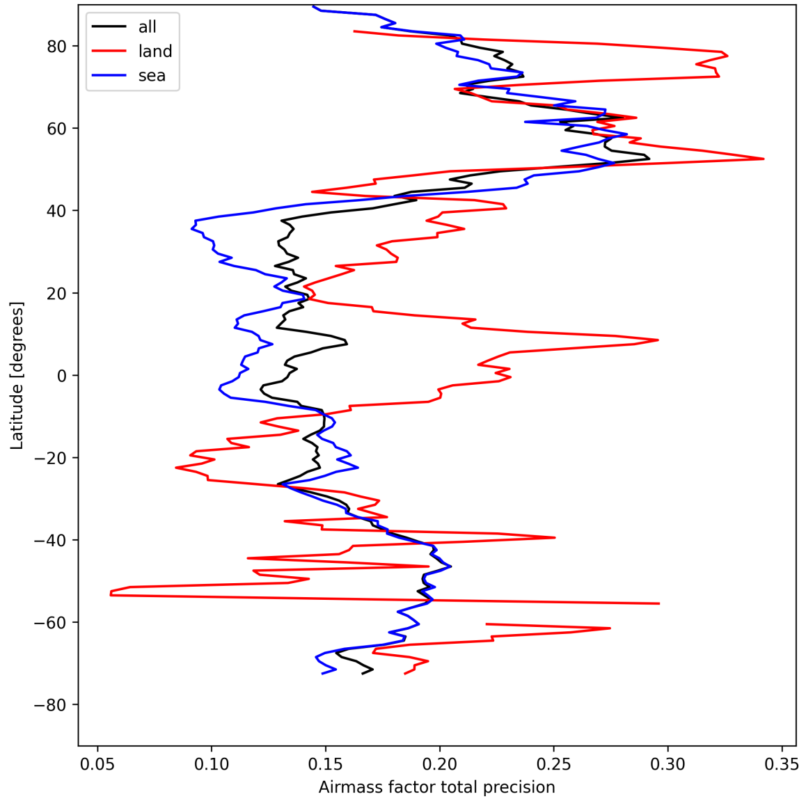
Figure 27: Zonal average of “Airmass factor total precision” for 2025-08-19 to 2025-08-21.
