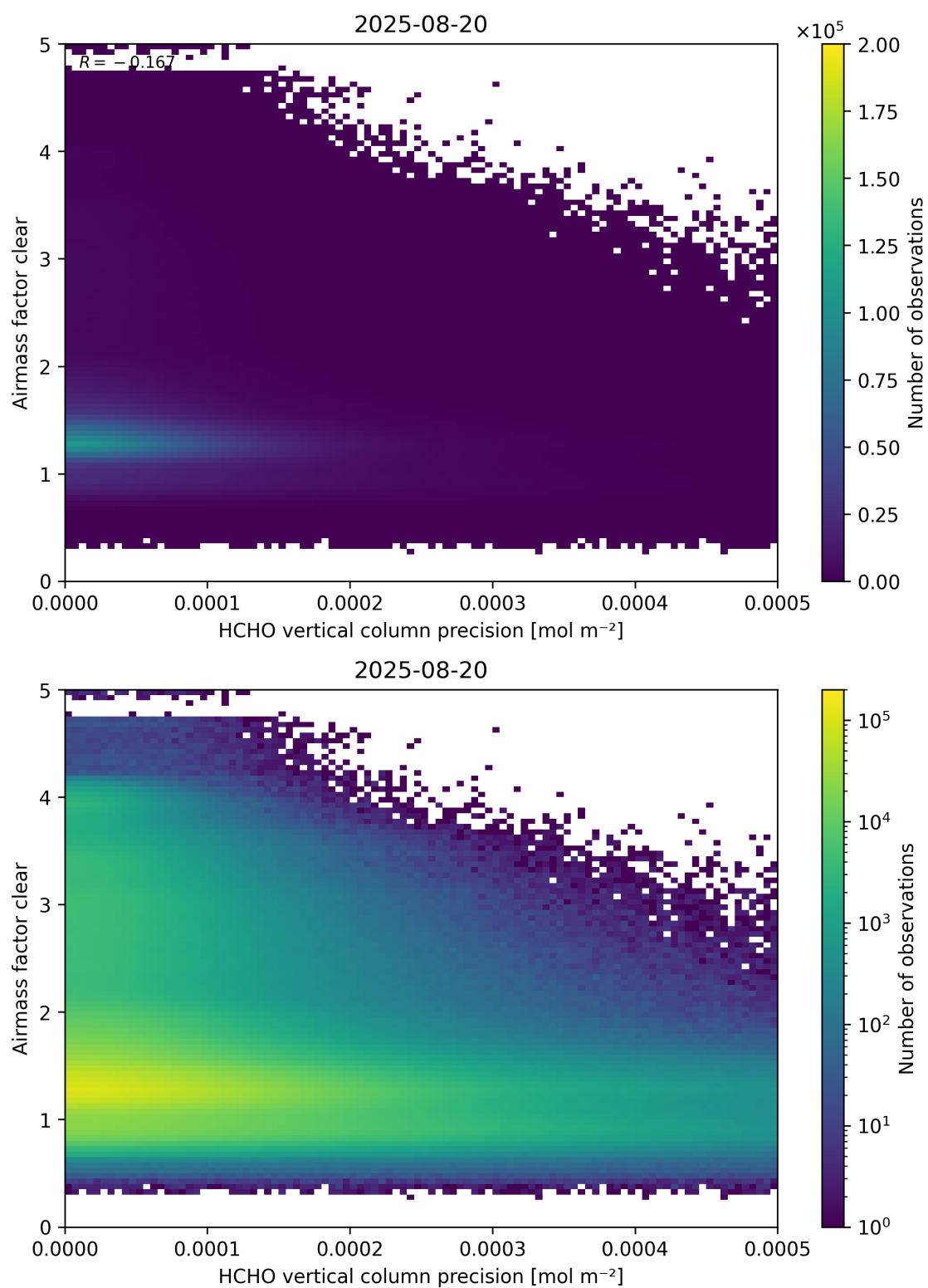
Figure 139: Scatter density plot of “HCHO vertical column precision” against “Airmass factor clear” for 2025-08-19 to 2025-08-21.
