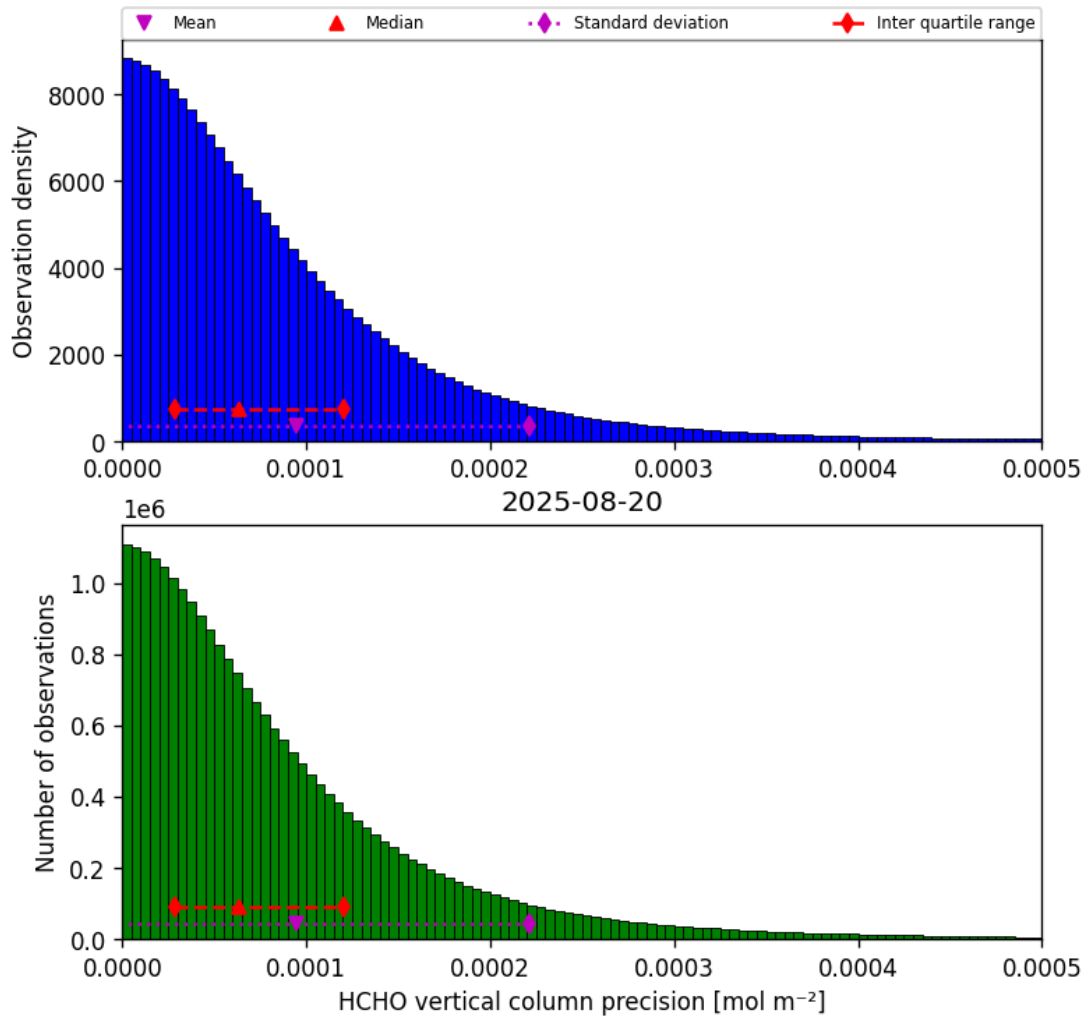
Figure 36: Histogram of “HCHO vertical column precision” for 2025-08-19 to 2025-08-21
