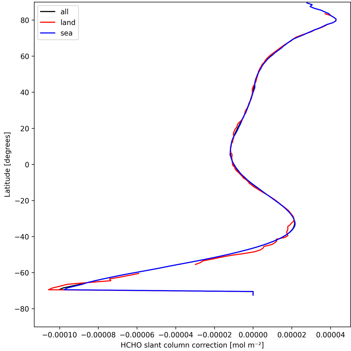
Figure 33: Zonal average of "HCHO slant column correction" for 2025-08-19 to 2025-08-21.
