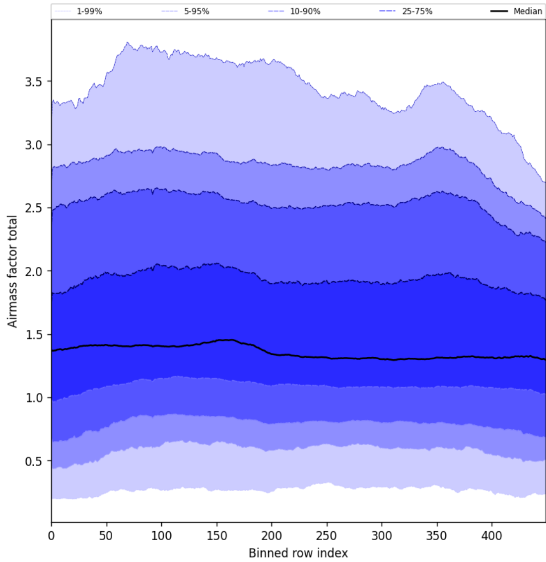
Figure 54: Along track statistics of “Airmass factor total” for 2025-08-19 to 2025-08-21
