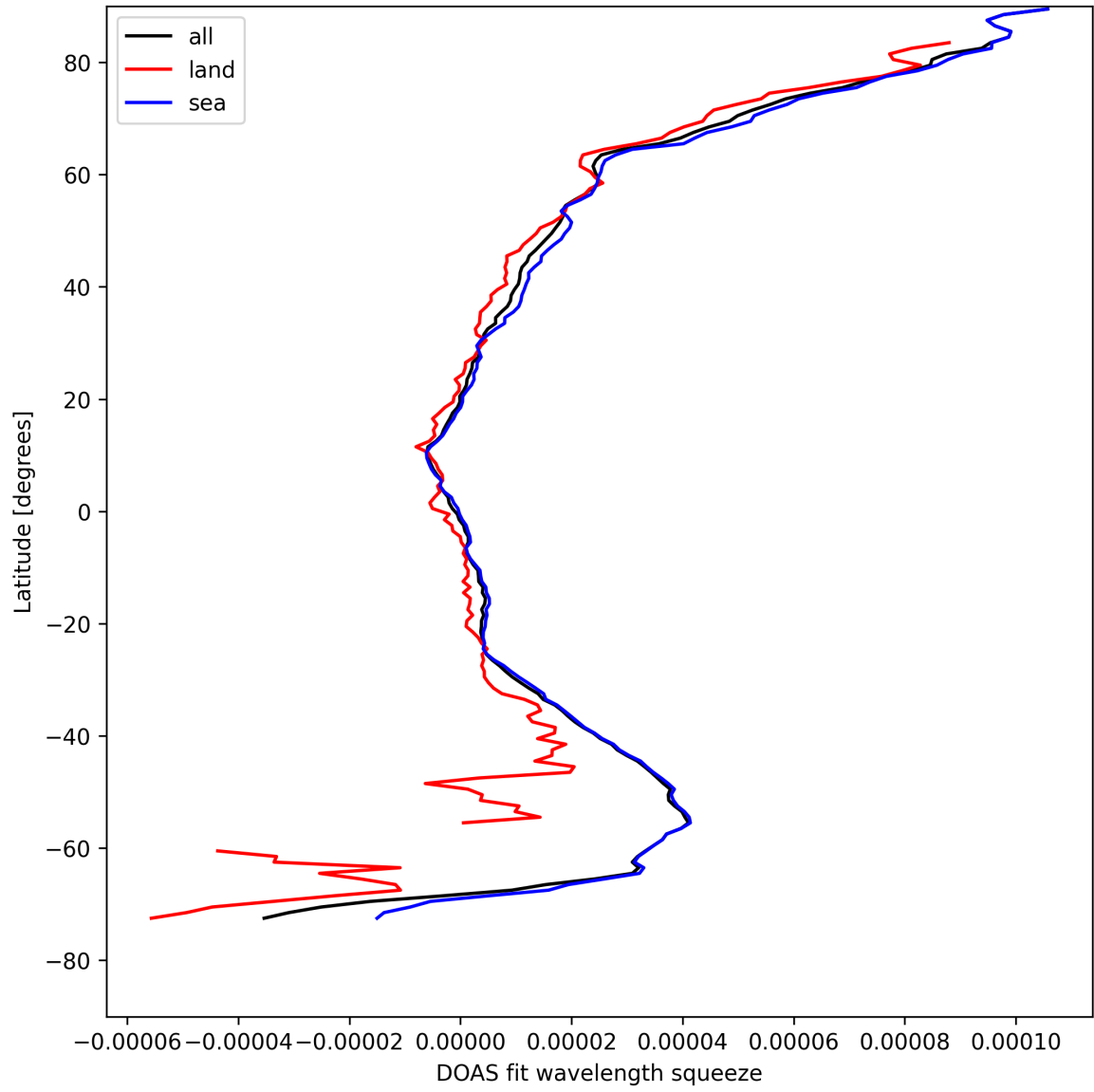
Figure 31: Zonal average of “DOAS fit wavelength squeeze” for 2025-08-19 to 2025-08-21.
