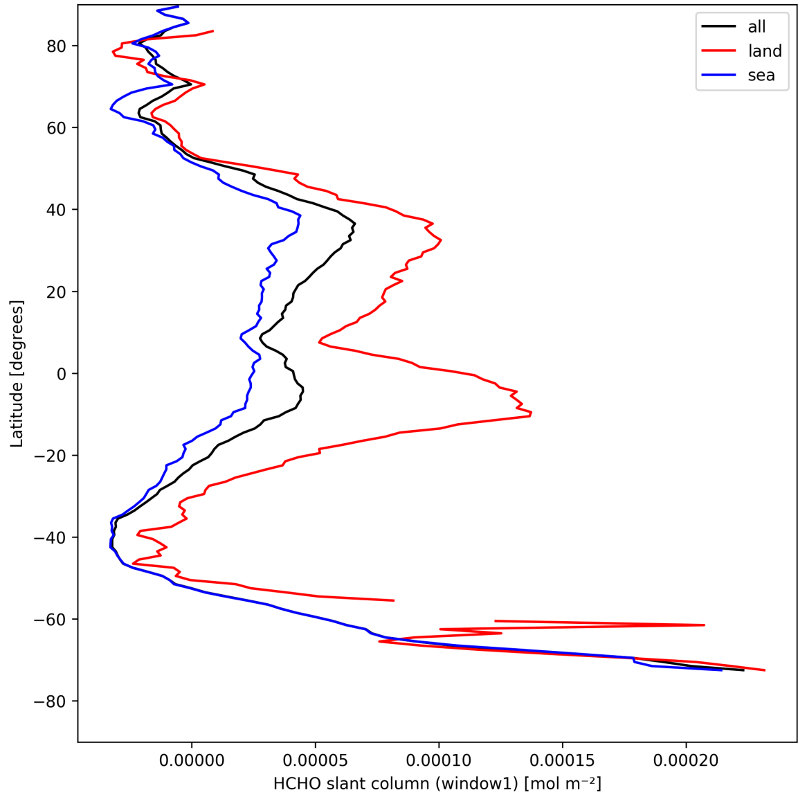
Figure 24: Zonal average of “HCHO slant column (window1)” for 2025-08-19 to 2025-08-21.
