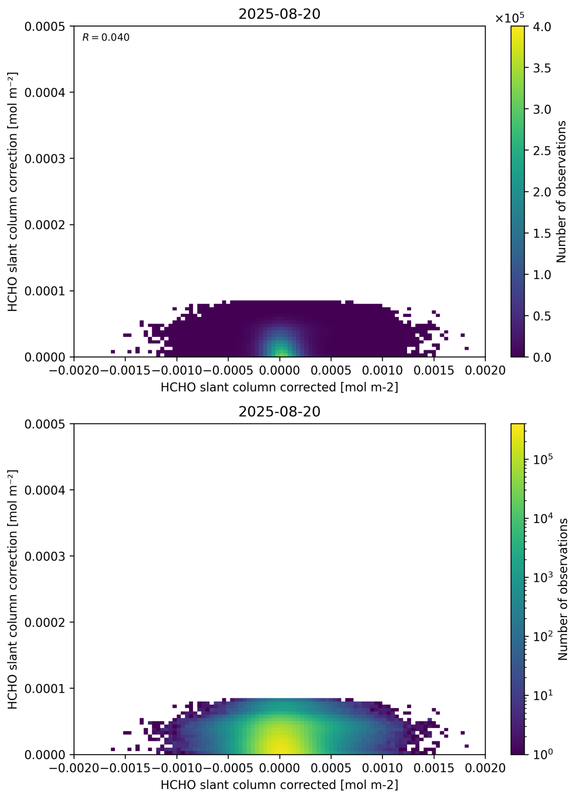
Figure 77: Scatter density plot of “HCHO slant column corrected” against “HCHO slant column correction” for 2025-08-19 to 2025-08-21.
