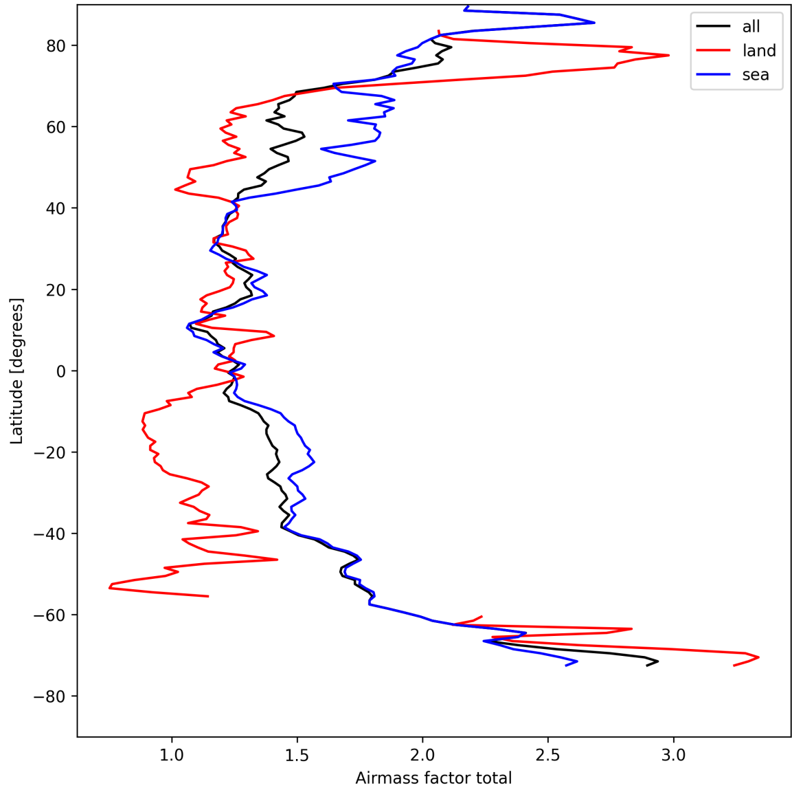
Figure 26: Zonal average of “Airmass factor total” for 2025-08-19 to 2025-08-21.
