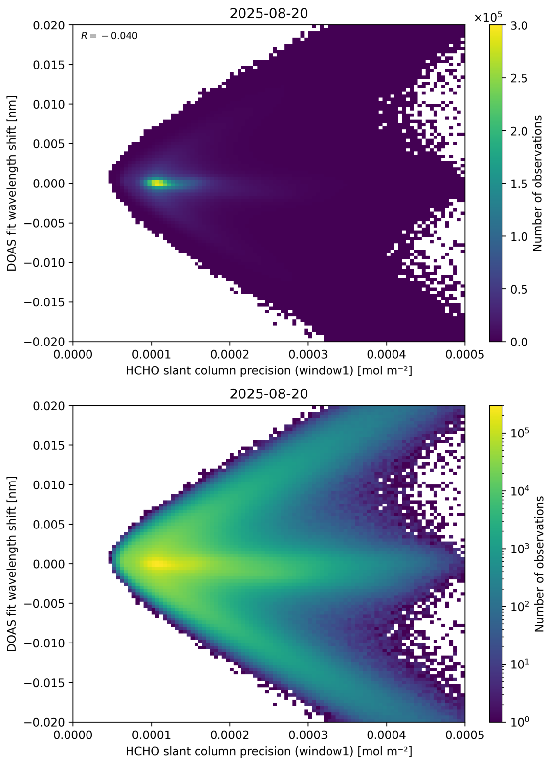
Figure 89: Scatter density plot of “HCHO slant column precision (window1)” against “DOAS fit wavelength shift” for 2025-08-19 to 2025-08-21.
