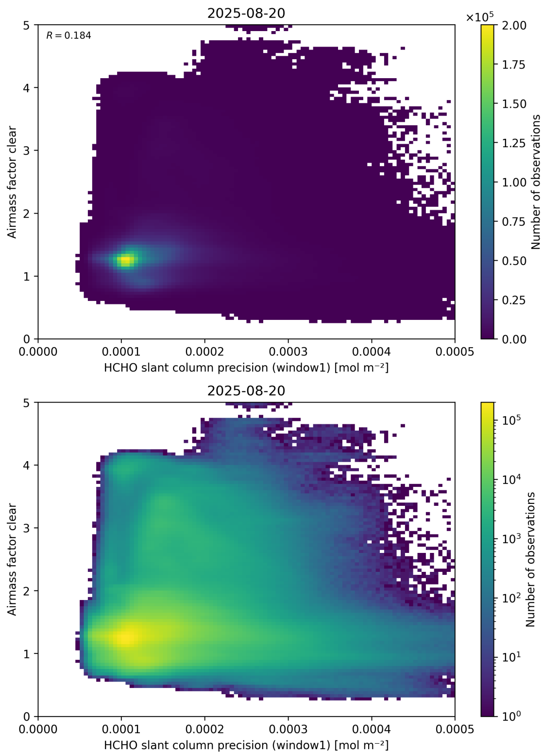
Figure 91: Scatter density plot of “HCHO slant column precision (window1)” against “Airmass factor clear” for 2025-08-19 to 2025-08-21.
