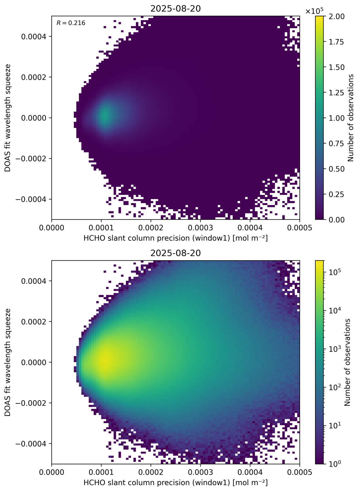
Figure 90: Scatter density plot of “HCHO slant column precision (window1)” against “DOAS fit wavelength squeeze” for 2025-08-19 to 2025-08-21.
