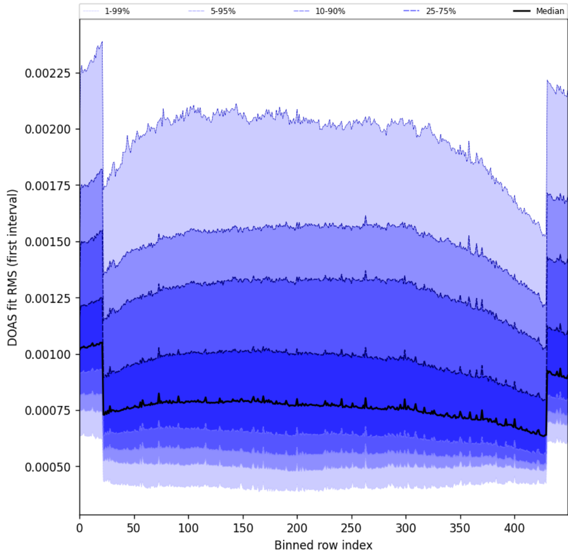
Figure 60: Along track statistics of “DOAS fit RMS (first interval)” for 2025-08-19 to 2025-08-21
