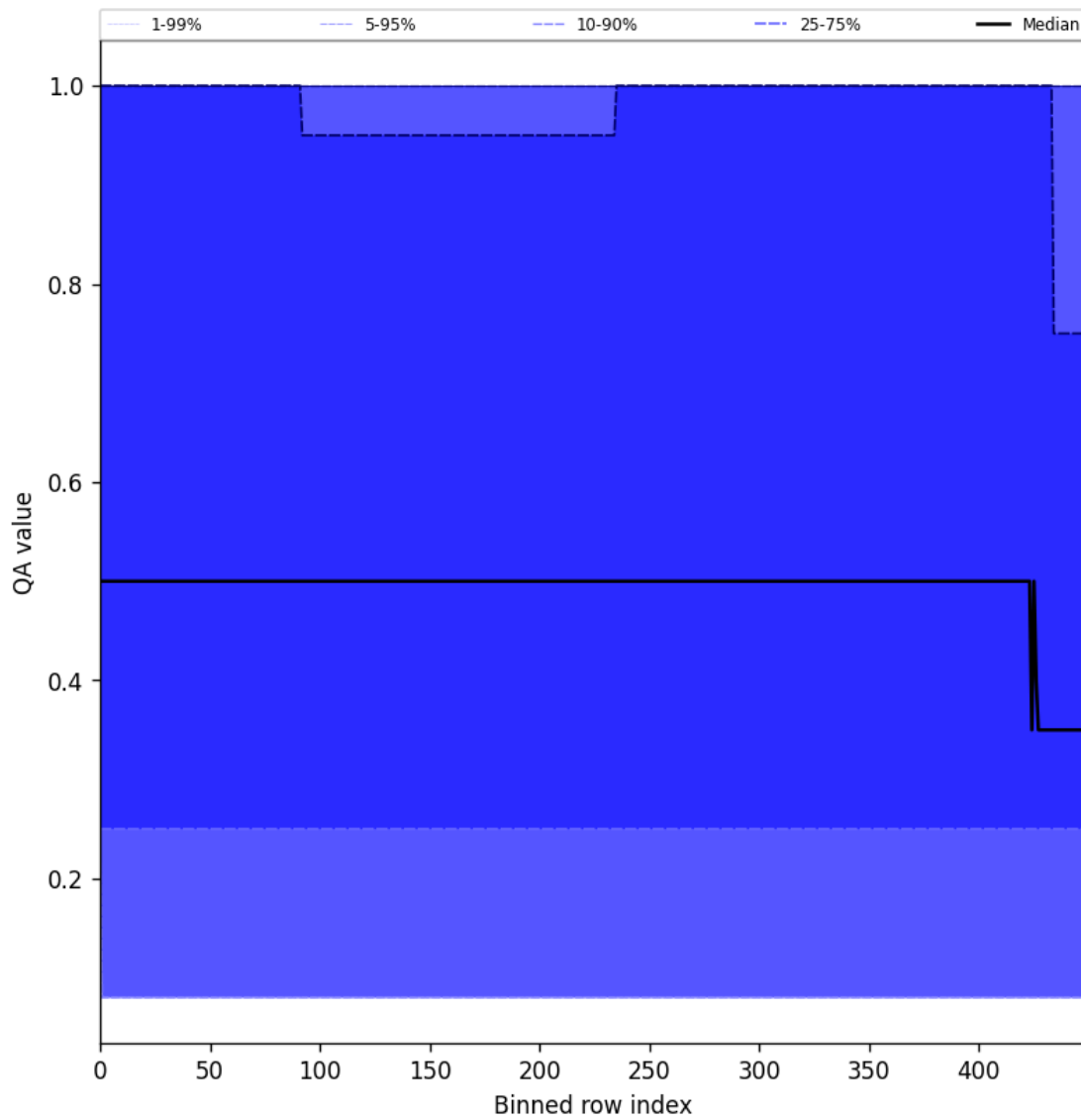
Figure 48: Along track statistics of “QA value” for 2025-08-19 to 2025-08-21
