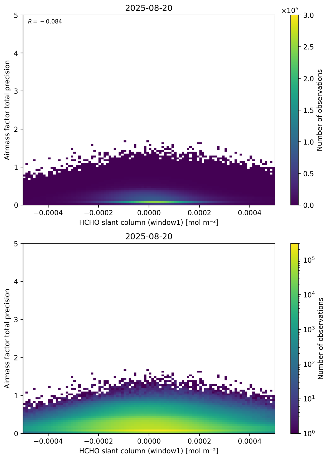
Figure 86: Scatter density plot of “HCHO slant column (window1)” against “Airmass factor total precision” for 2025-08-19 to 2025-08-21.
