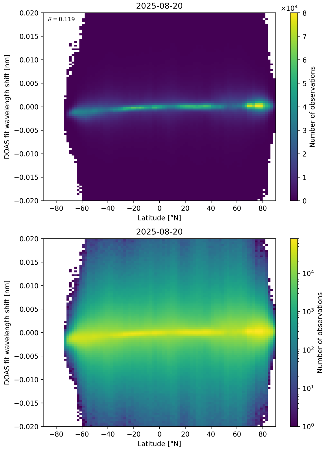
Figure 154: Scatter density plot of “Latitude” against “DOAS fit wavelength shift” for 2025-08-19 to 2025-08-21.
