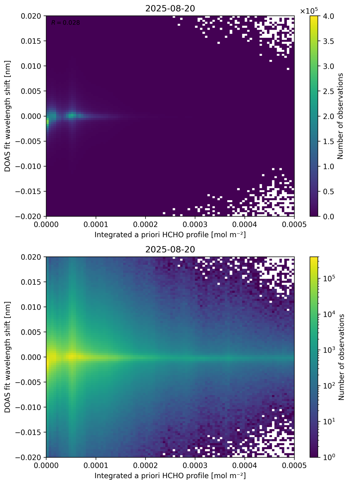
Figure 149: Scatter density plot of “Integrated a priori HCHO profile” against “DOAS fit wavelength shift” for 2025-08-19 to 2025-08-21.
