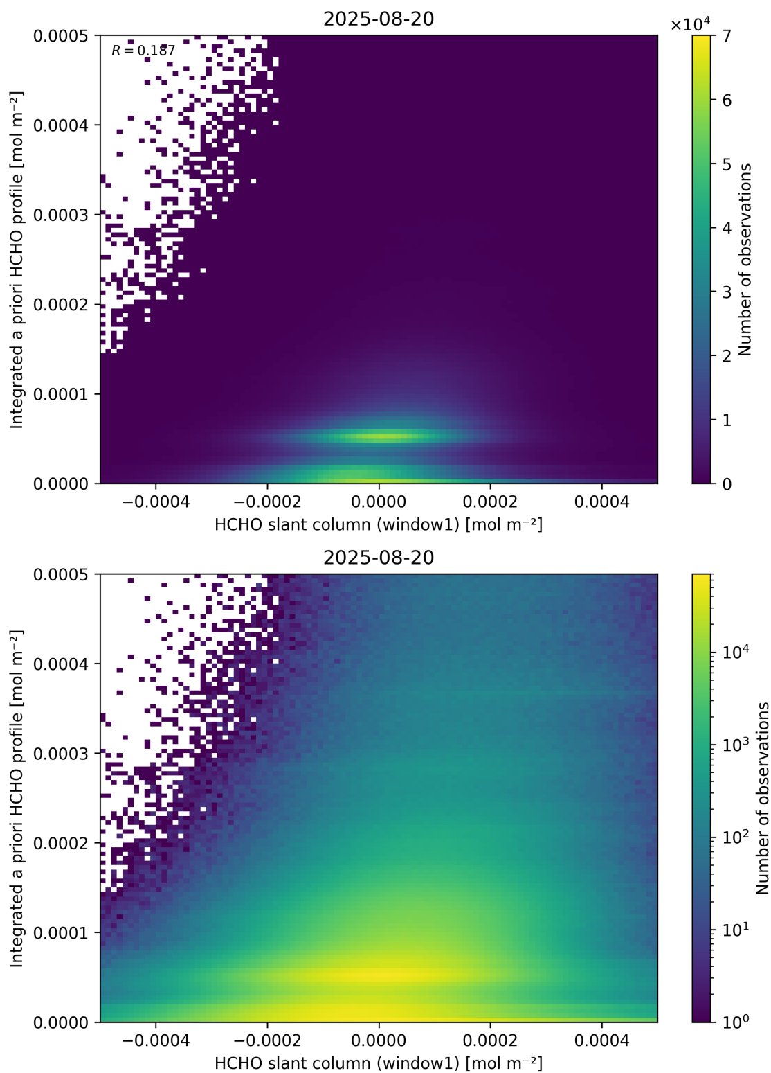
Figure 87: Scatter density plot of “HCHO slant column (window1)” against “Integrated a priori HCHO profile” for 2025-08-19 to 2025-08-21.
