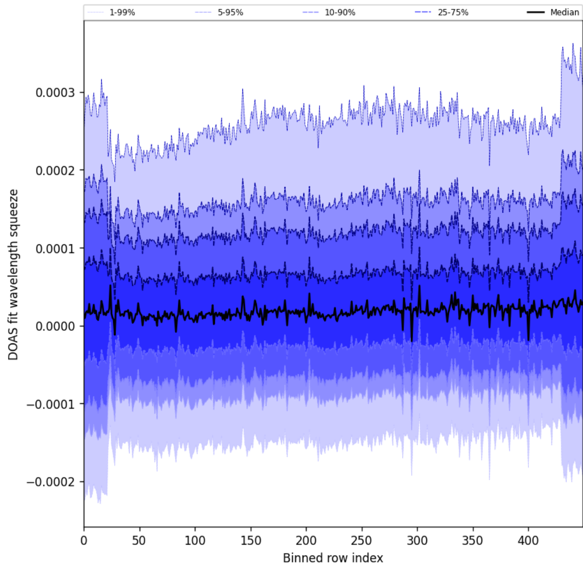
Figure 59: Along track statistics of “DOAS fit wavelength squeeze” for 2025-08-19 to 2025-08-21
