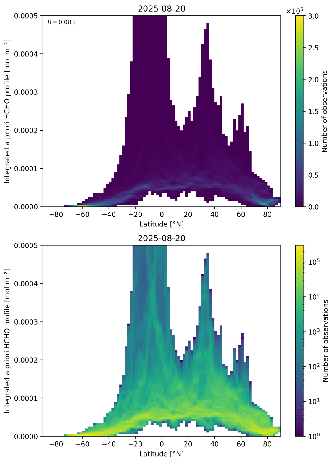
Figure 166: Scatter density plot of “Latitude” against “Integrated a priori HCHO profile” for 2025-08-19 to 2025-08-21.
