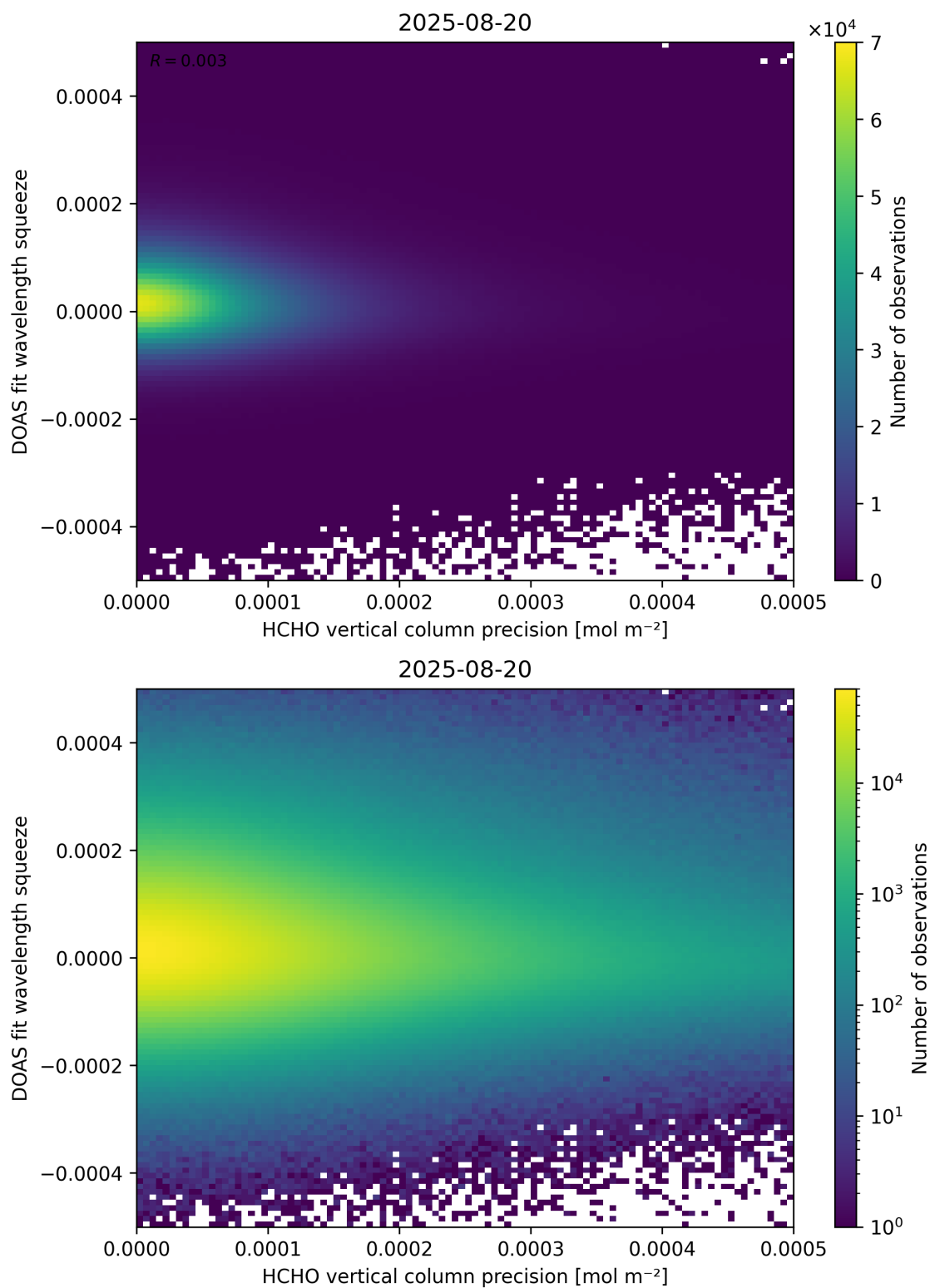
Figure 138: Scatter density plot of “HCHO vertical column precision” against “DOAS fit wavelength squeeze” for 2025-08-19 to 2025-08-21.
