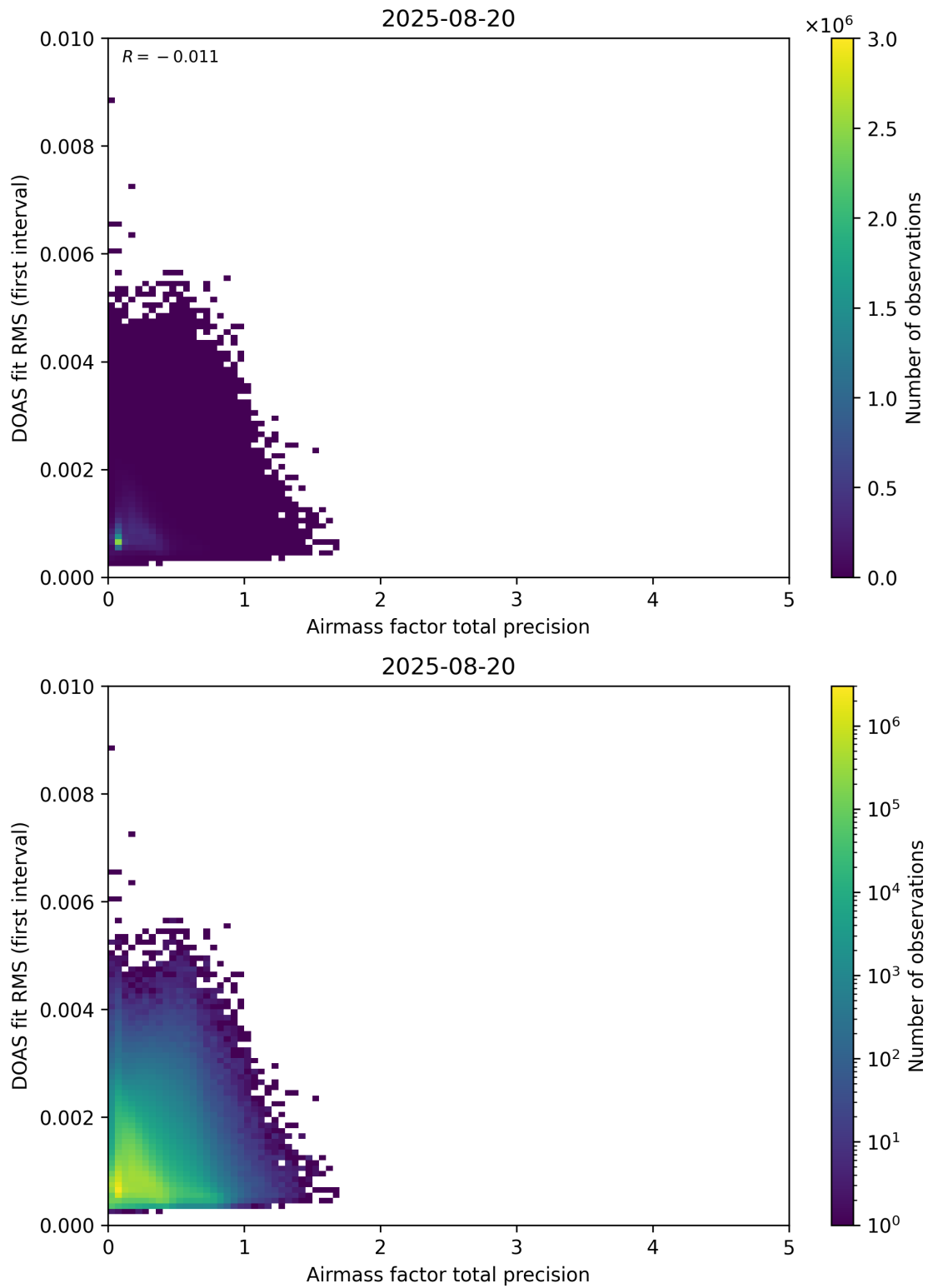
Figure 105: Scatter density plot of “Airmass factor total precision” against “DOAS fit RMS (first interval)” for 2025-08-19 to 2025-08-21.
