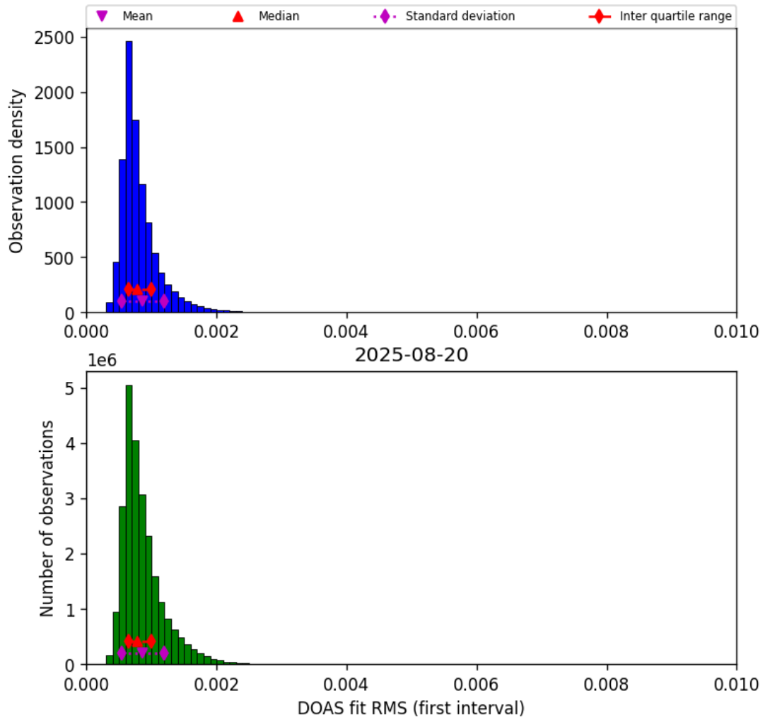
Figure 46: Histogram of “DOAS fit RMS (first interval)” for 2025-08-19 to 2025-08-21
