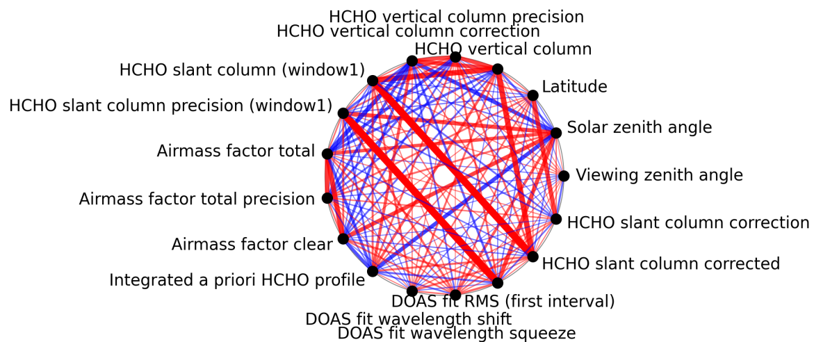
Figure 1: Map of correlation graph for 2025-08-19 to 2025-08-21.
