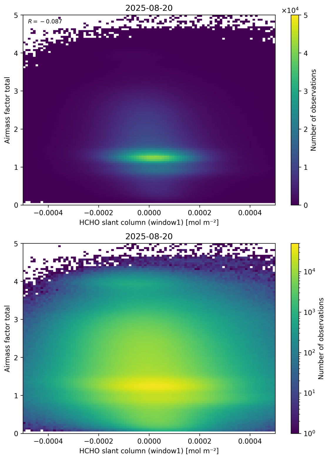
Figure 85: Scatter density plot of “HCHO slant column (window1)” against “Airmass factor total” for 2025-08-19 to 2025-08-21.
