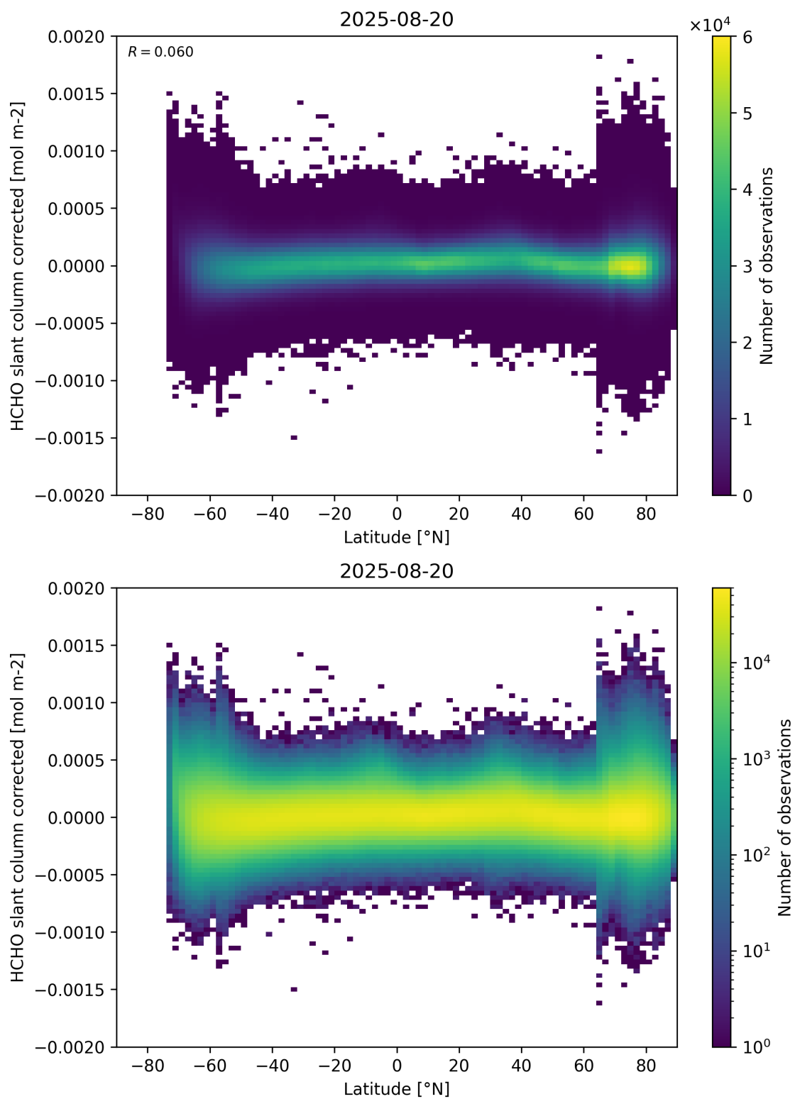
Figure 157: Scatter density plot of “Latitude” against “HCHO slant column corrected” for 2025-08-19 to 2025-08-21.
