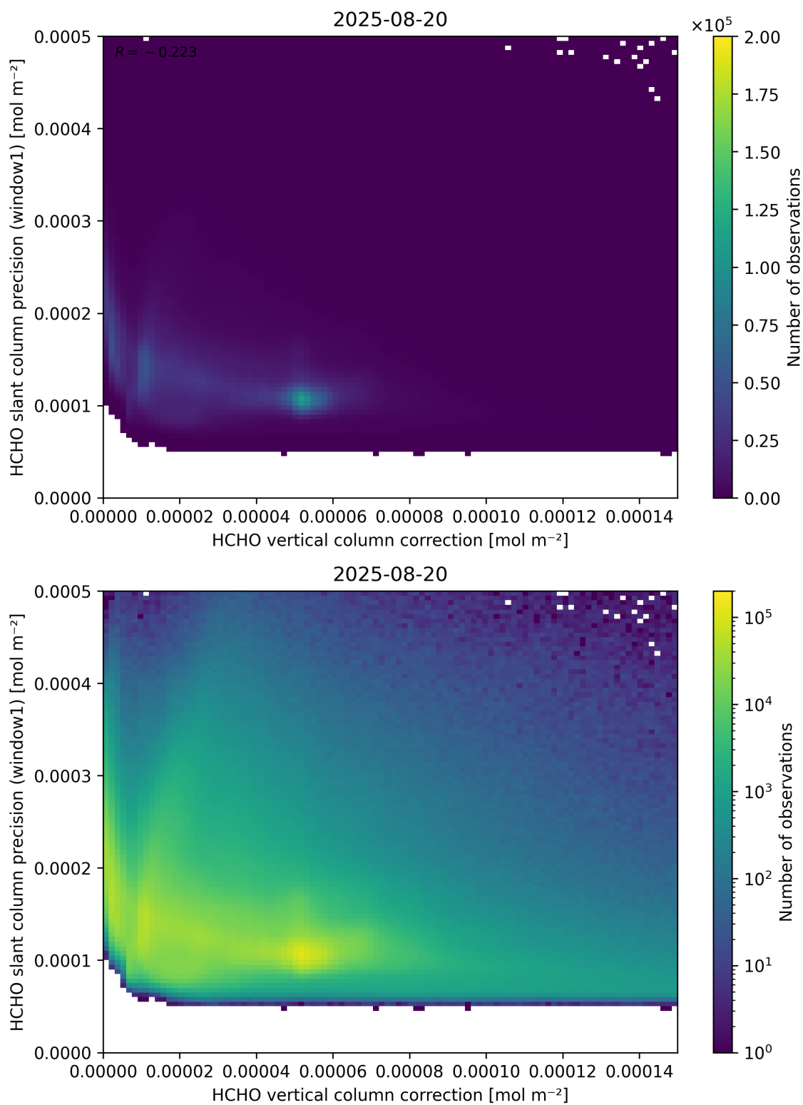
Figure 119: Scatter density plot of “HCHO vertical column correction” against “HCHO slant column precision (window1)” for 2025-08-19 to 2025-08-21.
