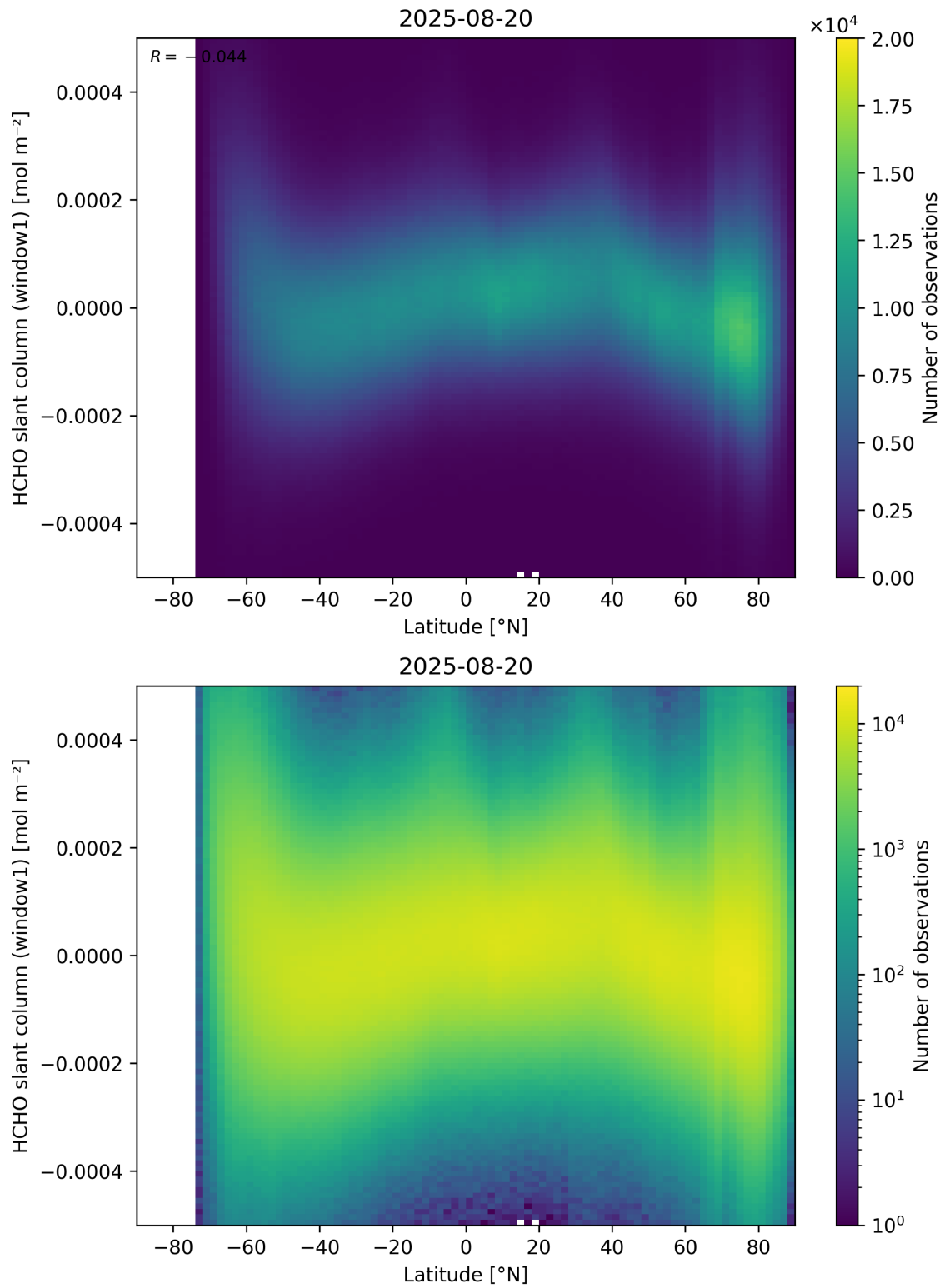
Figure 159: Scatter density plot of “Latitude” against “HCHO slant column (window1)” for 2025-08-19 to 2025-08-21.
