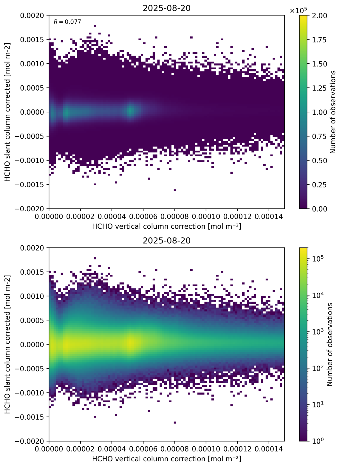
Figure 116: Scatter density plot of “HCHO vertical column correction” against “HCHO slant column corrected” for 2025-08-19 to 2025-08-21.
