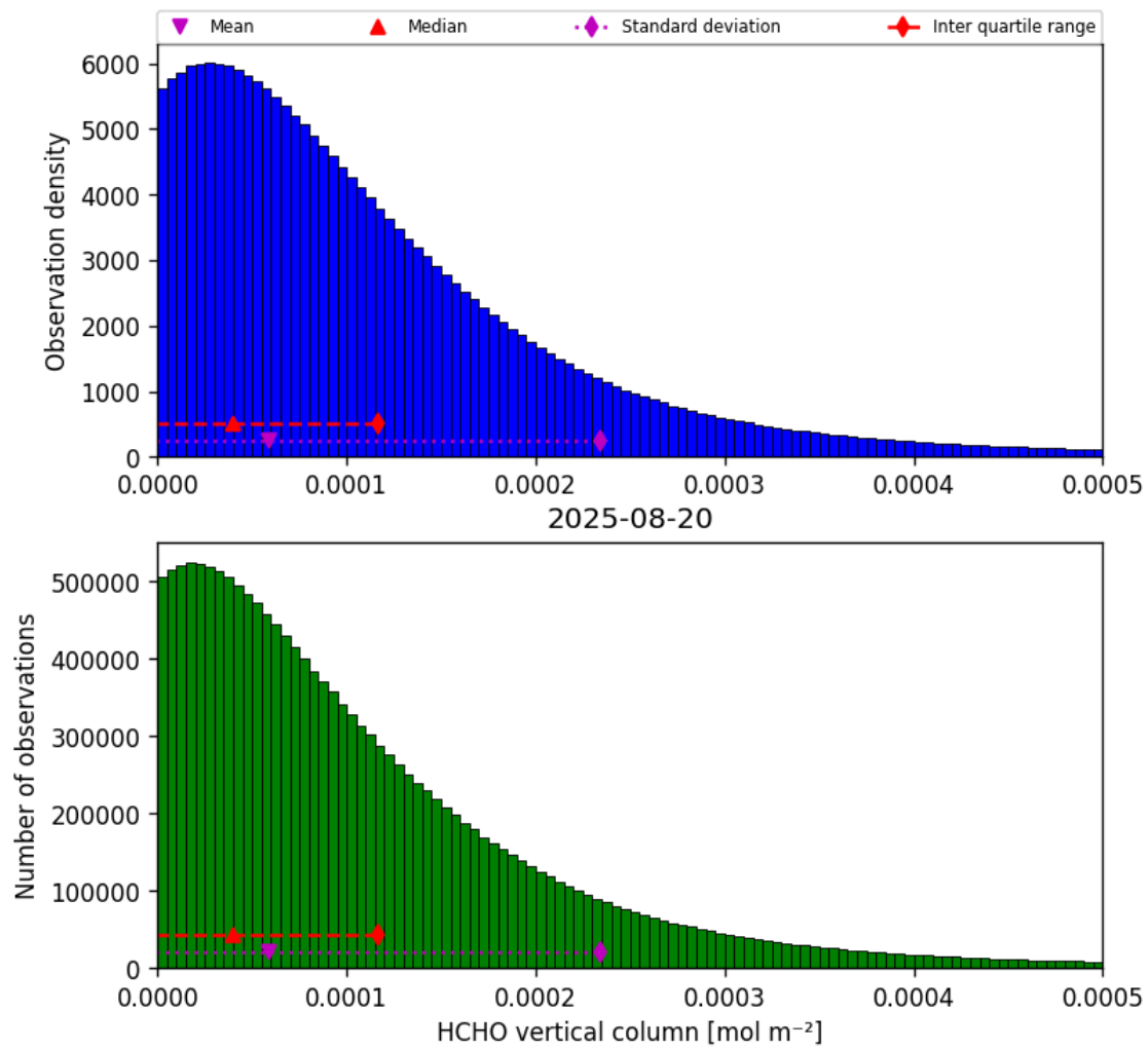
Figure 35: Histogram of “HCHO vertical column” for 2025-08-19 to 2025-08-21
