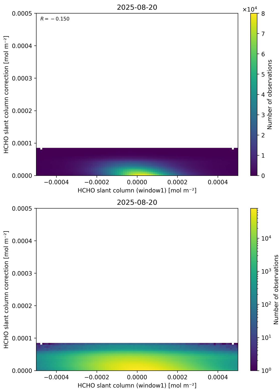
Figure 83: Scatter density plot of “HCHO slant column (window1)” against “HCHO slant column correction” for 2025-08-19 to 2025-08-21.
