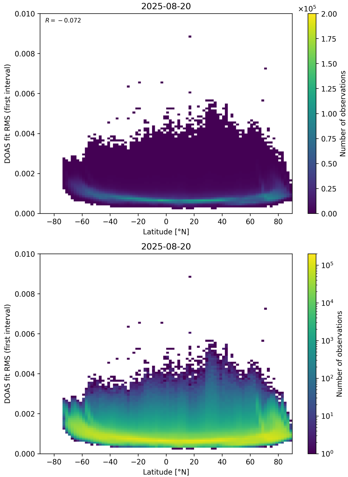
Figure 153: Scatter density plot of “Latitude” against “DOAS fit RMS (first interval)” for 2025-08-19 to 2025-08-21.
