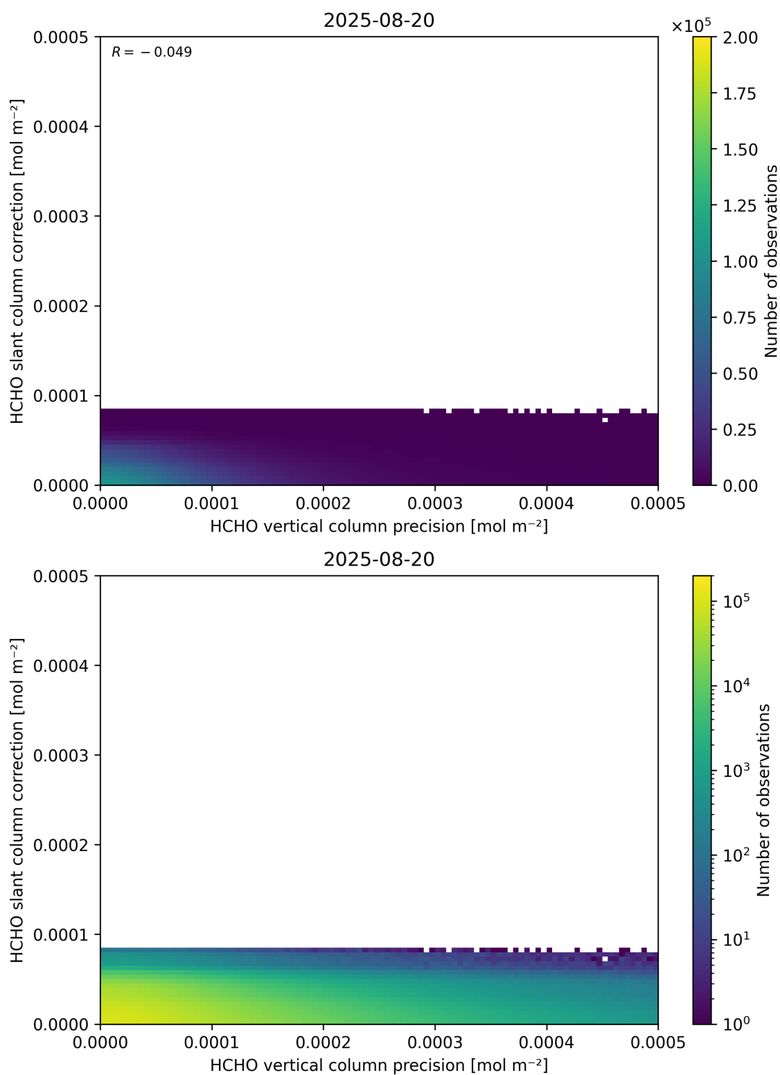
Figure 141: Scatter density plot of “HCHO vertical column precision” against “HCHO slant column correction” for 2025-08-19 to 2025-08-21.
