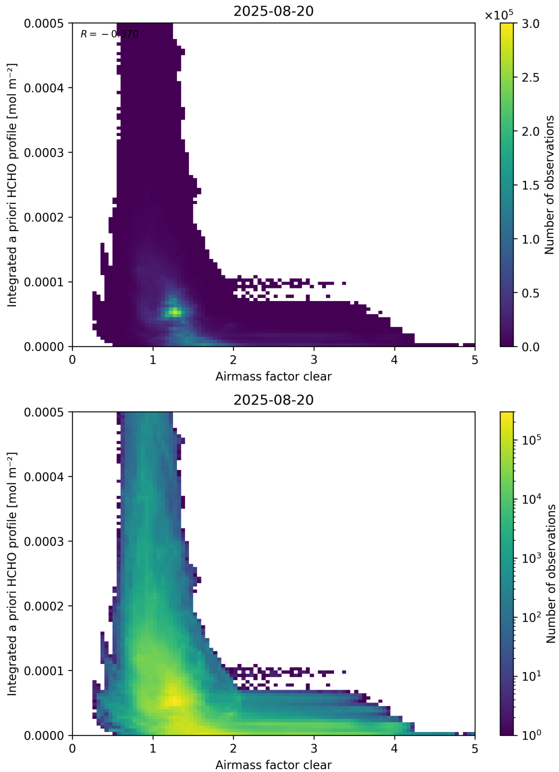
Figure 76: Scatter density plot of “Airmass factor clear” against “Integrated a priori HCHO profile” for 2025-08-19 to 2025-08-21.
