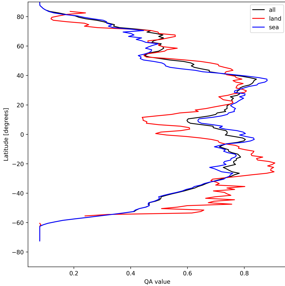
Figure 20: Zonal average of “QA value” for 2025-08-19 to 2025-08-21.
