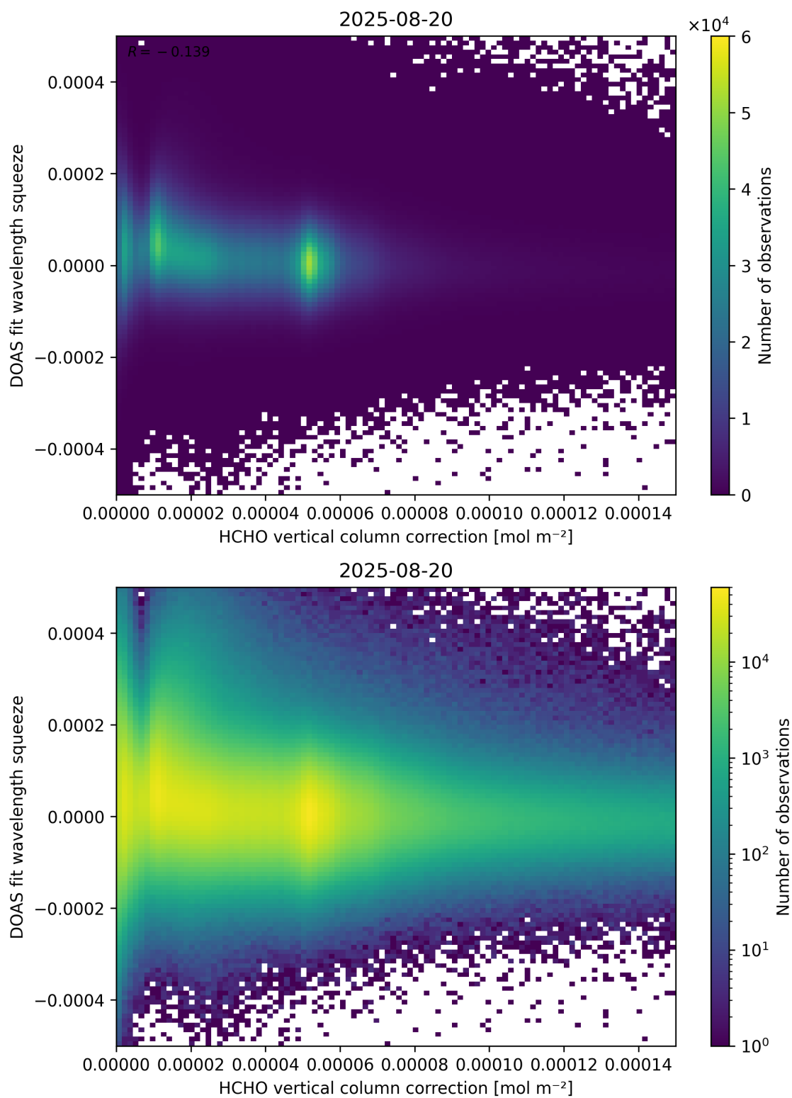
Figure 114: Scatter density plot of “HCHO vertical column correction” against “DOAS fit wavelength squeeze” for 2025-08-19 to 2025-08-21.
