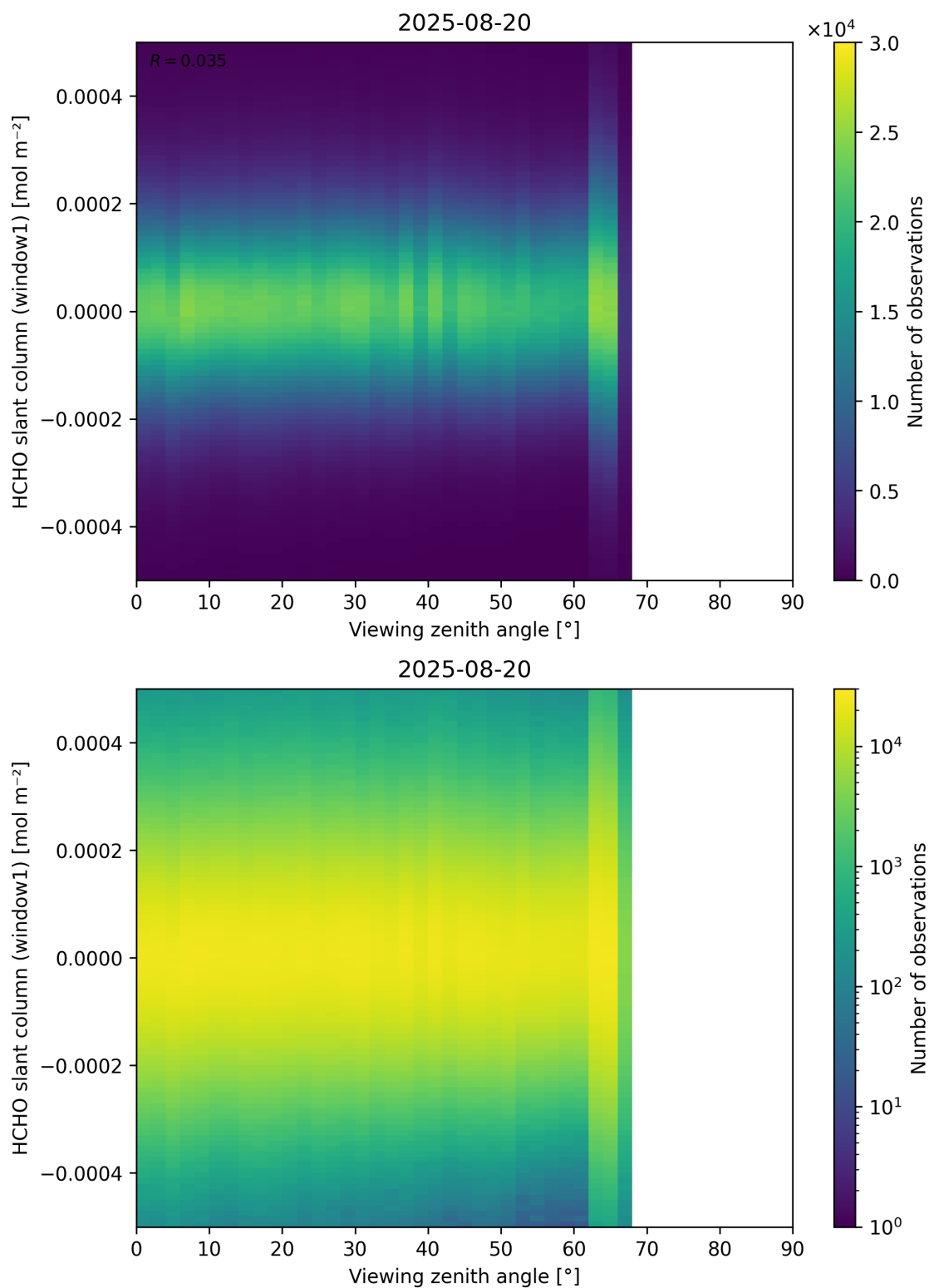
Figure 188: Scatter density plot of “Viewing zenith angle” against “HCHO slant column (window1)” for 2025-08-19 to 2025-08-21.
