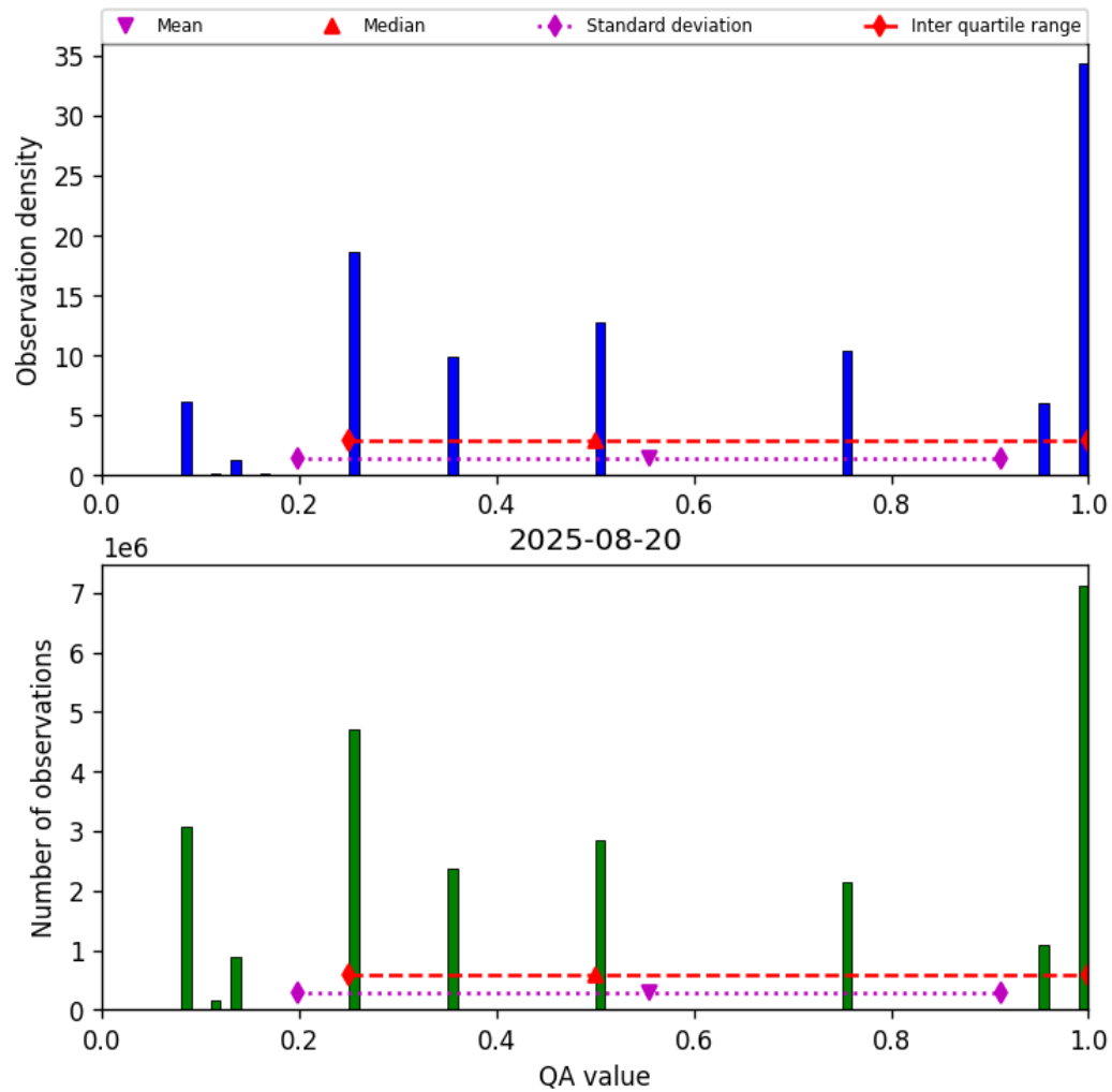
Figure 34: Histogram of “QA value” for 2025-08-19 to 2025-08-21
