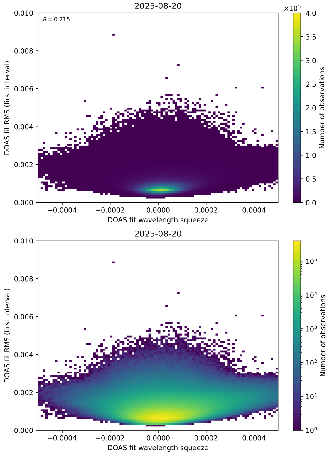
Figure 68: Scatter density plot of “DOAS fit wavelength squeeze” against “DOAS fit RMS (first interval)” for 2025-08-19 to 2025-08-21.
