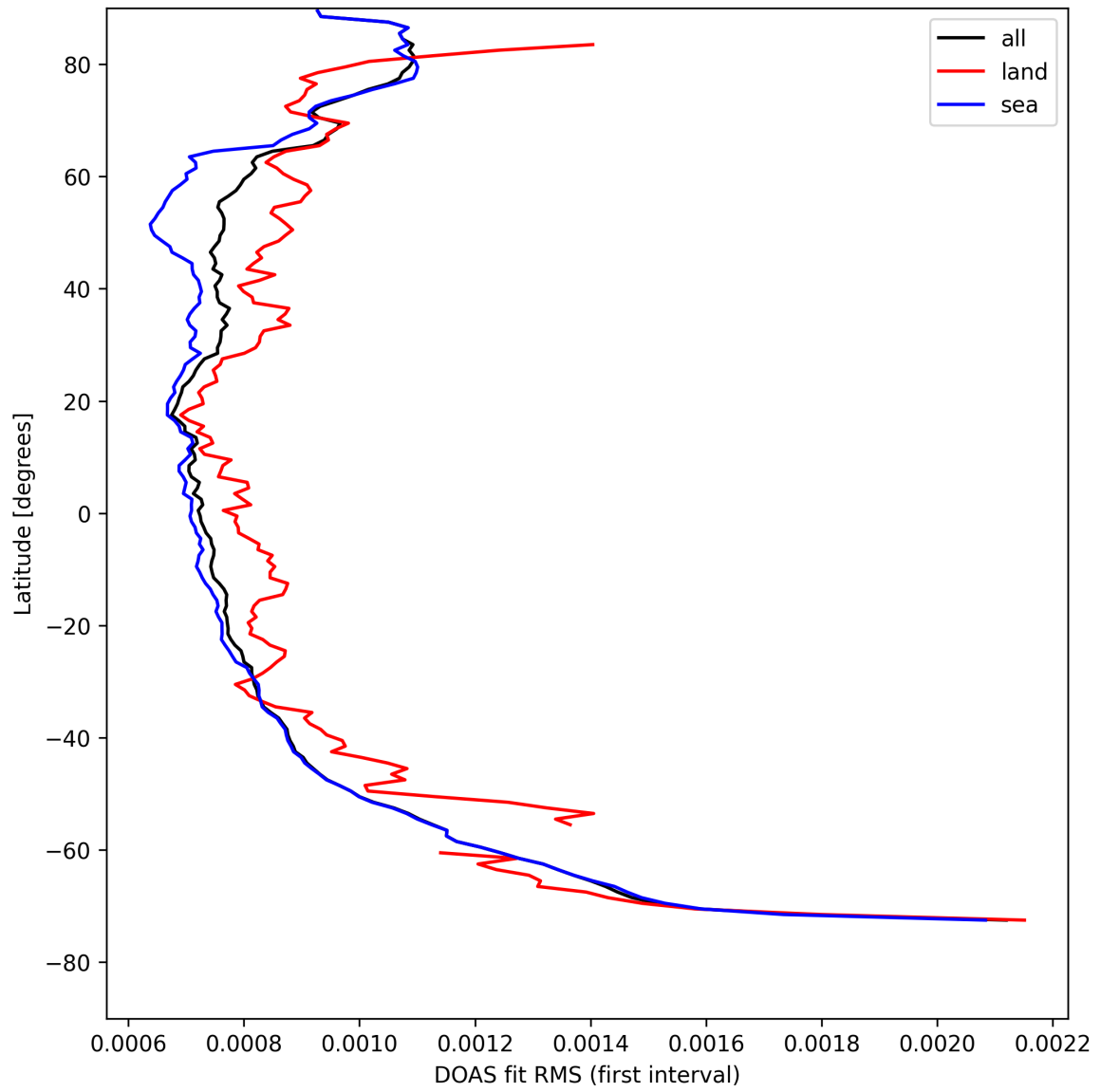
Figure 32: Zonal average of “DOAS fit RMS (first interval)” for 2025-08-19 to 2025-08-21.
