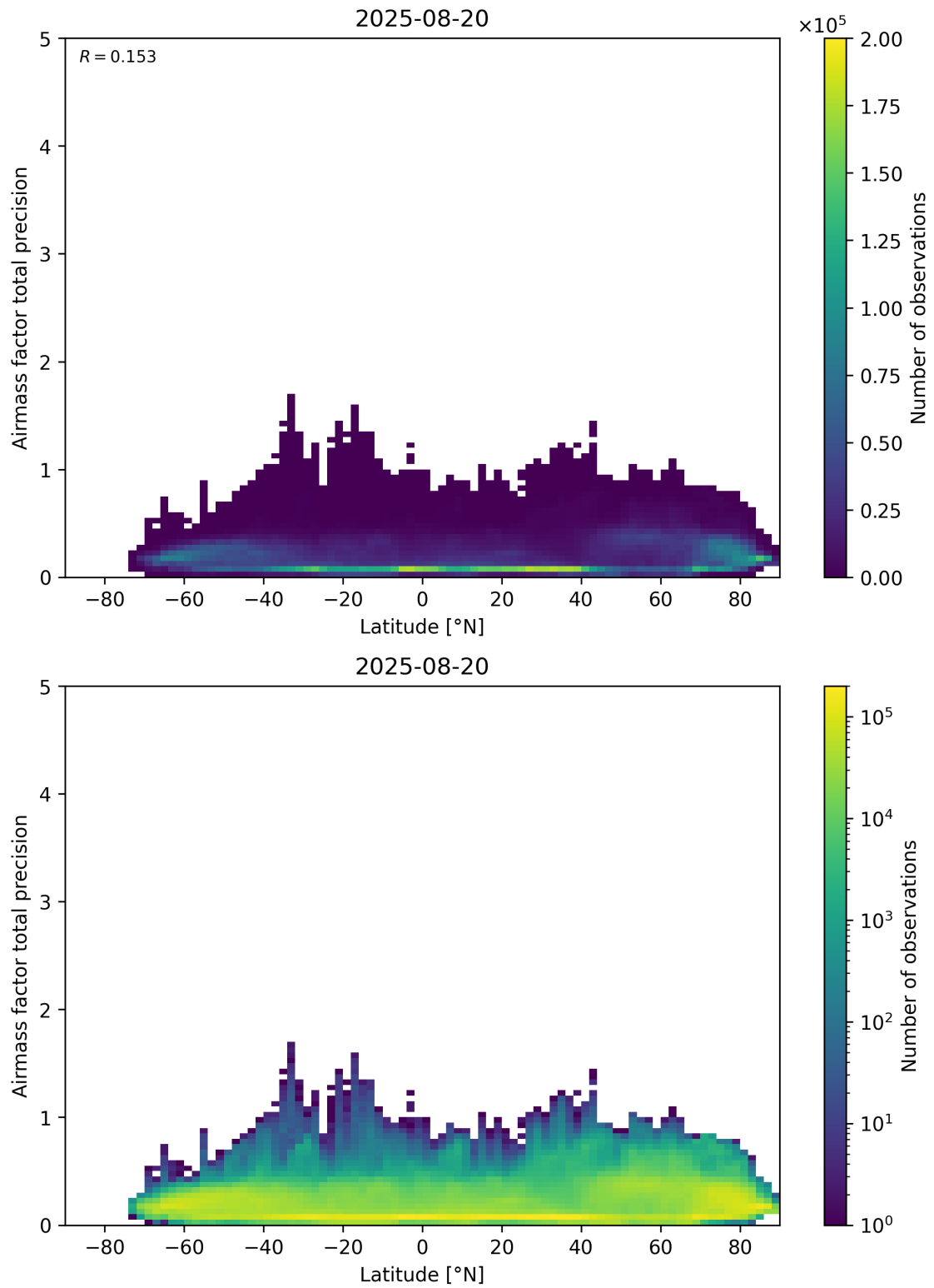
Figure 162: Scatter density plot of “Latitude” against “Airmass factor total precision” for 2025-08-19 to 2025-08-21.
