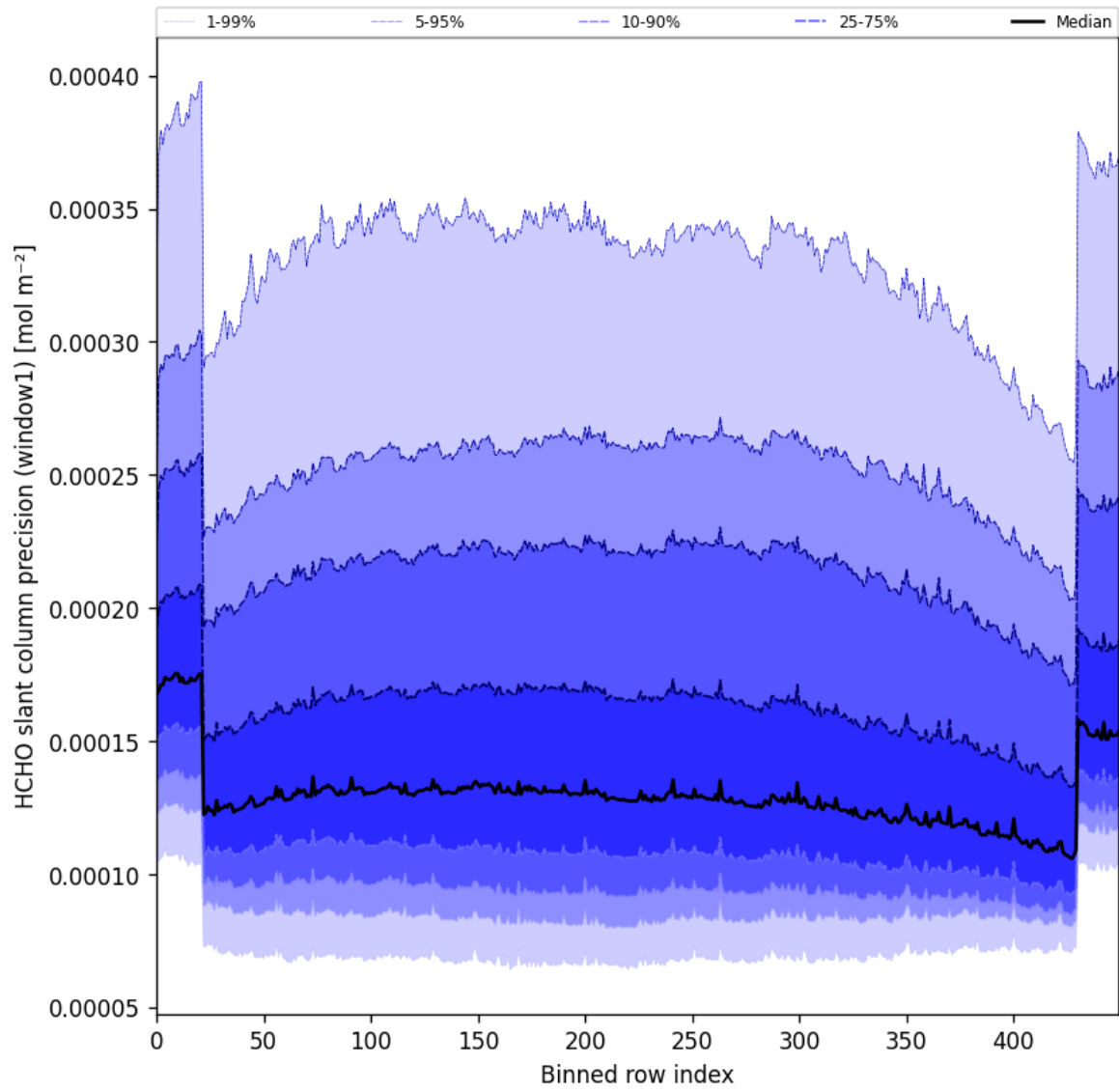
Figure 53: Along track statistics of “HCHO slant column precision (window1)” for 2025-08-19 to 2025-08-21
