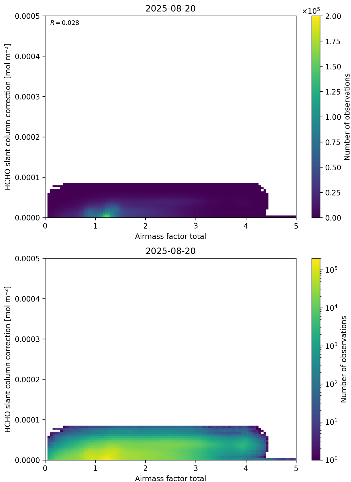
Figure 102: Scatter density plot of “Airmass factor total” against “HCHO slant column correction” for 2025-08-19 to 2025-08-21.
