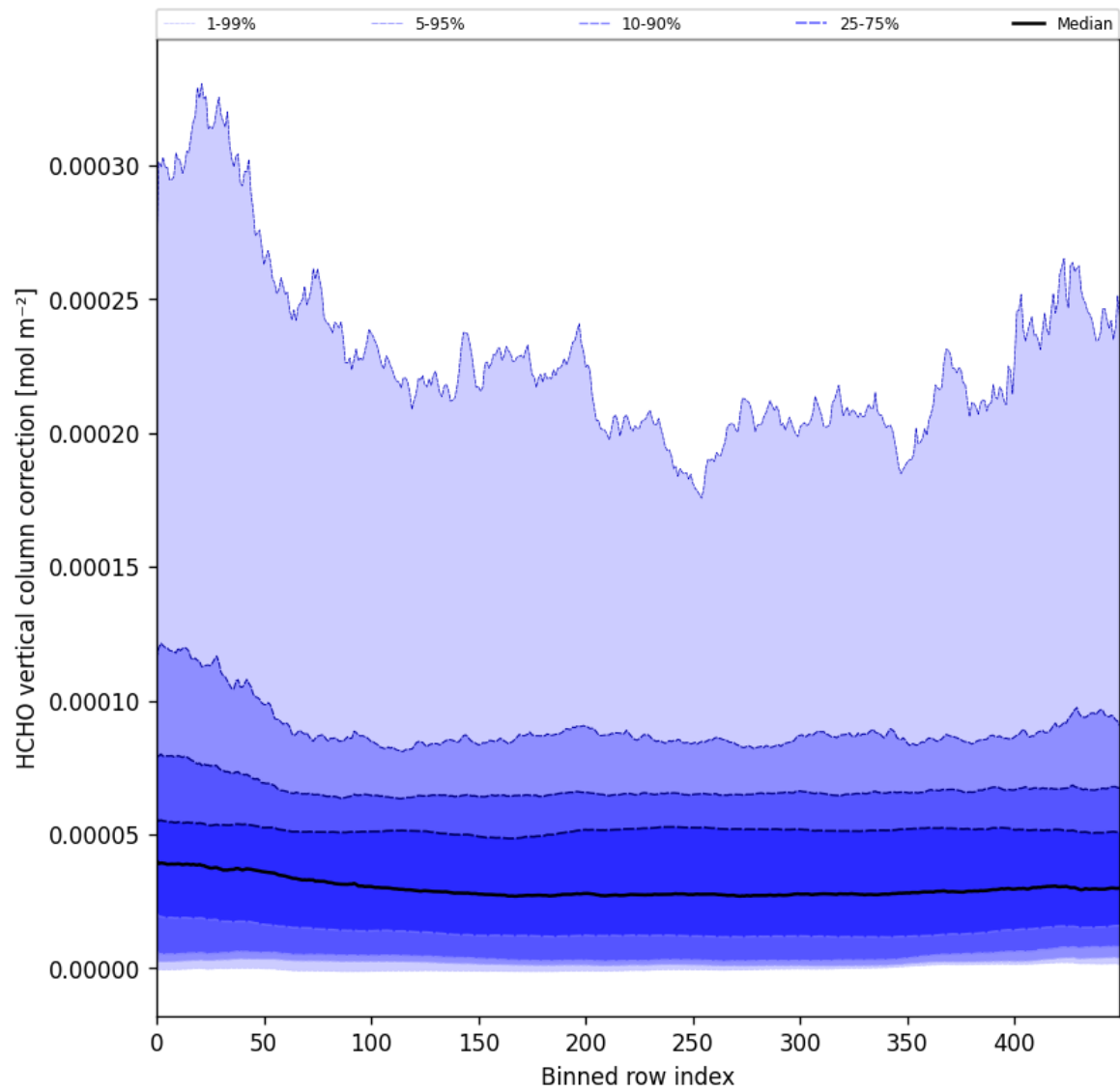
Figure 51: Along track statistics of “HCHO vertical column correction” for 2025-08-19 to 2025-08-21
