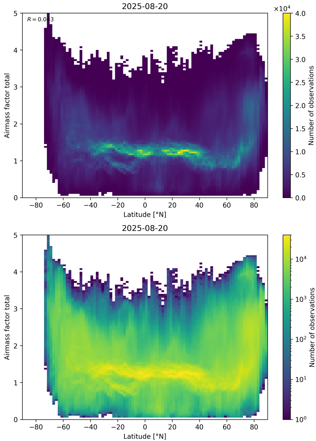
Figure 161: Scatter density plot of “Latitude” against “Airmass factor total” for 2025-08-19 to 2025-08-21.
