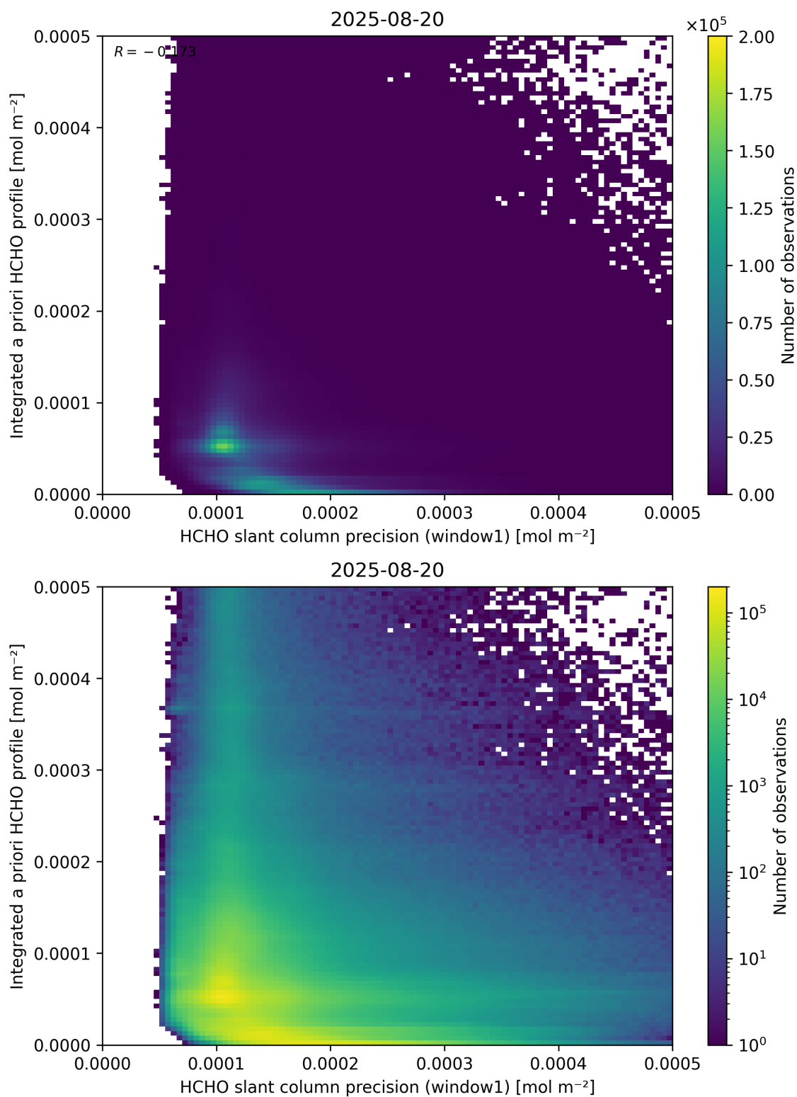
Figure 96: Scatter density plot of “HCHO slant column precision (window1)” against “Integrated a priori HCHO profile” for 2025-08-19 to 2025-08-21.
