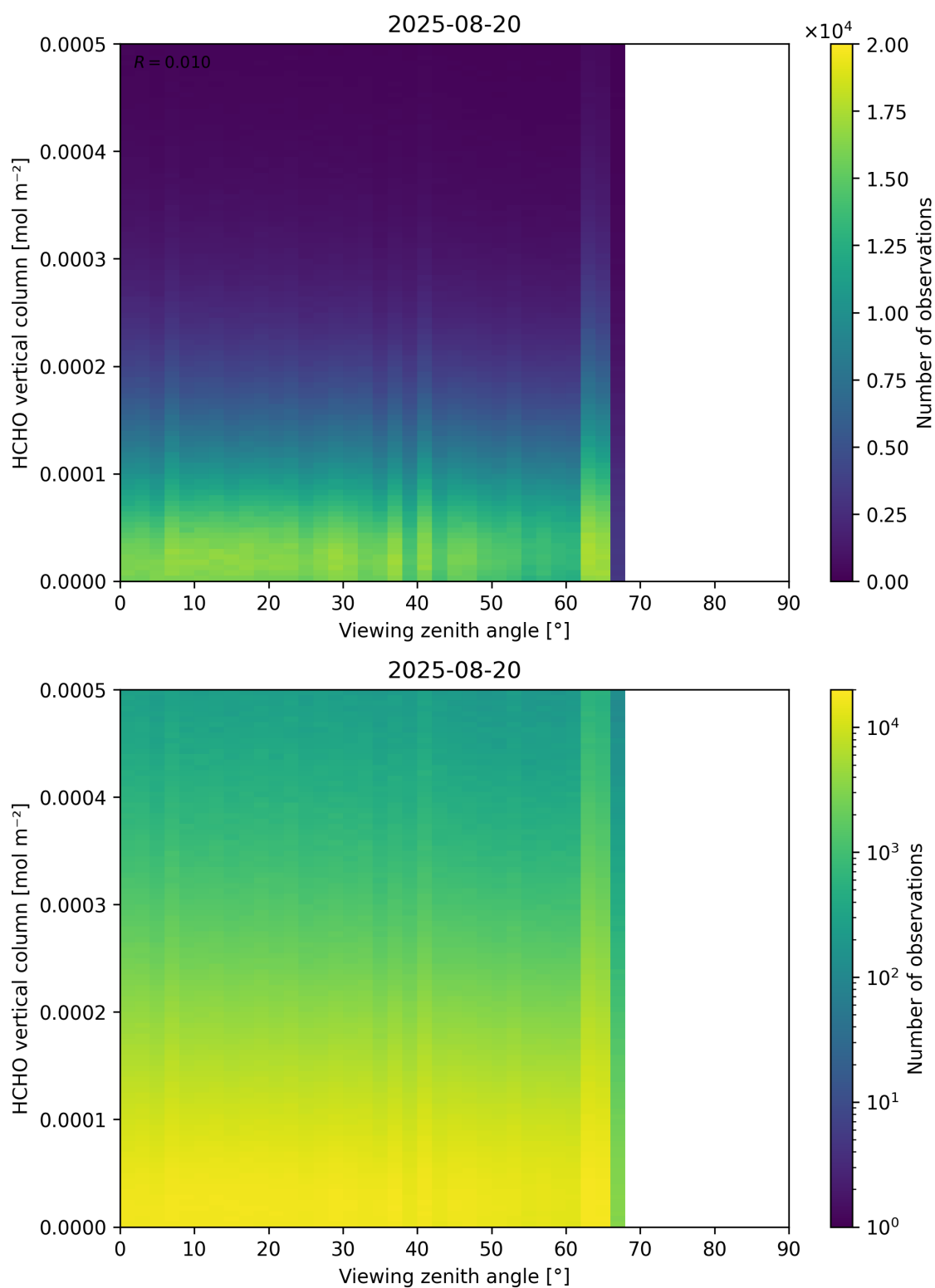
Figure 192: Scatter density plot of “Viewing zenith angle” against “HCHO vertical column” for 2025-08-19 to 2025-08-21.
