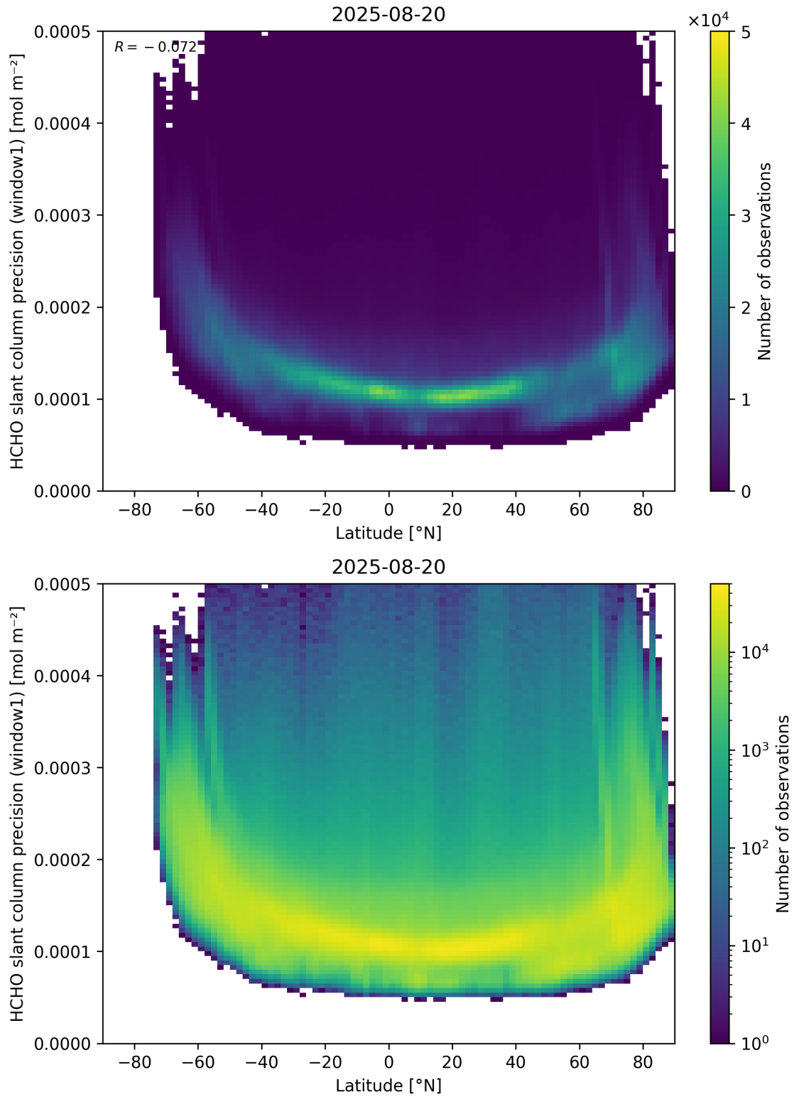
Figure 160: Scatter density plot of “Latitude” against “HCHO slant column precision (window1)” for 2025-08-19 to 2025-08-21.
