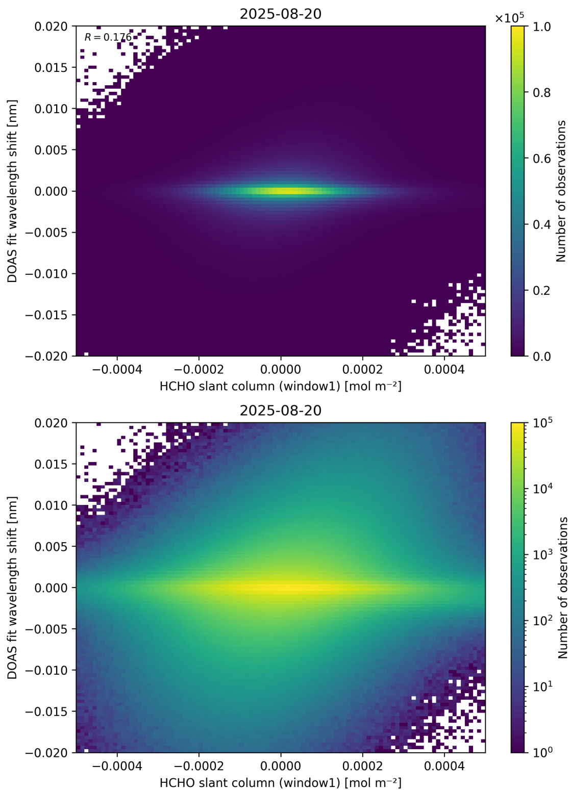
Figure 79: Scatter density plot of “HCHO slant column (window1)” against “DOAS fit wavelength shift” for 2025-08-19 to 2025-08-21.
