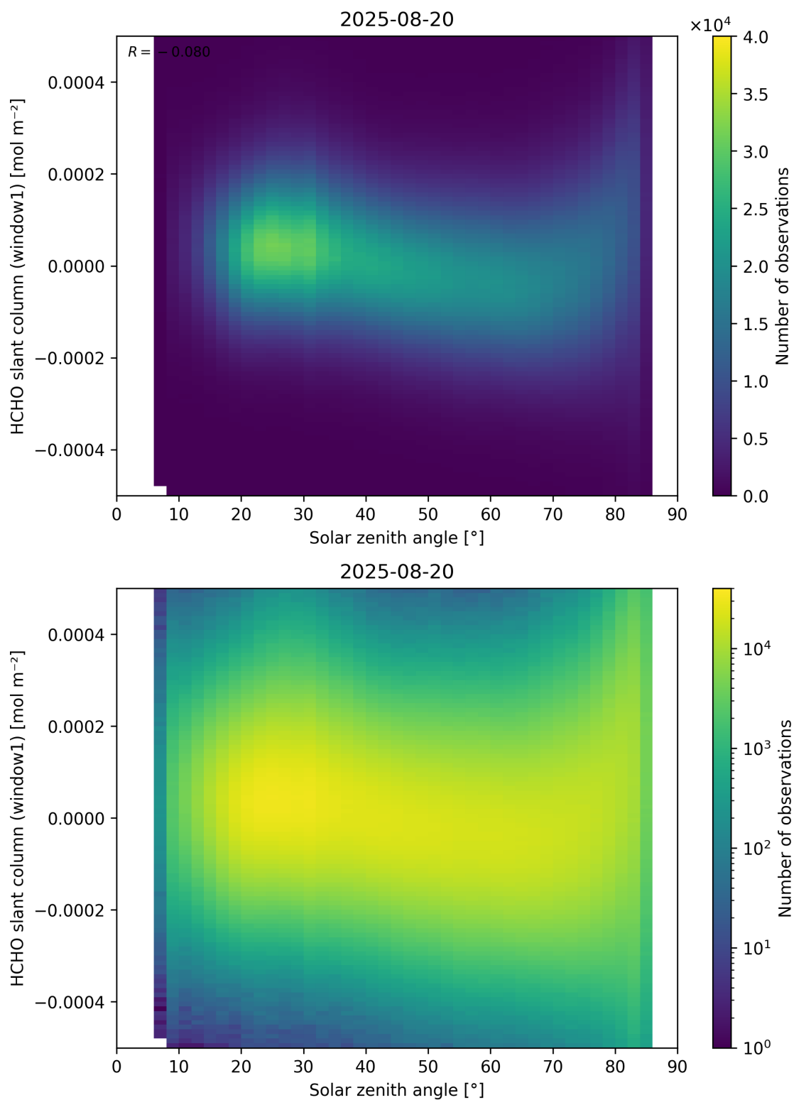
Figure 173: Scatter density plot of “Solar zenith angle” against “HCHO slant column (window1)” for 2025-08-19 to 2025-08-21.
