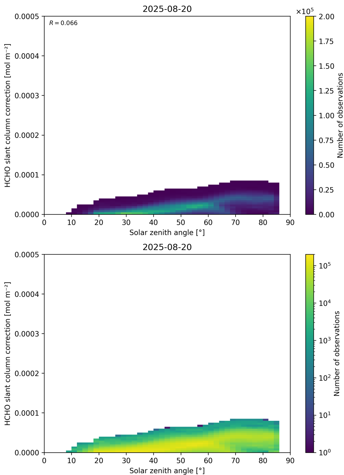
Figure 172: Scatter density plot of “Solar zenith angle” against “HCHO slant column correction” for 2025-08-19 to 2025-08-21.
