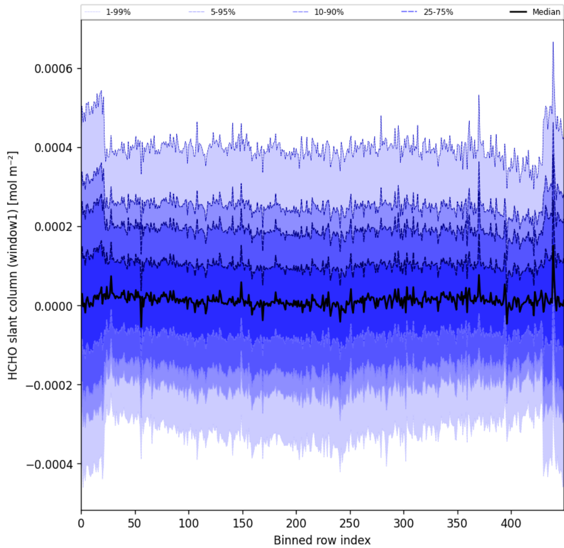
Figure 52: Along track statistics of "HCHO slant column (window1)" for 2025-08-19 to 2025-08-21
