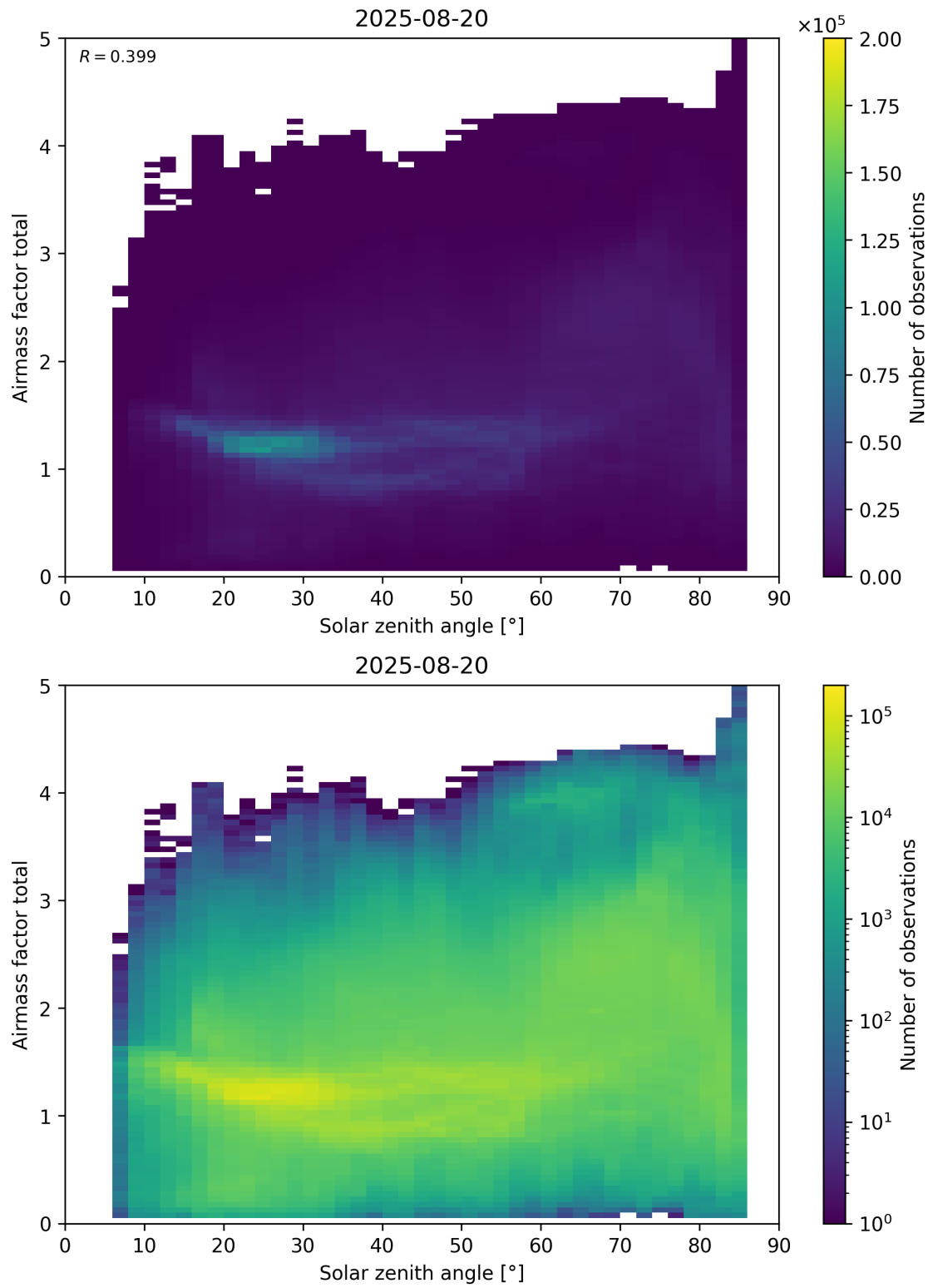
Figure 175: Scatter density plot of “Solar zenith angle” against “Airmass factor total” for 2025-08-19 to 2025-08-21.
