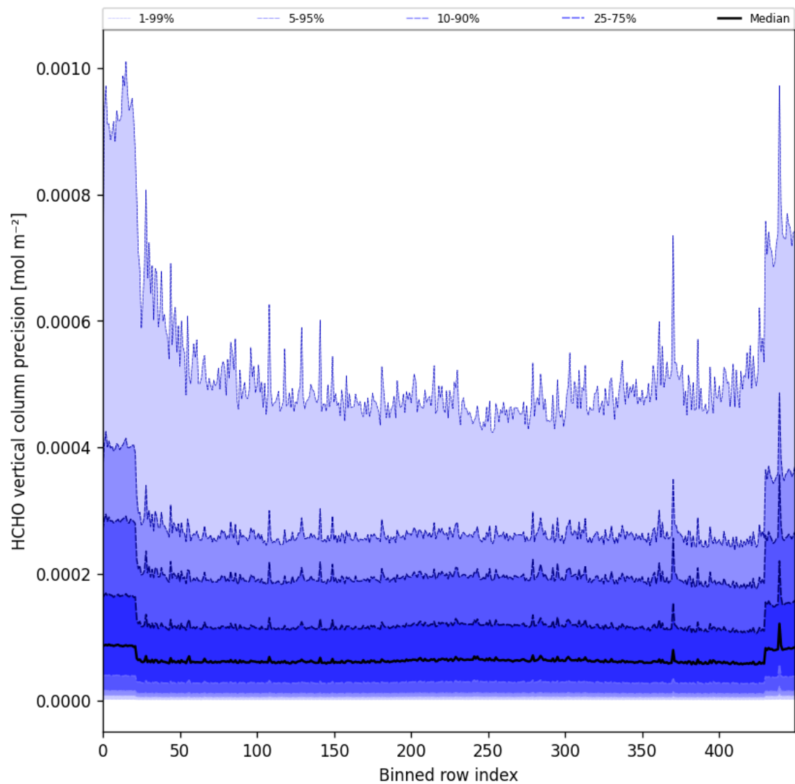
Figure 50: Along track statistics of “HCHO vertical column precision” for 2025-08-19 to 2025-08-21
