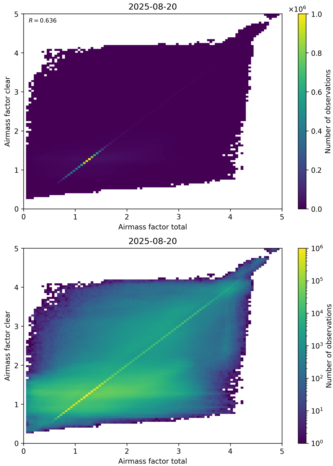
Figure 100: Scatter density plot of “Airmass factor total” against “Airmass factor clear” for 2025-08-19 to 2025-08-21.
