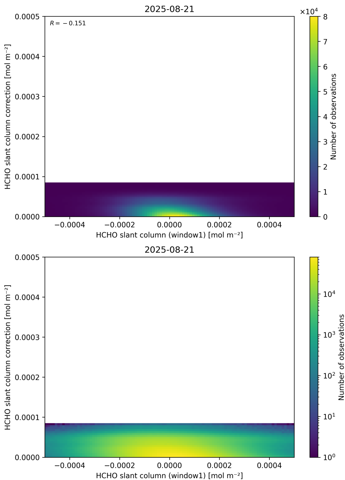
Figure 83: Scatter density plot of “HCHO slant column (window1)” against “HCHO slant column correction” for 2025-08-20 to 2025-08-22.
