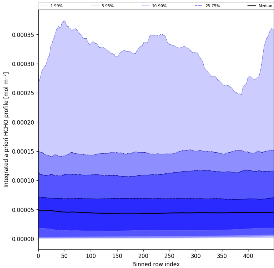
Figure 57: Along track statistics of "Integrated a priori HCHO profile" for 2025-08-20 to 2025-08-22
