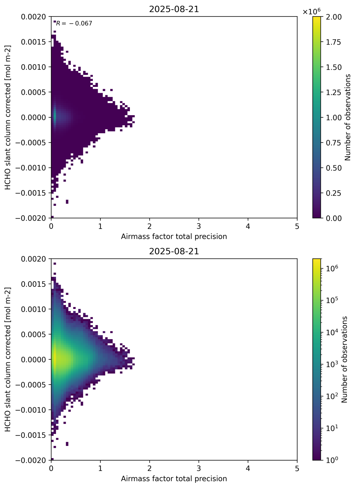
Figure 109: Scatter density plot of “Airmass factor total precision” against “HCHO slant column corrected” for 2025-08-20 to 2025-08-22.
