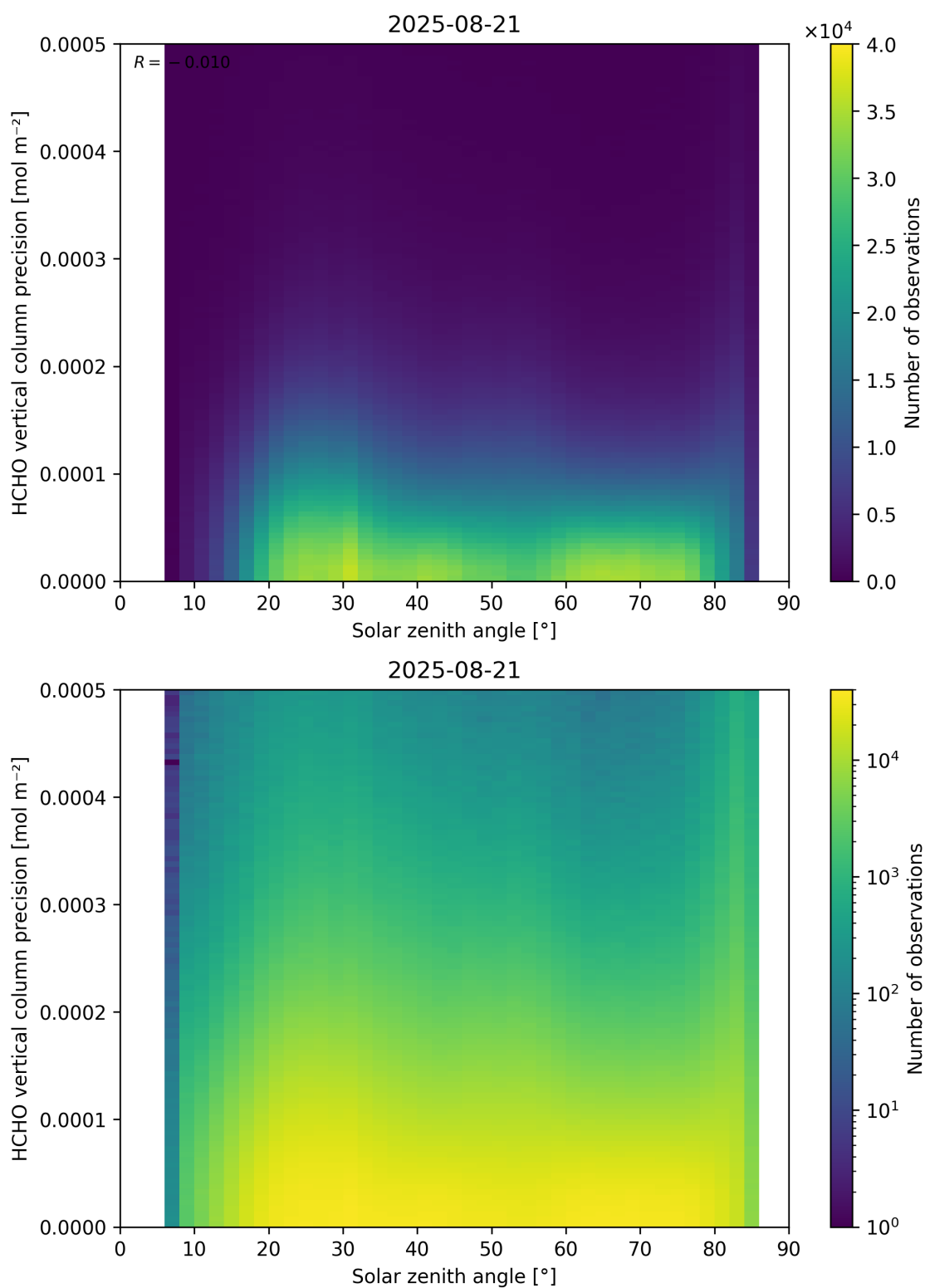
Figure 179: Scatter density plot of “Solar zenith angle” against “HCHO vertical column precision” for 2025-08-20 to 2025-08-22.
