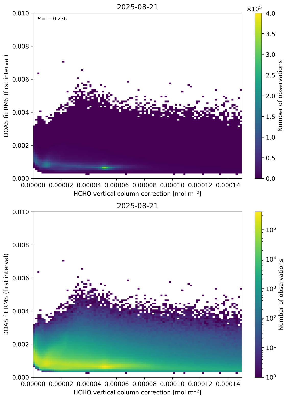
Figure 112: Scatter density plot of “HCHO vertical column correction” against “DOAS fit RMS (first interval)” for 2025-08-20 to 2025-08-22.
