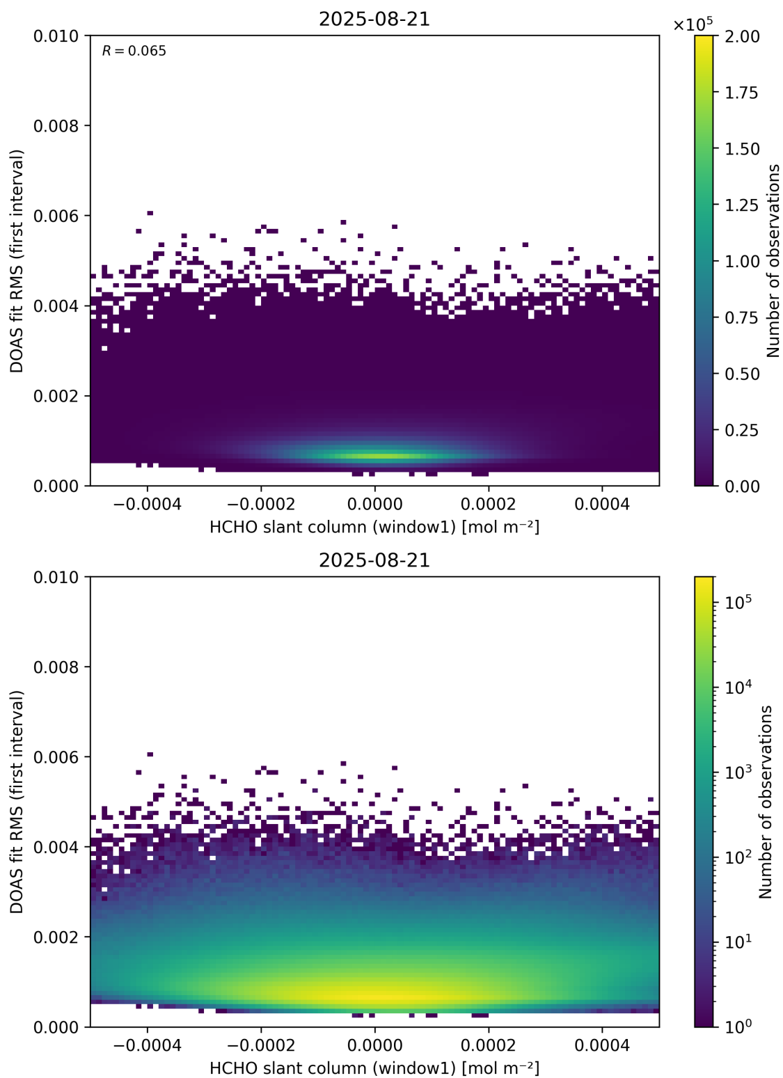
Figure 78: Scatter density plot of “HCHO slant column (window1)” against “DOAS fit RMS (first interval)” for 2025-08-20 to 2025-08-22.
