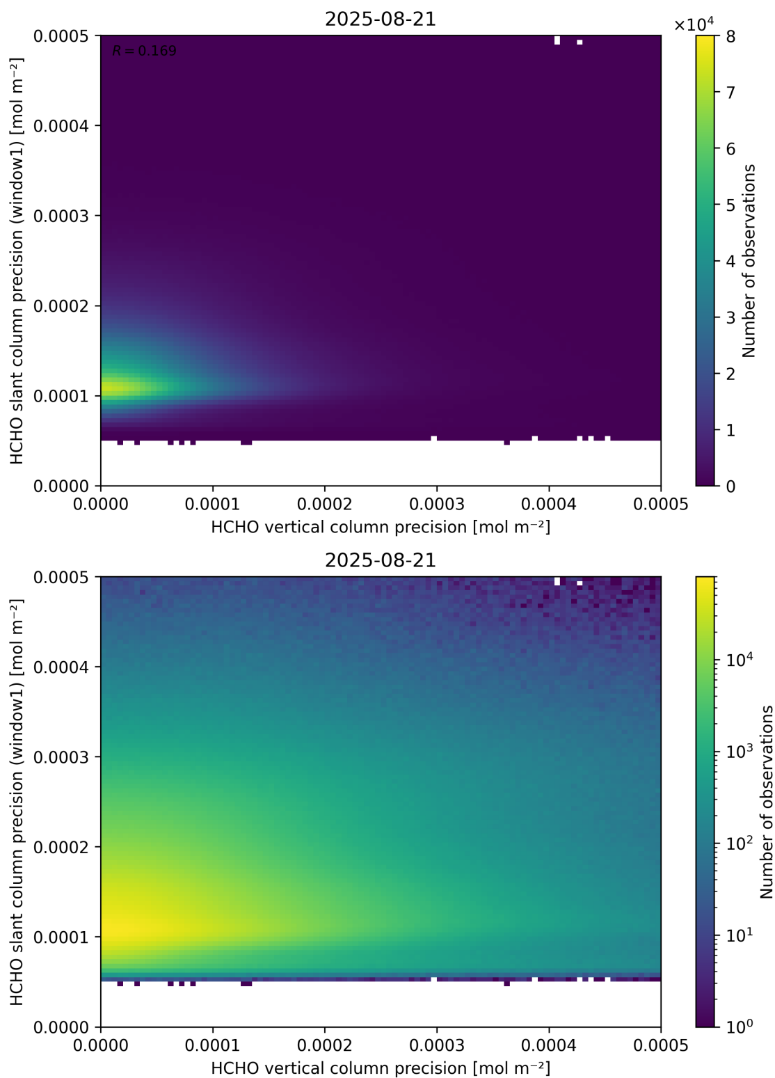
Figure 143: Scatter density plot of “HCHO vertical column precision” against “HCHO slant column precision (window1)” for 2025-08-20 to 2025-08-22.
