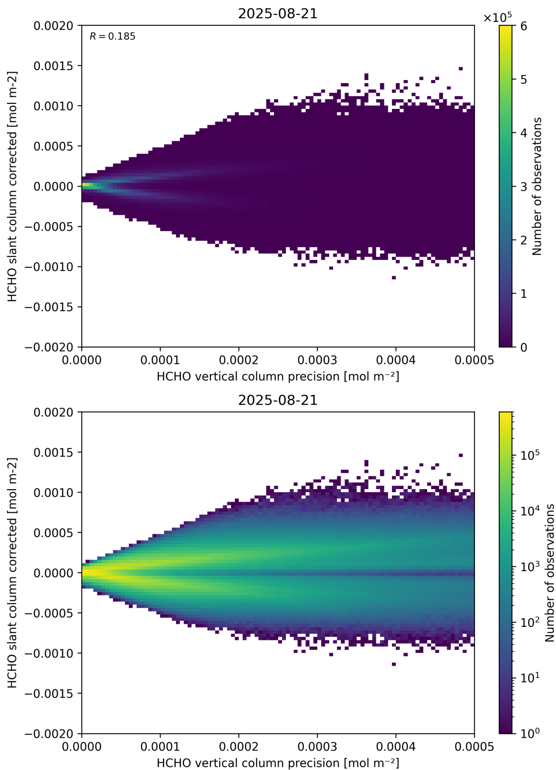
Figure 140: Scatter density plot of “HCHO vertical column precision” against “HCHO slant column corrected” for 2025-08-20 to 2025-08-22.
