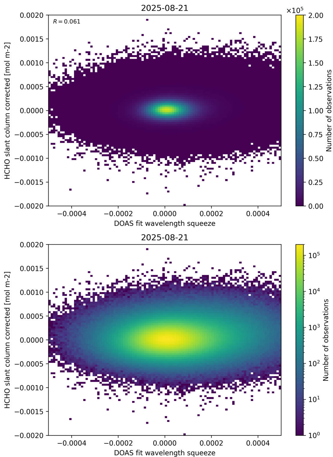
Figure 69: Scatter density plot of “DOAS fit wavelength squeeze” against “HCHO slant column corrected” for 2025-08-20 to 2025-08-22.
