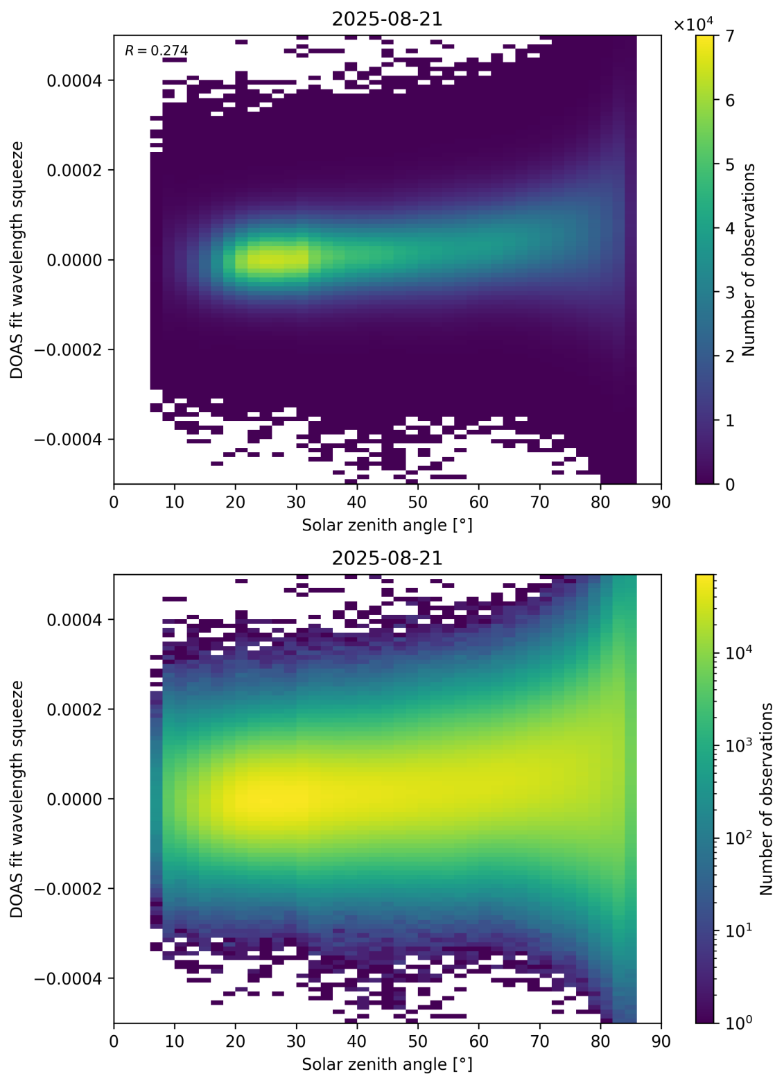
Figure 169: Scatter density plot of “Solar zenith angle” against “DOAS fit wavelength squeeze” for 2025-08-20 to 2025-08-22.
