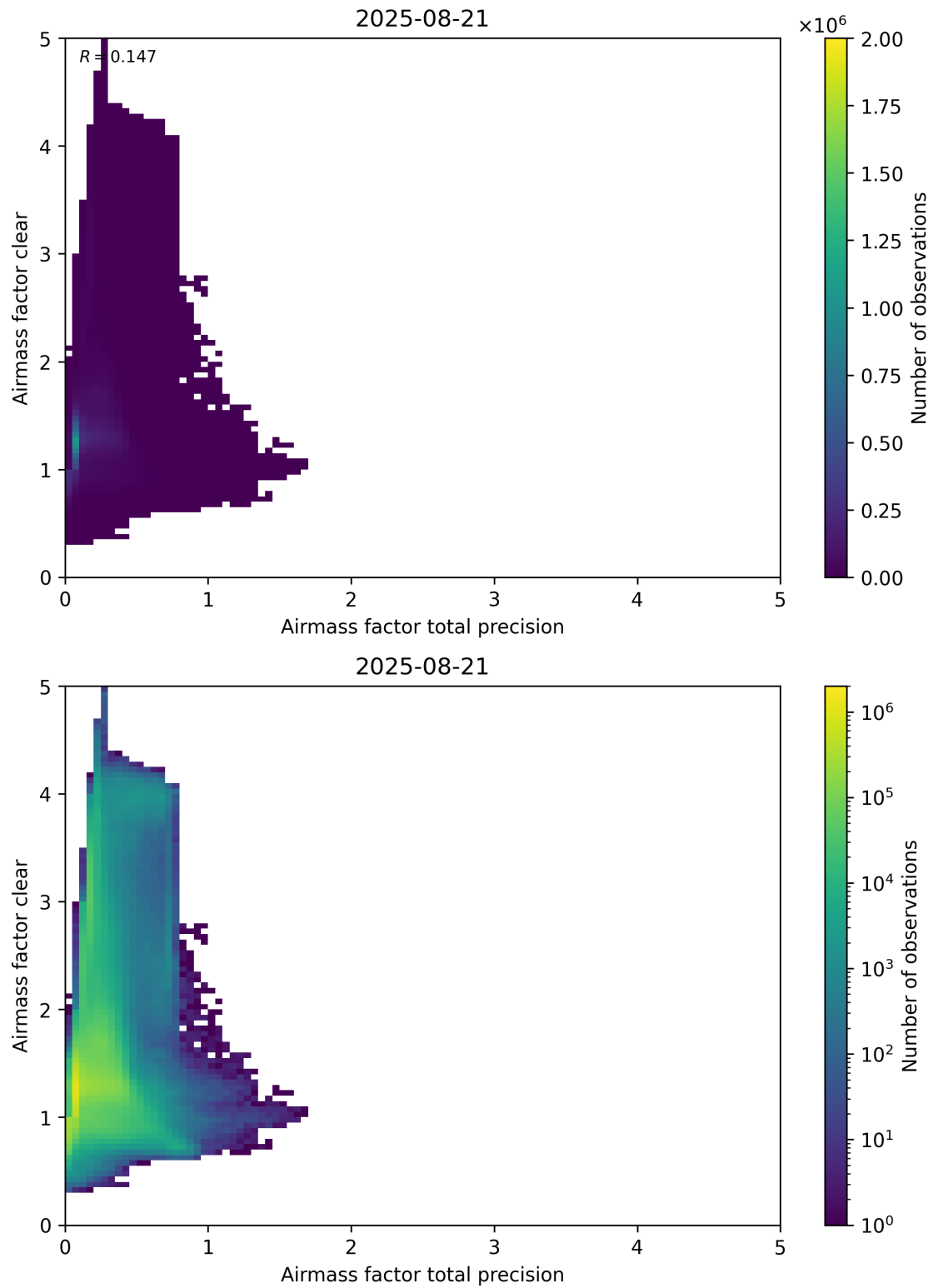
Figure 108: Scatter density plot of “Airmass factor total precision” against “Airmass factor clear” for 2025-08-20 to 2025-08-22.
