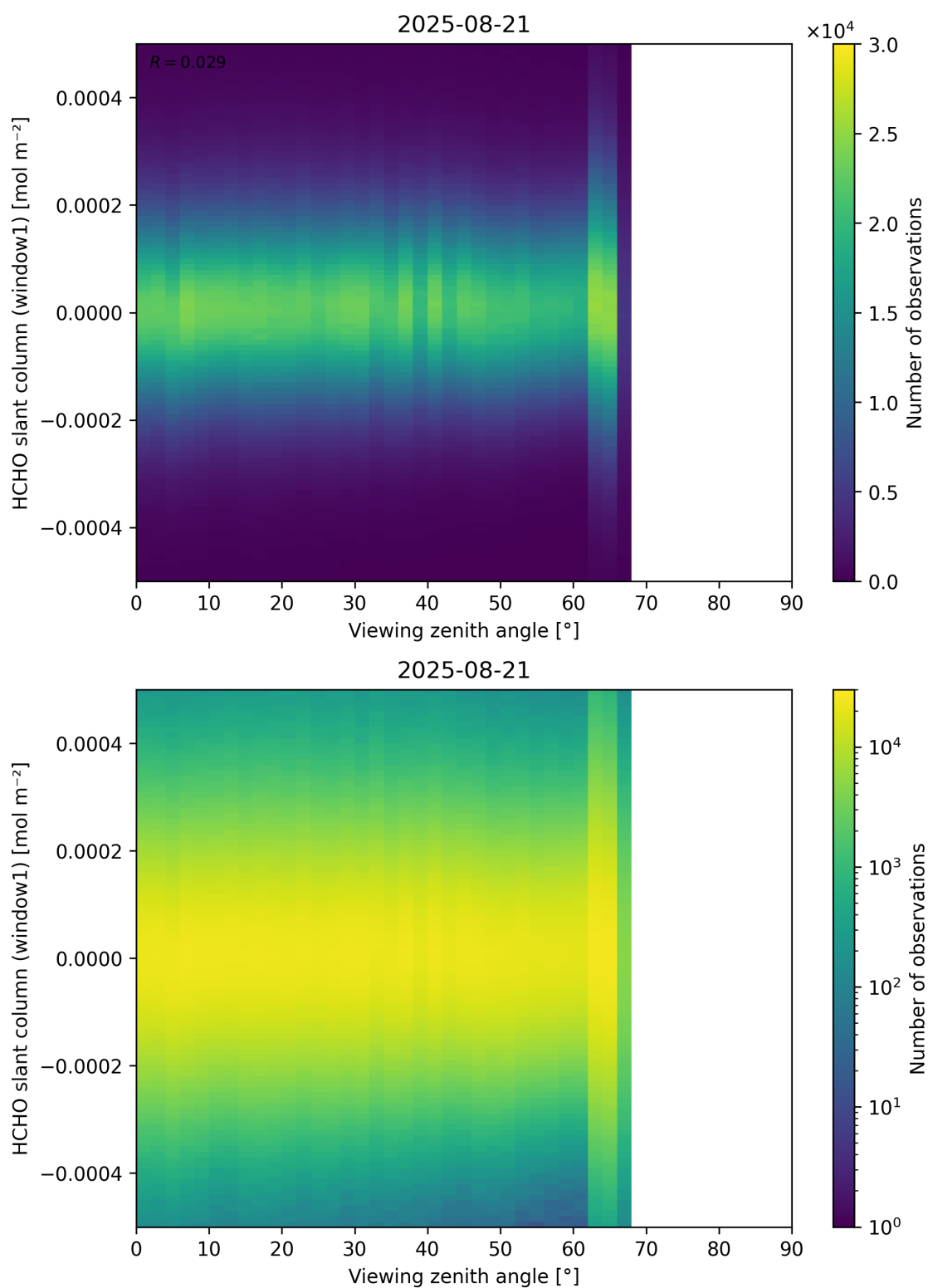
Figure 188: Scatter density plot of “Viewing zenith angle” against “HCHO slant column (window1)” for 2025-08-20 to 2025-08-22.
