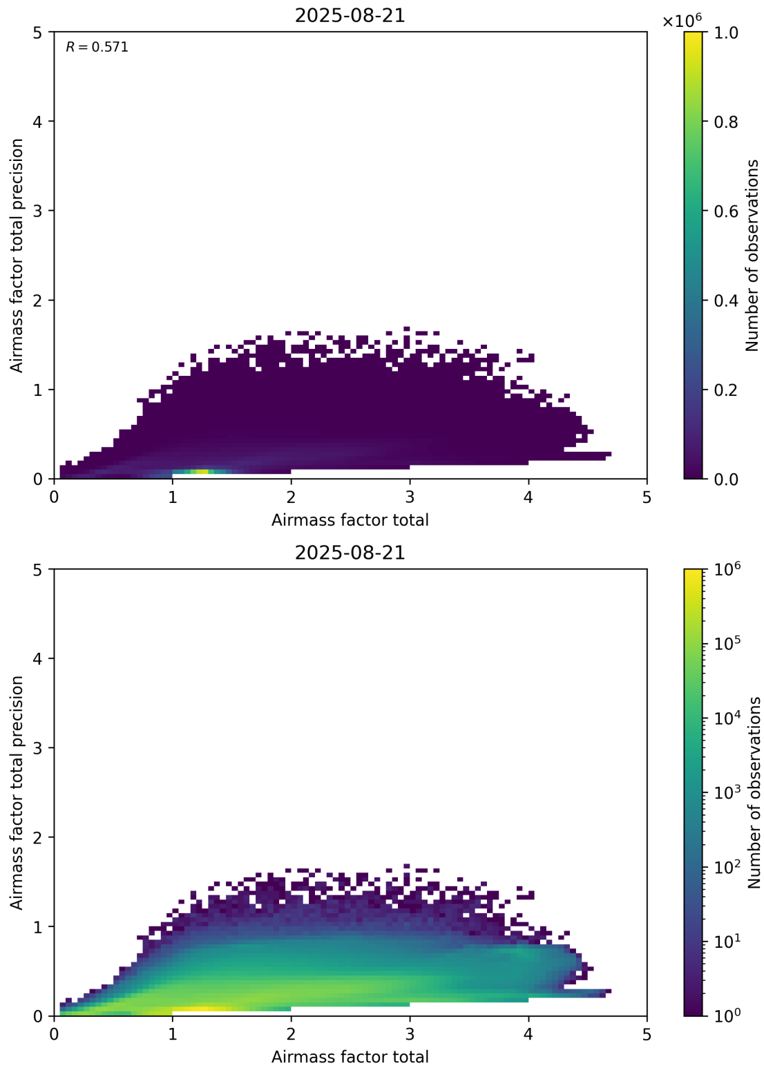
Figure 103: Scatter density plot of “Airmass factor total” against “Airmass factor total precision” for 2025-08-20 to 2025-08-22.
