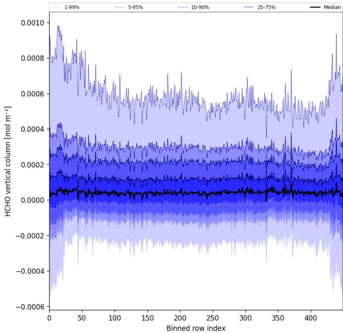
Figure 49: Along track statistics of “HCHO vertical column” for 2025-08-20 to 2025-08-22
