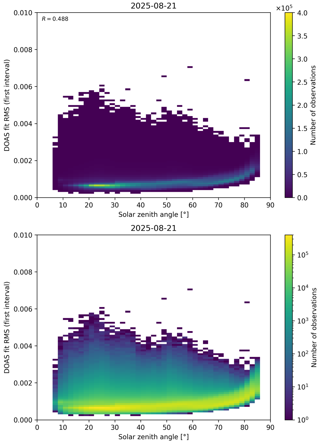
Figure 167: Scatter density plot of “Solar zenith angle” against “DOAS fit RMS (first interval)” for 2025-08-20 to 2025-08-22.
