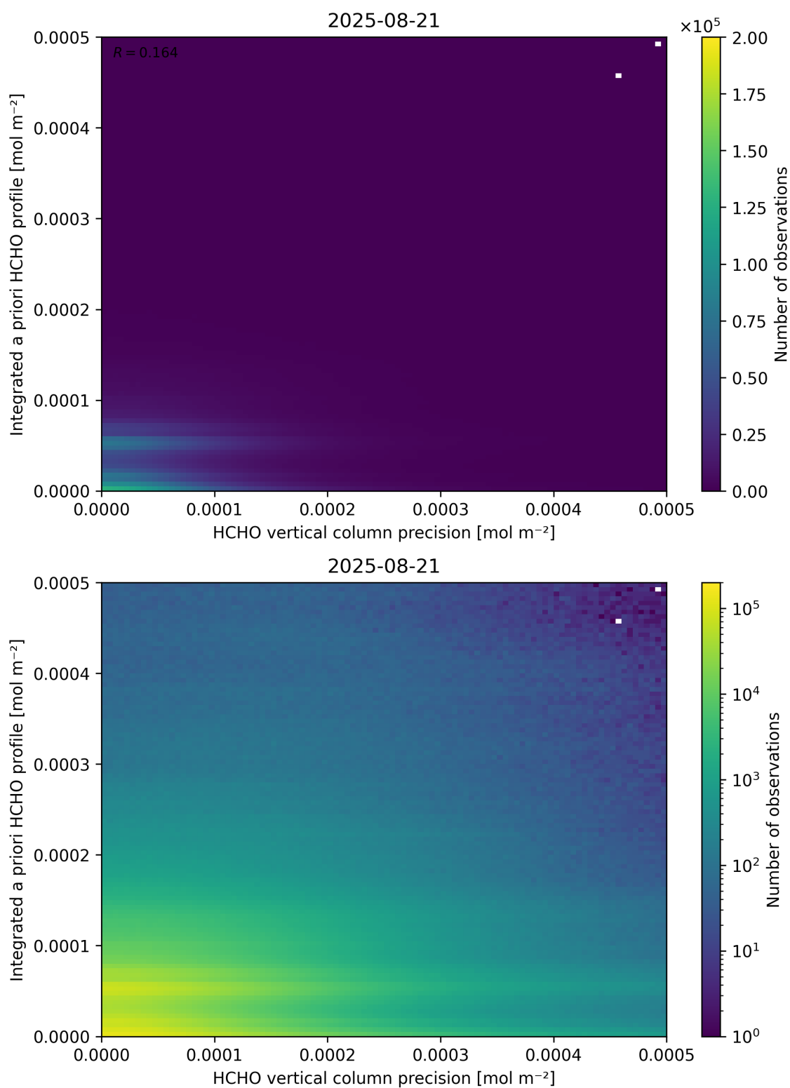
Figure 147: Scatter density plot of “HCHO vertical column precision” against “Integrated a priori HCHO profile” for 2025-08-20 to 2025-08-22.
