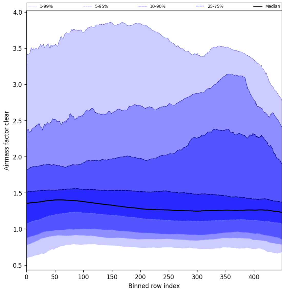
Figure 56: Along track statistics of “Airmass factor clear” for 2025-08-20 to 2025-08-22
