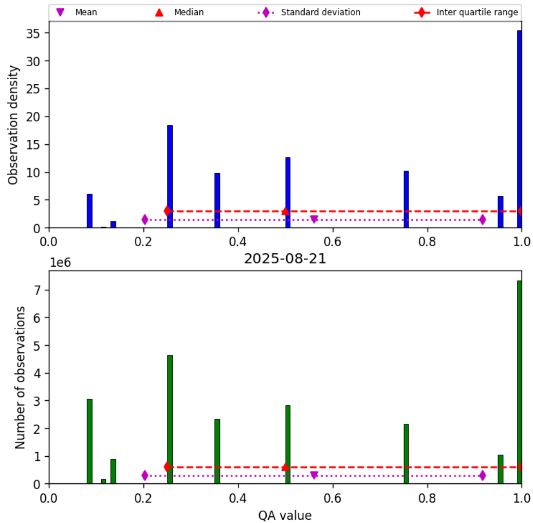
Figure 34: Histogram of “QA value” for 2025-08-20 to 2025-08-22
