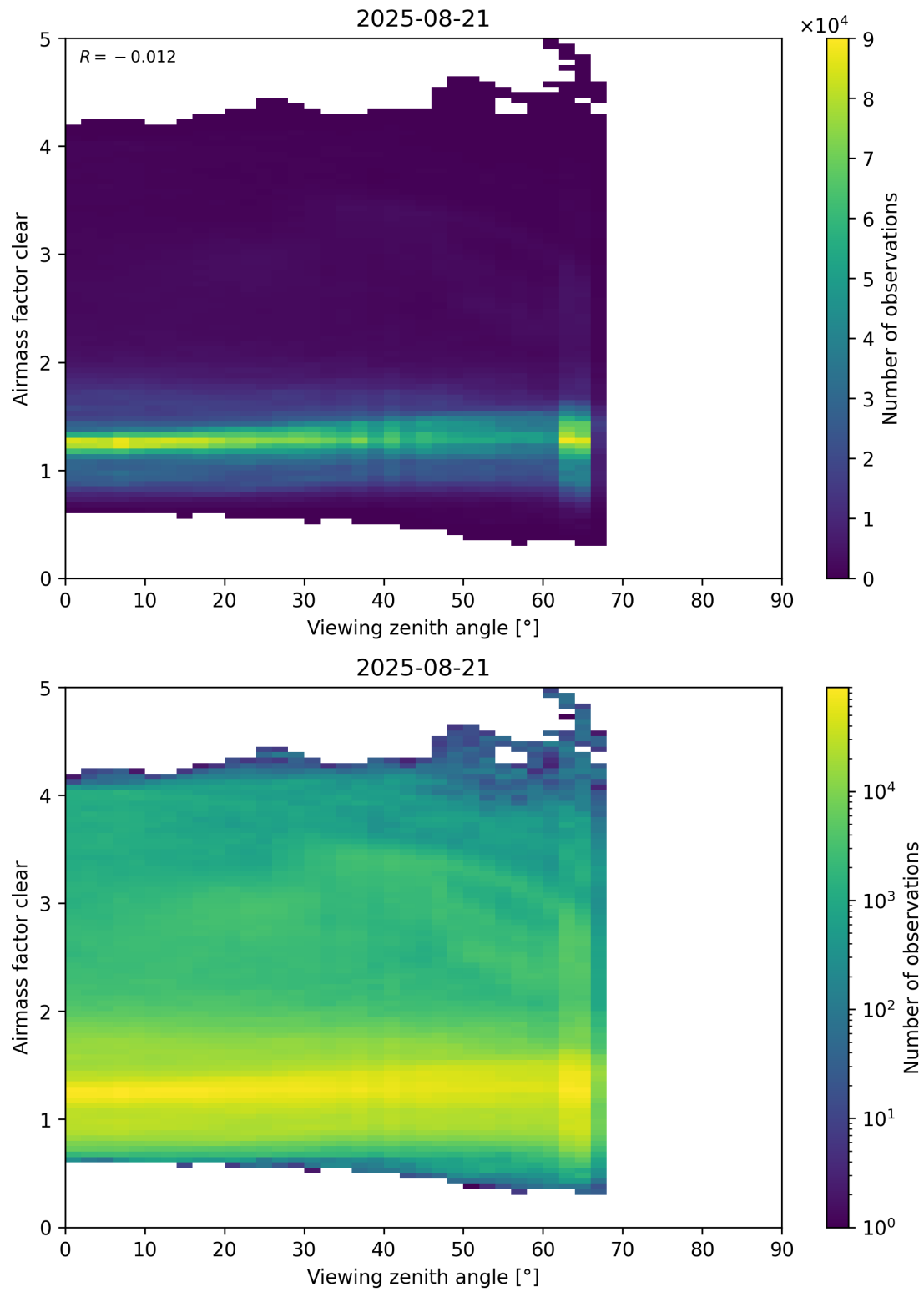
Figure 185: Scatter density plot of “Viewing zenith angle” against “Airmass factor clear” for 2025-08-20 to 2025-08-22.
