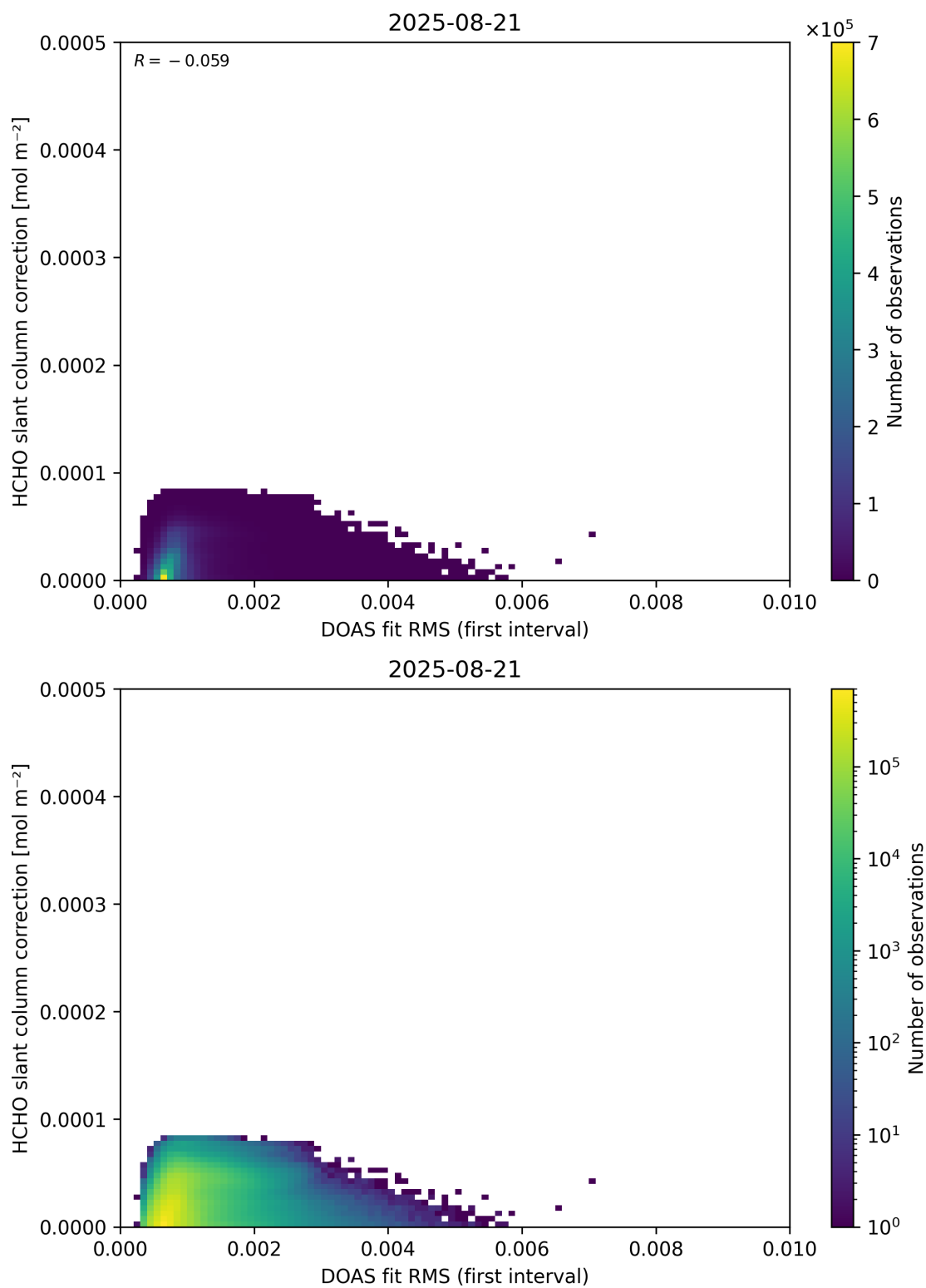
Figure 63: Scatter density plot of “DOAS fit RMS (first interval)” against “HCHO slant column correction” for 2025-08-20 to 2025-08-22.
