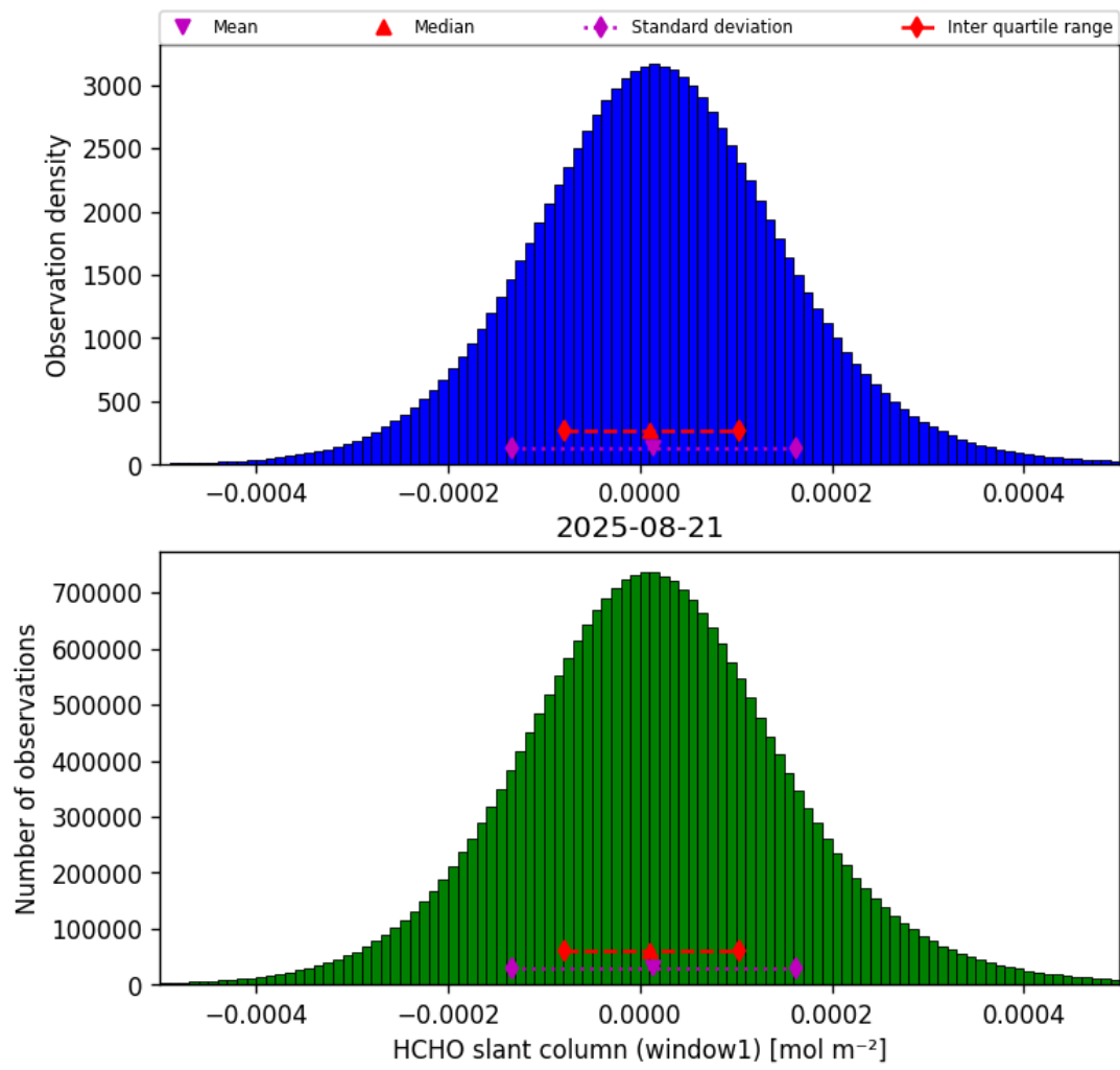
Figure 38: Histogram of “HCHO slant column (window1)” for 2025-08-20 to 2025-08-22
