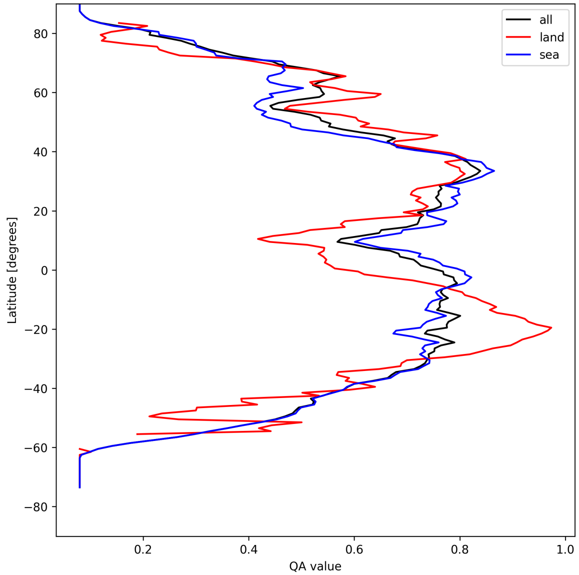
Figure 20: Zonal average of “QA value” for 2025-08-20 to 2025-08-22.
