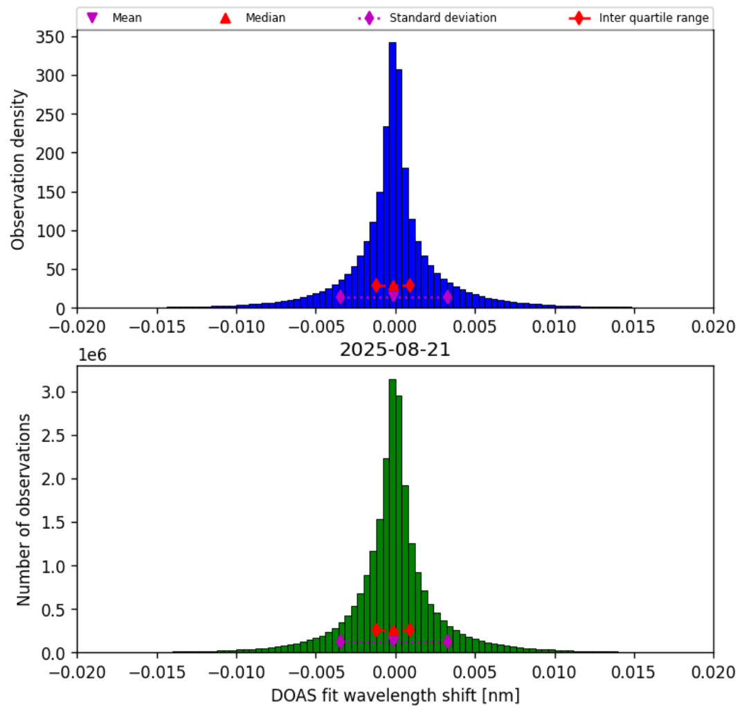
Figure 44: Histogram of “DOAS fit wavelength shift” for 2025-08-20 to 2025-08-22
