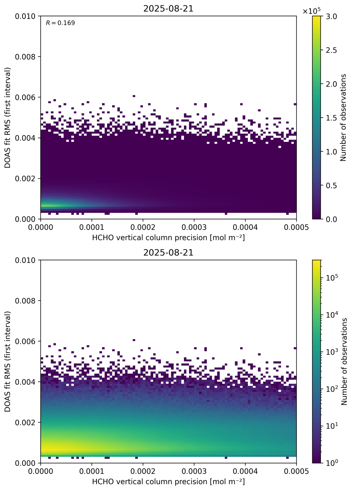
Figure 136: Scatter density plot of “HCHO vertical column precision” against “DOAS fit RMS (first interval)” for 2025-08-20 to 2025-08-22.
