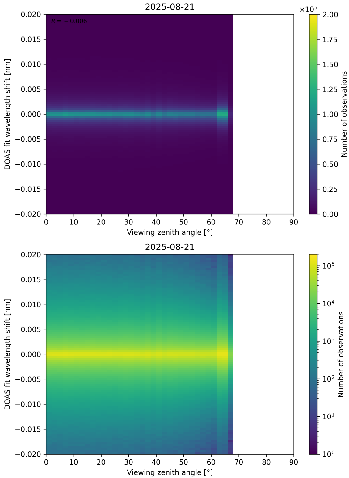
Figure 183: Scatter density plot of “Viewing zenith angle” against “DOAS fit wavelength shift” for 2025-08-20 to 2025-08-22.
