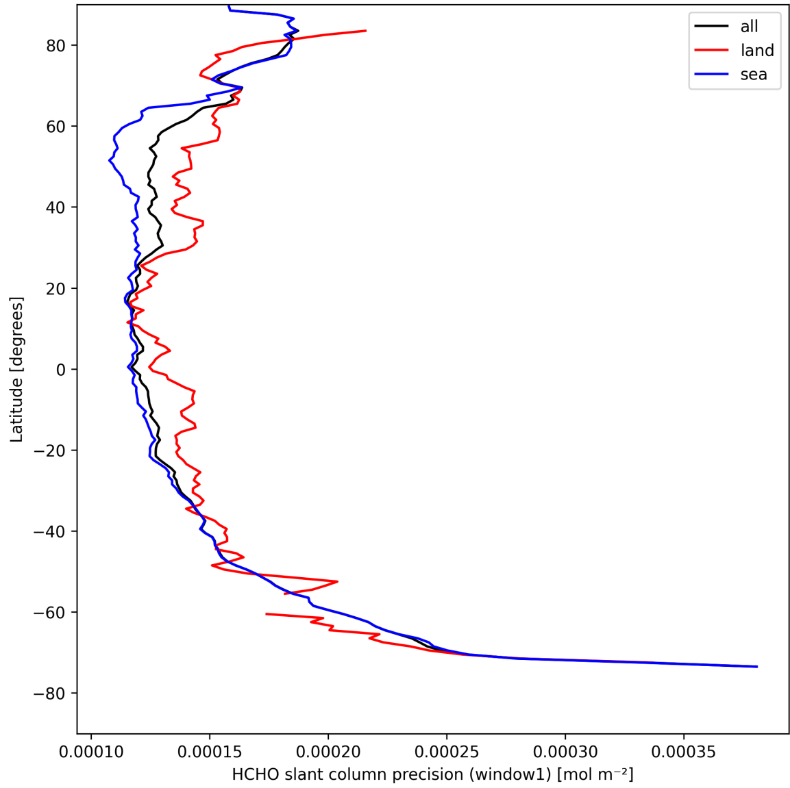
Figure 25: Zonal average of “HCHO slant column precision (window1)” for 2025-08-20 to 2025-08-22.
