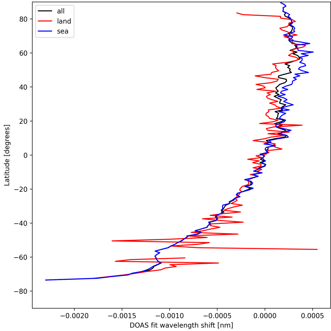
Figure 30: Zonal average of “DOAS fit wavelength shift” for 2025-08-20 to 2025-08-22.
