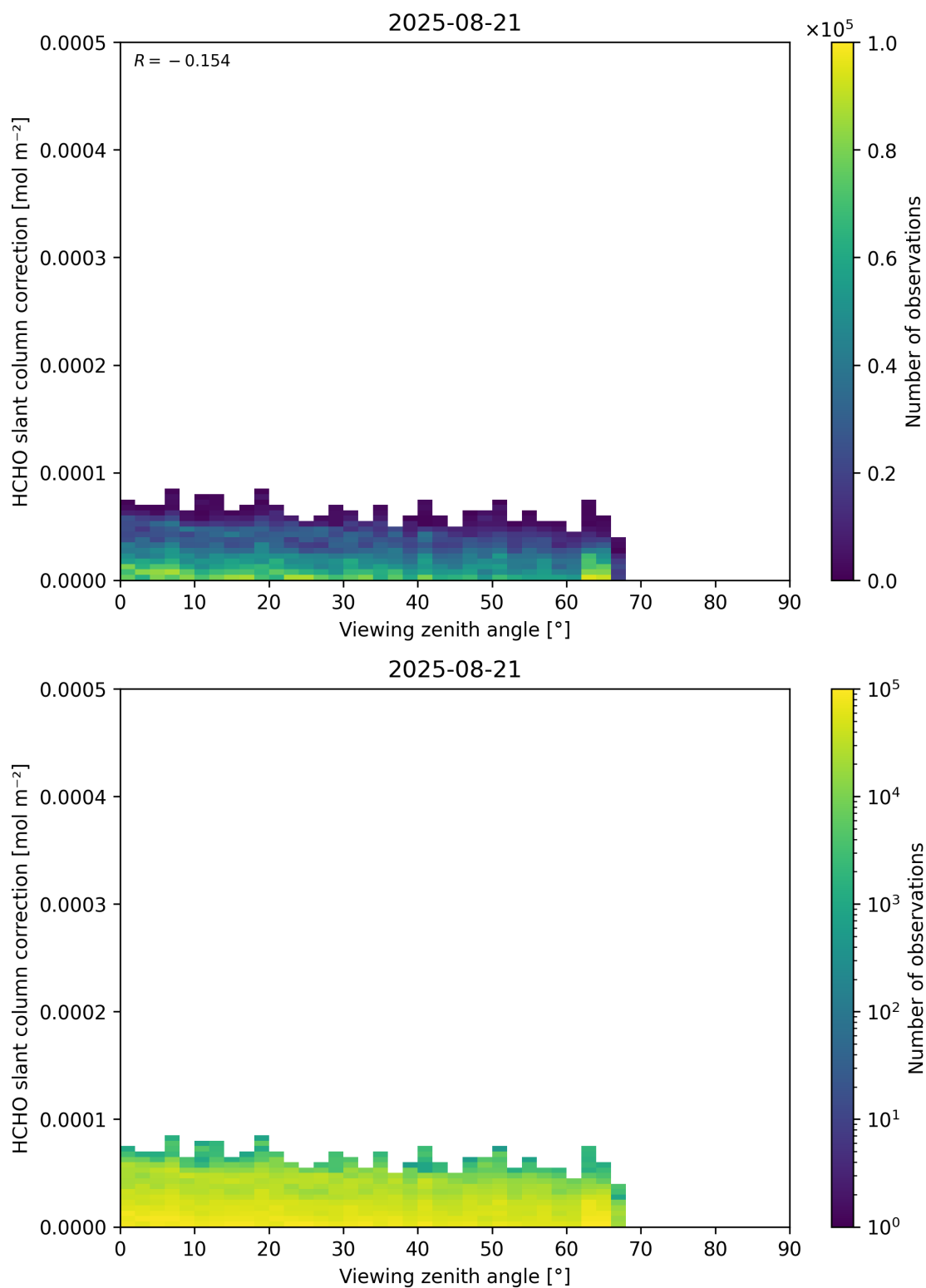
Figure 187: Scatter density plot of “Viewing zenith angle” against “HCHO slant column correction” for 2025-08-20 to 2025-08-22.
