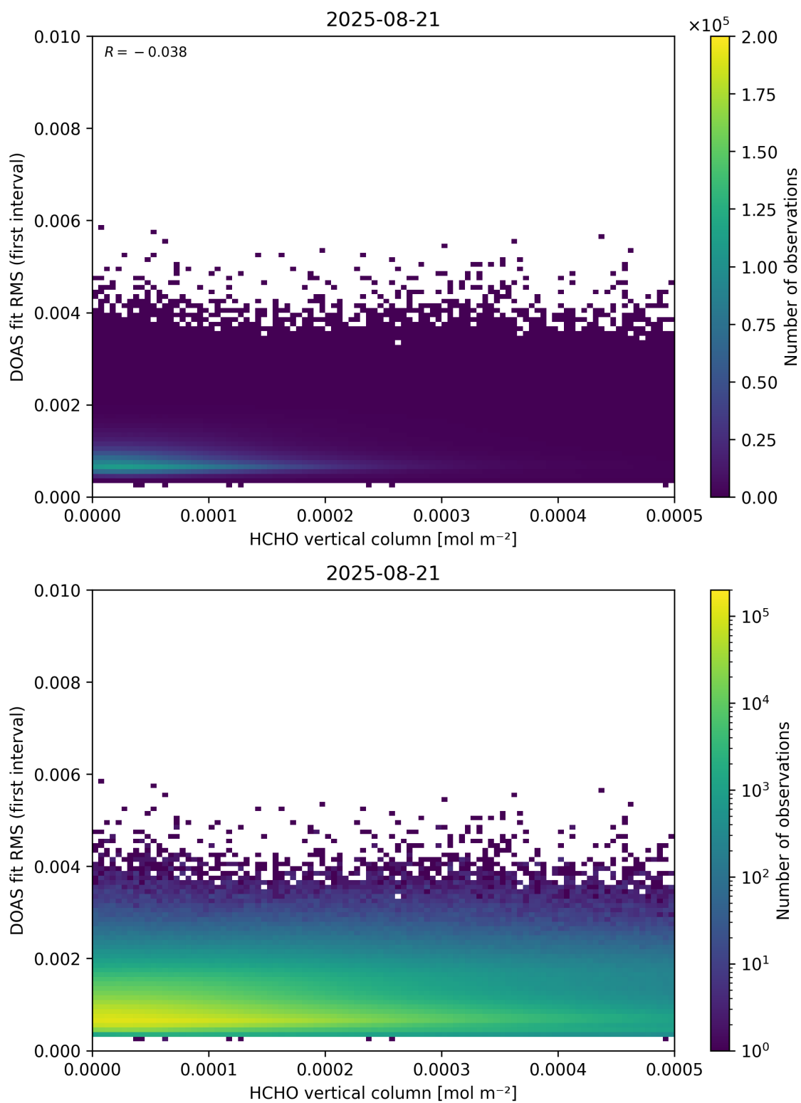
Figure 123: Scatter density plot of “HCHO vertical column” against “DOAS fit RMS (first interval)” for 2025-08-20 to 2025-08-22.
