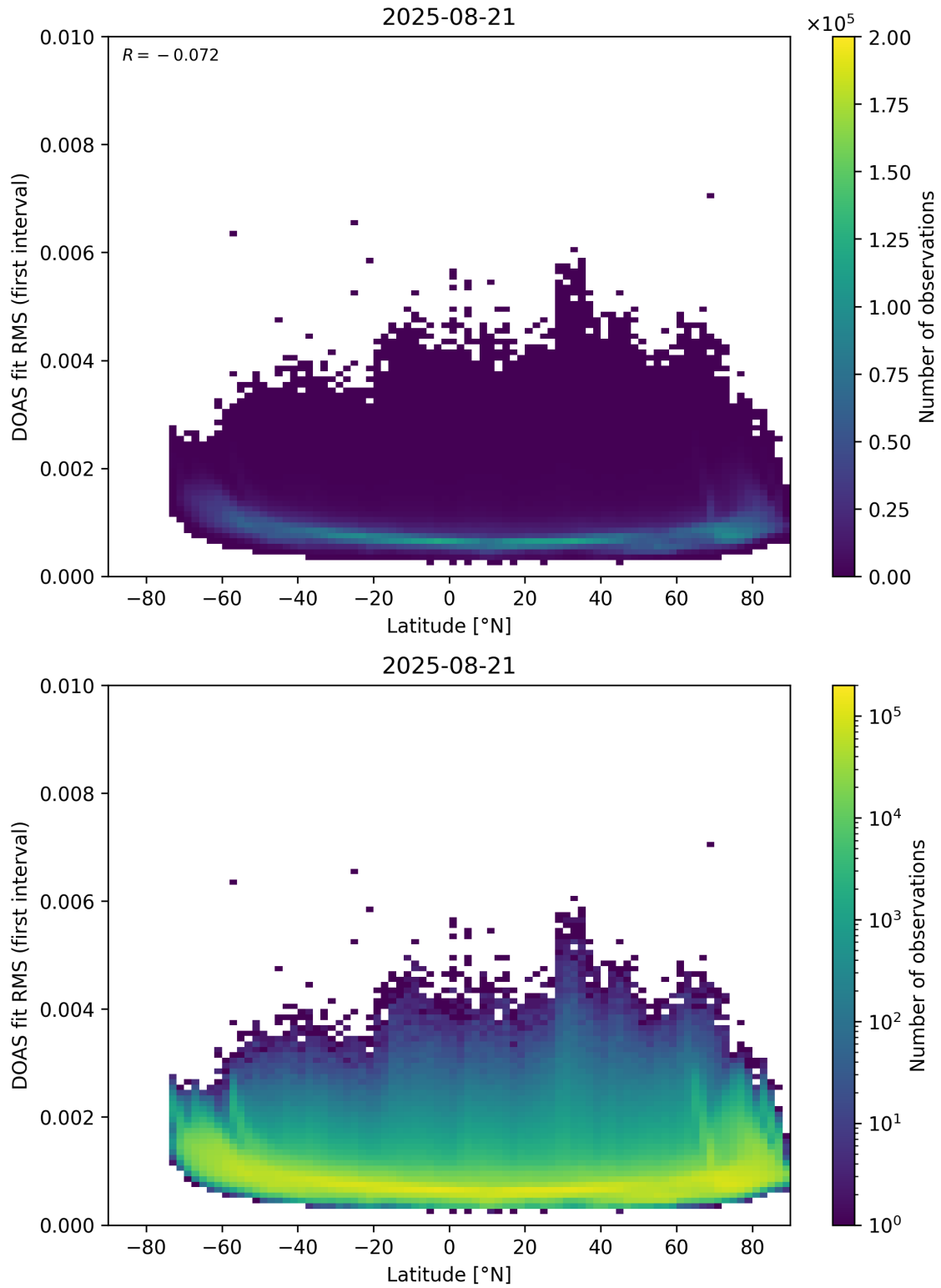
Figure 153: Scatter density plot of “Latitude” against “DOAS fit RMS (first interval)” for 2025-08-20 to 2025-08-22.
