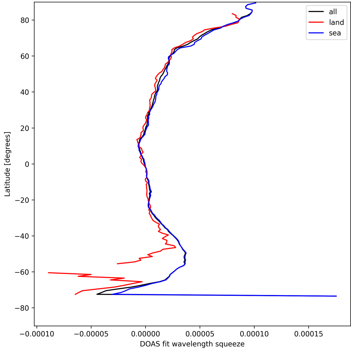
Figure 31: Zonal average of “DOAS fit wavelength squeeze” for 2025-08-20 to 2025-08-22.
