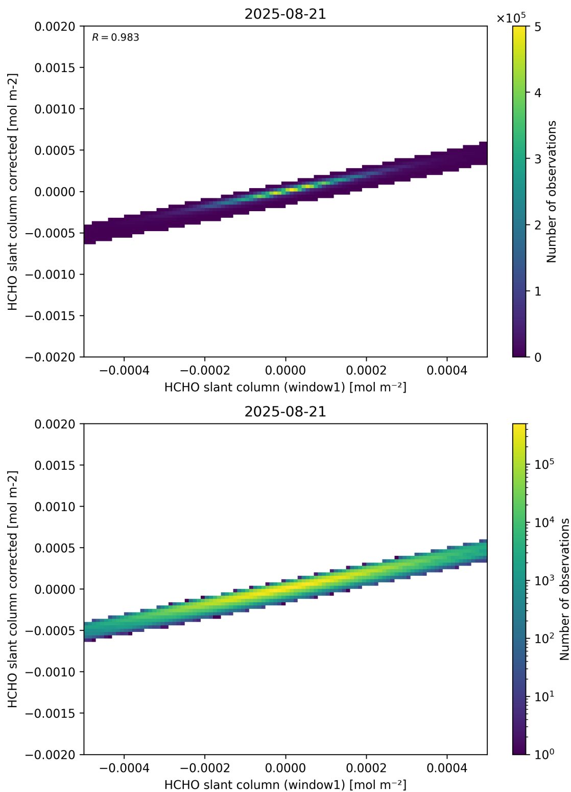
Figure 82: Scatter density plot of “HCHO slant column (window1)” against “HCHO slant column corrected” for 2025-08-20 to 2025-08-22.
