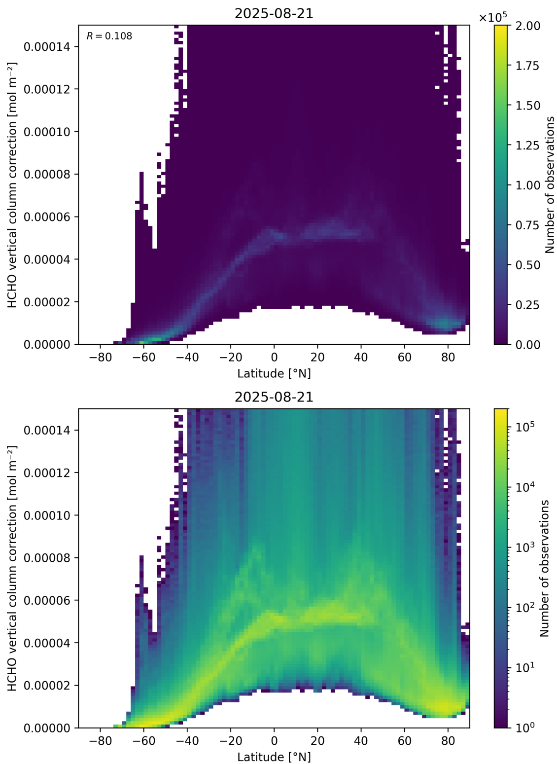
Figure 164: Scatter density plot of “Latitude” against “HCHO vertical column correction” for 2025-08-20 to 2025-08-22.
