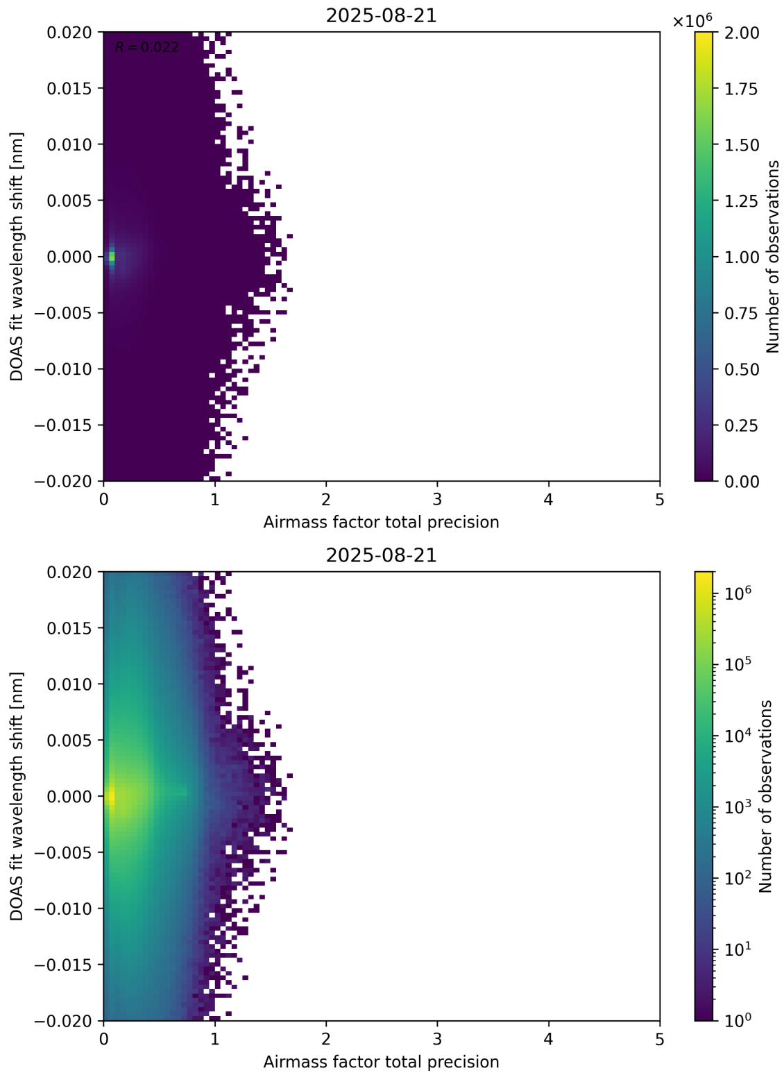
Figure 106: Scatter density plot of “Airmass factor total precision” against “DOAS fit wavelength shift” for 2025-08-20 to 2025-08-22.
