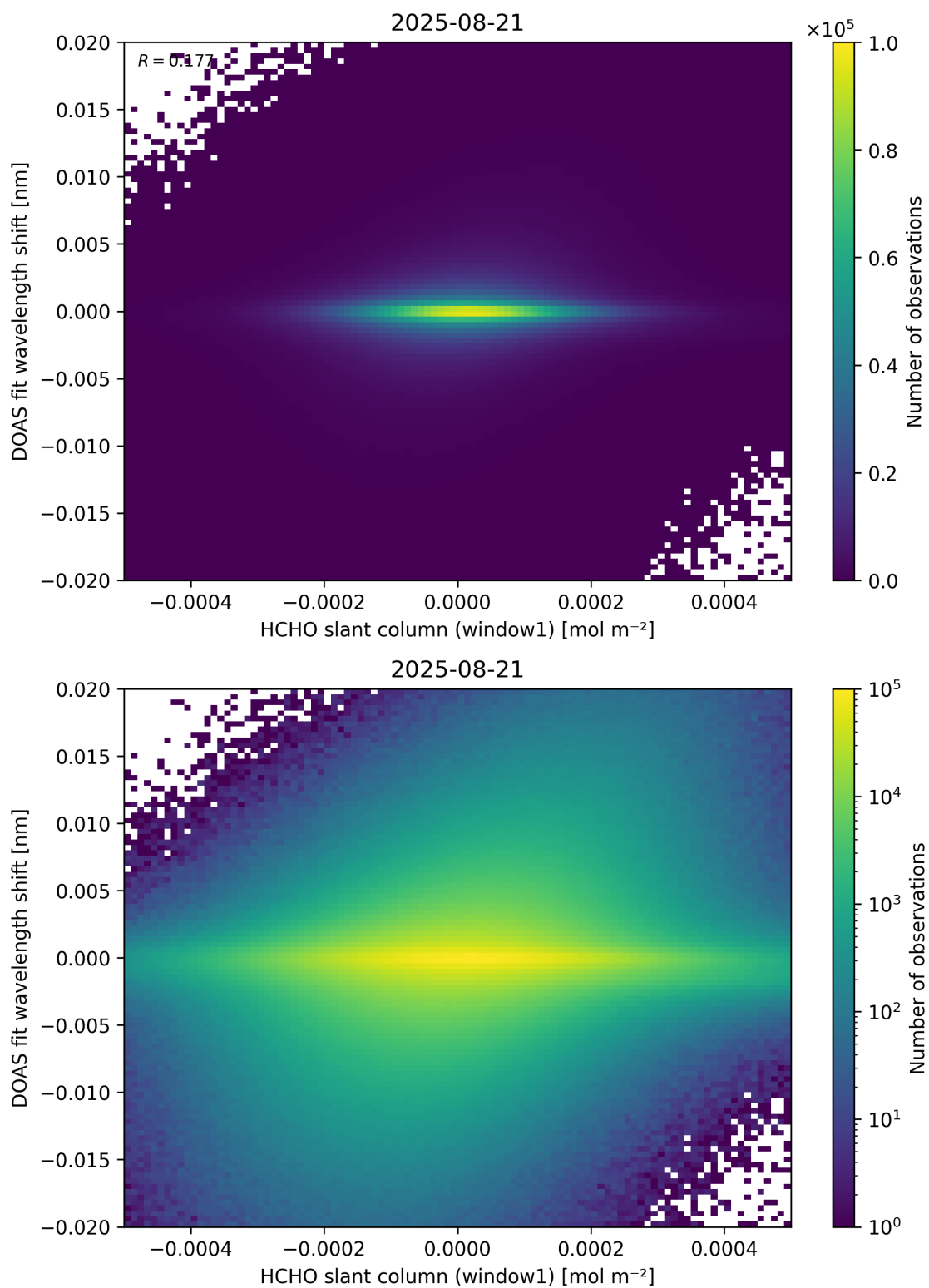
Figure 79: Scatter density plot of “HCHO slant column (window1)” against “DOAS fit wavelength shift” for 2025-08-20 to 2025-08-22.
