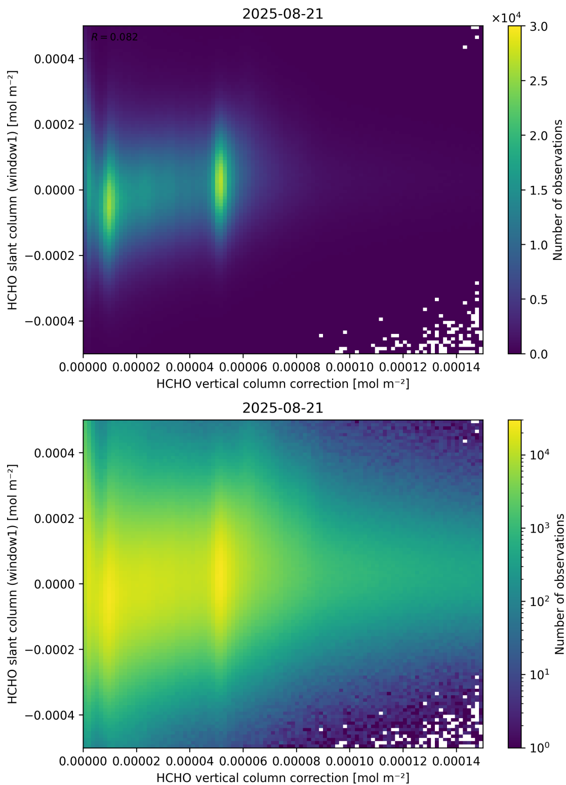
Figure 118: Scatter density plot of “HCHO vertical column correction” against “HCHO slant column (window1)” for 2025-08-20 to 2025-08-22.
