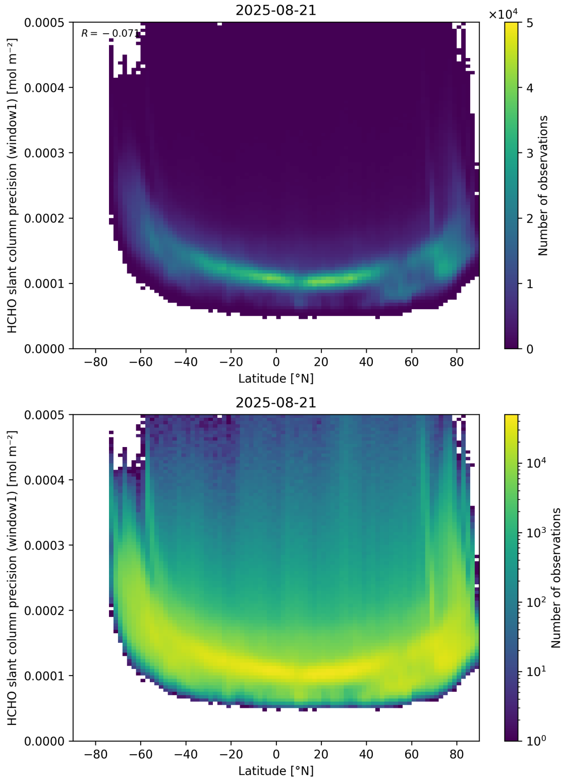
Figure 160: Scatter density plot of “Latitude” against “HCHO slant column precision (window1)” for 2025-08-20 to 2025-08-22.
