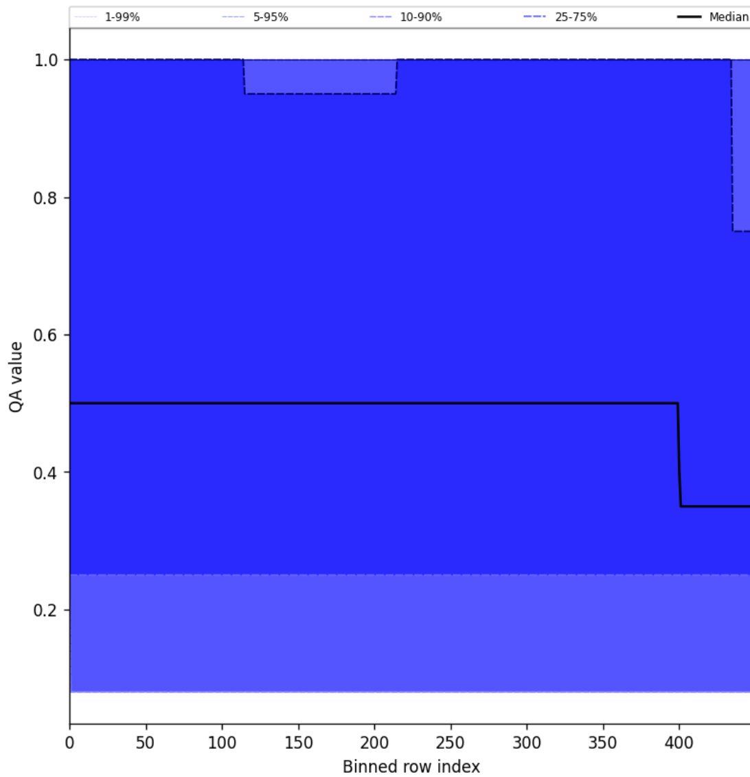
Figure 48: Along track statistics of “QA value” for 2025-08-20 to 2025-08-22
