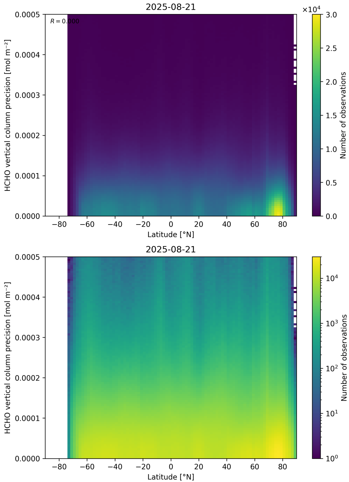
Figure 165: Scatter density plot of “Latitude” against “HCHO vertical column precision” for 2025-08-20 to 2025-08-22.
