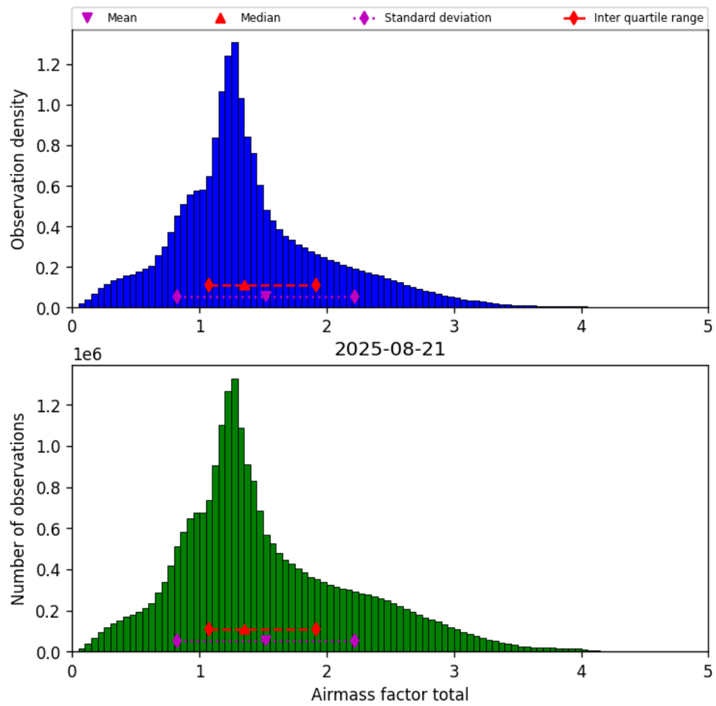
Figure 40: Histogram of “Airmass factor total” for 2025-08-20 to 2025-08-22
