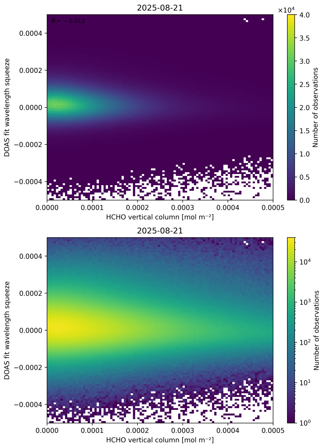
Figure 125: Scatter density plot of “HCHO vertical column” against “DOAS fit wavelength squeeze” for 2025-08-20 to 2025-08-22.
