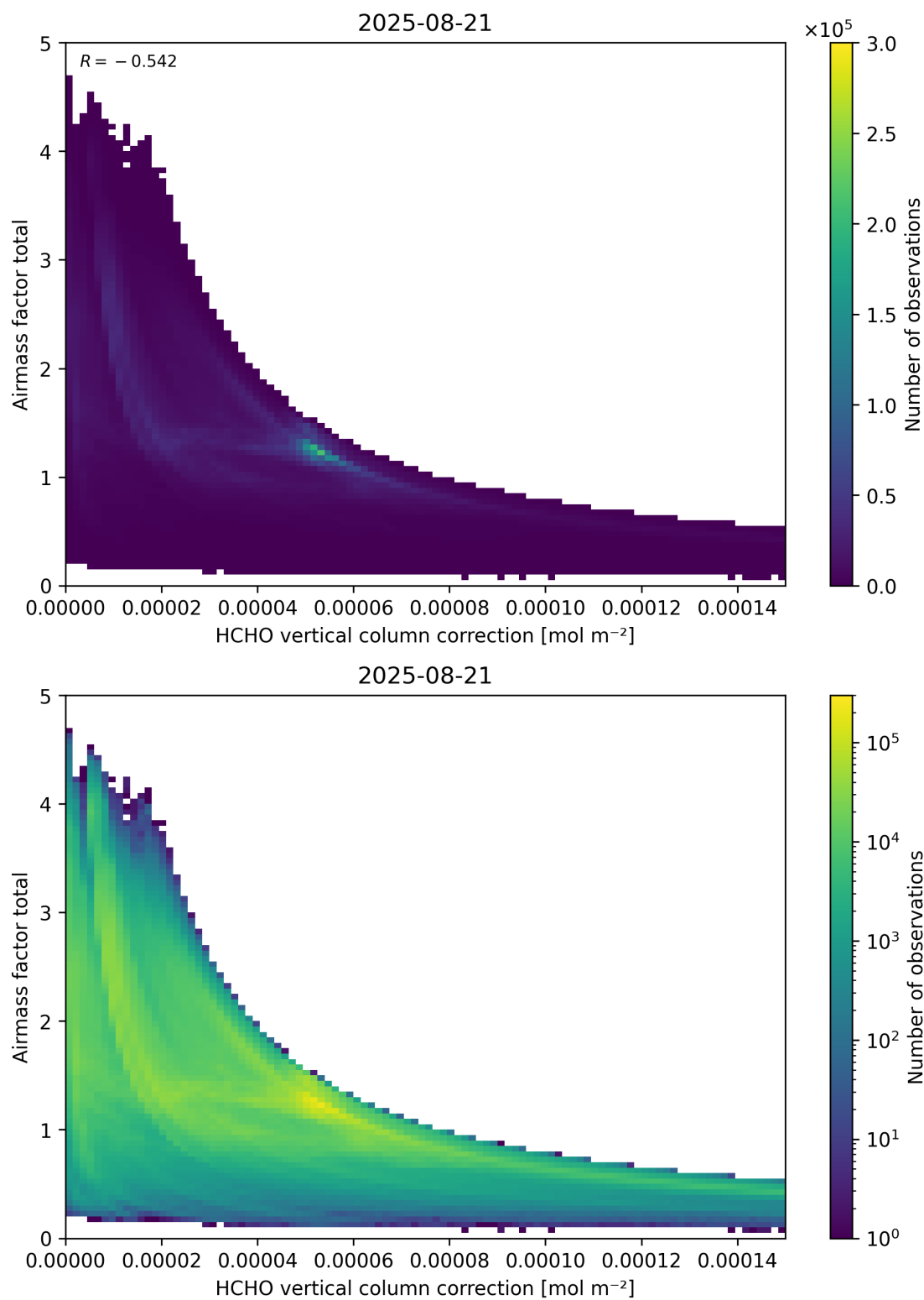
Figure 120: Scatter density plot of “HCHO vertical column correction” against “Airmass factor total” for 2025-08-20 to 2025-08-22.
