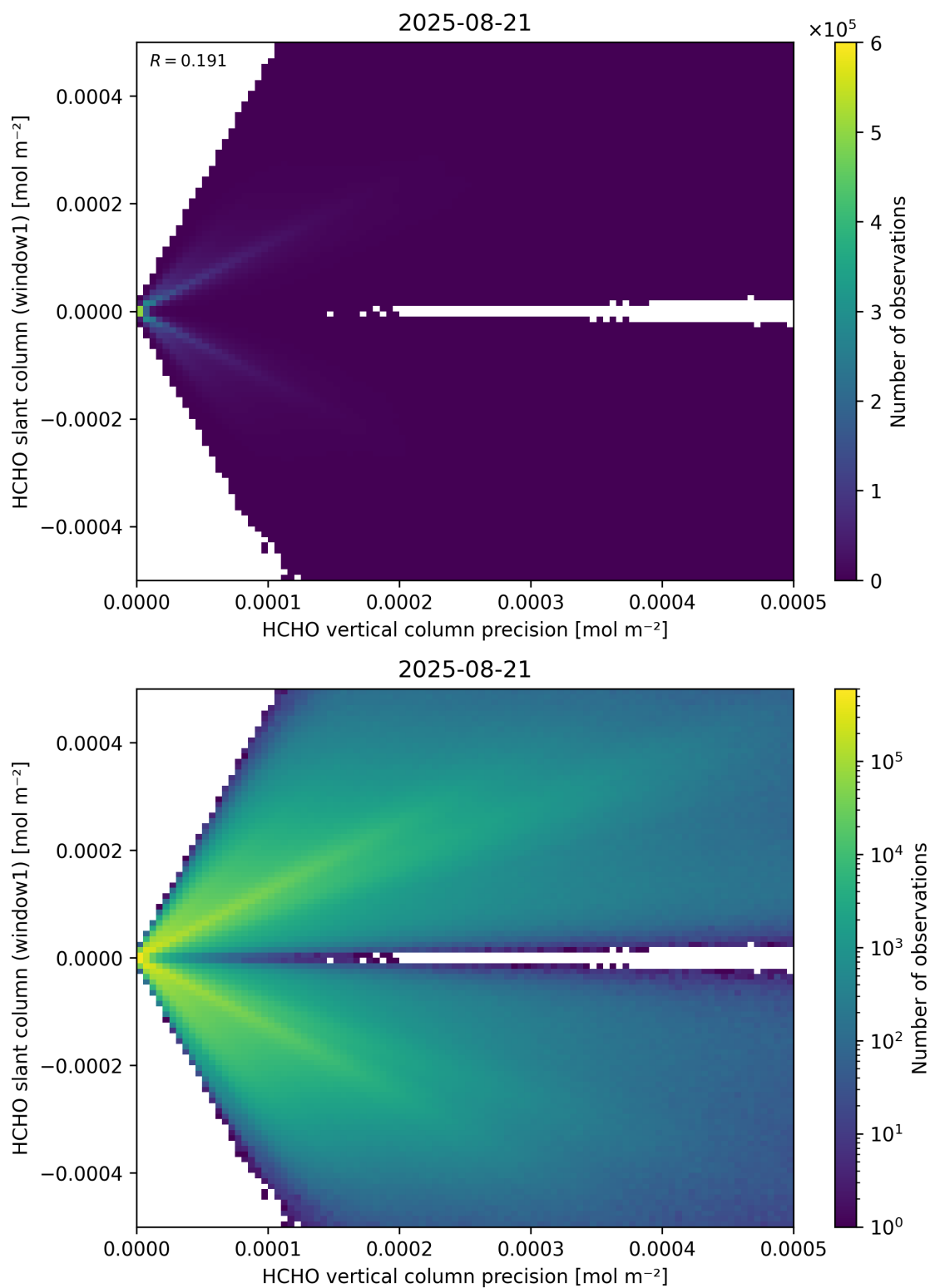
Figure 142: Scatter density plot of “HCHO vertical column precision” against “HCHO slant column (window1)” for 2025-08-20 to 2025-08-22.
