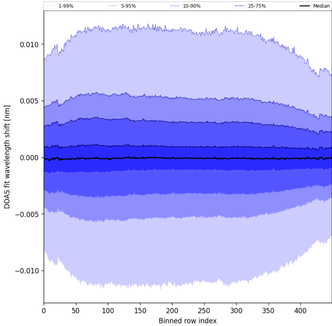
Figure 58: Along track statistics of “DOAS fit wavelength shift” for 2025-08-20 to 2025-08-22
