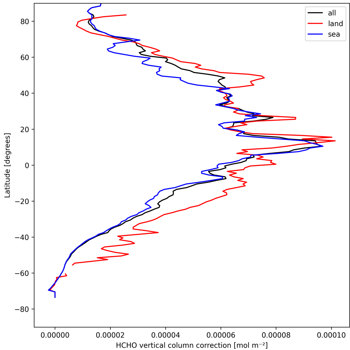
Figure 23: Zonal average of “HCHO vertical column correction” for 2025-08-20 to 2025-08-22.
