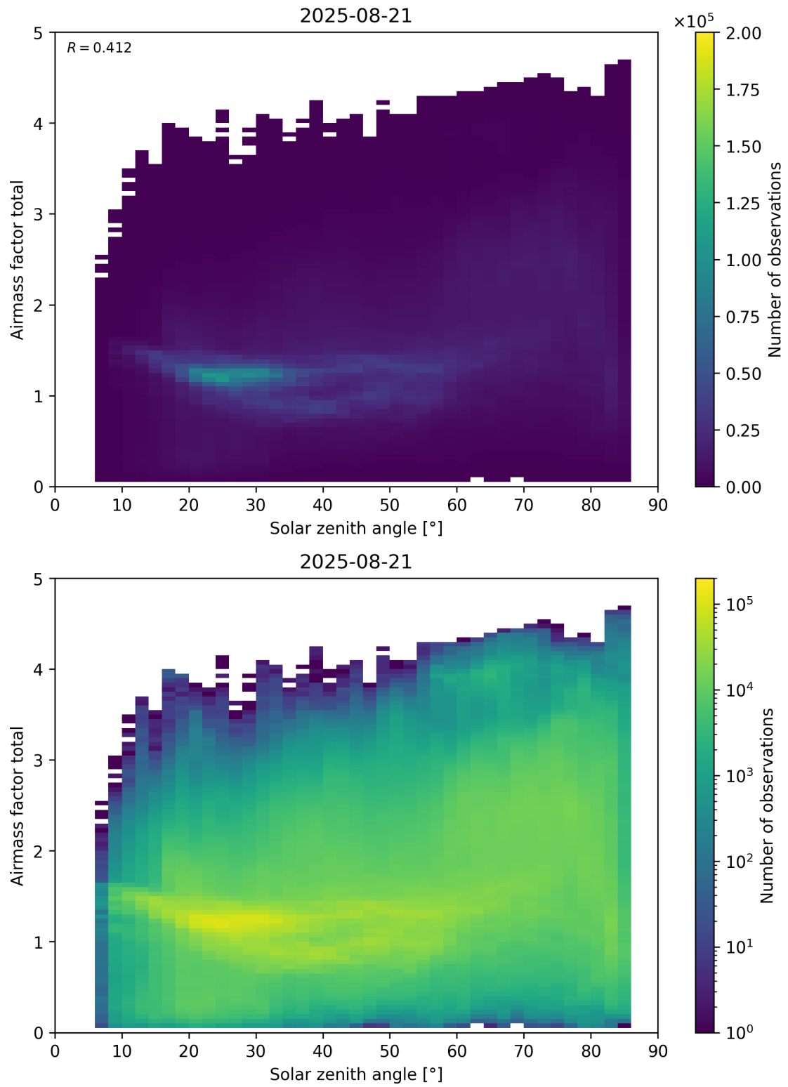
Figure 175: Scatter density plot of “Solar zenith angle” against “Airmass factor total” for 2025-08-20 to 2025-08-22.
