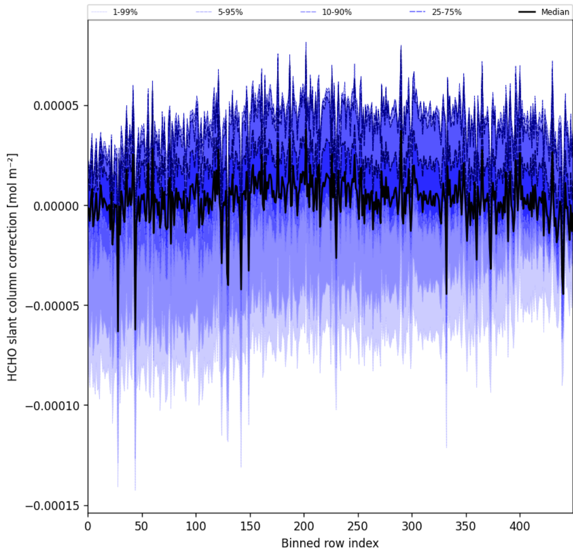
Figure 61: Along track statistics of “HCHO slant column correction” for 2025-08-20 to 2025-08-22
