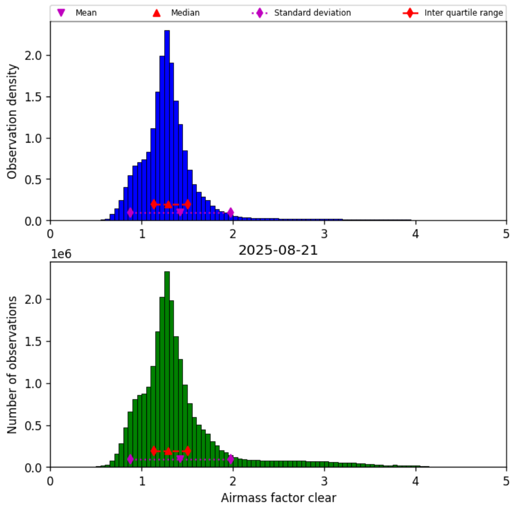
Figure 42: Histogram of “Airmass factor clear” for 2025-08-20 to 2025-08-22
