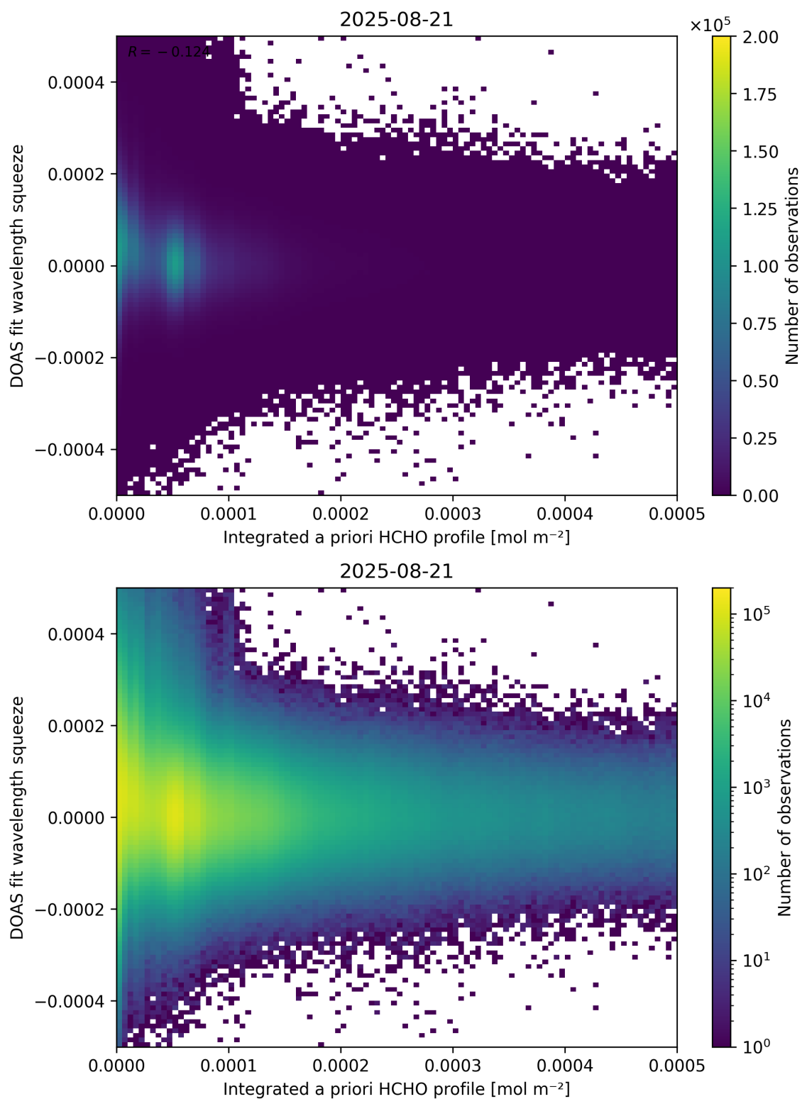
Figure 150: Scatter density plot of “Integrated a priori HCHO profile” against “DOAS fit wavelength squeeze” for 2025-08-20 to 2025-08-22.
