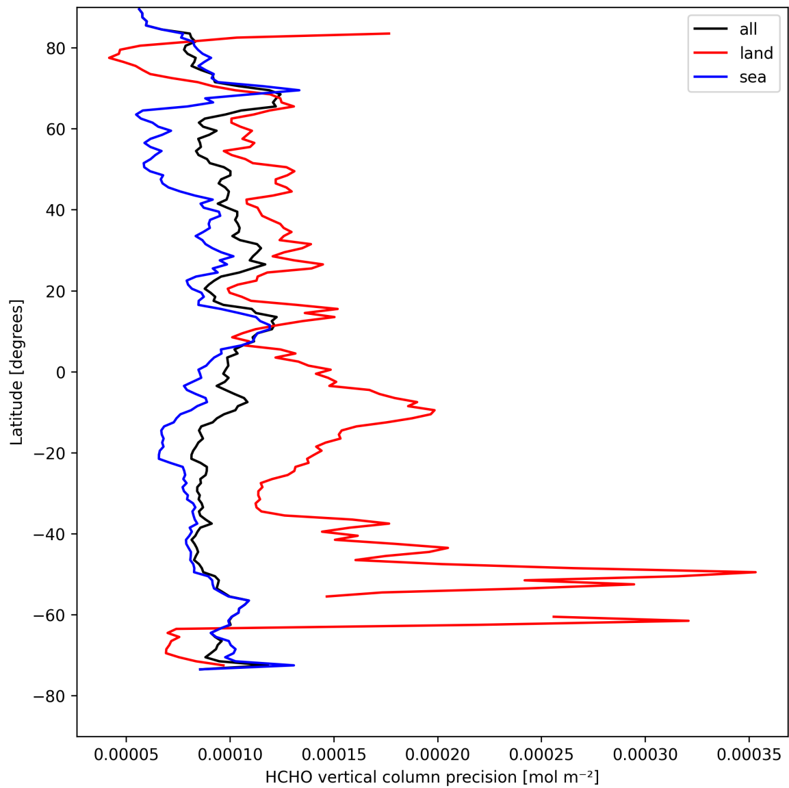
Figure 22: Zonal average of “HCHO vertical column precision” for 2025-08-20 to 2025-08-22.
