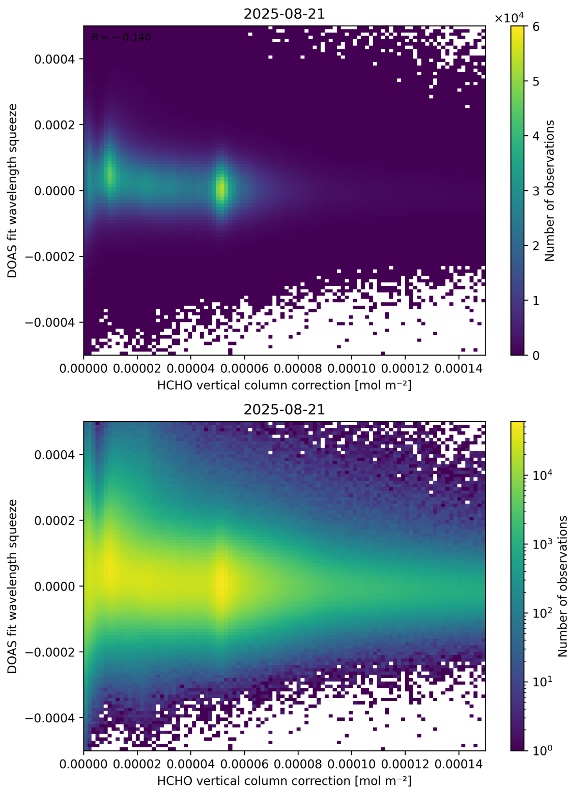
Figure 114: Scatter density plot of “HCHO vertical column correction” against “DOAS fit wavelength squeeze” for 2025-08-20 to 2025-08-22.
