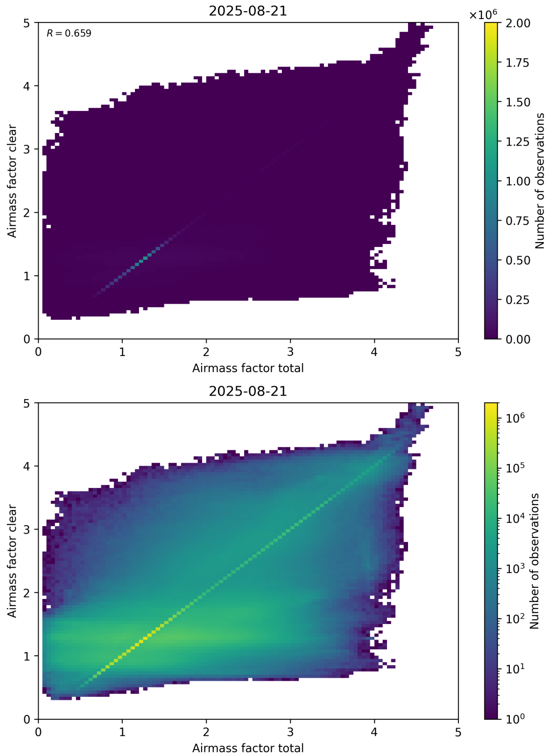
Figure 100: Scatter density plot of “Airmass factor total” against “Airmass factor clear” for 2025-08-20 to 2025-08-22.
