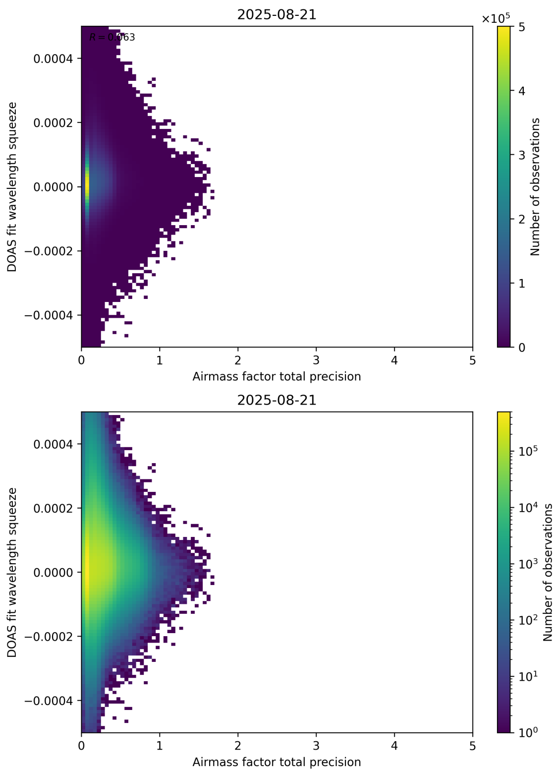
Figure 107: Scatter density plot of “Airmass factor total precision” against “DOAS fit wavelength squeeze” for 2025-08-20 to 2025-08-22.
