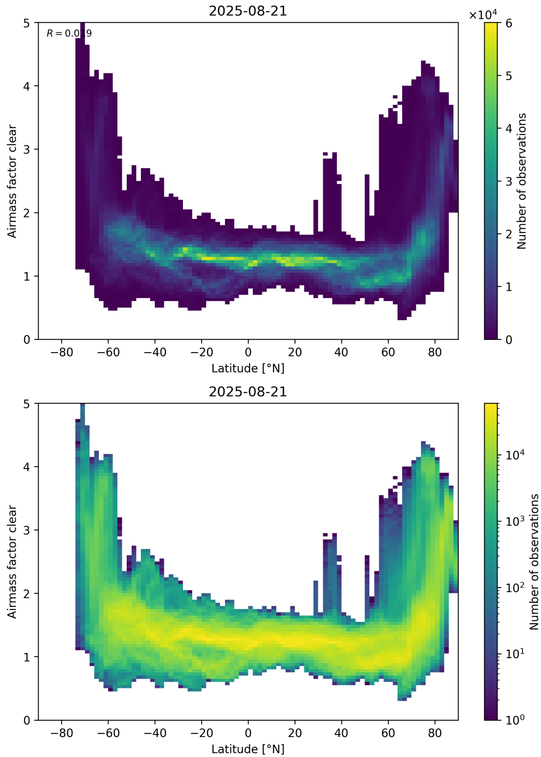
Figure 156: Scatter density plot of “Latitude” against “Airmass factor clear” for 2025-08-20 to 2025-08-22.
