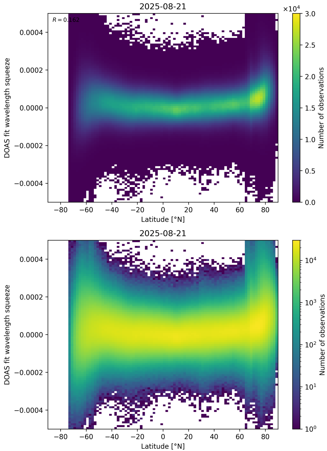
Figure 155: Scatter density plot of “Latitude” against “DOAS fit wavelength squeeze” for 2025-08-20 to 2025-08-22.
