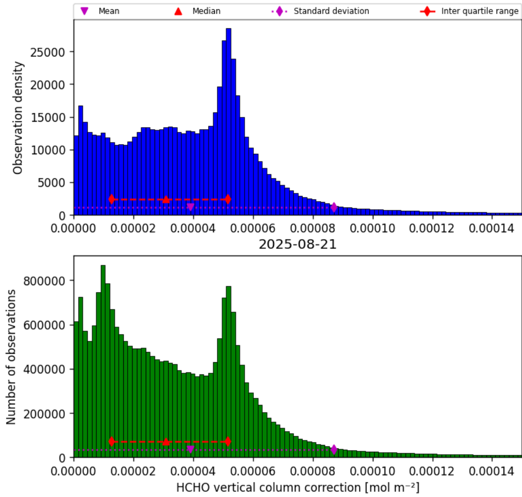
Figure 37: Histogram of “HCHO vertical column correction” for 2025-08-20 to 2025-08-22
