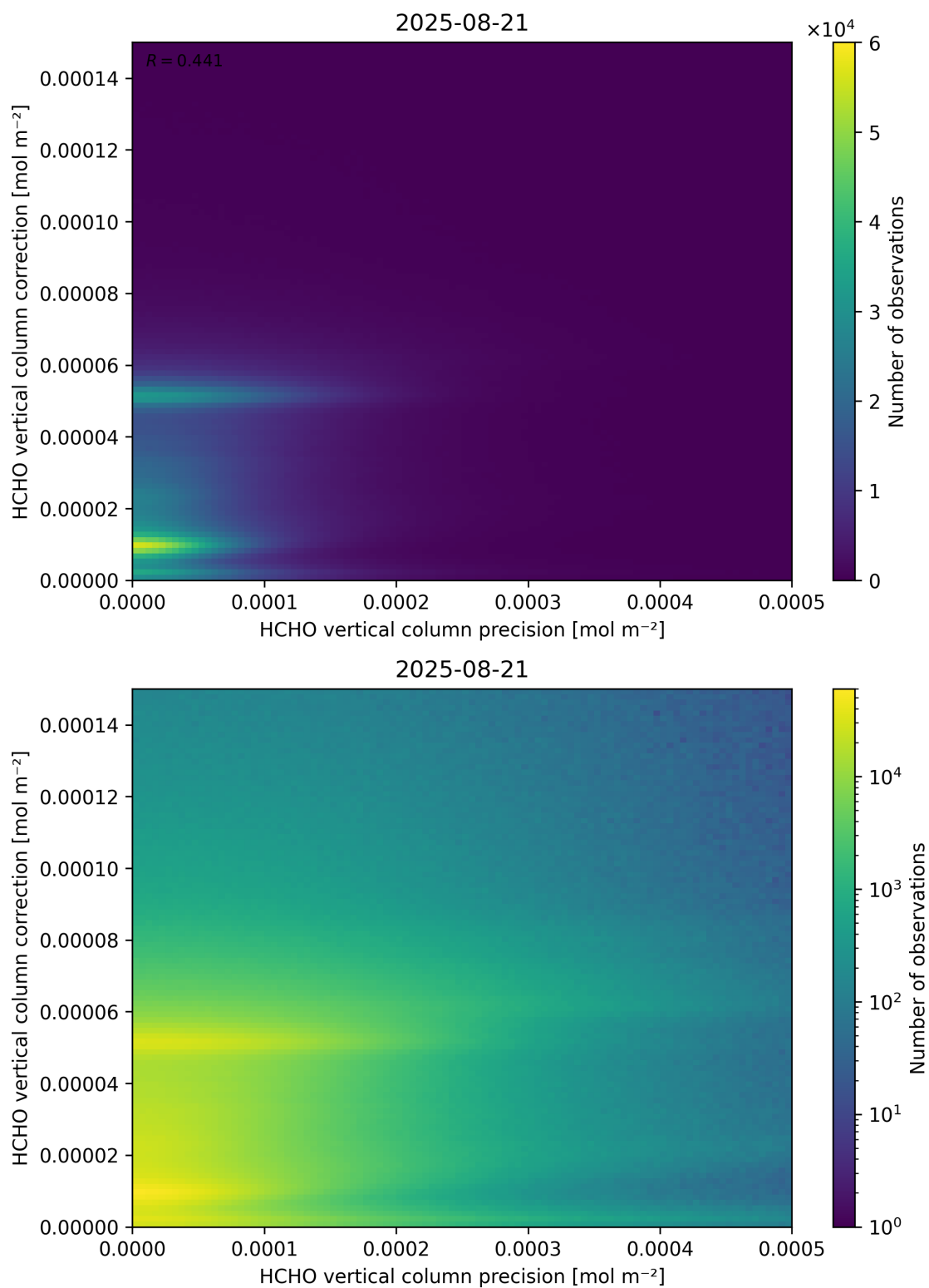
Figure 146: Scatter density plot of “HCHO vertical column precision” against “HCHO vertical column correction” for 2025-08-20 to 2025-08-22.
