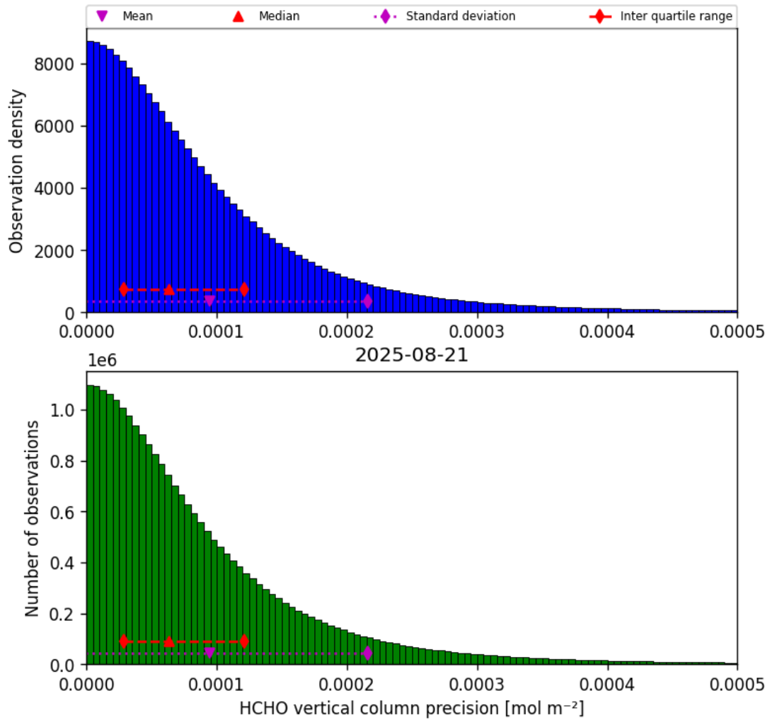
Figure 36: Histogram of “HCHO vertical column precision” for 2025-08-20 to 2025-08-22
