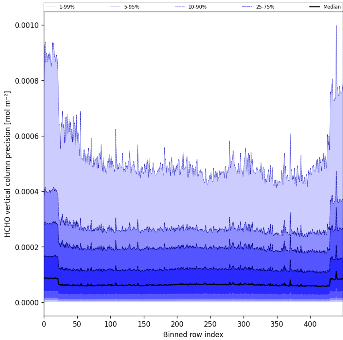
Figure 50: Along track statistics of “HCHO vertical column precision” for 2025-08-20 to 2025-08-22
