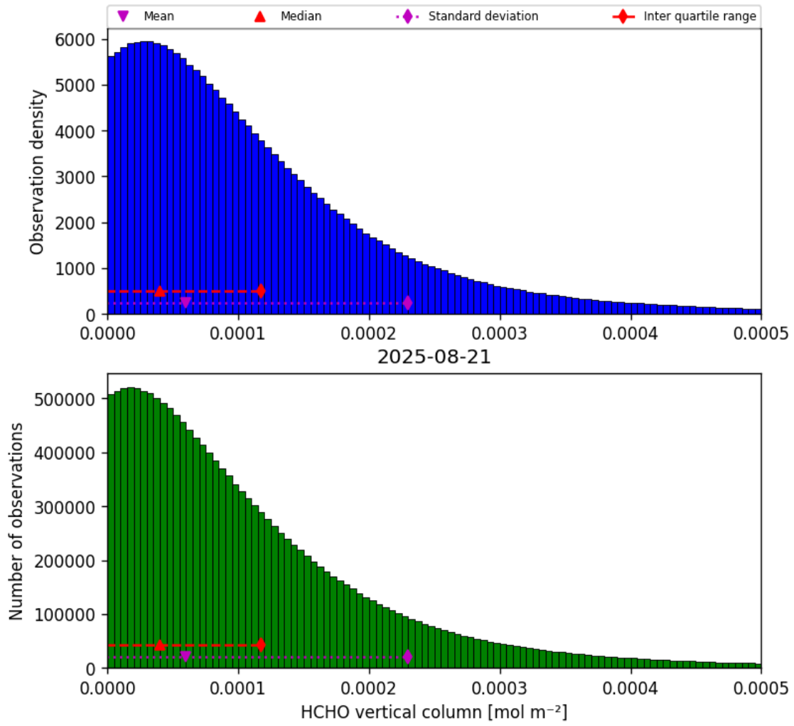
Figure 35: Histogram of “HCHO vertical column” for 2025-08-20 to 2025-08-22
