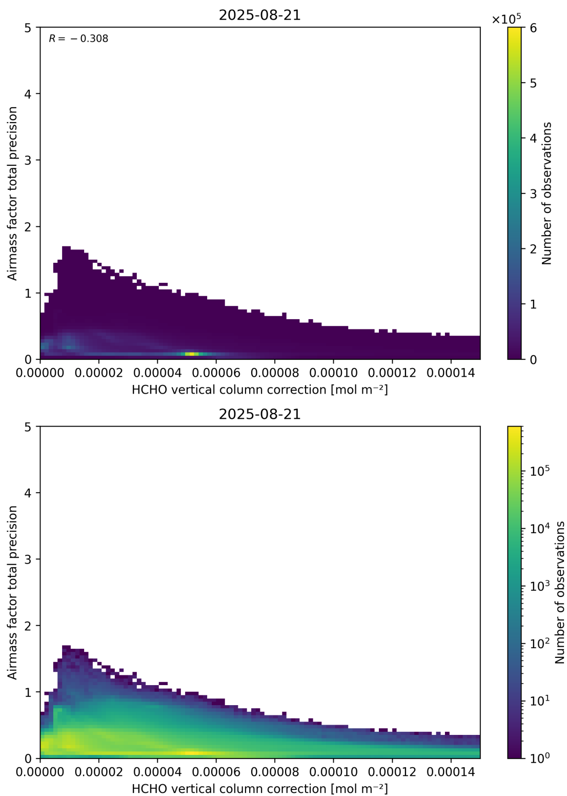
Figure 121: Scatter density plot of “HCHO vertical column correction” against “Airmass factor total precision” for 2025-08-20 to 2025-08-22.
