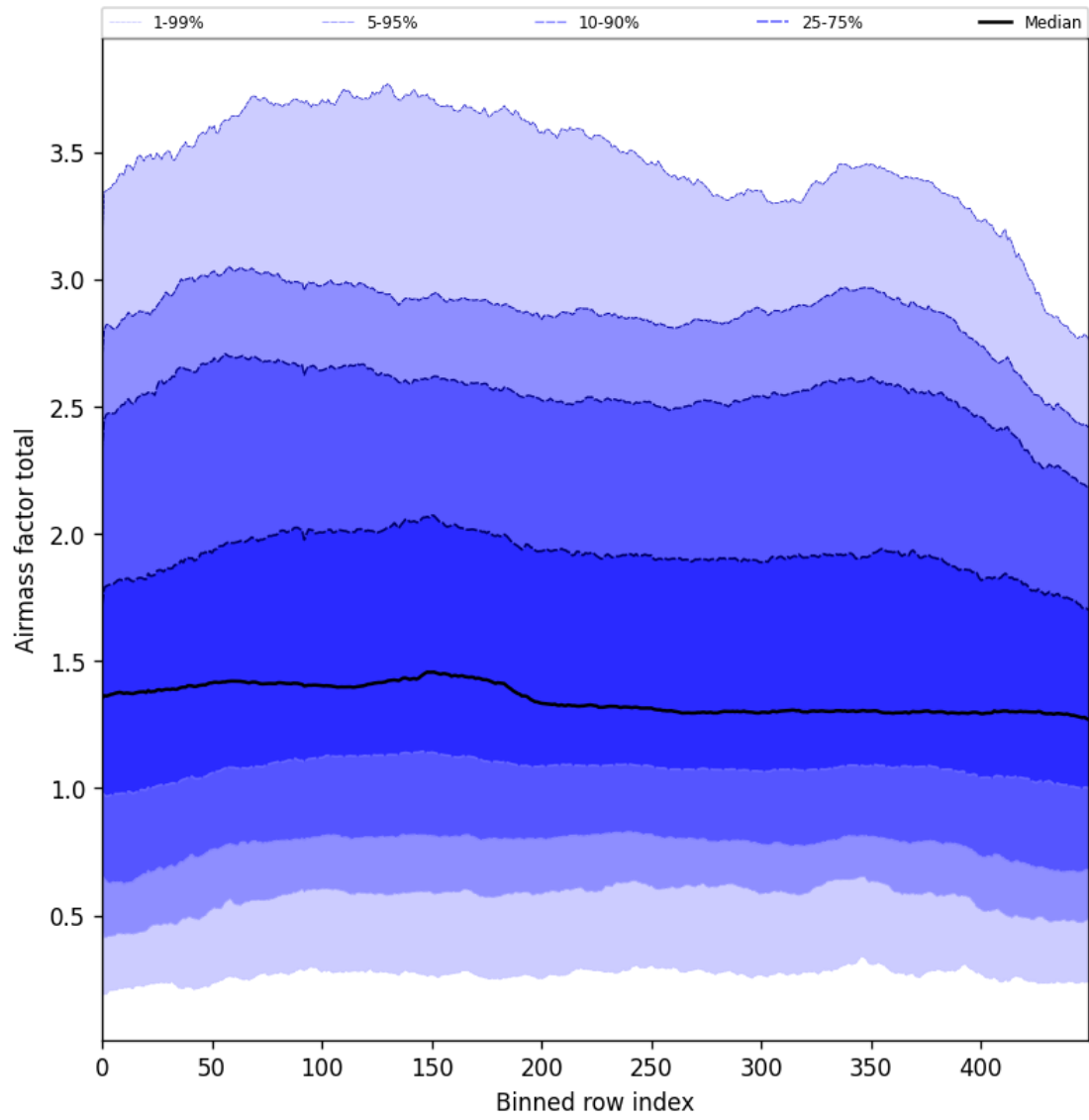
Figure 54: Along track statistics of “Airmass factor total” for 2025-08-20 to 2025-08-22
