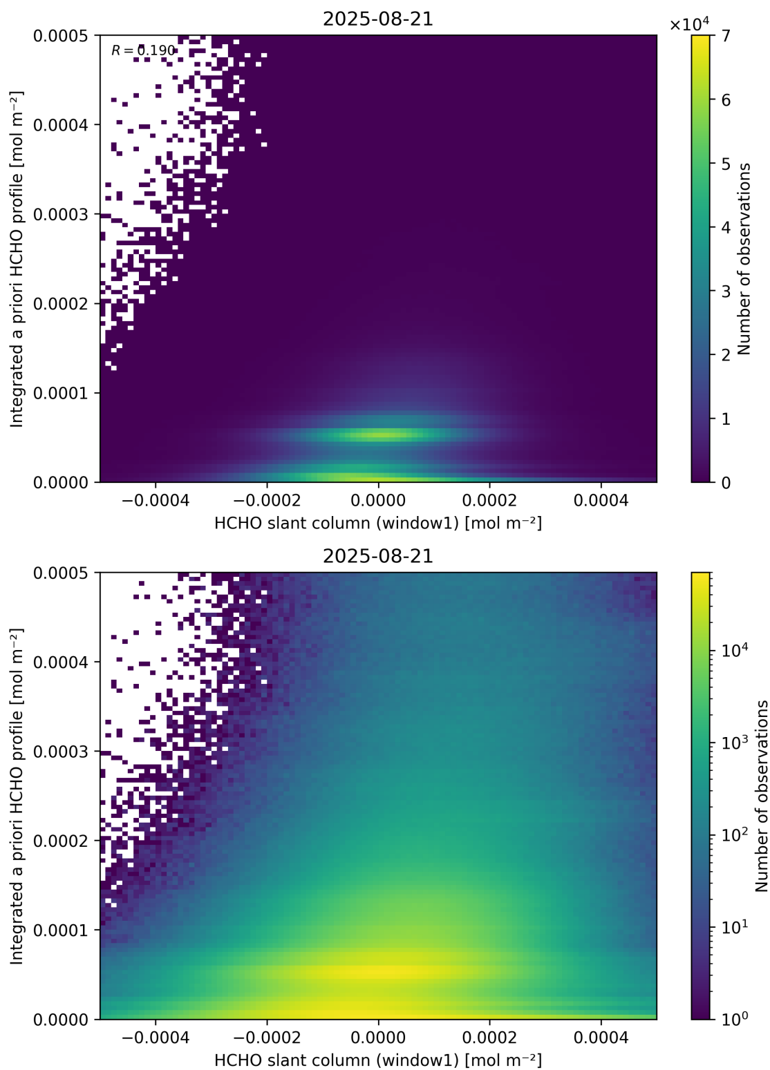
Figure 87: Scatter density plot of “HCHO slant column (window1)” against “Integrated a priori HCHO profile” for 2025-08-20 to 2025-08-22.
