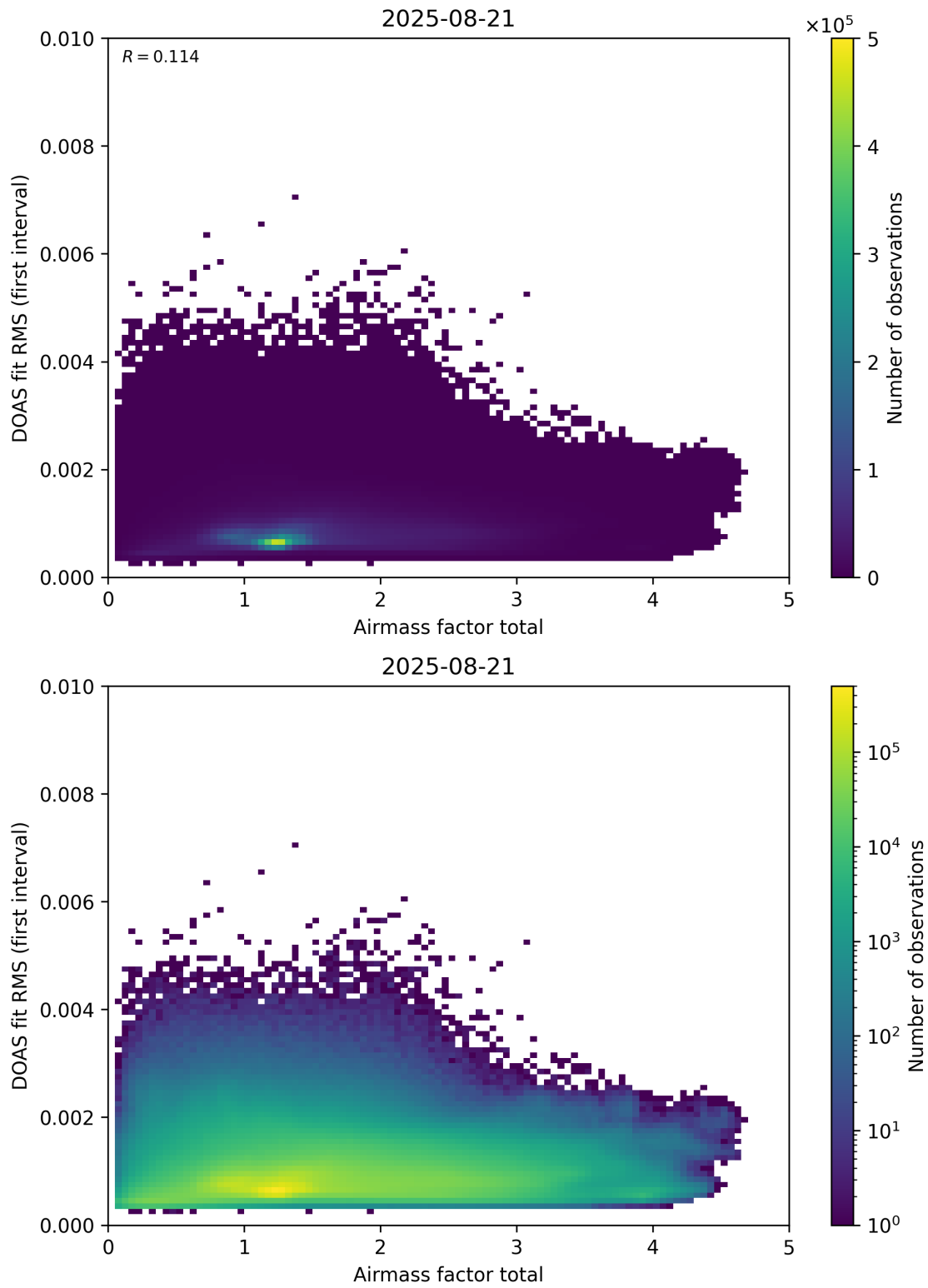
Figure 97: Scatter density plot of “Airmass factor total” against “DOAS fit RMS (first interval)” for 2025-08-20 to 2025-08-22.
