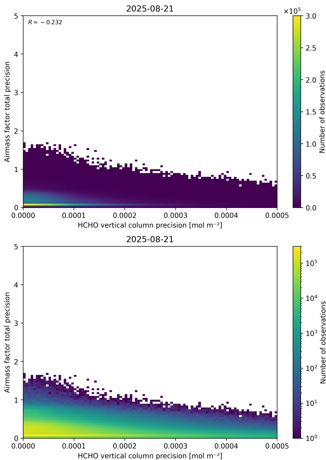
Figure 145: Scatter density plot of “HCHO vertical column precision” against “Airmass factor total precision” for 2025-08-20 to 2025-08-22.
