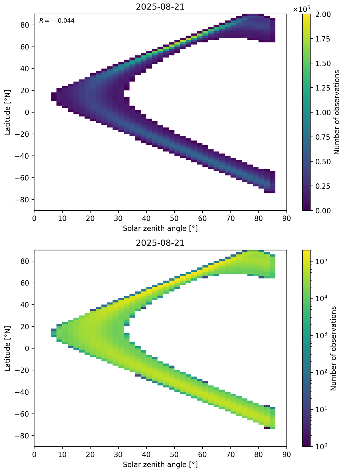
Figure 181: Scatter density plot of “Solar zenith angle” against “Latitude” for 2025-08-20 to 2025-08-22.
