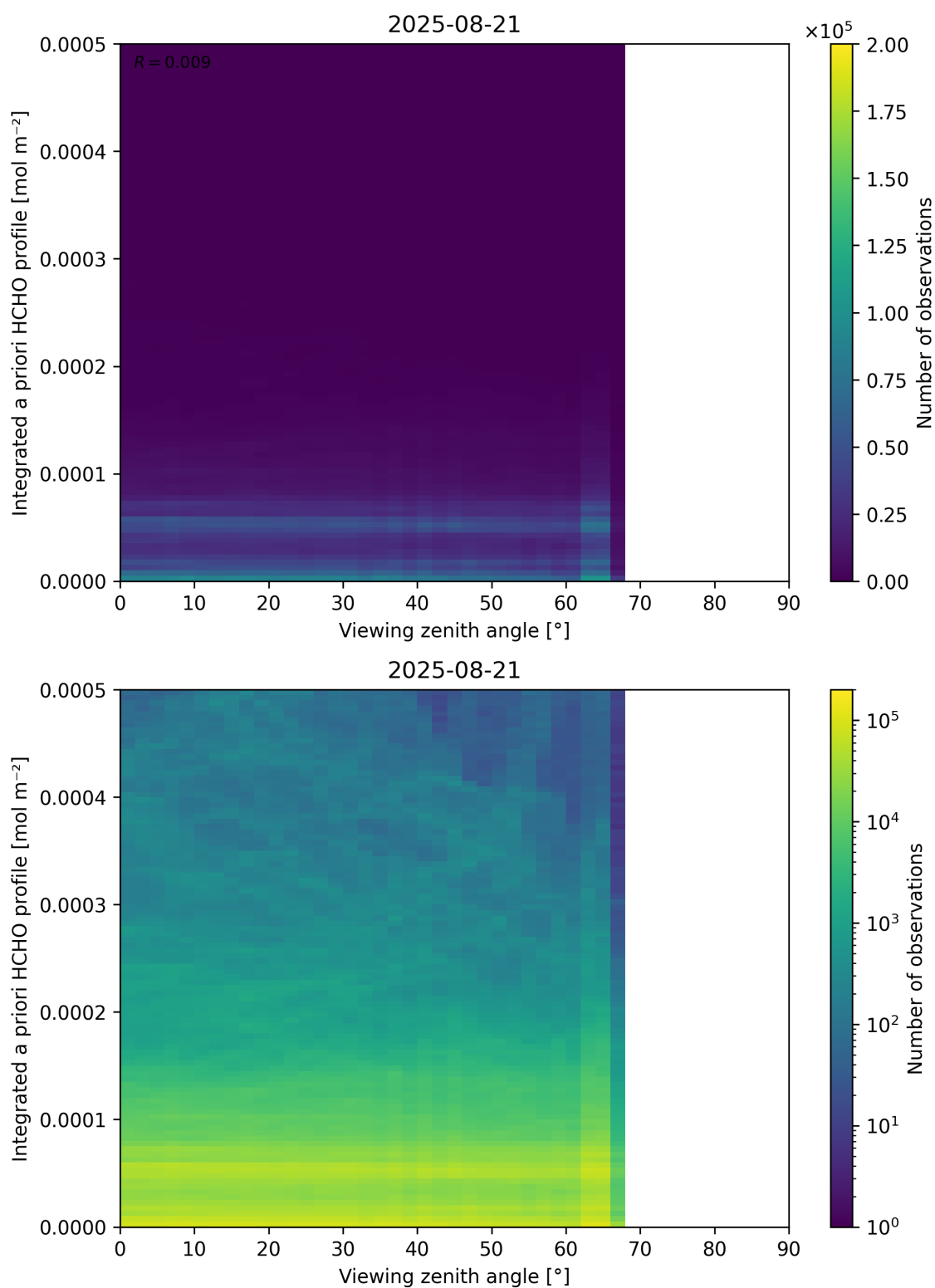
Figure 195: Scatter density plot of “Viewing zenith angle” against “Integrated a priori HCHO profile” for 2025-08-20 to 2025-08-22.
