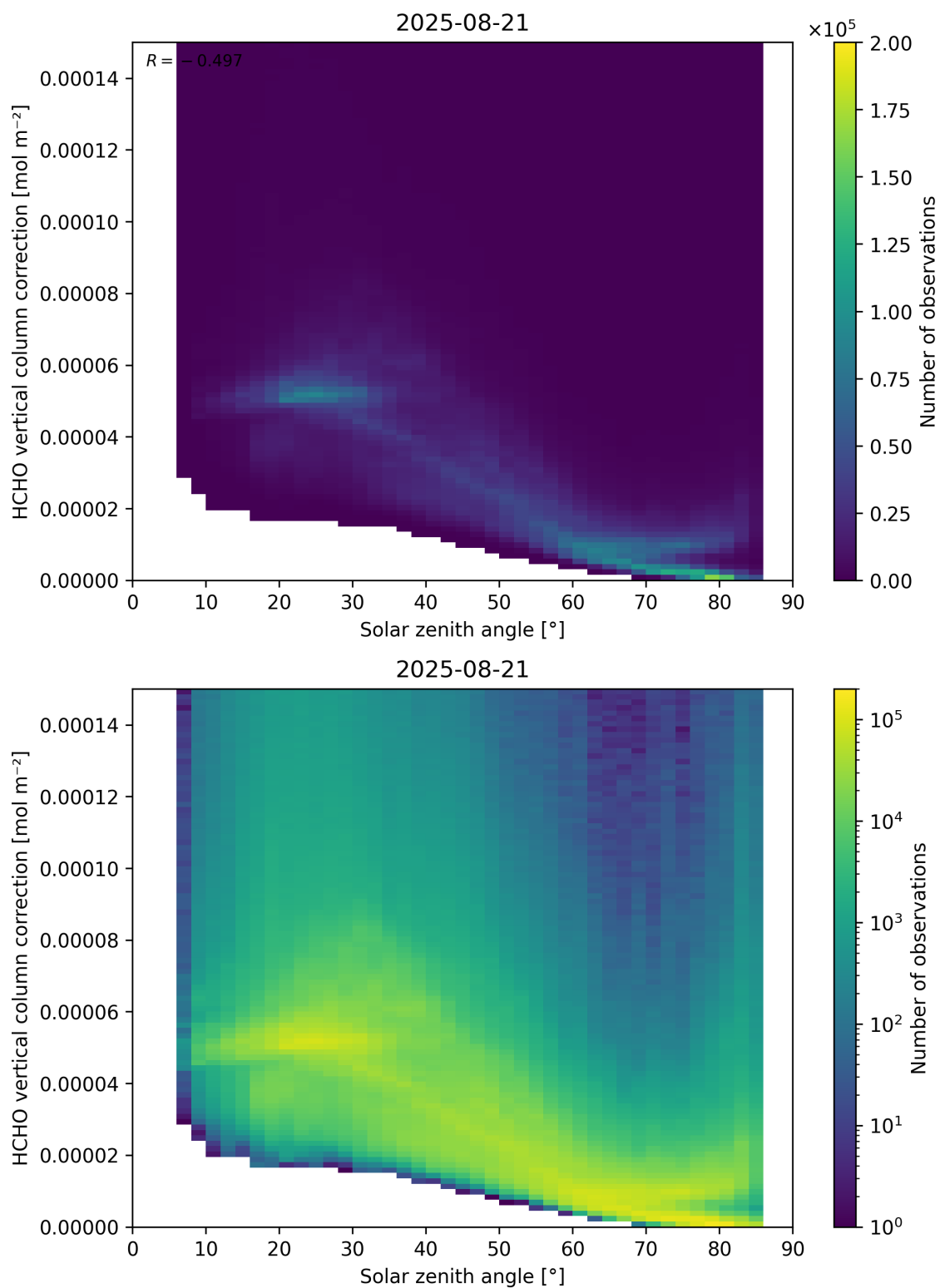
Figure 178: Scatter density plot of “Solar zenith angle” against “HCHO vertical column correction” for 2025-08-20 to 2025-08-22.
