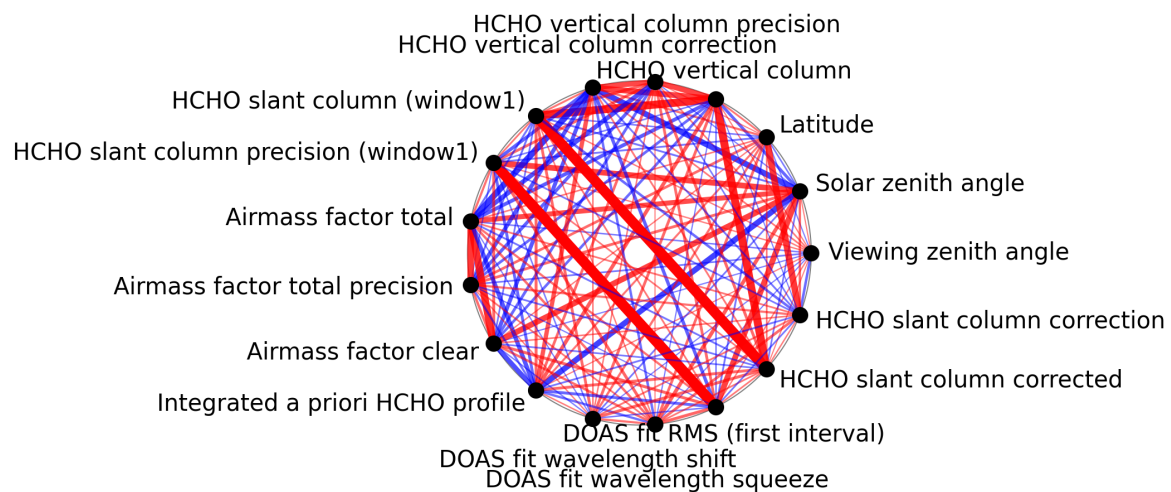
Figure 1: Map of correlation graph for 2025-08-20 to 2025-08-22.
