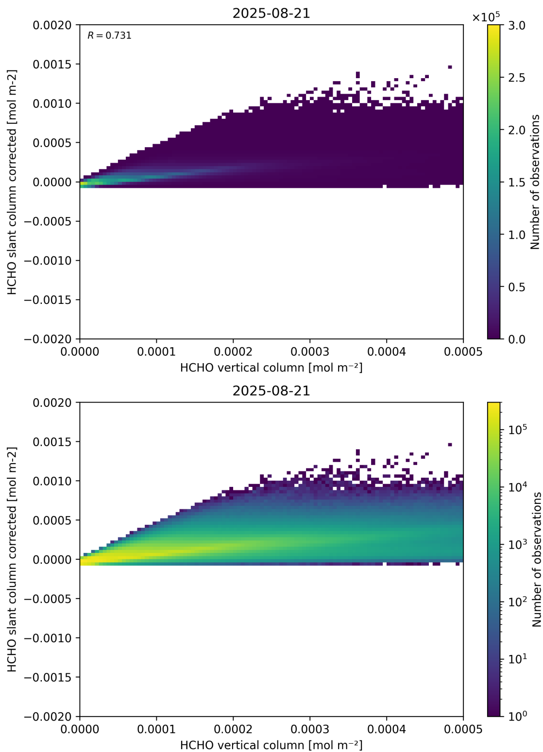
Figure 127: Scatter density plot of “HCHO vertical column” against “HCHO slant column corrected” for 2025-08-20 to 2025-08-22.
