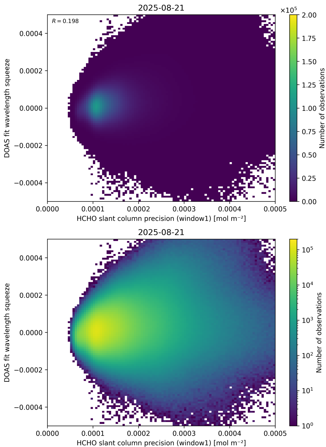
Figure 90: Scatter density plot of “HCHO slant column precision (window1)” against “DOAS fit wavelength squeeze” for 2025-08-20 to 2025-08-22.
