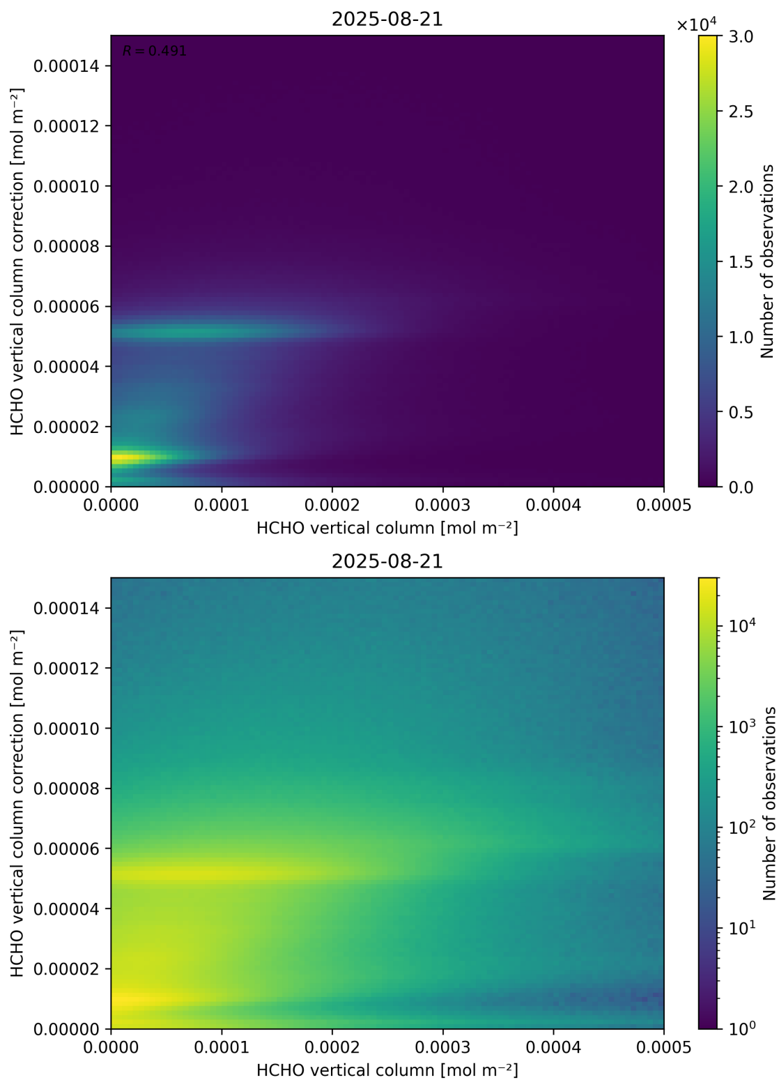
Figure 133: Scatter density plot of “HCHO vertical column” against “HCHO vertical column correction” for 2025-08-20 to 2025-08-22.
