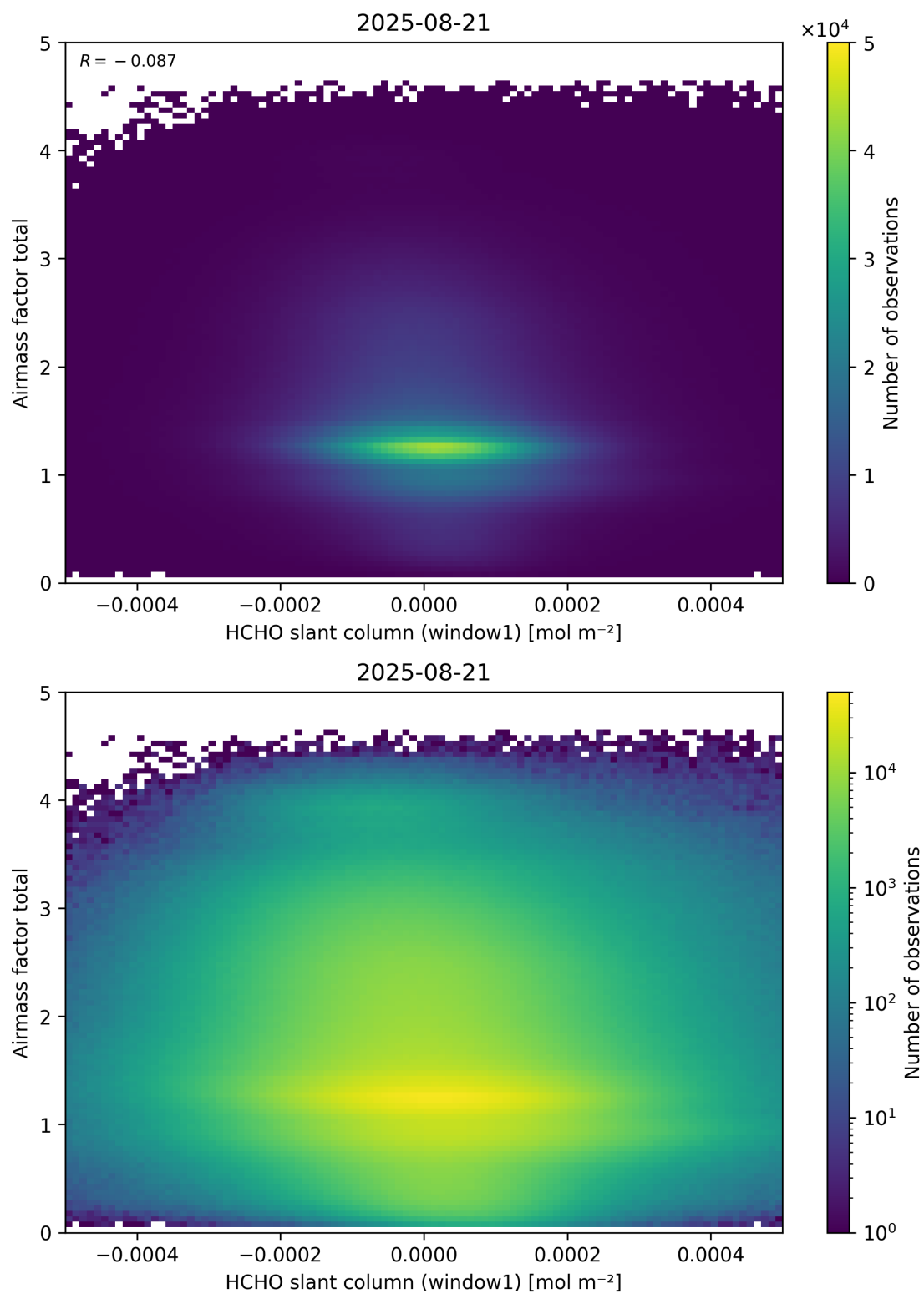
Figure 85: Scatter density plot of “HCHO slant column (window1)” against “Airmass factor total” for 2025-08-20 to 2025-08-22.
