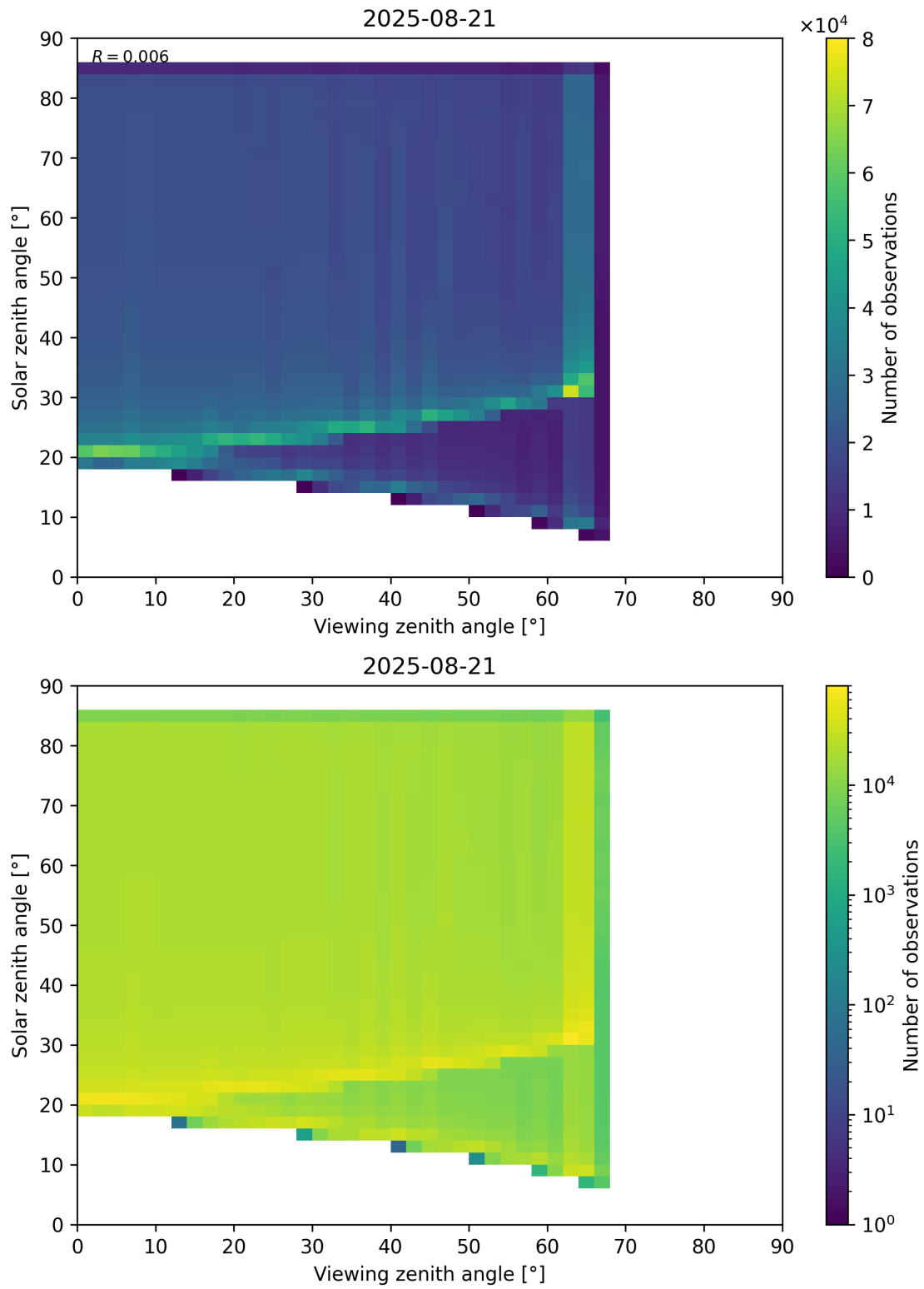
Figure 197: Scatter density plot of “Viewing zenith angle” against “Solar zenith angle” for 2025-08-20 to 2025-08-22.
