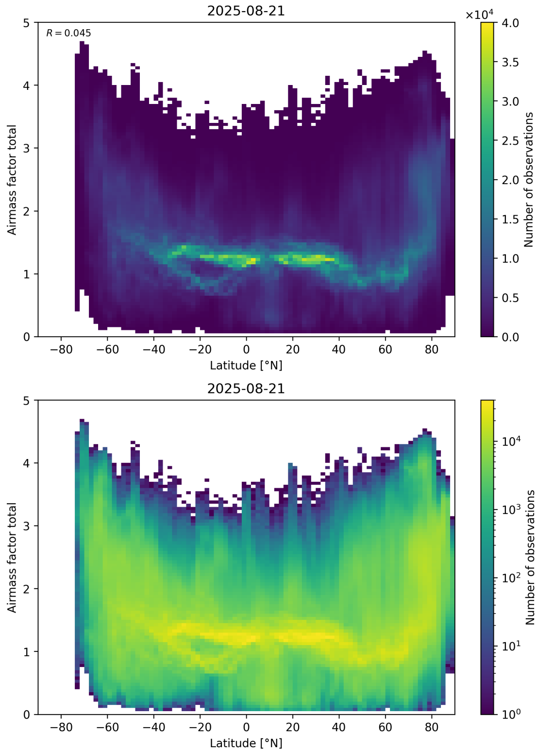
Figure 161: Scatter density plot of “Latitude” against “Airmass factor total” for 2025-08-20 to 2025-08-22.
