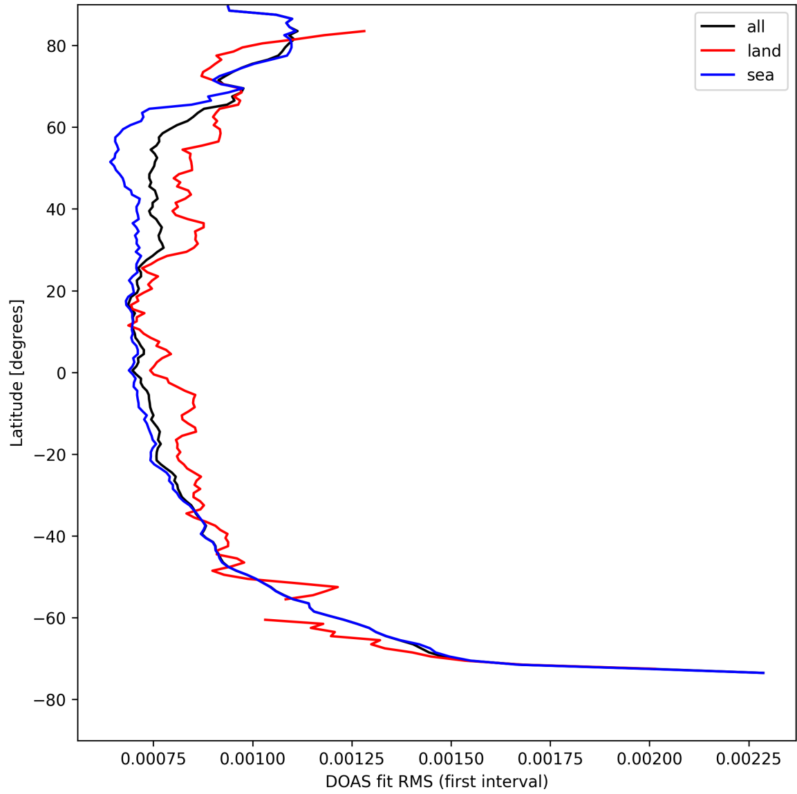
Figure 32: Zonal average of "DOAS fit RMS (first interval)" for 2025-08-20 to 2025-08-22.
