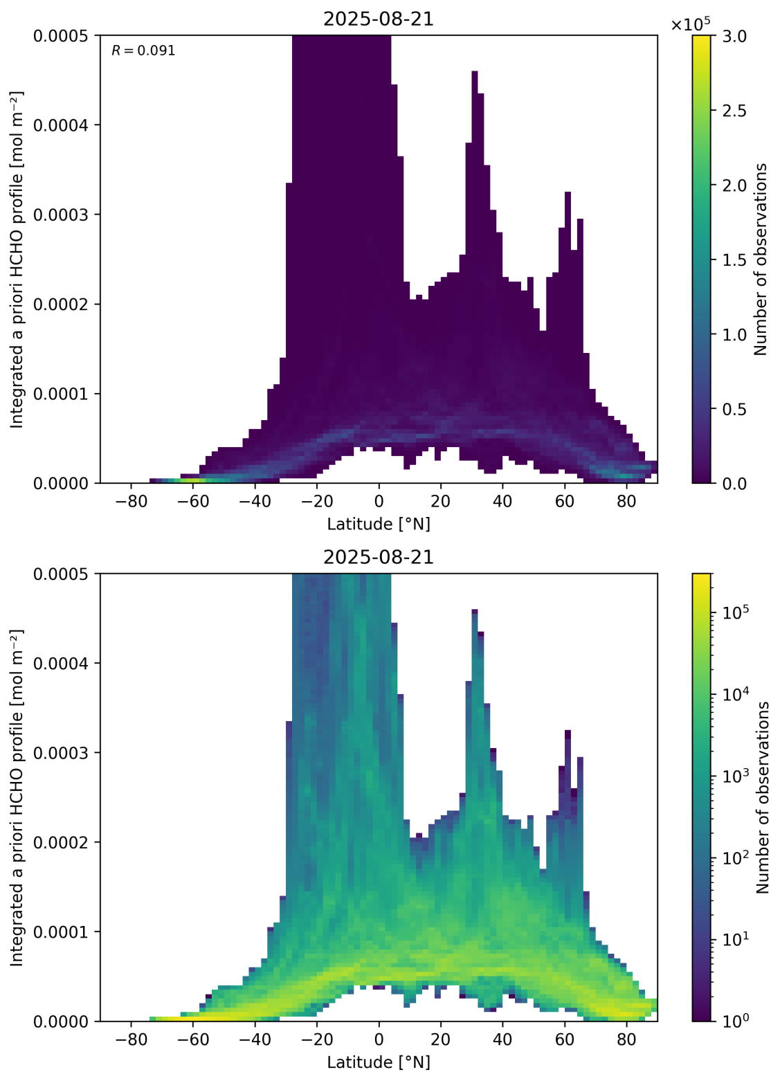
Figure 166: Scatter density plot of “Latitude” against “Integrated a priori HCHO profile” for 2025-08-20 to 2025-08-22.
