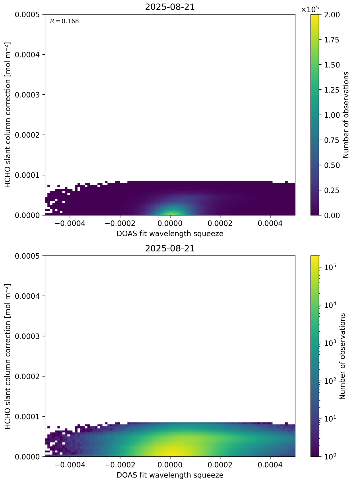
Figure 70: Scatter density plot of “DOAS fit wavelength squeeze” against “HCHO slant column correction” for 2025-08-20 to 2025-08-22.
