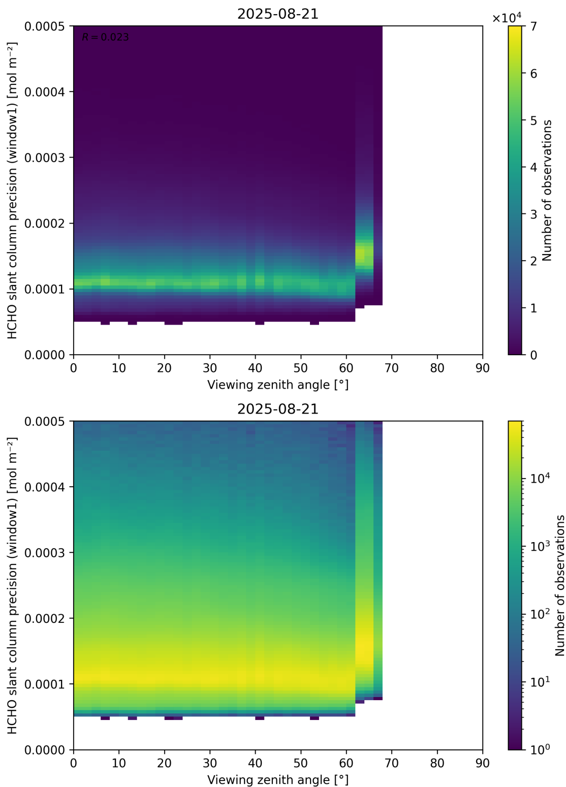
Figure 189: Scatter density plot of “Viewing zenith angle” against “HCHO slant column precision (window1)” for 2025-08-20 to 2025-08-22.
