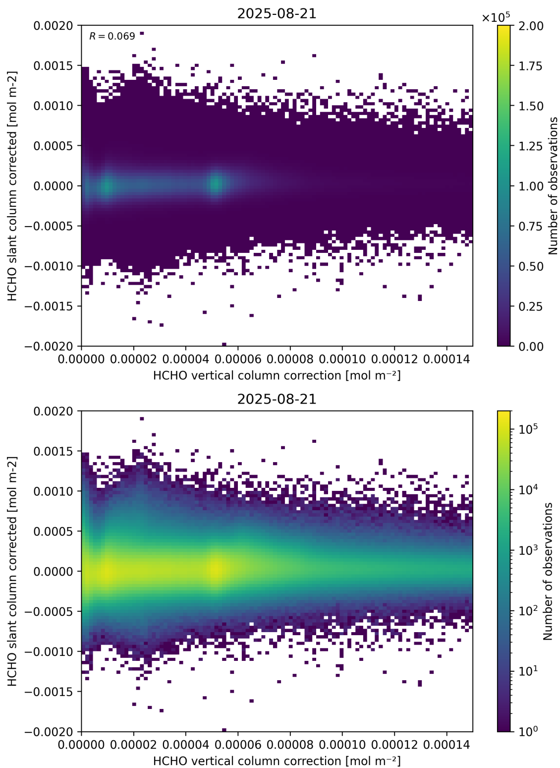
Figure 116: Scatter density plot of “HCHO vertical column correction” against “HCHO slant column corrected” for 2025-08-20 to 2025-08-22.
