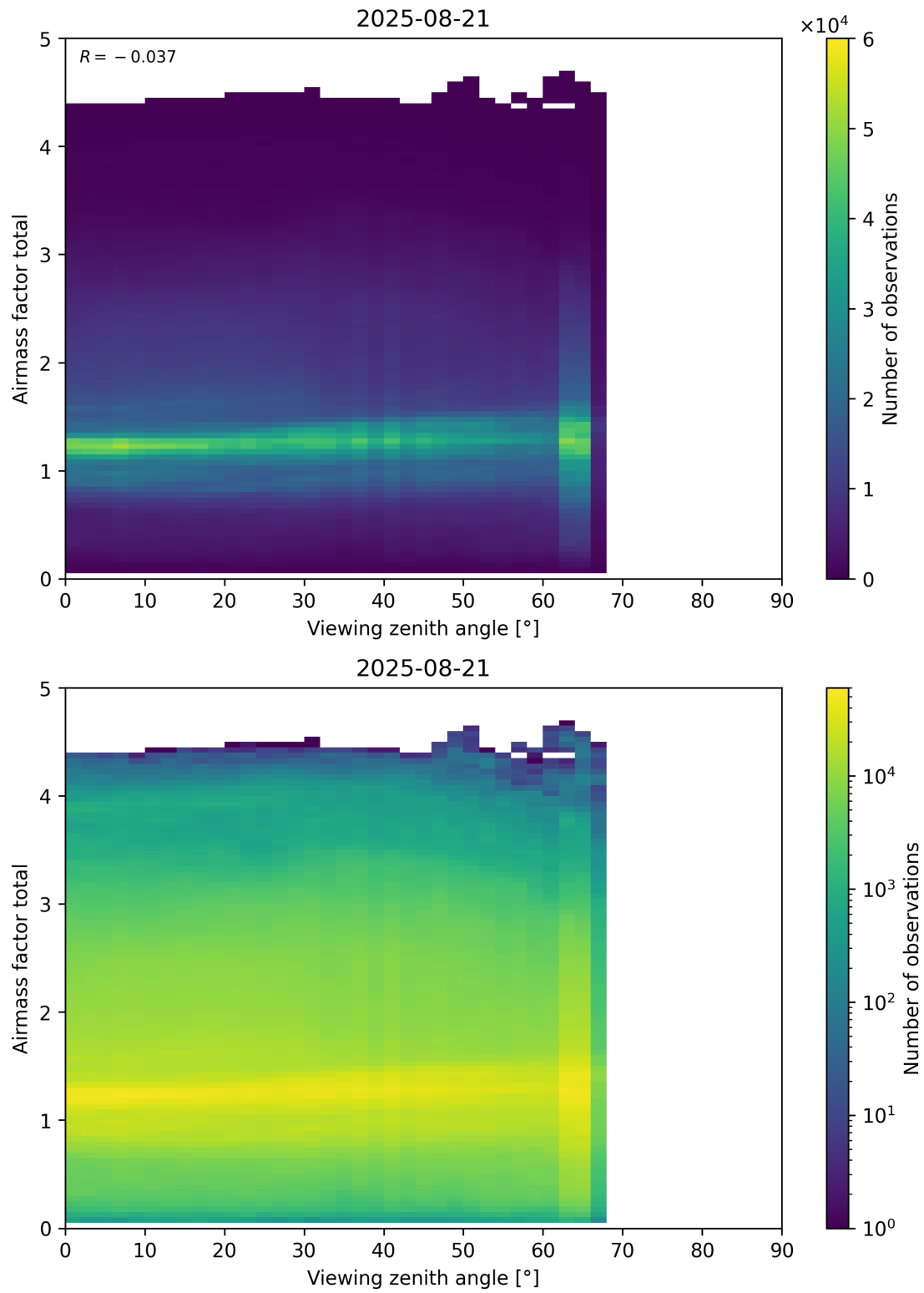
Figure 190: Scatter density plot of “Viewing zenith angle” against “Airmass factor total” for 2025-08-20 to 2025-08-22.
