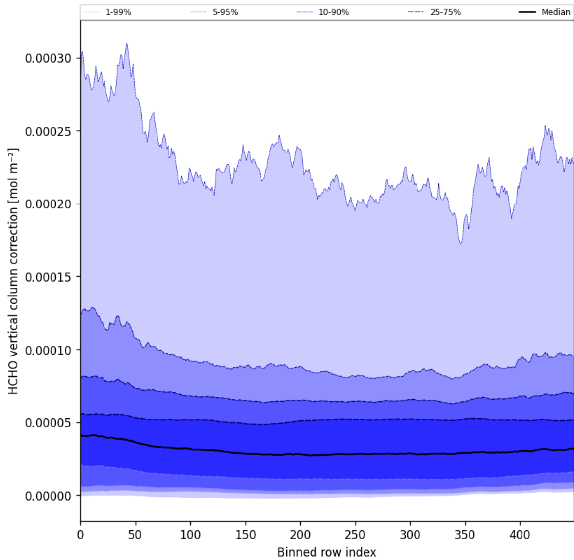
Figure 51: Along track statistics of “HCHO vertical column correction” for 2025-08-20 to 2025-08-22
