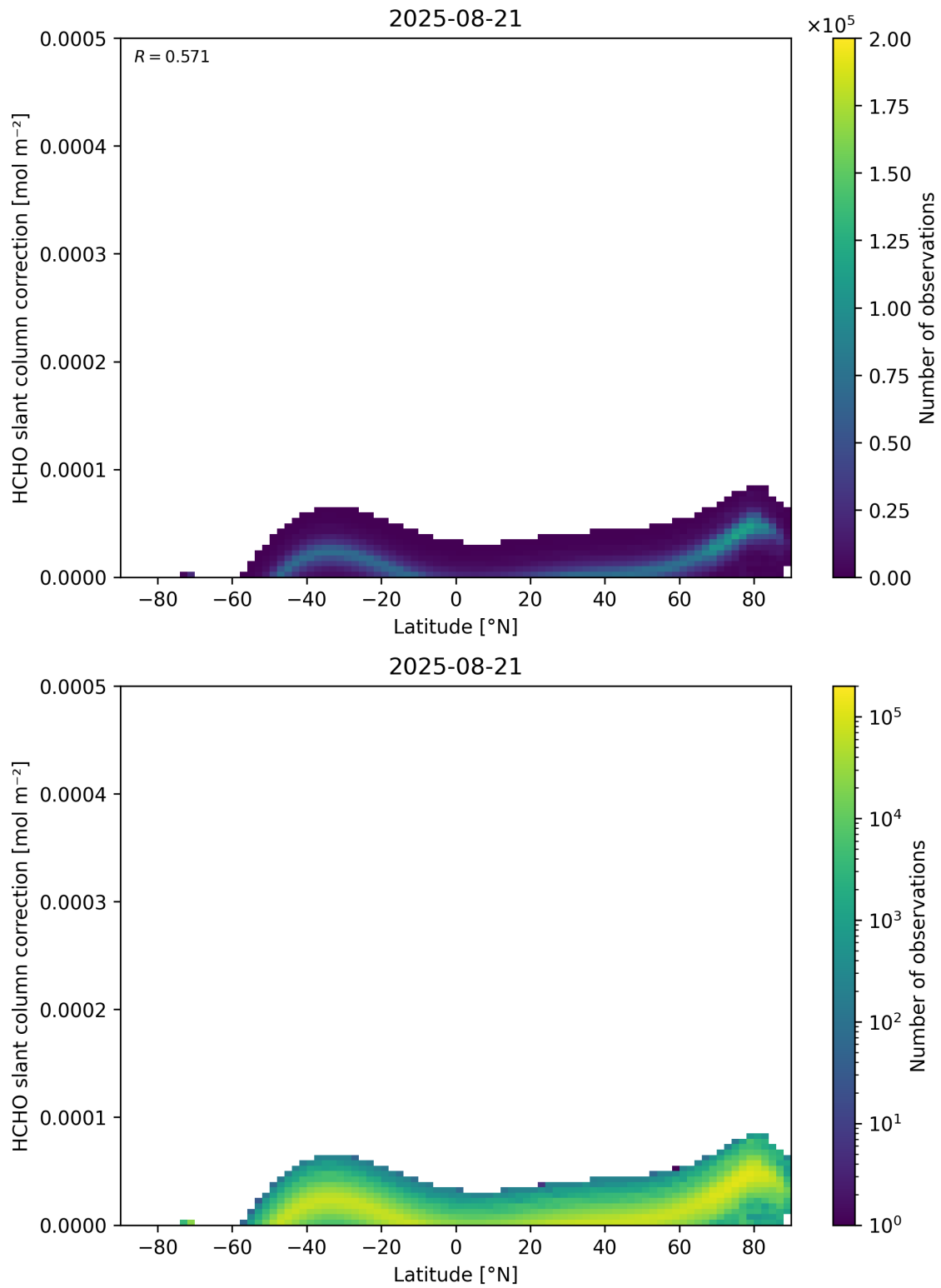
Figure 158: Scatter density plot of “Latitude” against “HCHO slant column correction” for 2025-08-20 to 2025-08-22.
