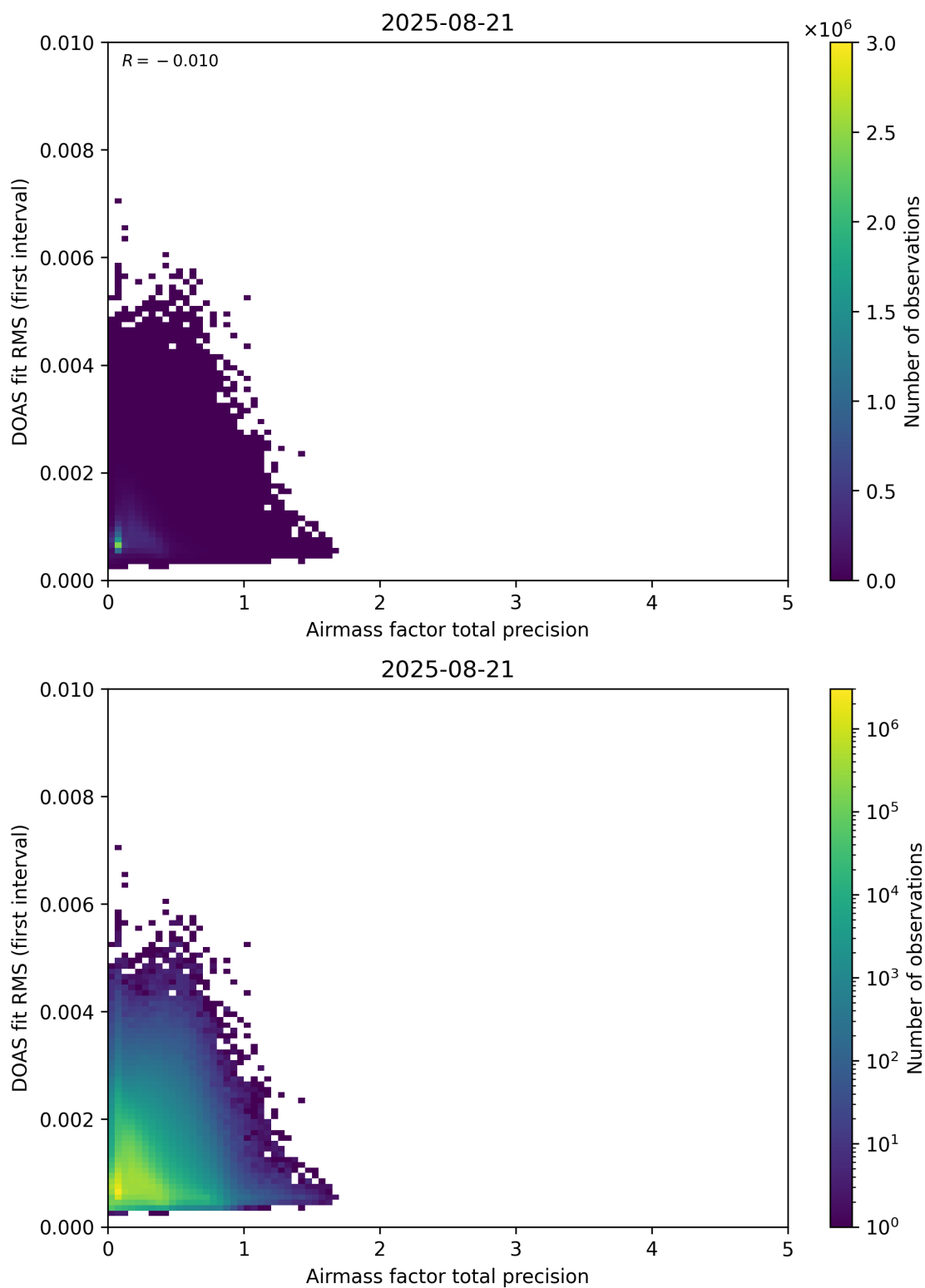
Figure 105: Scatter density plot of “Airmass factor total precision” against “DOAS fit RMS (first interval)” for 2025-08-20 to 2025-08-22.
