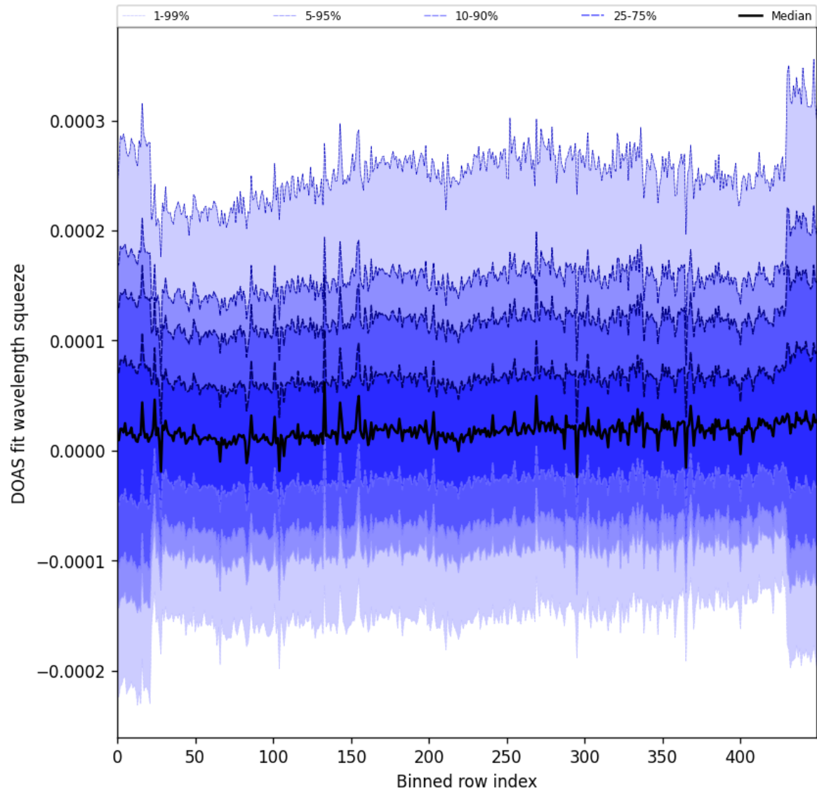
Figure 59: Along track statistics of “DOAS fit wavelength squeeze” for 2025-08-20 to 2025-08-22
