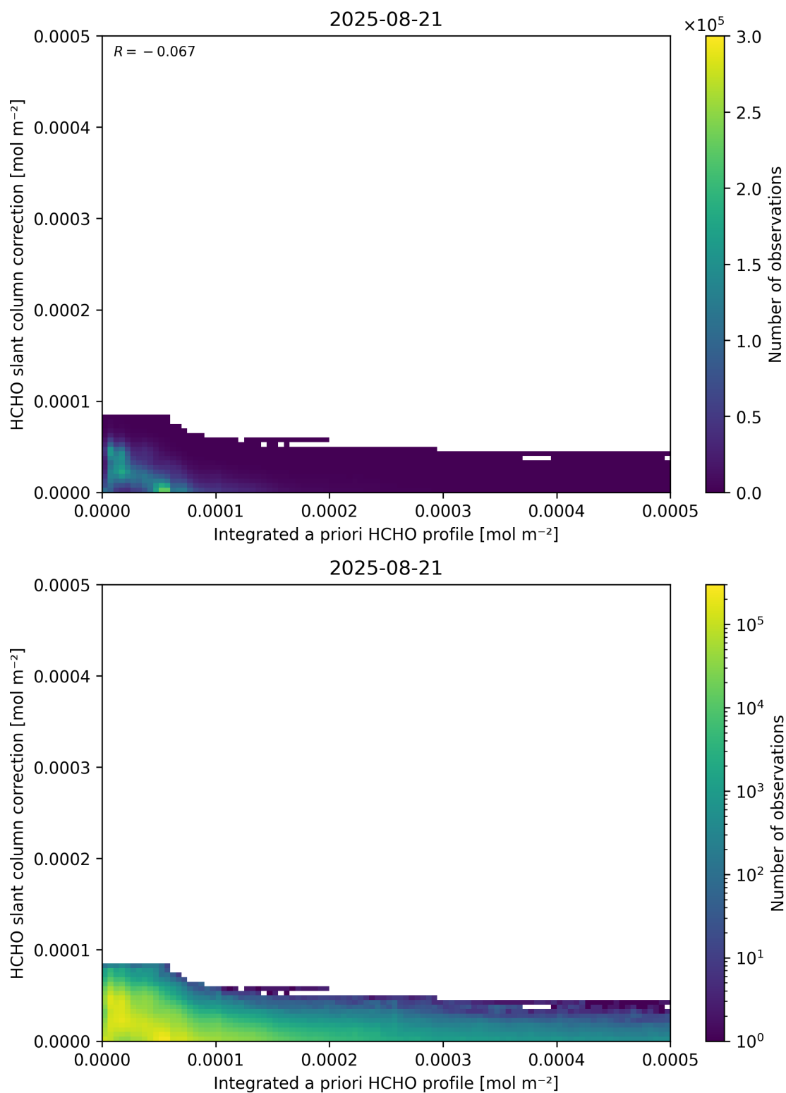
Figure 152: Scatter density plot of “Integrated a priori HCHO profile” against “HCHO slant column correction” for 2025-08-20 to 2025-08-22.
