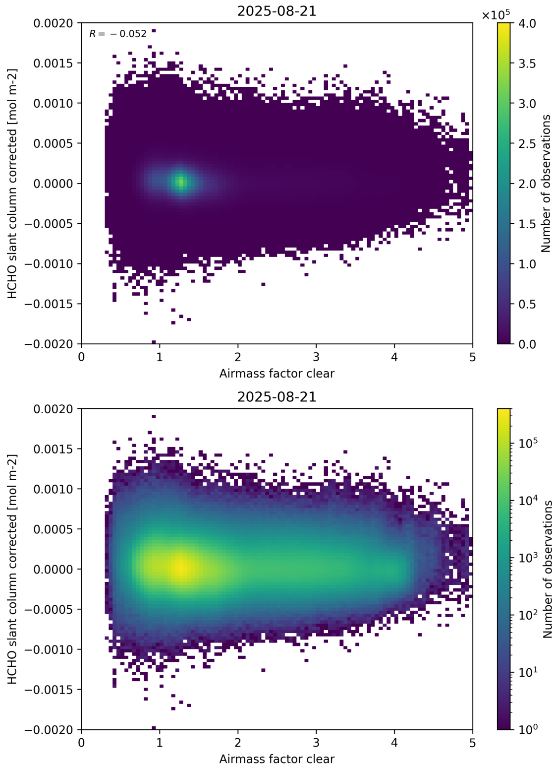
Figure 74: Scatter density plot of “Airmass factor clear” against “HCHO slant column corrected” for 2025-08-20 to 2025-08-22.
