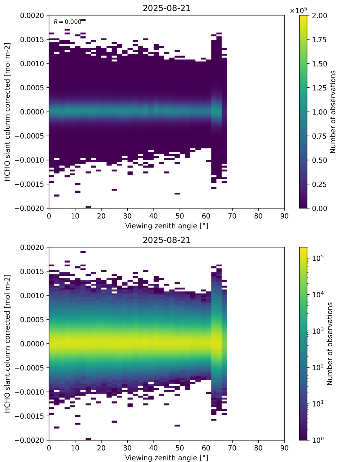
Figure 186: Scatter density plot of “Viewing zenith angle” against “HCHO slant column corrected” for 2025-08-20 to 2025-08-22.
