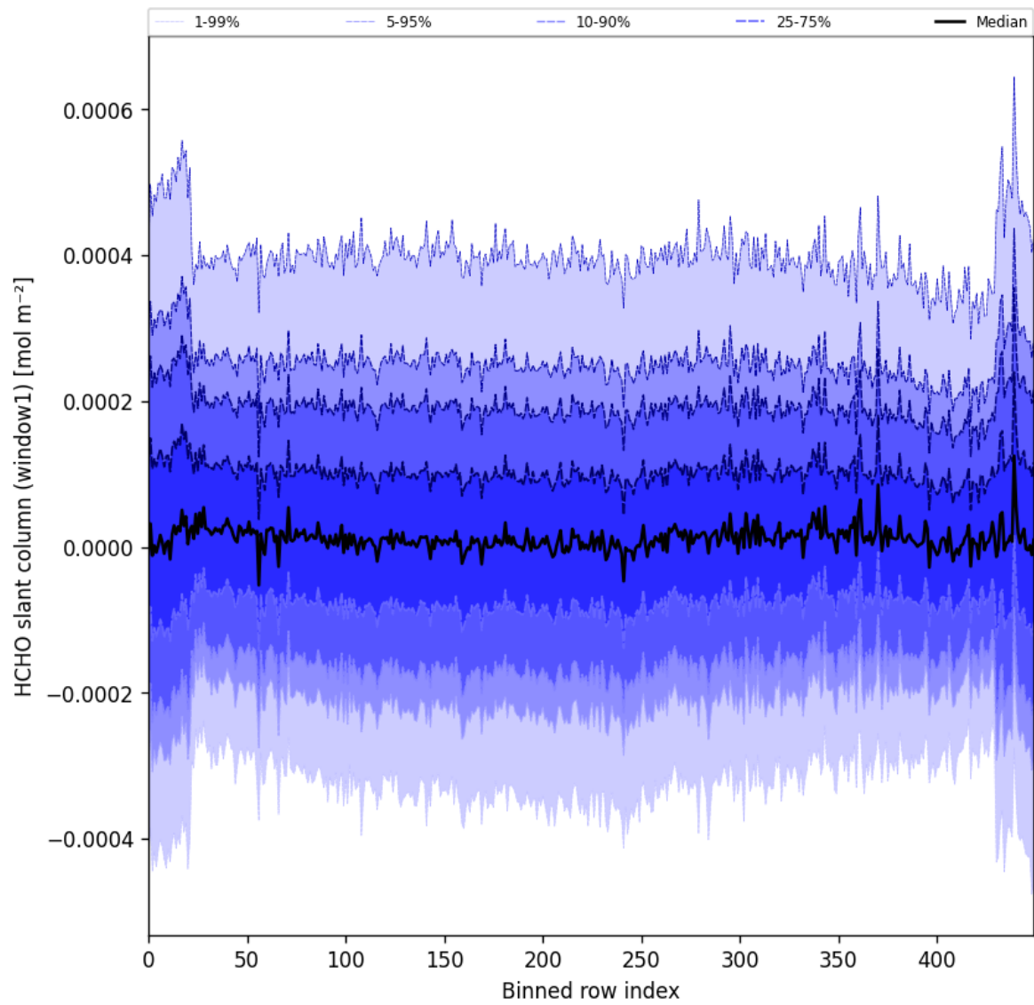
Figure 52: Along track statistics of “HCHO slant column (window1)” for 2025-08-20 to 2025-08-22
