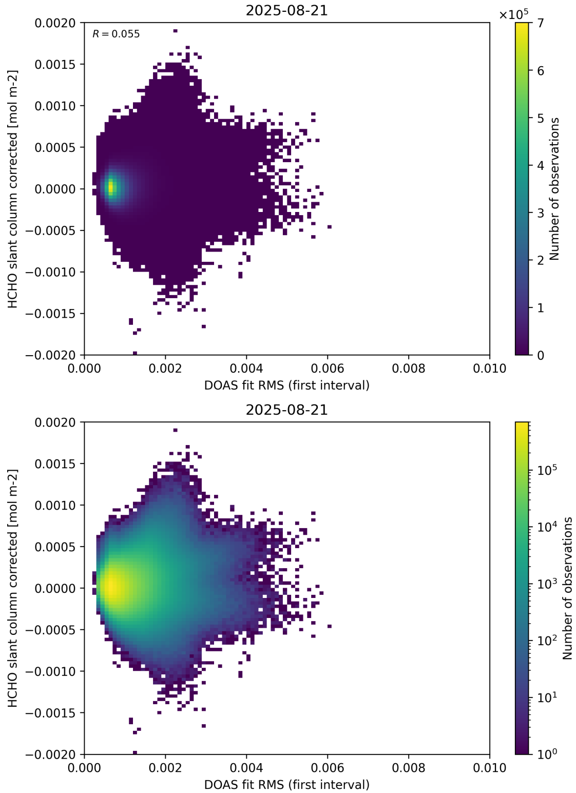
Figure 62: Scatter density plot of “DOAS fit RMS (first interval)” against “HCHO slant column corrected” for 2025-08-20 to 2025-08-22.
