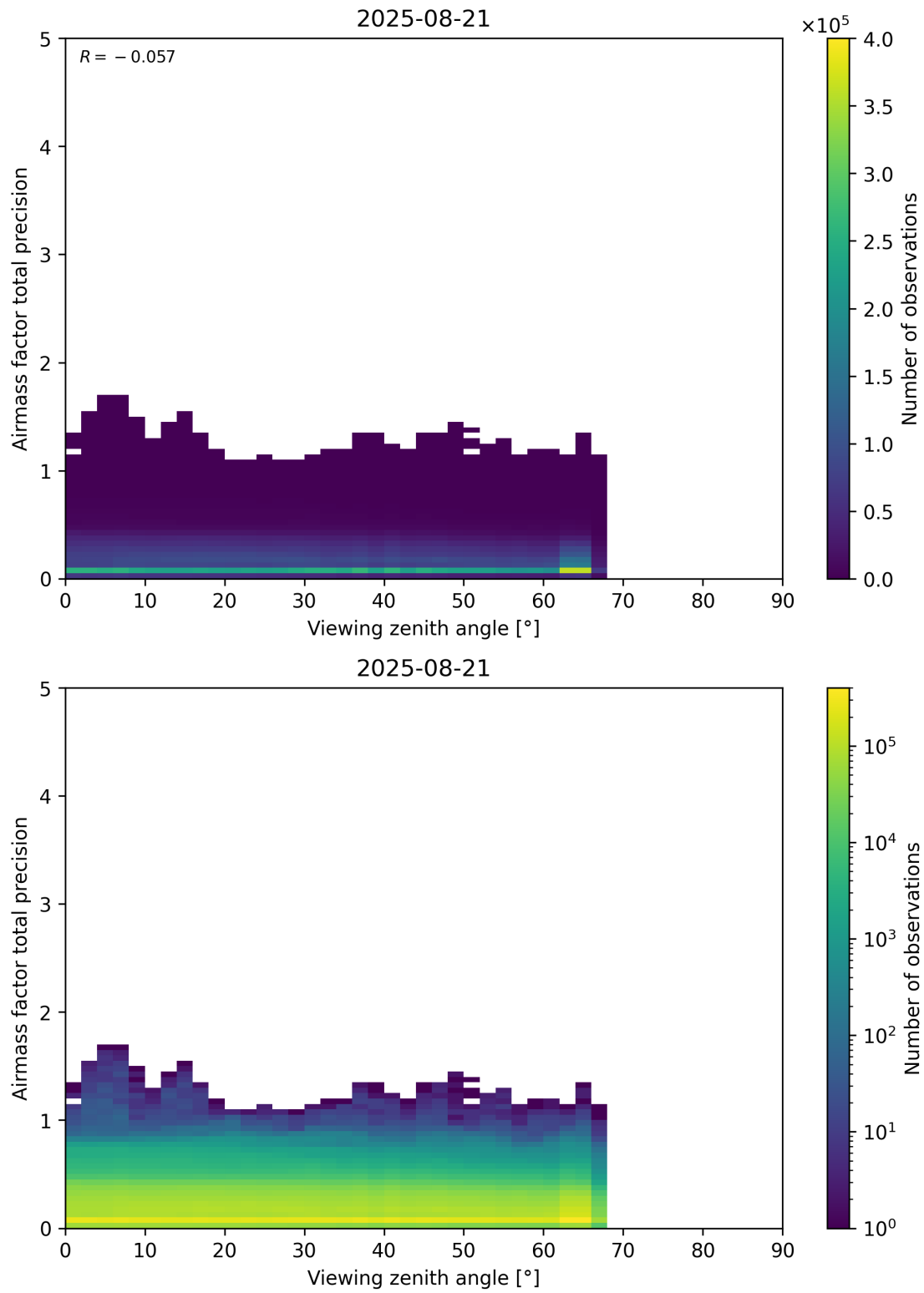
Figure 191: Scatter density plot of “Viewing zenith angle” against “Airmass factor total precision” for 2025-08-20 to 2025-08-22.
