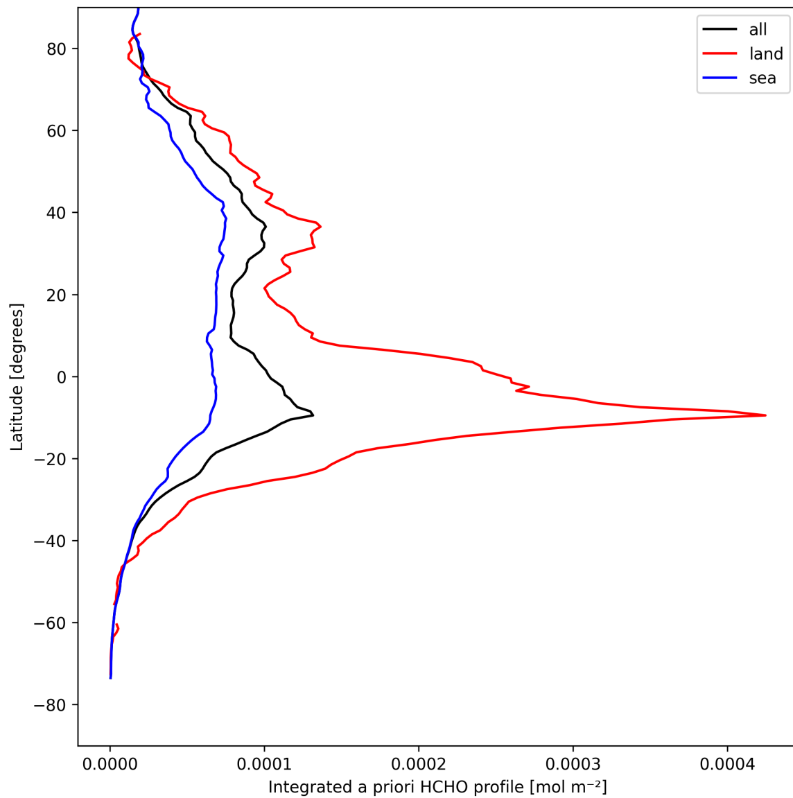
Figure 29: Zonal average of “Integrated a priori HCHO profile” for 2025-08-20 to 2025-08-22.
