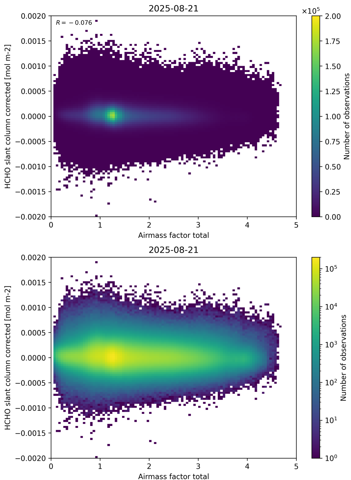
Figure 101: Scatter density plot of “Airmass factor total” against “HCHO slant column corrected” for 2025-08-20 to 2025-08-22.
