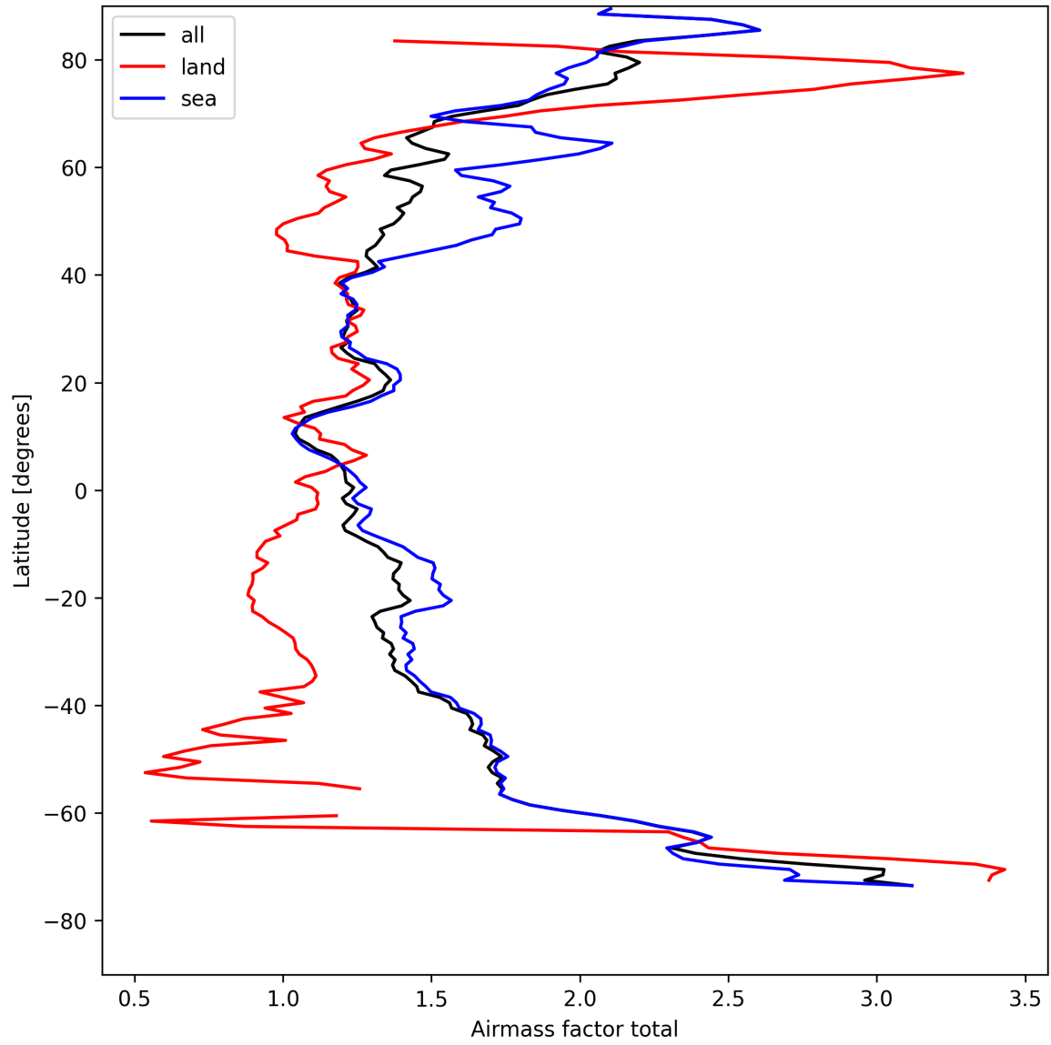
Figure 26: Zonal average of “Airmass factor total” for 2025-08-20 to 2025-08-22.
