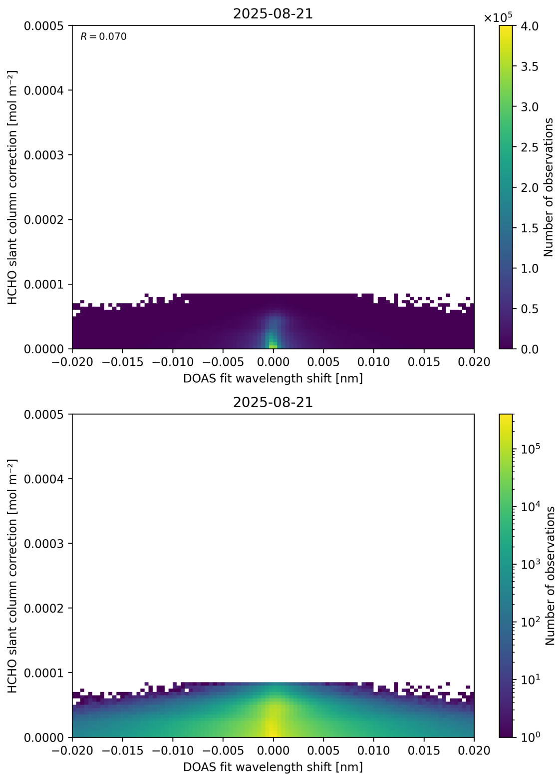
Figure 67: Scatter density plot of “DOAS fit wavelength shift” against “HCHO slant column correction” for 2025-08-20 to 2025-08-22.
