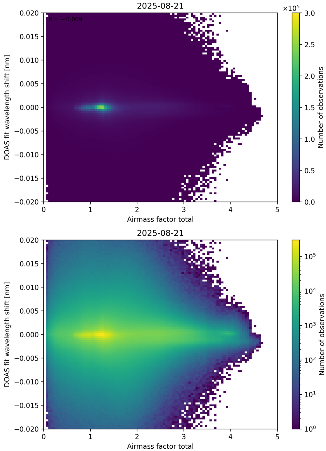
Figure 98: Scatter density plot of “Airmass factor total” against “DOAS fit wavelength shift” for 2025-08-20 to 2025-08-22.
