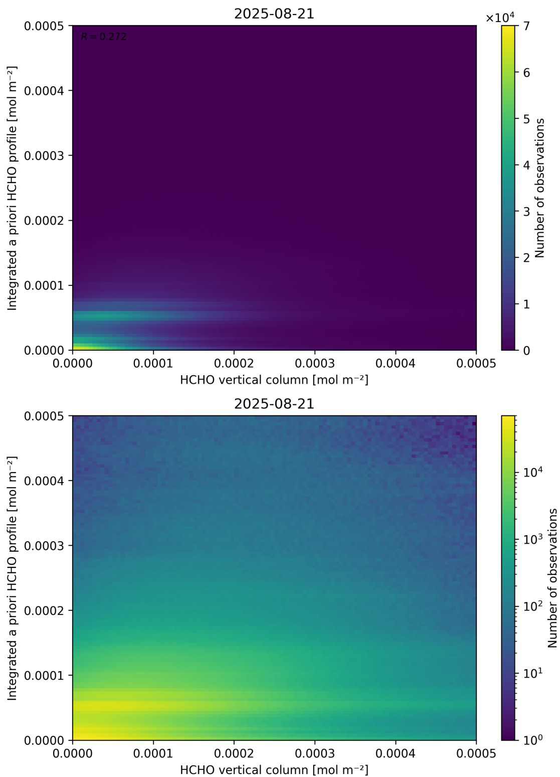
Figure 135: Scatter density plot of “HCHO vertical column” against “Integrated a priori HCHO profile” for 2025-08-20 to 2025-08-22.
