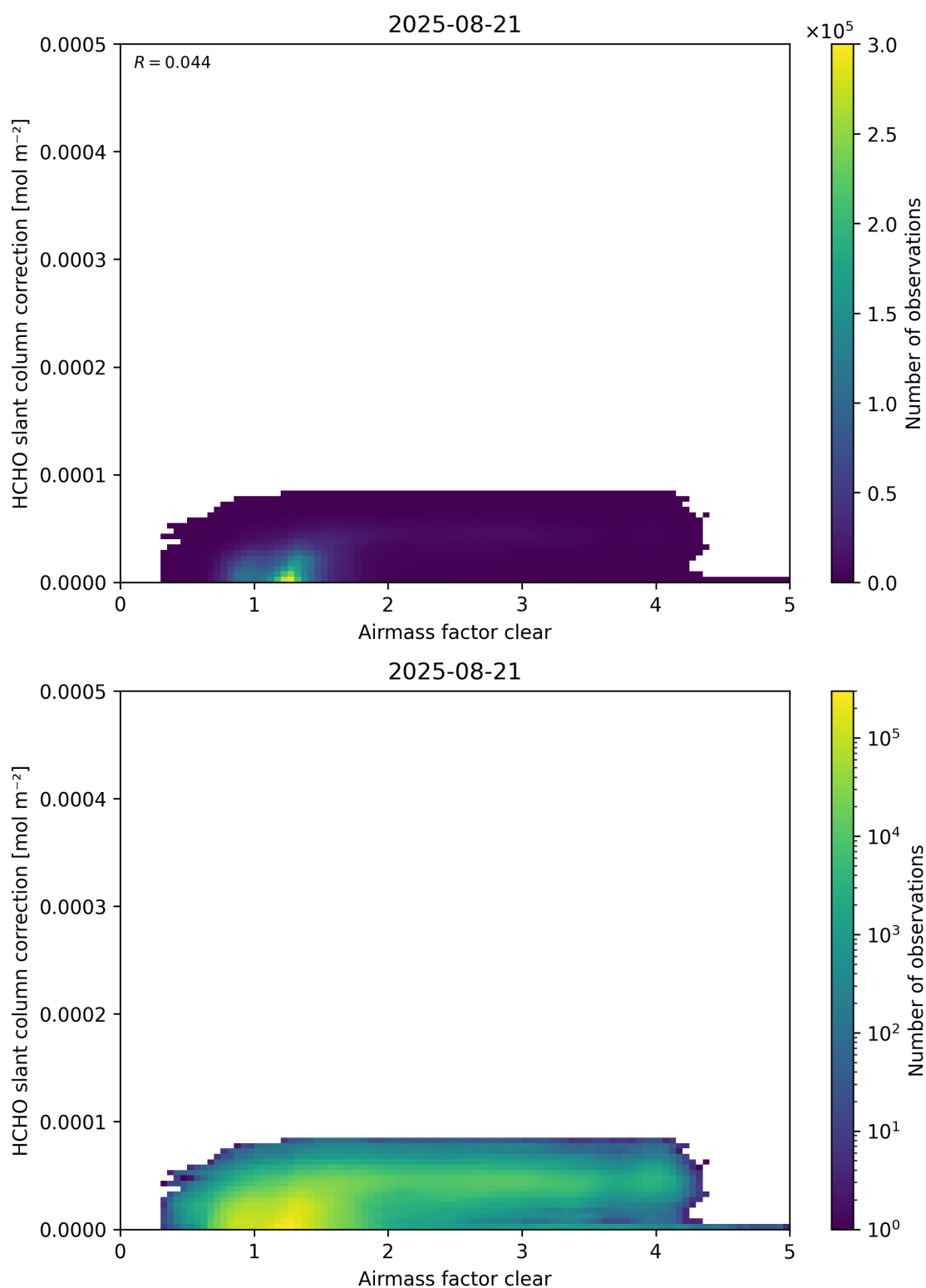
Figure 75: Scatter density plot of “Airmass factor clear” against “HCHO slant column correction” for 2025-08-20 to 2025-08-22.
