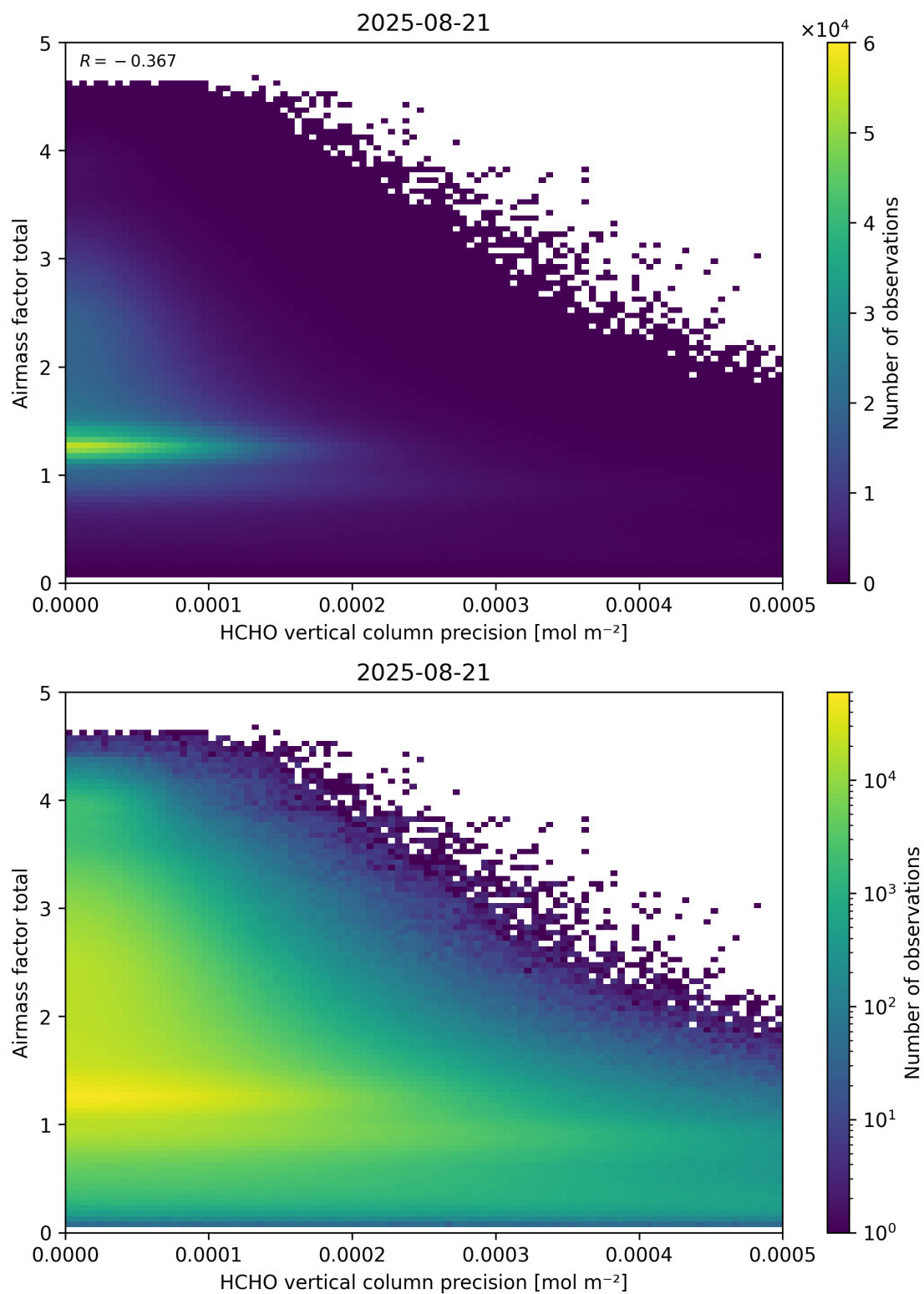
Figure 144: Scatter density plot of “HCHO vertical column precision” against “Airmass factor total” for 2025-08-20 to 2025-08-22.
