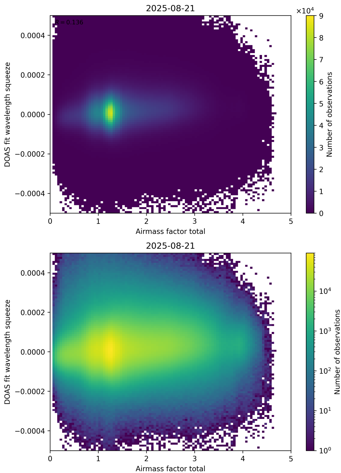
Figure 99: Scatter density plot of “Airmass factor total” against “DOAS fit wavelength squeeze” for 2025-08-20 to 2025-08-22.
