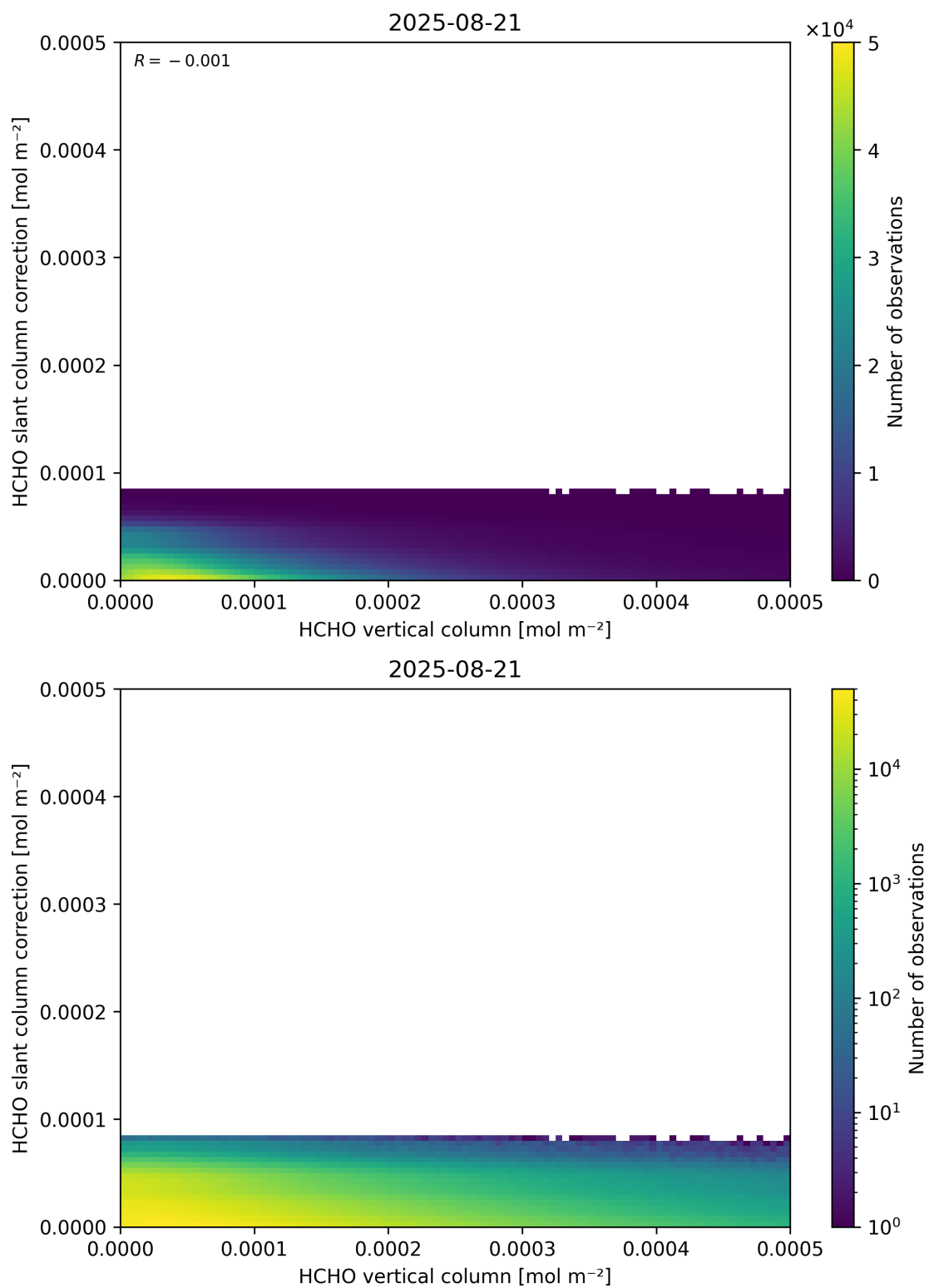
Figure 128: Scatter density plot of “HCHO vertical column” against “HCHO slant column correction” for 2025-08-20 to 2025-08-22.
