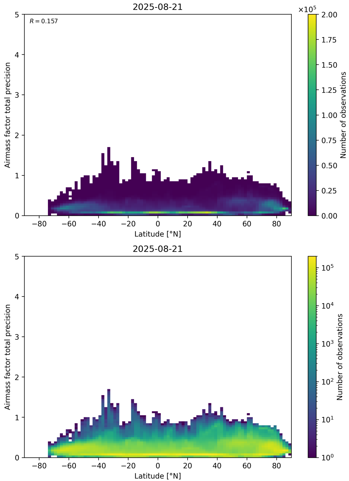
Figure 162: Scatter density plot of “Latitude” against “Airmass factor total precision” for 2025-08-20 to 2025-08-22.
