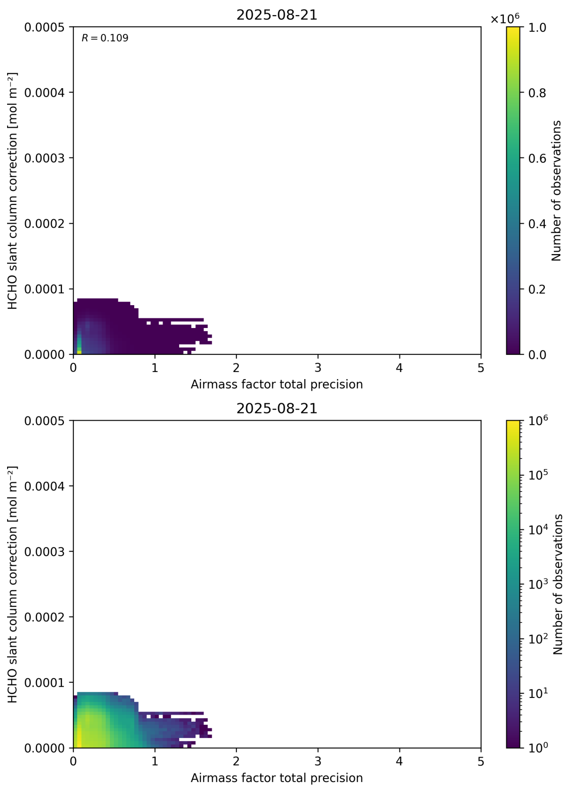
Figure 110: Scatter density plot of “Airmass factor total precision” against “HCHO slant column correction” for 2025-08-20 to 2025-08-22.
