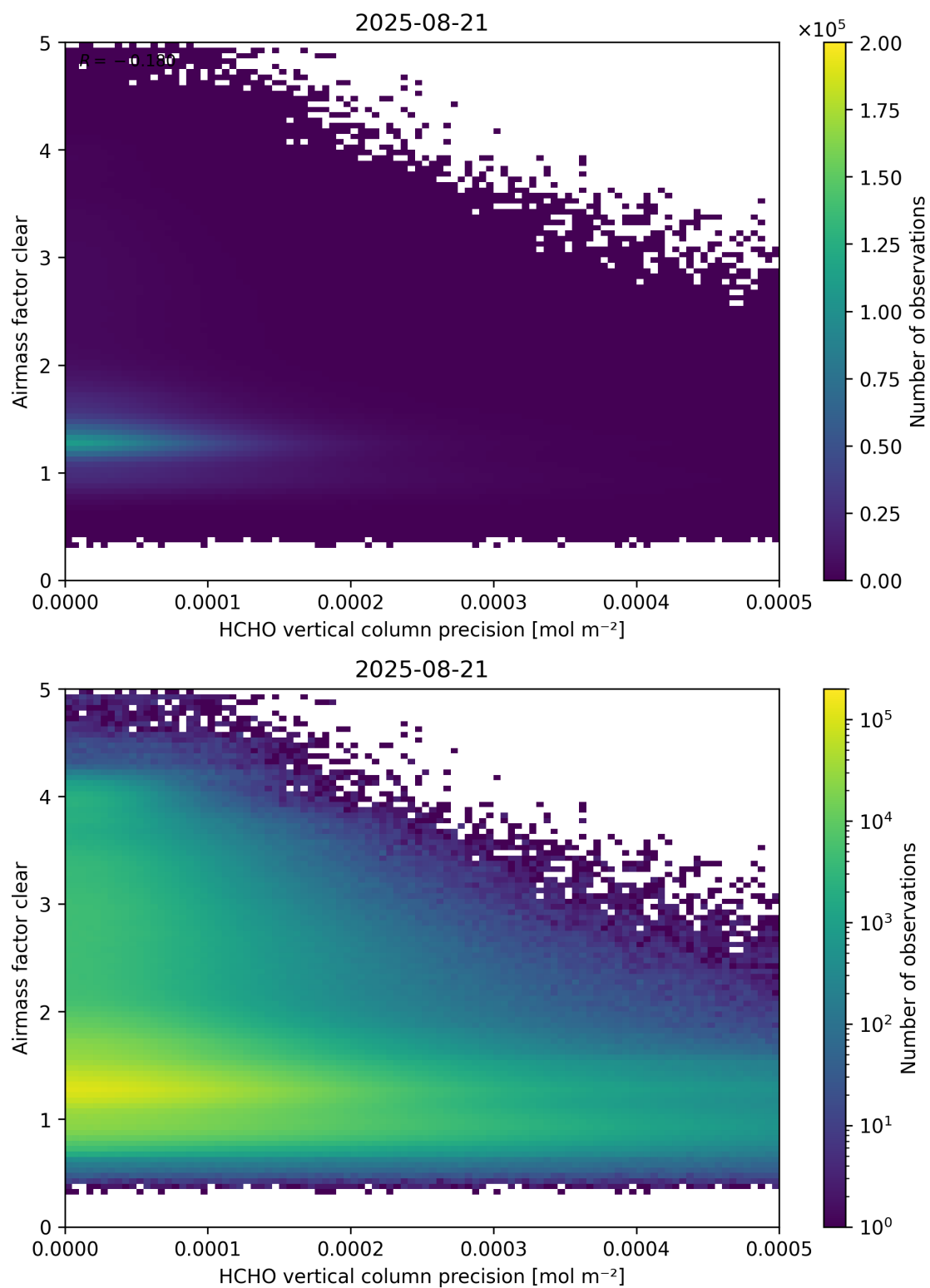
Figure 139: Scatter density plot of “HCHO vertical column precision” against “Airmass factor clear” for 2025-08-20 to 2025-08-22.
