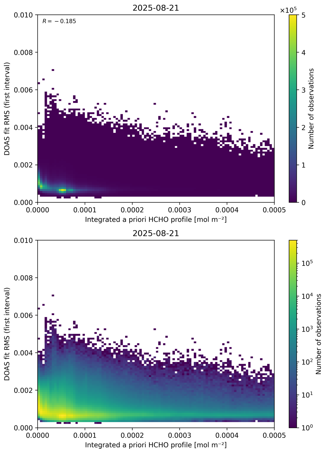
Figure 148: Scatter density plot of “Integrated a priori HCHO profile” against “DOAS fit RMS (first interval)” for 2025-08-20 to 2025-08-22.
