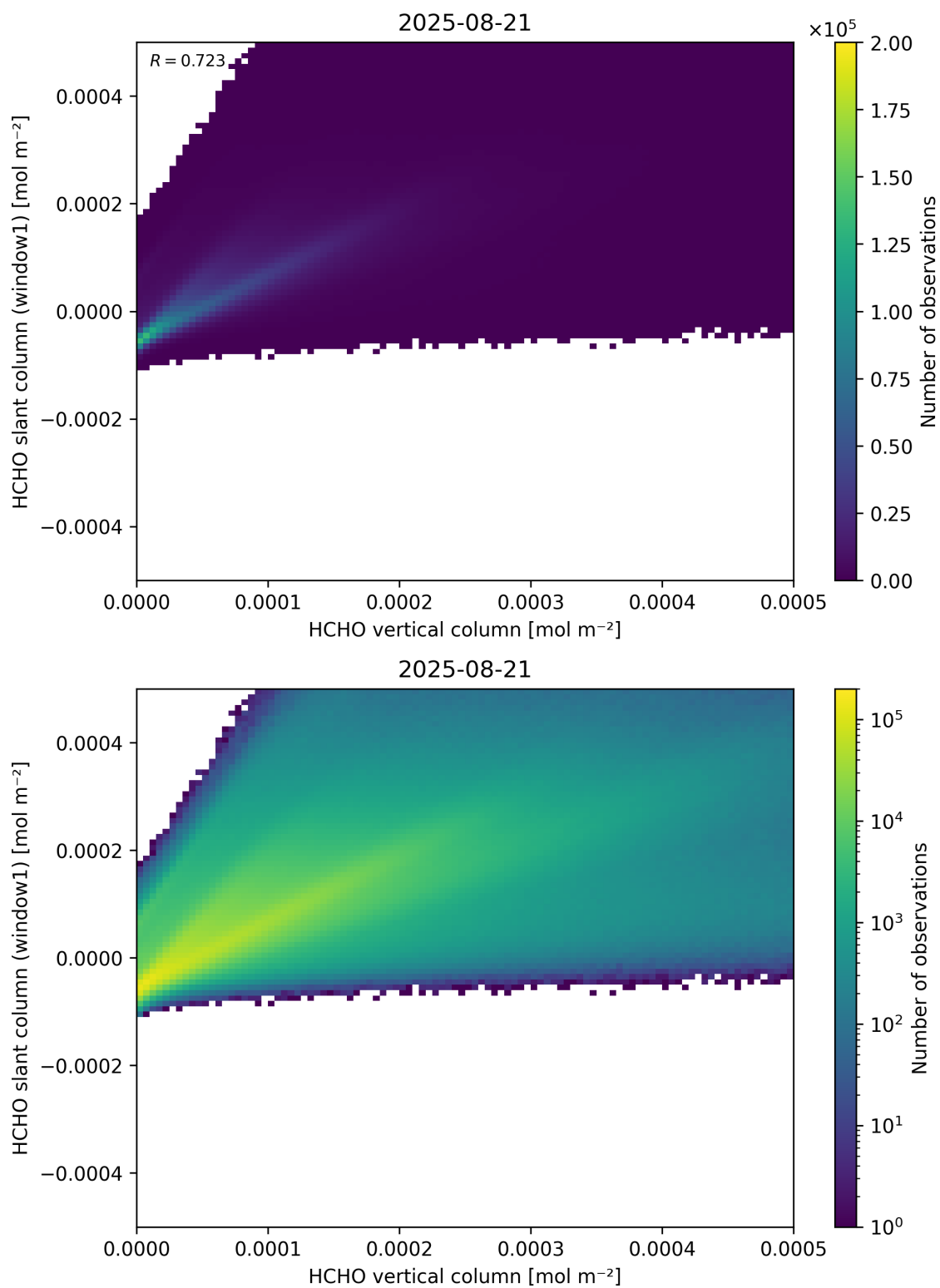
Figure 129: Scatter density plot of “HCHO vertical column” against “HCHO slant column (window1)” for 2025-08-20 to 2025-08-22.
