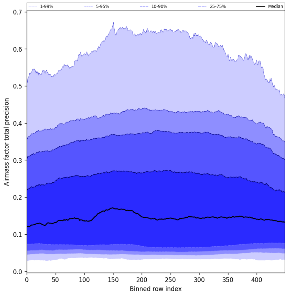
Figure 55: Along track statistics of “Airmass factor total precision” for 2025-08-20 to 2025-08-22
