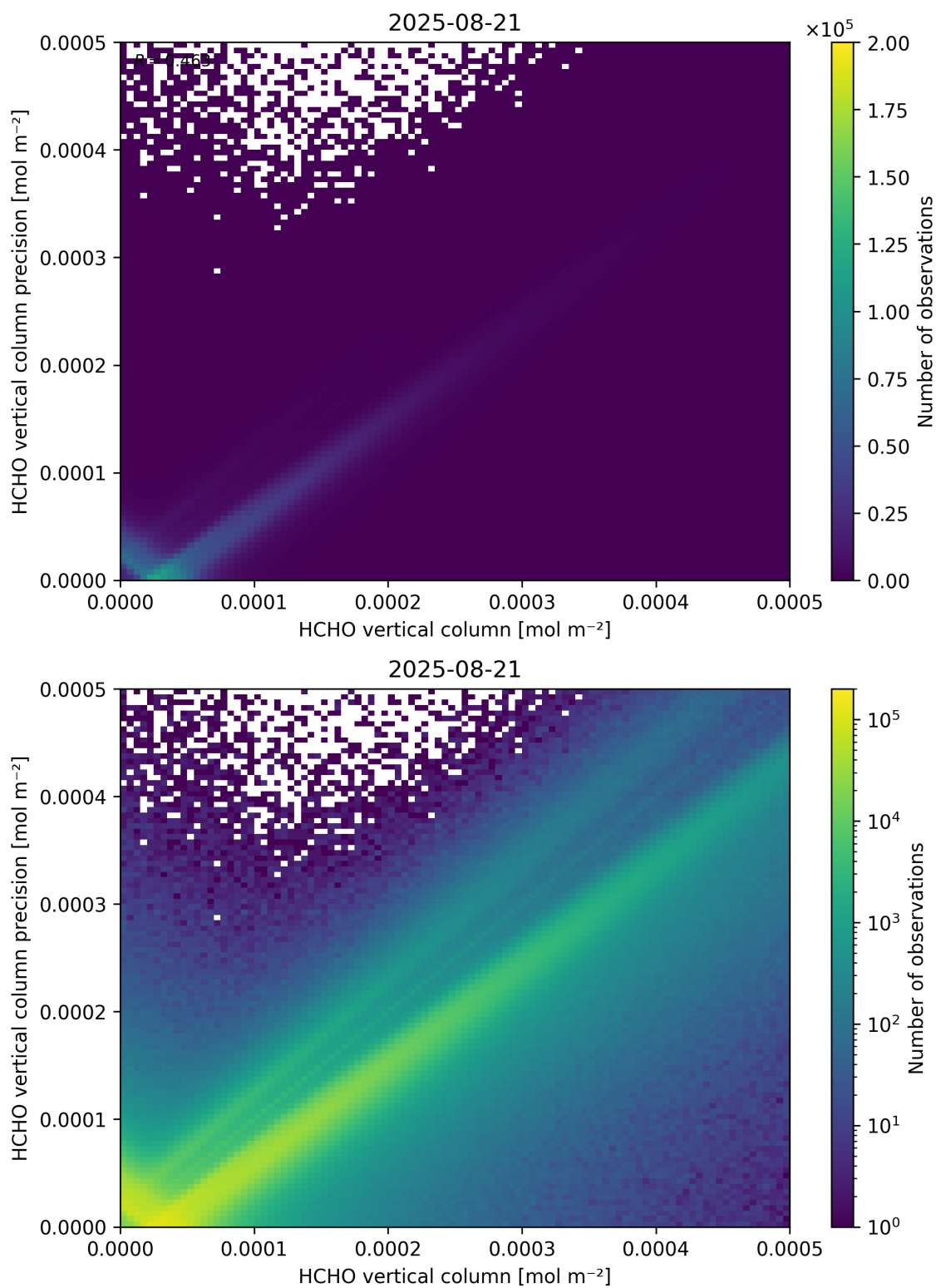
Figure 134: Scatter density plot of “HCHO vertical column” against “HCHO vertical column precision” for 2025-08-20 to 2025-08-22.
