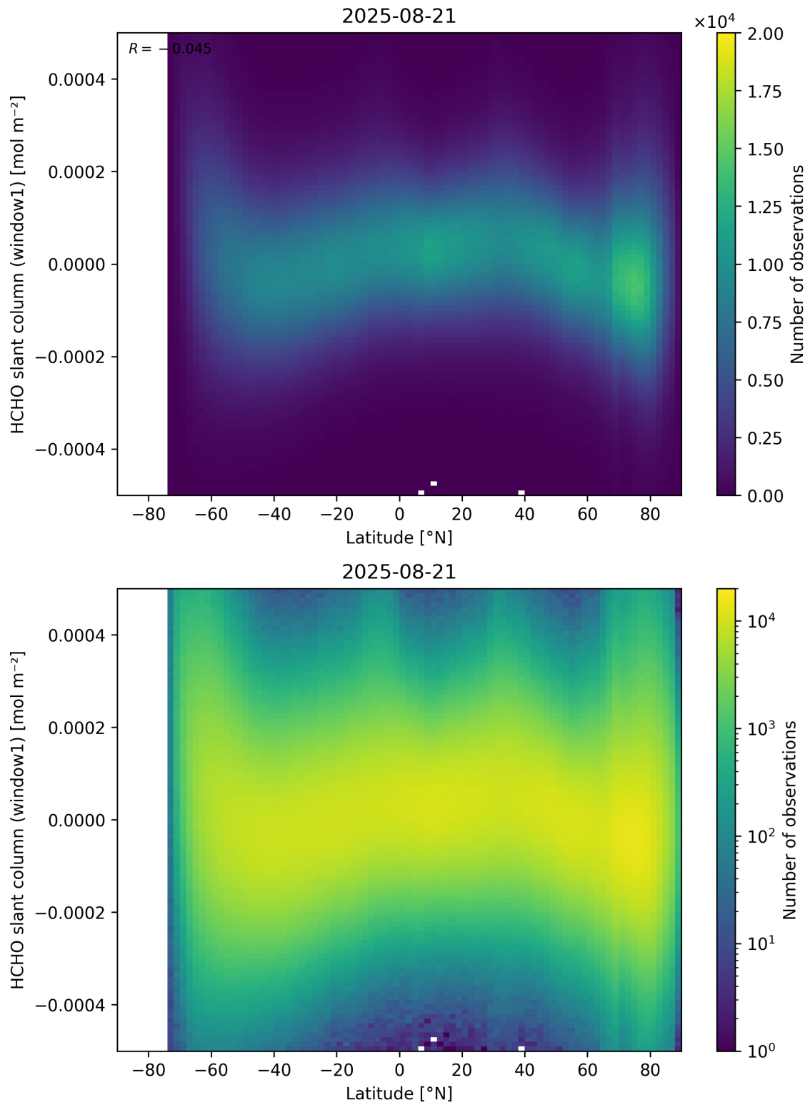
Figure 159: Scatter density plot of “Latitude” against “HCHO slant column (window1)” for 2025-08-20 to 2025-08-22.
