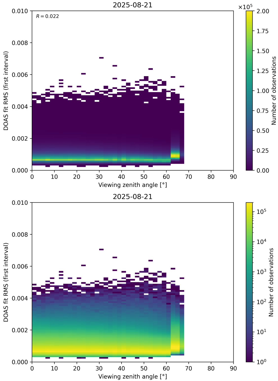
Figure 182: Scatter density plot of “Viewing zenith angle” against “DOAS fit RMS (first interval)” for 2025-08-20 to 2025-08-22.
