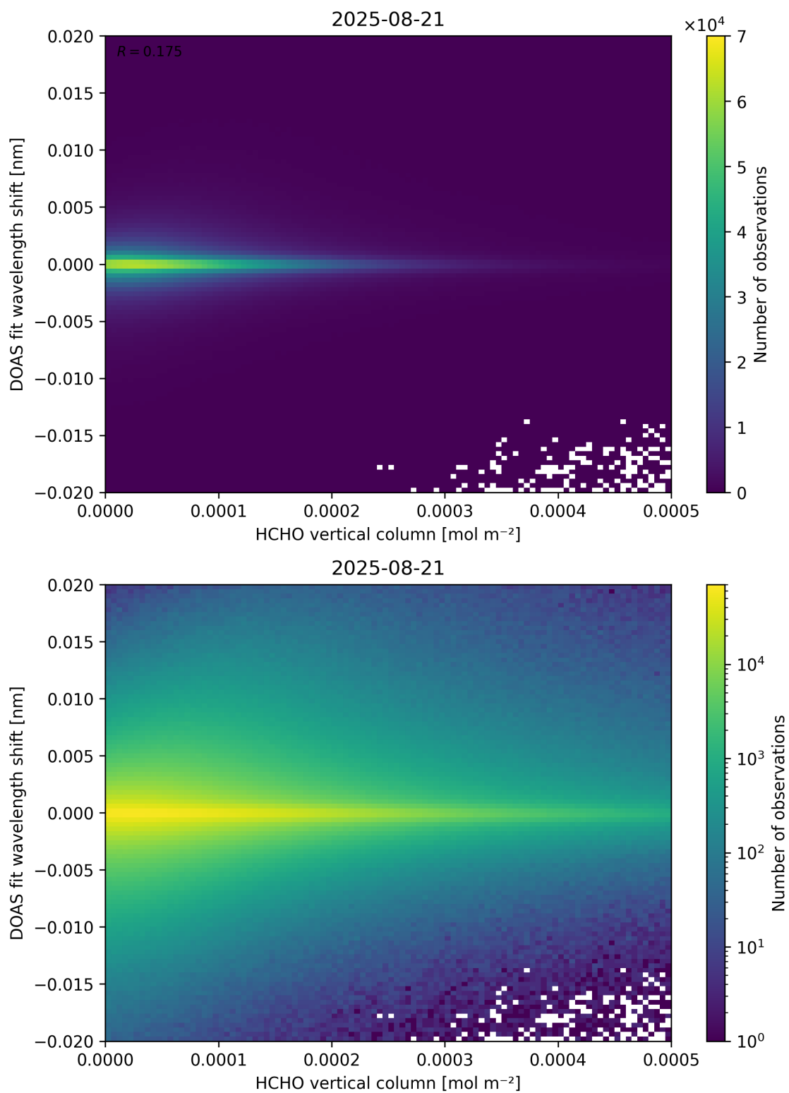
Figure 124: Scatter density plot of “HCHO vertical column” against “DOAS fit wavelength shift” for 2025-08-20 to 2025-08-22.
