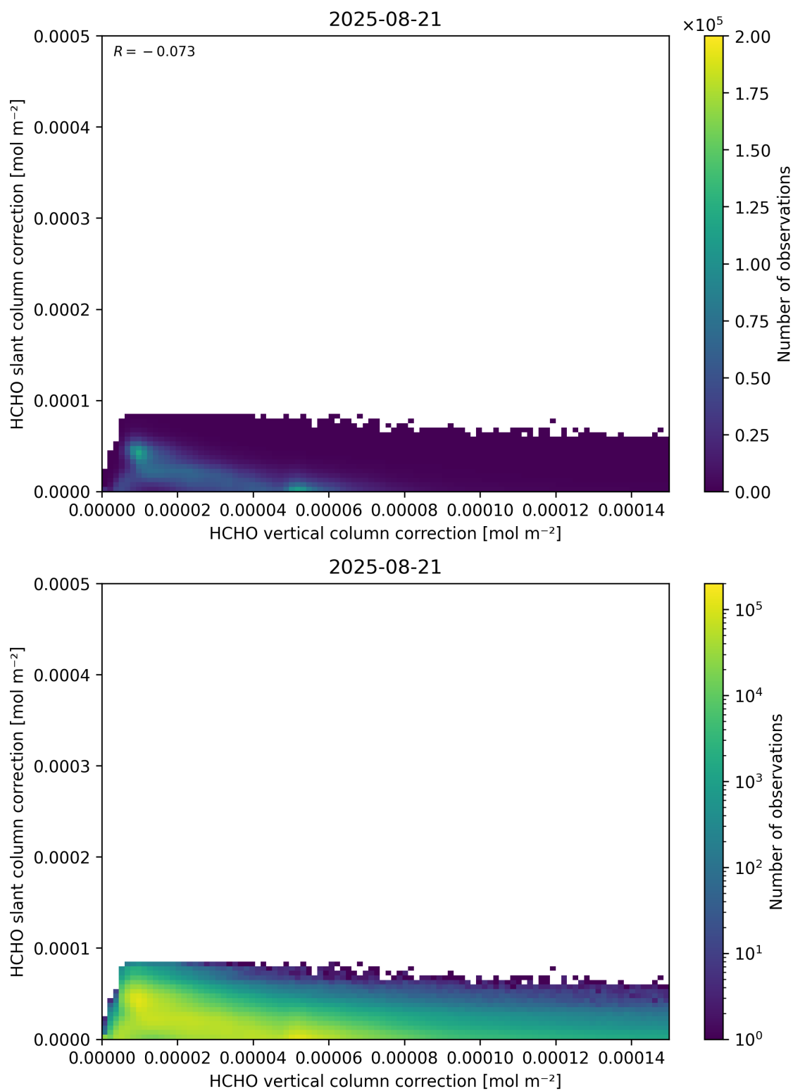
Figure 117: Scatter density plot of “HCHO vertical column correction” against “HCHO slant column correction” for 2025-08-20 to 2025-08-22.
