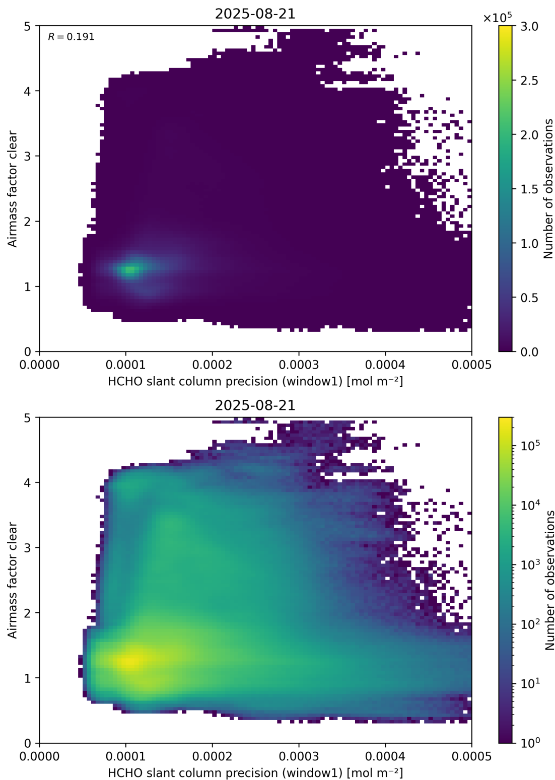
Figure 91: Scatter density plot of “HCHO slant column precision (window1)” against “Airmass factor clear” for 2025-08-20 to 2025-08-22.
