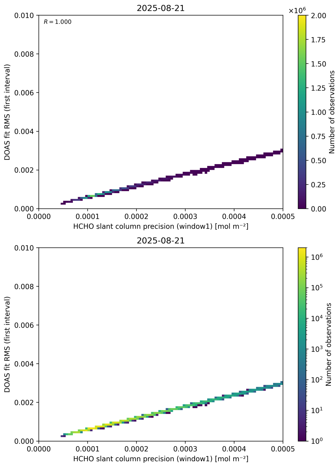
Figure 88: Scatter density plot of “HCHO slant column precision (window1)” against “DOAS fit RMS (first interval)” for 2025-08-20 to 2025-08-22.
