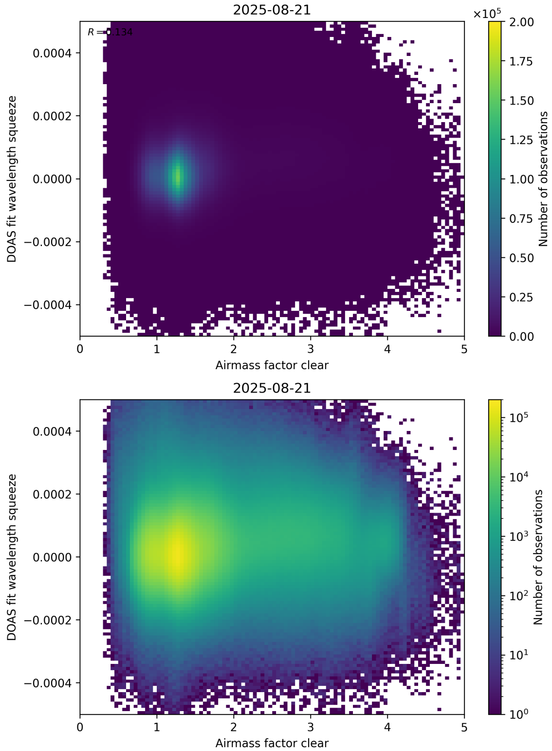
Figure 73: Scatter density plot of “Airmass factor clear” against “DOAS fit wavelength squeeze” for 2025-08-20 to 2025-08-22.
