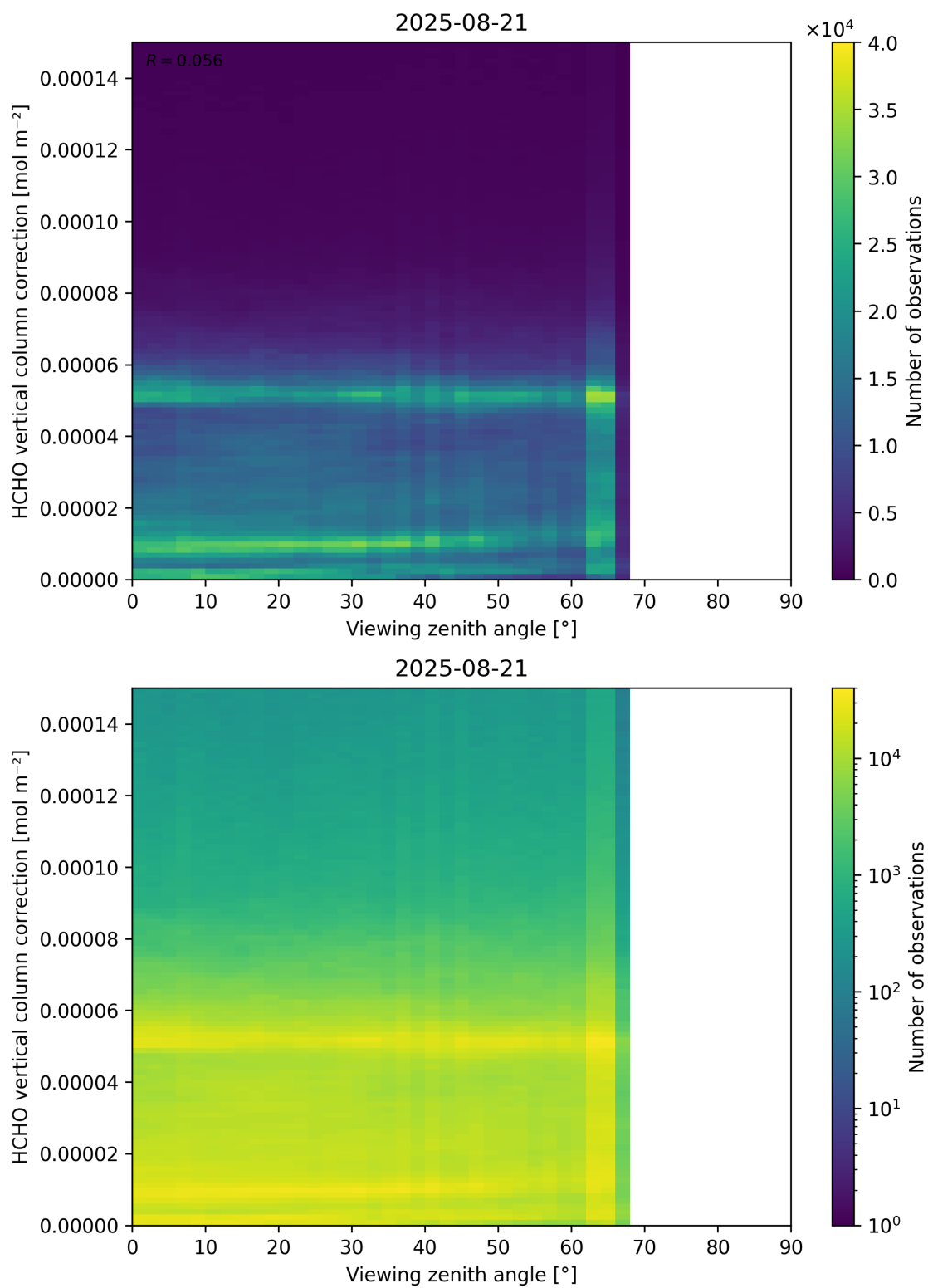
Figure 193: Scatter density plot of “Viewing zenith angle” against “HCHO vertical column correction” for 2025-08-20 to 2025-08-22.
