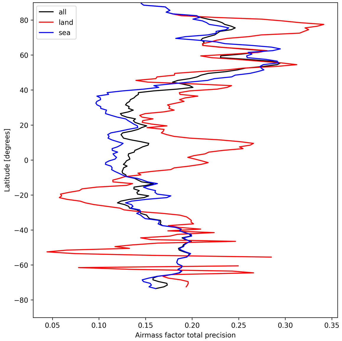
Figure 27: Zonal average of “Airmass factor total precision” for 2025-08-20 to 2025-08-22.
