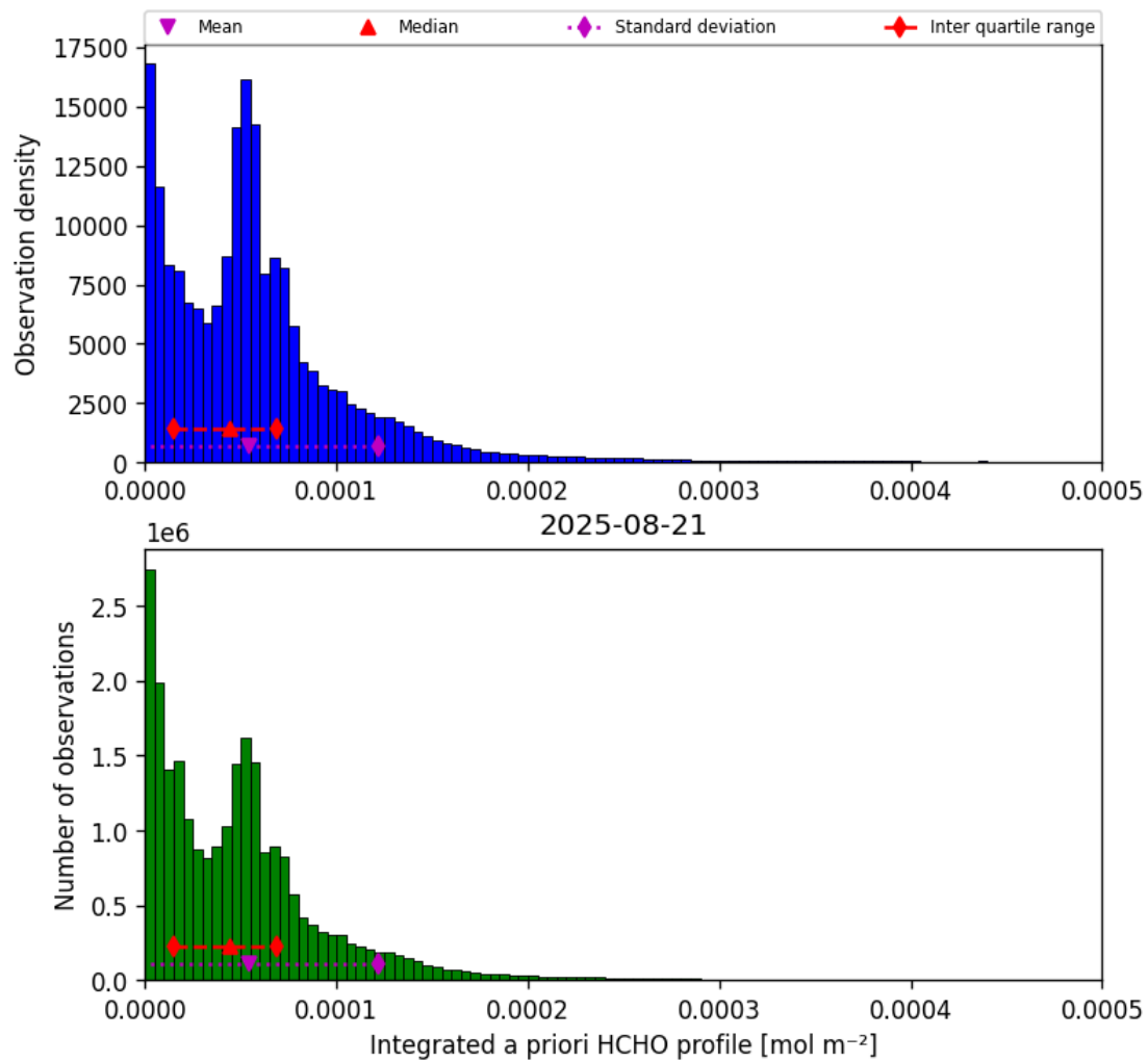
Figure 43: Histogram of “Integrated a priori HCHO profile” for 2025-08-20 to 2025-08-22
