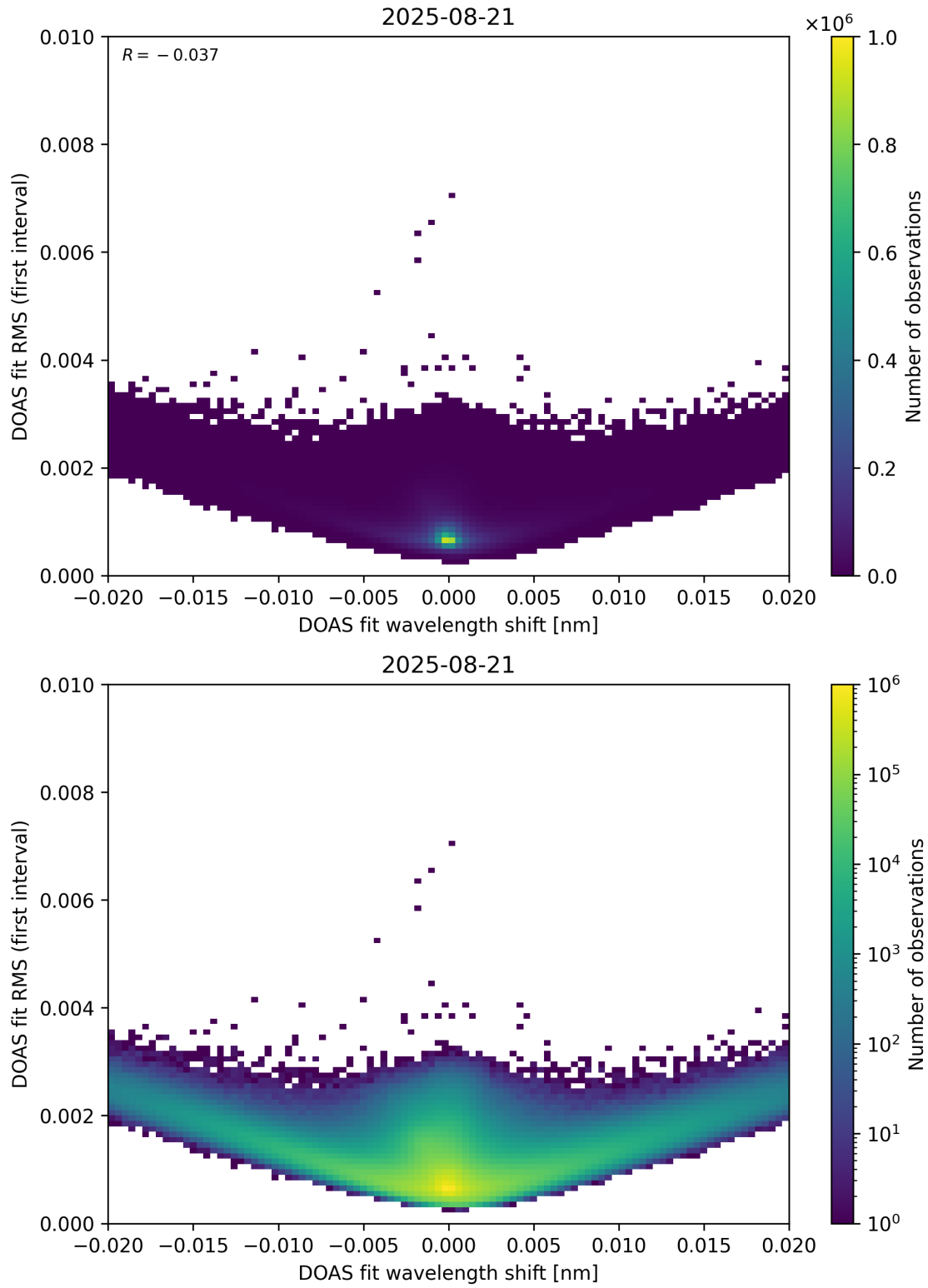
Figure 64: Scatter density plot of “DOAS fit wavelength shift” against “DOAS fit RMS (first interval)” for 2025-08-20 to 2025-08-22.
