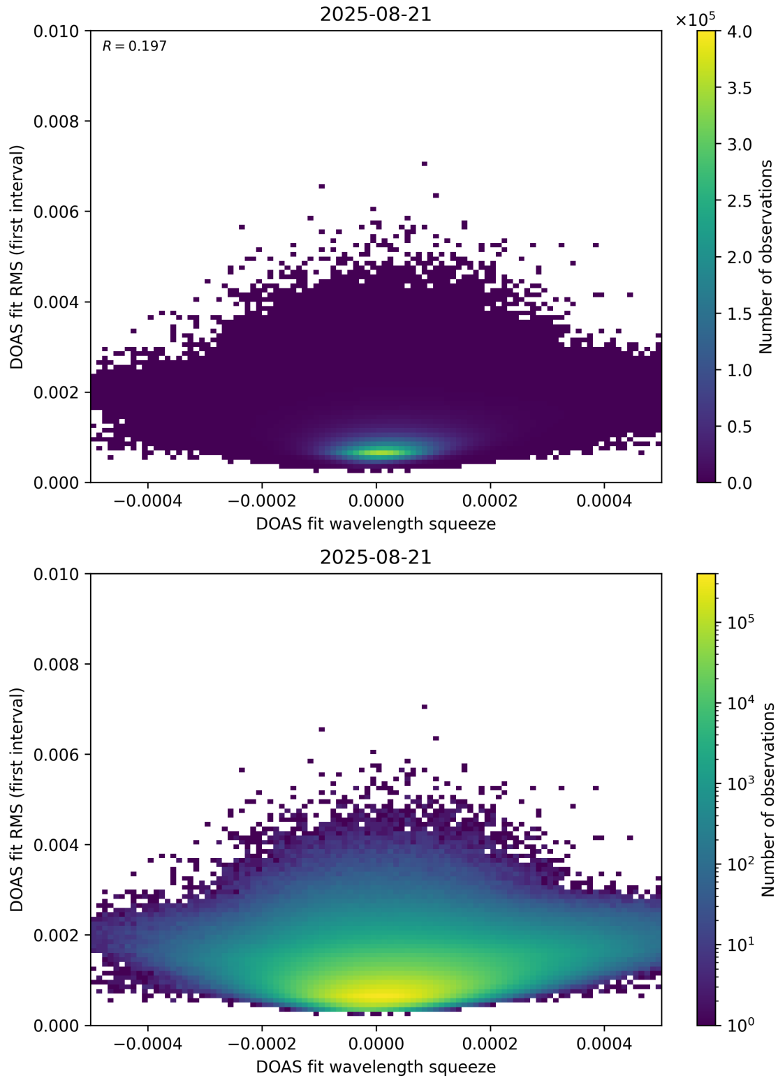
Figure 68: Scatter density plot of “DOAS fit wavelength squeeze” against “DOAS fit RMS (first interval)” for 2025-08-20 to 2025-08-22.
