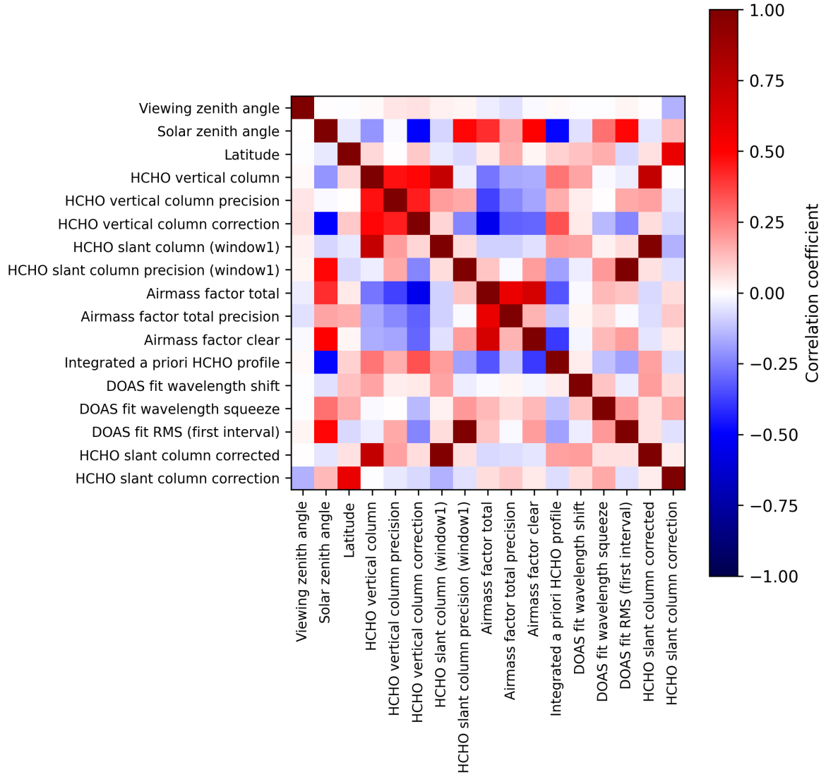
Figure 2: Map of correlation matrix for 2025-08-20 to 2025-08-22.
