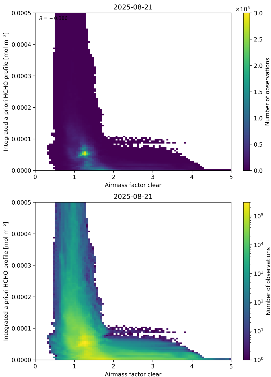
Figure 76: Scatter density plot of “Airmass factor clear” against “Integrated a priori HCHO profile” for 2025-08-20 to 2025-08-22.
