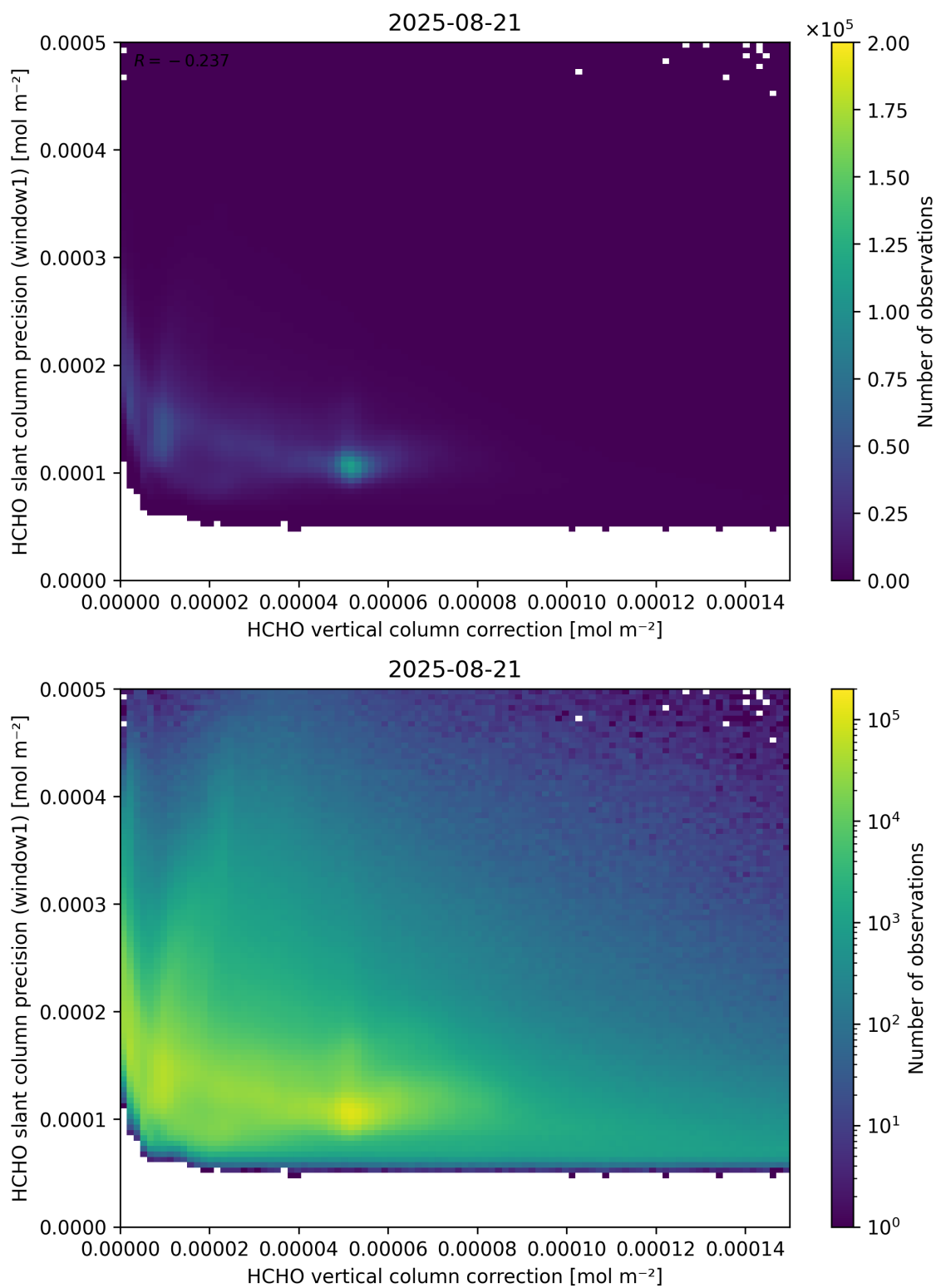
Figure 119: Scatter density plot of “HCHO vertical column correction” against “HCHO slant column precision (window1)” for 2025-08-20 to 2025-08-22.
