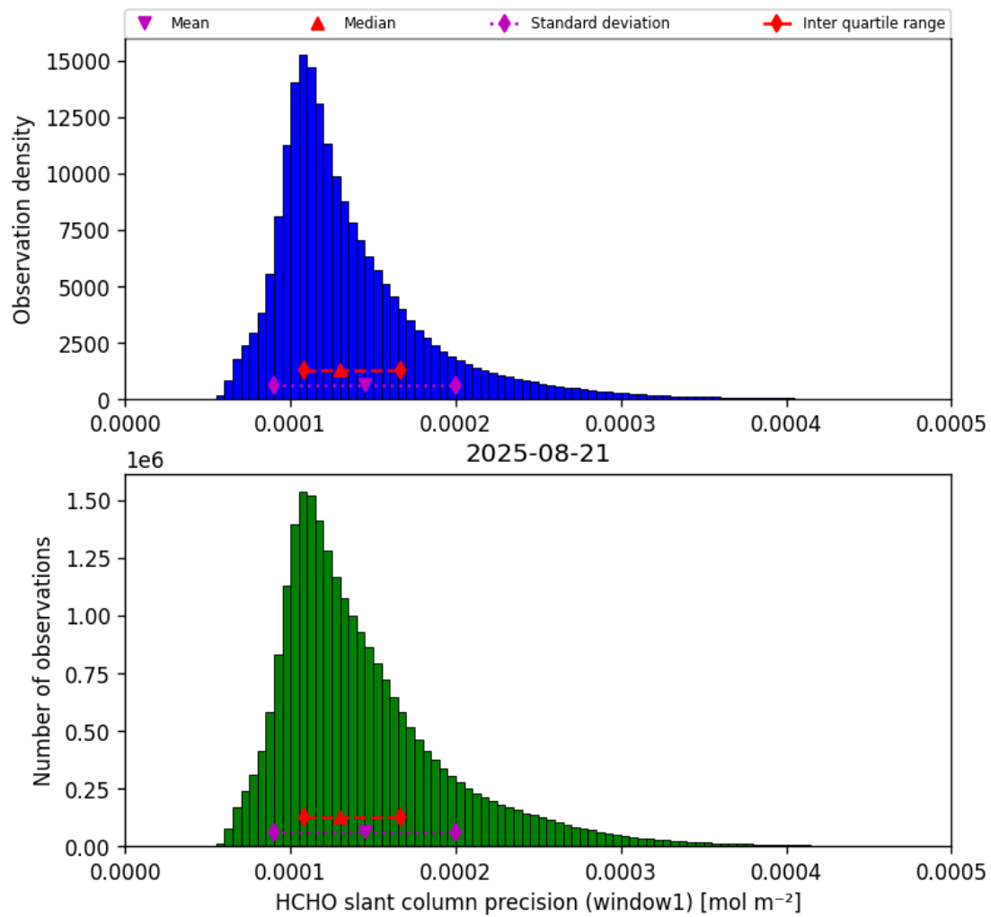
Figure 39: Histogram of “HCHO slant column precision (window1)” for 2025-08-20 to 2025-08-22
