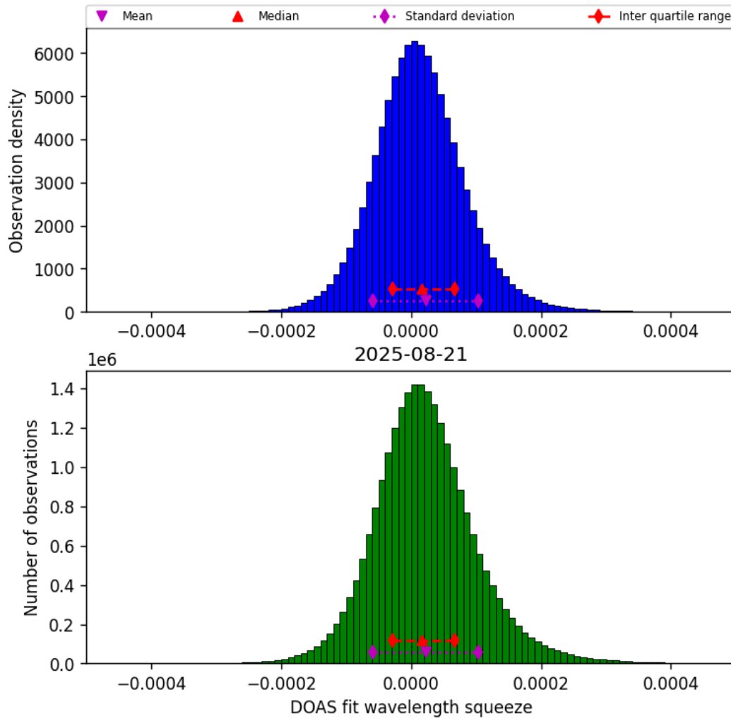
Figure 45: Histogram of “DOAS fit wavelength squeeze” for 2025-08-20 to 2025-08-22
