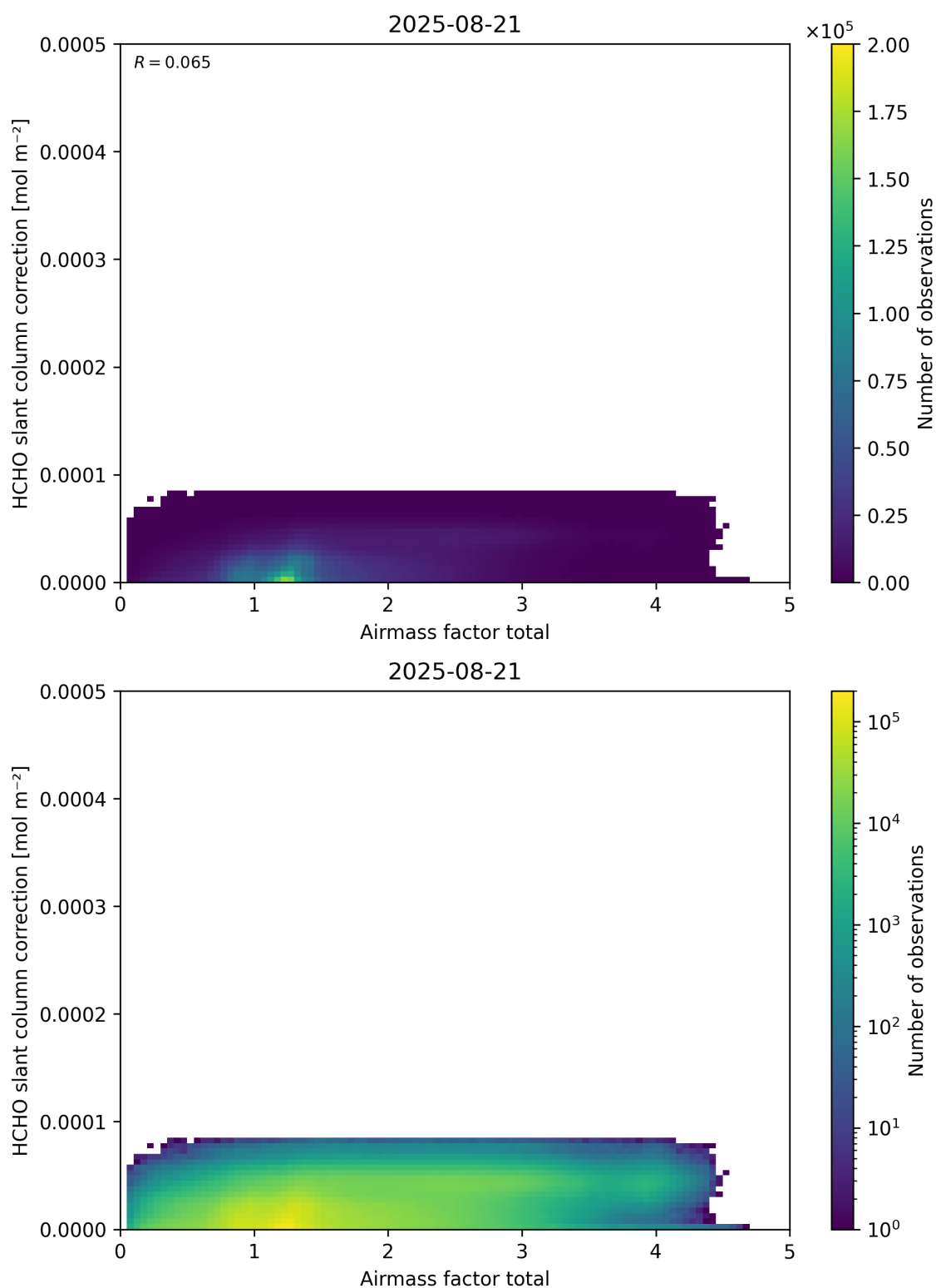
Figure 102: Scatter density plot of “Airmass factor total” against “HCHO slant column correction” for 2025-08-20 to 2025-08-22.
