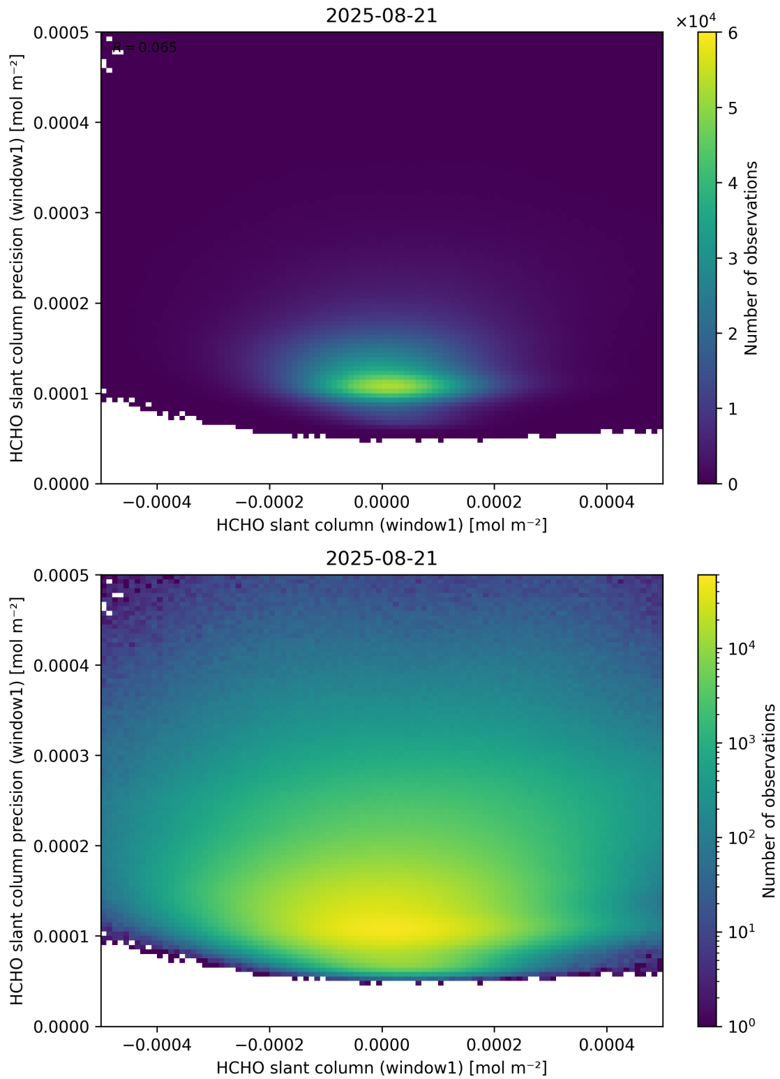
Figure 84: Scatter density plot of “HCHO slant column (window1)” against “HCHO slant column precision (window1)” for 2025-08-20 to 2025-08-22.
