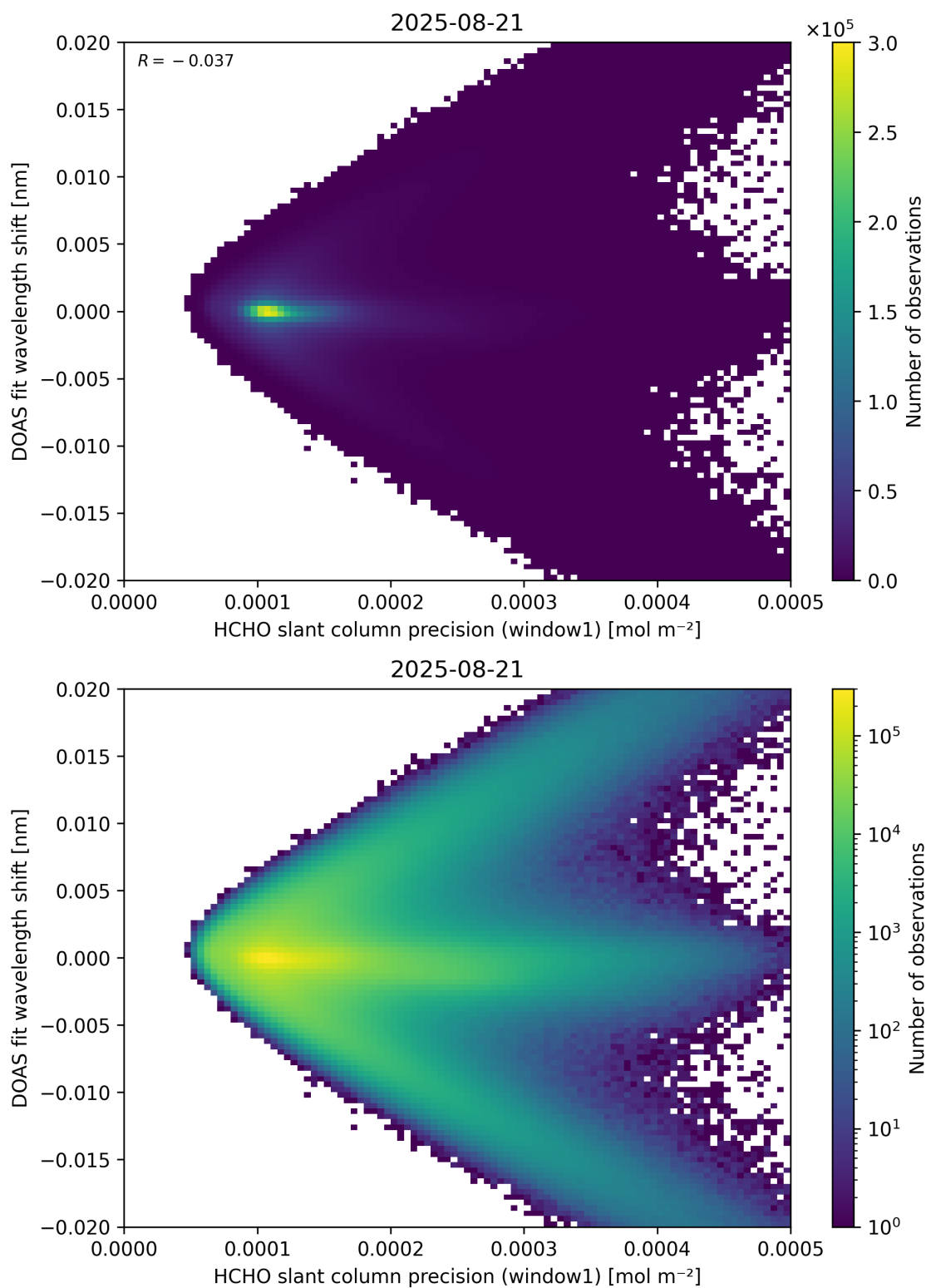
Figure 89: Scatter density plot of “HCHO slant column precision (window1)” against “DOAS fit wavelength shift” for 2025-08-20 to 2025-08-22.
