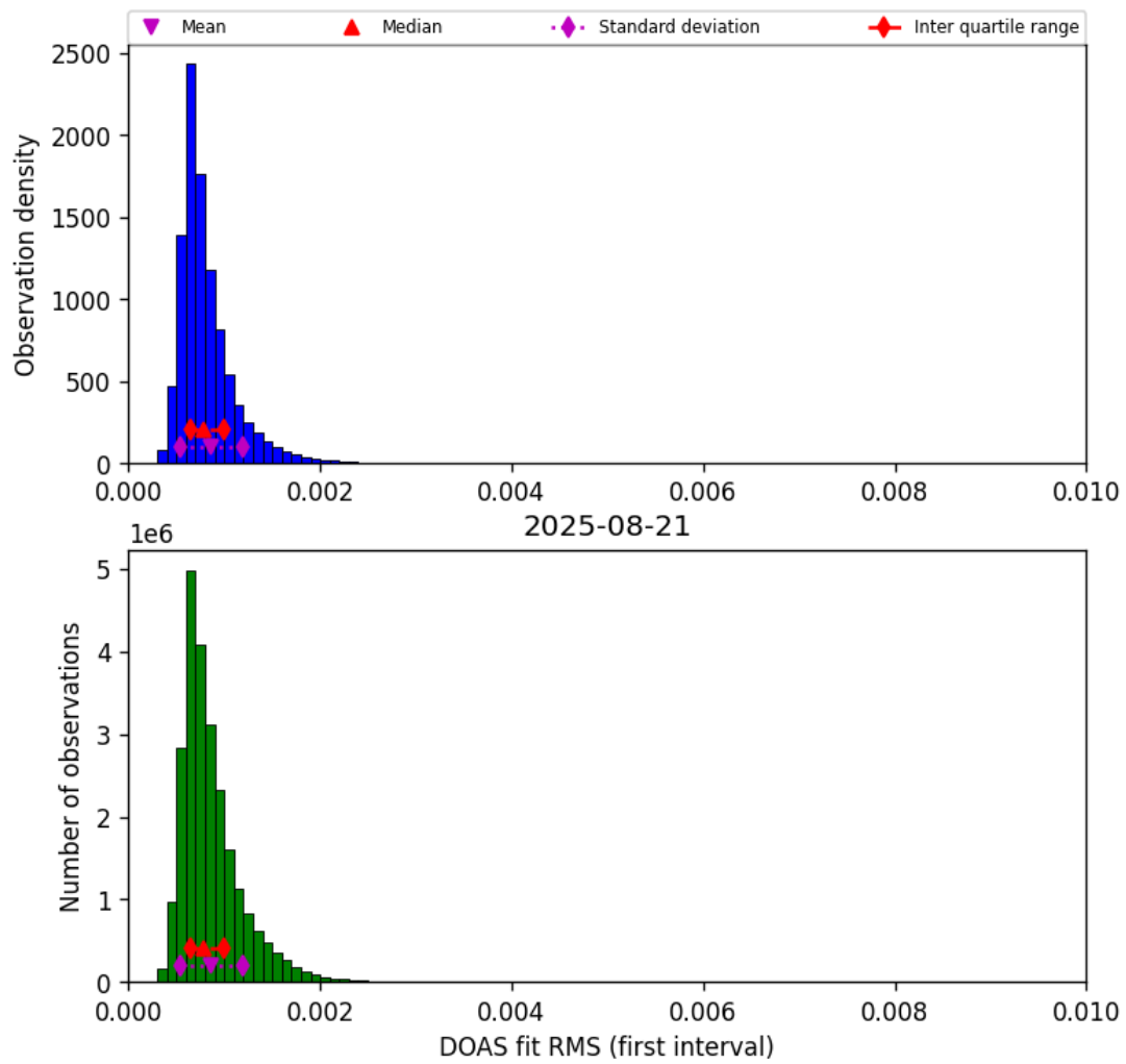
Figure 46: Histogram of “DOAS fit RMS (first interval)” for 2025-08-20 to 2025-08-22
