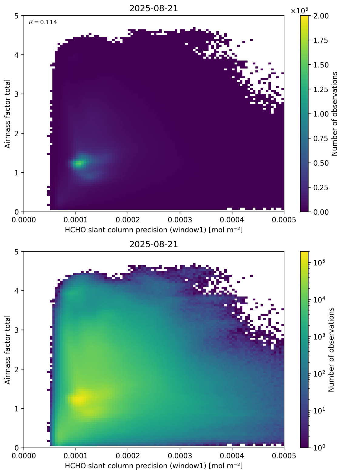
Figure 94: Scatter density plot of “HCHO slant column precision (window1)” against “Airmass factor total” for 2025-08-20 to 2025-08-22.
