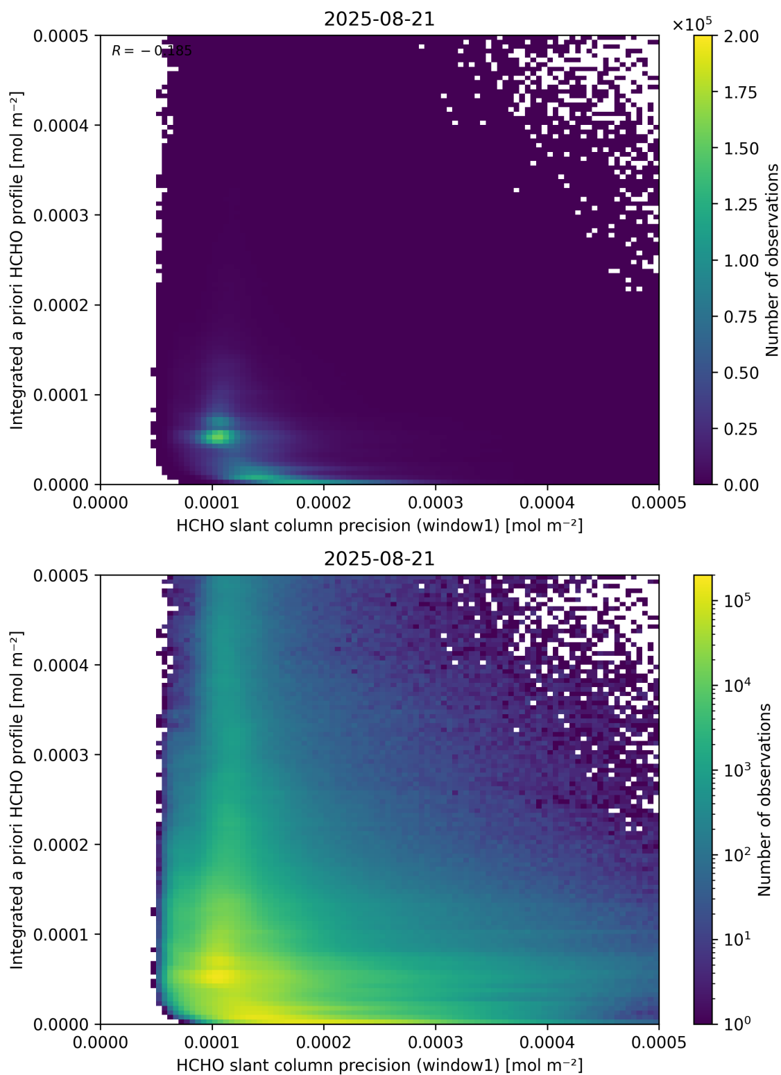
Figure 96: Scatter density plot of “HCHO slant column precision (window1)” against “Integrated a priori HCHO profile” for 2025-08-20 to 2025-08-22.
