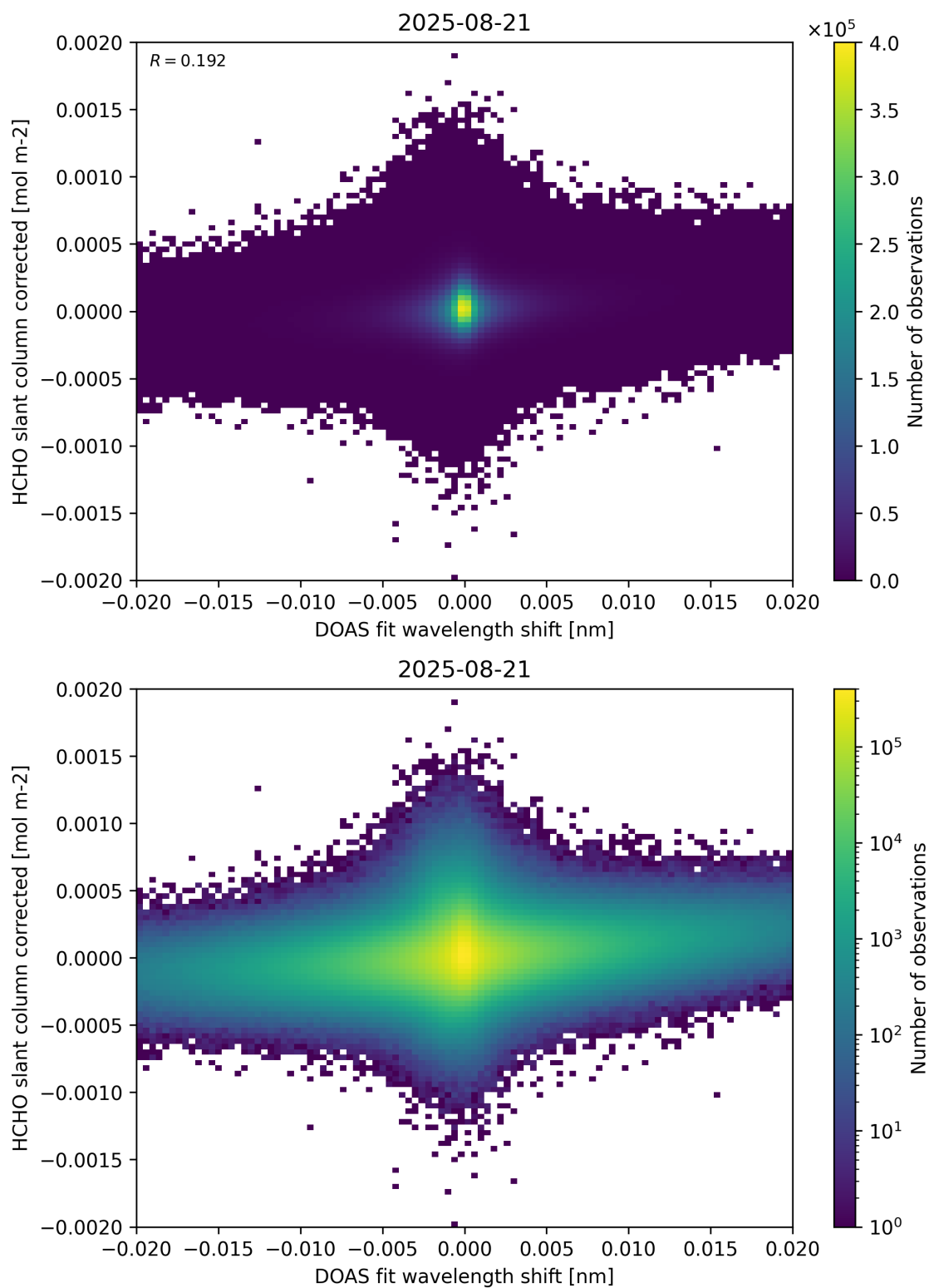
Figure 66: Scatter density plot of “DOAS fit wavelength shift” against “HCHO slant column corrected” for 2025-08-20 to 2025-08-22.
