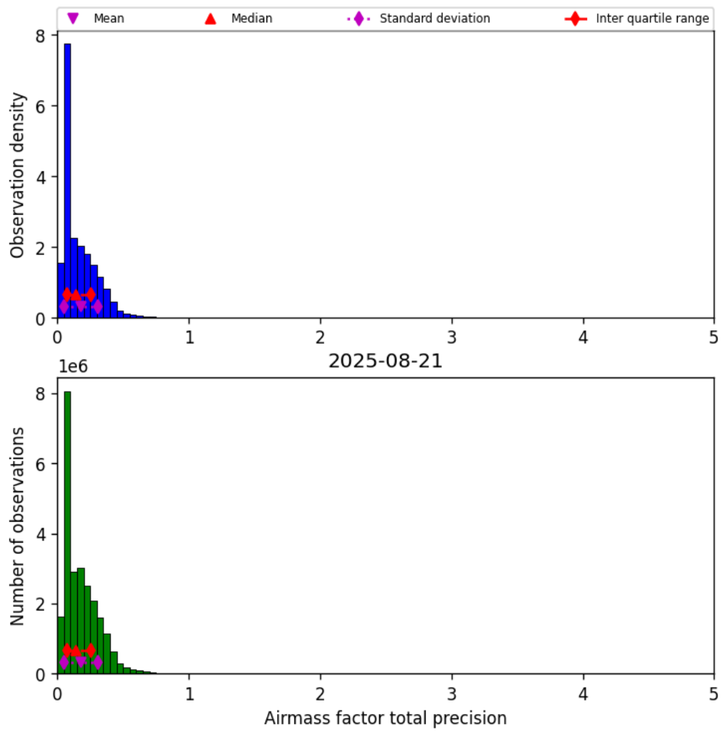
Figure 41: Histogram of “Airmass factor total precision” for 2025-08-20 to 2025-08-22
