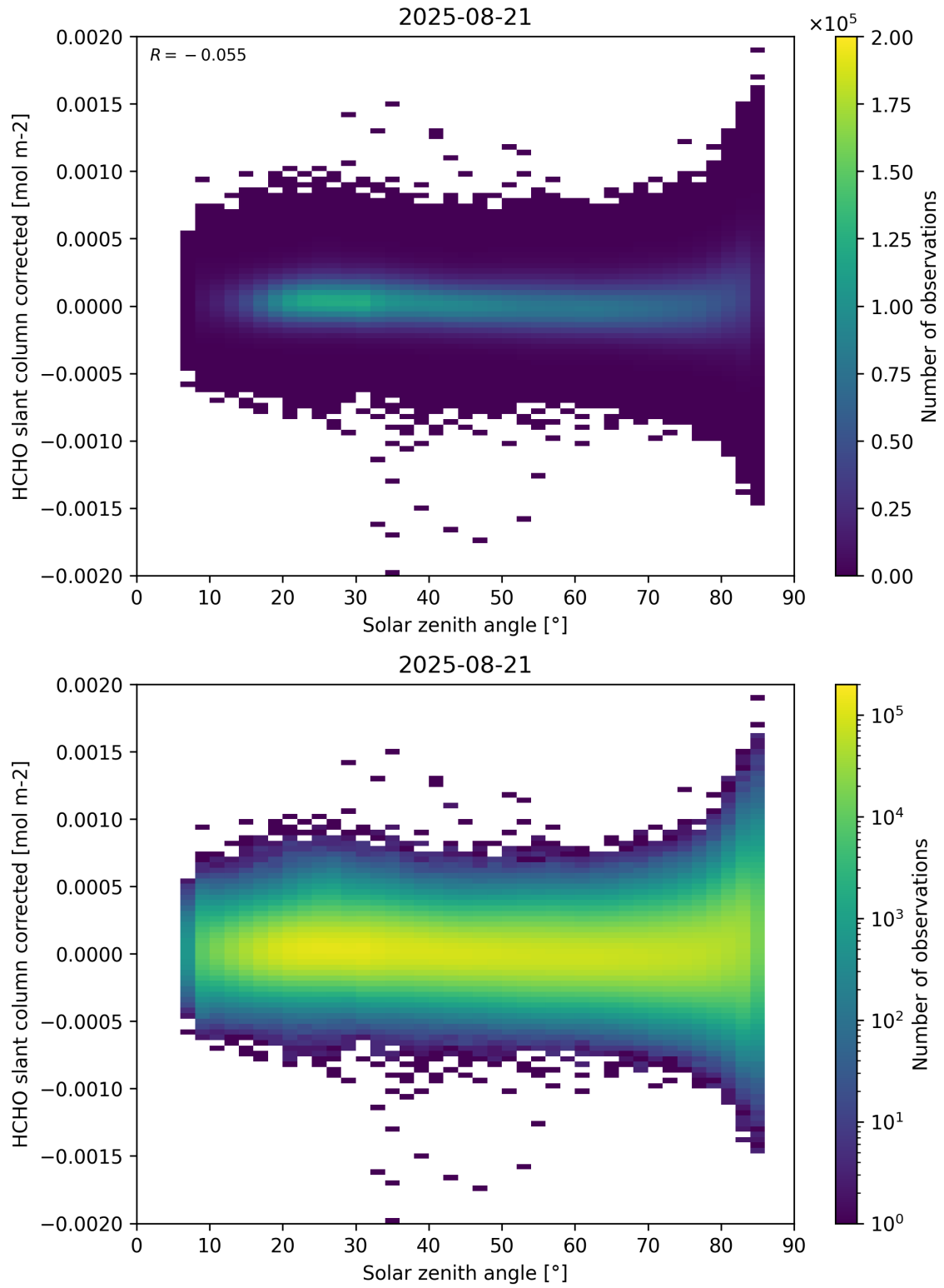
Figure 171: Scatter density plot of “Solar zenith angle” against “HCHO slant column corrected” for 2025-08-20 to 2025-08-22.
