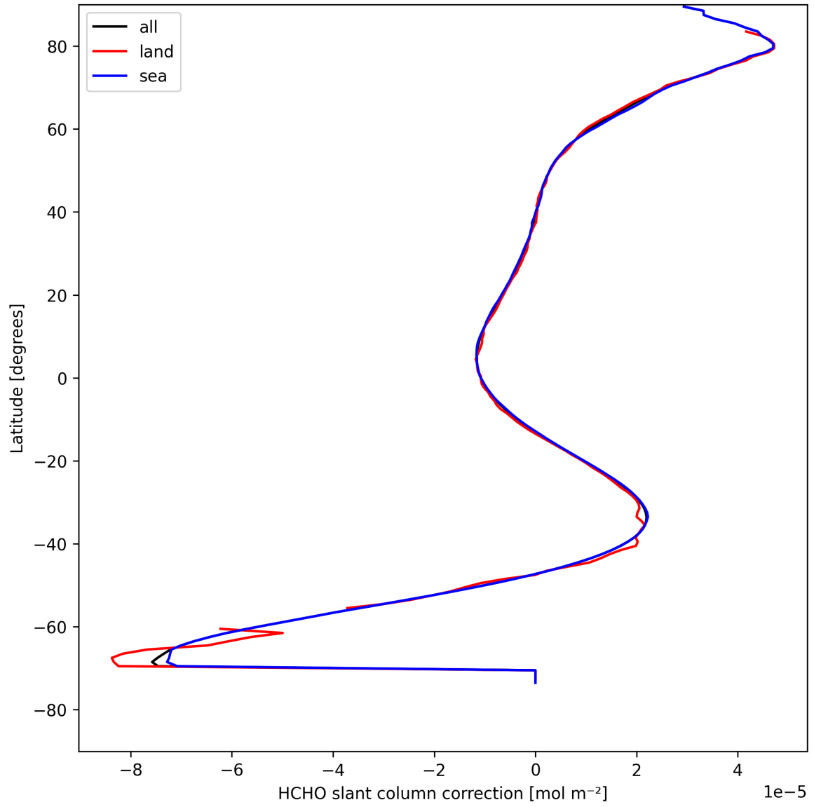
Figure 33: Zonal average of “HCHO slant column correction” for 2025-08-20 to 2025-08-22.
