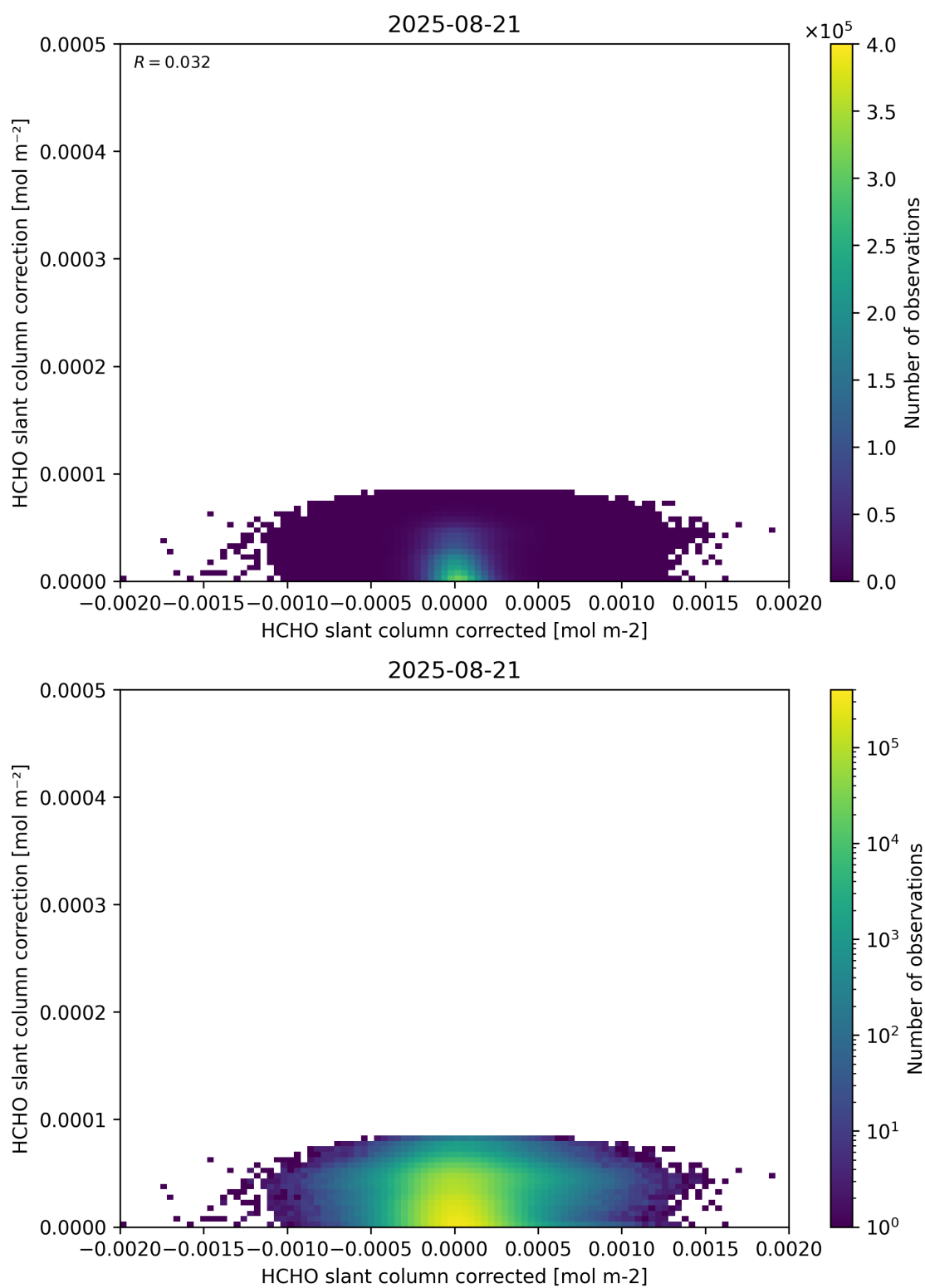
Figure 77: Scatter density plot of “HCHO slant column corrected” against “HCHO slant column correction” for 2025-08-20 to 2025-08-22.
