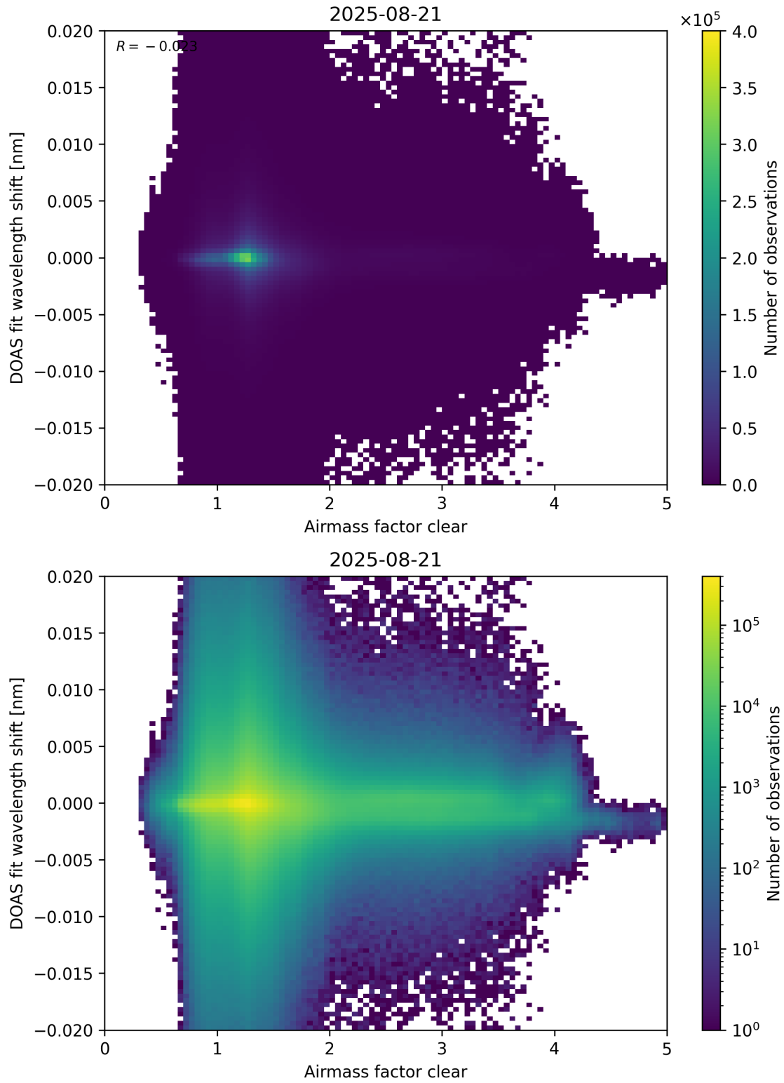
Figure 72: Scatter density plot of “Airmass factor clear” against “DOAS fit wavelength shift” for 2025-08-20 to 2025-08-22.
