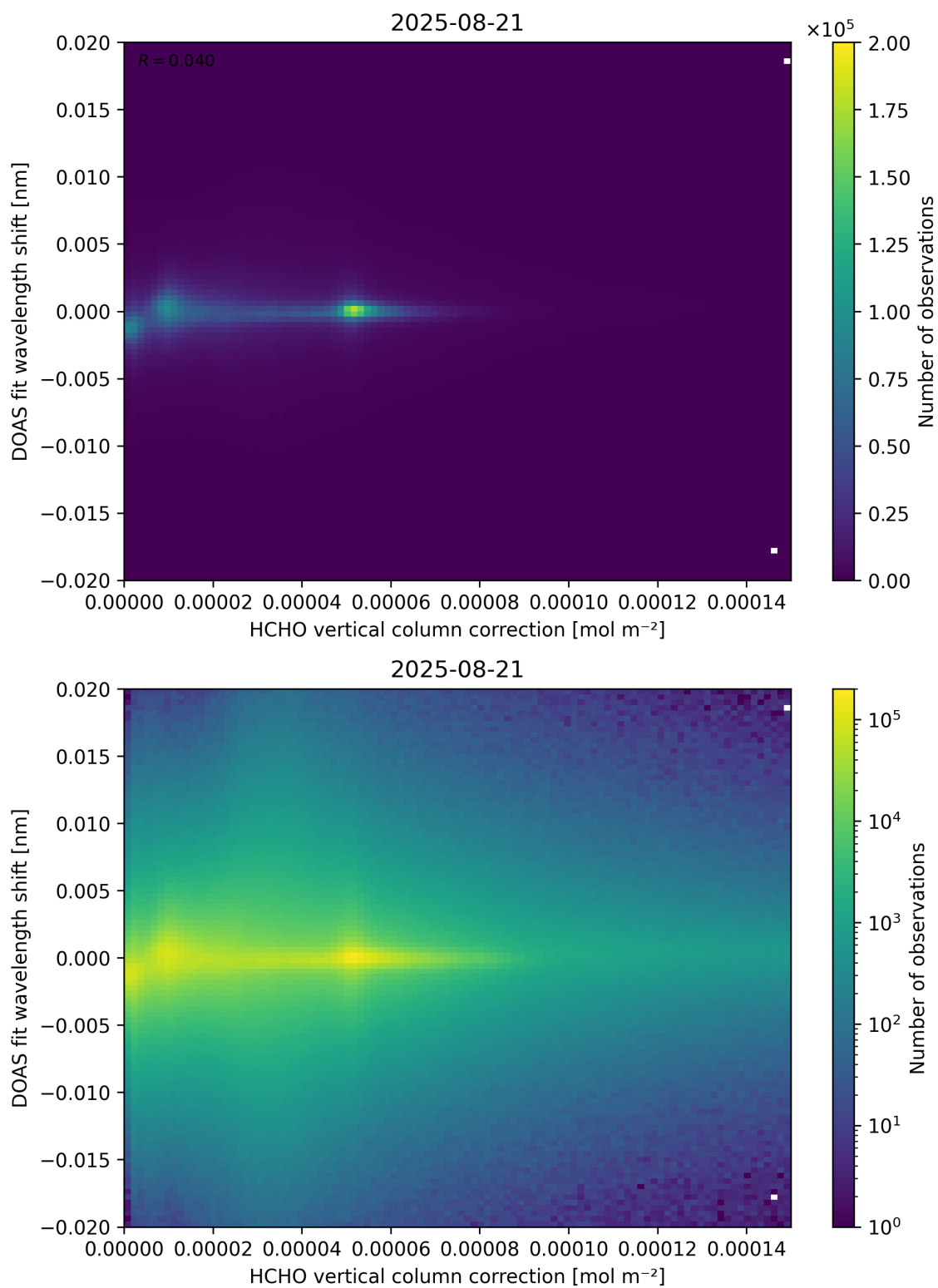
Figure 113: Scatter density plot of “HCHO vertical column correction” against “DOAS fit wavelength shift” for 2025-08-20 to 2025-08-22.
