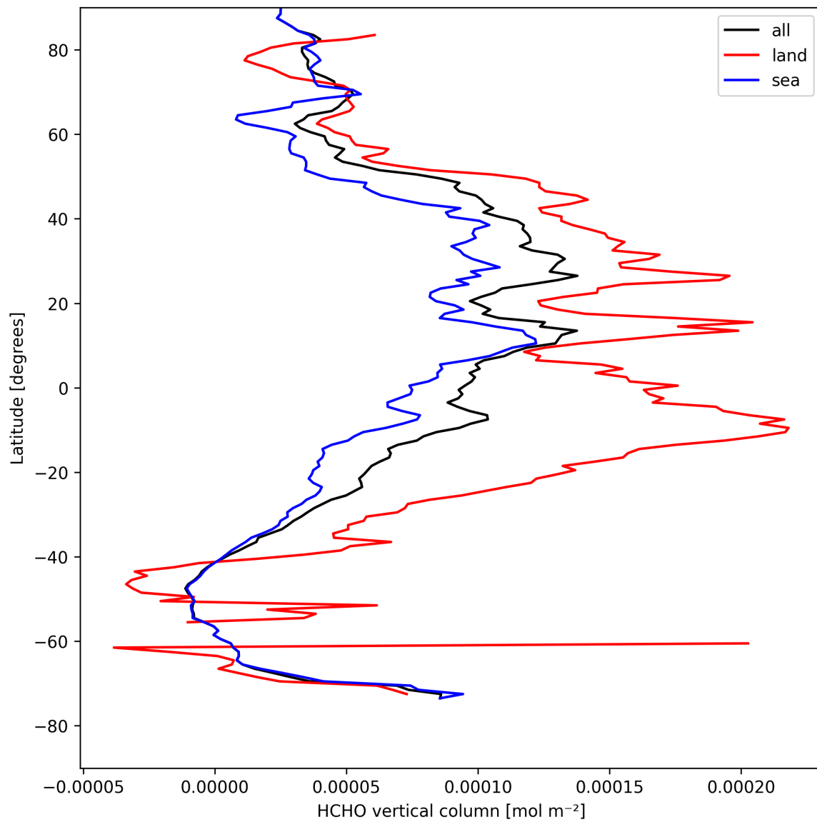
Figure 21: Zonal average of “HCHO vertical column” for 2025-08-20 to 2025-08-22.
