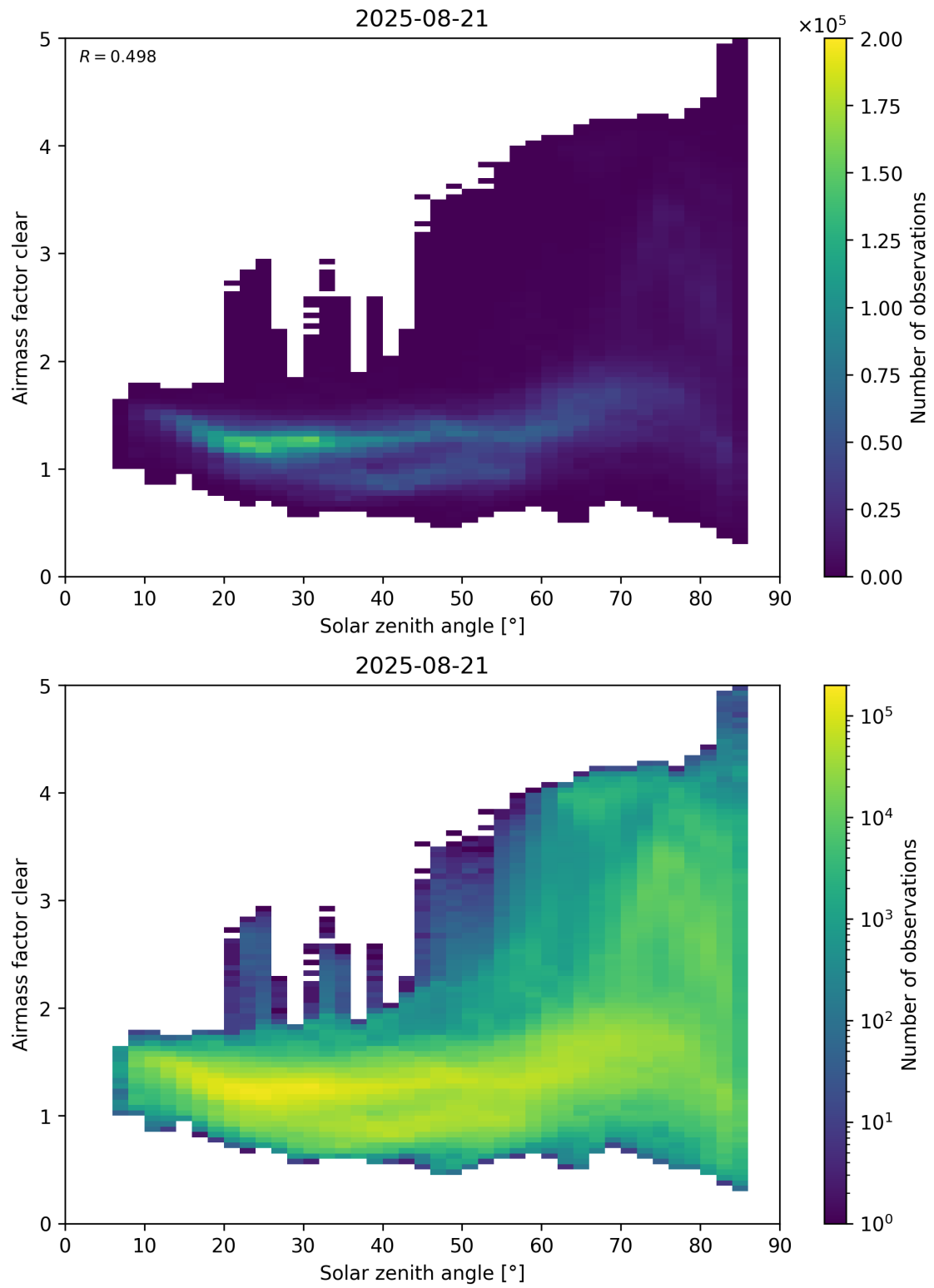
Figure 170: Scatter density plot of “Solar zenith angle” against “Airmass factor clear” for 2025-08-20 to 2025-08-22.
