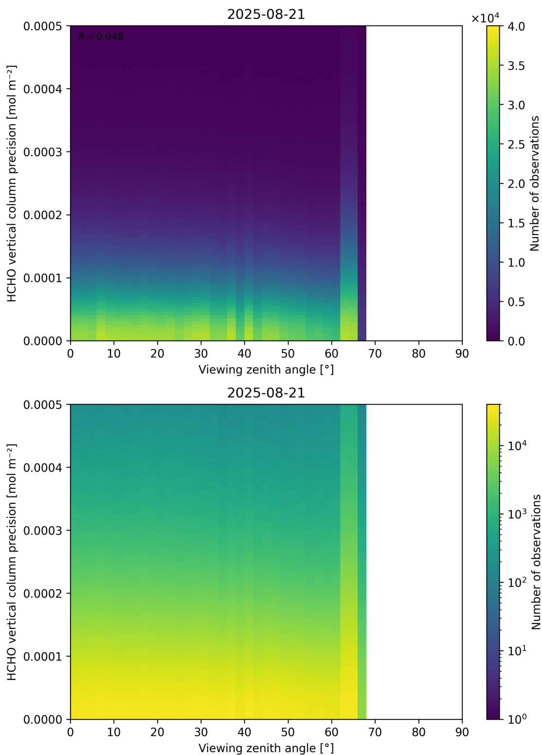
Figure 194: Scatter density plot of “Viewing zenith angle” against “HCHO vertical column precision” for 2025-08-20 to 2025-08-22.
