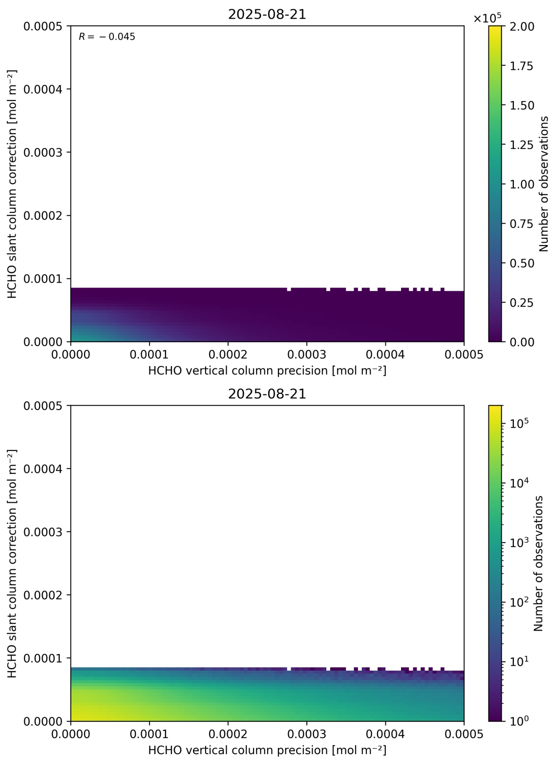
Figure 141: Scatter density plot of “HCHO vertical column precision” against “HCHO slant column correction” for 2025-08-20 to 2025-08-22.
