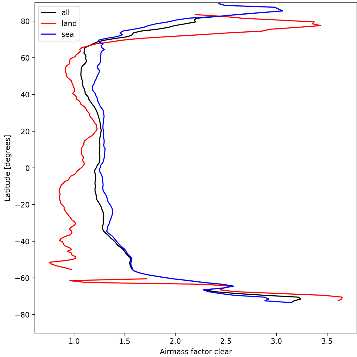
Figure 28: Zonal average of “Airmass factor clear” for 2025-08-20 to 2025-08-22.
