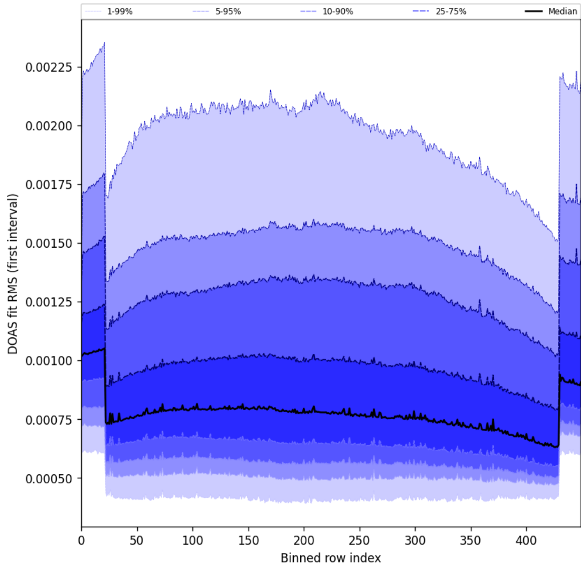
Figure 60: Along track statistics of “DOAS fit RMS (first interval)” for 2025-08-20 to 2025-08-22
