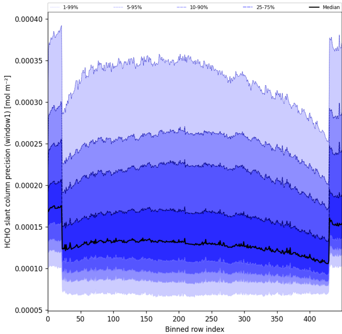
Figure 53: Along track statistics of “HCHO slant column precision (window1)” for 2025-08-20 to 2025-08-22
