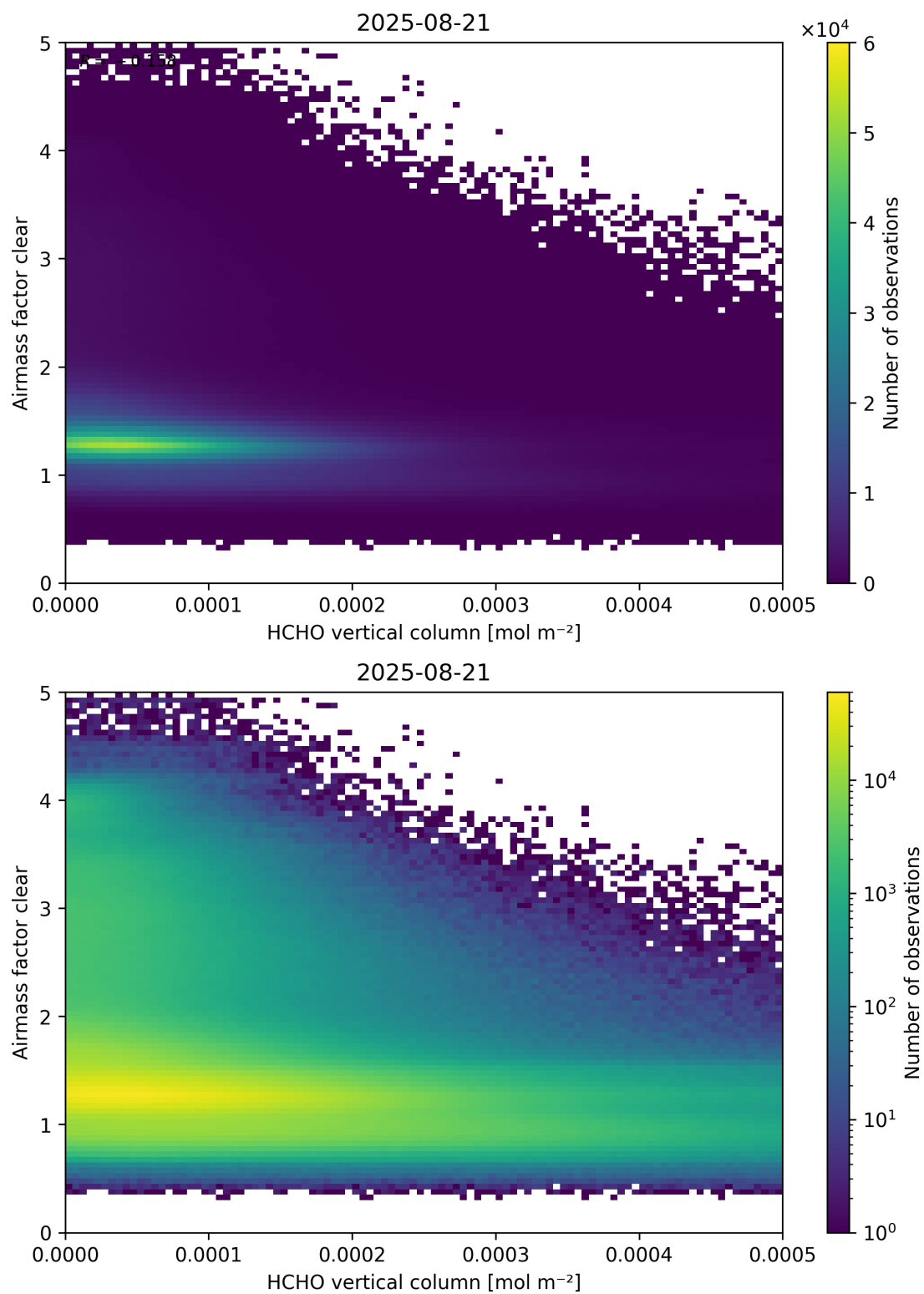
Figure 126: Scatter density plot of “HCHO vertical column” against “Airmass factor clear” for 2025-08-20 to 2025-08-22.
