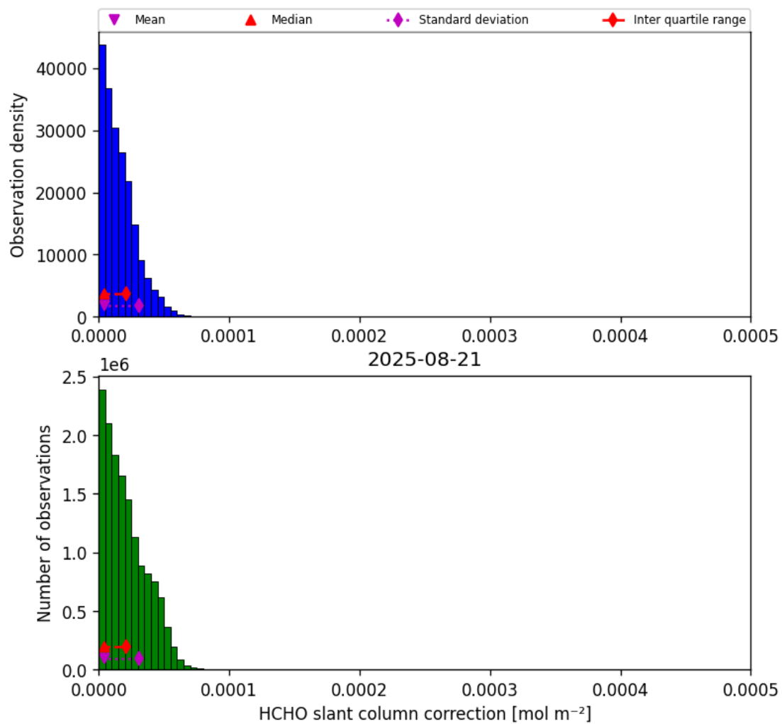
Figure 47: Histogram of “HCHO slant column correction” for 2025-08-20 to 2025-08-22
