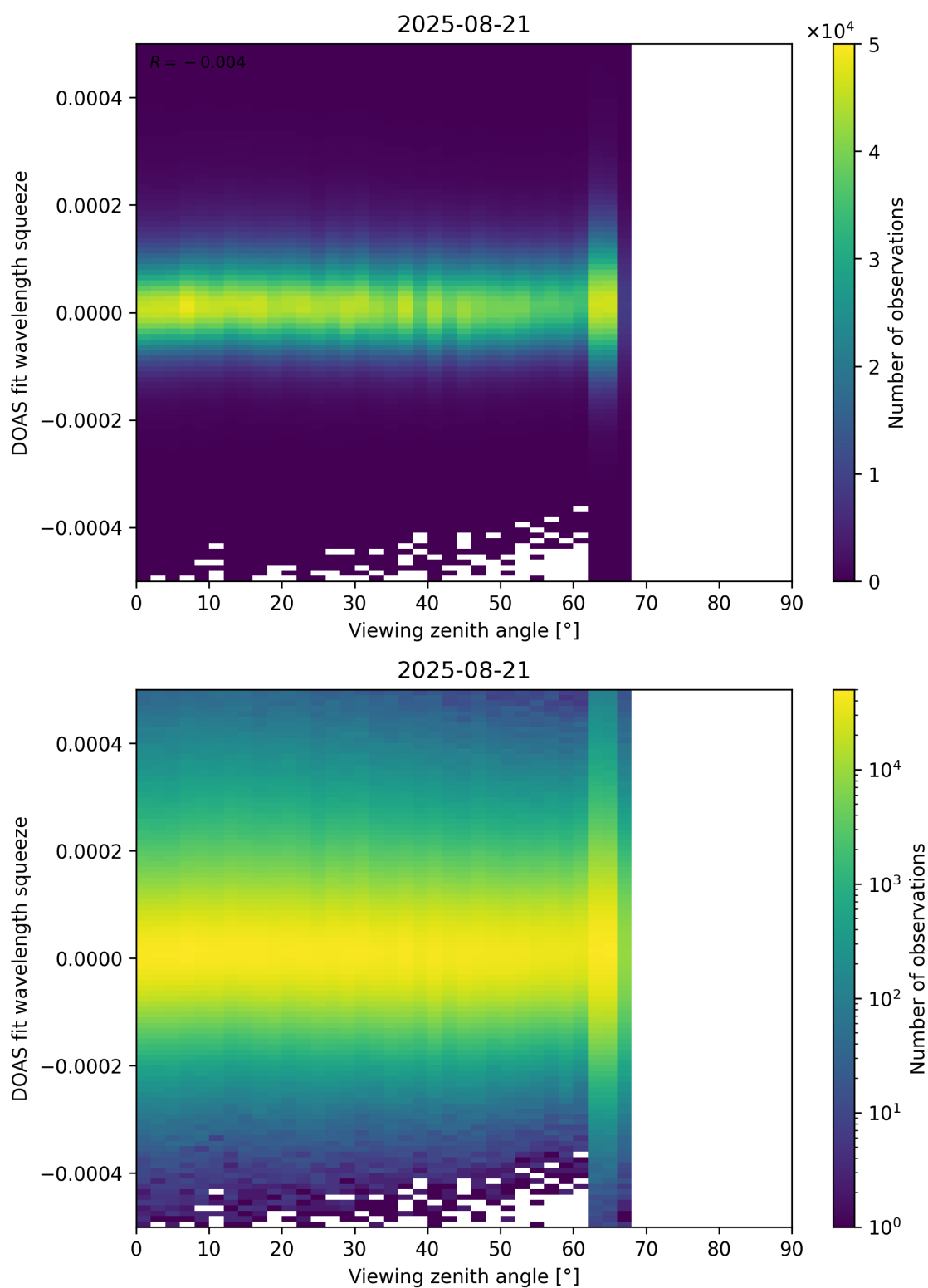
Figure 184: Scatter density plot of “Viewing zenith angle” against “DOAS fit wavelength squeeze” for 2025-08-20 to 2025-08-22.
