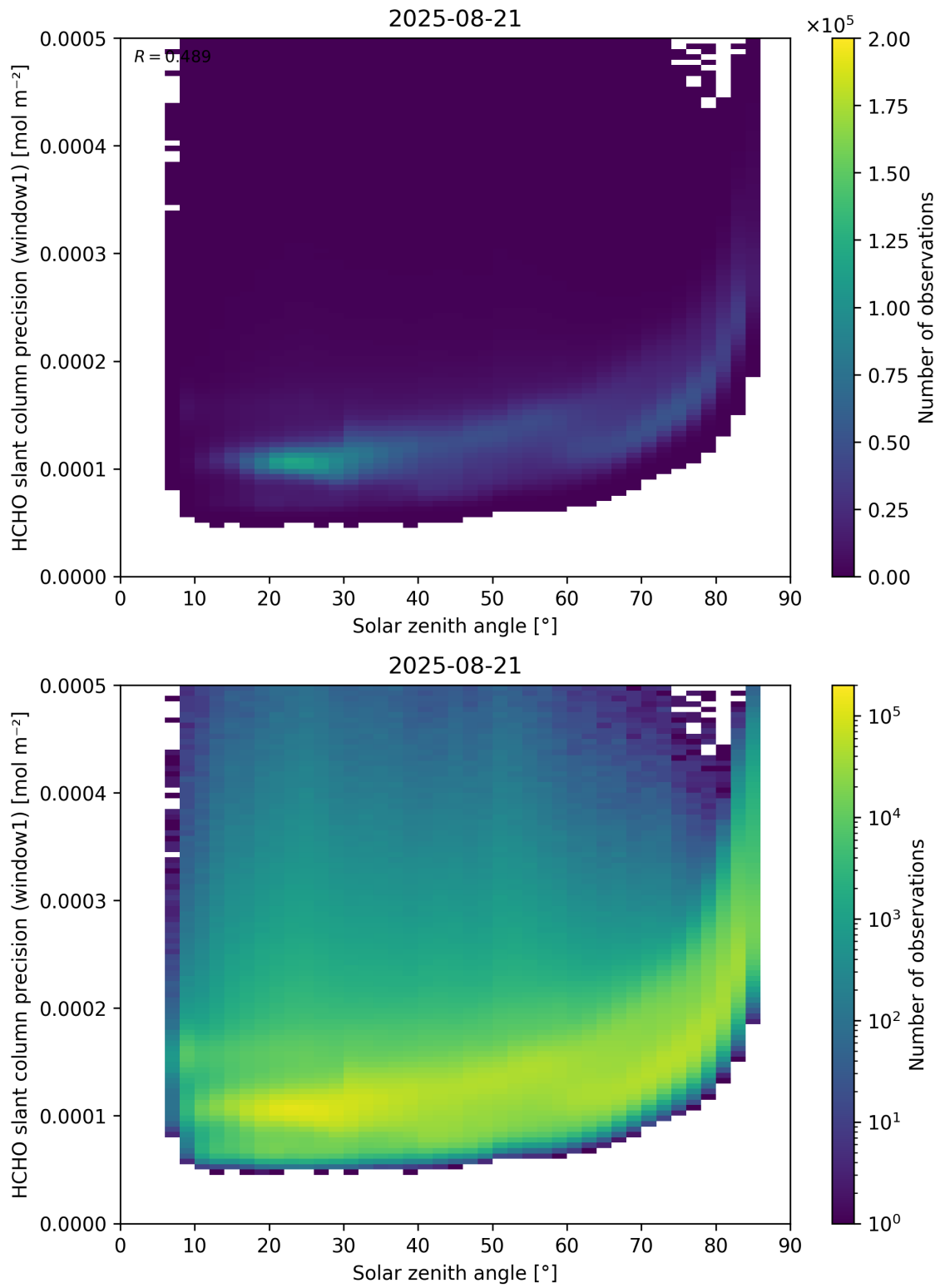
Figure 174: Scatter density plot of “Solar zenith angle” against “HCHO slant column precision (window1)” for 2025-08-20 to 2025-08-22.
