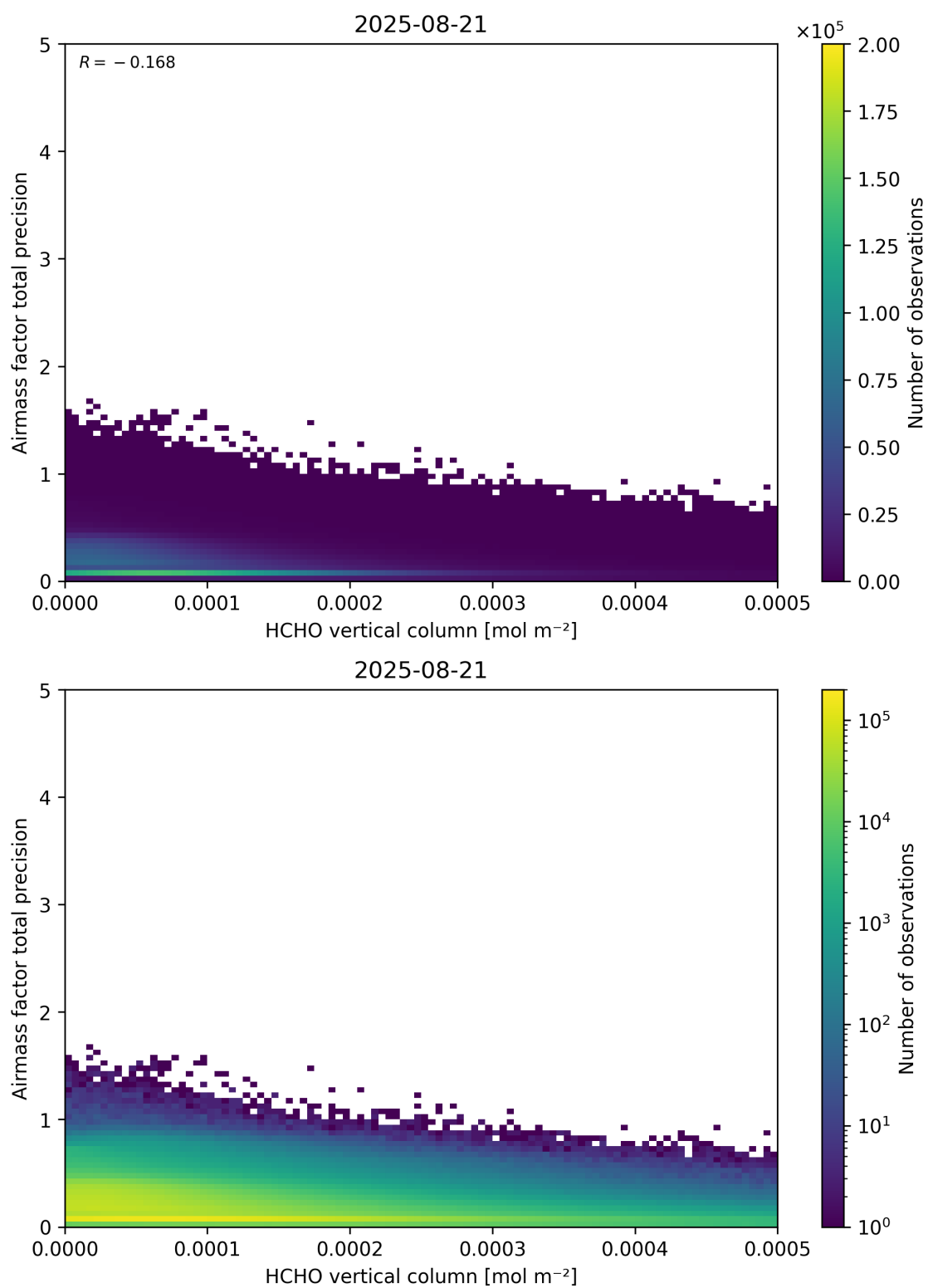
Figure 132: Scatter density plot of “HCHO vertical column” against “Airmass factor total precision” for 2025-08-20 to 2025-08-22.
