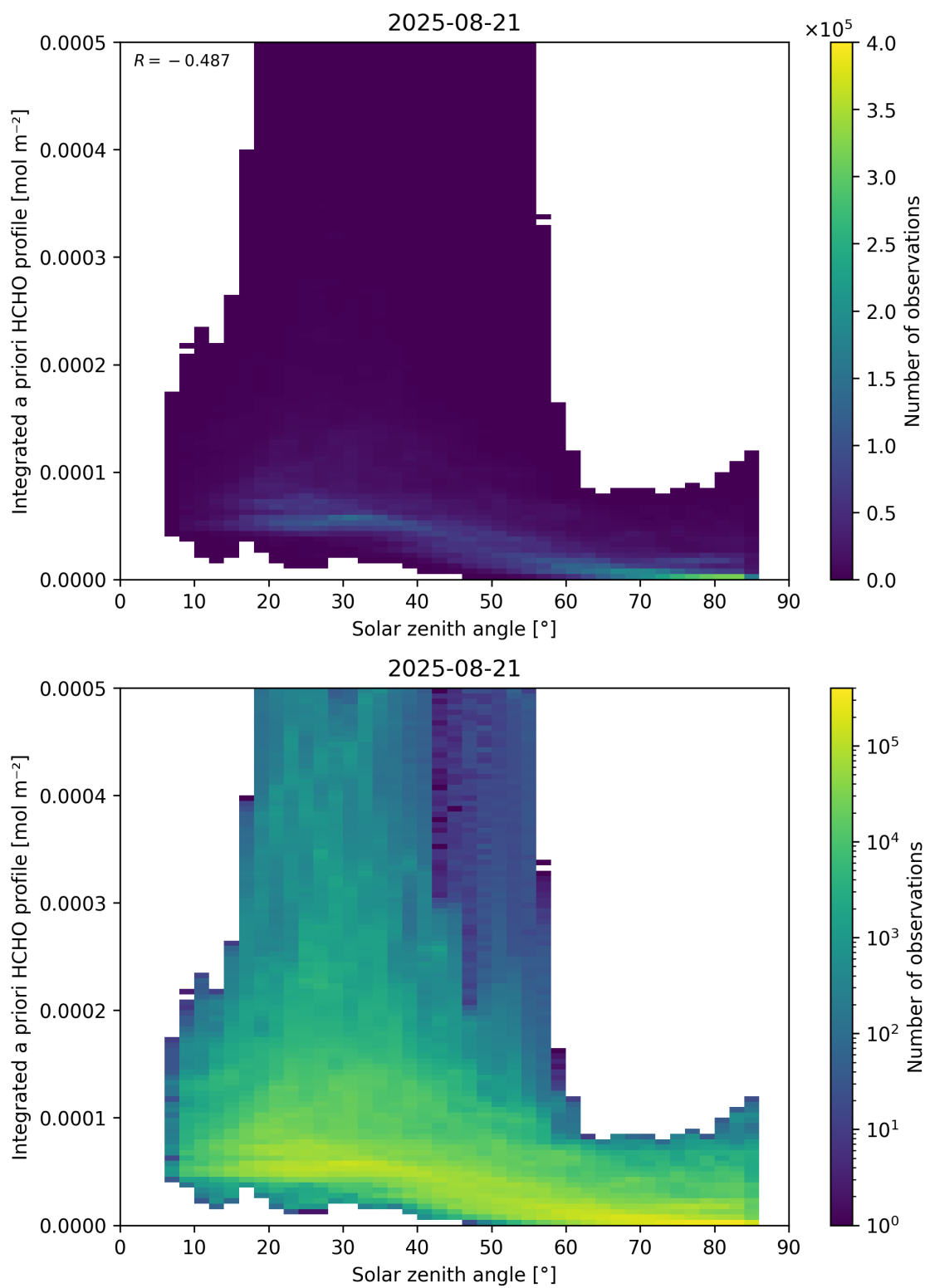
Figure 180: Scatter density plot of “Solar zenith angle” against “Integrated a priori HCHO profile” for 2025-08-20 to 2025-08-22.
