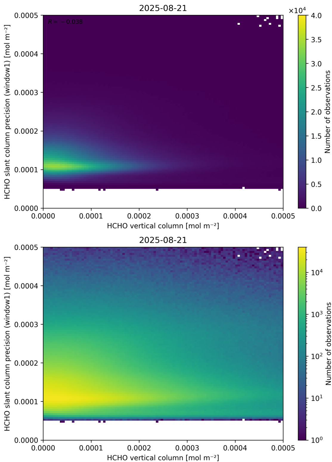
Figure 130: Scatter density plot of “HCHO vertical column” against “HCHO slant column precision (window1)” for 2025-08-20 to 2025-08-22.
