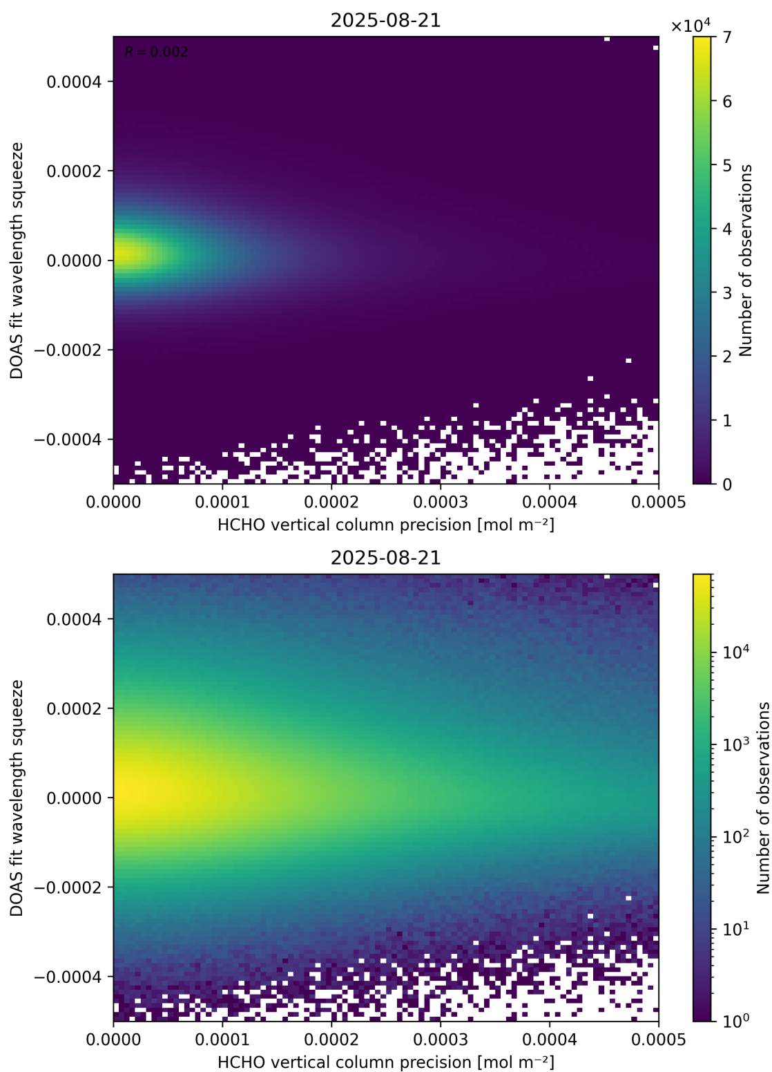
Figure 138: Scatter density plot of “HCHO vertical column precision” against “DOAS fit wavelength squeeze” for 2025-08-20 to 2025-08-22.
