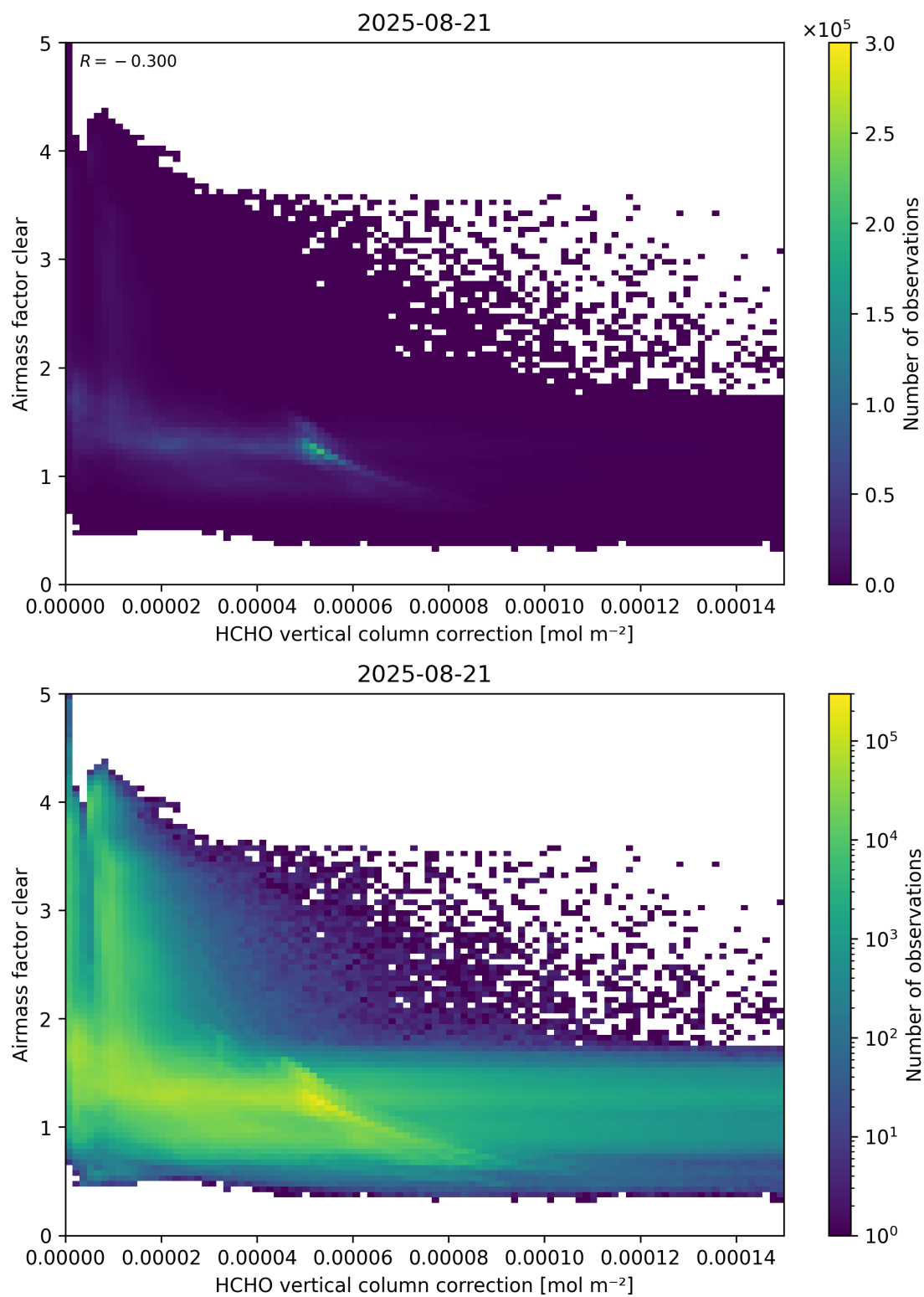
Figure 115: Scatter density plot of “HCHO vertical column correction” against “Airmass factor clear” for 2025-08-20 to 2025-08-22.
