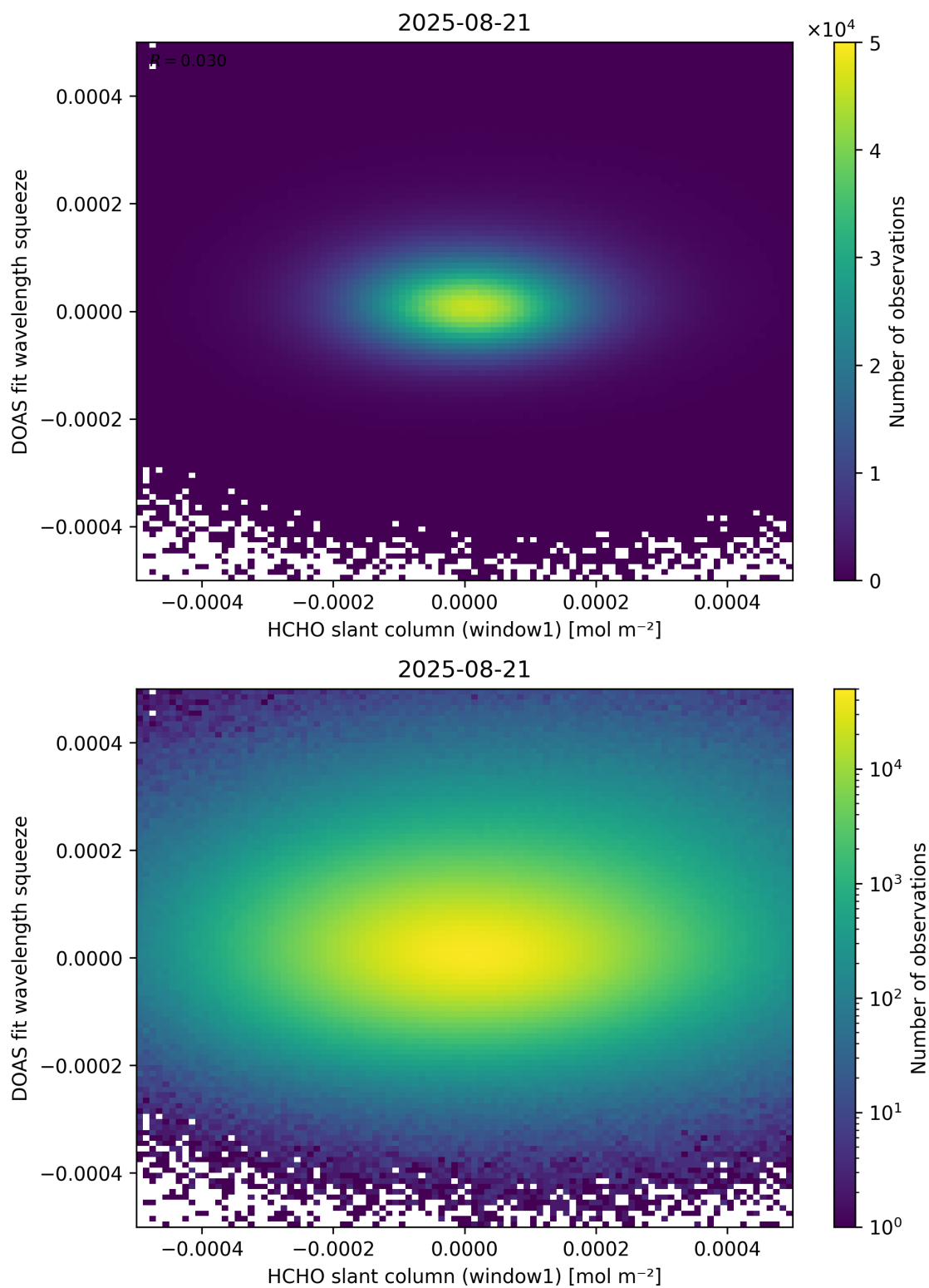
Figure 80: Scatter density plot of “HCHO slant column (window1)” against “DOAS fit wavelength squeeze” for 2025-08-20 to 2025-08-22.
