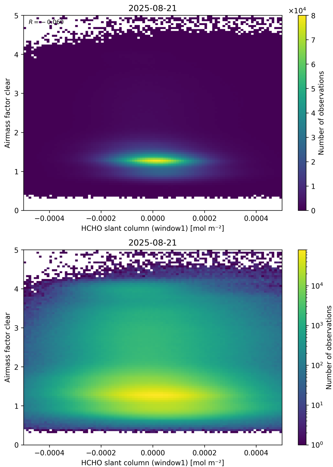
Figure 81: Scatter density plot of “HCHO slant column (window1)” against “Airmass factor clear” for 2025-08-20 to 2025-08-22.
