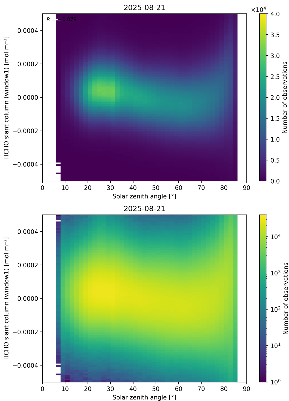
Figure 173: Scatter density plot of “Solar zenith angle” against “HCHO slant column (window1)” for 2025-08-20 to 2025-08-22.
