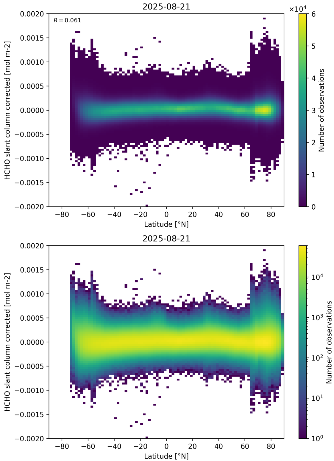
Figure 157: Scatter density plot of “Latitude” against “HCHO slant column corrected” for 2025-08-20 to 2025-08-22.
