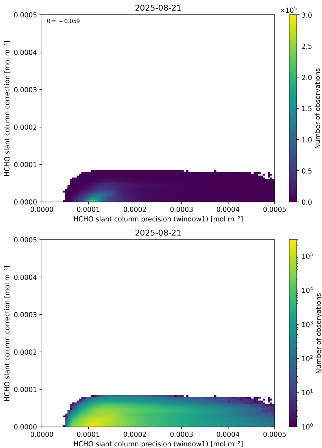
Figure 93: Scatter density plot of “HCHO slant column precision (window1)” against “HCHO slant column correction” for 2025-08-20 to 2025-08-22.
