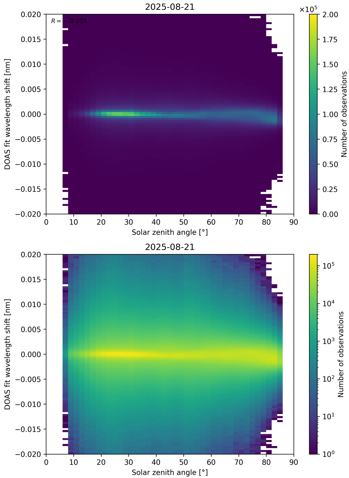
Figure 168: Scatter density plot of “Solar zenith angle” against “DOAS fit wavelength shift” for 2025-08-20 to 2025-08-22.
