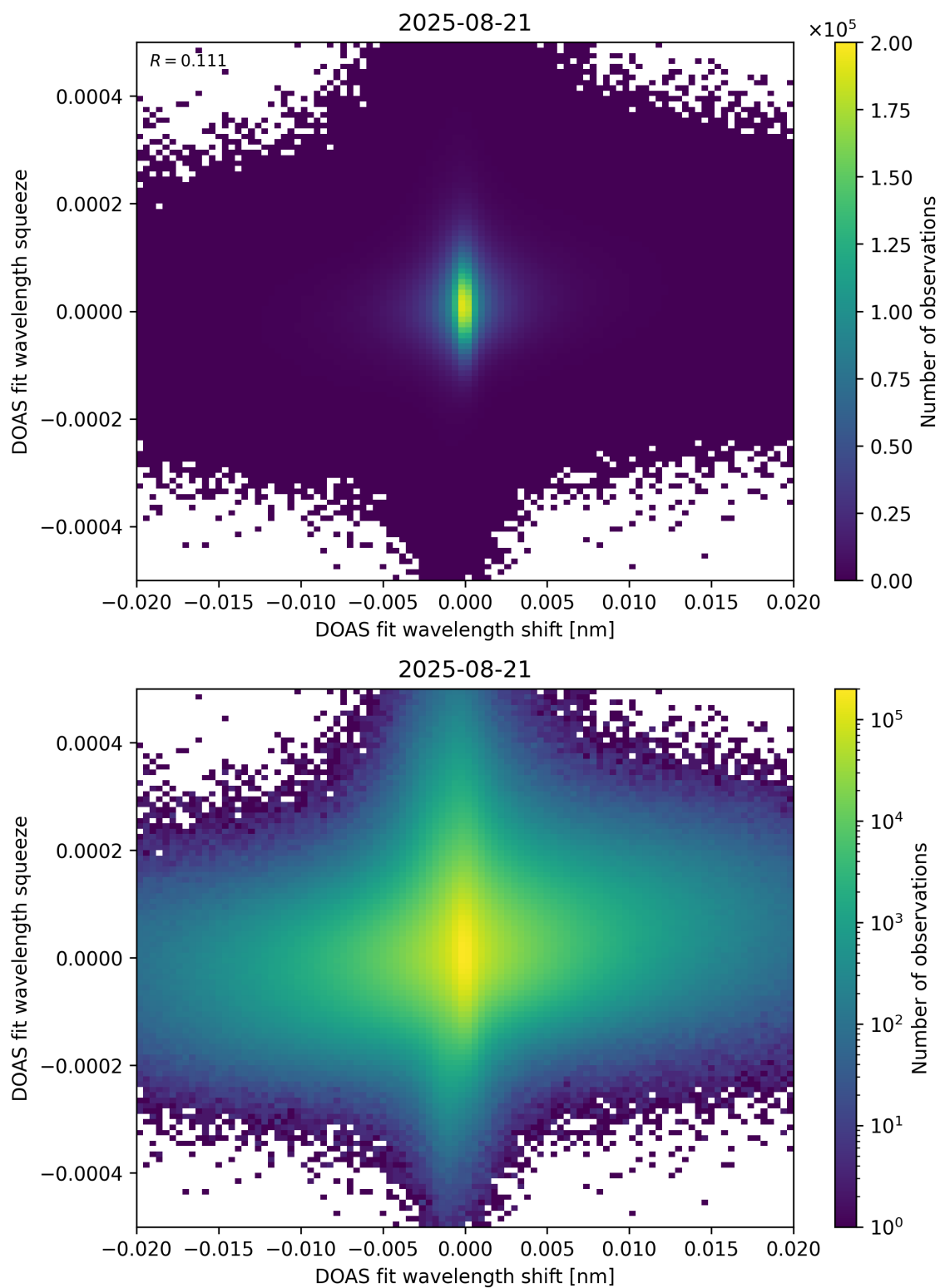
Figure 65: Scatter density plot of “DOAS fit wavelength shift” against “DOAS fit wavelength squeeze” for 2025-08-20 to 2025-08-22.
