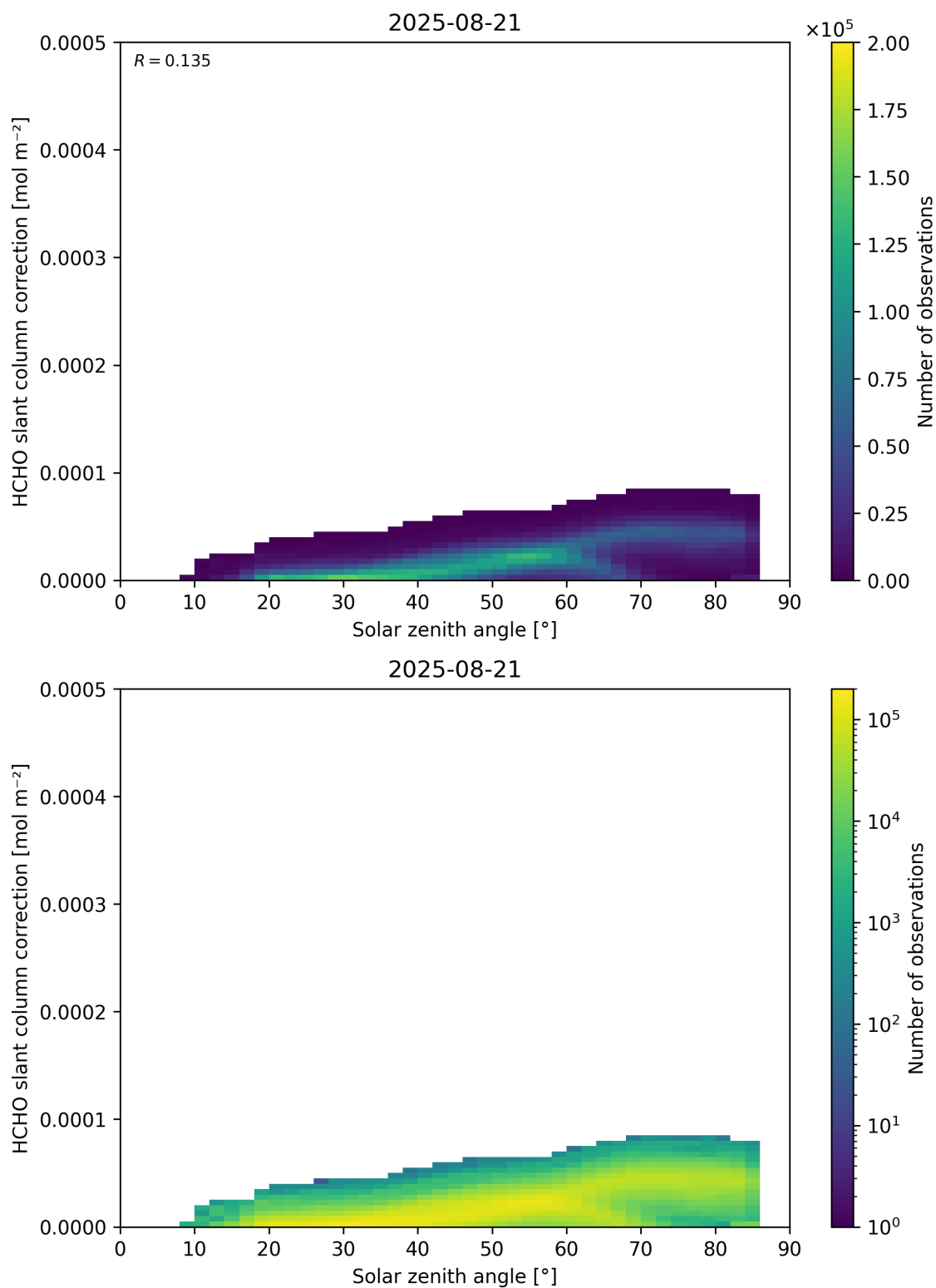
Figure 172: Scatter density plot of “Solar zenith angle” against “HCHO slant column correction” for 2025-08-20 to 2025-08-22.
