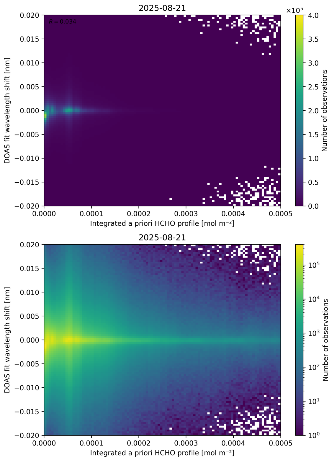
Figure 149: Scatter density plot of “Integrated a priori HCHO profile” against “DOAS fit wavelength shift” for 2025-08-20 to 2025-08-22.
