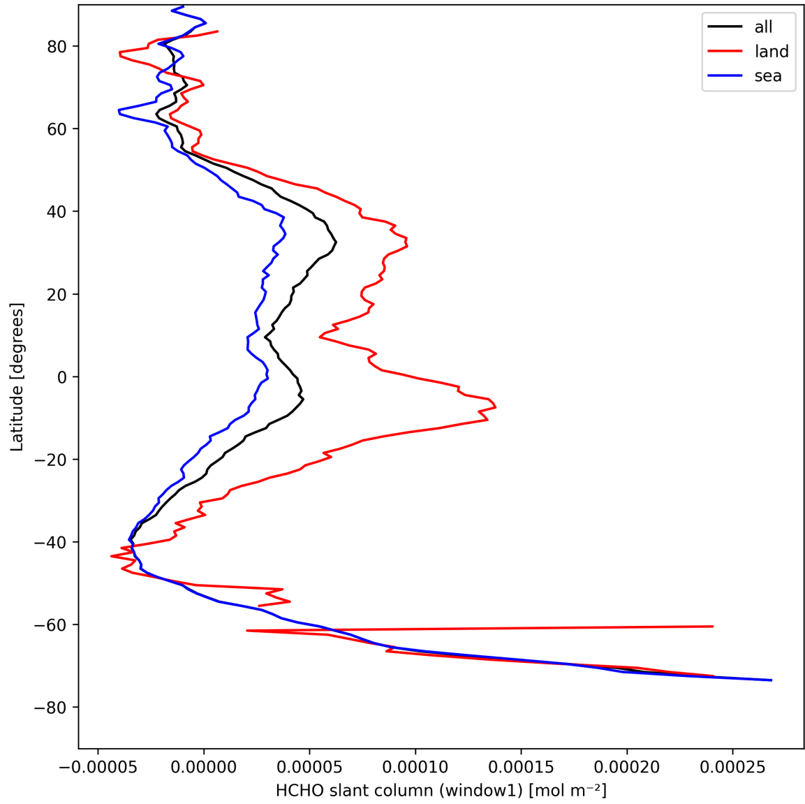
Figure 24: Zonal average of “HCHO slant column (window1)” for 2025-08-20 to 2025-08-22.
