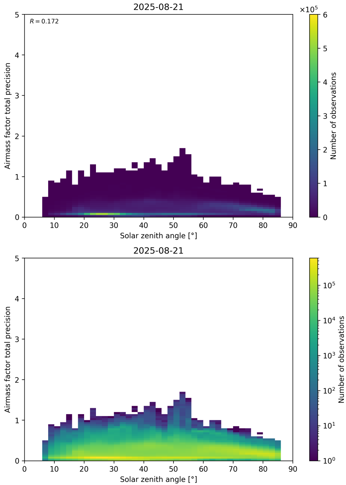
Figure 176: Scatter density plot of “Solar zenith angle” against “Airmass factor total precision” for 2025-08-20 to 2025-08-22.
