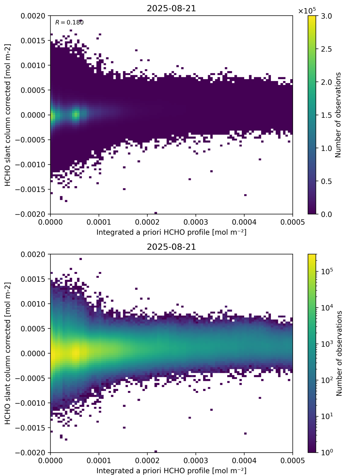
Figure 151: Scatter density plot of “Integrated a priori HCHO profile” against “HCHO slant column corrected” for 2025-08-20 to 2025-08-22.
