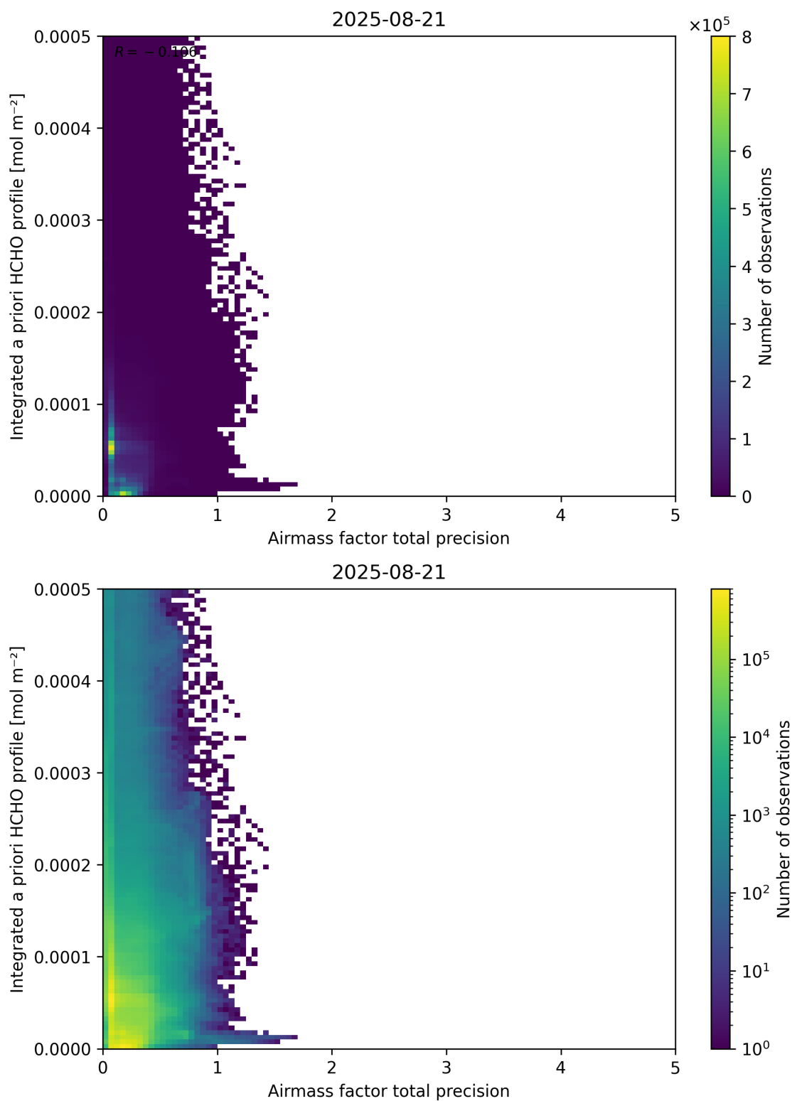
Figure 111: Scatter density plot of “Airmass factor total precision” against “Integrated a priori HCHO profile” for 2025-08-20 to 2025-08-22.
