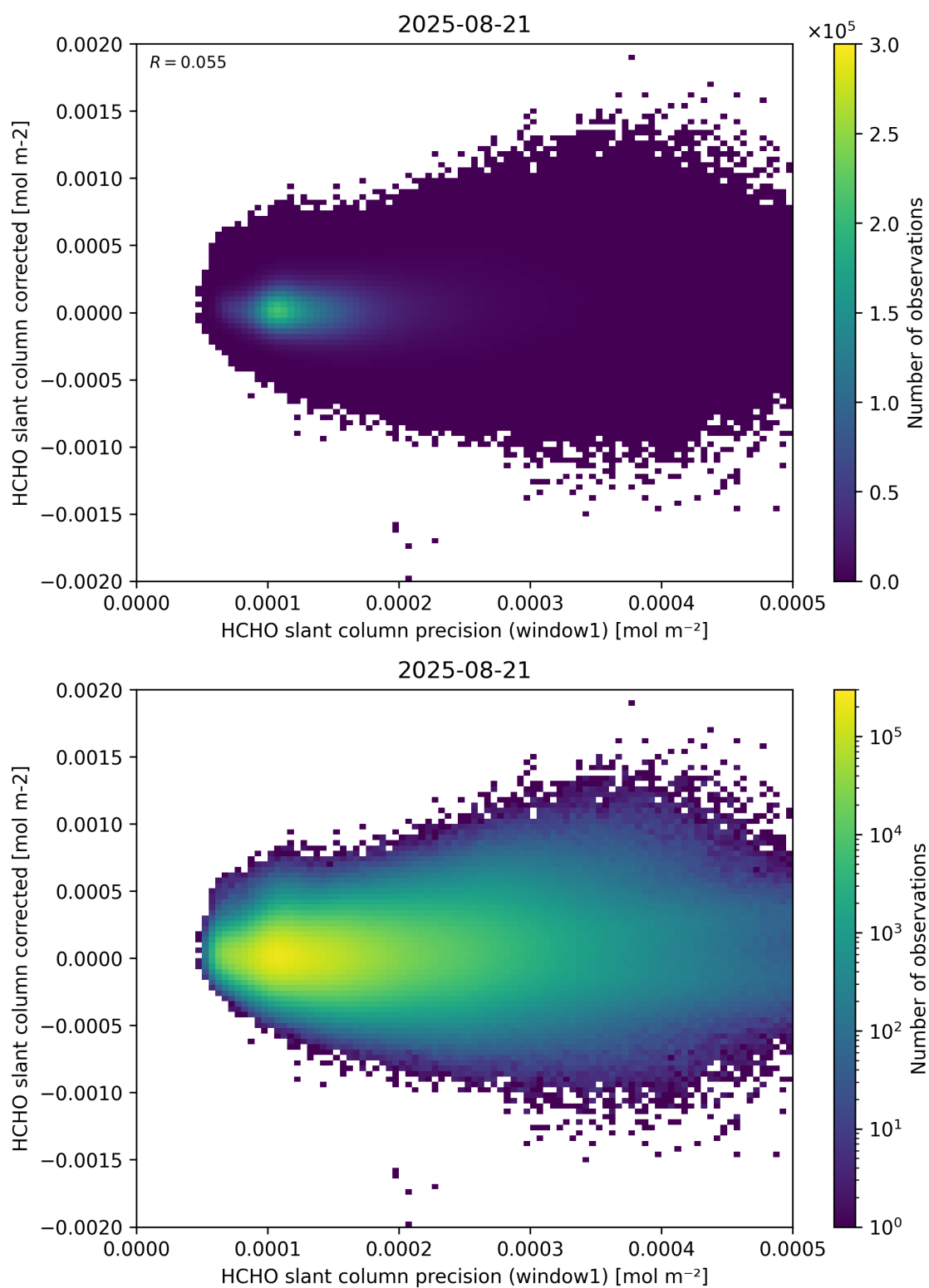
Figure 92: Scatter density plot of “HCHO slant column precision (window1)” against “HCHO slant column corrected” for 2025-08-20 to 2025-08-22.
