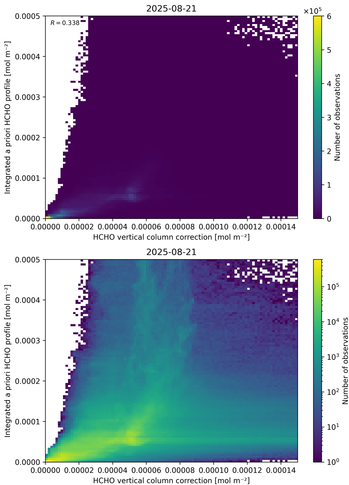
Figure 122: Scatter density plot of “HCHO vertical column correction” against “Integrated a priori HCHO profile” for 2025-08-20 to 2025-08-22.
