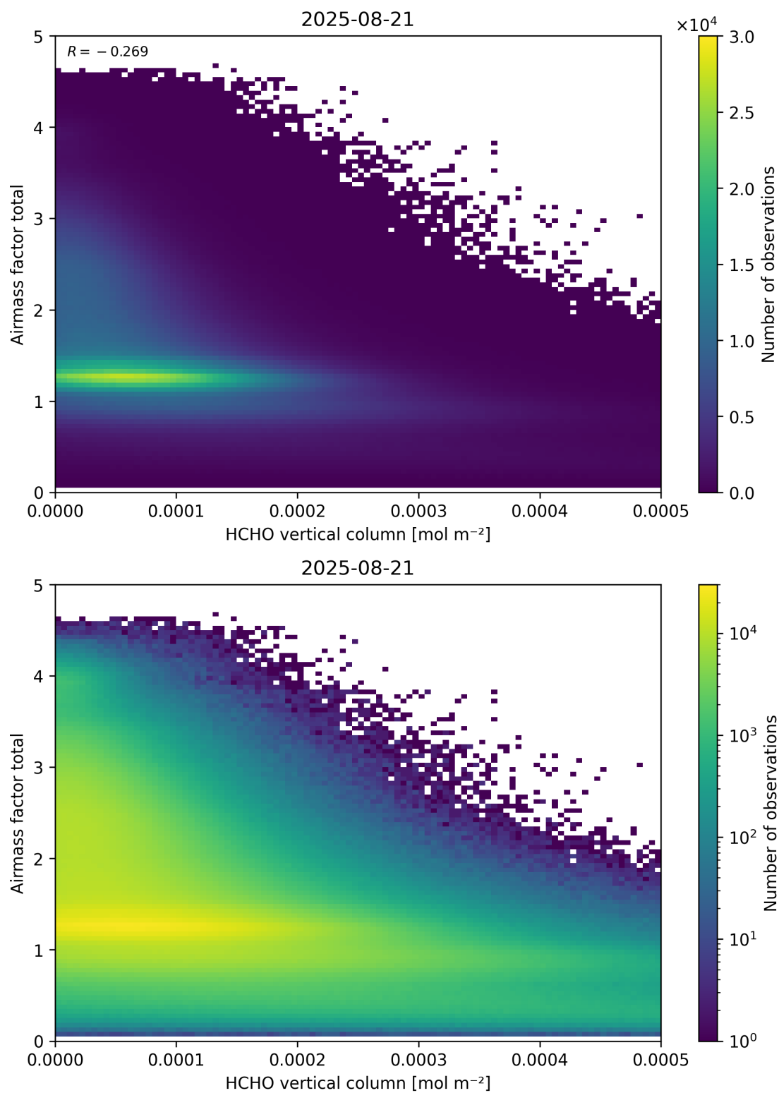
Figure 131: Scatter density plot of “HCHO vertical column” against “Airmass factor total” for 2025-08-20 to 2025-08-22.
