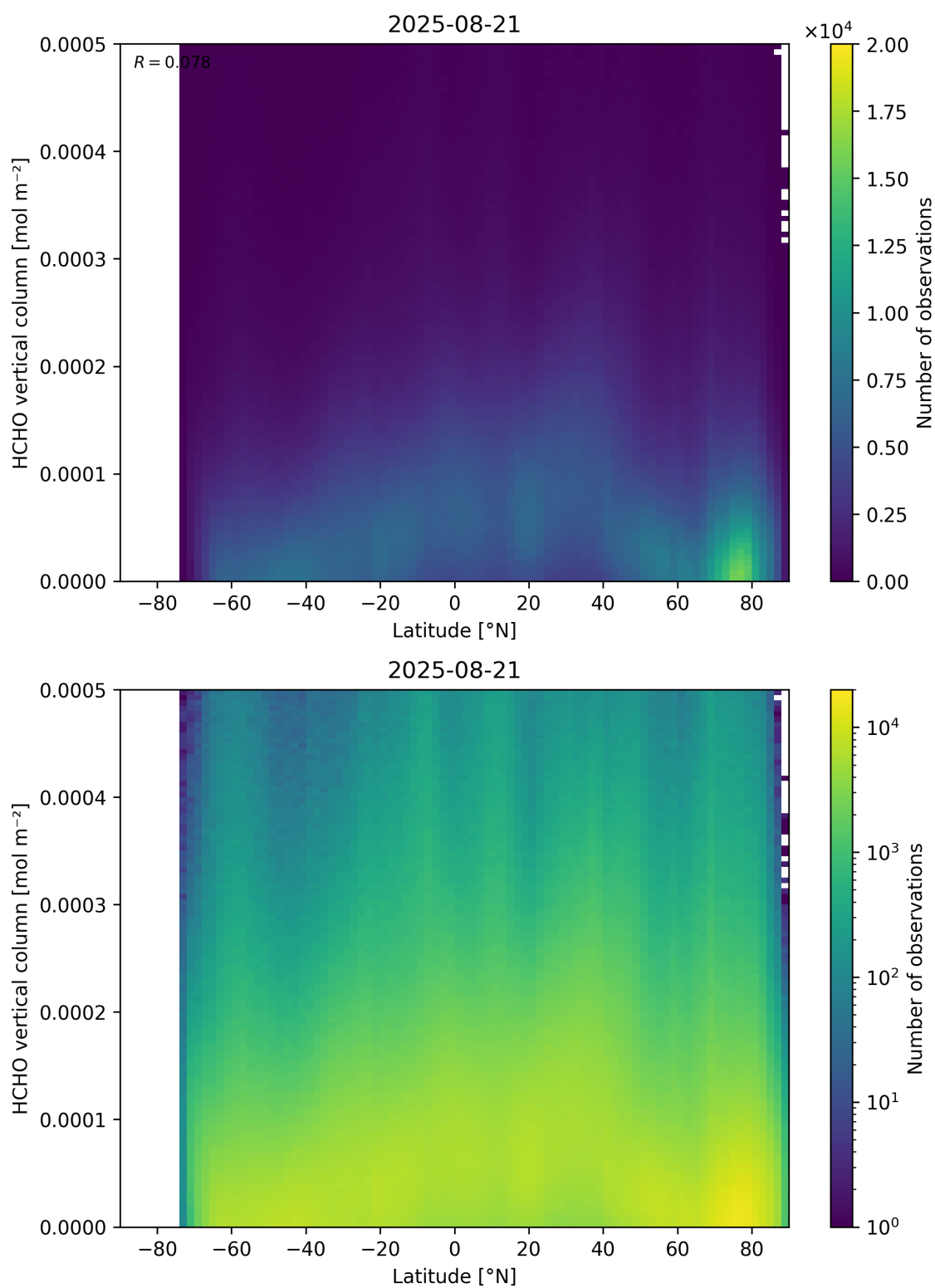
Figure 163: Scatter density plot of “Latitude” against “HCHO vertical column” for 2025-08-20 to 2025-08-22.
