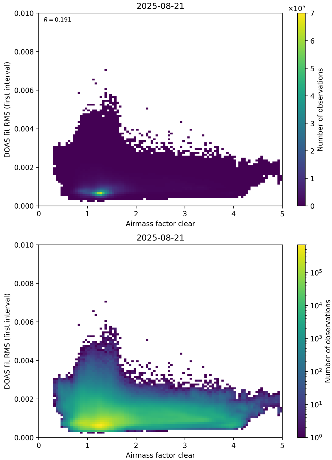
Figure 71: Scatter density plot of “Airmass factor clear” against “DOAS fit RMS (first interval)” for 2025-08-20 to 2025-08-22.
