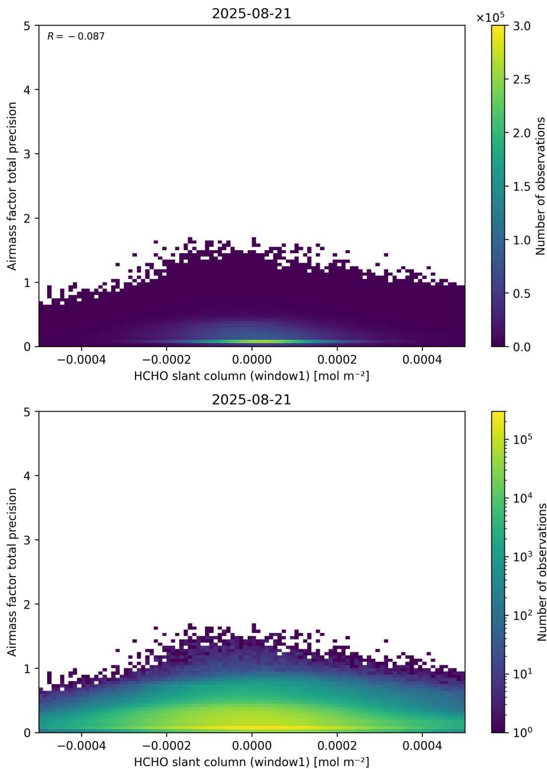
Figure 86: Scatter density plot of “HCHO slant column (window1)” against “Airmass factor total precision” for 2025-08-20 to 2025-08-22.
