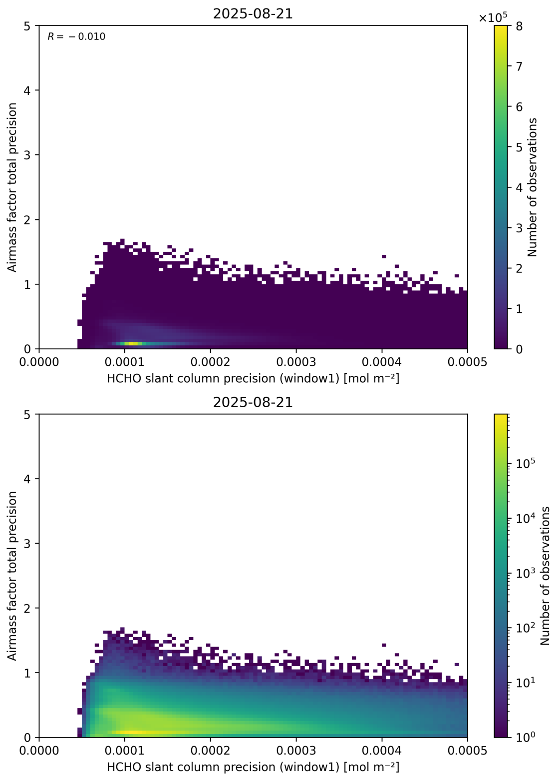
Figure 95: Scatter density plot of “HCHO slant column precision (window1)” against “Airmass factor total precision” for 2025-08-20 to 2025-08-22.
