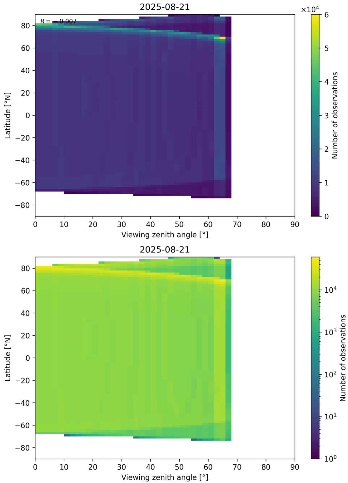
Figure 196: Scatter density plot of “Viewing zenith angle” against “Latitude” for 2025-08-20 to 2025-08-22.
