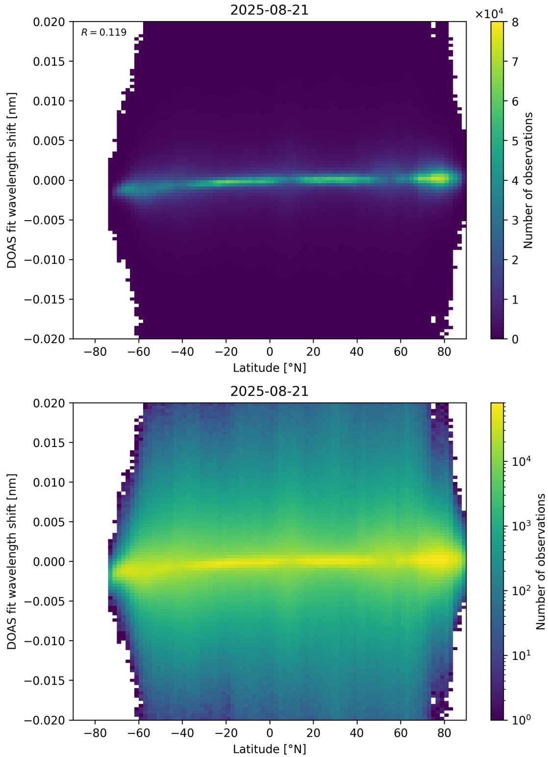
Figure 154: Scatter density plot of “Latitude” against “DOAS fit wavelength shift” for 2025-08-20 to 2025-08-22.
