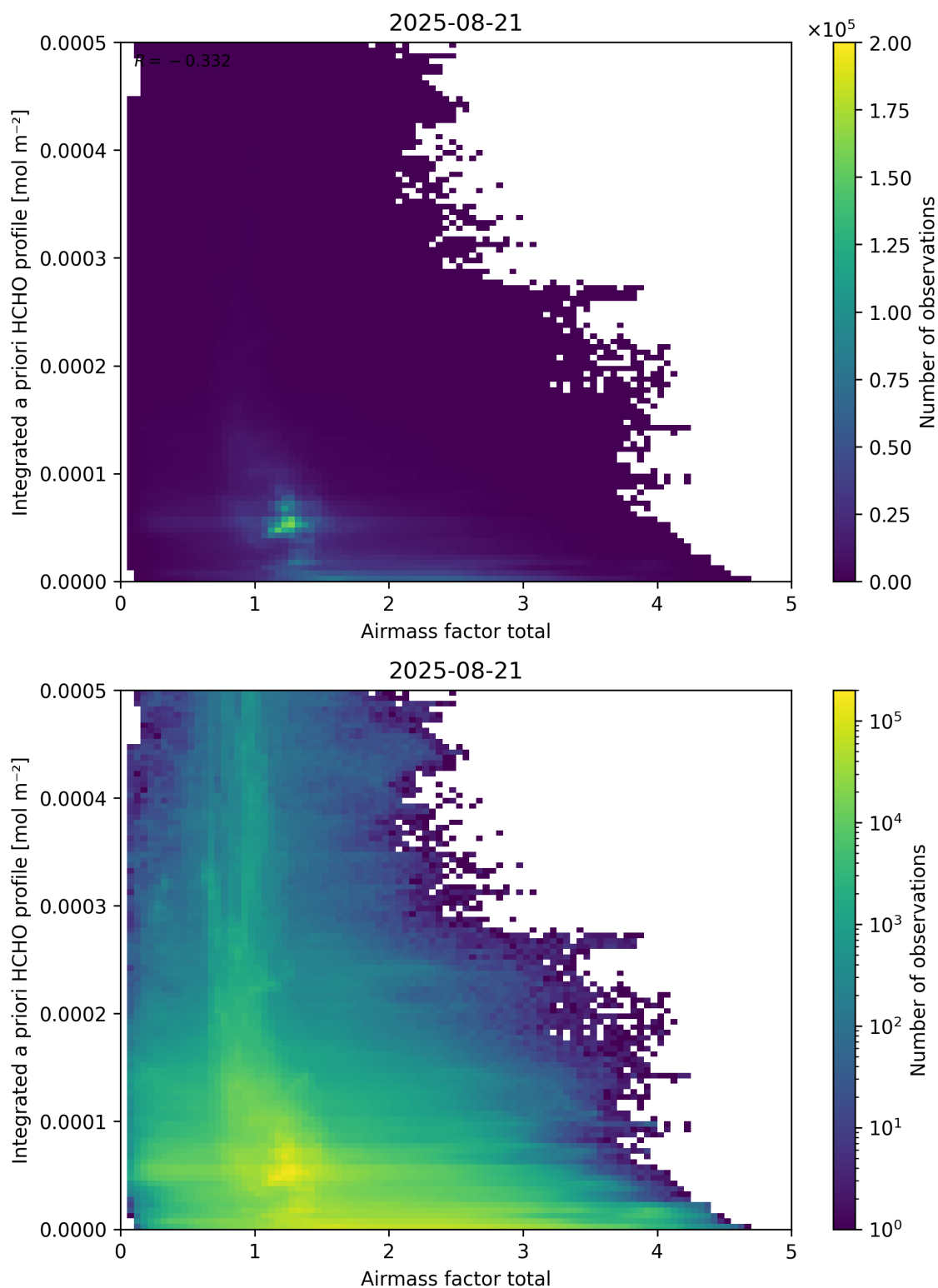
Figure 104: Scatter density plot of “Airmass factor total” against “Integrated a priori HCHO profile” for 2025-08-20 to 2025-08-22.
