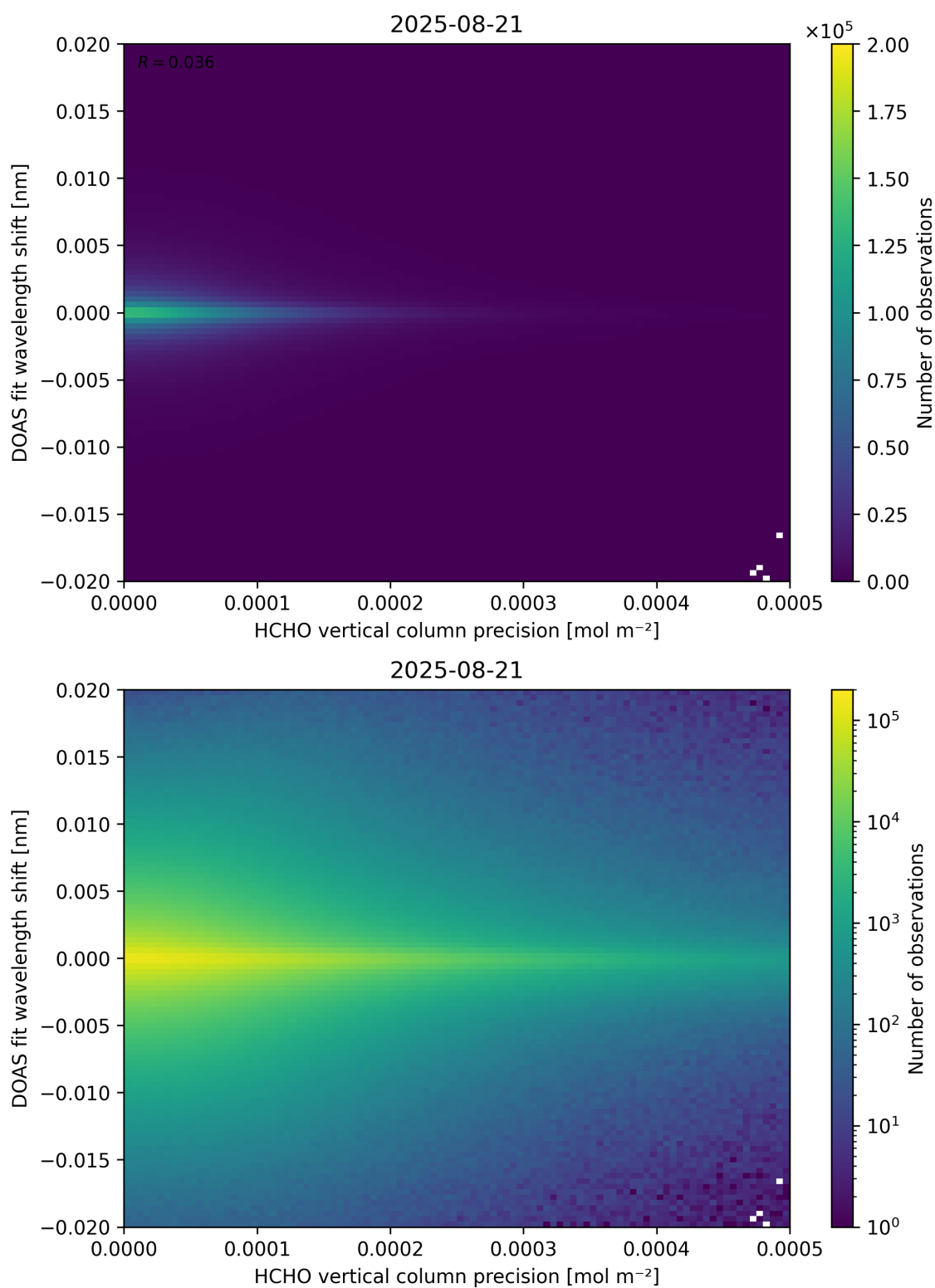
Figure 137: Scatter density plot of “HCHO vertical column precision” against “DOAS fit wavelength shift” for 2025-08-20 to 2025-08-22.
