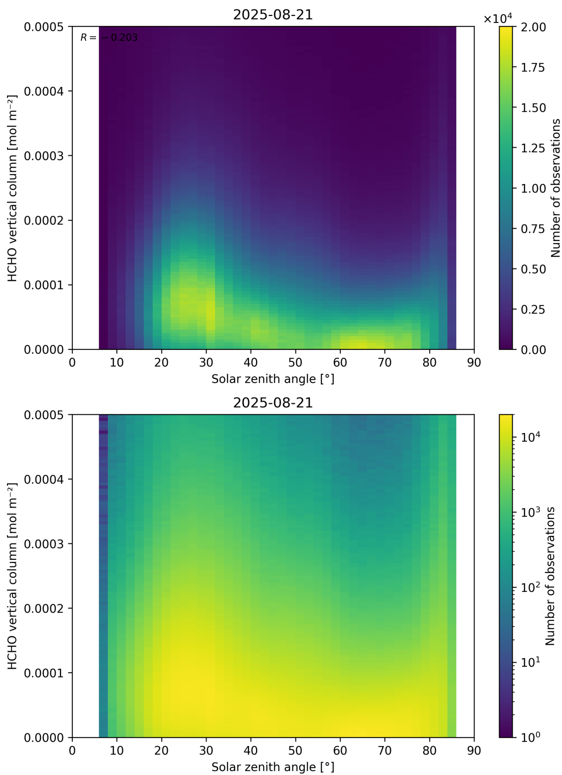
Figure 177: Scatter density plot of “Solar zenith angle” against “HCHO vertical column” for 2025-08-20 to 2025-08-22.
