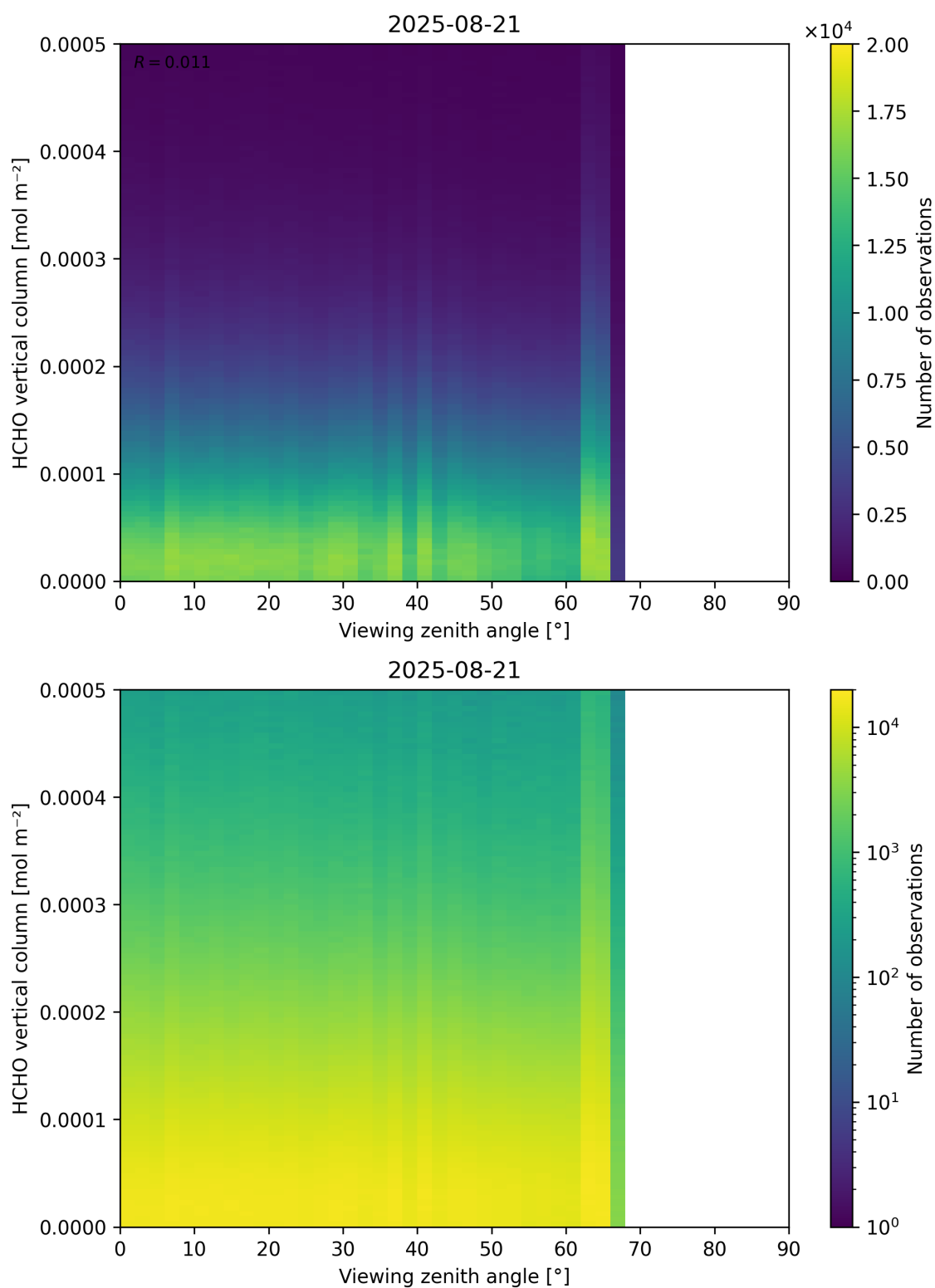
Figure 192: Scatter density plot of “Viewing zenith angle” against “HCHO vertical column” for 2025-08-20 to 2025-08-22.
