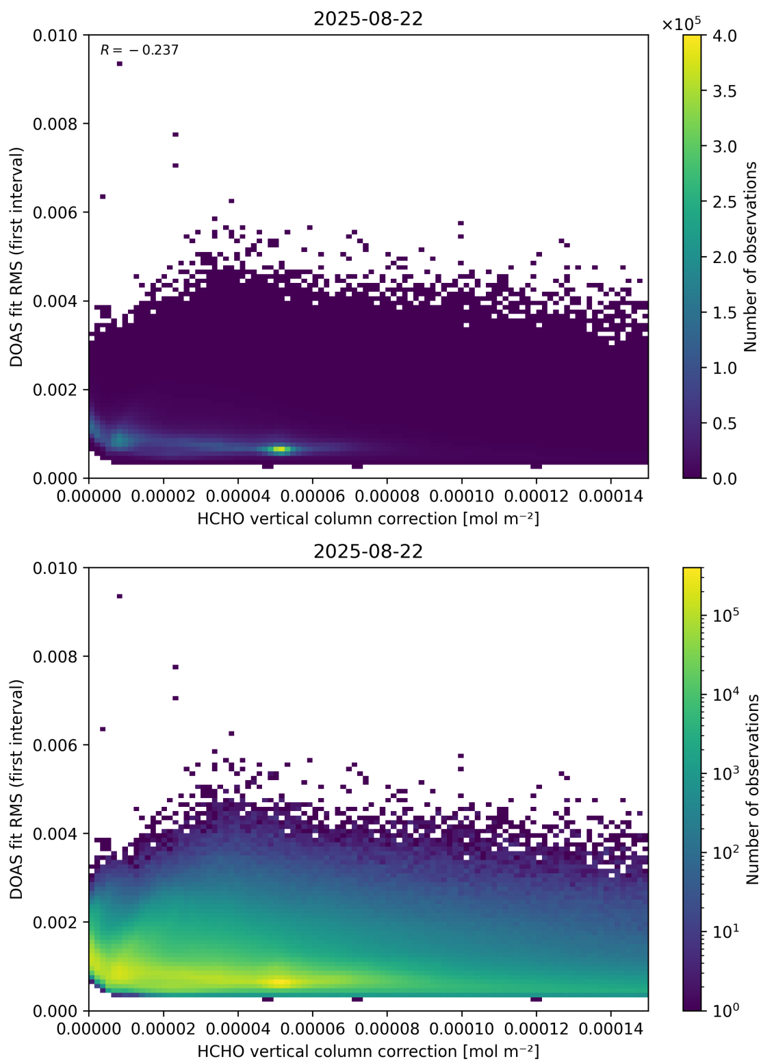
Figure 112: Scatter density plot of “HCHO vertical column correction” against “DOAS fit RMS (first interval)” for 2025-08-21 to 2025-08-23.
