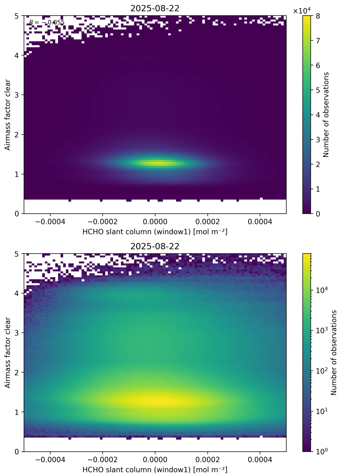
Figure 81: Scatter density plot of “HCHO slant column (window1)” against “Airmass factor clear” for 2025-08-21 to 2025-08-23.
