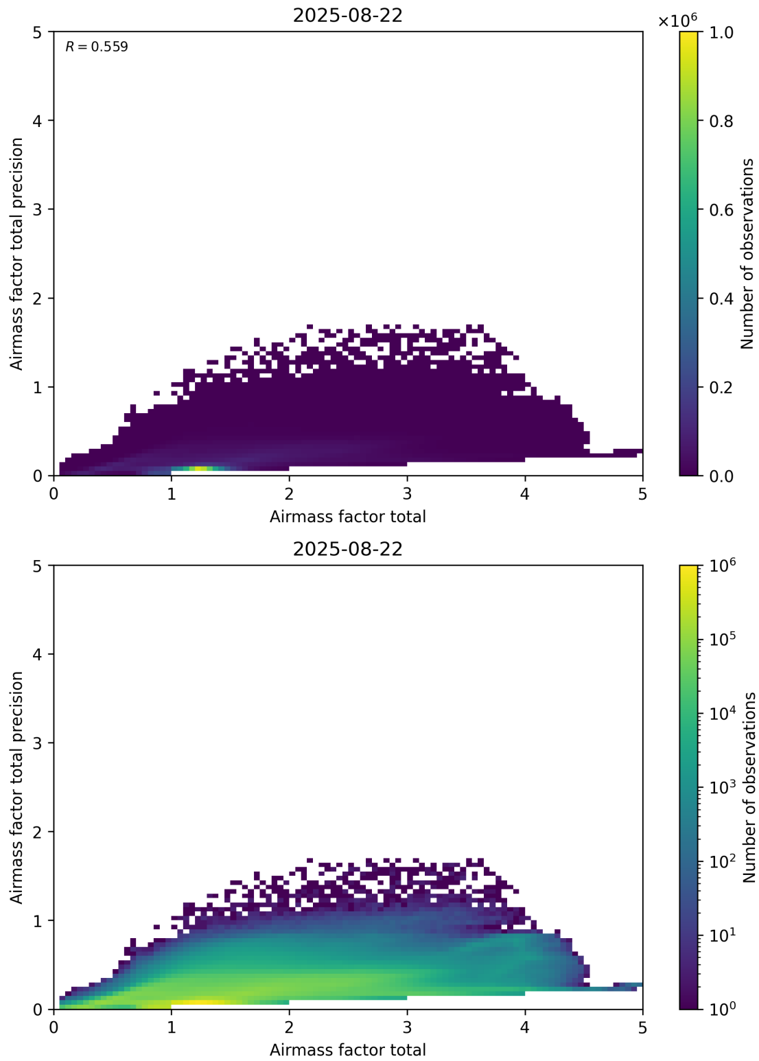
Figure 103: Scatter density plot of “Airmass factor total” against “Airmass factor total precision” for 2025-08-21 to 2025-08-23.
