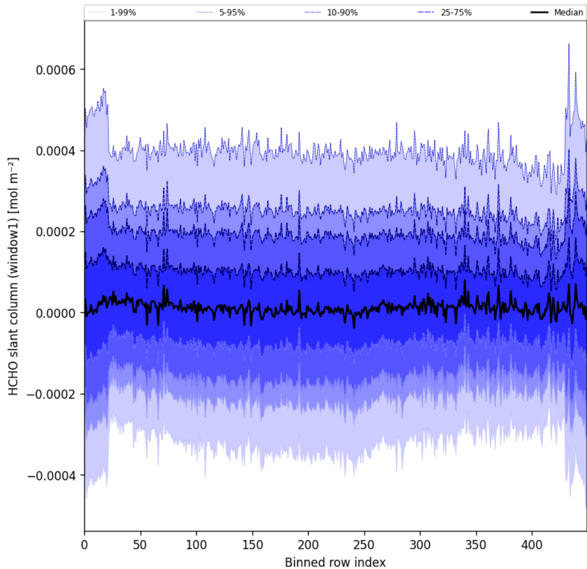
Figure 52: Along track statistics of “HCHO slant column (window1)” for 2025-08-21 to 2025-08-23
