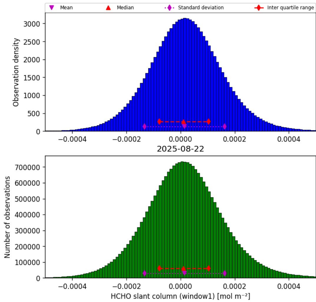
Figure 38: Histogram of “HCHO slant column (window1)” for 2025-08-21 to 2025-08-23
