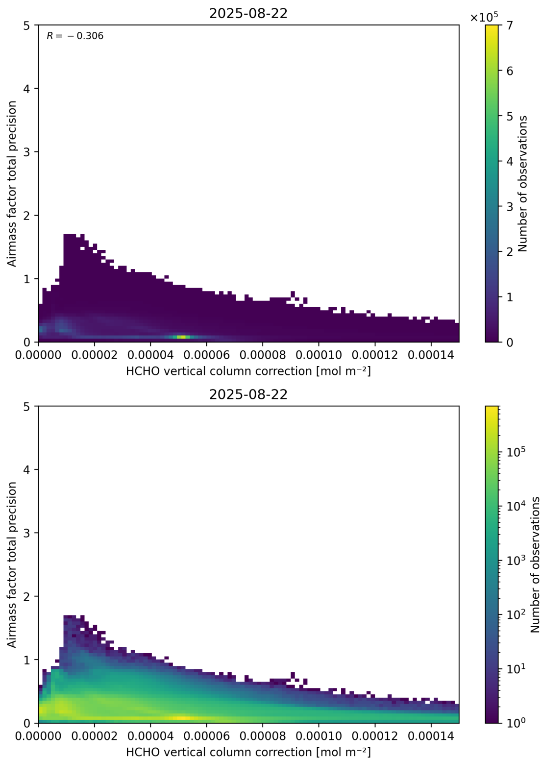
Figure 121: Scatter density plot of “HCHO vertical column correction” against “Airmass factor total precision” for 2025-08-21 to 2025-08-23.
