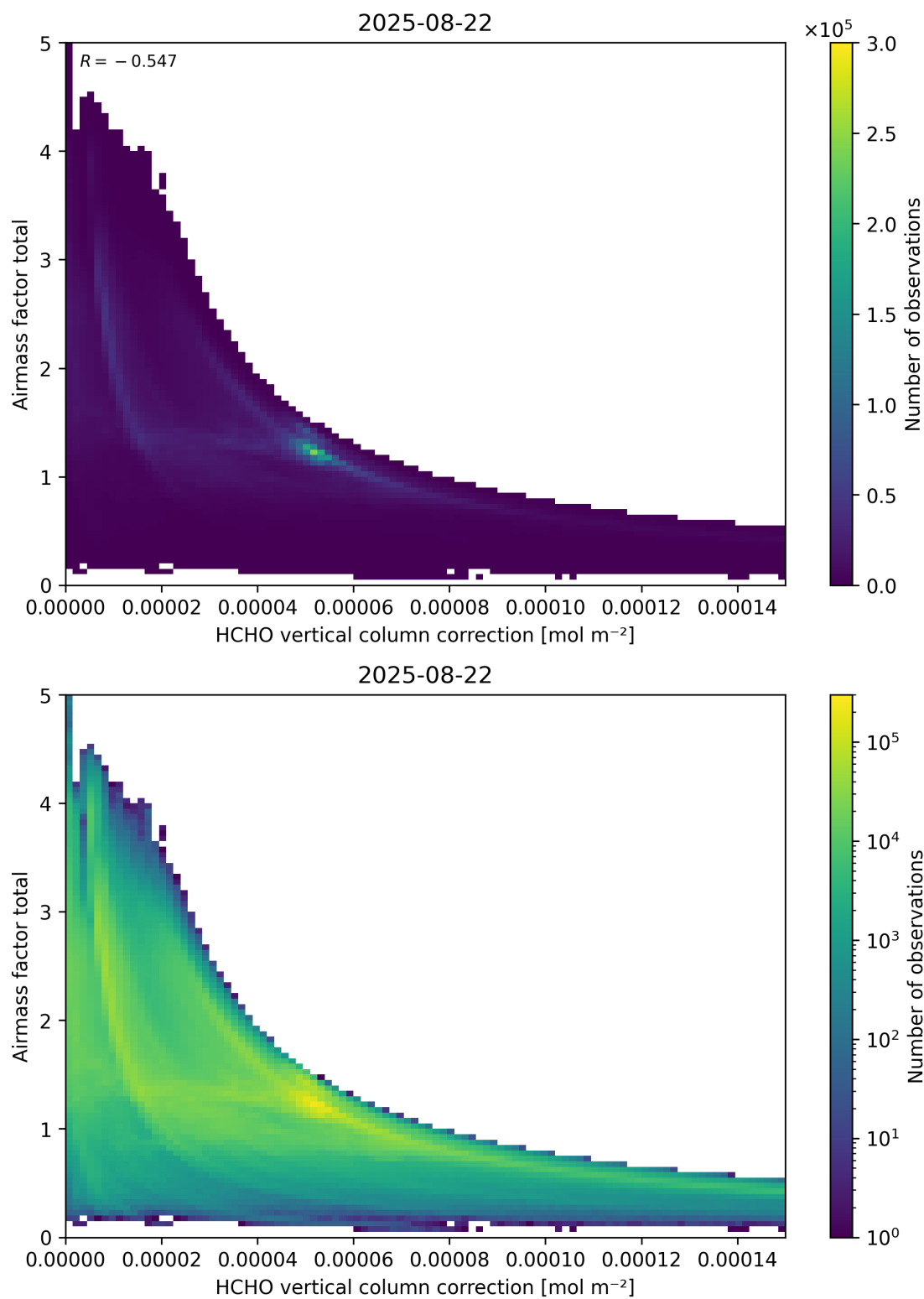
Figure 120: Scatter density plot of “HCHO vertical column correction” against “Airmass factor total” for 2025-08-21 to 2025-08-23.
