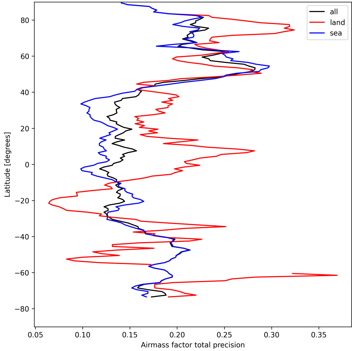
Figure 27: Zonal average of “Airmass factor total precision” for 2025-08-21 to 2025-08-23.
