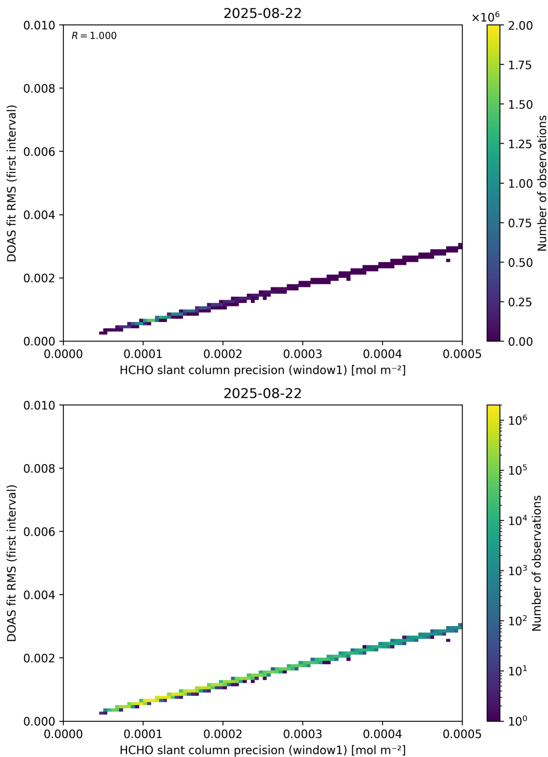
Figure 88: Scatter density plot of “HCHO slant column precision (window1)” against “DOAS fit RMS (first interval)” for 2025-08-21 to 2025-08-23.
