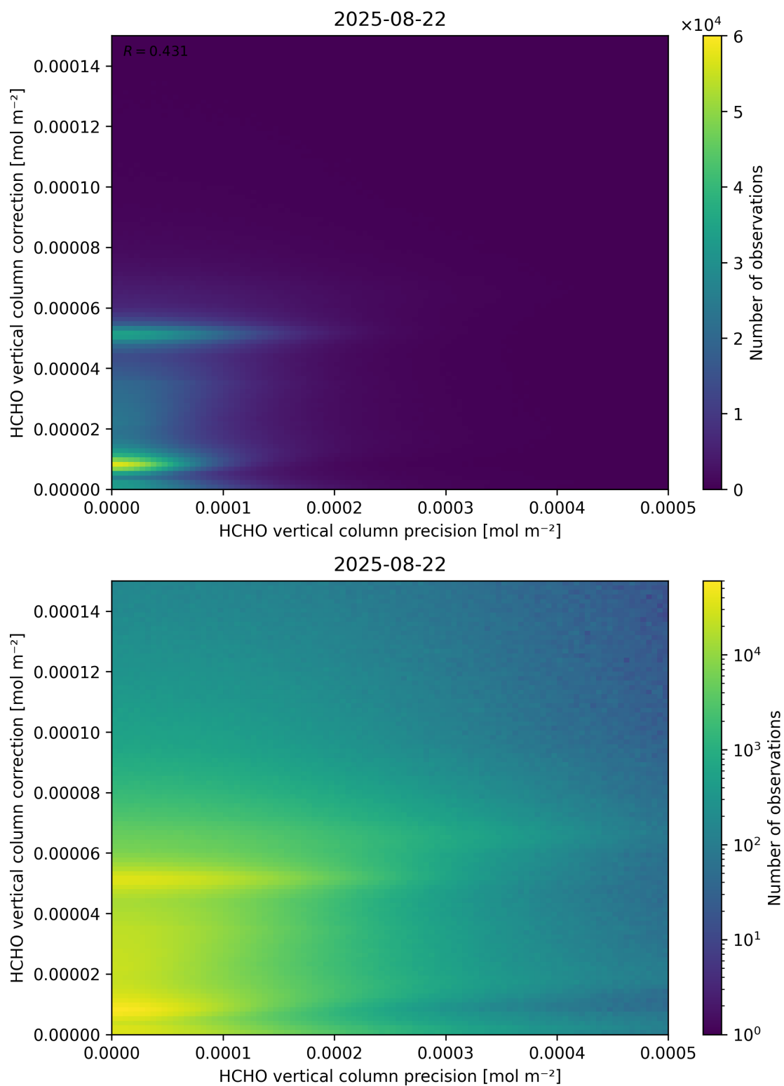
Figure 146: Scatter density plot of “HCHO vertical column precision” against “HCHO vertical column correction” for 2025-08-21 to 2025-08-23.
