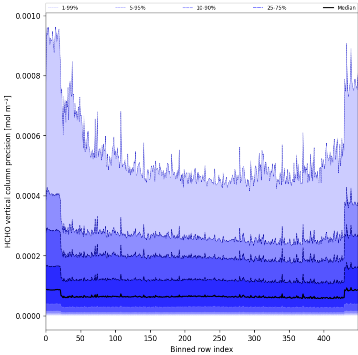
Figure 50: Along track statistics of “HCHO vertical column precision” for 2025-08-21 to 2025-08-23
