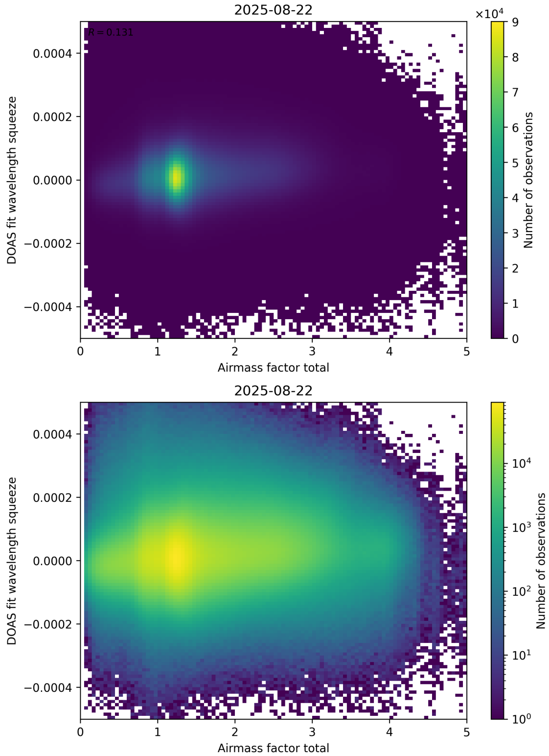
Figure 99: Scatter density plot of “Airmass factor total” against “DOAS fit wavelength squeeze” for 2025-08-21 to 2025-08-23.
