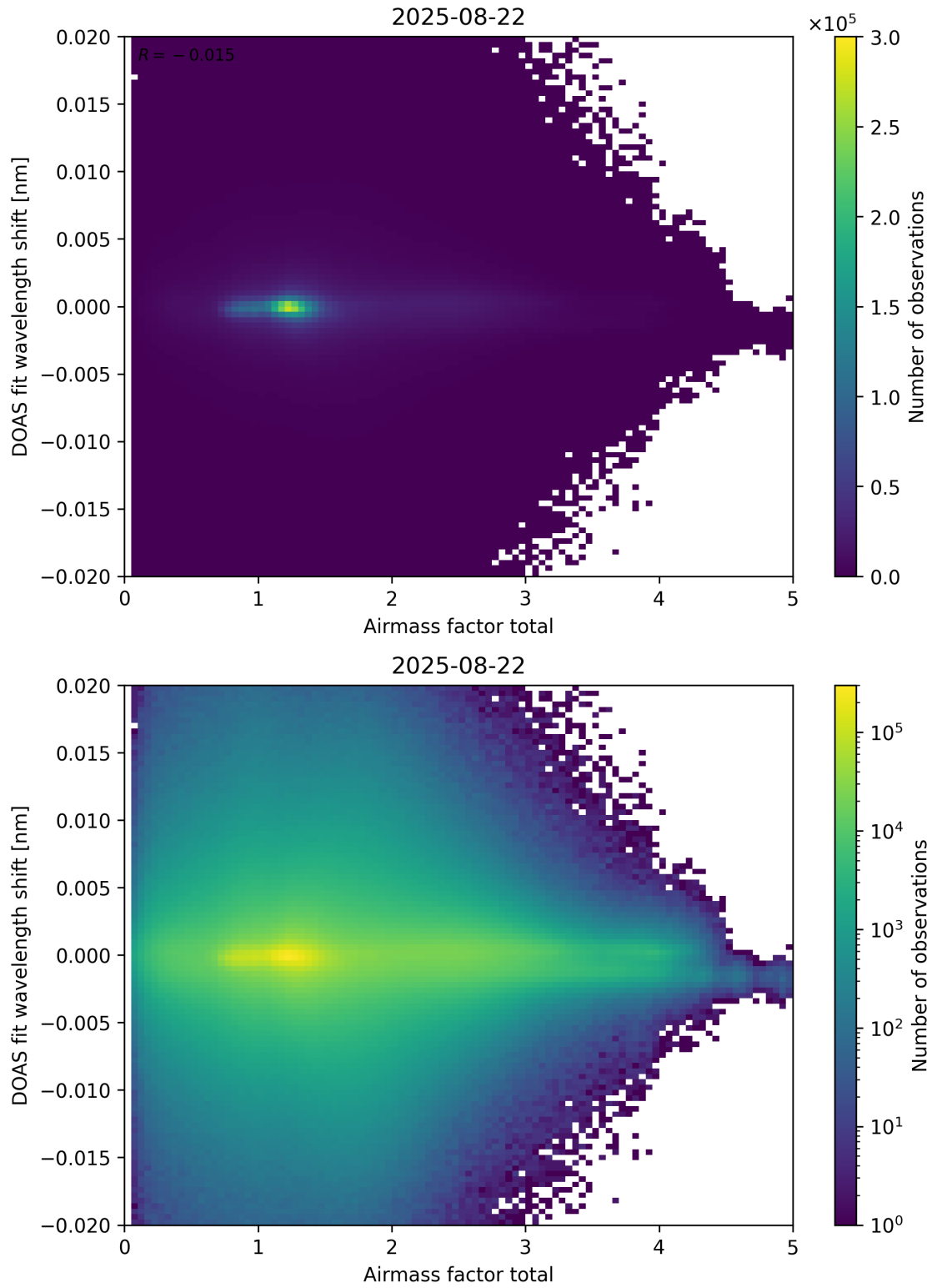
Figure 98: Scatter density plot of “Airmass factor total” against “DOAS fit wavelength shift” for 2025-08-21 to 2025-08-23.
