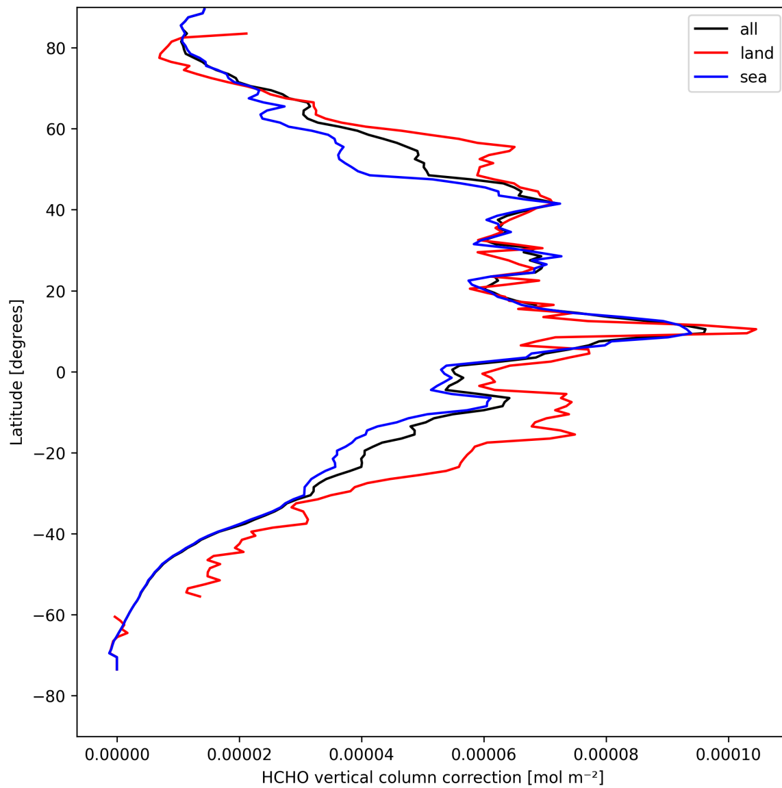
Figure 23: Zonal average of “HCHO vertical column correction” for 2025-08-21 to 2025-08-23.
