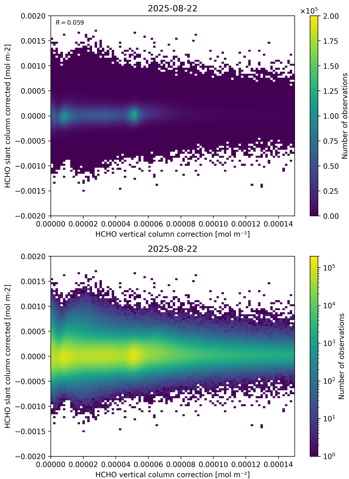
Figure 116: Scatter density plot of “HCHO vertical column correction” against “HCHO slant column corrected” for 2025-08-21 to 2025-08-23.
