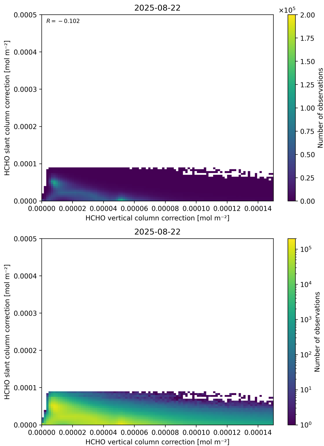
Figure 117: Scatter density plot of “HCHO vertical column correction” against “HCHO slant column correction” for 2025-08-21 to 2025-08-23.
