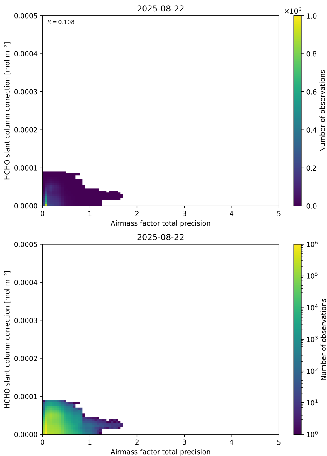
Figure 110: Scatter density plot of “Airmass factor total precision” against “HCHO slant column correction” for 2025-08-21 to 2025-08-23.
