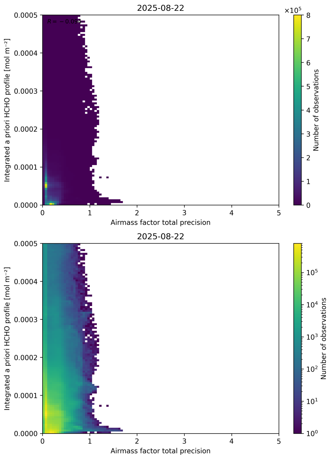
Figure 111: Scatter density plot of “Airmass factor total precision” against “Integrated a priori HCHO profile” for 2025-08-21 to 2025-08-23.
