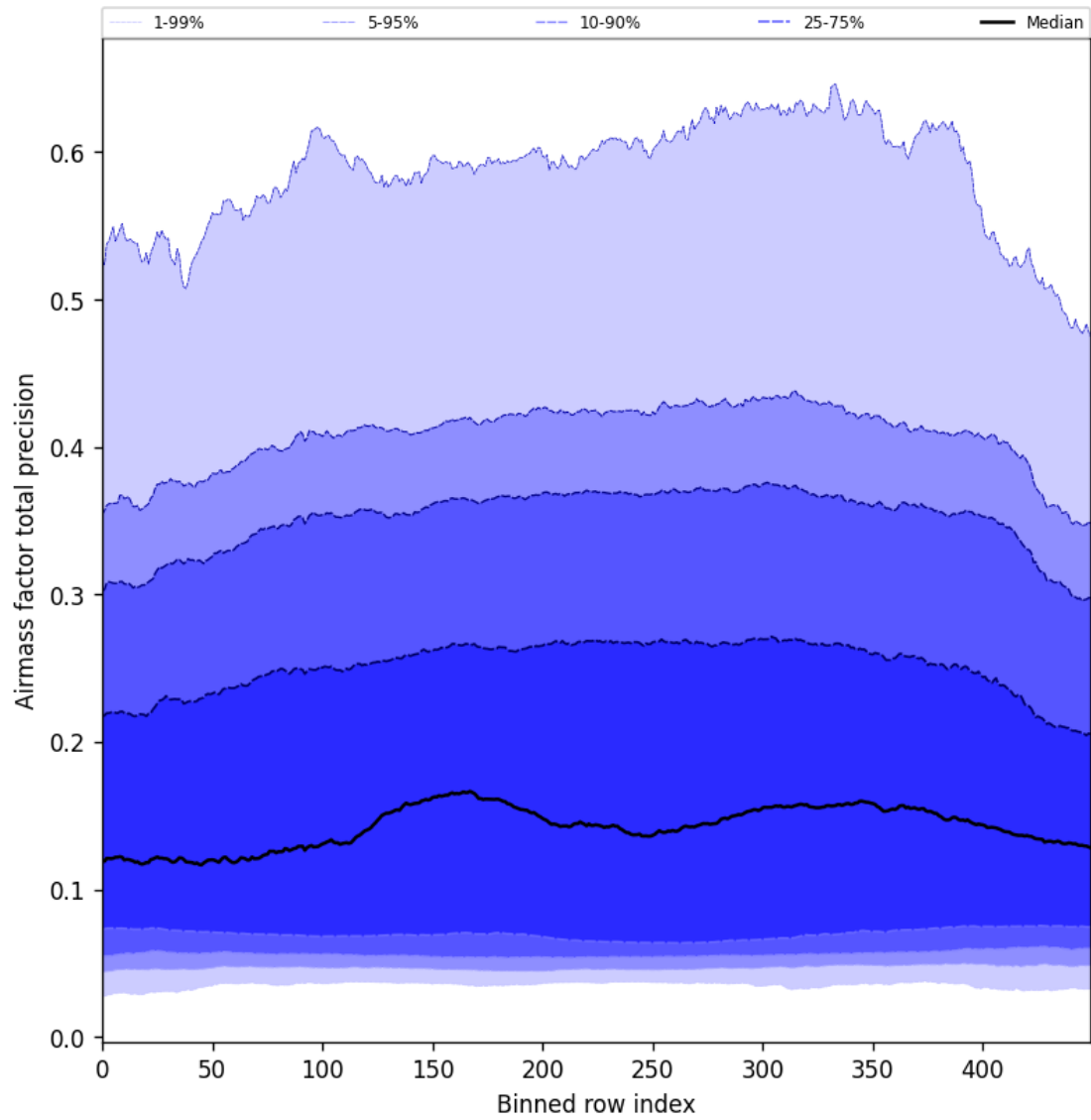
Figure 55: Along track statistics of “Airmass factor total precision” for 2025-08-21 to 2025-08-23
