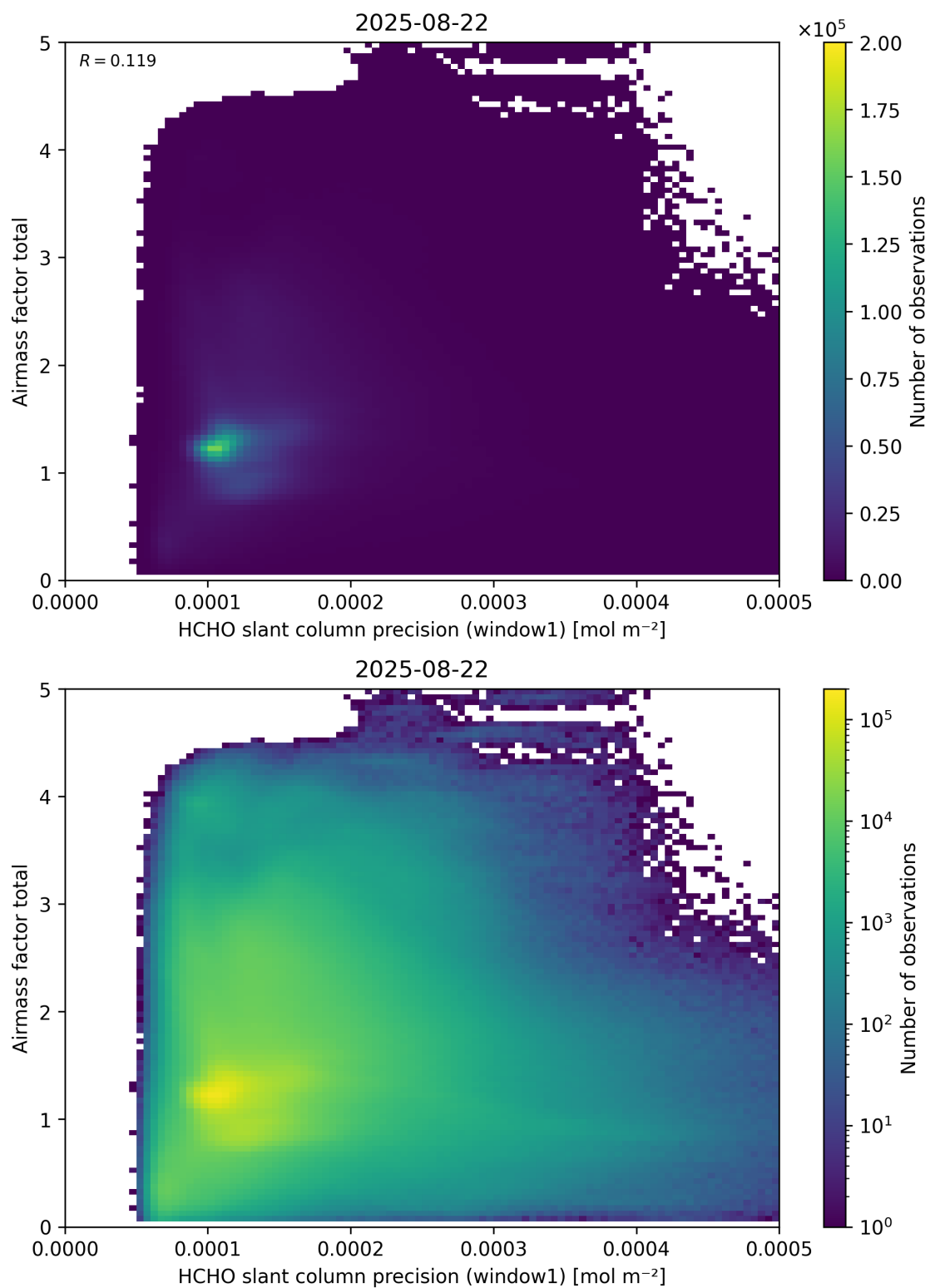
Figure 94: Scatter density plot of “HCHO slant column precision (window1)” against “Airmass factor total” for 2025-08-21 to 2025-08-23.
