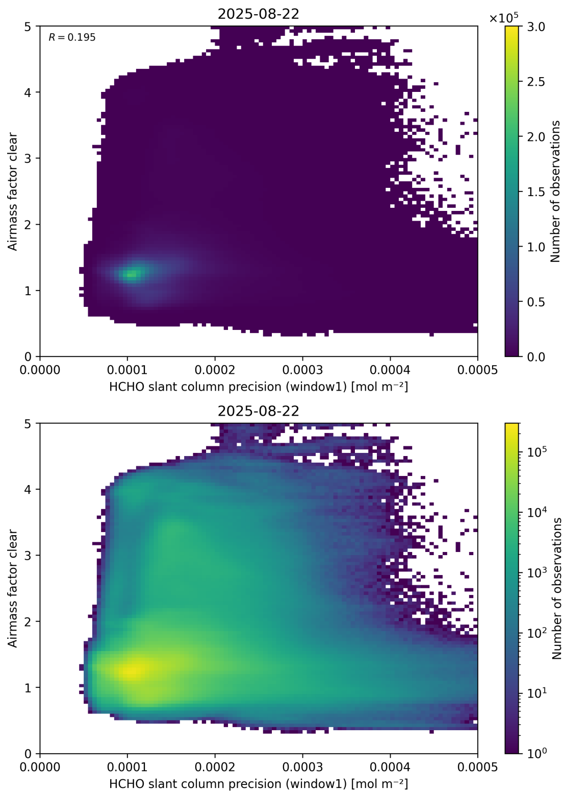
Figure 91: Scatter density plot of “HCHO slant column precision (window1)” against “Airmass factor clear” for 2025-08-21 to 2025-08-23.
