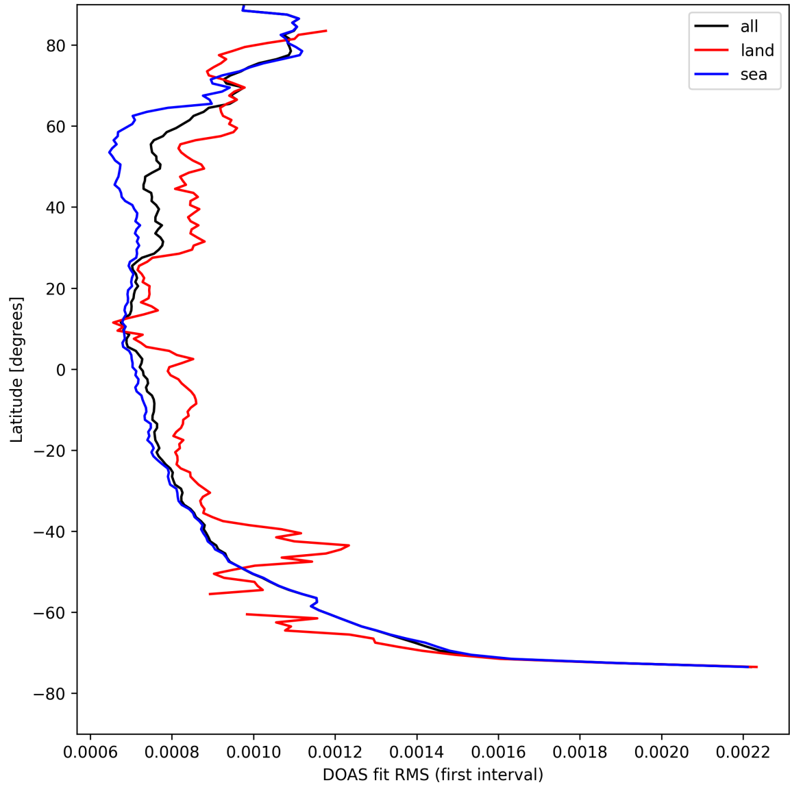
Figure 32: Zonal average of “DOAS fit RMS (first interval)” for 2025-08-21 to 2025-08-23.
