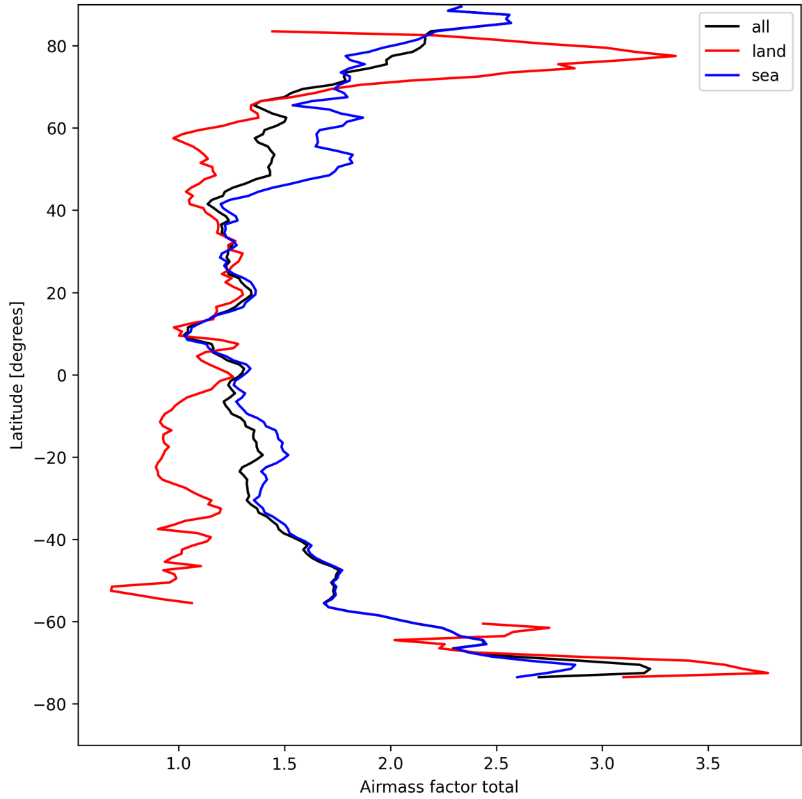
Figure 26: Zonal average of “Airmass factor total” for 2025-08-21 to 2025-08-23.
