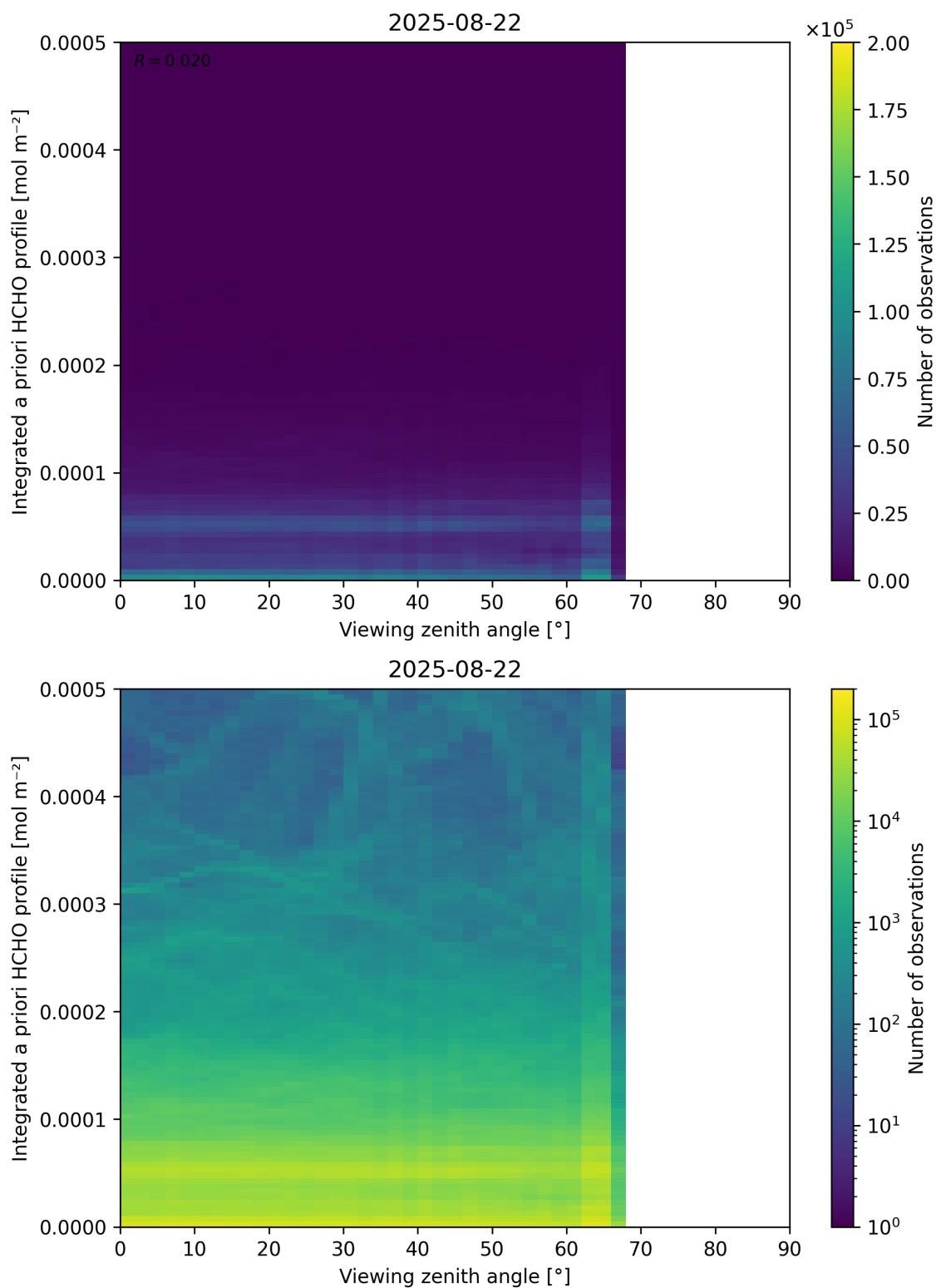
Figure 195: Scatter density plot of “Viewing zenith angle” against “Integrated a priori HCHO profile” for 2025-08-21 to 2025-08-23.
