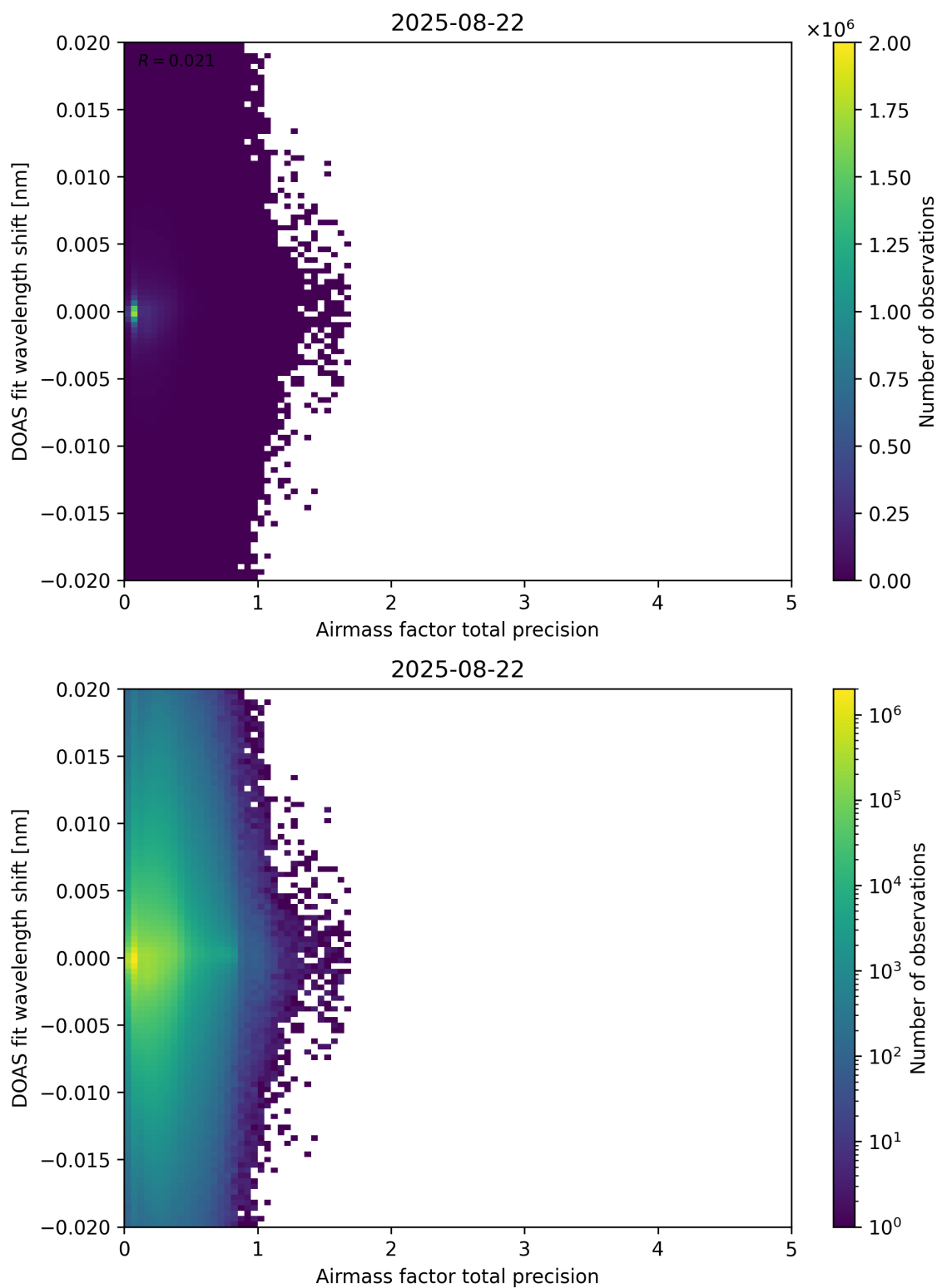
Figure 106: Scatter density plot of “Airmass factor total precision” against “DOAS fit wavelength shift” for 2025-08-21 to 2025-08-23.
