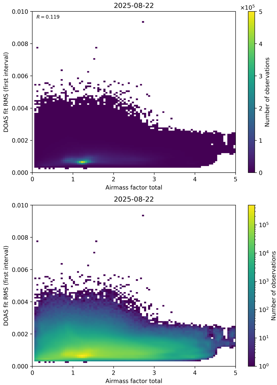
Figure 97: Scatter density plot of “Airmass factor total” against “DOAS fit RMS (first interval)” for 2025-08-21 to 2025-08-23.
