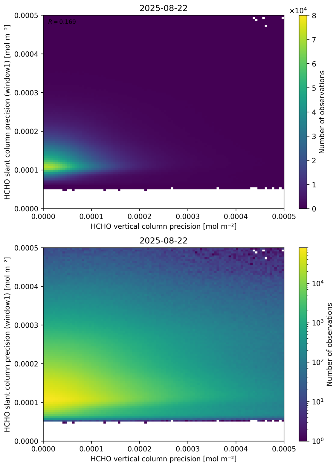
Figure 143: Scatter density plot of “HCHO vertical column precision” against “HCHO slant column precision (window1)” for 2025-08-21 to 2025-08-23.
