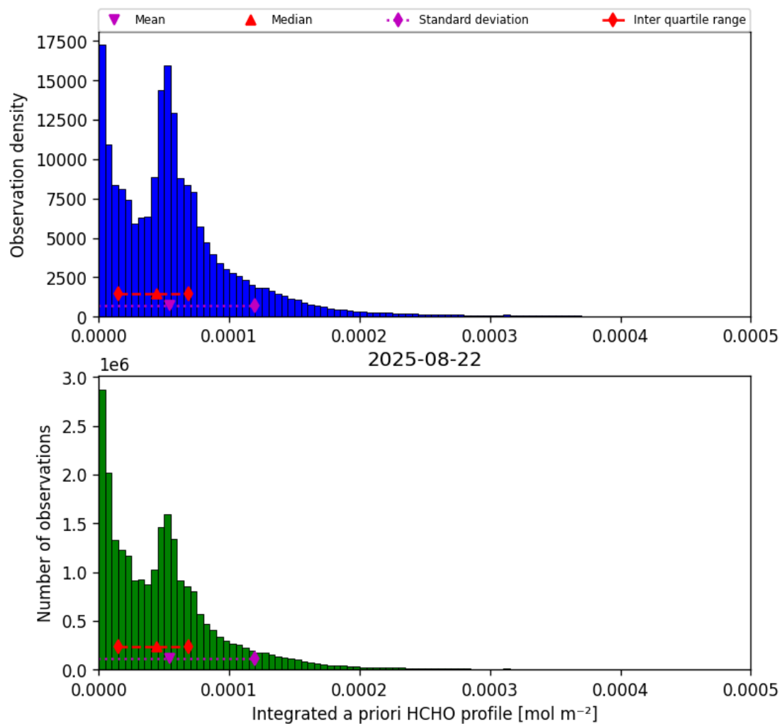
Figure 43: Histogram of “Integrated a priori HCHO profile” for 2025-08-21 to 2025-08-23
