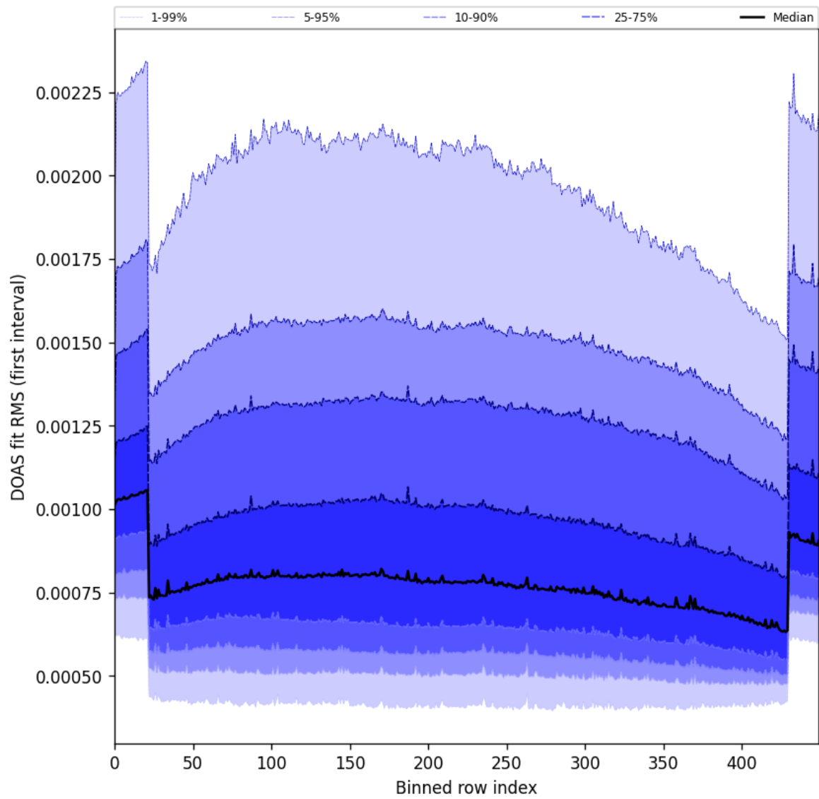
Figure 60: Along track statistics of “DOAS fit RMS (first interval)” for 2025-08-21 to 2025-08-23
