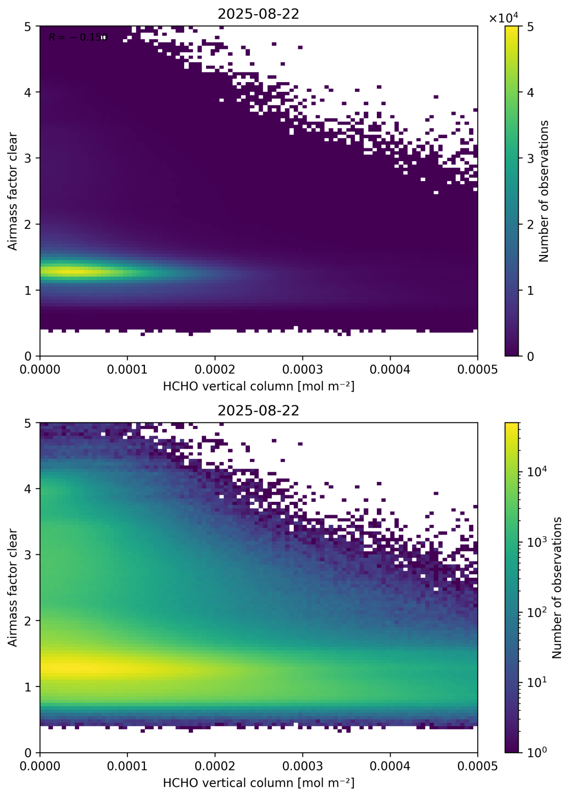
Figure 126: Scatter density plot of “HCHO vertical column” against “Airmass factor clear” for 2025-08-21 to 2025-08-23.
