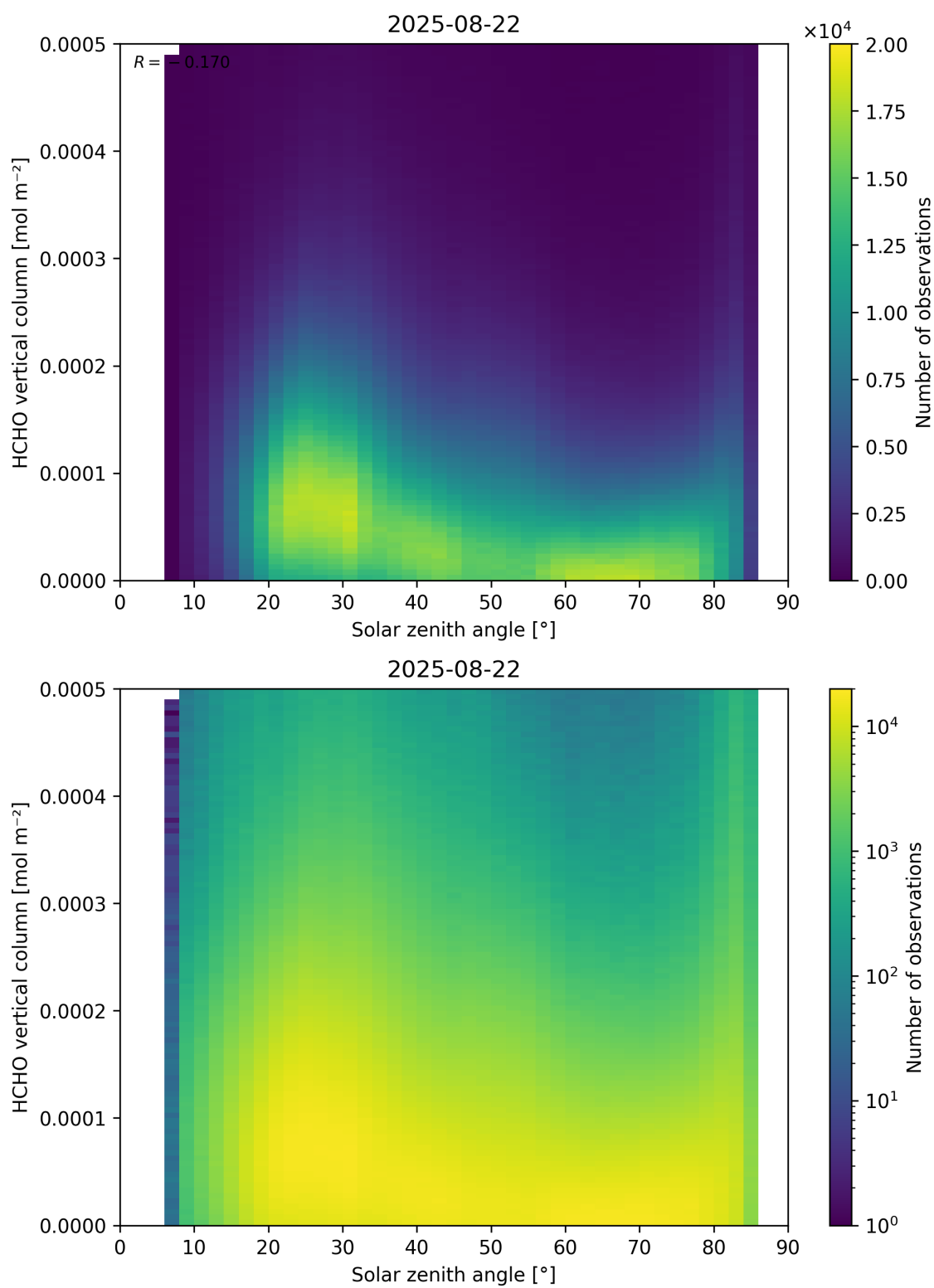
Figure 177: Scatter density plot of “Solar zenith angle” against “HCHO vertical column” for 2025-08-21 to 2025-08-23.
