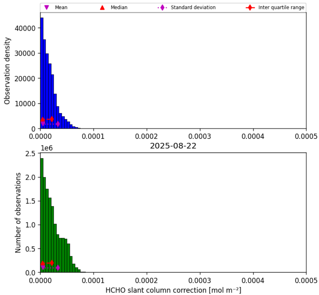
Figure 47: Histogram of “HCHO slant column correction” for 2025-08-21 to 2025-08-23
