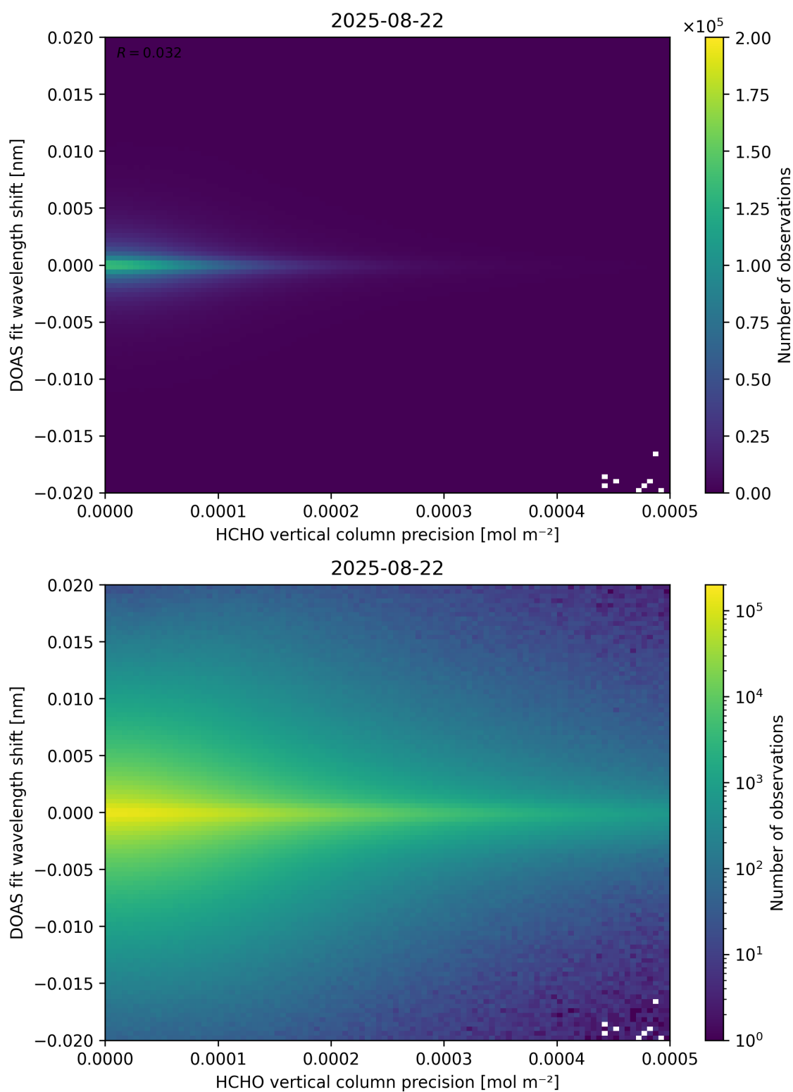
Figure 137: Scatter density plot of “HCHO vertical column precision” against “DOAS fit wavelength shift” for 2025-08-21 to 2025-08-23.
