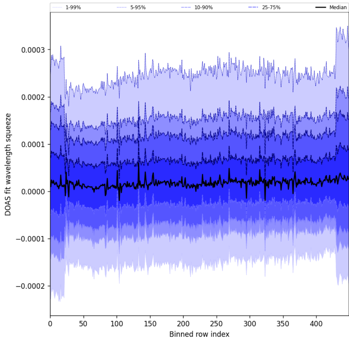
Figure 59: Along track statistics of “DOAS fit wavelength squeeze” for 2025-08-21 to 2025-08-23
