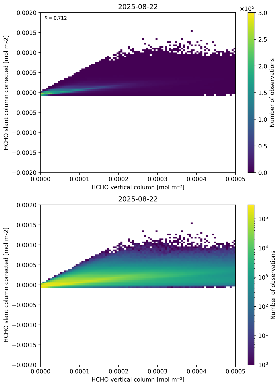
Figure 127: Scatter density plot of “HCHO vertical column” against “HCHO slant column corrected” for 2025-08-21 to 2025-08-23.
