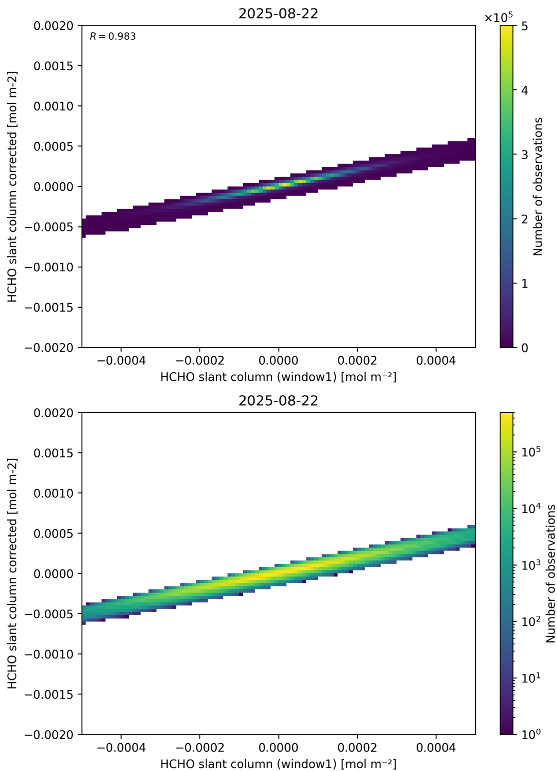
Figure 82: Scatter density plot of “HCHO slant column (window1)” against “HCHO slant column corrected” for 2025-08-21 to 2025-08-23.
