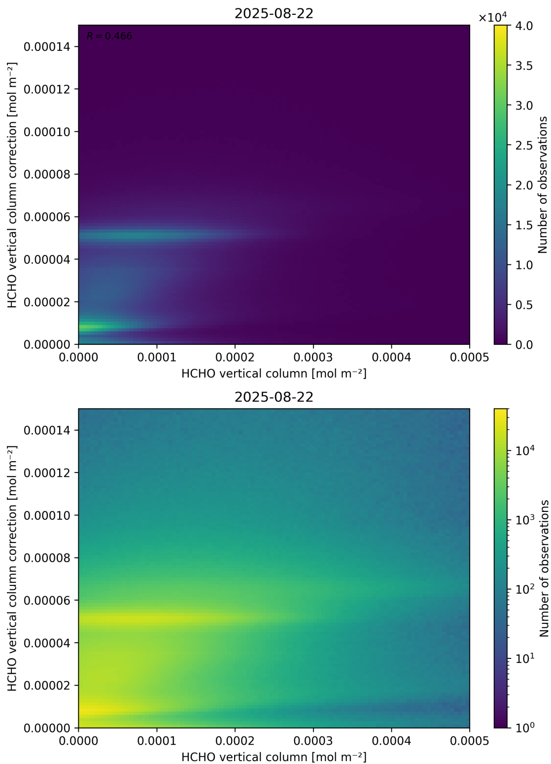
Figure 133: Scatter density plot of “HCHO vertical column” against “HCHO vertical column correction” for 2025-08-21 to 2025-08-23.
