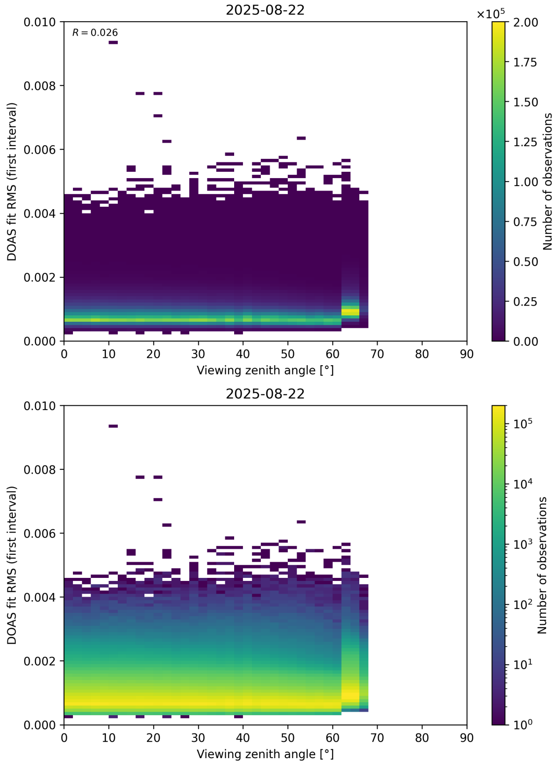
Figure 182: Scatter density plot of “Viewing zenith angle” against “DOAS fit RMS (first interval)” for 2025-08-21 to 2025-08-23.
