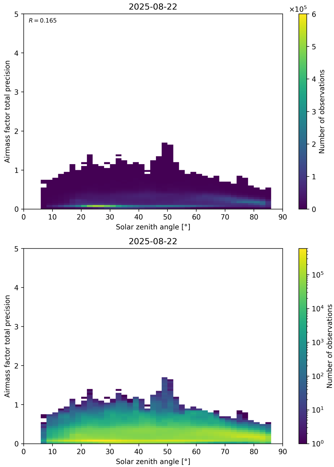
Figure 176: Scatter density plot of “Solar zenith angle” against “Airmass factor total precision” for 2025-08-21 to 2025-08-23.
