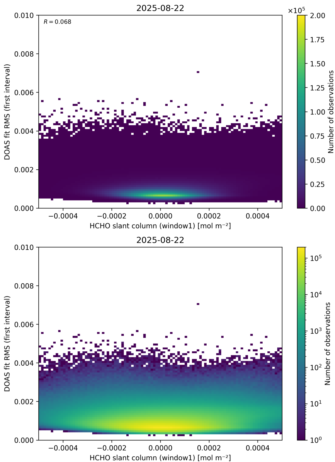
Figure 78: Scatter density plot of “HCHO slant column (window1)” against “DOAS fit RMS (first interval)” for 2025-08-21 to 2025-08-23.
