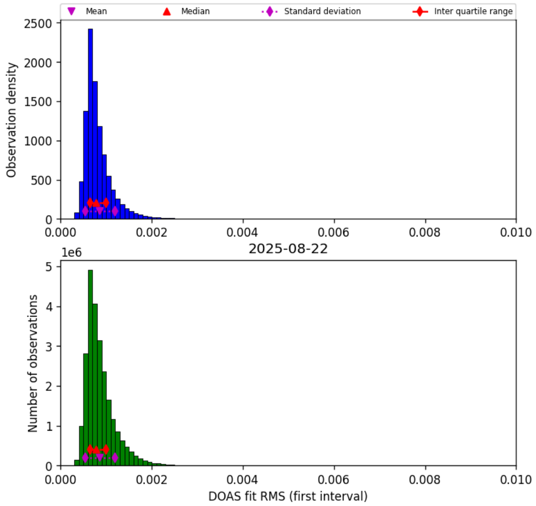
Figure 46: Histogram of “DOAS fit RMS (first interval)” for 2025-08-21 to 2025-08-23
