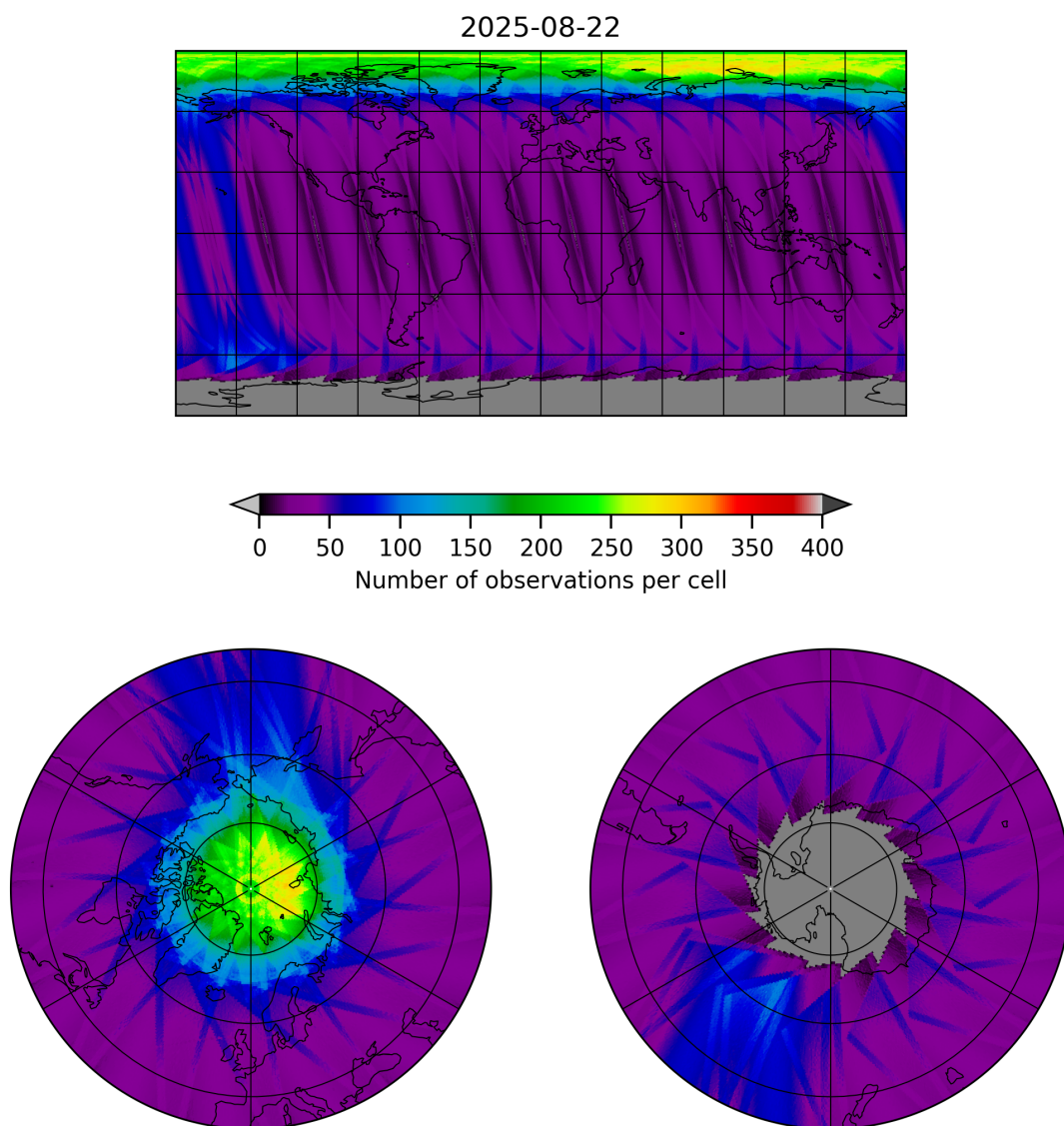
Figure 19: Map of the number of observations for 2025-08-21 to 2025-08-23
