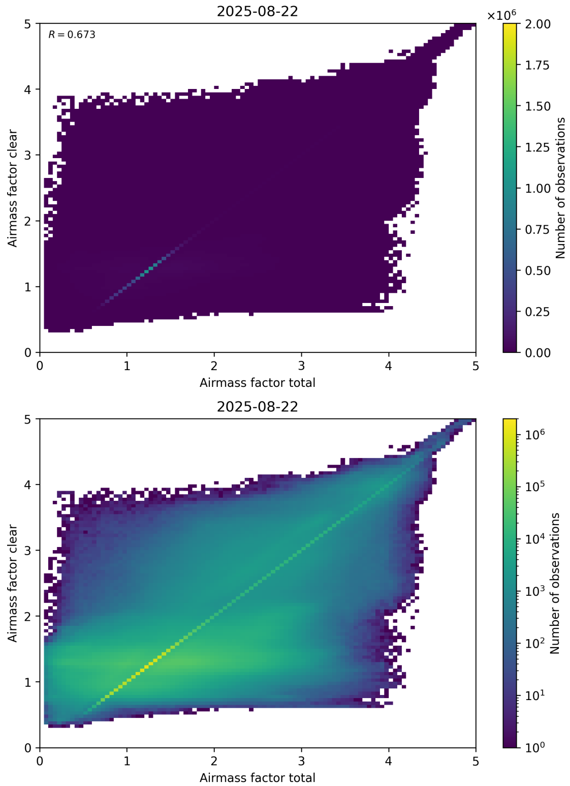
Figure 100: Scatter density plot of “Airmass factor total” against “Airmass factor clear” for 2025-08-21 to 2025-08-23.
