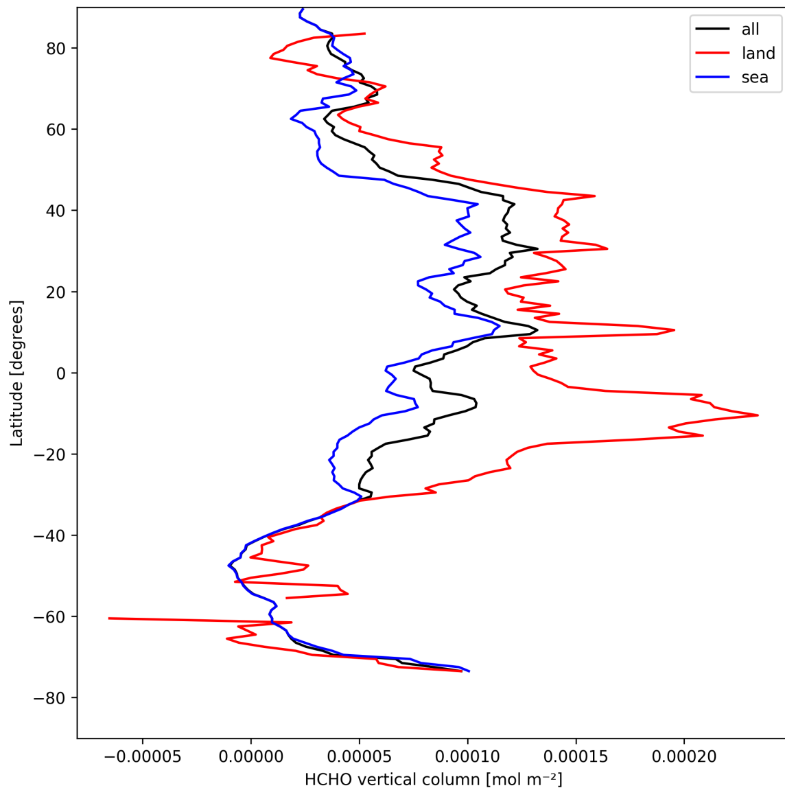
Figure 21: Zonal average of “HCHO vertical column” for 2025-08-21 to 2025-08-23.
