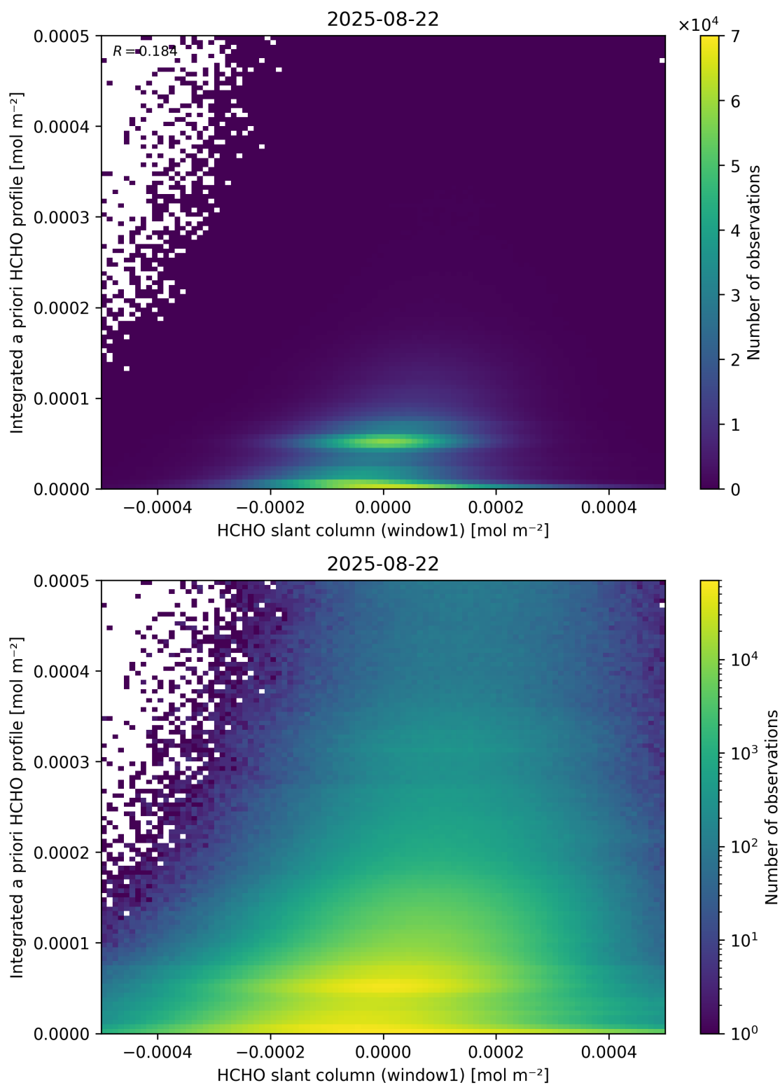
Figure 87: Scatter density plot of “HCHO slant column (window1)” against “Integrated a priori HCHO profile” for 2025-08-21 to 2025-08-23.
