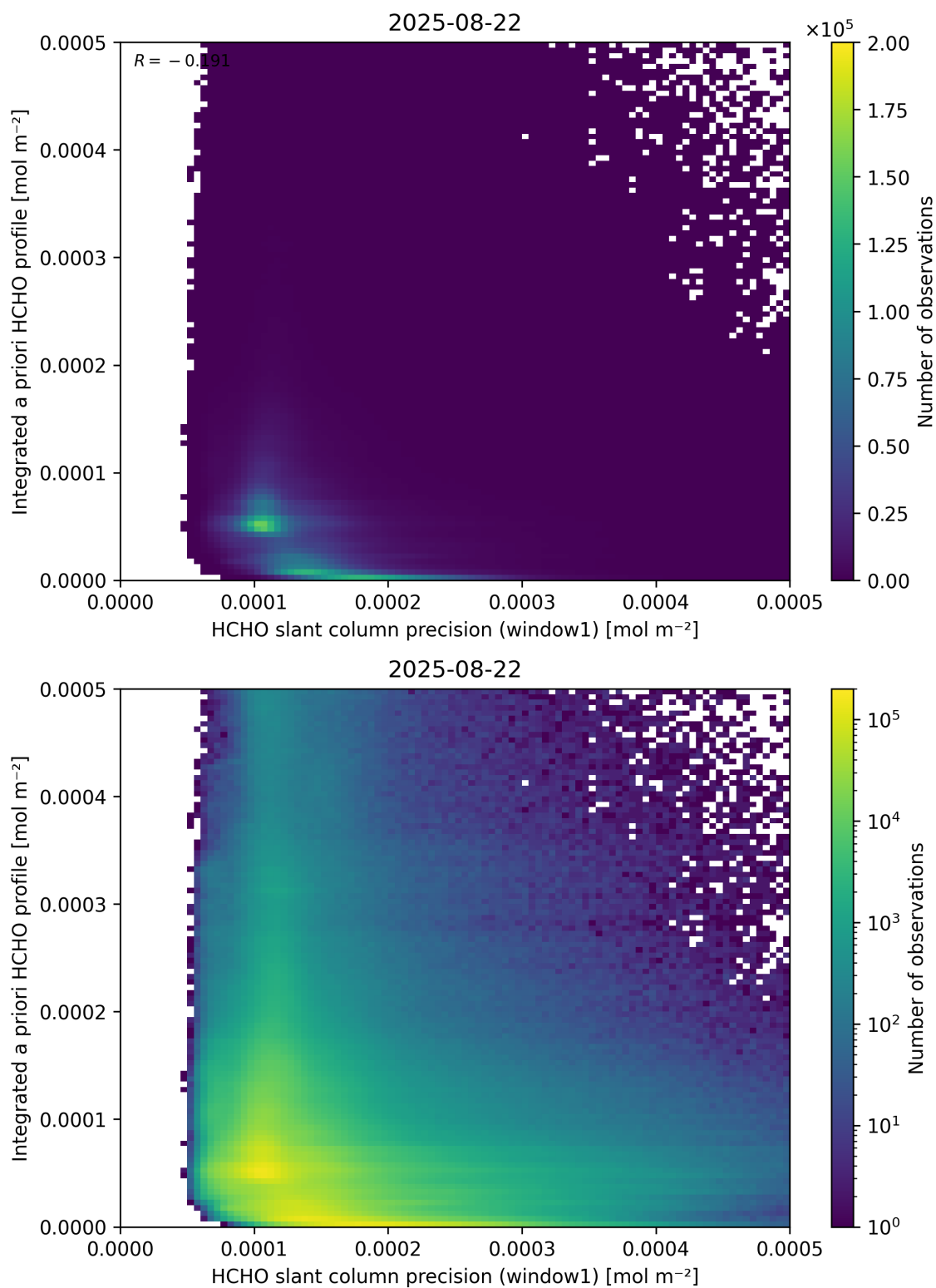
Figure 96: Scatter density plot of “HCHO slant column precision (window1)” against “Integrated a priori HCHO profile” for 2025-08-21 to 2025-08-23.
