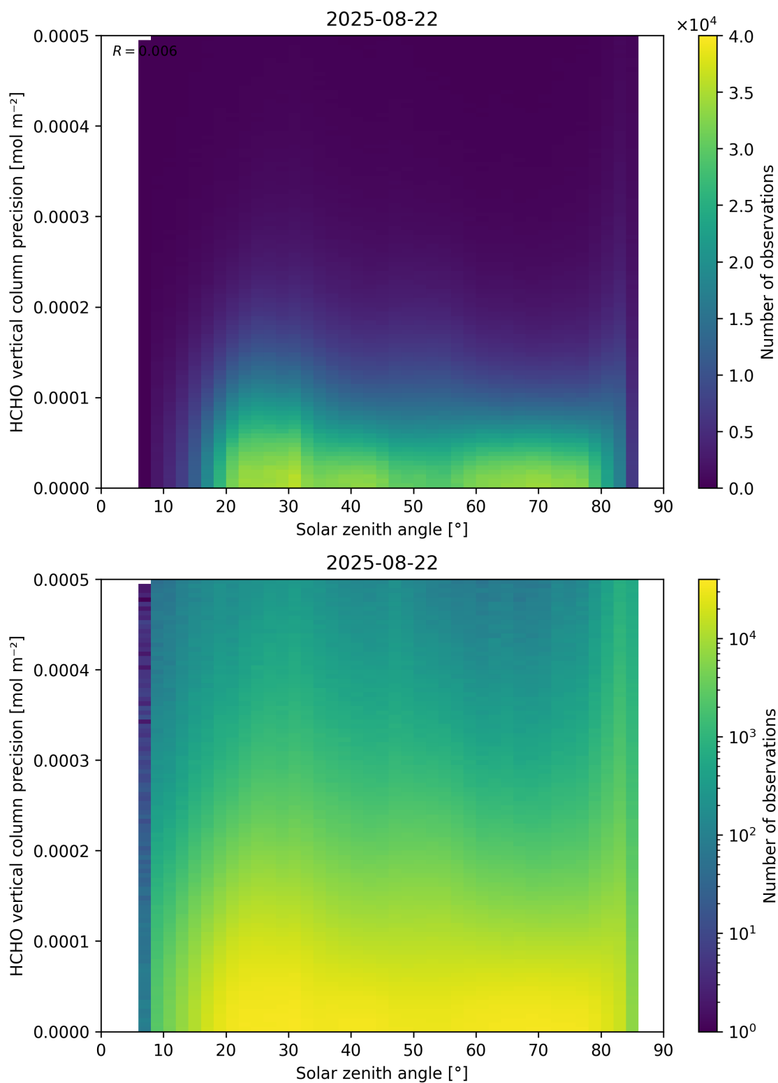
Figure 179: Scatter density plot of “Solar zenith angle” against “HCHO vertical column precision” for 2025-08-21 to 2025-08-23.
