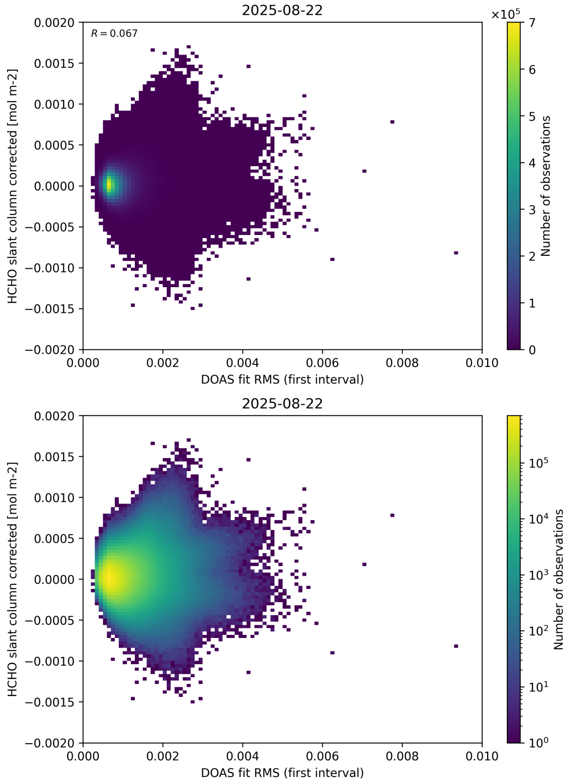
Figure 62: Scatter density plot of “DOAS fit RMS (first interval)” against “HCHO slant column corrected” for 2025-08-21 to 2025-08-23.
