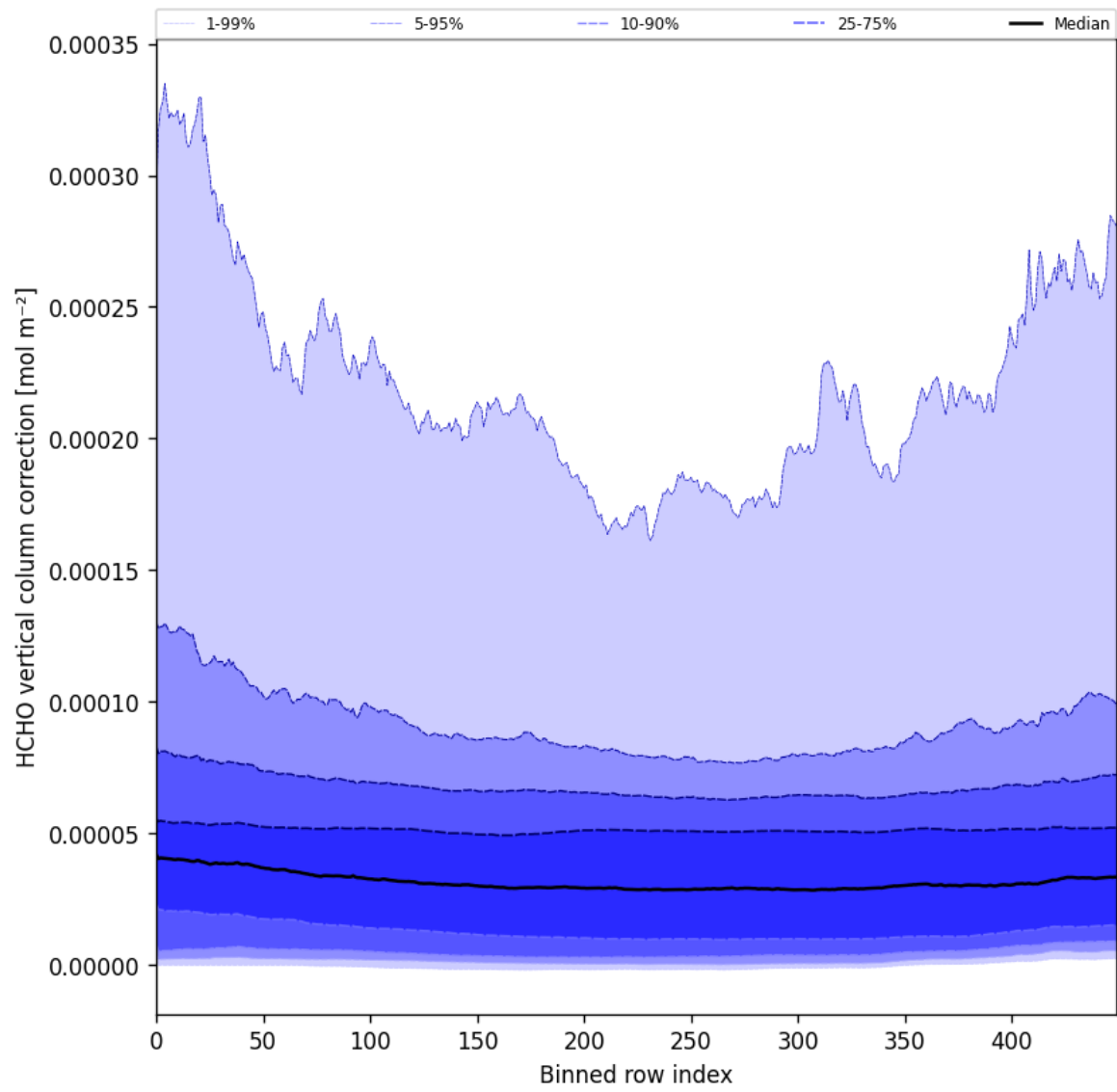
Figure 51: Along track statistics of “HCHO vertical column correction” for 2025-08-21 to 2025-08-23
