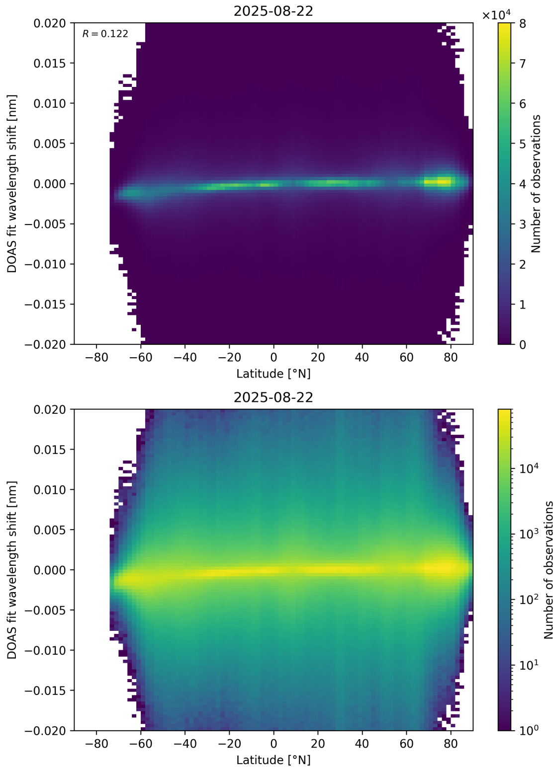
Figure 154: Scatter density plot of “Latitude” against “DOAS fit wavelength shift” for 2025-08-21 to 2025-08-23.
