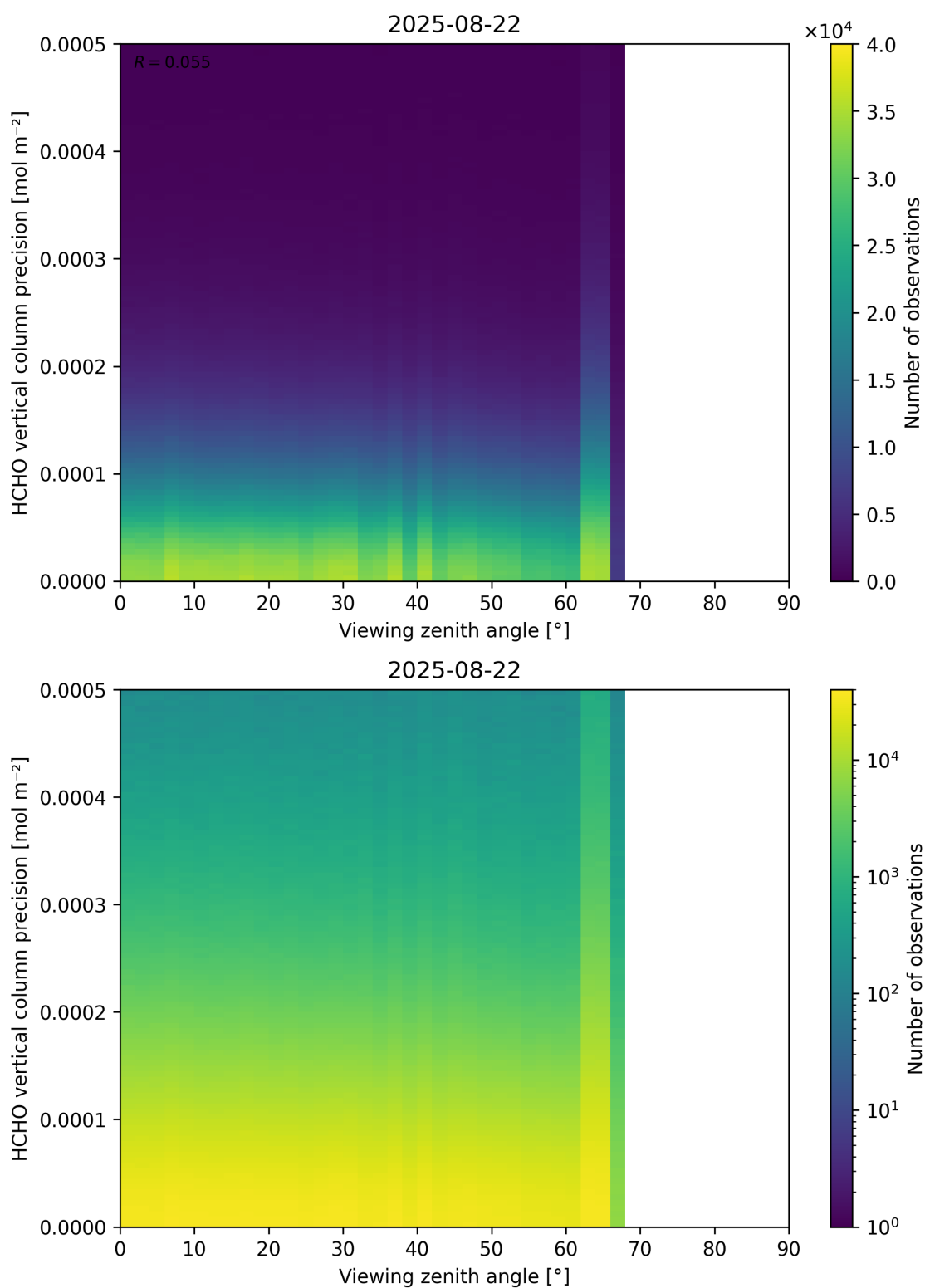
Figure 194: Scatter density plot of “Viewing zenith angle” against “HCHO vertical column precision” for 2025-08-21 to 2025-08-23.
