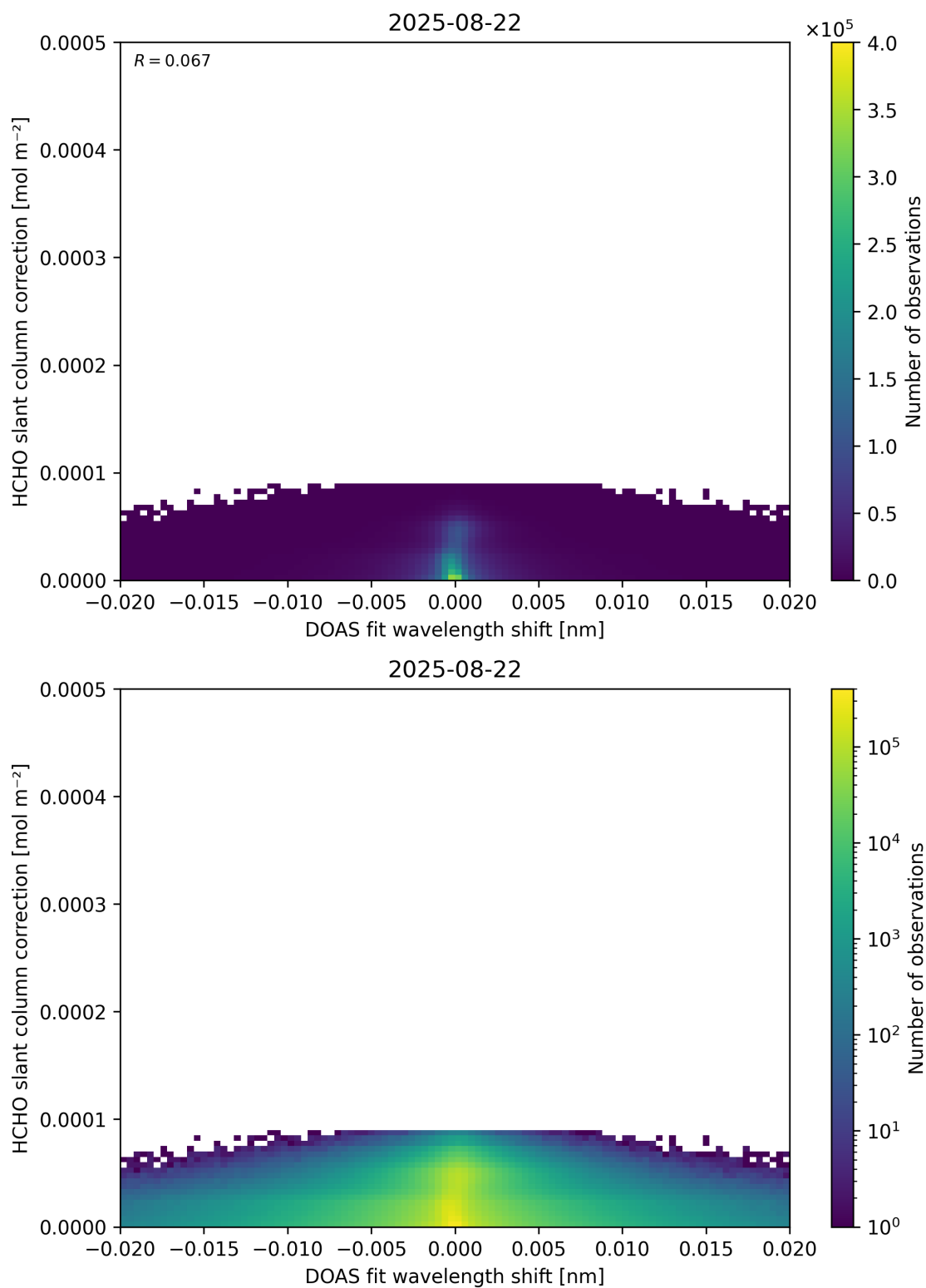
Figure 67: Scatter density plot of “DOAS fit wavelength shift” against “HCHO slant column correction” for 2025-08-21 to 2025-08-23.
