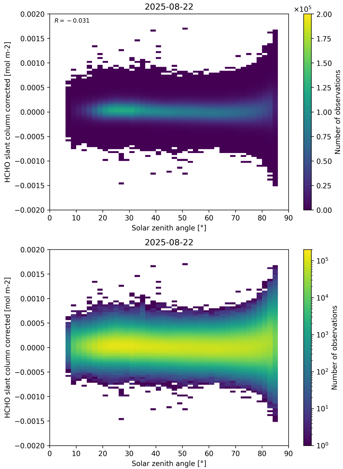
Figure 171: Scatter density plot of “Solar zenith angle” against “HCHO slant column corrected” for 2025-08-21 to 2025-08-23.
