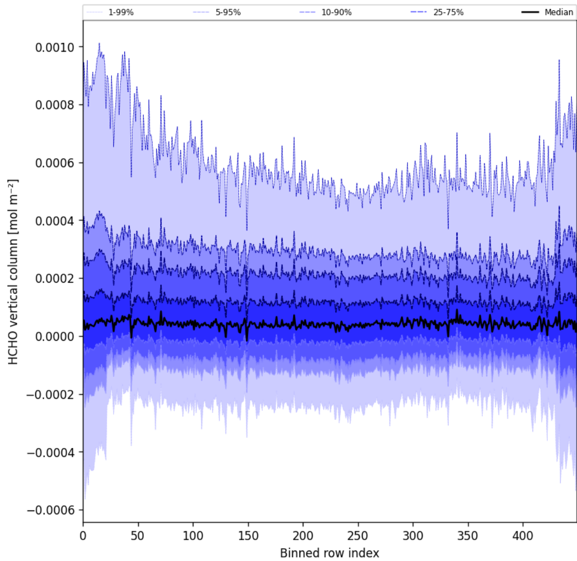
Figure 49: Along track statistics of “HCHO vertical column” for 2025-08-21 to 2025-08-23
