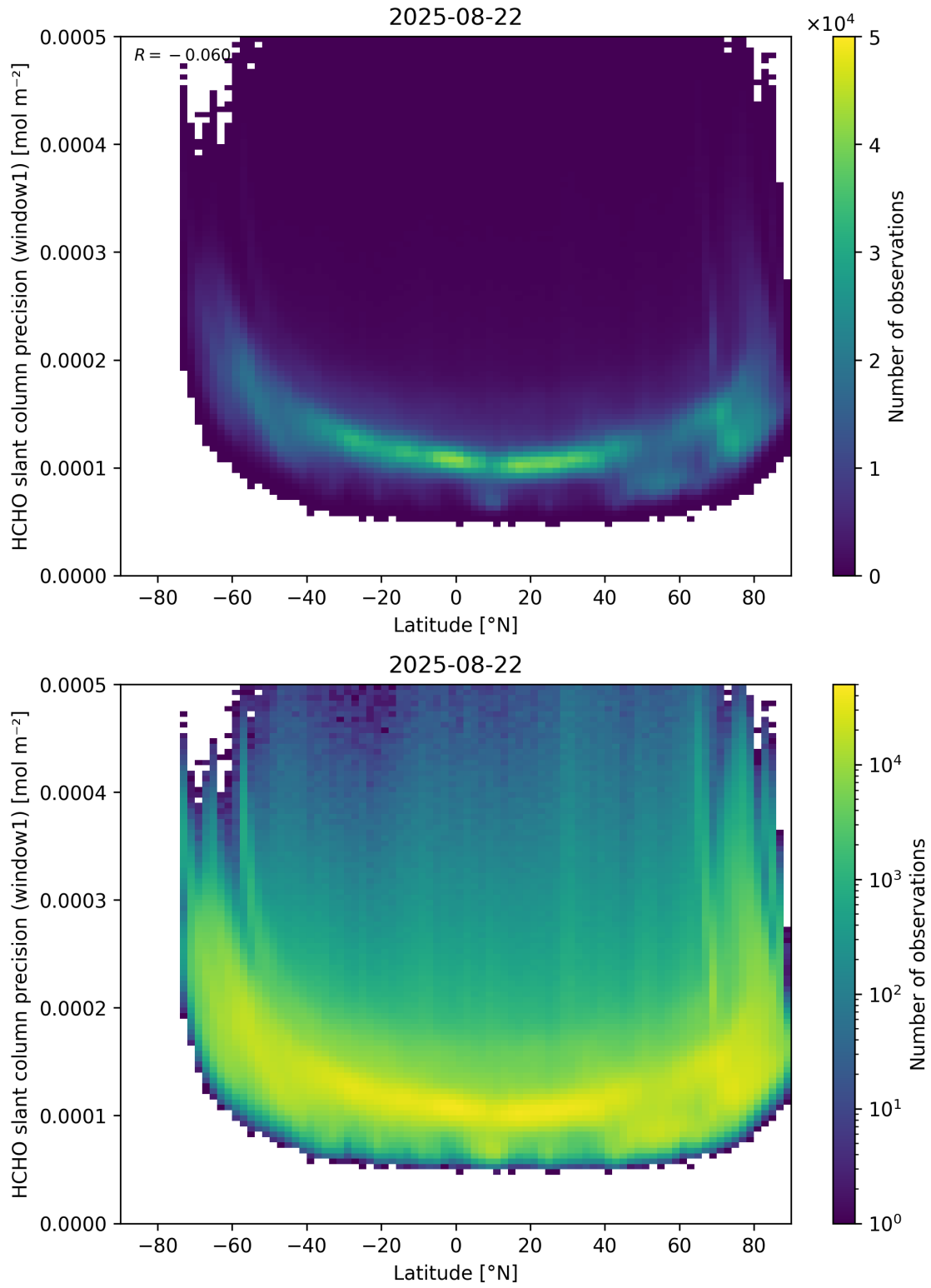
Figure 160: Scatter density plot of “Latitude” against “HCHO slant column precision (window1)” for 2025-08-21 to 2025-08-23.
