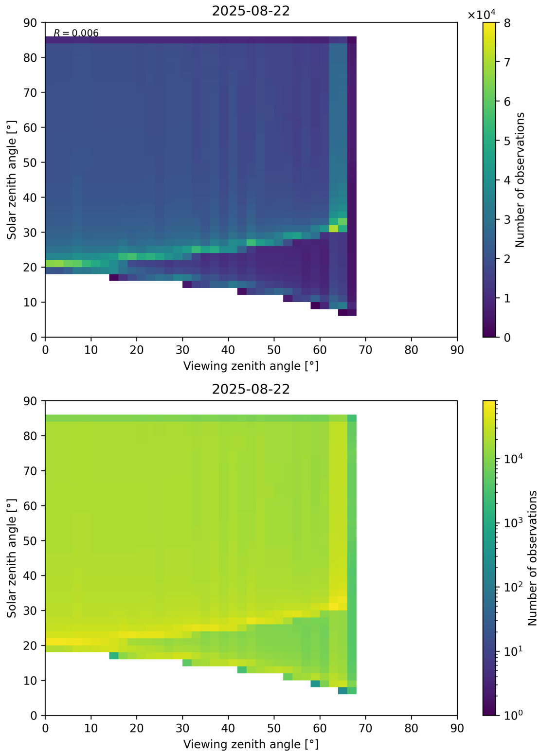
Figure 197: Scatter density plot of “Viewing zenith angle” against “Solar zenith angle” for 2025-08-21 to 2025-08-23.
