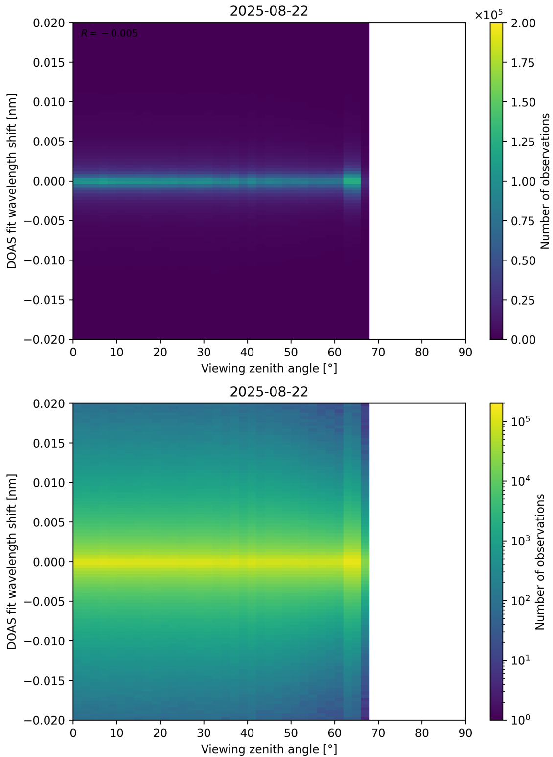
Figure 183: Scatter density plot of “Viewing zenith angle” against “DOAS fit wavelength shift” for 2025-08-21 to 2025-08-23.
