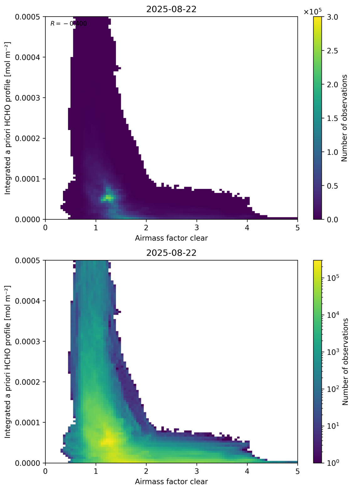
Figure 76: Scatter density plot of “Airmass factor clear” against “Integrated a priori HCHO profile” for 2025-08-21 to 2025-08-23.
