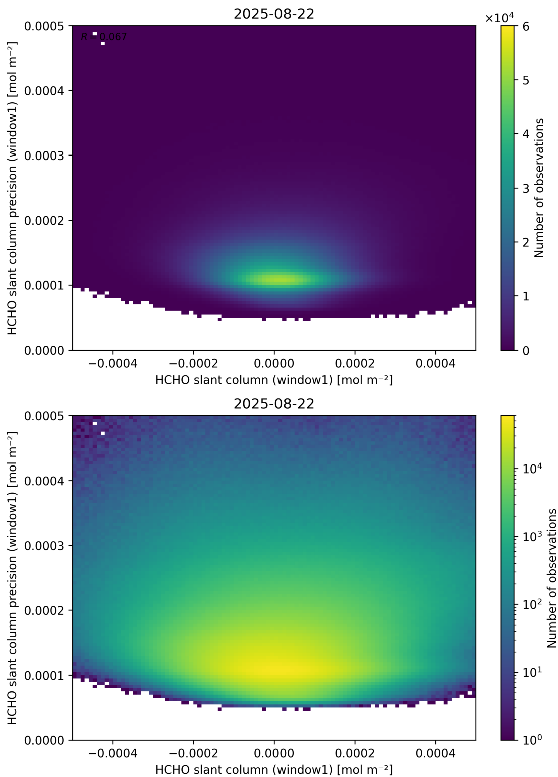
Figure 84: Scatter density plot of “HCHO slant column (window1)” against “HCHO slant column precision (window1)” for 2025-08-21 to 2025-08-23.
