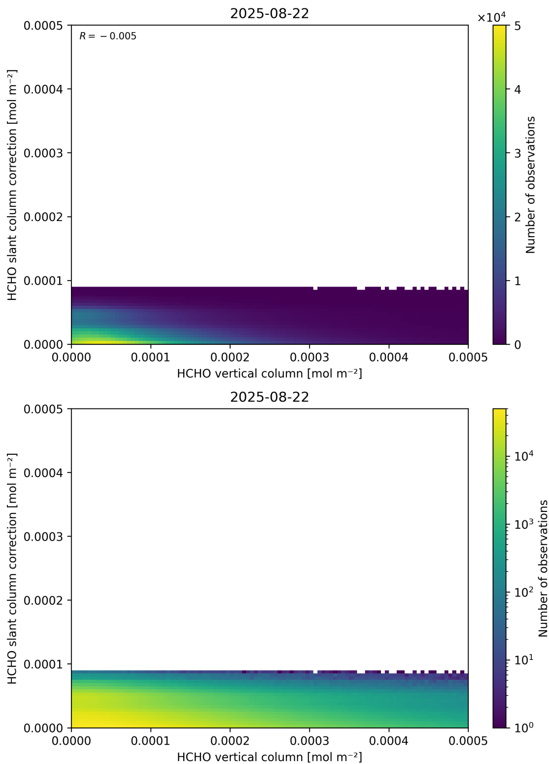
Figure 128: Scatter density plot of “HCHO vertical column” against “HCHO slant column correction” for 2025-08-21 to 2025-08-23.
