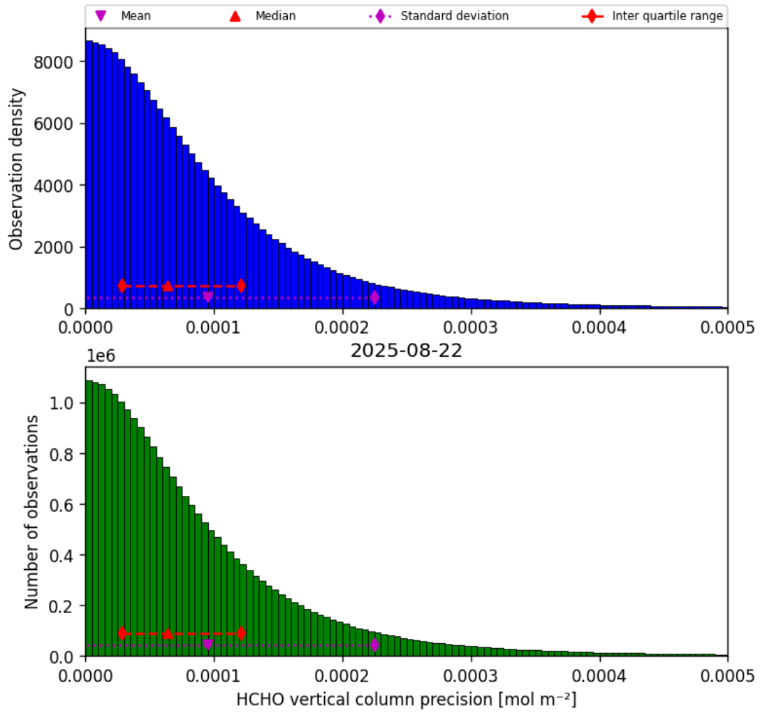
Figure 36: Histogram of “HCHO vertical column precision” for 2025-08-21 to 2025-08-23
