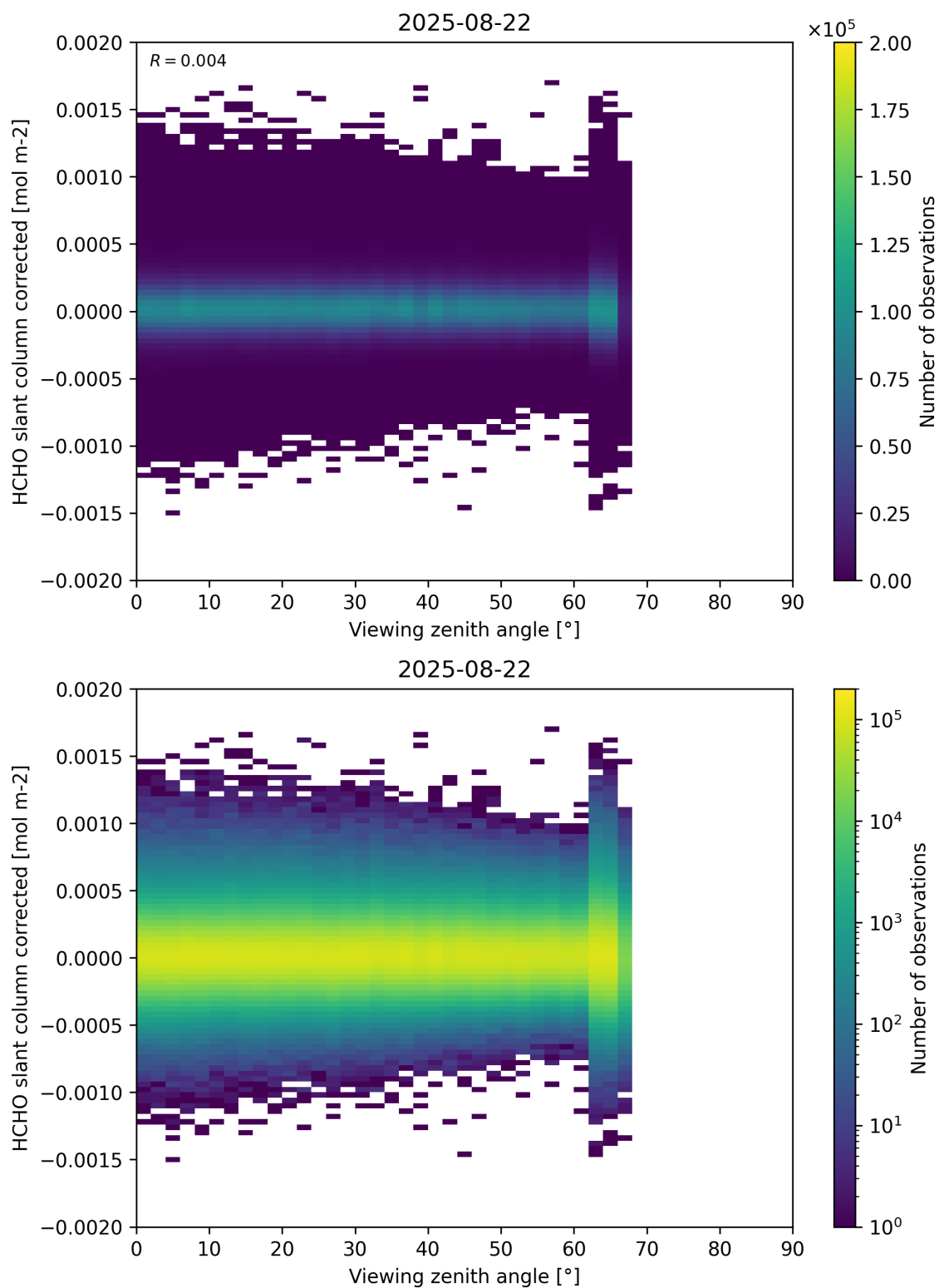
Figure 186: Scatter density plot of “Viewing zenith angle” against “HCHO slant column corrected” for 2025-08-21 to 2025-08-23.
