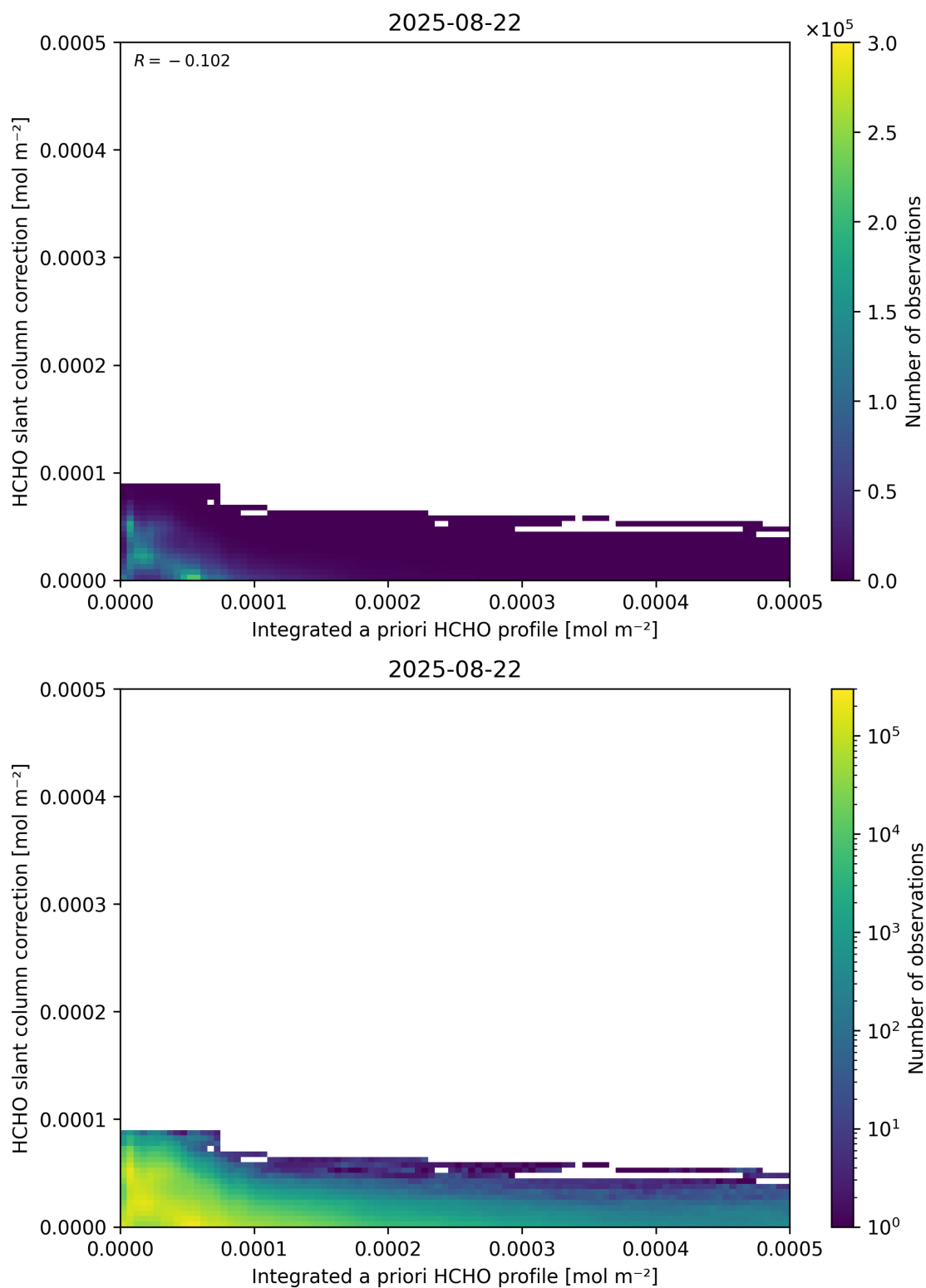
Figure 152: Scatter density plot of “Integrated a priori HCHO profile” against “HCHO slant column correction” for 2025-08-21 to 2025-08-23.
