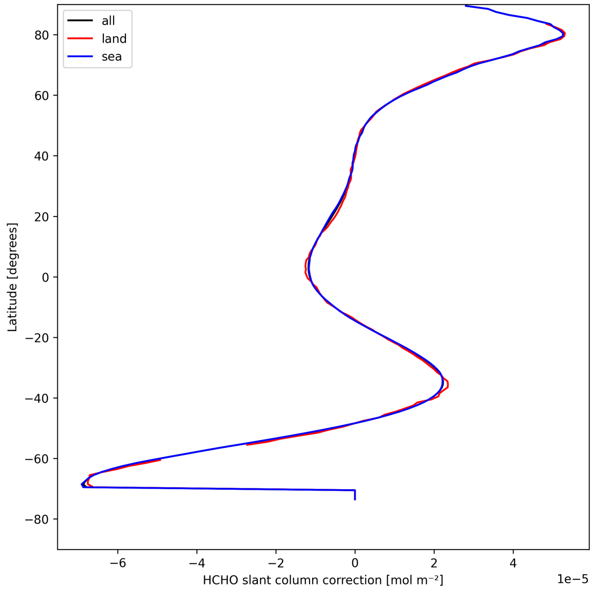
Figure 33: Zonal average of “HCHO slant column correction” for 2025-08-21 to 2025-08-23.
