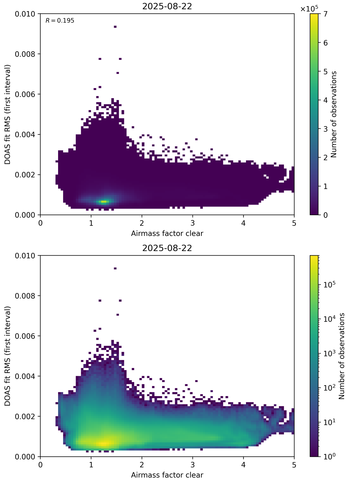
Figure 71: Scatter density plot of “Airmass factor clear” against “DOAS fit RMS (first interval)” for 2025-08-21 to 2025-08-23.
