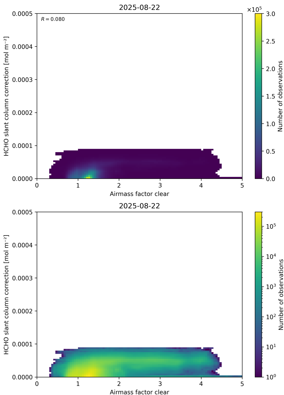
Figure 75: Scatter density plot of “Airmass factor clear” against “HCHO slant column correction” for 2025-08-21 to 2025-08-23.
