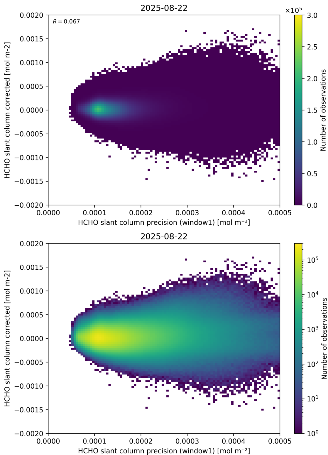
Figure 92: Scatter density plot of “HCHO slant column precision (window1)” against “HCHO slant column corrected” for 2025-08-21 to 2025-08-23.
