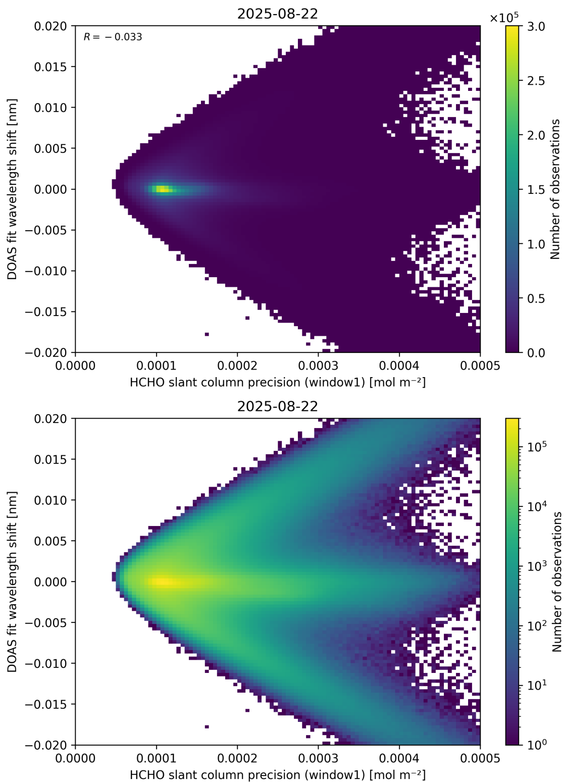
Figure 89: Scatter density plot of “HCHO slant column precision (window1)” against “DOAS fit wavelength shift” for 2025-08-21 to 2025-08-23.
