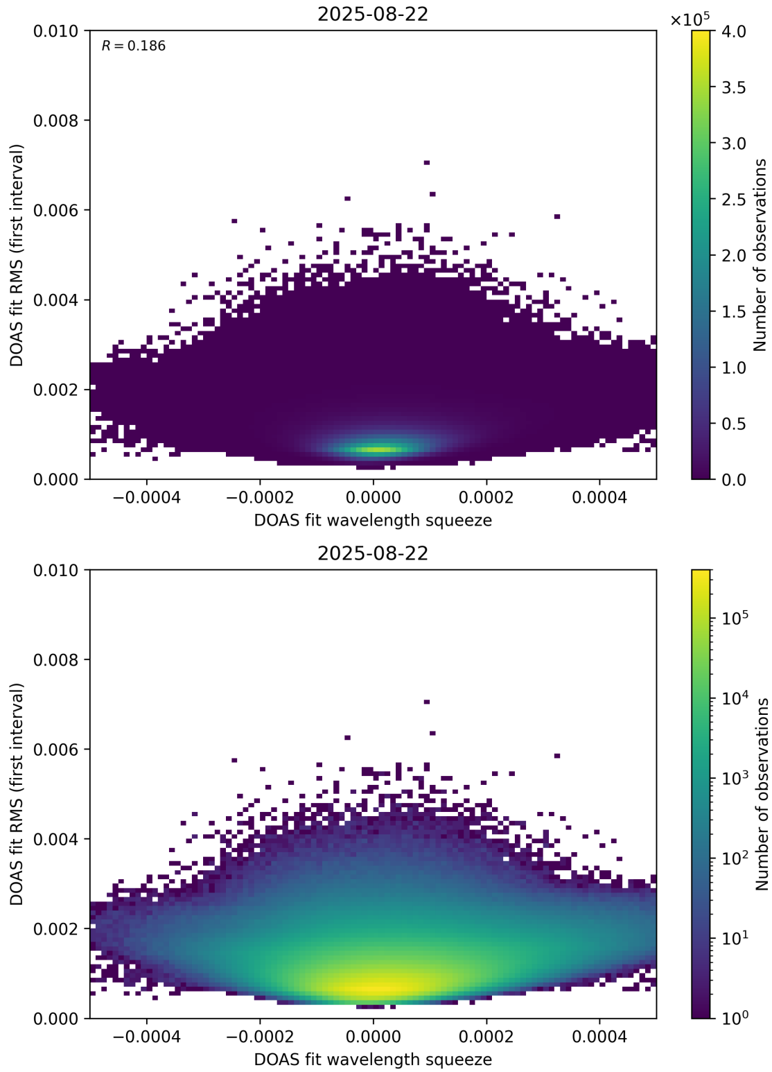
Figure 68: Scatter density plot of “DOAS fit wavelength squeeze” against “DOAS fit RMS (first interval)” for 2025-08-21 to 2025-08-23.
