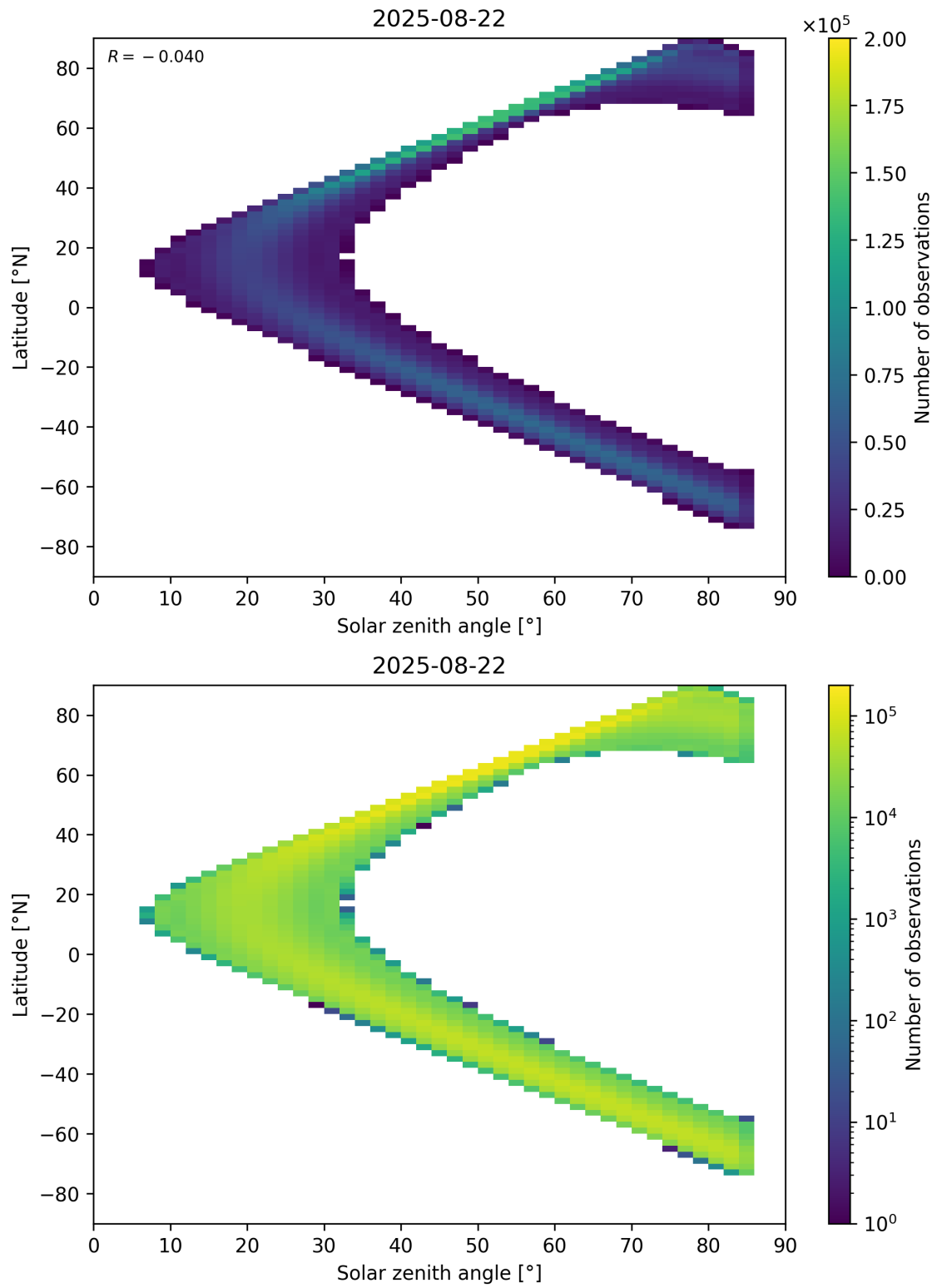
Figure 181: Scatter density plot of “Solar zenith angle” against “Latitude” for 2025-08-21 to 2025-08-23.
