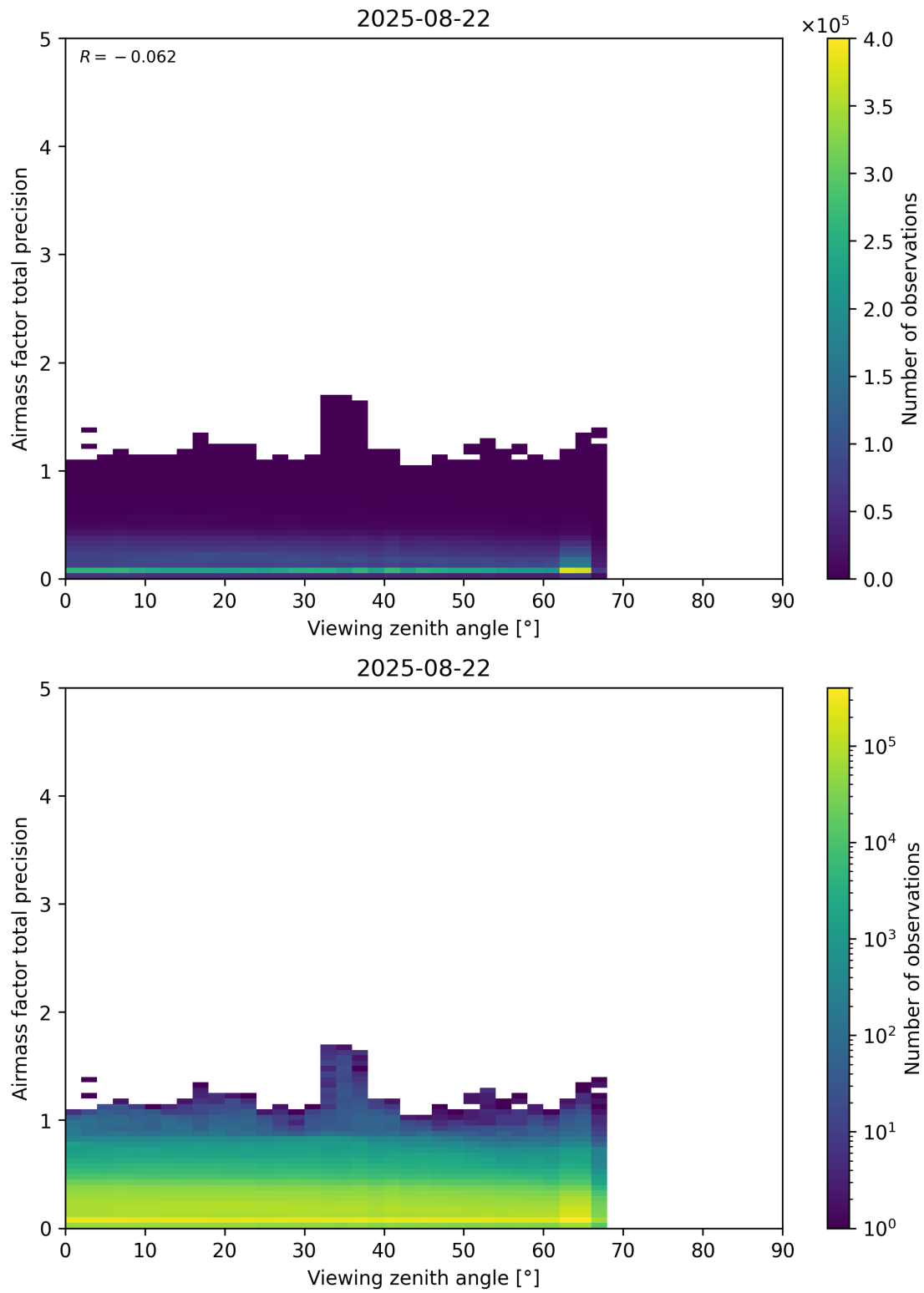
Figure 191: Scatter density plot of “Viewing zenith angle” against “Airmass factor total precision” for 2025-08-21 to 2025-08-23.
