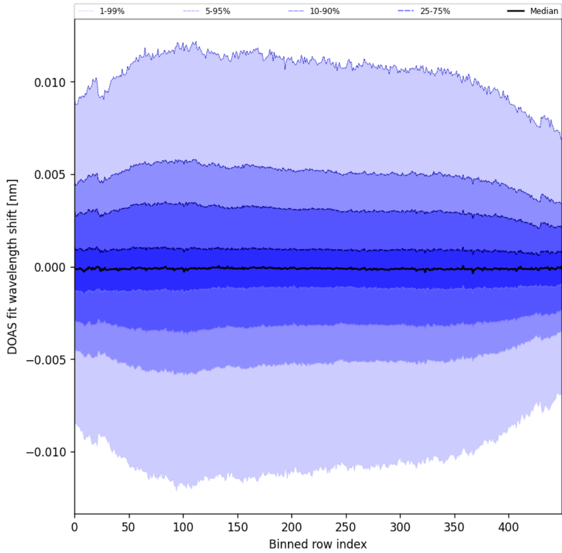
Figure 58: Along track statistics of “DOAS fit wavelength shift” for 2025-08-21 to 2025-08-23
