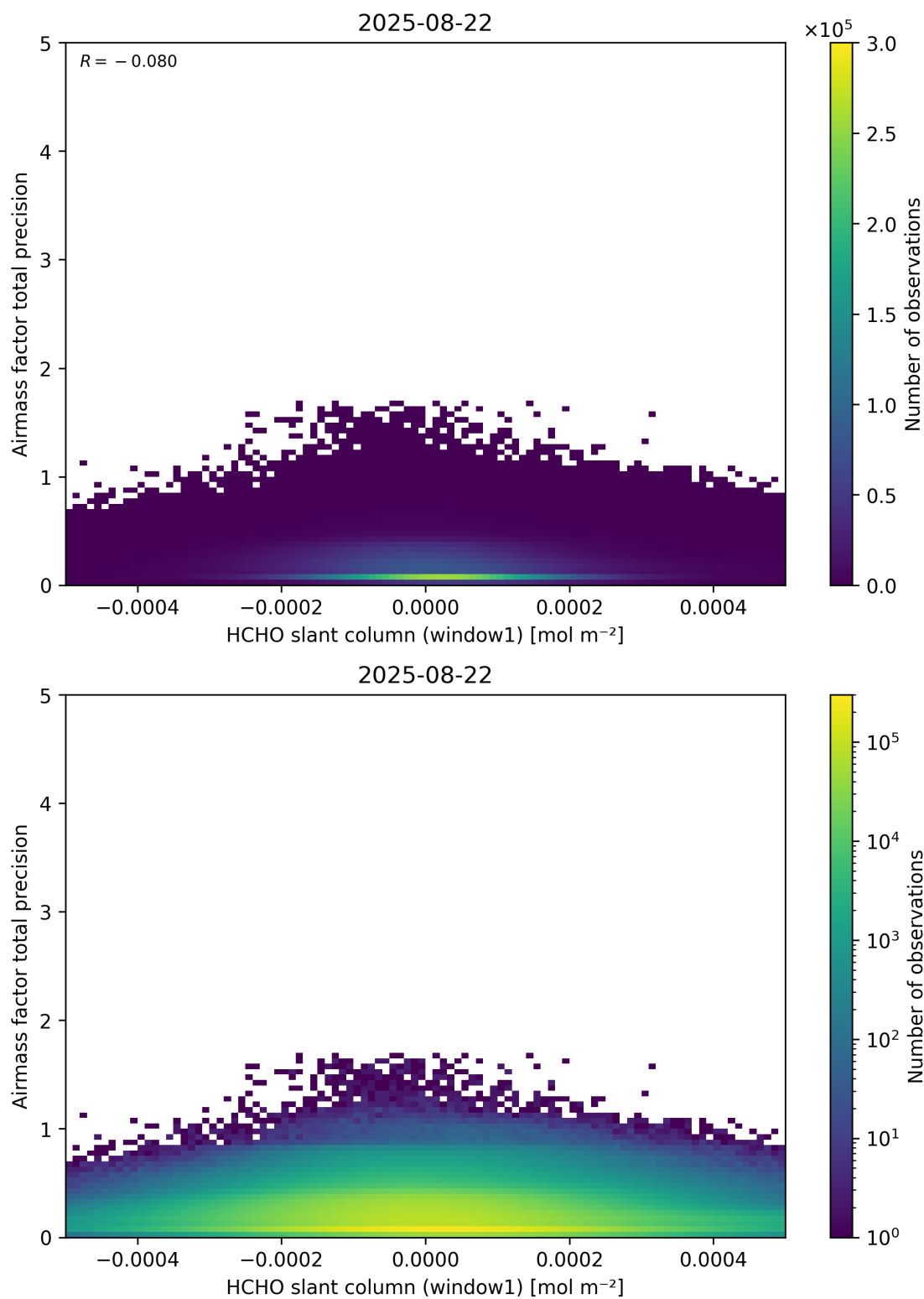
Figure 86: Scatter density plot of “HCHO slant column (window1)” against “Airmass factor total precision” for 2025-08-21 to 2025-08-23.
