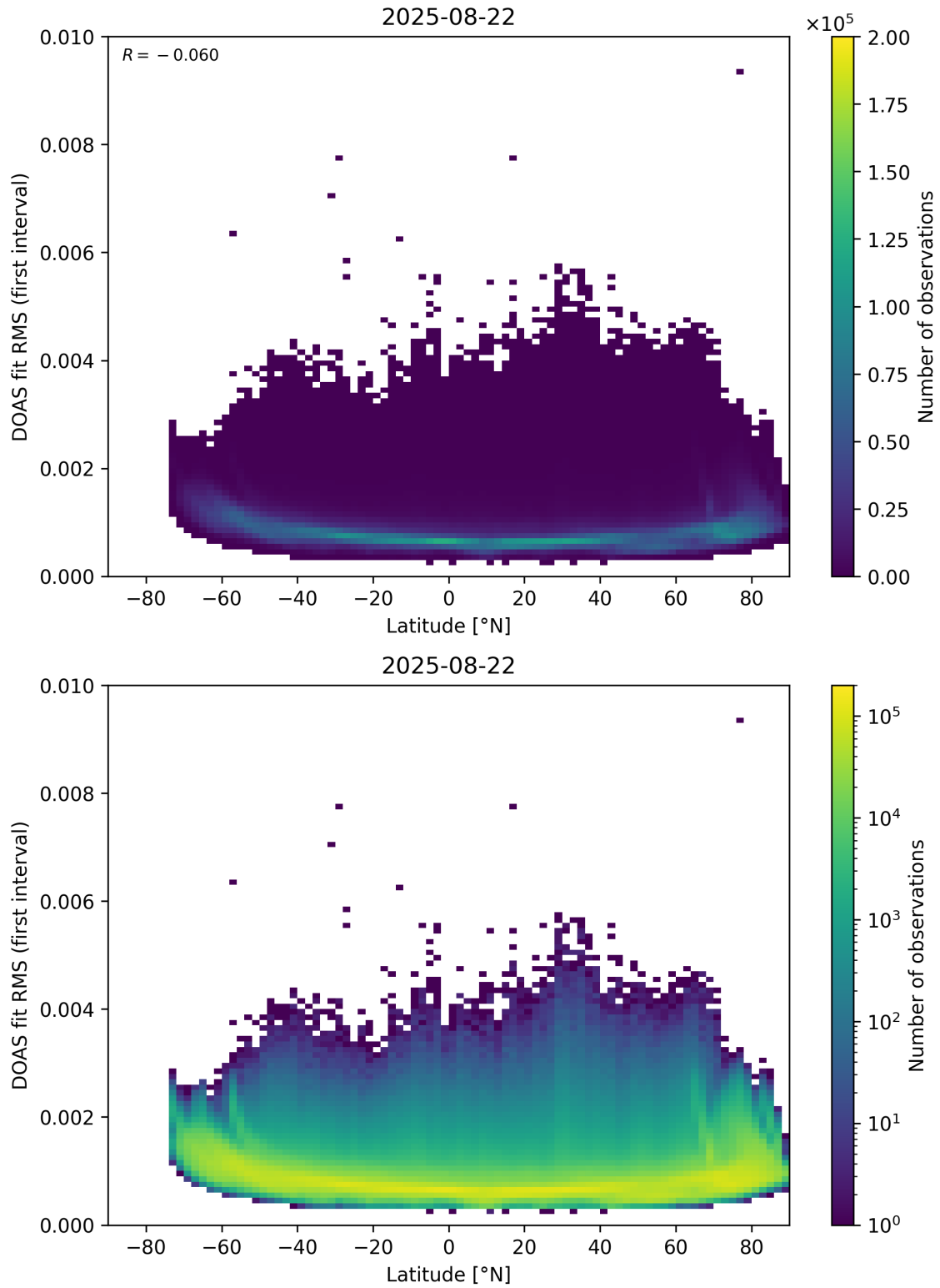
Figure 153: Scatter density plot of “Latitude” against “DOAS fit RMS (first interval)” for 2025-08-21 to 2025-08-23.
