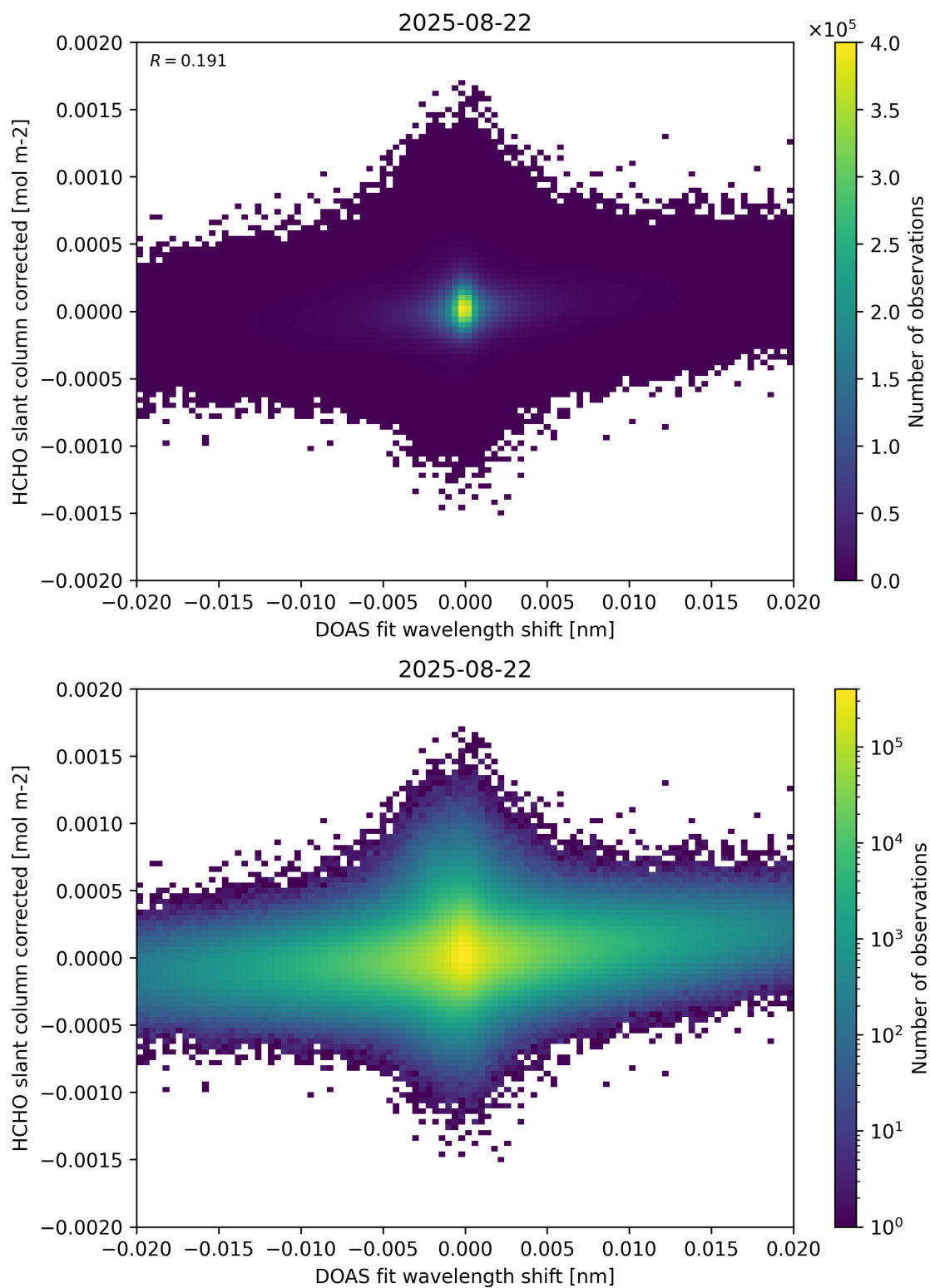
Figure 66: Scatter density plot of “DOAS fit wavelength shift” against “HCHO slant column corrected” for 2025-08-21 to 2025-08-23.
