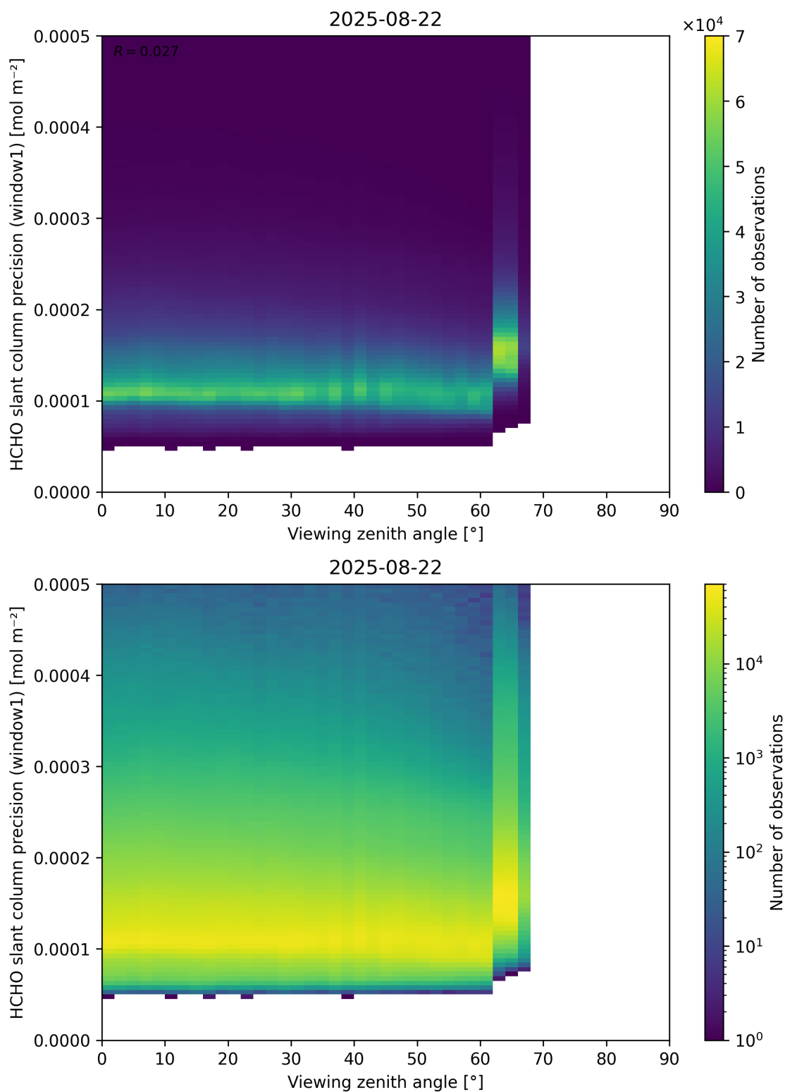
Figure 189: Scatter density plot of “Viewing zenith angle” against “HCHO slant column precision (window1)” for 2025-08-21 to 2025-08-23.
