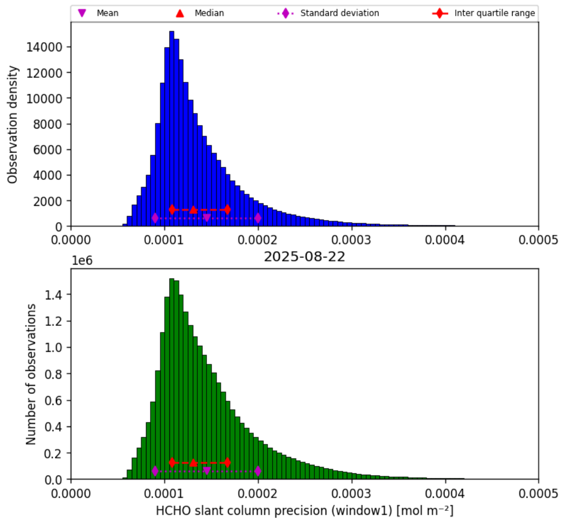
Figure 39: Histogram of “HCHO slant column precision (window1)” for 2025-08-21 to 2025-08-23
