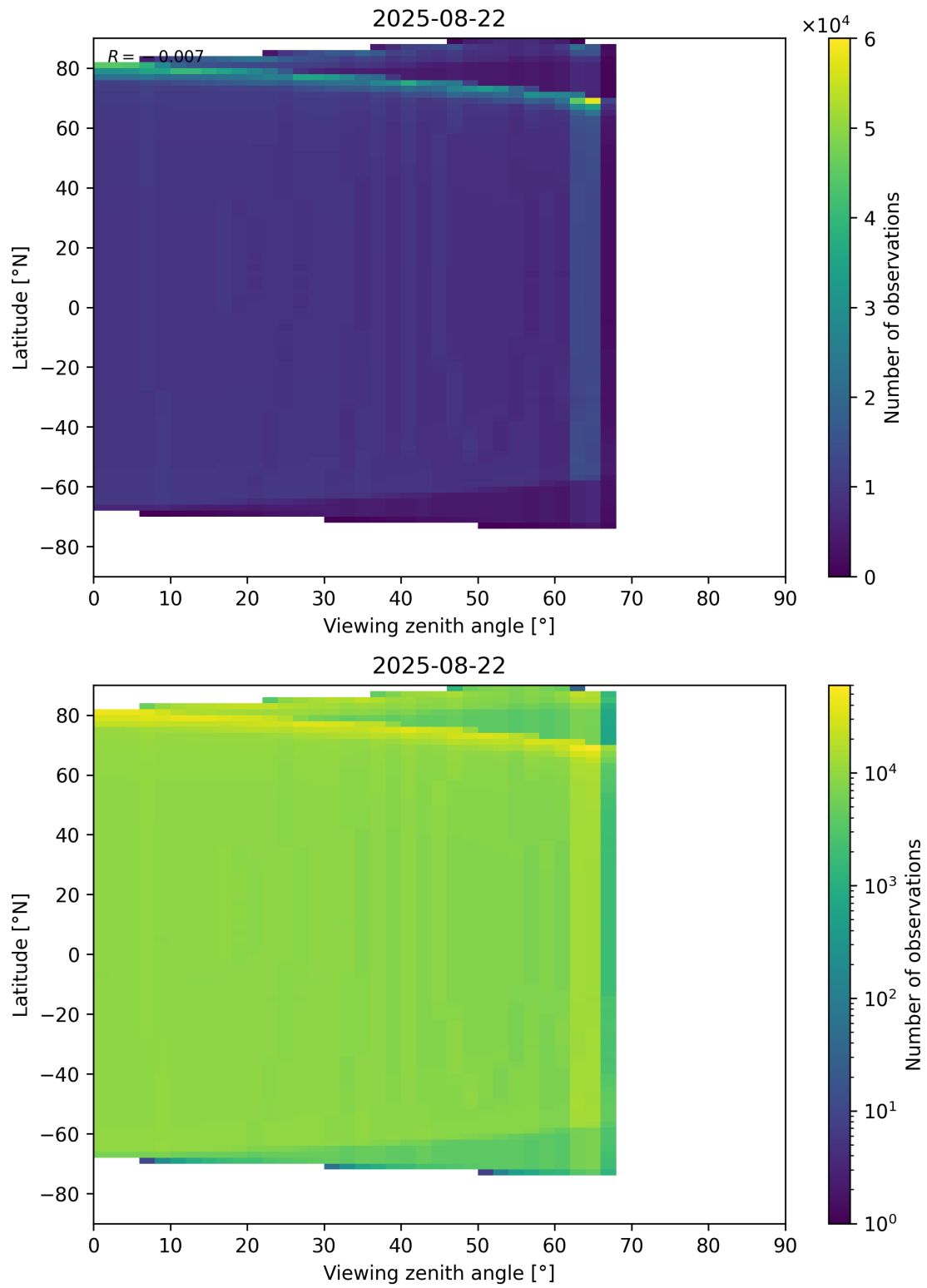
Figure 196: Scatter density plot of “Viewing zenith angle” against “Latitude” for 2025-08-21 to 2025-08-23.
