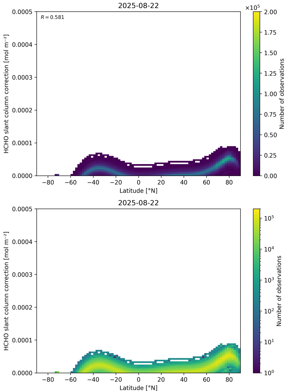
Figure 158: Scatter density plot of “Latitude” against “HCHO slant column correction” for 2025-08-21 to 2025-08-23.
