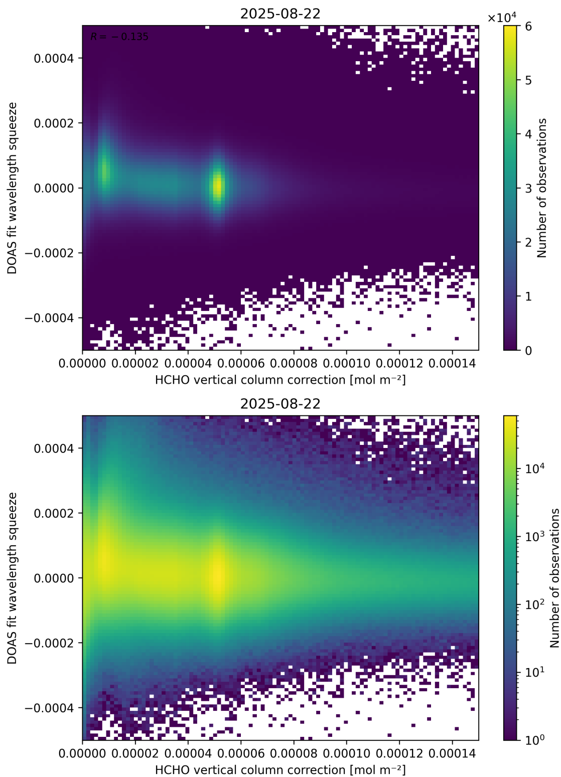
Figure 114: Scatter density plot of “HCHO vertical column correction” against “DOAS fit wavelength squeeze” for 2025-08-21 to 2025-08-23.
