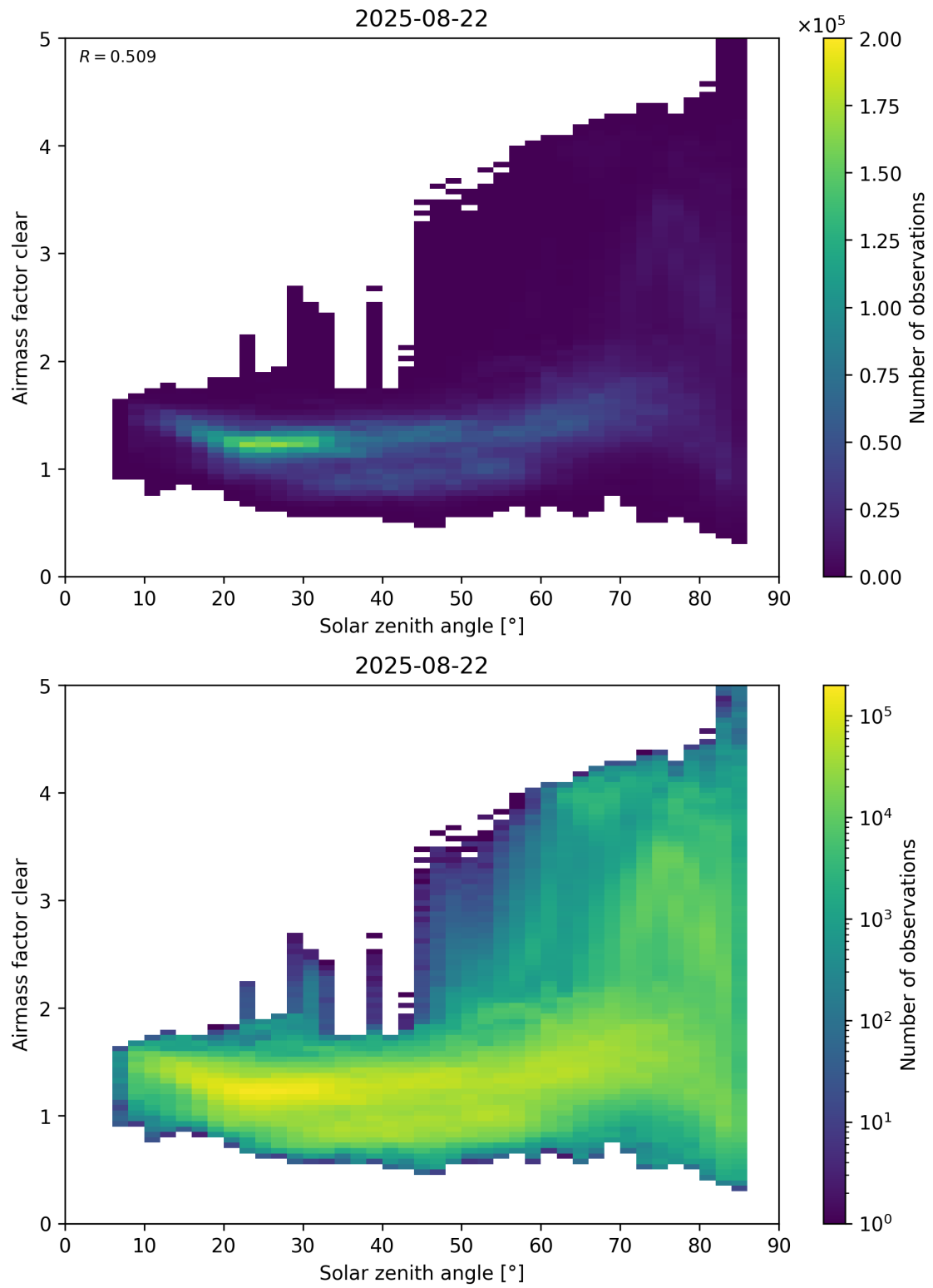
Figure 170: Scatter density plot of “Solar zenith angle” against “Airmass factor clear” for 2025-08-21 to 2025-08-23.
