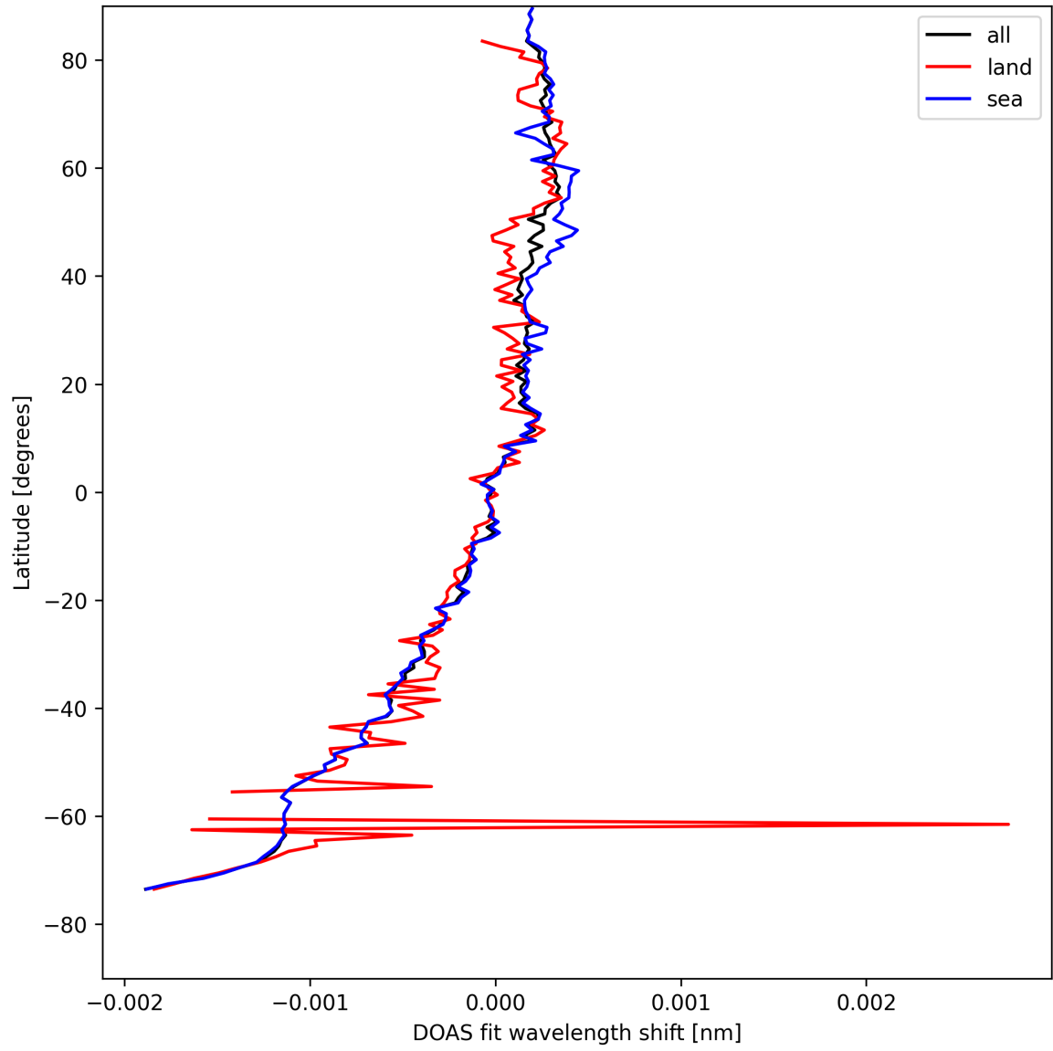
Figure 30: Zonal average of "DOAS fit wavelength shift" for 2025-08-21 to 2025-08-23.
