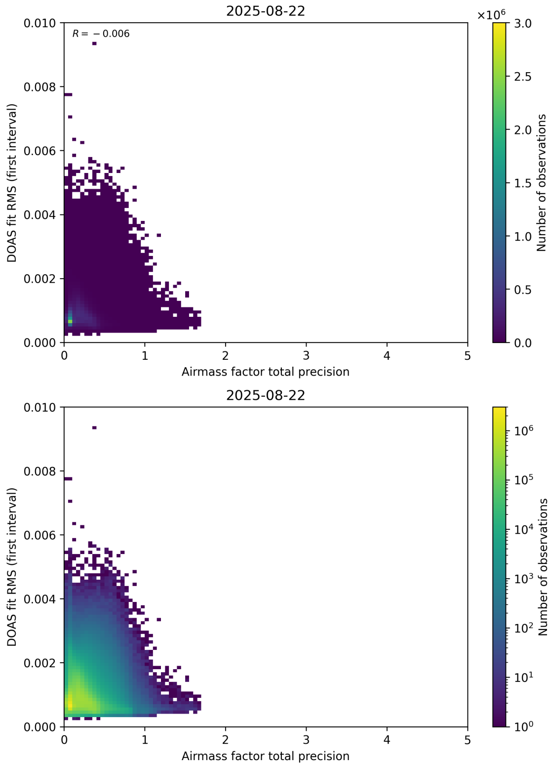
Figure 105: Scatter density plot of “Airmass factor total precision” against “DOAS fit RMS (first interval)” for 2025-08-21 to 2025-08-23.
