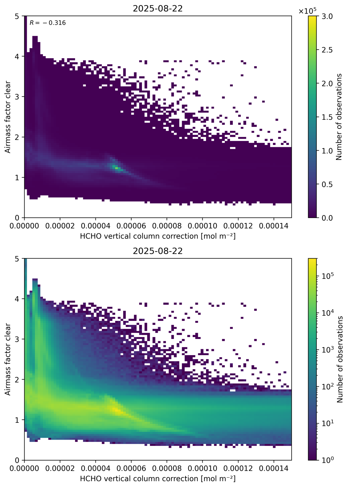
Figure 115: Scatter density plot of “HCHO vertical column correction” against “Airmass factor clear” for 2025-08-21 to 2025-08-23.
