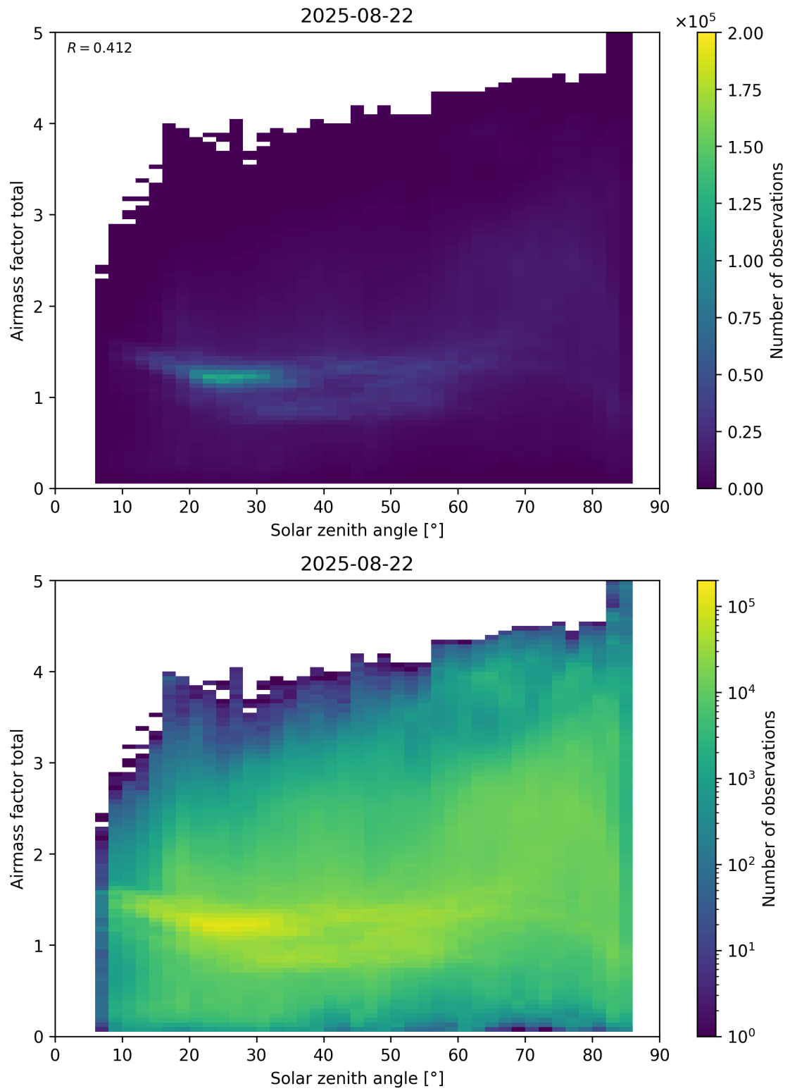
Figure 175: Scatter density plot of “Solar zenith angle” against “Airmass factor total” for 2025-08-21 to 2025-08-23.
