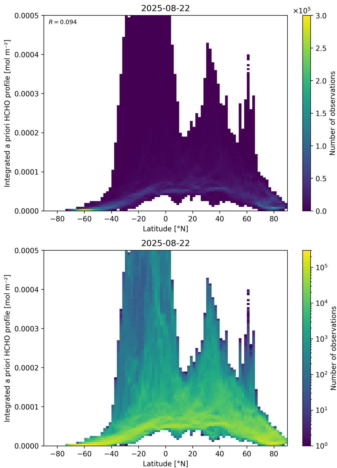
Figure 166: Scatter density plot of “Latitude” against “Integrated a priori HCHO profile” for 2025-08-21 to 2025-08-23.
