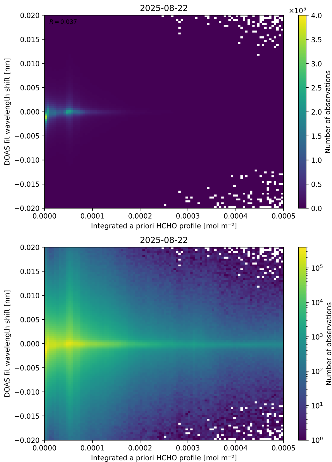
Figure 149: Scatter density plot of “Integrated a priori HCHO profile” against “DOAS fit wavelength shift” for 2025-08-21 to 2025-08-23.
