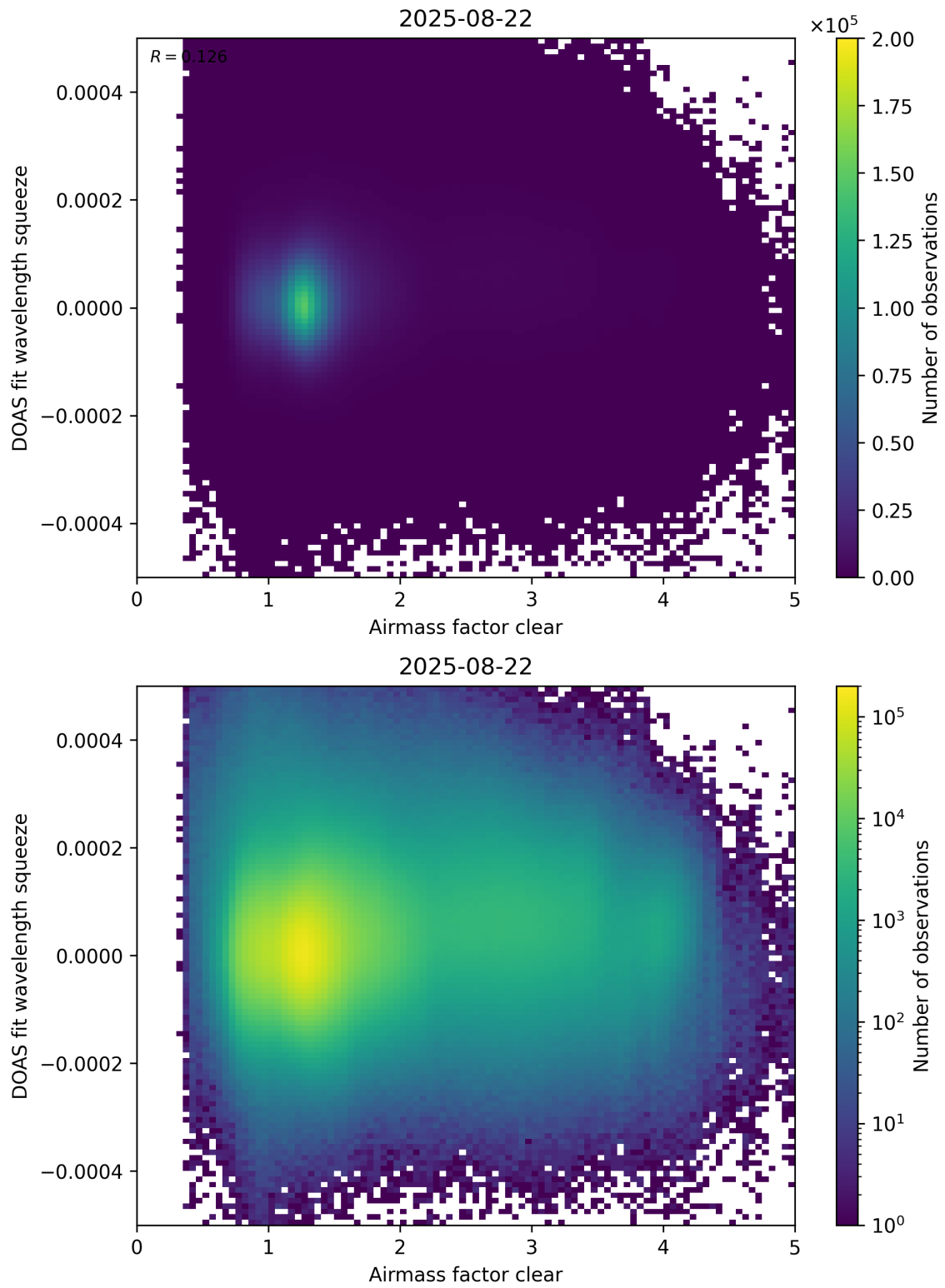
Figure 73: Scatter density plot of “Airmass factor clear” against “DOAS fit wavelength squeeze” for 2025-08-21 to 2025-08-23.
