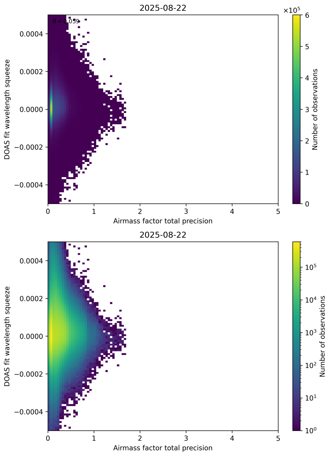
Figure 107: Scatter density plot of “Airmass factor total precision” against “DOAS fit wavelength squeeze” for 2025-08-21 to 2025-08-23.
