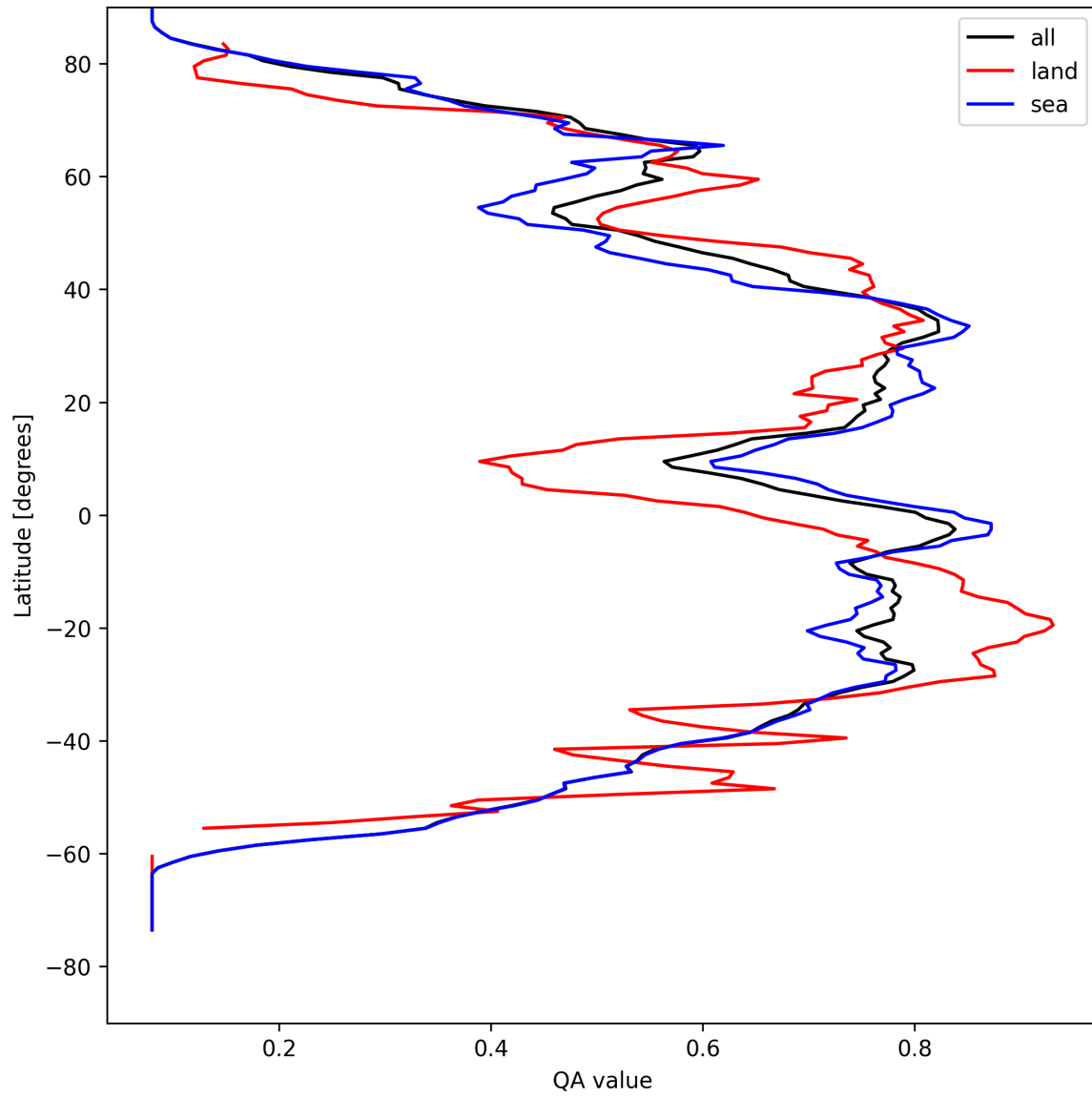
Figure 20: Zonal average of “QA value” for 2025-08-21 to 2025-08-23.
