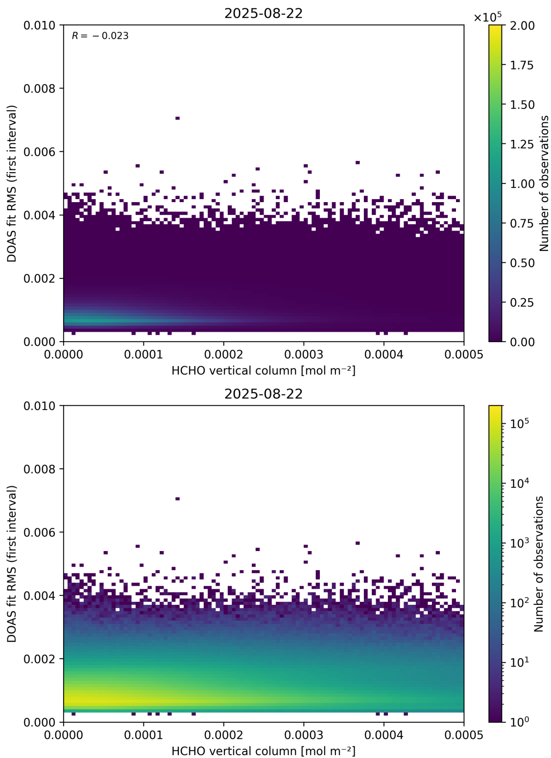
Figure 123: Scatter density plot of “HCHO vertical column” against “DOAS fit RMS (first interval)” for 2025-08-21 to 2025-08-23.
