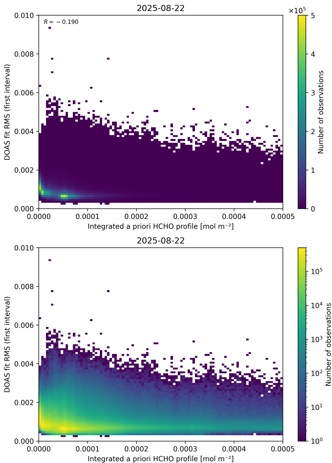
Figure 148: Scatter density plot of “Integrated a priori HCHO profile” against “DOAS fit RMS (first interval)” for 2025-08-21 to 2025-08-23.
