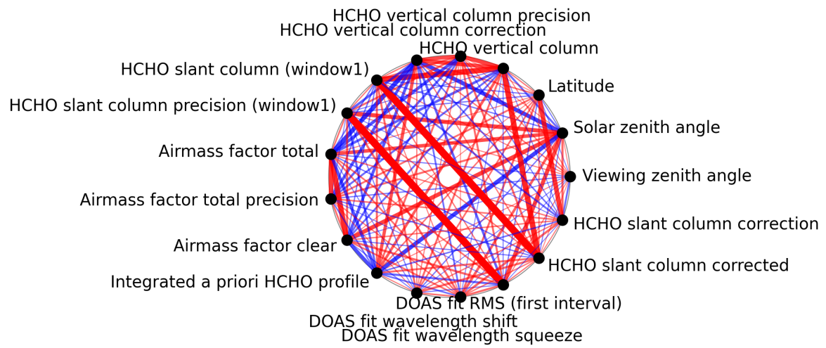
Figure 1: Map of correlation graph for 2025-08-21 to 2025-08-23.
