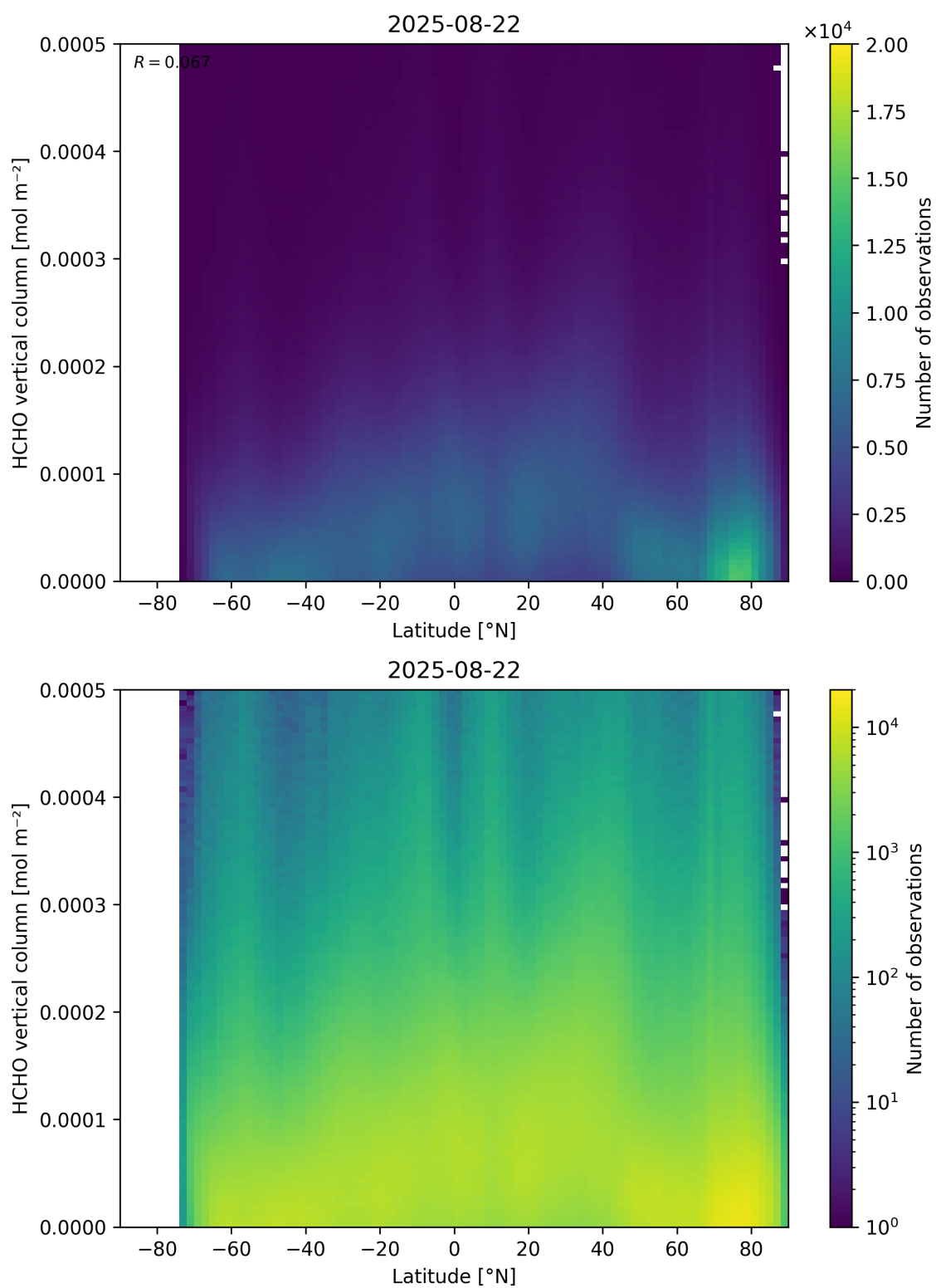
Figure 163: Scatter density plot of “Latitude” against “HCHO vertical column” for 2025-08-21 to 2025-08-23.
