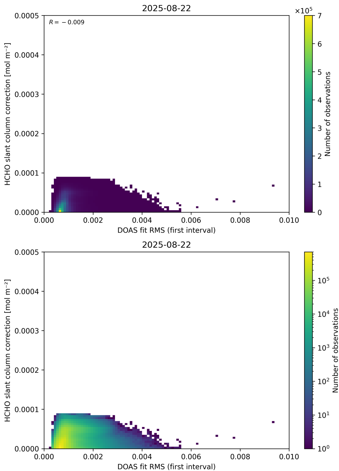
Figure 63: Scatter density plot of “DOAS fit RMS (first interval)” against “HCHO slant column correction” for 2025-08-21 to 2025-08-23.
