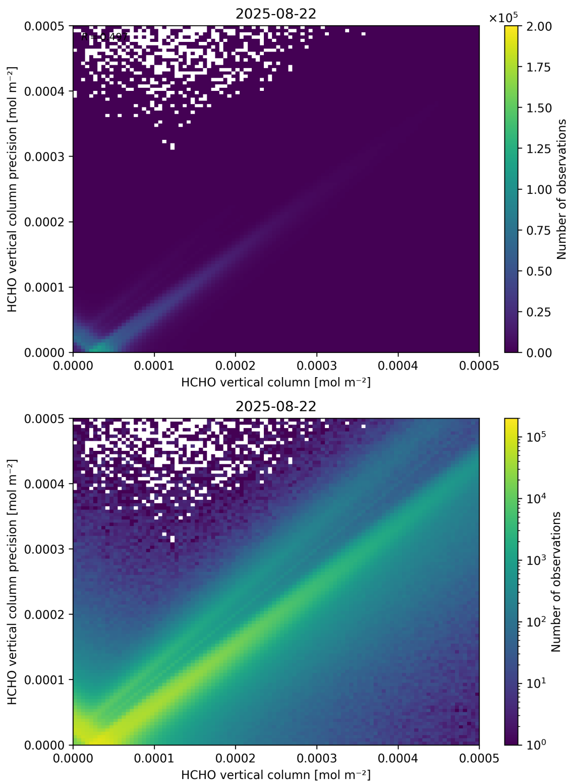
Figure 134: Scatter density plot of “HCHO vertical column” against “HCHO vertical column precision” for 2025-08-21 to 2025-08-23.
