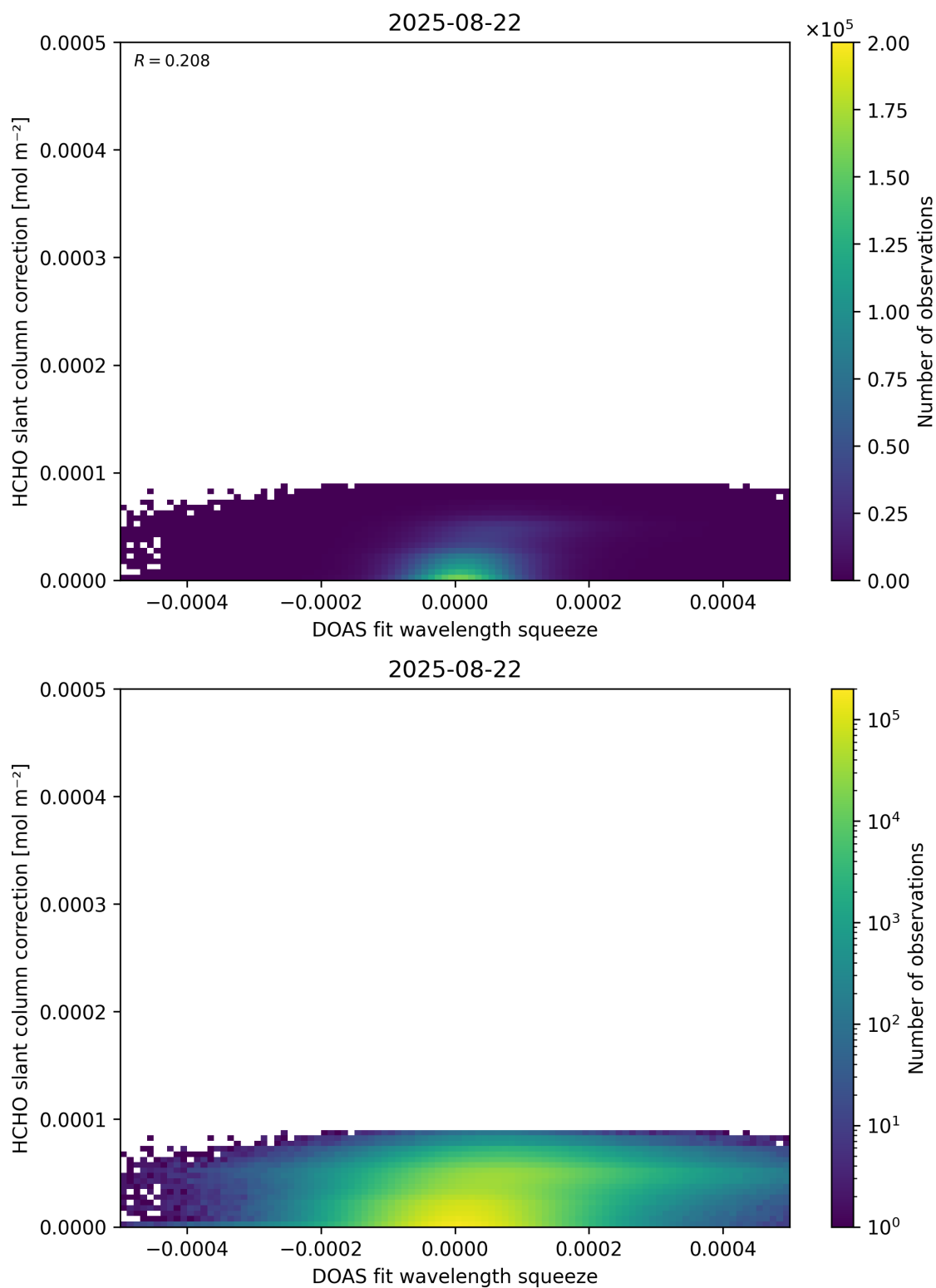
Figure 70: Scatter density plot of “DOAS fit wavelength squeeze” against “HCHO slant column correction” for 2025-08-21 to 2025-08-23.
