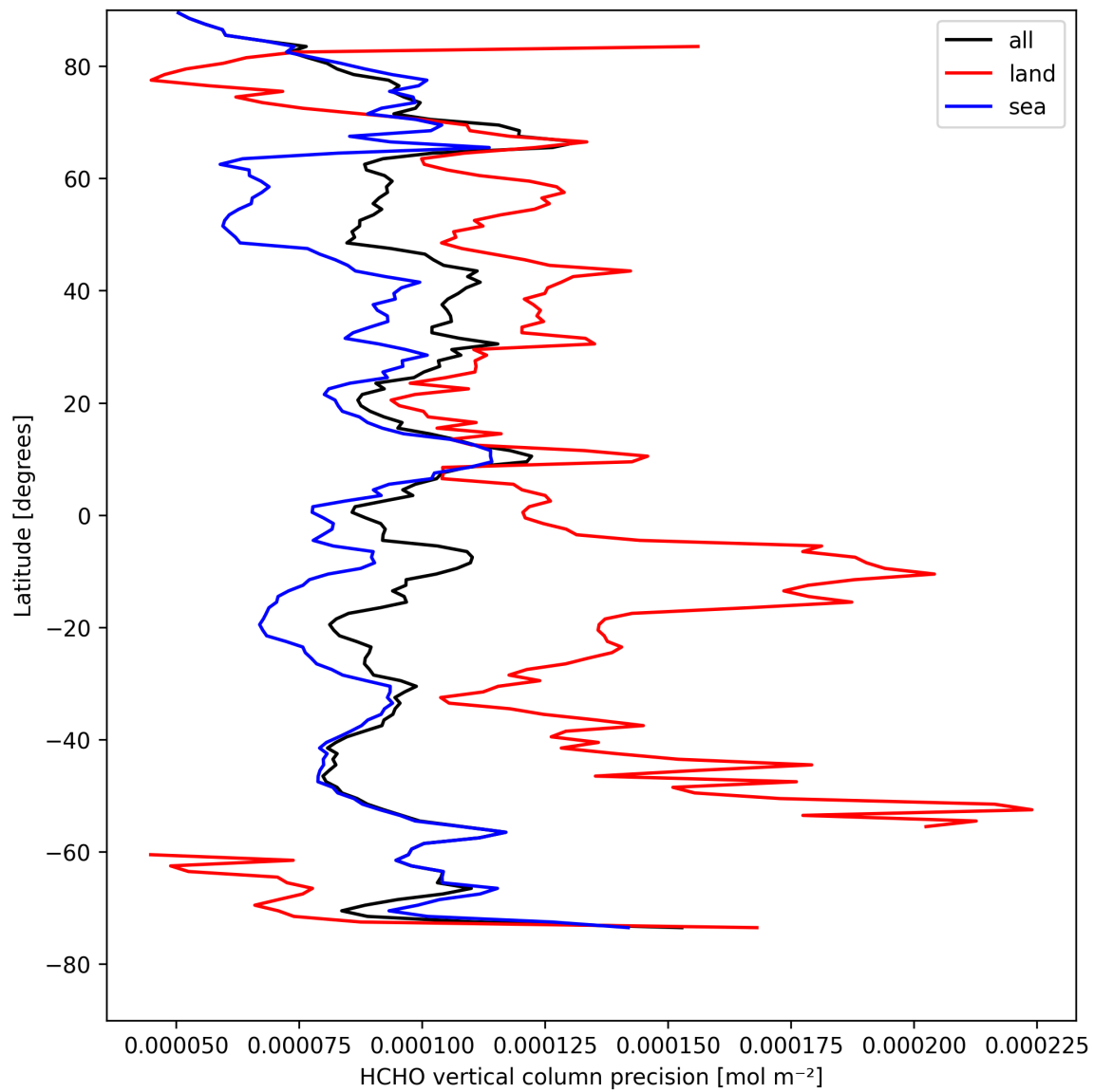
Figure 22: Zonal average of “HCHO vertical column precision” for 2025-08-21 to 2025-08-23.
