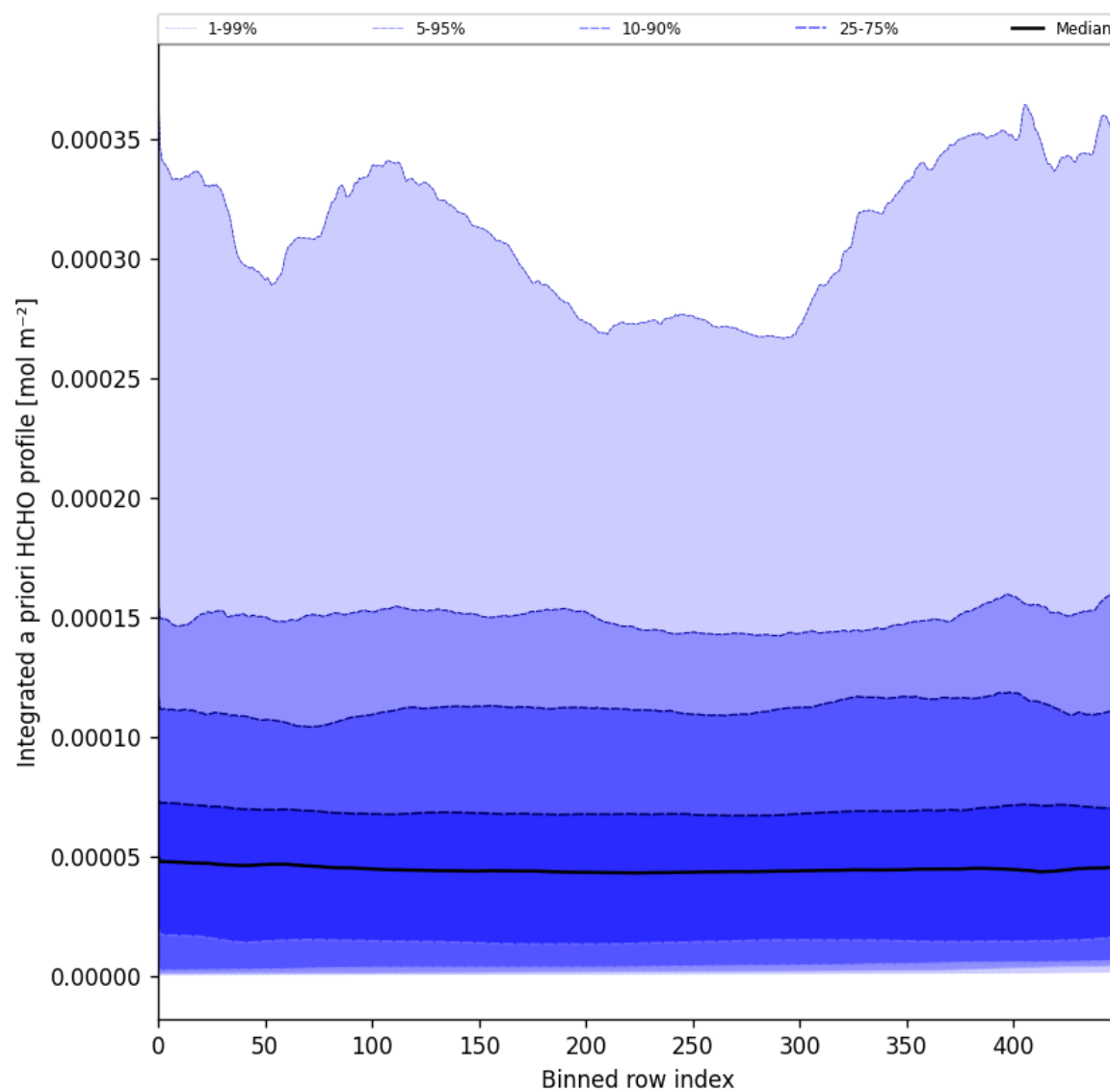
Figure 57: Along track statistics of “Integrated a priori HCHO profile” for 2025-08-21 to 2025-08-23
