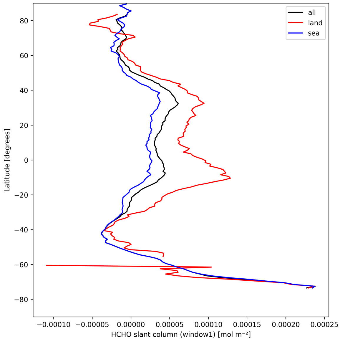
Figure 24: Zonal average of “HCHO slant column (window1)” for 2025-08-21 to 2025-08-23.
