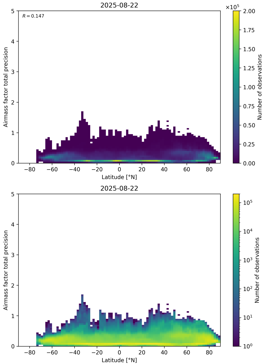
Figure 162: Scatter density plot of “Latitude” against “Airmass factor total precision” for 2025-08-21 to 2025-08-23.
