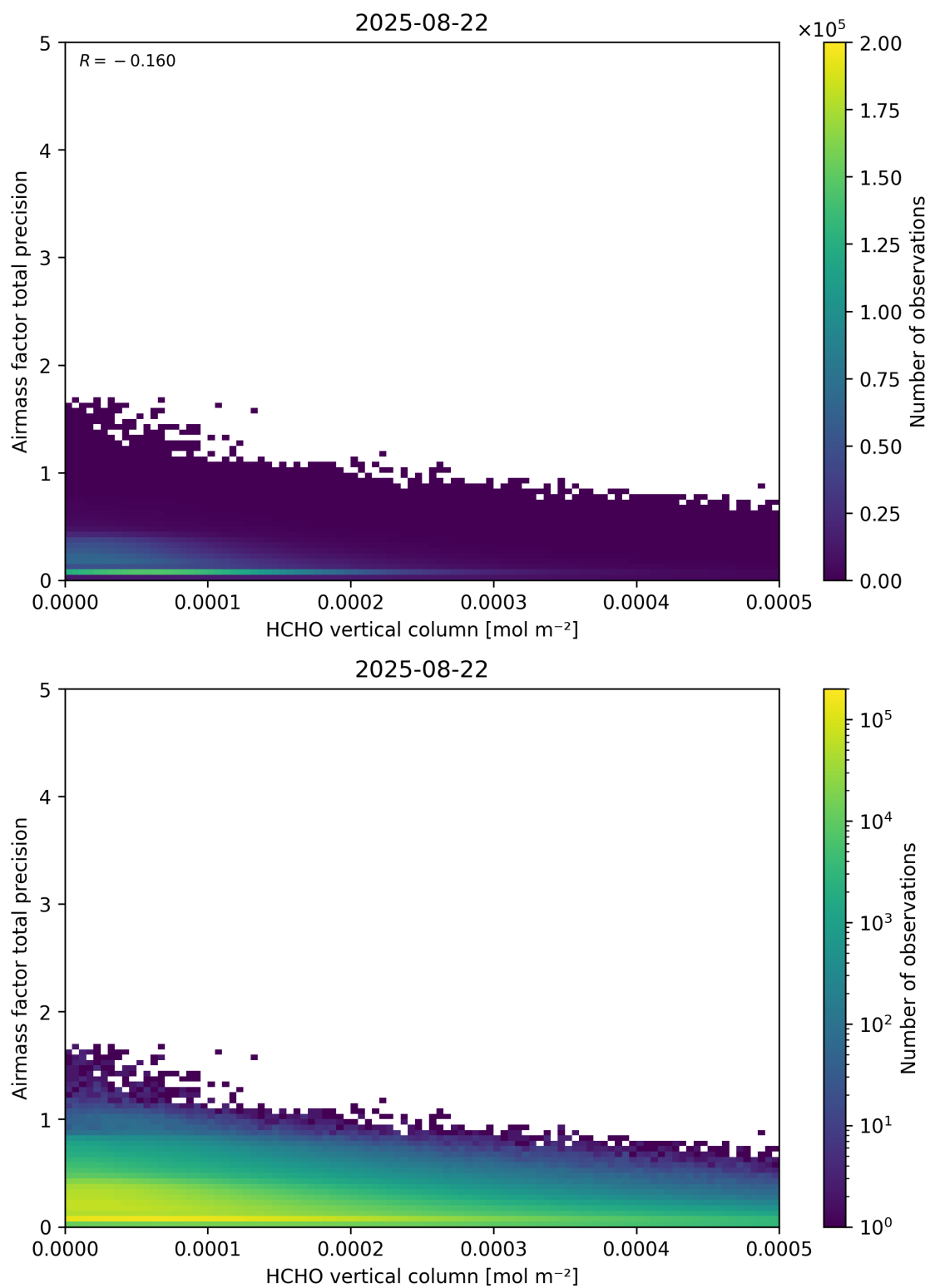
Figure 132: Scatter density plot of “HCHO vertical column” against “Airmass factor total precision” for 2025-08-21 to 2025-08-23.
