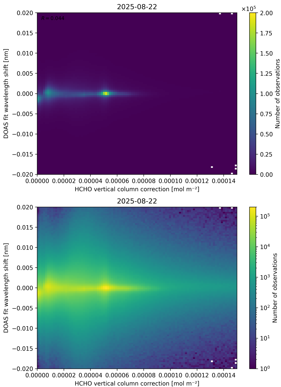
Figure 113: Scatter density plot of “HCHO vertical column correction” against “DOAS fit wavelength shift” for 2025-08-21 to 2025-08-23.
