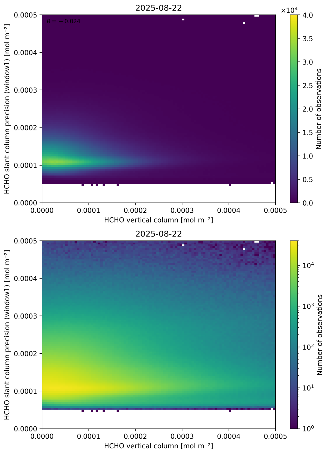
Figure 130: Scatter density plot of “HCHO vertical column” against “HCHO slant column precision (window1)” for 2025-08-21 to 2025-08-23.
