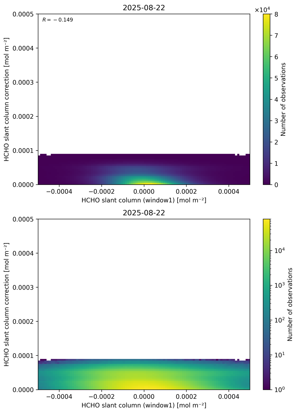
Figure 83: Scatter density plot of “HCHO slant column (window1)” against “HCHO slant column correction” for 2025-08-21 to 2025-08-23.
