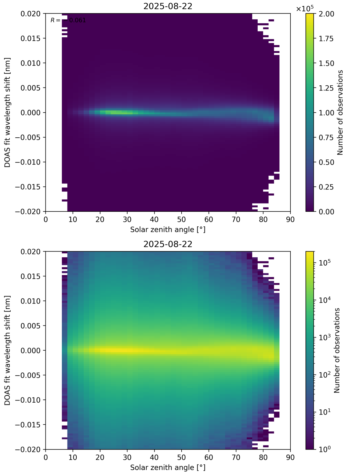
Figure 168: Scatter density plot of “Solar zenith angle” against “DOAS fit wavelength shift” for 2025-08-21 to 2025-08-23.
