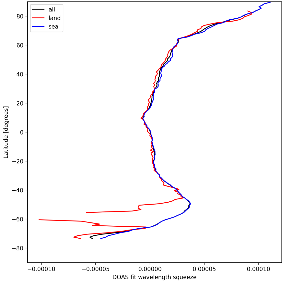
Figure 31: Zonal average of “DOAS fit wavelength squeeze” for 2025-08-21 to 2025-08-23.
