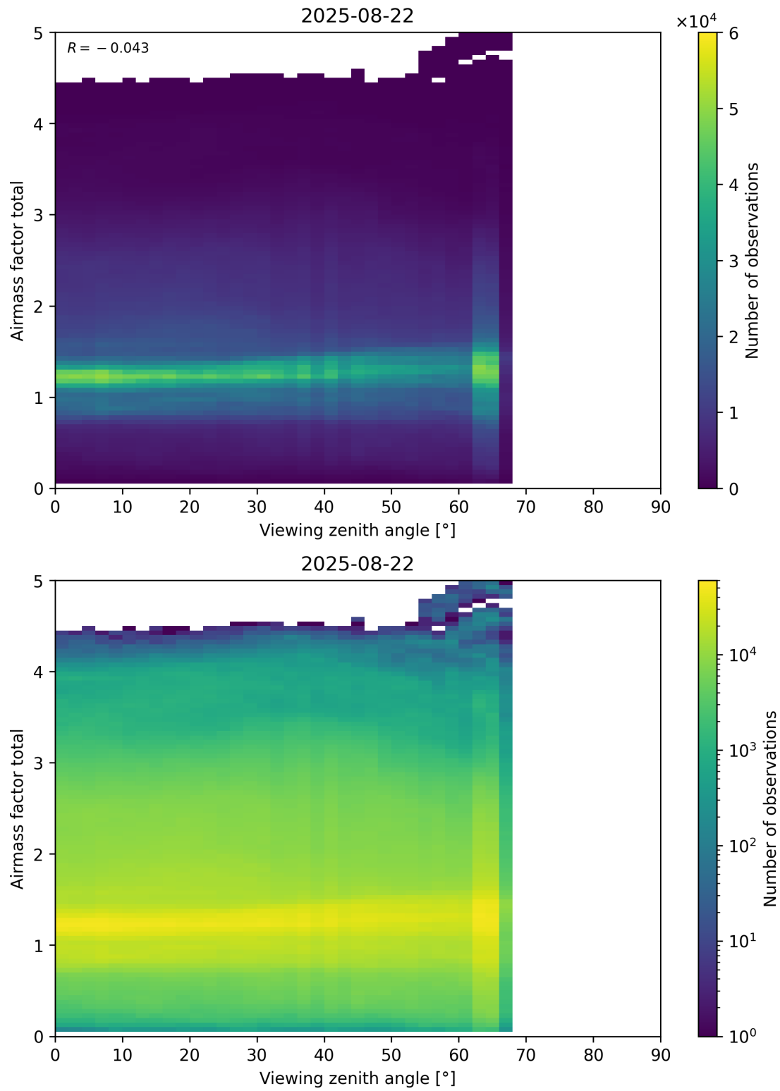
Figure 190: Scatter density plot of “Viewing zenith angle” against “Airmass factor total” for 2025-08-21 to 2025-08-23.
