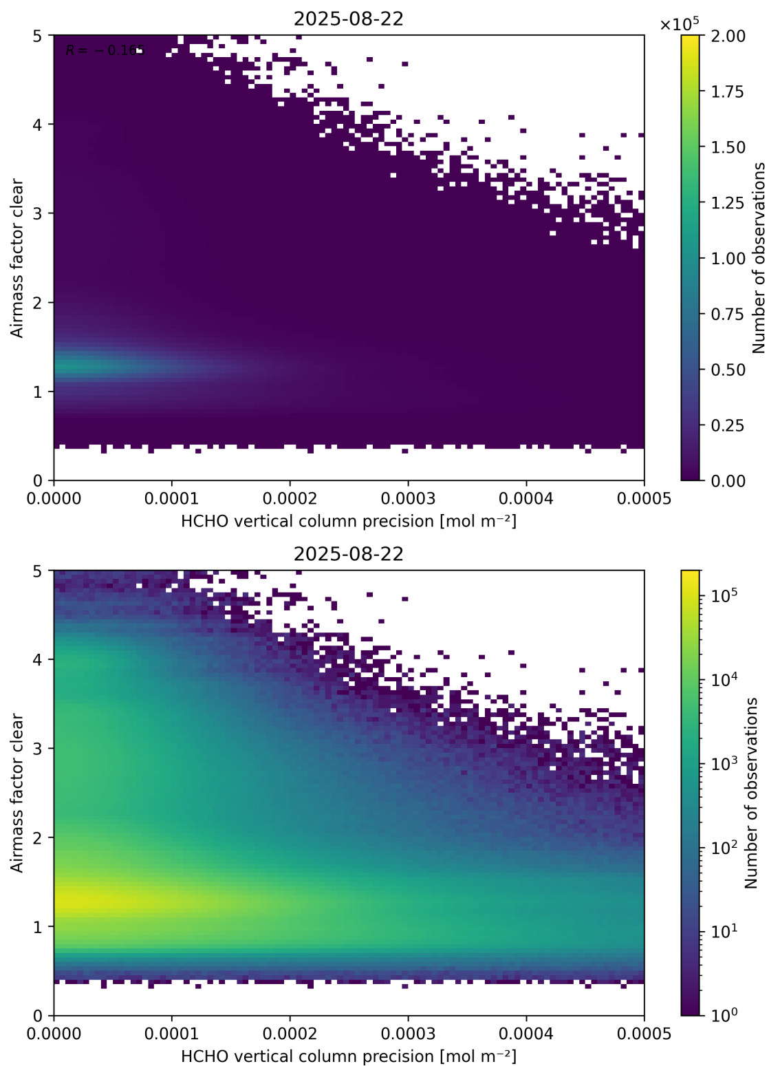
Figure 139: Scatter density plot of “HCHO vertical column precision” against “Airmass factor clear” for 2025-08-21 to 2025-08-23.
