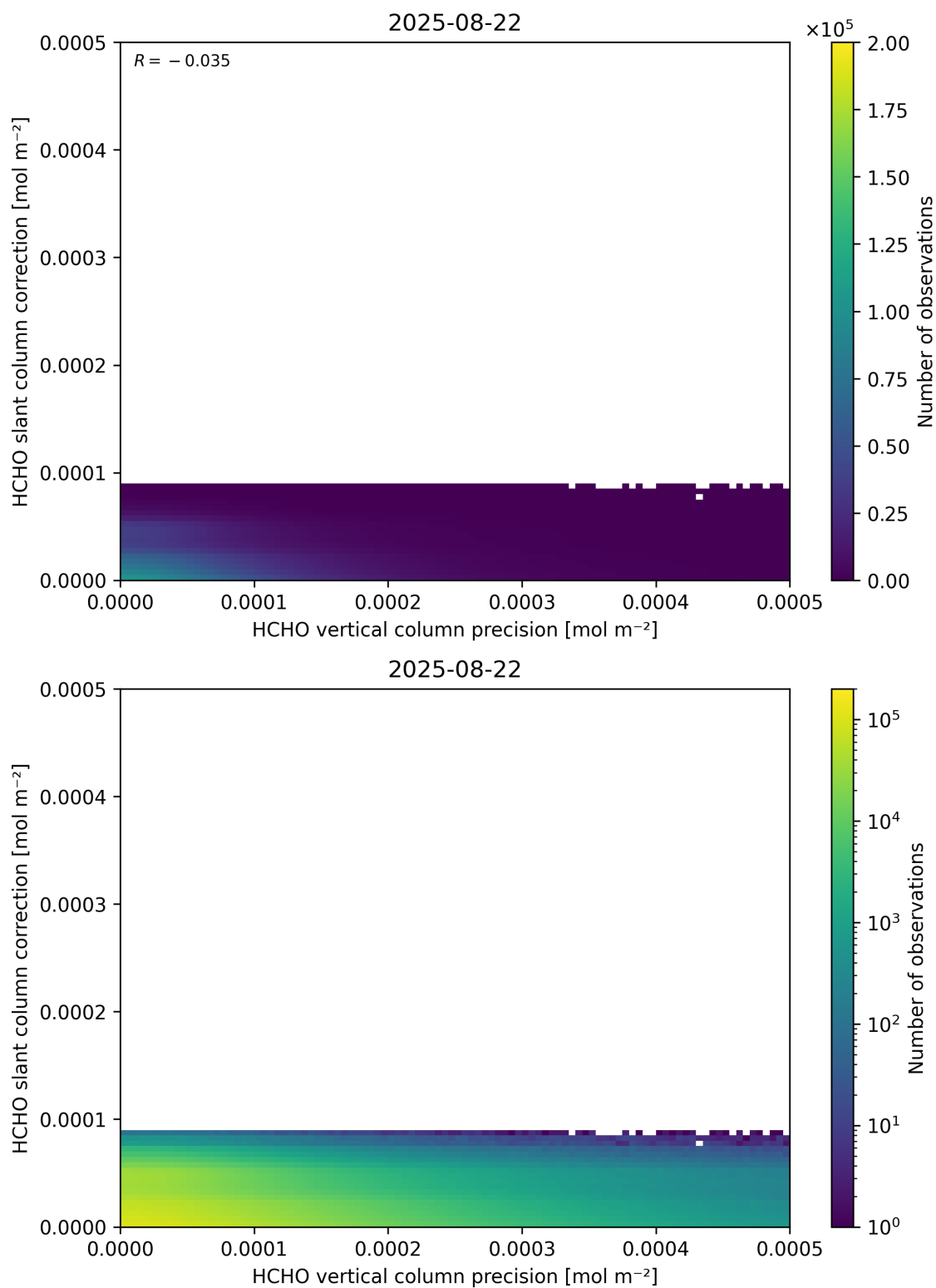
Figure 141: Scatter density plot of “HCHO vertical column precision” against “HCHO slant column correction” for 2025-08-21 to 2025-08-23.
