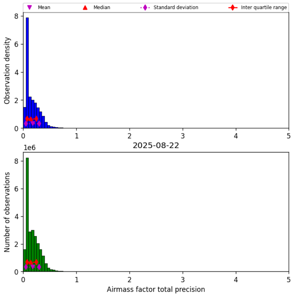
Figure 41: Histogram of “Airmass factor total precision” for 2025-08-21 to 2025-08-23
