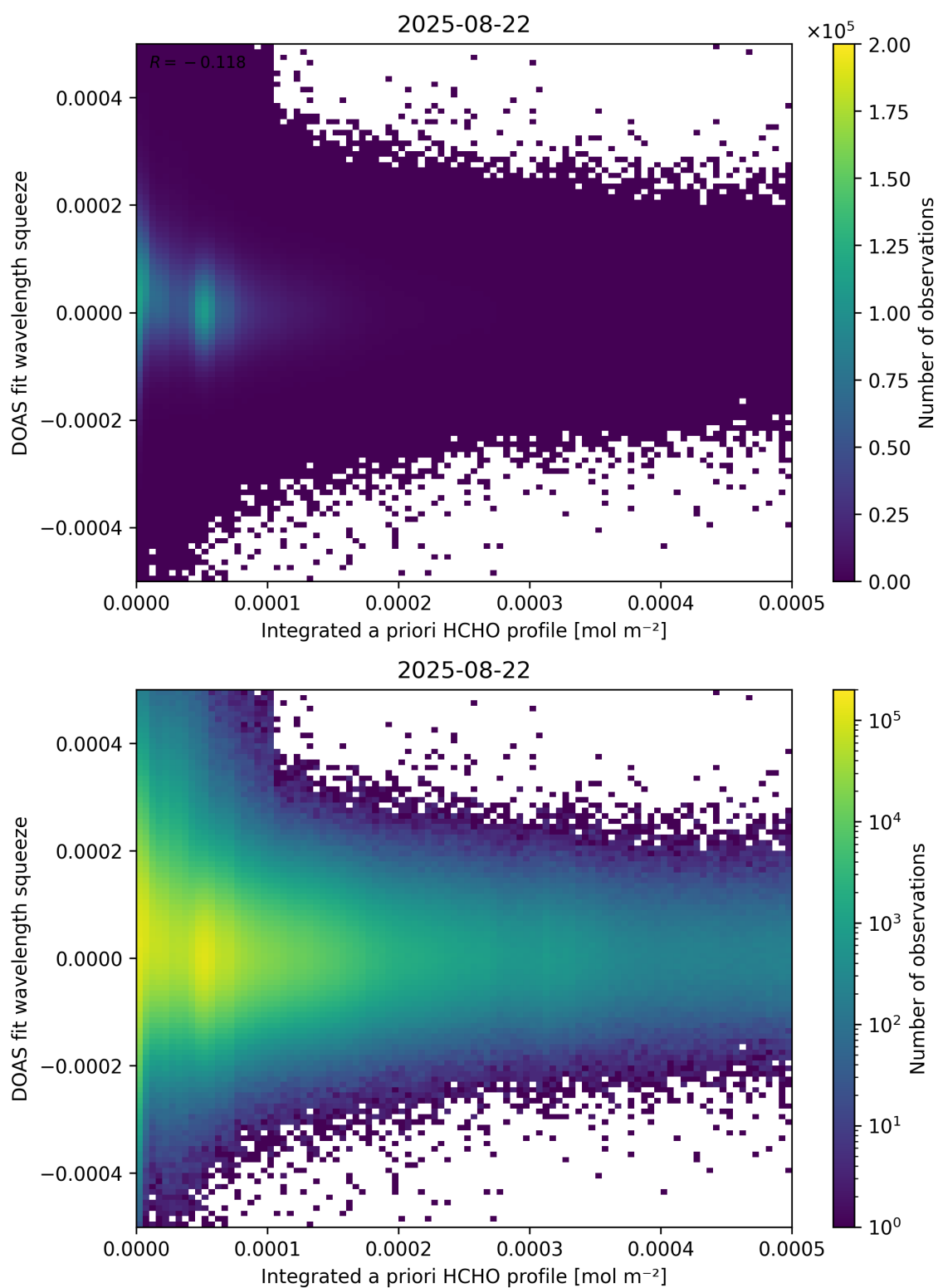
Figure 150: Scatter density plot of “Integrated a priori HCHO profile” against “DOAS fit wavelength squeeze” for 2025-08-21 to 2025-08-23.
