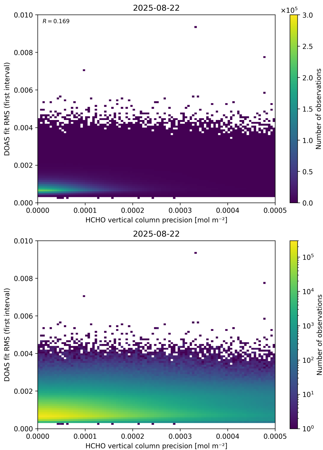
Figure 136: Scatter density plot of “HCHO vertical column precision” against “DOAS fit RMS (first interval)” for 2025-08-21 to 2025-08-23.
