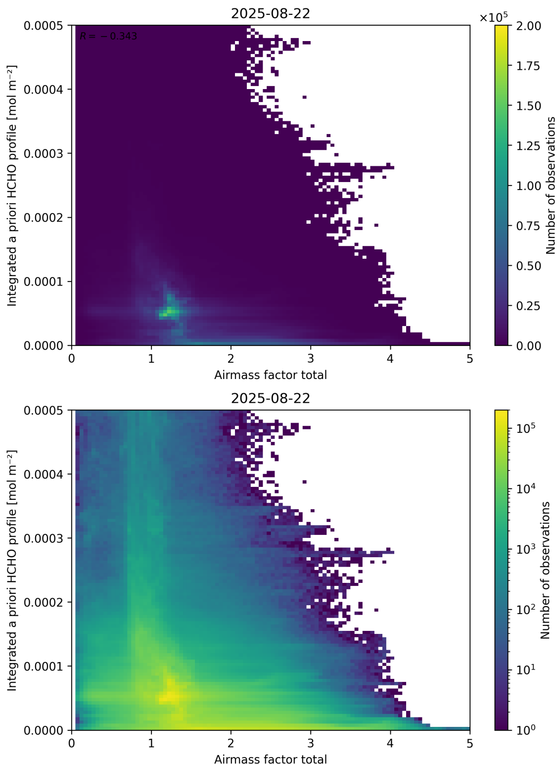
Figure 104: Scatter density plot of “Airmass factor total” against “Integrated a priori HCHO profile” for 2025-08-21 to 2025-08-23.
