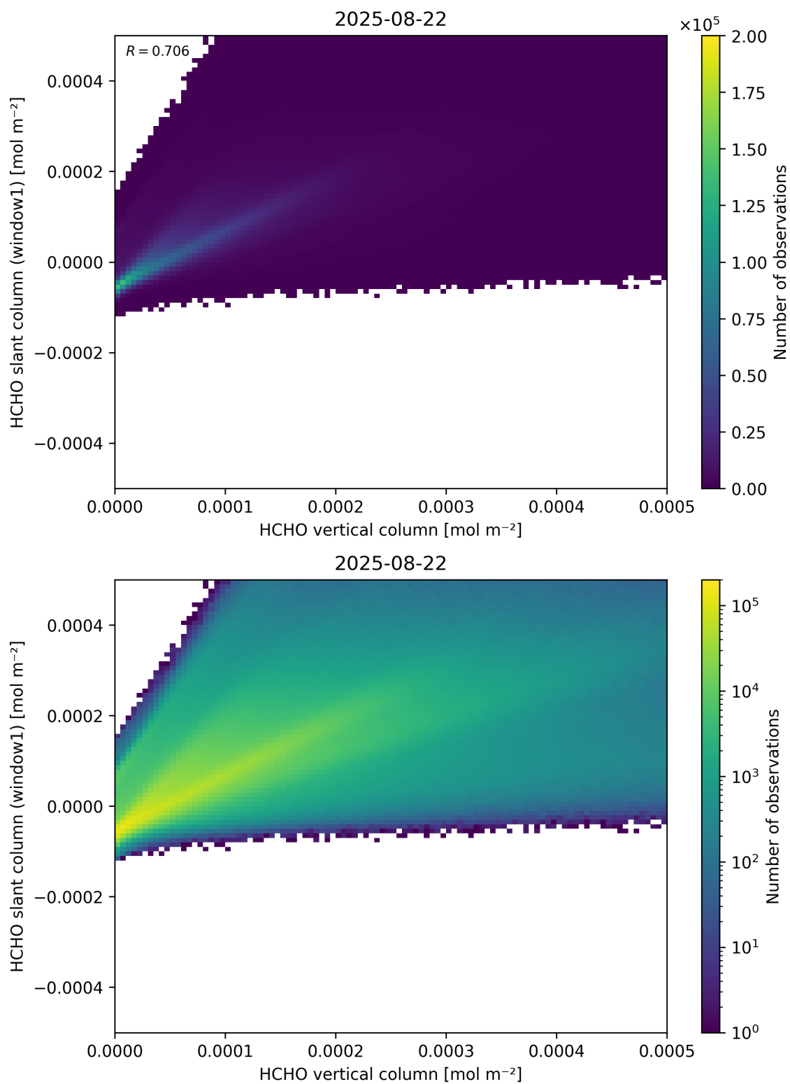
Figure 129: Scatter density plot of “HCHO vertical column” against “HCHO slant column (window1)” for 2025-08-21 to 2025-08-23.
