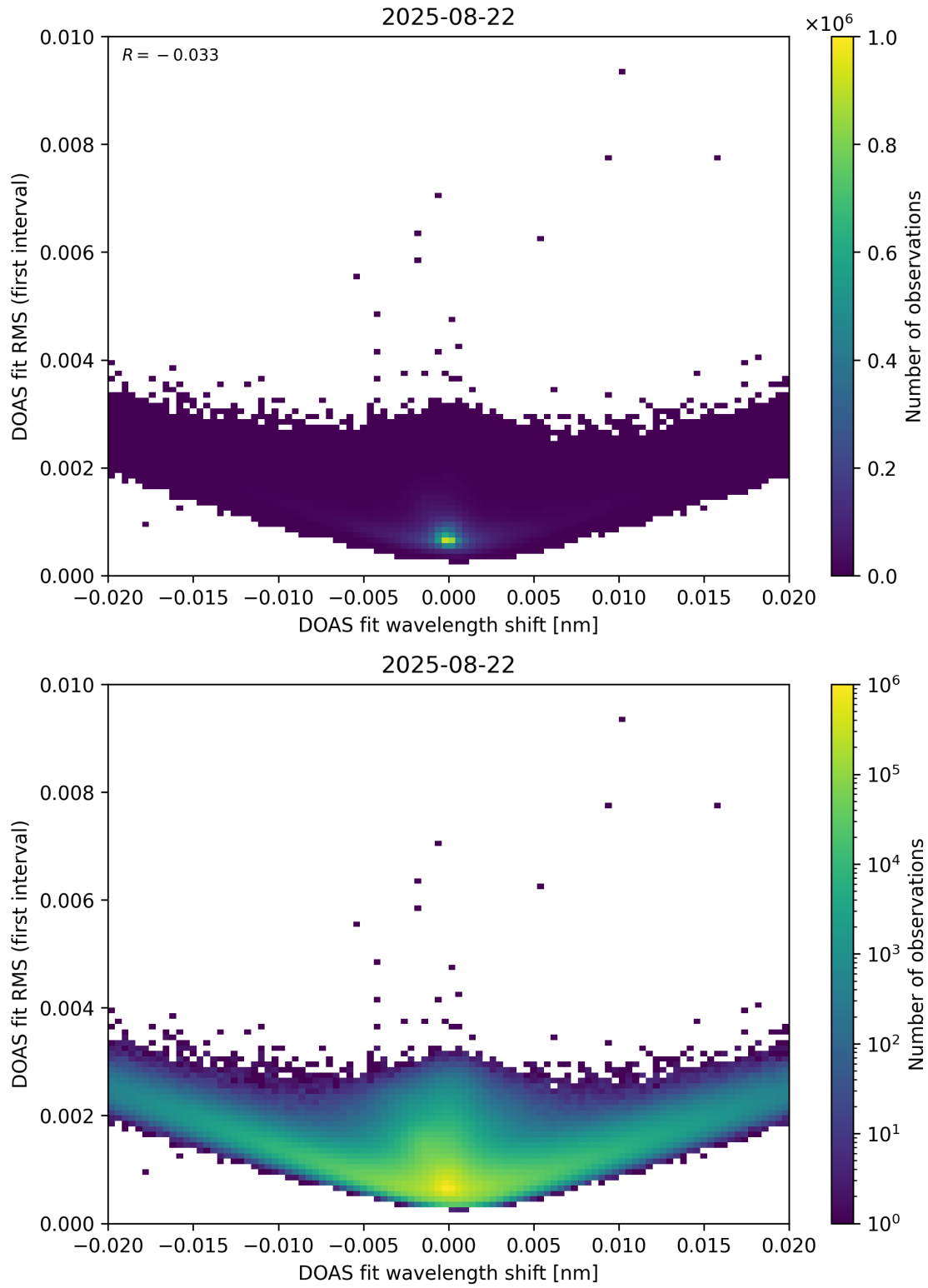
Figure 64: Scatter density plot of “DOAS fit wavelength shift” against “DOAS fit RMS (first interval)” for 2025-08-21 to 2025-08-23.
