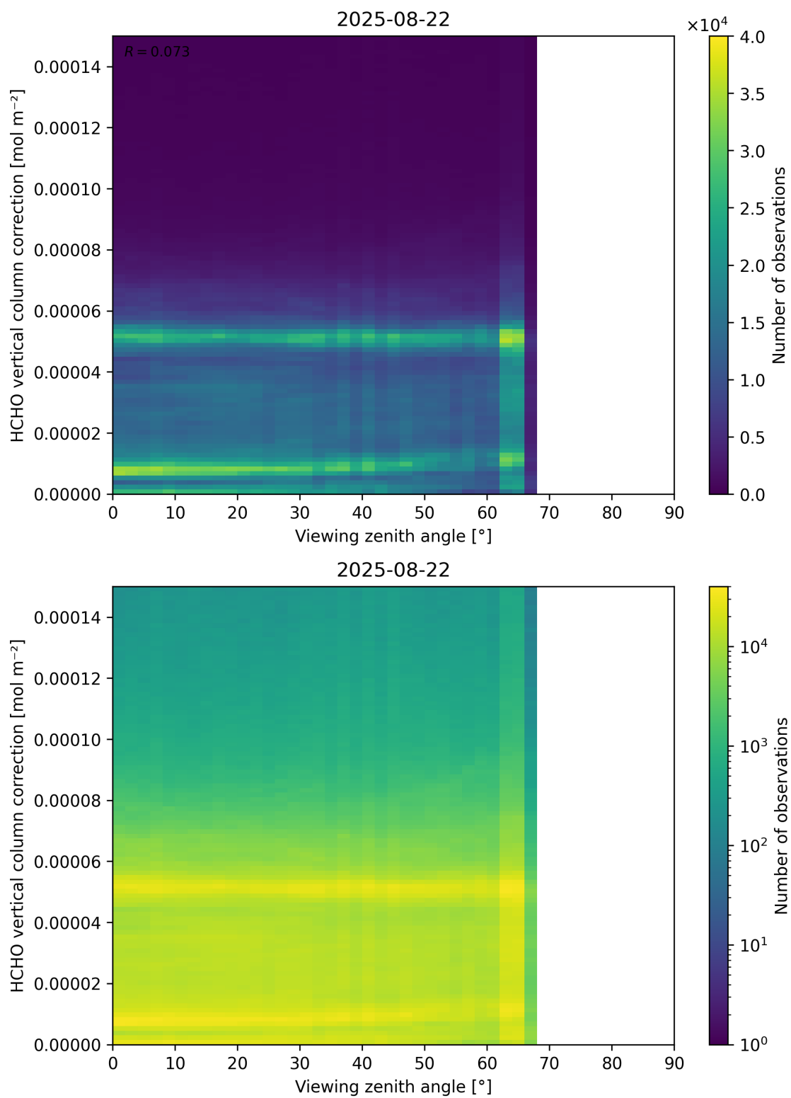
Figure 193: Scatter density plot of “Viewing zenith angle” against “HCHO vertical column correction” for 2025-08-21 to 2025-08-23.
