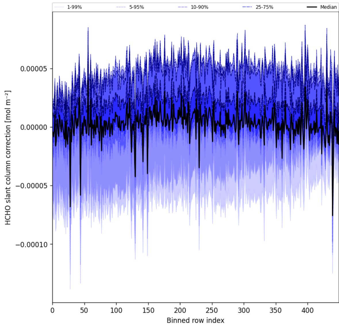
Figure 61: Along track statistics of “HCHO slant column correction” for 2025-08-21 to 2025-08-23
