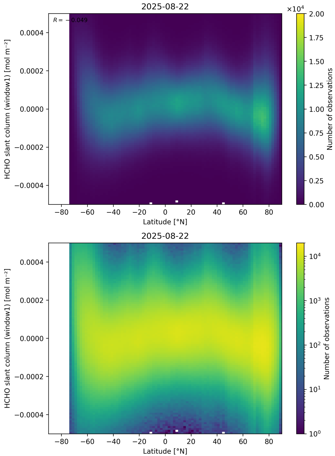
Figure 159: Scatter density plot of “Latitude” against “HCHO slant column (window1)” for 2025-08-21 to 2025-08-23.
