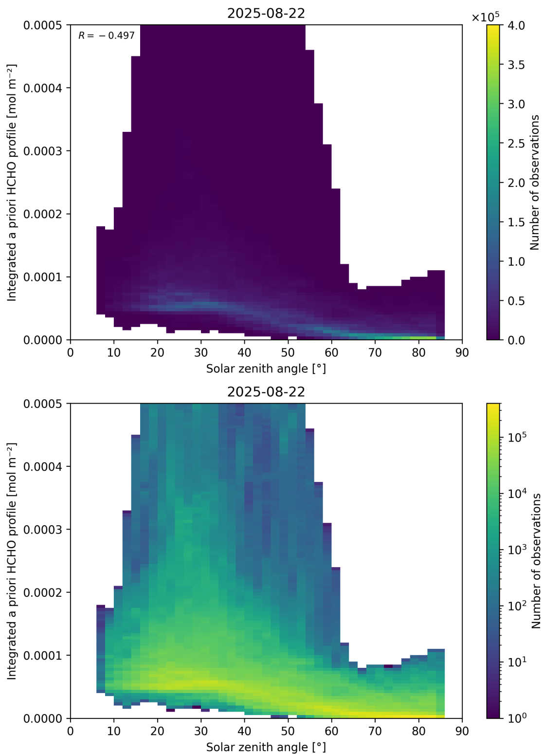
Figure 180: Scatter density plot of “Solar zenith angle” against “Integrated a priori HCHO profile” for 2025-08-21 to 2025-08-23.
