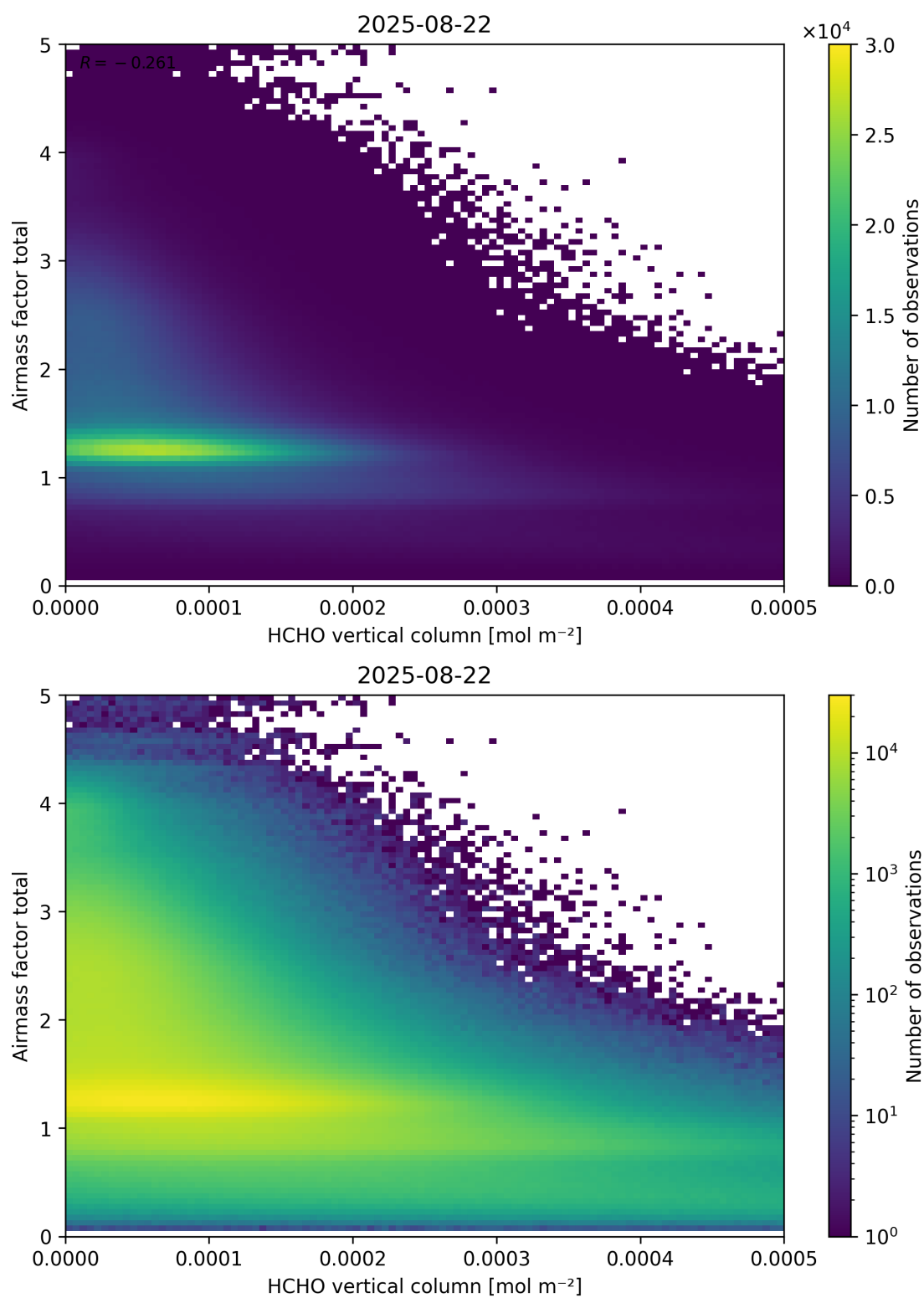
Figure 131: Scatter density plot of “HCHO vertical column” against “Airmass factor total” for 2025-08-21 to 2025-08-23.
