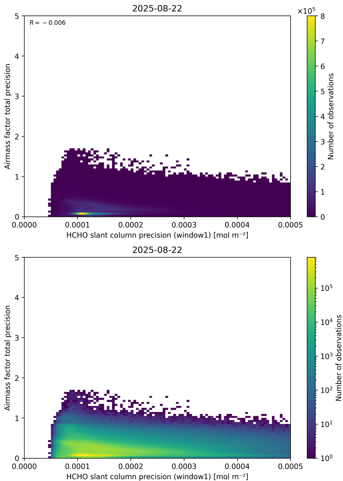
Figure 95: Scatter density plot of “HCHO slant column precision (window1)” against “Airmass factor total precision” for 2025-08-21 to 2025-08-23.
