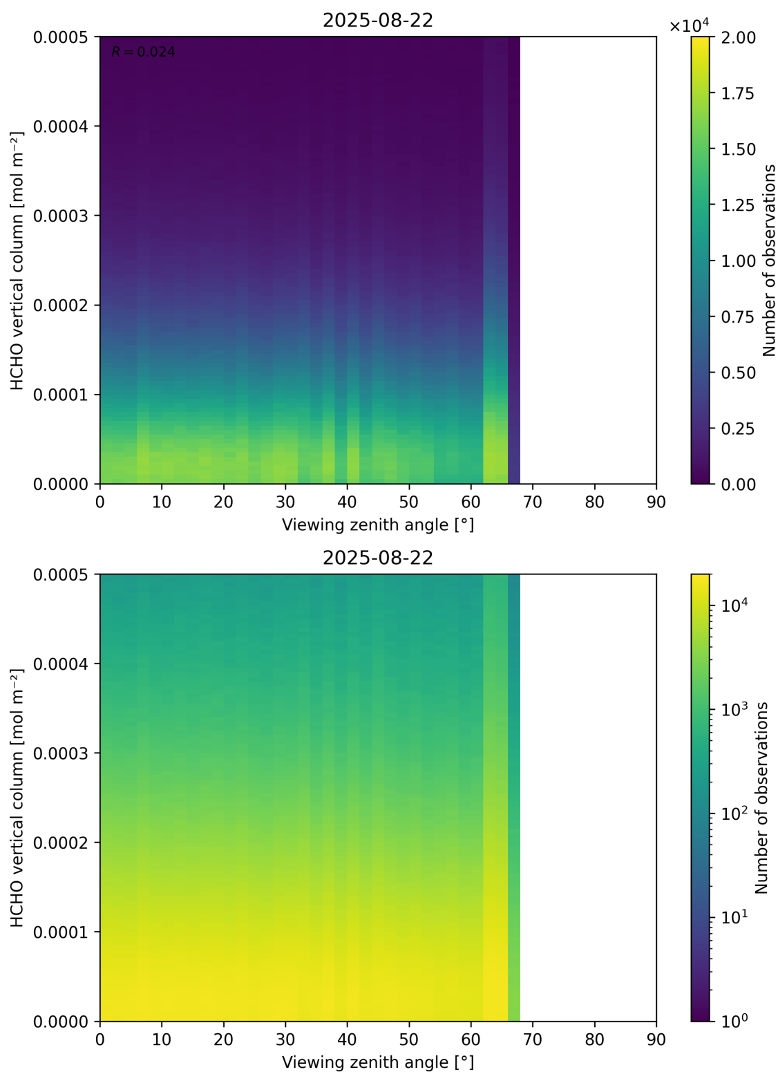
Figure 192: Scatter density plot of “Viewing zenith angle” against “HCHO vertical column” for 2025-08-21 to 2025-08-23.
