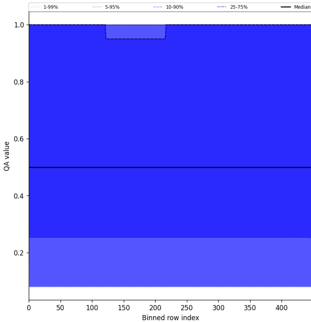
Figure 48: Along track statistics of “QA value” for 2025-08-21 to 2025-08-23
