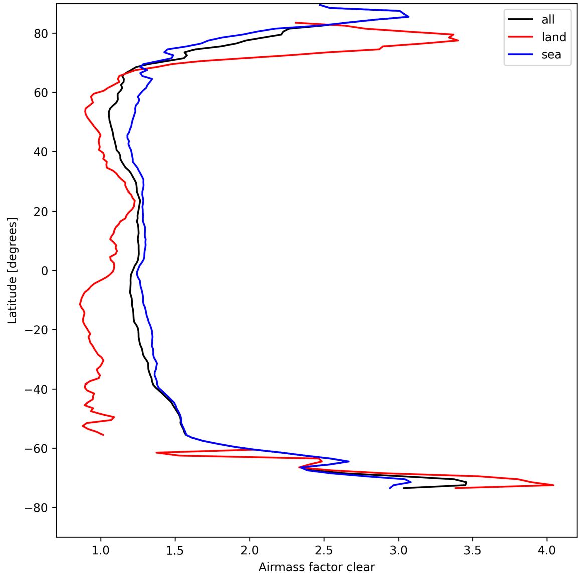
Figure 28: Zonal average of “Airmass factor clear” for 2025-08-21 to 2025-08-23.
