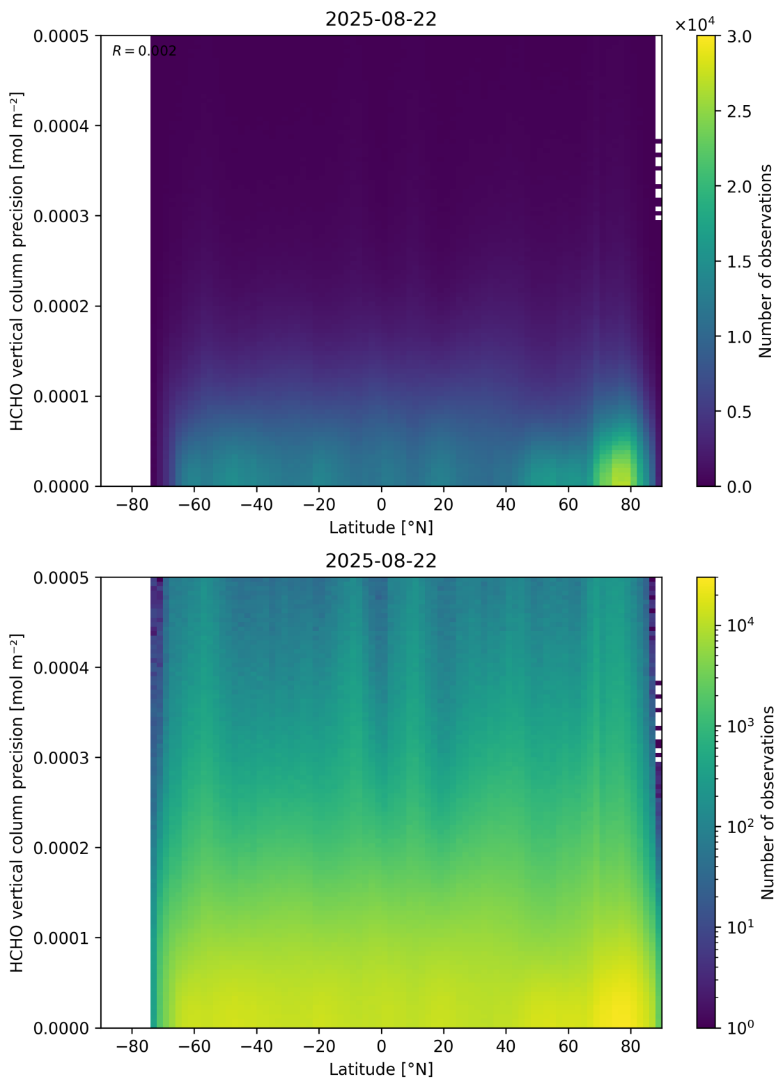
Figure 165: Scatter density plot of “Latitude” against “HCHO vertical column precision” for 2025-08-21 to 2025-08-23.
