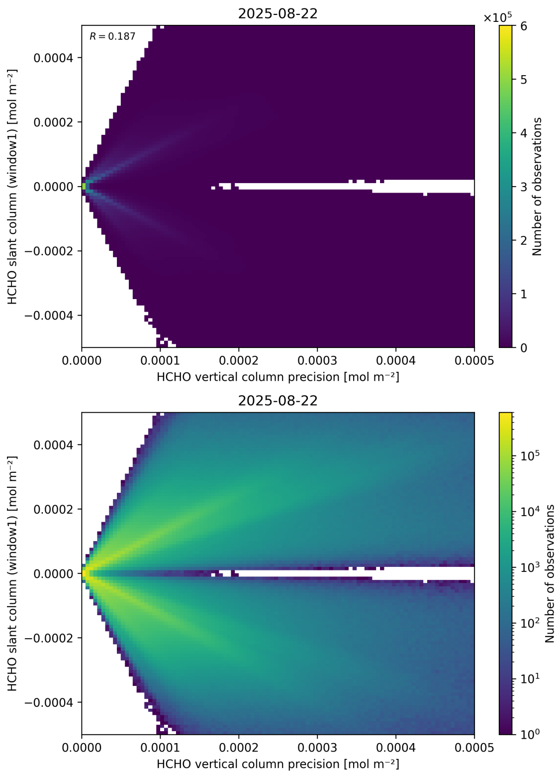
Figure 142: Scatter density plot of “HCHO vertical column precision” against “HCHO slant column (window1)” for 2025-08-21 to 2025-08-23.
