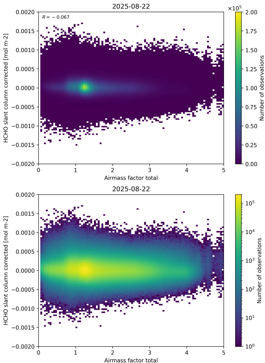
Figure 101: Scatter density plot of “Airmass factor total” against “HCHO slant column corrected” for 2025-08-21 to 2025-08-23.
