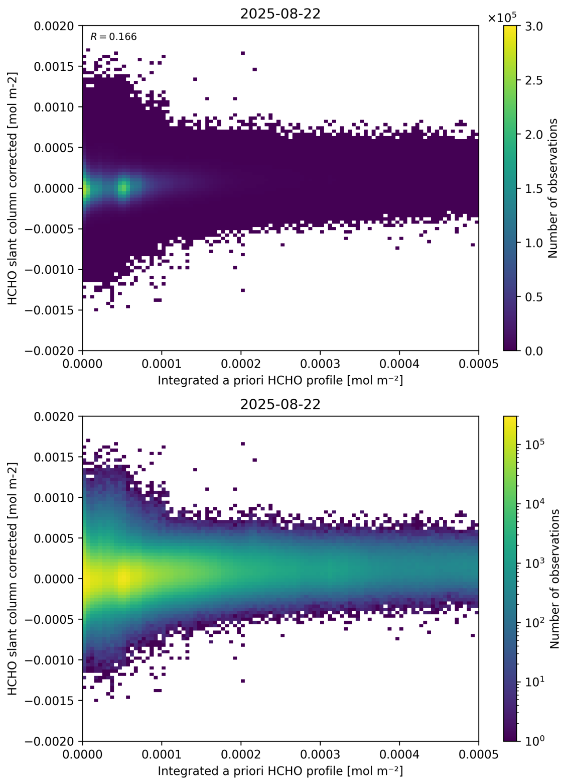
Figure 151: Scatter density plot of “Integrated a priori HCHO profile” against “HCHO slant column corrected” for 2025-08-21 to 2025-08-23.
