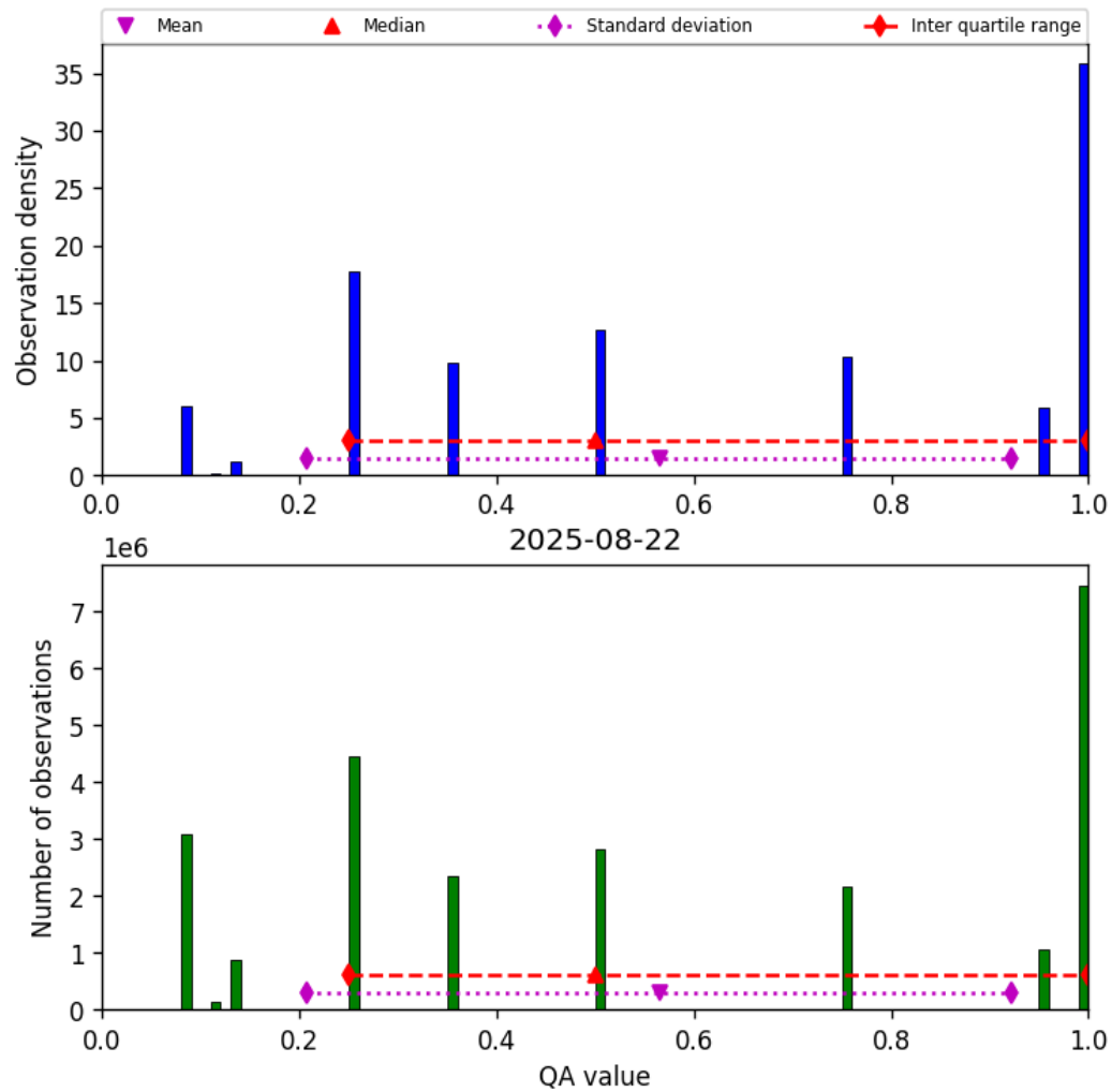
Figure 34: Histogram of “QA value” for 2025-08-21 to 2025-08-23
