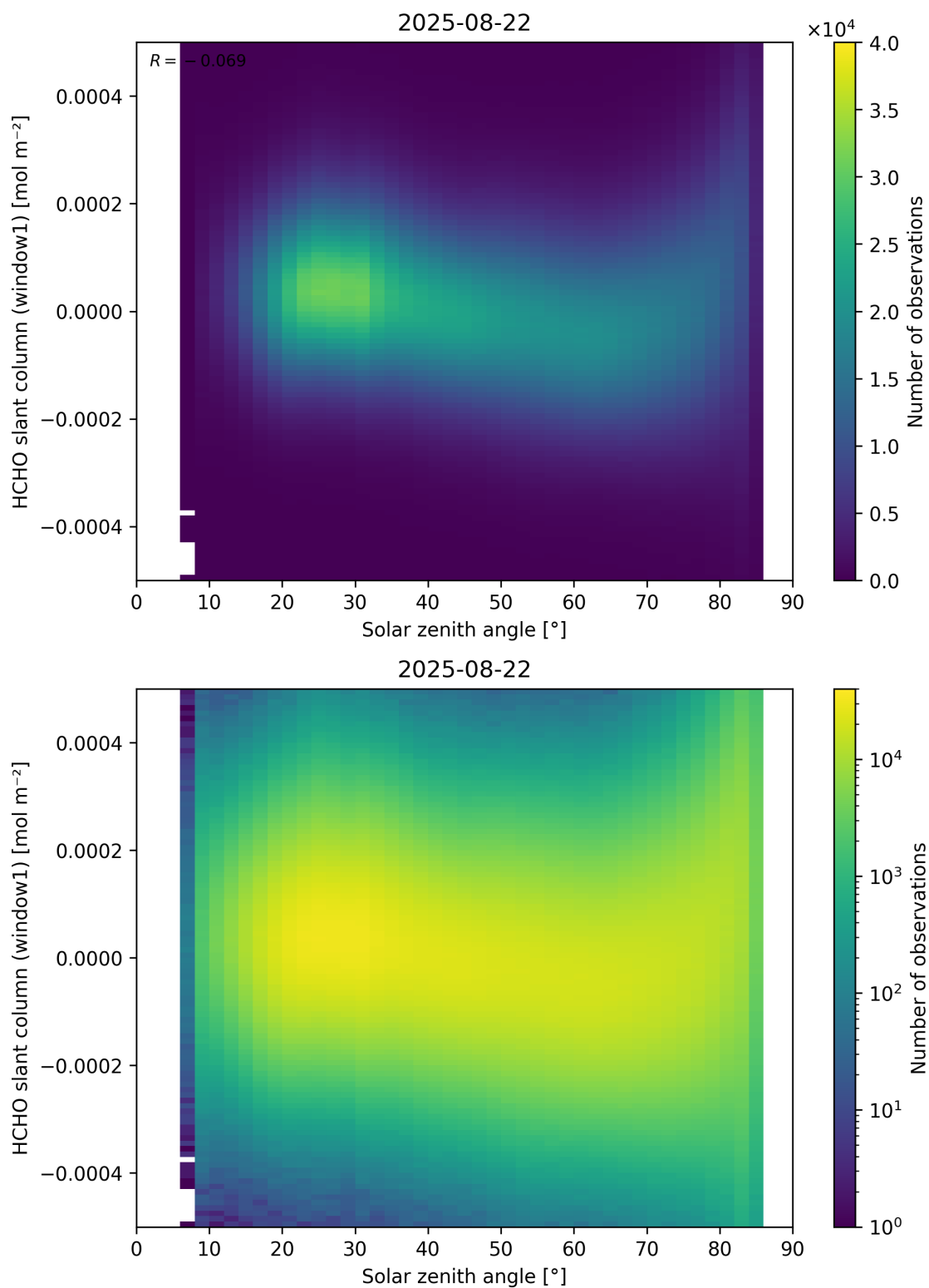
Figure 173: Scatter density plot of “Solar zenith angle” against “HCHO slant column (window1)” for 2025-08-21 to 2025-08-23.
