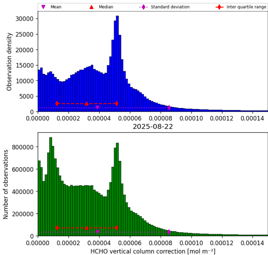
Figure 37: Histogram of “HCHO vertical column correction” for 2025-08-21 to 2025-08-23
