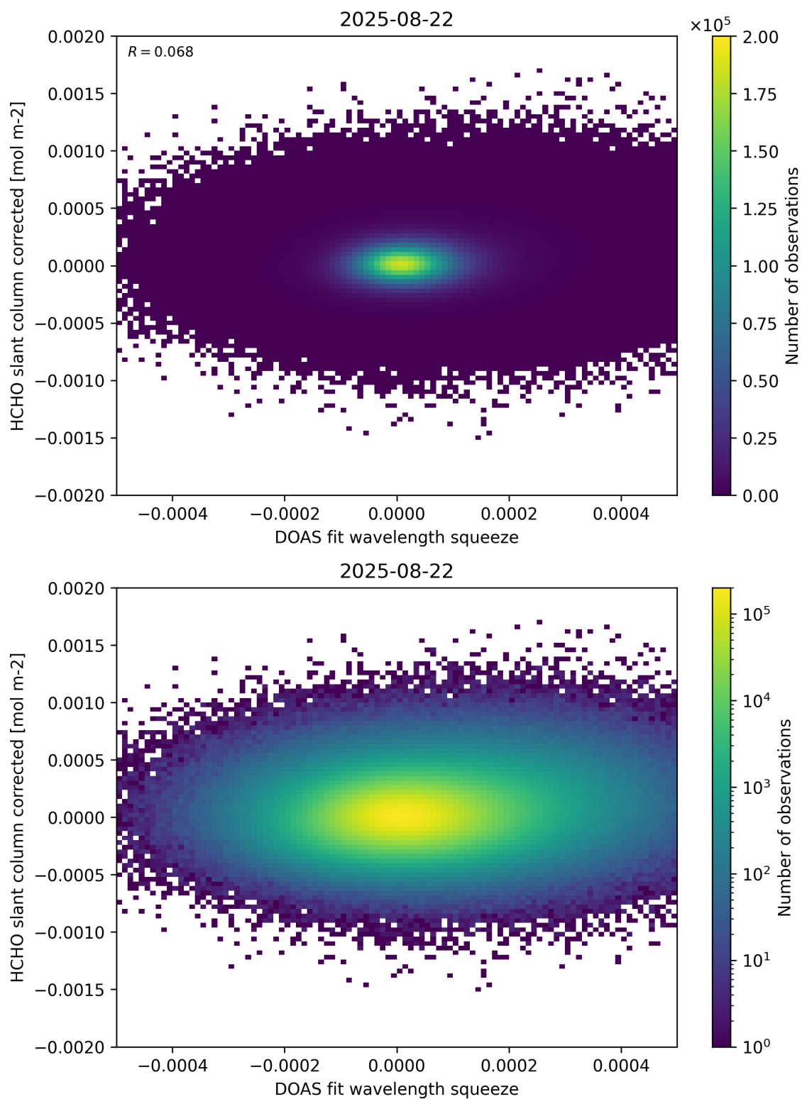
Figure 69: Scatter density plot of “DOAS fit wavelength squeeze” against “HCHO slant column corrected” for 2025-08-21 to 2025-08-23.
