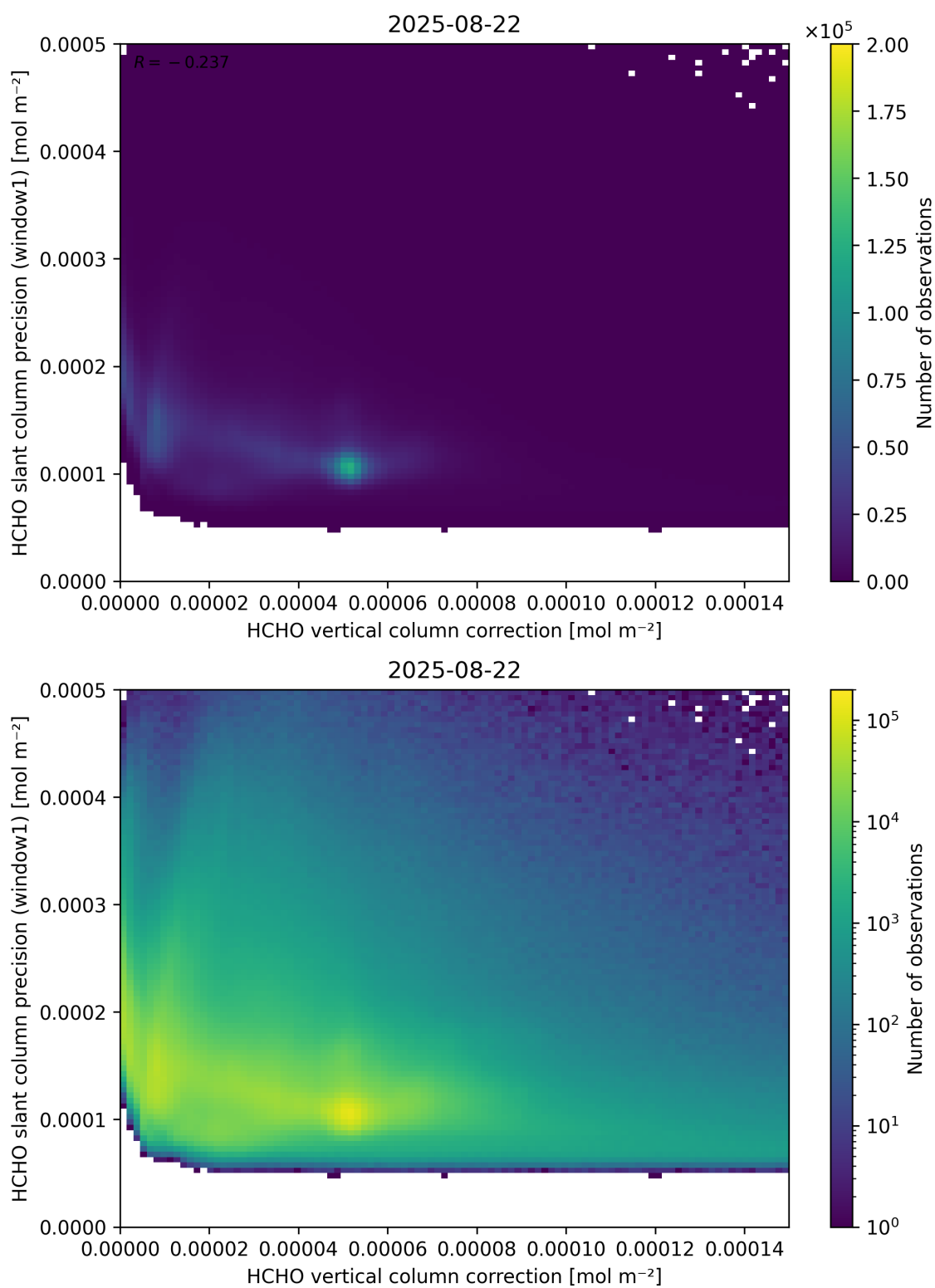
Figure 119: Scatter density plot of “HCHO vertical column correction” against “HCHO slant column precision (window1)” for 2025-08-21 to 2025-08-23.
