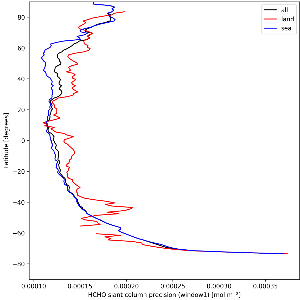
Figure 25: Zonal average of “HCHO slant column precision (window1)” for 2025-08-21 to 2025-08-23.
