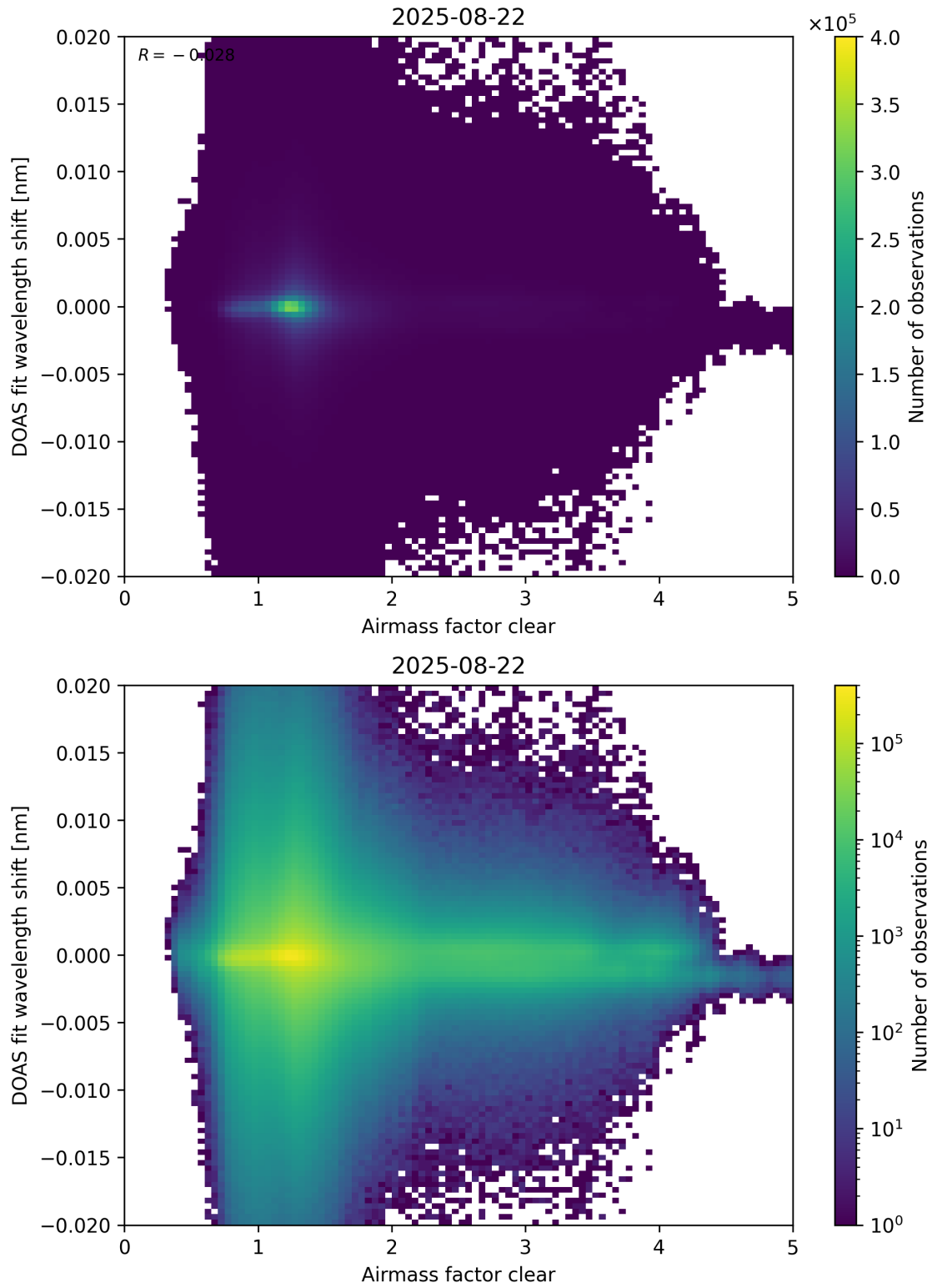
Figure 72: Scatter density plot of “Airmass factor clear” against “DOAS fit wavelength shift” for 2025-08-21 to 2025-08-23.
