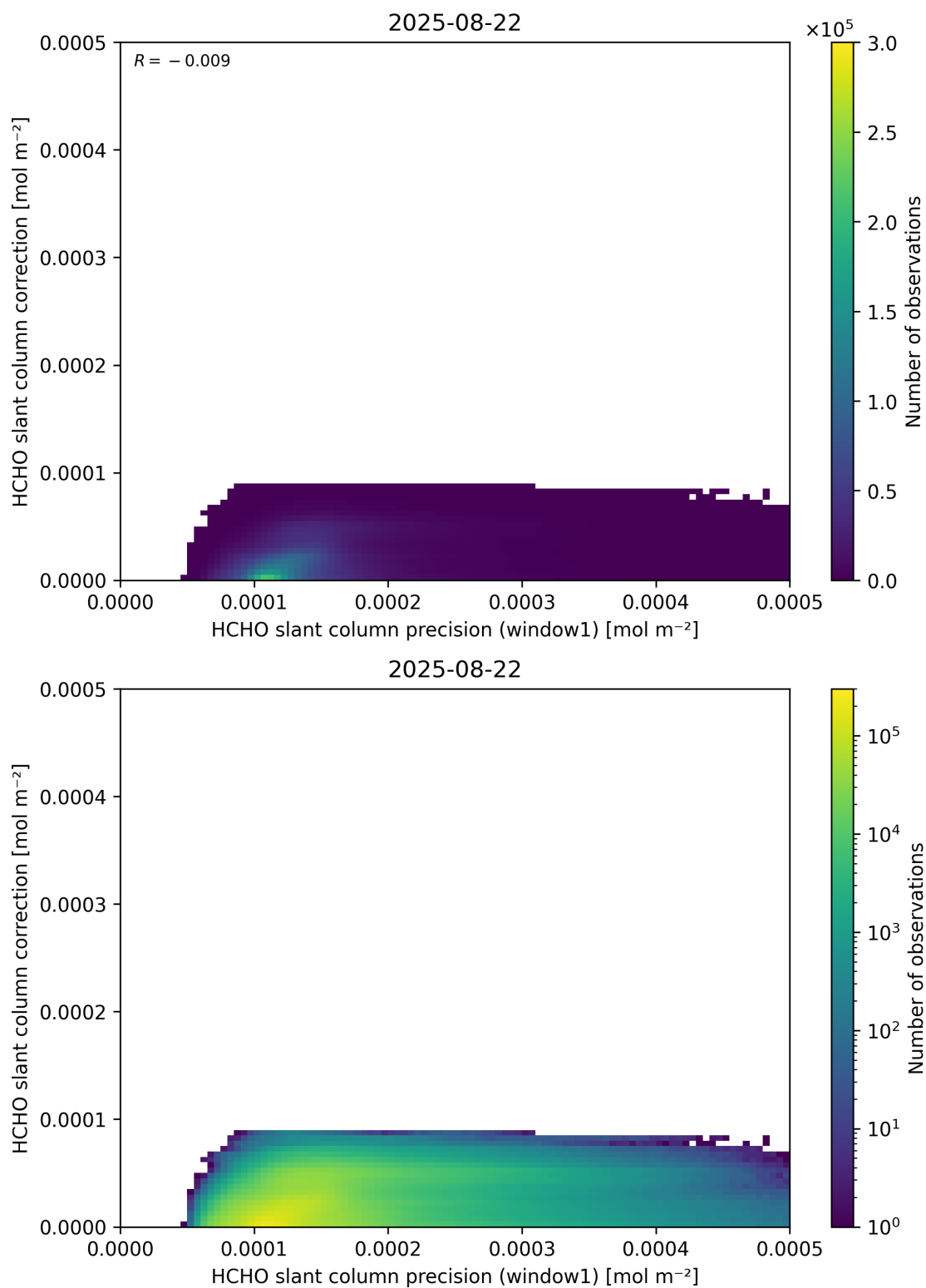
Figure 93: Scatter density plot of “HCHO slant column precision (window1)” against “HCHO slant column correction” for 2025-08-21 to 2025-08-23.
