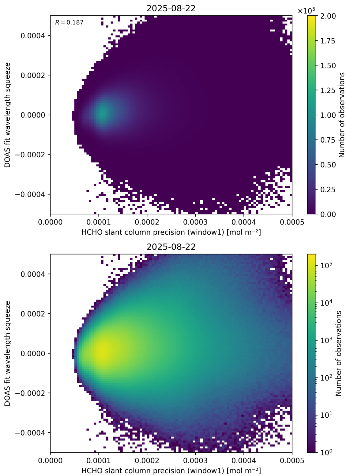
Figure 90: Scatter density plot of “HCHO slant column precision (window1)” against “DOAS fit wavelength squeeze” for 2025-08-21 to 2025-08-23.
