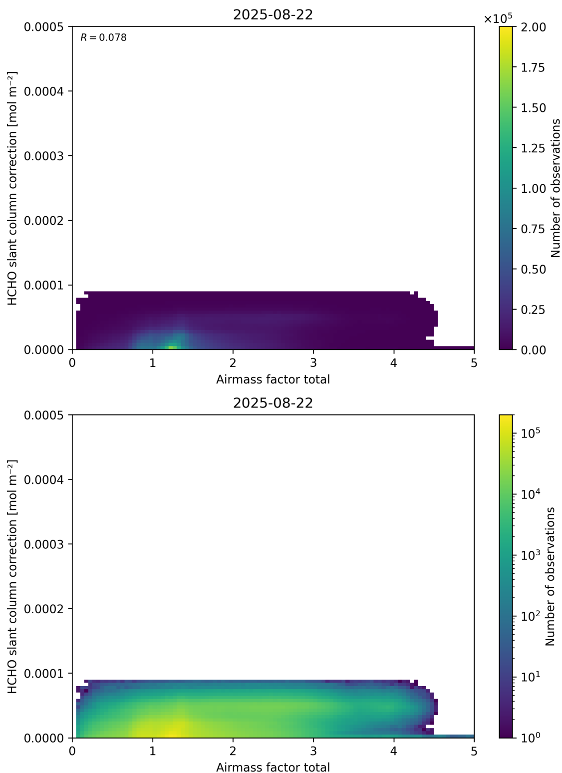
Figure 102: Scatter density plot of “Airmass factor total” against “HCHO slant column correction” for 2025-08-21 to 2025-08-23.
