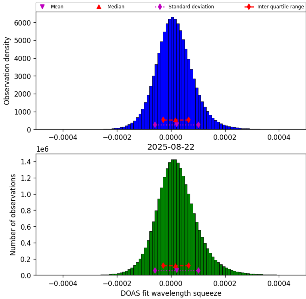
Figure 45: Histogram of “DOAS fit wavelength squeeze” for 2025-08-21 to 2025-08-23
