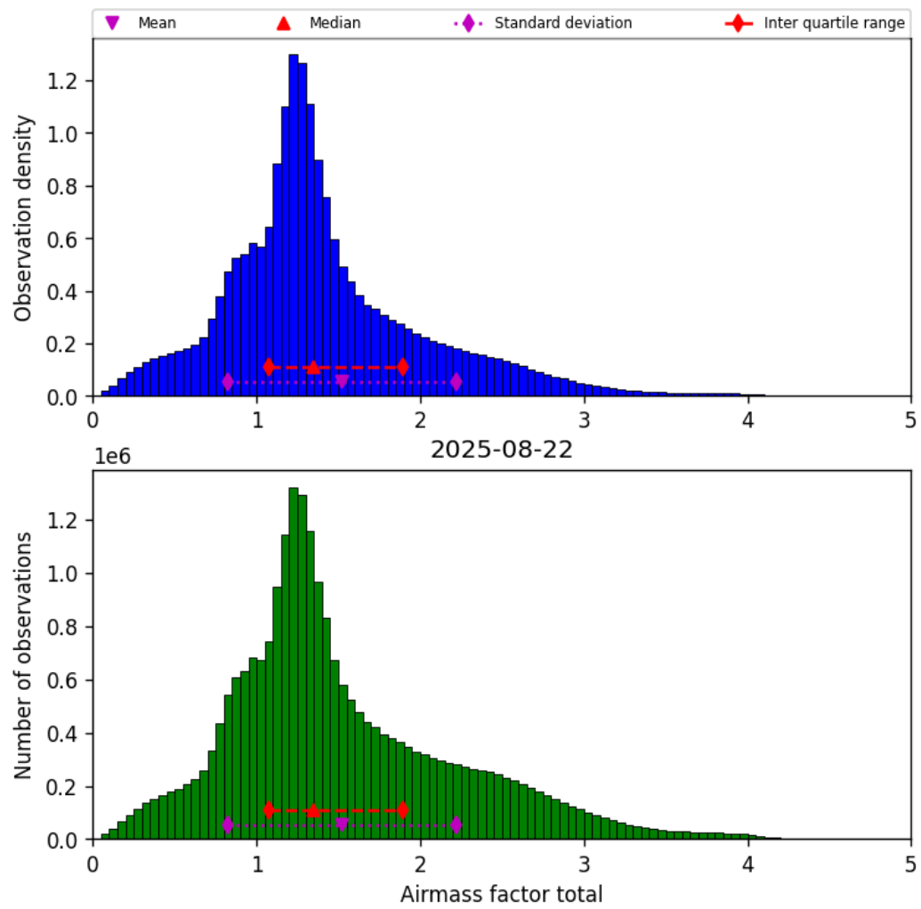
Figure 40: Histogram of “Airmass factor total” for 2025-08-21 to 2025-08-23
