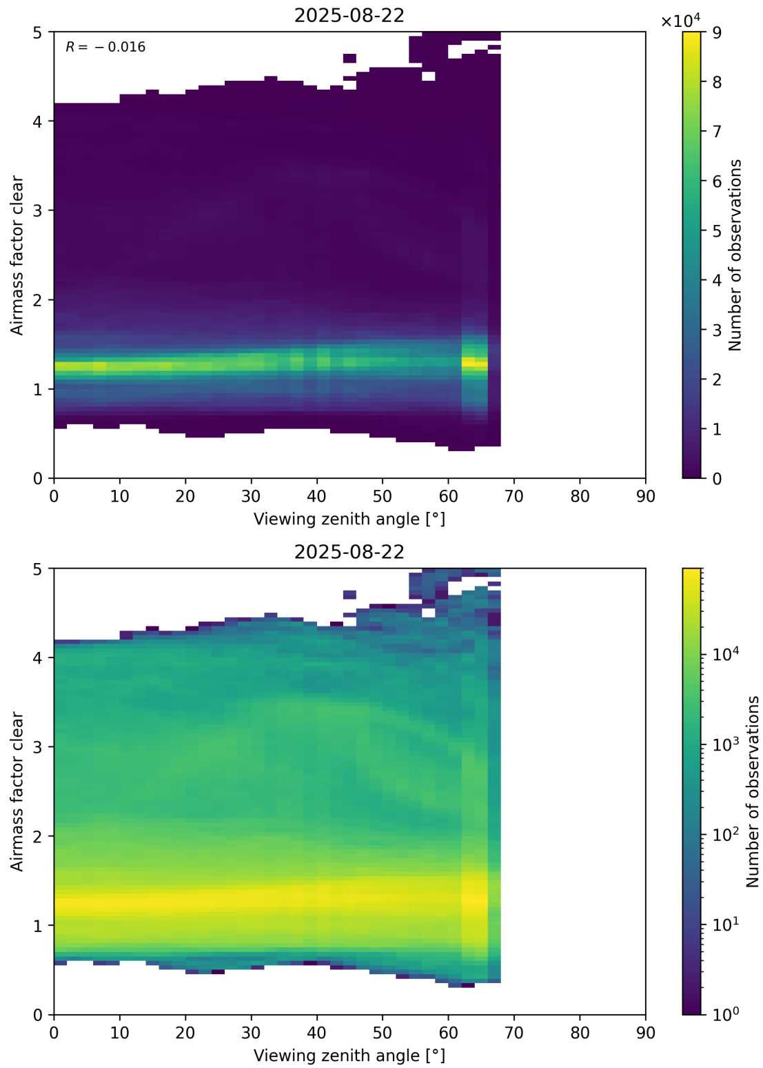
Figure 185: Scatter density plot of “Viewing zenith angle” against “Airmass factor clear” for 2025-08-21 to 2025-08-23.
