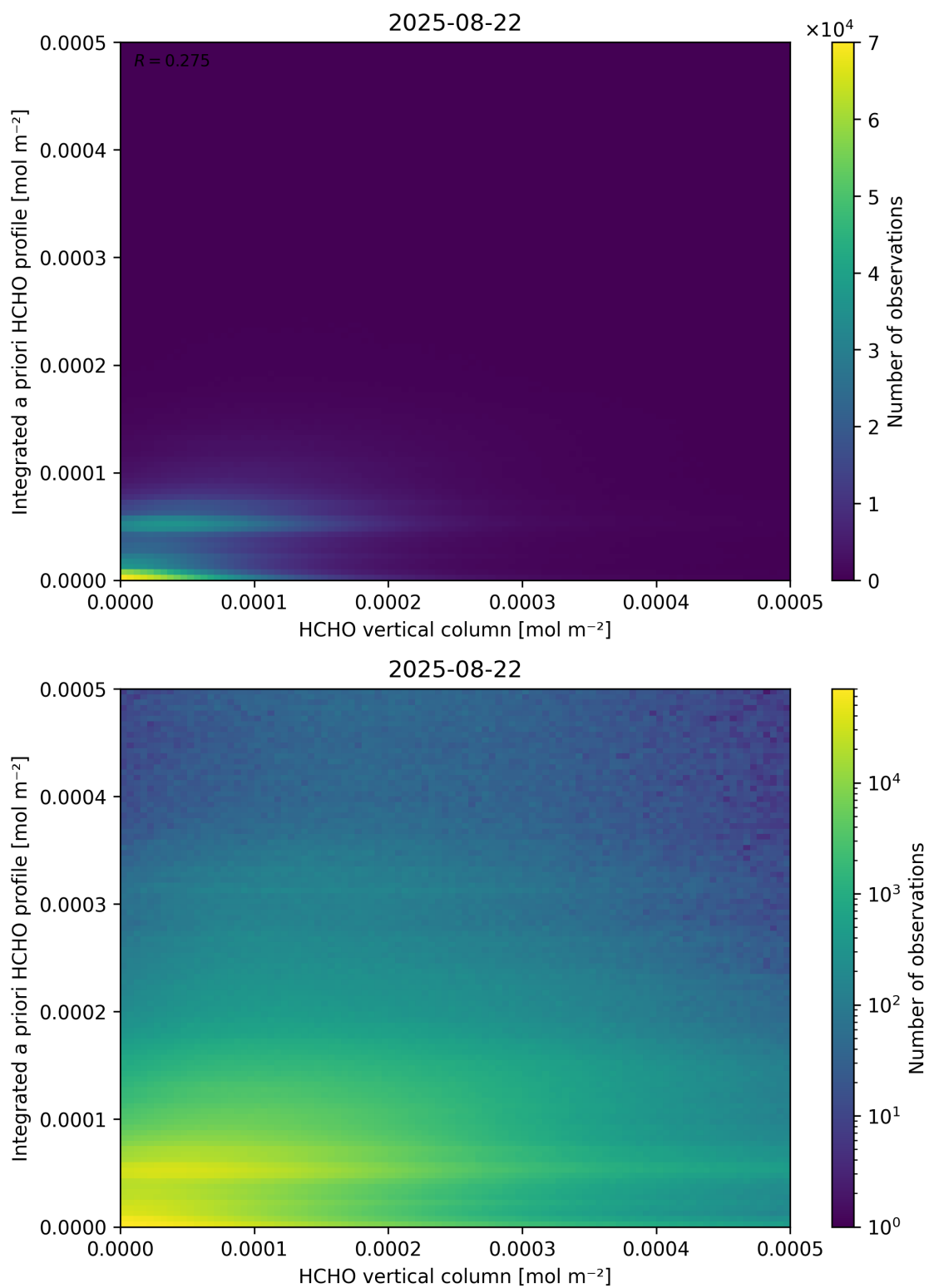
Figure 135: Scatter density plot of “HCHO vertical column” against “Integrated a priori HCHO profile” for 2025-08-21 to 2025-08-23.
