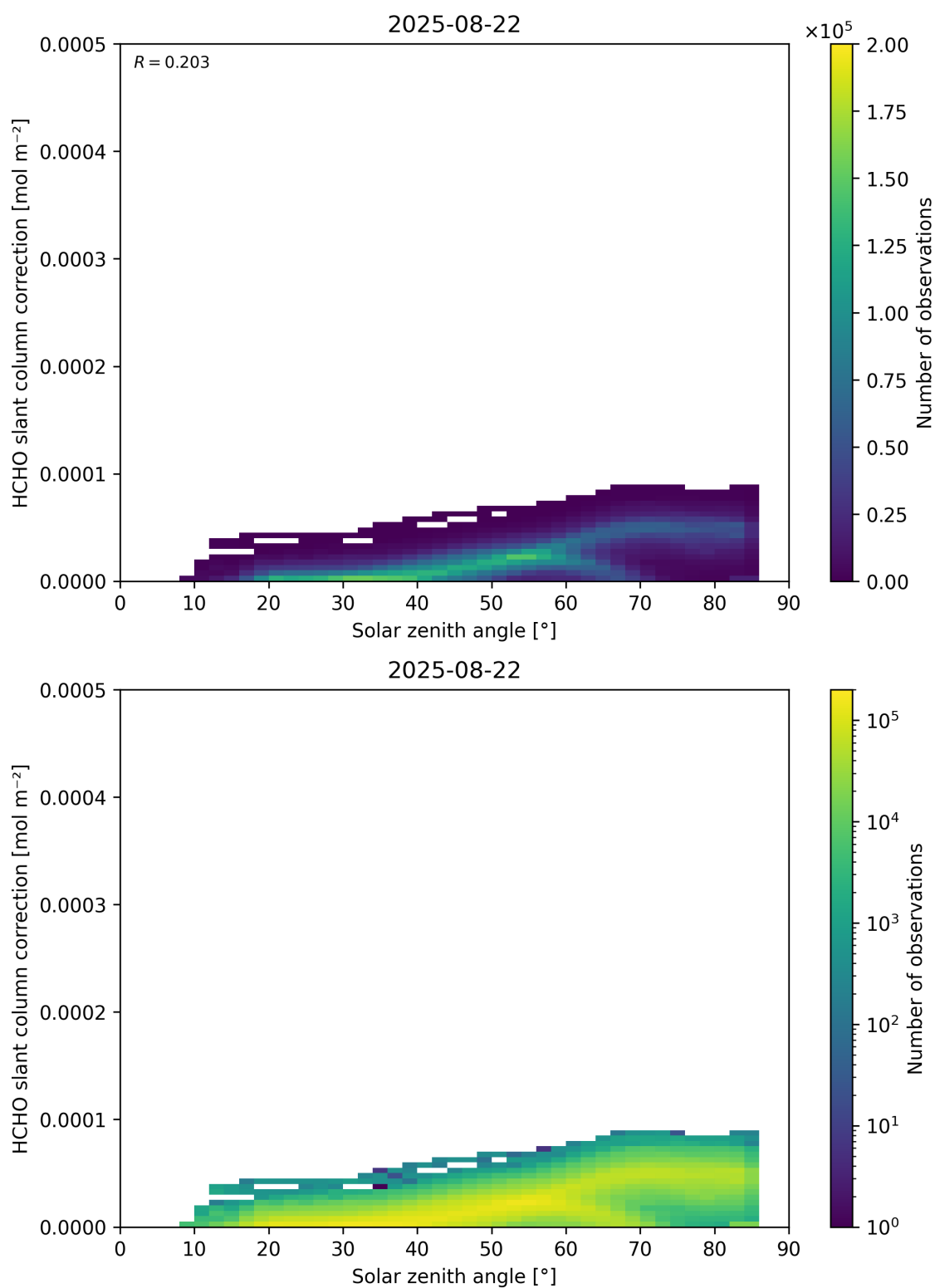
Figure 172: Scatter density plot of “Solar zenith angle” against “HCHO slant column correction” for 2025-08-21 to 2025-08-23.
