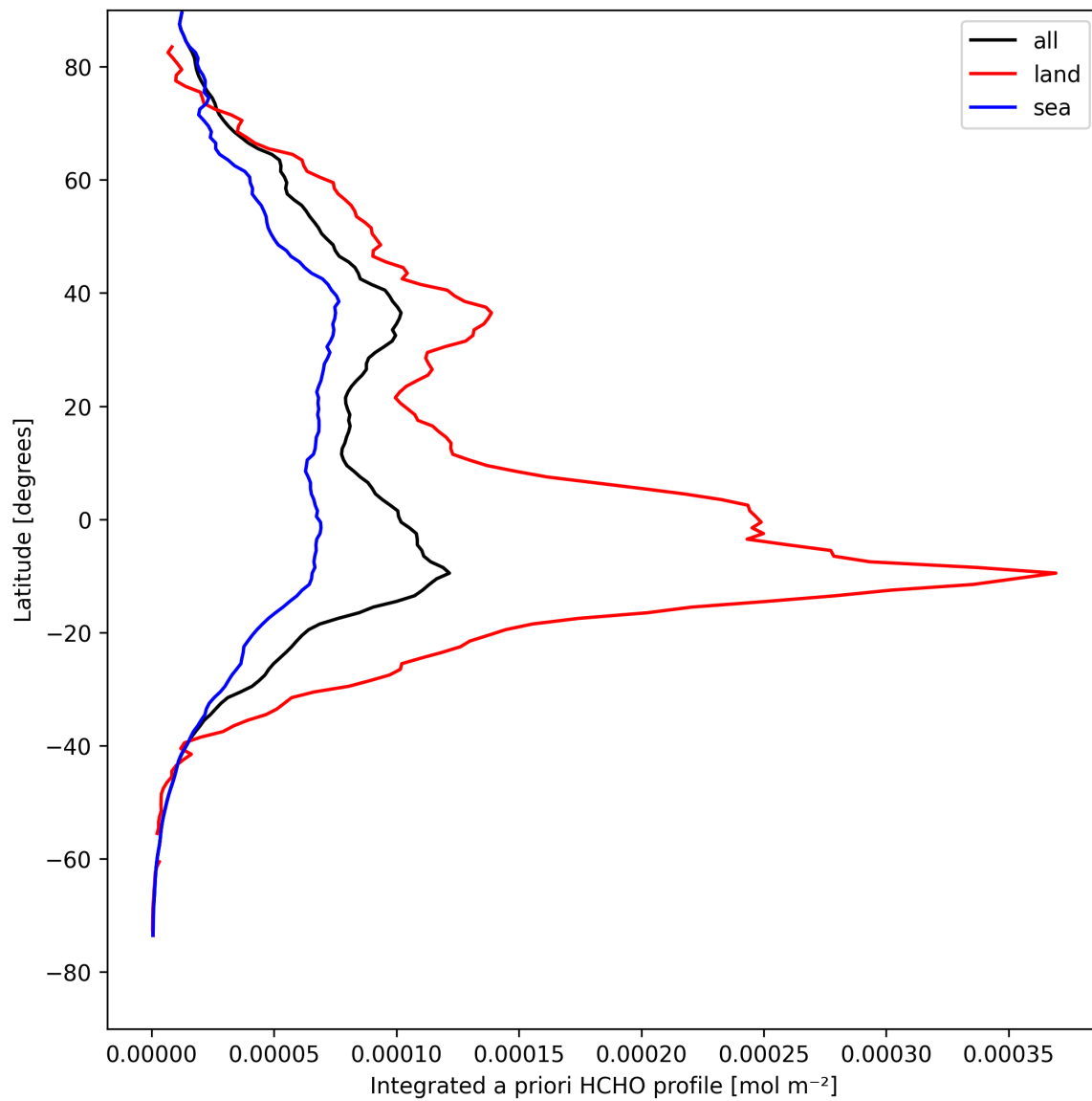
Figure 29: Zonal average of “Integrated a priori HCHO profile” for 2025-08-21 to 2025-08-23.
