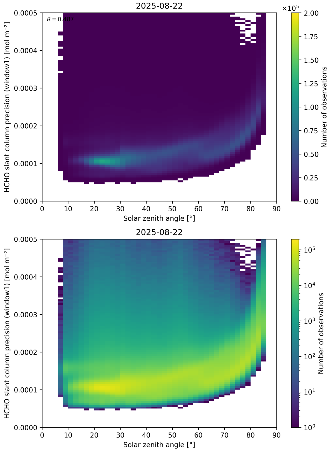
Figure 174: Scatter density plot of “Solar zenith angle” against “HCHO slant column precision (window1)” for 2025-08-21 to 2025-08-23.
