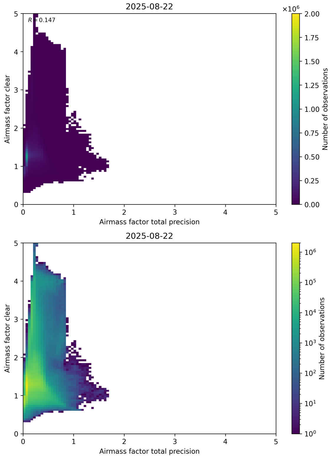
Figure 108: Scatter density plot of “Airmass factor total precision” against “Airmass factor clear” for 2025-08-21 to 2025-08-23.
