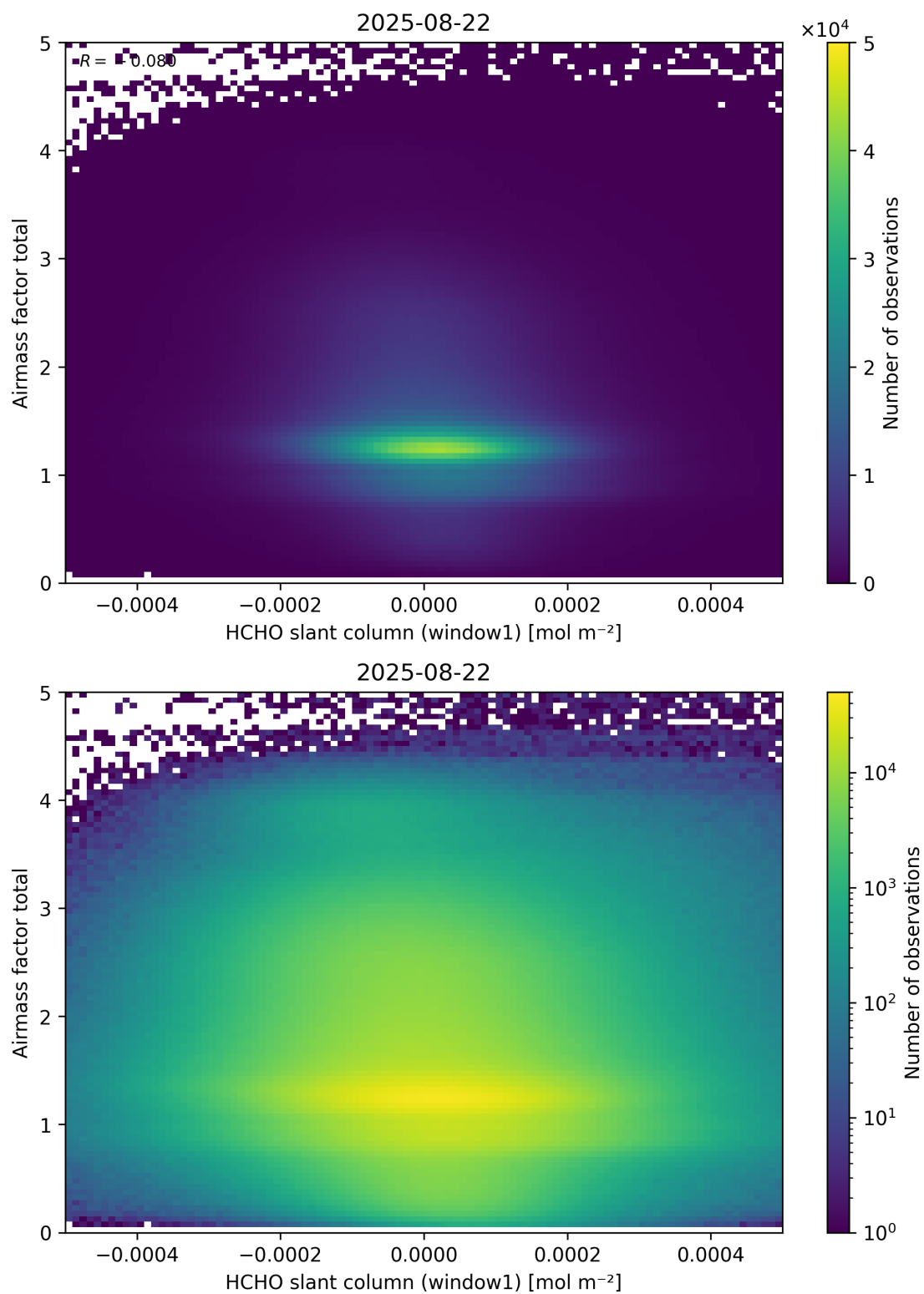
Figure 85: Scatter density plot of “HCHO slant column (window1)” against “Airmass factor total” for 2025-08-21 to 2025-08-23.
