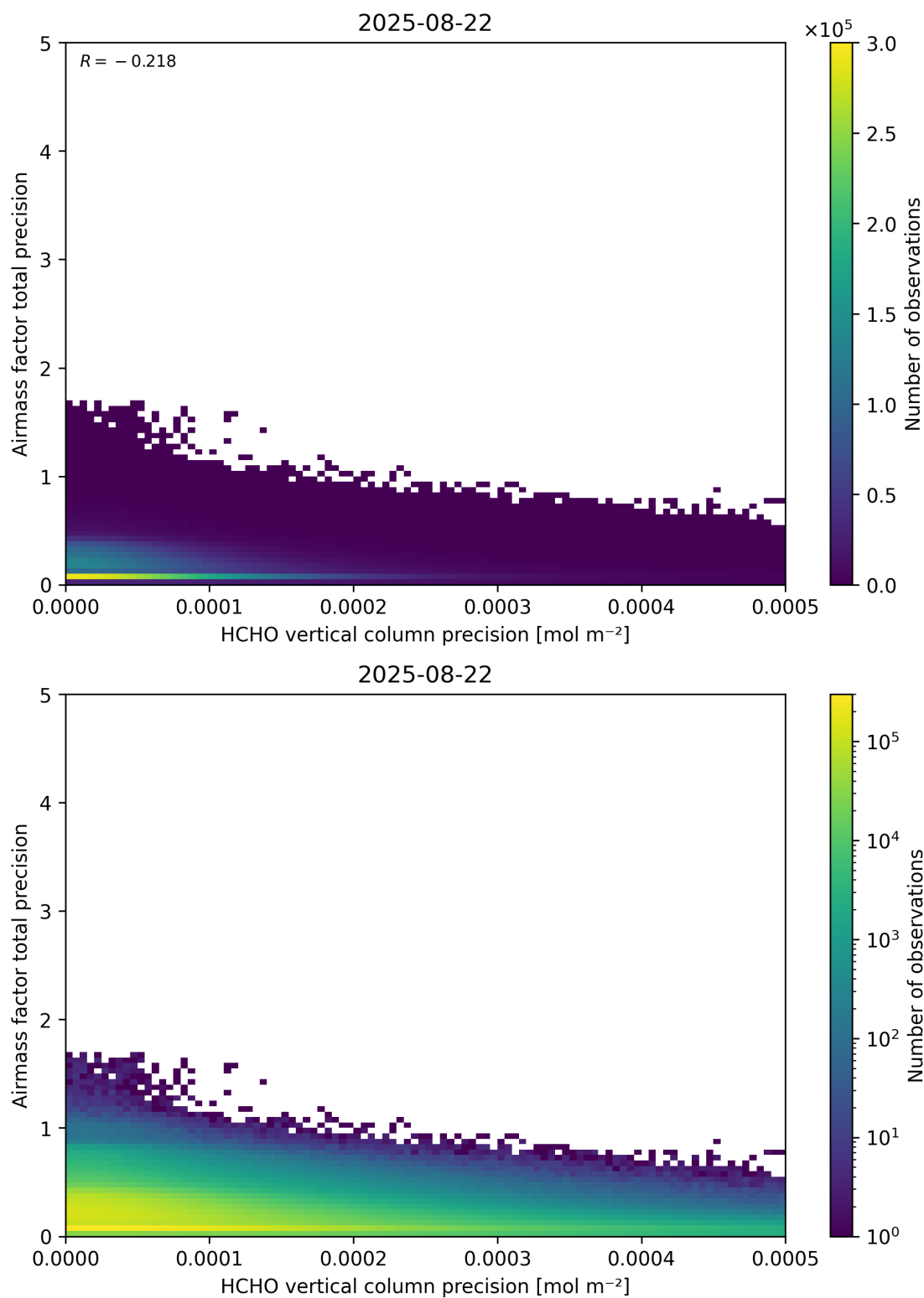
Figure 145: Scatter density plot of “HCHO vertical column precision” against “Airmass factor total precision” for 2025-08-21 to 2025-08-23.
