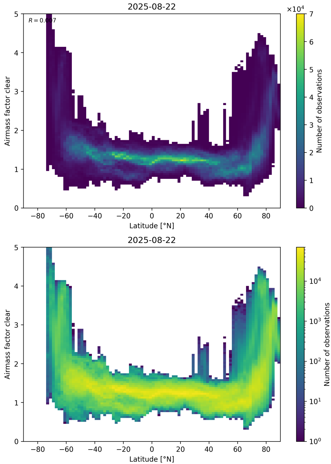
Figure 156: Scatter density plot of “Latitude” against “Airmass factor clear” for 2025-08-21 to 2025-08-23.
