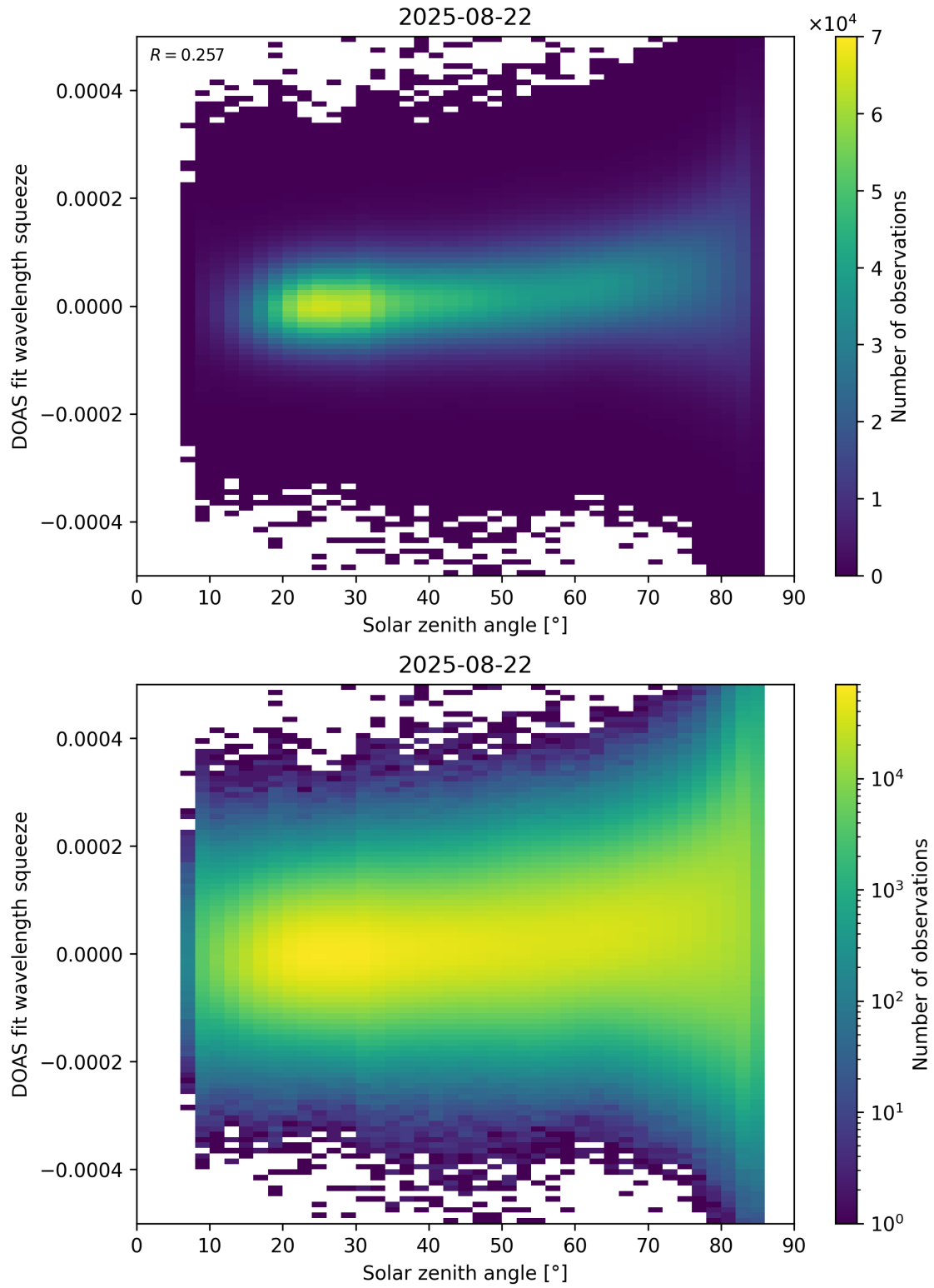
Figure 169: Scatter density plot of “Solar zenith angle” against “DOAS fit wavelength squeeze” for 2025-08-21 to 2025-08-23.
