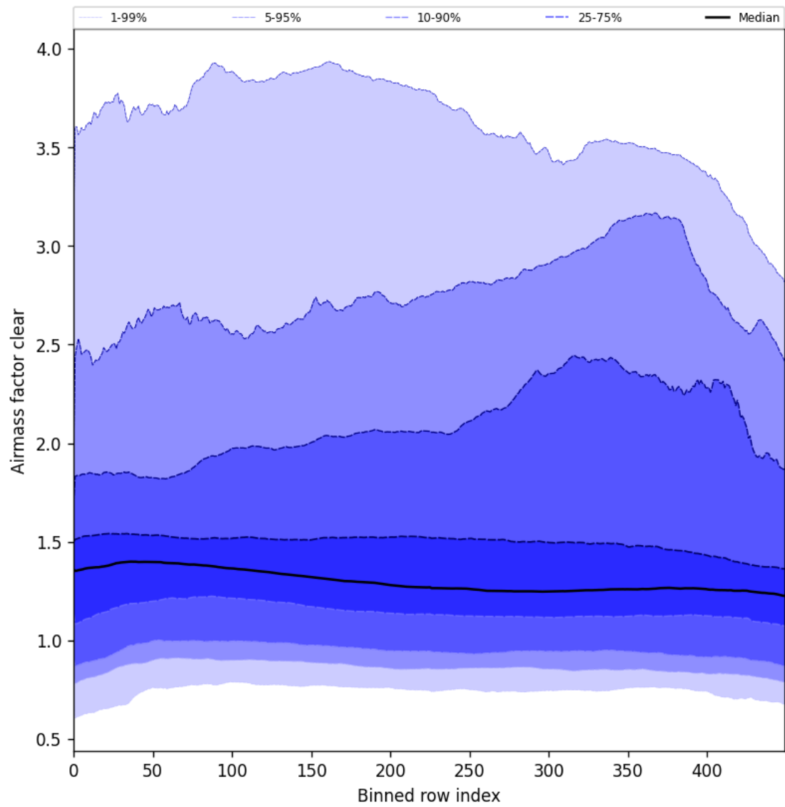
Figure 56: Along track statistics of “Airmass factor clear” for 2025-08-21 to 2025-08-23
