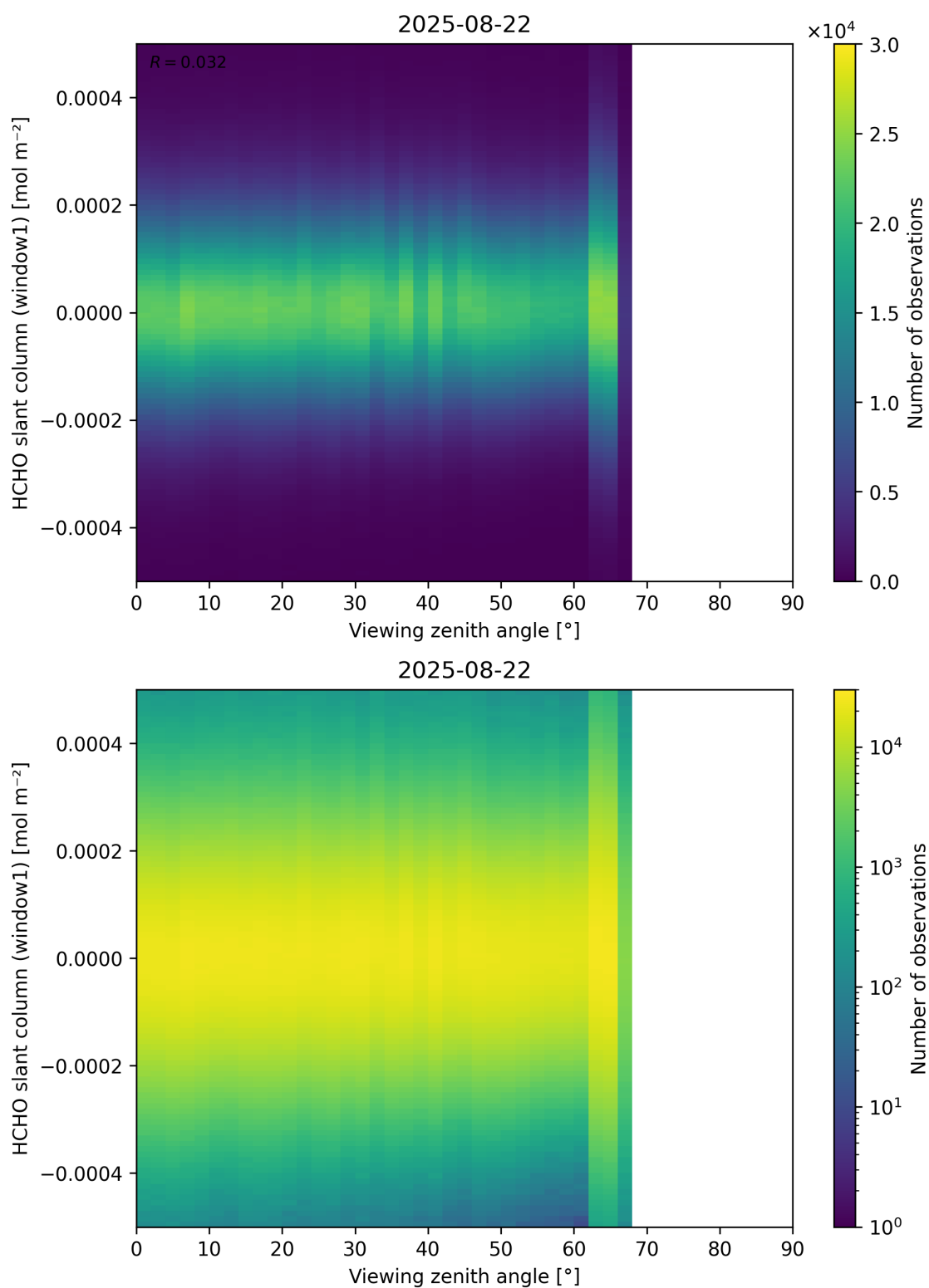
Figure 188: Scatter density plot of “Viewing zenith angle” against “HCHO slant column (window1)” for 2025-08-21 to 2025-08-23.
