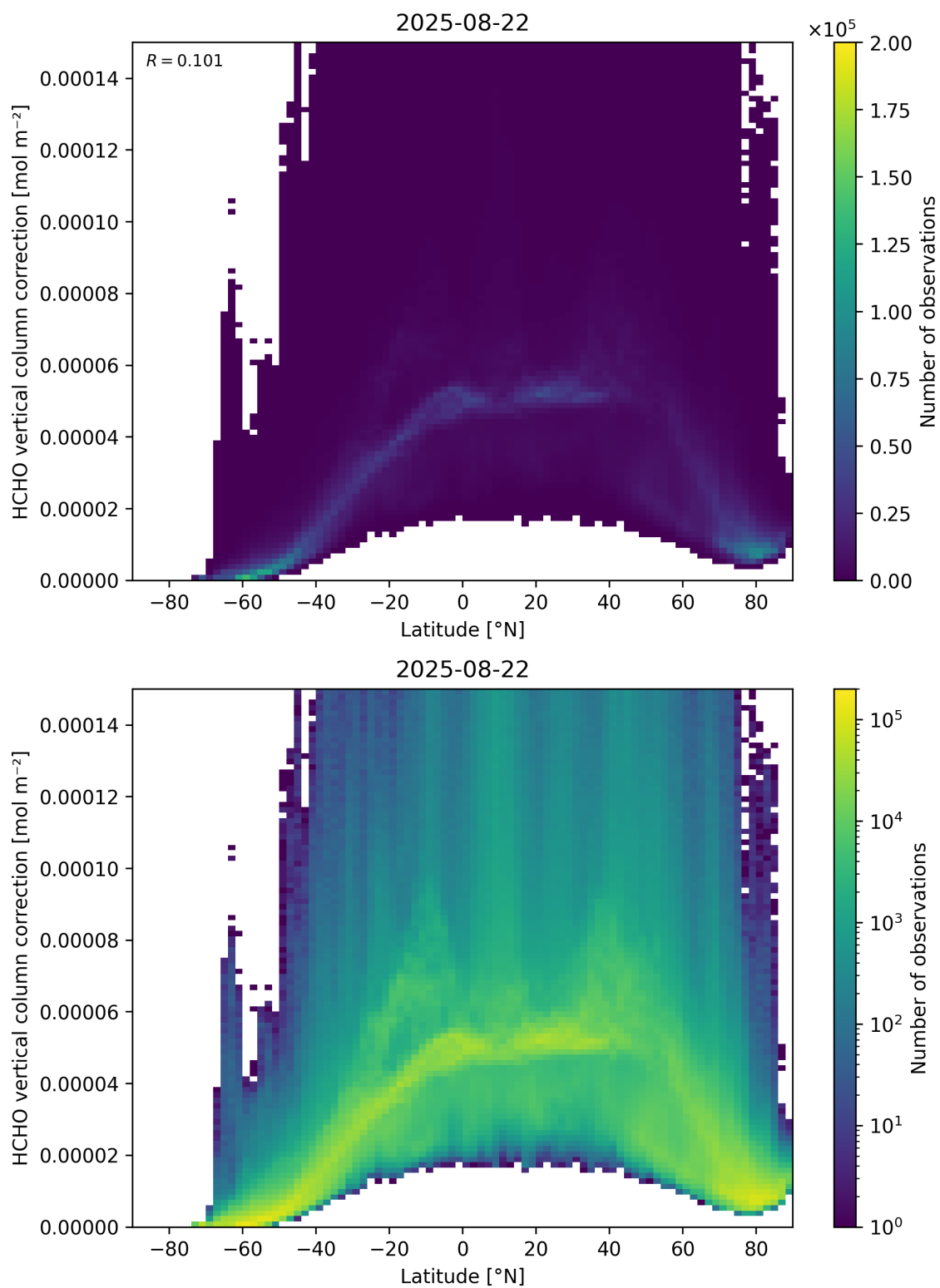
Figure 164: Scatter density plot of “Latitude” against “HCHO vertical column correction” for 2025-08-21 to 2025-08-23.
