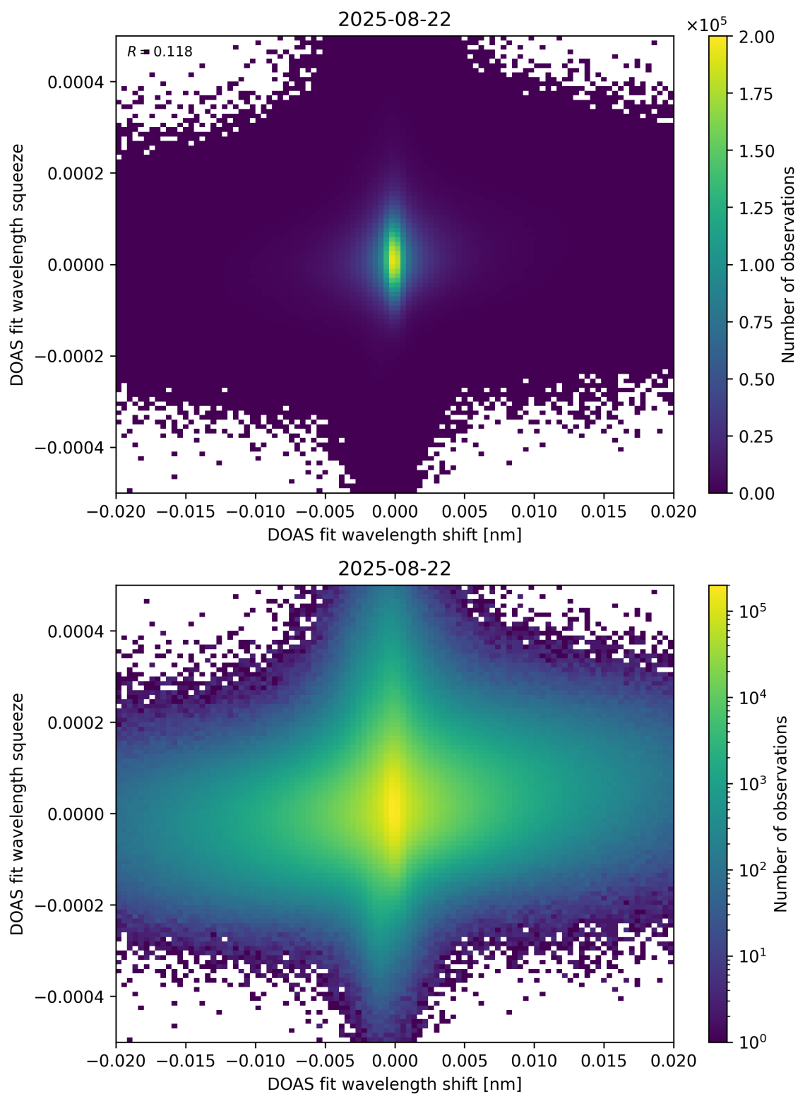
Figure 65: Scatter density plot of “DOAS fit wavelength shift” against “DOAS fit wavelength squeeze” for 2025-08-21 to 2025-08-23.
