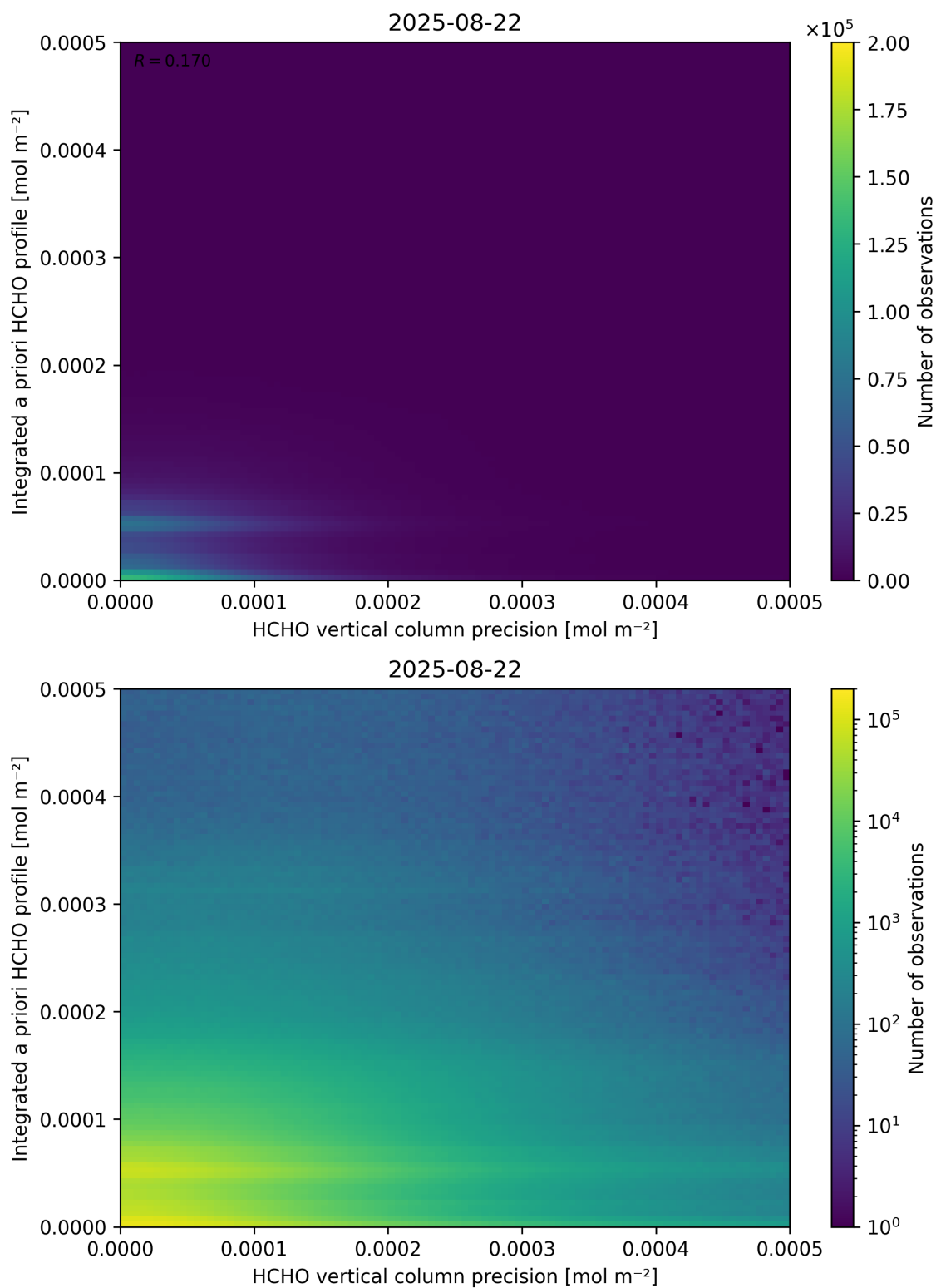
Figure 147: Scatter density plot of “HCHO vertical column precision” against “Integrated a priori HCHO profile” for 2025-08-21 to 2025-08-23.
