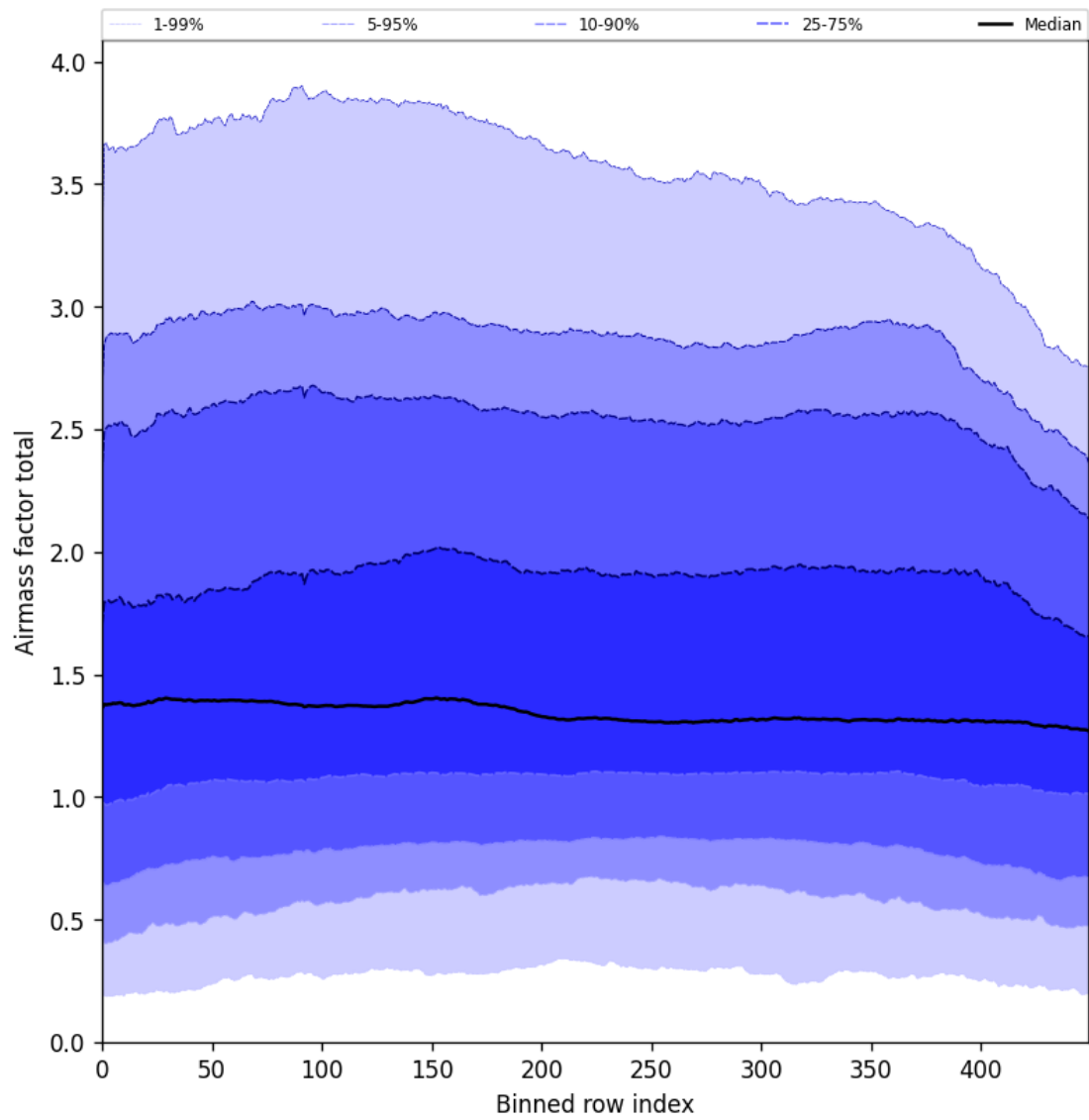
Figure 54: Along track statistics of “Airmass factor total” for 2025-08-21 to 2025-08-23
