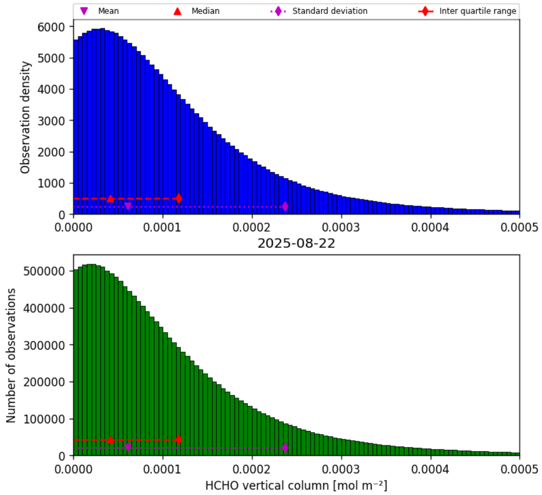
Figure 35: Histogram of “HCHO vertical column” for 2025-08-21 to 2025-08-23
