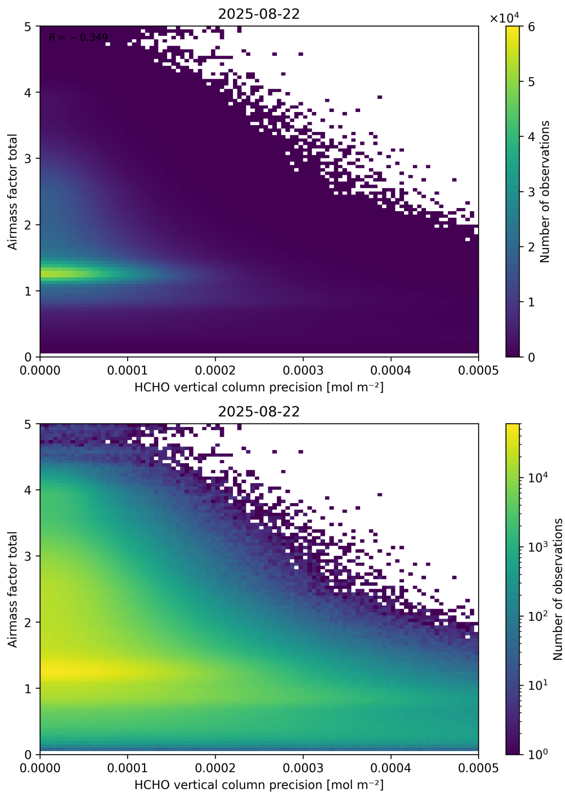
Figure 144: Scatter density plot of “HCHO vertical column precision” against “Airmass factor total” for 2025-08-21 to 2025-08-23.
