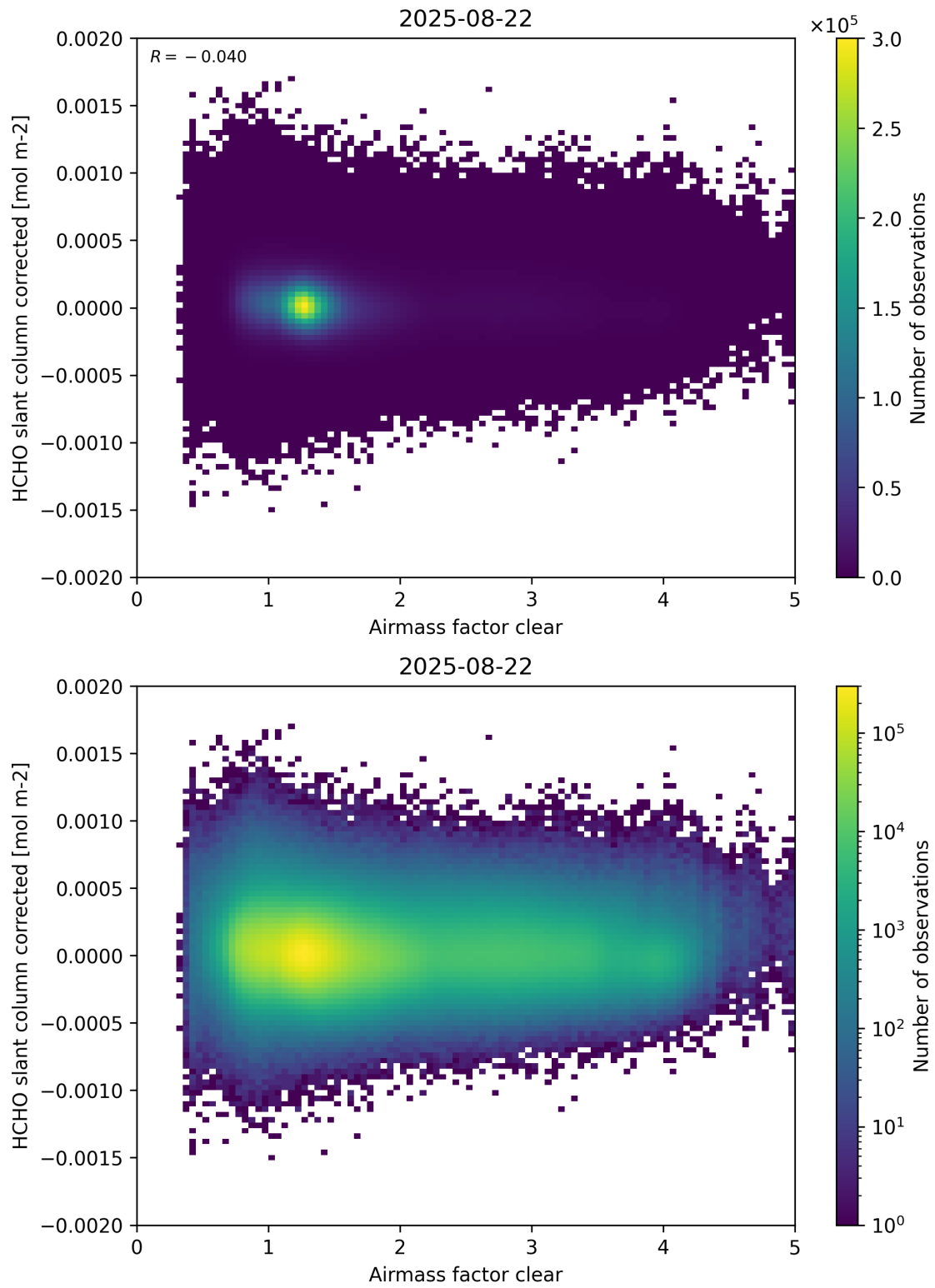
Figure 74: Scatter density plot of “Airmass factor clear” against “HCHO slant column corrected” for 2025-08-21 to 2025-08-23.
