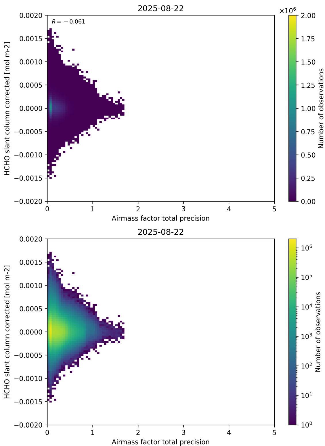
Figure 109: Scatter density plot of “Airmass factor total precision” against “HCHO slant column corrected” for 2025-08-21 to 2025-08-23.
