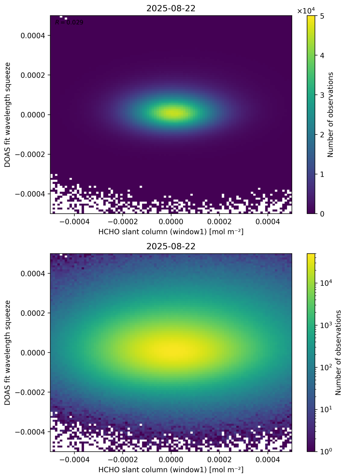
Figure 80: Scatter density plot of “HCHO slant column (window1)” against “DOAS fit wavelength squeeze” for 2025-08-21 to 2025-08-23.
