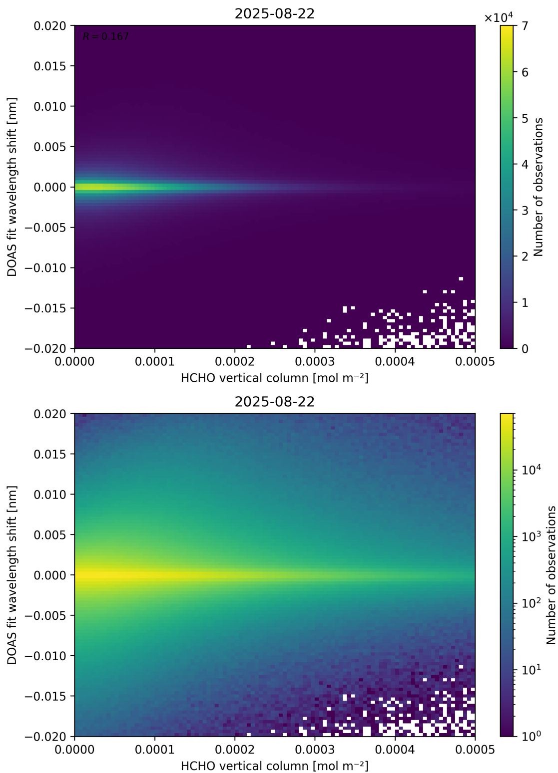
Figure 124: Scatter density plot of “HCHO vertical column” against “DOAS fit wavelength shift” for 2025-08-21 to 2025-08-23.
