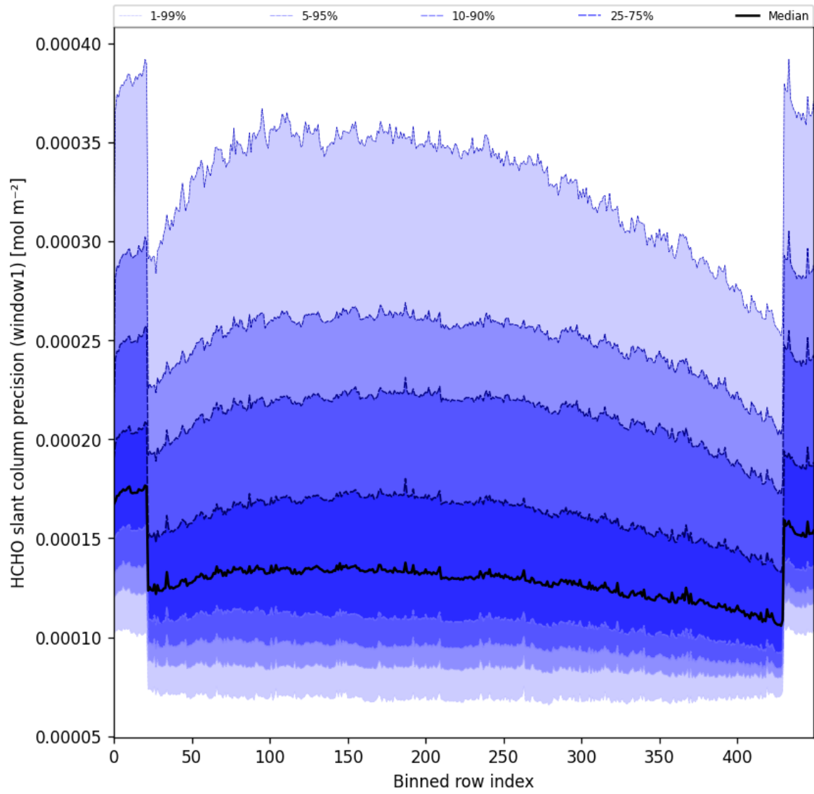
Figure 53: Along track statistics of “HCHO slant column precision (window1)” for 2025-08-21 to 2025-08-23
