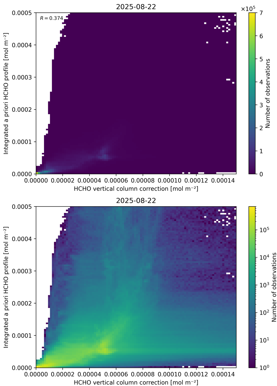
Figure 122: Scatter density plot of “HCHO vertical column correction” against “Integrated a priori HCHO profile” for 2025-08-21 to 2025-08-23.
