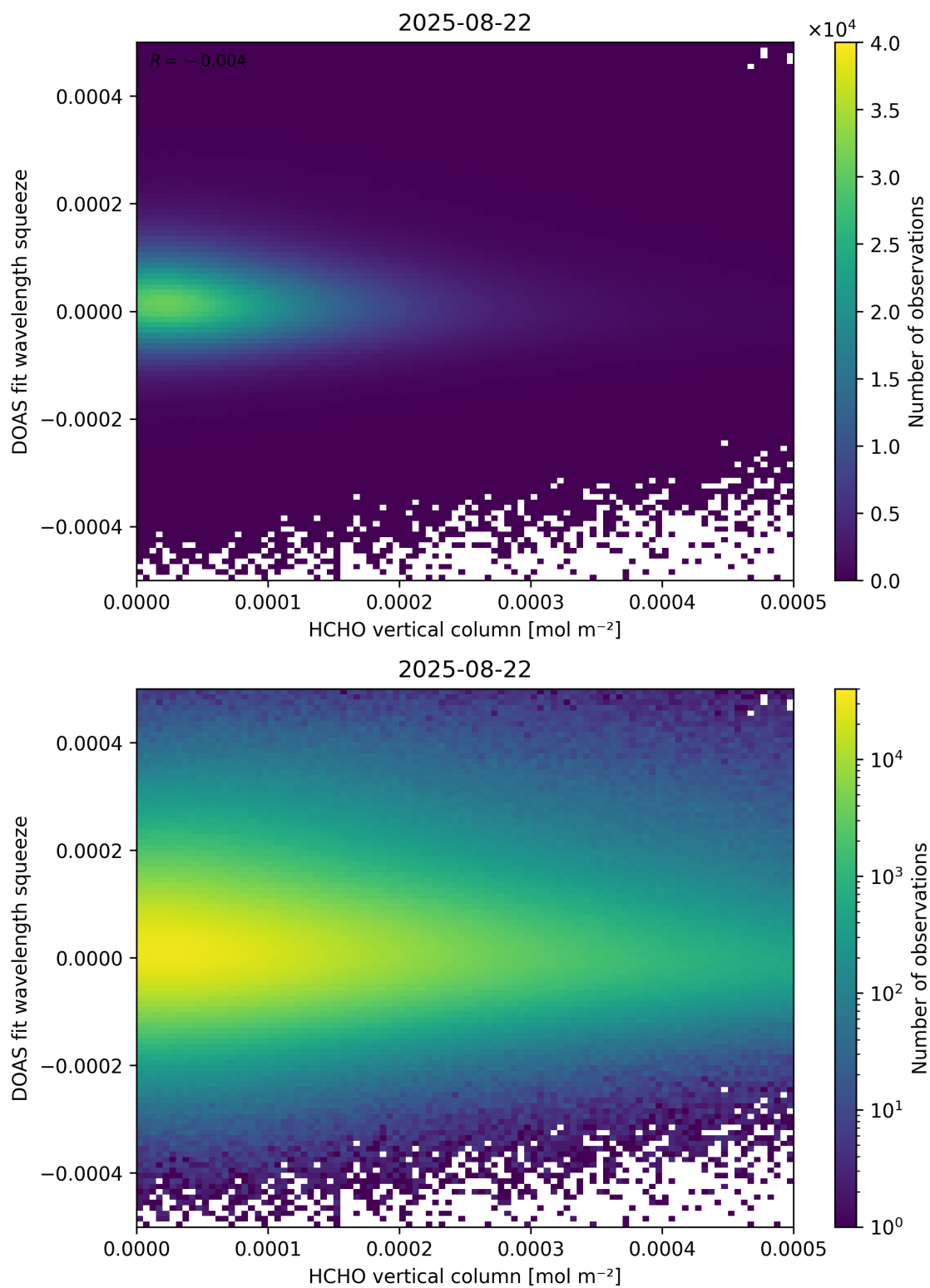
Figure 125: Scatter density plot of “HCHO vertical column” against “DOAS fit wavelength squeeze” for 2025-08-21 to 2025-08-23.
