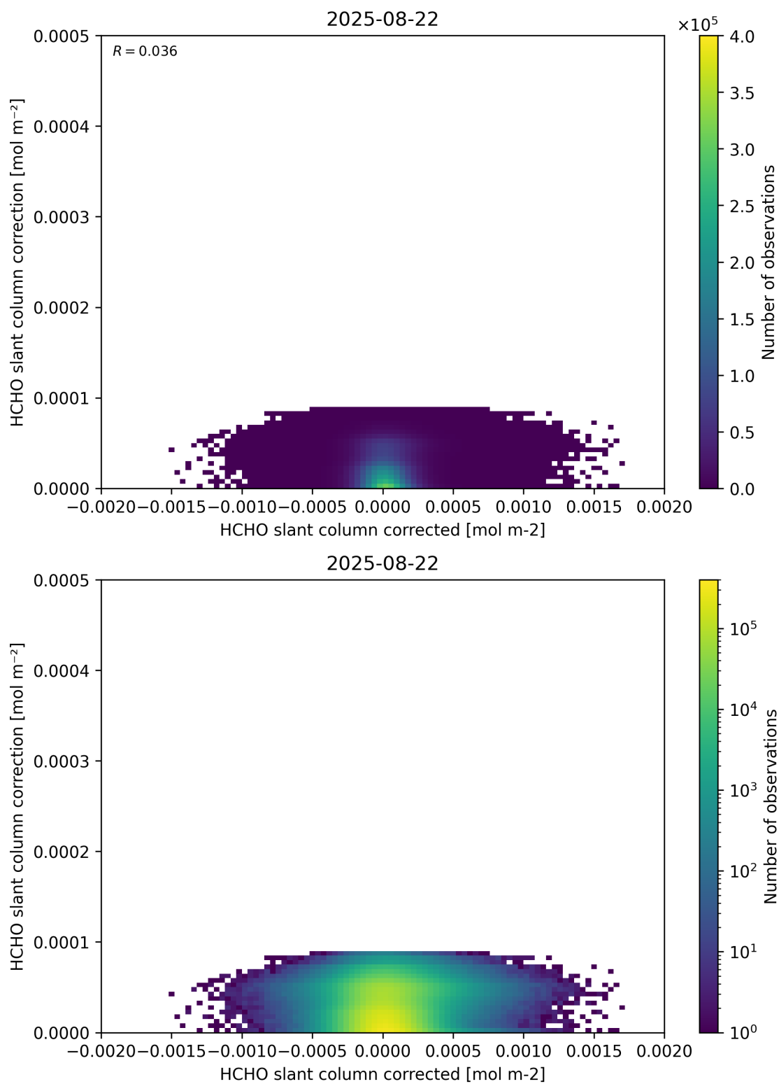
Figure 77: Scatter density plot of “HCHO slant column corrected” against “HCHO slant column correction” for 2025-08-21 to 2025-08-23.
