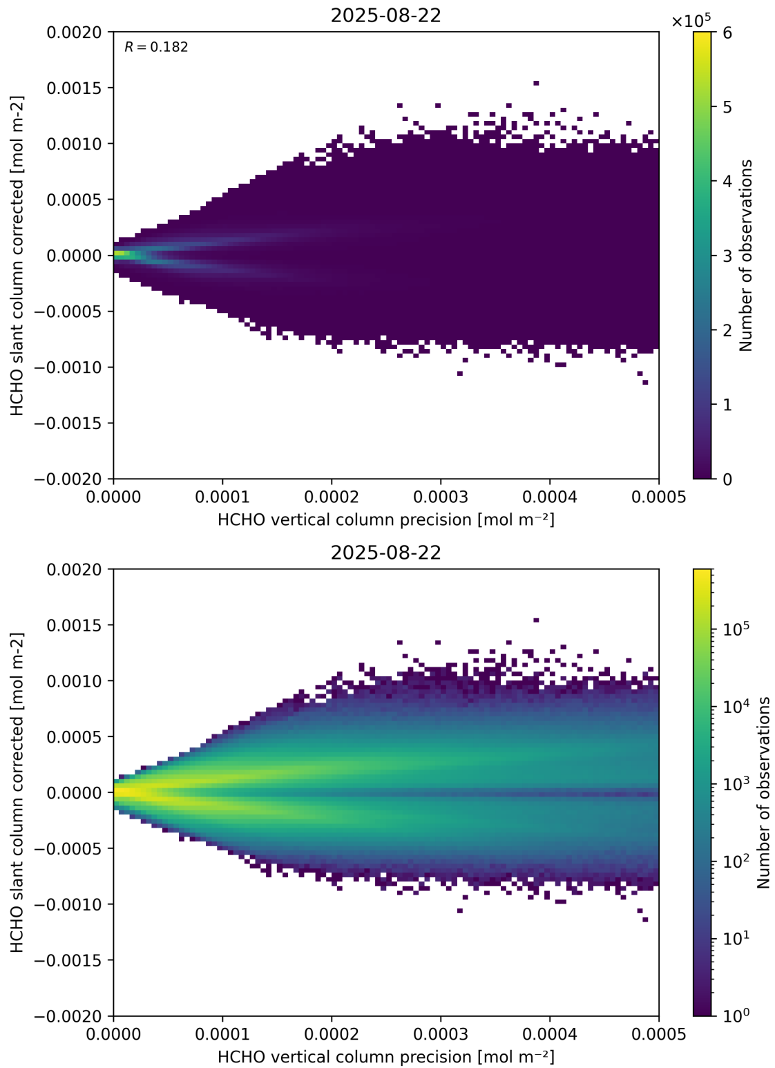
Figure 140: Scatter density plot of “HCHO vertical column precision” against “HCHO slant column corrected” for 2025-08-21 to 2025-08-23.
