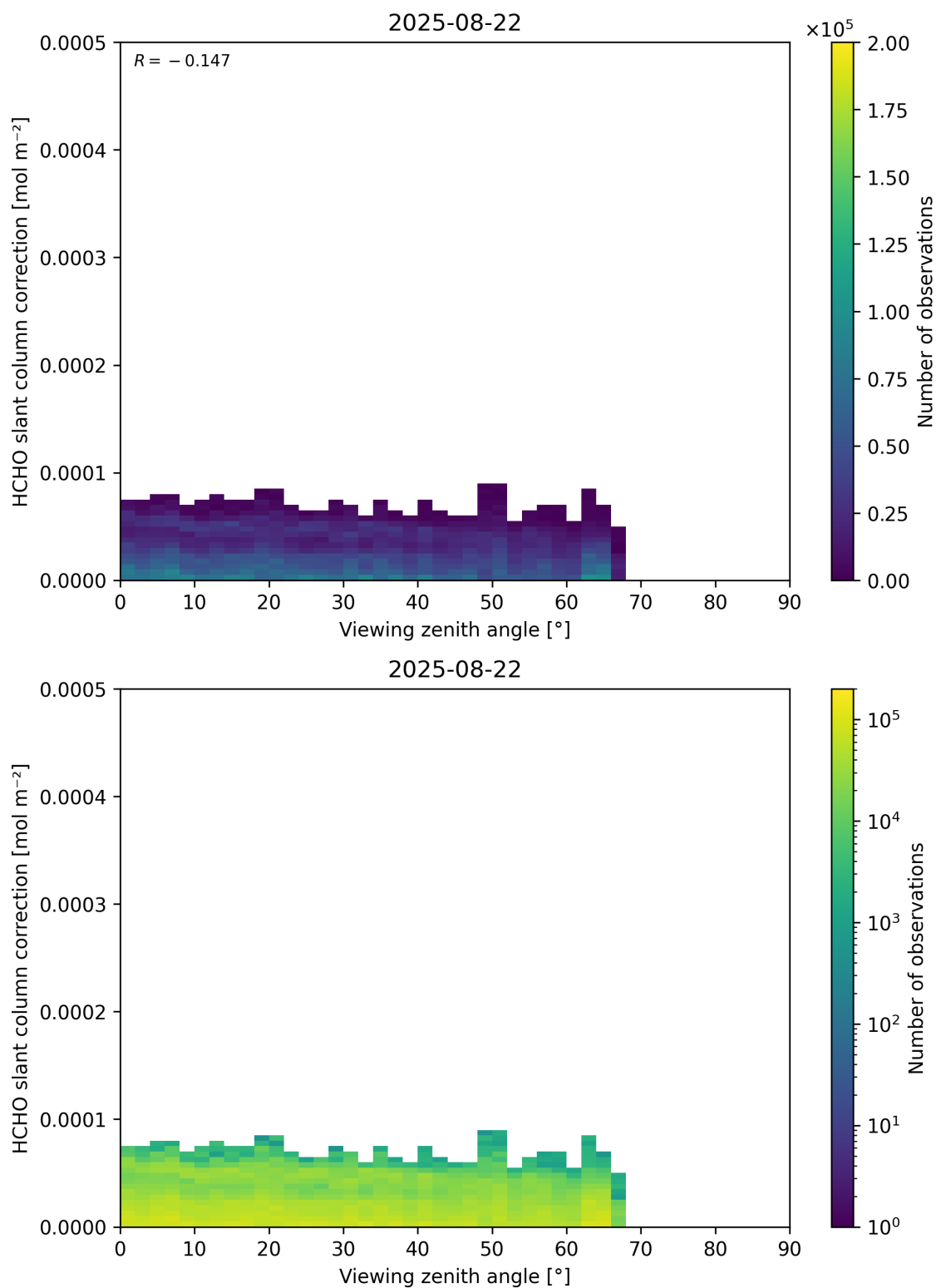
Figure 187: Scatter density plot of “Viewing zenith angle” against “HCHO slant column correction” for 2025-08-21 to 2025-08-23.
