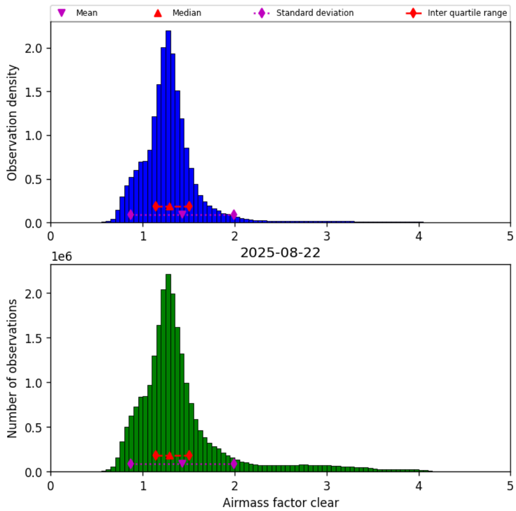
Figure 42: Histogram of “Airmass factor clear” for 2025-08-21 to 2025-08-23
