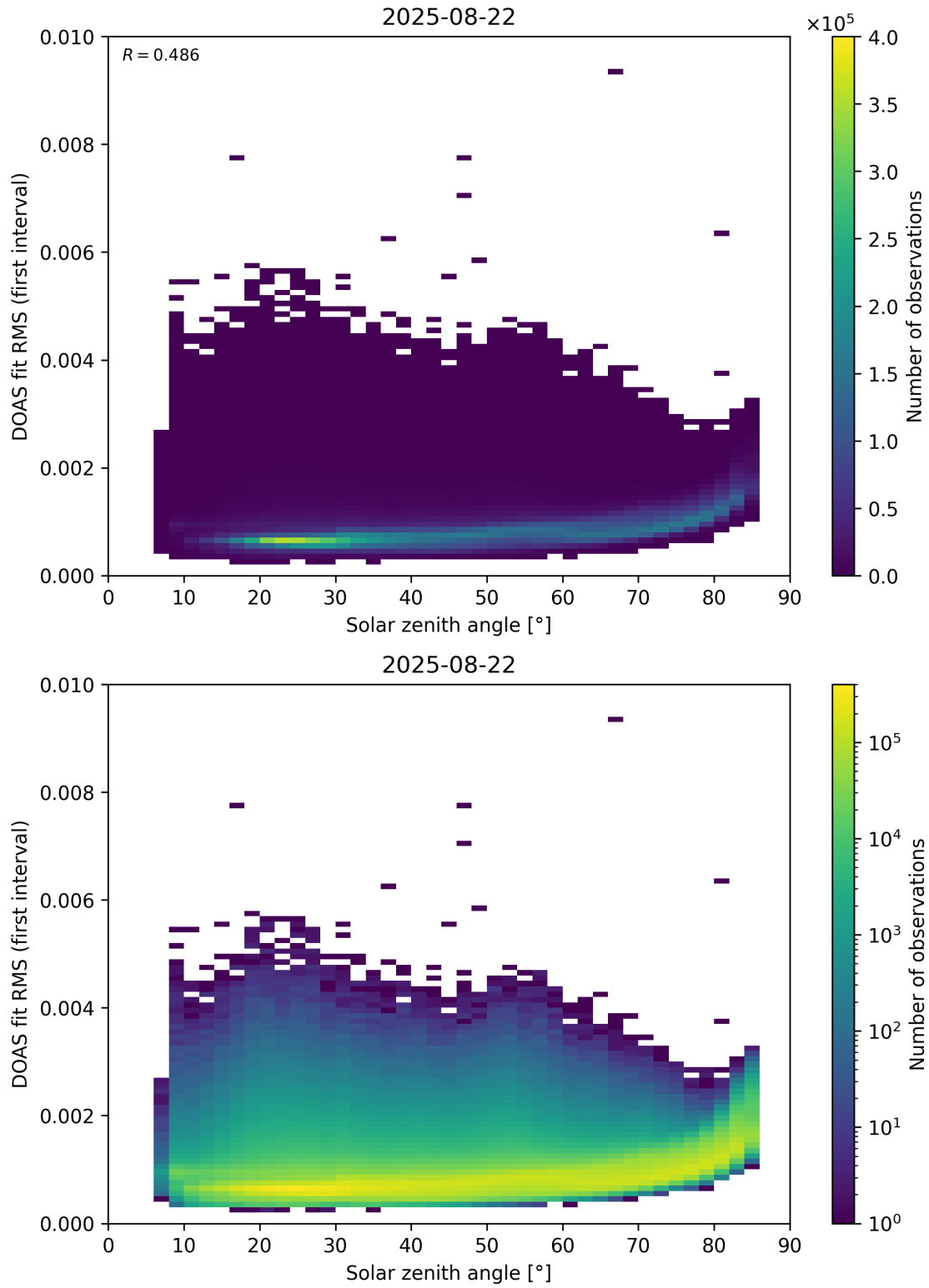
Figure 167: Scatter density plot of “Solar zenith angle” against “DOAS fit RMS (first interval)” for 2025-08-21 to 2025-08-23.
