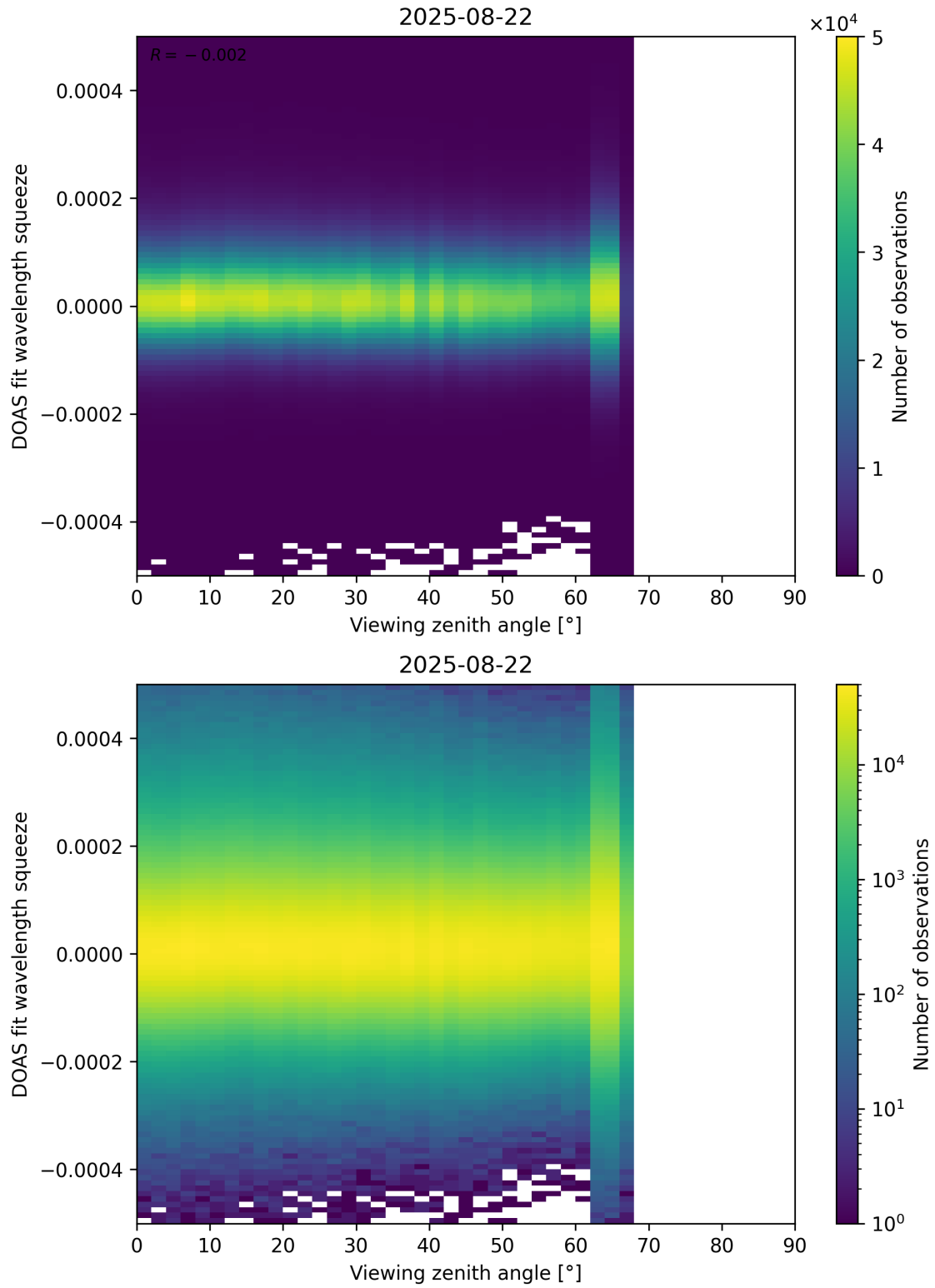
Figure 184: Scatter density plot of “Viewing zenith angle” against “DOAS fit wavelength squeeze” for 2025-08-21 to 2025-08-23.
