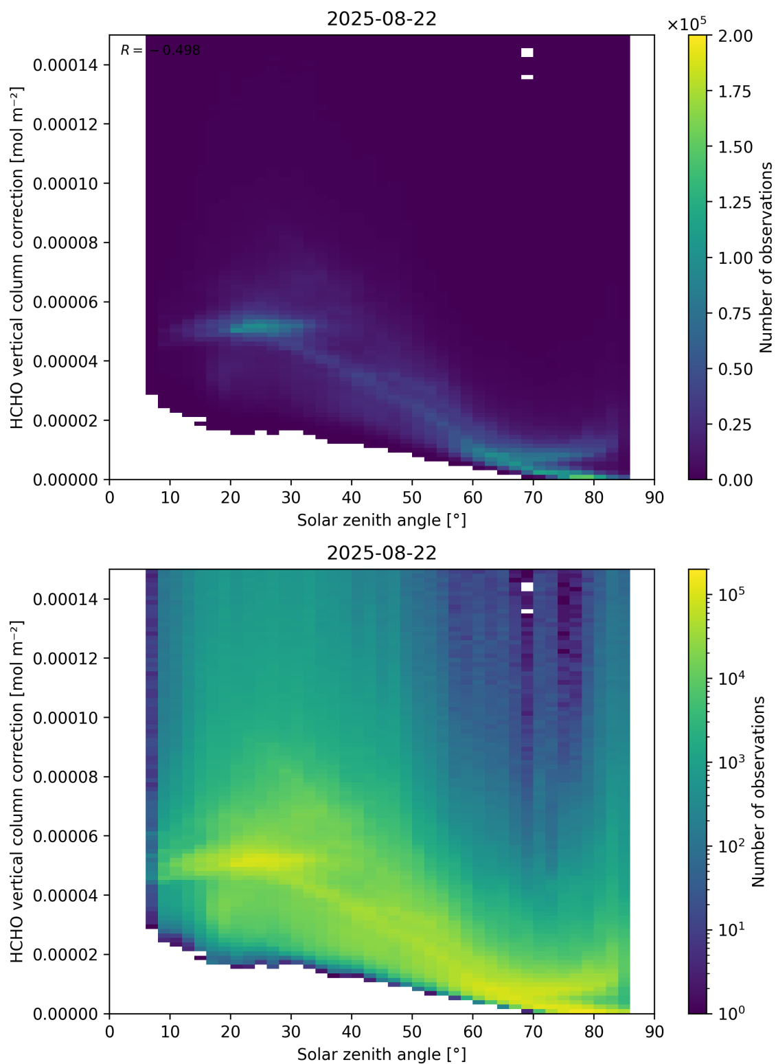
Figure 178: Scatter density plot of “Solar zenith angle” against “HCHO vertical column correction” for 2025-08-21 to 2025-08-23.
