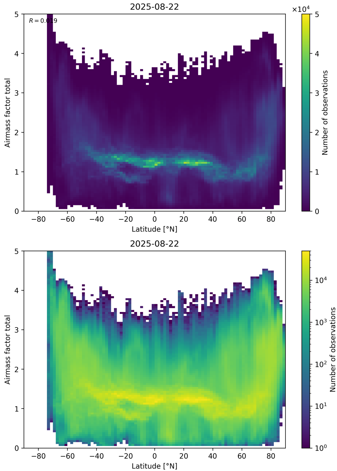
Figure 161: Scatter density plot of “Latitude” against “Airmass factor total” for 2025-08-21 to 2025-08-23.
