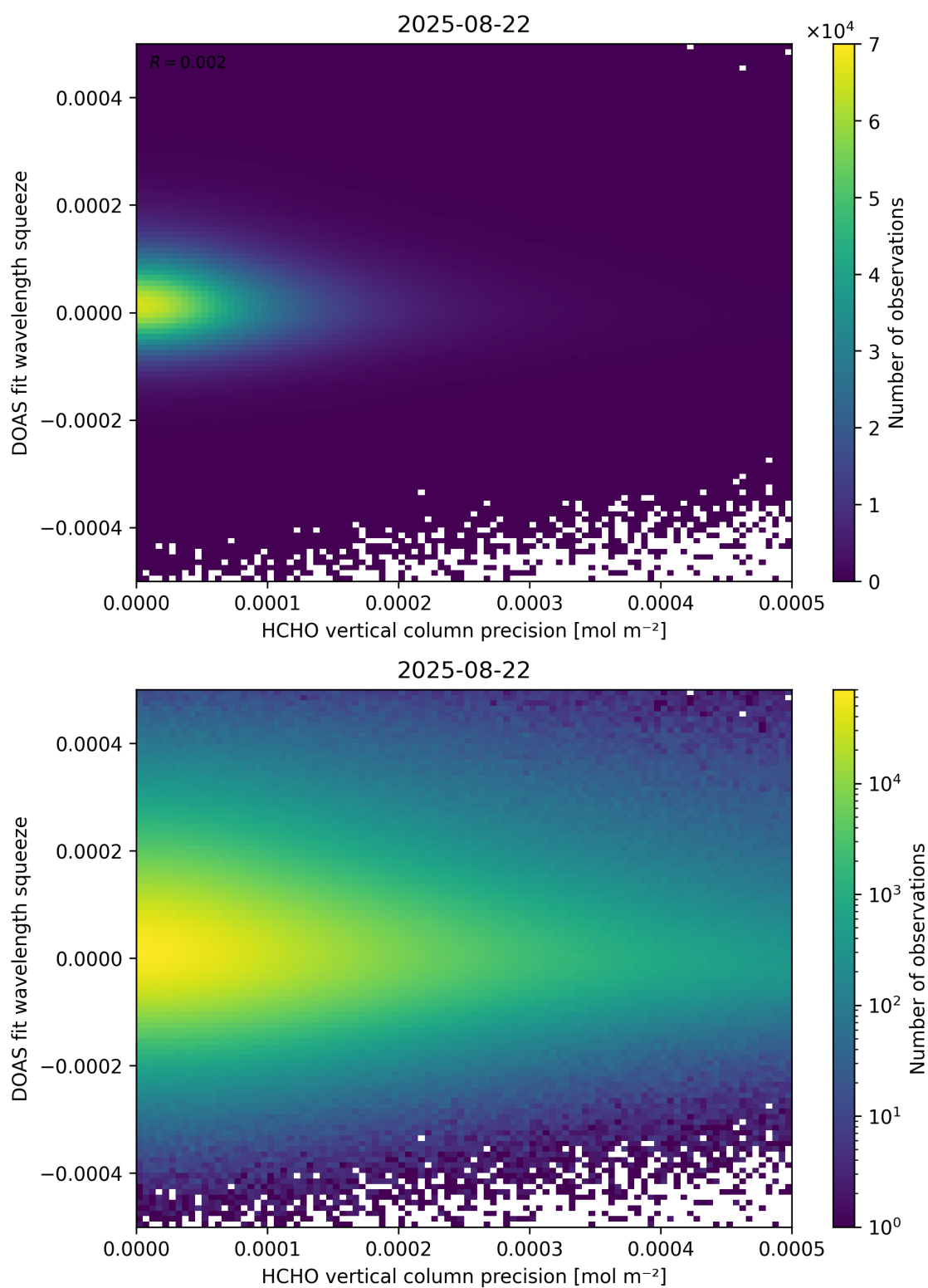
Figure 138: Scatter density plot of “HCHO vertical column precision” against “DOAS fit wavelength squeeze” for 2025-08-21 to 2025-08-23.
