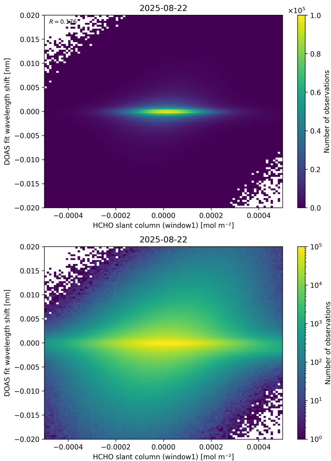
Figure 79: Scatter density plot of “HCHO slant column (window1)” against “DOAS fit wavelength shift” for 2025-08-21 to 2025-08-23.
