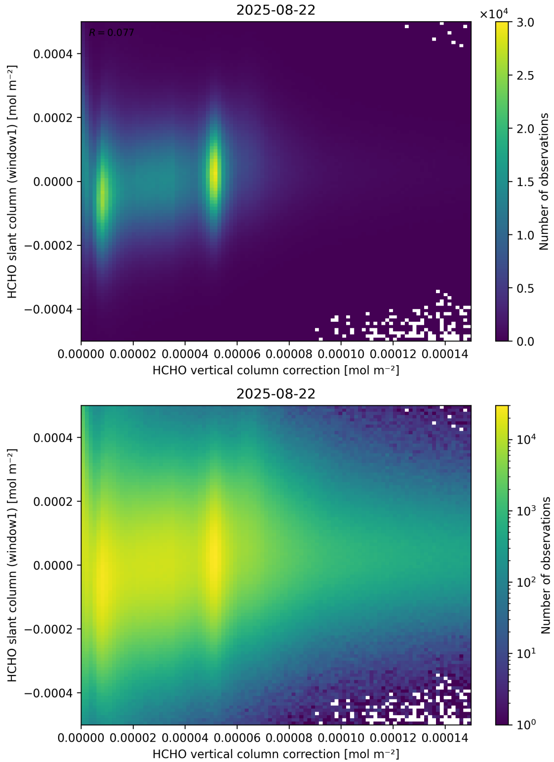
Figure 118: Scatter density plot of “HCHO vertical column correction” against “HCHO slant column (window1)” for 2025-08-21 to 2025-08-23.
