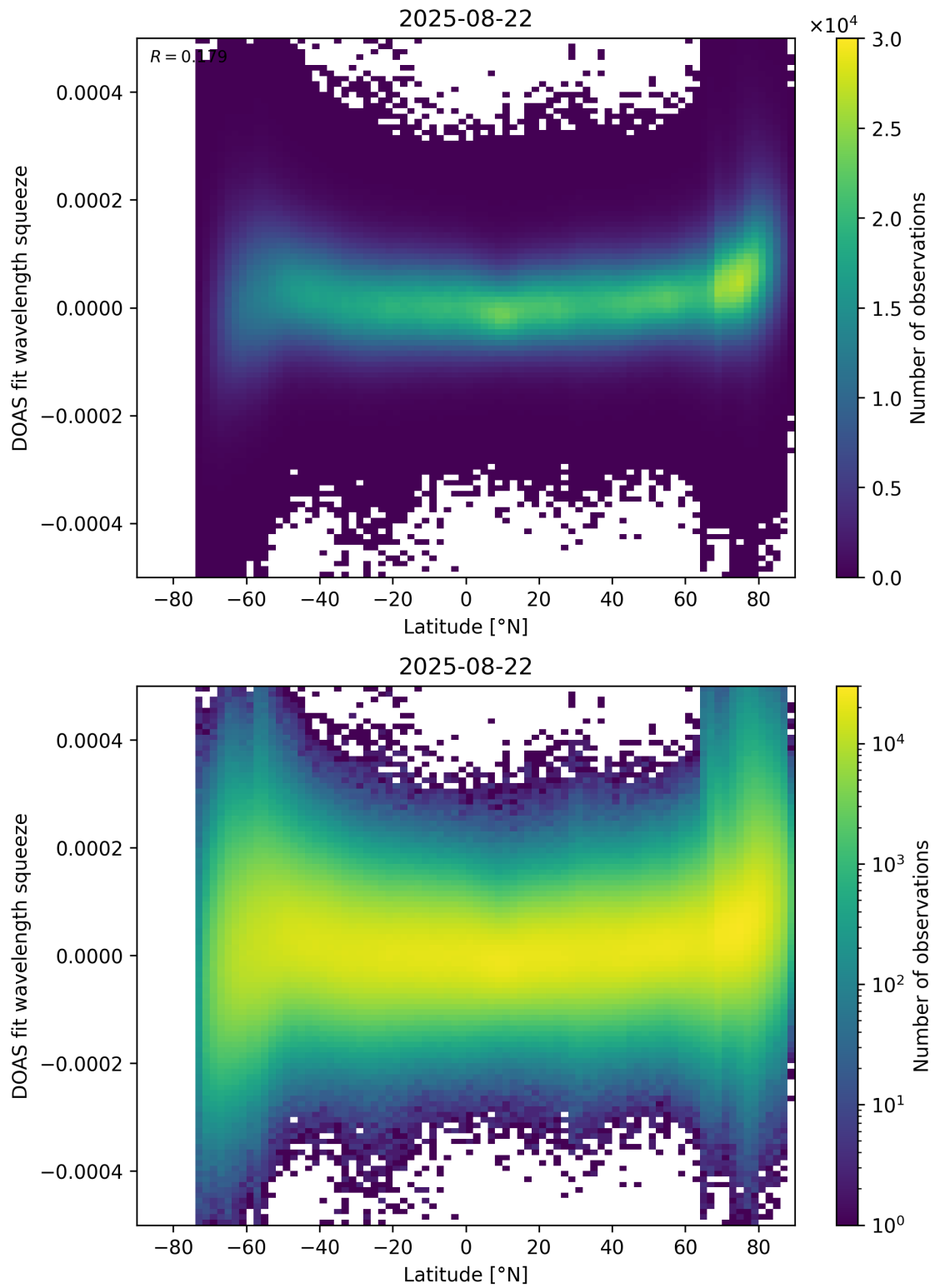
Figure 155: Scatter density plot of “Latitude” against “DOAS fit wavelength squeeze” for 2025-08-21 to 2025-08-23.
