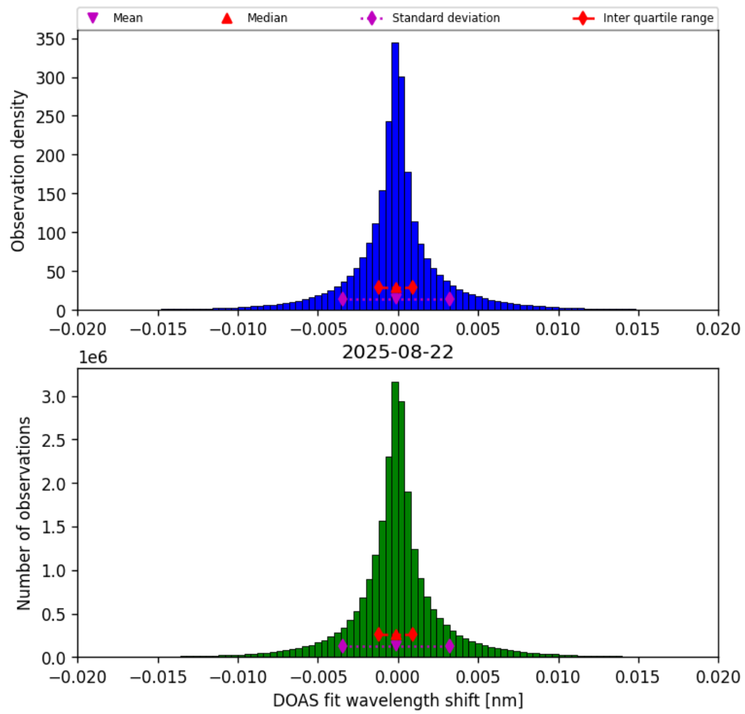
Figure 44: Histogram of “DOAS fit wavelength shift” for 2025-08-21 to 2025-08-23
