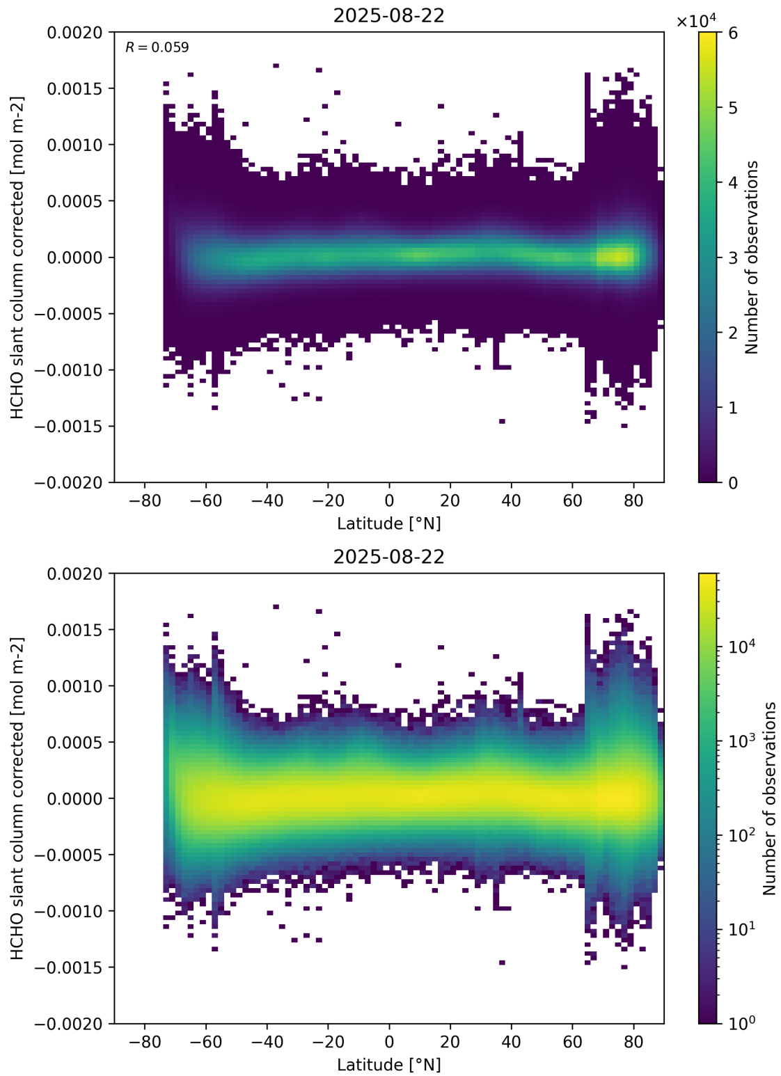
Figure 157: Scatter density plot of “Latitude” against “HCHO slant column corrected” for 2025-08-21 to 2025-08-23.
