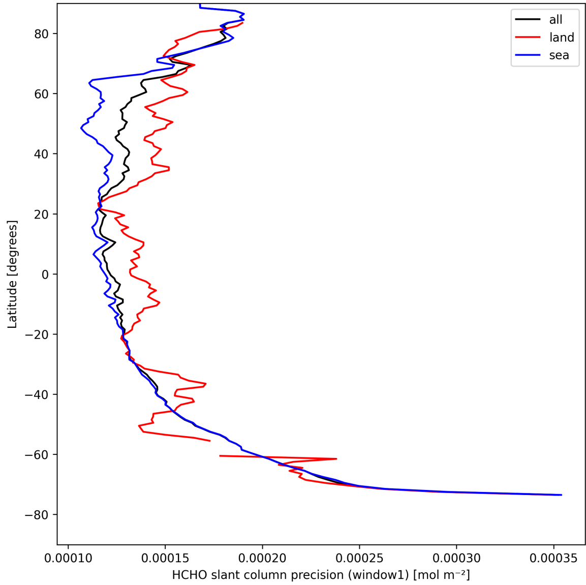
Figure 25: Zonal average of “HCHO slant column precision (window1)” for 2025-08-22 to 2025-08-24.
