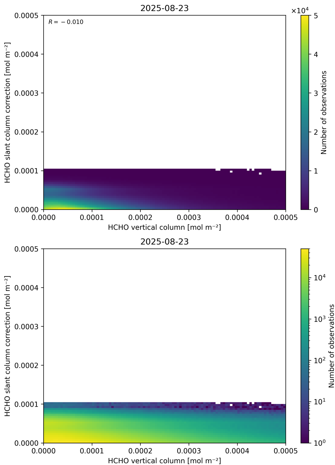
Figure 128: Scatter density plot of “HCHO vertical column” against “HCHO slant column correction” for 2025-08-22 to 2025-08-24.
