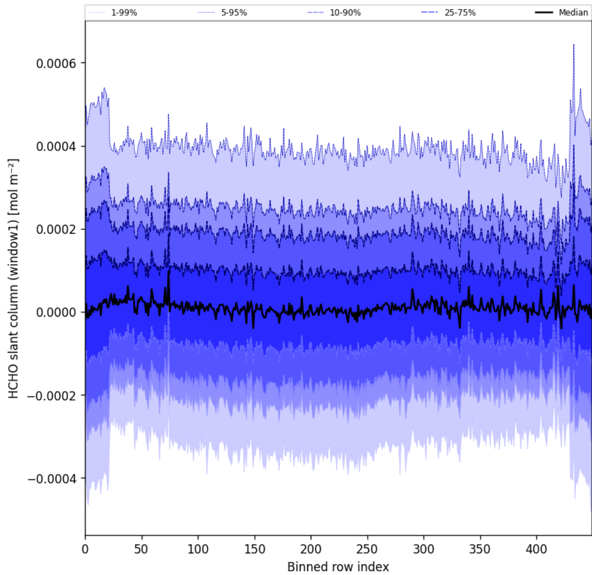
Figure 52: Along track statistics of “HCHO slant column (window1)” for 2025-08-22 to 2025-08-24
