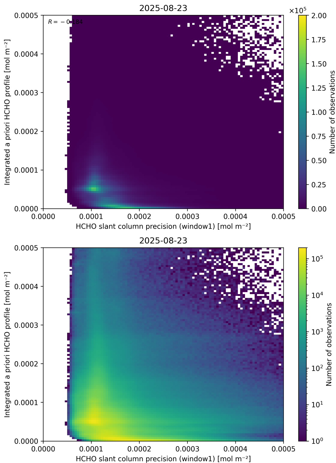
Figure 96: Scatter density plot of “HCHO slant column precision (window1)” against “Integrated a priori HCHO profile” for 2025-08-22 to 2025-08-24.
