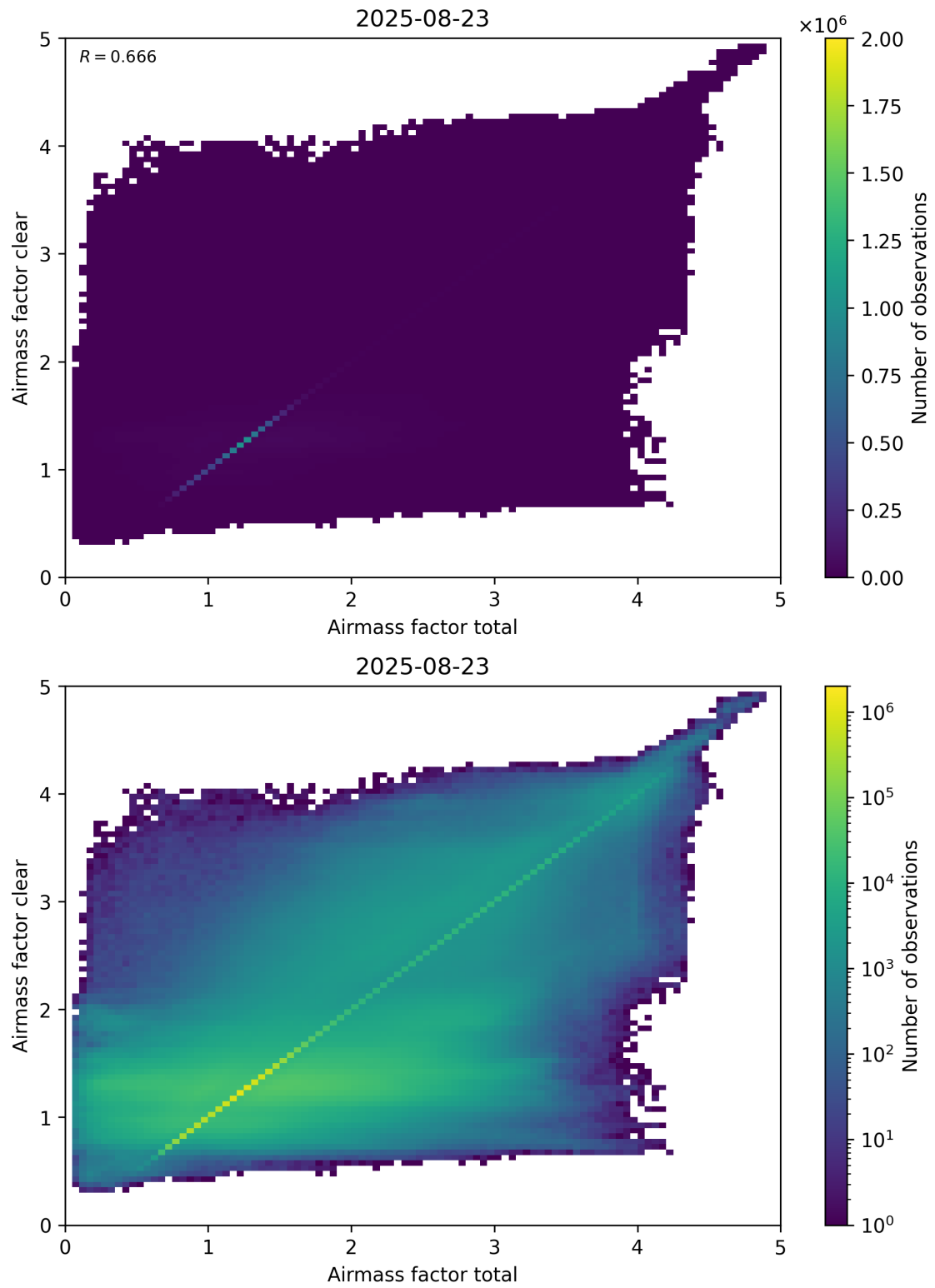
Figure 100: Scatter density plot of “Airmass factor total” against “Airmass factor clear” for 2025-08-22 to 2025-08-24.
