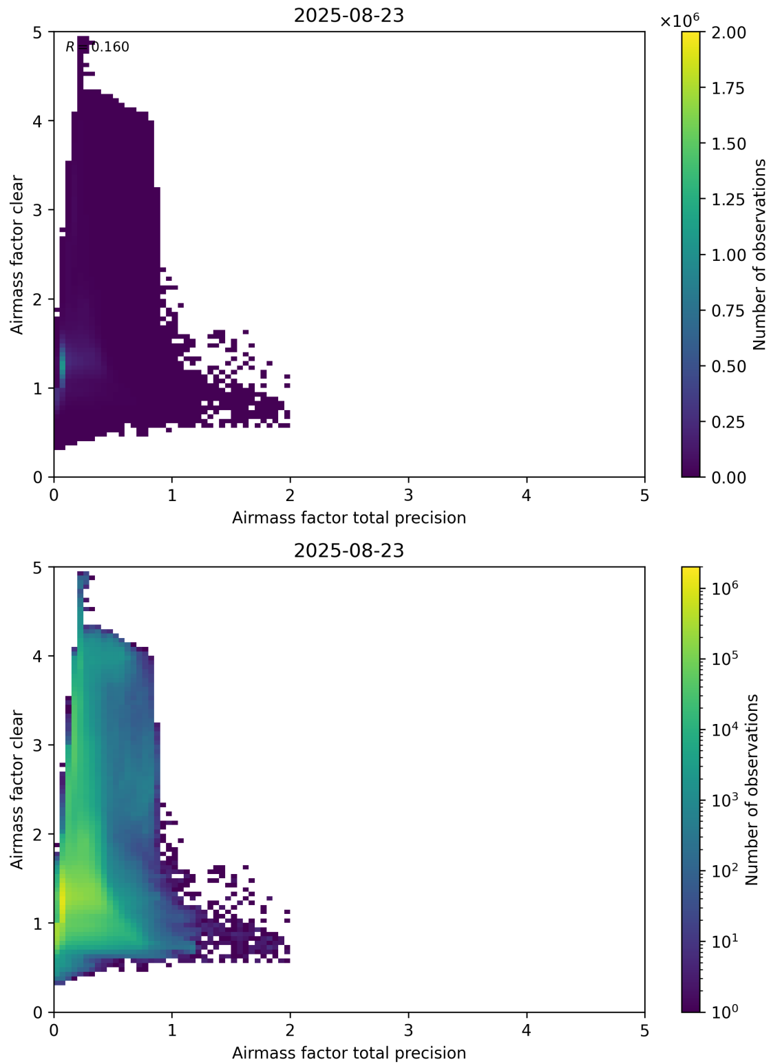
Figure 108: Scatter density plot of “Airmass factor total precision” against “Airmass factor clear” for 2025-08-22 to 2025-08-24.
