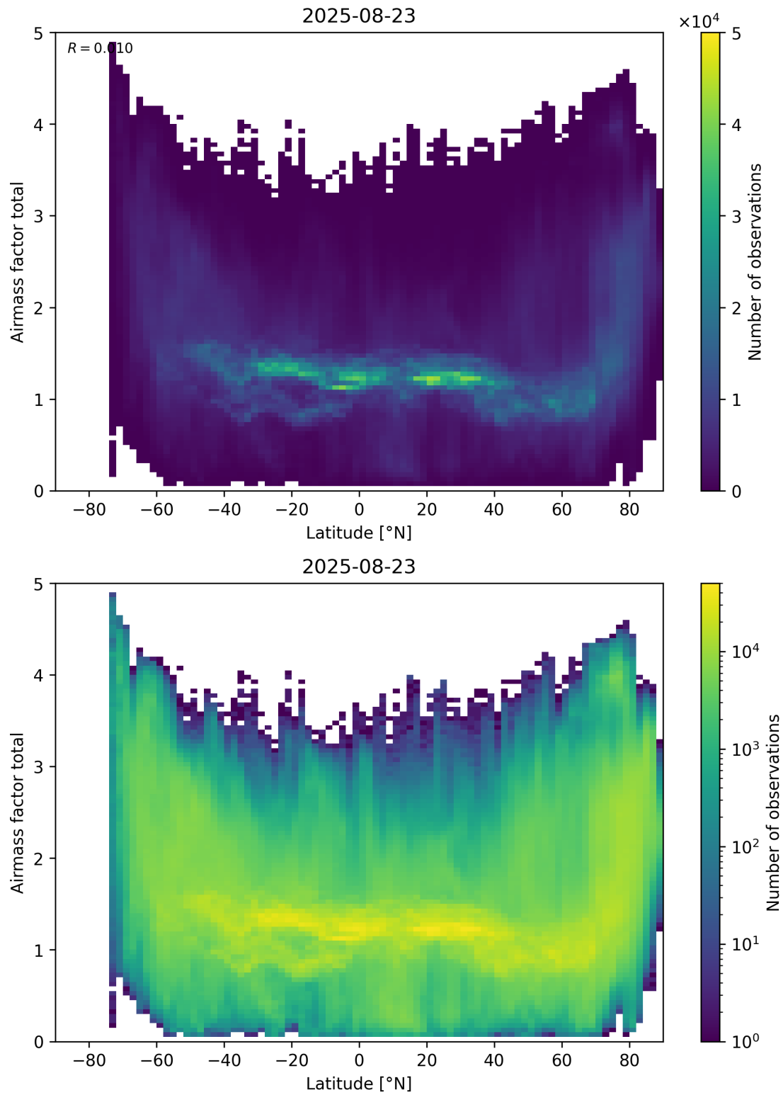
Figure 161: Scatter density plot of “Latitude” against “Airmass factor total” for 2025-08-22 to 2025-08-24.
