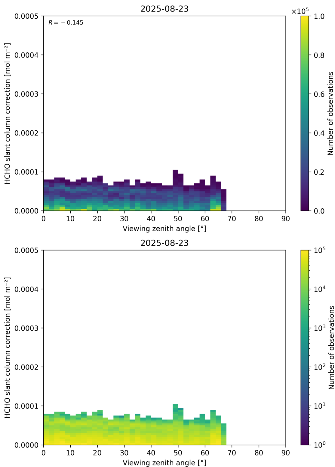
Figure 187: Scatter density plot of “Viewing zenith angle” against “HCHO slant column correction” for 2025-08-22 to 2025-08-24.
