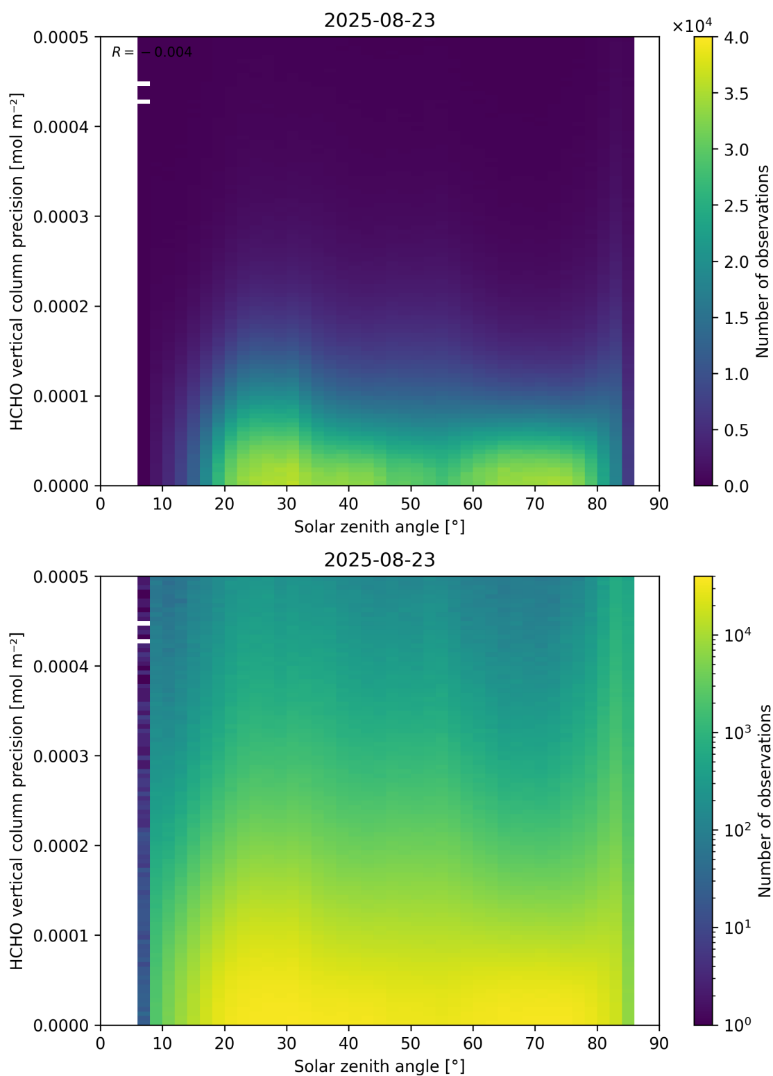
Figure 179: Scatter density plot of “Solar zenith angle” against “HCHO vertical column precision” for 2025-08-22 to 2025-08-24.
