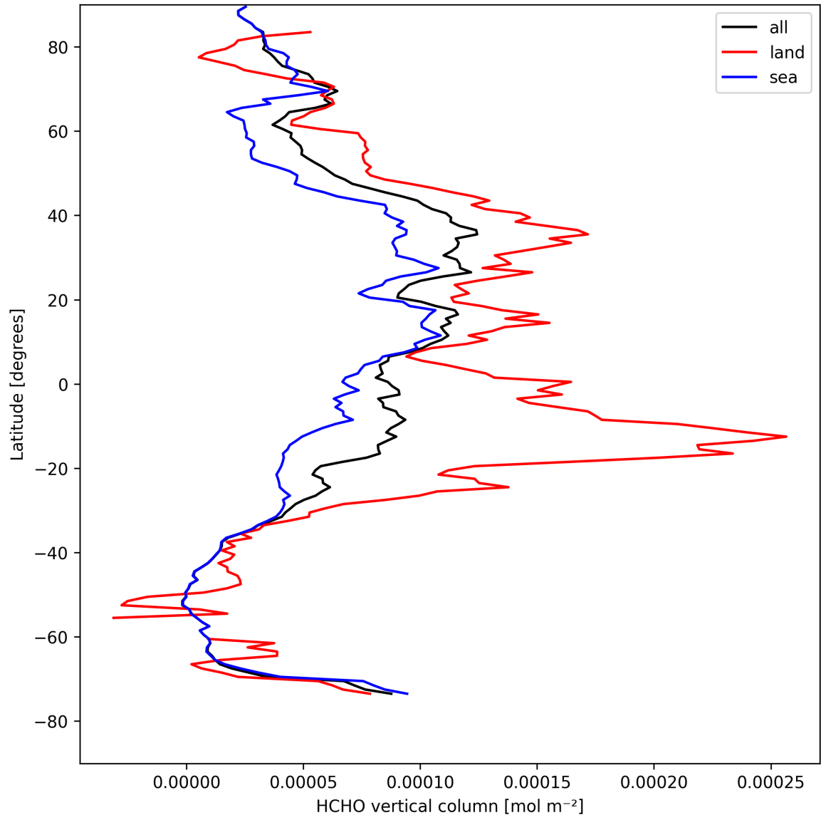
Figure 21: Zonal average of “HCHO vertical column” for 2025-08-22 to 2025-08-24.
