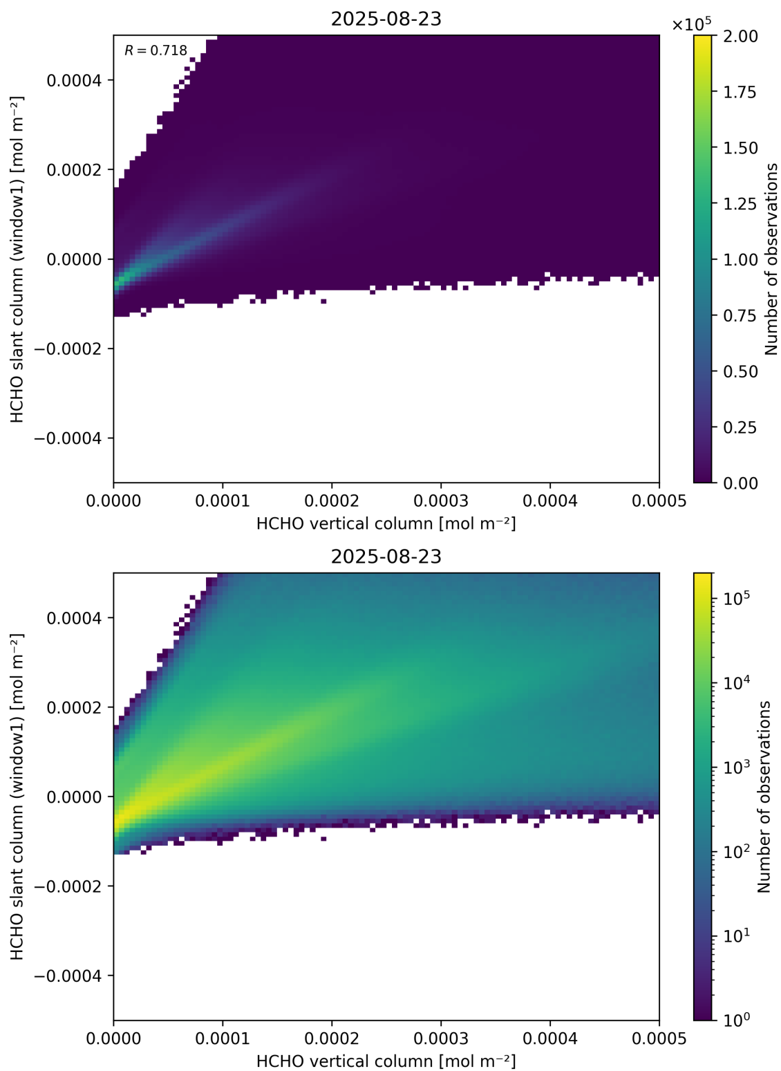
Figure 129: Scatter density plot of “HCHO vertical column” against “HCHO slant column (window1)” for 2025-08-22 to 2025-08-24.
