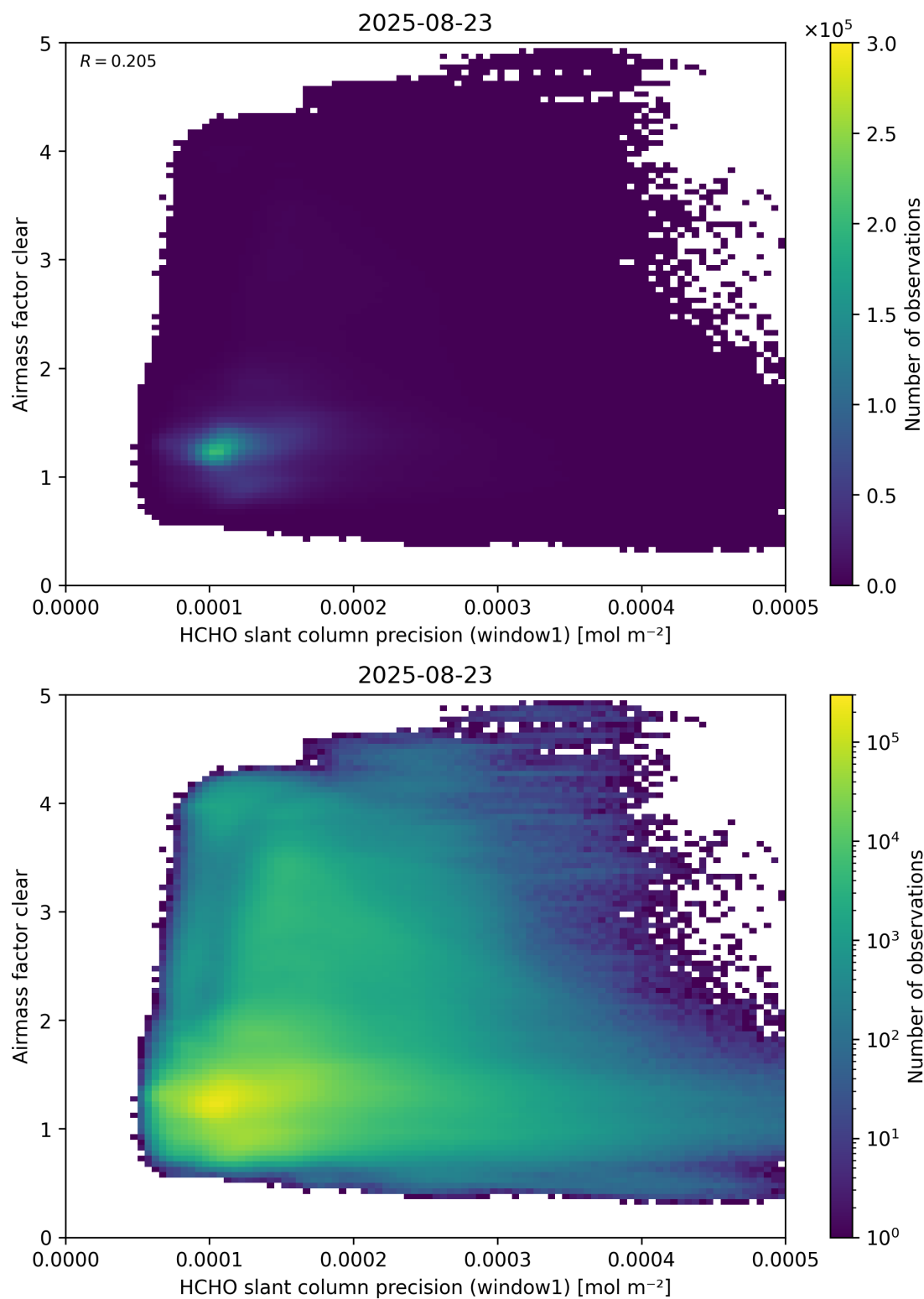
Figure 91: Scatter density plot of “HCHO slant column precision (window1)” against “Airmass factor clear” for 2025-08-22 to 2025-08-24.
