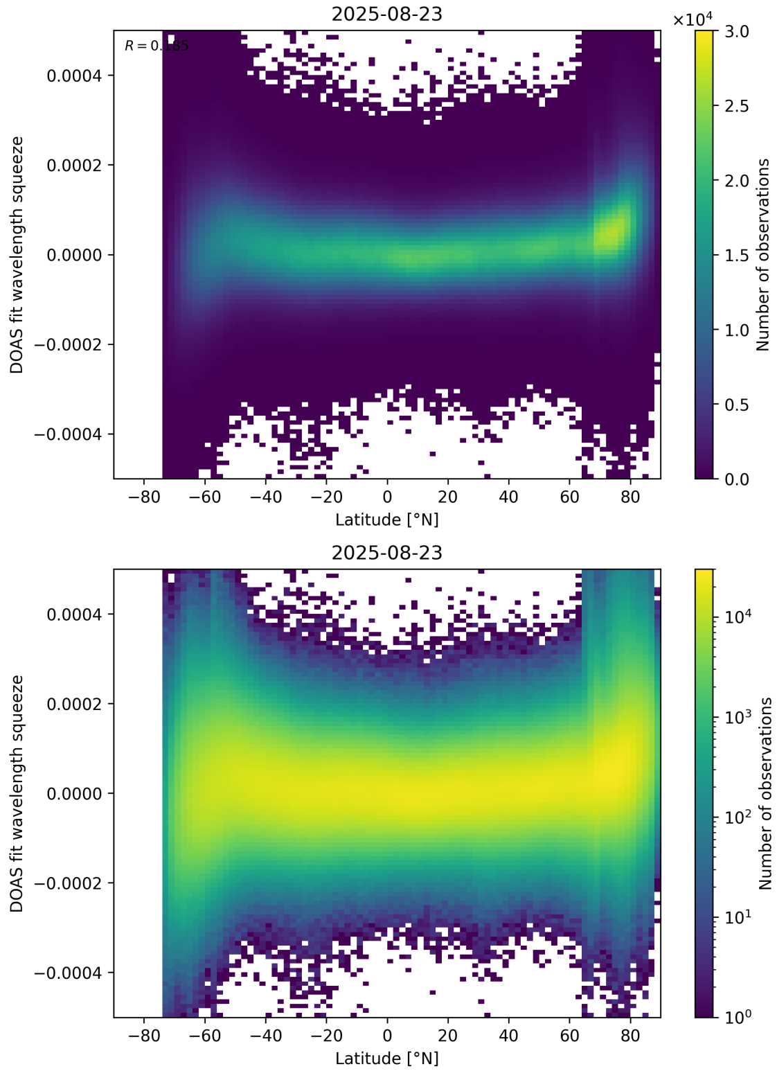
Figure 155: Scatter density plot of “Latitude” against “DOAS fit wavelength squeeze” for 2025-08-22 to 2025-08-24.
