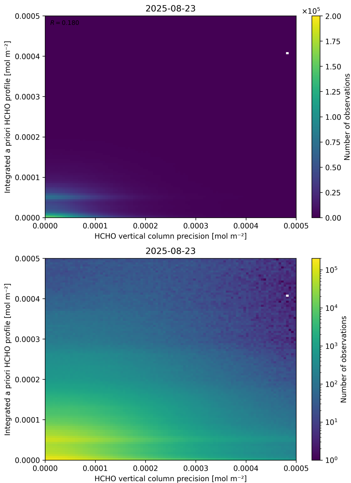
Figure 147: Scatter density plot of “HCHO vertical column precision” against “Integrated a priori HCHO profile” for 2025-08-22 to 2025-08-24.
