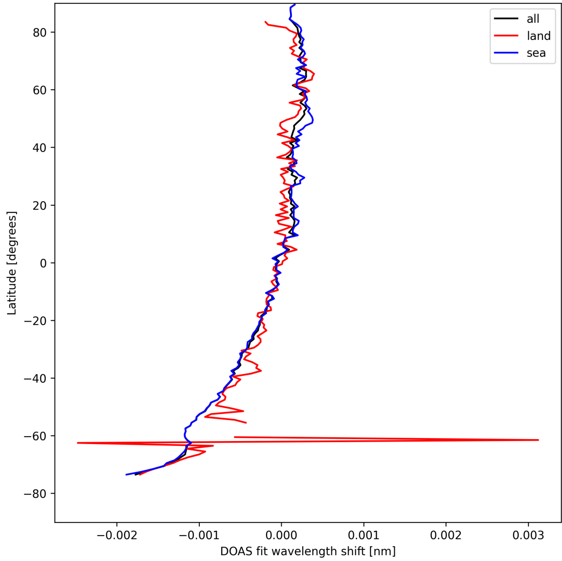
Figure 30: Zonal average of "DOAS fit wavelength shift" for 2025-08-22 to 2025-08-24.
