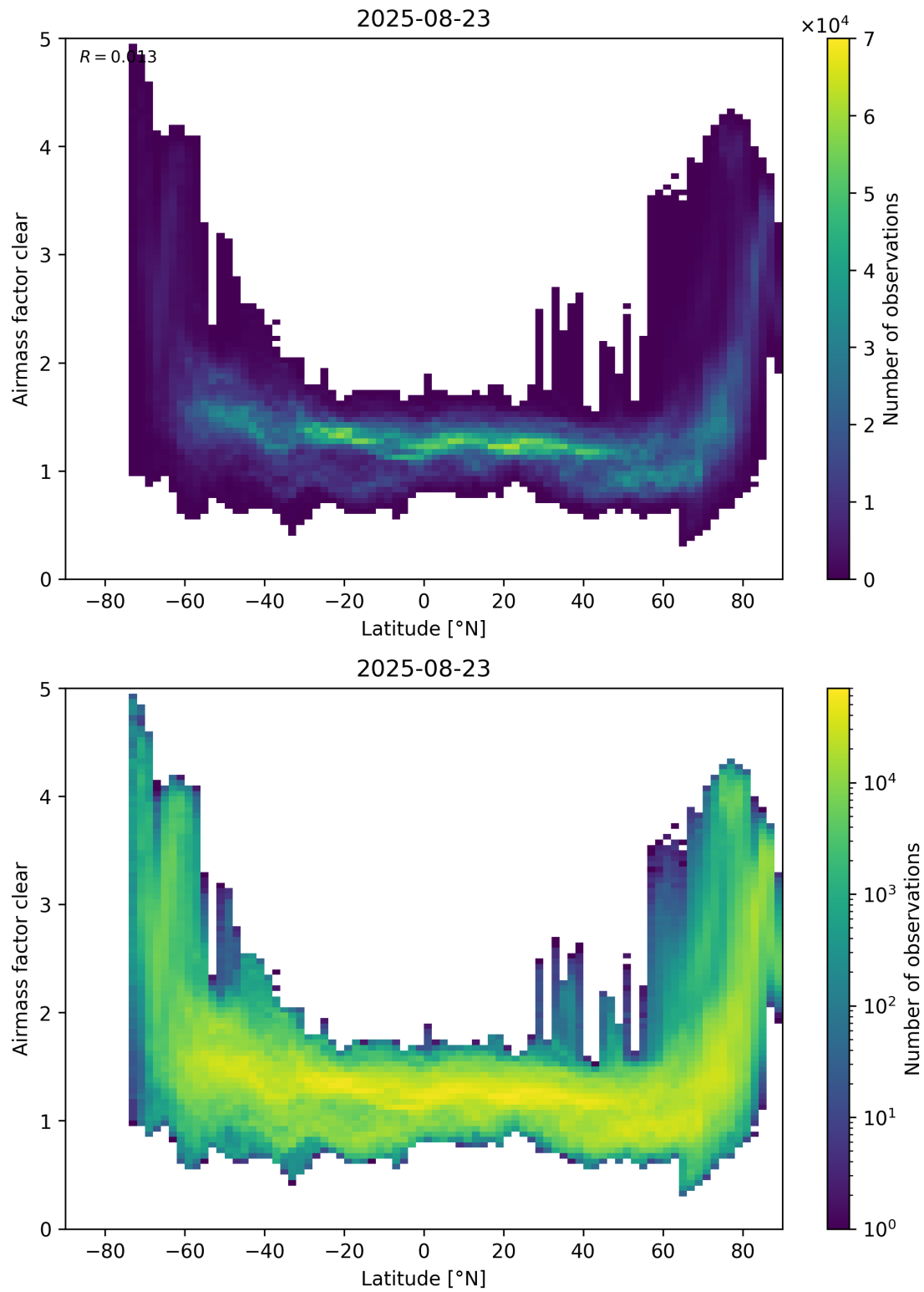
Figure 156: Scatter density plot of “Latitude” against “Airmass factor clear” for 2025-08-22 to 2025-08-24.
