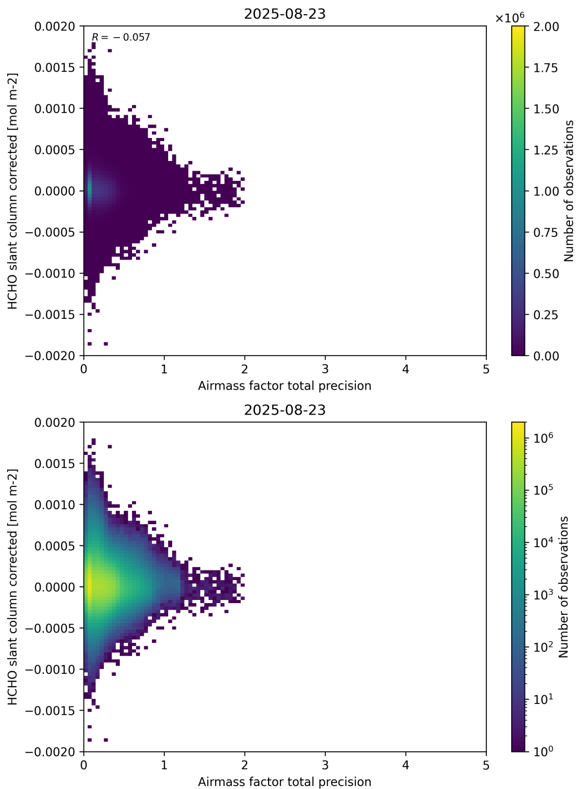
Figure 109: Scatter density plot of “Airmass factor total precision” against “HCHO slant column corrected” for 2025-08-22 to 2025-08-24.
