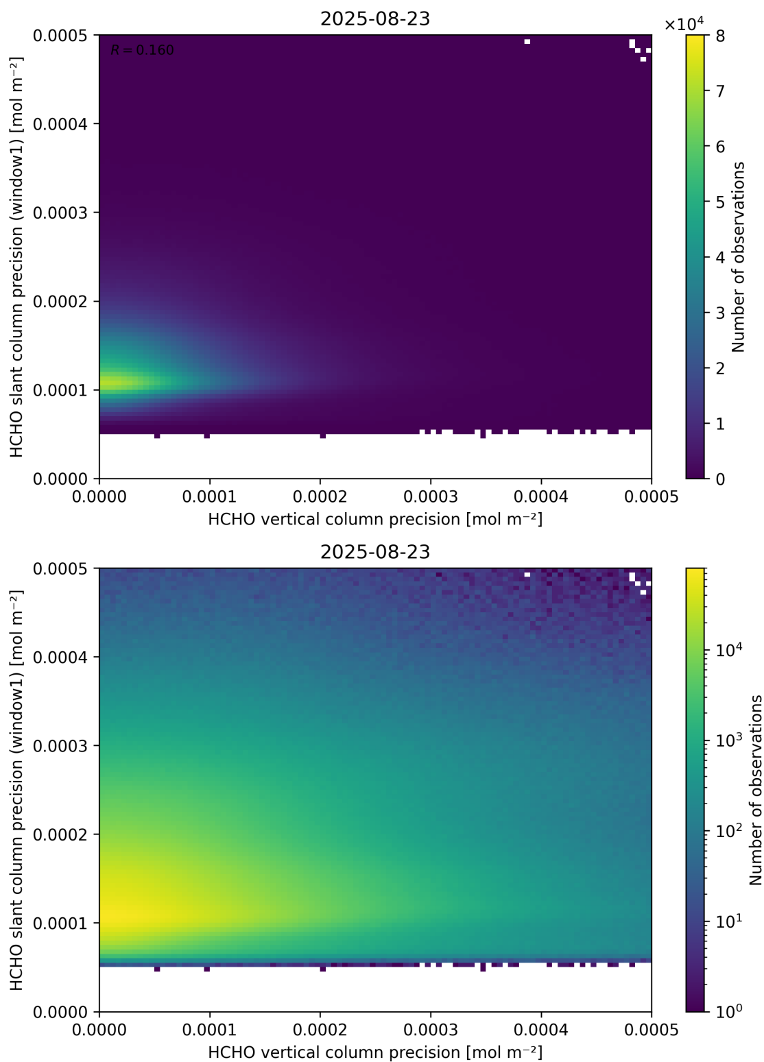
Figure 143: Scatter density plot of “HCHO vertical column precision” against “HCHO slant column precision (window1)” for 2025-08-22 to 2025-08-24.
