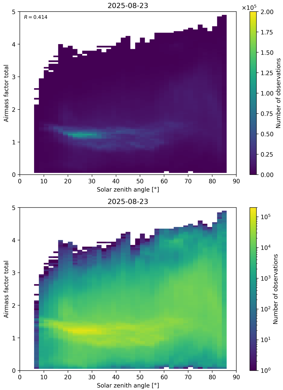
Figure 175: Scatter density plot of “Solar zenith angle” against “Airmass factor total” for 2025-08-22 to 2025-08-24.
