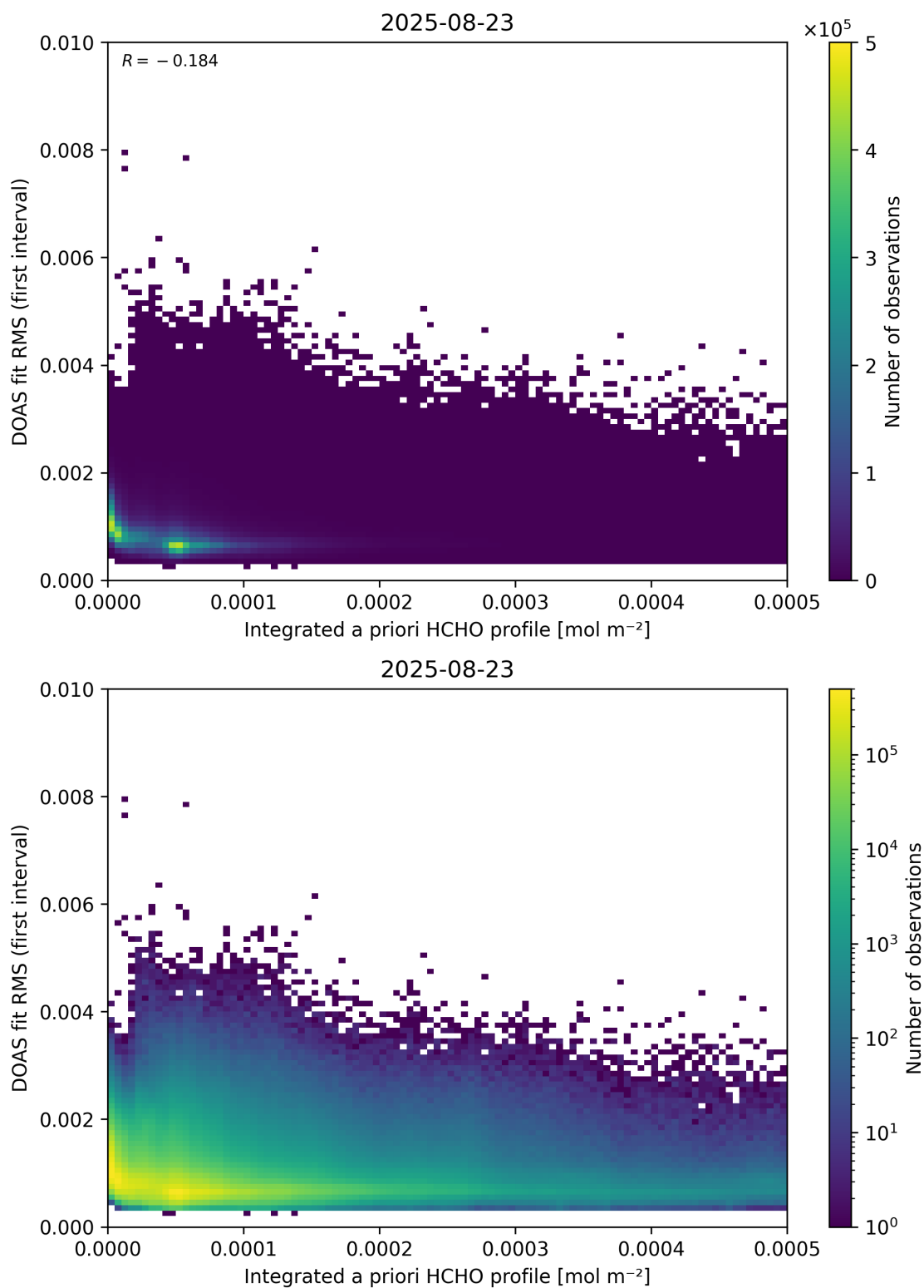
Figure 148: Scatter density plot of “Integrated a priori HCHO profile” against “DOAS fit RMS (first interval)” for 2025-08-22 to 2025-08-24.
