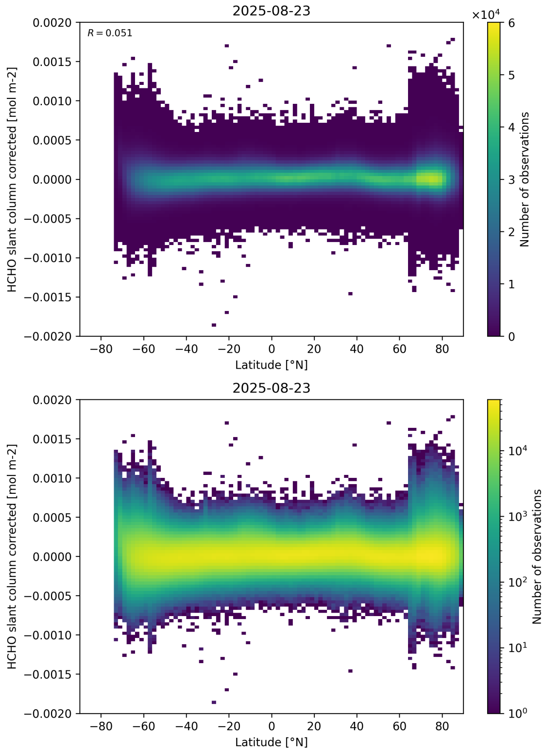
Figure 157: Scatter density plot of “Latitude” against “HCHO slant column corrected” for 2025-08-22 to 2025-08-24.
