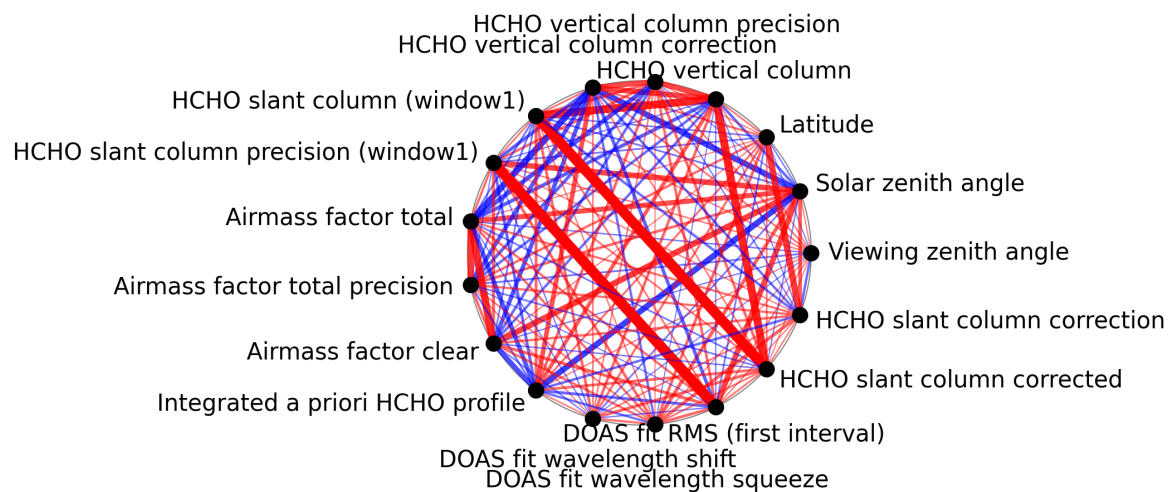
Figure 1: Map of correlation graph for 2025-08-22 to 2025-08-24.
