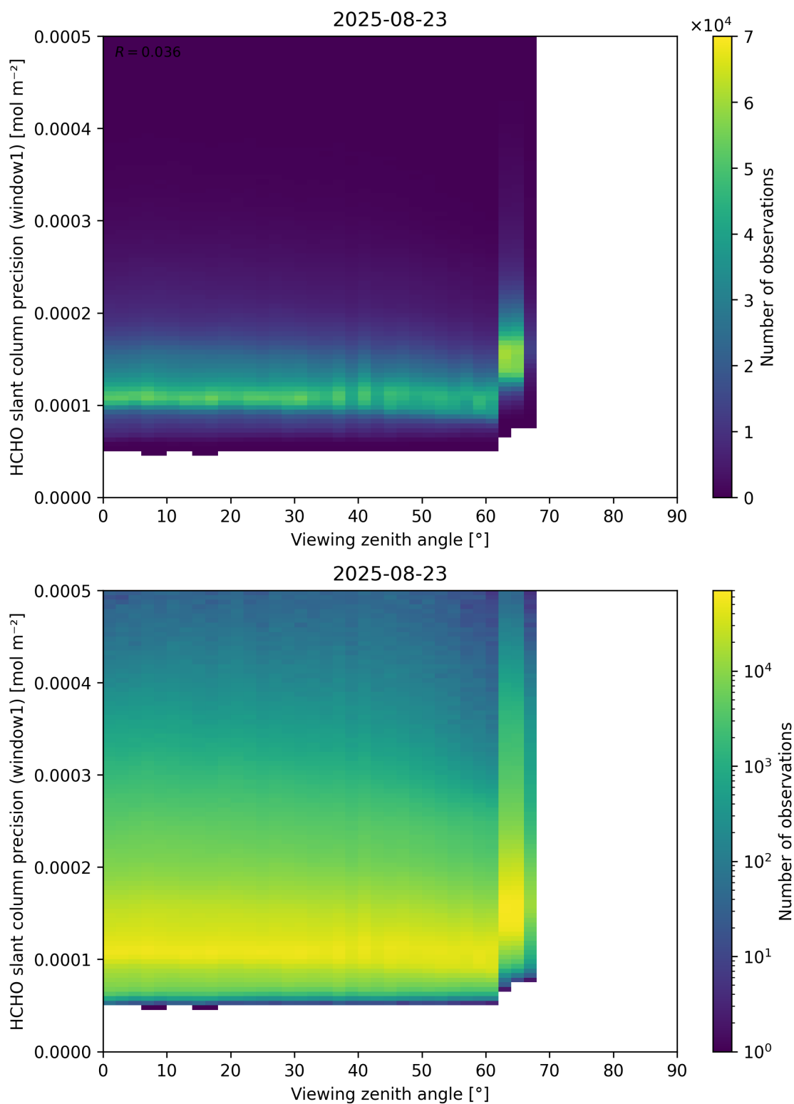
Figure 189: Scatter density plot of “Viewing zenith angle” against “HCHO slant column precision (window1)” for 2025-08-22 to 2025-08-24.
