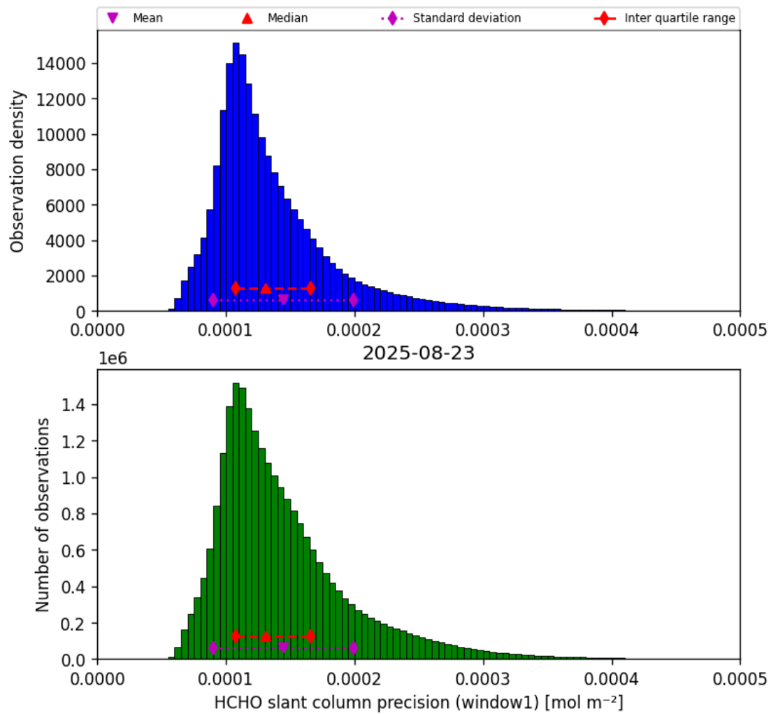
Figure 39: Histogram of “HCHO slant column precision (window1)” for 2025-08-22 to 2025-08-24
