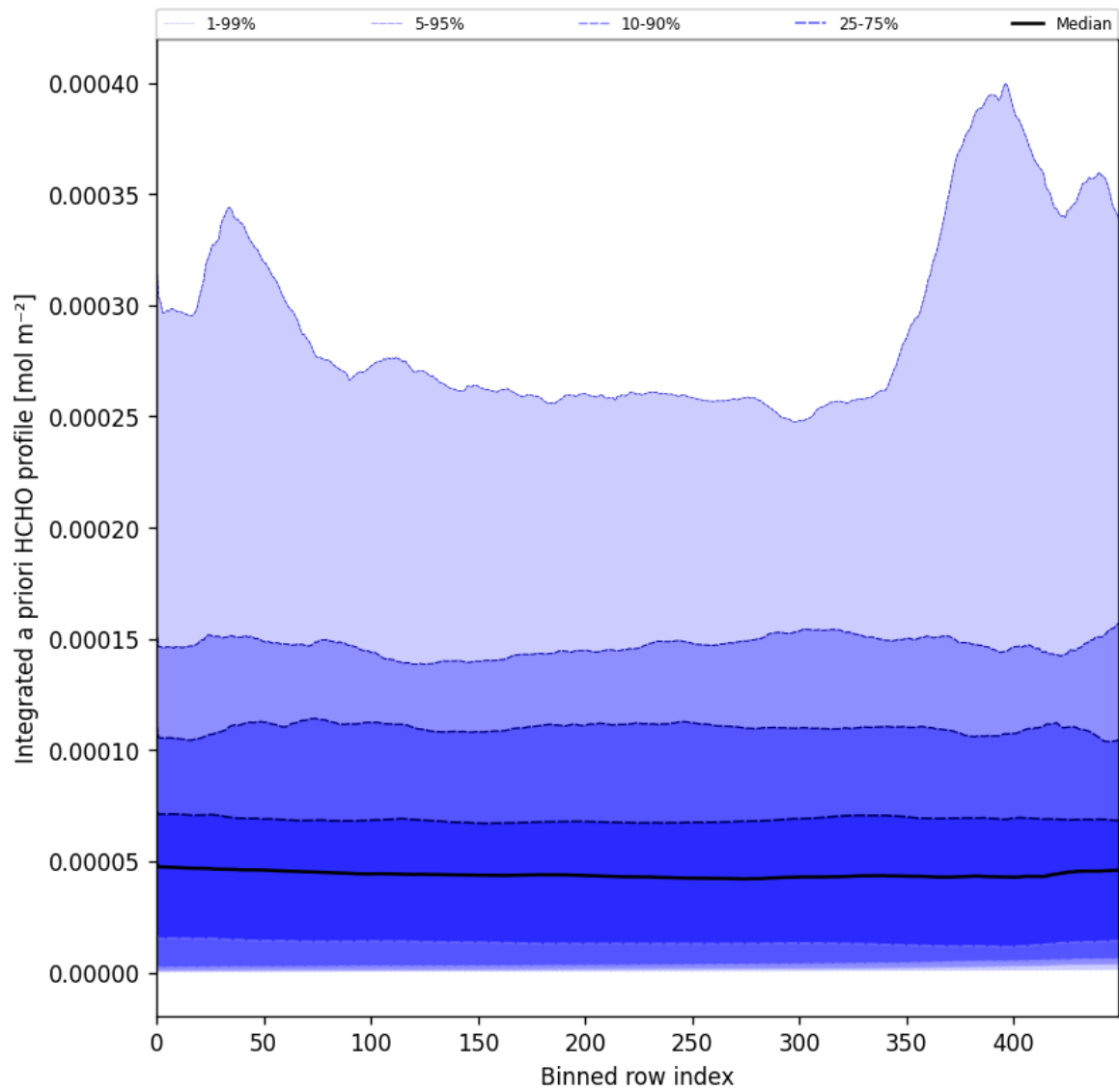
Figure 57: Along track statistics of “Integrated a priori HCHO profile” for 2025-08-22 to 2025-08-24
