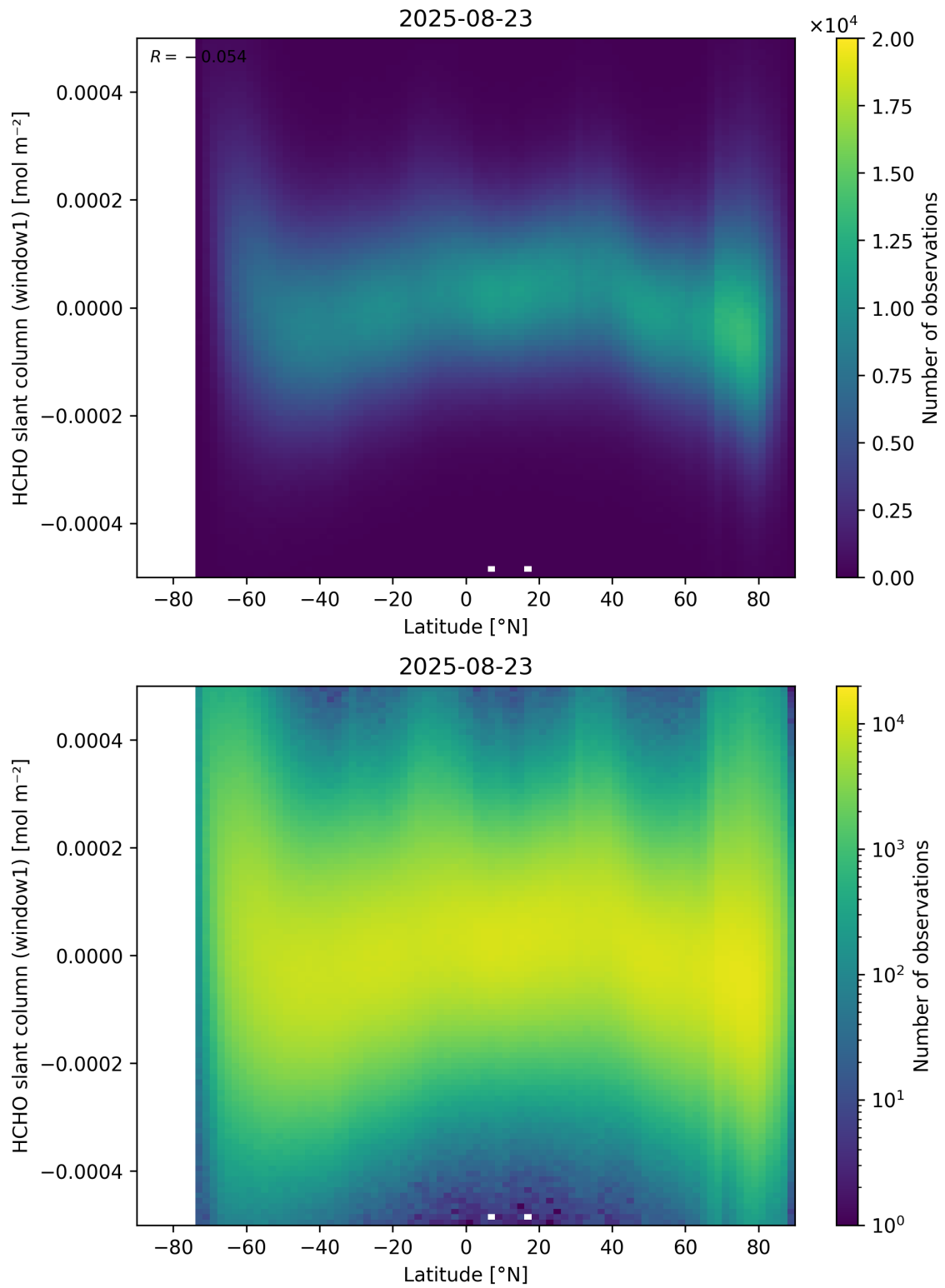
Figure 159: Scatter density plot of “Latitude” against “HCHO slant column (window1)” for 2025-08-22 to 2025-08-24.
