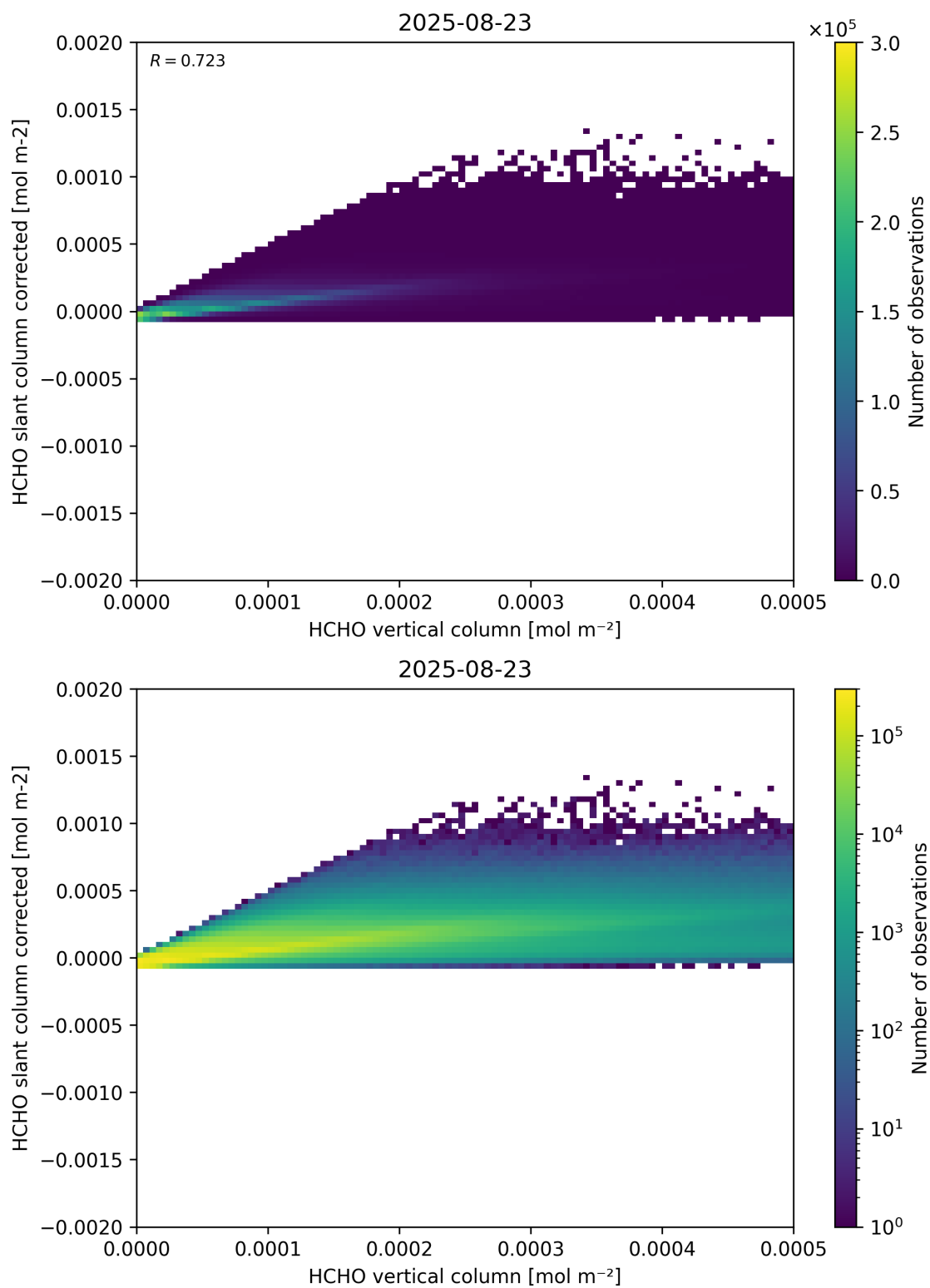
Figure 127: Scatter density plot of “HCHO vertical column” against “HCHO slant column corrected” for 2025-08-22 to 2025-08-24.
