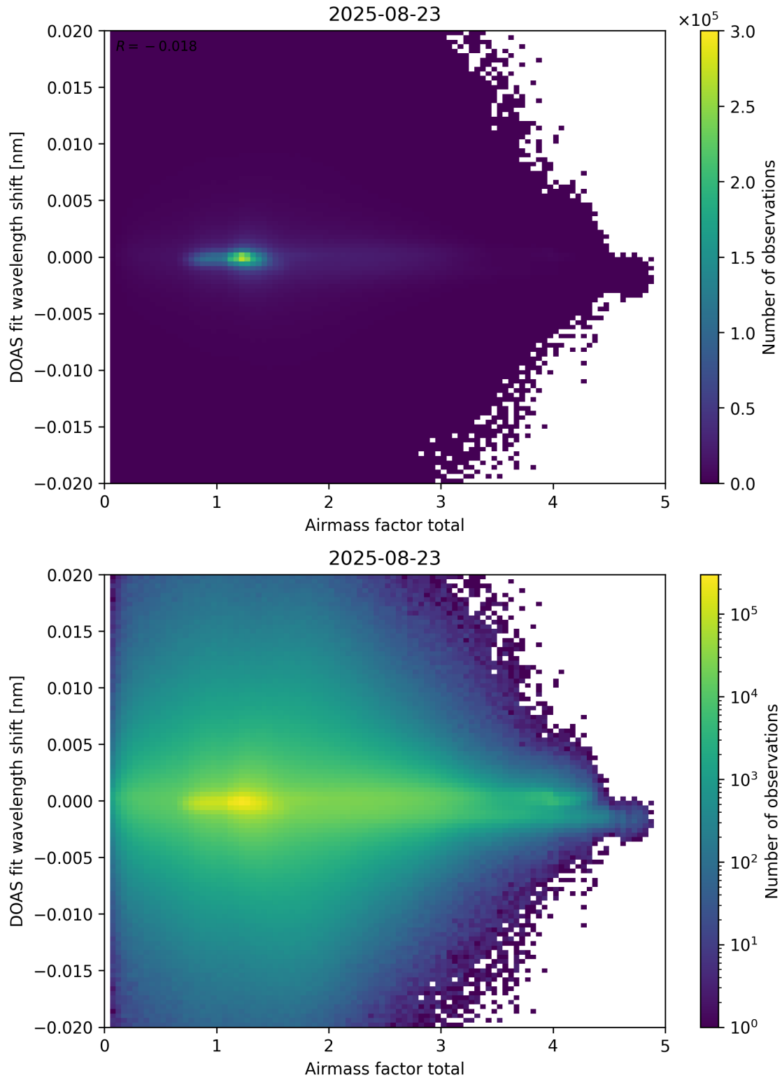
Figure 98: Scatter density plot of “Airmass factor total” against “DOAS fit wavelength shift” for 2025-08-22 to 2025-08-24.
