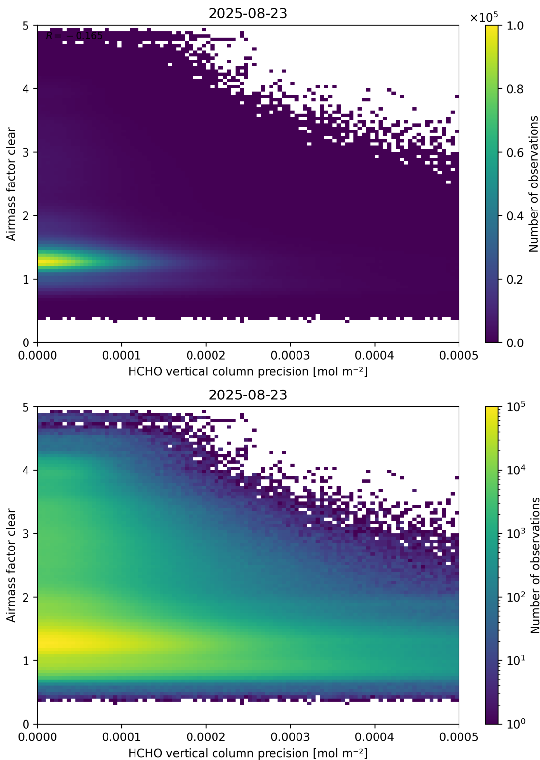
Figure 139: Scatter density plot of “HCHO vertical column precision” against “Airmass factor clear” for 2025-08-22 to 2025-08-24.
