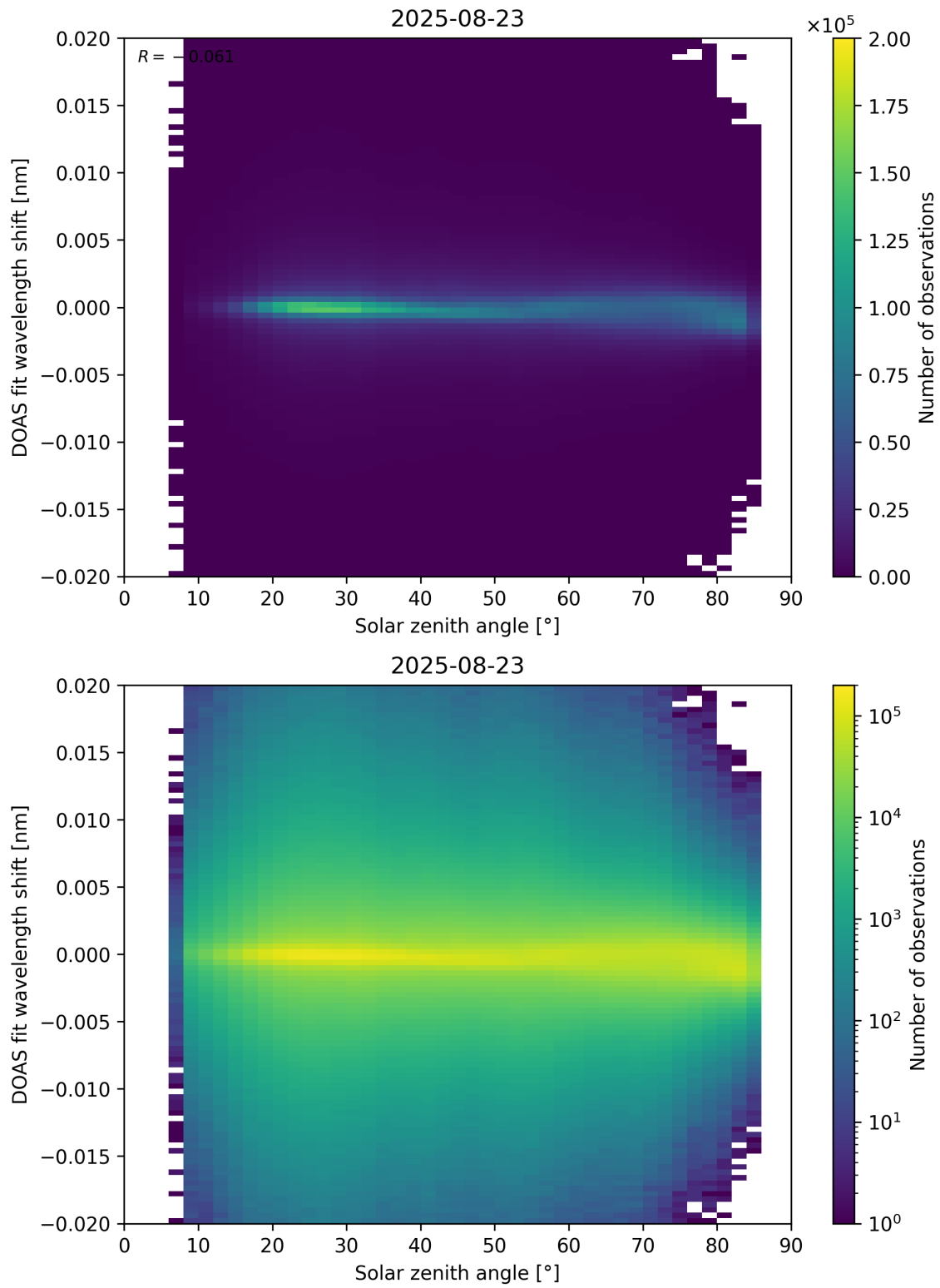
Figure 168: Scatter density plot of “Solar zenith angle” against “DOAS fit wavelength shift” for 2025-08-22 to 2025-08-24.
