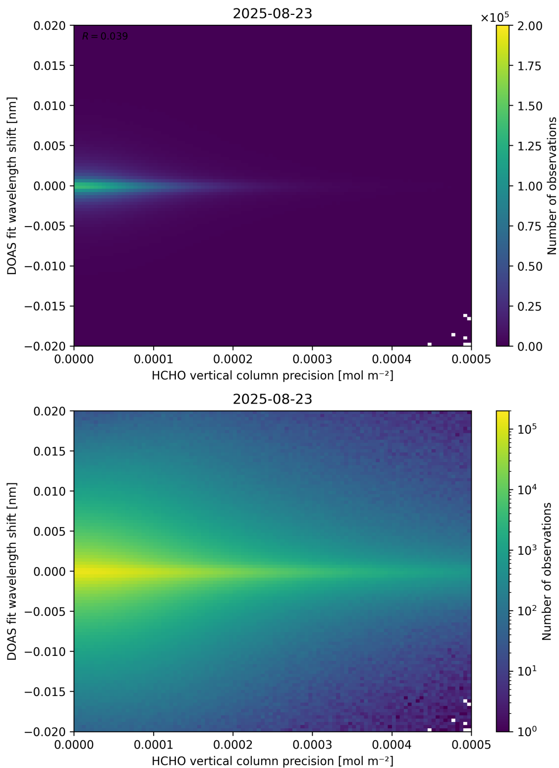
Figure 137: Scatter density plot of “HCHO vertical column precision” against “DOAS fit wavelength shift” for 2025-08-22 to 2025-08-24.
