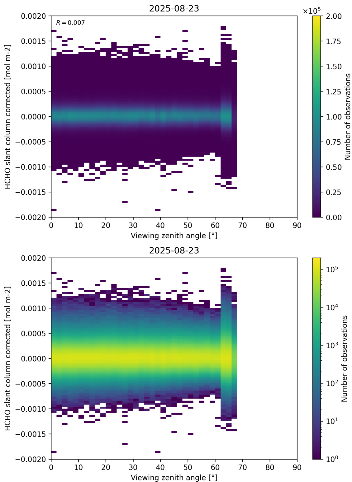
Figure 186: Scatter density plot of “Viewing zenith angle” against “HCHO slant column corrected” for 2025-08-22 to 2025-08-24.
