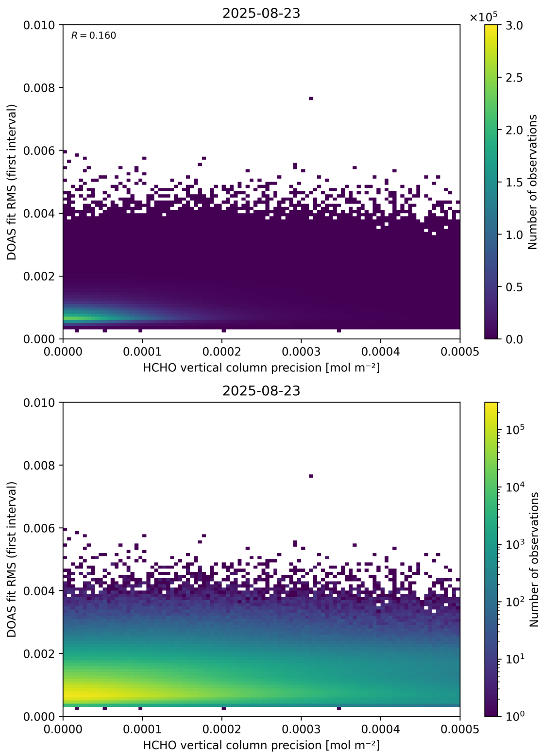
Figure 136: Scatter density plot of “HCHO vertical column precision” against “DOAS fit RMS (first interval)” for 2025-08-22 to 2025-08-24.
