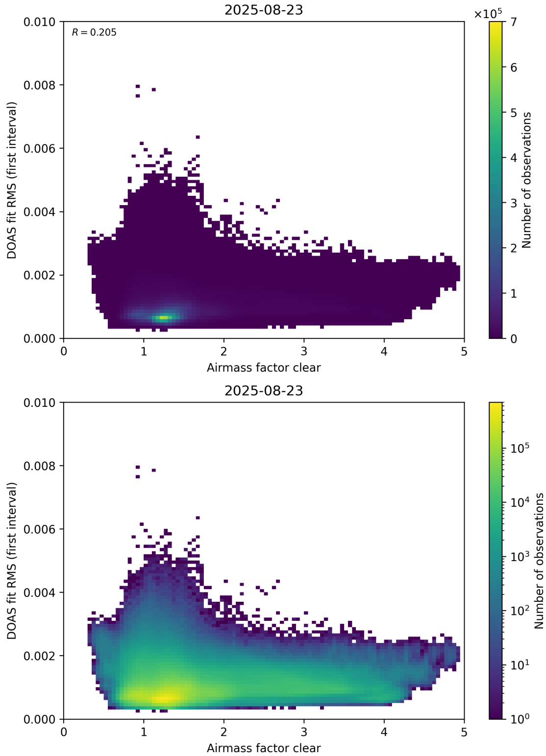
Figure 71: Scatter density plot of “Airmass factor clear” against “DOAS fit RMS (first interval)” for 2025-08-22 to 2025-08-24.
