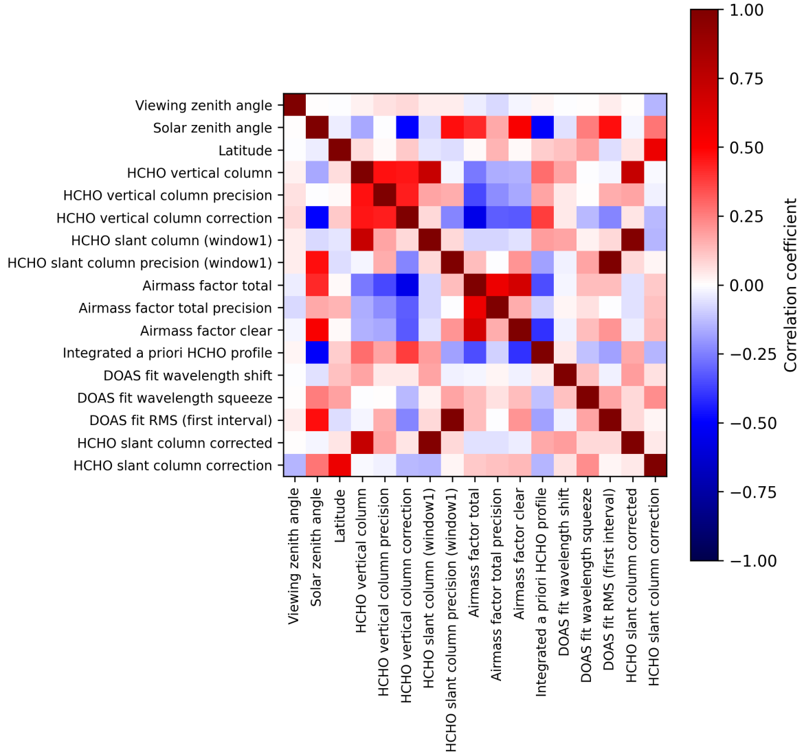
Figure 2: Map of correlation matrix for 2025-08-22 to 2025-08-24.
