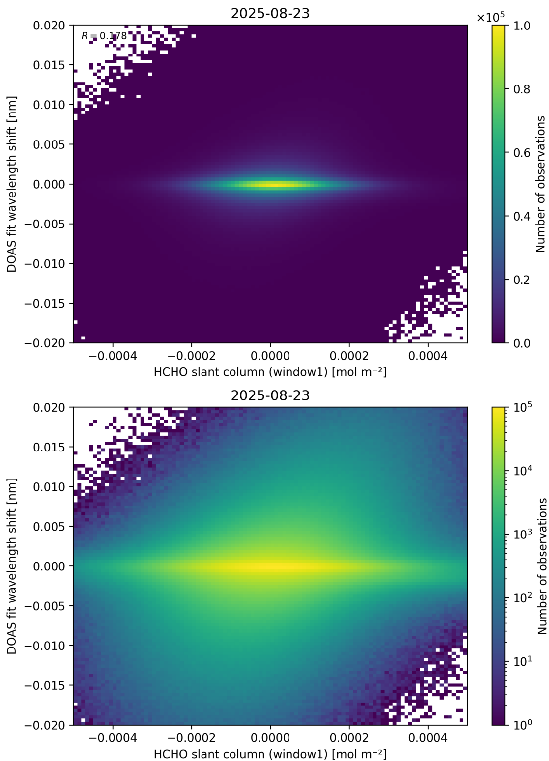
Figure 79: Scatter density plot of “HCHO slant column (window1)” against “DOAS fit wavelength shift” for 2025-08-22 to 2025-08-24.
