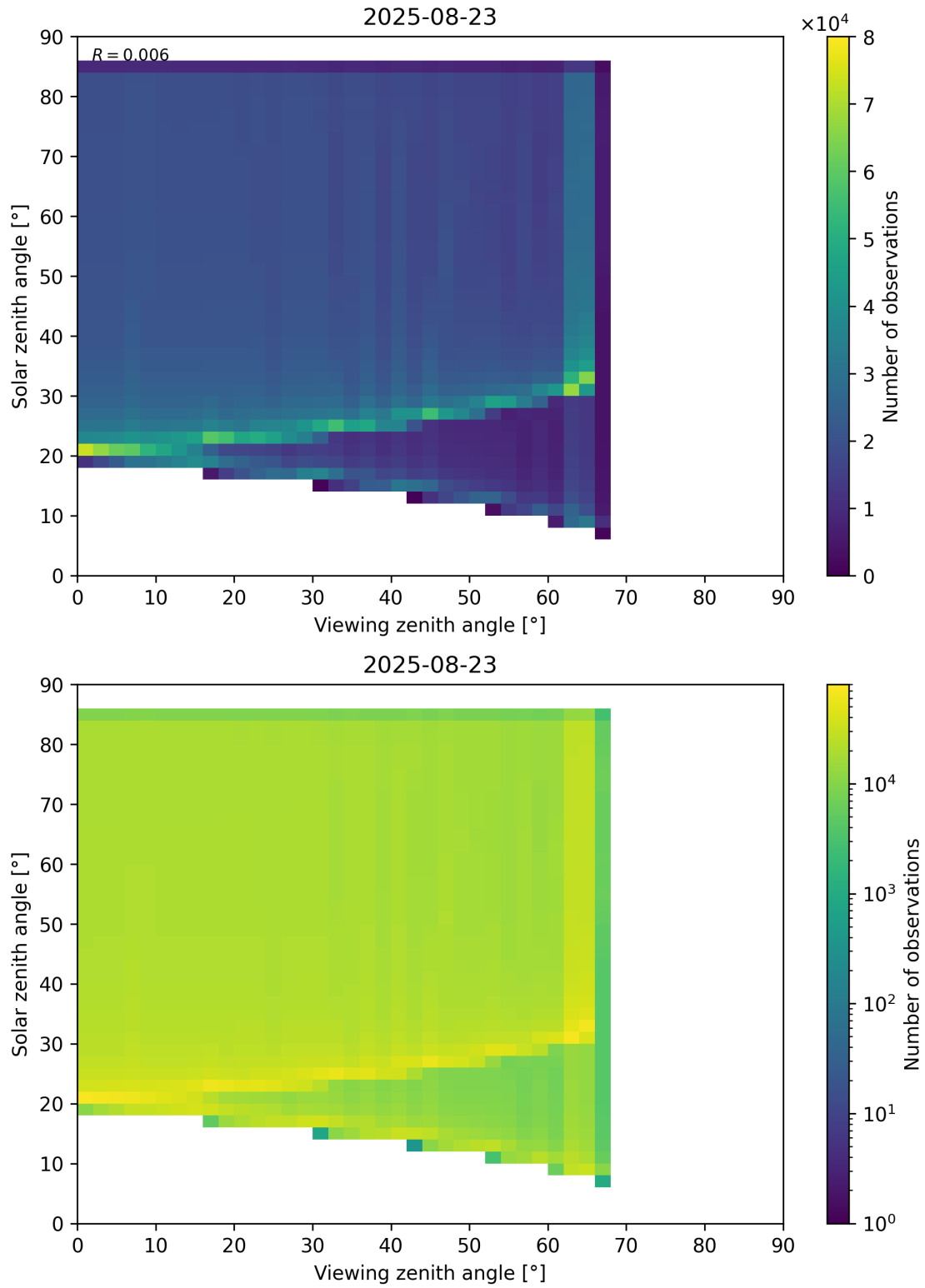
Figure 197: Scatter density plot of “Viewing zenith angle” against “Solar zenith angle” for 2025-08-22 to 2025-08-24.
