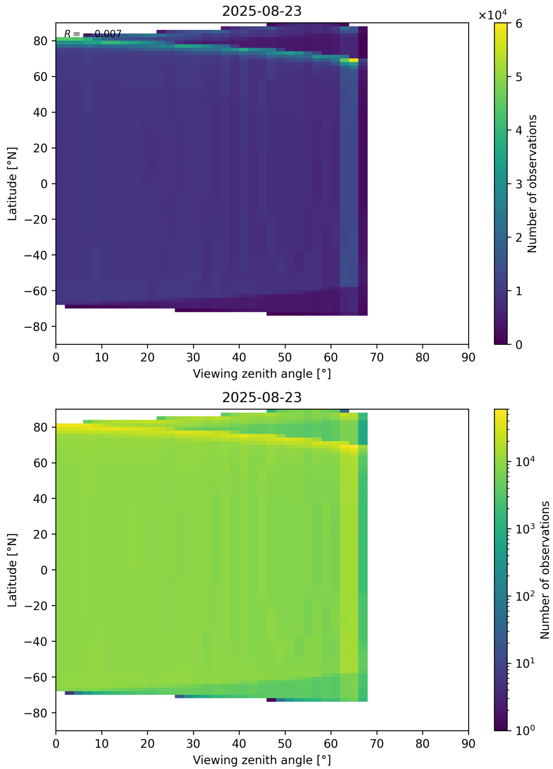
Figure 196: Scatter density plot of “Viewing zenith angle” against “Latitude” for 2025-08-22 to 2025-08-24.
