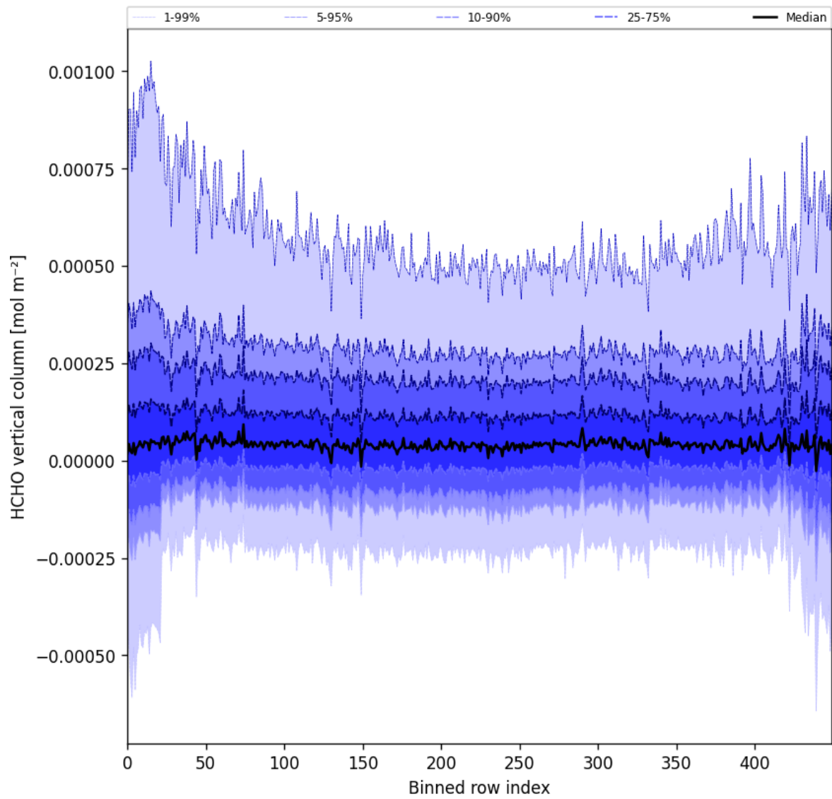
Figure 49: Along track statistics of “HCHO vertical column” for 2025-08-22 to 2025-08-24
