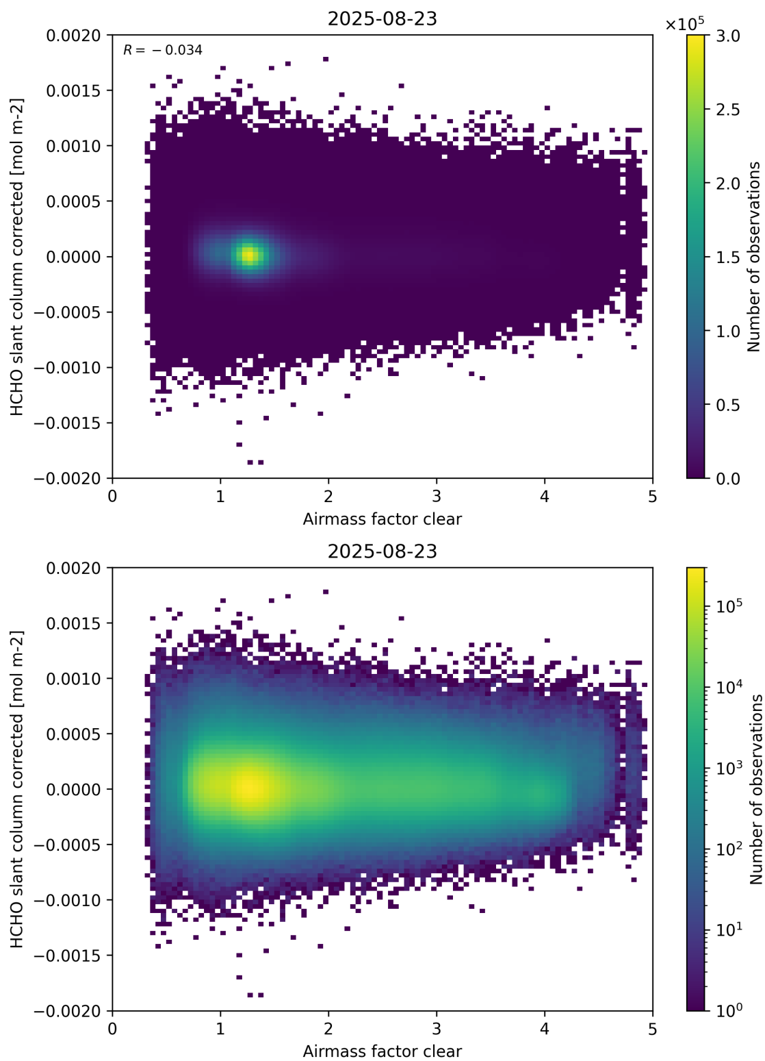
Figure 74: Scatter density plot of “Airmass factor clear” against “HCHO slant column corrected” for 2025-08-22 to 2025-08-24.
