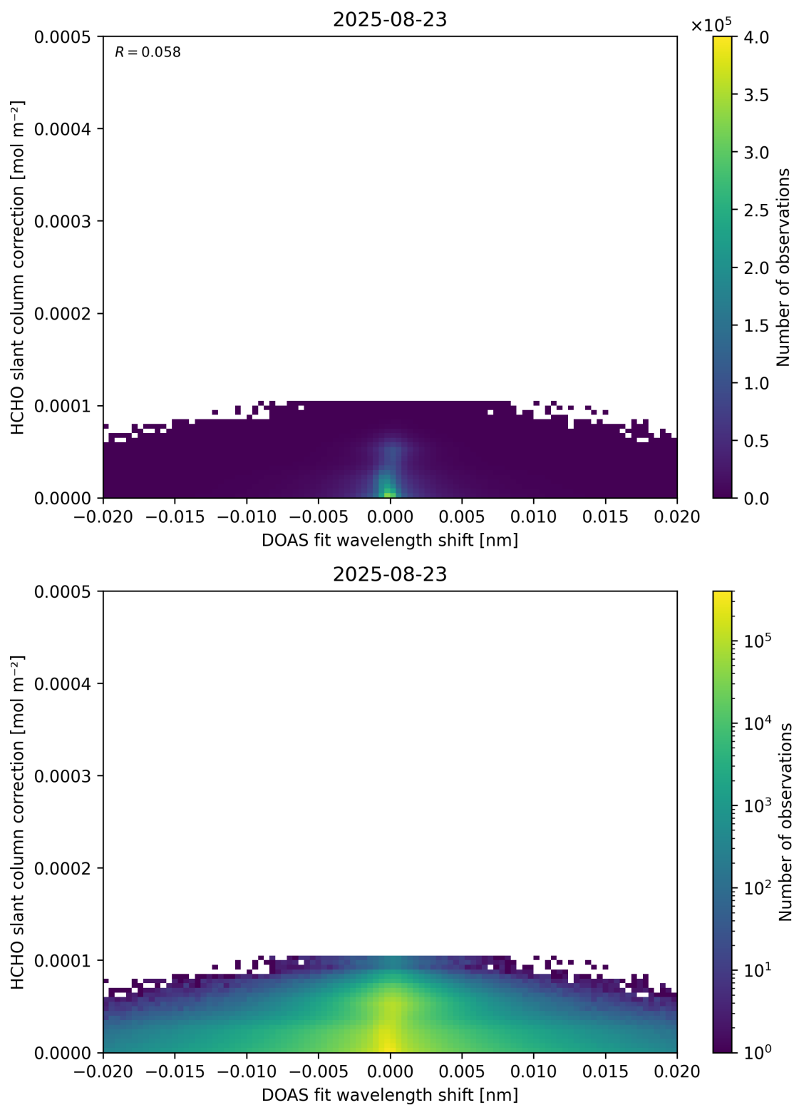
Figure 67: Scatter density plot of “DOAS fit wavelength shift” against “HCHO slant column correction” for 2025-08-22 to 2025-08-24.
