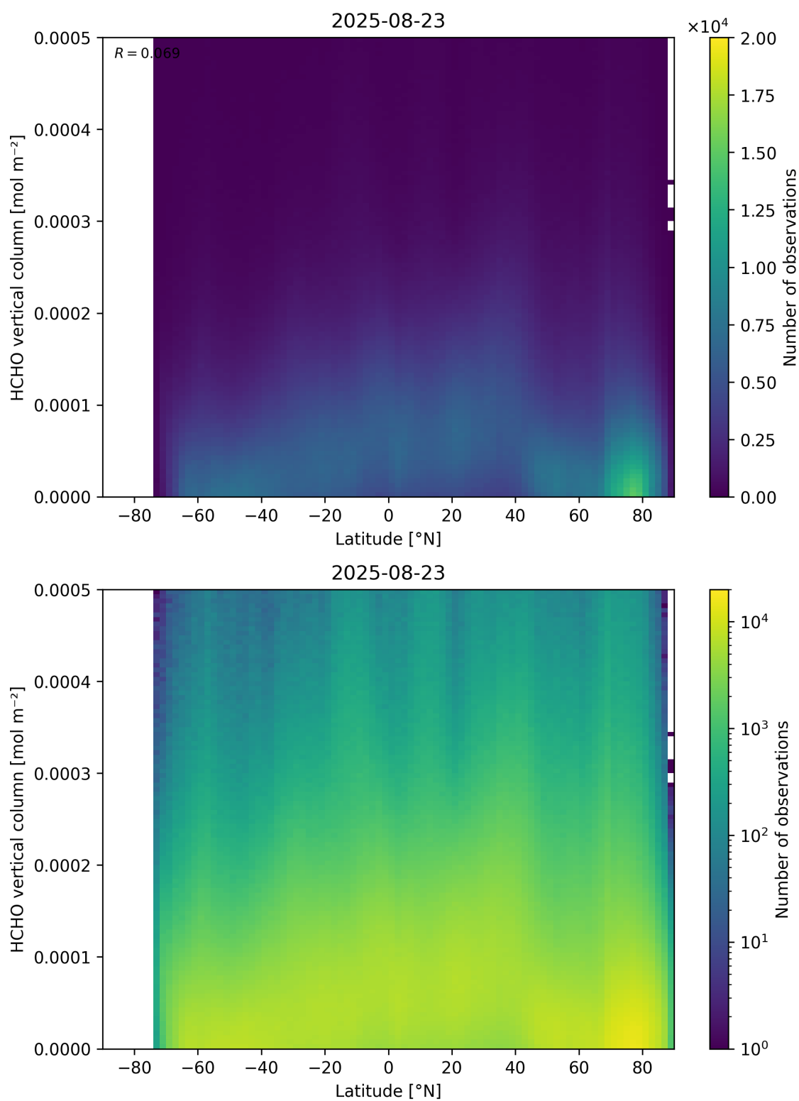
Figure 163: Scatter density plot of “Latitude” against “HCHO vertical column” for 2025-08-22 to 2025-08-24.
