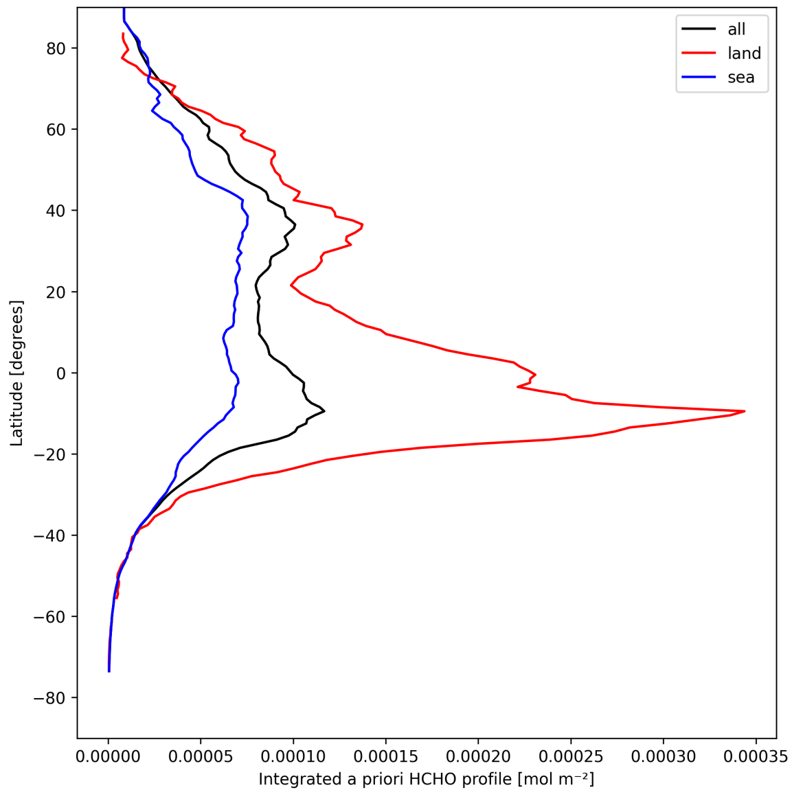
Figure 29: Zonal average of “Integrated a priori HCHO profile” for 2025-08-22 to 2025-08-24.
