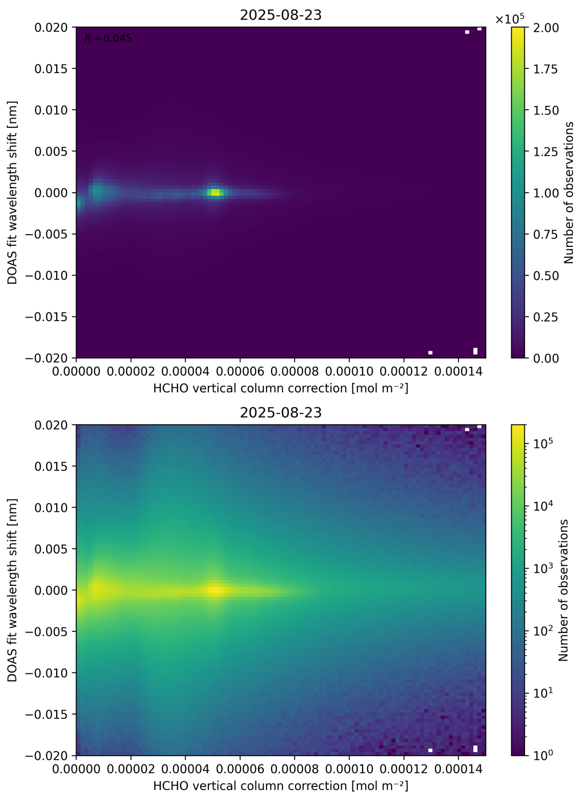
Figure 113: Scatter density plot of “HCHO vertical column correction” against “DOAS fit wavelength shift” for 2025-08-22 to 2025-08-24.
