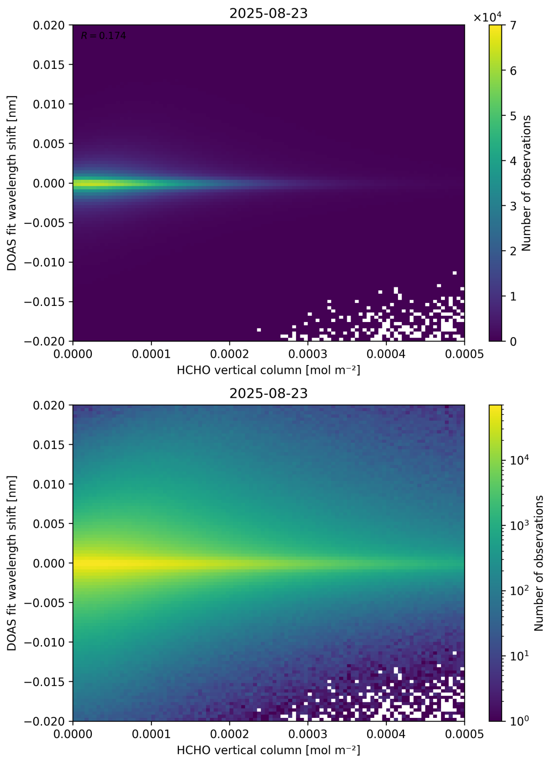
Figure 124: Scatter density plot of “HCHO vertical column” against “DOAS fit wavelength shift” for 2025-08-22 to 2025-08-24.
