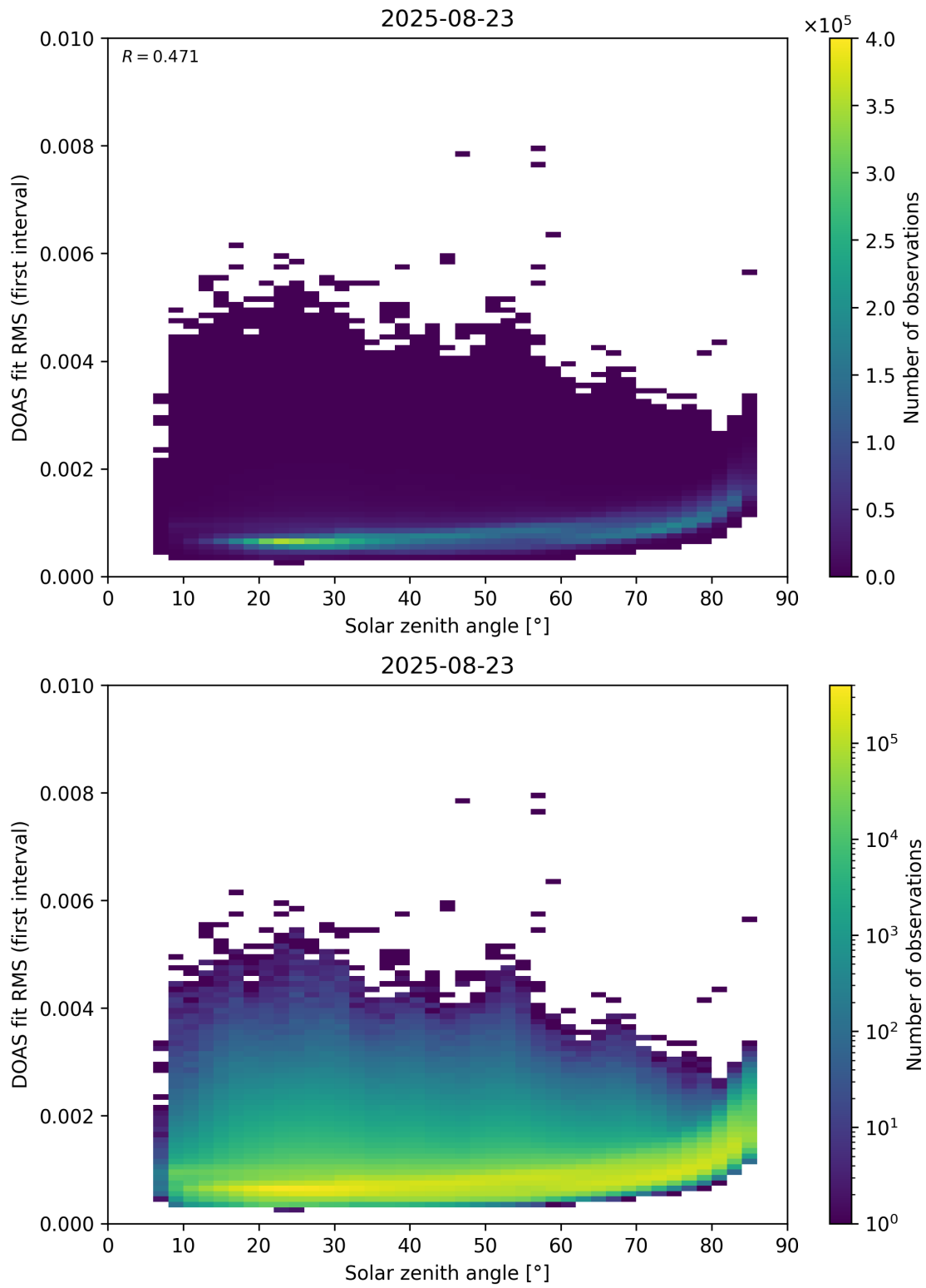
Figure 167: Scatter density plot of “Solar zenith angle” against “DOAS fit RMS (first interval)” for 2025-08-22 to 2025-08-24.
