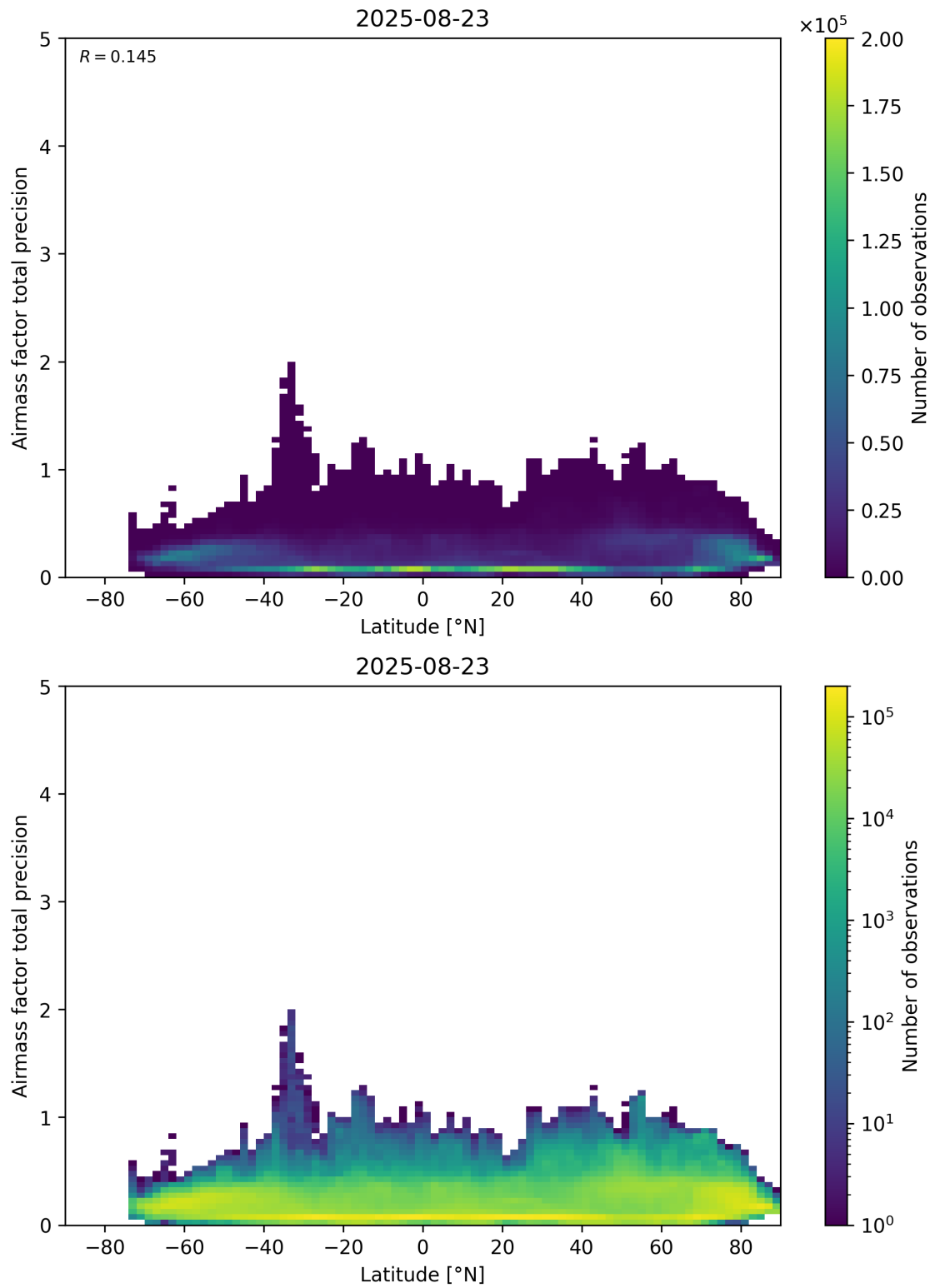
Figure 162: Scatter density plot of “Latitude” against “Airmass factor total precision” for 2025-08-22 to 2025-08-24.
