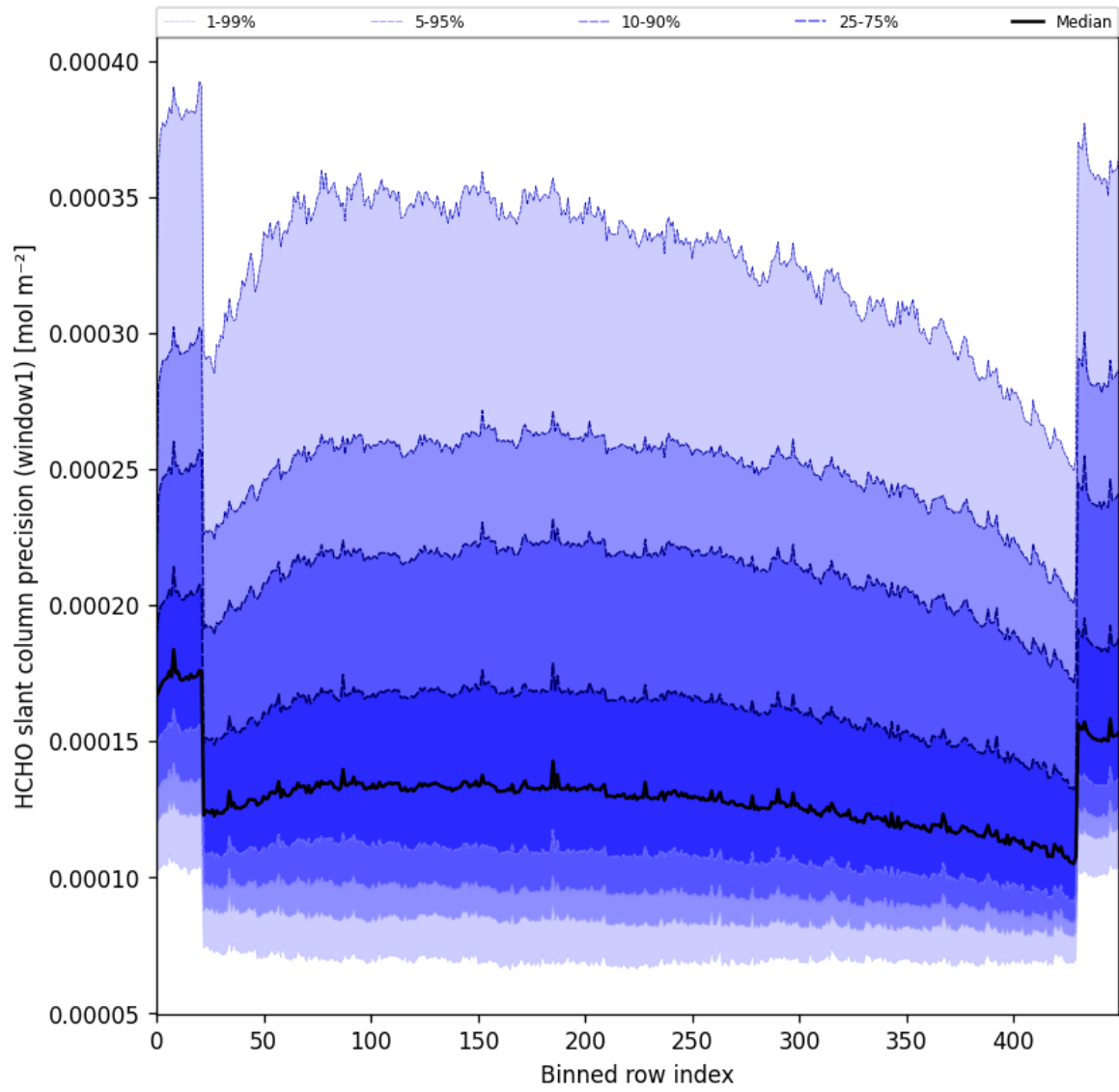
Figure 53: Along track statistics of “HCHO slant column precision (window1)” for 2025-08-22 to 2025-08-24
