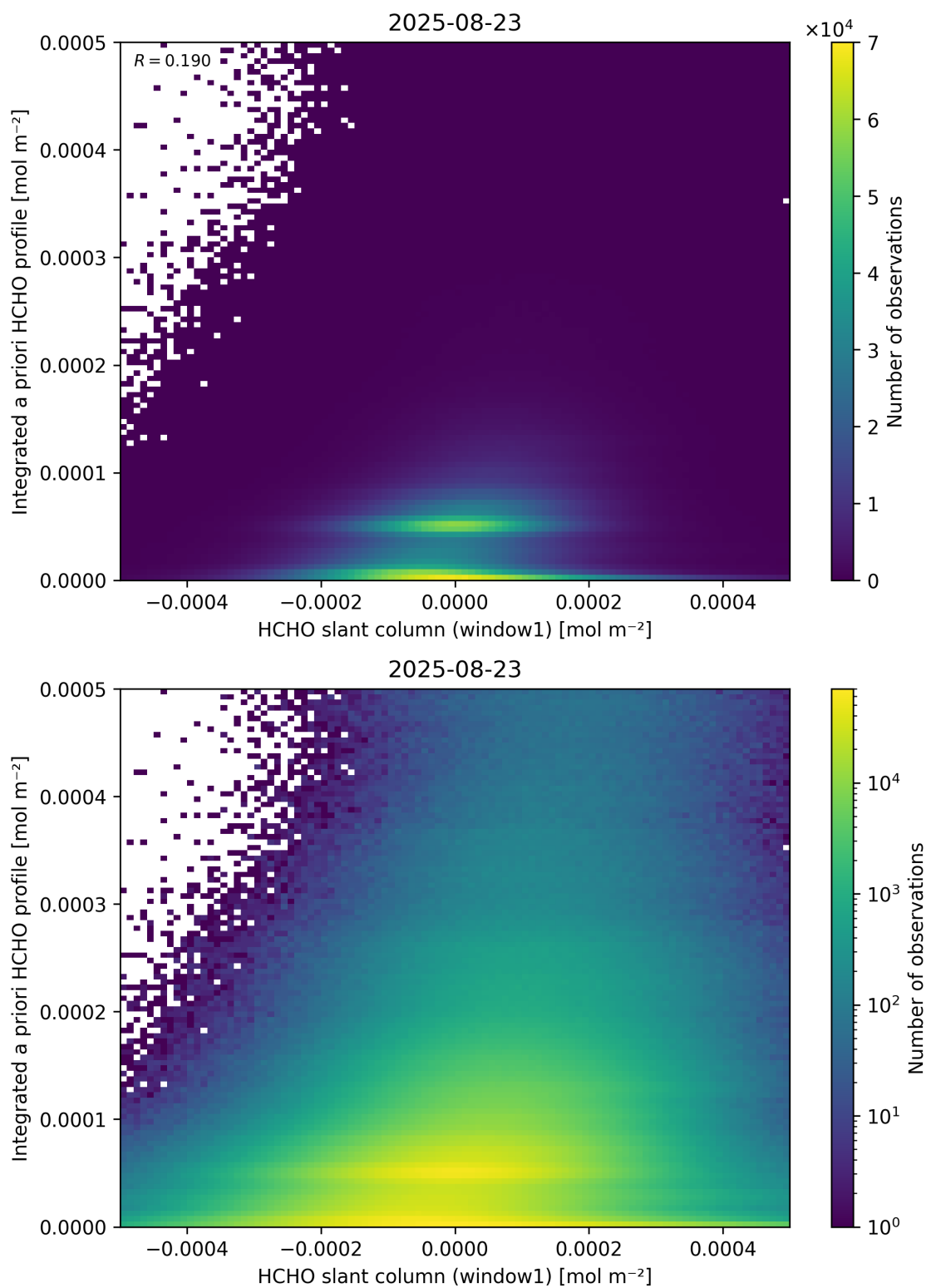
Figure 87: Scatter density plot of “HCHO slant column (window1)” against “Integrated a priori HCHO profile” for 2025-08-22 to 2025-08-24.
