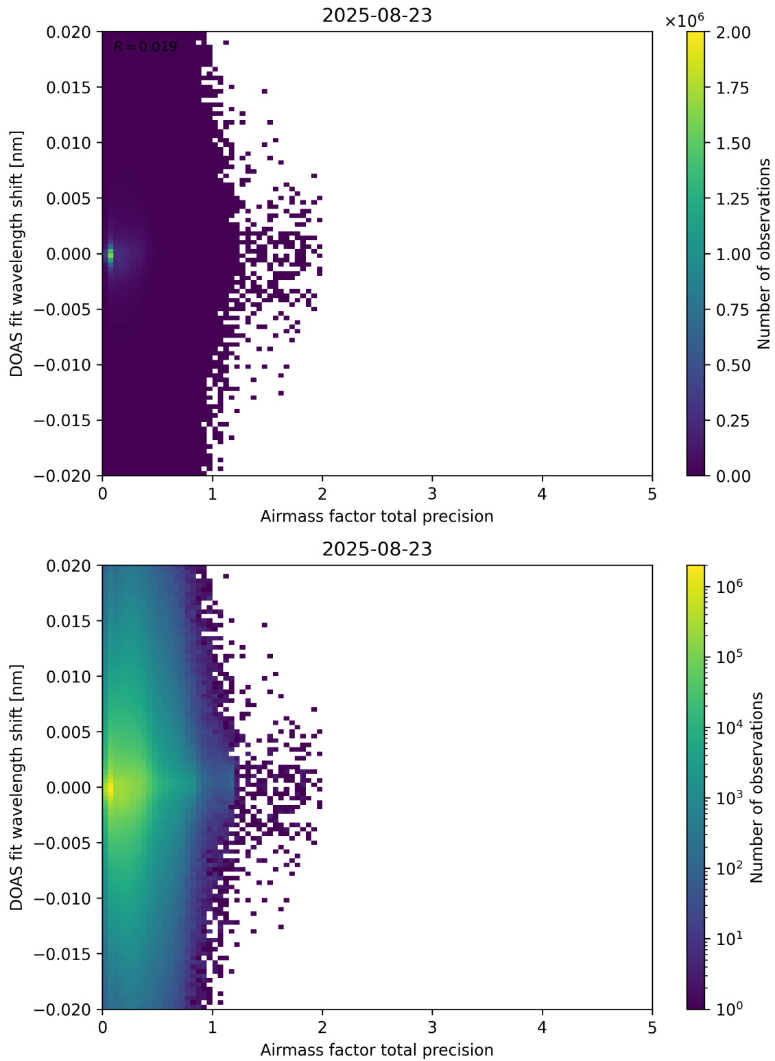
Figure 106: Scatter density plot of “Airmass factor total precision” against “DOAS fit wavelength shift” for 2025-08-22 to 2025-08-24.
