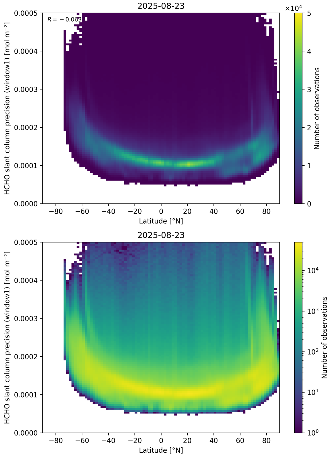
Figure 160: Scatter density plot of “Latitude” against “HCHO slant column precision (window1)” for 2025-08-22 to 2025-08-24.
