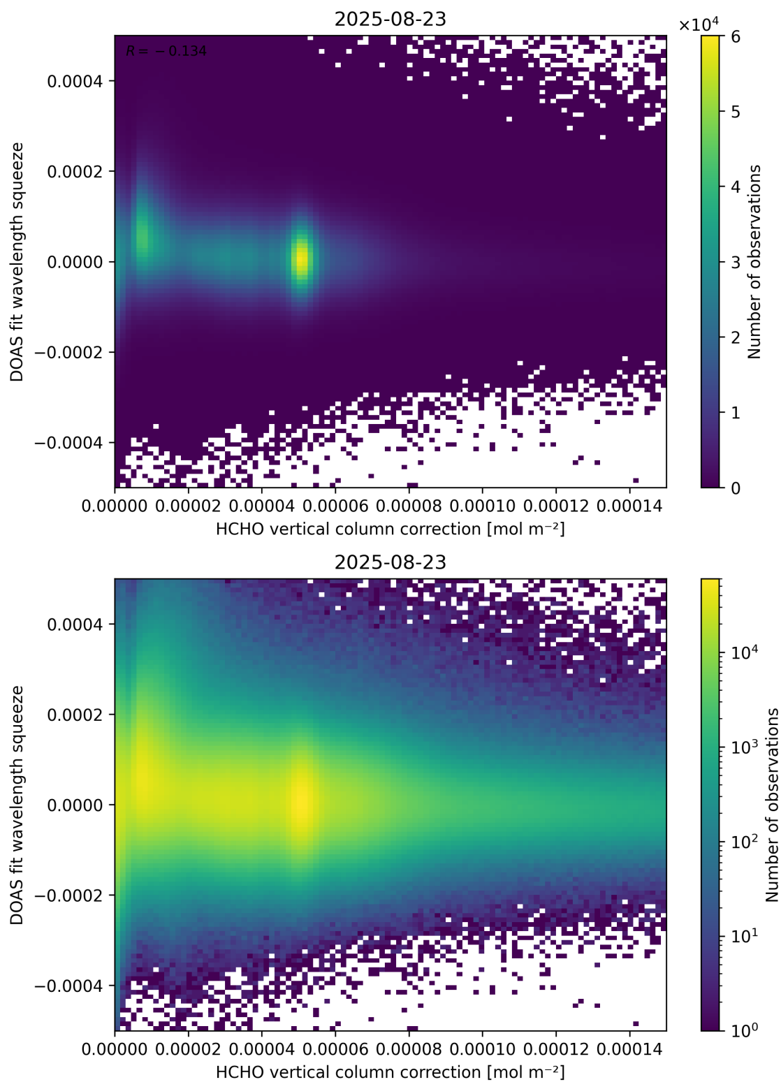
Figure 114: Scatter density plot of “HCHO vertical column correction” against “DOAS fit wavelength squeeze” for 2025-08-22 to 2025-08-24.
