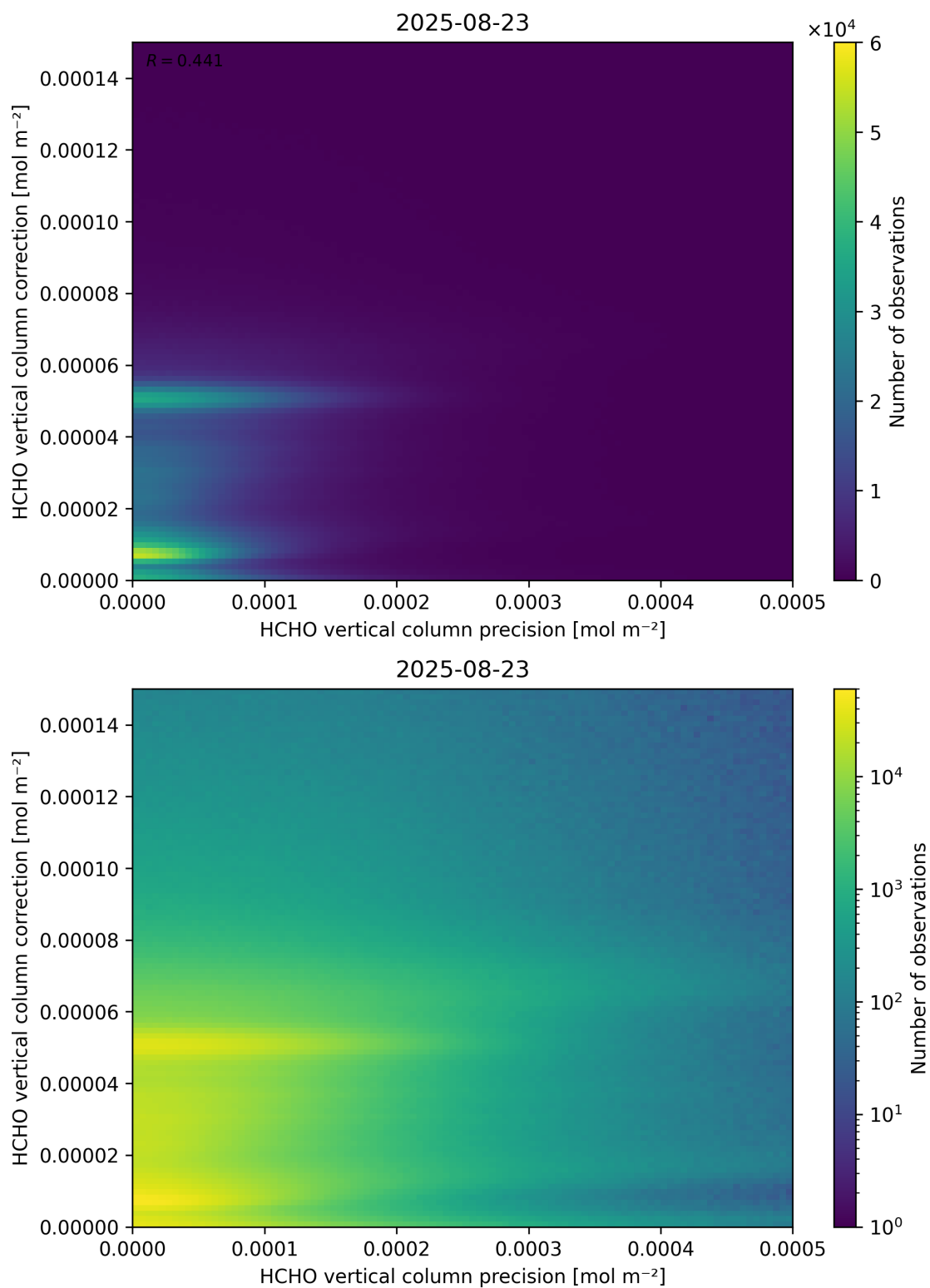
Figure 146: Scatter density plot of “HCHO vertical column precision” against “HCHO vertical column correction” for 2025-08-22 to 2025-08-24.
