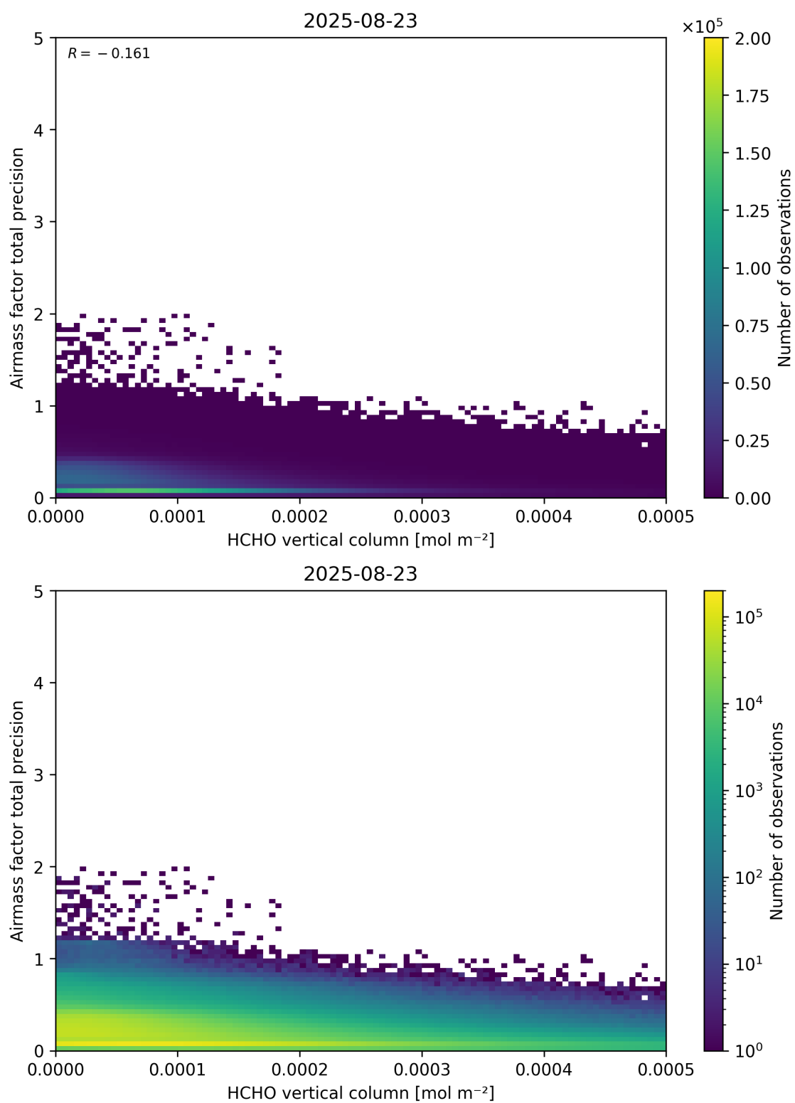
Figure 132: Scatter density plot of “HCHO vertical column” against “Airmass factor total precision” for 2025-08-22 to 2025-08-24.
