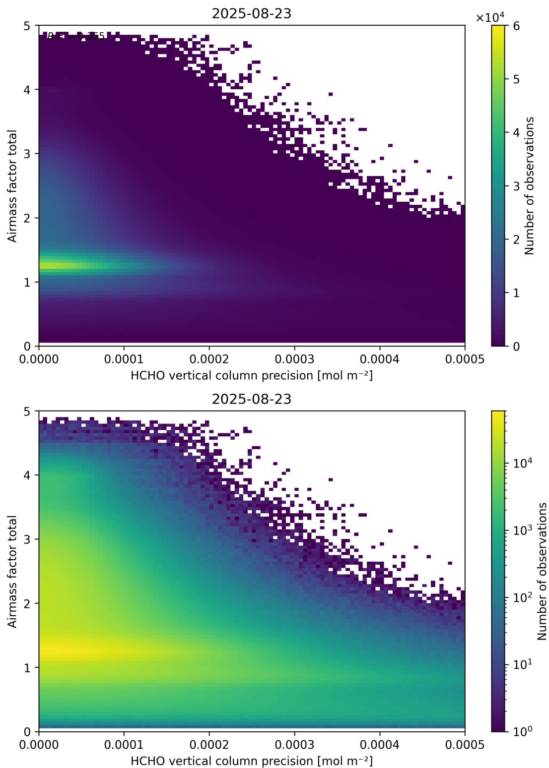
Figure 144: Scatter density plot of “HCHO vertical column precision” against “Airmass factor total” for 2025-08-22 to 2025-08-24.
