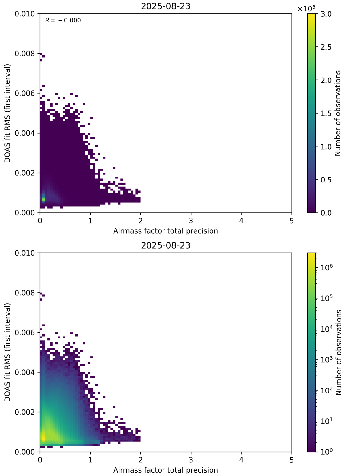
Figure 105: Scatter density plot of “Airmass factor total precision” against “DOAS fit RMS (first interval)” for 2025-08-22 to 2025-08-24.
