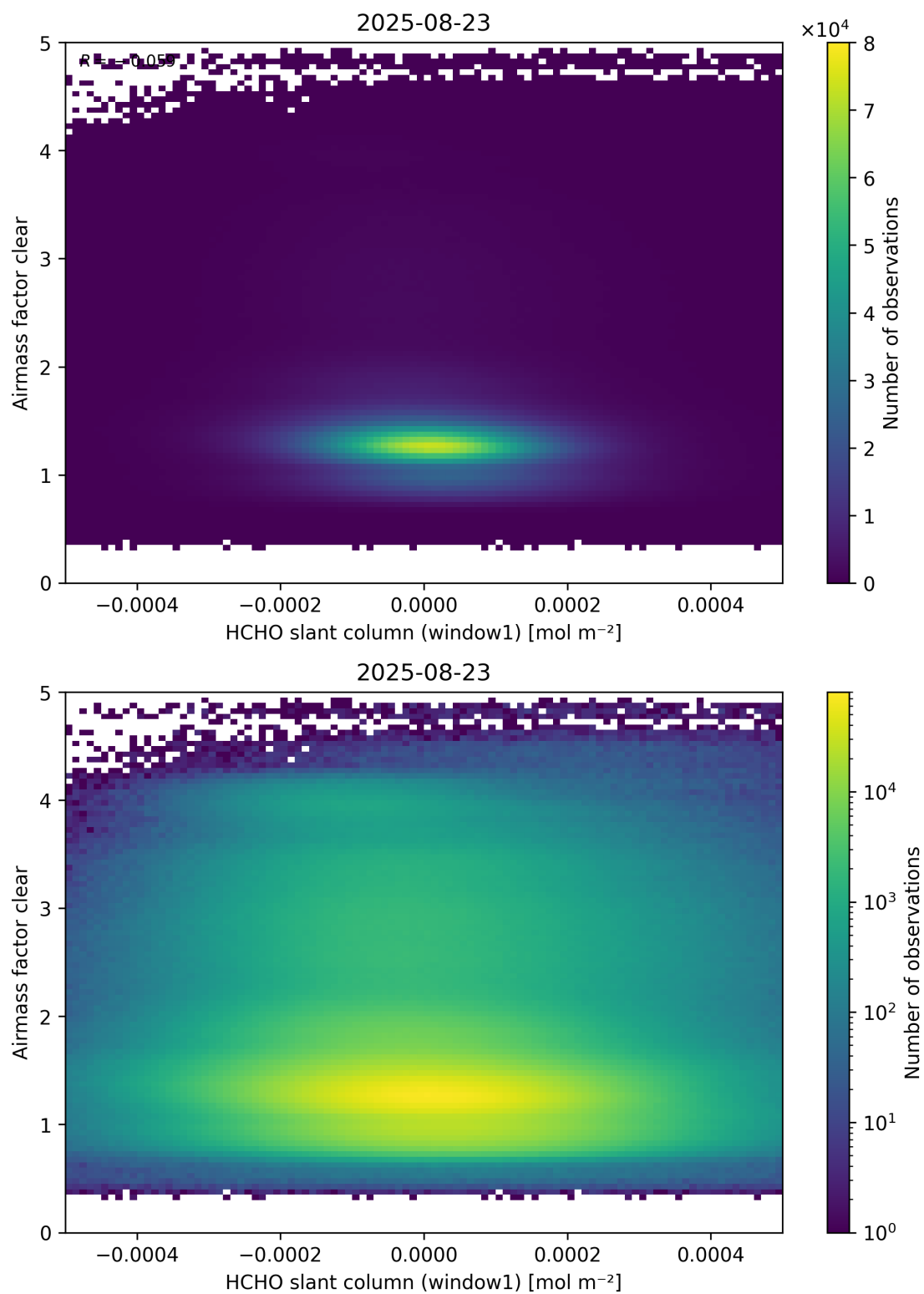
Figure 81: Scatter density plot of “HCHO slant column (window1)” against “Airmass factor clear” for 2025-08-22 to 2025-08-24.
