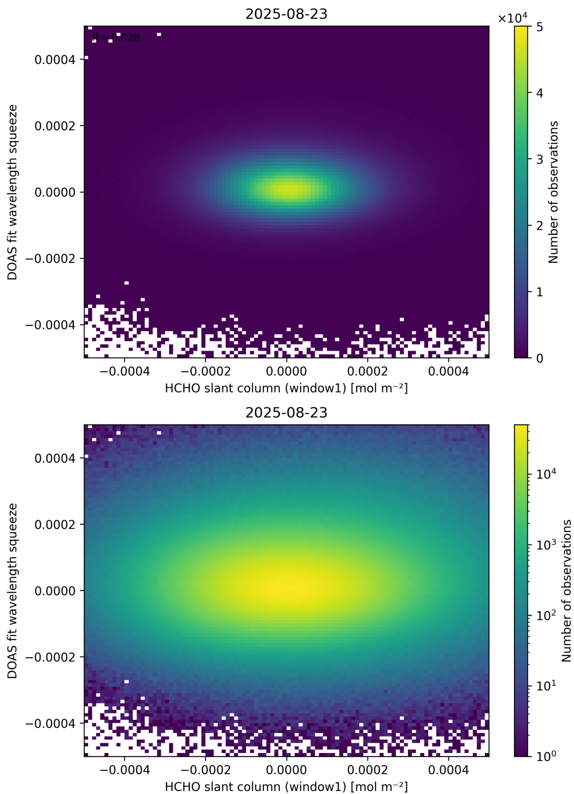
Figure 80: Scatter density plot of “HCHO slant column (window1)” against “DOAS fit wavelength squeeze” for 2025-08-22 to 2025-08-24.
