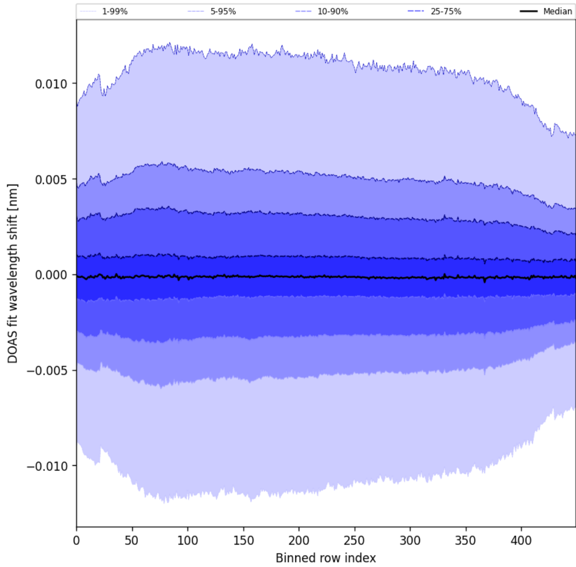
Figure 58: Along track statistics of “DOAS fit wavelength shift” for 2025-08-22 to 2025-08-24
