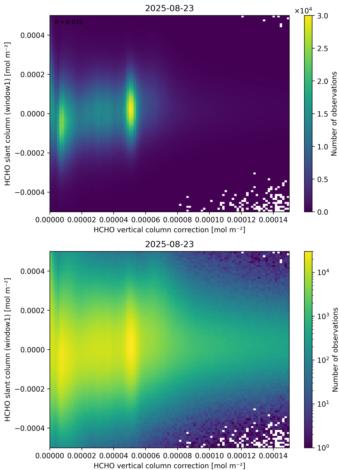
Figure 118: Scatter density plot of “HCHO vertical column correction” against “HCHO slant column (window1)” for 2025-08-22 to 2025-08-24.
