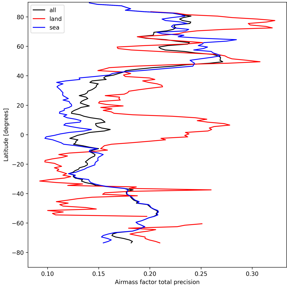
Figure 27: Zonal average of “Airmass factor total precision” for 2025-08-22 to 2025-08-24.
