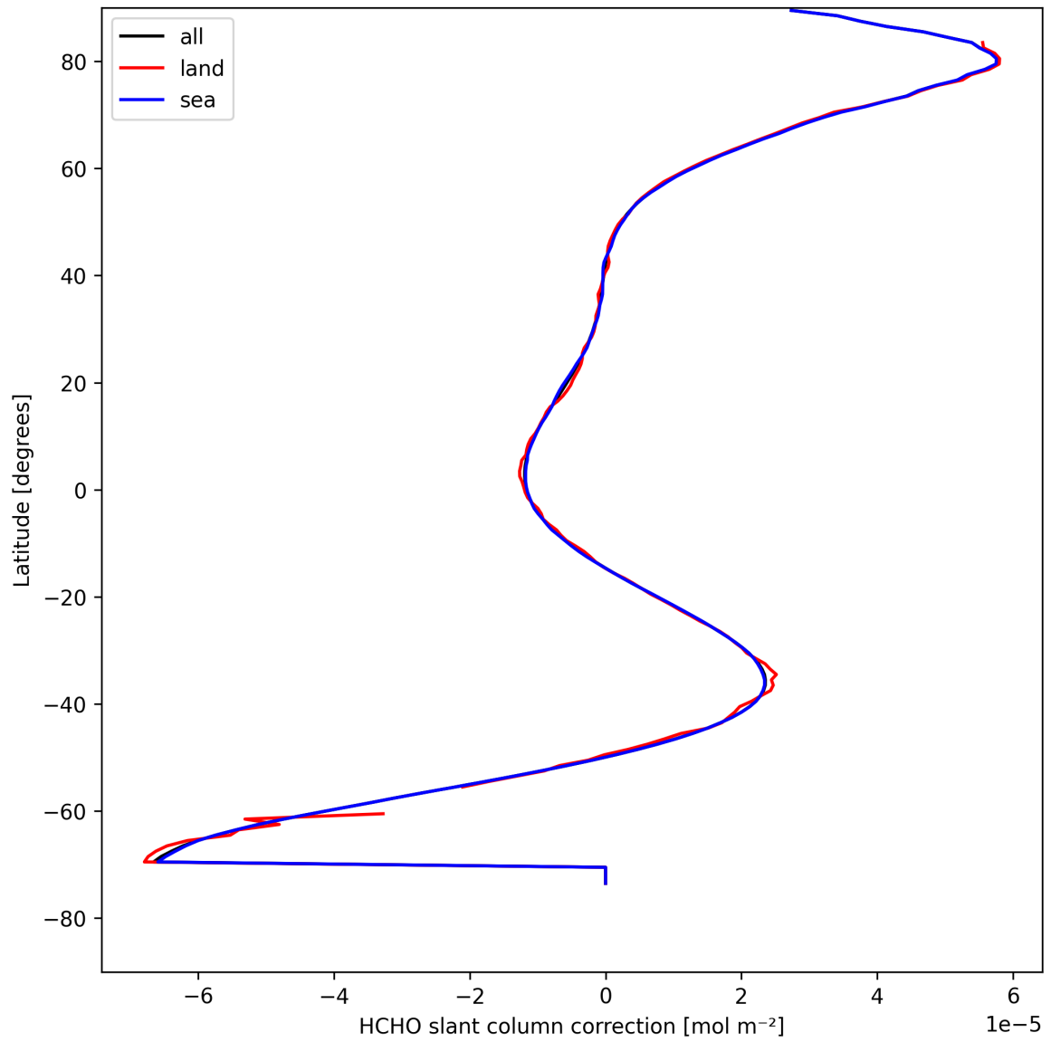
Figure 33: Zonal average of “HCHO slant column correction” for 2025-08-22 to 2025-08-24.
