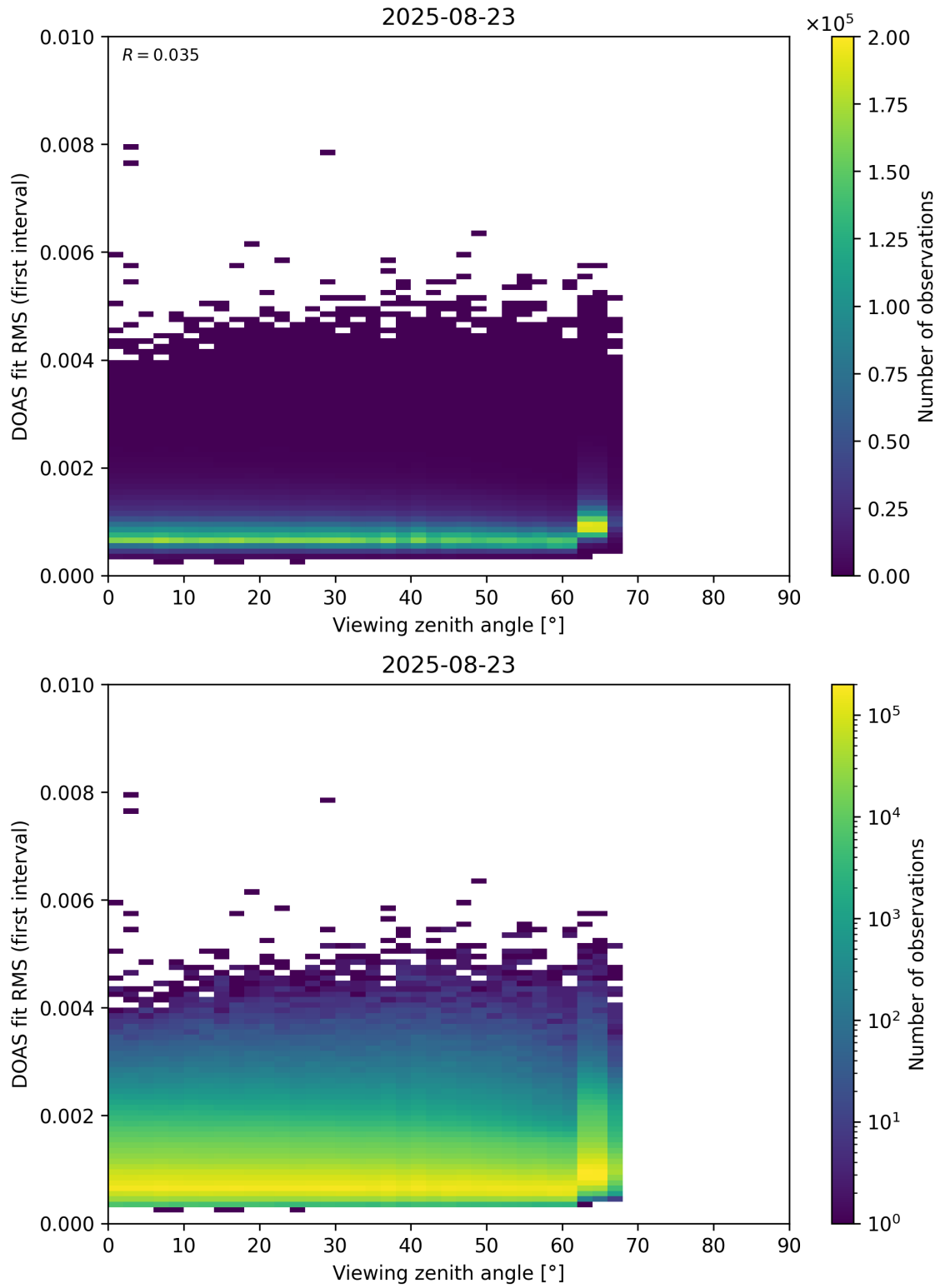
Figure 182: Scatter density plot of “Viewing zenith angle” against “DOAS fit RMS (first interval)” for 2025-08-22 to 2025-08-24.
