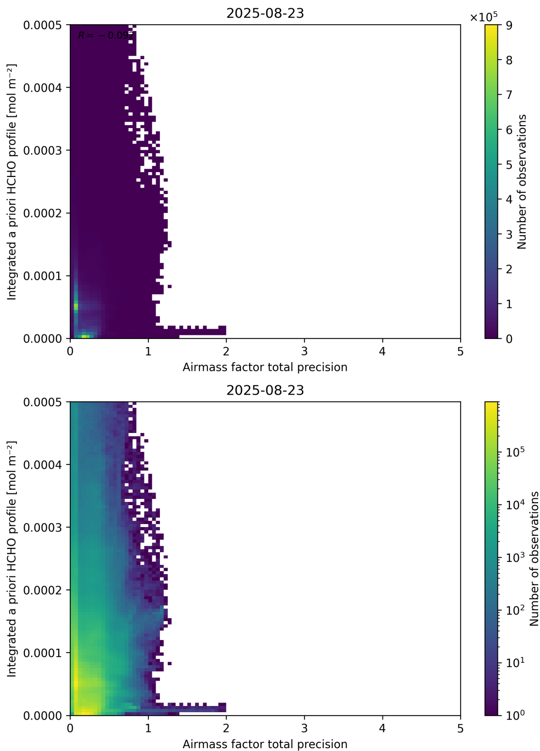
Figure 111: Scatter density plot of “Airmass factor total precision” against “Integrated a priori HCHO profile” for 2025-08-22 to 2025-08-24.
