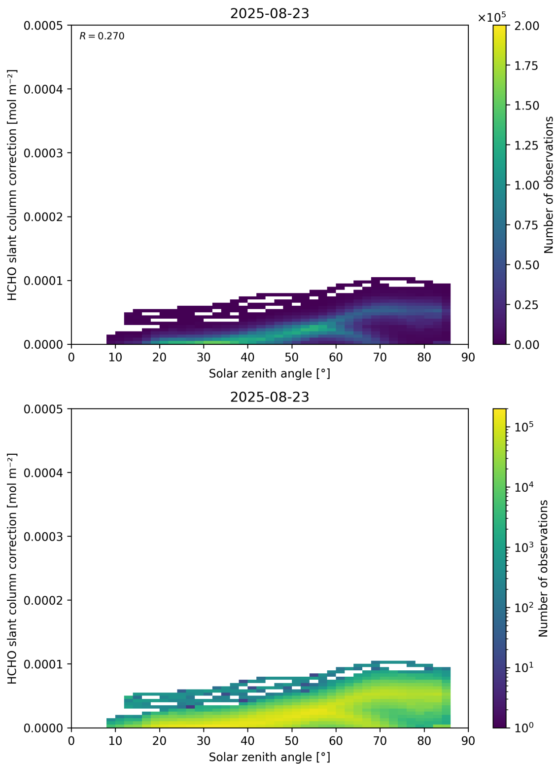
Figure 172: Scatter density plot of “Solar zenith angle” against “HCHO slant column correction” for 2025-08-22 to 2025-08-24.
