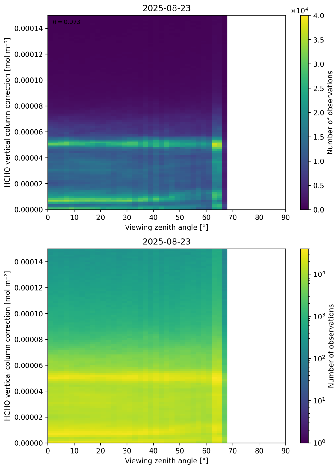
Figure 193: Scatter density plot of “Viewing zenith angle” against “HCHO vertical column correction” for 2025-08-22 to 2025-08-24.
