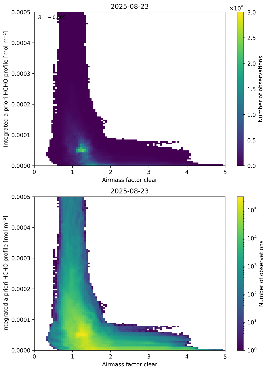
Figure 76: Scatter density plot of “Airmass factor clear” against “Integrated a priori HCHO profile” for 2025-08-22 to 2025-08-24.
