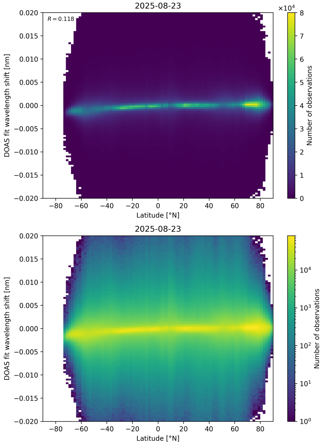
Figure 154: Scatter density plot of “Latitude” against “DOAS fit wavelength shift” for 2025-08-22 to 2025-08-24.
