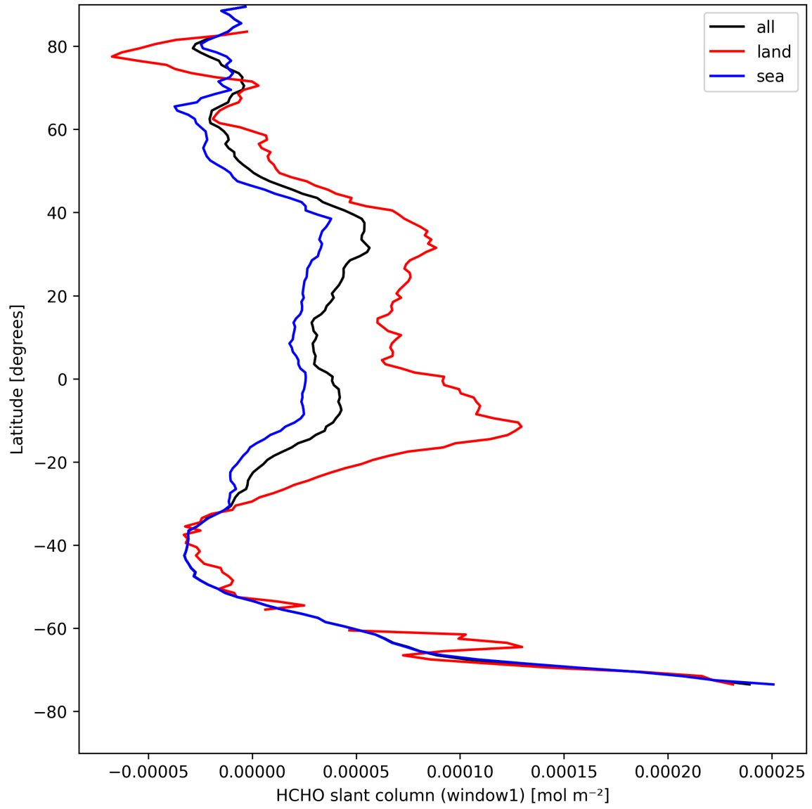
Figure 24: Zonal average of “HCHO slant column (window1)” for 2025-08-22 to 2025-08-24.
