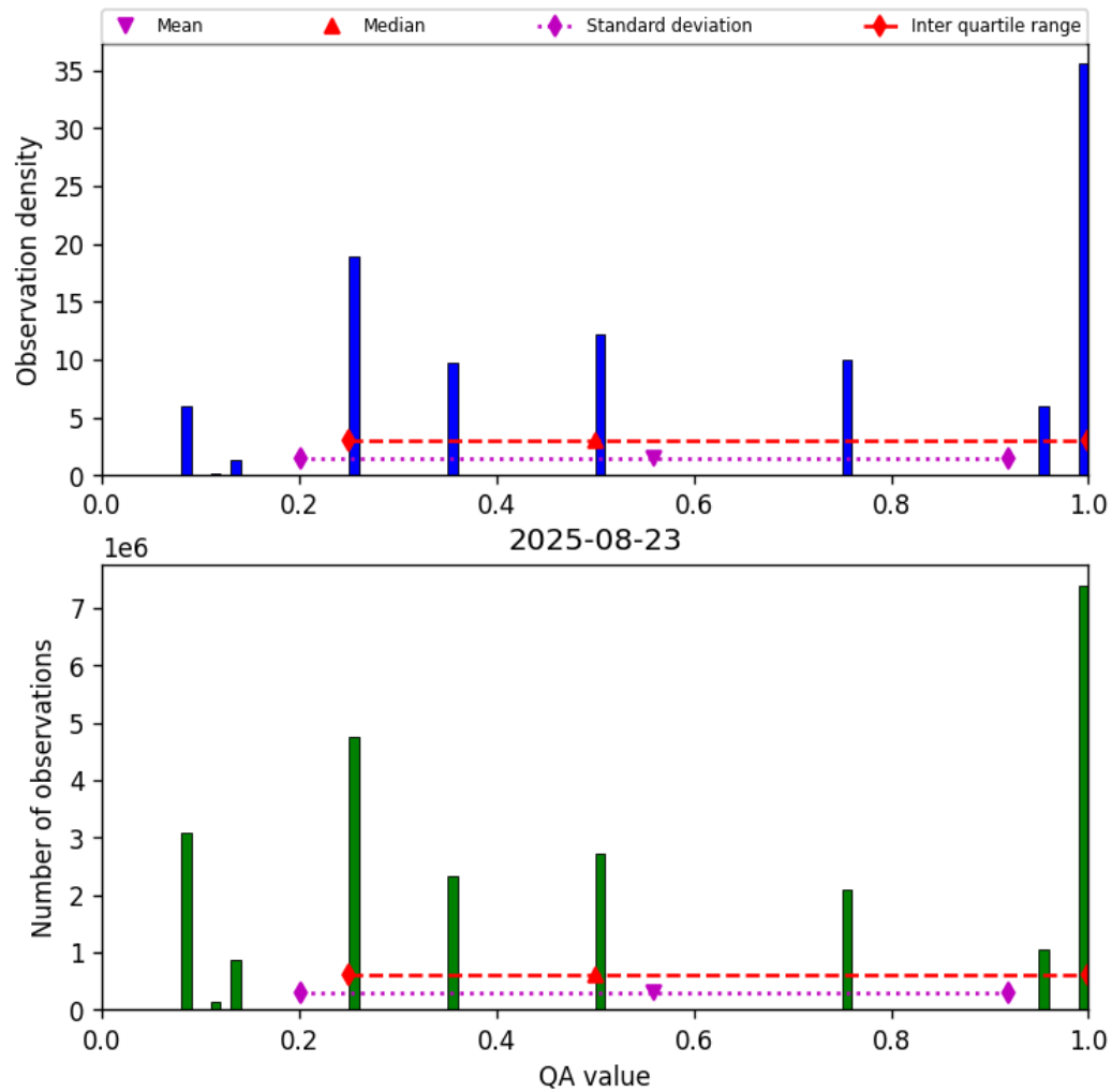
Figure 34: Histogram of “QA value” for 2025-08-22 to 2025-08-24
