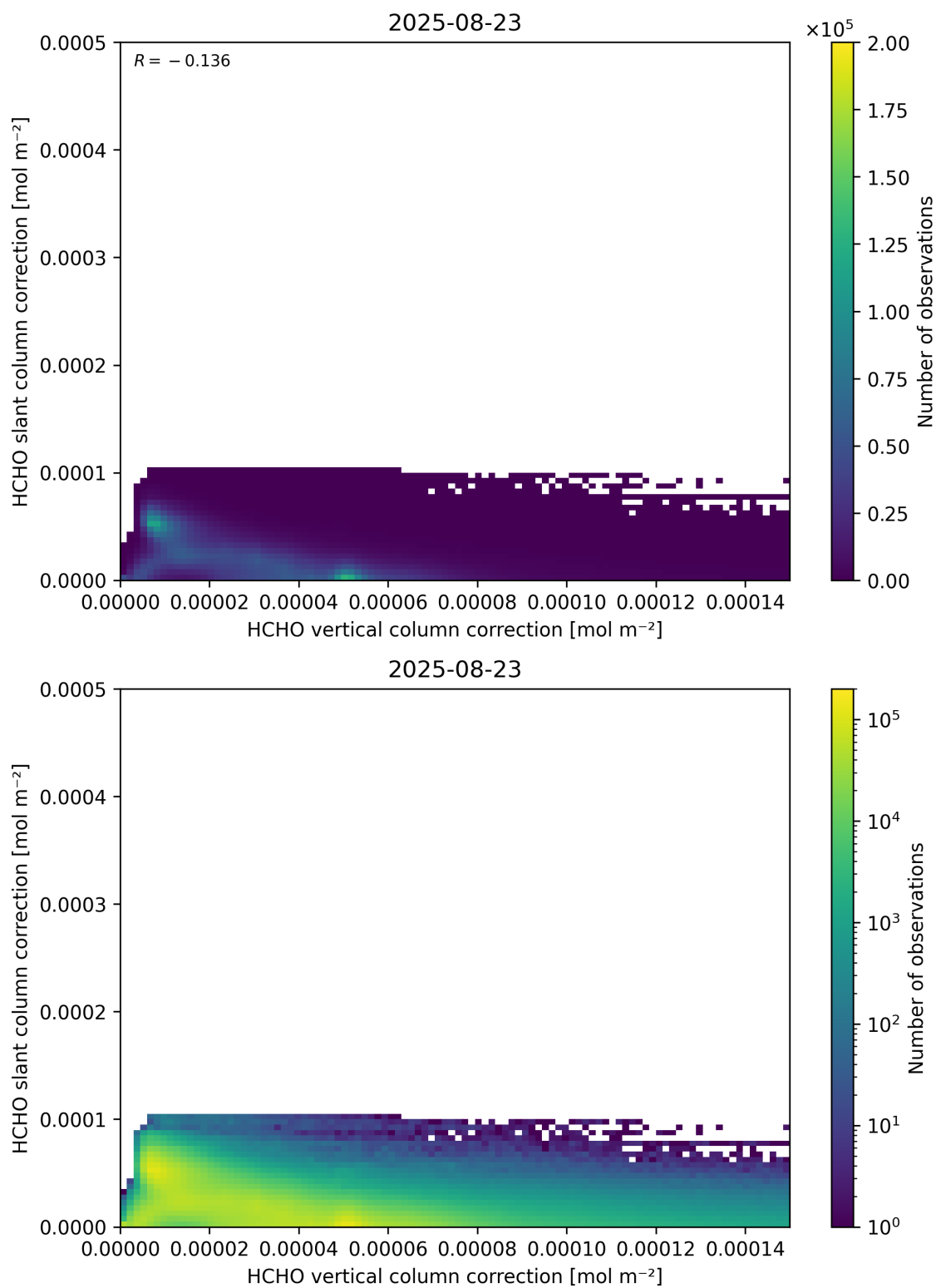
Figure 117: Scatter density plot of “HCHO vertical column correction” against “HCHO slant column correction” for 2025-08-22 to 2025-08-24.
