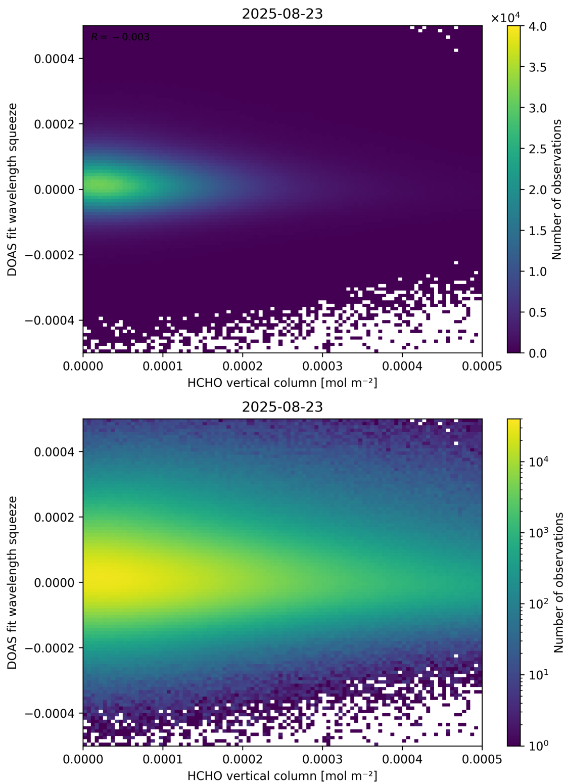
Figure 125: Scatter density plot of “HCHO vertical column” against “DOAS fit wavelength squeeze” for 2025-08-22 to 2025-08-24.
