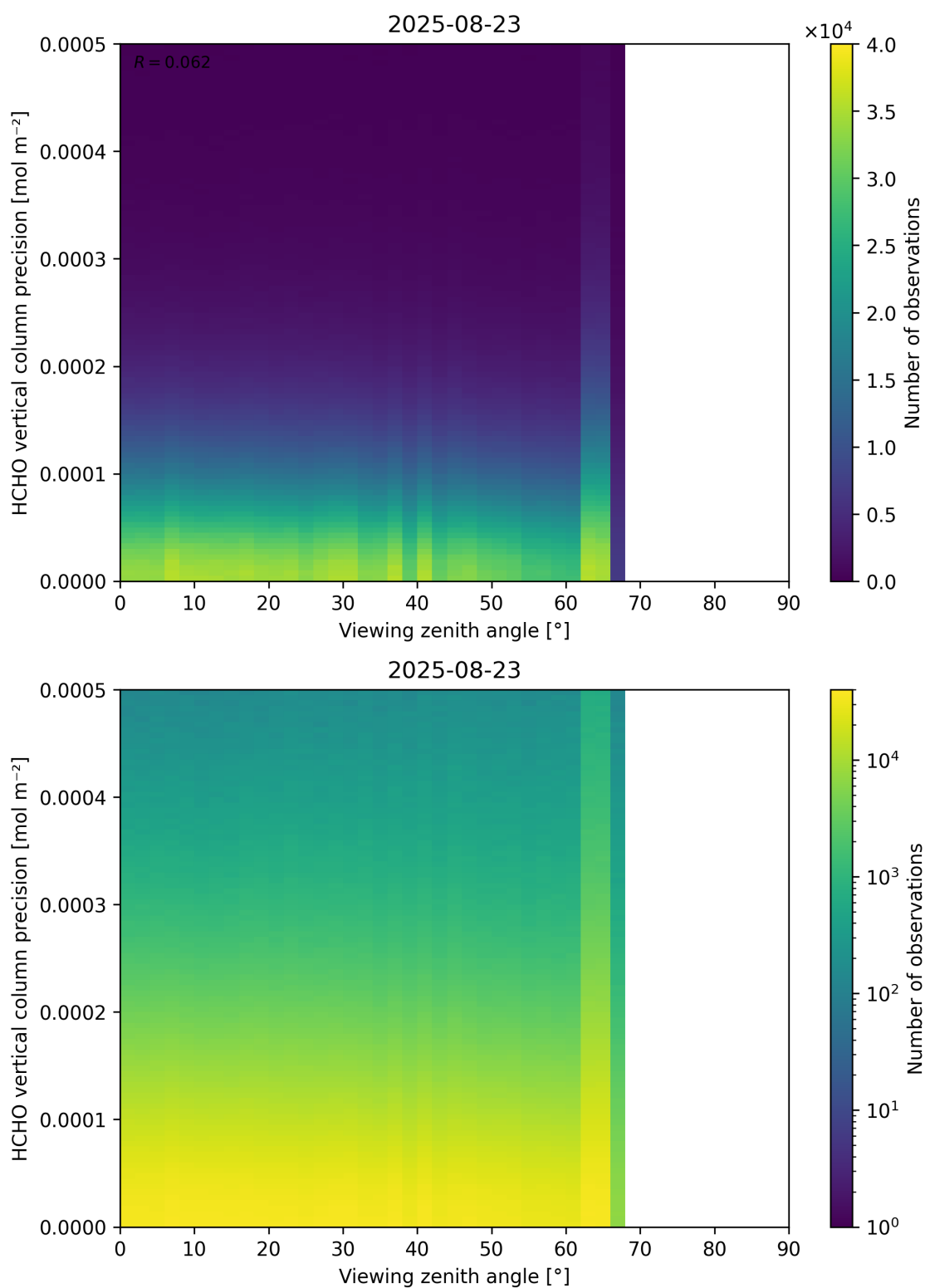
Figure 194: Scatter density plot of “Viewing zenith angle” against “HCHO vertical column precision” for 2025-08-22 to 2025-08-24.
