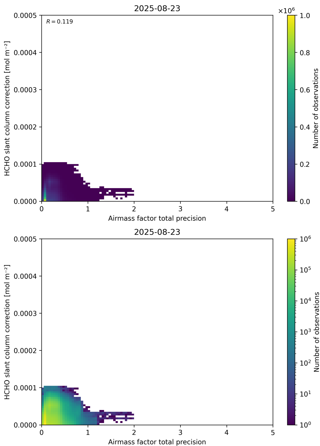
Figure 110: Scatter density plot of “Airmass factor total precision” against “HCHO slant column correction” for 2025-08-22 to 2025-08-24.
