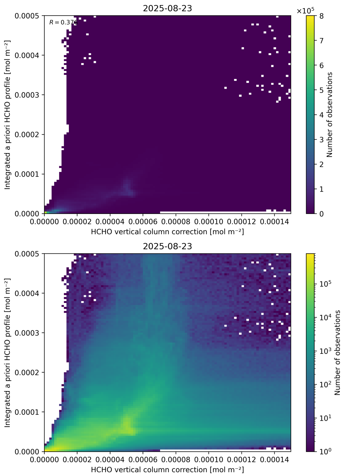
Figure 122: Scatter density plot of “HCHO vertical column correction” against “Integrated a priori HCHO profile” for 2025-08-22 to 2025-08-24.
