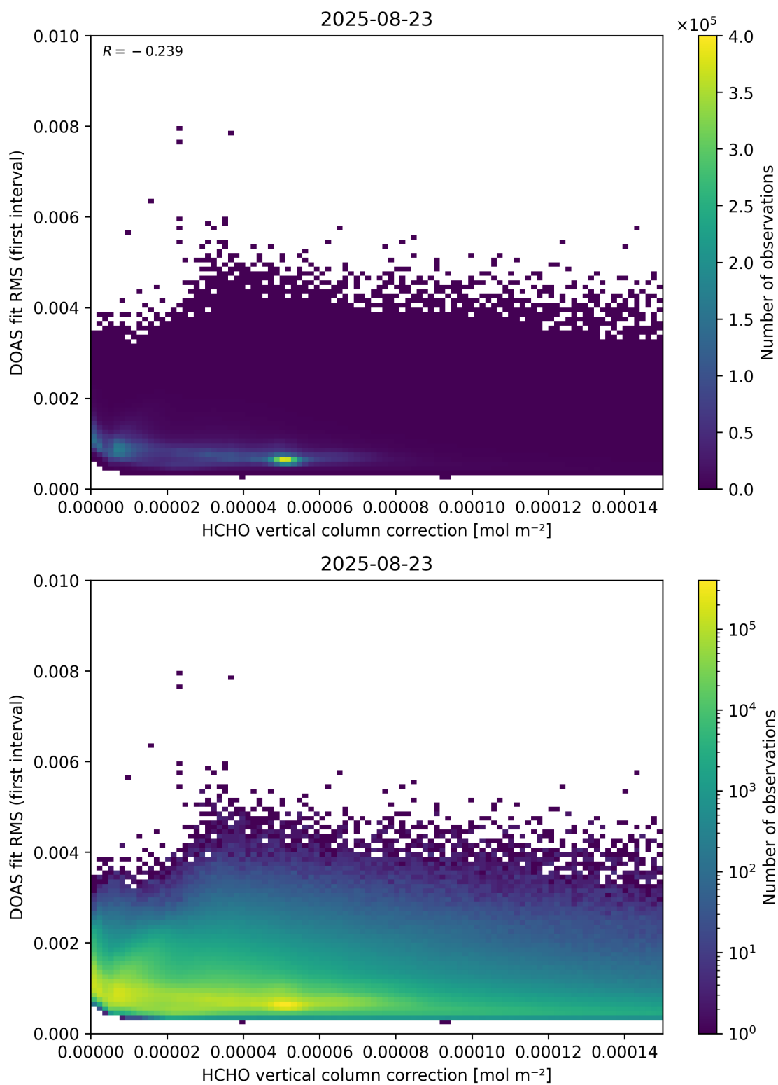
Figure 112: Scatter density plot of “HCHO vertical column correction” against “DOAS fit RMS (first interval)” for 2025-08-22 to 2025-08-24.
