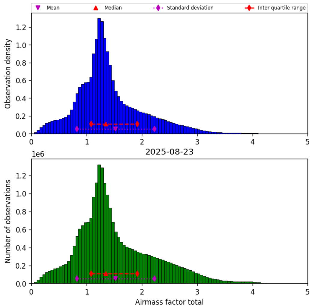
Figure 40: Histogram of “Airmass factor total” for 2025-08-22 to 2025-08-24
