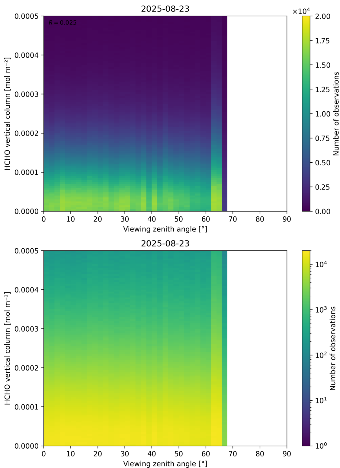
Figure 192: Scatter density plot of “Viewing zenith angle” against “HCHO vertical column” for 2025-08-22 to 2025-08-24.
