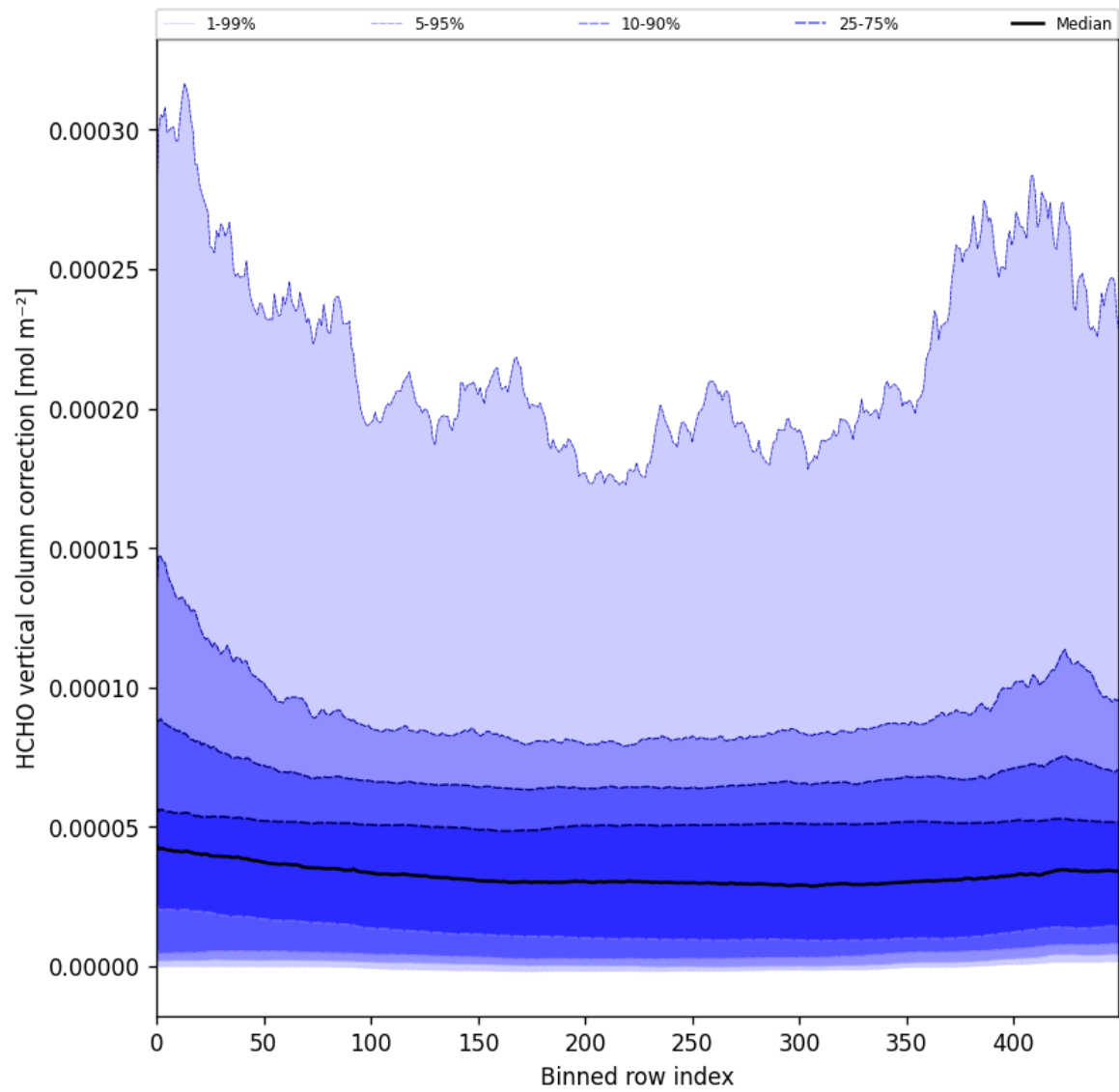
Figure 51: Along track statistics of “HCHO vertical column correction” for 2025-08-22 to 2025-08-24
