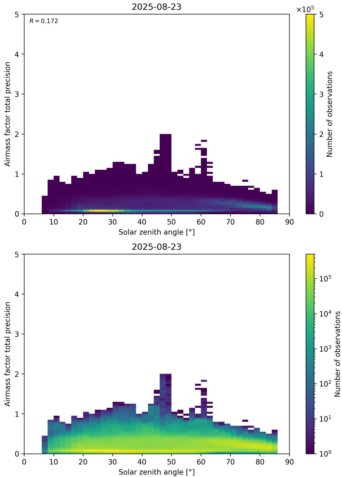
Figure 176: Scatter density plot of “Solar zenith angle” against “Airmass factor total precision” for 2025-08-22 to 2025-08-24.
