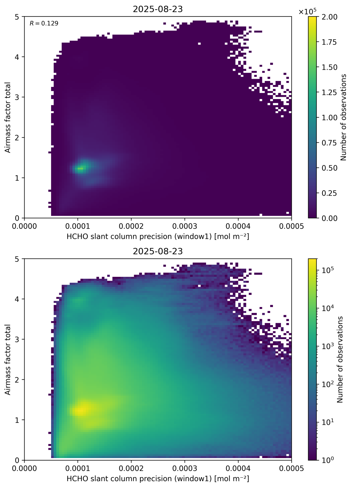
Figure 94: Scatter density plot of “HCHO slant column precision (window1)” against “Airmass factor total” for 2025-08-22 to 2025-08-24.
