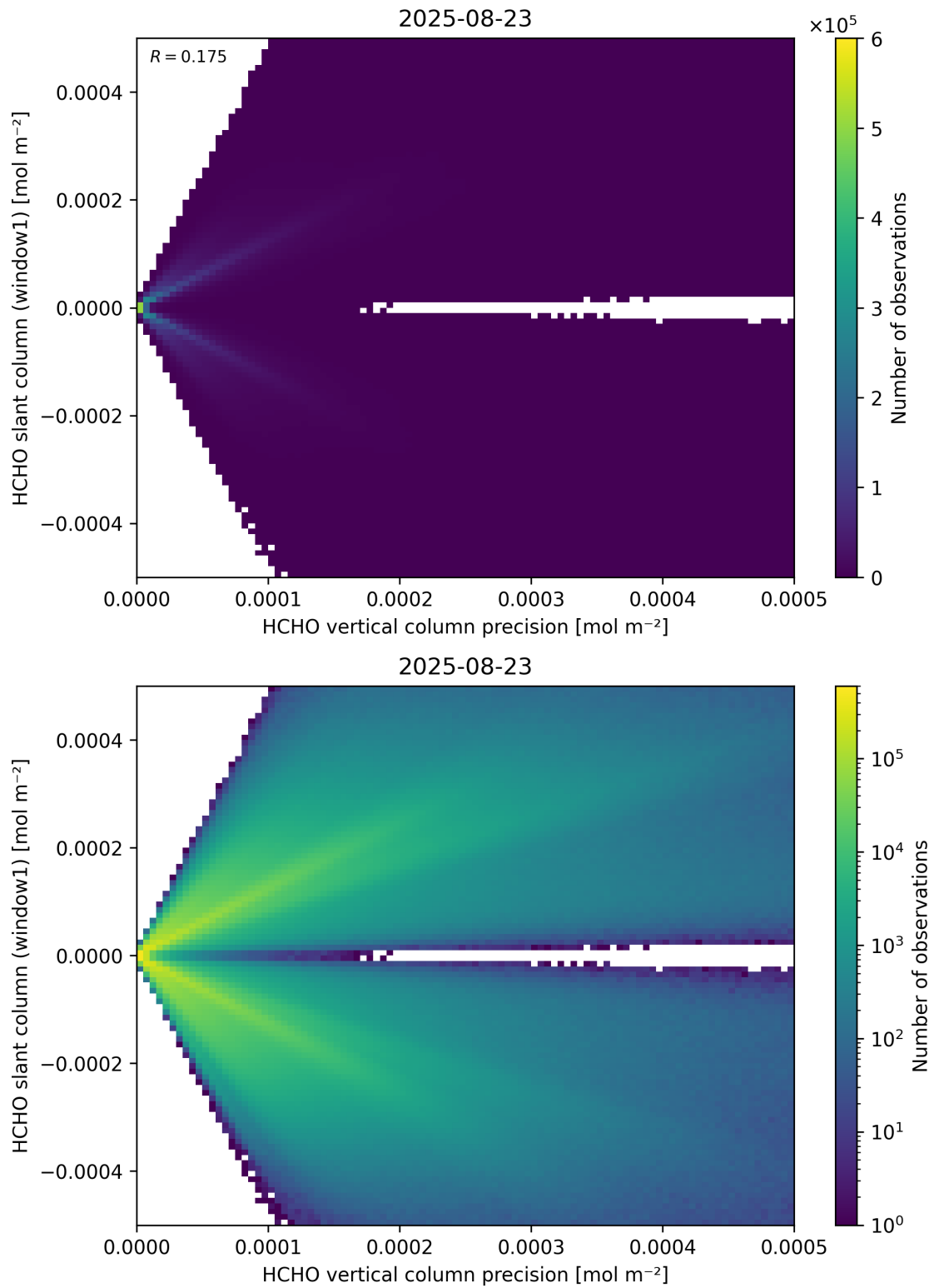
Figure 142: Scatter density plot of “HCHO vertical column precision” against “HCHO slant column (window1)” for 2025-08-22 to 2025-08-24.
