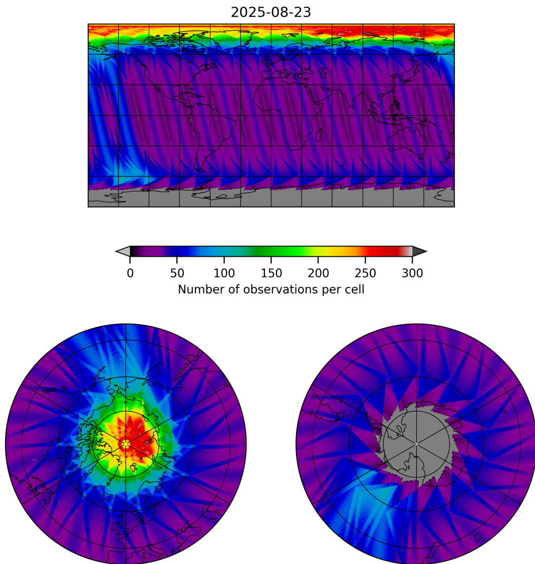
Figure 19: Map of the number of observations for 2025-08-22 to 2025-08-24
