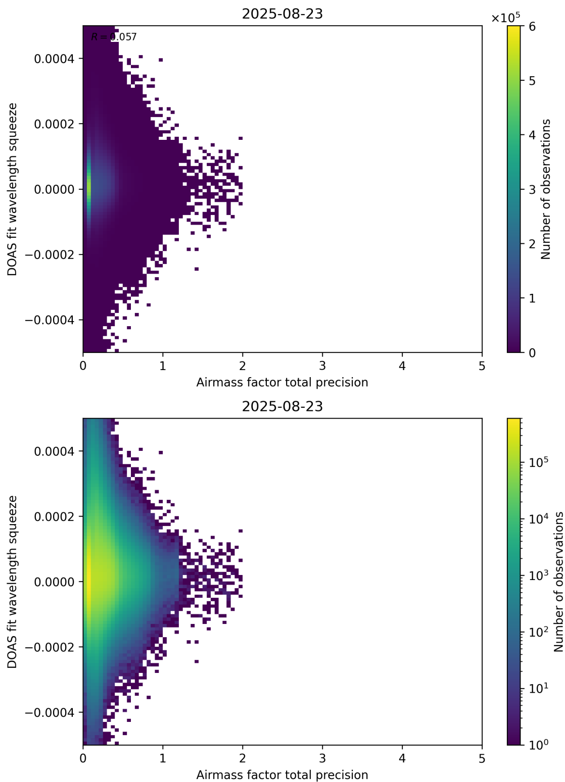
Figure 107: Scatter density plot of “Airmass factor total precision” against “DOAS fit wavelength squeeze” for 2025-08-22 to 2025-08-24.
