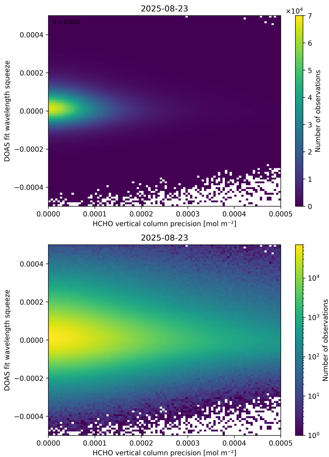
Figure 138: Scatter density plot of “HCHO vertical column precision” against “DOAS fit wavelength squeeze” for 2025-08-22 to 2025-08-24.
