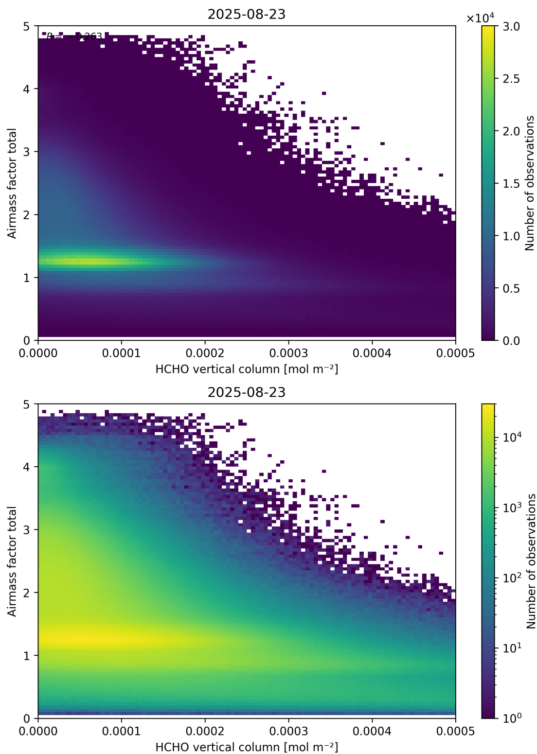
Figure 131: Scatter density plot of “HCHO vertical column” against “Airmass factor total” for 2025-08-22 to 2025-08-24.
