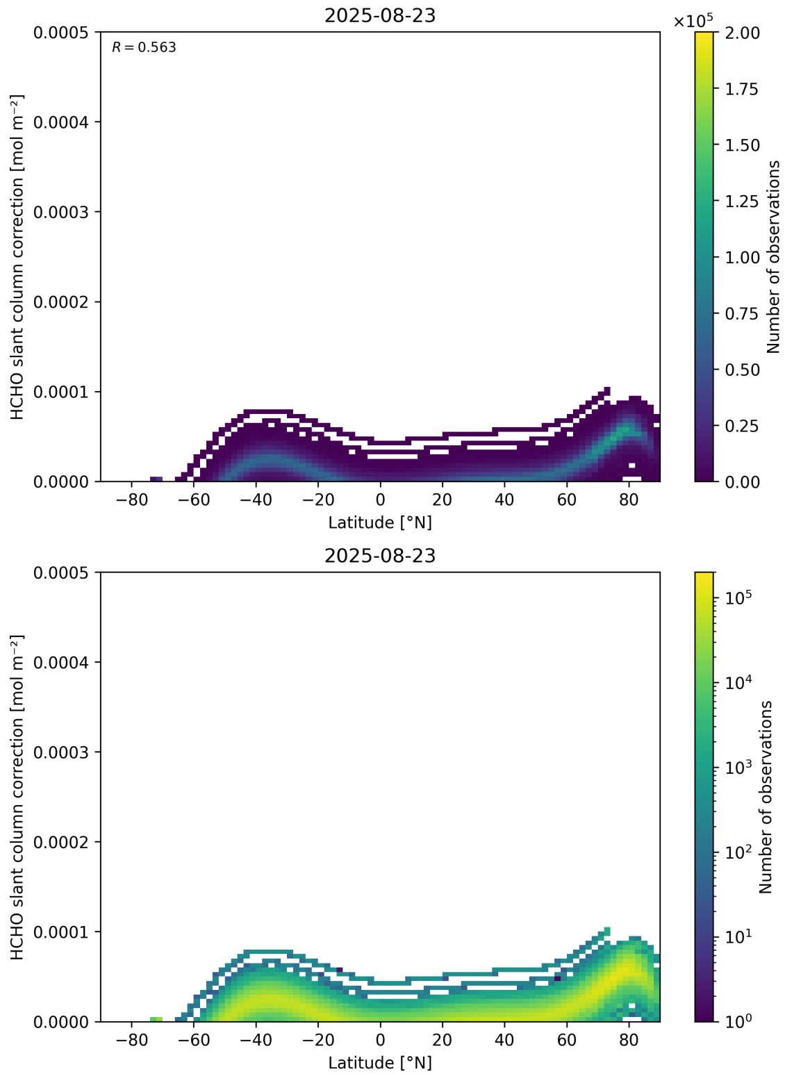
Figure 158: Scatter density plot of “Latitude” against “HCHO slant column correction” for 2025-08-22 to 2025-08-24.
