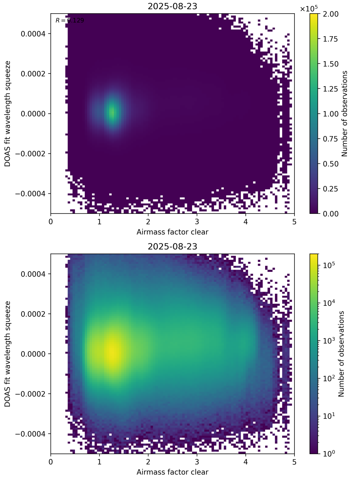
Figure 73: Scatter density plot of “Airmass factor clear” against “DOAS fit wavelength squeeze” for 2025-08-22 to 2025-08-24.
