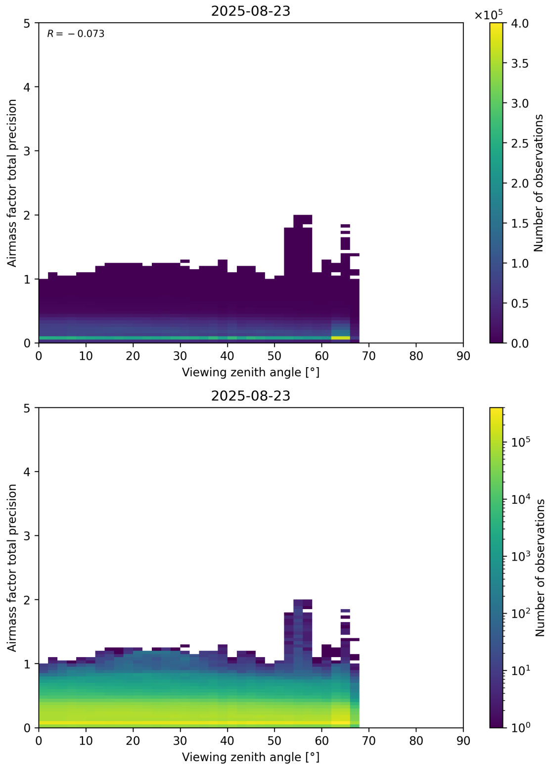
Figure 191: Scatter density plot of “Viewing zenith angle” against “Airmass factor total precision” for 2025-08-22 to 2025-08-24.
