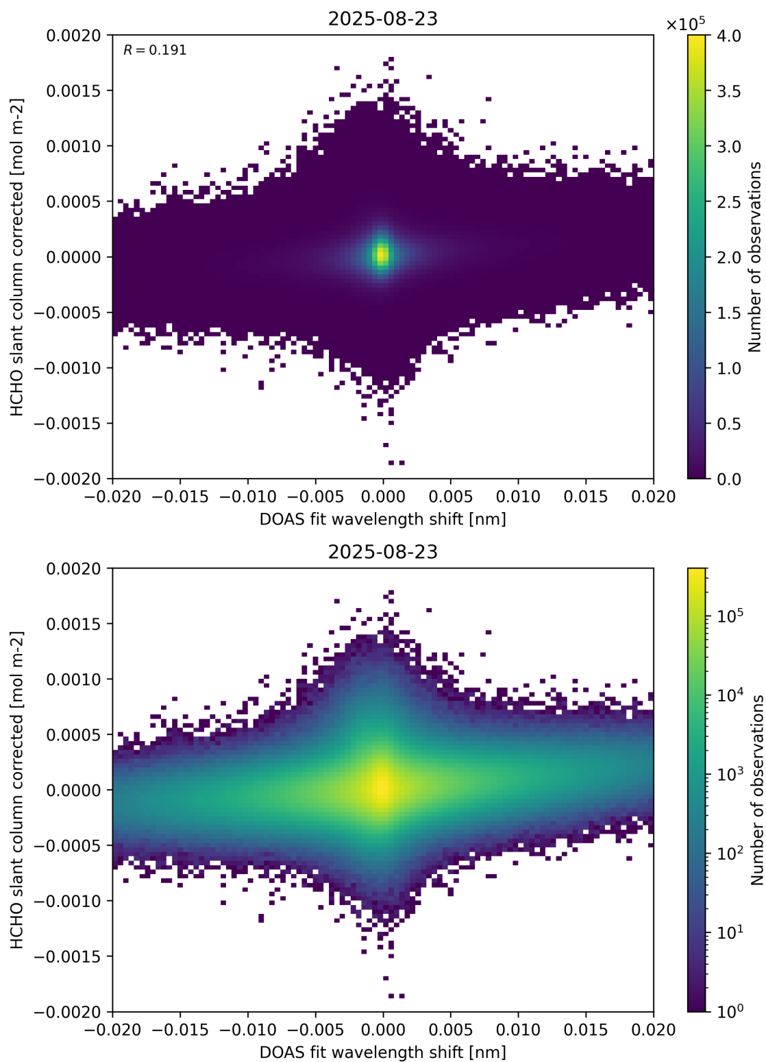
Figure 66: Scatter density plot of “DOAS fit wavelength shift” against “HCHO slant column corrected” for 2025-08-22 to 2025-08-24.
