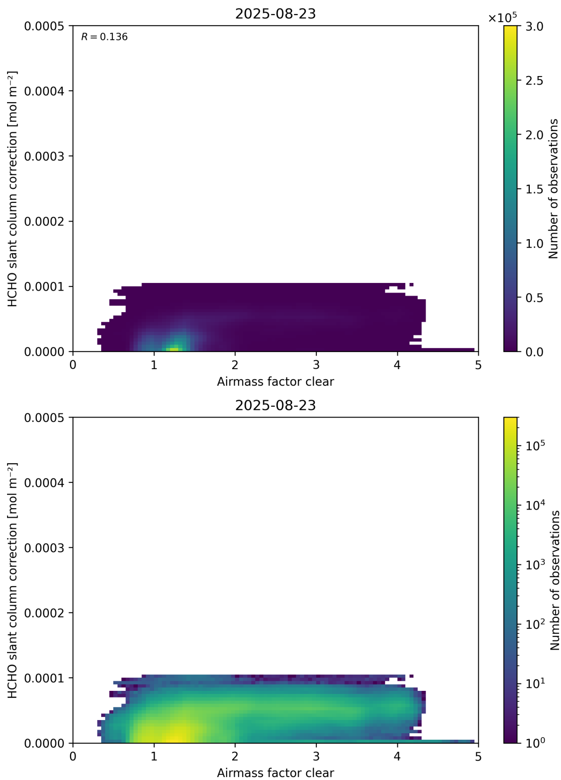
Figure 75: Scatter density plot of “Airmass factor clear” against “HCHO slant column correction” for 2025-08-22 to 2025-08-24.
