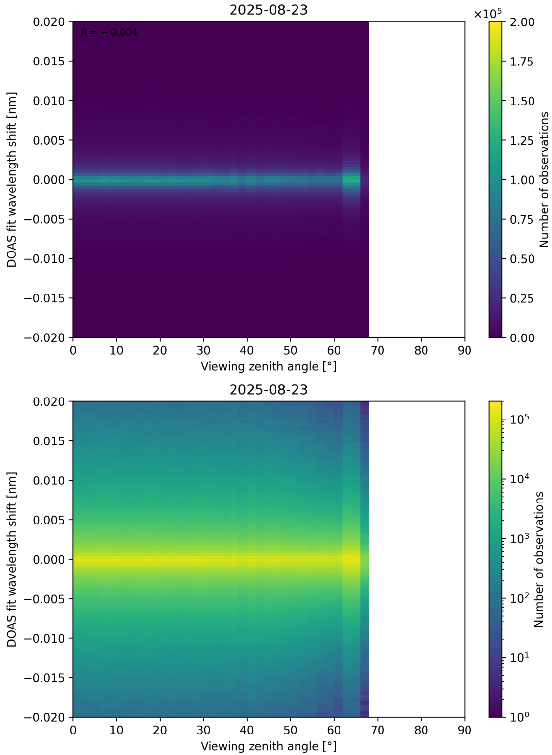
Figure 183: Scatter density plot of “Viewing zenith angle” against “DOAS fit wavelength shift” for 2025-08-22 to 2025-08-24.
