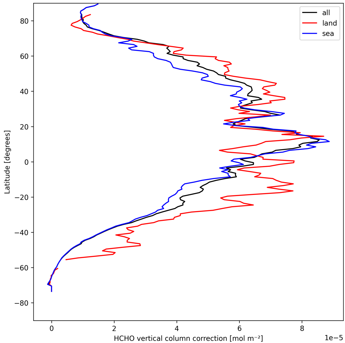
Figure 23: Zonal average of “HCHO vertical column correction” for 2025-08-22 to 2025-08-24.
