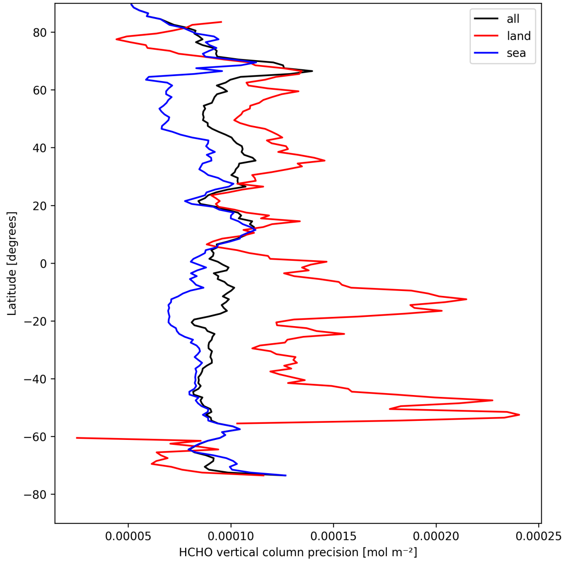
Figure 22: Zonal average of “HCHO vertical column precision” for 2025-08-22 to 2025-08-24.
