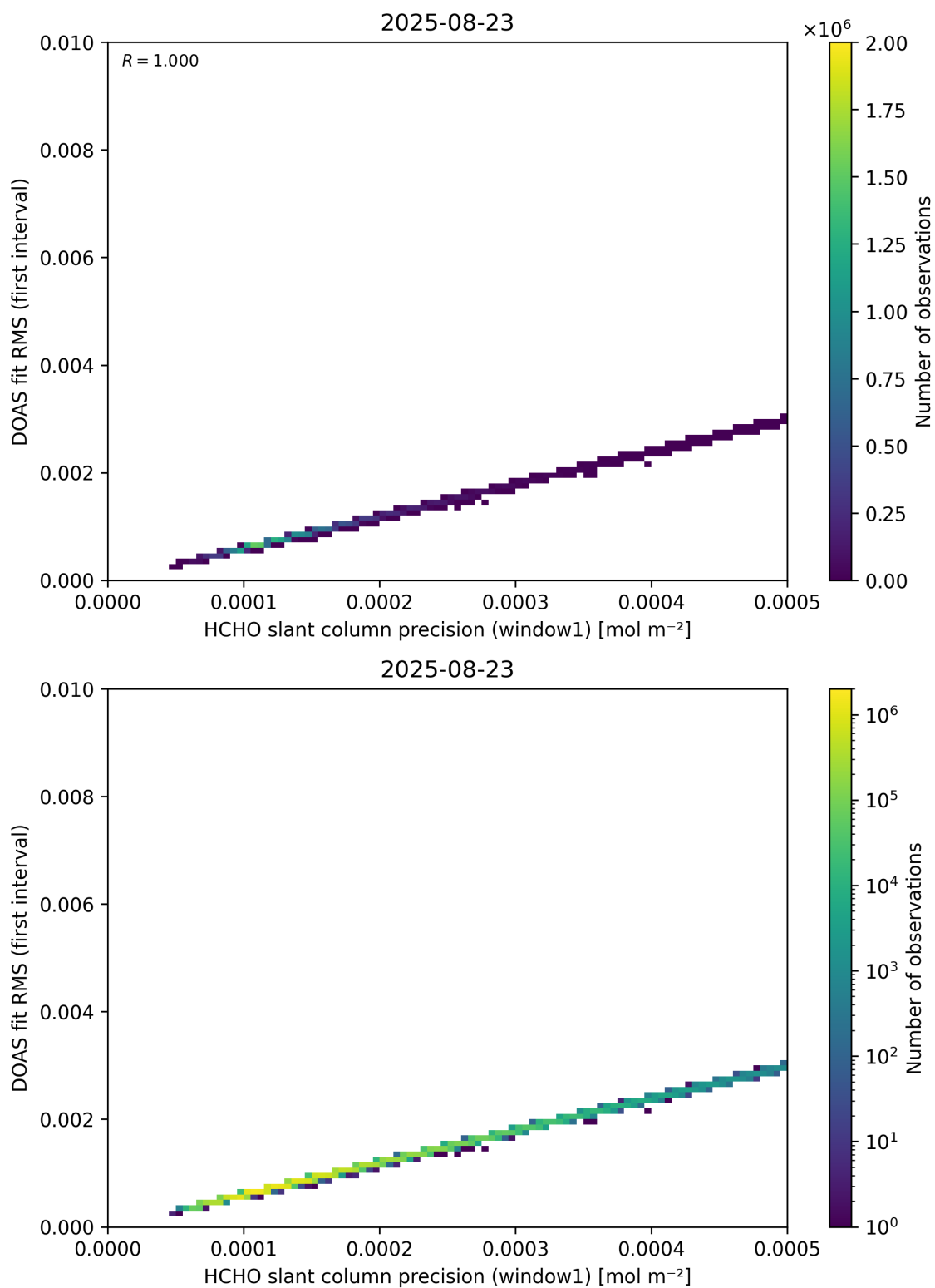
Figure 88: Scatter density plot of “HCHO slant column precision (window1)” against “DOAS fit RMS (first interval)” for 2025-08-22 to 2025-08-24.
