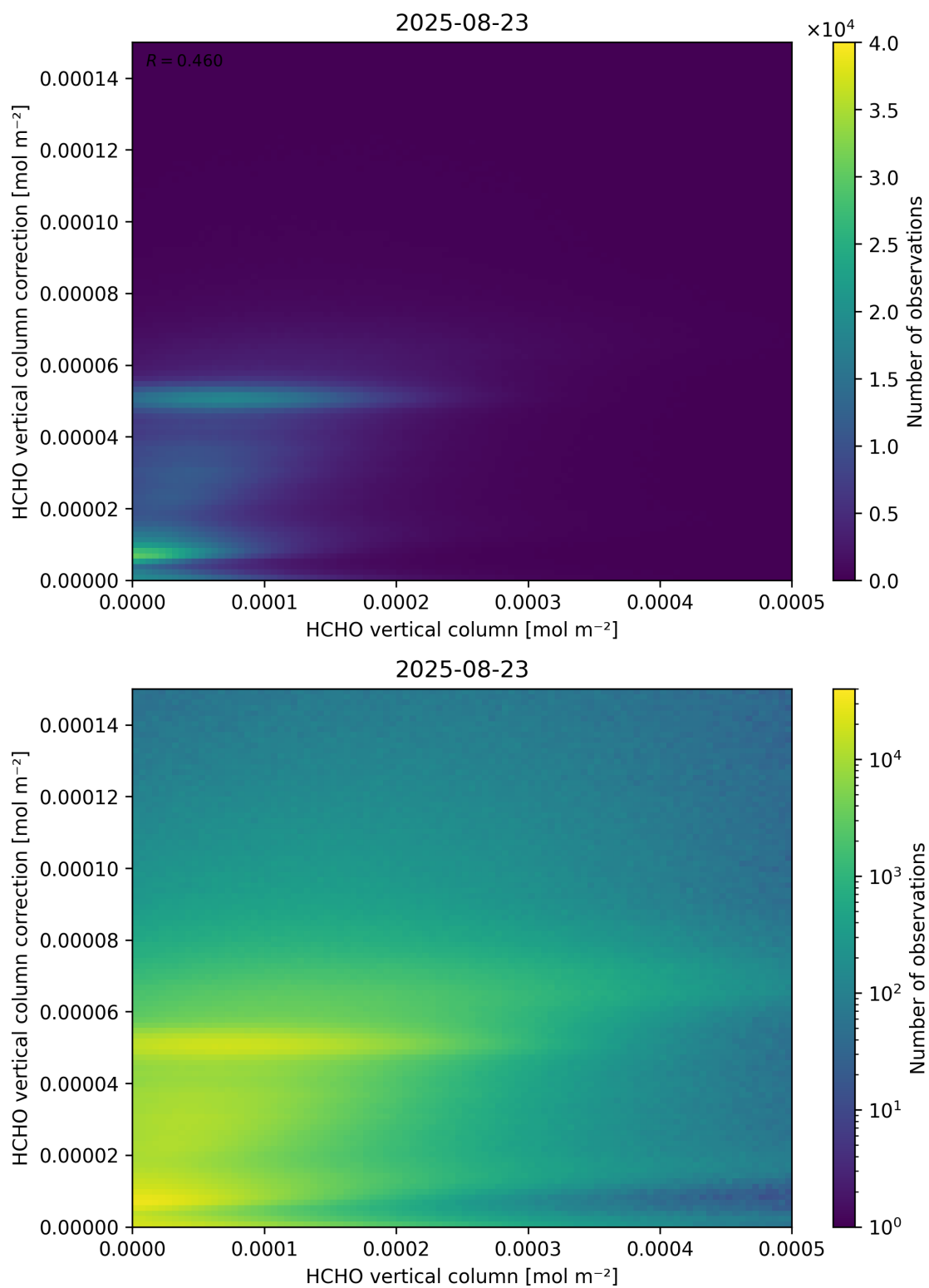
Figure 133: Scatter density plot of “HCHO vertical column” against “HCHO vertical column correction” for 2025-08-22 to 2025-08-24.
