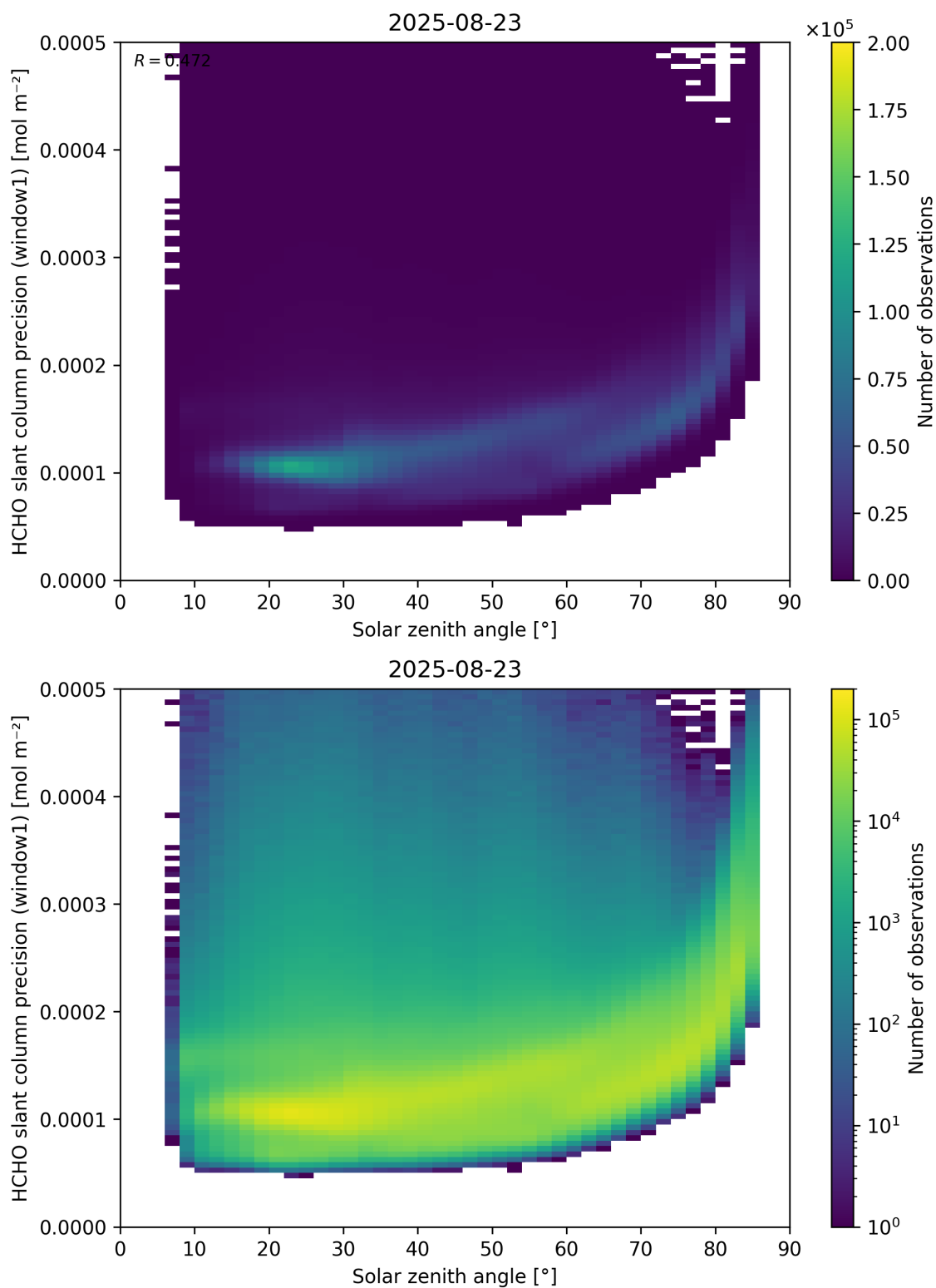
Figure 174: Scatter density plot of “Solar zenith angle” against “HCHO slant column precision (window1)” for 2025-08-22 to 2025-08-24.
