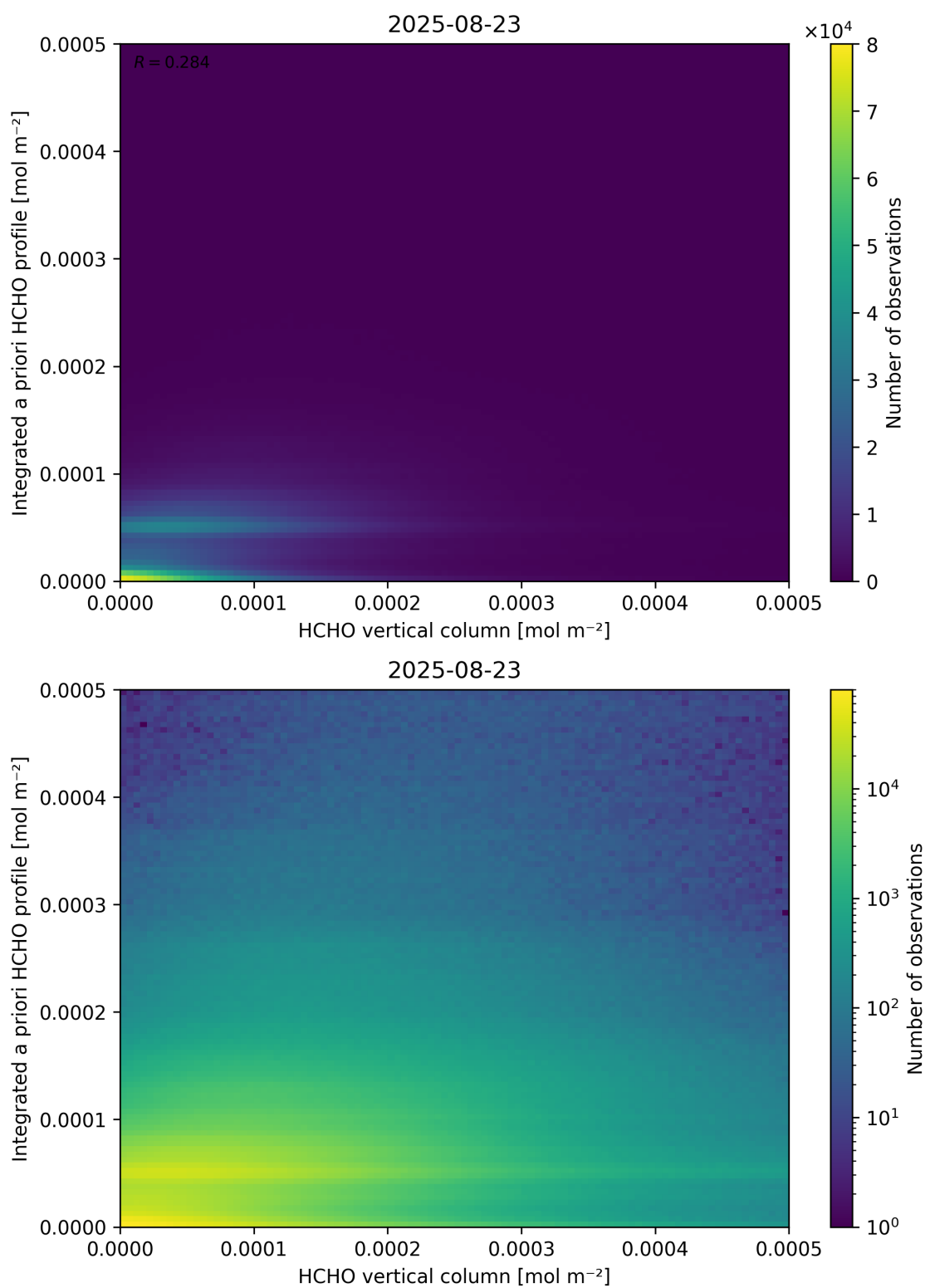
Figure 135: Scatter density plot of “HCHO vertical column” against “Integrated a priori HCHO profile” for 2025-08-22 to 2025-08-24.
