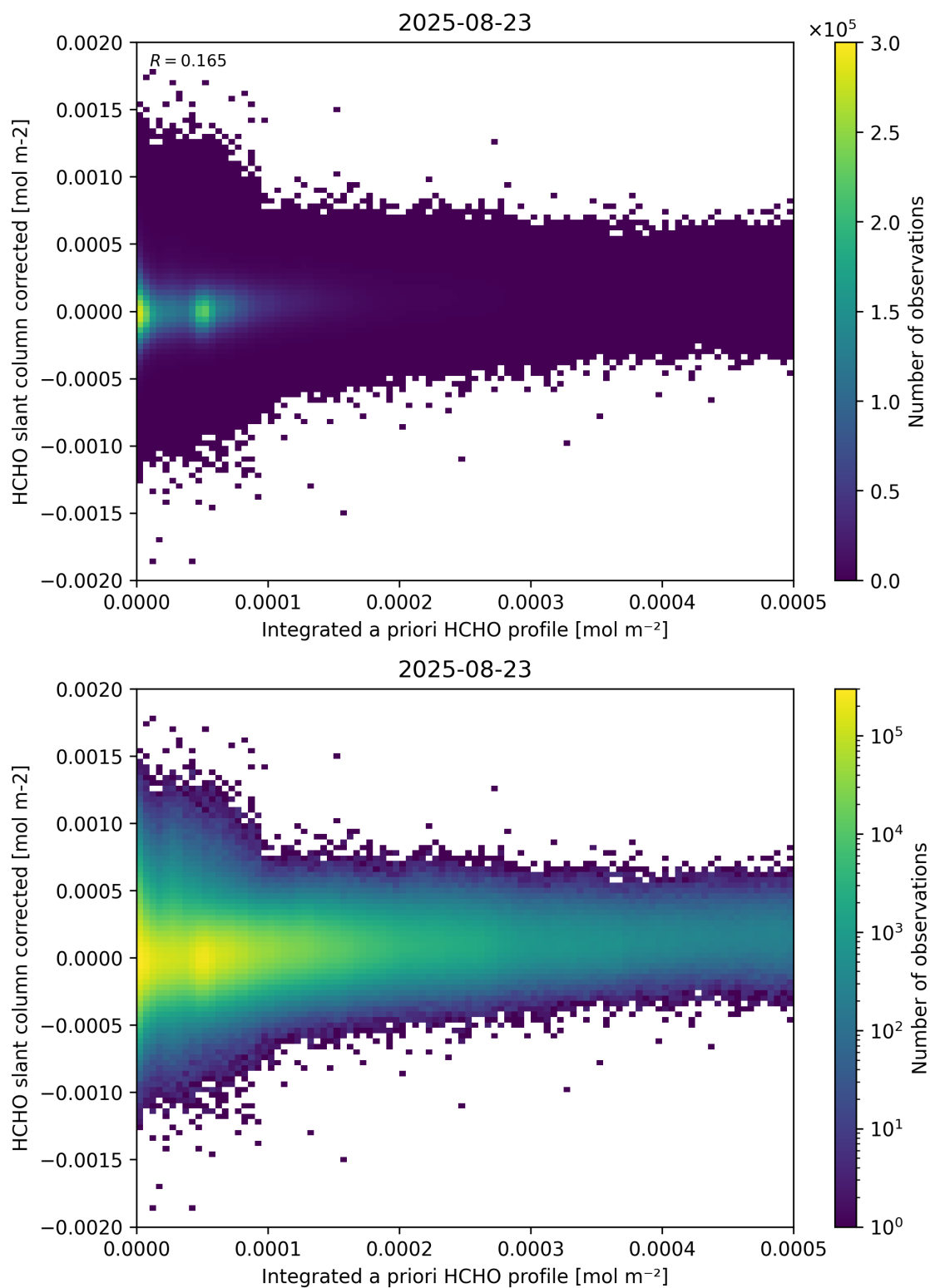
Figure 151: Scatter density plot of “Integrated a priori HCHO profile” against “HCHO slant column corrected” for 2025-08-22 to 2025-08-24.
