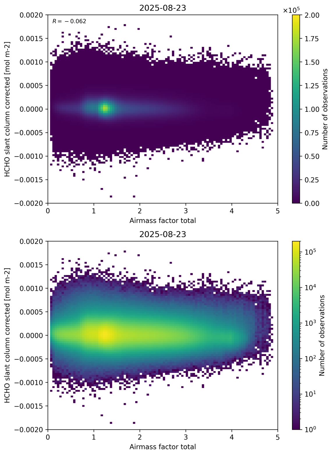
Figure 101: Scatter density plot of “Airmass factor total” against “HCHO slant column corrected” for 2025-08-22 to 2025-08-24.
