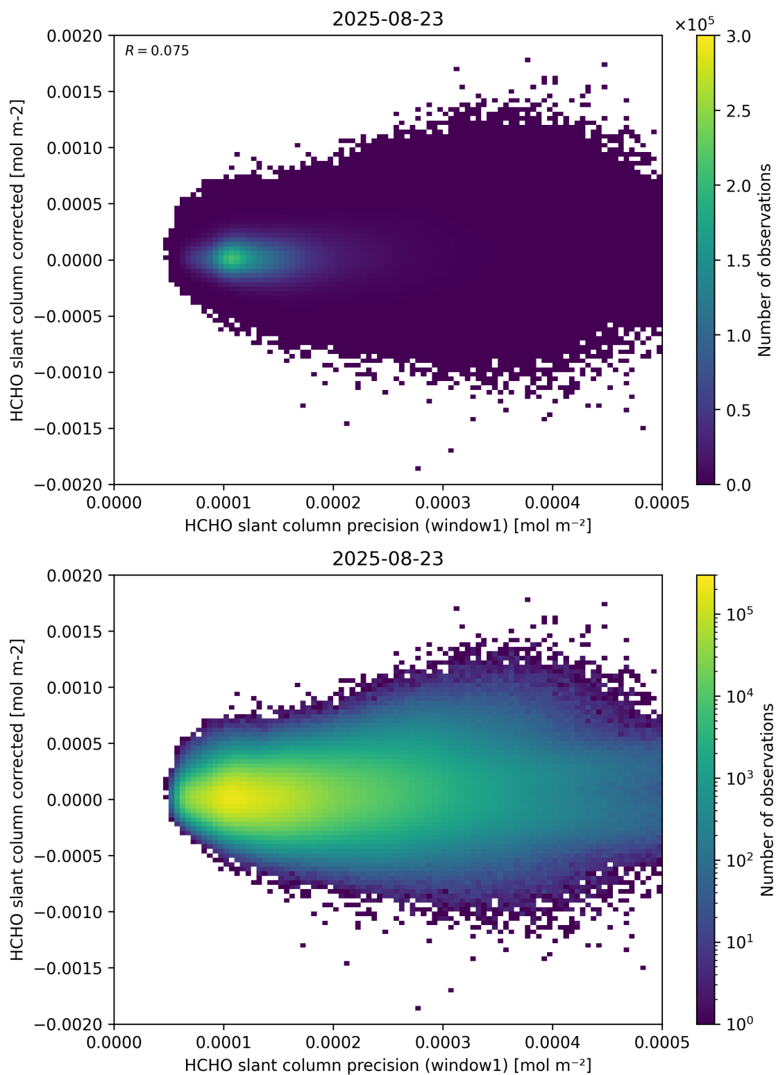
Figure 92: Scatter density plot of “HCHO slant column precision (window1)” against “HCHO slant column corrected” for 2025-08-22 to 2025-08-24.
