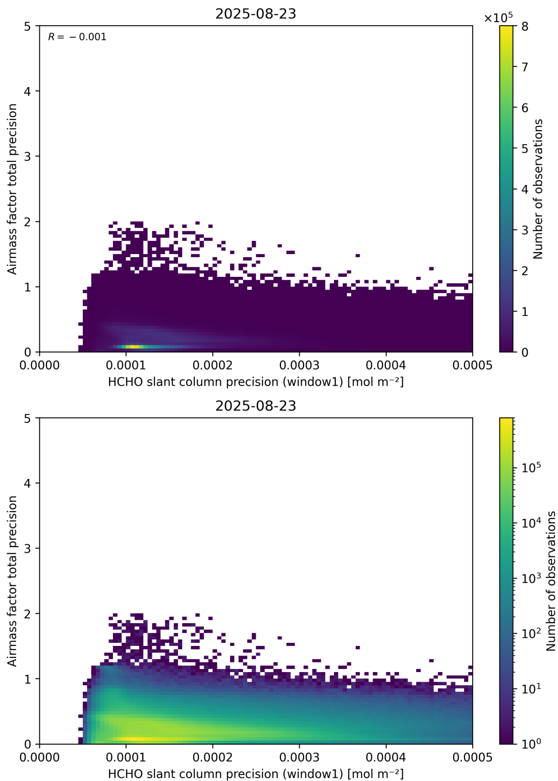
Figure 95: Scatter density plot of “HCHO slant column precision (window1)” against “Airmass factor total precision” for 2025-08-22 to 2025-08-24.
