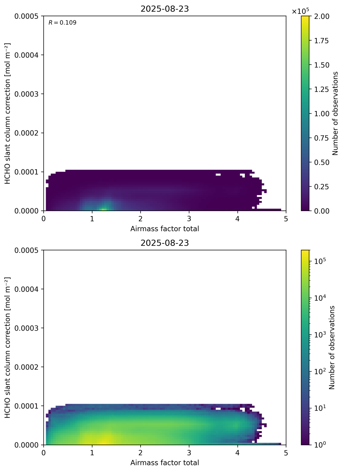
Figure 102: Scatter density plot of “Airmass factor total” against “HCHO slant column correction” for 2025-08-22 to 2025-08-24.
