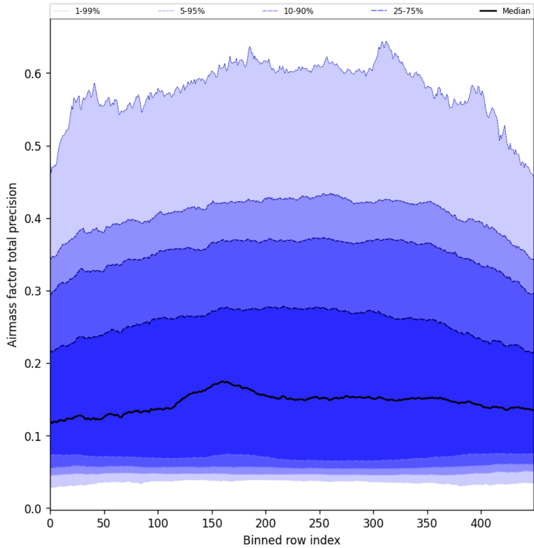
Figure 55: Along track statistics of “Airmass factor total precision” for 2025-08-22 to 2025-08-24
