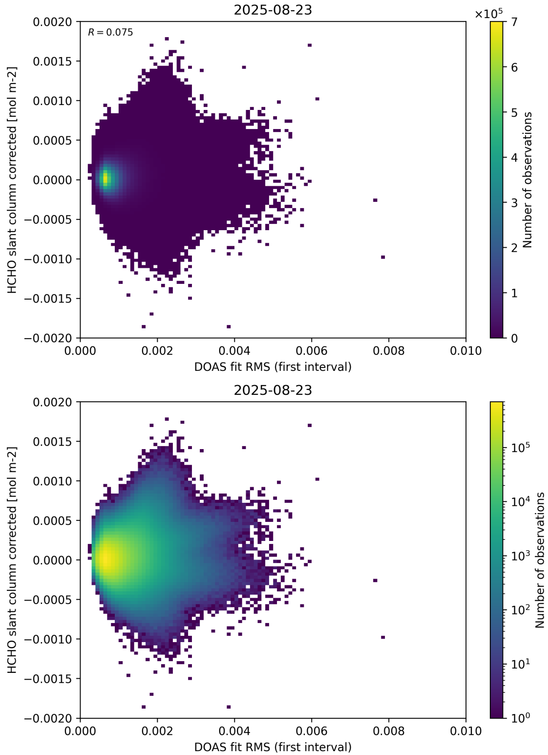
Figure 62: Scatter density plot of “DOAS fit RMS (first interval)” against “HCHO slant column corrected” for 2025-08-22 to 2025-08-24.
