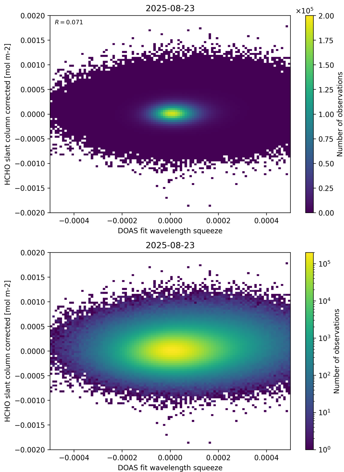
Figure 69: Scatter density plot of “DOAS fit wavelength squeeze” against “HCHO slant column corrected” for 2025-08-22 to 2025-08-24.
