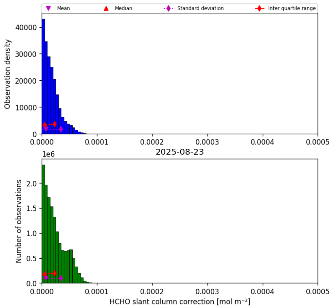
Figure 47: Histogram of “HCHO slant column correction” for 2025-08-22 to 2025-08-24
