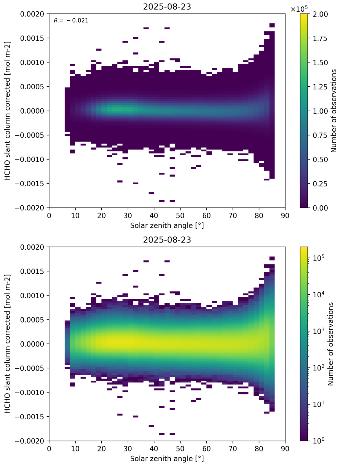
Figure 171: Scatter density plot of “Solar zenith angle” against “HCHO slant column corrected” for 2025-08-22 to 2025-08-24.
