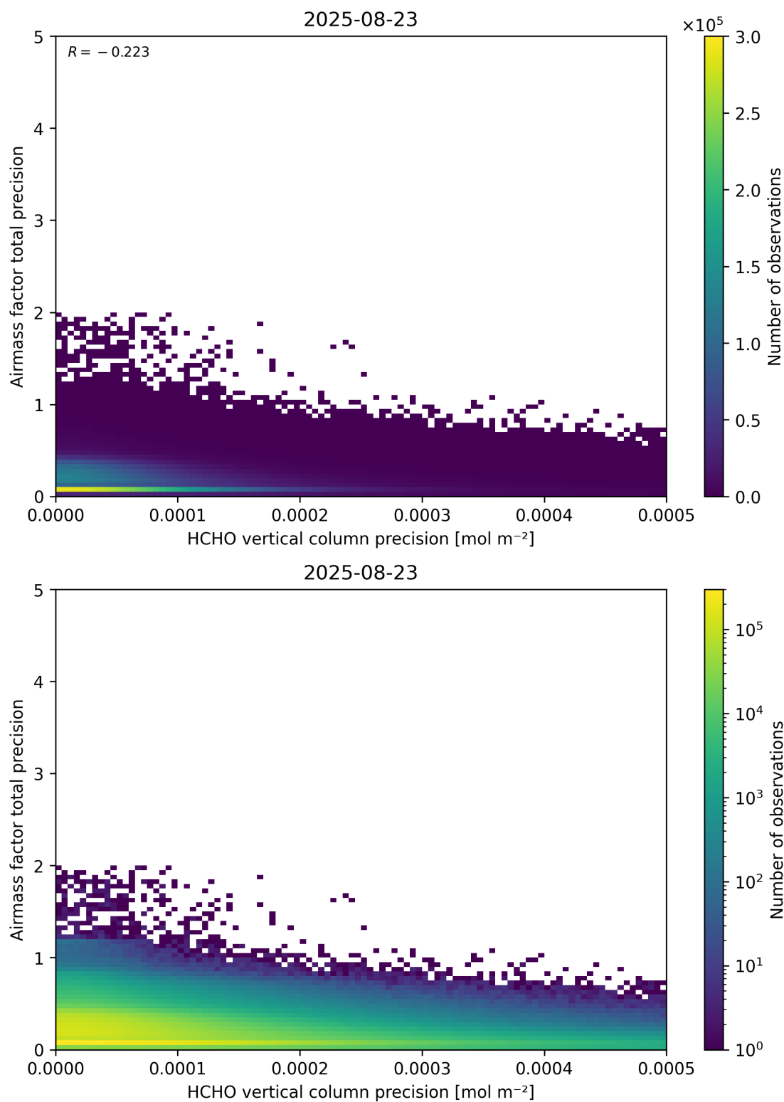
Figure 145: Scatter density plot of “HCHO vertical column precision” against “Airmass factor total precision” for 2025-08-22 to 2025-08-24.
