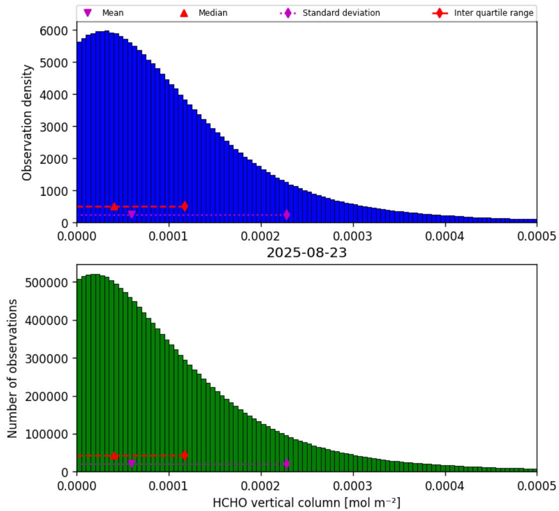
Figure 35: Histogram of “HCHO vertical column” for 2025-08-22 to 2025-08-24
