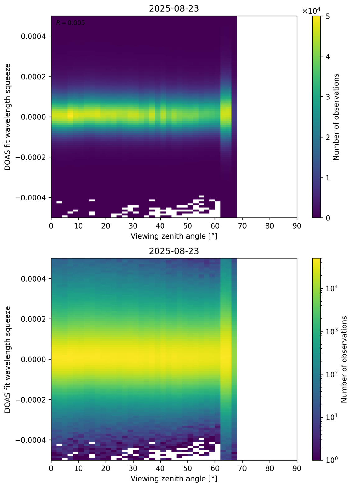
Figure 184: Scatter density plot of “Viewing zenith angle” against “DOAS fit wavelength squeeze” for 2025-08-22 to 2025-08-24.
