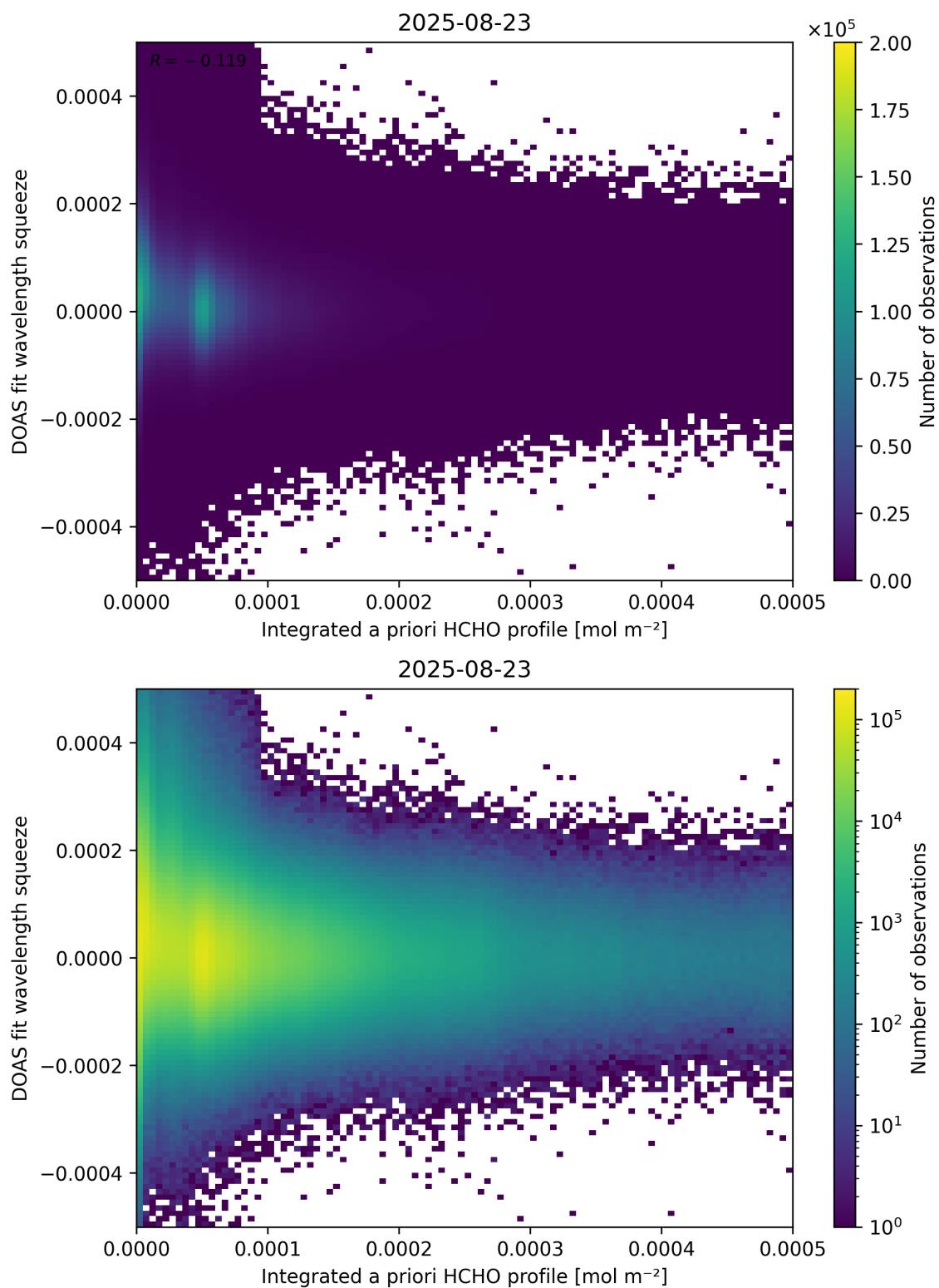
Figure 150: Scatter density plot of “Integrated a priori HCHO profile” against “DOAS fit wavelength squeeze” for 2025-08-22 to 2025-08-24.
