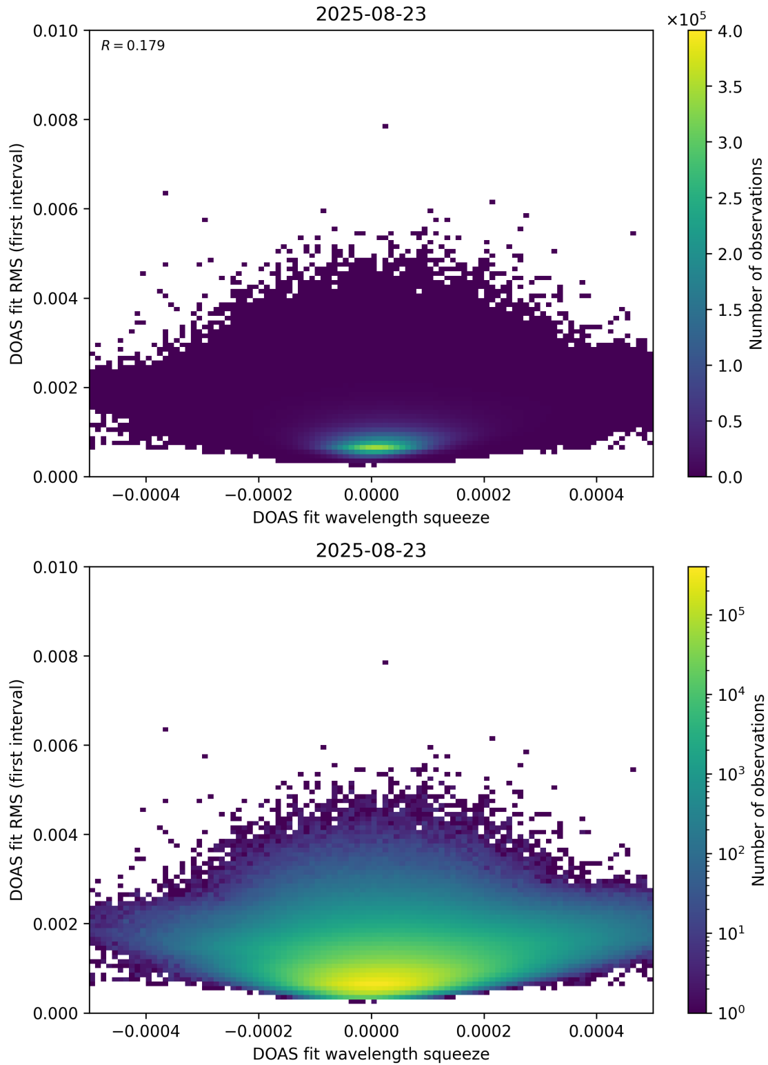
Figure 68: Scatter density plot of “DOAS fit wavelength squeeze” against “DOAS fit RMS (first interval)” for 2025-08-22 to 2025-08-24.
