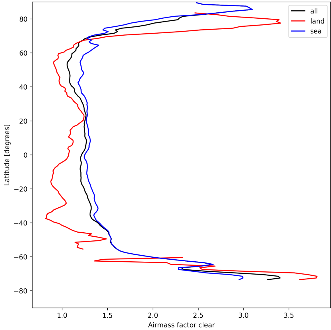
Figure 28: Zonal average of “Airmass factor clear” for 2025-08-22 to 2025-08-24.
