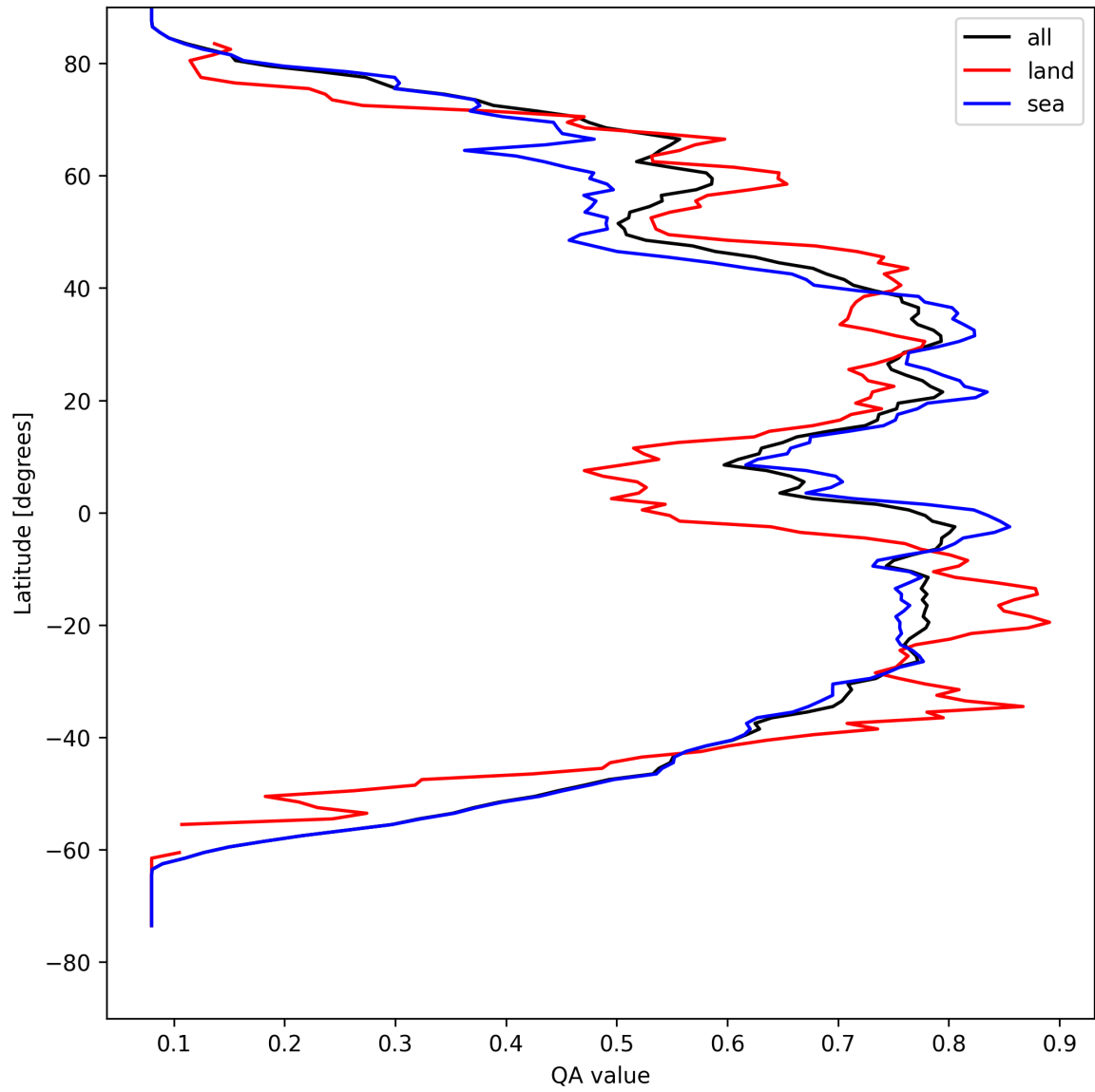
Figure 20: Zonal average of “QA value” for 2025-08-22 to 2025-08-24.
