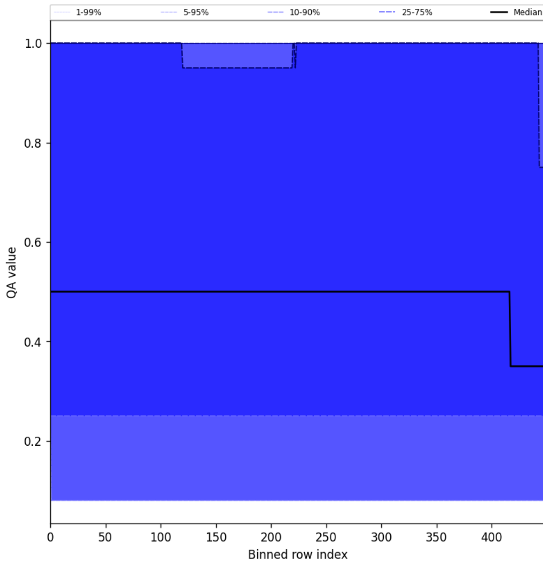
Figure 48: Along track statistics of “QA value” for 2025-08-22 to 2025-08-24
