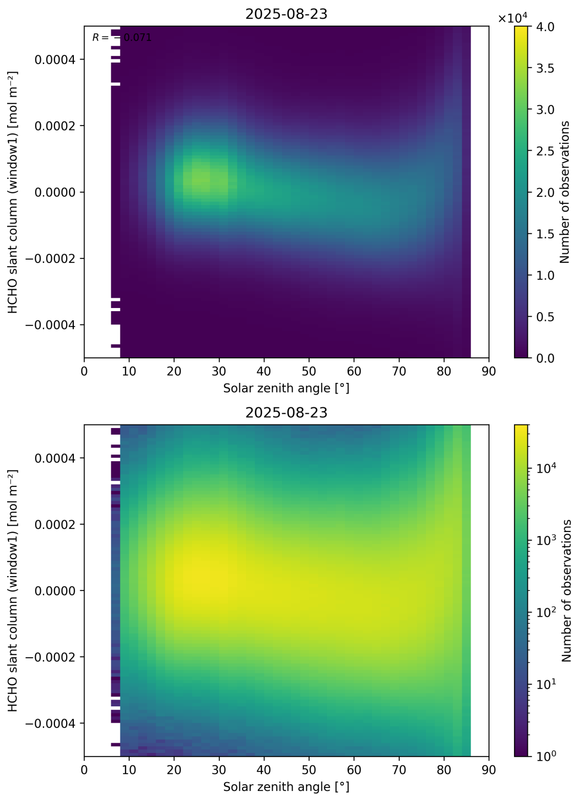
Figure 173: Scatter density plot of “Solar zenith angle” against “HCHO slant column (window1)” for 2025-08-22 to 2025-08-24.
