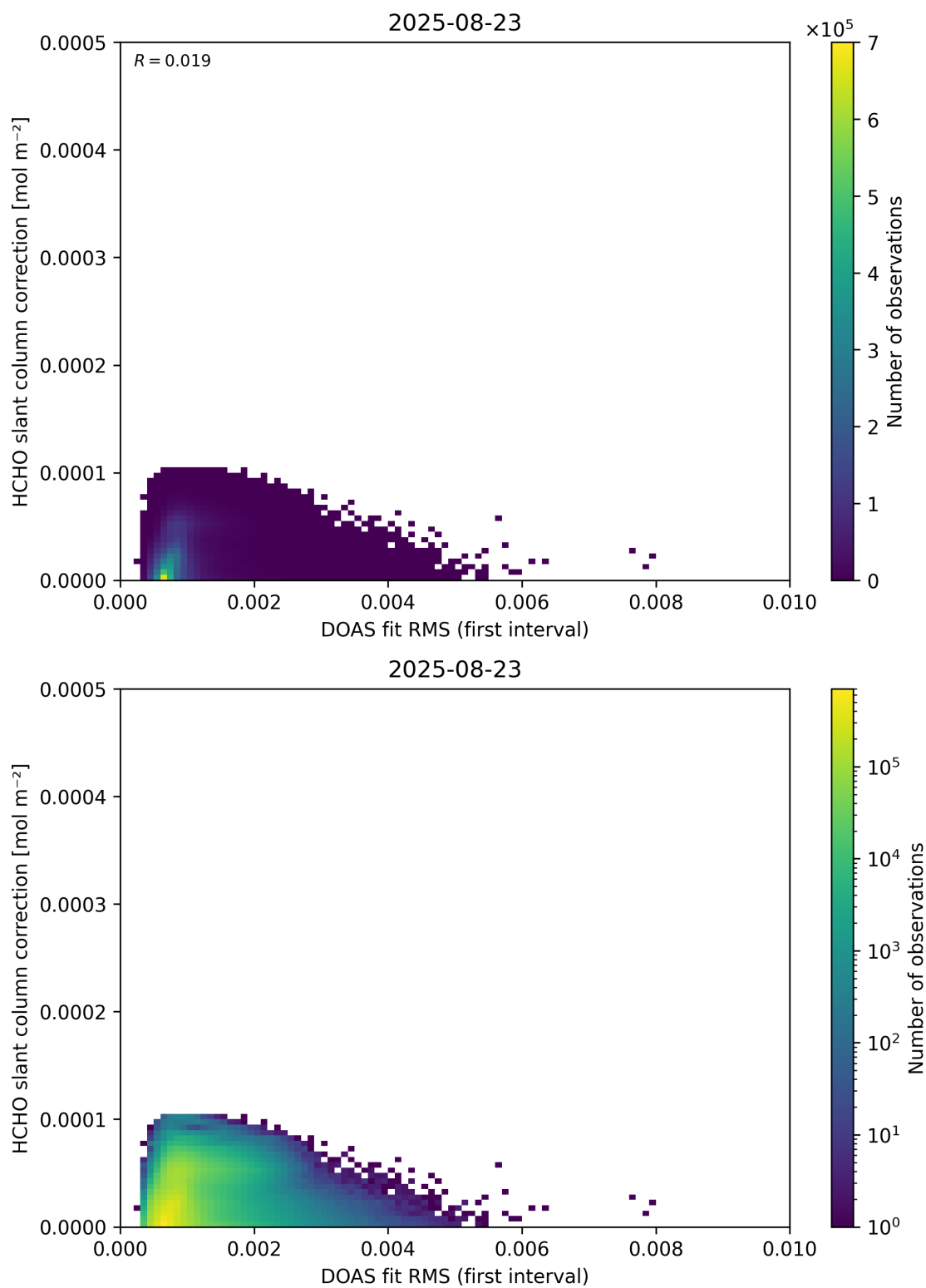
Figure 63: Scatter density plot of “DOAS fit RMS (first interval)” against “HCHO slant column correction” for 2025-08-22 to 2025-08-24.
