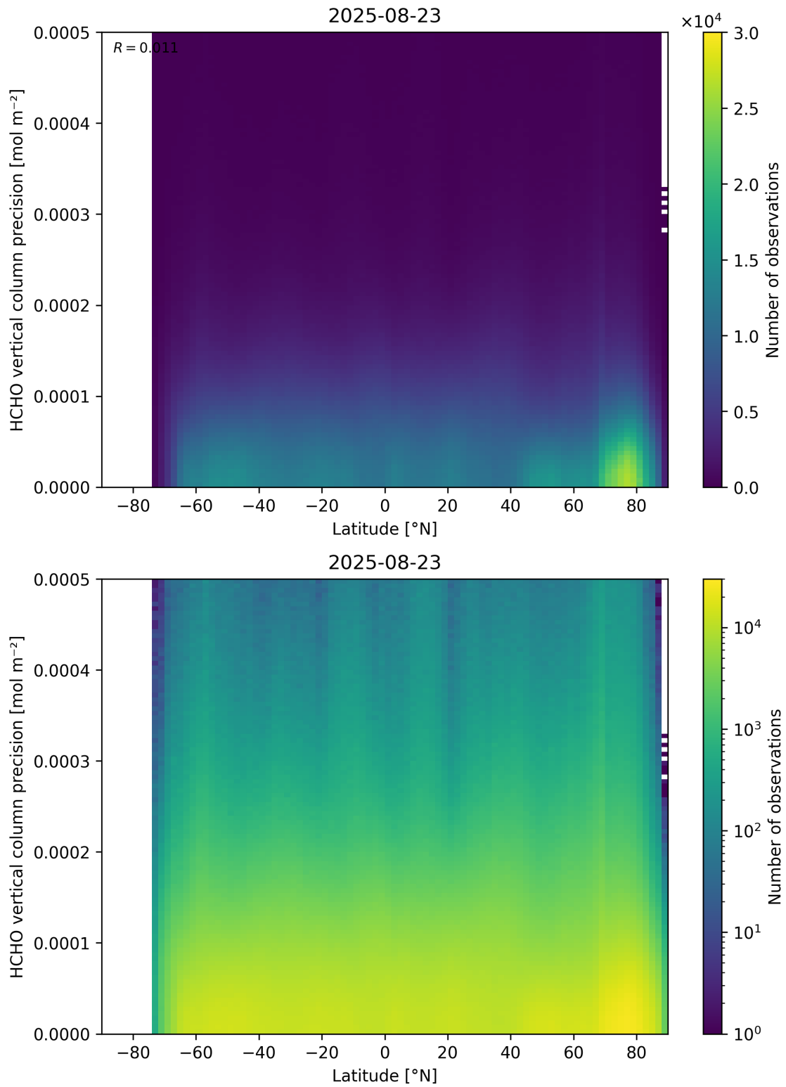
Figure 165: Scatter density plot of “Latitude” against “HCHO vertical column precision” for 2025-08-22 to 2025-08-24.
