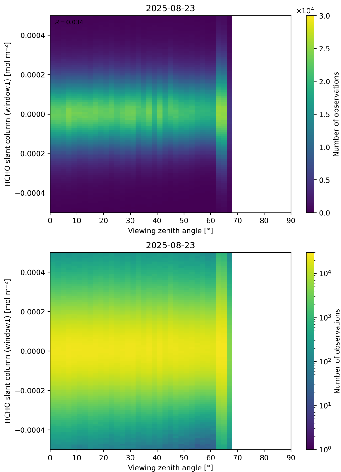
Figure 188: Scatter density plot of “Viewing zenith angle” against “HCHO slant column (window1)” for 2025-08-22 to 2025-08-24.
