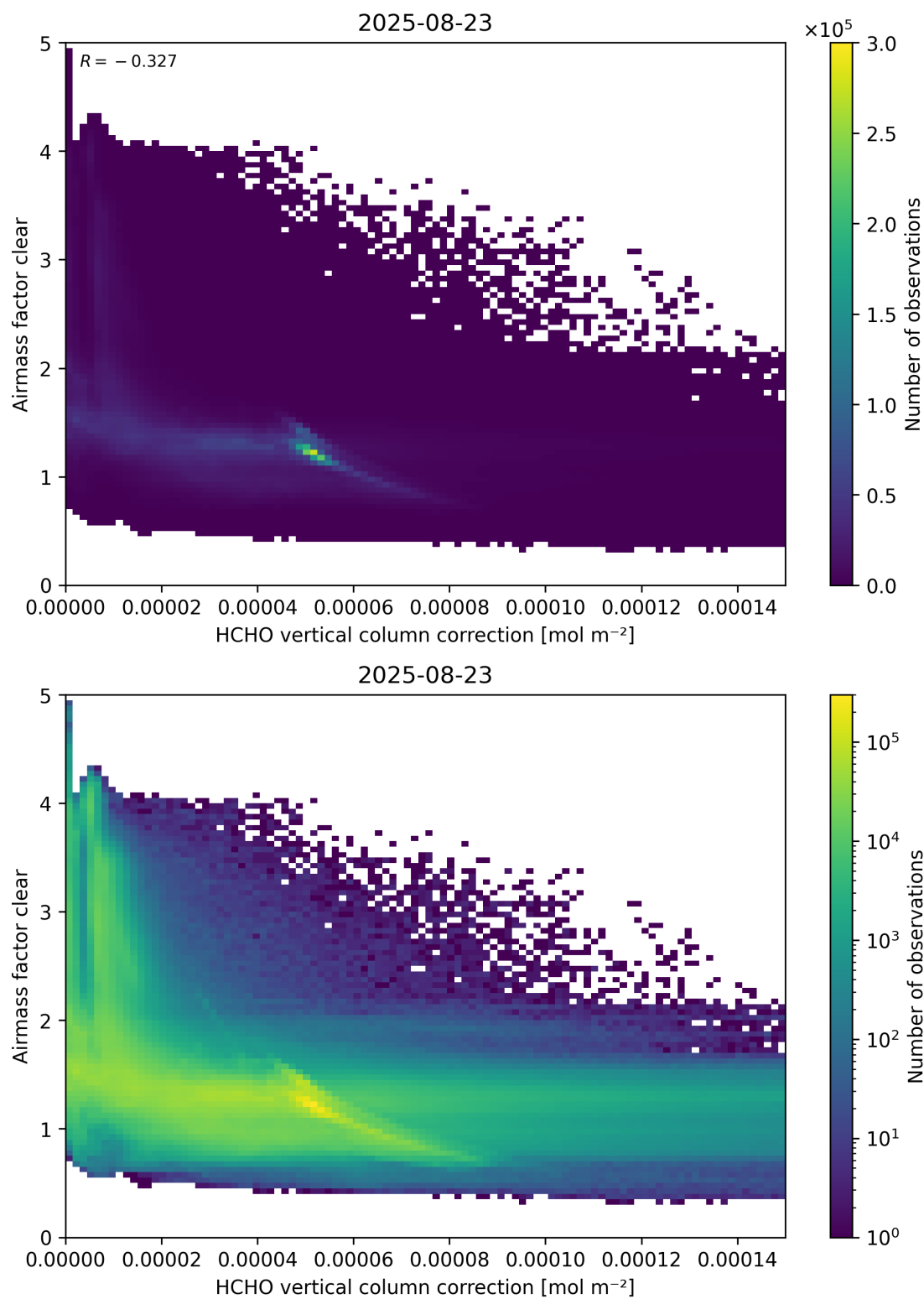
Figure 115: Scatter density plot of “HCHO vertical column correction” against “Airmass factor clear” for 2025-08-22 to 2025-08-24.
