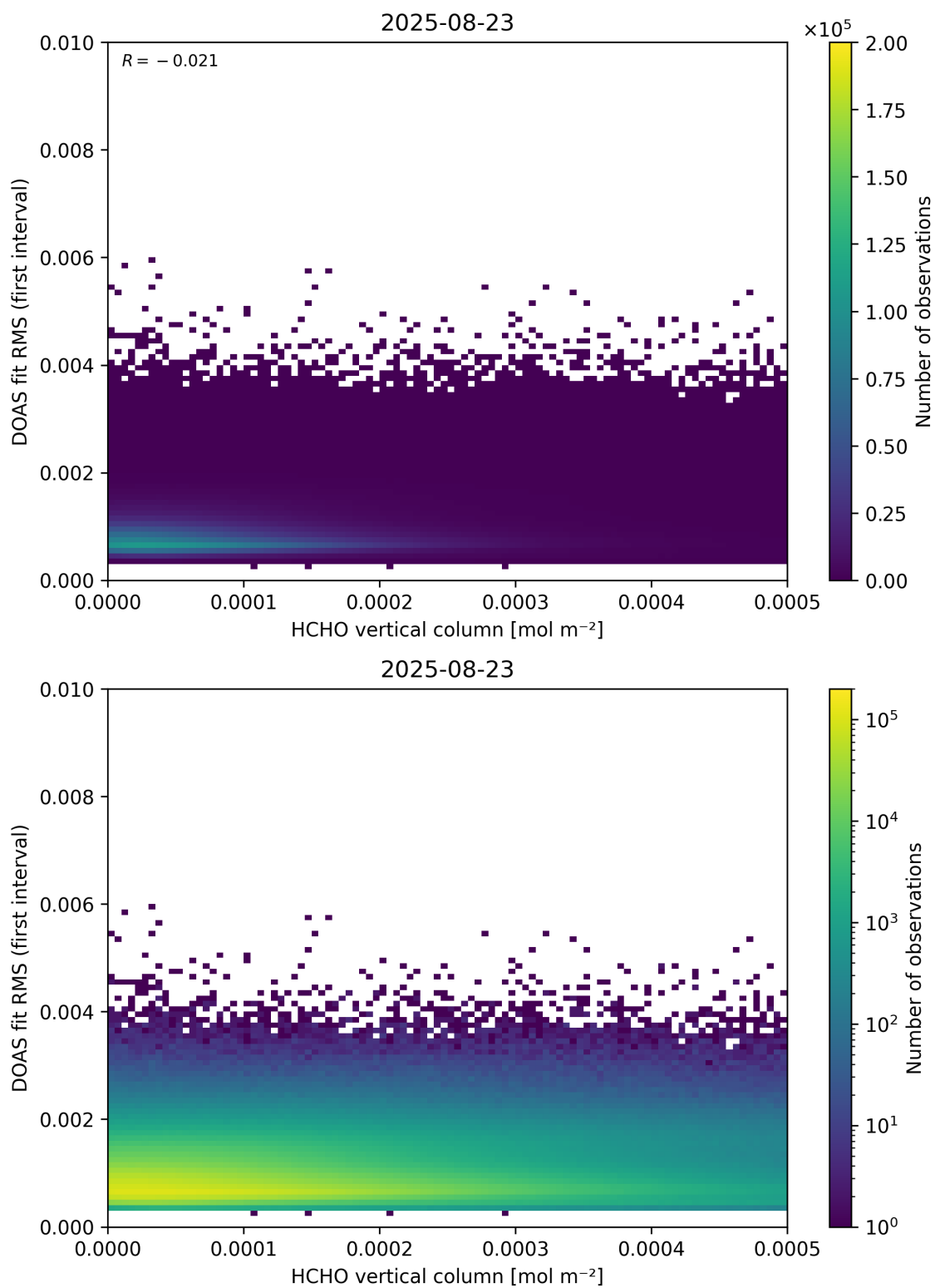
Figure 123: Scatter density plot of “HCHO vertical column” against “DOAS fit RMS (first interval)” for 2025-08-22 to 2025-08-24.
