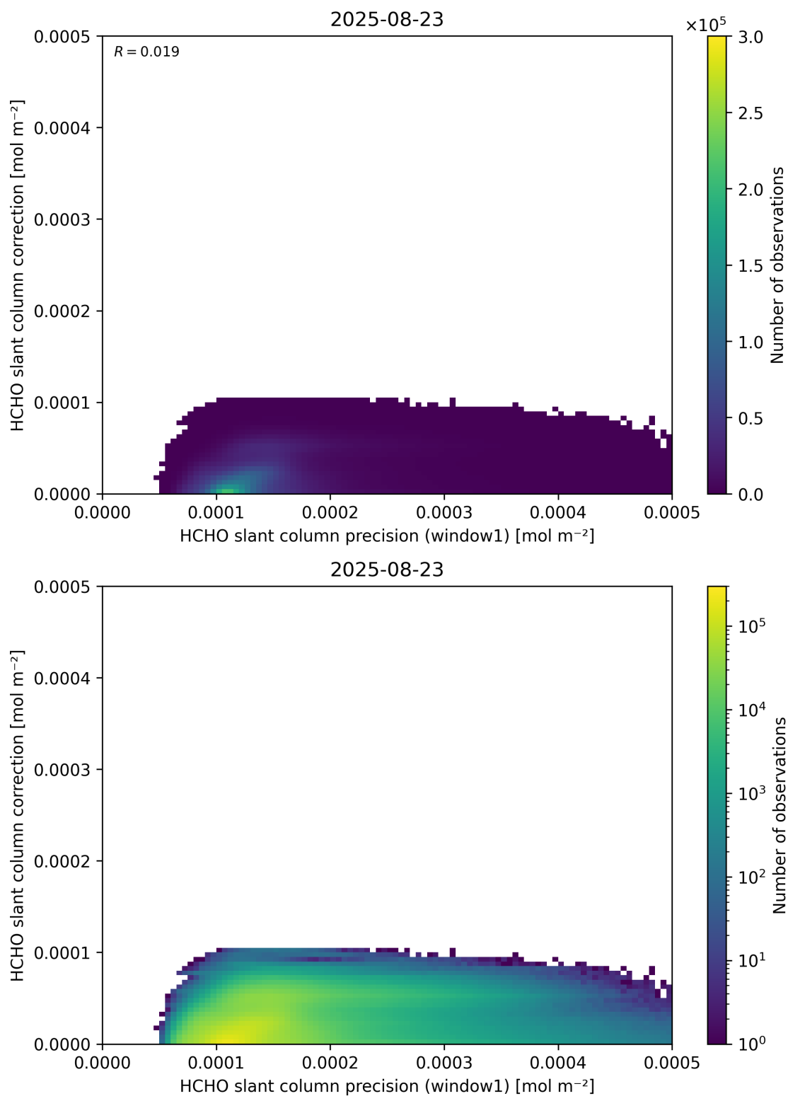
Figure 93: Scatter density plot of “HCHO slant column precision (window1)” against “HCHO slant column correction” for 2025-08-22 to 2025-08-24.
