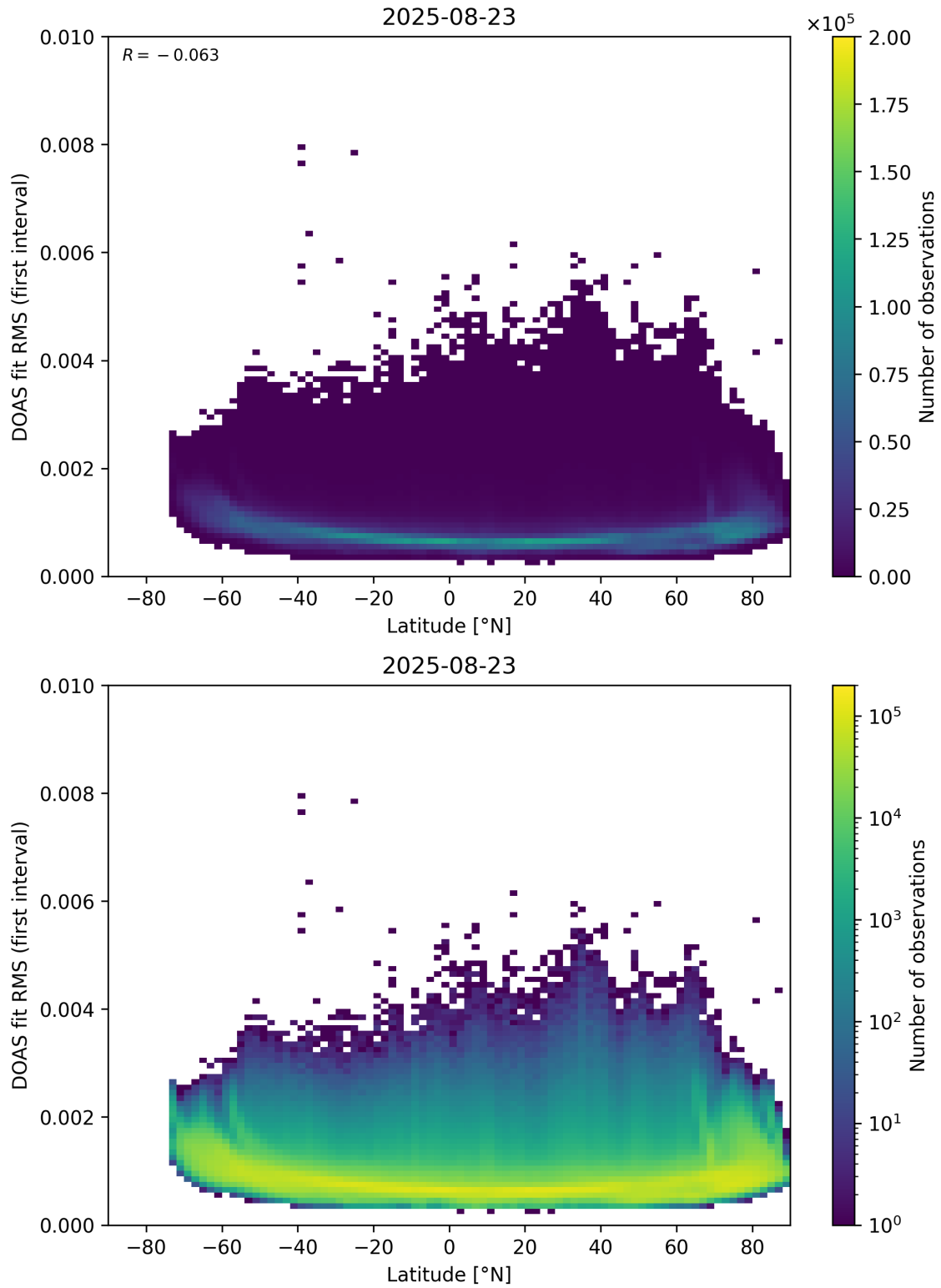
Figure 153: Scatter density plot of “Latitude” against “DOAS fit RMS (first interval)” for 2025-08-22 to 2025-08-24.
