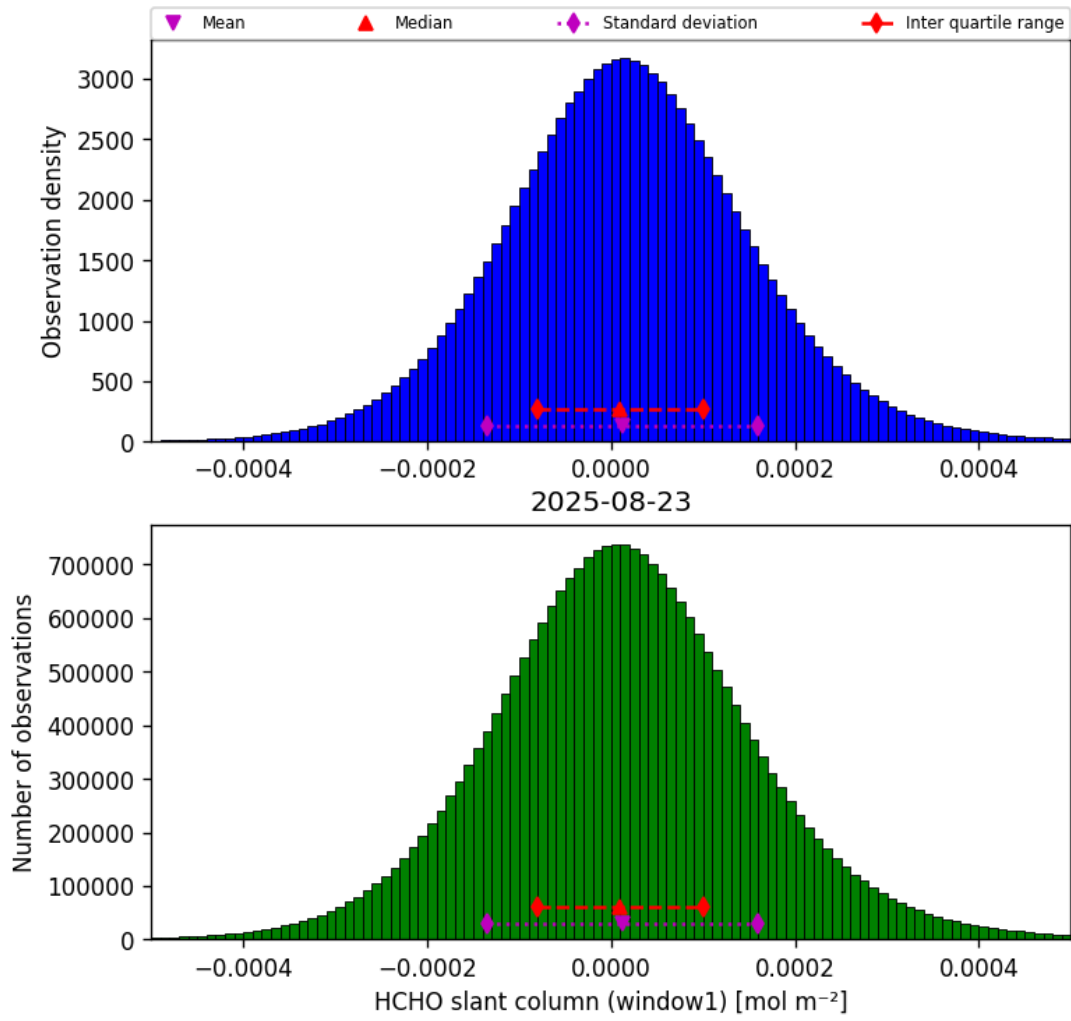
Figure 38: Histogram of “HCHO slant column (window1)” for 2025-08-22 to 2025-08-24
