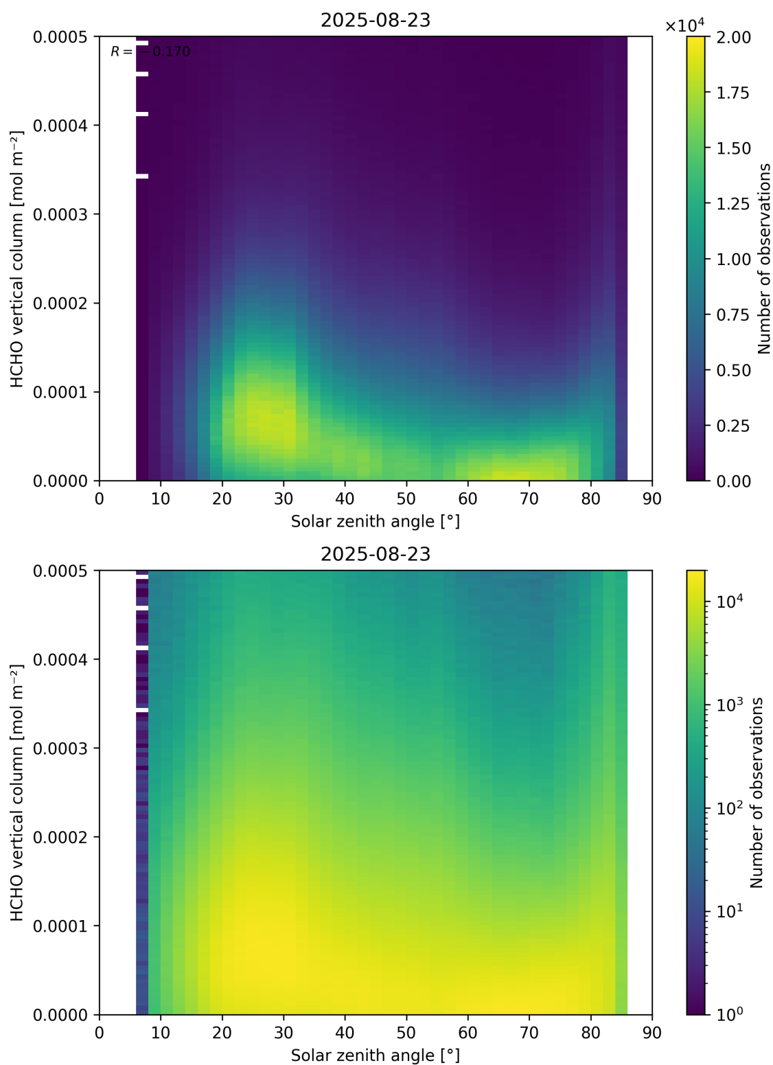
Figure 177: Scatter density plot of “Solar zenith angle” against “HCHO vertical column” for 2025-08-22 to 2025-08-24.
