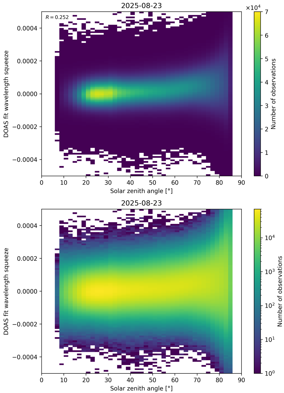
Figure 169: Scatter density plot of “Solar zenith angle” against “DOAS fit wavelength squeeze” for 2025-08-22 to 2025-08-24.
