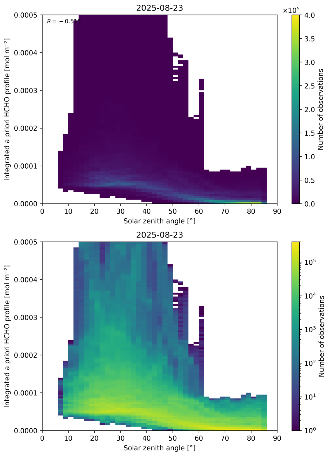
Figure 180: Scatter density plot of “Solar zenith angle” against “Integrated a priori HCHO profile” for 2025-08-22 to 2025-08-24.
