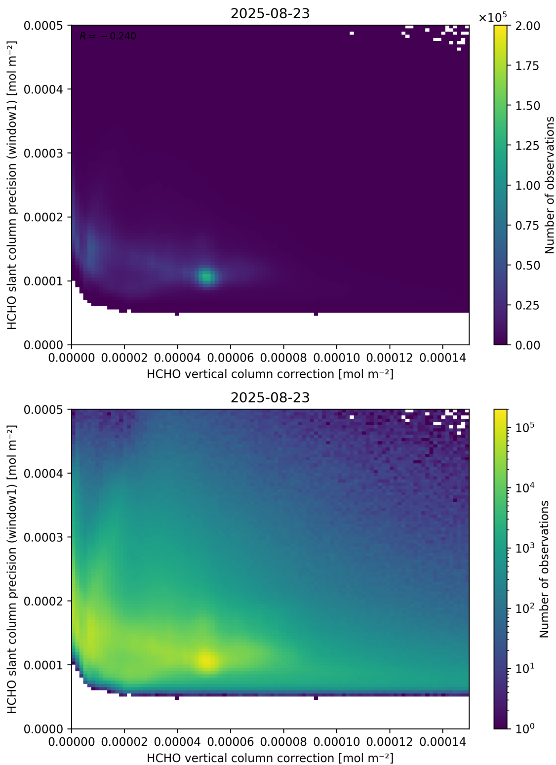
Figure 119: Scatter density plot of “HCHO vertical column correction” against “HCHO slant column precision (window1)” for 2025-08-22 to 2025-08-24.
