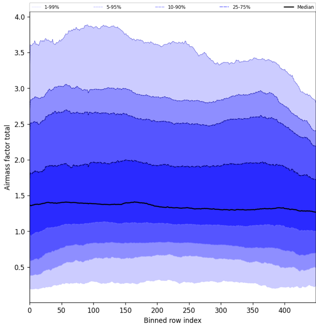
Figure 54: Along track statistics of “Airmass factor total” for 2025-08-22 to 2025-08-24
