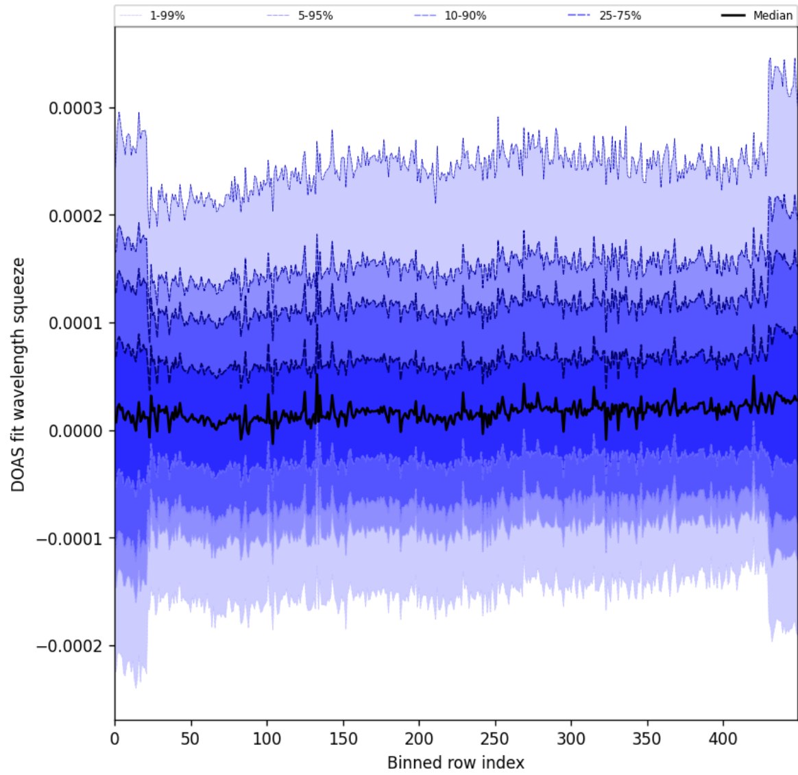
Figure 59: Along track statistics of “DOAS fit wavelength squeeze” for 2025-08-22 to 2025-08-24
