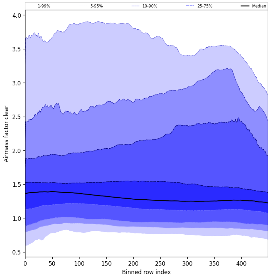
Figure 56: Along track statistics of “Airmass factor clear” for 2025-08-22 to 2025-08-24
