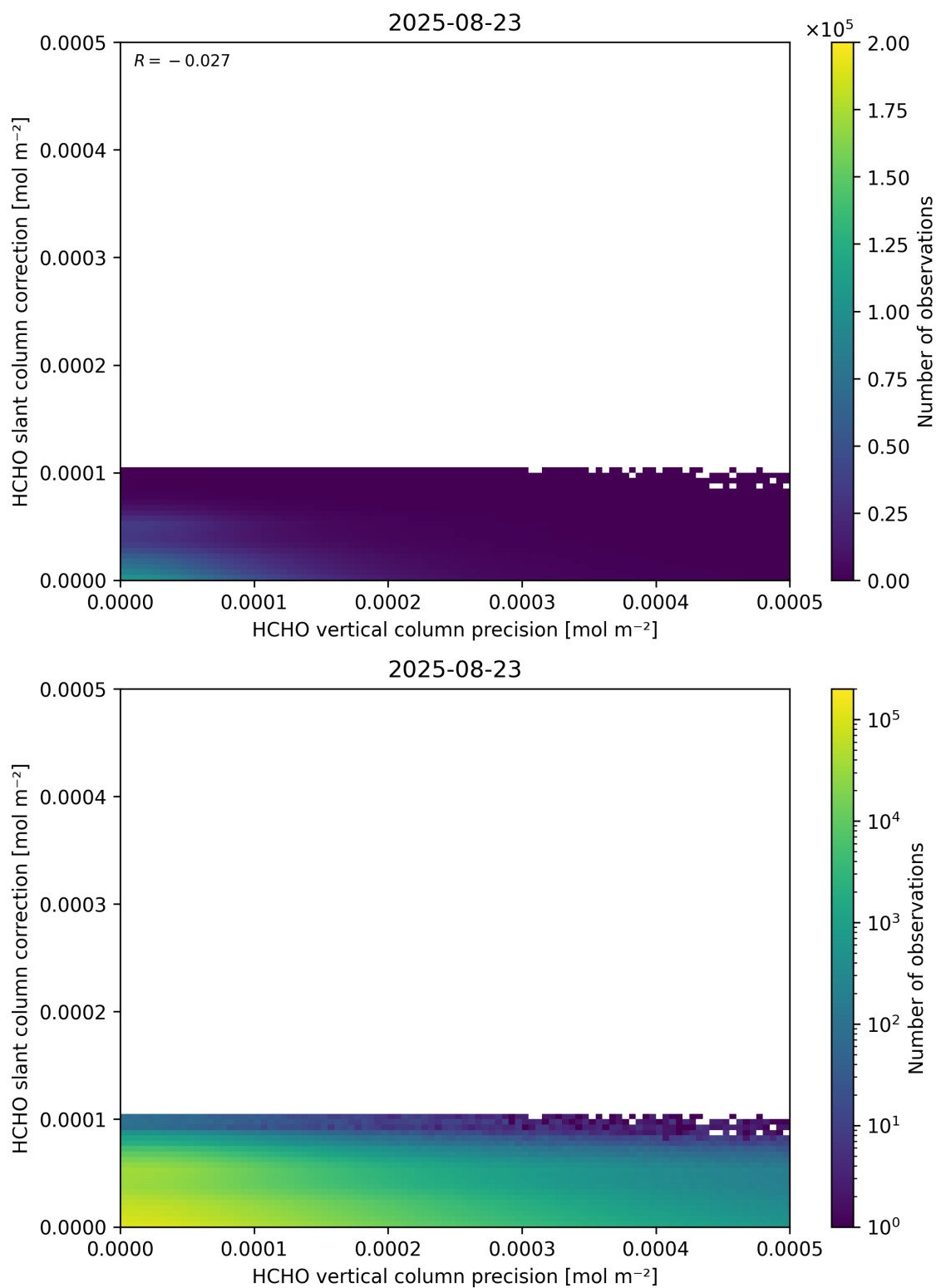
Figure 141: Scatter density plot of “HCHO vertical column precision” against “HCHO slant column correction” for 2025-08-22 to 2025-08-24.
