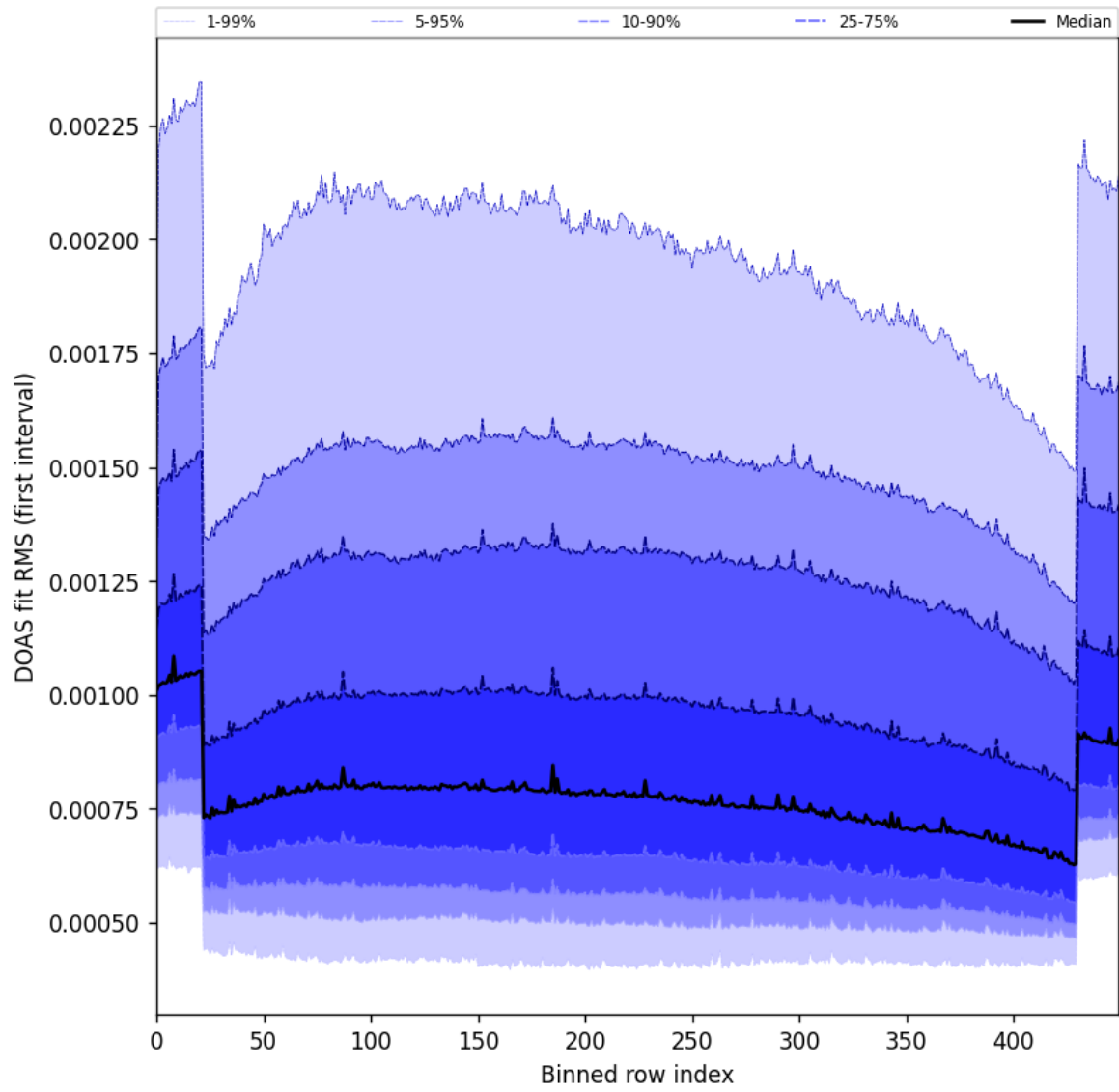
Figure 60: Along track statistics of “DOAS fit RMS (first interval)” for 2025-08-22 to 2025-08-24
