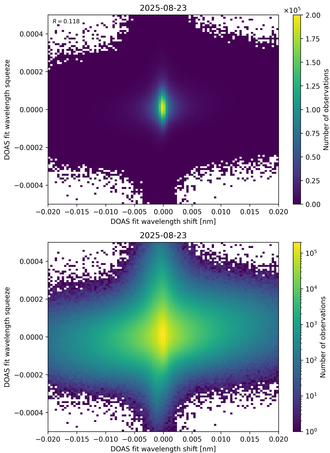
Figure 65: Scatter density plot of “DOAS fit wavelength shift” against “DOAS fit wavelength squeeze” for 2025-08-22 to 2025-08-24.
