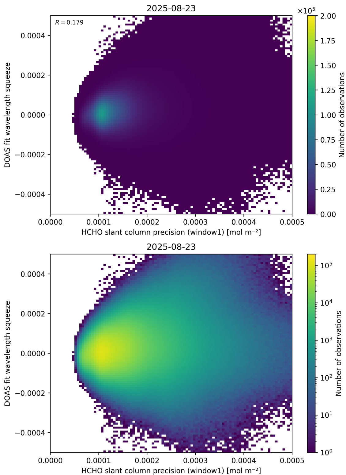
Figure 90: Scatter density plot of “HCHO slant column precision (window1)” against “DOAS fit wavelength squeeze” for 2025-08-22 to 2025-08-24.
