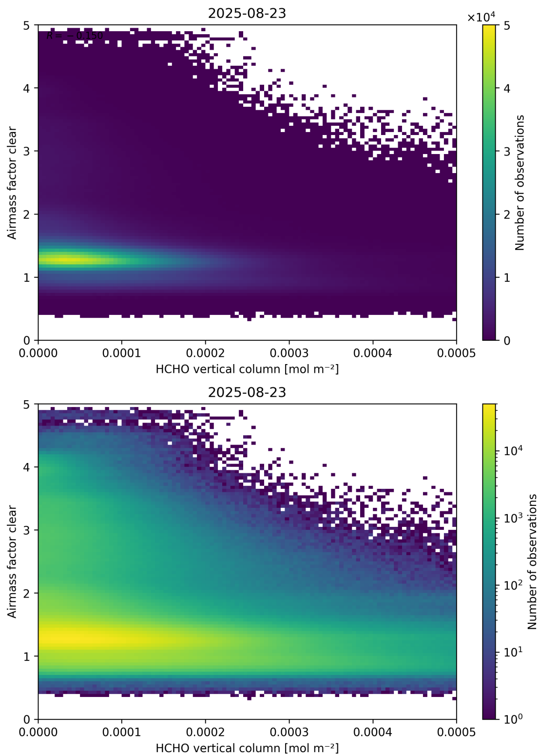
Figure 126: Scatter density plot of “HCHO vertical column” against “Airmass factor clear” for 2025-08-22 to 2025-08-24.
