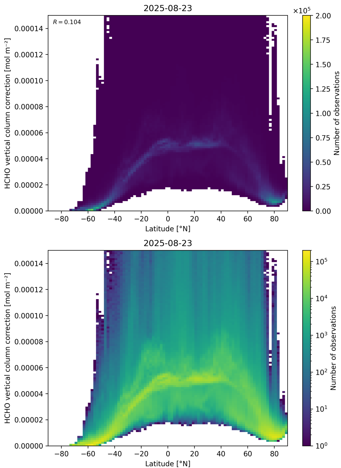
Figure 164: Scatter density plot of “Latitude” against “HCHO vertical column correction” for 2025-08-22 to 2025-08-24.
