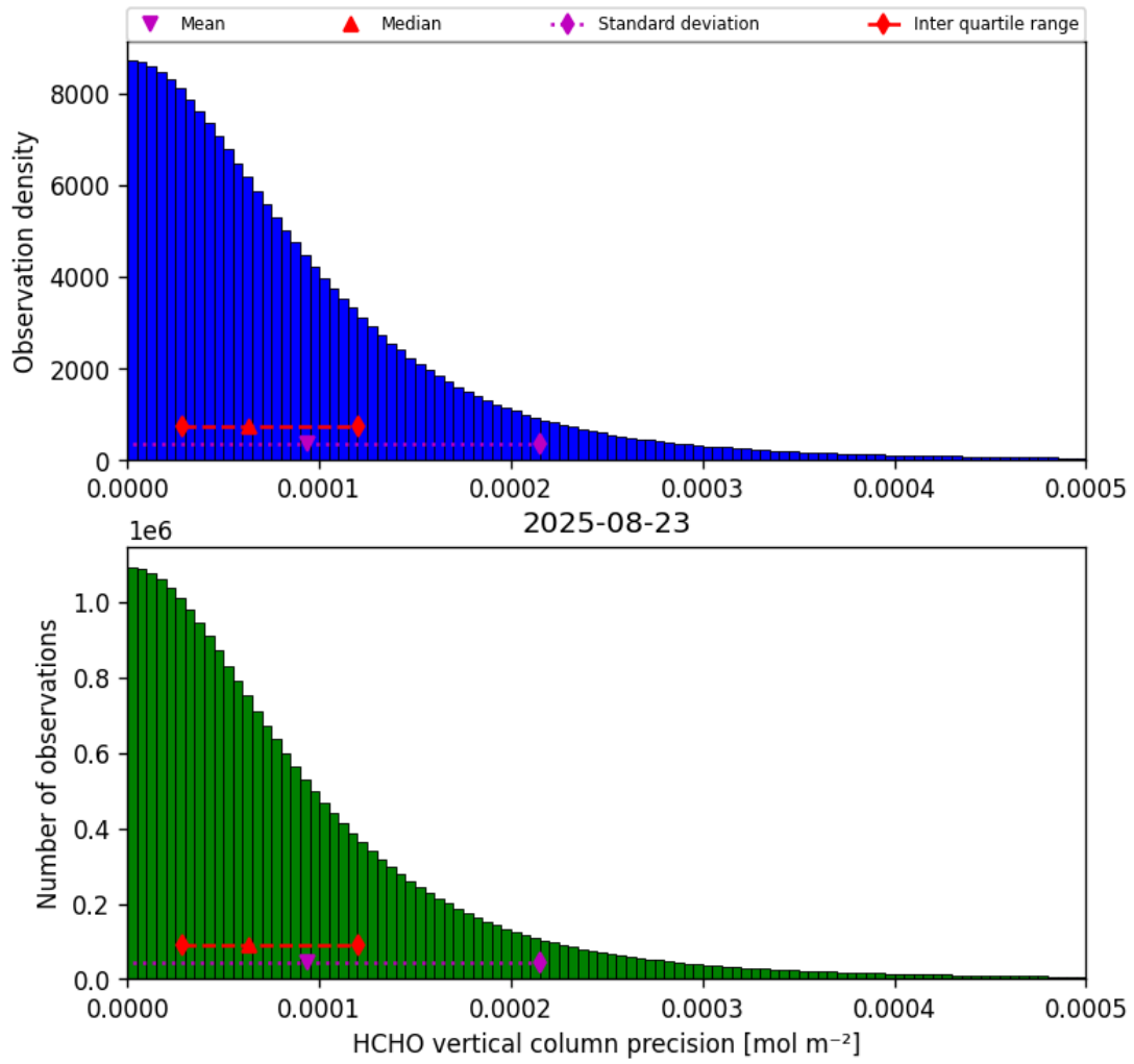
Figure 36: Histogram of “HCHO vertical column precision” for 2025-08-22 to 2025-08-24
