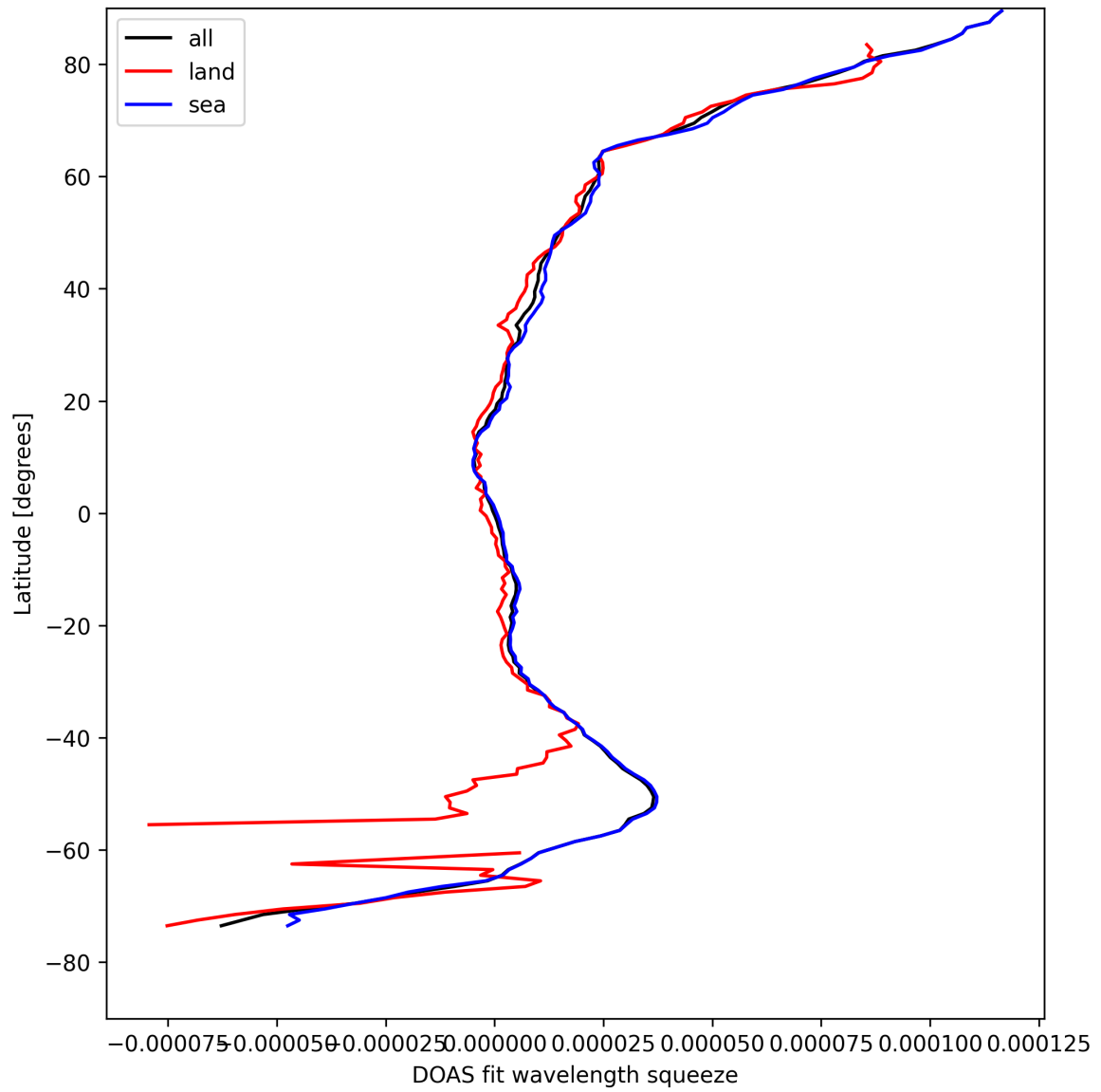
Figure 31: Zonal average of “DOAS fit wavelength squeeze” for 2025-08-22 to 2025-08-24.
