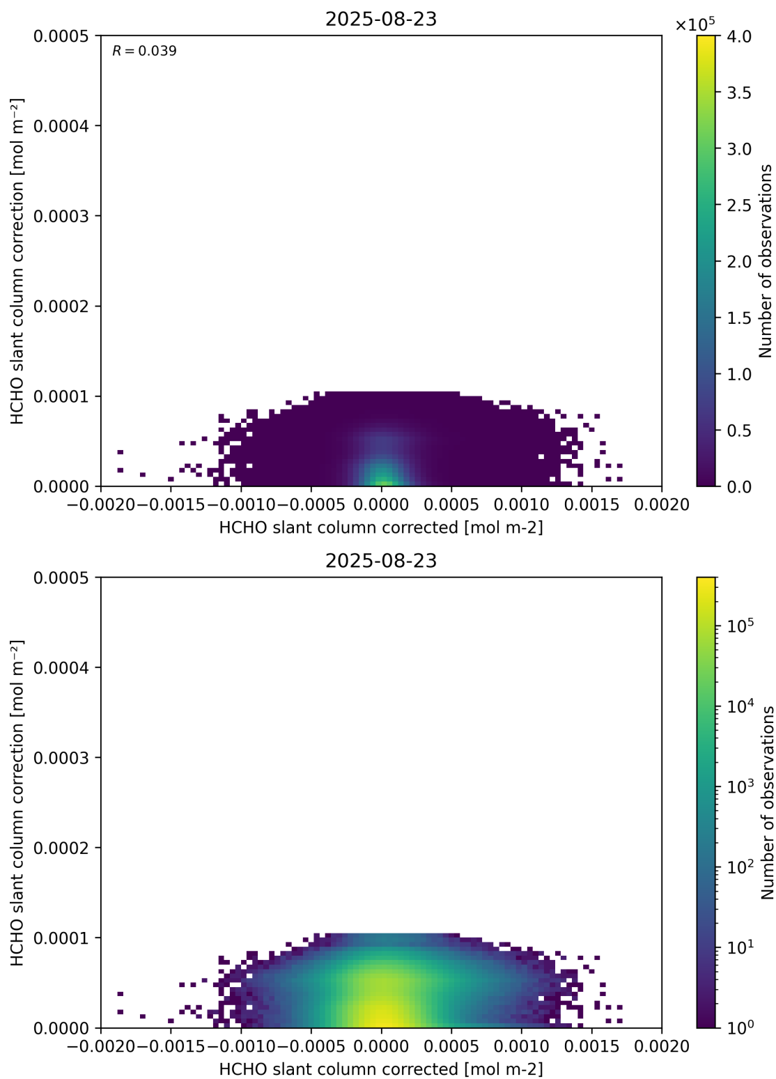
Figure 77: Scatter density plot of “HCHO slant column corrected” against “HCHO slant column correction” for 2025-08-22 to 2025-08-24.
