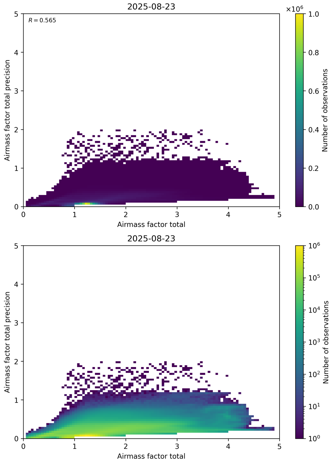
Figure 103: Scatter density plot of “Airmass factor total” against “Airmass factor total precision” for 2025-08-22 to 2025-08-24.
