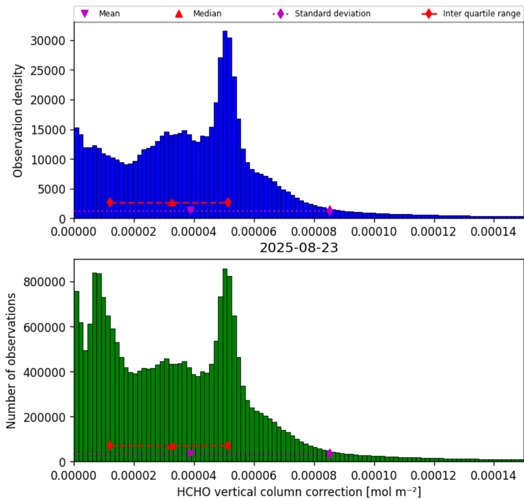
Figure 37: Histogram of “HCHO vertical column correction” for 2025-08-22 to 2025-08-24
