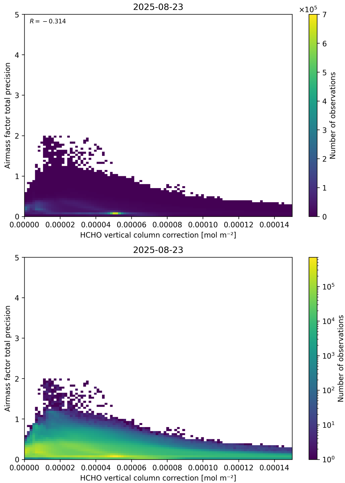
Figure 121: Scatter density plot of “HCHO vertical column correction” against “Airmass factor total precision” for 2025-08-22 to 2025-08-24.
