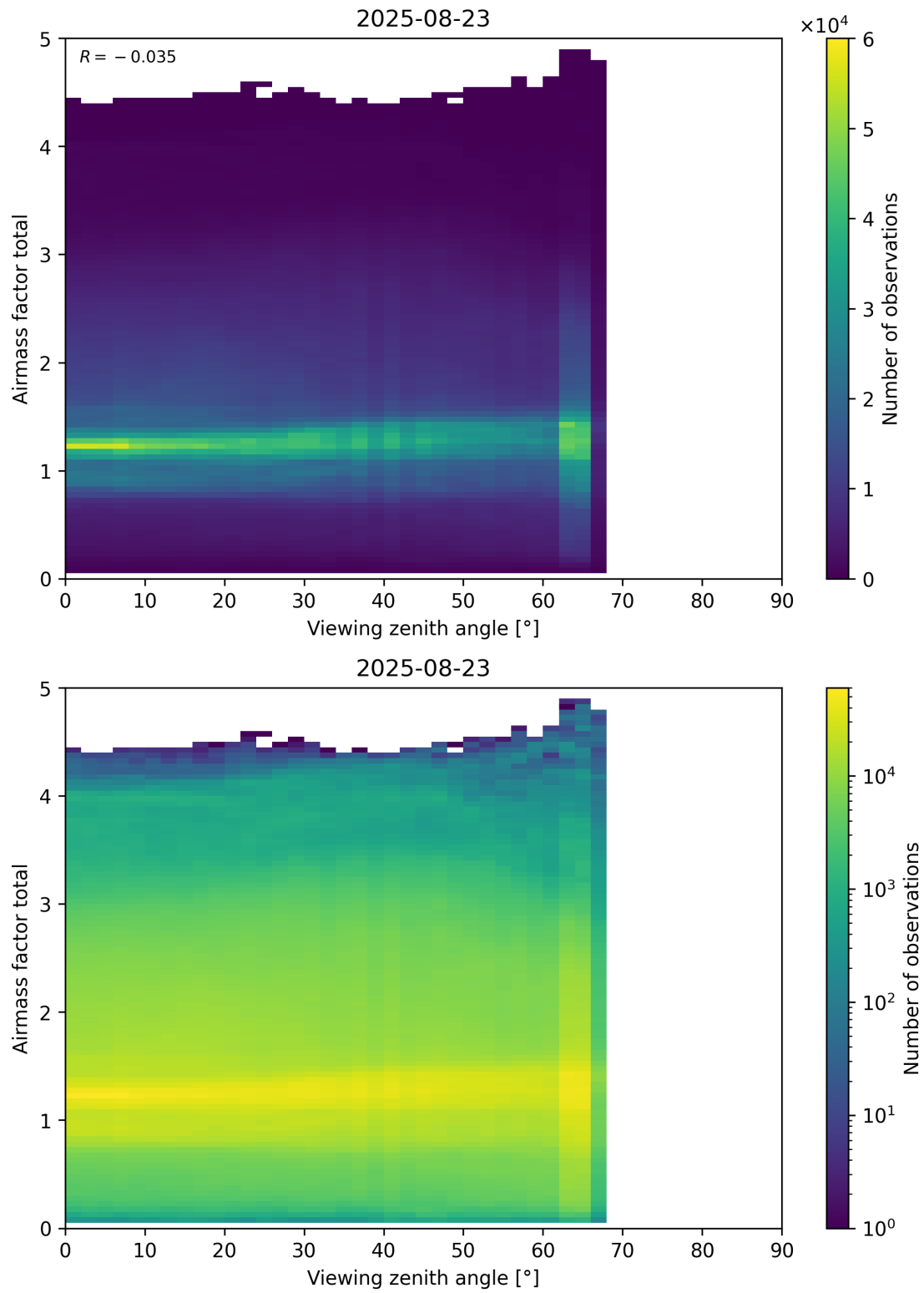
Figure 190: Scatter density plot of “Viewing zenith angle” against “Airmass factor total” for 2025-08-22 to 2025-08-24.
