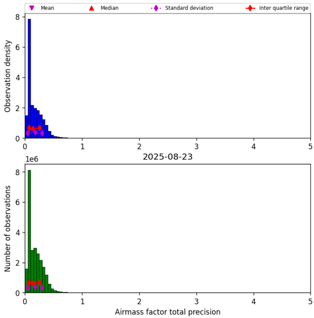
Figure 41: Histogram of “Airmass factor total precision” for 2025-08-22 to 2025-08-24
