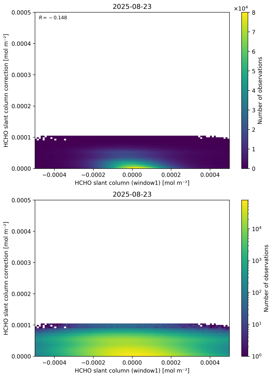
Figure 83: Scatter density plot of “HCHO slant column (window1)” against “HCHO slant column correction” for 2025-08-22 to 2025-08-24.
