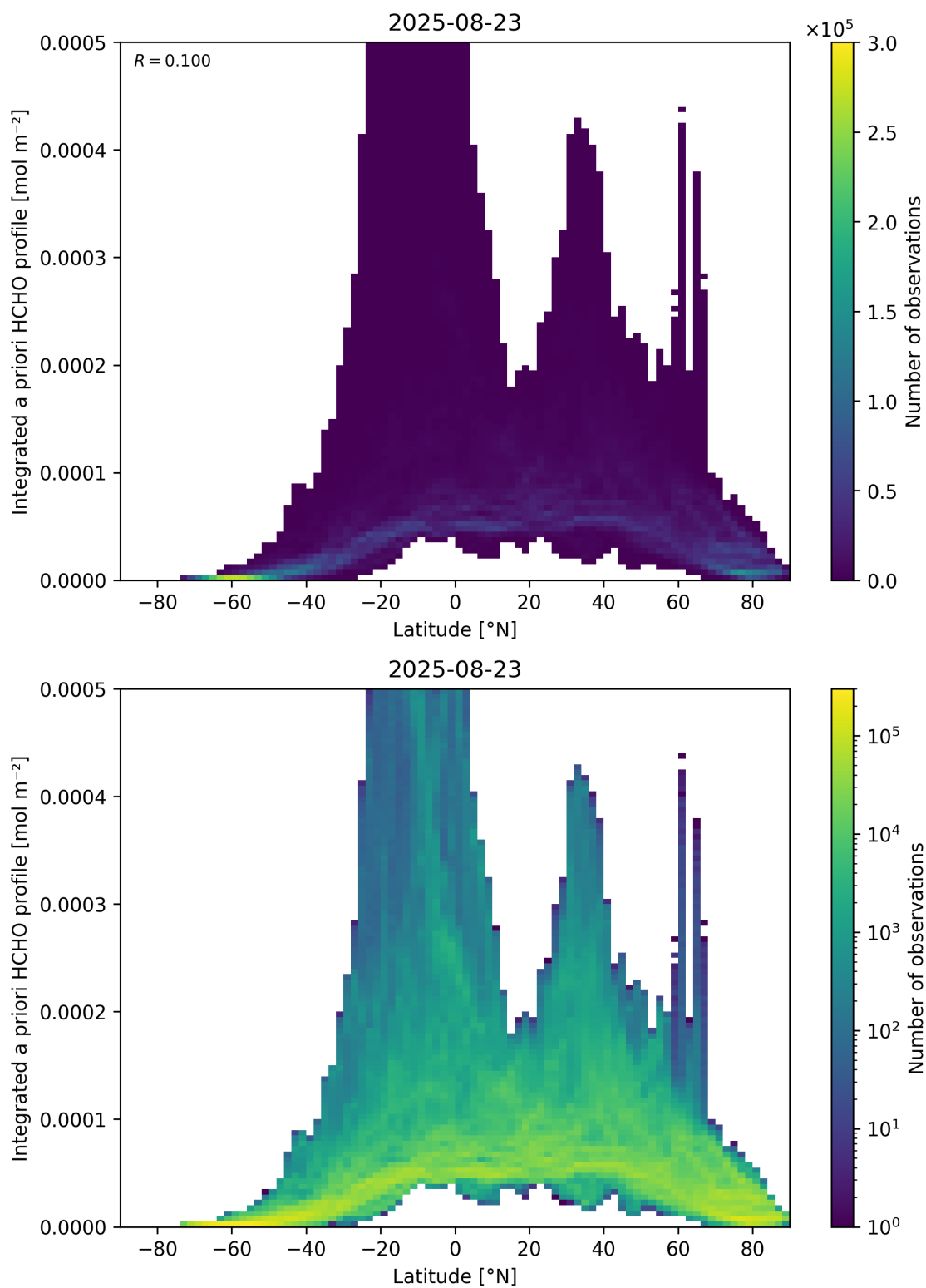
Figure 166: Scatter density plot of “Latitude” against “Integrated a priori HCHO profile” for 2025-08-22 to 2025-08-24.
