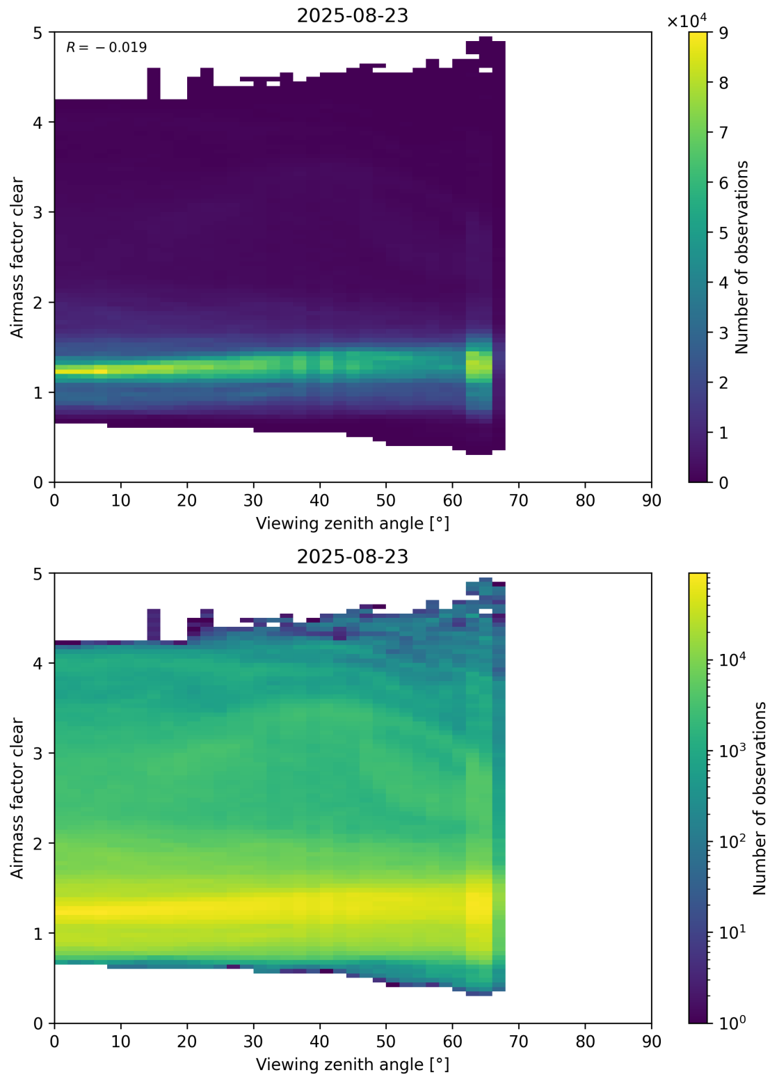
Figure 185: Scatter density plot of “Viewing zenith angle” against “Airmass factor clear” for 2025-08-22 to 2025-08-24.
