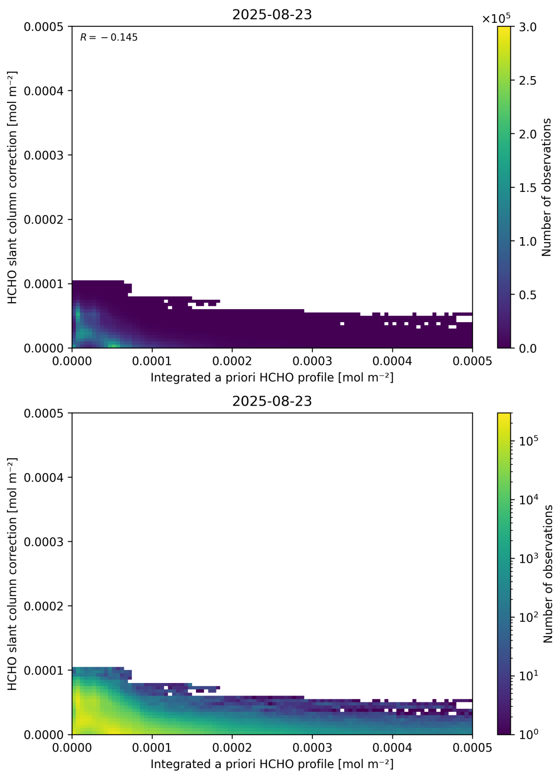
Figure 152: Scatter density plot of “Integrated a priori HCHO profile” against “HCHO slant column correction” for 2025-08-22 to 2025-08-24.
