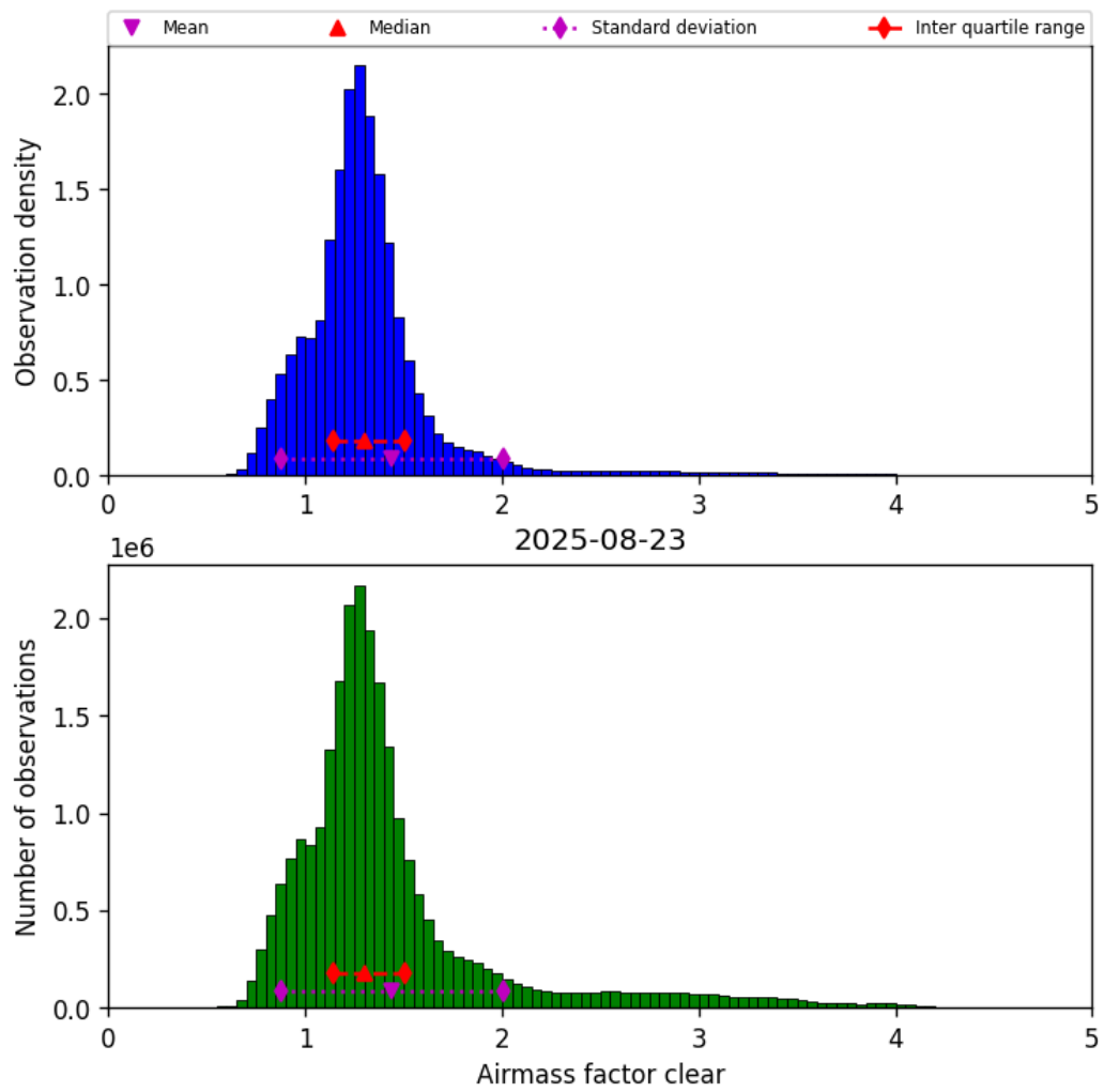
Figure 42: Histogram of “Airmass factor clear” for 2025-08-22 to 2025-08-24
