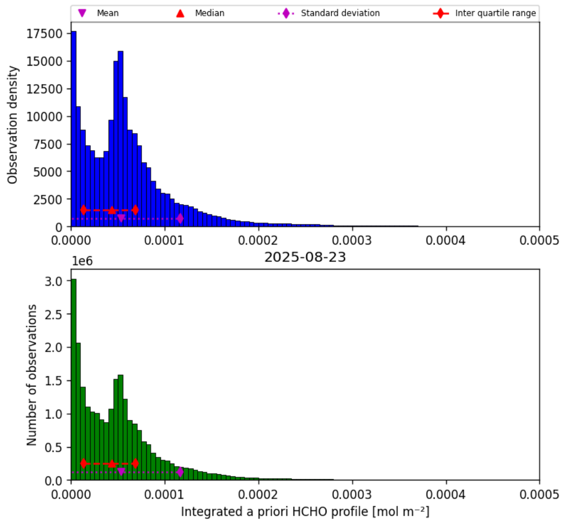
Figure 43: Histogram of “Integrated a priori HCHO profile” for 2025-08-22 to 2025-08-24
