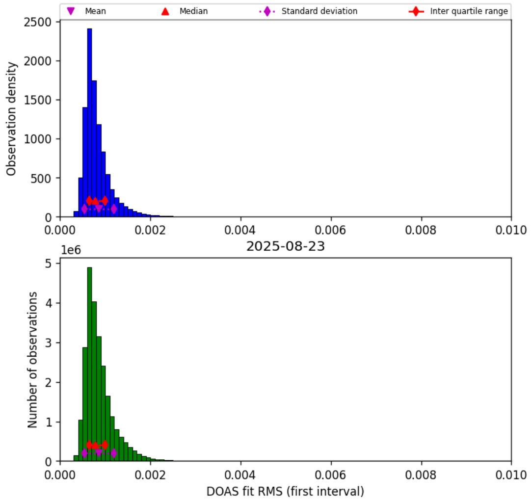
Figure 46: Histogram of “DOAS fit RMS (first interval)” for 2025-08-22 to 2025-08-24
