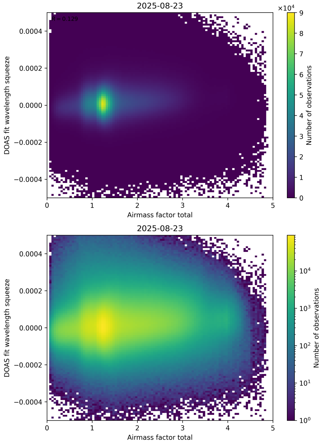
Figure 99: Scatter density plot of “Airmass factor total” against “DOAS fit wavelength squeeze” for 2025-08-22 to 2025-08-24.
