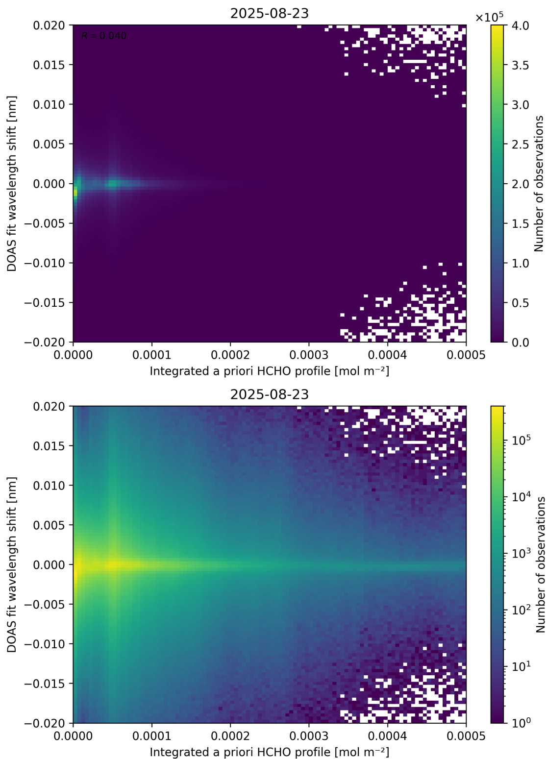
Figure 149: Scatter density plot of “Integrated a priori HCHO profile” against “DOAS fit wavelength shift” for 2025-08-22 to 2025-08-24.
