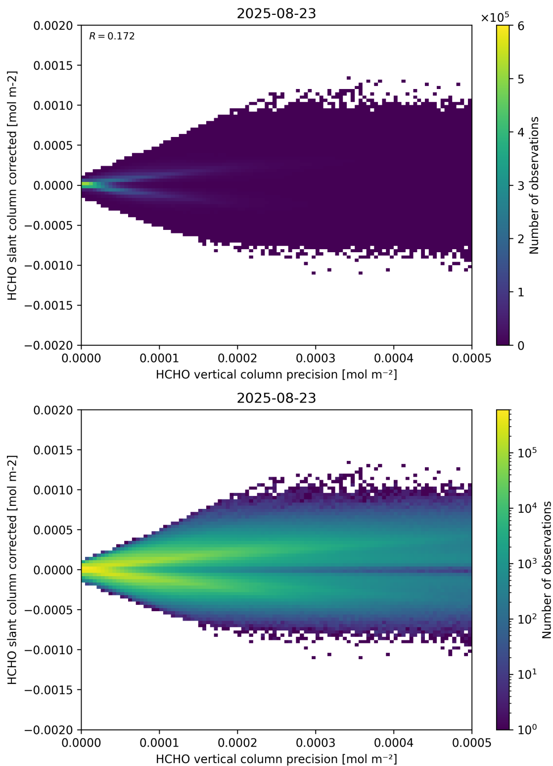
Figure 140: Scatter density plot of “HCHO vertical column precision” against “HCHO slant column corrected” for 2025-08-22 to 2025-08-24.
