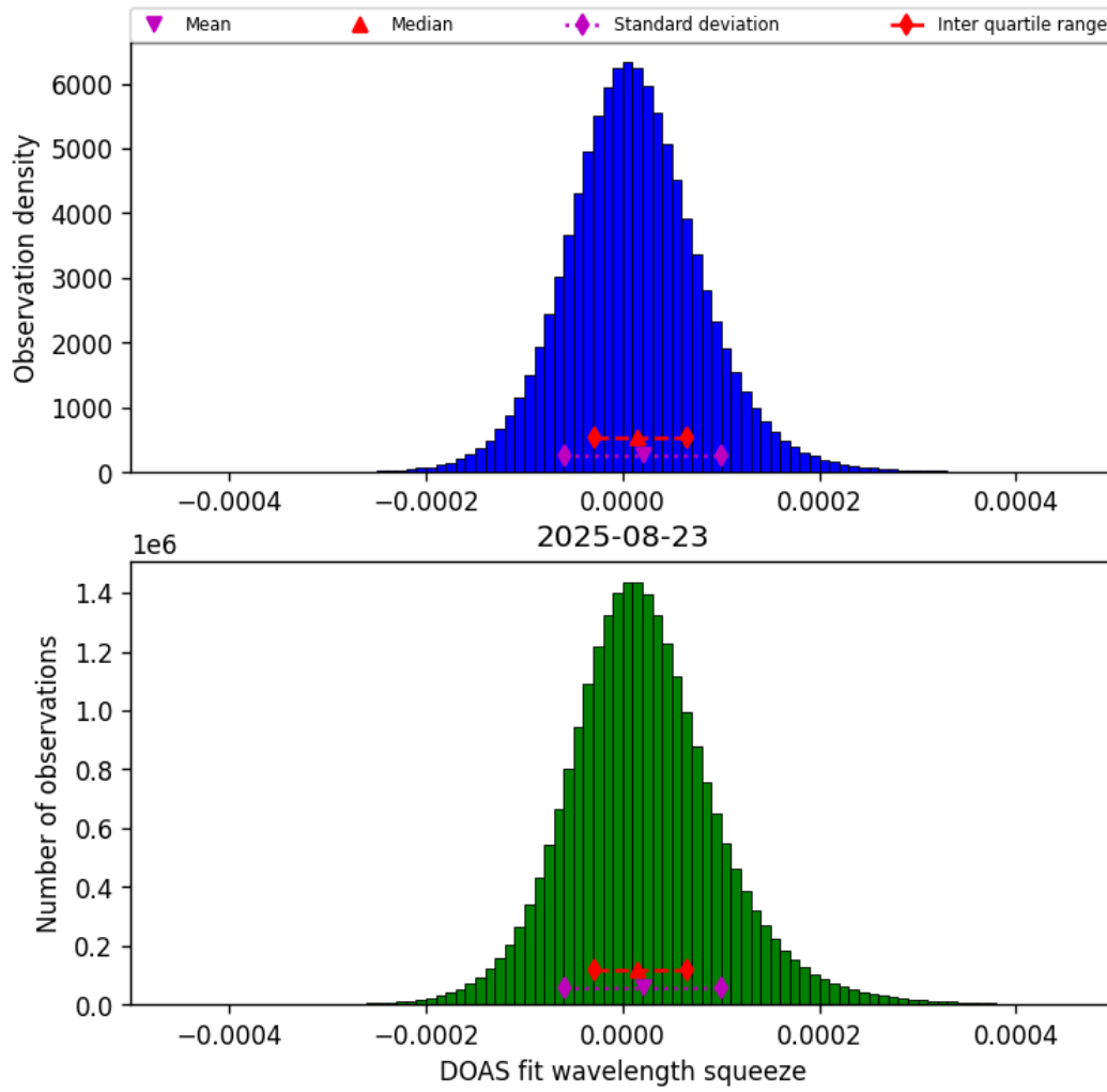
Figure 45: Histogram of “DOAS fit wavelength squeeze” for 2025-08-22 to 2025-08-24
