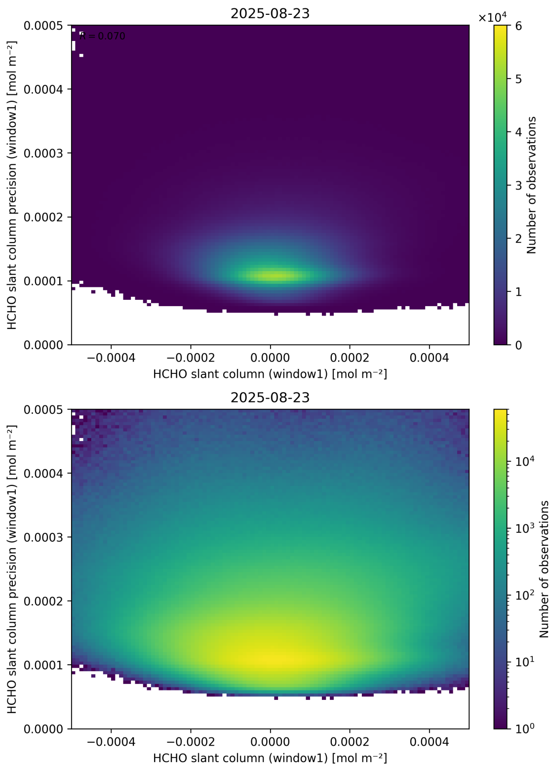
Figure 84: Scatter density plot of “HCHO slant column (window1)” against “HCHO slant column precision (window1)” for 2025-08-22 to 2025-08-24.
