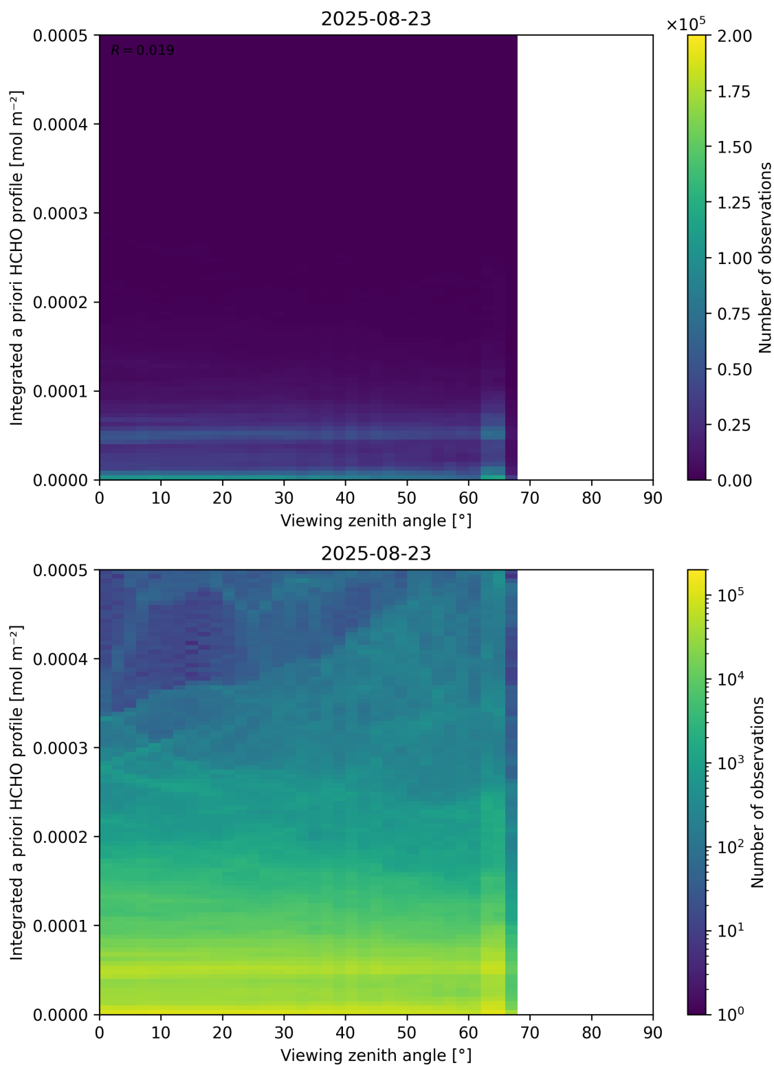
Figure 195: Scatter density plot of “Viewing zenith angle” against “Integrated a priori HCHO profile” for 2025-08-22 to 2025-08-24.
