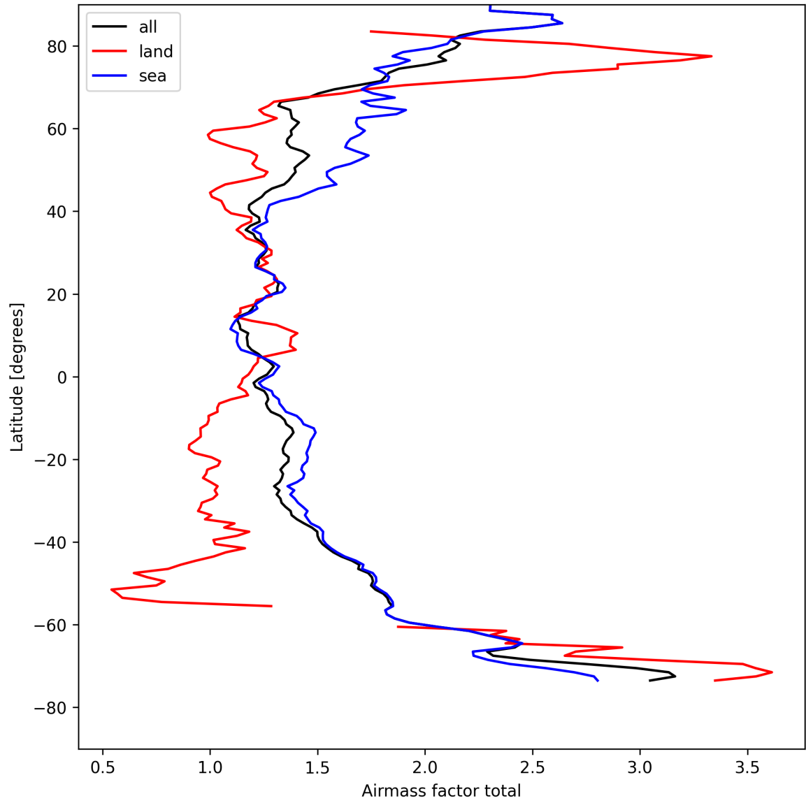
Figure 26: Zonal average of “Airmass factor total” for 2025-08-22 to 2025-08-24.
