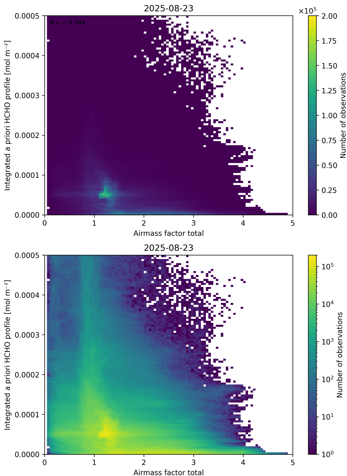
Figure 104: Scatter density plot of “Airmass factor total” against “Integrated a priori HCHO profile” for 2025-08-22 to 2025-08-24.
