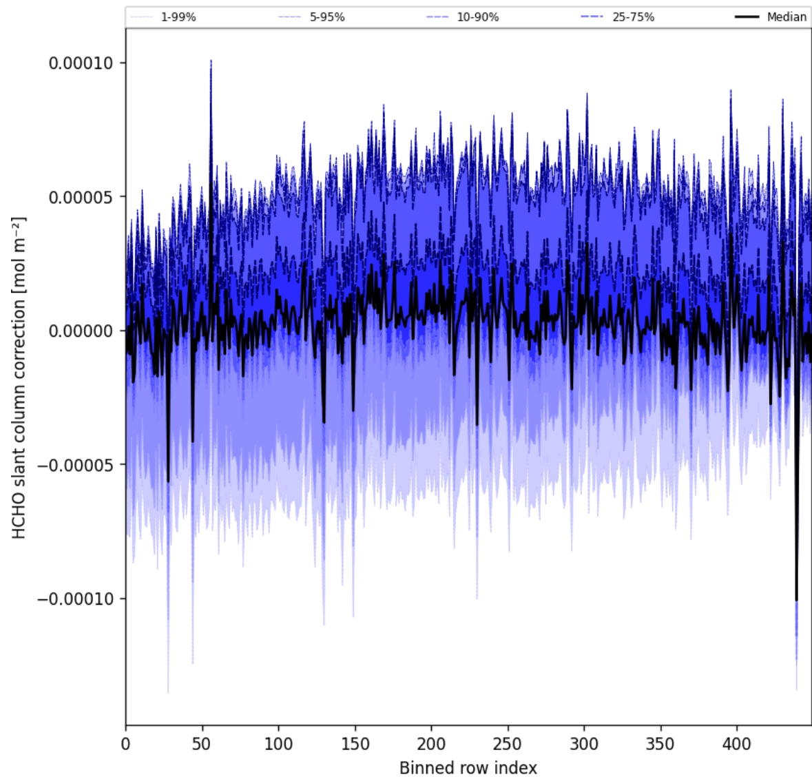
Figure 61: Along track statistics of "HCHO slant column correction" for 2025-08-22 to 2025-08-24
