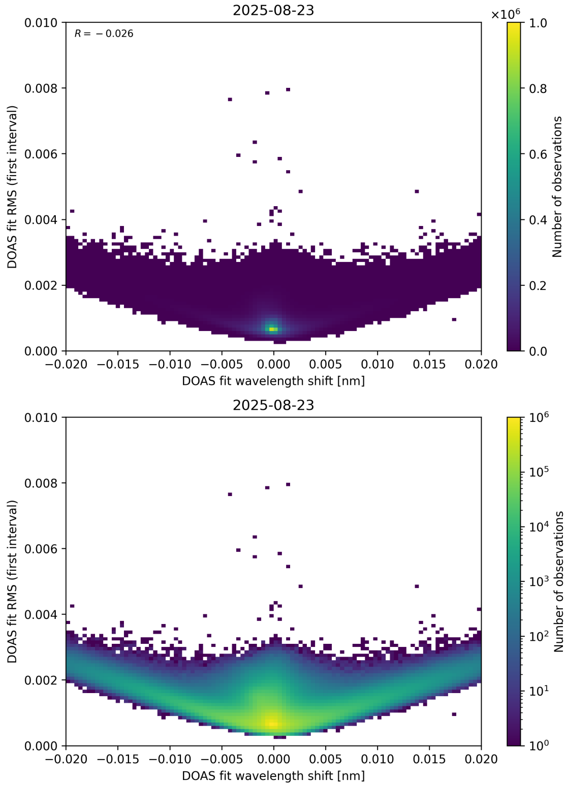
Figure 64: Scatter density plot of “DOAS fit wavelength shift” against “DOAS fit RMS (first interval)” for 2025-08-22 to 2025-08-24.
