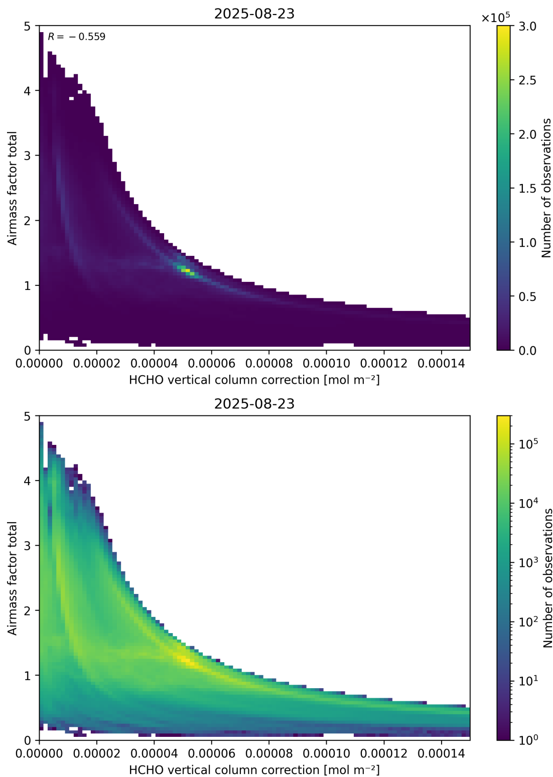
Figure 120: Scatter density plot of “HCHO vertical column correction” against “Airmass factor total” for 2025-08-22 to 2025-08-24.
