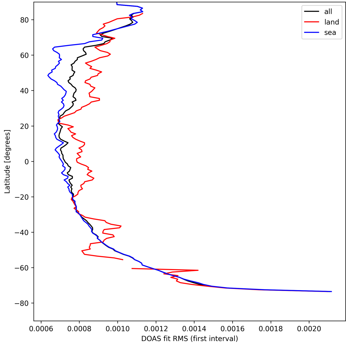
Figure 32: Zonal average of “DOAS fit RMS (first interval)” for 2025-08-22 to 2025-08-24.
