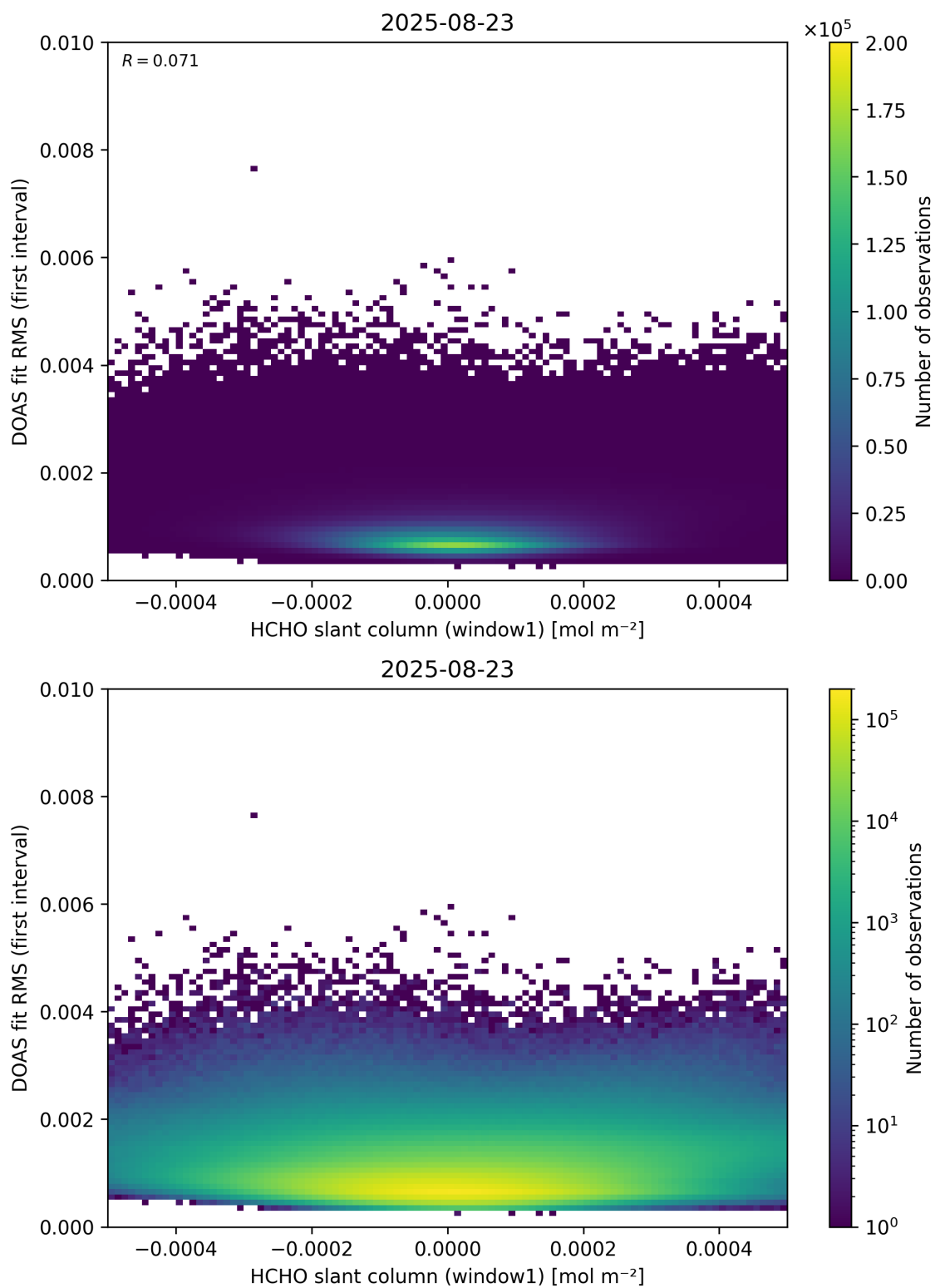
Figure 78: Scatter density plot of “HCHO slant column (window1)” against “DOAS fit RMS (first interval)” for 2025-08-22 to 2025-08-24.
