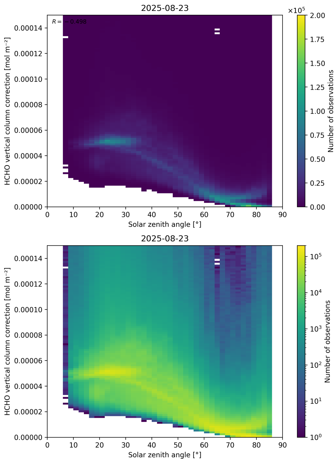
Figure 178: Scatter density plot of “Solar zenith angle” against “HCHO vertical column correction” for 2025-08-22 to 2025-08-24.
