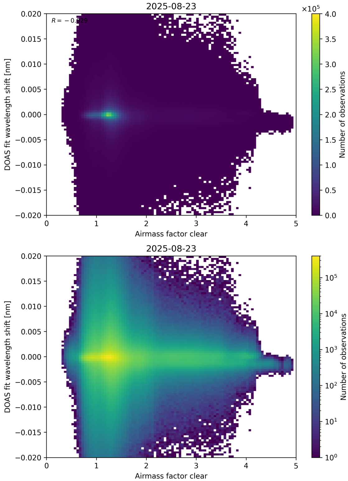
Figure 72: Scatter density plot of “Airmass factor clear” against “DOAS fit wavelength shift” for 2025-08-22 to 2025-08-24.
