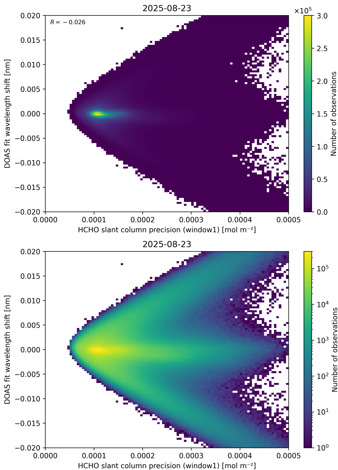
Figure 89: Scatter density plot of “HCHO slant column precision (window1)” against “DOAS fit wavelength shift” for 2025-08-22 to 2025-08-24.
