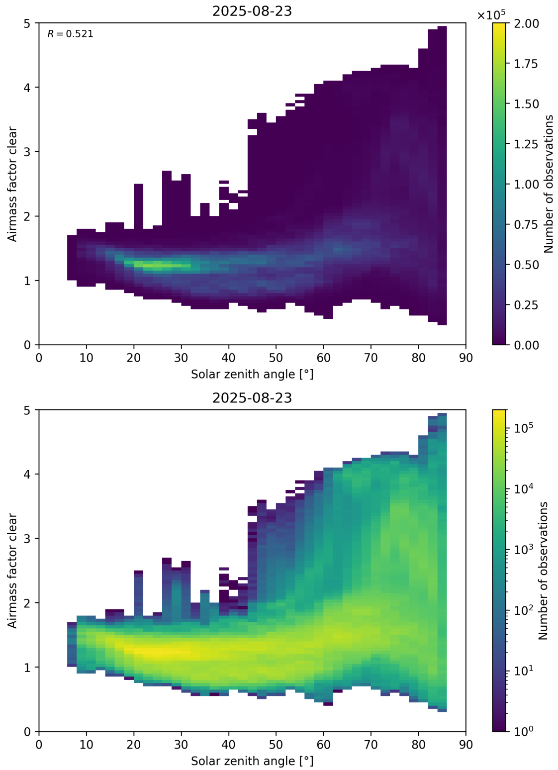
Figure 170: Scatter density plot of “Solar zenith angle” against “Airmass factor clear” for 2025-08-22 to 2025-08-24.
