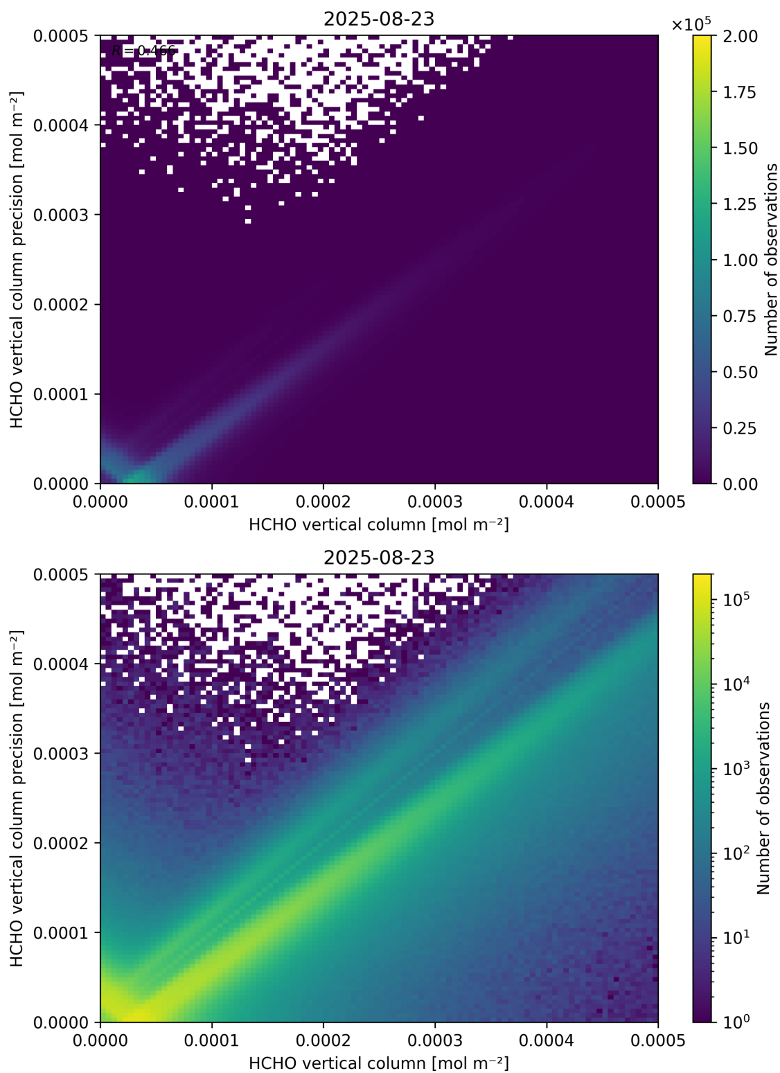
Figure 134: Scatter density plot of “HCHO vertical column” against “HCHO vertical column precision” for 2025-08-22 to 2025-08-24.
