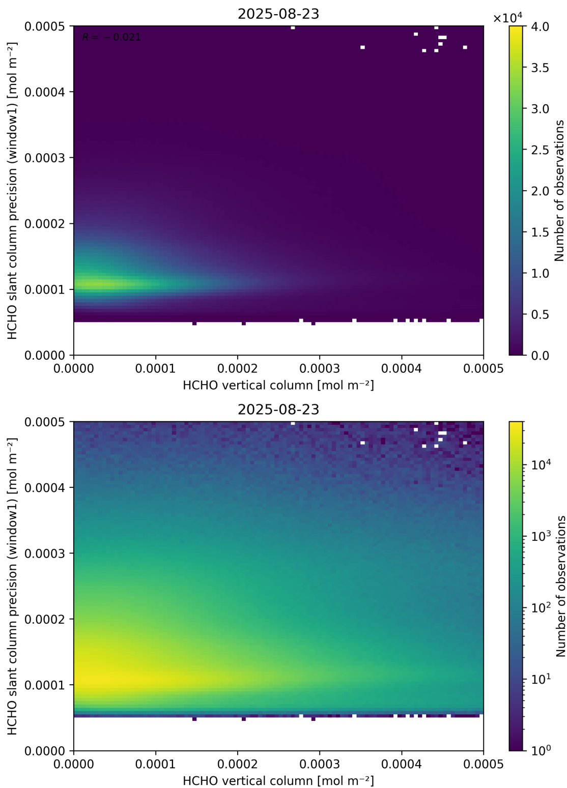
Figure 130: Scatter density plot of “HCHO vertical column” against “HCHO slant column precision (window1)” for 2025-08-22 to 2025-08-24.
