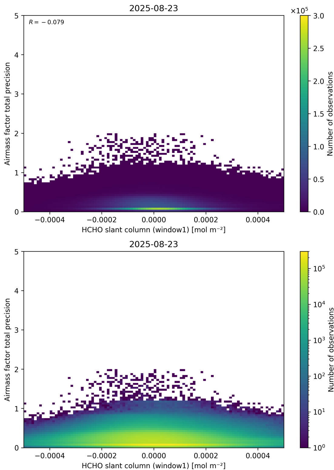
Figure 86: Scatter density plot of “HCHO slant column (window1)” against “Airmass factor total precision” for 2025-08-22 to 2025-08-24.
