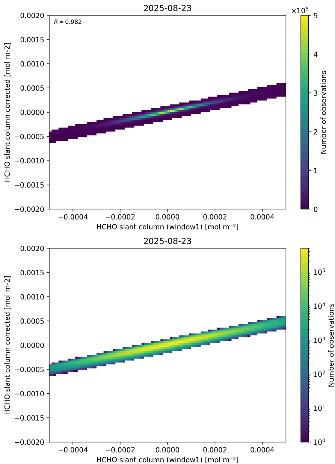
Figure 82: Scatter density plot of “HCHO slant column (window1)” against “HCHO slant column corrected” for 2025-08-22 to 2025-08-24.
