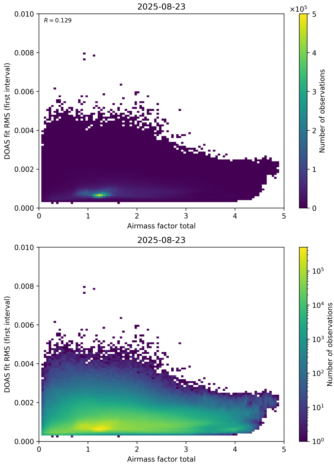
Figure 97: Scatter density plot of “Airmass factor total” against “DOAS fit RMS (first interval)” for 2025-08-22 to 2025-08-24.
