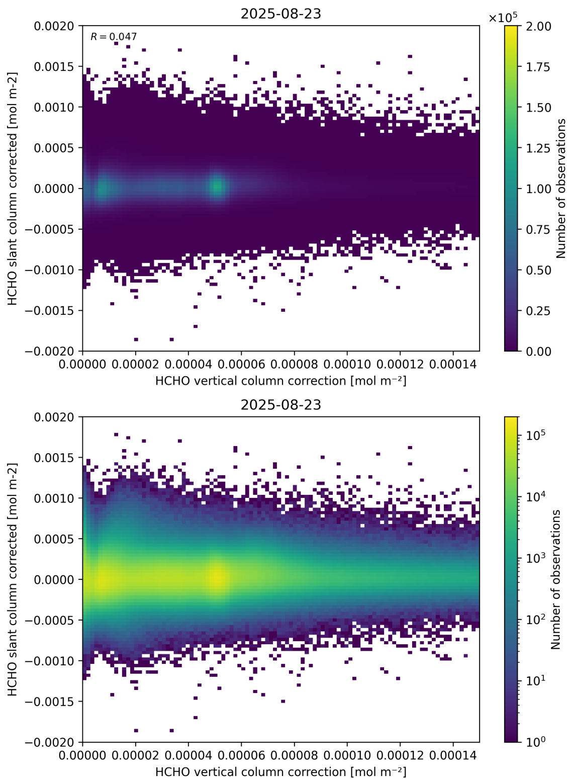
Figure 116: Scatter density plot of “HCHO vertical column correction” against “HCHO slant column corrected” for 2025-08-22 to 2025-08-24.
