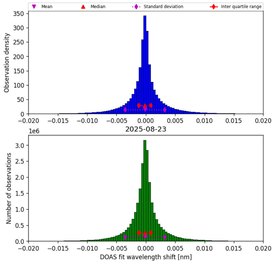
Figure 44: Histogram of “DOAS fit wavelength shift” for 2025-08-22 to 2025-08-24
