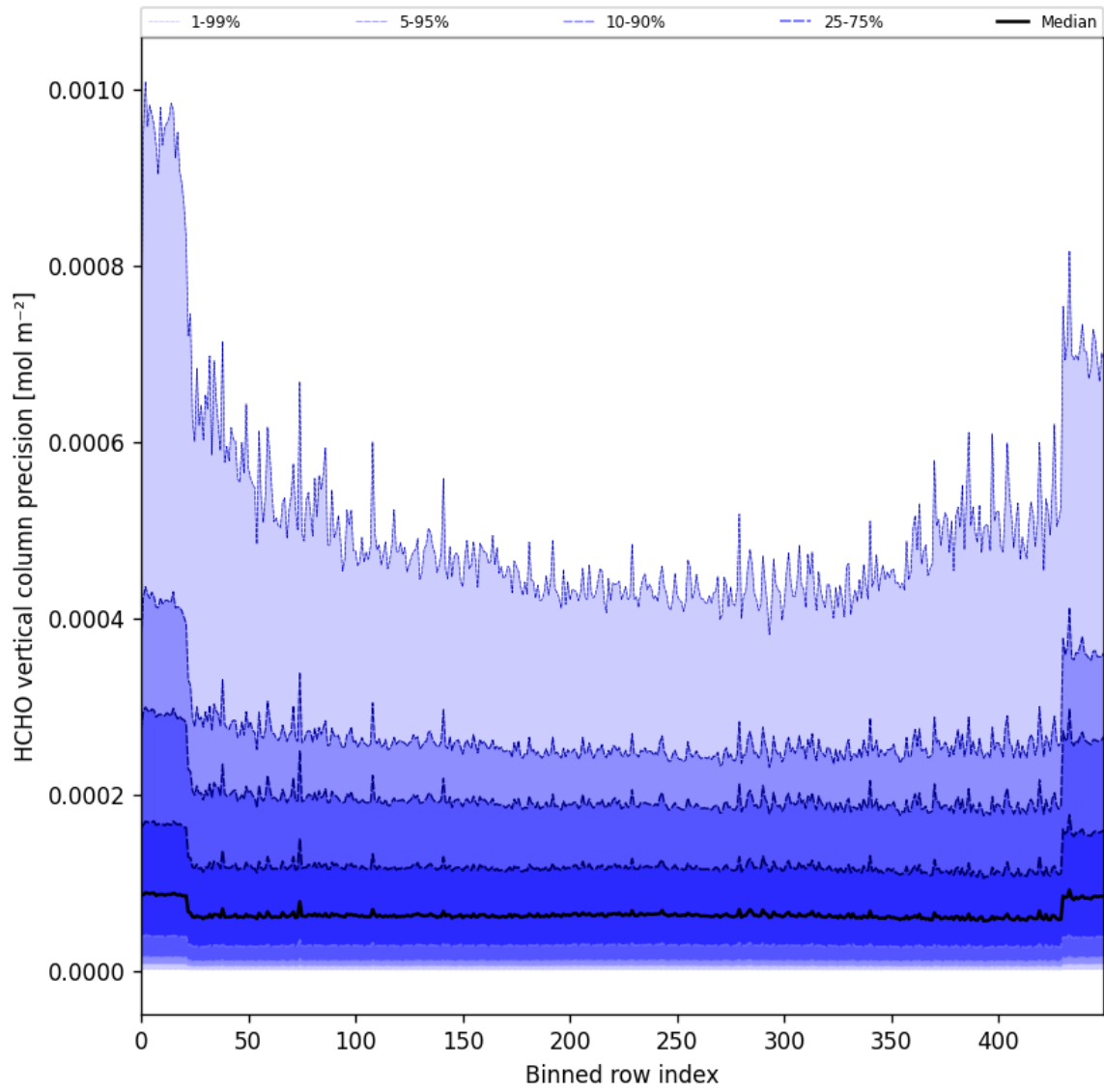
Figure 50: Along track statistics of “HCHO vertical column precision” for 2025-08-22 to 2025-08-24
