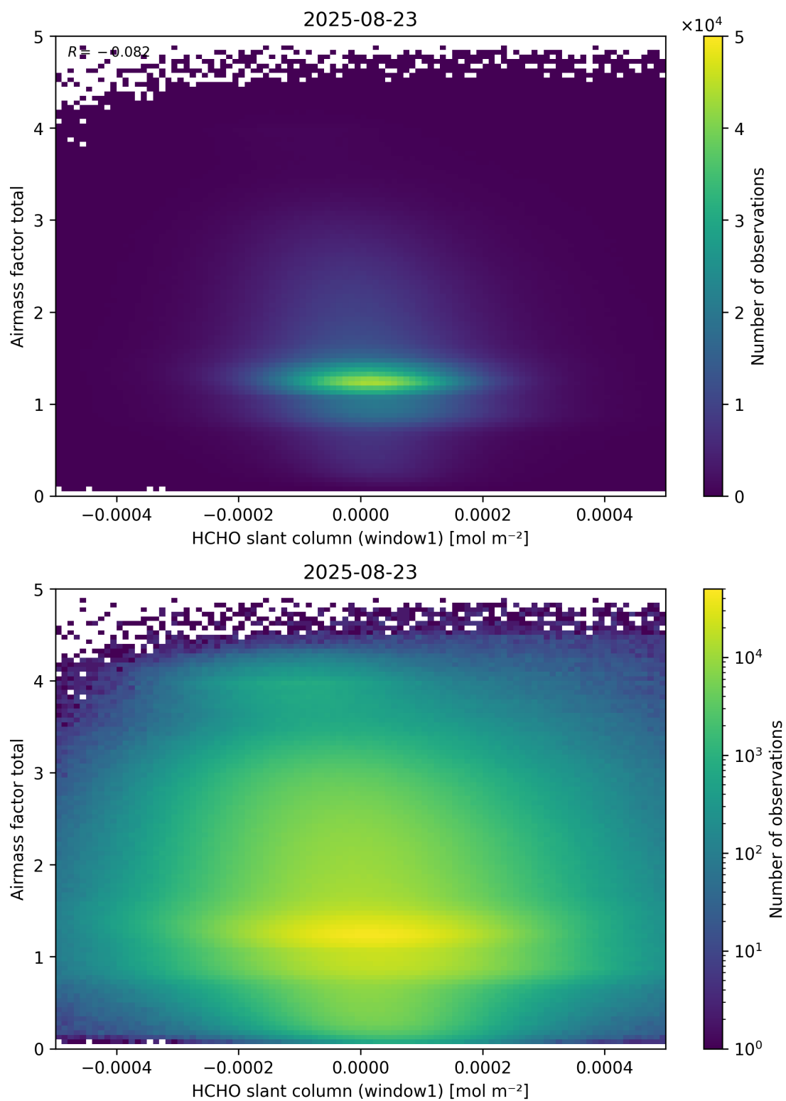
Figure 85: Scatter density plot of “HCHO slant column (window1)” against “Airmass factor total” for 2025-08-22 to 2025-08-24.
