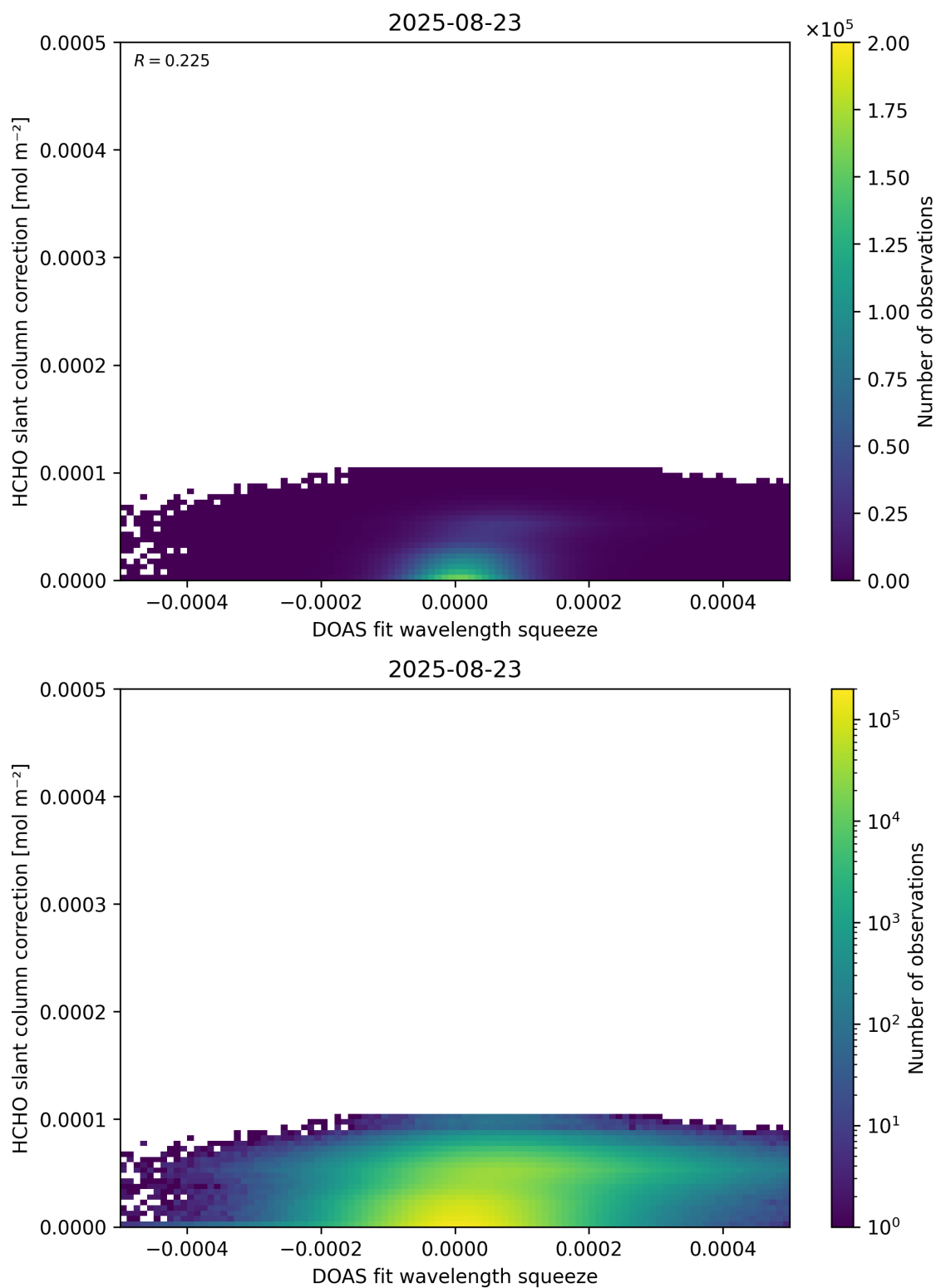
Figure 70: Scatter density plot of “DOAS fit wavelength squeeze” against “HCHO slant column correction” for 2025-08-22 to 2025-08-24.
