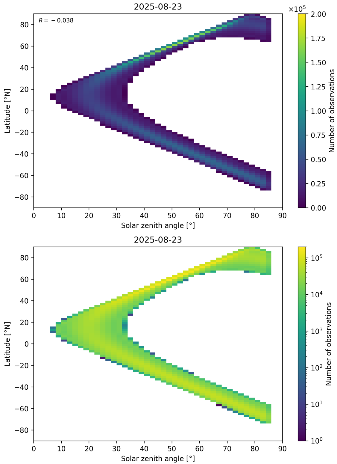
Figure 181: Scatter density plot of “Solar zenith angle” against “Latitude” for 2025-08-22 to 2025-08-24.
