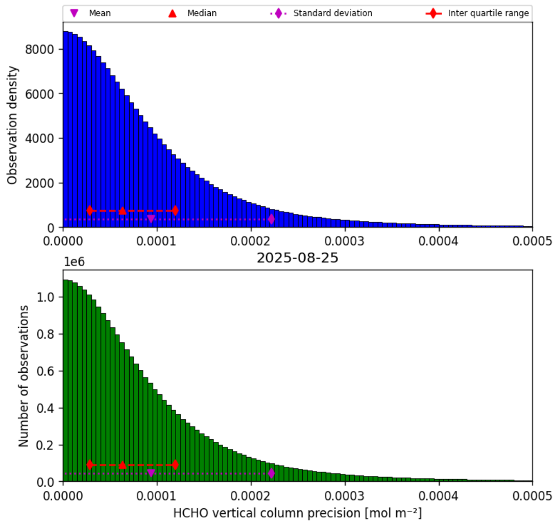
Figure 36: Histogram of “HCHO vertical column precision” for 2025-08-25 to 2025-08-26
