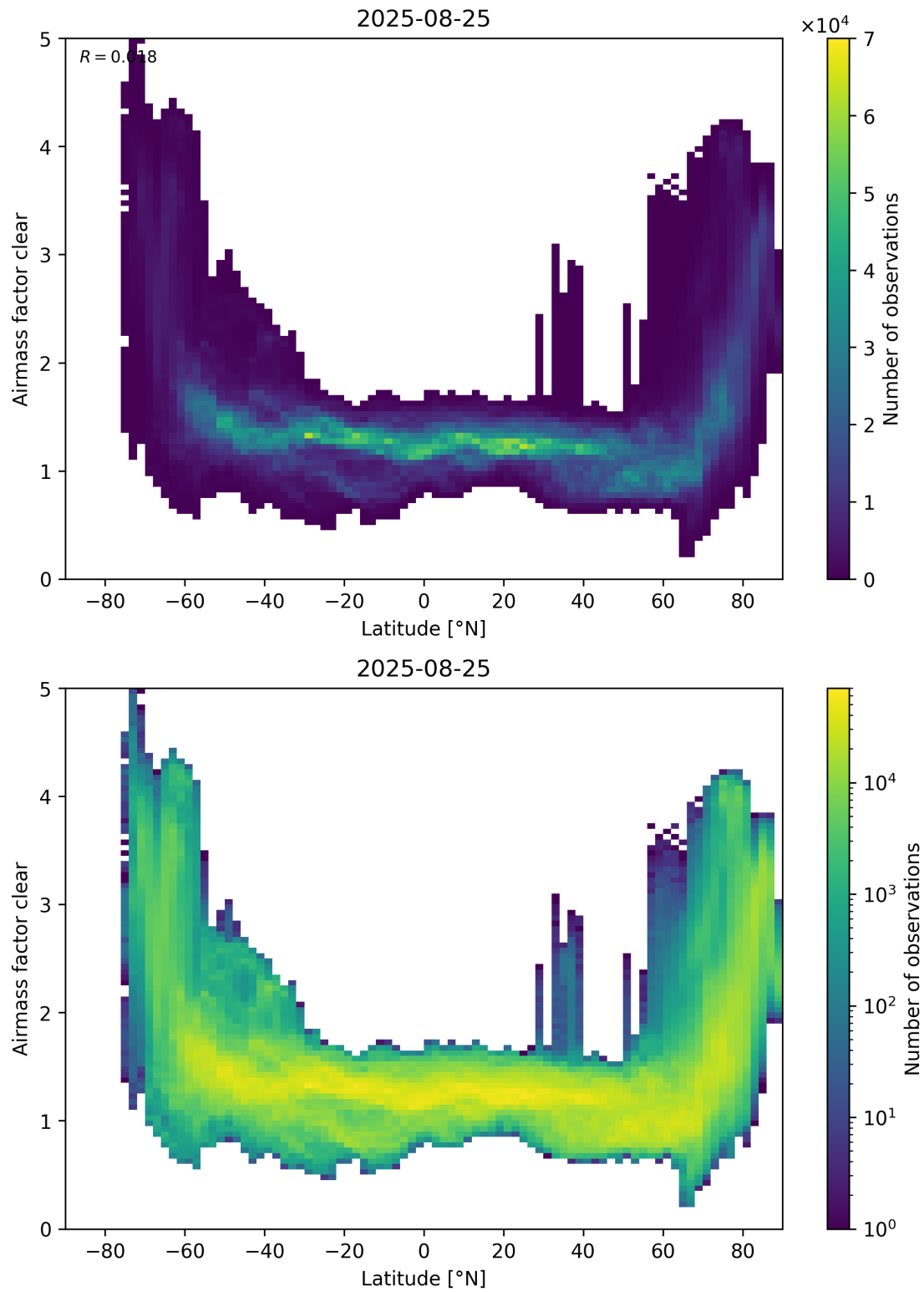
Figure 156: Scatter density plot of “Latitude” against “Airmass factor clear” for 2025-08-25 to 2025-08-26.
