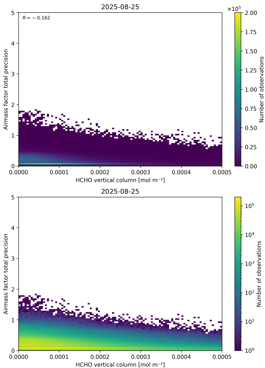
Figure 132: Scatter density plot of “HCHO vertical column” against “Airmass factor total precision” for 2025-08-25 to 2025-08-26.
