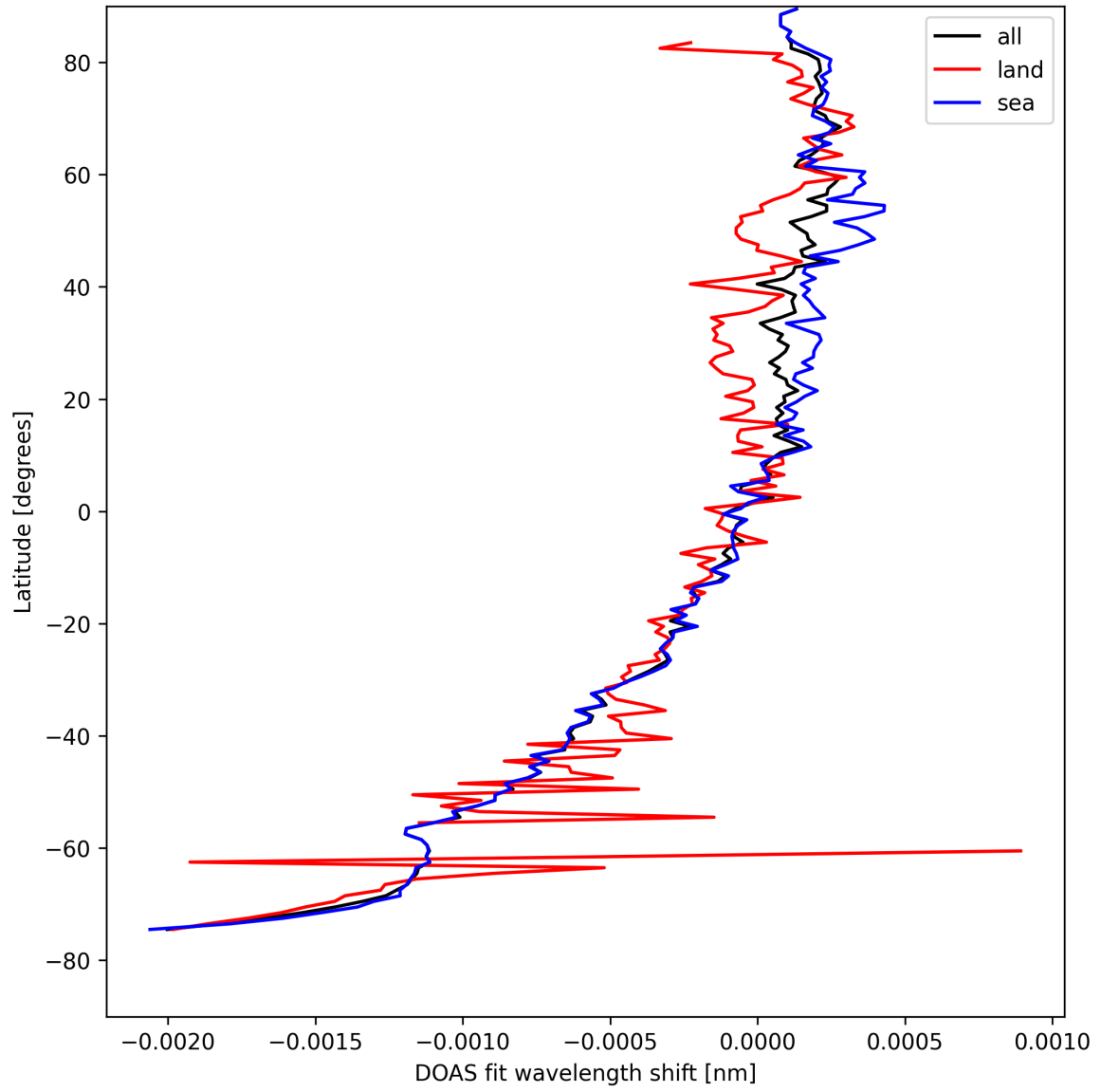
Figure 30: Zonal average of “DOAS fit wavelength shift” for 2025-08-25 to 2025-08-26.
