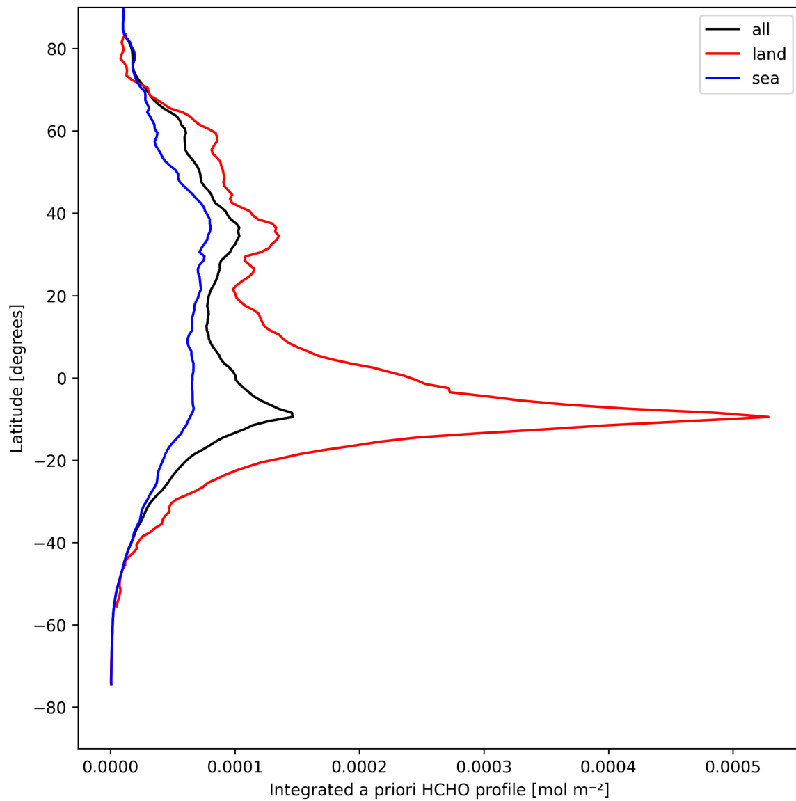
Figure 29: Zonal average of “Integrated a priori HCHO profile” for 2025-08-25 to 2025-08-26.
