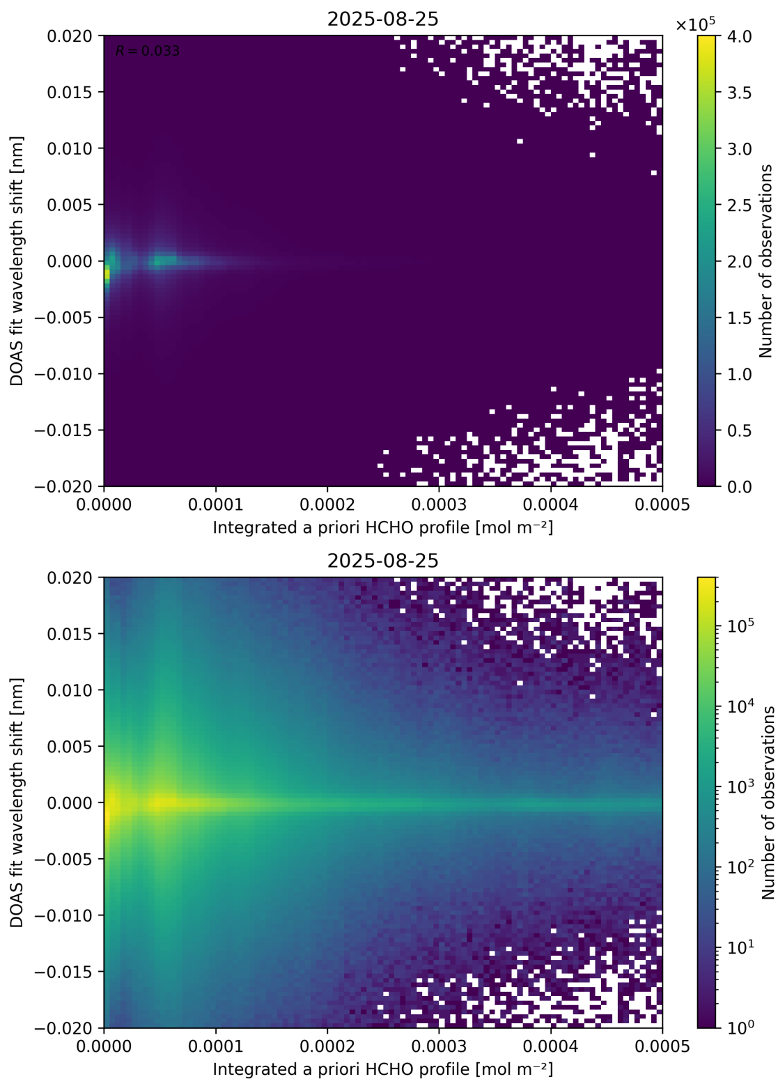
Figure 149: Scatter density plot of “Integrated a priori HCHO profile” against “DOAS fit wavelength shift” for 2025-08-25 to 2025-08-26.
