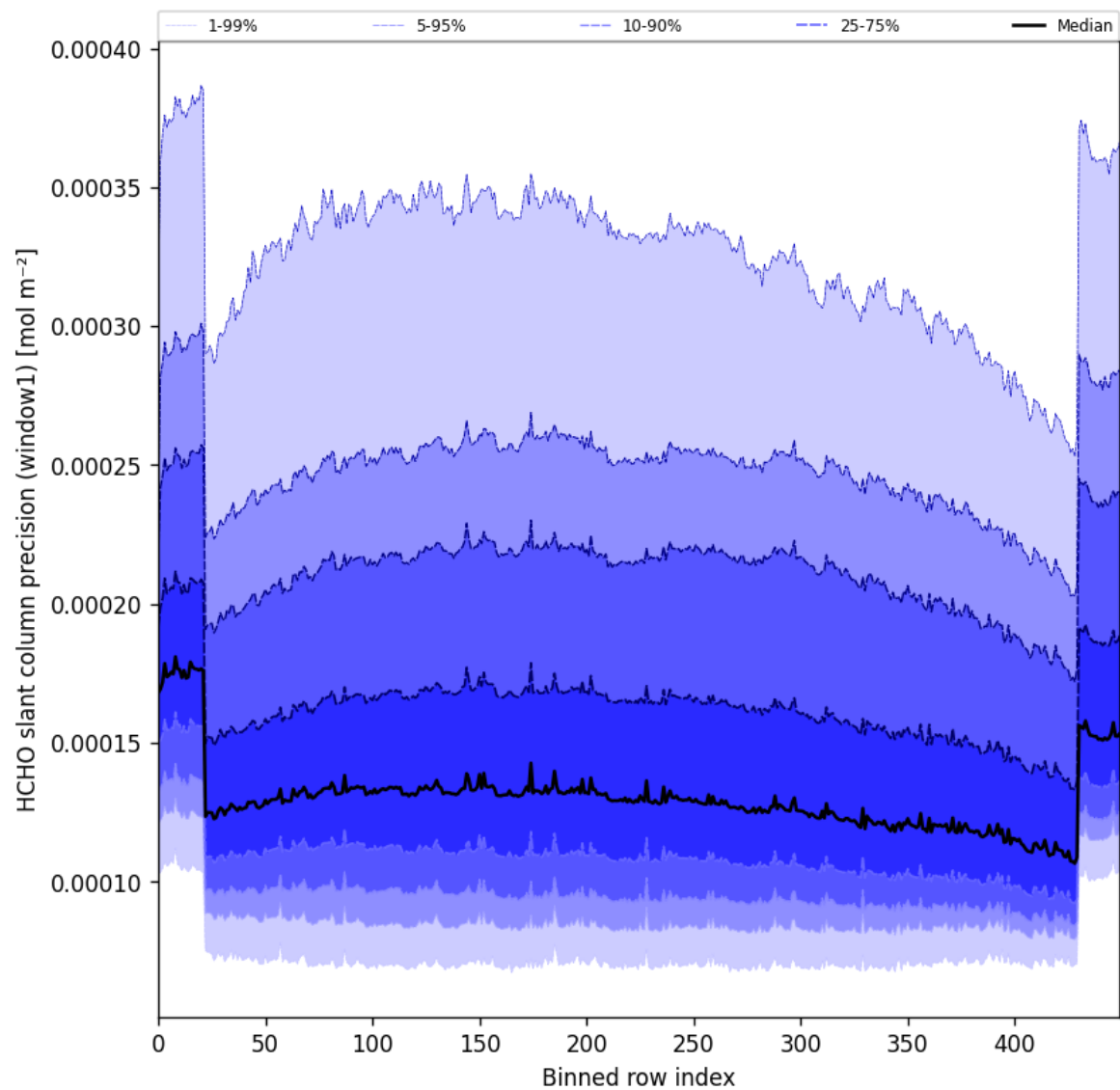
Figure 53: Along track statistics of “HCHO slant column precision (window1)” for 2025-08-25 to 2025-08-26
