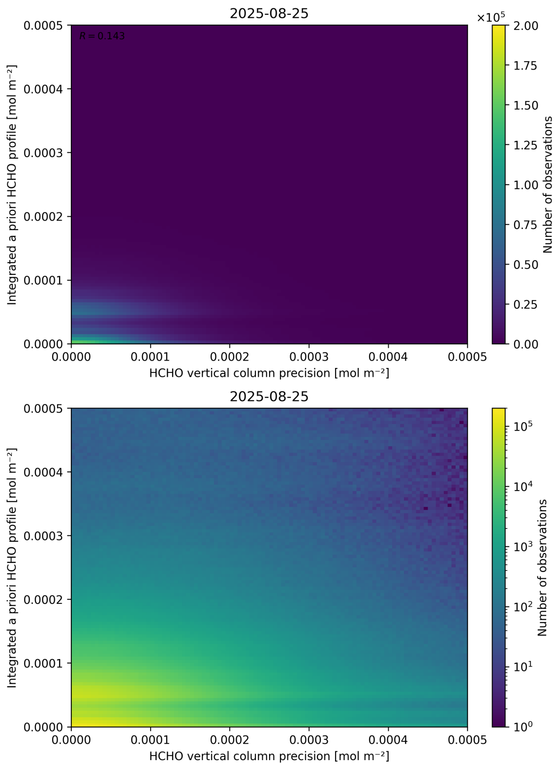
Figure 147: Scatter density plot of “HCHO vertical column precision” against “Integrated a priori HCHO profile” for 2025-08-25 to 2025-08-26.
