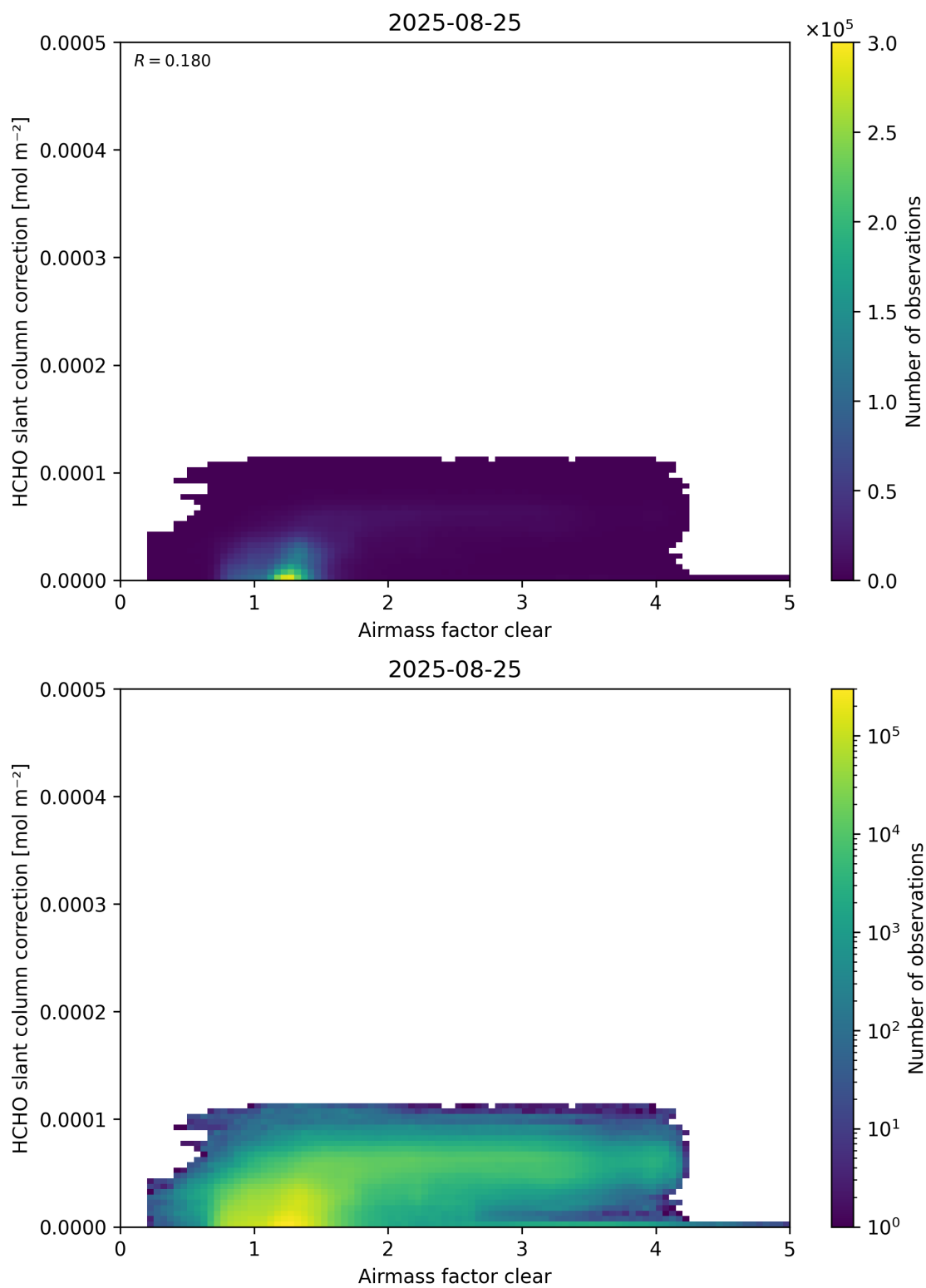
Figure 75: Scatter density plot of “Airmass factor clear” against “HCHO slant column correction” for 2025-08-25 to 2025-08-26.
