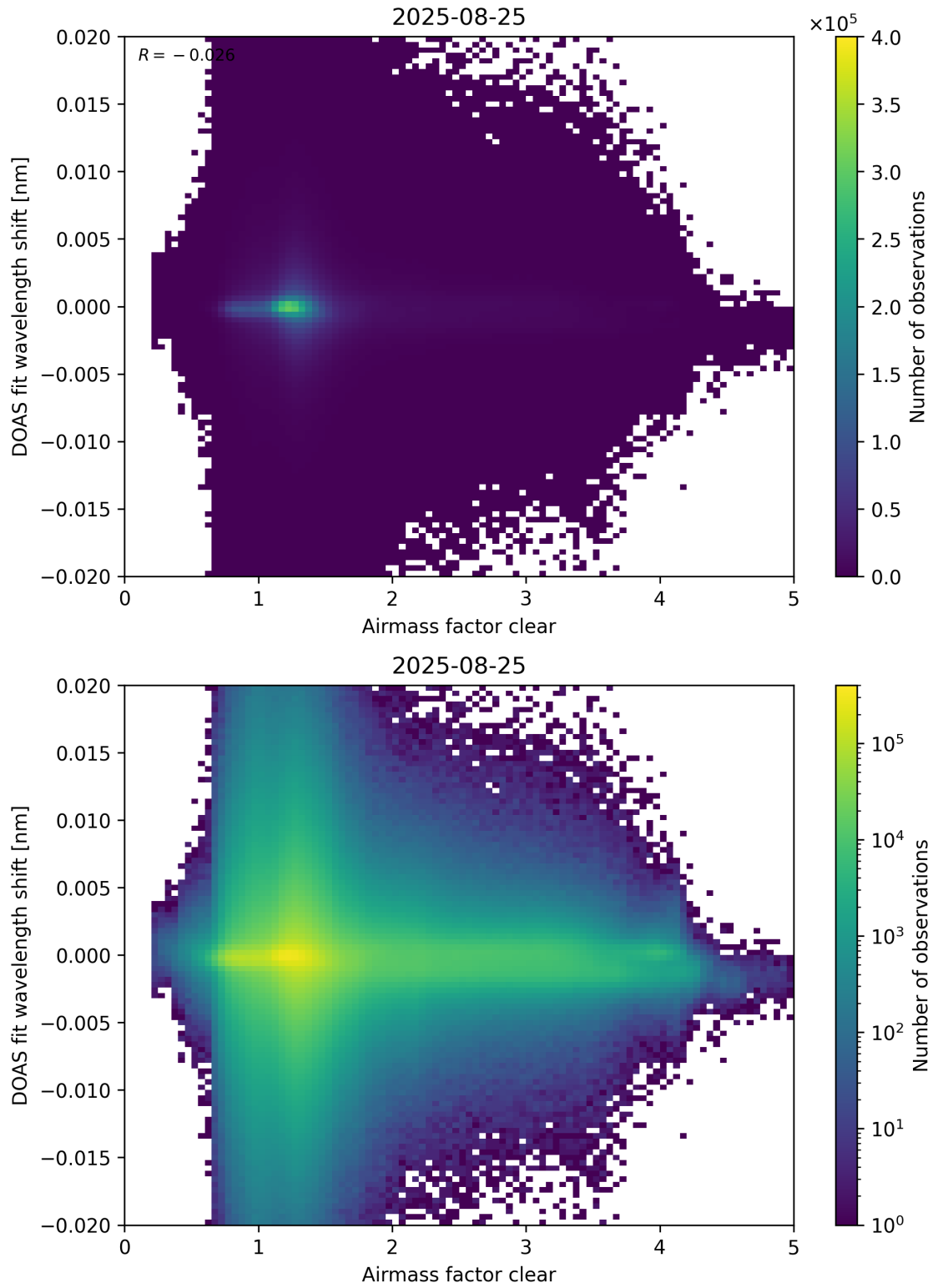
Figure 72: Scatter density plot of “Airmass factor clear” against “DOAS fit wavelength shift” for 2025-08-25 to 2025-08-26.
