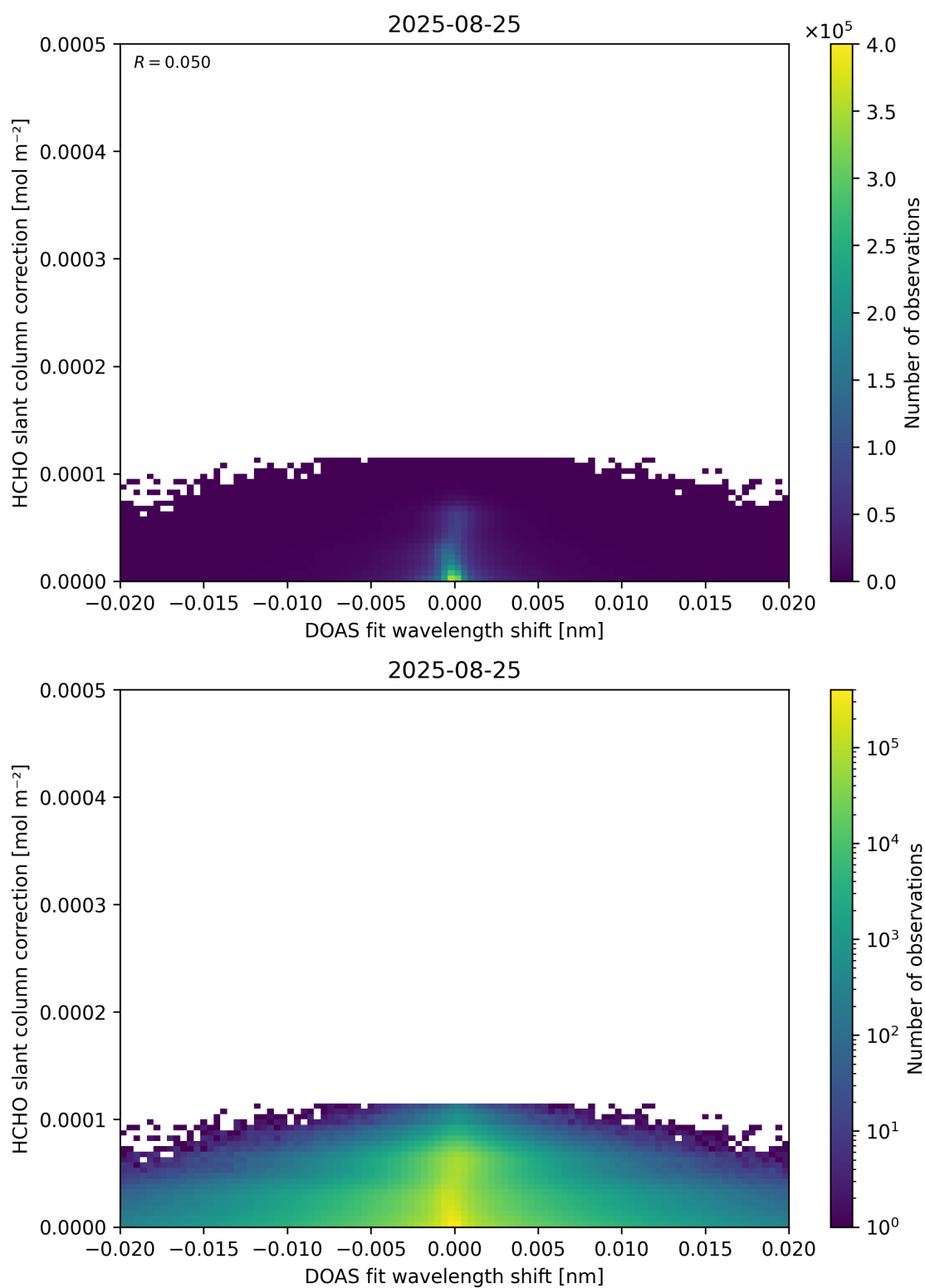
Figure 67: Scatter density plot of “DOAS fit wavelength shift” against “HCHO slant column correction” for 2025-08-25 to 2025-08-26.
