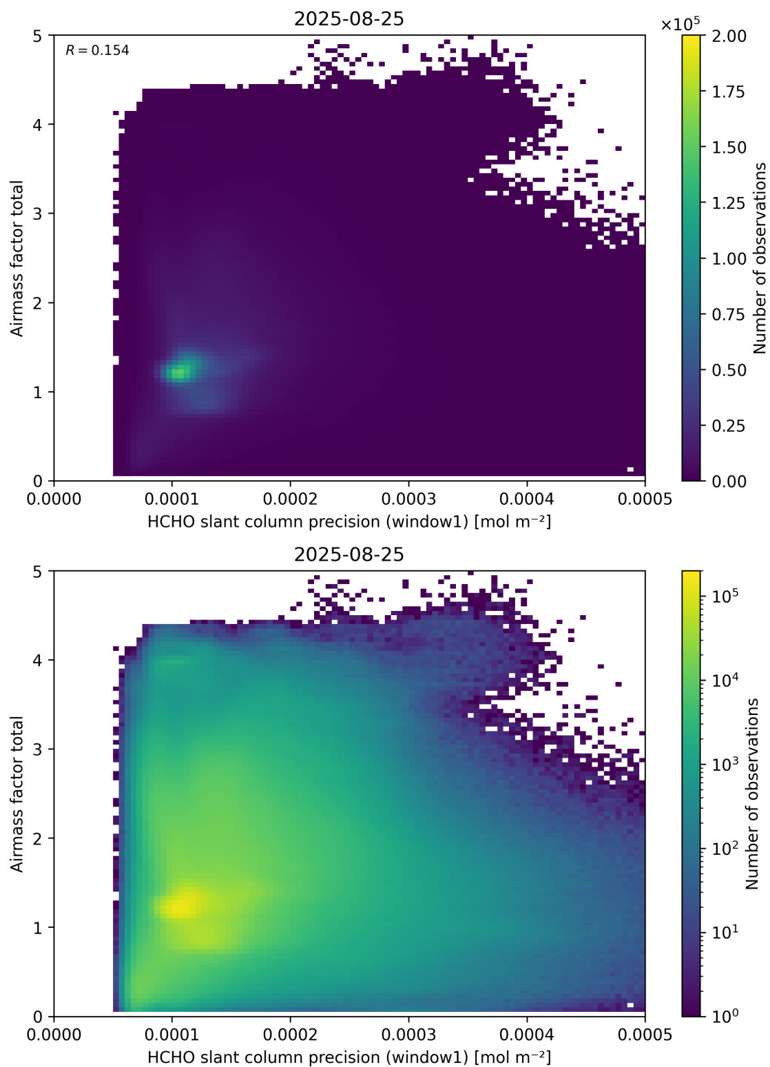
Figure 94: Scatter density plot of “HCHO slant column precision (window1)” against “Airmass factor total” for 2025-08-25 to 2025-08-26.
