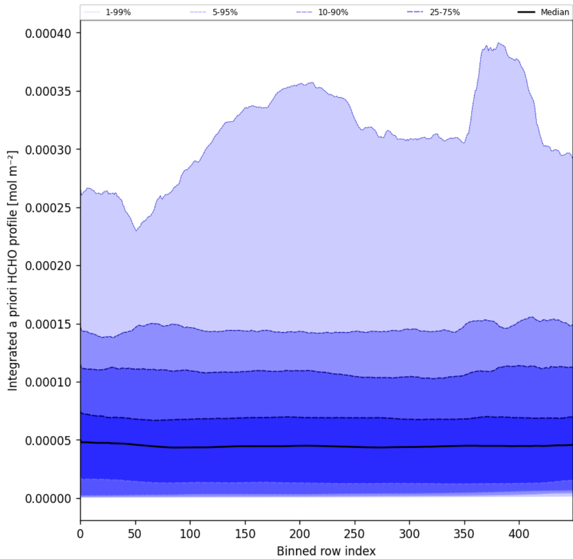
Figure 57: Along track statistics of "Integrated a priori HCHO profile" for 2025-08-25 to 2025-08-26
