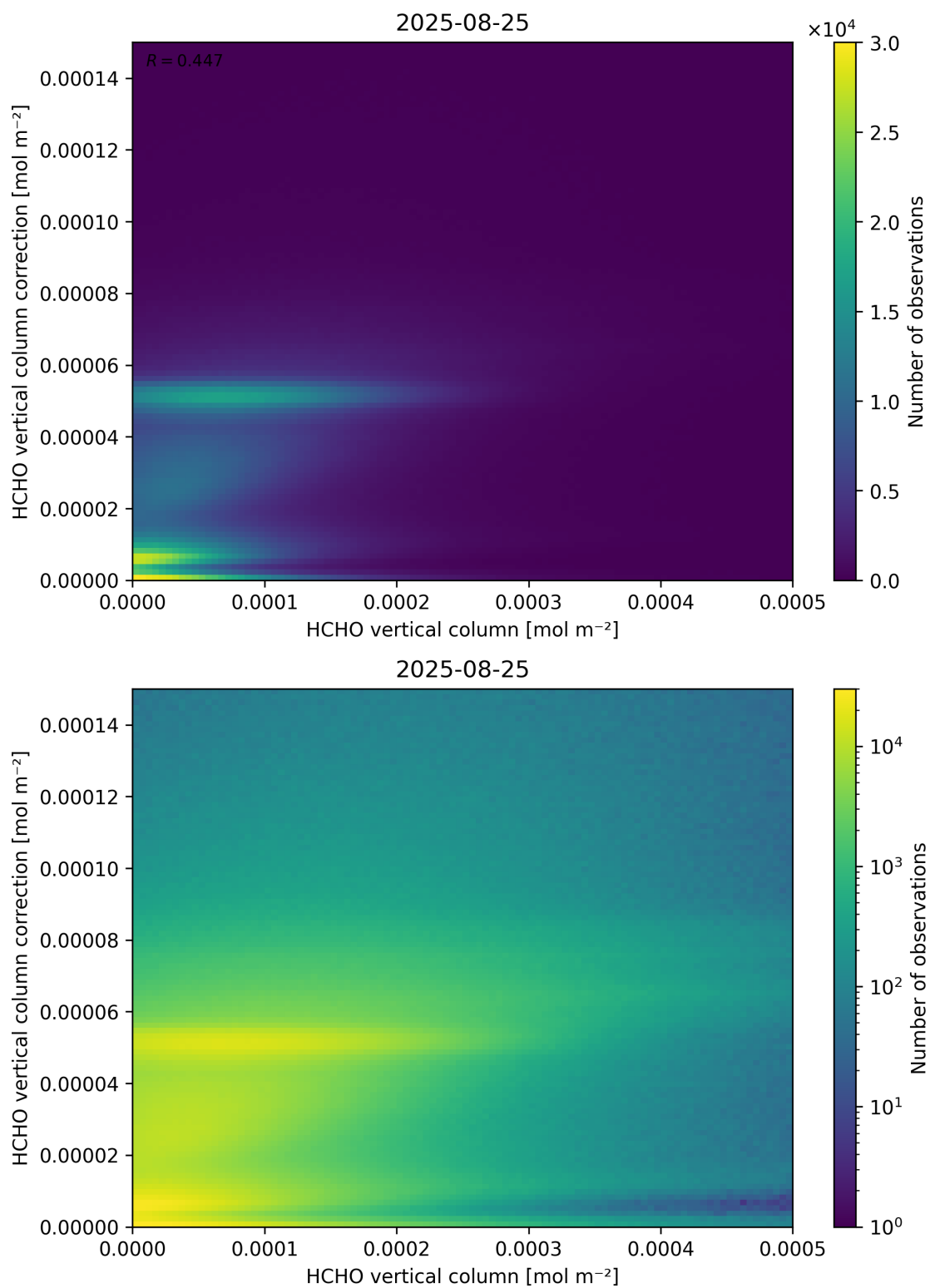
Figure 133: Scatter density plot of “HCHO vertical column” against “HCHO vertical column correction” for 2025-08-25 to 2025-08-26.
