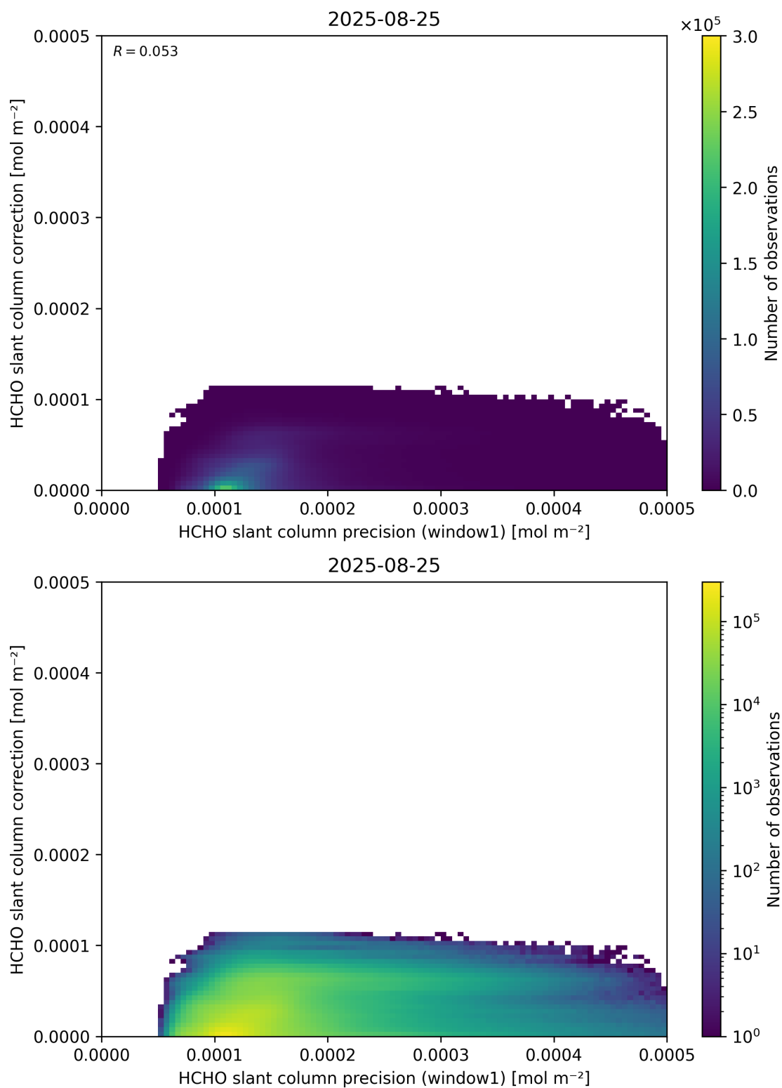
Figure 93: Scatter density plot of “HCHO slant column precision (window1)” against “HCHO slant column correction” for 2025-08-25 to 2025-08-26.
