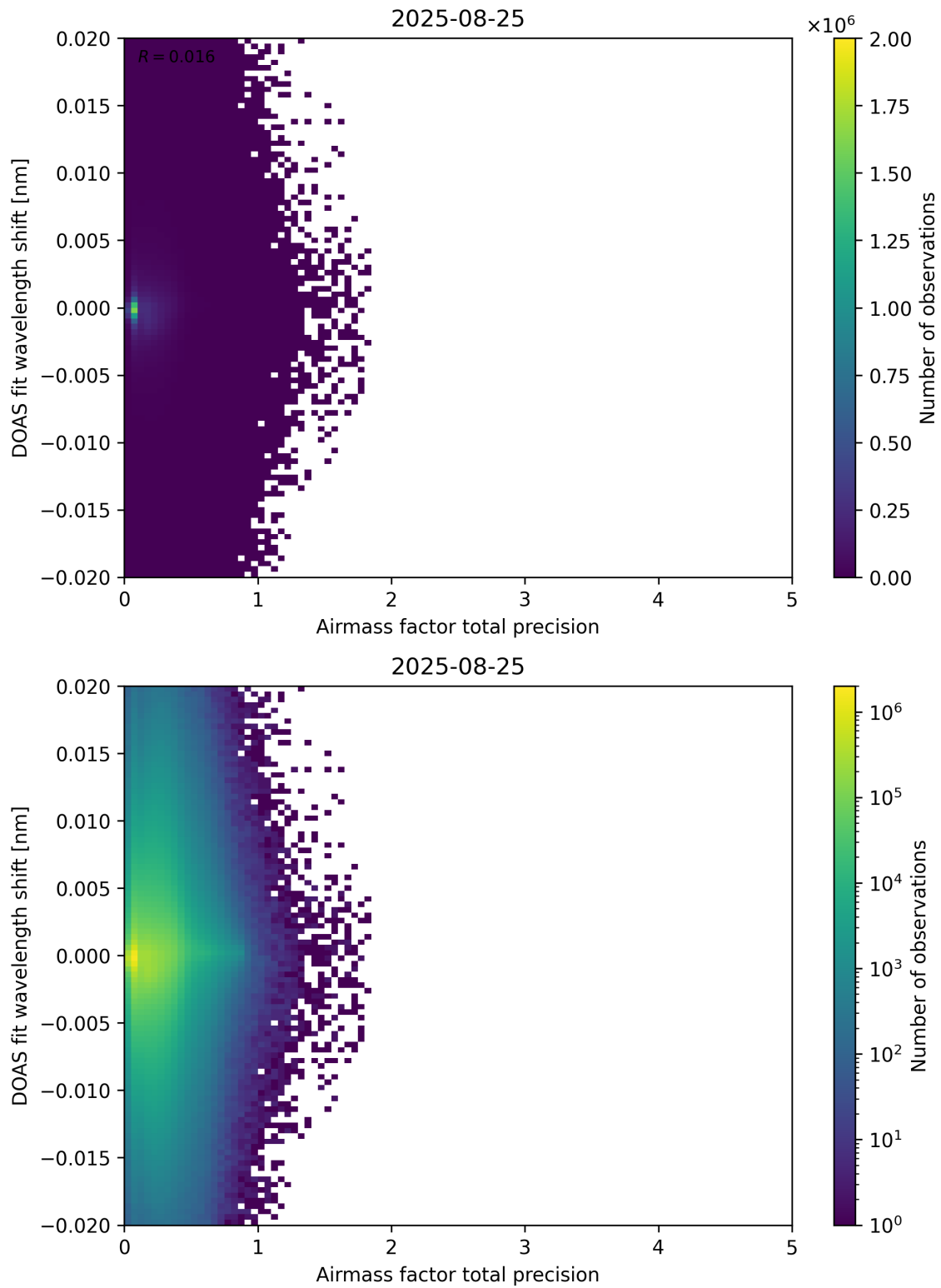
Figure 106: Scatter density plot of “Airmass factor total precision” against “DOAS fit wavelength shift” for 2025-08-25 to 2025-08-26.
