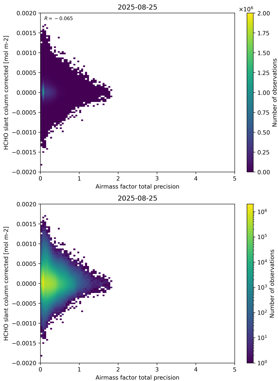
Figure 109: Scatter density plot of “Airmass factor total precision” against “HCHO slant column corrected” for 2025-08-25 to 2025-08-26.
