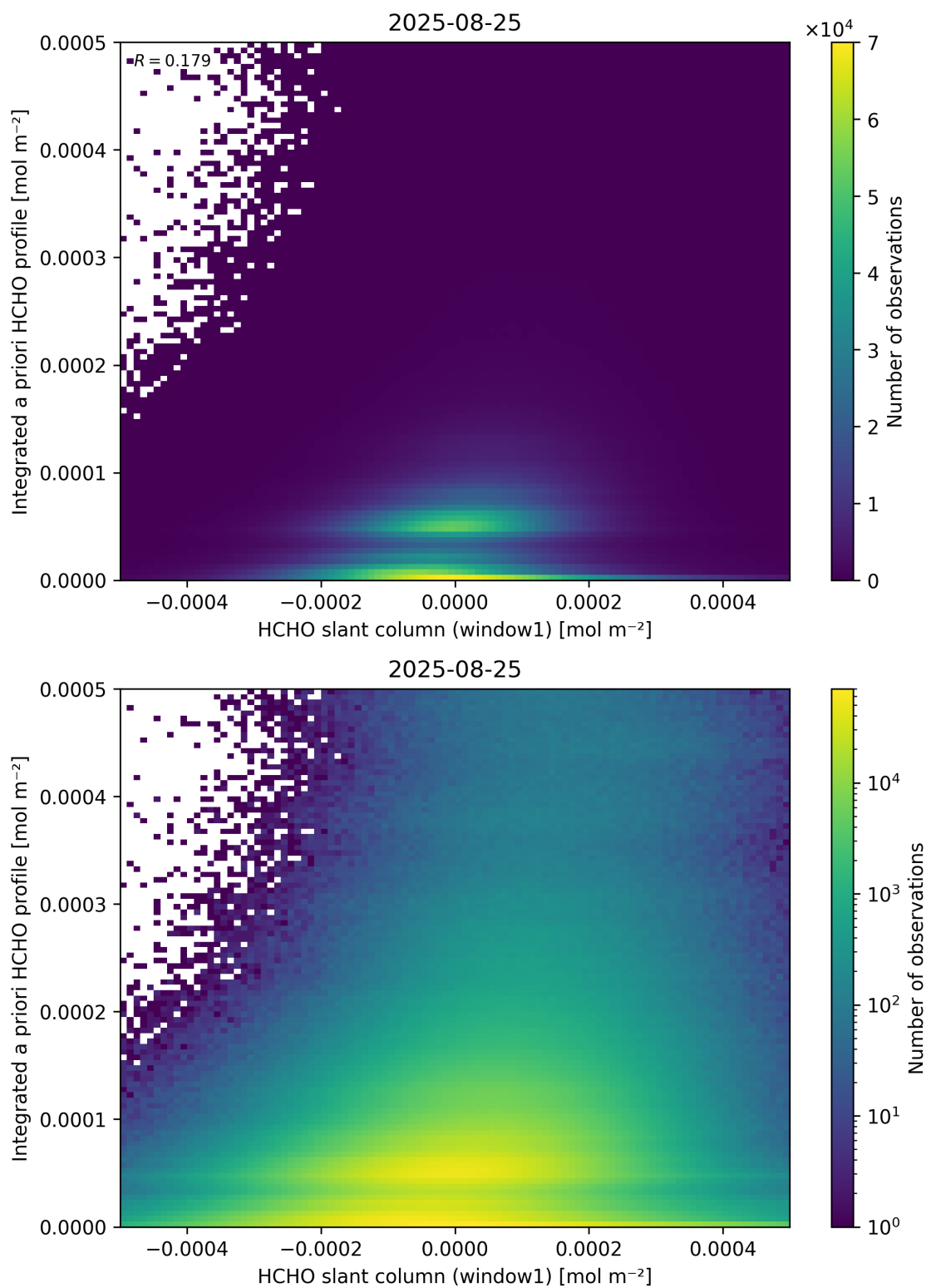
Figure 87: Scatter density plot of “HCHO slant column (window1)” against “Integrated a priori HCHO profile” for 2025-08-25 to 2025-08-26.
