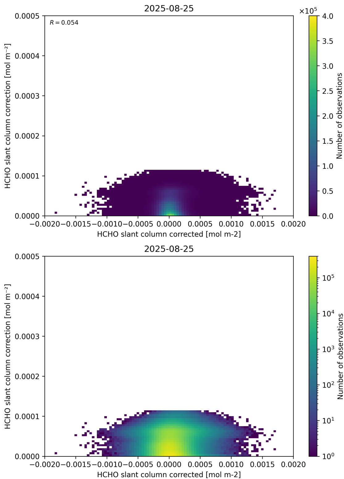
Figure 77: Scatter density plot of “HCHO slant column corrected” against “HCHO slant column correction” for 2025-08-25 to 2025-08-26.
