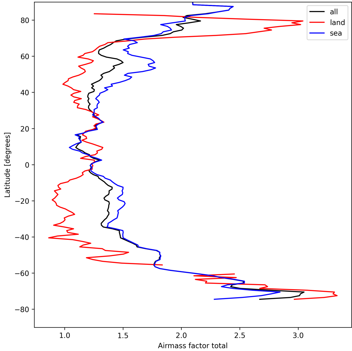
Figure 26: Zonal average of “Airmass factor total” for 2025-08-25 to 2025-08-26.
