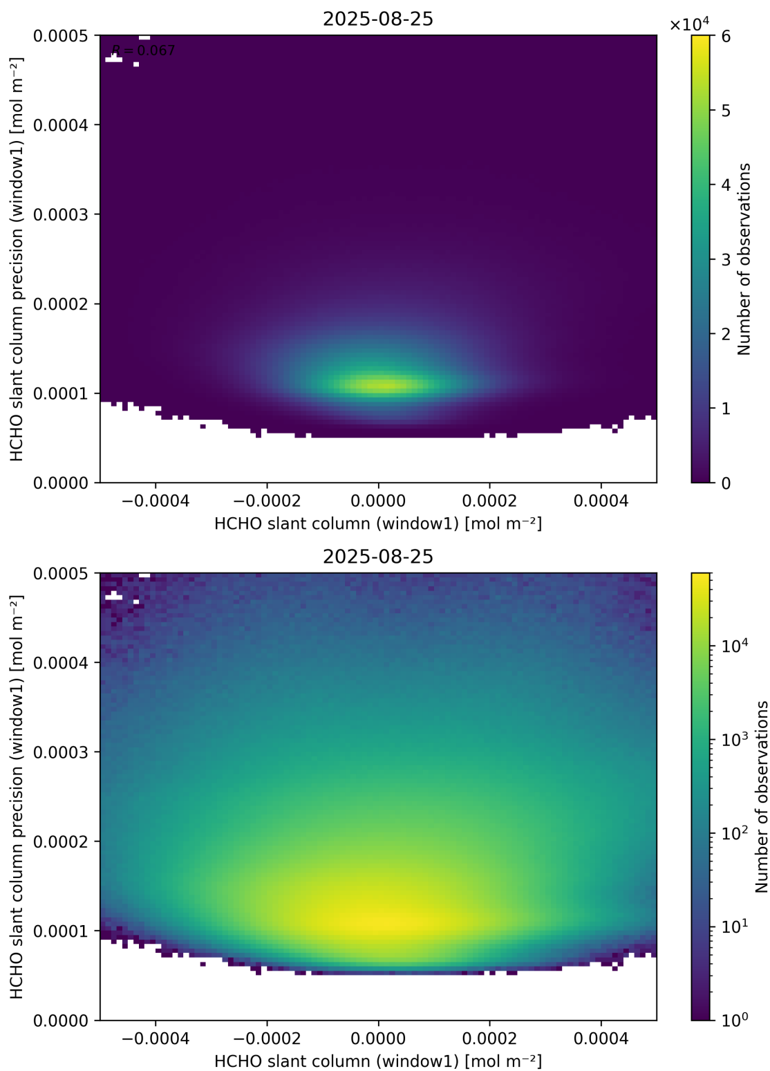
Figure 84: Scatter density plot of “HCHO slant column (window1)” against “HCHO slant column precision (window1)” for 2025-08-25 to 2025-08-26.
