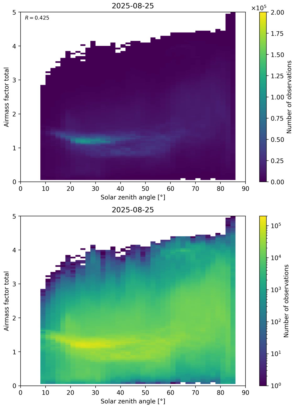
Figure 175: Scatter density plot of “Solar zenith angle” against “Airmass factor total” for 2025-08-25 to 2025-08-26.
