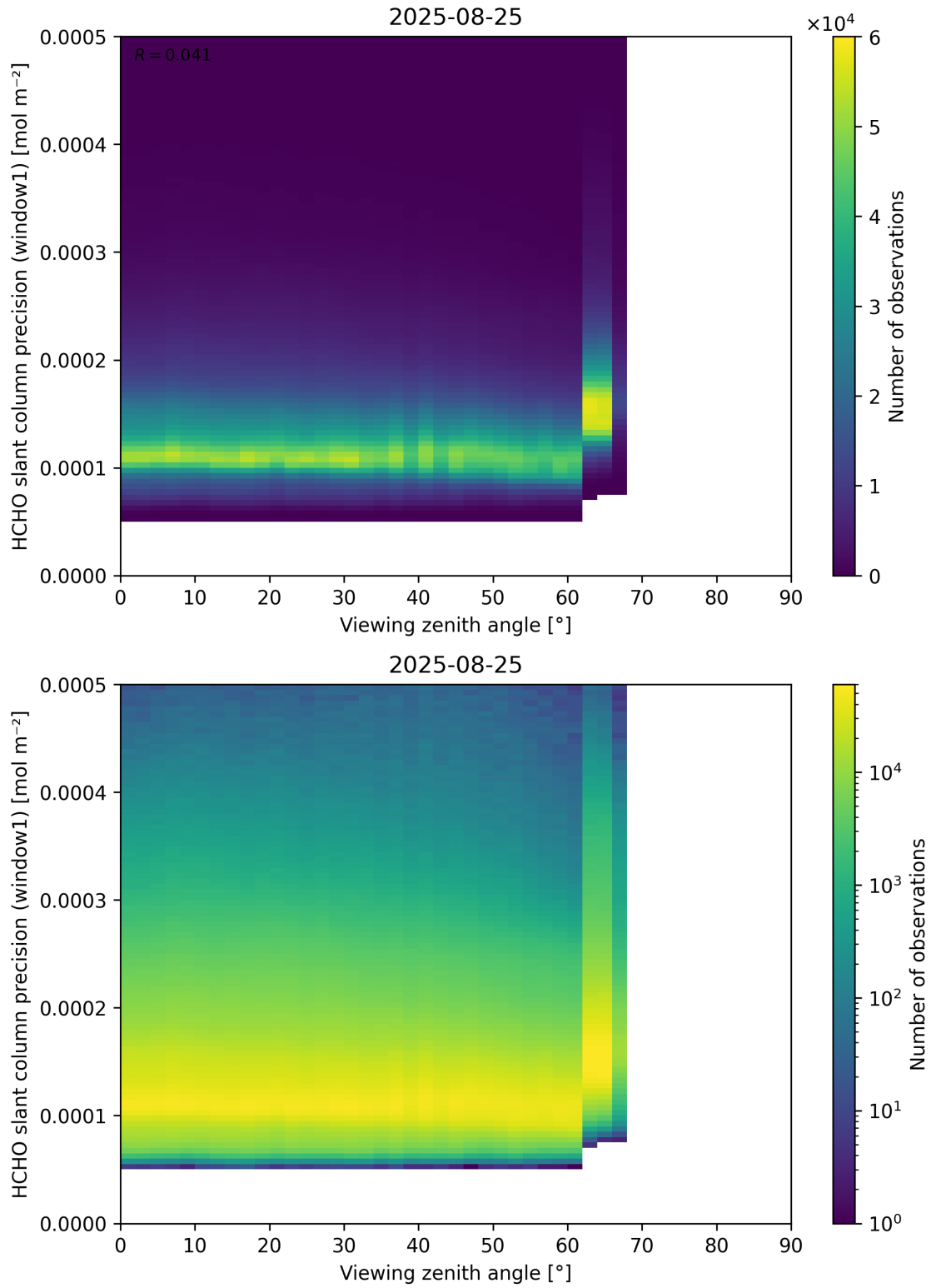
Figure 189: Scatter density plot of “Viewing zenith angle” against “HCHO slant column precision (window1)” for 2025-08-25 to 2025-08-26.
