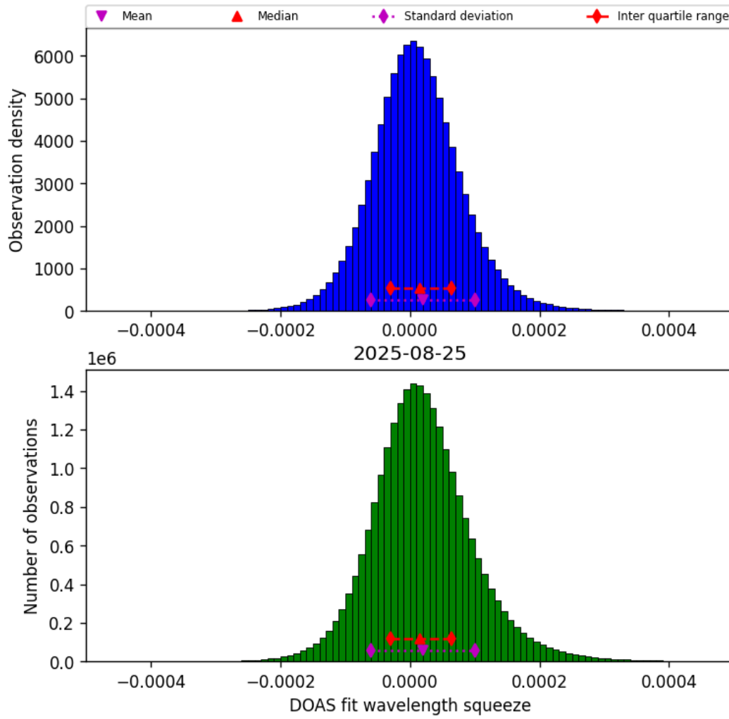
Figure 45: Histogram of “DOAS fit wavelength squeeze” for 2025-08-25 to 2025-08-26
