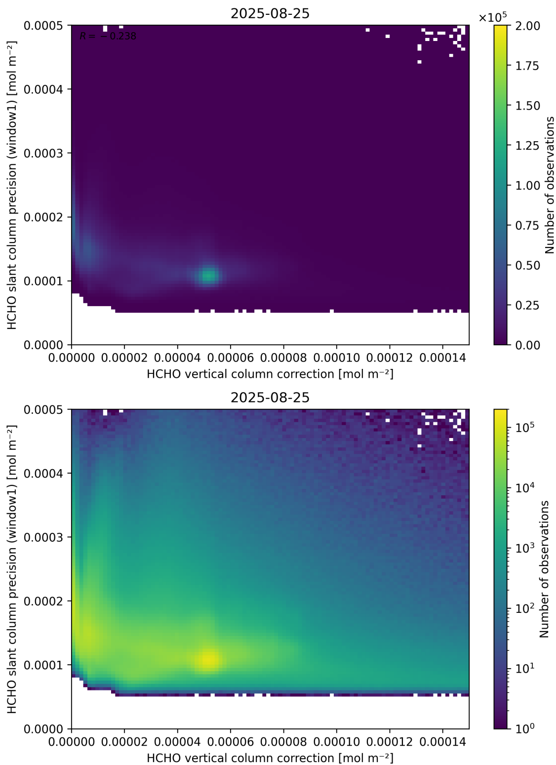
Figure 119: Scatter density plot of “HCHO vertical column correction” against “HCHO slant column precision (window1)” for 2025-08-25 to 2025-08-26.
