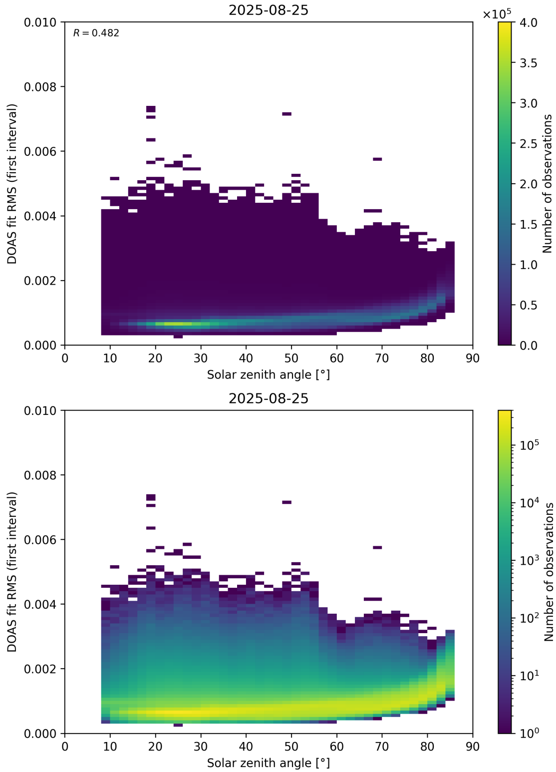
Figure 167: Scatter density plot of “Solar zenith angle” against “DOAS fit RMS (first interval)” for 2025-08-25 to 2025-08-26.
