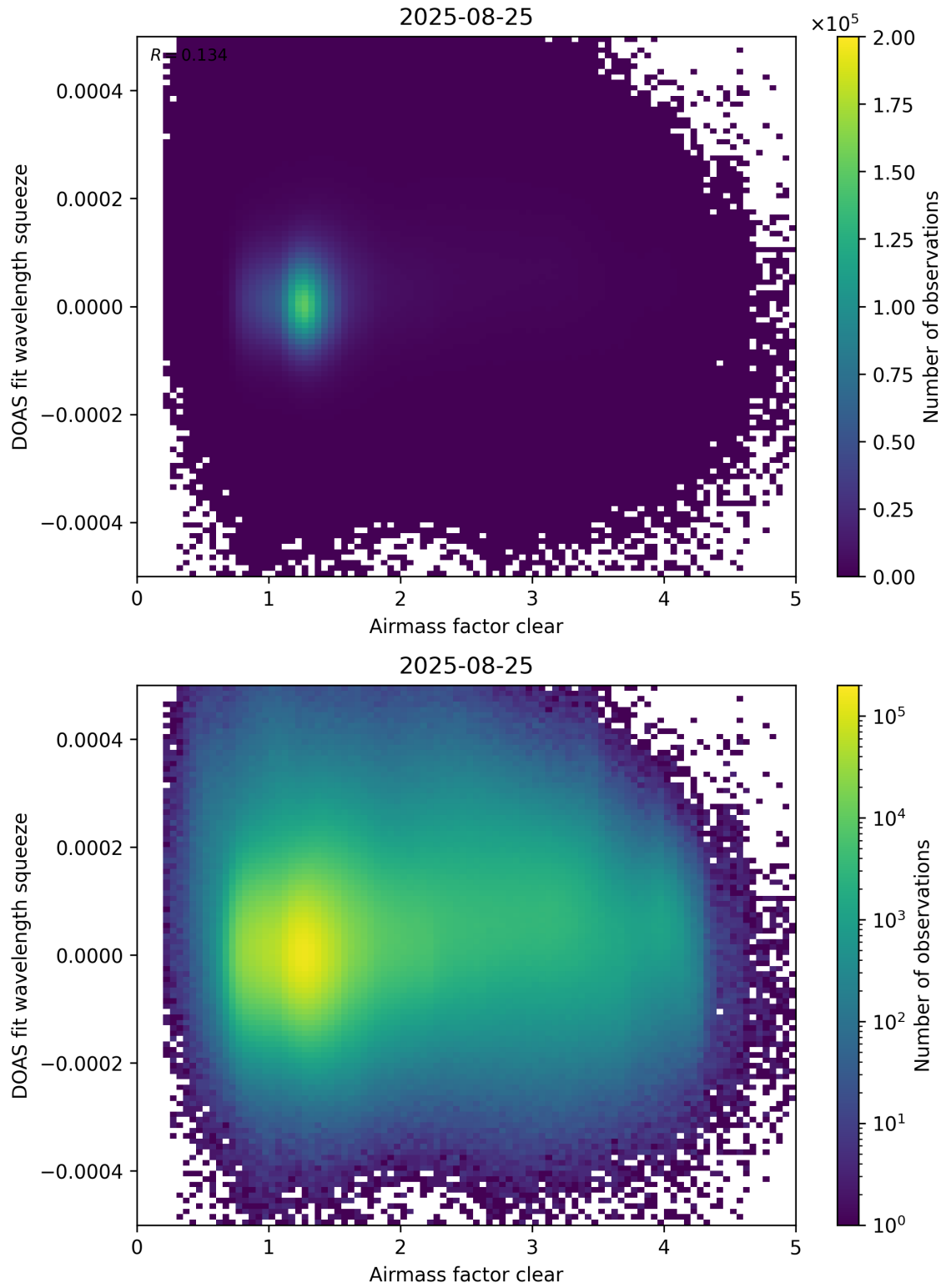
Figure 73: Scatter density plot of “Airmass factor clear” against “DOAS fit wavelength squeeze” for 2025-08-25 to 2025-08-26.
