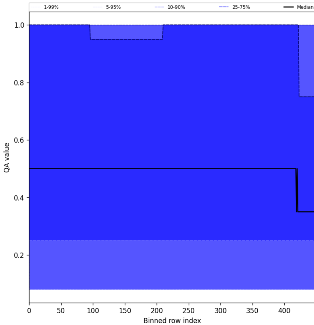
Figure 48: Along track statistics of “QA value” for 2025-08-25 to 2025-08-26
