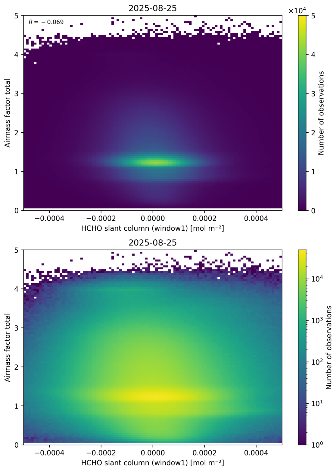
Figure 85: Scatter density plot of “HCHO slant column (window1)” against “Airmass factor total” for 2025-08-25 to 2025-08-26.
