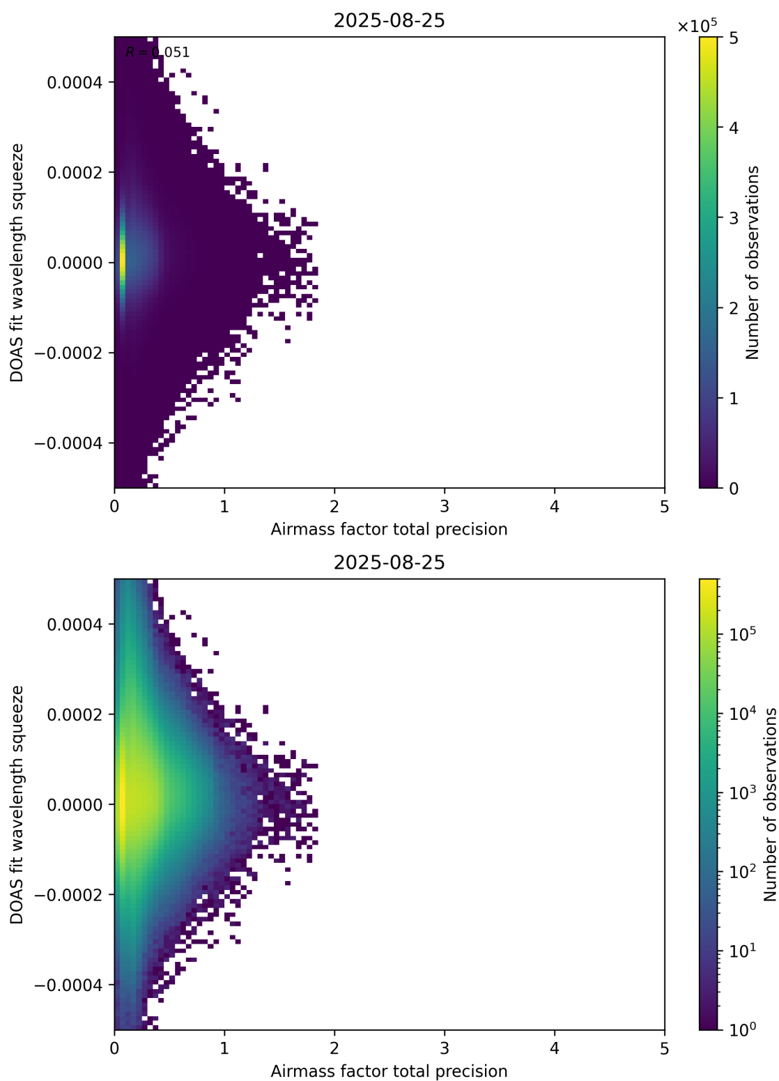
Figure 107: Scatter density plot of “Airmass factor total precision” against “DOAS fit wavelength squeeze” for 2025-08-25 to 2025-08-26.
