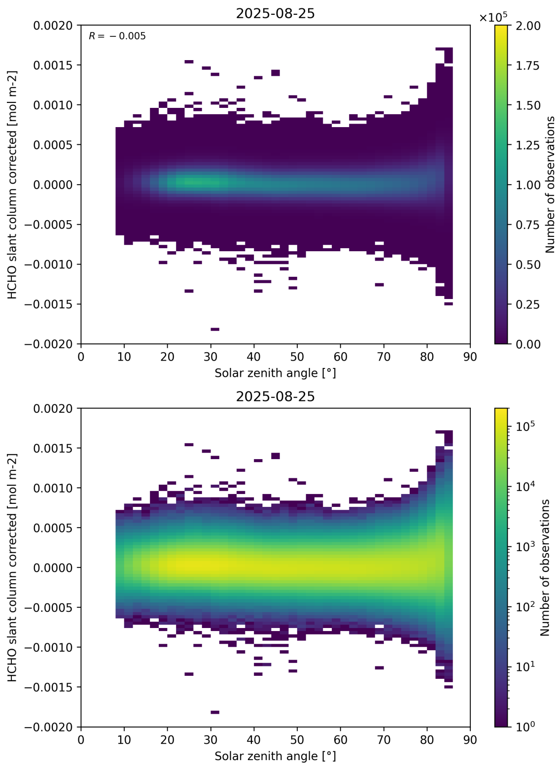
Figure 171: Scatter density plot of “Solar zenith angle” against “HCHO slant column corrected” for 2025-08-25 to 2025-08-26.
