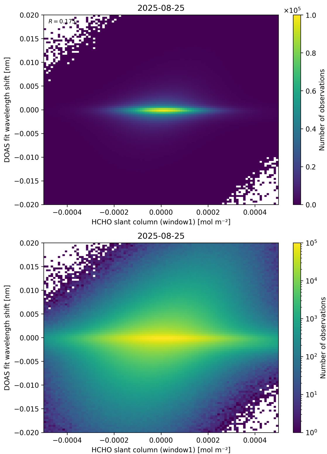
Figure 79: Scatter density plot of “HCHO slant column (window1)” against “DOAS fit wavelength shift” for 2025-08-25 to 2025-08-26.
