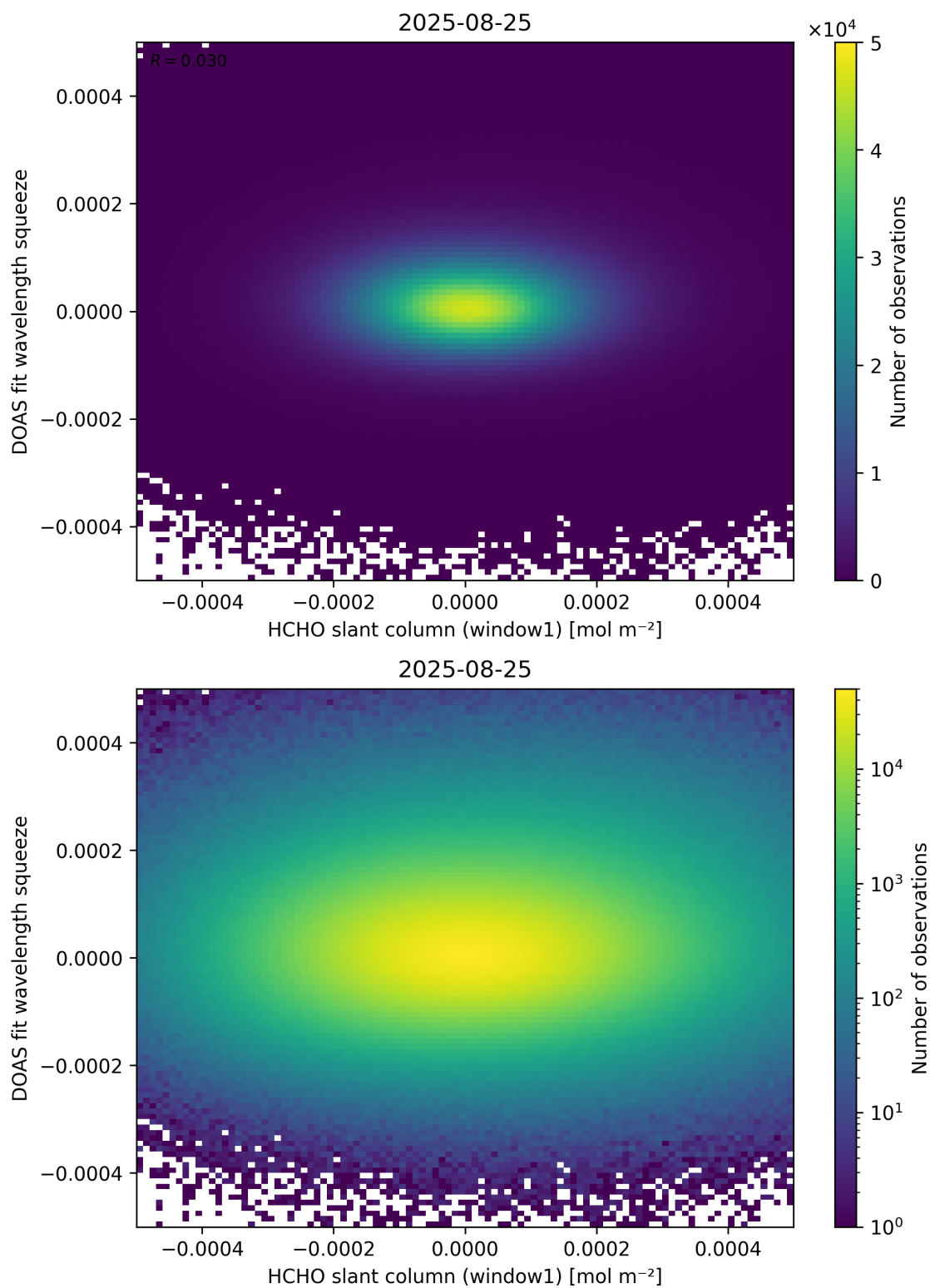
Figure 80: Scatter density plot of “HCHO slant column (window1)” against “DOAS fit wavelength squeeze” for 2025-08-25 to 2025-08-26.
