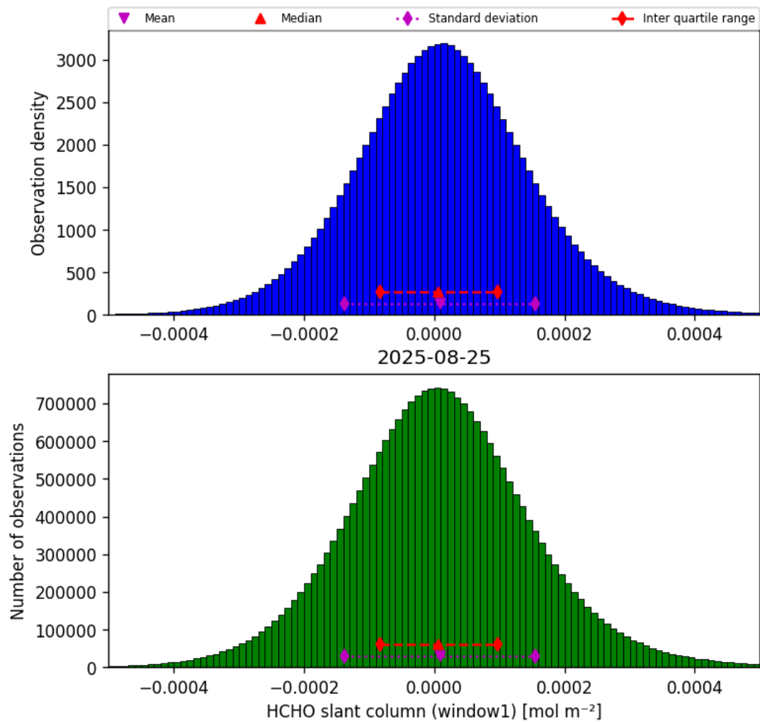
Figure 38: Histogram of “HCHO slant column (window1)” for 2025-08-25 to 2025-08-26
