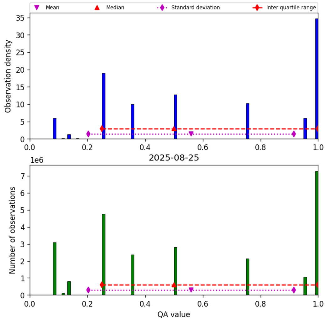
Figure 34: Histogram of “QA value” for 2025-08-25 to 2025-08-26
