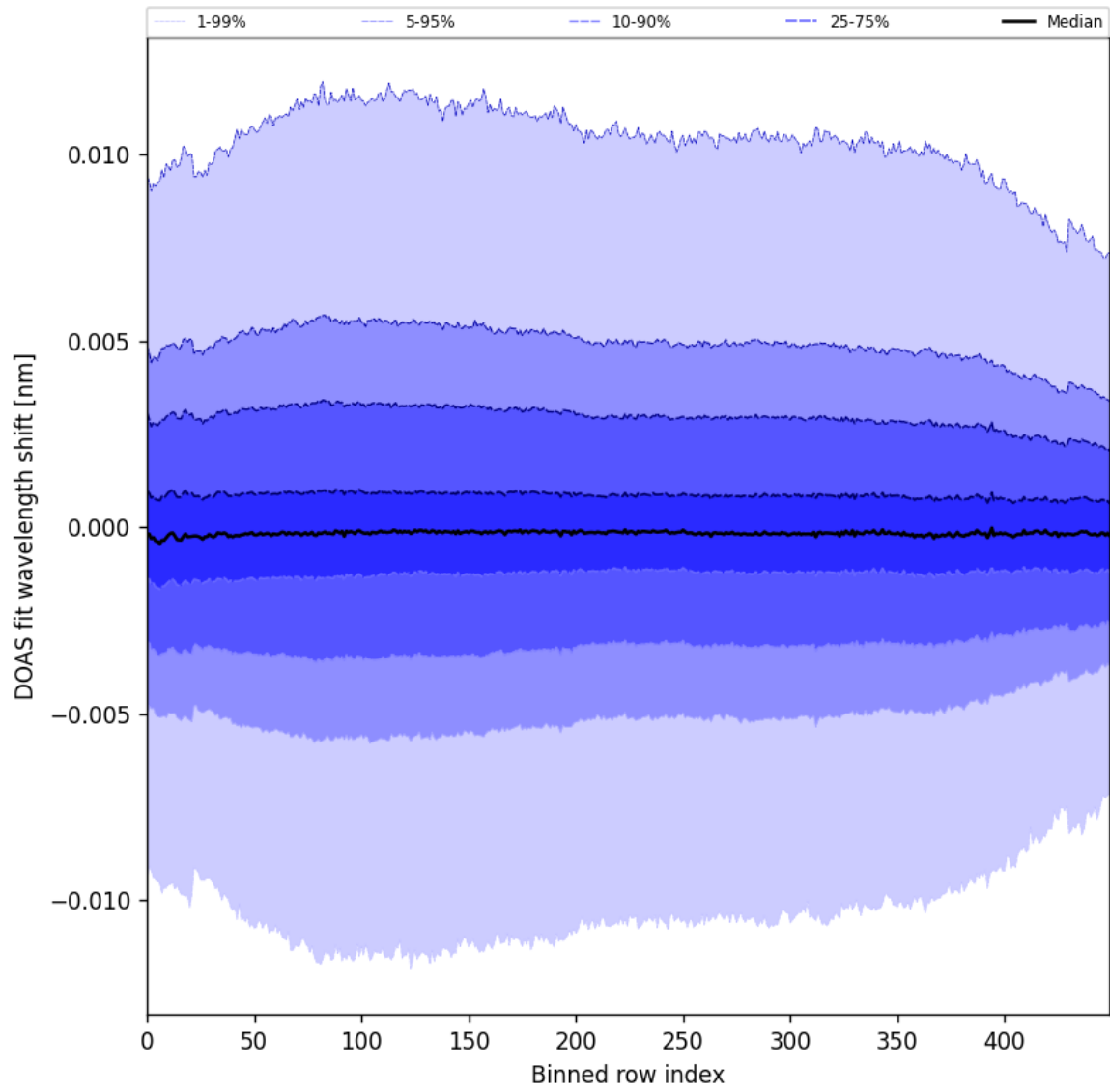
Figure 58: Along track statistics of “DOAS fit wavelength shift” for 2025-08-25 to 2025-08-26
