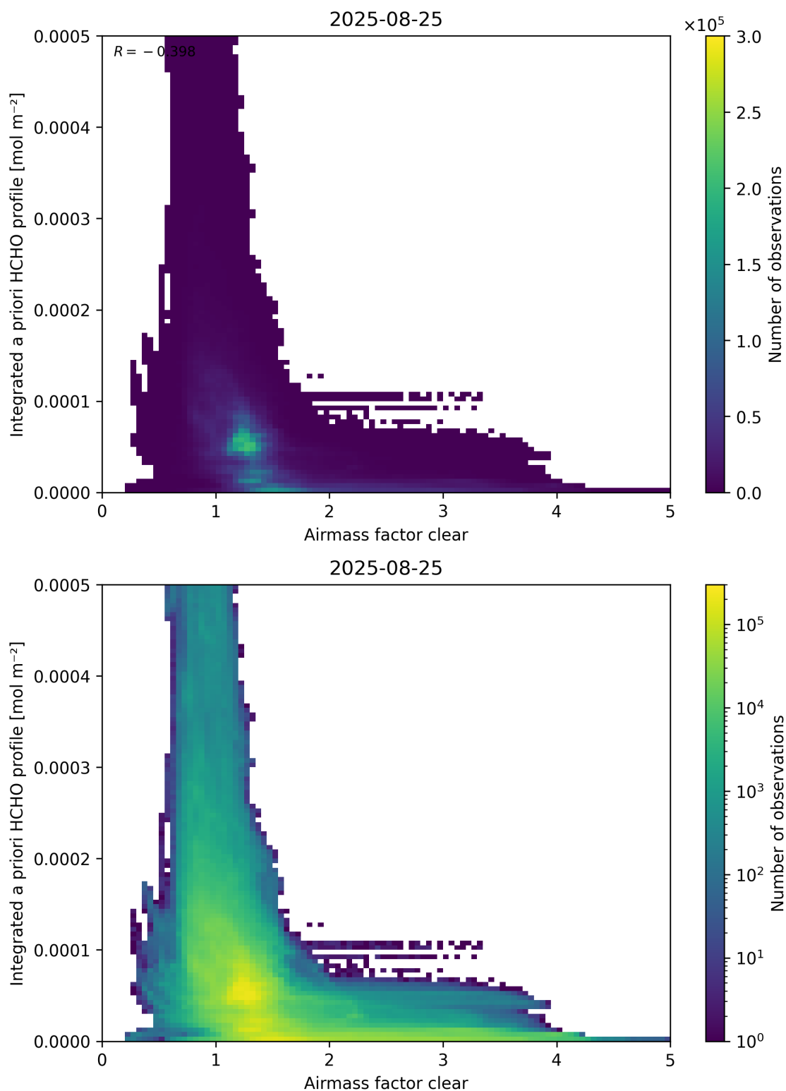
Figure 76: Scatter density plot of “Airmass factor clear” against “Integrated a priori HCHO profile” for 2025-08-25 to 2025-08-26.
