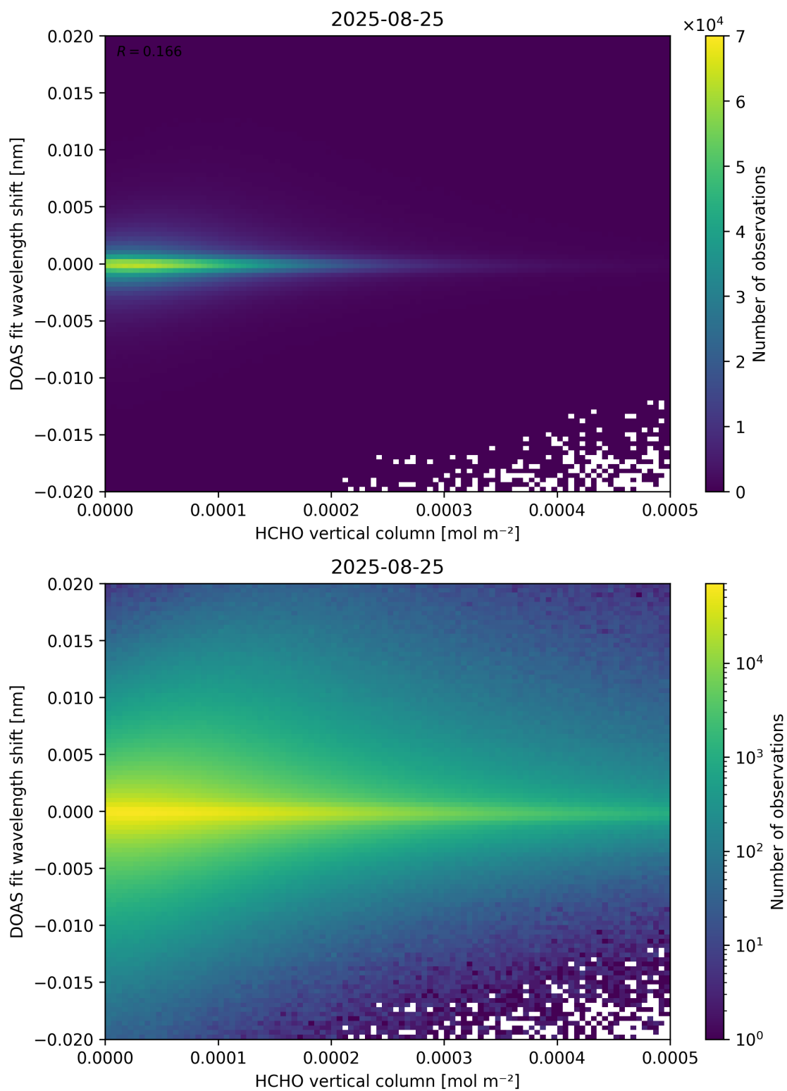
Figure 124: Scatter density plot of “HCHO vertical column” against “DOAS fit wavelength shift” for 2025-08-25 to 2025-08-26.
