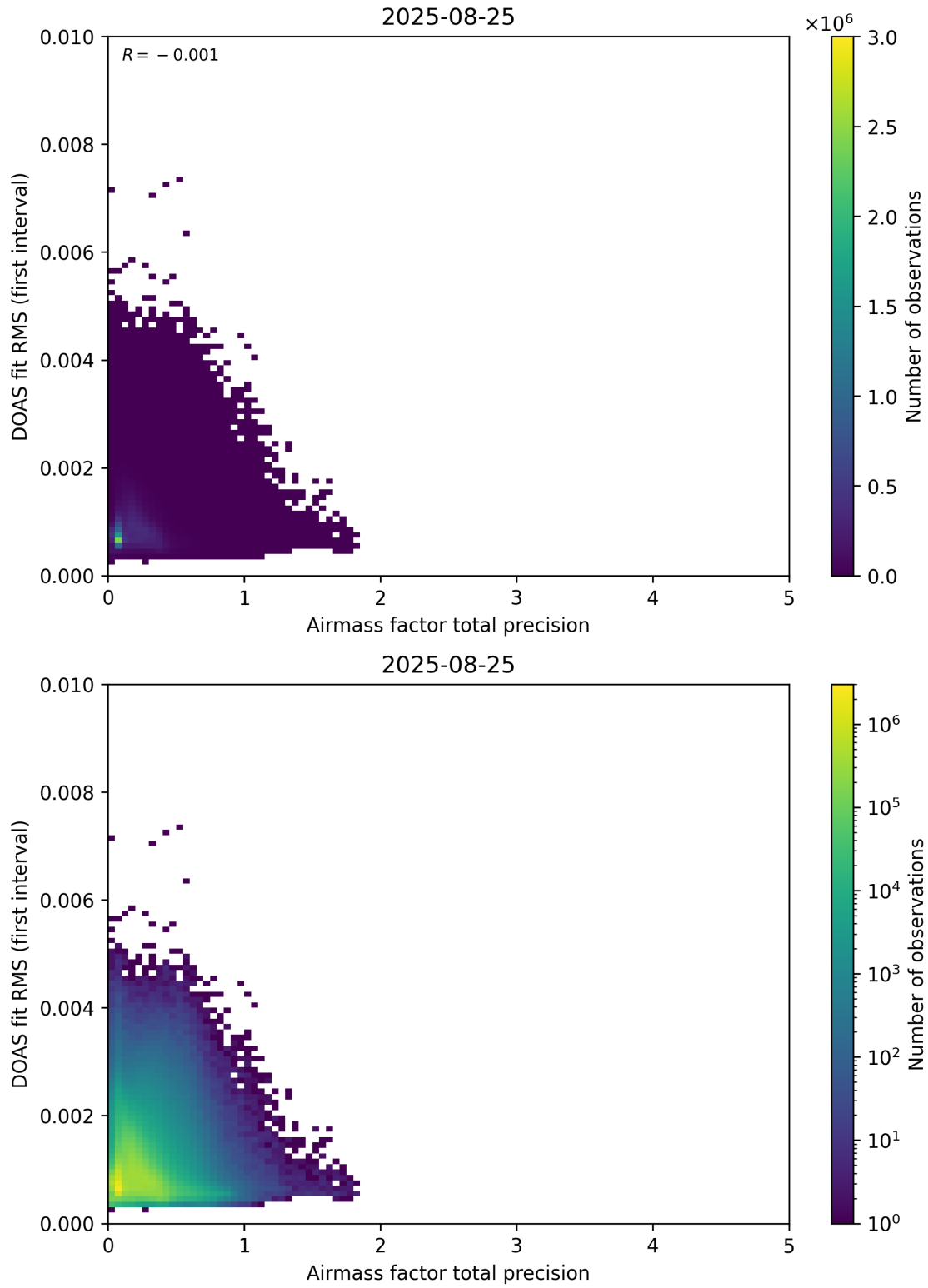
Figure 105: Scatter density plot of “Airmass factor total precision” against “DOAS fit RMS (first interval)” for 2025-08-25 to 2025-08-26.
