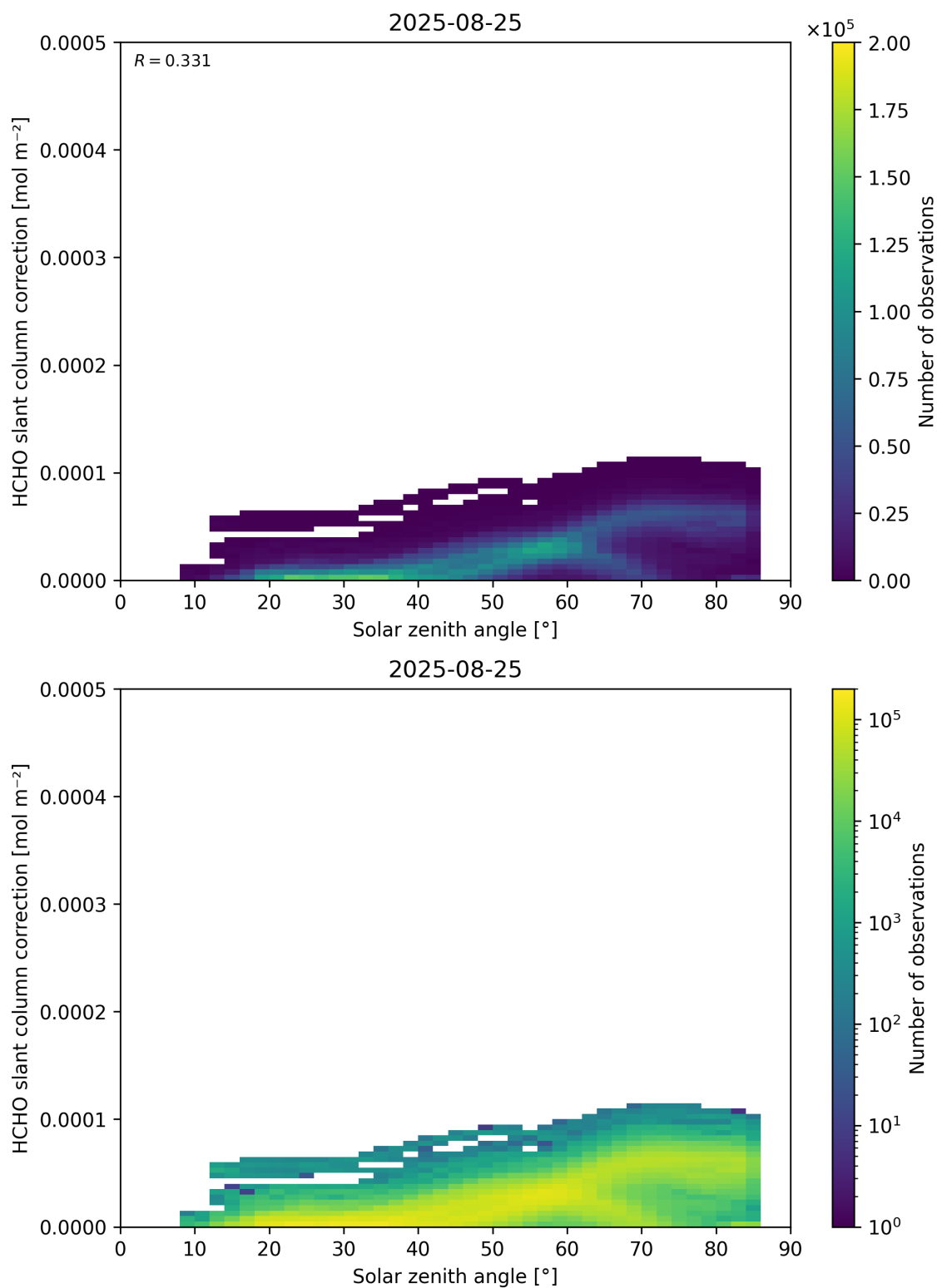
Figure 172: Scatter density plot of “Solar zenith angle” against “HCHO slant column correction” for 2025-08-25 to 2025-08-26.
