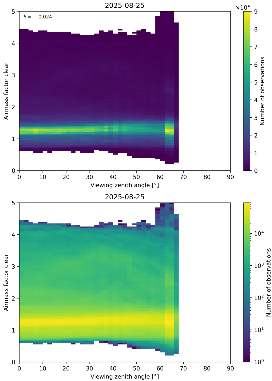
Figure 185: Scatter density plot of “Viewing zenith angle” against “Airmass factor clear” for 2025-08-25 to 2025-08-26.
