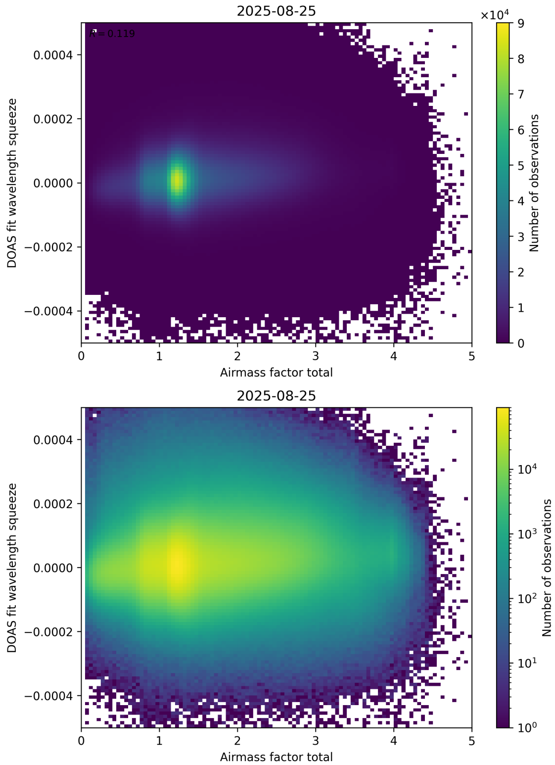
Figure 99: Scatter density plot of “Airmass factor total” against “DOAS fit wavelength squeeze” for 2025-08-25 to 2025-08-26.
