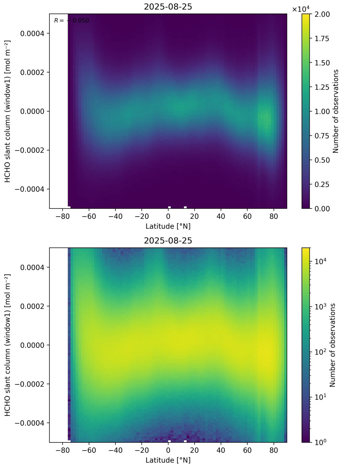
Figure 159: Scatter density plot of “Latitude” against “HCHO slant column (window1)” for 2025-08-25 to 2025-08-26.
