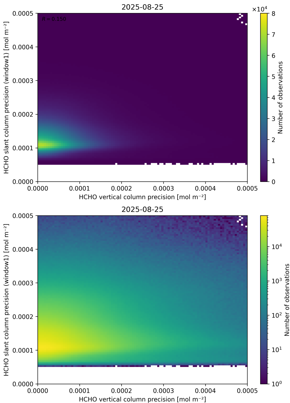
Figure 143: Scatter density plot of “HCHO vertical column precision” against “HCHO slant column precision (window1)” for 2025-08-25 to 2025-08-26.
