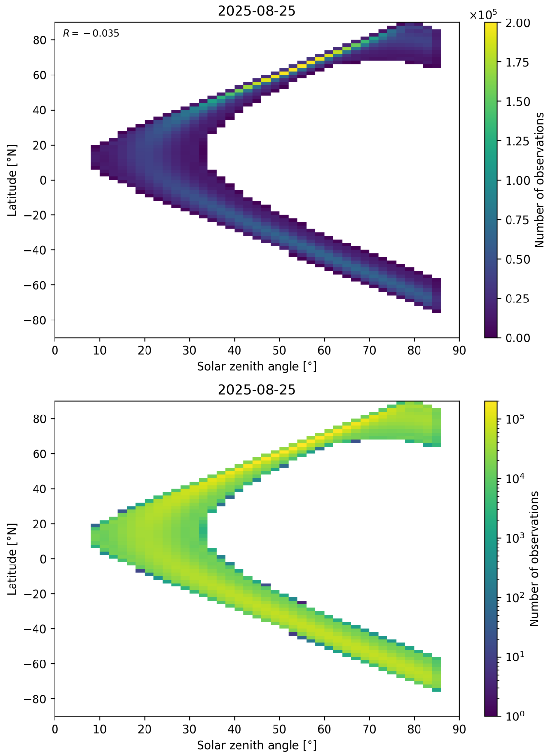
Figure 181: Scatter density plot of “Solar zenith angle” against “Latitude” for 2025-08-25 to 2025-08-26.
