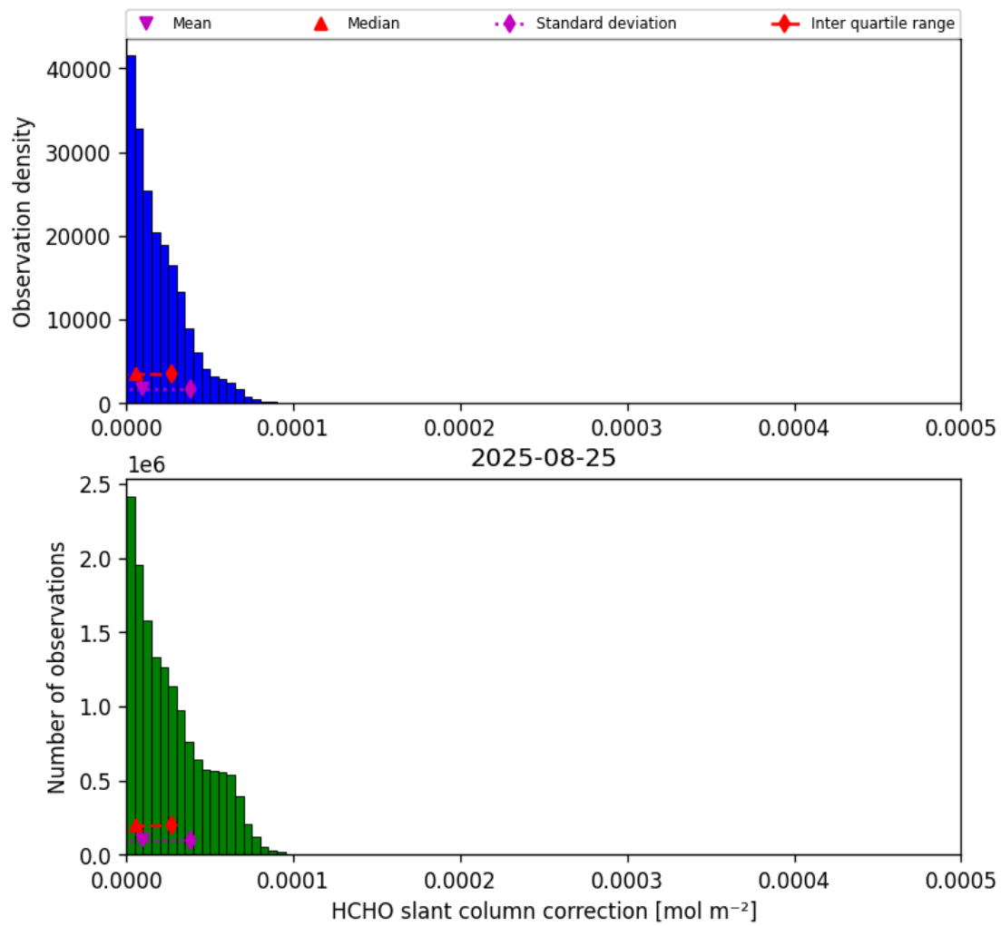
Figure 47: Histogram of “HCHO slant column correction” for 2025-08-25 to 2025-08-26
