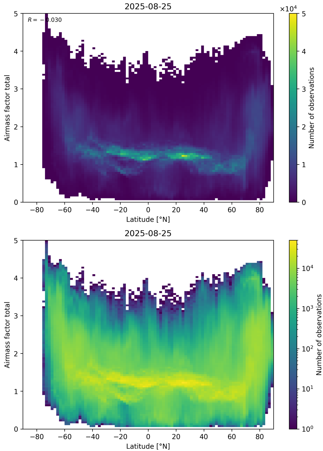
Figure 161: Scatter density plot of “Latitude” against “Airmass factor total” for 2025-08-25 to 2025-08-26.
