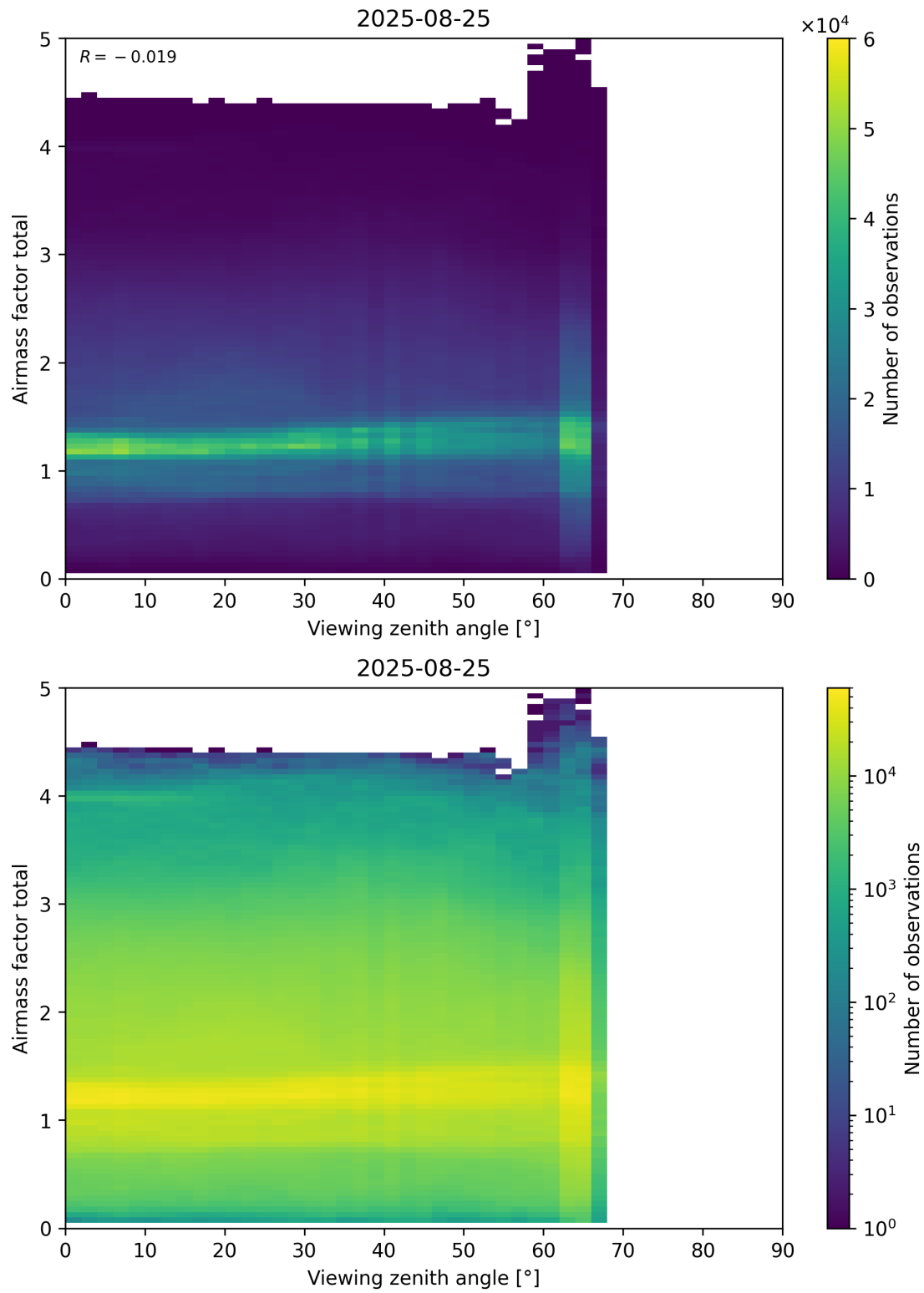
Figure 190: Scatter density plot of “Viewing zenith angle” against “Airmass factor total” for 2025-08-25 to 2025-08-26.
