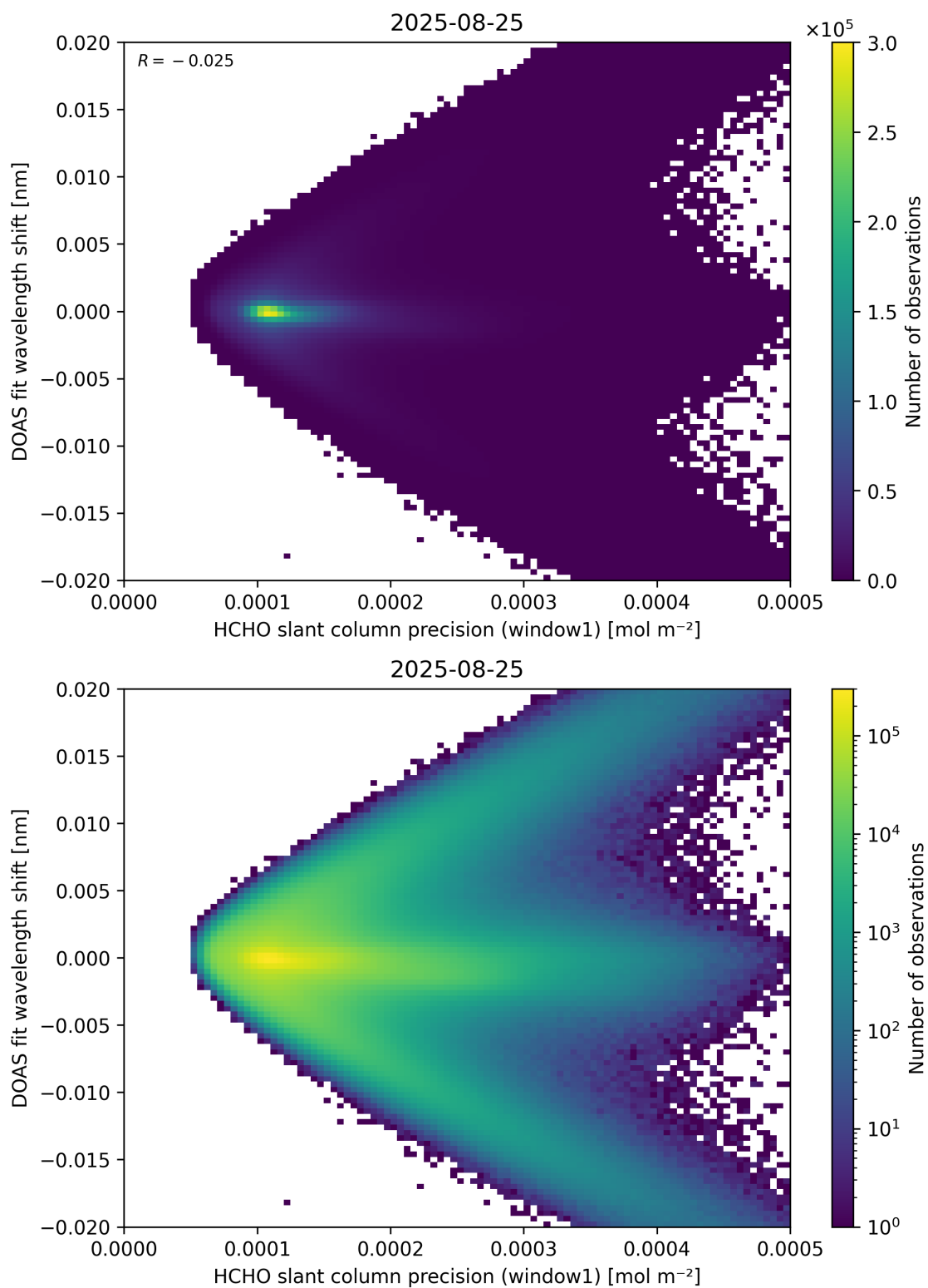
Figure 89: Scatter density plot of “HCHO slant column precision (window1)” against “DOAS fit wavelength shift” for 2025-08-25 to 2025-08-26.
