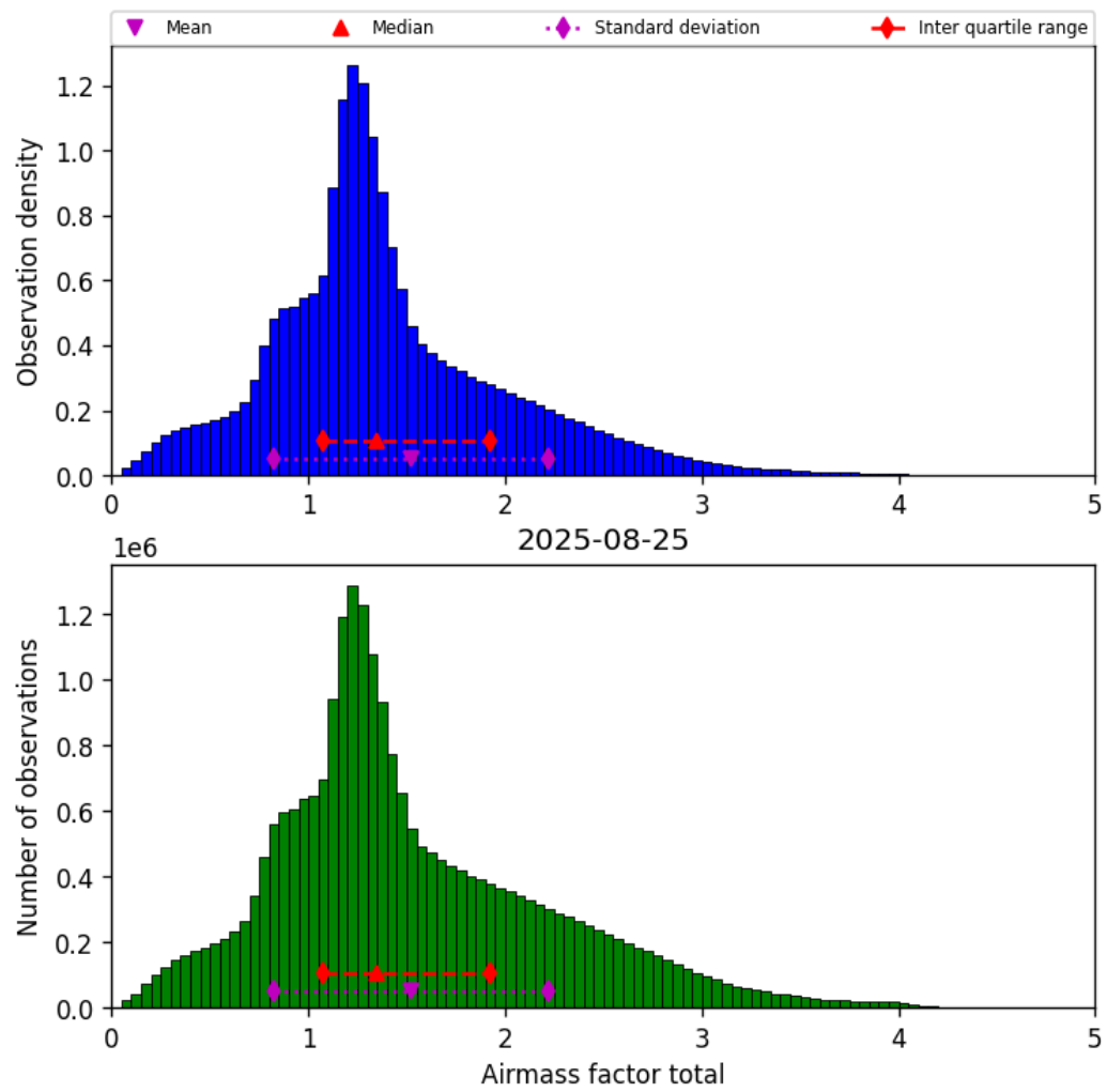
Figure 40: Histogram of “Airmass factor total” for 2025-08-25 to 2025-08-26
