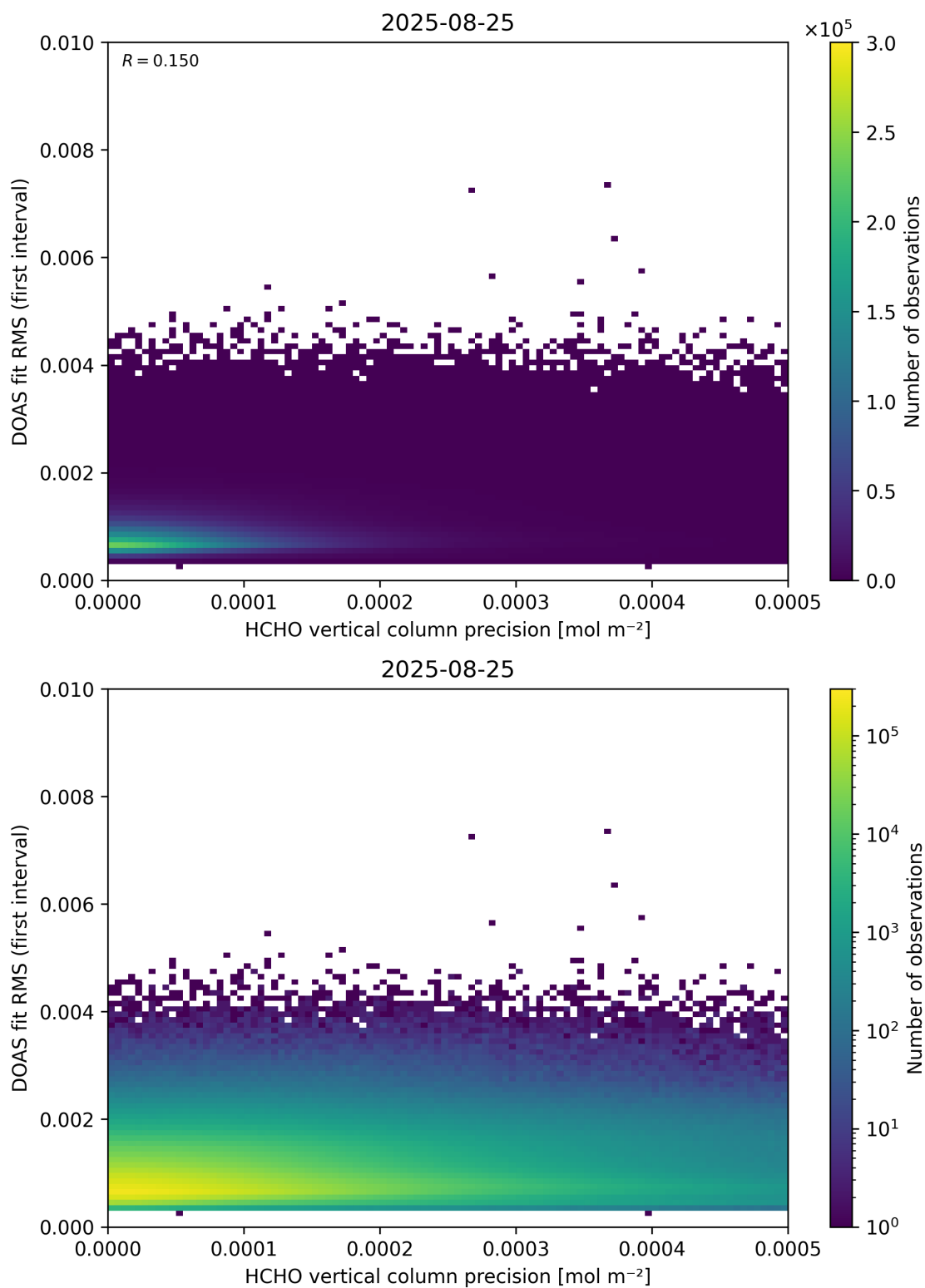
Figure 136: Scatter density plot of “HCHO vertical column precision” against “DOAS fit RMS (first interval)” for 2025-08-25 to 2025-08-26.
