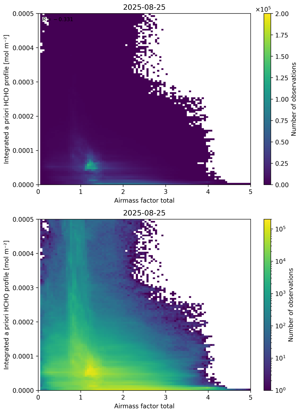
Figure 104: Scatter density plot of “Airmass factor total” against “Integrated a priori HCHO profile” for 2025-08-25 to 2025-08-26.
