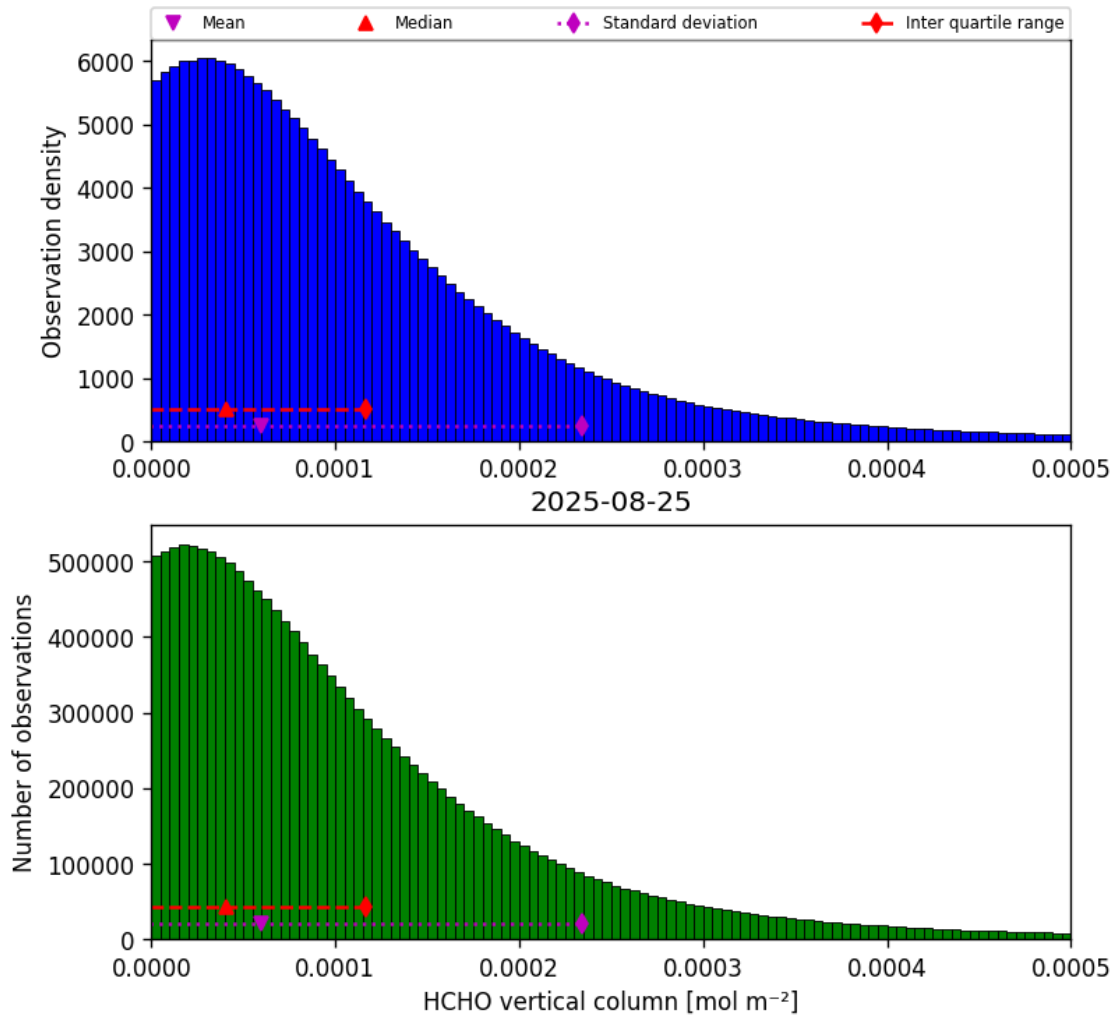
Figure 35: Histogram of “HCHO vertical column” for 2025-08-25 to 2025-08-26
