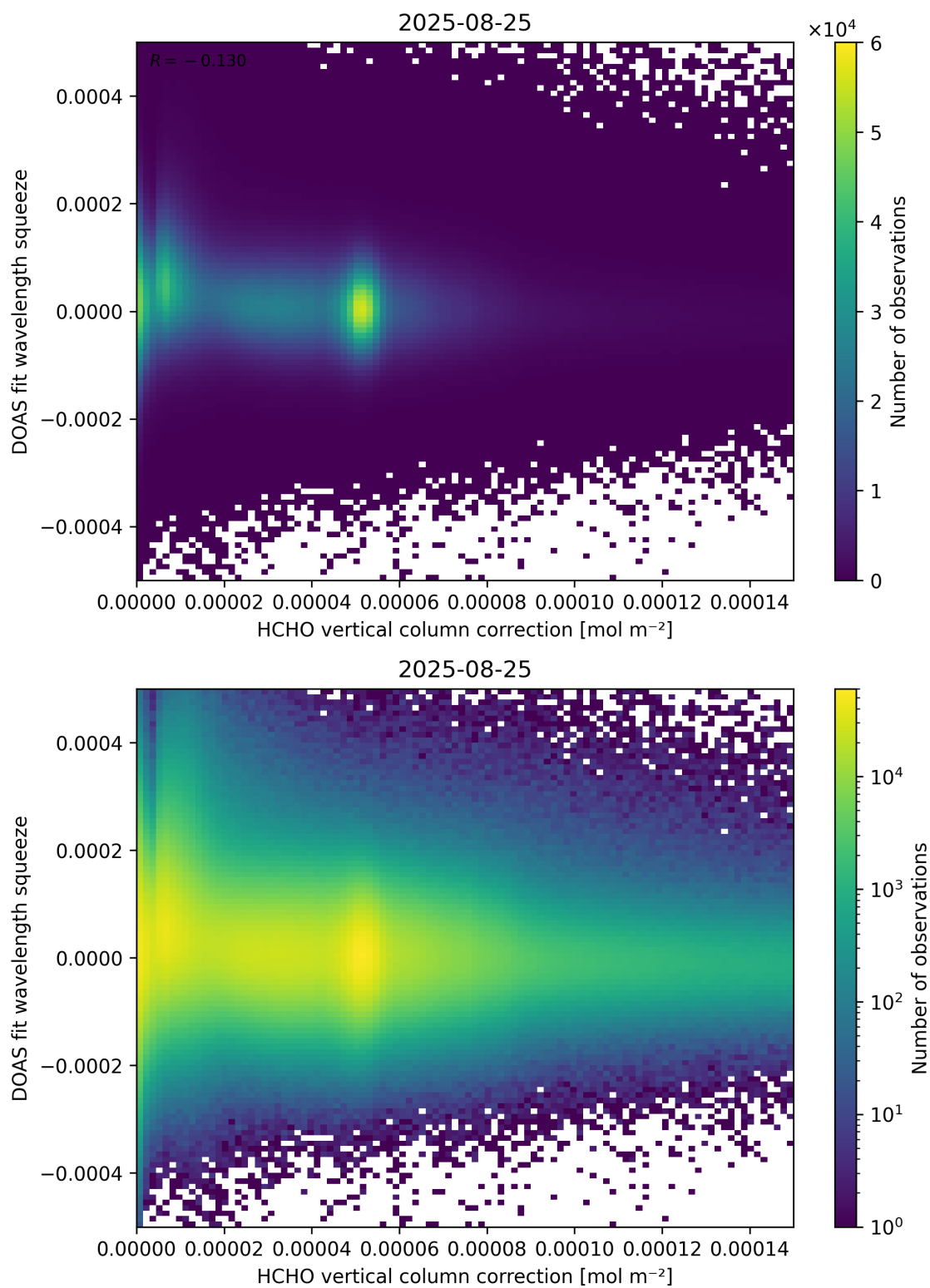
Figure 114: Scatter density plot of “HCHO vertical column correction” against “DOAS fit wavelength squeeze” for 2025-08-25 to 2025-08-26.
