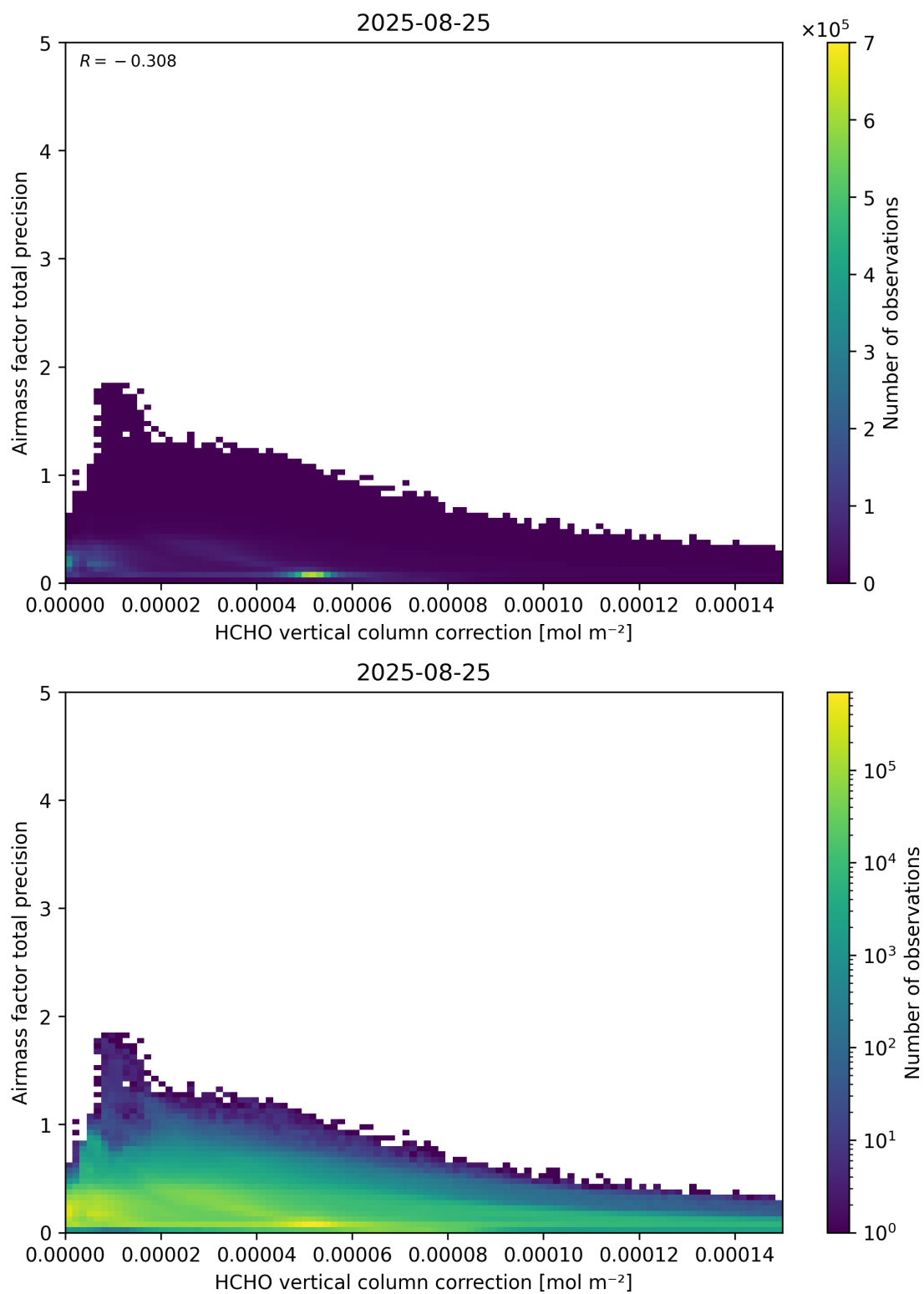
Figure 121: Scatter density plot of “HCHO vertical column correction” against “Airmass factor total precision” for 2025-08-25 to 2025-08-26.
