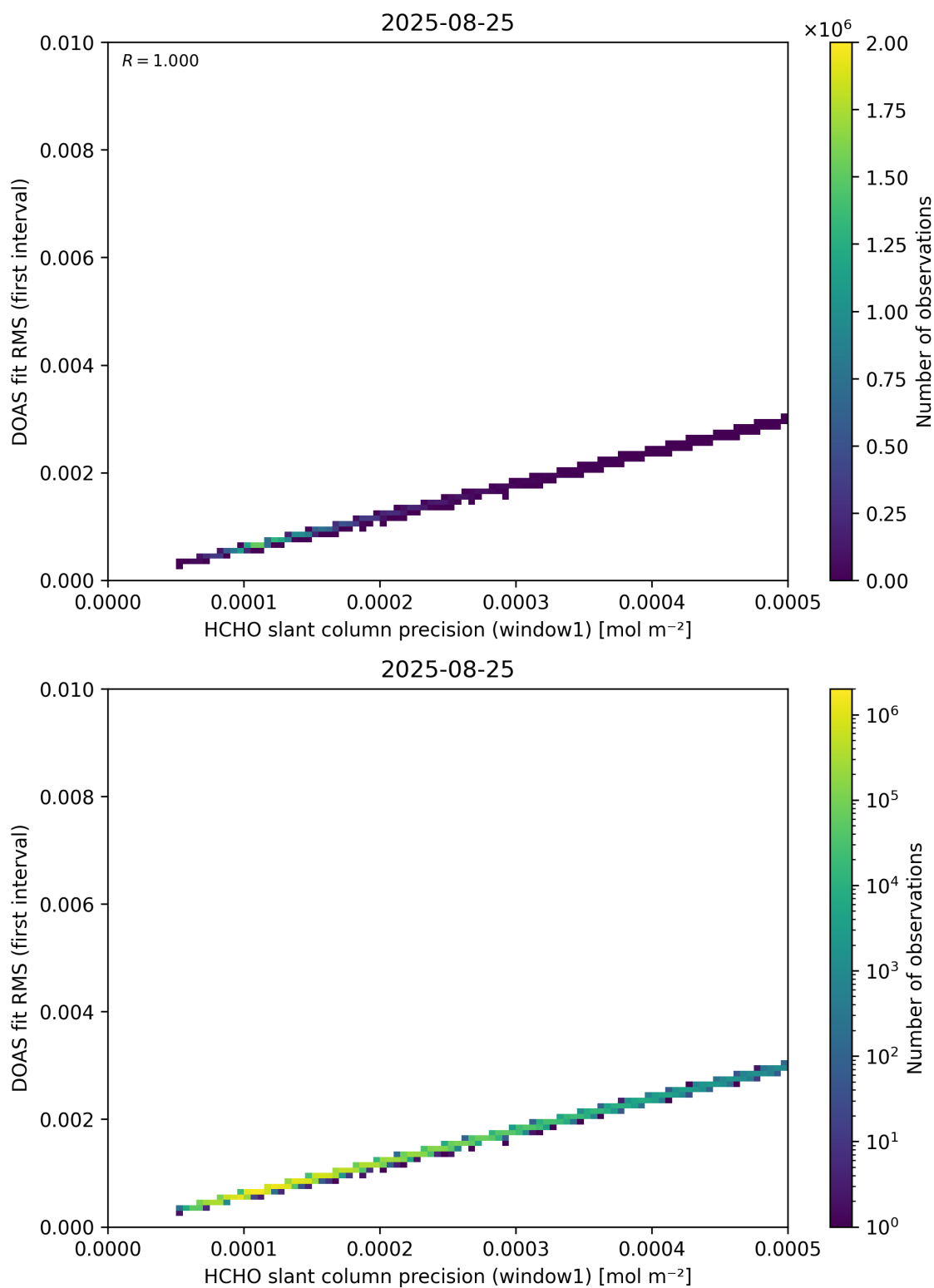
Figure 88: Scatter density plot of “HCHO slant column precision (window1)” against “DOAS fit RMS (first interval)” for 2025-08-25 to 2025-08-26.
