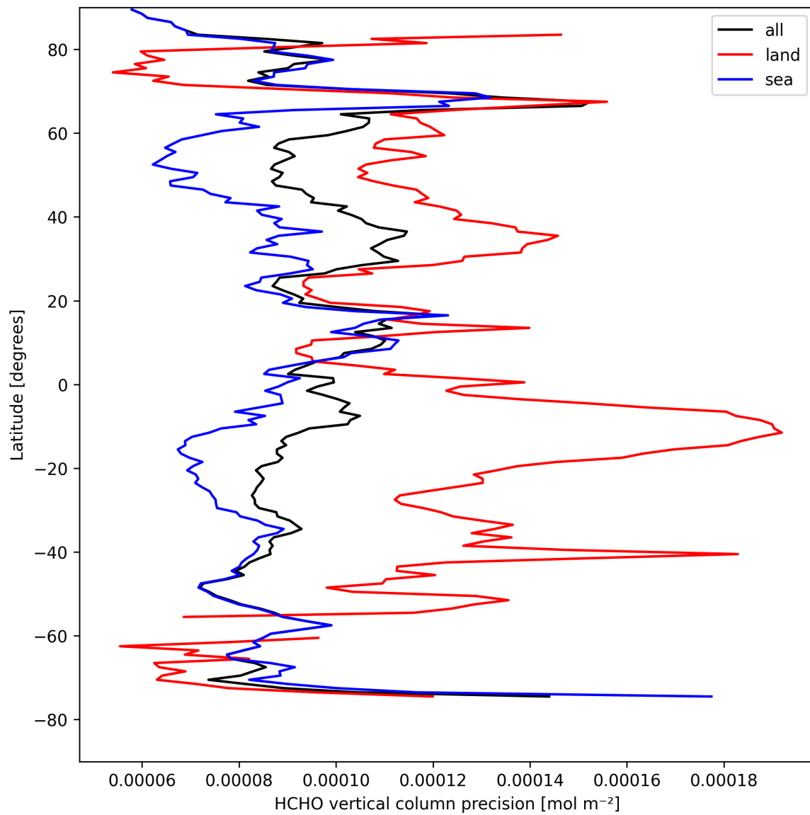
Figure 22: Zonal average of “HCHO vertical column precision” for 2025-08-25 to 2025-08-26.
