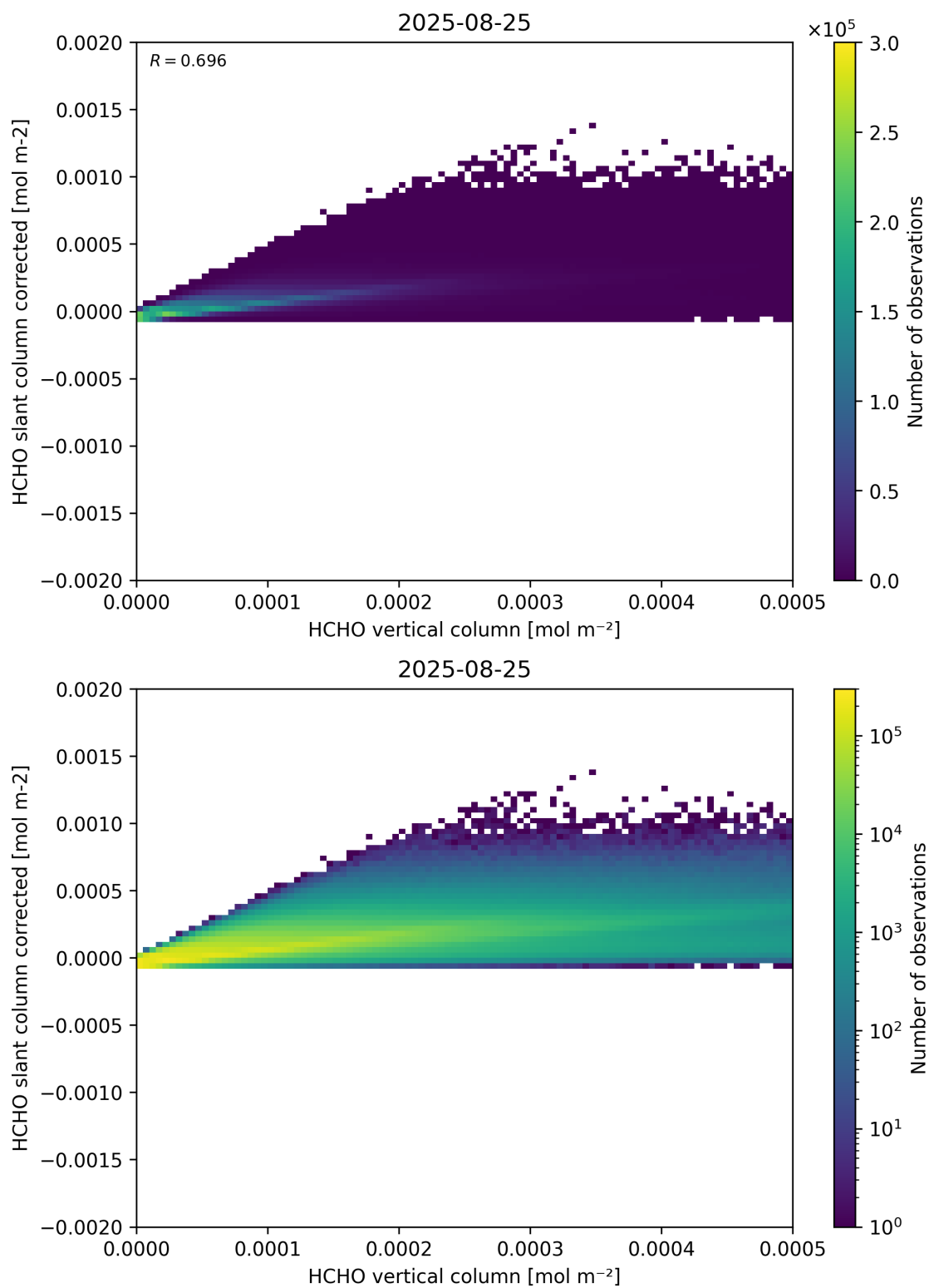
Figure 127: Scatter density plot of “HCHO vertical column” against “HCHO slant column corrected” for 2025-08-25 to 2025-08-26.
