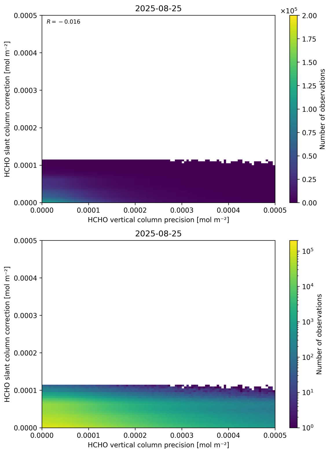
Figure 141: Scatter density plot of “HCHO vertical column precision” against “HCHO slant column correction” for 2025-08-25 to 2025-08-26.
