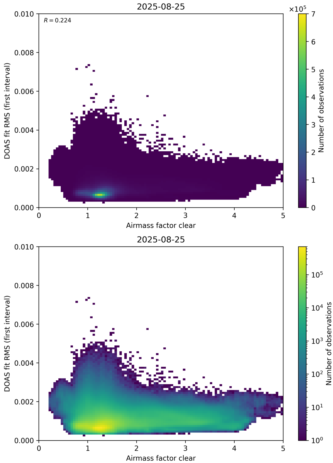
Figure 71: Scatter density plot of “Airmass factor clear” against “DOAS fit RMS (first interval)” for 2025-08-25 to 2025-08-26.
