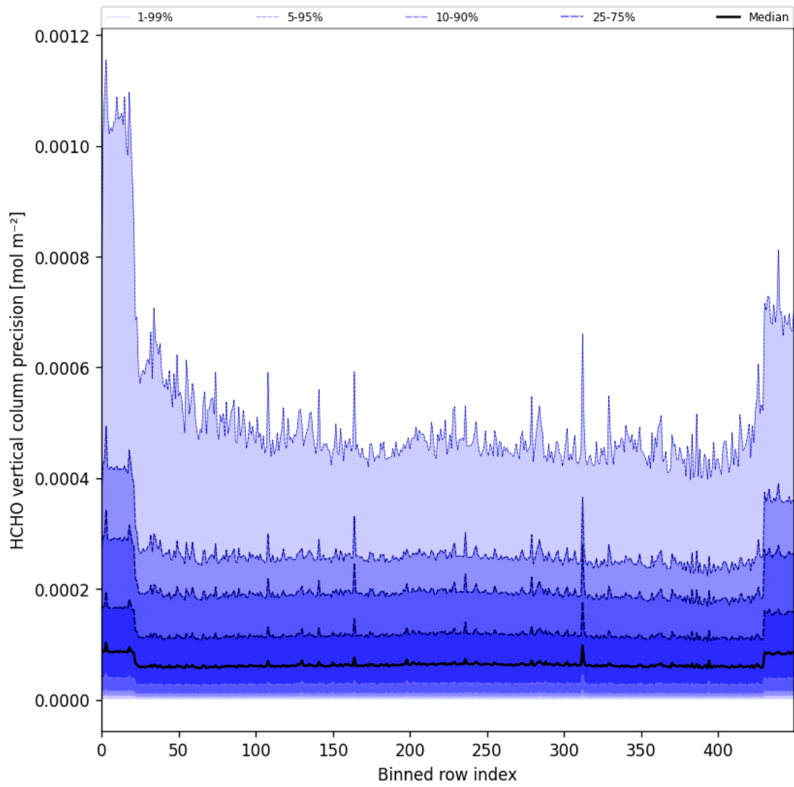
Figure 50: Along track statistics of “HCHO vertical column precision” for 2025-08-25 to 2025-08-26
