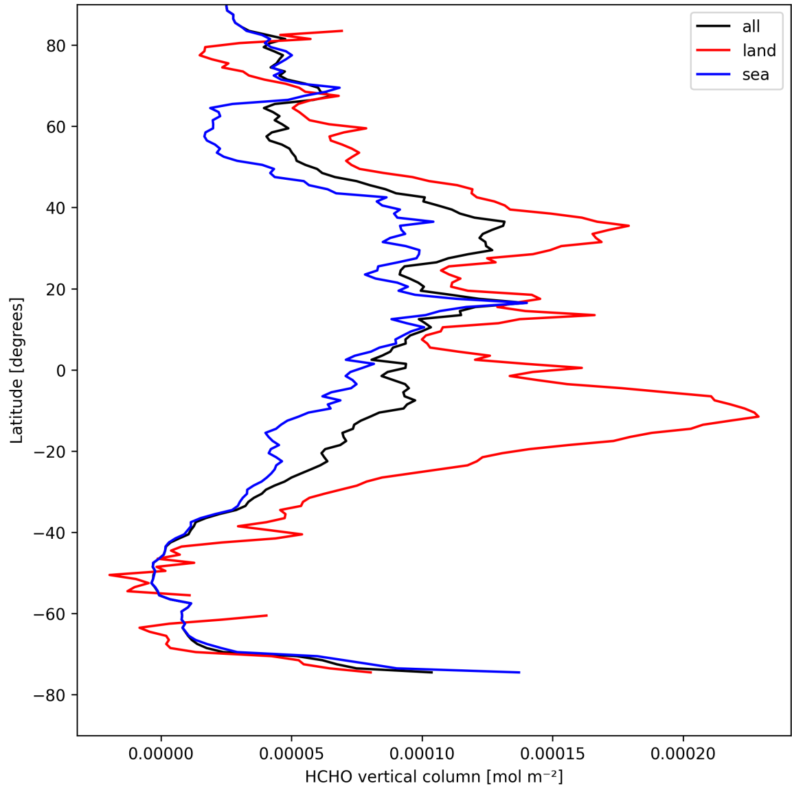
Figure 21: Zonal average of “HCHO vertical column” for 2025-08-25 to 2025-08-26.
