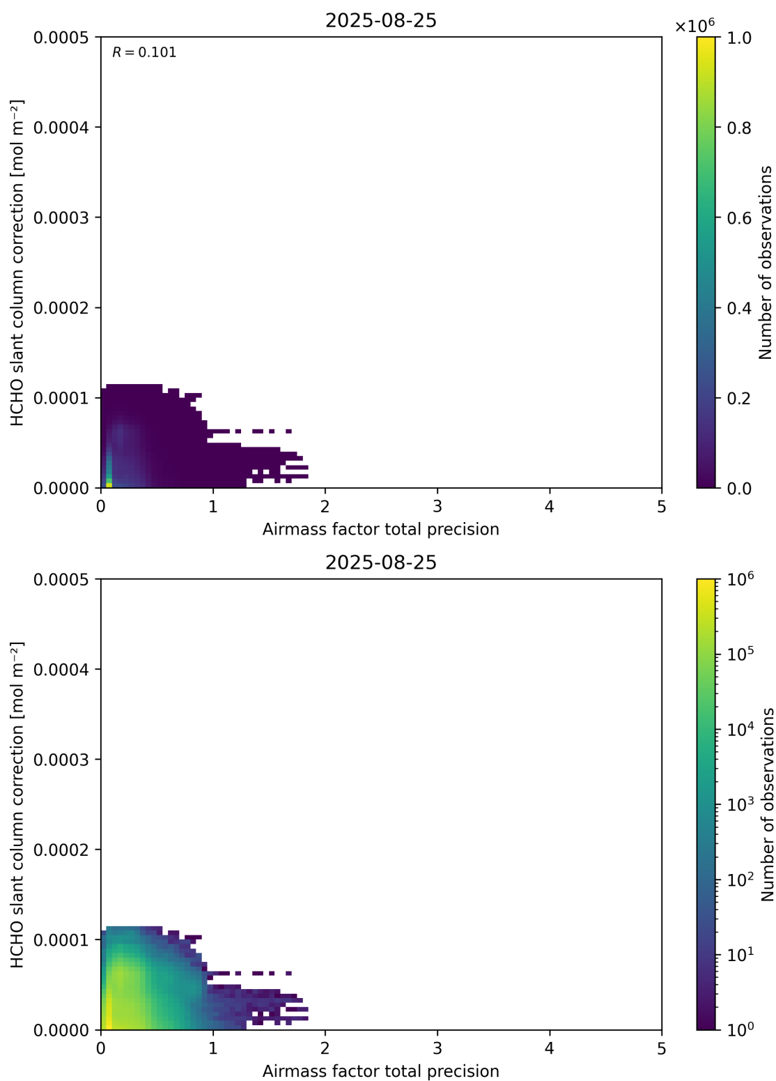
Figure 110: Scatter density plot of “Airmass factor total precision” against “HCHO slant column correction” for 2025-08-25 to 2025-08-26.
