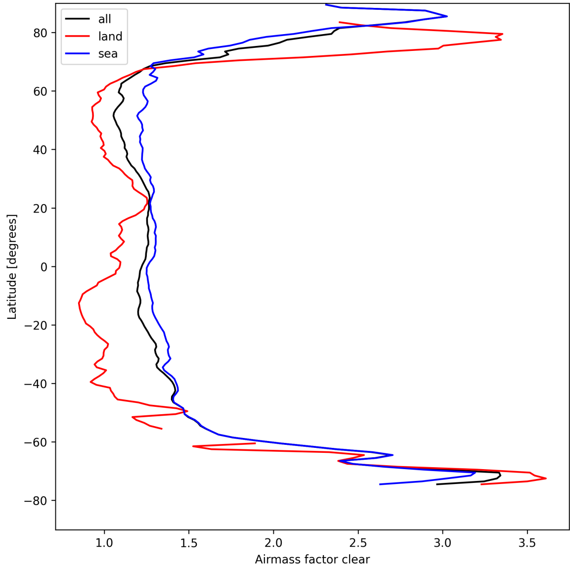
Figure 28: Zonal average of “Airmass factor clear” for 2025-08-25 to 2025-08-26.
