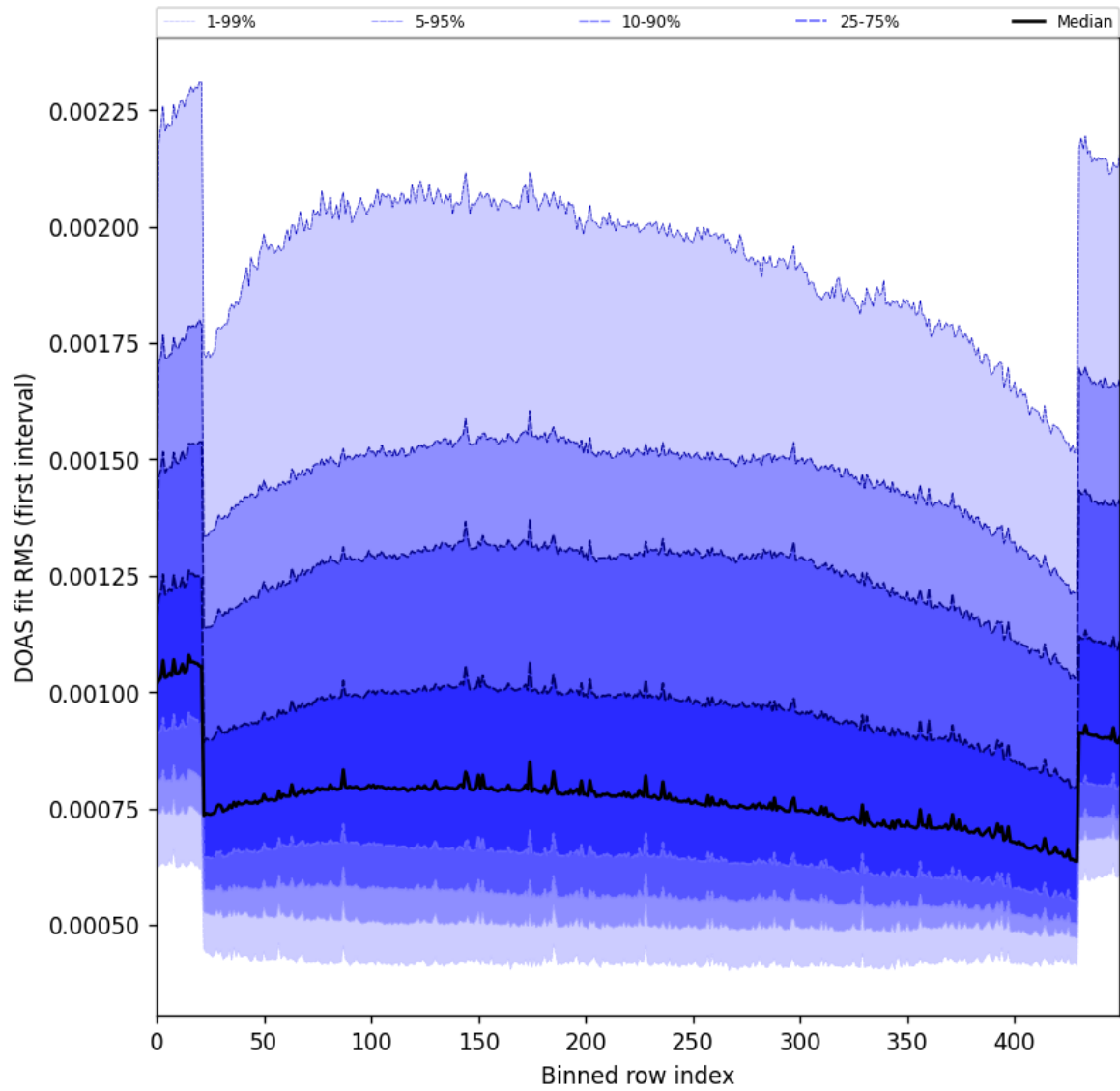
Figure 60: Along track statistics of “DOAS fit RMS (first interval)” for 2025-08-25 to 2025-08-26
