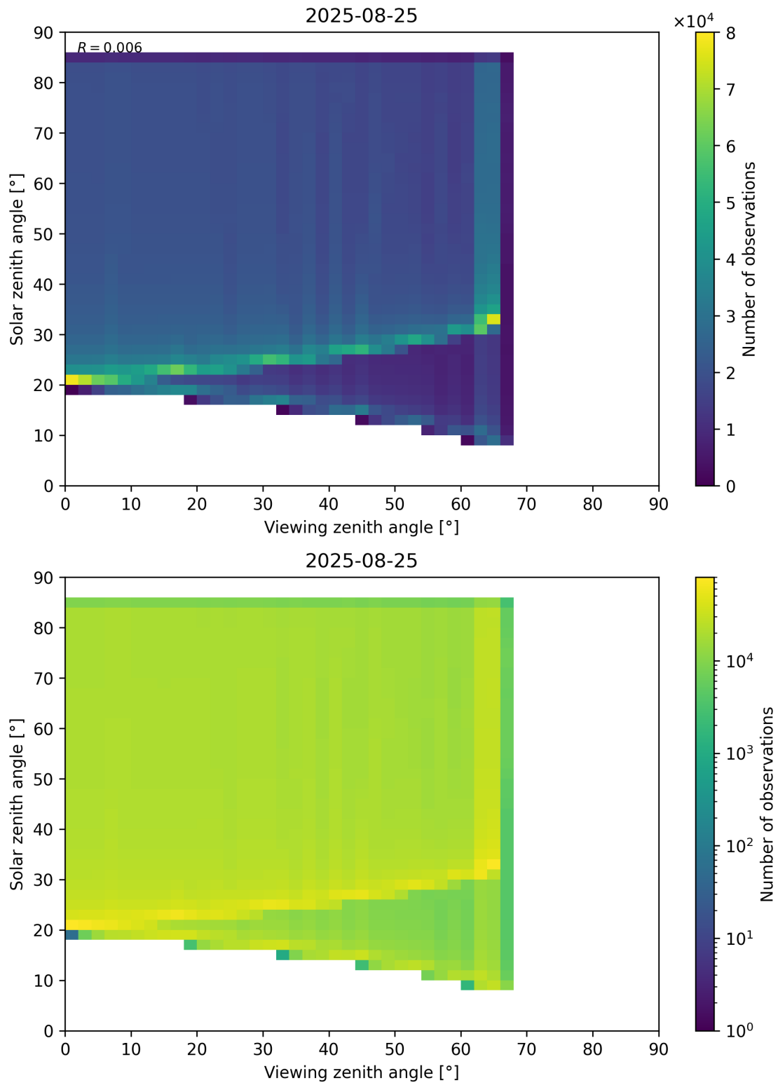
Figure 197: Scatter density plot of “Viewing zenith angle” against “Solar zenith angle” for 2025-08-25 to 2025-08-26.
