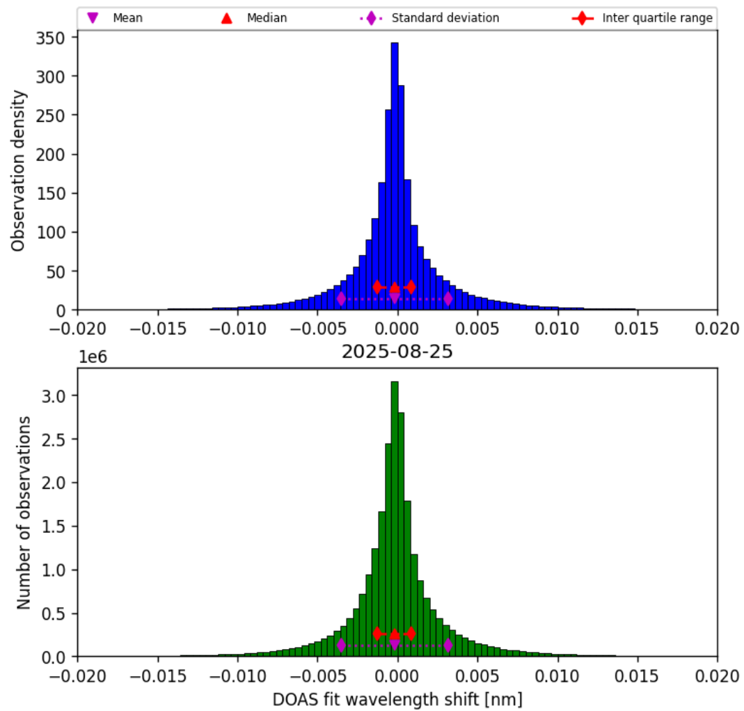
Figure 44: Histogram of “DOAS fit wavelength shift” for 2025-08-25 to 2025-08-26
