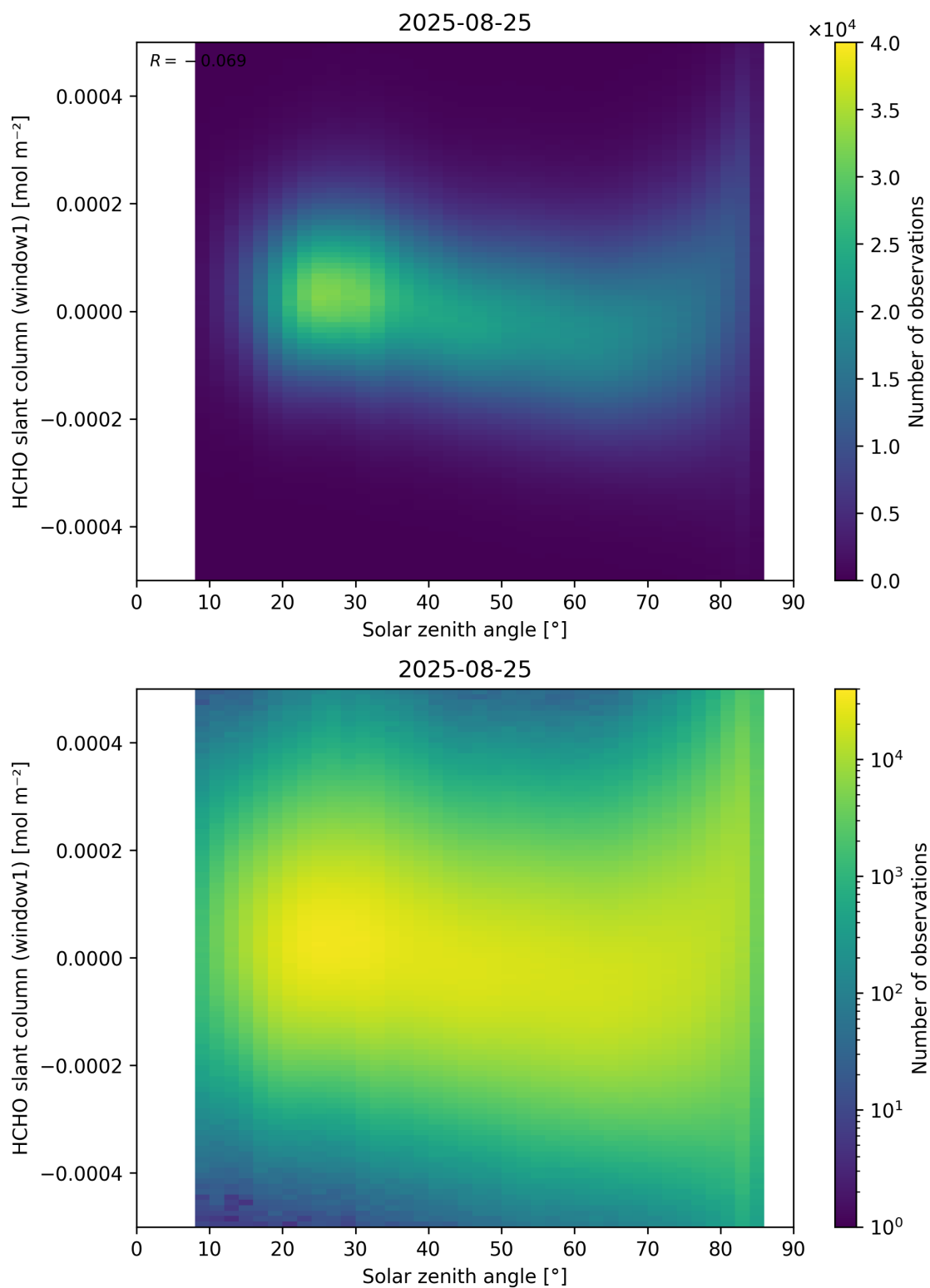
Figure 173: Scatter density plot of “Solar zenith angle” against “HCHO slant column (window1)” for 2025-08-25 to 2025-08-26.
