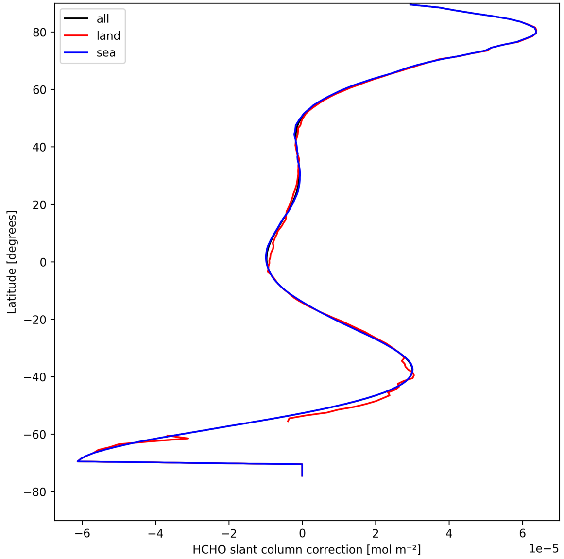
Figure 33: Zonal average of “HCHO slant column correction” for 2025-08-25 to 2025-08-26.
