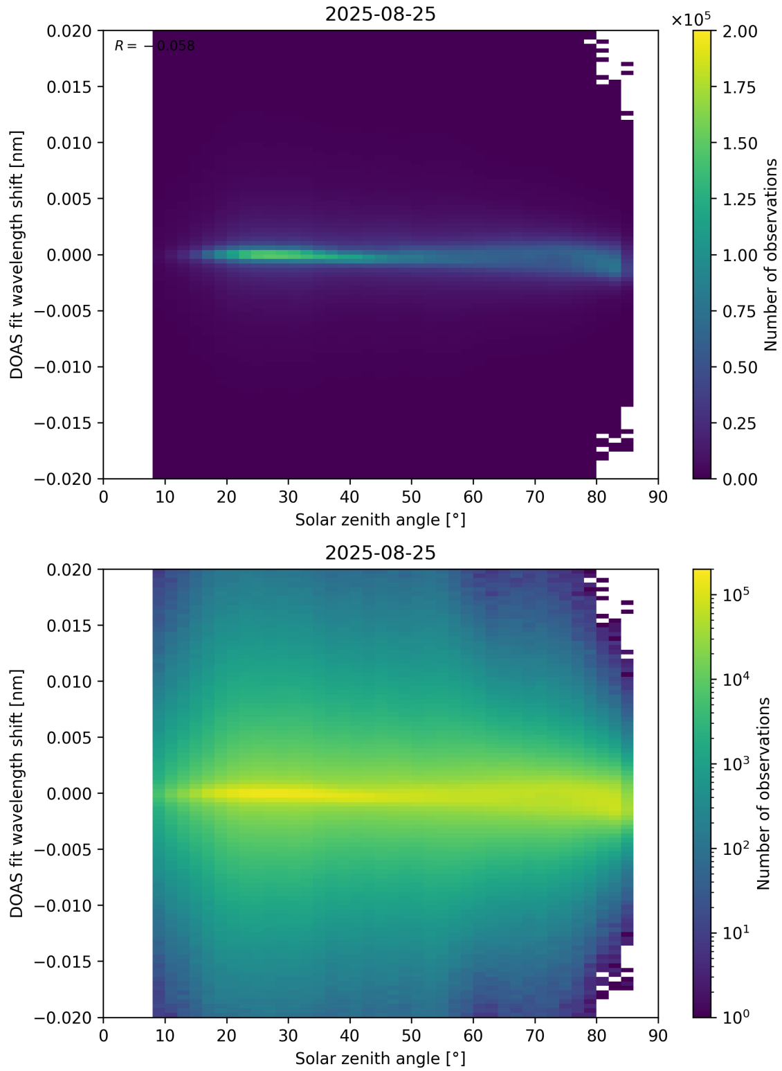
Figure 168: Scatter density plot of “Solar zenith angle” against “DOAS fit wavelength shift” for 2025-08-25 to 2025-08-26.
