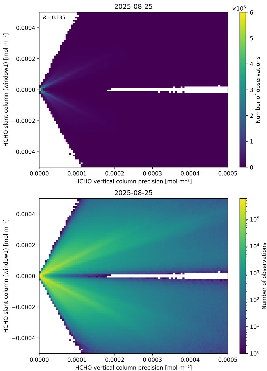
Figure 142: Scatter density plot of “HCHO vertical column precision” against “HCHO slant column (window1)” for 2025-08-25 to 2025-08-26.
