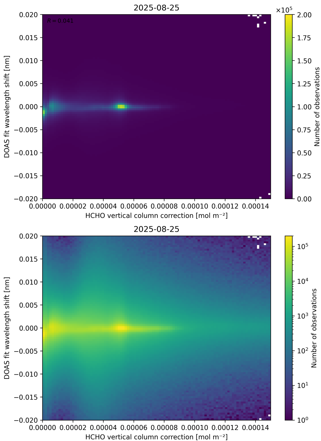
Figure 113: Scatter density plot of “HCHO vertical column correction” against “DOAS fit wavelength shift” for 2025-08-25 to 2025-08-26.
