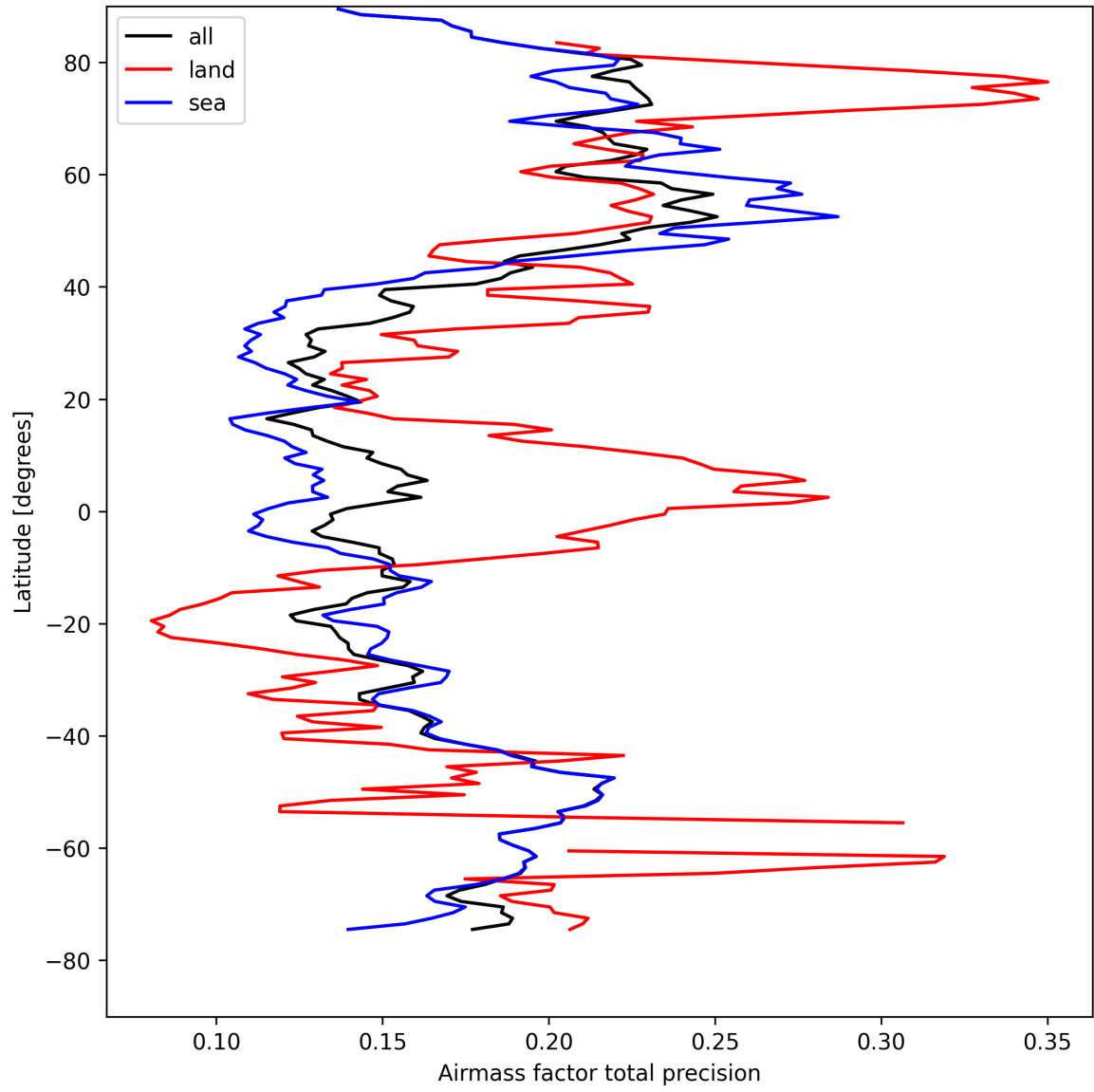
Figure 27: Zonal average of “Airmass factor total precision” for 2025-08-25 to 2025-08-26.
