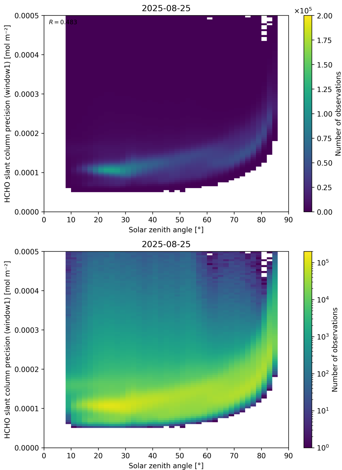
Figure 174: Scatter density plot of “Solar zenith angle” against “HCHO slant column precision (window1)” for 2025-08-25 to 2025-08-26.
