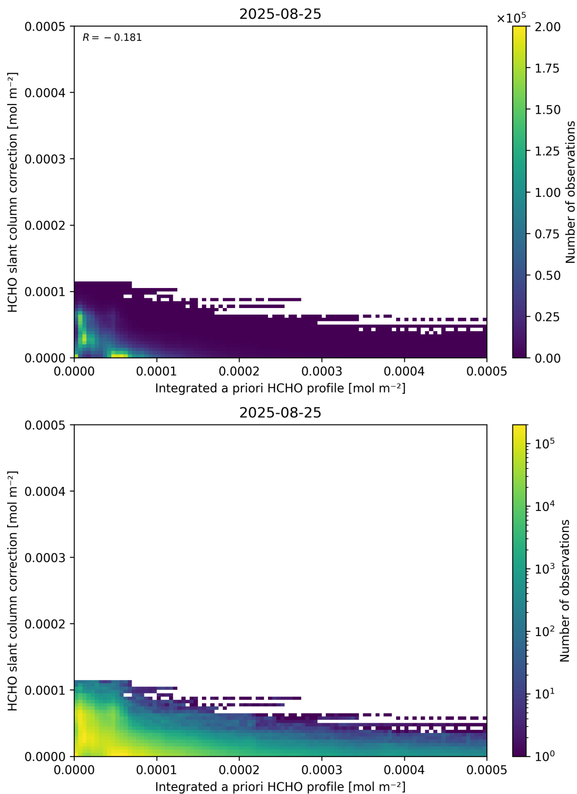
Figure 152: Scatter density plot of “Integrated a priori HCHO profile” against “HCHO slant column correction” for 2025-08-25 to 2025-08-26.
