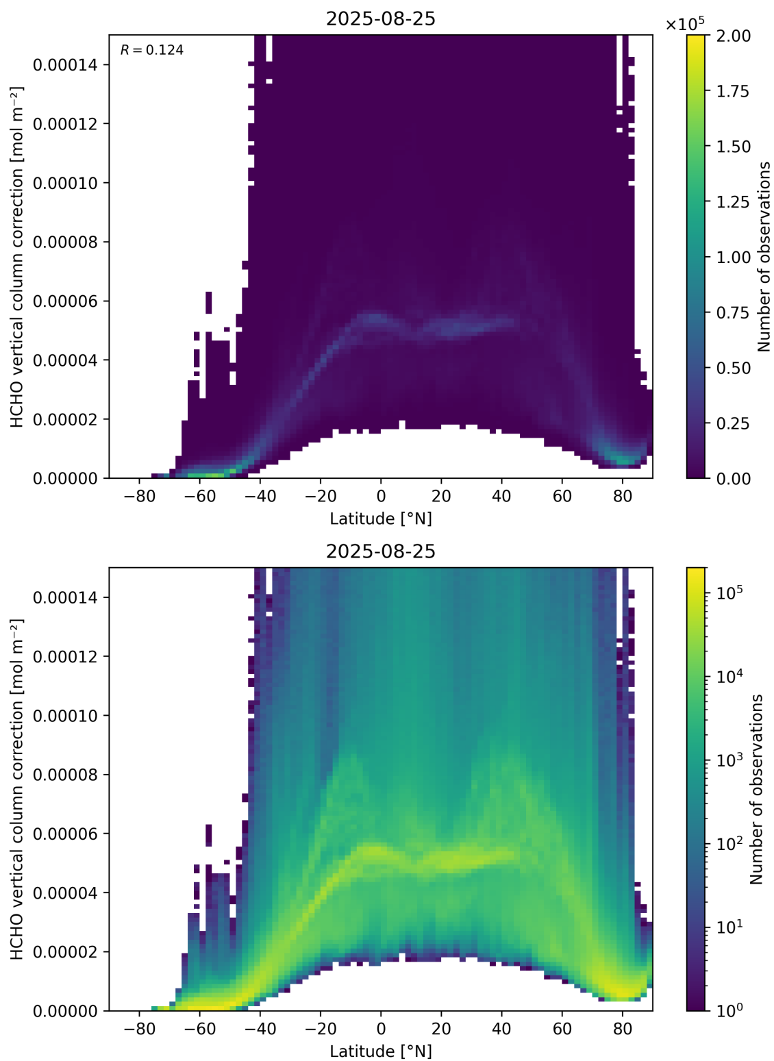
Figure 164: Scatter density plot of “Latitude” against “HCHO vertical column correction” for 2025-08-25 to 2025-08-26.
