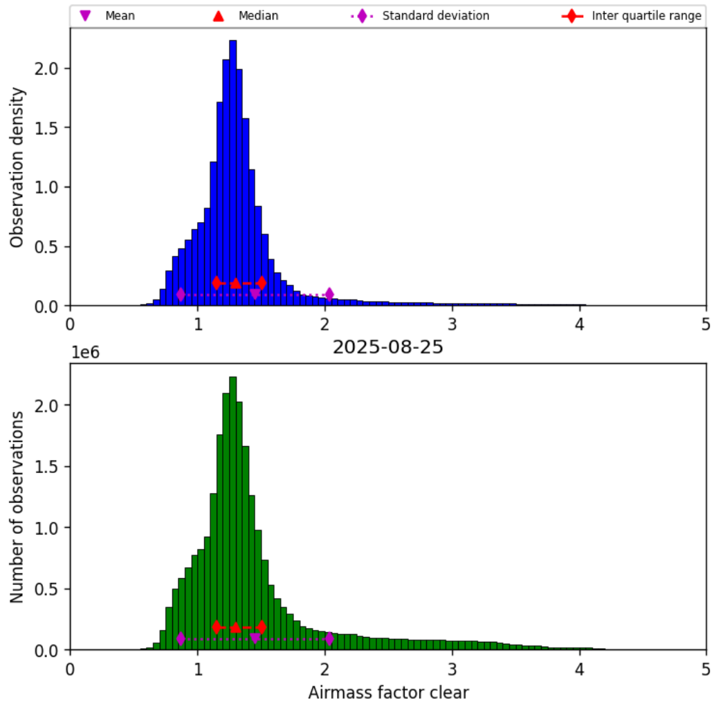
Figure 42: Histogram of “Airmass factor clear” for 2025-08-25 to 2025-08-26
