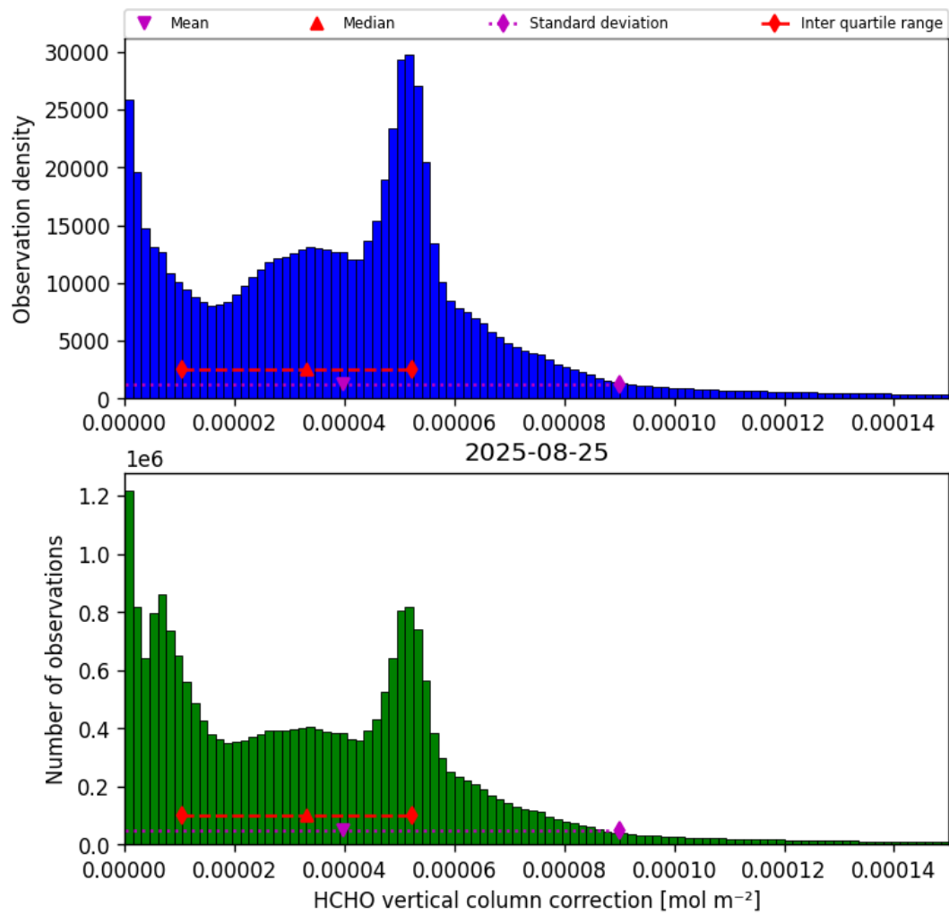
Figure 37: Histogram of “HCHO vertical column correction” for 2025-08-25 to 2025-08-26
