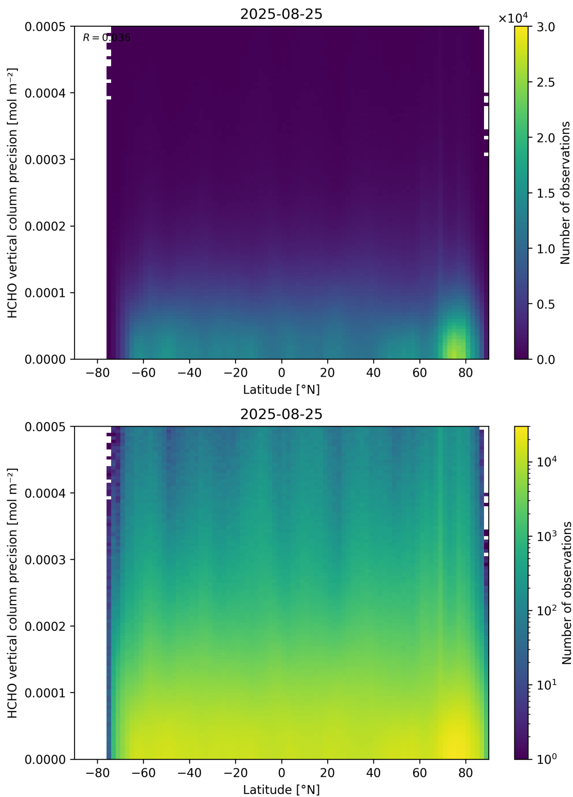
Figure 165: Scatter density plot of “Latitude” against “HCHO vertical column precision” for 2025-08-25 to 2025-08-26.
