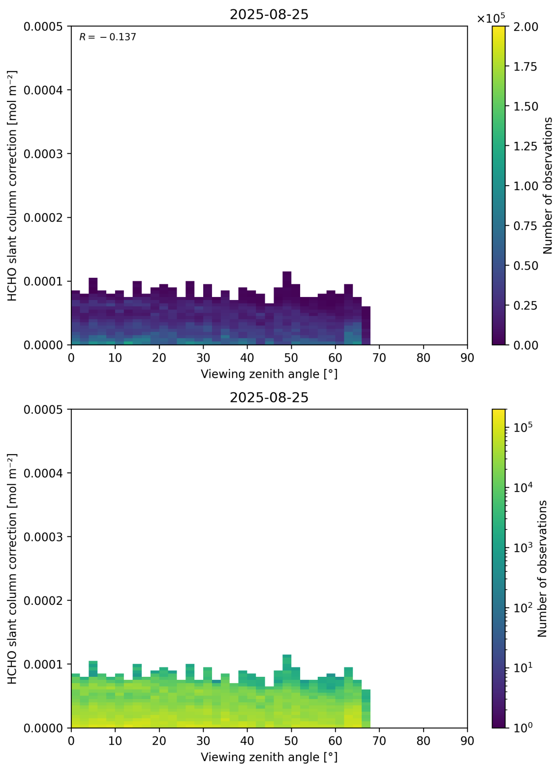
Figure 187: Scatter density plot of “Viewing zenith angle” against “HCHO slant column correction” for 2025-08-25 to 2025-08-26.
