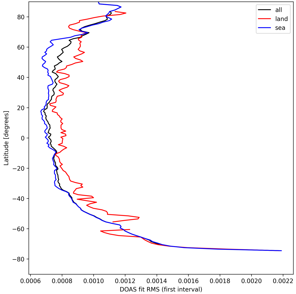
Figure 32: Zonal average of "DOAS fit RMS (first interval)" for 2025-08-25 to 2025-08-26.
