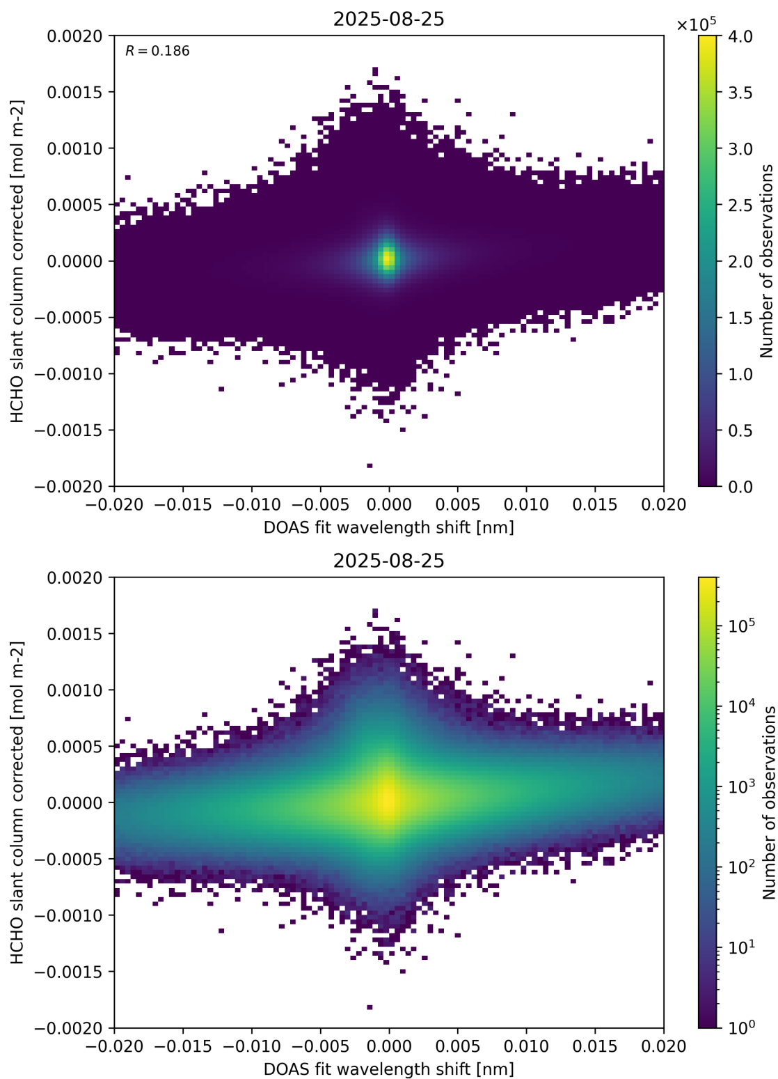
Figure 66: Scatter density plot of “DOAS fit wavelength shift” against “HCHO slant column corrected” for 2025-08-25 to 2025-08-26.
