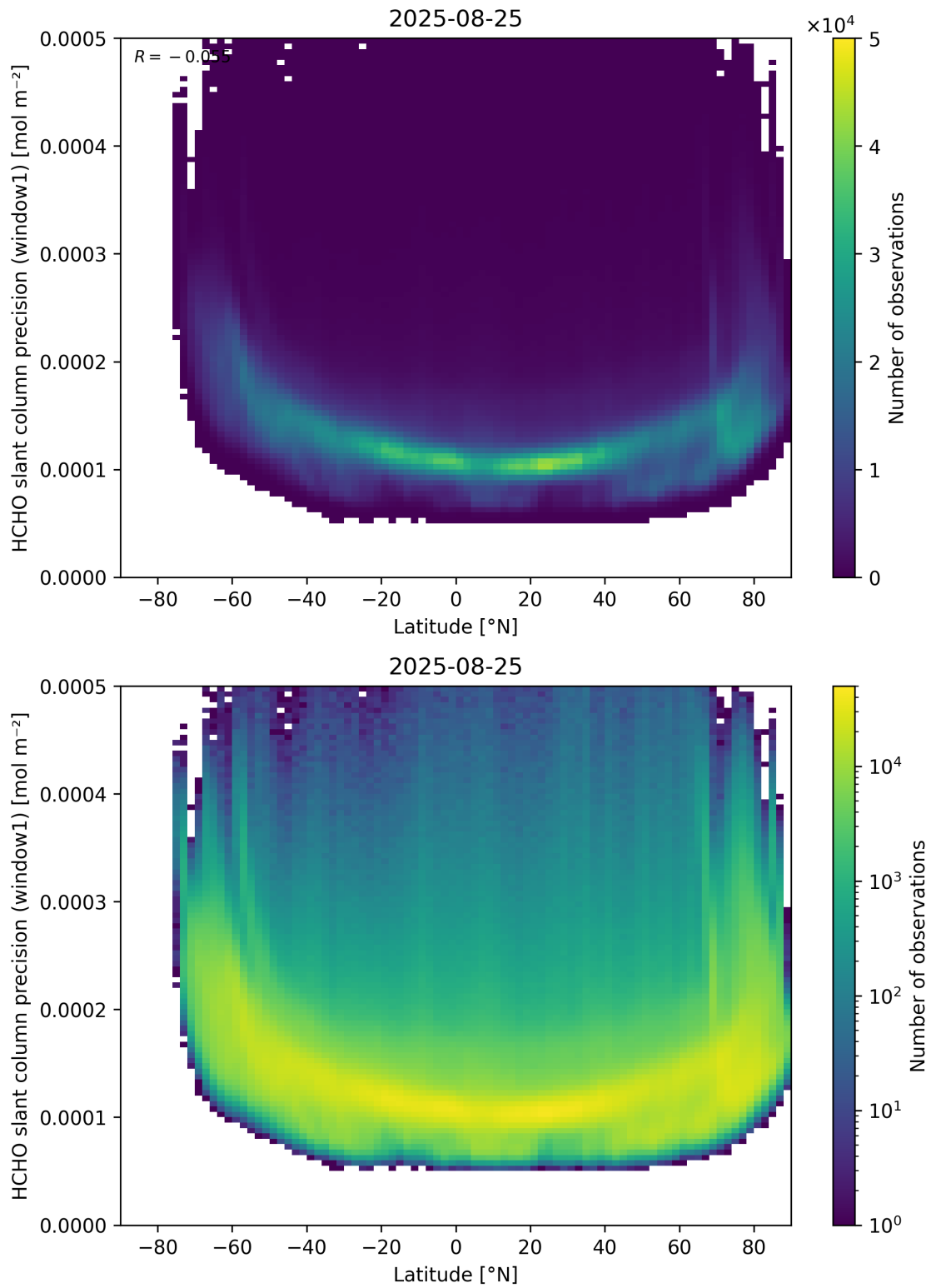
Figure 160: Scatter density plot of “Latitude” against “HCHO slant column precision (window1)” for 2025-08-25 to 2025-08-26.
