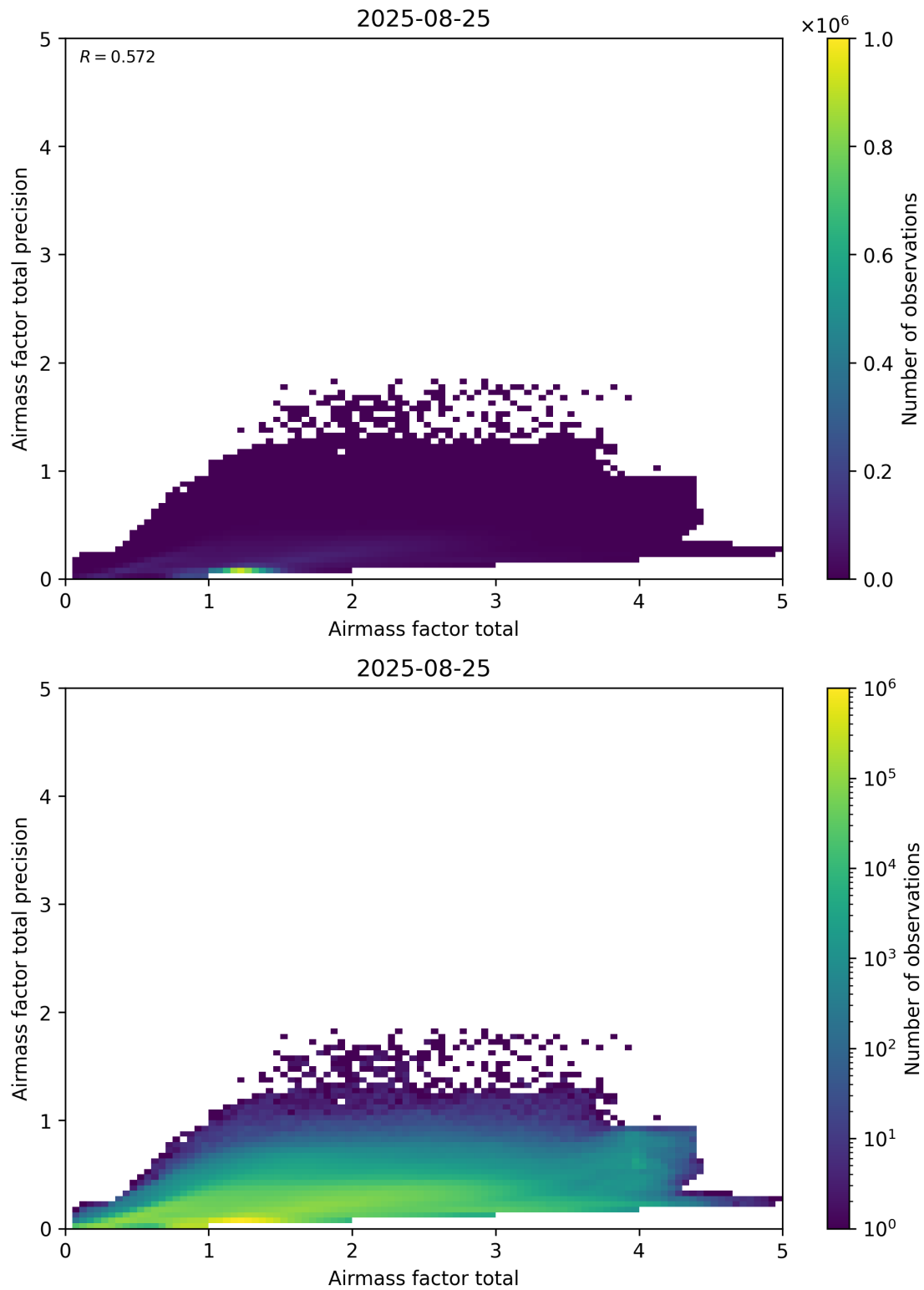
Figure 103: Scatter density plot of “Airmass factor total” against “Airmass factor total precision” for 2025-08-25 to 2025-08-26.
