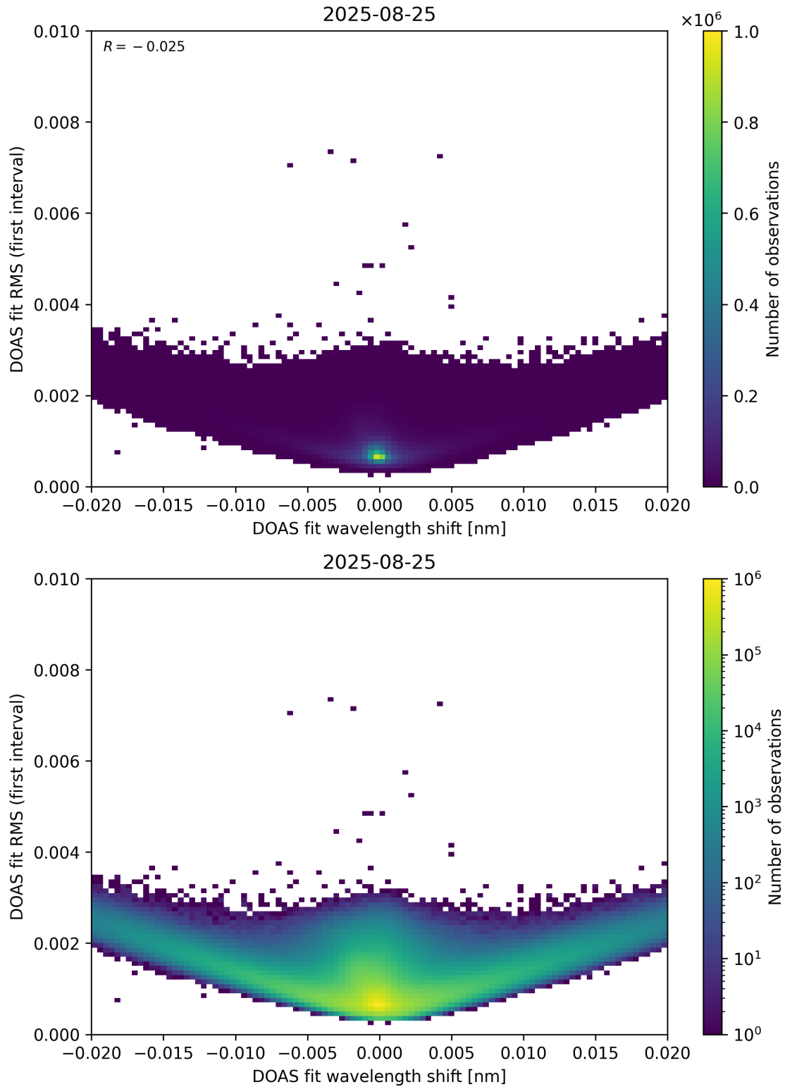
Figure 64: Scatter density plot of “DOAS fit wavelength shift” against “DOAS fit RMS (first interval)” for 2025-08-25 to 2025-08-26.
