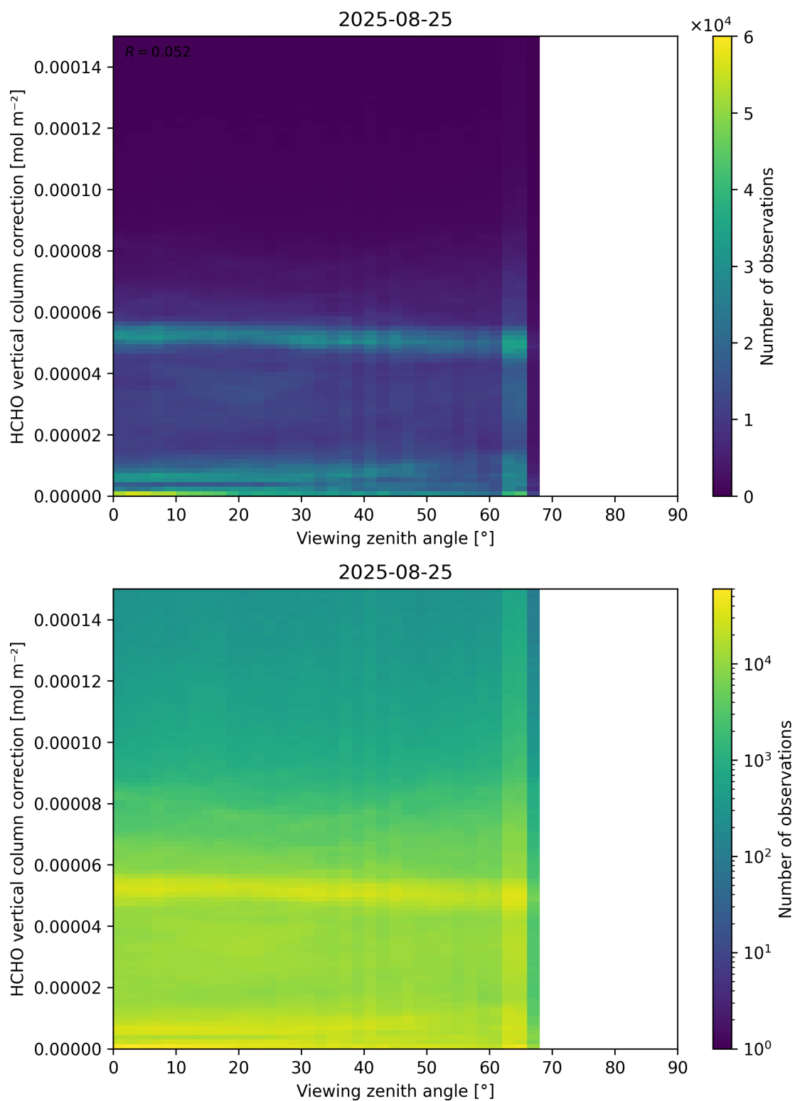
Figure 193: Scatter density plot of “Viewing zenith angle” against “HCHO vertical column correction” for 2025-08-25 to 2025-08-26.
