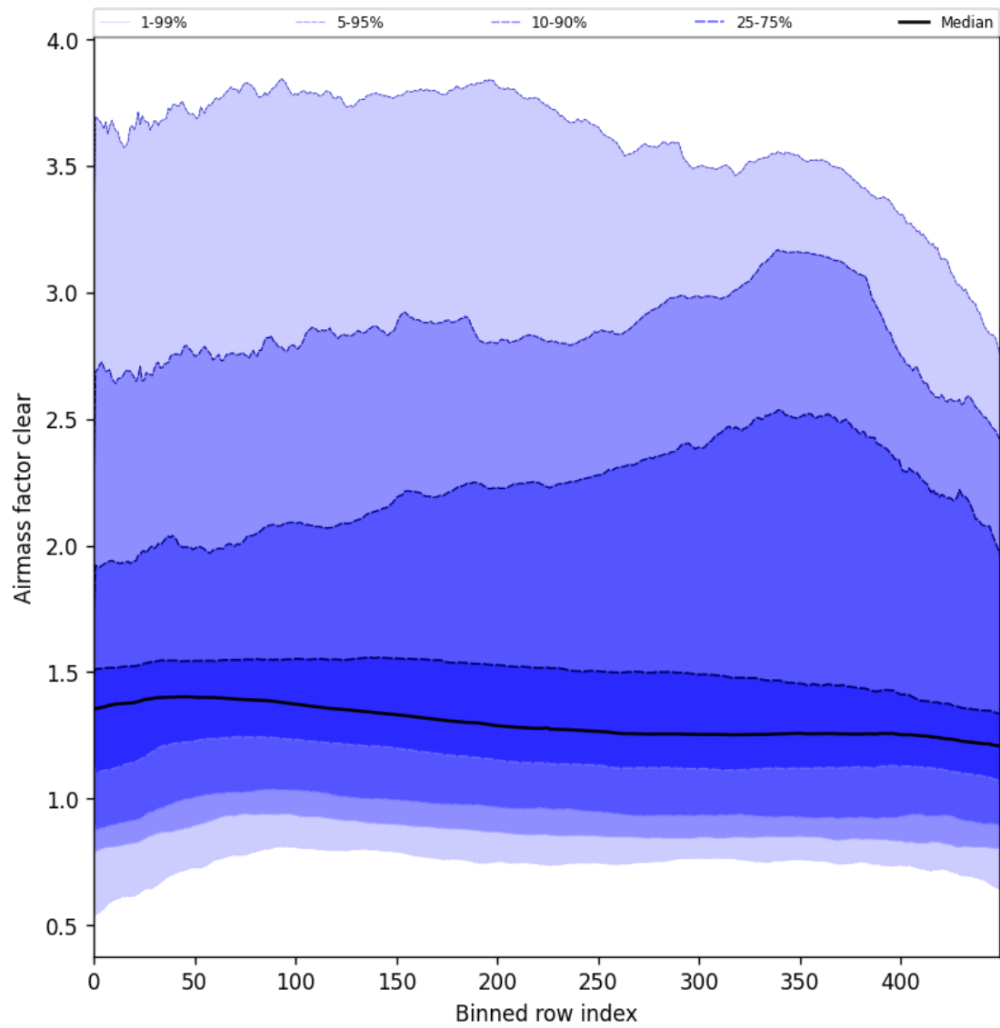
Figure 56: Along track statistics of “Airmass factor clear” for 2025-08-25 to 2025-08-26
