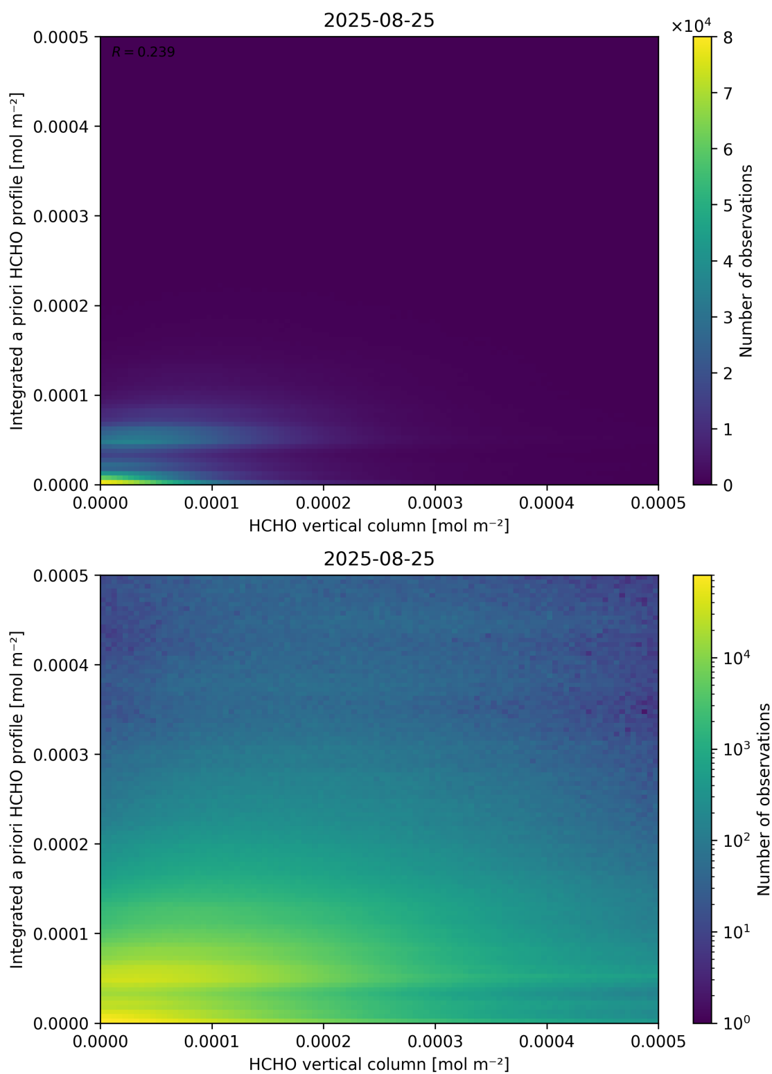
Figure 135: Scatter density plot of “HCHO vertical column” against “Integrated a priori HCHO profile” for 2025-08-25 to 2025-08-26.
