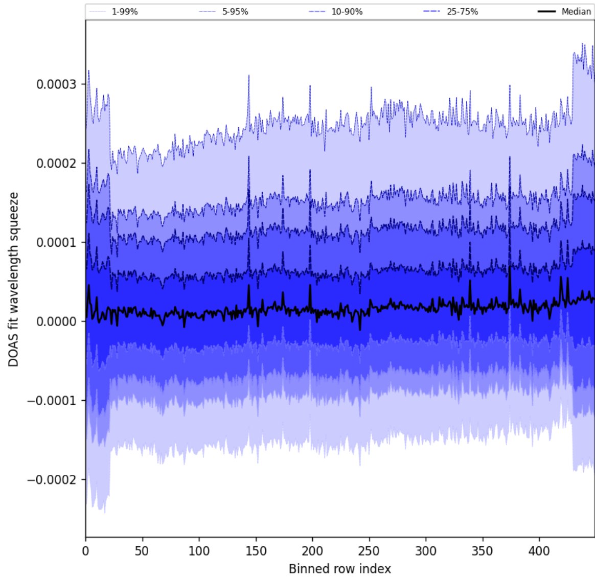
Figure 59: Along track statistics of “DOAS fit wavelength squeeze” for 2025-08-25 to 2025-08-26
