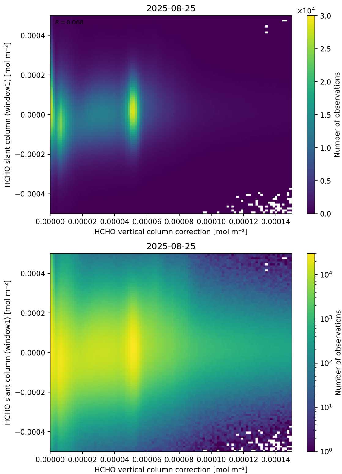
Figure 118: Scatter density plot of “HCHO vertical column correction” against “HCHO slant column (window1)” for 2025-08-25 to 2025-08-26.
