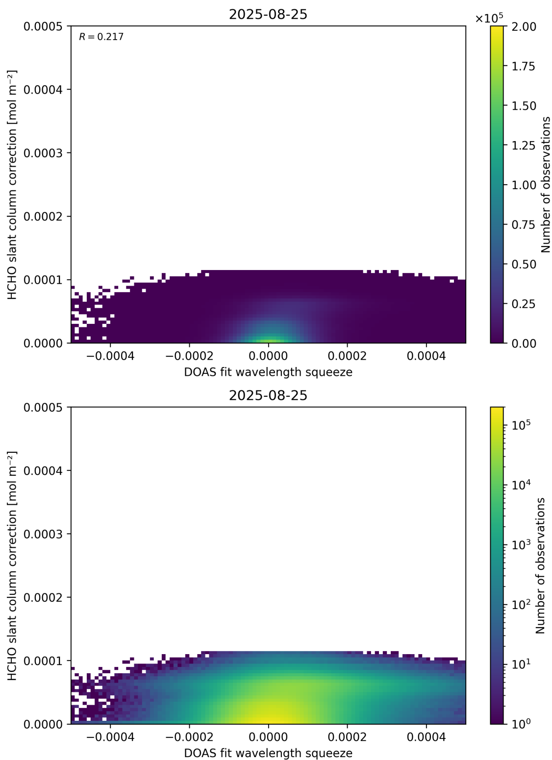
Figure 70: Scatter density plot of “DOAS fit wavelength squeeze” against “HCHO slant column correction” for 2025-08-25 to 2025-08-26.
