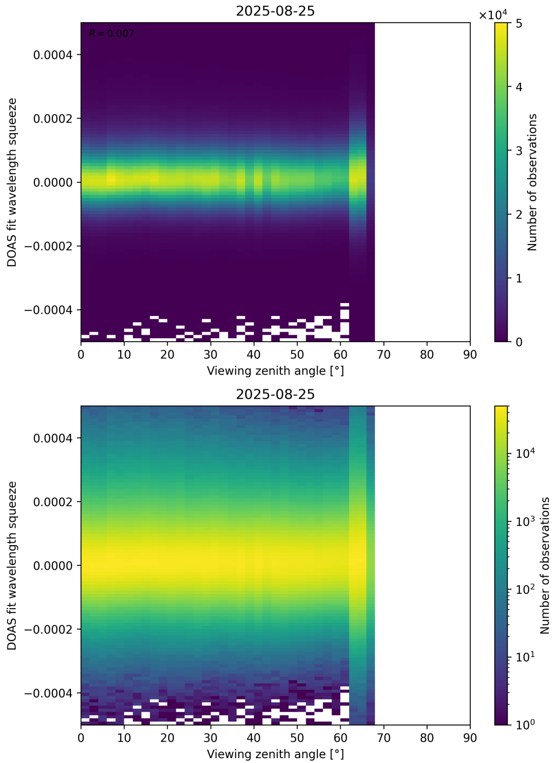
Figure 184: Scatter density plot of “Viewing zenith angle” against “DOAS fit wavelength squeeze” for 2025-08-25 to 2025-08-26.
