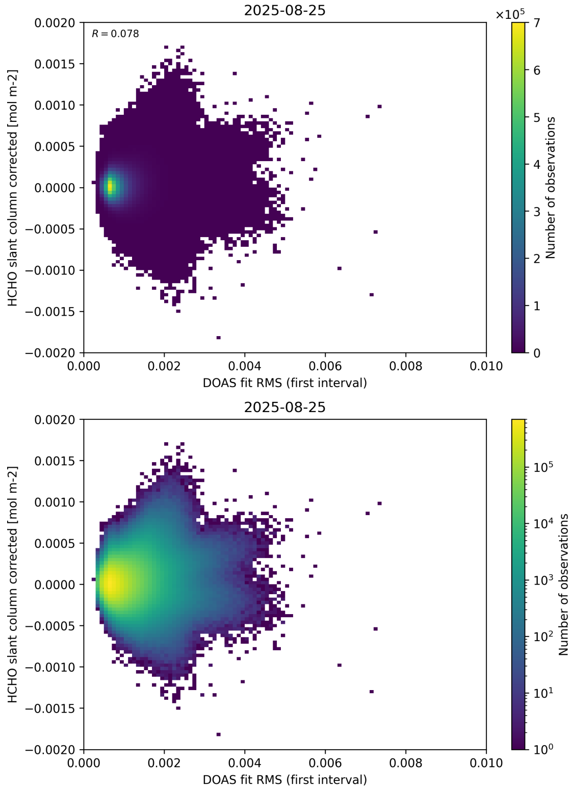
Figure 62: Scatter density plot of “DOAS fit RMS (first interval)” against “HCHO slant column corrected” for 2025-08-25 to 2025-08-26.
