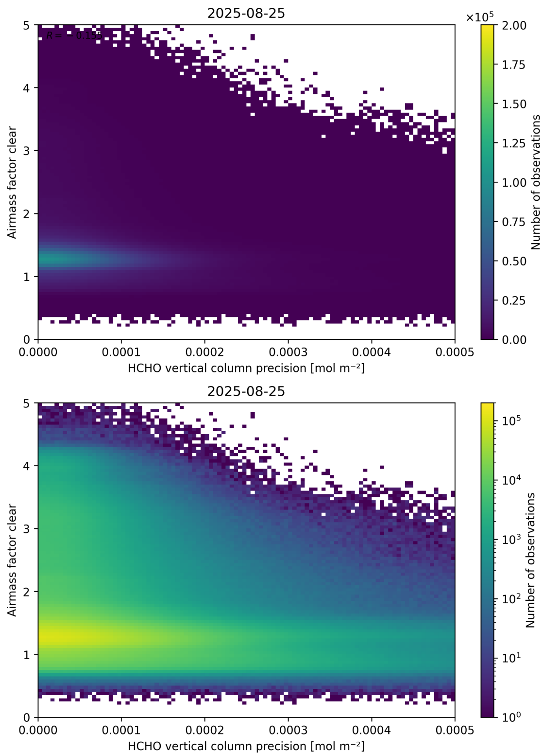
Figure 139: Scatter density plot of “HCHO vertical column precision” against “Airmass factor clear” for 2025-08-25 to 2025-08-26.
