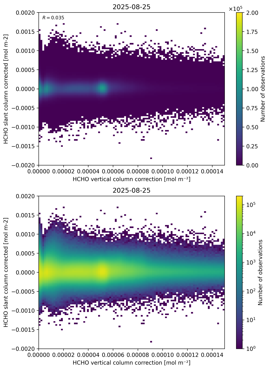
Figure 116: Scatter density plot of “HCHO vertical column correction” against “HCHO slant column corrected” for 2025-08-25 to 2025-08-26.
