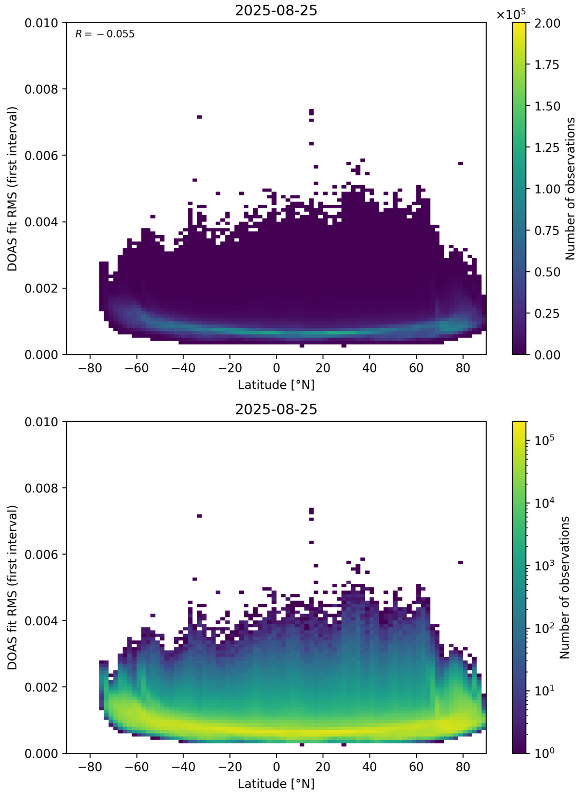
Figure 153: Scatter density plot of “Latitude” against “DOAS fit RMS (first interval)” for 2025-08-25 to 2025-08-26.
