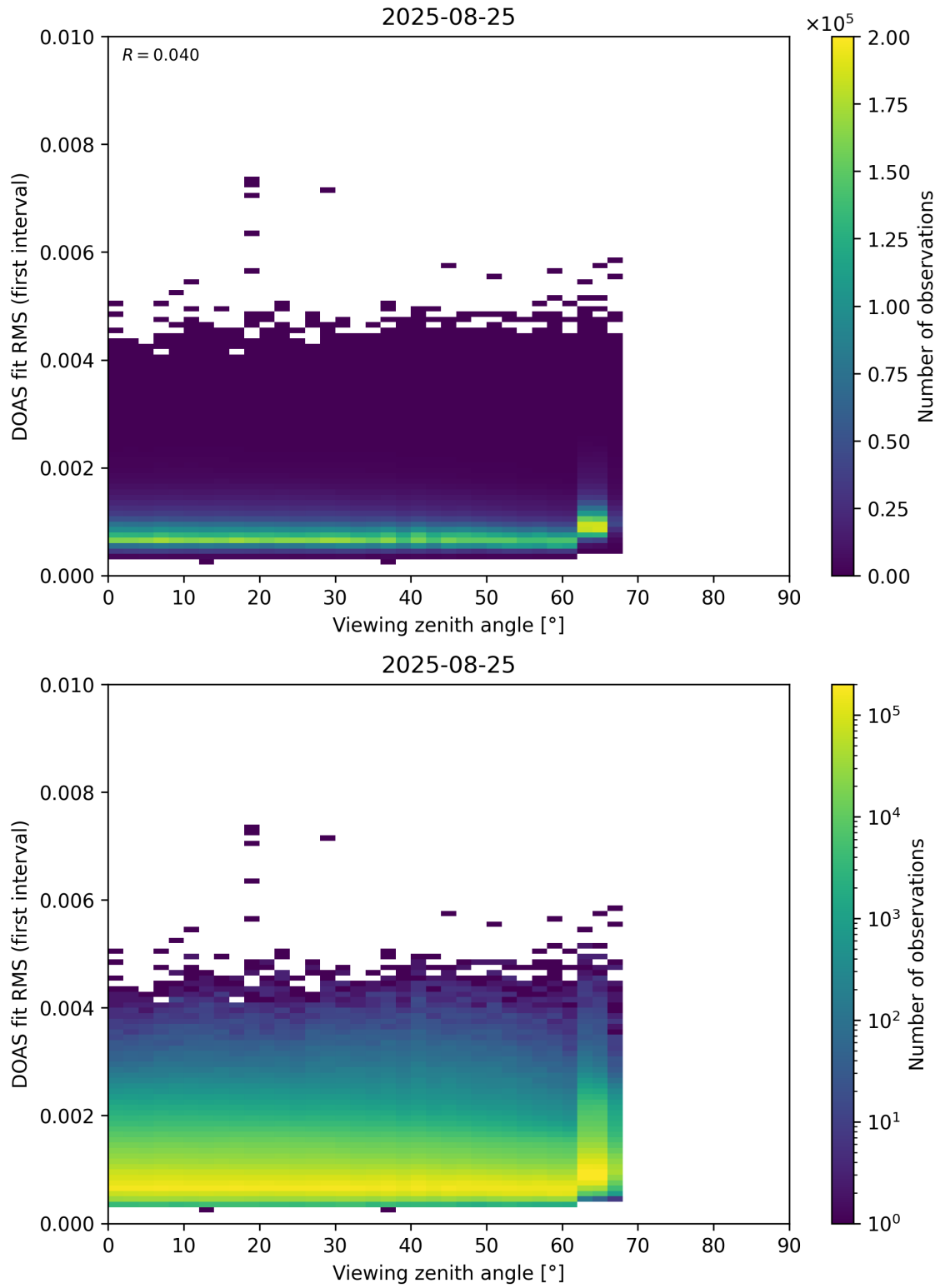
Figure 182: Scatter density plot of “Viewing zenith angle” against “DOAS fit RMS (first interval)” for 2025-08-25 to 2025-08-26.
