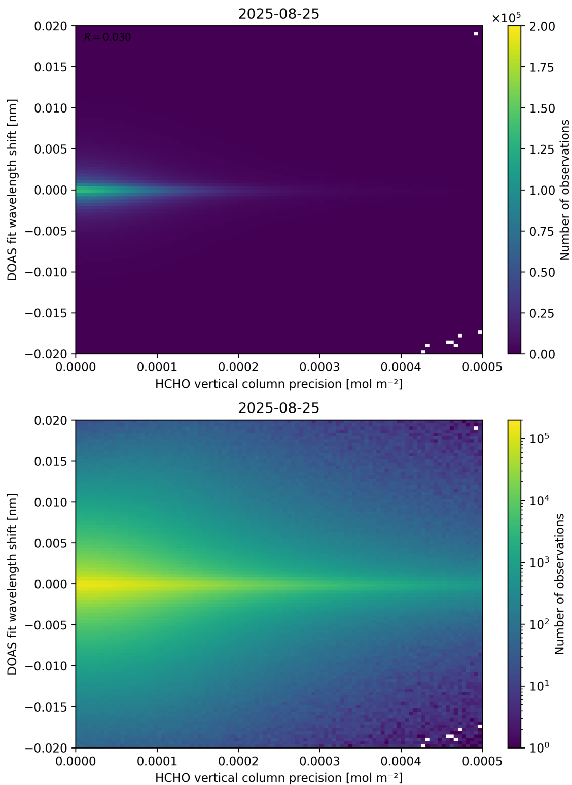
Figure 137: Scatter density plot of “HCHO vertical column precision” against “DOAS fit wavelength shift” for 2025-08-25 to 2025-08-26.
