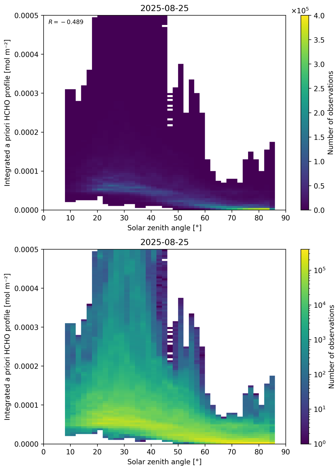
Figure 180: Scatter density plot of “Solar zenith angle” against “Integrated a priori HCHO profile” for 2025-08-25 to 2025-08-26.
