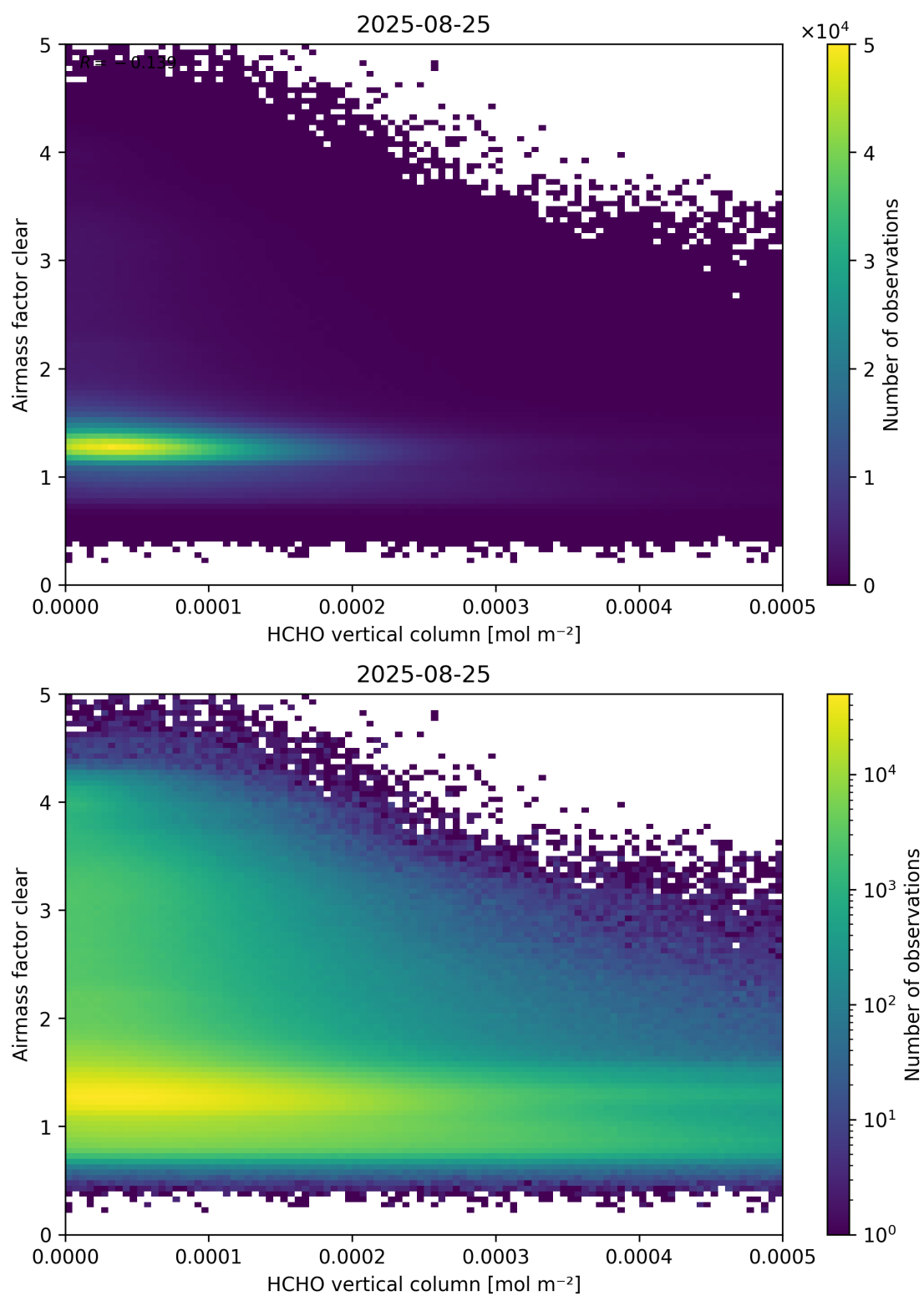
Figure 126: Scatter density plot of “HCHO vertical column” against “Airmass factor clear” for 2025-08-25 to 2025-08-26.
