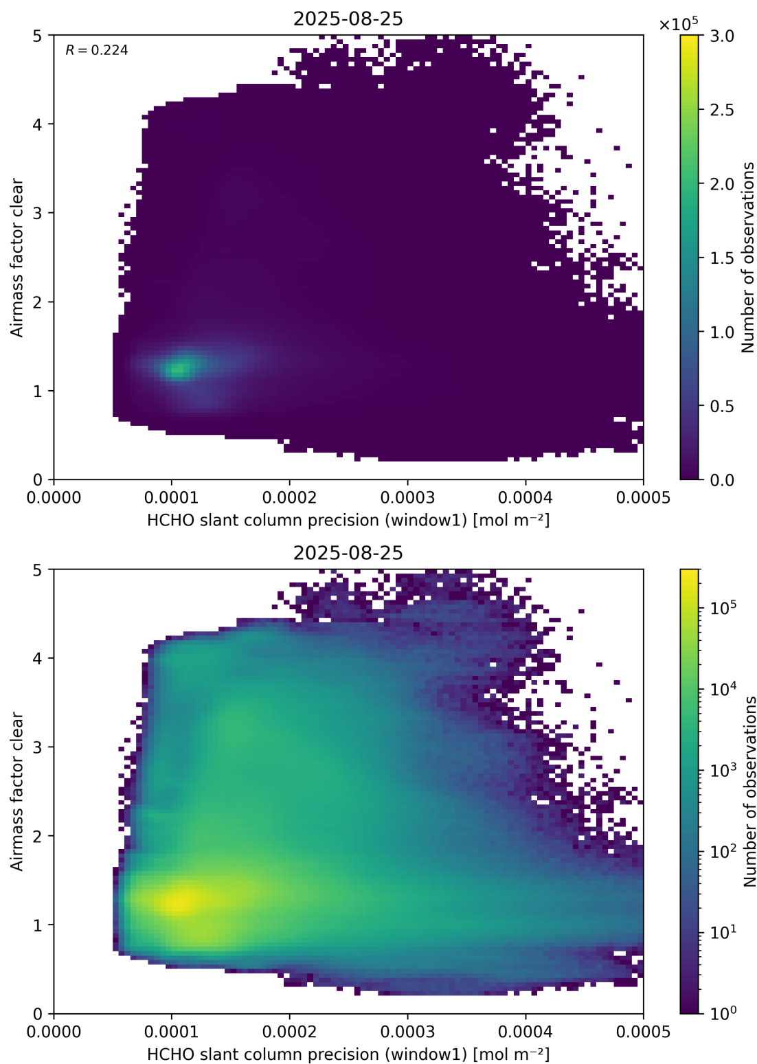
Figure 91: Scatter density plot of “HCHO slant column precision (window1)” against “Airmass factor clear” for 2025-08-25 to 2025-08-26.
