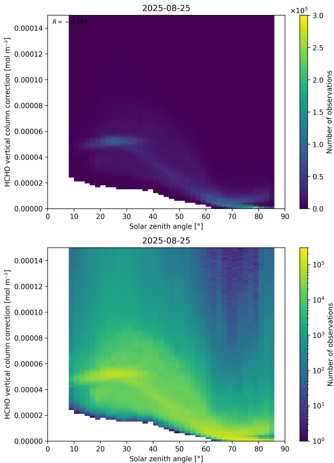
Figure 178: Scatter density plot of “Solar zenith angle” against “HCHO vertical column correction” for 2025-08-25 to 2025-08-26.
