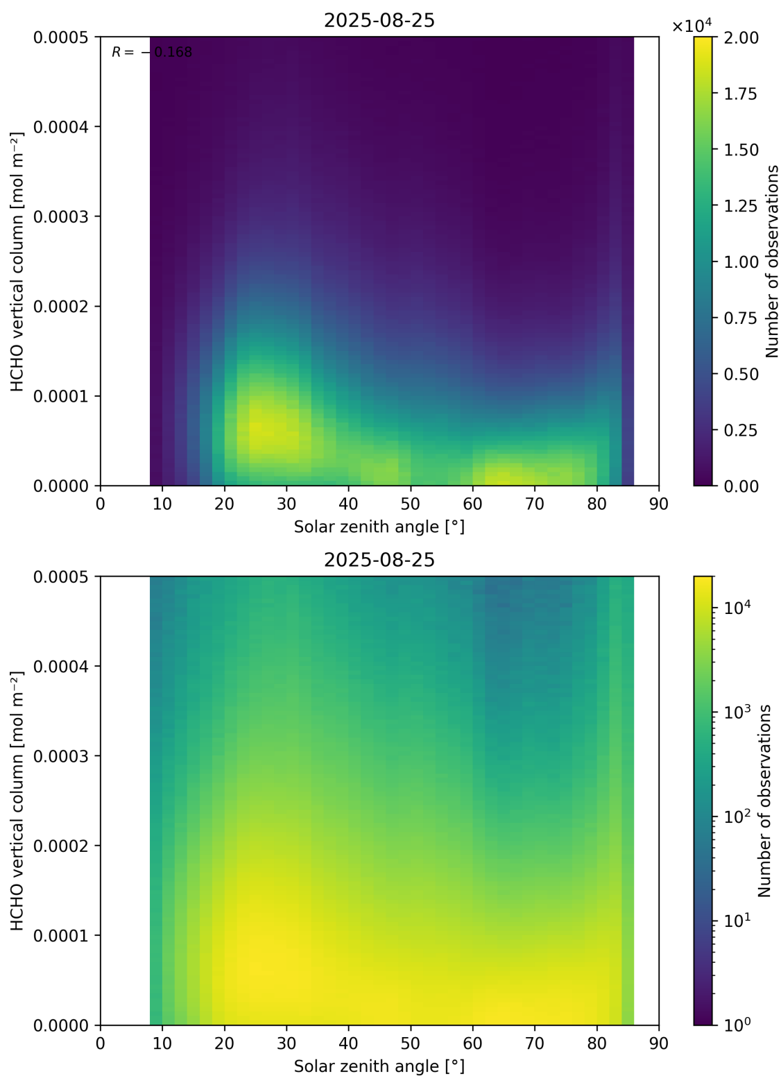
Figure 177: Scatter density plot of “Solar zenith angle” against “HCHO vertical column” for 2025-08-25 to 2025-08-26.
