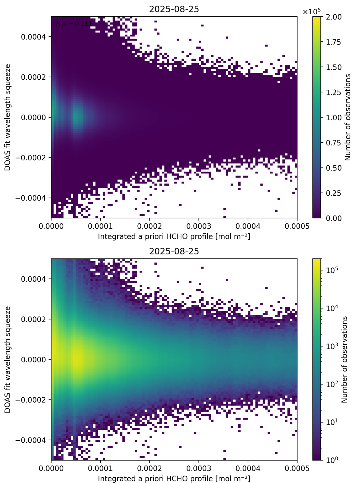
Figure 150: Scatter density plot of “Integrated a priori HCHO profile” against “DOAS fit wavelength squeeze” for 2025-08-25 to 2025-08-26.
