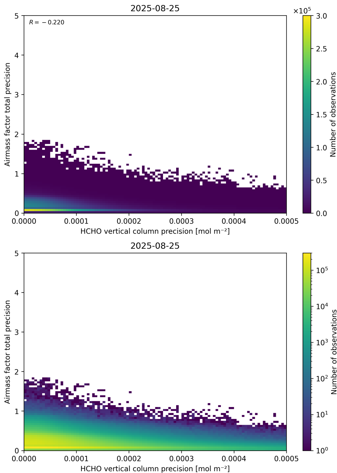
Figure 145: Scatter density plot of “HCHO vertical column precision” against “Airmass factor total precision” for 2025-08-25 to 2025-08-26.
