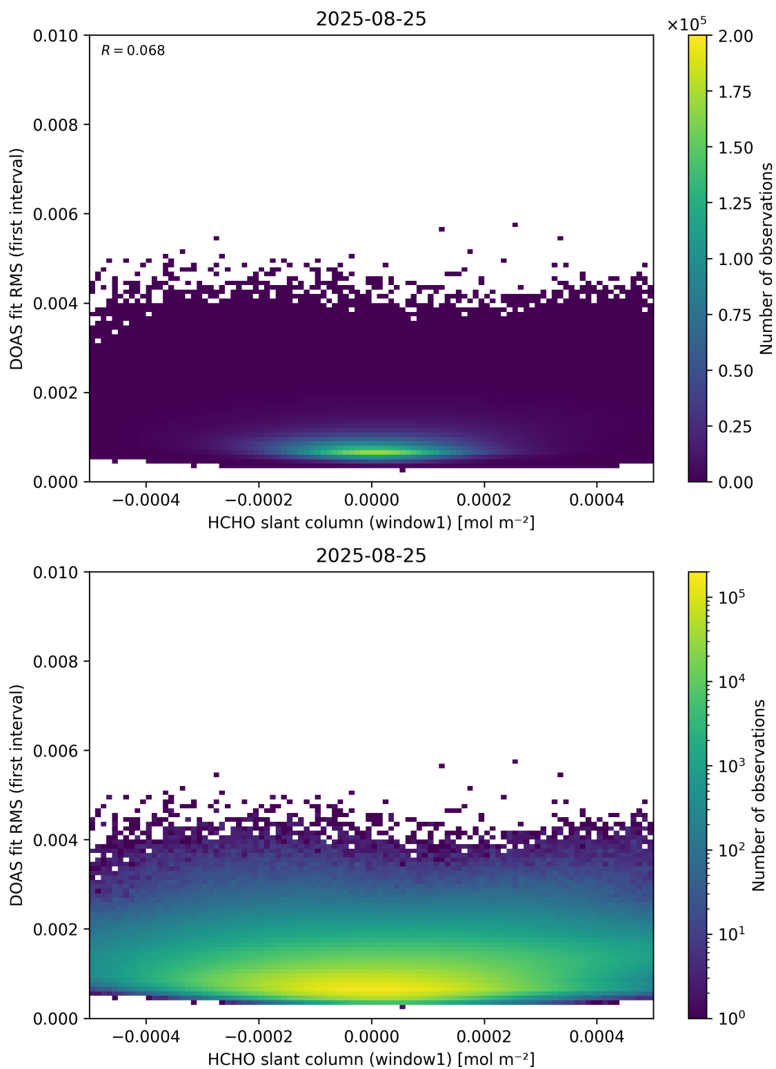
Figure 78: Scatter density plot of “HCHO slant column (window1)” against “DOAS fit RMS (first interval)” for 2025-08-25 to 2025-08-26.
