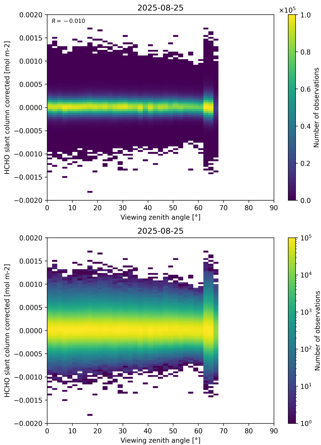
Figure 186: Scatter density plot of “Viewing zenith angle” against “HCHO slant column corrected” for 2025-08-25 to 2025-08-26.
