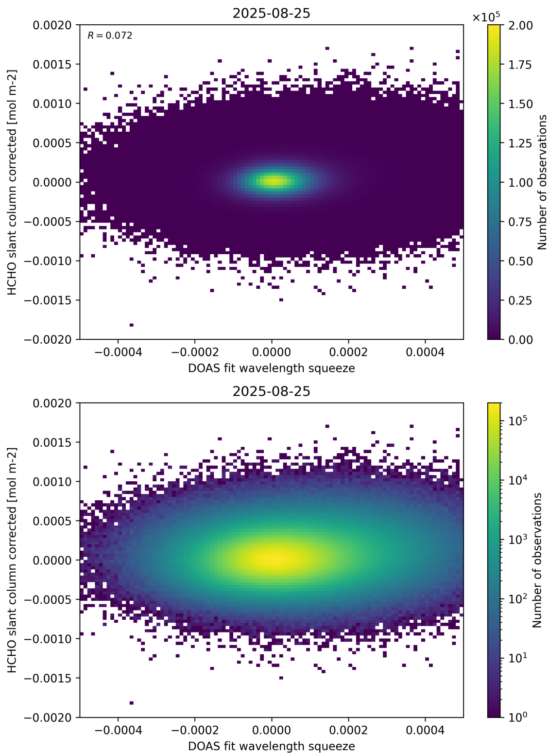
Figure 69: Scatter density plot of “DOAS fit wavelength squeeze” against “HCHO slant column corrected” for 2025-08-25 to 2025-08-26.
