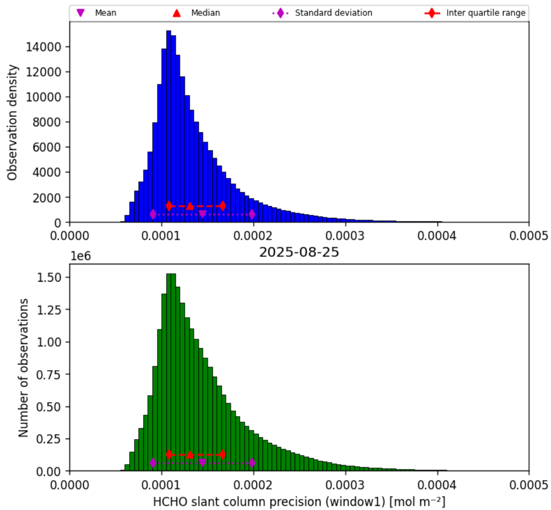
Figure 39: Histogram of “HCHO slant column precision (window1)” for 2025-08-25 to 2025-08-26
