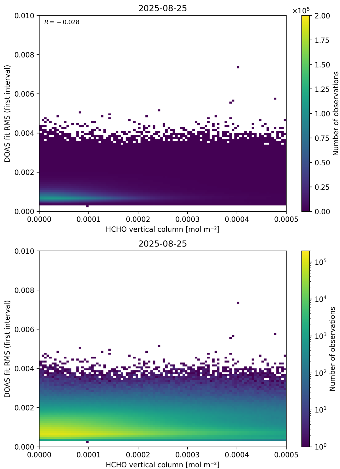
Figure 123: Scatter density plot of “HCHO vertical column” against “DOAS fit RMS (first interval)” for 2025-08-25 to 2025-08-26.
