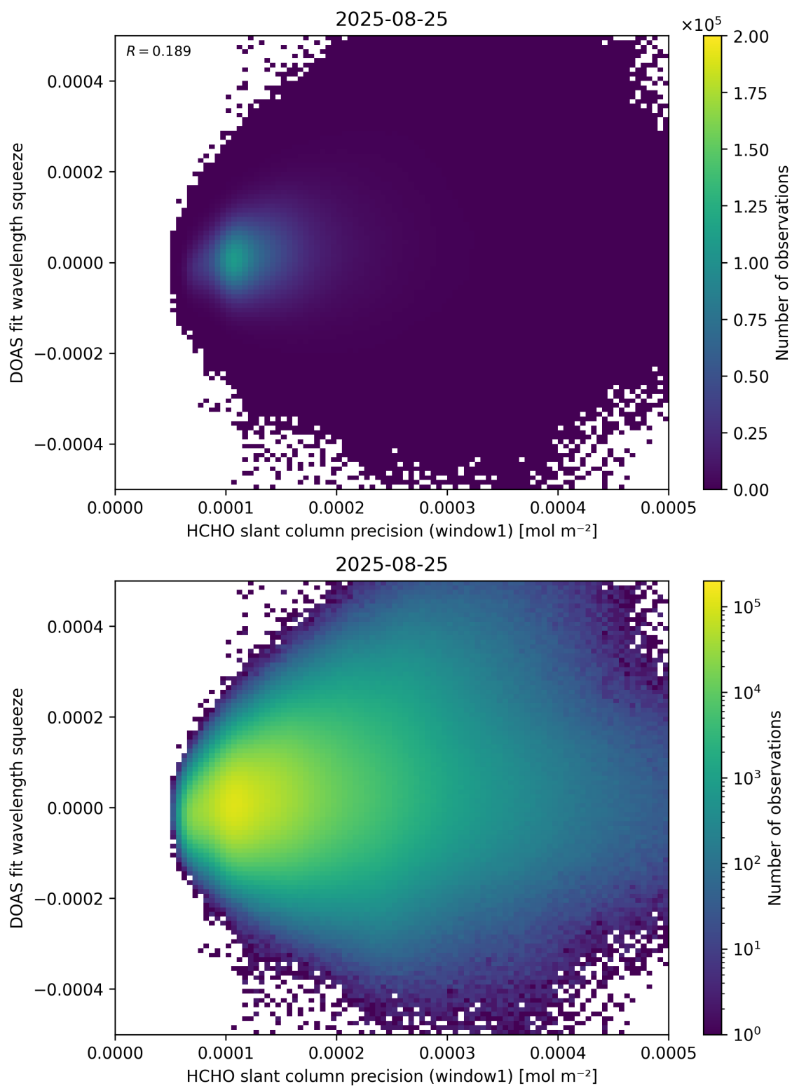
Figure 90: Scatter density plot of “HCHO slant column precision (window1)” against “DOAS fit wavelength squeeze” for 2025-08-25 to 2025-08-26.
