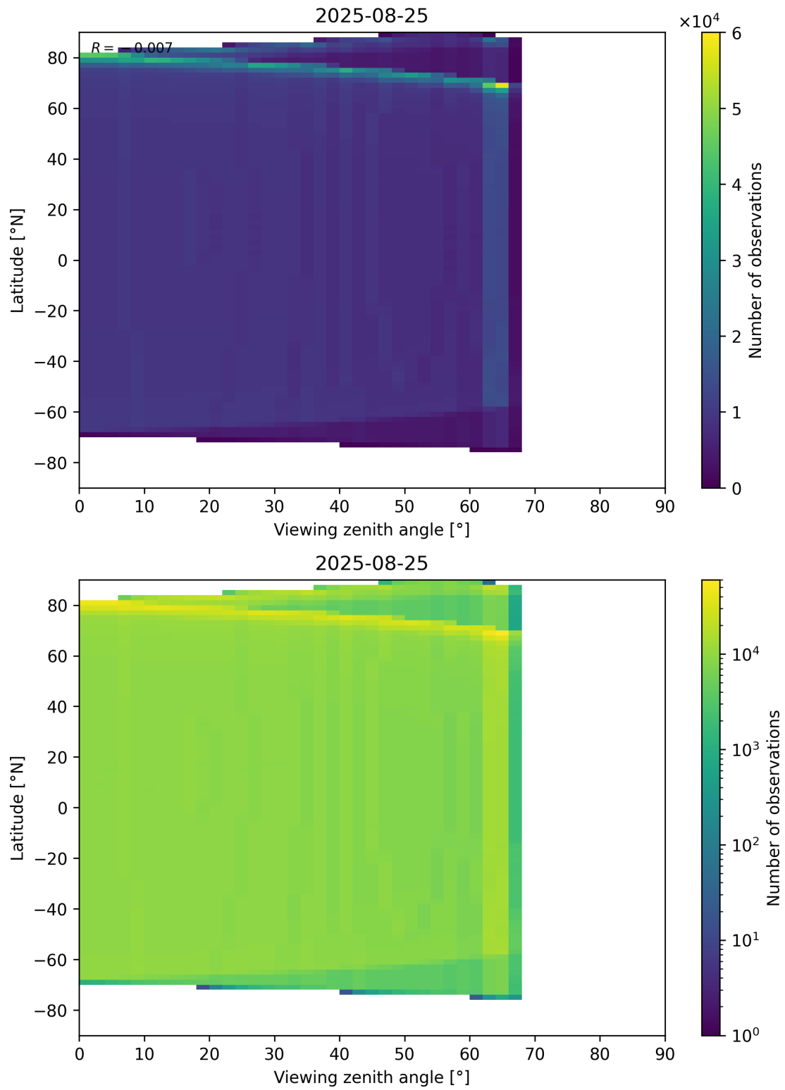
Figure 196: Scatter density plot of “Viewing zenith angle” against “Latitude” for 2025-08-25 to 2025-08-26.
