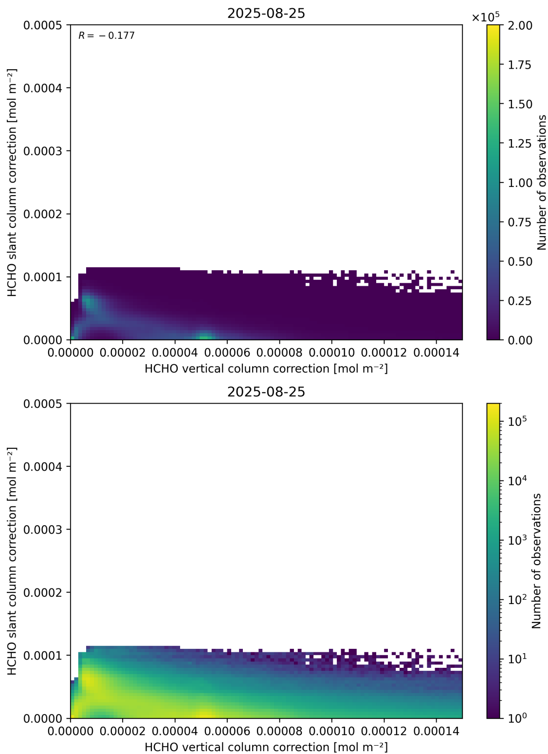
Figure 117: Scatter density plot of “HCHO vertical column correction” against “HCHO slant column correction” for 2025-08-25 to 2025-08-26.
