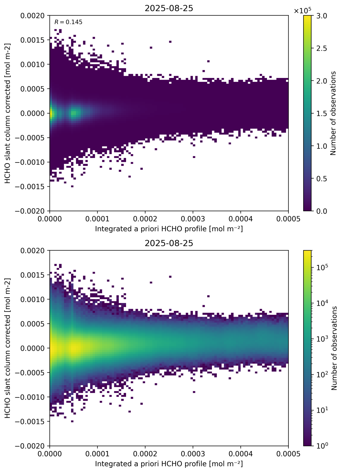
Figure 151: Scatter density plot of “Integrated a priori HCHO profile” against “HCHO slant column corrected” for 2025-08-25 to 2025-08-26.
