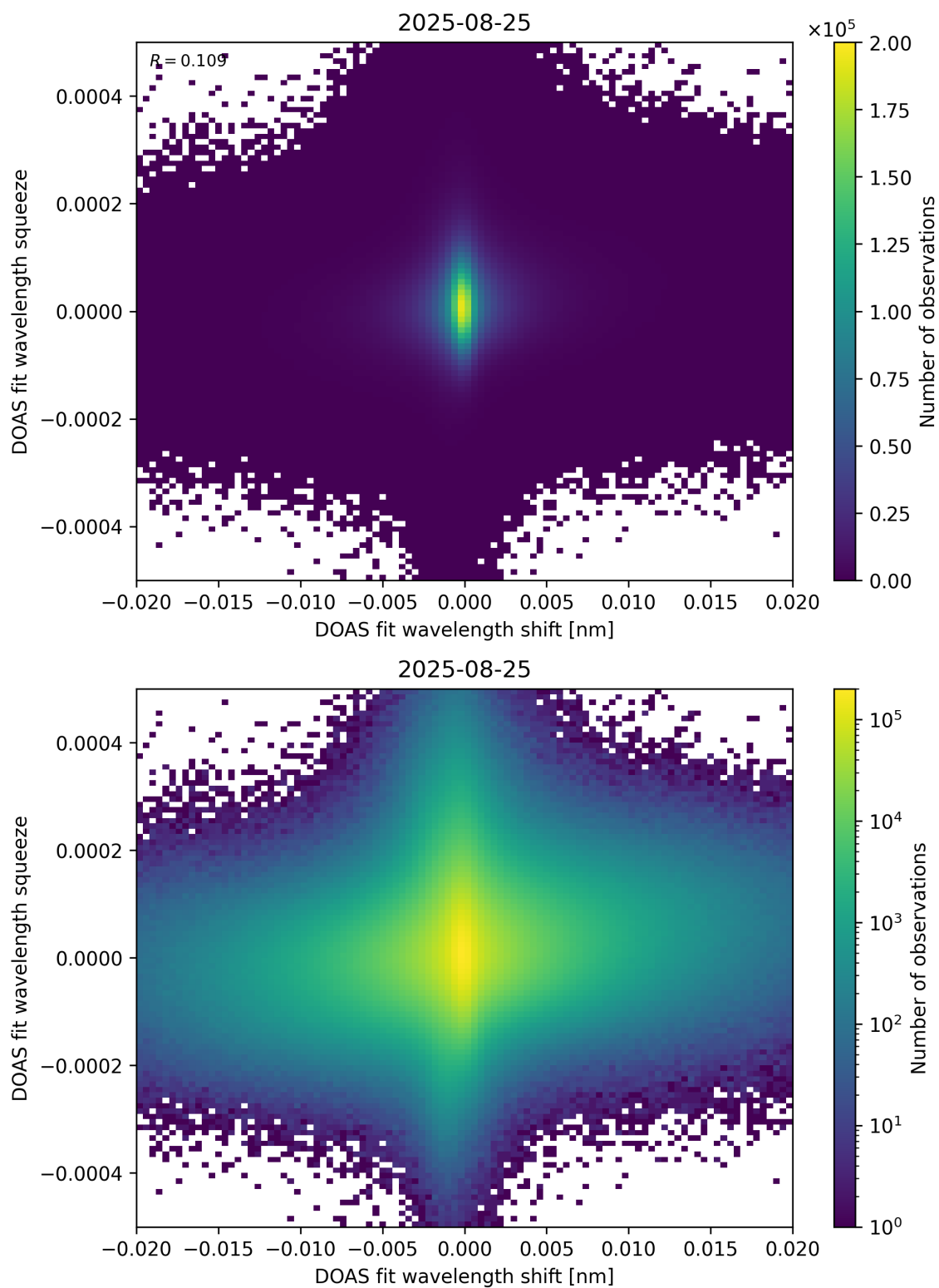
Figure 65: Scatter density plot of “DOAS fit wavelength shift” against “DOAS fit wavelength squeeze” for 2025-08-25 to 2025-08-26.
