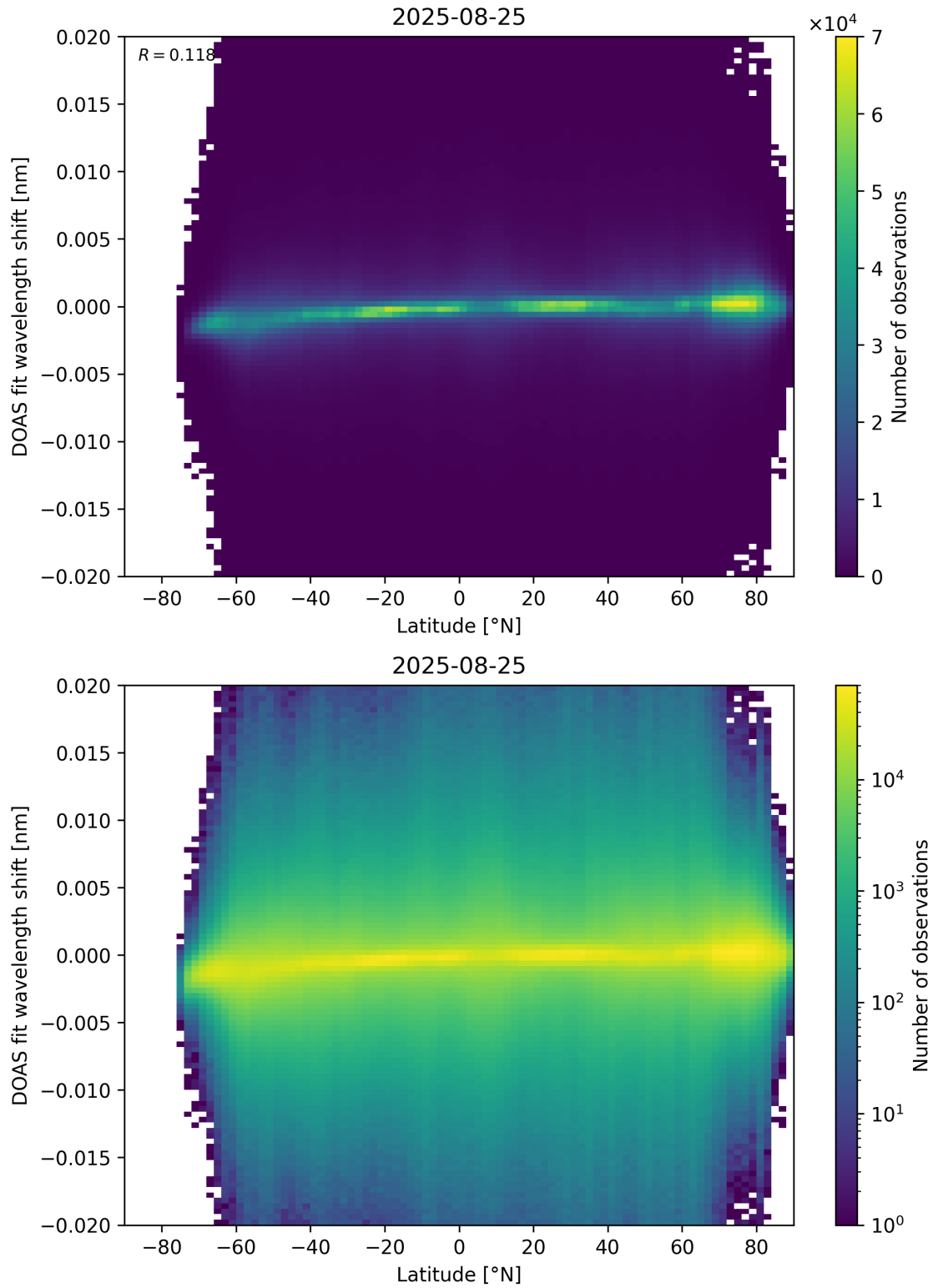
Figure 154: Scatter density plot of “Latitude” against “DOAS fit wavelength shift” for 2025-08-25 to 2025-08-26.
