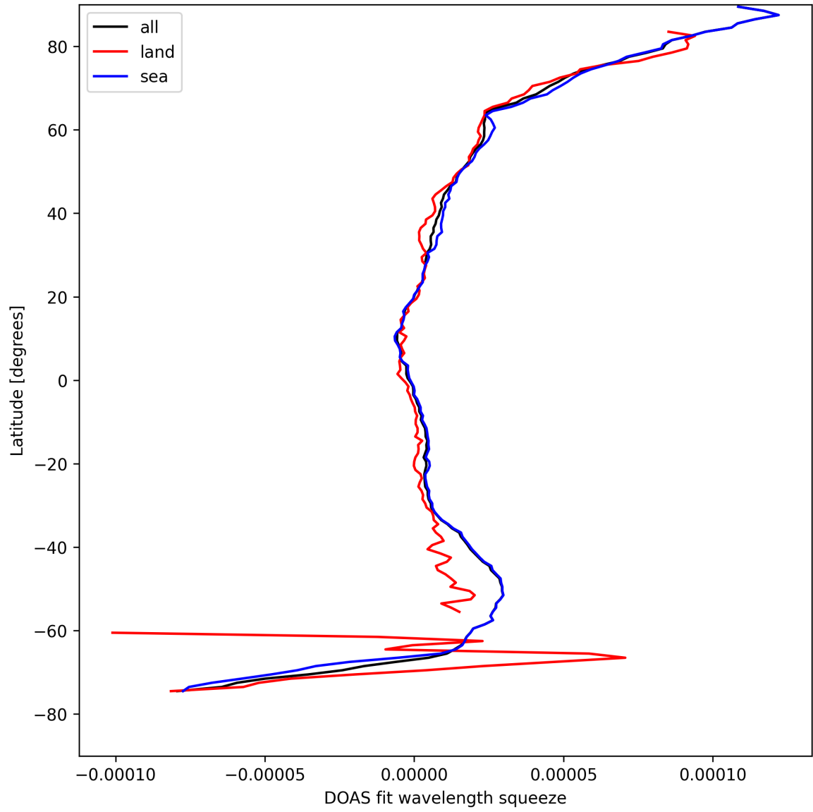
Figure 31: Zonal average of “DOAS fit wavelength squeeze” for 2025-08-25 to 2025-08-26.
