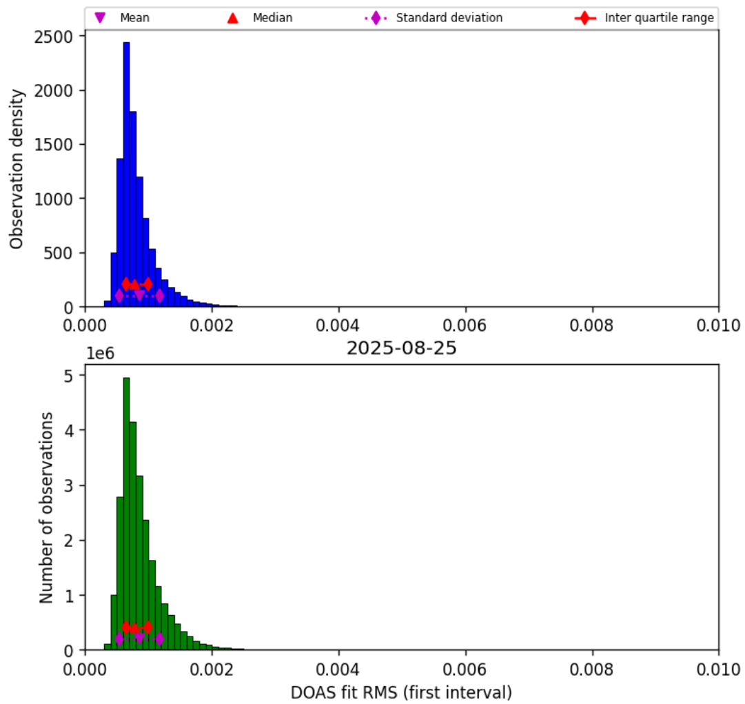
Figure 46: Histogram of “DOAS fit RMS (first interval)” for 2025-08-25 to 2025-08-26
