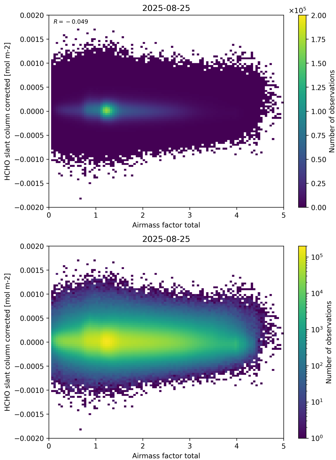
Figure 101: Scatter density plot of “Airmass factor total” against “HCHO slant column corrected” for 2025-08-25 to 2025-08-26.
