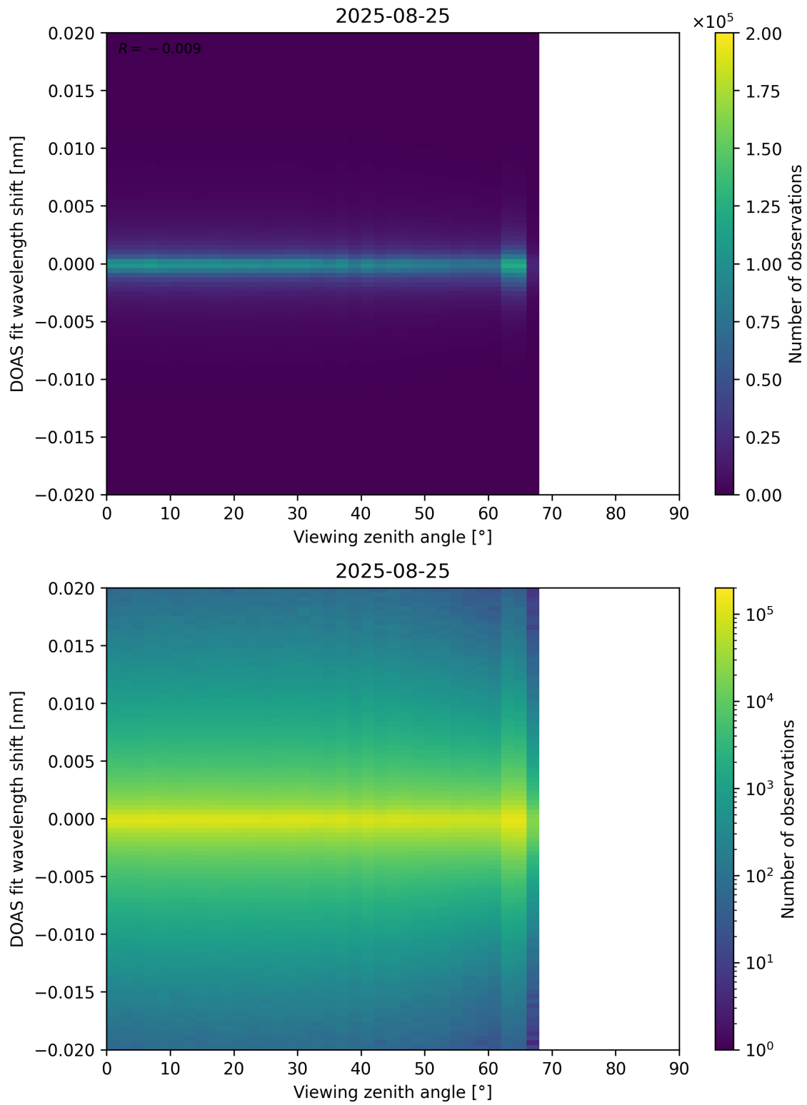
Figure 183: Scatter density plot of “Viewing zenith angle” against “DOAS fit wavelength shift” for 2025-08-25 to 2025-08-26.
