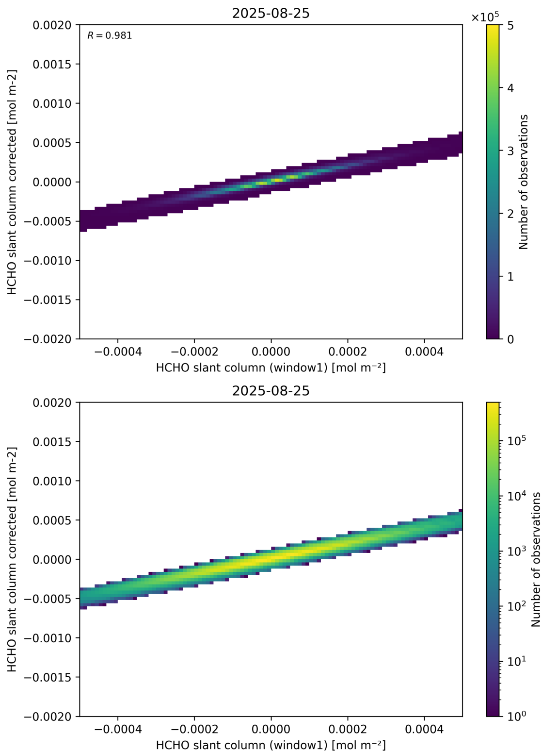
Figure 82: Scatter density plot of “HCHO slant column (window1)” against “HCHO slant column corrected” for 2025-08-25 to 2025-08-26.
