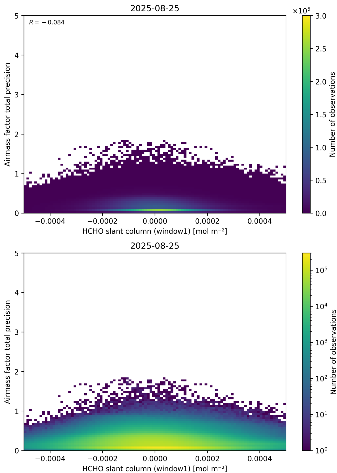
Figure 86: Scatter density plot of “HCHO slant column (window1)” against “Airmass factor total precision” for 2025-08-25 to 2025-08-26.
