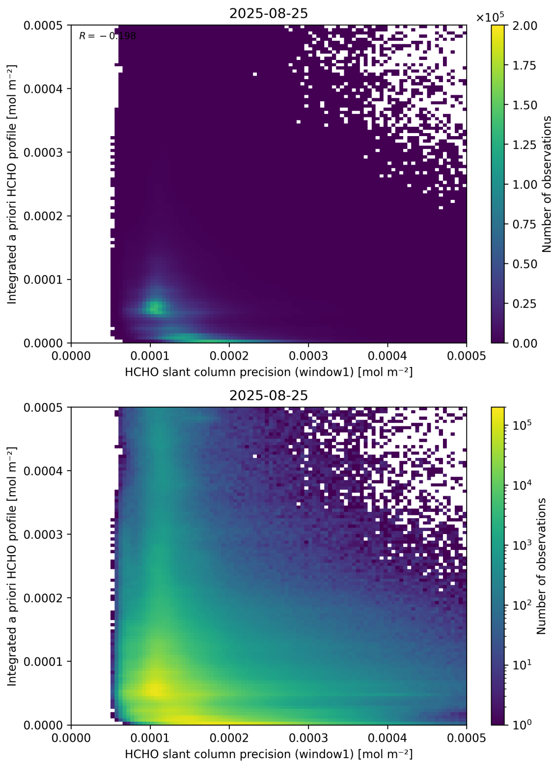
Figure 96: Scatter density plot of “HCHO slant column precision (window1)” against “Integrated a priori HCHO profile” for 2025-08-25 to 2025-08-26.
