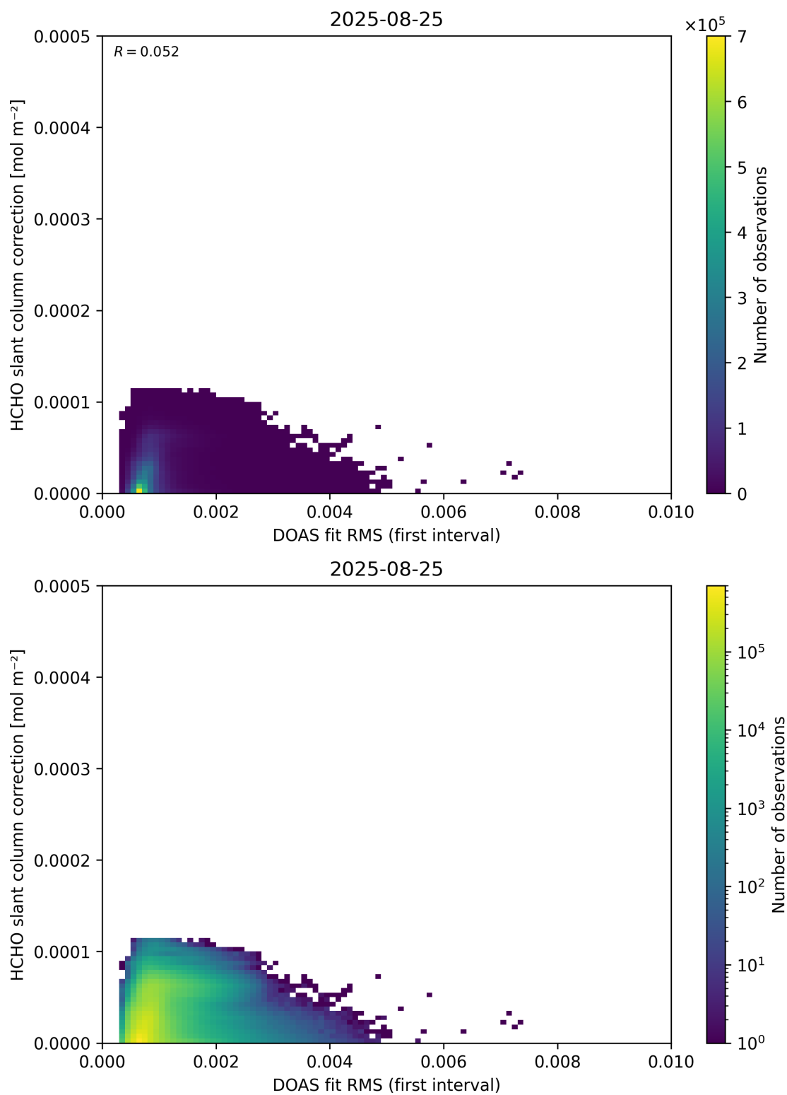
Figure 63: Scatter density plot of “DOAS fit RMS (first interval)” against “HCHO slant column correction” for 2025-08-25 to 2025-08-26.
