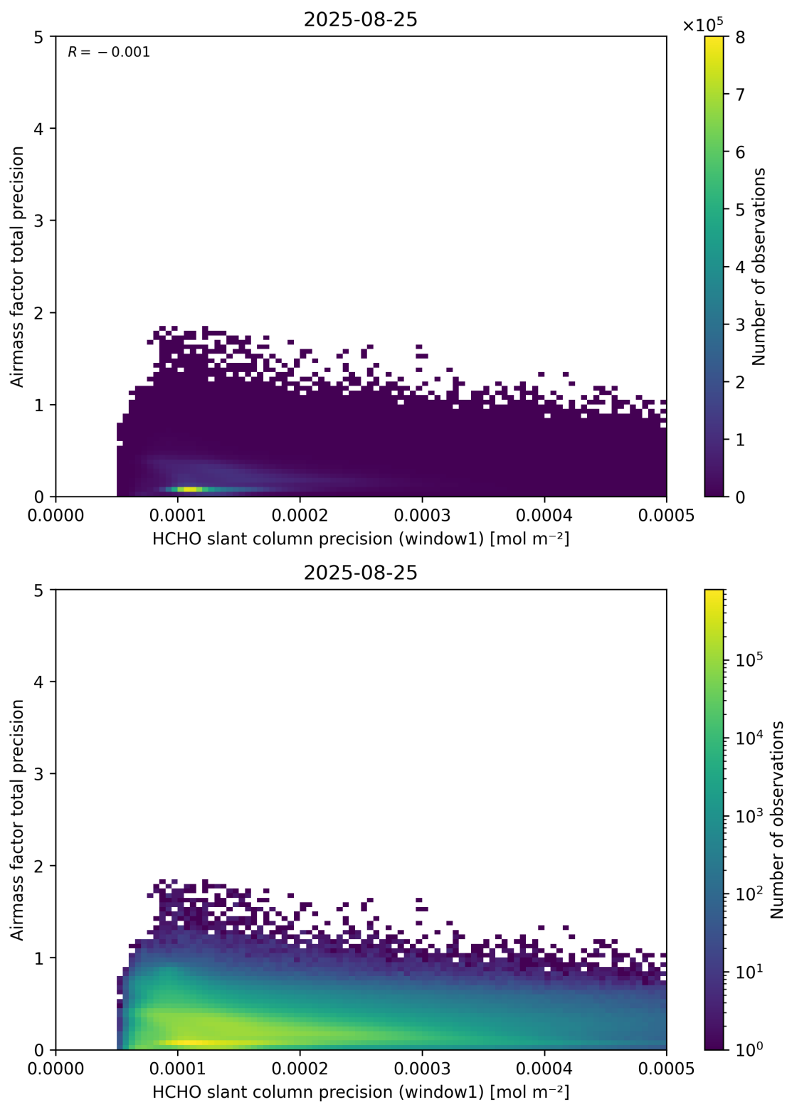
Figure 95: Scatter density plot of “HCHO slant column precision (window1)” against “Airmass factor total precision” for 2025-08-25 to 2025-08-26.
