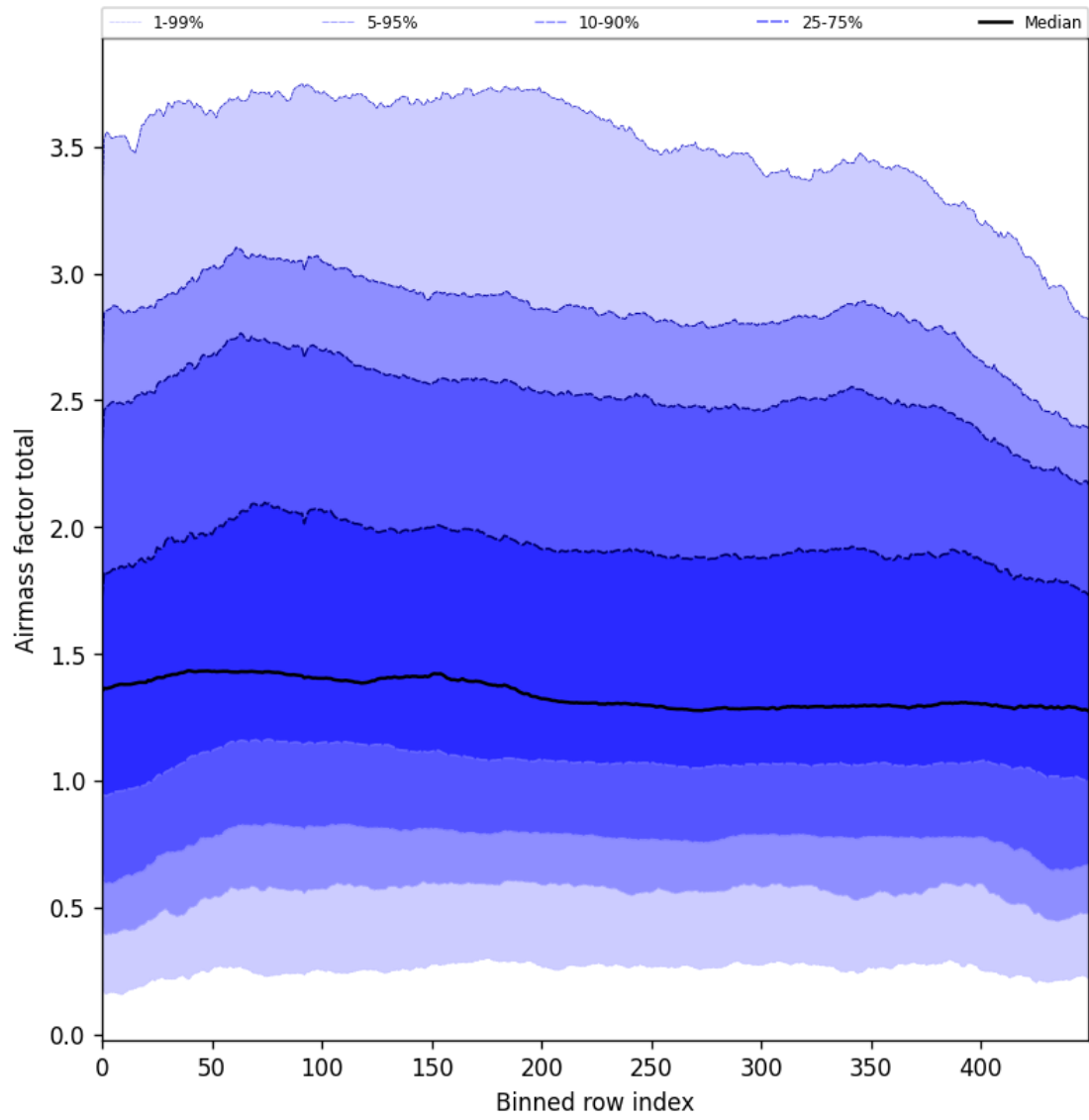
Figure 54: Along track statistics of “Airmass factor total” for 2025-08-25 to 2025-08-26
