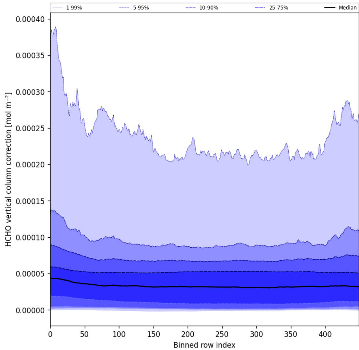
Figure 51: Along track statistics of “HCHO vertical column correction” for 2025-08-25 to 2025-08-26
