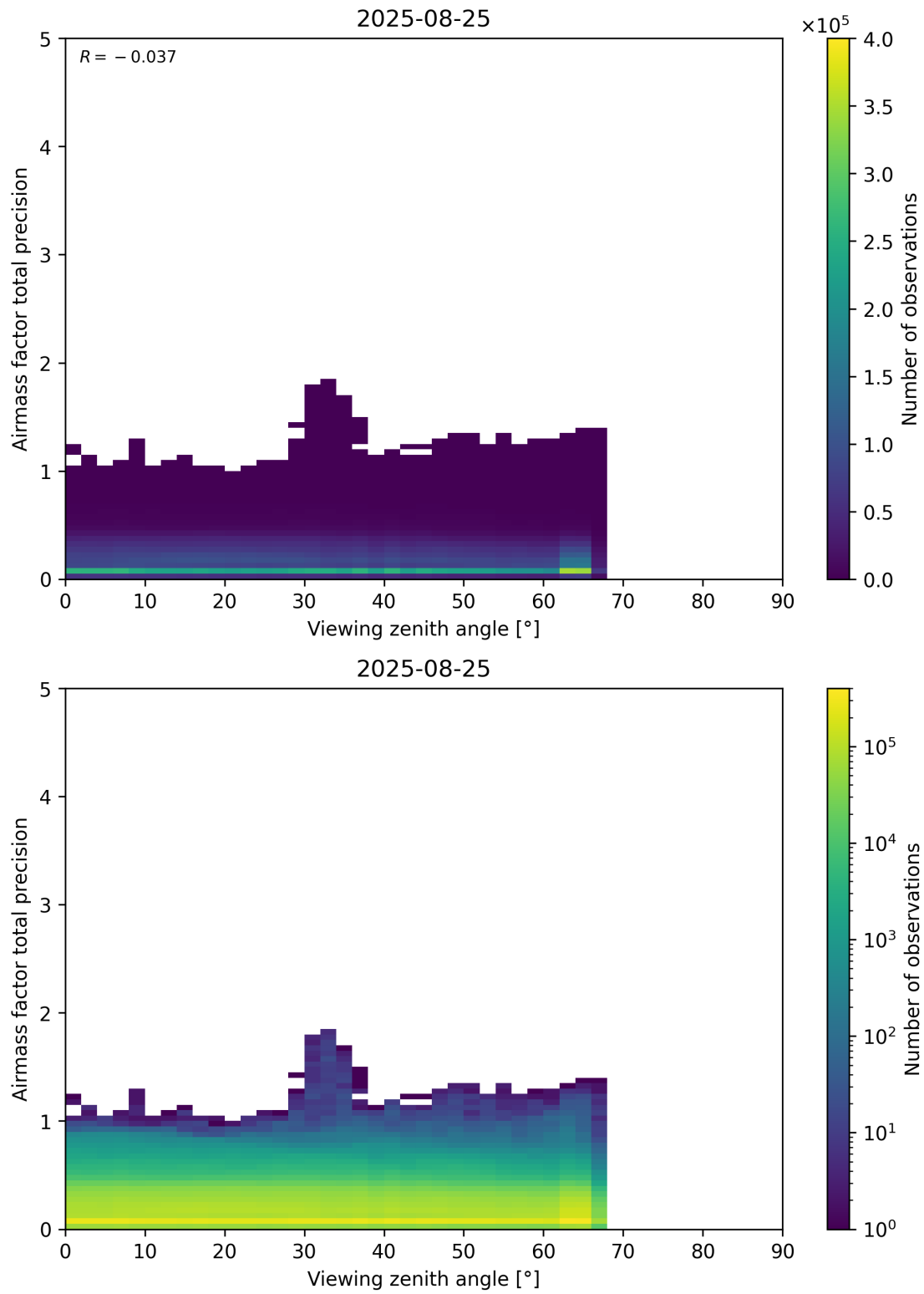
Figure 191: Scatter density plot of “Viewing zenith angle” against “Airmass factor total precision” for 2025-08-25 to 2025-08-26.
