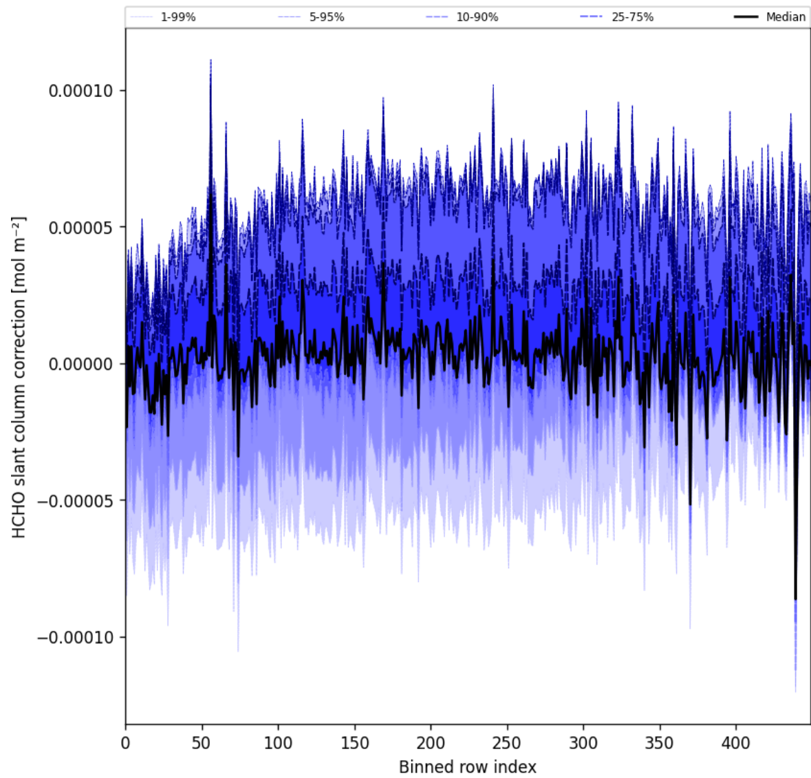
Figure 61: Along track statistics of "HCHO slant column correction" for 2025-08-25 to 2025-08-26
