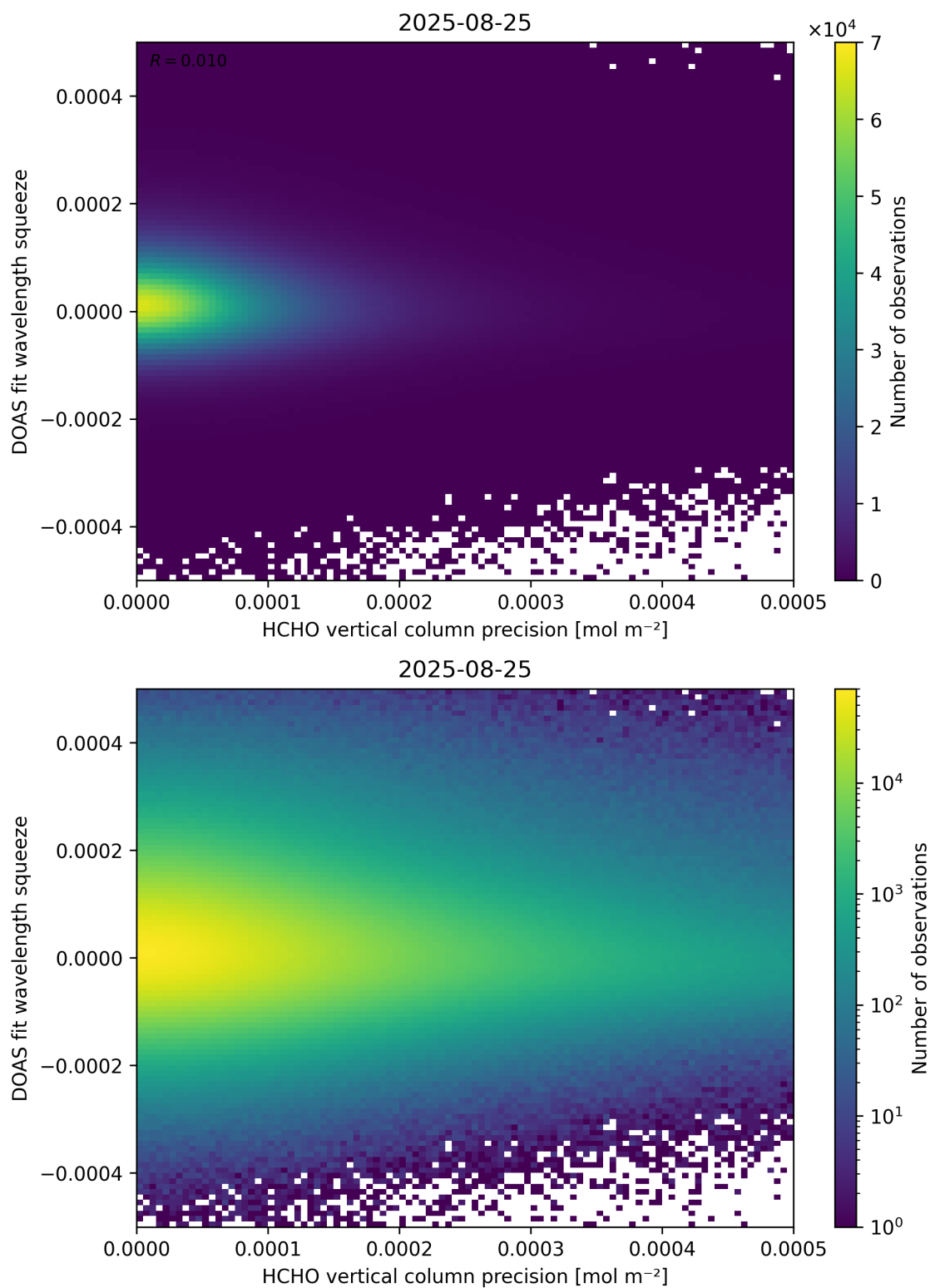
Figure 138: Scatter density plot of “HCHO vertical column precision” against “DOAS fit wavelength squeeze” for 2025-08-25 to 2025-08-26.
