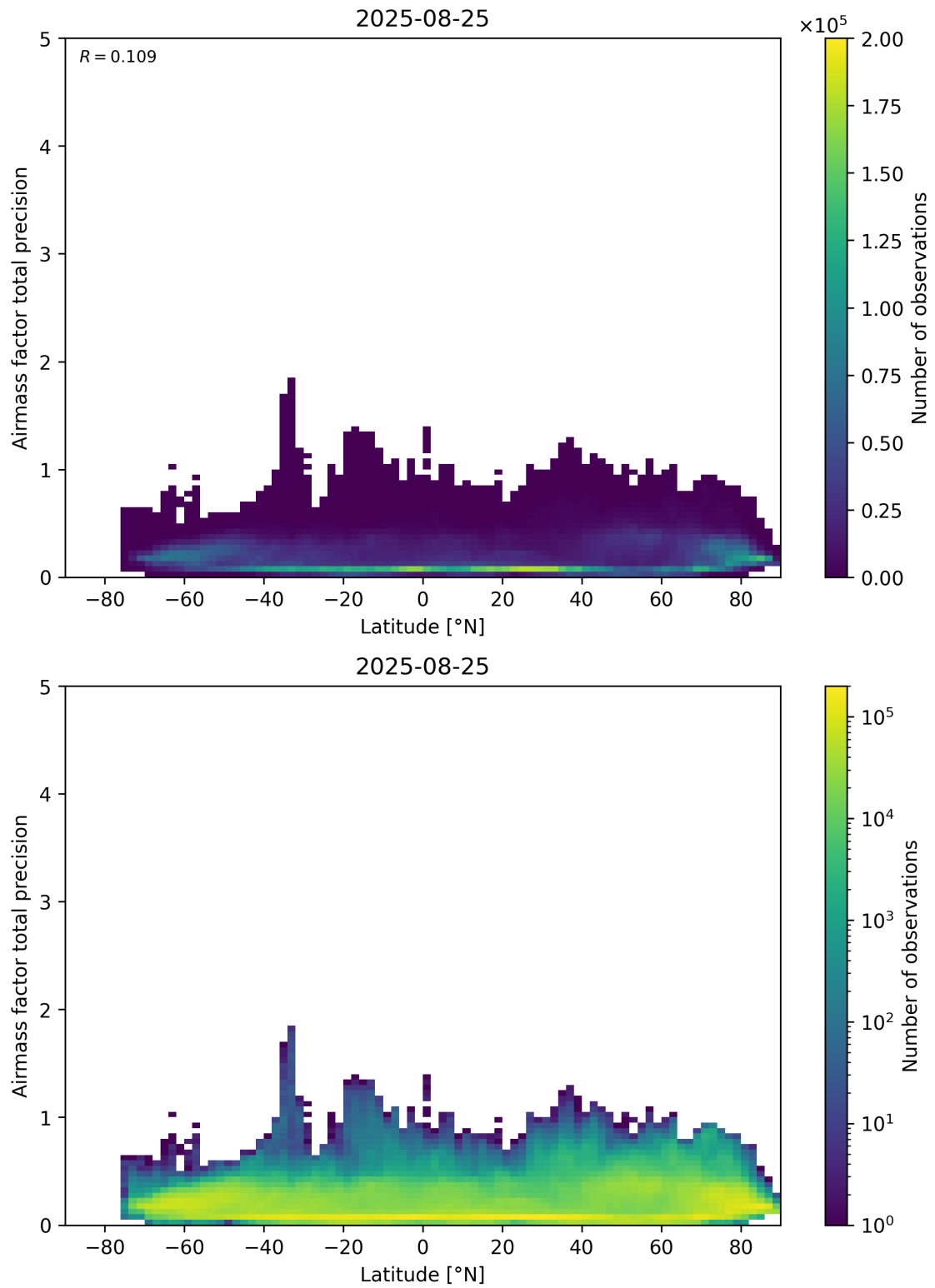
Figure 162: Scatter density plot of “Latitude” against “Airmass factor total precision” for 2025-08-25 to 2025-08-26.
