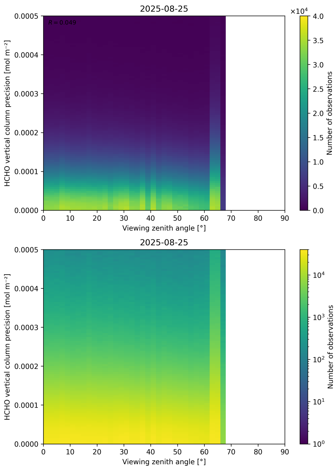
Figure 194: Scatter density plot of “Viewing zenith angle” against “HCHO vertical column precision” for 2025-08-25 to 2025-08-26.
