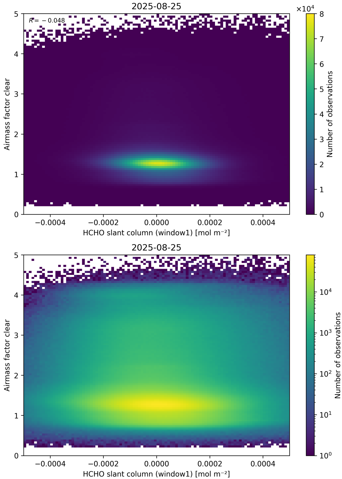
Figure 81: Scatter density plot of “HCHO slant column (window1)” against “Airmass factor clear” for 2025-08-25 to 2025-08-26.
