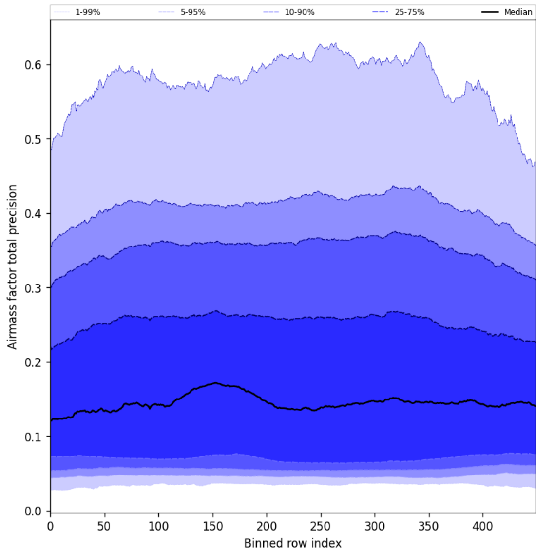
Figure 55: Along track statistics of “Airmass factor total precision” for 2025-08-25 to 2025-08-26
