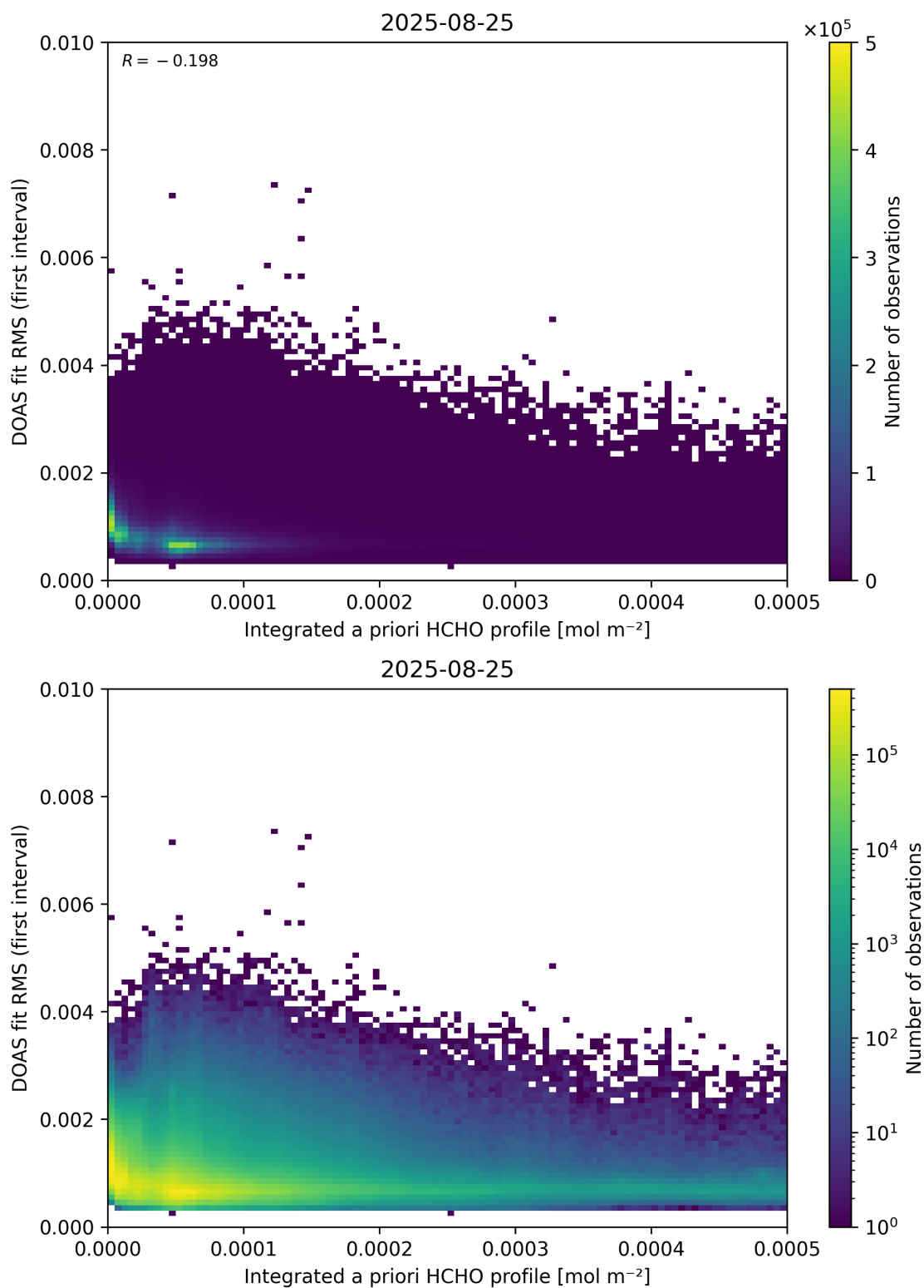
Figure 148: Scatter density plot of “Integrated a priori HCHO profile” against “DOAS fit RMS (first interval)” for 2025-08-25 to 2025-08-26.
