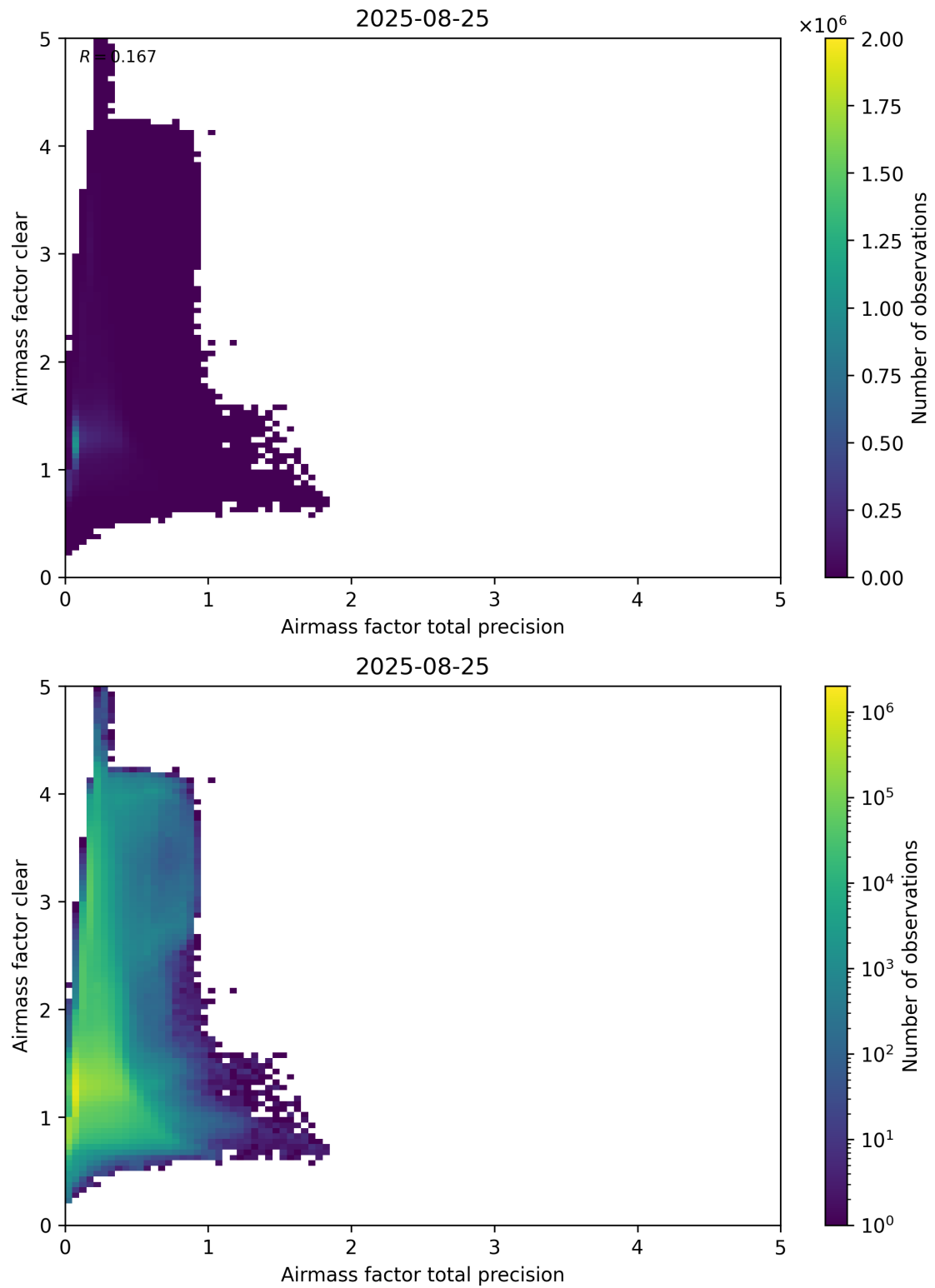
Figure 108: Scatter density plot of “Airmass factor total precision” against “Airmass factor clear” for 2025-08-25 to 2025-08-26.
