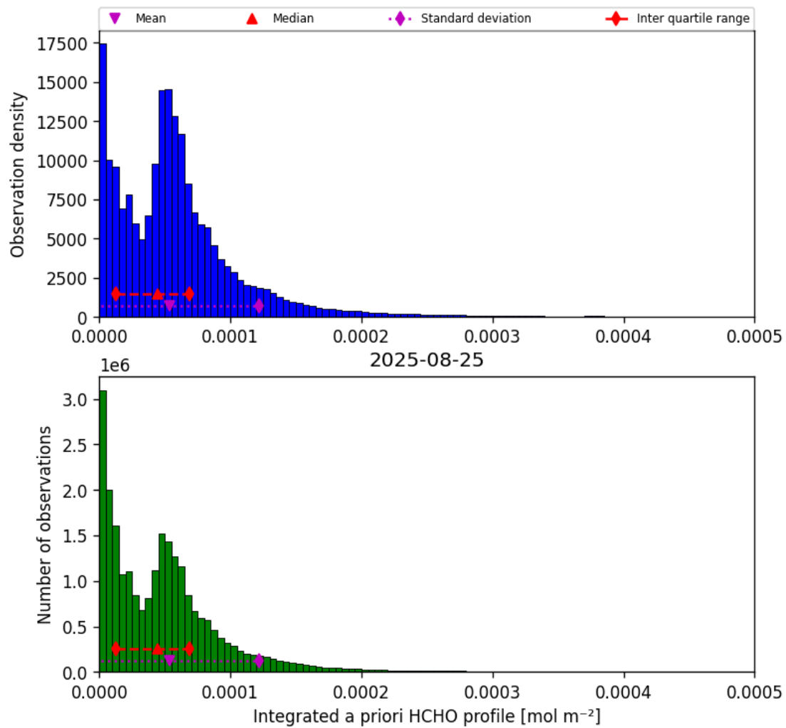
Figure 43: Histogram of “Integrated a priori HCHO profile” for 2025-08-25 to 2025-08-26
