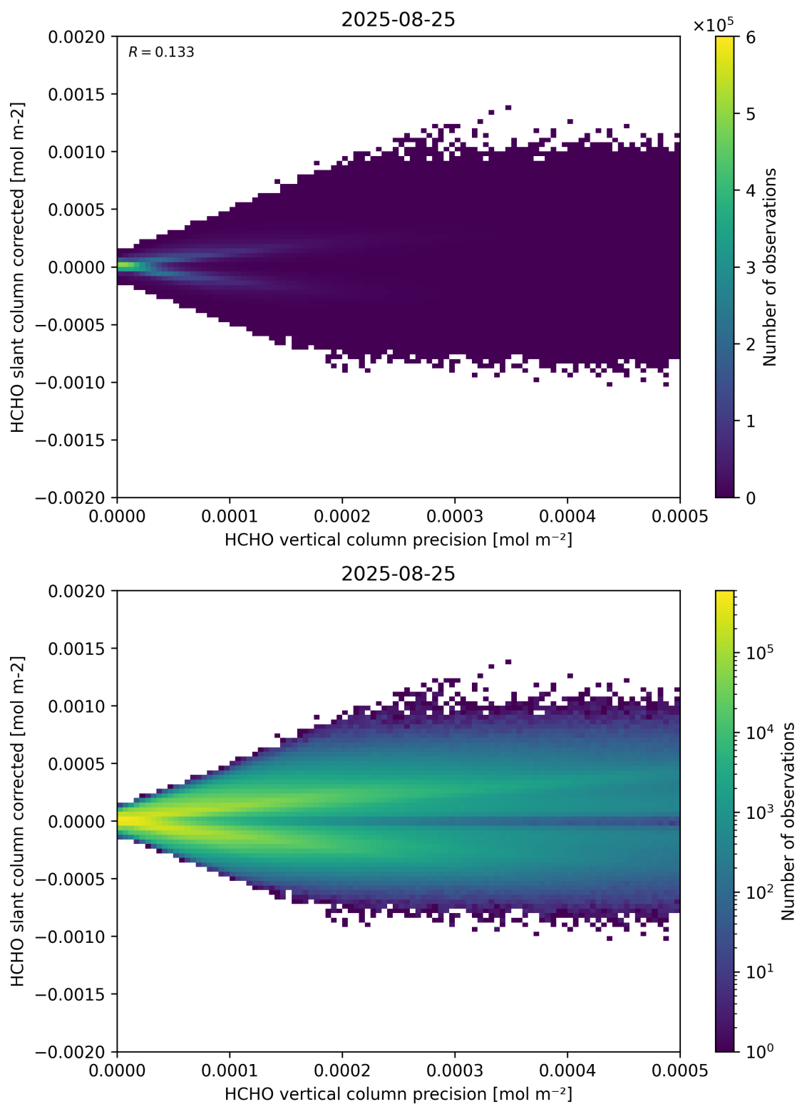
Figure 140: Scatter density plot of “HCHO vertical column precision” against “HCHO slant column corrected” for 2025-08-25 to 2025-08-26.
