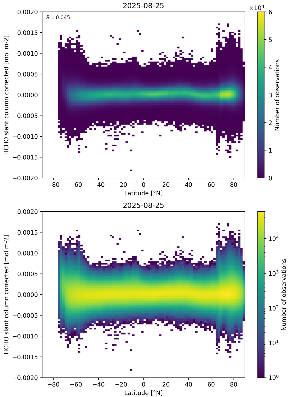
Figure 157: Scatter density plot of “Latitude” against “HCHO slant column corrected” for 2025-08-25 to 2025-08-26.
