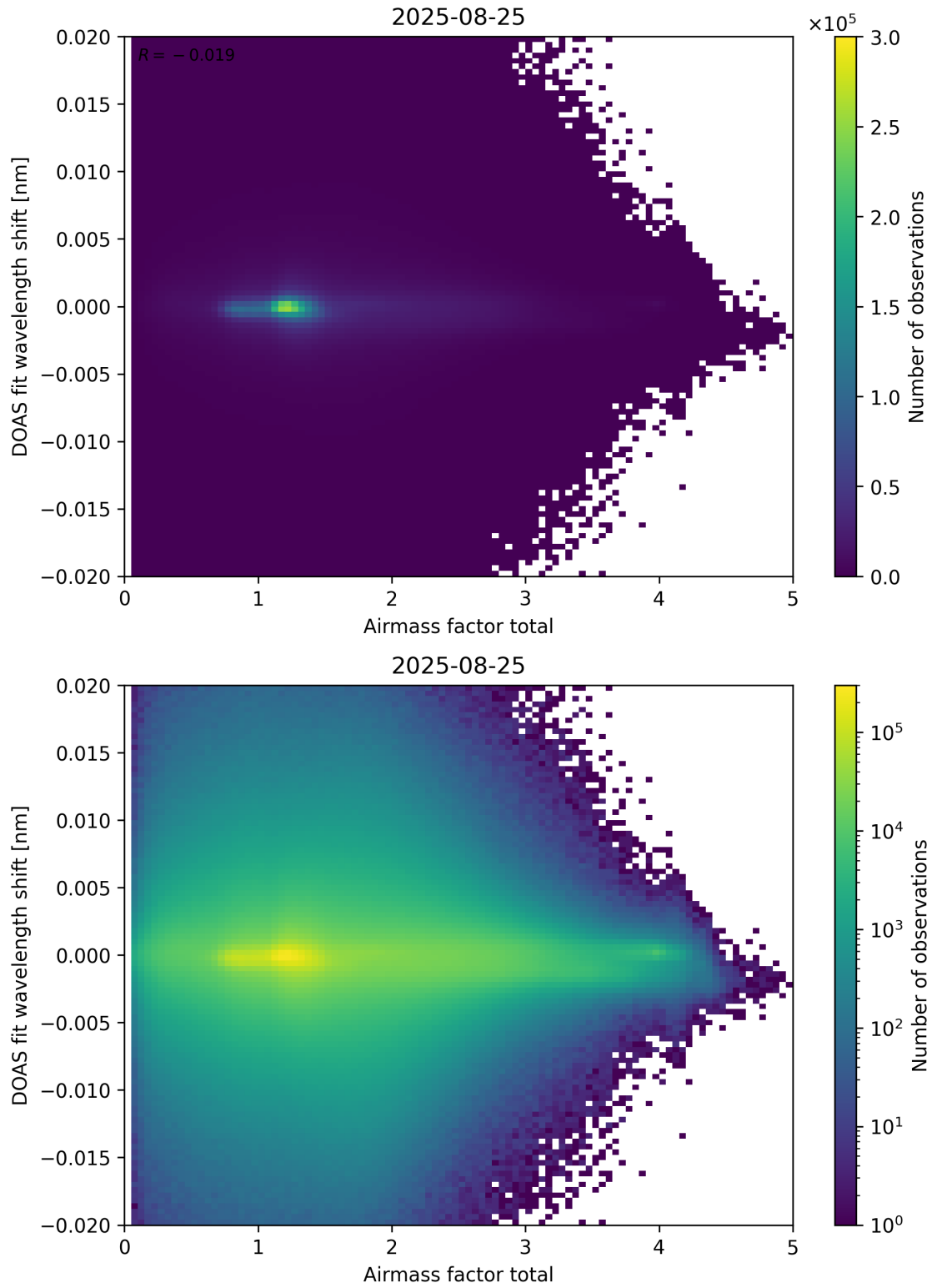
Figure 98: Scatter density plot of “Airmass factor total” against “DOAS fit wavelength shift” for 2025-08-25 to 2025-08-26.
