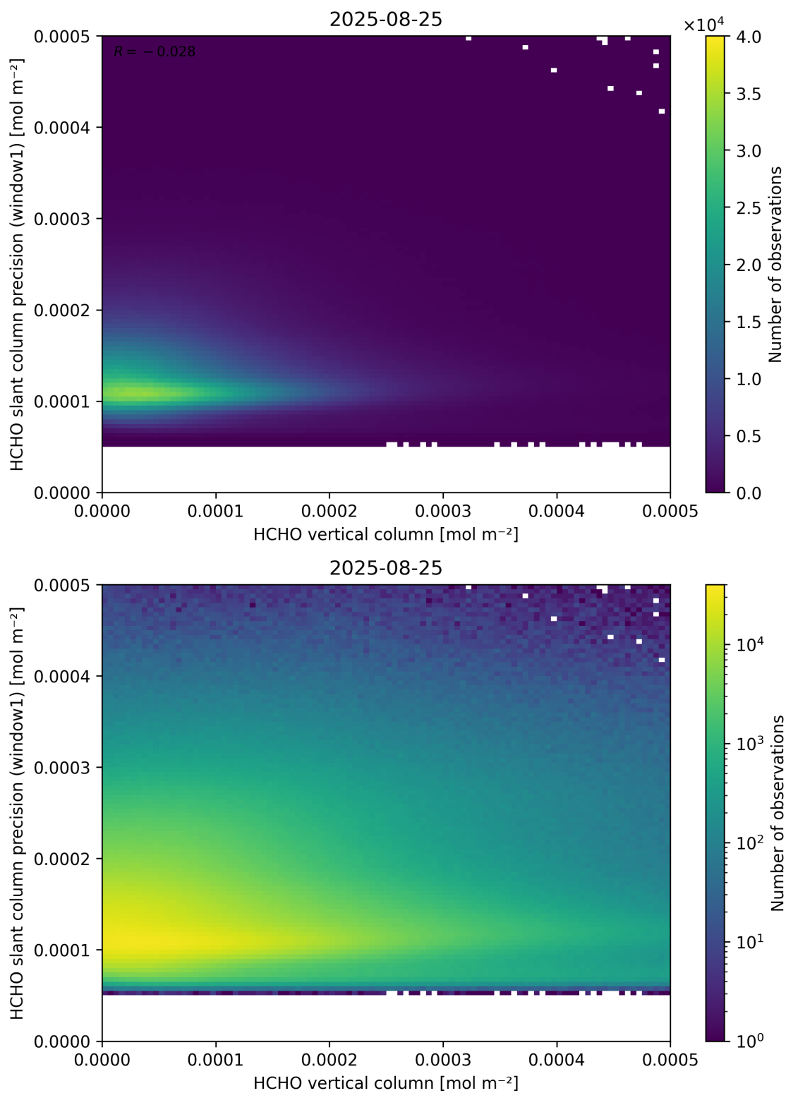
Figure 130: Scatter density plot of “HCHO vertical column” against “HCHO slant column precision (window1)” for 2025-08-25 to 2025-08-26.
