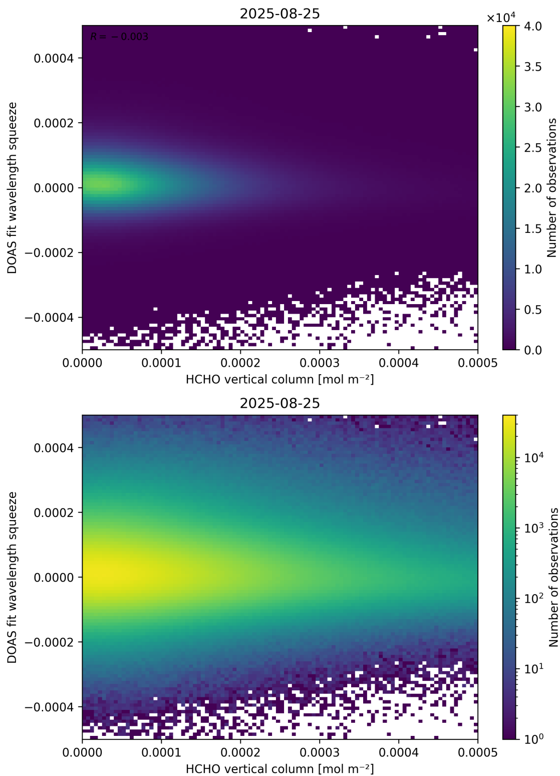
Figure 125: Scatter density plot of “HCHO vertical column” against “DOAS fit wavelength squeeze” for 2025-08-25 to 2025-08-26.
