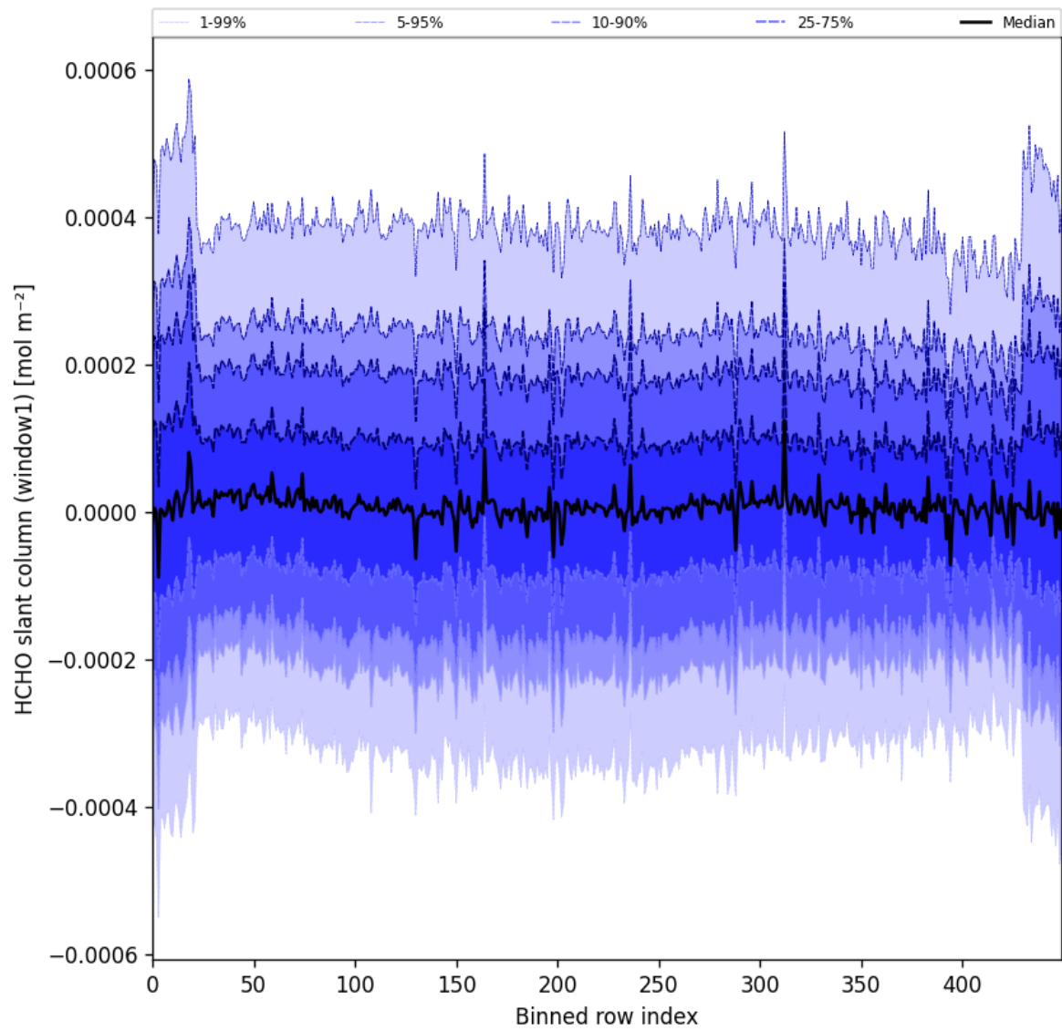
Figure 52: Along track statistics of “HCHO slant column (window1)” for 2025-08-25 to 2025-08-26
