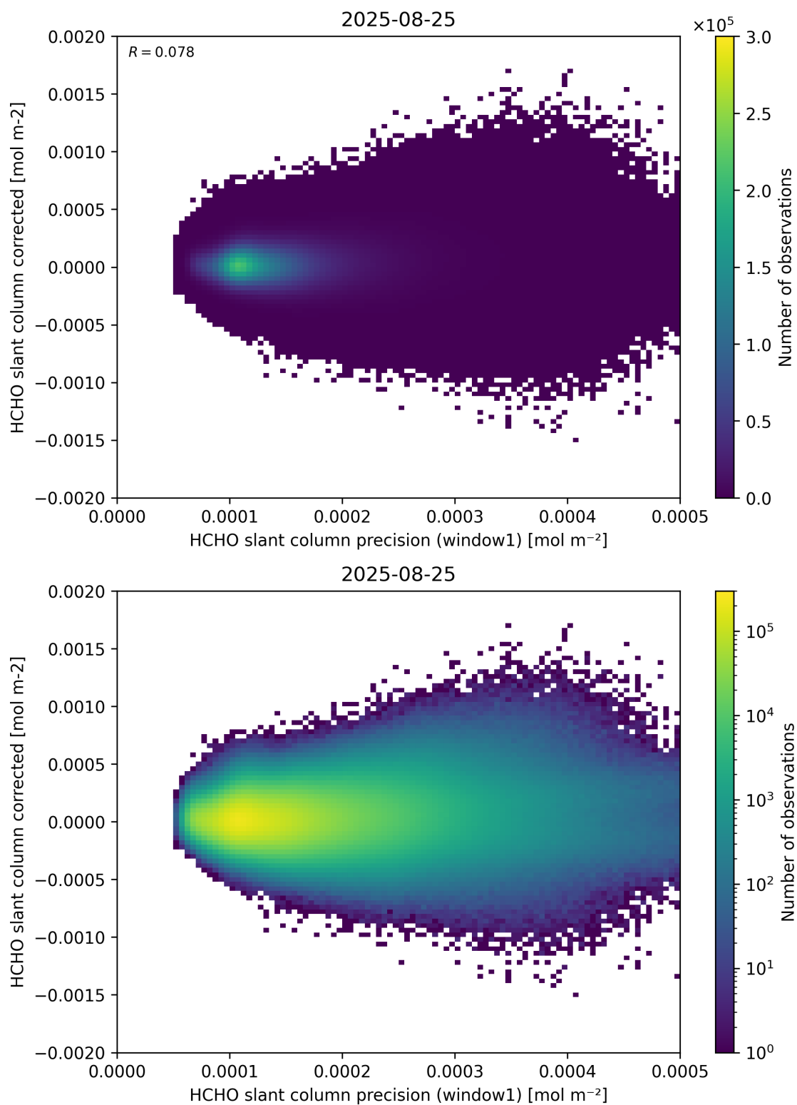
Figure 92: Scatter density plot of “HCHO slant column precision (window1)” against “HCHO slant column corrected” for 2025-08-25 to 2025-08-26.
