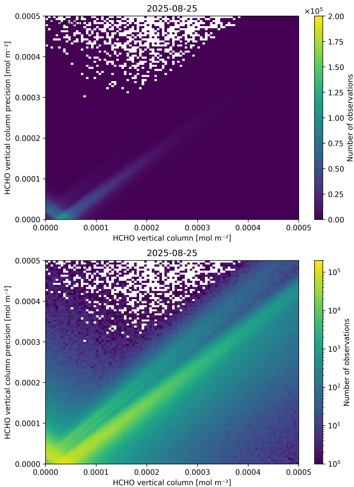
Figure 134: Scatter density plot of “HCHO vertical column” against “HCHO vertical column precision” for 2025-08-25 to 2025-08-26.
