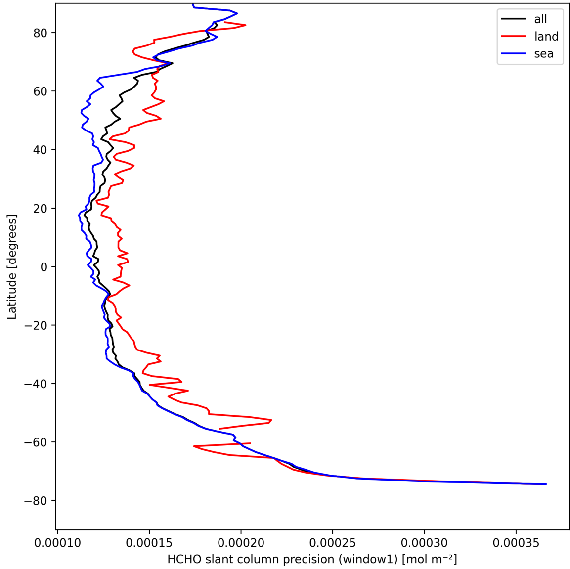
Figure 25: Zonal average of “HCHO slant column precision (window1)” for 2025-08-25 to 2025-08-26.
