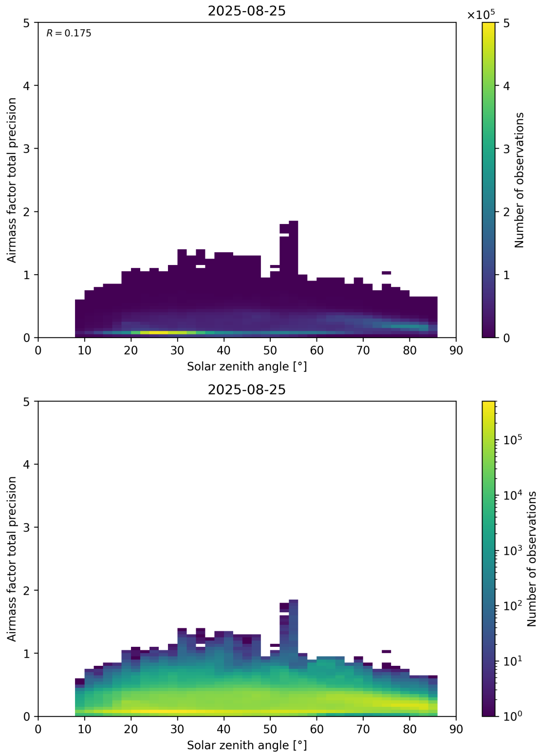
Figure 176: Scatter density plot of “Solar zenith angle” against “Airmass factor total precision” for 2025-08-25 to 2025-08-26.
