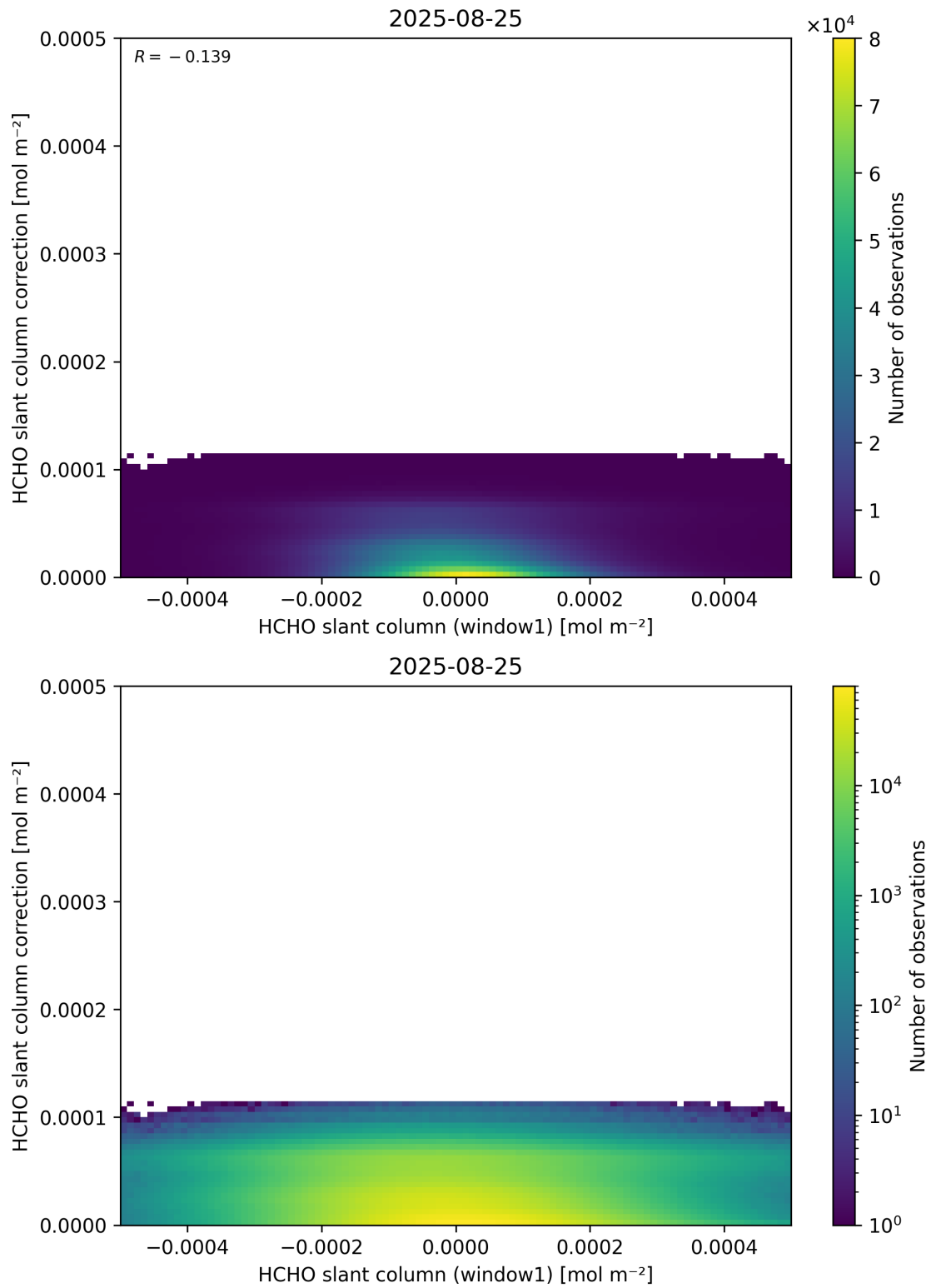
Figure 83: Scatter density plot of “HCHO slant column (window1)” against “HCHO slant column correction” for 2025-08-25 to 2025-08-26.
