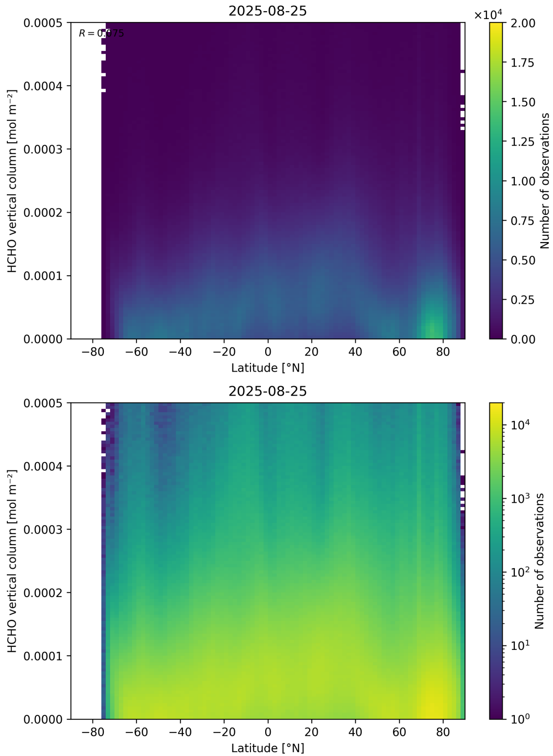
Figure 163: Scatter density plot of “Latitude” against “HCHO vertical column” for 2025-08-25 to 2025-08-26.
