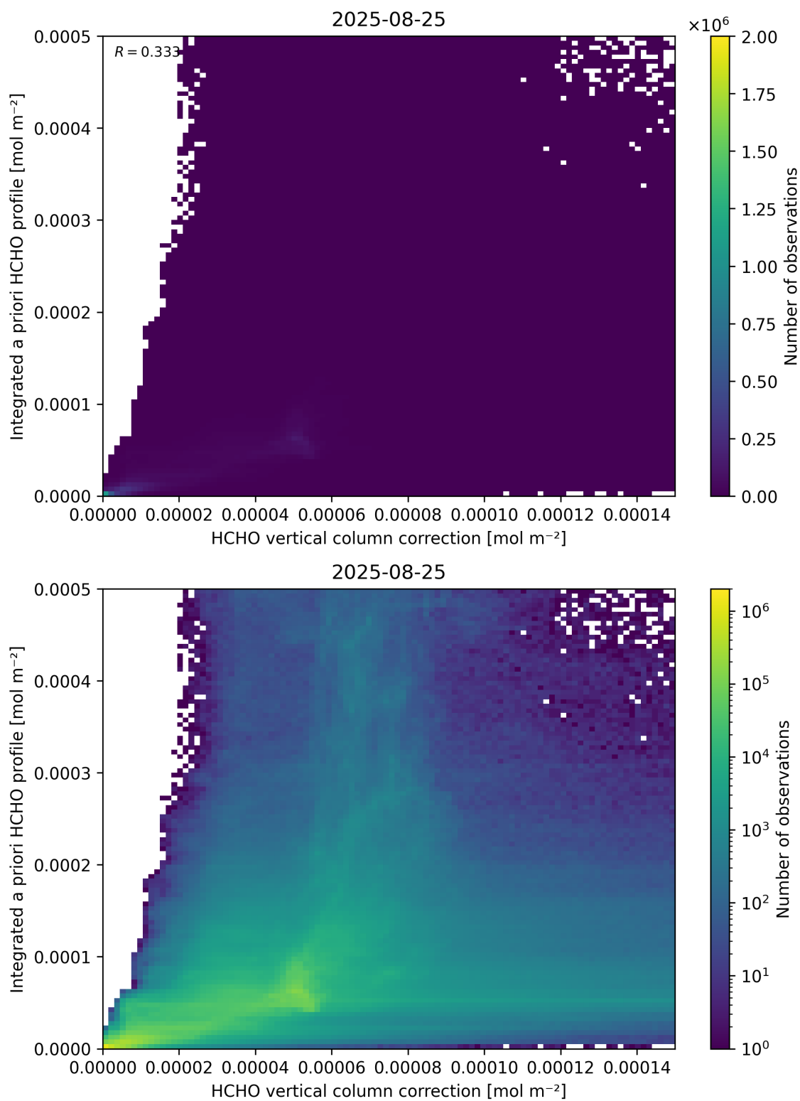
Figure 122: Scatter density plot of “HCHO vertical column correction” against “Integrated a priori HCHO profile” for 2025-08-25 to 2025-08-26.
