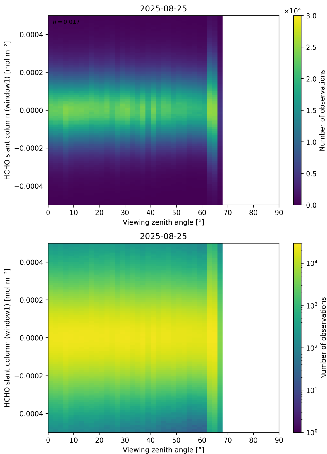
Figure 188: Scatter density plot of “Viewing zenith angle” against “HCHO slant column (window1)” for 2025-08-25 to 2025-08-26.
