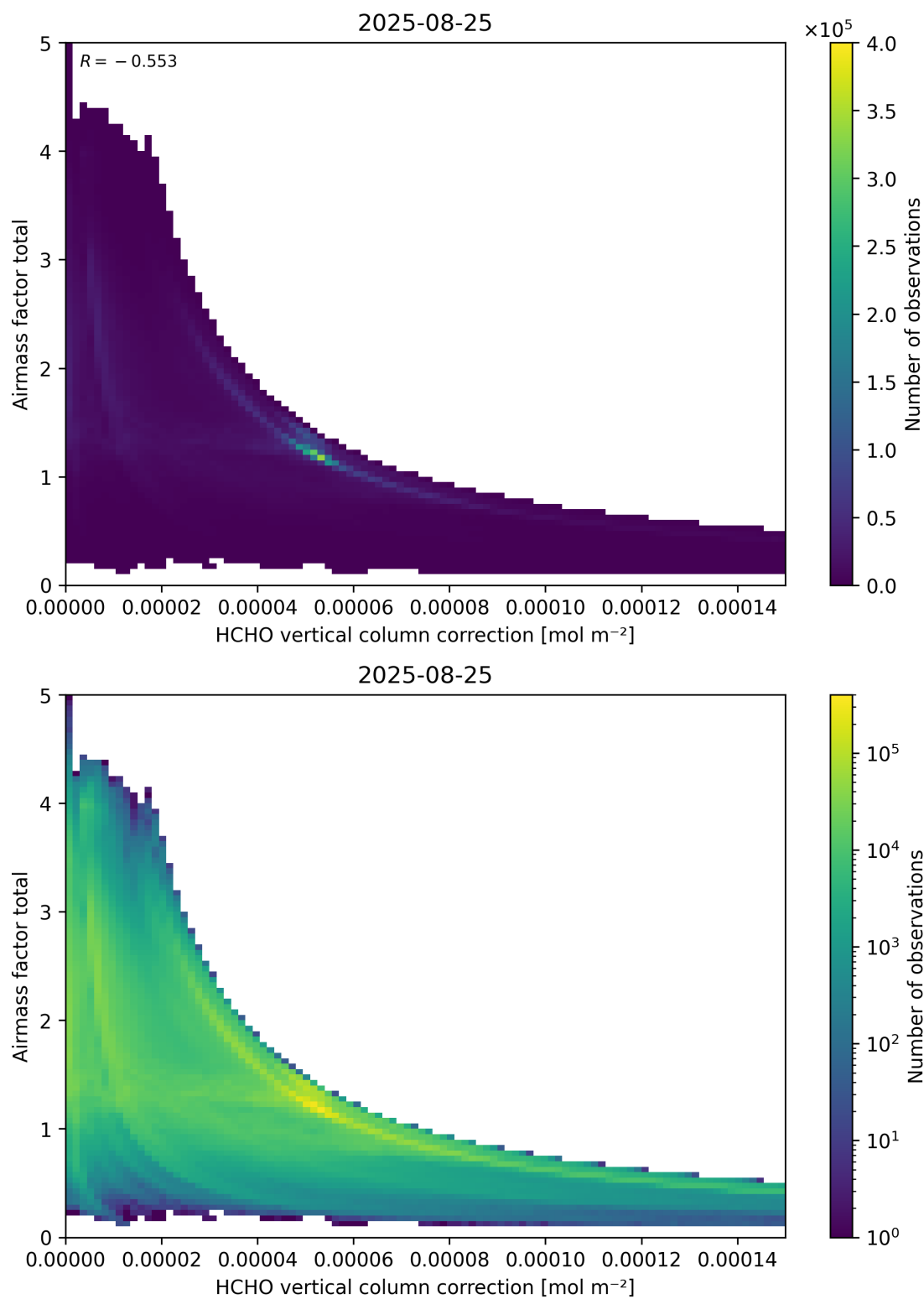
Figure 120: Scatter density plot of “HCHO vertical column correction” against “Airmass factor total” for 2025-08-25 to 2025-08-26.
