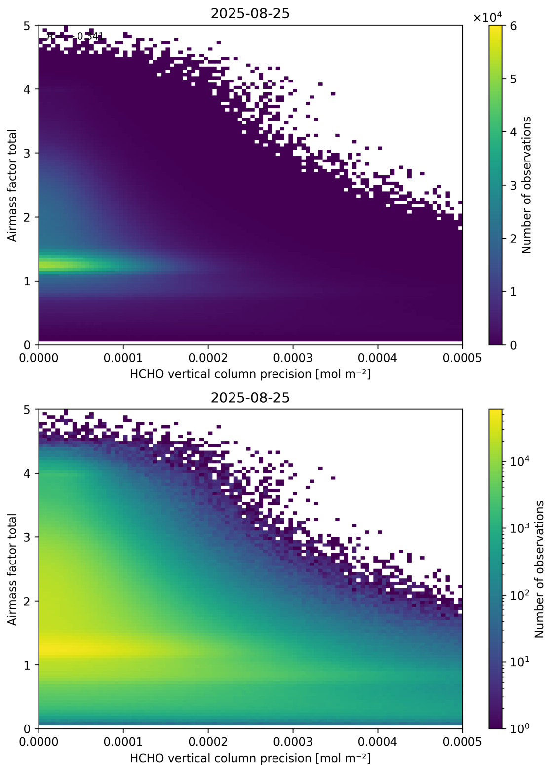
Figure 144: Scatter density plot of “HCHO vertical column precision” against “Airmass factor total” for 2025-08-25 to 2025-08-26.
