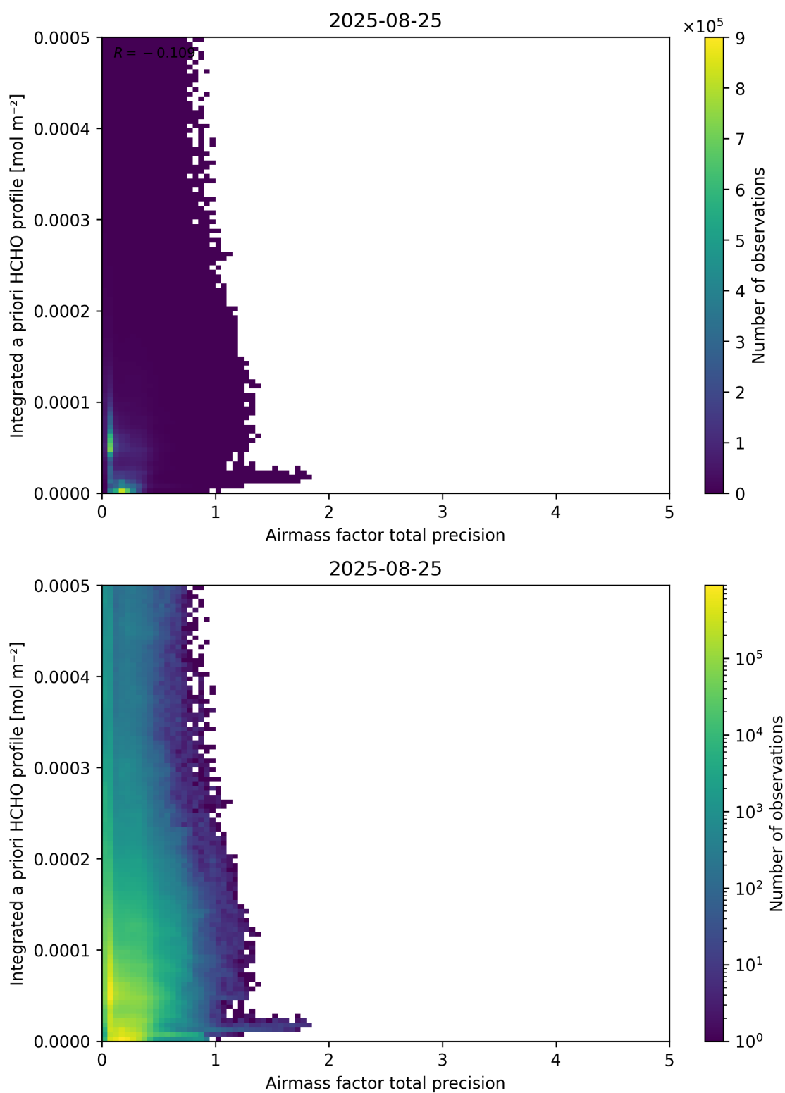
Figure 111: Scatter density plot of “Airmass factor total precision” against “Integrated a priori HCHO profile” for 2025-08-25 to 2025-08-26.
