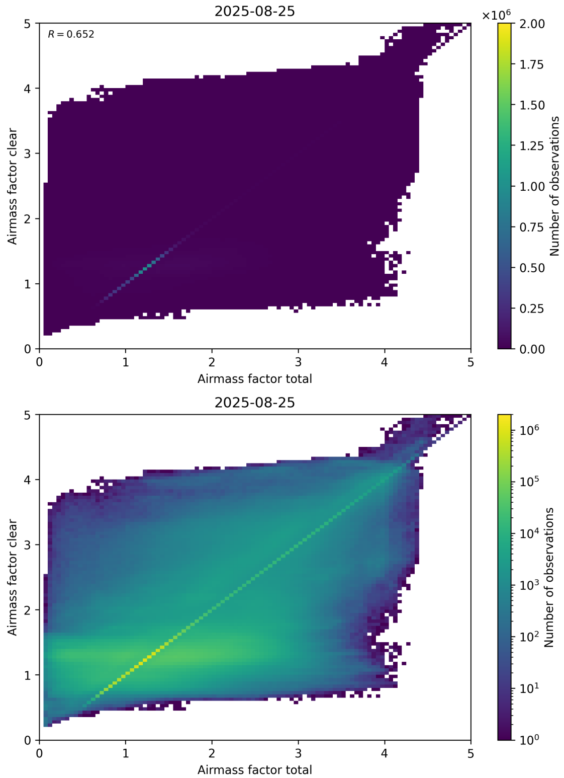
Figure 100: Scatter density plot of “Airmass factor total” against “Airmass factor clear” for 2025-08-25 to 2025-08-26.
