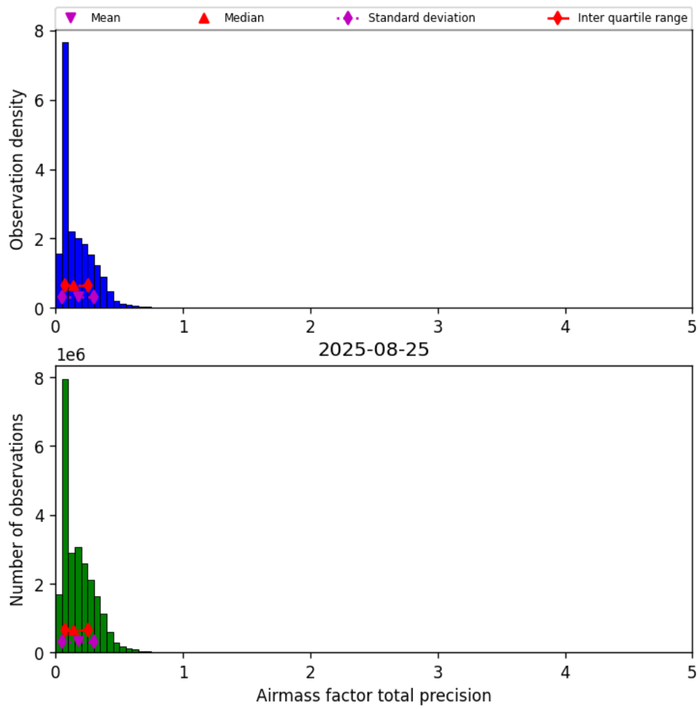
Figure 41: Histogram of “Airmass factor total precision” for 2025-08-25 to 2025-08-26
