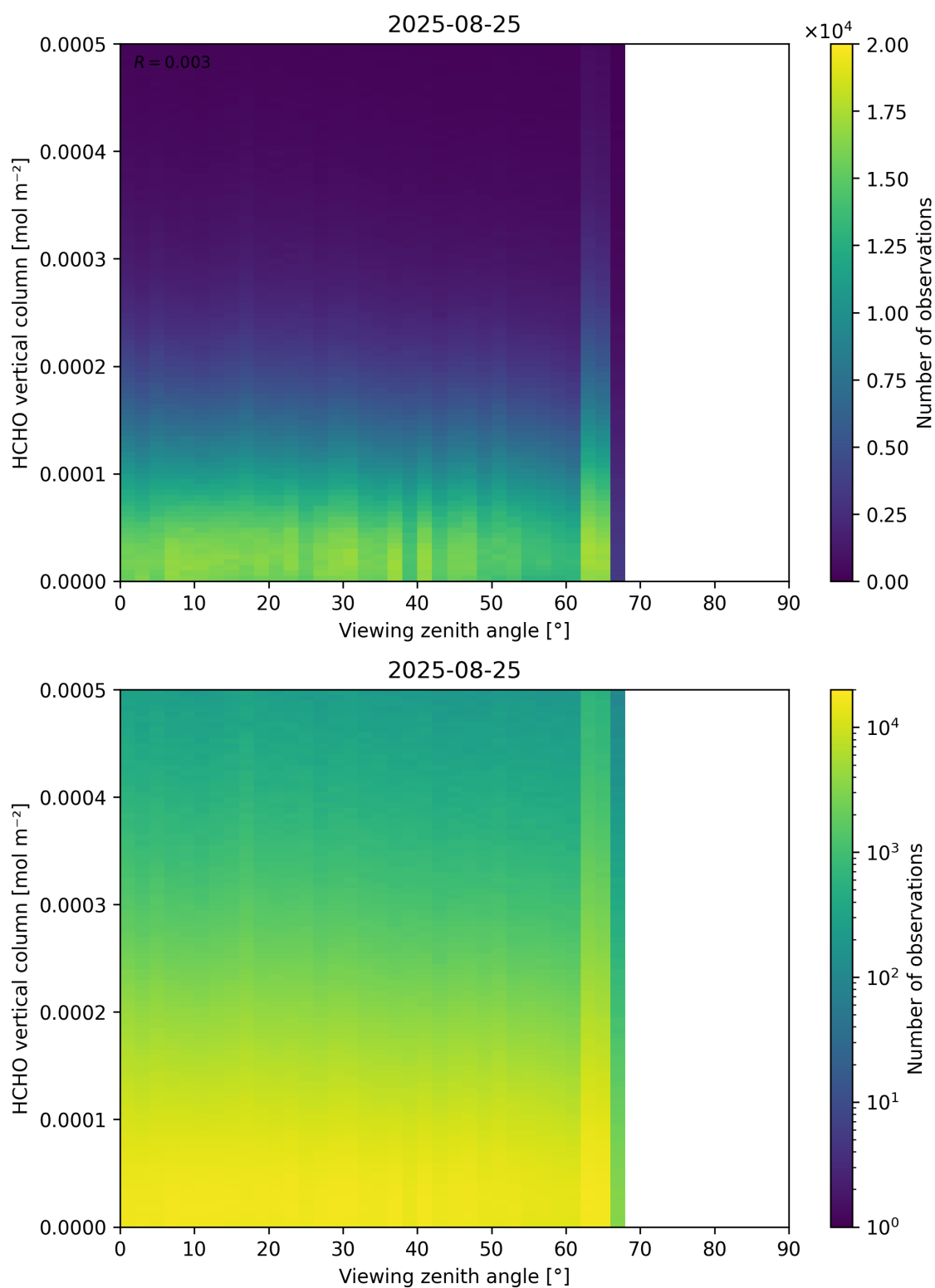
Figure 192: Scatter density plot of “Viewing zenith angle” against “HCHO vertical column” for 2025-08-25 to 2025-08-26.
