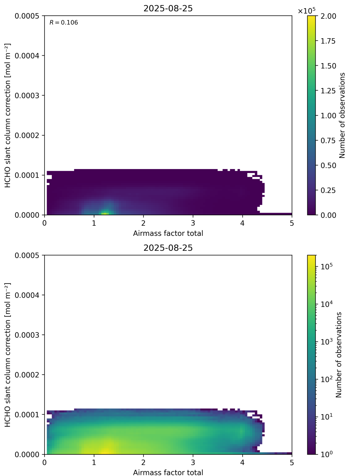
Figure 102: Scatter density plot of “Airmass factor total” against “HCHO slant column correction” for 2025-08-25 to 2025-08-26.
