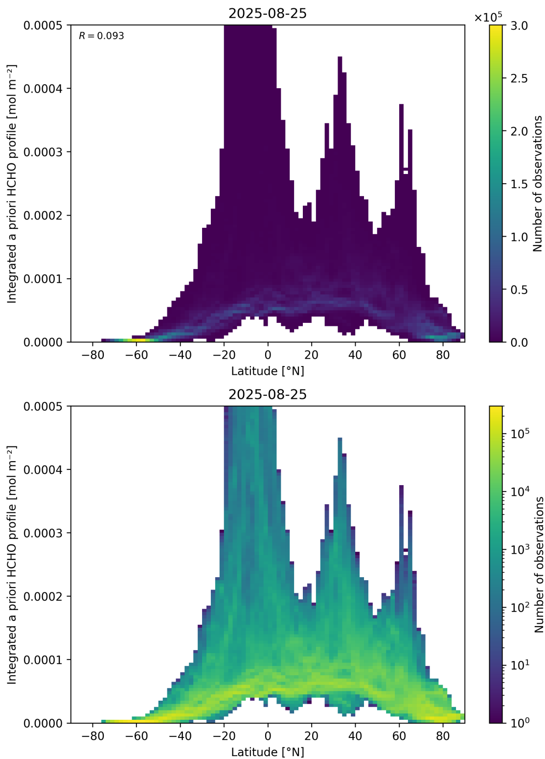
Figure 166: Scatter density plot of “Latitude” against “Integrated a priori HCHO profile” for 2025-08-25 to 2025-08-26.
