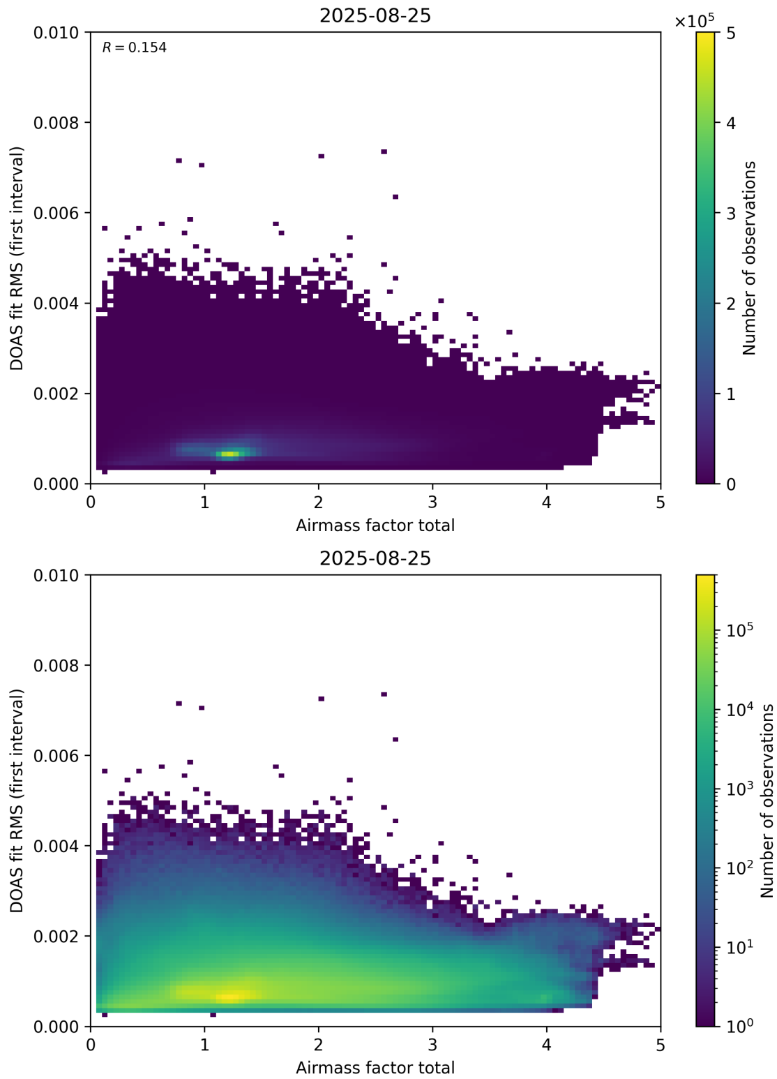
Figure 97: Scatter density plot of “Airmass factor total” against “DOAS fit RMS (first interval)” for 2025-08-25 to 2025-08-26.
