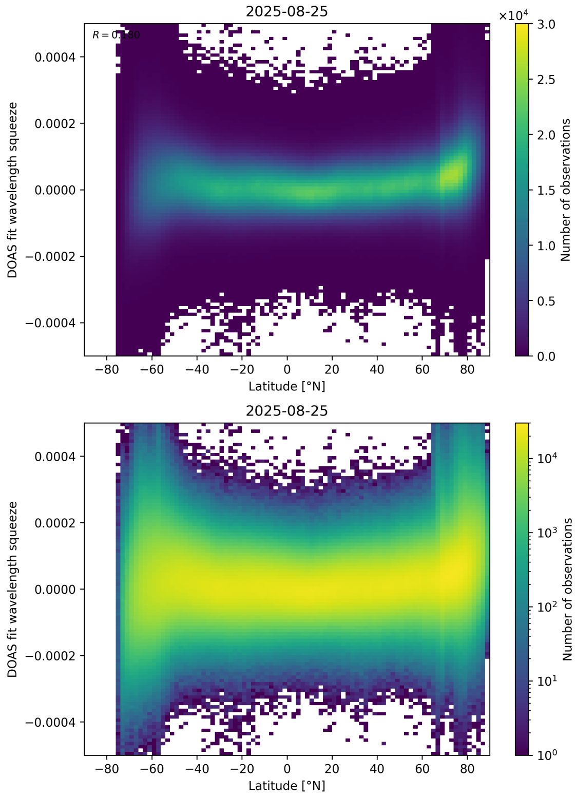
Figure 155: Scatter density plot of “Latitude” against “DOAS fit wavelength squeeze” for 2025-08-25 to 2025-08-26.
