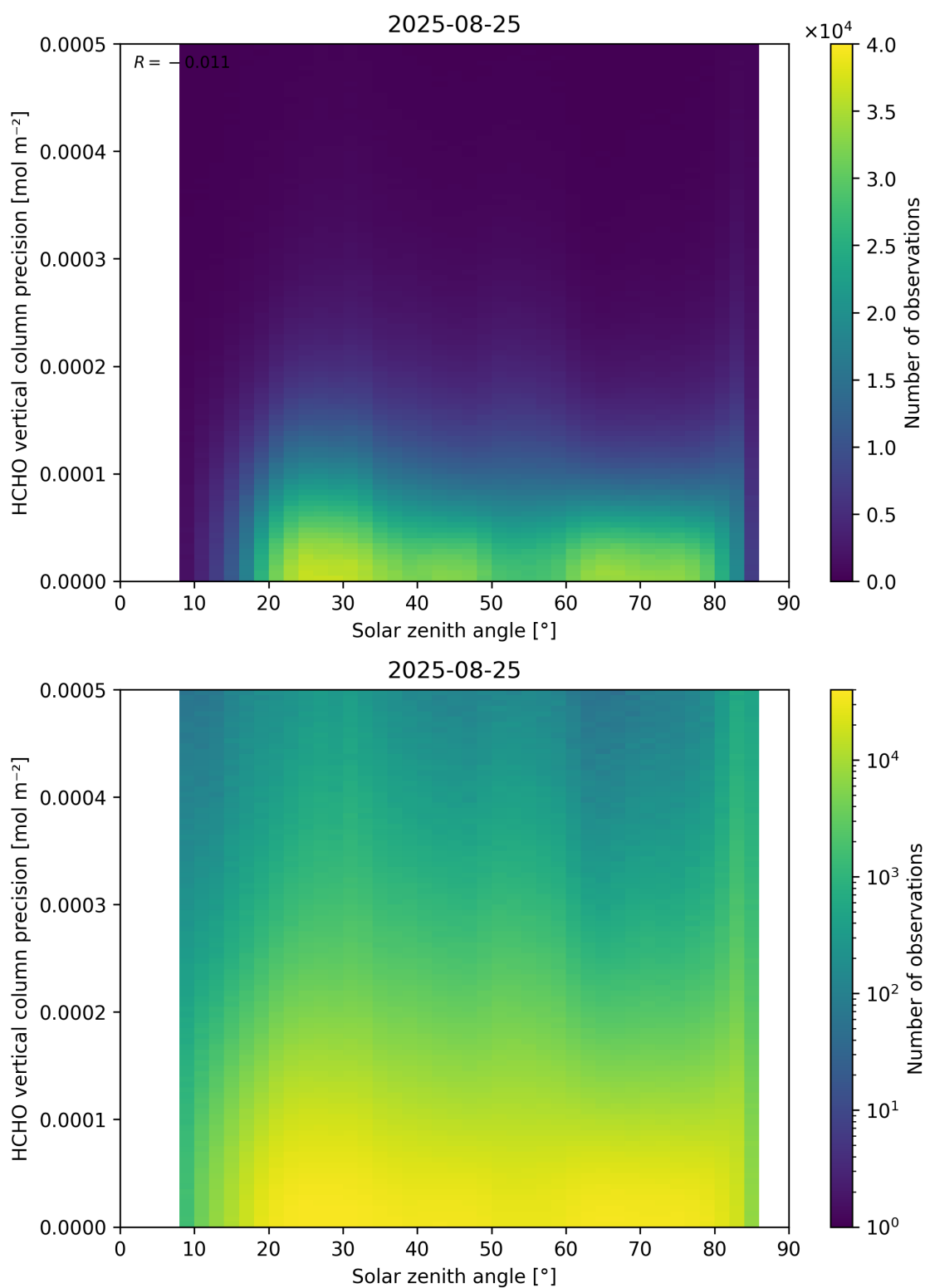
Figure 179: Scatter density plot of “Solar zenith angle” against “HCHO vertical column precision” for 2025-08-25 to 2025-08-26.
