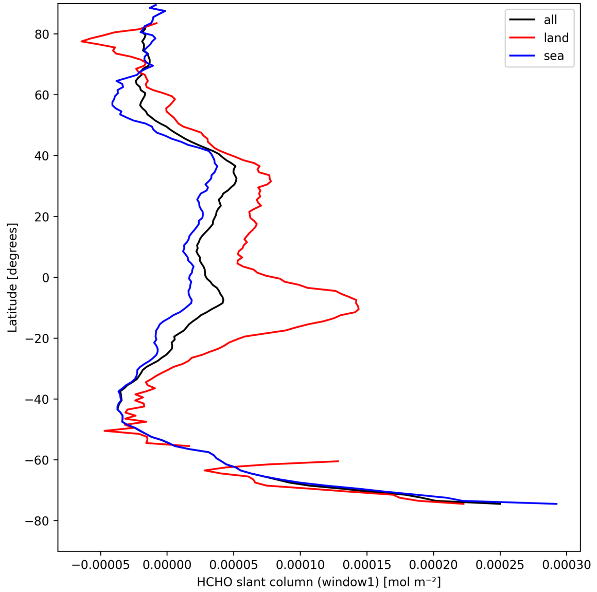
Figure 24: Zonal average of “HCHO slant column (window1)” for 2025-08-25 to 2025-08-26.
