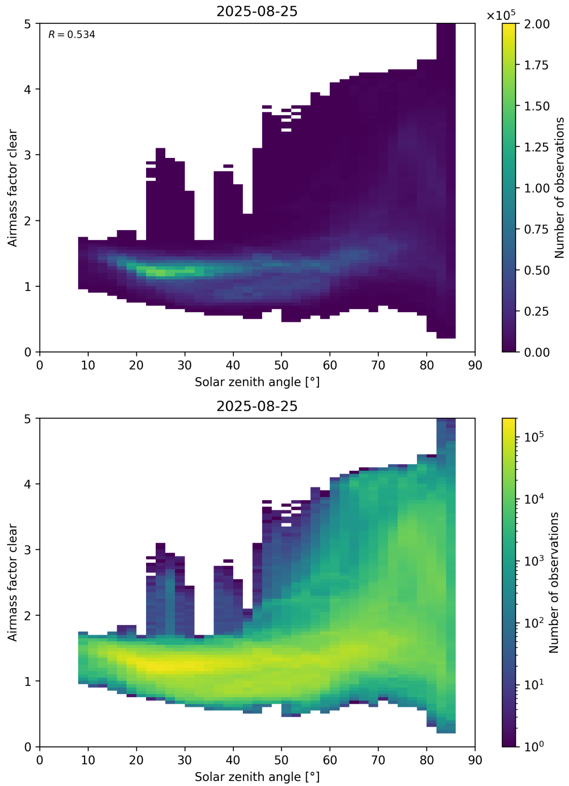
Figure 170: Scatter density plot of “Solar zenith angle” against “Airmass factor clear” for 2025-08-25 to 2025-08-26.
