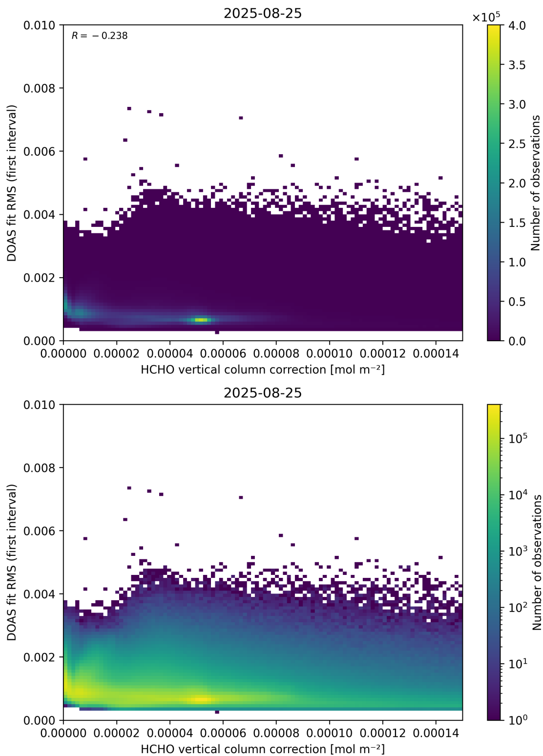
Figure 112: Scatter density plot of “HCHO vertical column correction” against “DOAS fit RMS (first interval)” for 2025-08-25 to 2025-08-26.
