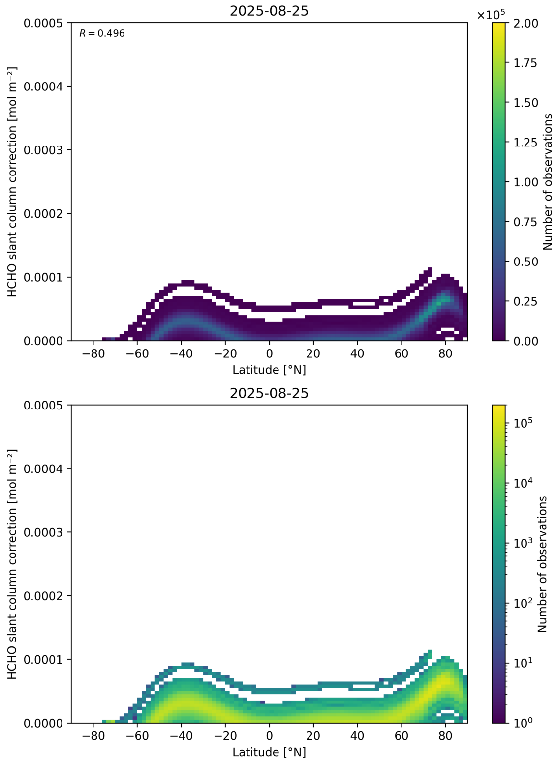
Figure 158: Scatter density plot of “Latitude” against “HCHO slant column correction” for 2025-08-25 to 2025-08-26.
