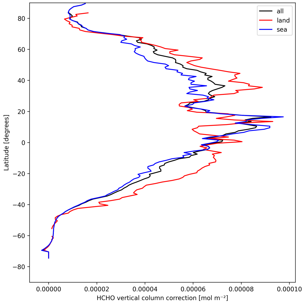
Figure 23: Zonal average of “HCHO vertical column correction” for 2025-08-25 to 2025-08-26.
