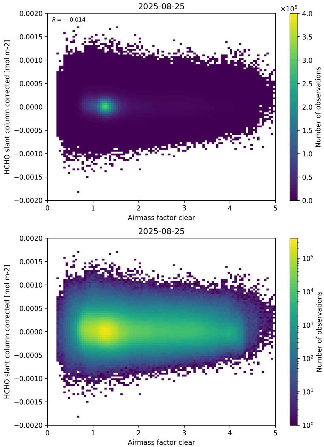
Figure 74: Scatter density plot of “Airmass factor clear” against “HCHO slant column corrected” for 2025-08-25 to 2025-08-26.
