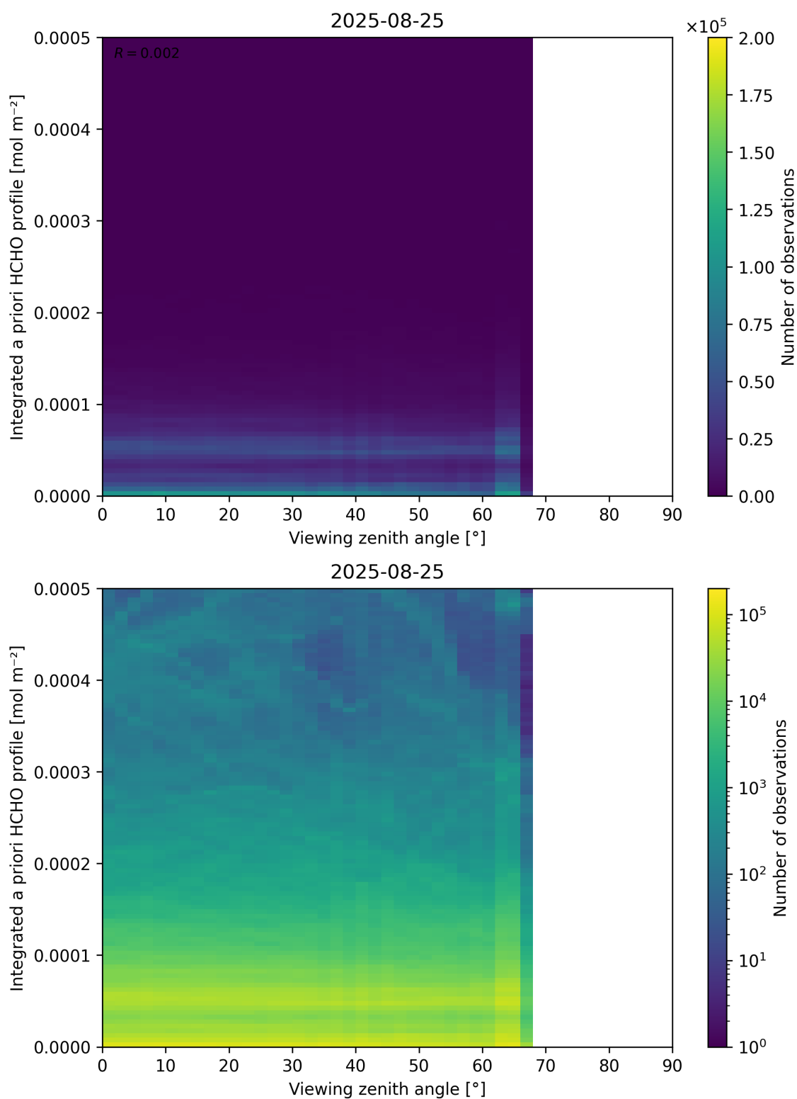
Figure 195: Scatter density plot of “Viewing zenith angle” against “Integrated a priori HCHO profile” for 2025-08-25 to 2025-08-26.
