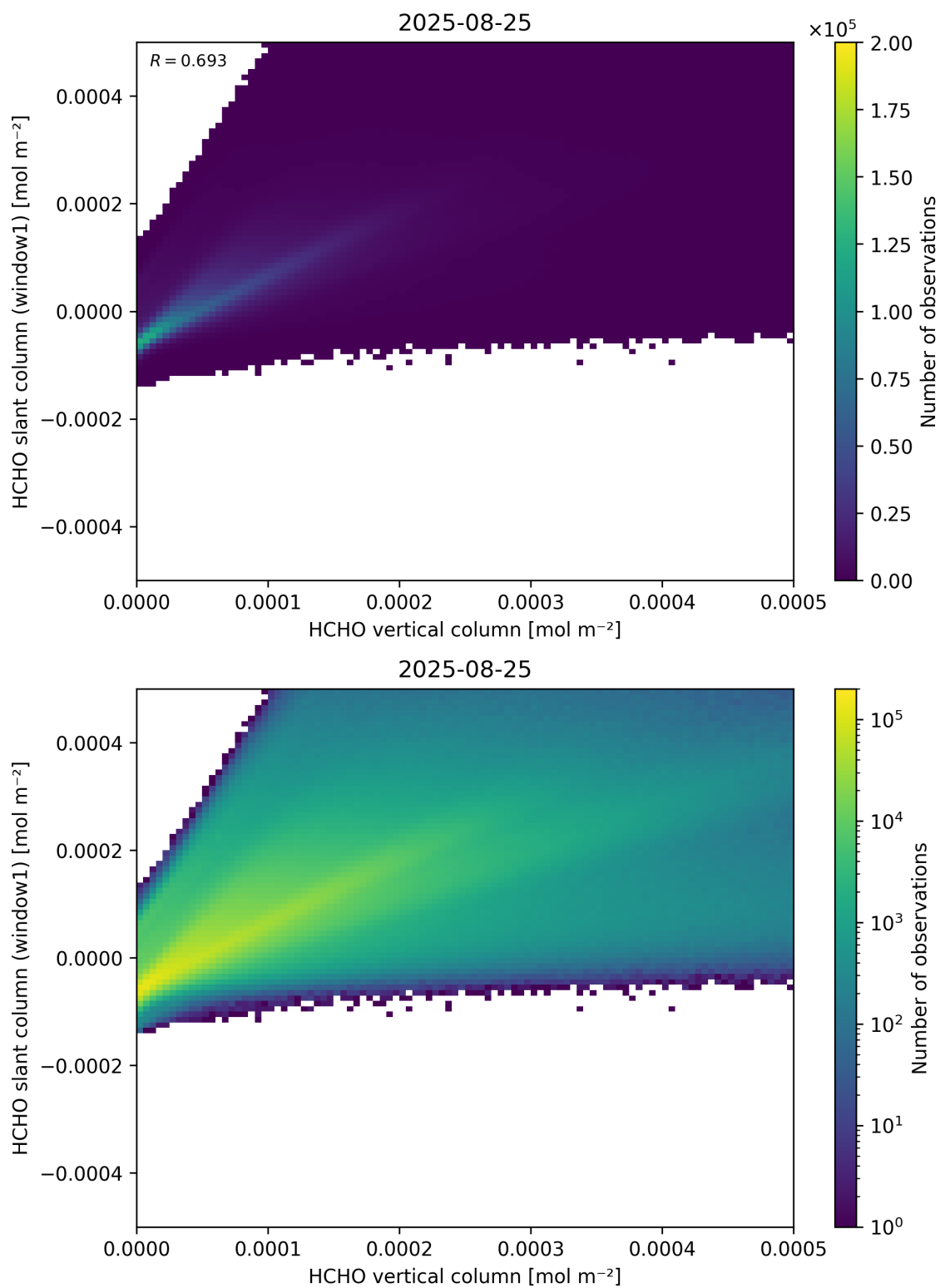
Figure 129: Scatter density plot of “HCHO vertical column” against “HCHO slant column (window1)” for 2025-08-25 to 2025-08-26.
