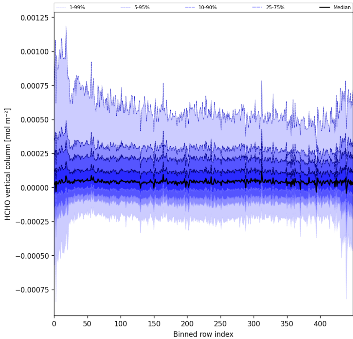
Figure 49: Along track statistics of “HCHO vertical column” for 2025-08-25 to 2025-08-26
