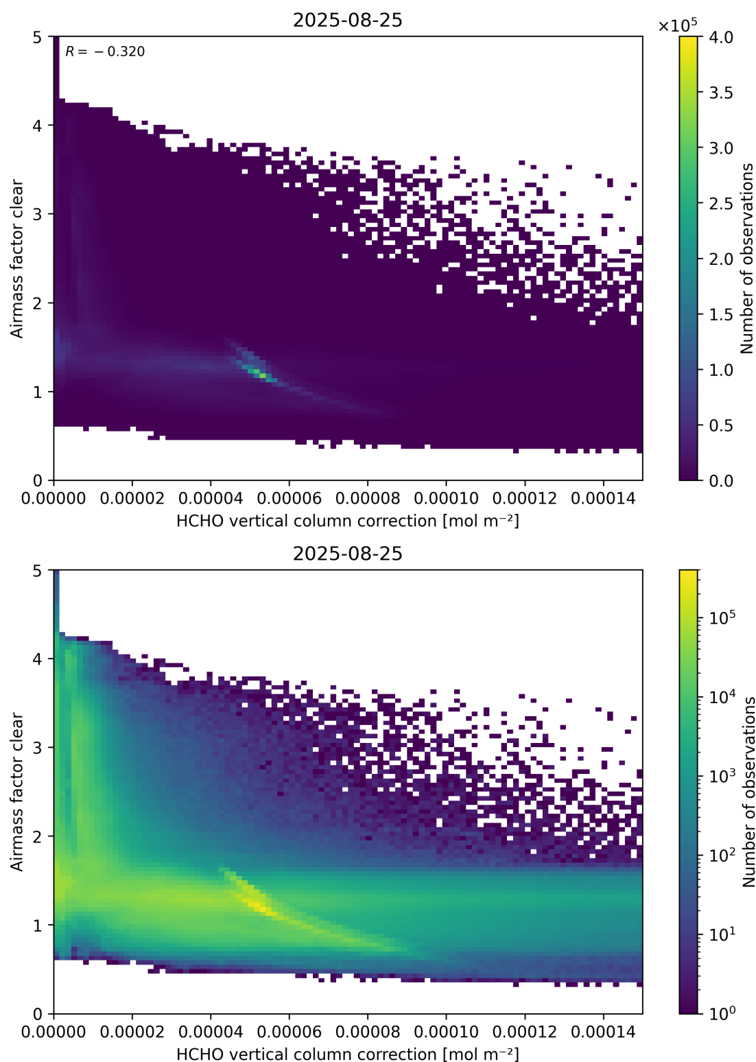
Figure 115: Scatter density plot of “HCHO vertical column correction” against “Airmass factor clear” for 2025-08-25 to 2025-08-26.
