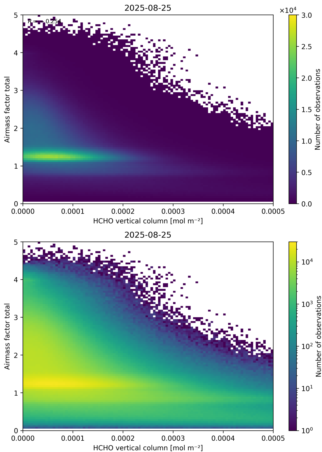
Figure 131: Scatter density plot of “HCHO vertical column” against “Airmass factor total” for 2025-08-25 to 2025-08-26.
