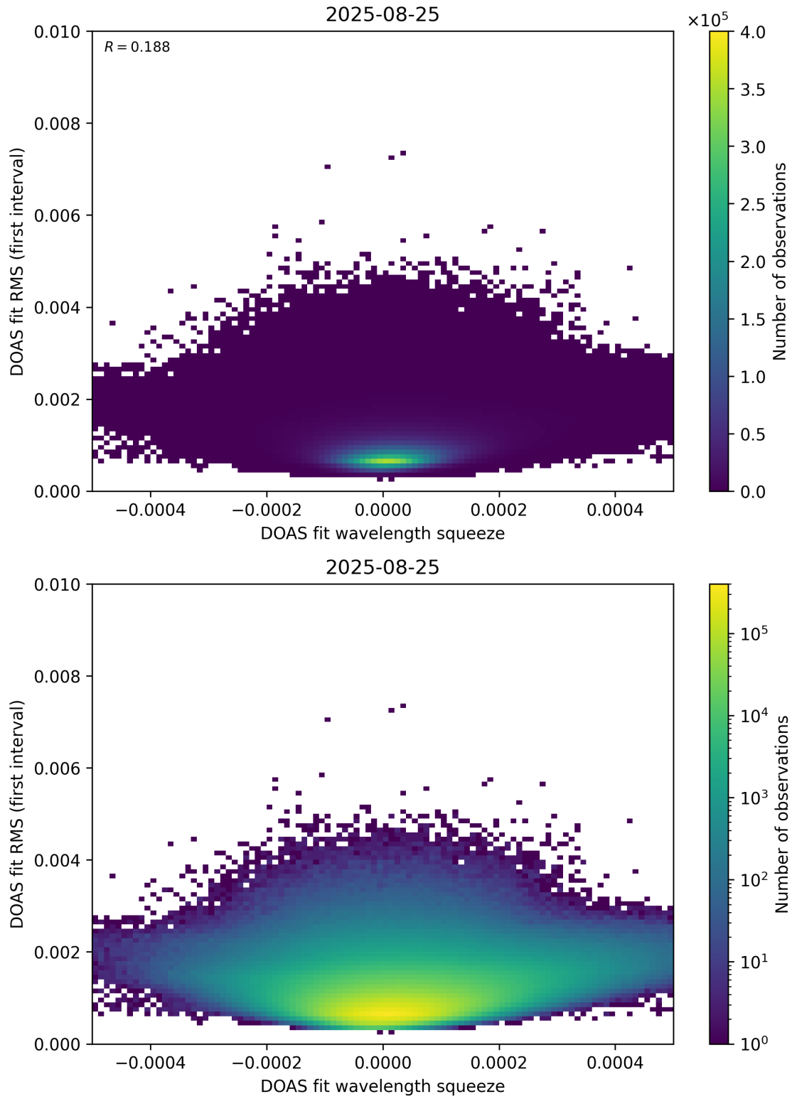
Figure 68: Scatter density plot of “DOAS fit wavelength squeeze” against “DOAS fit RMS (first interval)” for 2025-08-25 to 2025-08-26.
