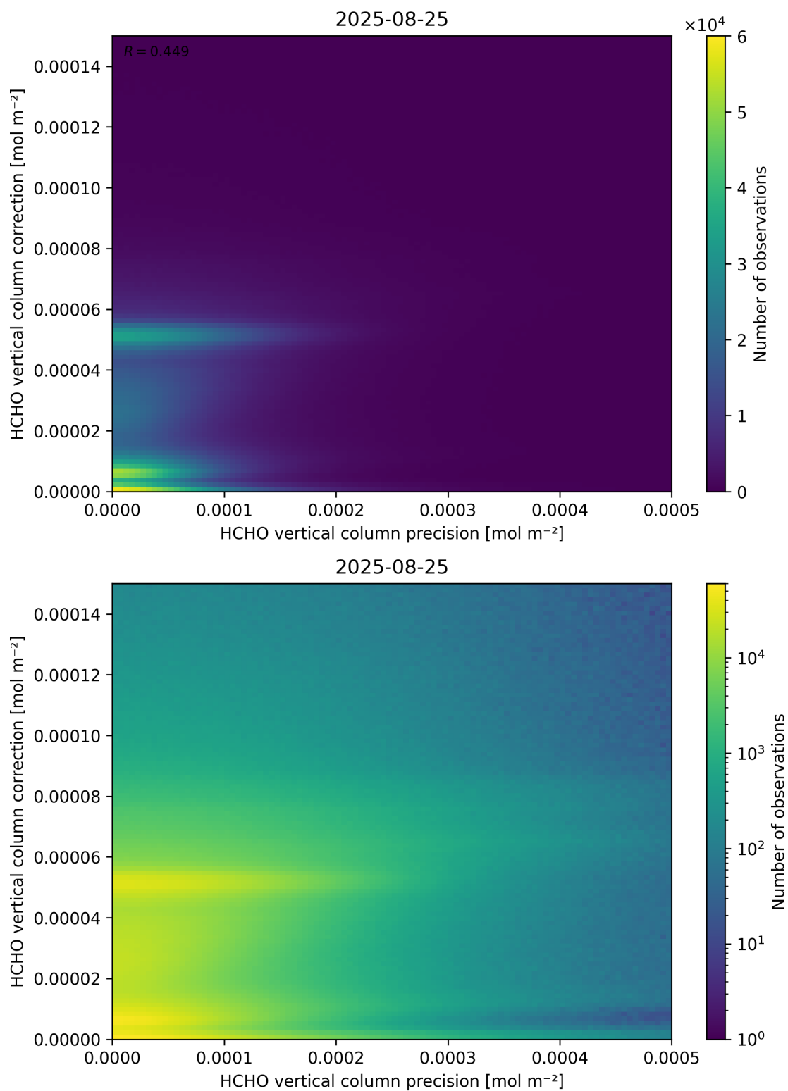
Figure 146: Scatter density plot of “HCHO vertical column precision” against “HCHO vertical column correction” for 2025-08-25 to 2025-08-26.
