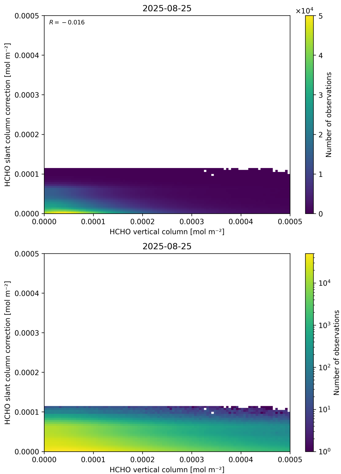
Figure 128: Scatter density plot of “HCHO vertical column” against “HCHO slant column correction” for 2025-08-25 to 2025-08-26.
