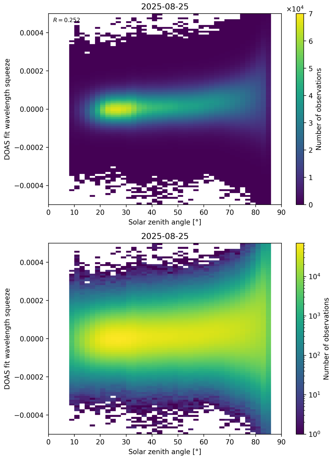
Figure 169: Scatter density plot of “Solar zenith angle” against “DOAS fit wavelength squeeze” for 2025-08-25 to 2025-08-26.
