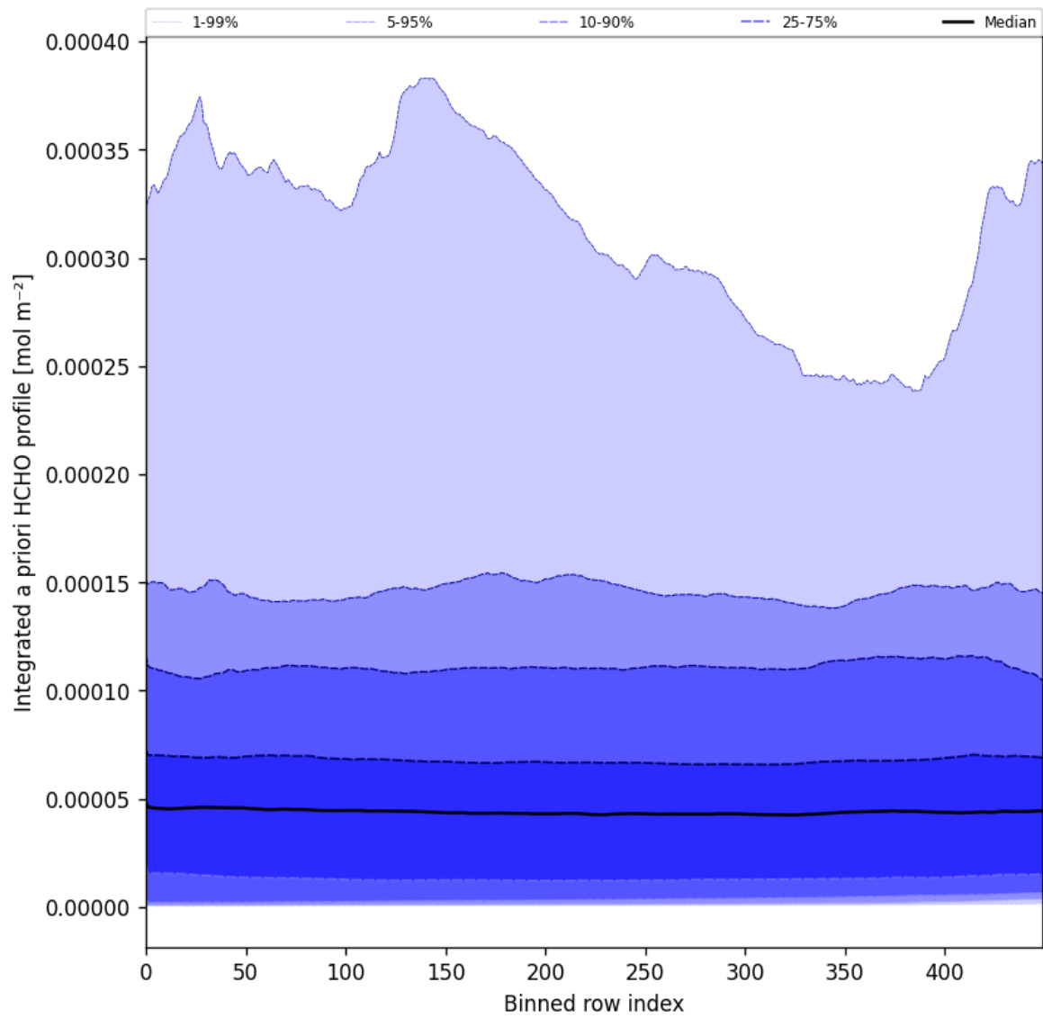
Figure 57: Along track statistics of "Integrated a priori HCHO profile" for 2025-08-26 to 2025-08-28
