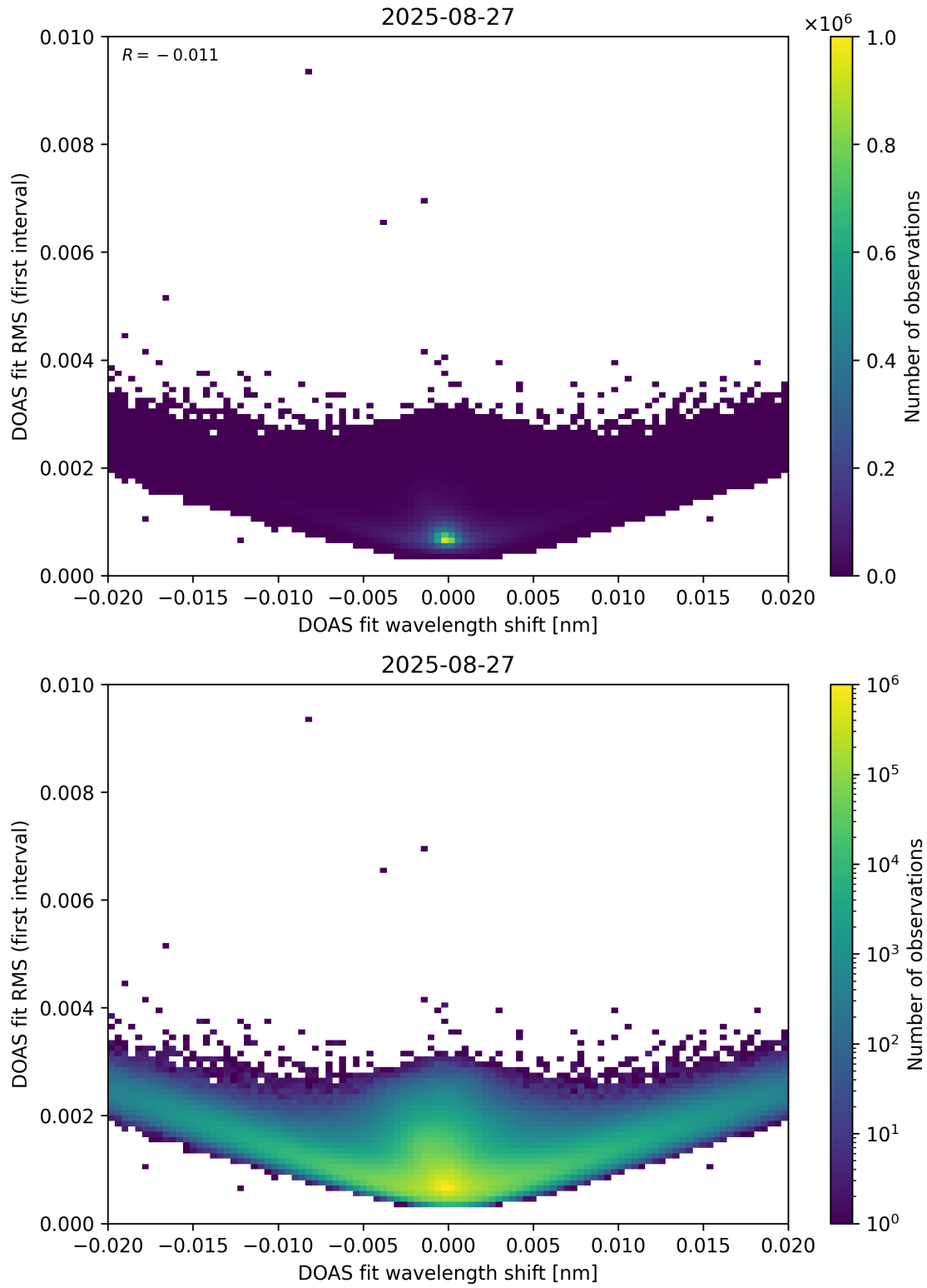
Figure 64: Scatter density plot of “DOAS fit wavelength shift” against “DOAS fit RMS (first interval)” for 2025-08-26 to 2025-08-28.
