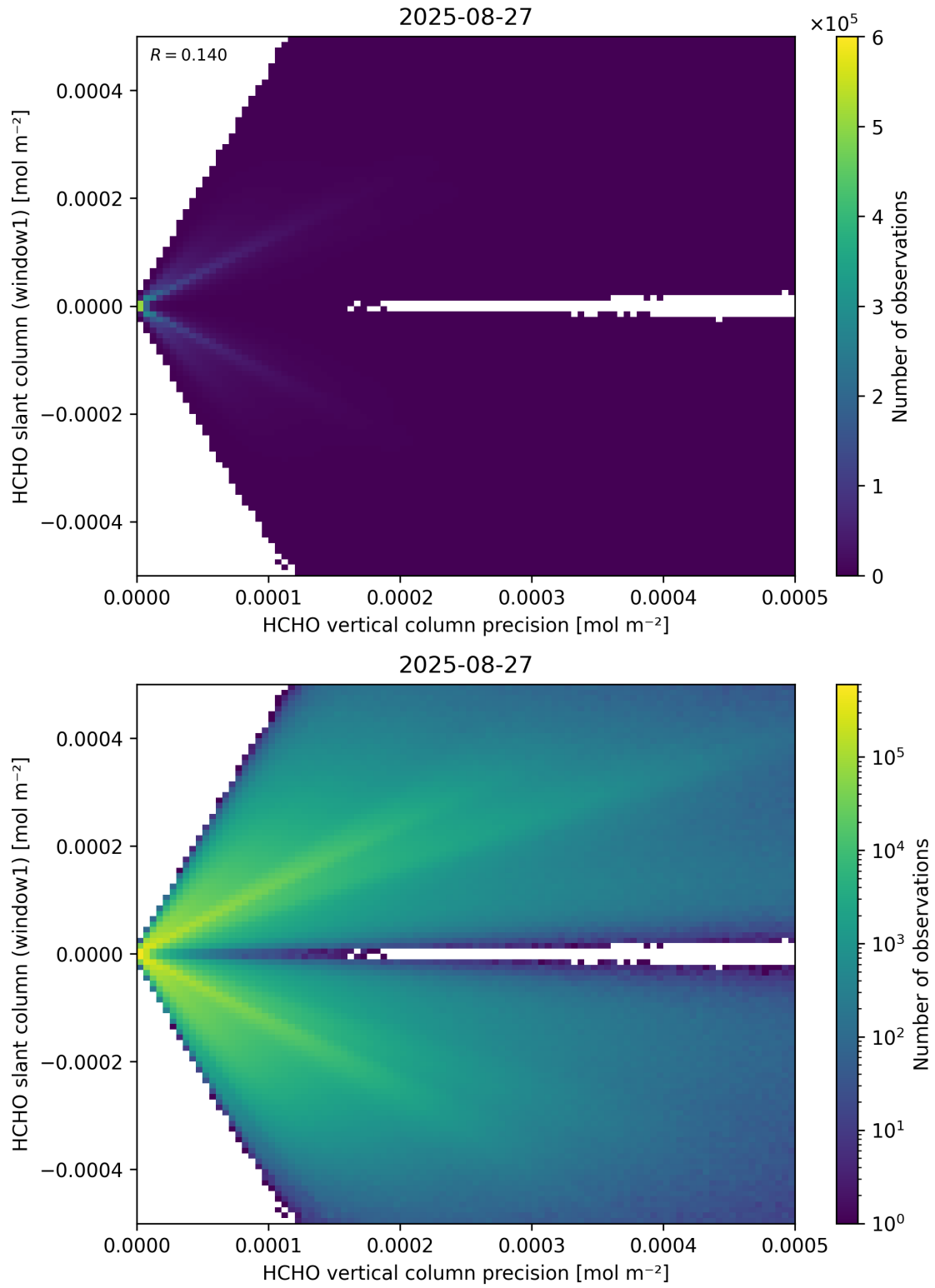
Figure 142: Scatter density plot of “HCHO vertical column precision” against “HCHO slant column (window1)” for 2025-08-26 to 2025-08-28.
