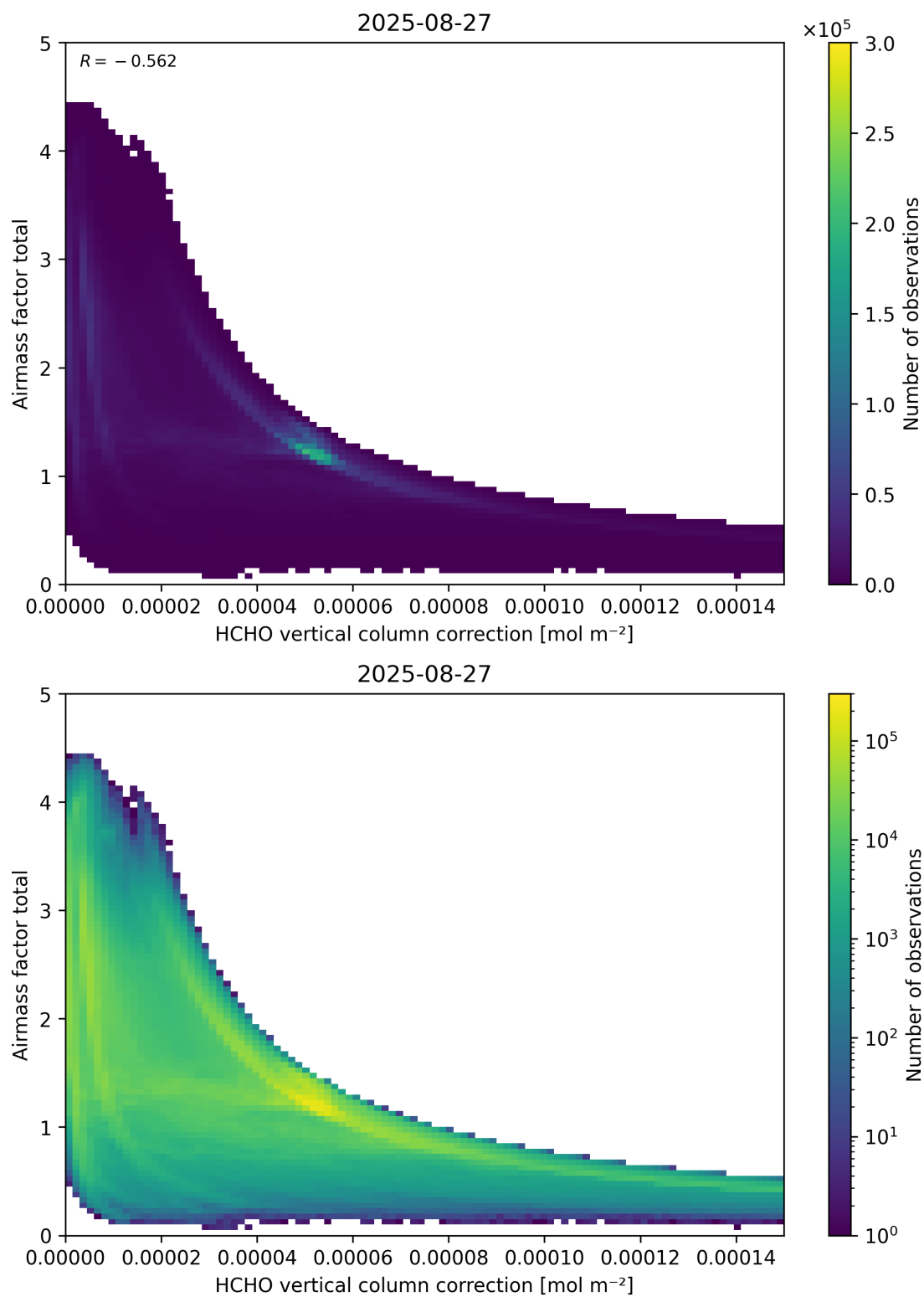
Figure 120: Scatter density plot of “HCHO vertical column correction” against “Airmass factor total” for 2025-08-26 to 2025-08-28.
