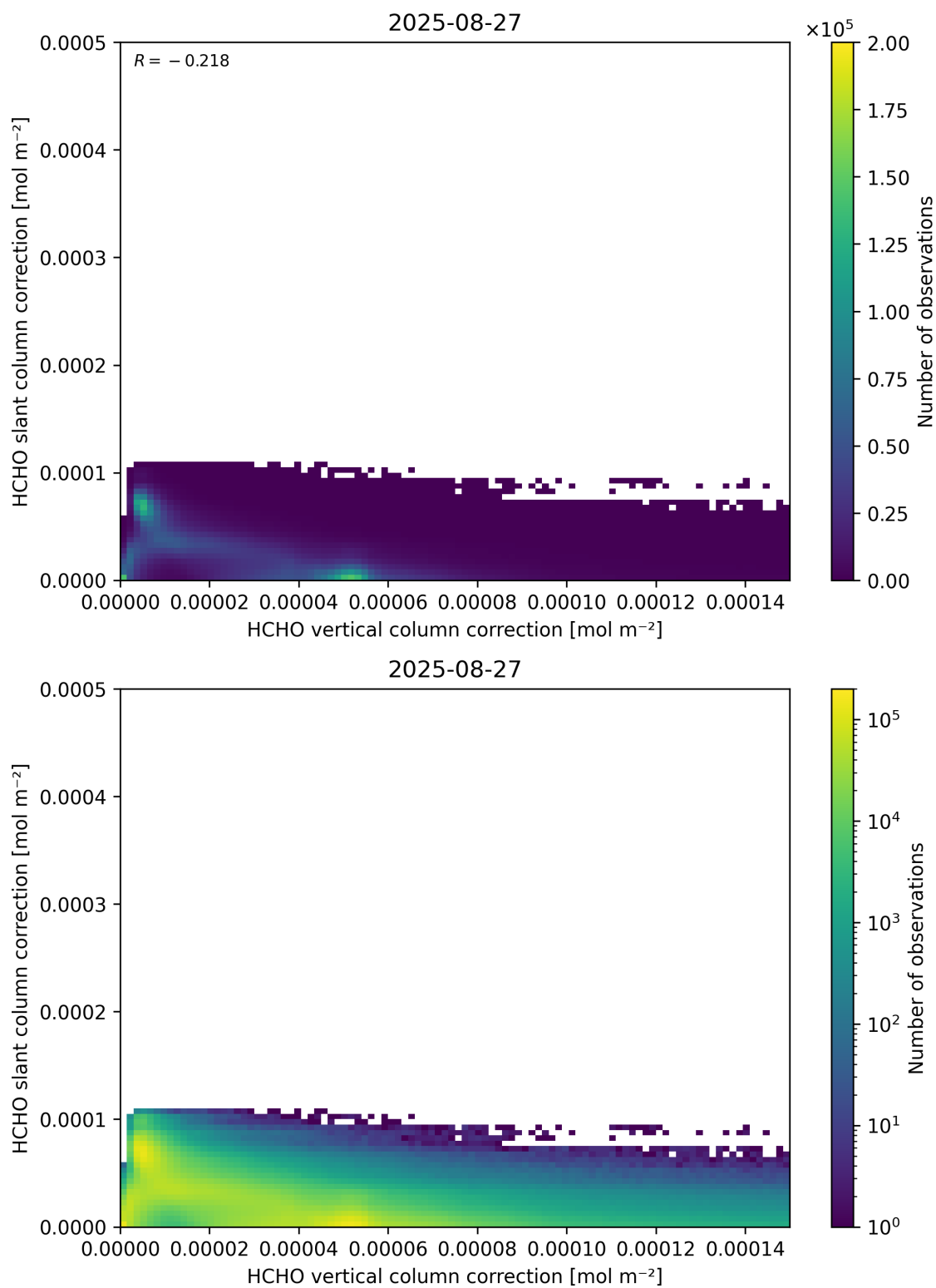
Figure 117: Scatter density plot of “HCHO vertical column correction” against “HCHO slant column correction” for 2025-08-26 to 2025-08-28.
