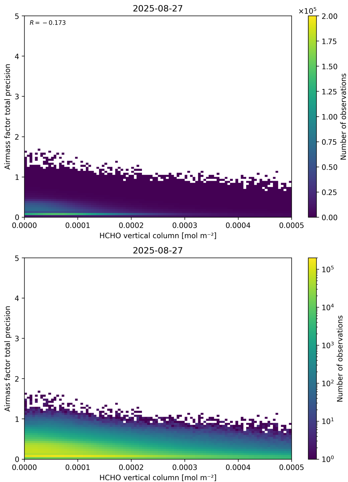
Figure 132: Scatter density plot of “HCHO vertical column” against “Airmass factor total precision” for 2025-08-26 to 2025-08-28.
