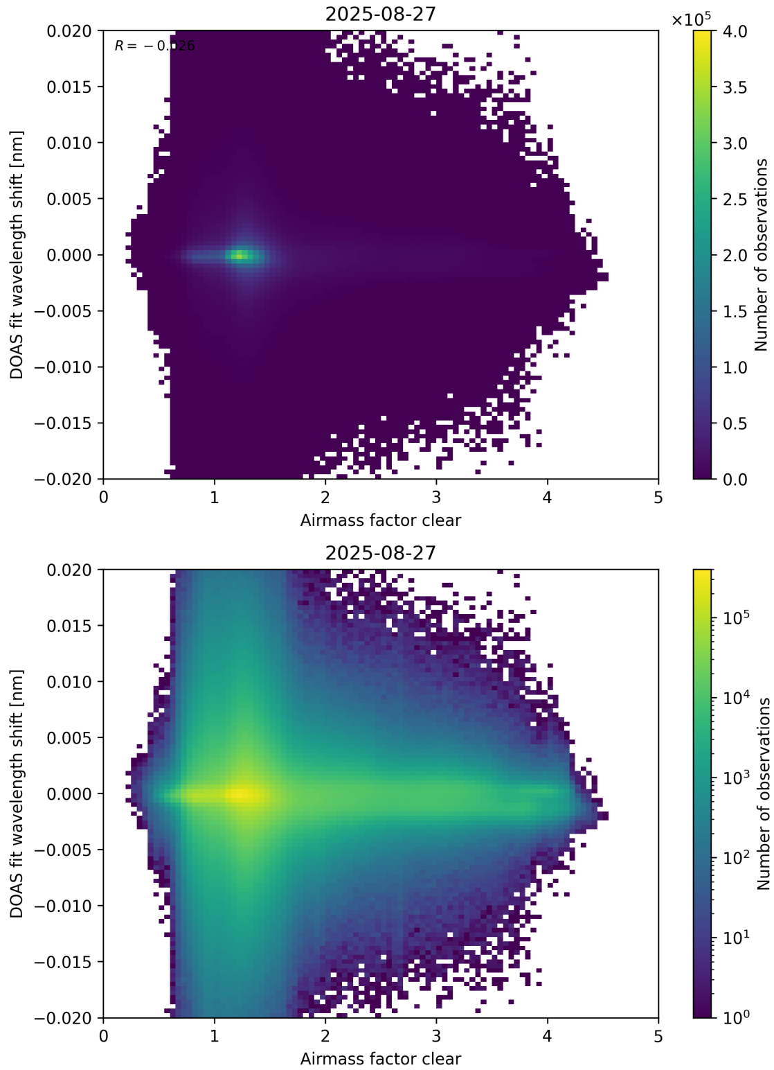
Figure 72: Scatter density plot of “Airmass factor clear” against “DOAS fit wavelength shift” for 2025-08-26 to 2025-08-28.
