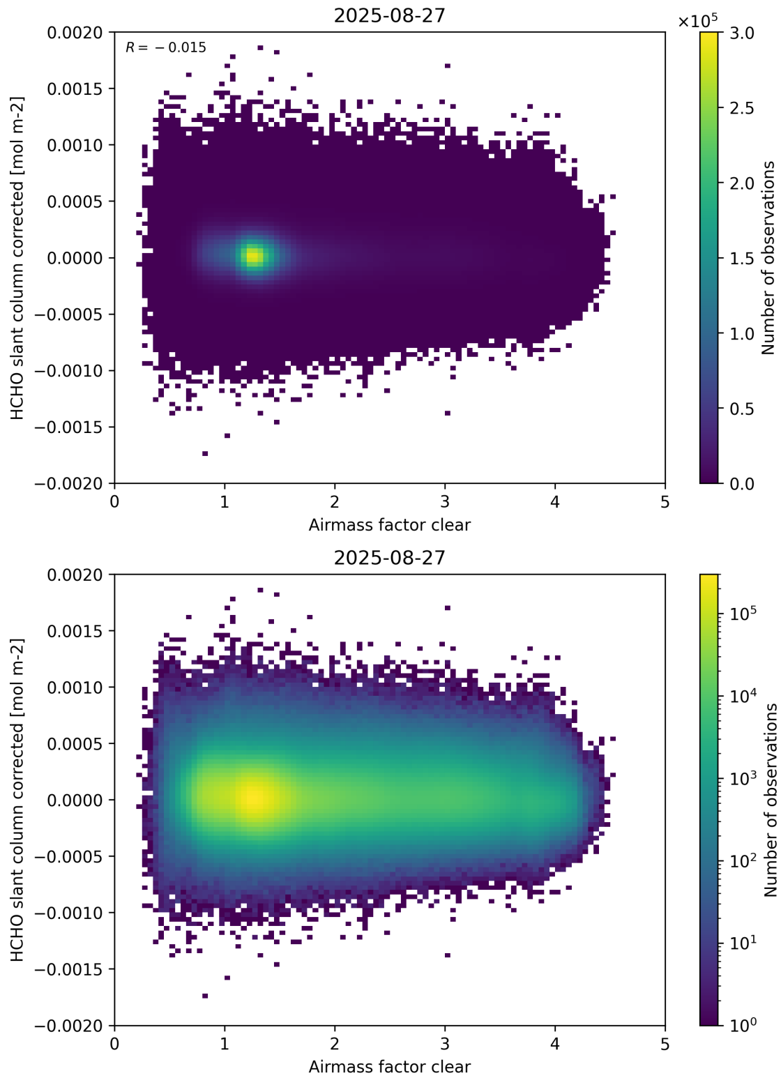
Figure 74: Scatter density plot of “Airmass factor clear” against “HCHO slant column corrected” for 2025-08-26 to 2025-08-28.
