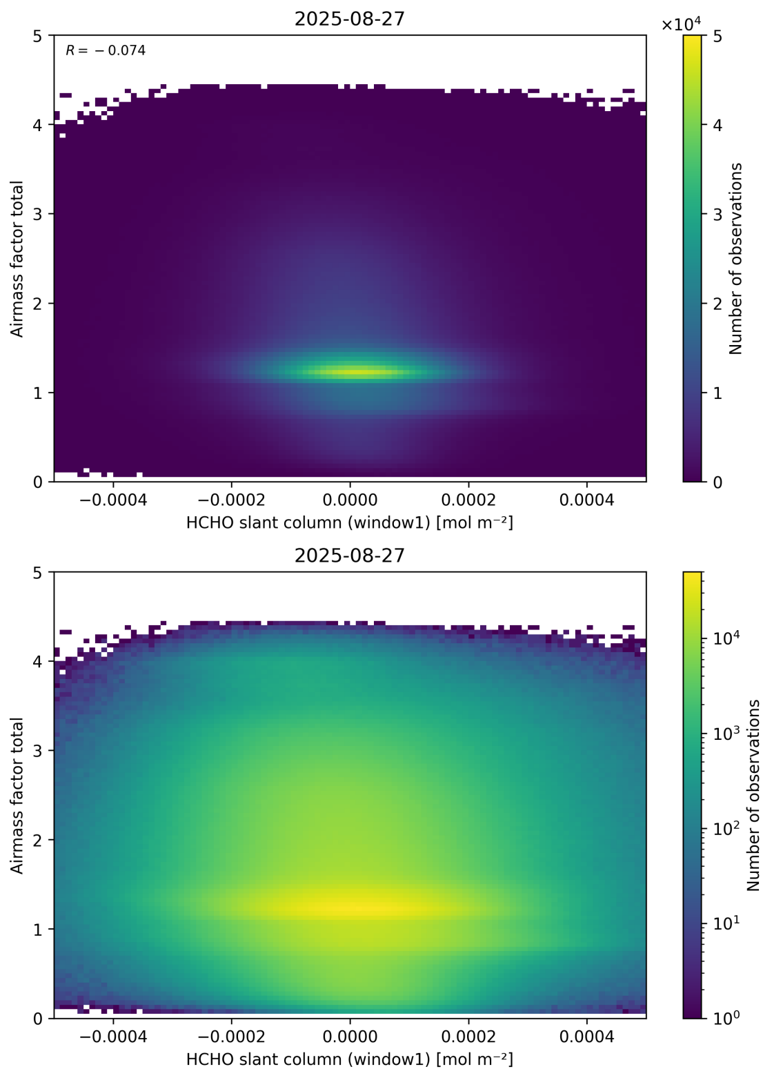
Figure 85: Scatter density plot of “HCHO slant column (window1)” against “Airmass factor total” for 2025-08-26 to 2025-08-28.
