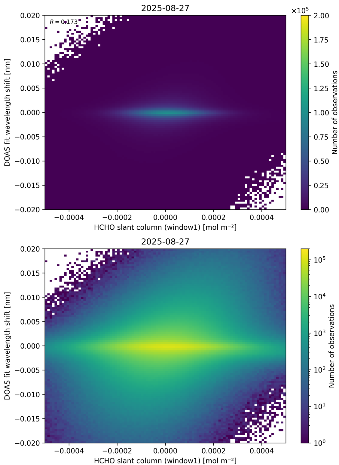
Figure 79: Scatter density plot of “HCHO slant column (window1)” against “DOAS fit wavelength shift” for 2025-08-26 to 2025-08-28.
