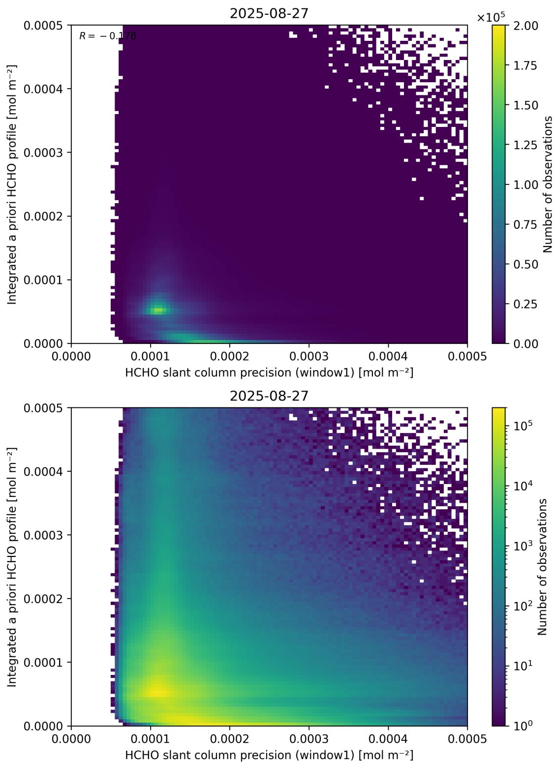
Figure 96: Scatter density plot of “HCHO slant column precision (window1)” against “Integrated a priori HCHO profile” for 2025-08-26 to 2025-08-28.
