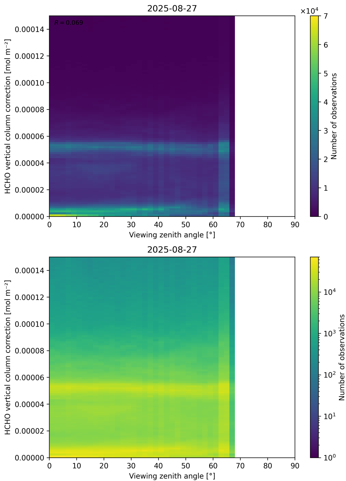
Figure 193: Scatter density plot of “Viewing zenith angle” against “HCHO vertical column correction” for 2025-08-26 to 2025-08-28.
