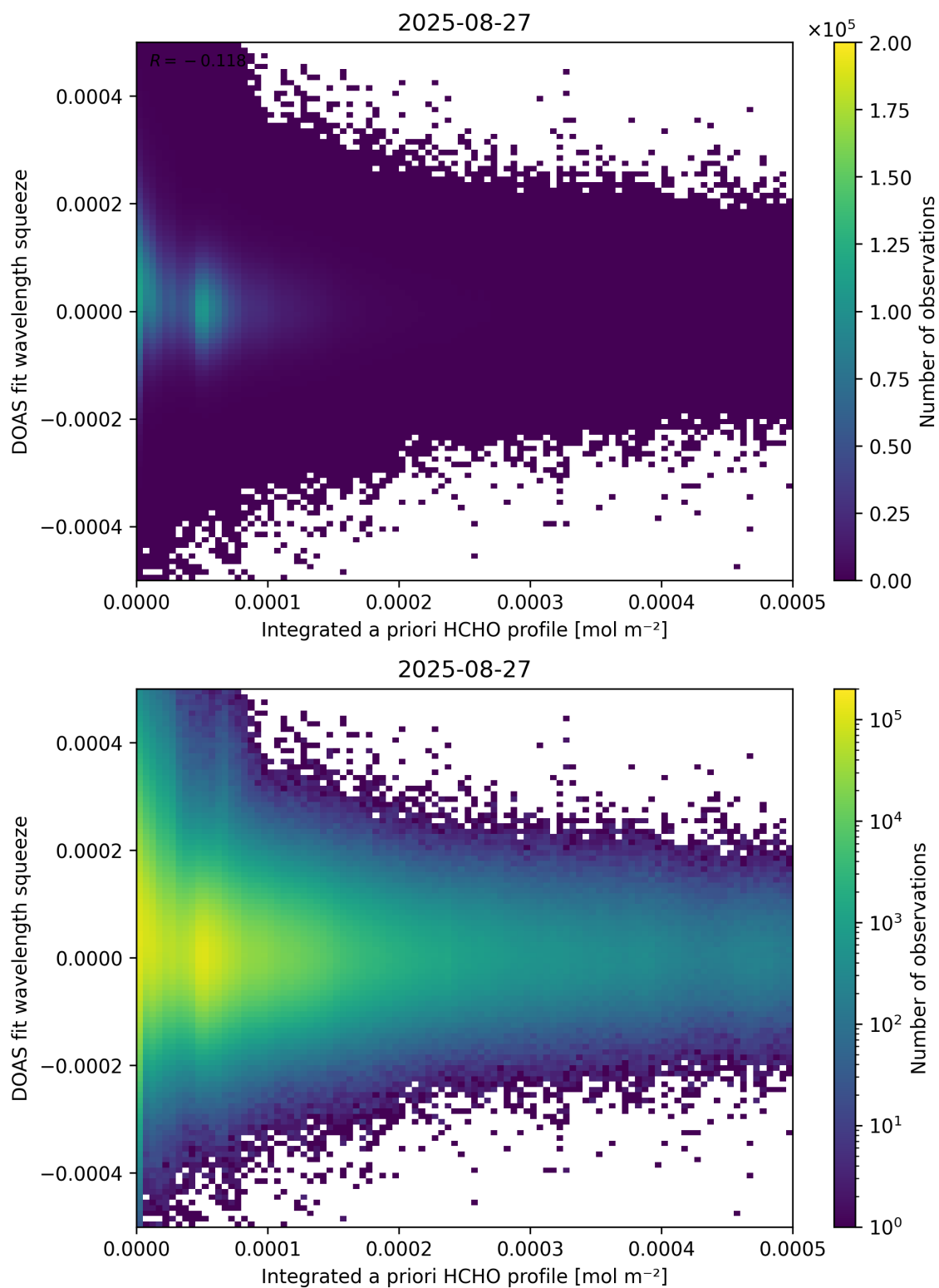
Figure 150: Scatter density plot of “Integrated a priori HCHO profile” against “DOAS fit wavelength squeeze” for 2025-08-26 to 2025-08-28.
