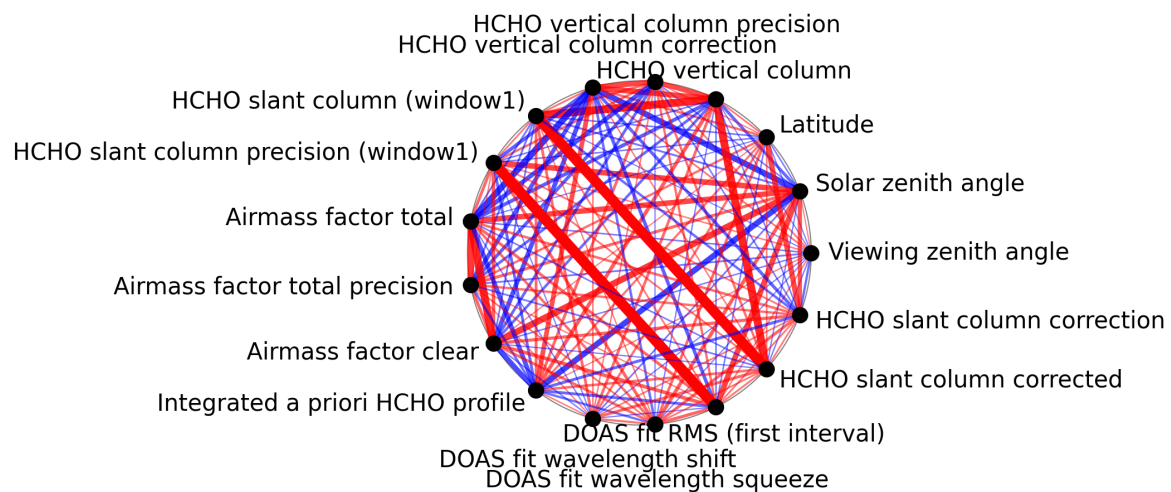
Figure 1: Map of correlation graph for 2025-08-26 to 2025-08-28.
