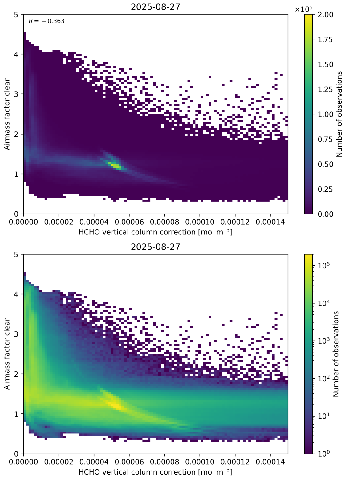
Figure 115: Scatter density plot of “HCHO vertical column correction” against “Airmass factor clear” for 2025-08-26 to 2025-08-28.
