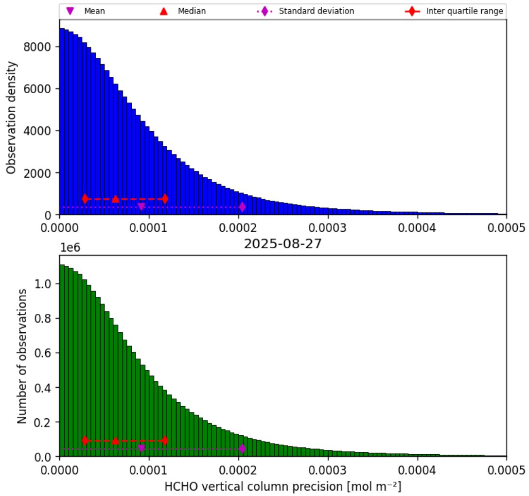
Figure 36: Histogram of “HCHO vertical column precision” for 2025-08-26 to 2025-08-28
