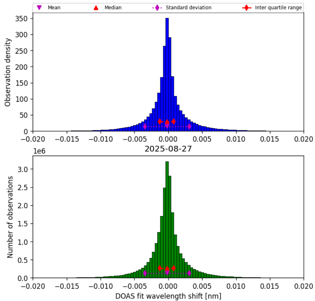
Figure 44: Histogram of “DOAS fit wavelength shift” for 2025-08-26 to 2025-08-28
