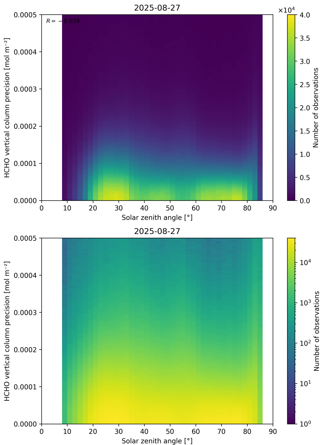
Figure 179: Scatter density plot of “Solar zenith angle” against “HCHO vertical column precision” for 2025-08-26 to 2025-08-28.
