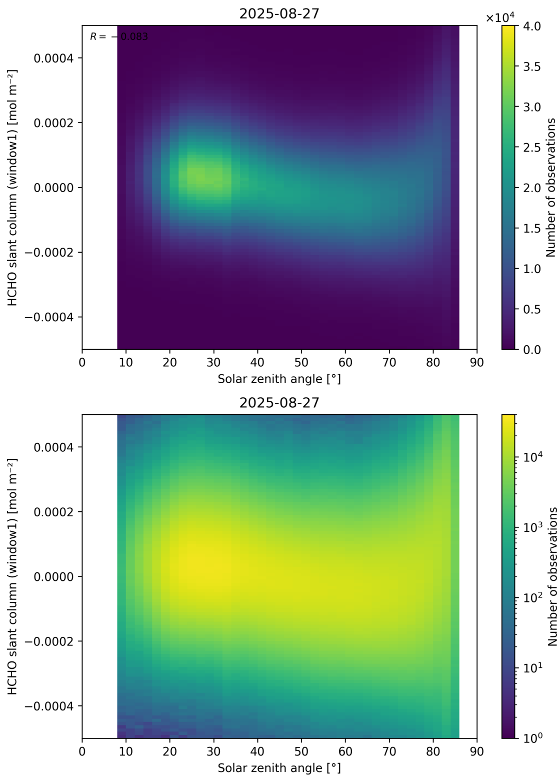
Figure 173: Scatter density plot of “Solar zenith angle” against “HCHO slant column (window1)” for 2025-08-26 to 2025-08-28.
