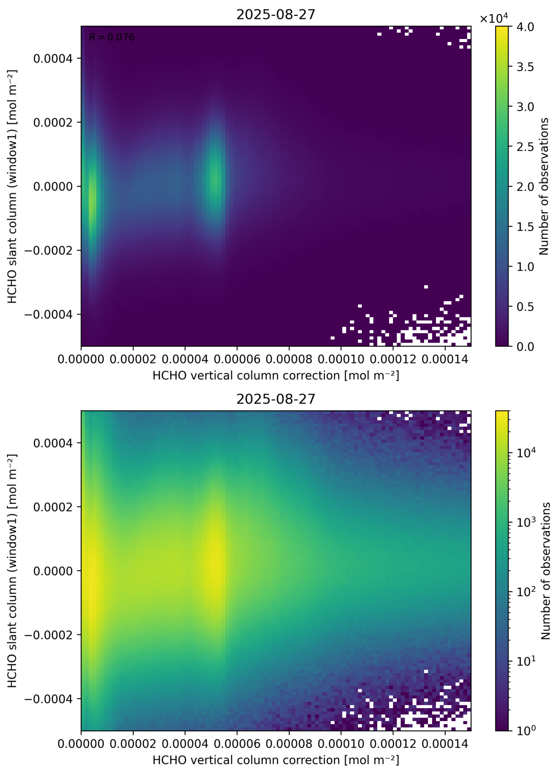
Figure 118: Scatter density plot of “HCHO vertical column correction” against “HCHO slant column (window1)” for 2025-08-26 to 2025-08-28.
