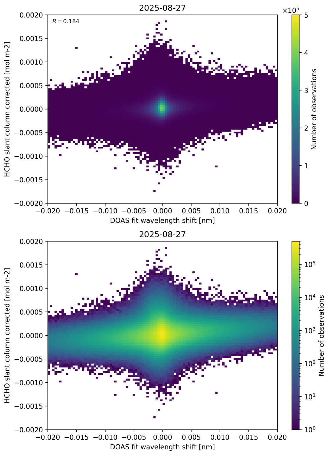
Figure 66: Scatter density plot of “DOAS fit wavelength shift” against “HCHO slant column corrected” for 2025-08-26 to 2025-08-28.
