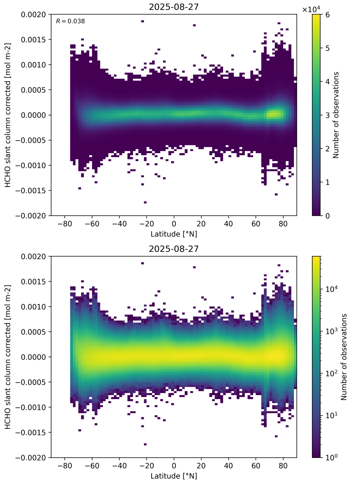
Figure 157: Scatter density plot of “Latitude” against “HCHO slant column corrected” for 2025-08-26 to 2025-08-28.
