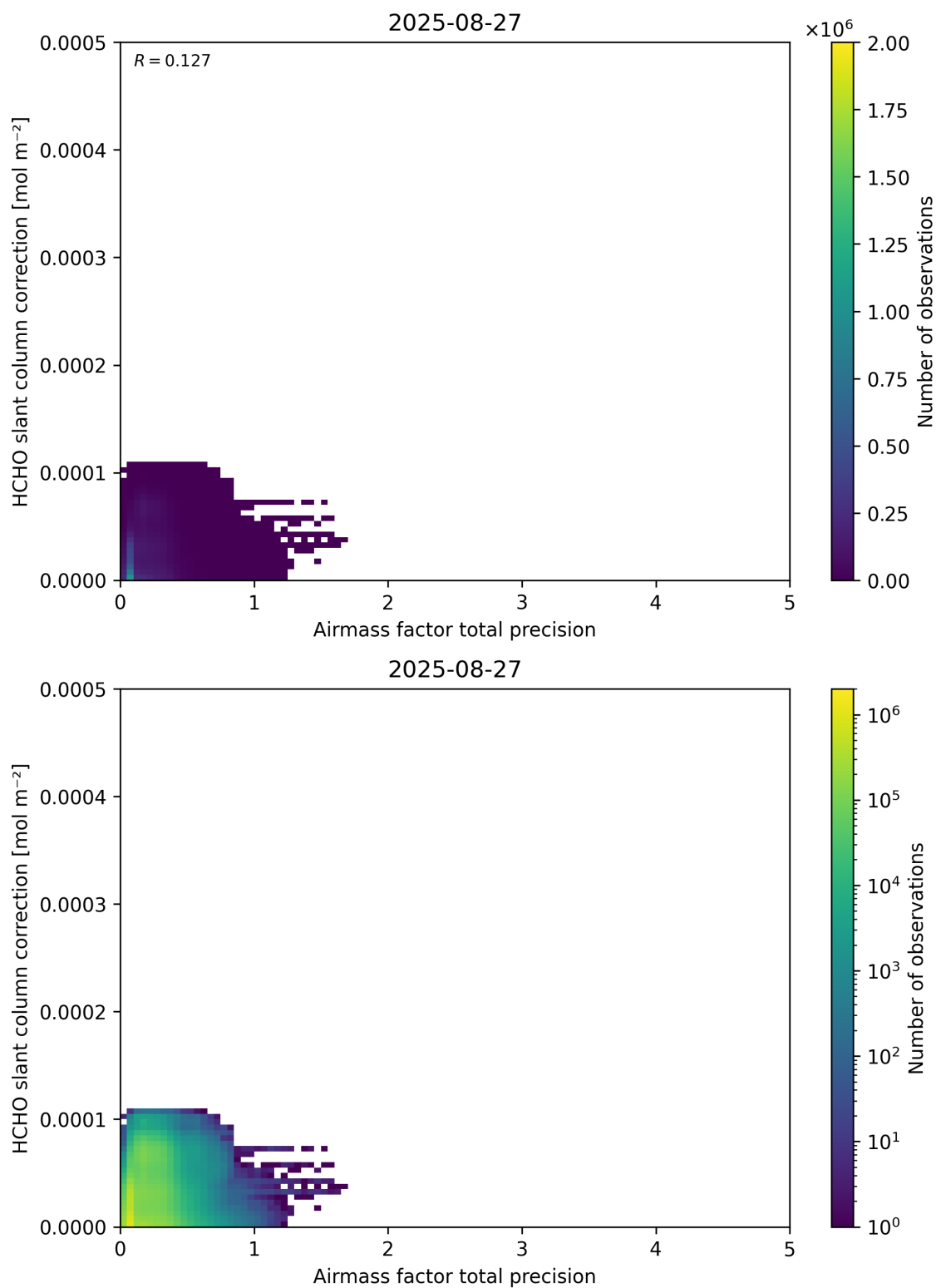
Figure 110: Scatter density plot of “Airmass factor total precision” against “HCHO slant column correction” for 2025-08-26 to 2025-08-28.
