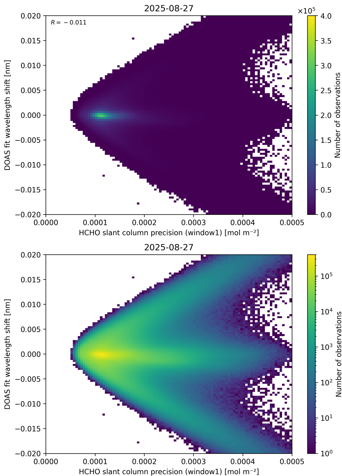
Figure 89: Scatter density plot of “HCHO slant column precision (window1)” against “DOAS fit wavelength shift” for 2025-08-26 to 2025-08-28.
