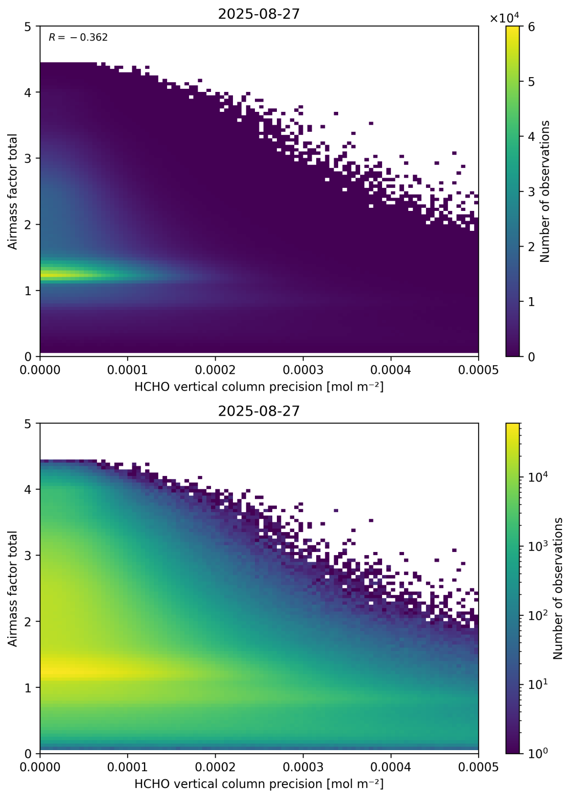
Figure 144: Scatter density plot of “HCHO vertical column precision” against “Airmass factor total” for 2025-08-26 to 2025-08-28.
