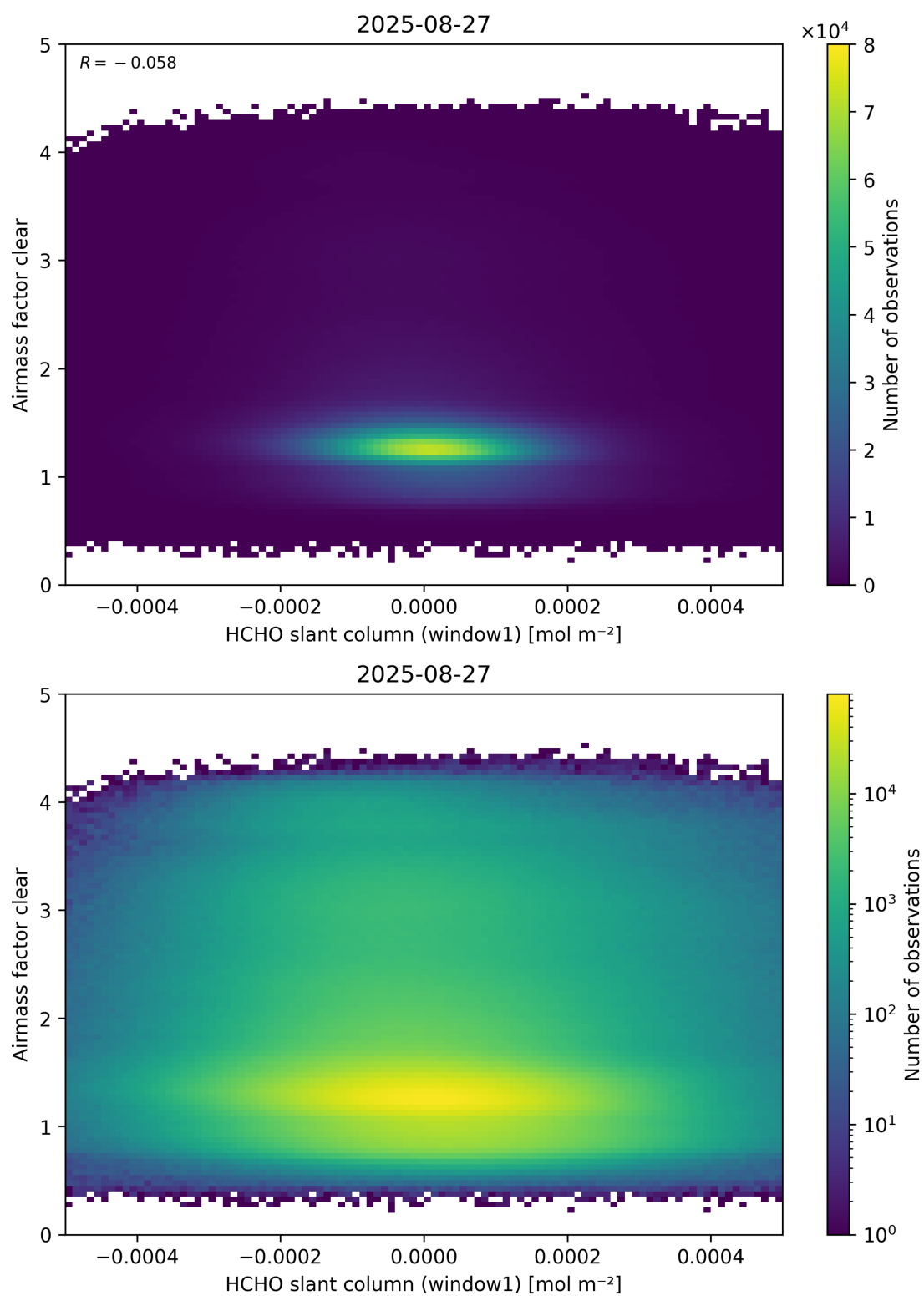
Figure 81: Scatter density plot of “HCHO slant column (window1)” against “Airmass factor clear” for 2025-08-26 to 2025-08-28.
