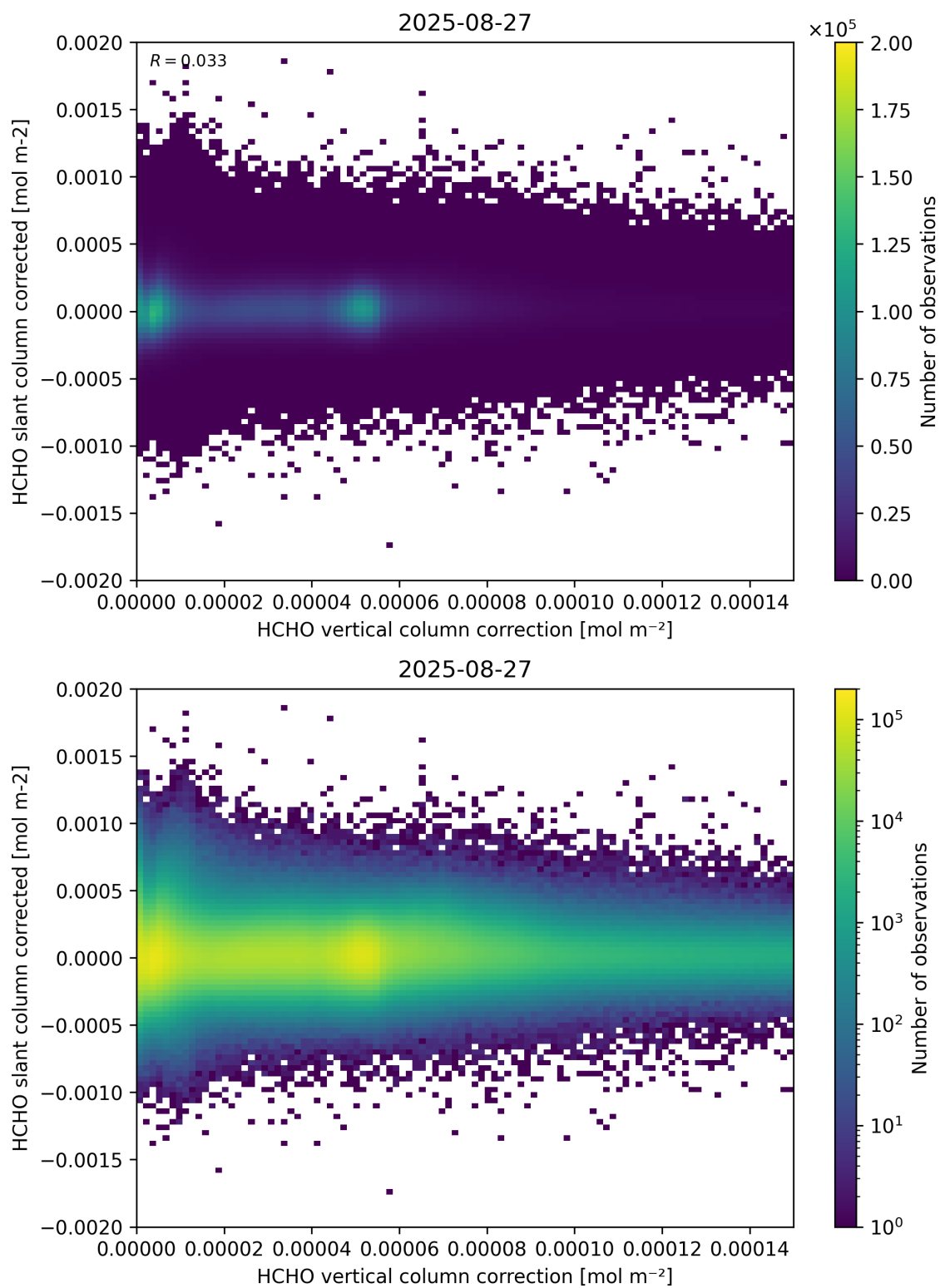
Figure 116: Scatter density plot of “HCHO vertical column correction” against “HCHO slant column corrected” for 2025-08-26 to 2025-08-28.
