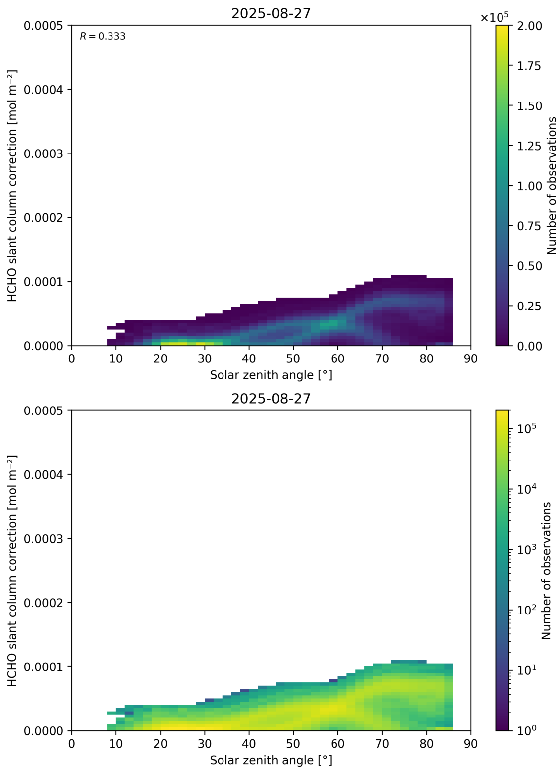
Figure 172: Scatter density plot of “Solar zenith angle” against “HCHO slant column correction” for 2025-08-26 to 2025-08-28.
