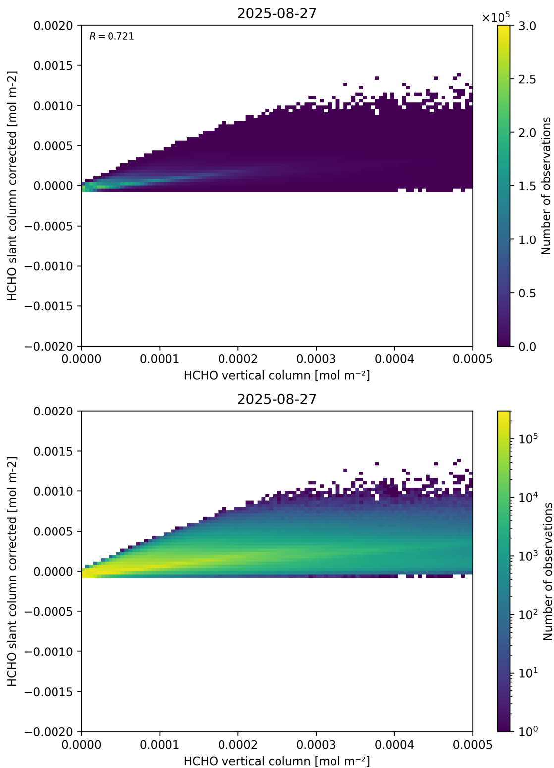
Figure 127: Scatter density plot of “HCHO vertical column” against “HCHO slant column corrected” for 2025-08-26 to 2025-08-28.
