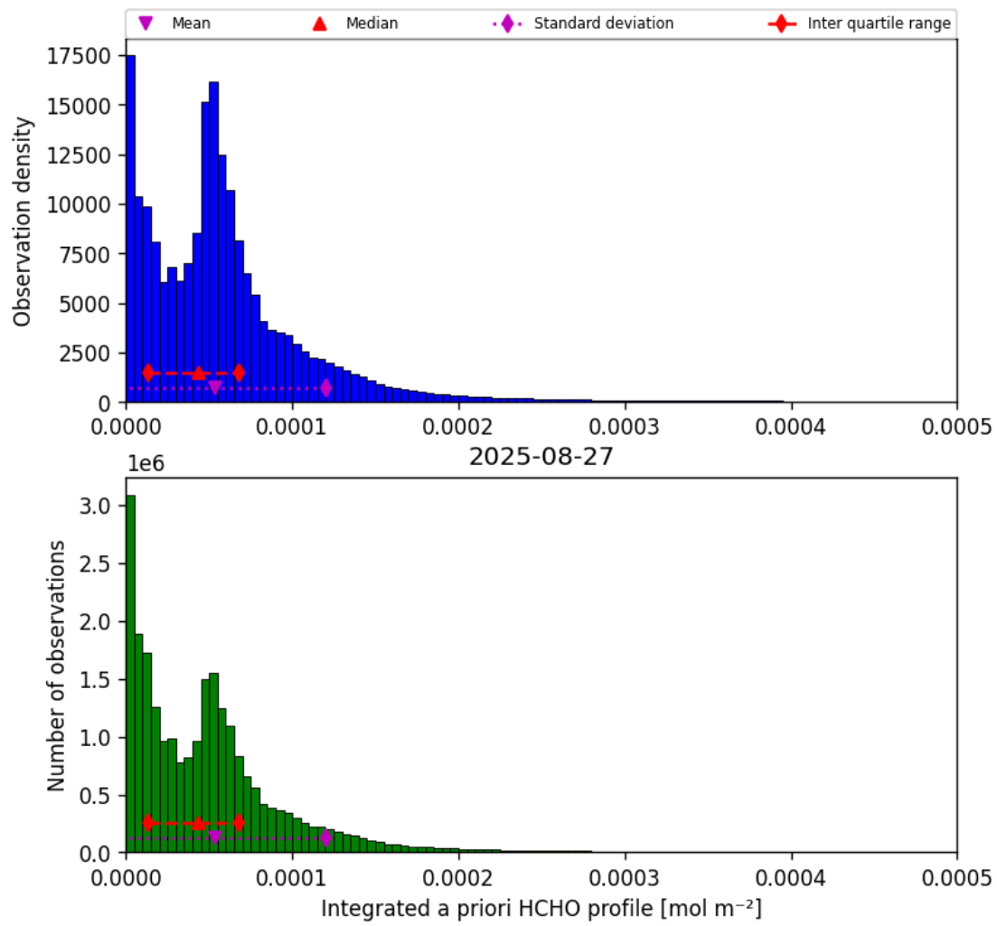
Figure 43: Histogram of “Integrated a priori HCHO profile” for 2025-08-26 to 2025-08-28
