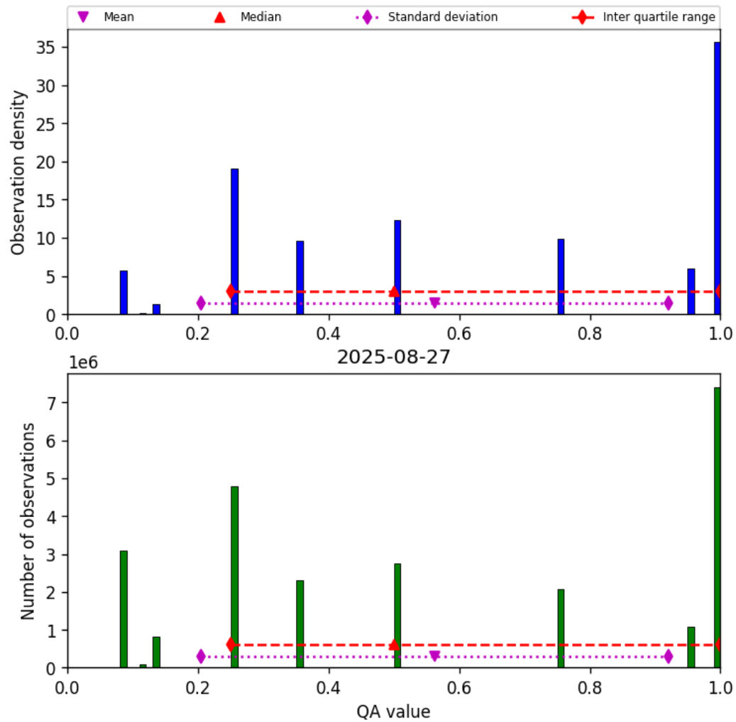
Figure 34: Histogram of “QA value” for 2025-08-26 to 2025-08-28
