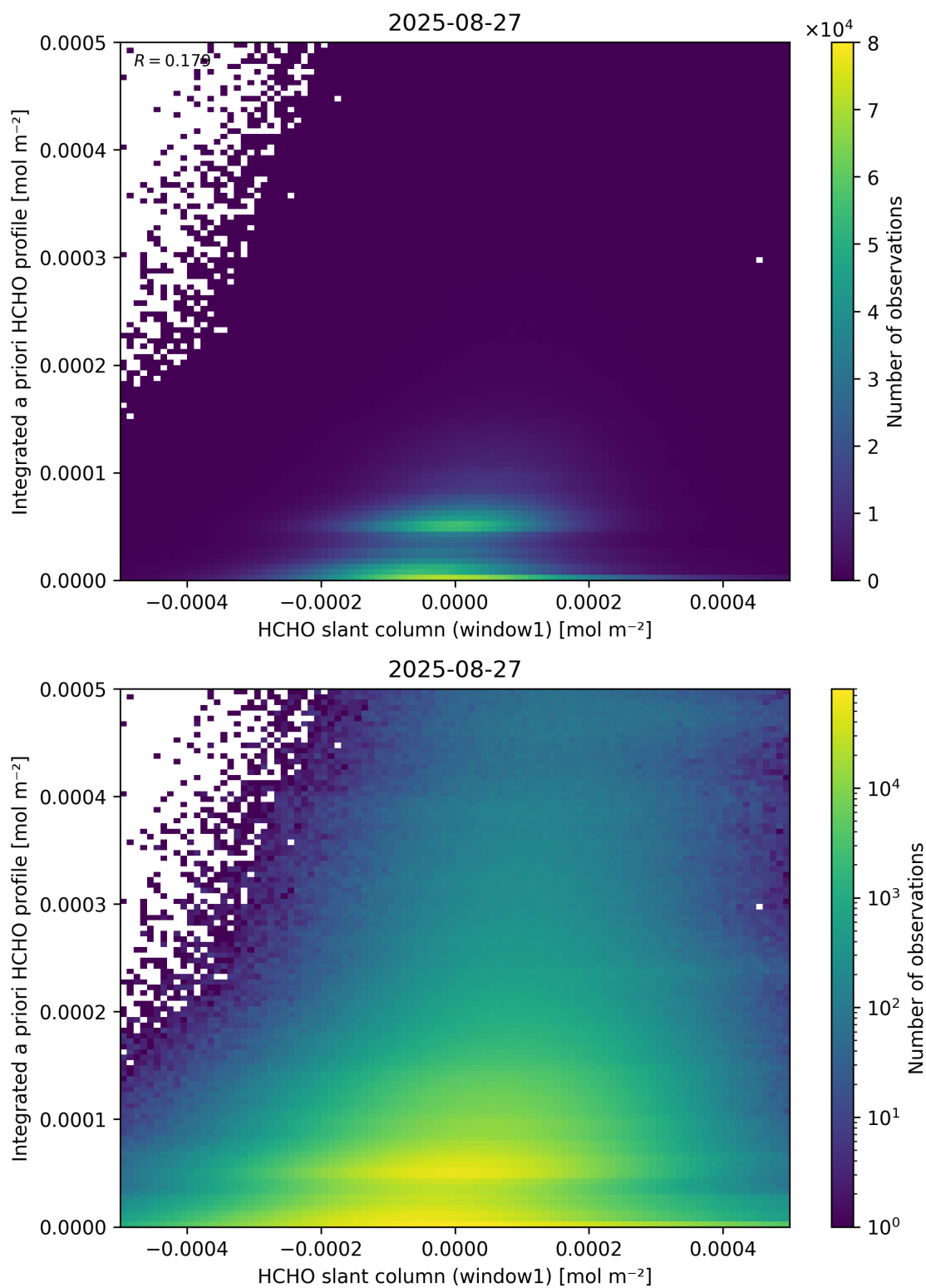
Figure 87: Scatter density plot of “HCHO slant column (window1)” against “Integrated a priori HCHO profile” for 2025-08-26 to 2025-08-28.
