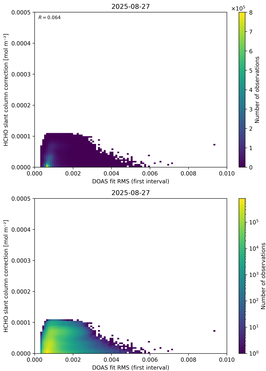
Figure 63: Scatter density plot of “DOAS fit RMS (first interval)” against “HCHO slant column correction” for 2025-08-26 to 2025-08-28.
