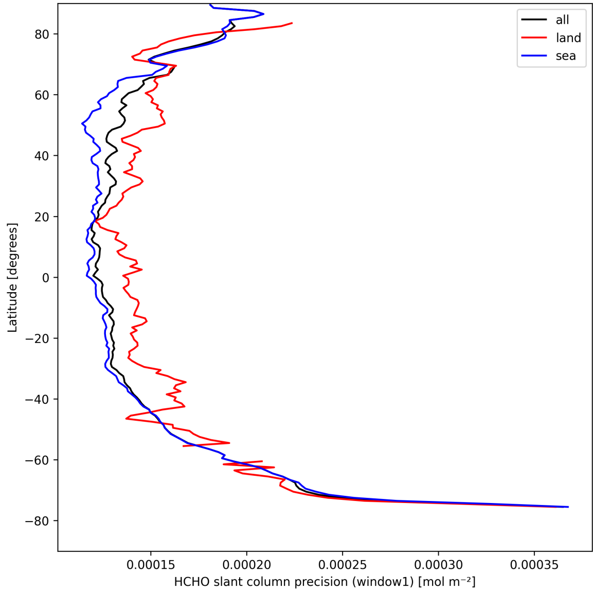
Figure 25: Zonal average of “HCHO slant column precision (window1)” for 2025-08-26 to 2025-08-28.
