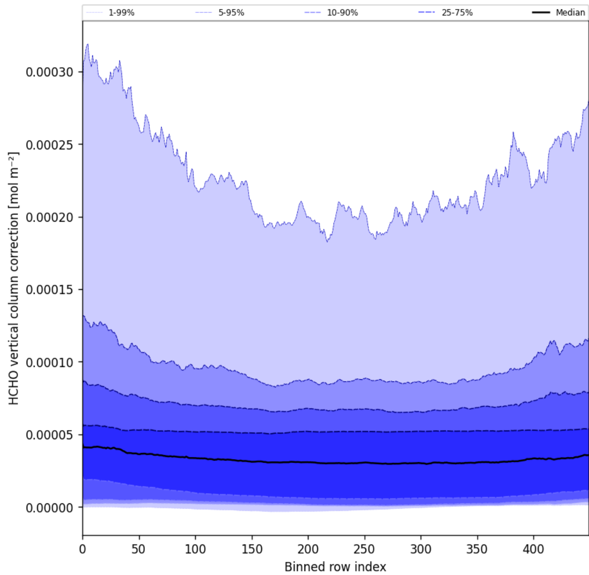
Figure 51: Along track statistics of “HCHO vertical column correction” for 2025-08-26 to 2025-08-28
