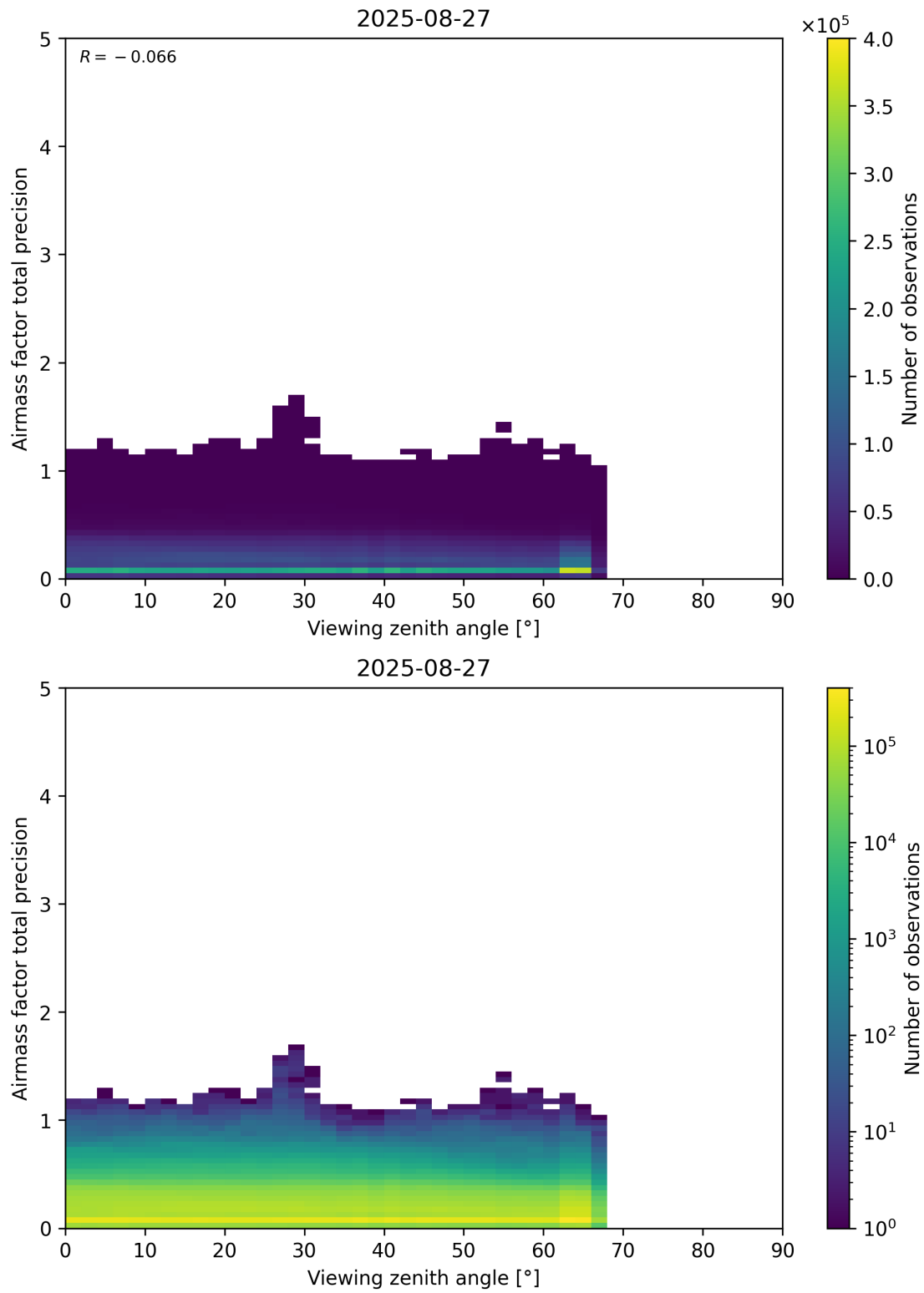
Figure 191: Scatter density plot of “Viewing zenith angle” against “Airmass factor total precision” for 2025-08-26 to 2025-08-28.
