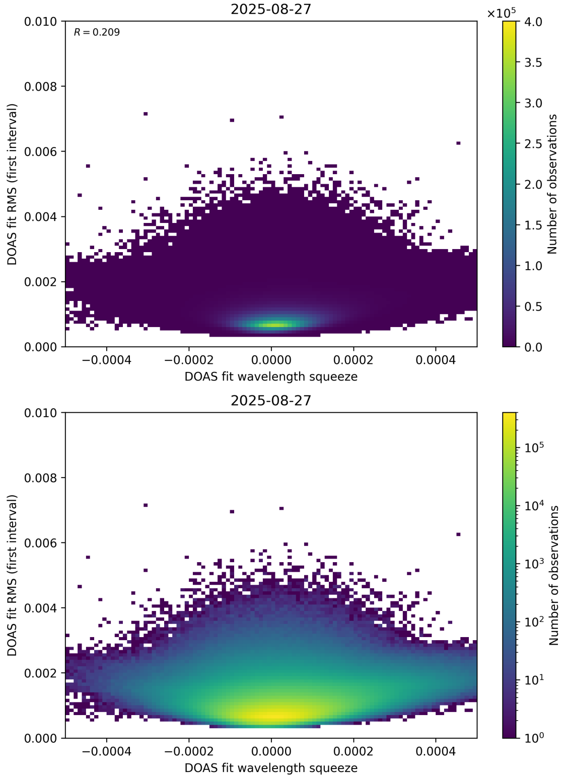
Figure 68: Scatter density plot of “DOAS fit wavelength squeeze” against “DOAS fit RMS (first interval)” for 2025-08-26 to 2025-08-28.
