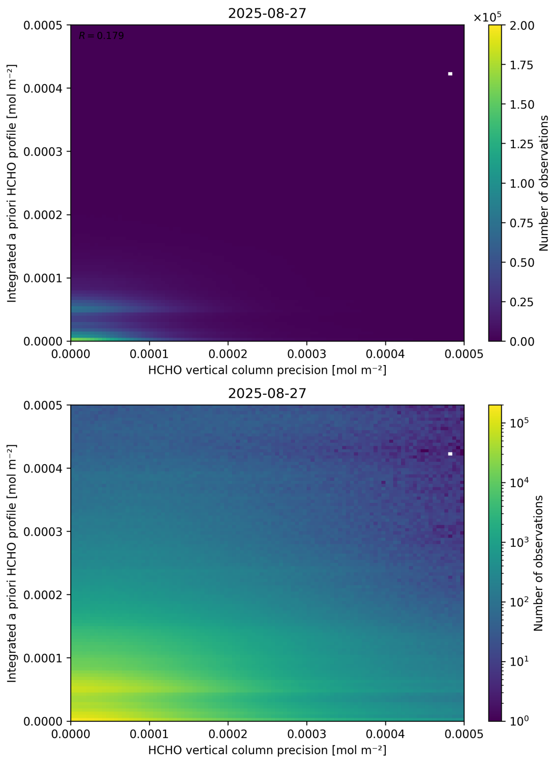
Figure 147: Scatter density plot of “HCHO vertical column precision” against “Integrated a priori HCHO profile” for 2025-08-26 to 2025-08-28.
