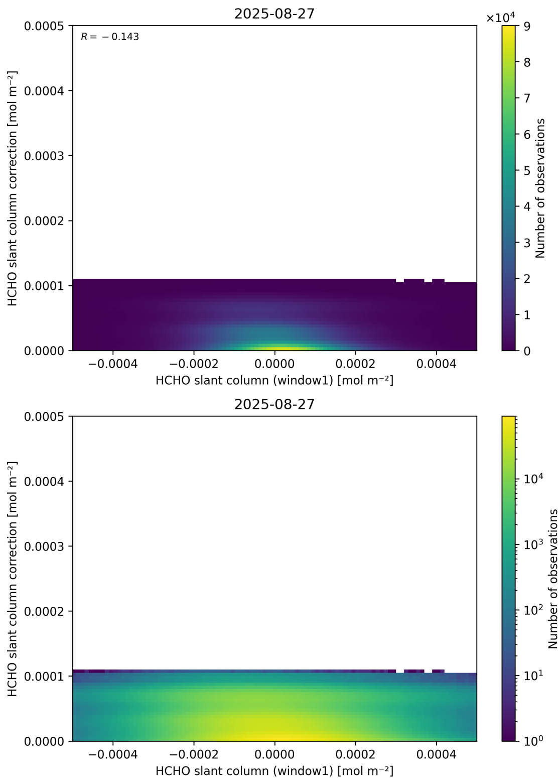
Figure 83: Scatter density plot of “HCHO slant column (window1)” against “HCHO slant column correction” for 2025-08-26 to 2025-08-28.
