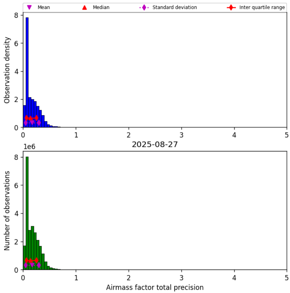
Figure 41: Histogram of “Airmass factor total precision” for 2025-08-26 to 2025-08-28
