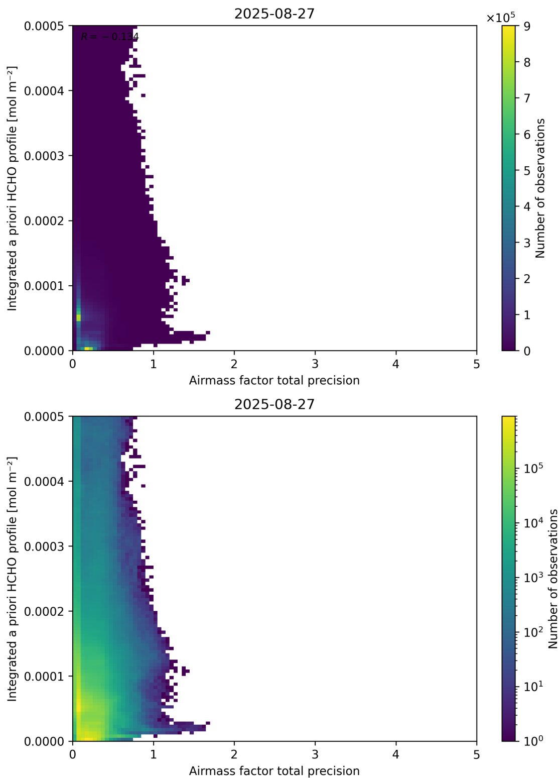
Figure 111: Scatter density plot of “Airmass factor total precision” against “Integrated a priori HCHO profile” for 2025-08-26 to 2025-08-28.
