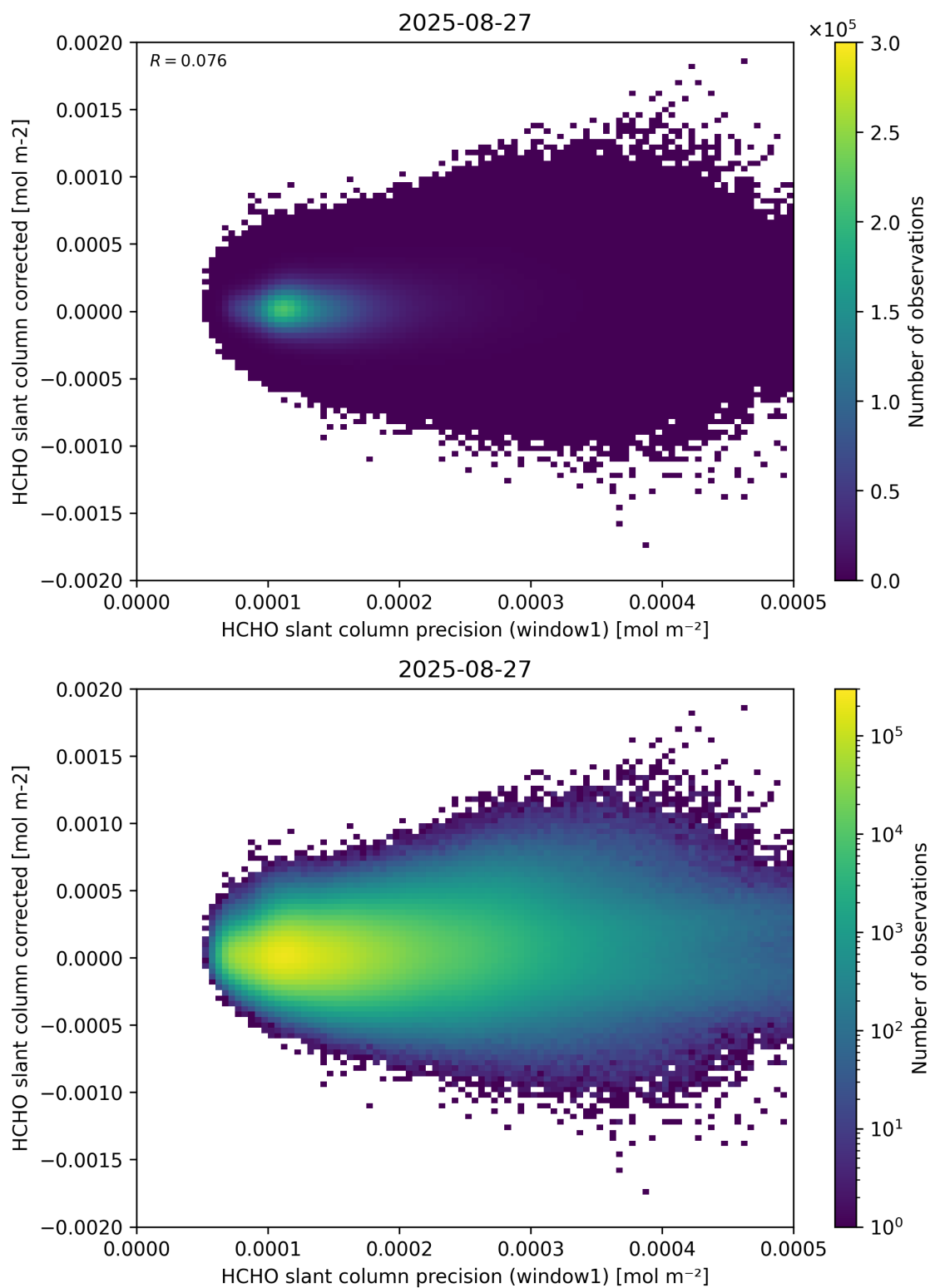
Figure 92: Scatter density plot of “HCHO slant column precision (window1)” against “HCHO slant column corrected” for 2025-08-26 to 2025-08-28.
