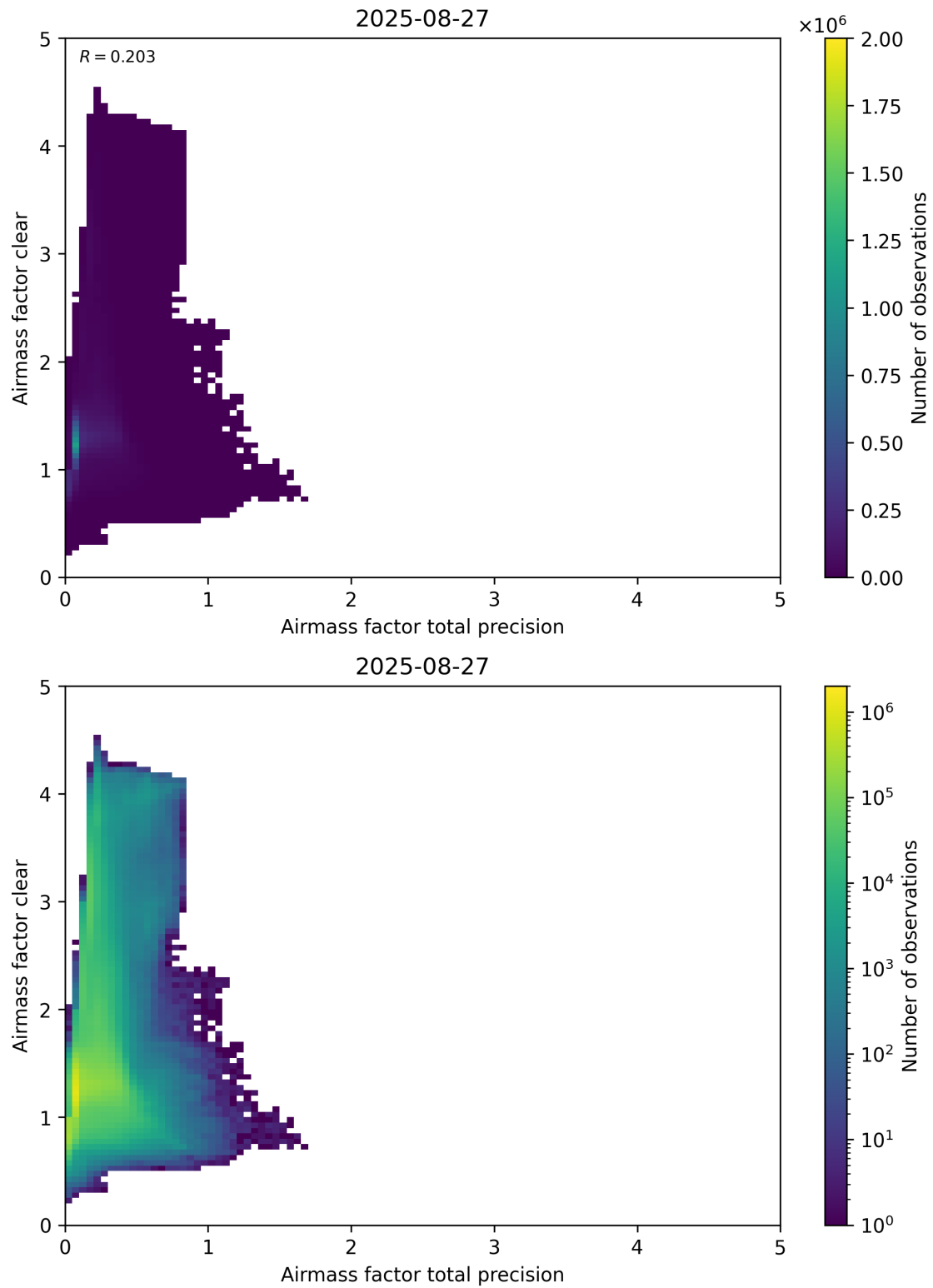
Figure 108: Scatter density plot of “Airmass factor total precision” against “Airmass factor clear” for 2025-08-26 to 2025-08-28.
