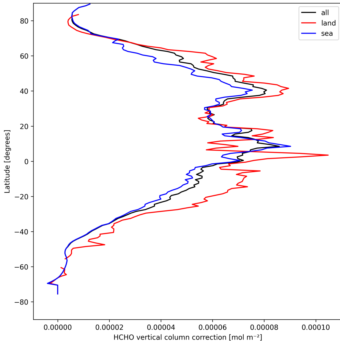
Figure 23: Zonal average of “HCHO vertical column correction” for 2025-08-26 to 2025-08-28.
