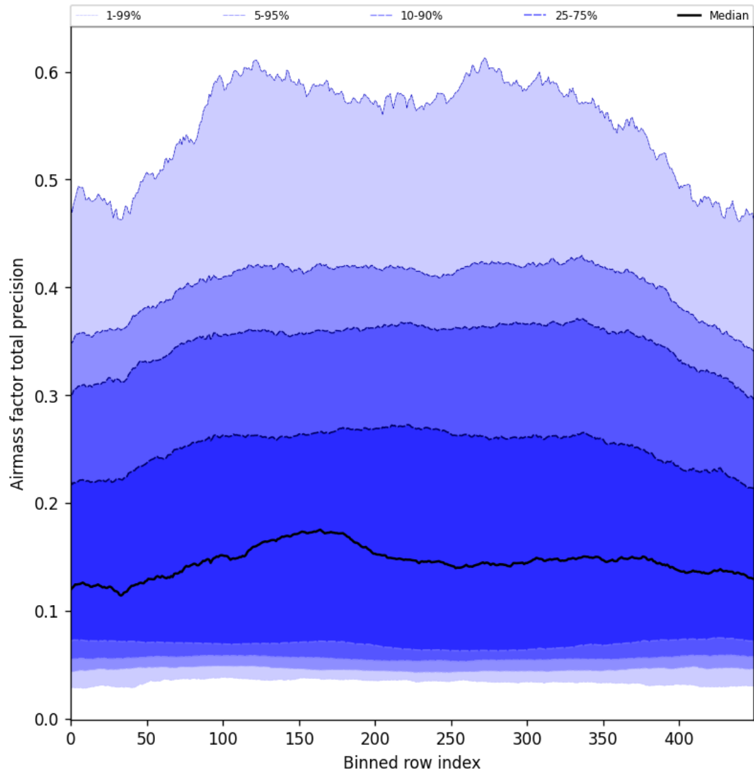
Figure 55: Along track statistics of “Airmass factor total precision” for 2025-08-26 to 2025-08-28
