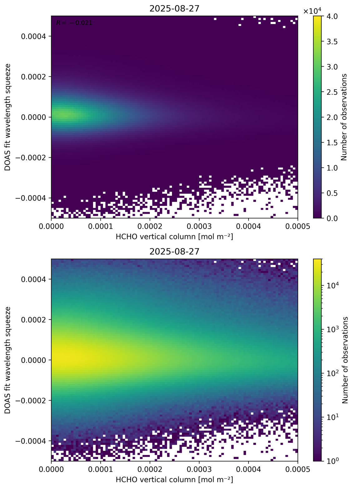
Figure 125: Scatter density plot of “HCHO vertical column” against “DOAS fit wavelength squeeze” for 2025-08-26 to 2025-08-28.
