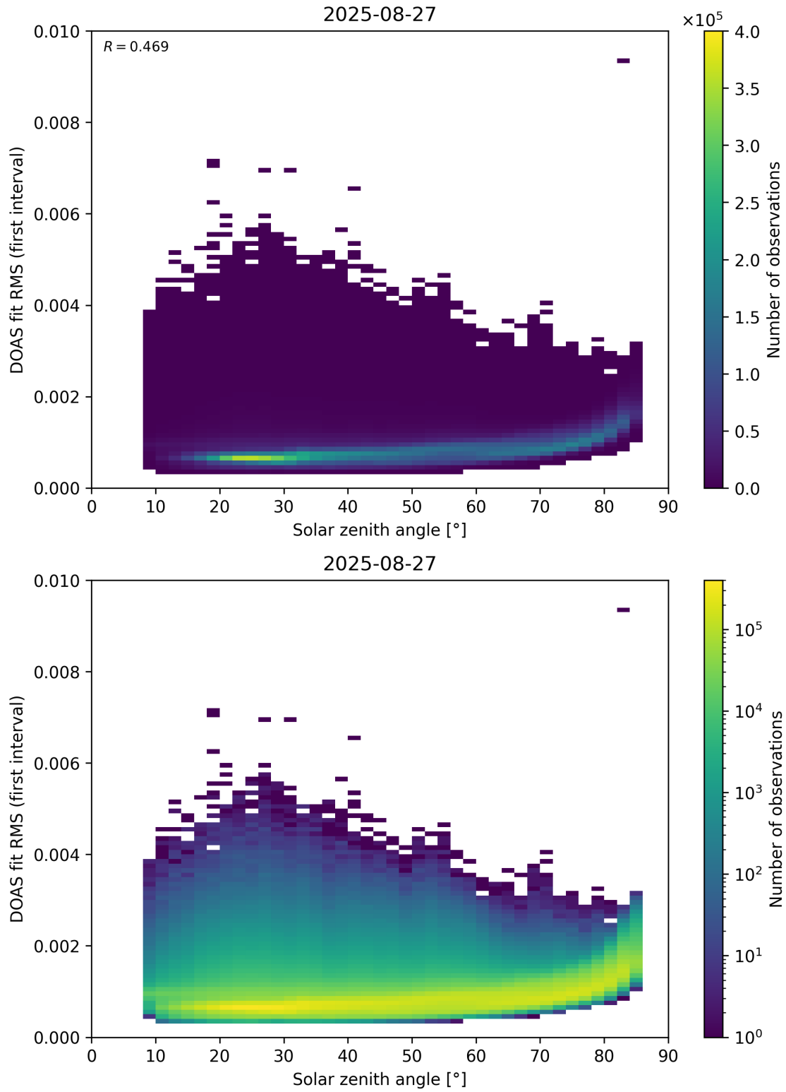
Figure 167: Scatter density plot of “Solar zenith angle” against “DOAS fit RMS (first interval)” for 2025-08-26 to 2025-08-28.
