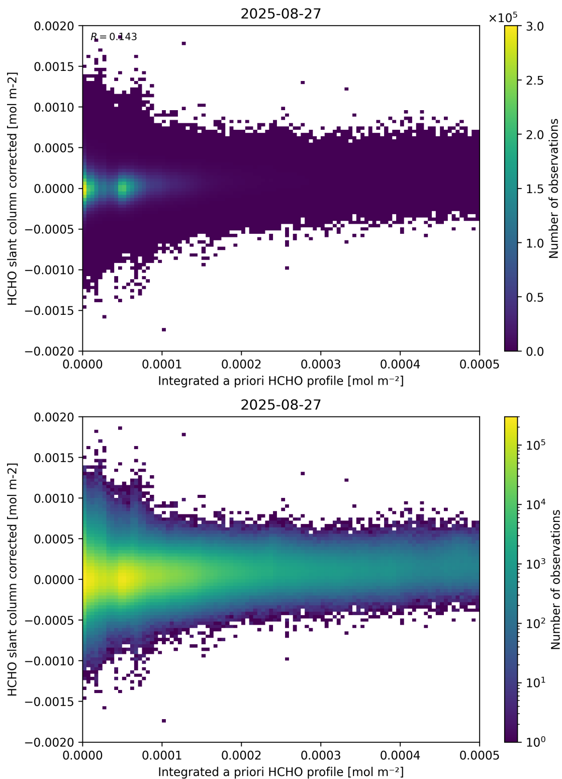
Figure 151: Scatter density plot of “Integrated a priori HCHO profile” against “HCHO slant column corrected” for 2025-08-26 to 2025-08-28.
