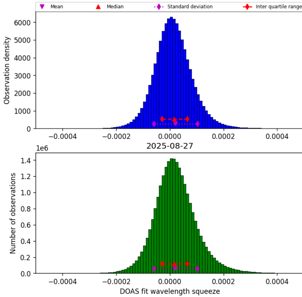
Figure 45: Histogram of “DOAS fit wavelength squeeze” for 2025-08-26 to 2025-08-28
