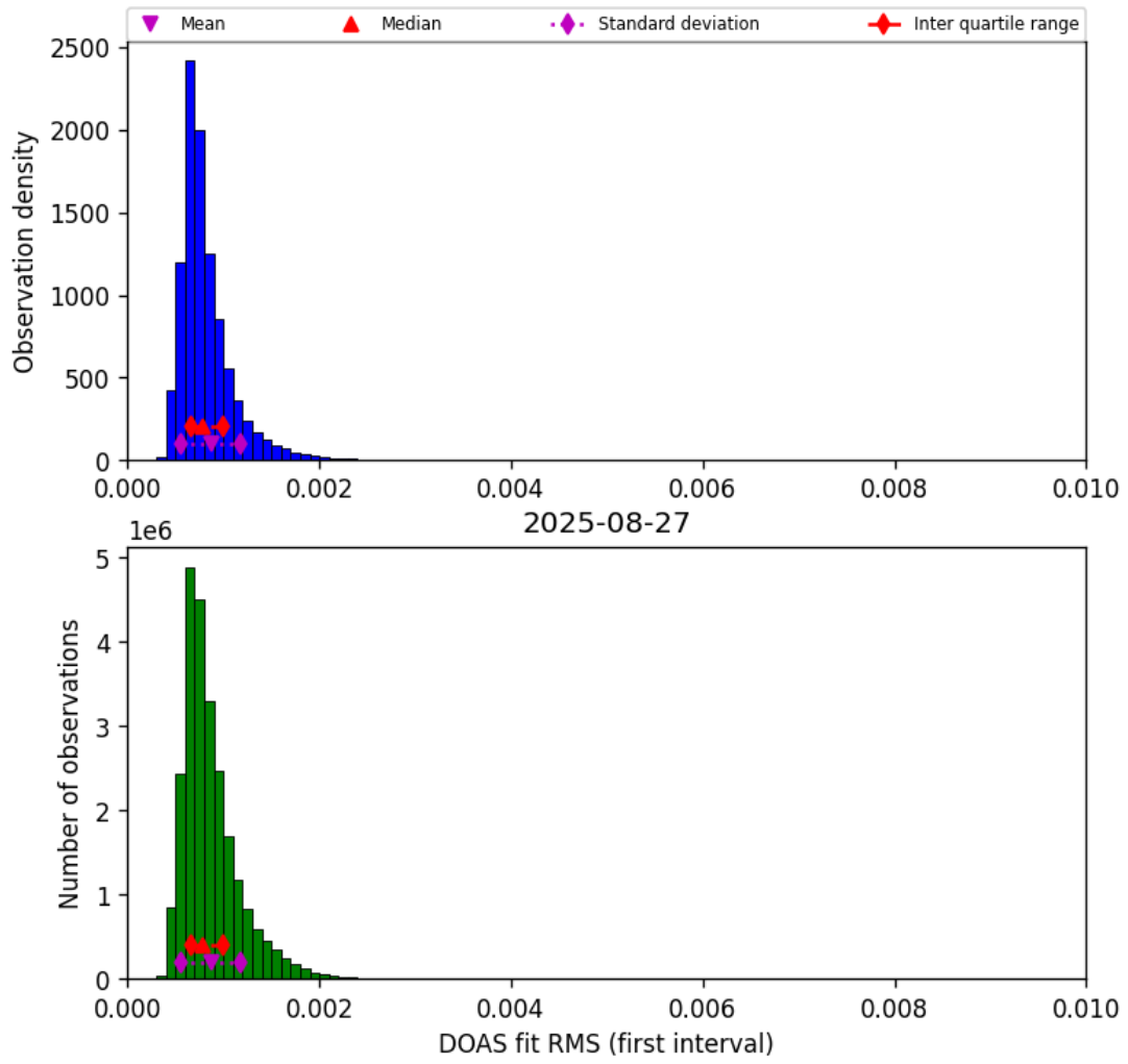
Figure 46: Histogram of “DOAS fit RMS (first interval)” for 2025-08-26 to 2025-08-28
