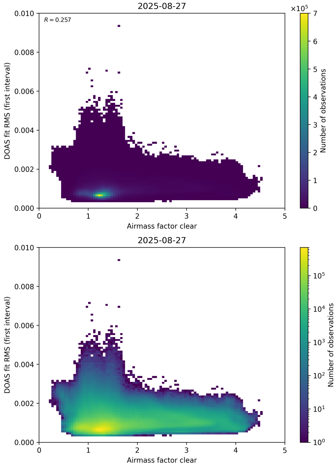
Figure 71: Scatter density plot of “Airmass factor clear” against “DOAS fit RMS (first interval)” for 2025-08-26 to 2025-08-28.
