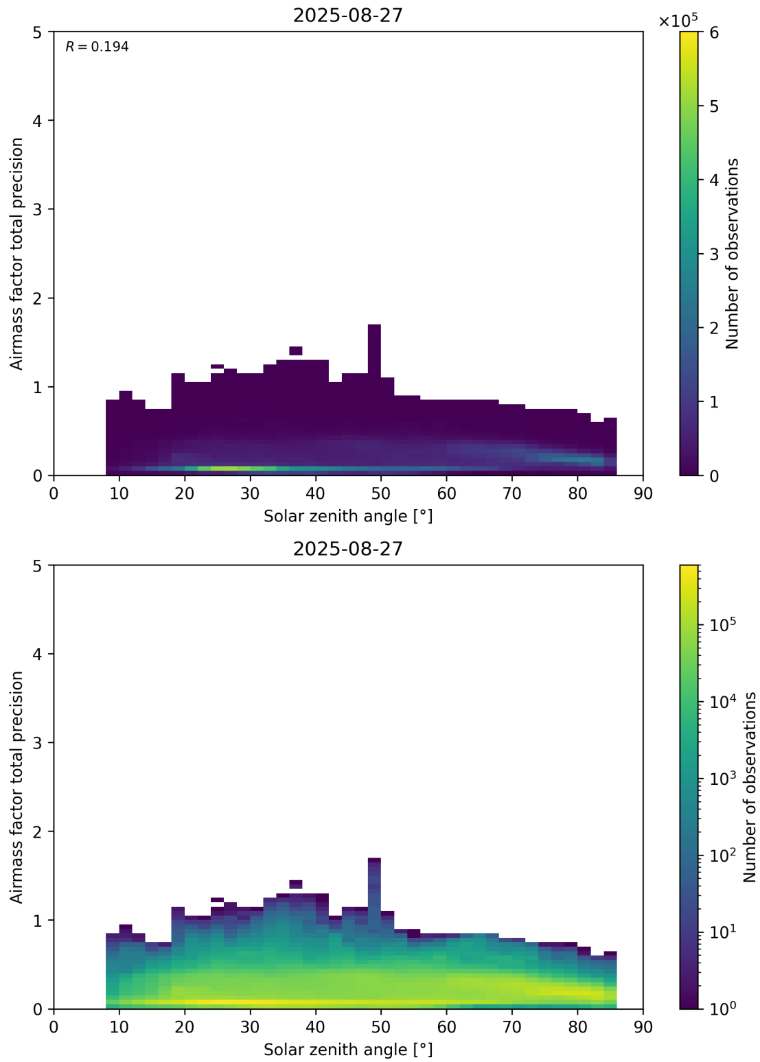
Figure 176: Scatter density plot of “Solar zenith angle” against “Airmass factor total precision” for 2025-08-26 to 2025-08-28.
