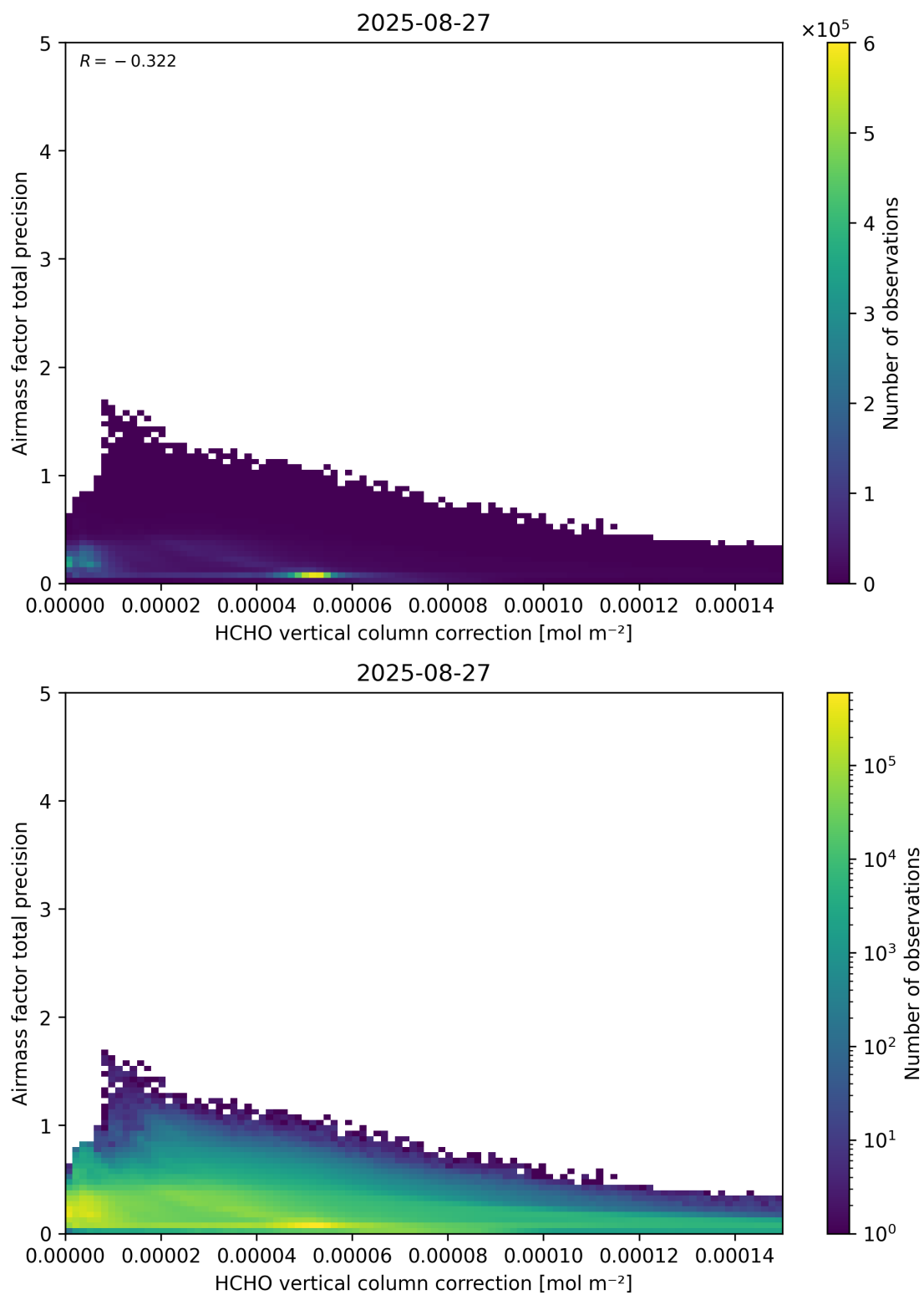
Figure 121: Scatter density plot of “HCHO vertical column correction” against “Airmass factor total precision” for 2025-08-26 to 2025-08-28.
