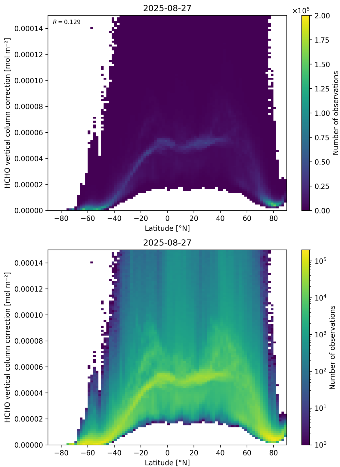
Figure 164: Scatter density plot of “Latitude” against “HCHO vertical column correction” for 2025-08-26 to 2025-08-28.
