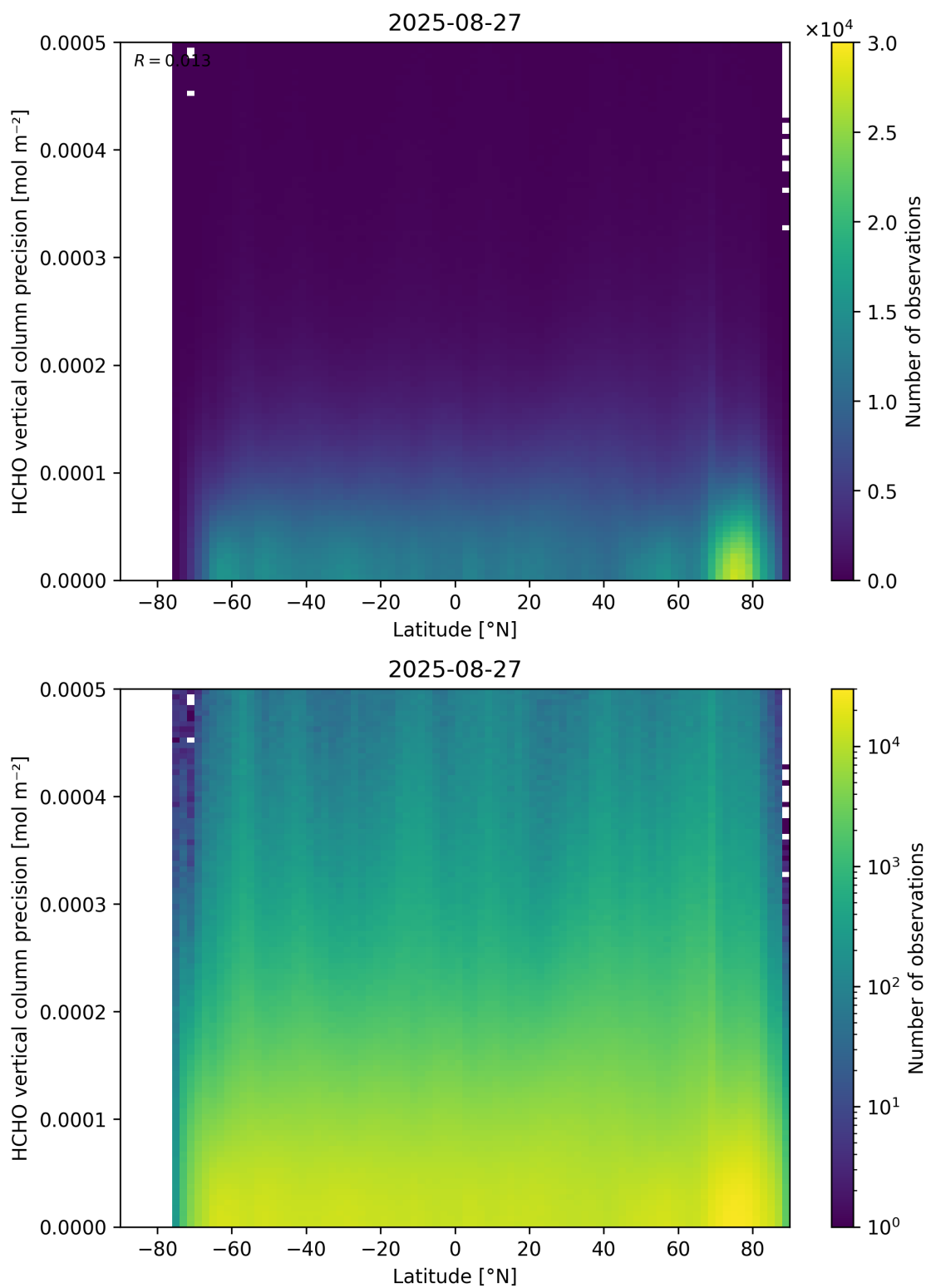
Figure 165: Scatter density plot of “Latitude” against “HCHO vertical column precision” for 2025-08-26 to 2025-08-28.
