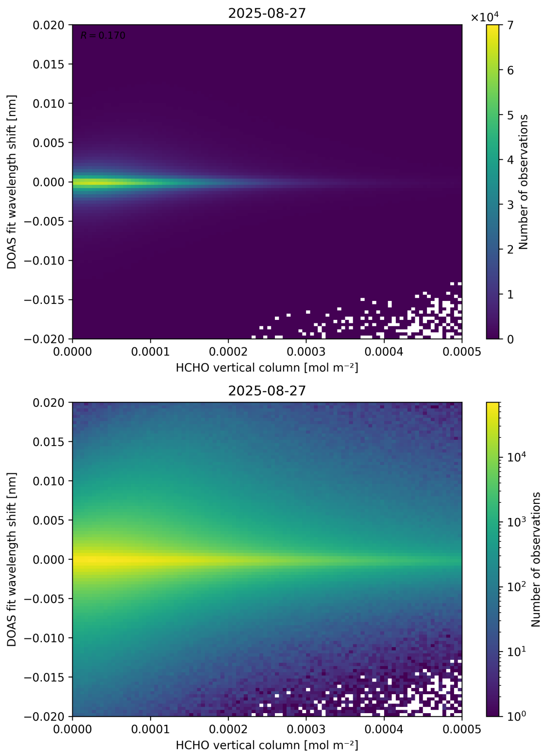
Figure 124: Scatter density plot of “HCHO vertical column” against “DOAS fit wavelength shift” for 2025-08-26 to 2025-08-28.
