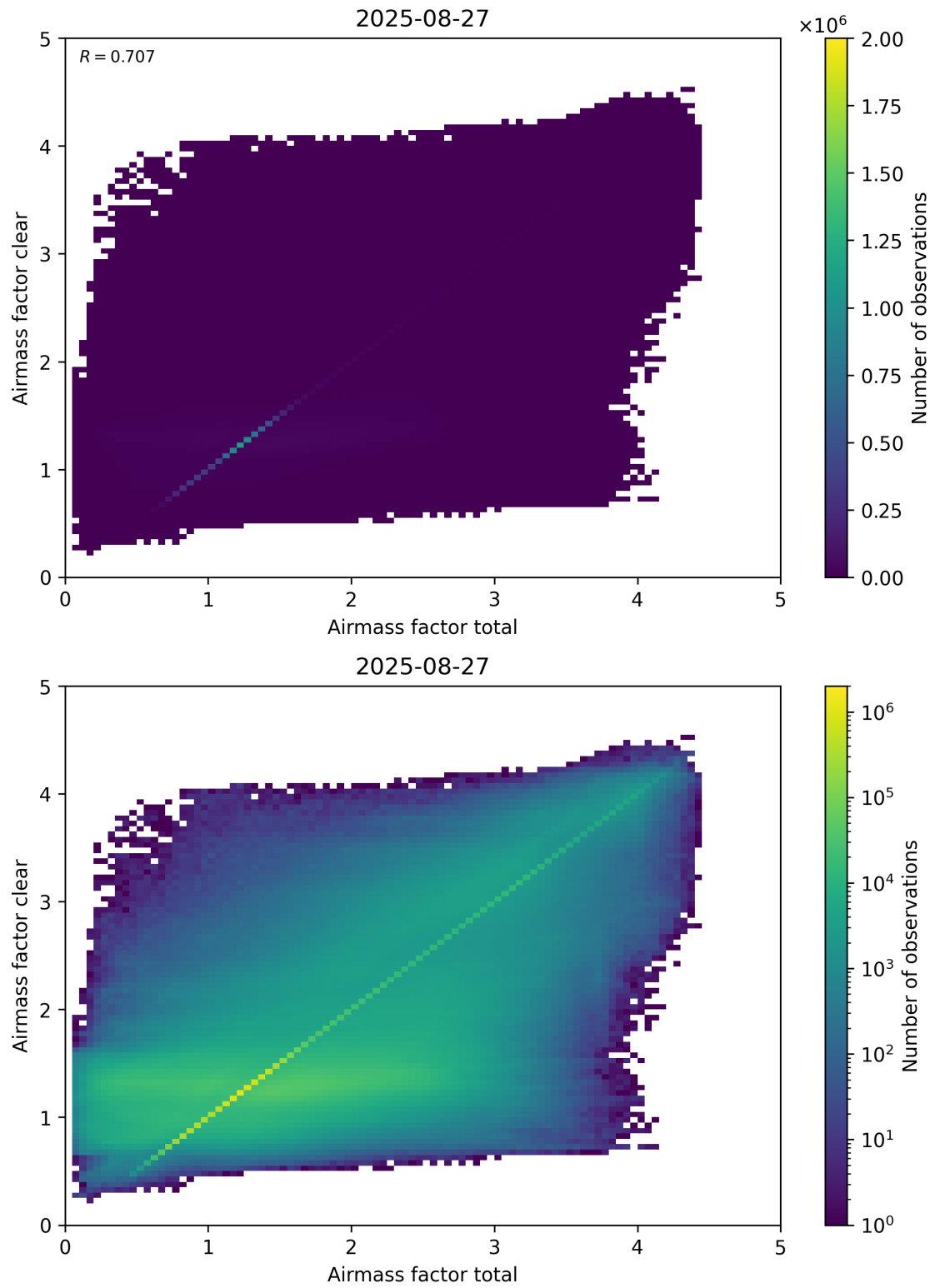
Figure 100: Scatter density plot of “Airmass factor total” against “Airmass factor clear” for 2025-08-26 to 2025-08-28.
