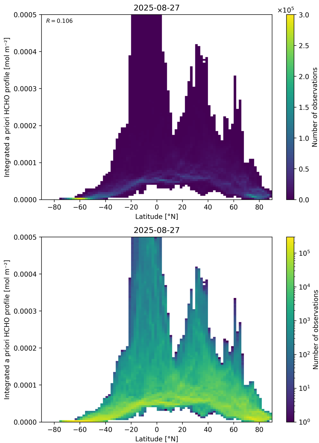
Figure 166: Scatter density plot of “Latitude” against “Integrated a priori HCHO profile” for 2025-08-26 to 2025-08-28.
