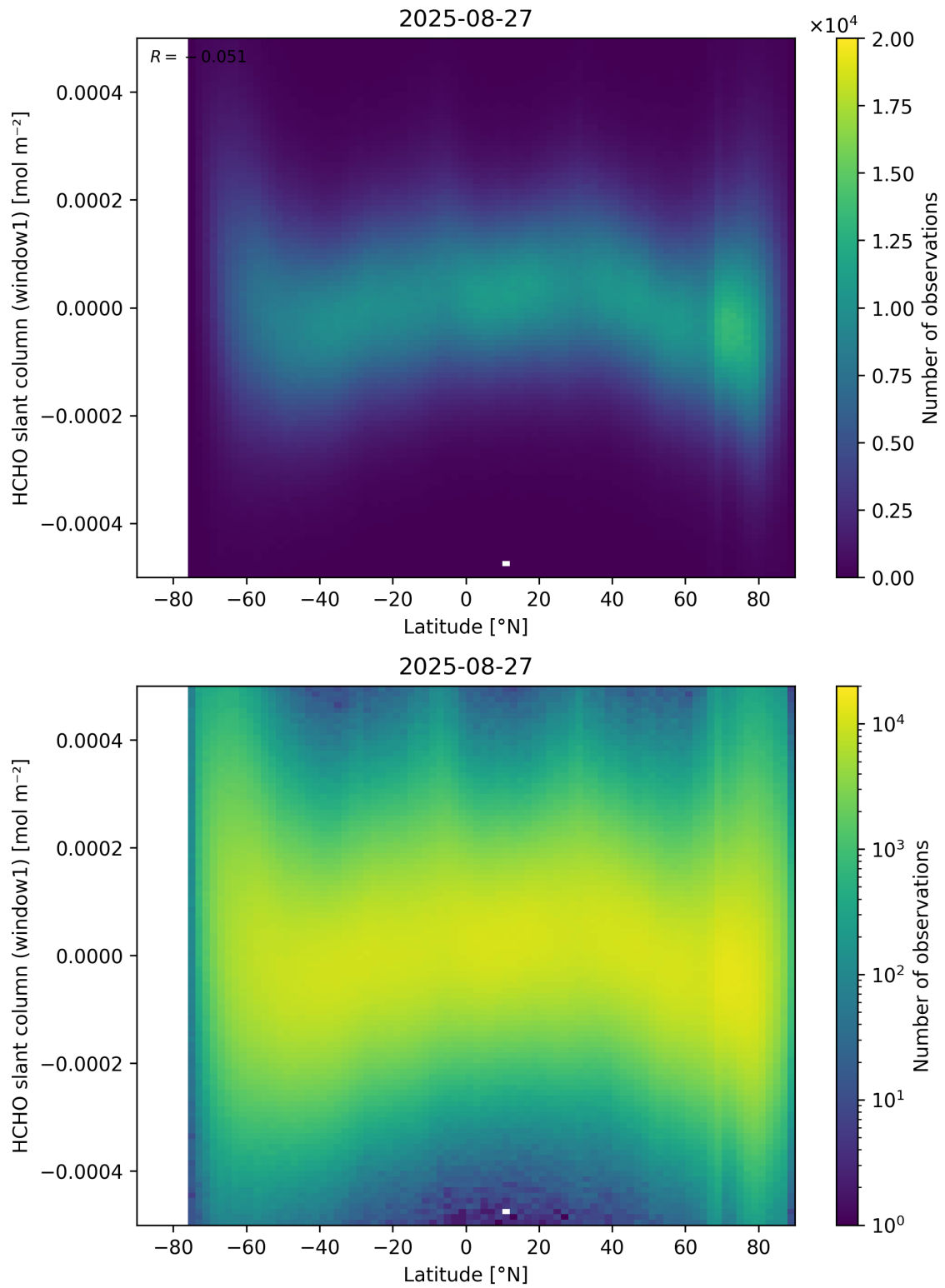
Figure 159: Scatter density plot of “Latitude” against “HCHO slant column (window1)” for 2025-08-26 to 2025-08-28.
