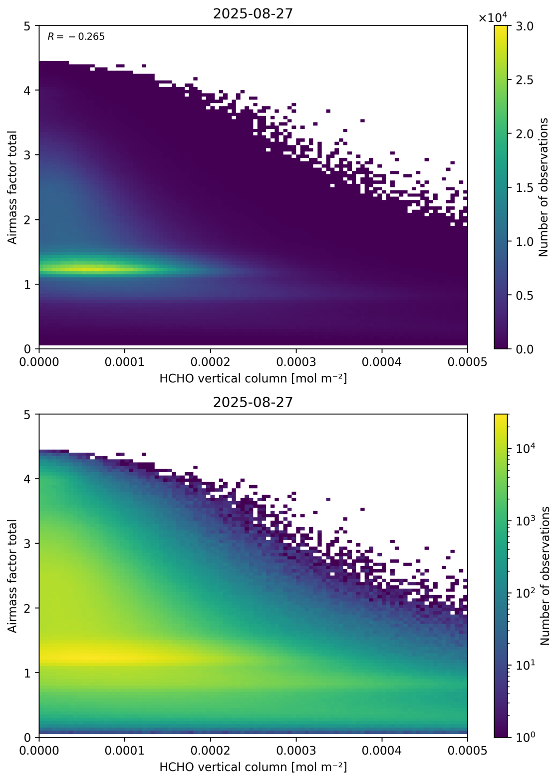
Figure 131: Scatter density plot of “HCHO vertical column” against “Airmass factor total” for 2025-08-26 to 2025-08-28.
