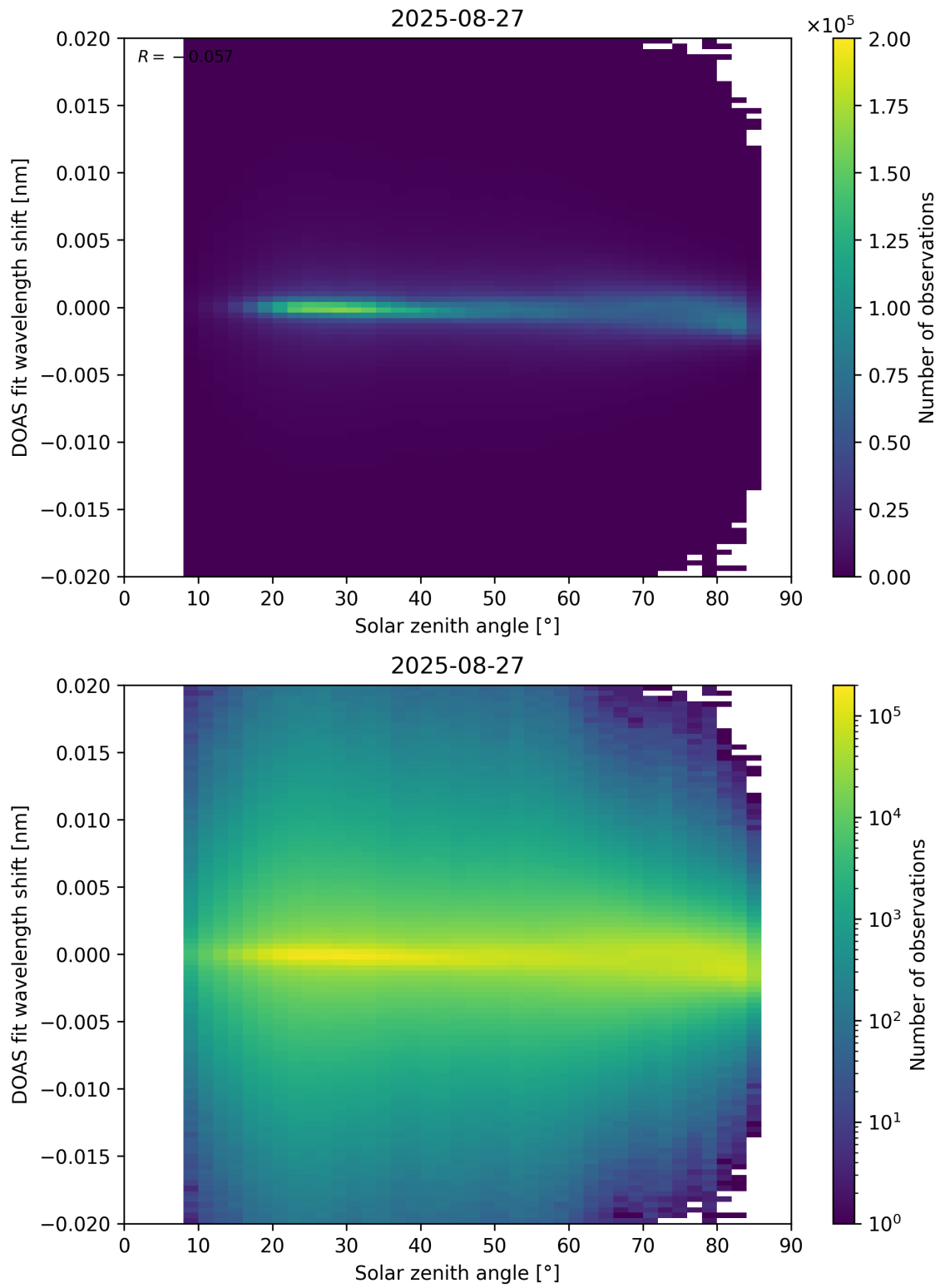
Figure 168: Scatter density plot of “Solar zenith angle” against “DOAS fit wavelength shift” for 2025-08-26 to 2025-08-28.
