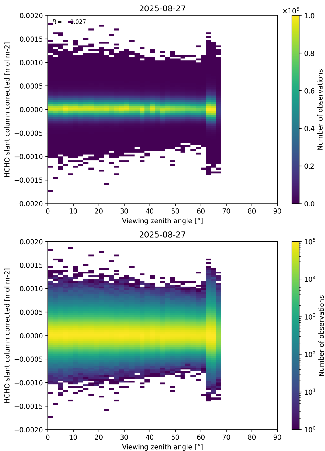
Figure 186: Scatter density plot of “Viewing zenith angle” against “HCHO slant column corrected” for 2025-08-26 to 2025-08-28.
