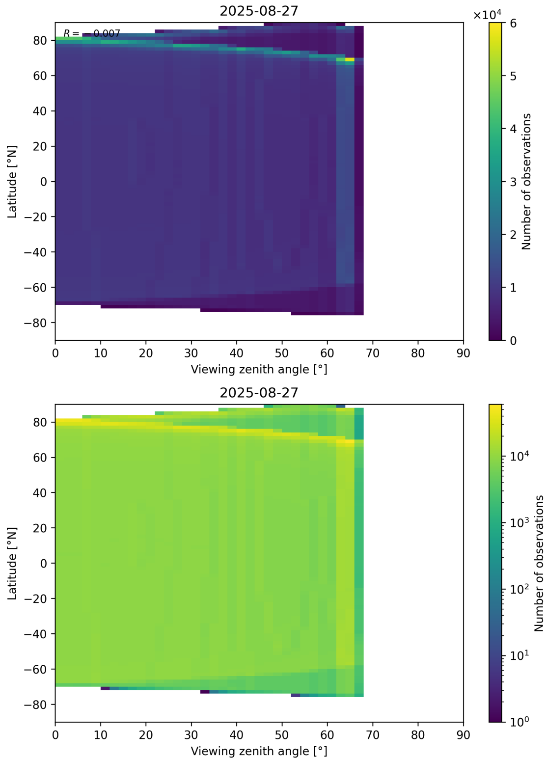
Figure 196: Scatter density plot of “Viewing zenith angle” against “Latitude” for 2025-08-26 to 2025-08-28.
