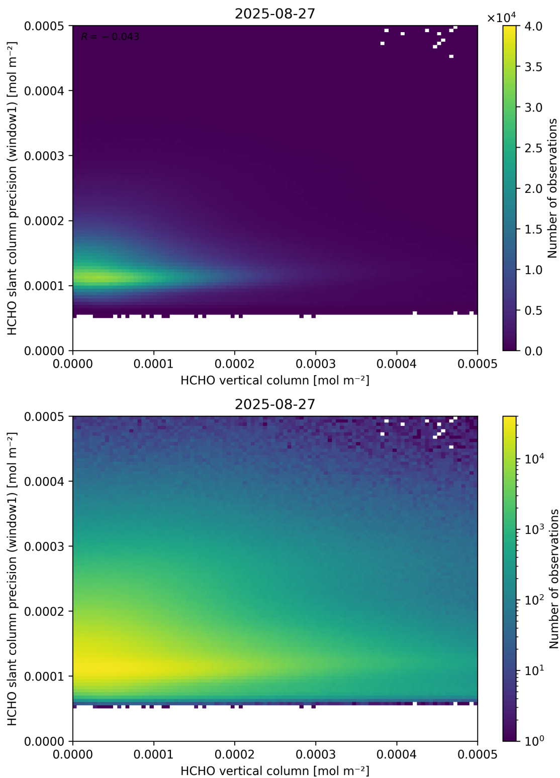
Figure 130: Scatter density plot of “HCHO vertical column” against “HCHO slant column precision (window1)” for 2025-08-26 to 2025-08-28.
