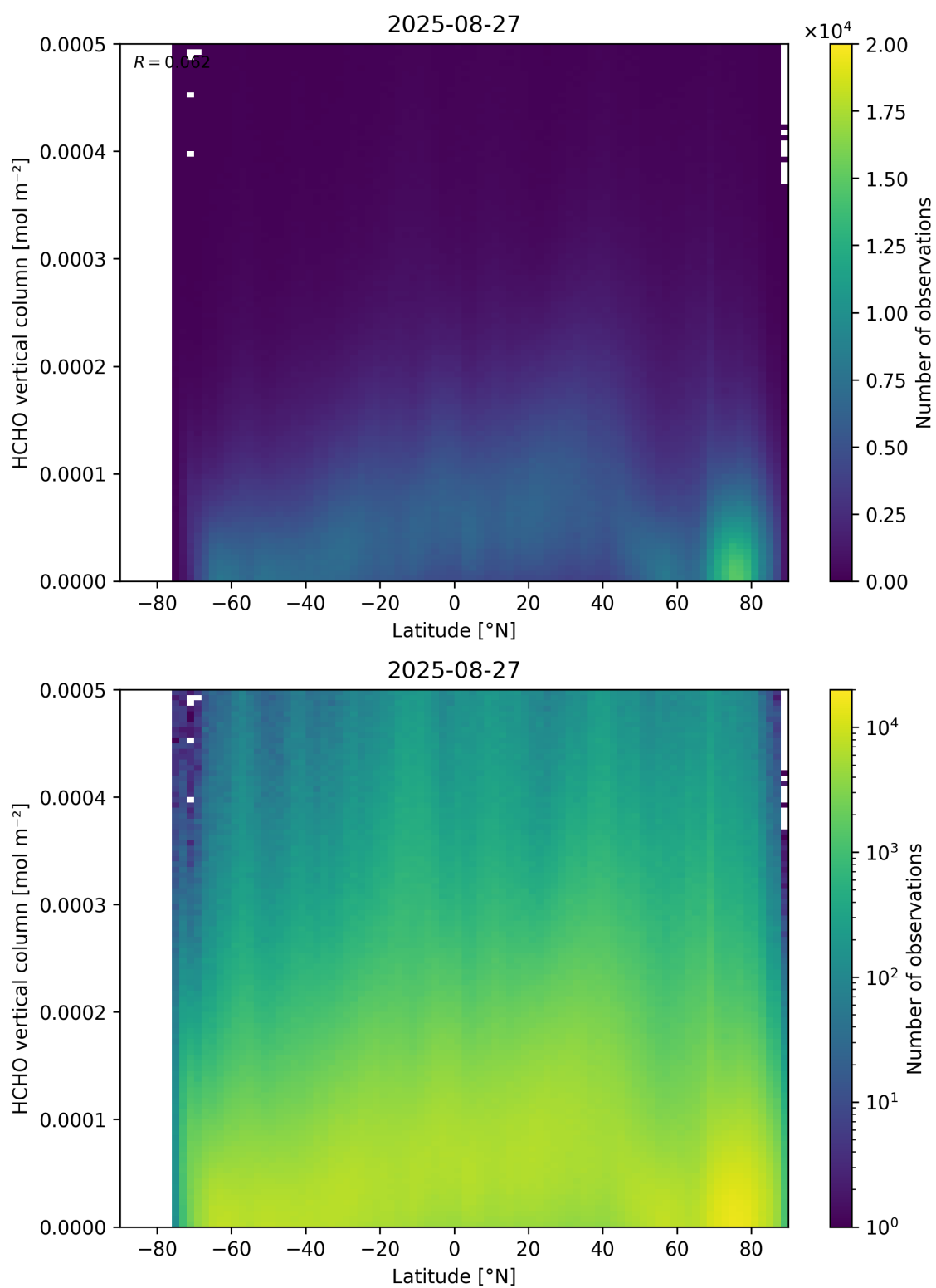
Figure 163: Scatter density plot of “Latitude” against “HCHO vertical column” for 2025-08-26 to 2025-08-28.
