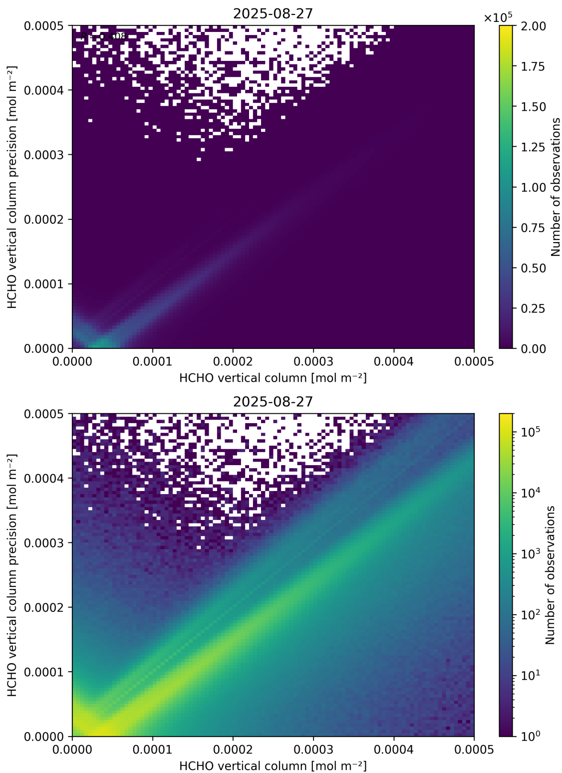
Figure 134: Scatter density plot of “HCHO vertical column” against “HCHO vertical column precision” for 2025-08-26 to 2025-08-28.
