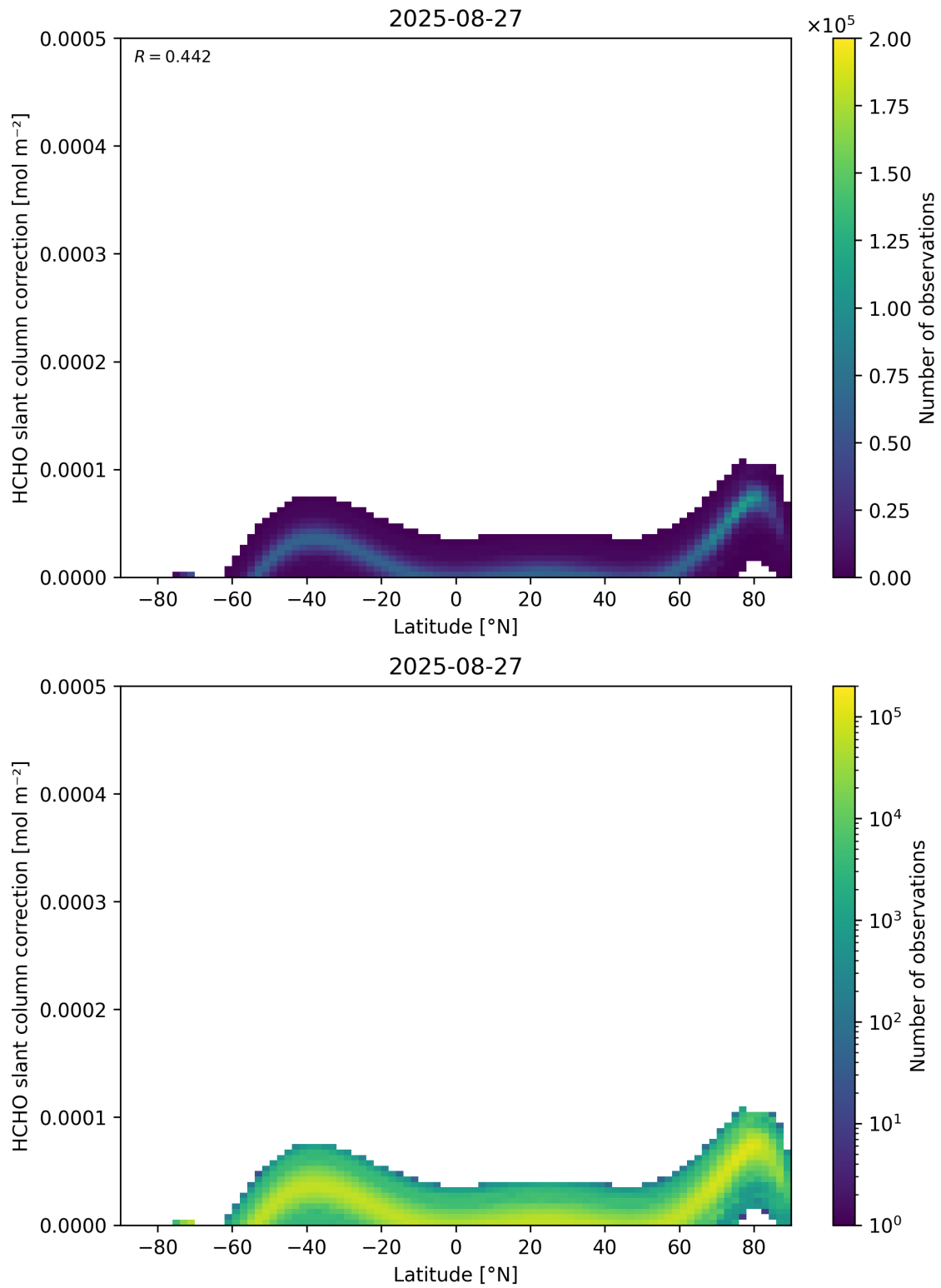
Figure 158: Scatter density plot of “Latitude” against “HCHO slant column correction” for 2025-08-26 to 2025-08-28.
