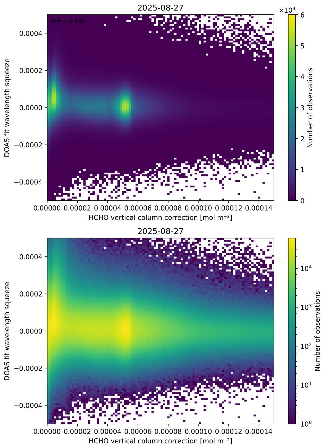
Figure 114: Scatter density plot of “HCHO vertical column correction” against “DOAS fit wavelength squeeze” for 2025-08-26 to 2025-08-28.
