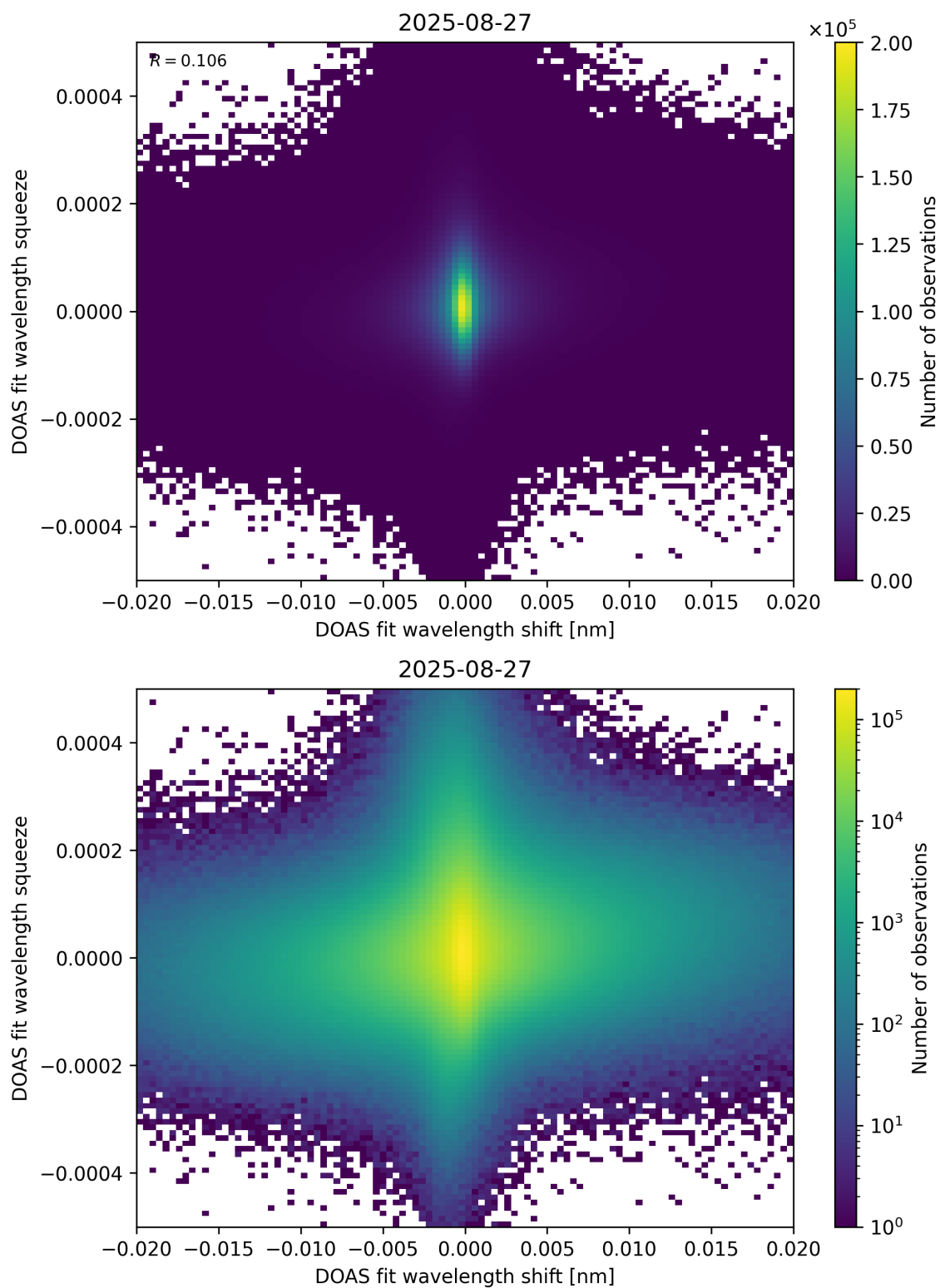
Figure 65: Scatter density plot of “DOAS fit wavelength shift” against “DOAS fit wavelength squeeze” for 2025-08-26 to 2025-08-28.
