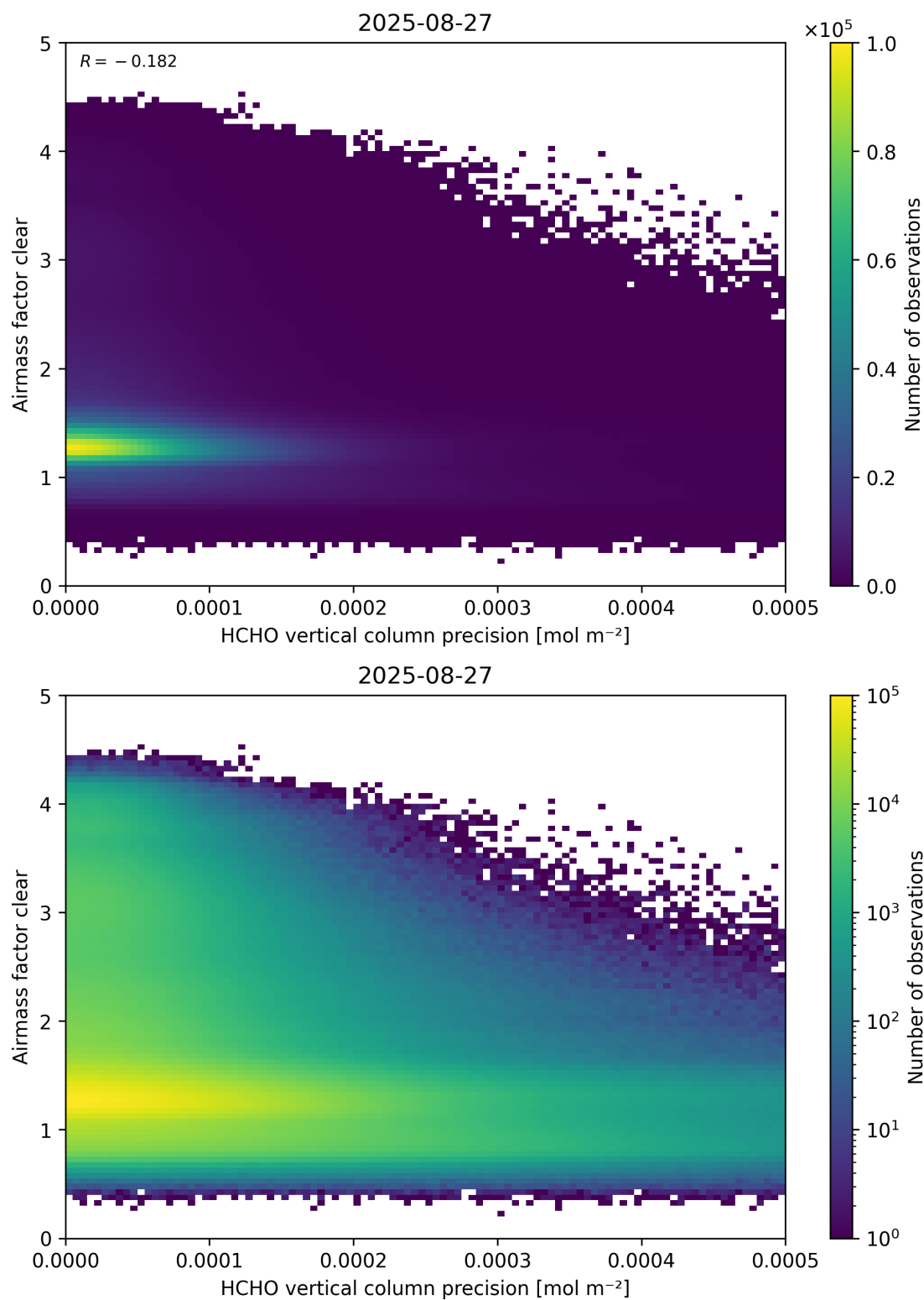
Figure 139: Scatter density plot of “HCHO vertical column precision” against “Airmass factor clear” for 2025-08-26 to 2025-08-28.
