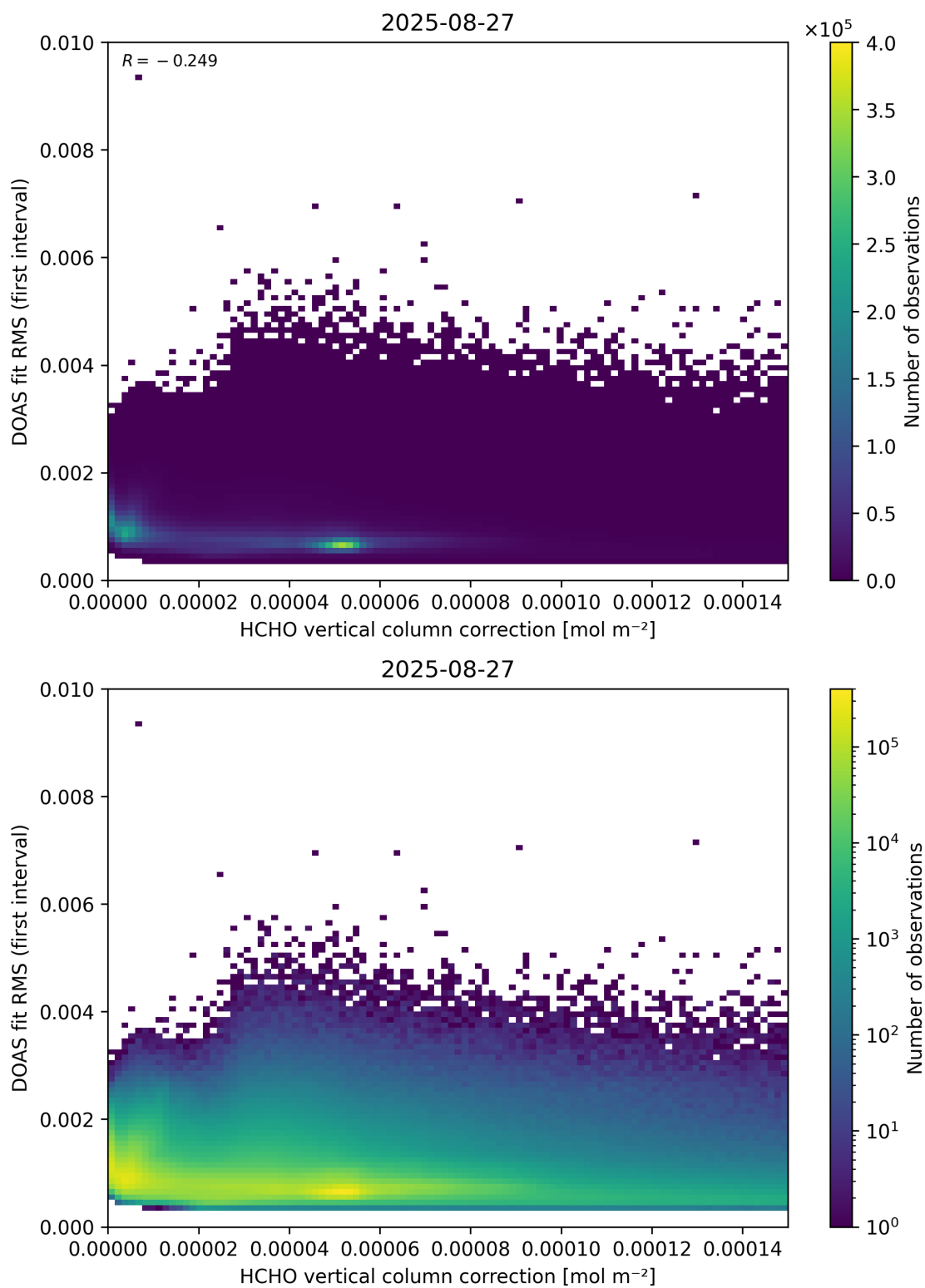
Figure 112: Scatter density plot of “HCHO vertical column correction” against “DOAS fit RMS (first interval)” for 2025-08-26 to 2025-08-28.
