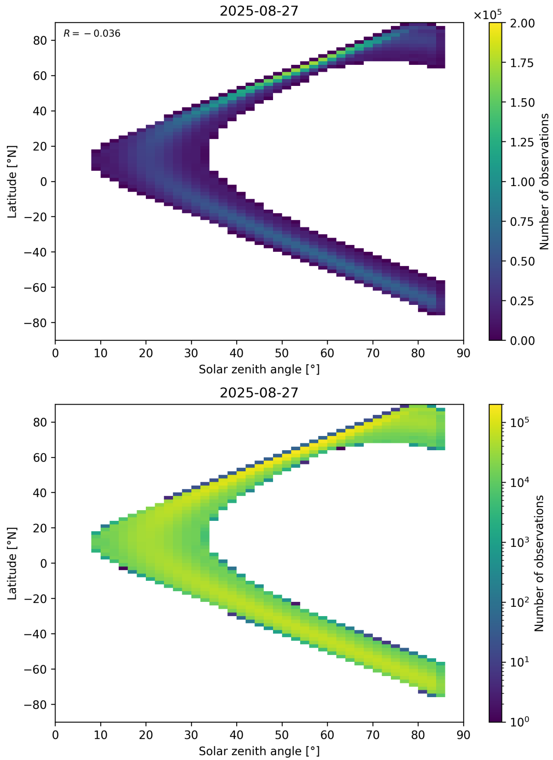
Figure 181: Scatter density plot of “Solar zenith angle” against “Latitude” for 2025-08-26 to 2025-08-28.
