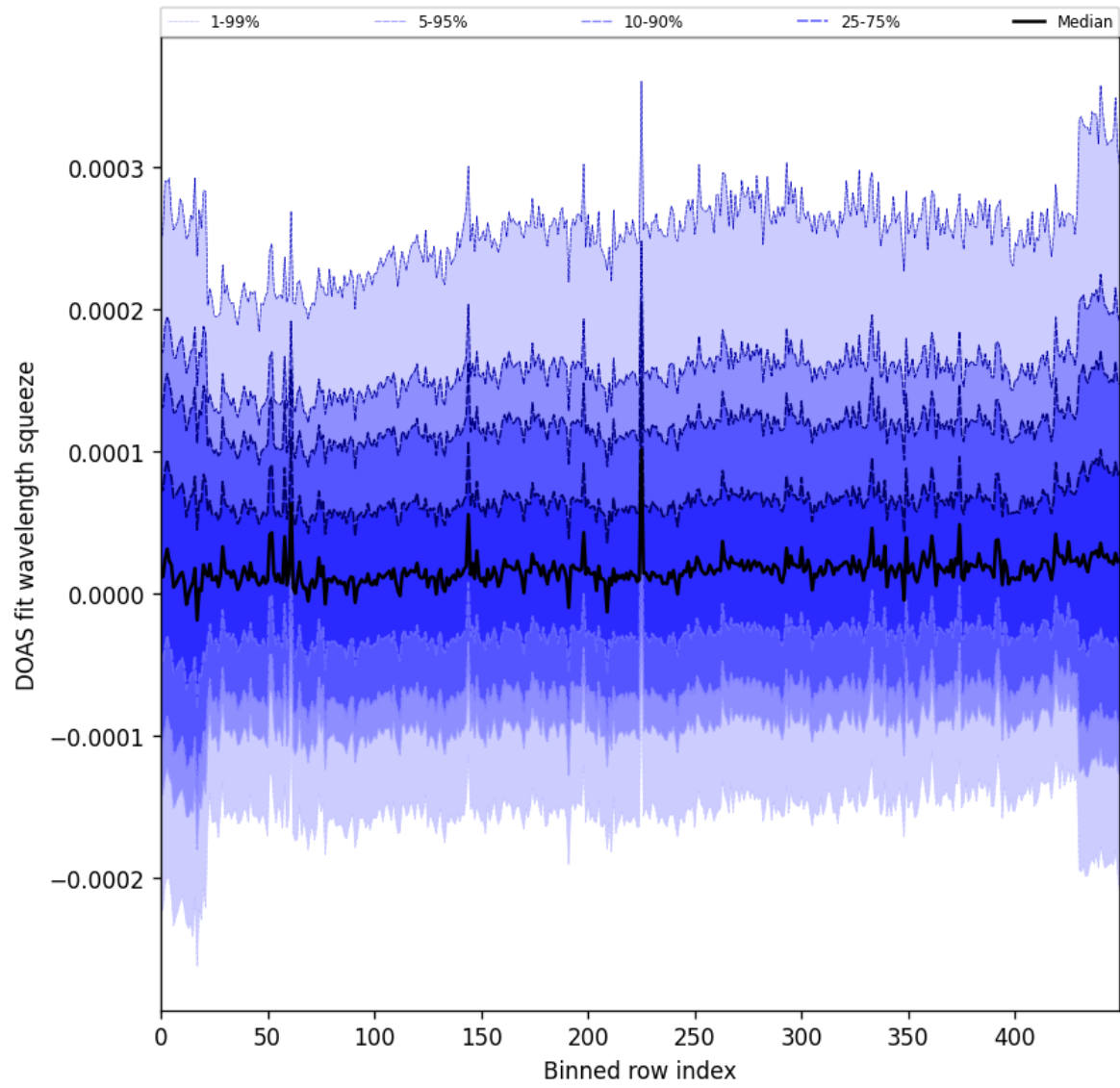
Figure 59: Along track statistics of “DOAS fit wavelength squeeze” for 2025-08-26 to 2025-08-28
