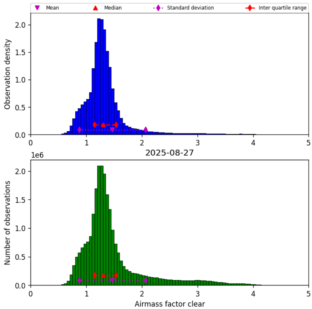
Figure 42: Histogram of “Airmass factor clear” for 2025-08-26 to 2025-08-28
