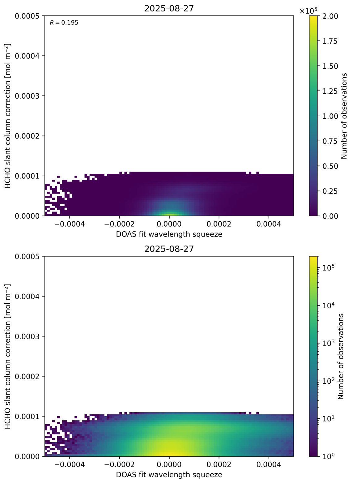
Figure 70: Scatter density plot of “DOAS fit wavelength squeeze” against “HCHO slant column correction” for 2025-08-26 to 2025-08-28.
