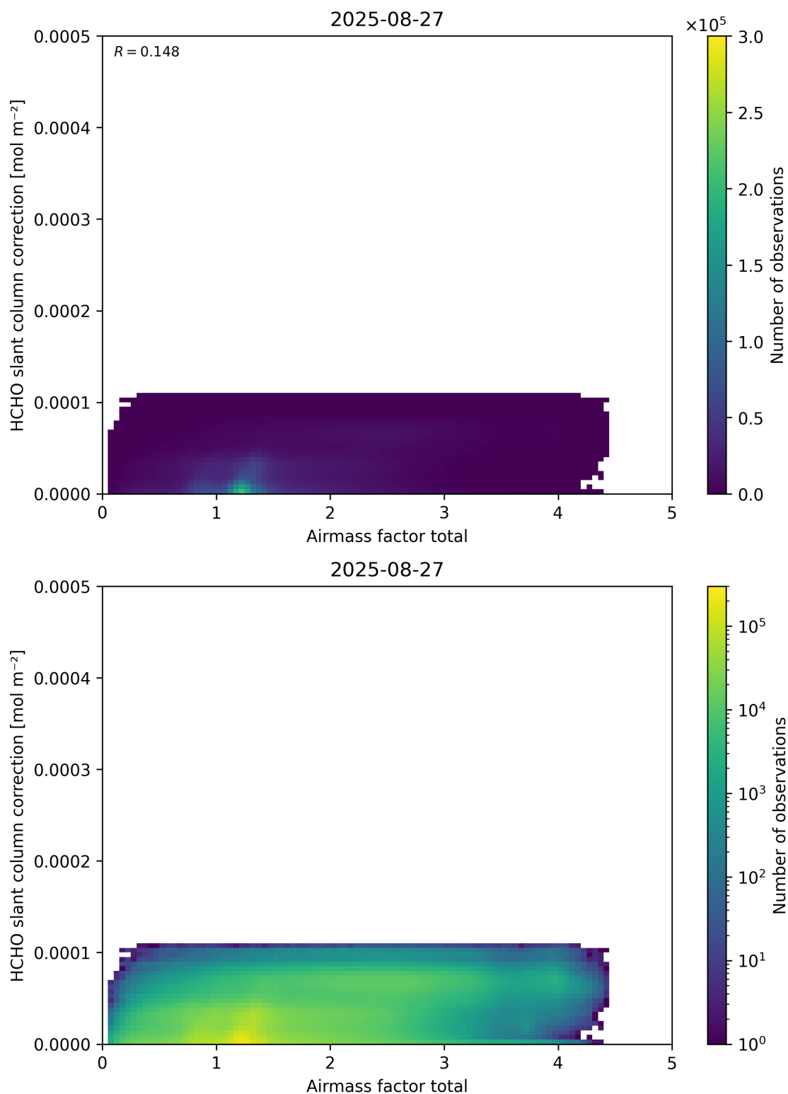
Figure 102: Scatter density plot of “Airmass factor total” against “HCHO slant column correction” for 2025-08-26 to 2025-08-28.
