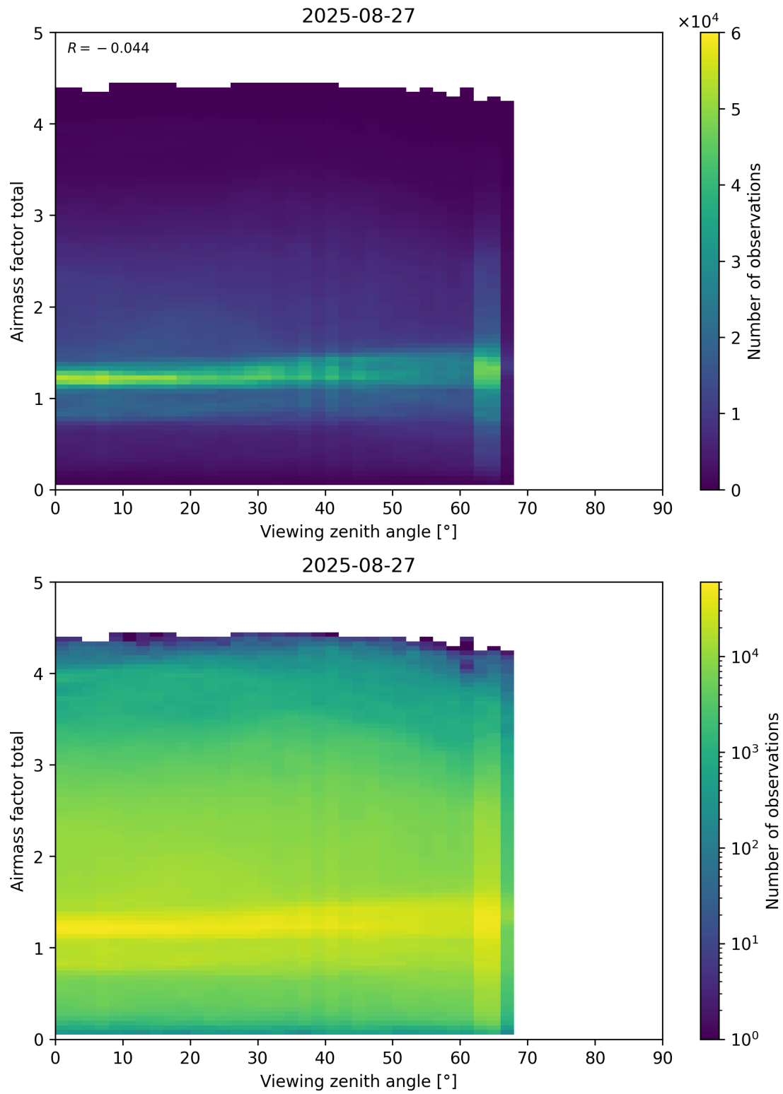
Figure 190: Scatter density plot of “Viewing zenith angle” against “Airmass factor total” for 2025-08-26 to 2025-08-28.
