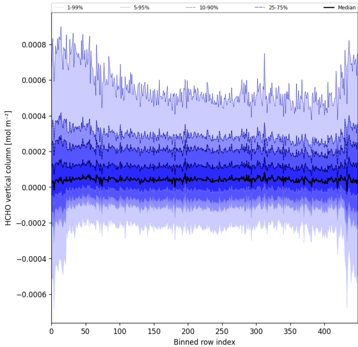
Figure 49: Along track statistics of “HCHO vertical column” for 2025-08-26 to 2025-08-28
