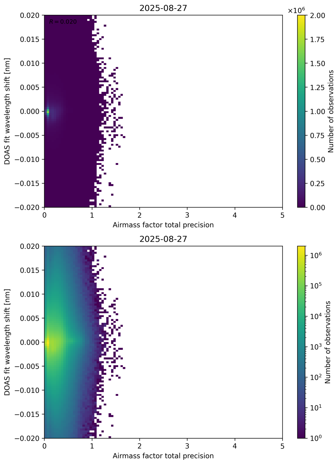
Figure 106: Scatter density plot of “Airmass factor total precision” against “DOAS fit wavelength shift” for 2025-08-26 to 2025-08-28.
