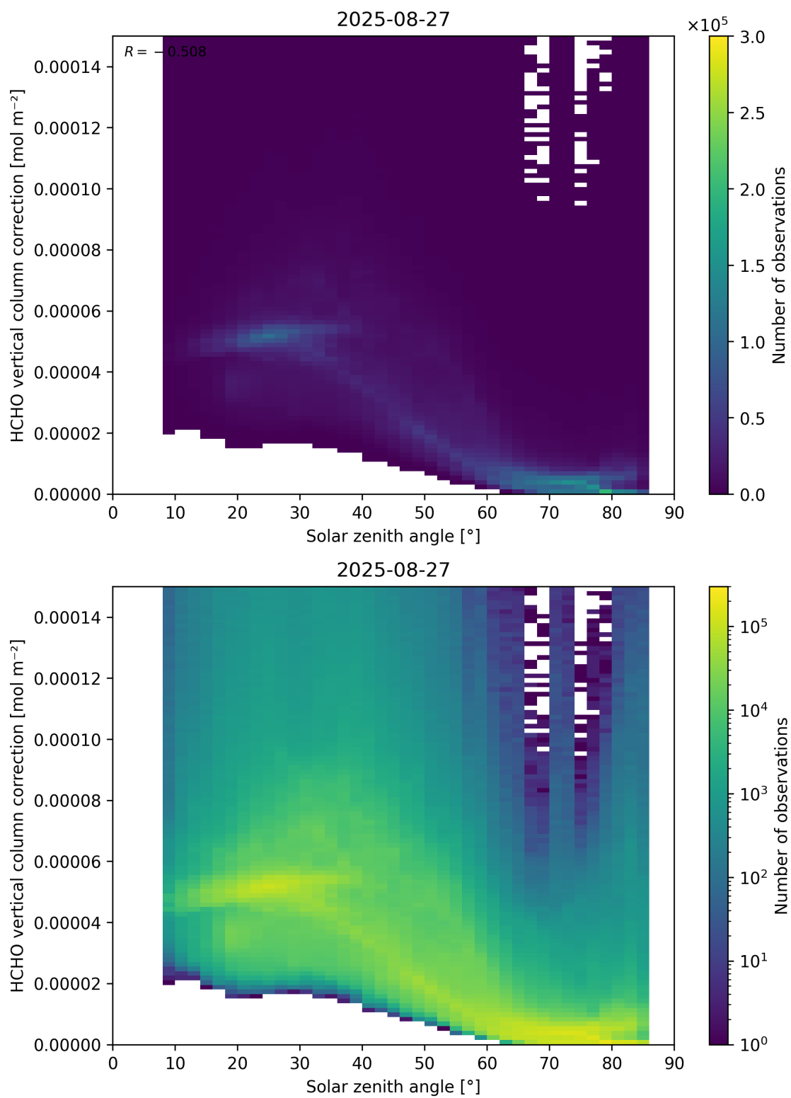
Figure 178: Scatter density plot of “Solar zenith angle” against “HCHO vertical column correction” for 2025-08-26 to 2025-08-28.
