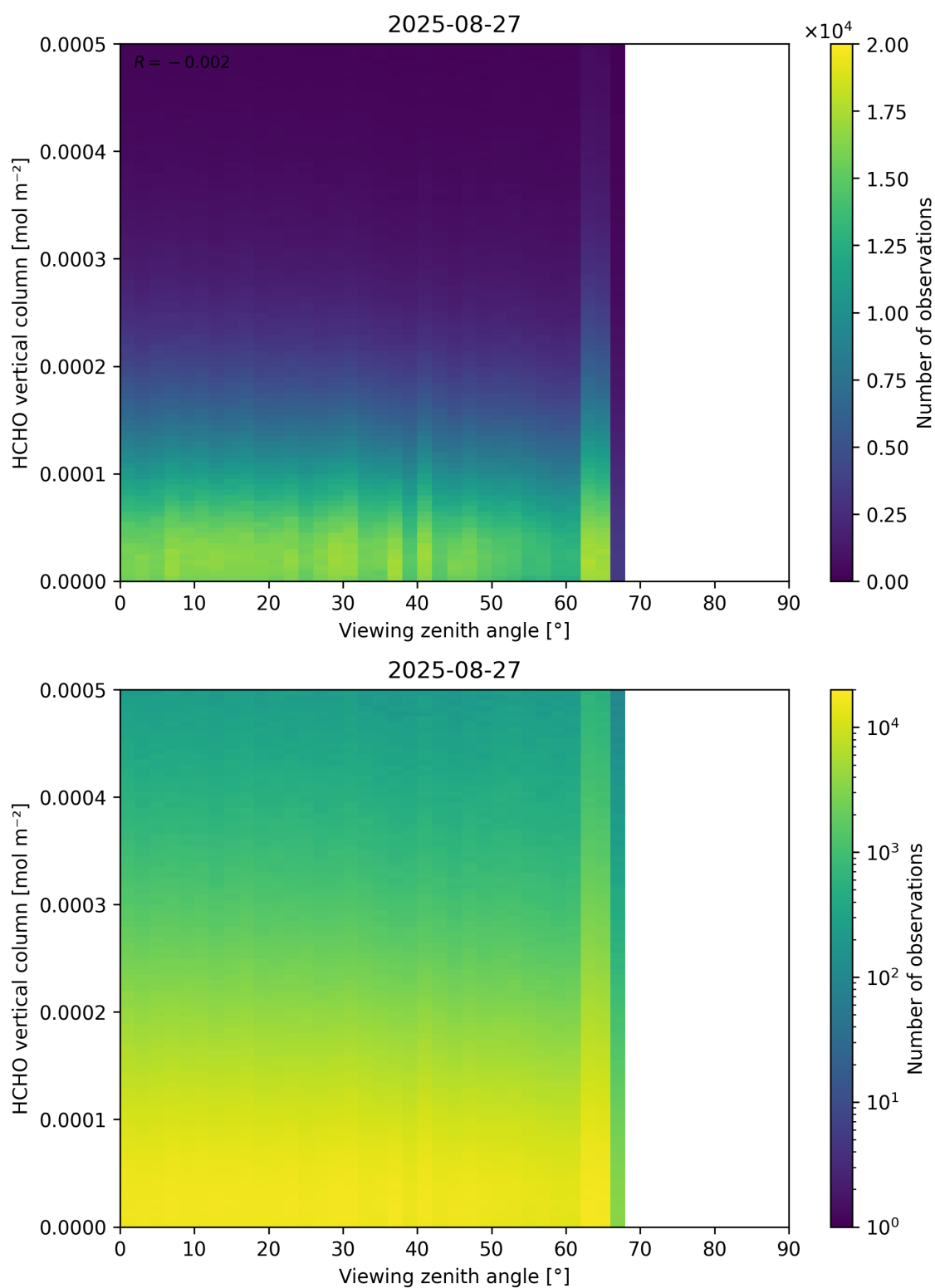
Figure 192: Scatter density plot of “Viewing zenith angle” against “HCHO vertical column” for 2025-08-26 to 2025-08-28.
