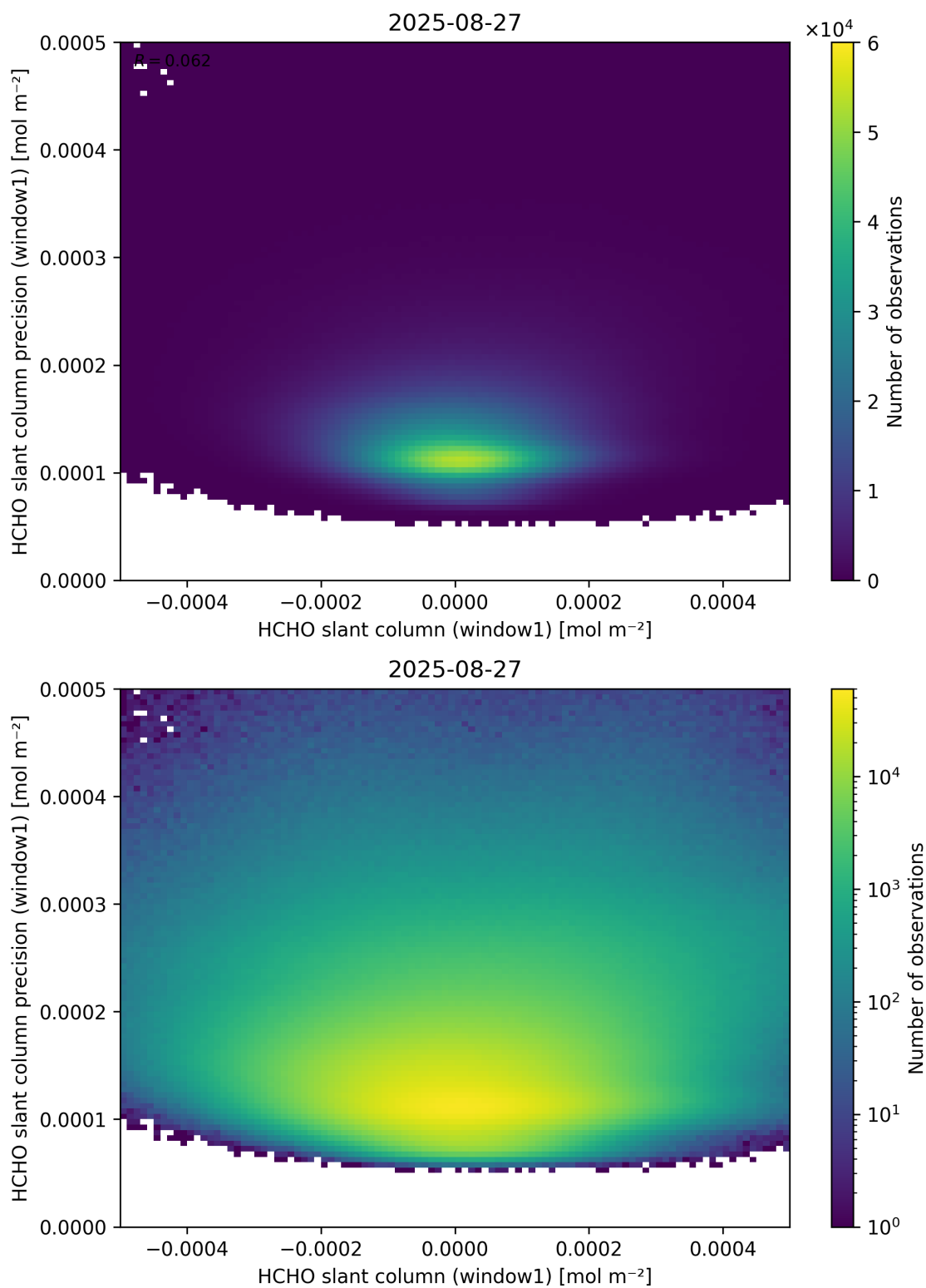
Figure 84: Scatter density plot of “HCHO slant column (window1)” against “HCHO slant column precision (window1)” for 2025-08-26 to 2025-08-28.
