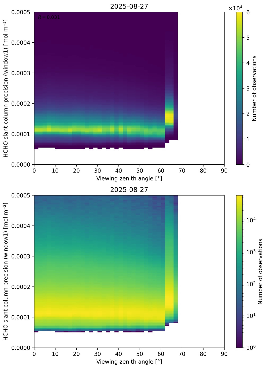
Figure 189: Scatter density plot of “Viewing zenith angle” against “HCHO slant column precision (window1)” for 2025-08-26 to 2025-08-28.
