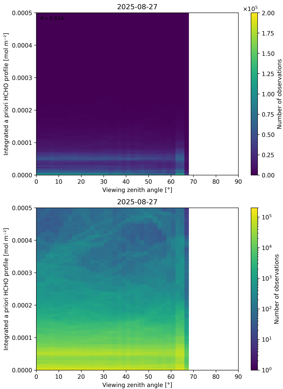
Figure 195: Scatter density plot of “Viewing zenith angle” against “Integrated a priori HCHO profile” for 2025-08-26 to 2025-08-28.
