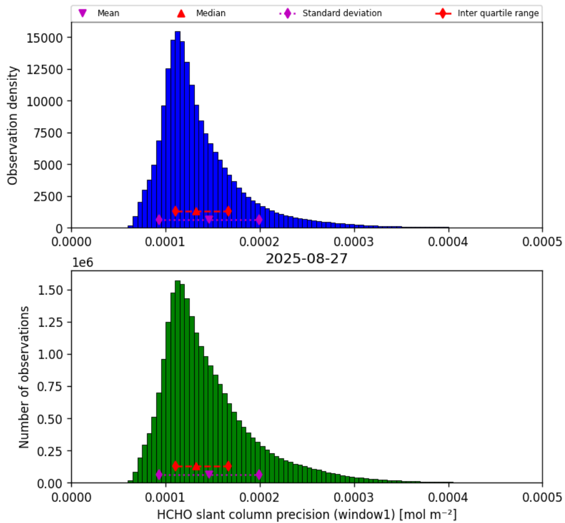
Figure 39: Histogram of “HCHO slant column precision (window1)” for 2025-08-26 to 2025-08-28
