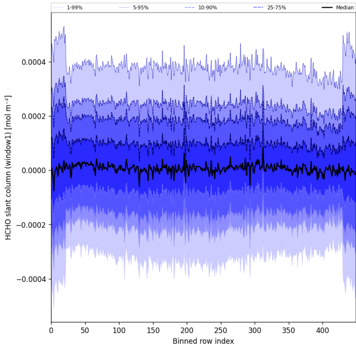
Figure 52: Along track statistics of “HCHO slant column (window1)” for 2025-08-26 to 2025-08-28
