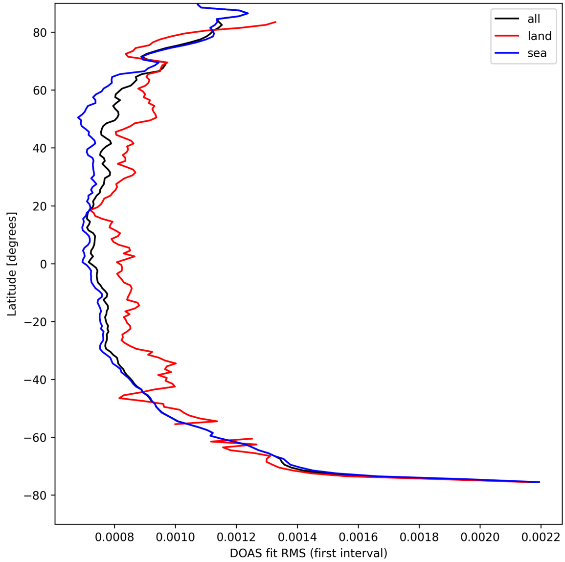
Figure 32: Zonal average of “DOAS fit RMS (first interval)” for 2025-08-26 to 2025-08-28.
