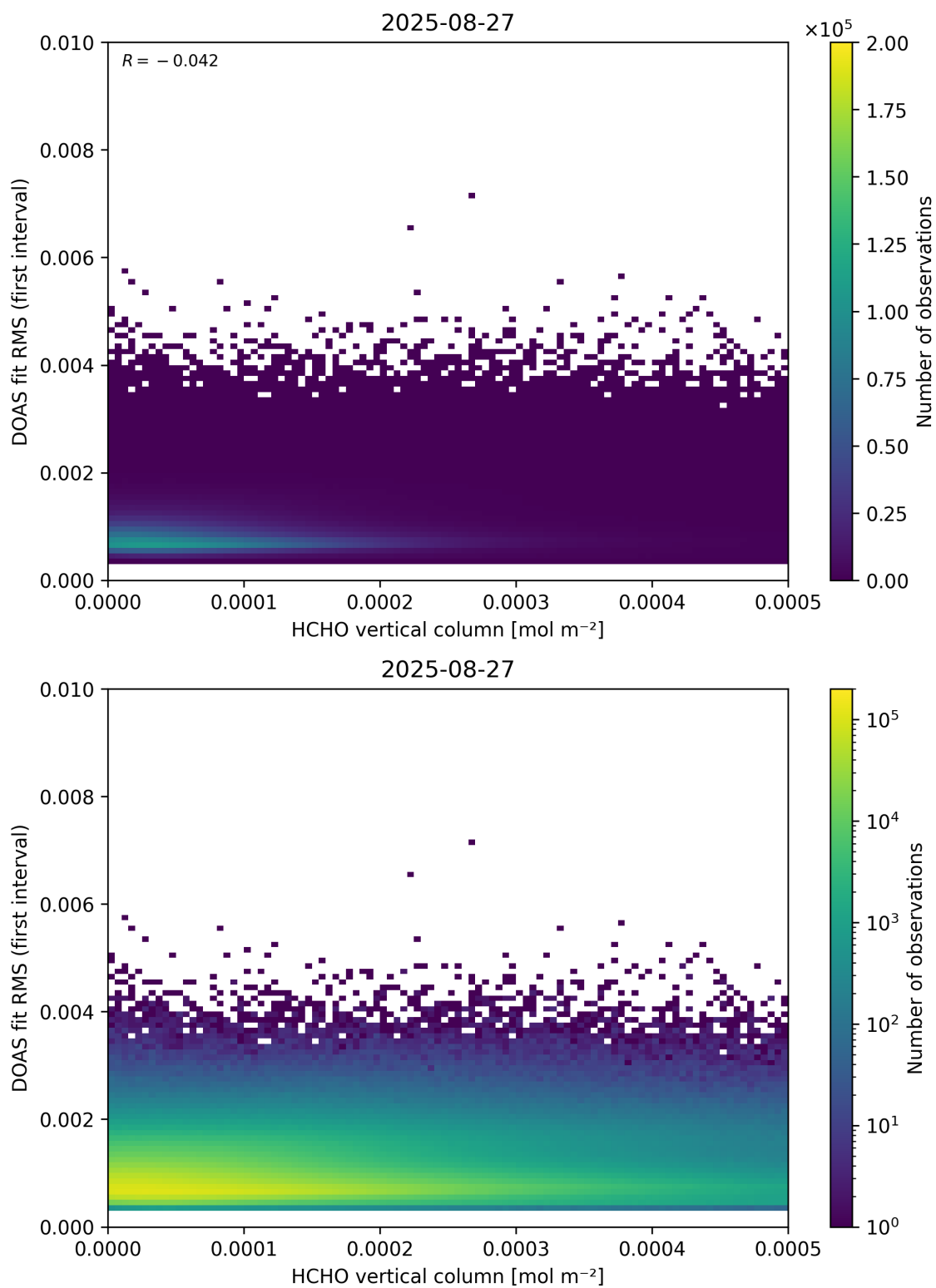
Figure 123: Scatter density plot of “HCHO vertical column” against “DOAS fit RMS (first interval)” for 2025-08-26 to 2025-08-28.
