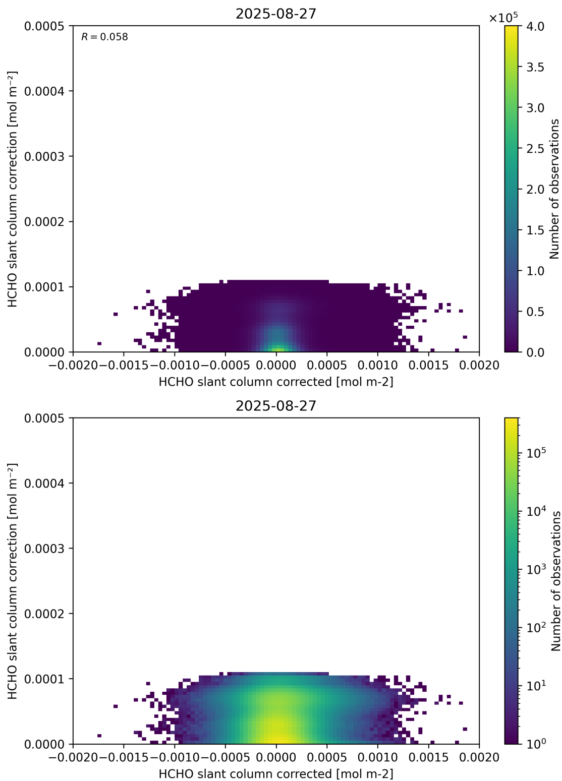
Figure 77: Scatter density plot of “HCHO slant column corrected” against “HCHO slant column correction” for 2025-08-26 to 2025-08-28.
