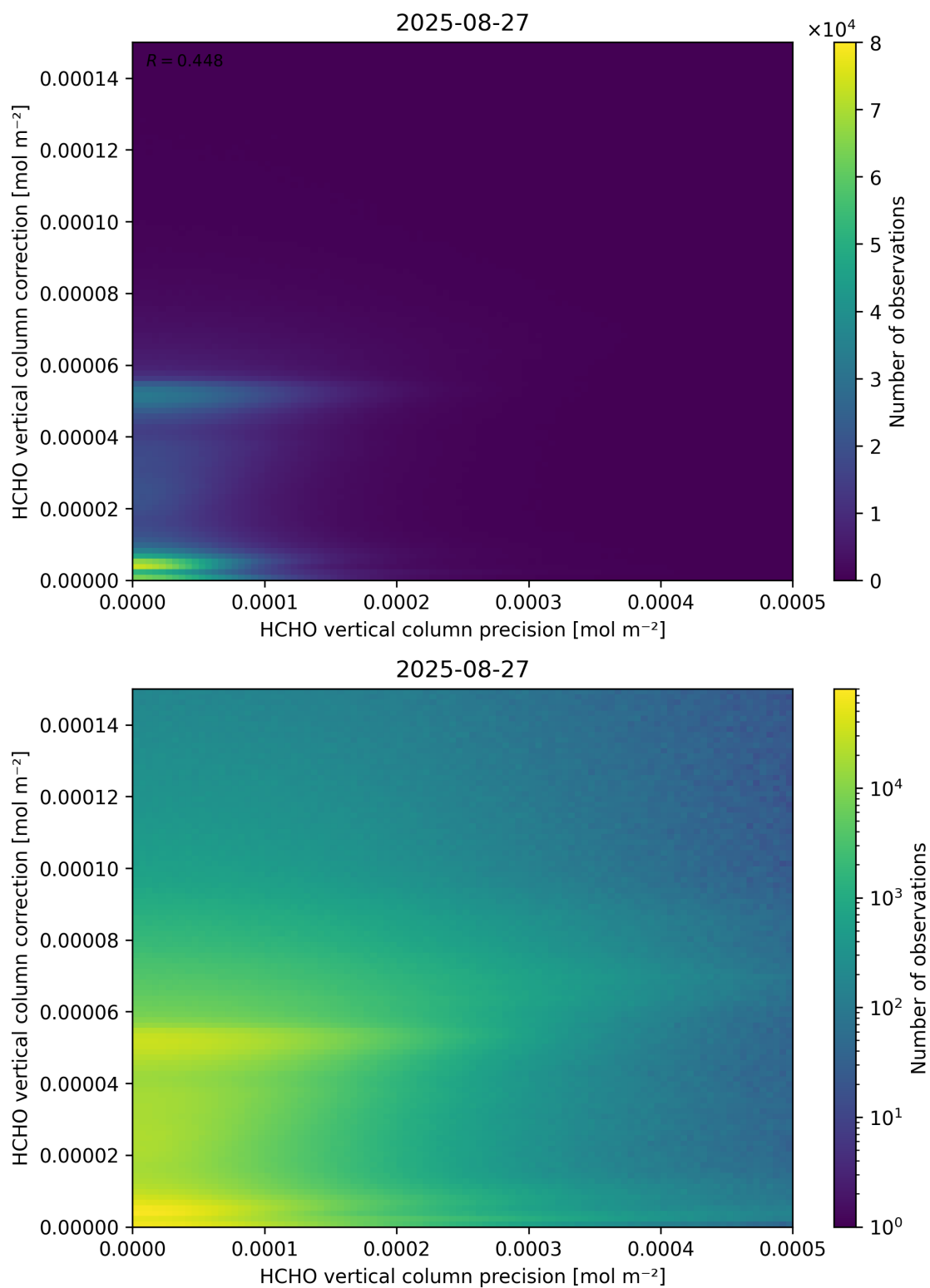
Figure 146: Scatter density plot of “HCHO vertical column precision” against “HCHO vertical column correction” for 2025-08-26 to 2025-08-28.
