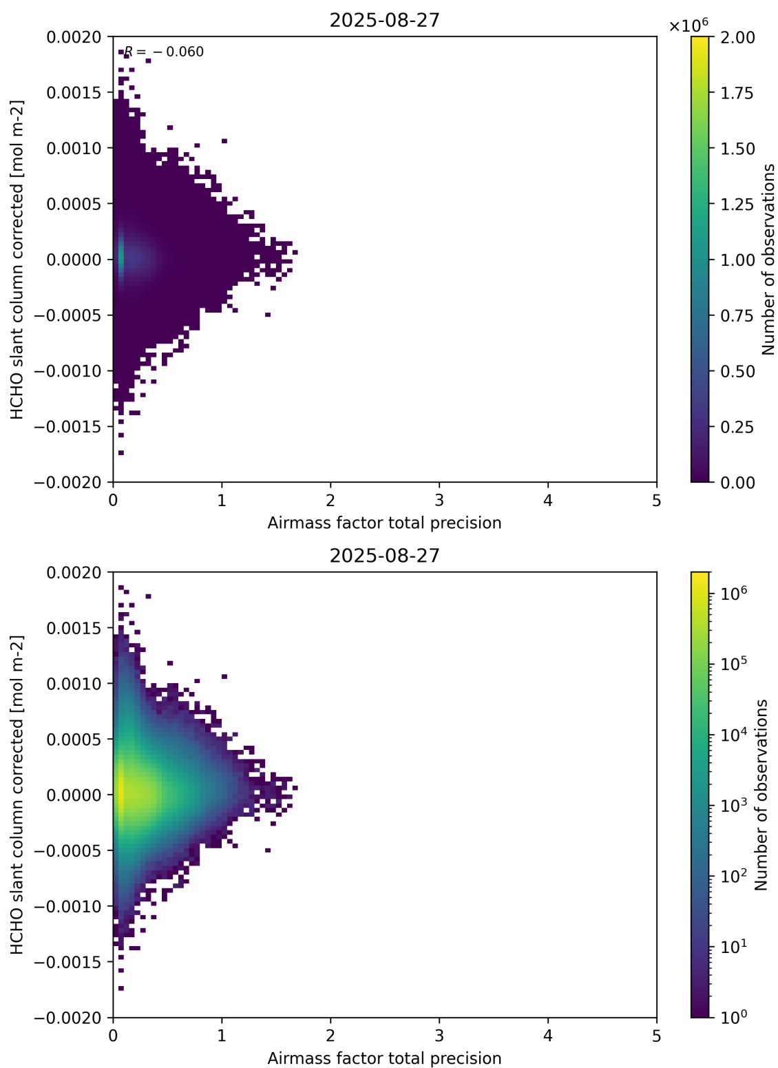
Figure 109: Scatter density plot of “Airmass factor total precision” against “HCHO slant column corrected” for 2025-08-26 to 2025-08-28.
