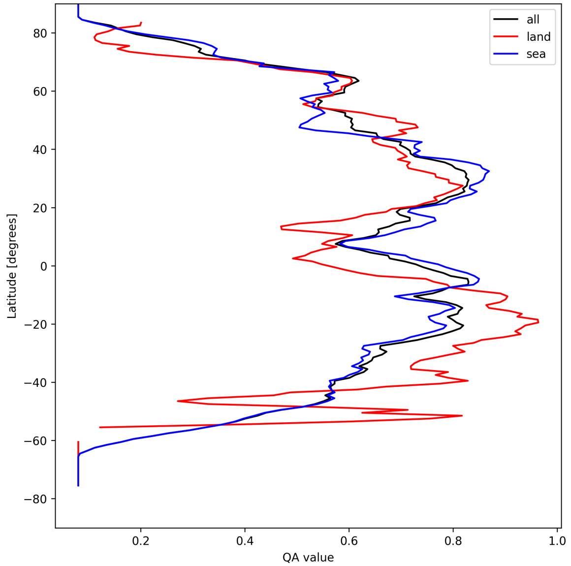
Figure 20: Zonal average of “QA value” for 2025-08-26 to 2025-08-28.
