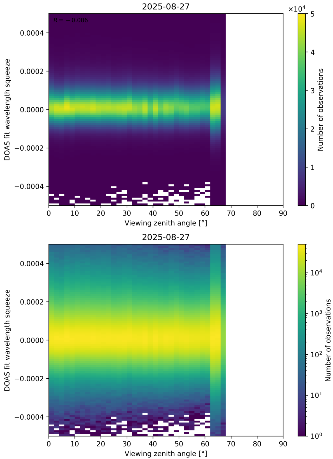
Figure 184: Scatter density plot of “Viewing zenith angle” against “DOAS fit wavelength squeeze” for 2025-08-26 to 2025-08-28.
