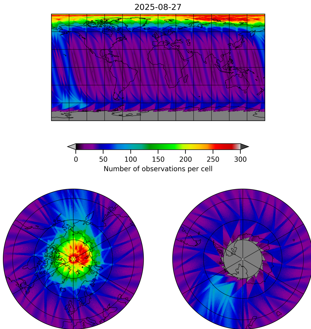
Figure 19: Map of the number of observations for 2025-08-26 to 2025-08-28
