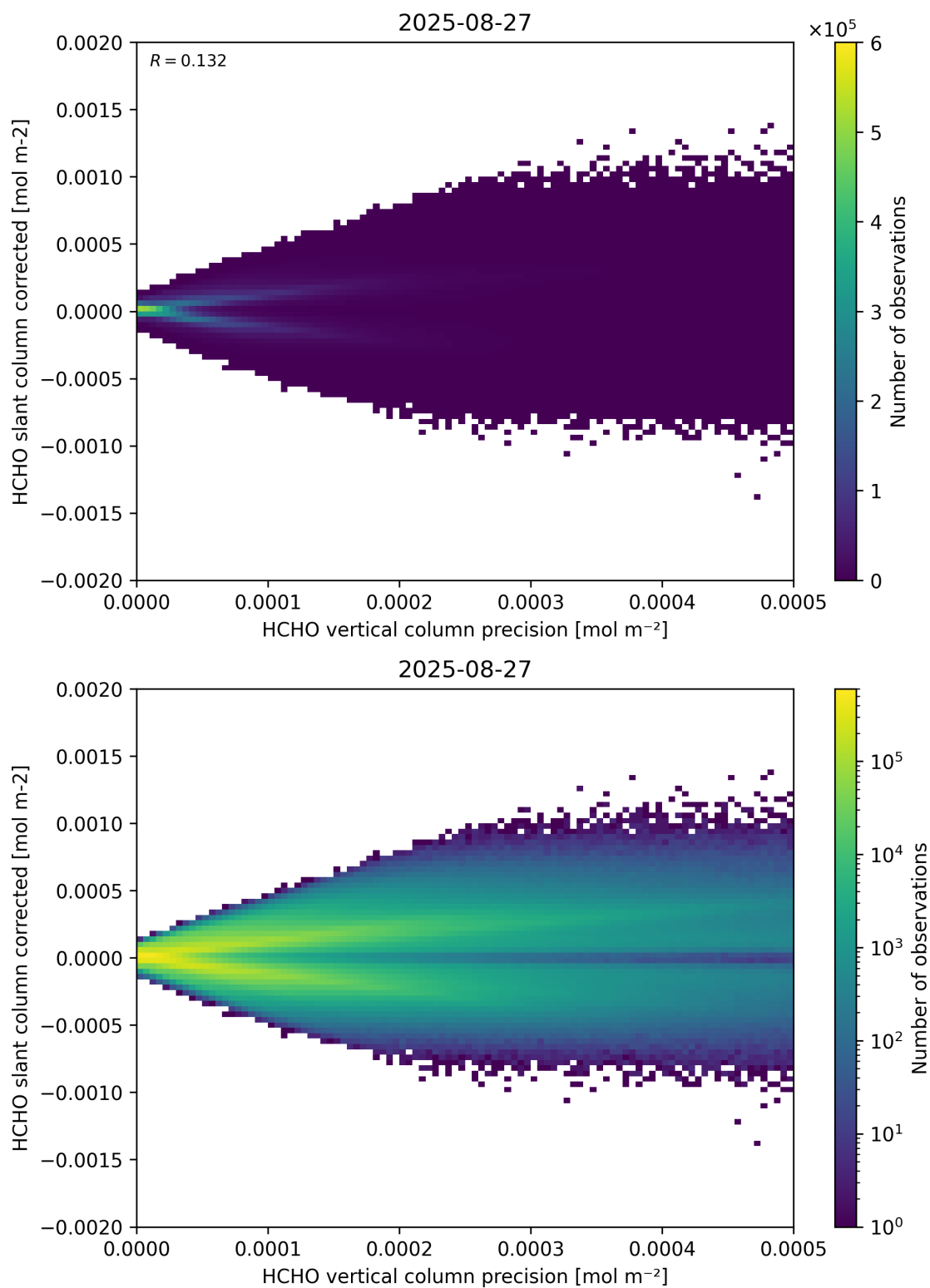
Figure 140: Scatter density plot of “HCHO vertical column precision” against “HCHO slant column corrected” for 2025-08-26 to 2025-08-28.
