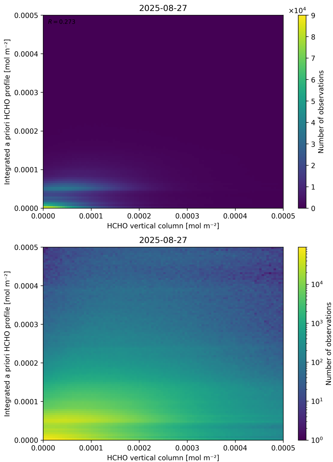
Figure 135: Scatter density plot of “HCHO vertical column” against “Integrated a priori HCHO profile” for 2025-08-26 to 2025-08-28.
