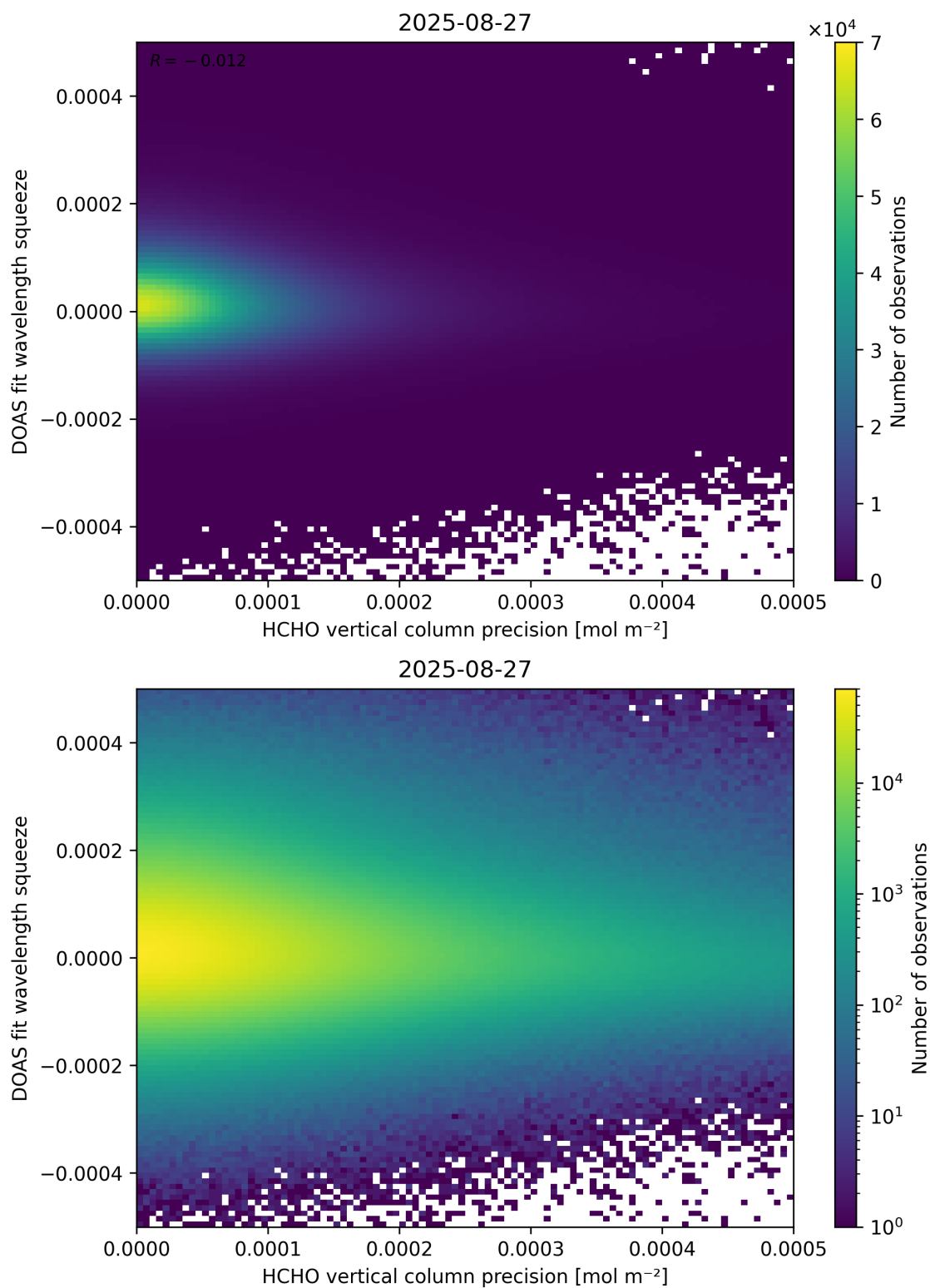
Figure 138: Scatter density plot of “HCHO vertical column precision” against “DOAS fit wavelength squeeze” for 2025-08-26 to 2025-08-28.
