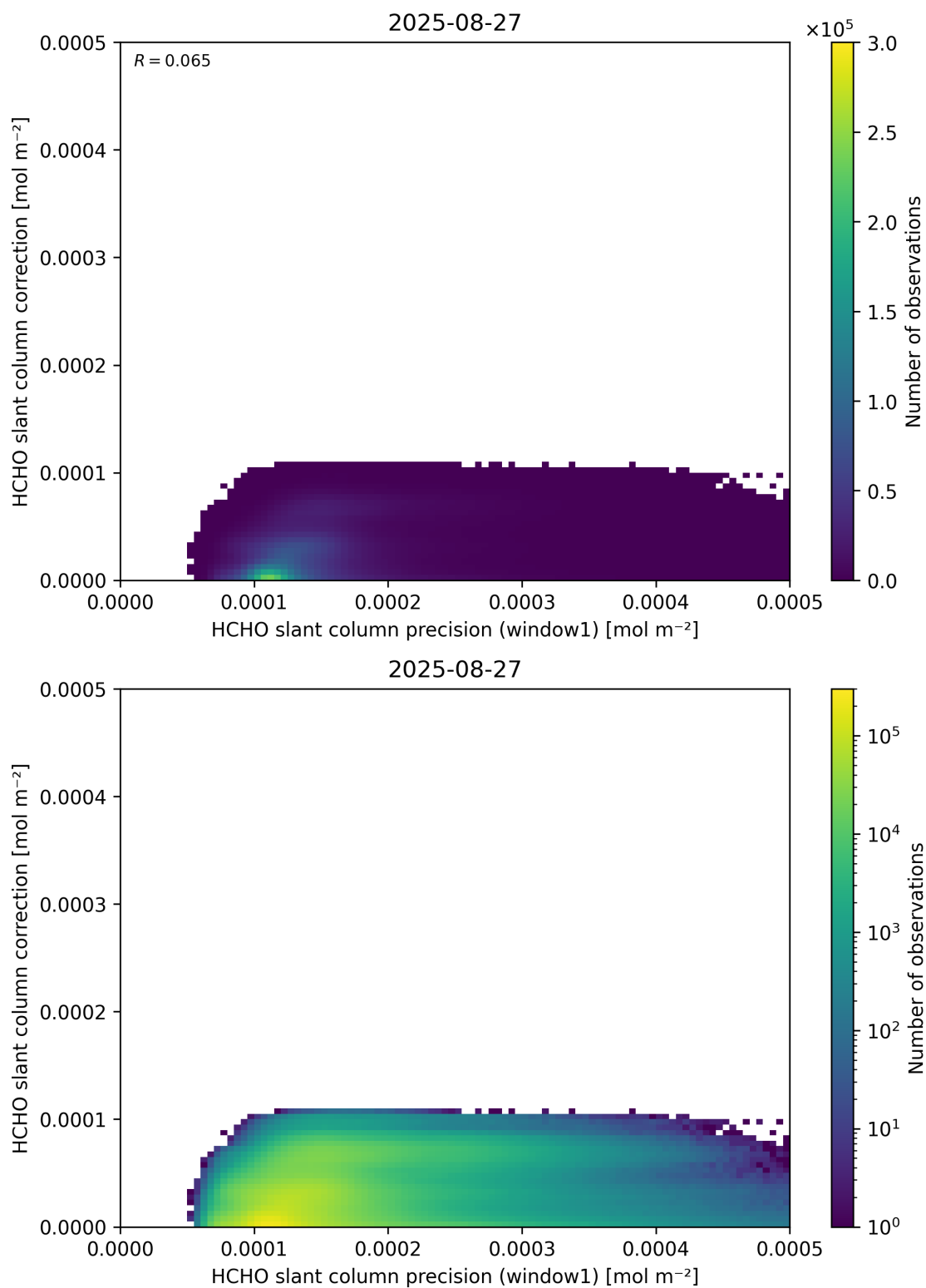
Figure 93: Scatter density plot of “HCHO slant column precision (window1)” against “HCHO slant column correction” for 2025-08-26 to 2025-08-28.
