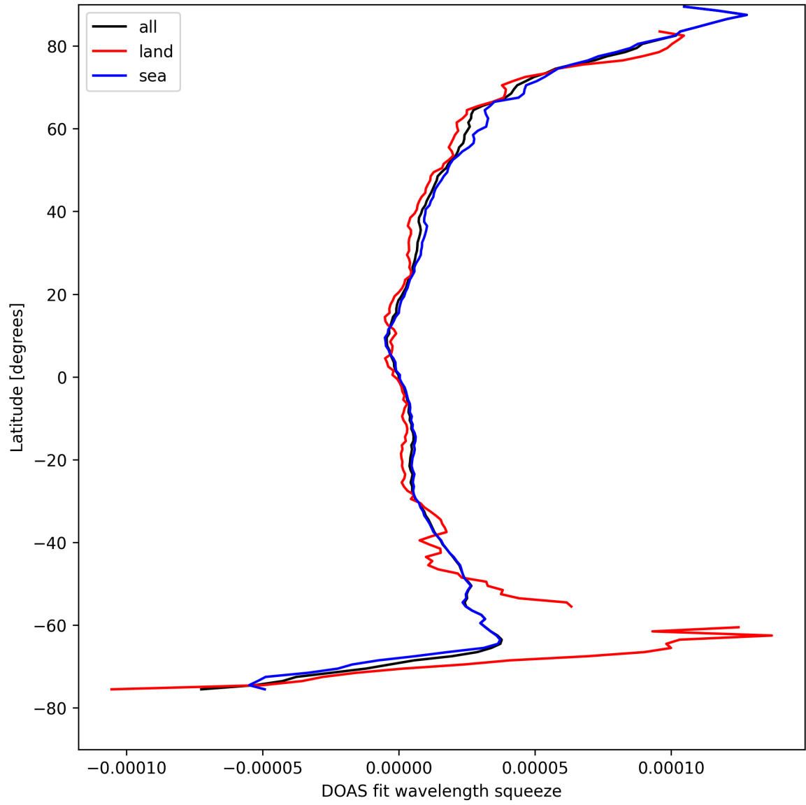
Figure 31: Zonal average of “DOAS fit wavelength squeeze” for 2025-08-26 to 2025-08-28.
