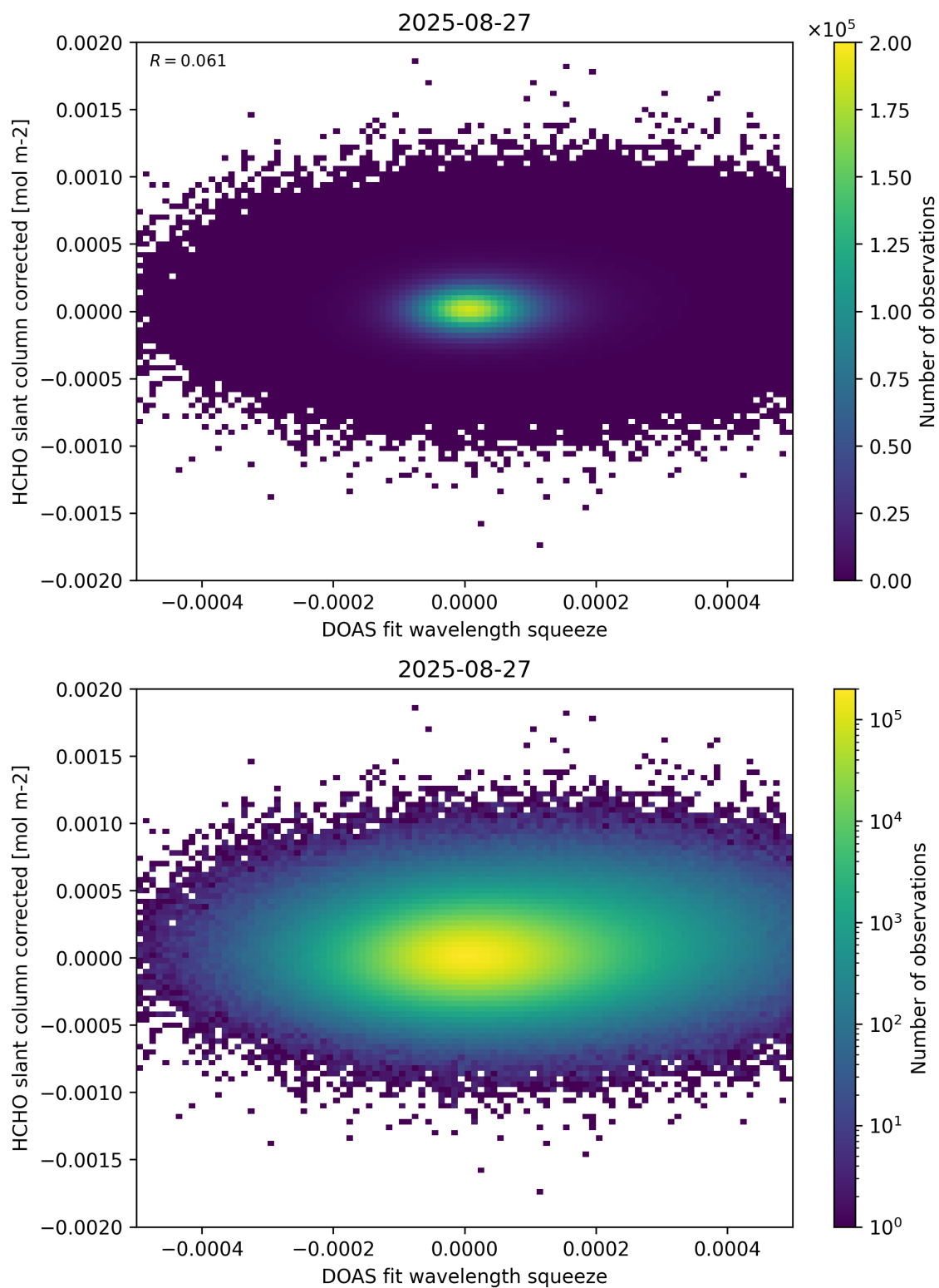
Figure 69: Scatter density plot of “DOAS fit wavelength squeeze” against “HCHO slant column corrected” for 2025-08-26 to 2025-08-28.
