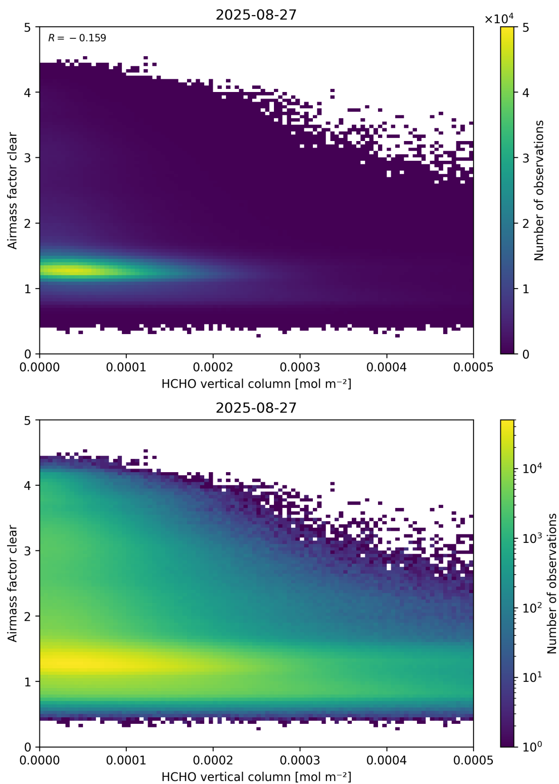
Figure 126: Scatter density plot of “HCHO vertical column” against “Airmass factor clear” for 2025-08-26 to 2025-08-28.
