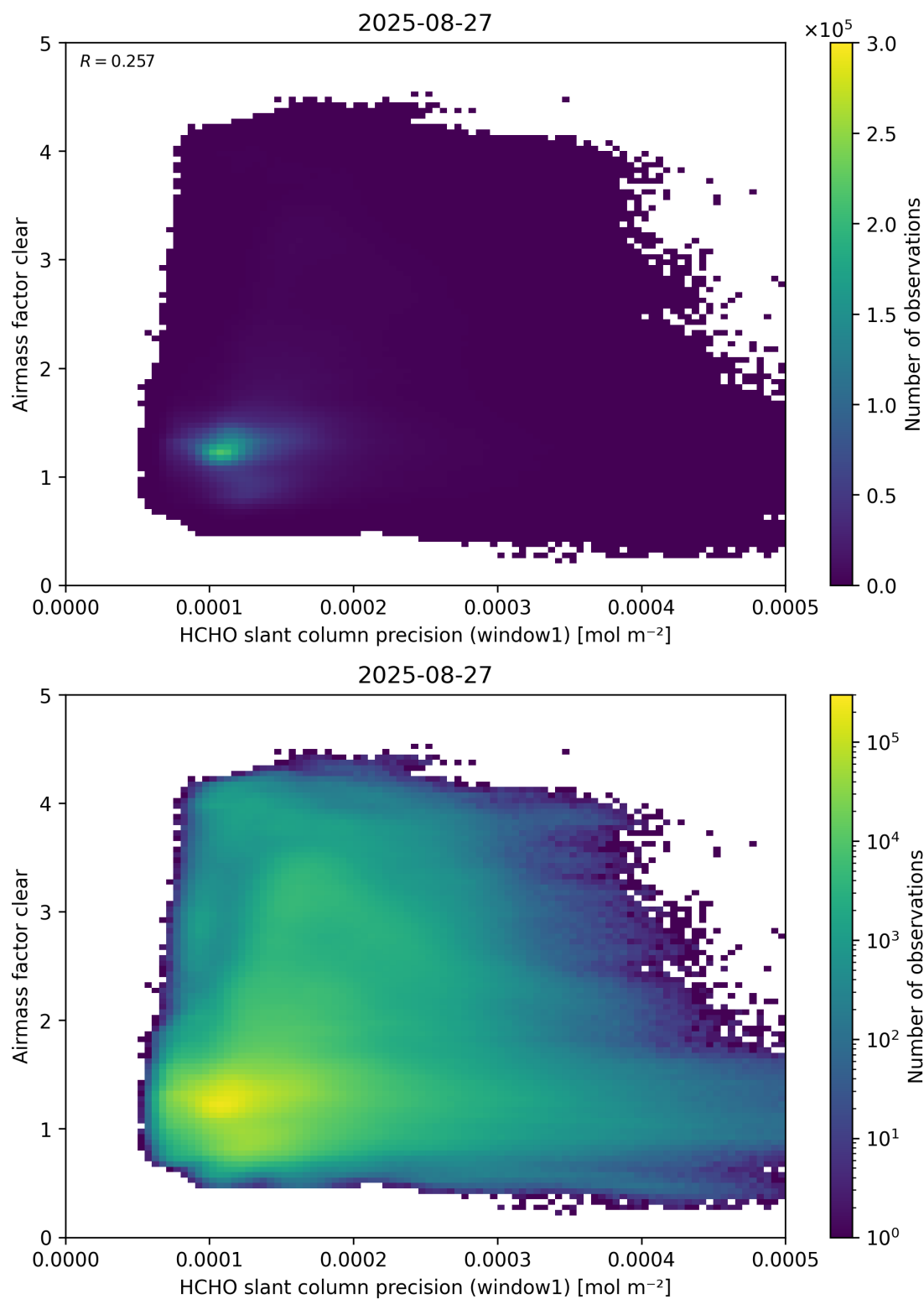
Figure 91: Scatter density plot of “HCHO slant column precision (window1)” against “Airmass factor clear” for 2025-08-26 to 2025-08-28.
