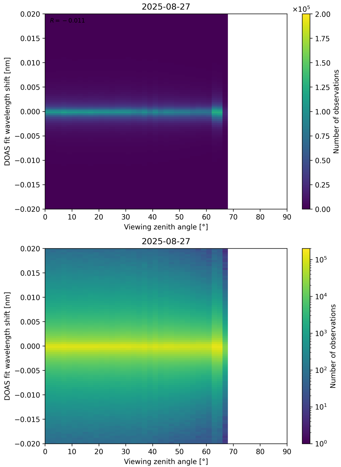
Figure 183: Scatter density plot of “Viewing zenith angle” against “DOAS fit wavelength shift” for 2025-08-26 to 2025-08-28.
