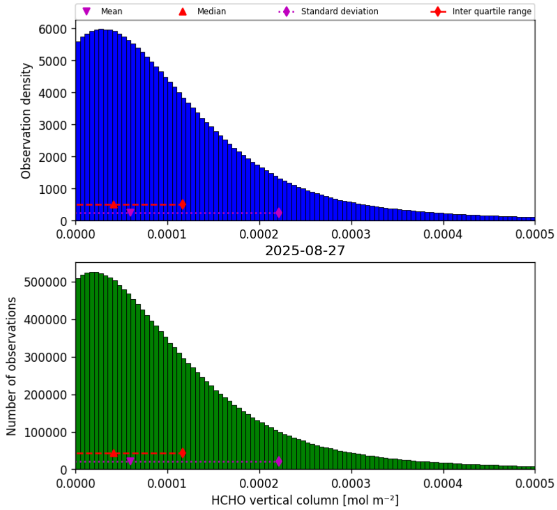
Figure 35: Histogram of “HCHO vertical column” for 2025-08-26 to 2025-08-28
