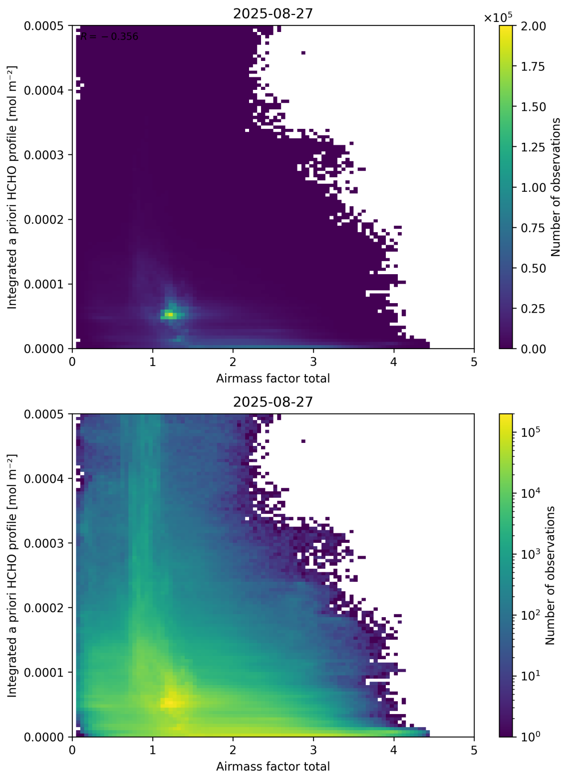
Figure 104: Scatter density plot of “Airmass factor total” against “Integrated a priori HCHO profile” for 2025-08-26 to 2025-08-28.
