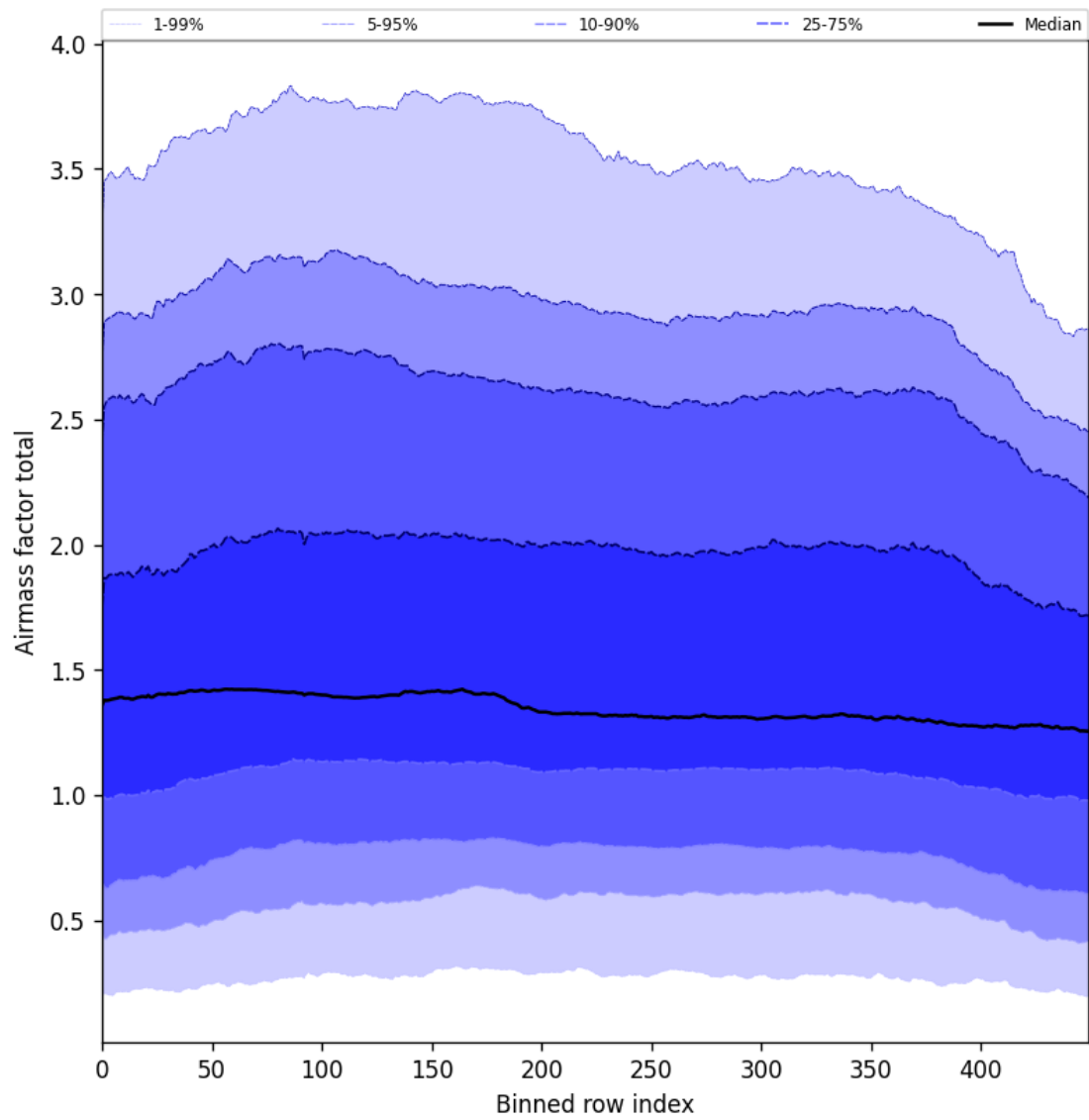
Figure 54: Along track statistics of “Airmass factor total” for 2025-08-26 to 2025-08-28
