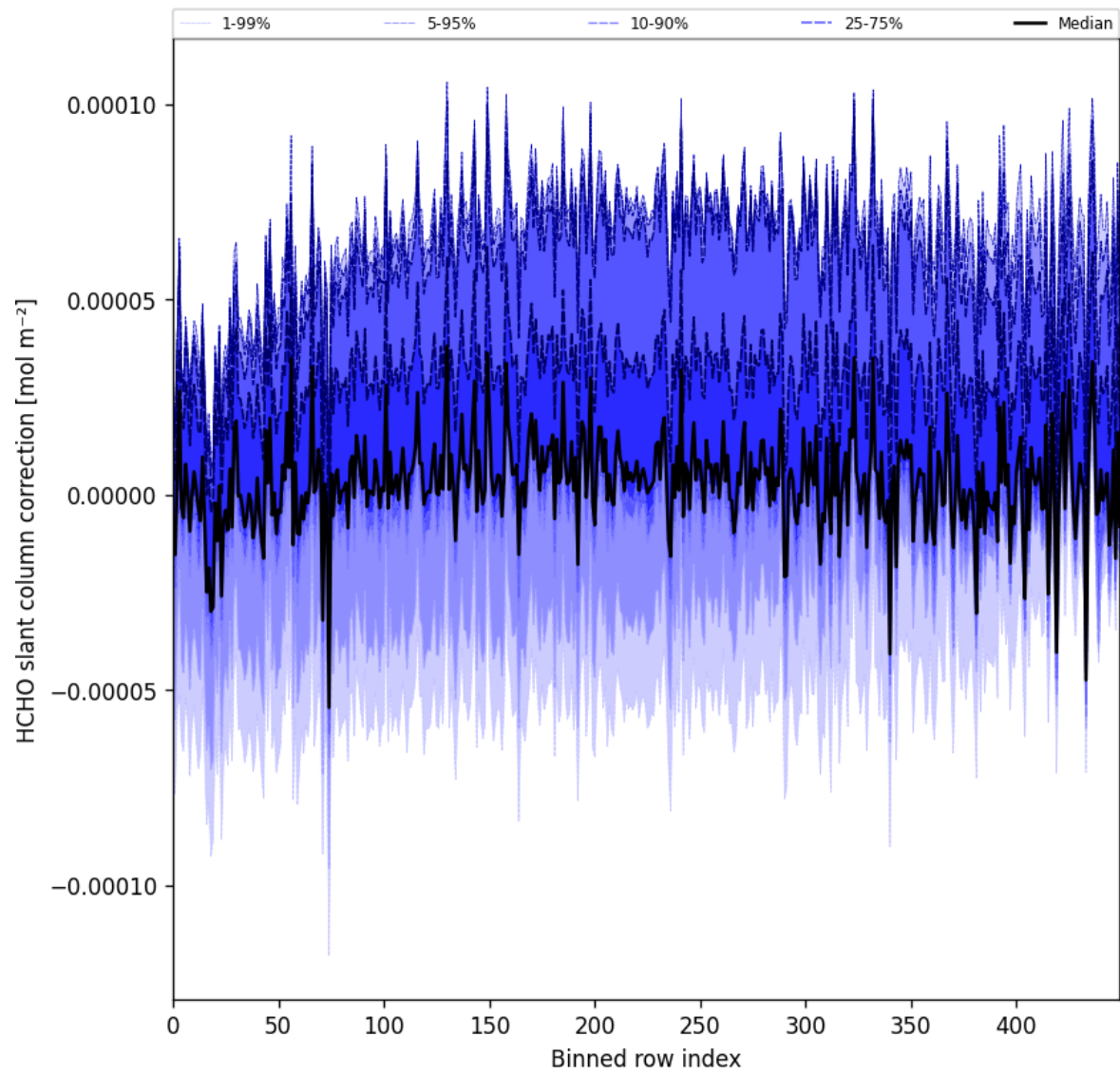
Figure 61: Along track statistics of “HCHO slant column correction” for 2025-08-26 to 2025-08-28
