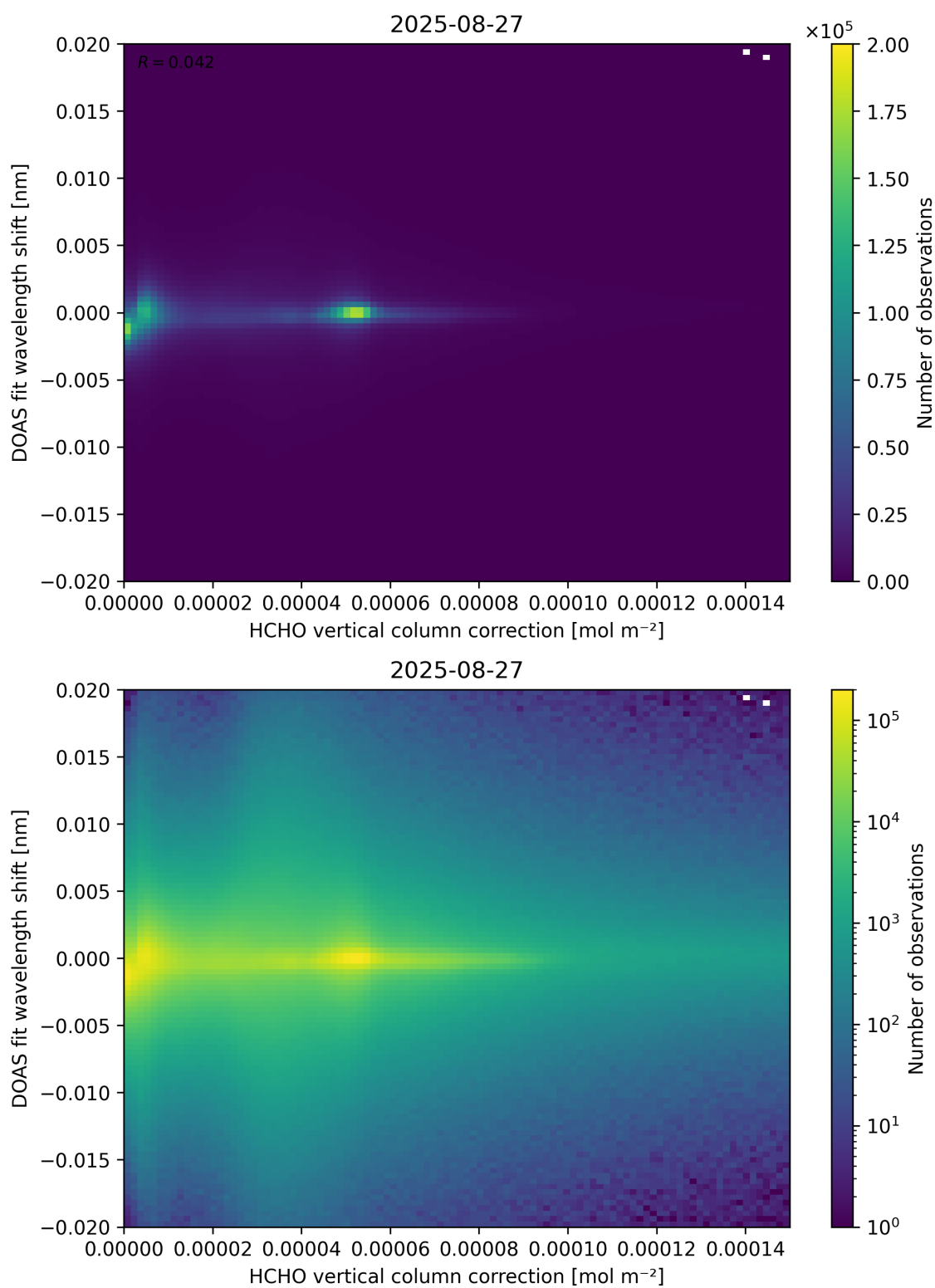
Figure 113: Scatter density plot of “HCHO vertical column correction” against “DOAS fit wavelength shift” for 2025-08-26 to 2025-08-28.
