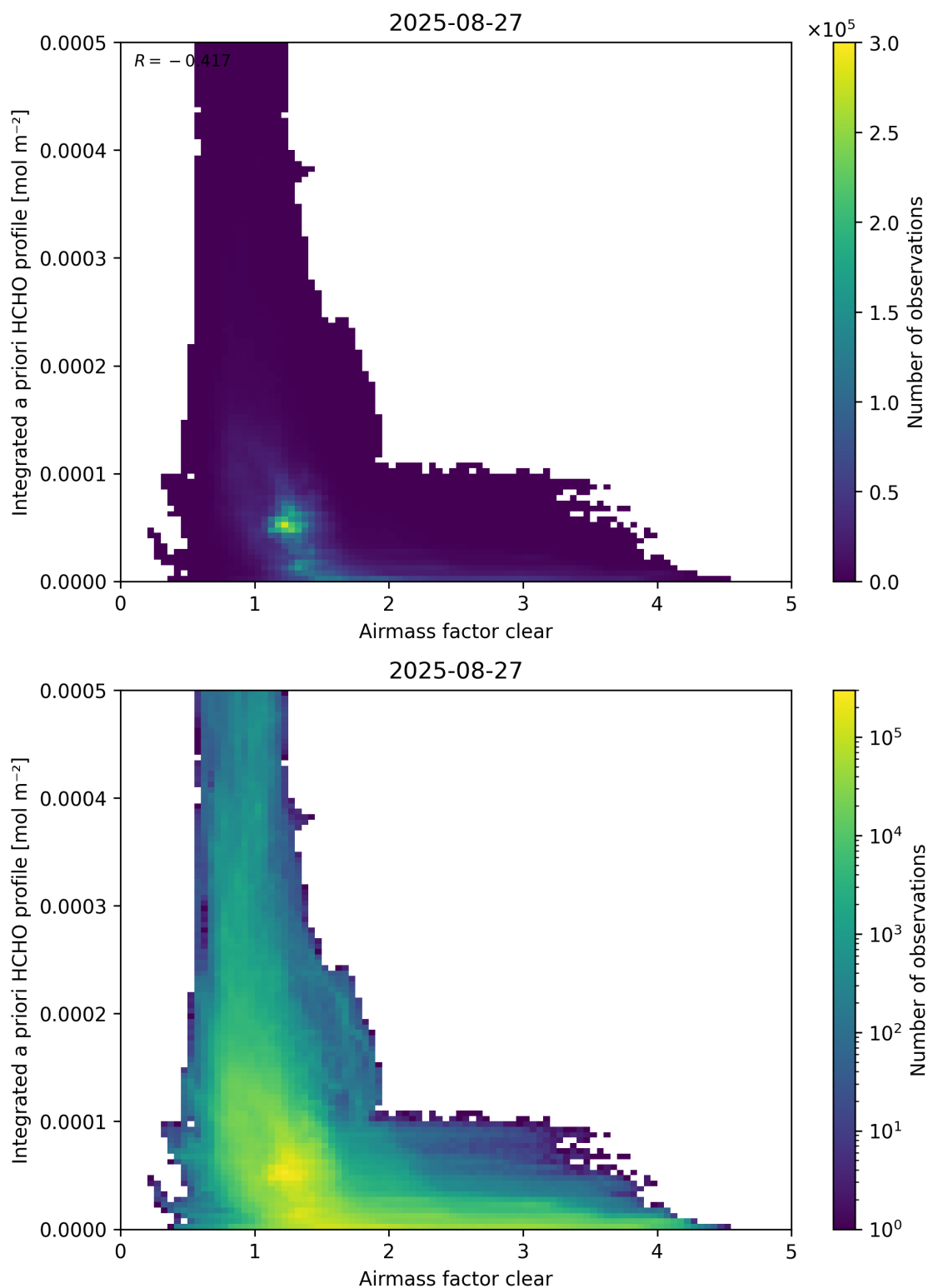
Figure 76: Scatter density plot of “Airmass factor clear” against “Integrated a priori HCHO profile” for 2025-08-26 to 2025-08-28.
