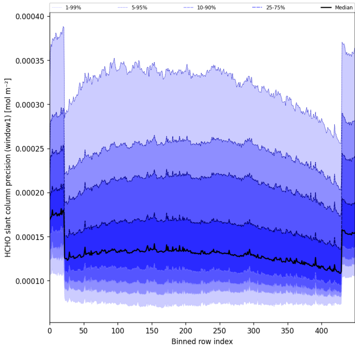
Figure 53: Along track statistics of “HCHO slant column precision (window1)” for 2025-08-26 to 2025-08-28
