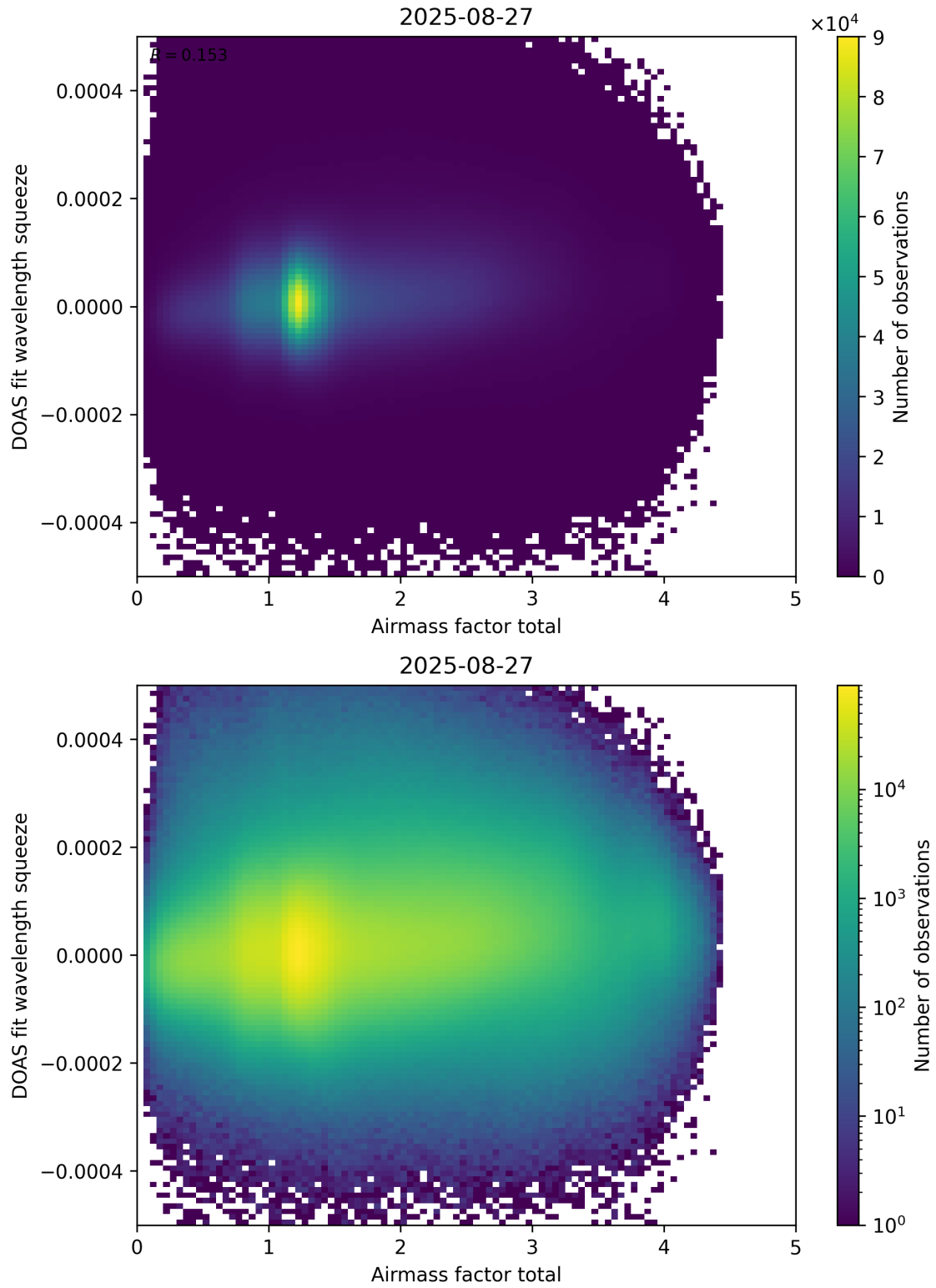
Figure 99: Scatter density plot of “Airmass factor total” against “DOAS fit wavelength squeeze” for 2025-08-26 to 2025-08-28.
