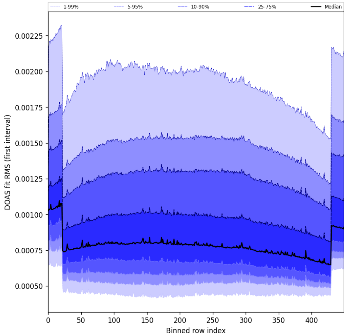
Figure 60: Along track statistics of “DOAS fit RMS (first interval)” for 2025-08-26 to 2025-08-28
