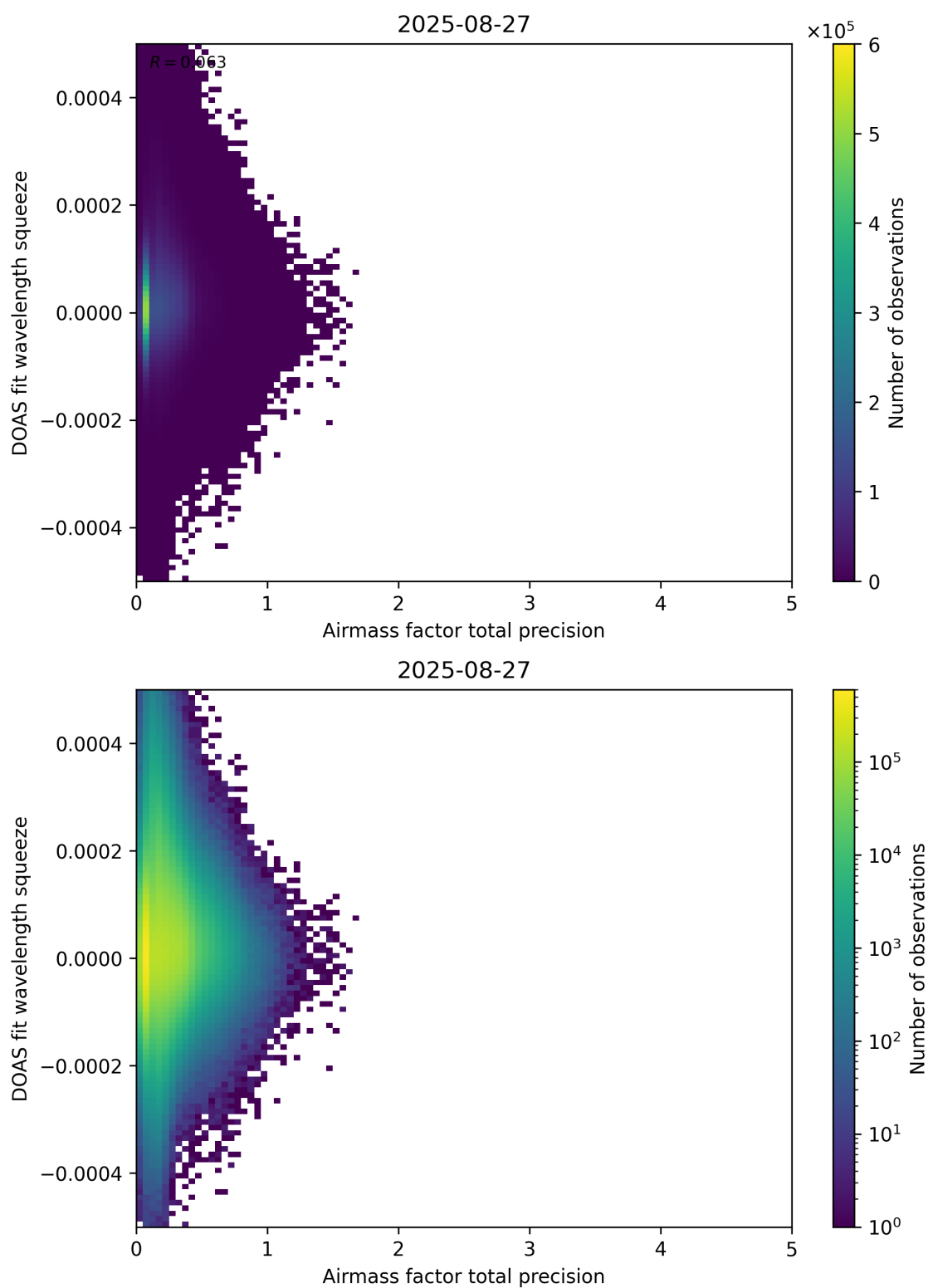
Figure 107: Scatter density plot of “Airmass factor total precision” against “DOAS fit wavelength squeeze” for 2025-08-26 to 2025-08-28.
