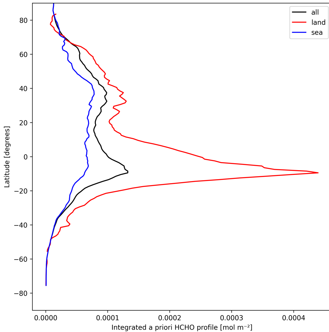
Figure 29: Zonal average of “Integrated a priori HCHO profile” for 2025-08-26 to 2025-08-28.
