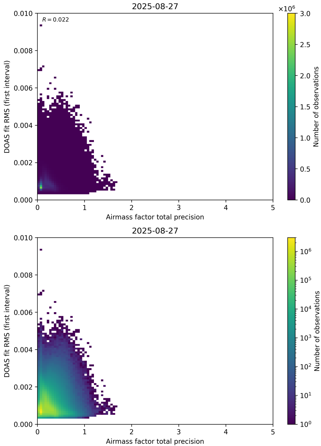
Figure 105: Scatter density plot of “Airmass factor total precision” against “DOAS fit RMS (first interval)” for 2025-08-26 to 2025-08-28.
