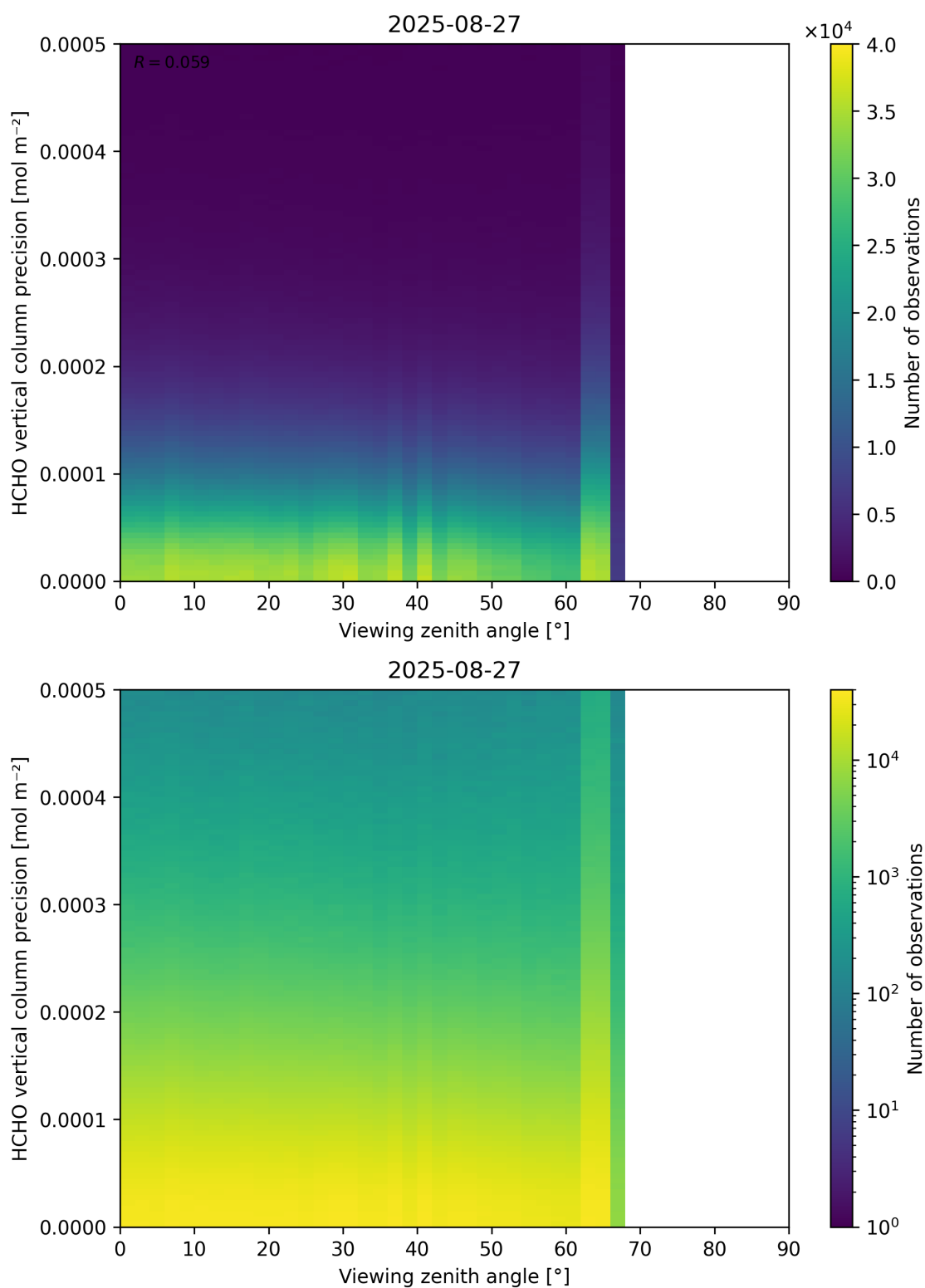
Figure 194: Scatter density plot of “Viewing zenith angle” against “HCHO vertical column precision” for 2025-08-26 to 2025-08-28.
