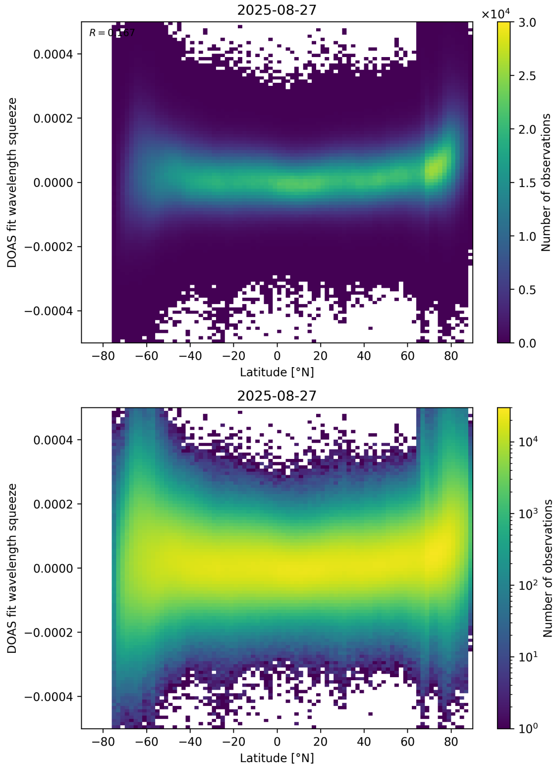
Figure 155: Scatter density plot of “Latitude” against “DOAS fit wavelength squeeze” for 2025-08-26 to 2025-08-28.
