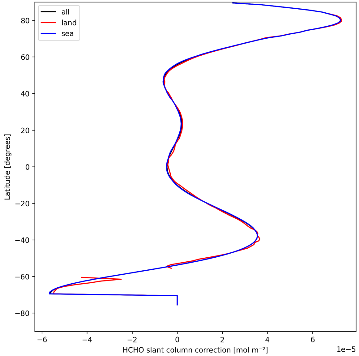
Figure 33: Zonal average of “HCHO slant column correction” for 2025-08-26 to 2025-08-28.
