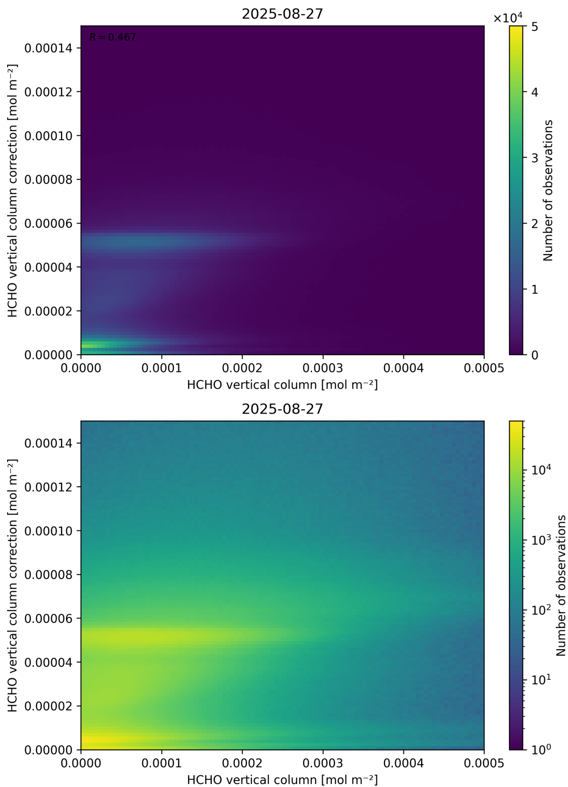
Figure 133: Scatter density plot of “HCHO vertical column” against “HCHO vertical column correction” for 2025-08-26 to 2025-08-28.
