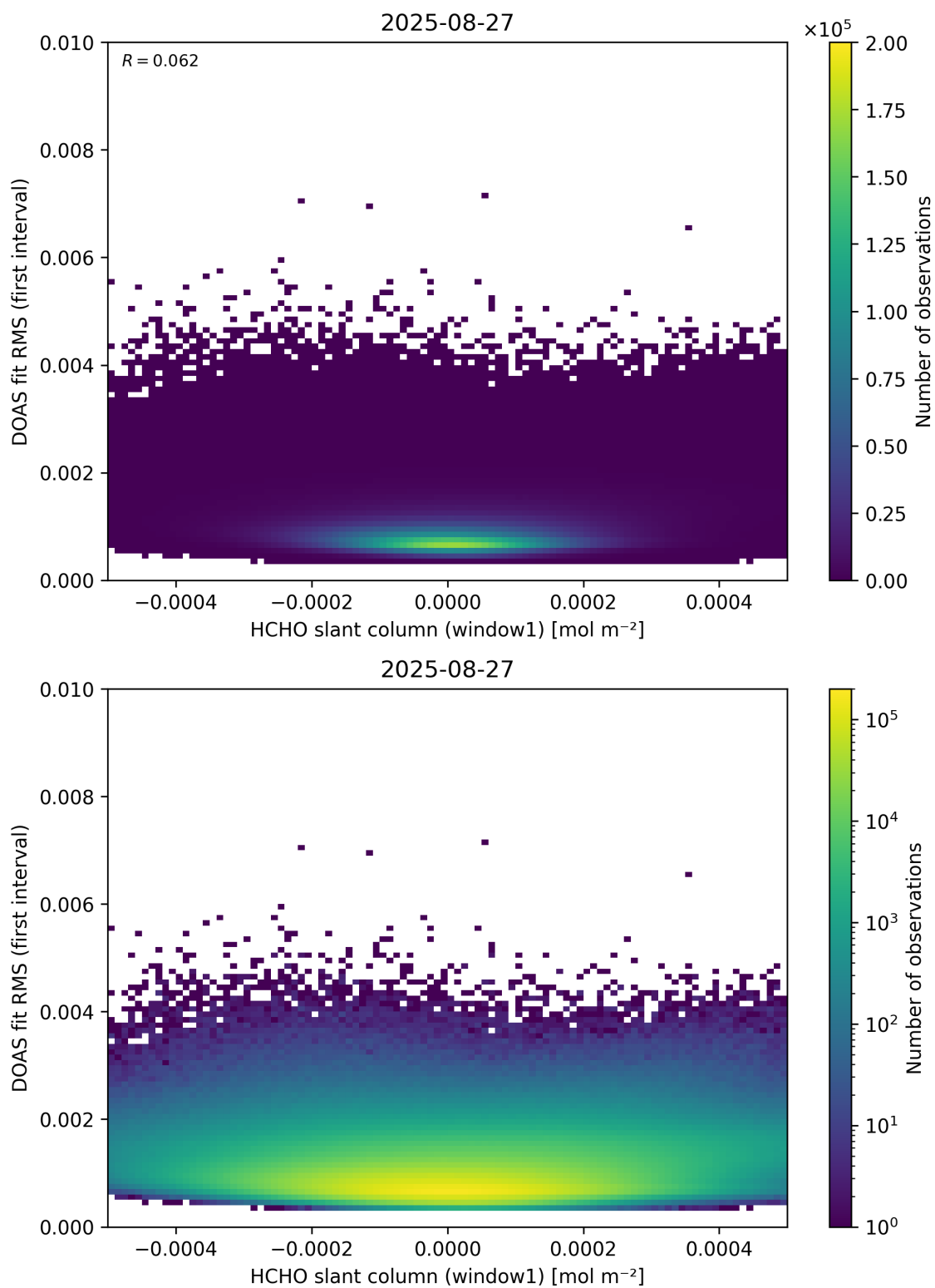
Figure 78: Scatter density plot of “HCHO slant column (window1)” against “DOAS fit RMS (first interval)” for 2025-08-26 to 2025-08-28.
