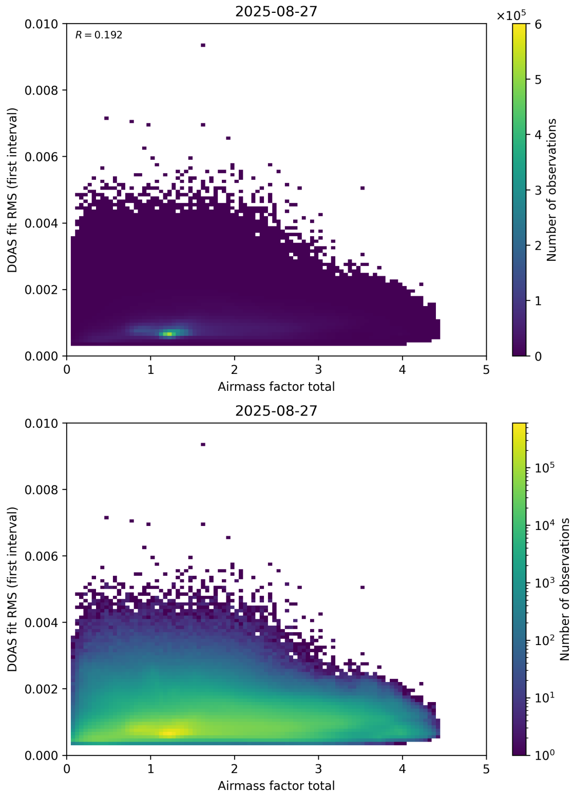
Figure 97: Scatter density plot of “Airmass factor total” against “DOAS fit RMS (first interval)” for 2025-08-26 to 2025-08-28.
