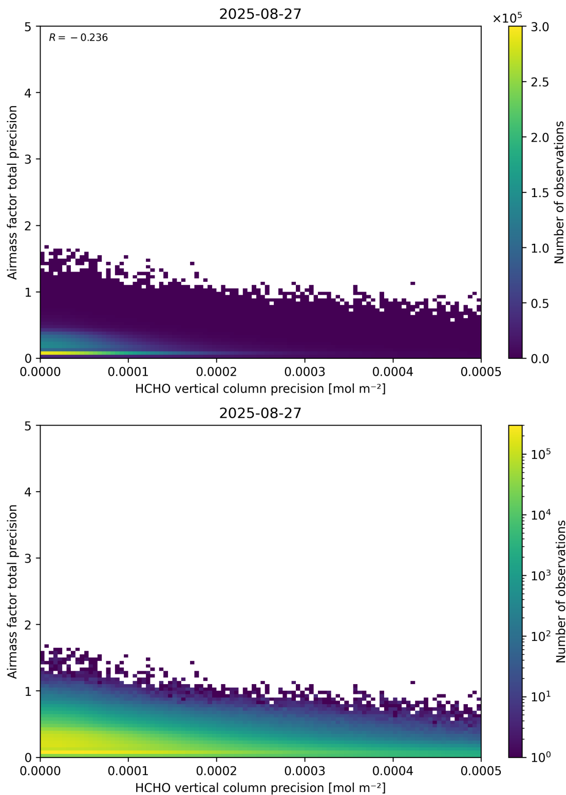
Figure 145: Scatter density plot of “HCHO vertical column precision” against “Airmass factor total precision” for 2025-08-26 to 2025-08-28.
