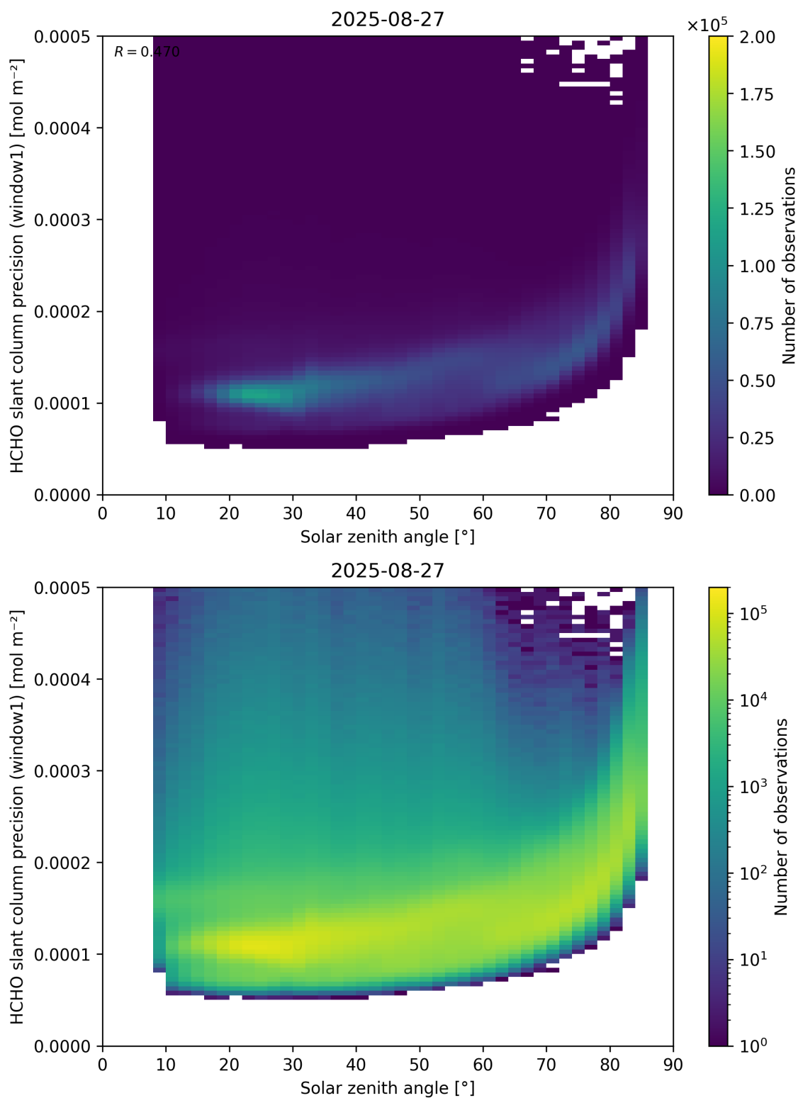
Figure 174: Scatter density plot of “Solar zenith angle” against “HCHO slant column precision (window1)” for 2025-08-26 to 2025-08-28.
