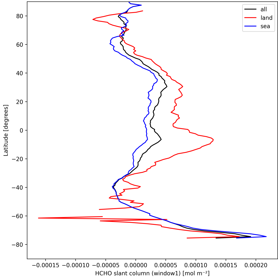
Figure 24: Zonal average of “HCHO slant column (window1)” for 2025-08-26 to 2025-08-28.
