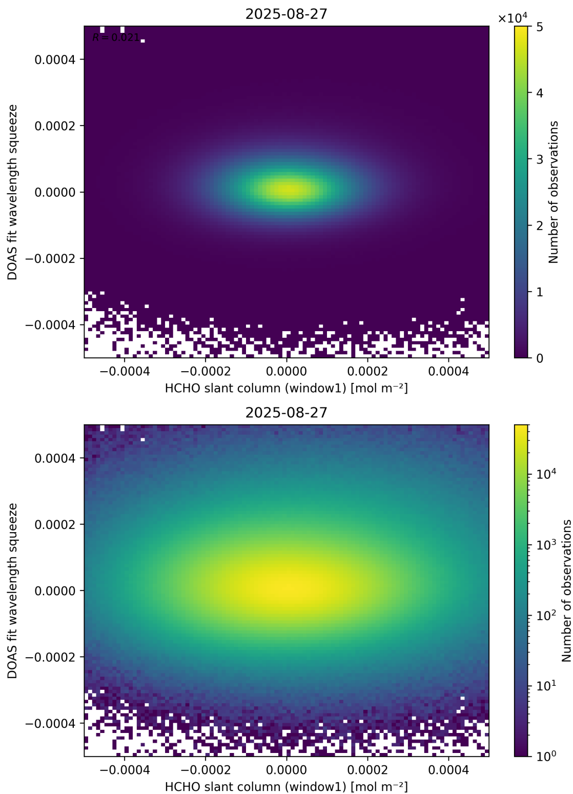
Figure 80: Scatter density plot of “HCHO slant column (window1)” against “DOAS fit wavelength squeeze” for 2025-08-26 to 2025-08-28.
