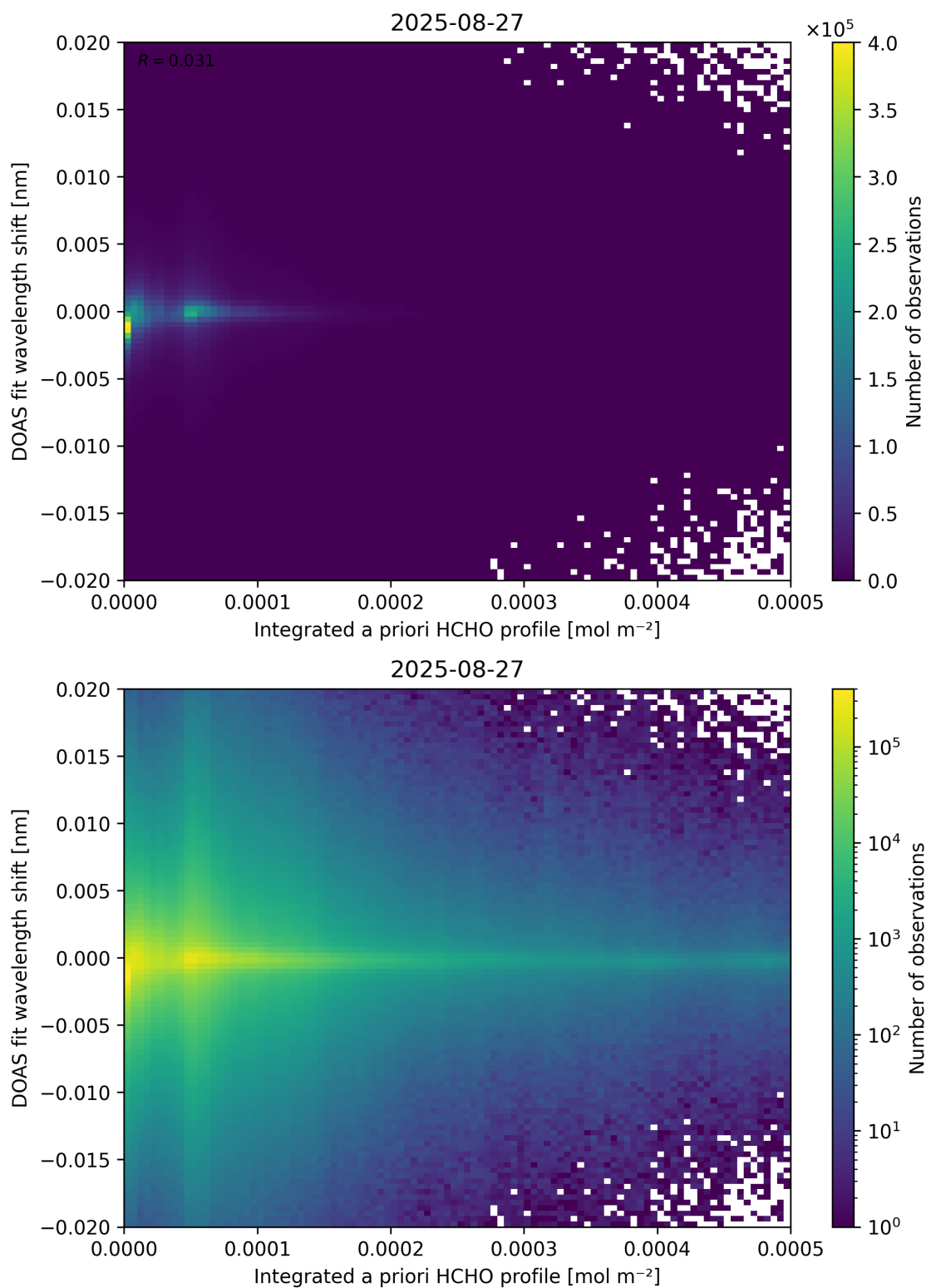
Figure 149: Scatter density plot of “Integrated a priori HCHO profile” against “DOAS fit wavelength shift” for 2025-08-26 to 2025-08-28.
