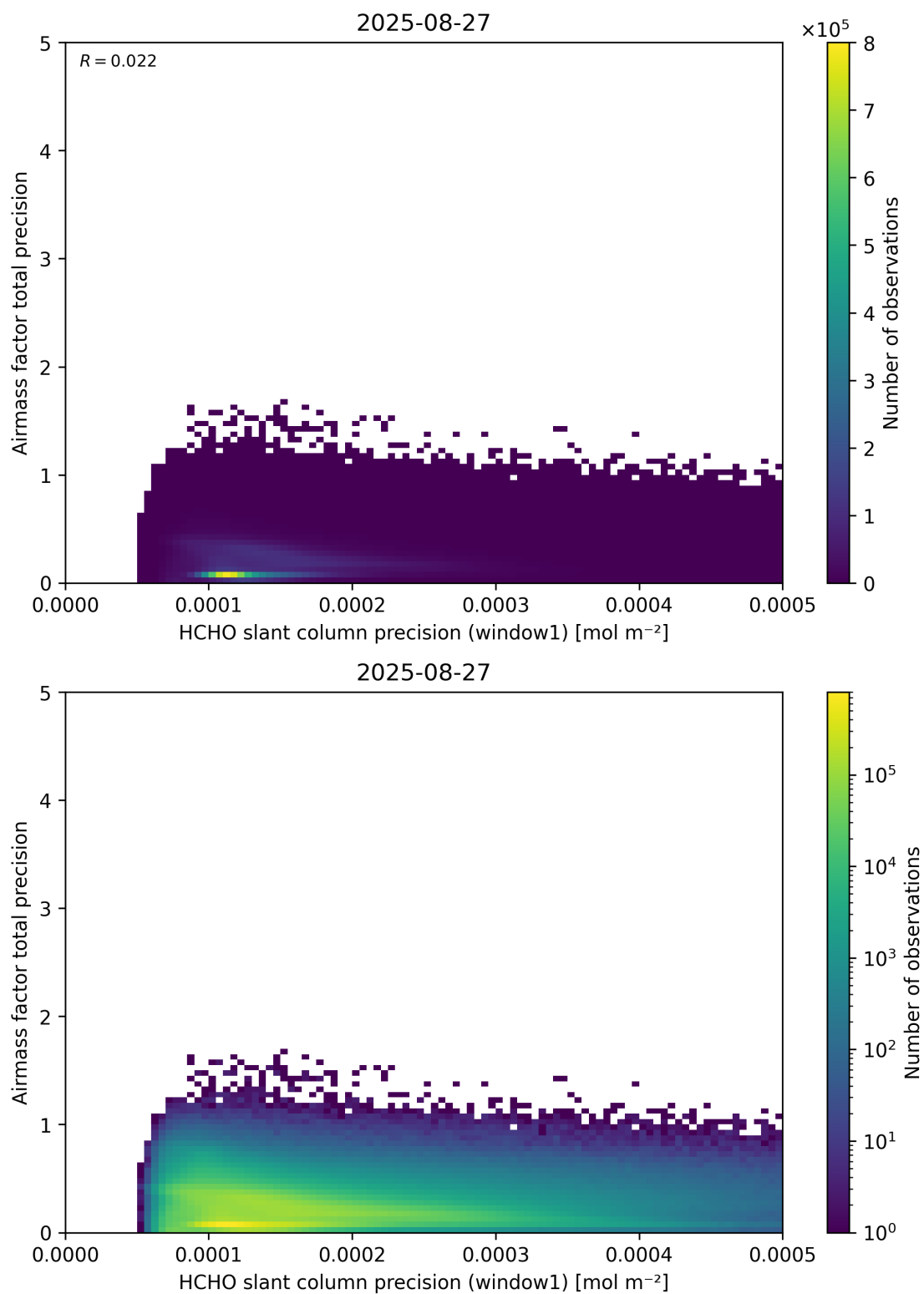
Figure 95: Scatter density plot of “HCHO slant column precision (window1)” against “Airmass factor total precision” for 2025-08-26 to 2025-08-28.
