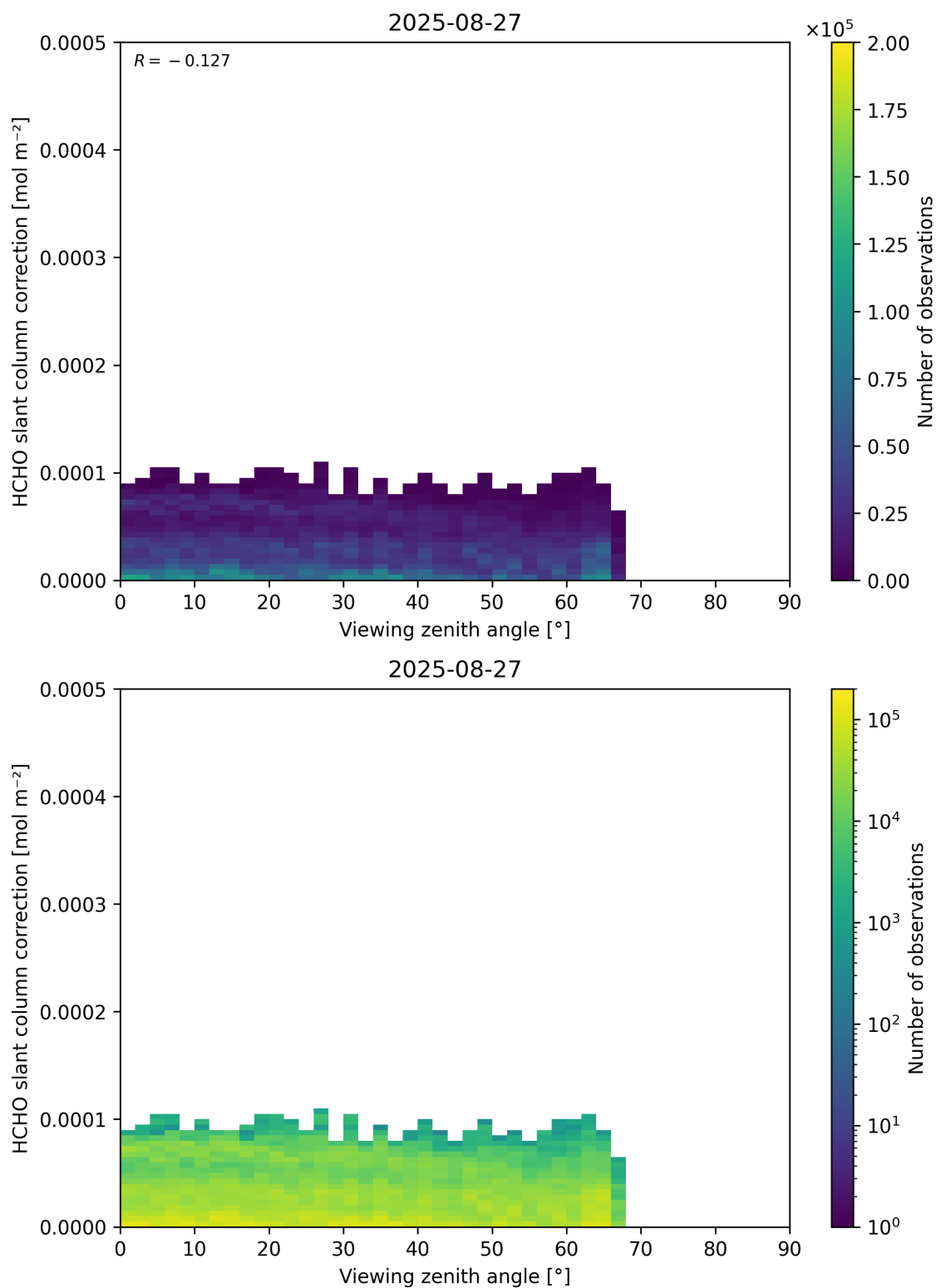
Figure 187: Scatter density plot of “Viewing zenith angle” against “HCHO slant column correction” for 2025-08-26 to 2025-08-28.
