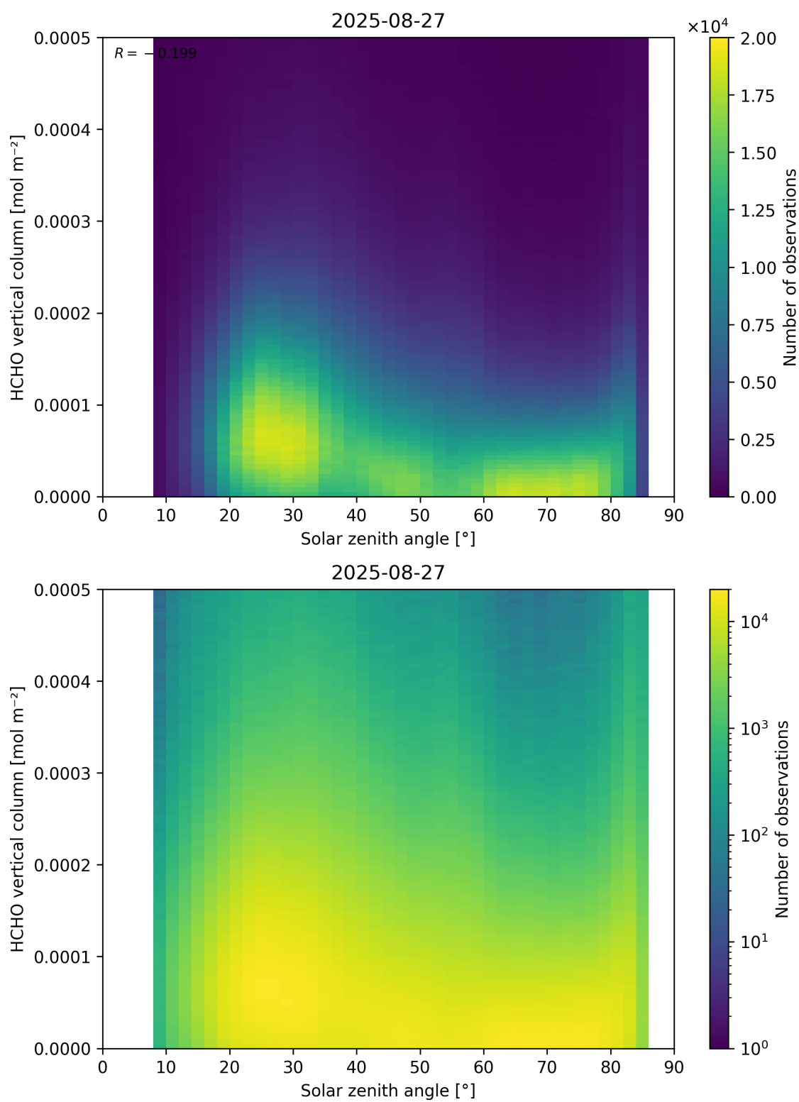
Figure 177: Scatter density plot of “Solar zenith angle” against “HCHO vertical column” for 2025-08-26 to 2025-08-28.
