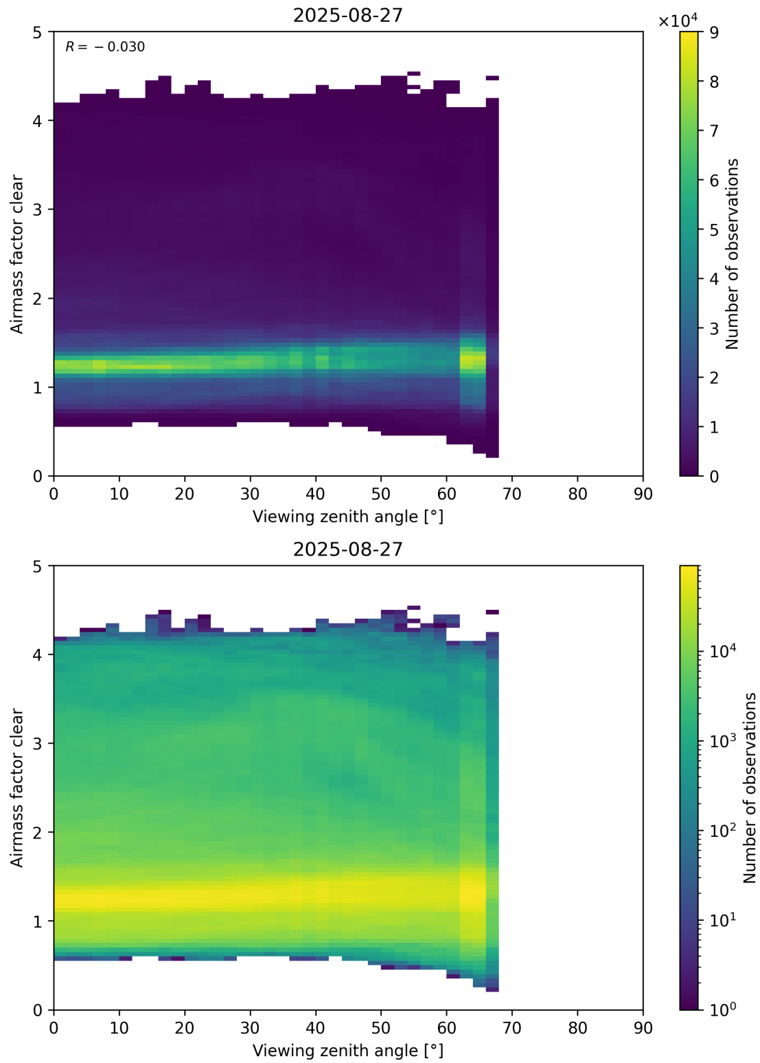
Figure 185: Scatter density plot of “Viewing zenith angle” against “Airmass factor clear” for 2025-08-26 to 2025-08-28.
