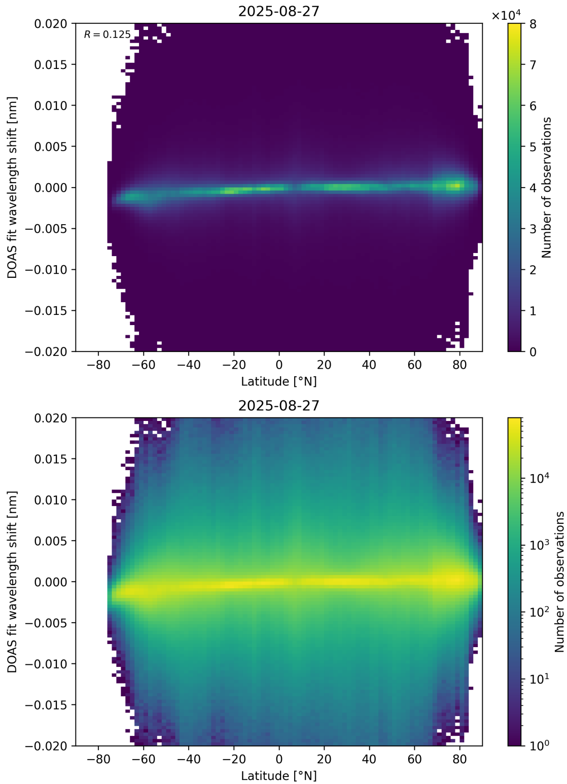
Figure 154: Scatter density plot of “Latitude” against “DOAS fit wavelength shift” for 2025-08-26 to 2025-08-28.
