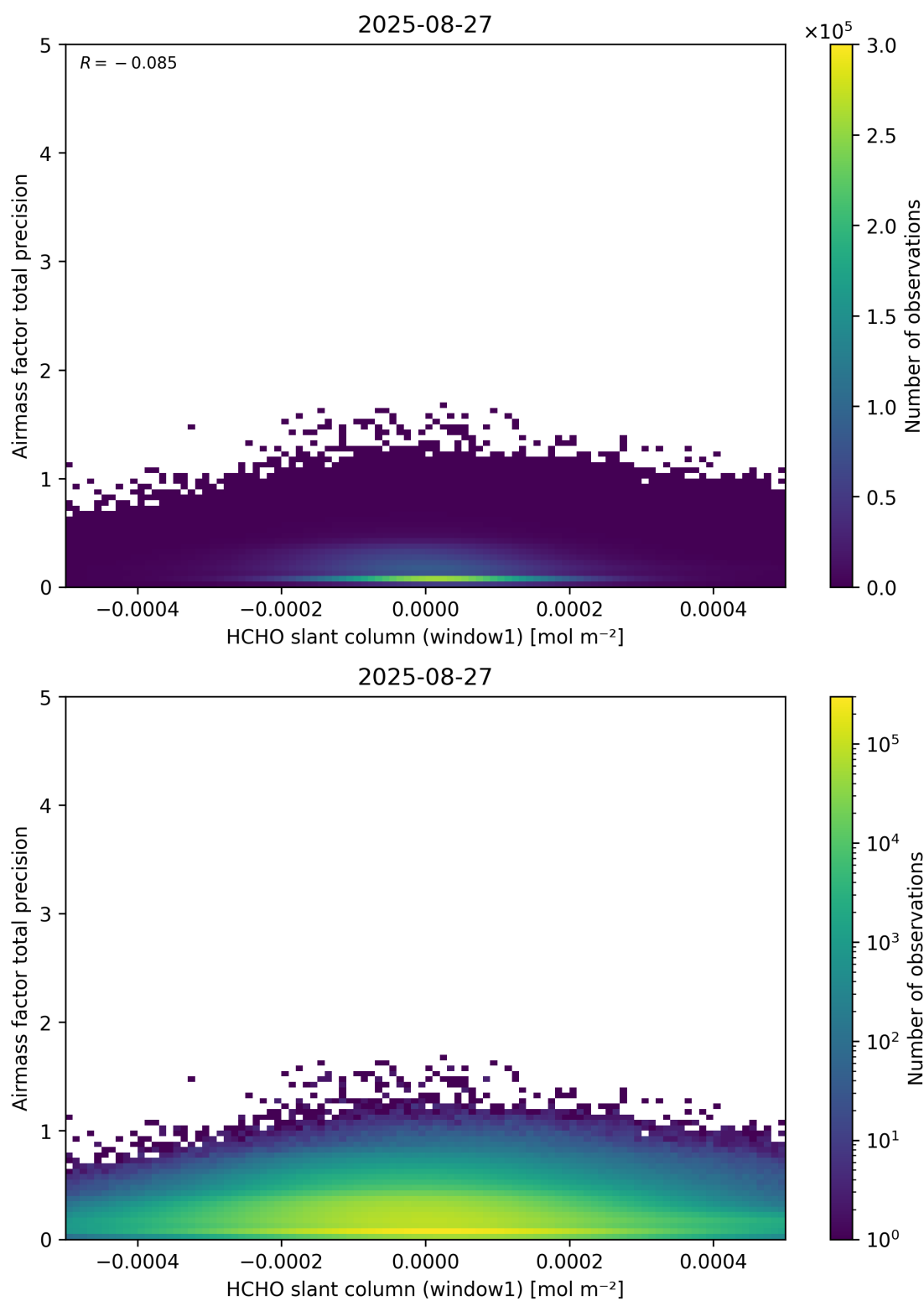
Figure 86: Scatter density plot of “HCHO slant column (window1)” against “Airmass factor total precision” for 2025-08-26 to 2025-08-28.
