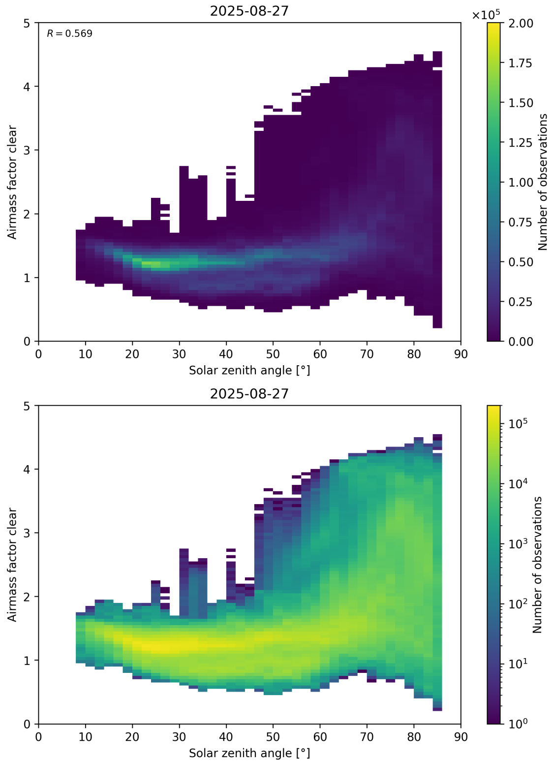
Figure 170: Scatter density plot of “Solar zenith angle” against “Airmass factor clear” for 2025-08-26 to 2025-08-28.
