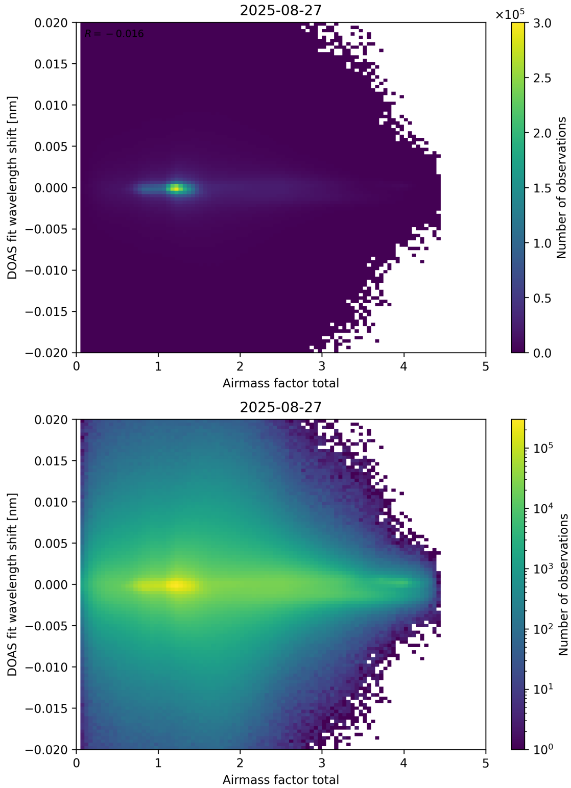
Figure 98: Scatter density plot of “Airmass factor total” against “DOAS fit wavelength shift” for 2025-08-26 to 2025-08-28.
