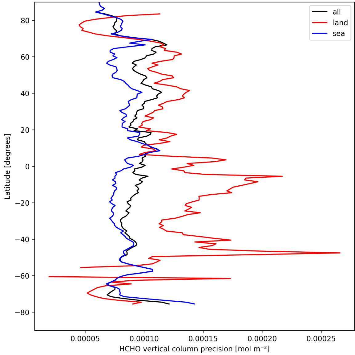
Figure 22: Zonal average of “HCHO vertical column precision” for 2025-08-26 to 2025-08-28.
