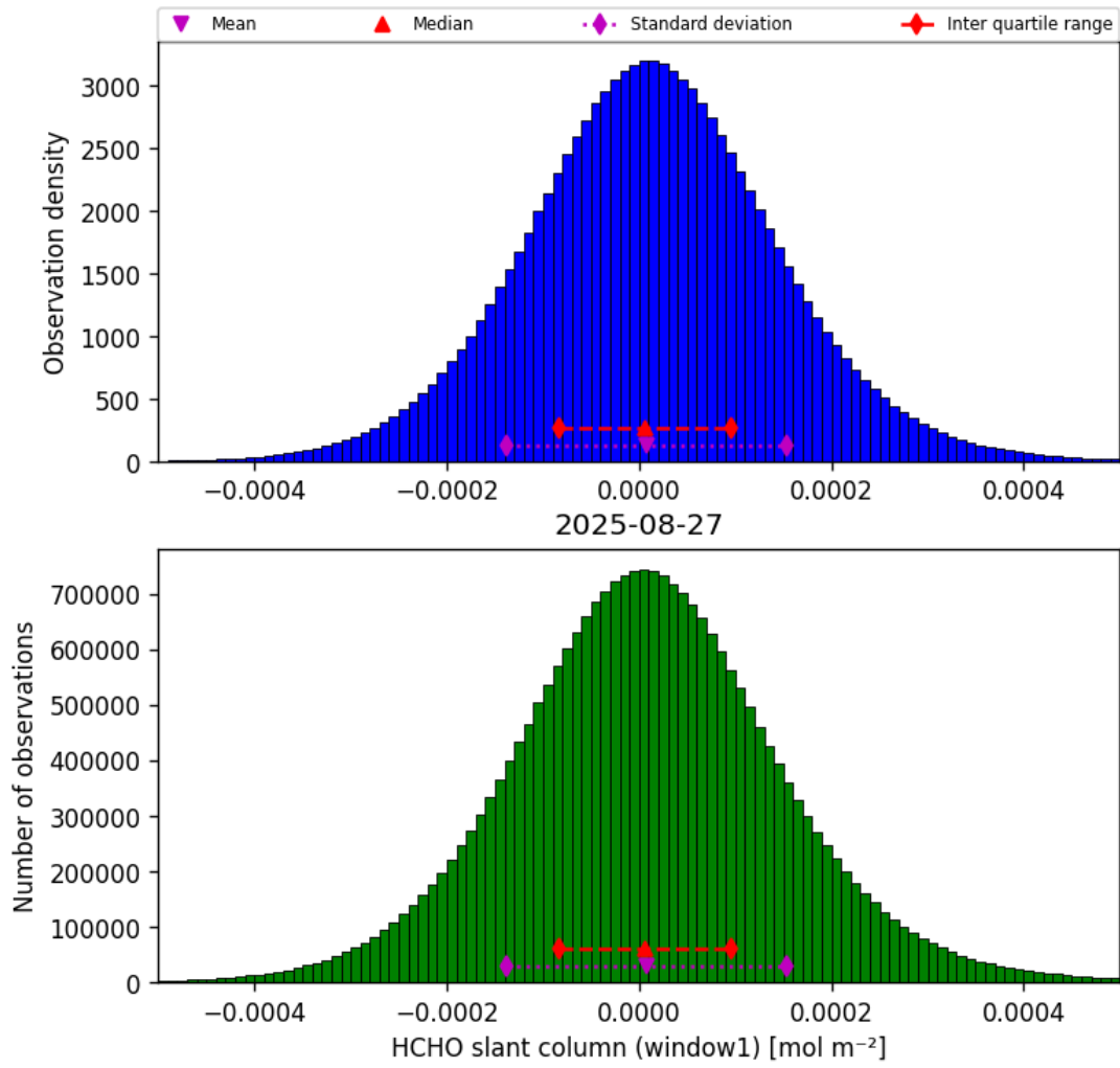
Figure 38: Histogram of “HCHO slant column (window1)” for 2025-08-26 to 2025-08-28
