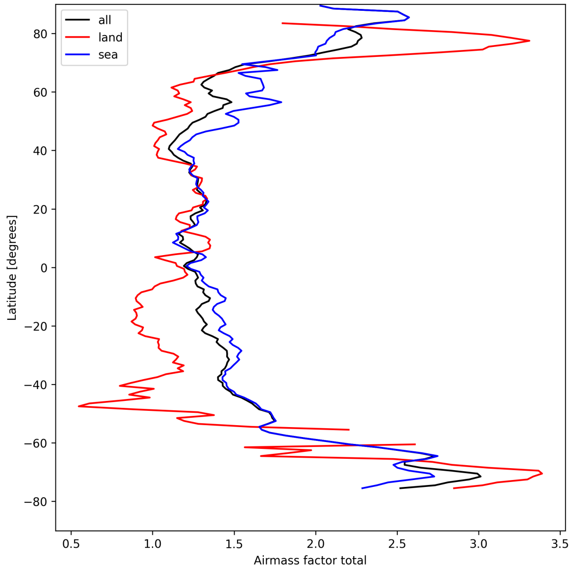
Figure 26: Zonal average of “Airmass factor total” for 2025-08-26 to 2025-08-28.
