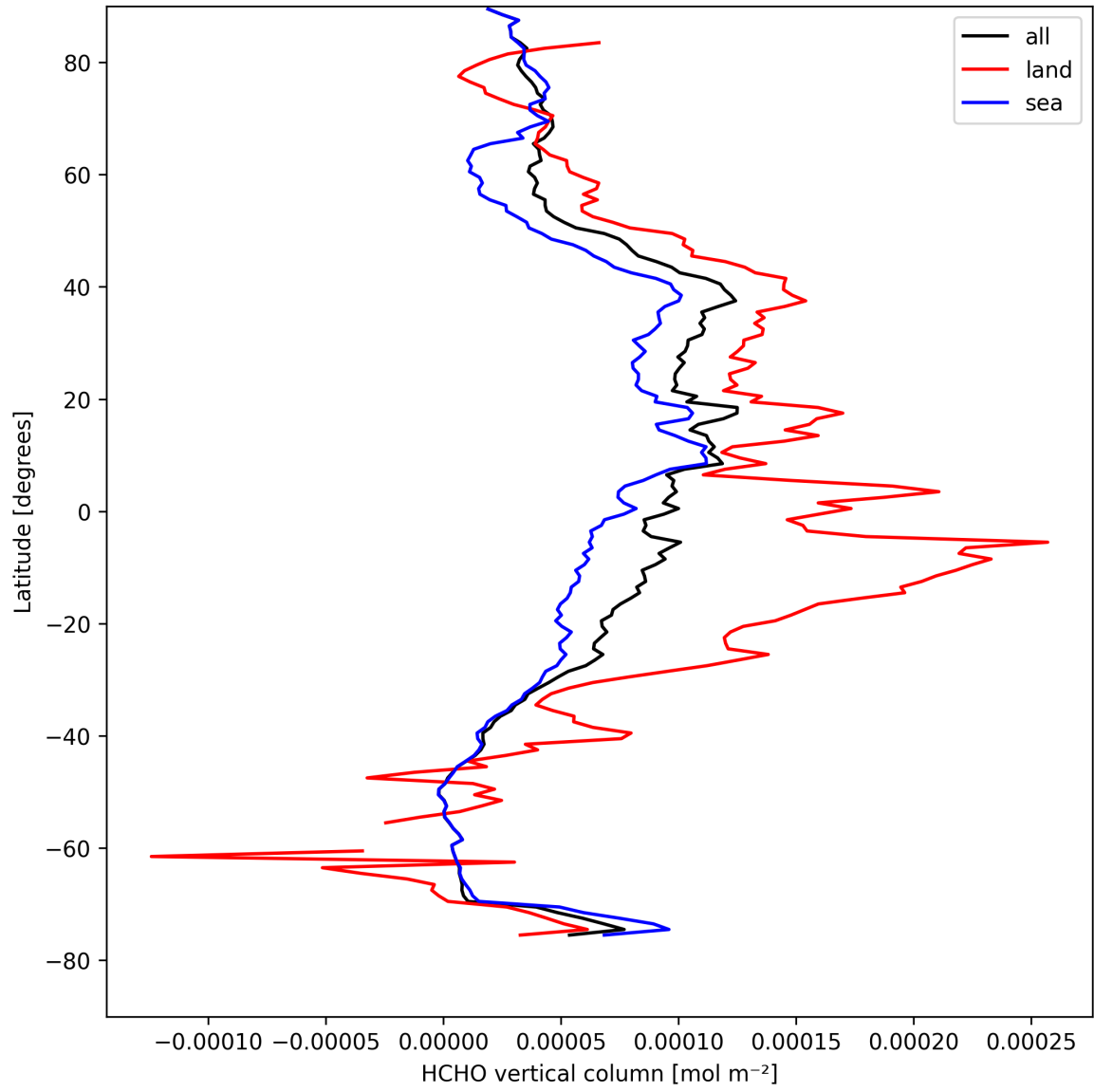
Figure 21: Zonal average of “HCHO vertical column” for 2025-08-26 to 2025-08-28.
