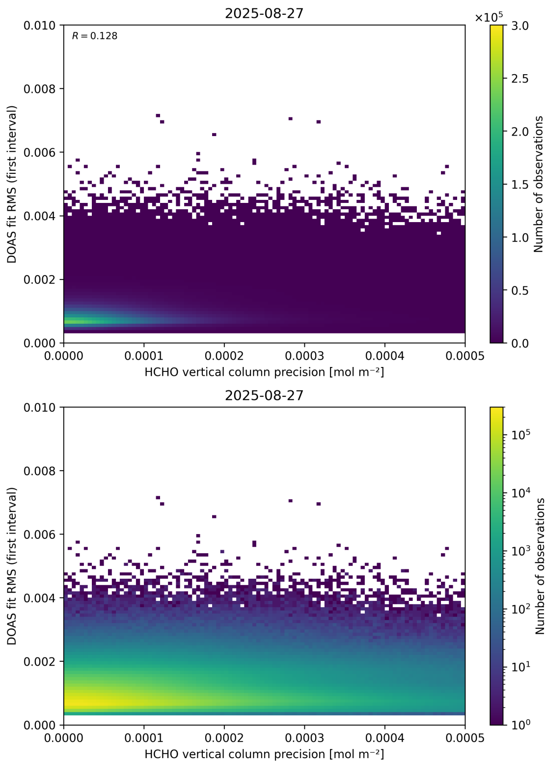
Figure 136: Scatter density plot of “HCHO vertical column precision” against “DOAS fit RMS (first interval)” for 2025-08-26 to 2025-08-28.
