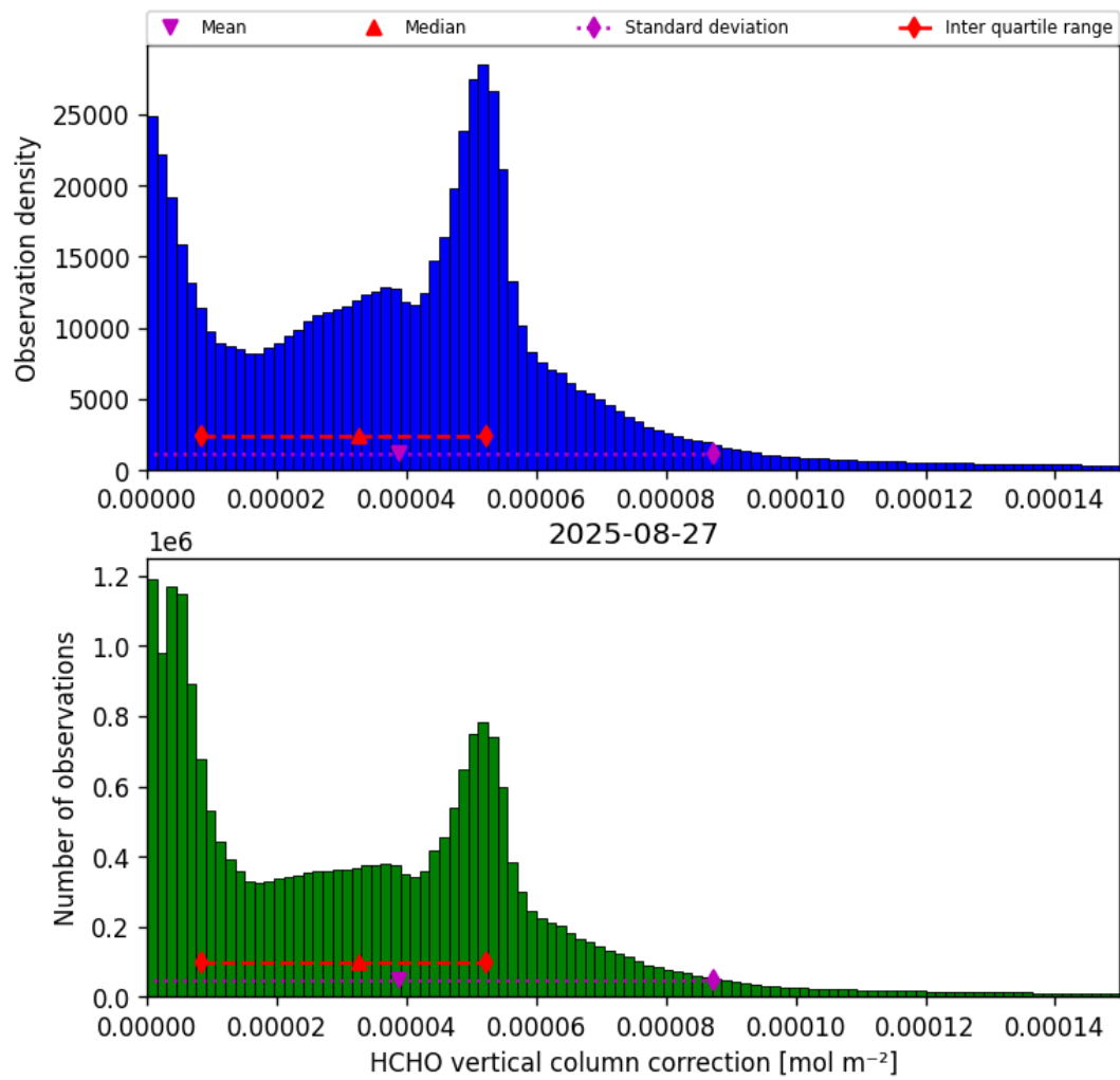
Figure 37: Histogram of “HCHO vertical column correction” for 2025-08-26 to 2025-08-28
