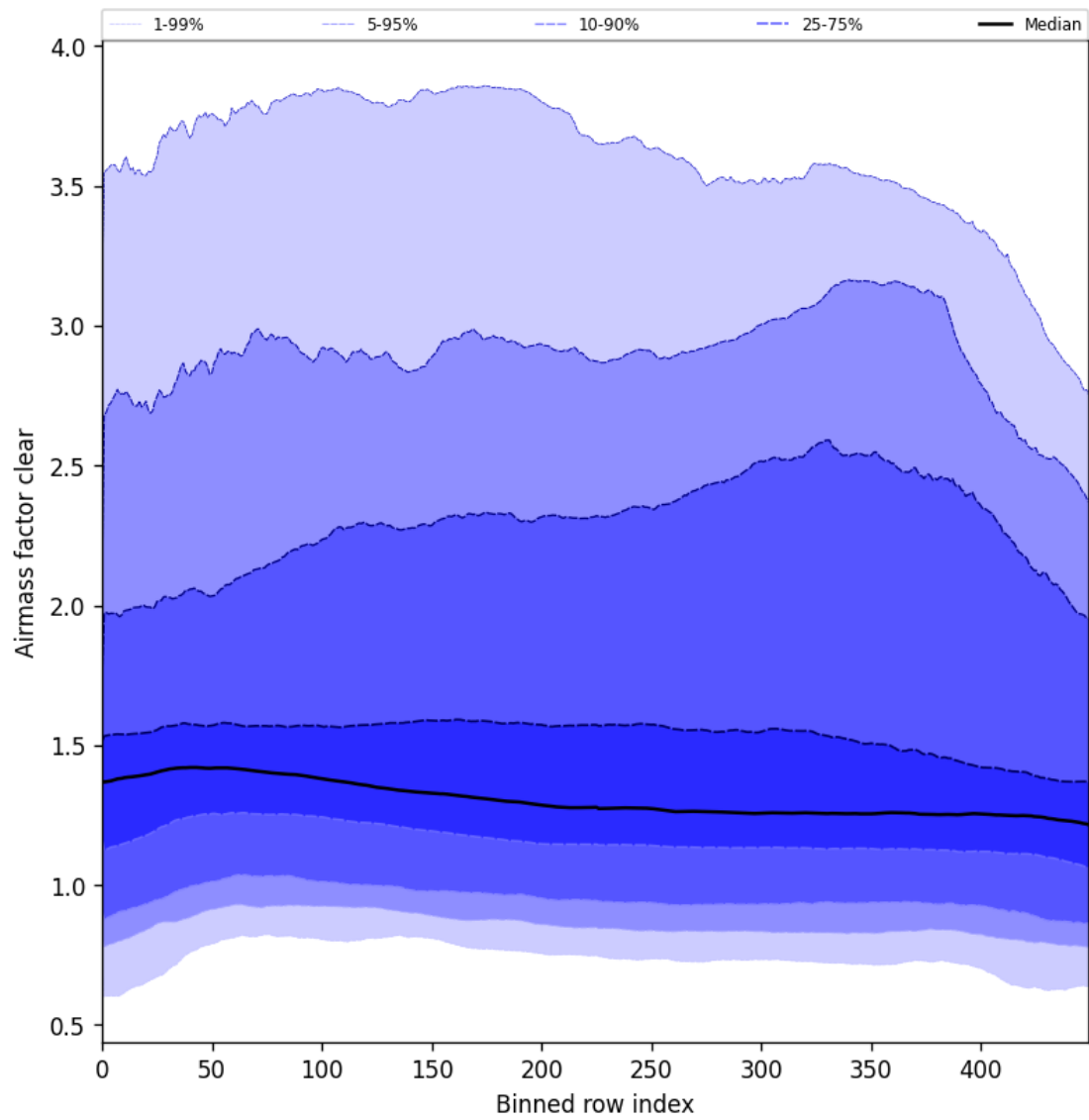
Figure 56: Along track statistics of “Airmass factor clear” for 2025-08-26 to 2025-08-28
