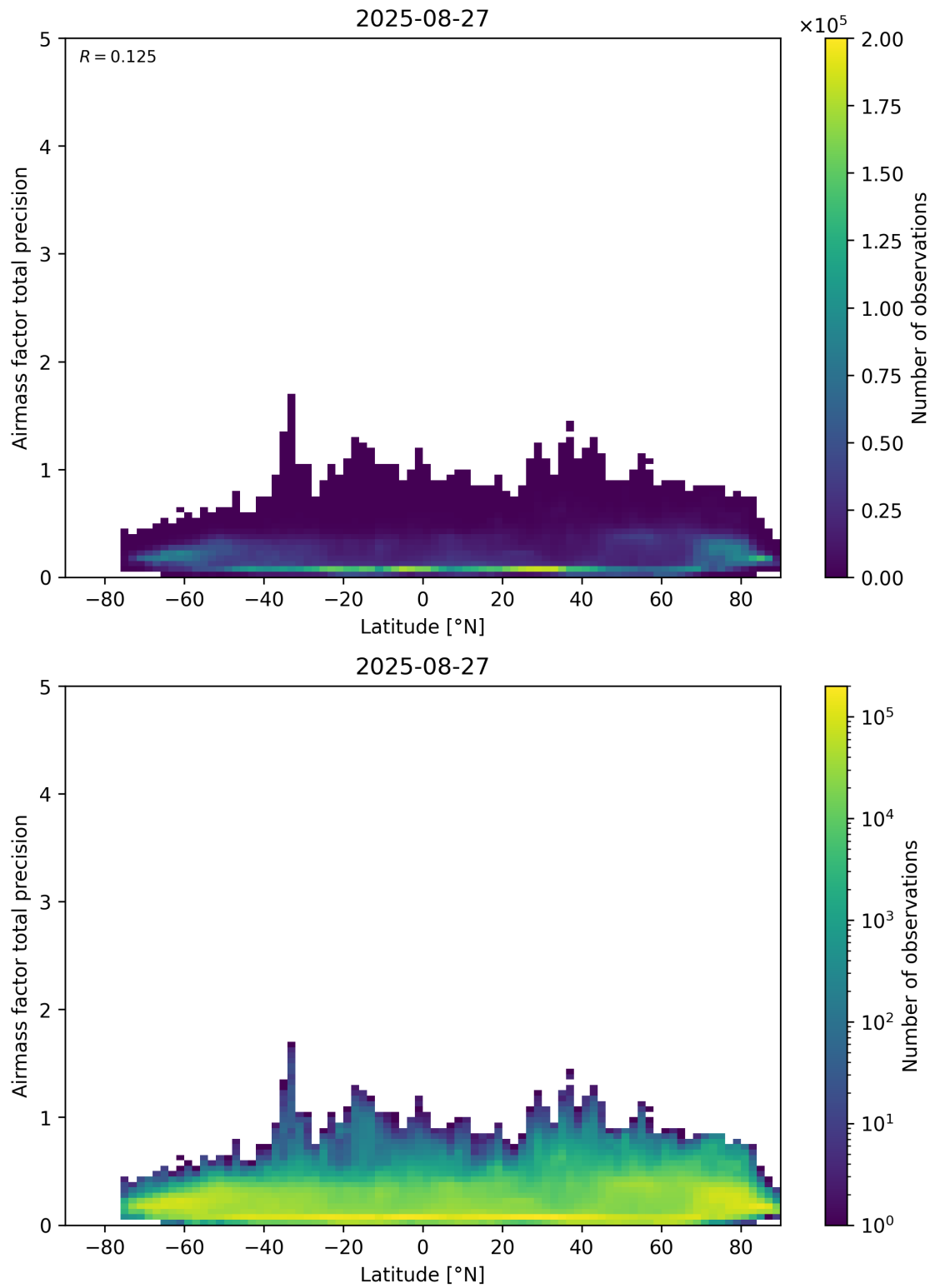
Figure 162: Scatter density plot of “Latitude” against “Airmass factor total precision” for 2025-08-26 to 2025-08-28.
