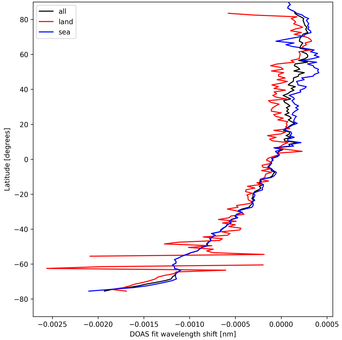
Figure 30: Zonal average of “DOAS fit wavelength shift” for 2025-08-26 to 2025-08-28.
