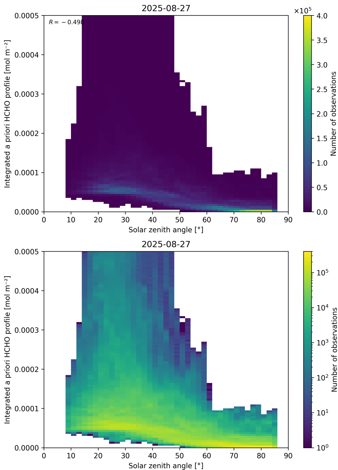
Figure 180: Scatter density plot of “Solar zenith angle” against “Integrated a priori HCHO profile” for 2025-08-26 to 2025-08-28.
