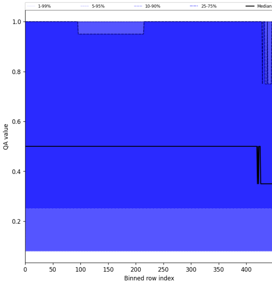
Figure 48: Along track statistics of “QA value” for 2025-08-26 to 2025-08-28
