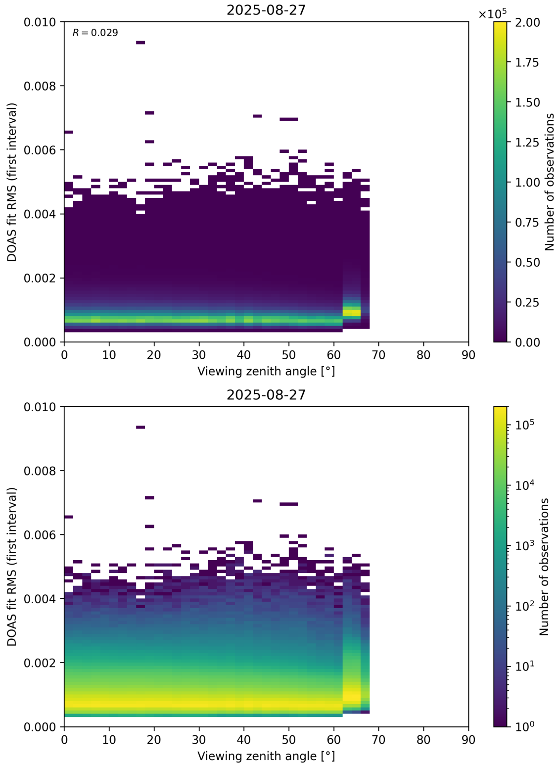
Figure 182: Scatter density plot of “Viewing zenith angle” against “DOAS fit RMS (first interval)” for 2025-08-26 to 2025-08-28.
