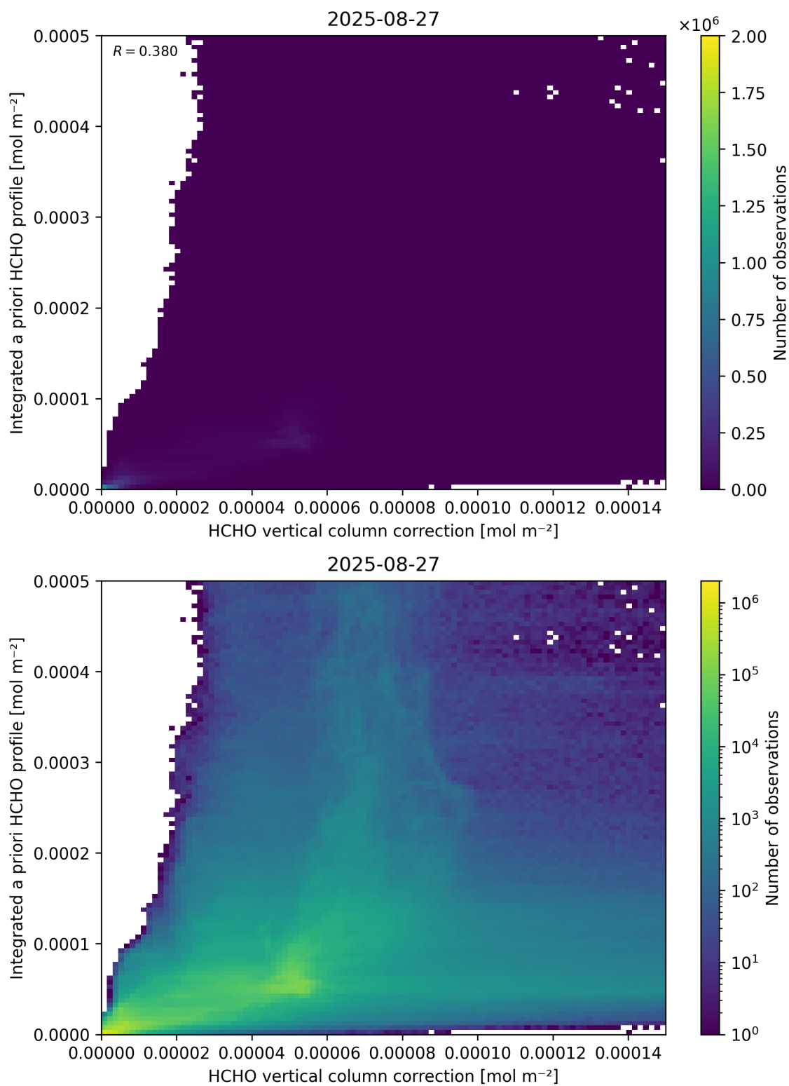
Figure 122: Scatter density plot of “HCHO vertical column correction” against “Integrated a priori HCHO profile” for 2025-08-26 to 2025-08-28.
