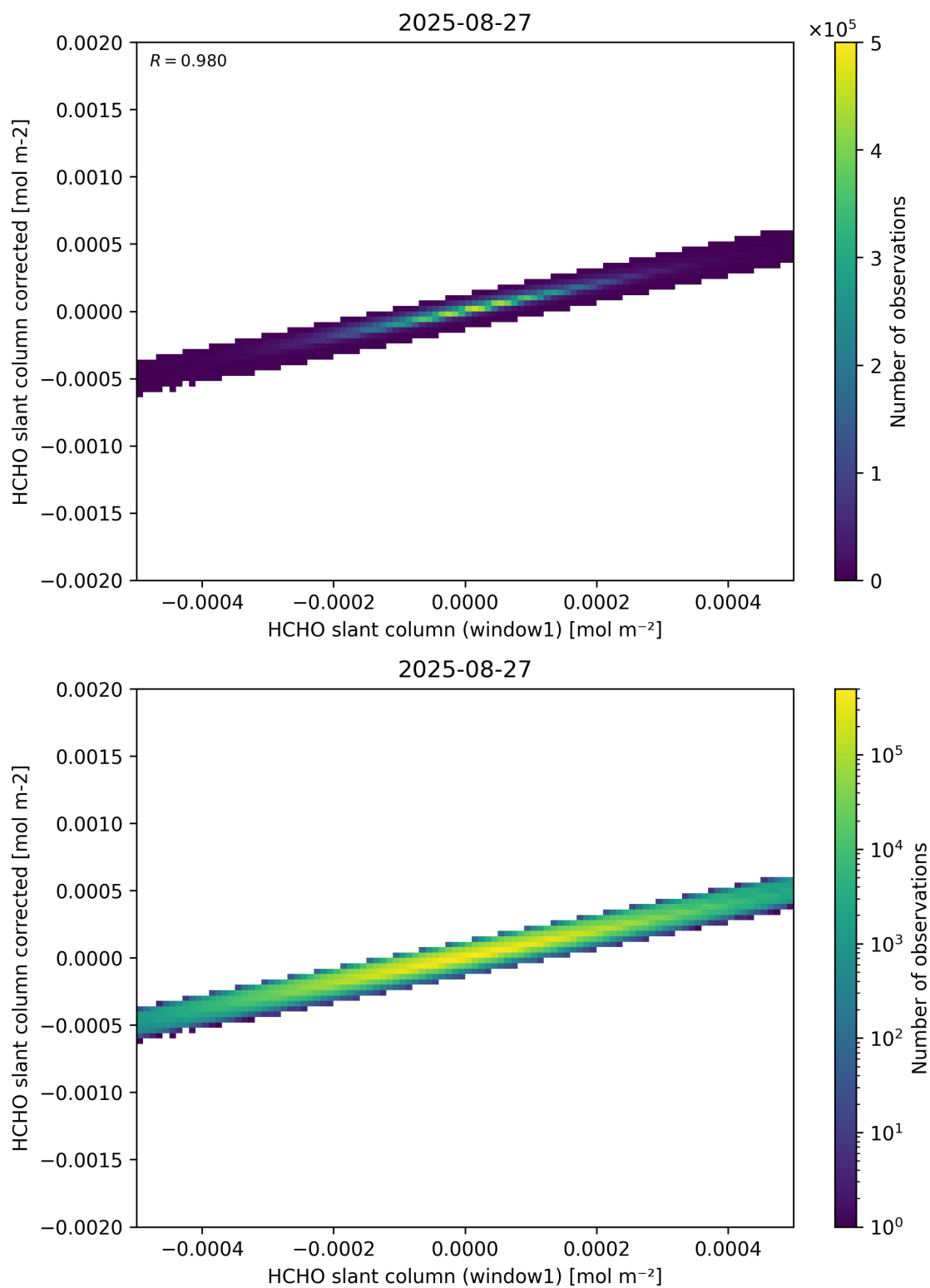
Figure 82: Scatter density plot of “HCHO slant column (window1)” against “HCHO slant column corrected” for 2025-08-26 to 2025-08-28.
