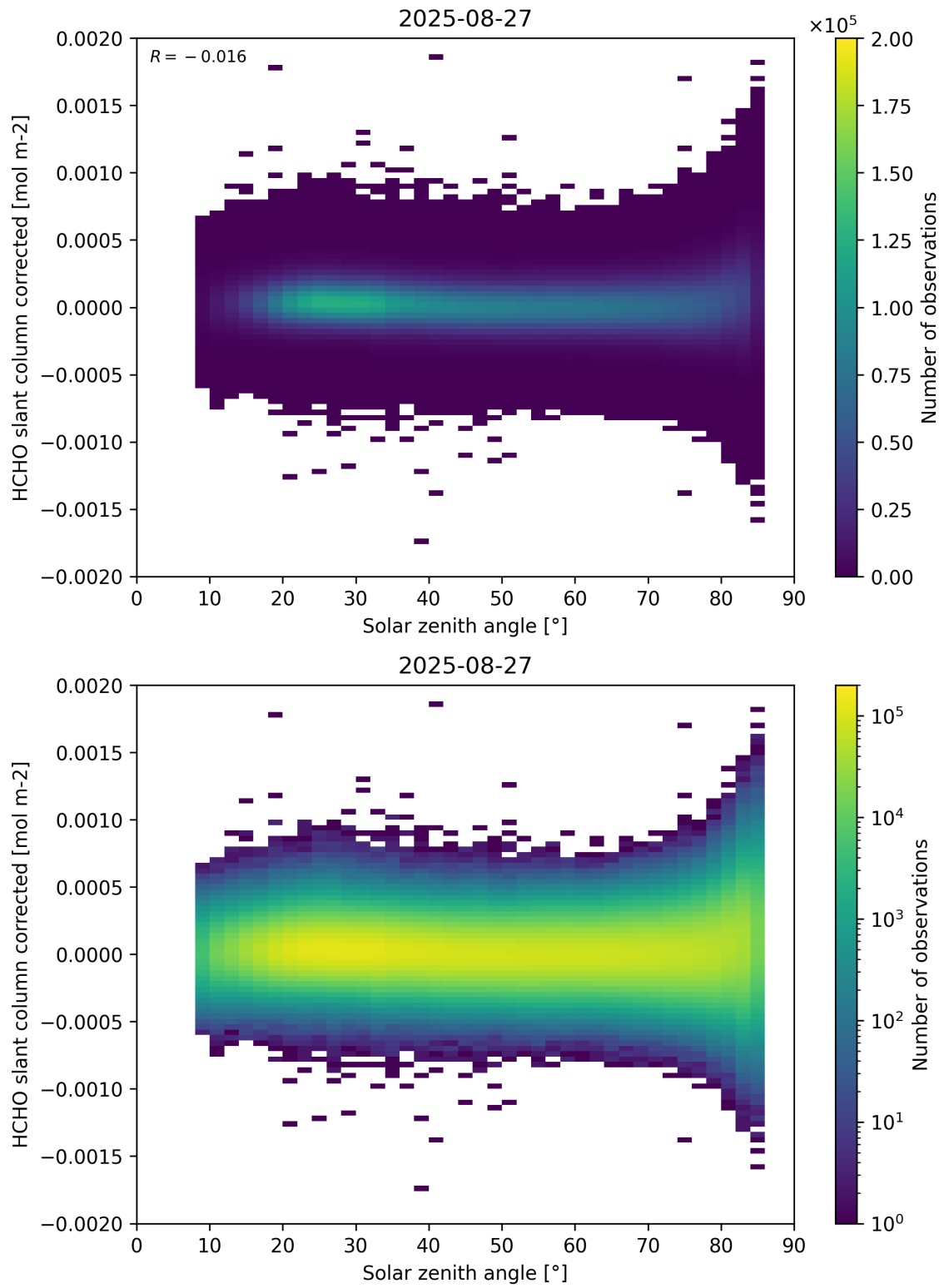
Figure 171: Scatter density plot of “Solar zenith angle” against “HCHO slant column corrected” for 2025-08-26 to 2025-08-28.
