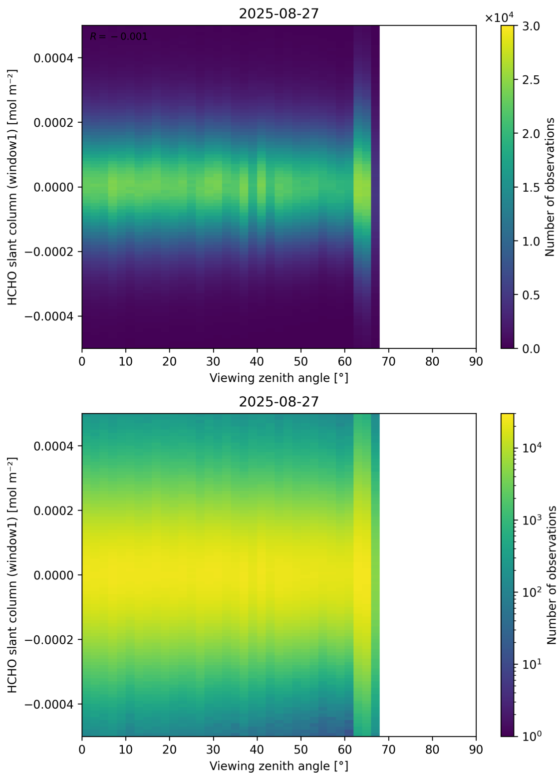
Figure 188: Scatter density plot of “Viewing zenith angle” against “HCHO slant column (window1)” for 2025-08-26 to 2025-08-28.
