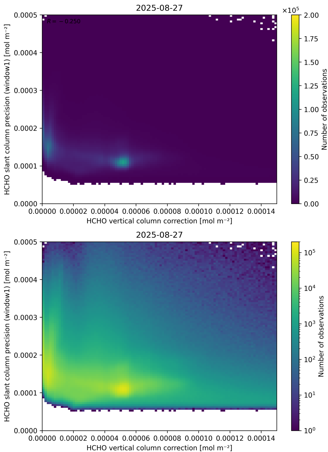
Figure 119: Scatter density plot of “HCHO vertical column correction” against “HCHO slant column precision (window1)” for 2025-08-26 to 2025-08-28.
