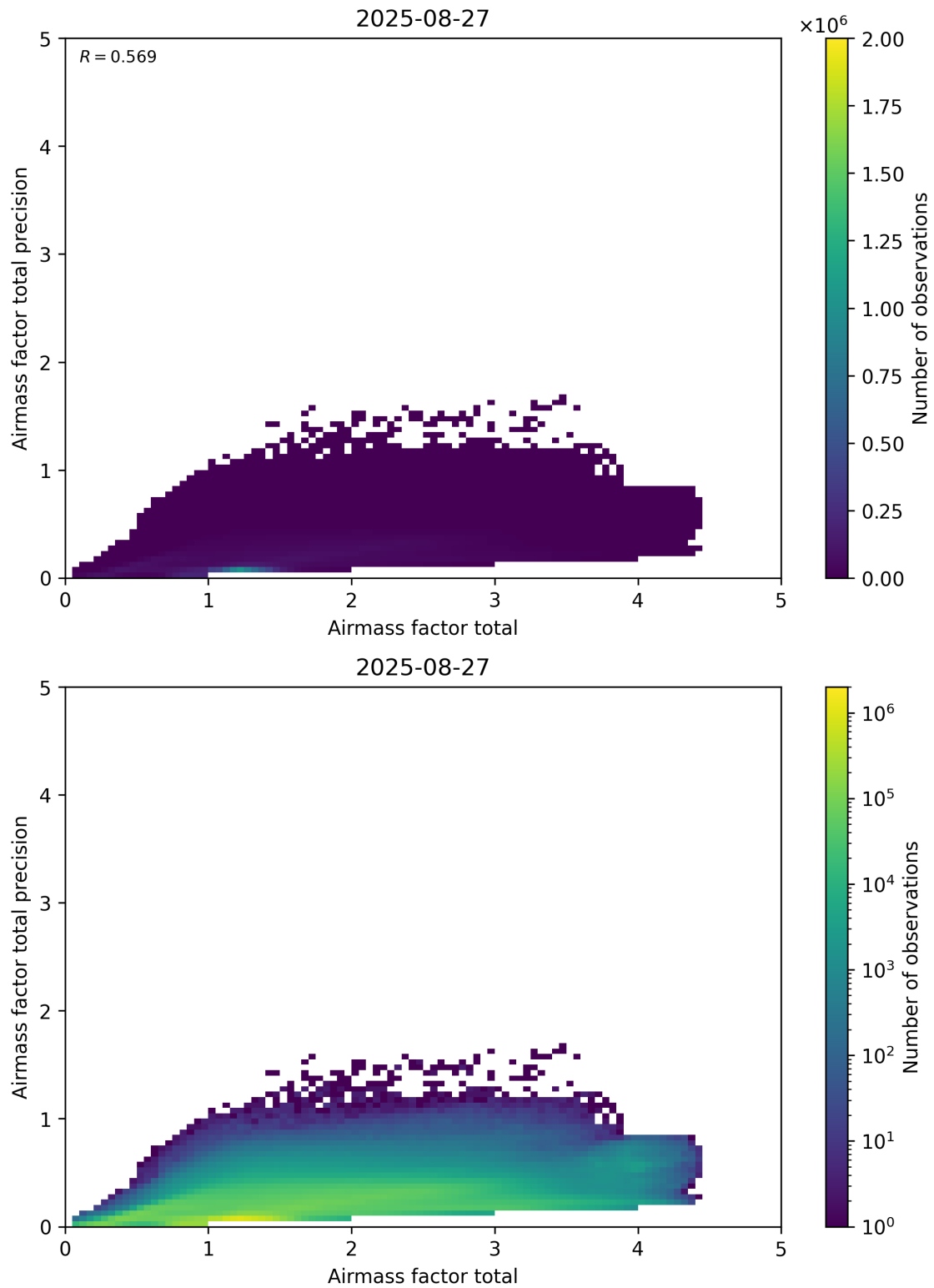
Figure 103: Scatter density plot of “Airmass factor total” against “Airmass factor total precision” for 2025-08-26 to 2025-08-28.
