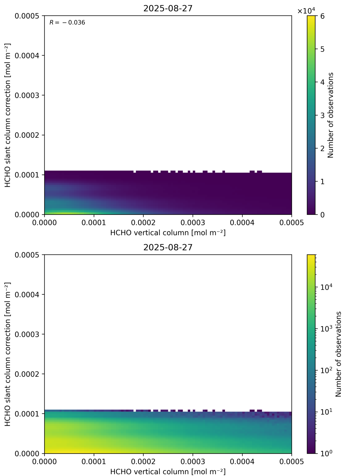
Figure 128: Scatter density plot of “HCHO vertical column” against “HCHO slant column correction” for 2025-08-26 to 2025-08-28.
