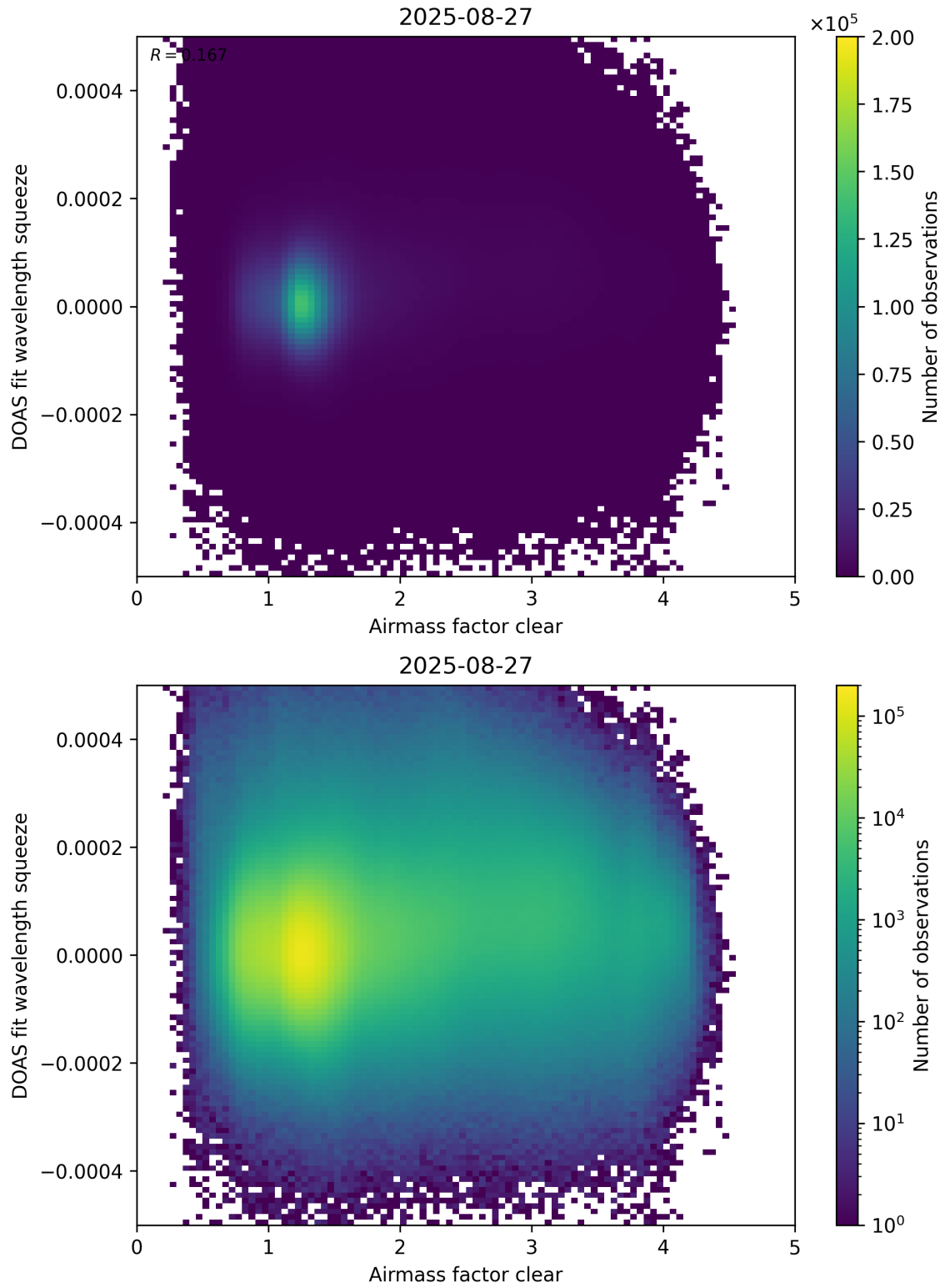
Figure 73: Scatter density plot of “Airmass factor clear” against “DOAS fit wavelength squeeze” for 2025-08-26 to 2025-08-28.
