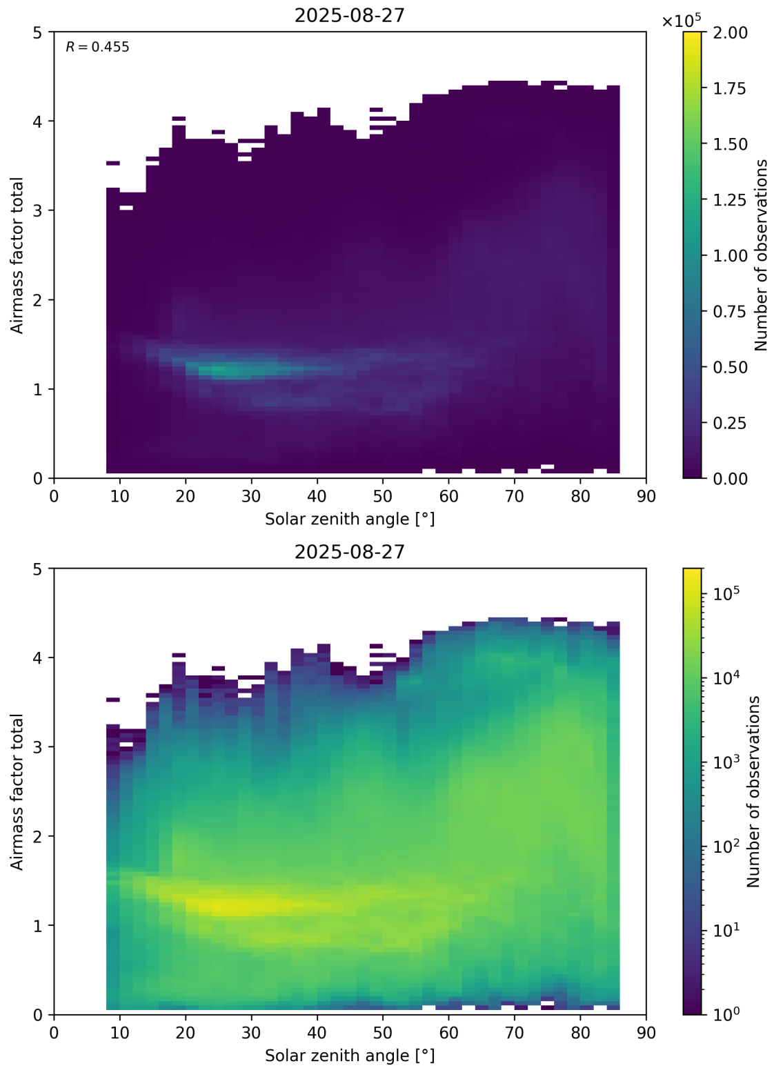
Figure 175: Scatter density plot of “Solar zenith angle” against “Airmass factor total” for 2025-08-26 to 2025-08-28.
