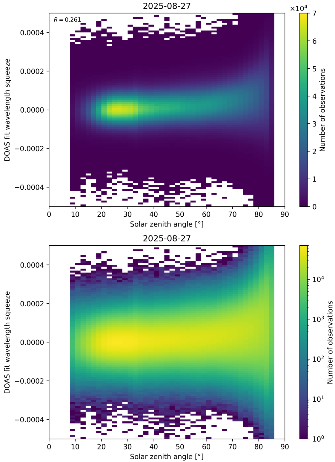
Figure 169: Scatter density plot of “Solar zenith angle” against “DOAS fit wavelength squeeze” for 2025-08-26 to 2025-08-28.
