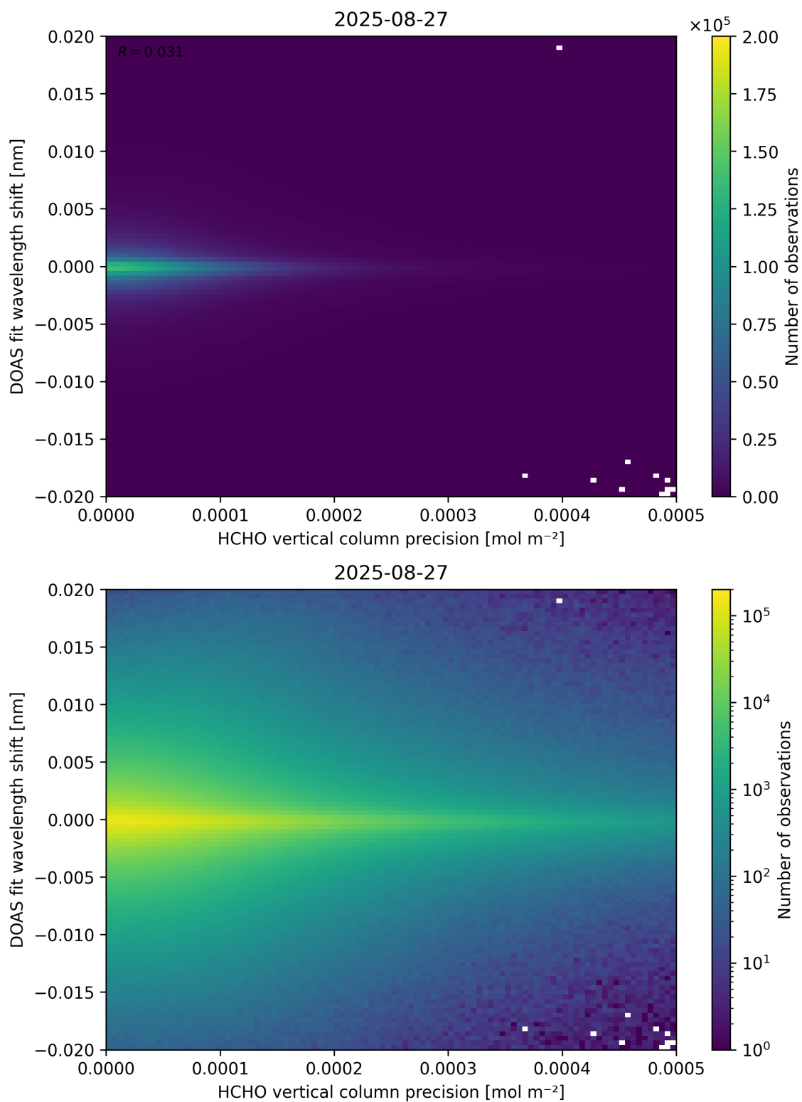
Figure 137: Scatter density plot of “HCHO vertical column precision” against “DOAS fit wavelength shift” for 2025-08-26 to 2025-08-28.
