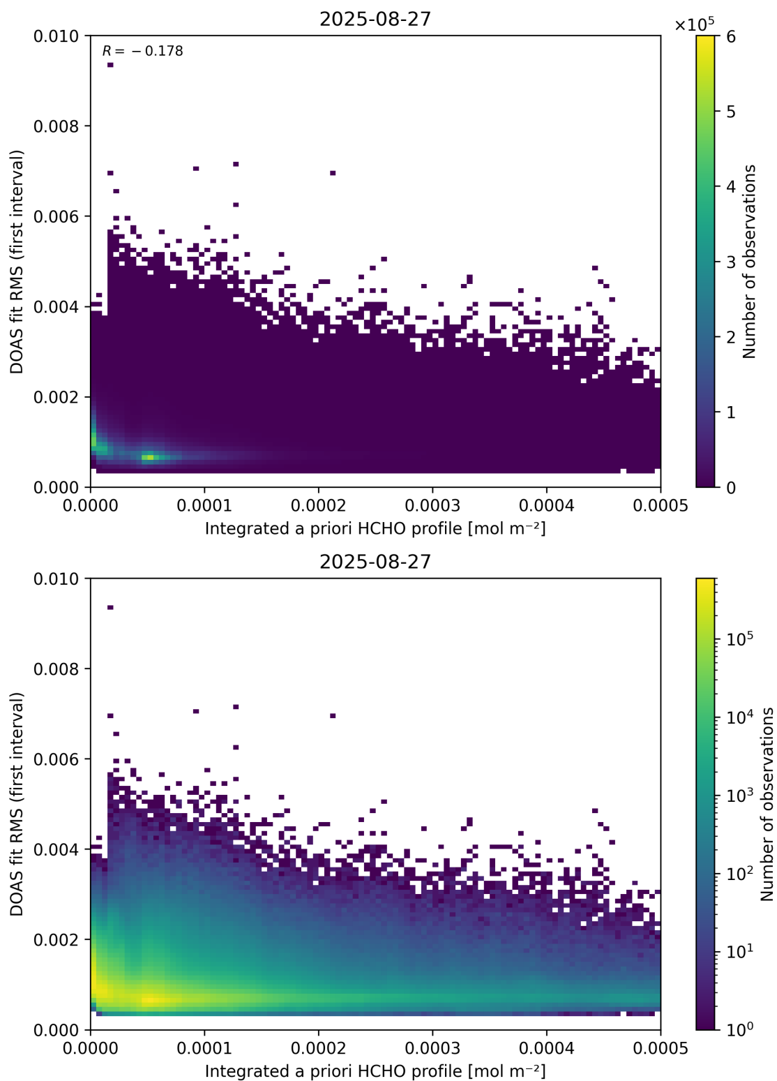
Figure 148: Scatter density plot of “Integrated a priori HCHO profile” against “DOAS fit RMS (first interval)” for 2025-08-26 to 2025-08-28.
