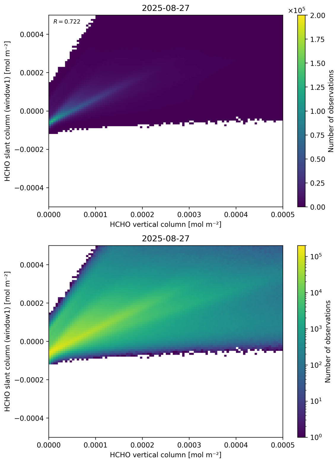
Figure 129: Scatter density plot of “HCHO vertical column” against “HCHO slant column (window1)” for 2025-08-26 to 2025-08-28.
