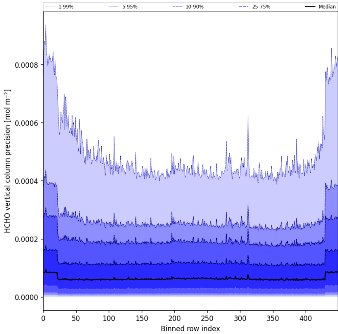
Figure 50: Along track statistics of “HCHO vertical column precision” for 2025-08-26 to 2025-08-28
