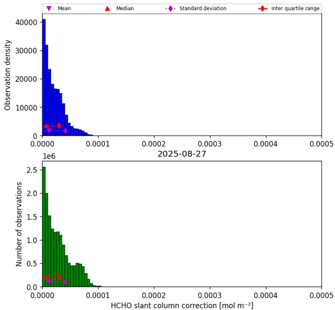
Figure 47: Histogram of “HCHO slant column correction” for 2025-08-26 to 2025-08-28
