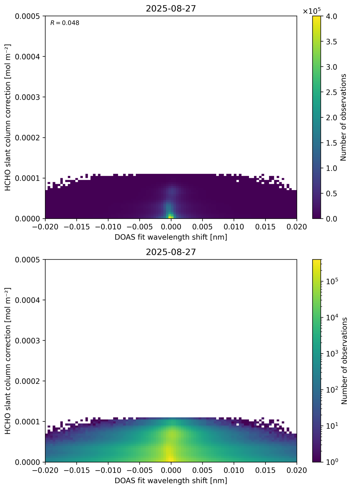
Figure 67: Scatter density plot of “DOAS fit wavelength shift” against “HCHO slant column correction” for 2025-08-26 to 2025-08-28.
