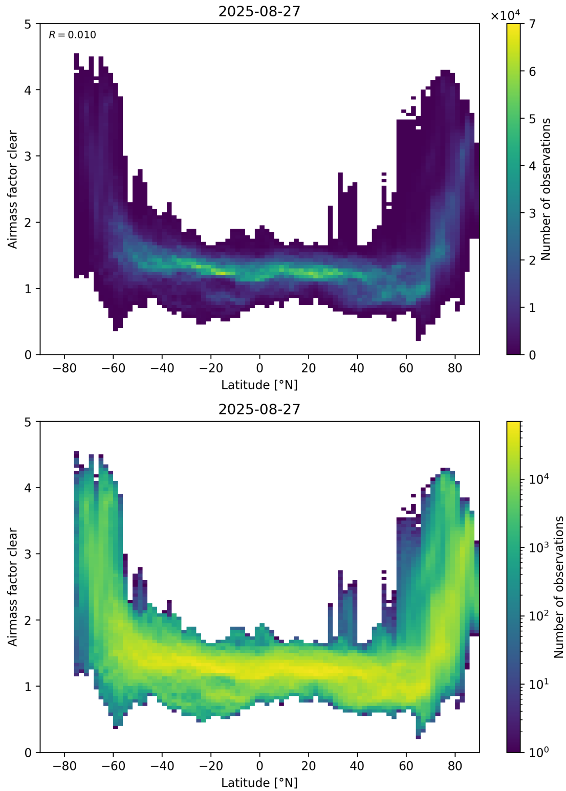
Figure 156: Scatter density plot of “Latitude” against “Airmass factor clear” for 2025-08-26 to 2025-08-28.
