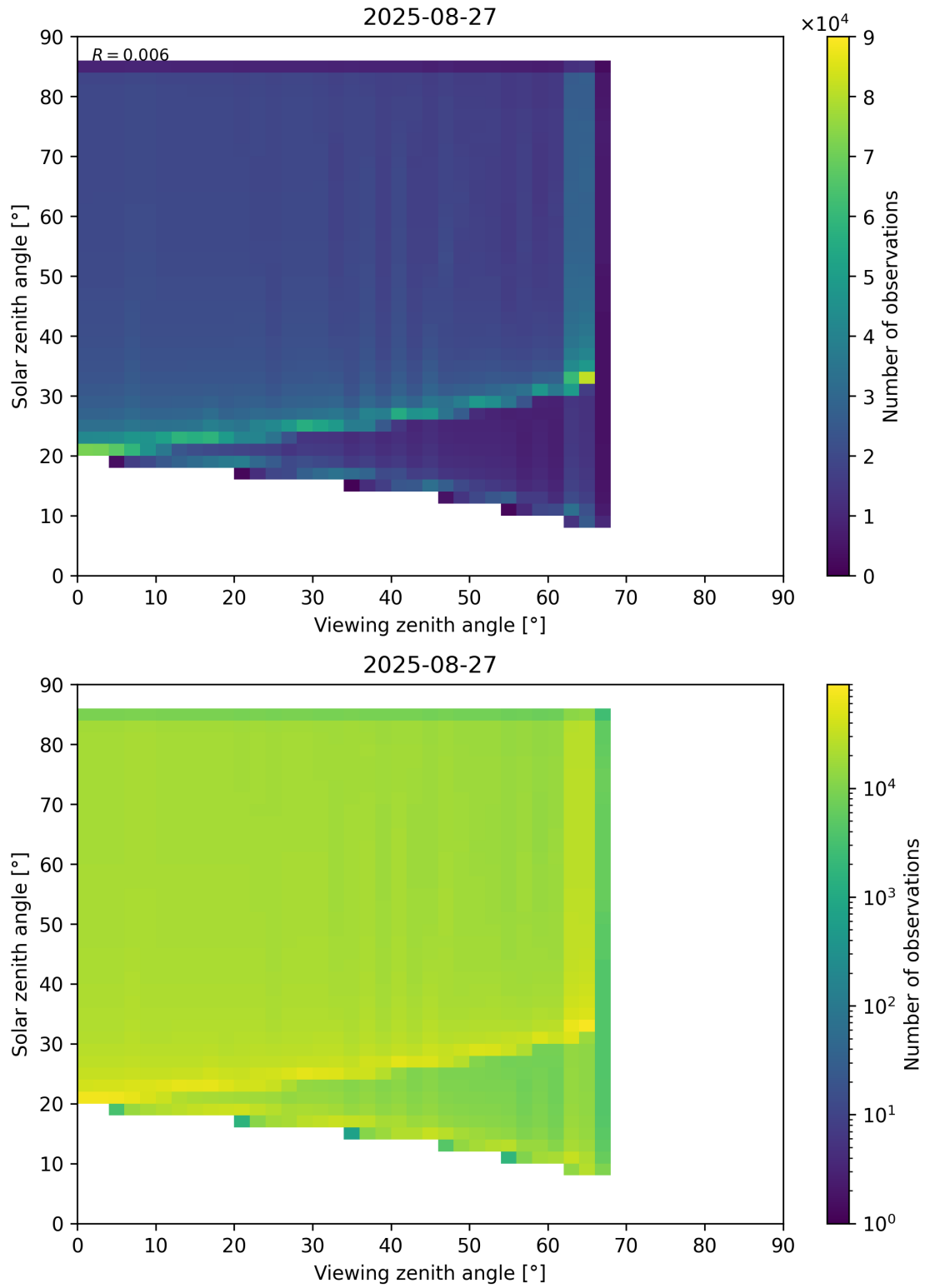
Figure 197: Scatter density plot of “Viewing zenith angle” against “Solar zenith angle” for 2025-08-26 to 2025-08-28.
