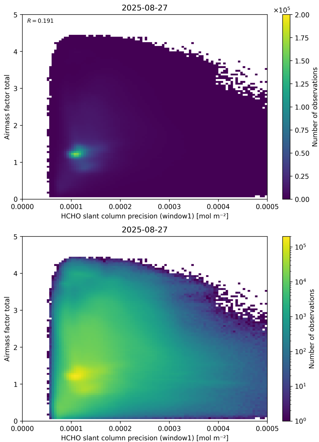
Figure 94: Scatter density plot of “HCHO slant column precision (window1)” against “Airmass factor total” for 2025-08-26 to 2025-08-28.
