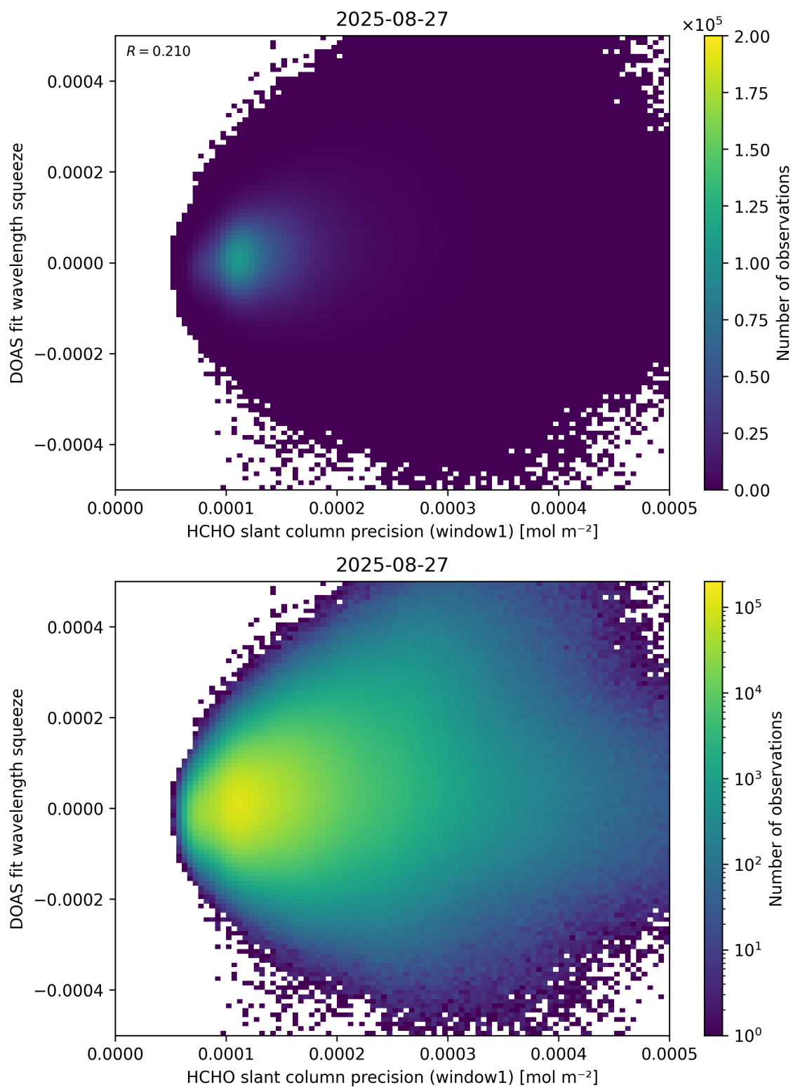
Figure 90: Scatter density plot of “HCHO slant column precision (window1)” against “DOAS fit wavelength squeeze” for 2025-08-26 to 2025-08-28.
