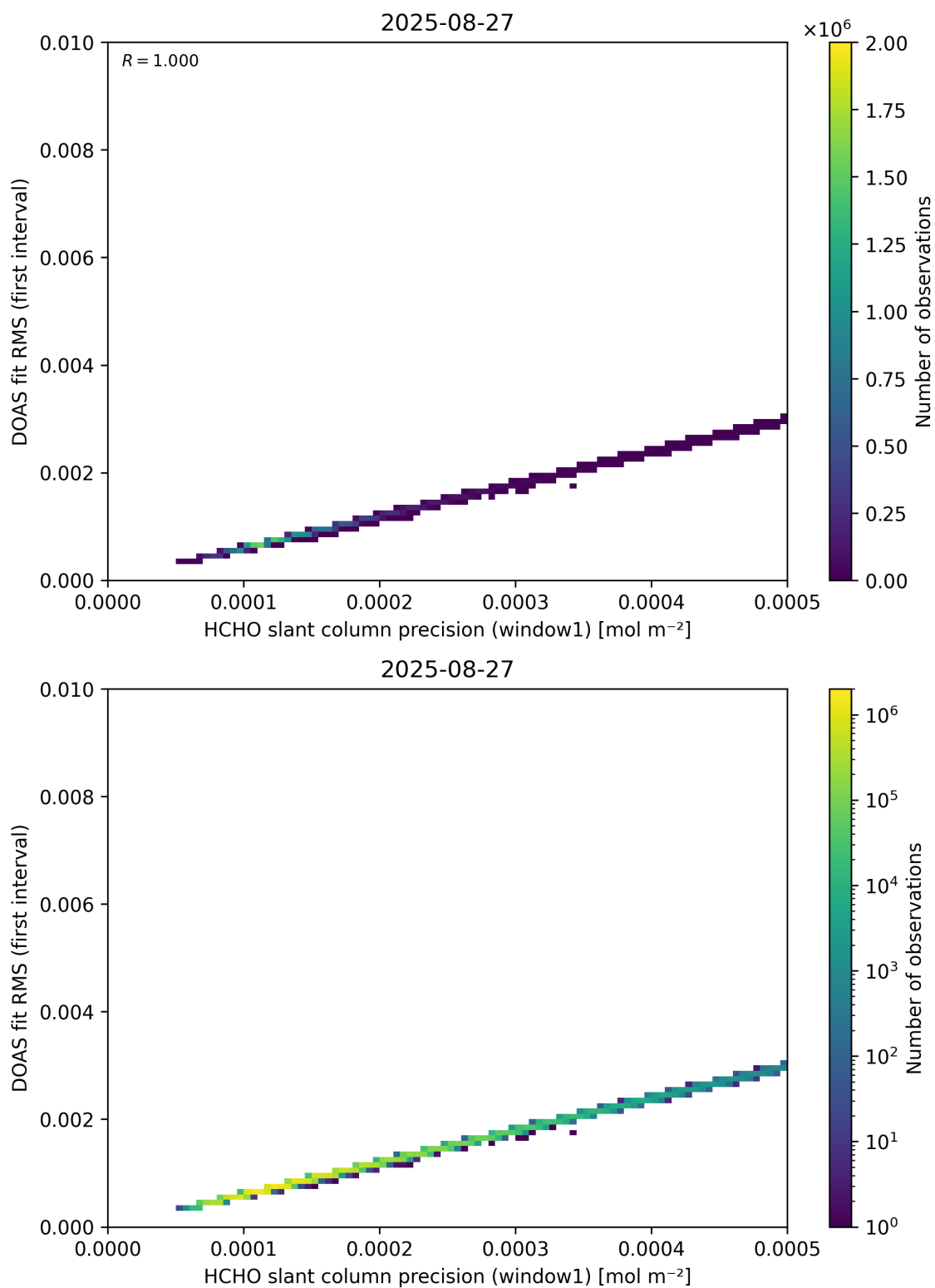
Figure 88: Scatter density plot of “HCHO slant column precision (window1)” against “DOAS fit RMS (first interval)” for 2025-08-26 to 2025-08-28.
