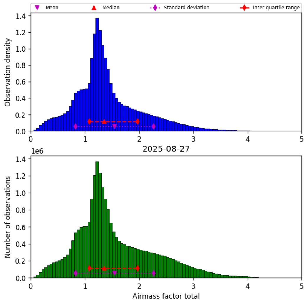
Figure 40: Histogram of “Airmass factor total” for 2025-08-26 to 2025-08-28
