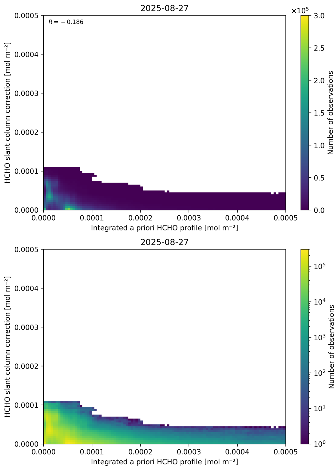
Figure 152: Scatter density plot of “Integrated a priori HCHO profile” against “HCHO slant column correction” for 2025-08-26 to 2025-08-28.
