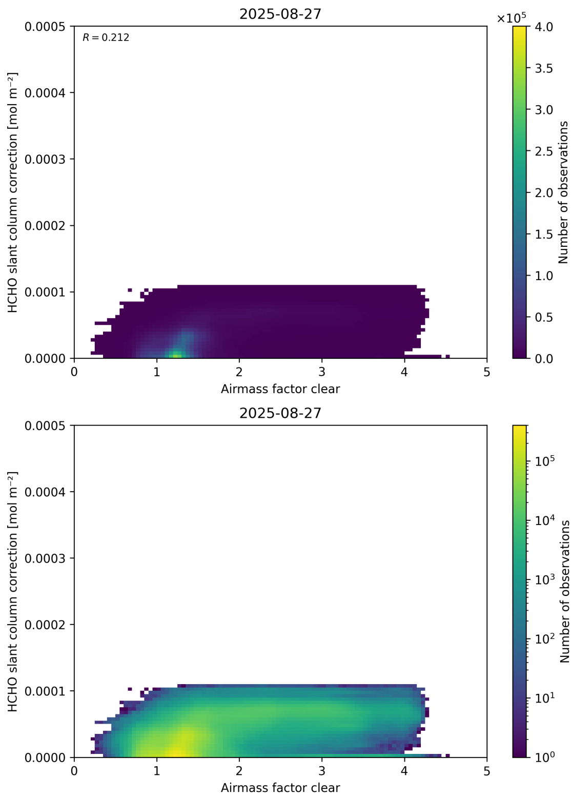
Figure 75: Scatter density plot of “Airmass factor clear” against “HCHO slant column correction” for 2025-08-26 to 2025-08-28.
