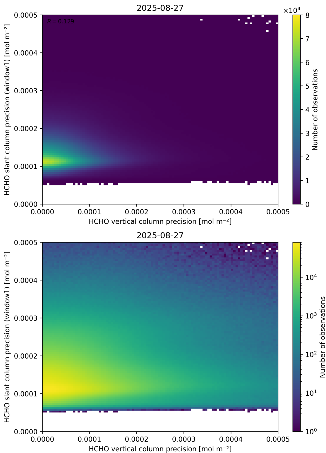
Figure 143: Scatter density plot of “HCHO vertical column precision” against “HCHO slant column precision (window1)” for 2025-08-26 to 2025-08-28.
