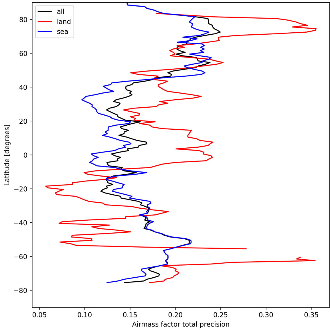
Figure 27: Zonal average of “Airmass factor total precision” for 2025-08-26 to 2025-08-28.
