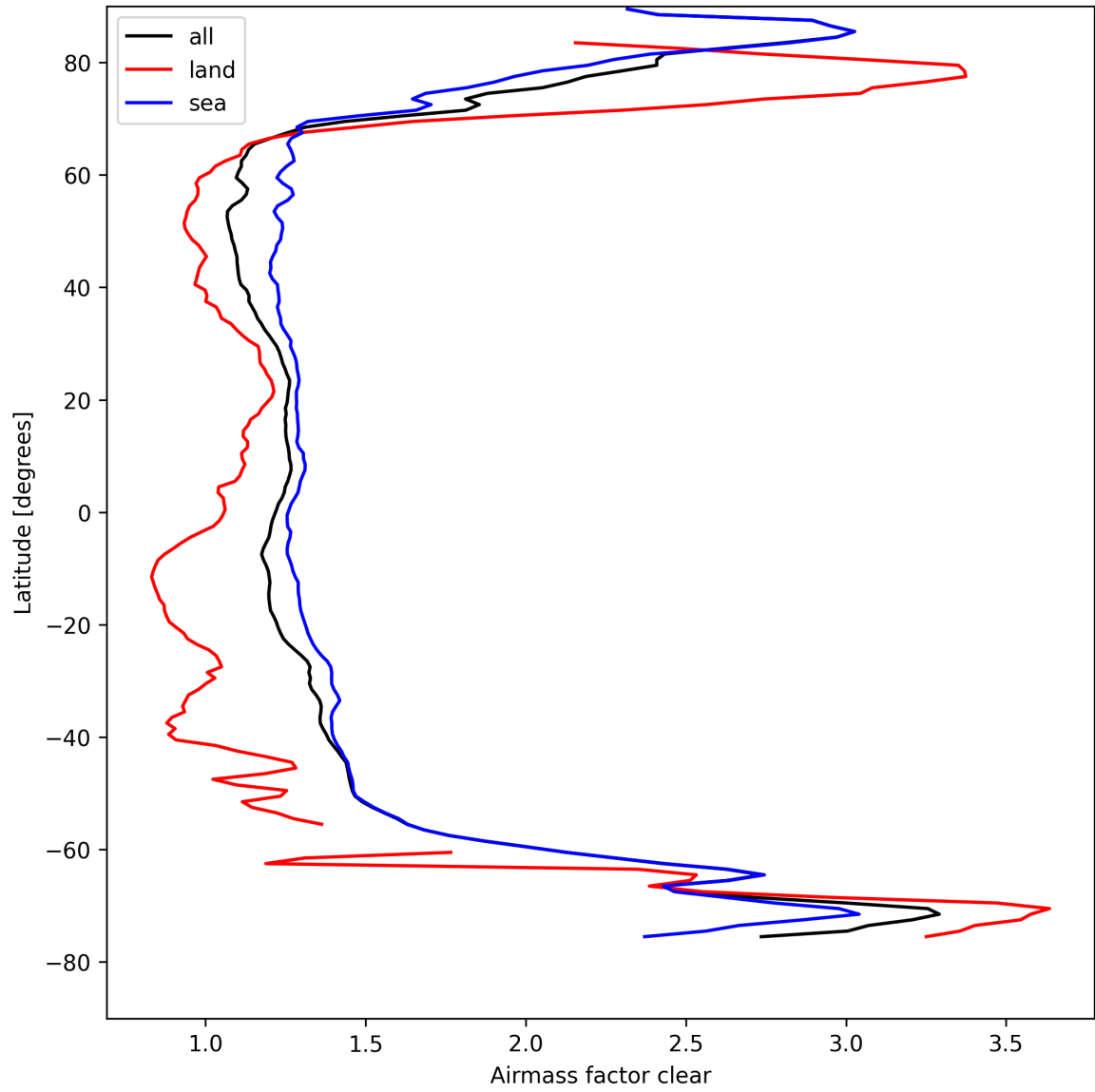
Figure 28: Zonal average of “Airmass factor clear” for 2025-08-26 to 2025-08-28.
