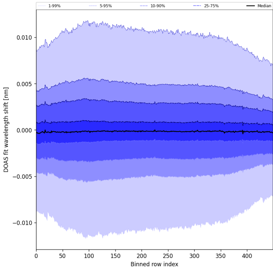
Figure 58: Along track statistics of “DOAS fit wavelength shift” for 2025-08-26 to 2025-08-28
