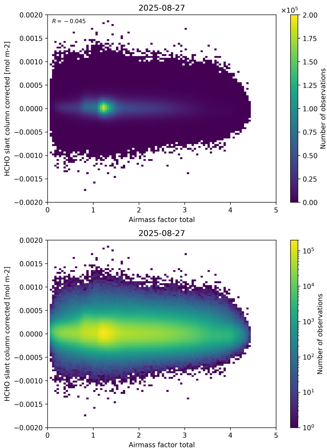
Figure 101: Scatter density plot of “Airmass factor total” against “HCHO slant column corrected” for 2025-08-26 to 2025-08-28.
