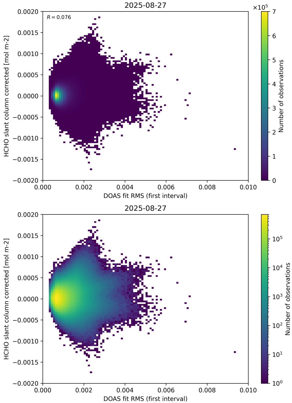
Figure 62: Scatter density plot of “DOAS fit RMS (first interval)” against “HCHO slant column corrected” for 2025-08-26 to 2025-08-28.
