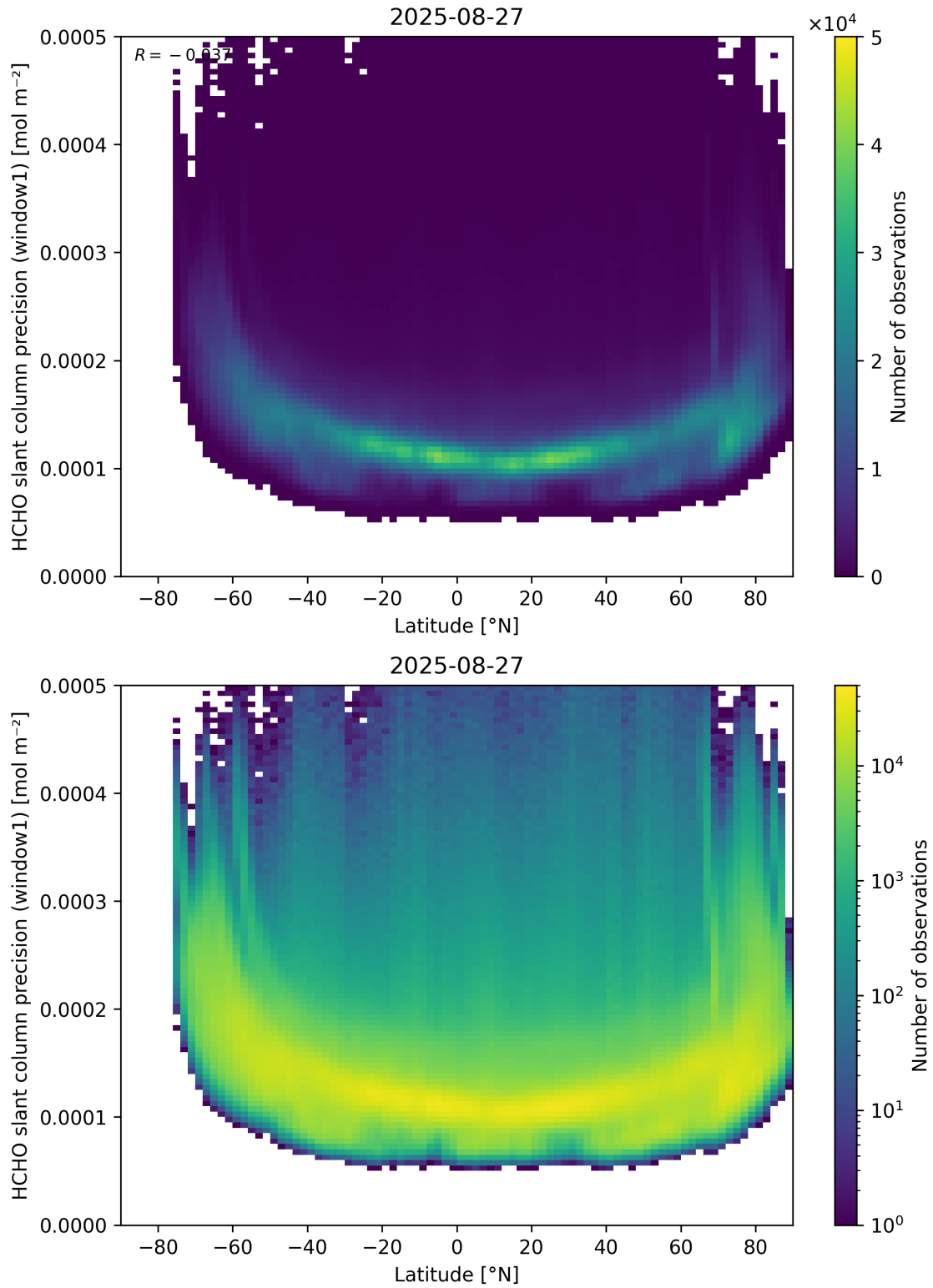
Figure 160: Scatter density plot of “Latitude” against “HCHO slant column precision (window1)” for 2025-08-26 to 2025-08-28.
