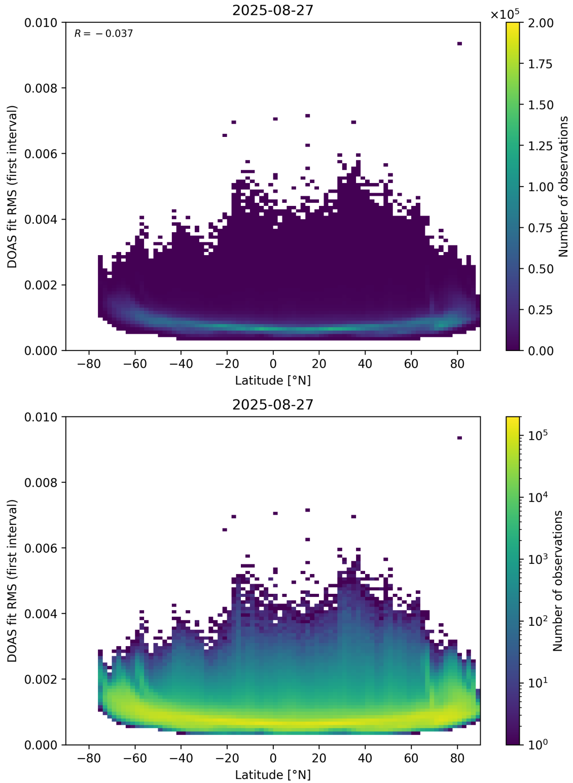
Figure 153: Scatter density plot of “Latitude” against “DOAS fit RMS (first interval)” for 2025-08-26 to 2025-08-28.
