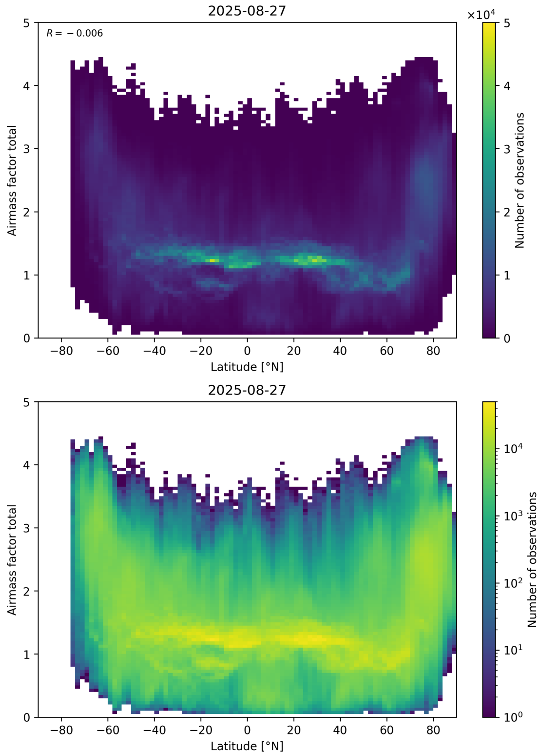
Figure 161: Scatter density plot of “Latitude” against “Airmass factor total” for 2025-08-26 to 2025-08-28.
