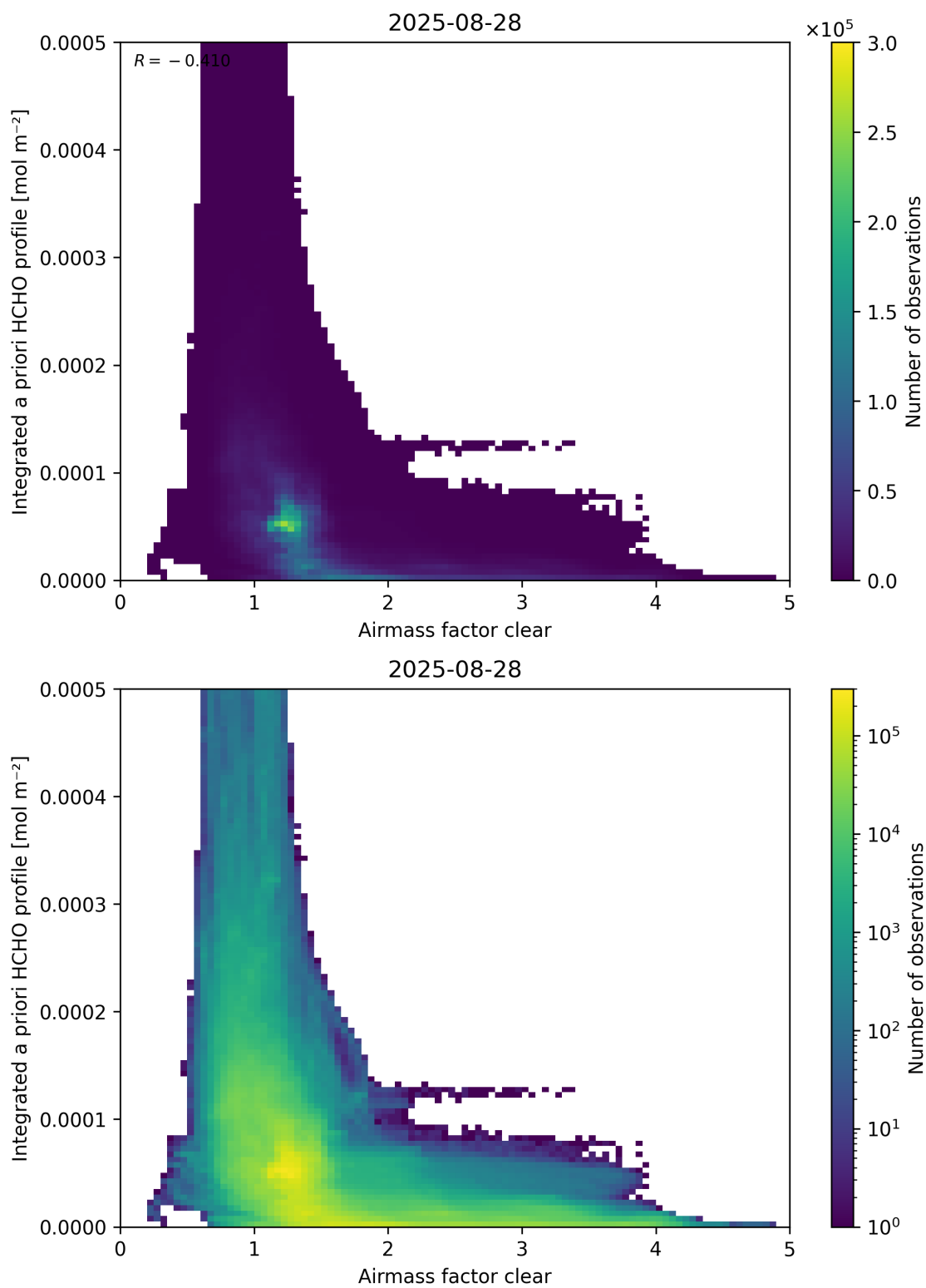
Figure 76: Scatter density plot of “Airmass factor clear” against “Integrated a priori HCHO profile” for 2025-08-27 to 2025-08-29.
