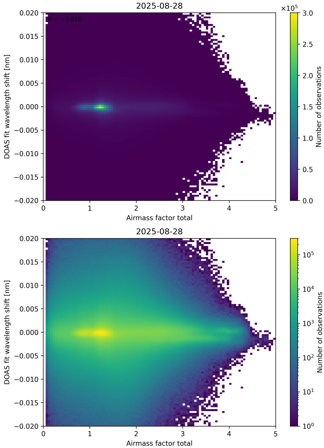
Figure 98: Scatter density plot of “Airmass factor total” against “DOAS fit wavelength shift” for 2025-08-27 to 2025-08-29.
