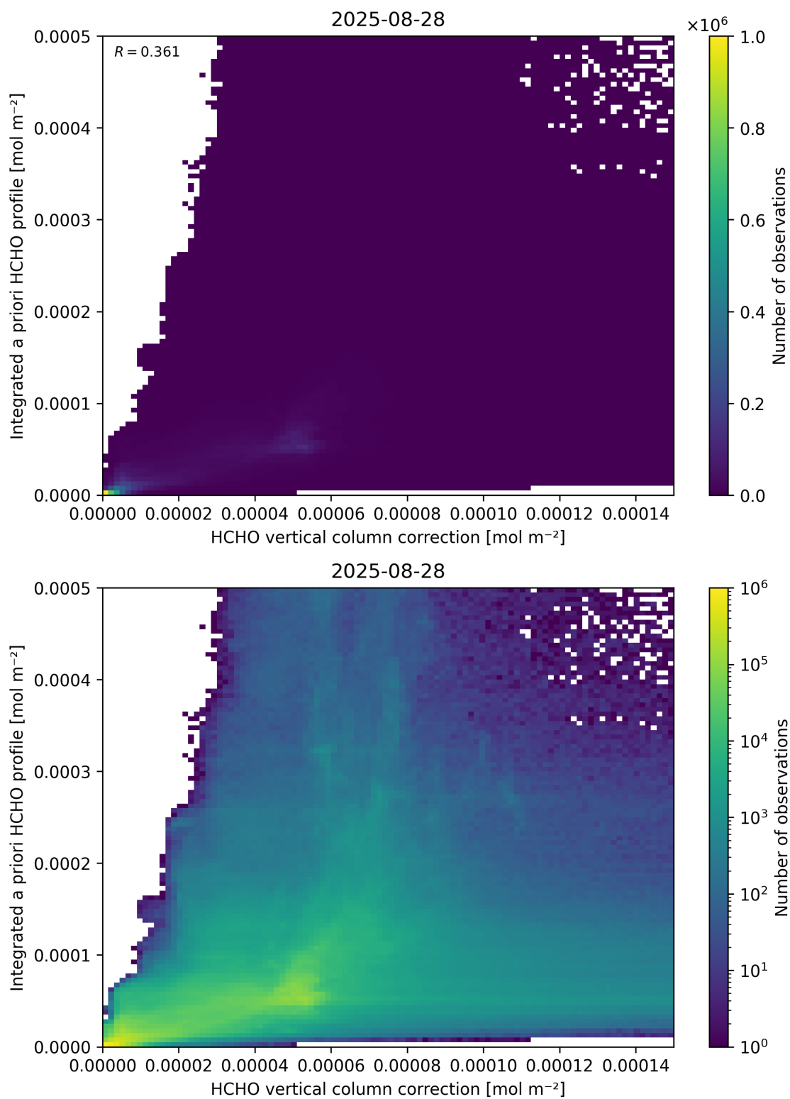
Figure 122: Scatter density plot of “HCHO vertical column correction” against “Integrated a priori HCHO profile” for 2025-08-27 to 2025-08-29.
