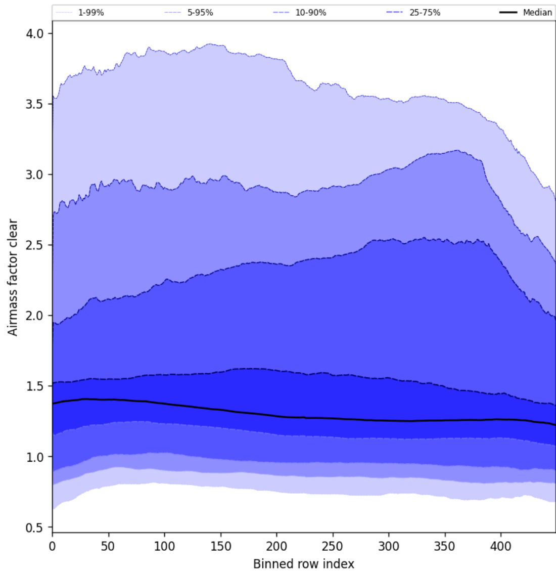
Figure 56: Along track statistics of “Airmass factor clear” for 2025-08-27 to 2025-08-29
