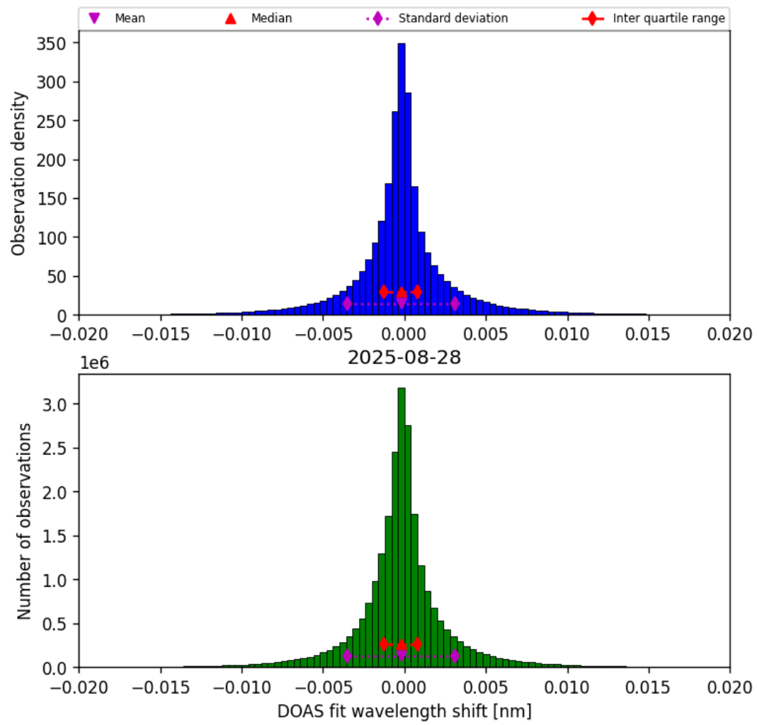
Figure 44: Histogram of “DOAS fit wavelength shift” for 2025-08-27 to 2025-08-29
