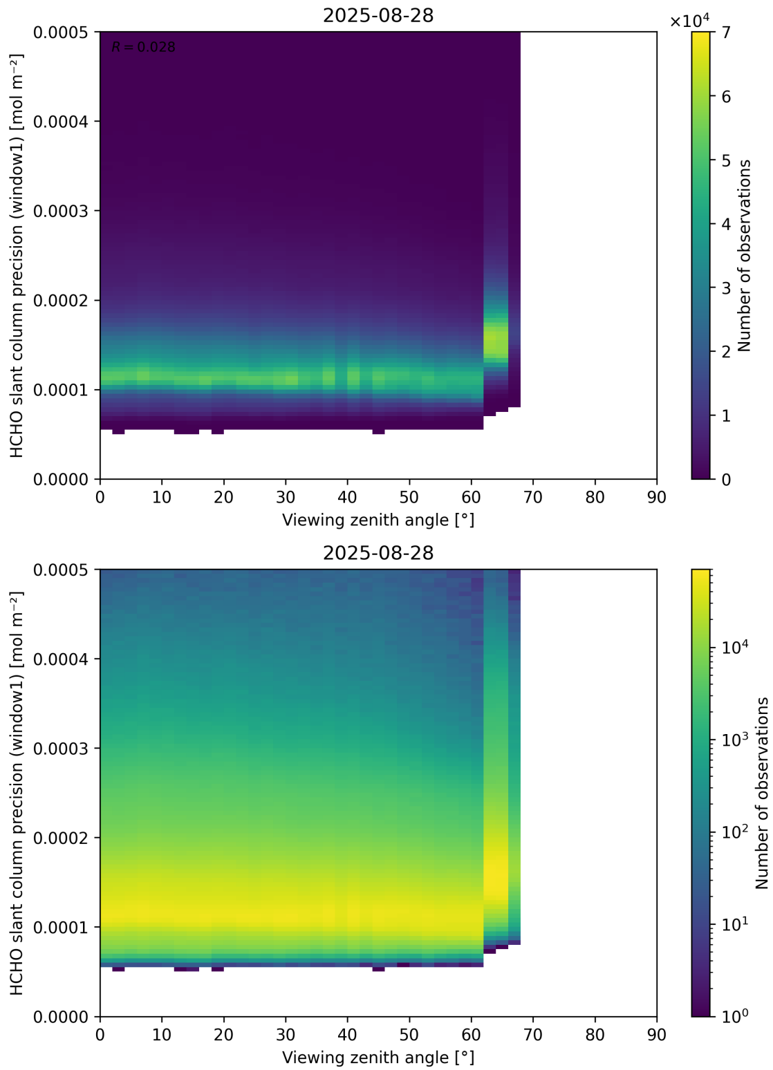
Figure 189: Scatter density plot of “Viewing zenith angle” against “HCHO slant column precision (window1)” for 2025-08-27 to 2025-08-29.
