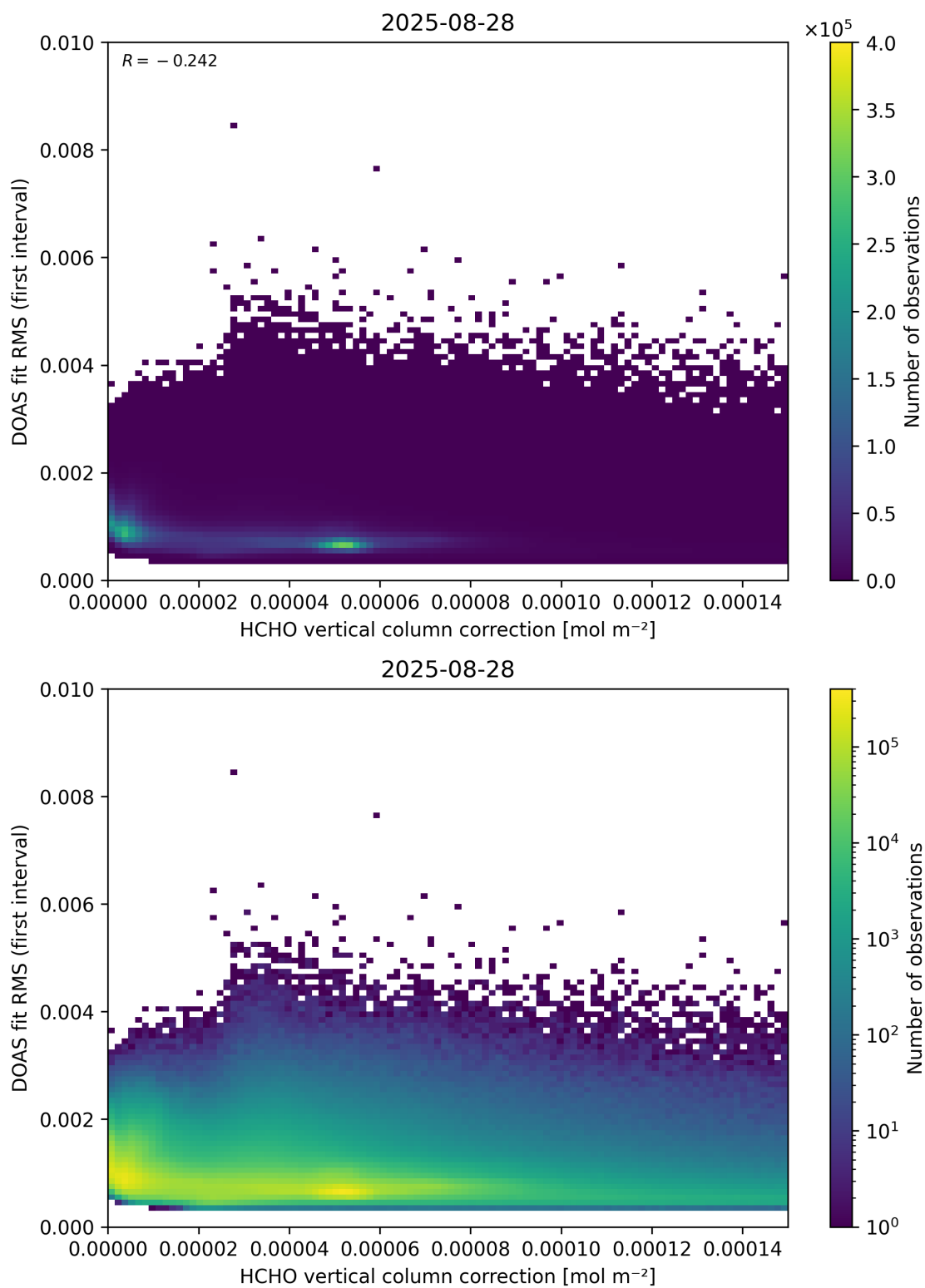
Figure 112: Scatter density plot of “HCHO vertical column correction” against “DOAS fit RMS (first interval)” for 2025-08-27 to 2025-08-29.
