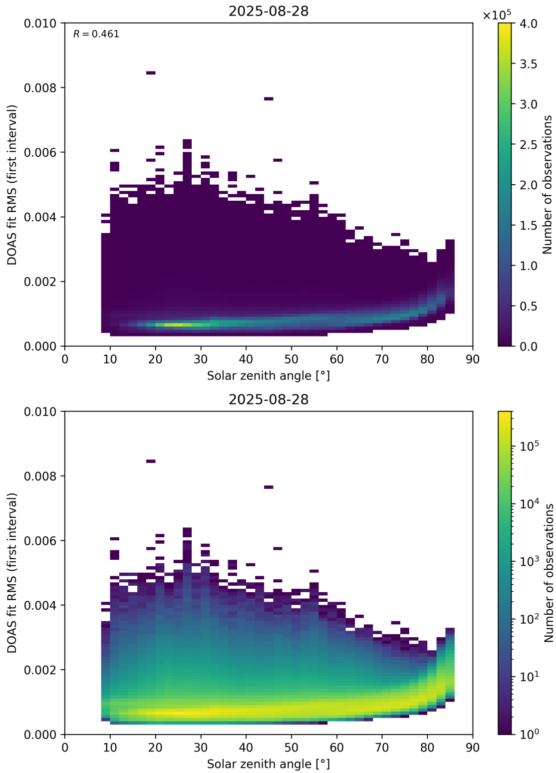
Figure 167: Scatter density plot of “Solar zenith angle” against “DOAS fit RMS (first interval)” for 2025-08-27 to 2025-08-29.
