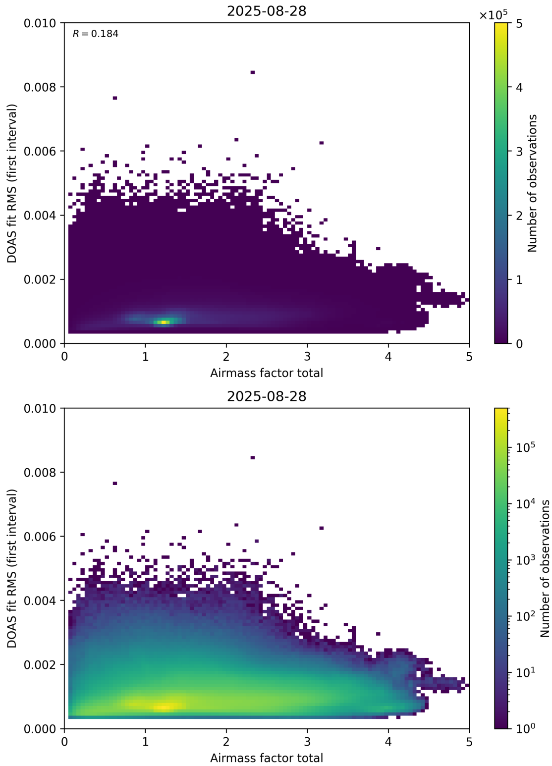
Figure 97: Scatter density plot of “Airmass factor total” against “DOAS fit RMS (first interval)” for 2025-08-27 to 2025-08-29.
