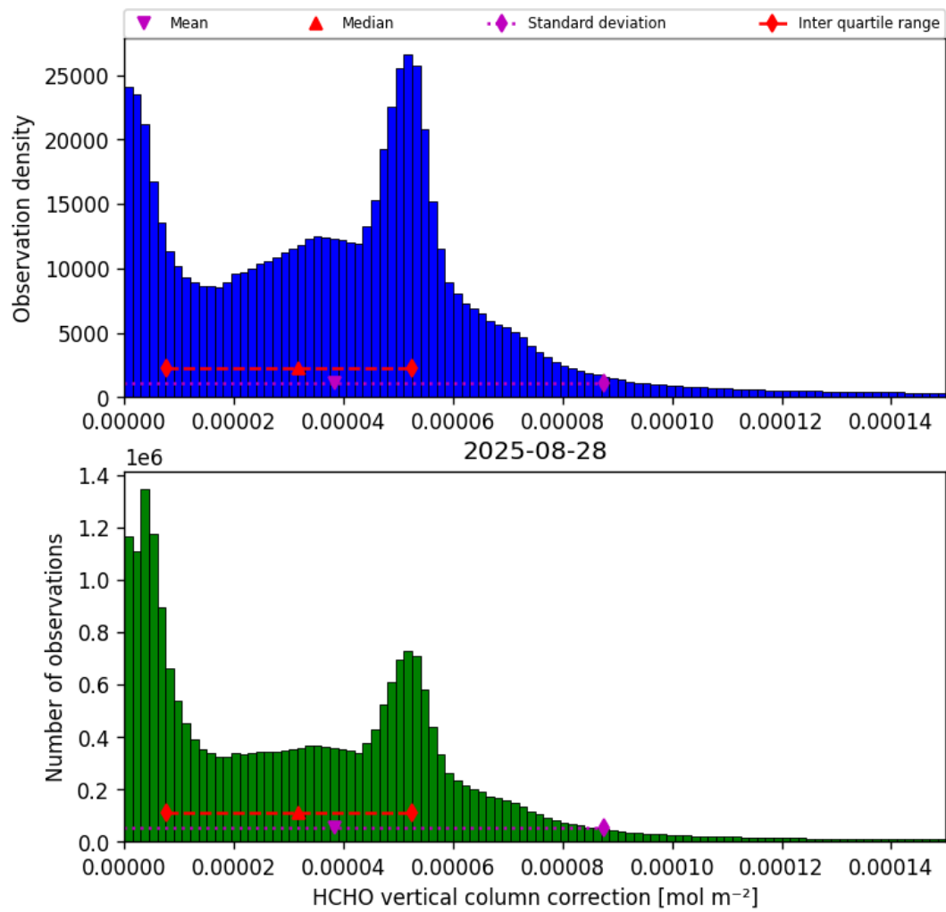
Figure 37: Histogram of “HCHO vertical column correction” for 2025-08-27 to 2025-08-29
