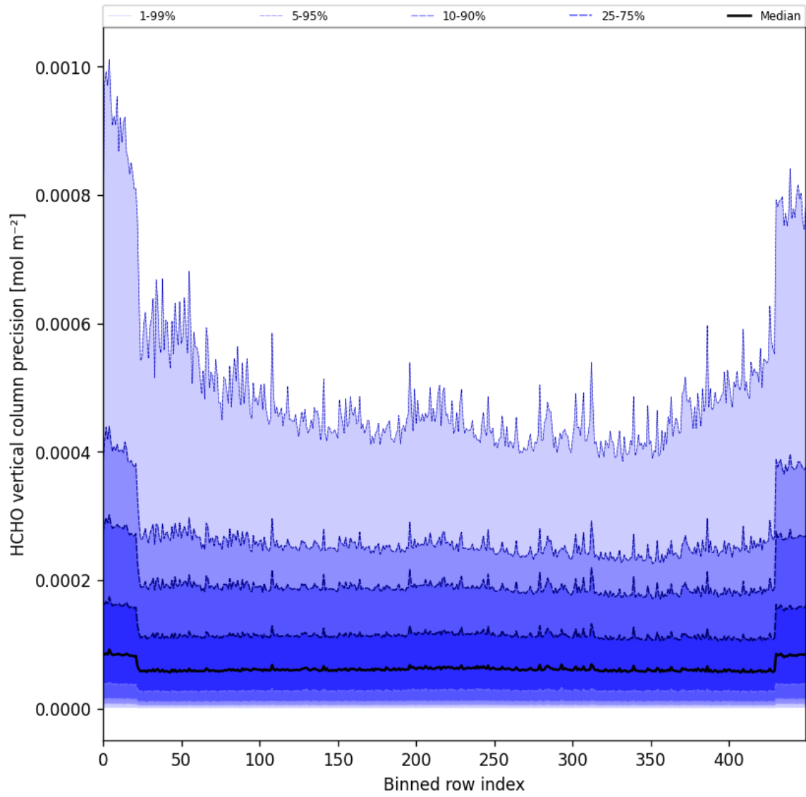
Figure 50: Along track statistics of “HCHO vertical column precision” for 2025-08-27 to 2025-08-29
