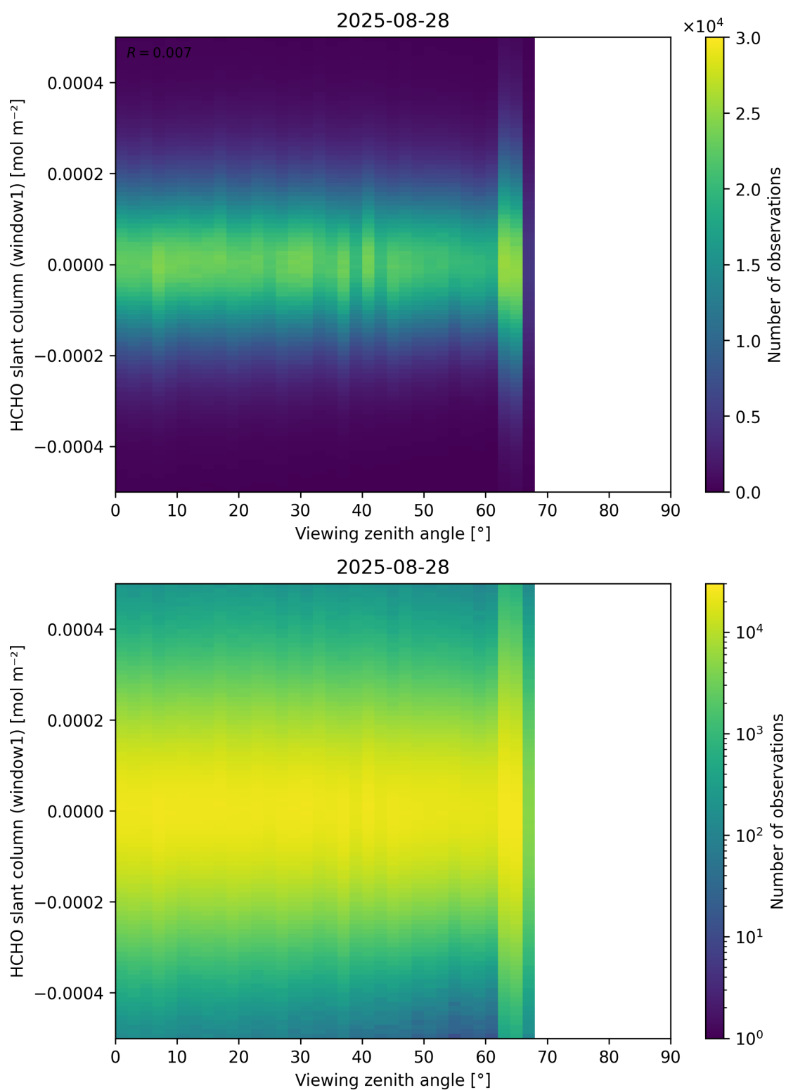
Figure 188: Scatter density plot of “Viewing zenith angle” against “HCHO slant column (window1)” for 2025-08-27 to 2025-08-29.
