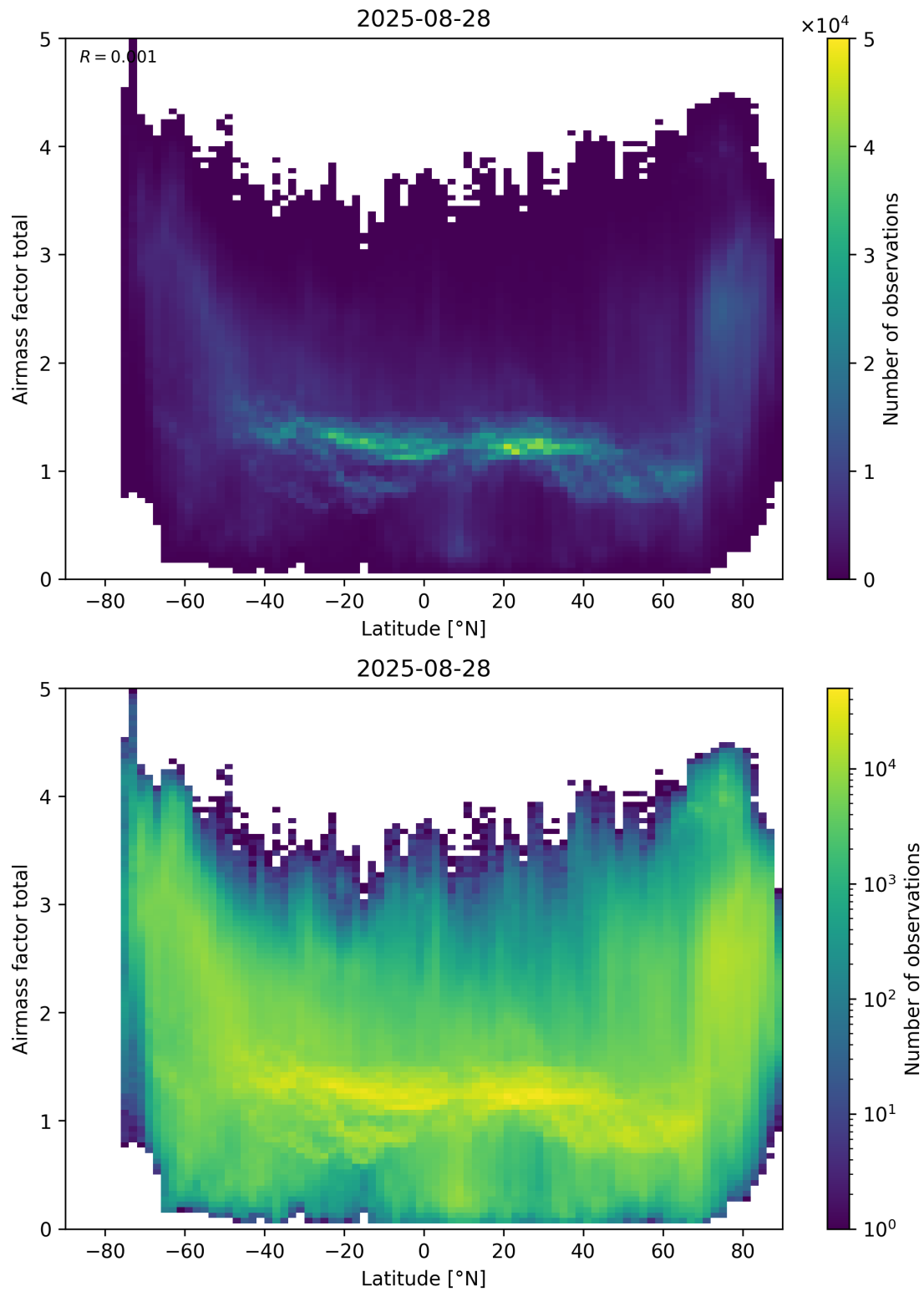
Figure 161: Scatter density plot of “Latitude” against “Airmass factor total” for 2025-08-27 to 2025-08-29.
