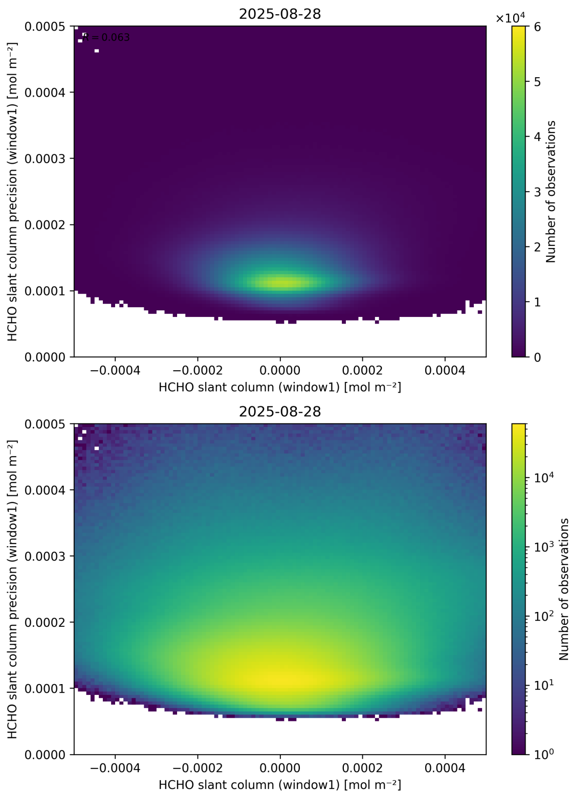
Figure 84: Scatter density plot of “HCHO slant column (window1)” against “HCHO slant column precision (window1)” for 2025-08-27 to 2025-08-29.
