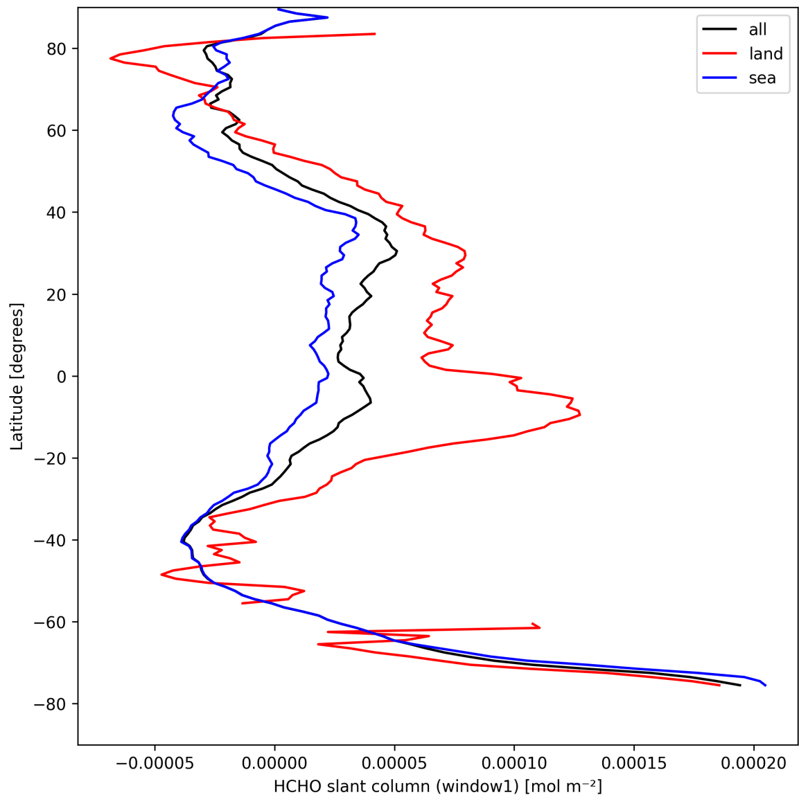
Figure 24: Zonal average of “HCHO slant column (window1)” for 2025-08-27 to 2025-08-29.
