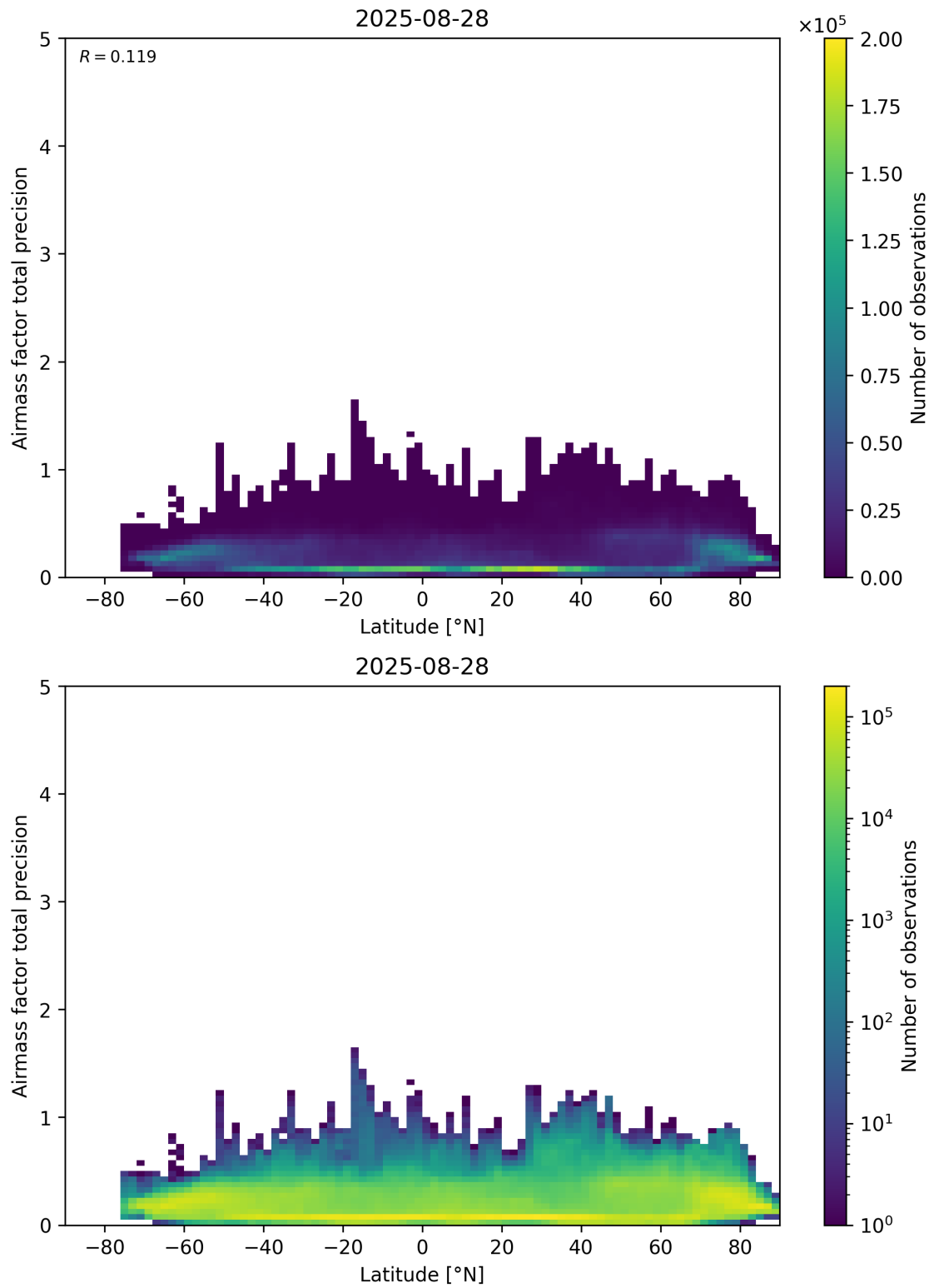
Figure 162: Scatter density plot of “Latitude” against “Airmass factor total precision” for 2025-08-27 to 2025-08-29.
