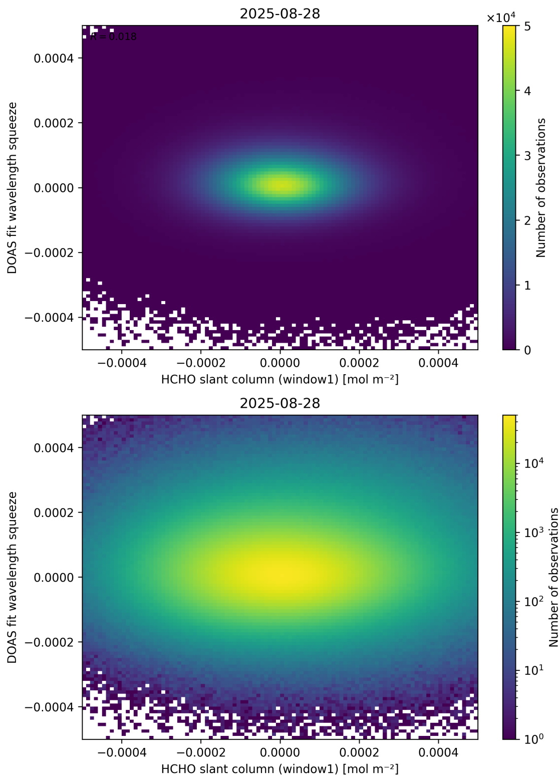
Figure 80: Scatter density plot of “HCHO slant column (window1)” against “DOAS fit wavelength squeeze” for 2025-08-27 to 2025-08-29.
