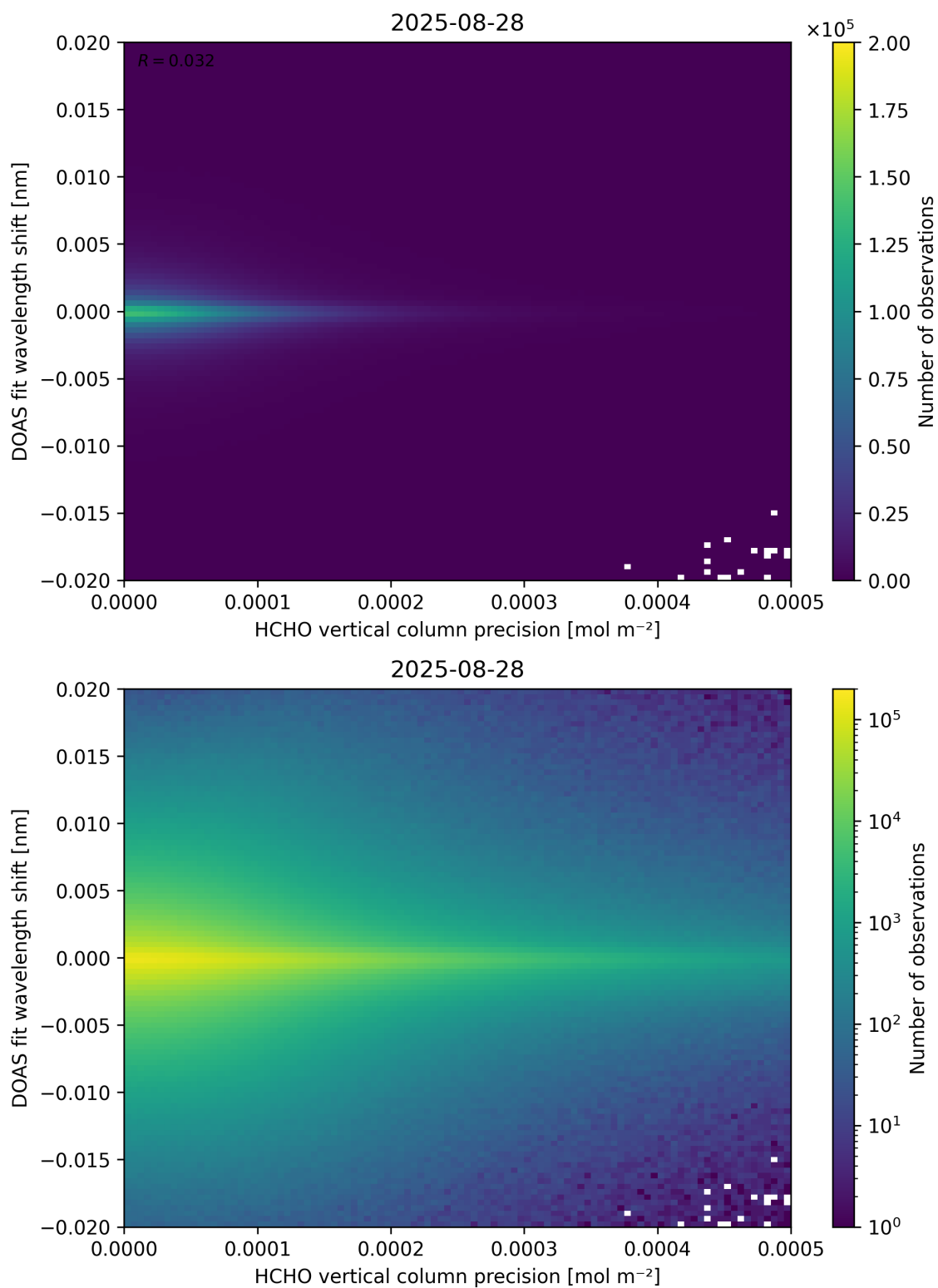
Figure 137: Scatter density plot of “HCHO vertical column precision” against “DOAS fit wavelength shift” for 2025-08-27 to 2025-08-29.
