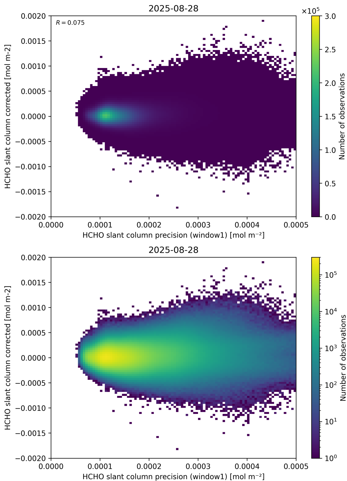
Figure 92: Scatter density plot of “HCHO slant column precision (window1)” against “HCHO slant column corrected” for 2025-08-27 to 2025-08-29.
