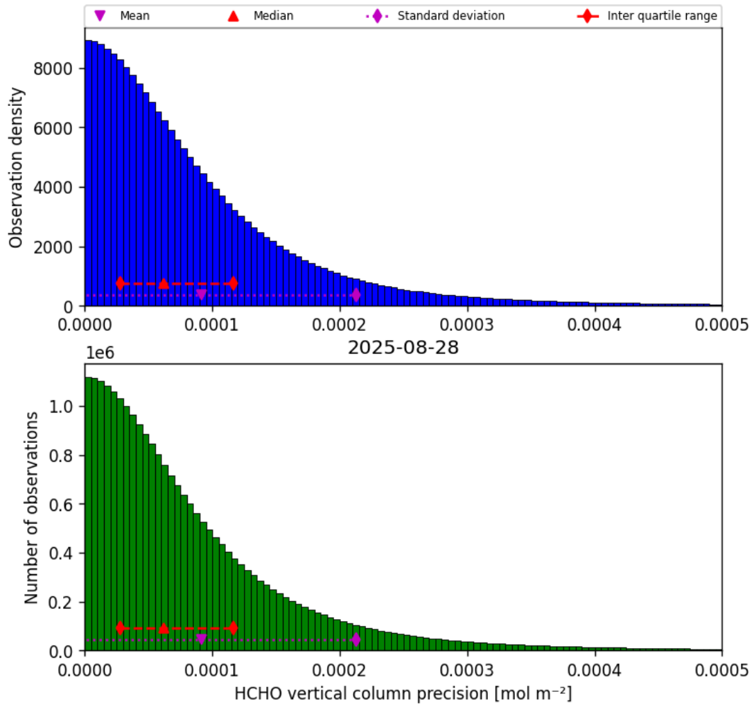
Figure 36: Histogram of “HCHO vertical column precision” for 2025-08-27 to 2025-08-29
