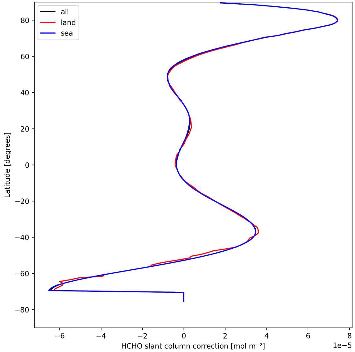
Figure 33: Zonal average of “HCHO slant column correction” for 2025-08-27 to 2025-08-29.
