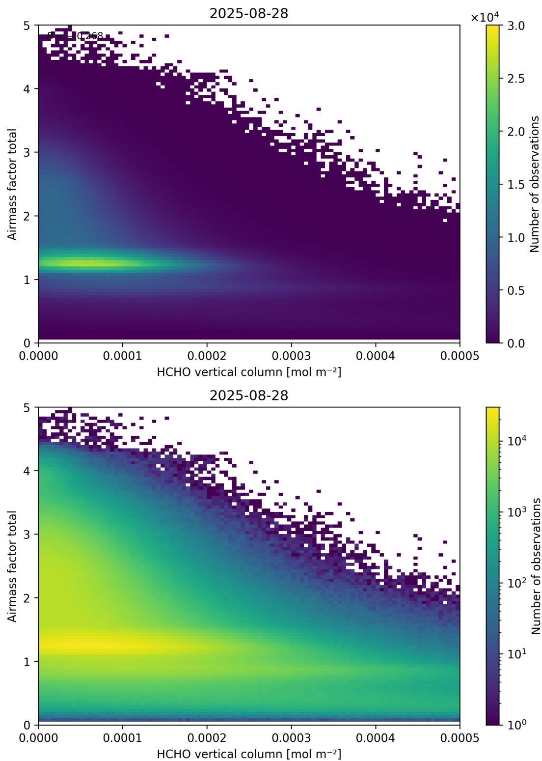
Figure 131: Scatter density plot of “HCHO vertical column” against “Airmass factor total” for 2025-08-27 to 2025-08-29.
