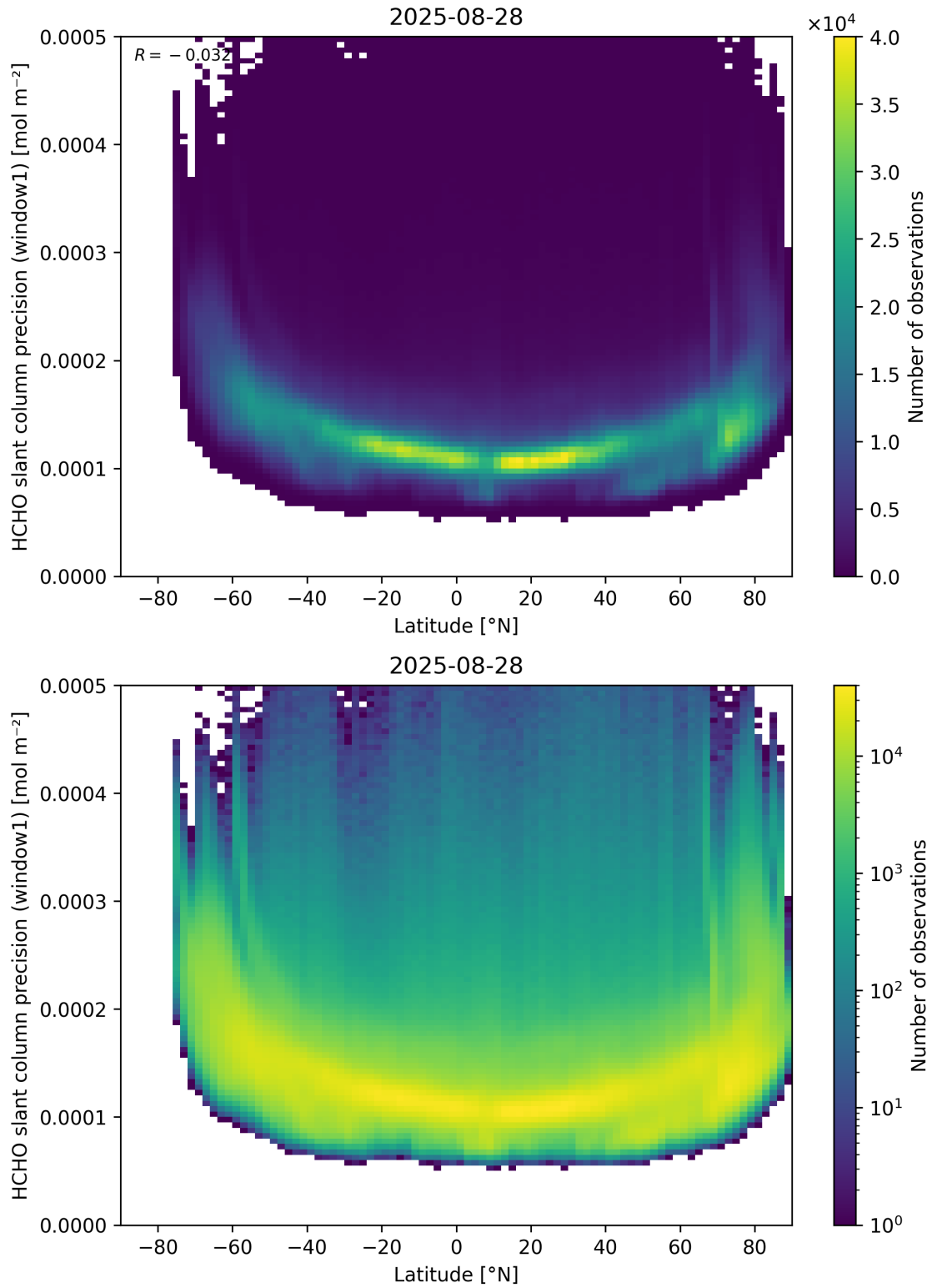
Figure 160: Scatter density plot of “Latitude” against “HCHO slant column precision (window1)” for 2025-08-27 to 2025-08-29.
