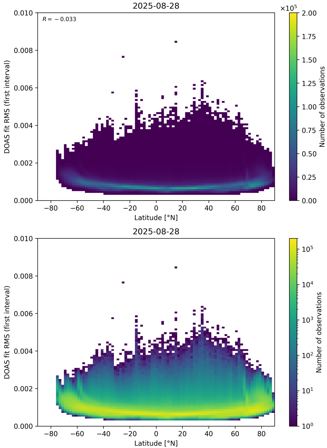
Figure 153: Scatter density plot of “Latitude” against “DOAS fit RMS (first interval)” for 2025-08-27 to 2025-08-29.
