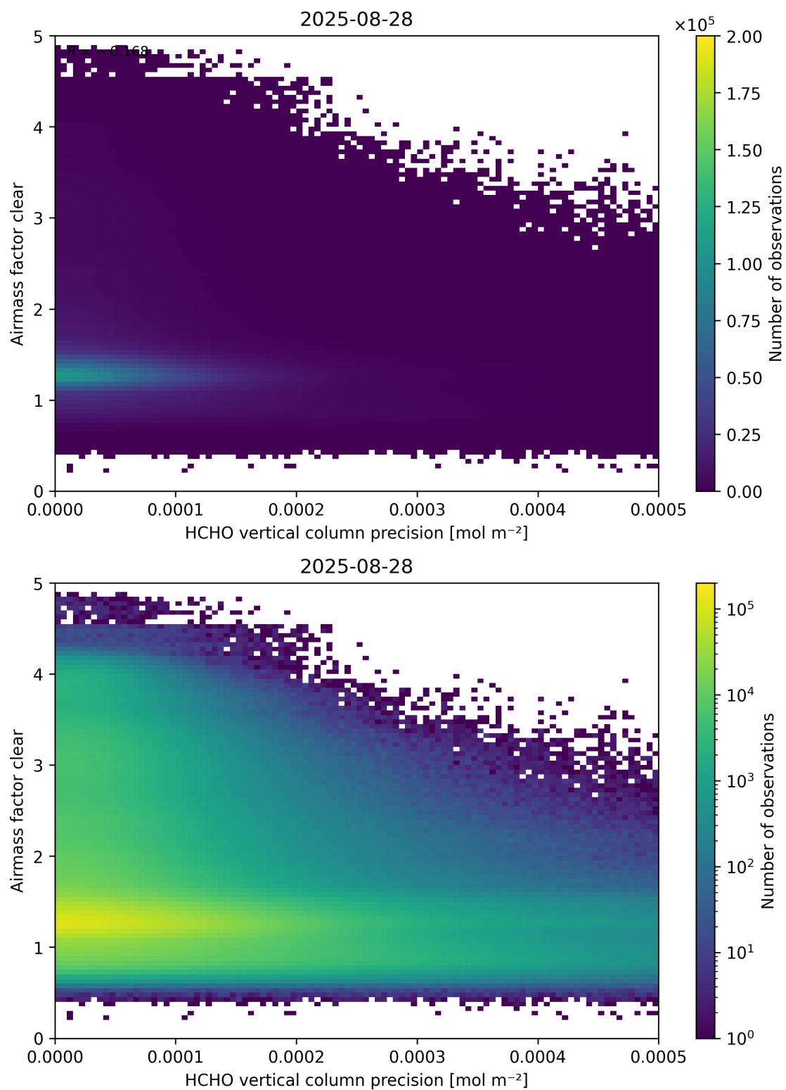
Figure 139: Scatter density plot of “HCHO vertical column precision” against “Airmass factor clear” for 2025-08-27 to 2025-08-29.
