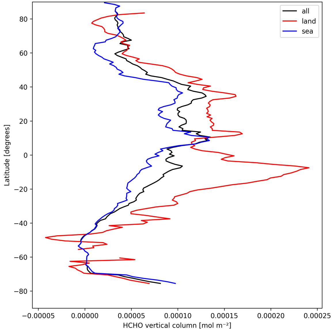
Figure 21: Zonal average of “HCHO vertical column” for 2025-08-27 to 2025-08-29.
