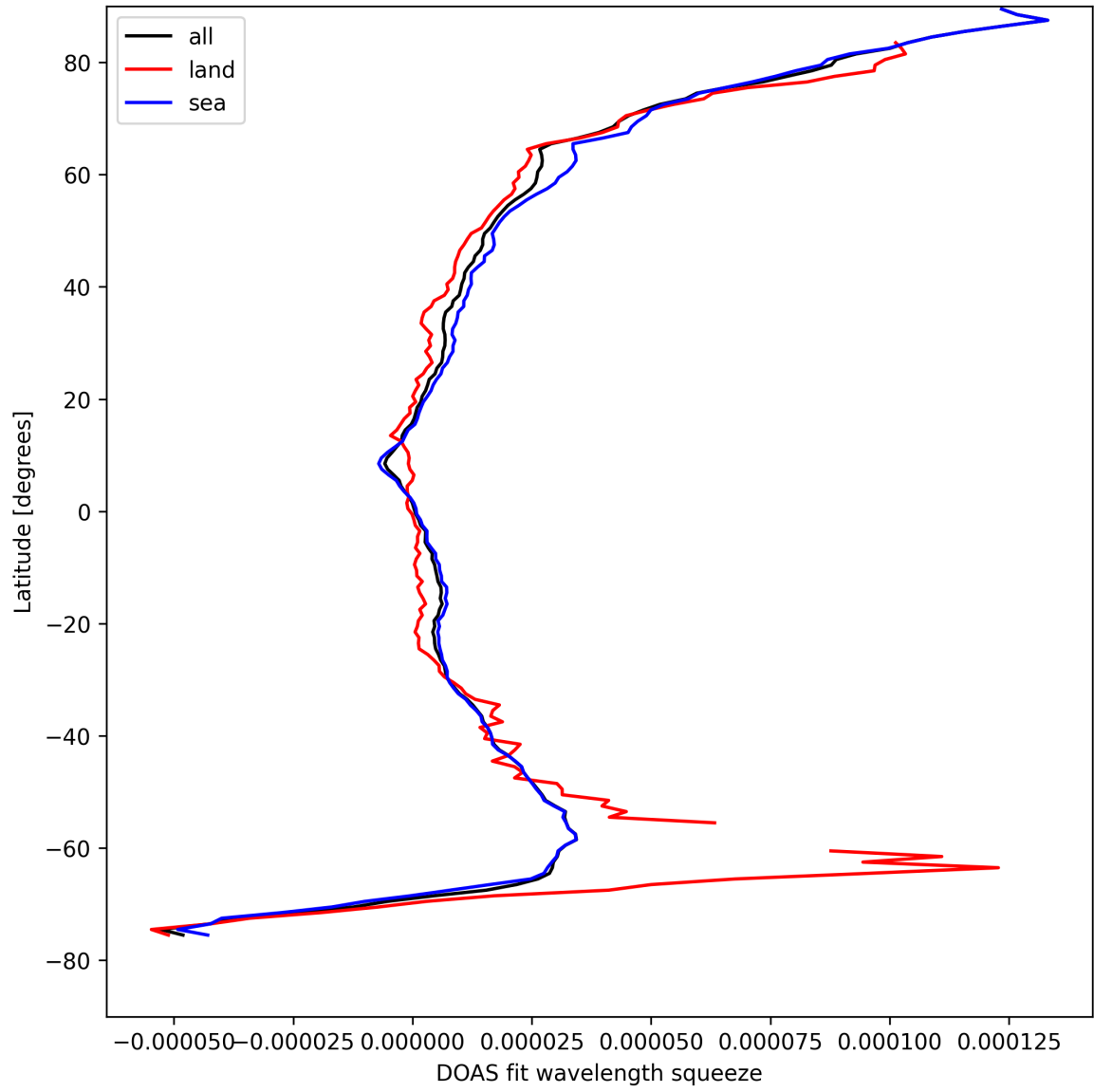
Figure 31: Zonal average of “DOAS fit wavelength squeeze” for 2025-08-27 to 2025-08-29.
