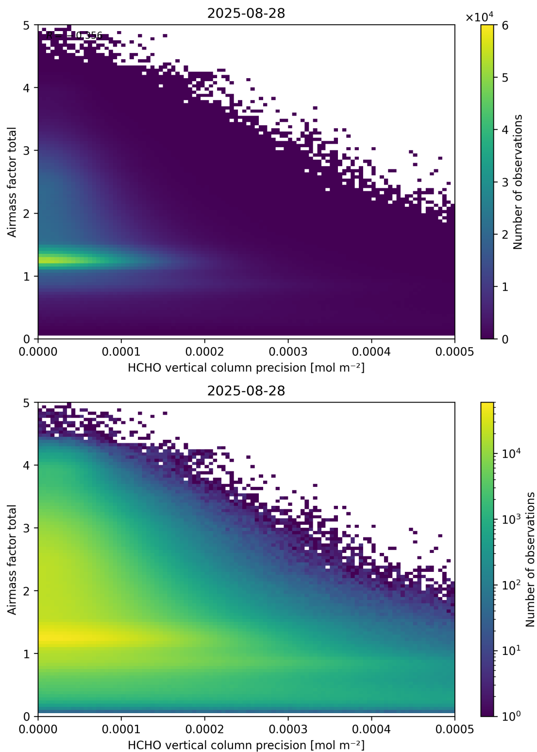
Figure 144: Scatter density plot of “HCHO vertical column precision” against “Airmass factor total” for 2025-08-27 to 2025-08-29.
