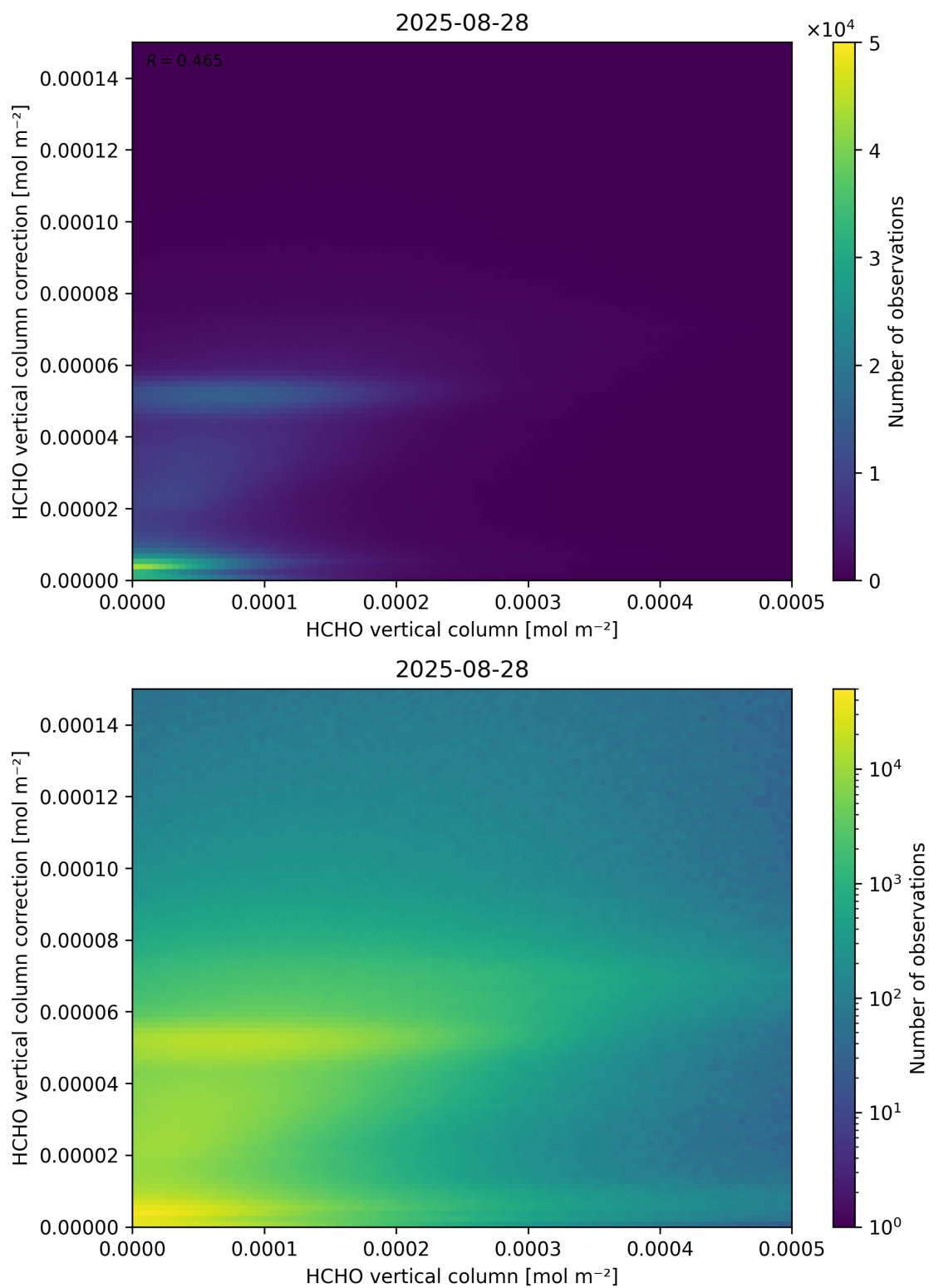
Figure 133: Scatter density plot of “HCHO vertical column” against “HCHO vertical column correction” for 2025-08-27 to 2025-08-29.
