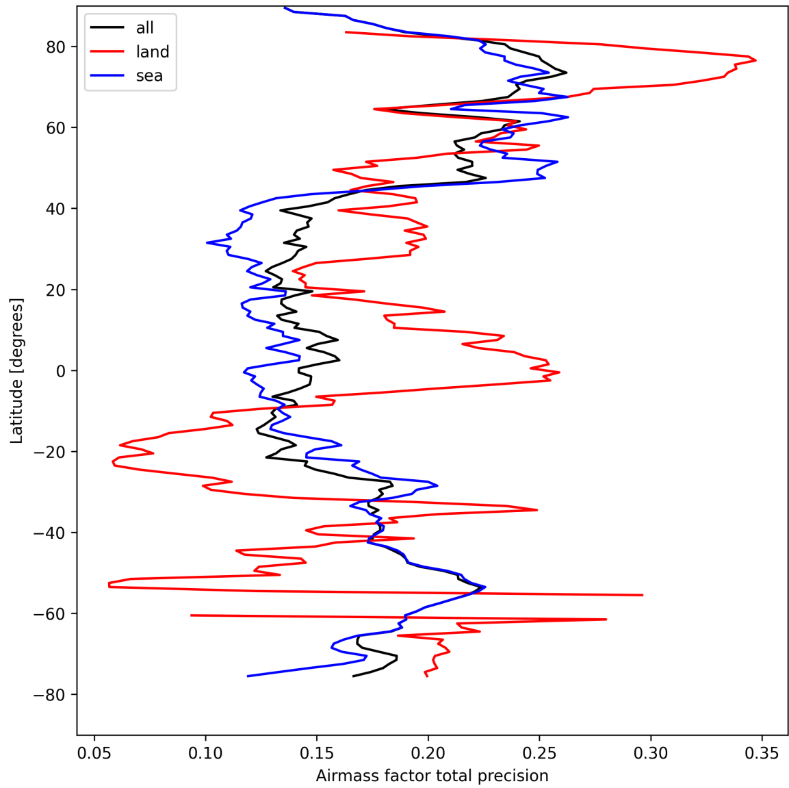
Figure 27: Zonal average of “Airmass factor total precision” for 2025-08-27 to 2025-08-29.
