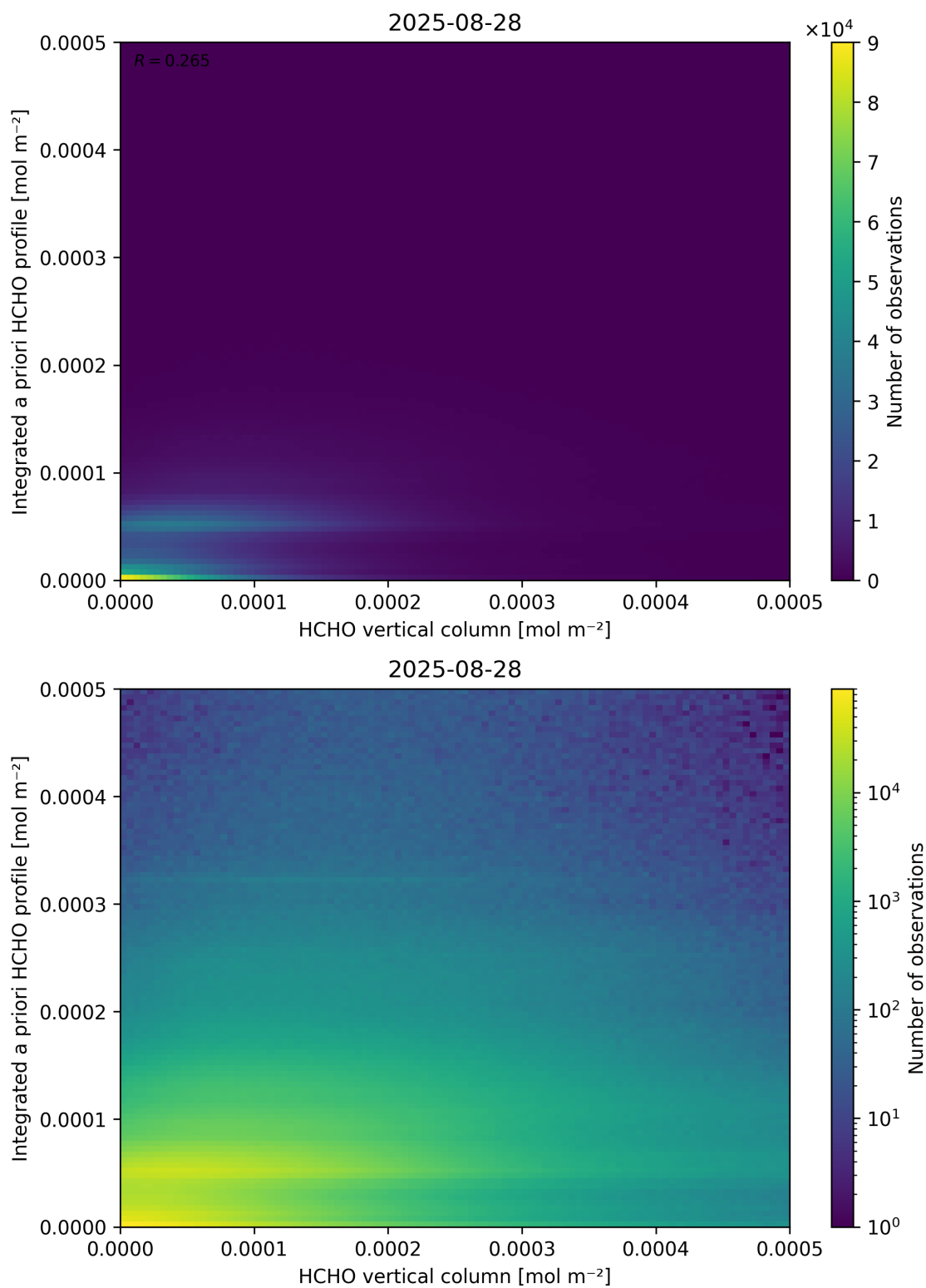
Figure 135: Scatter density plot of “HCHO vertical column” against “Integrated a priori HCHO profile” for 2025-08-27 to 2025-08-29.
