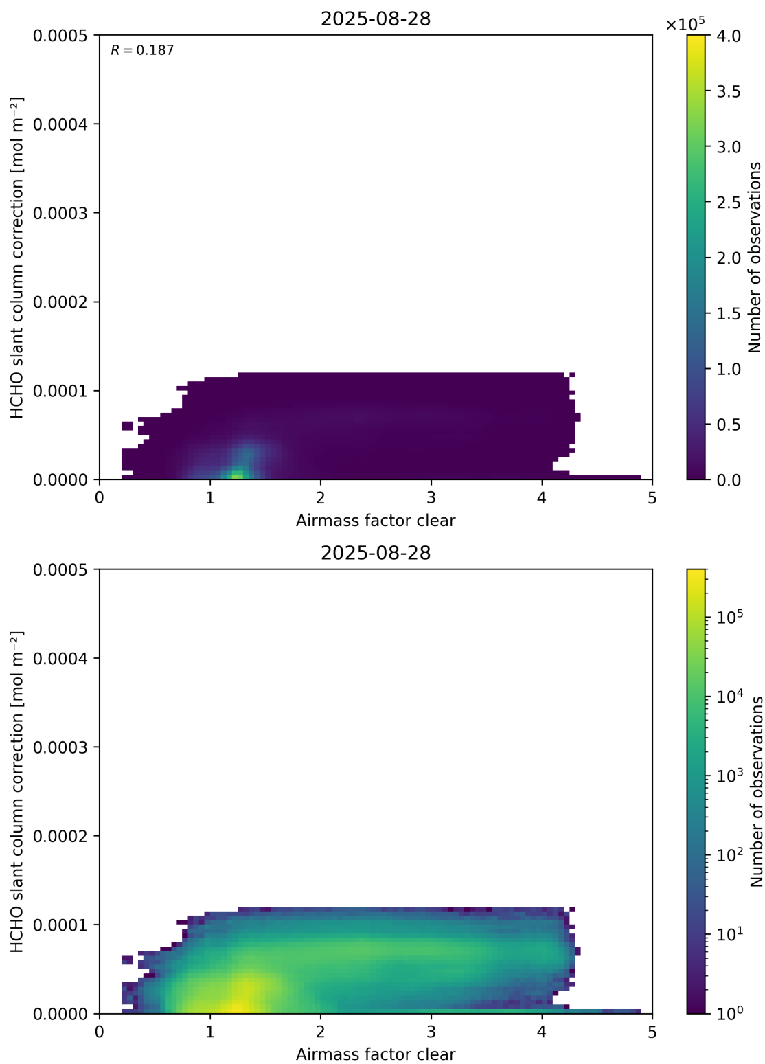
Figure 75: Scatter density plot of “Airmass factor clear” against “HCHO slant column correction” for 2025-08-27 to 2025-08-29.
