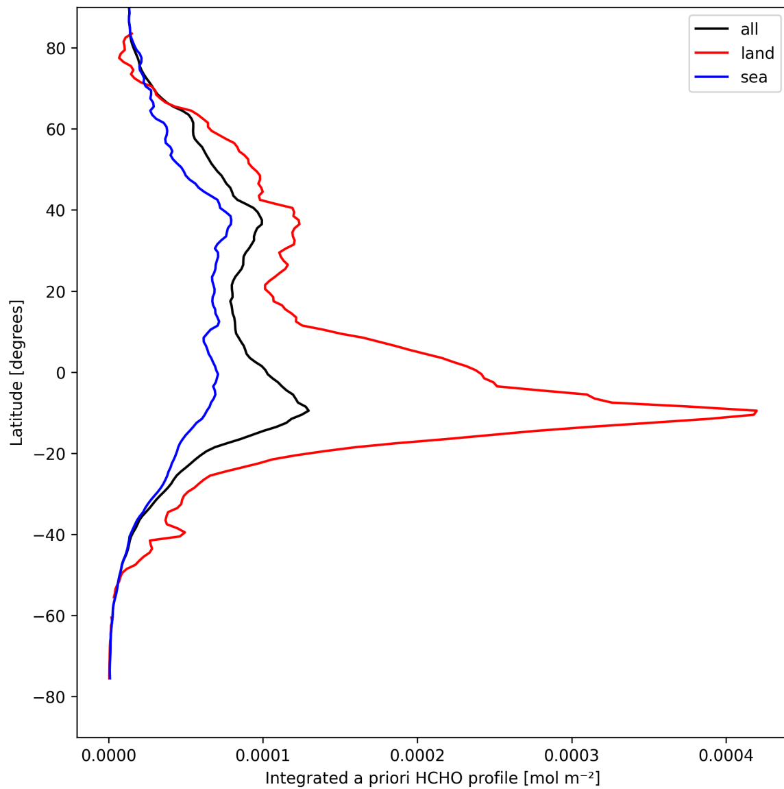
Figure 29: Zonal average of “Integrated a priori HCHO profile” for 2025-08-27 to 2025-08-29.
