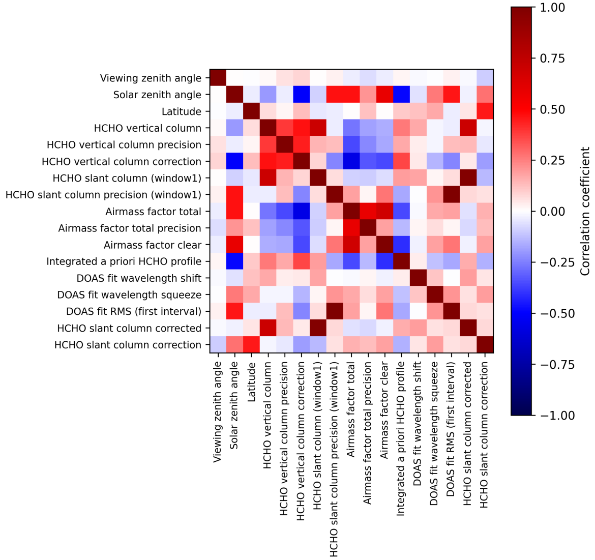
Figure 2: Map of correlation matrix for 2025-08-27 to 2025-08-29.
