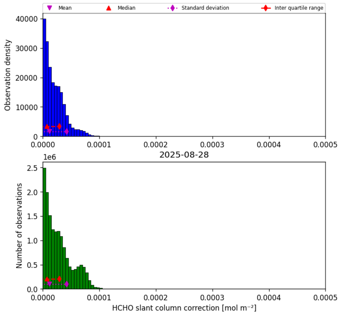
Figure 47: Histogram of “HCHO slant column correction” for 2025-08-27 to 2025-08-29
