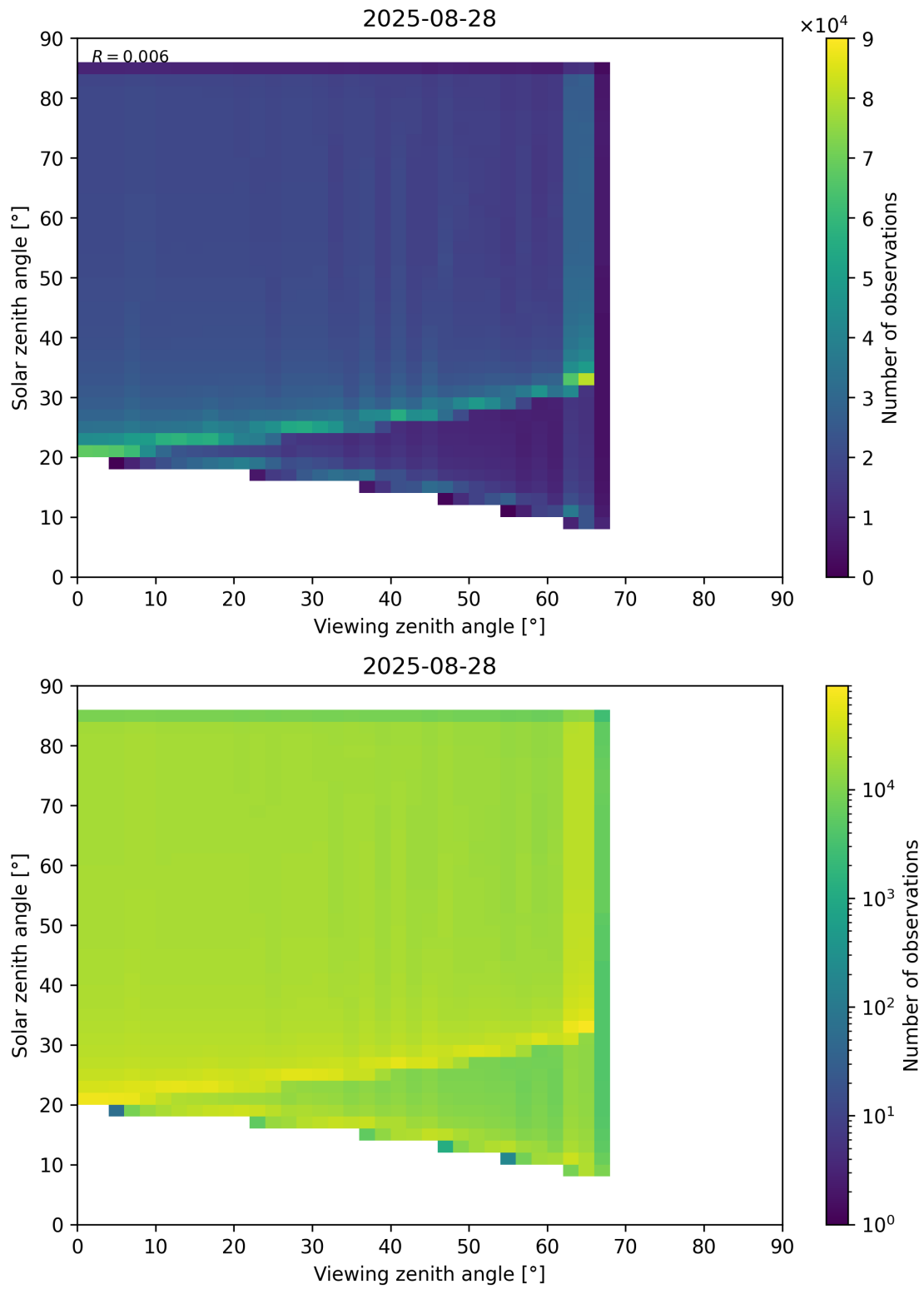
Figure 197: Scatter density plot of “Viewing zenith angle” against “Solar zenith angle” for 2025-08-27 to 2025-08-29.
