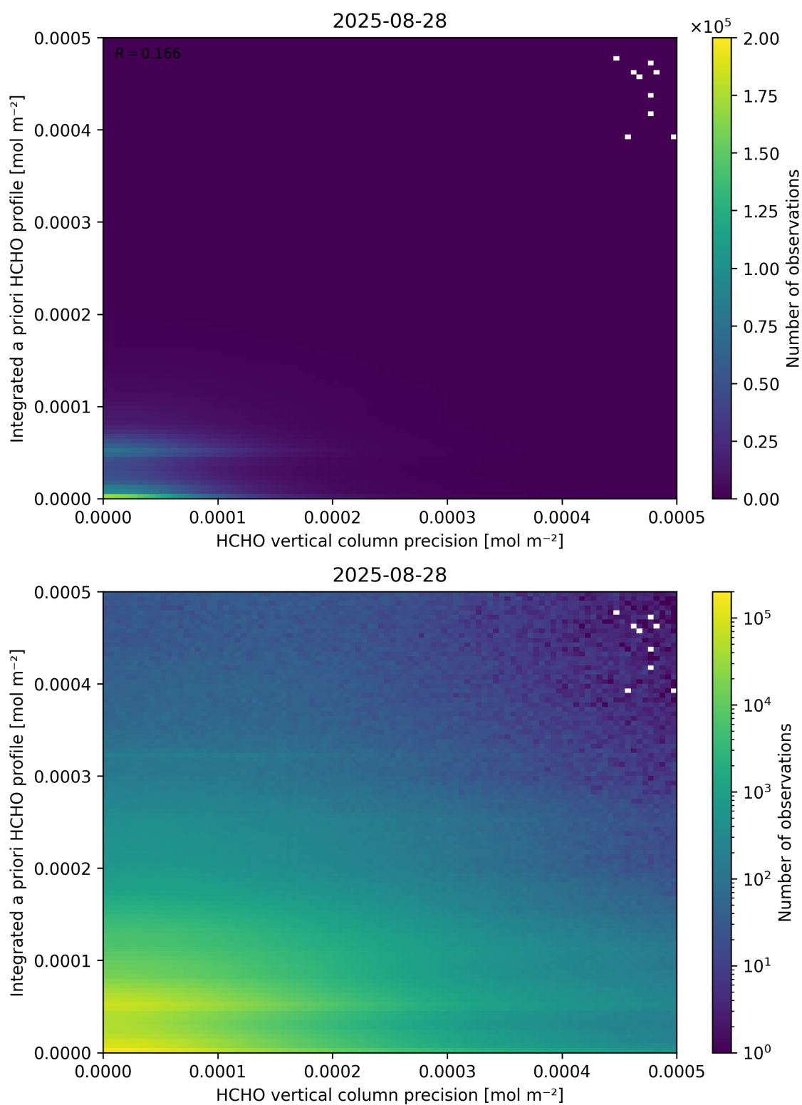
Figure 147: Scatter density plot of “HCHO vertical column precision” against “Integrated a priori HCHO profile” for 2025-08-27 to 2025-08-29.
