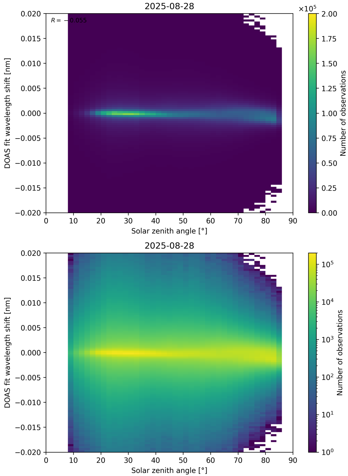
Figure 168: Scatter density plot of “Solar zenith angle” against “DOAS fit wavelength shift” for 2025-08-27 to 2025-08-29.
