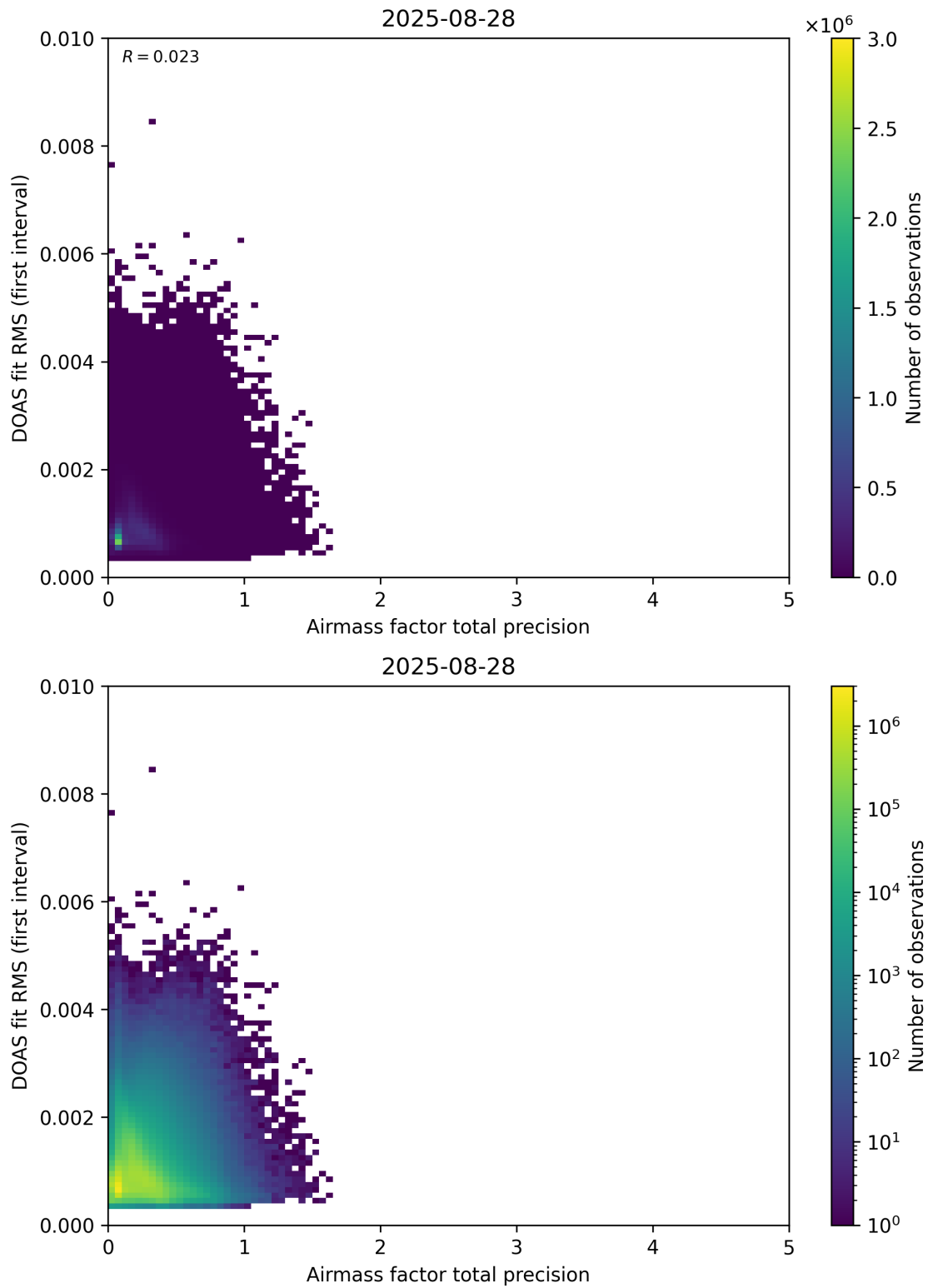
Figure 105: Scatter density plot of “Airmass factor total precision” against “DOAS fit RMS (first interval)” for 2025-08-27 to 2025-08-29.
