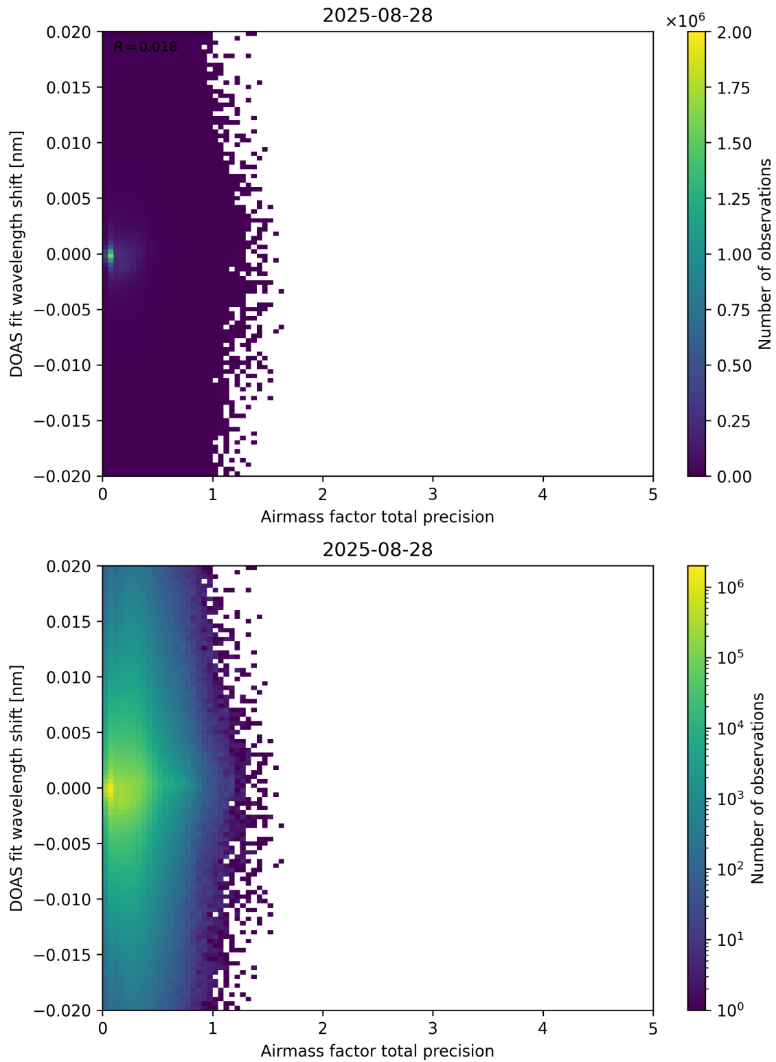
Figure 106: Scatter density plot of “Airmass factor total precision” against “DOAS fit wavelength shift” for 2025-08-27 to 2025-08-29.
