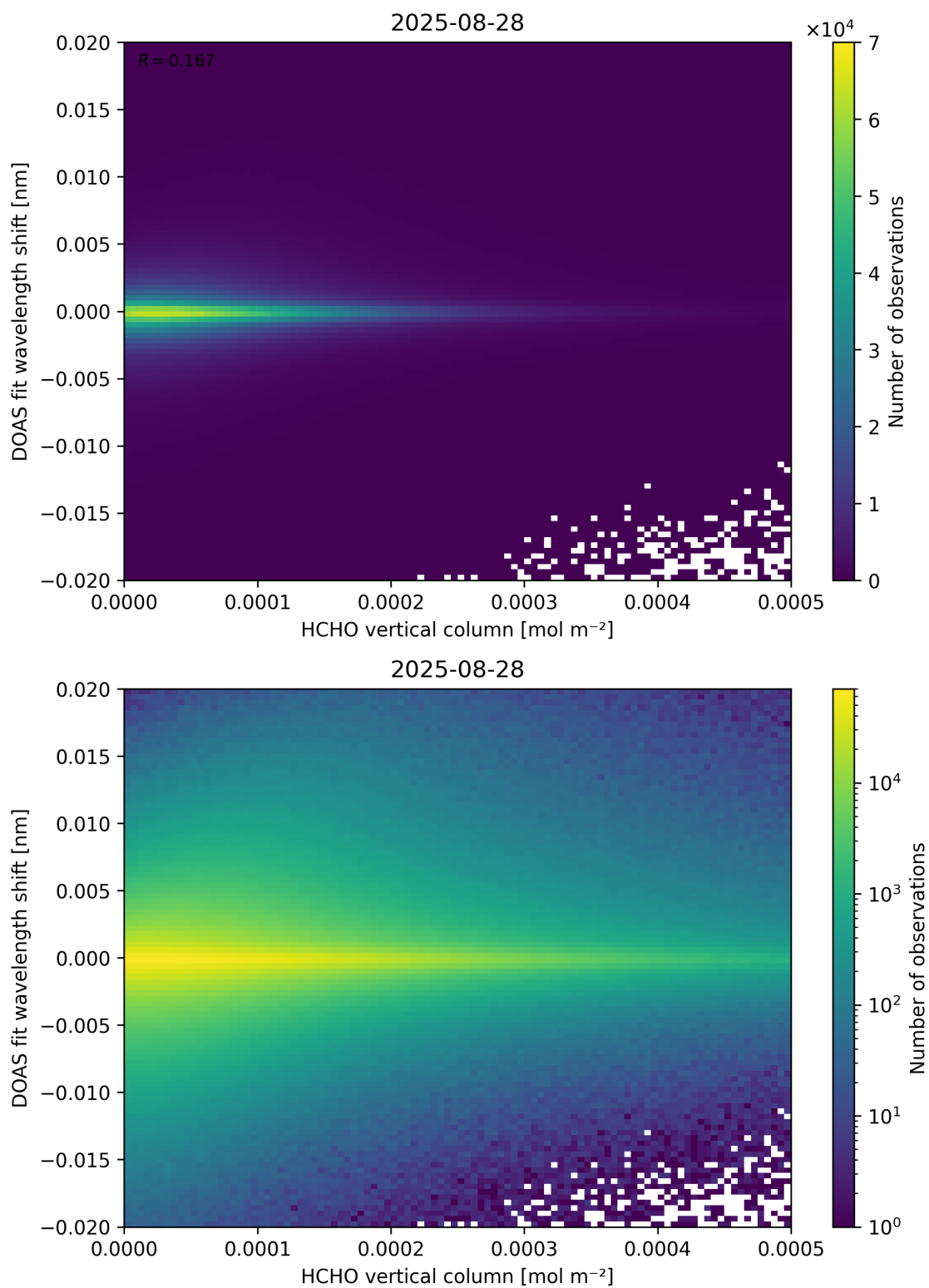
Figure 124: Scatter density plot of “HCHO vertical column” against “DOAS fit wavelength shift” for 2025-08-27 to 2025-08-29.
