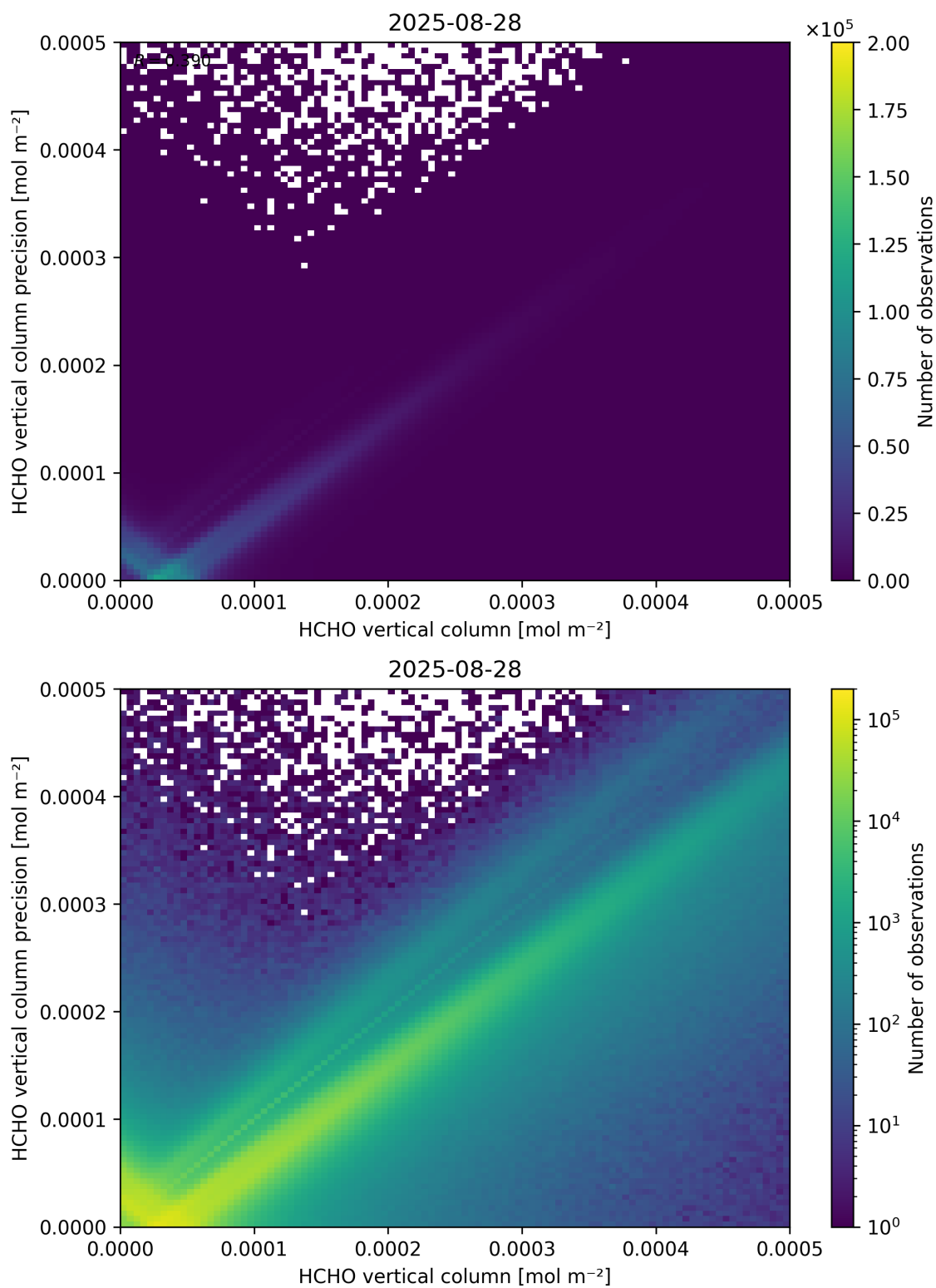
Figure 134: Scatter density plot of “HCHO vertical column” against “HCHO vertical column precision” for 2025-08-27 to 2025-08-29.
