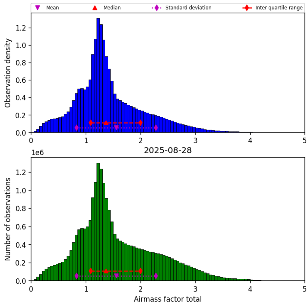
Figure 40: Histogram of “Airmass factor total” for 2025-08-27 to 2025-08-29
