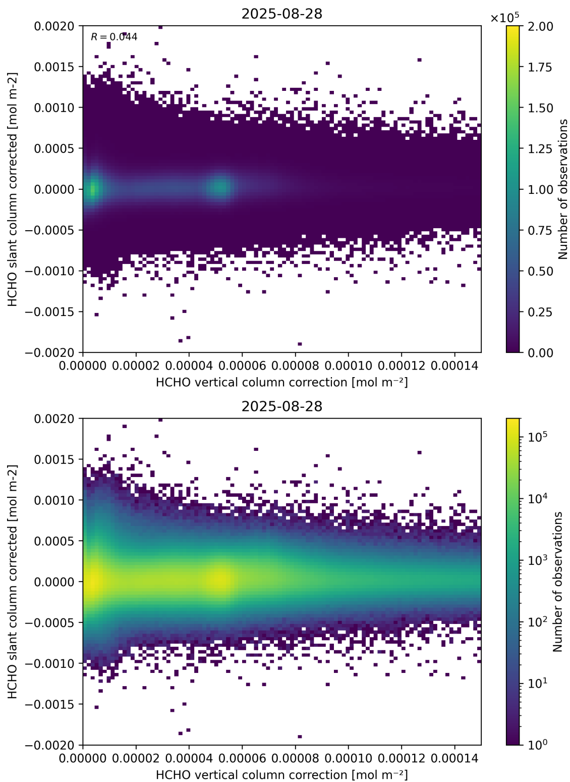
Figure 116: Scatter density plot of “HCHO vertical column correction” against “HCHO slant column corrected” for 2025-08-27 to 2025-08-29.
