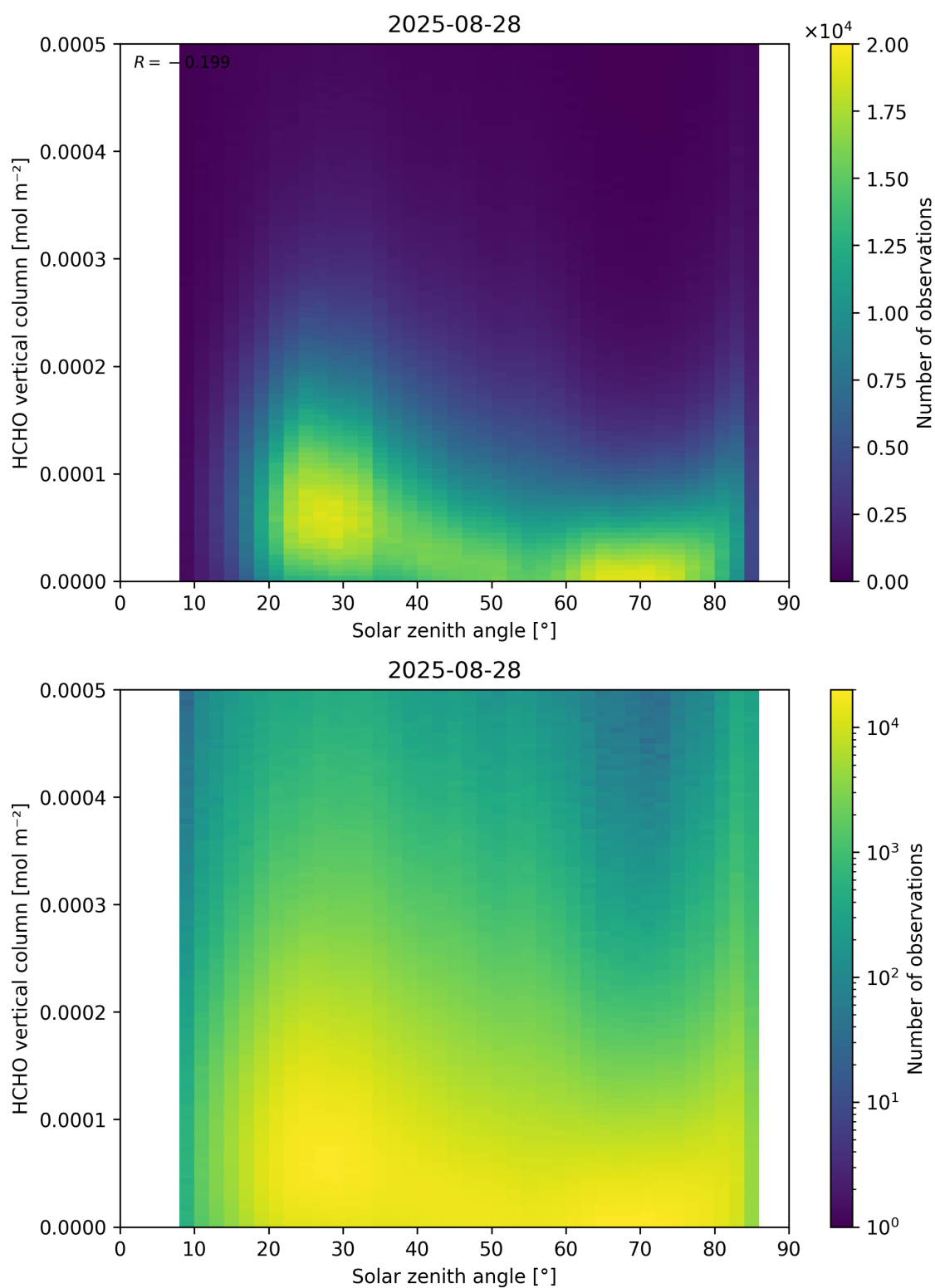
Figure 177: Scatter density plot of “Solar zenith angle” against “HCHO vertical column” for 2025-08-27 to 2025-08-29.
