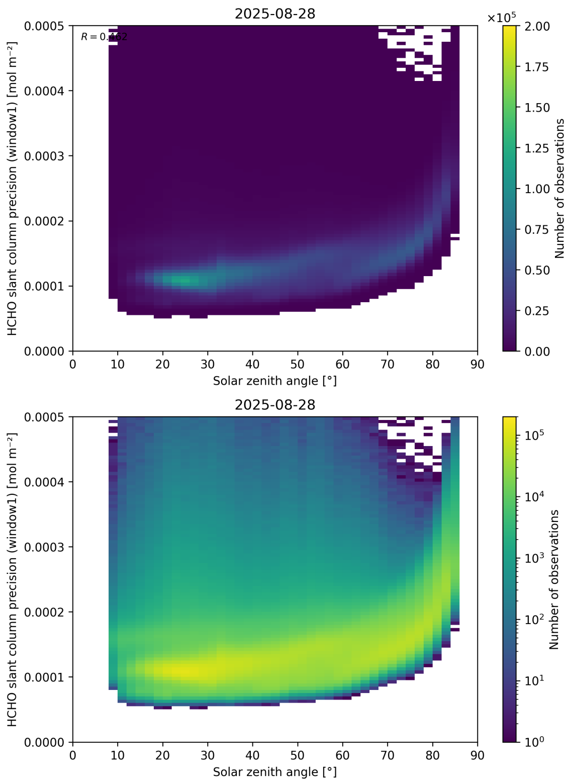
Figure 174: Scatter density plot of “Solar zenith angle” against “HCHO slant column precision (window1)” for 2025-08-27 to 2025-08-29.
