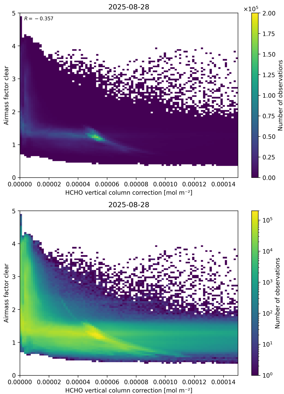
Figure 115: Scatter density plot of “HCHO vertical column correction” against “Airmass factor clear” for 2025-08-27 to 2025-08-29.
