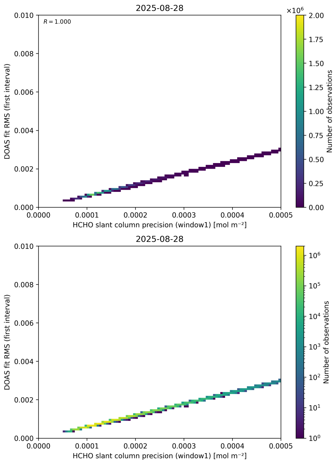
Figure 88: Scatter density plot of “HCHO slant column precision (window1)” against “DOAS fit RMS (first interval)” for 2025-08-27 to 2025-08-29.
