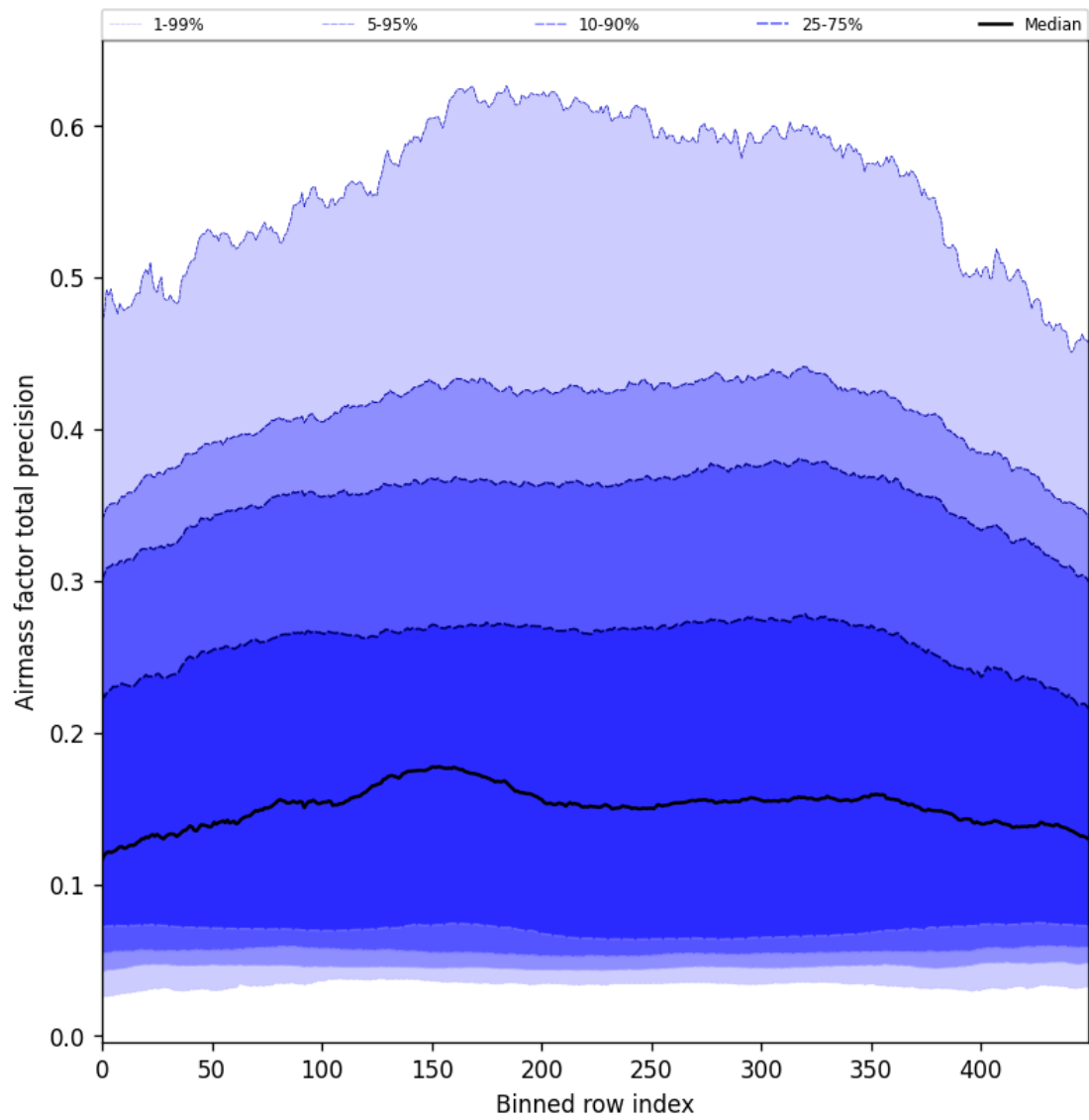
Figure 55: Along track statistics of “Airmass factor total precision” for 2025-08-27 to 2025-08-29
