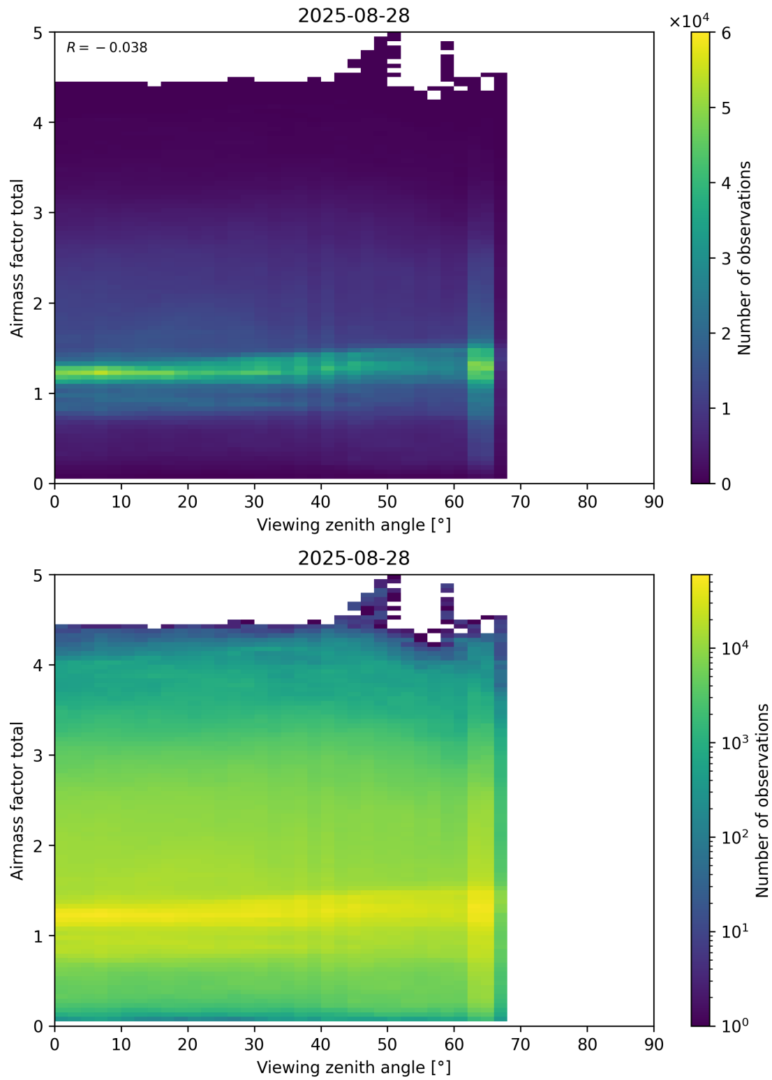
Figure 190: Scatter density plot of “Viewing zenith angle” against “Airmass factor total” for 2025-08-27 to 2025-08-29.
