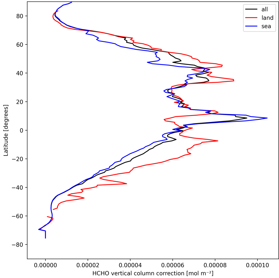
Figure 23: Zonal average of “HCHO vertical column correction” for 2025-08-27 to 2025-08-29.
