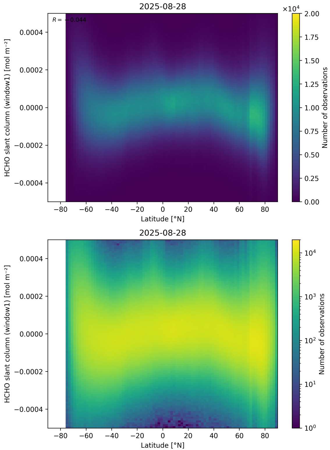
Figure 159: Scatter density plot of “Latitude” against “HCHO slant column (window1)” for 2025-08-27 to 2025-08-29.
