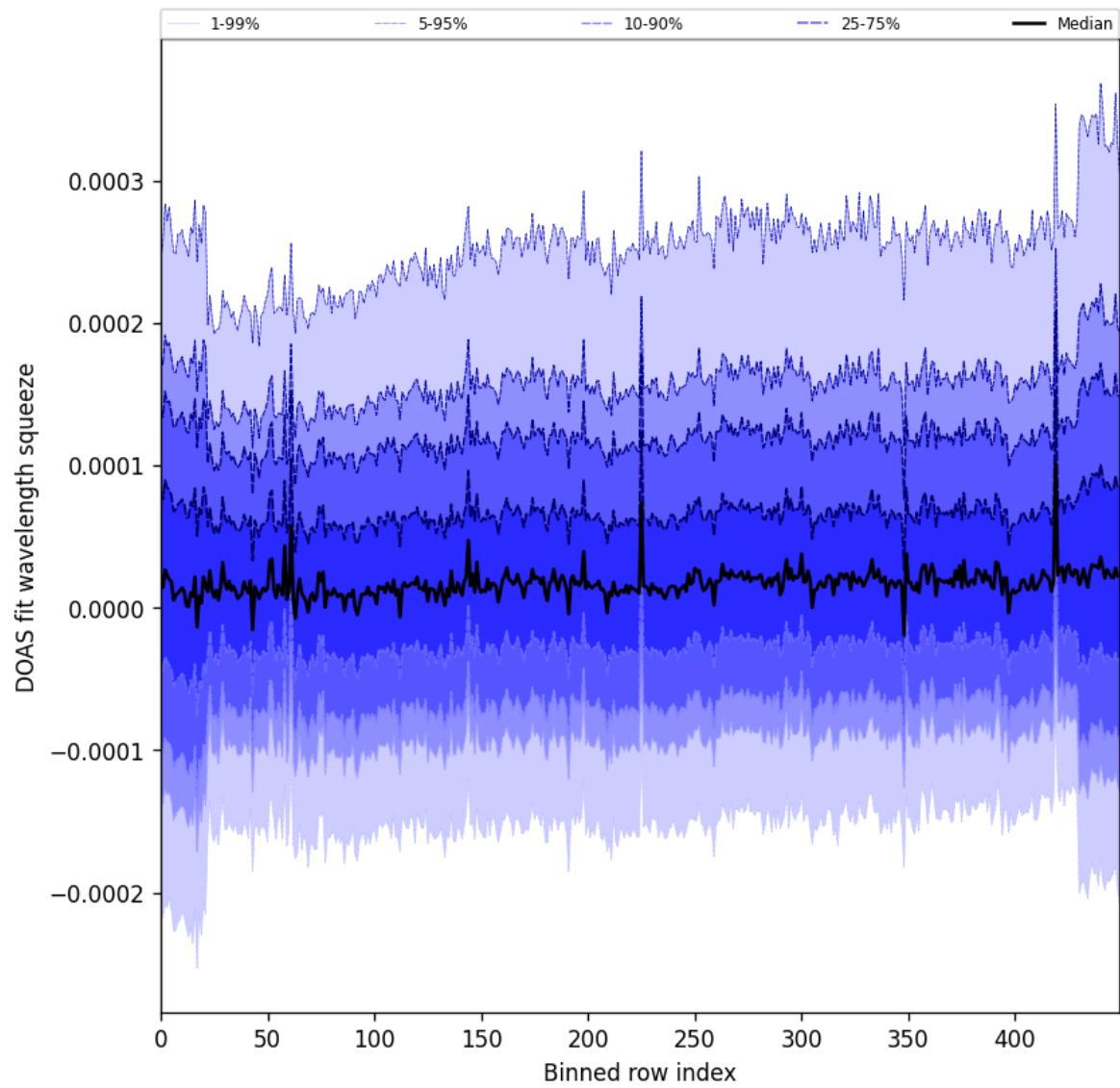
Figure 59: Along track statistics of “DOAS fit wavelength squeeze” for 2025-08-27 to 2025-08-29
