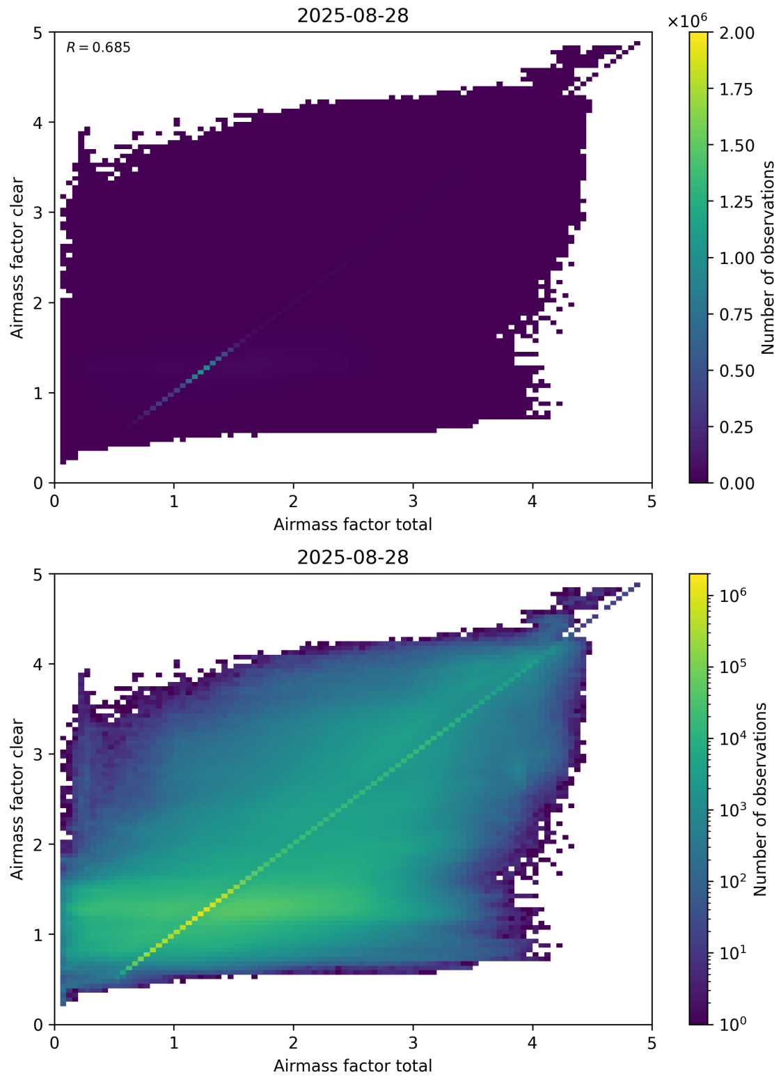
Figure 100: Scatter density plot of “Airmass factor total” against “Airmass factor clear” for 2025-08-27 to 2025-08-29.
