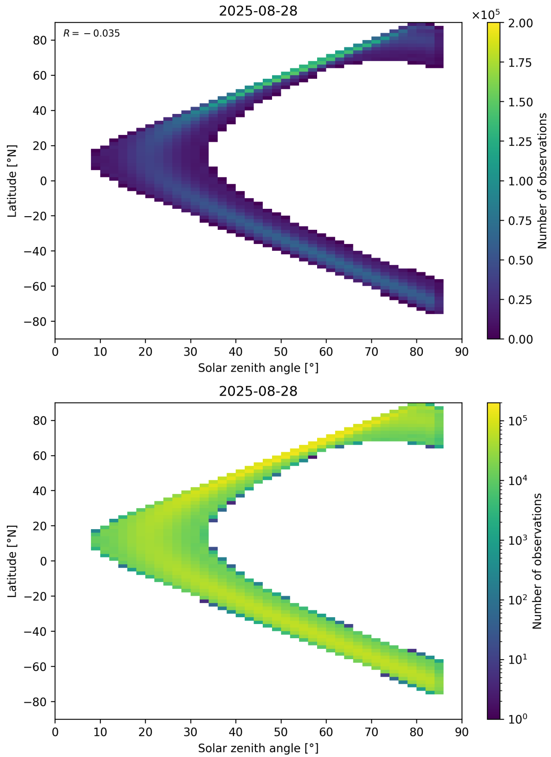
Figure 181: Scatter density plot of “Solar zenith angle” against “Latitude” for 2025-08-27 to 2025-08-29.
