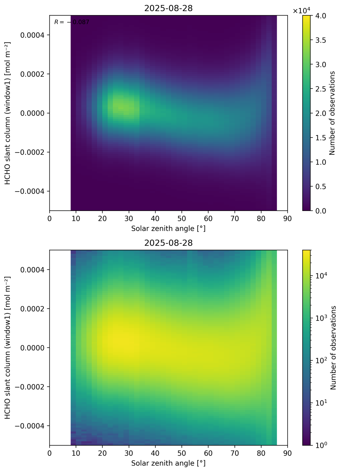
Figure 173: Scatter density plot of “Solar zenith angle” against “HCHO slant column (window1)” for 2025-08-27 to 2025-08-29.
