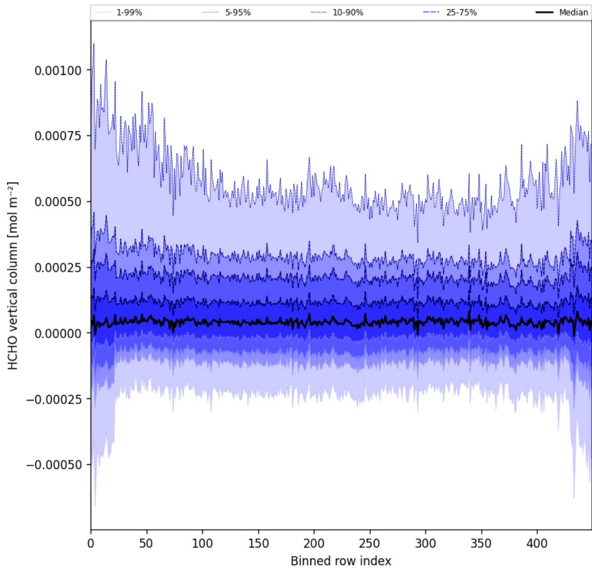
Figure 49: Along track statistics of “HCHO vertical column” for 2025-08-27 to 2025-08-29
