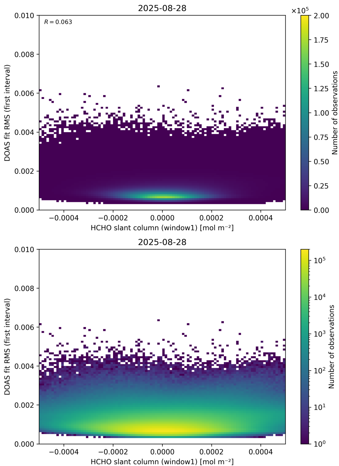
Figure 78: Scatter density plot of “HCHO slant column (window1)” against “DOAS fit RMS (first interval)” for 2025-08-27 to 2025-08-29.
