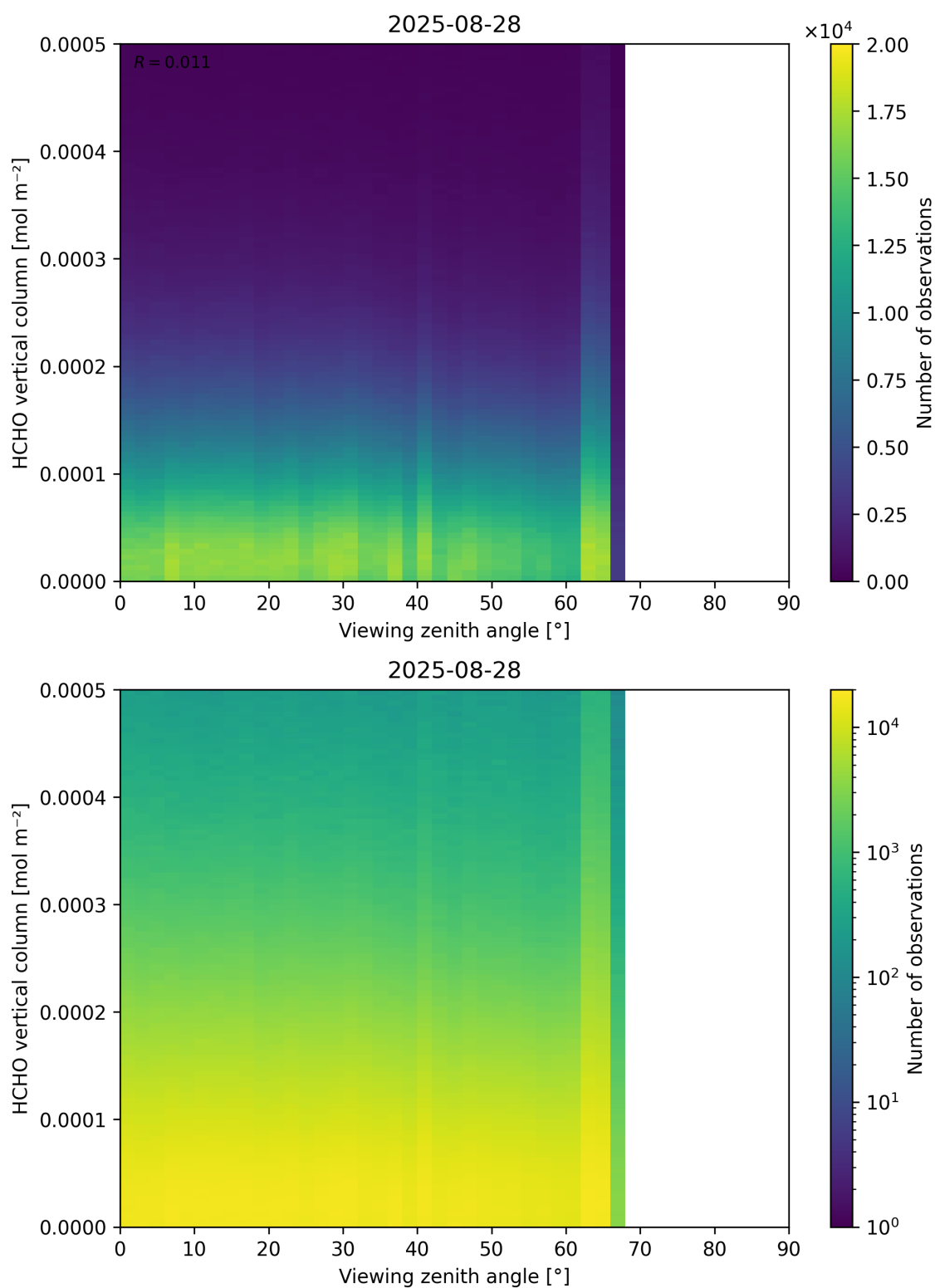
Figure 192: Scatter density plot of “Viewing zenith angle” against “HCHO vertical column” for 2025-08-27 to 2025-08-29.
