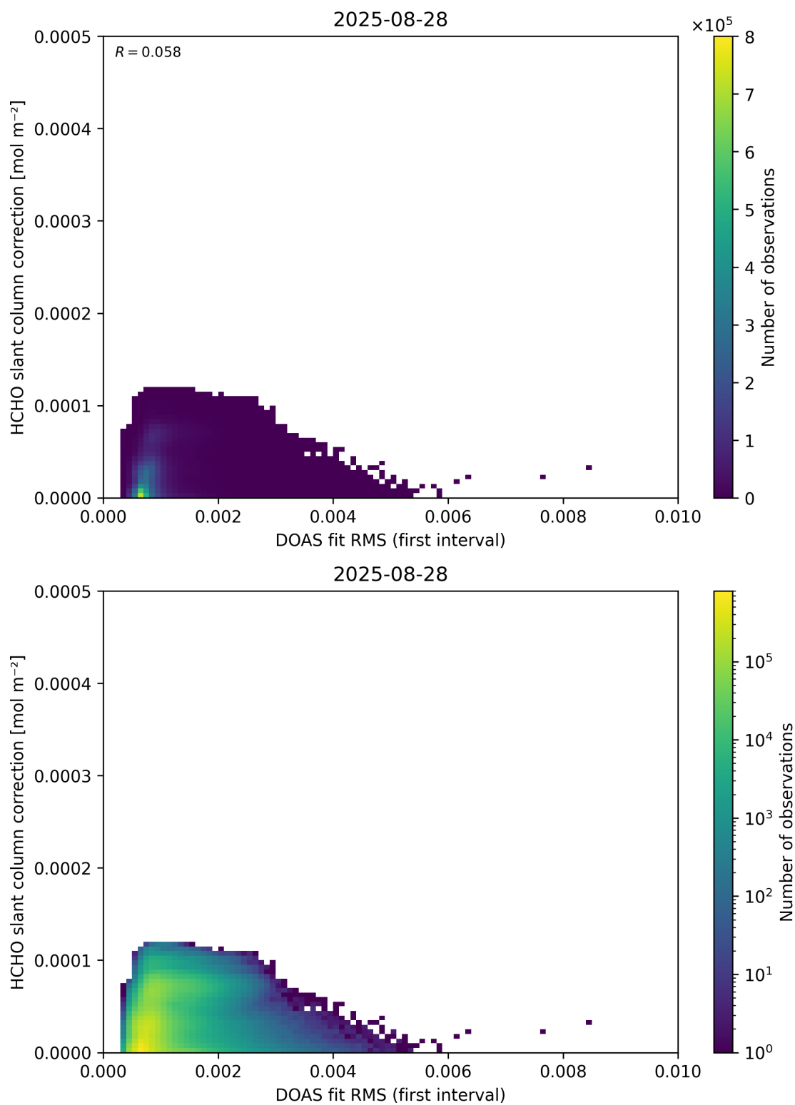
Figure 63: Scatter density plot of “DOAS fit RMS (first interval)” against “HCHO slant column correction” for 2025-08-27 to 2025-08-29.
