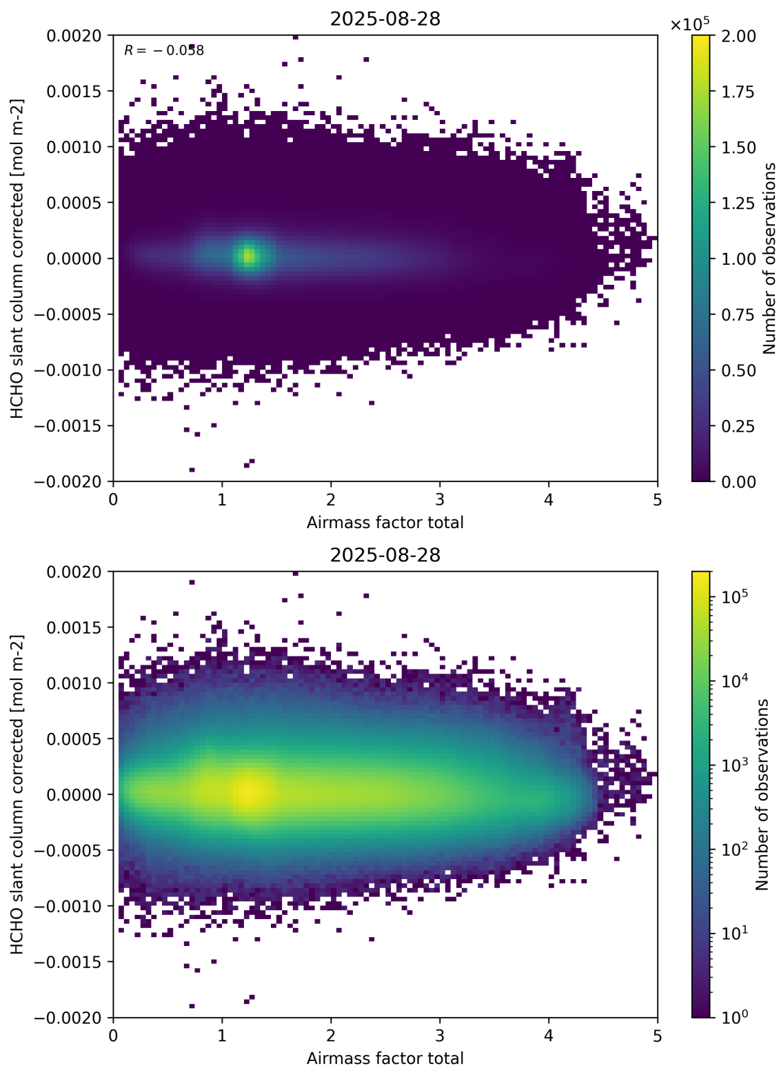
Figure 101: Scatter density plot of “Airmass factor total” against “HCHO slant column corrected” for 2025-08-27 to 2025-08-29.
