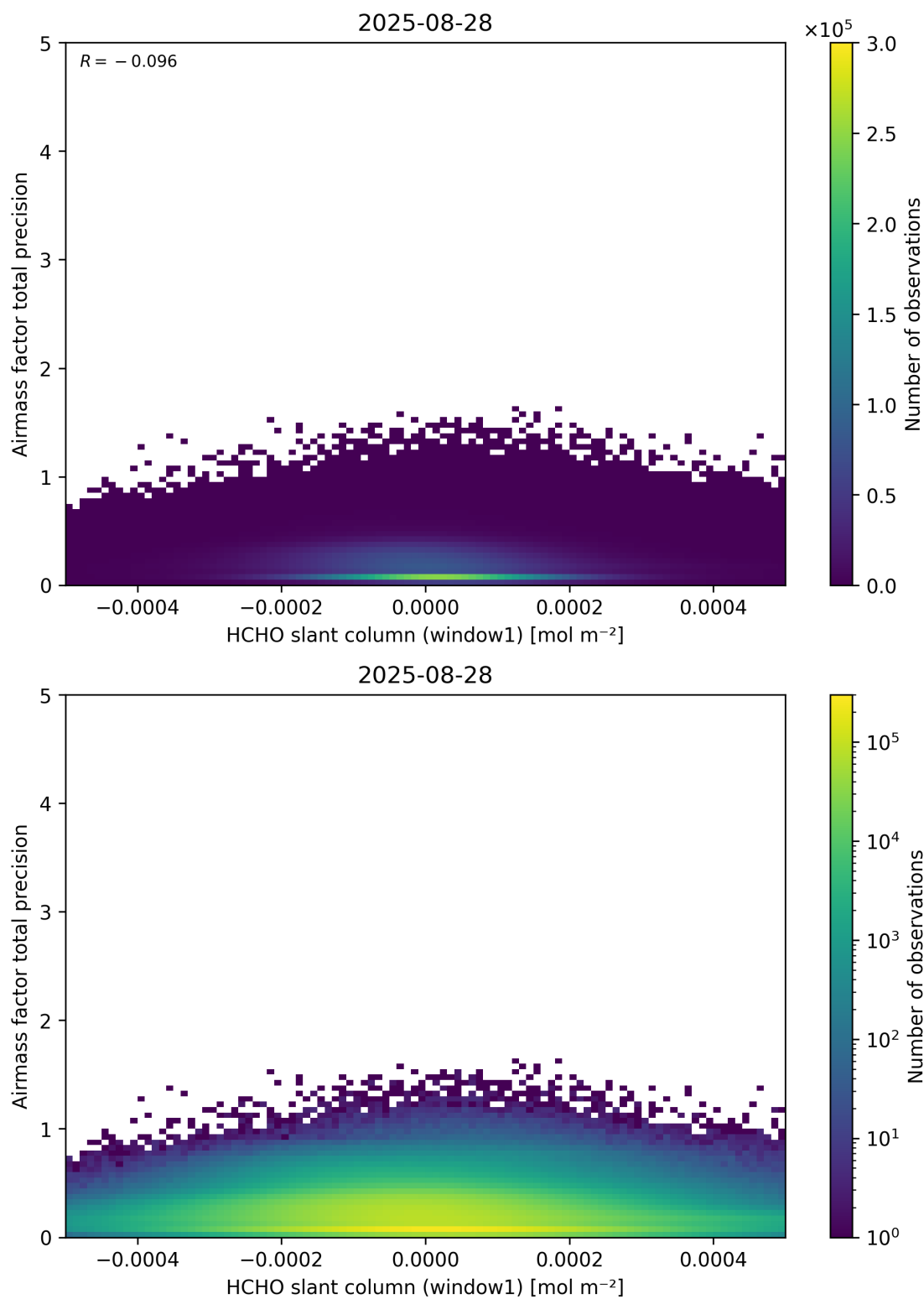
Figure 86: Scatter density plot of “HCHO slant column (window1)” against “Airmass factor total precision” for 2025-08-27 to 2025-08-29.
