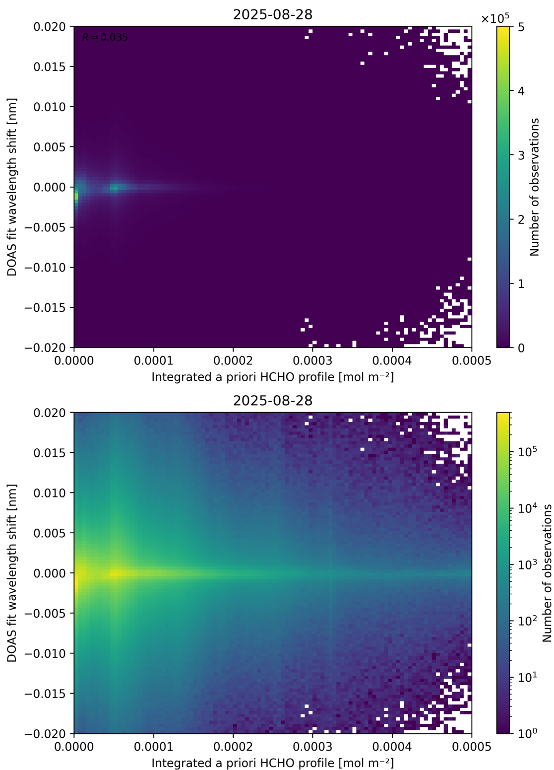
Figure 149: Scatter density plot of “Integrated a priori HCHO profile” against “DOAS fit wavelength shift” for 2025-08-27 to 2025-08-29.
