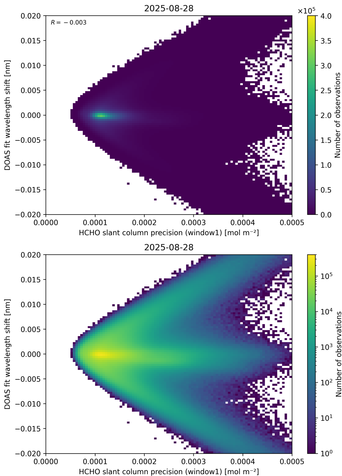
Figure 89: Scatter density plot of “HCHO slant column precision (window1)” against “DOAS fit wavelength shift” for 2025-08-27 to 2025-08-29.
