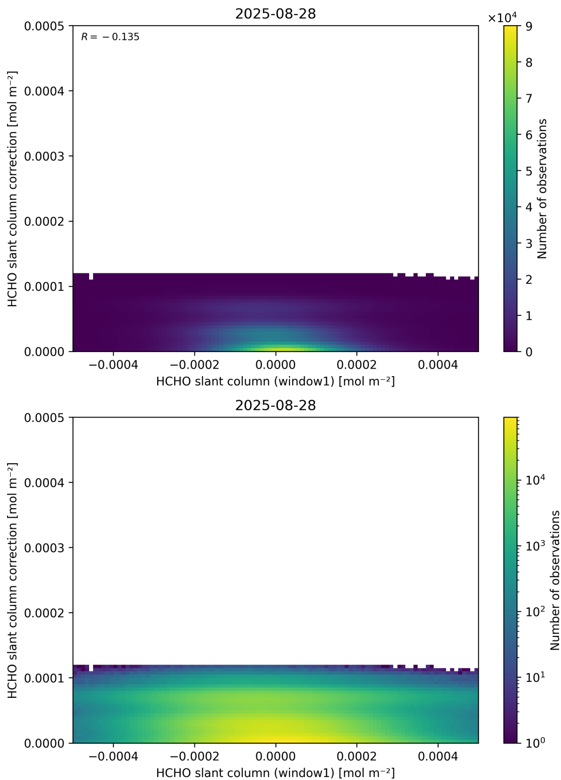
Figure 83: Scatter density plot of “HCHO slant column (window1)” against “HCHO slant column correction” for 2025-08-27 to 2025-08-29.
