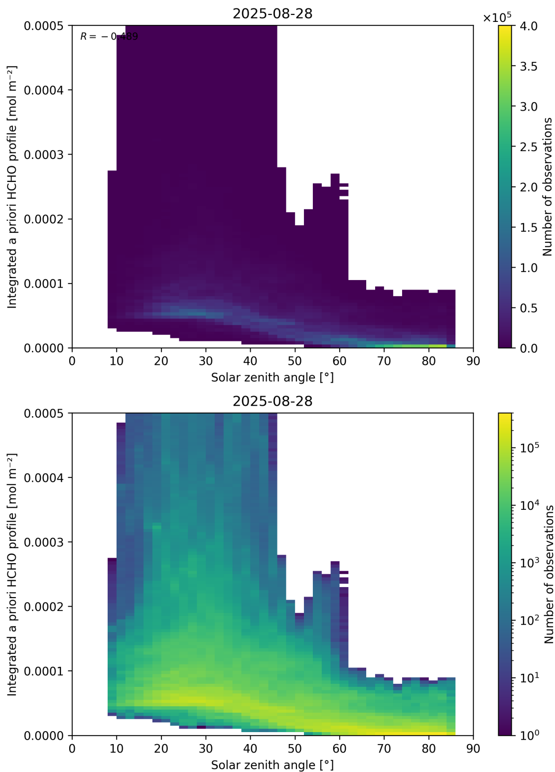
Figure 180: Scatter density plot of “Solar zenith angle” against “Integrated a priori HCHO profile” for 2025-08-27 to 2025-08-29.
