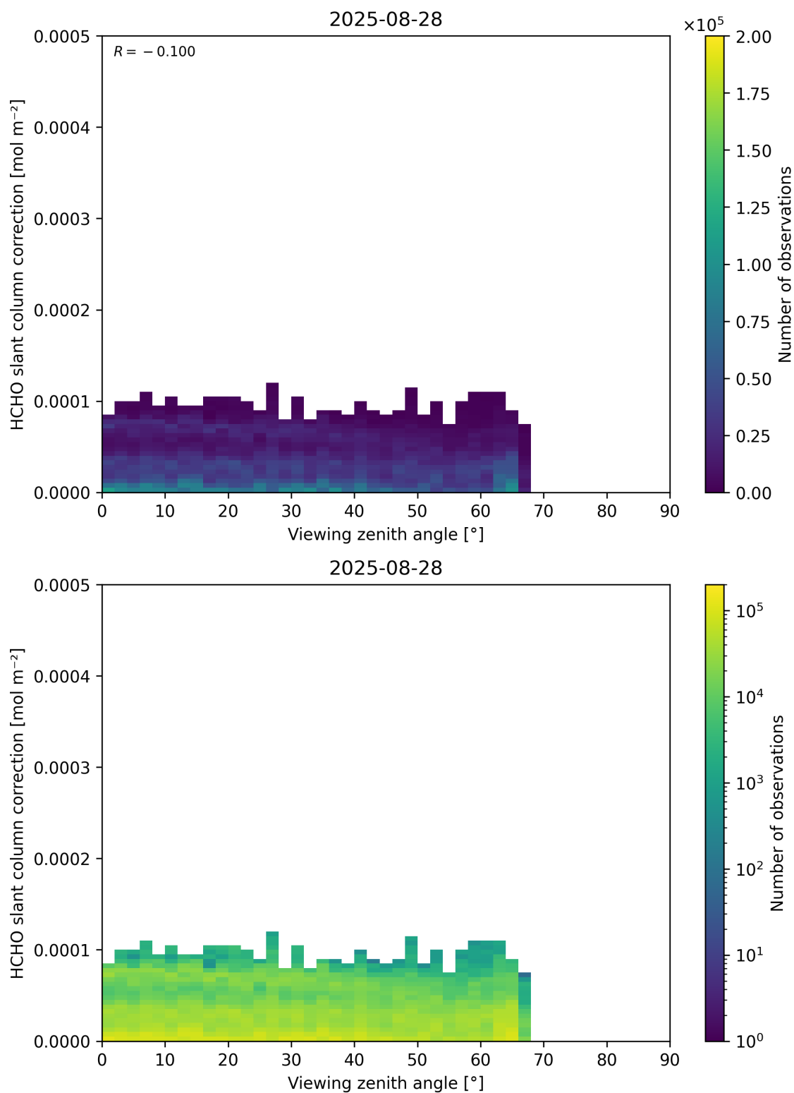
Figure 187: Scatter density plot of “Viewing zenith angle” against “HCHO slant column correction” for 2025-08-27 to 2025-08-29.
