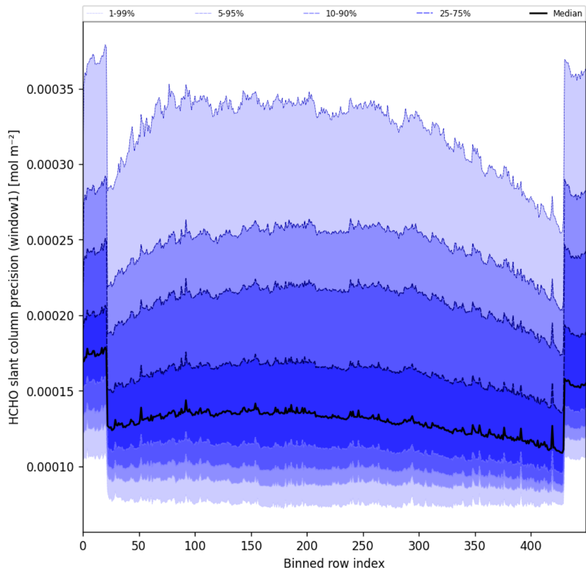
Figure 53: Along track statistics of “HCHO slant column precision (window1)” for 2025-08-27 to 2025-08-29
