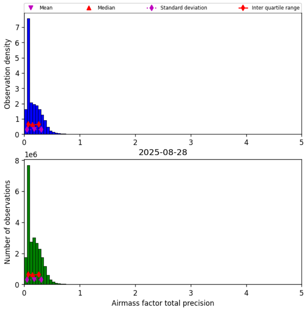
Figure 41: Histogram of “Airmass factor total precision” for 2025-08-27 to 2025-08-29
