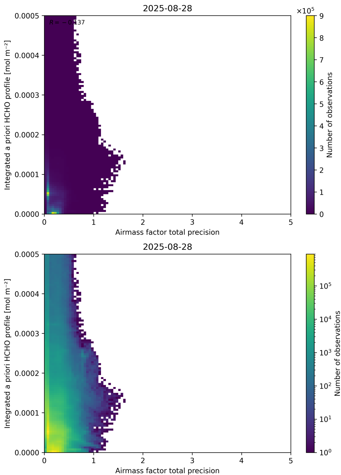
Figure 111: Scatter density plot of “Airmass factor total precision” against “Integrated a priori HCHO profile” for 2025-08-27 to 2025-08-29.
