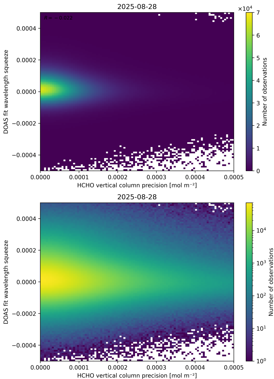
Figure 138: Scatter density plot of “HCHO vertical column precision” against “DOAS fit wavelength squeeze” for 2025-08-27 to 2025-08-29.
