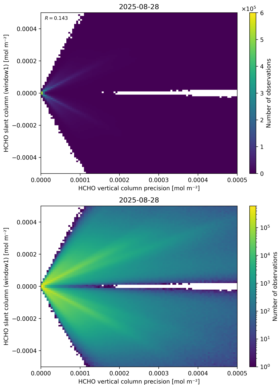
Figure 142: Scatter density plot of “HCHO vertical column precision” against “HCHO slant column (window1)” for 2025-08-27 to 2025-08-29.
