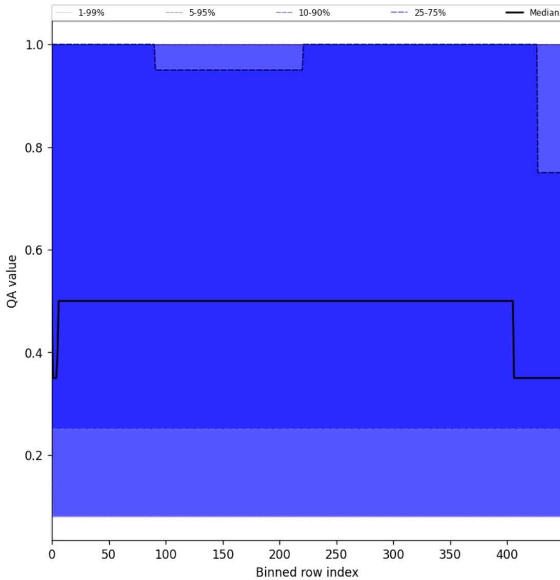
Figure 48: Along track statistics of “QA value” for 2025-08-27 to 2025-08-29
