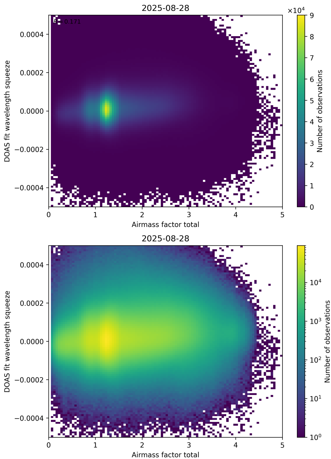
Figure 99: Scatter density plot of “Airmass factor total” against “DOAS fit wavelength squeeze” for 2025-08-27 to 2025-08-29.
