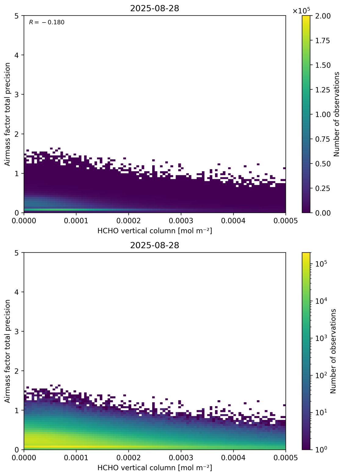
Figure 132: Scatter density plot of “HCHO vertical column” against “Airmass factor total precision” for 2025-08-27 to 2025-08-29.
