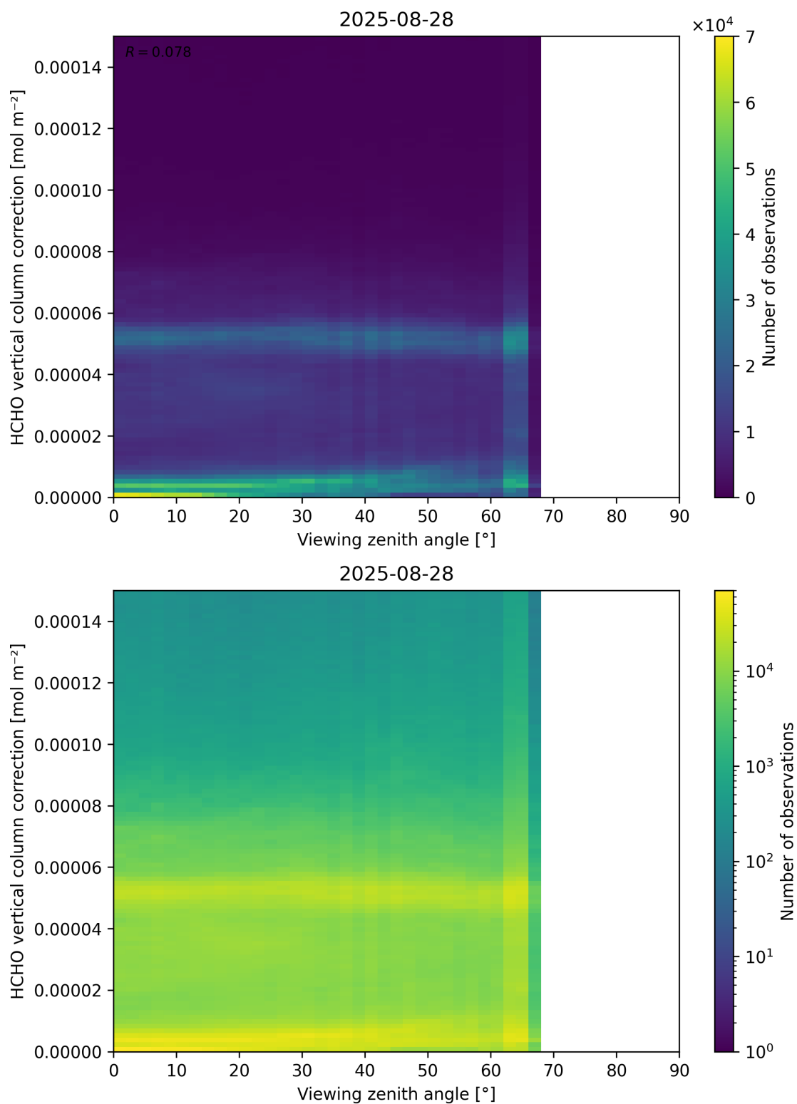
Figure 193: Scatter density plot of “Viewing zenith angle” against “HCHO vertical column correction” for 2025-08-27 to 2025-08-29.
