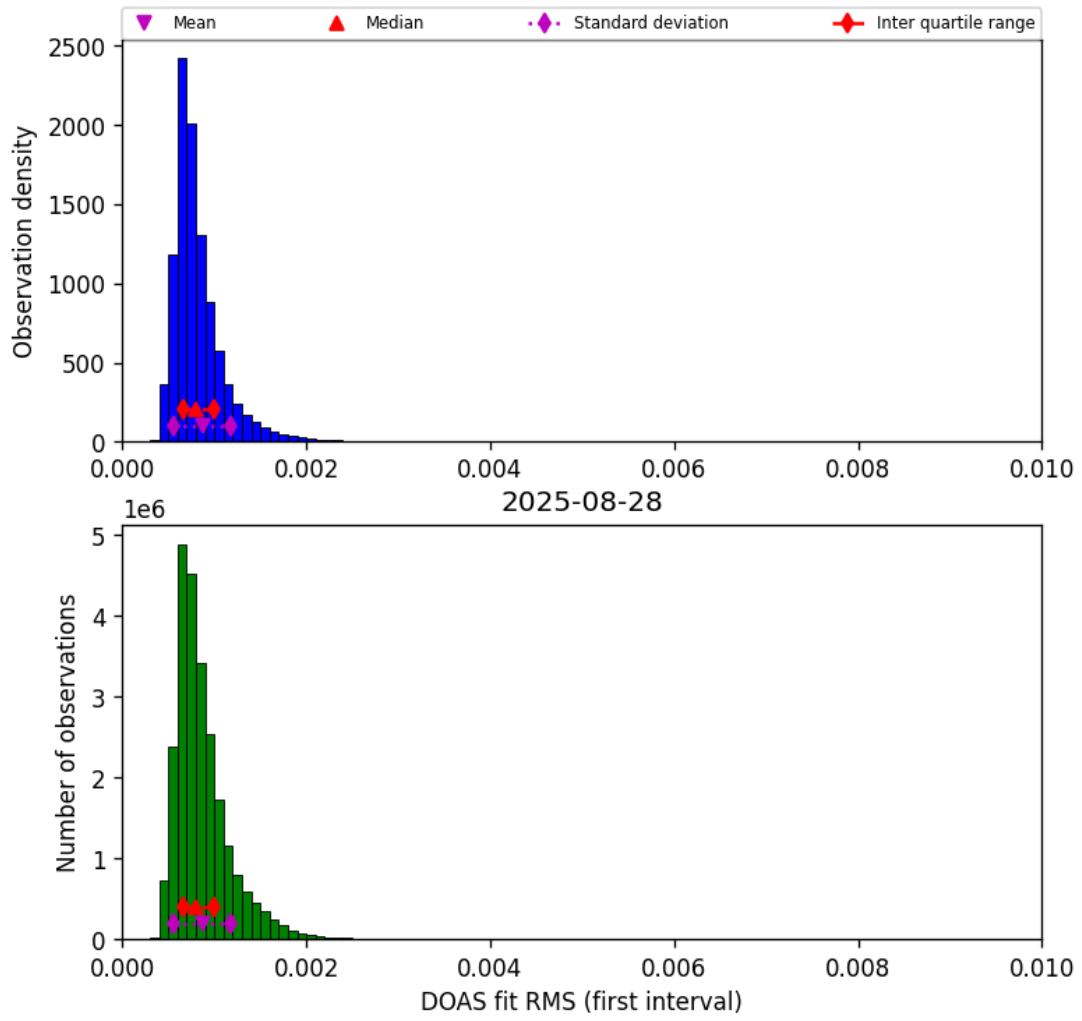
Figure 46: Histogram of “DOAS fit RMS (first interval)” for 2025-08-27 to 2025-08-29
