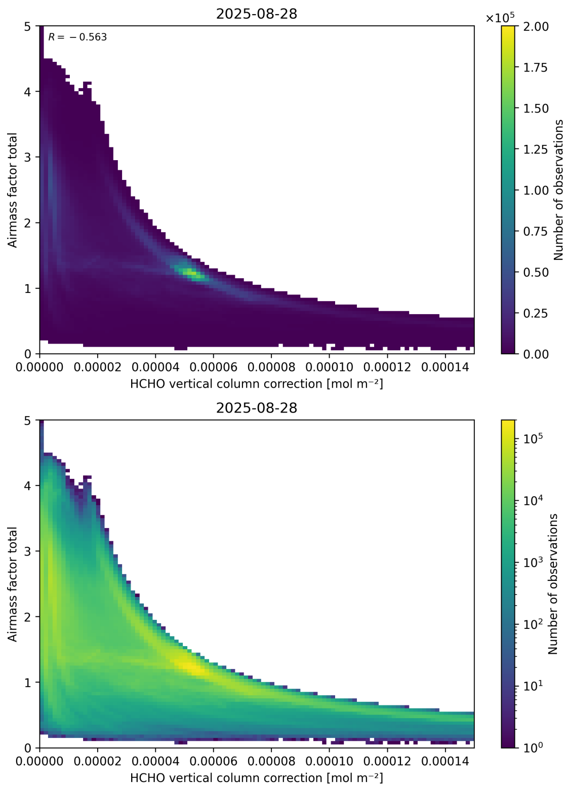
Figure 120: Scatter density plot of “HCHO vertical column correction” against “Airmass factor total” for 2025-08-27 to 2025-08-29.
