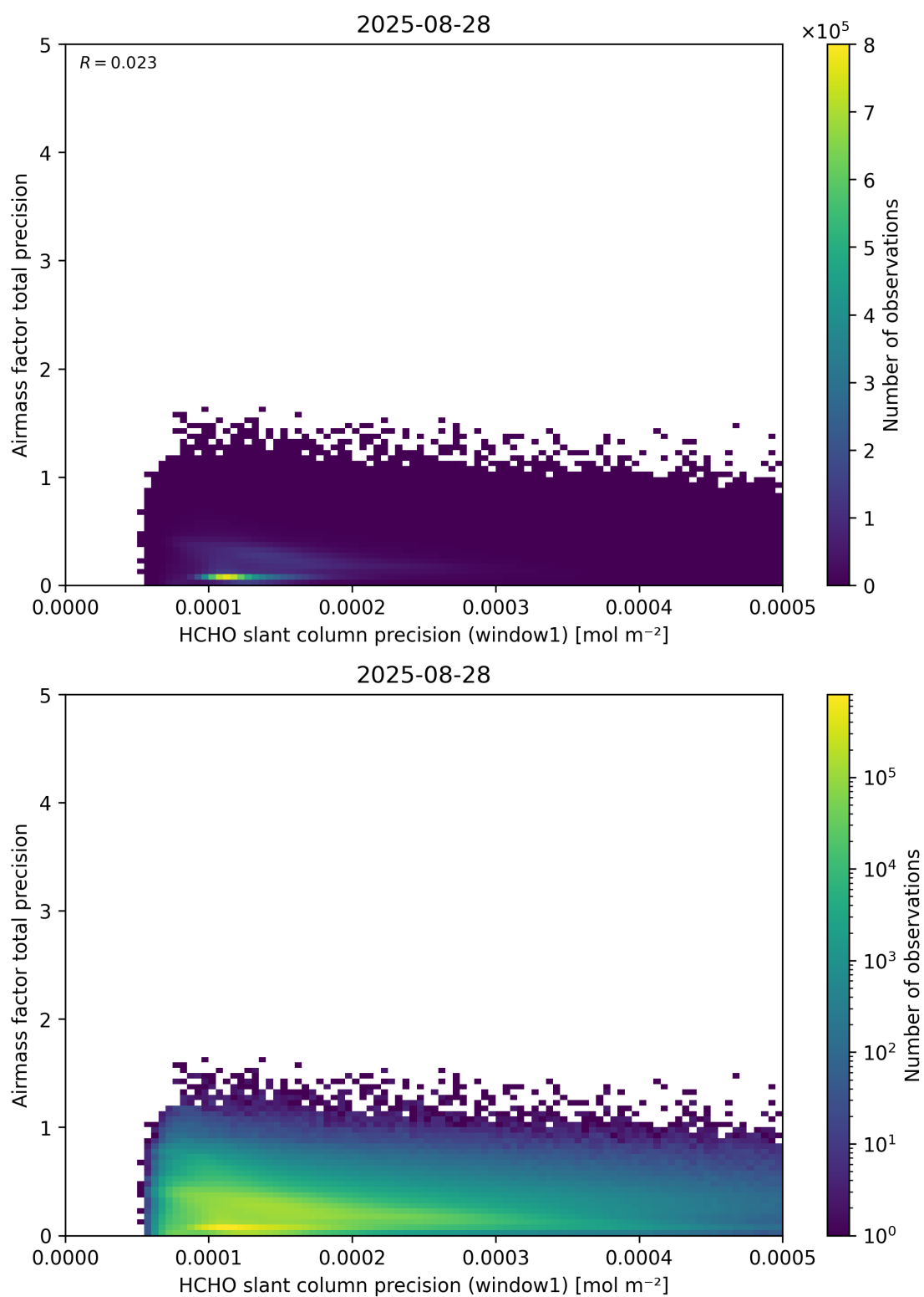
Figure 95: Scatter density plot of “HCHO slant column precision (window1)” against “Airmass factor total precision” for 2025-08-27 to 2025-08-29.
