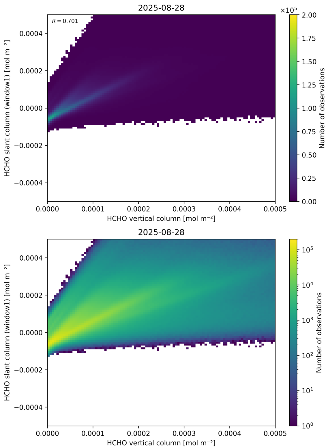
Figure 129: Scatter density plot of “HCHO vertical column” against “HCHO slant column (window1)” for 2025-08-27 to 2025-08-29.
