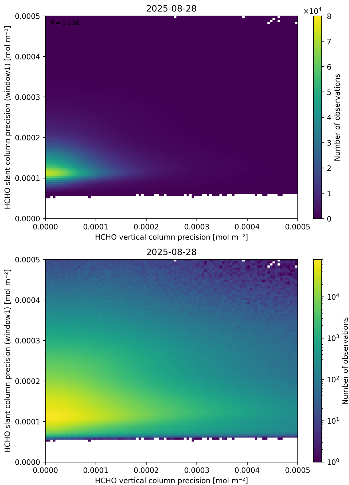
Figure 143: Scatter density plot of “HCHO vertical column precision” against “HCHO slant column precision (window1)” for 2025-08-27 to 2025-08-29.
