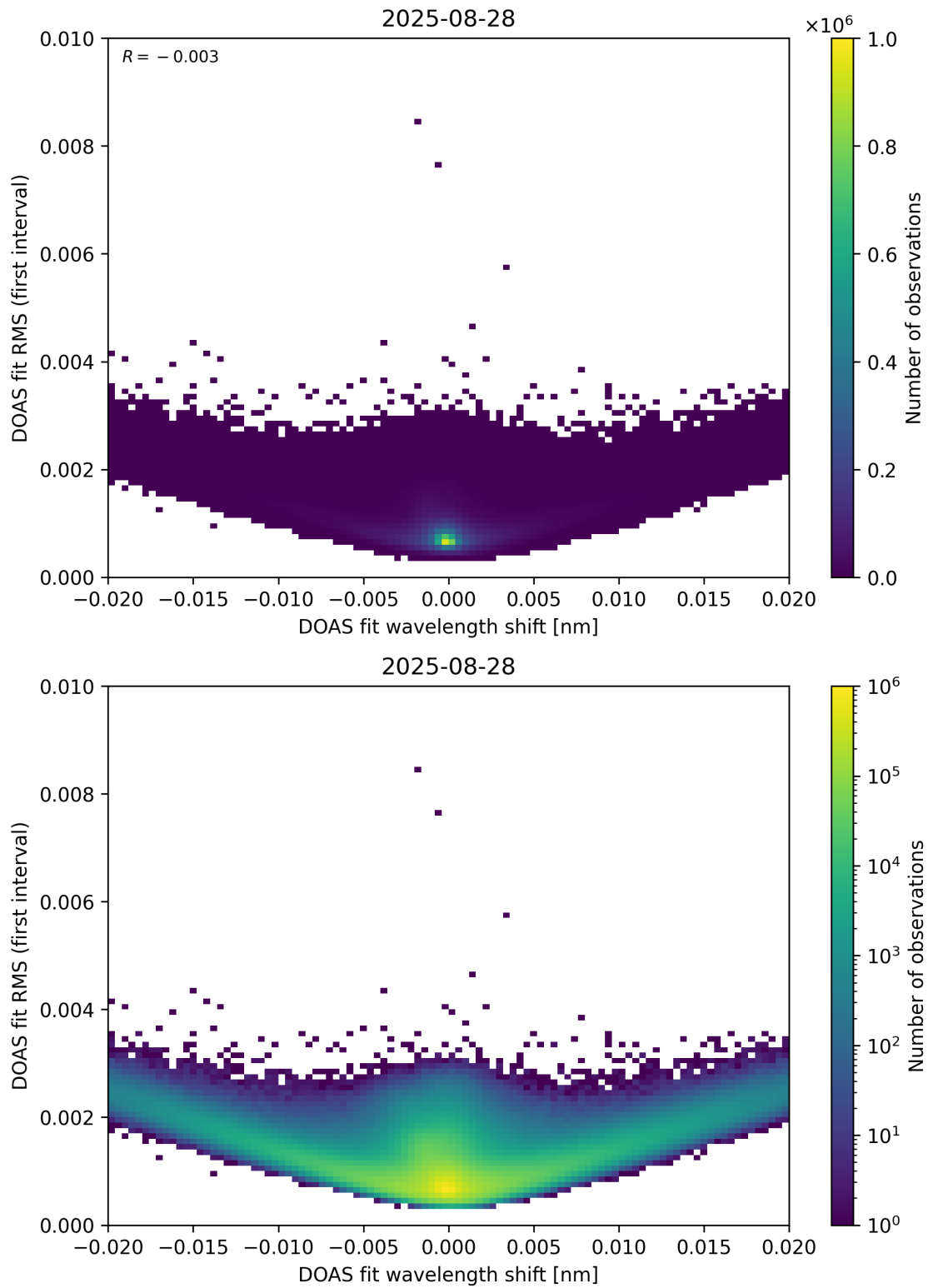
Figure 64: Scatter density plot of “DOAS fit wavelength shift” against “DOAS fit RMS (first interval)” for 2025-08-27 to 2025-08-29.
