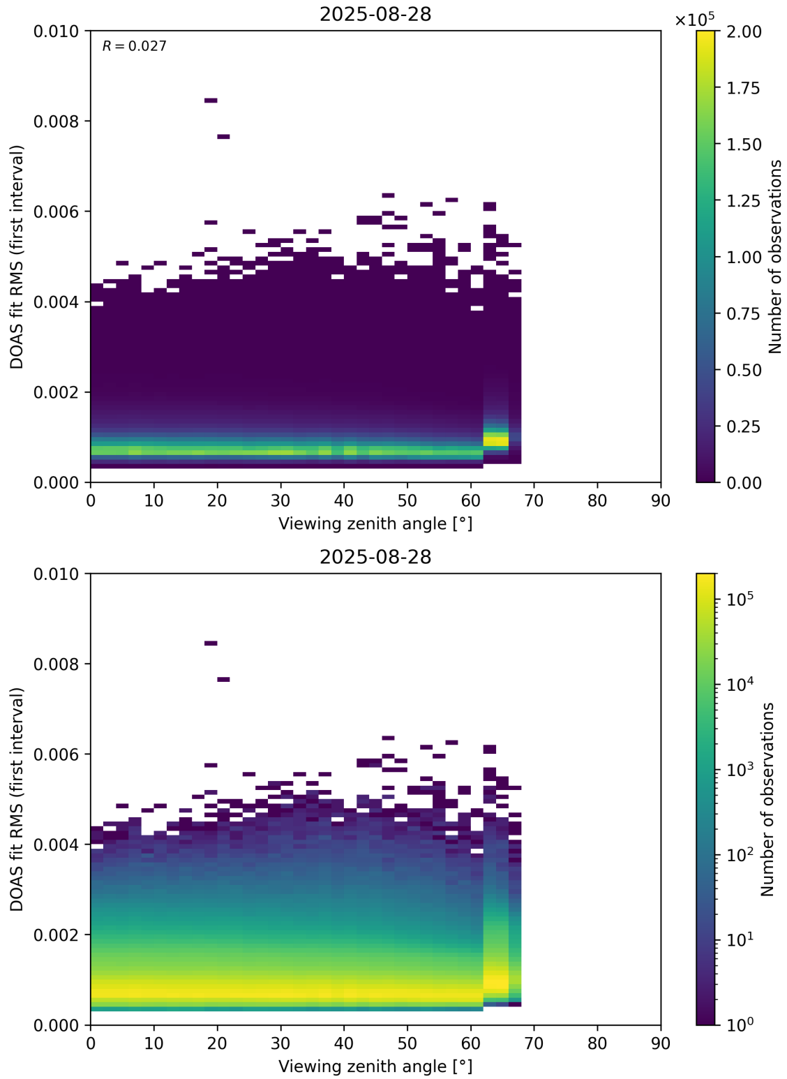
Figure 182: Scatter density plot of “Viewing zenith angle” against “DOAS fit RMS (first interval)” for 2025-08-27 to 2025-08-29.
