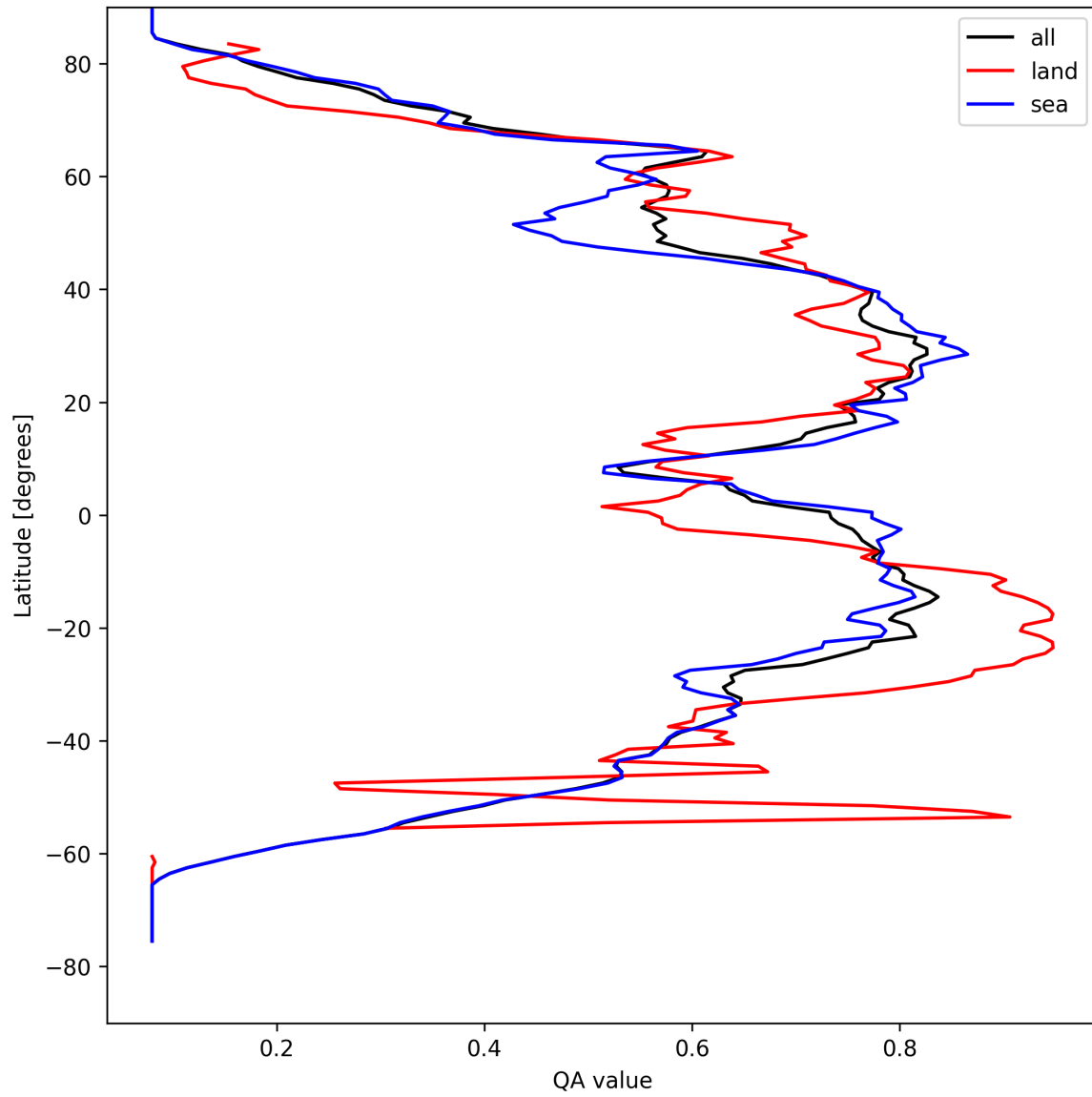
Figure 20: Zonal average of “QA value” for 2025-08-27 to 2025-08-29.
