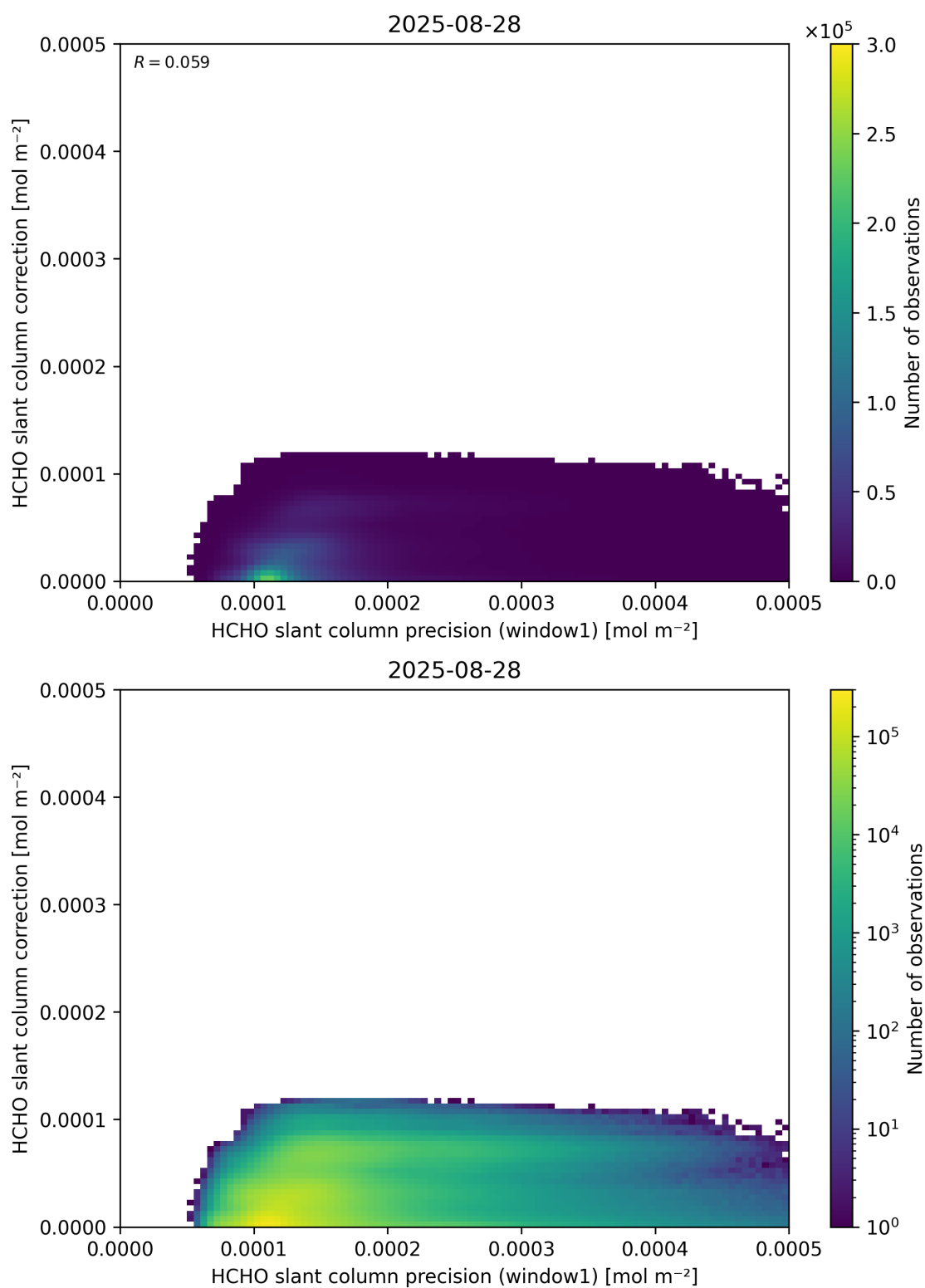
Figure 93: Scatter density plot of “HCHO slant column precision (window1)” against “HCHO slant column correction” for 2025-08-27 to 2025-08-29.
