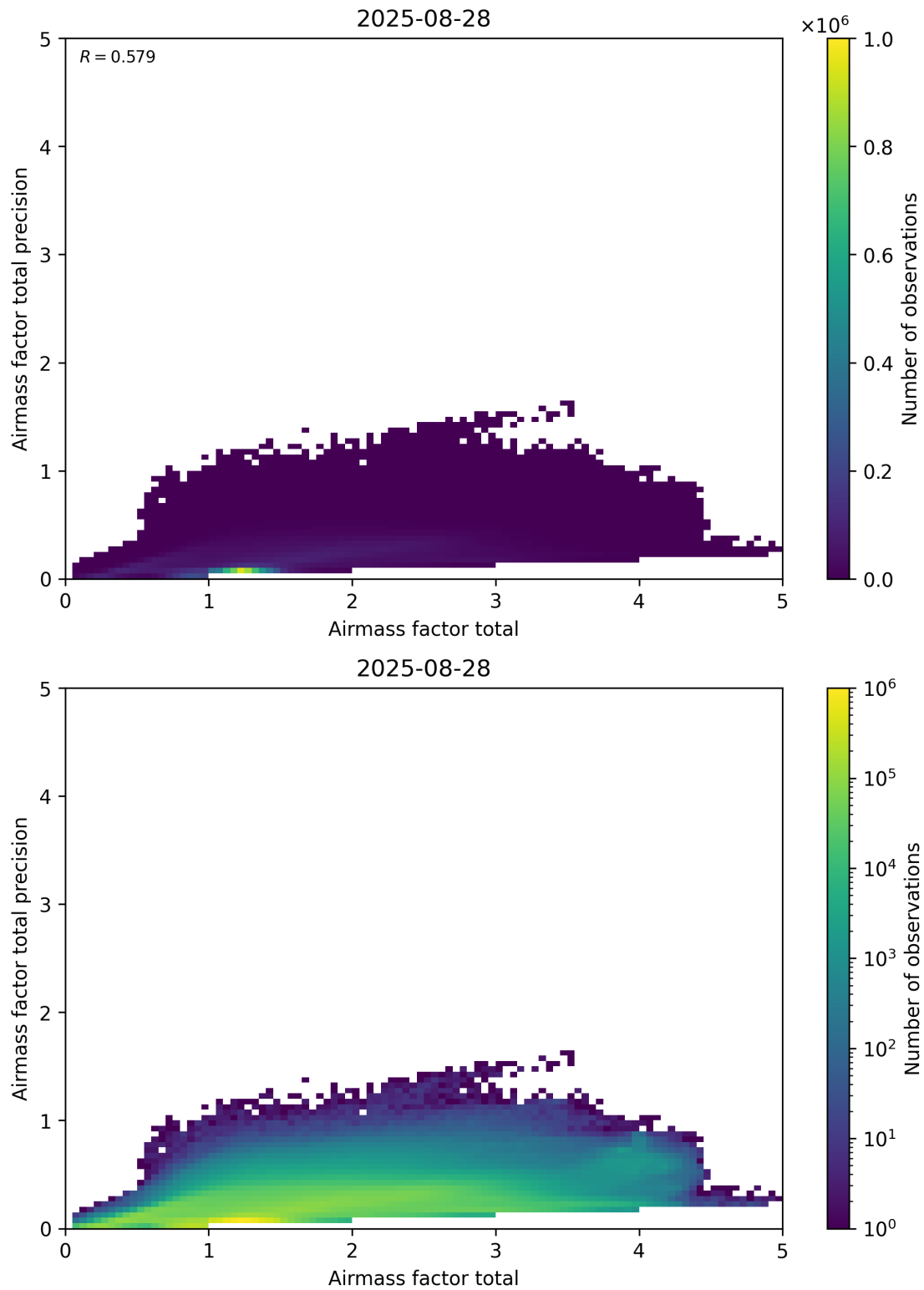
Figure 103: Scatter density plot of “Airmass factor total” against “Airmass factor total precision” for 2025-08-27 to 2025-08-29.
