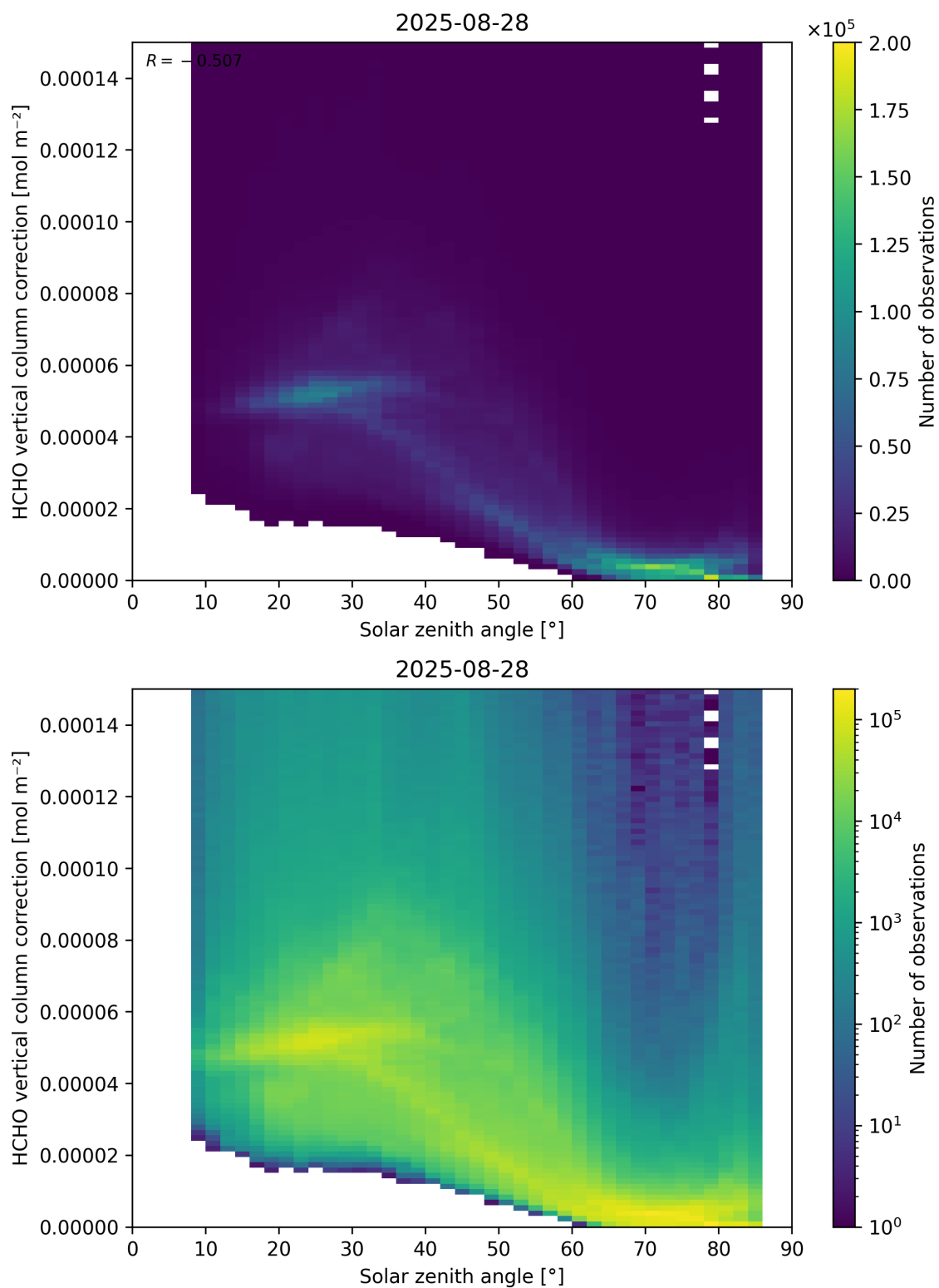
Figure 178: Scatter density plot of “Solar zenith angle” against “HCHO vertical column correction” for 2025-08-27 to 2025-08-29.
