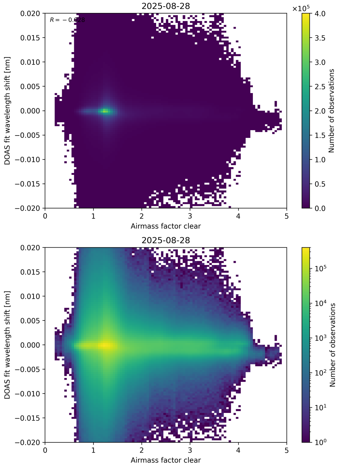
Figure 72: Scatter density plot of “Airmass factor clear” against “DOAS fit wavelength shift” for 2025-08-27 to 2025-08-29.
