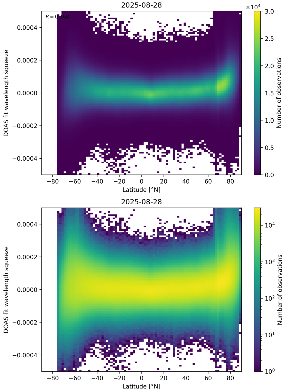
Figure 155: Scatter density plot of “Latitude” against “DOAS fit wavelength squeeze” for 2025-08-27 to 2025-08-29.
