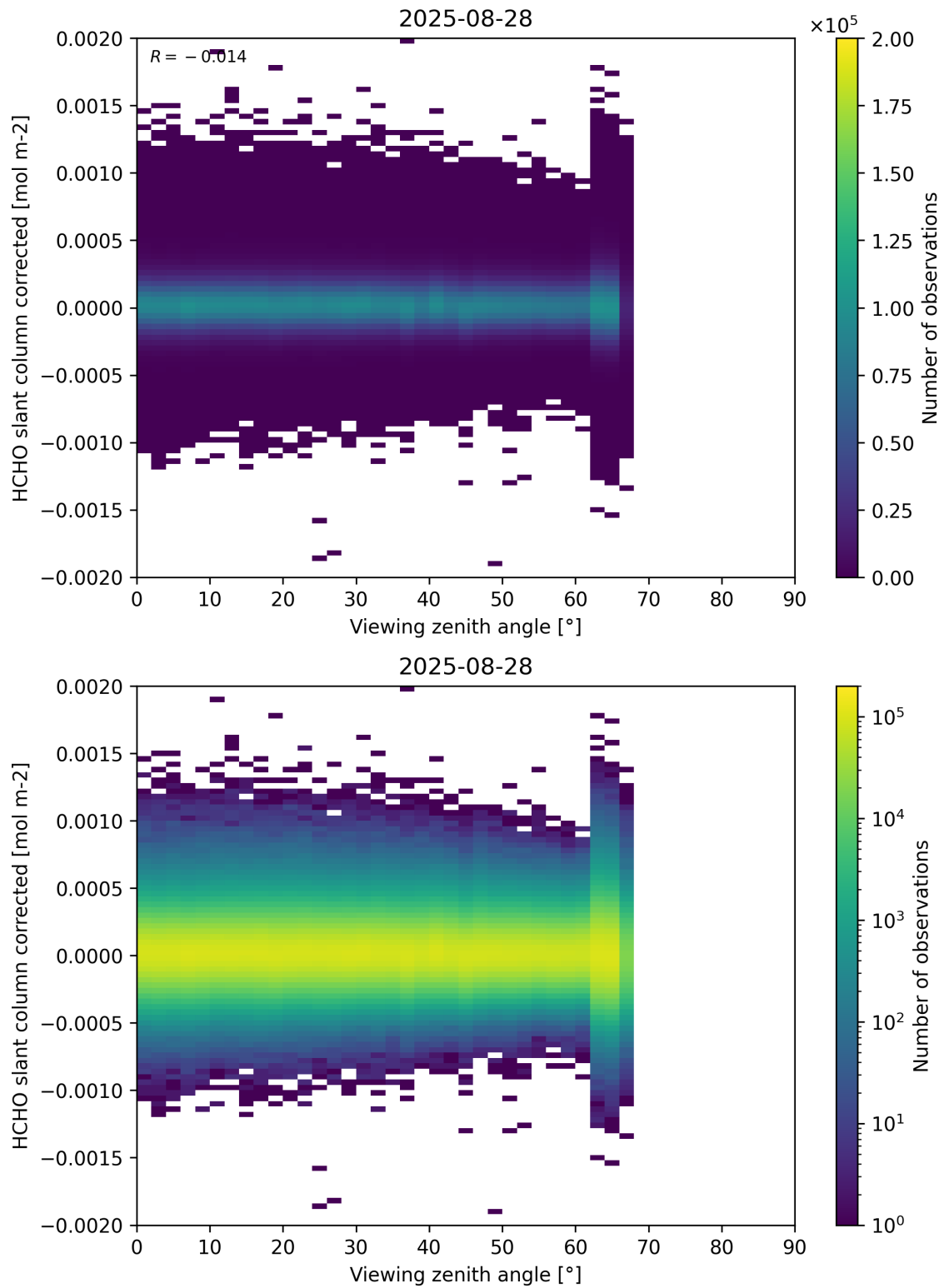
Figure 186: Scatter density plot of “Viewing zenith angle” against “HCHO slant column corrected” for 2025-08-27 to 2025-08-29.
