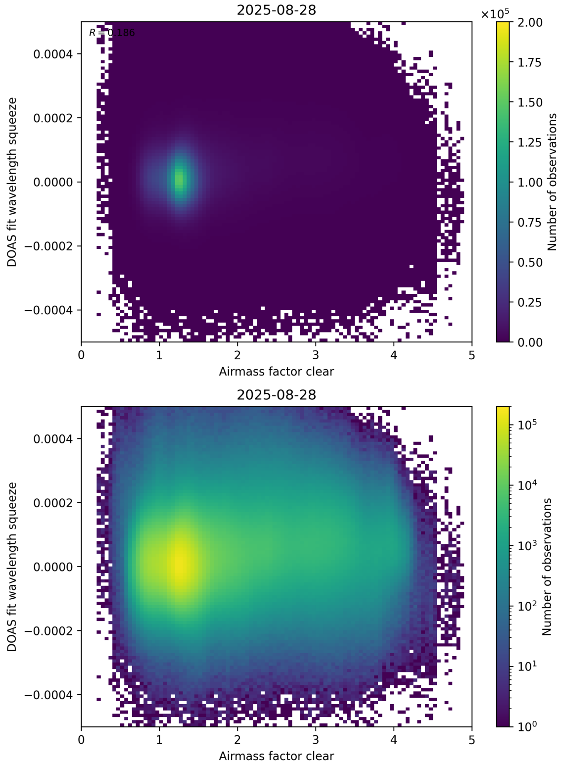
Figure 73: Scatter density plot of “Airmass factor clear” against “DOAS fit wavelength squeeze” for 2025-08-27 to 2025-08-29.
