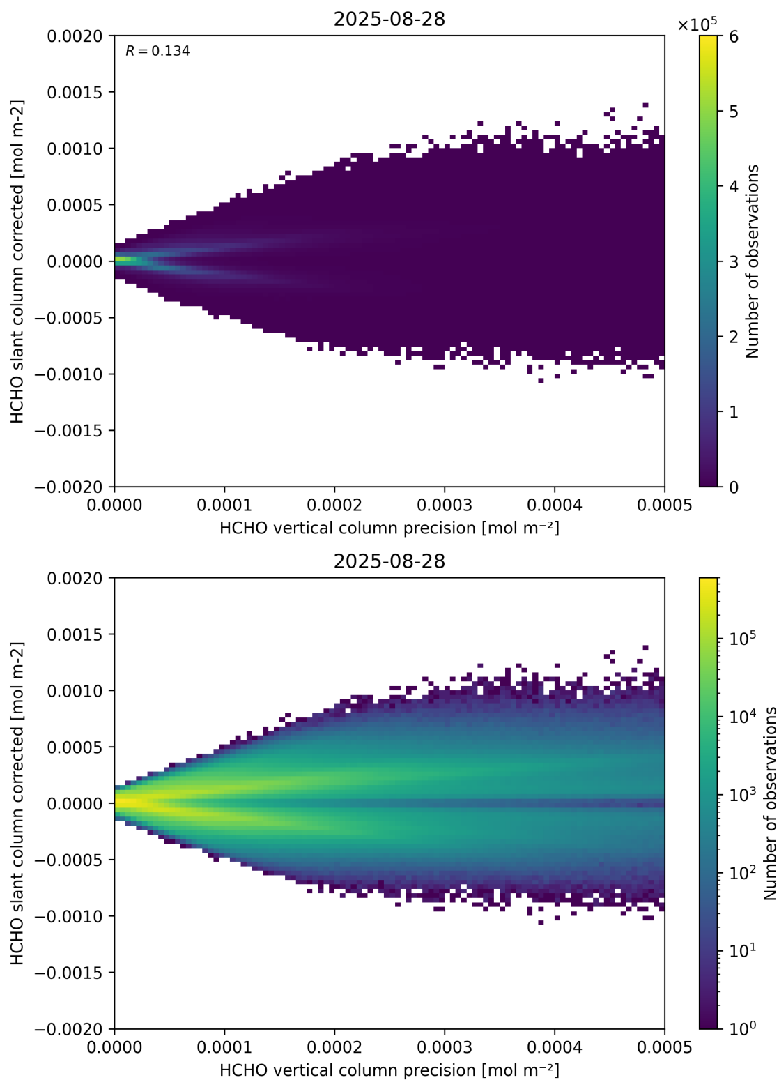
Figure 140: Scatter density plot of “HCHO vertical column precision” against “HCHO slant column corrected” for 2025-08-27 to 2025-08-29.
