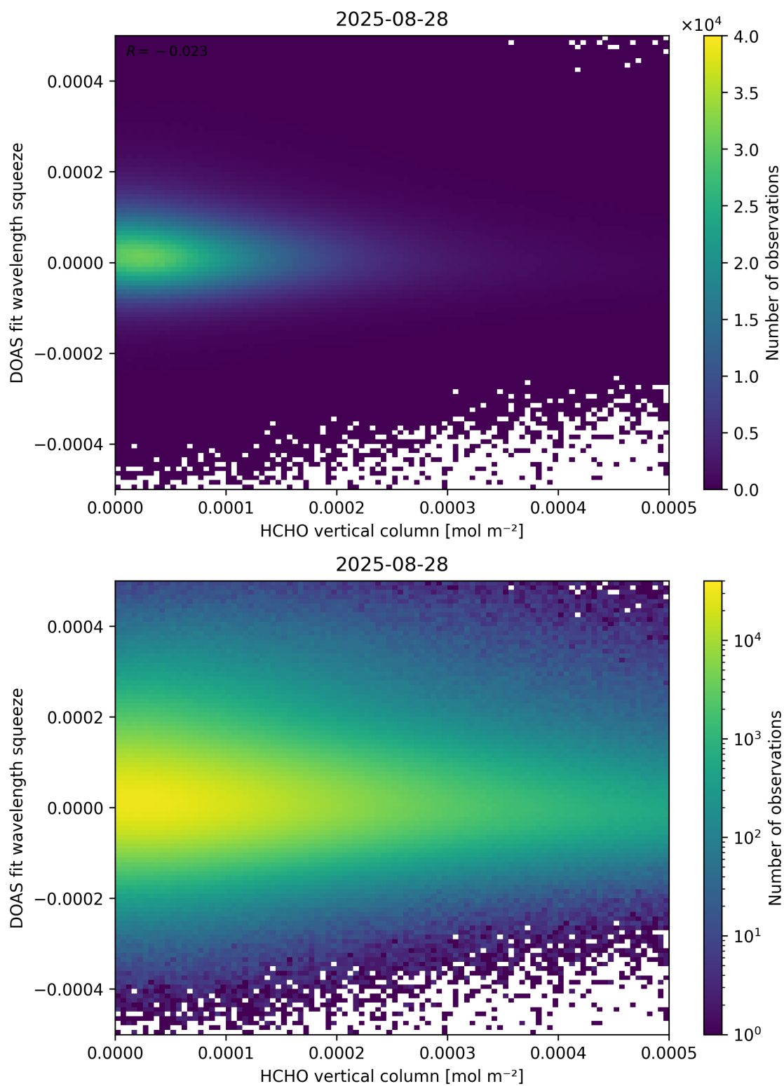
Figure 125: Scatter density plot of “HCHO vertical column” against “DOAS fit wavelength squeeze” for 2025-08-27 to 2025-08-29.
