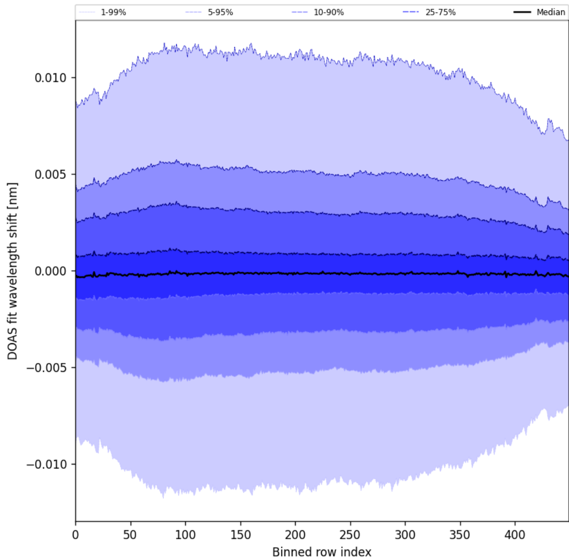
Figure 58: Along track statistics of “DOAS fit wavelength shift” for 2025-08-27 to 2025-08-29
