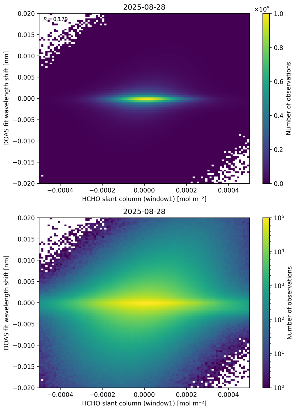
Figure 79: Scatter density plot of “HCHO slant column (window1)” against “DOAS fit wavelength shift” for 2025-08-27 to 2025-08-29.
