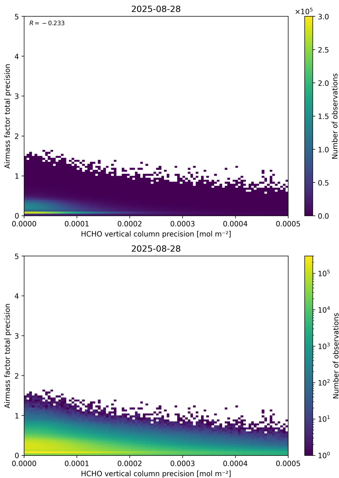
Figure 145: Scatter density plot of “HCHO vertical column precision” against “Airmass factor total precision” for 2025-08-27 to 2025-08-29.
