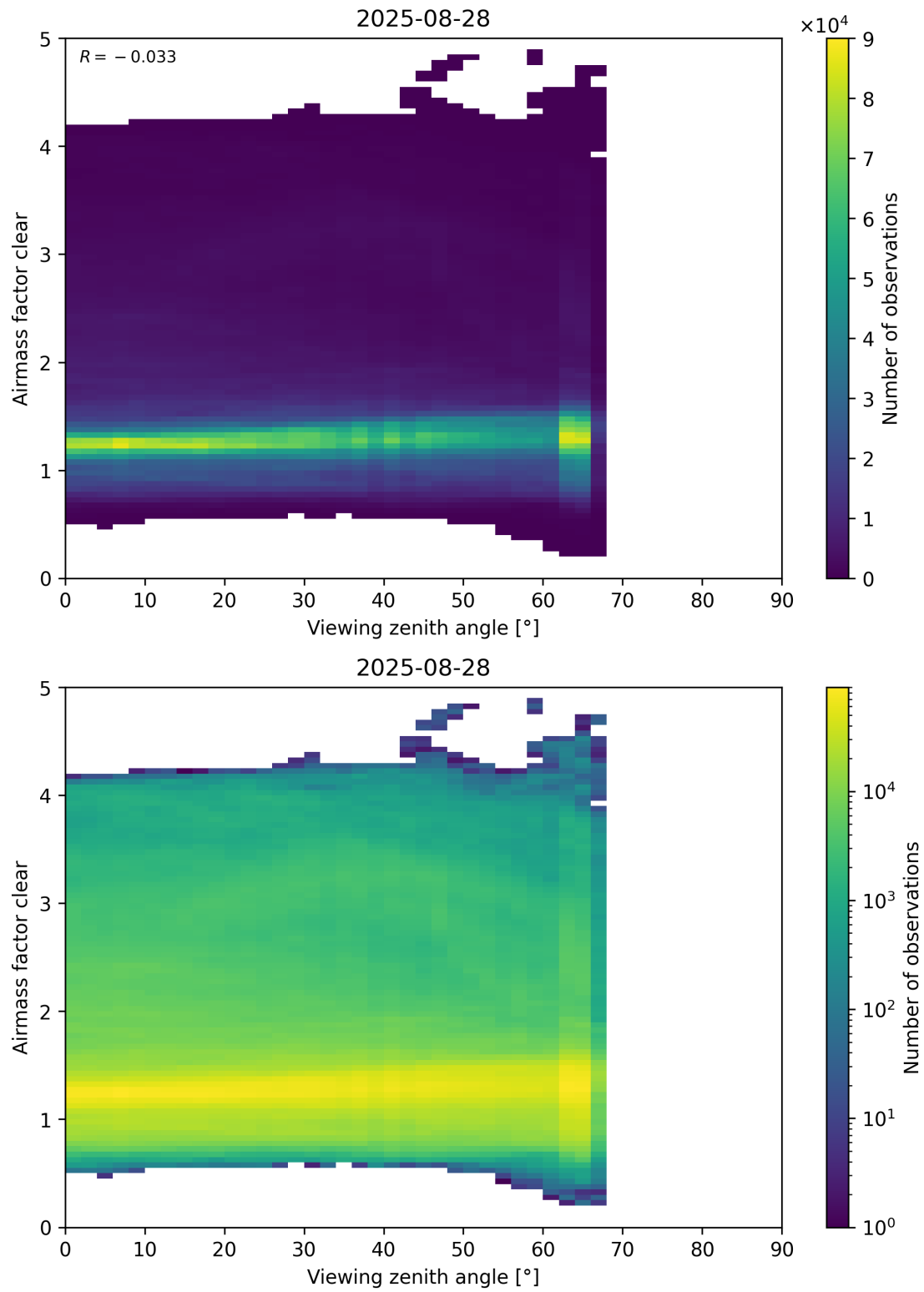
Figure 185: Scatter density plot of “Viewing zenith angle” against “Airmass factor clear” for 2025-08-27 to 2025-08-29.
