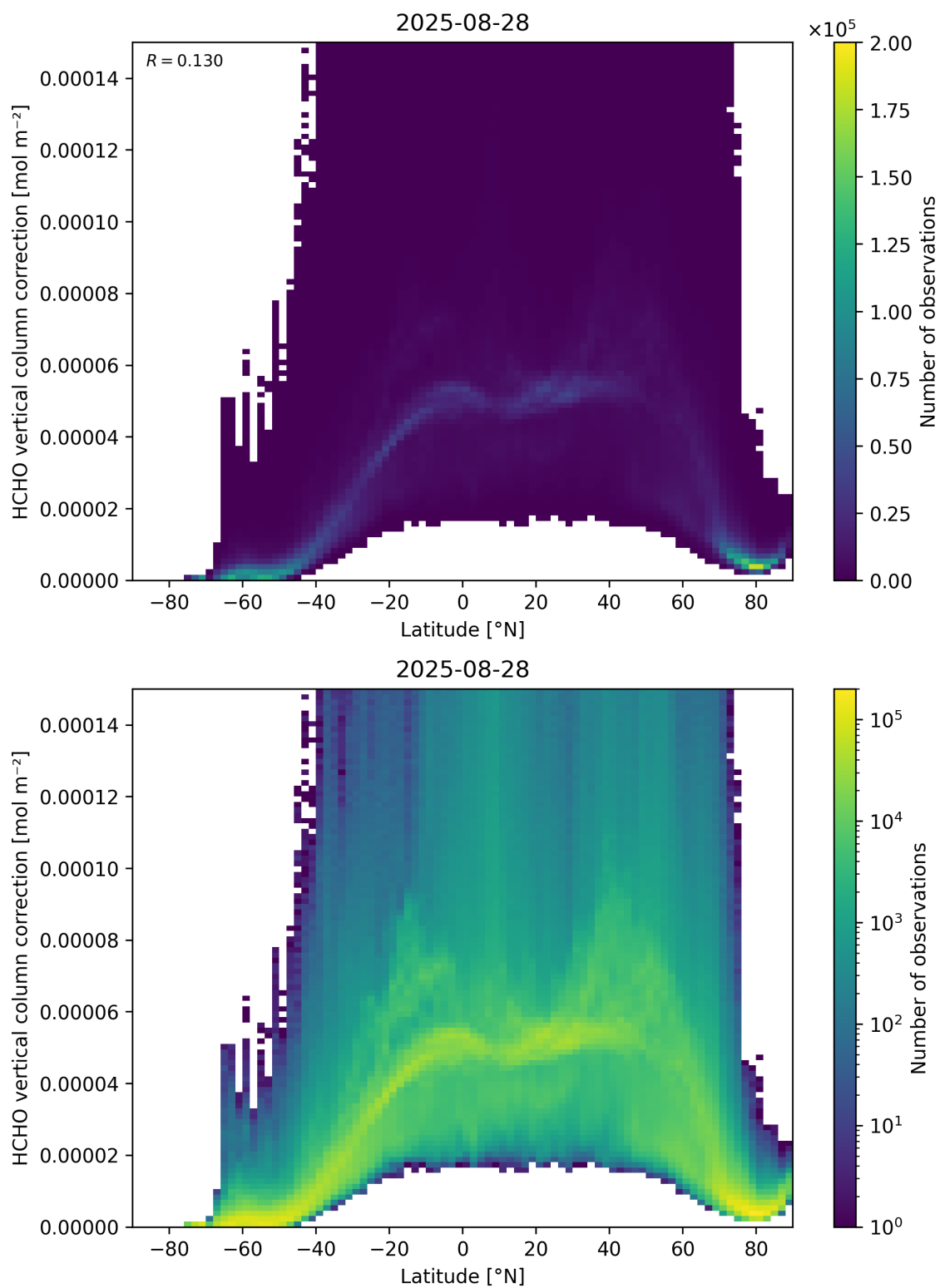
Figure 164: Scatter density plot of “Latitude” against “HCHO vertical column correction” for 2025-08-27 to 2025-08-29.
