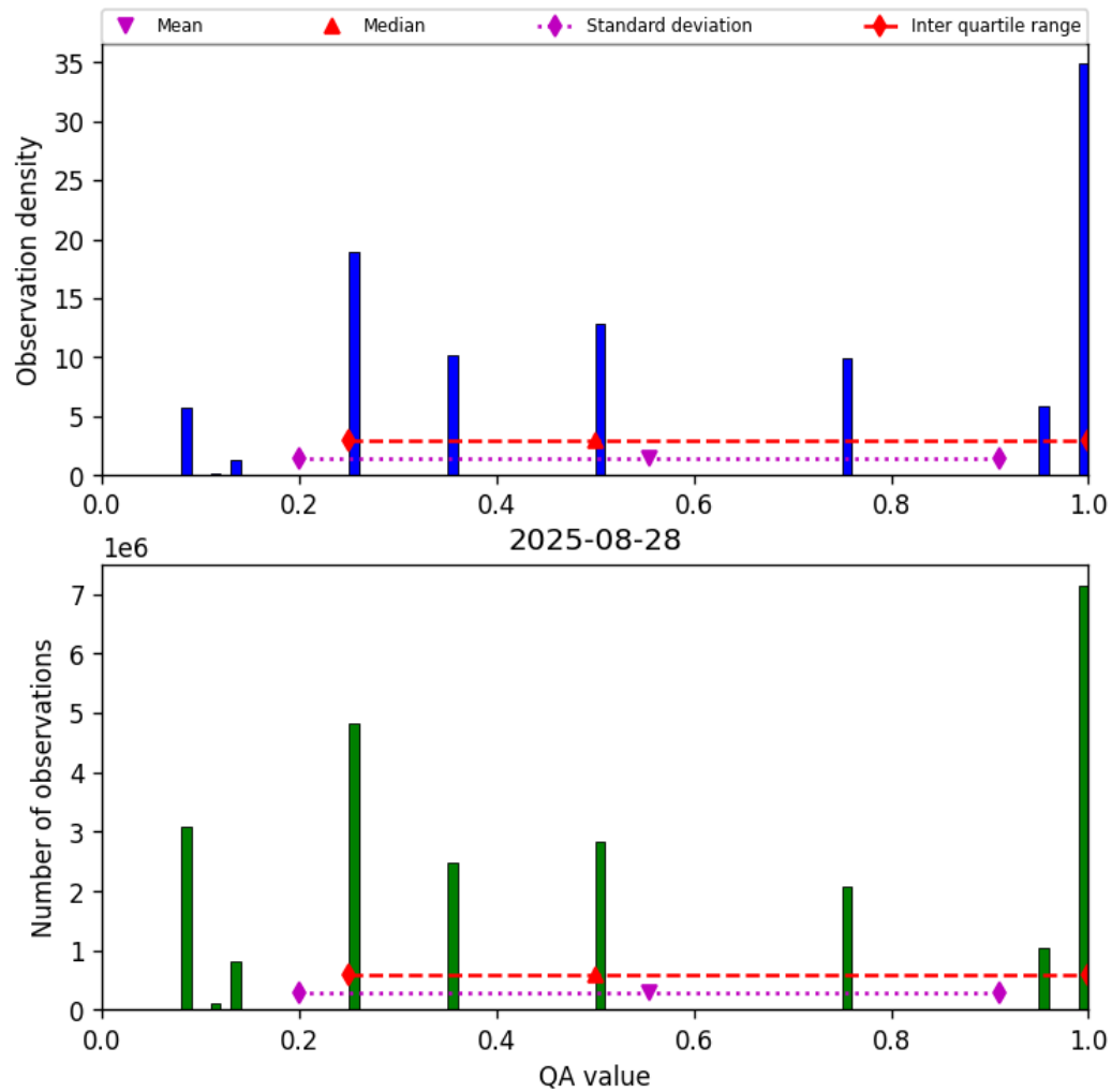
Figure 34: Histogram of “QA value” for 2025-08-27 to 2025-08-29
