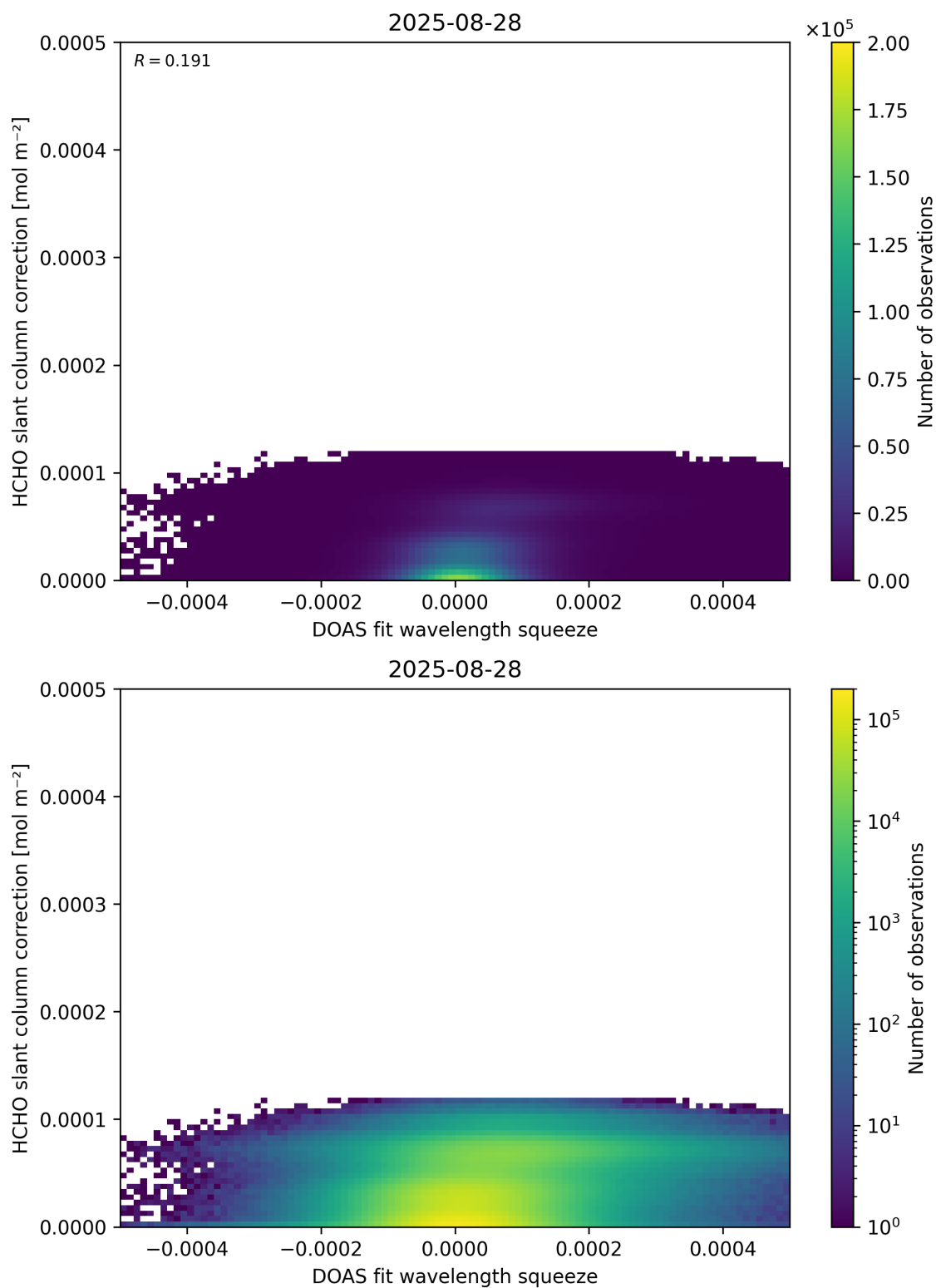
Figure 70: Scatter density plot of “DOAS fit wavelength squeeze” against “HCHO slant column correction” for 2025-08-27 to 2025-08-29.
