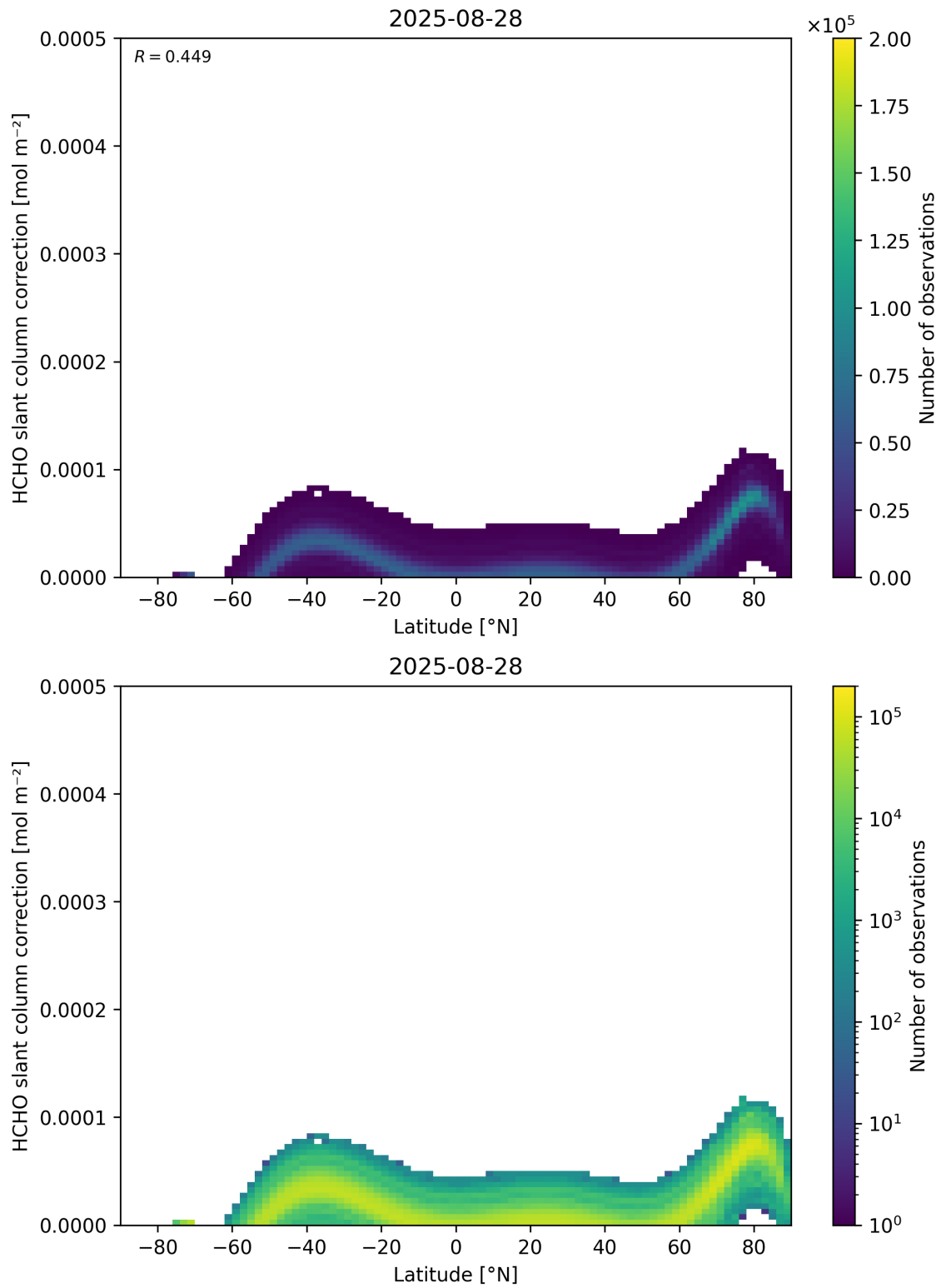
Figure 158: Scatter density plot of “Latitude” against “HCHO slant column correction” for 2025-08-27 to 2025-08-29.
