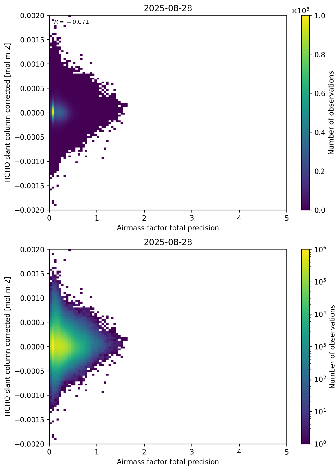
Figure 109: Scatter density plot of “Airmass factor total precision” against “HCHO slant column corrected” for 2025-08-27 to 2025-08-29.
