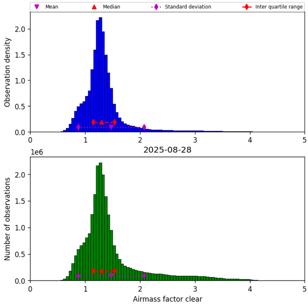
Figure 42: Histogram of “Airmass factor clear” for 2025-08-27 to 2025-08-29
