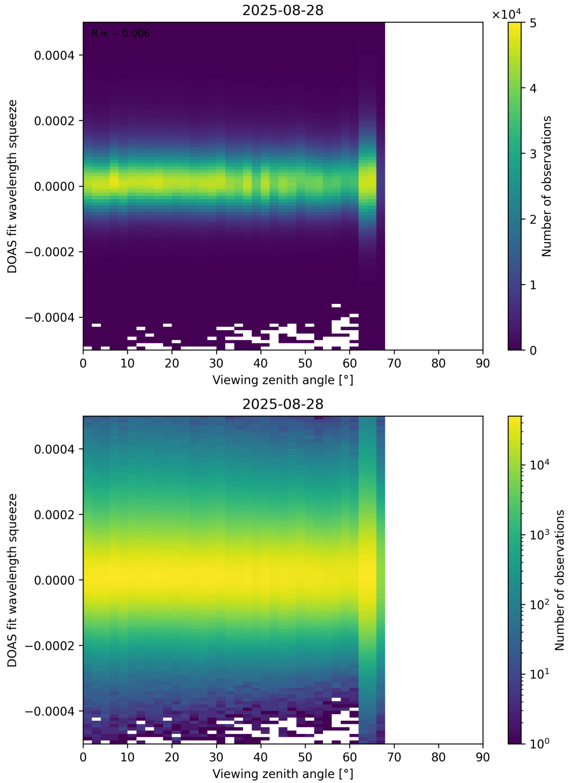
Figure 184: Scatter density plot of “Viewing zenith angle” against “DOAS fit wavelength squeeze” for 2025-08-27 to 2025-08-29.
