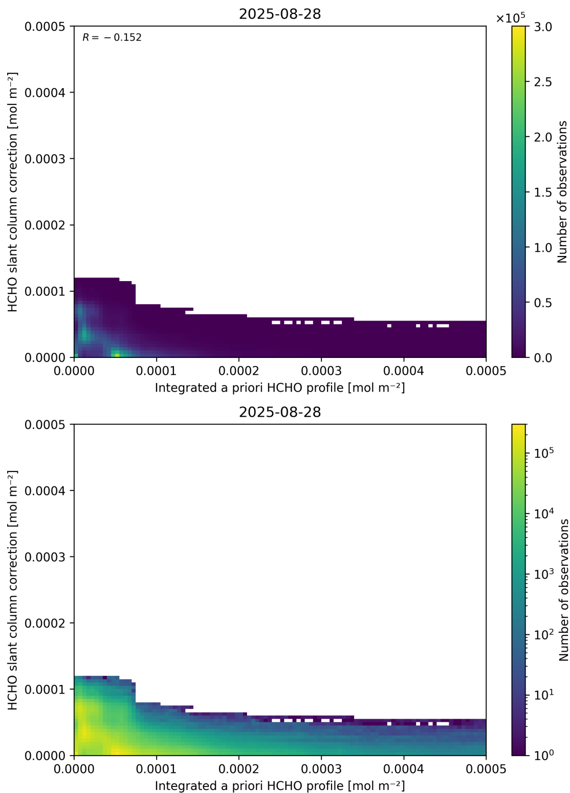
Figure 152: Scatter density plot of “Integrated a priori HCHO profile” against “HCHO slant column correction” for 2025-08-27 to 2025-08-29.
