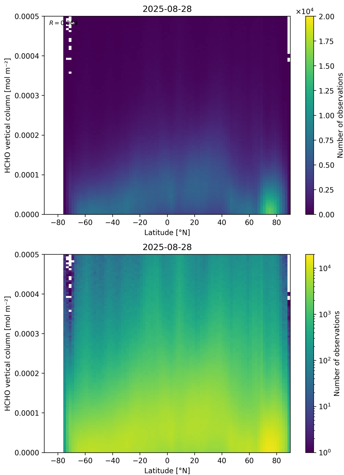
Figure 163: Scatter density plot of “Latitude” against “HCHO vertical column” for 2025-08-27 to 2025-08-29.
