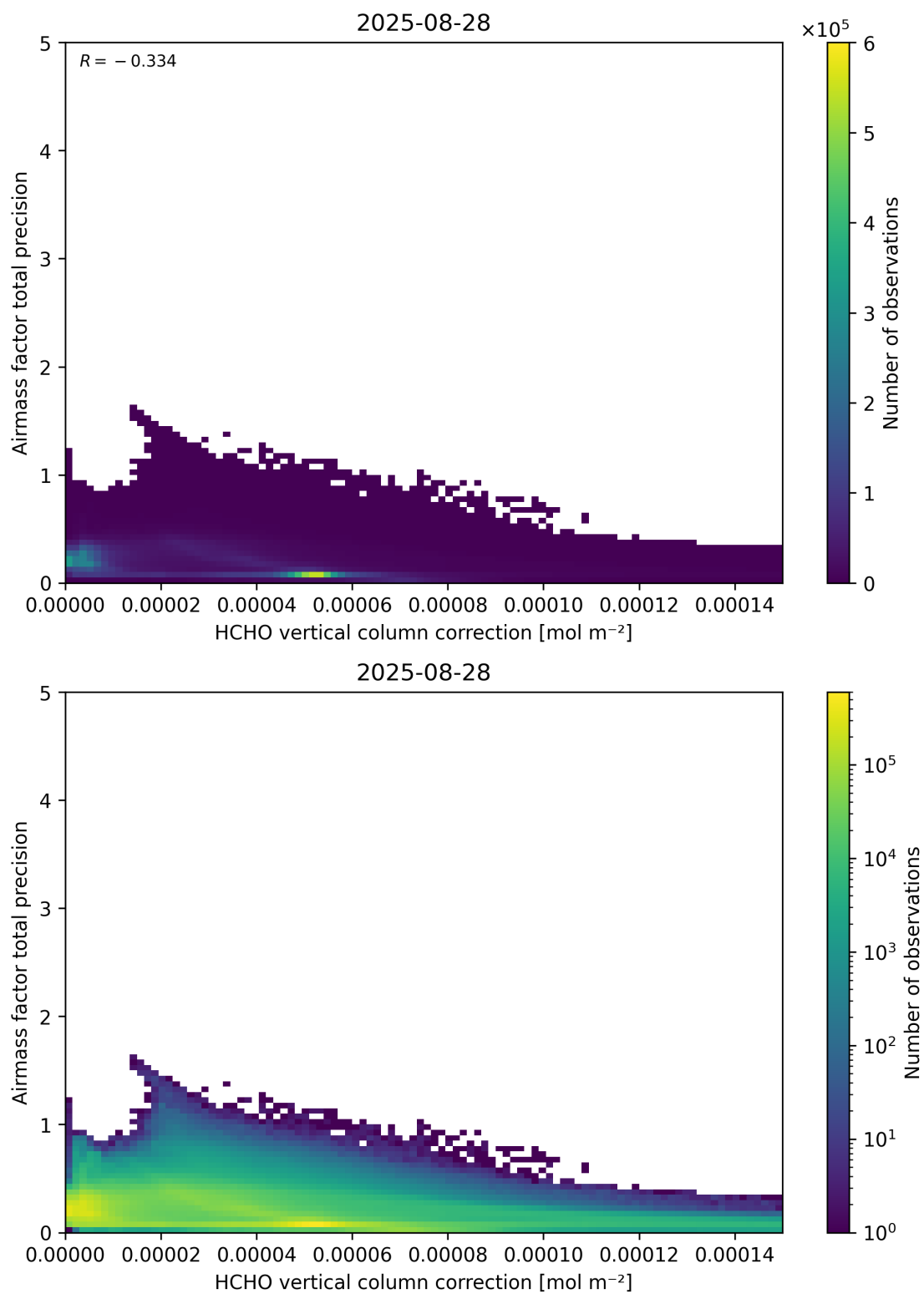
Figure 121: Scatter density plot of “HCHO vertical column correction” against “Airmass factor total precision” for 2025-08-27 to 2025-08-29.
