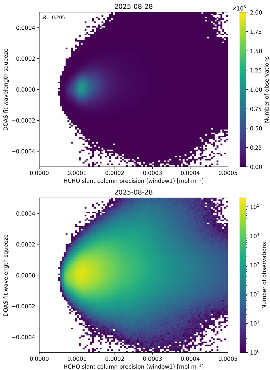
Figure 90: Scatter density plot of “HCHO slant column precision (window1)” against “DOAS fit wavelength squeeze” for 2025-08-27 to 2025-08-29.
