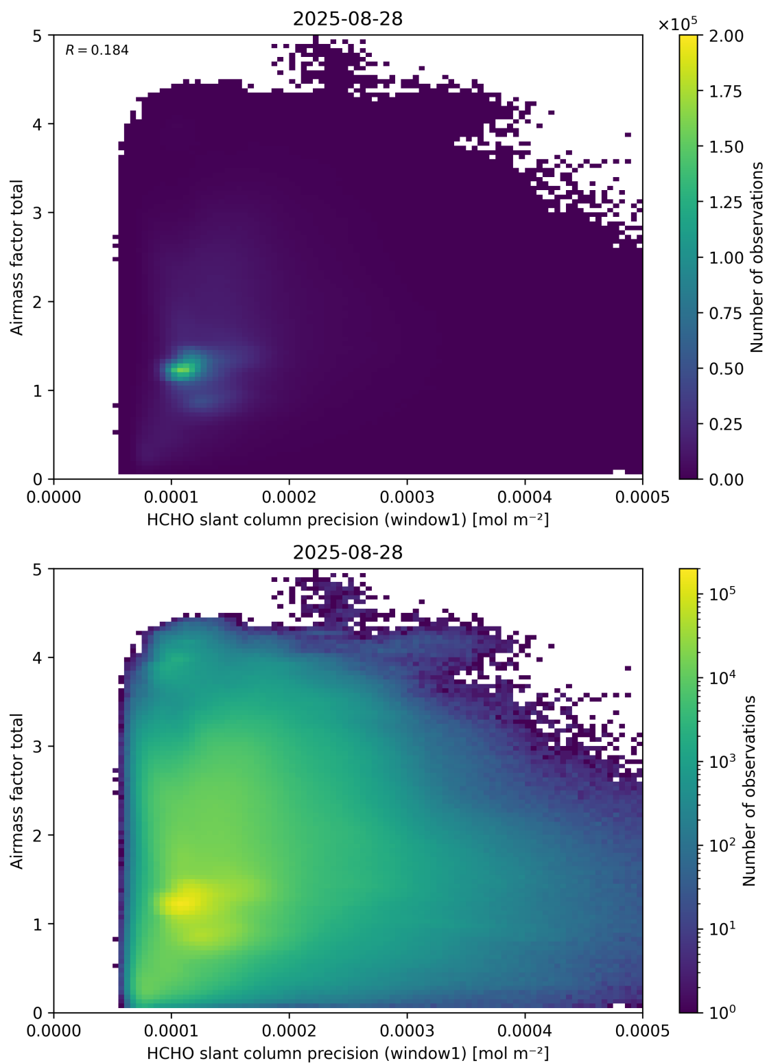
Figure 94: Scatter density plot of “HCHO slant column precision (window1)” against “Airmass factor total” for 2025-08-27 to 2025-08-29.
