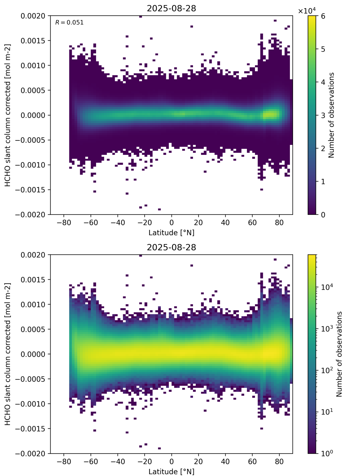
Figure 157: Scatter density plot of “Latitude” against “HCHO slant column corrected” for 2025-08-27 to 2025-08-29.
