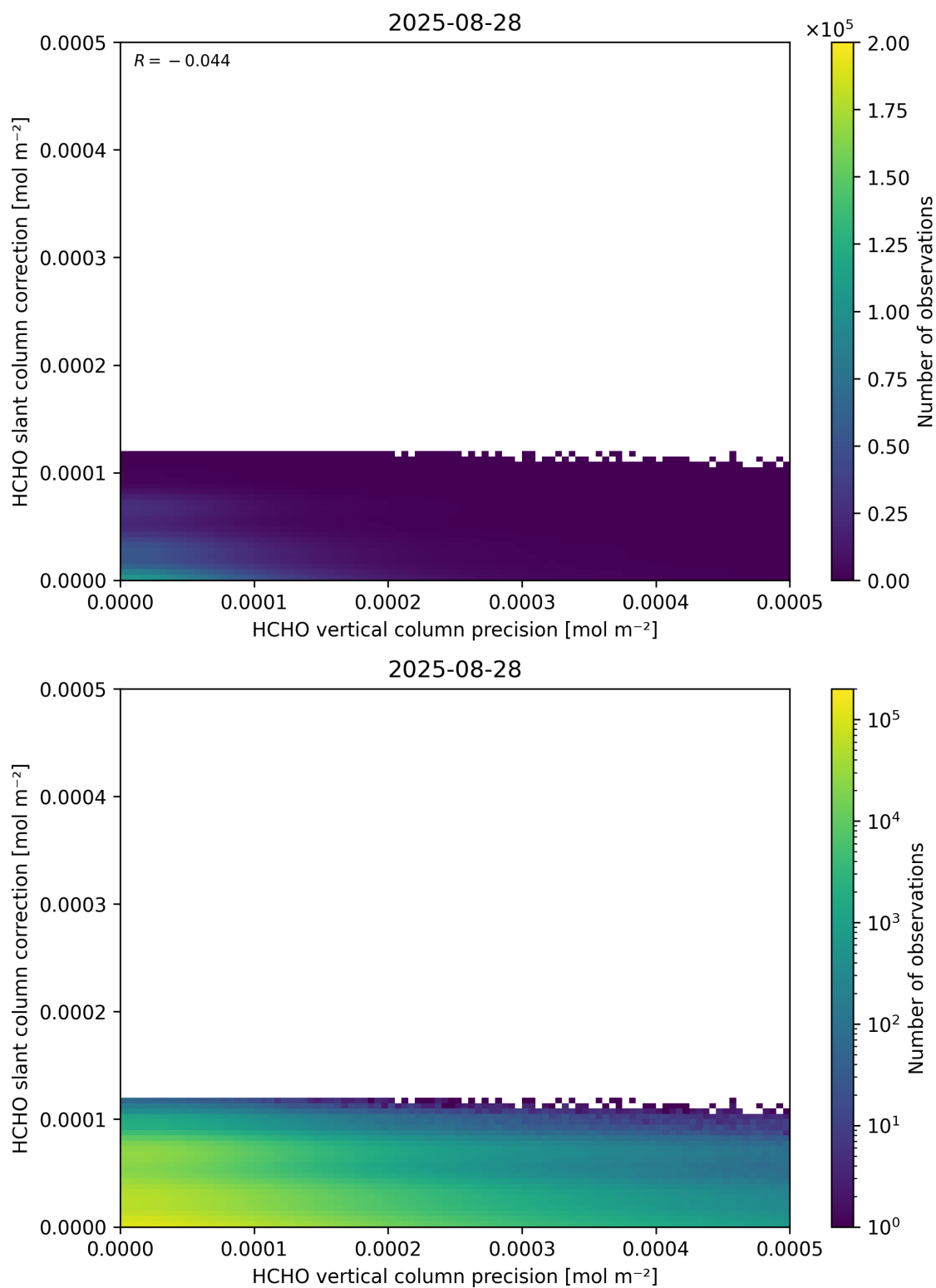
Figure 141: Scatter density plot of “HCHO vertical column precision” against “HCHO slant column correction” for 2025-08-27 to 2025-08-29.
