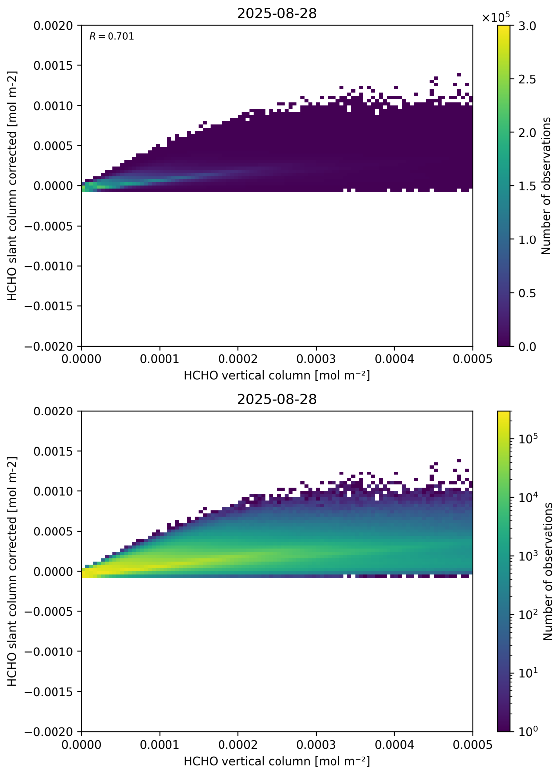
Figure 127: Scatter density plot of “HCHO vertical column” against “HCHO slant column corrected” for 2025-08-27 to 2025-08-29.
