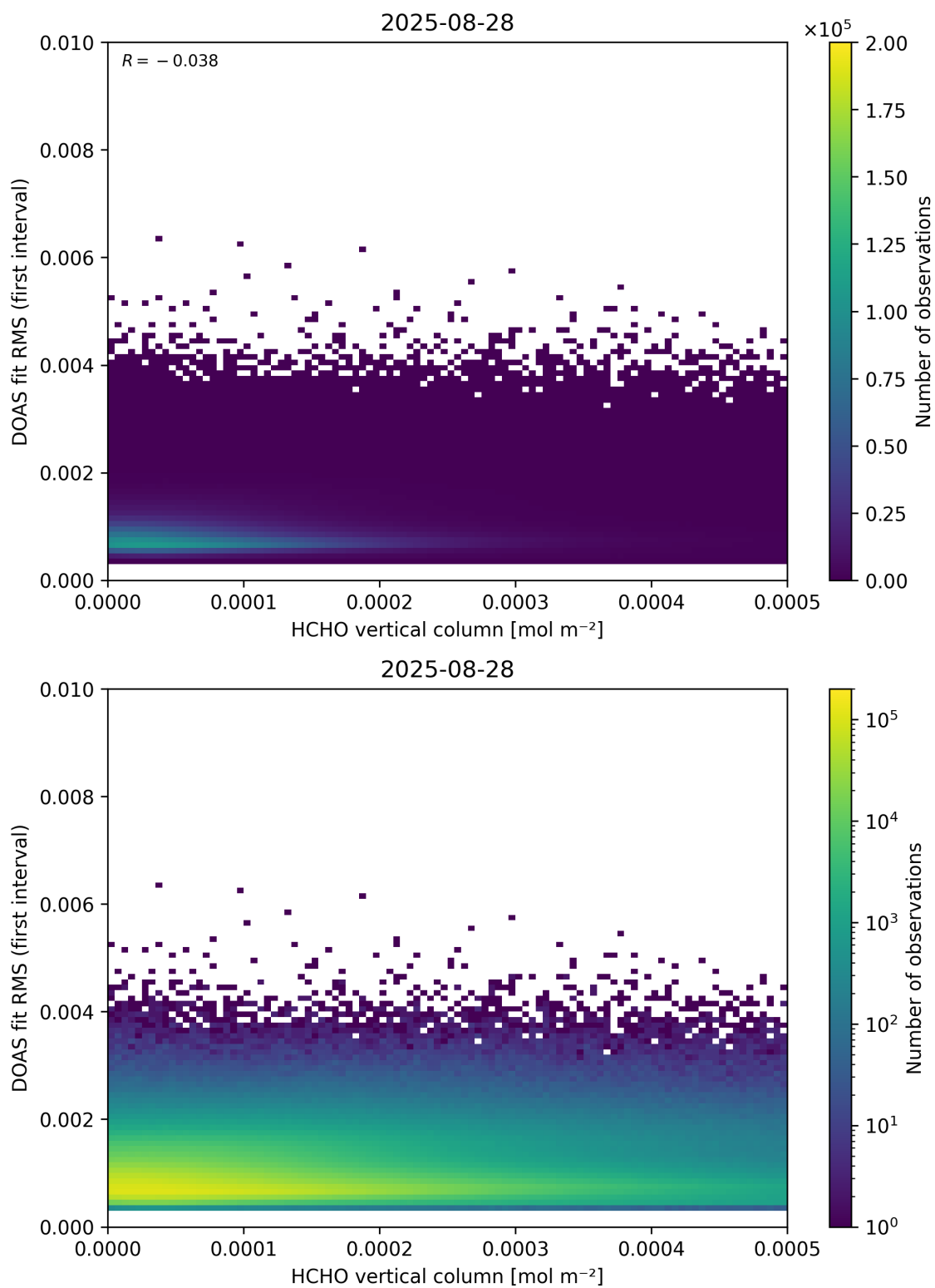
Figure 123: Scatter density plot of “HCHO vertical column” against “DOAS fit RMS (first interval)” for 2025-08-27 to 2025-08-29.
