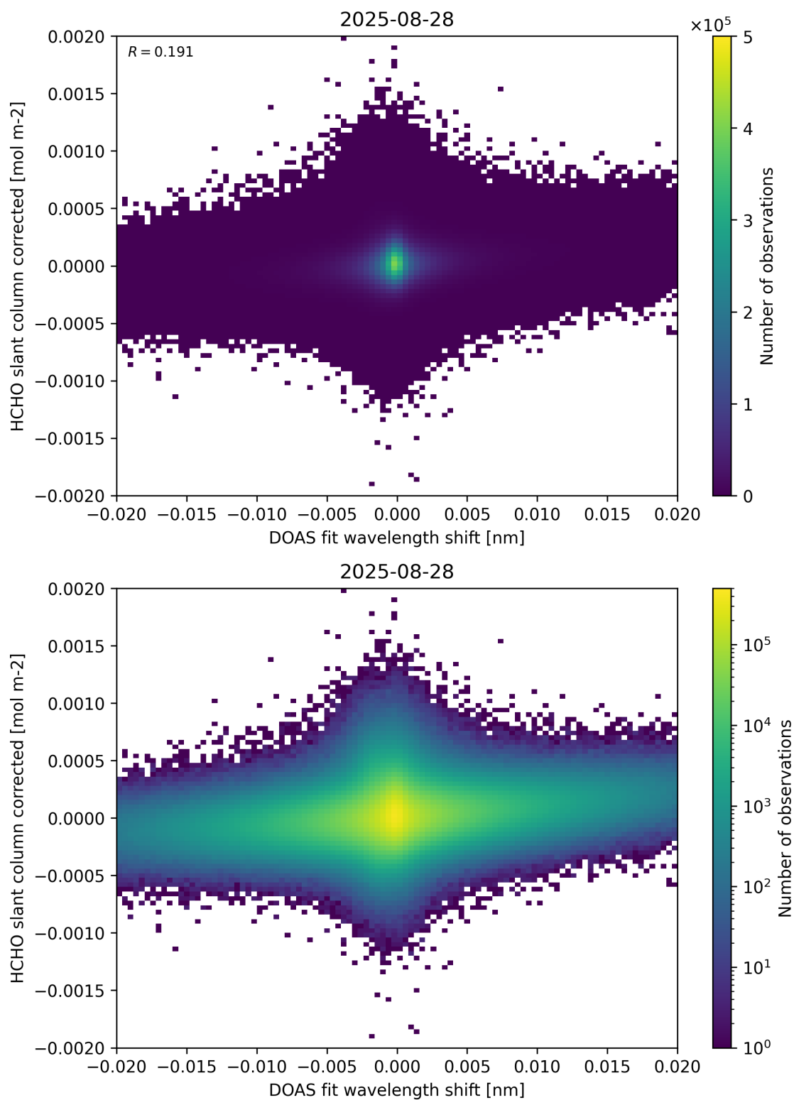
Figure 66: Scatter density plot of “DOAS fit wavelength shift” against “HCHO slant column corrected” for 2025-08-27 to 2025-08-29.
