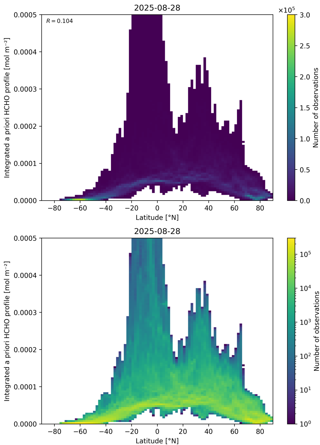
Figure 166: Scatter density plot of “Latitude” against “Integrated a priori HCHO profile” for 2025-08-27 to 2025-08-29.
