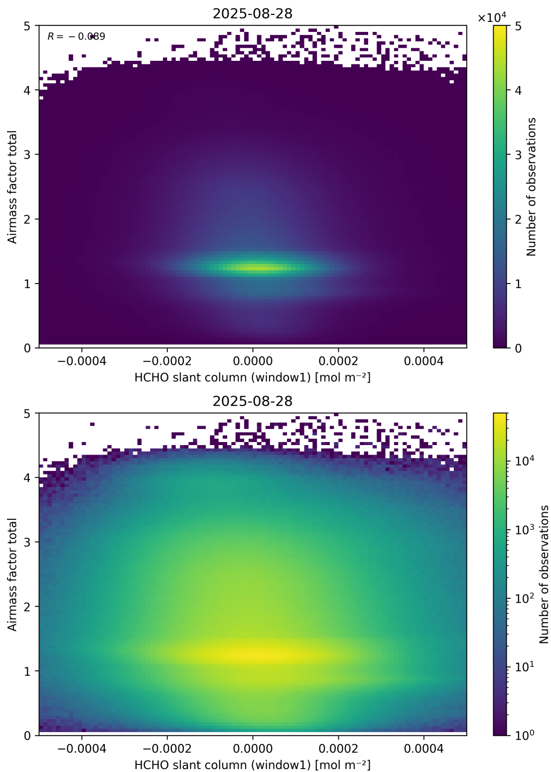
Figure 85: Scatter density plot of “HCHO slant column (window1)” against “Airmass factor total” for 2025-08-27 to 2025-08-29.
