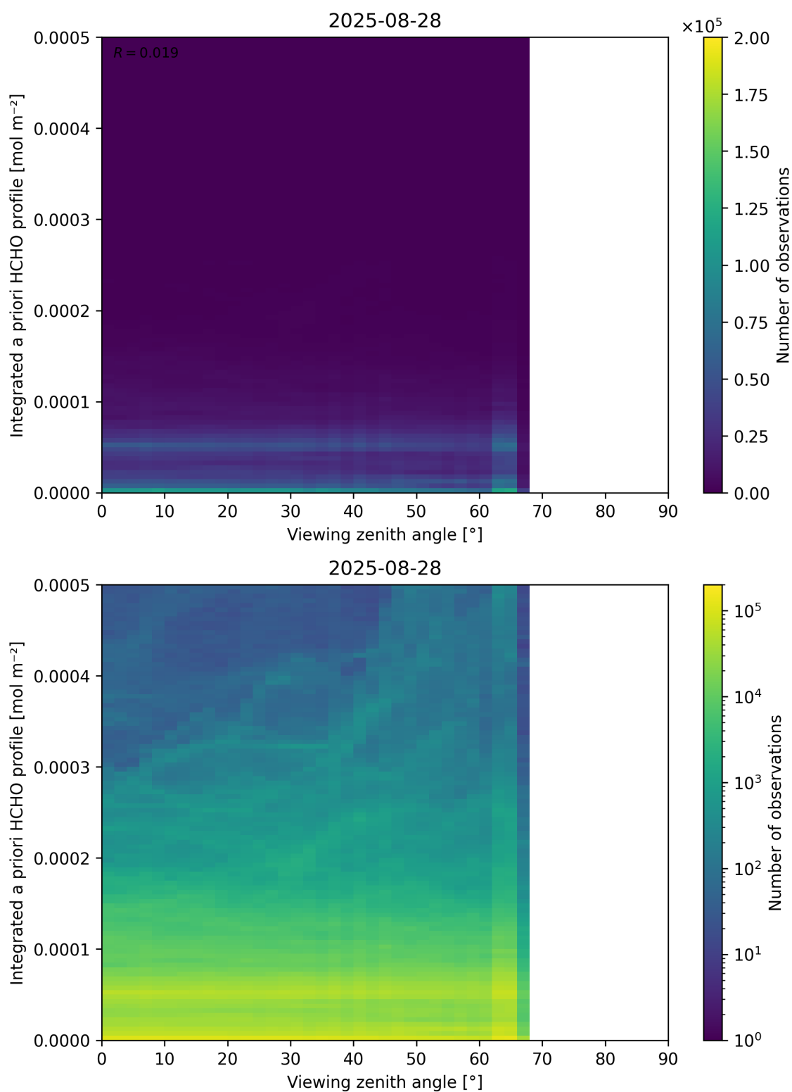
Figure 195: Scatter density plot of “Viewing zenith angle” against “Integrated a priori HCHO profile” for 2025-08-27 to 2025-08-29.
