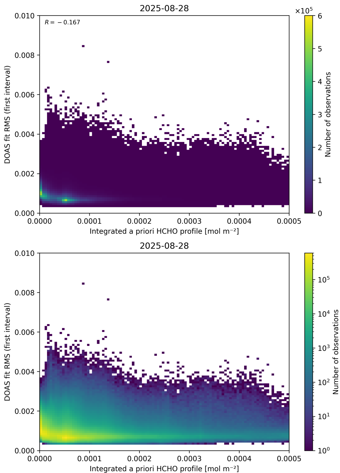
Figure 148: Scatter density plot of “Integrated a priori HCHO profile” against “DOAS fit RMS (first interval)” for 2025-08-27 to 2025-08-29.
