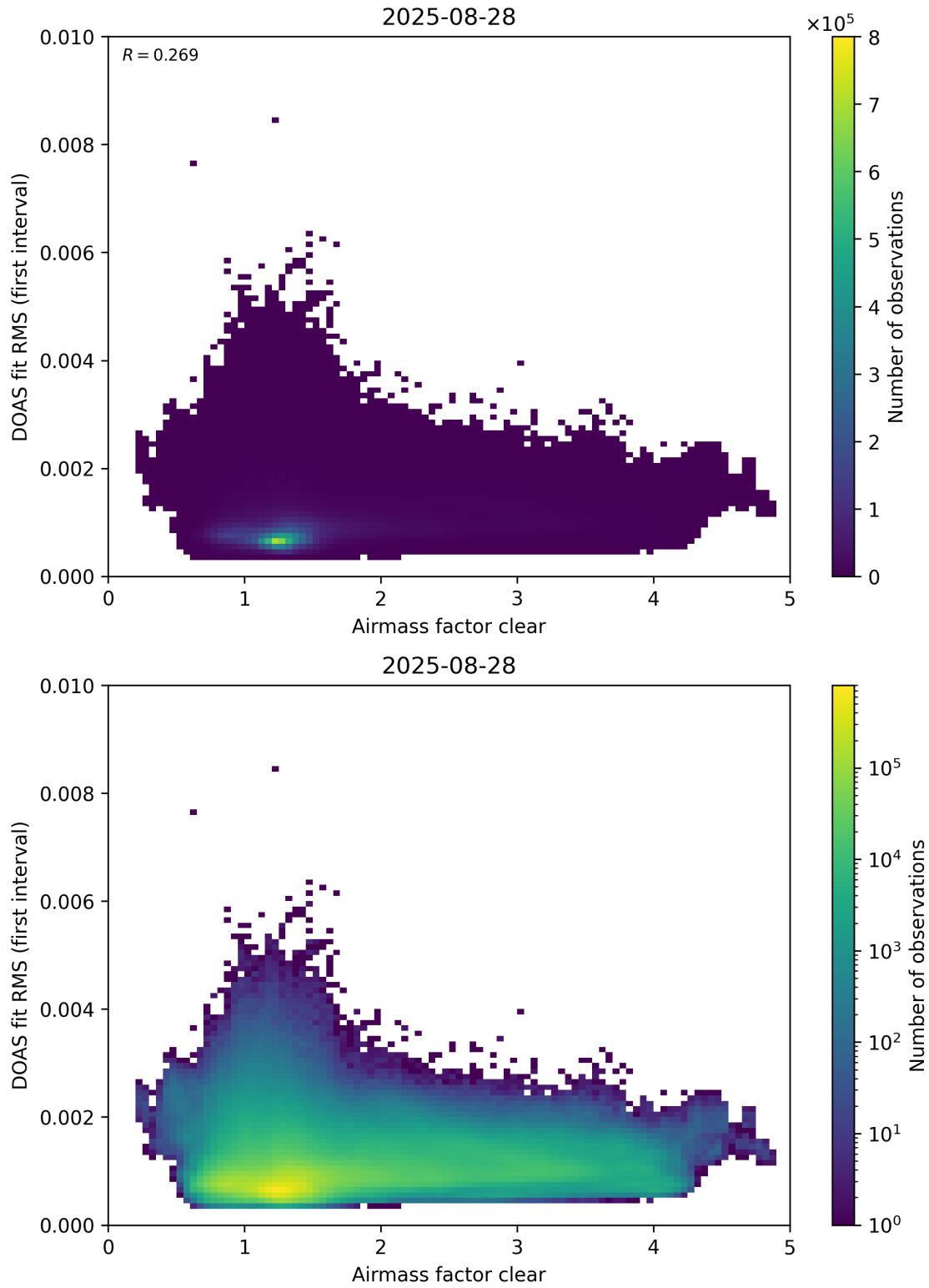
Figure 71: Scatter density plot of “Airmass factor clear” against “DOAS fit RMS (first interval)” for 2025-08-27 to 2025-08-29.
