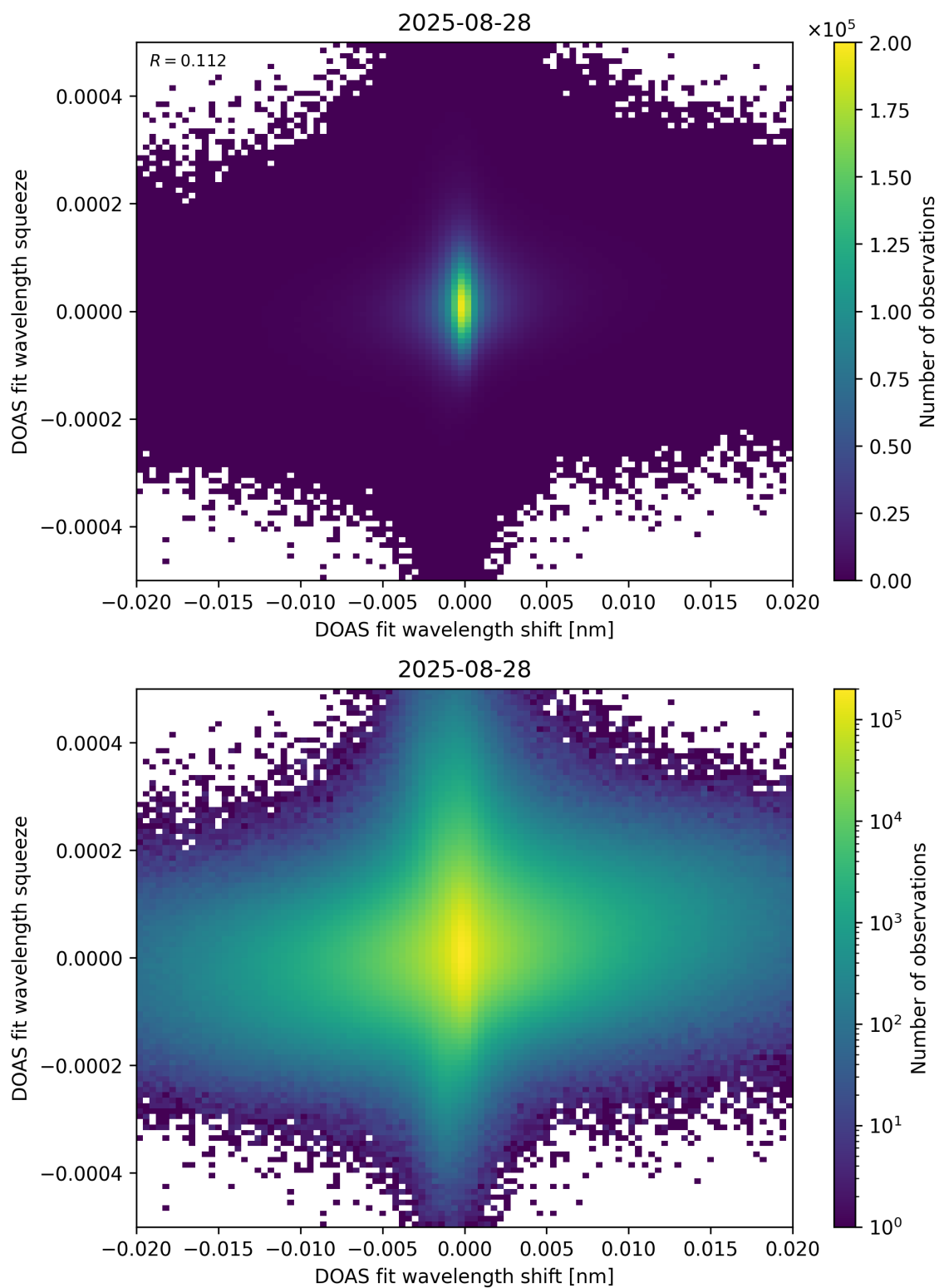
Figure 65: Scatter density plot of “DOAS fit wavelength shift” against “DOAS fit wavelength squeeze” for 2025-08-27 to 2025-08-29.
