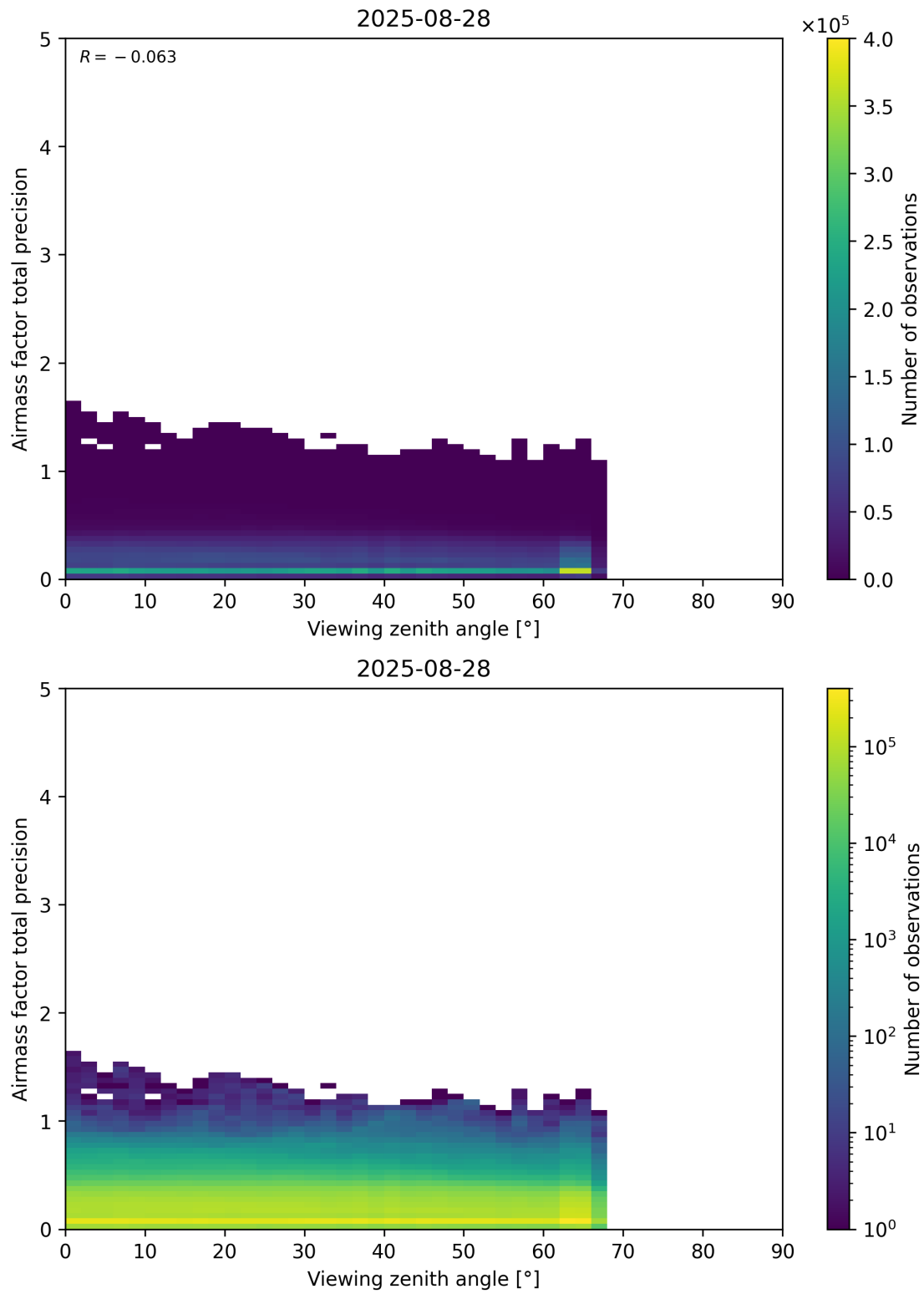
Figure 191: Scatter density plot of “Viewing zenith angle” against “Airmass factor total precision” for 2025-08-27 to 2025-08-29.
