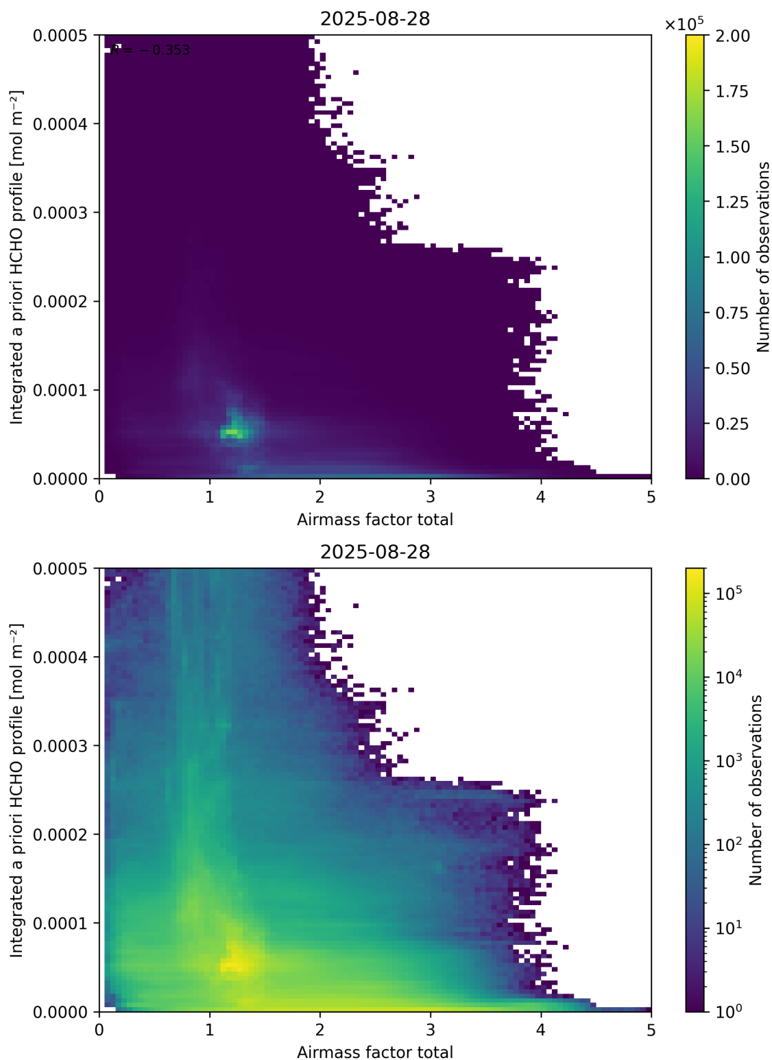
Figure 104: Scatter density plot of “Airmass factor total” against “Integrated a priori HCHO profile” for 2025-08-27 to 2025-08-29.
