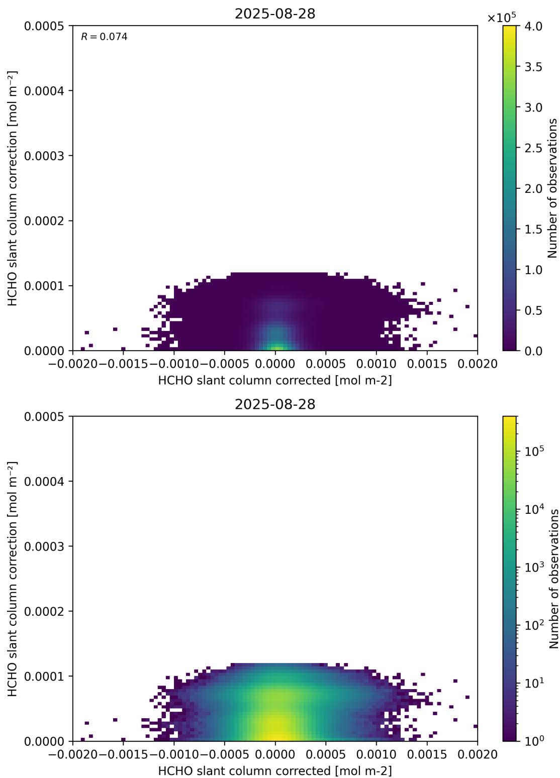
Figure 77: Scatter density plot of “HCHO slant column corrected” against “HCHO slant column correction” for 2025-08-27 to 2025-08-29.
