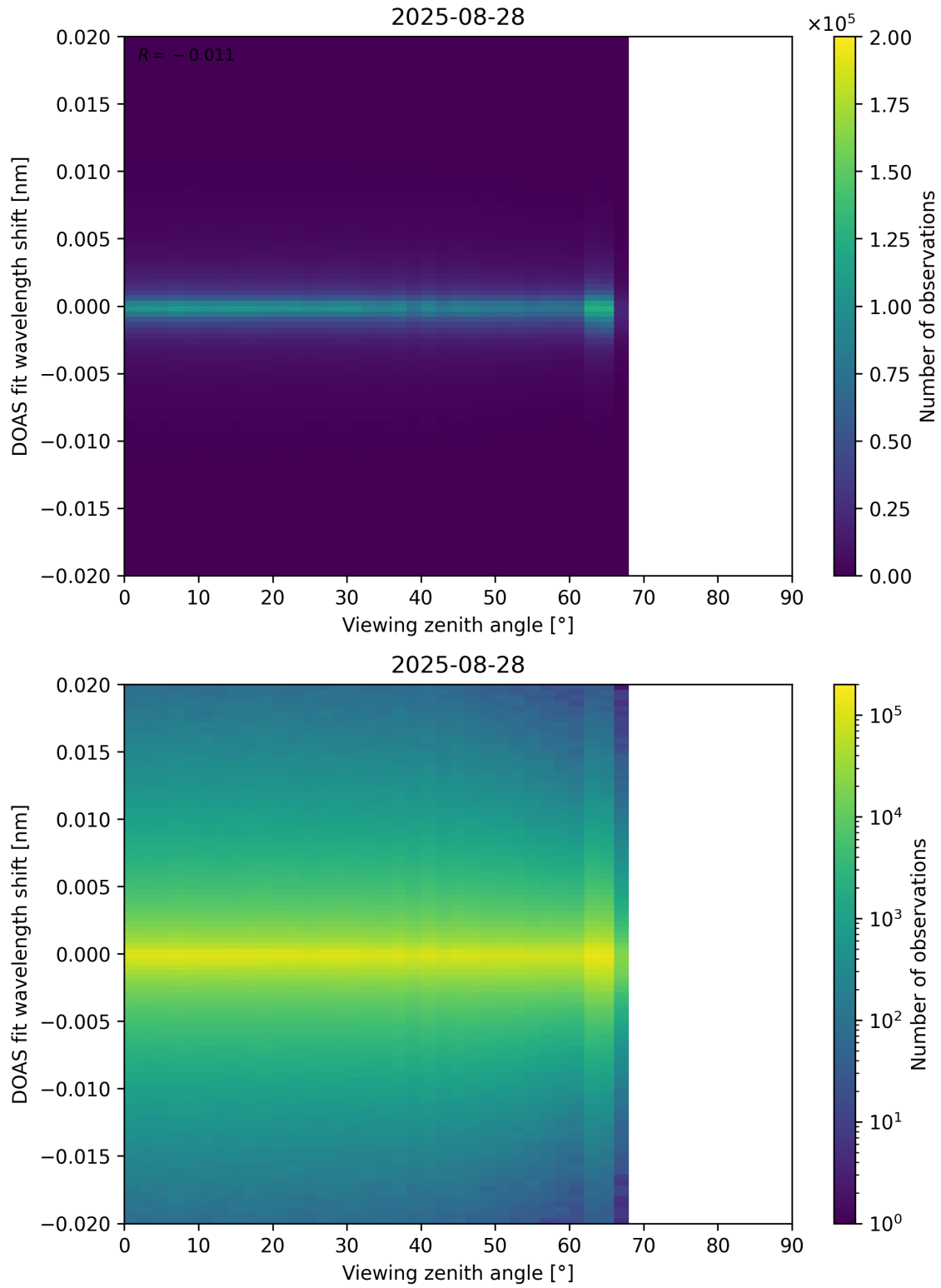
Figure 183: Scatter density plot of “Viewing zenith angle” against “DOAS fit wavelength shift” for 2025-08-27 to 2025-08-29.
