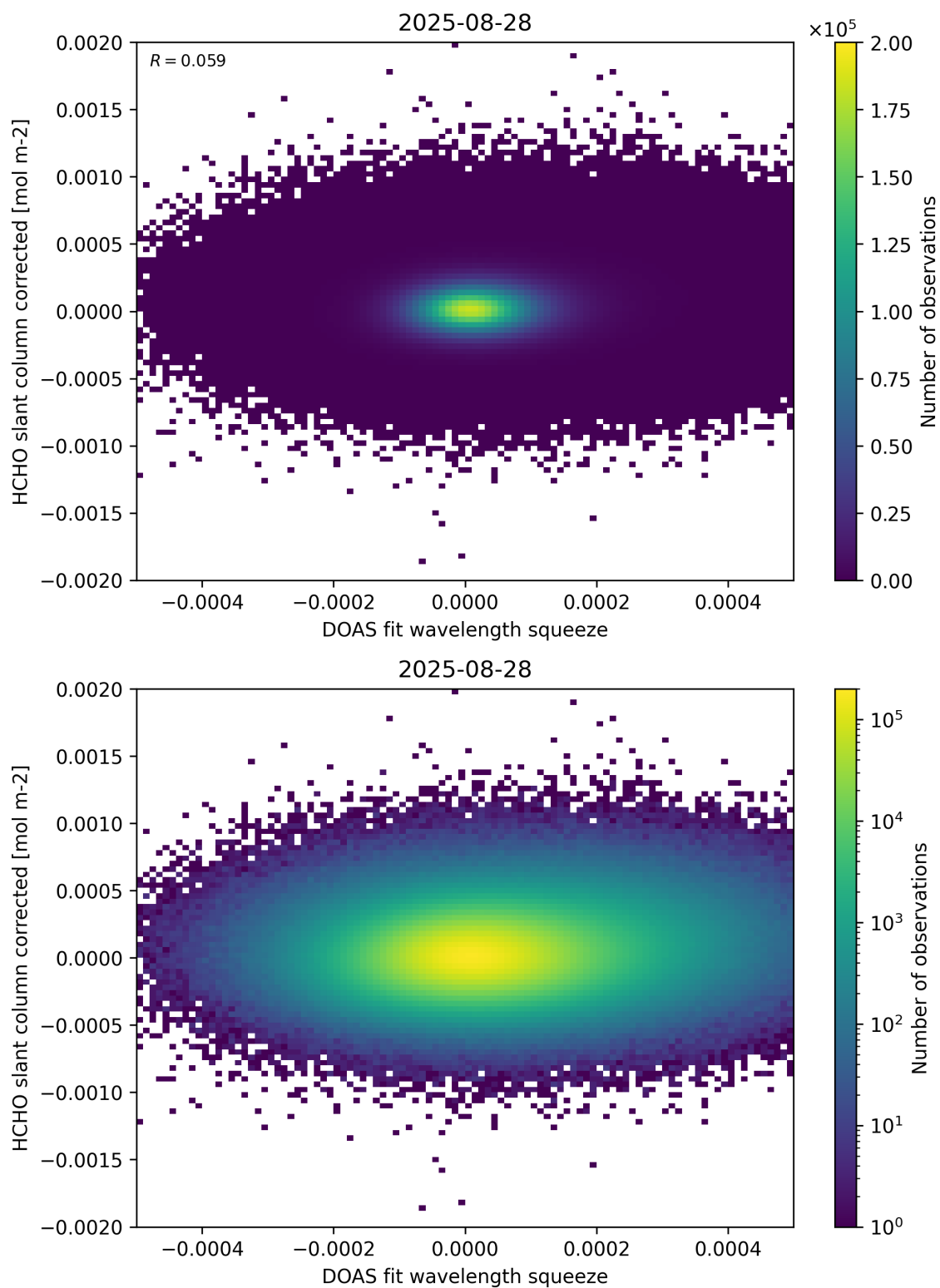
Figure 69: Scatter density plot of “DOAS fit wavelength squeeze” against “HCHO slant column corrected” for 2025-08-27 to 2025-08-29.
