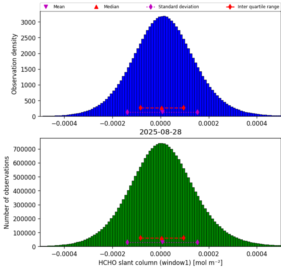
Figure 38: Histogram of “HCHO slant column (window1)” for 2025-08-27 to 2025-08-29
