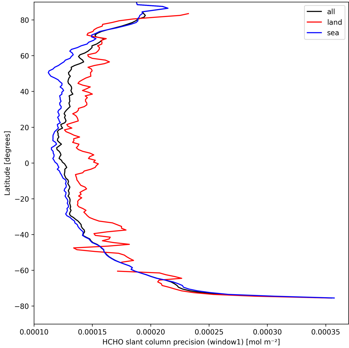
Figure 25: Zonal average of “HCHO slant column precision (window1)” for 2025-08-27 to 2025-08-29.
