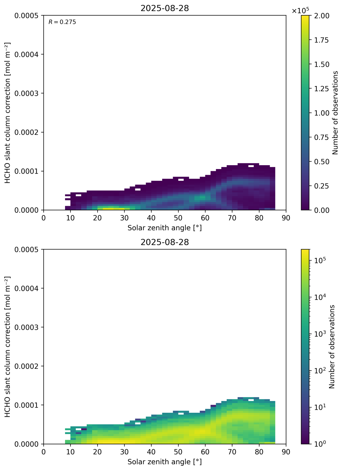
Figure 172: Scatter density plot of “Solar zenith angle” against “HCHO slant column correction” for 2025-08-27 to 2025-08-29.
