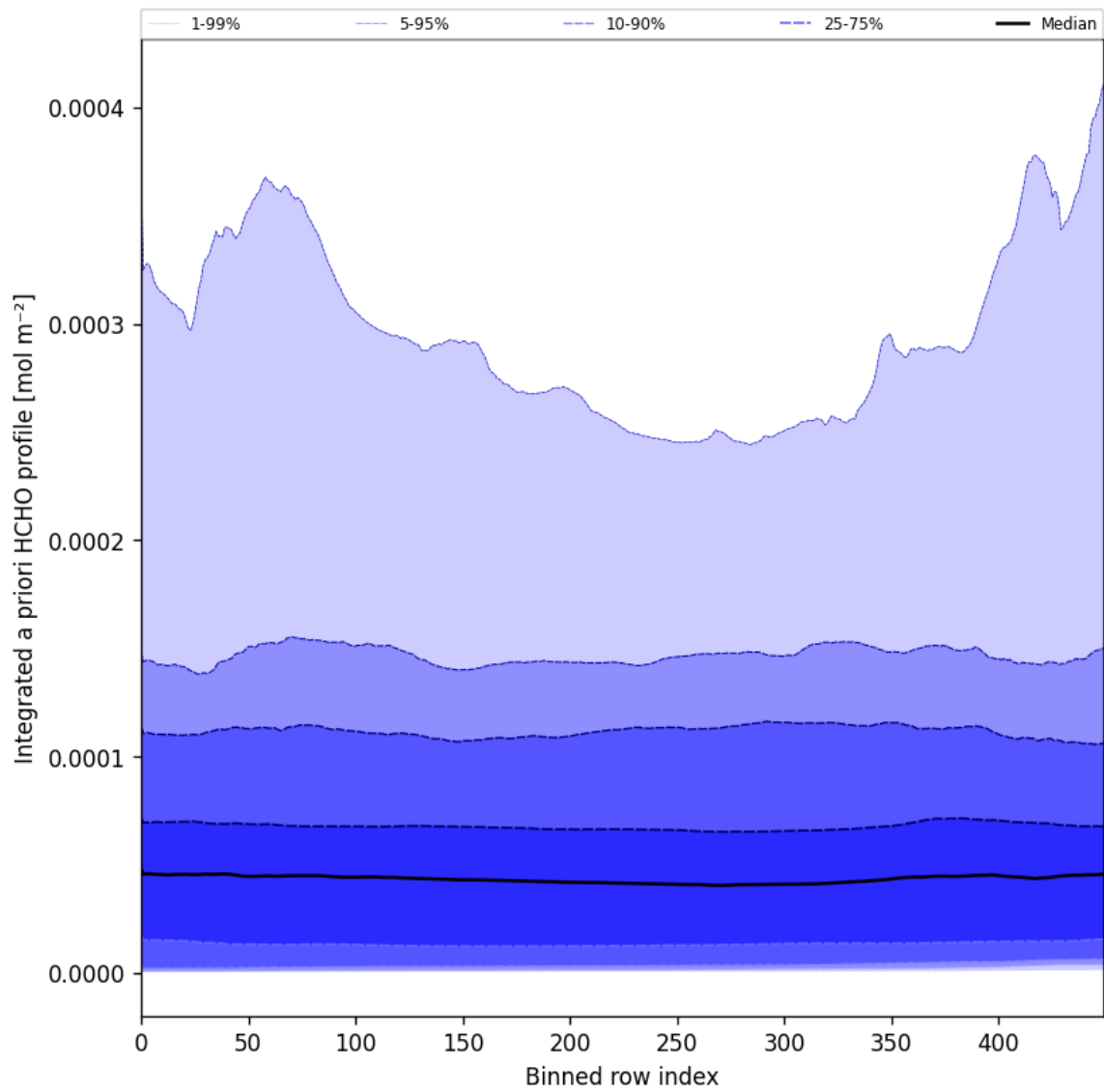
Figure 57: Along track statistics of "Integrated a priori HCHO profile" for 2025-08-27 to 2025-08-29
