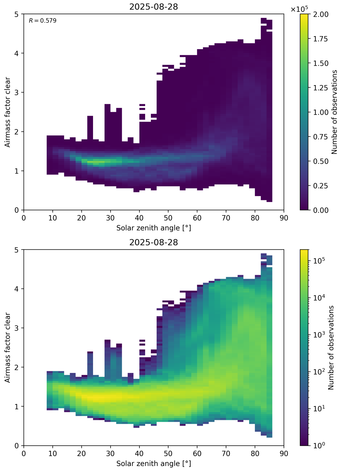
Figure 170: Scatter density plot of “Solar zenith angle” against “Airmass factor clear” for 2025-08-27 to 2025-08-29.
