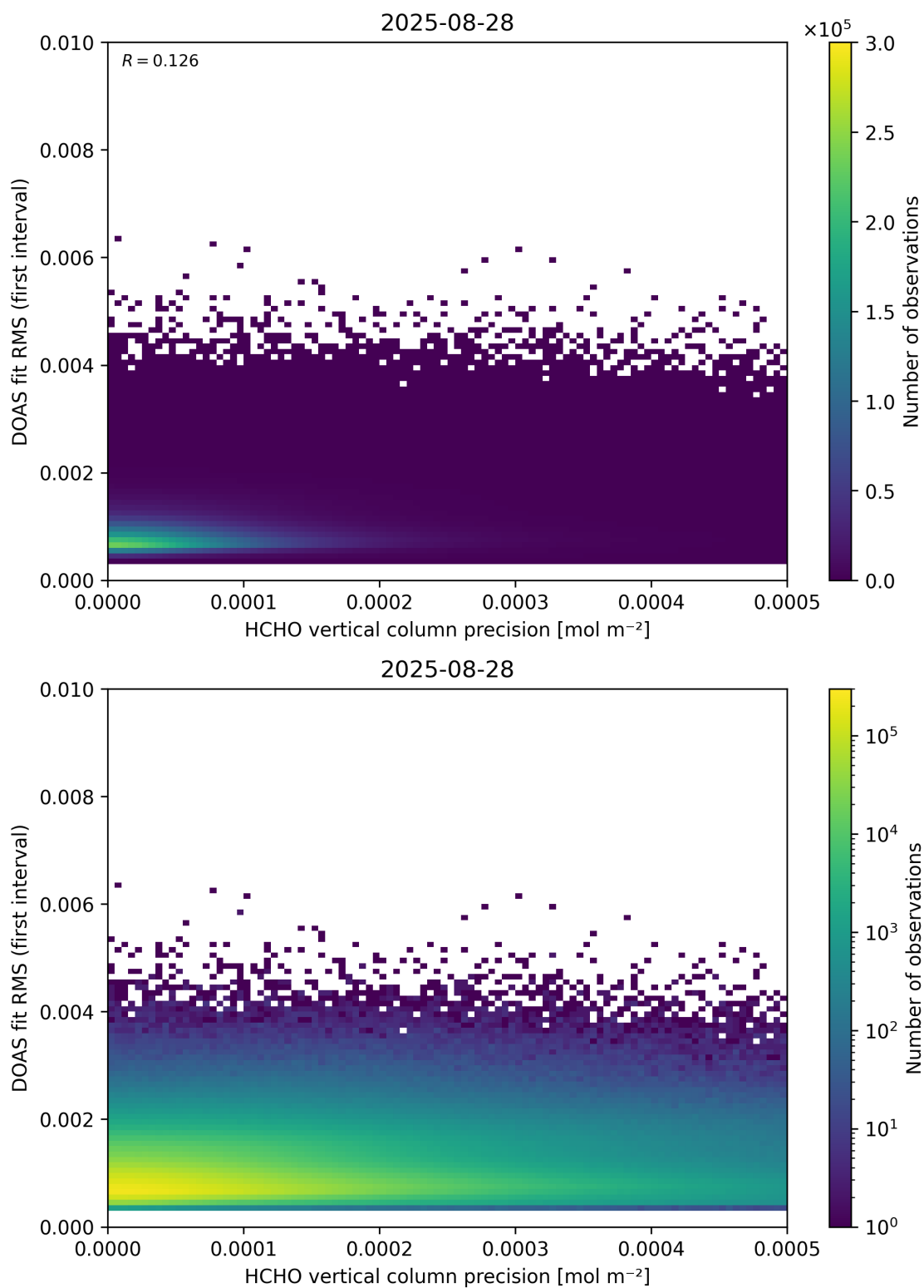
Figure 136: Scatter density plot of “HCHO vertical column precision” against “DOAS fit RMS (first interval)” for 2025-08-27 to 2025-08-29.
