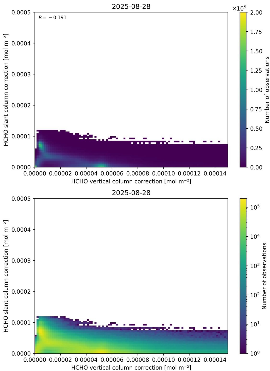
Figure 117: Scatter density plot of “HCHO vertical column correction” against “HCHO slant column correction” for 2025-08-27 to 2025-08-29.
