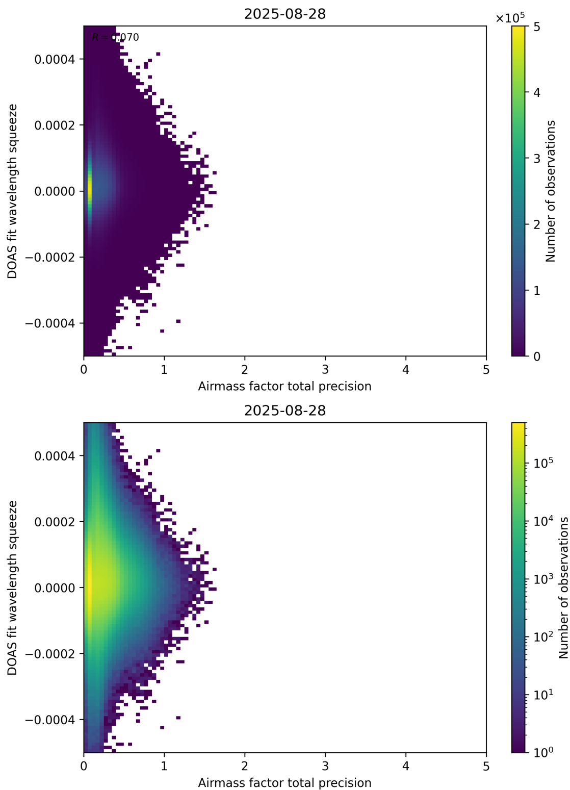
Figure 107: Scatter density plot of “Airmass factor total precision” against “DOAS fit wavelength squeeze” for 2025-08-27 to 2025-08-29.
