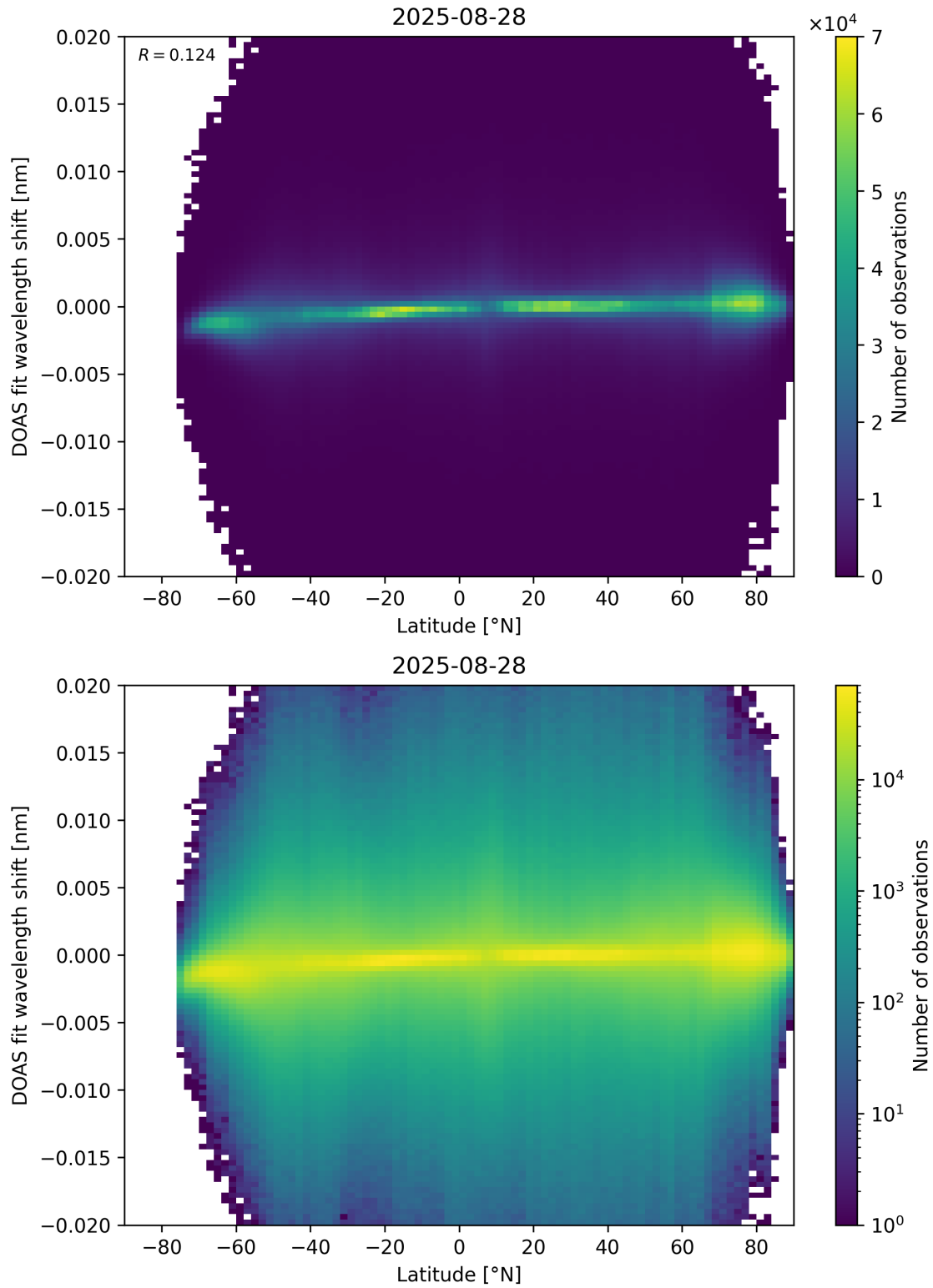
Figure 154: Scatter density plot of “Latitude” against “DOAS fit wavelength shift” for 2025-08-27 to 2025-08-29.
