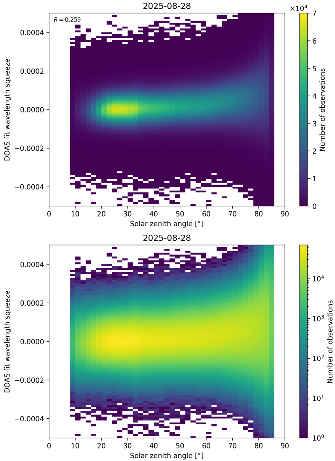
Figure 169: Scatter density plot of “Solar zenith angle” against “DOAS fit wavelength squeeze” for 2025-08-27 to 2025-08-29.
