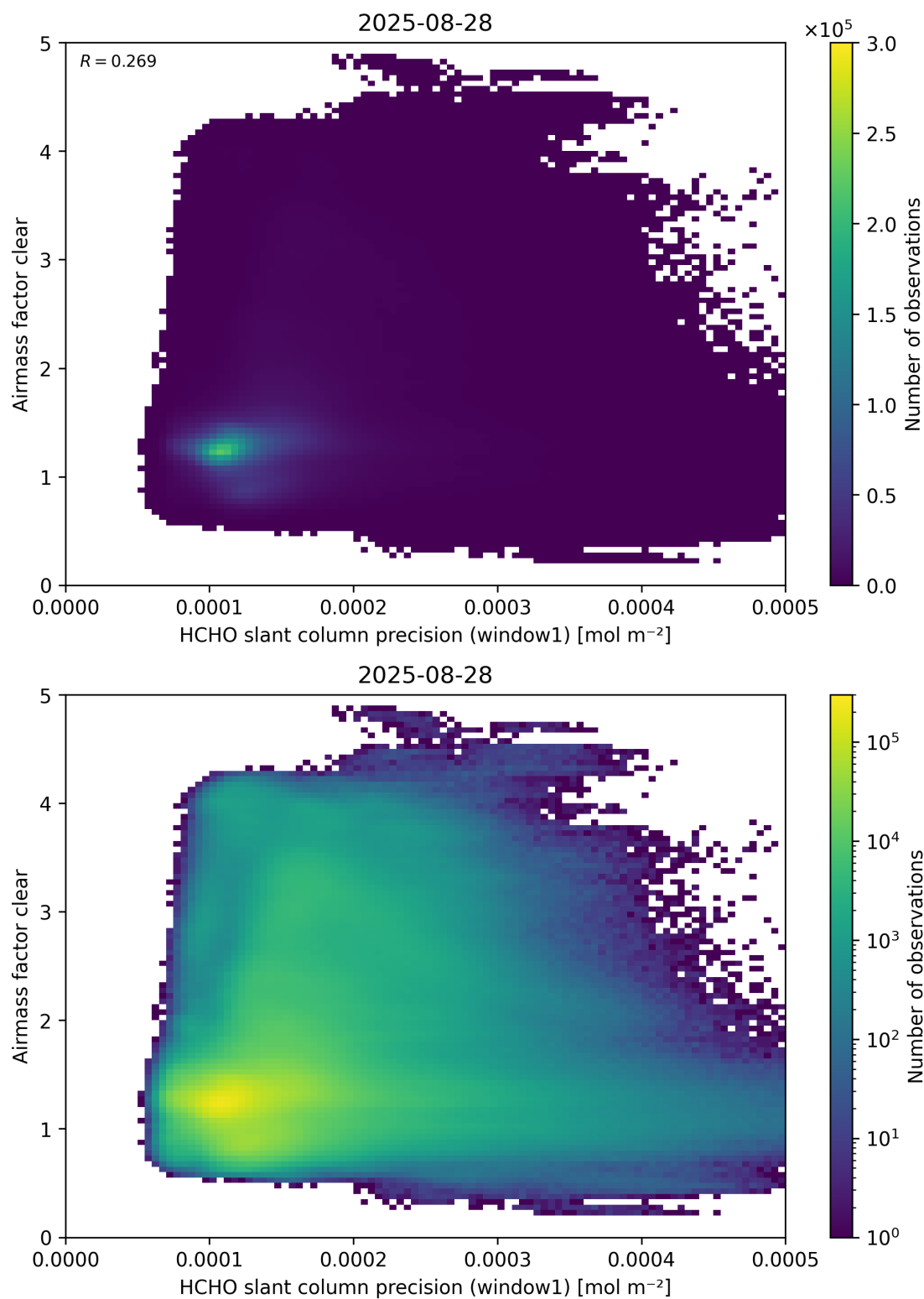
Figure 91: Scatter density plot of “HCHO slant column precision (window1)” against “Airmass factor clear” for 2025-08-27 to 2025-08-29.
