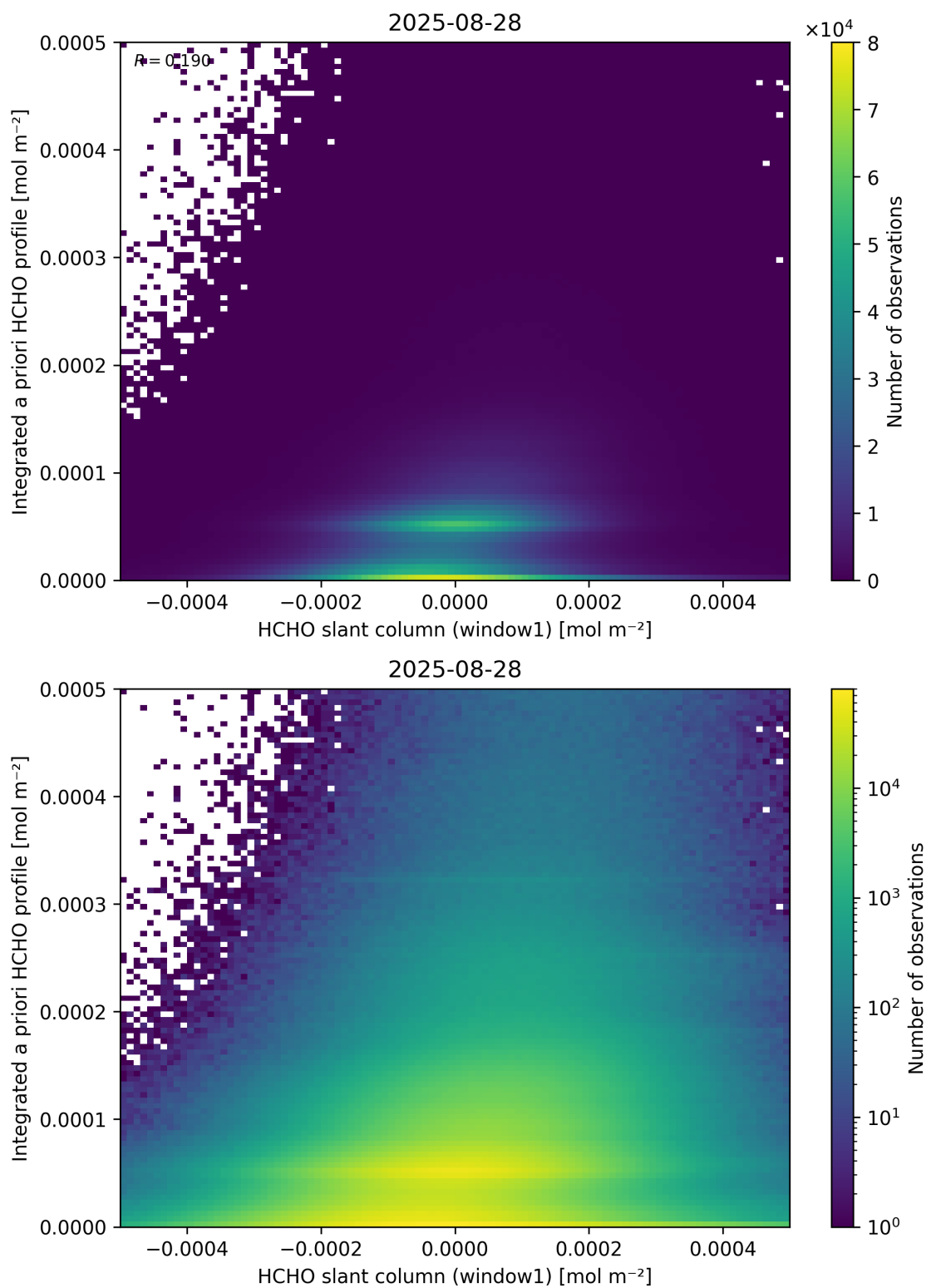
Figure 87: Scatter density plot of “HCHO slant column (window1)” against “Integrated a priori HCHO profile” for 2025-08-27 to 2025-08-29.
