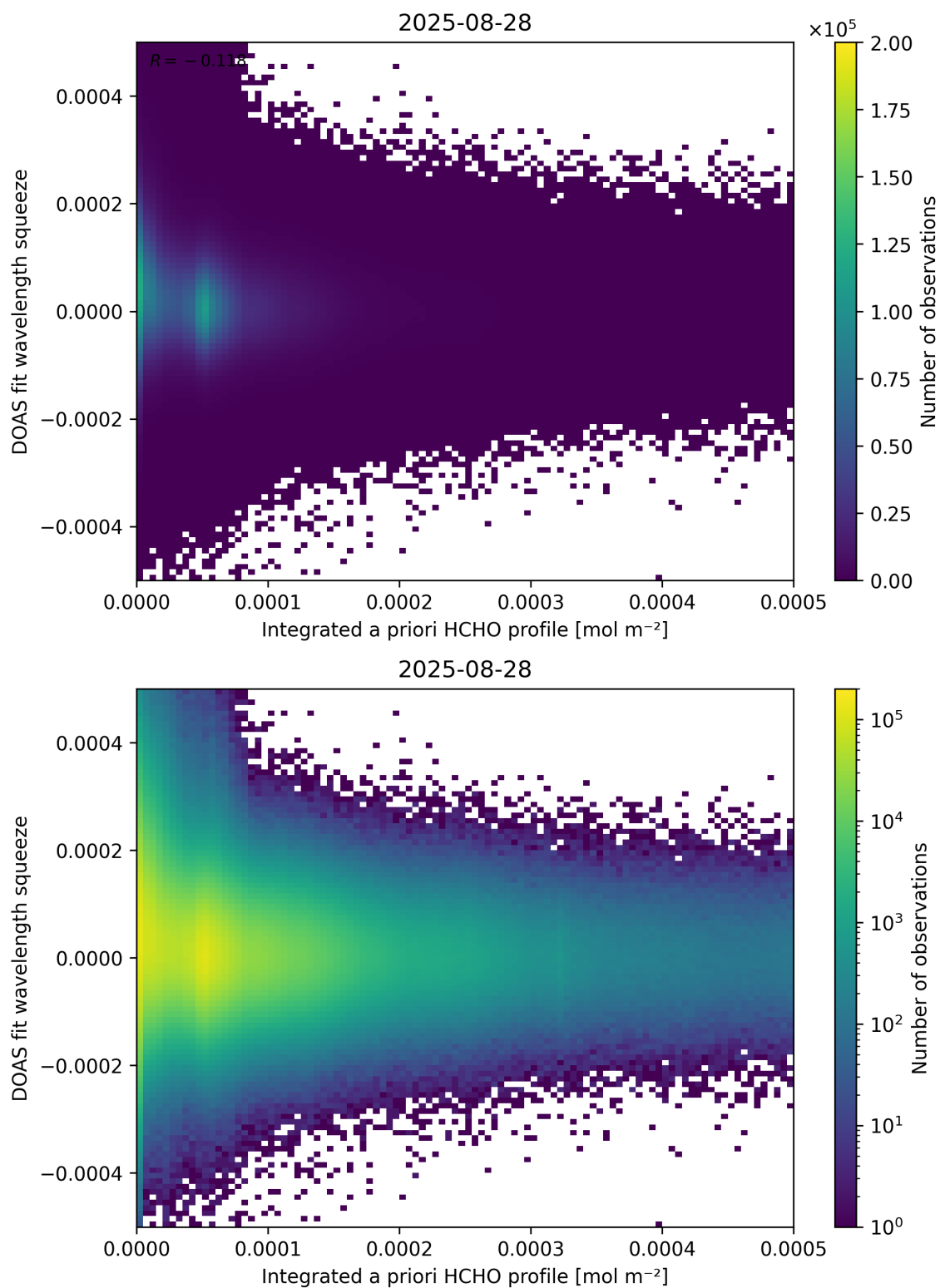
Figure 150: Scatter density plot of “Integrated a priori HCHO profile” against “DOAS fit wavelength squeeze” for 2025-08-27 to 2025-08-29.
