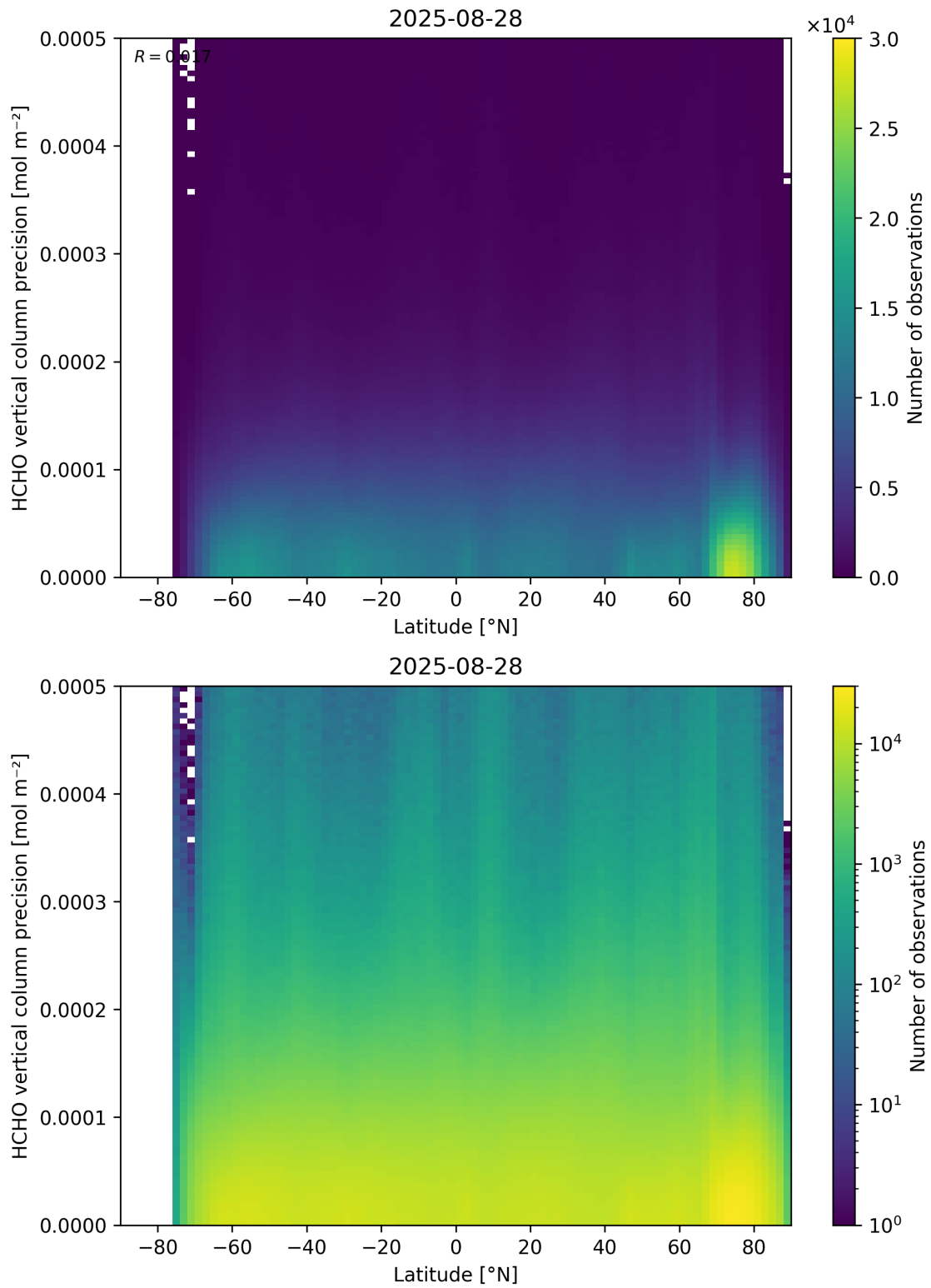
Figure 165: Scatter density plot of “Latitude” against “HCHO vertical column precision” for 2025-08-27 to 2025-08-29.
