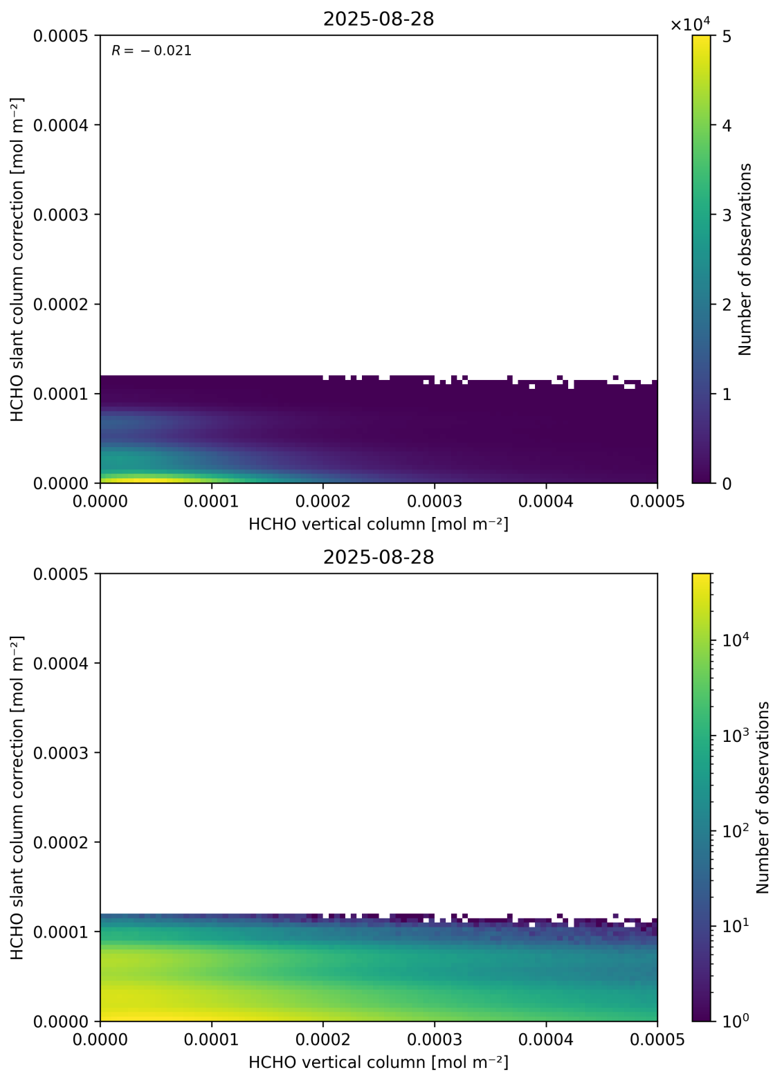
Figure 128: Scatter density plot of “HCHO vertical column” against “HCHO slant column correction” for 2025-08-27 to 2025-08-29.
