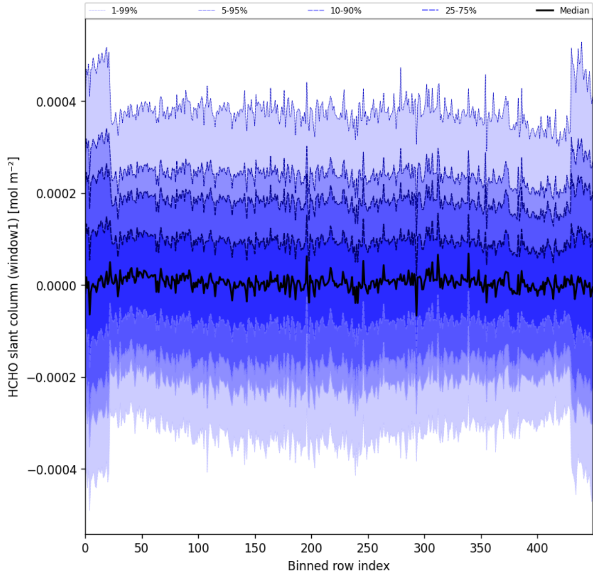
Figure 52: Along track statistics of “HCHO slant column (window1)” for 2025-08-27 to 2025-08-29
