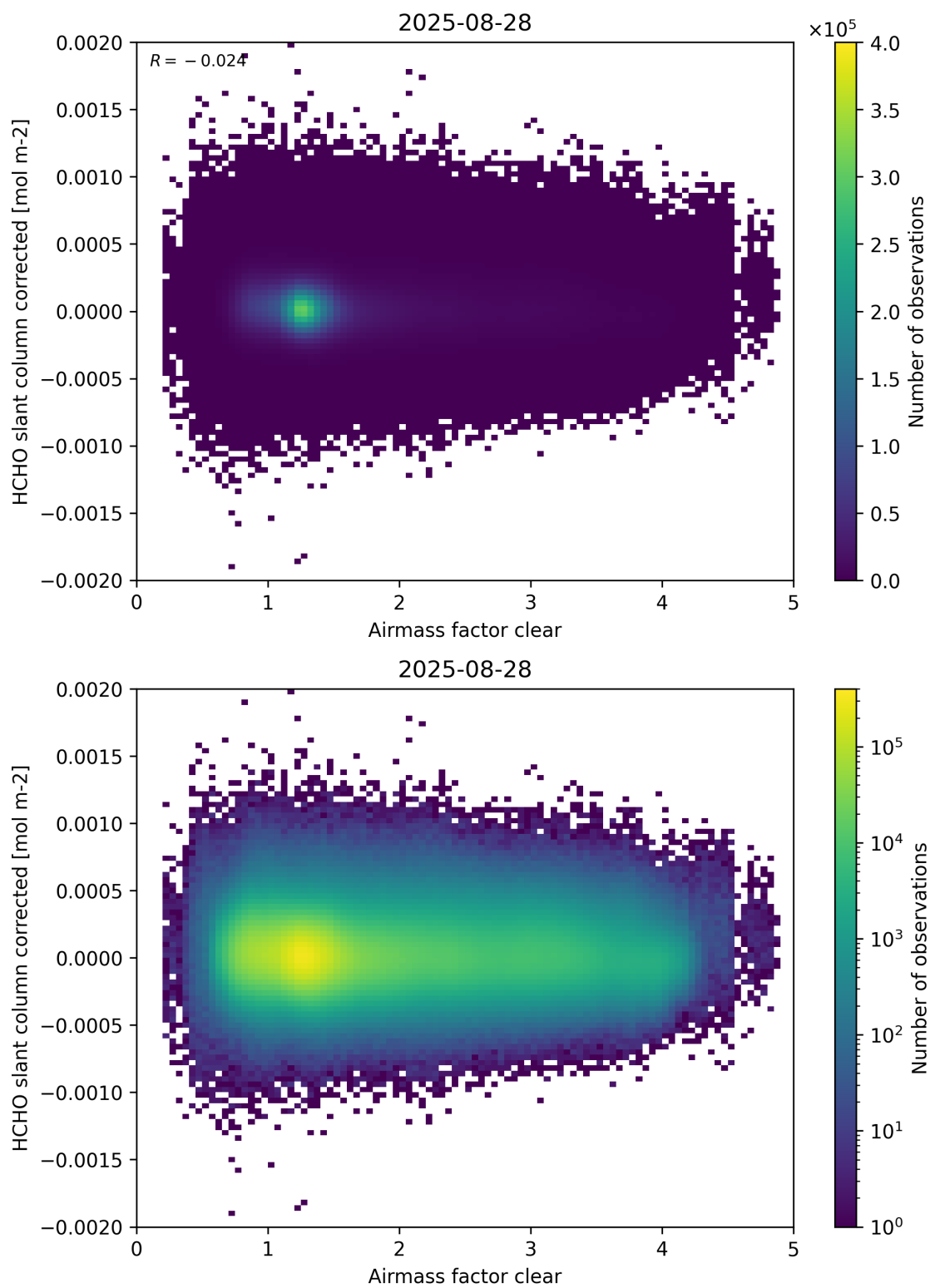
Figure 74: Scatter density plot of “Airmass factor clear” against “HCHO slant column corrected” for 2025-08-27 to 2025-08-29.
