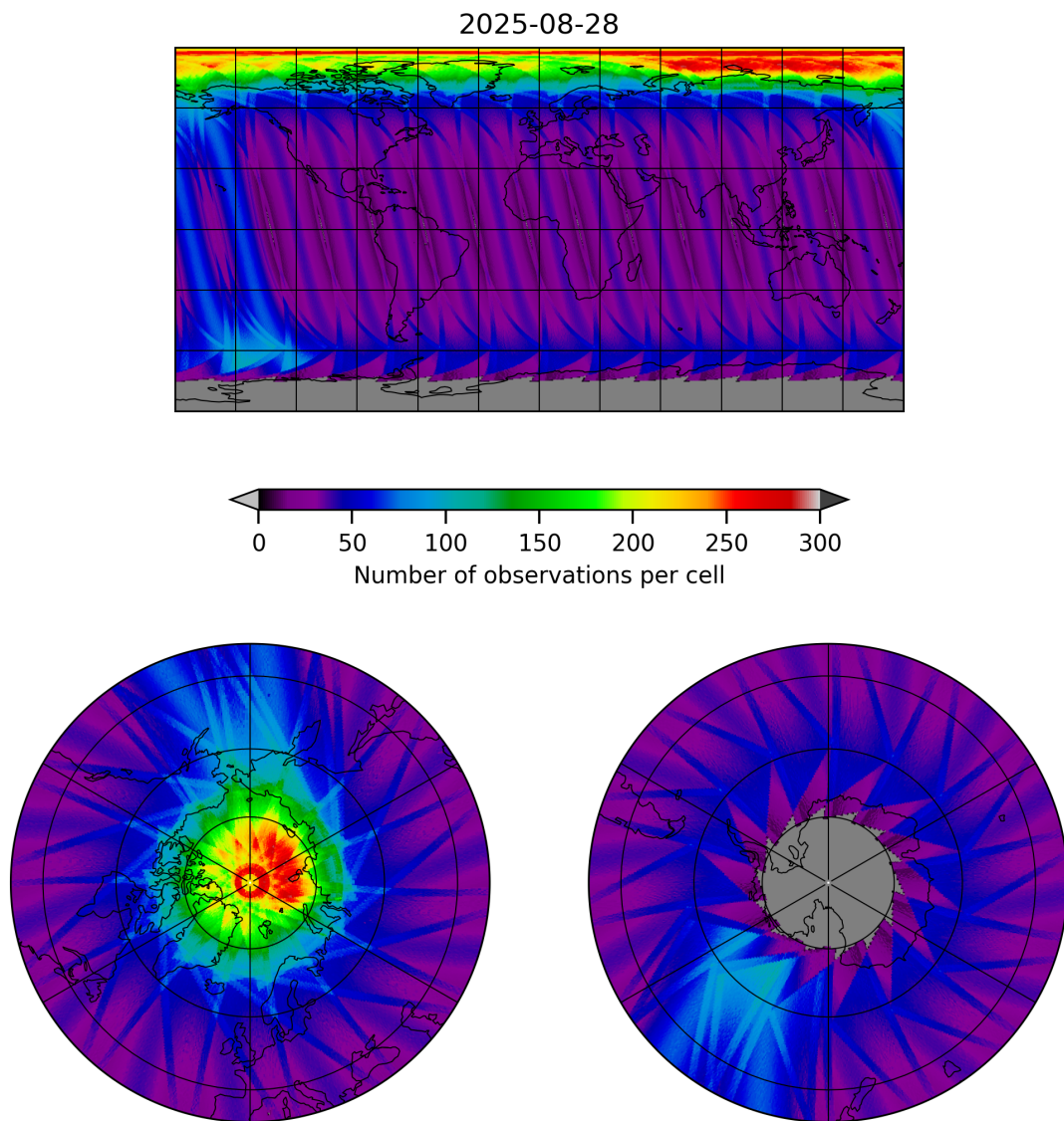
Figure 19: Map of the number of observations for 2025-08-27 to 2025-08-29
