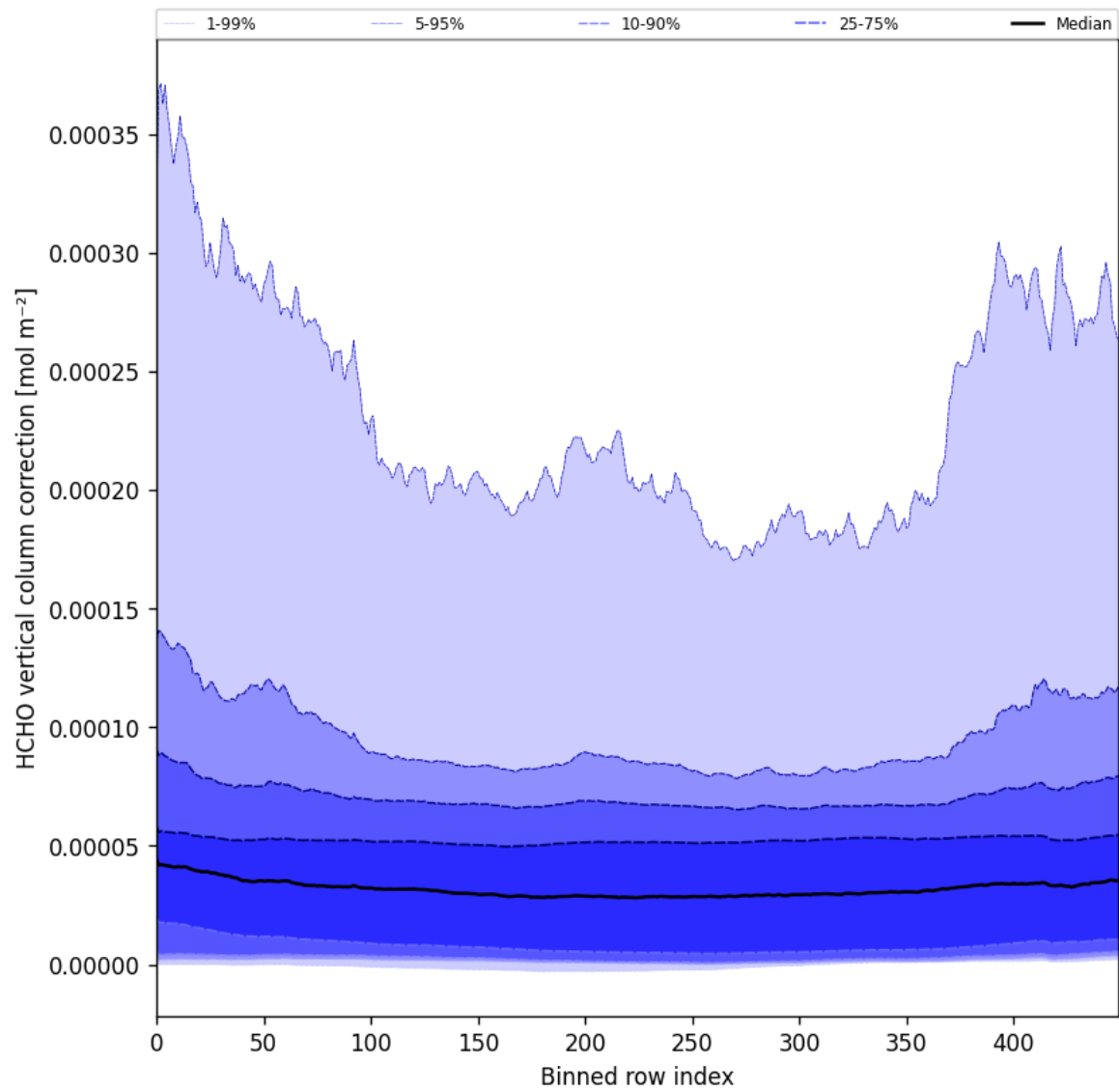
Figure 51: Along track statistics of “HCHO vertical column correction” for 2025-08-27 to 2025-08-29
