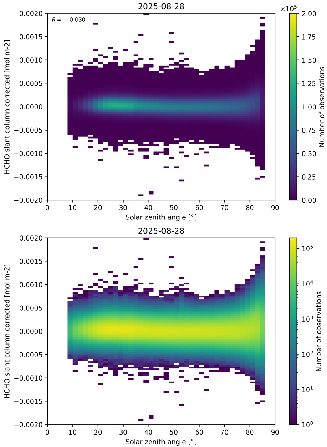
Figure 171: Scatter density plot of “Solar zenith angle” against “HCHO slant column corrected” for 2025-08-27 to 2025-08-29.
