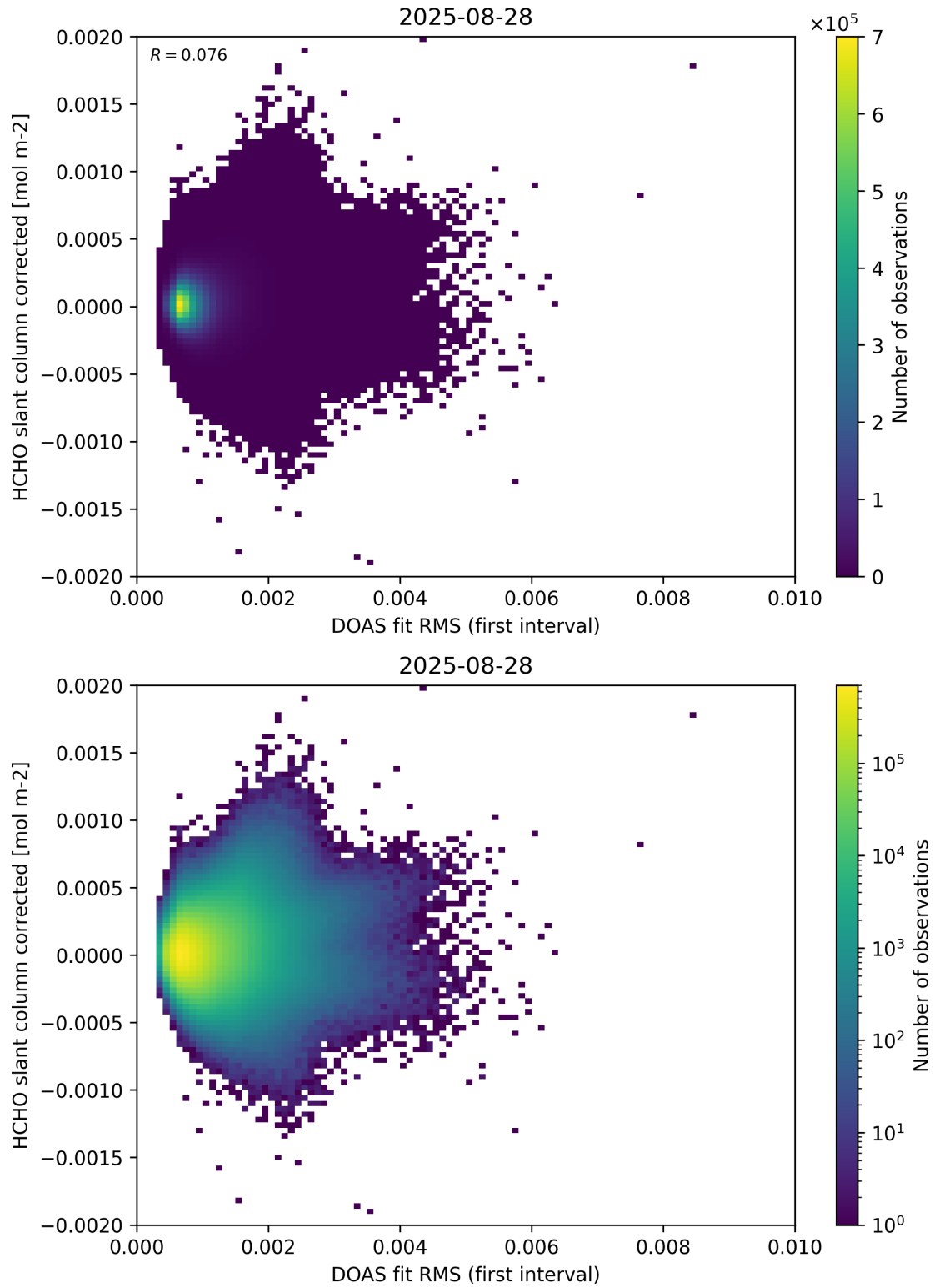
Figure 62: Scatter density plot of “DOAS fit RMS (first interval)” against “HCHO slant column corrected” for 2025-08-27 to 2025-08-29.
