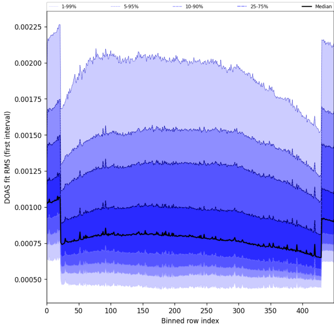
Figure 60: Along track statistics of “DOAS fit RMS (first interval)” for 2025-08-27 to 2025-08-29
