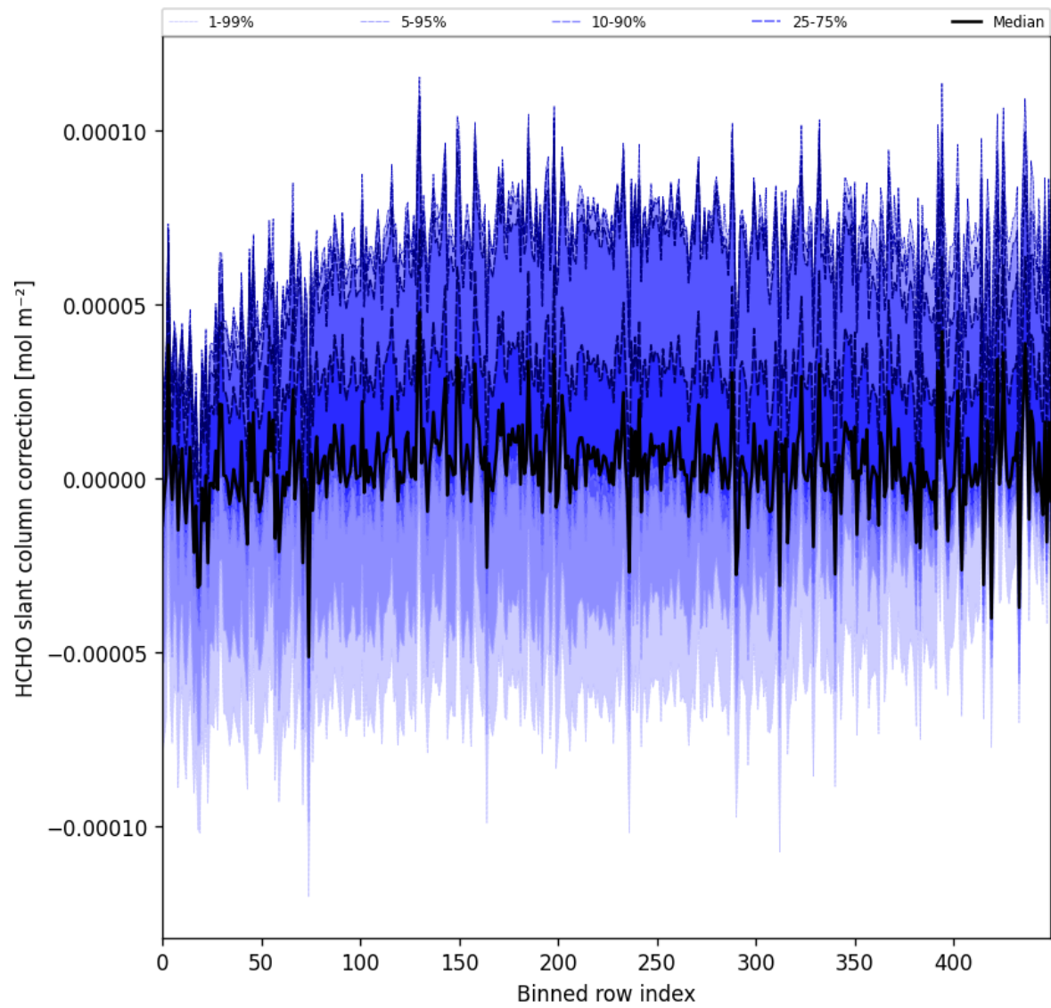
Figure 61: Along track statistics of “HCHO slant column correction” for 2025-08-27 to 2025-08-29
