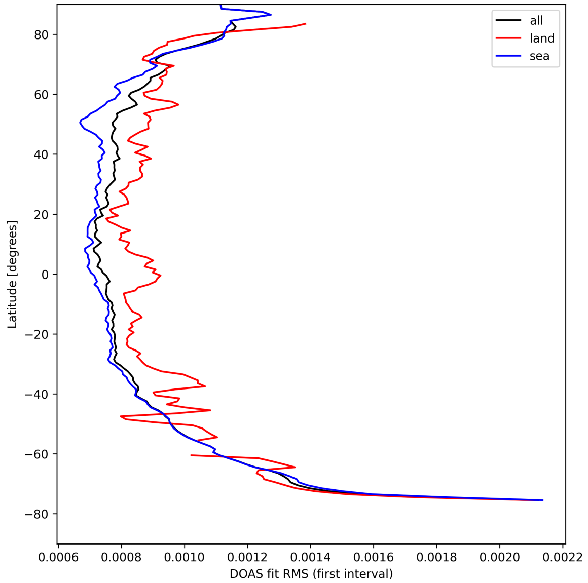
Figure 32: Zonal average of “DOAS fit RMS (first interval)” for 2025-08-27 to 2025-08-29.
