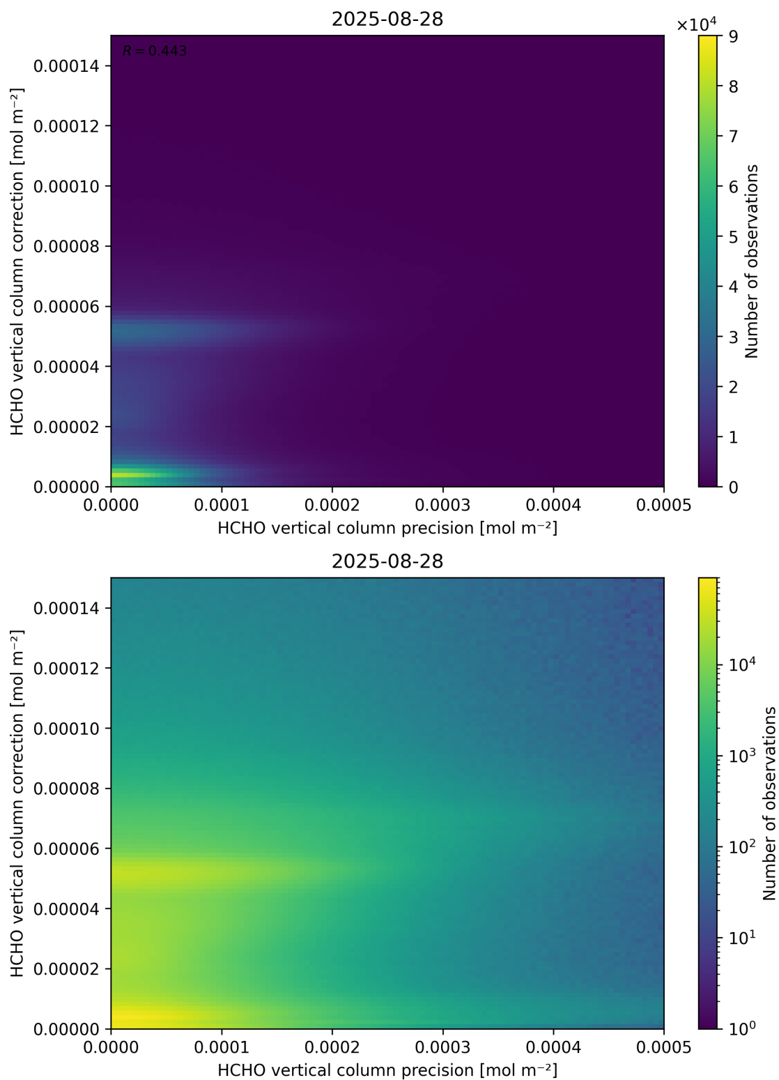
Figure 146: Scatter density plot of “HCHO vertical column precision” against “HCHO vertical column correction” for 2025-08-27 to 2025-08-29.
