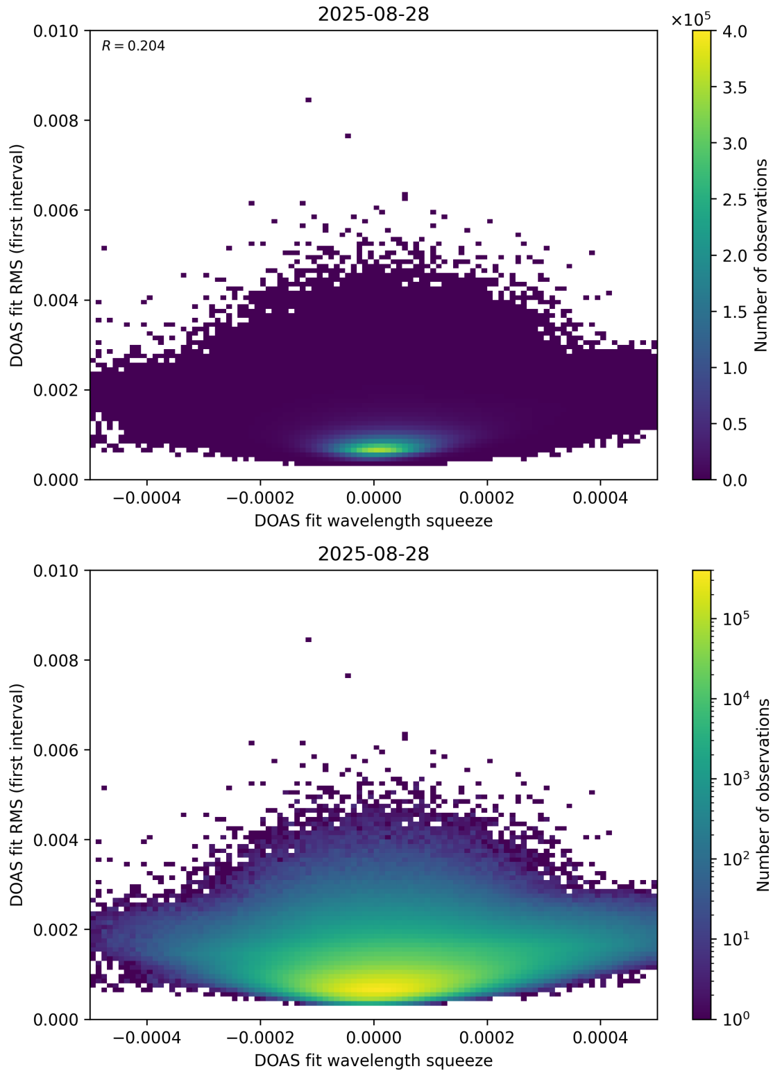
Figure 68: Scatter density plot of “DOAS fit wavelength squeeze” against “DOAS fit RMS (first interval)” for 2025-08-27 to 2025-08-29.
