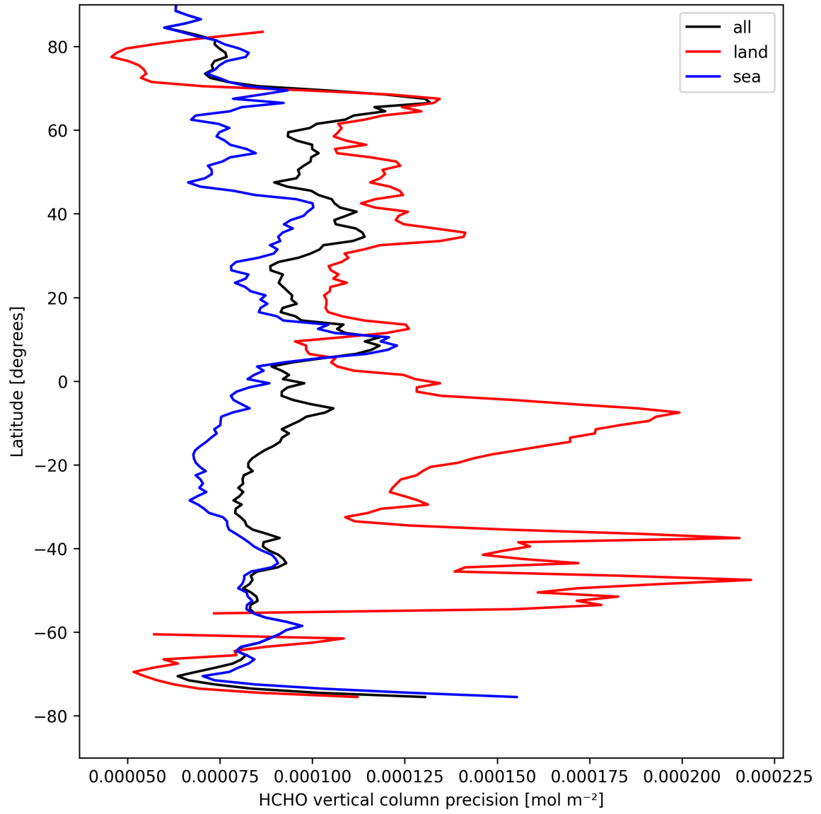
Figure 22: Zonal average of “HCHO vertical column precision” for 2025-08-27 to 2025-08-29.
