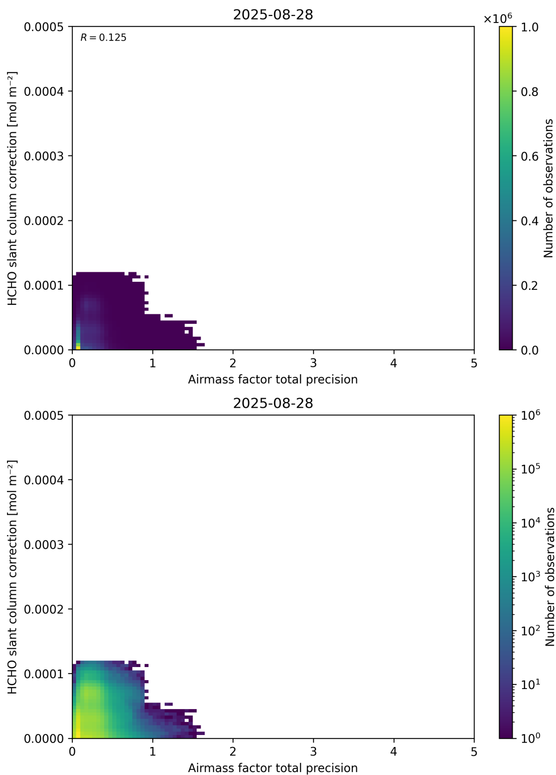
Figure 110: Scatter density plot of “Airmass factor total precision” against “HCHO slant column correction” for 2025-08-27 to 2025-08-29.
