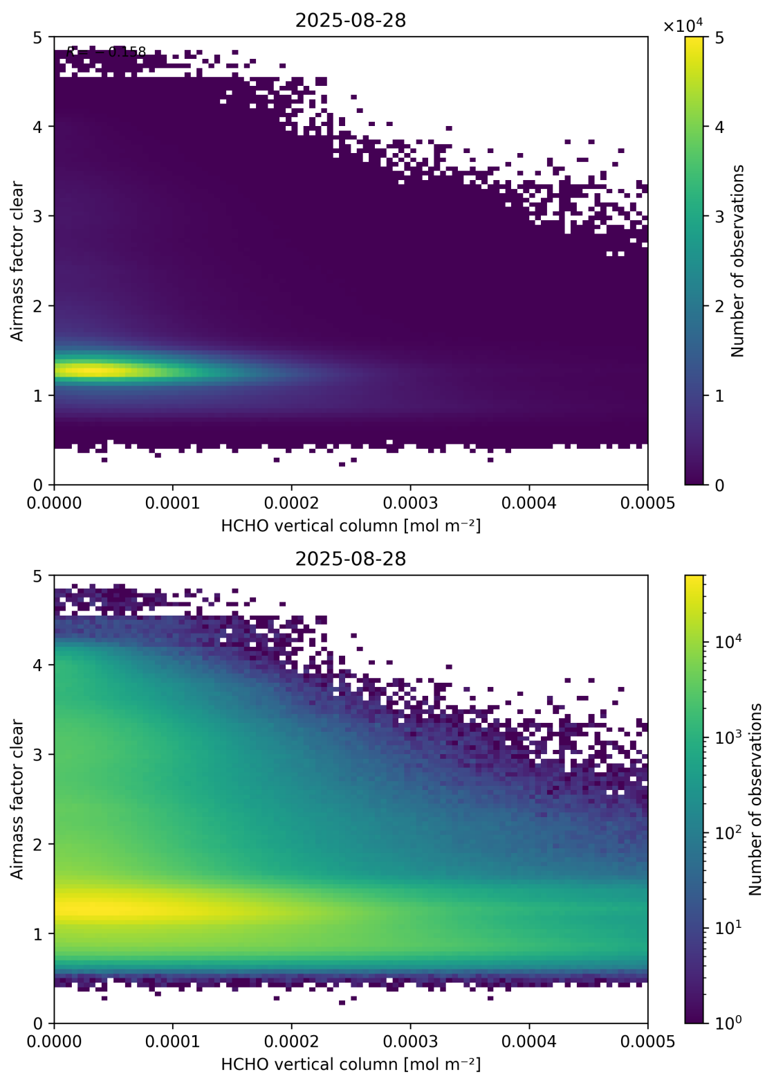
Figure 126: Scatter density plot of “HCHO vertical column” against “Airmass factor clear” for 2025-08-27 to 2025-08-29.
