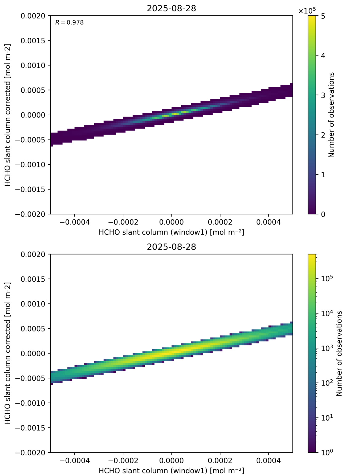
Figure 82: Scatter density plot of “HCHO slant column (window1)” against “HCHO slant column corrected” for 2025-08-27 to 2025-08-29.
