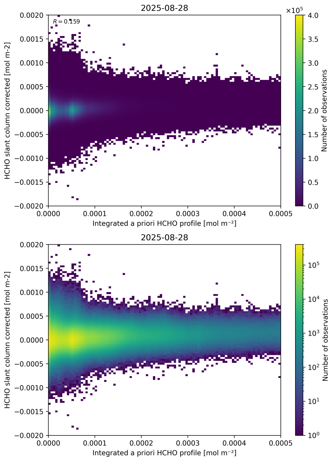
Figure 151: Scatter density plot of “Integrated a priori HCHO profile” against “HCHO slant column corrected” for 2025-08-27 to 2025-08-29.
