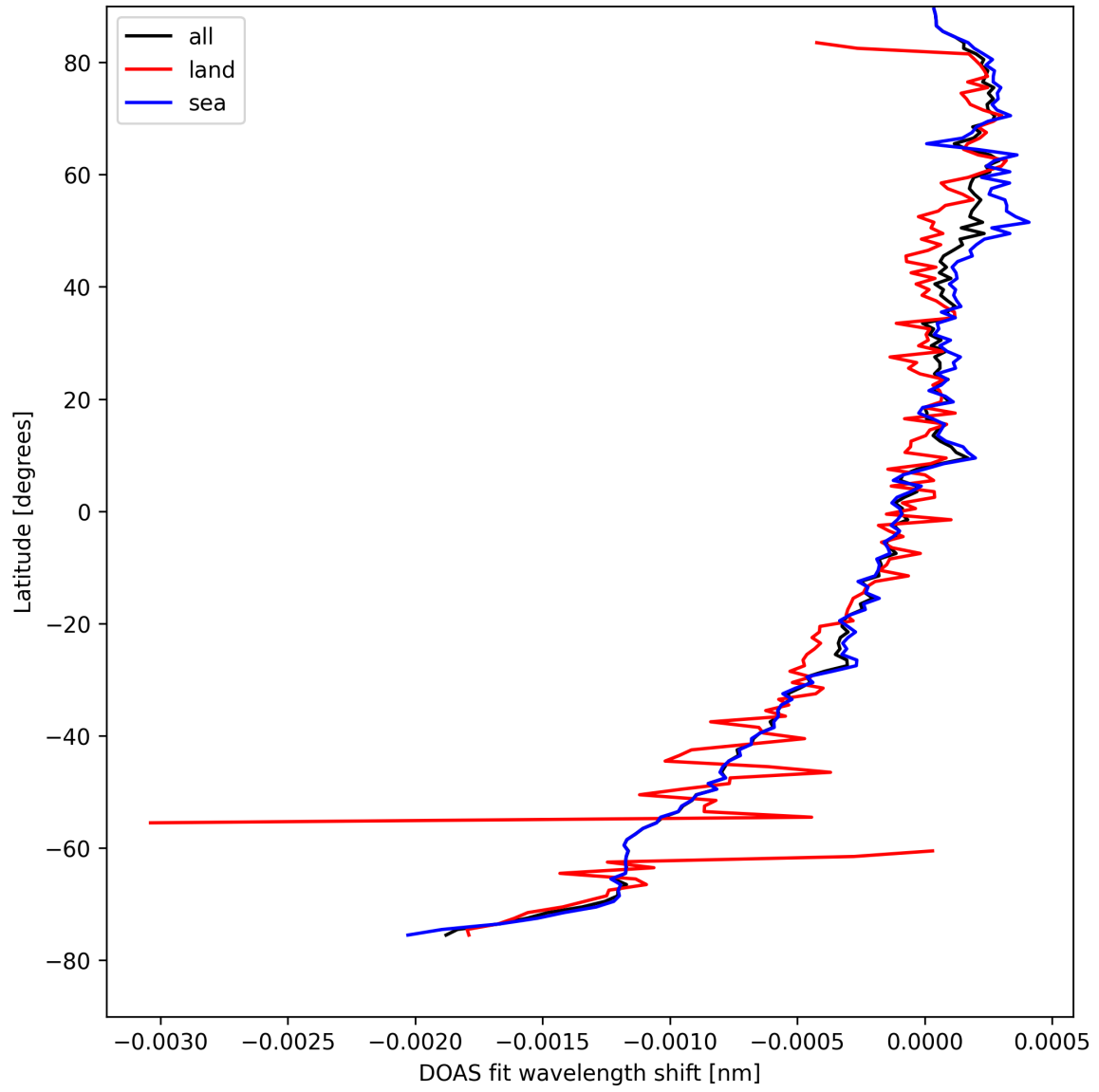
Figure 30: Zonal average of “DOAS fit wavelength shift” for 2025-08-27 to 2025-08-29.
