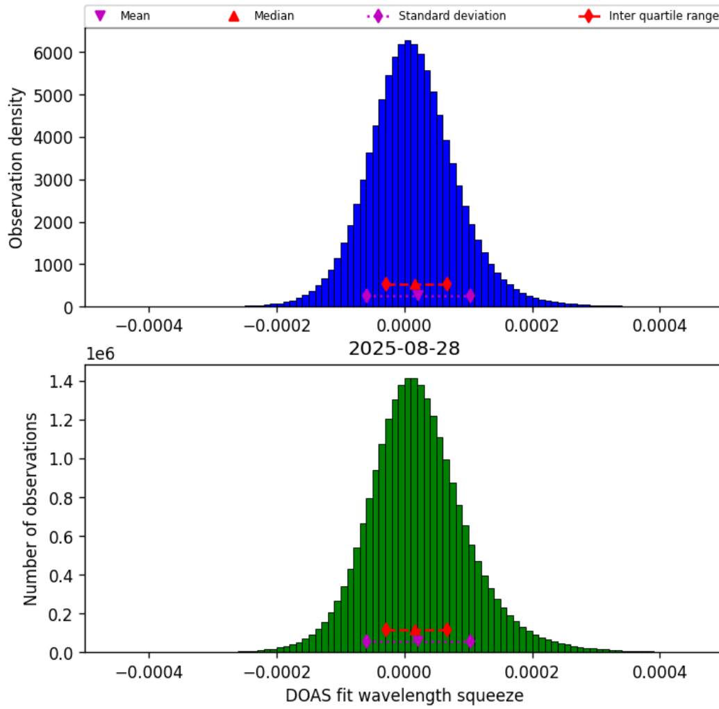
Figure 45: Histogram of “DOAS fit wavelength squeeze” for 2025-08-27 to 2025-08-29
