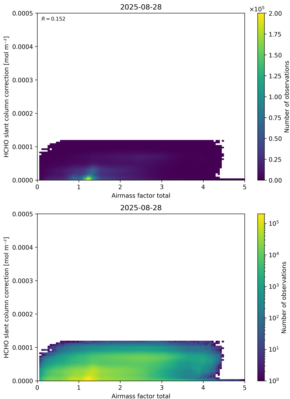
Figure 102: Scatter density plot of “Airmass factor total” against “HCHO slant column correction” for 2025-08-27 to 2025-08-29.
