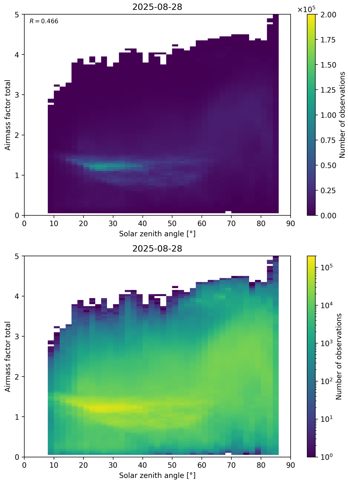
Figure 175: Scatter density plot of “Solar zenith angle” against “Airmass factor total” for 2025-08-27 to 2025-08-29.
