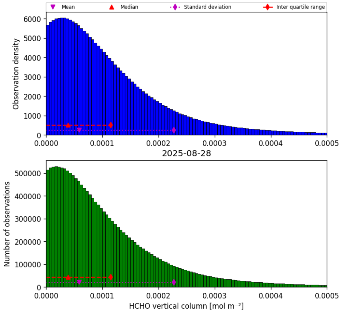
Figure 35: Histogram of “HCHO vertical column” for 2025-08-27 to 2025-08-29
