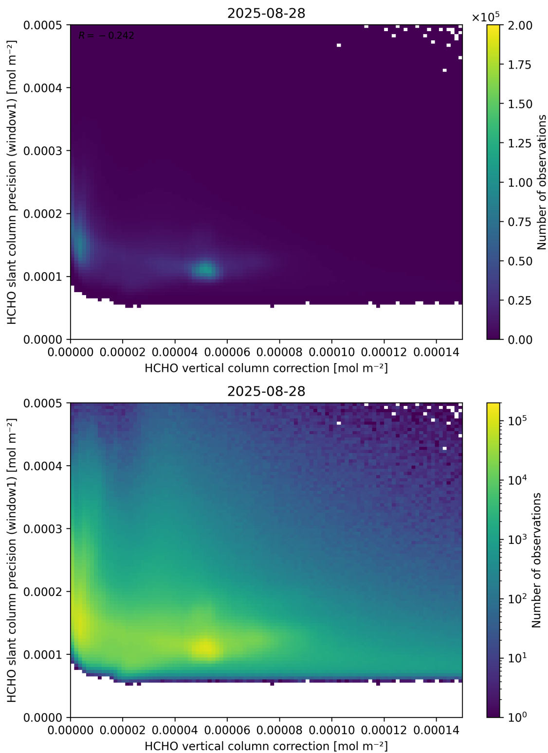
Figure 119: Scatter density plot of “HCHO vertical column correction” against “HCHO slant column precision (window1)” for 2025-08-27 to 2025-08-29.
