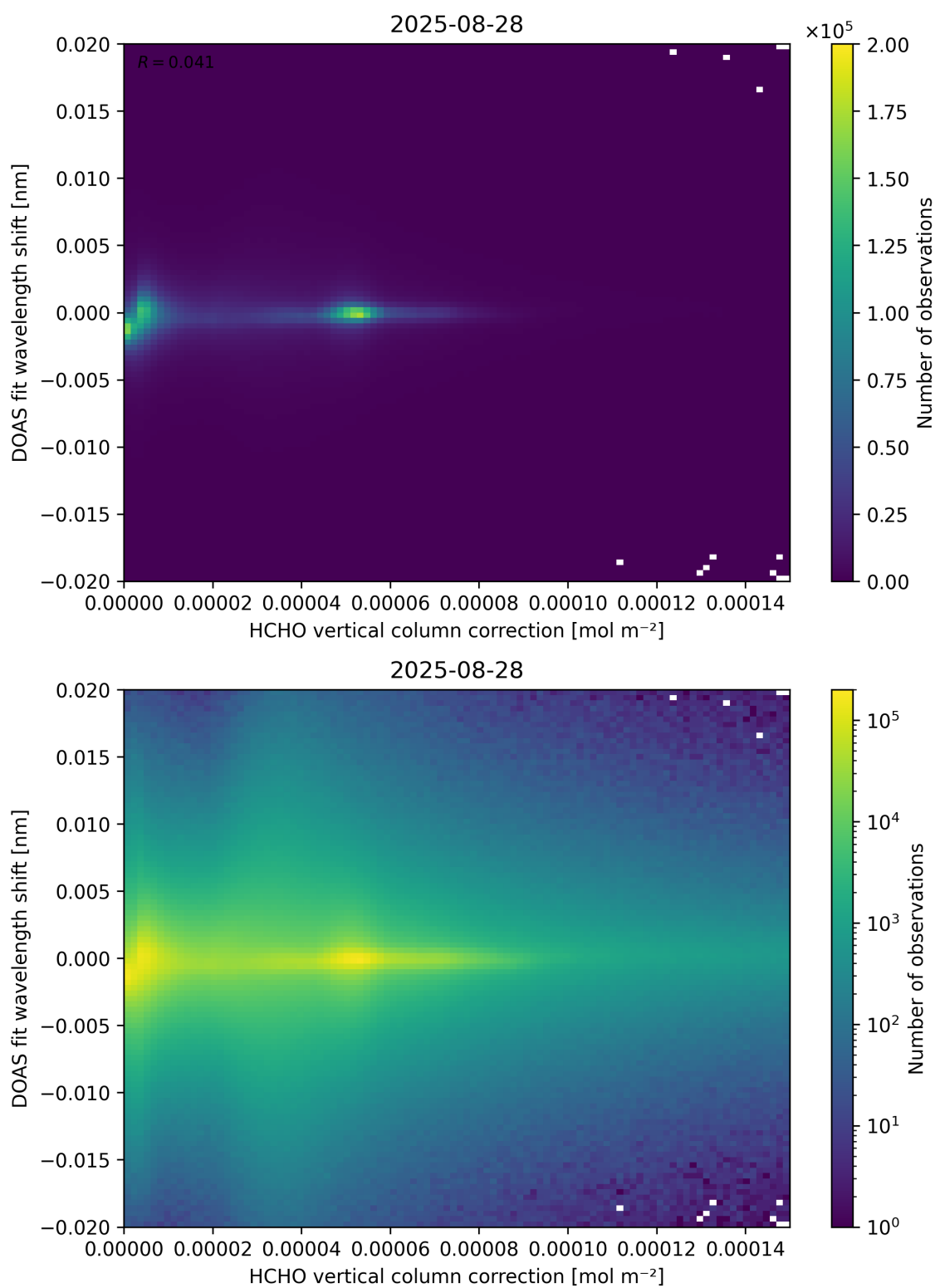
Figure 113: Scatter density plot of “HCHO vertical column correction” against “DOAS fit wavelength shift” for 2025-08-27 to 2025-08-29.
