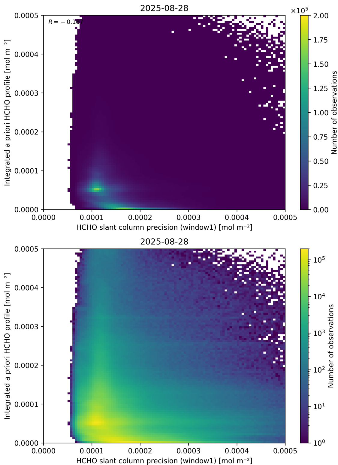
Figure 96: Scatter density plot of “HCHO slant column precision (window1)” against “Integrated a priori HCHO profile” for 2025-08-27 to 2025-08-29.
