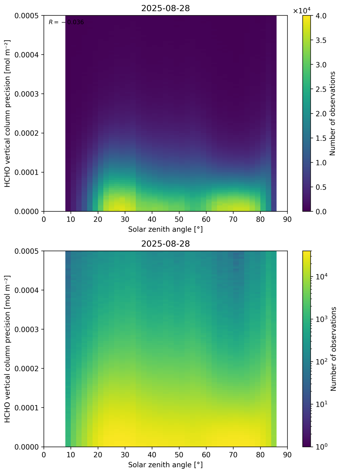
Figure 179: Scatter density plot of “Solar zenith angle” against “HCHO vertical column precision” for 2025-08-27 to 2025-08-29.
