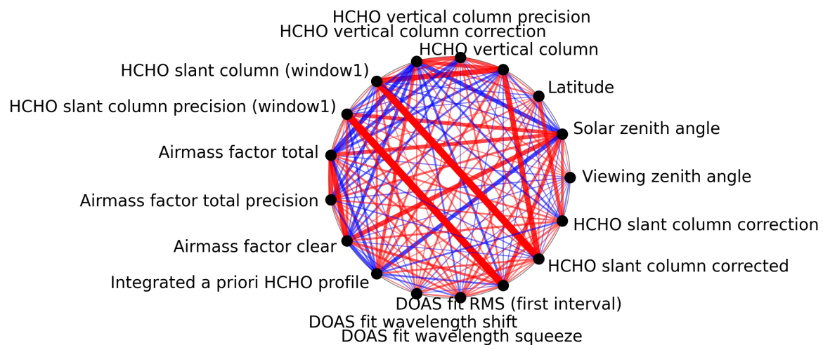
Figure 1: Map of correlation graph for 2025-08-27 to 2025-08-29.
