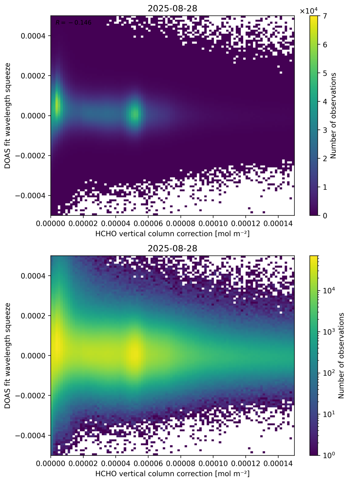
Figure 114: Scatter density plot of “HCHO vertical column correction” against “DOAS fit wavelength squeeze” for 2025-08-27 to 2025-08-29.
