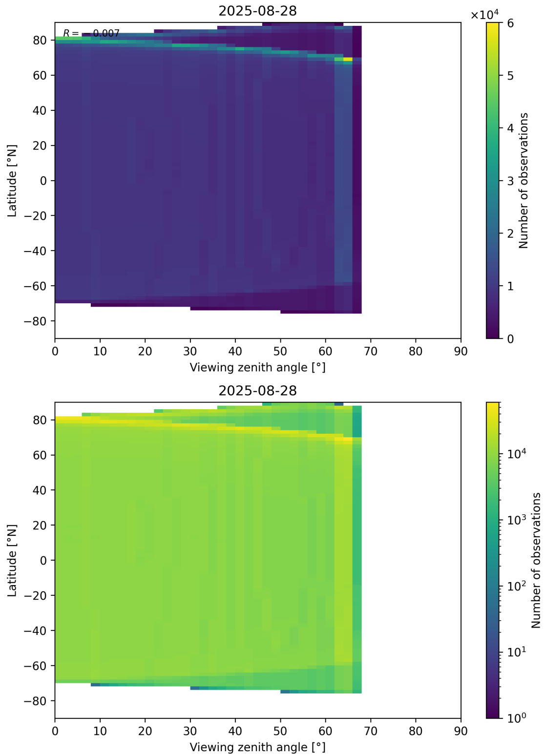
Figure 196: Scatter density plot of “Viewing zenith angle” against “Latitude” for 2025-08-27 to 2025-08-29.
