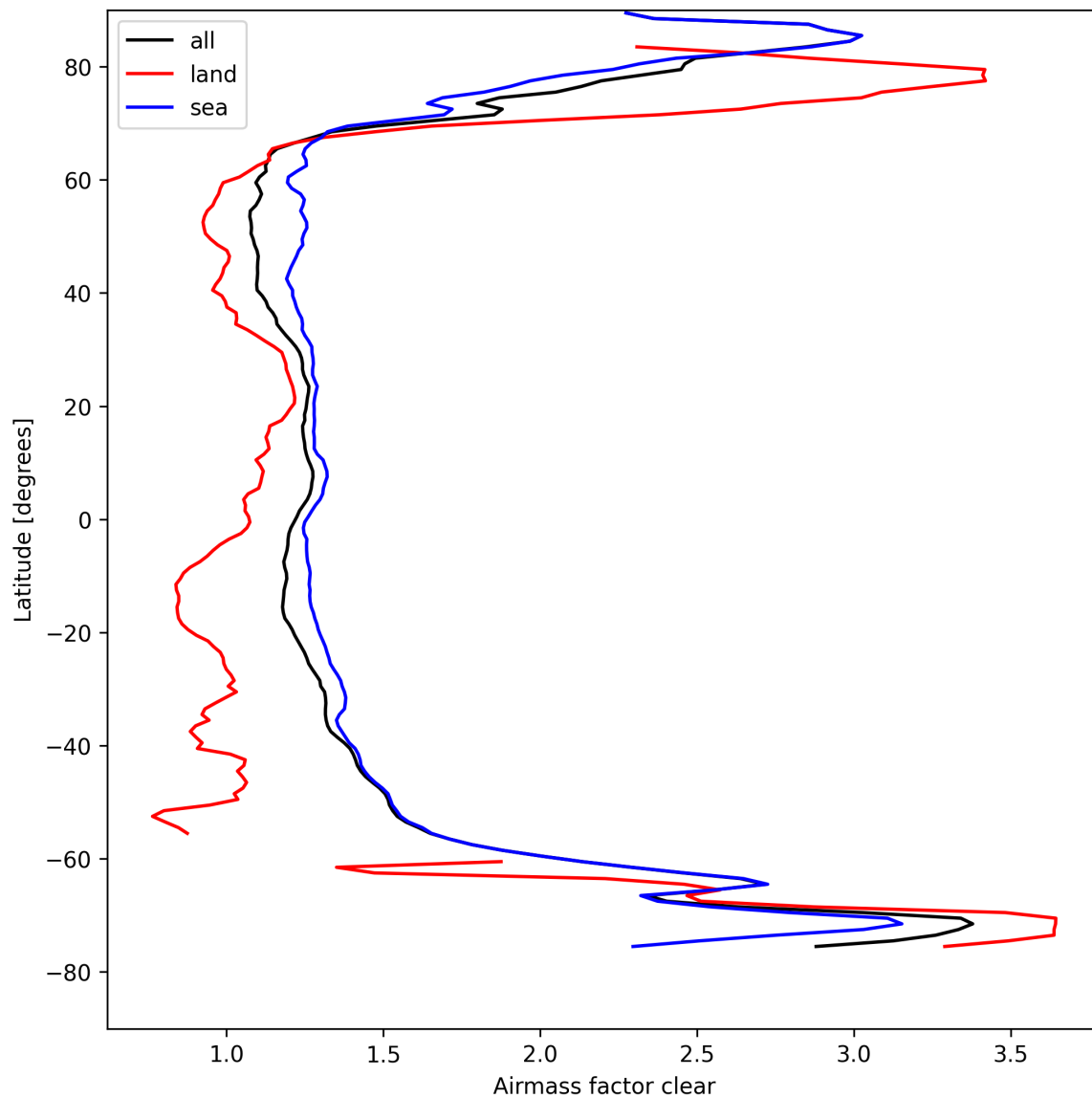
Figure 28: Zonal average of “Airmass factor clear” for 2025-08-27 to 2025-08-29.
