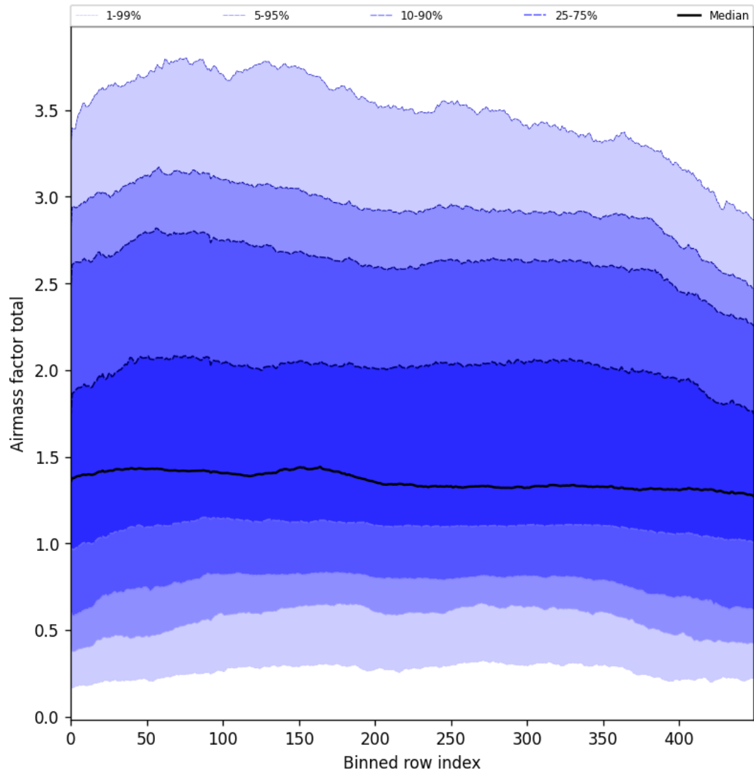
Figure 54: Along track statistics of “Airmass factor total” for 2025-08-27 to 2025-08-29
