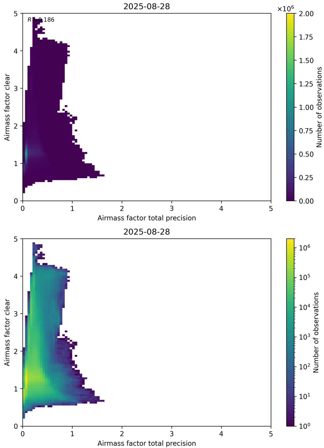
Figure 108: Scatter density plot of “Airmass factor total precision” against “Airmass factor clear” for 2025-08-27 to 2025-08-29.
