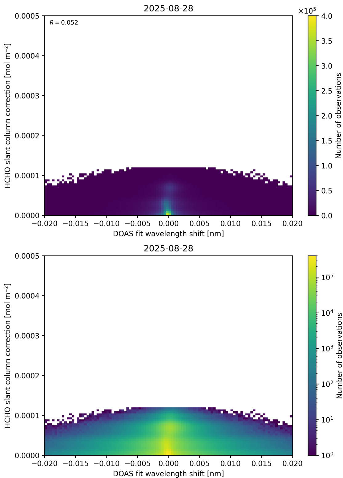
Figure 67: Scatter density plot of “DOAS fit wavelength shift” against “HCHO slant column correction” for 2025-08-27 to 2025-08-29.
