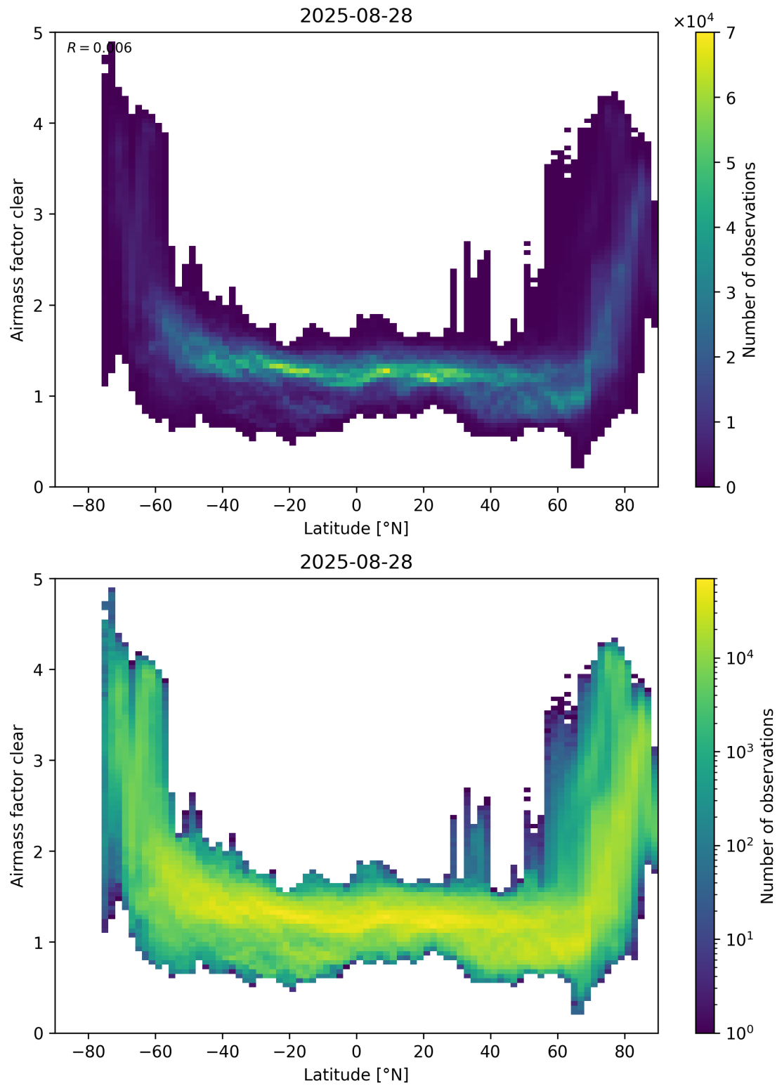
Figure 156: Scatter density plot of “Latitude” against “Airmass factor clear” for 2025-08-27 to 2025-08-29.
