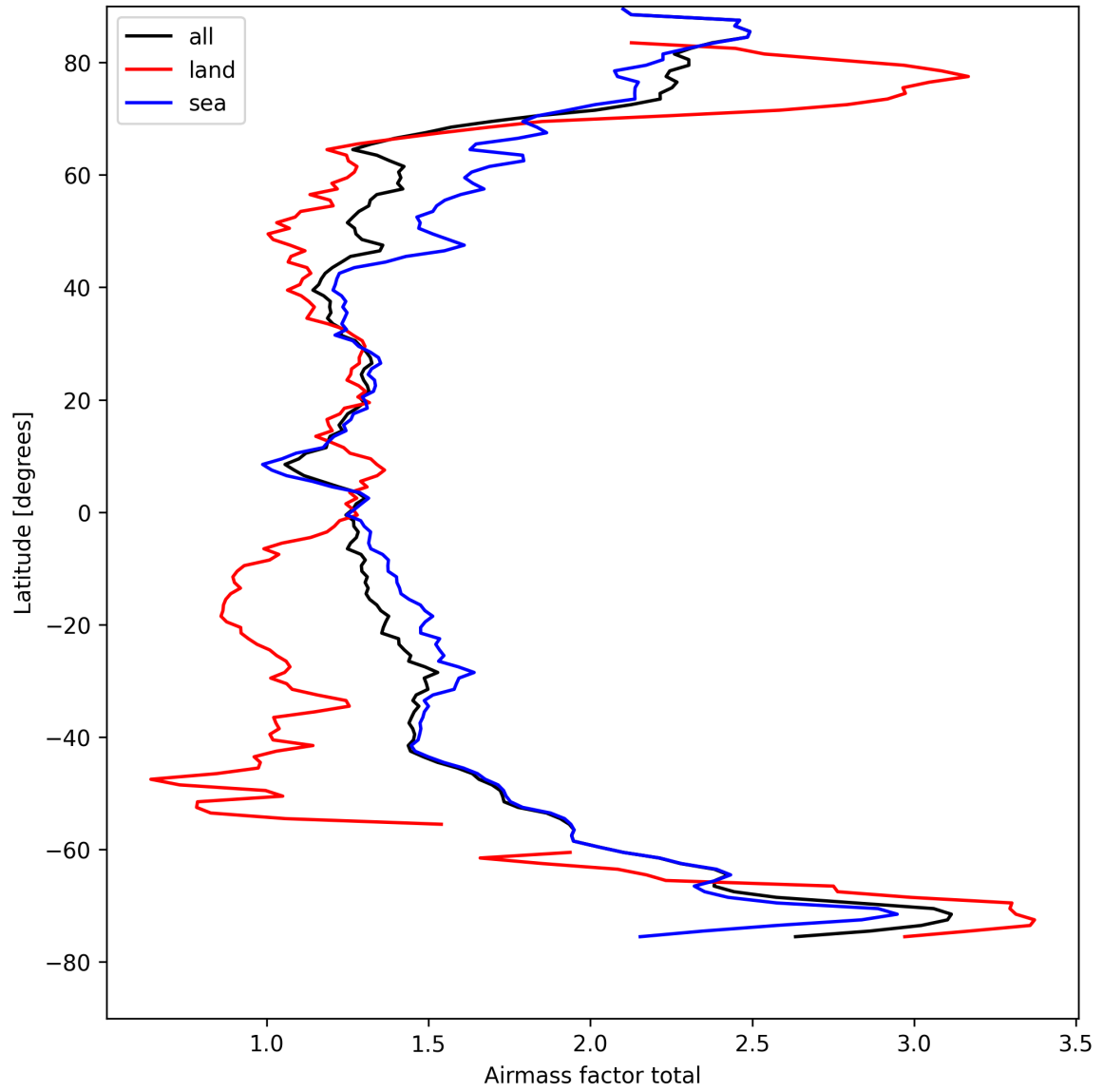
Figure 26: Zonal average of “Airmass factor total” for 2025-08-27 to 2025-08-29.
