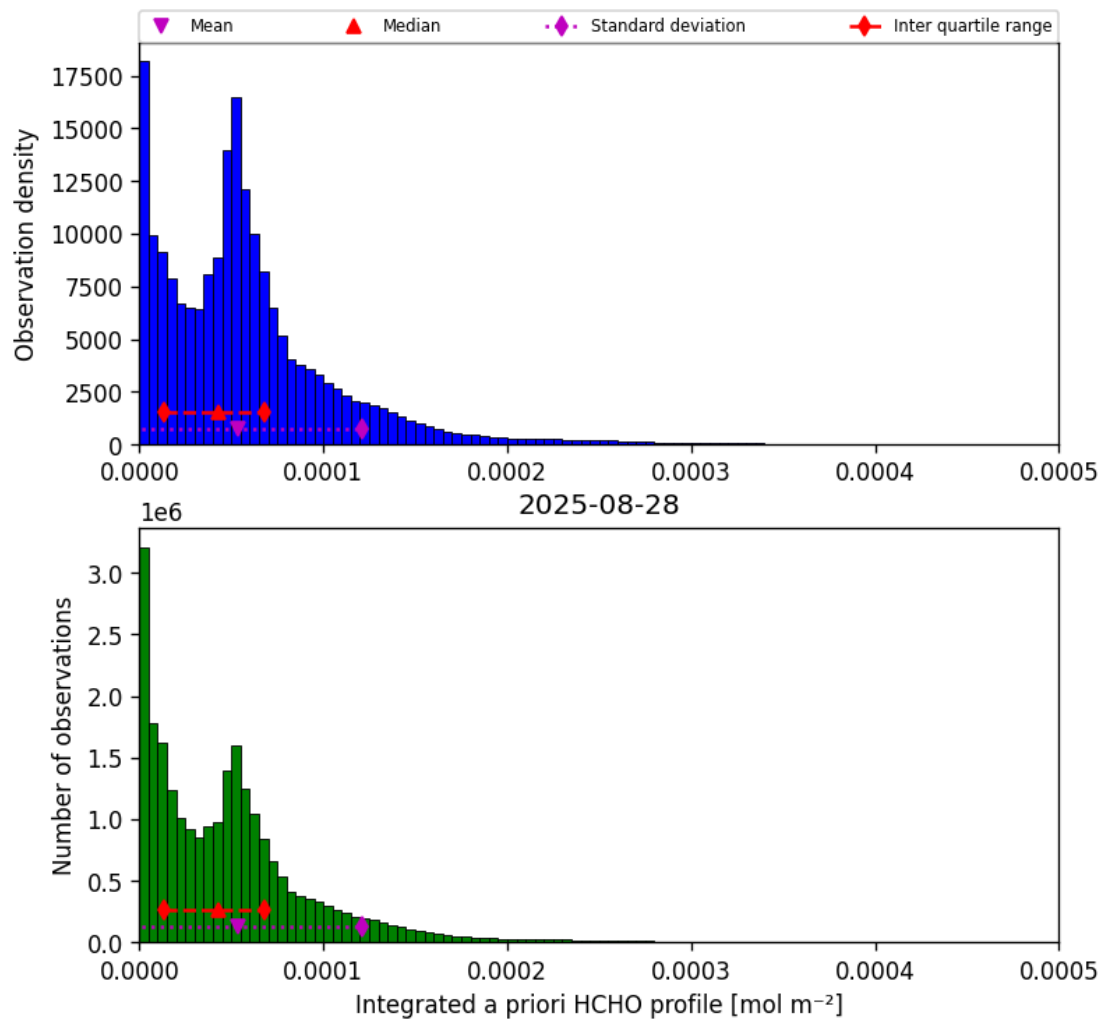
Figure 43: Histogram of “Integrated a priori HCHO profile” for 2025-08-27 to 2025-08-29
