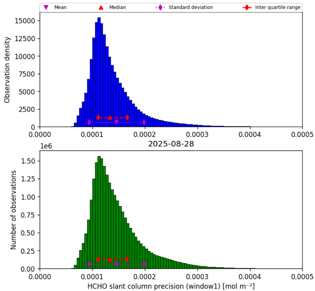
Figure 39: Histogram of “HCHO slant column precision (window1)” for 2025-08-27 to 2025-08-29
