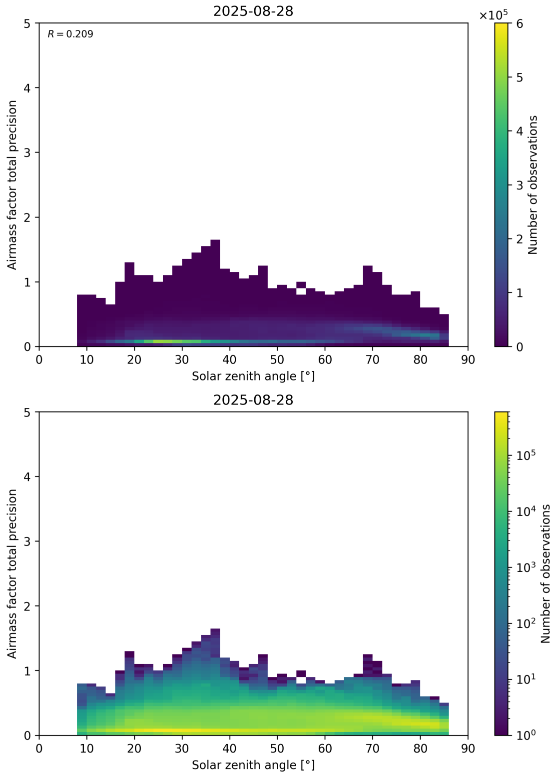
Figure 176: Scatter density plot of “Solar zenith angle” against “Airmass factor total precision” for 2025-08-27 to 2025-08-29.
