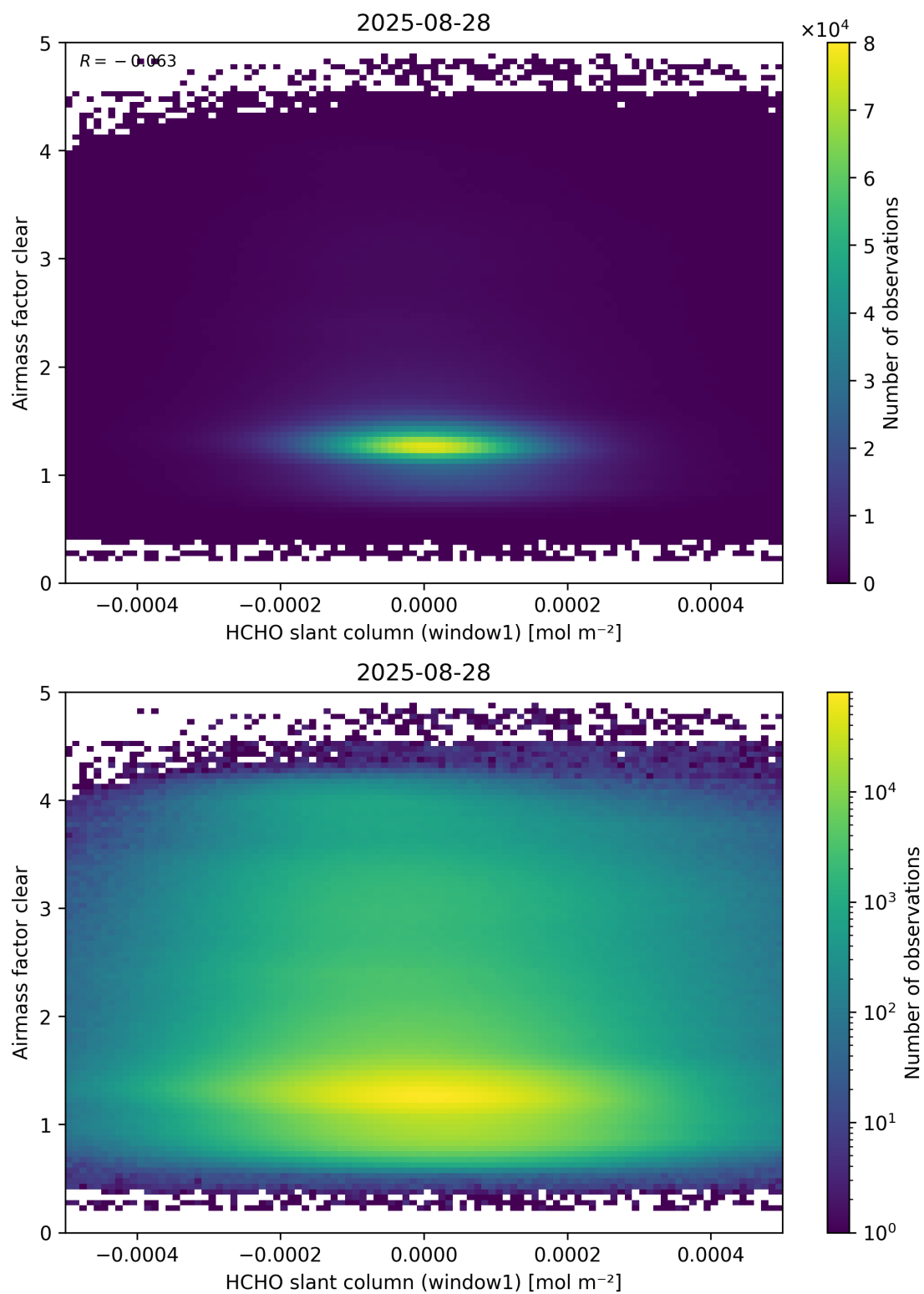
Figure 81: Scatter density plot of “HCHO slant column (window1)” against “Airmass factor clear” for 2025-08-27 to 2025-08-29.
