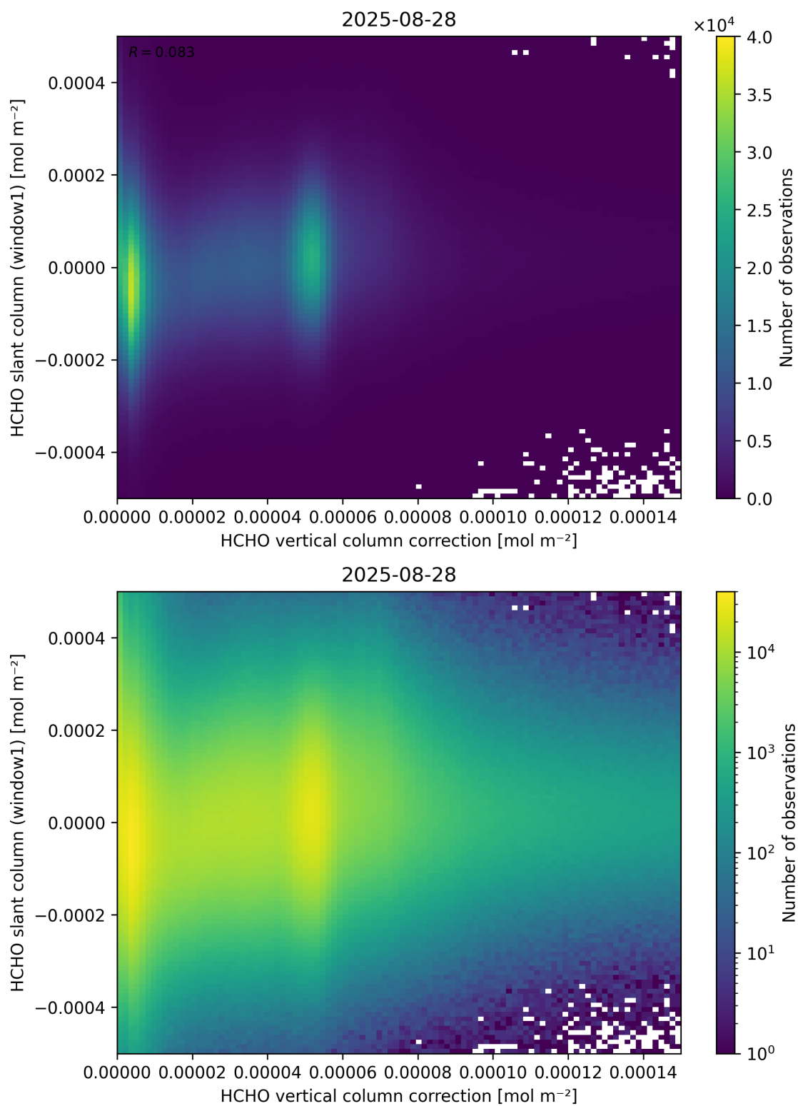
Figure 118: Scatter density plot of “HCHO vertical column correction” against “HCHO slant column (window1)” for 2025-08-27 to 2025-08-29.
