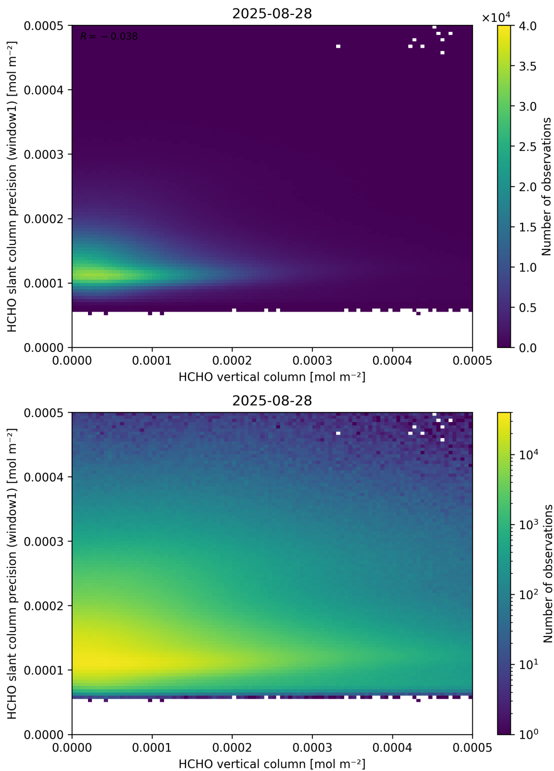
Figure 130: Scatter density plot of “HCHO vertical column” against “HCHO slant column precision (window1)” for 2025-08-27 to 2025-08-29.
