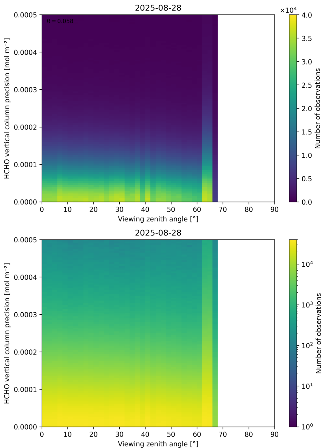
Figure 194: Scatter density plot of “Viewing zenith angle” against “HCHO vertical column precision” for 2025-08-27 to 2025-08-29.
