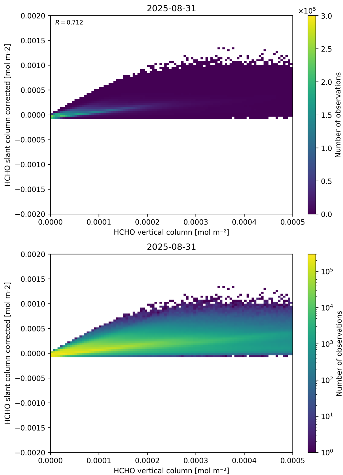
Figure 127: Scatter density plot of “HCHO vertical column” against “HCHO slant column corrected” for 2025-08-30 to 2025-09-01.
