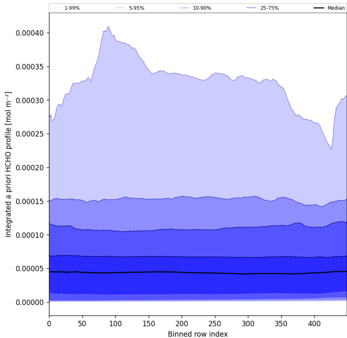
Figure 57: Along track statistics of “Integrated a priori HCHO profile” for 2025-08-30 to 2025-09-01
