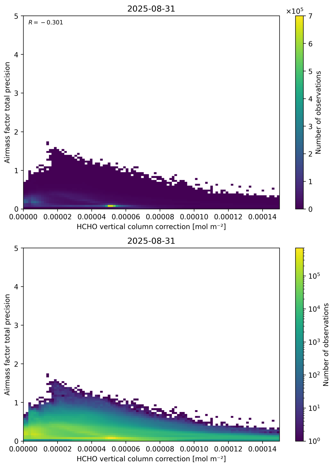
Figure 121: Scatter density plot of “HCHO vertical column correction” against “Airmass factor total precision” for 2025-08-30 to 2025-09-01.
