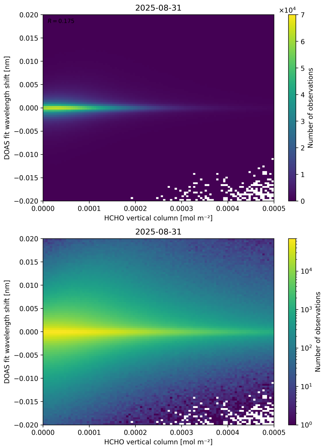
Figure 124: Scatter density plot of “HCHO vertical column” against “DOAS fit wavelength shift” for 2025-08-30 to 2025-09-01.
