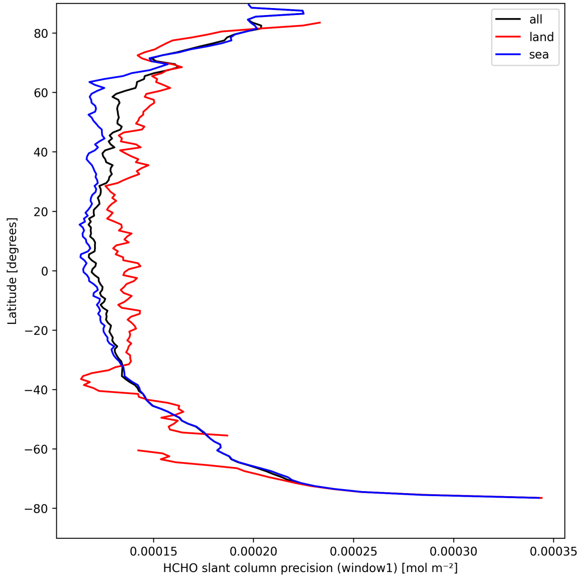
Figure 25: Zonal average of "HCHO slant column precision (window1)" for 2025-08-30 to 2025-09-01.
