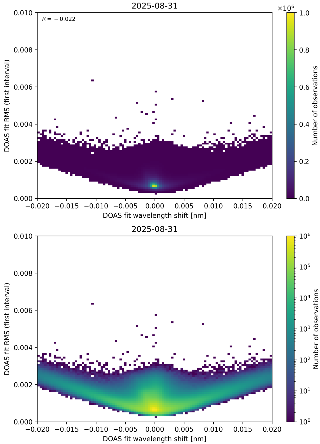
Figure 64: Scatter density plot of “DOAS fit wavelength shift” against “DOAS fit RMS (first interval)” for 2025-08-30 to 2025-09-01.
