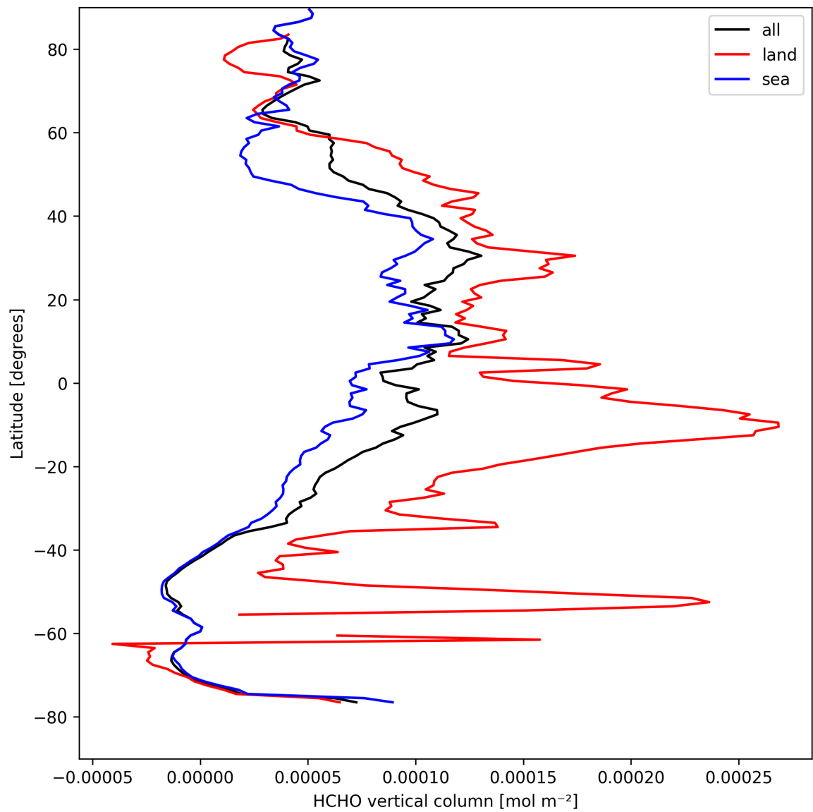
Figure 21: Zonal average of “HCHO vertical column” for 2025-08-30 to 2025-09-01.
