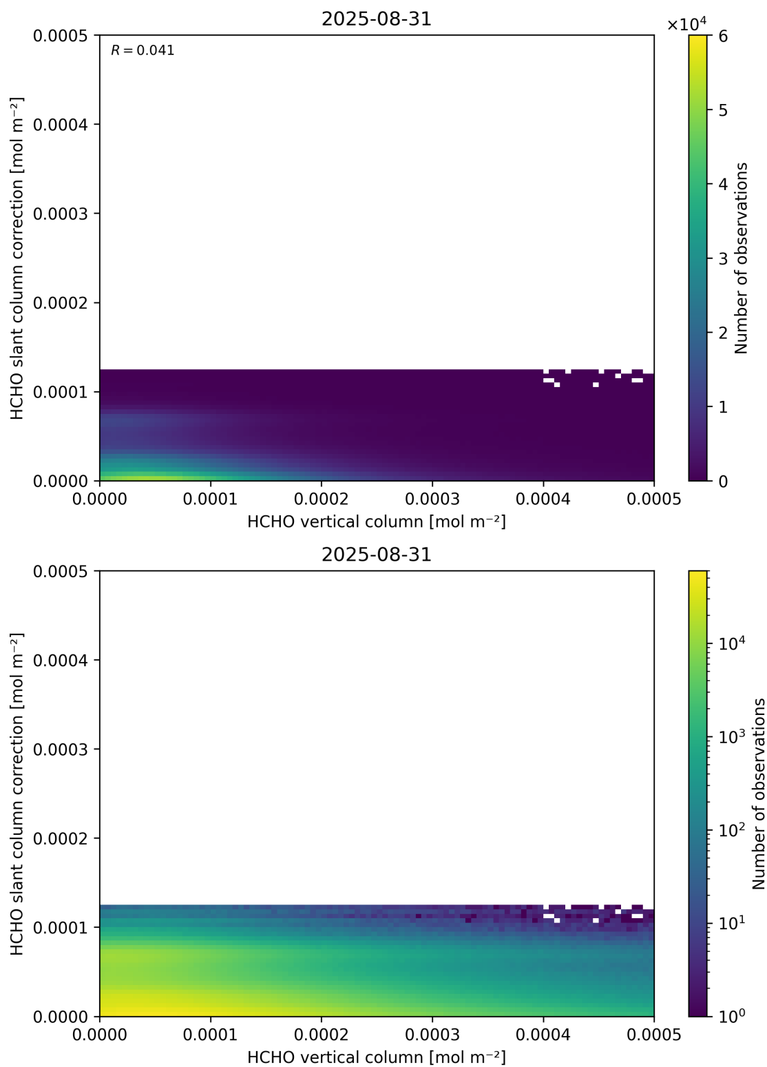
Figure 128: Scatter density plot of “HCHO vertical column” against “HCHO slant column correction” for 2025-08-30 to 2025-09-01.
