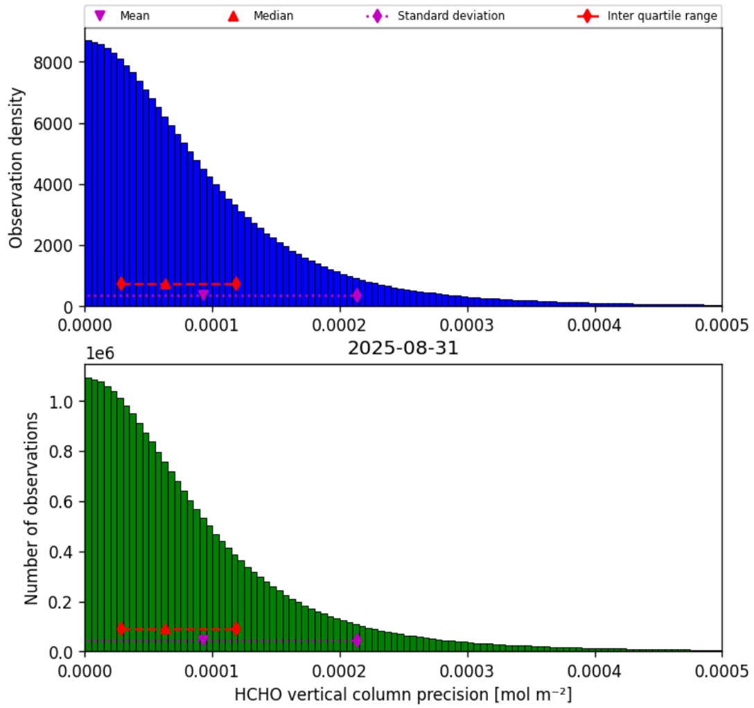
Figure 36: Histogram of “HCHO vertical column precision” for 2025-08-30 to 2025-09-01
