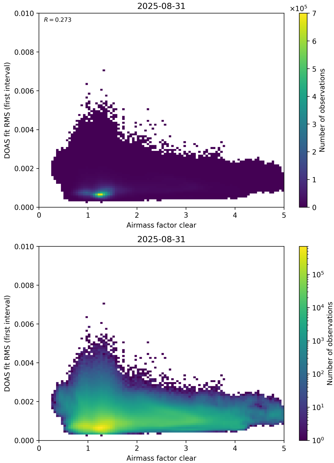
Figure 71: Scatter density plot of “Airmass factor clear” against “DOAS fit RMS (first interval)” for 2025-08-30 to 2025-09-01.
