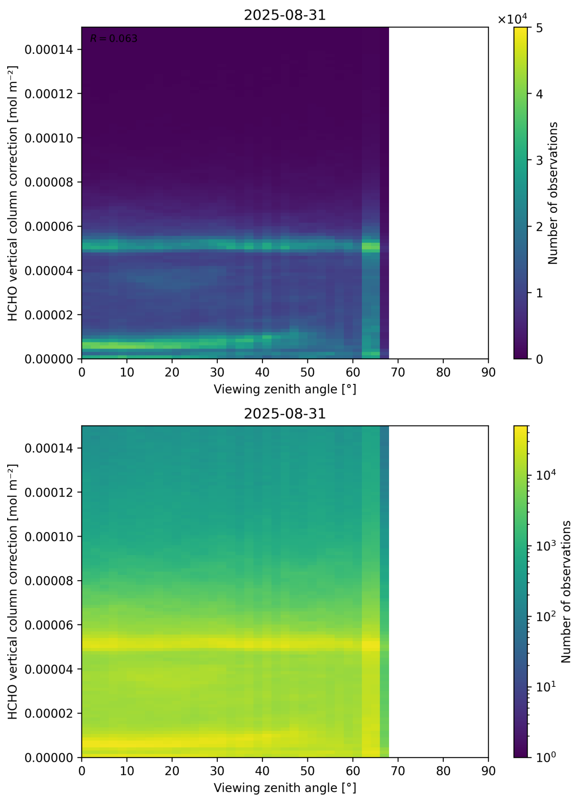
Figure 193: Scatter density plot of “Viewing zenith angle” against “HCHO vertical column correction” for 2025-08-30 to 2025-09-01.
