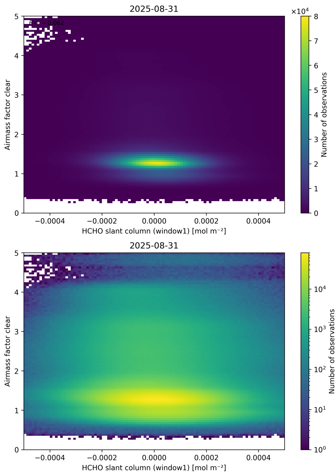
Figure 81: Scatter density plot of “HCHO slant column (window1)” against “Airmass factor clear” for 2025-08-30 to 2025-09-01.
