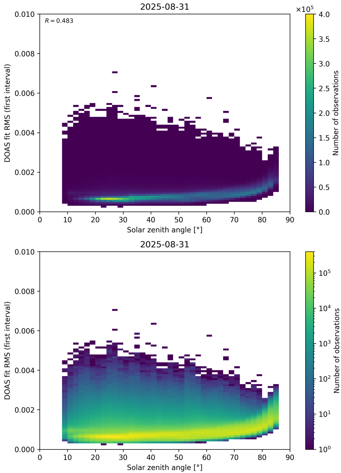
Figure 167: Scatter density plot of “Solar zenith angle” against “DOAS fit RMS (first interval)” for 2025-08-30 to 2025-09-01.
