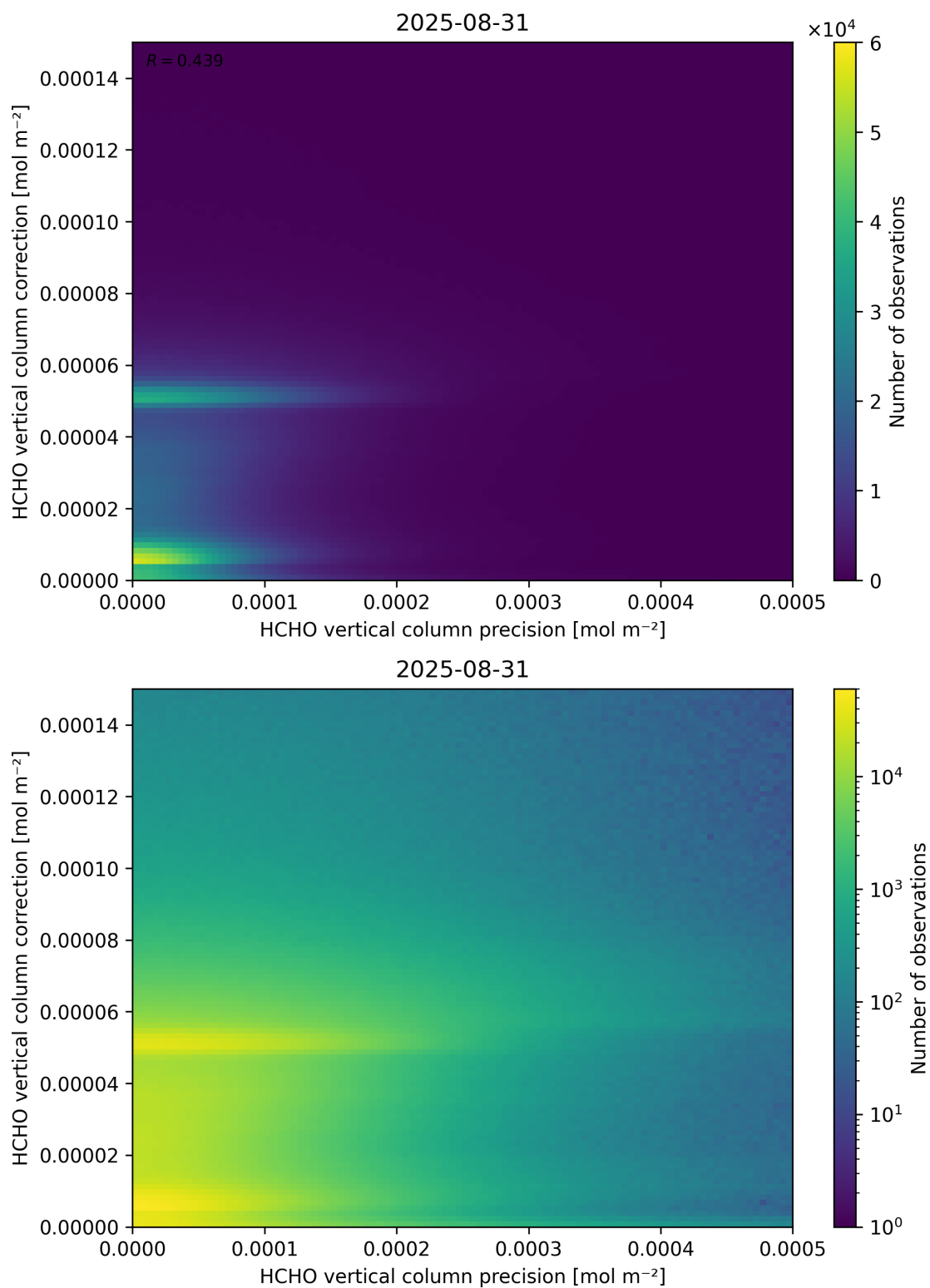
Figure 146: Scatter density plot of “HCHO vertical column precision” against “HCHO vertical column correction” for 2025-08-30 to 2025-09-01.
