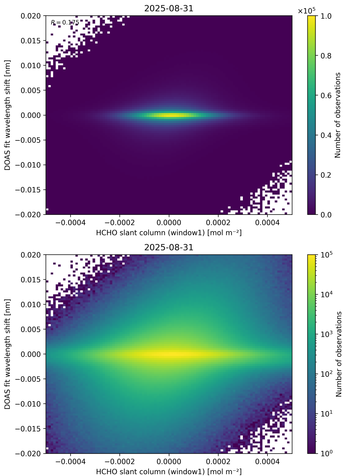
Figure 79: Scatter density plot of “HCHO slant column (window1)” against “DOAS fit wavelength shift” for 2025-08-30 to 2025-09-01.
