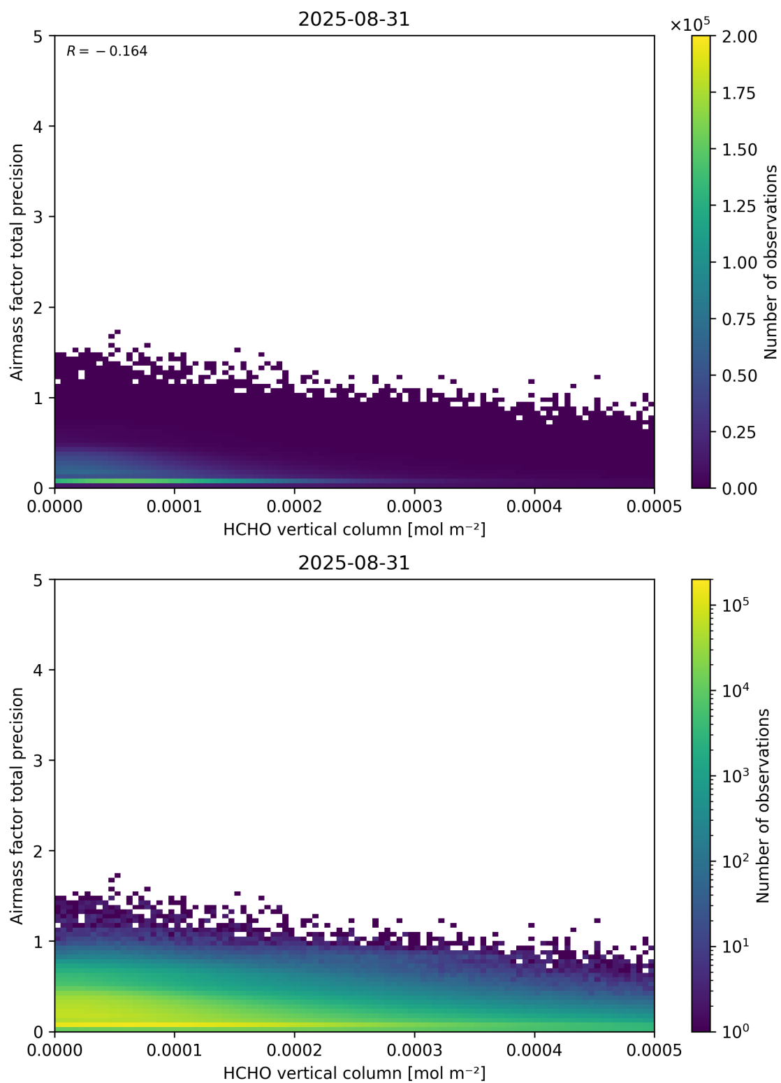
Figure 132: Scatter density plot of “HCHO vertical column” against “Airmass factor total precision” for 2025-08-30 to 2025-09-01.
