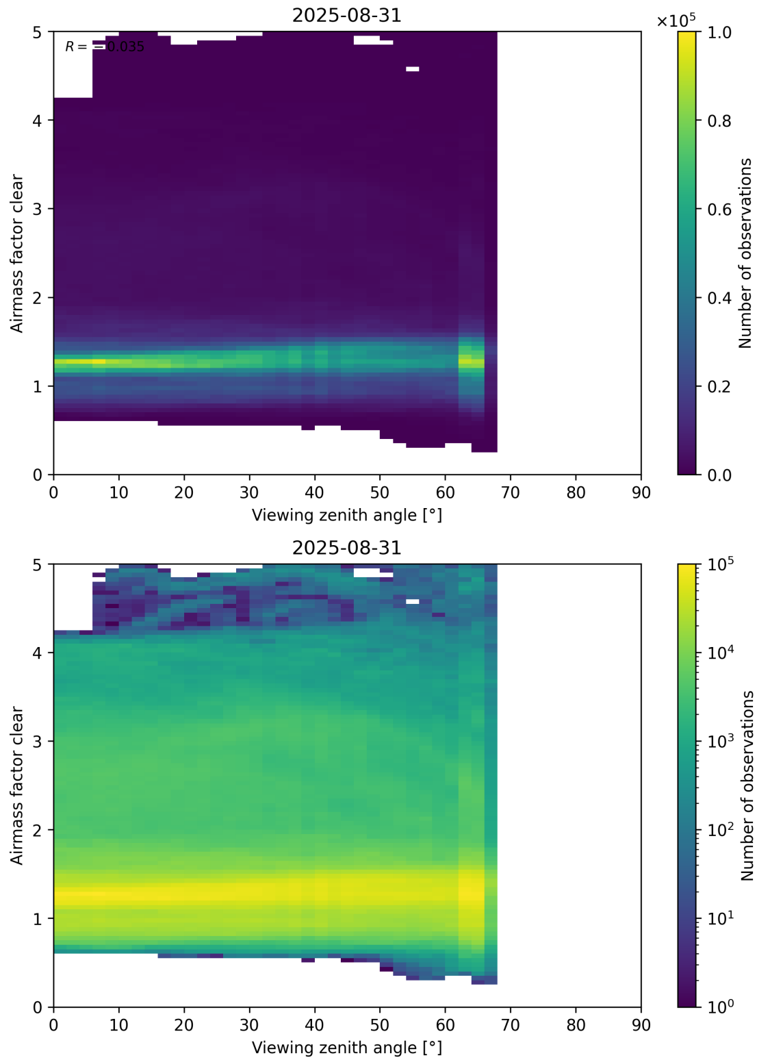
Figure 185: Scatter density plot of “Viewing zenith angle” against “Airmass factor clear” for 2025-08-30 to 2025-09-01.
