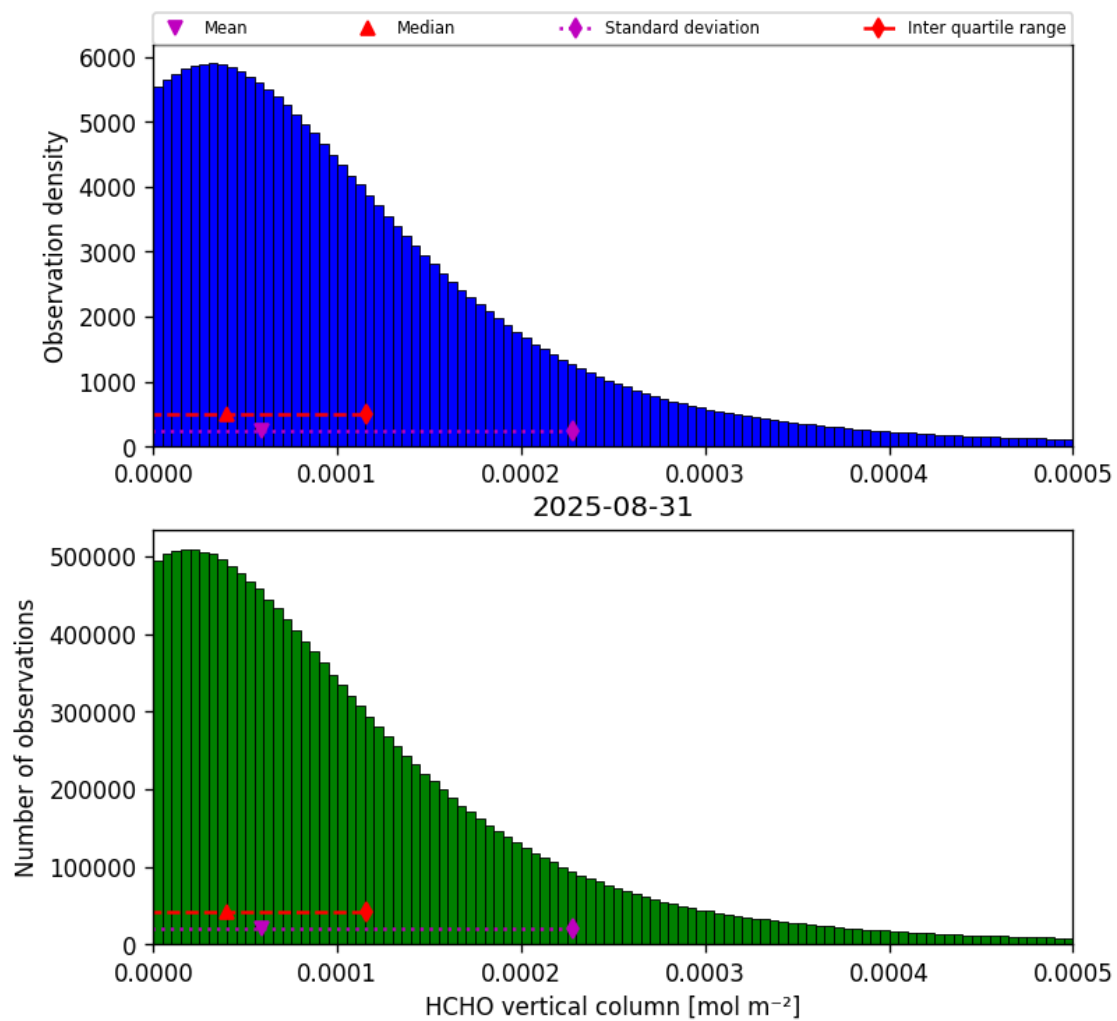
Figure 35: Histogram of “HCHO vertical column” for 2025-08-30 to 2025-09-01
