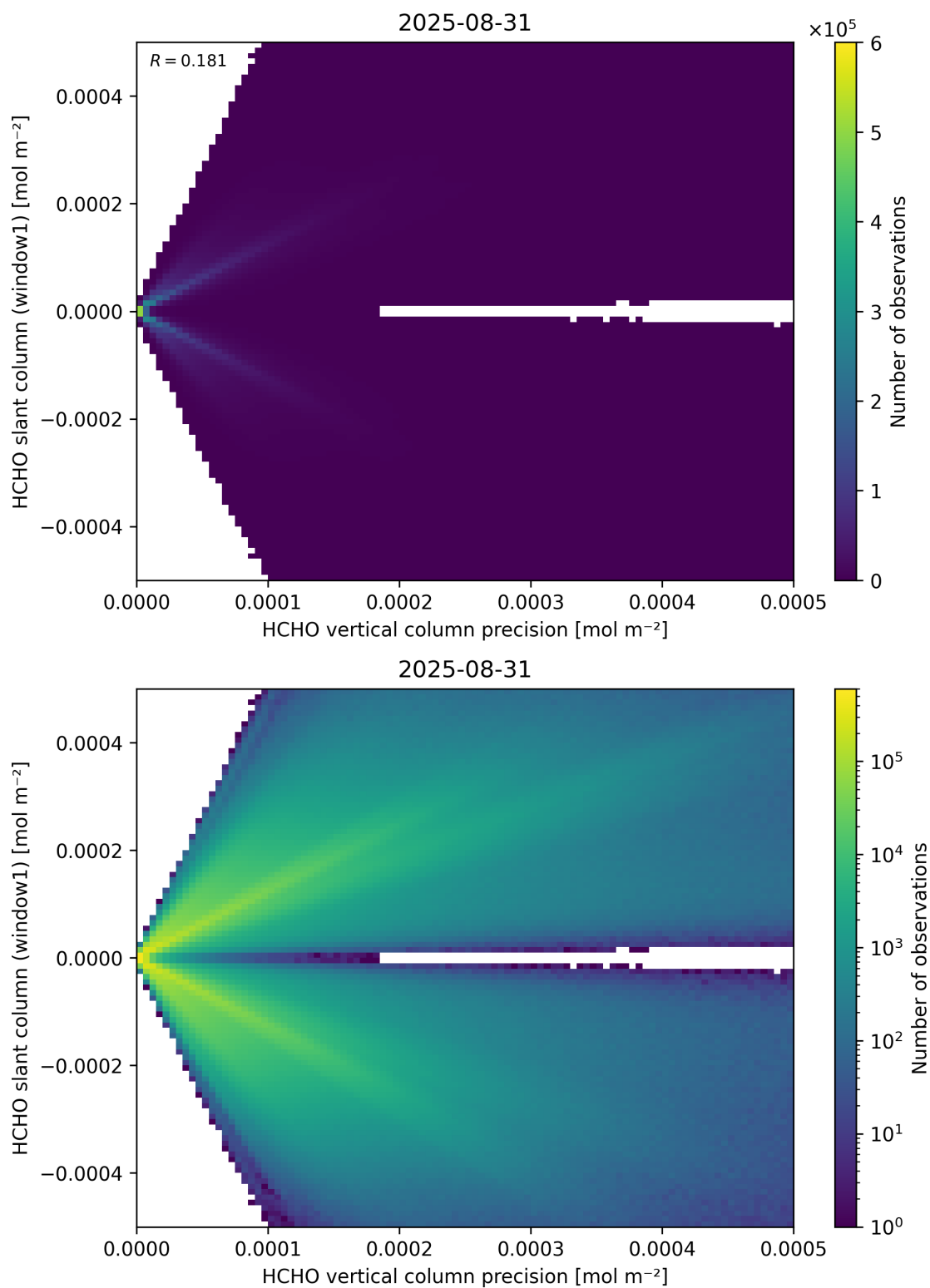
Figure 142: Scatter density plot of “HCHO vertical column precision” against “HCHO slant column (window1)” for 2025-08-30 to 2025-09-01.
