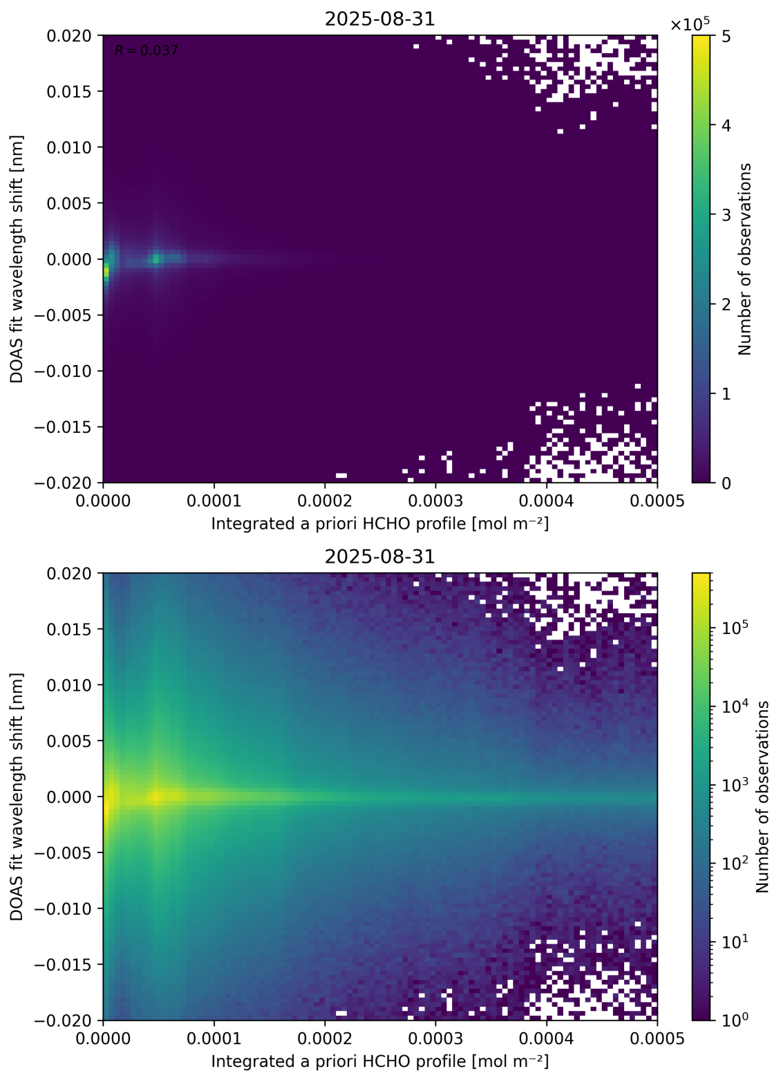
Figure 149: Scatter density plot of “Integrated a priori HCHO profile” against “DOAS fit wavelength shift” for 2025-08-30 to 2025-09-01.
