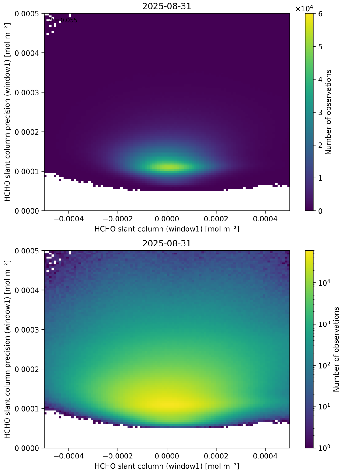
Figure 84: Scatter density plot of “HCHO slant column (window1)” against “HCHO slant column precision (window1)” for 2025-08-30 to 2025-09-01.
