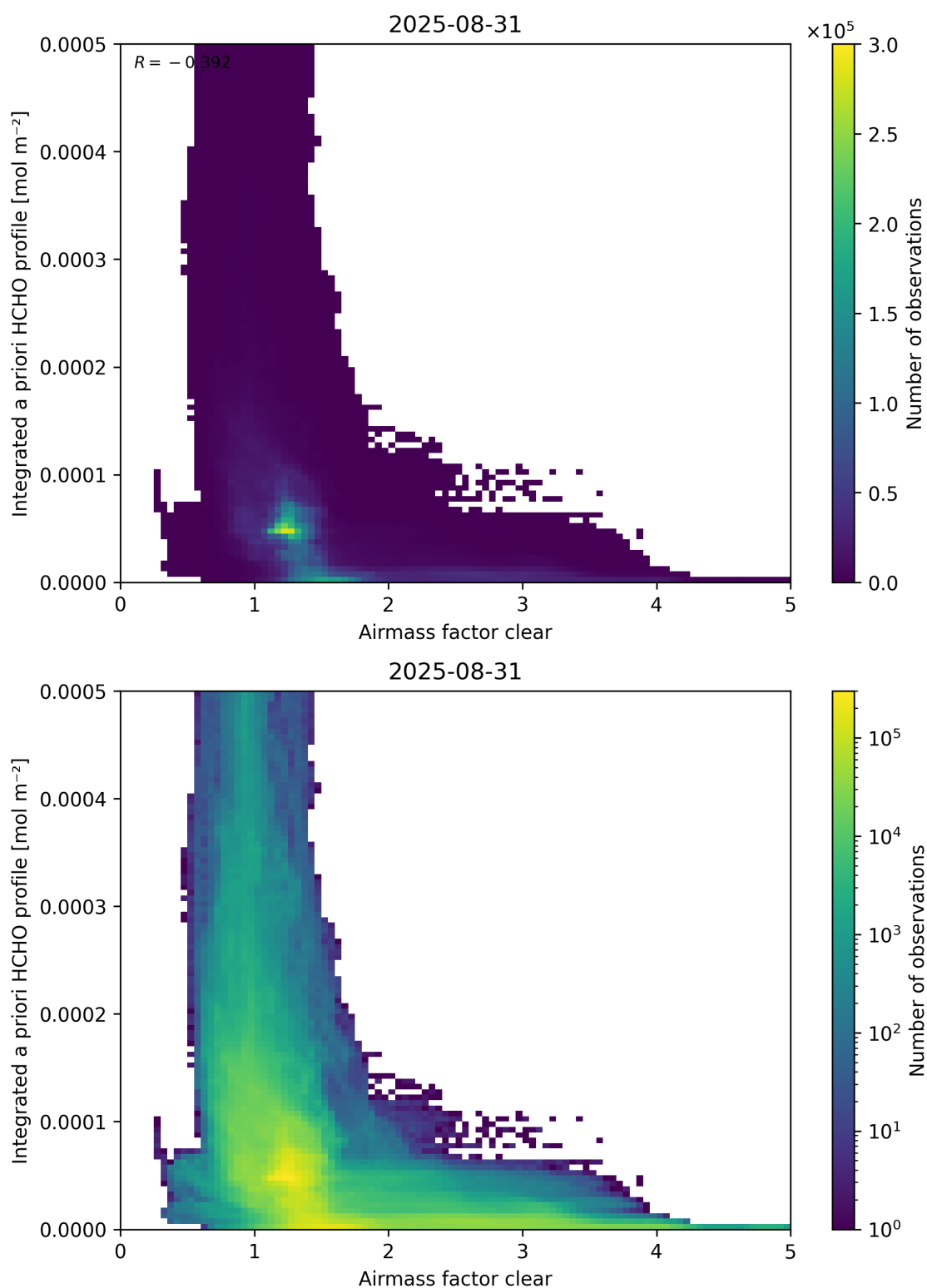
Figure 76: Scatter density plot of “Airmass factor clear” against “Integrated a priori HCHO profile” for 2025-08-30 to 2025-09-01.
