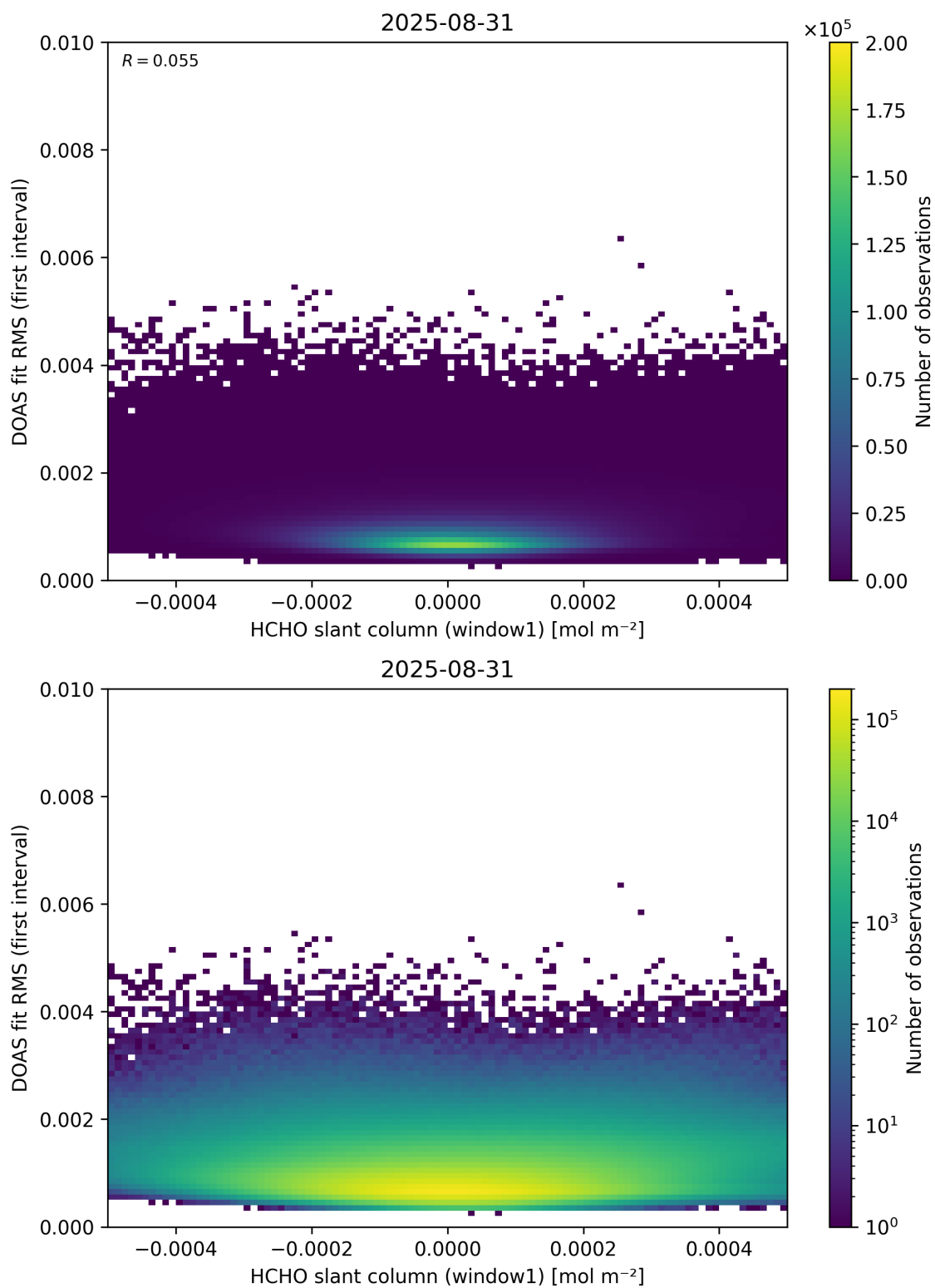
Figure 78: Scatter density plot of “HCHO slant column (window1)” against “DOAS fit RMS (first interval)” for 2025-08-30 to 2025-09-01.
