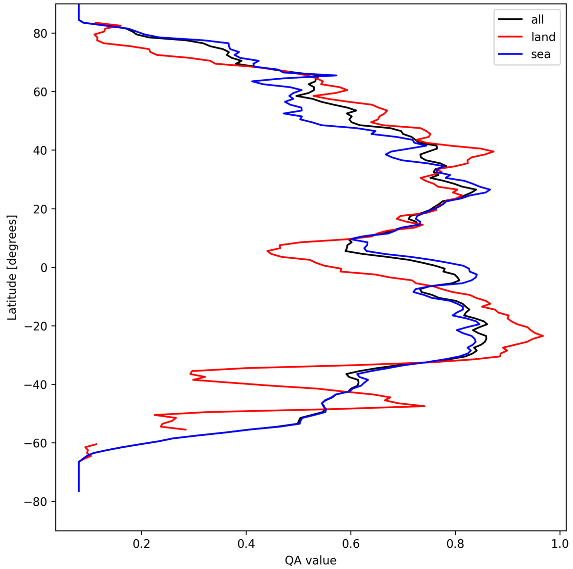
Figure 20: Zonal average of “QA value” for 2025-08-30 to 2025-09-01.
