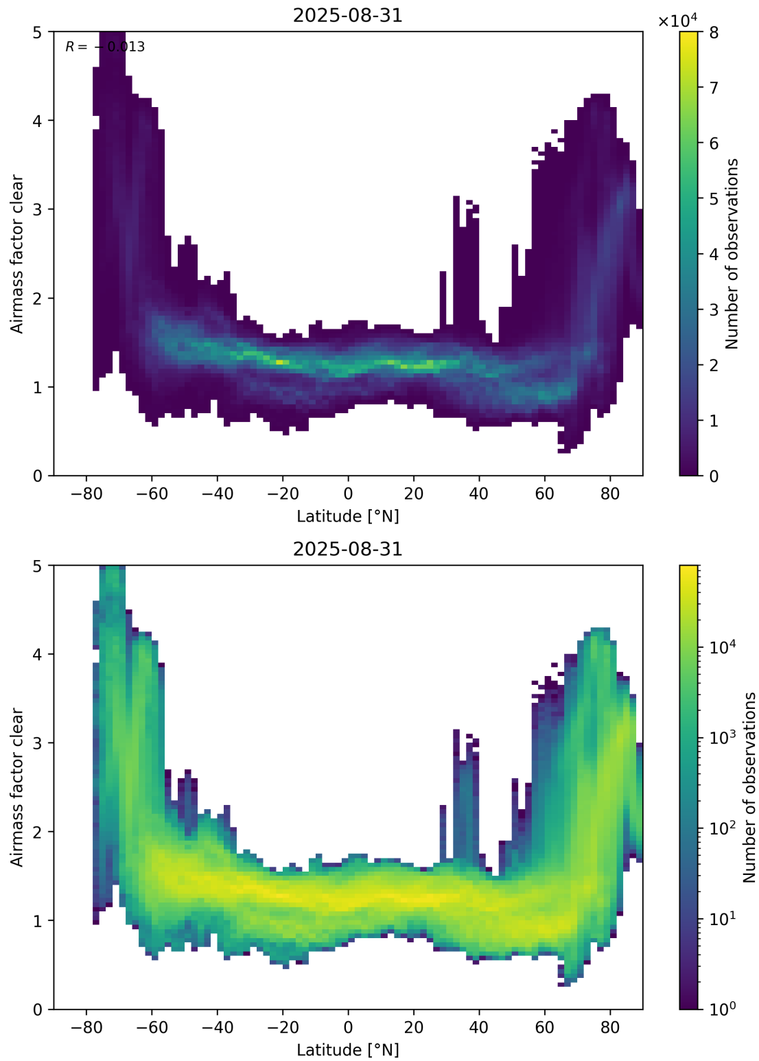
Figure 156: Scatter density plot of “Latitude” against “Airmass factor clear” for 2025-08-30 to 2025-09-01.
