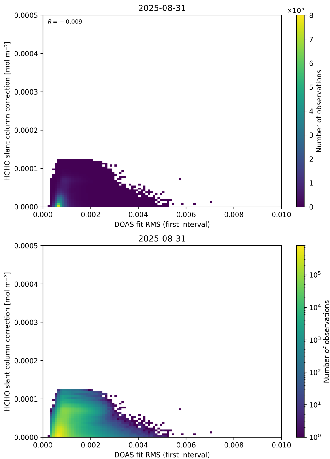
Figure 63: Scatter density plot of “DOAS fit RMS (first interval)” against “HCHO slant column correction” for 2025-08-30 to 2025-09-01.
