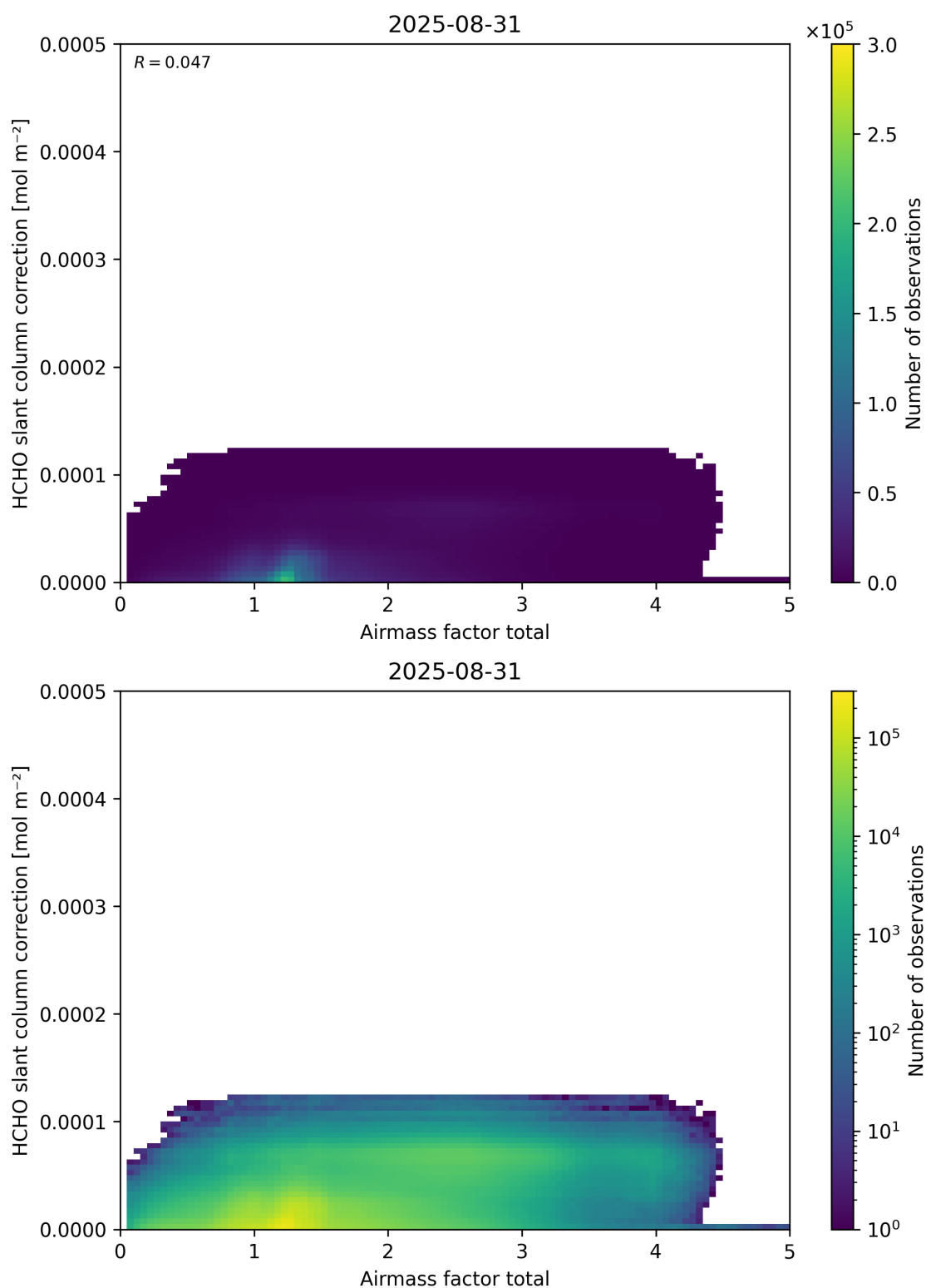
Figure 102: Scatter density plot of “Airmass factor total” against “HCHO slant column correction” for 2025-08-30 to 2025-09-01.
