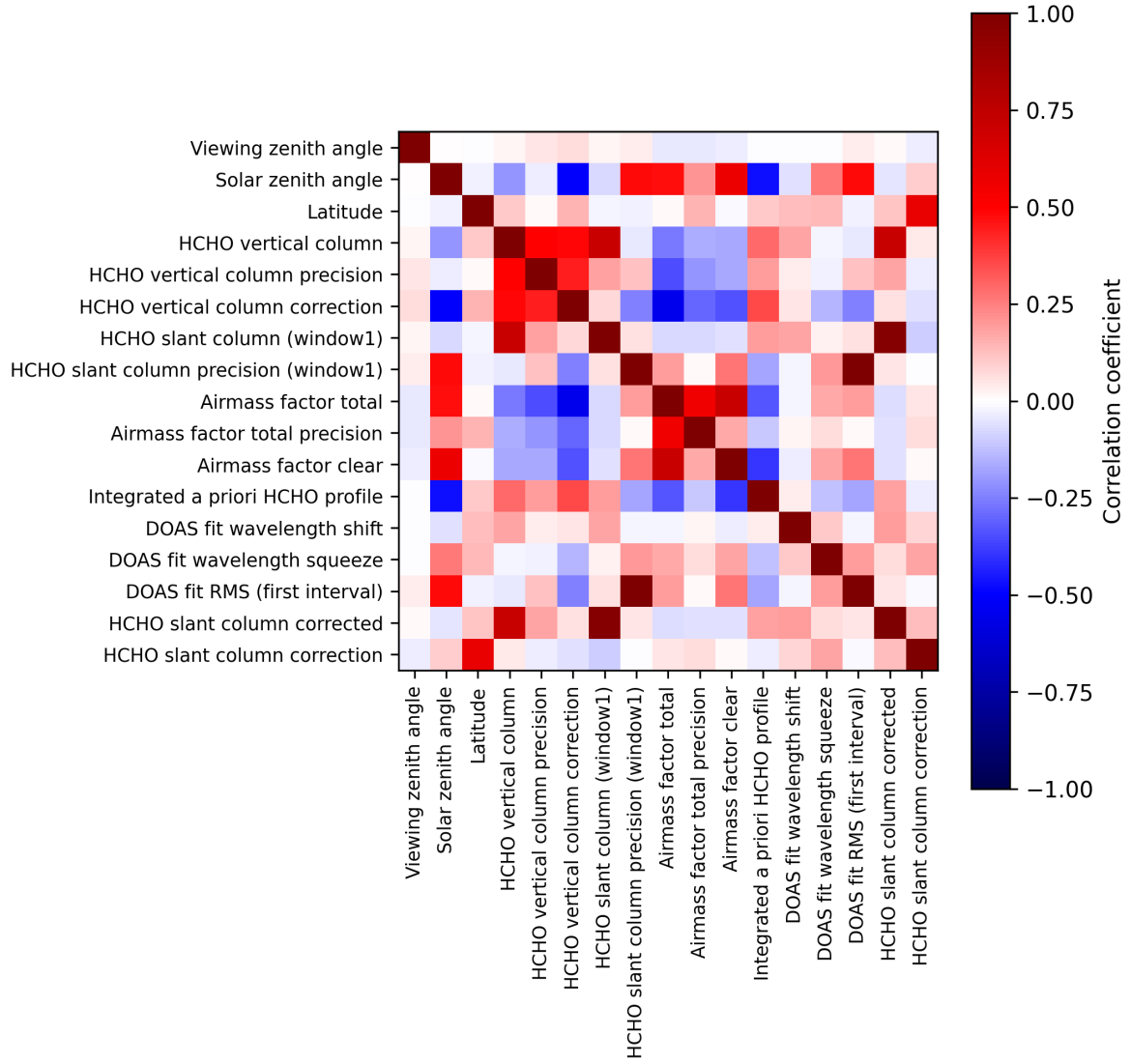
Figure 2: Map of correlation matrix for 2025-08-30 to 2025-09-01.
