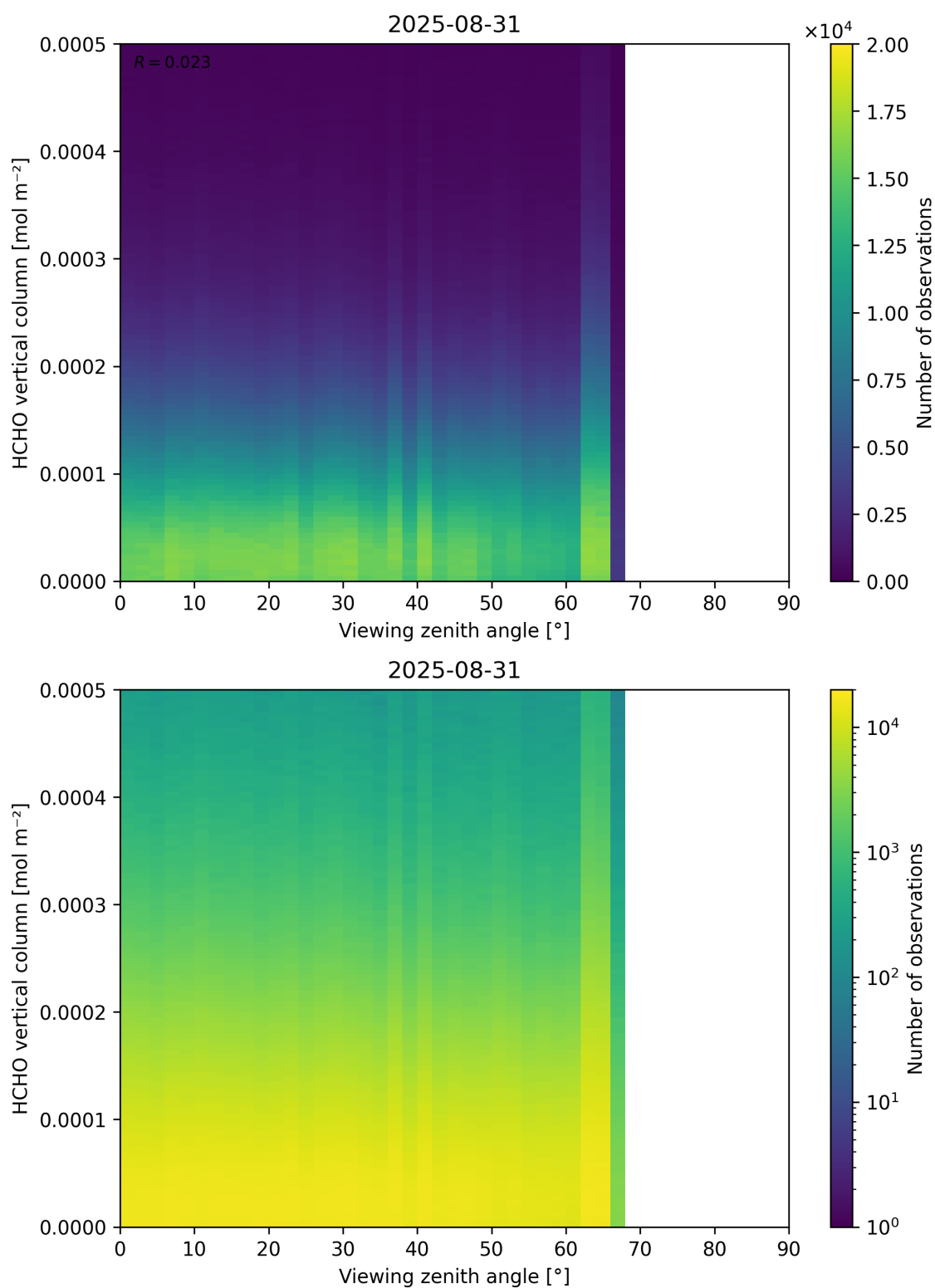
Figure 192: Scatter density plot of “Viewing zenith angle” against “HCHO vertical column” for 2025-08-30 to 2025-09-01.
