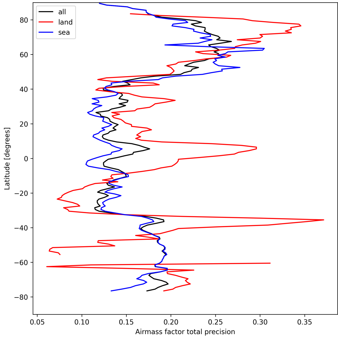
Figure 27: Zonal average of “Airmass factor total precision” for 2025-08-30 to 2025-09-01.
