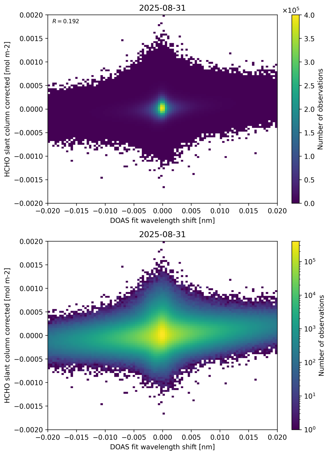
Figure 66: Scatter density plot of “DOAS fit wavelength shift” against “HCHO slant column corrected” for 2025-08-30 to 2025-09-01.
