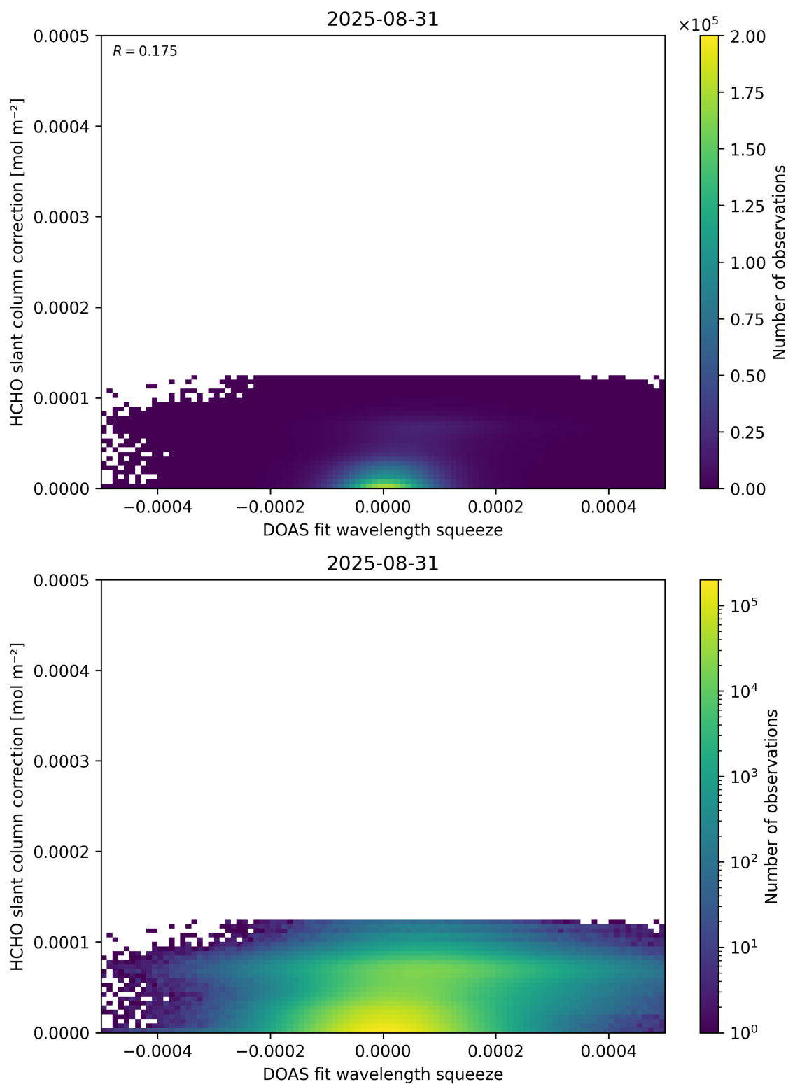
Figure 70: Scatter density plot of “DOAS fit wavelength squeeze” against “HCHO slant column correction” for 2025-08-30 to 2025-09-01.
