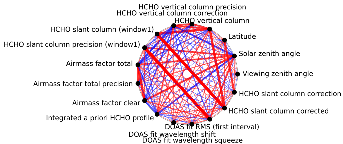
Figure 1: Map of correlation graph for 2025-08-30 to 2025-09-01.
