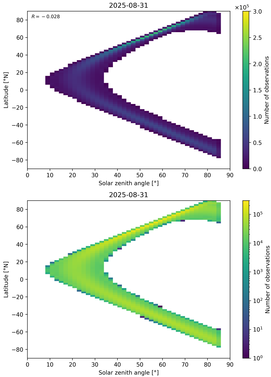
Figure 181: Scatter density plot of “Solar zenith angle” against “Latitude” for 2025-08-30 to 2025-09-01.
