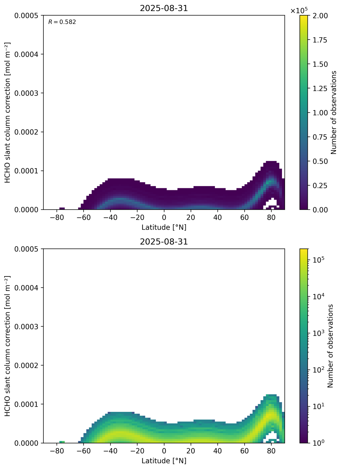
Figure 158: Scatter density plot of “Latitude” against “HCHO slant column correction” for 2025-08-30 to 2025-09-01.
