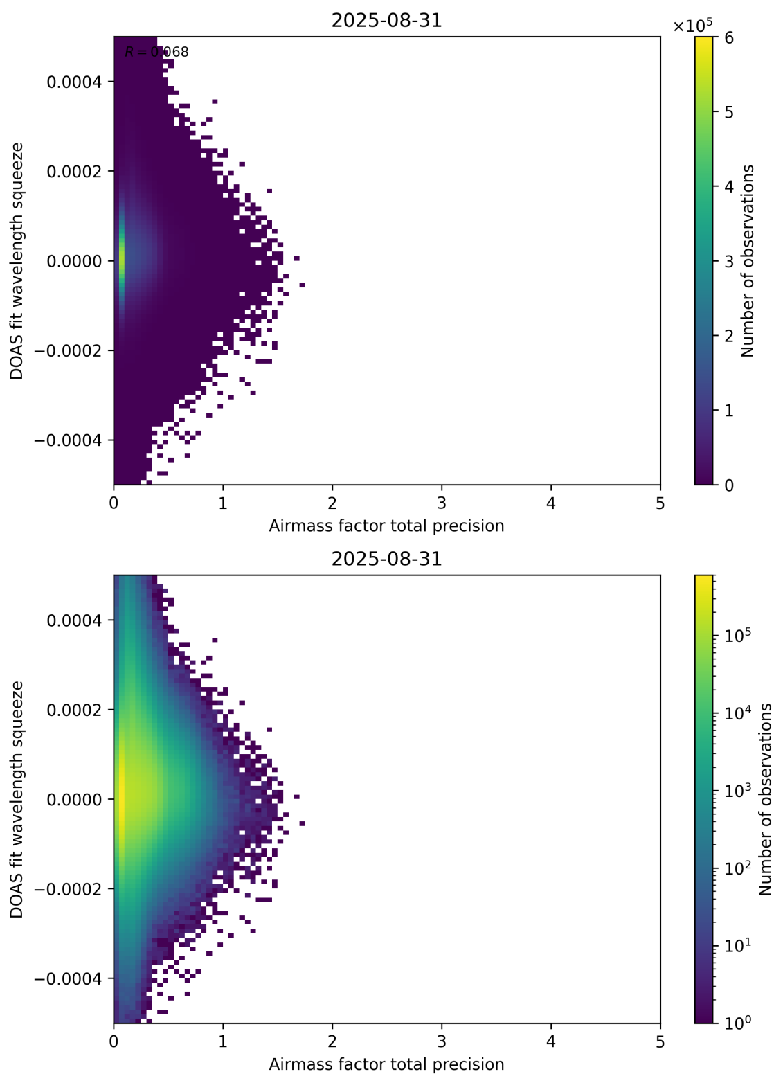
Figure 107: Scatter density plot of “Airmass factor total precision” against “DOAS fit wavelength squeeze” for 2025-08-30 to 2025-09-01.
