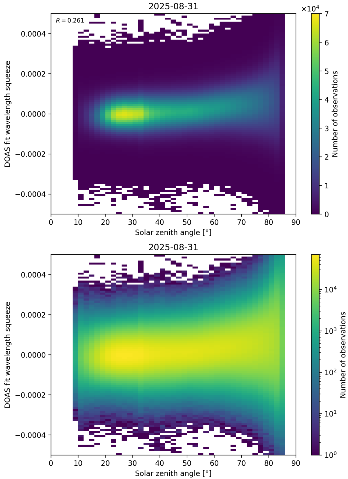
Figure 169: Scatter density plot of “Solar zenith angle” against “DOAS fit wavelength squeeze” for 2025-08-30 to 2025-09-01.
