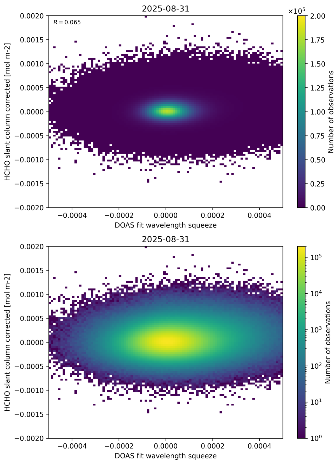
Figure 69: Scatter density plot of “DOAS fit wavelength squeeze” against “HCHO slant column corrected” for 2025-08-30 to 2025-09-01.
