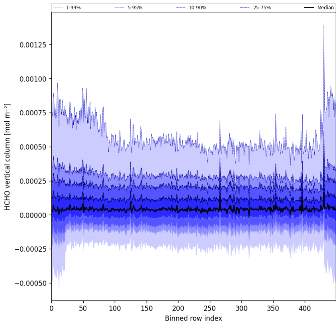
Figure 49: Along track statistics of “HCHO vertical column” for 2025-08-30 to 2025-09-01
