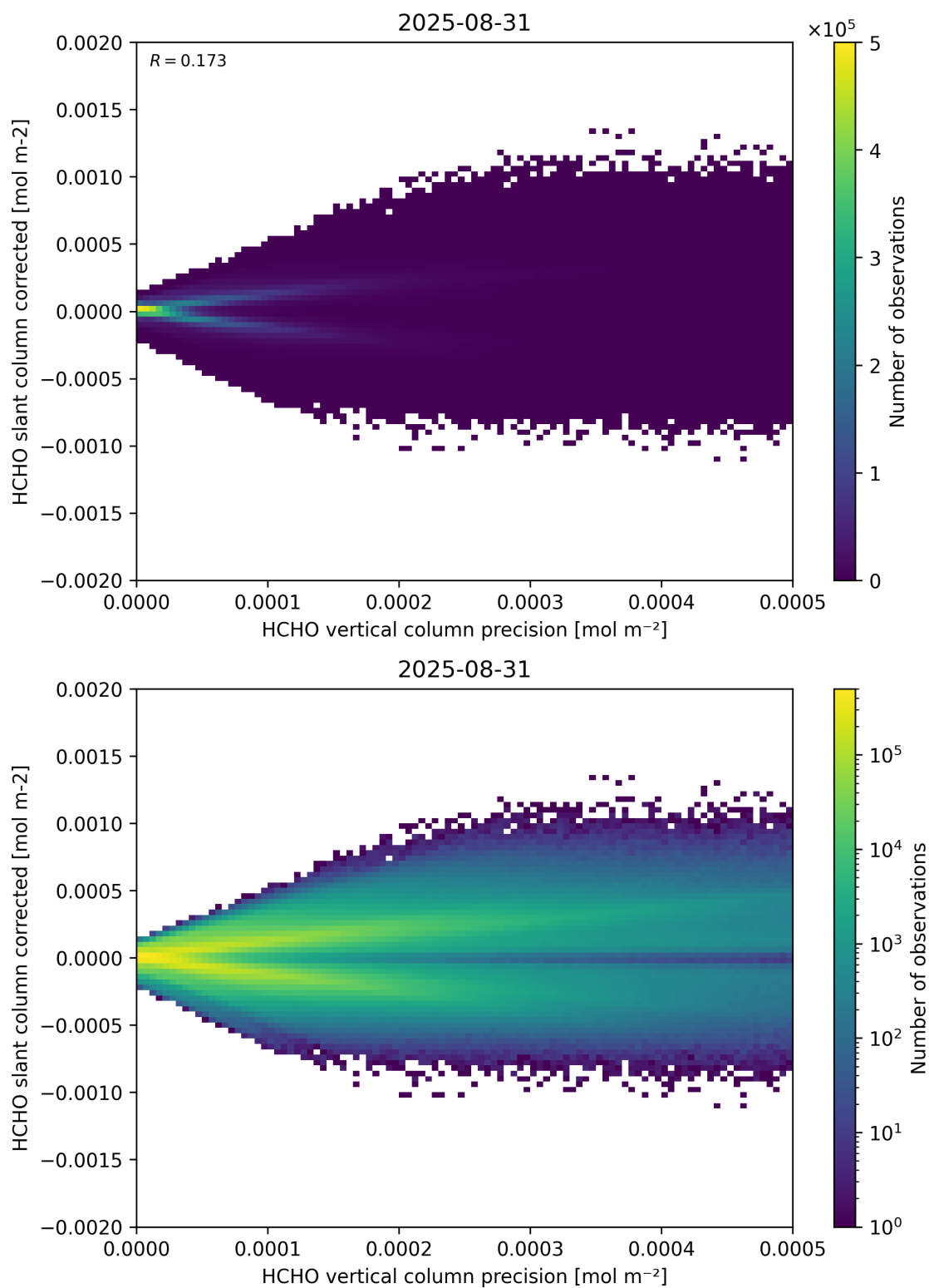
Figure 140: Scatter density plot of “HCHO vertical column precision” against “HCHO slant column corrected” for 2025-08-30 to 2025-09-01.
