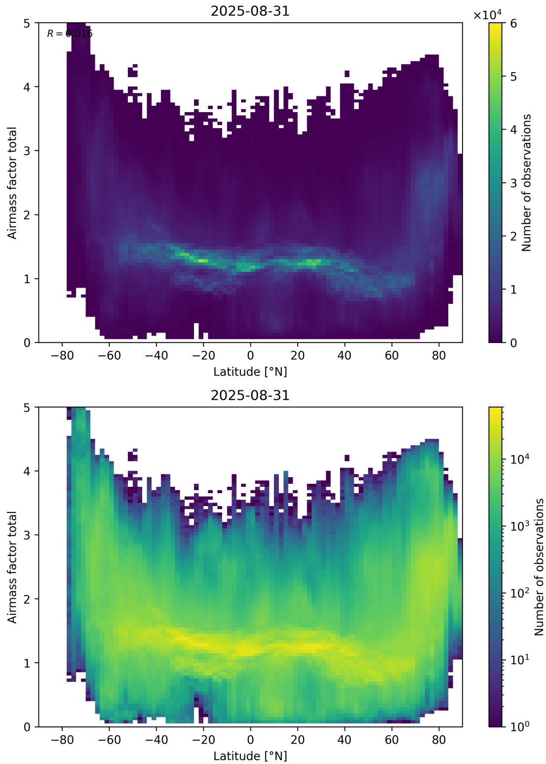
Figure 161: Scatter density plot of “Latitude” against “Airmass factor total” for 2025-08-30 to 2025-09-01.
