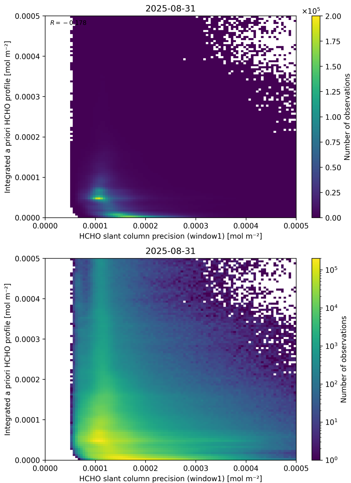
Figure 96: Scatter density plot of “HCHO slant column precision (window1)” against “Integrated a priori HCHO profile” for 2025-08-30 to 2025-09-01.
