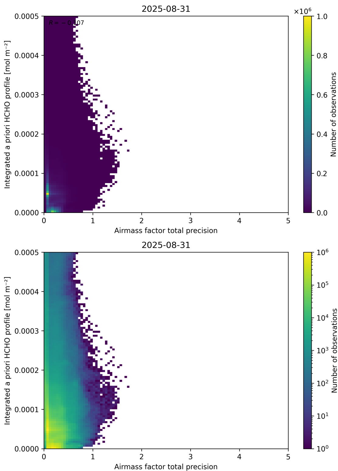
Figure 111: Scatter density plot of “Airmass factor total precision” against “Integrated a priori HCHO profile” for 2025-08-30 to 2025-09-01.
