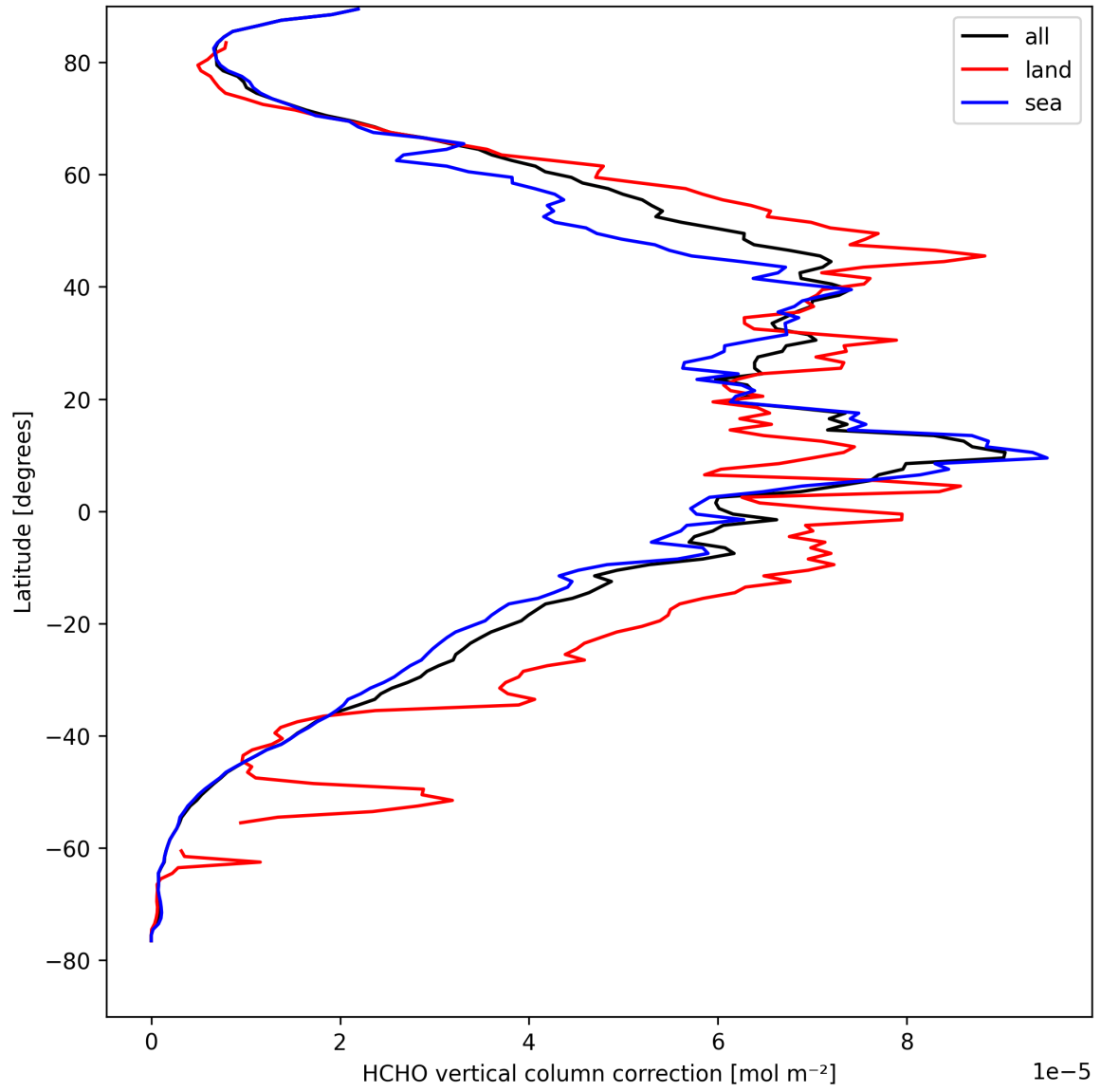
Figure 23: Zonal average of "HCHO vertical column correction" for 2025-08-30 to 2025-09-01.
