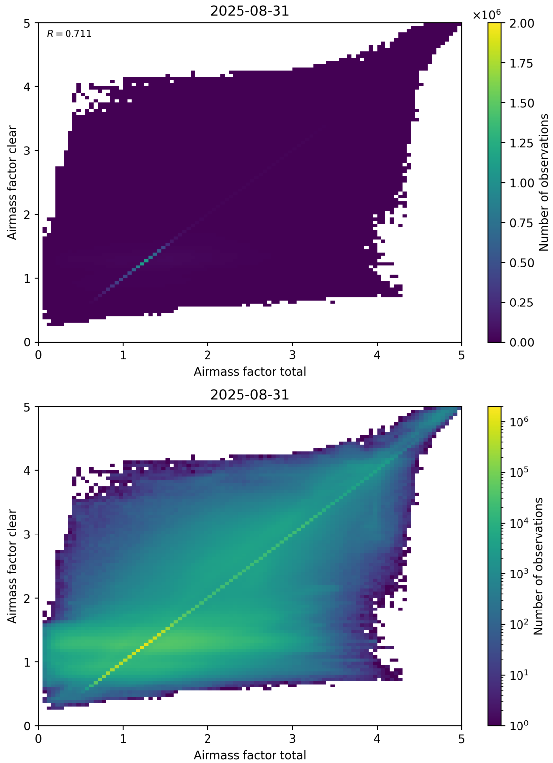
Figure 100: Scatter density plot of “Airmass factor total” against “Airmass factor clear” for 2025-08-30 to 2025-09-01.
