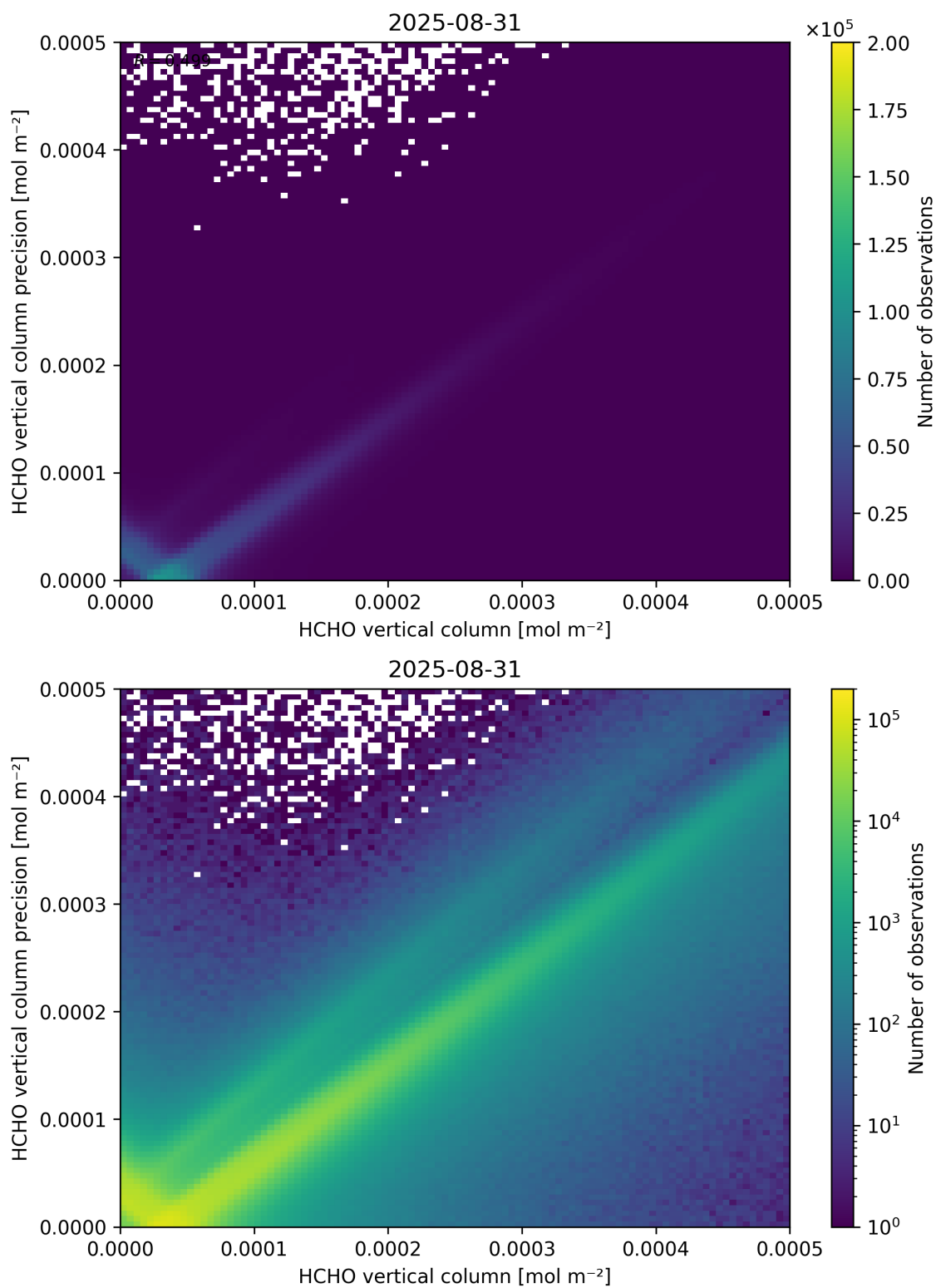
Figure 134: Scatter density plot of “HCHO vertical column” against “HCHO vertical column precision” for 2025-08-30 to 2025-09-01.
