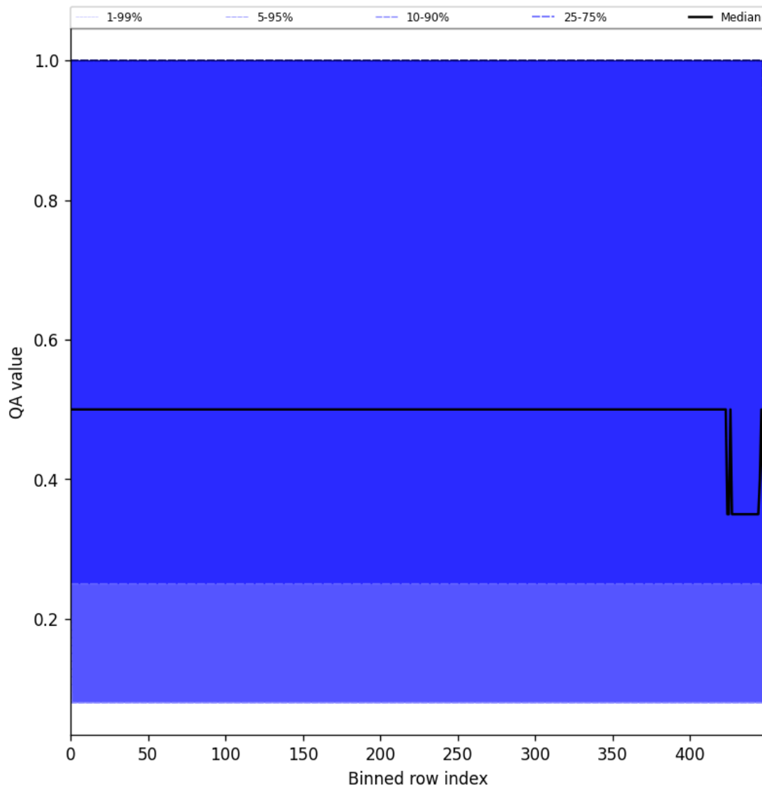
Figure 48: Along track statistics of “QA value” for 2025-08-30 to 2025-09-01
