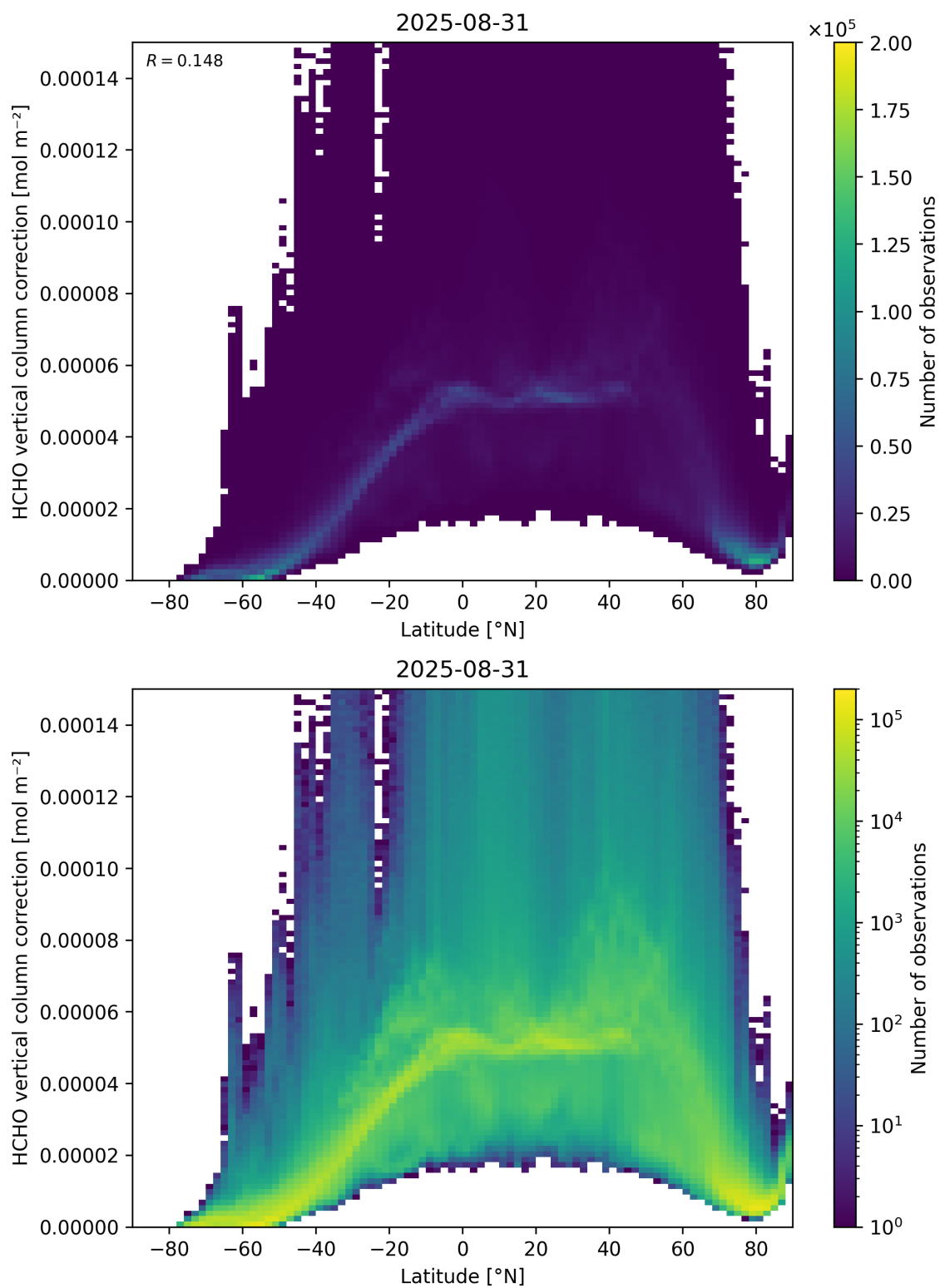
Figure 164: Scatter density plot of “Latitude” against “HCHO vertical column correction” for 2025-08-30 to 2025-09-01.
