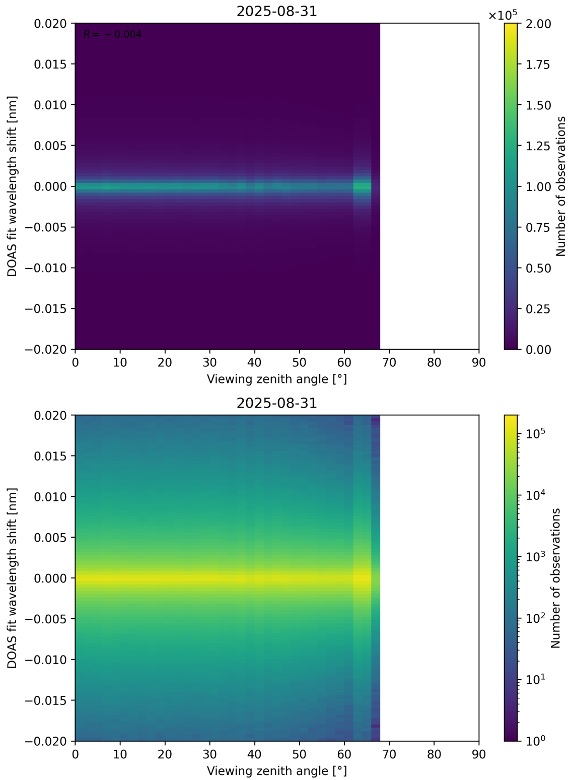
Figure 183: Scatter density plot of “Viewing zenith angle” against “DOAS fit wavelength shift” for 2025-08-30 to 2025-09-01.
