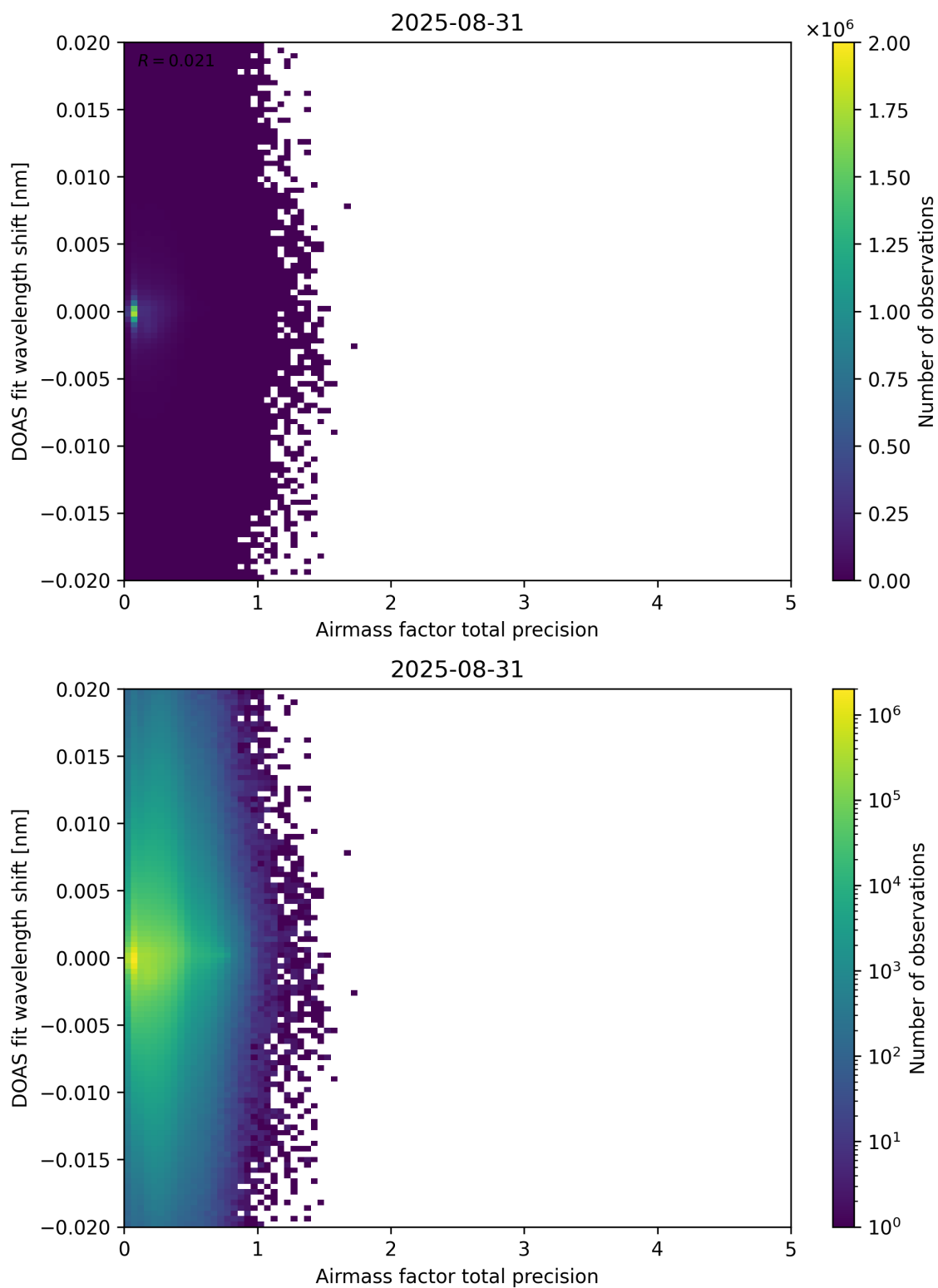
Figure 106: Scatter density plot of “Airmass factor total precision” against “DOAS fit wavelength shift” for 2025-08-30 to 2025-09-01.
