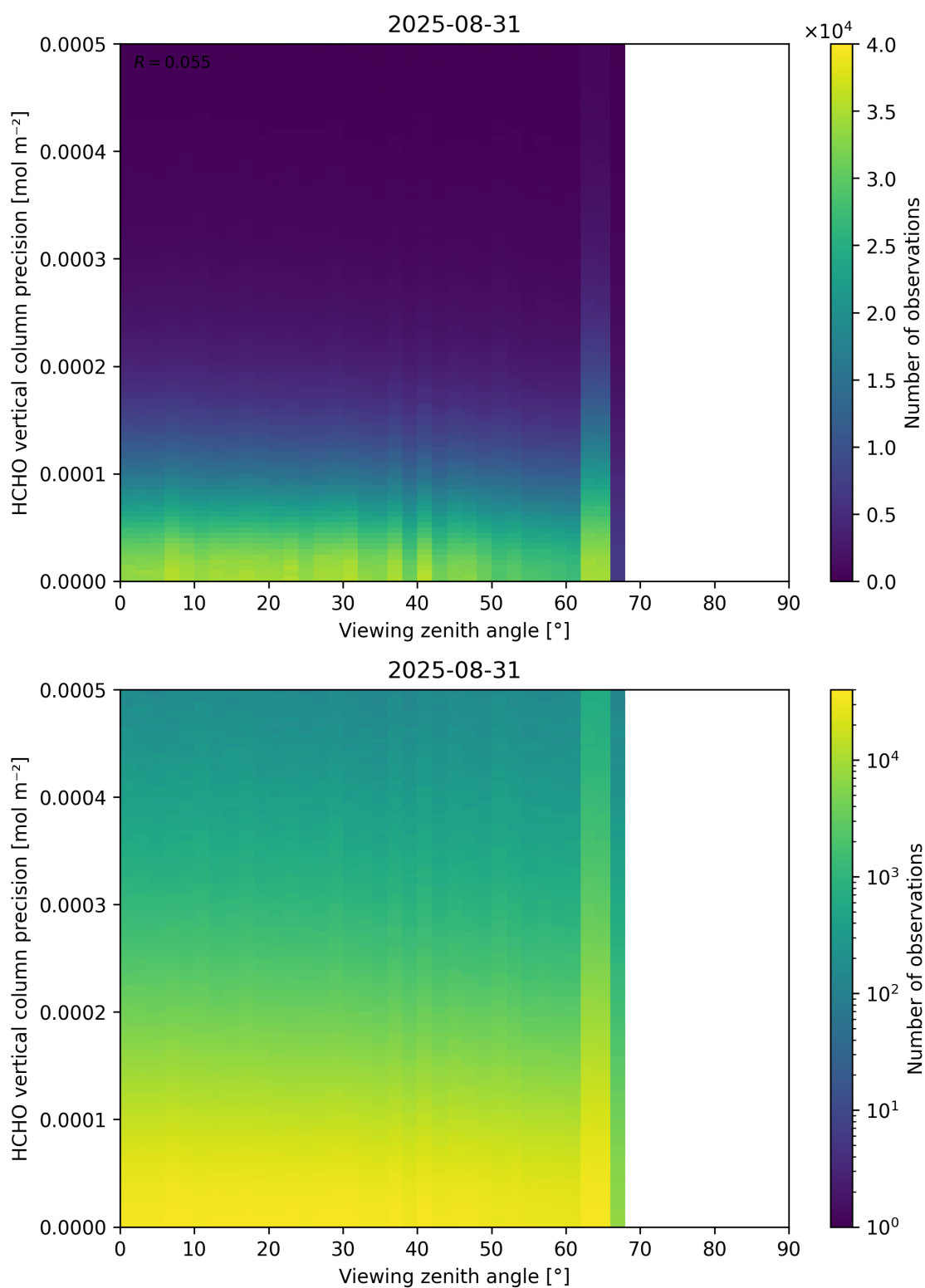
Figure 194: Scatter density plot of “Viewing zenith angle” against “HCHO vertical column precision” for 2025-08-30 to 2025-09-01.
