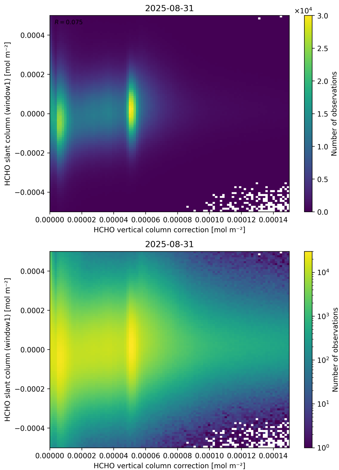
Figure 118: Scatter density plot of “HCHO vertical column correction” against “HCHO slant column (window1)” for 2025-08-30 to 2025-09-01.
