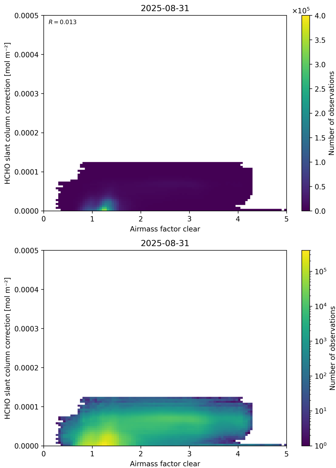
Figure 75: Scatter density plot of “Air mass factor clear” against “HCHO slant column correction” for 2025-08-30 to 2025-09-01.
