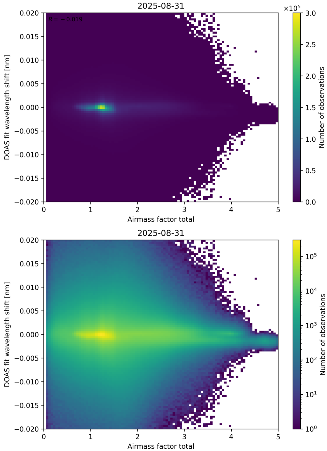
Figure 98: Scatter density plot of “Airmass factor total” against “DOAS fit wavelength shift” for 2025-08-30 to 2025-09-01.
