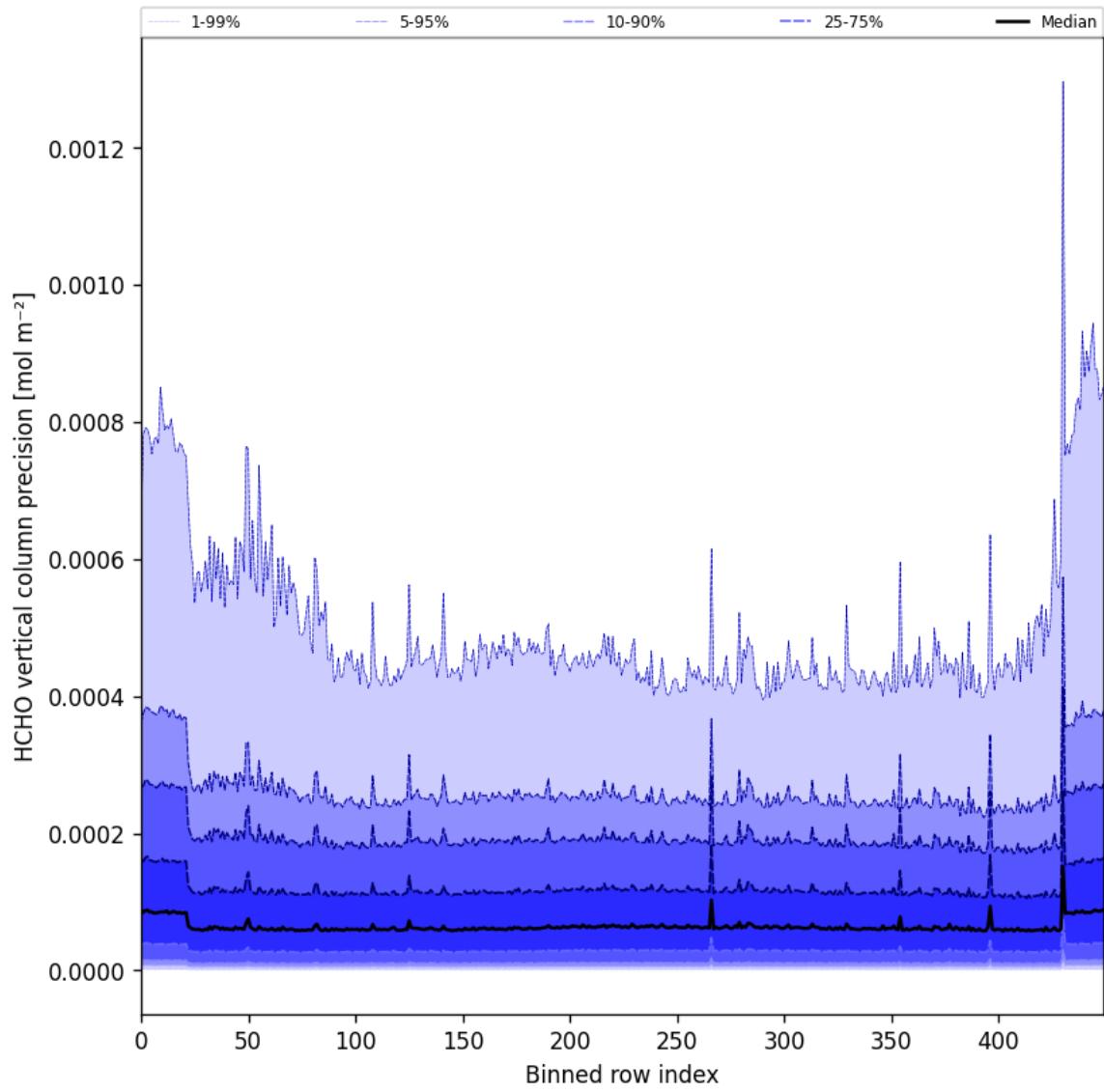
Figure 50: Along track statistics of “HCHO vertical column precision” for 2025-08-30 to 2025-09-01
