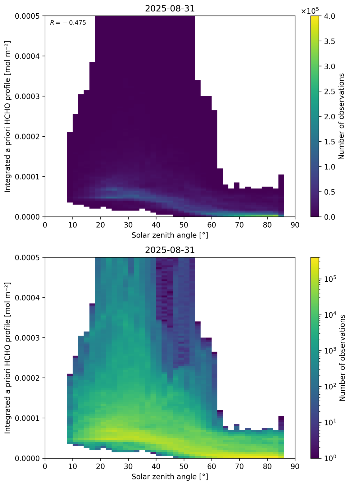
Figure 180: Scatter density plot of “Solar zenith angle” against “Integrated a priori HCHO profile” for 2025-08-30 to 2025-09-01.
