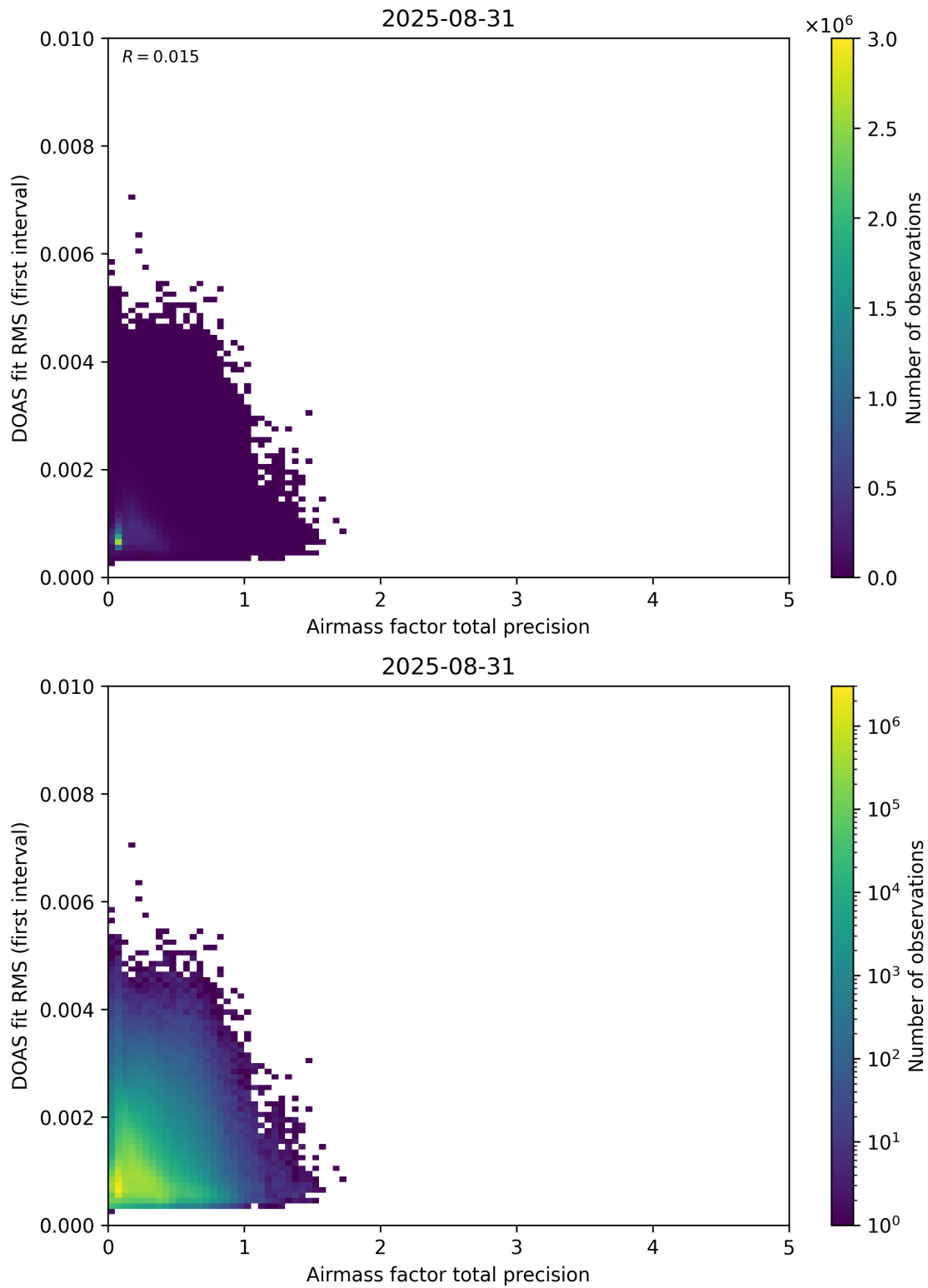
Figure 105: Scatter density plot of “Airmass factor total precision” against “DOAS fit RMS (first interval)” for 2025-08-30 to 2025-09-01.
