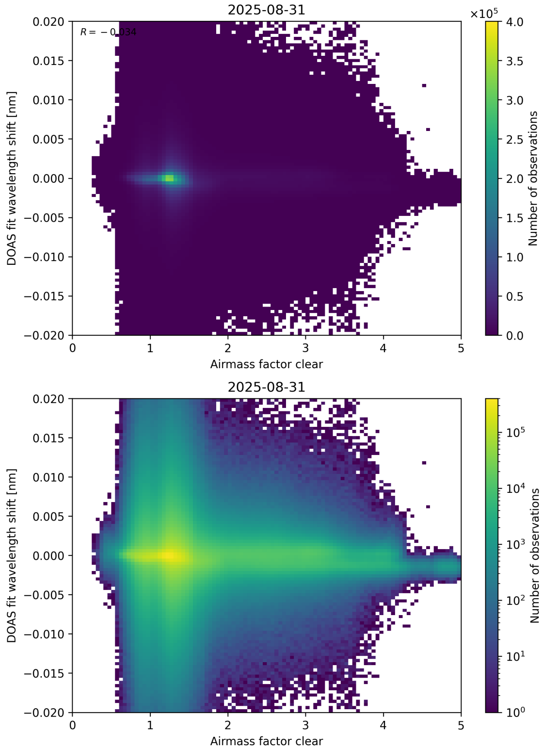
Figure 72: Scatter density plot of “Airmass factor clear” against “DOAS fit wavelength shift” for 2025-08-30 to 2025-09-01.
