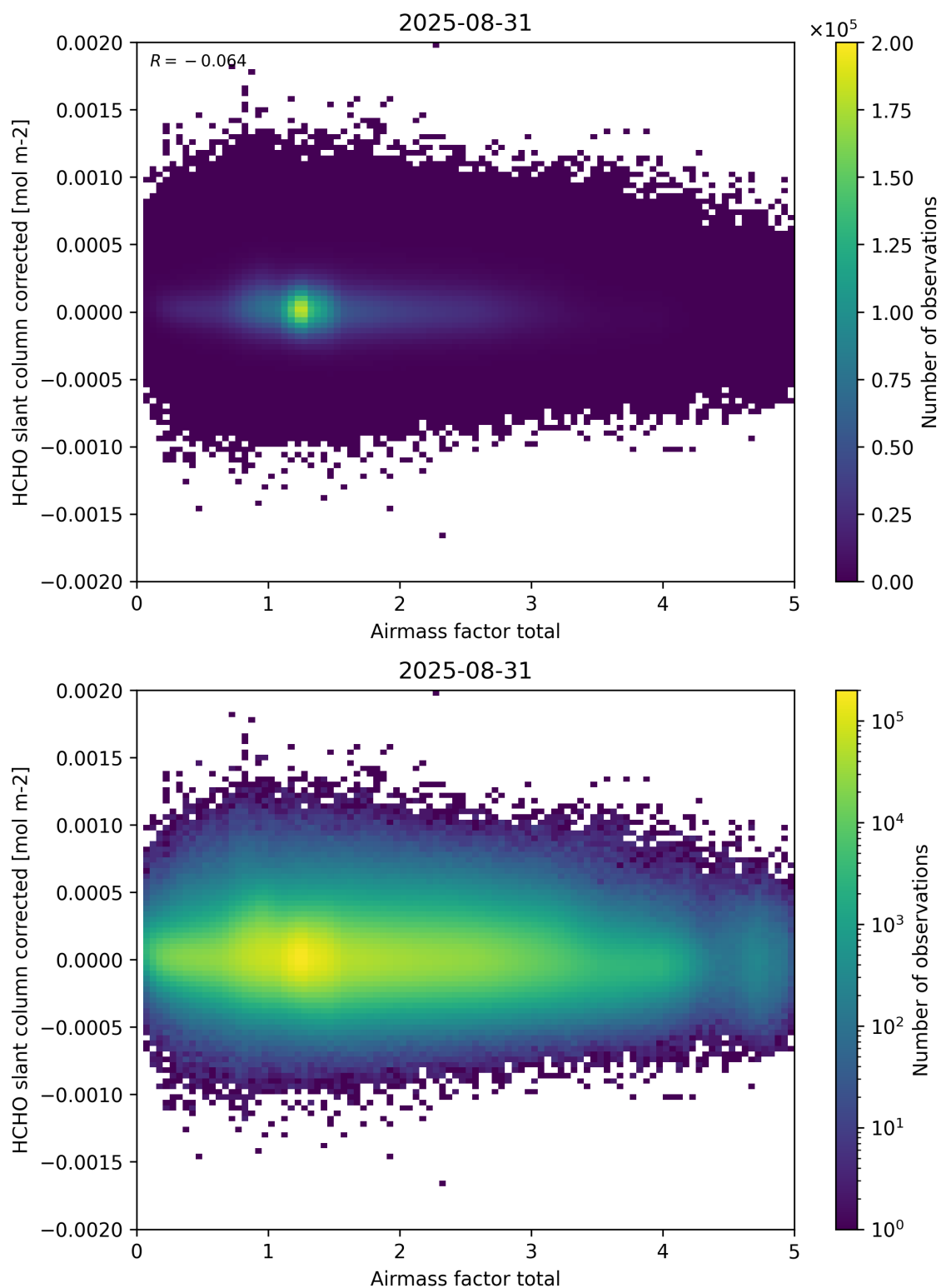
Figure 101: Scatter density plot of “Airmass factor total” against “HCHO slant column corrected” for 2025-08-30 to 2025-09-01.
