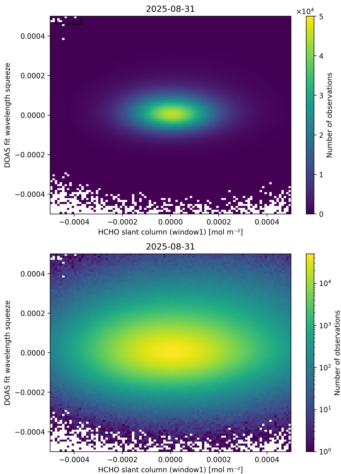
Figure 80: Scatter density plot of “HCHO slant column (window1)” against “DOAS fit wavelength squeeze” for 2025-08-30 to 2025-09-01.
