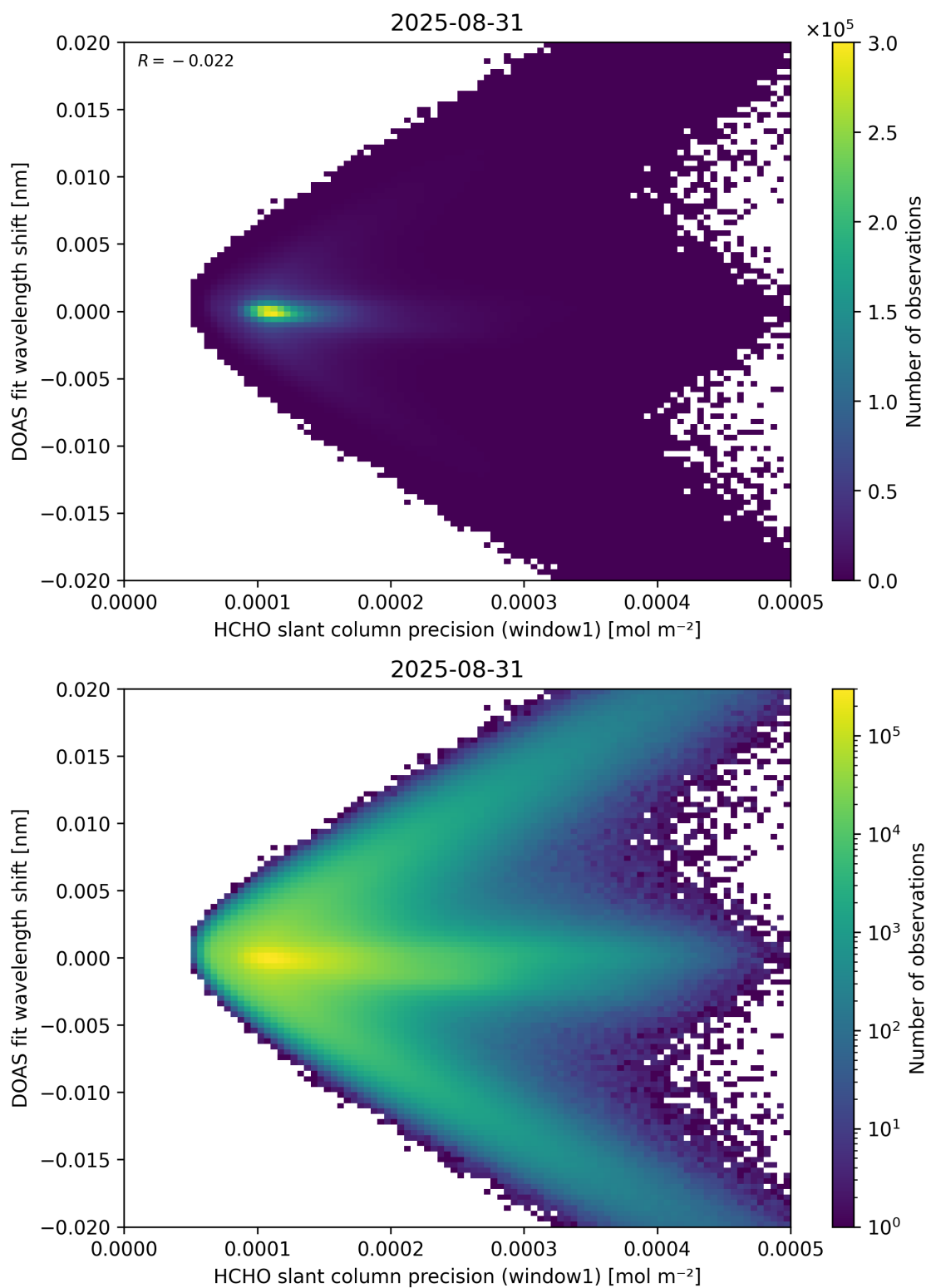
Figure 89: Scatter density plot of “HCHO slant column precision (window1)” against “DOAS fit wavelength shift” for 2025-08-30 to 2025-09-01.
