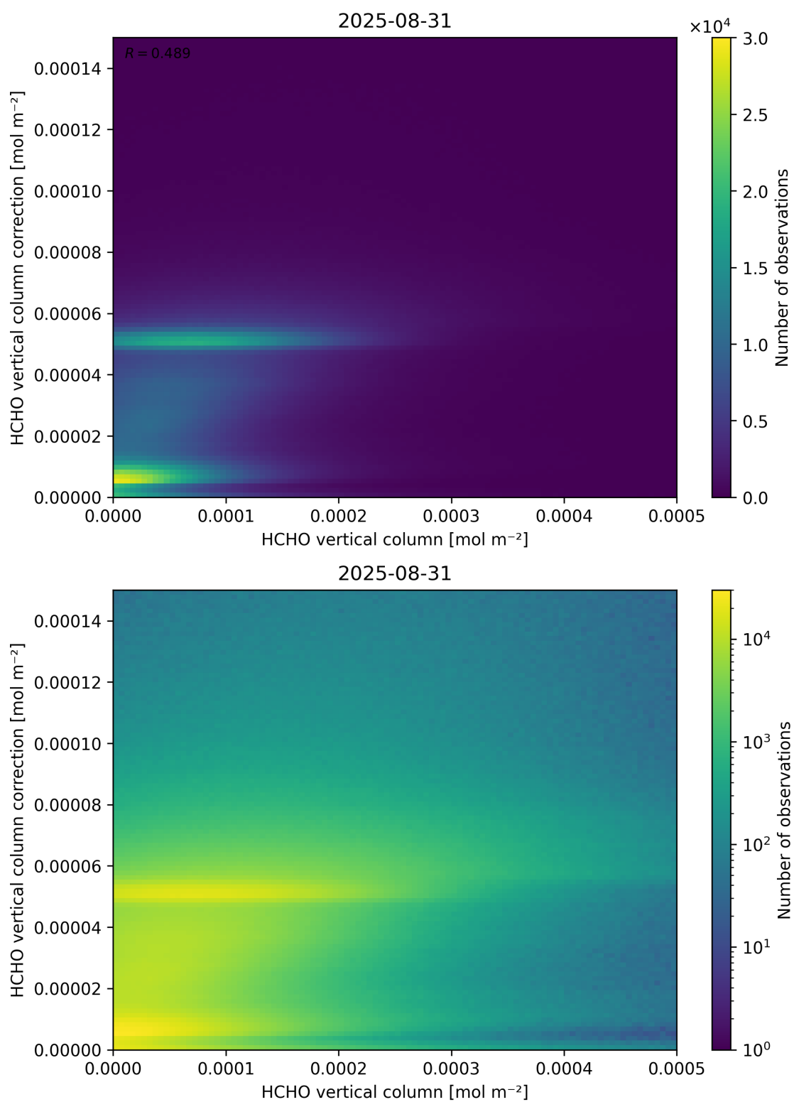
Figure 133: Scatter density plot of “HCHO vertical column” against “HCHO vertical column correction” for 2025-08-30 to 2025-09-01.
