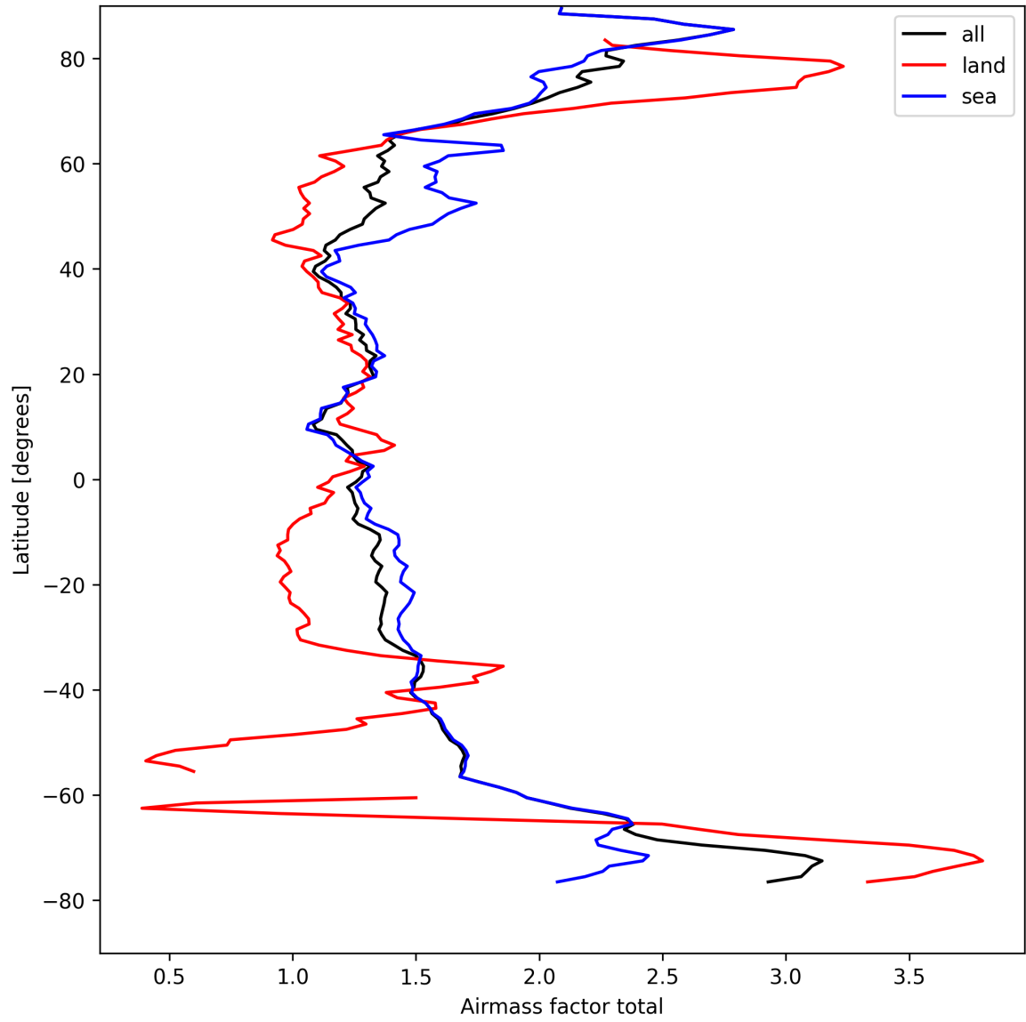
Figure 26: Zonal average of “Airmass factor total” for 2025-08-30 to 2025-09-01.
