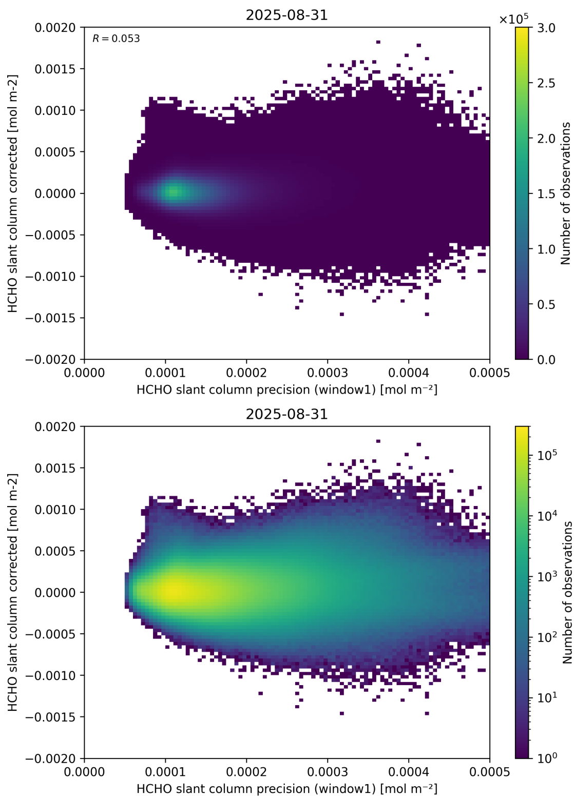
Figure 92: Scatter density plot of “HCHO slant column precision (window1)” against “HCHO slant column corrected” for 2025-08-30 to 2025-09-01.
