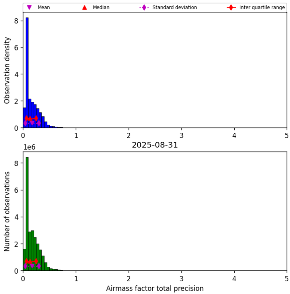
Figure 41: Histogram of “Airmass factor total precision” for 2025-08-30 to 2025-09-01
