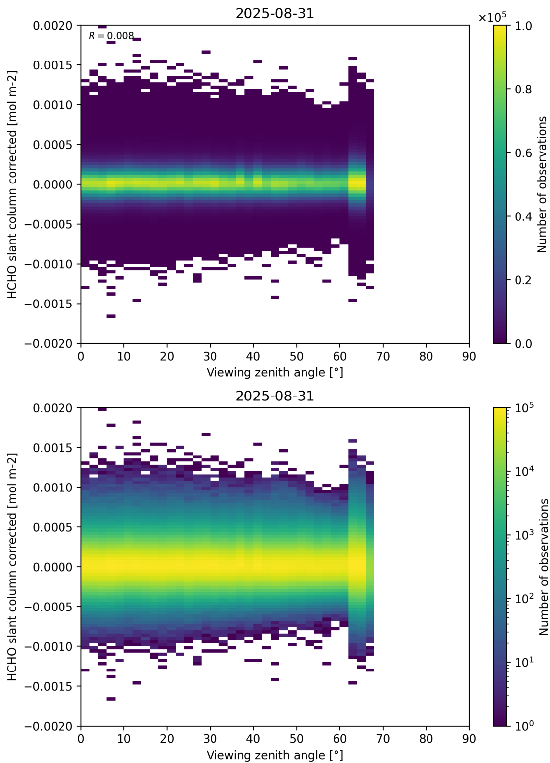
Figure 186: Scatter density plot of “Viewing zenith angle” against “HCHO slant column corrected” for 2025-08-30 to 2025-09-01.
