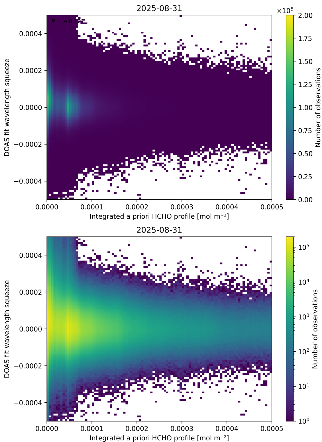
Figure 150: Scatter density plot of “Integrated a priori HCHO profile” against “DOAS fit wavelength squeeze” for 2025-08-30 to 2025-09-01.
