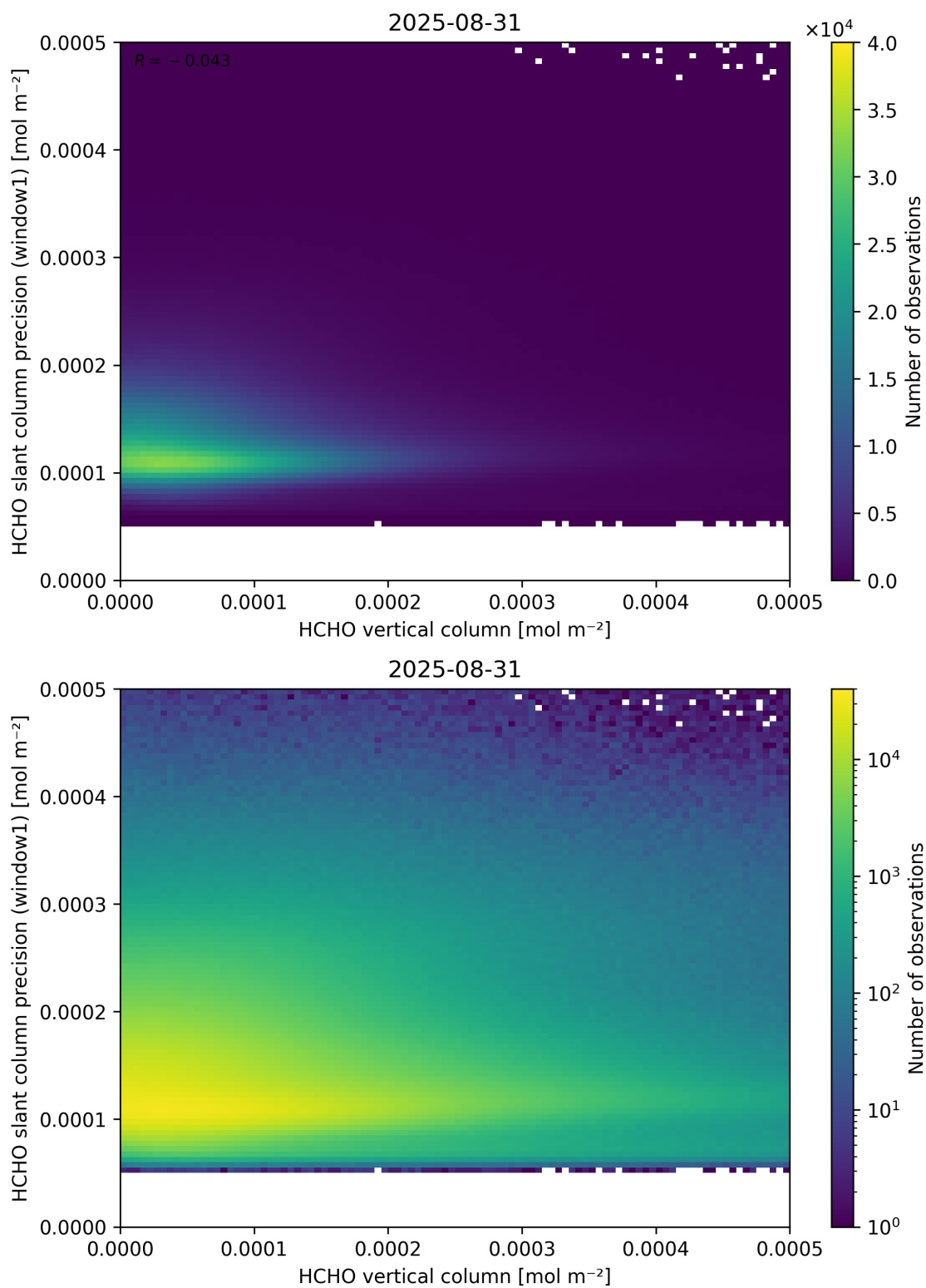
Figure 130: Scatter density plot of “HCHO vertical column” against “HCHO slant column precision (window1)” for 2025-08-30 to 2025-09-01.
