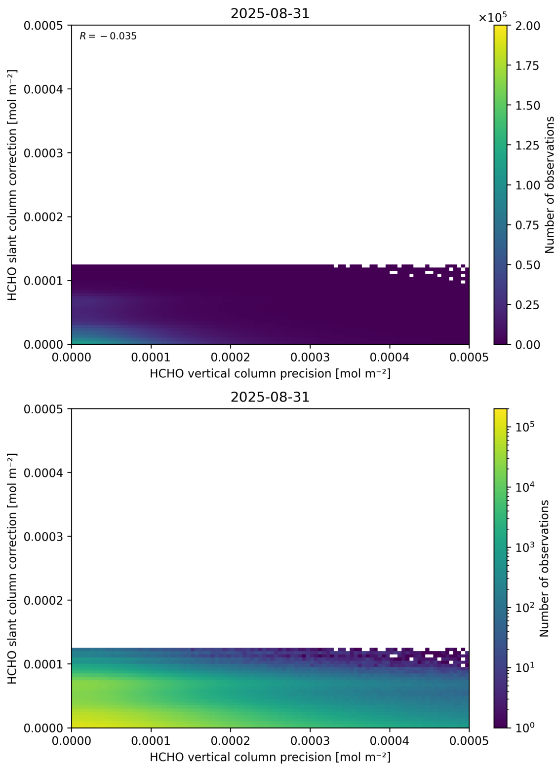
Figure 141: Scatter density plot of “HCHO vertical column precision” against “HCHO slant column correction” for 2025-08-30 to 2025-09-01.
