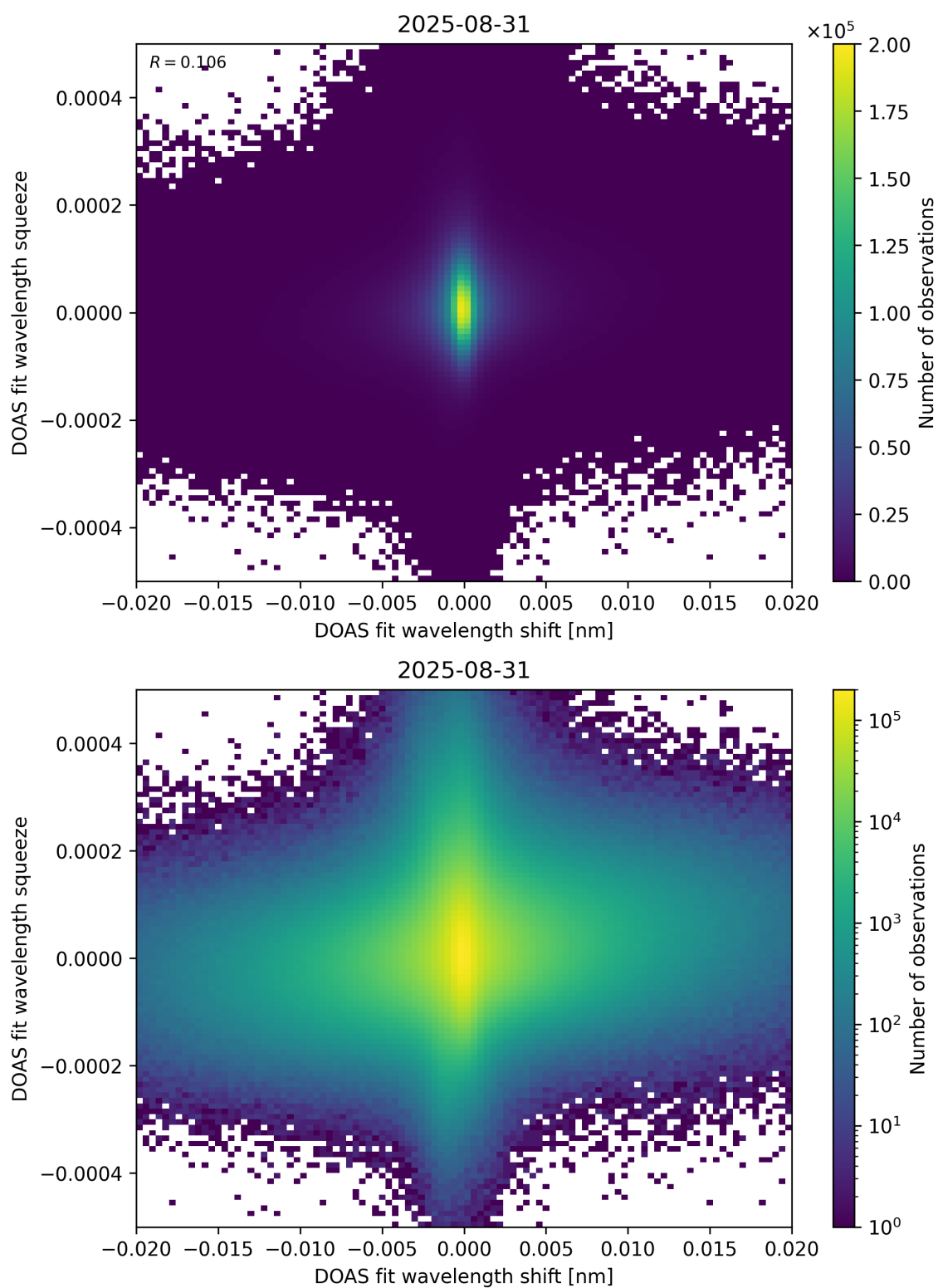
Figure 65: Scatter density plot of “DOAS fit wavelength shift” against “DOAS fit wavelength squeeze” for 2025-08-30 to 2025-09-01.
