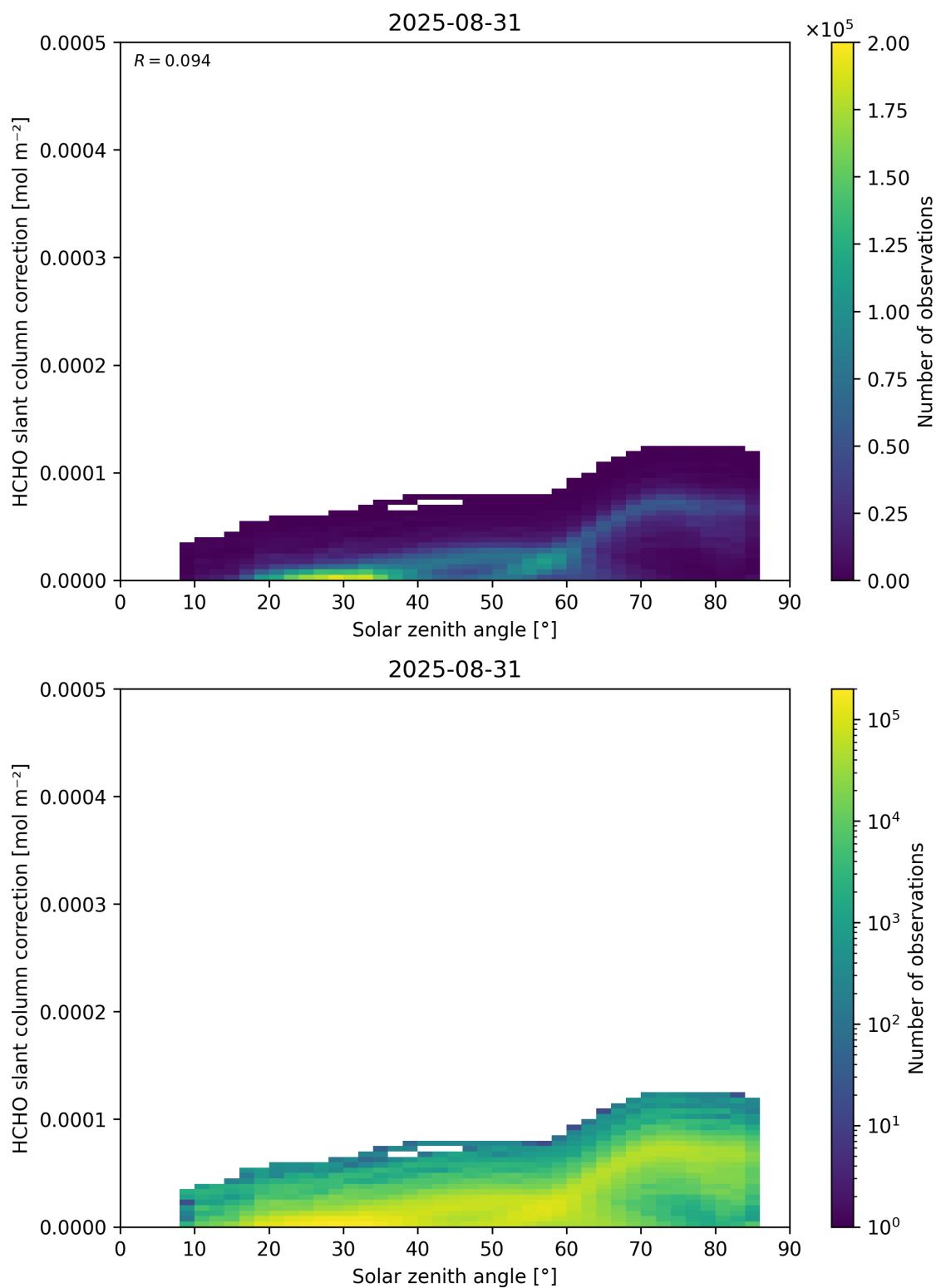
Figure 172: Scatter density plot of “Solar zenith angle” against “HCHO slant column correction” for 2025-08-30 to 2025-09-01.
