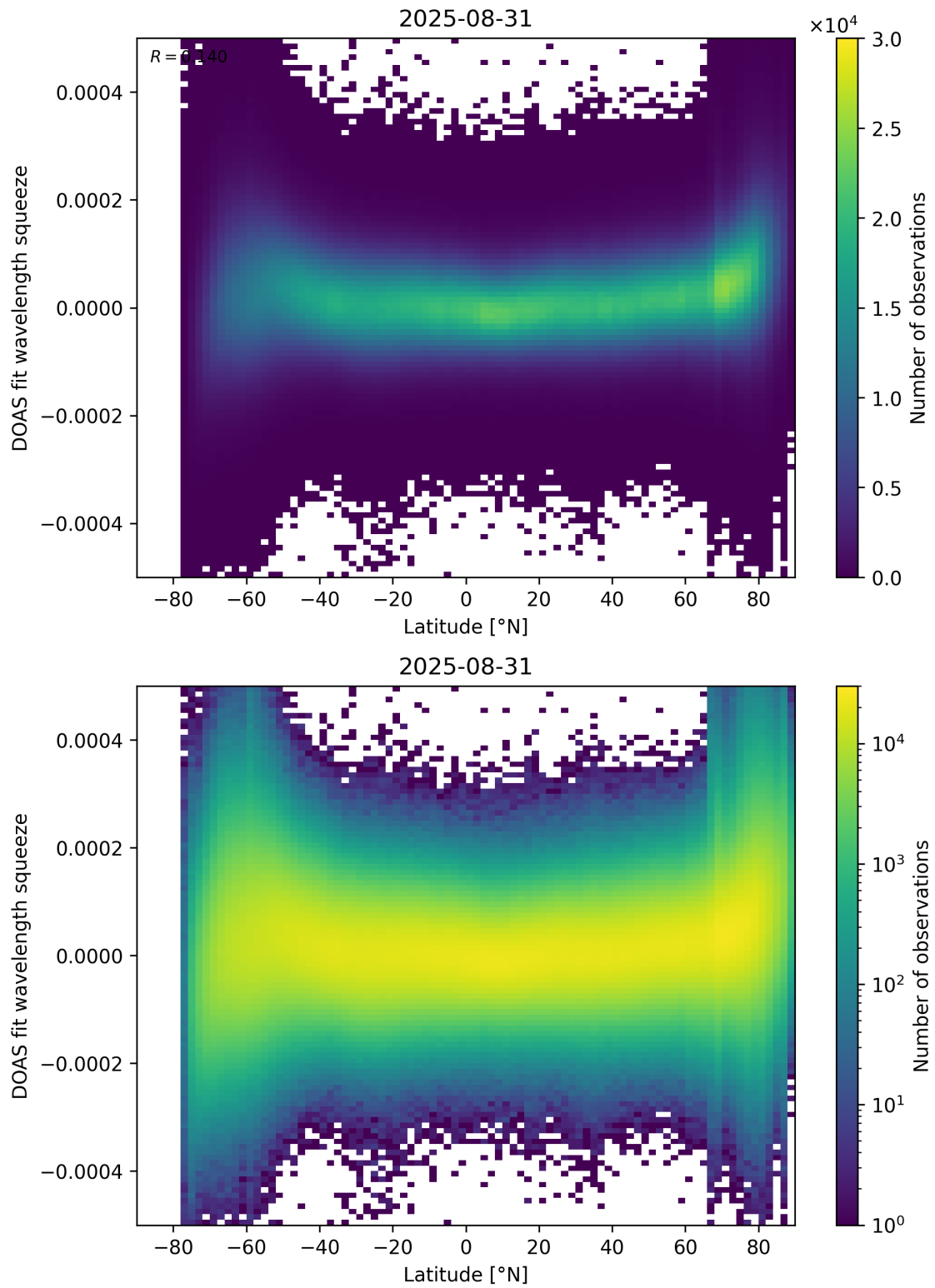
Figure 155: Scatter density plot of “Latitude” against “DOAS fit wavelength squeeze” for 2025-08-30 to 2025-09-01.
