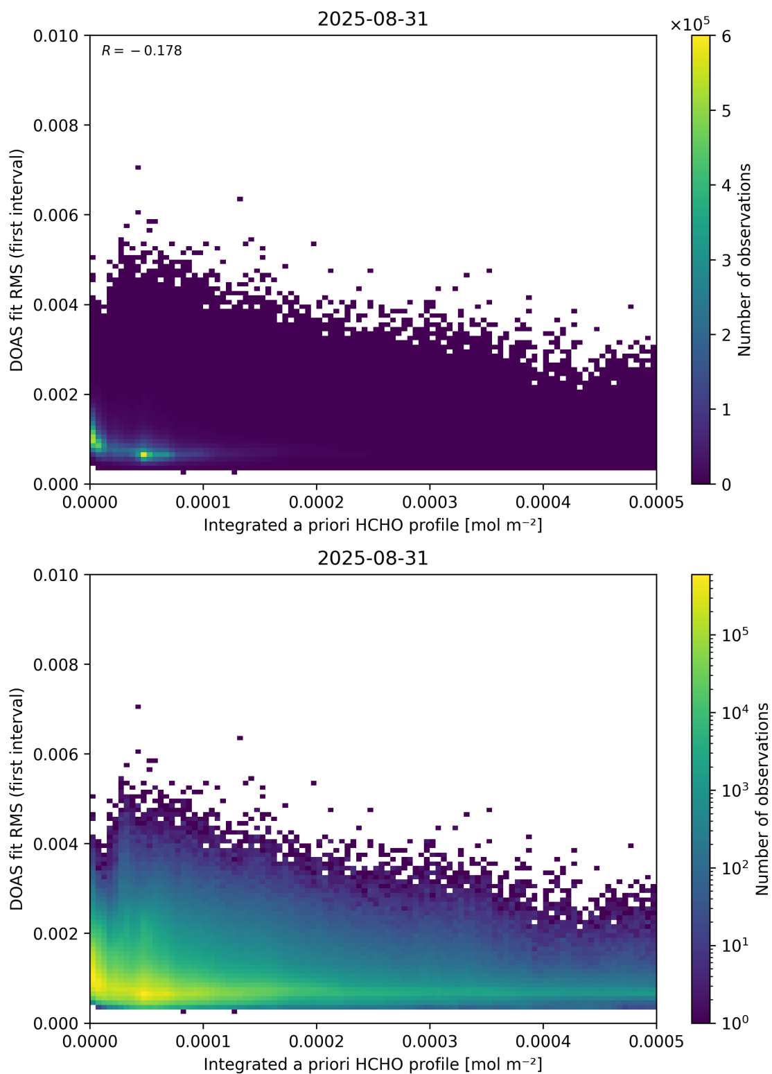
Figure 148: Scatter density plot of “Integrated a priori HCHO profile” against “DOAS fit RMS (first interval)” for 2025-08-30 to 2025-09-01.
