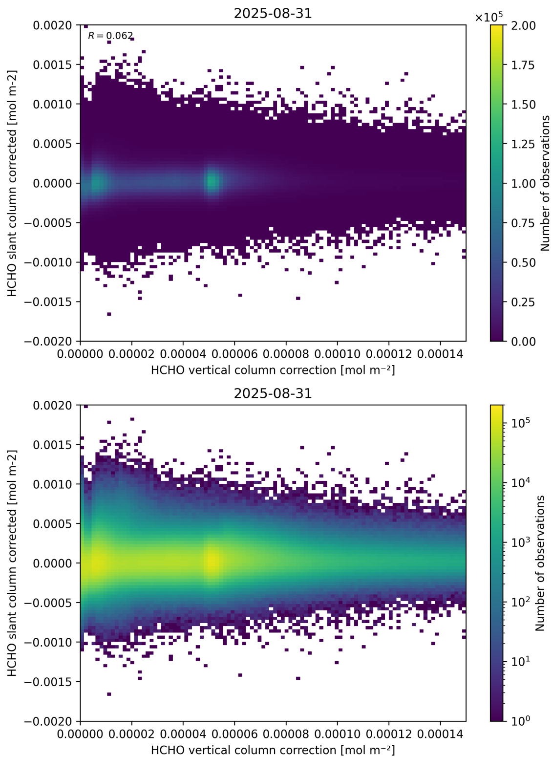
Figure 116: Scatter density plot of “HCHO vertical column correction” against “HCHO slant column corrected” for 2025-08-30 to 2025-09-01.
