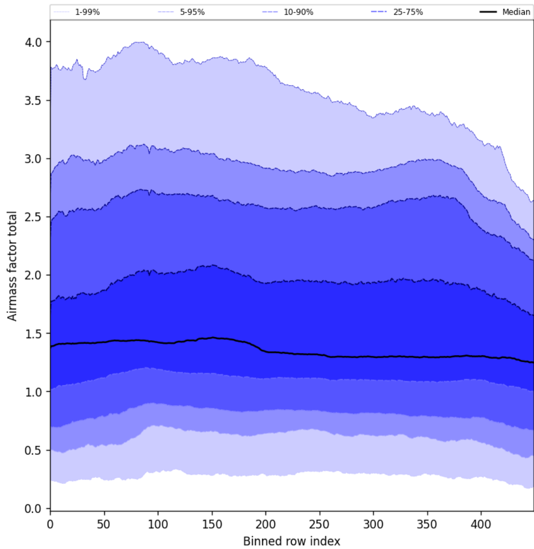
Figure 54: Along track statistics of “Airmass factor total” for 2025-08-30 to 2025-09-01
