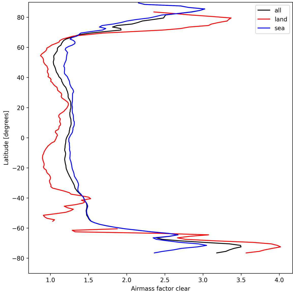
Figure 28: Zonal average of “Airmass factor clear” for 2025-08-30 to 2025-09-01.
