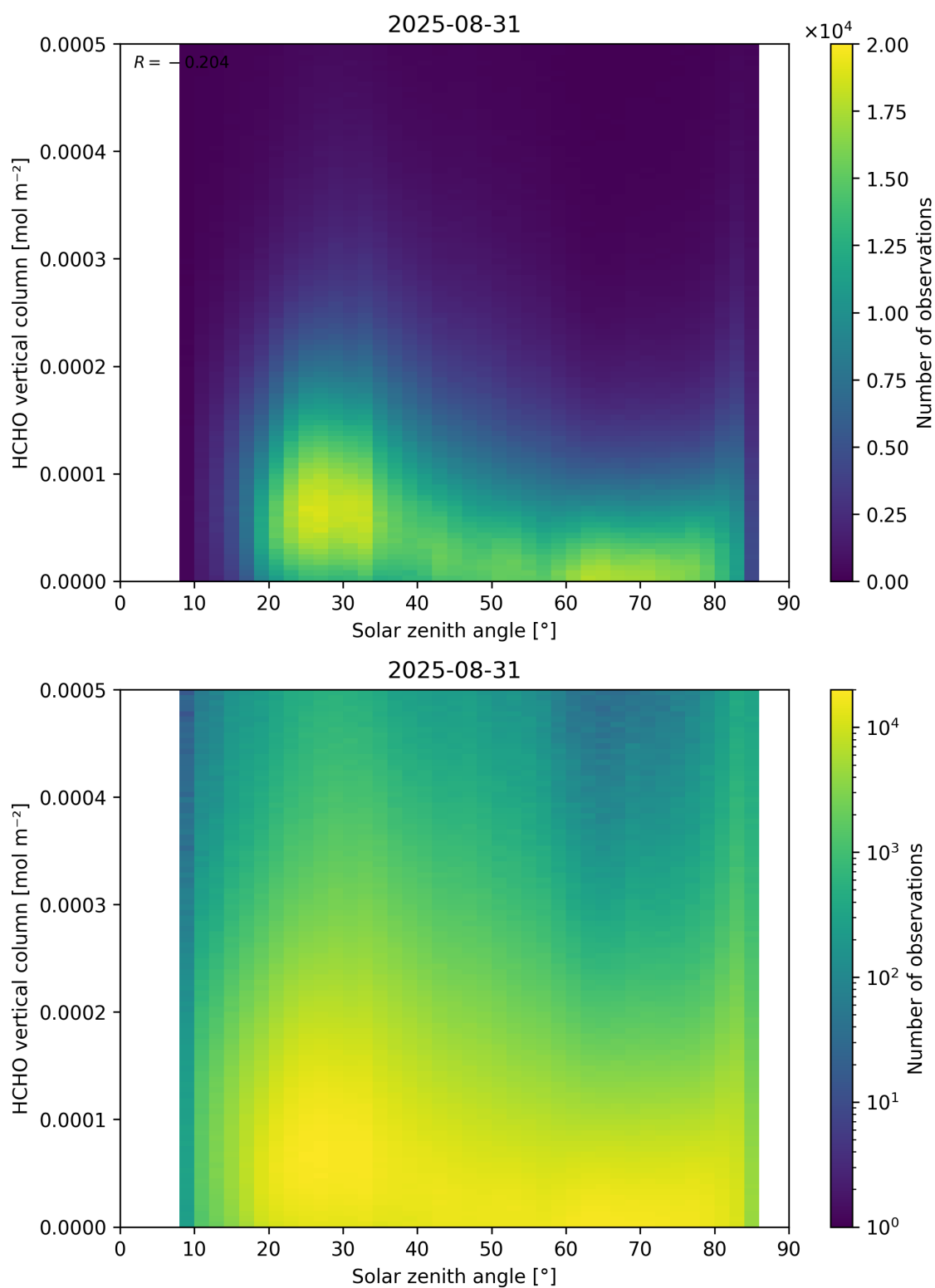
Figure 177: Scatter density plot of “Solar zenith angle” against “HCHO vertical column” for 2025-08-30 to 2025-09-01.
