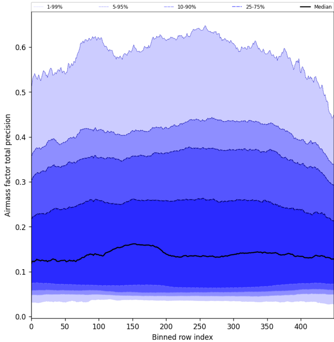
Figure 55: Along track statistics of “Airmass factor total precision” for 2025-08-30 to 2025-09-01
