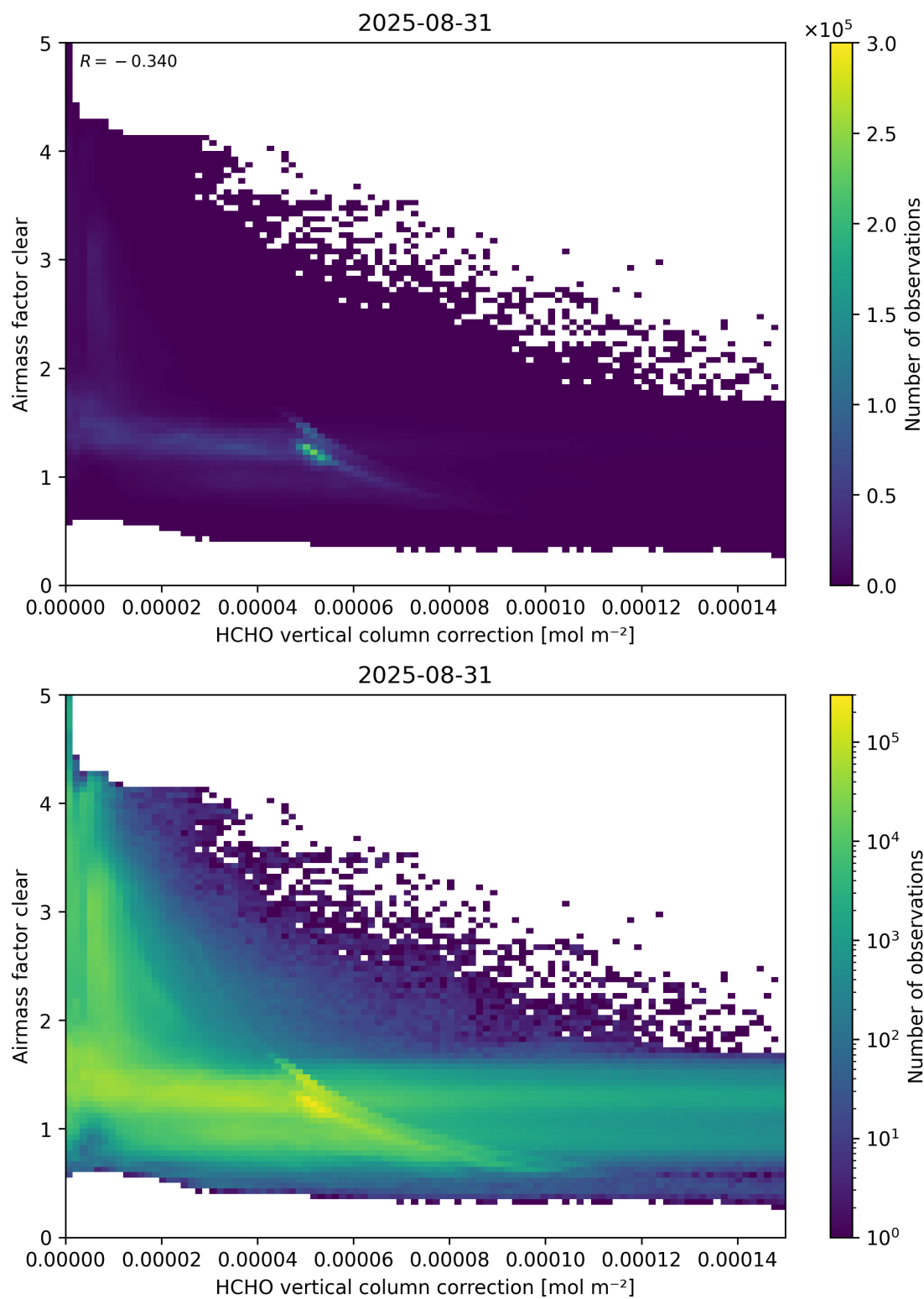
Figure 115: Scatter density plot of “HCHO vertical column correction” against “Airmass factor clear” for 2025-08-30 to 2025-09-01.
