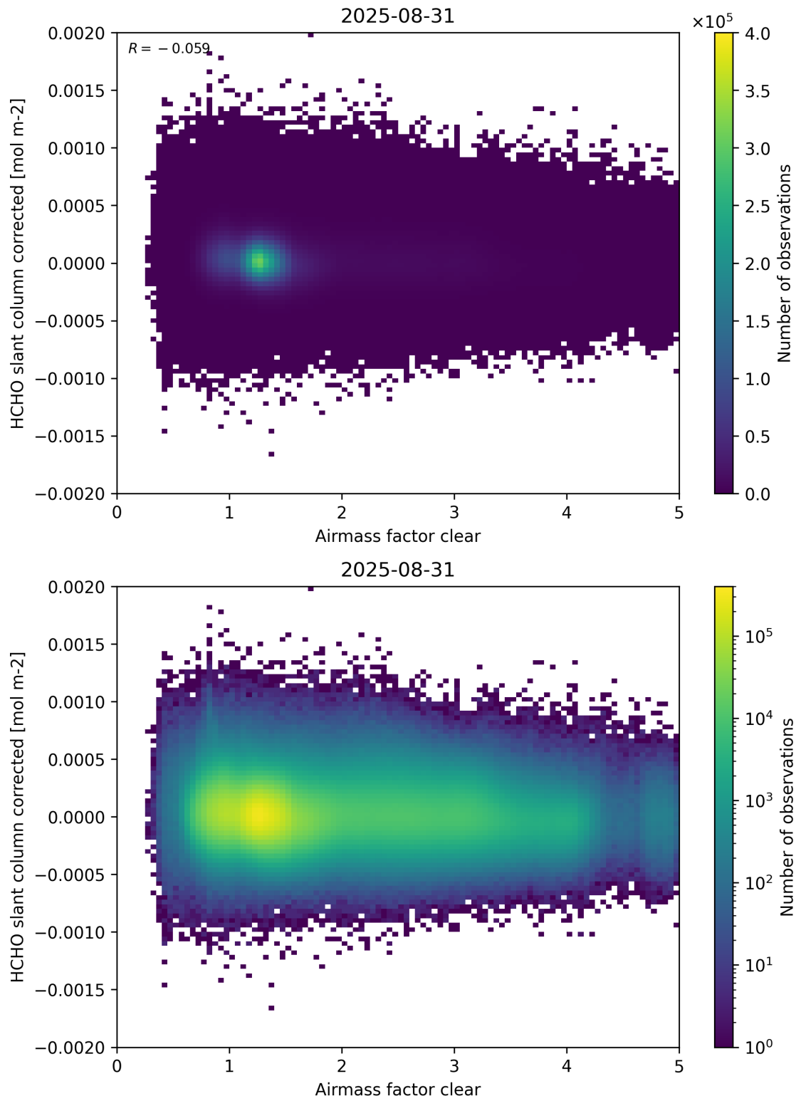
Figure 74: Scatter density plot of “Airmass factor clear” against “HCHO slant column corrected” for 2025-08-30 to 2025-09-01.
