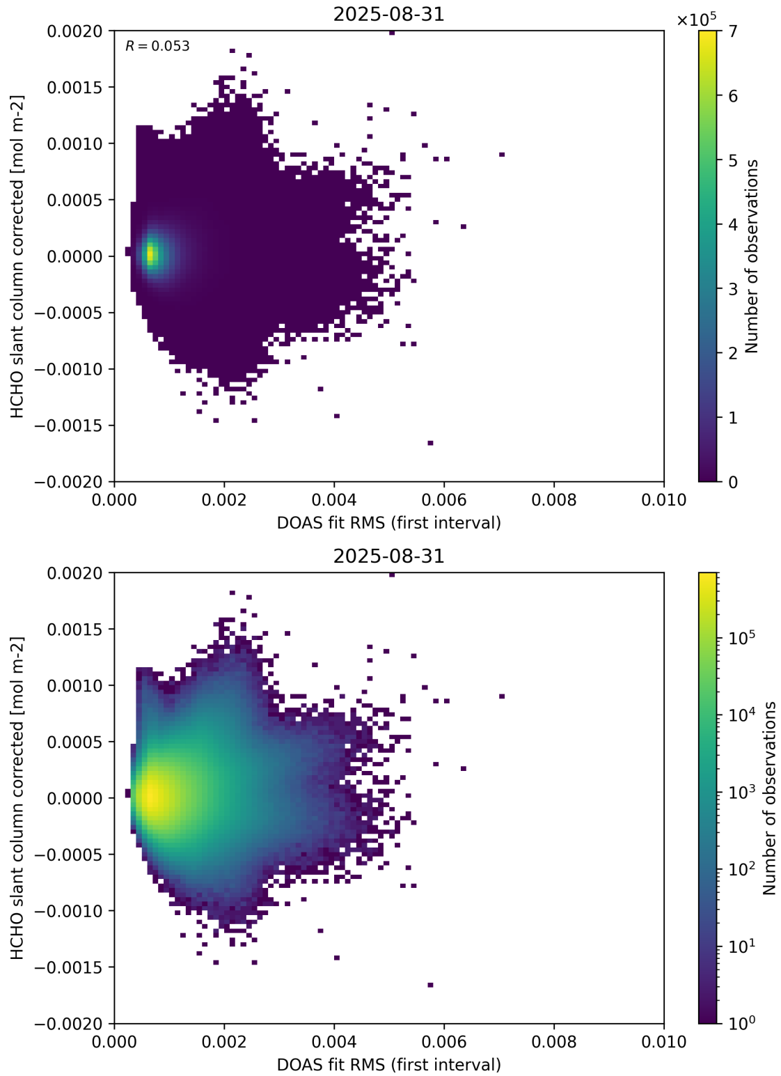
Figure 62: Scatter density plot of “DOAS fit RMS (first interval)” against “HCHO slant column corrected” for 2025-08-30 to 2025-09-01.
