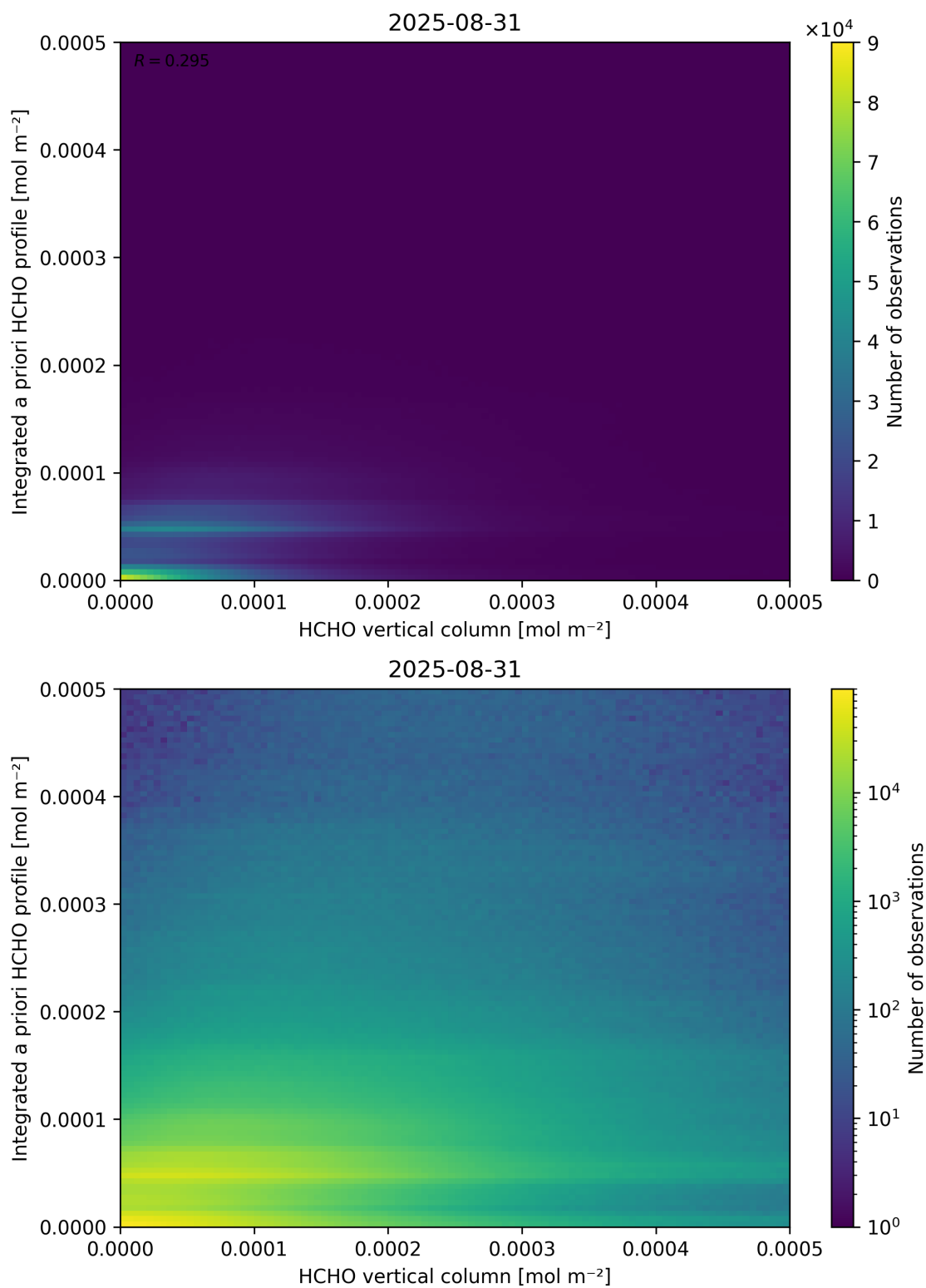
Figure 135: Scatter density plot of “HCHO vertical column” against “Integrated a priori HCHO profile” for 2025-08-30 to 2025-09-01.
