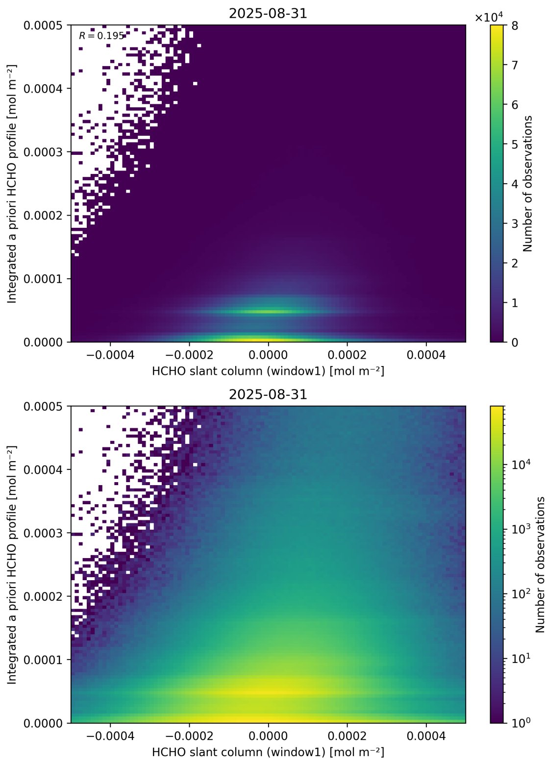
Figure 87: Scatter density plot of “HCHO slant column (window1)” against “Integrated a priori HCHO profile” for 2025-08-30 to 2025-09-01.
