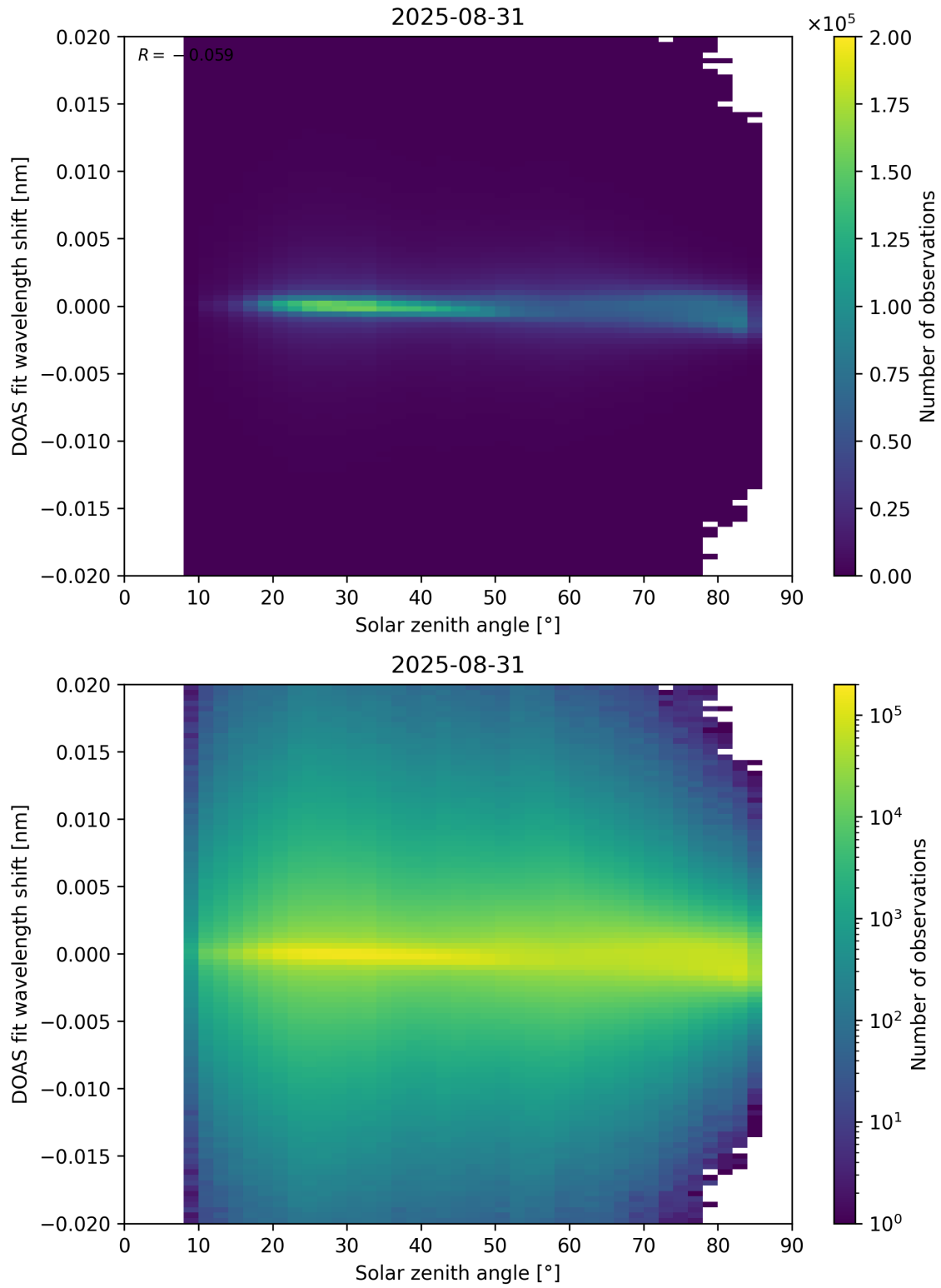
Figure 168: Scatter density plot of “Solar zenith angle” against “DOAS fit wavelength shift” for 2025-08-30 to 2025-09-01.
