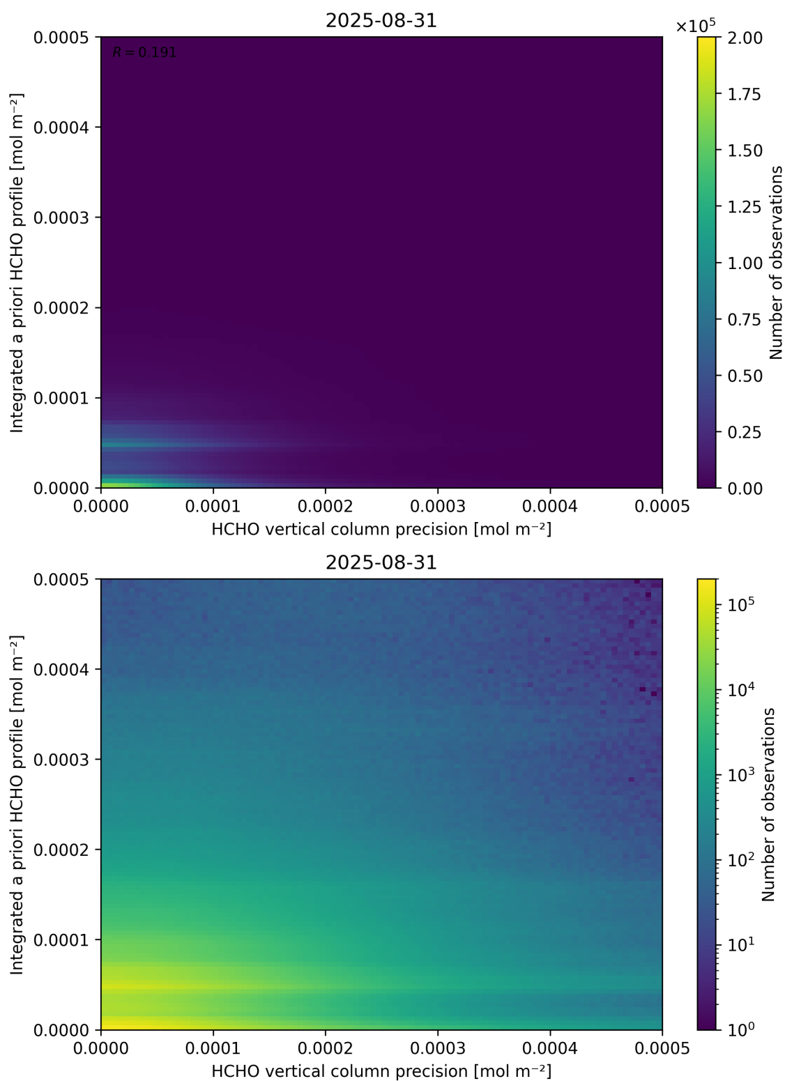
Figure 147: Scatter density plot of “HCHO vertical column precision” against “Integrated a priori HCHO profile” for 2025-08-30 to 2025-09-01.
