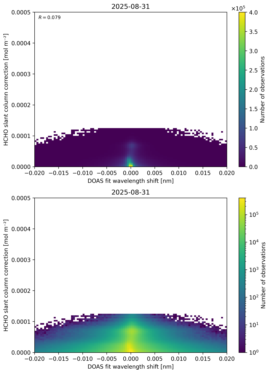
Figure 67: Scatter density plot of “DOAS fit wavelength shift” against “HCHO slant column correction” for 2025-08-30 to 2025-09-01.
