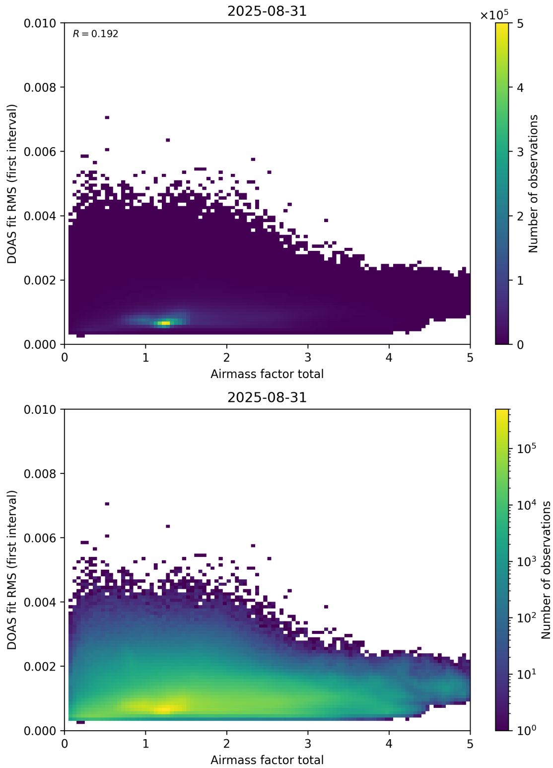
Figure 97: Scatter density plot of “Airmass factor total” against “DOAS fit RMS (first interval)” for 2025-08-30 to 2025-09-01.
