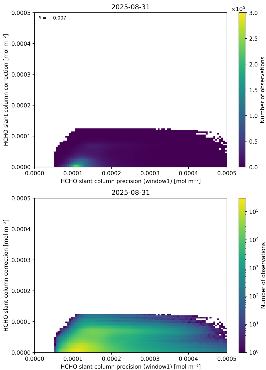
Figure 93: Scatter density plot of “HCHO slant column precision (window1)” against “HCHO slant column correction” for 2025-08-30 to 2025-09-01.
