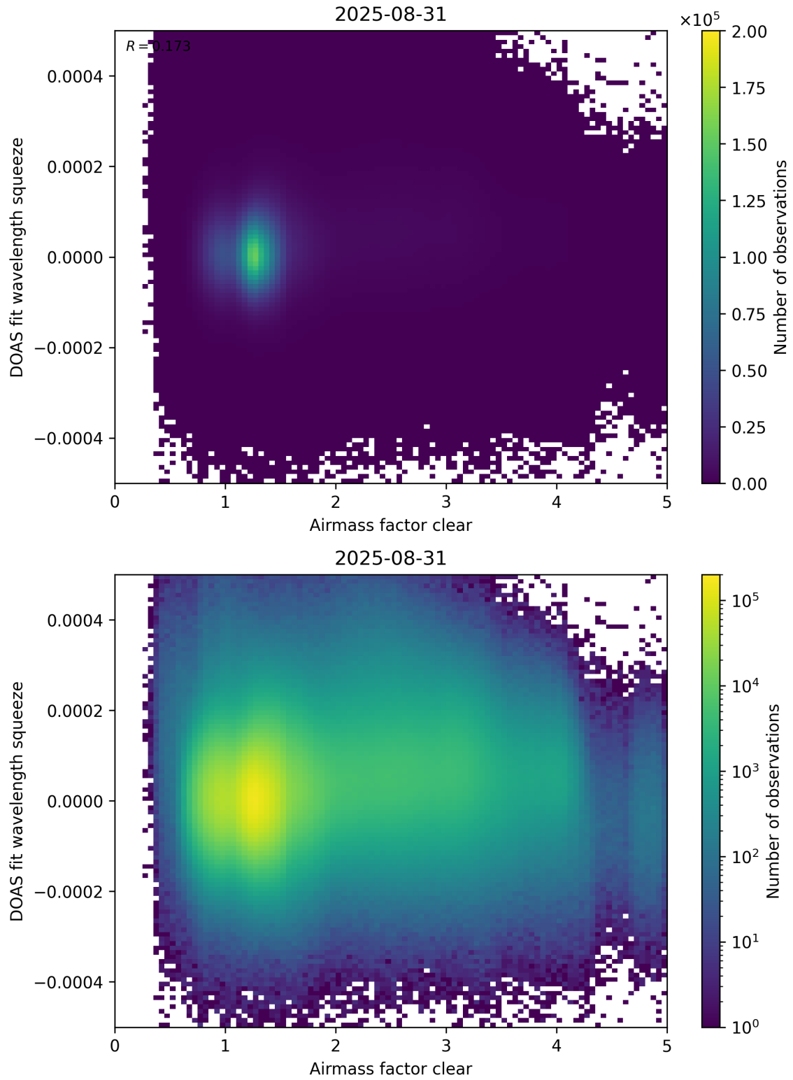
Figure 73: Scatter density plot of “Airmass factor clear” against “DOAS fit wavelength squeeze” for 2025-08-30 to 2025-09-01.
