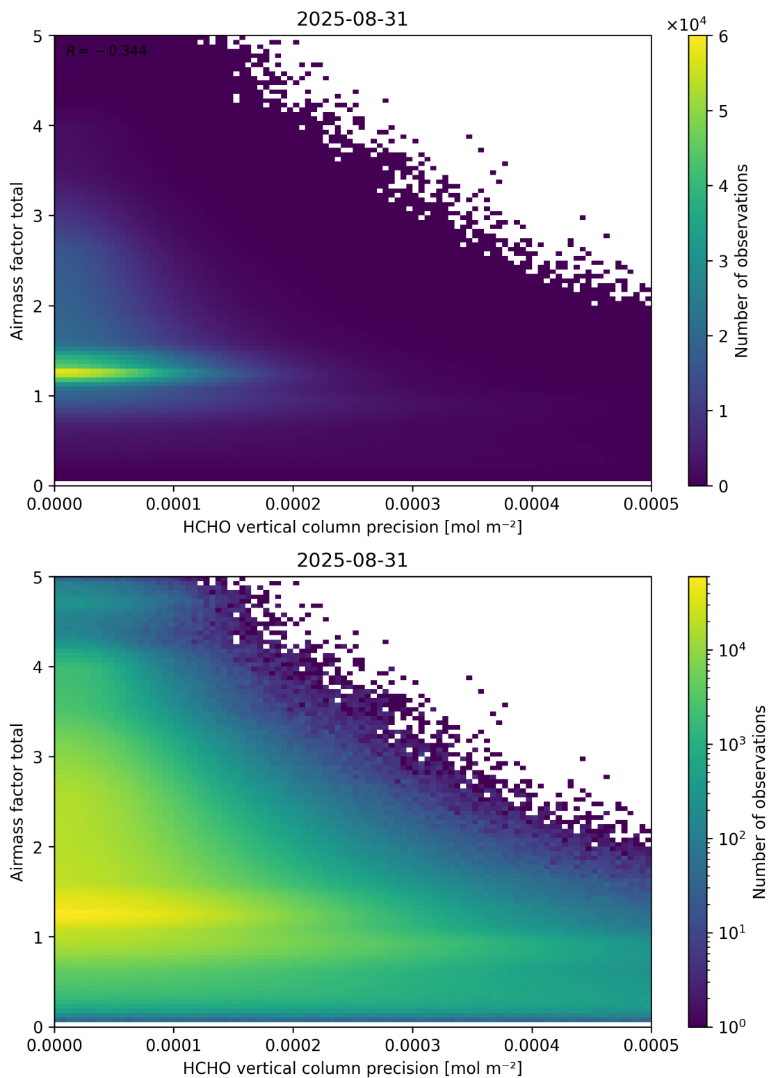
Figure 144: Scatter density plot of “HCHO vertical column precision” against “Airmass factor total” for 2025-08-30 to 2025-09-01.
