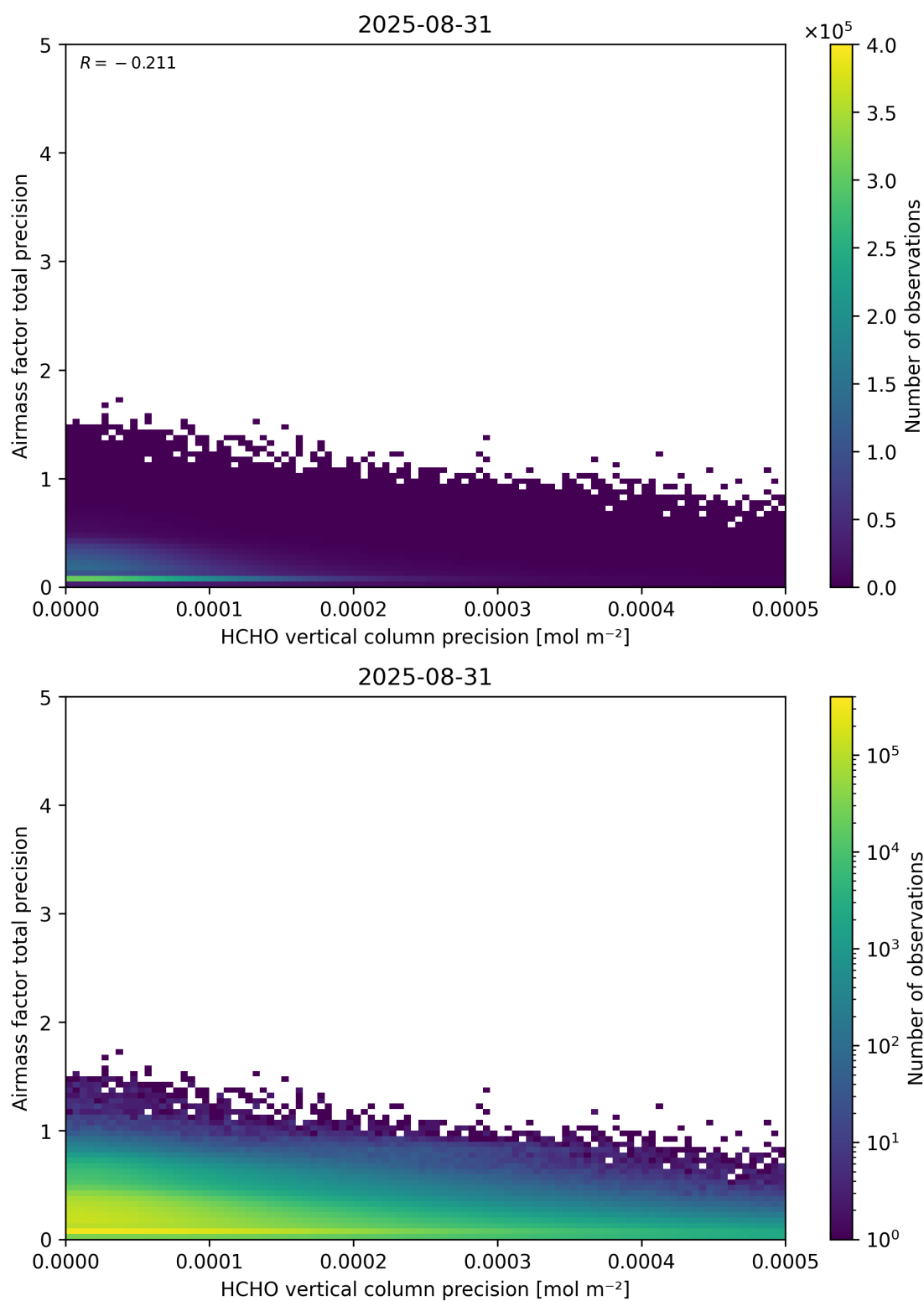
Figure 145: Scatter density plot of “HCHO vertical column precision” against “Airmass factor total precision” for 2025-08-30 to 2025-09-01.
