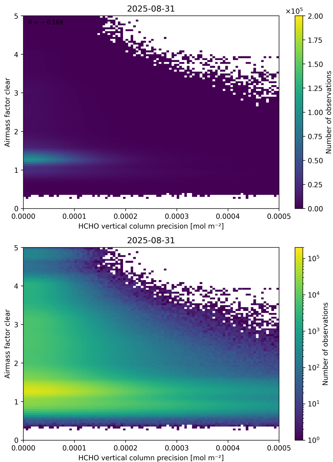
Figure 139: Scatter density plot of “HCHO vertical column precision” against “Airmass factor clear” for 2025-08-30 to 2025-09-01.
