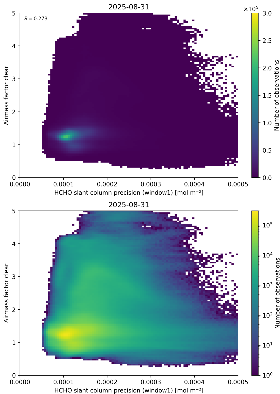
Figure 91: Scatter density plot of “HCHO slant column precision (window1)” against “Airmass factor clear” for 2025-08-30 to 2025-09-01.
