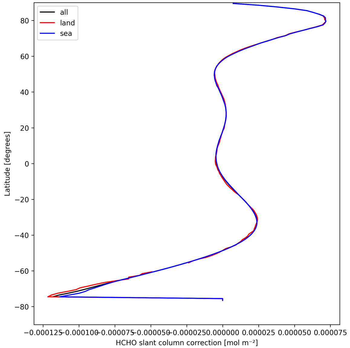
Figure 33: Zonal average of “HCHO slant column correction” for 2025-08-30 to 2025-09-01.
