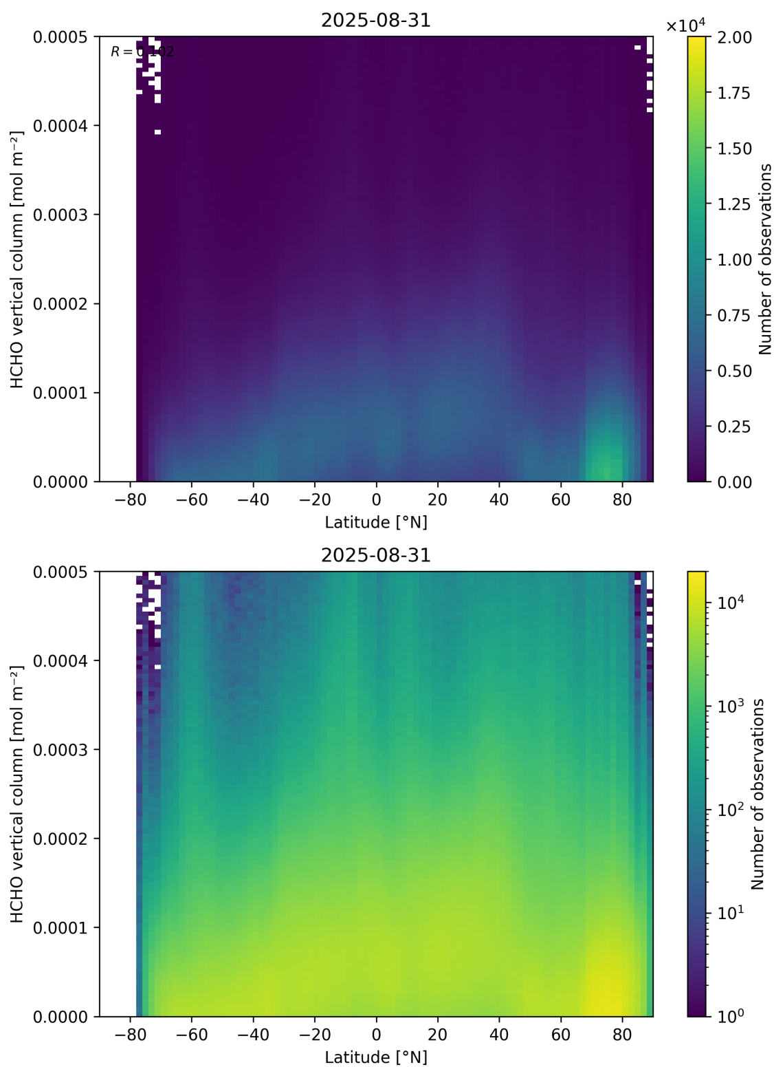
Figure 163: Scatter density plot of “Latitude” against “HCHO vertical column” for 2025-08-30 to 2025-09-01.
