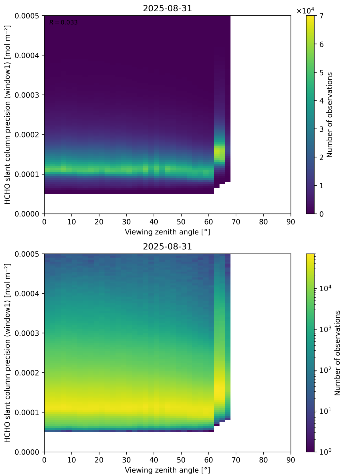
Figure 189: Scatter density plot of “Viewing zenith angle” against “HCHO slant column precision (window1)” for 2025-08-30 to 2025-09-01.
