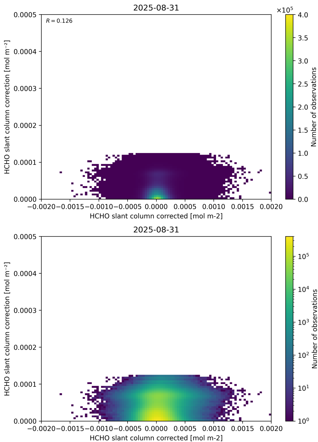
Figure 77: Scatter density plot of “HCHO slant column corrected” against “HCHO slant column correction” for 2025-08-30 to 2025-09-01.
