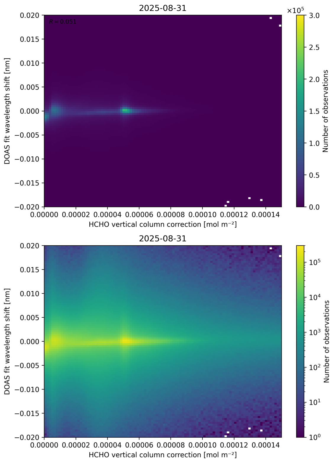
Figure 113: Scatter density plot of “HCHO vertical column correction” against “DOAS fit wavelength shift” for 2025-08-30 to 2025-09-01.
