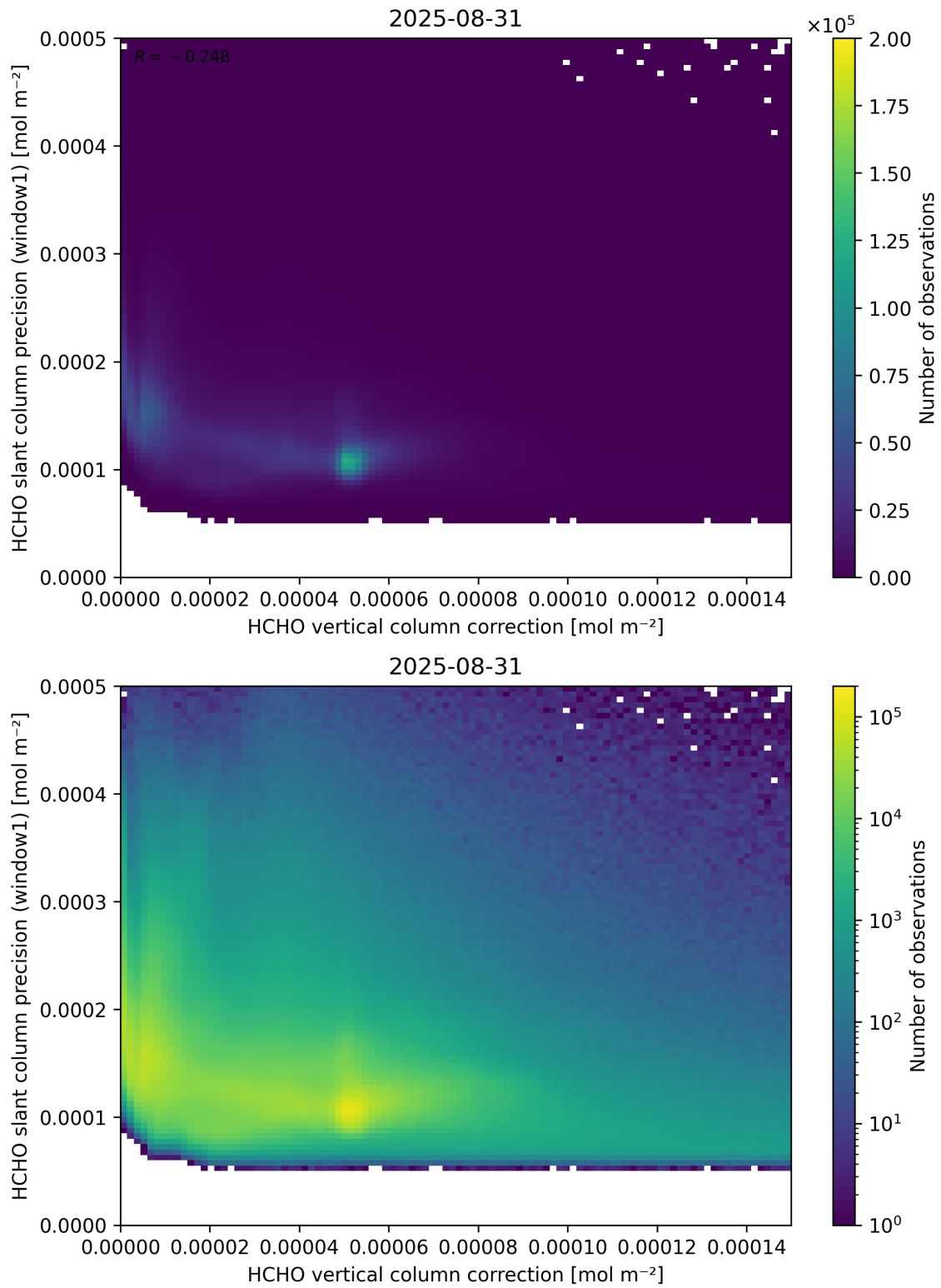
Figure 119: Scatter density plot of “HCHO vertical column correction” against “HCHO slant column precision (window1)” for 2025-08-30 to 2025-09-01.
