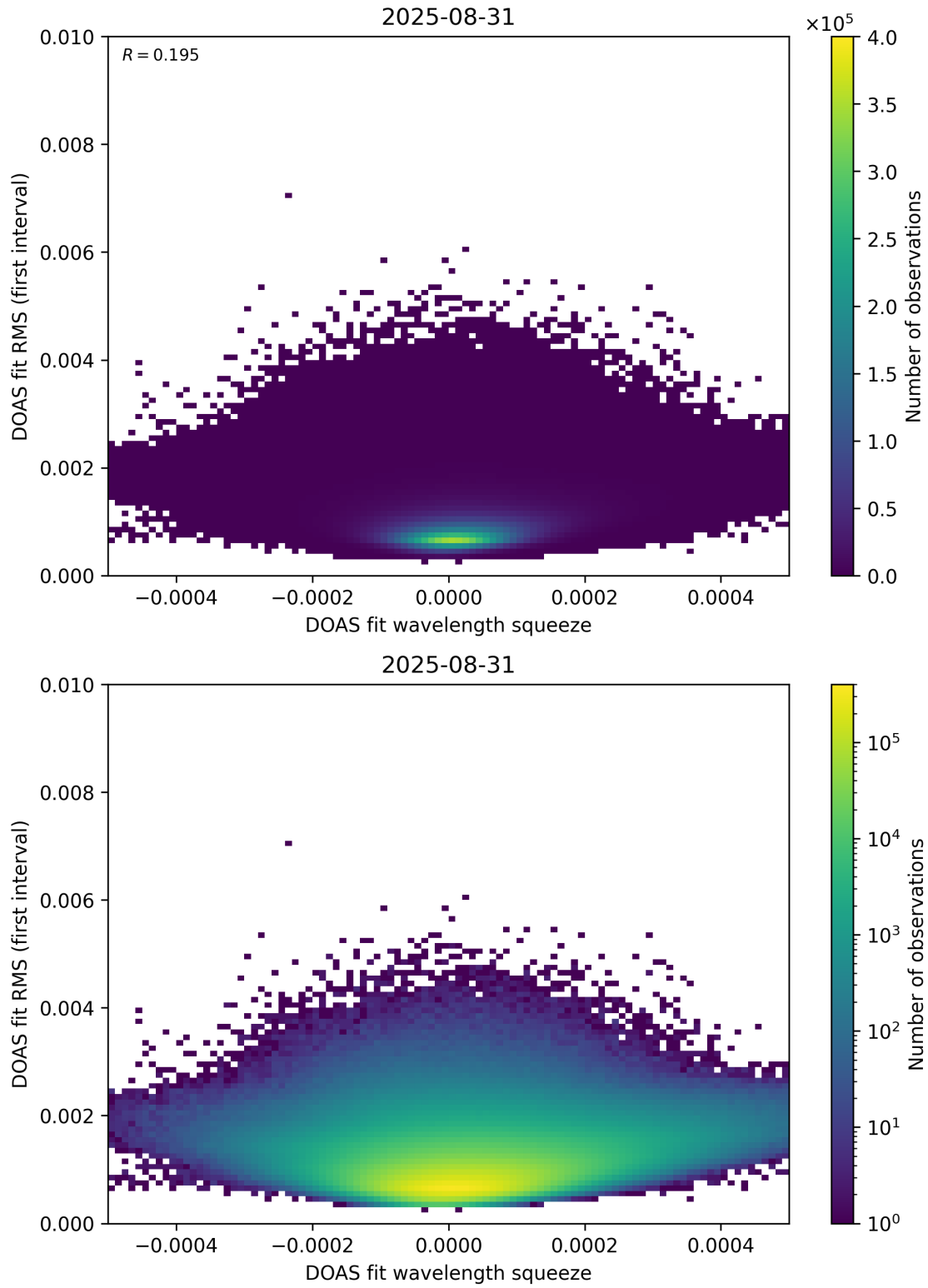
Figure 68: Scatter density plot of “DOAS fit wavelength squeeze” against “DOAS fit RMS (first interval)” for 2025-08-30 to 2025-09-01.
