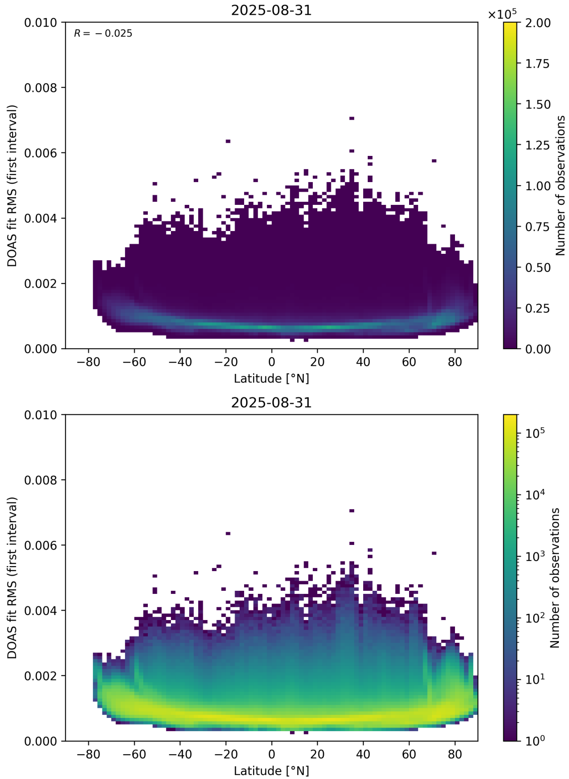
Figure 153: Scatter density plot of “Latitude” against “DOAS fit RMS (first interval)” for 2025-08-30 to 2025-09-01.
