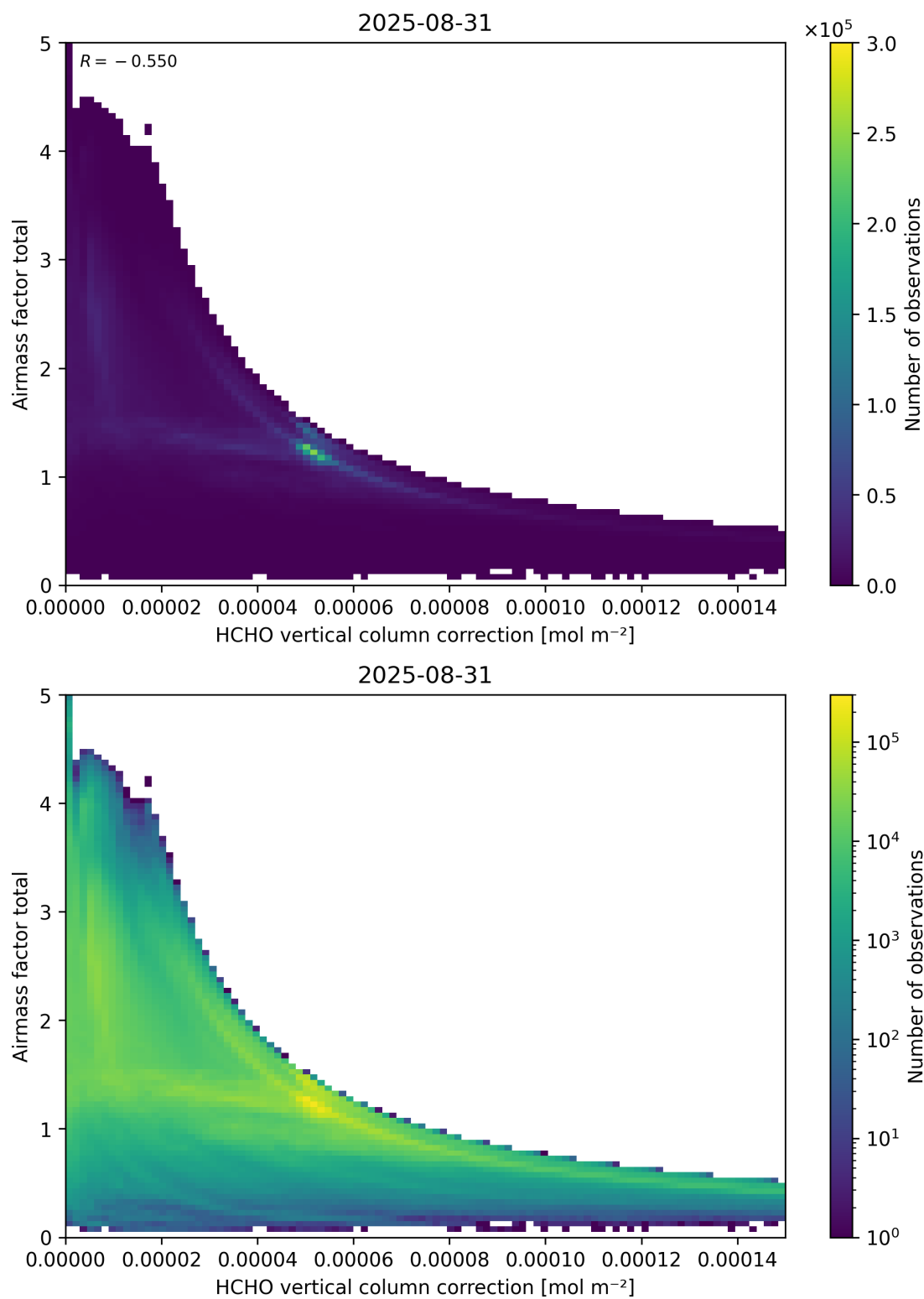
Figure 120: Scatter density plot of “HCHO vertical column correction” against “Airmass factor total” for 2025-08-30 to 2025-09-01.
