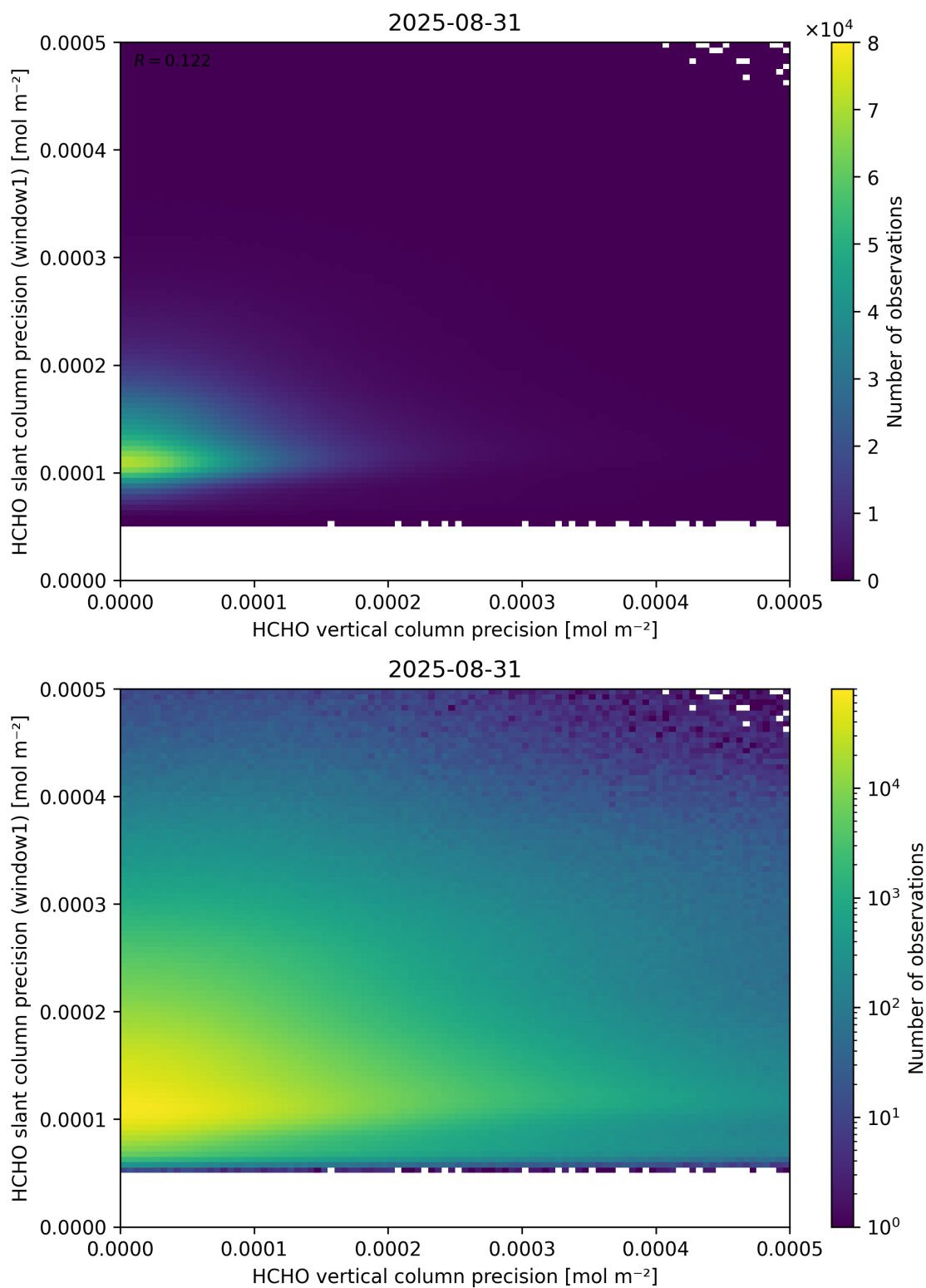
Figure 143: Scatter density plot of “HCHO vertical column precision” against “HCHO slant column precision (window1)” for 2025-08-30 to 2025-09-01.
