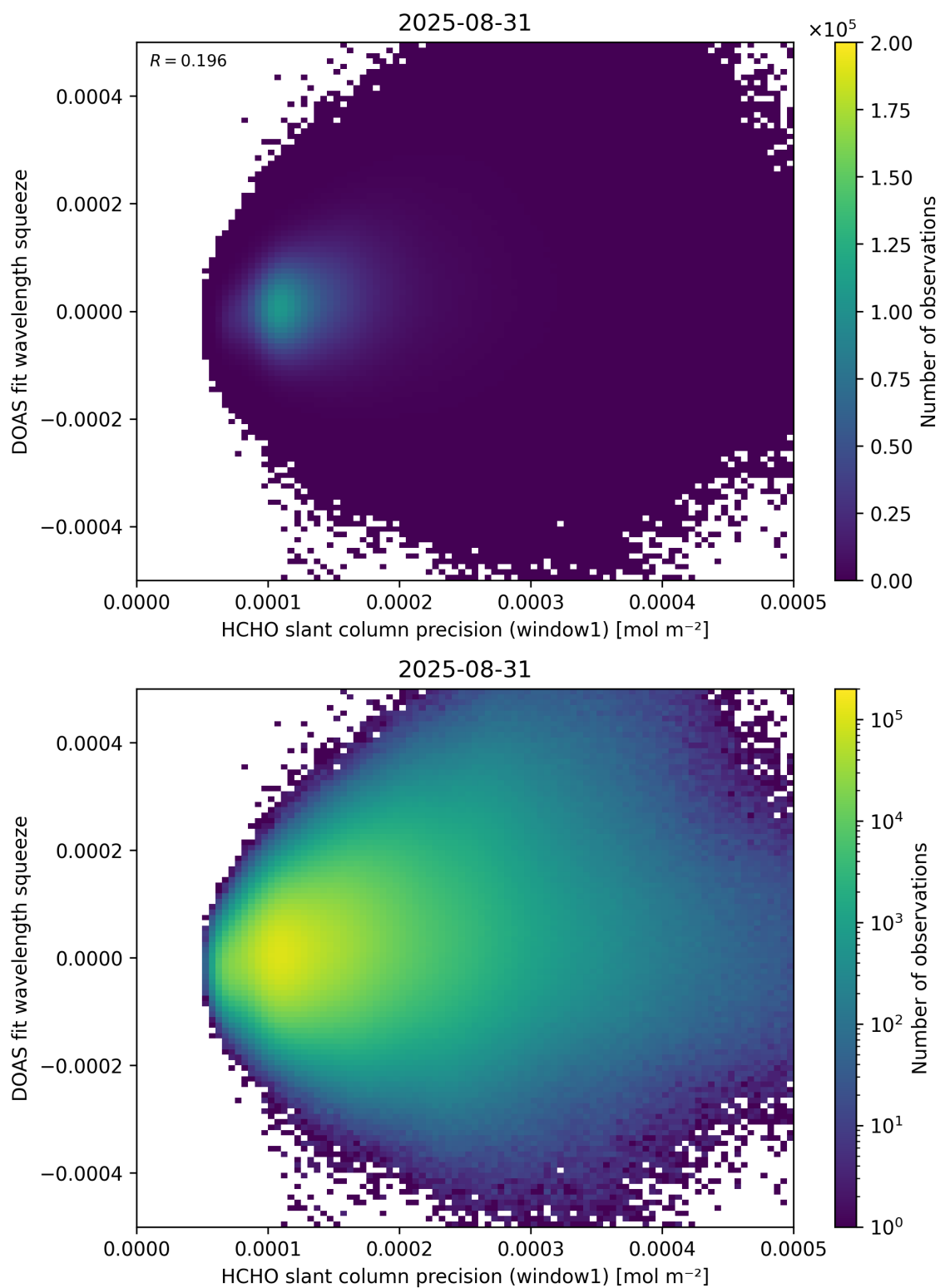
Figure 90: Scatter density plot of “HCHO slant column precision (window1)” against “DOAS fit wavelength squeeze” for 2025-08-30 to 2025-09-01.
