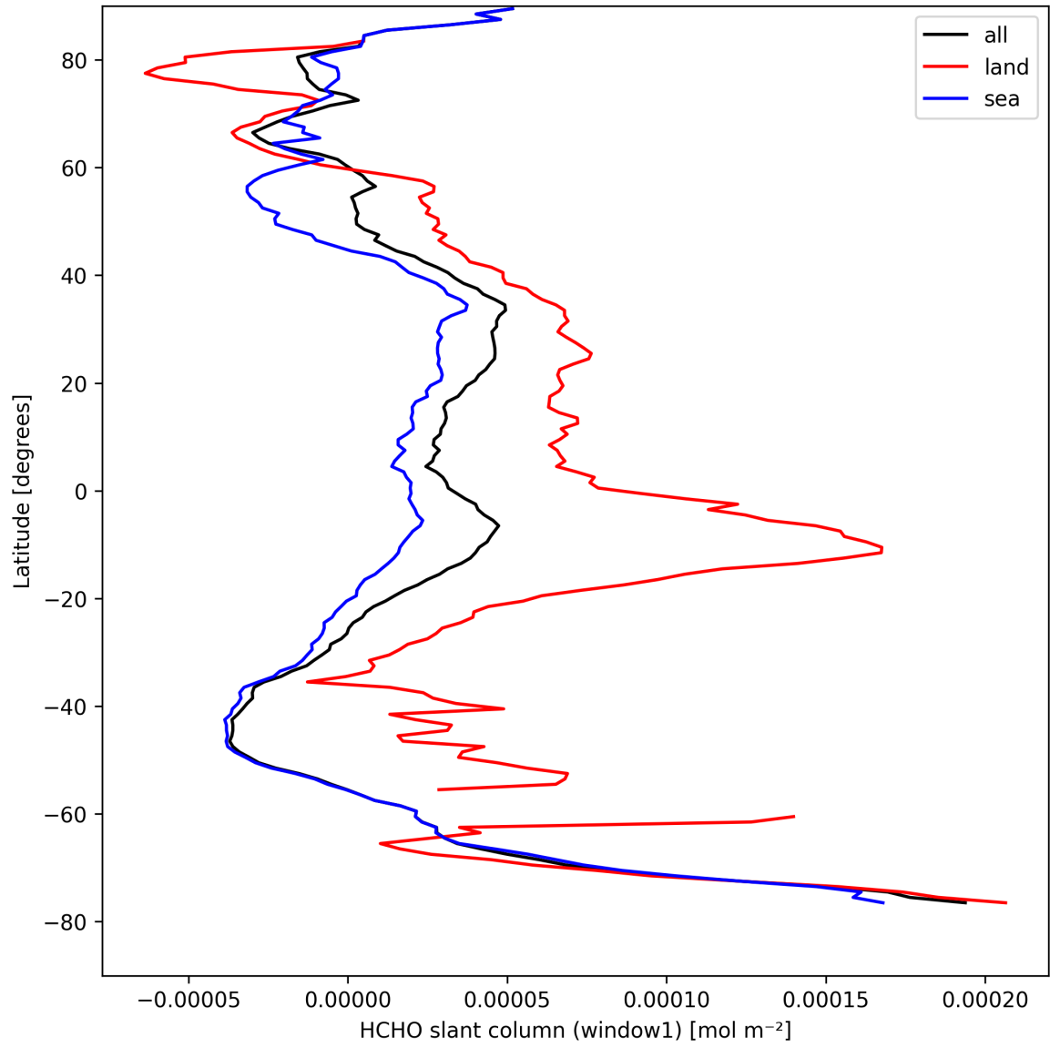
Figure 24: Zonal average of “HCHO slant column (window1)” for 2025-08-30 to 2025-09-01.
