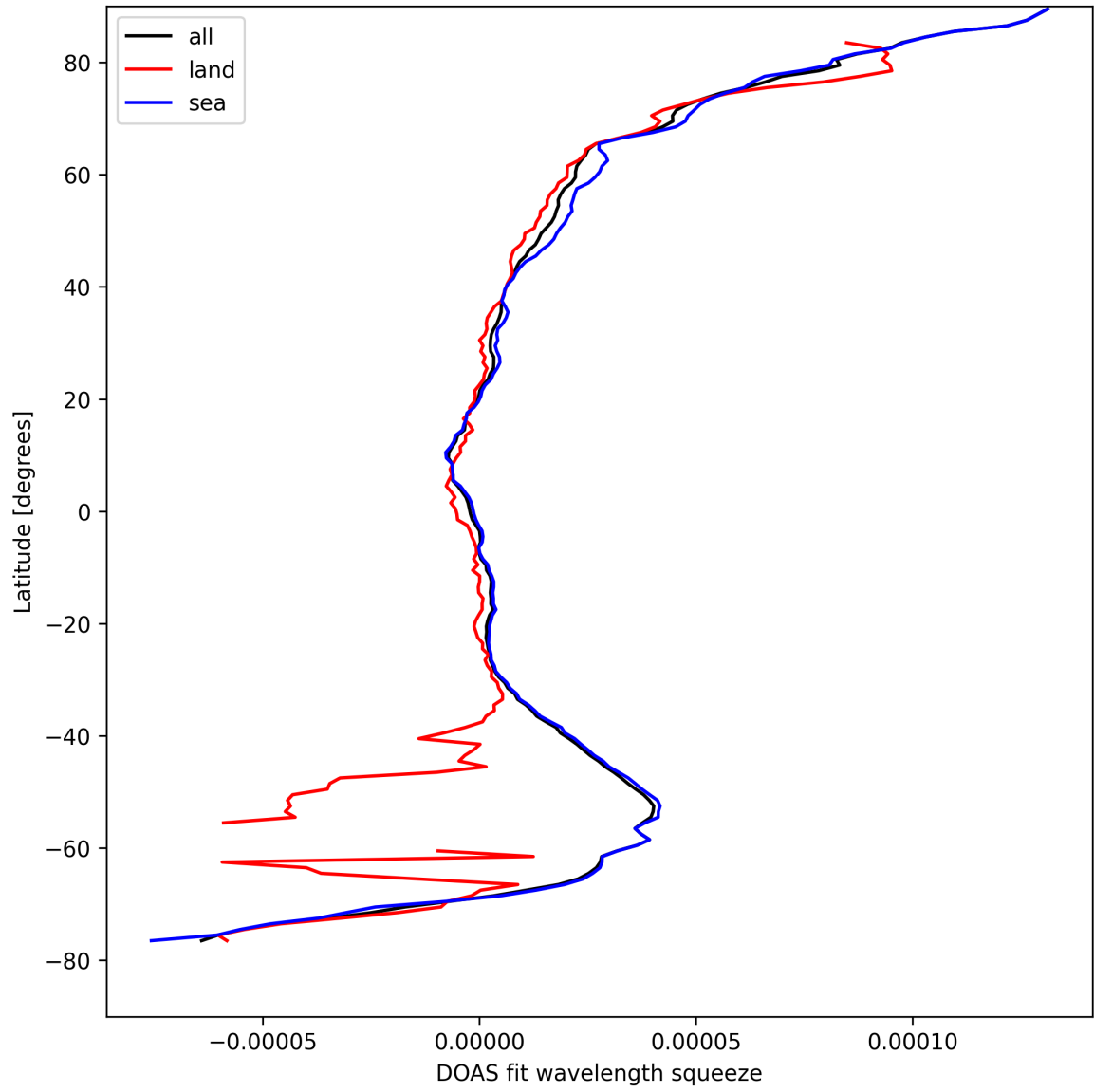
Figure 31: Zonal average of “DOAS fit wavelength squeeze” for 2025-08-30 to 2025-09-01.
