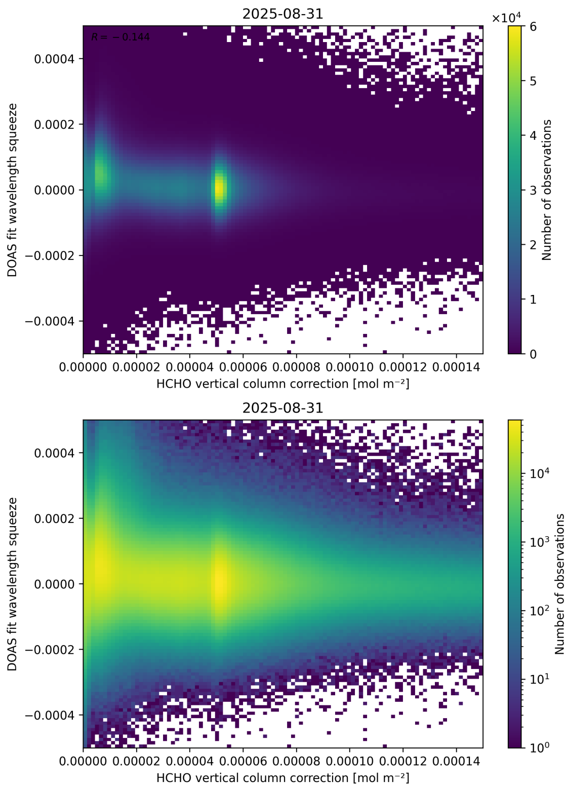
Figure 114: Scatter density plot of “HCHO vertical column correction” against “DOAS fit wavelength squeeze” for 2025-08-30 to 2025-09-01.
