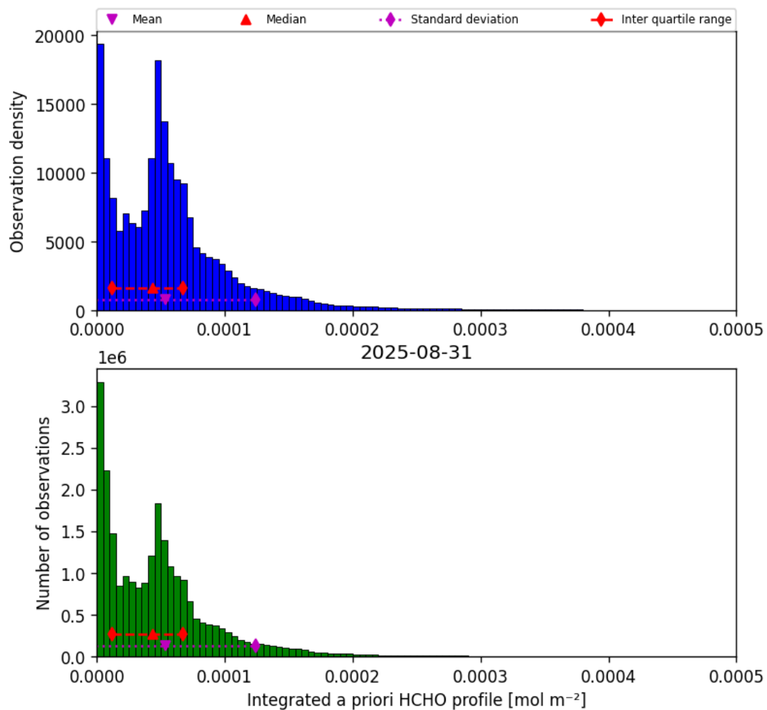
Figure 43: Histogram of “Integrated a priori HCHO profile” for 2025-08-30 to 2025-09-01
