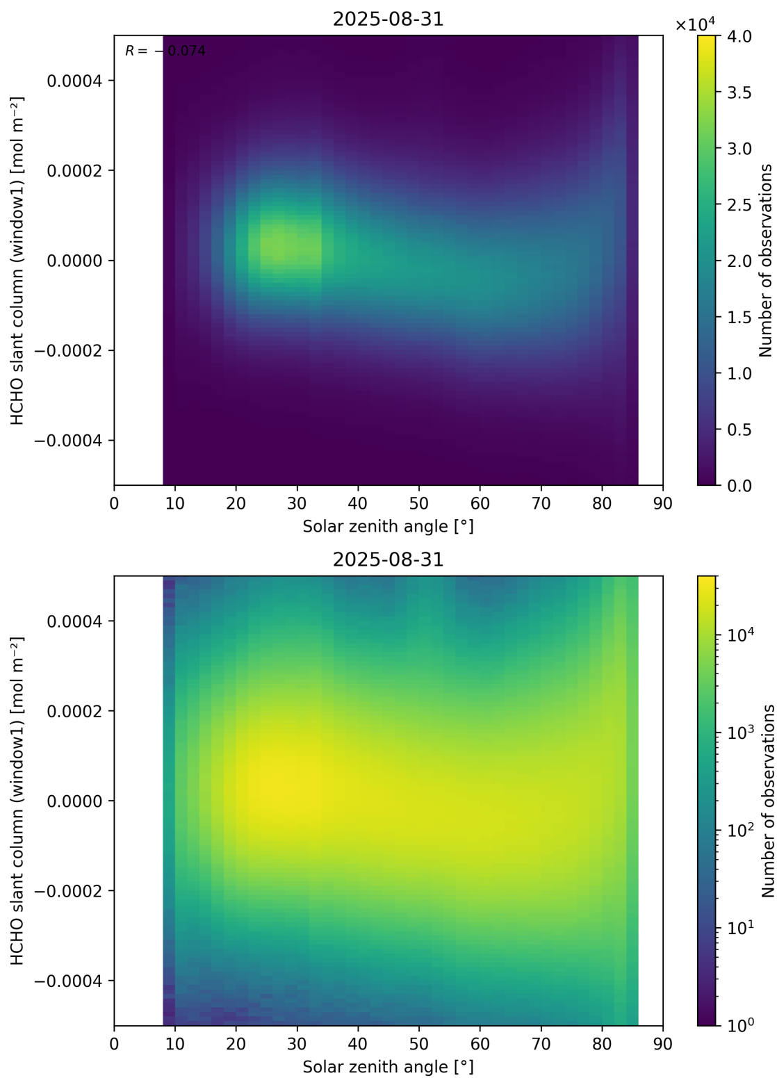
Figure 173: Scatter density plot of “Solar zenith angle” against “HCHO slant column (window1)” for 2025-08-30 to 2025-09-01.
