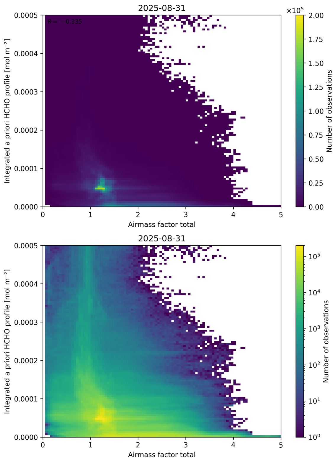
Figure 104: Scatter density plot of “Airmass factor total” against “Integrated a priori HCHO profile” for 2025-08-30 to 2025-09-01.
