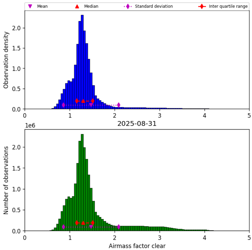
Figure 42: Histogram of “Airmass factor clear” for 2025-08-30 to 2025-09-01
