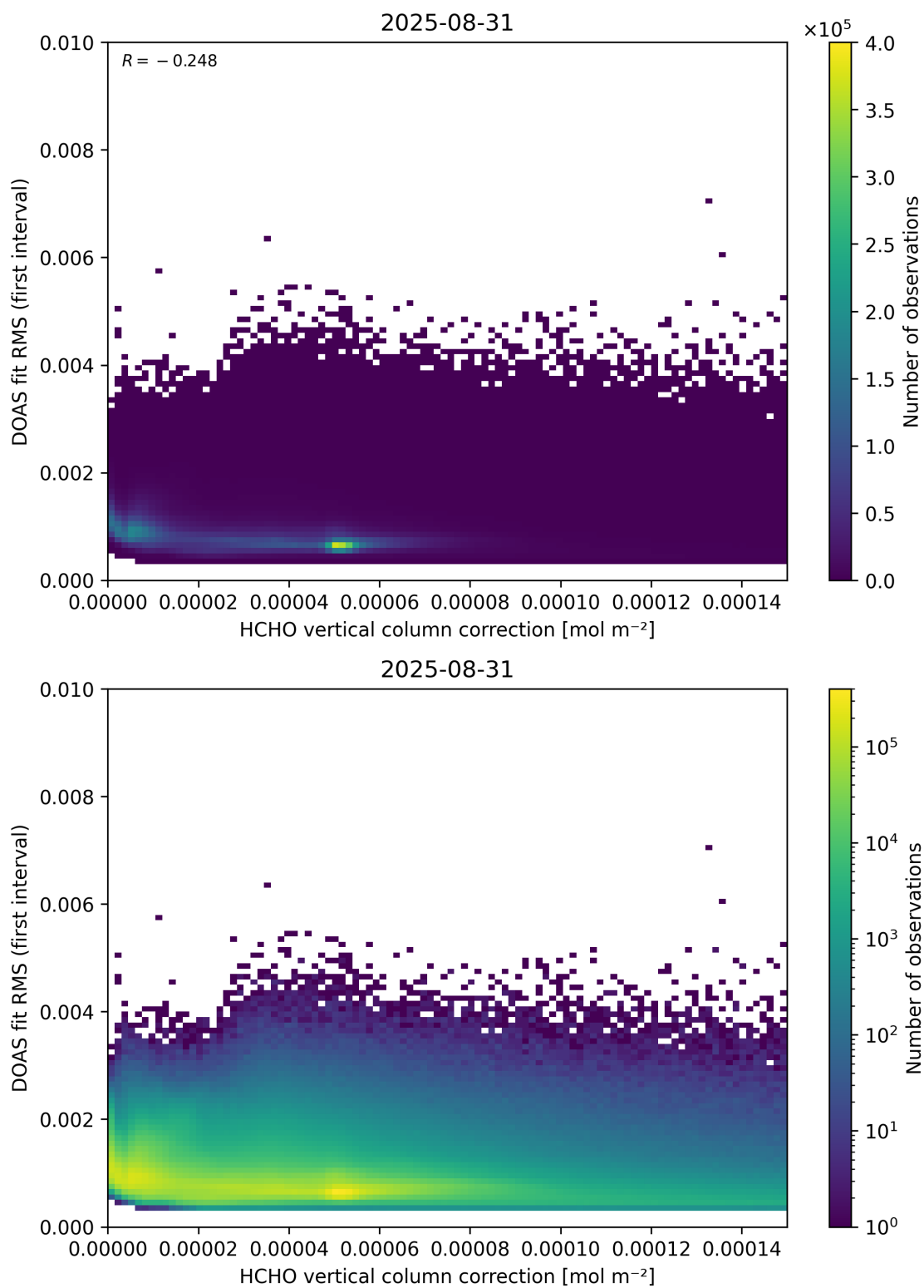
Figure 112: Scatter density plot of “HCHO vertical column correction” against “DOAS fit RMS (first interval)” for 2025-08-30 to 2025-09-01.
