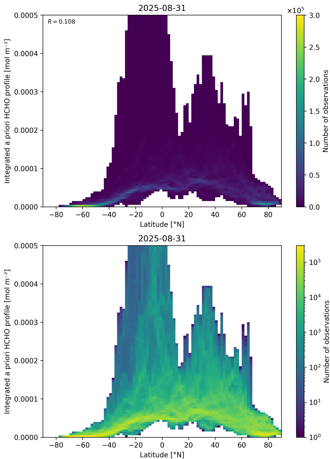
Figure 166: Scatter density plot of “Latitude” against “Integrated a priori HCHO profile” for 2025-08-30 to 2025-09-01.
