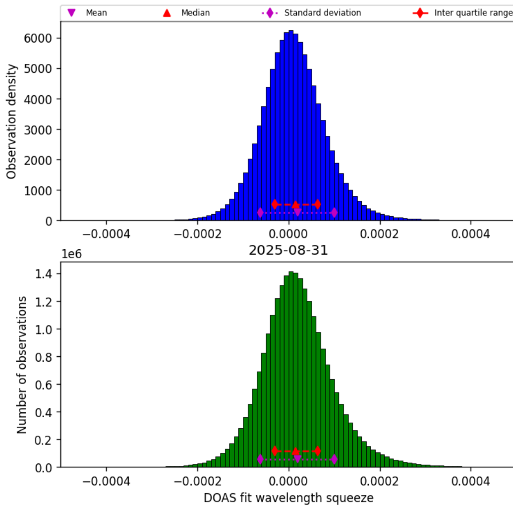
Figure 45: Histogram of “DOAS fit wavelength squeeze” for 2025-08-30 to 2025-09-01
