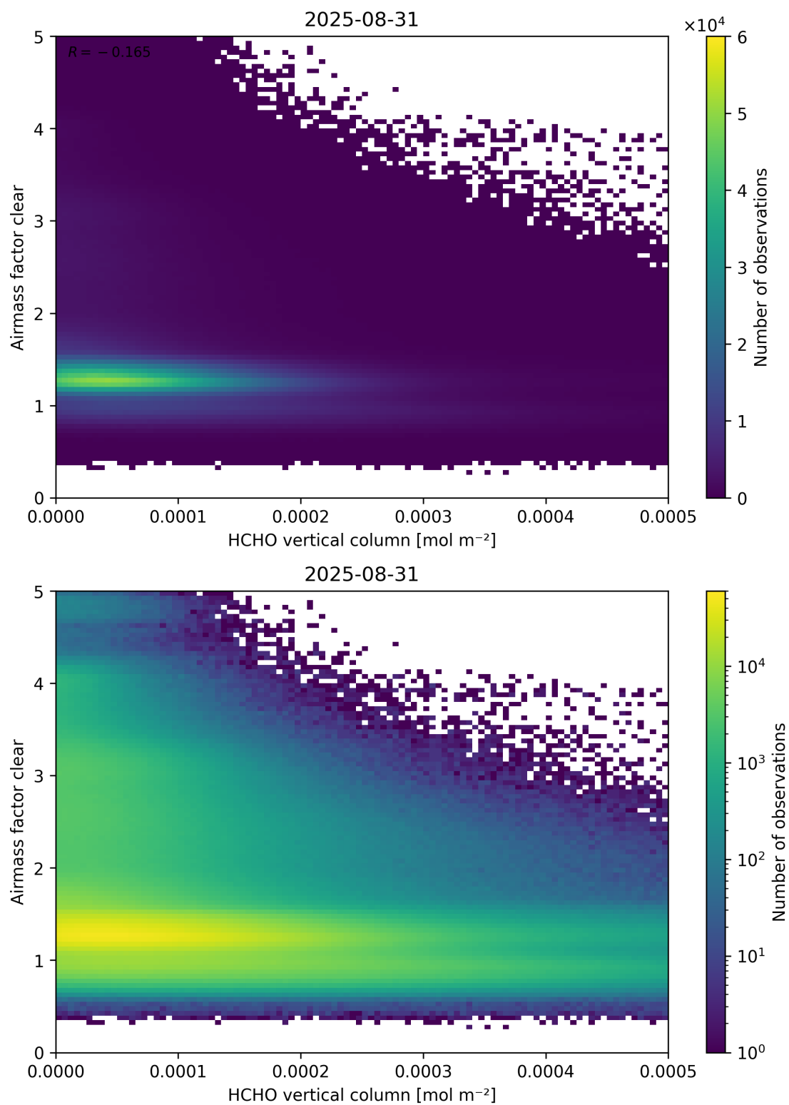
Figure 126: Scatter density plot of “HCHO vertical column” against “Airmass factor clear” for 2025-08-30 to 2025-09-01.
