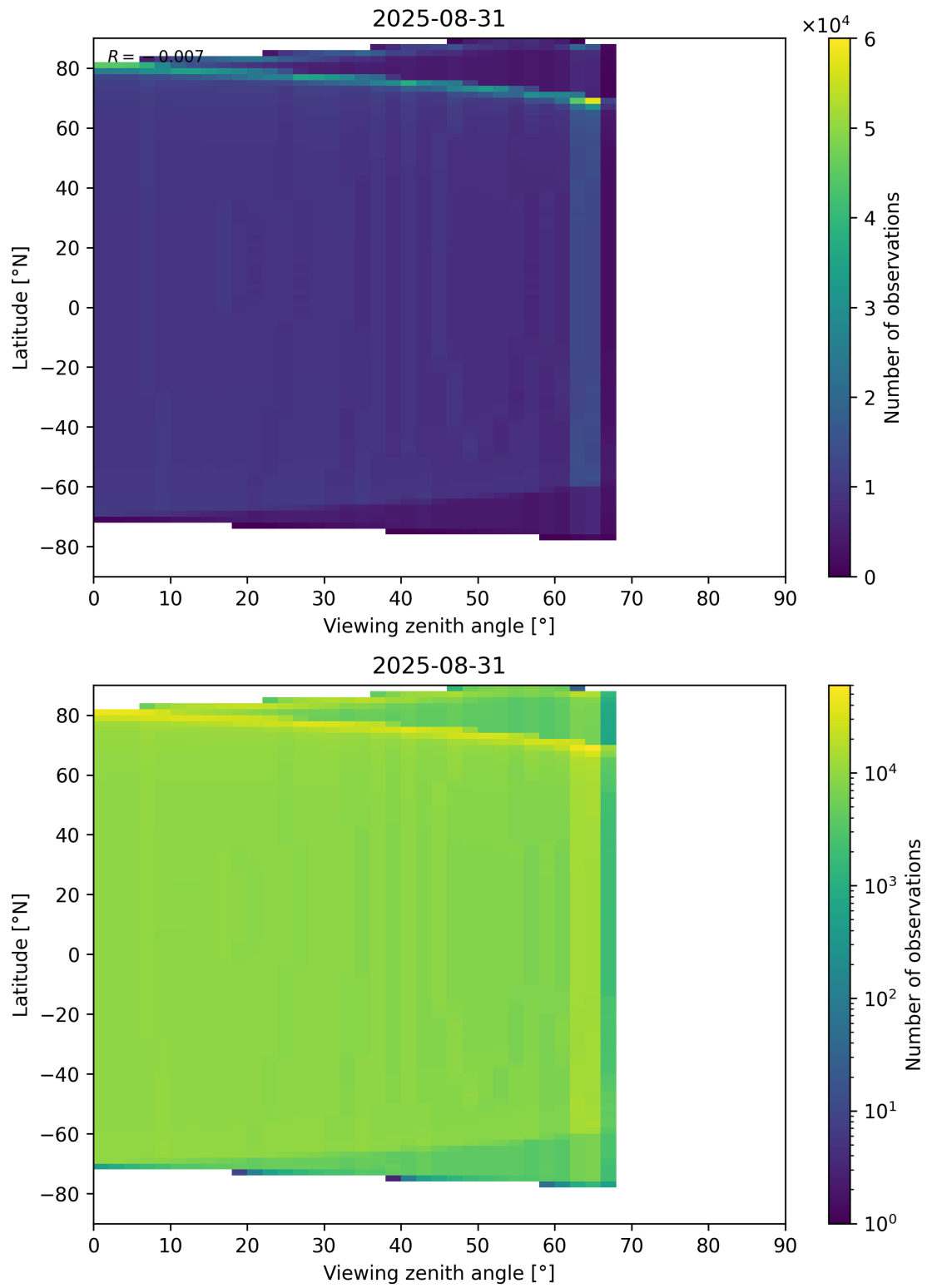
Figure 196: Scatter density plot of “Viewing zenith angle” against “Latitude” for 2025-08-30 to 2025-09-01.
