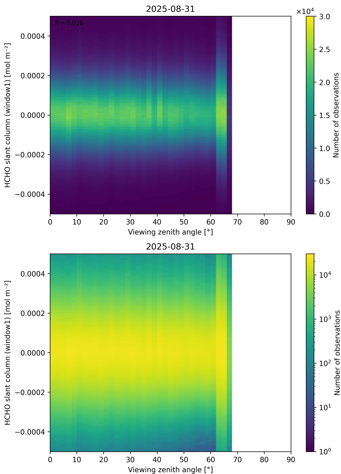
Figure 188: Scatter density plot of “Viewing zenith angle” against “HCHO slant column (window1)” for 2025-08-30 to 2025-09-01.
