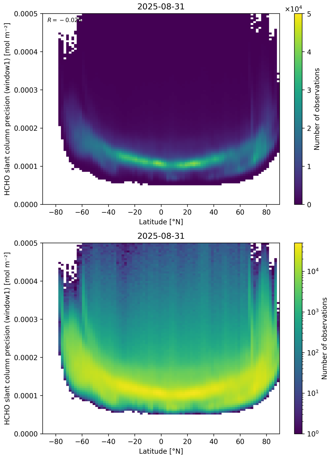
Figure 160: Scatter density plot of “Latitude” against “HCHO slant column precision (window1)” for 2025-08-30 to 2025-09-01.
