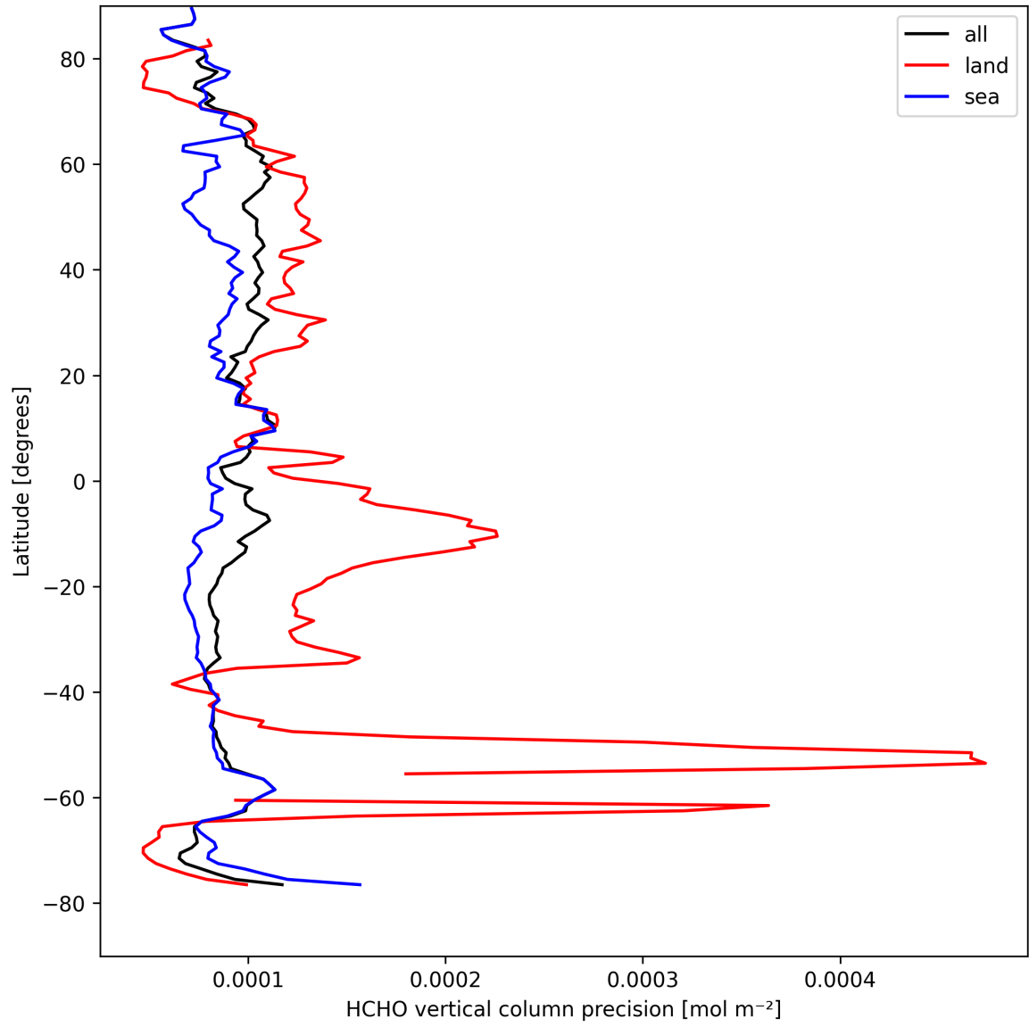
Figure 22: Zonal average of “HCHO vertical column precision” for 2025-08-30 to 2025-09-01.
