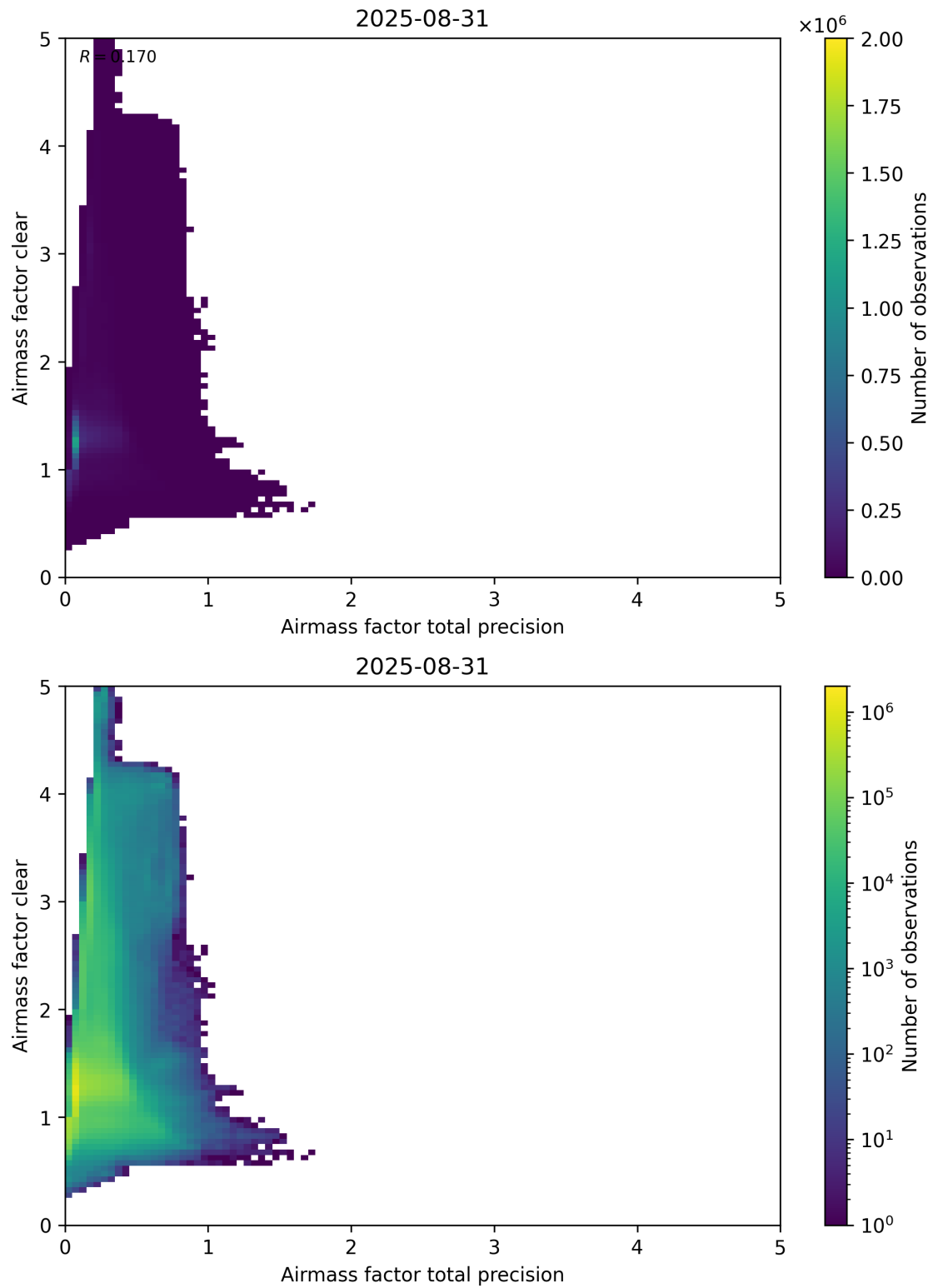
Figure 108: Scatter density plot of “Airmass factor total precision” against “Airmass factor clear” for 2025-08-30 to 2025-09-01.
