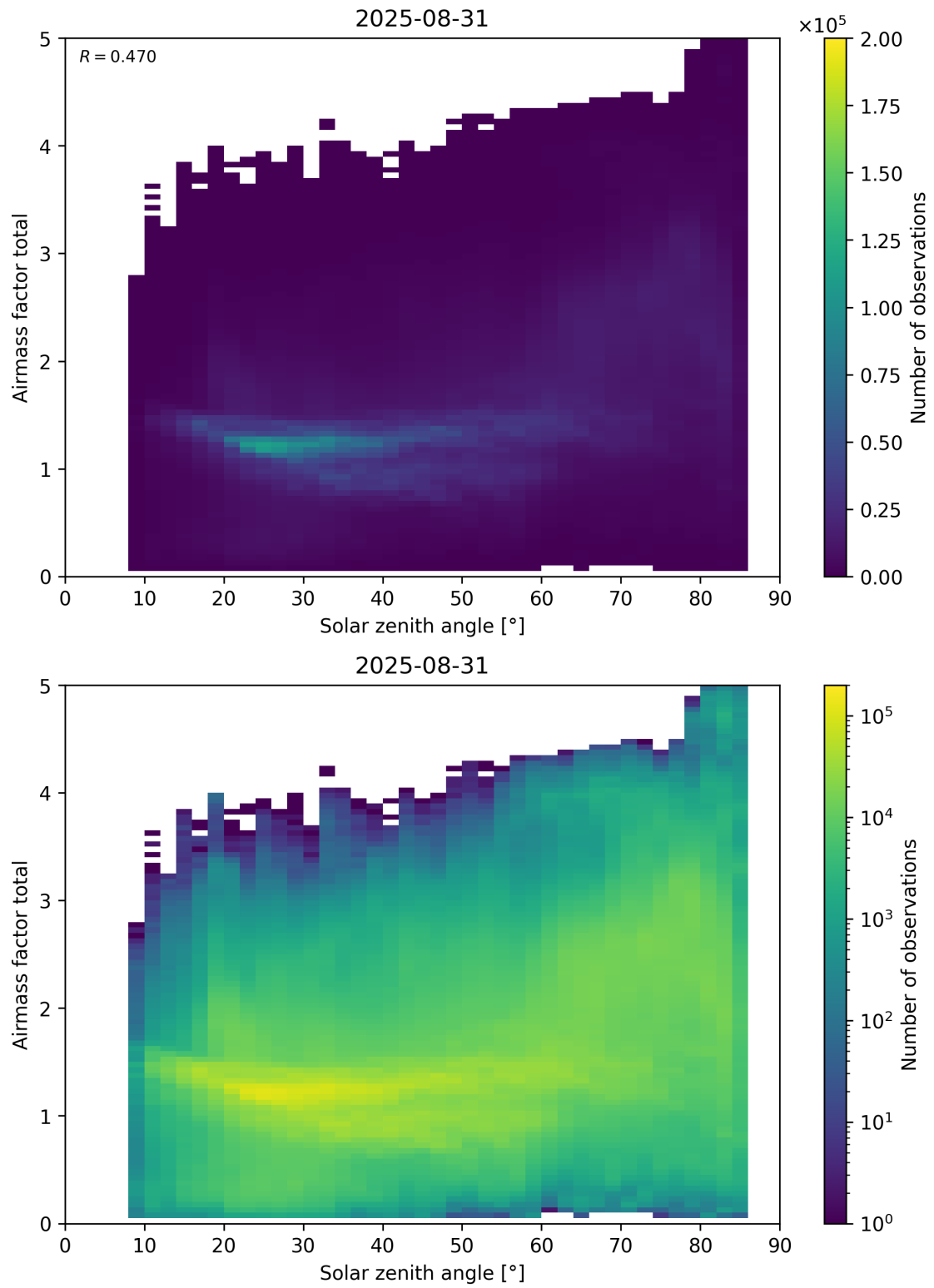
Figure 175: Scatter density plot of “Solar zenith angle” against “Airmass factor total” for 2025-08-30 to 2025-09-01.
