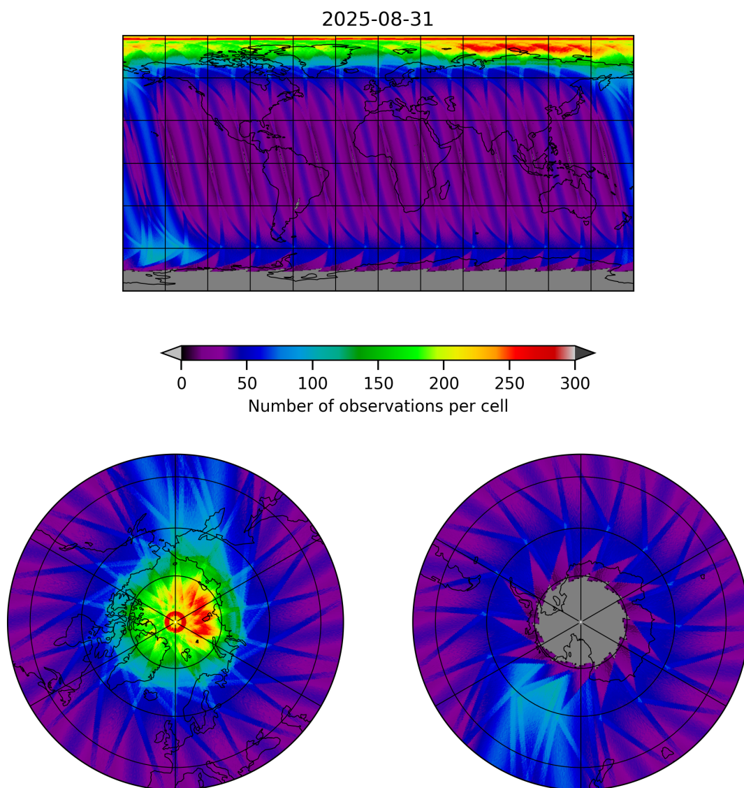
Figure 19: Map of the number of observations for 2025-08-30 to 2025-09-01
