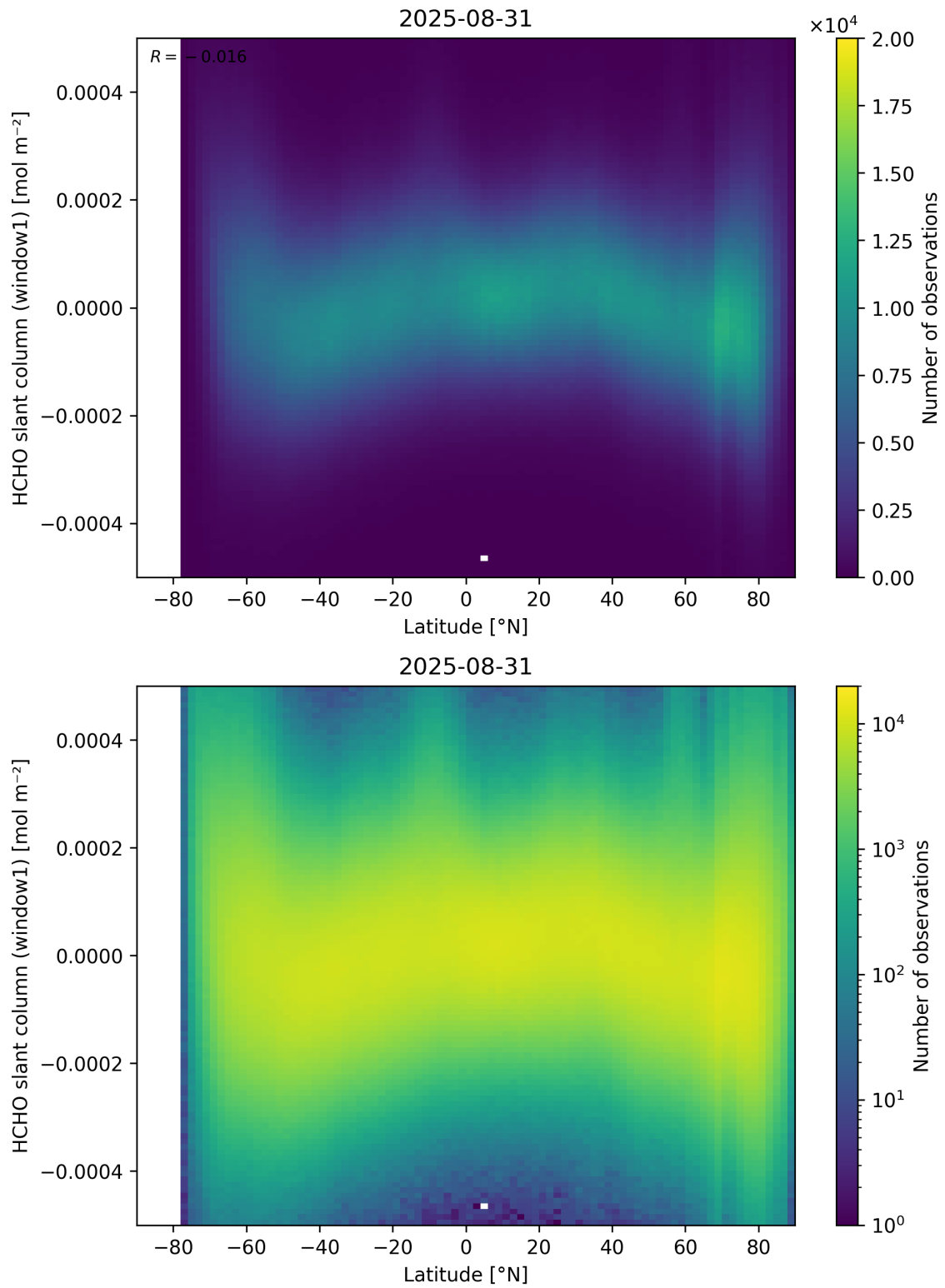
Figure 159: Scatter density plot of “Latitude” against “HCHO slant column (window1)” for 2025-08-30 to 2025-09-01.
