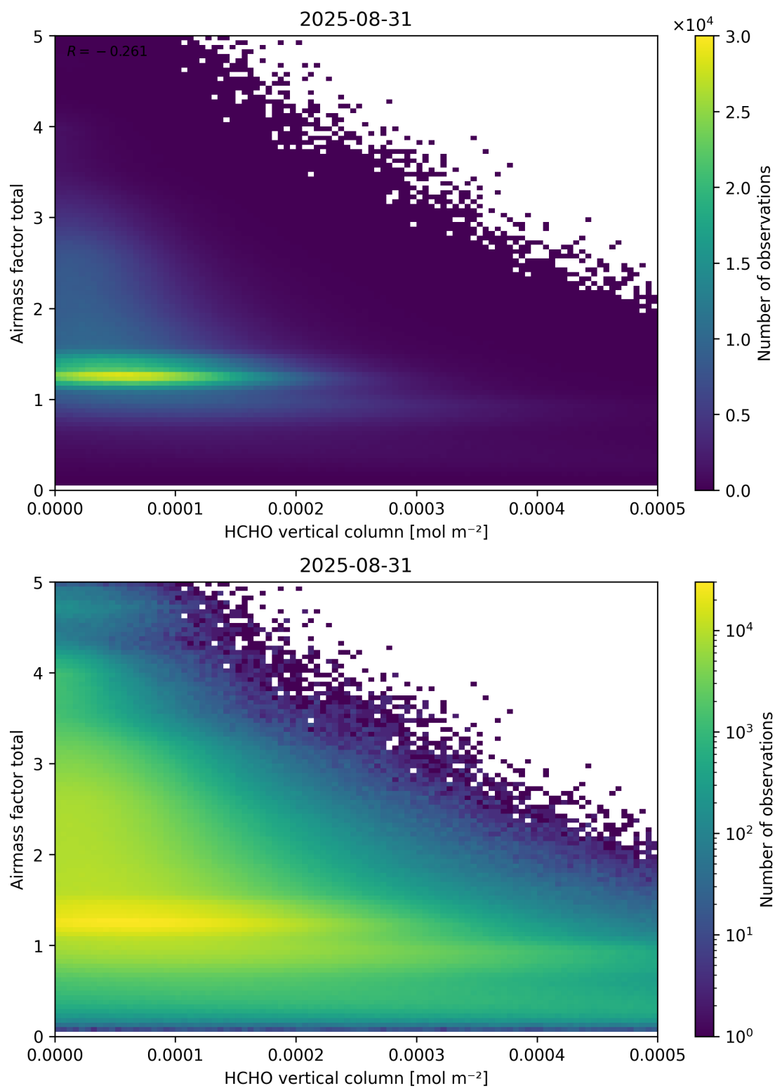
Figure 131: Scatter density plot of “HCHO vertical column” against “Airmass factor total” for 2025-08-30 to 2025-09-01.
