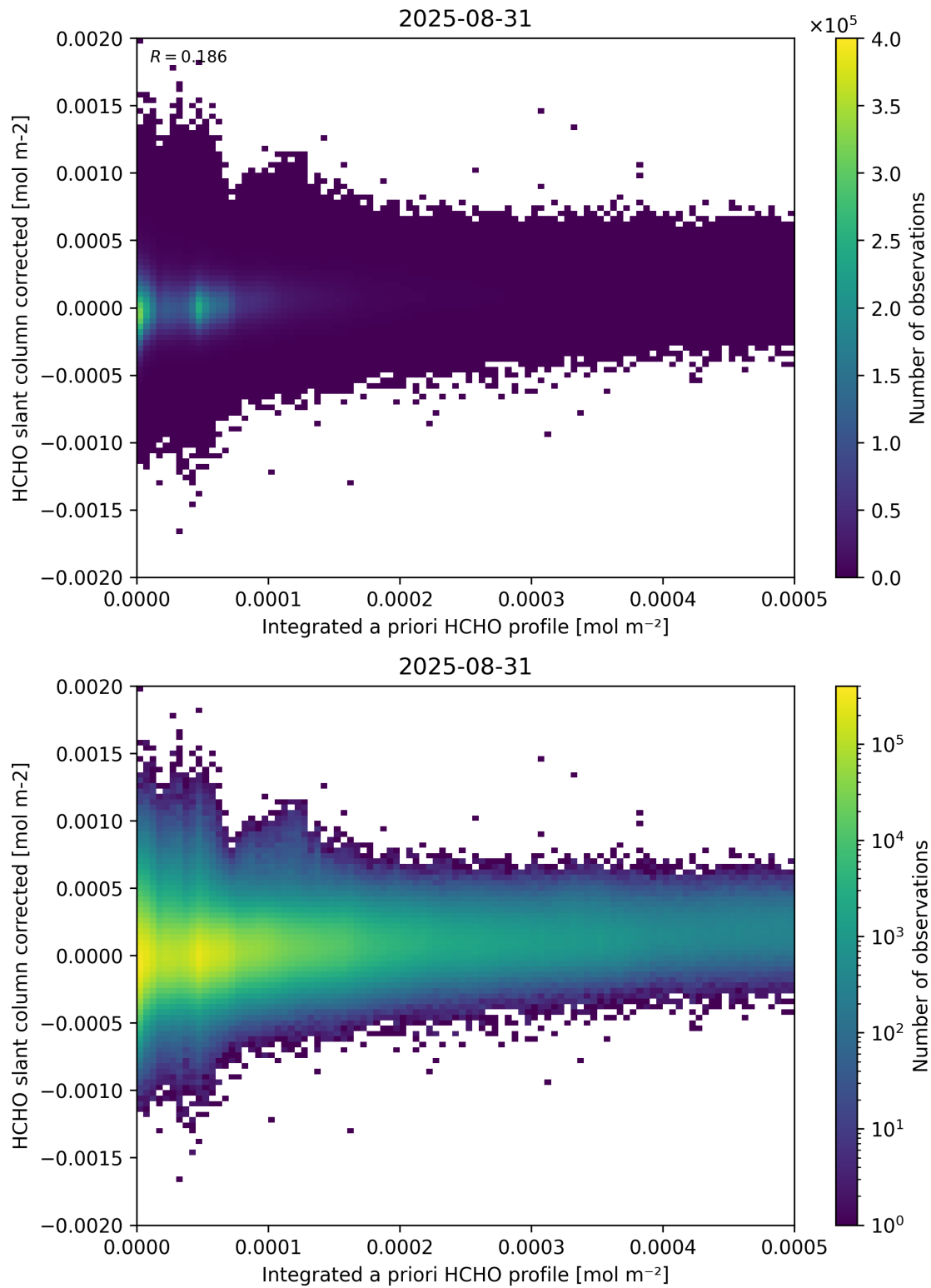
Figure 151: Scatter density plot of “Integrated a priori HCHO profile” against “HCHO slant column corrected” for 2025-08-30 to 2025-09-01.
