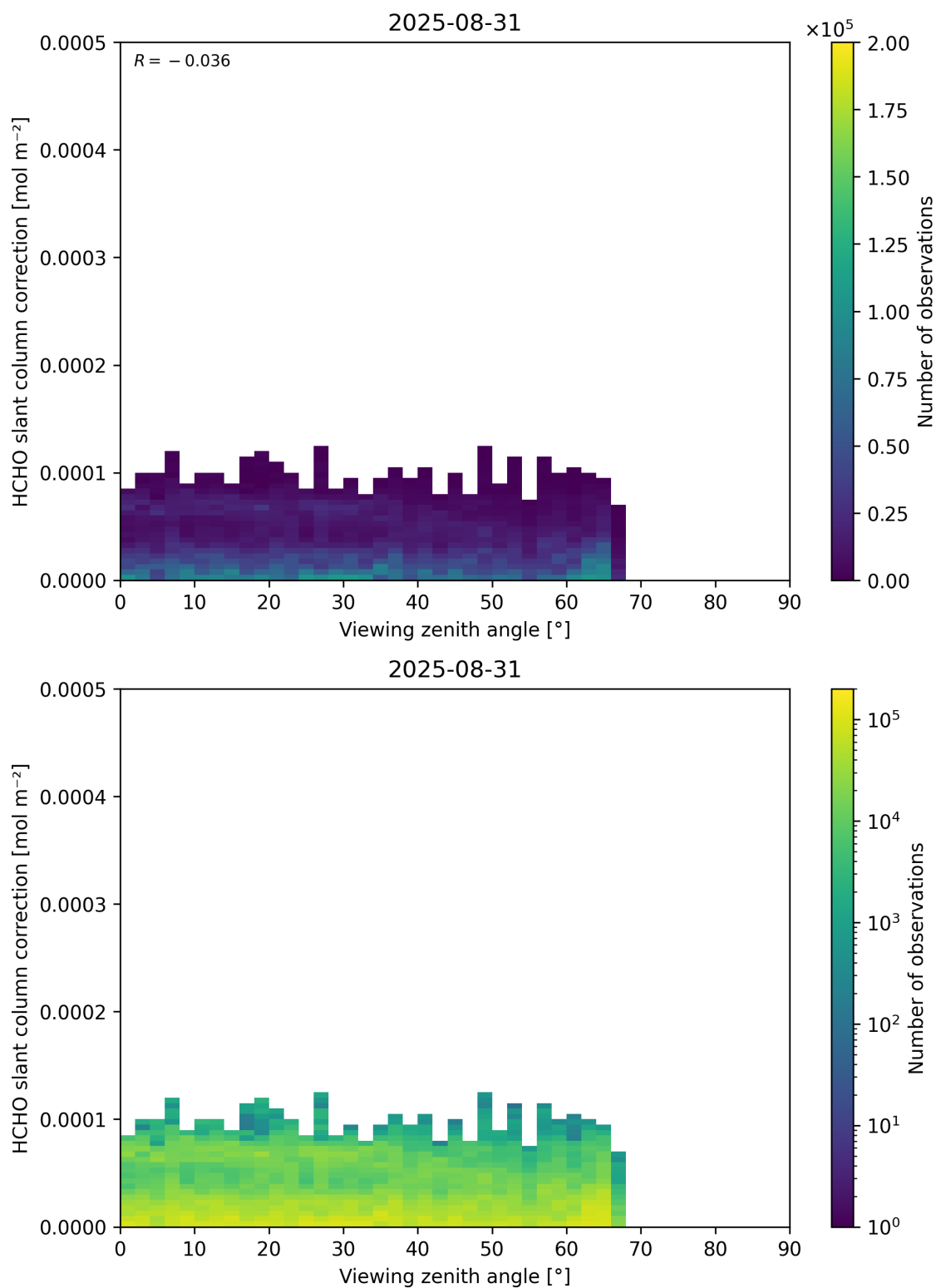
Figure 187: Scatter density plot of “Viewing zenith angle” against “HCHO slant column correction” for 2025-08-30 to 2025-09-01.
