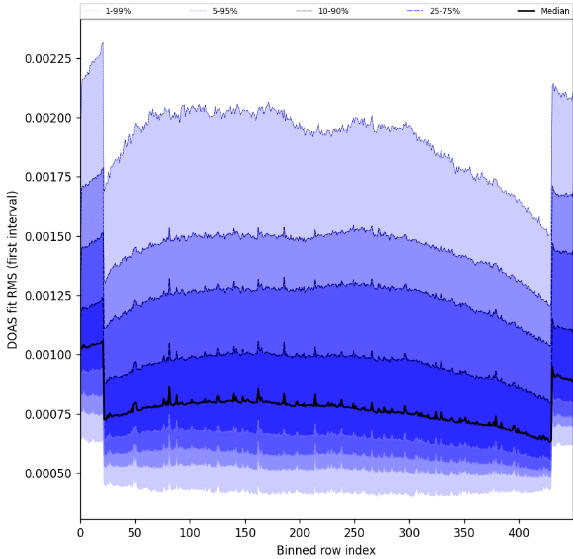
Figure 60: Along track statistics of “DOAS fit RMS (first interval)” for 2025-08-30 to 2025-09-01
