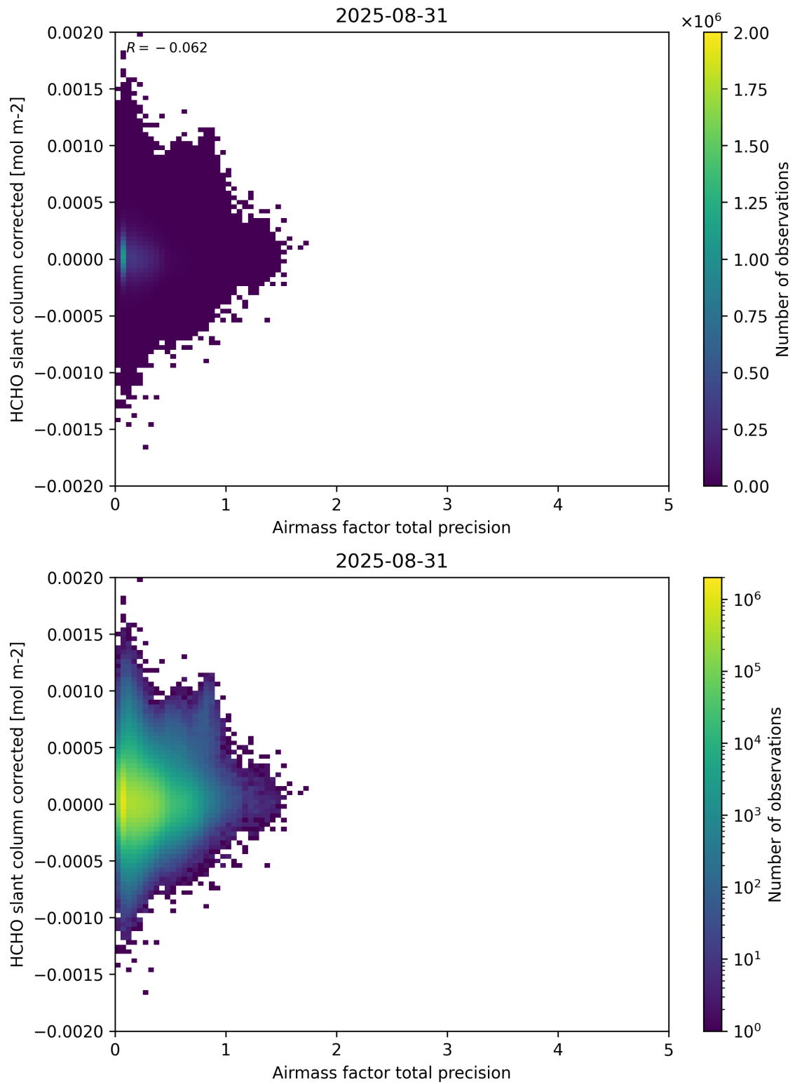
Figure 109: Scatter density plot of “Airmass factor total precision” against “HCHO slant column corrected” for 2025-08-30 to 2025-09-01.
