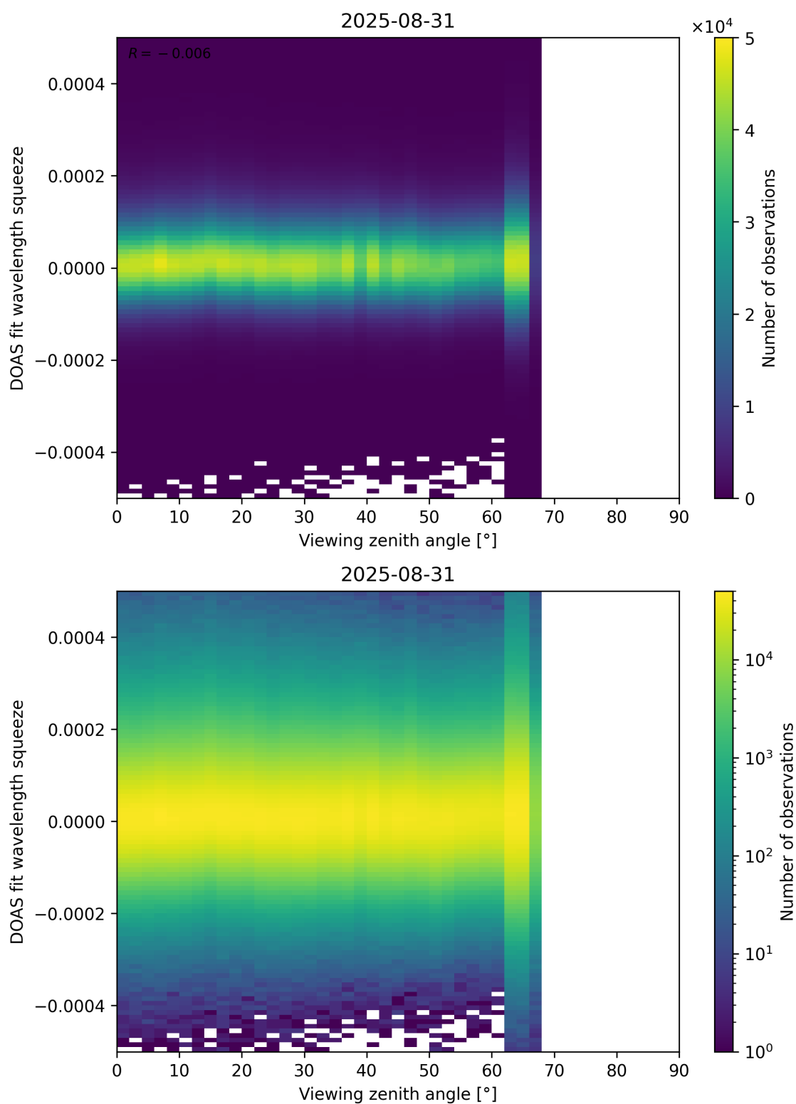
Figure 184: Scatter density plot of “Viewing zenith angle” against “DOAS fit wavelength squeeze” for 2025-08-30 to 2025-09-01.
