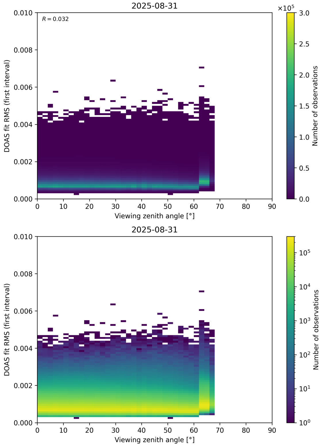
Figure 182: Scatter density plot of “Viewing zenith angle” against “DOAS fit RMS (first interval)” for 2025-08-30 to 2025-09-01.
