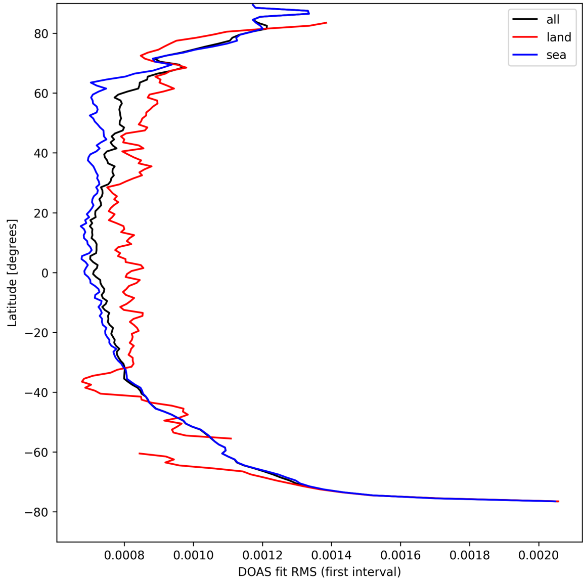
Figure 32: Zonal average of “DOAS fit RMS (first interval)” for 2025-08-30 to 2025-09-01.
