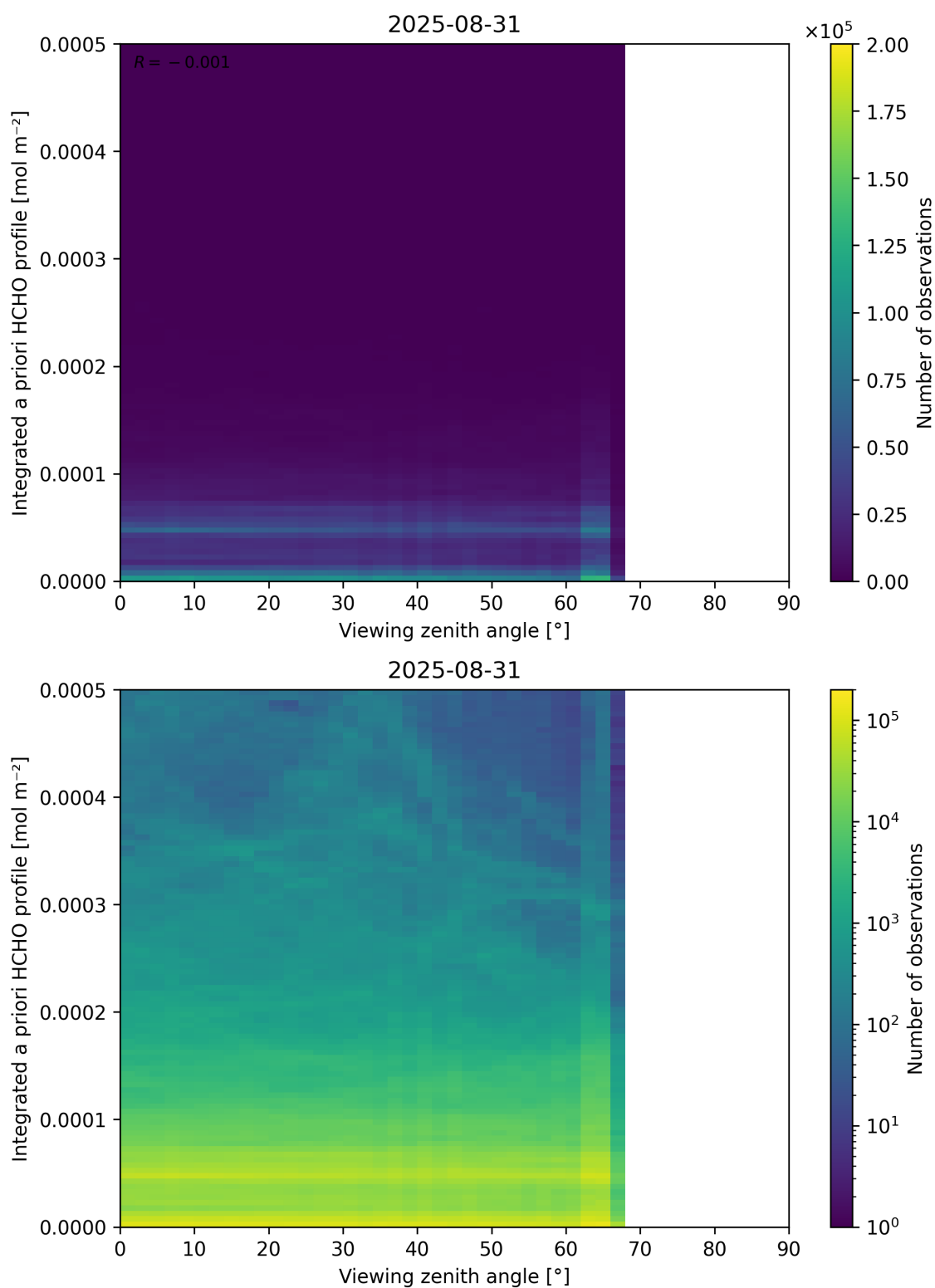
Figure 195: Scatter density plot of “Viewing zenith angle” against “Integrated a priori HCHO profile” for 2025-08-30 to 2025-09-01.
