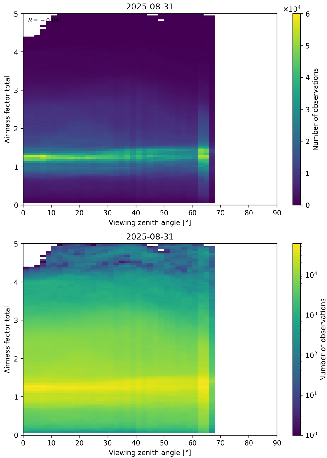
Figure 190: Scatter density plot of “Viewing zenith angle” against “Airmass factor total” for 2025-08-30 to 2025-09-01.
