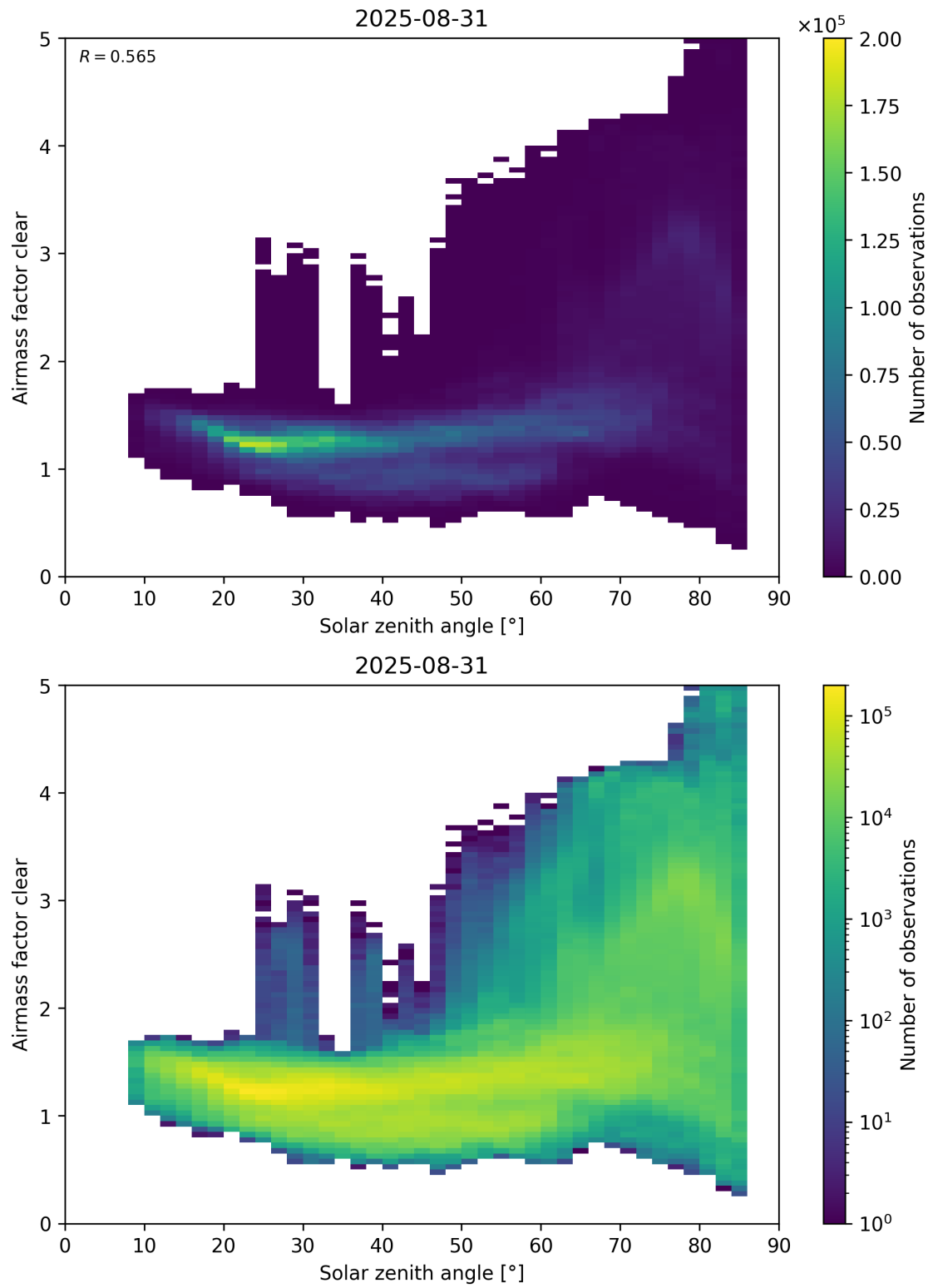
Figure 170: Scatter density plot of “Solar zenith angle” against “Airmass factor clear” for 2025-08-30 to 2025-09-01.
