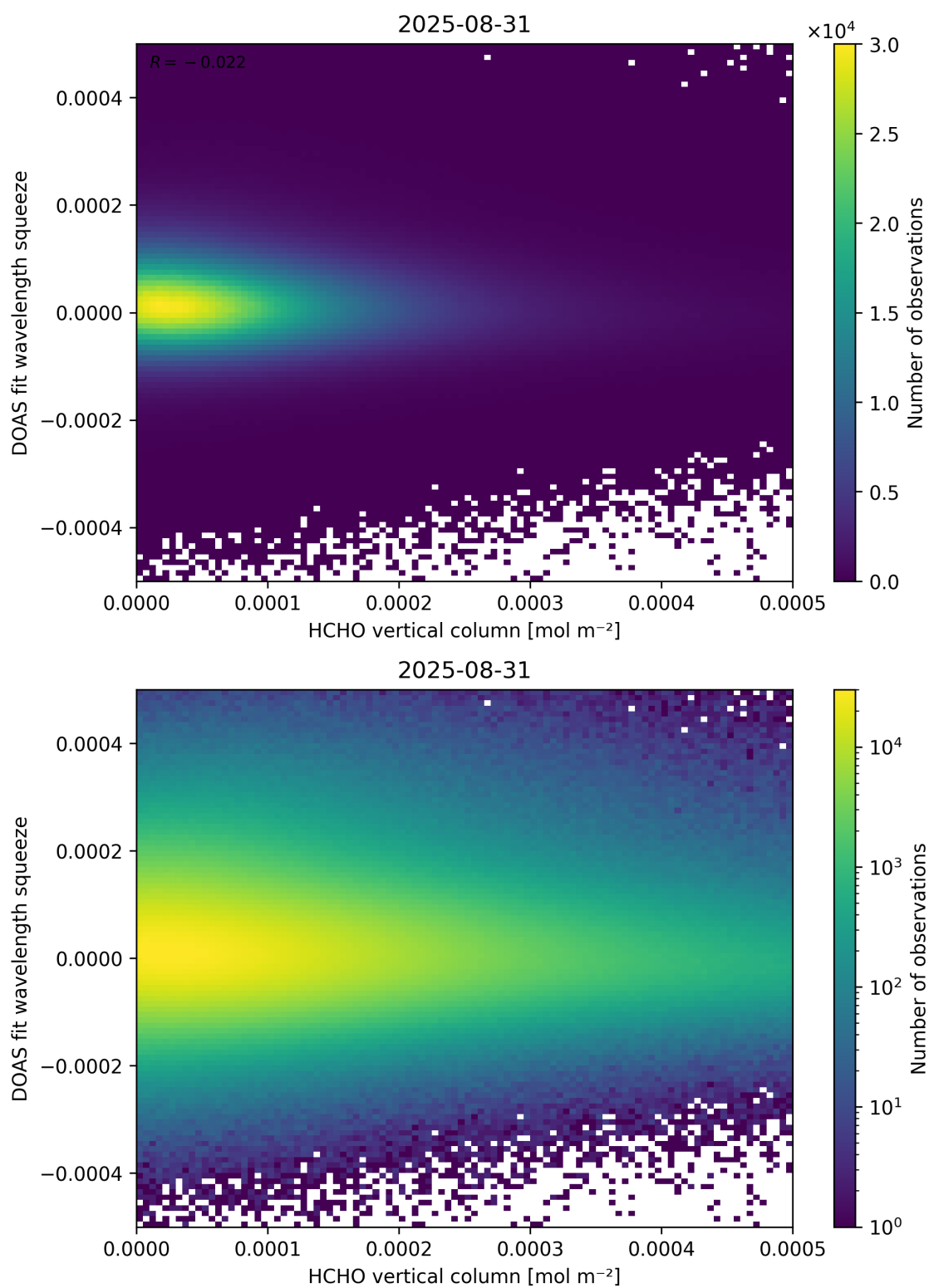
Figure 125: Scatter density plot of “HCHO vertical column” against “DOAS fit wavelength squeeze” for 2025-08-30 to 2025-09-01.
