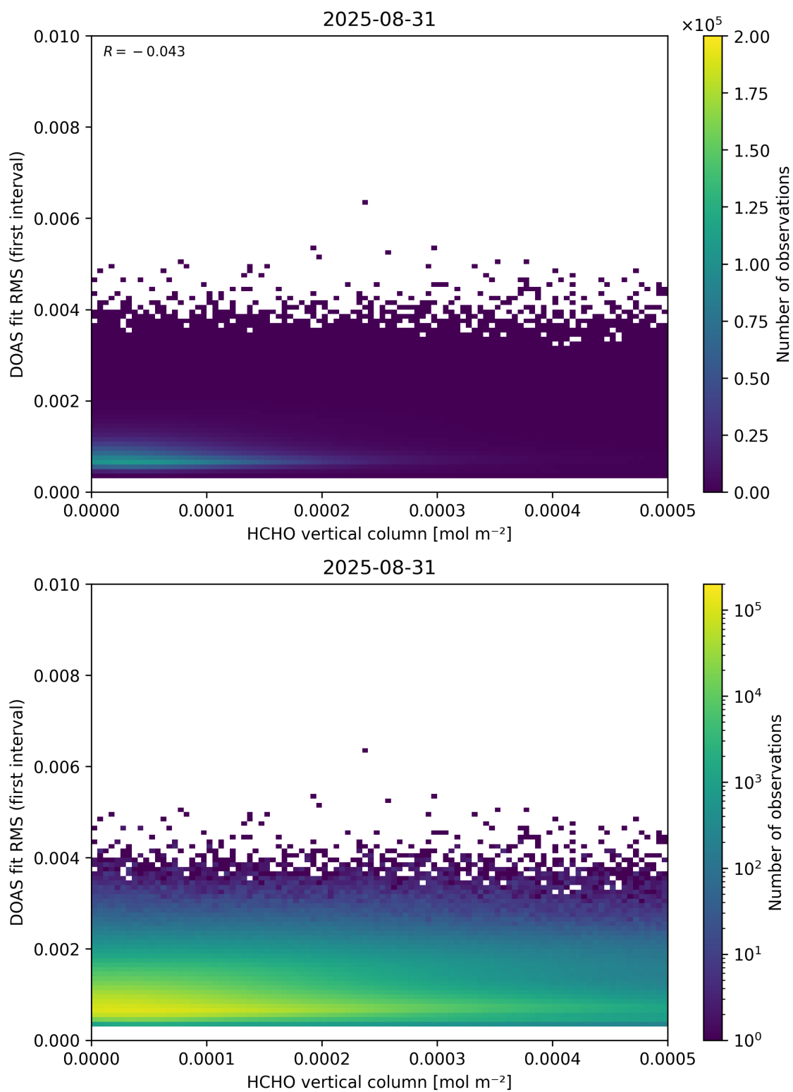
Figure 123: Scatter density plot of “HCHO vertical column” against “DOAS fit RMS (first interval)” for 2025-08-30 to 2025-09-01.
