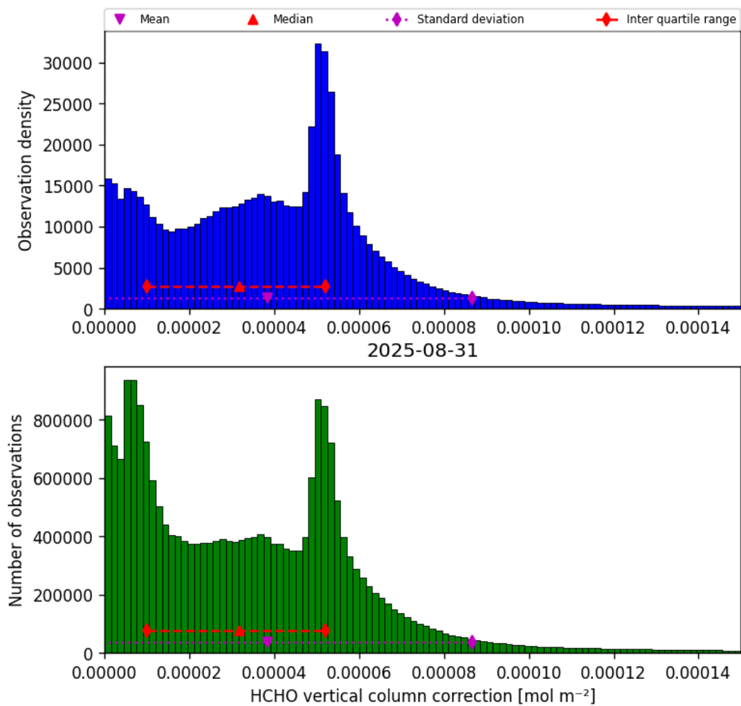
Figure 37: Histogram of “HCHO vertical column correction” for 2025-08-30 to 2025-09-01
