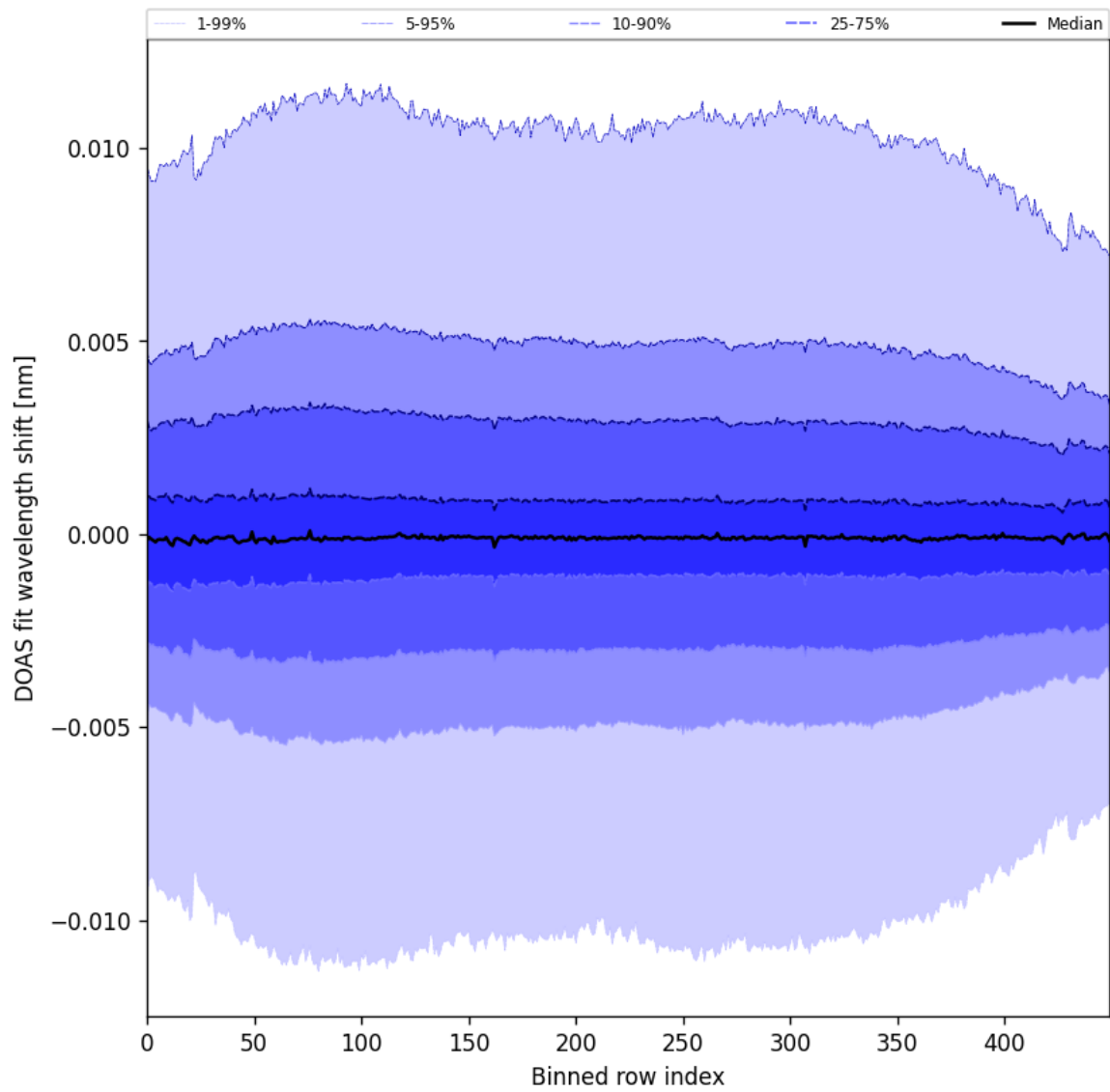
Figure 58: Along track statistics of “DOAS fit wavelength shift” for 2025-08-30 to 2025-09-01
