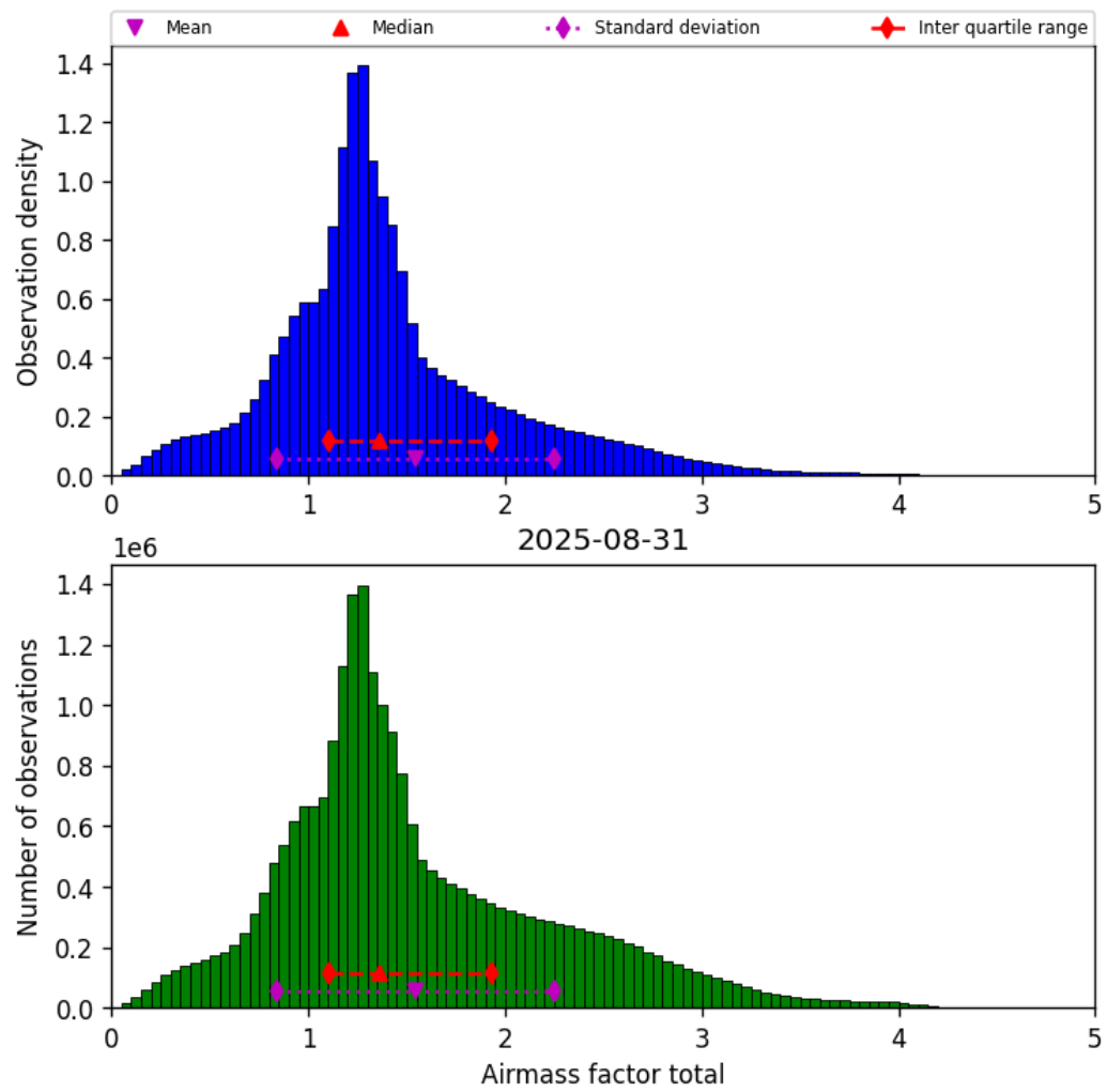
Figure 40: Histogram of “Airmass factor total” for 2025-08-30 to 2025-09-01
