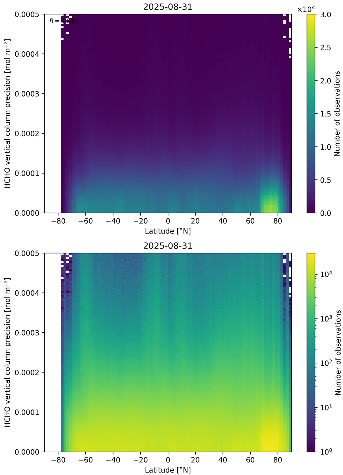
Figure 165: Scatter density plot of “Latitude” against “HCHO vertical column precision” for 2025-08-30 to 2025-09-01.
