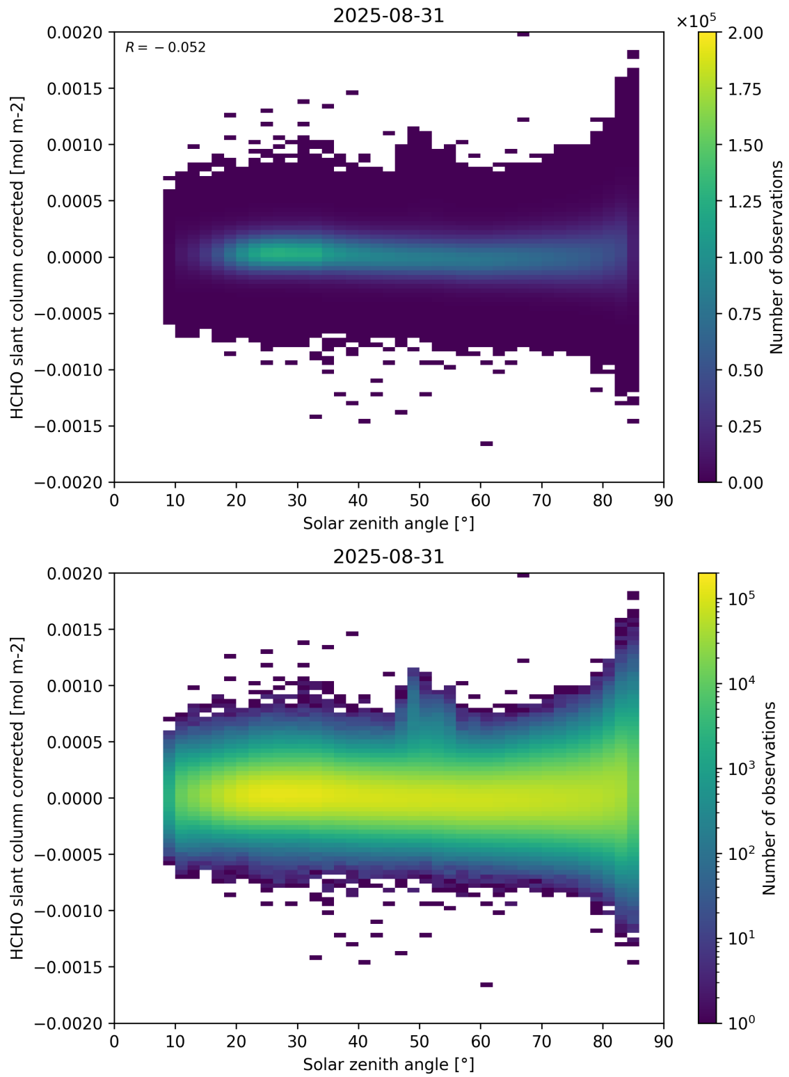
Figure 171: Scatter density plot of “Solar zenith angle” against “HCHO slant column corrected” for 2025-08-30 to 2025-09-01.
