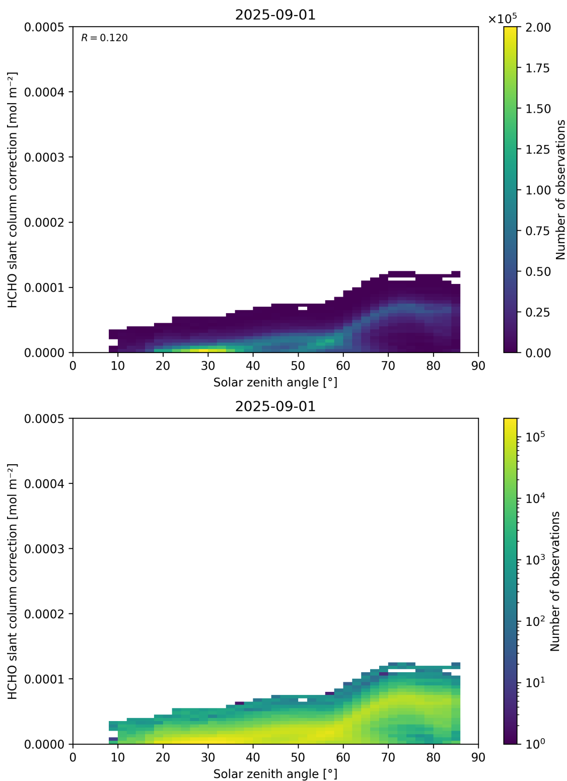
Figure 172: Scatter density plot of “Solar zenith angle” against “HCHO slant column correction” for 2025-08-31 to 2025-09-02.
