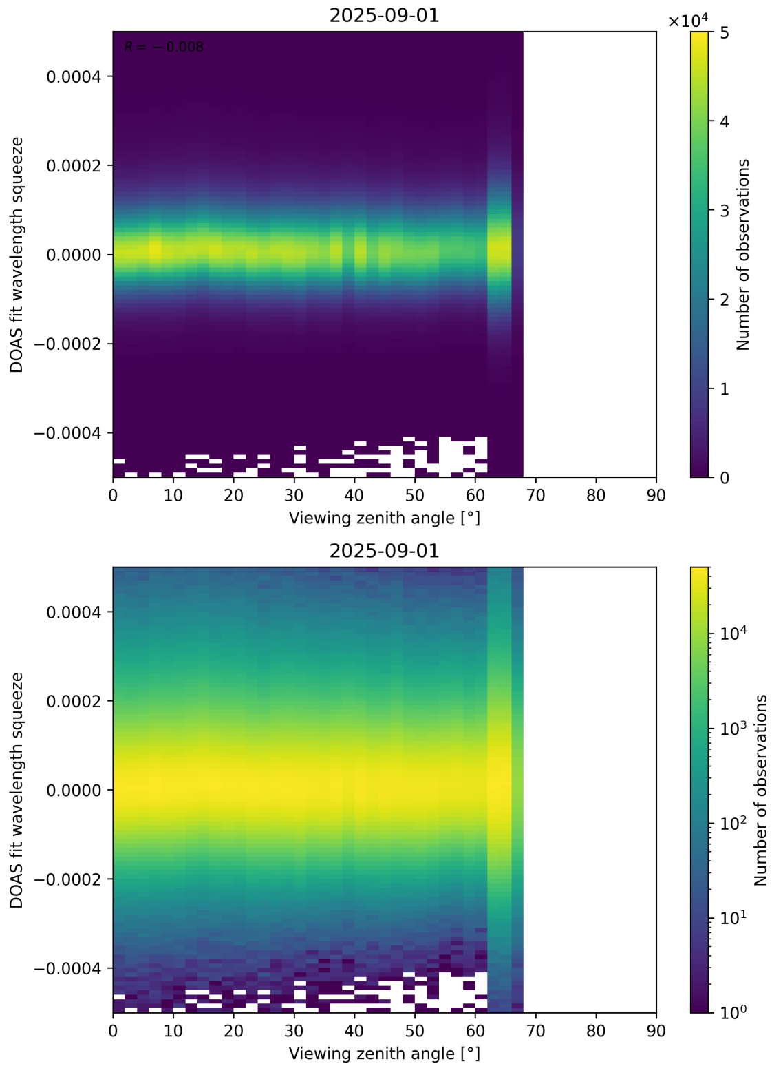
Figure 184: Scatter density plot of “Viewing zenith angle” against “DOAS fit wavelength squeeze” for 2025-08-31 to 2025-09-02.
