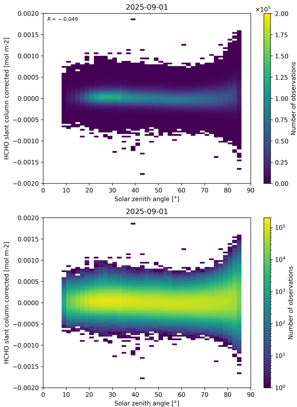
Figure 171: Scatter density plot of “Solar zenith angle” against “HCHO slant column corrected” for 2025-08-31 to 2025-09-02.
