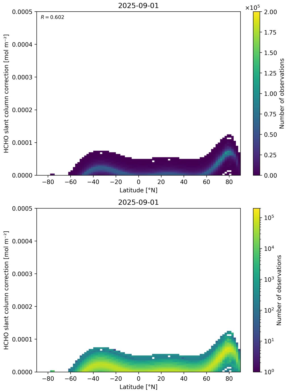
Figure 158: Scatter density plot of “Latitude” against “HCHO slant column correction” for 2025-08-31 to 2025-09-02.
