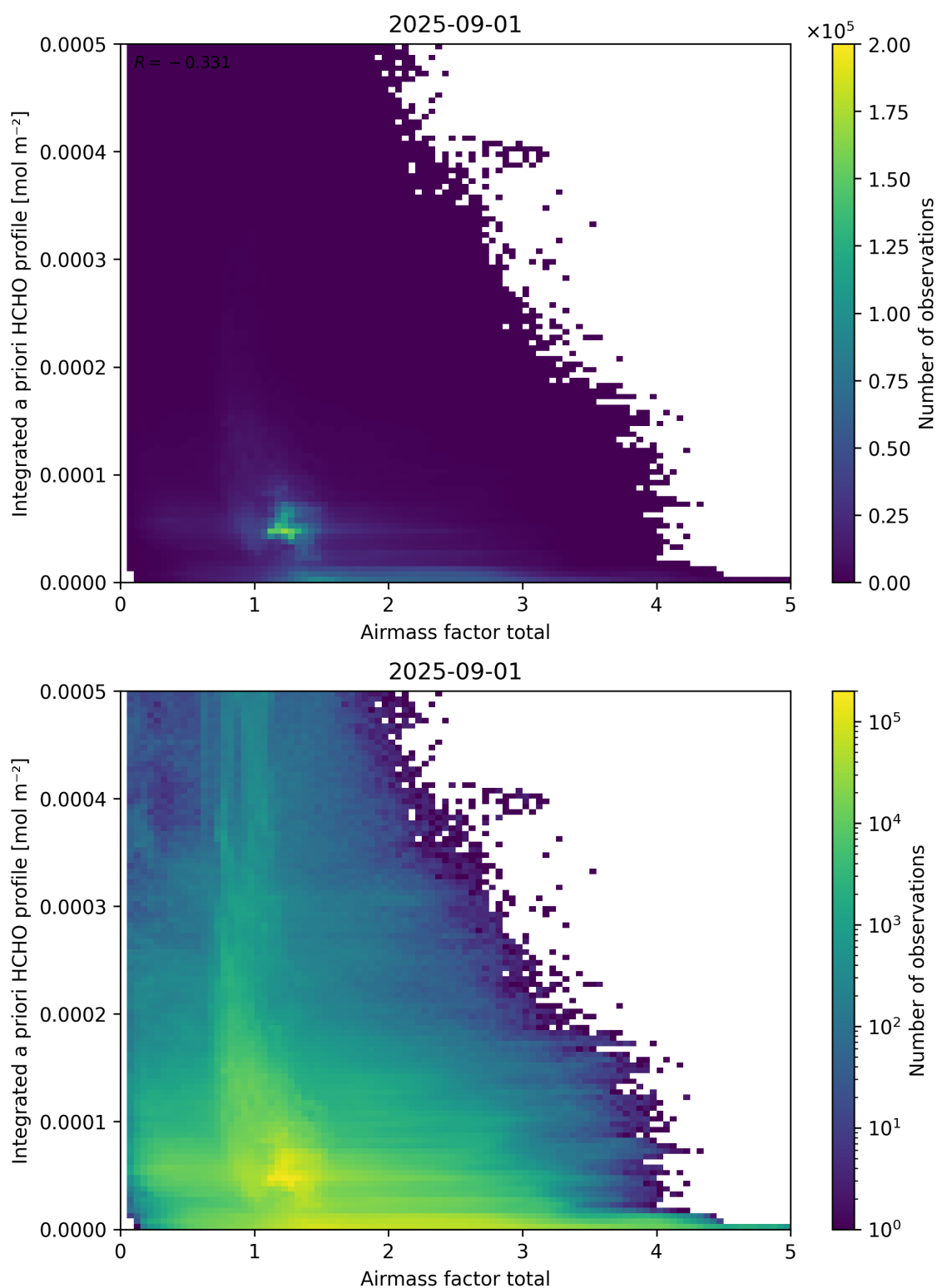
Figure 104: Scatter density plot of “Airmass factor total” against “Integrated a priori HCHO profile” for 2025-08-31 to 2025-09-02.
