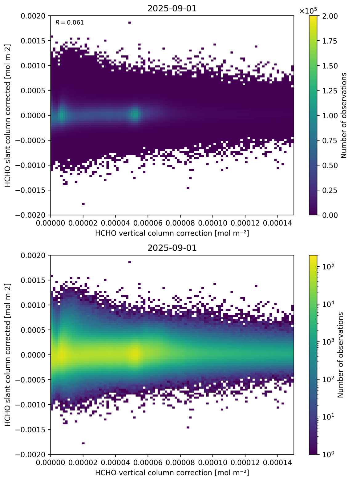
Figure 116: Scatter density plot of “HCHO vertical column correction” against “HCHO slant column corrected” for 2025-08-31 to 2025-09-02.
