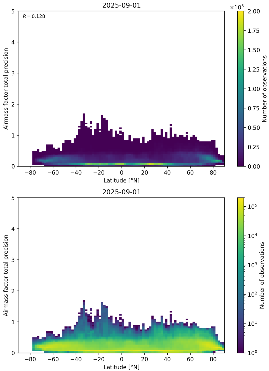
Figure 162: Scatter density plot of “Latitude” against “Airmass factor total precision” for 2025-08-31 to 2025-09-02.
