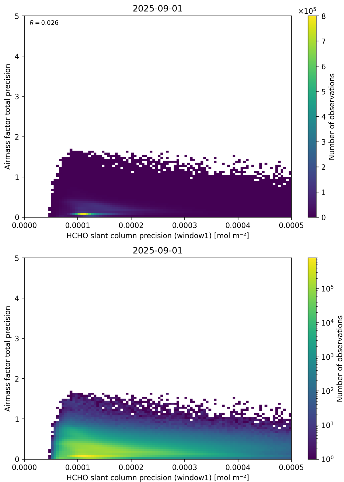
Figure 95: Scatter density plot of “HCHO slant column precision (window1)” against “Airmass factor total precision” for 2025-08-31 to 2025-09-02.
