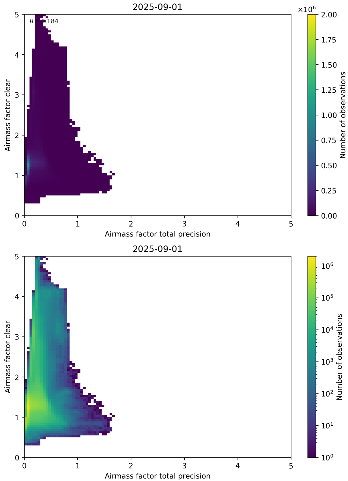
Figure 108: Scatter density plot of “Airmass factor total precision” against “Airmass factor clear” for 2025-08-31 to 2025-09-02.
