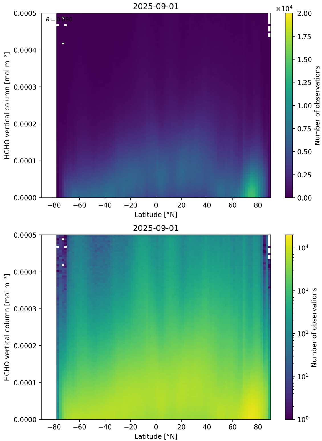
Figure 163: Scatter density plot of “Latitude” against “HCHO vertical column” for 2025-08-31 to 2025-09-02.
