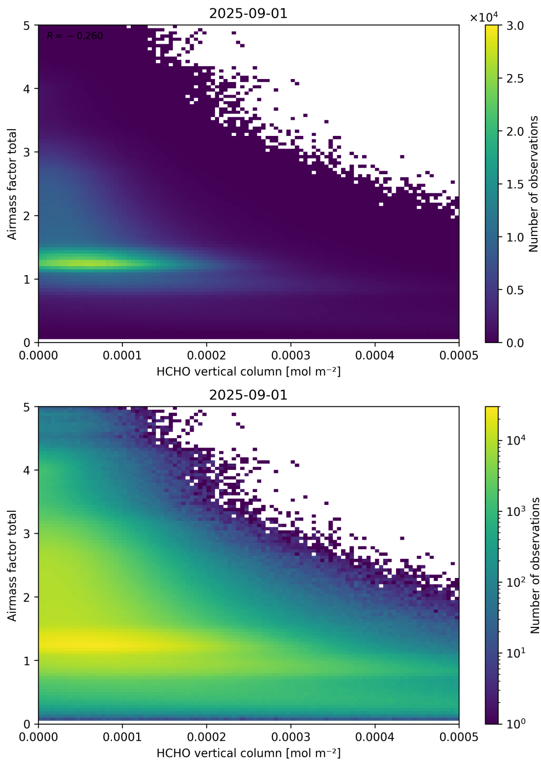
Figure 131: Scatter density plot of “HCHO vertical column” against “Airmass factor total” for 2025-08-31 to 2025-09-02.
