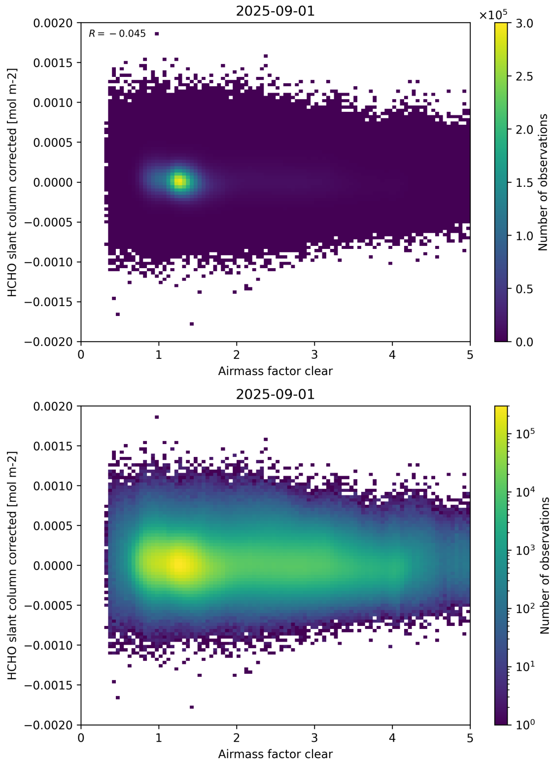
Figure 74: Scatter density plot of “Airmass factor clear” against “HCHO slant column corrected” for 2025-08-31 to 2025-09-02.
