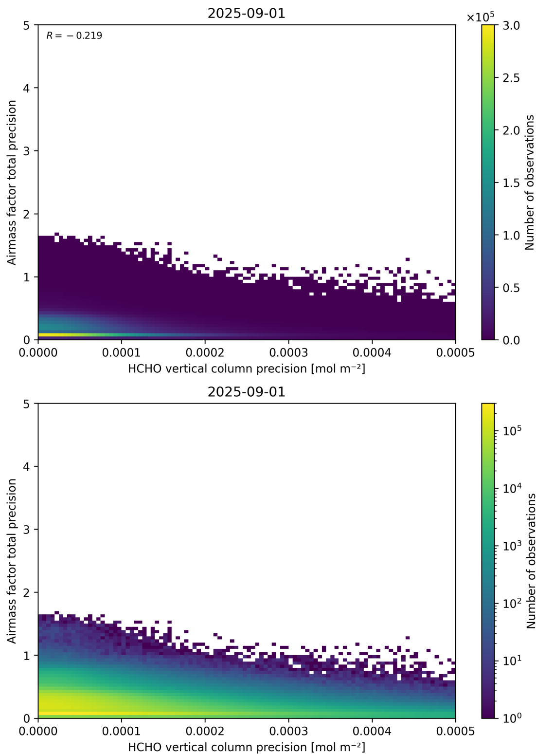
Figure 145: Scatter density plot of “HCHO vertical column precision” against “Airmass factor total precision” for 2025-08-31 to 2025-09-02.
