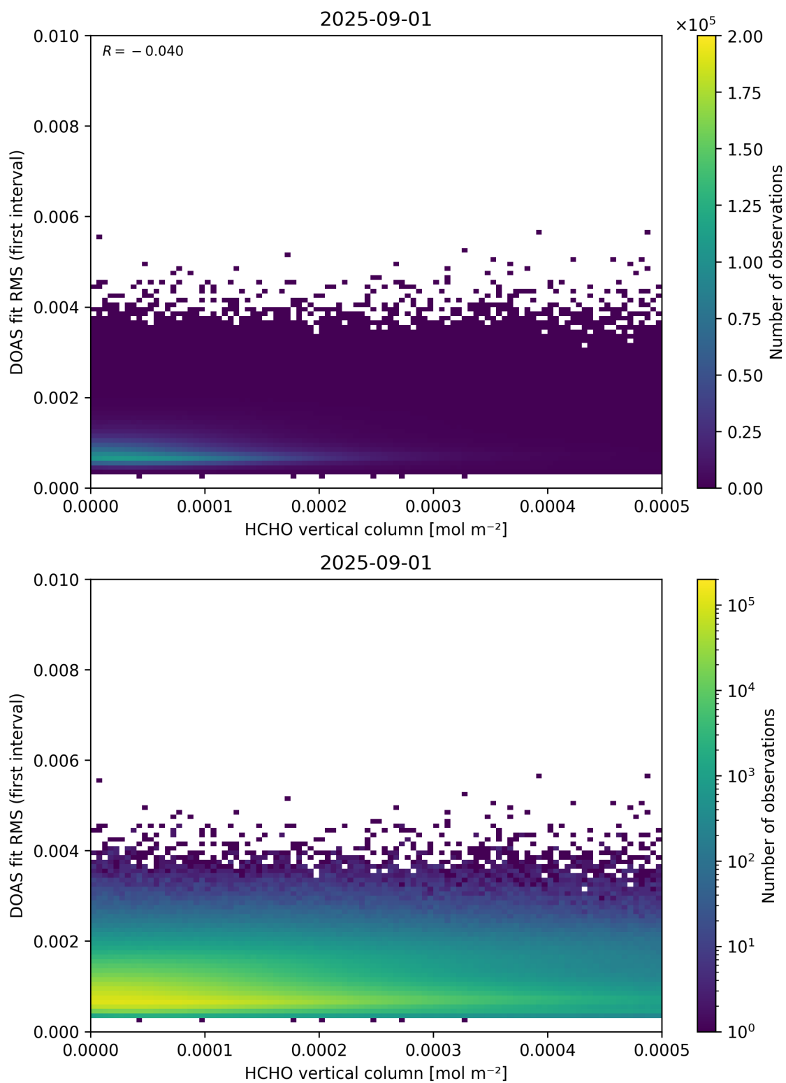
Figure 123: Scatter density plot of “HCHO vertical column” against “DOAS fit RMS (first interval)” for 2025-08-31 to 2025-09-02.
