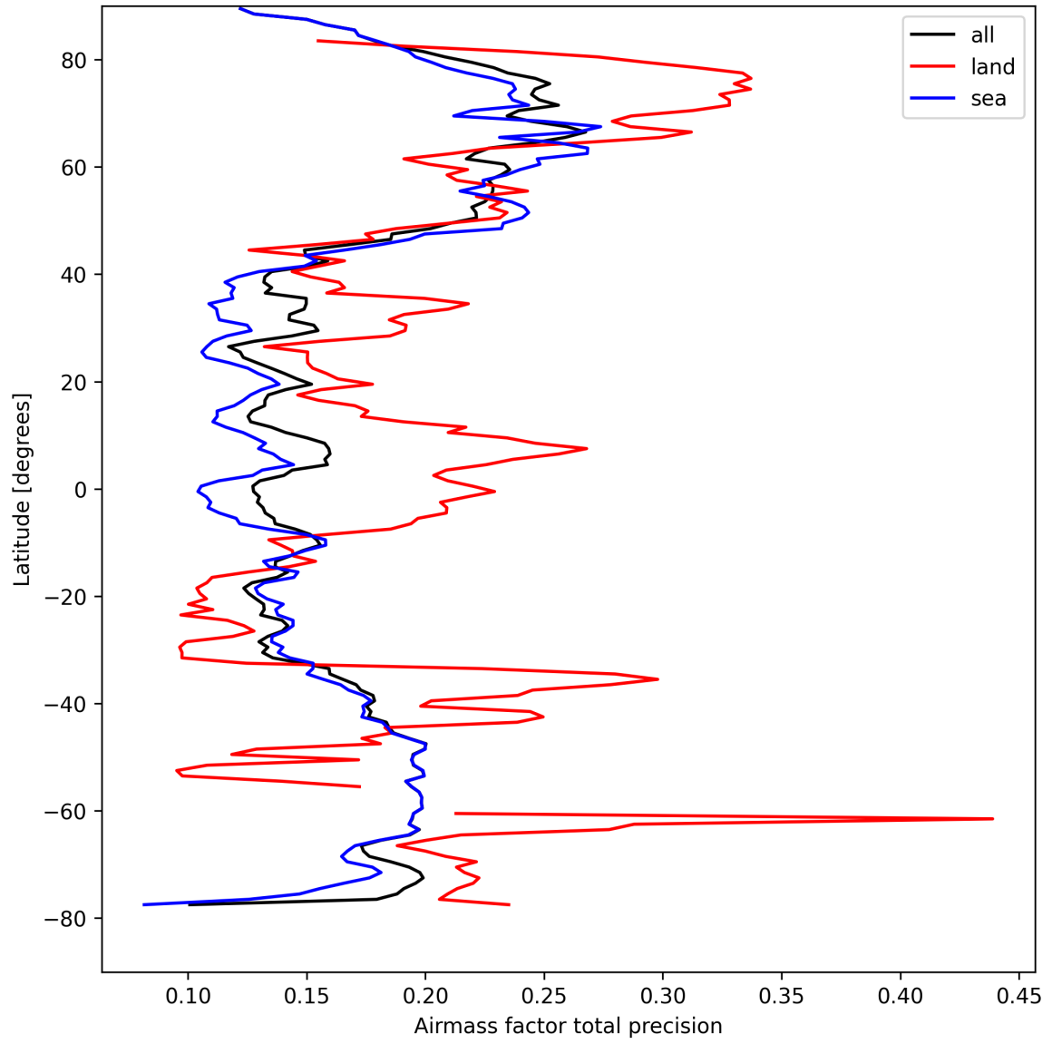
Figure 27: Zonal average of “Airmass factor total precision” for 2025-08-31 to 2025-09-02.
