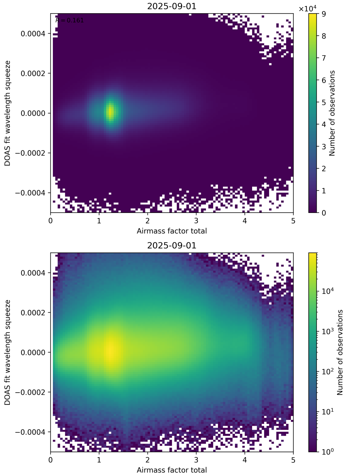
Figure 99: Scatter density plot of “Airmass factor total” against “DOAS fit wavelength squeeze” for 2025-08-31 to 2025-09-02.
