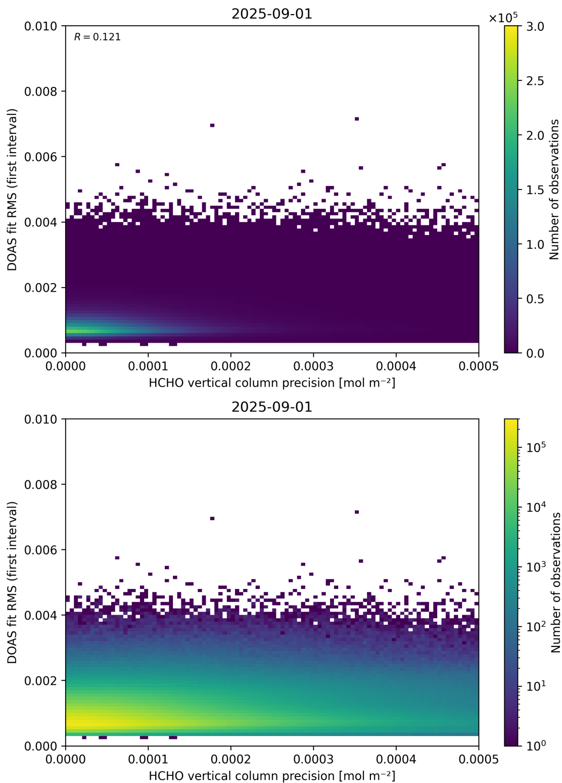
Figure 136: Scatter density plot of “HCHO vertical column precision” against “DOAS fit RMS (first interval)” for 2025-08-31 to 2025-09-02.
