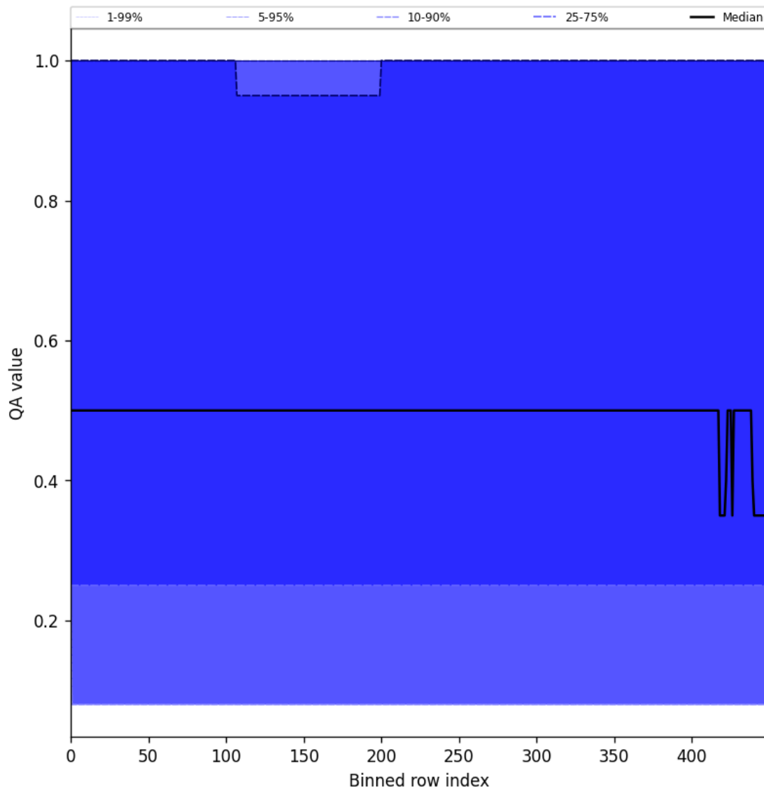
Figure 48: Along track statistics of “QA value” for 2025-08-31 to 2025-09-02
