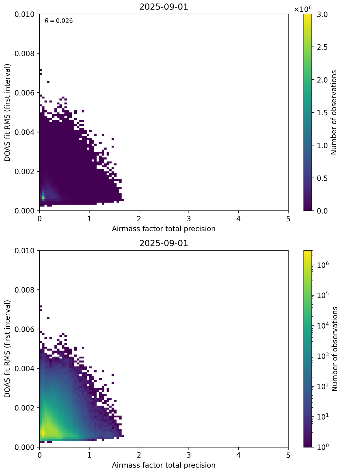
Figure 105: Scatter density plot of “Airmass factor total precision” against “DOAS fit RMS (first interval)” for 2025-08-31 to 2025-09-02.
