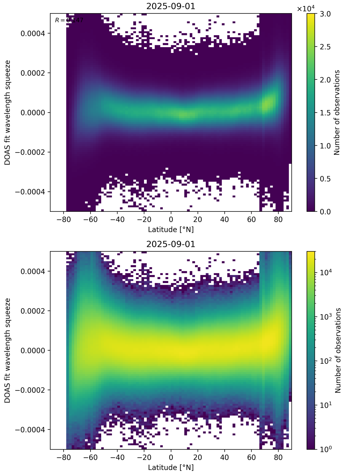
Figure 155: Scatter density plot of “Latitude” against “DOAS fit wavelength squeeze” for 2025-08-31 to 2025-09-02.
