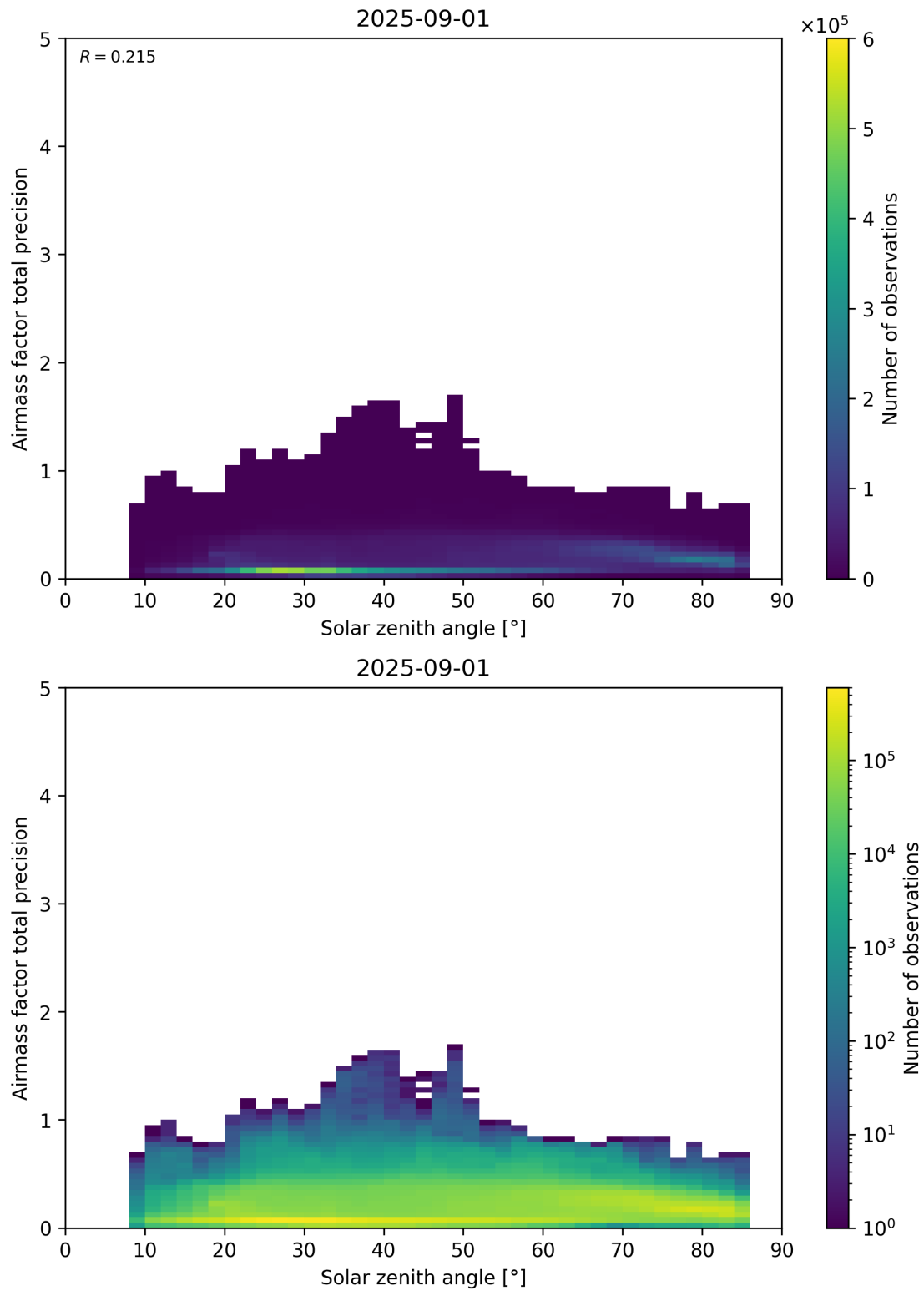
Figure 176: Scatter density plot of “Solar zenith angle” against “Airmass factor total precision” for 2025-08-31 to 2025-09-02.
