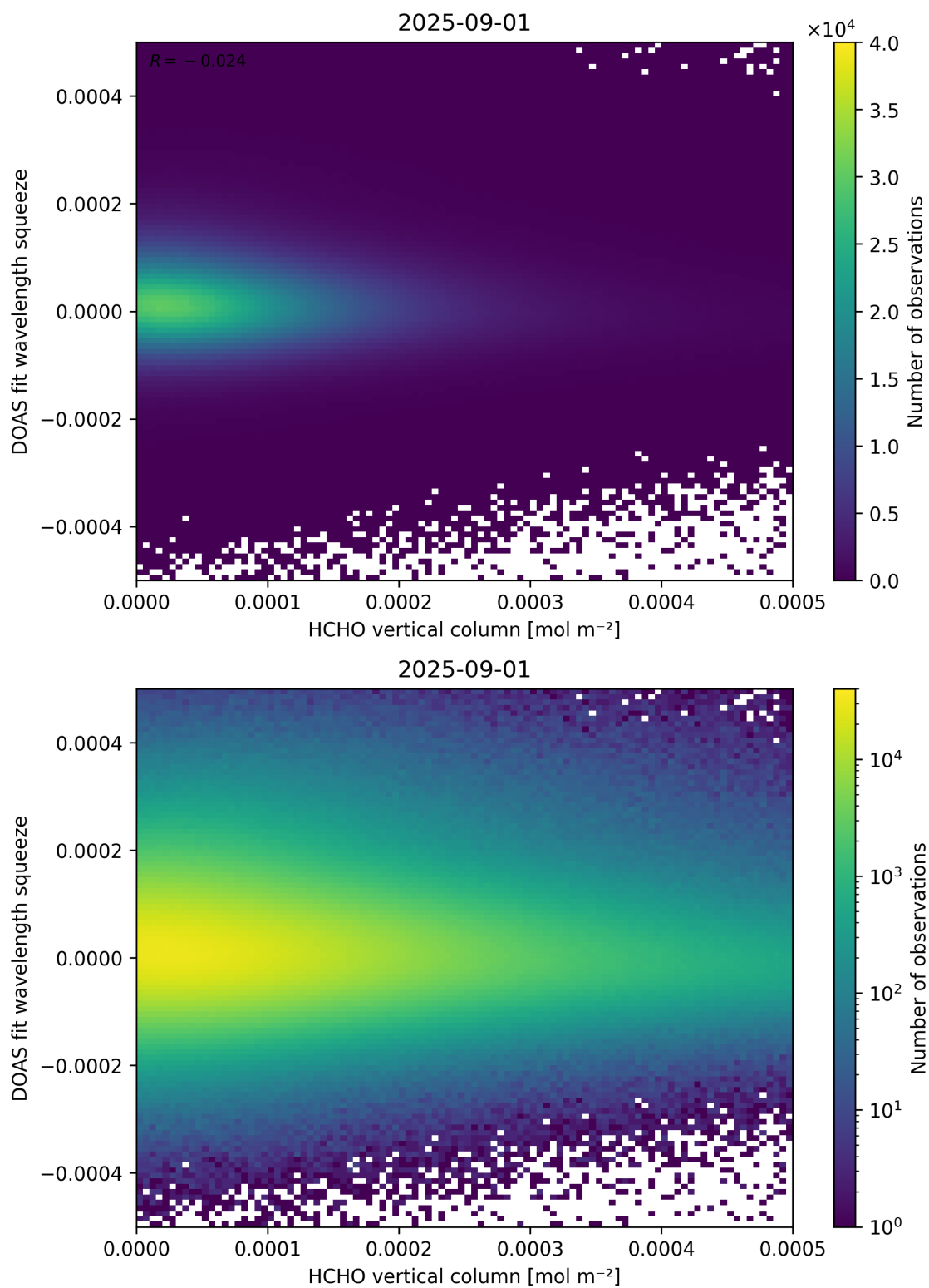
Figure 125: Scatter density plot of “HCHO vertical column” against “DOAS fit wavelength squeeze” for 2025-08-31 to 2025-09-02.
