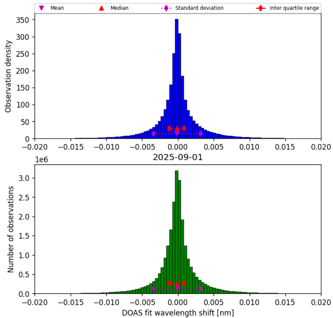
Figure 44: Histogram of “DOAS fit wavelength shift” for 2025-08-31 to 2025-09-02
