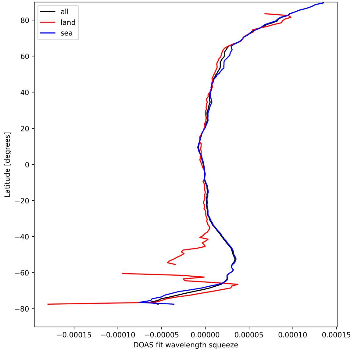
Figure 31: Zonal average of “DOAS fit wavelength squeeze” for 2025-08-31 to 2025-09-02.
