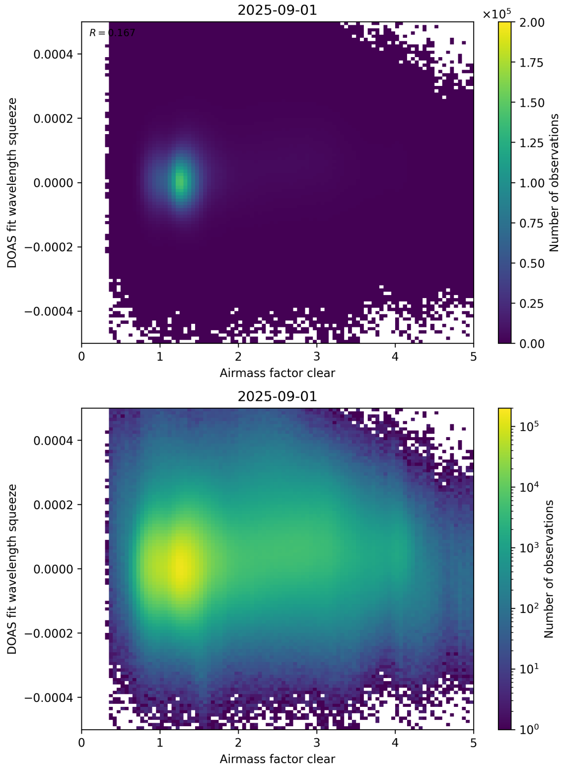
Figure 73: Scatter density plot of “Airmass factor clear” against “DOAS fit wavelength squeeze” for 2025-08-31 to 2025-09-02.
