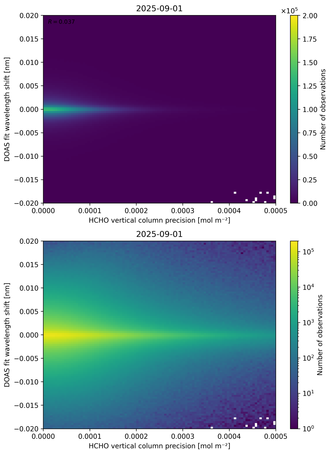
Figure 137: Scatter density plot of “HCHO vertical column precision” against “DOAS fit wavelength shift” for 2025-08-31 to 2025-09-02.
