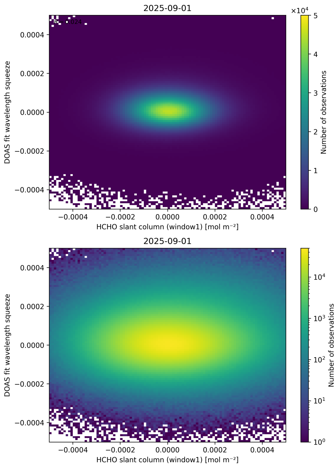
Figure 80: Scatter density plot of “HCHO slant column (window1)” against “DOAS fit wavelength squeeze” for 2025-08-31 to 2025-09-02.
