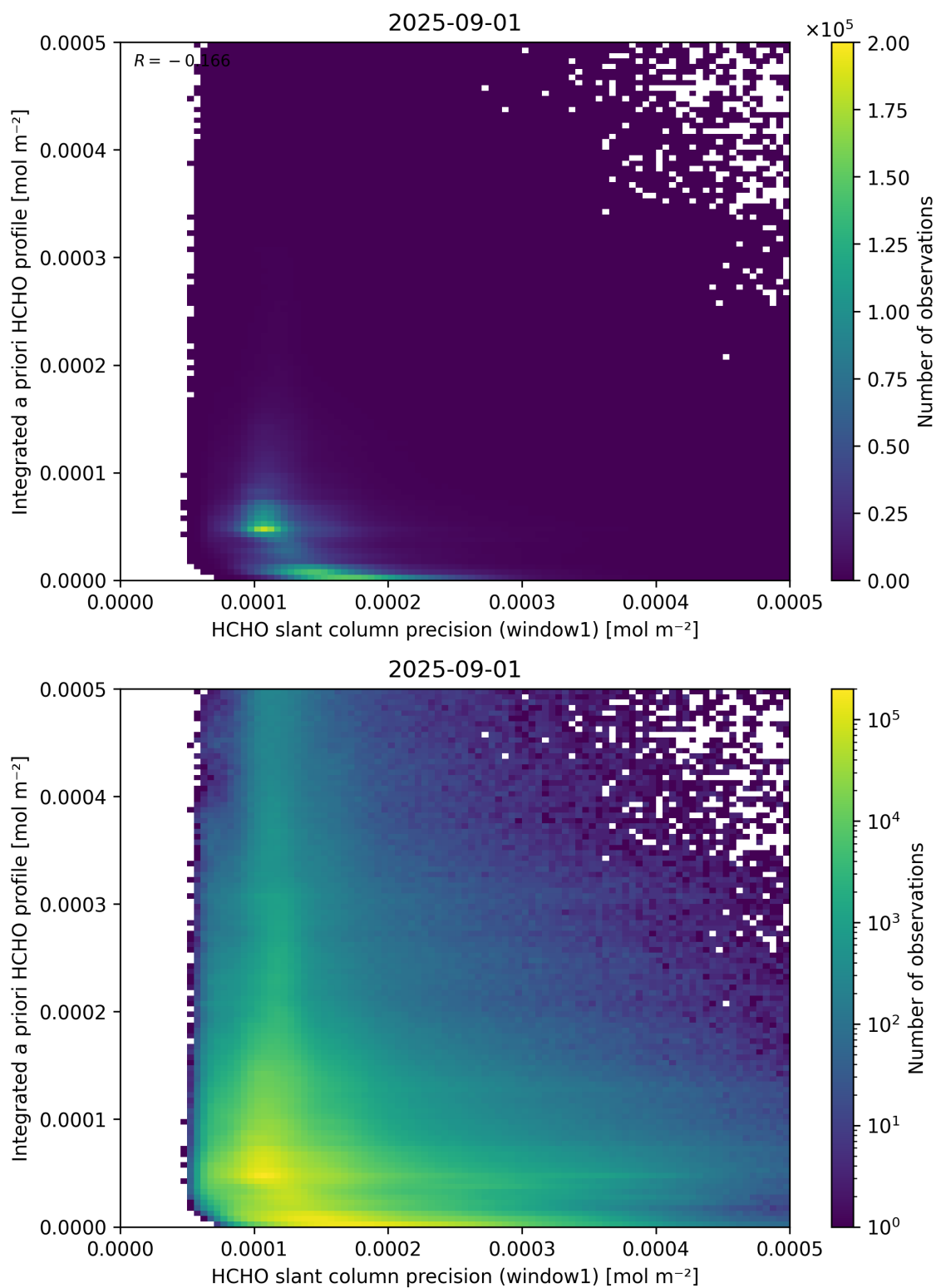
Figure 96: Scatter density plot of “HCHO slant column precision (window1)” against “Integrated a priori HCHO profile” for 2025-08-31 to 2025-09-02.
