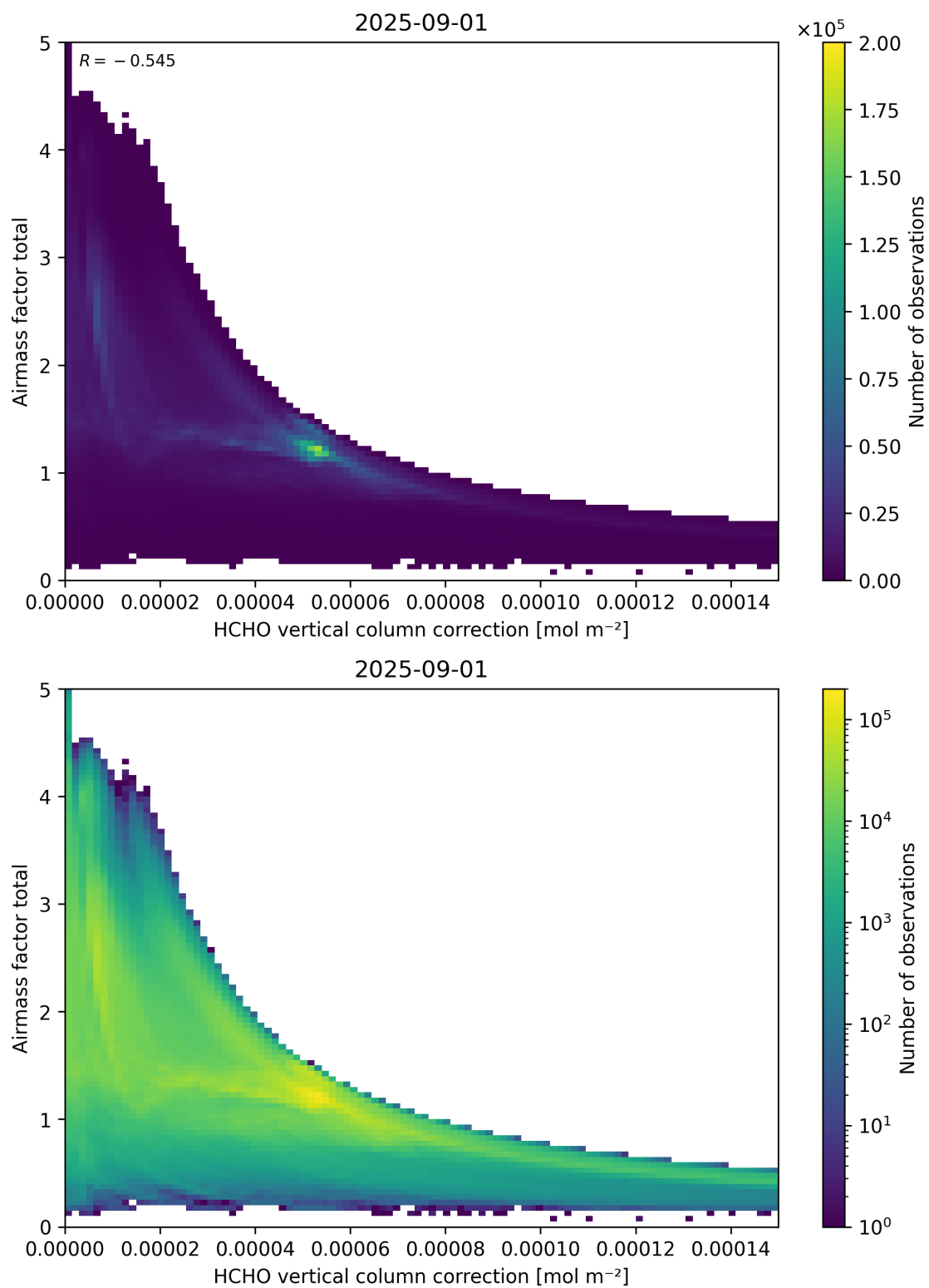
Figure 120: Scatter density plot of “HCHO vertical column correction” against “Airmass factor total” for 2025-08-31 to 2025-09-02.
