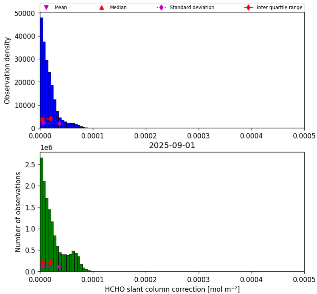
Figure 47: Histogram of “HCHO slant column correction” for 2025-08-31 to 2025-09-02
