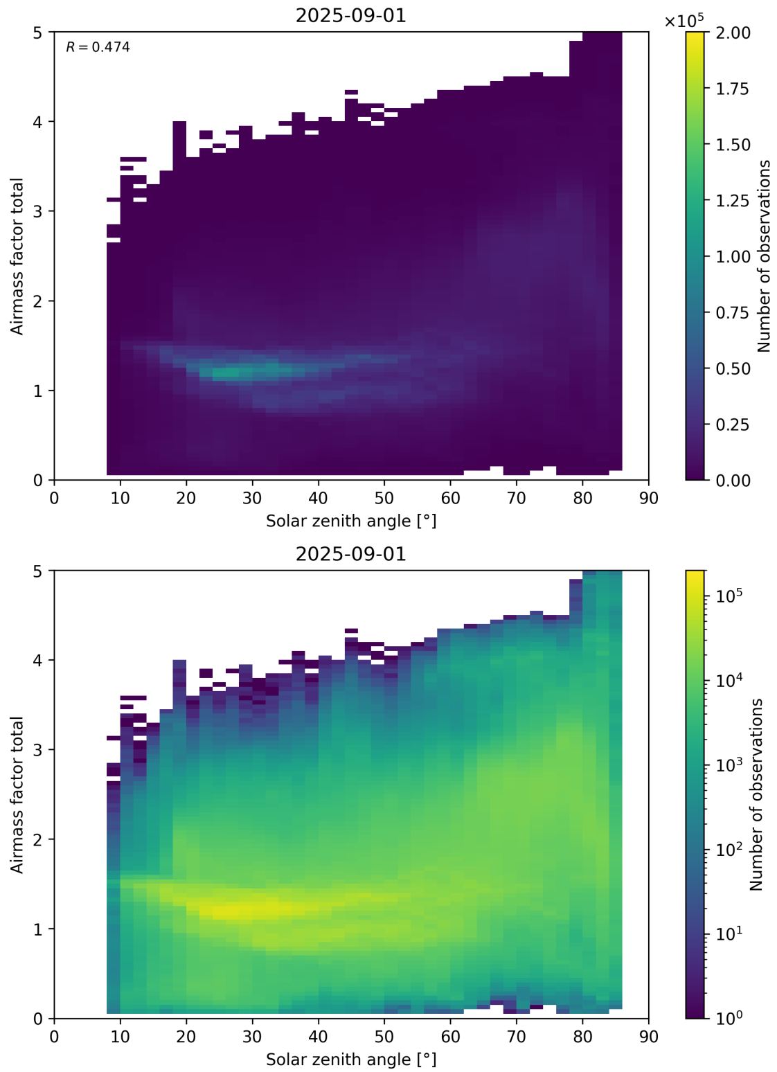
Figure 175: Scatter density plot of “Solar zenith angle” against “Airmass factor total” for 2025-08-31 to 2025-09-02.
