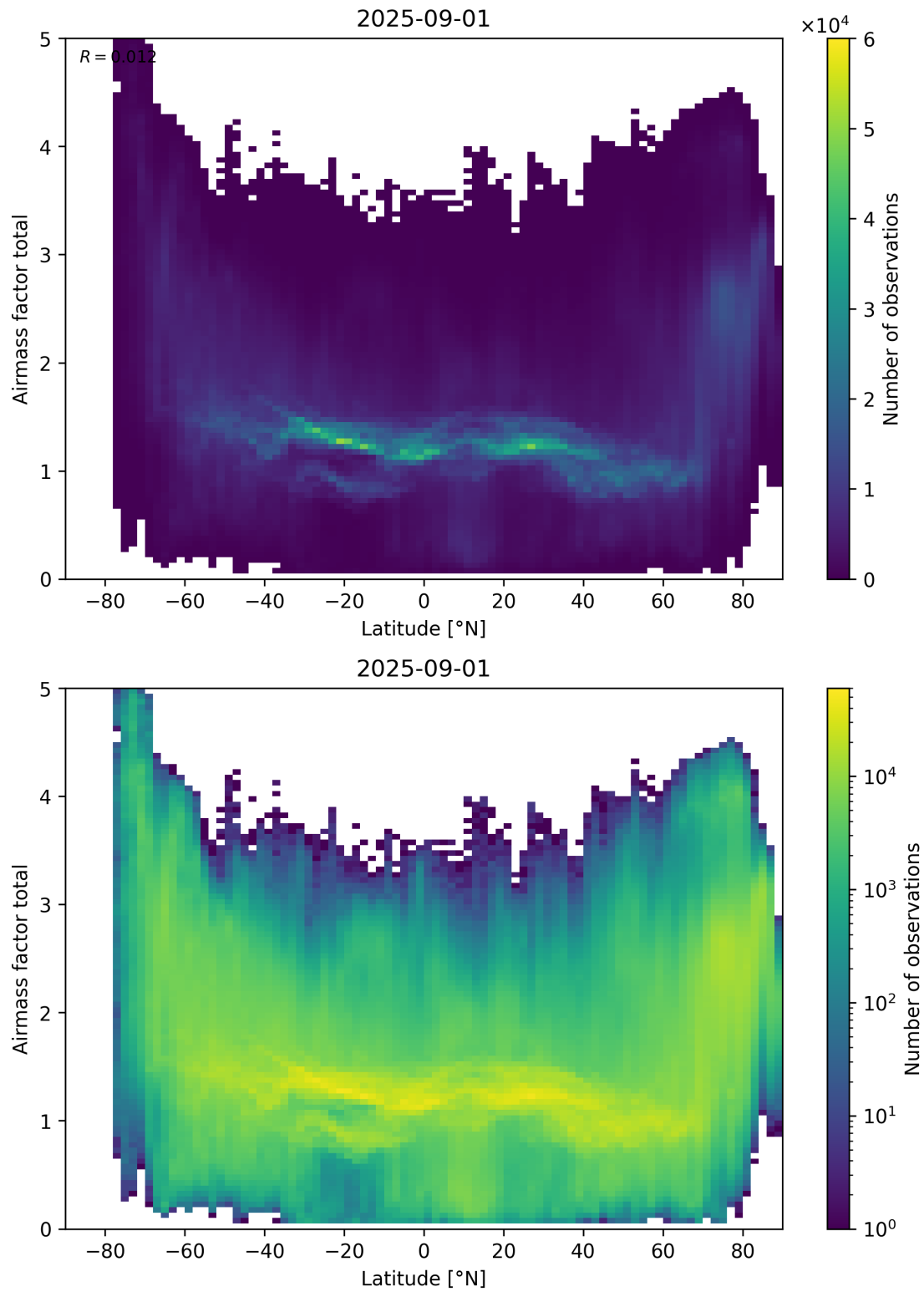
Figure 161: Scatter density plot of “Latitude” against “Airmass factor total” for 2025-08-31 to 2025-09-02.
