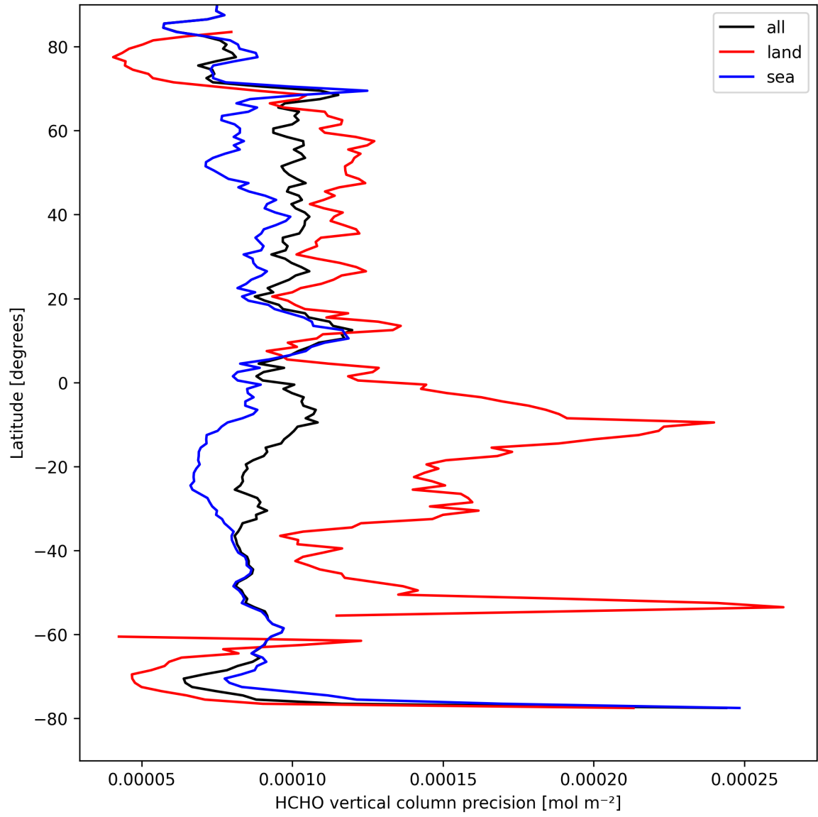
Figure 22: Zonal average of "HCHO vertical column precision" for 2025-08-31 to 2025-09-02.
