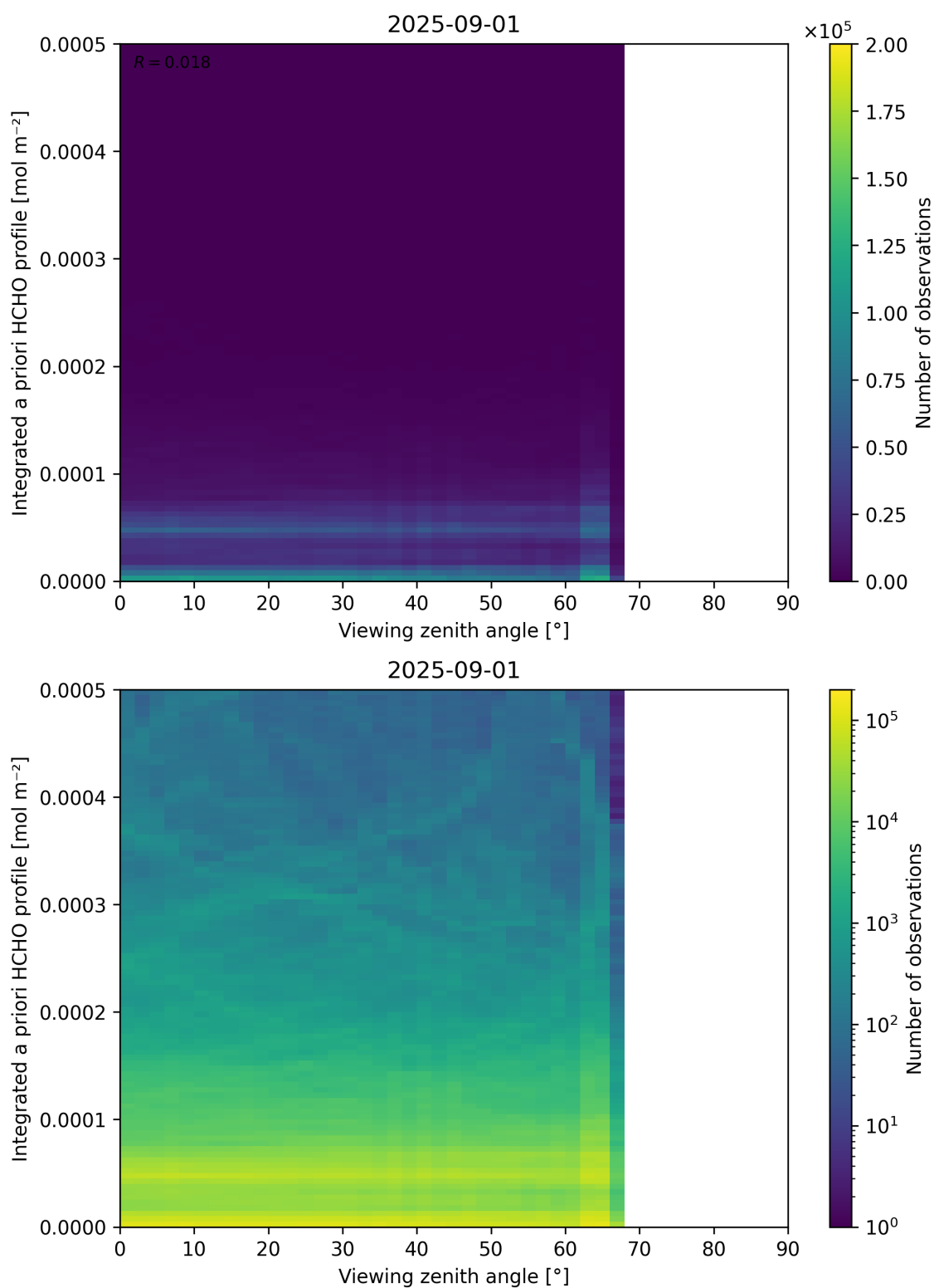
Figure 195: Scatter density plot of “Viewing zenith angle” against “Integrated a priori HCHO profile” for 2025-08-31 to 2025-09-02.
