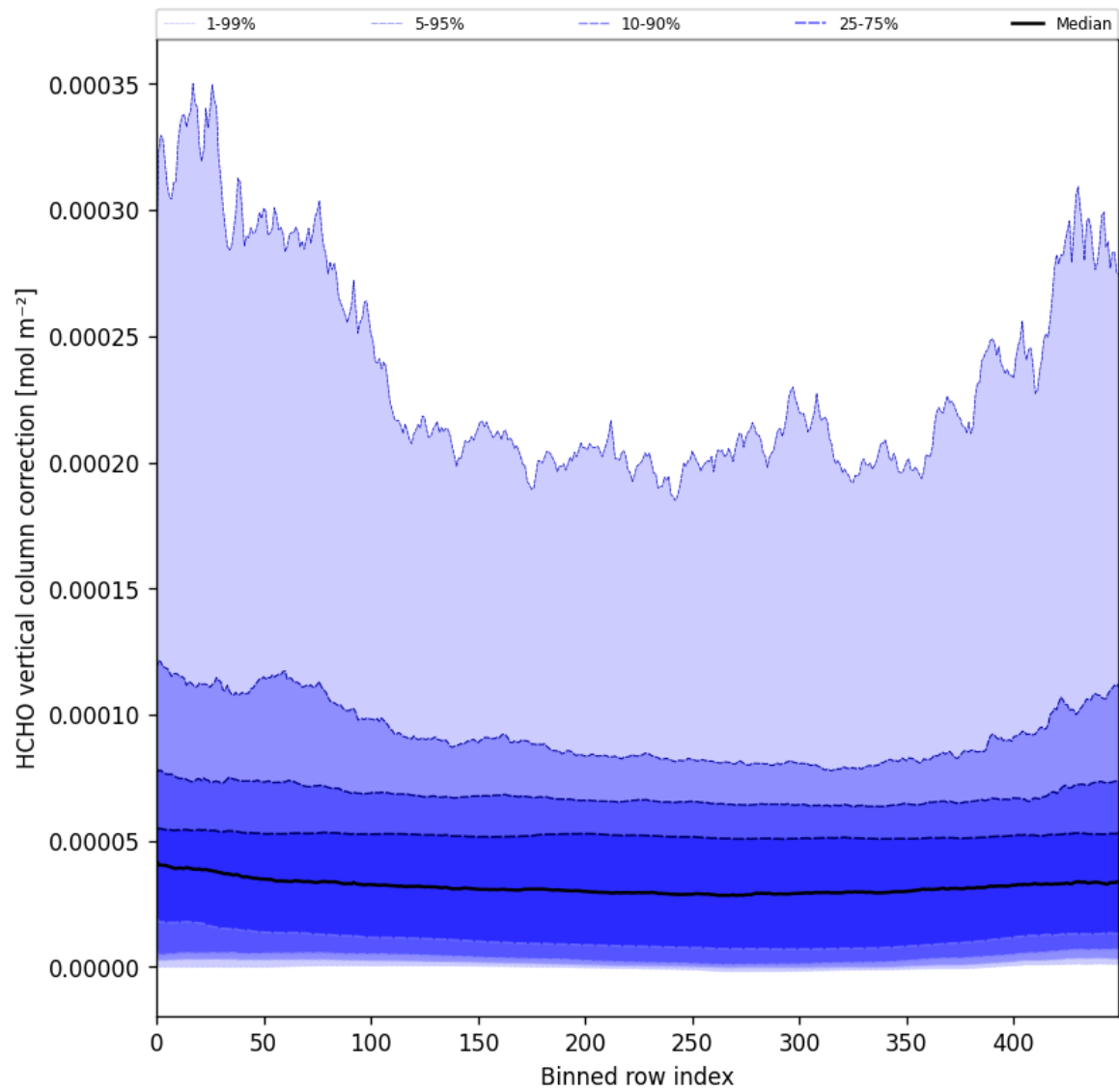
Figure 51: Along track statistics of “HCHO vertical column correction” for 2025-08-31 to 2025-09-02
