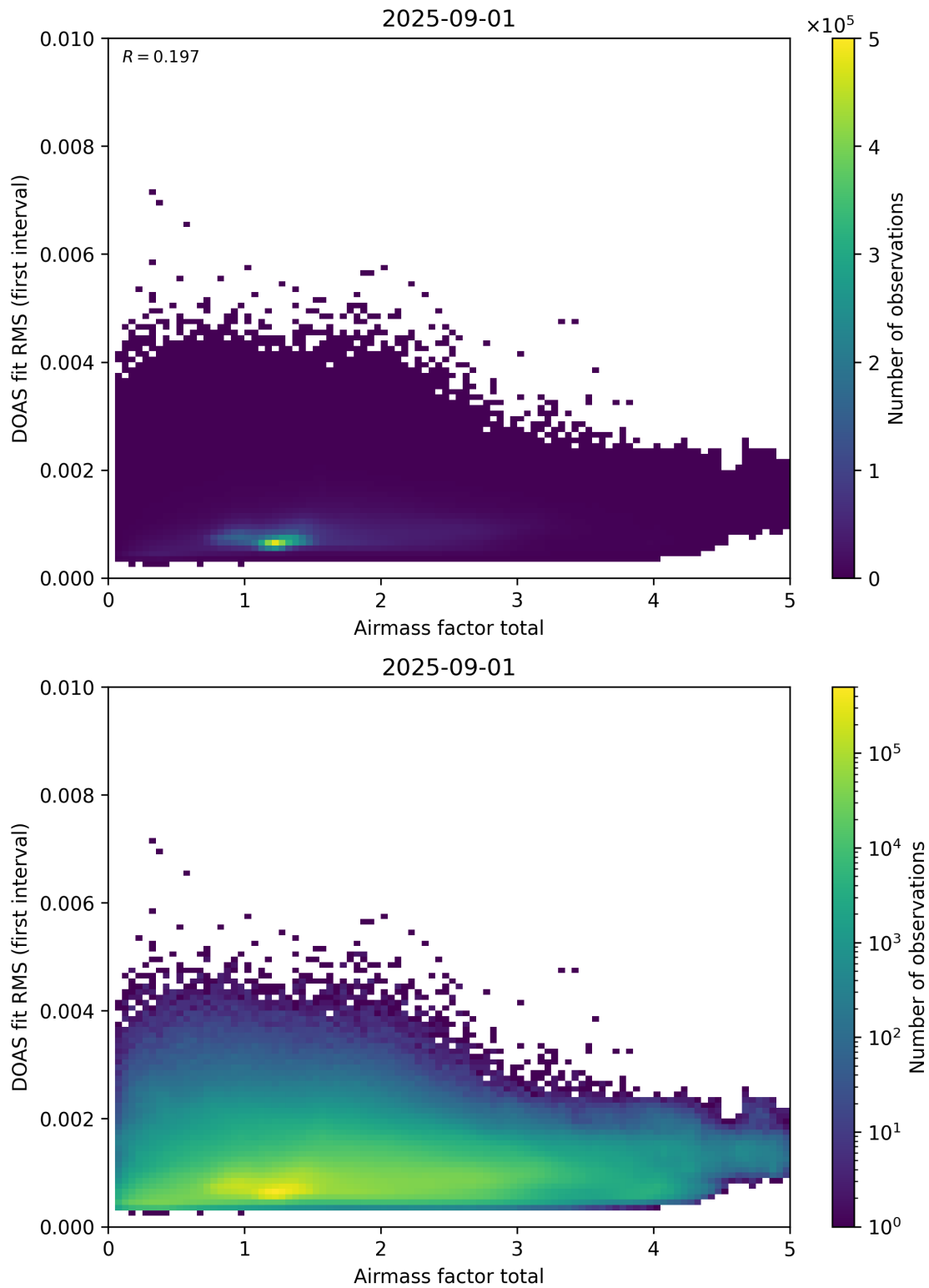
Figure 97: Scatter density plot of “Airmass factor total” against “DOAS fit RMS (first interval)” for 2025-08-31 to 2025-09-02.
