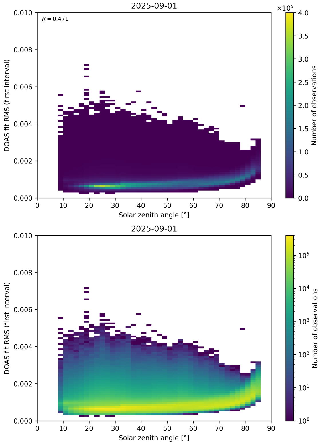
Figure 167: Scatter density plot of “Solar zenith angle” against “DOAS fit RMS (first interval)” for 2025-08-31 to 2025-09-02.
