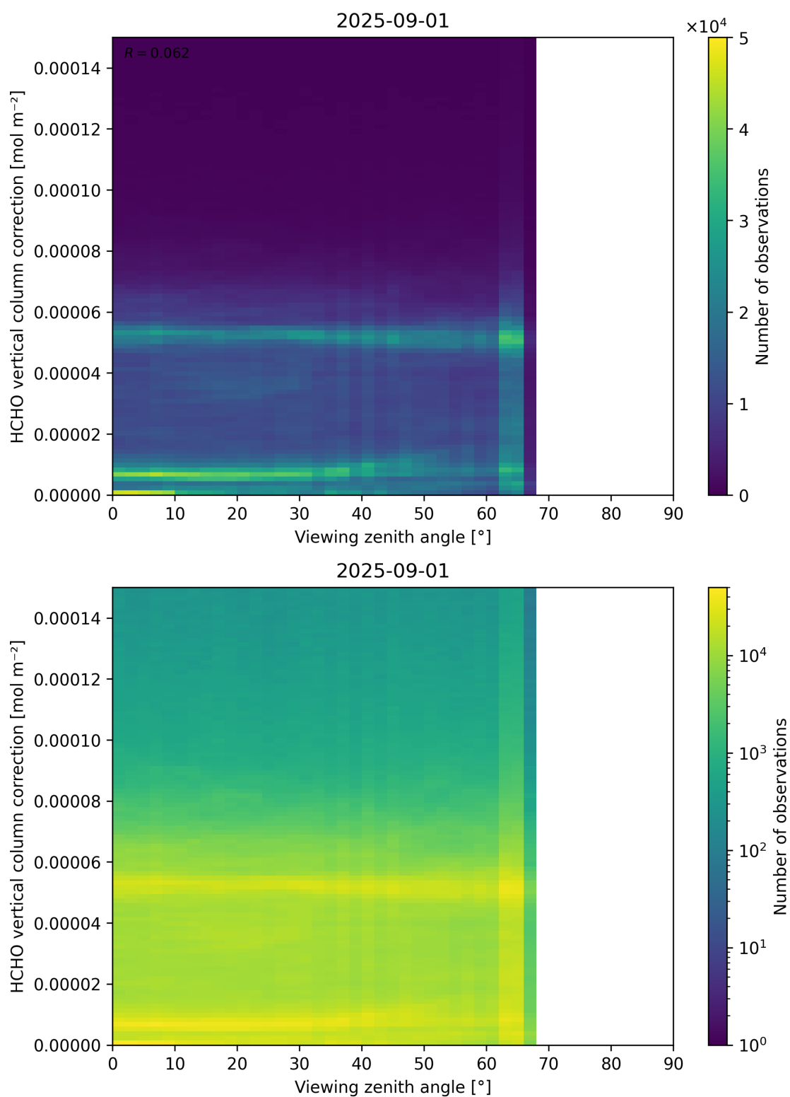
Figure 193: Scatter density plot of “Viewing zenith angle” against “HCHO vertical column correction” for 2025-08-31 to 2025-09-02.
