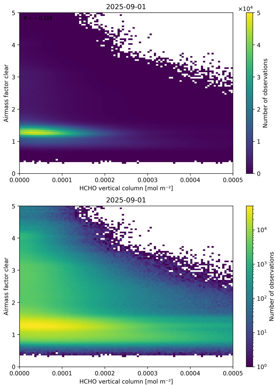
Figure 126: Scatter density plot of “HCHO vertical column” against “Airmass factor clear” for 2025-08-31 to 2025-09-02.
