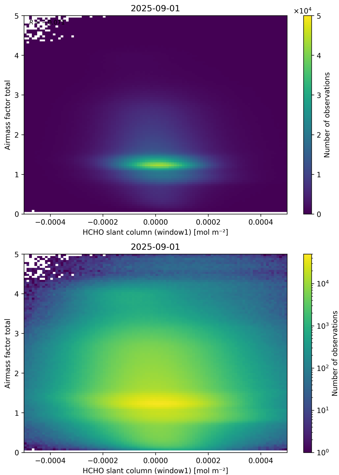
Figure 85: Scatter density plot of “HCHO slant column (window1)” against “Airmass factor total” for 2025-08-31 to 2025-09-02.
