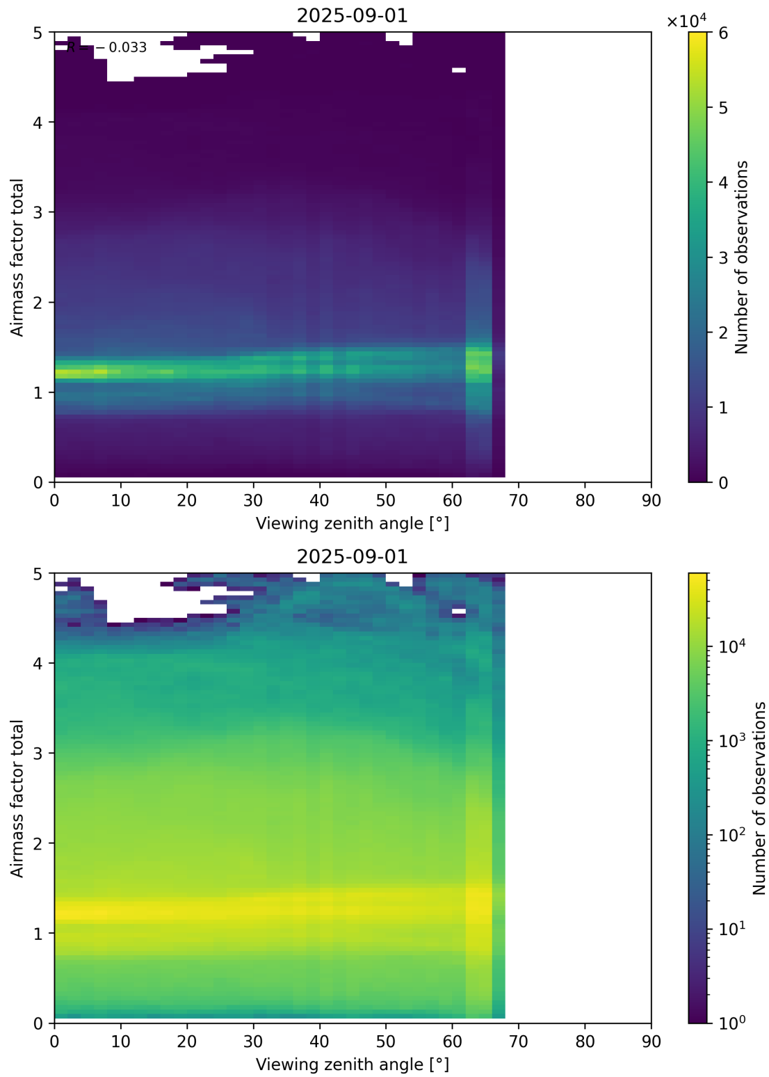
Figure 190: Scatter density plot of “Viewing zenith angle” against “Airmass factor total” for 2025-08-31 to 2025-09-02.
