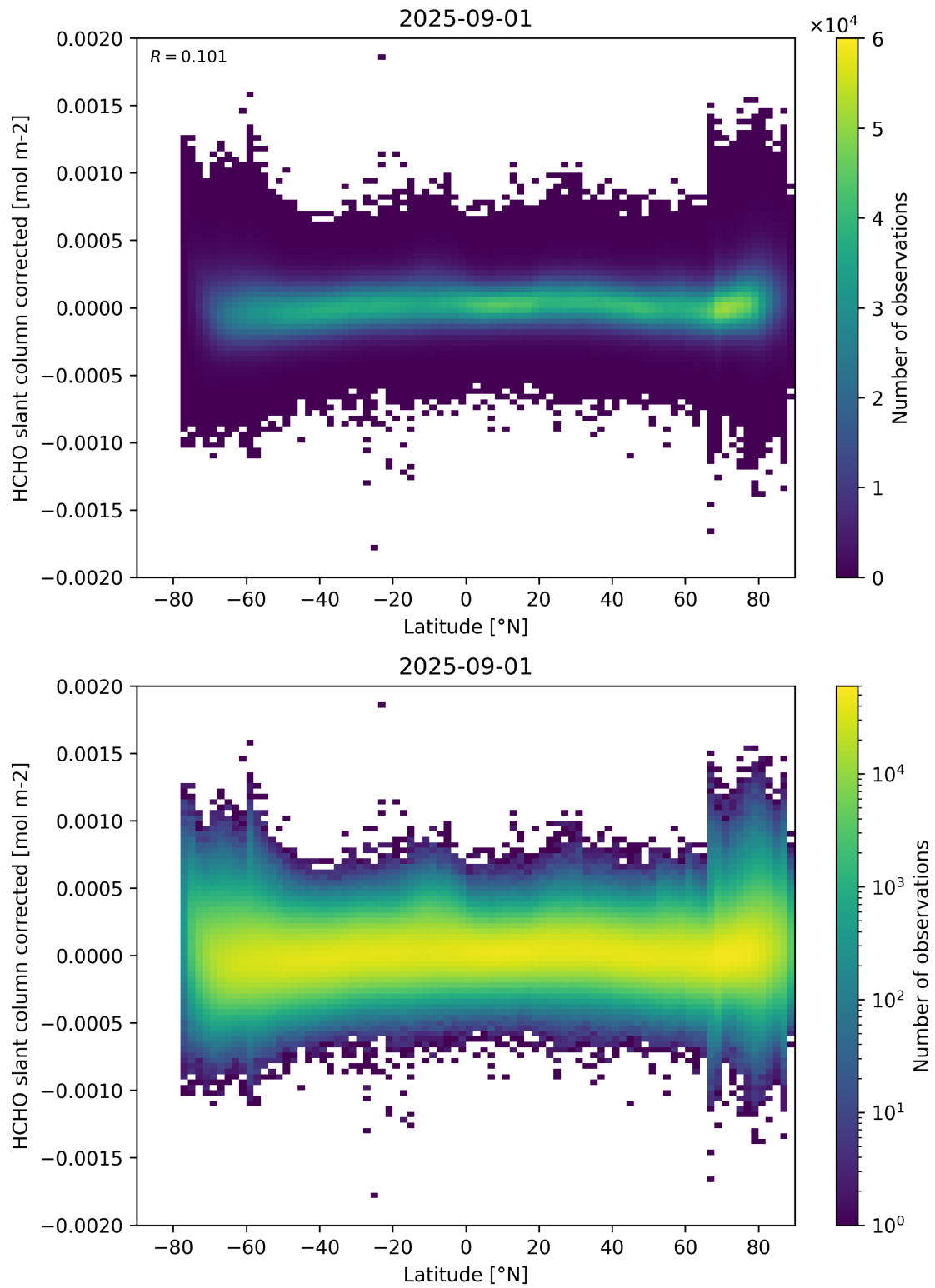
Figure 157: Scatter density plot of “Latitude” against “HCHO slant column corrected” for 2025-08-31 to 2025-09-02.
