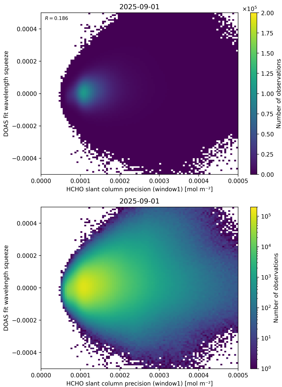
Figure 90: Scatter density plot of “HCHO slant column precision (window1)” against “DOAS fit wavelength squeeze” for 2025-08-31 to 2025-09-02.
