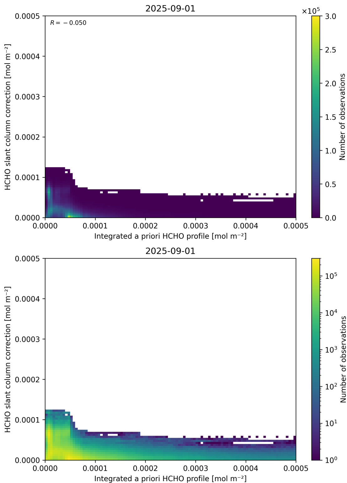
Figure 152: Scatter density plot of “Integrated a priori HCHO profile” against “HCHO slant column correction” for 2025-08-31 to 2025-09-02.
