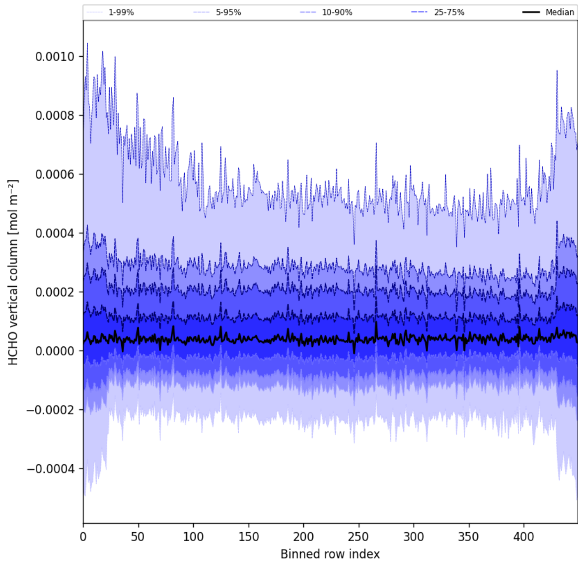
Figure 49: Along track statistics of “HCHO vertical column” for 2025-08-31 to 2025-09-02
