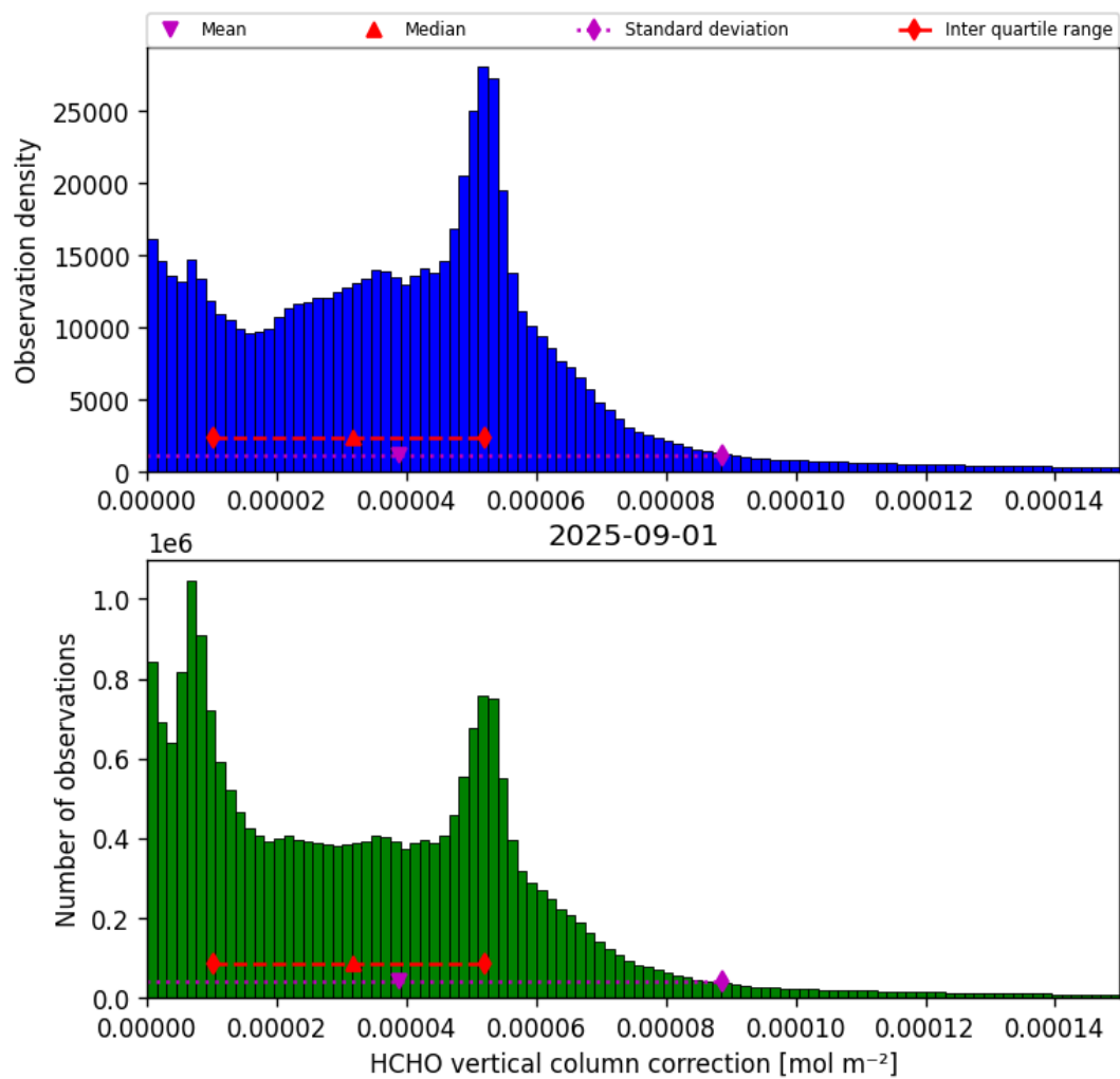
Figure 37: Histogram of “HCHO vertical column correction” for 2025-08-31 to 2025-09-02
