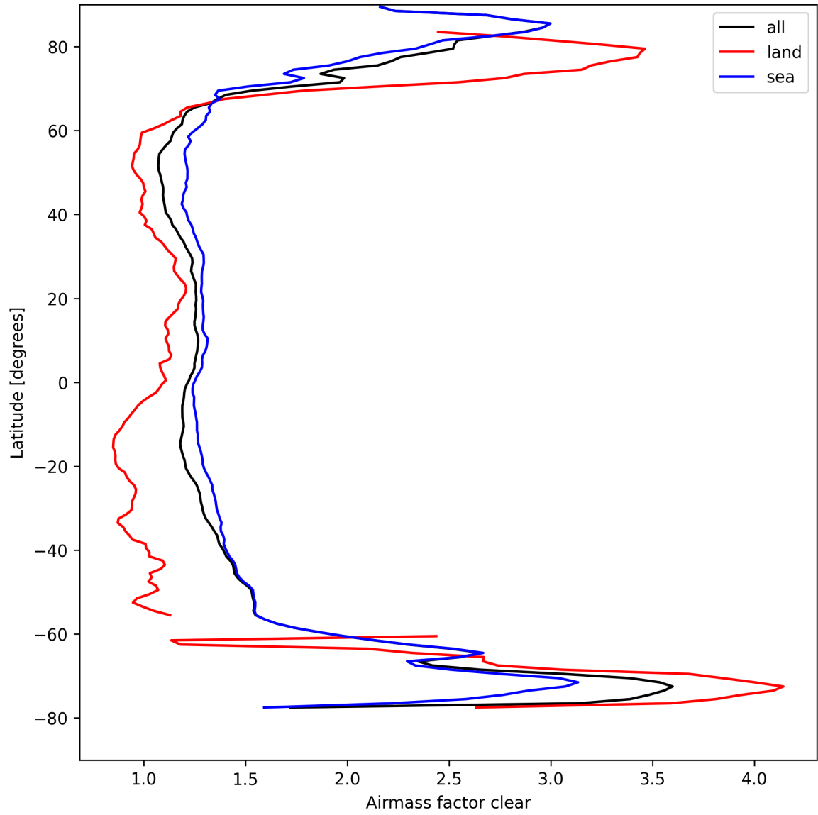
Figure 28: Zonal average of “Airmass factor clear” for 2025-08-31 to 2025-09-02.
