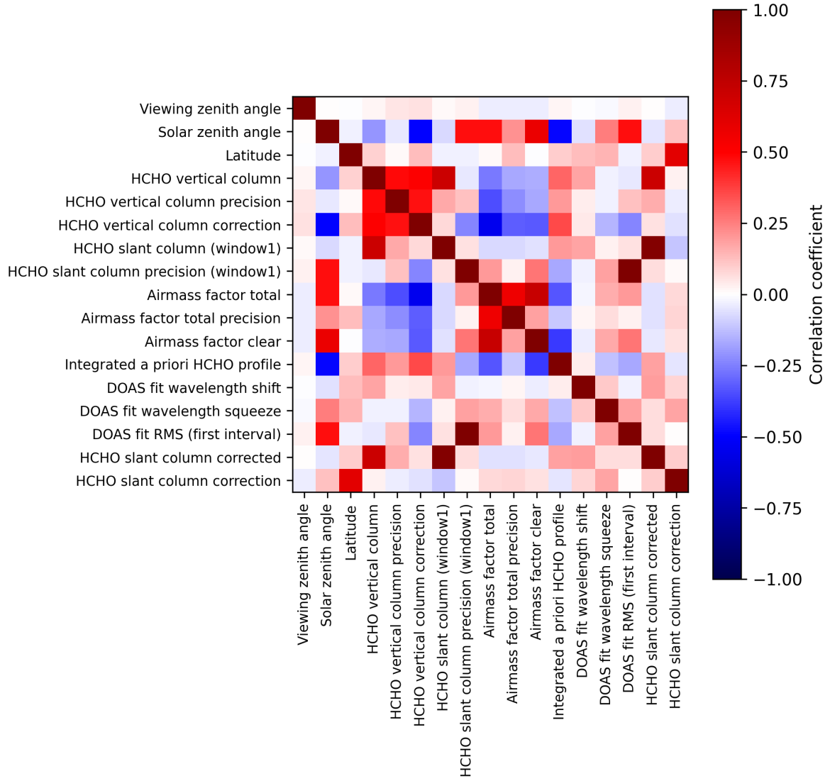
Figure 2: Map of correlation matrix for 2025-08-31 to 2025-09-02.
