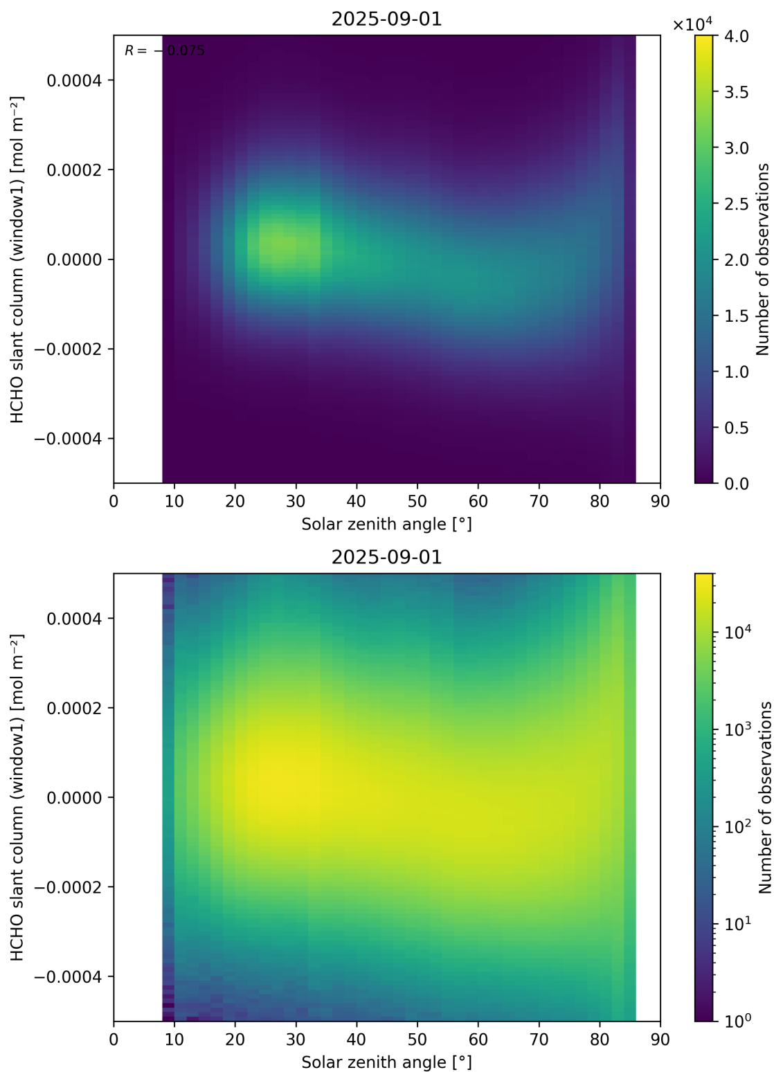
Figure 173: Scatter density plot of “Solar zenith angle” against “HCHO slant column (window1)” for 2025-08-31 to 2025-09-02.
