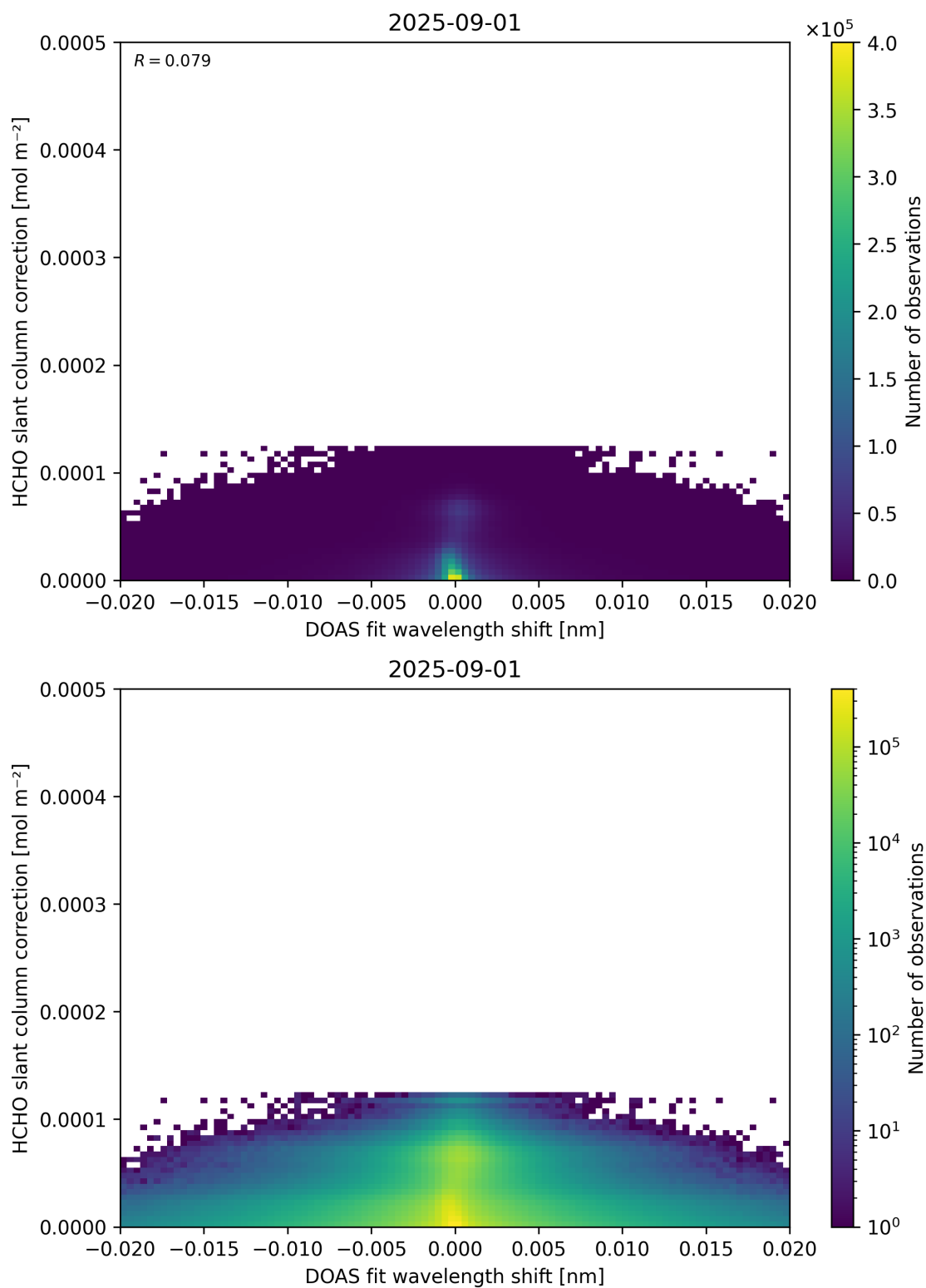
Figure 67: Scatter density plot of “DOAS fit wavelength shift” against “HCHO slant column correction” for 2025-08-31 to 2025-09-02.
