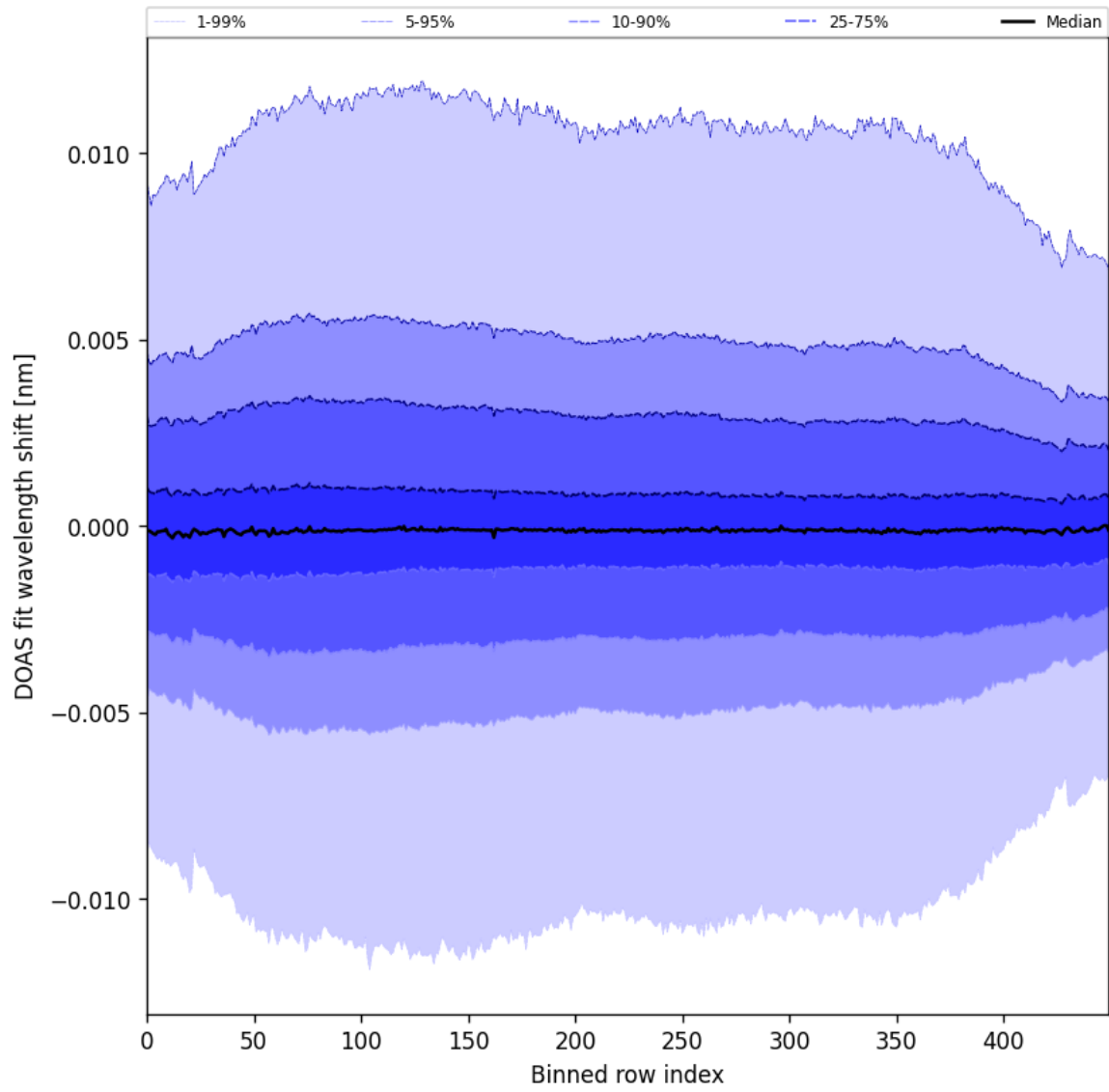
Figure 58: Along track statistics of “DOAS fit wavelength shift” for 2025-08-31 to 2025-09-02
