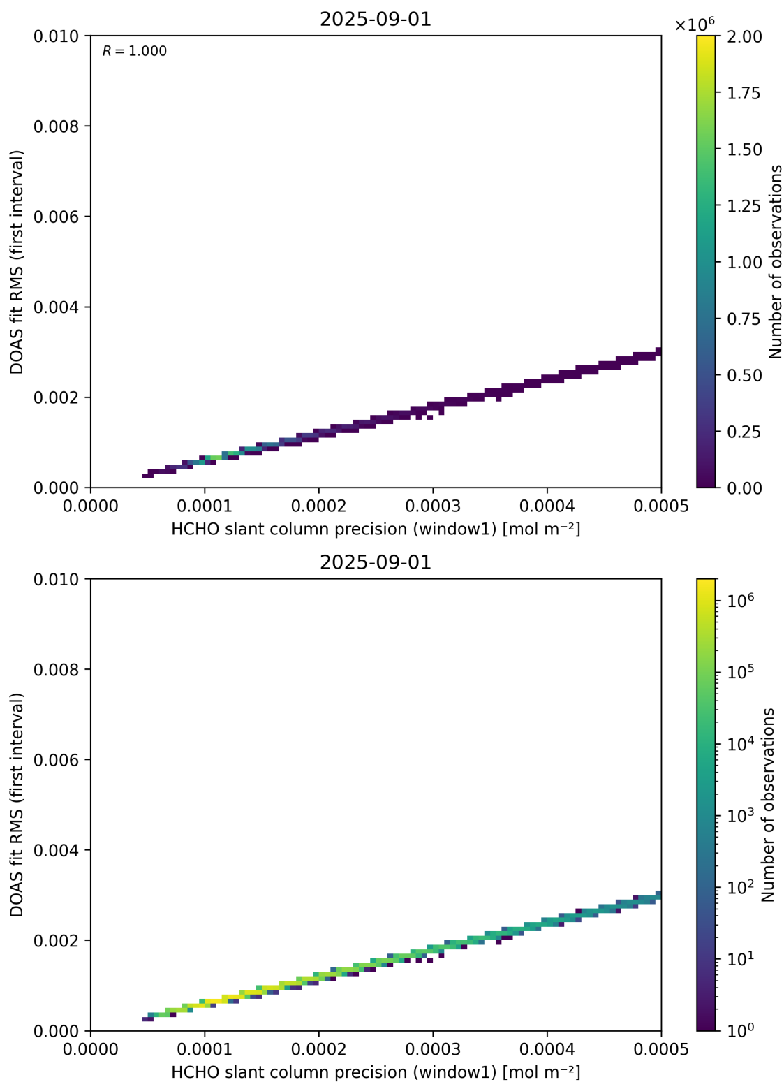
Figure 88: Scatter density plot of “HCHO slant column precision (window1)” against “DOAS fit RMS (first interval)” for 2025-08-31 to 2025-09-02.
