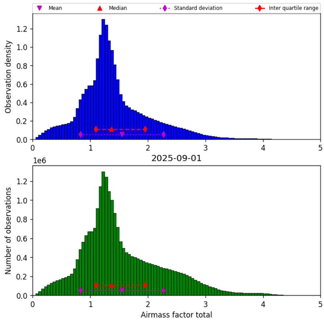
Figure 40: Histogram of “Airmass factor total” for 2025-08-31 to 2025-09-02
