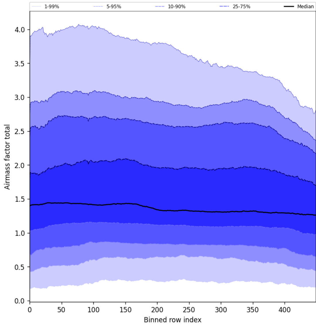
Figure 54: Along track statistics of “Airmass factor total” for 2025-08-31 to 2025-09-02
