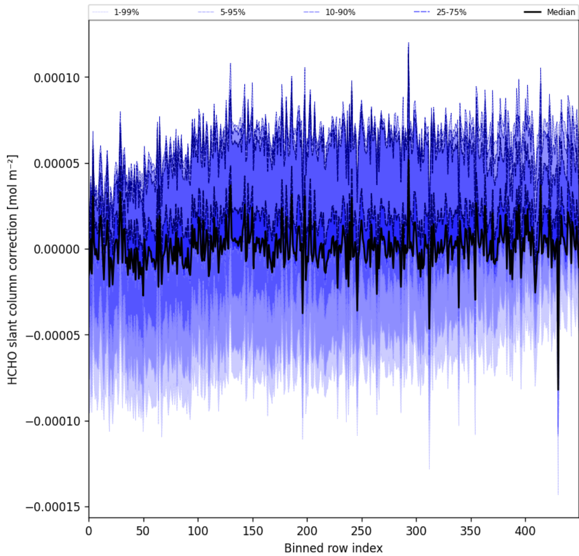
Figure 61: Along track statistics of “HCHO slant column correction” for 2025-08-31 to 2025-09-02
