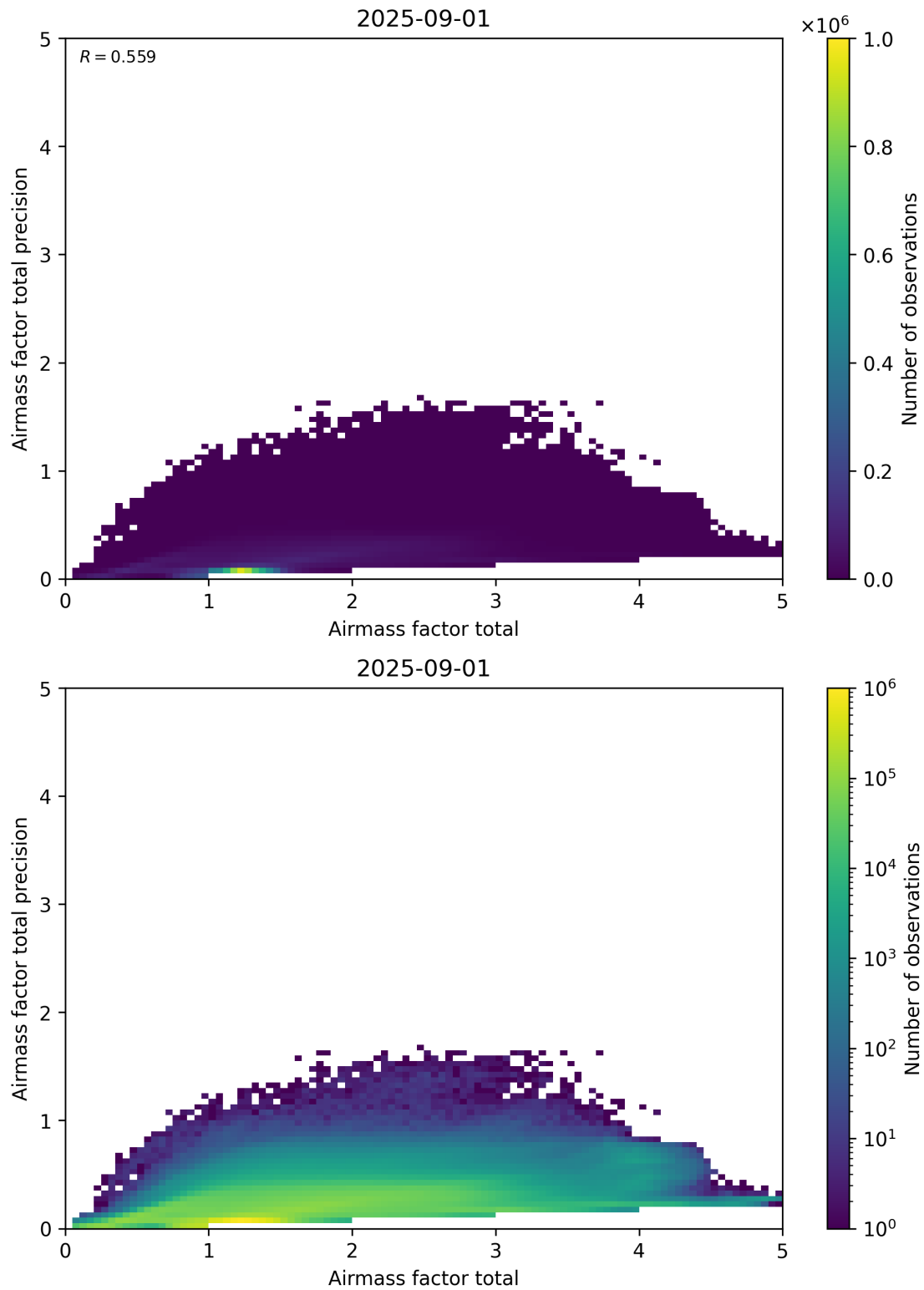
Figure 103: Scatter density plot of “Airmass factor total” against “Airmass factor total precision” for 2025-08-31 to 2025-09-02.
