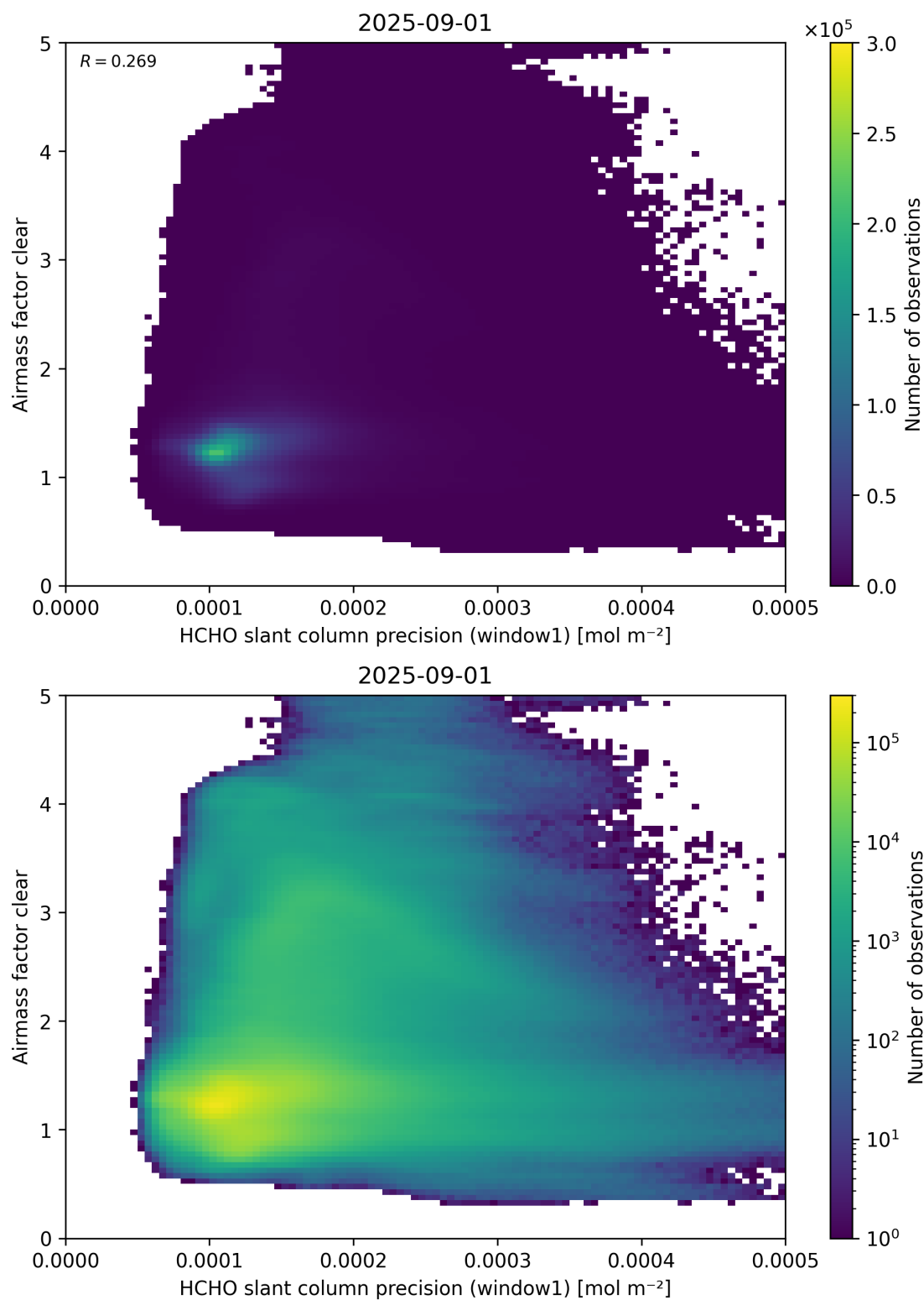
Figure 91: Scatter density plot of “HCHO slant column precision (window1)” against “Airmass factor clear” for 2025-08-31 to 2025-09-02.
