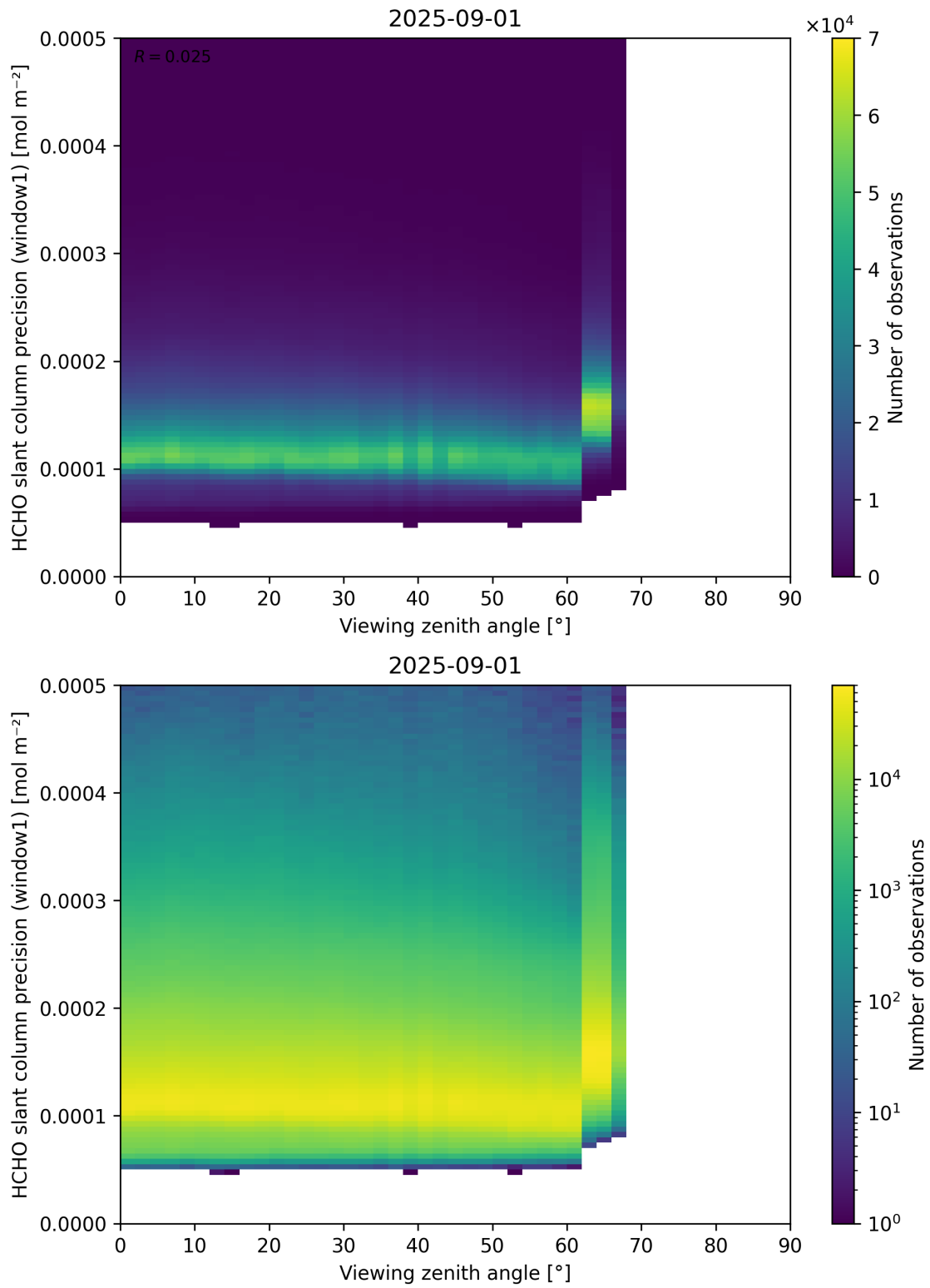
Figure 189: Scatter density plot of “Viewing zenith angle” against “HCHO slant column precision (window1)” for 2025-08-31 to 2025-09-02.
