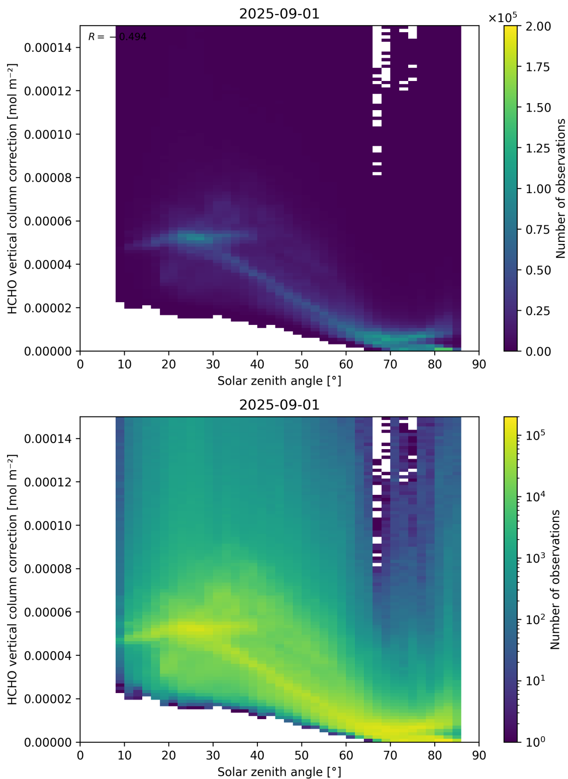
Figure 178: Scatter density plot of “Solar zenith angle” against “HCHO vertical column correction” for 2025-08-31 to 2025-09-02.
