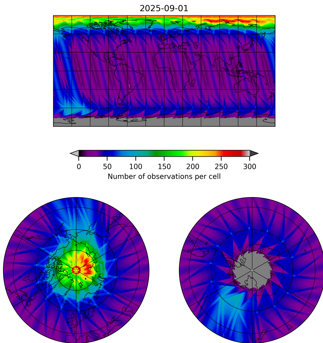
Figure 19: Map of the number of observations for 2025-08-31 to 2025-09-02
