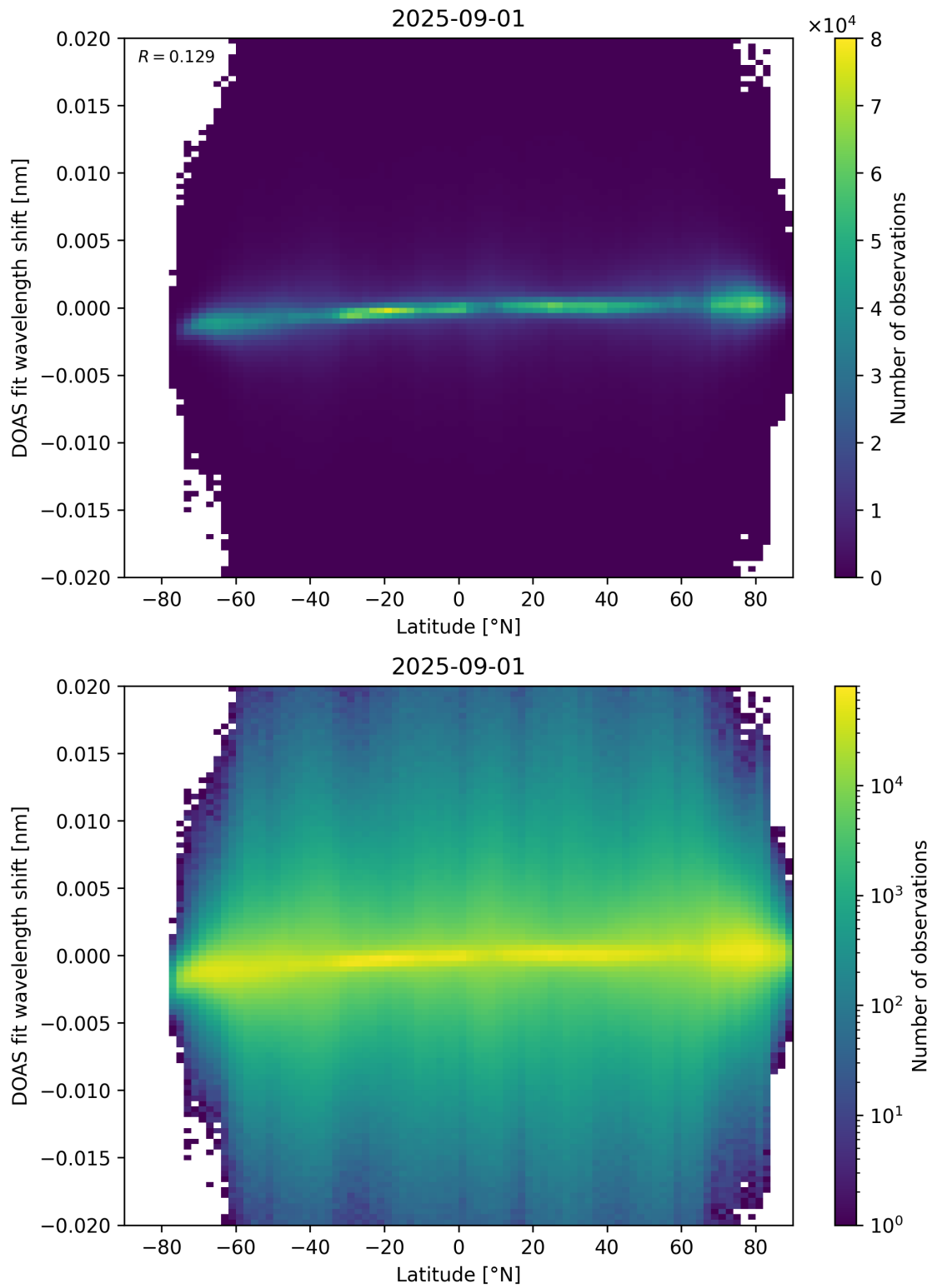
Figure 154: Scatter density plot of “Latitude” against “DOAS fit wavelength shift” for 2025-08-31 to 2025-09-02.
