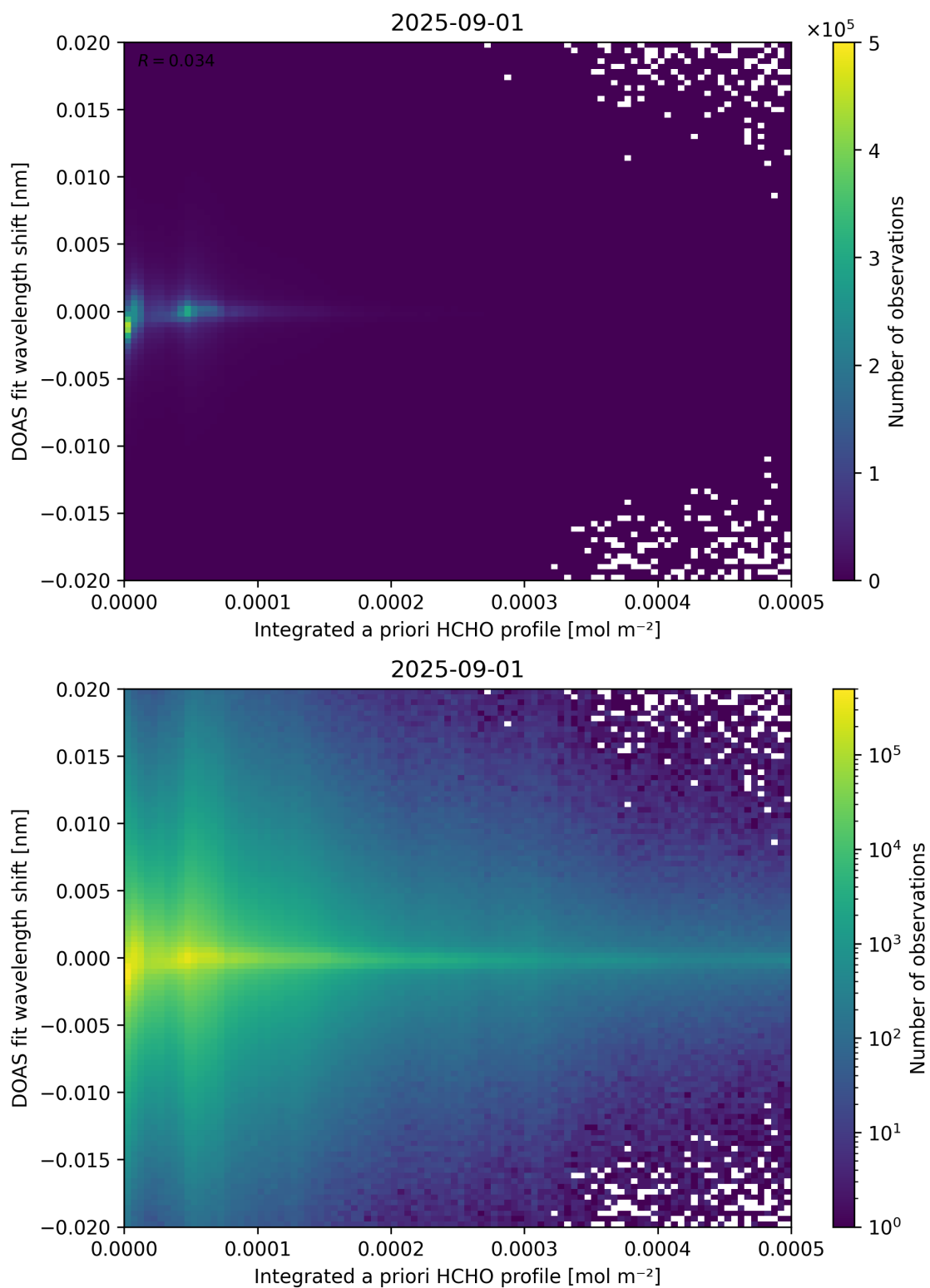
Figure 149: Scatter density plot of “Integrated a priori HCHO profile” against “DOAS fit wavelength shift” for 2025-08-31 to 2025-09-02.
