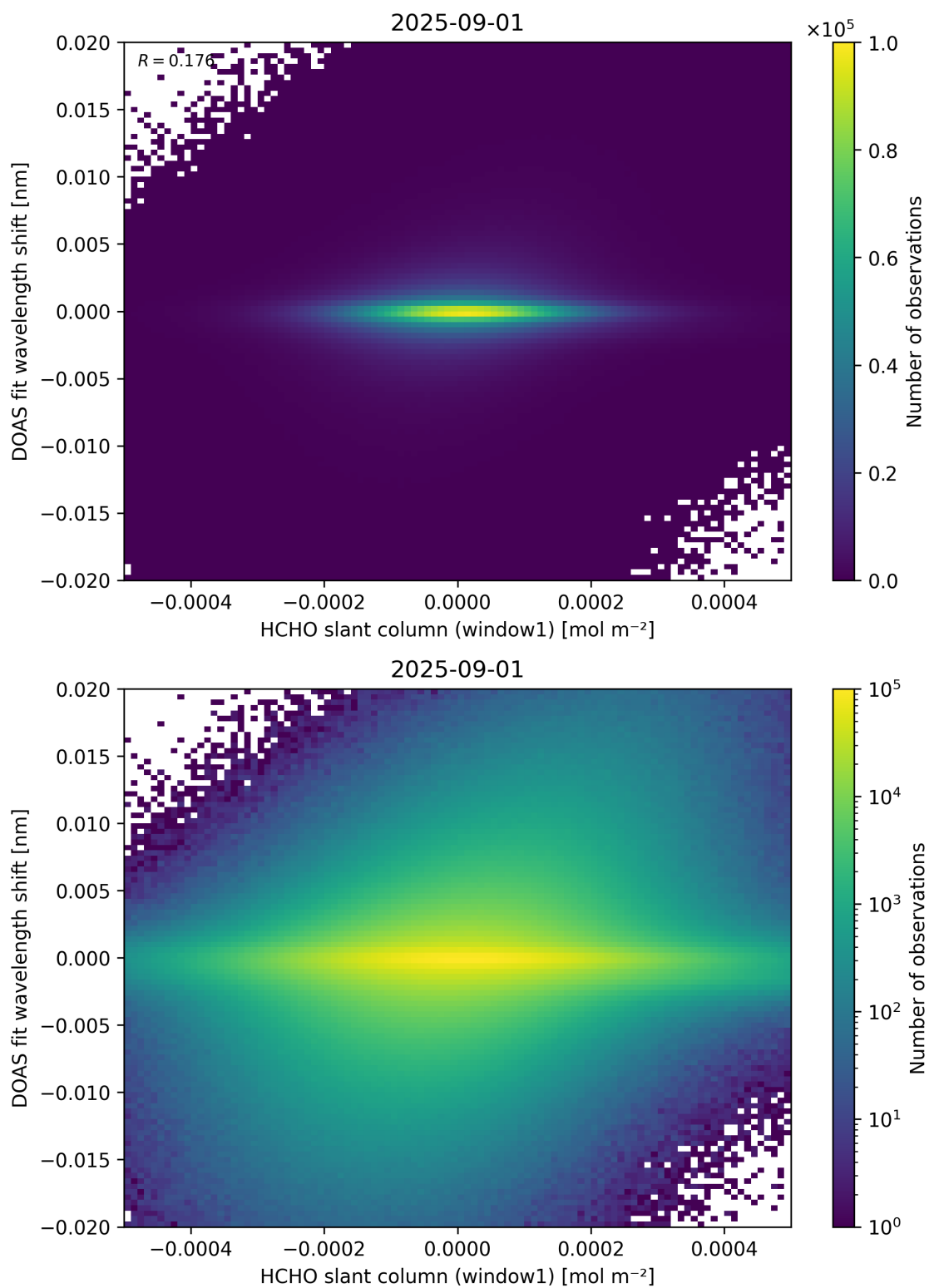
Figure 79: Scatter density plot of “HCHO slant column (window1)” against “DOAS fit wavelength shift” for 2025-08-31 to 2025-09-02.
