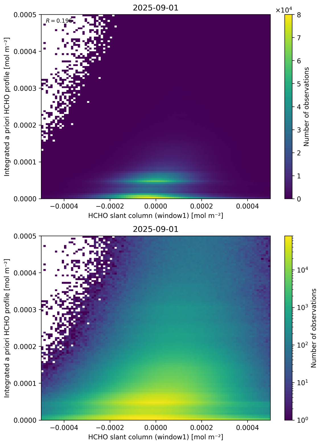
Figure 87: Scatter density plot of “HCHO slant column (window1)” against “Integrated a priori HCHO profile” for 2025-08-31 to 2025-09-02.
