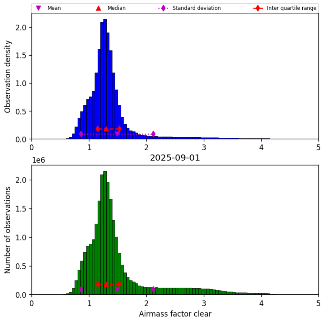
Figure 42: Histogram of “Airmass factor clear” for 2025-08-31 to 2025-09-02
