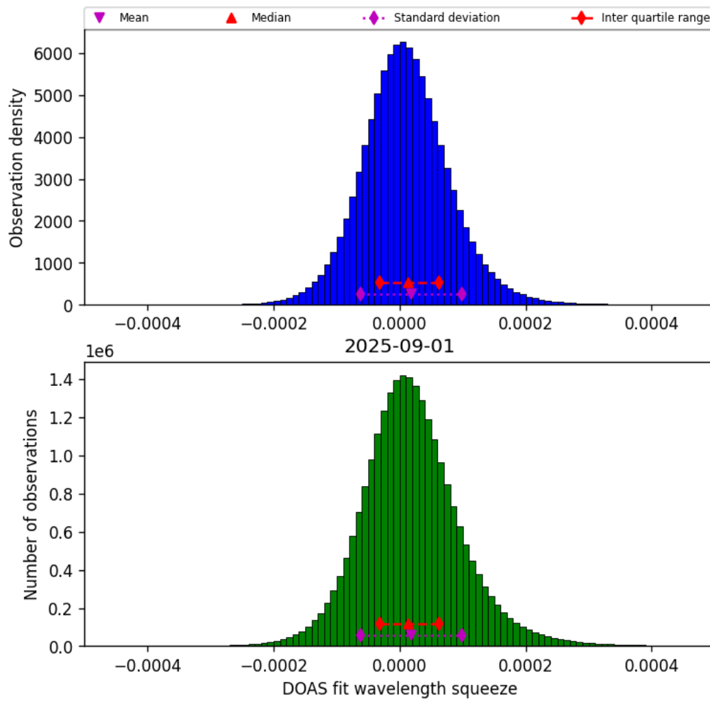
Figure 45: Histogram of “DOAS fit wavelength squeeze” for 2025-08-31 to 2025-09-02
