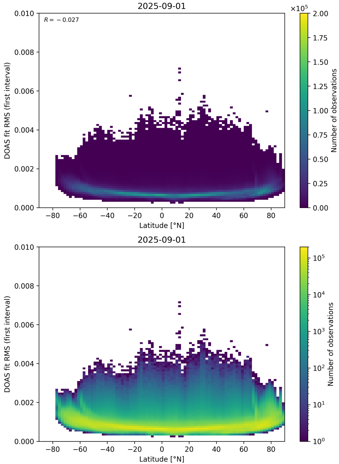
Figure 153: Scatter density plot of “Latitude” against “DOAS fit RMS (first interval)” for 2025-08-31 to 2025-09-02.
