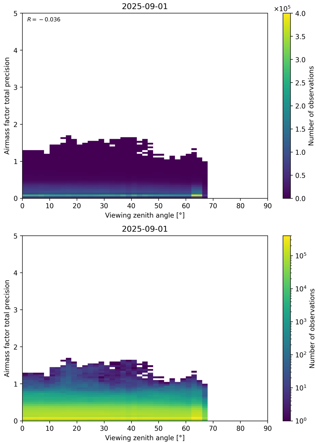
Figure 191: Scatter density plot of “Viewing zenith angle” against “Airmass factor total precision” for 2025-08-31 to 2025-09-02.
