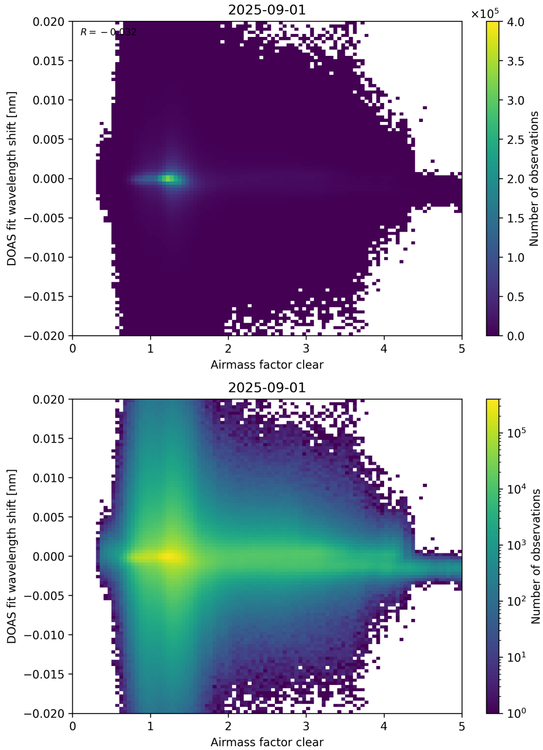
Figure 72: Scatter density plot of “Airmass factor clear” against “DOAS fit wavelength shift” for 2025-08-31 to 2025-09-02.
