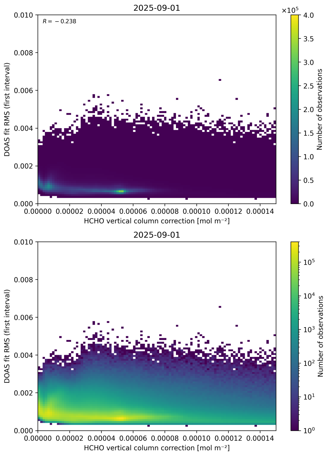
Figure 112: Scatter density plot of “HCHO vertical column correction” against “DOAS fit RMS (first interval)” for 2025-08-31 to 2025-09-02.
