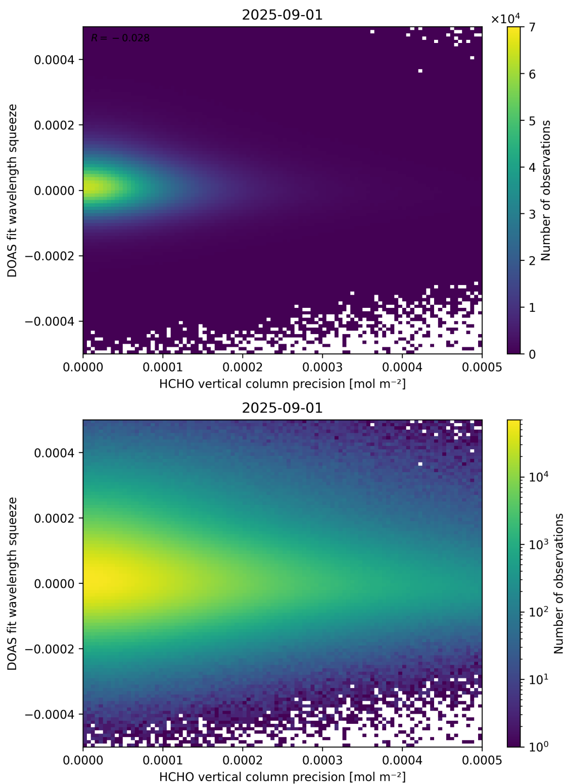
Figure 138: Scatter density plot of “HCHO vertical column precision” against “DOAS fit wavelength squeeze” for 2025-08-31 to 2025-09-02.
