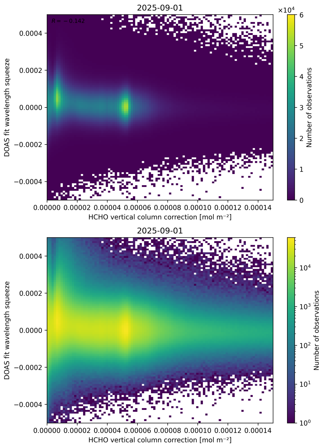
Figure 114: Scatter density plot of “HCHO vertical column correction” against “DOAS fit wavelength squeeze” for 2025-08-31 to 2025-09-02.
