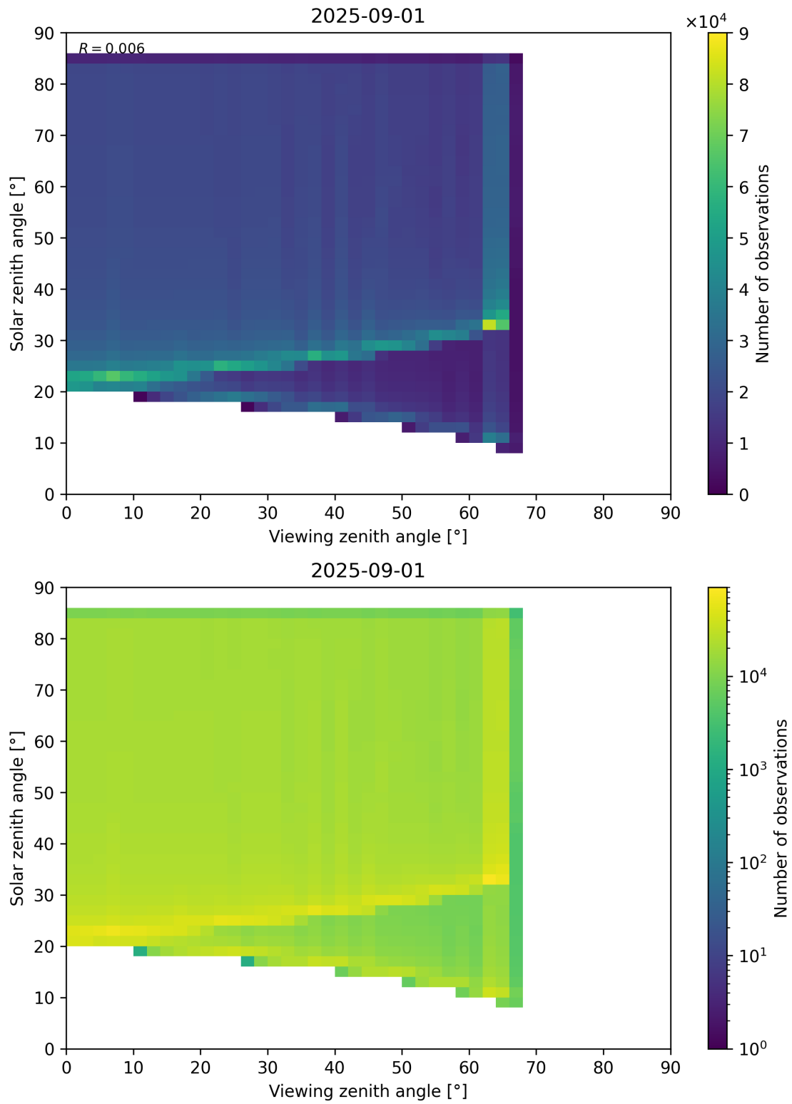
Figure 197: Scatter density plot of “Viewing zenith angle” against “Solar zenith angle” for 2025-08-31 to 2025-09-02.
