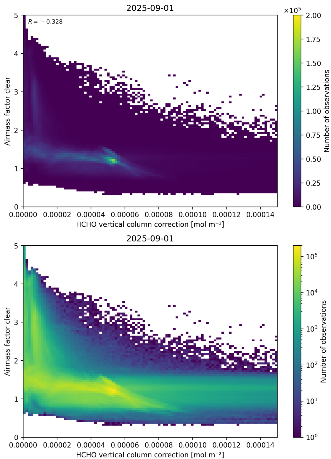
Figure 115: Scatter density plot of “HCHO vertical column correction” against “Airmass factor clear” for 2025-08-31 to 2025-09-02.
