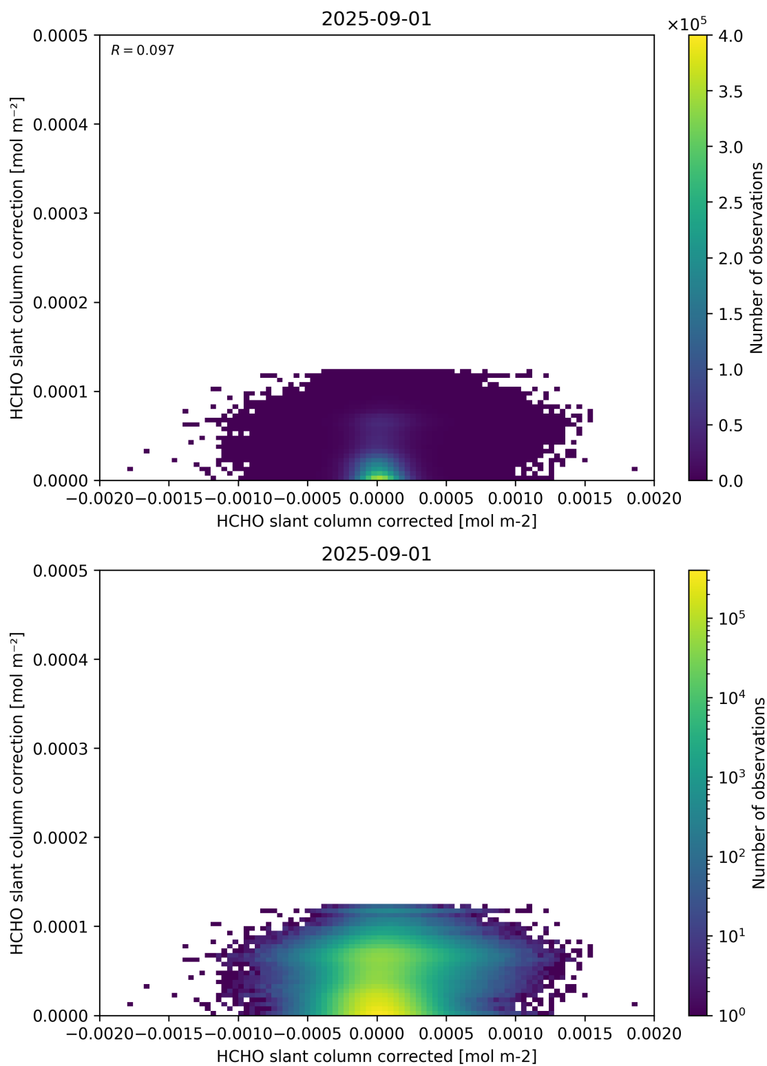
Figure 77: Scatter density plot of “HCHO slant column corrected” against “HCHO slant column correction” for 2025-08-31 to 2025-09-02.
