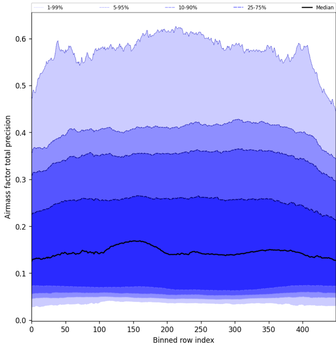
Figure 55: Along track statistics of “Airmass factor total precision” for 2025-08-31 to 2025-09-02
