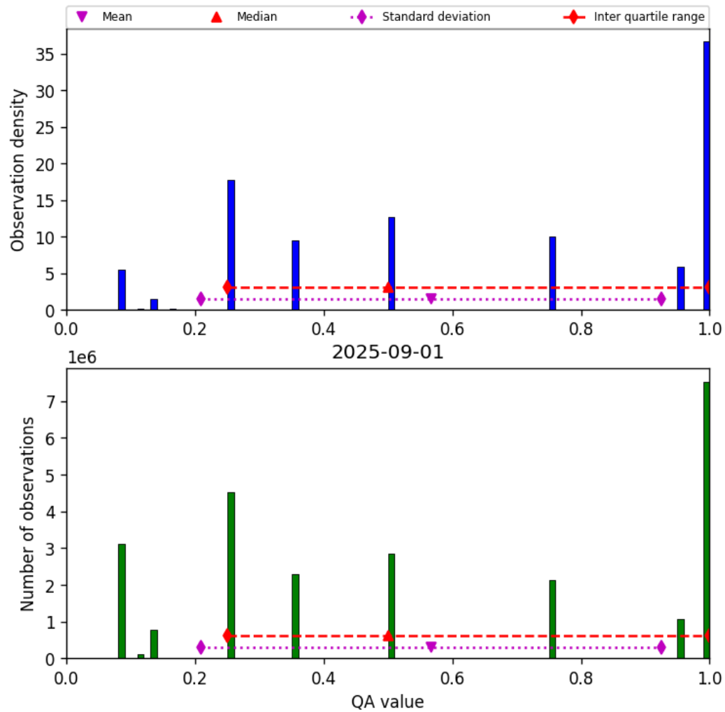
Figure 34: Histogram of “QA value” for 2025-08-31 to 2025-09-02
