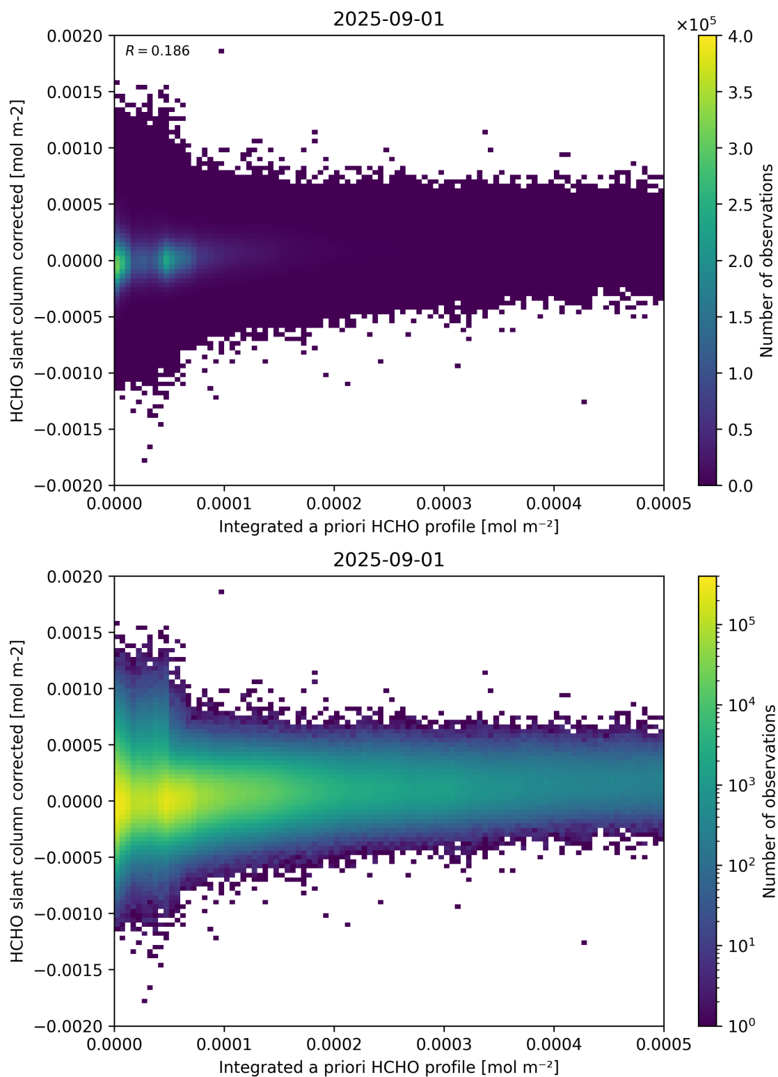
Figure 151: Scatter density plot of “Integrated a priori HCHO profile” against “HCHO slant column corrected” for 2025-08-31 to 2025-09-02.
