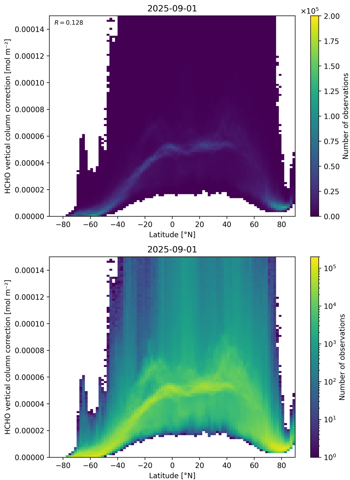
Figure 164: Scatter density plot of “Latitude” against “HCHO vertical column correction” for 2025-08-31 to 2025-09-02.
