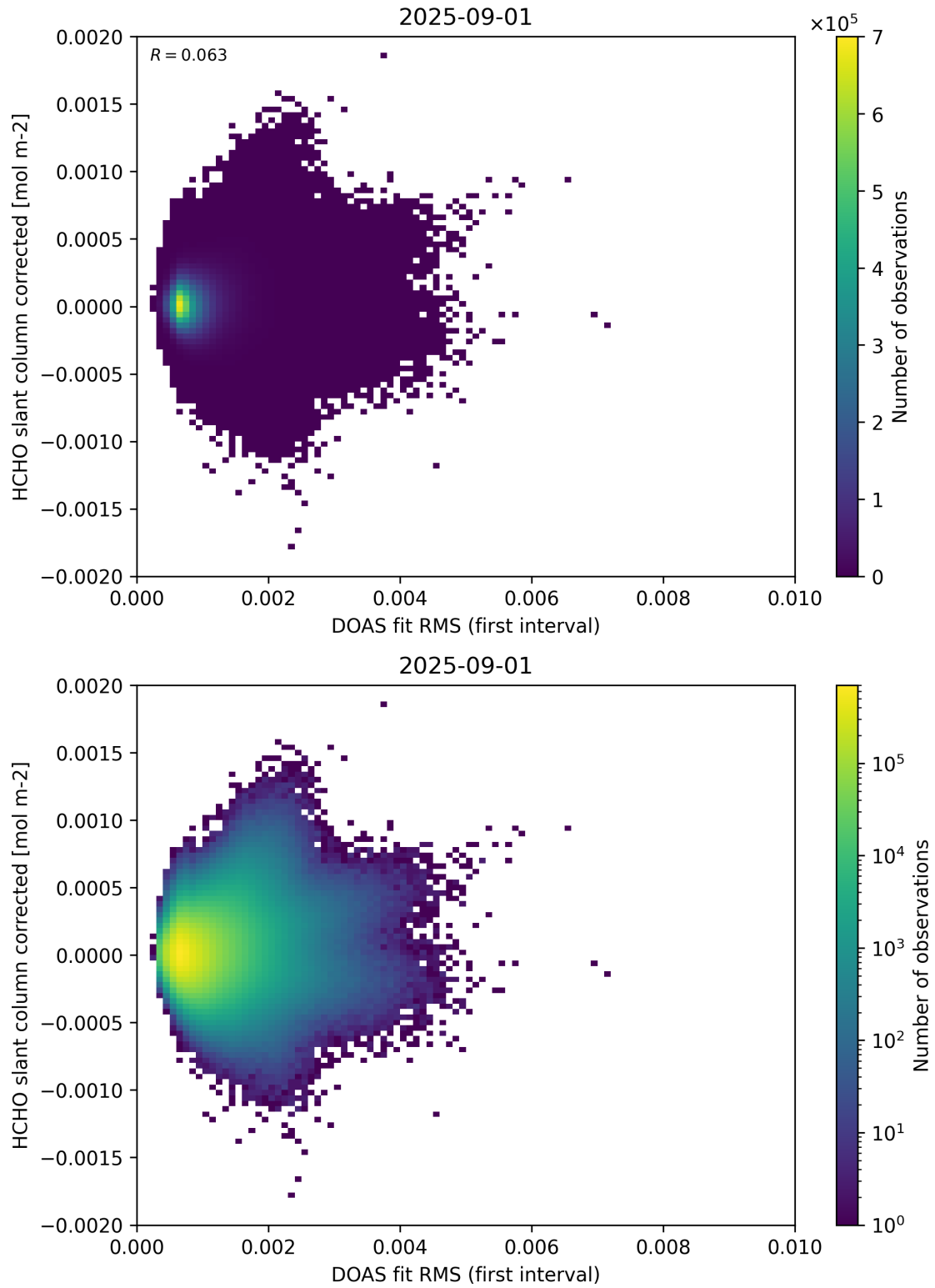
Figure 62: Scatter density plot of “DOAS fit RMS (first interval)” against “HCHO slant column corrected” for 2025-08-31 to 2025-09-02.
