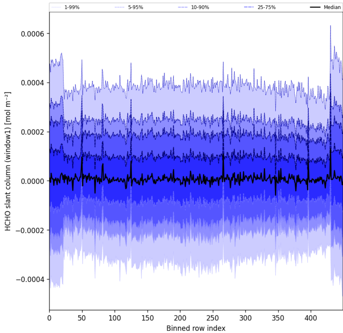
Figure 52: Along track statistics of “HCHO slant column (window1)” for 2025-08-31 to 2025-09-02
