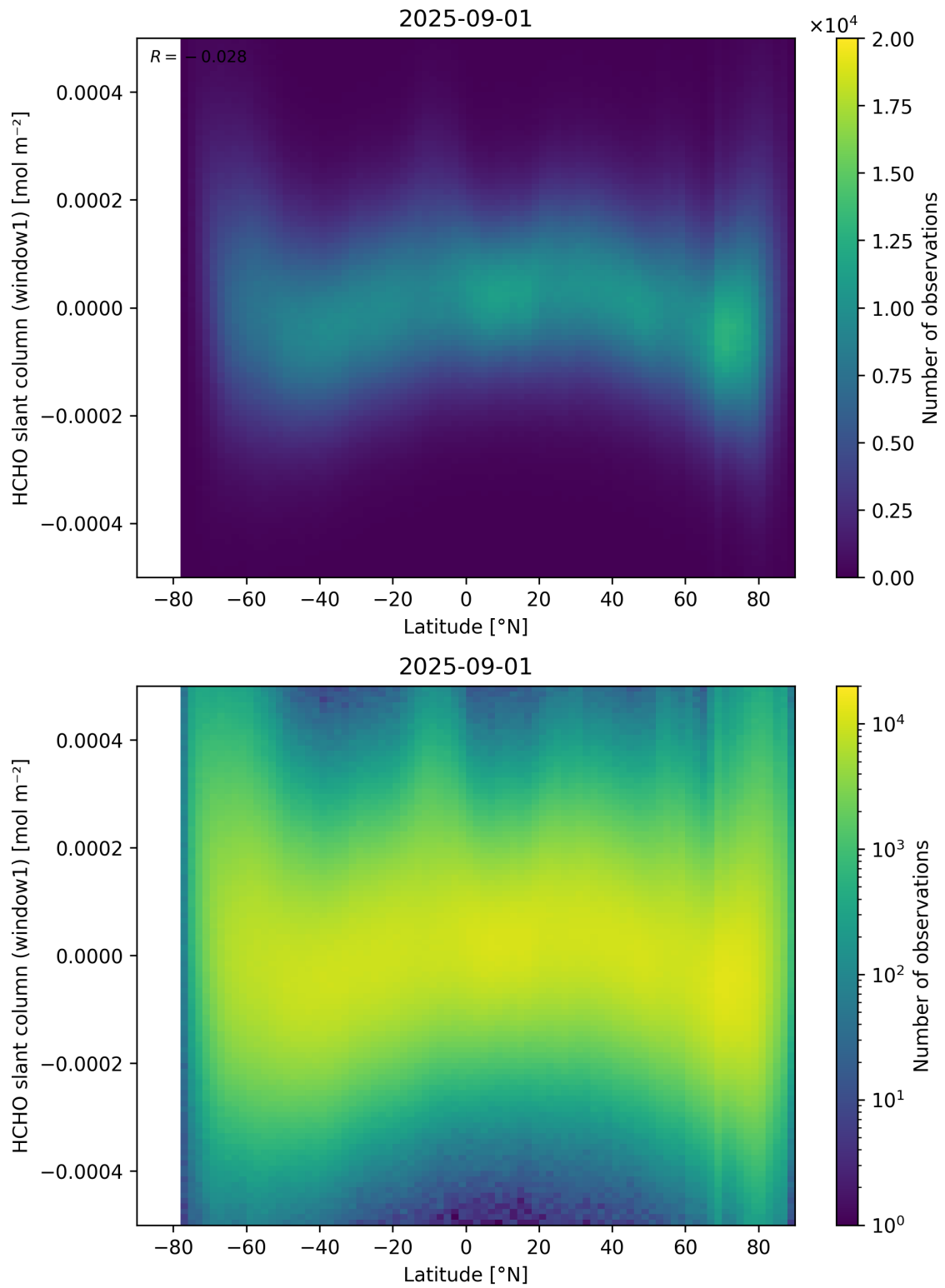
Figure 159: Scatter density plot of “Latitude” against “HCHO slant column (window1)” for 2025-08-31 to 2025-09-02.
