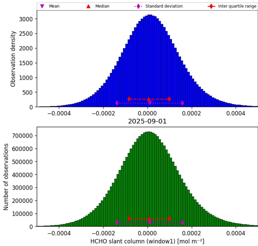
Figure 38: Histogram of “HCHO slant column (window1)” for 2025-08-31 to 2025-09-02
