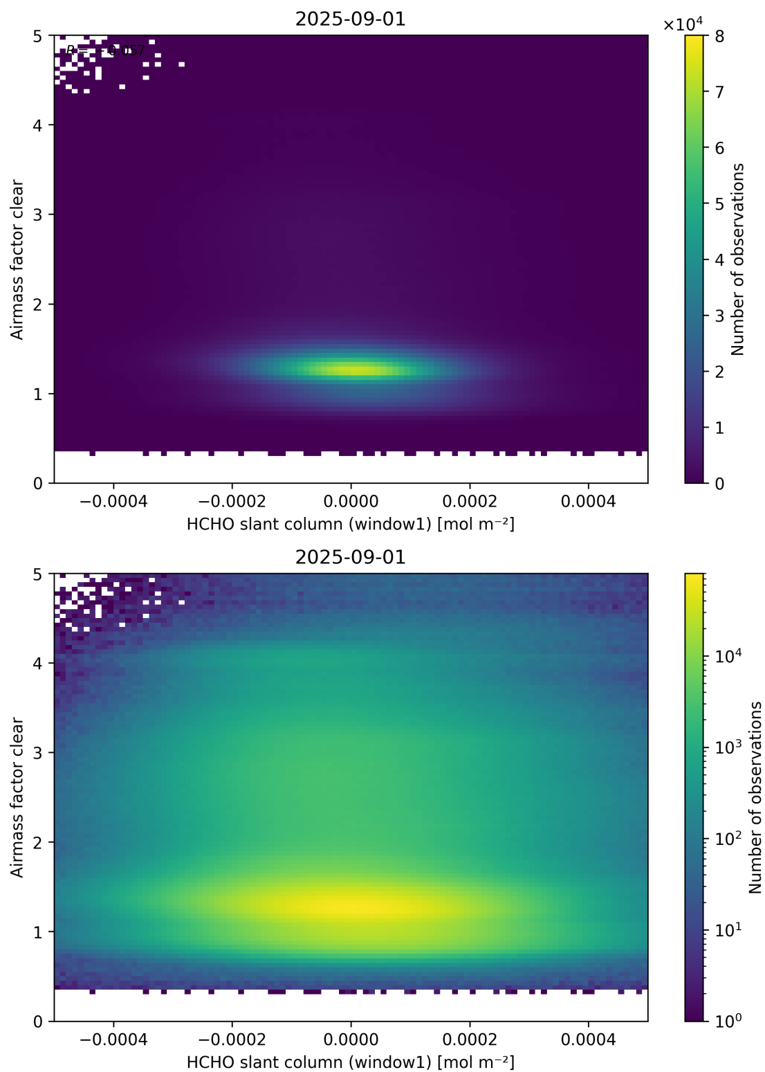
Figure 81: Scatter density plot of “HCHO slant column (window1)” against “Airmass factor clear” for 2025-08-31 to 2025-09-02.
