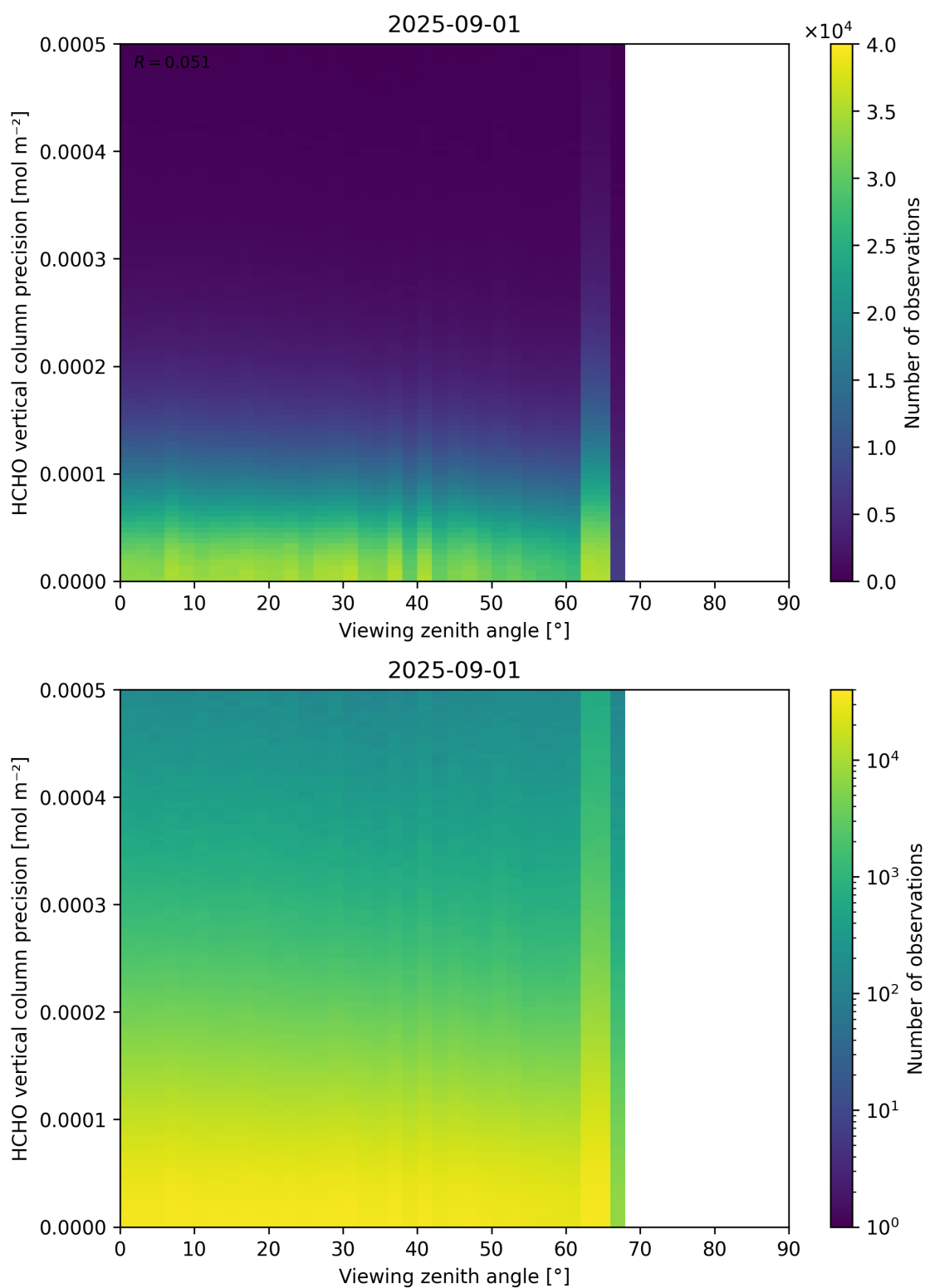
Figure 194: Scatter density plot of “Viewing zenith angle” against “HCHO vertical column precision” for 2025-08-31 to 2025-09-02.
