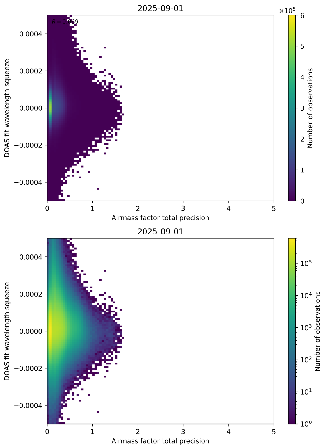
Figure 107: Scatter density plot of “Airmass factor total precision” against “DOAS fit wavelength squeeze” for 2025-08-31 to 2025-09-02.
