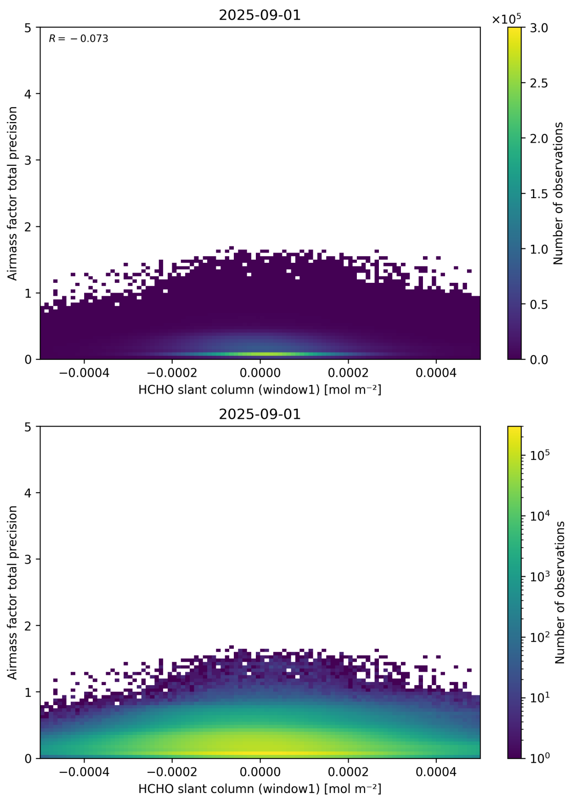
Figure 86: Scatter density plot of “HCHO slant column (window1)” against “Airmass factor total precision” for 2025-08-31 to 2025-09-02.
