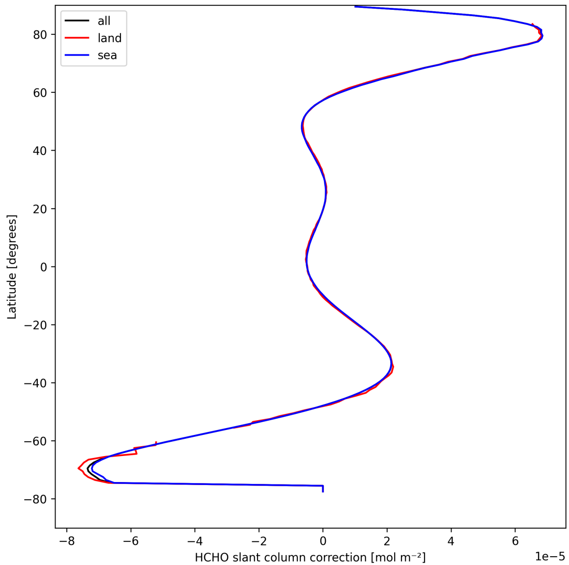
Figure 33: Zonal average of “HCHO slant column correction” for 2025-08-31 to 2025-09-02.
