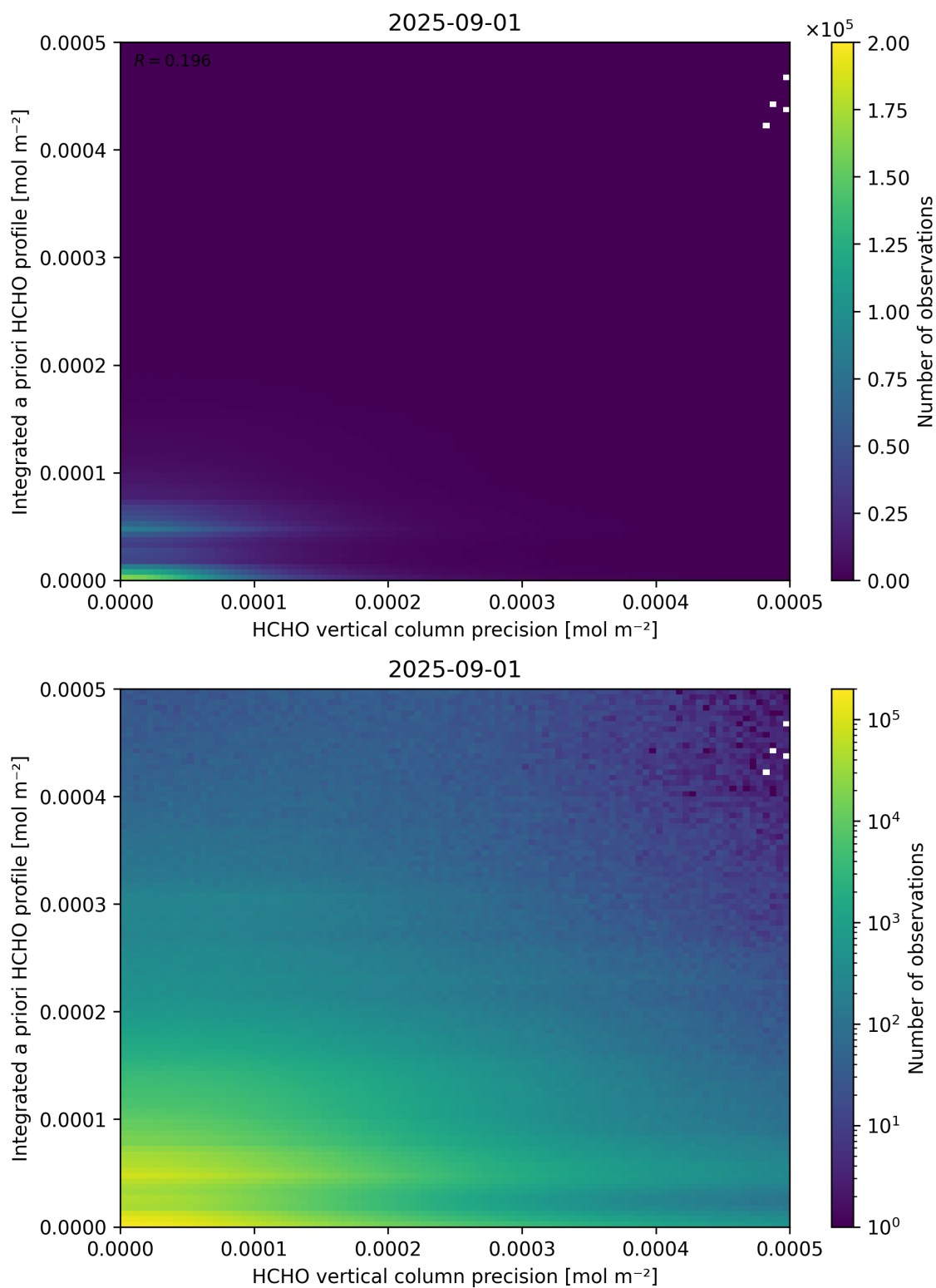
Figure 147: Scatter density plot of “HCHO vertical column precision” against “Integrated a priori HCHO profile” for 2025-08-31 to 2025-09-02.
