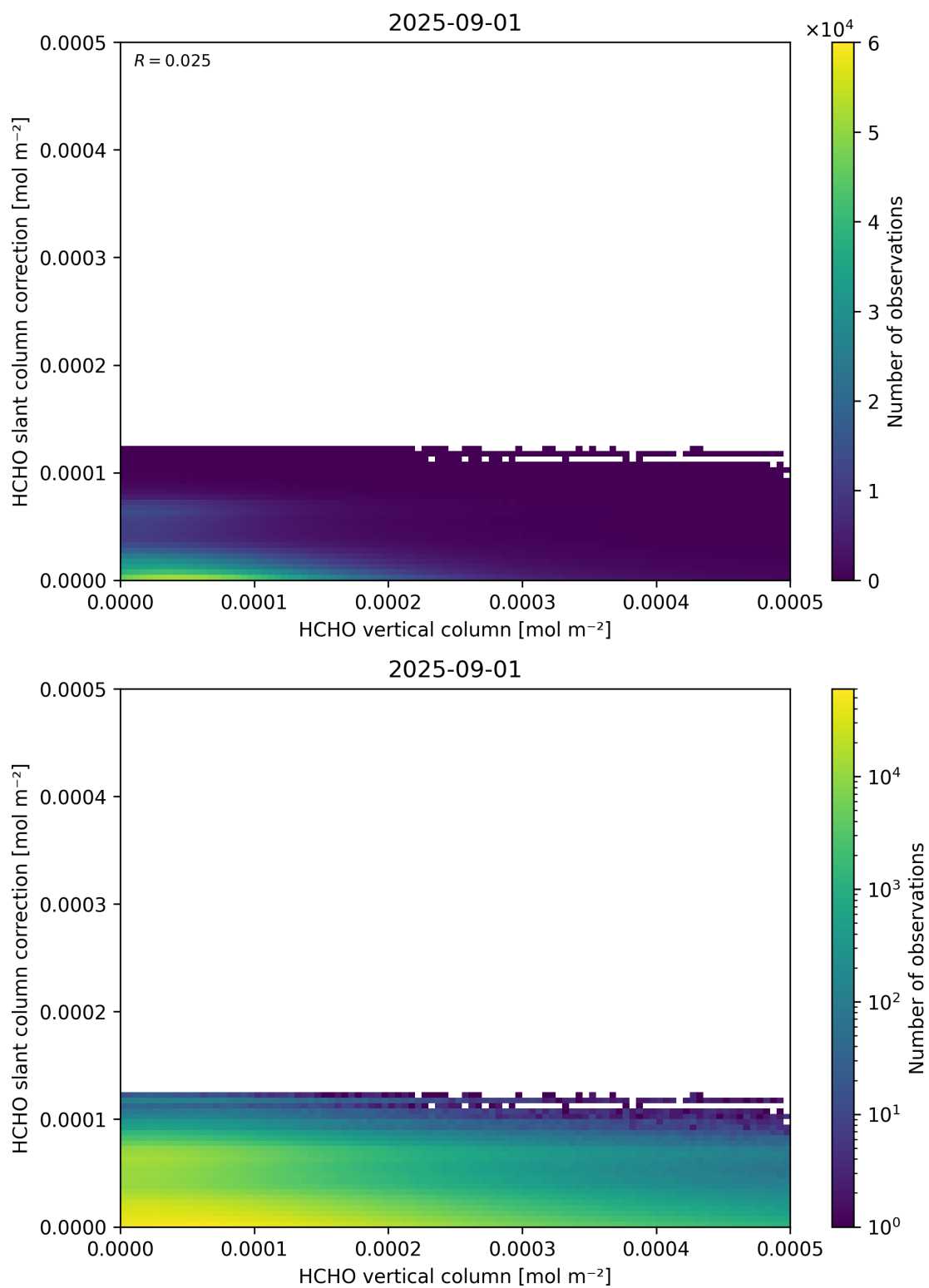
Figure 128: Scatter density plot of “HCHO vertical column” against “HCHO slant column correction” for 2025-08-31 to 2025-09-02.
