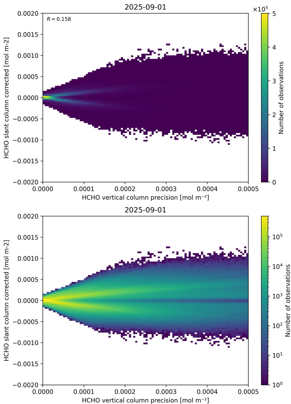
Figure 140: Scatter density plot of “HCHO vertical column precision” against “HCHO slant column corrected” for 2025-08-31 to 2025-09-02.
