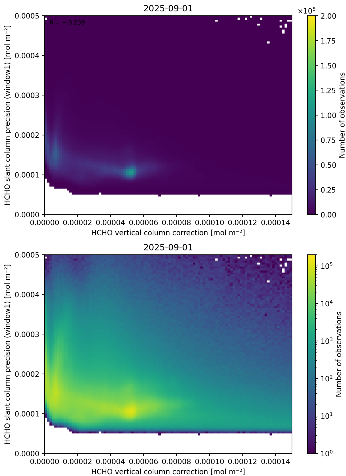
Figure 119: Scatter density plot of “HCHO vertical column correction” against “HCHO slant column precision (window1)” for 2025-08-31 to 2025-09-02.
