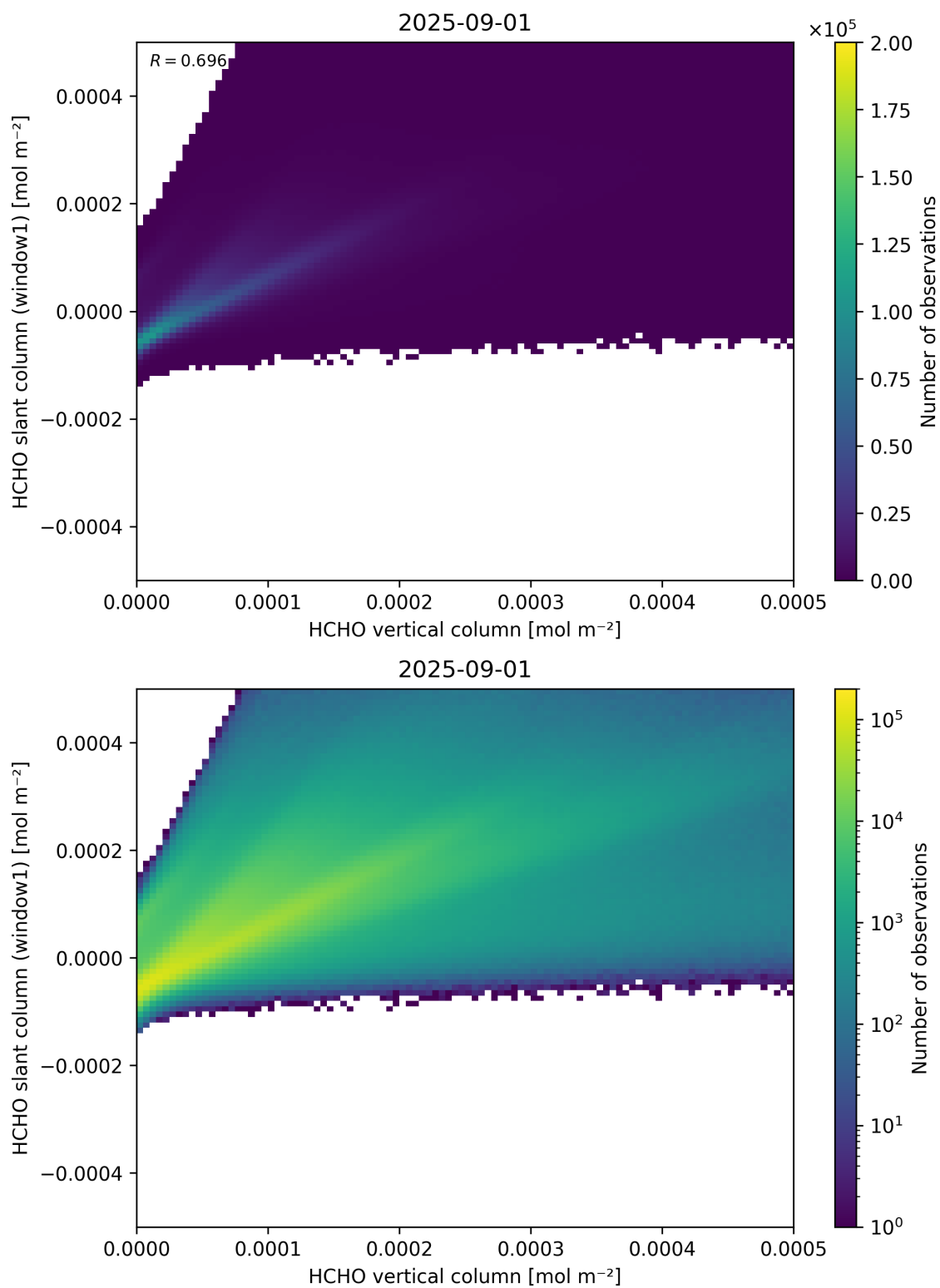
Figure 129: Scatter density plot of “HCHO vertical column” against “HCHO slant column (window1)” for 2025-08-31 to 2025-09-02.
