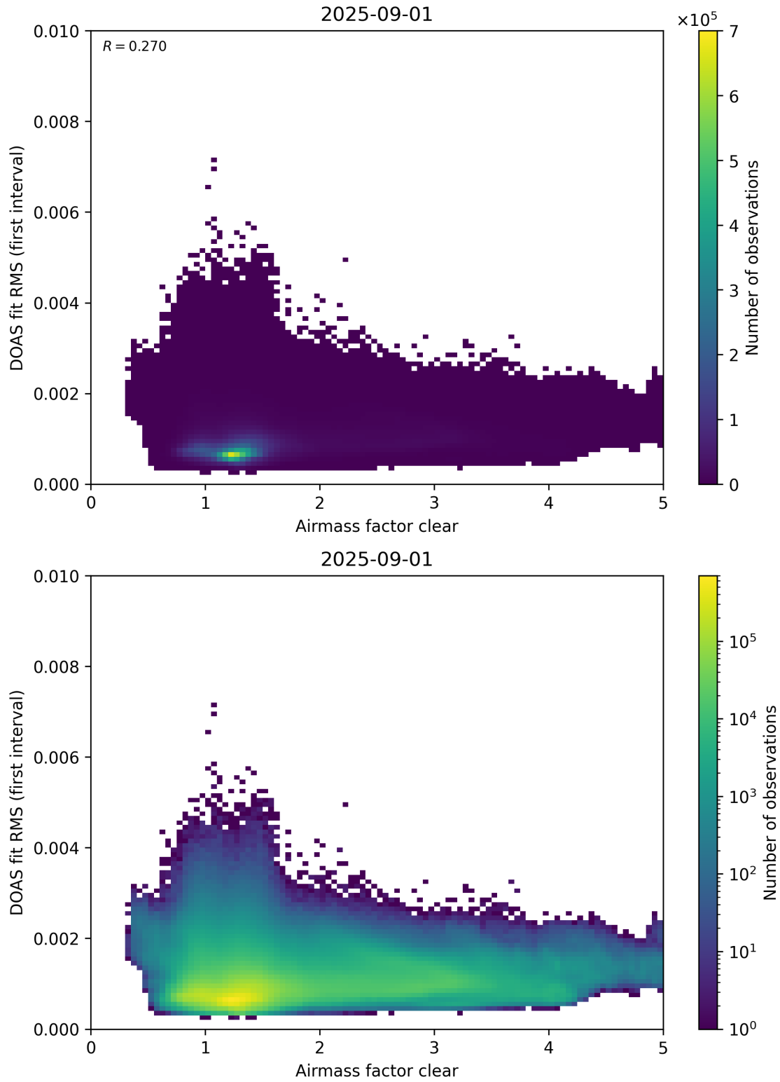
Figure 71: Scatter density plot of “Airmass factor clear” against “DOAS fit RMS (first interval)” for 2025-08-31 to 2025-09-02.
