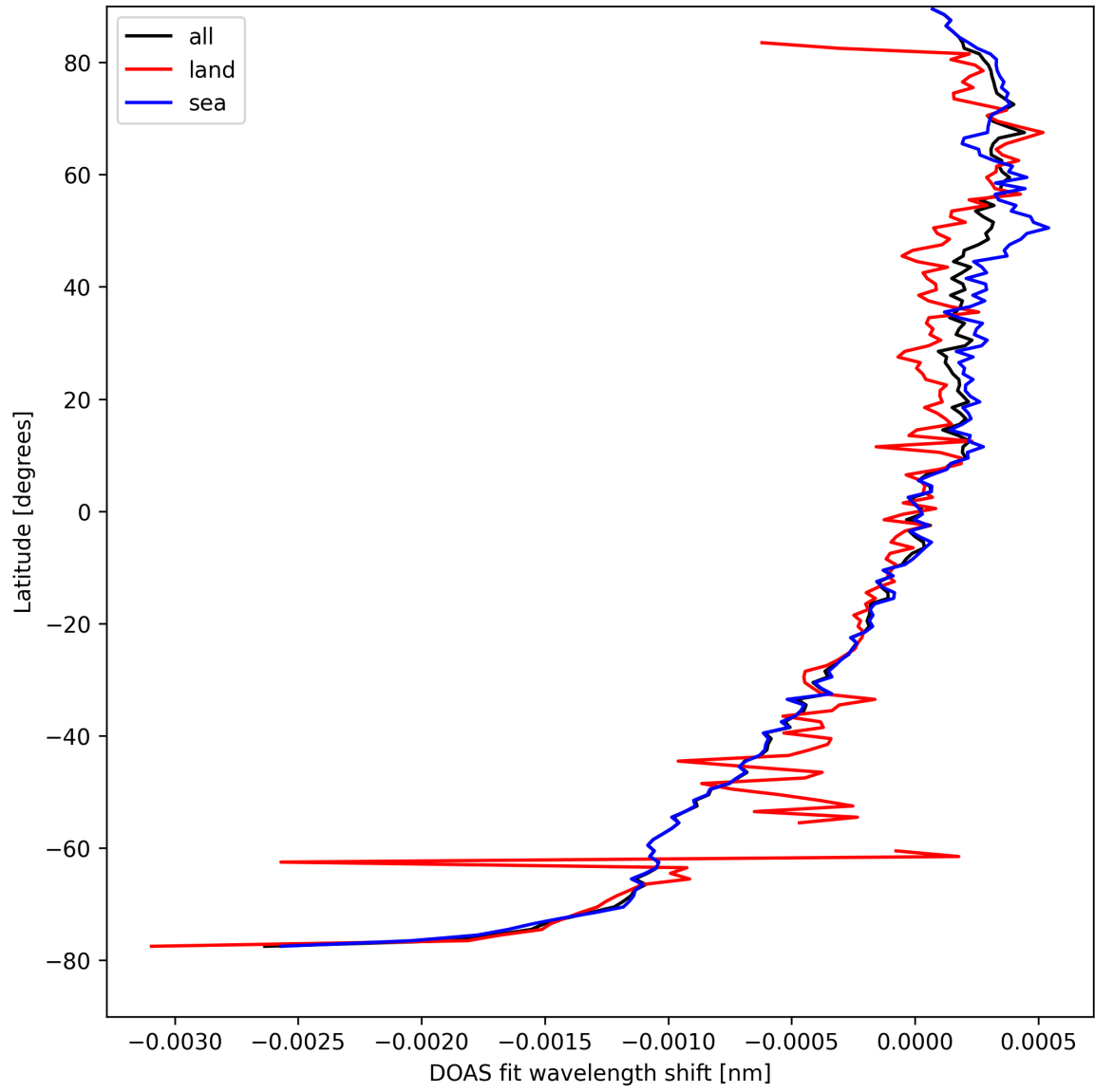
Figure 30: Zonal average of “DOAS fit wavelength shift” for 2025-08-31 to 2025-09-02.
