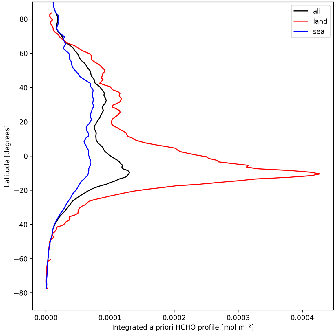
Figure 29: Zonal average of “Integrated a priori HCHO profile” for 2025-08-31 to 2025-09-02.
