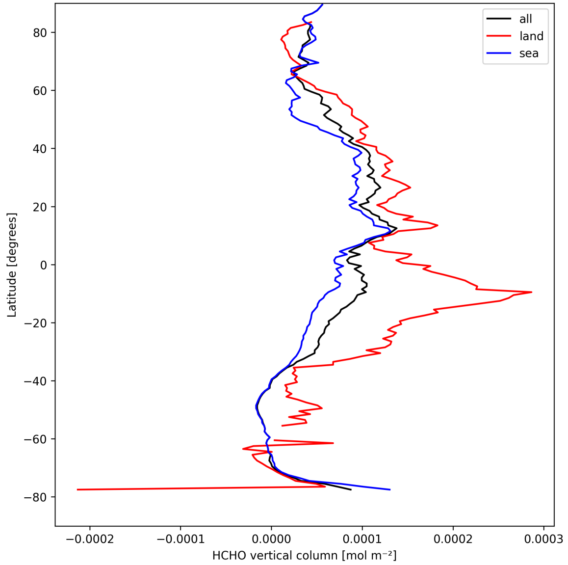
Figure 21: Zonal average of “HCHO vertical column” for 2025-08-31 to 2025-09-02.
