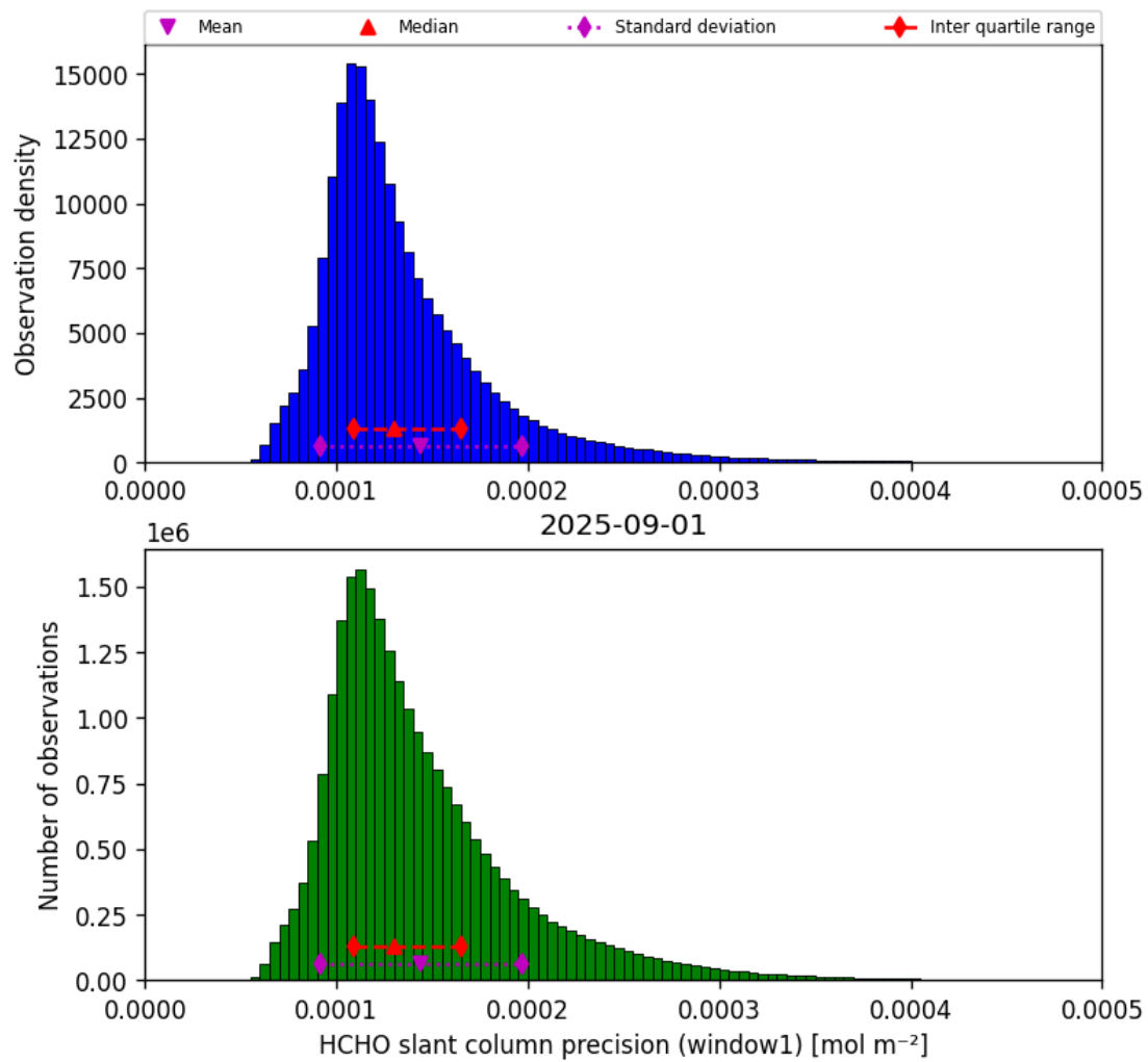
Figure 39: Histogram of “HCHO slant column precision (window1)” for 2025-08-31 to 2025-09-02
