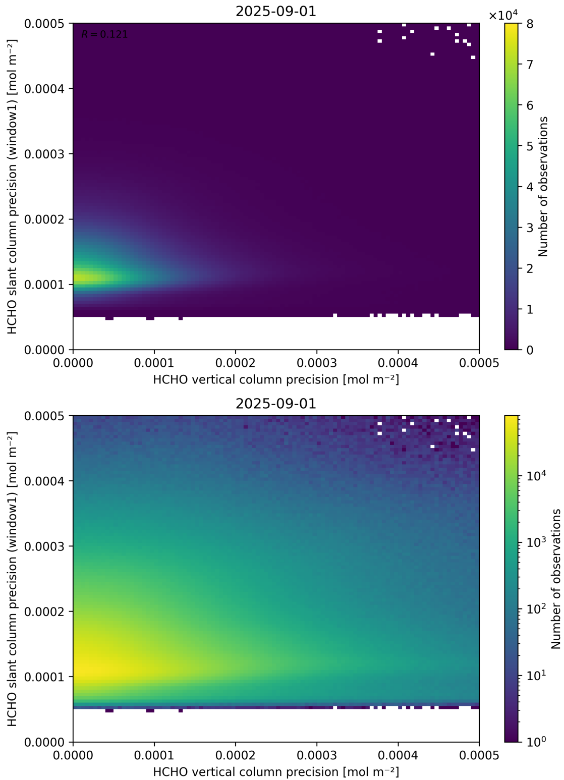
Figure 143: Scatter density plot of “HCHO vertical column precision” against “HCHO slant column precision (window1)” for 2025-08-31 to 2025-09-02.
