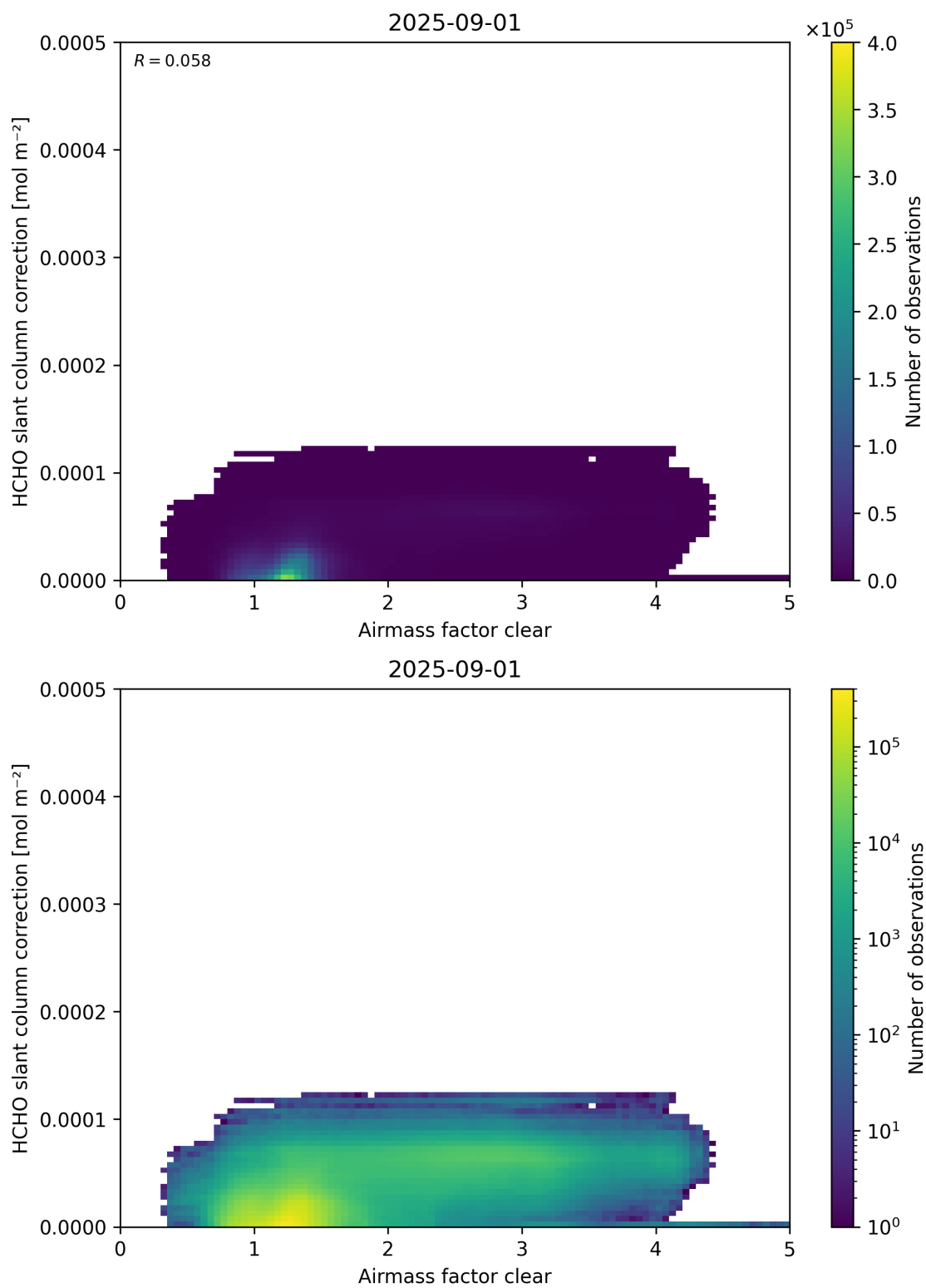
Figure 75: Scatter density plot of “Airmass factor clear” against “HCHO slant column correction” for 2025-08-31 to 2025-09-02.
