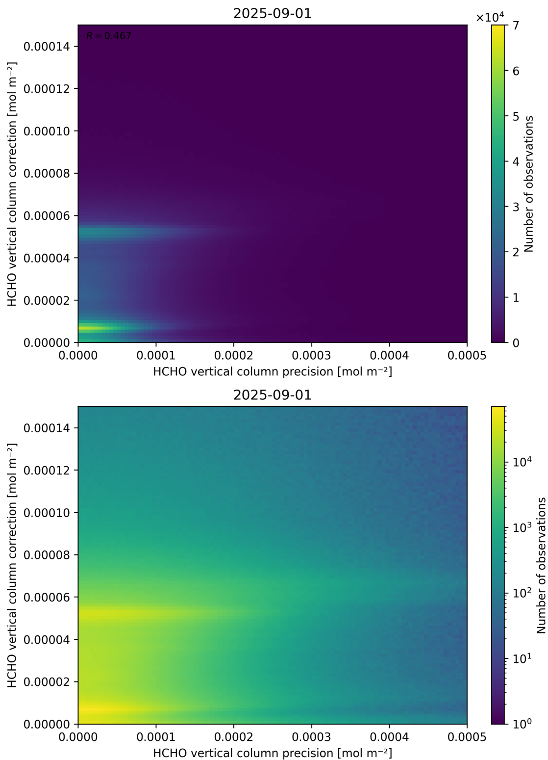
Figure 146: Scatter density plot of “HCHO vertical column precision” against “HCHO vertical column correction” for 2025-08-31 to 2025-09-02.
