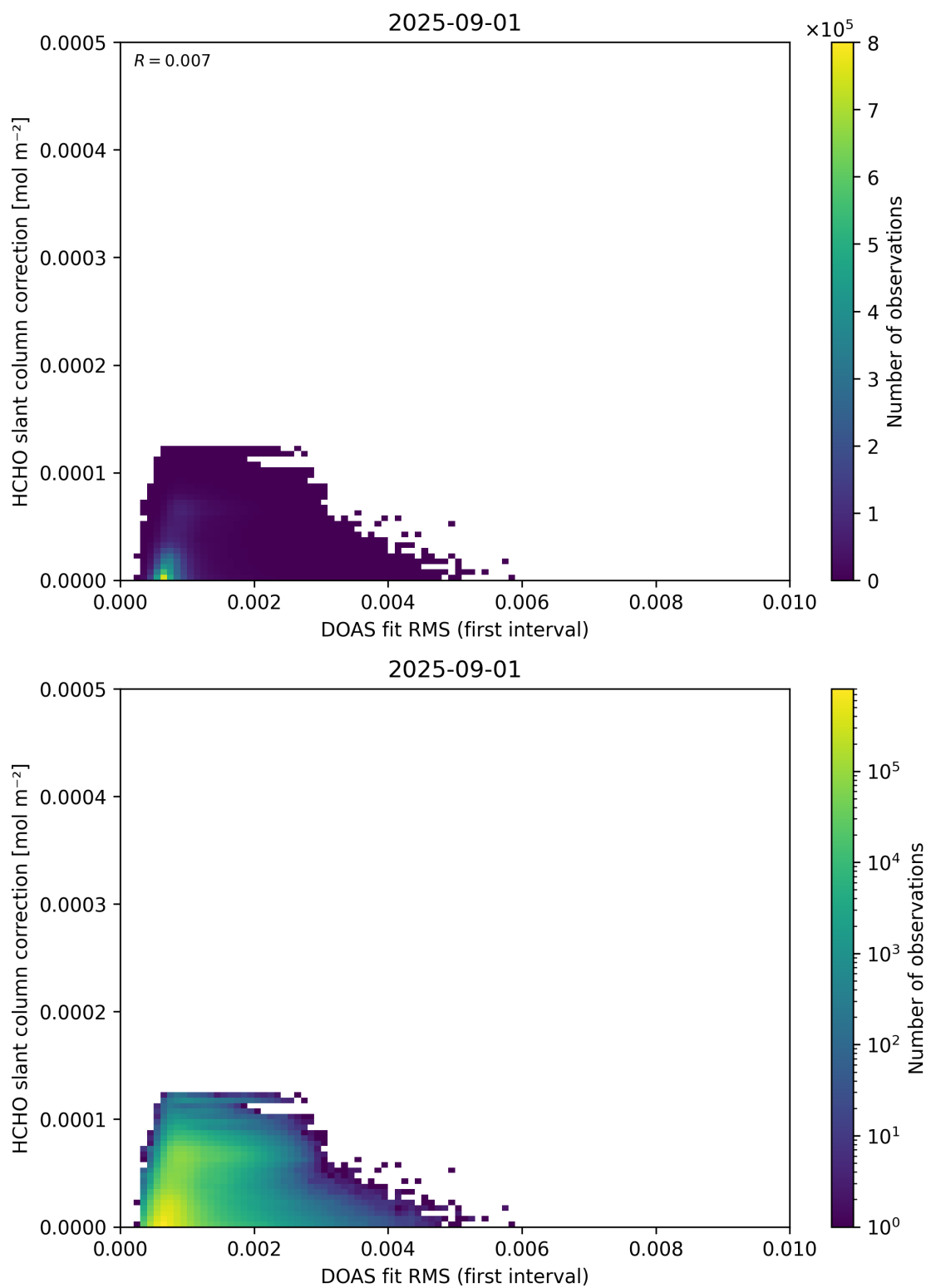
Figure 63: Scatter density plot of “DOAS fit RMS (first interval)” against “HCHO slant column correction” for 2025-08-31 to 2025-09-02.
