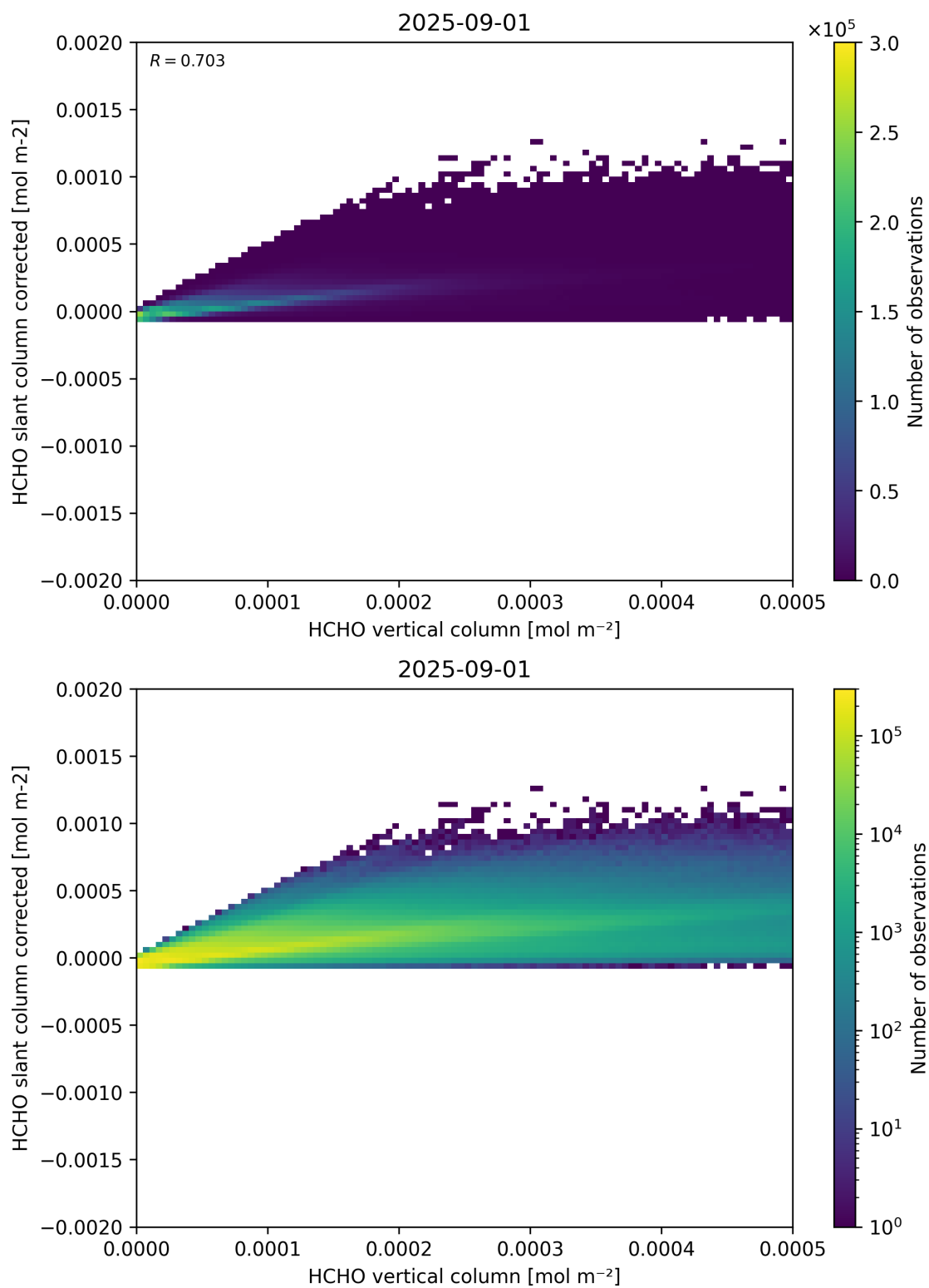
Figure 127: Scatter density plot of “HCHO vertical column” against “HCHO slant column corrected” for 2025-08-31 to 2025-09-02.
