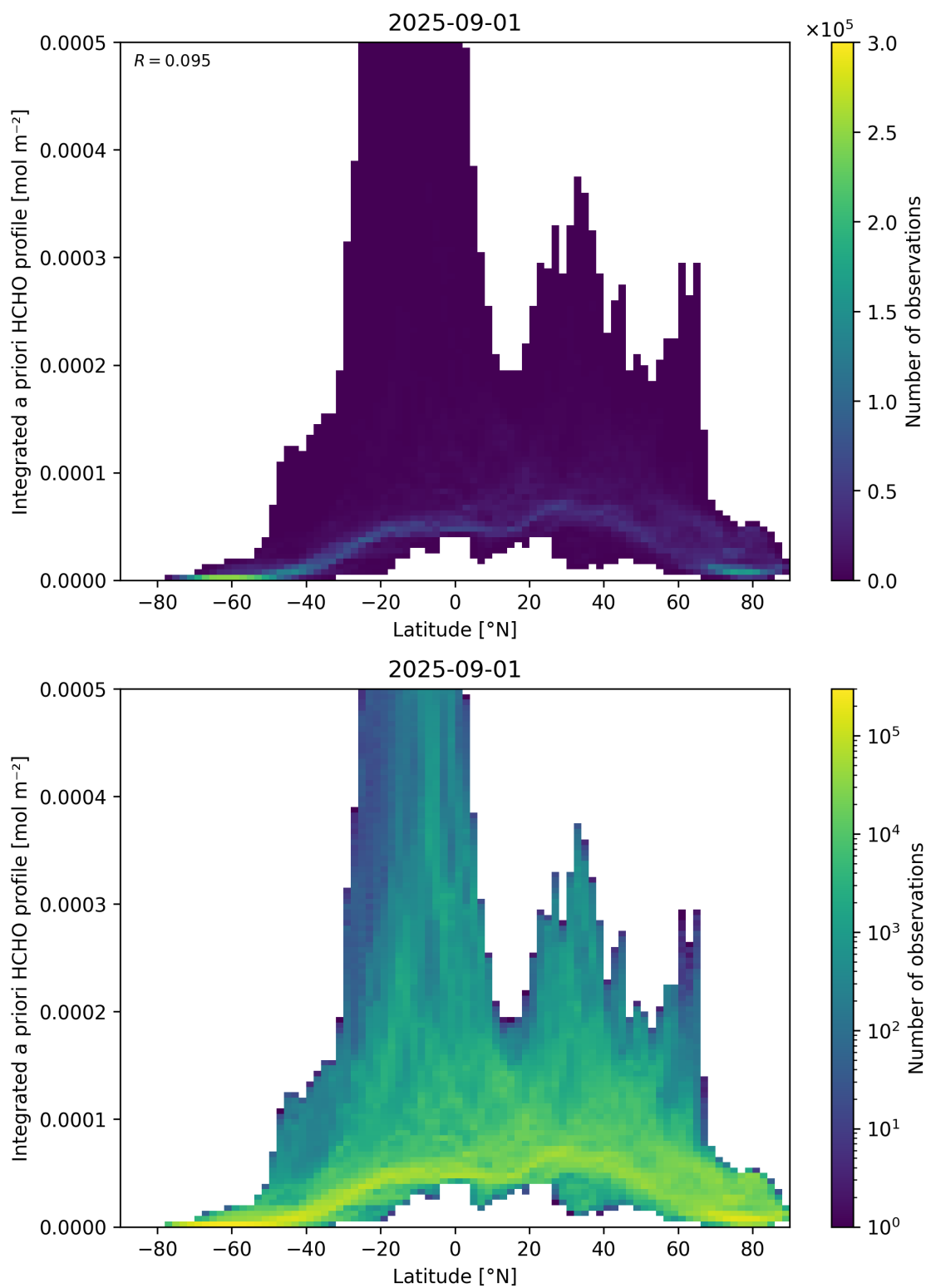
Figure 166: Scatter density plot of “Latitude” against “Integrated a priori HCHO profile” for 2025-08-31 to 2025-09-02.
