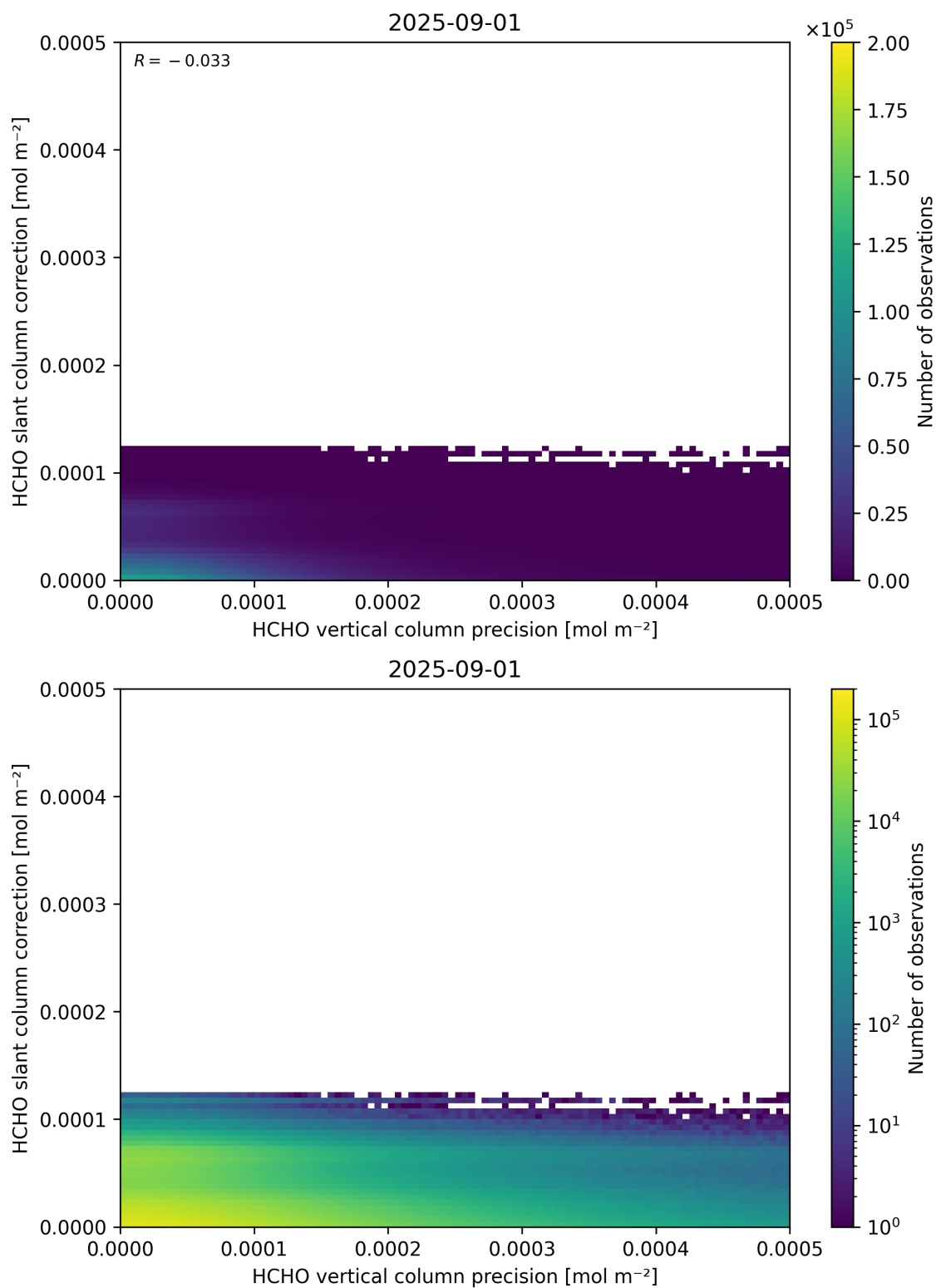
Figure 141: Scatter density plot of “HCHO vertical column precision” against “HCHO slant column correction” for 2025-08-31 to 2025-09-02.
