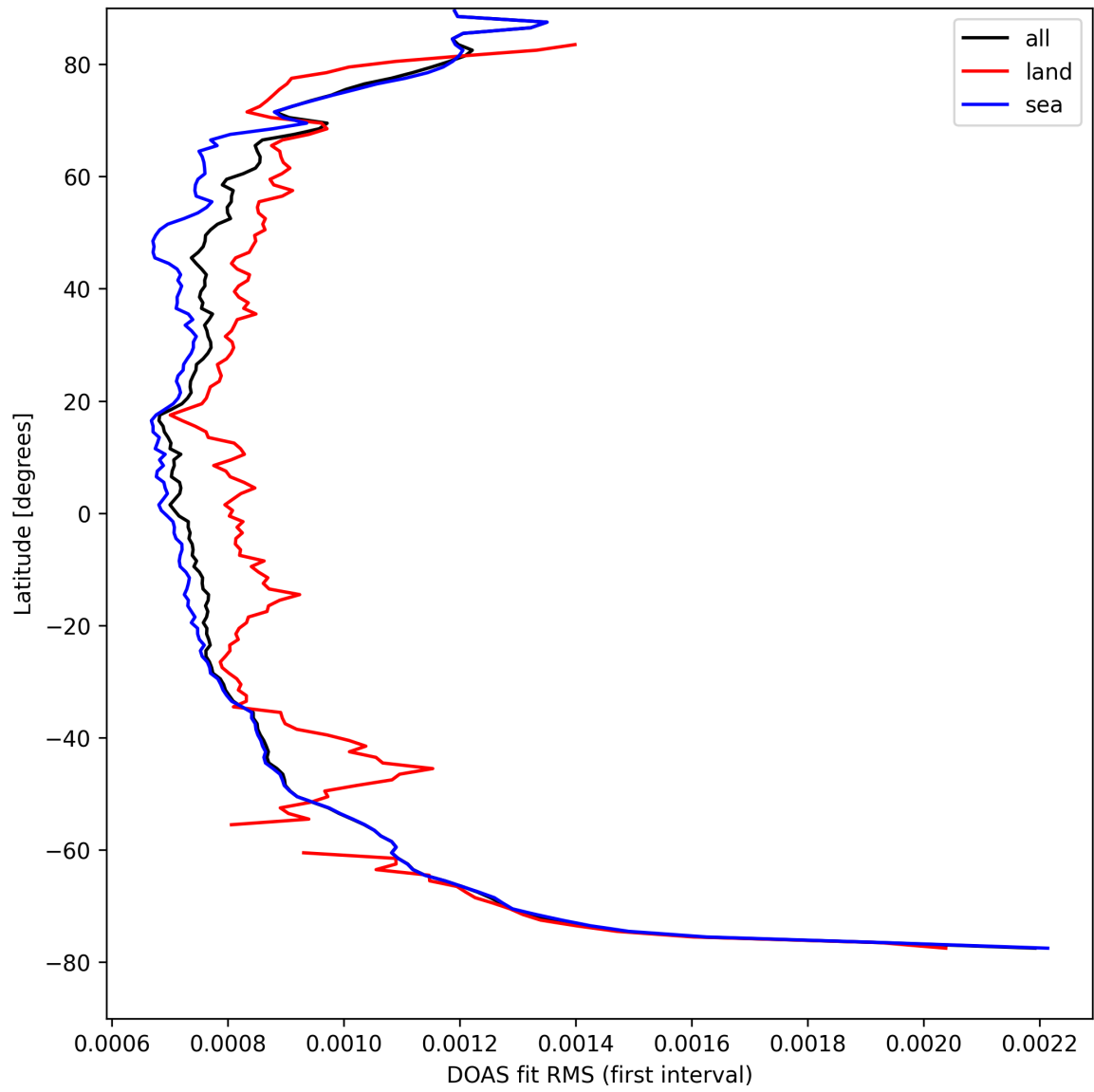
Figure 32: Zonal average of “DOAS fit RMS (first interval)” for 2025-08-31 to 2025-09-02.
