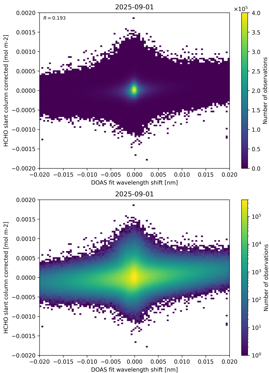
Figure 66: Scatter density plot of “DOAS fit wavelength shift” against “HCHO slant column corrected” for 2025-08-31 to 2025-09-02.
