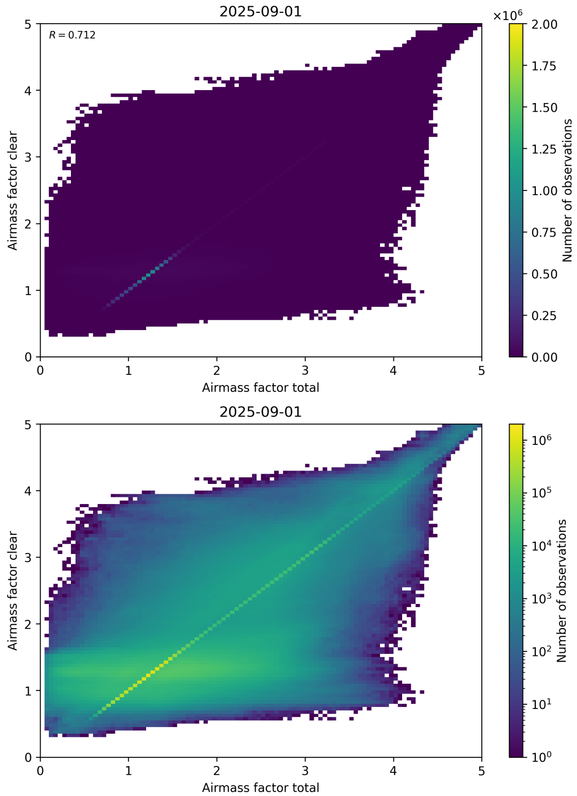
Figure 100: Scatter density plot of “Airmass factor total” against “Airmass factor clear” for 2025-08-31 to 2025-09-02.
