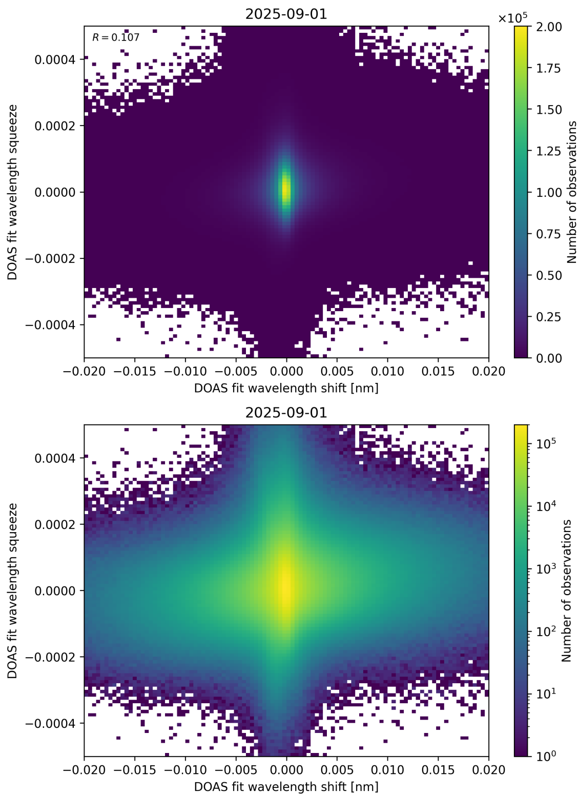
Figure 65: Scatter density plot of “DOAS fit wavelength shift” against “DOAS fit wavelength squeeze” for 2025-08-31 to 2025-09-02.
