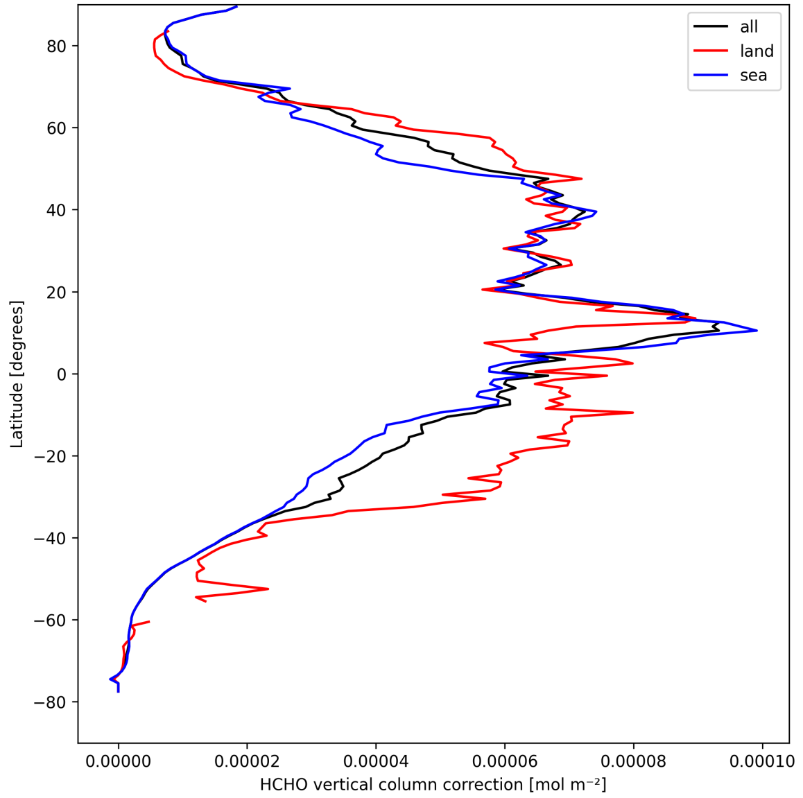
Figure 23: Zonal average of “HCHO vertical column correction” for 2025-08-31 to 2025-09-02.
