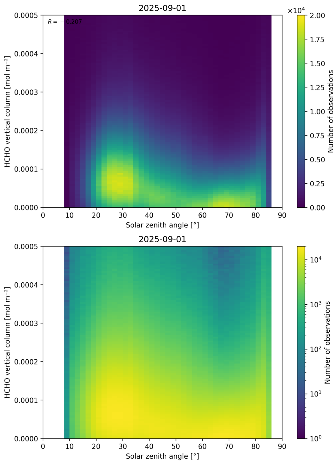
Figure 177: Scatter density plot of “Solar zenith angle” against “HCHO vertical column” for 2025-08-31 to 2025-09-02.
