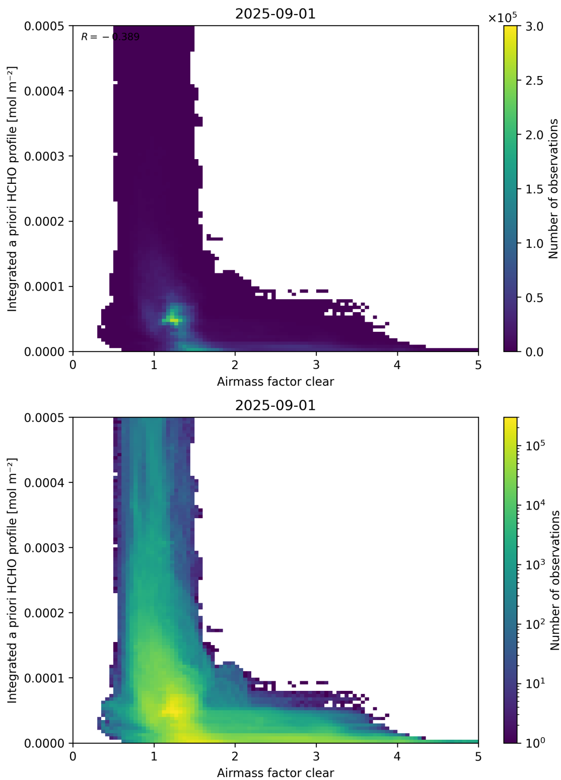
Figure 76: Scatter density plot of “Airmass factor clear” against “Integrated a priori HCHO profile” for 2025-08-31 to 2025-09-02.
