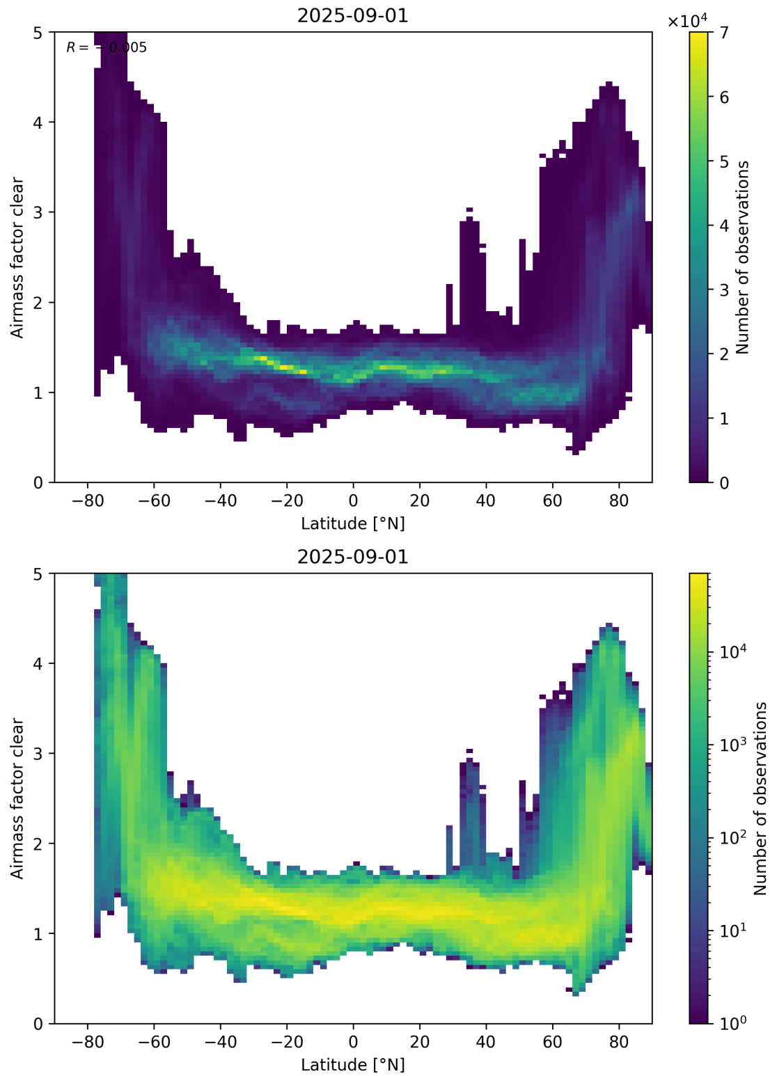
Figure 156: Scatter density plot of “Latitude” against “Airmass factor clear” for 2025-08-31 to 2025-09-02.
