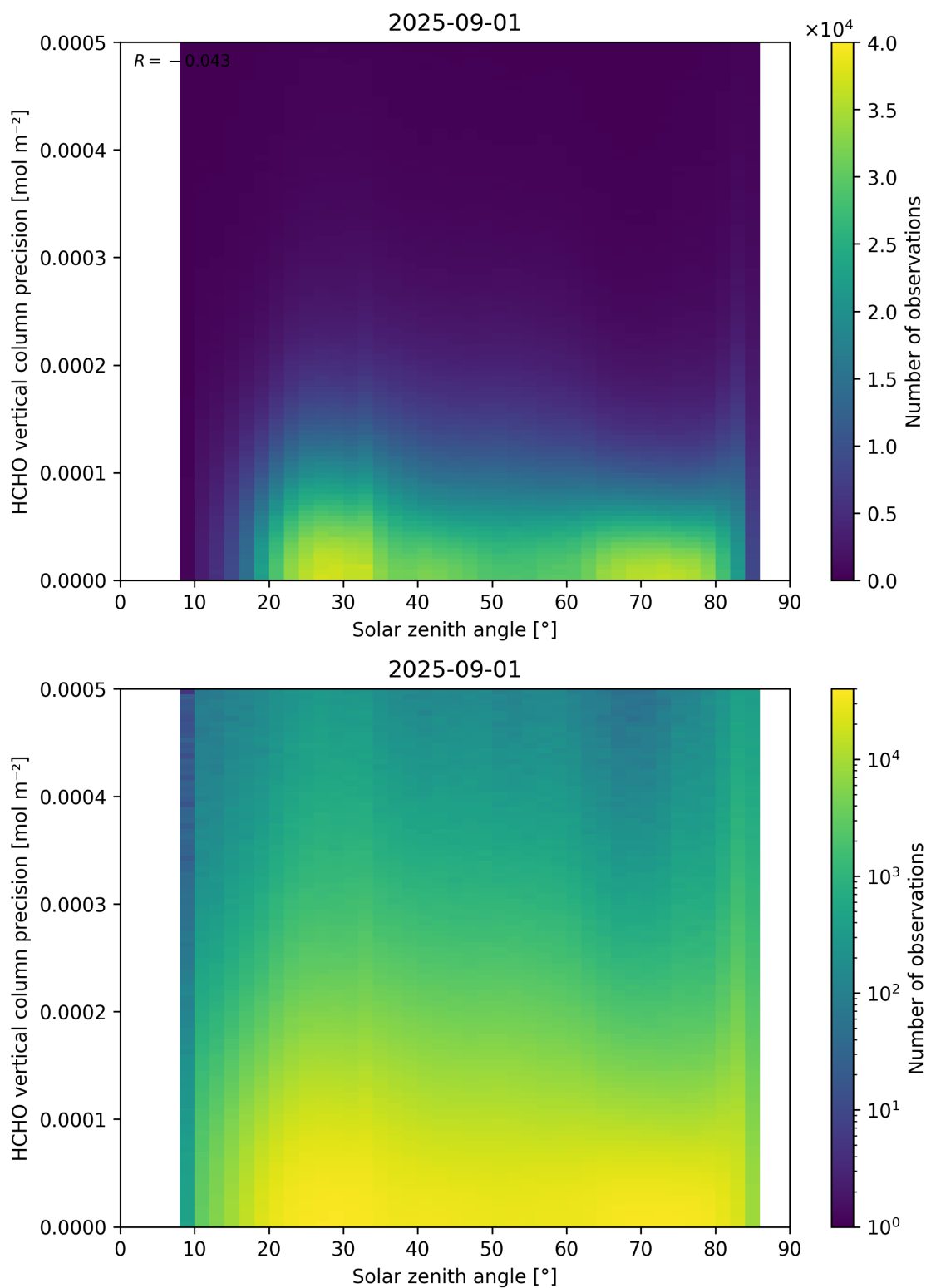
Figure 179: Scatter density plot of “Solar zenith angle” against “HCHO vertical column precision” for 2025-08-31 to 2025-09-02.
