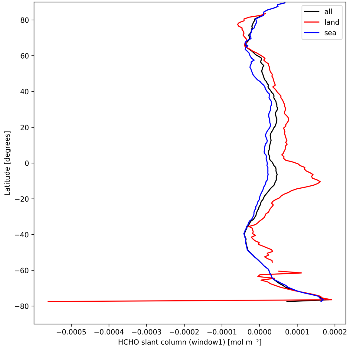
Figure 24: Zonal average of “HCHO slant column (window1)” for 2025-08-31 to 2025-09-02.
