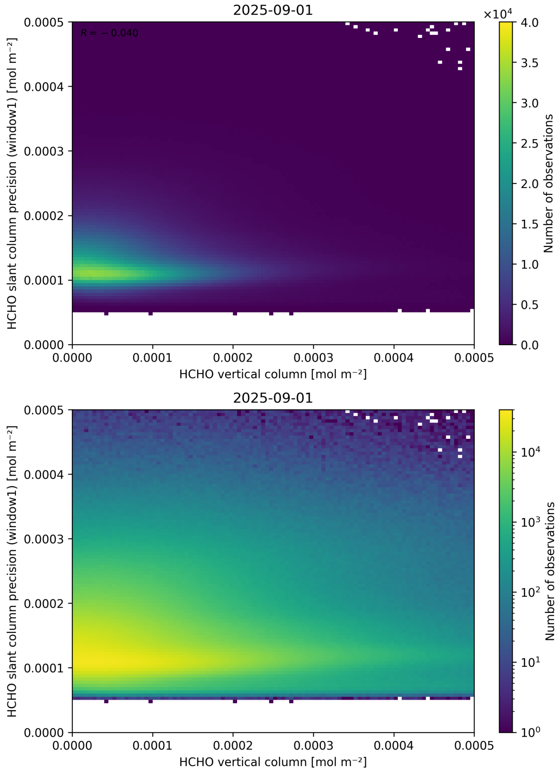
Figure 130: Scatter density plot of “HCHO vertical column” against “HCHO slant column precision (window1)” for 2025-08-31 to 2025-09-02.
