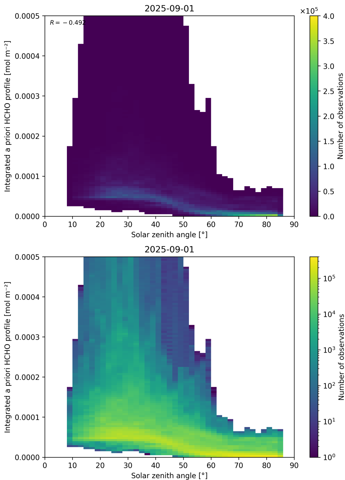
Figure 180: Scatter density plot of “Solar zenith angle” against “Integrated a priori HCHO profile” for 2025-08-31 to 2025-09-02.
