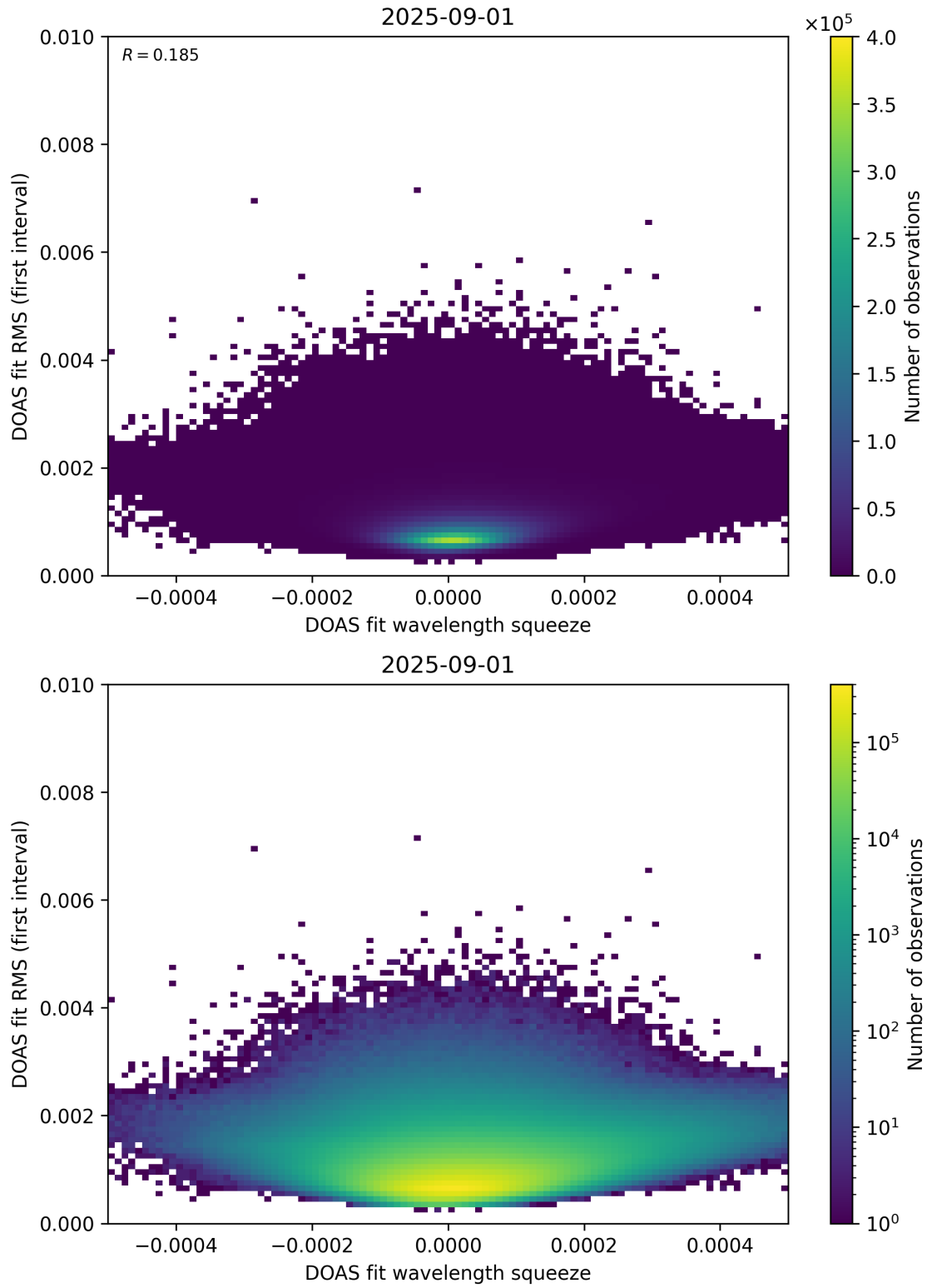
Figure 68: Scatter density plot of “DOAS fit wavelength squeeze” against “DOAS fit RMS (first interval)” for 2025-08-31 to 2025-09-02.
