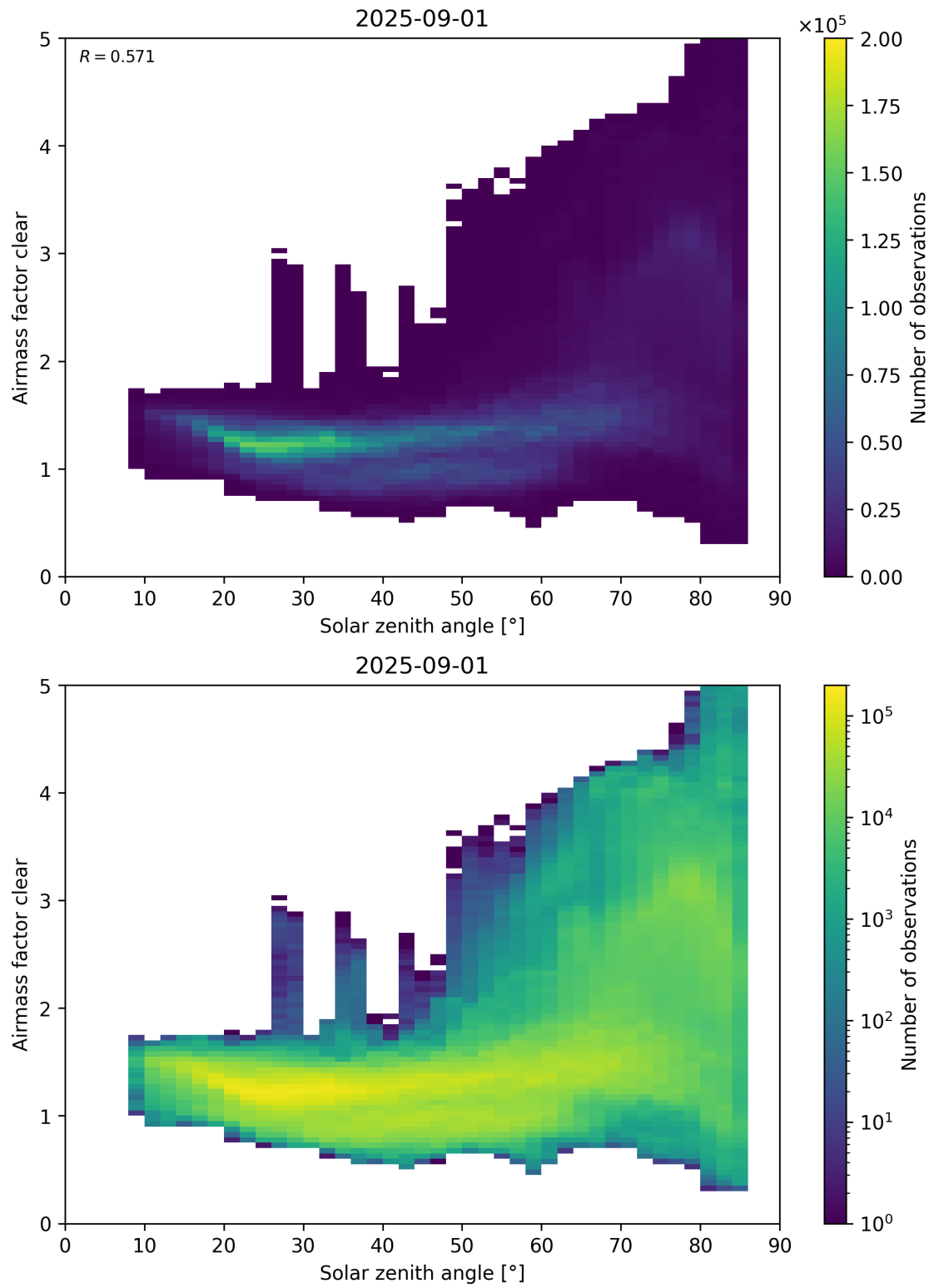
Figure 170: Scatter density plot of “Solar zenith angle” against “Airmass factor clear” for 2025-08-31 to 2025-09-02.
