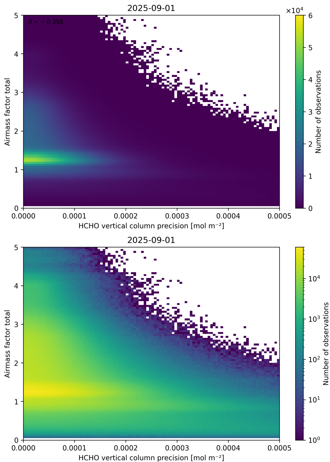
Figure 144: Scatter density plot of “HCHO vertical column precision” against “Airmass factor total” for 2025-08-31 to 2025-09-02.
