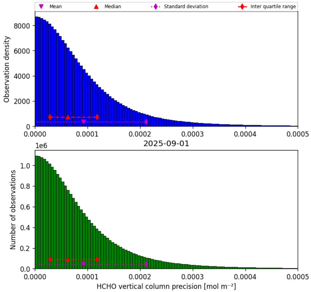
Figure 36: Histogram of “HCHO vertical column precision” for 2025-08-31 to 2025-09-02
