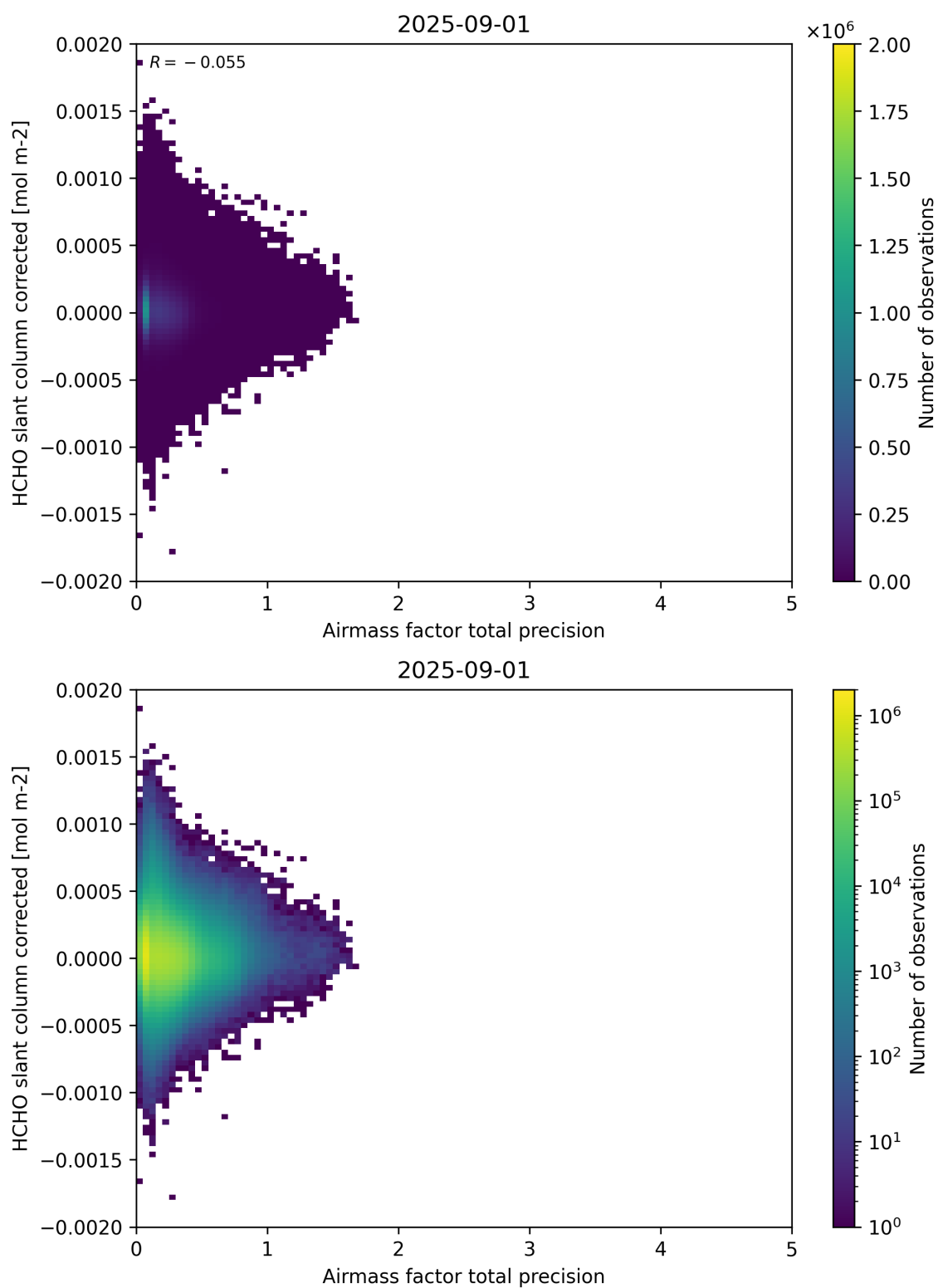
Figure 109: Scatter density plot of “Airmass factor total precision” against “HCHO slant column corrected” for 2025-08-31 to 2025-09-02.
