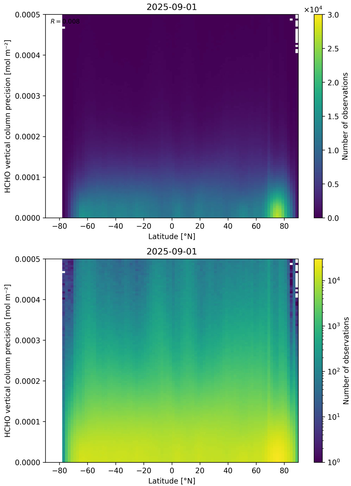
Figure 165: Scatter density plot of “Latitude” against “HCHO vertical column precision” for 2025-08-31 to 2025-09-02.
