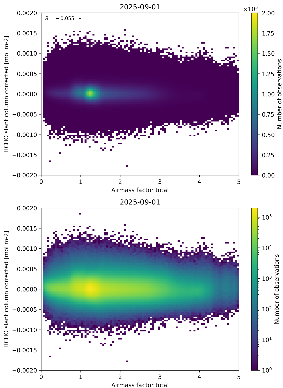
Figure 101: Scatter density plot of “Airmass factor total” against “HCHO slant column corrected” for 2025-08-31 to 2025-09-02.
