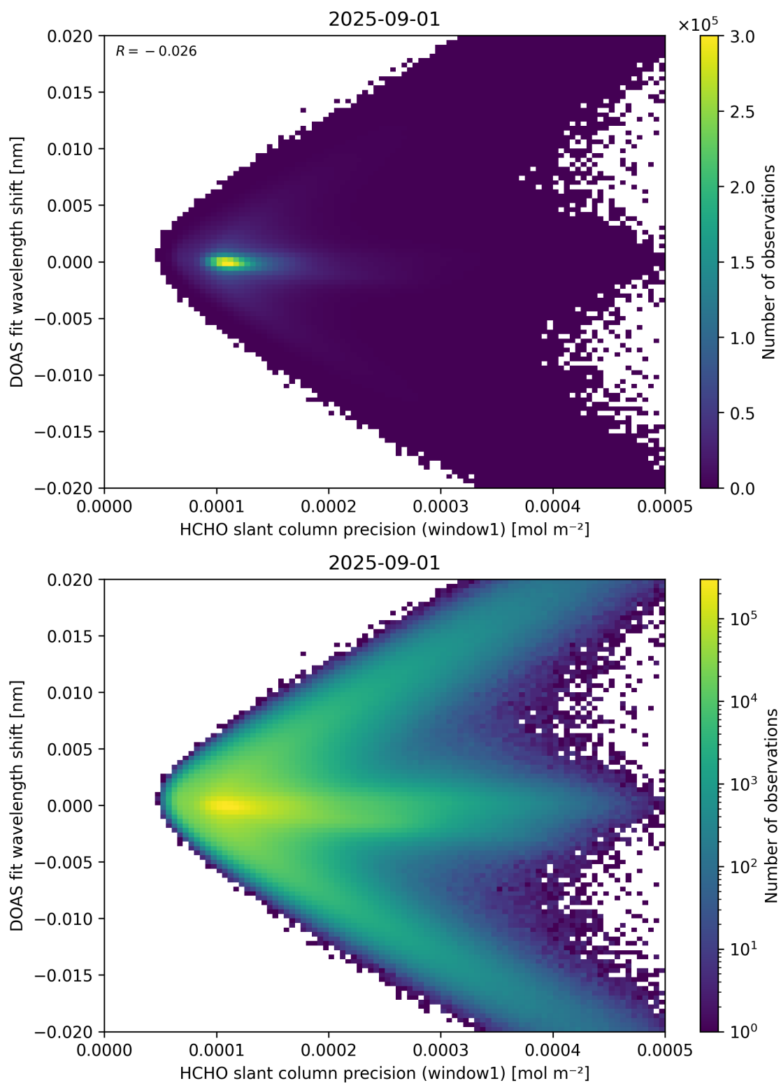
Figure 89: Scatter density plot of “HCHO slant column precision (window1)” against “DOAS fit wavelength shift” for 2025-08-31 to 2025-09-02.
