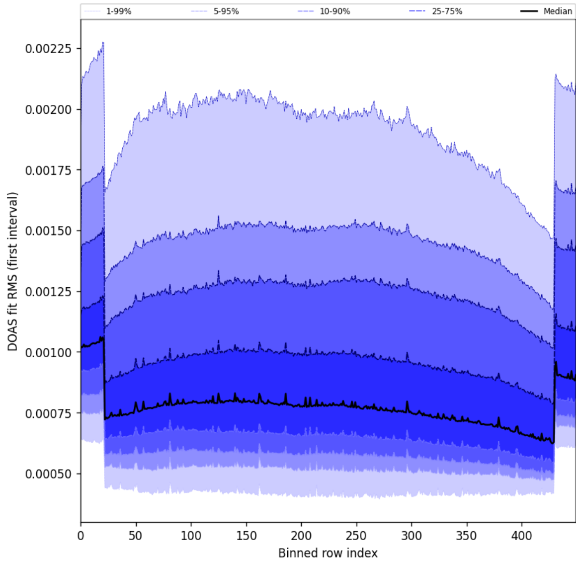
Figure 60: Along track statistics of “DOAS fit RMS (first interval)” for 2025-08-31 to 2025-09-02
