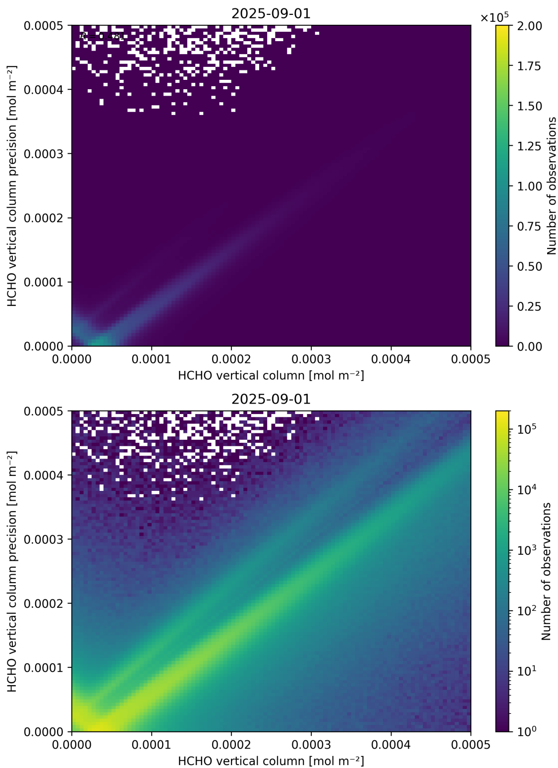
Figure 134: Scatter density plot of “HCHO vertical column” against “HCHO vertical column precision” for 2025-08-31 to 2025-09-02.
