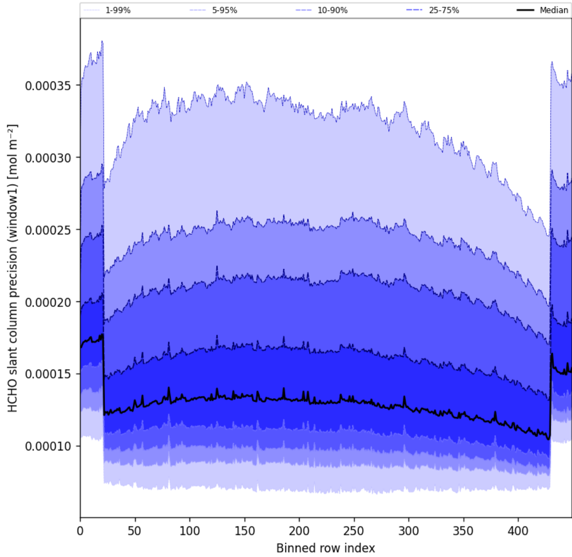
Figure 53: Along track statistics of “HCHO slant column precision (window1)” for 2025-08-31 to 2025-09-02
