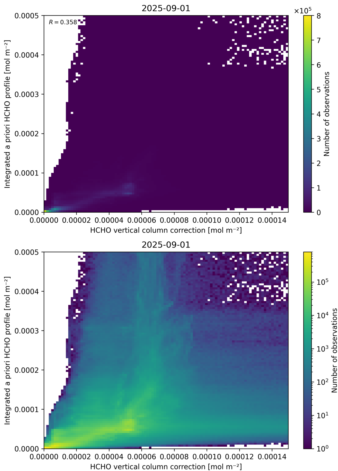
Figure 122: Scatter density plot of “HCHO vertical column correction” against “Integrated a priori HCHO profile” for 2025-08-31 to 2025-09-02.
