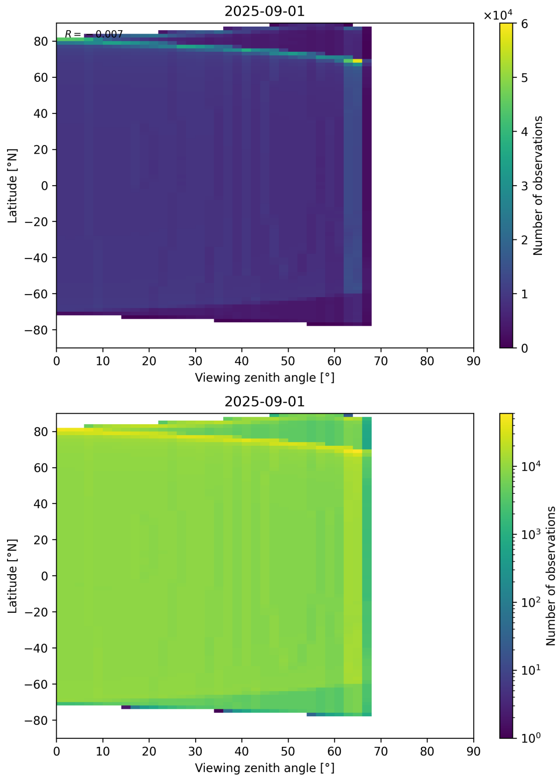
Figure 196: Scatter density plot of “Viewing zenith angle” against “Latitude” for 2025-08-31 to 2025-09-02.
