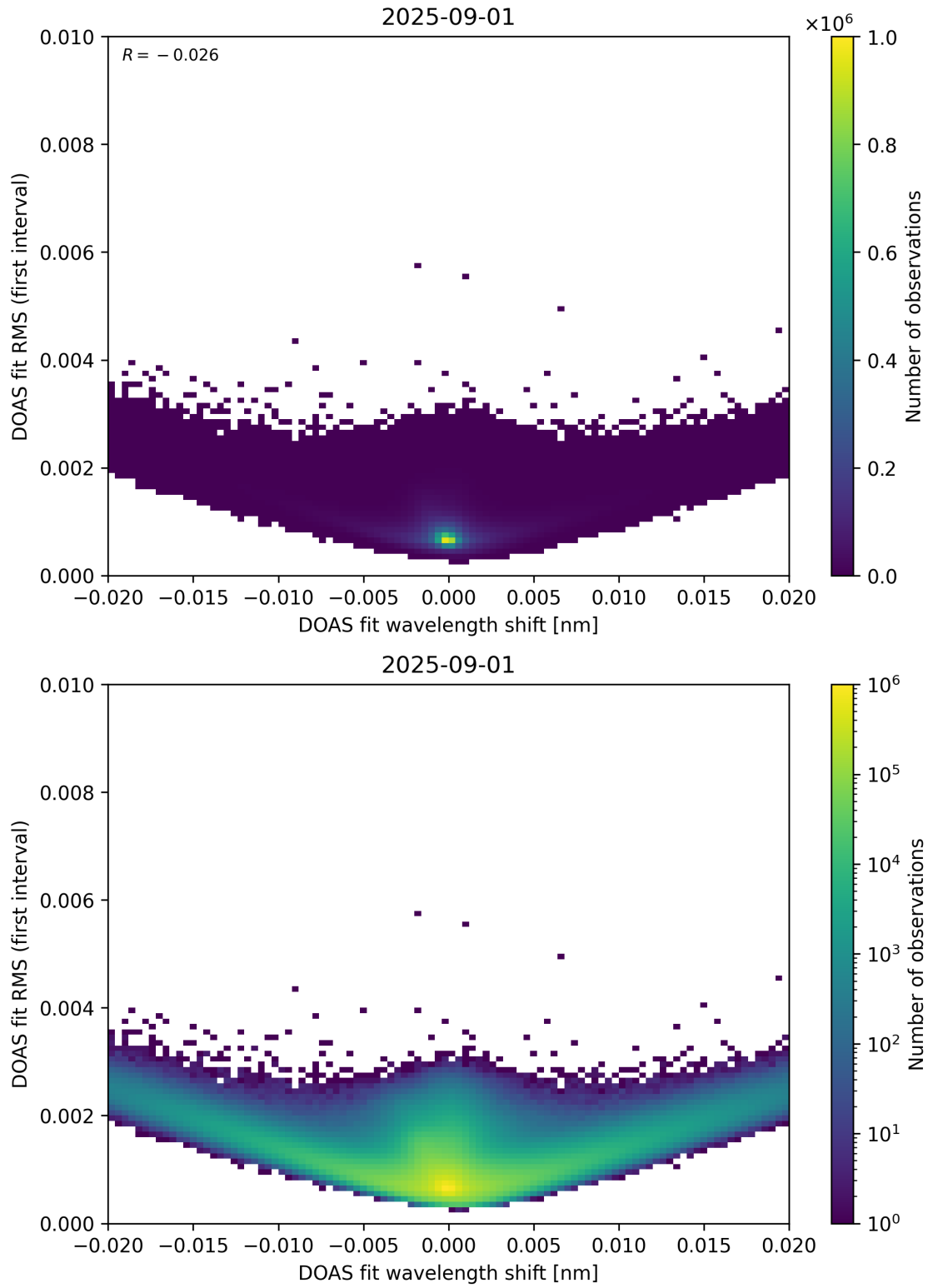
Figure 64: Scatter density plot of “DOAS fit wavelength shift” against “DOAS fit RMS (first interval)” for 2025-08-31 to 2025-09-02.
