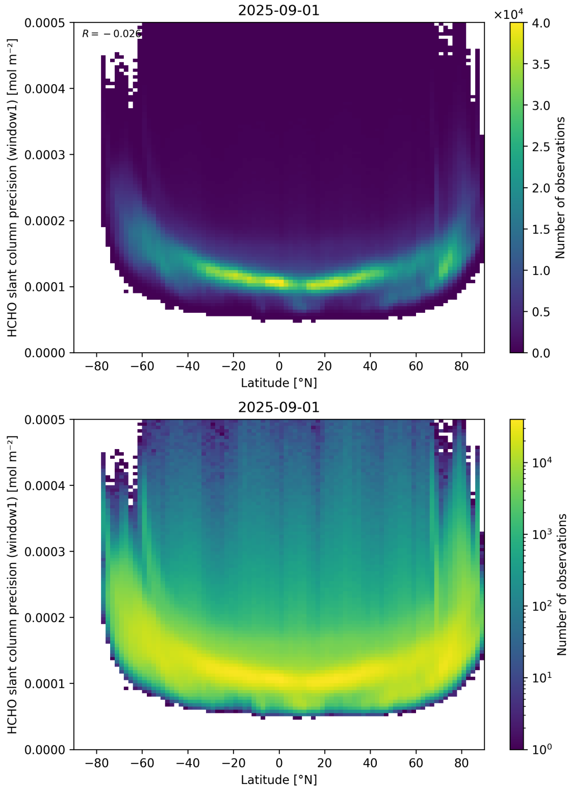
Figure 160: Scatter density plot of “Latitude” against “HCHO slant column precision (window1)” for 2025-08-31 to 2025-09-02.
