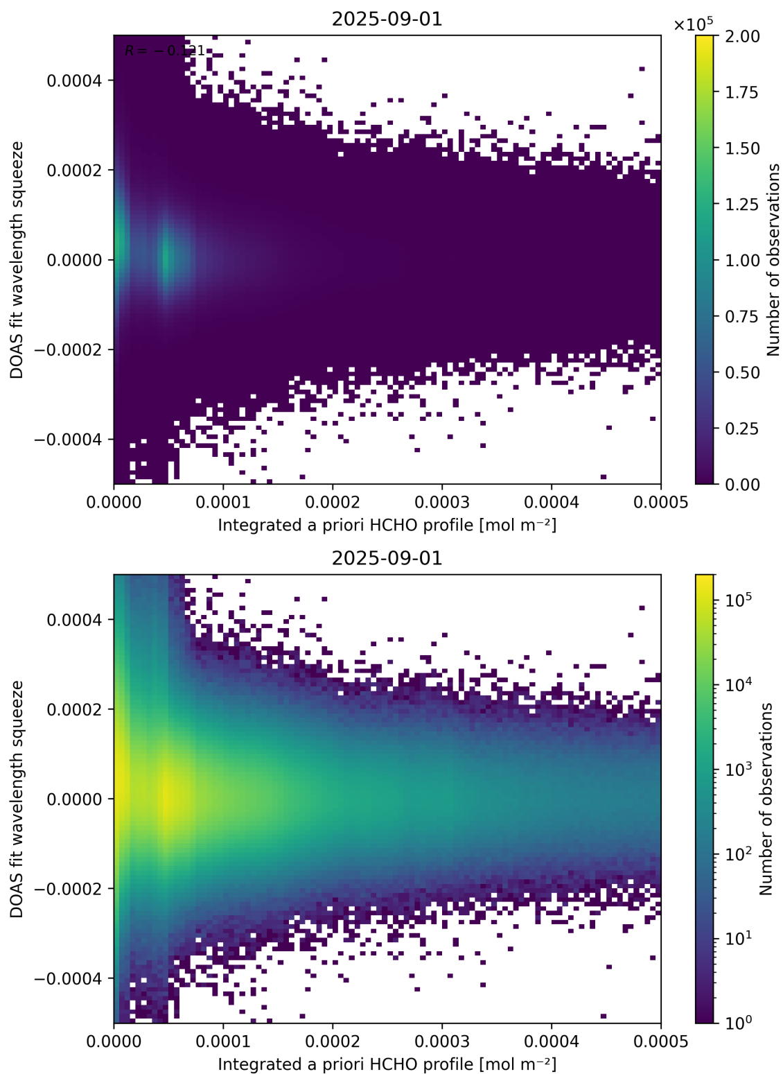
Figure 150: Scatter density plot of “Integrated a priori HCHO profile” against “DOAS fit wavelength squeeze” for 2025-08-31 to 2025-09-02.
