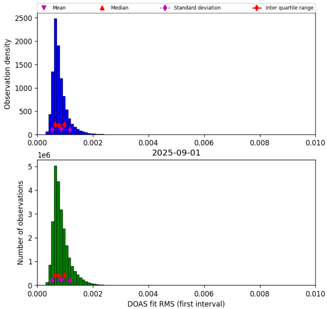
Figure 46: Histogram of “DOAS fit RMS (first interval)” for 2025-08-31 to 2025-09-02
