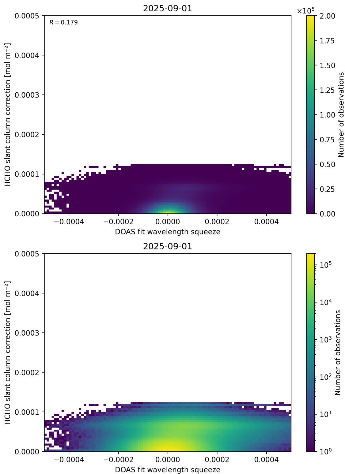
Figure 70: Scatter density plot of “DOAS fit wavelength squeeze” against “HCHO slant column correction” for 2025-08-31 to 2025-09-02.
