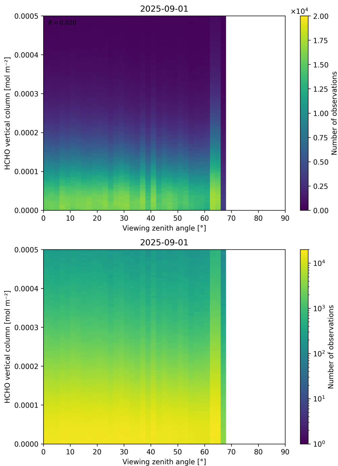
Figure 192: Scatter density plot of “Viewing zenith angle” against “HCHO vertical column” for 2025-08-31 to 2025-09-02.
