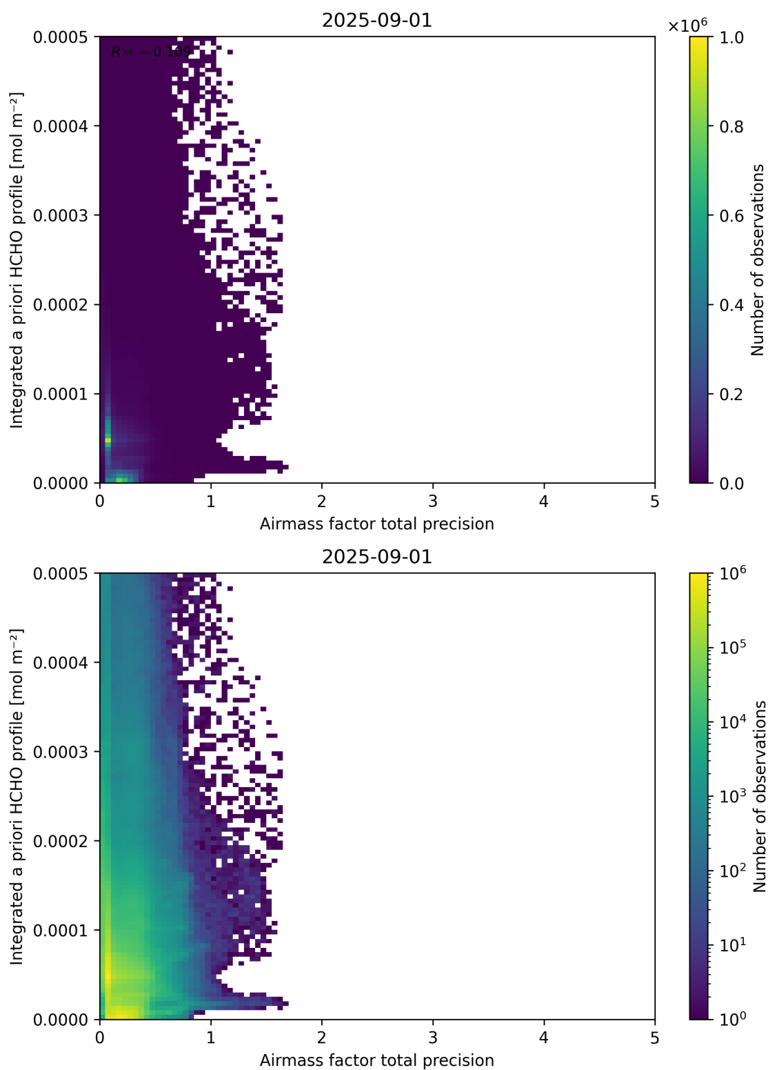
Figure 111: Scatter density plot of “Airmass factor total precision” against “Integrated a priori HCHO profile” for 2025-08-31 to 2025-09-02.
