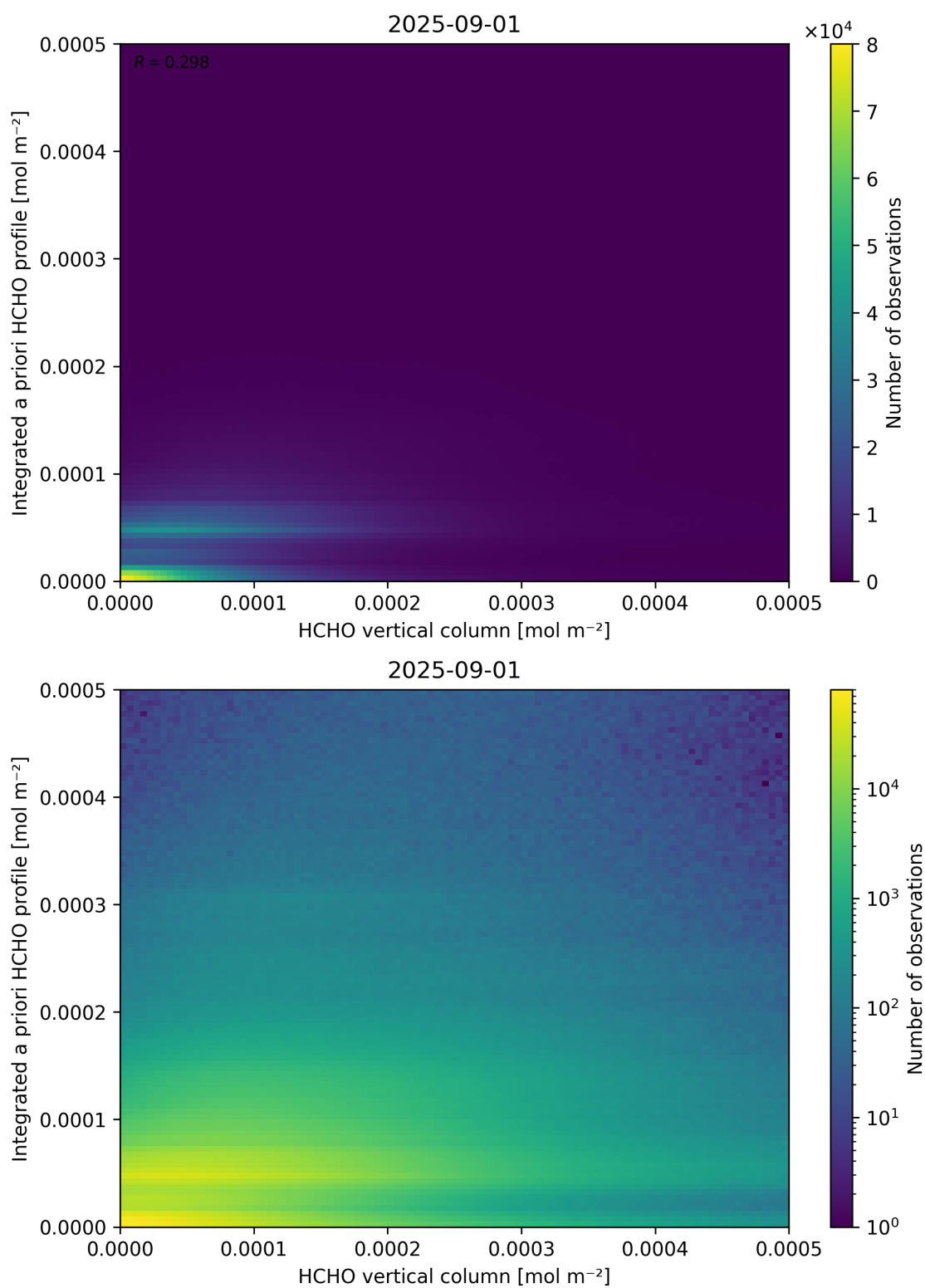
Figure 135: Scatter density plot of “HCHO vertical column” against “Integrated a priori HCHO profile” for 2025-08-31 to 2025-09-02.
