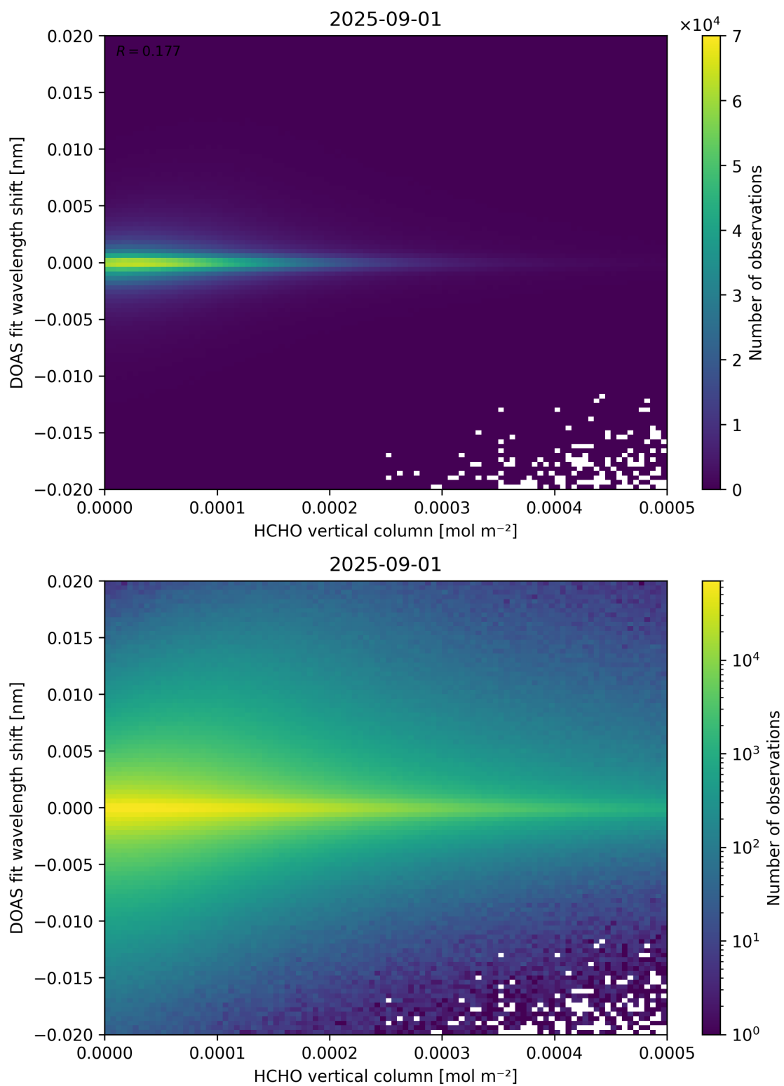
Figure 124: Scatter density plot of “HCHO vertical column” against “DOAS fit wavelength shift” for 2025-08-31 to 2025-09-02.
