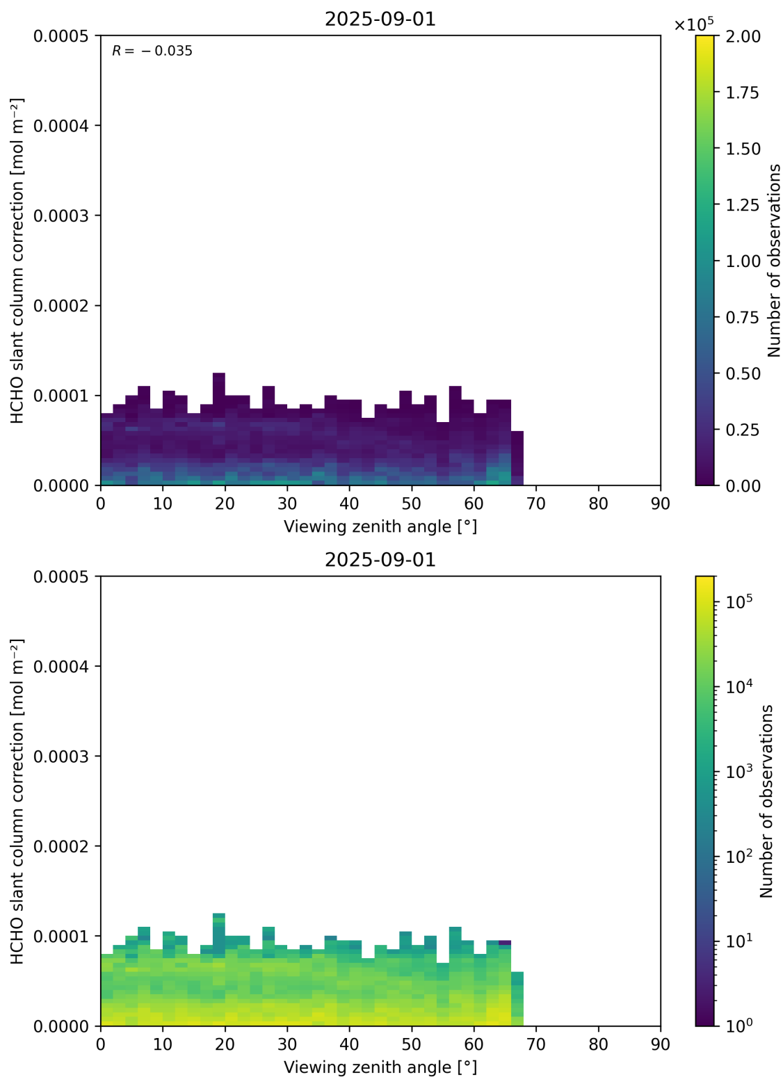
Figure 187: Scatter density plot of “Viewing zenith angle” against “HCHO slant column correction” for 2025-08-31 to 2025-09-02.
