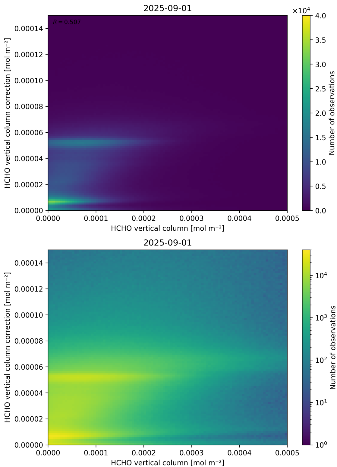
Figure 133: Scatter density plot of “HCHO vertical column” against “HCHO vertical column correction” for 2025-08-31 to 2025-09-02.
