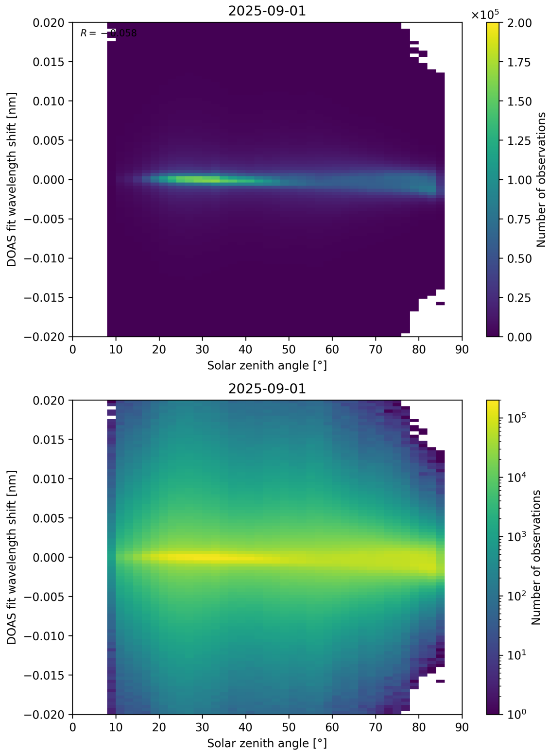
Figure 168: Scatter density plot of “Solar zenith angle” against “DOAS fit wavelength shift” for 2025-08-31 to 2025-09-02.
