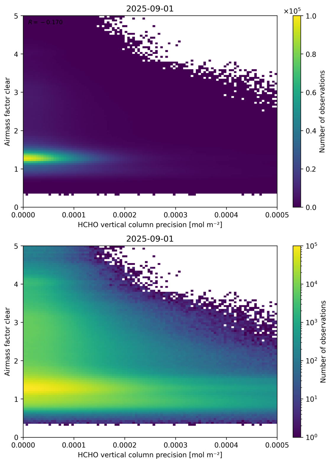
Figure 139: Scatter density plot of “HCHO vertical column precision” against “Airmass factor clear” for 2025-08-31 to 2025-09-02.
