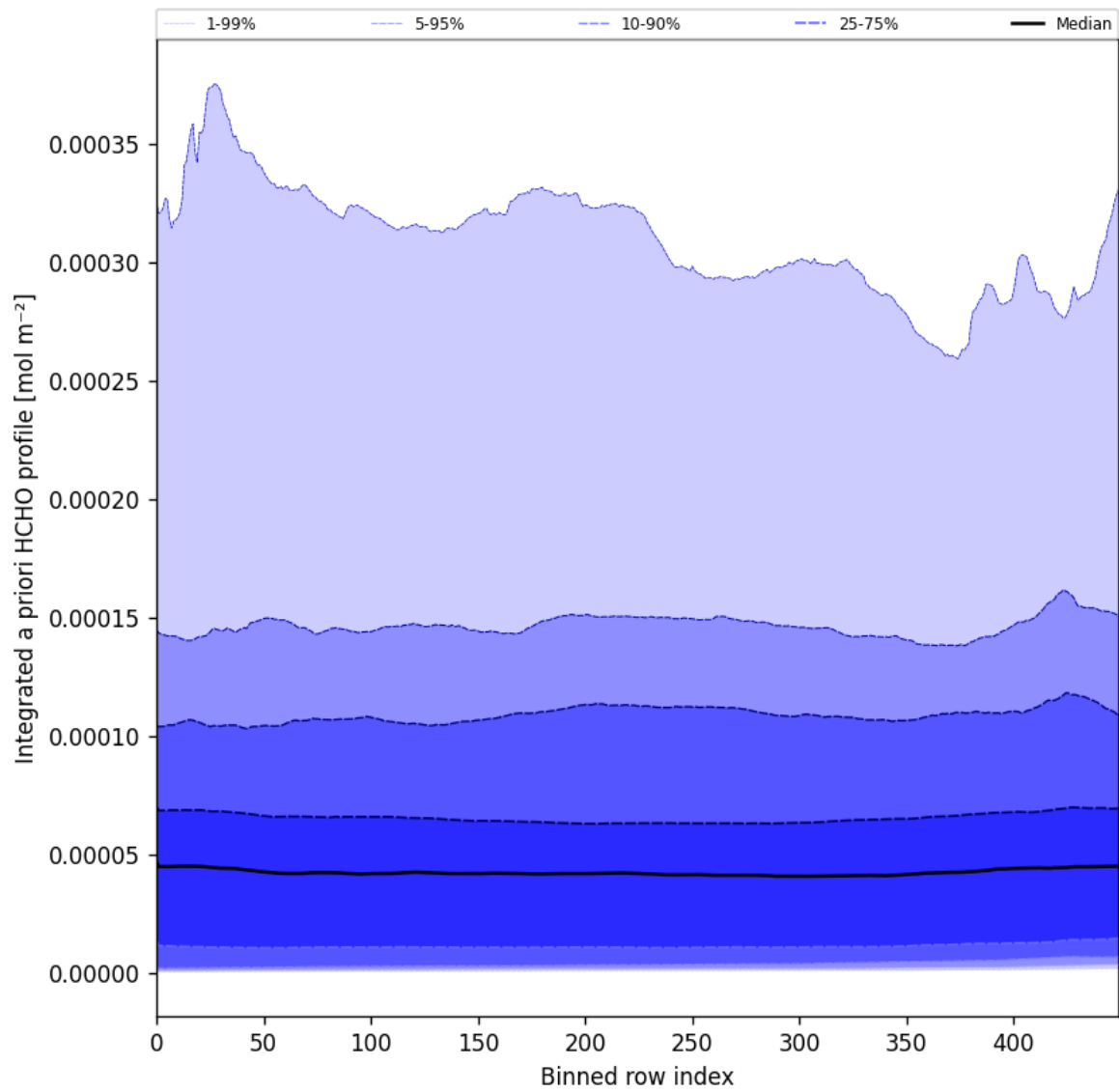
Figure 57: Along track statistics of “Integrated a priori HCHO profile” for 2025-08-31 to 2025-09-02
