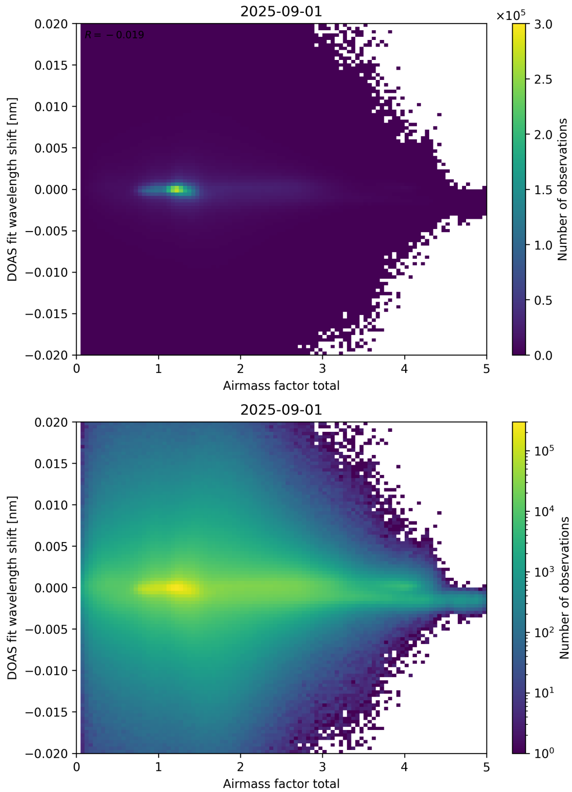
Figure 98: Scatter density plot of “Airmass factor total” against “DOAS fit wavelength shift” for 2025-08-31 to 2025-09-02.
