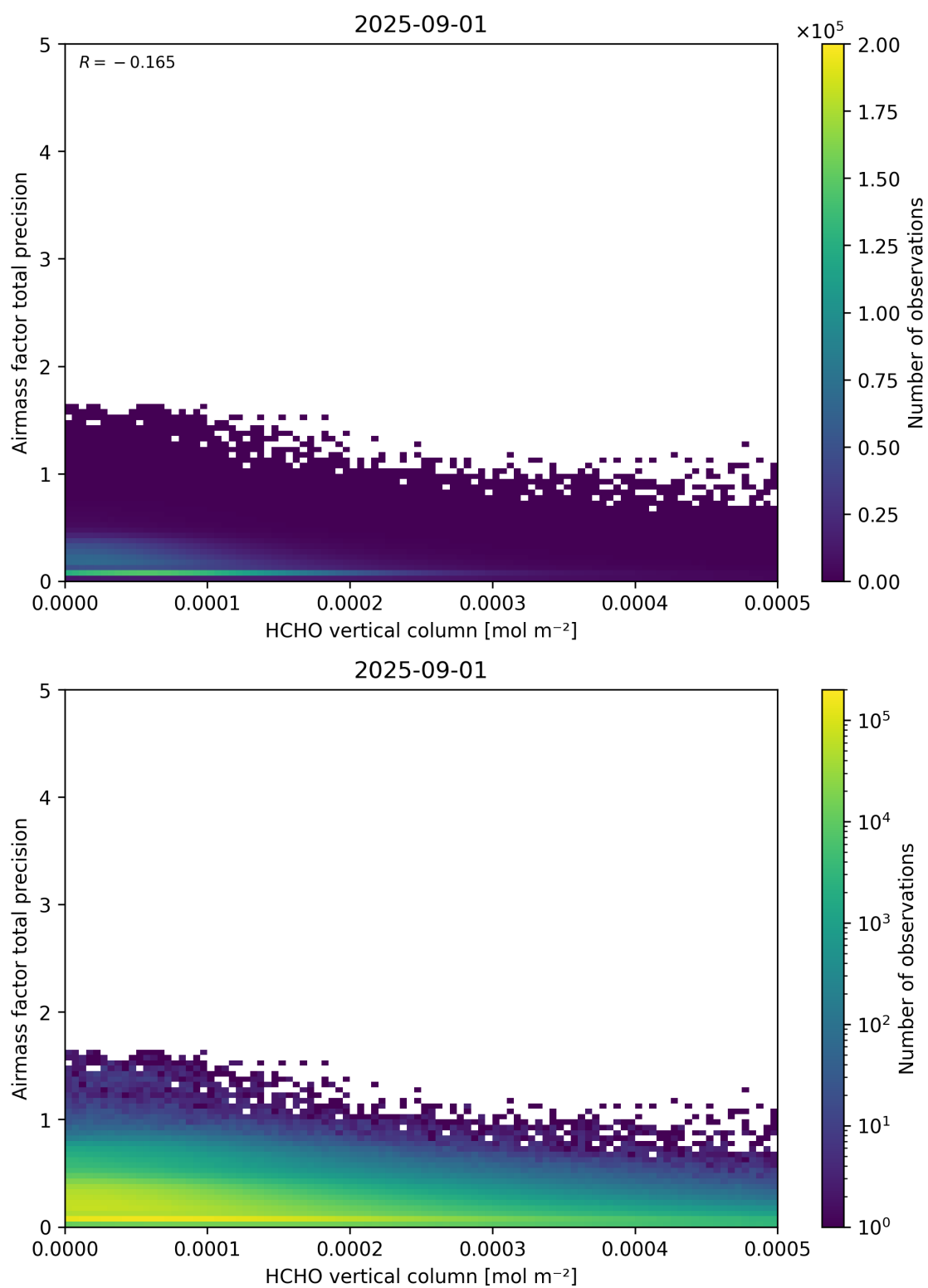
Figure 132: Scatter density plot of “HCHO vertical column” against “Airmass factor total precision” for 2025-08-31 to 2025-09-02.
