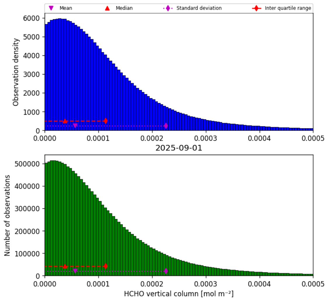
Figure 35: Histogram of “HCHO vertical column” for 2025-08-31 to 2025-09-02
