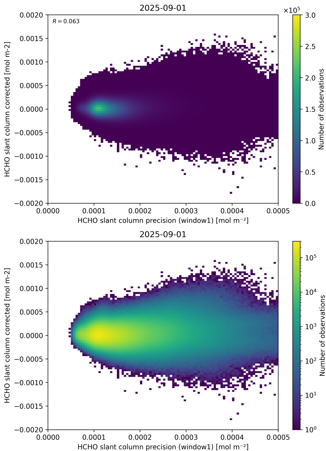
Figure 92: Scatter density plot of “HCHO slant column precision (window1)” against “HCHO slant column corrected” for 2025-08-31 to 2025-09-02.
