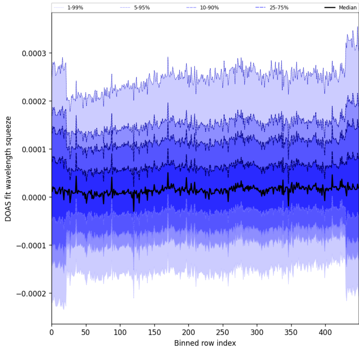
Figure 59: Along track statistics of “DOAS fit wavelength squeeze” for 2025-08-31 to 2025-09-02
