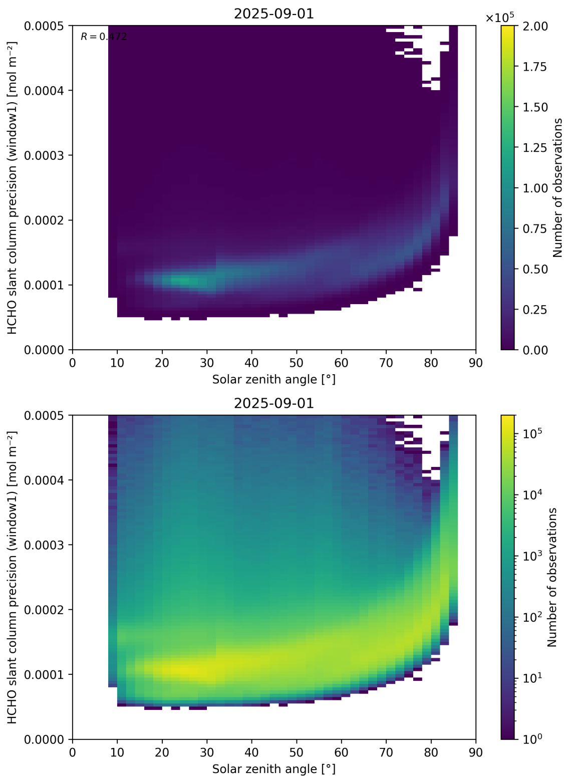
Figure 174: Scatter density plot of “Solar zenith angle” against “HCHO slant column precision (window1)” for 2025-08-31 to 2025-09-02.
