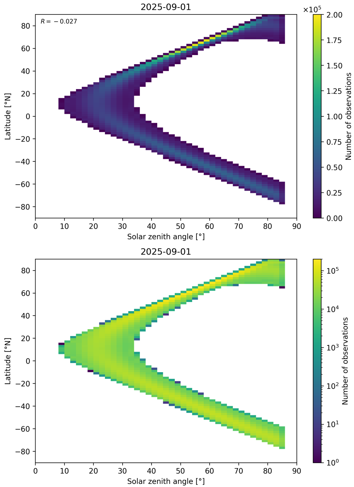
Figure 181: Scatter density plot of “Solar zenith angle” against “Latitude” for 2025-08-31 to 2025-09-02.
