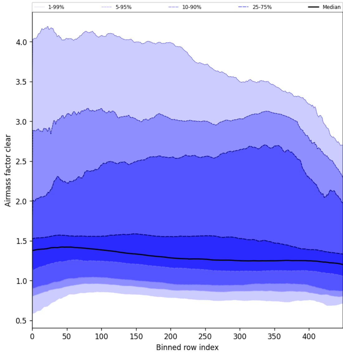
Figure 56: Along track statistics of “Air mass factor clear” for 2025-08-31 to 2025-09-02
