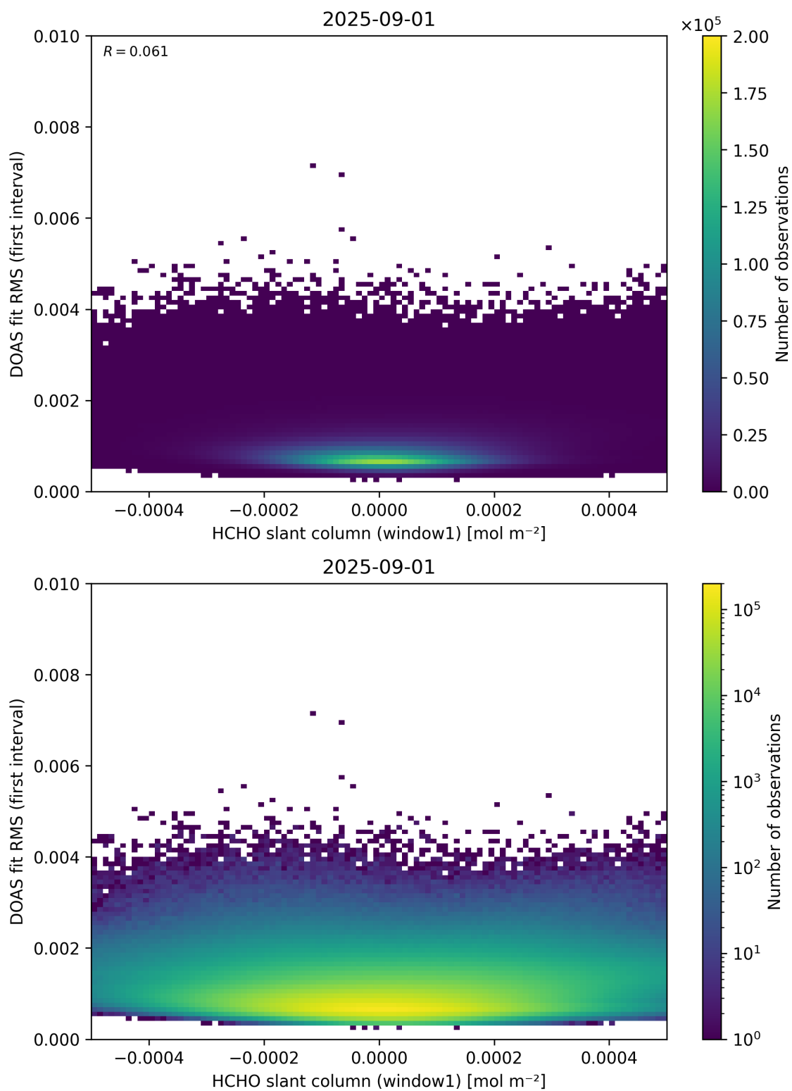
Figure 78: Scatter density plot of “HCHO slant column (window1)” against “DOAS fit RMS (first interval)” for 2025-08-31 to 2025-09-02.
