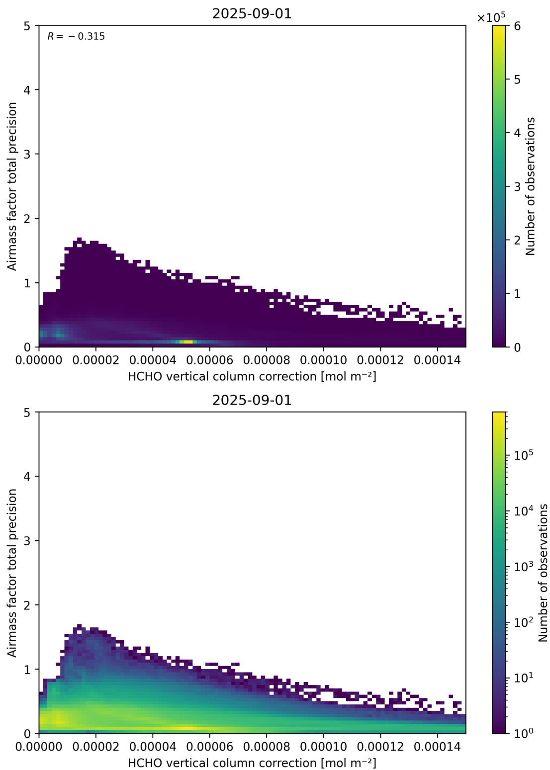
Figure 121: Scatter density plot of “HCHO vertical column correction” against “Airmass factor total precision” for 2025-08-31 to 2025-09-02.
