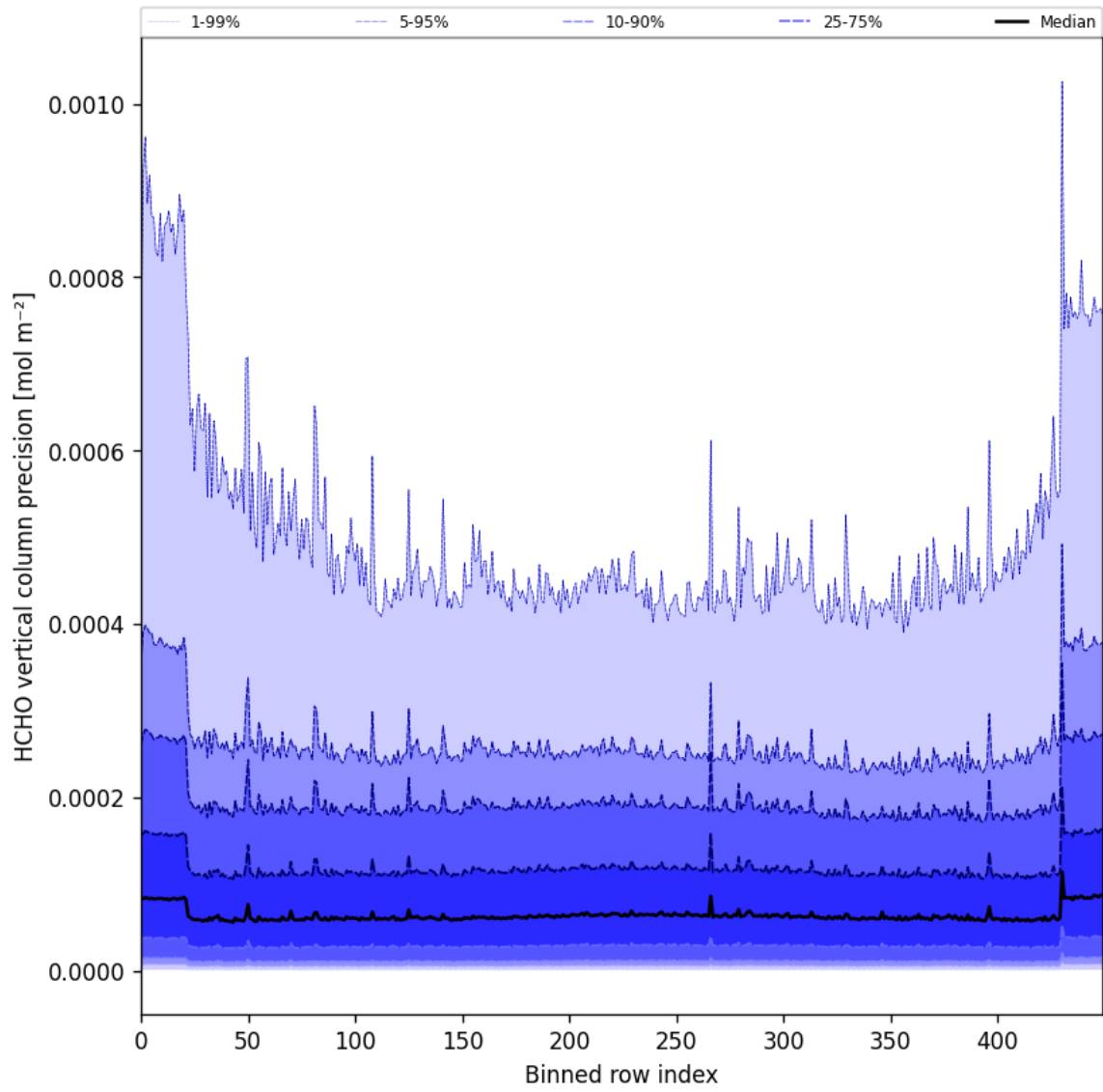
Figure 50: Along track statistics of “HCHO vertical column precision” for 2025-08-31 to 2025-09-02
