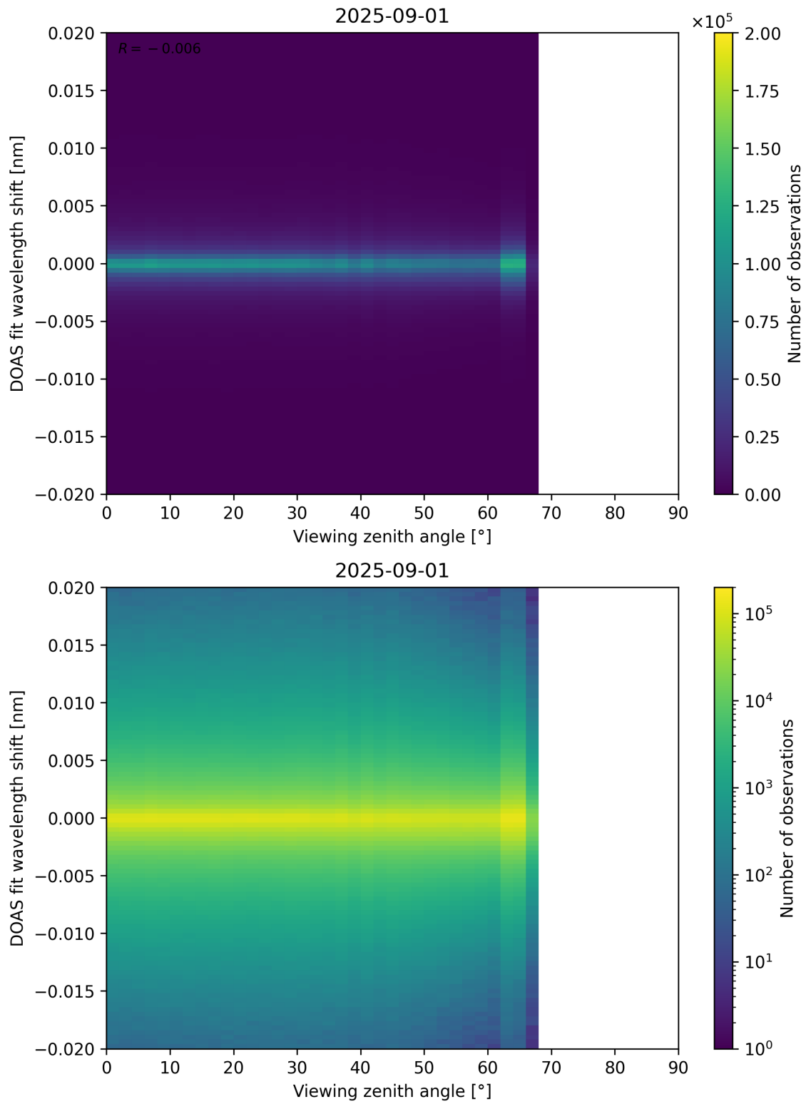
Figure 183: Scatter density plot of “Viewing zenith angle” against “DOAS fit wavelength shift” for 2025-08-31 to 2025-09-02.
