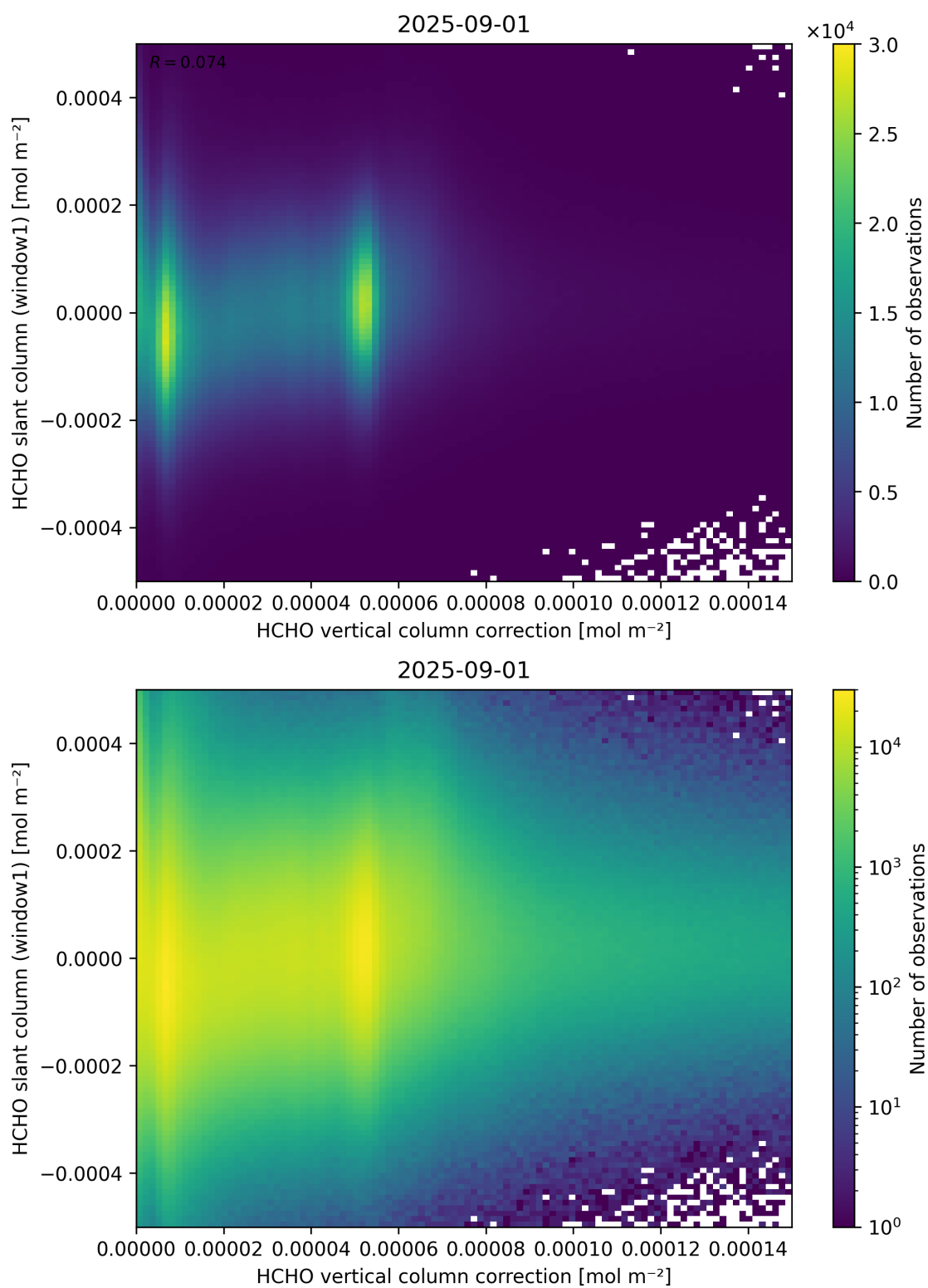
Figure 118: Scatter density plot of “HCHO vertical column correction” against “HCHO slant column (window1)” for 2025-08-31 to 2025-09-02.
