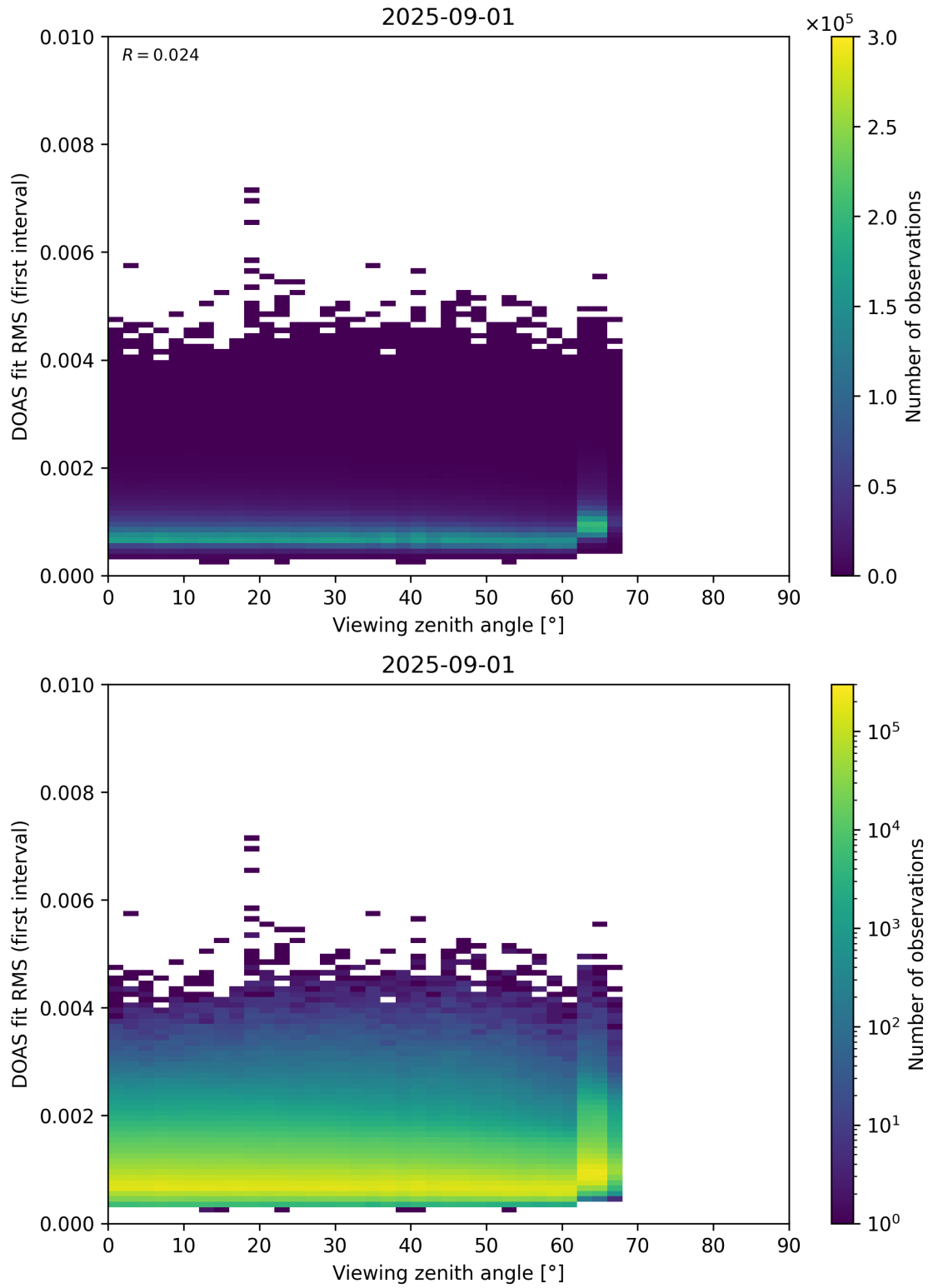
Figure 182: Scatter density plot of “Viewing zenith angle” against “DOAS fit RMS (first interval)” for 2025-08-31 to 2025-09-02.
