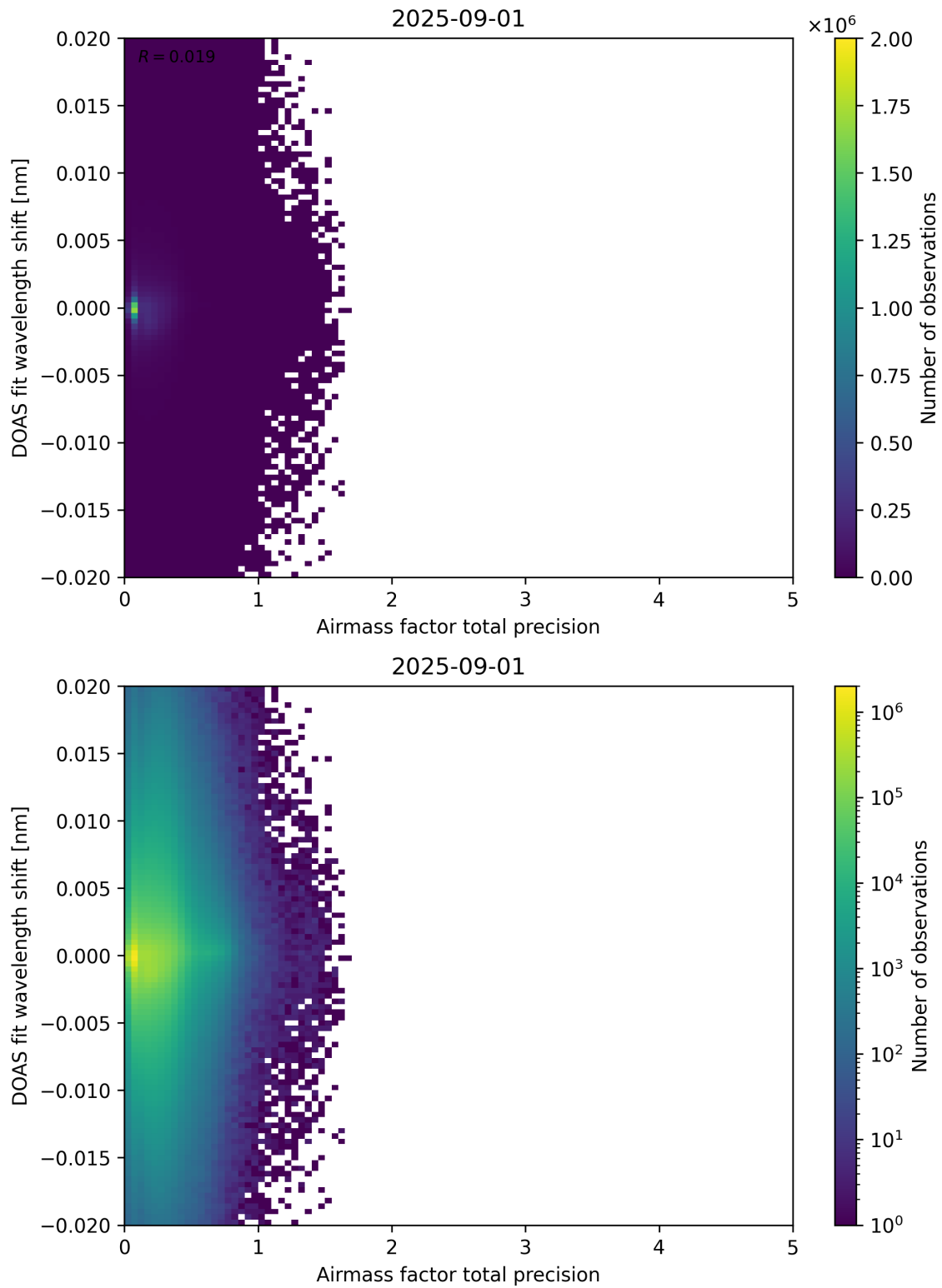
Figure 106: Scatter density plot of “Airmass factor total precision” against “DOAS fit wavelength shift” for 2025-08-31 to 2025-09-02.
