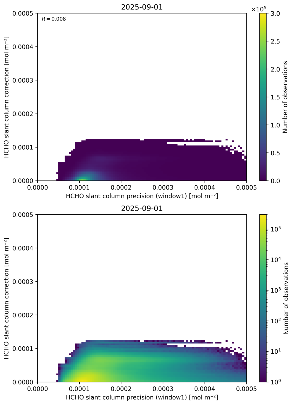
Figure 93: Scatter density plot of “HCHO slant column precision (window1)” against “HCHO slant column correction” for 2025-08-31 to 2025-09-02.
