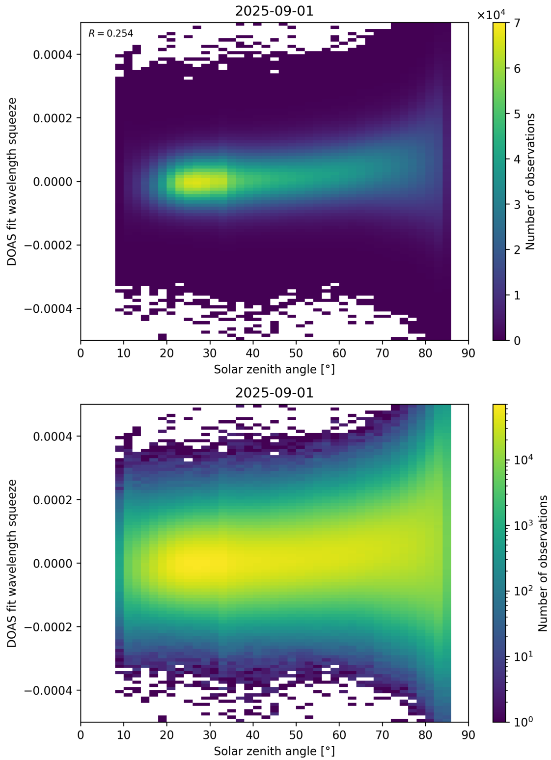
Figure 169: Scatter density plot of “Solar zenith angle” against “DOAS fit wavelength squeeze” for 2025-08-31 to 2025-09-02.
