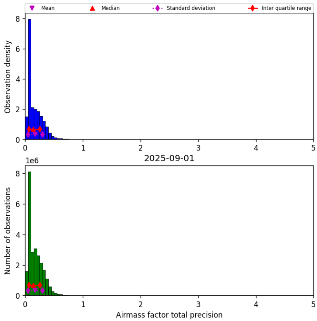
Figure 41: Histogram of “Airmass factor total precision” for 2025-08-31 to 2025-09-02
