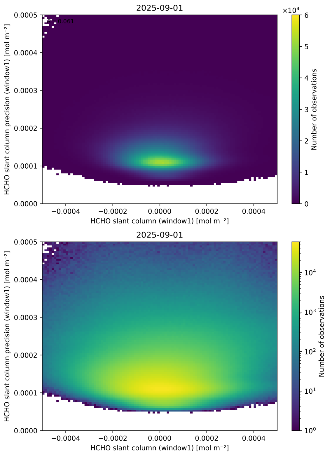
Figure 84: Scatter density plot of “HCHO slant column (window1)” against “HCHO slant column precision (window1)” for 2025-08-31 to 2025-09-02.
