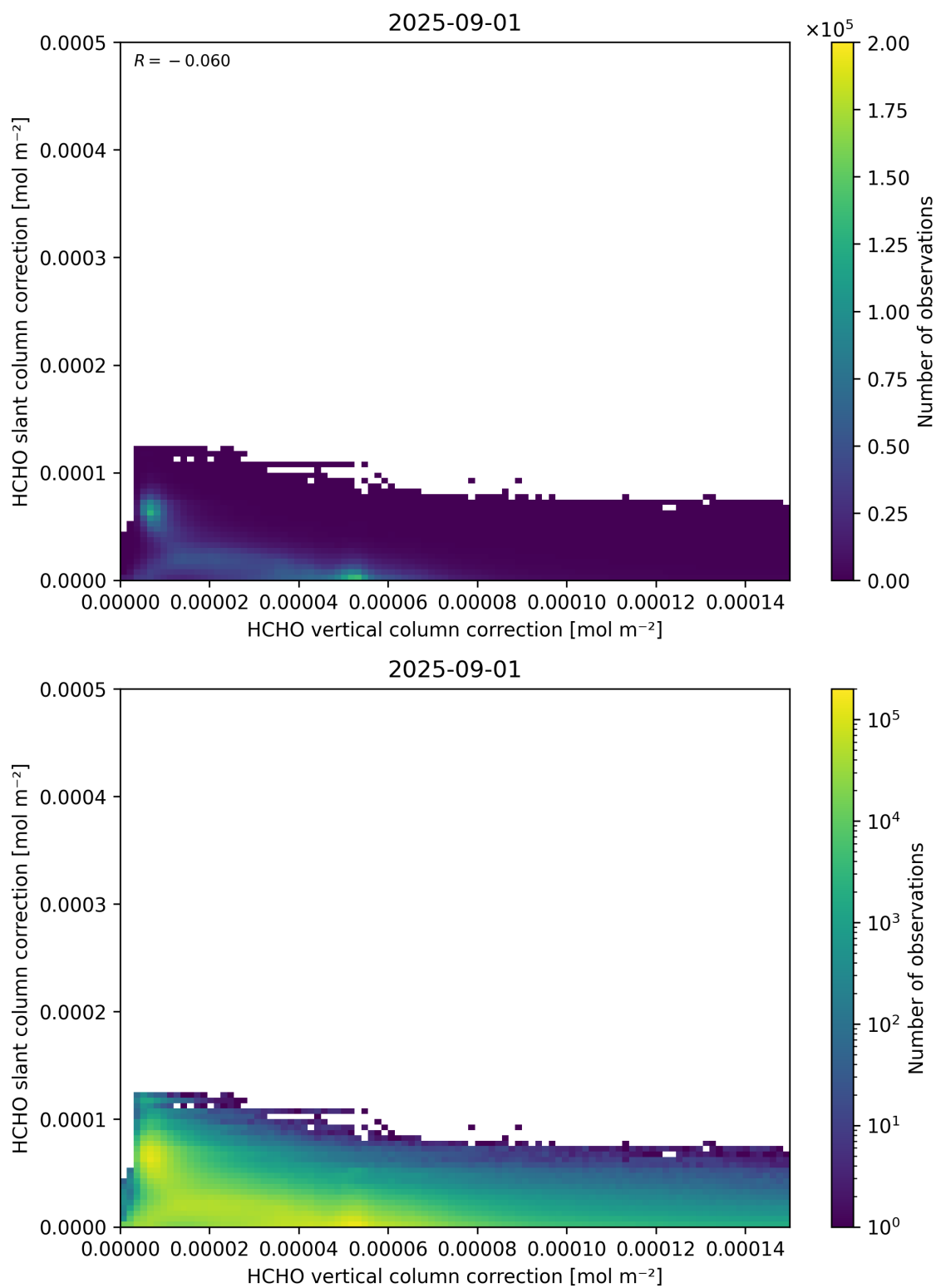
Figure 117: Scatter density plot of “HCHO vertical column correction” against “HCHO slant column correction” for 2025-08-31 to 2025-09-02.
