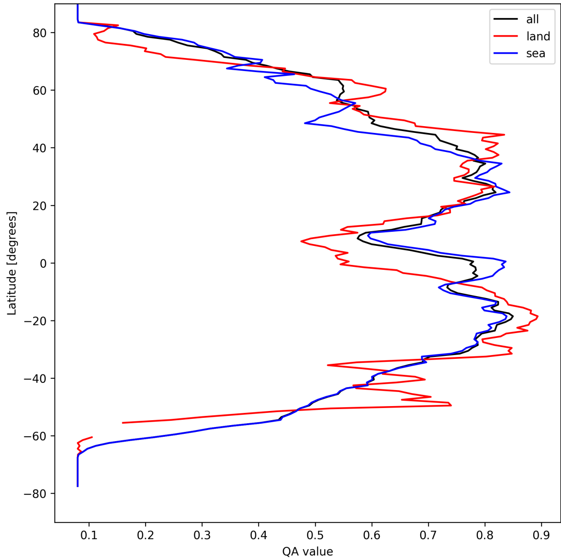
Figure 20: Zonal average of “QA value” for 2025-08-31 to 2025-09-02.
