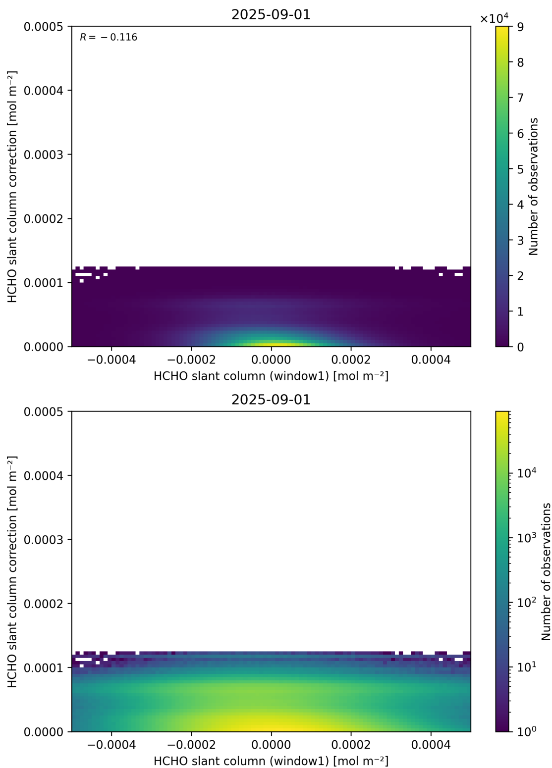
Figure 83: Scatter density plot of “HCHO slant column (window1)” against “HCHO slant column correction” for 2025-08-31 to 2025-09-02.
