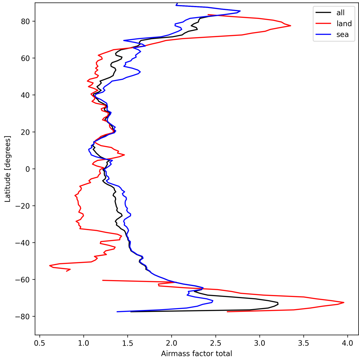
Figure 26: Zonal average of “Airmass factor total” for 2025-08-31 to 2025-09-02.
