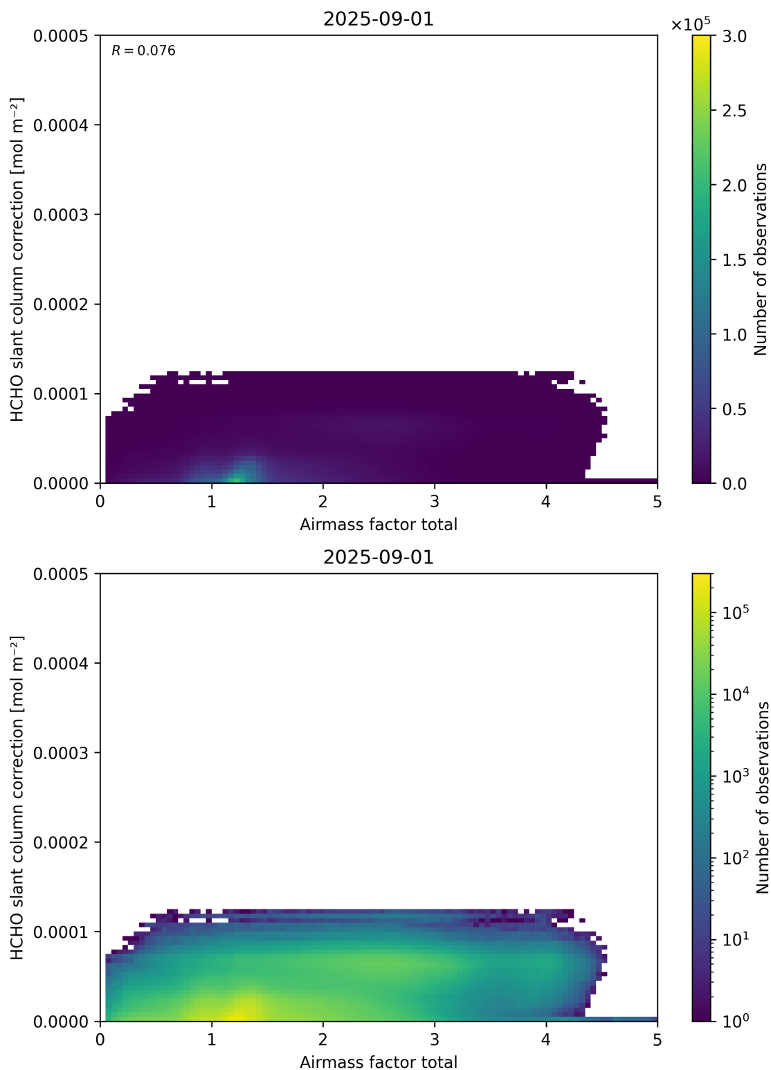
Figure 102: Scatter density plot of “Airmass factor total” against “HCHO slant column correction” for 2025-08-31 to 2025-09-02.
