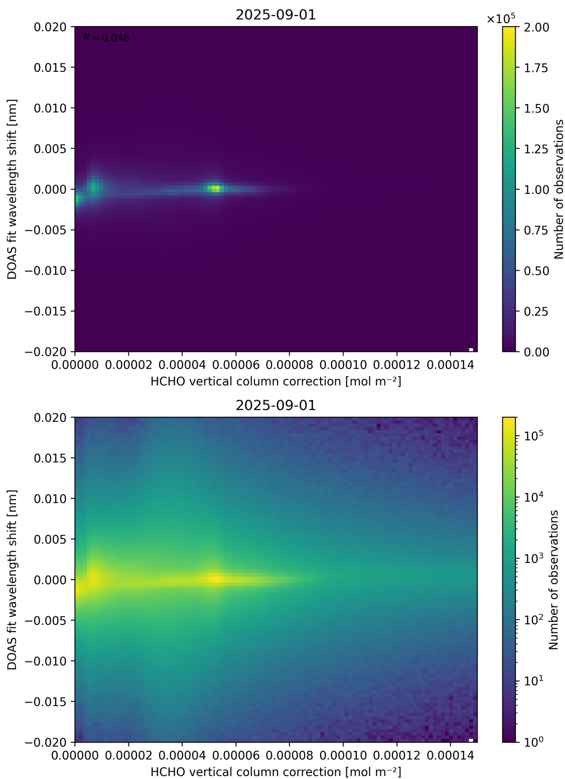
Figure 113: Scatter density plot of “HCHO vertical column correction” against “DOAS fit wavelength shift” for 2025-08-31 to 2025-09-02.
