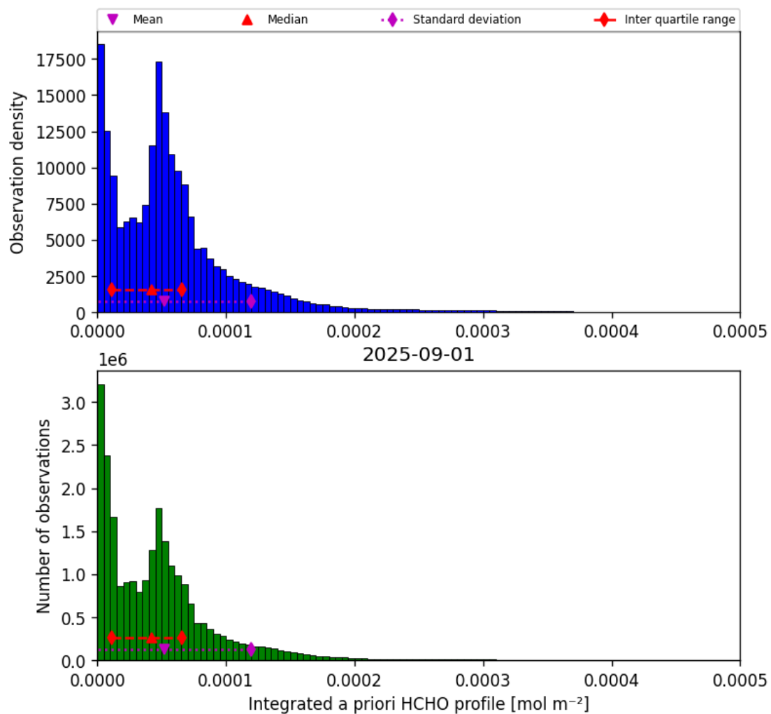
Figure 43: Histogram of “Integrated a priori HCHO profile” for 2025-08-31 to 2025-09-02
