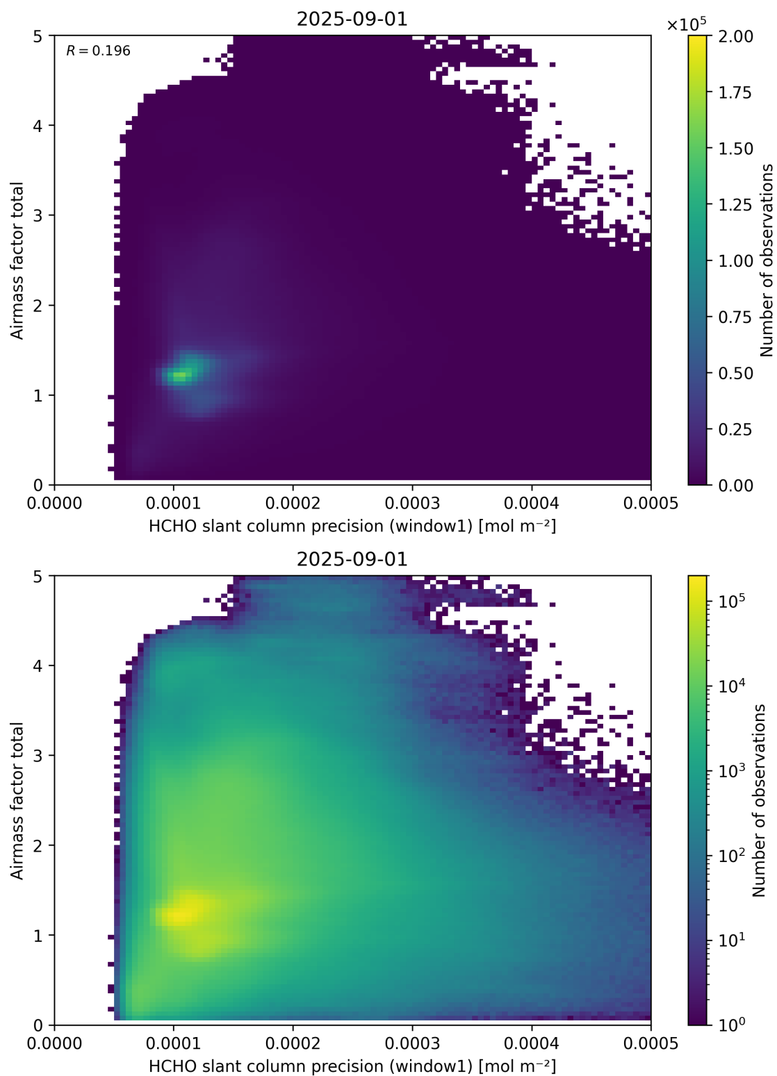
Figure 94: Scatter density plot of “HCHO slant column precision (window1)” against “Airmass factor total” for 2025-08-31 to 2025-09-02.
