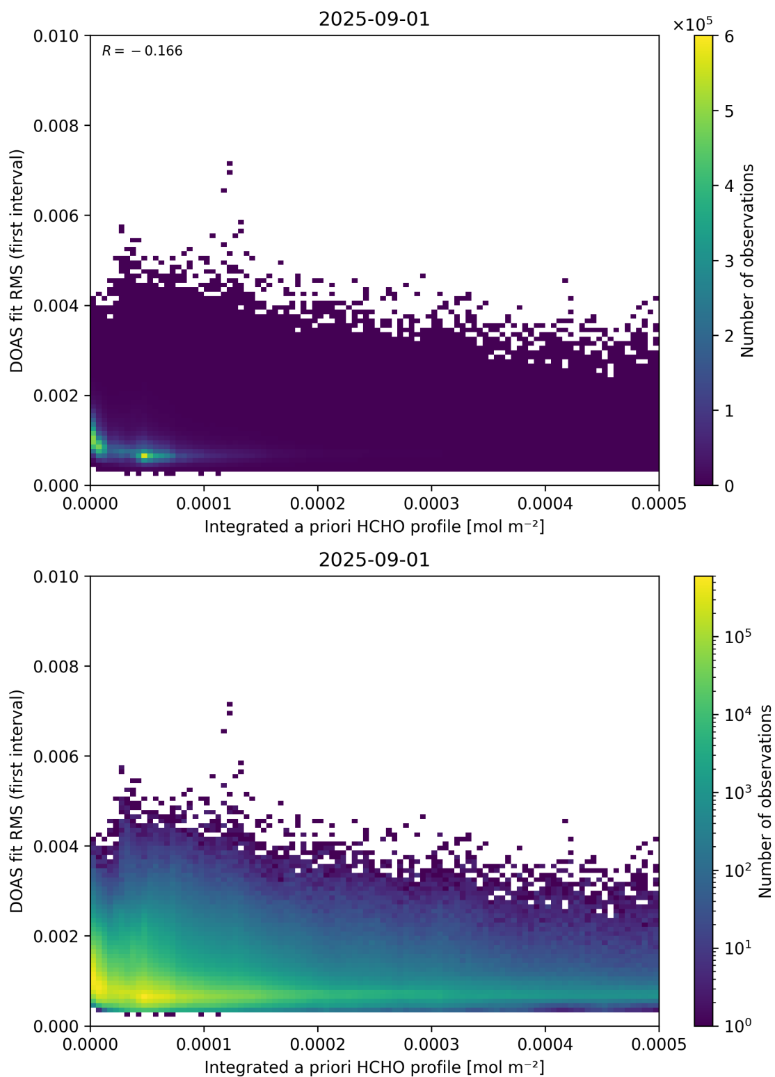
Figure 148: Scatter density plot of “Integrated a priori HCHO profile” against “DOAS fit RMS (first interval)” for 2025-08-31 to 2025-09-02.
