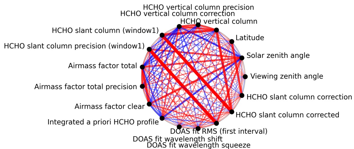
Figure 1: Map of correlation graph for 2025-08-31 to 2025-09-02.
