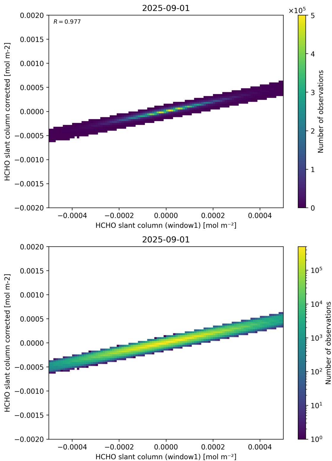
Figure 82: Scatter density plot of “HCHO slant column (window1)” against “HCHO slant column corrected” for 2025-08-31 to 2025-09-02.
