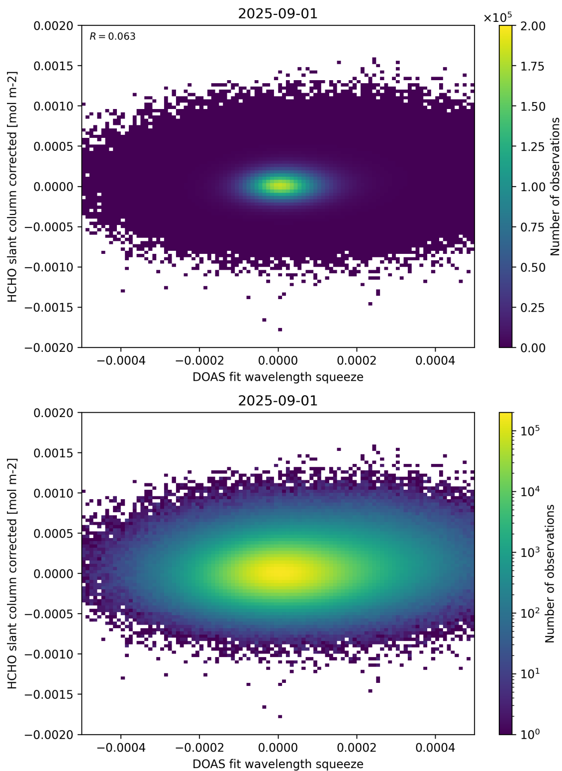
Figure 69: Scatter density plot of “DOAS fit wavelength squeeze” against “HCHO slant column corrected” for 2025-08-31 to 2025-09-02.
