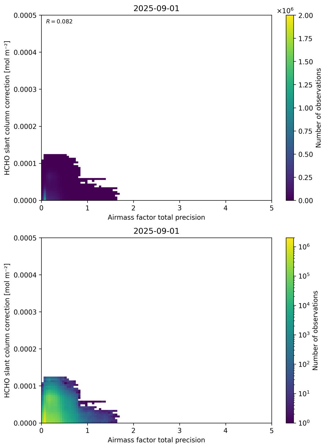
Figure 110: Scatter density plot of “Airmass factor total precision” against “HCHO slant column correction” for 2025-08-31 to 2025-09-02.
