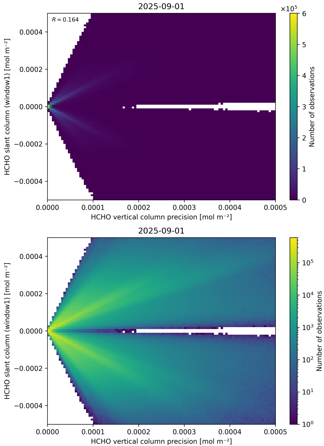
Figure 142: Scatter density plot of “HCHO vertical column precision” against “HCHO slant column (window1)” for 2025-08-31 to 2025-09-02.
