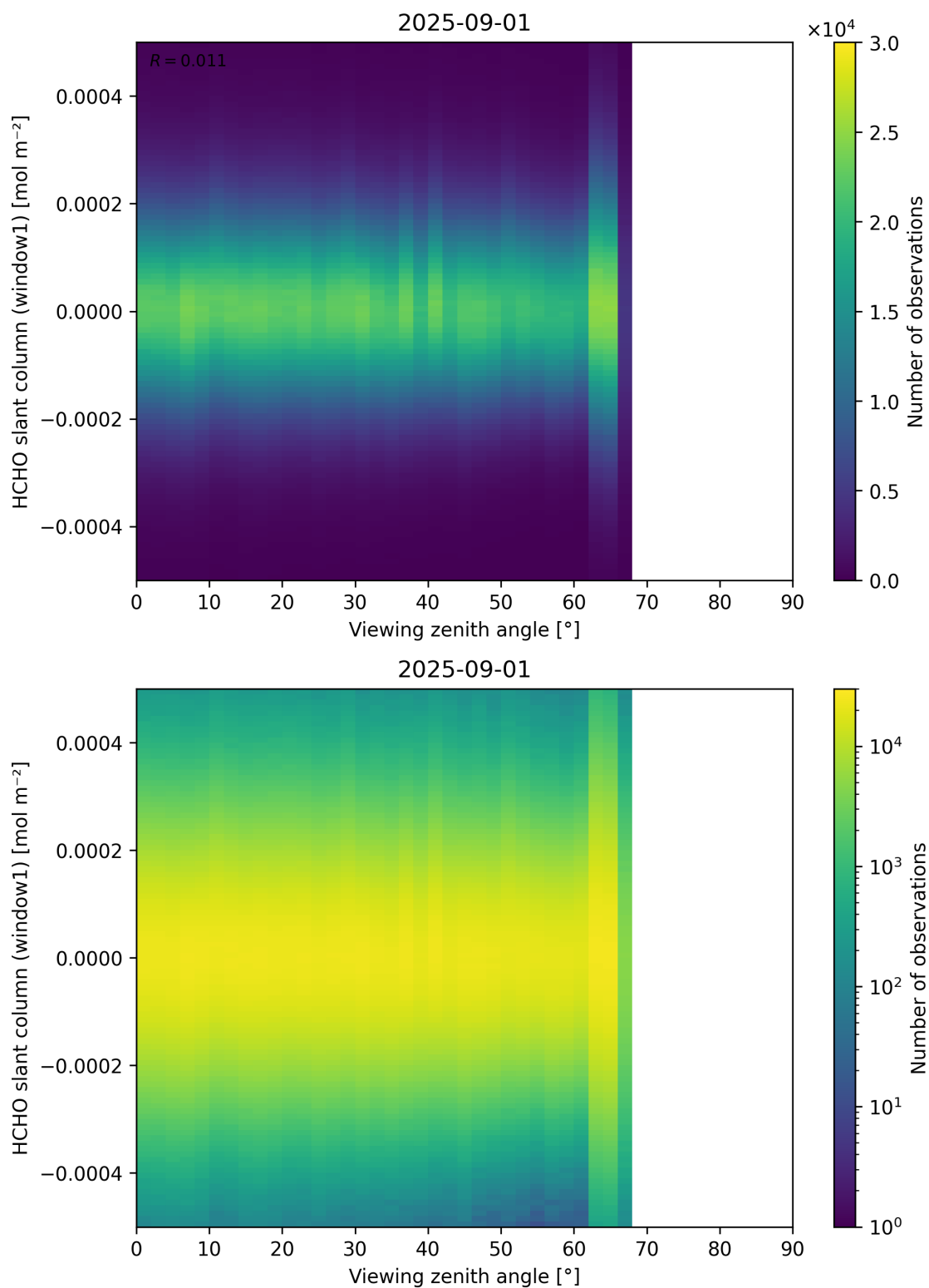
Figure 188: Scatter density plot of “Viewing zenith angle” against “HCHO slant column (window1)” for 2025-08-31 to 2025-09-02.
