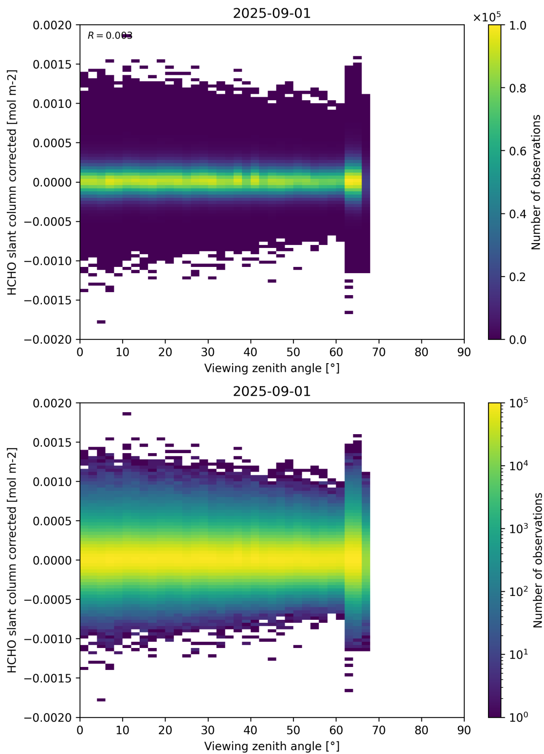
Figure 186: Scatter density plot of “Viewing zenith angle” against “HCHO slant column corrected” for 2025-08-31 to 2025-09-02.
