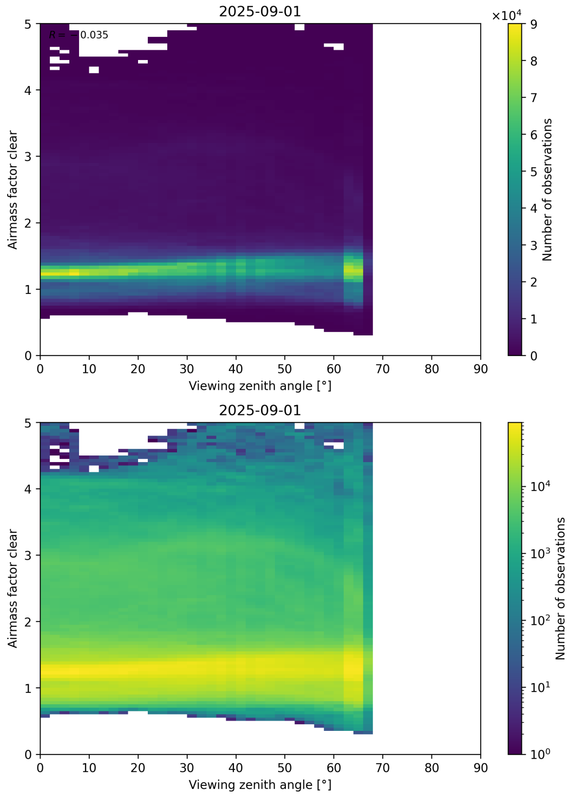
Figure 185: Scatter density plot of “Viewing zenith angle” against “Airmass factor clear” for 2025-08-31 to 2025-09-02.
