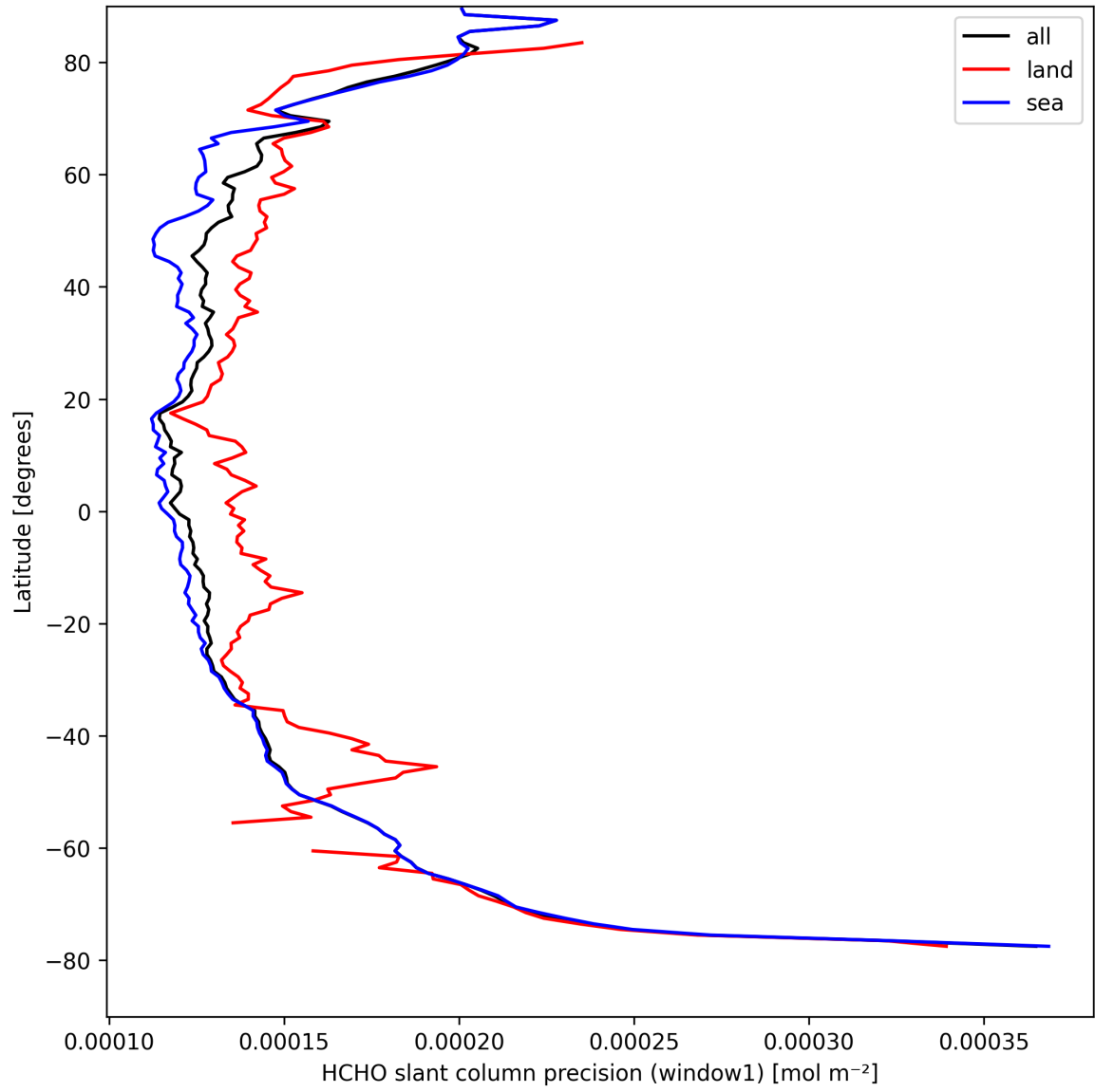
Figure 25: Zonal average of "HCHO slant column precision (window1)" for 2025-08-31 to 2025-09-02.
