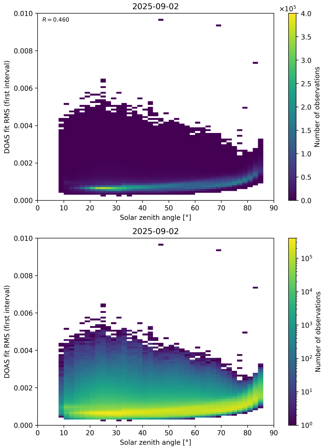
Figure 167: Scatter density plot of “Solar zenith angle” against “DOAS fit RMS (first interval)” for 2025-09-01 to 2025-09-03.
