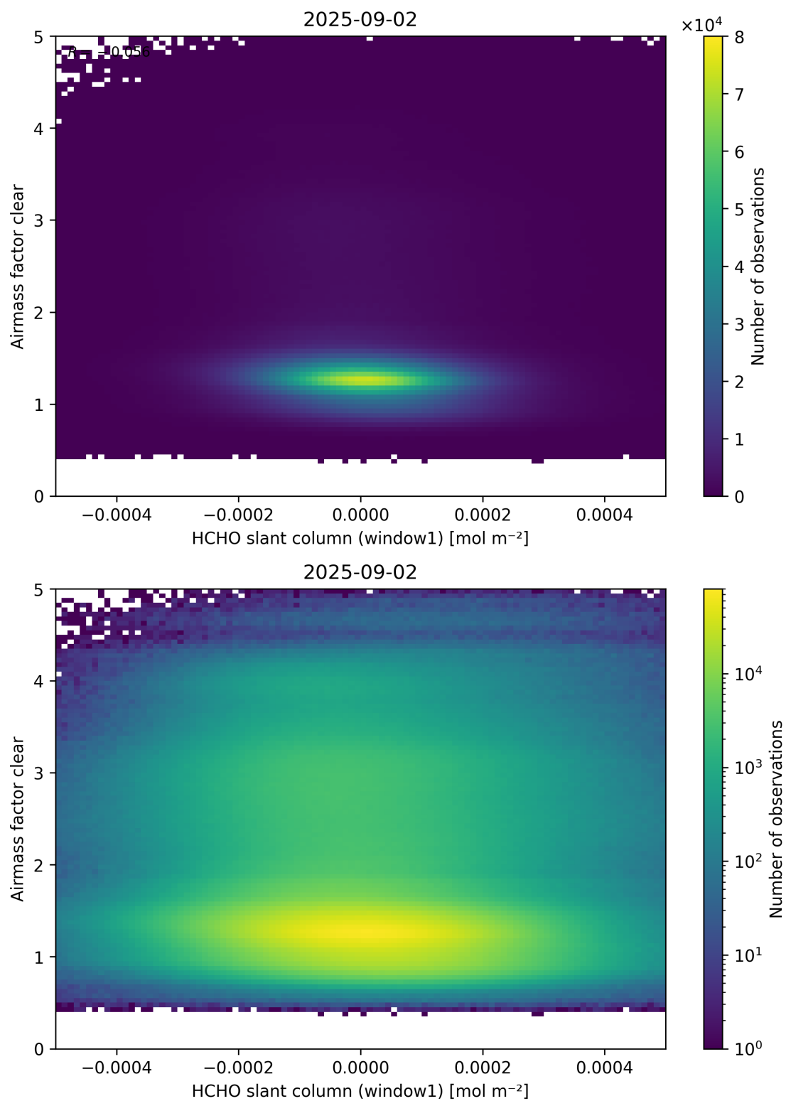
Figure 81: Scatter density plot of “HCHO slant column (window1)” against “Airmass factor clear” for 2025-09-01 to 2025-09-03.
