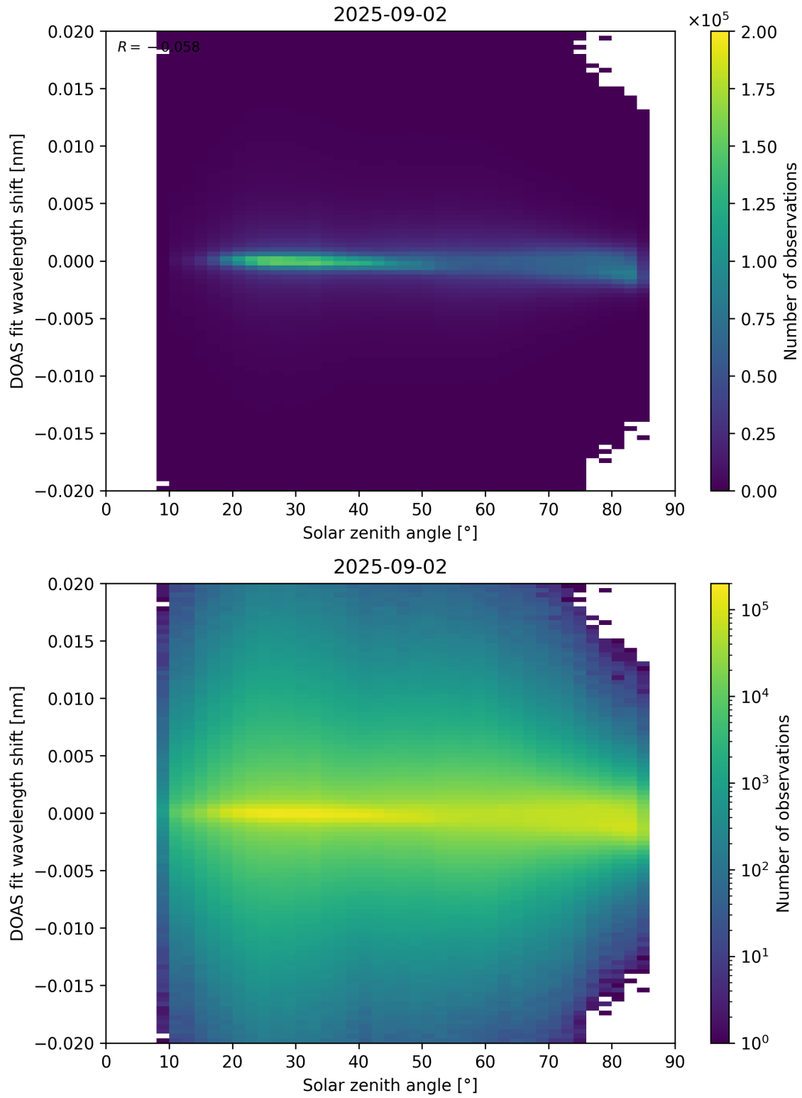
Figure 168: Scatter density plot of “Solar zenith angle” against “DOAS fit wavelength shift” for 2025-09-01 to 2025-09-03.
