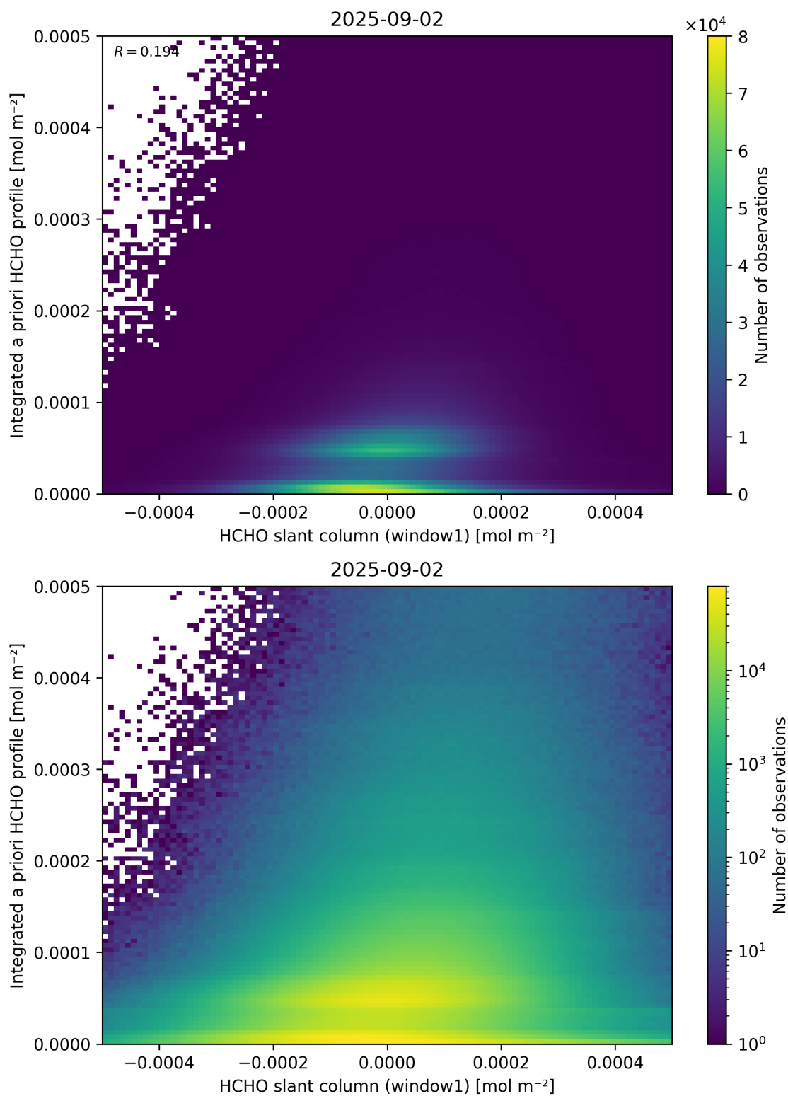
Figure 87: Scatter density plot of “HCHO slant column (window1)” against “Integrated a priori HCHO profile” for 2025-09-01 to 2025-09-03.
