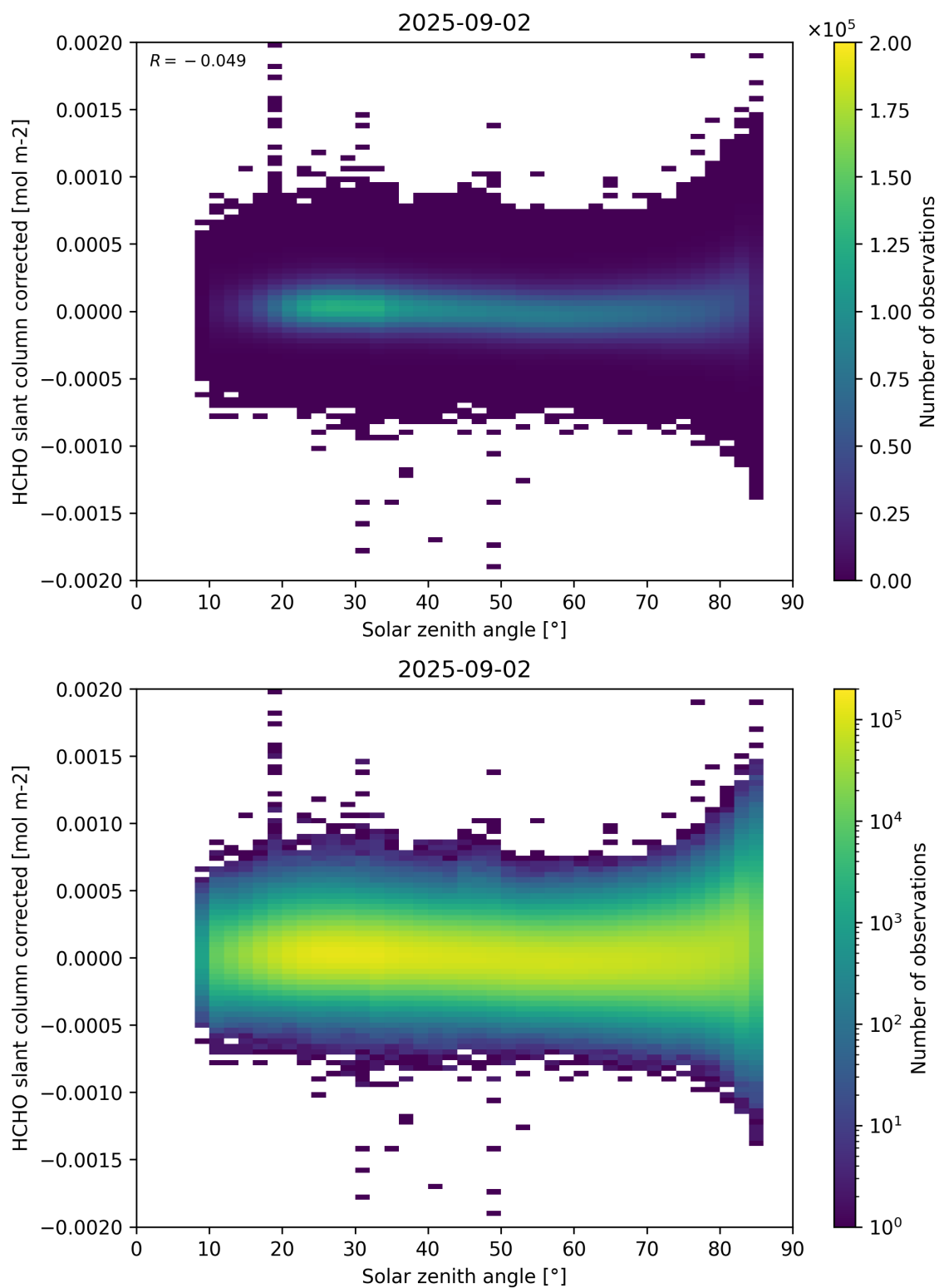
Figure 171: Scatter density plot of “Solar zenith angle” against “HCHO slant column corrected” for 2025-09-01 to 2025-09-03.
