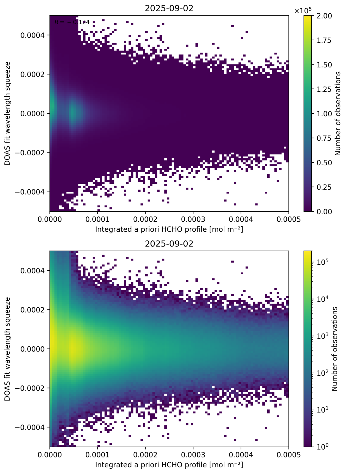
Figure 150: Scatter density plot of “Integrated a priori HCHO profile” against “DOAS fit wavelength squeeze” for 2025-09-01 to 2025-09-03.
