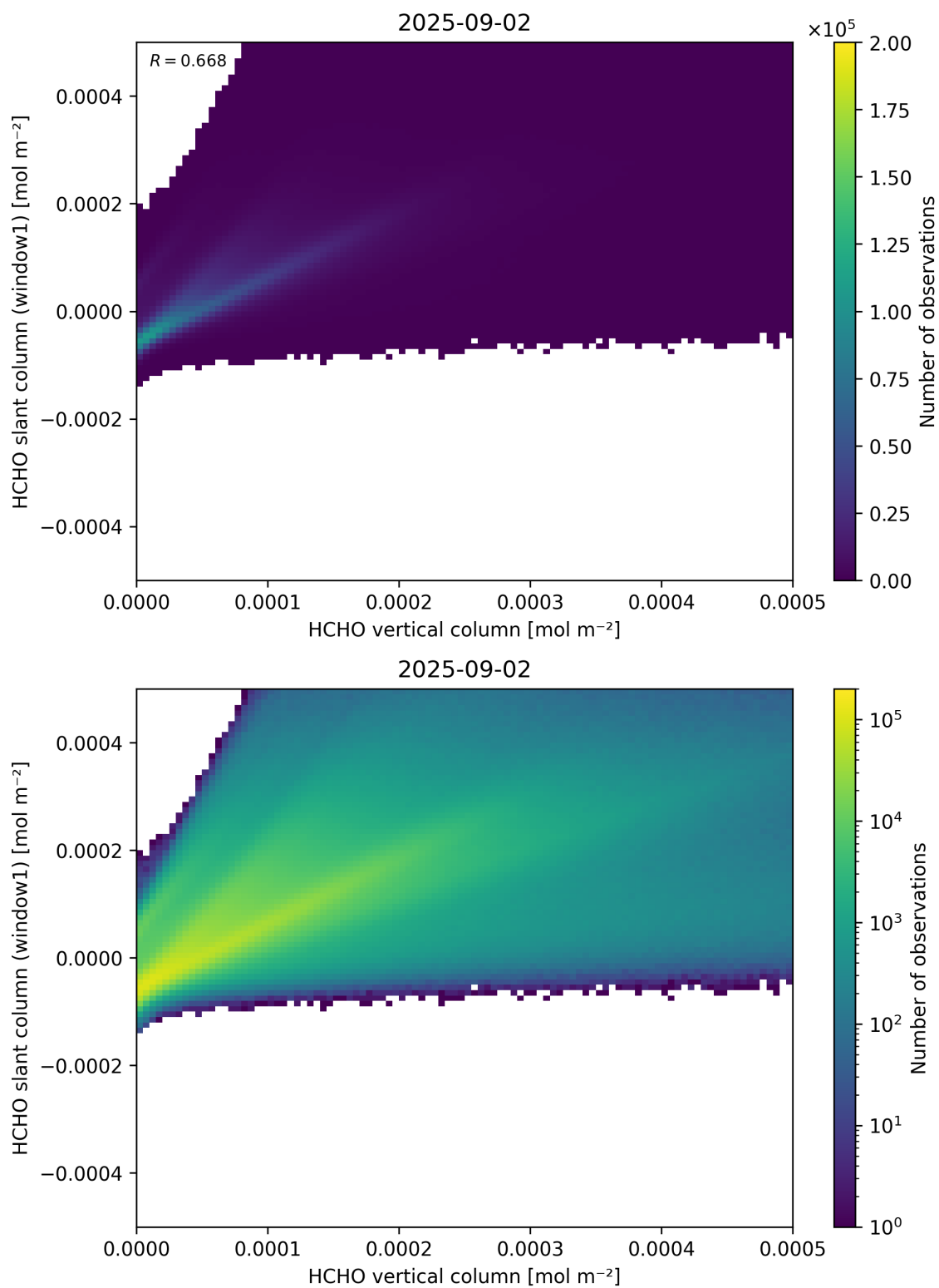
Figure 129: Scatter density plot of “HCHO vertical column” against “HCHO slant column (window1)” for 2025-09-01 to 2025-09-03.
