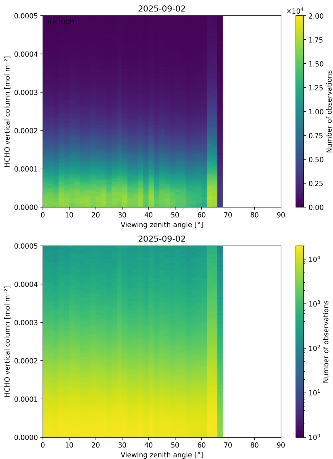
Figure 192: Scatter density plot of “Viewing zenith angle” against “HCHO vertical column” for 2025-09-01 to 2025-09-03.
