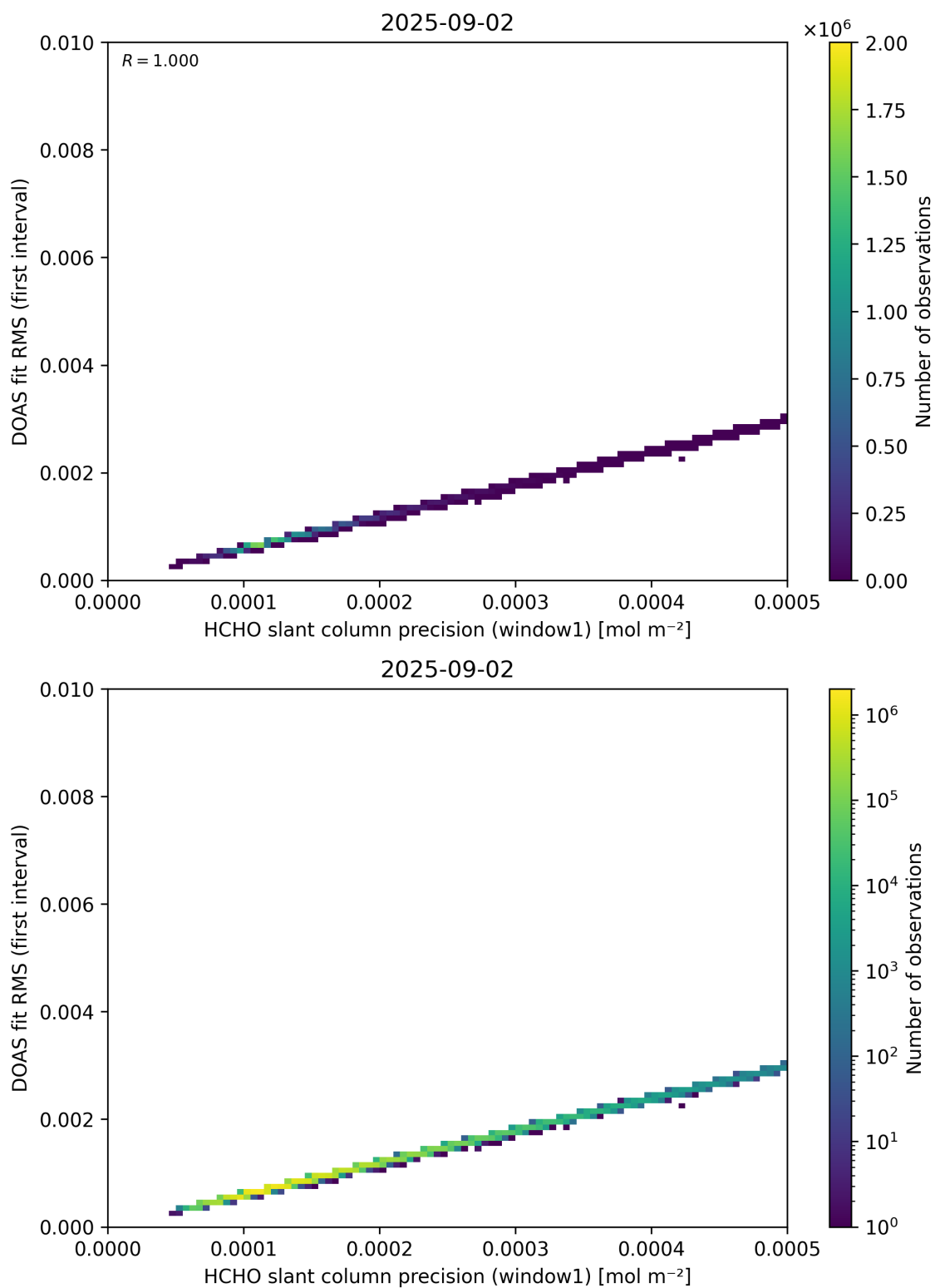
Figure 88: Scatter density plot of “HCHO slant column precision (window1)” against “DOAS fit RMS (first interval)” for 2025-09-01 to 2025-09-03.
