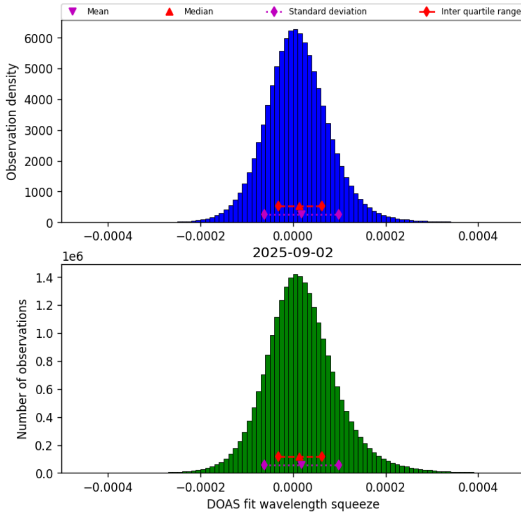
Figure 45: Histogram of “DOAS fit wavelength squeeze” for 2025-09-01 to 2025-09-03
