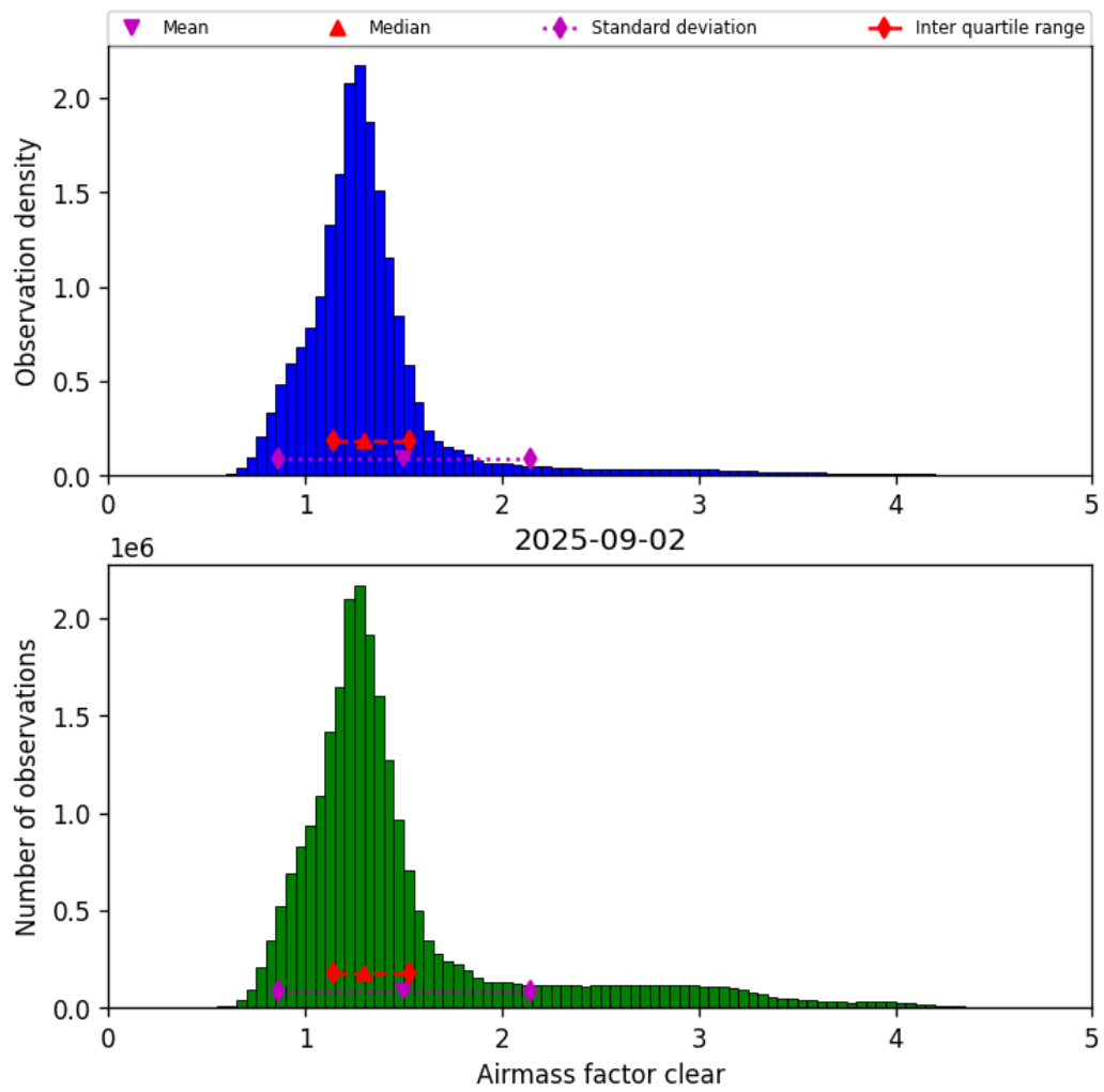
Figure 42: Histogram of “Airmass factor clear” for 2025-09-01 to 2025-09-03
