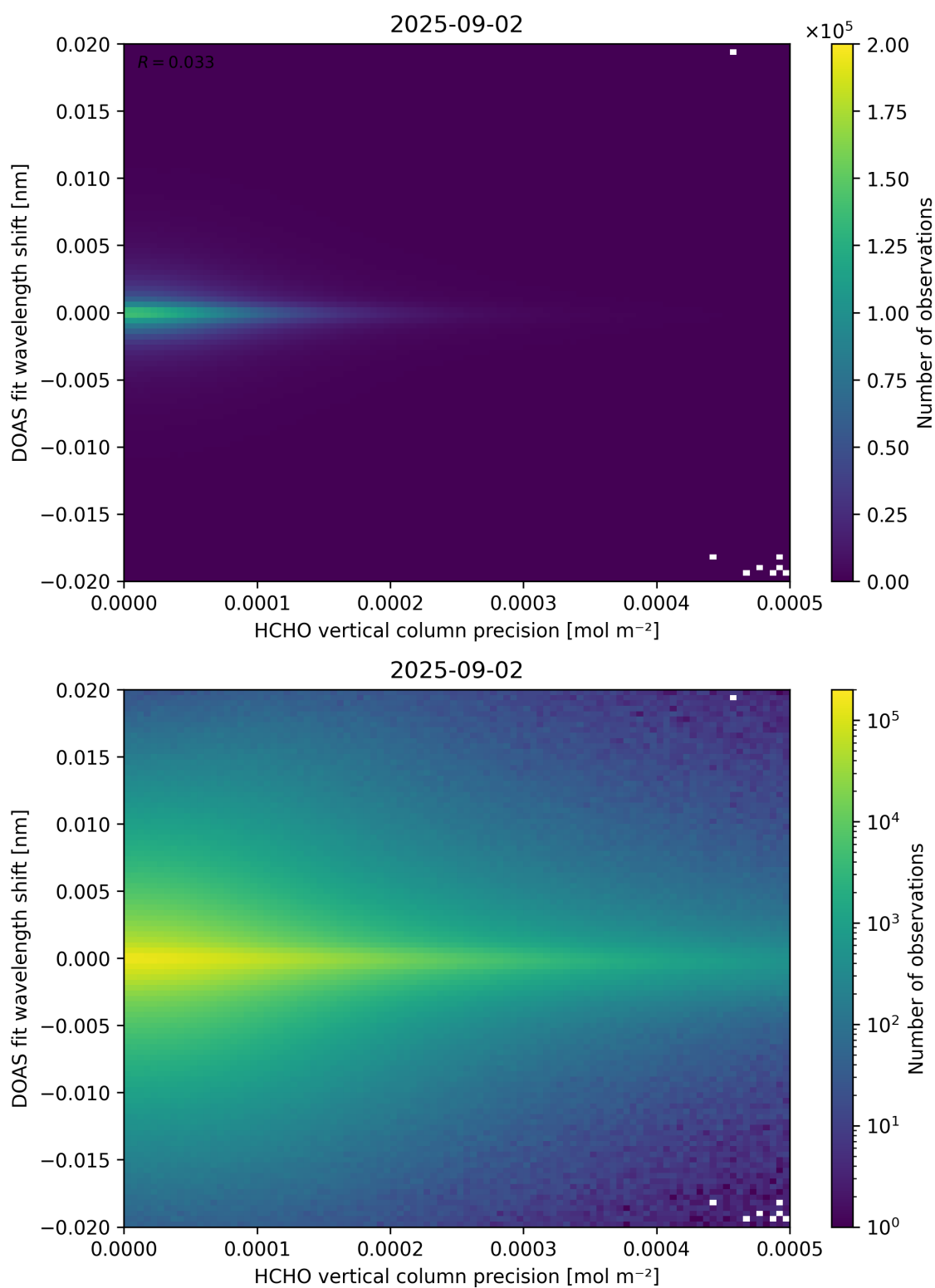
Figure 137: Scatter density plot of “HCHO vertical column precision” against “DOAS fit wavelength shift” for 2025-09-01 to 2025-09-03.
