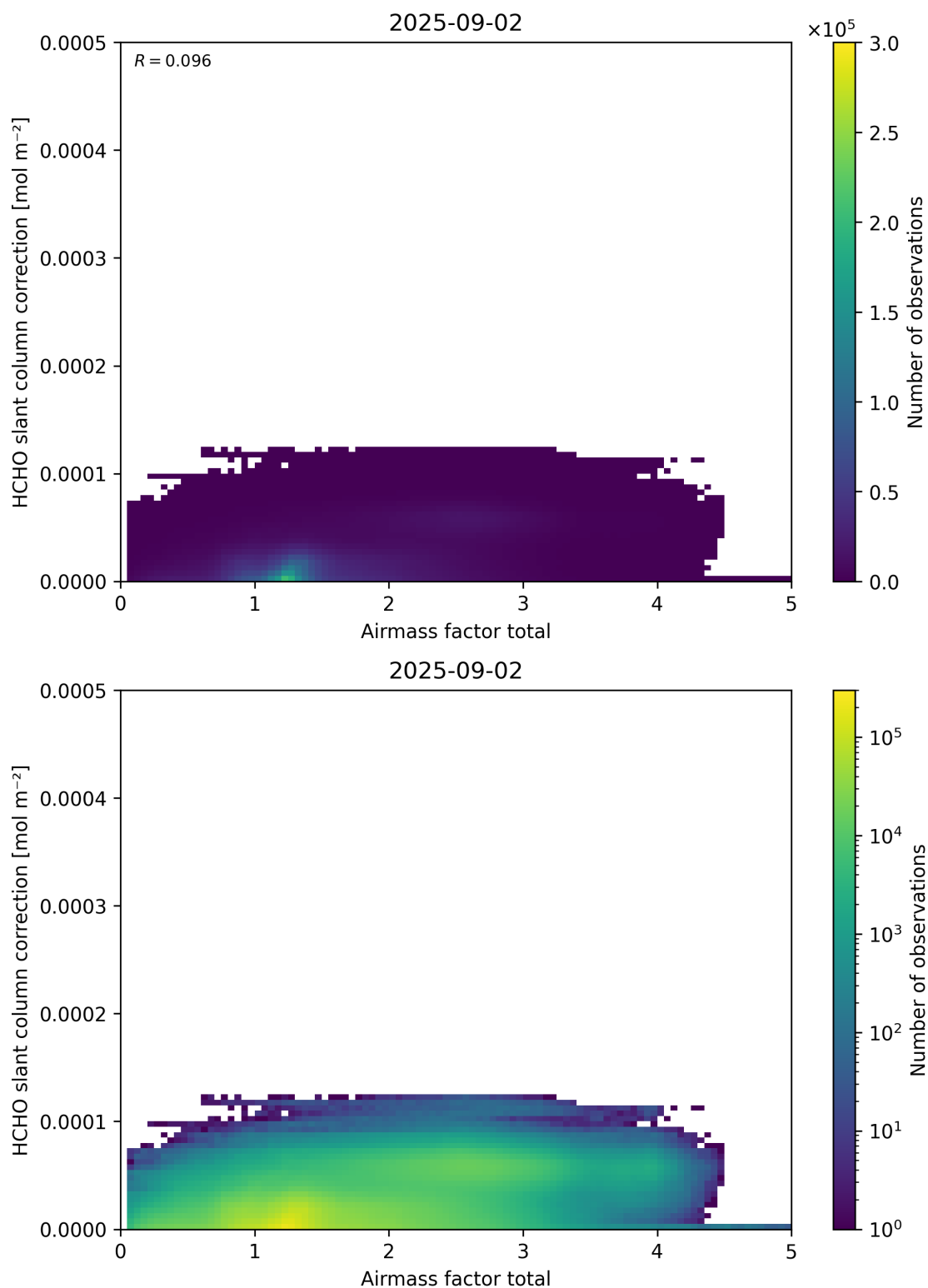
Figure 102: Scatter density plot of “Airmass factor total” against “HCHO slant column correction” for 2025-09-01 to 2025-09-03.
