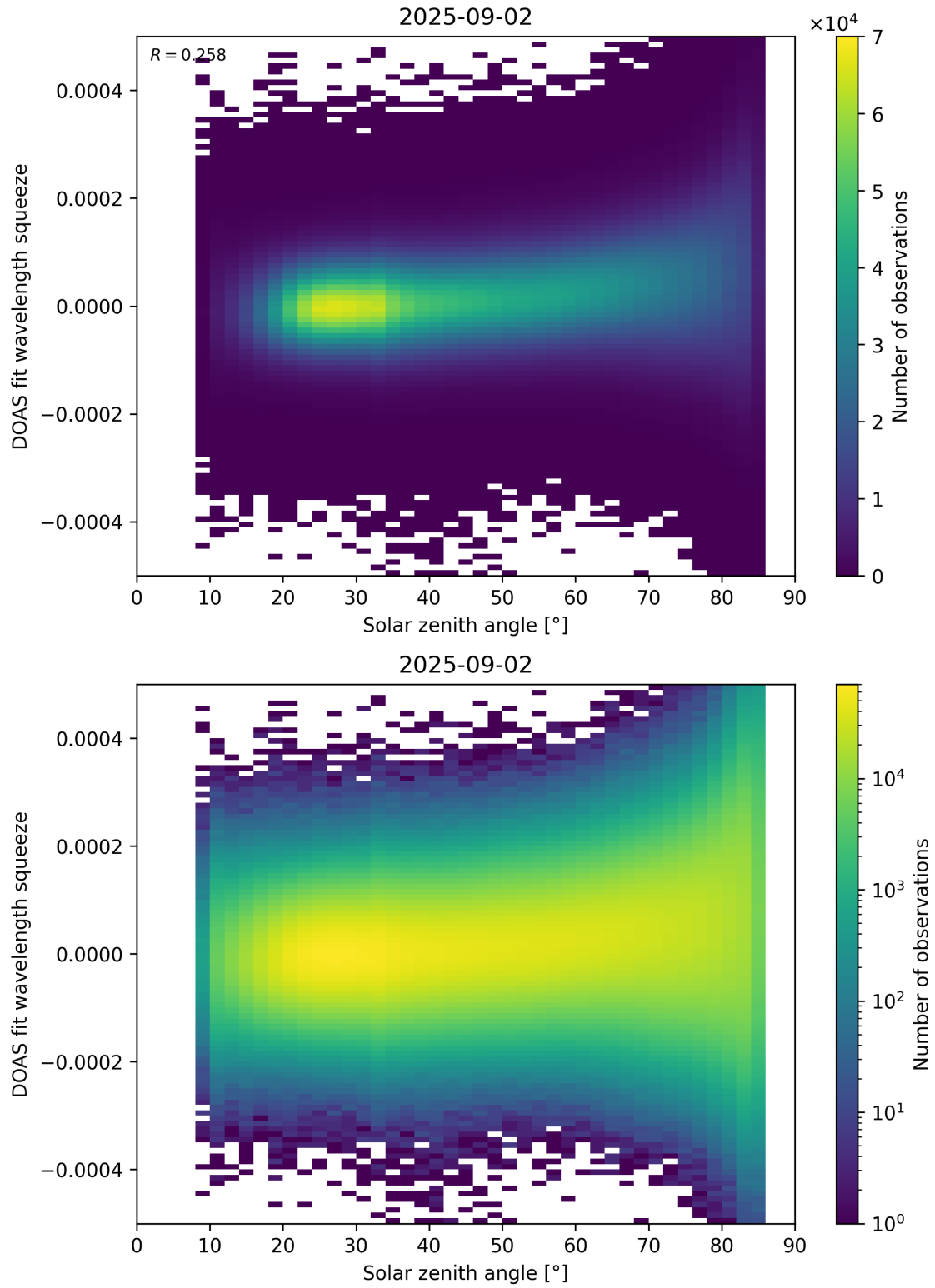
Figure 169: Scatter density plot of “Solar zenith angle” against “DOAS fit wavelength squeeze” for 2025-09-01 to 2025-09-03.
