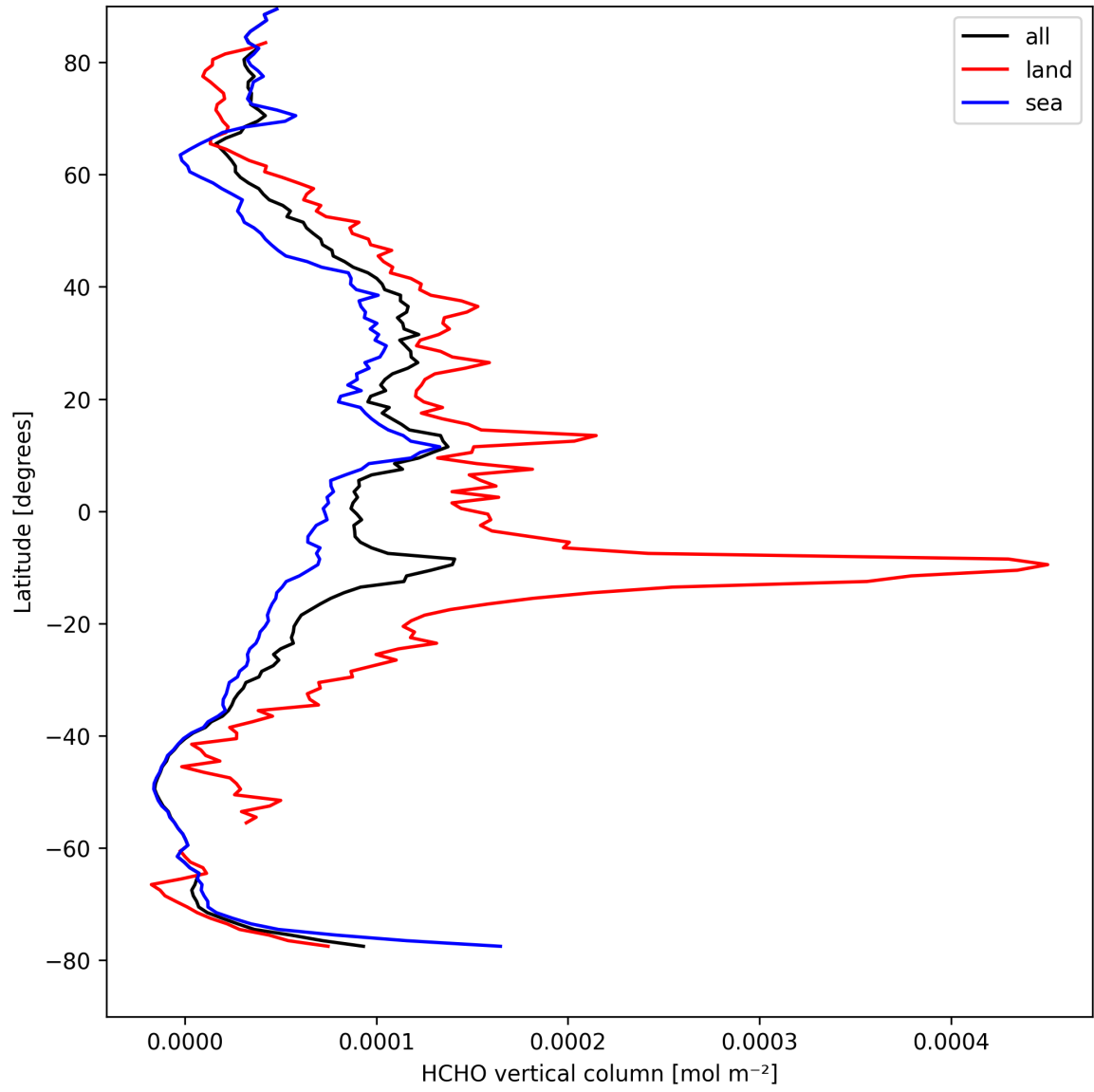
Figure 21: Zonal average of “HCHO vertical column” for 2025-09-01 to 2025-09-03.
