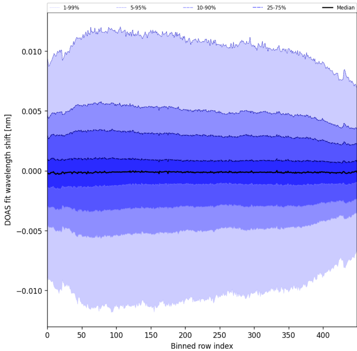
Figure 58: Along track statistics of “DOAS fit wavelength shift” for 2025-09-01 to 2025-09-03
