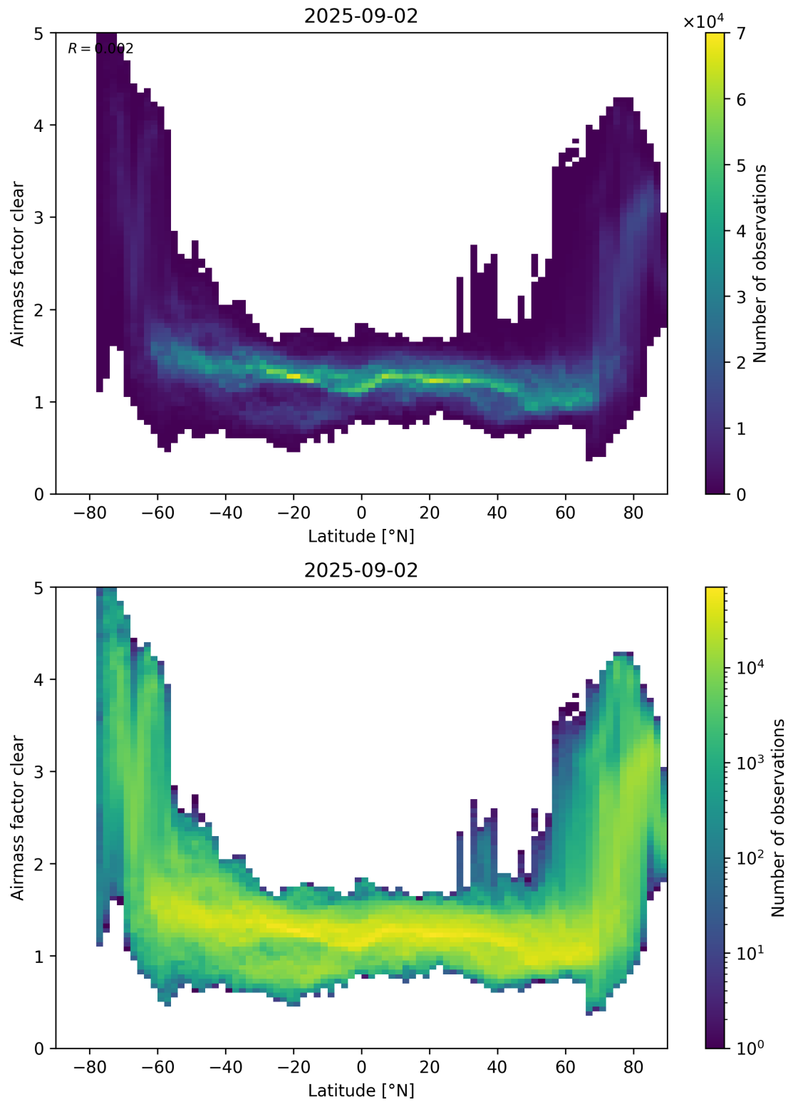
Figure 156: Scatter density plot of “Latitude” against “Airmass factor clear” for 2025-09-01 to 2025-09-03.
