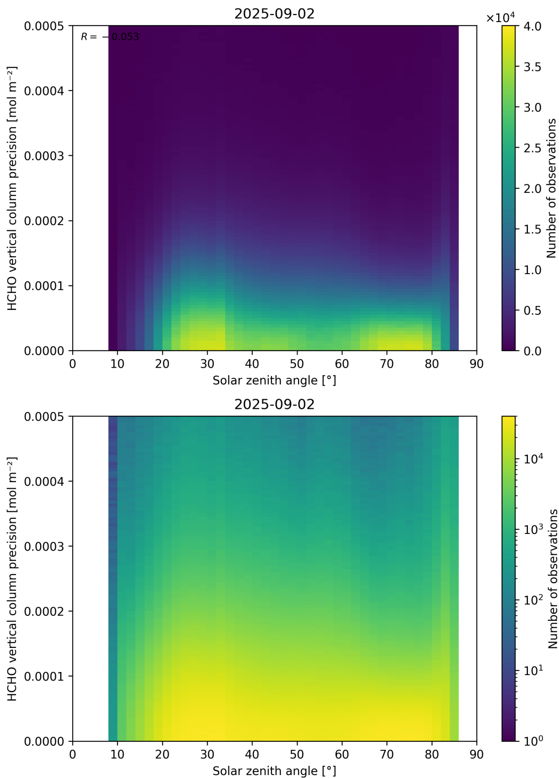
Figure 179: Scatter density plot of “Solar zenith angle” against “HCHO vertical column precision” for 2025-09-01 to 2025-09-03.
