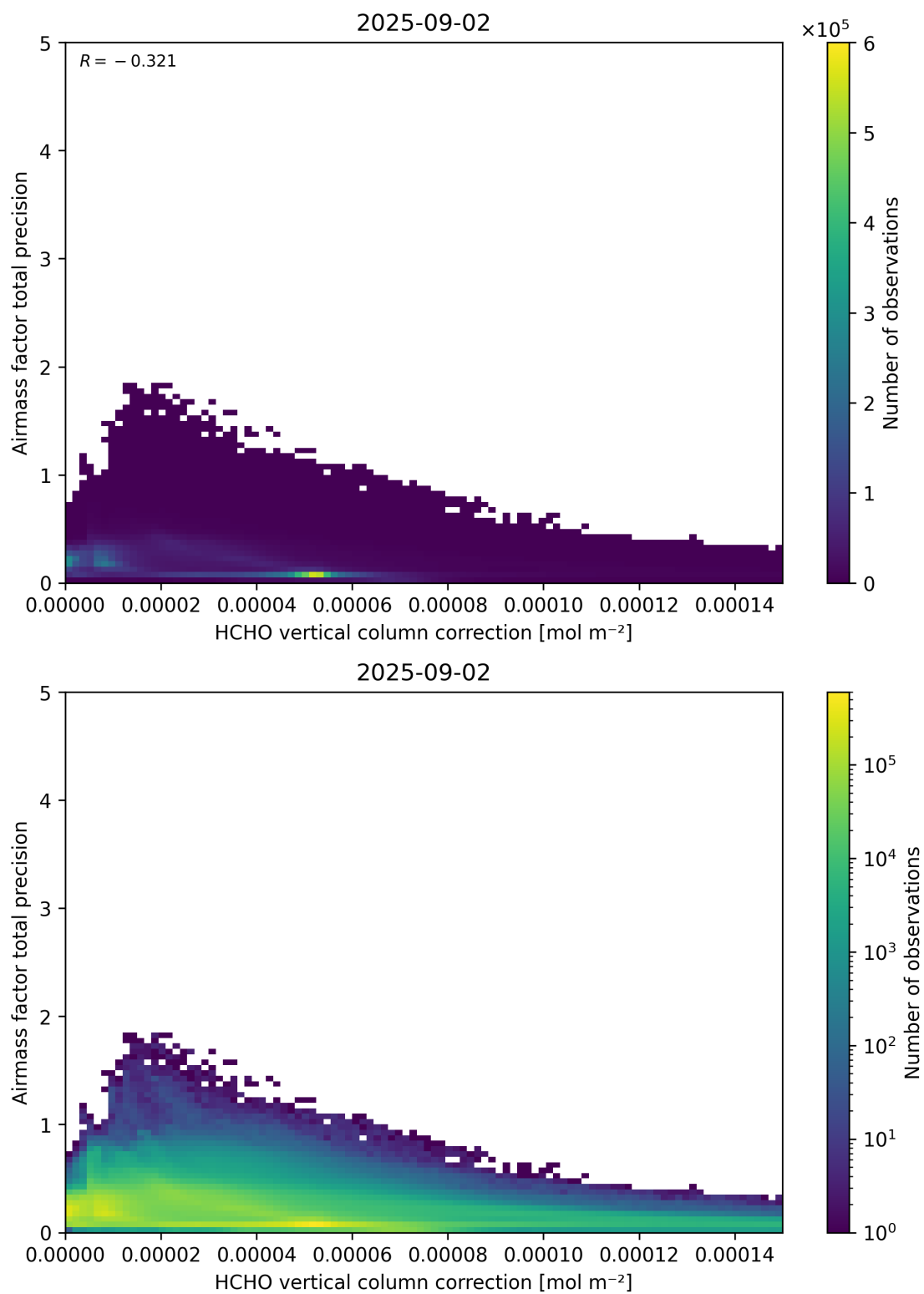
Figure 121: Scatter density plot of “HCHO vertical column correction” against “Airmass factor total precision” for 2025-09-01 to 2025-09-03.
