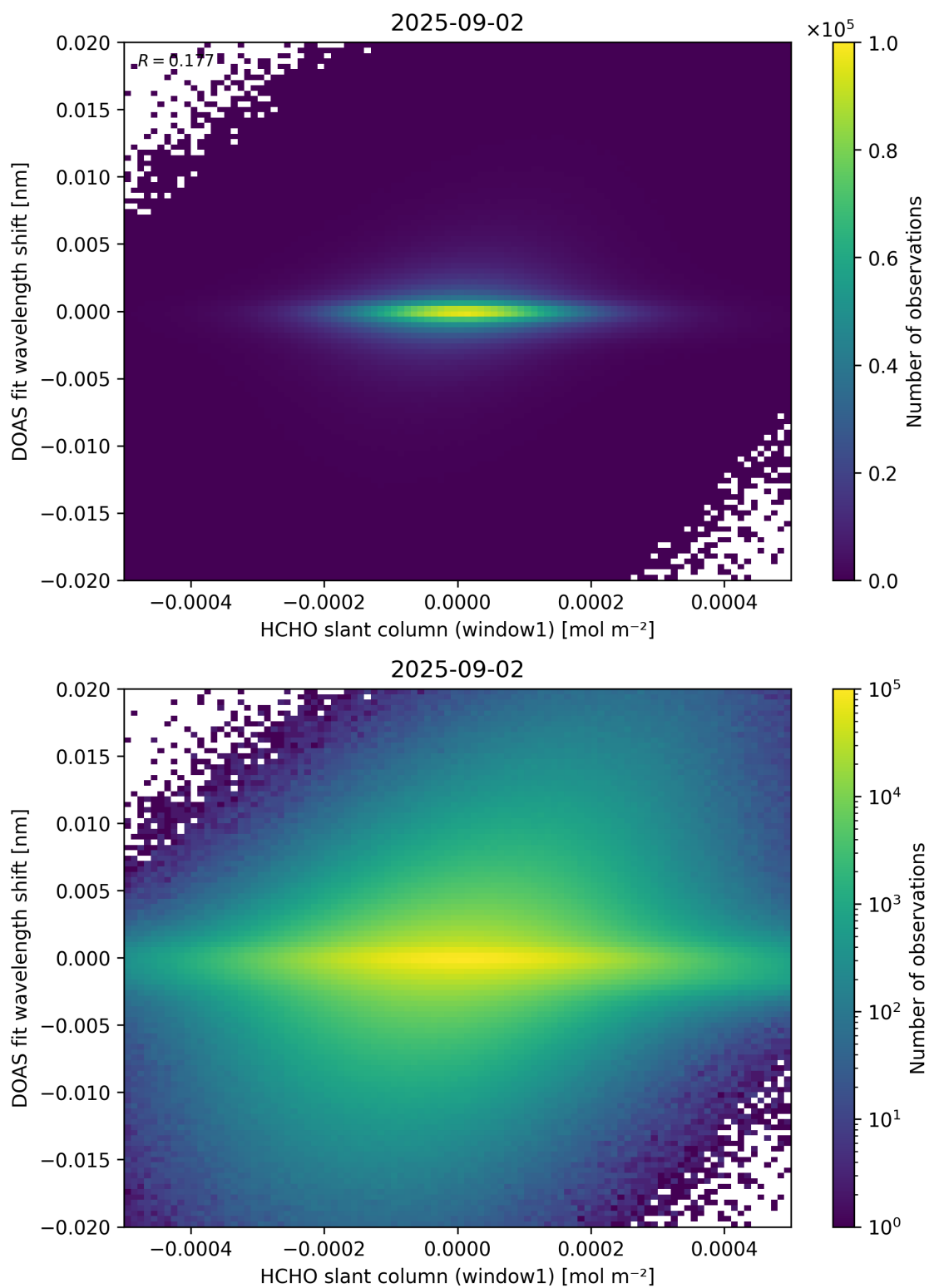
Figure 79: Scatter density plot of “HCHO slant column (window1)” against “DOAS fit wavelength shift” for 2025-09-01 to 2025-09-03.
