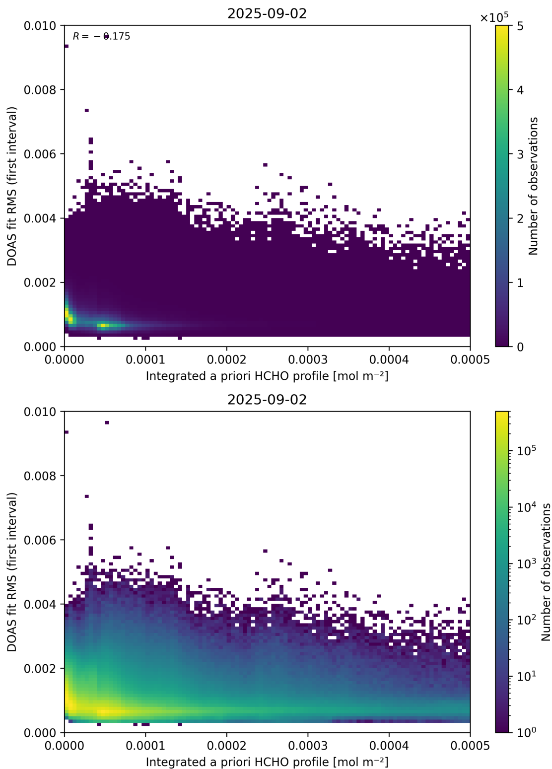
Figure 148: Scatter density plot of “Integrated a priori HCHO profile” against “DOAS fit RMS (first interval)” for 2025-09-01 to 2025-09-03.
