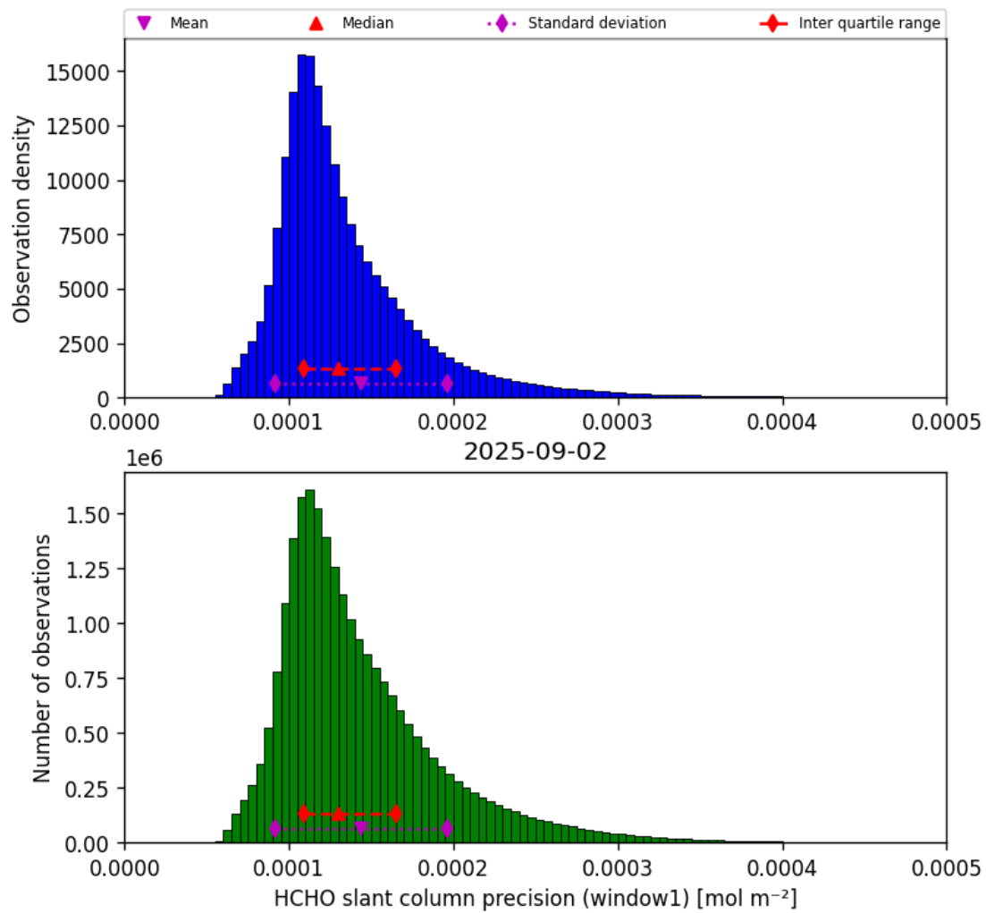
Figure 39: Histogram of “HCHO slant column precision (window1)” for 2025-09-01 to 2025-09-03
