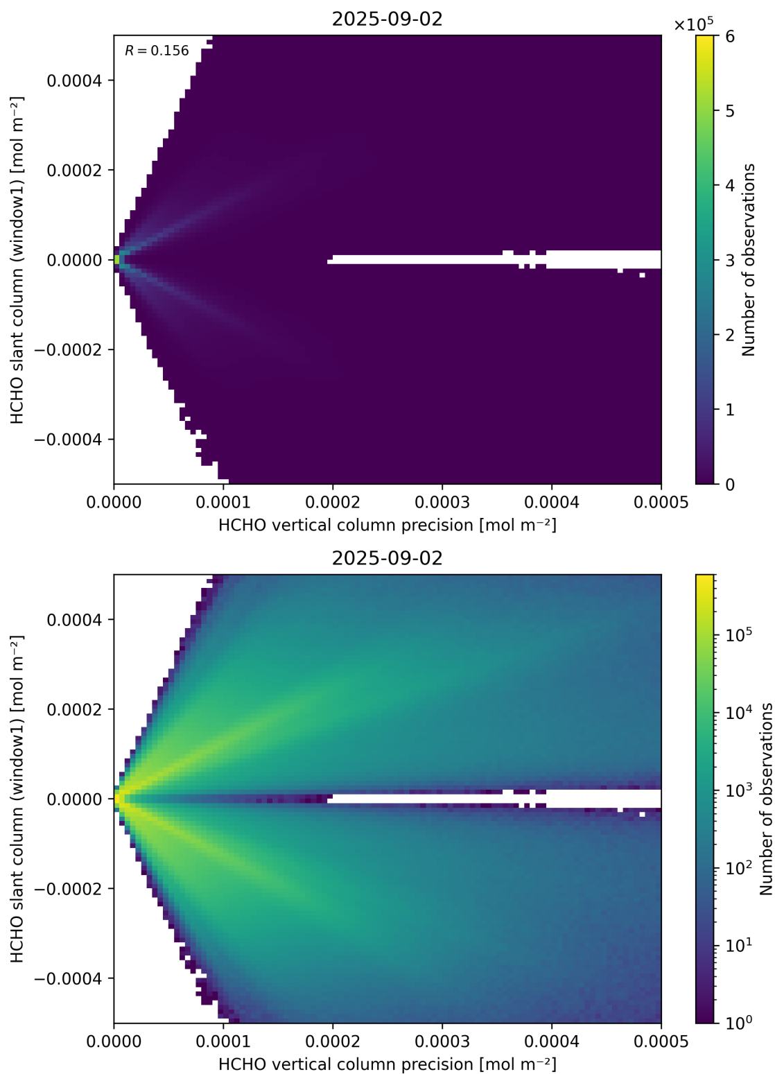
Figure 142: Scatter density plot of “HCHO vertical column precision” against “HCHO slant column (window1)” for 2025-09-01 to 2025-09-03.
