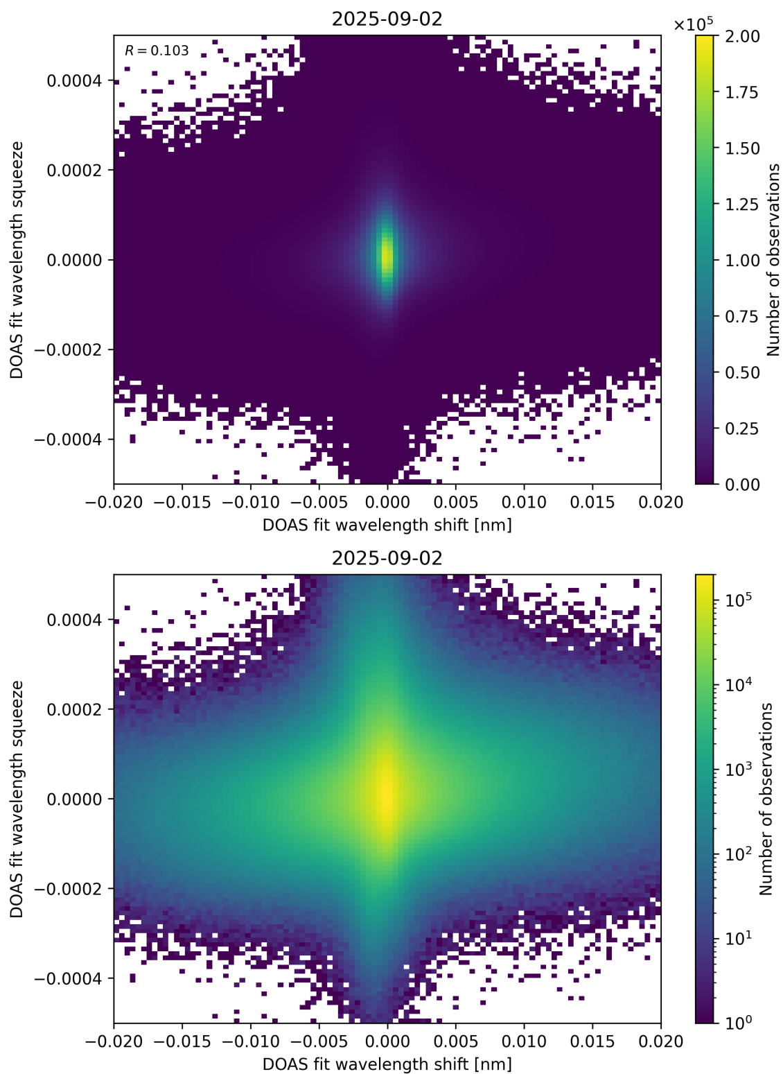
Figure 65: Scatter density plot of “DOAS fit wavelength shift” against “DOAS fit wavelength squeeze” for 2025-09-01 to 2025-09-03.
