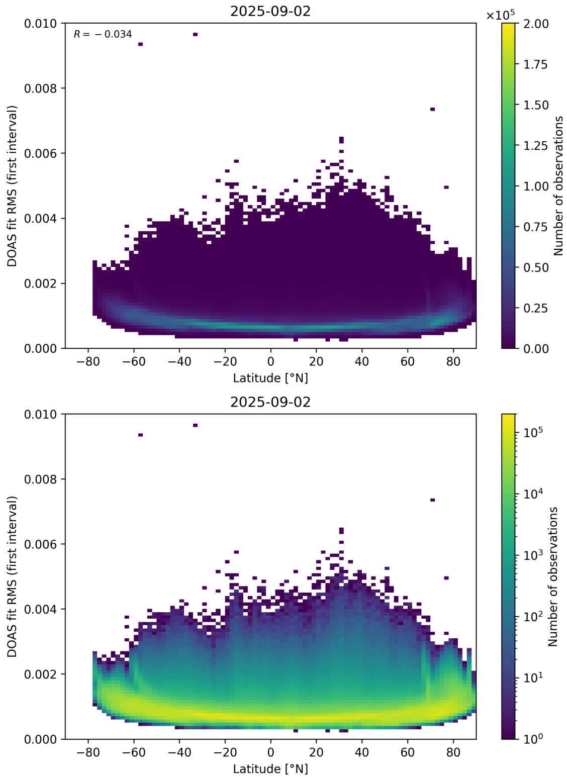
Figure 153: Scatter density plot of “Latitude” against “DOAS fit RMS (first interval)” for 2025-09-01 to 2025-09-03.
