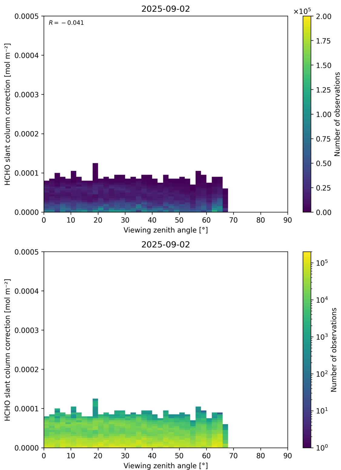
Figure 187: Scatter density plot of “Viewing zenith angle” against “HCHO slant column correction” for 2025-09-01 to 2025-09-03.
