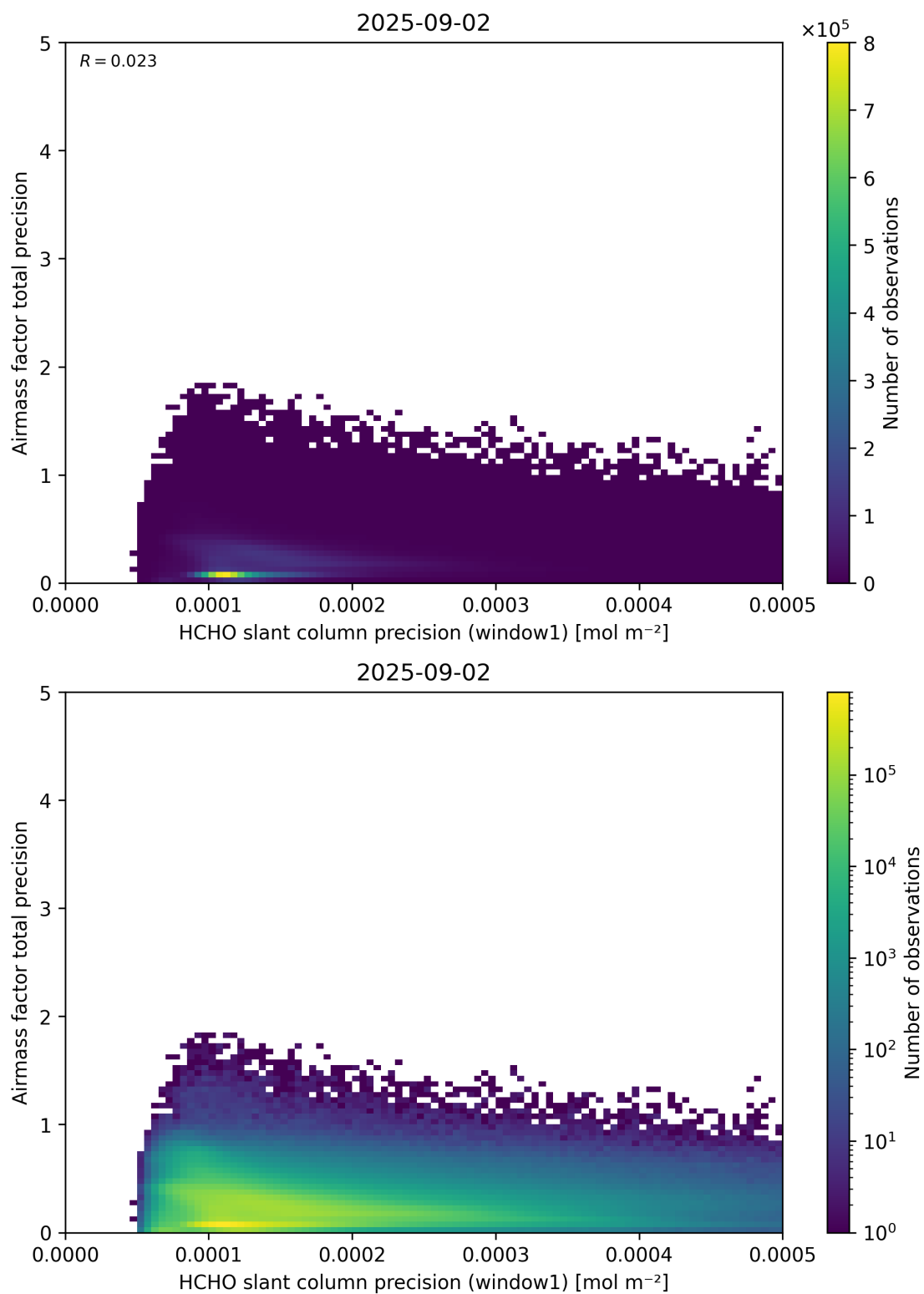
Figure 95: Scatter density plot of “HCHO slant column precision (window1)” against “Airmass factor total precision” for 2025-09-01 to 2025-09-03.
