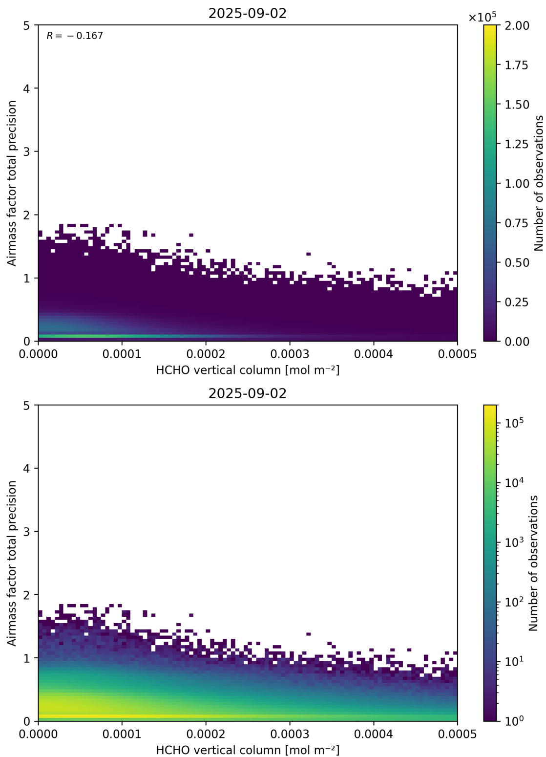
Figure 132: Scatter density plot of “HCHO vertical column” against “Airmass factor total precision” for 2025-09-01 to 2025-09-03.
