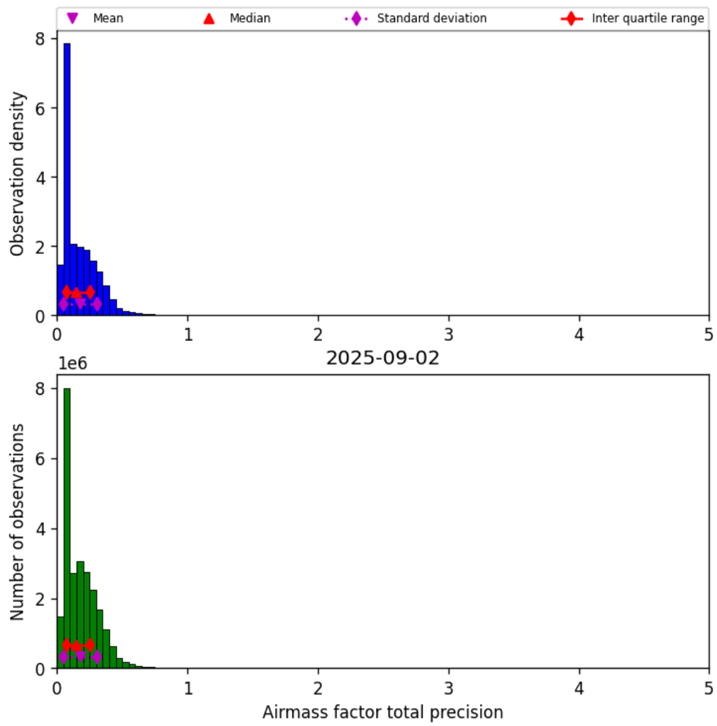
Figure 41: Histogram of “Airmass factor total precision” for 2025-09-01 to 2025-09-03
