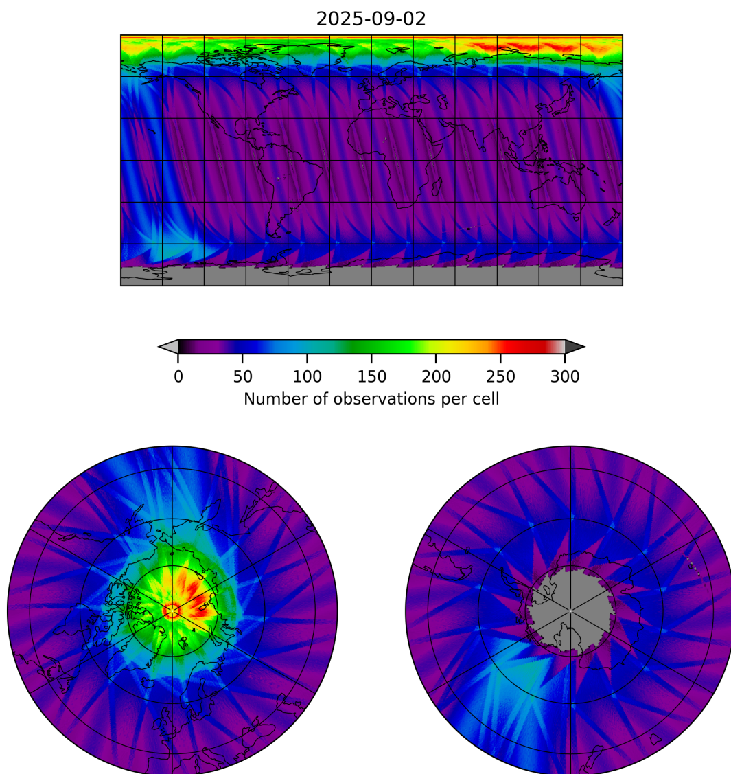
Figure 19: Map of the number of observations for 2025-09-01 to 2025-09-03
