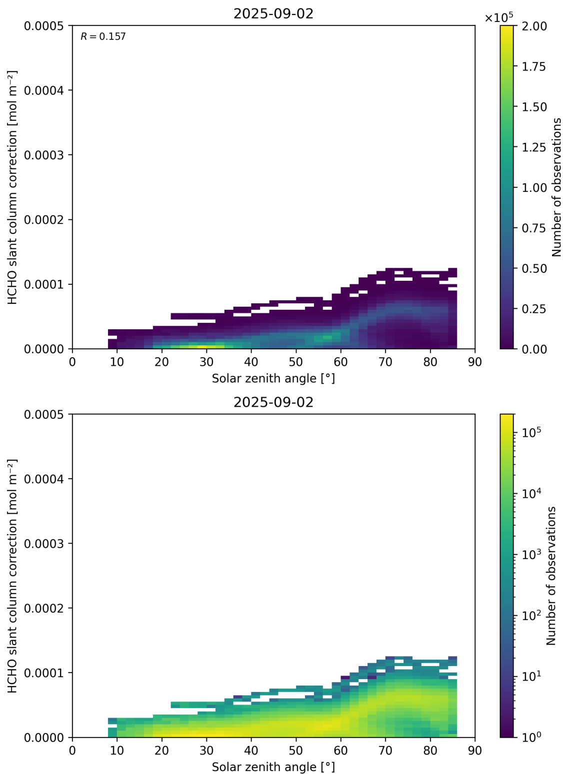
Figure 172: Scatter density plot of “Solar zenith angle” against “HCHO slant column correction” for 2025-09-01 to 2025-09-03.
