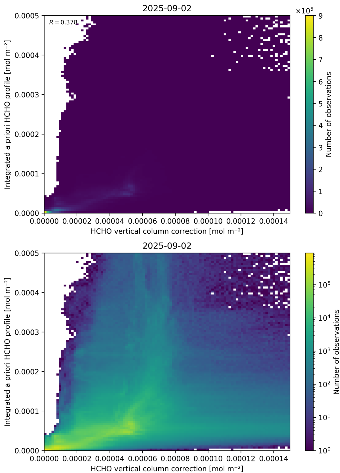
Figure 122: Scatter density plot of “HCHO vertical column correction” against “Integrated a priori HCHO profile” for 2025-09-01 to 2025-09-03.
