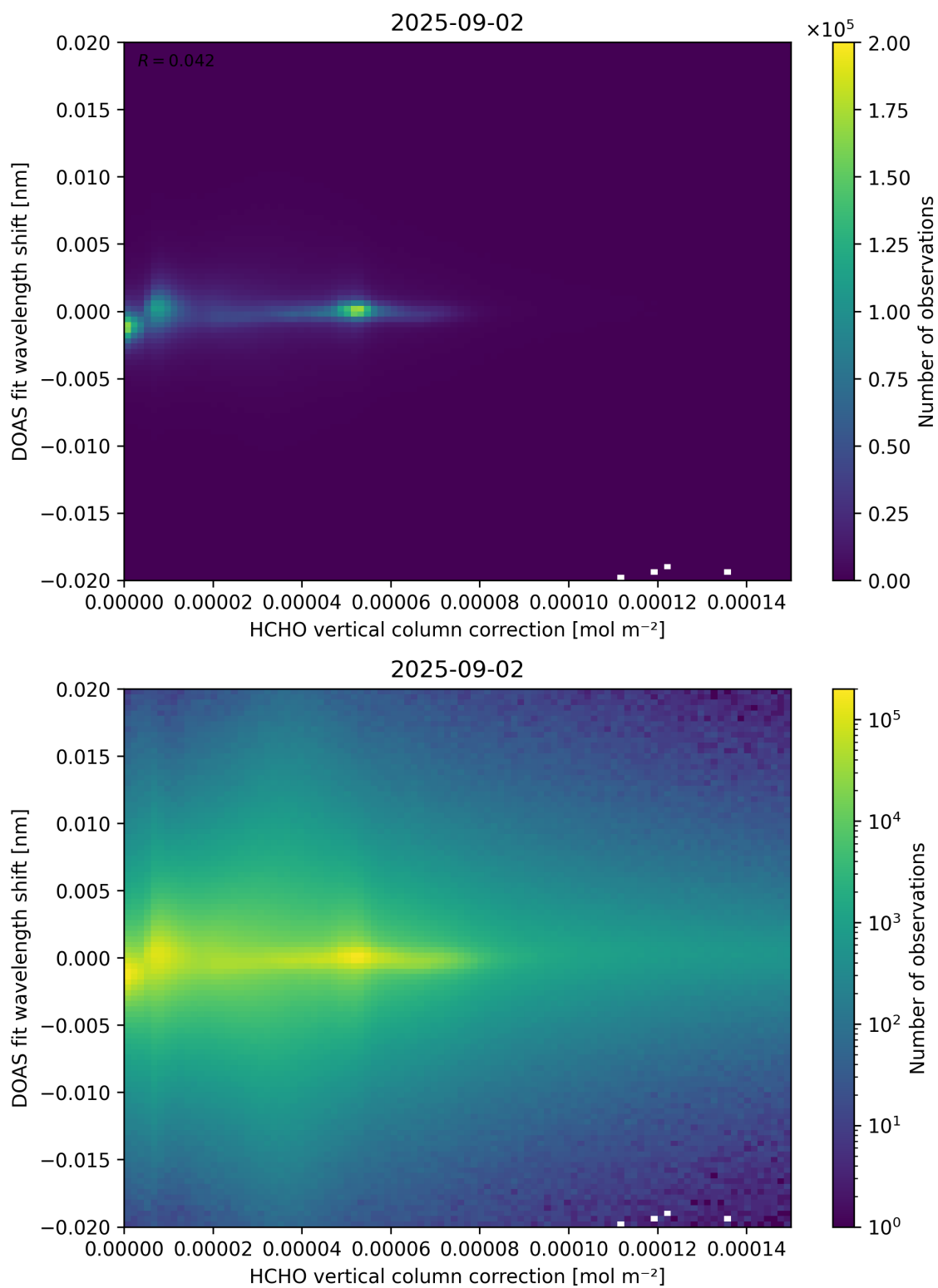
Figure 113: Scatter density plot of “HCHO vertical column correction” against “DOAS fit wavelength shift” for 2025-09-01 to 2025-09-03.
