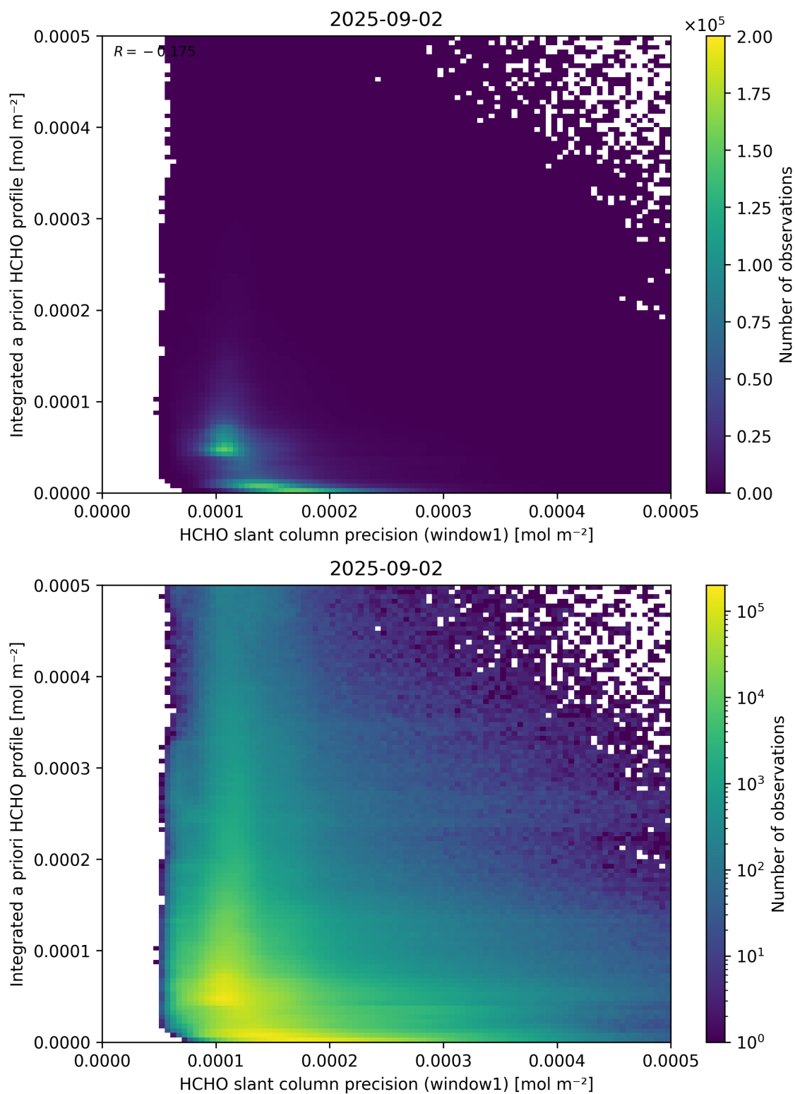
Figure 96: Scatter density plot of “HCHO slant column precision (window1)” against “Integrated a priori HCHO profile” for 2025-09-01 to 2025-09-03.
