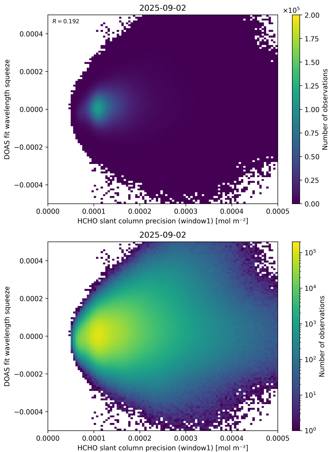
Figure 90: Scatter density plot of “HCHO slant column precision (window1)” against “DOAS fit wavelength squeeze” for 2025-09-01 to 2025-09-03.
