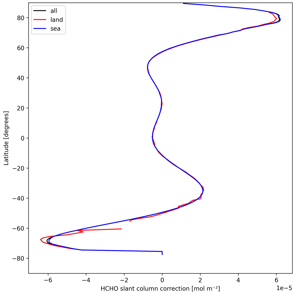
Figure 33: Zonal average of “HCHO slant column correction” for 2025-09-01 to 2025-09-03.
