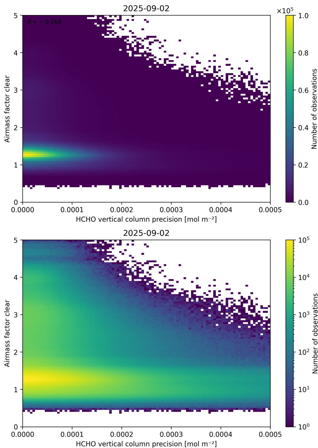
Figure 139: Scatter density plot of “HCHO vertical column precision” against “Airmass factor clear” for 2025-09-01 to 2025-09-03.
