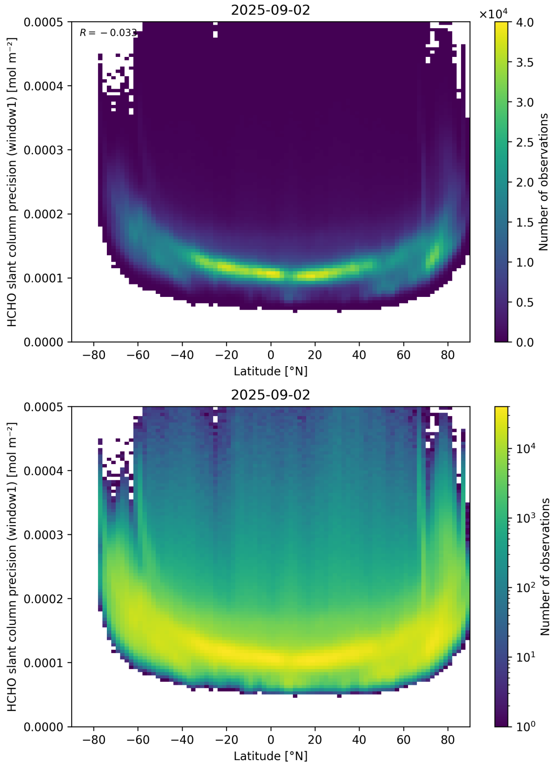
Figure 160: Scatter density plot of “Latitude” against “HCHO slant column precision (window1)” for 2025-09-01 to 2025-09-03.
