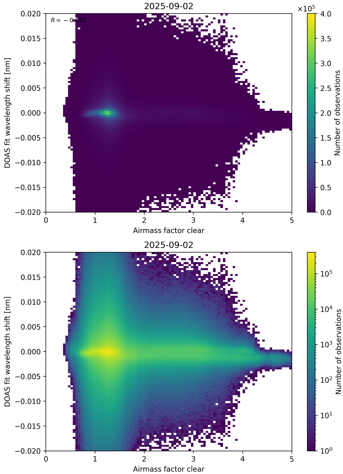
Figure 72: Scatter density plot of “Airmass factor clear” against “DOAS fit wavelength shift” for 2025-09-01 to 2025-09-03.
