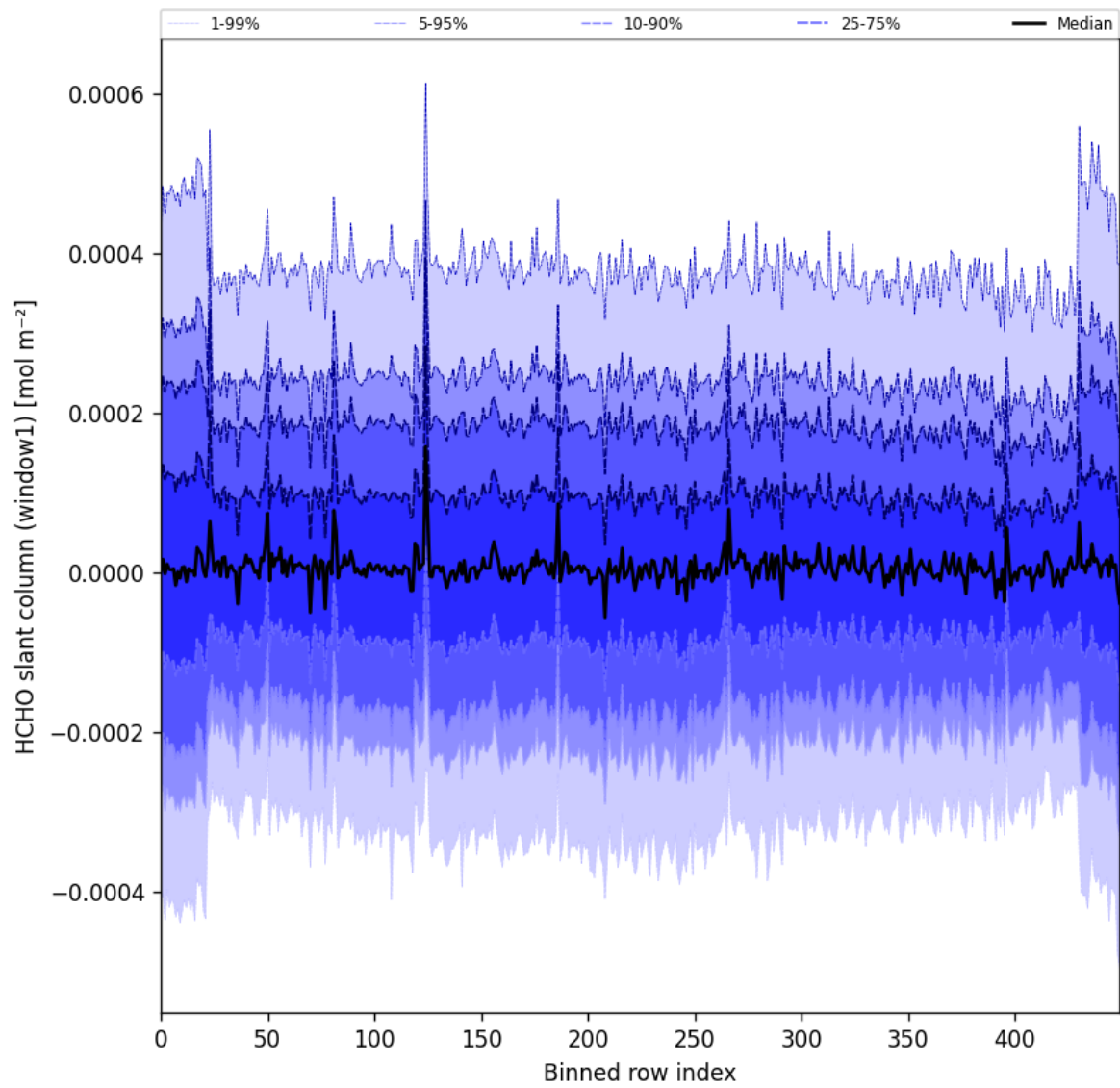
Figure 52: Along track statistics of “HCHO slant column (window1)” for 2025-09-01 to 2025-09-03
