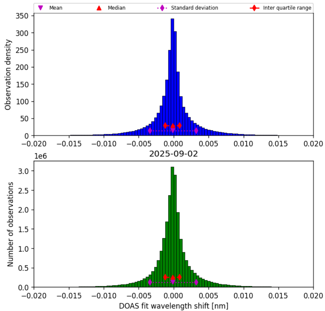
Figure 44: Histogram of “DOAS fit wavelength shift” for 2025-09-01 to 2025-09-03
