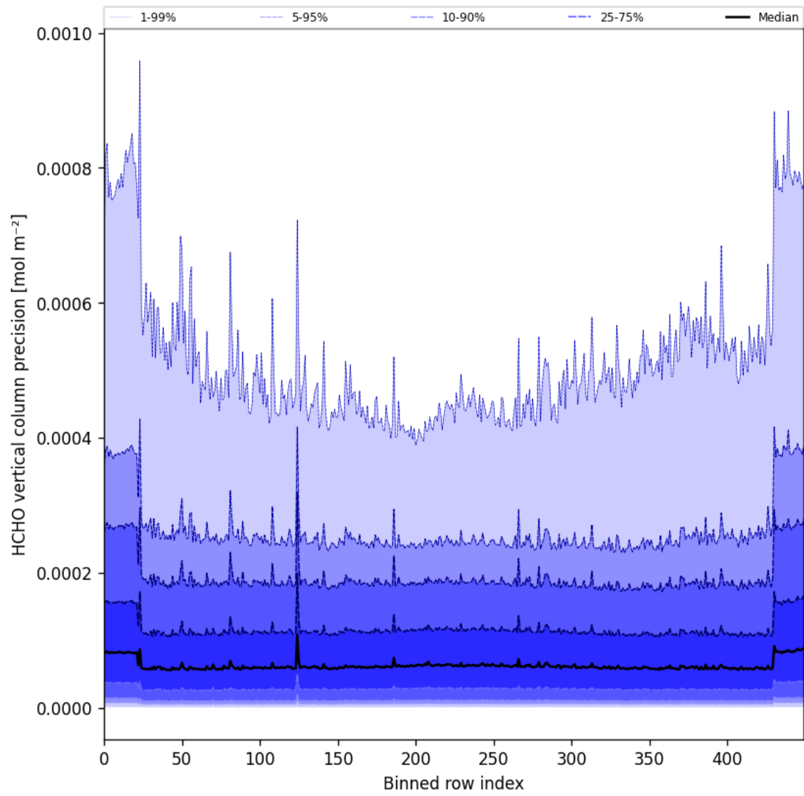
Figure 50: Along track statistics of “HCHO vertical column precision” for 2025-09-01 to 2025-09-03
