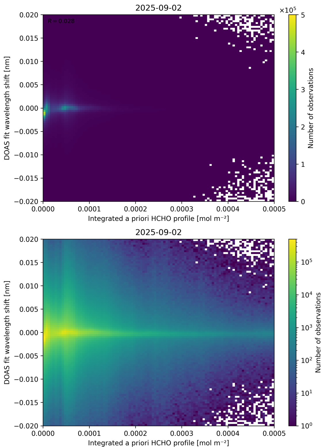
Figure 149: Scatter density plot of “Integrated a priori HCHO profile” against “DOAS fit wavelength shift” for 2025-09-01 to 2025-09-03.
