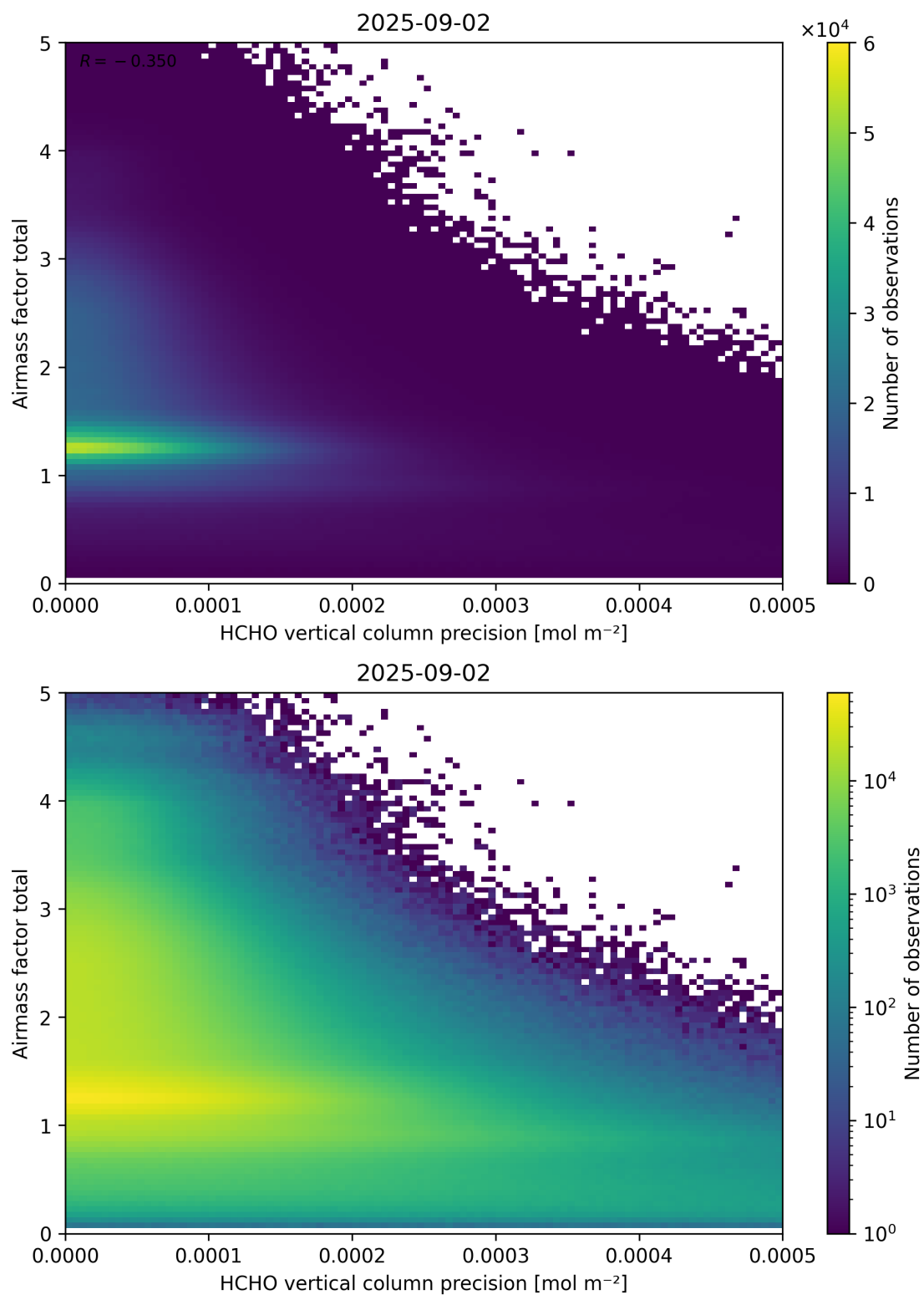
Figure 144: Scatter density plot of “HCHO vertical column precision” against “Airmass factor total” for 2025-09-01 to 2025-09-03.
