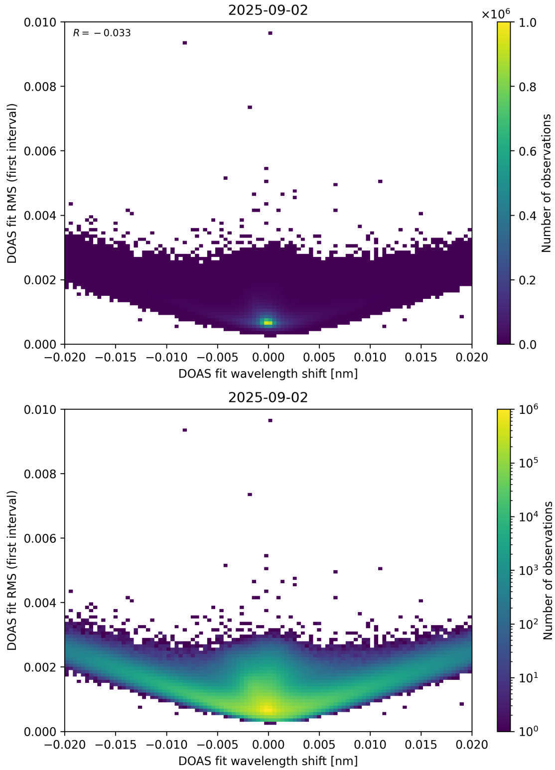
Figure 64: Scatter density plot of “DOAS fit wavelength shift” against “DOAS fit RMS (first interval)” for 2025-09-01 to 2025-09-03.
