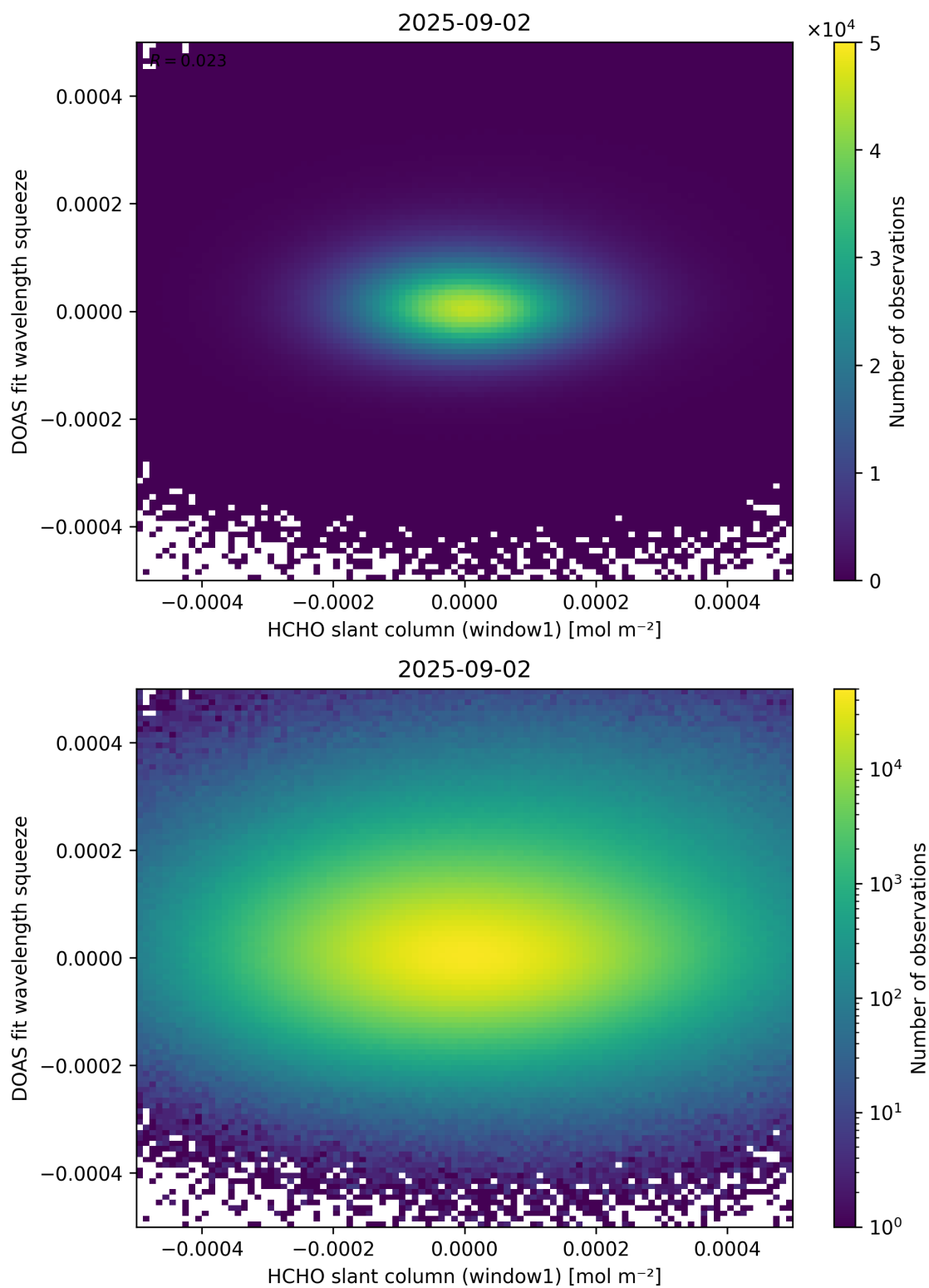
Figure 80: Scatter density plot of “HCHO slant column (window1)” against “DOAS fit wavelength squeeze” for 2025-09-01 to 2025-09-03.
