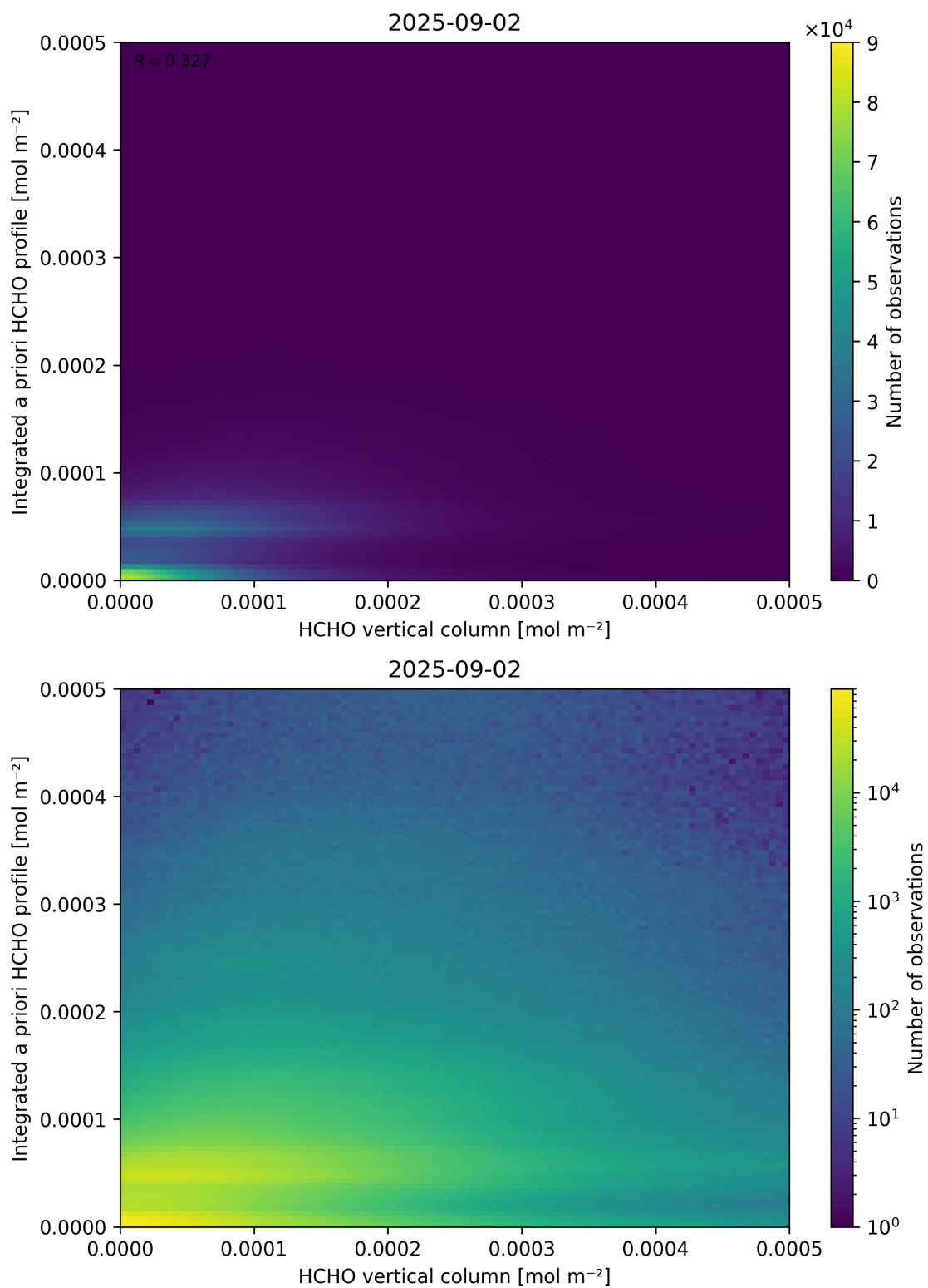
Figure 135: Scatter density plot of “HCHO vertical column” against “Integrated a priori HCHO profile” for 2025-09-01 to 2025-09-03.
