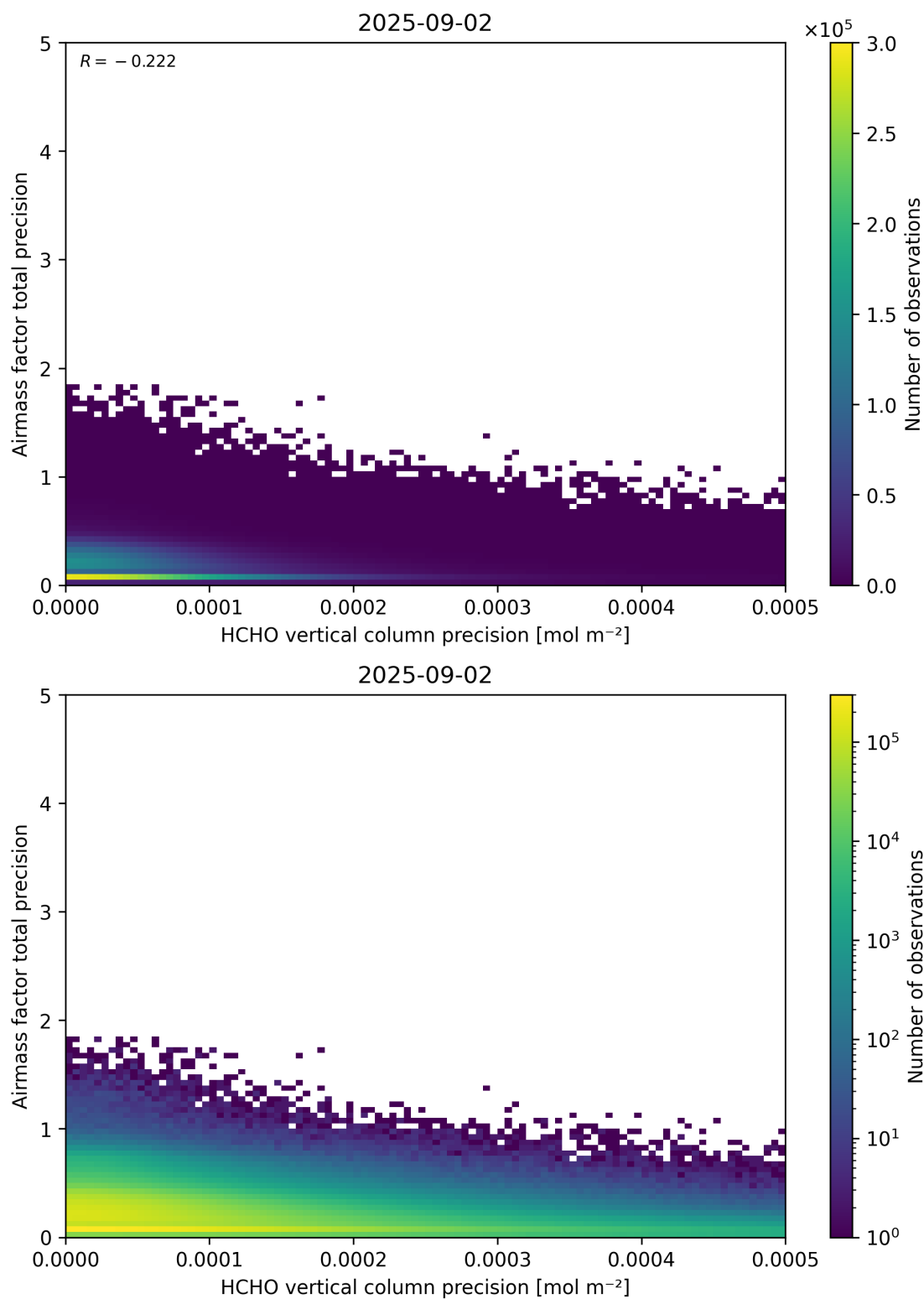
Figure 145: Scatter density plot of “HCHO vertical column precision” against “Airmass factor total precision” for 2025-09-01 to 2025-09-03.
