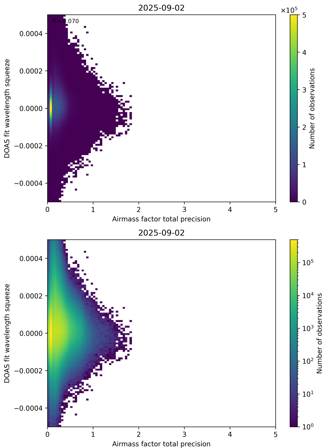
Figure 107: Scatter density plot of “Airmass factor total precision” against “DOAS fit wavelength squeeze” for 2025-09-01 to 2025-09-03.
