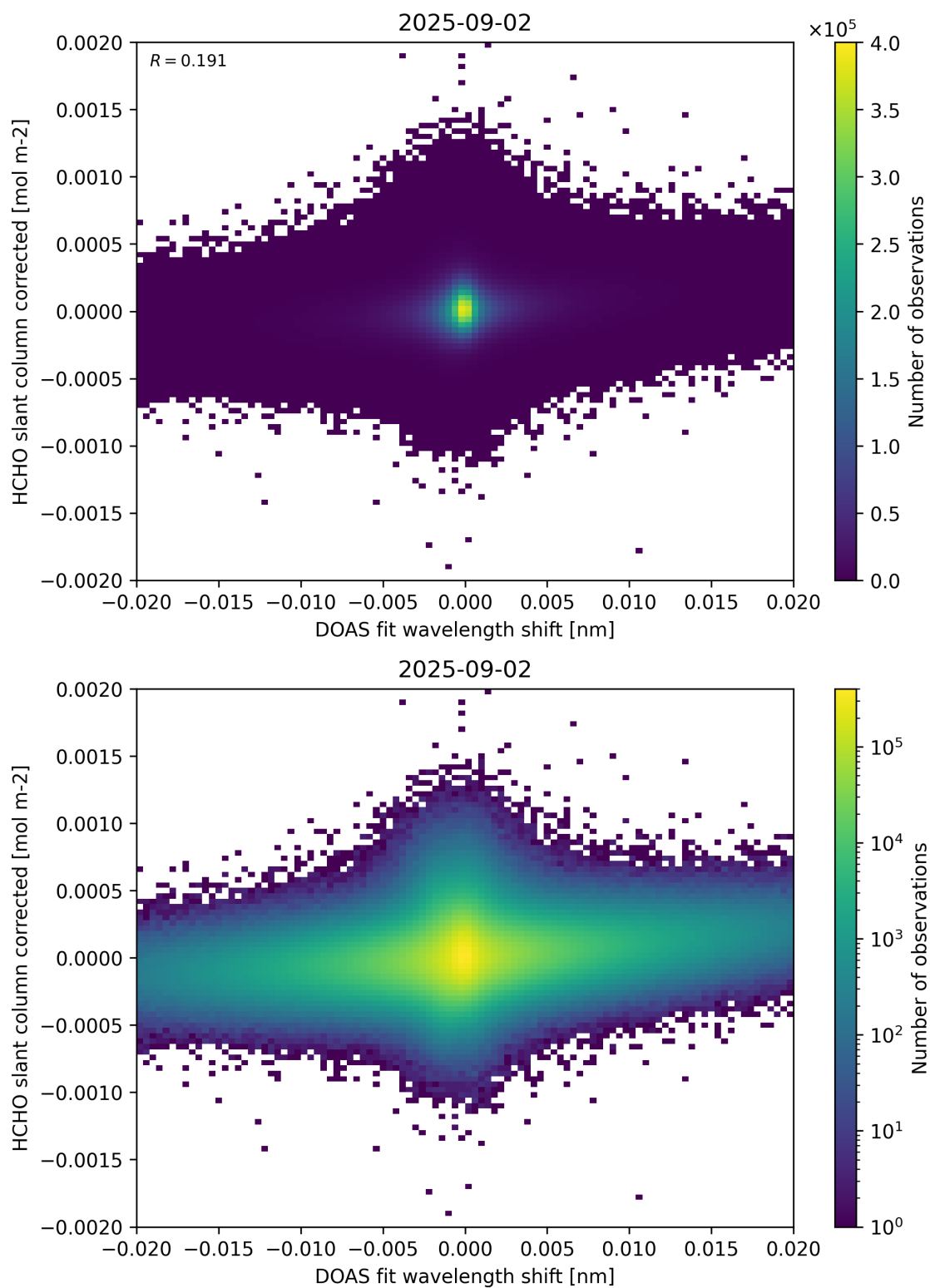
Figure 66: Scatter density plot of “DOAS fit wavelength shift” against “HCHO slant column corrected” for 2025-09-01 to 2025-09-03.
