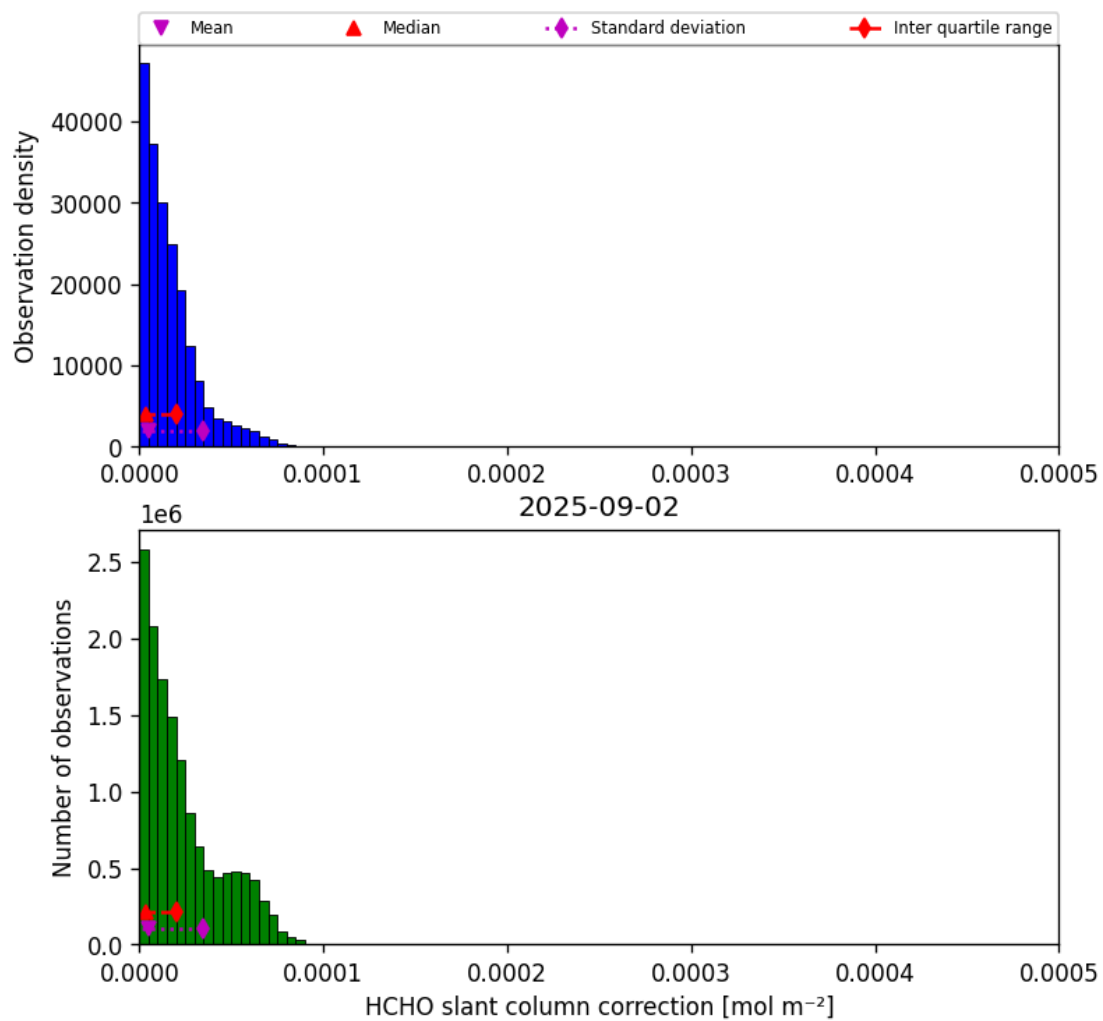
Figure 47: Histogram of “HCHO slant column correction” for 2025-09-01 to 2025-09-03
