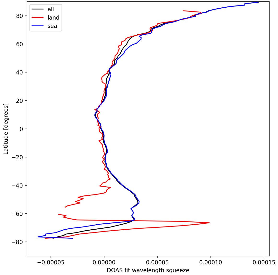
Figure 31: Zonal average of “DOAS fit wavelength squeeze” for 2025-09-01 to 2025-09-03.
