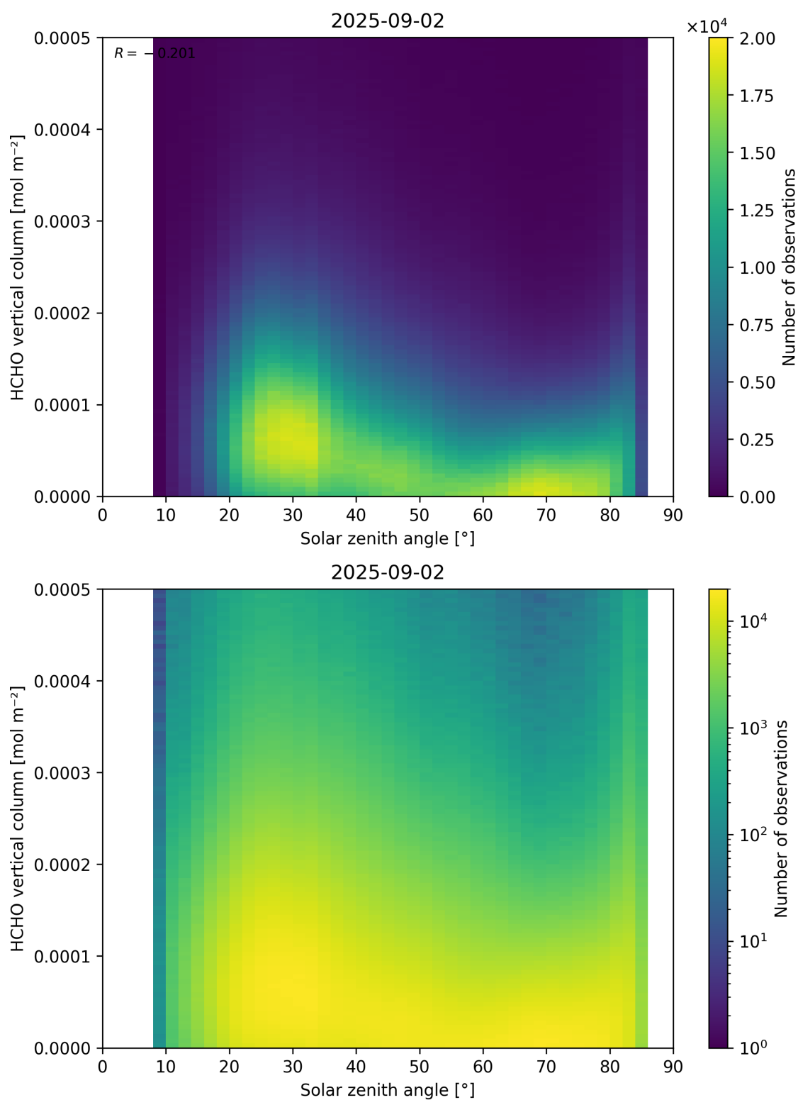
Figure 177: Scatter density plot of “Solar zenith angle” against “HCHO vertical column” for 2025-09-01 to 2025-09-03.
