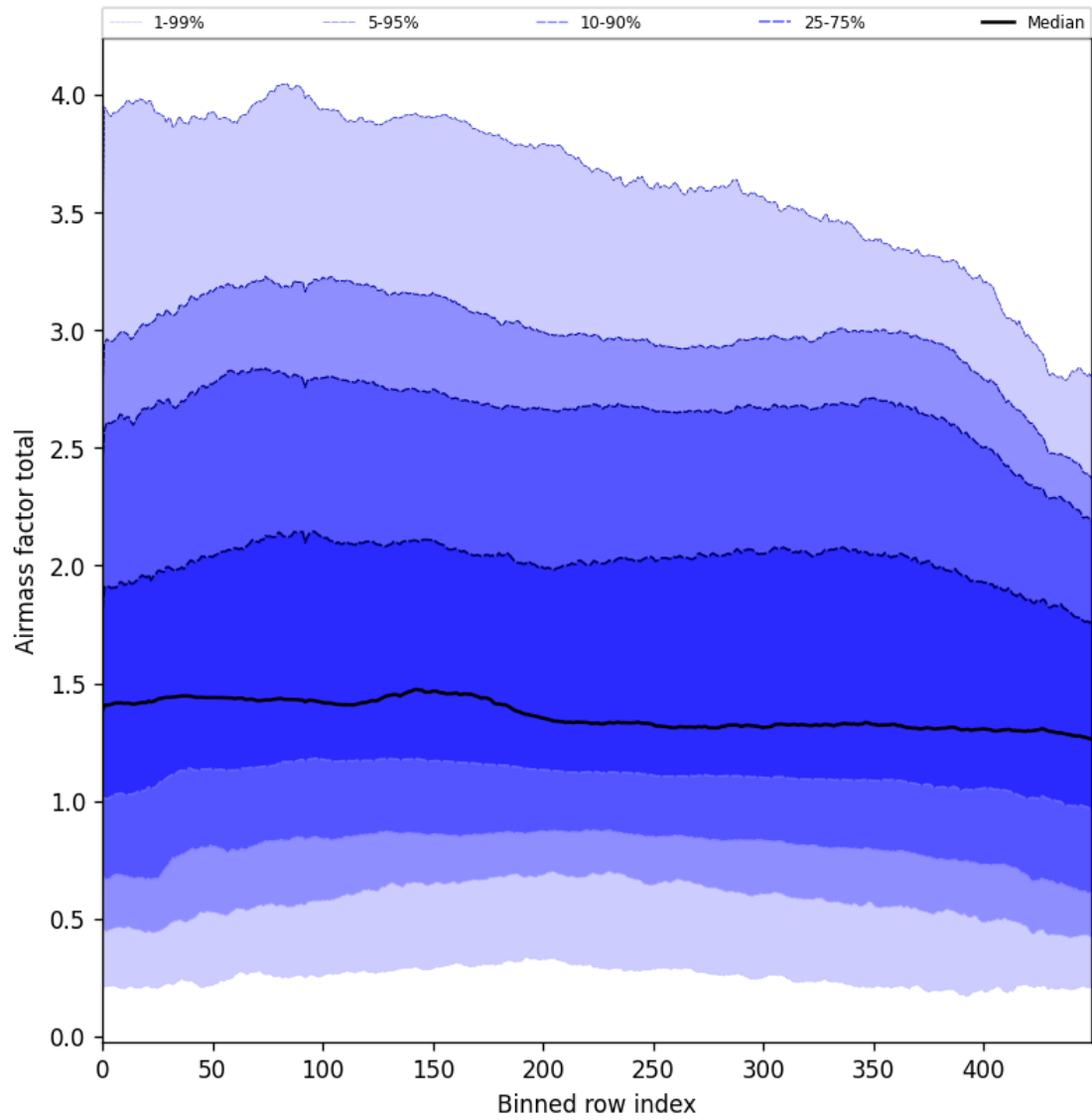
Figure 54: Along track statistics of “Airmass factor total” for 2025-09-01 to 2025-09-03
