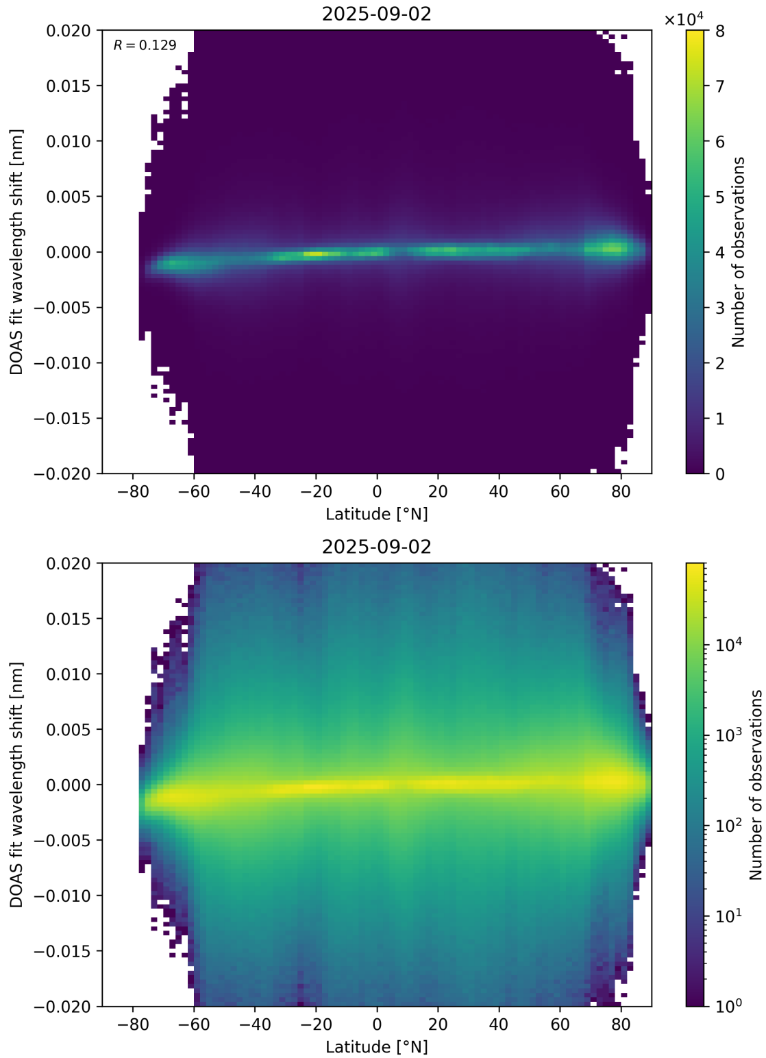
Figure 154: Scatter density plot of “Latitude” against “DOAS fit wavelength shift” for 2025-09-01 to 2025-09-03.
