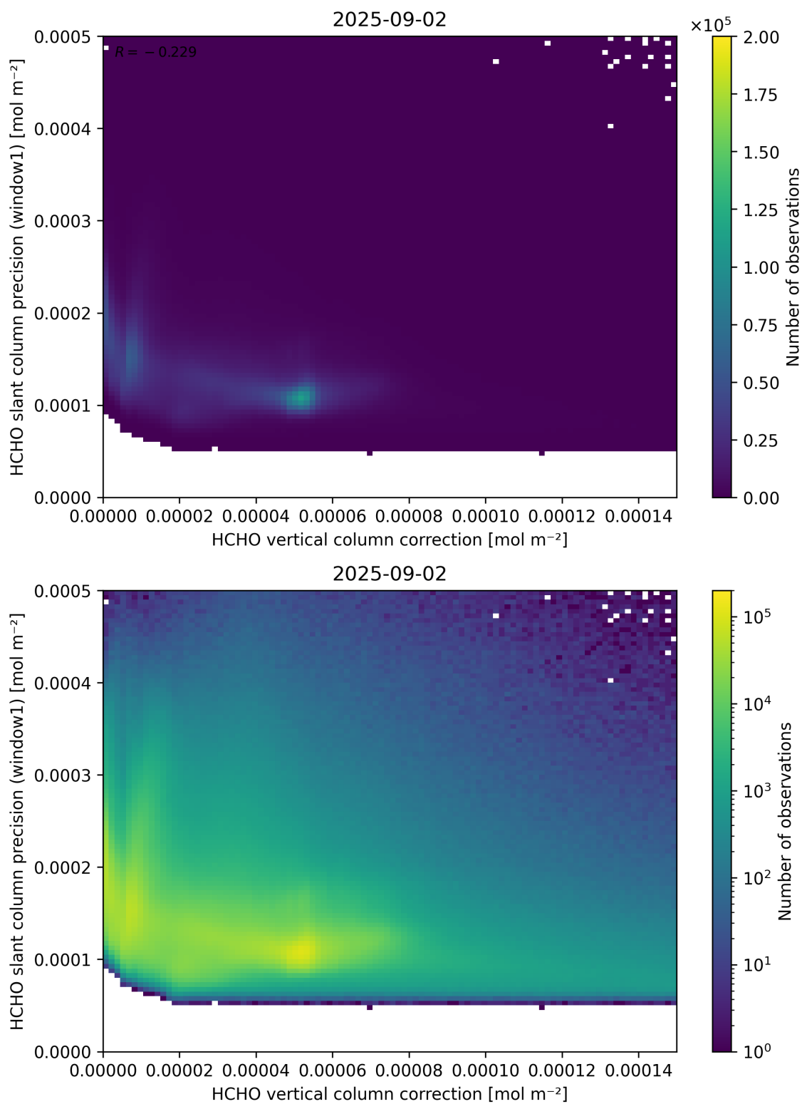
Figure 119: Scatter density plot of “HCHO vertical column correction” against “HCHO slant column precision (window1)” for 2025-09-01 to 2025-09-03.
