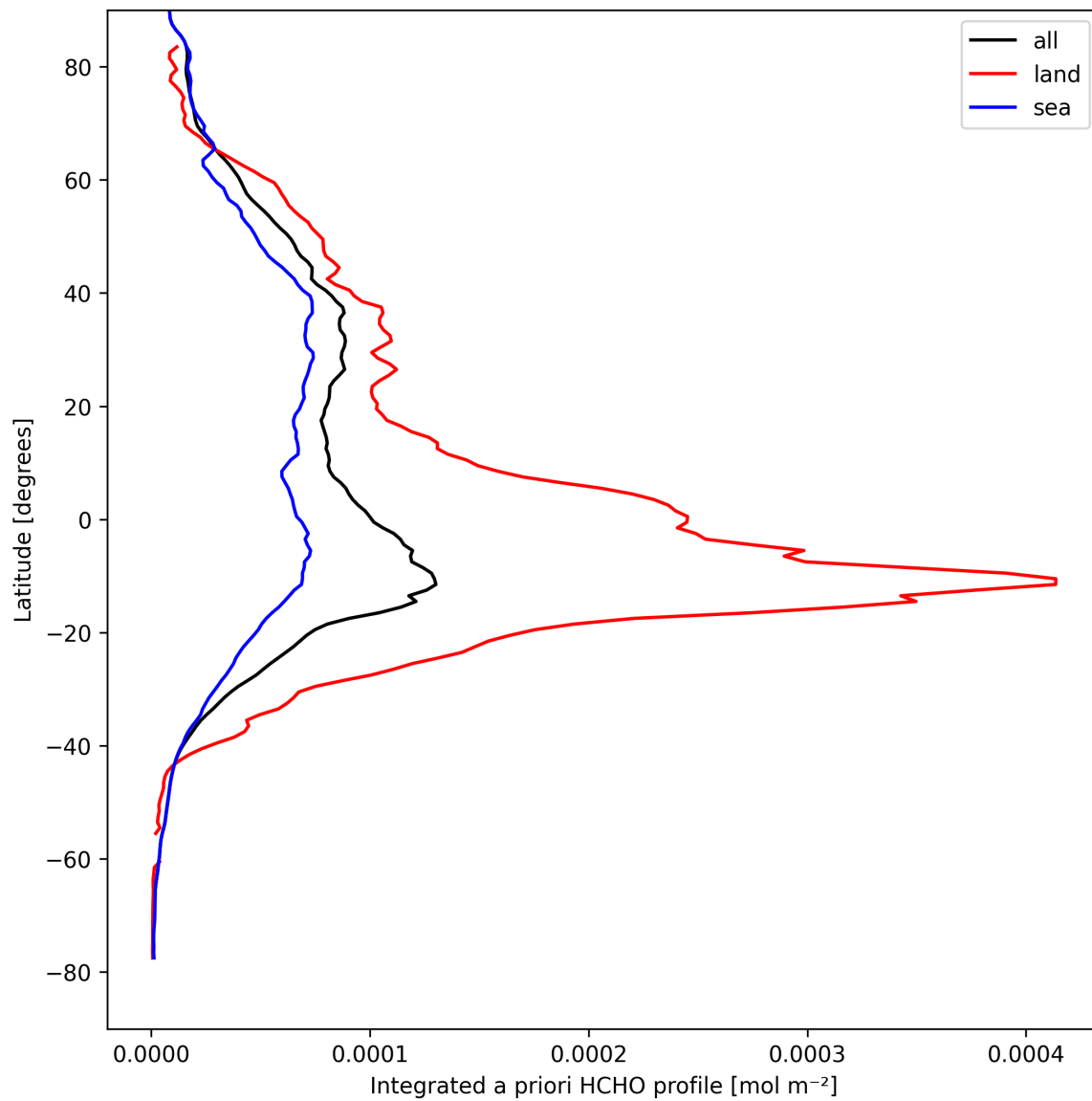
Figure 29: Zonal average of “Integrated a priori HCHO profile” for 2025-09-01 to 2025-09-03.
