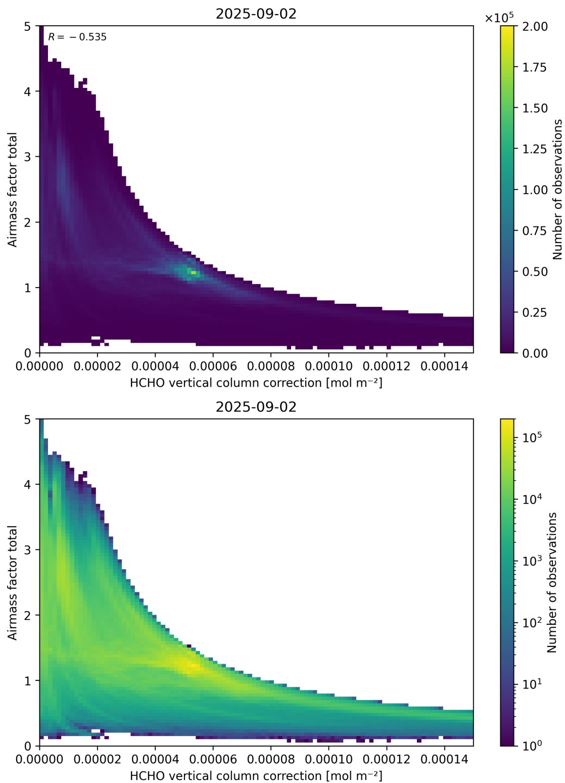
Figure 120: Scatter density plot of “HCHO vertical column correction” against “Airmass factor total” for 2025-09-01 to 2025-09-03.
