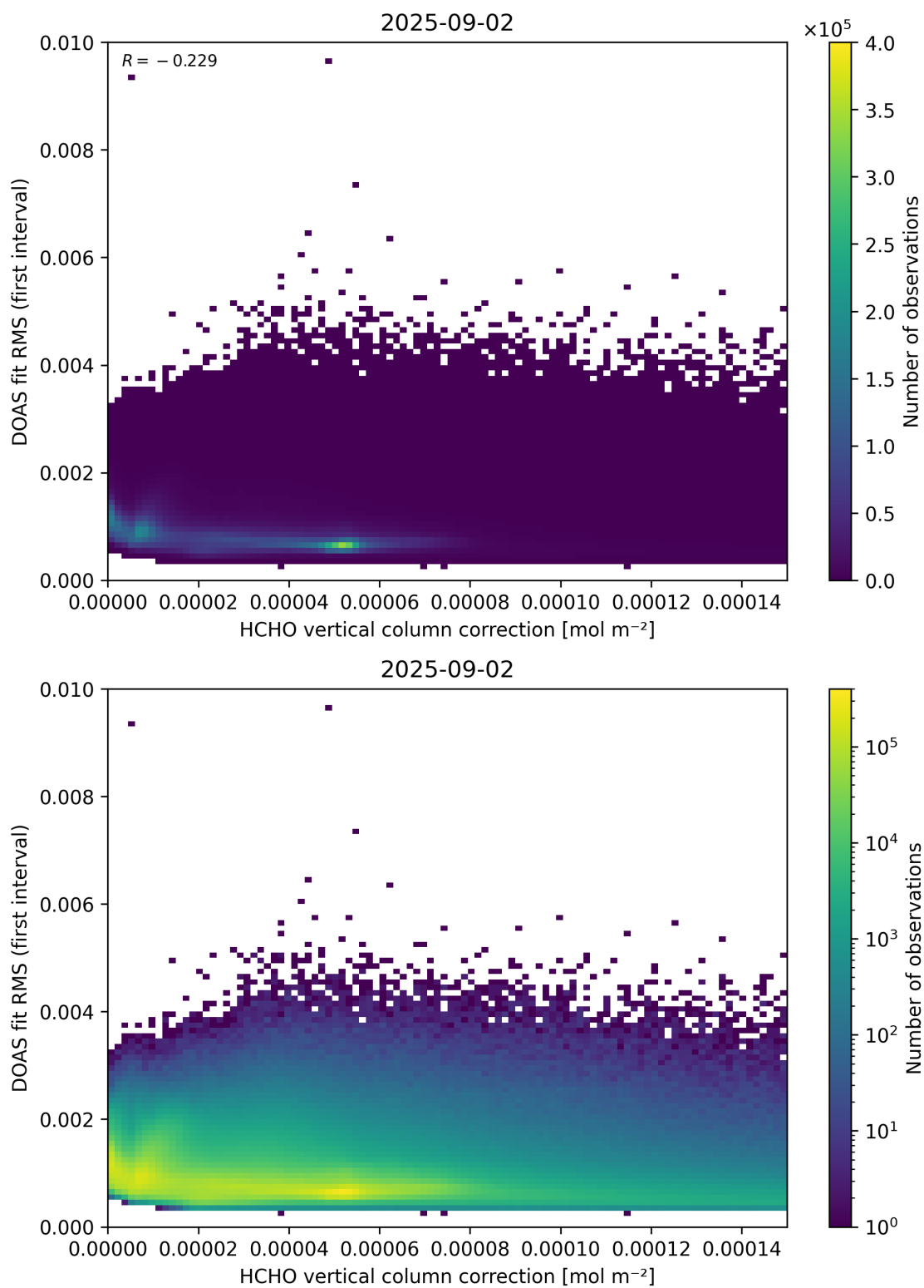
Figure 112: Scatter density plot of “HCHO vertical column correction” against “DOAS fit RMS (first interval)” for 2025-09-01 to 2025-09-03.
