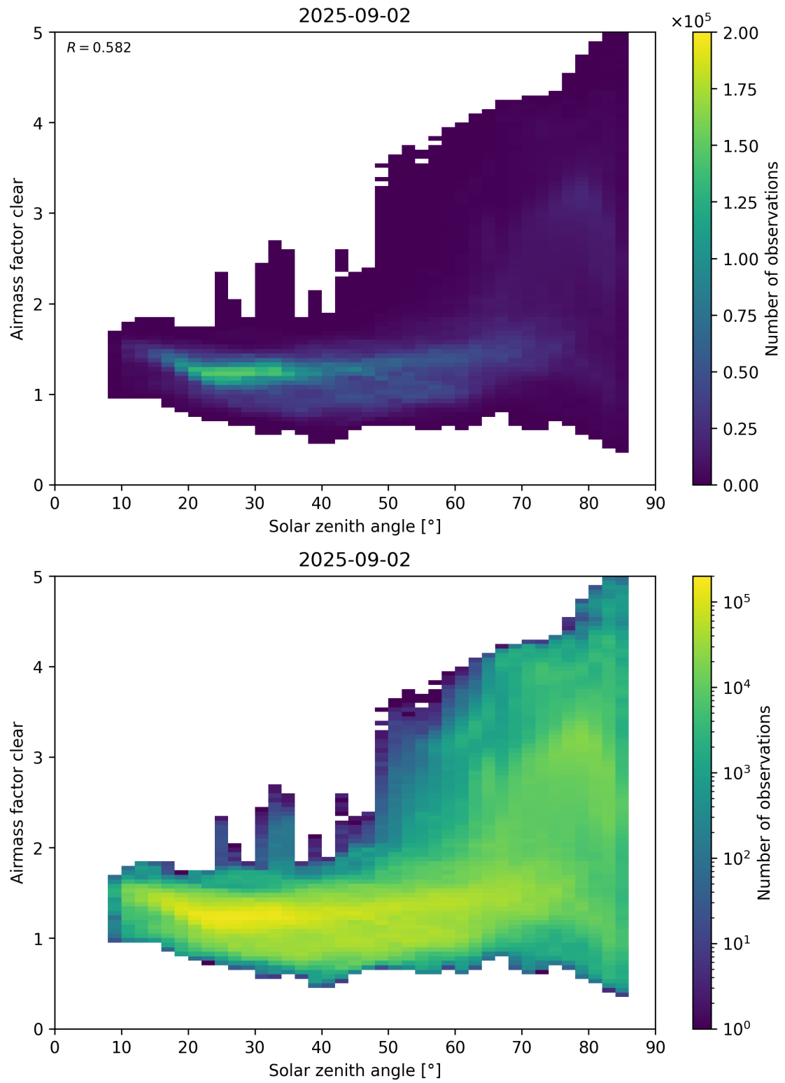
Figure 170: Scatter density plot of “Solar zenith angle” against “Airmass factor clear” for 2025-09-01 to 2025-09-03.
