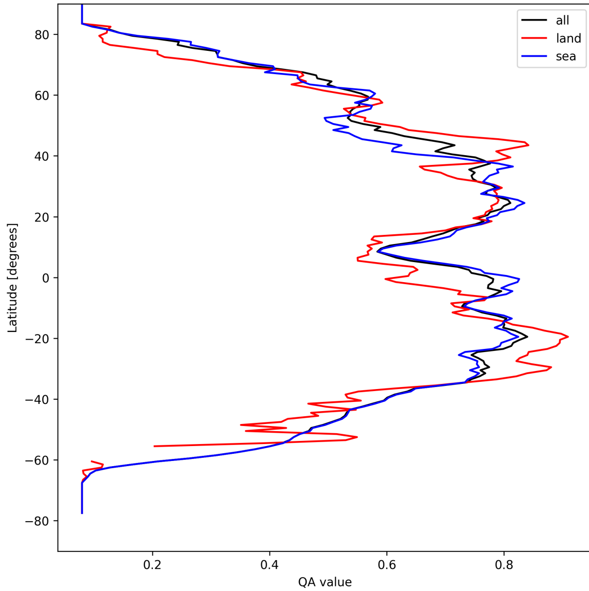
Figure 20: Zonal average of “QA value” for 2025-09-01 to 2025-09-03.
