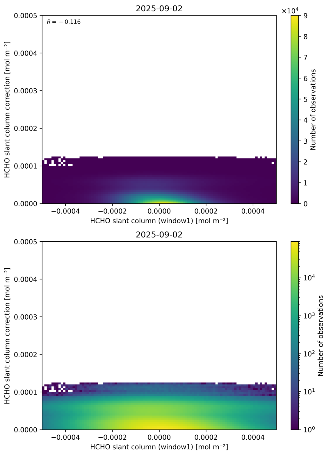
Figure 83: Scatter density plot of “HCHO slant column (window1)” against “HCHO slant column correction” for 2025-09-01 to 2025-09-03.
