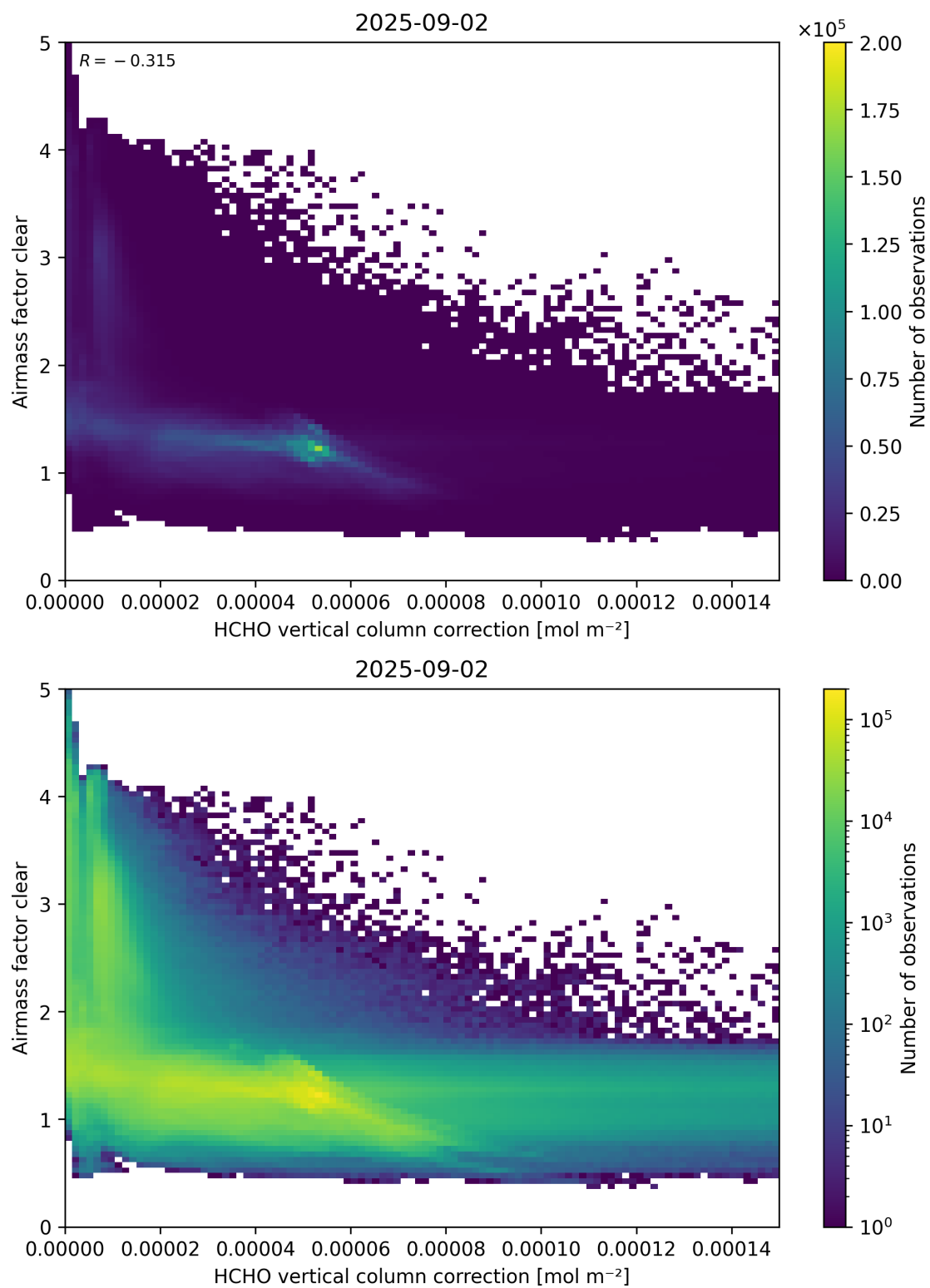
Figure 115: Scatter density plot of “HCHO vertical column correction” against “Airmass factor clear” for 2025-09-01 to 2025-09-03.
