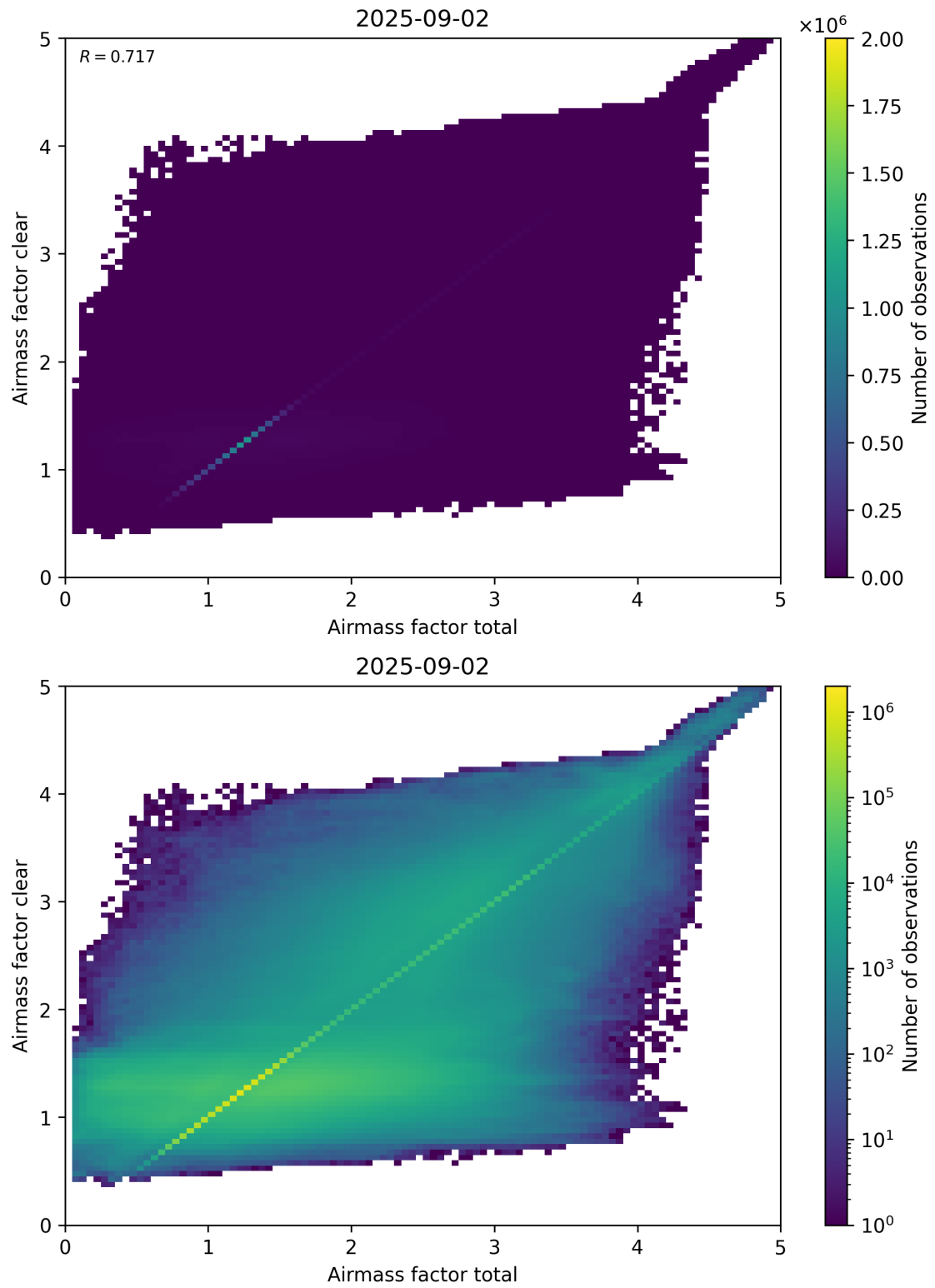
Figure 100: Scatter density plot of “Airmass factor total” against “Airmass factor clear” for 2025-09-01 to 2025-09-03.
