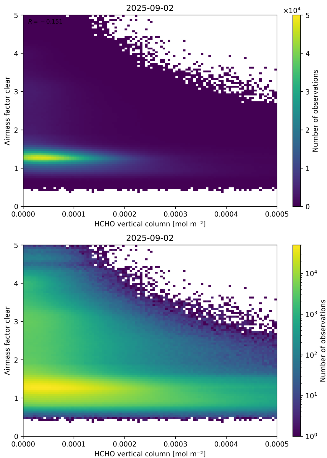
Figure 126: Scatter density plot of “HCHO vertical column” against “Airmass factor clear” for 2025-09-01 to 2025-09-03.
