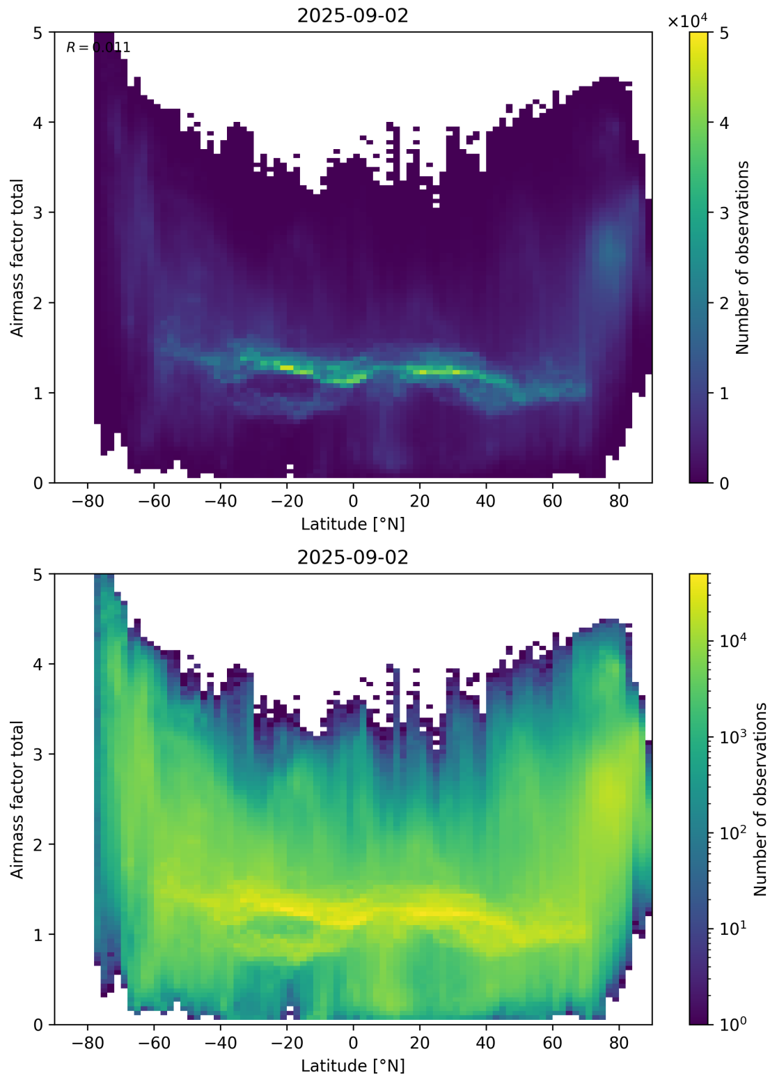
Figure 161: Scatter density plot of “Latitude” against “Airmass factor total” for 2025-09-01 to 2025-09-03.
