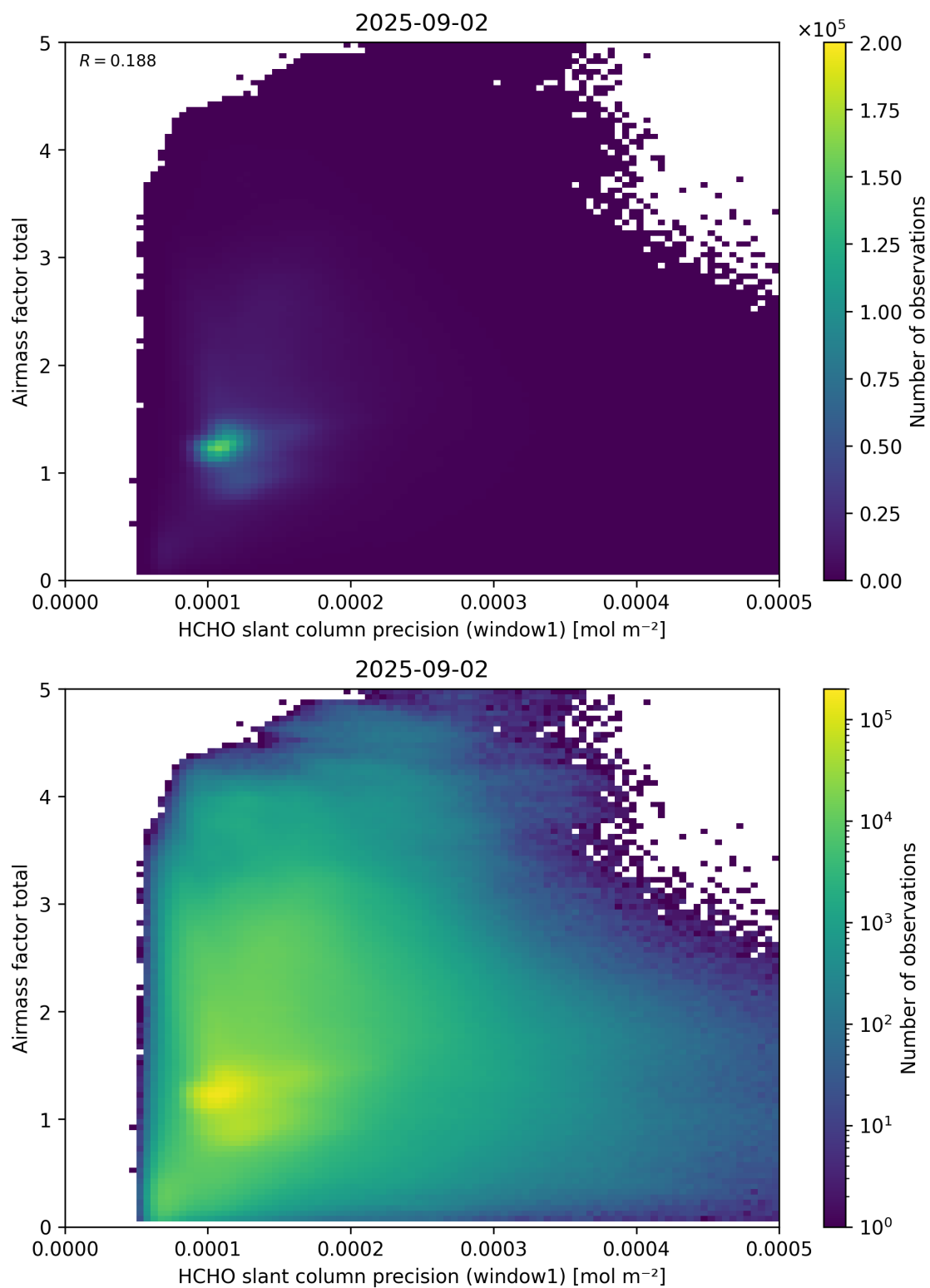
Figure 94: Scatter density plot of “HCHO slant column precision (window1)” against “Airmass factor total” for 2025-09-01 to 2025-09-03.
