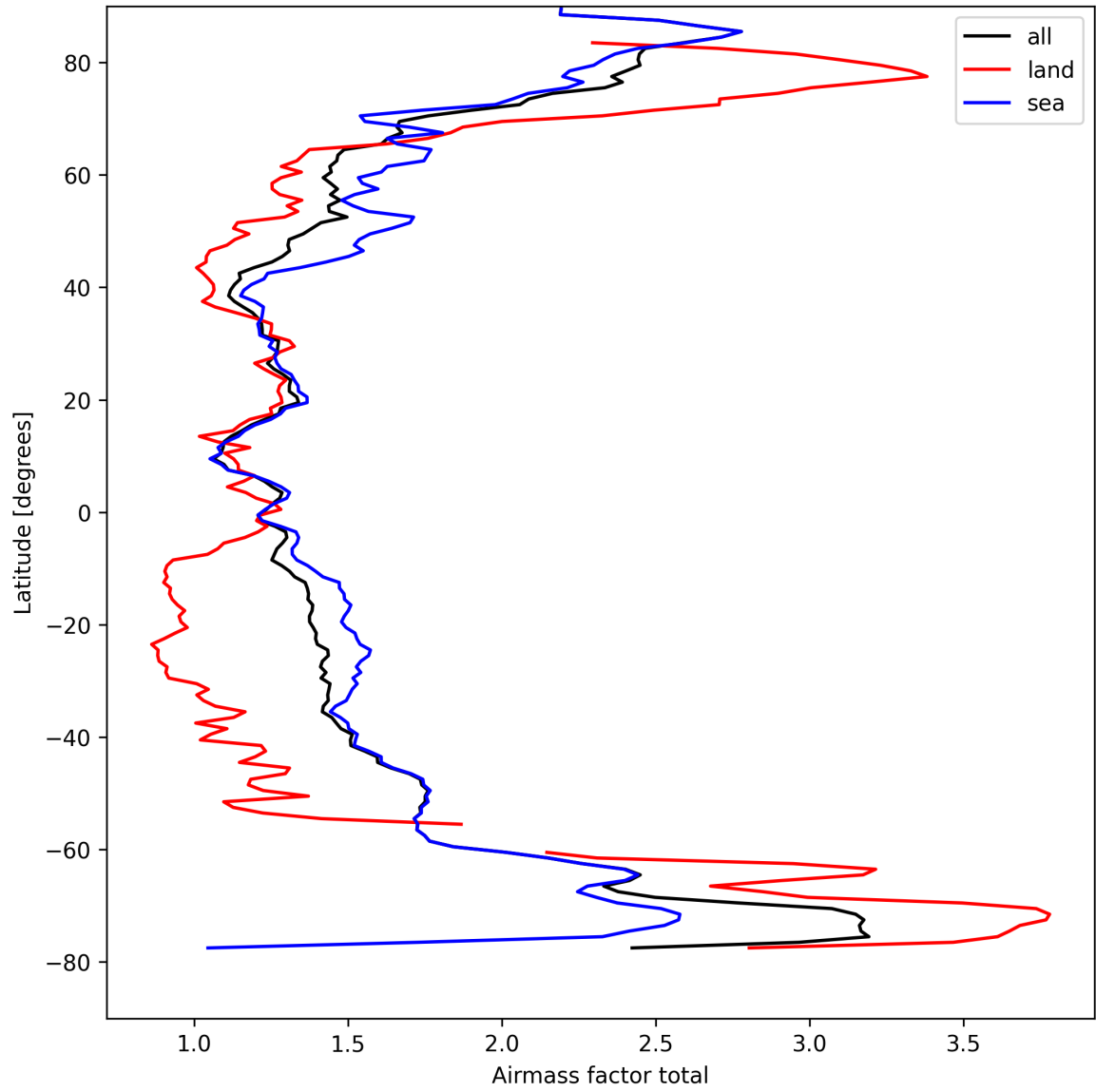
Figure 26: Zonal average of “Airmass factor total” for 2025-09-01 to 2025-09-03.
