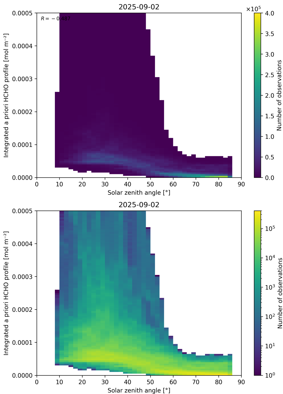
Figure 180: Scatter density plot of “Solar zenith angle” against “Integrated a priori HCHO profile” for 2025-09-01 to 2025-09-03.
