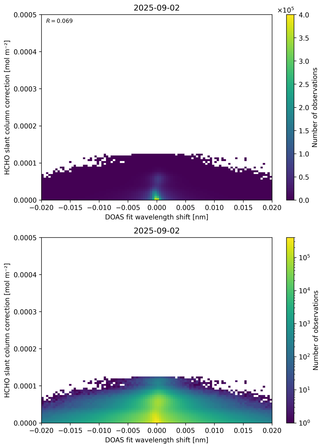
Figure 67: Scatter density plot of “DOAS fit wavelength shift” against “HCHO slant column correction” for 2025-09-01 to 2025-09-03.
