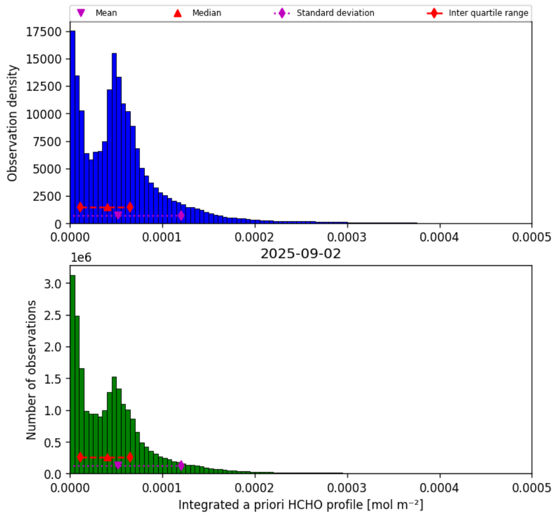
Figure 43: Histogram of “Integrated a priori HCHO profile” for 2025-09-01 to 2025-09-03
