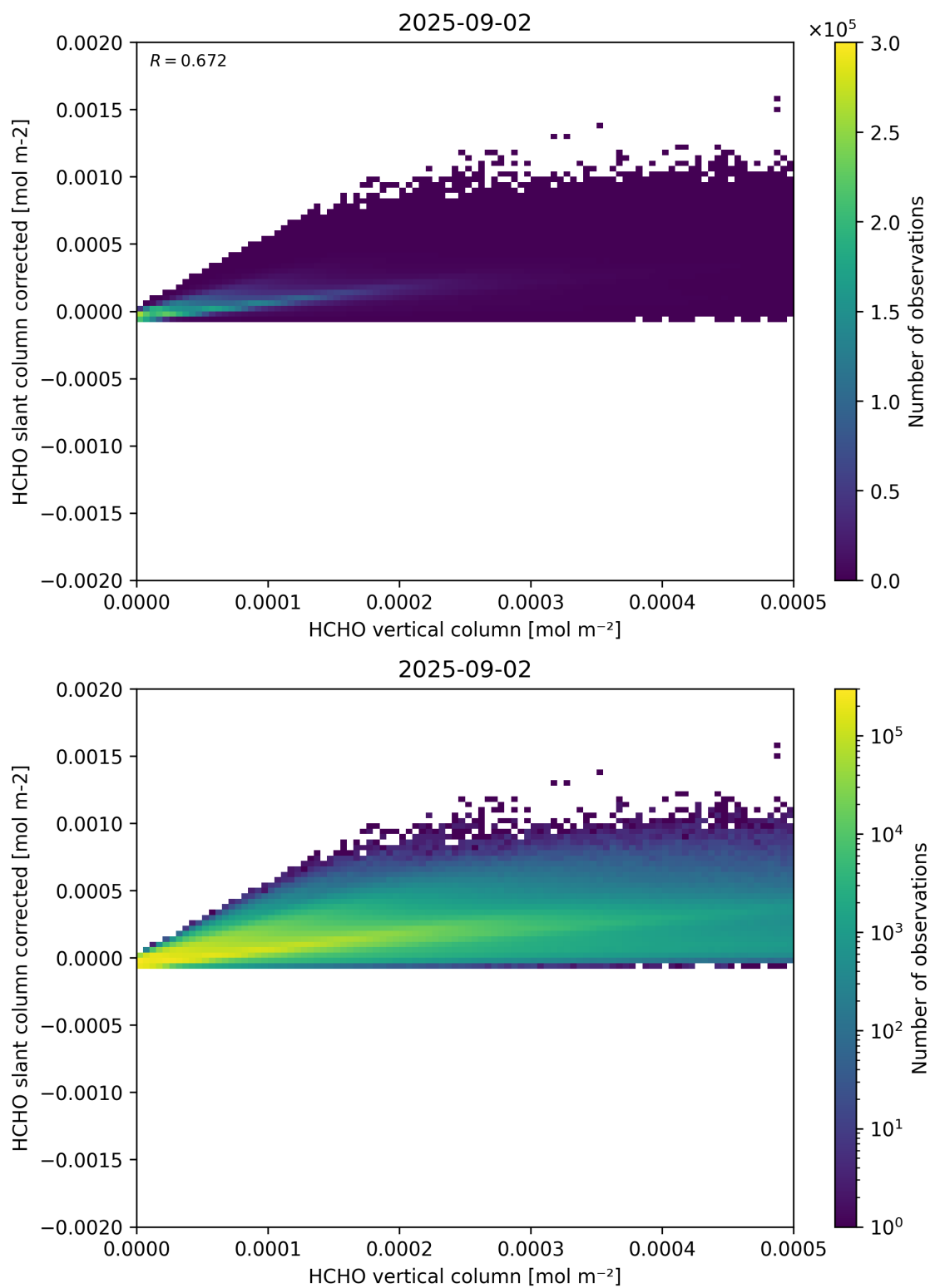
Figure 127: Scatter density plot of “HCHO vertical column” against “HCHO slant column corrected” for 2025-09-01 to 2025-09-03.
