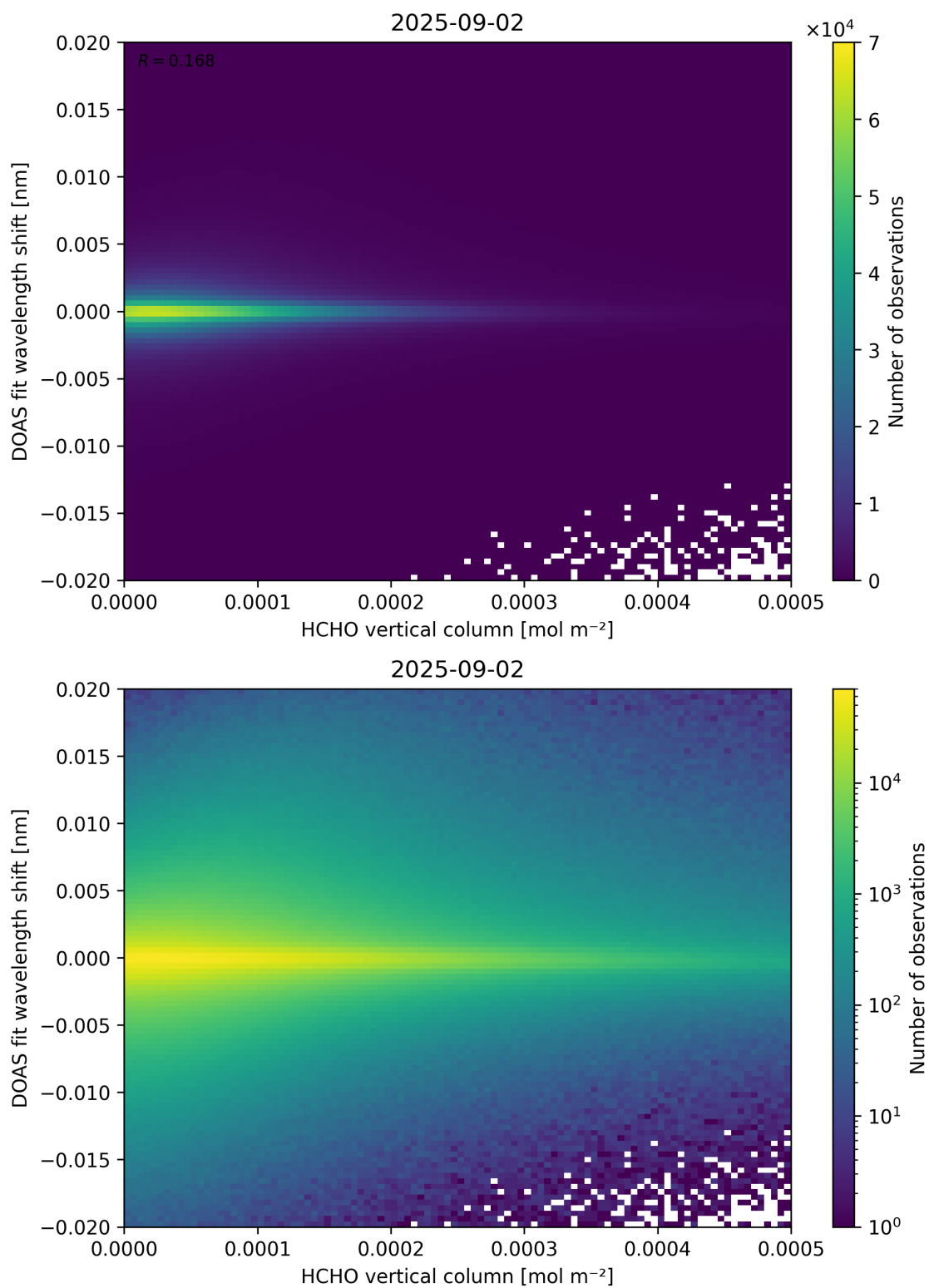
Figure 124: Scatter density plot of “HCHO vertical column” against “DOAS fit wavelength shift” for 2025-09-01 to 2025-09-03.
