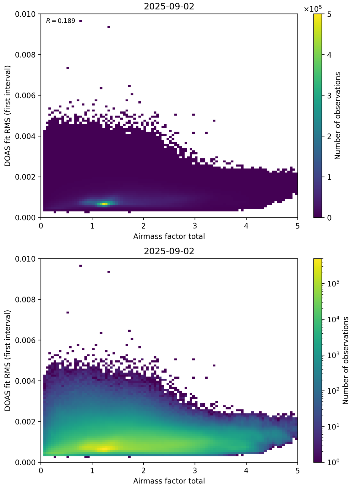
Figure 97: Scatter density plot of “Airmass factor total” against “DOAS fit RMS (first interval)” for 2025-09-01 to 2025-09-03.
