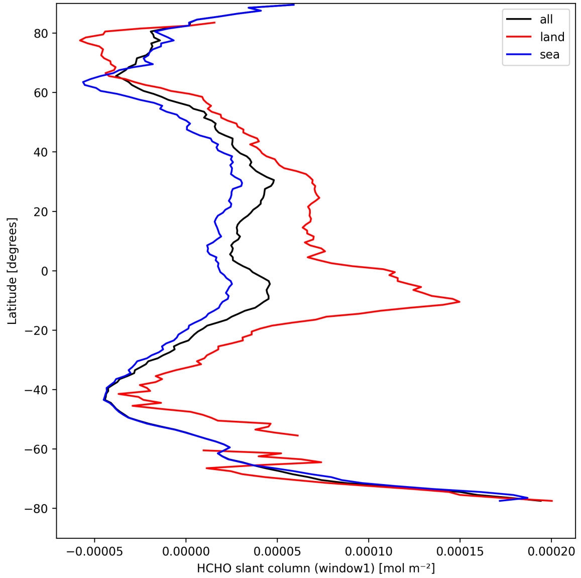
Figure 24: Zonal average of “HCHO slant column (window1)” for 2025-09-01 to 2025-09-03.
