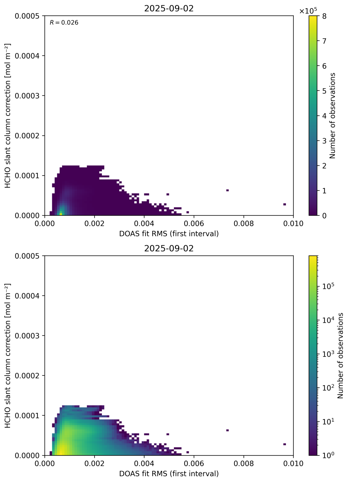
Figure 63: Scatter density plot of “DOAS fit RMS (first interval)” against “HCHO slant column correction” for 2025-09-01 to 2025-09-03.
