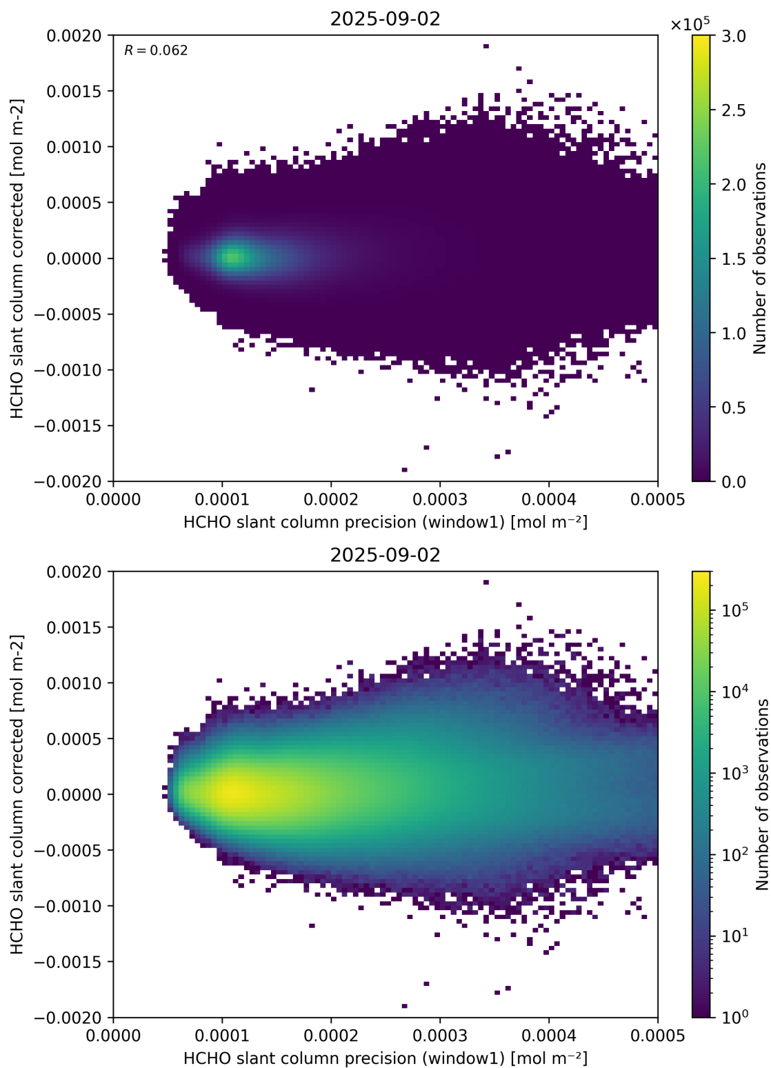
Figure 92: Scatter density plot of “HCHO slant column precision (window1)” against “HCHO slant column corrected” for 2025-09-01 to 2025-09-03.
