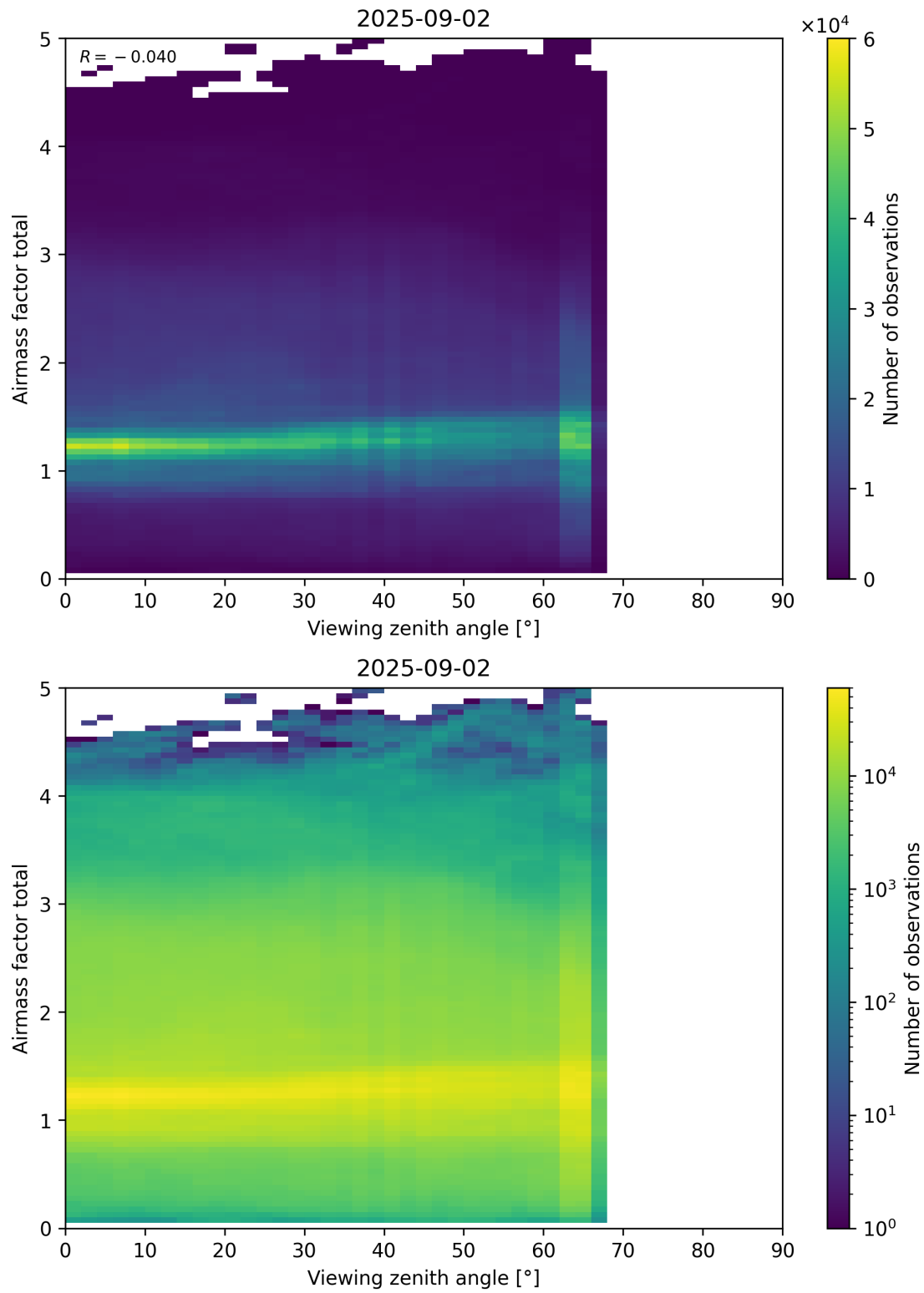
Figure 190: Scatter density plot of “Viewing zenith angle” against “Airmass factor total” for 2025-09-01 to 2025-09-03.
