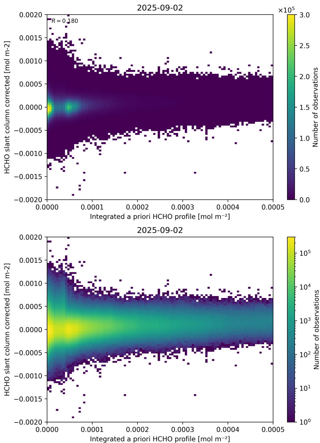
Figure 151: Scatter density plot of “Integrated a priori HCHO profile” against “HCHO slant column corrected” for 2025-09-01 to 2025-09-03.
