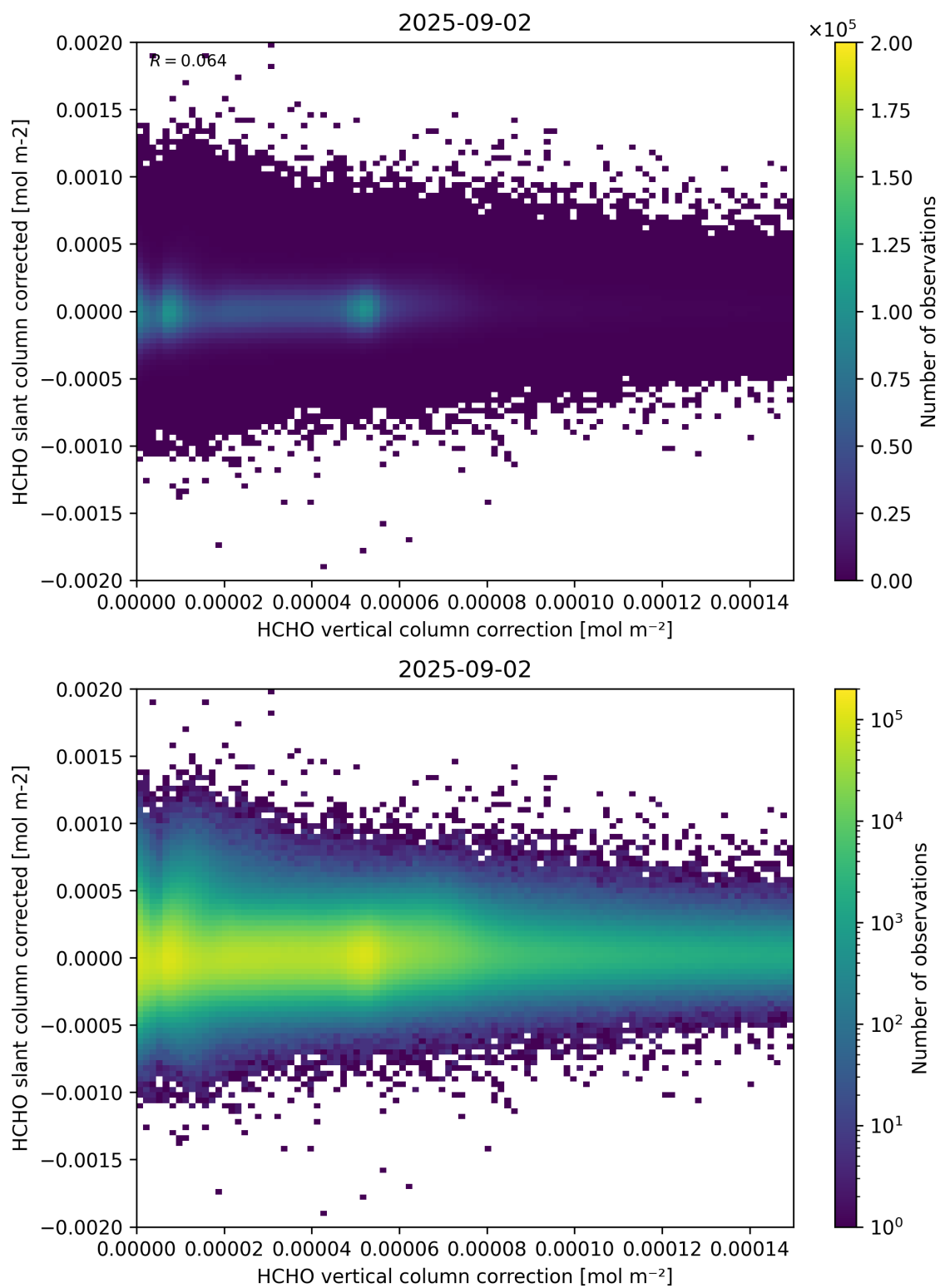
Figure 116: Scatter density plot of “HCHO vertical column correction” against “HCHO slant column corrected” for 2025-09-01 to 2025-09-03.
