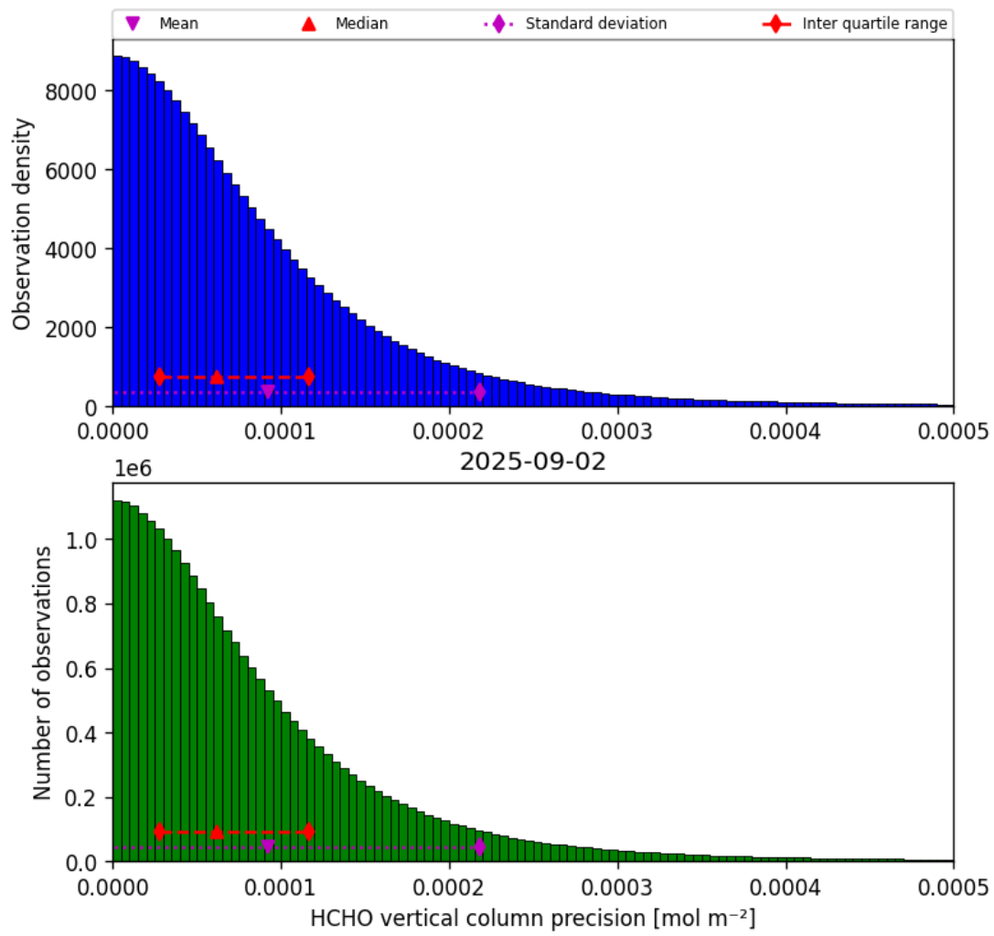
Figure 36: Histogram of “HCHO vertical column precision” for 2025-09-01 to 2025-09-03
