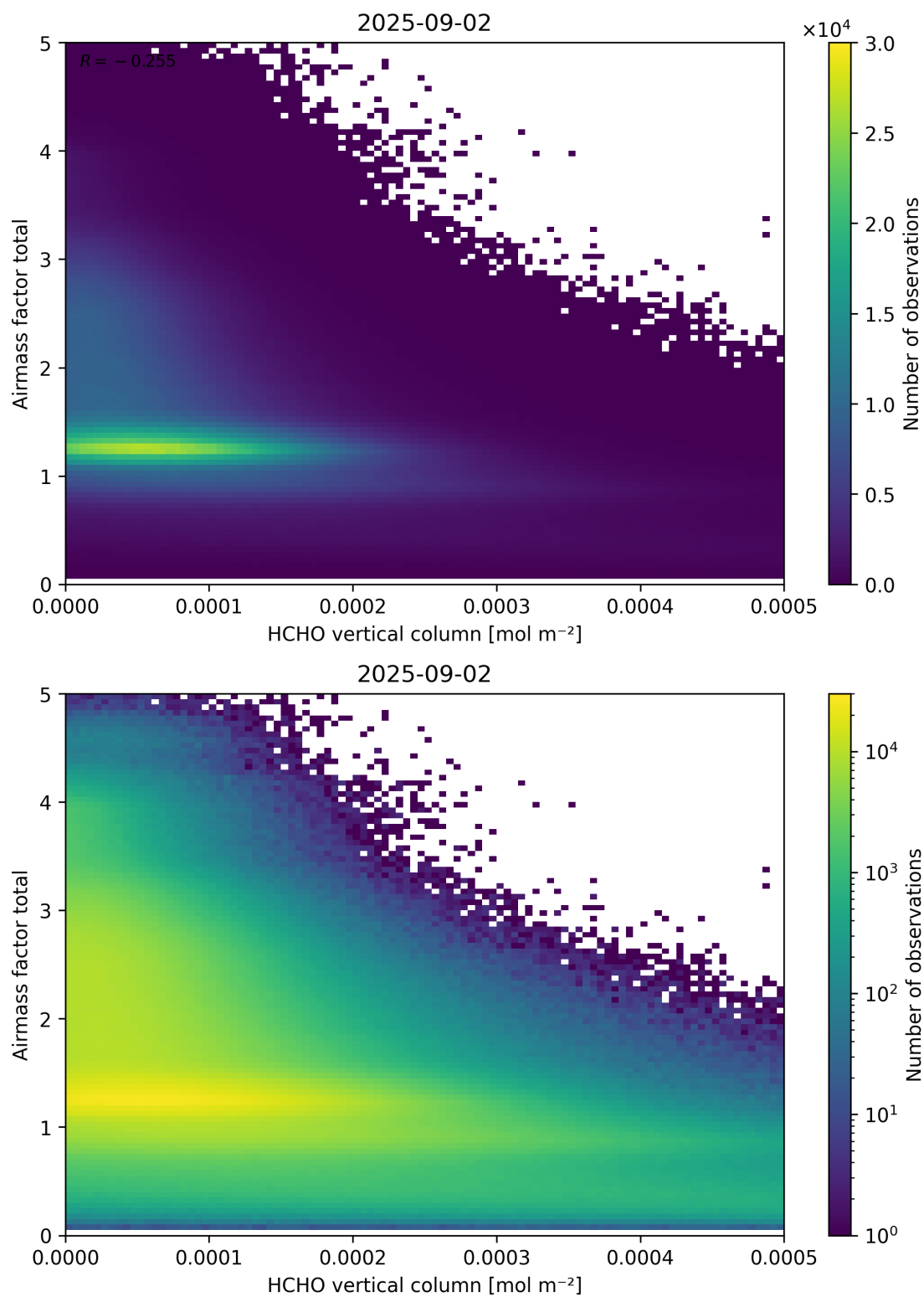
Figure 131: Scatter density plot of “HCHO vertical column” against “Airmass factor total” for 2025-09-01 to 2025-09-03.
