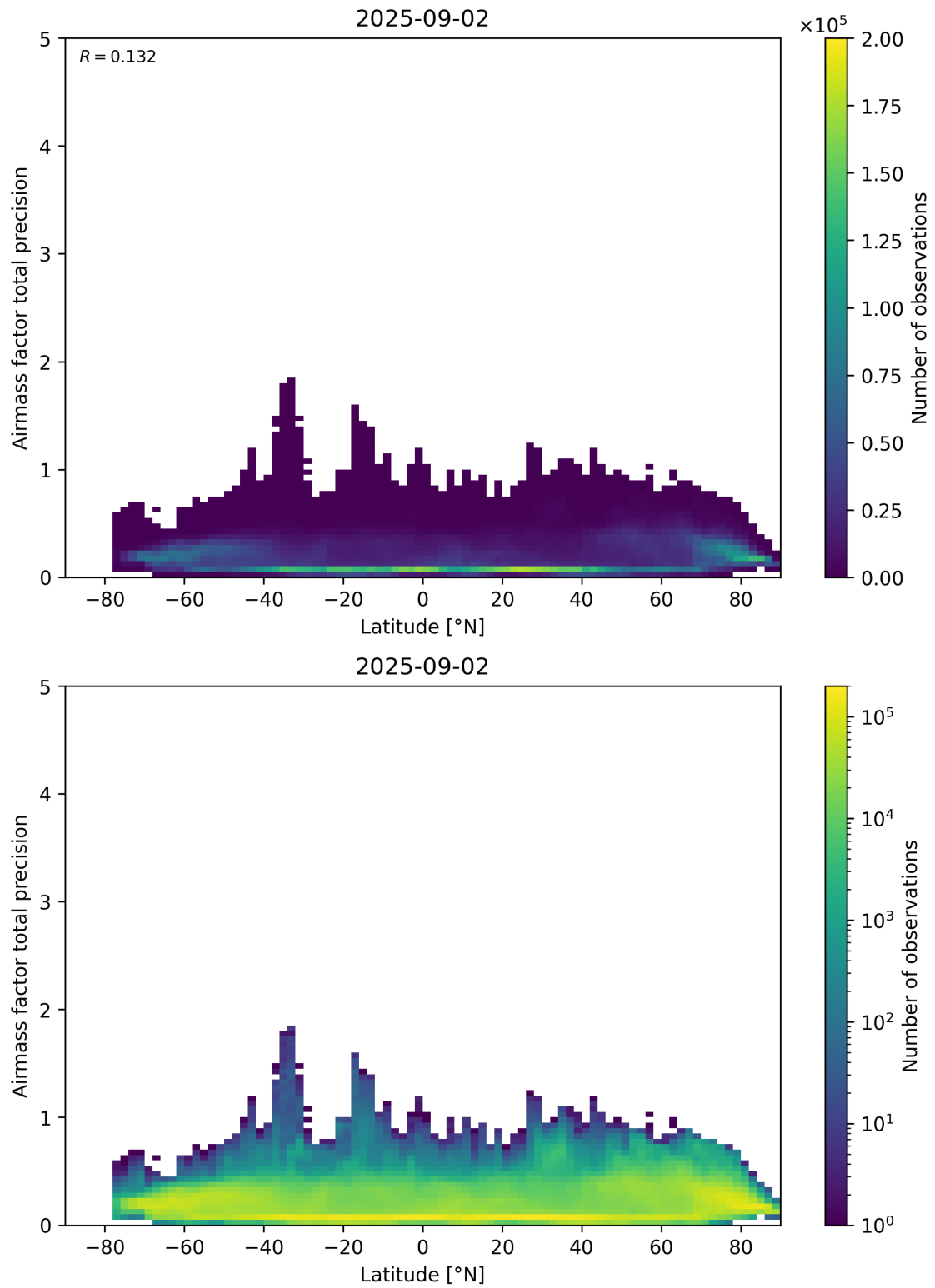
Figure 162: Scatter density plot of “Latitude” against “Airmass factor total precision” for 2025-09-01 to 2025-09-03.
