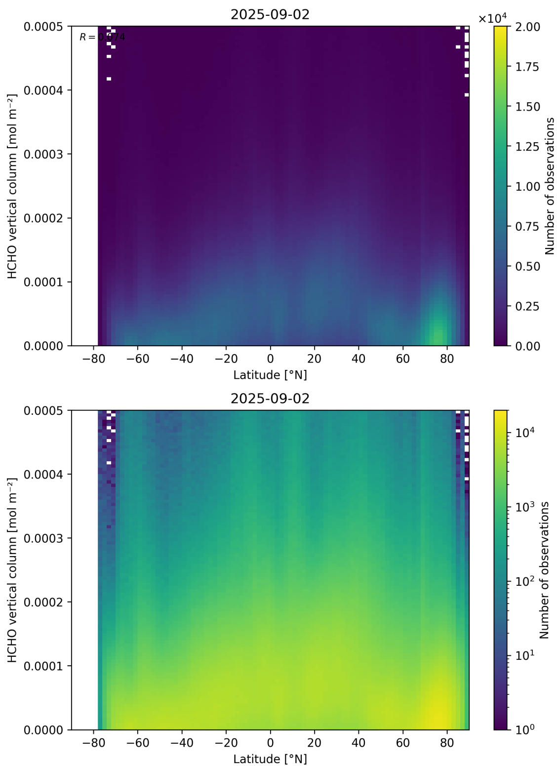
Figure 163: Scatter density plot of “Latitude” against “HCHO vertical column” for 2025-09-01 to 2025-09-03.
