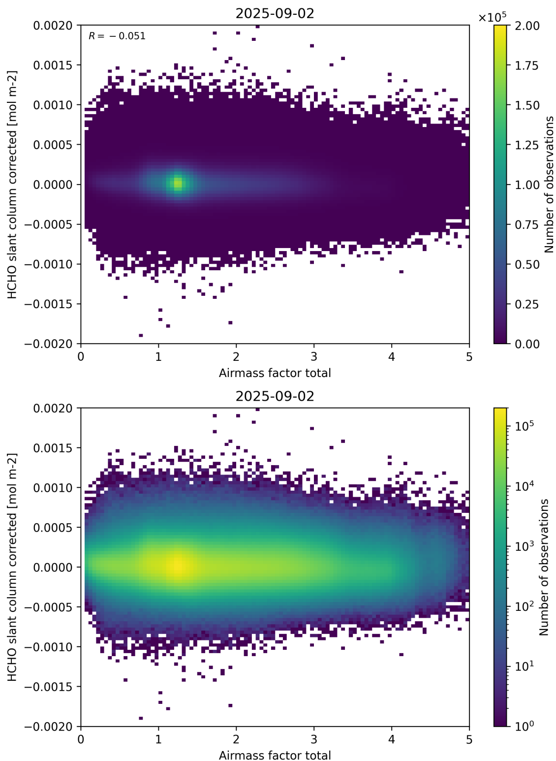
Figure 101: Scatter density plot of “Airmass factor total” against “HCHO slant column corrected” for 2025-09-01 to 2025-09-03.
