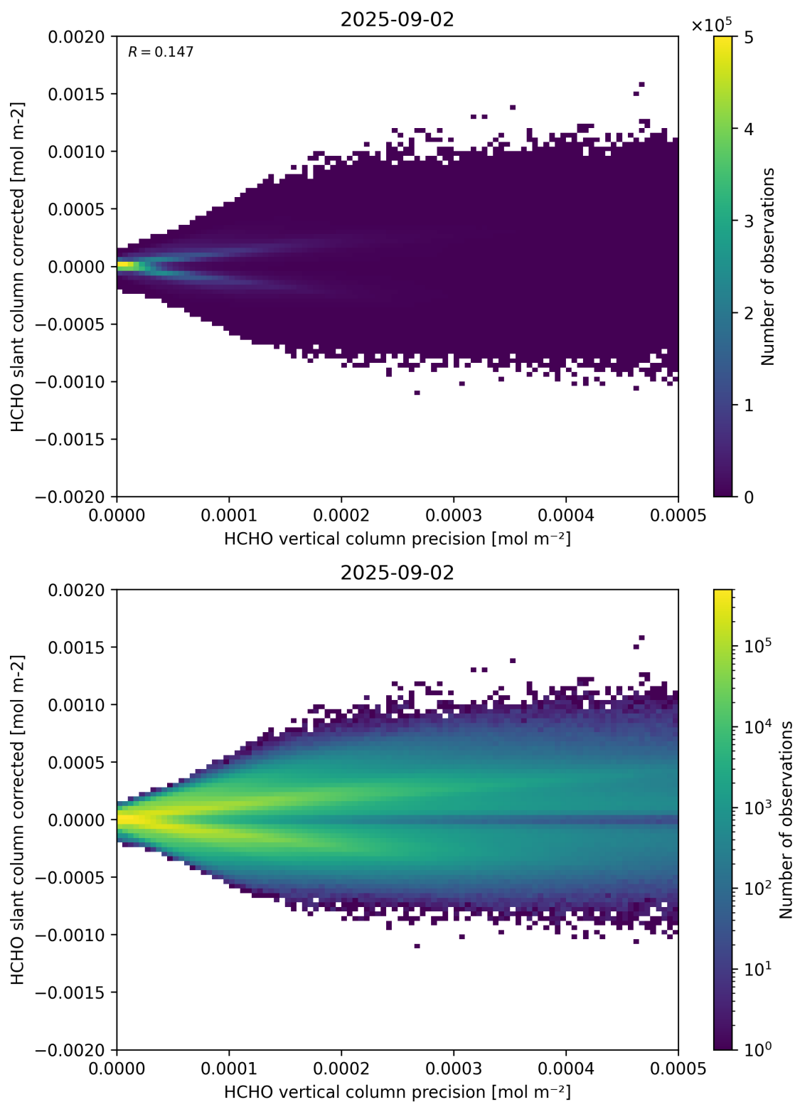
Figure 140: Scatter density plot of “HCHO vertical column precision” against “HCHO slant column corrected” for 2025-09-01 to 2025-09-03.
