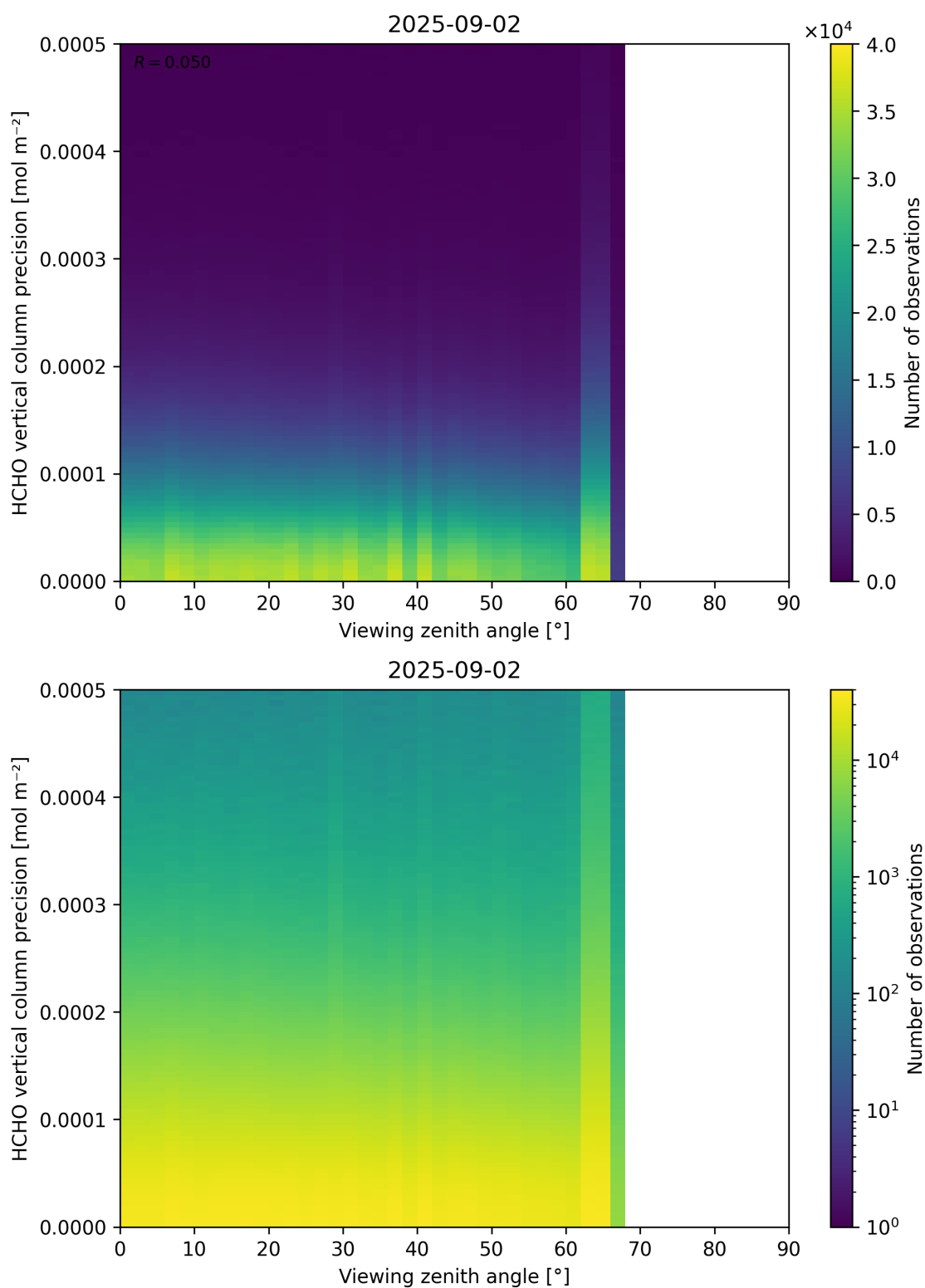
Figure 194: Scatter density plot of “Viewing zenith angle” against “HCHO vertical column precision” for 2025-09-01 to 2025-09-03.
