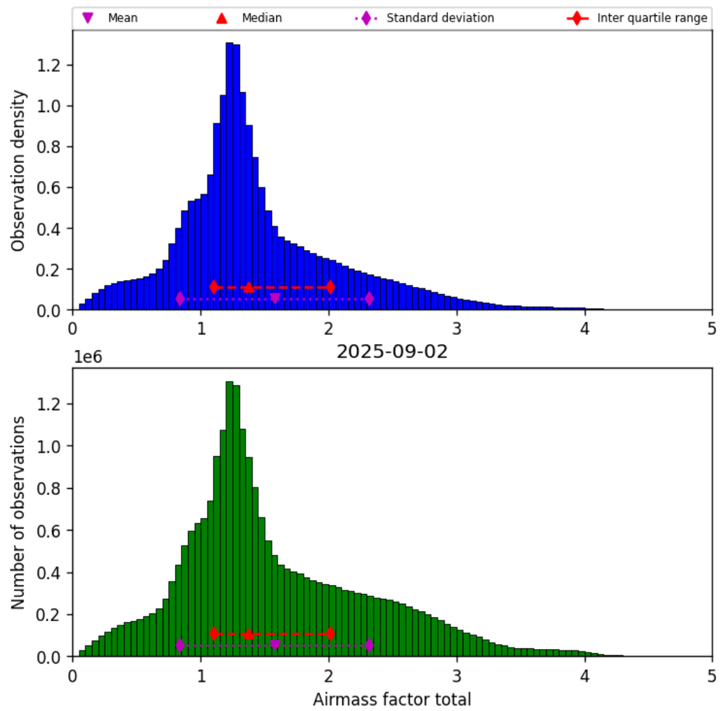
Figure 40: Histogram of “Airmass factor total” for 2025-09-01 to 2025-09-03
