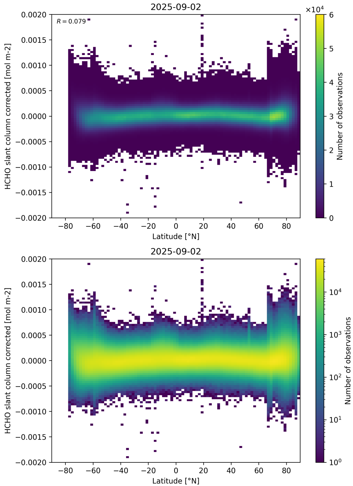
Figure 157: Scatter density plot of “Latitude” against “HCHO slant column corrected” for 2025-09-01 to 2025-09-03.
