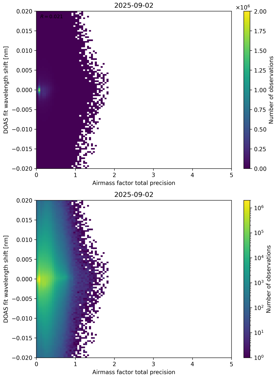
Figure 106: Scatter density plot of “Airmass factor total precision” against “DOAS fit wavelength shift” for 2025-09-01 to 2025-09-03.
