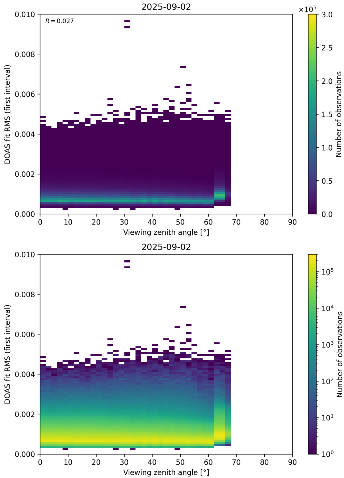
Figure 182: Scatter density plot of “Viewing zenith angle” against “DOAS fit RMS (first interval)” for 2025-09-01 to 2025-09-03.
