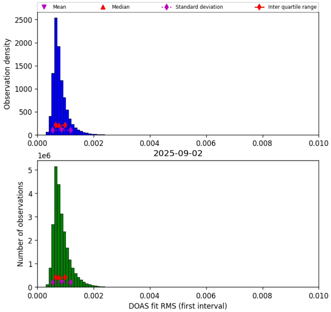
Figure 46: Histogram of “DOAS fit RMS (first interval)” for 2025-09-01 to 2025-09-03
