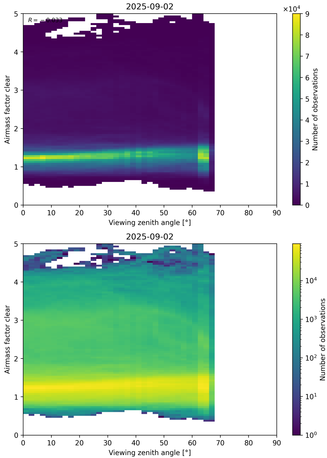
Figure 185: Scatter density plot of “Viewing zenith angle” against “Airmass factor clear” for 2025-09-01 to 2025-09-03.
