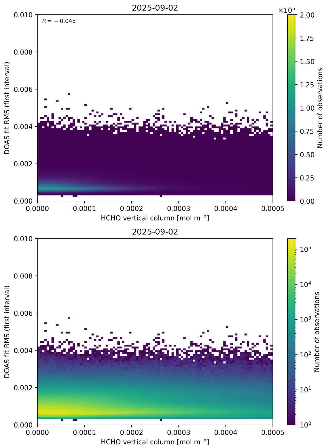
Figure 123: Scatter density plot of “HCHO vertical column” against “DOAS fit RMS (first interval)” for 2025-09-01 to 2025-09-03.
