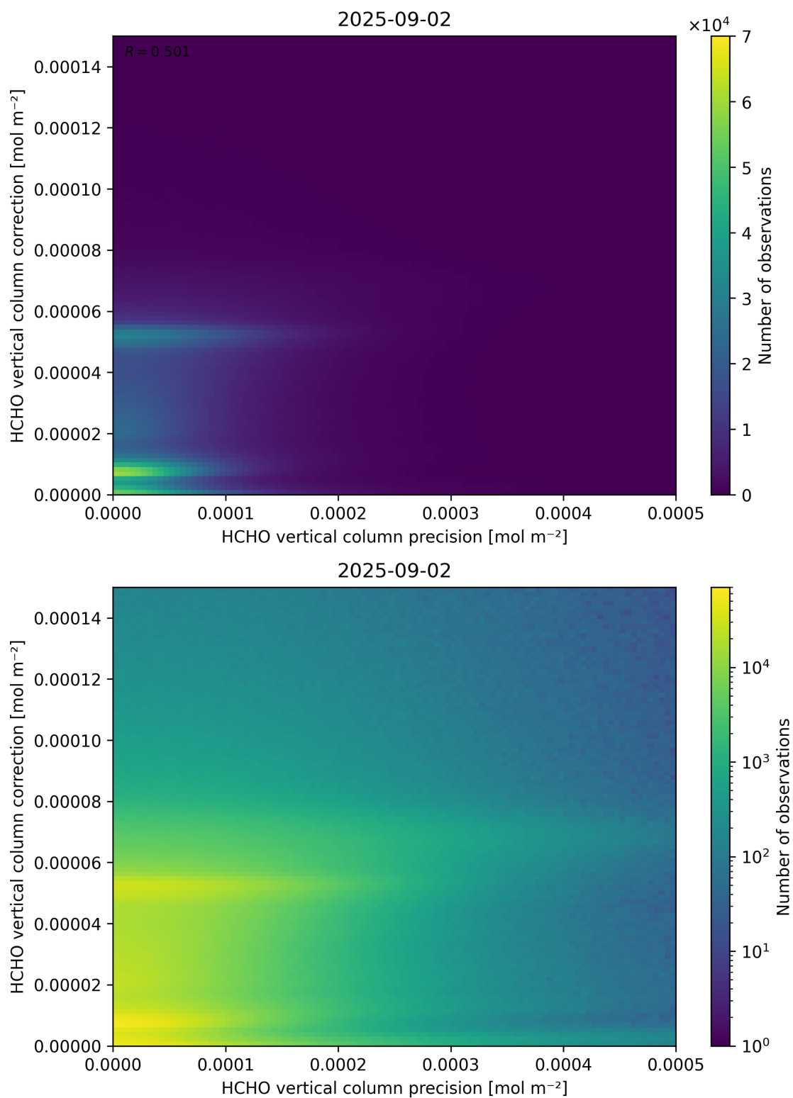
Figure 146: Scatter density plot of “HCHO vertical column precision” against “HCHO vertical column correction” for 2025-09-01 to 2025-09-03.
