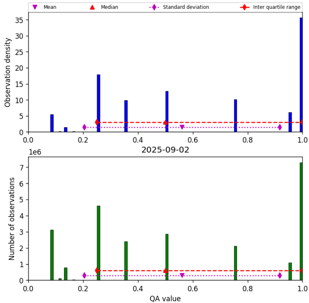
Figure 34: Histogram of “QA value” for 2025-09-01 to 2025-09-03
