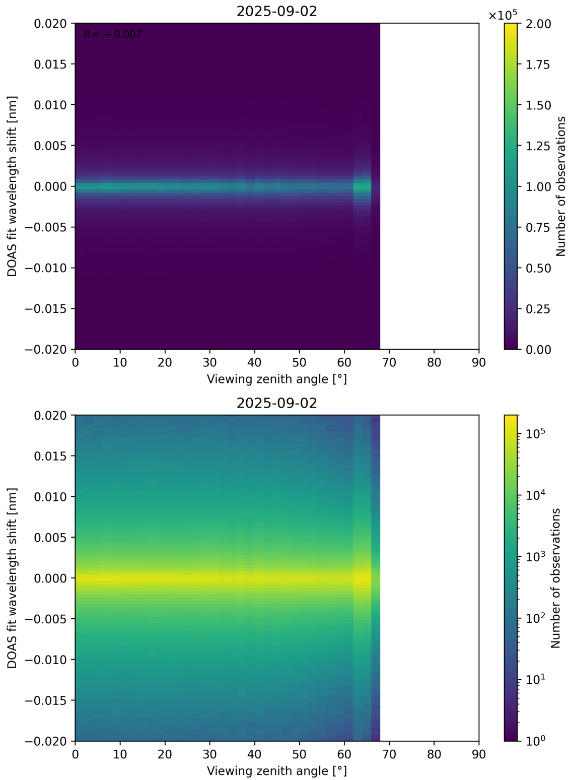
Figure 183: Scatter density plot of “Viewing zenith angle” against “DOAS fit wavelength shift” for 2025-09-01 to 2025-09-03.
