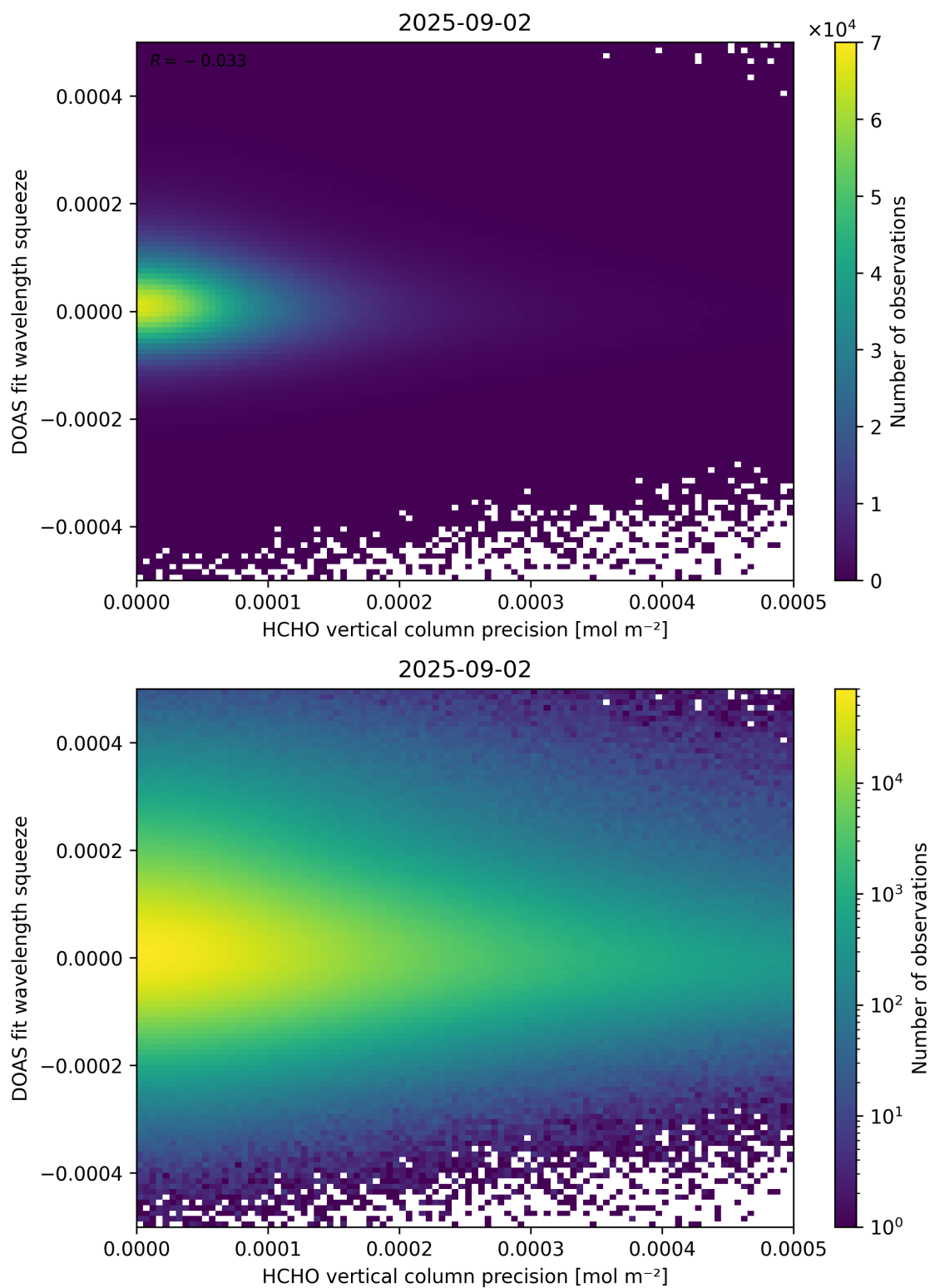
Figure 138: Scatter density plot of “HCHO vertical column precision” against “DOAS fit wavelength squeeze” for 2025-09-01 to 2025-09-03.
