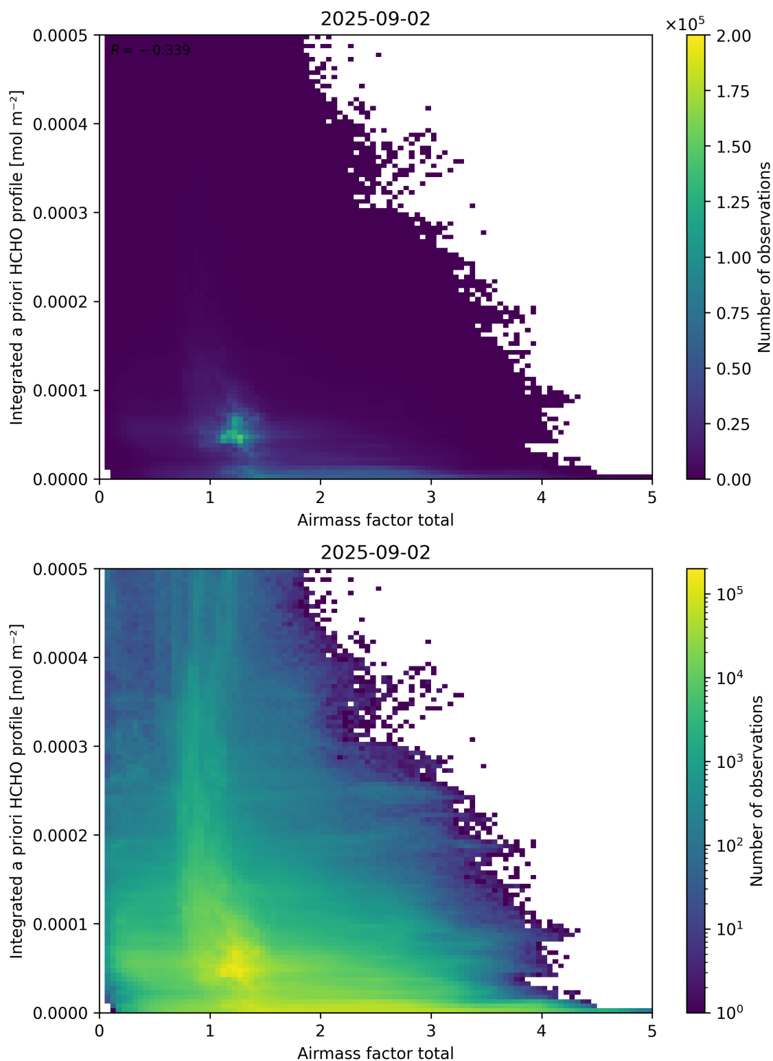
Figure 104: Scatter density plot of “Airmass factor total” against “Integrated a priori HCHO profile” for 2025-09-01 to 2025-09-03.
