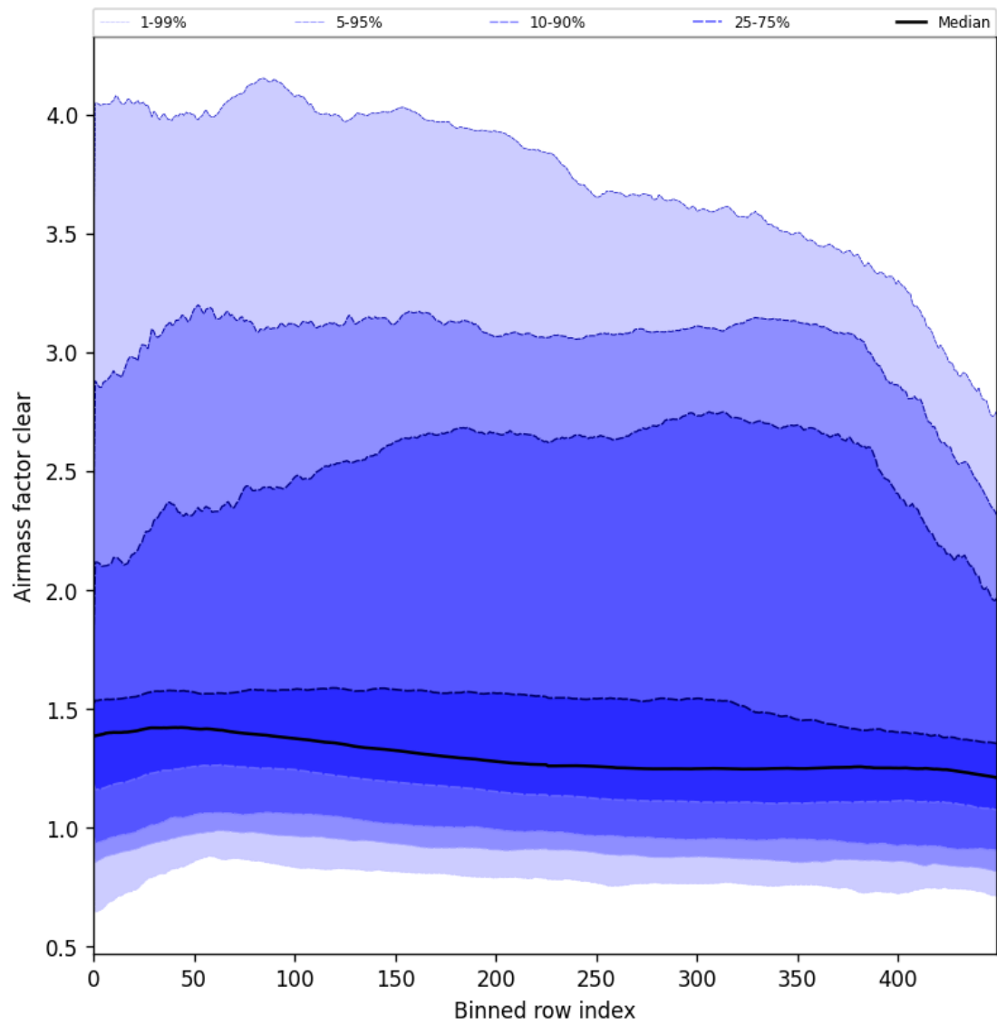
Figure 56: Along track statistics of “Air mass factor clear” for 2025-09-01 to 2025-09-03
