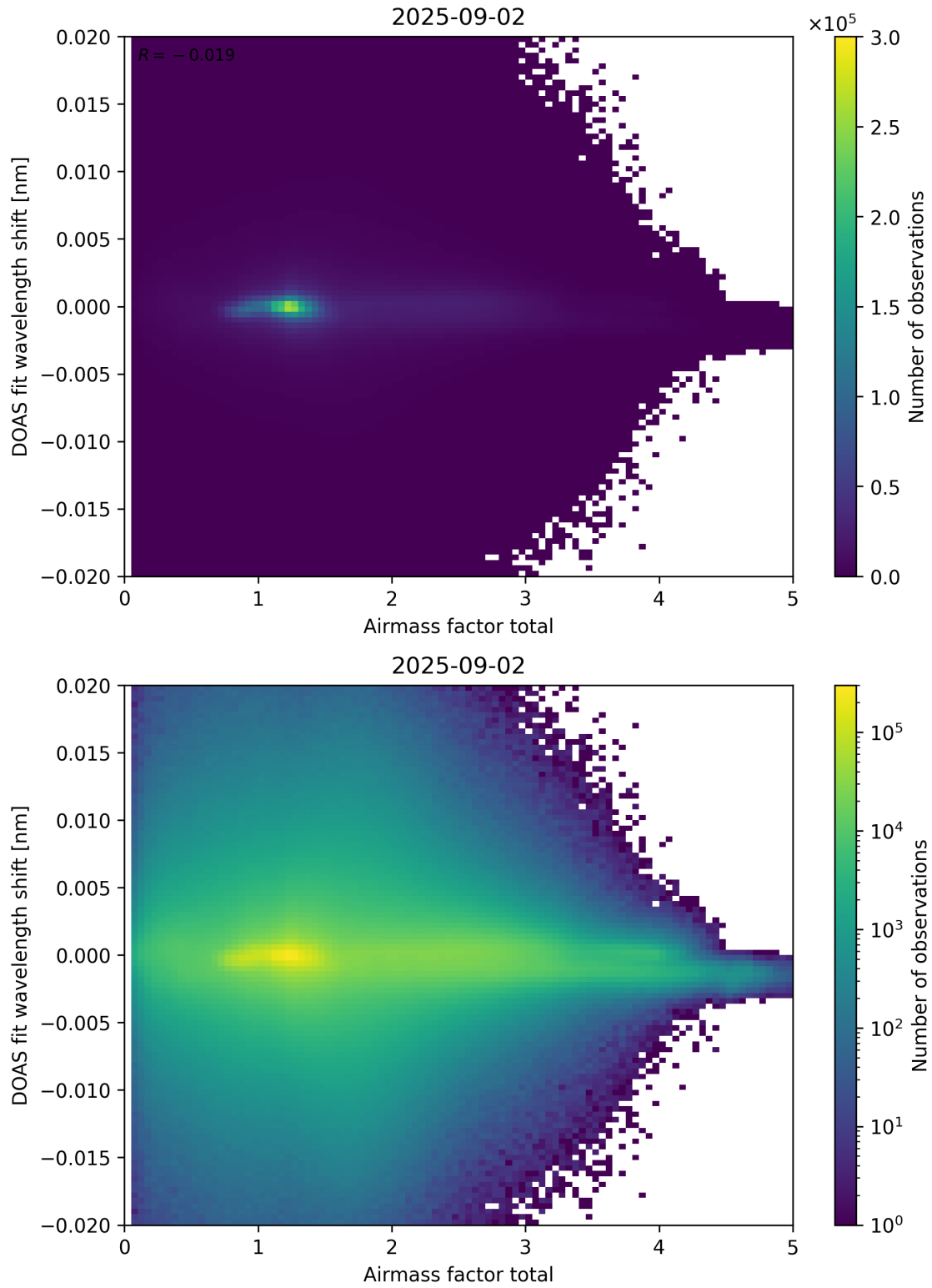
Figure 98: Scatter density plot of “Airmass factor total” against “DOAS fit wavelength shift” for 2025-09-01 to 2025-09-03.
