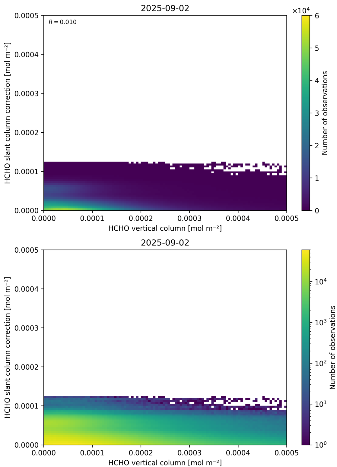
Figure 128: Scatter density plot of “HCHO vertical column” against “HCHO slant column correction” for 2025-09-01 to 2025-09-03.
