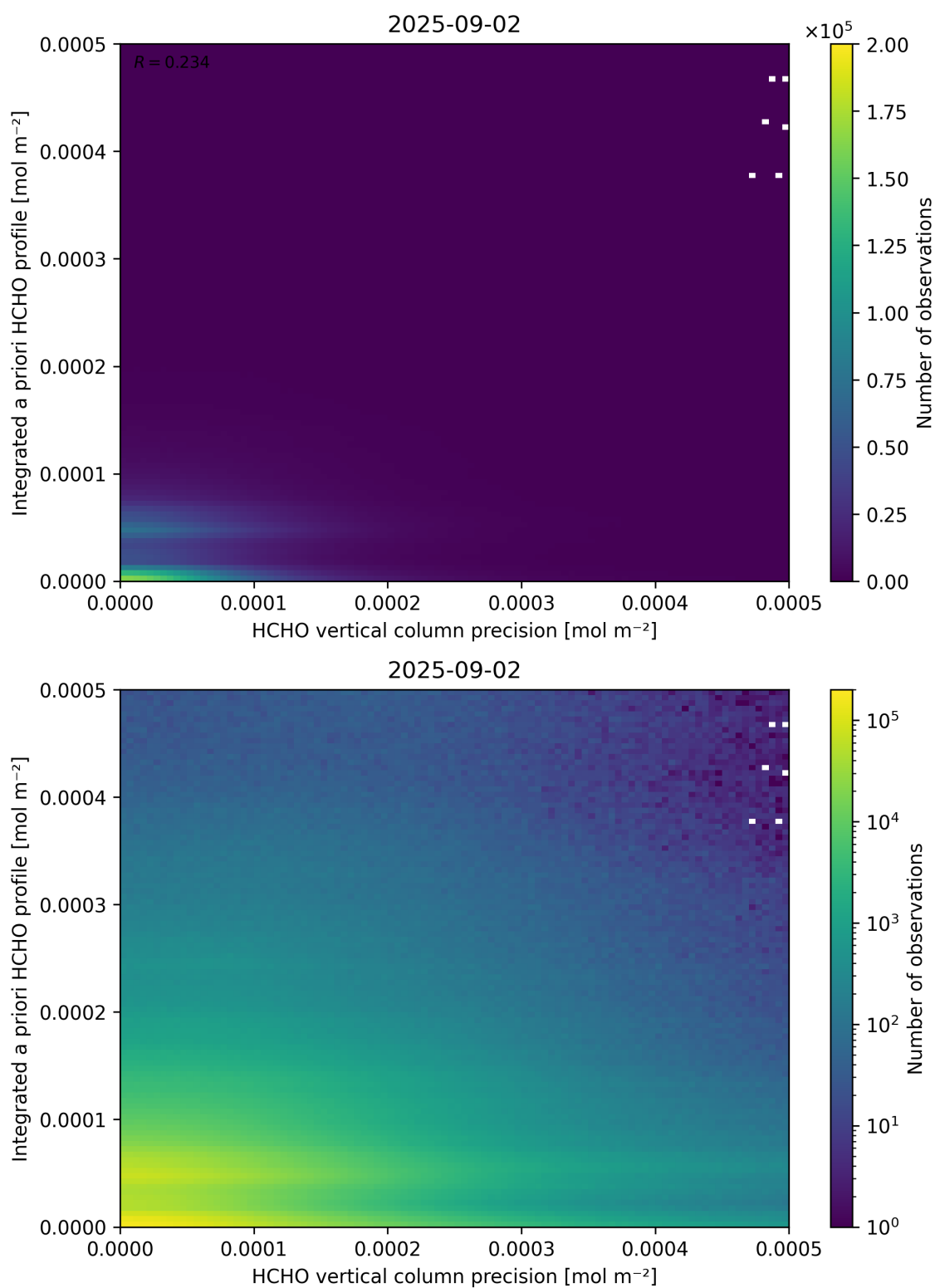
Figure 147: Scatter density plot of “HCHO vertical column precision” against “Integrated a priori HCHO profile” for 2025-09-01 to 2025-09-03.
