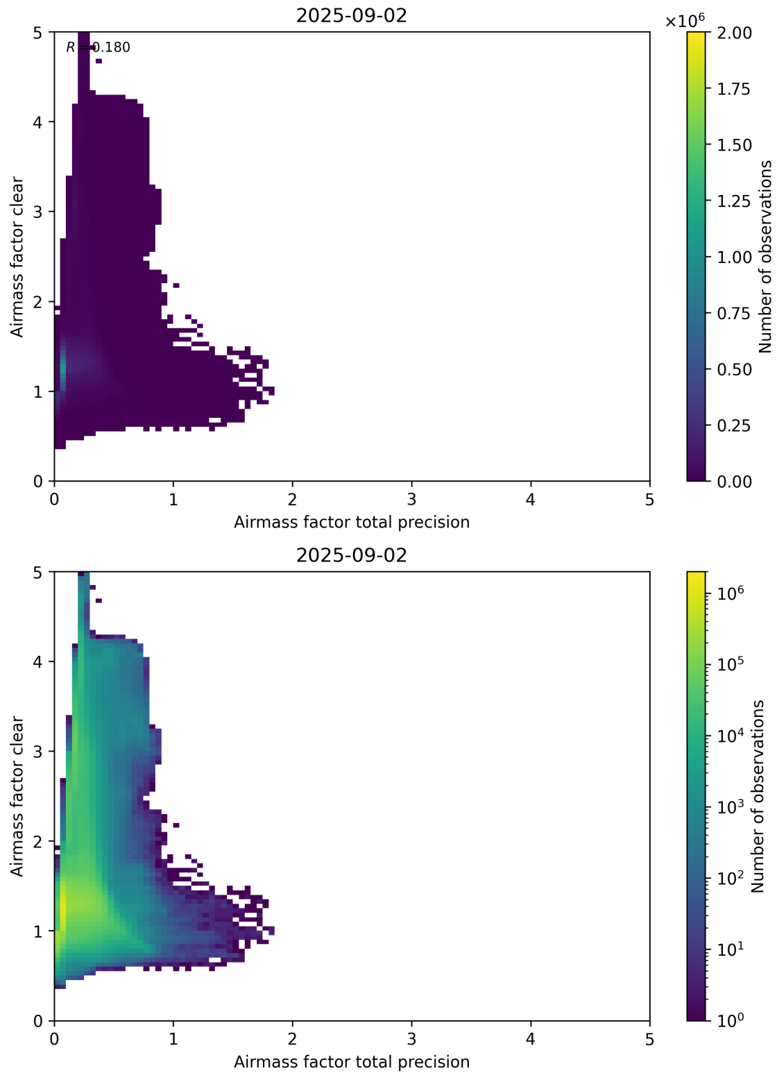
Figure 108: Scatter density plot of “Airmass factor total precision” against “Airmass factor clear” for 2025-09-01 to 2025-09-03.
