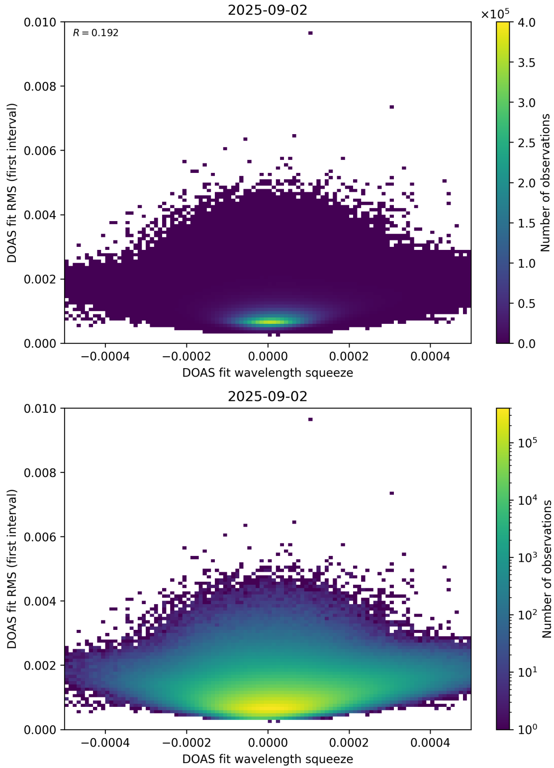
Figure 68: Scatter density plot of “DOAS fit wavelength squeeze” against “DOAS fit RMS (first interval)” for 2025-09-01 to 2025-09-03.
