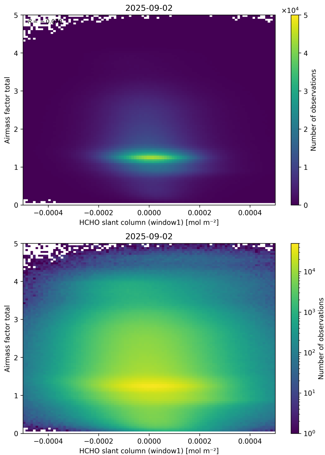
Figure 85: Scatter density plot of “HCHO slant column (window1)” against “Airmass factor total” for 2025-09-01 to 2025-09-03.
