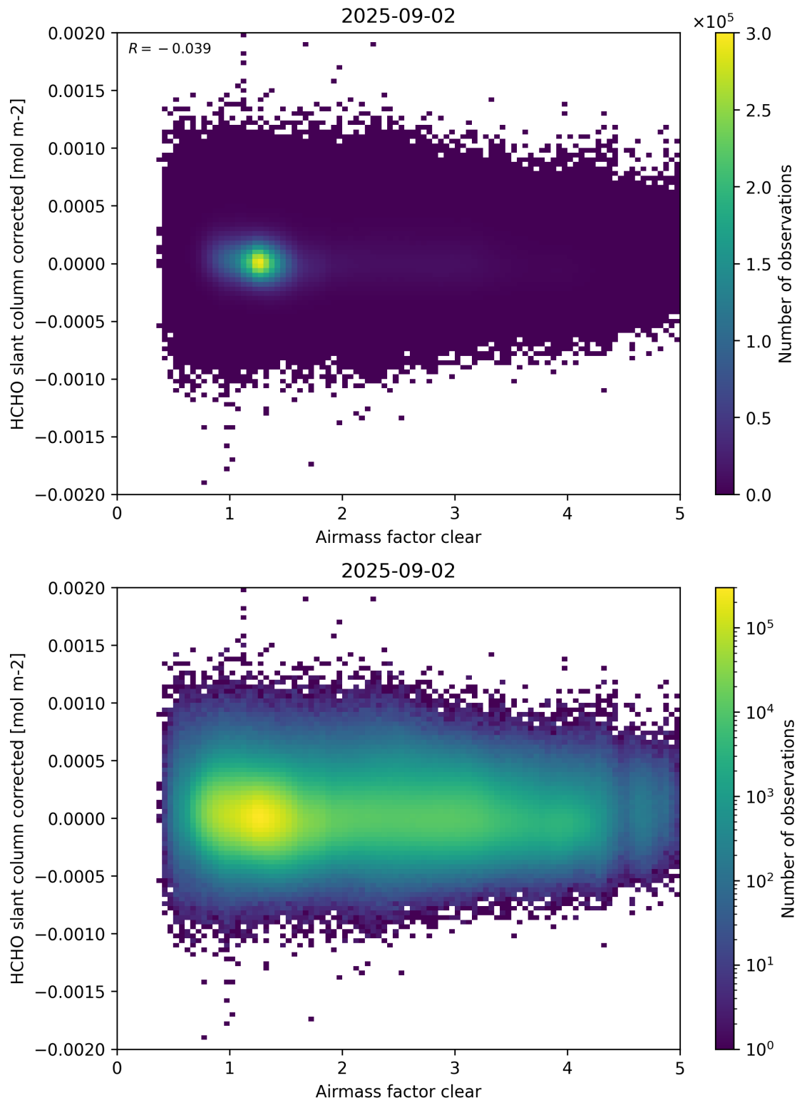
Figure 74: Scatter density plot of “Airmass factor clear” against “HCHO slant column corrected” for 2025-09-01 to 2025-09-03.
