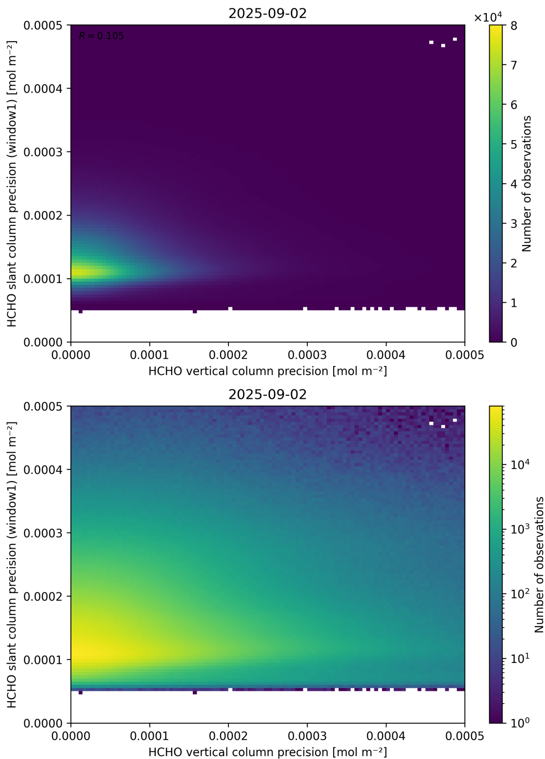
Figure 143: Scatter density plot of “HCHO vertical column precision” against “HCHO slant column precision (window1)” for 2025-09-01 to 2025-09-03.
