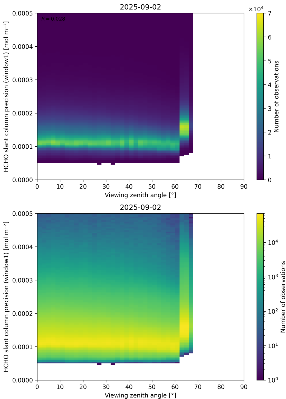
Figure 189: Scatter density plot of “Viewing zenith angle” against “HCHO slant column precision (window1)” for 2025-09-01 to 2025-09-03.
