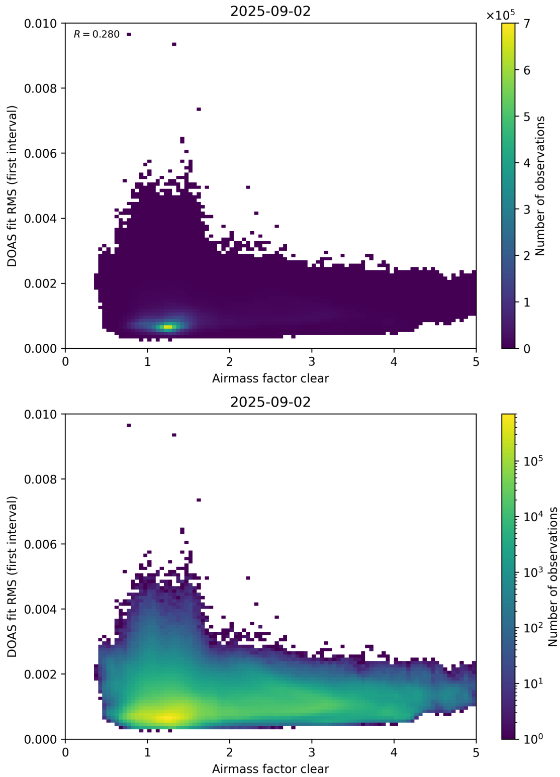
Figure 71: Scatter density plot of “Airmass factor clear” against “DOAS fit RMS (first interval)” for 2025-09-01 to 2025-09-03.
