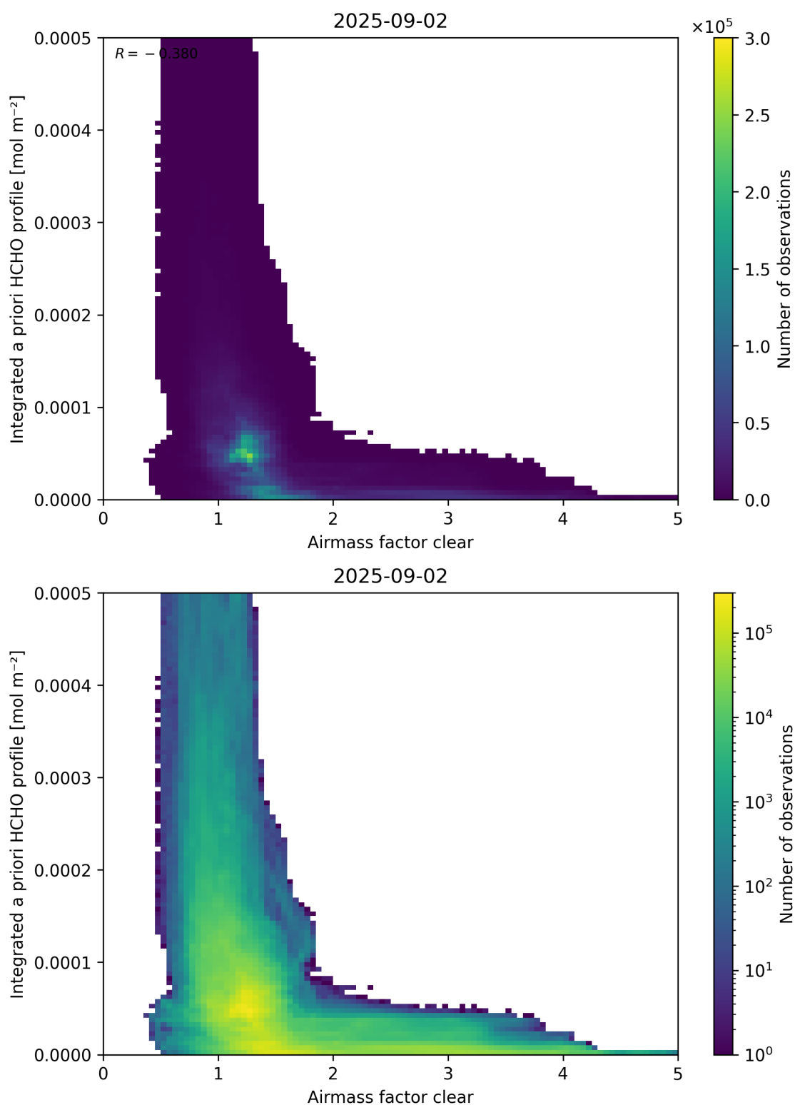
Figure 76: Scatter density plot of “Airmass factor clear” against “Integrated a priori HCHO profile” for 2025-09-01 to 2025-09-03.
