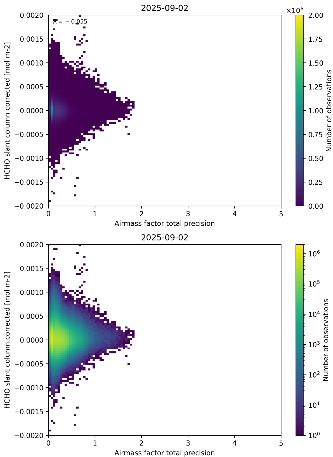
Figure 109: Scatter density plot of “Airmass factor total precision” against “HCHO slant column corrected” for 2025-09-01 to 2025-09-03.
