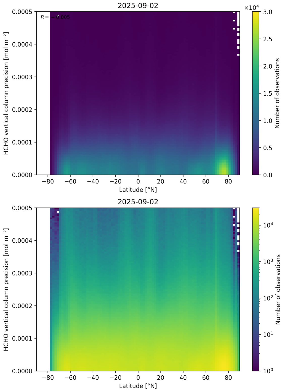
Figure 165: Scatter density plot of “Latitude” against “HCHO vertical column precision” for 2025-09-01 to 2025-09-03.
