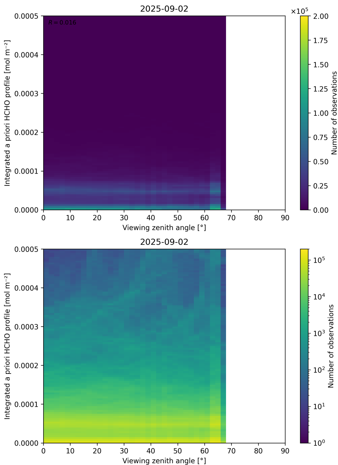
Figure 195: Scatter density plot of “Viewing zenith angle” against “Integrated a priori HCHO profile” for 2025-09-01 to 2025-09-03.
