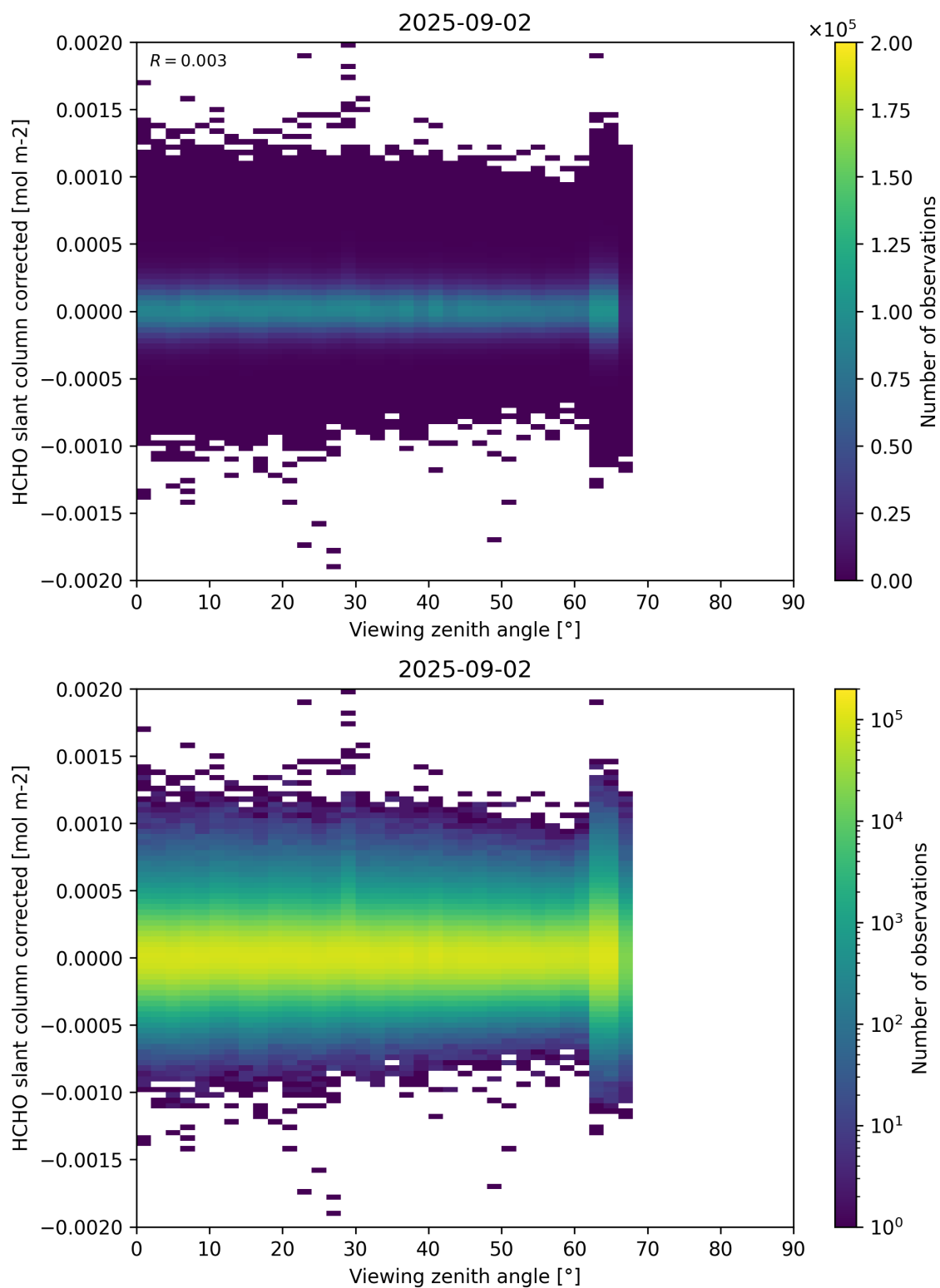
Figure 186: Scatter density plot of “Viewing zenith angle” against “HCHO slant column corrected” for 2025-09-01 to 2025-09-03.
