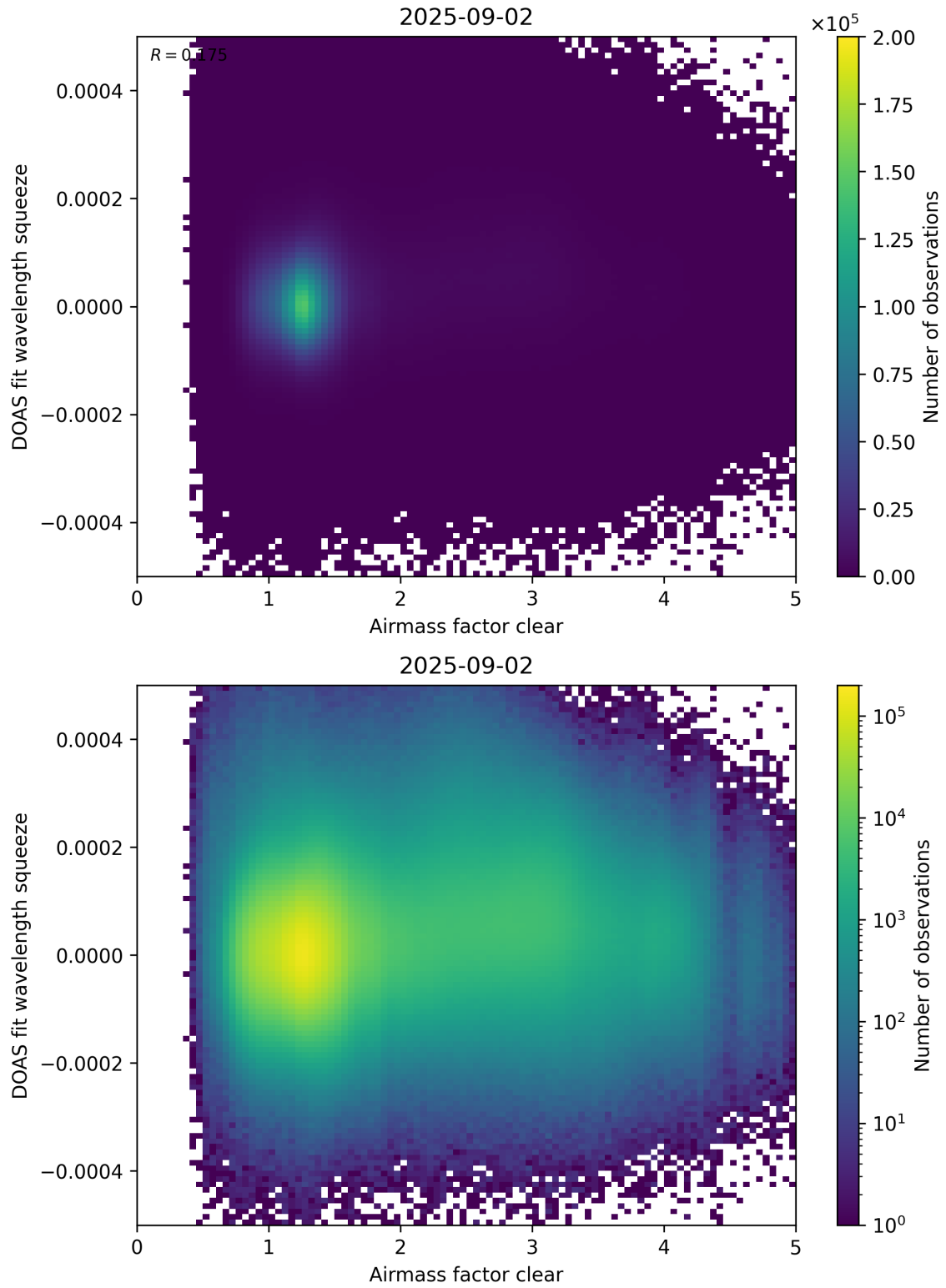
Figure 73: Scatter density plot of “Airmass factor clear” against “DOAS fit wavelength squeeze” for 2025-09-01 to 2025-09-03.
