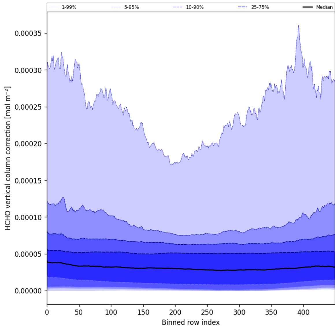
Figure 51: Along track statistics of “HCHO vertical column correction” for 2025-09-01 to 2025-09-03
