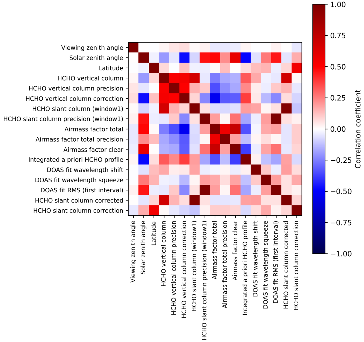
Figure 2: Map of correlation matrix for 2025-09-01 to 2025-09-03.
