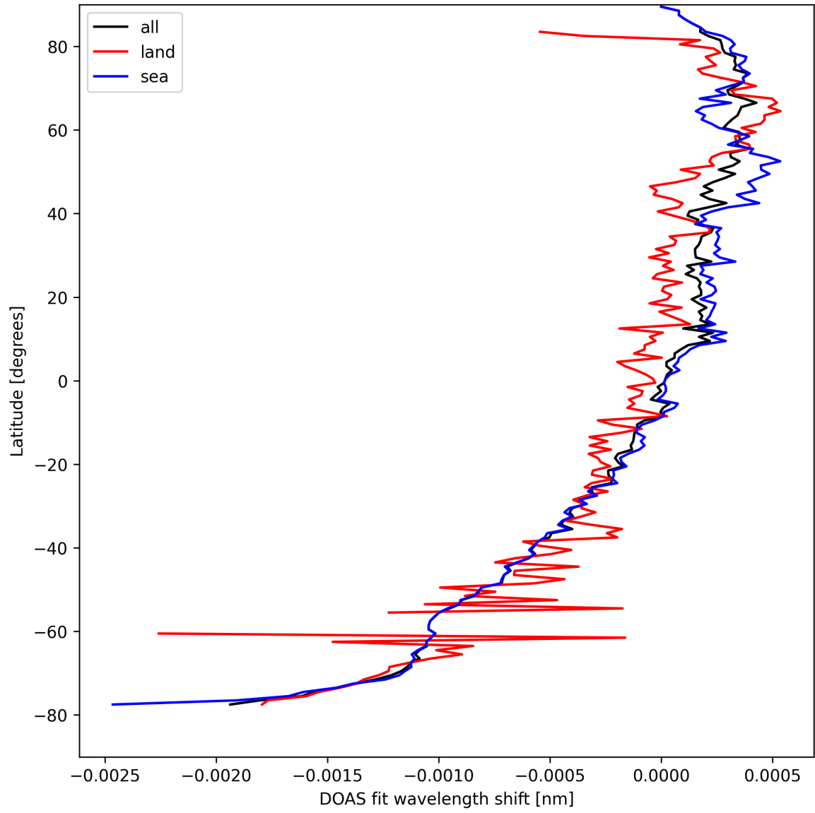
Figure 30: Zonal average of "DOAS fit wavelength shift" for 2025-09-01 to 2025-09-03.
