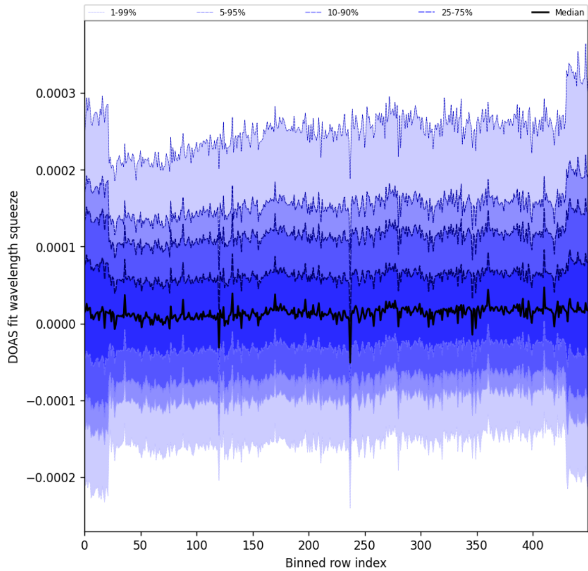
Figure 59: Along track statistics of “DOAS fit wavelength squeeze” for 2025-09-01 to 2025-09-03
