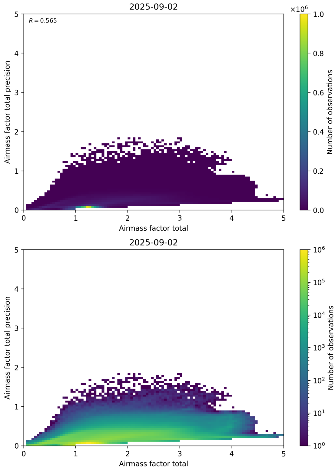
Figure 103: Scatter density plot of “Airmass factor total” against “Airmass factor total precision” for 2025-09-01 to 2025-09-03.
