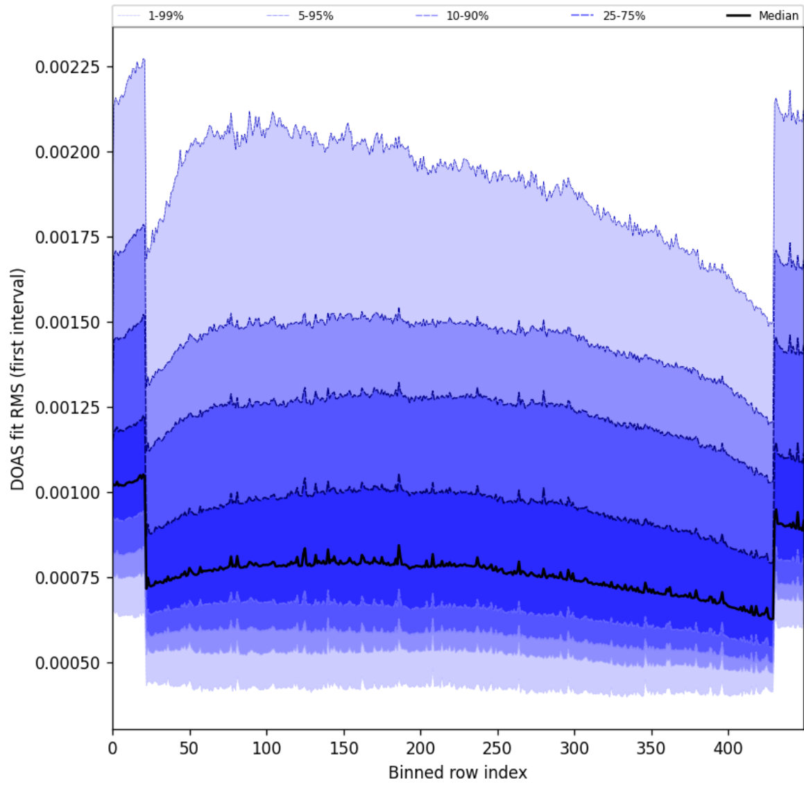
Figure 60: Along track statistics of “DOAS fit RMS (first interval)” for 2025-09-01 to 2025-09-03
