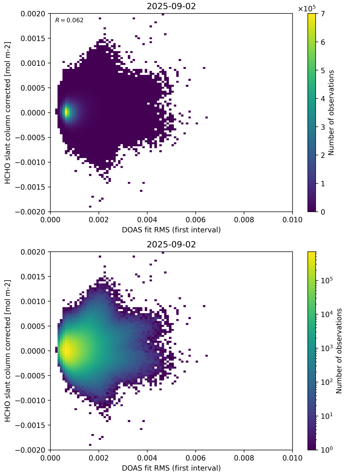
Figure 62: Scatter density plot of “DOAS fit RMS (first interval)” against “HCHO slant column corrected” for 2025-09-01 to 2025-09-03.
