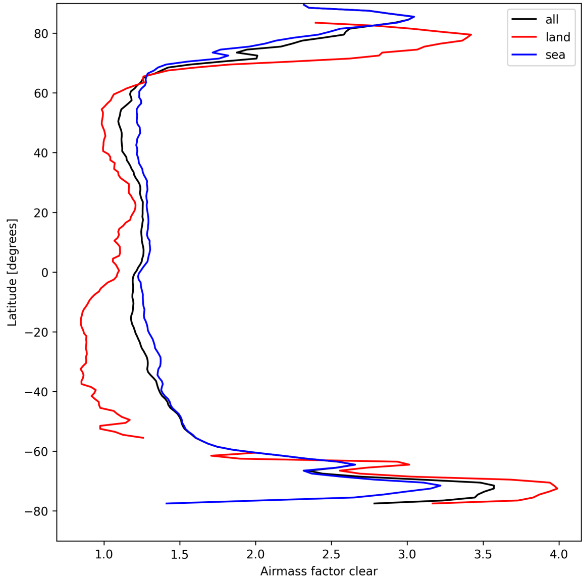
Figure 28: Zonal average of “Airmass factor clear” for 2025-09-01 to 2025-09-03.
