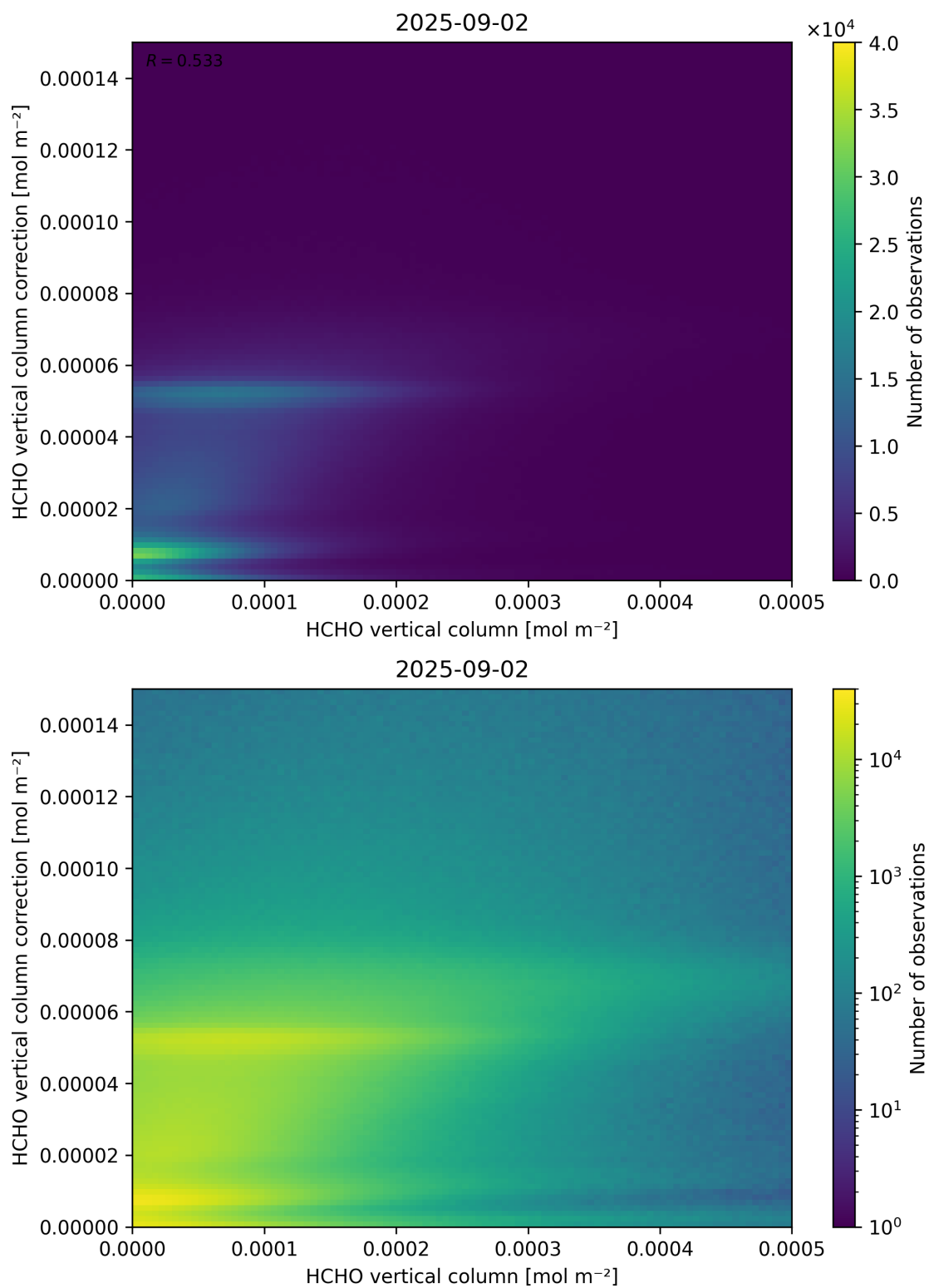
Figure 133: Scatter density plot of “HCHO vertical column” against “HCHO vertical column correction” for 2025-09-01 to 2025-09-03.
