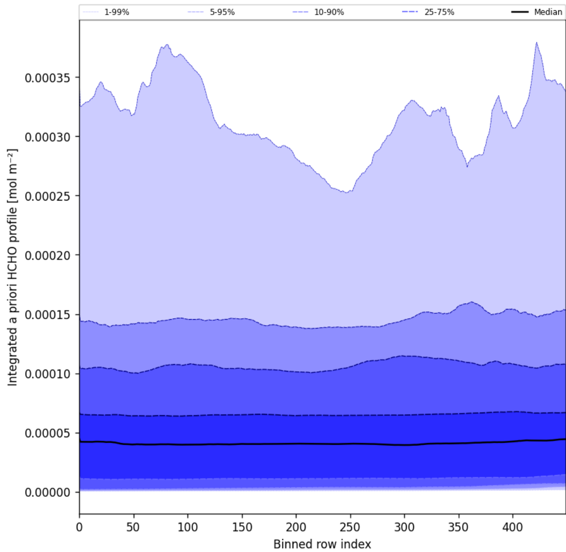
Figure 57: Along track statistics of “Integrated a priori HCHO profile” for 2025-09-01 to 2025-09-03
