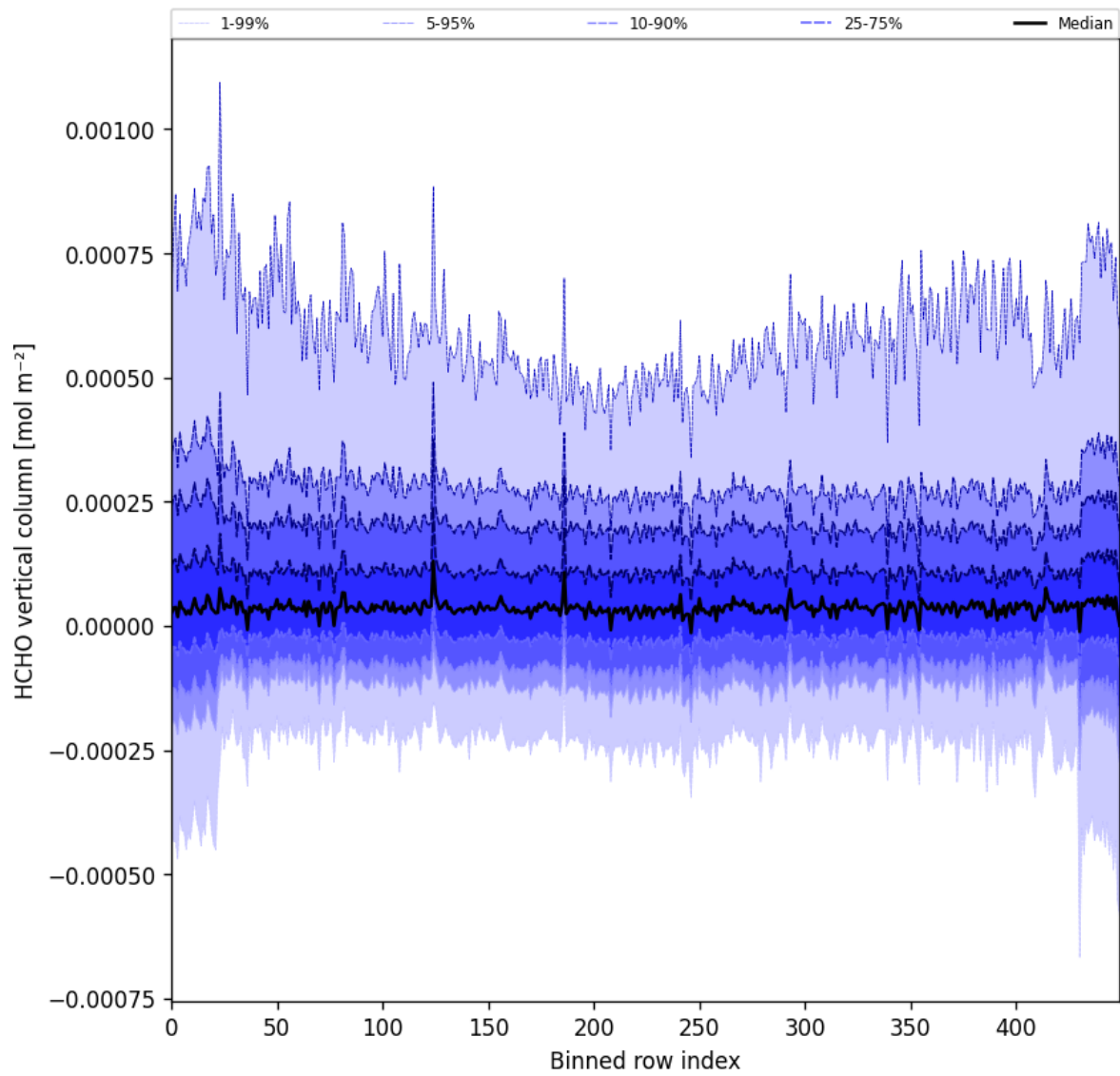
Figure 49: Along track statistics of “HCHO vertical column” for 2025-09-01 to 2025-09-03
