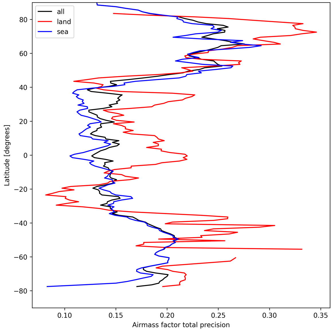
Figure 27: Zonal average of “Airmass factor total precision” for 2025-09-01 to 2025-09-03.
