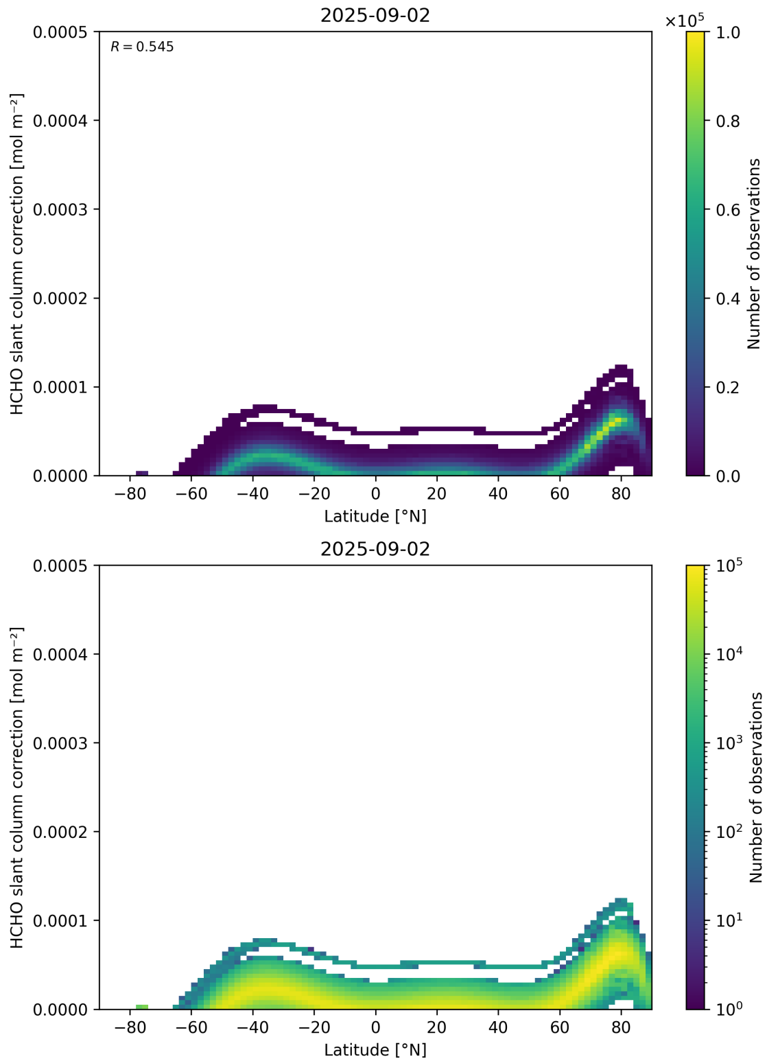
Figure 158: Scatter density plot of “Latitude” against “HCHO slant column correction” for 2025-09-01 to 2025-09-03.
