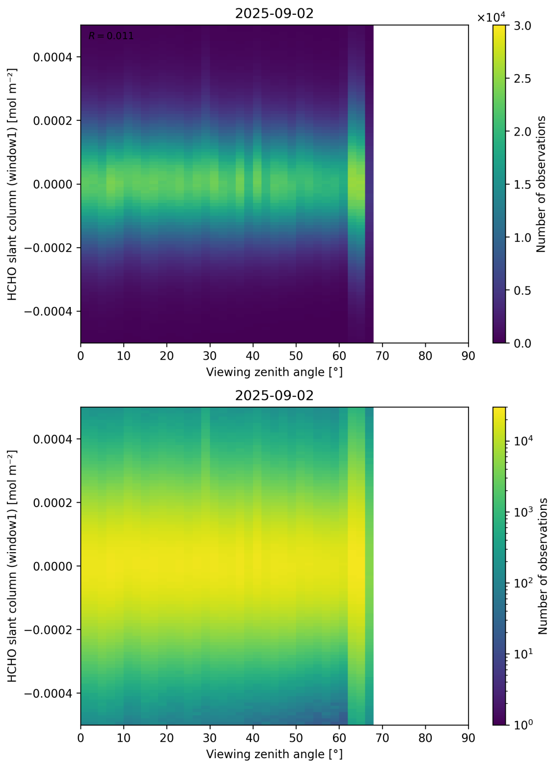
Figure 188: Scatter density plot of “Viewing zenith angle” against “HCHO slant column (window1)” for 2025-09-01 to 2025-09-03.
