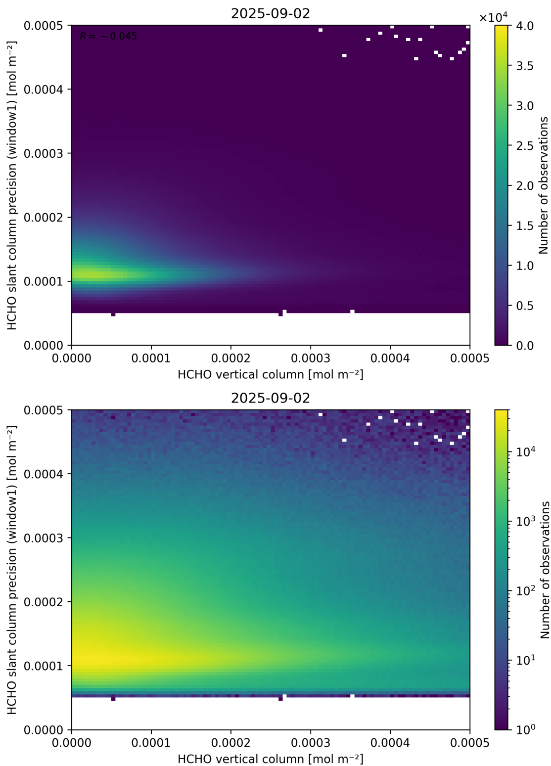
Figure 130: Scatter density plot of “HCHO vertical column” against “HCHO slant column precision (window1)” for 2025-09-01 to 2025-09-03.
