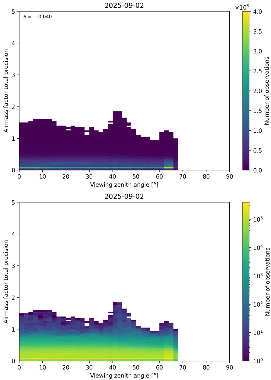
Figure 191: Scatter density plot of “Viewing zenith angle” against “Airmass factor total precision” for 2025-09-01 to 2025-09-03.
