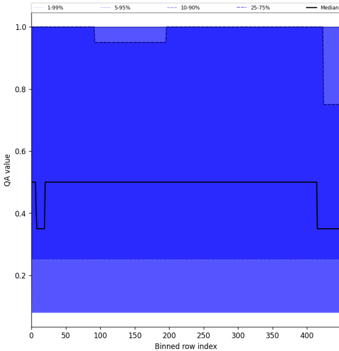
Figure 48: Along track statistics of “QA value” for 2025-09-01 to 2025-09-03
