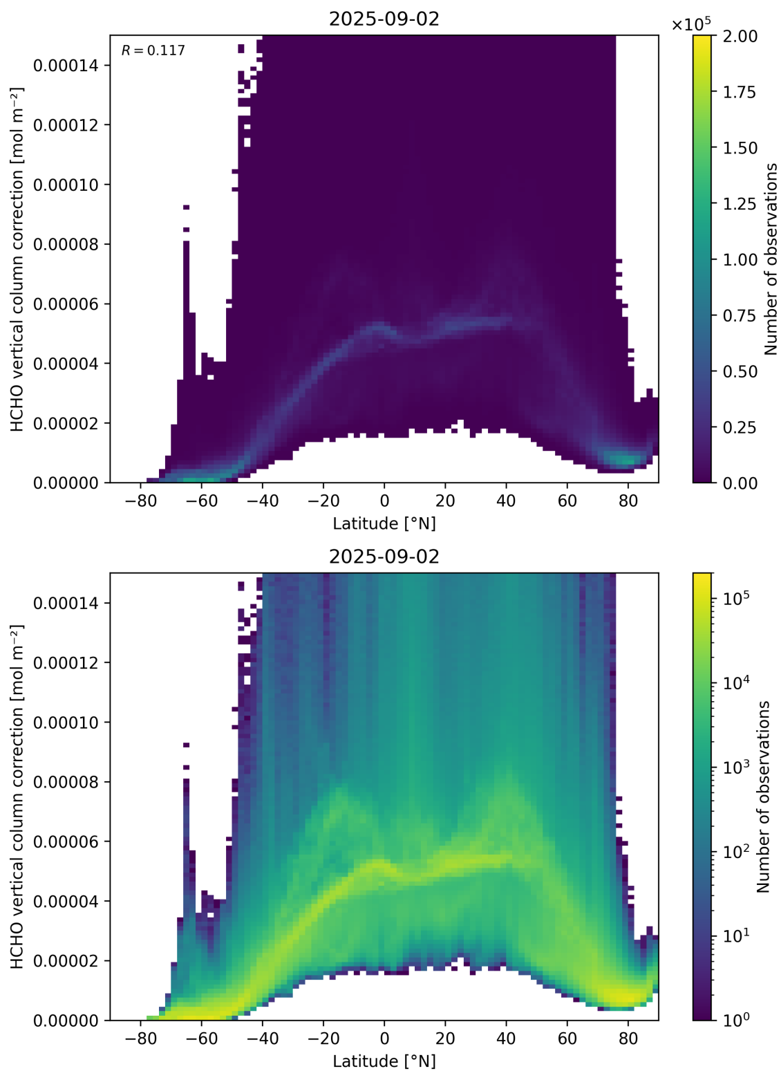
Figure 164: Scatter density plot of “Latitude” against “HCHO vertical column correction” for 2025-09-01 to 2025-09-03.
