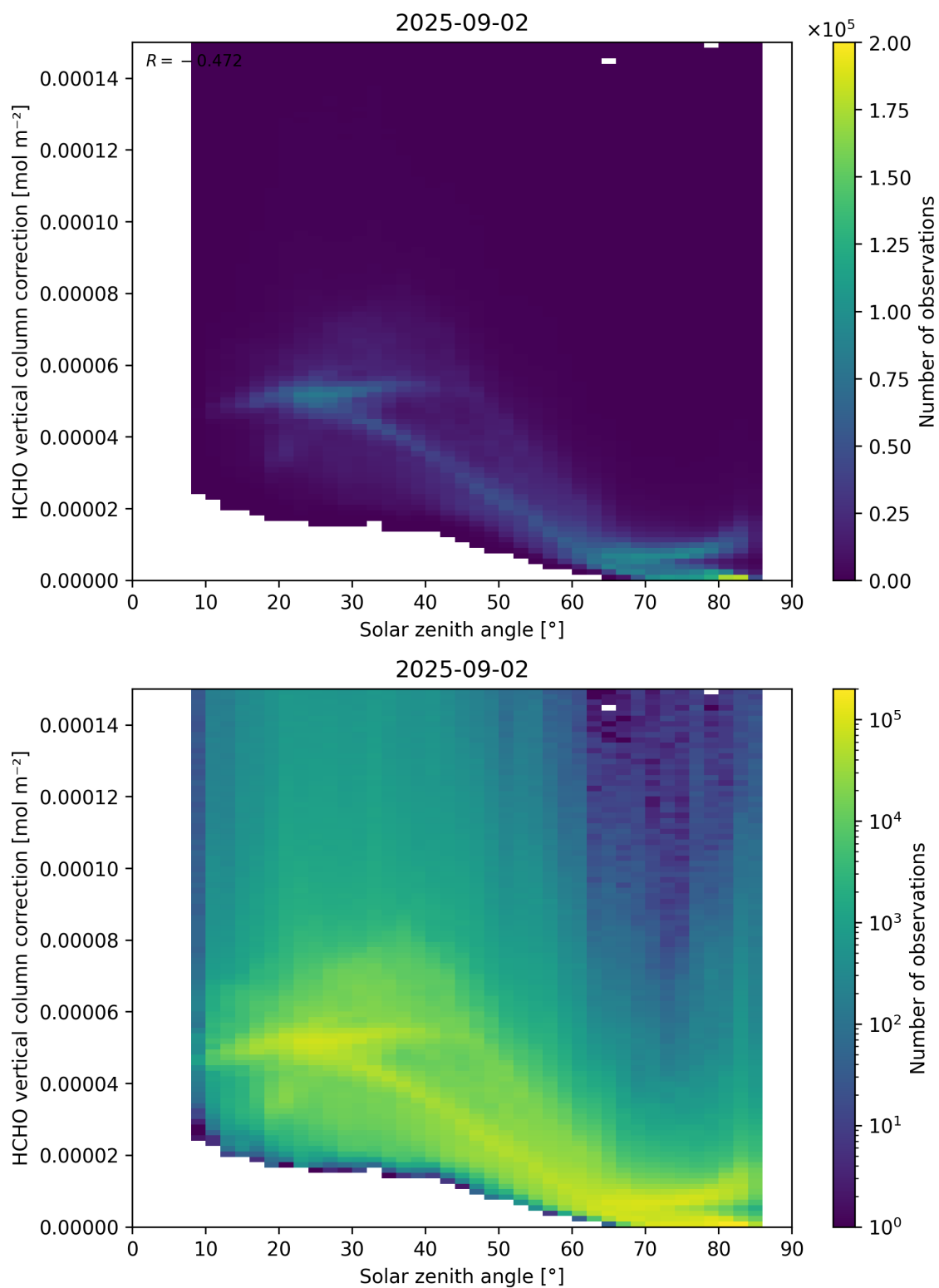
Figure 178: Scatter density plot of “Solar zenith angle” against “HCHO vertical column correction” for 2025-09-01 to 2025-09-03.
