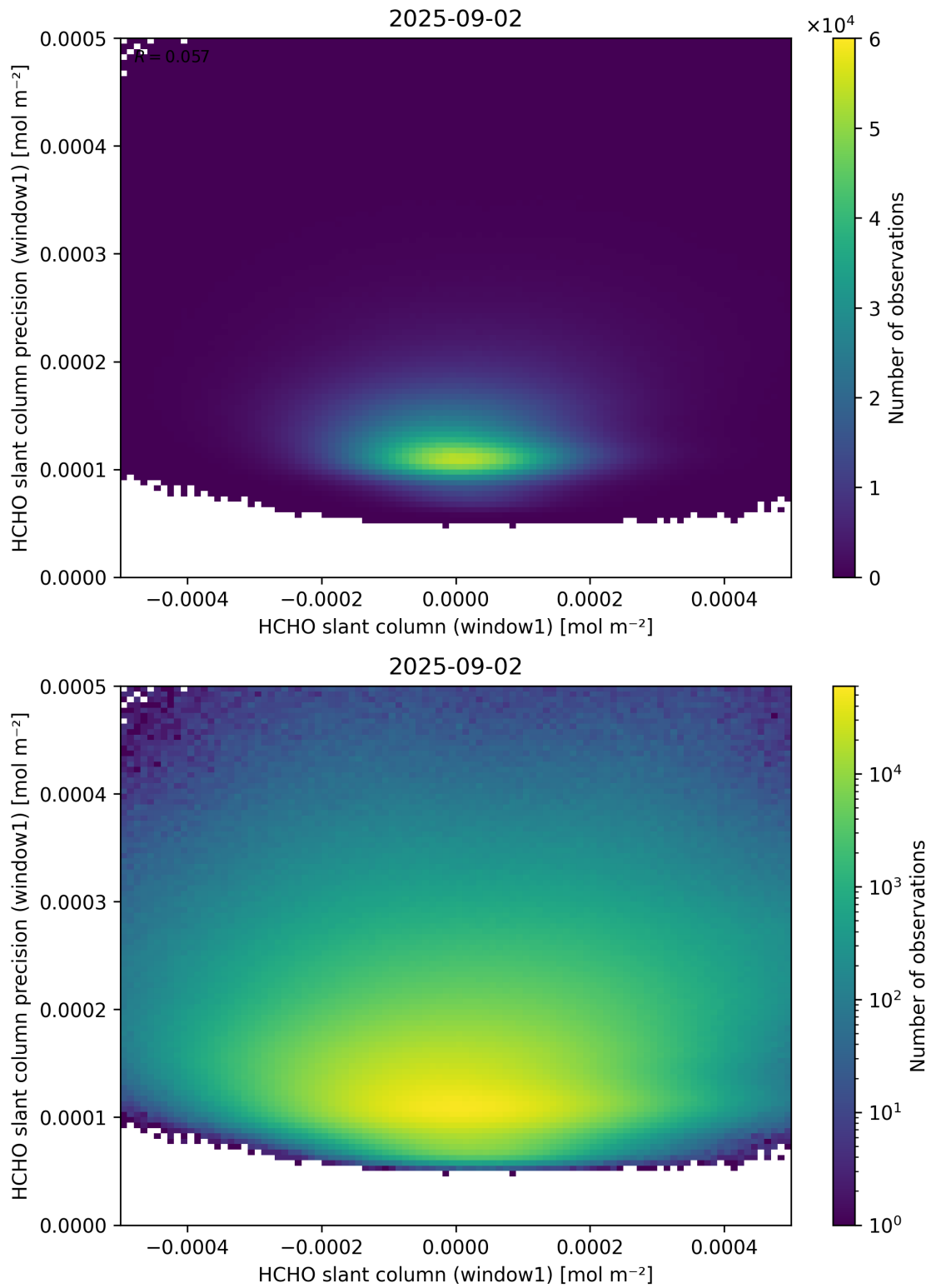
Figure 84: Scatter density plot of “HCHO slant column (window1)” against “HCHO slant column precision (window1)” for 2025-09-01 to 2025-09-03.
