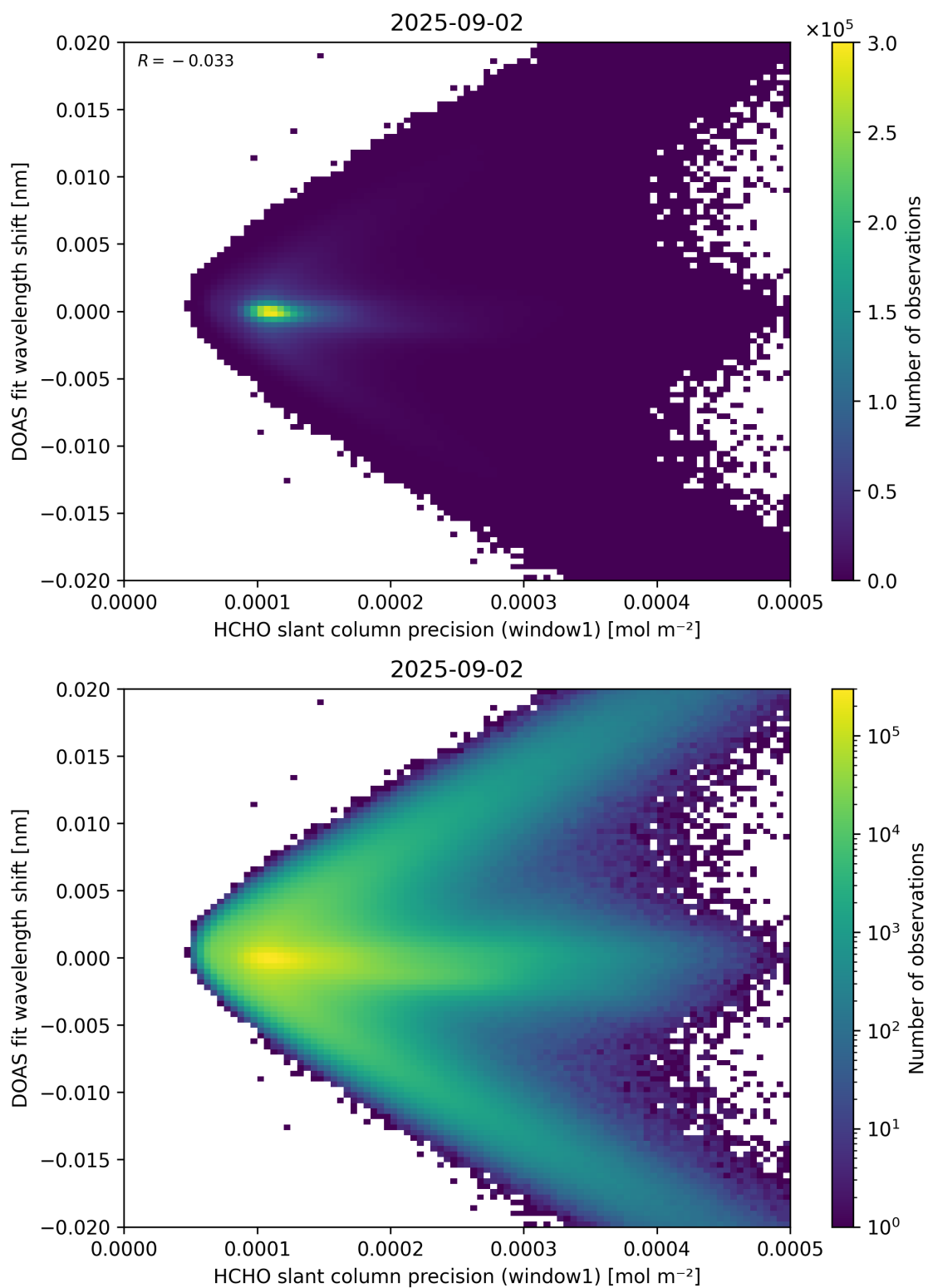
Figure 89: Scatter density plot of “HCHO slant column precision (window1)” against “DOAS fit wavelength shift” for 2025-09-01 to 2025-09-03.
