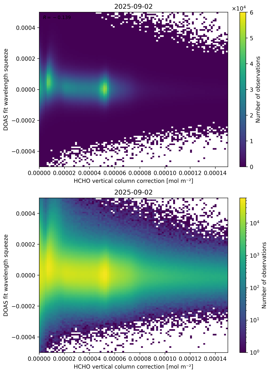
Figure 114: Scatter density plot of “HCHO vertical column correction” against “DOAS fit wavelength squeeze” for 2025-09-01 to 2025-09-03.
