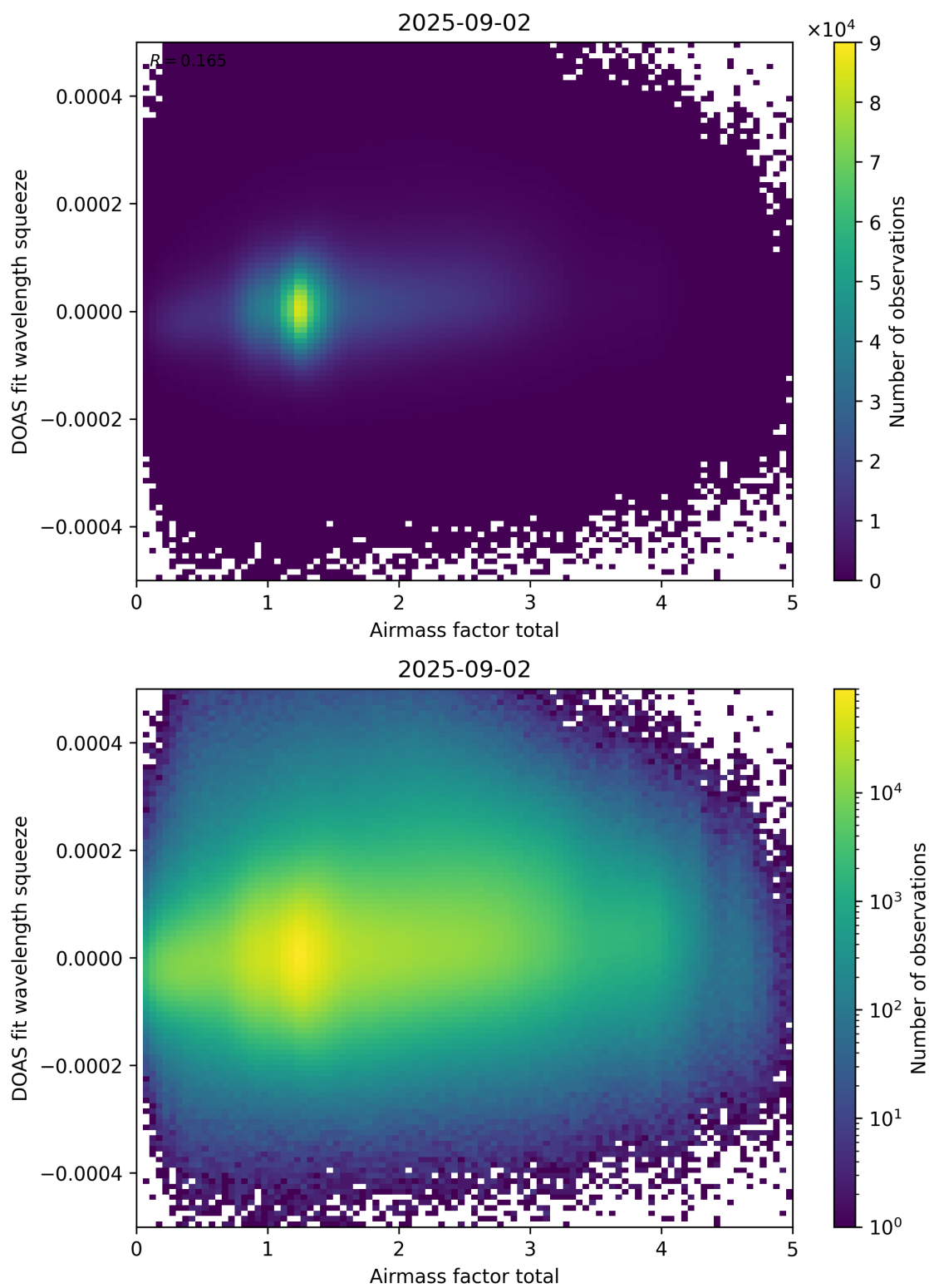
Figure 99: Scatter density plot of “Airmass factor total” against “DOAS fit wavelength squeeze” for 2025-09-01 to 2025-09-03.
