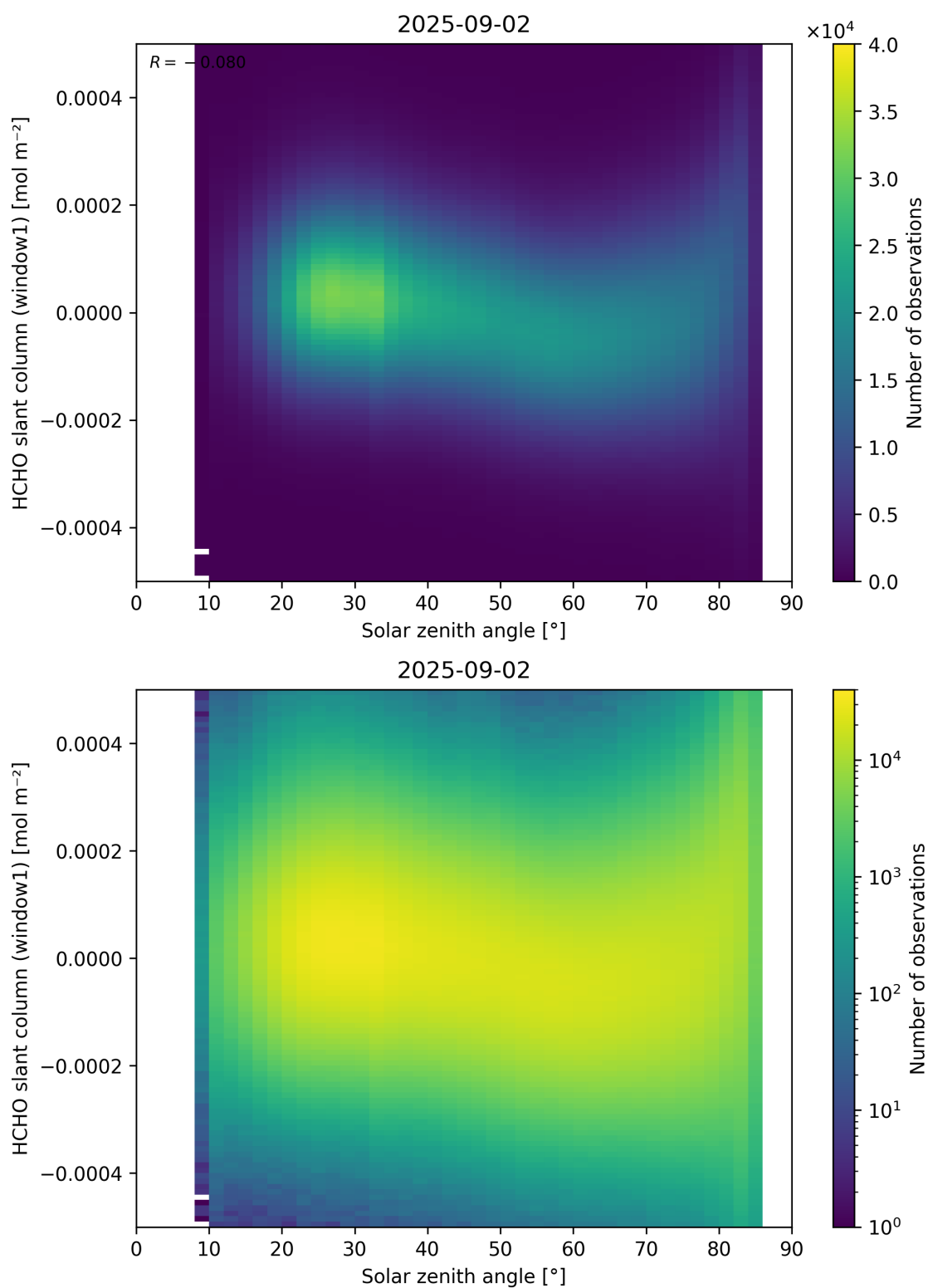
Figure 173: Scatter density plot of “Solar zenith angle” against “HCHO slant column (window1)” for 2025-09-01 to 2025-09-03.
