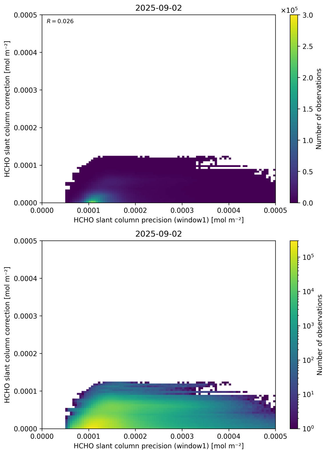
Figure 93: Scatter density plot of “HCHO slant column precision (window1)” against “HCHO slant column correction” for 2025-09-01 to 2025-09-03.
