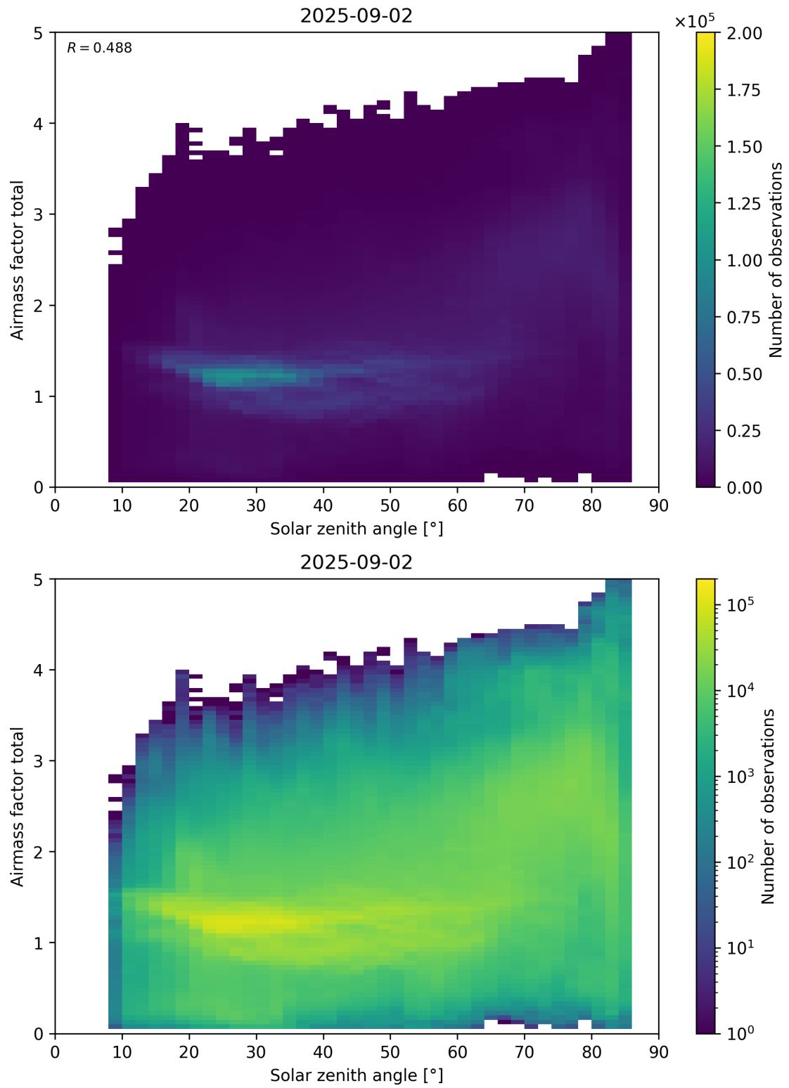
Figure 175: Scatter density plot of “Solar zenith angle” against “Airmass factor total” for 2025-09-01 to 2025-09-03.
