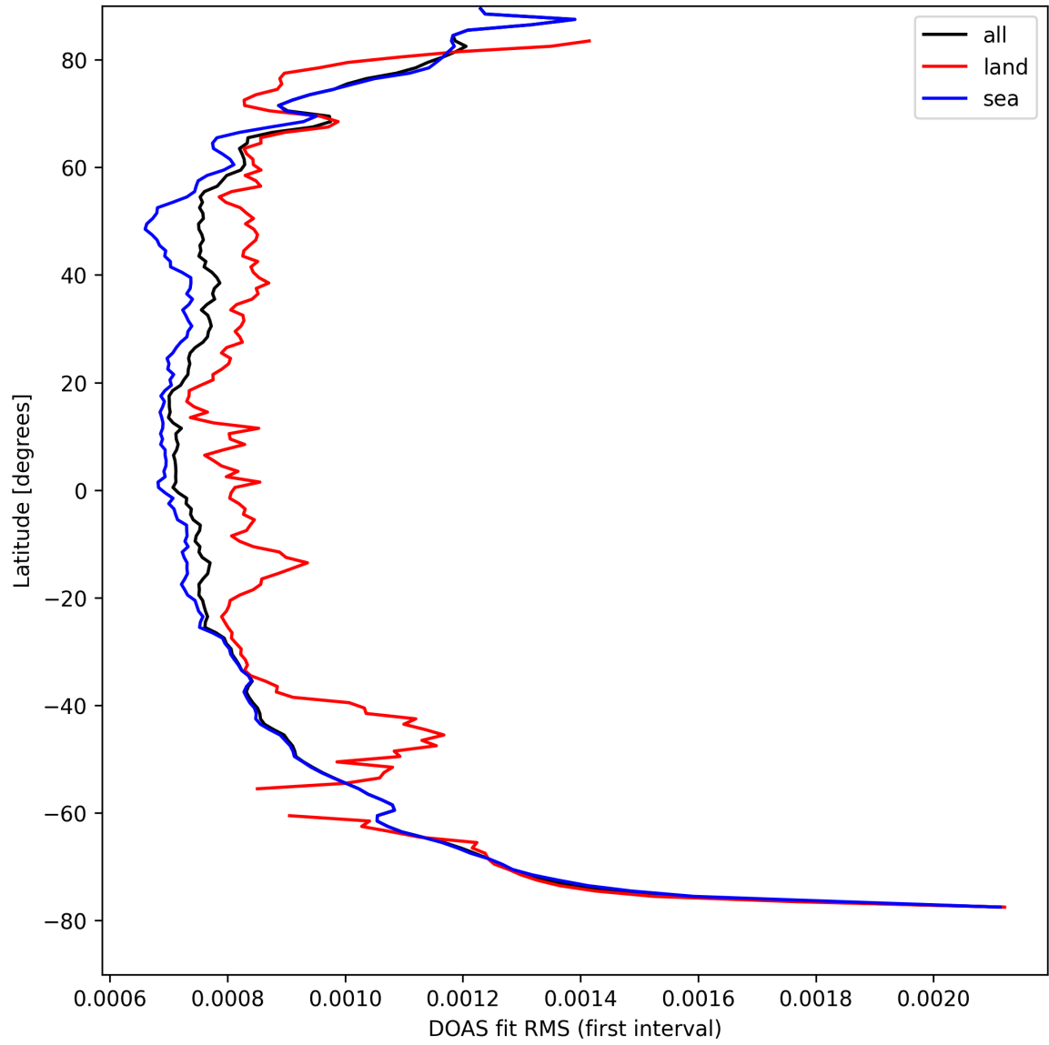
Figure 32: Zonal average of "DOAS fit RMS (first interval)" for 2025-09-01 to 2025-09-03.
