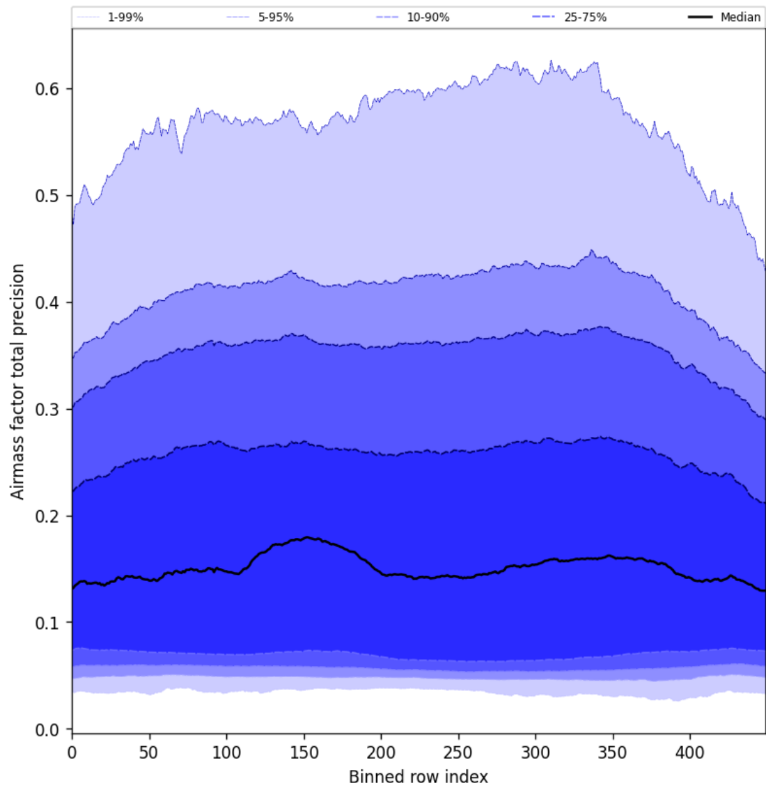
Figure 55: Along track statistics of “Airmass factor total precision” for 2025-09-01 to 2025-09-03
