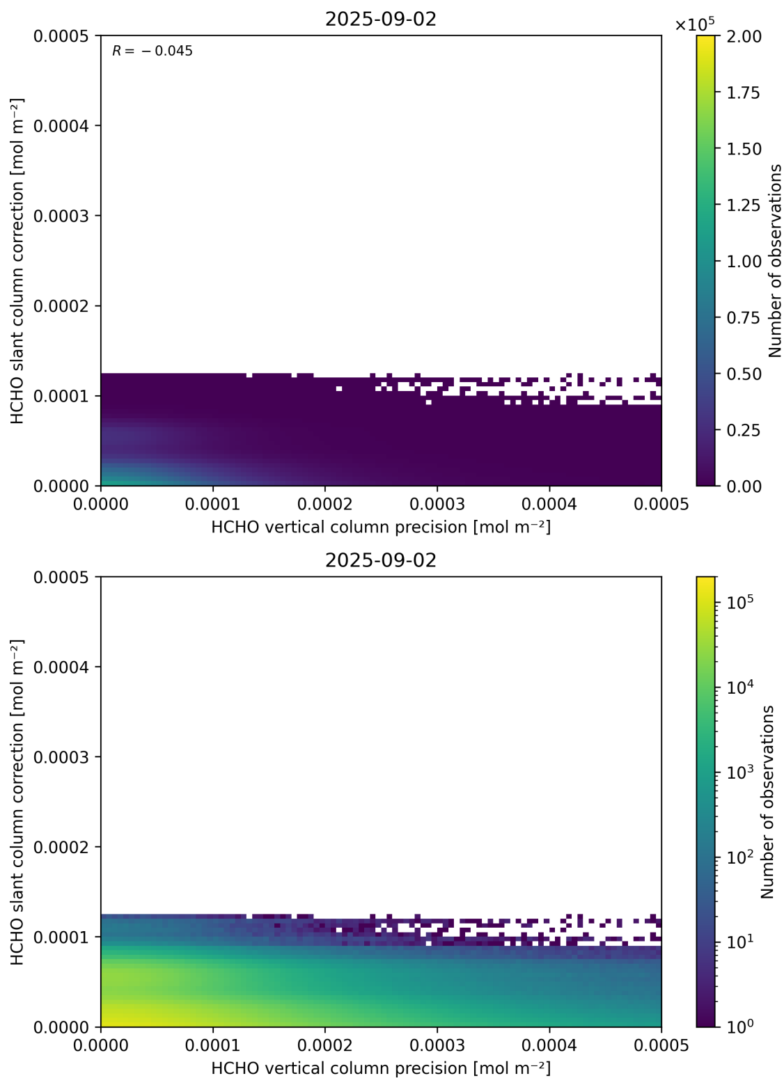
Figure 141: Scatter density plot of “HCHO vertical column precision” against “HCHO slant column correction” for 2025-09-01 to 2025-09-03.
