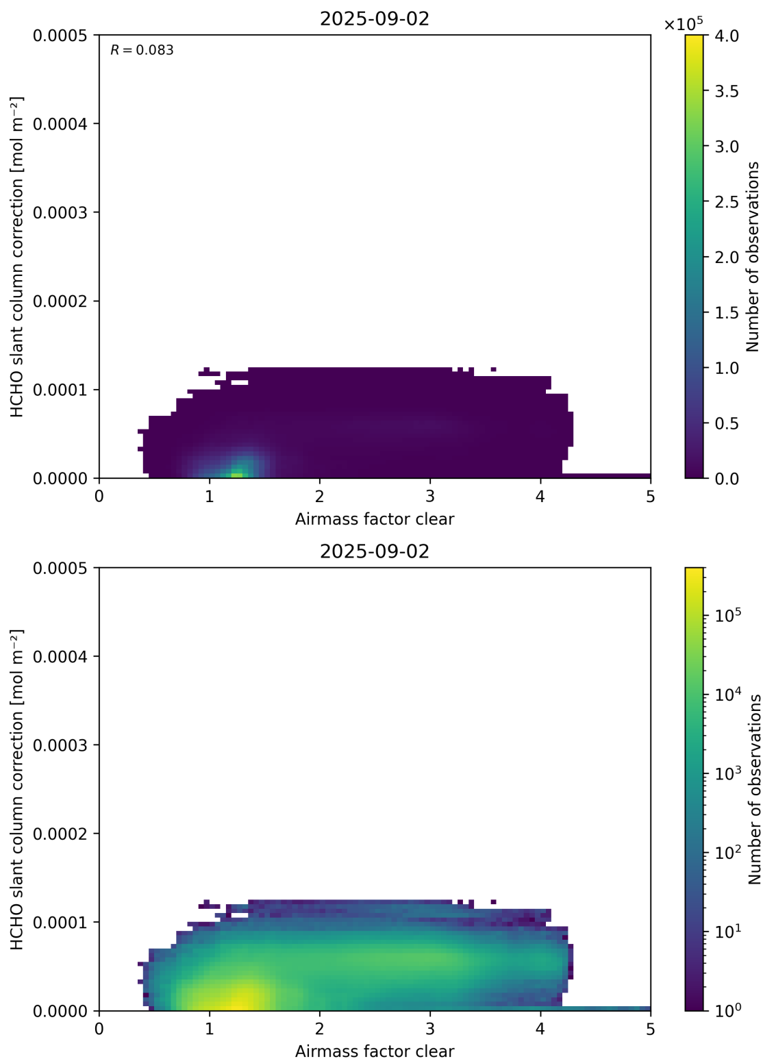
Figure 75: Scatter density plot of “Airmass factor clear” against “HCHO slant column correction” for 2025-09-01 to 2025-09-03.
