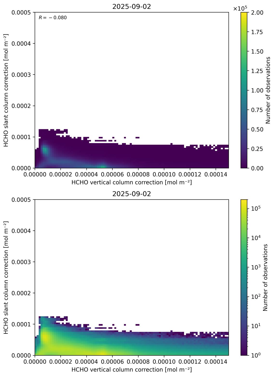
Figure 117: Scatter density plot of “HCHO vertical column correction” against “HCHO slant column correction” for 2025-09-01 to 2025-09-03.
