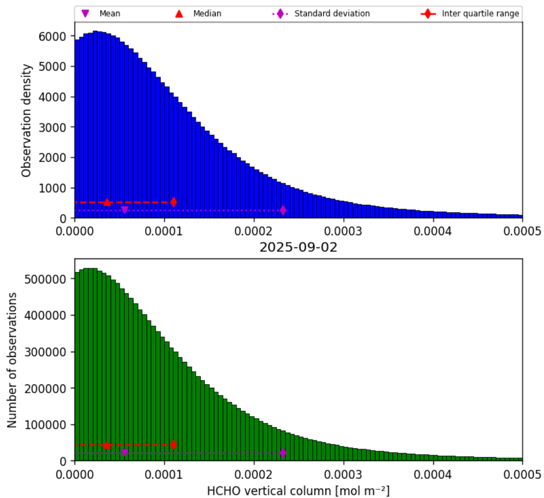
Figure 35: Histogram of “HCHO vertical column” for 2025-09-01 to 2025-09-03
