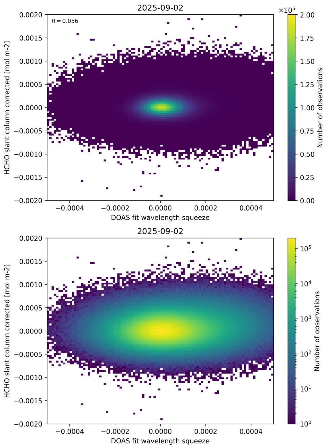
Figure 69: Scatter density plot of “DOAS fit wavelength squeeze” against “HCHO slant column corrected” for 2025-09-01 to 2025-09-03.
