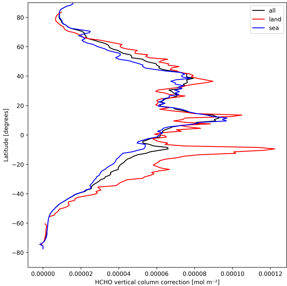
Figure 23: Zonal average of “HCHO vertical column correction” for 2025-09-01 to 2025-09-03.
