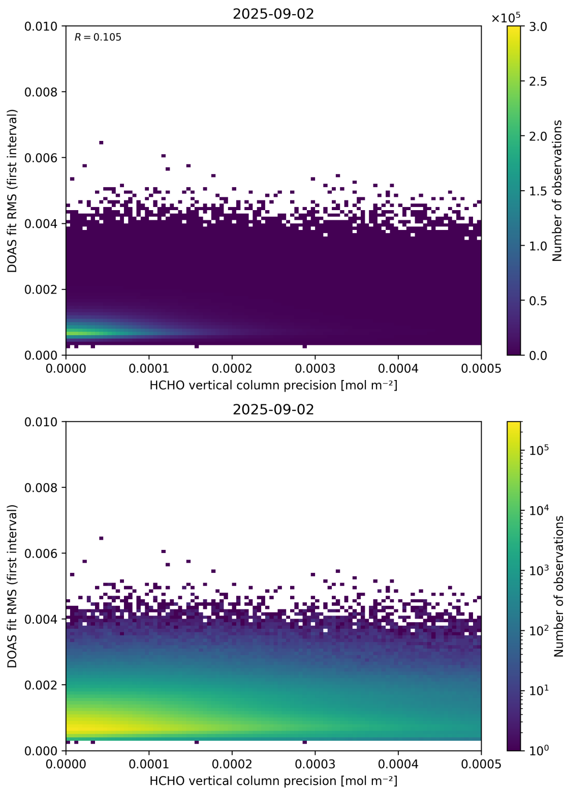
Figure 136: Scatter density plot of “HCHO vertical column precision” against “DOAS fit RMS (first interval)” for 2025-09-01 to 2025-09-03.
