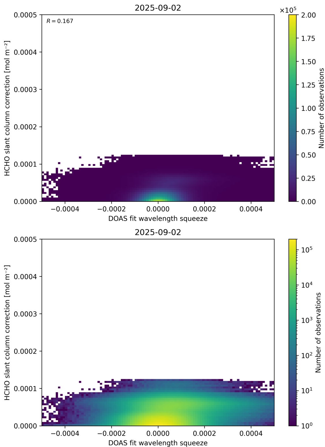
Figure 70: Scatter density plot of “DOAS fit wavelength squeeze” against “HCHO slant column correction” for 2025-09-01 to 2025-09-03.
