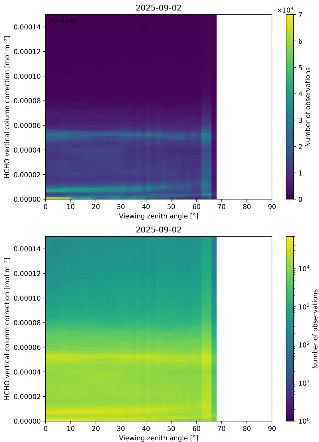
Figure 193: Scatter density plot of “Viewing zenith angle” against “HCHO vertical column correction” for 2025-09-01 to 2025-09-03.
