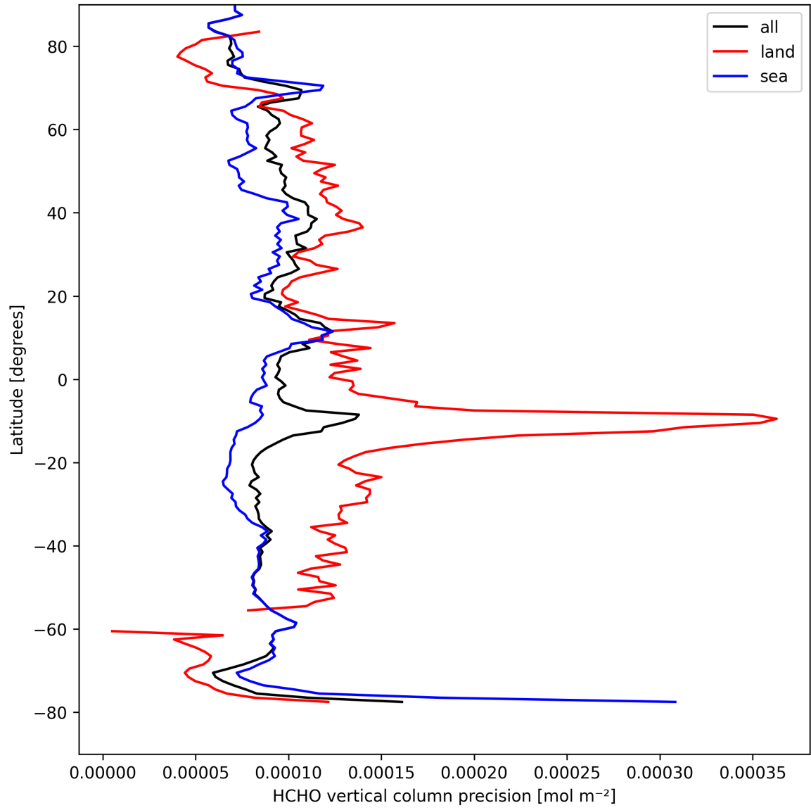
Figure 22: Zonal average of “HCHO vertical column precision” for 2025-09-01 to 2025-09-03.
