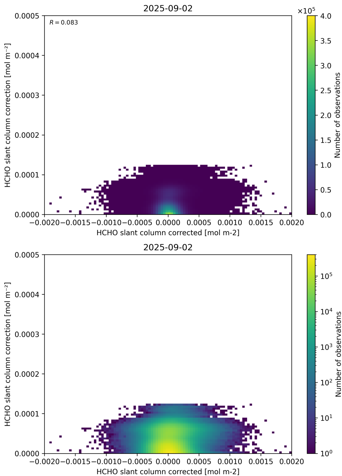
Figure 77: Scatter density plot of “HCHO slant column corrected” against “HCHO slant column correction” for 2025-09-01 to 2025-09-03.
