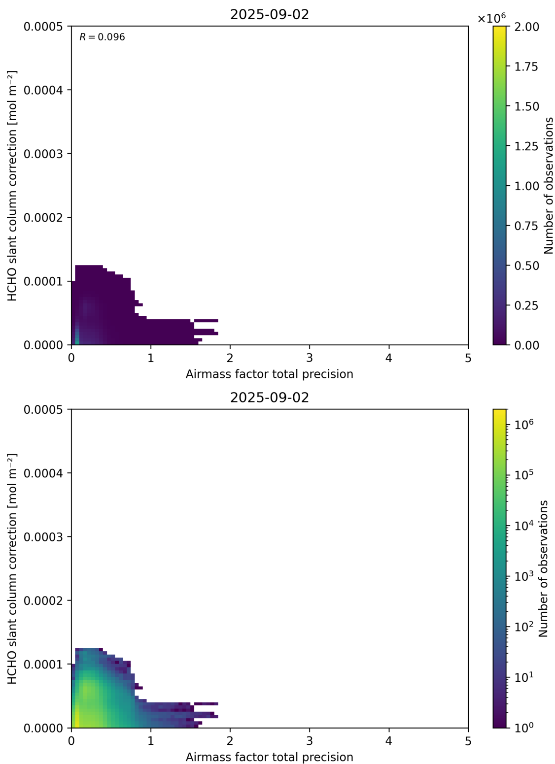
Figure 110: Scatter density plot of “Airmass factor total precision” against “HCHO slant column correction” for 2025-09-01 to 2025-09-03.
