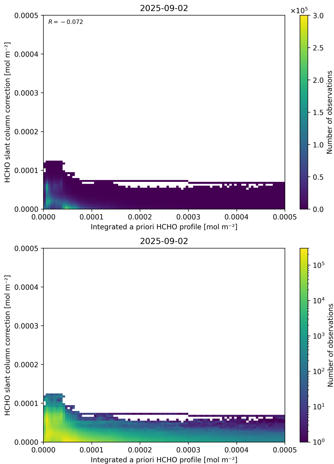
Figure 152: Scatter density plot of “Integrated a priori HCHO profile” against “HCHO slant column correction” for 2025-09-01 to 2025-09-03.
