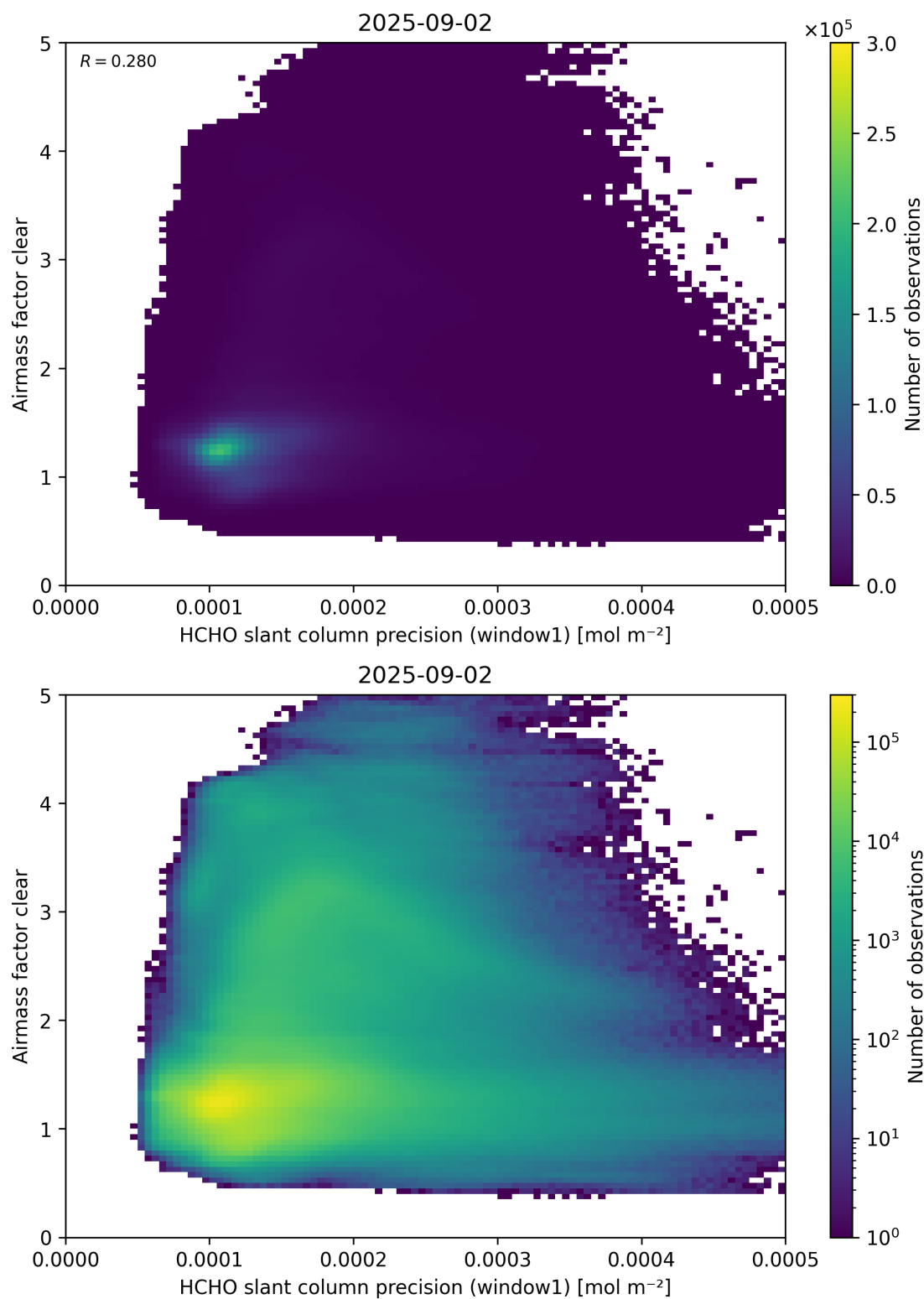
Figure 91: Scatter density plot of “HCHO slant column precision (window1)” against “Airmass factor clear” for 2025-09-01 to 2025-09-03.
