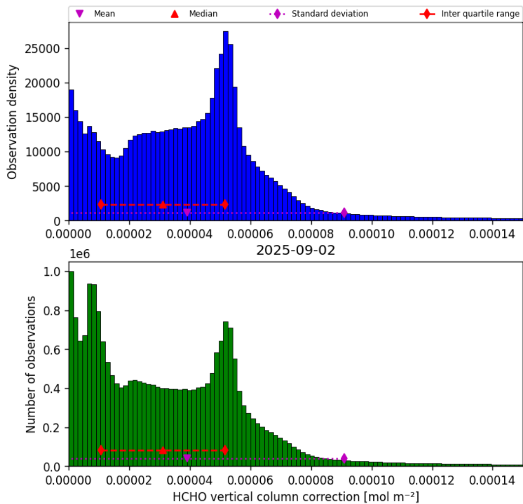
Figure 37: Histogram of “HCHO vertical column correction” for 2025-09-01 to 2025-09-03
