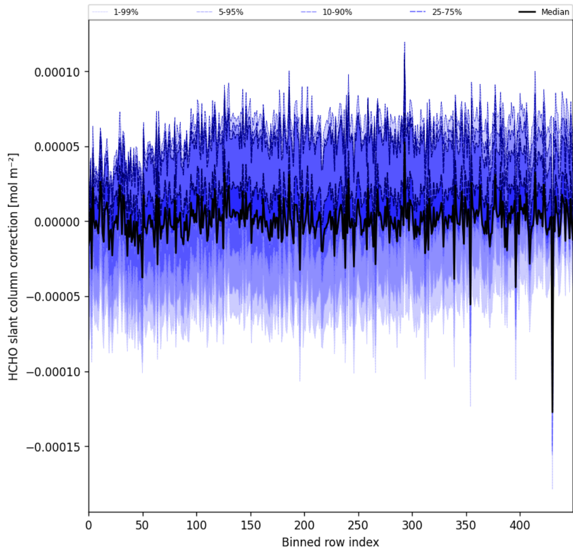
Figure 61: Along track statistics of “HCHO slant column correction” for 2025-09-01 to 2025-09-03
