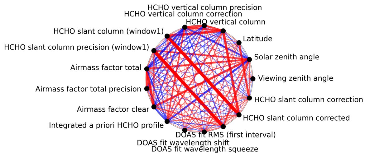
Figure 1: Map of correlation graph for 2025-09-01 to 2025-09-03.
