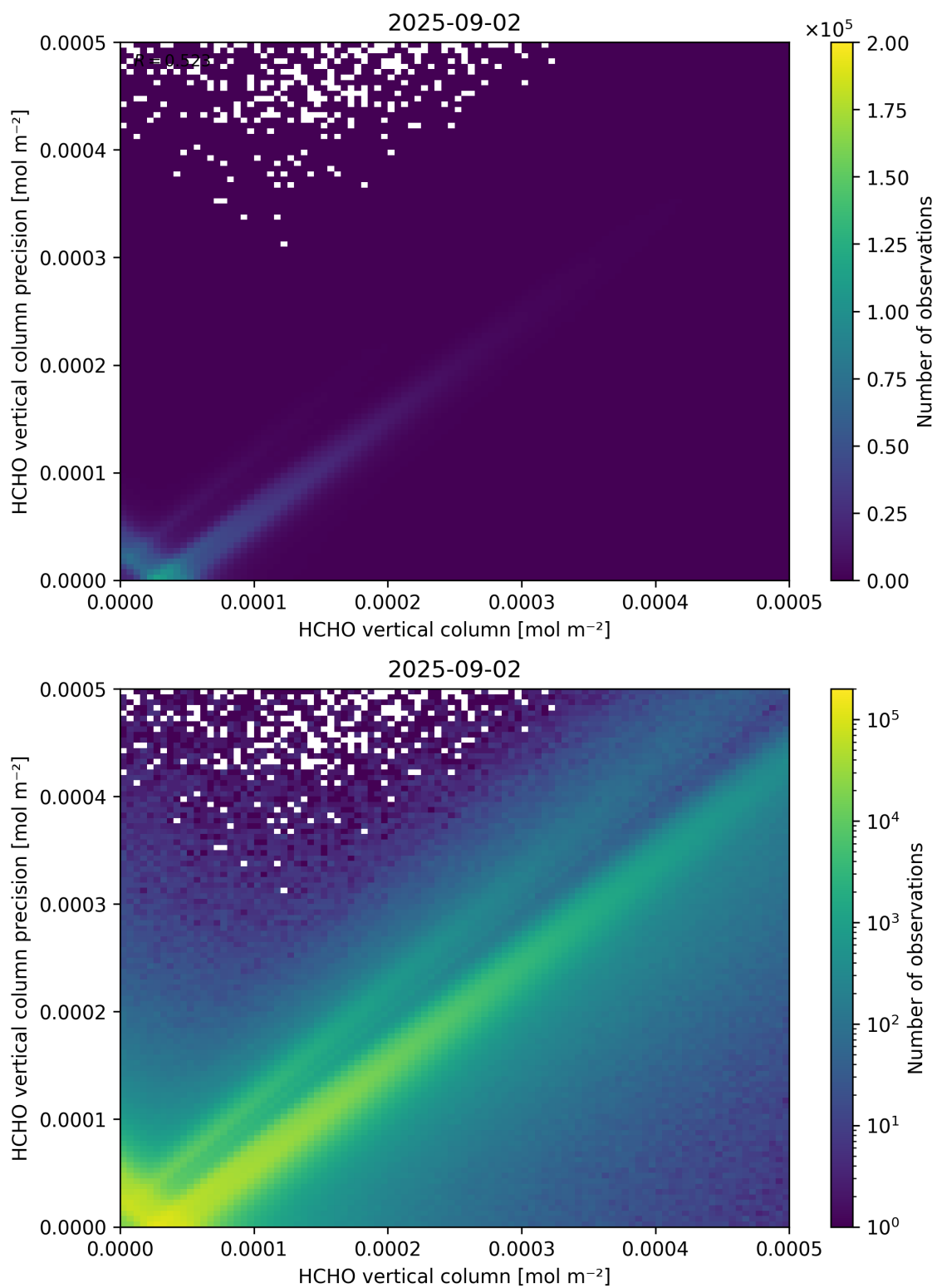
Figure 134: Scatter density plot of “HCHO vertical column” against “HCHO vertical column precision” for 2025-09-01 to 2025-09-03.
