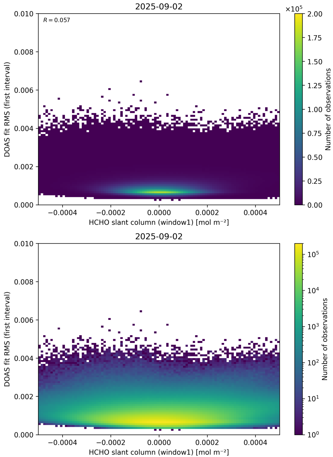
Figure 78: Scatter density plot of “HCHO slant column (window1)” against “DOAS fit RMS (first interval)” for 2025-09-01 to 2025-09-03.
