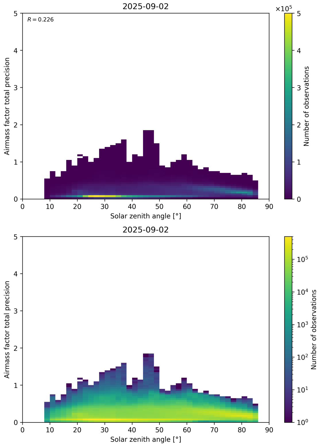
Figure 176: Scatter density plot of “Solar zenith angle” against “Airmass factor total precision” for 2025-09-01 to 2025-09-03.
