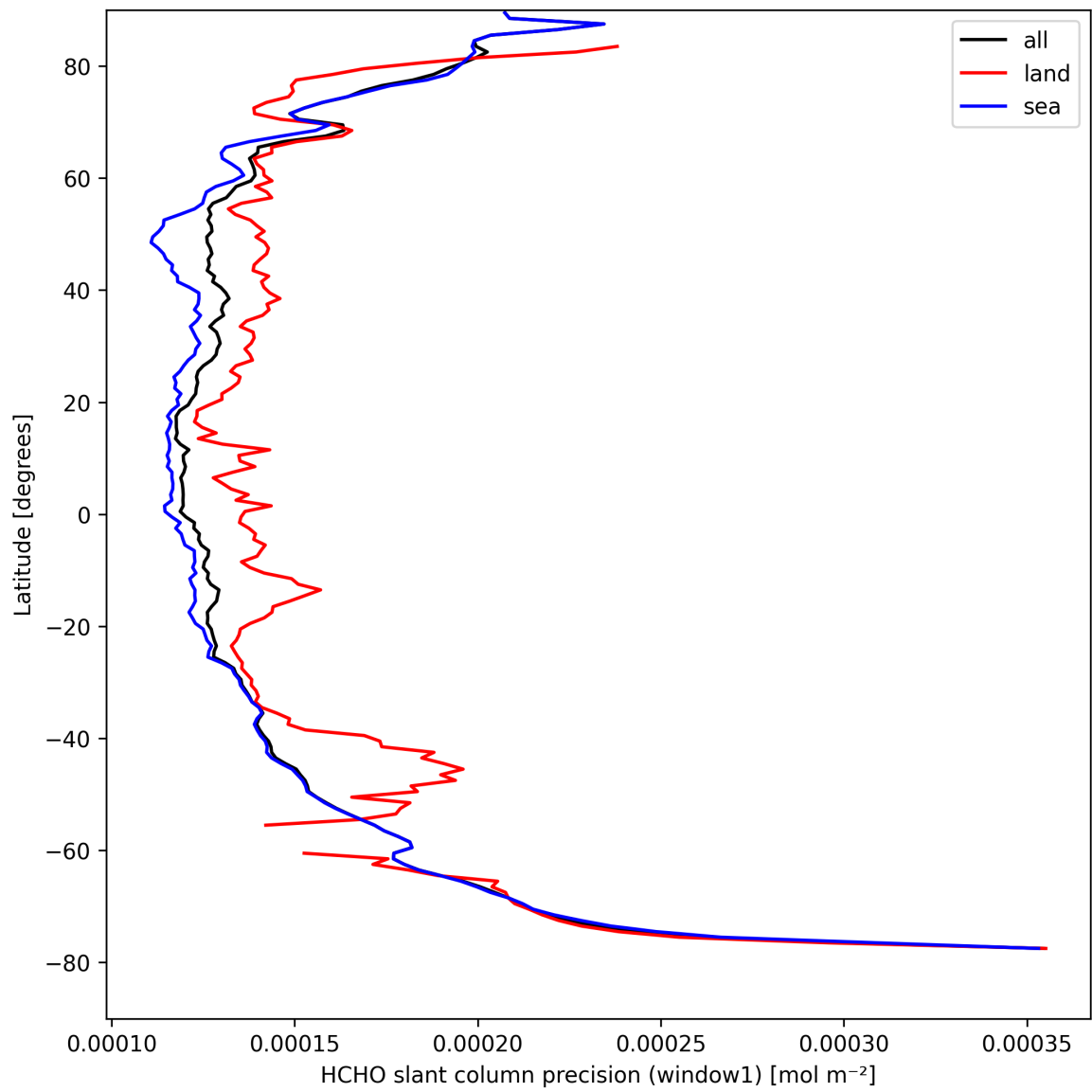
Figure 25: Zonal average of “HCHO slant column precision (window1)” for 2025-09-01 to 2025-09-03.
