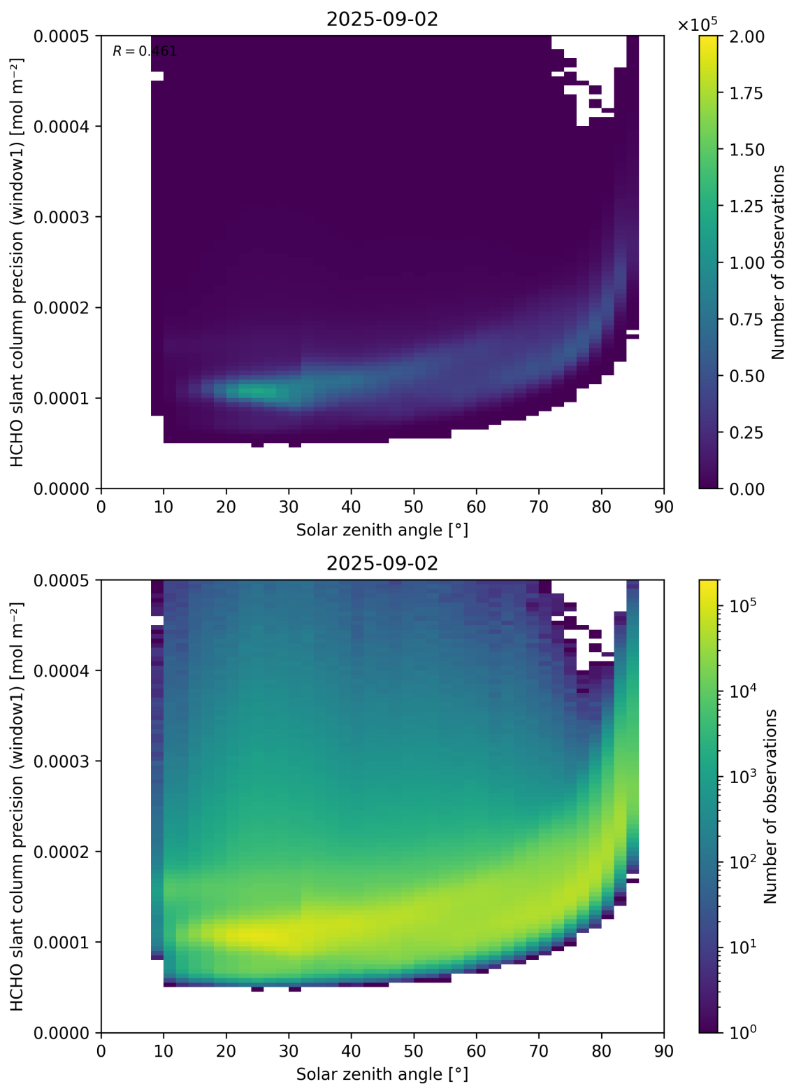
Figure 174: Scatter density plot of “Solar zenith angle” against “HCHO slant column precision (window1)” for 2025-09-01 to 2025-09-03.
