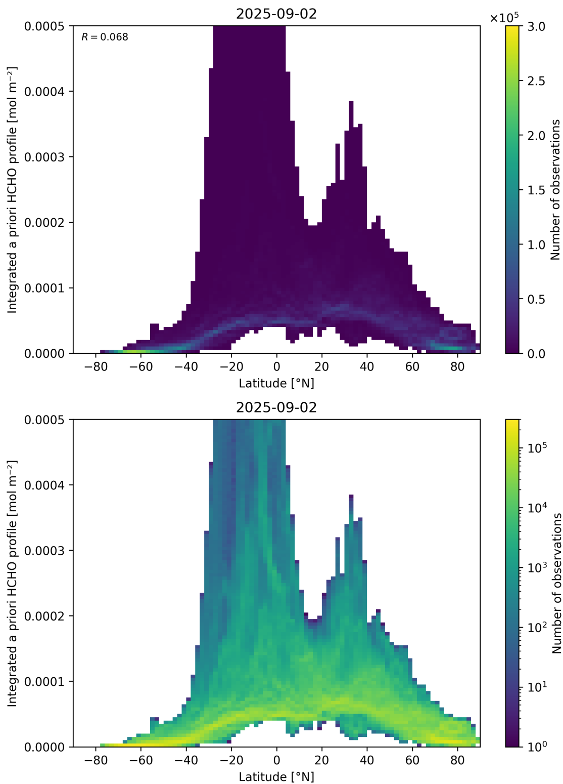
Figure 166: Scatter density plot of “Latitude” against “Integrated a priori HCHO profile” for 2025-09-01 to 2025-09-03.
