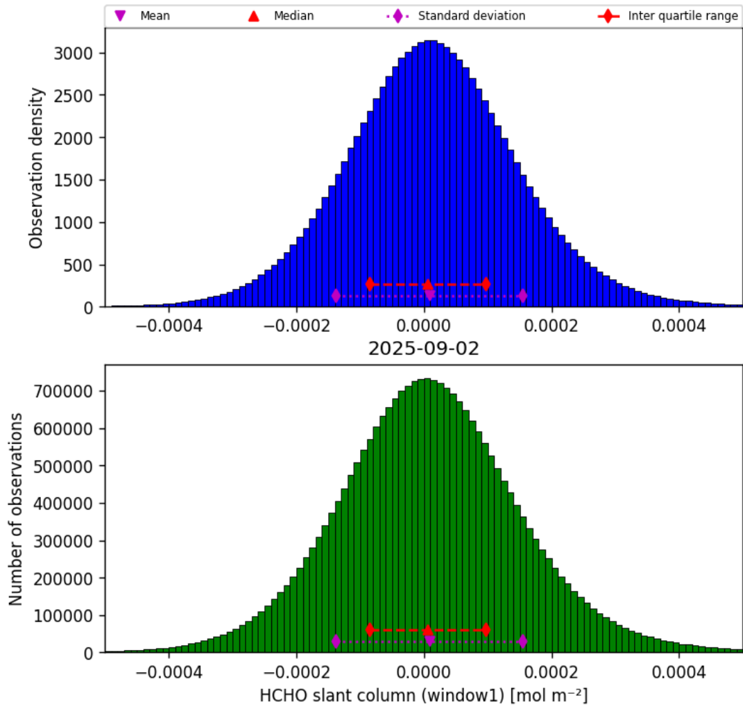
Figure 38: Histogram of “HCHO slant column (window1)” for 2025-09-01 to 2025-09-03
