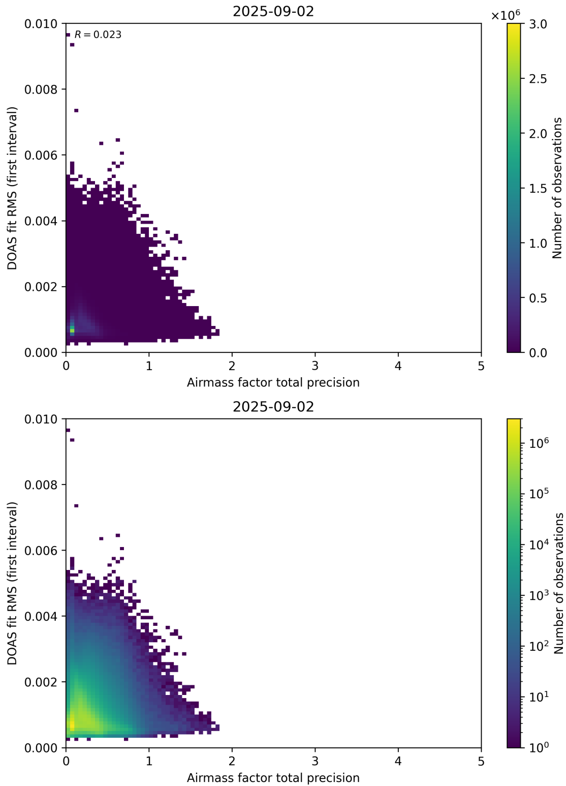
Figure 105: Scatter density plot of “Airmass factor total precision” against “DOAS fit RMS (first interval)” for 2025-09-01 to 2025-09-03.
