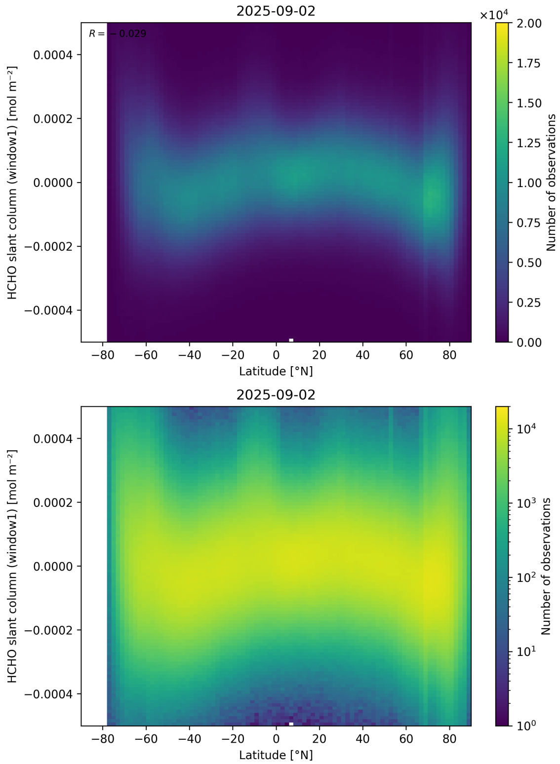
Figure 159: Scatter density plot of “Latitude” against “HCHO slant column (window1)” for 2025-09-01 to 2025-09-03.
