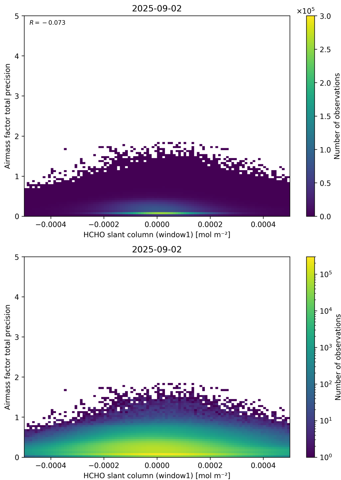
Figure 86: Scatter density plot of “HCHO slant column (window1)” against “Airmass factor total precision” for 2025-09-01 to 2025-09-03.
