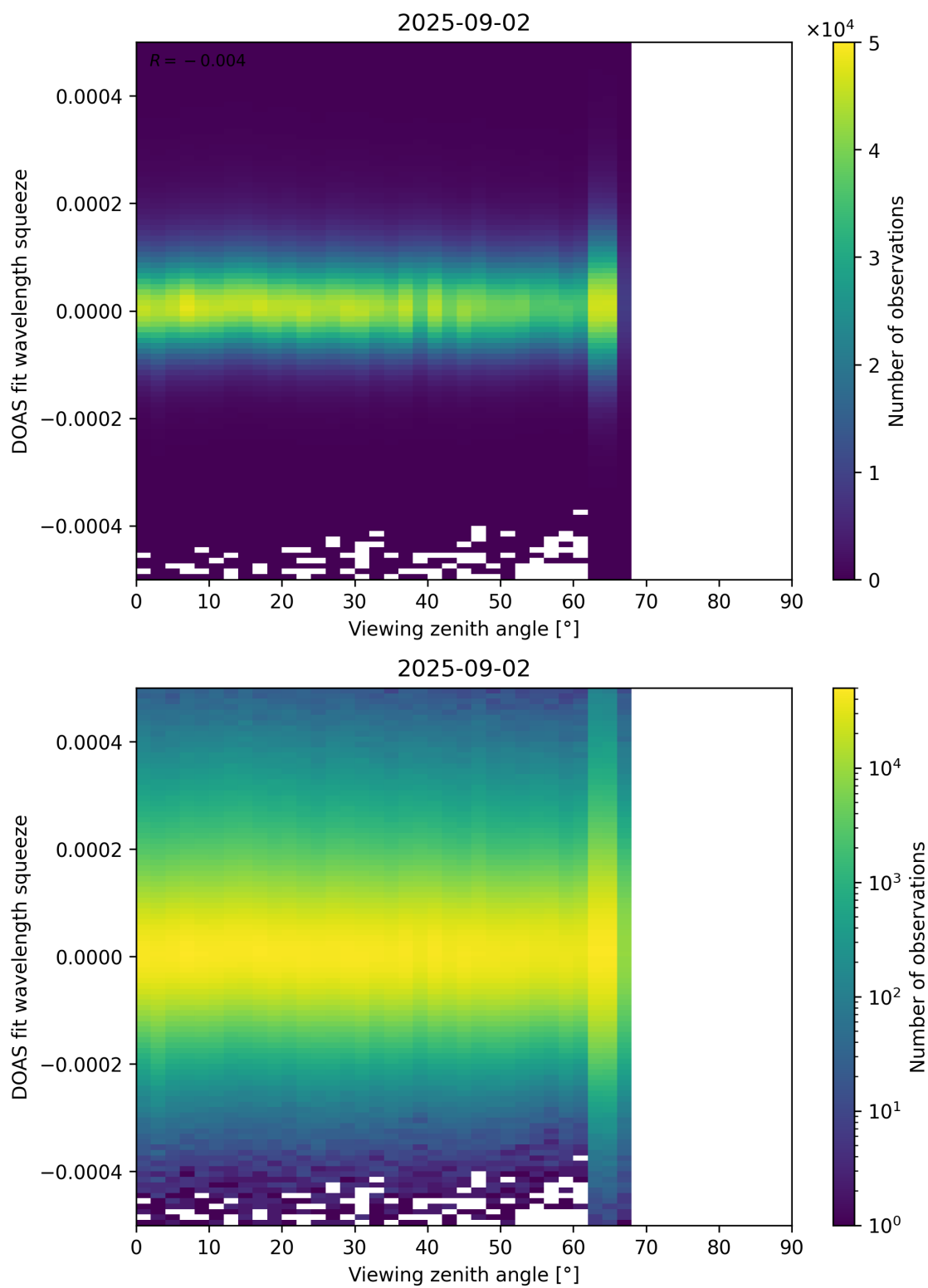
Figure 184: Scatter density plot of “Viewing zenith angle” against “DOAS fit wavelength squeeze” for 2025-09-01 to 2025-09-03.
