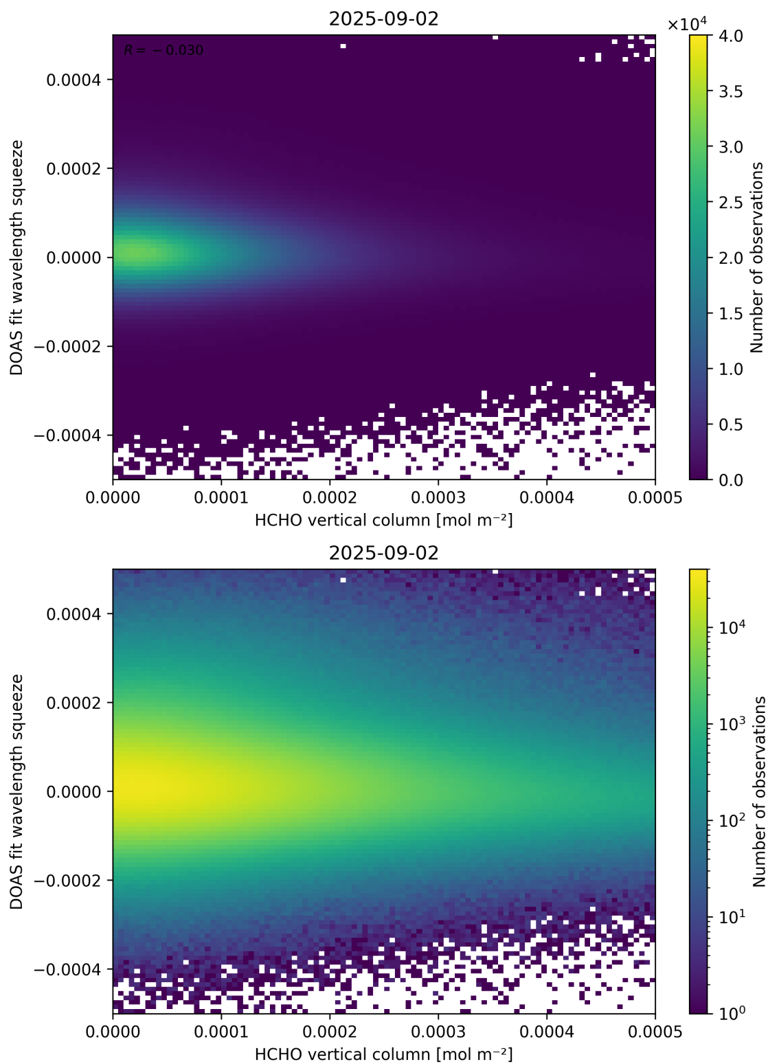
Figure 125: Scatter density plot of “HCHO vertical column” against “DOAS fit wavelength squeeze” for 2025-09-01 to 2025-09-03.
