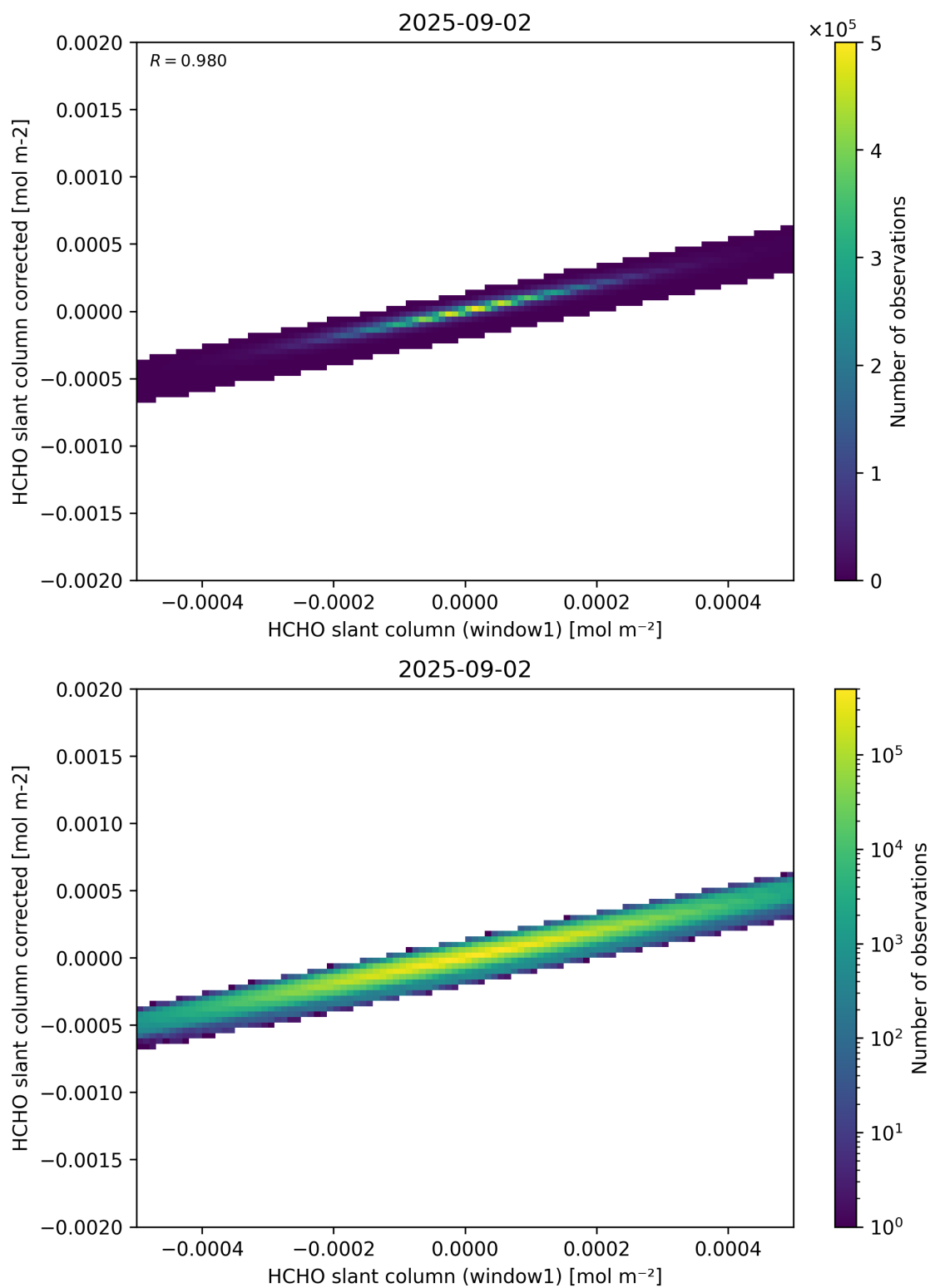
Figure 82: Scatter density plot of “HCHO slant column (window1)” against “HCHO slant column corrected” for 2025-09-01 to 2025-09-03.
