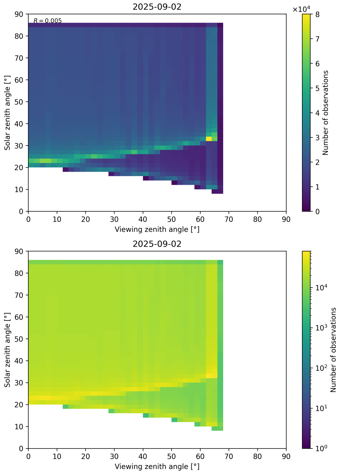
Figure 197: Scatter density plot of “Viewing zenith angle” against “Solar zenith angle” for 2025-09-01 to 2025-09-03.
