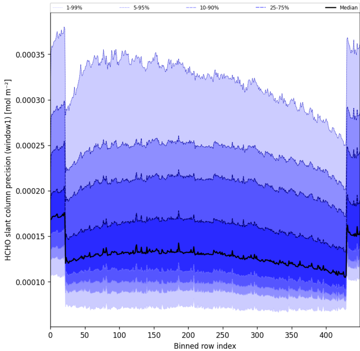
Figure 53: Along track statistics of “HCHO slant column precision (window1)” for 2025-09-01 to 2025-09-03
