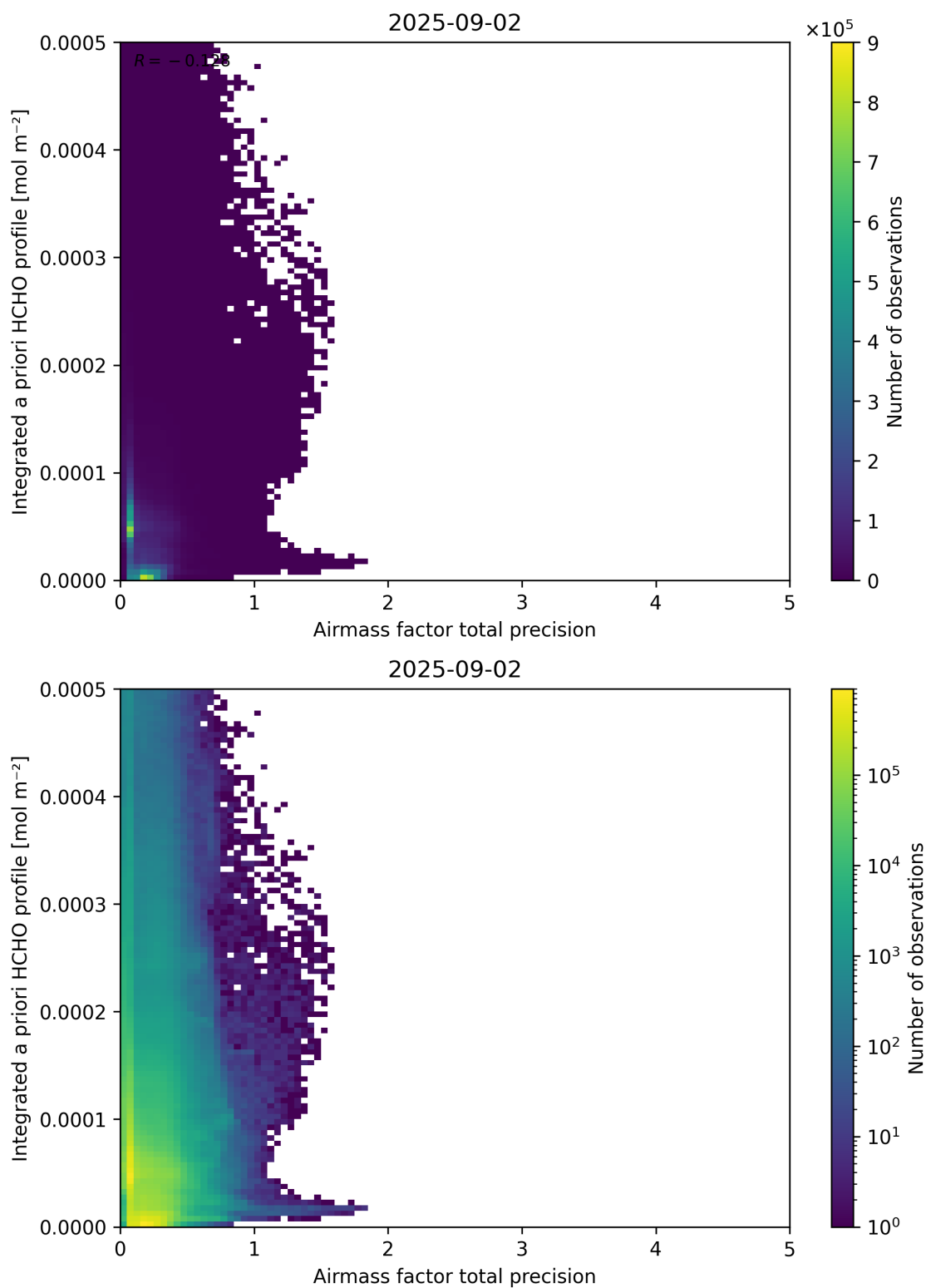
Figure 111: Scatter density plot of “Airmass factor total precision” against “Integrated a priori HCHO profile” for 2025-09-01 to 2025-09-03.
