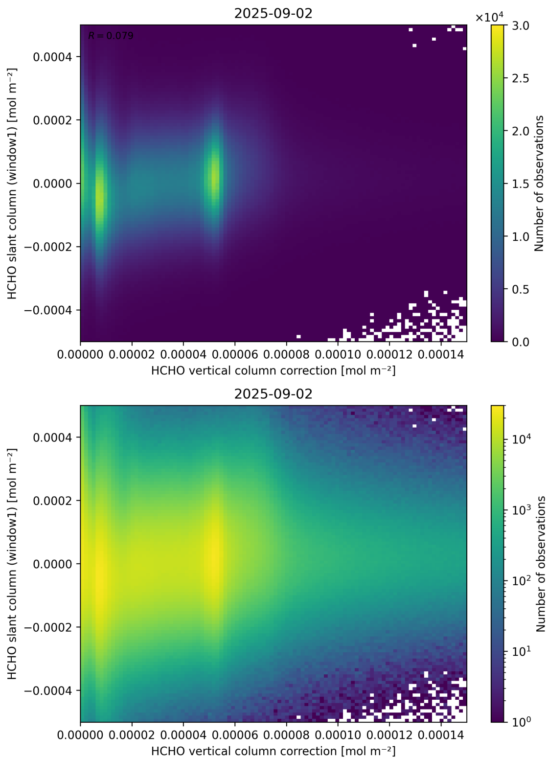
Figure 118: Scatter density plot of “HCHO vertical column correction” against “HCHO slant column (window1)” for 2025-09-01 to 2025-09-03.
