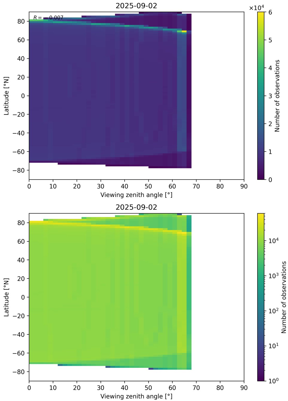
Figure 196: Scatter density plot of “Viewing zenith angle” against “Latitude” for 2025-09-01 to 2025-09-03.
