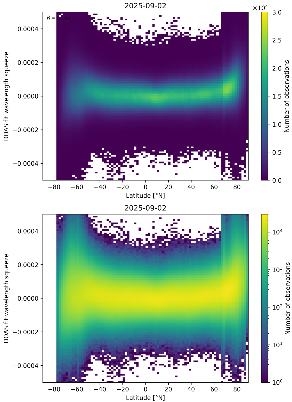
Figure 155: Scatter density plot of “Latitude” against “DOAS fit wavelength squeeze” for 2025-09-01 to 2025-09-03.
