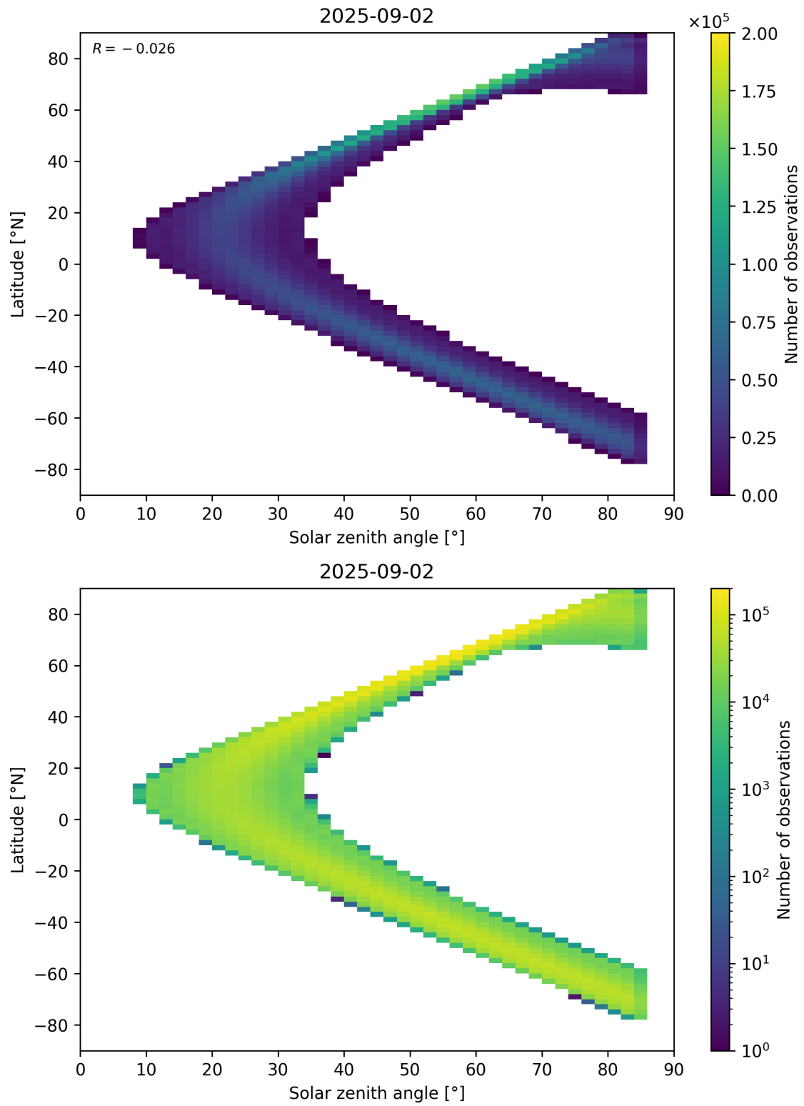
Figure 181: Scatter density plot of “Solar zenith angle” against “Latitude” for 2025-09-01 to 2025-09-03.
