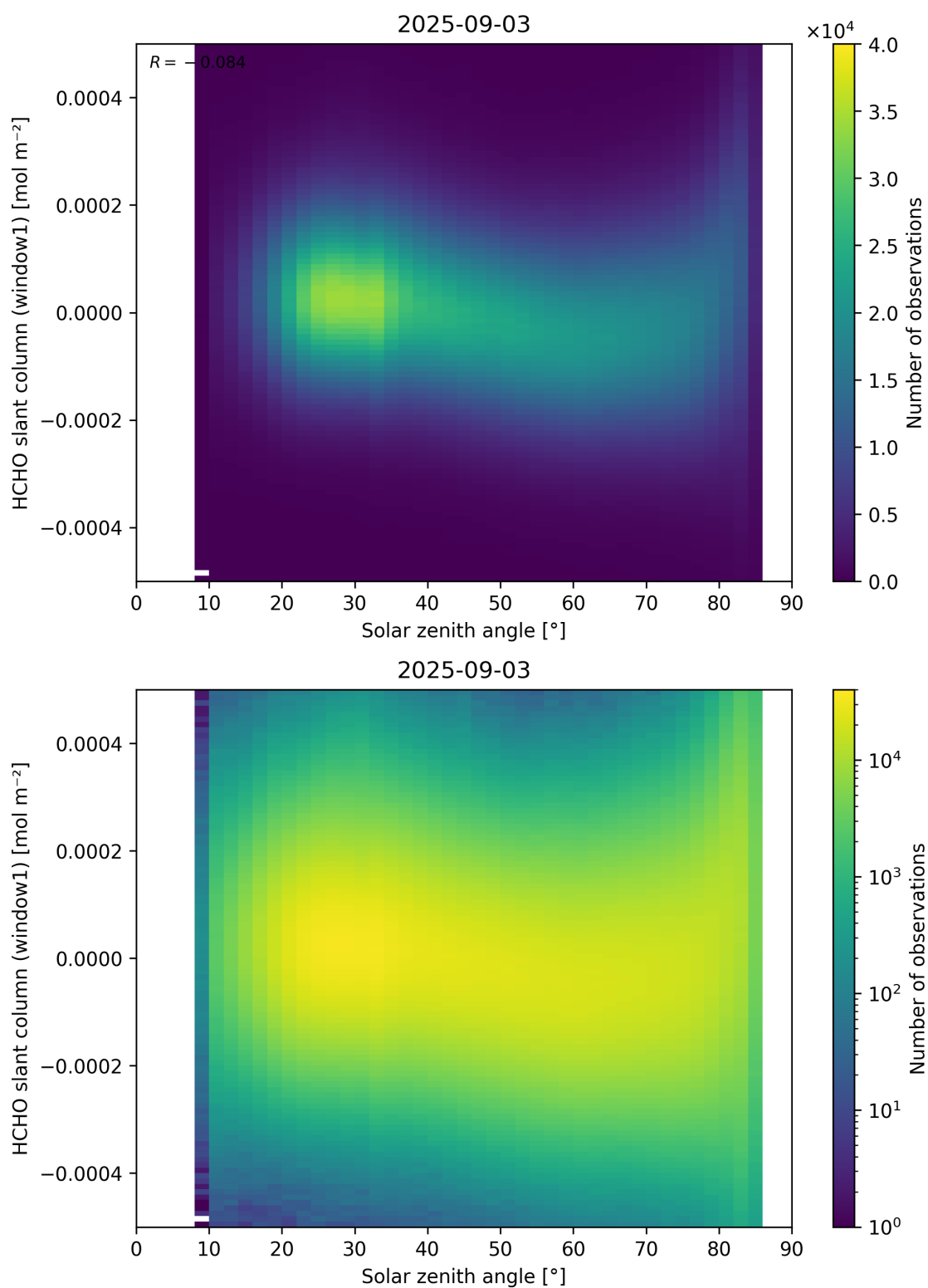
Figure 173: Scatter density plot of “Solar zenith angle” against “HCHO slant column (window1)” for 2025-09-02 to 2025-09-04.
