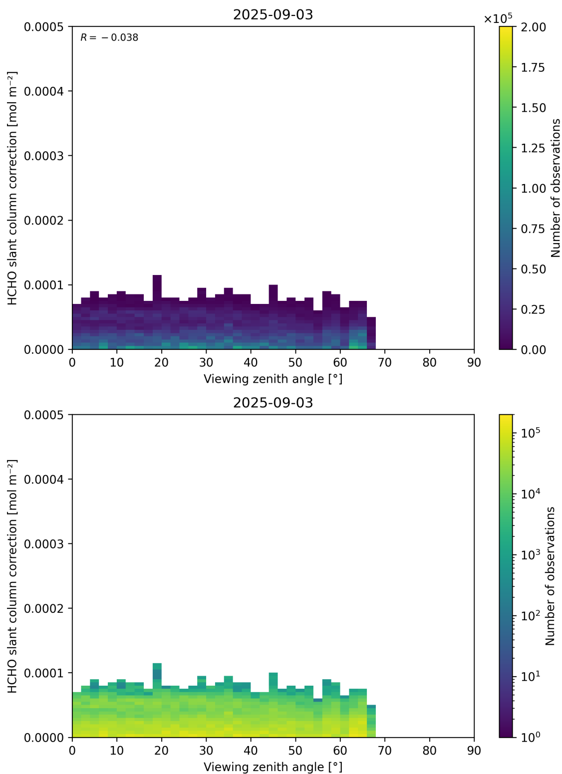
Figure 187: Scatter density plot of “Viewing zenith angle” against “HCHO slant column correction” for 2025-09-02 to 2025-09-04.
