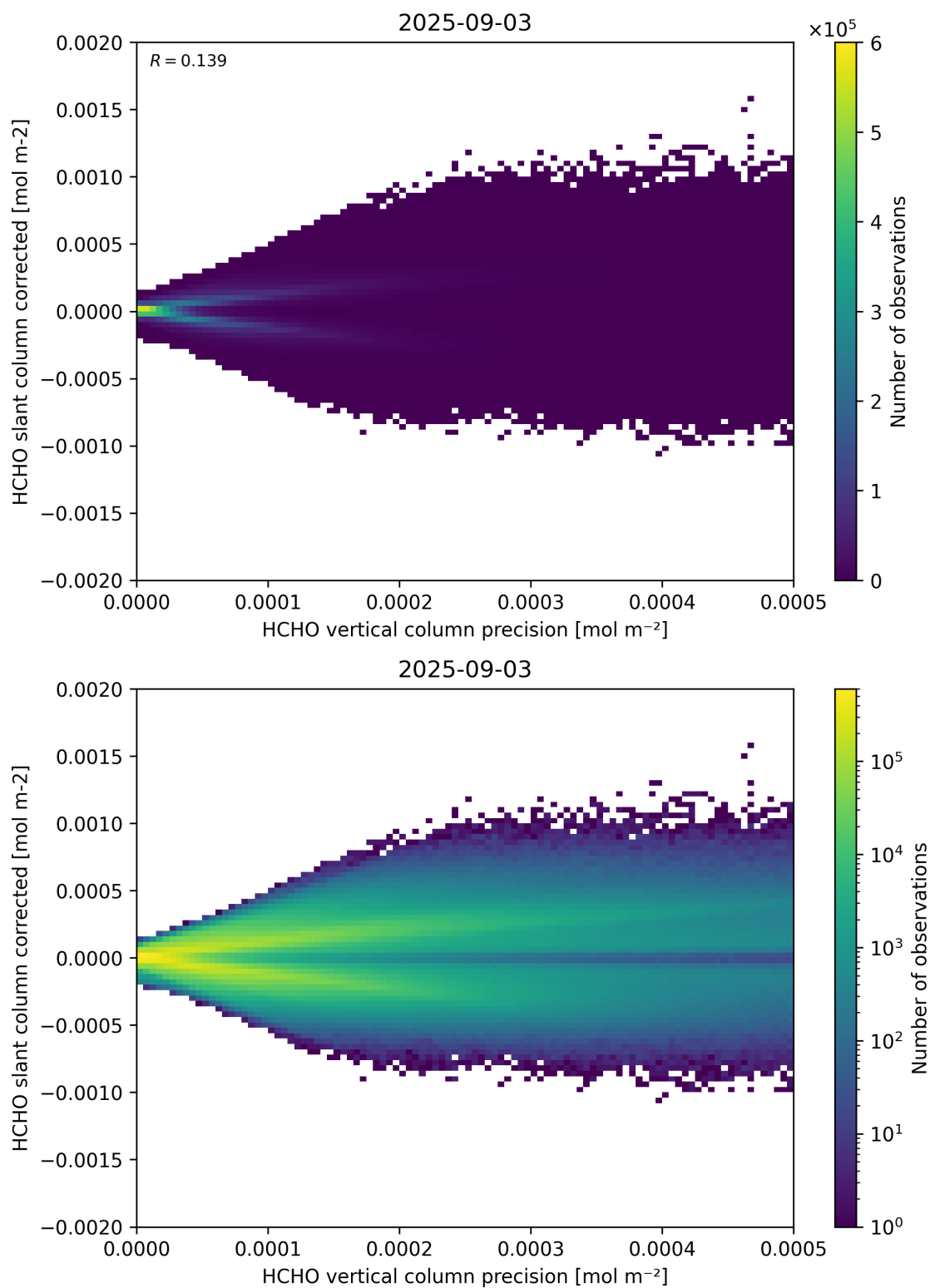
Figure 140: Scatter density plot of “HCHO vertical column precision” against “HCHO slant column corrected” for 2025-09-02 to 2025-09-04.
