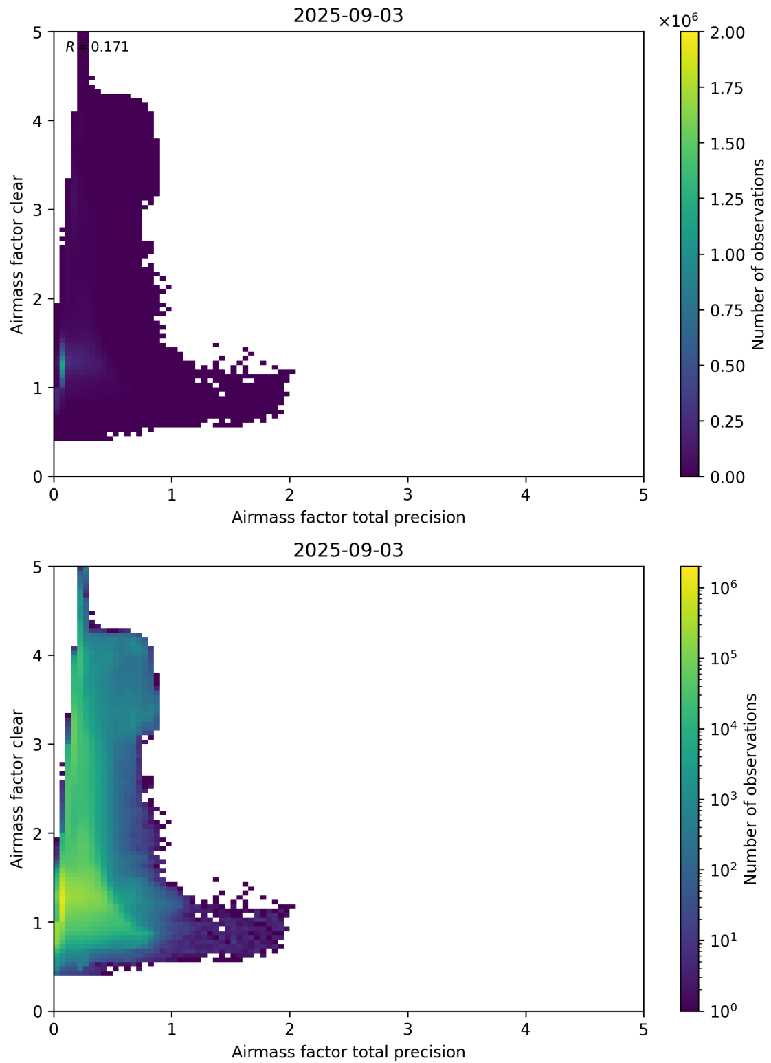
Figure 108: Scatter density plot of “Airmass factor total precision” against “Airmass factor clear” for 2025-09-02 to 2025-09-04.
