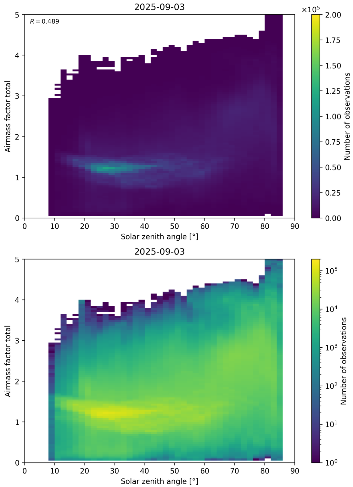
Figure 175: Scatter density plot of “Solar zenith angle” against “Airmass factor total” for 2025-09-02 to 2025-09-04.
