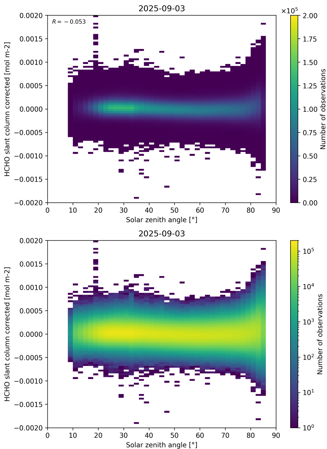
Figure 171: Scatter density plot of “Solar zenith angle” against “HCHO slant column corrected” for 2025-09-02 to 2025-09-04.
