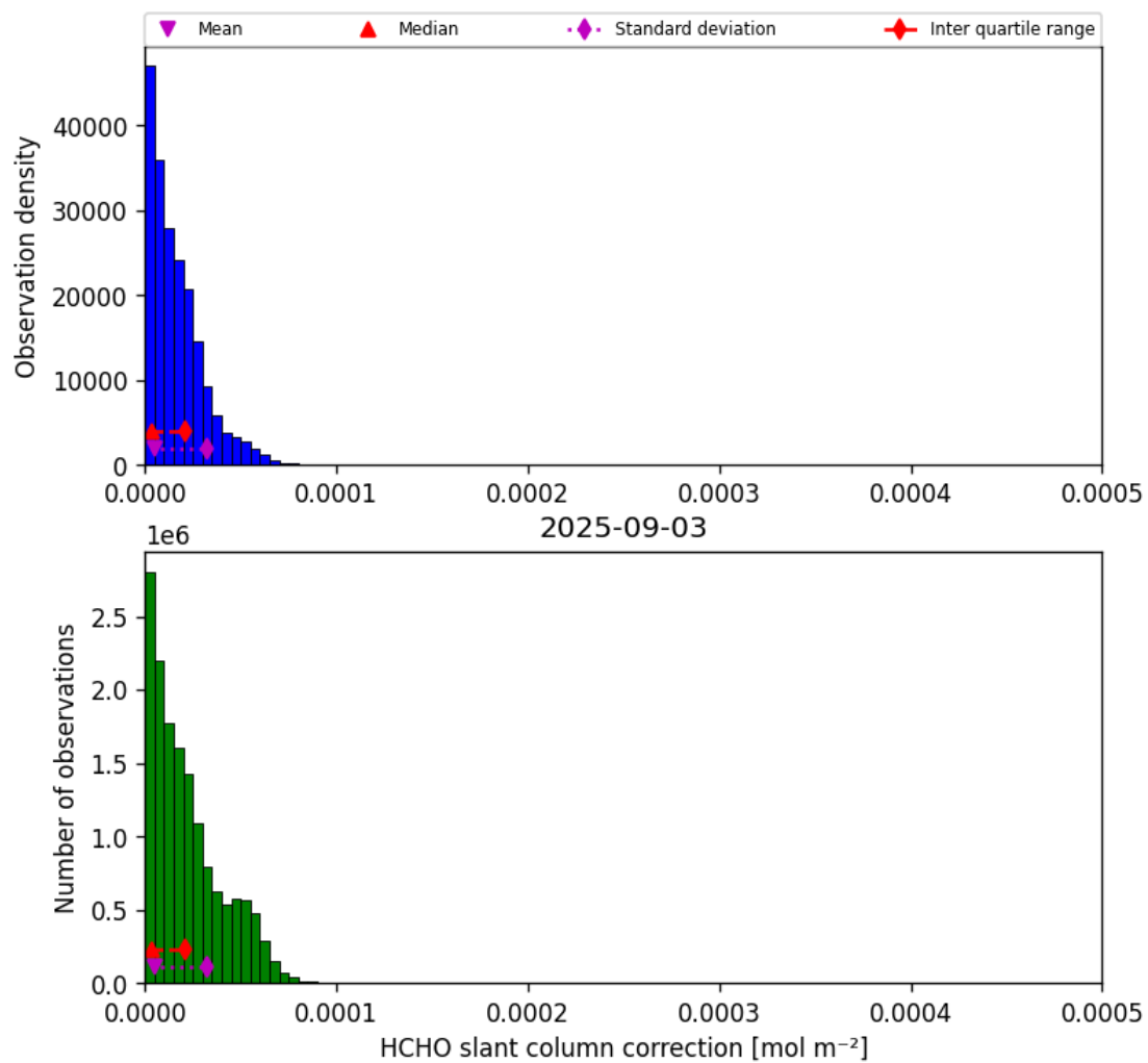
Figure 47: Histogram of “HCHO slant column correction” for 2025-09-02 to 2025-09-04
