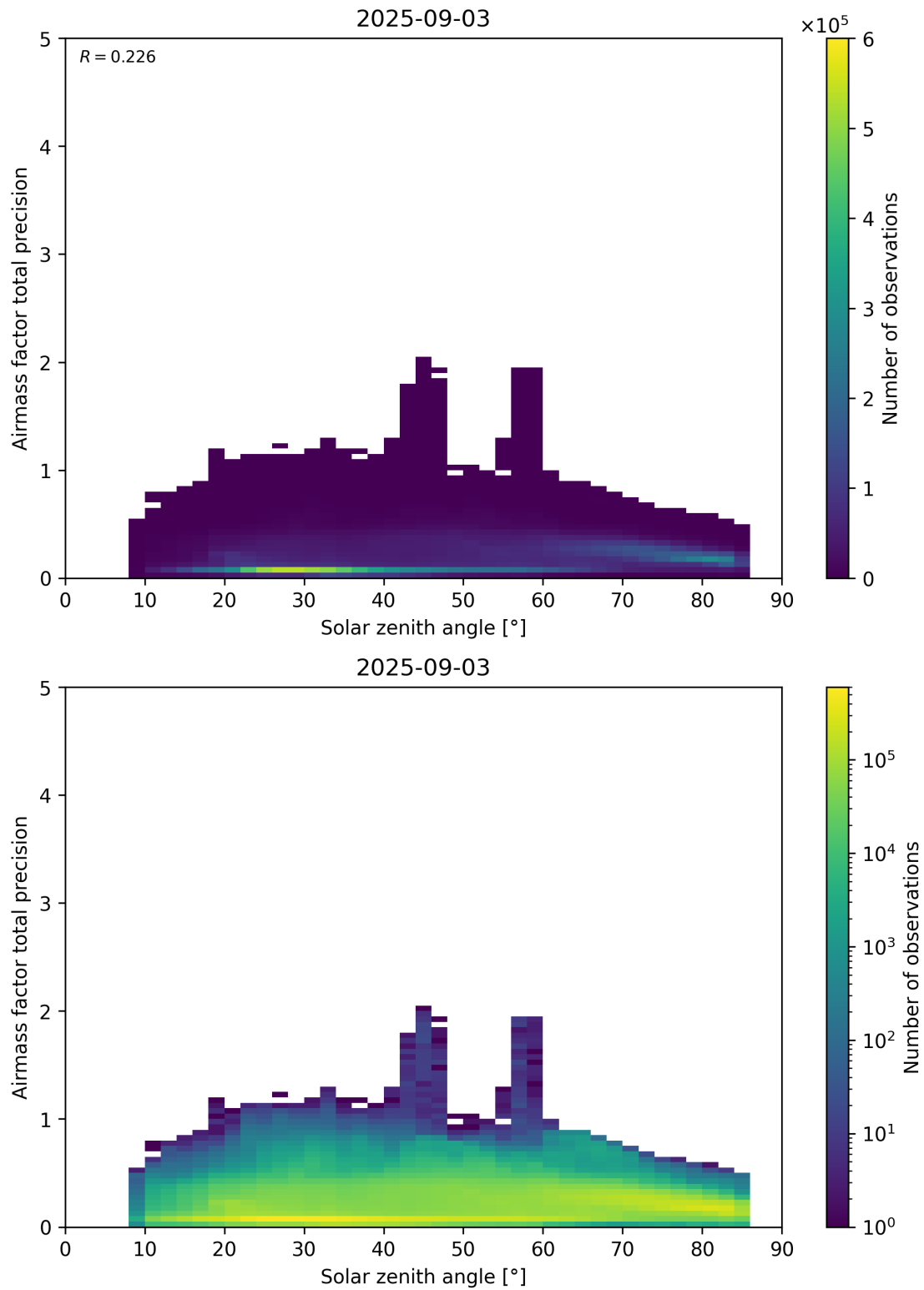
Figure 176: Scatter density plot of “Solar zenith angle” against “Airmass factor total precision” for 2025-09-02 to 2025-09-04.
