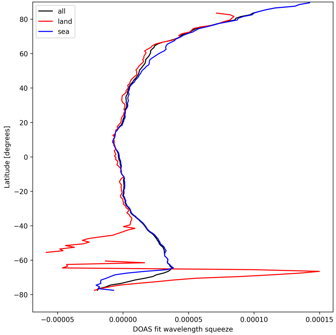
Figure 31: Zonal average of “DOAS fit wavelength squeeze” for 2025-09-02 to 2025-09-04.
