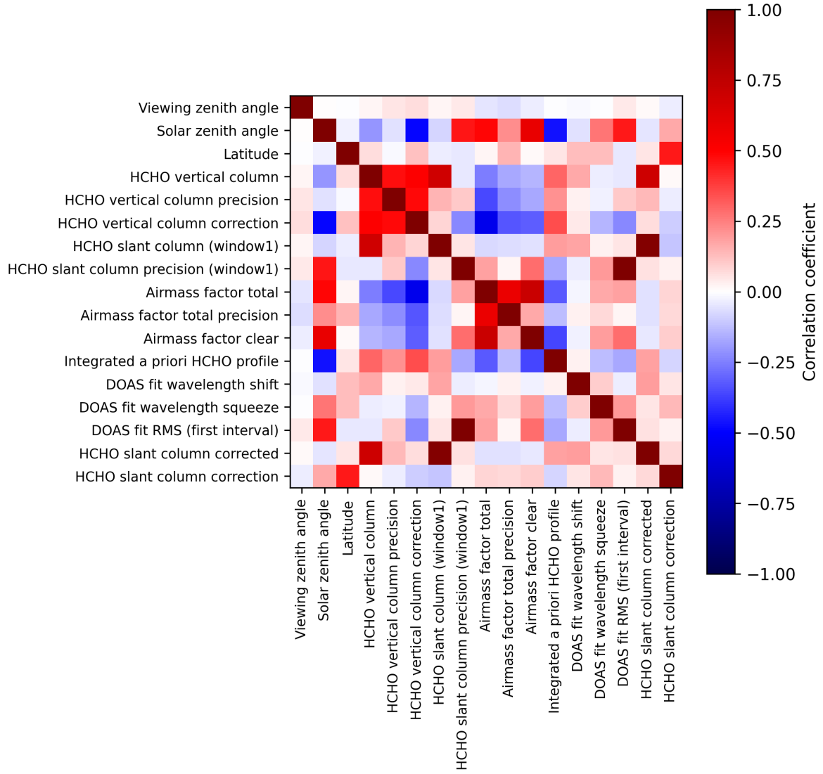
Figure 2: Map of correlation matrix for 2025-09-02 to 2025-09-04.
