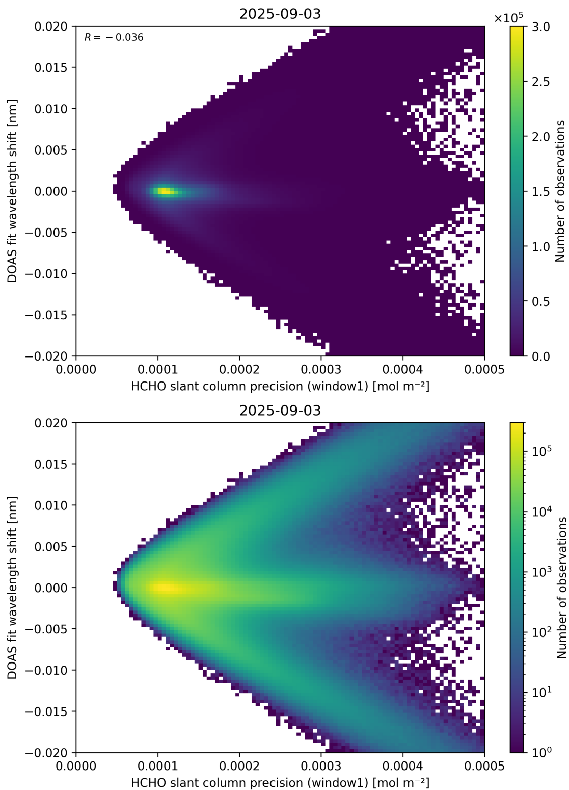
Figure 89: Scatter density plot of “HCHO slant column precision (window1)” against “DOAS fit wavelength shift” for 2025-09-02 to 2025-09-04.
