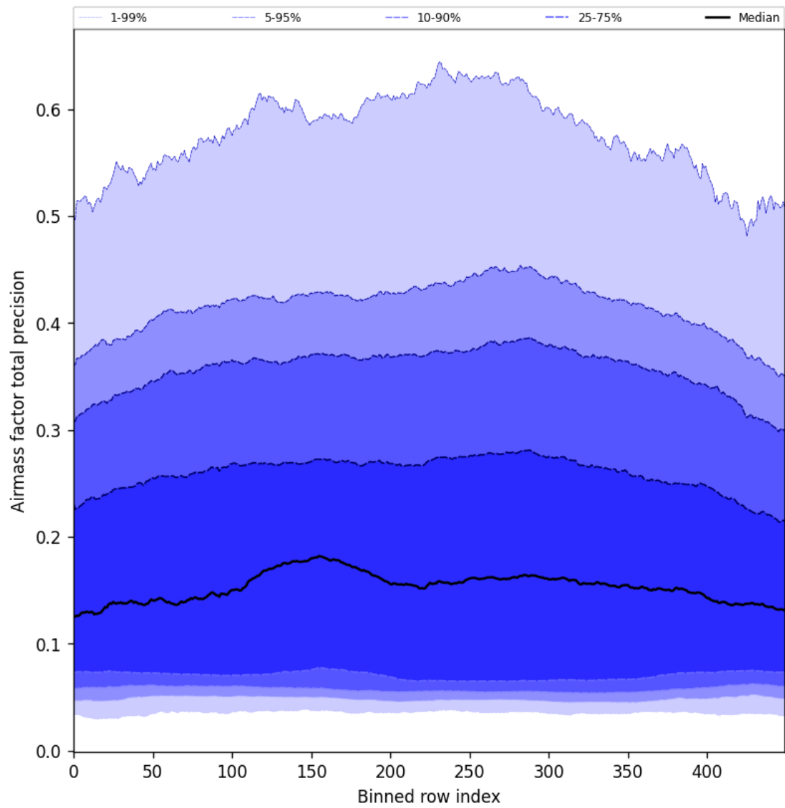
Figure 55: Along track statistics of “Airmass factor total precision” for 2025-09-02 to 2025-09-04
