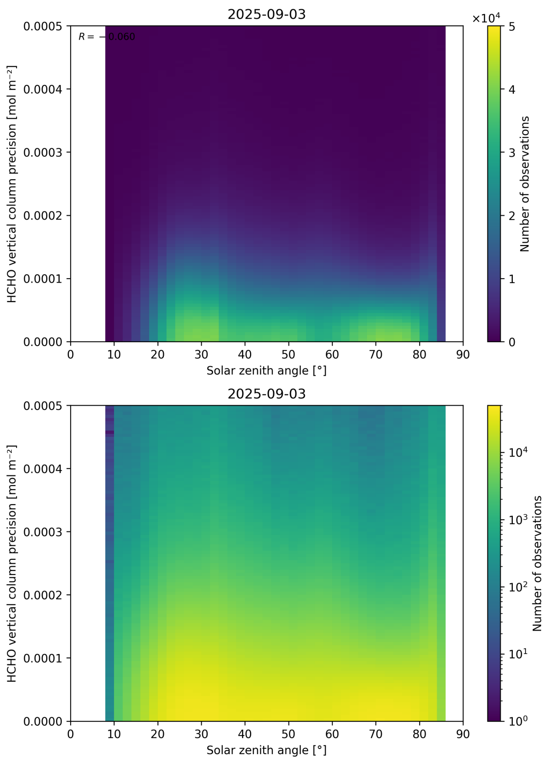
Figure 179: Scatter density plot of “Solar zenith angle” against “HCHO vertical column precision” for 2025-09-02 to 2025-09-04.
