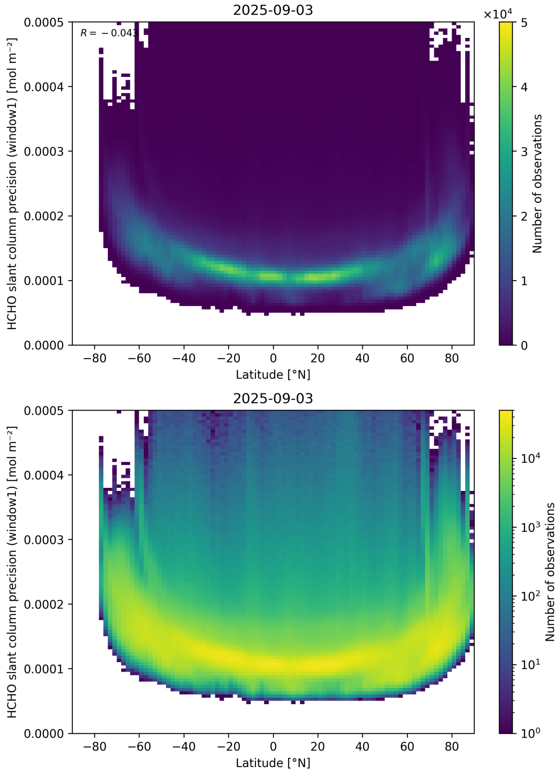
Figure 160: Scatter density plot of “Latitude” against “HCHO slant column precision (window1)” for 2025-09-02 to 2025-09-04.
