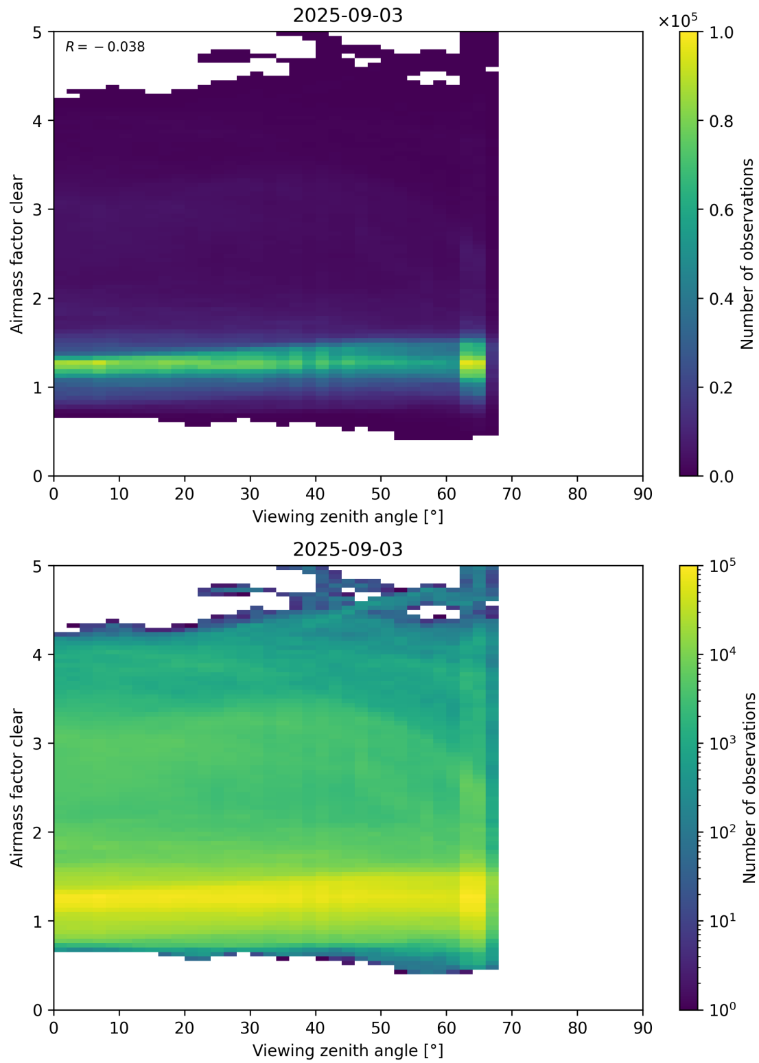
Figure 185: Scatter density plot of “Viewing zenith angle” against “Airmass factor clear” for 2025-09-02 to 2025-09-04.
