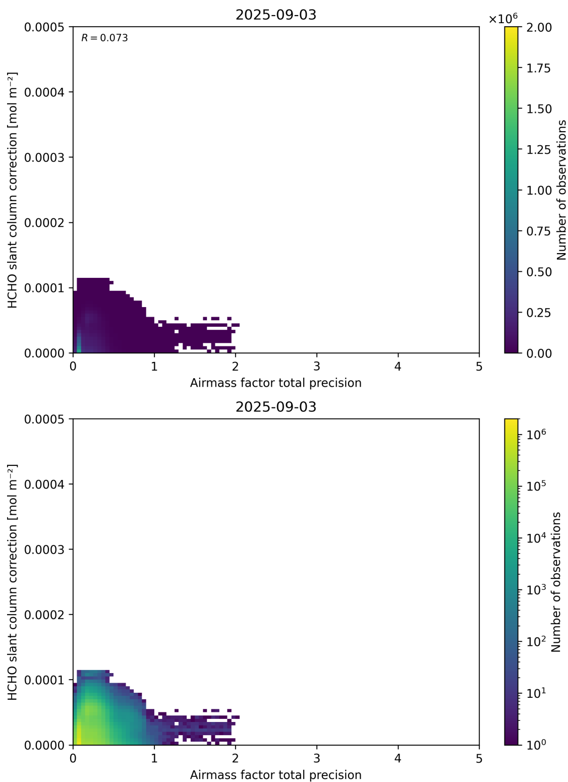
Figure 110: Scatter density plot of “Airmass factor total precision” against “HCHO slant column correction” for 2025-09-02 to 2025-09-04.
