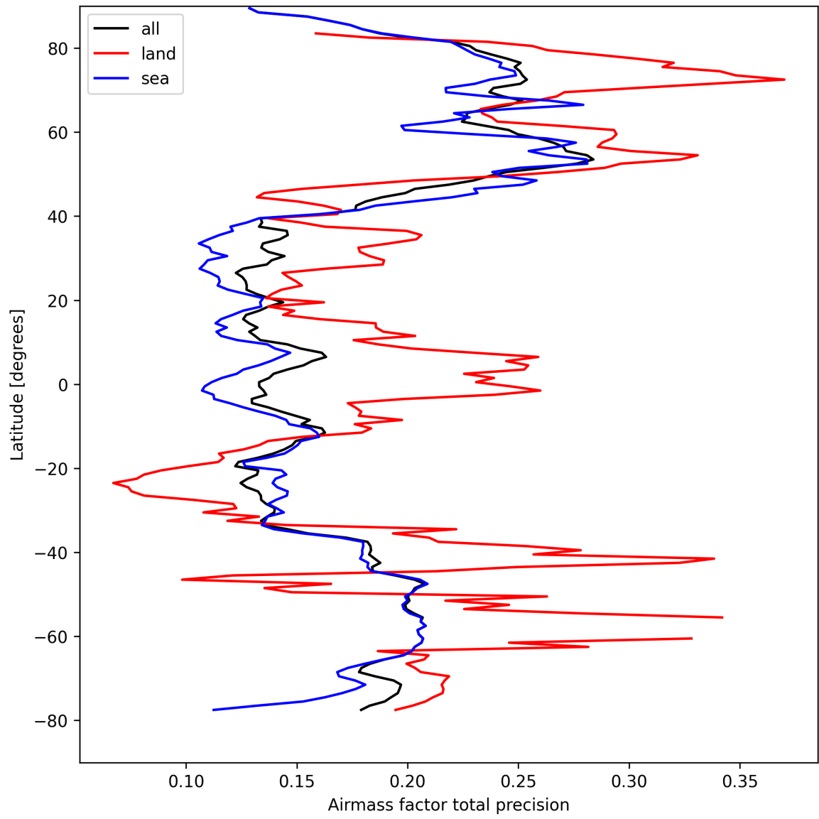
Figure 27: Zonal average of “Airmass factor total precision” for 2025-09-02 to 2025-09-04.
