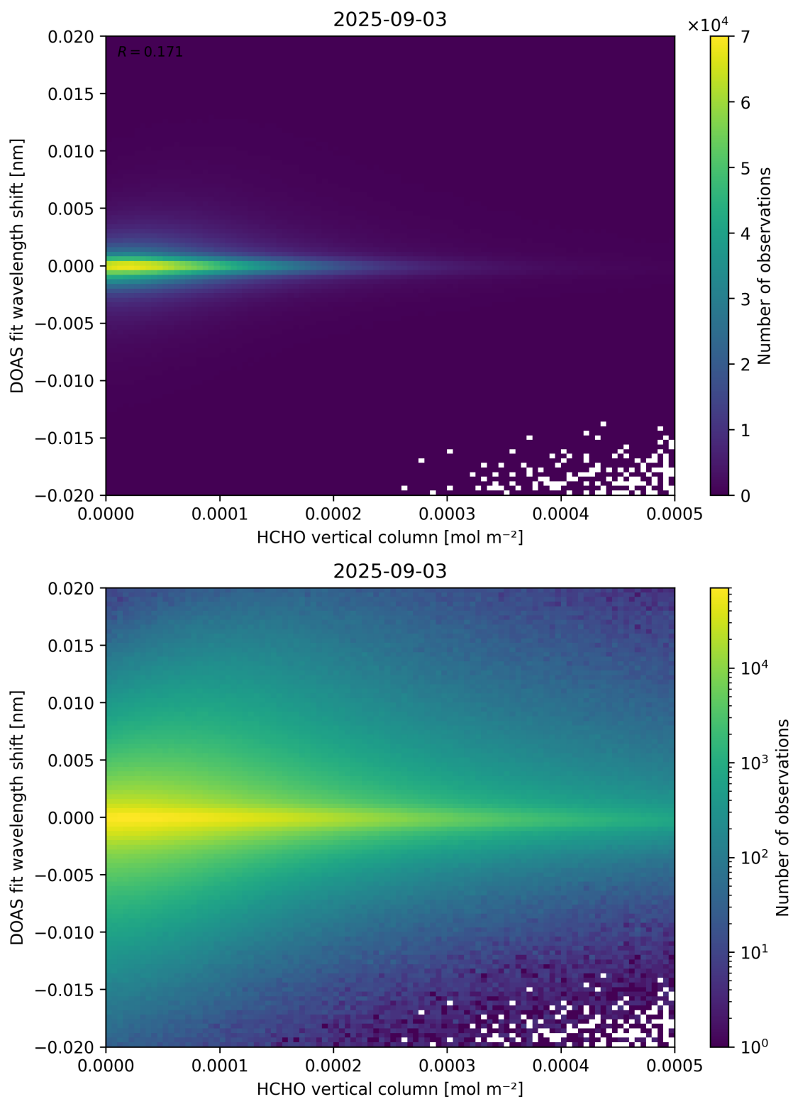
Figure 124: Scatter density plot of “HCHO vertical column” against “DOAS fit wavelength shift” for 2025-09-02 to 2025-09-04.
