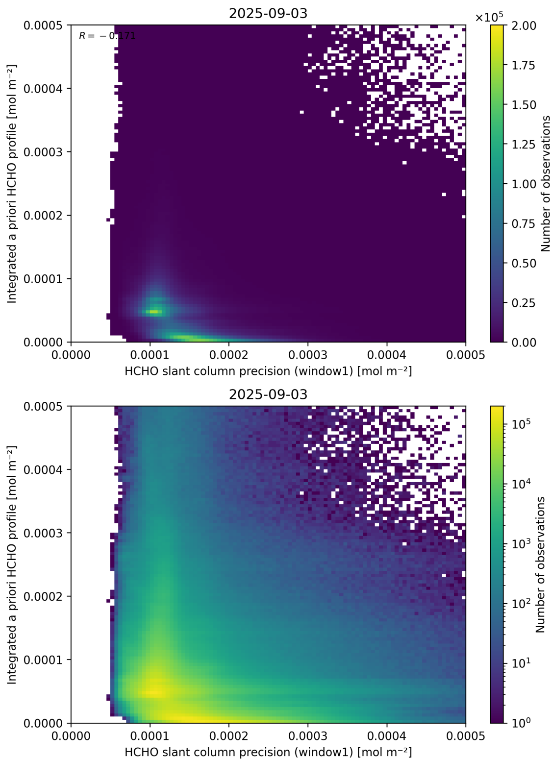
Figure 96: Scatter density plot of “HCHO slant column precision (window1)” against “Integrated a priori HCHO profile” for 2025-09-02 to 2025-09-04.
