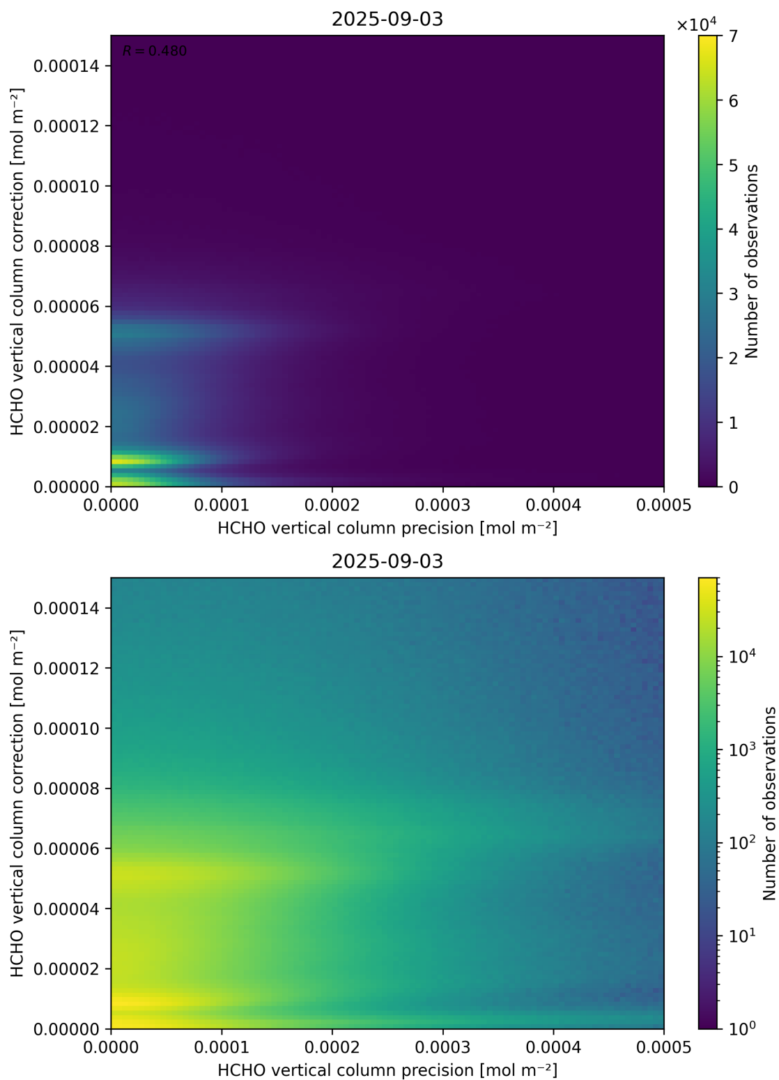
Figure 146: Scatter density plot of “HCHO vertical column precision” against “HCHO vertical column correction” for 2025-09-02 to 2025-09-04.
