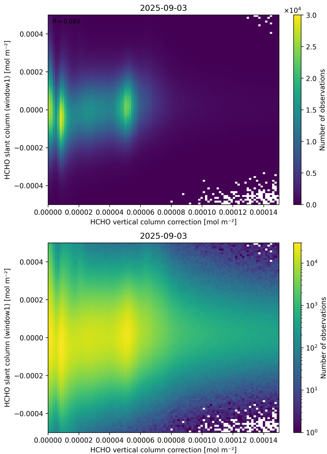
Figure 118: Scatter density plot of “HCHO vertical column correction” against “HCHO slant column (window1)” for 2025-09-02 to 2025-09-04.
