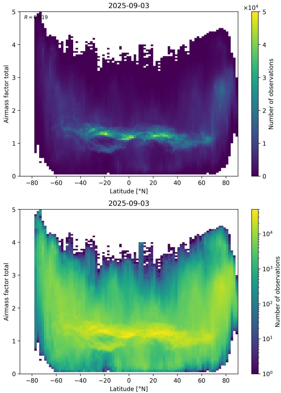
Figure 161: Scatter density plot of “Latitude” against “Airmass factor total” for 2025-09-02 to 2025-09-04.
