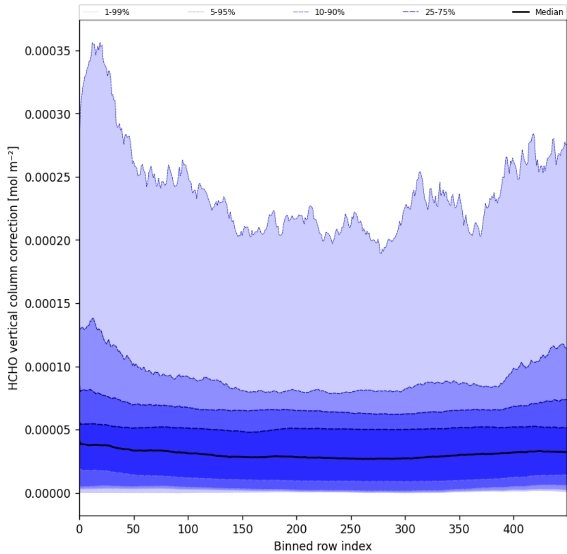
Figure 51: Along track statistics of “HCHO vertical column correction” for 2025-09-02 to 2025-09-04
