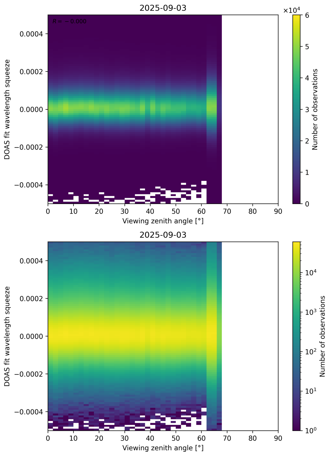
Figure 184: Scatter density plot of “Viewing zenith angle” against “DOAS fit wavelength squeeze” for 2025-09-02 to 2025-09-04.
