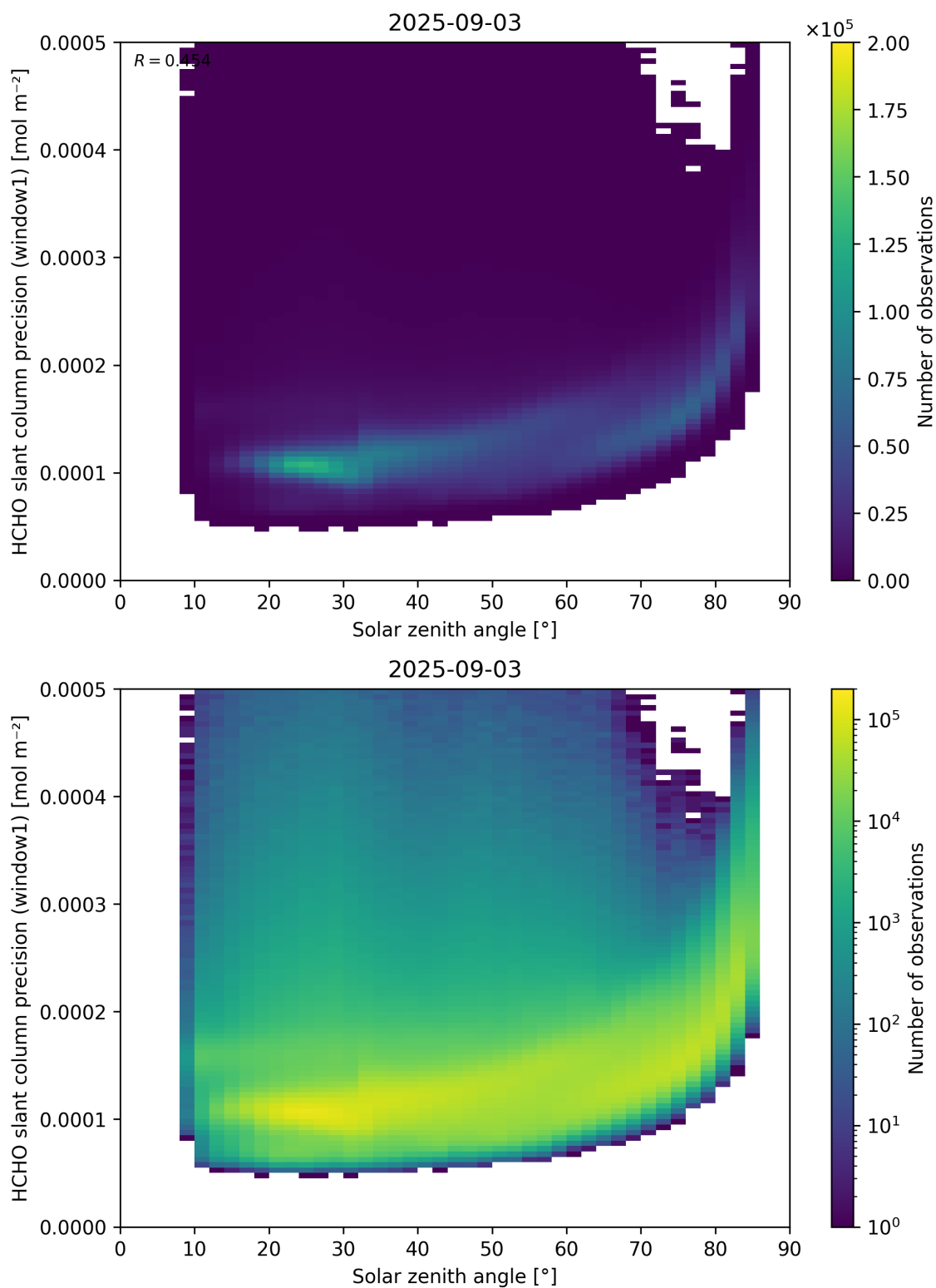
Figure 174: Scatter density plot of “Solar zenith angle” against “HCHO slant column precision (window1)” for 2025-09-02 to 2025-09-04.
