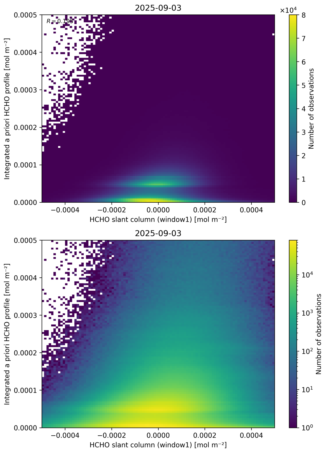
Figure 87: Scatter density plot of “HCHO slant column (window1)” against “Integrated a priori HCHO profile” for 2025-09-02 to 2025-09-04.
