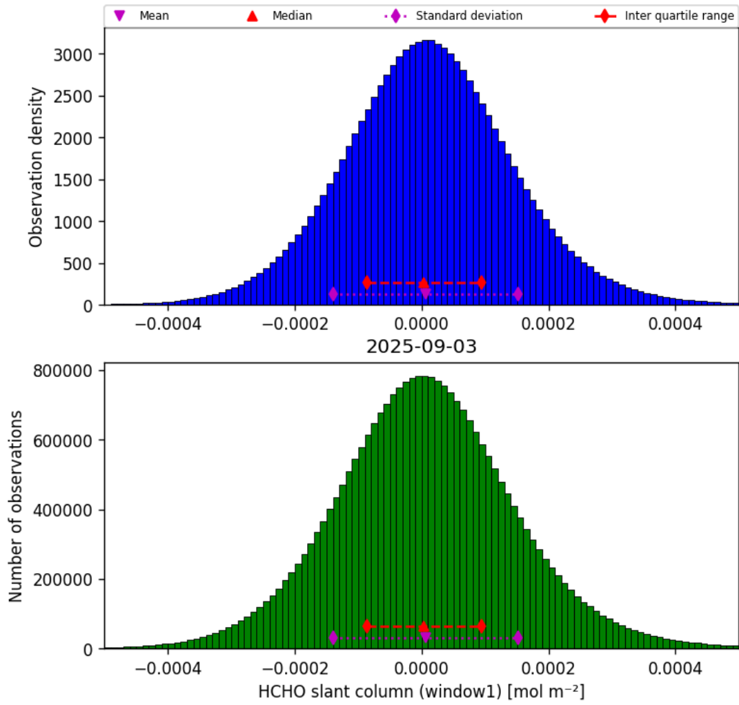
Figure 38: Histogram of “HCHO slant column (window1)” for 2025-09-02 to 2025-09-04
