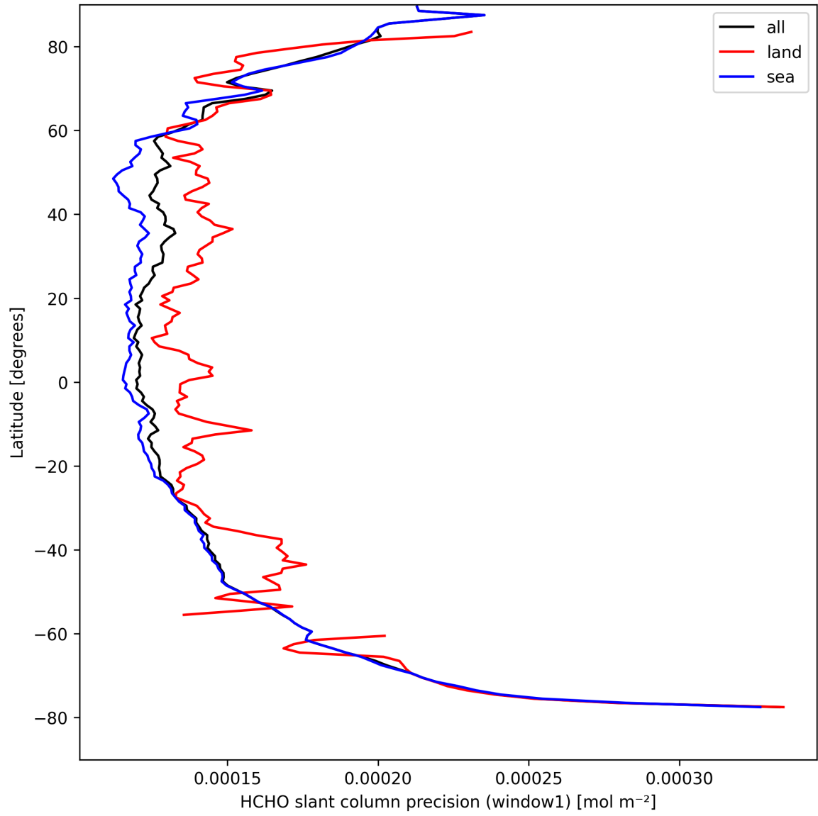
Figure 25: Zonal average of "HCHO slant column precision (window1)" for 2025-09-02 to 2025-09-04.
