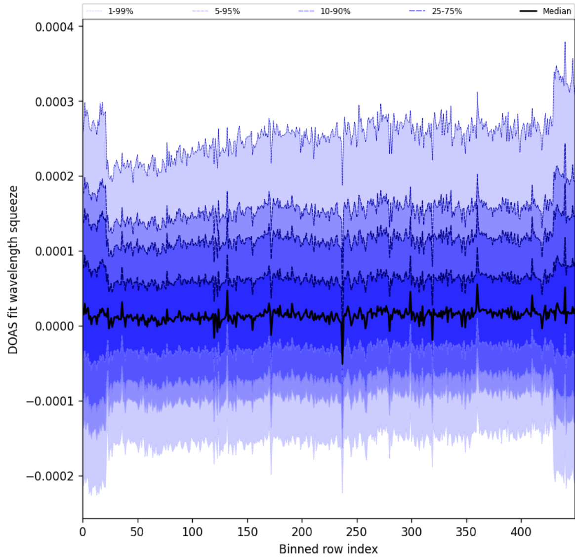
Figure 59: Along track statistics of “DOAS fit wavelength squeeze” for 2025-09-02 to 2025-09-04
