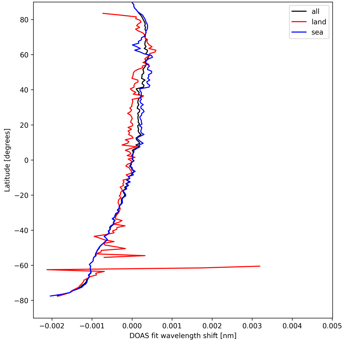
Figure 30: Zonal average of “DOAS fit wavelength shift” for 2025-09-02 to 2025-09-04.
