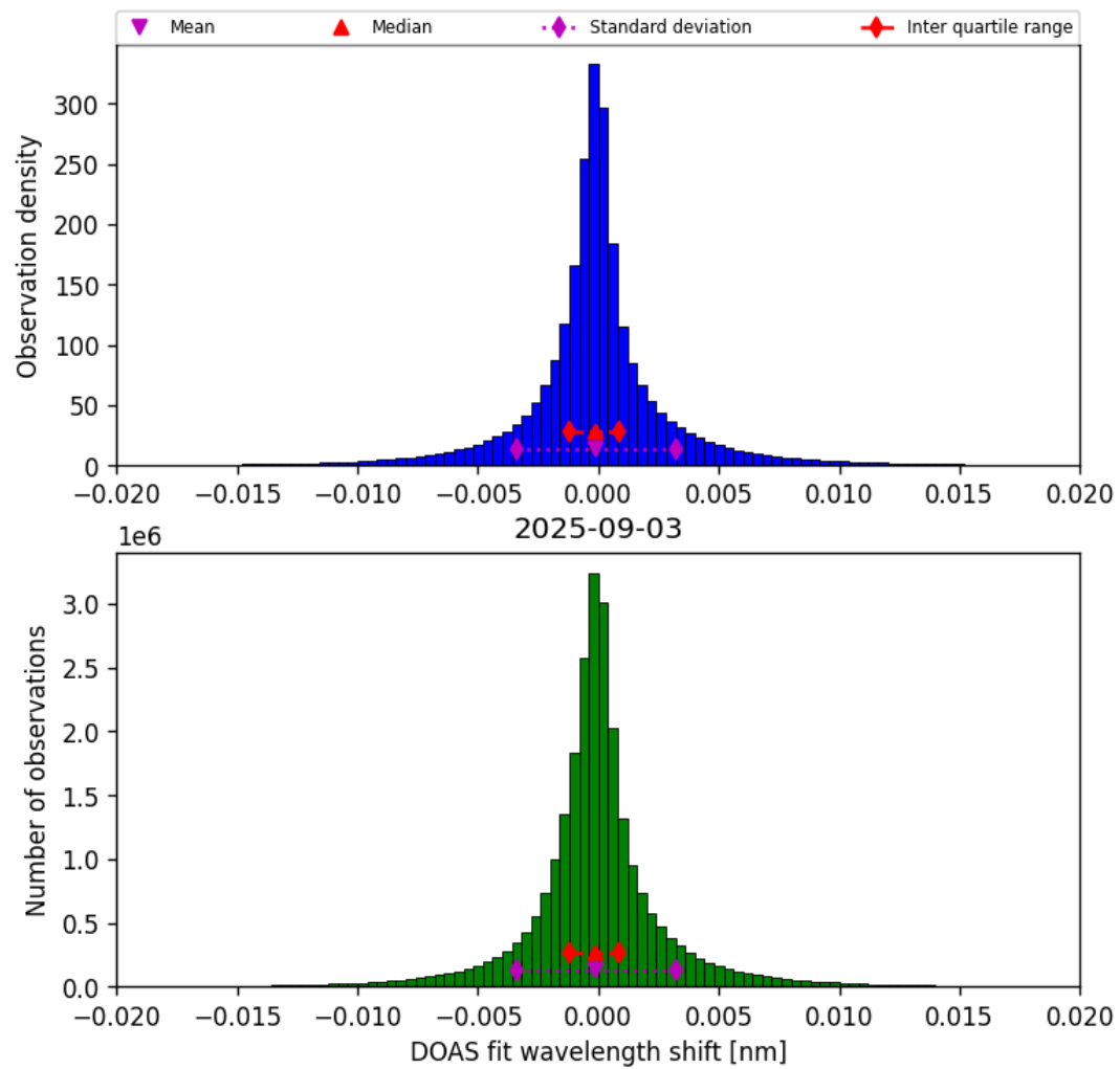
Figure 44: Histogram of “DOAS fit wavelength shift” for 2025-09-02 to 2025-09-04
