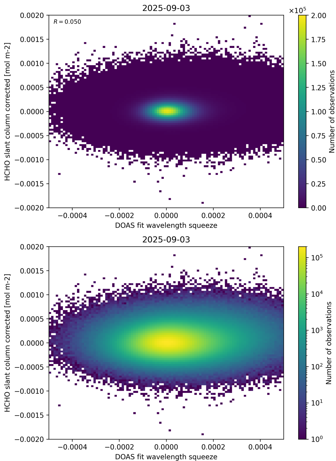
Figure 69: Scatter density plot of “DOAS fit wavelength squeeze” against “HCHO slant column corrected” for 2025-09-02 to 2025-09-04.
