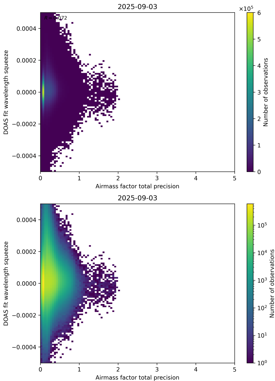
Figure 107: Scatter density plot of “Airmass factor total precision” against “DOAS fit wavelength squeeze” for 2025-09-02 to 2025-09-04.
