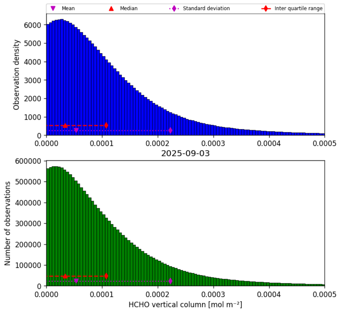
Figure 35: Histogram of “HCHO vertical column” for 2025-09-02 to 2025-09-04
