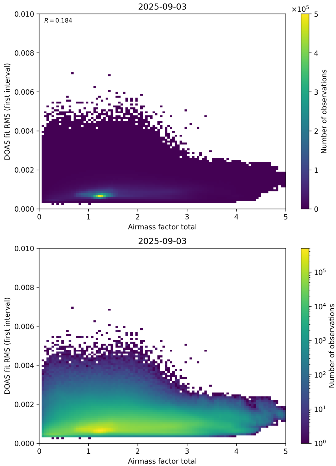
Figure 97: Scatter density plot of “Airmass factor total” against “DOAS fit RMS (first interval)” for 2025-09-02 to 2025-09-04.
