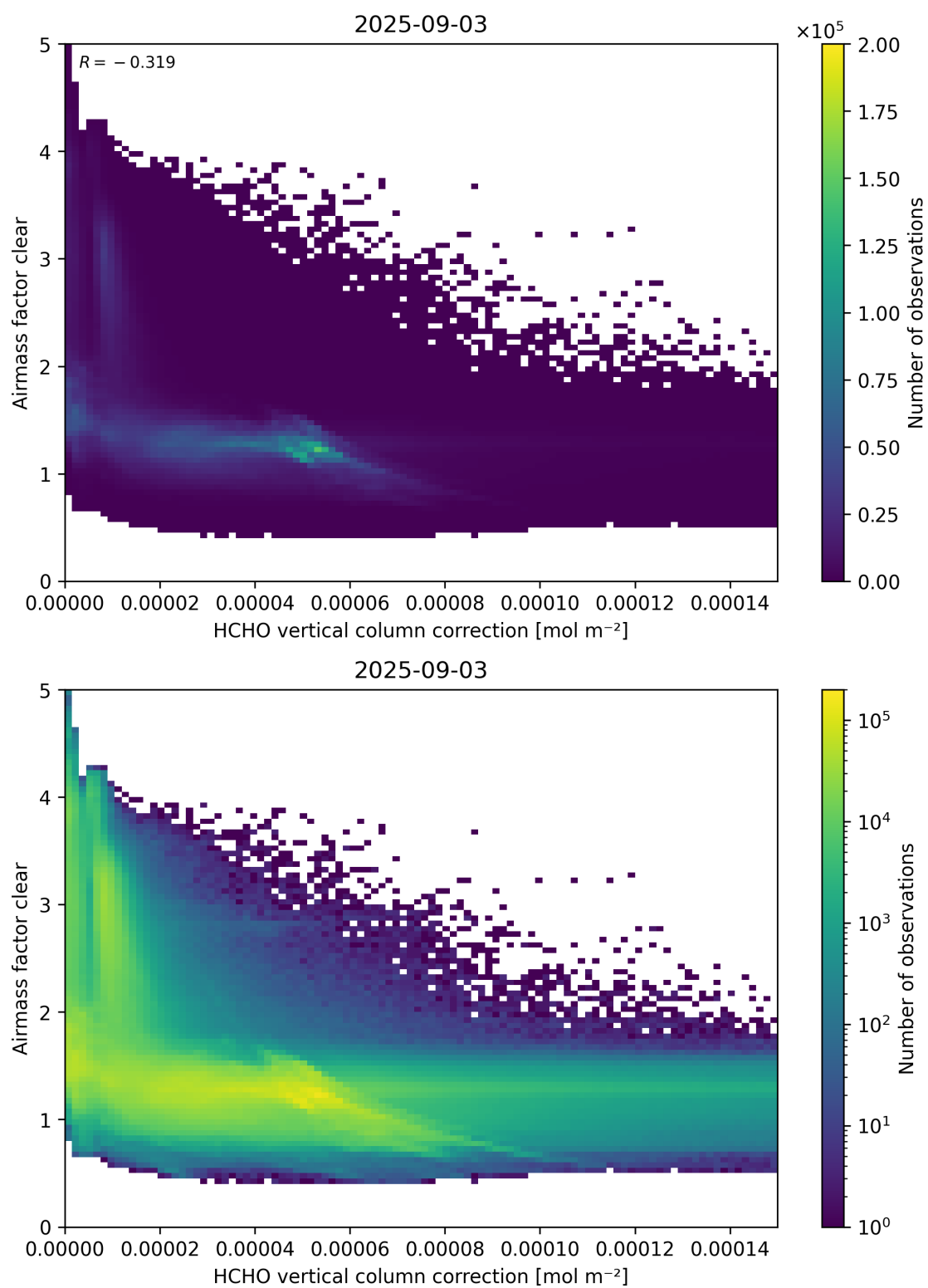
Figure 115: Scatter density plot of “HCHO vertical column correction” against “Airmass factor clear” for 2025-09-02 to 2025-09-04.
