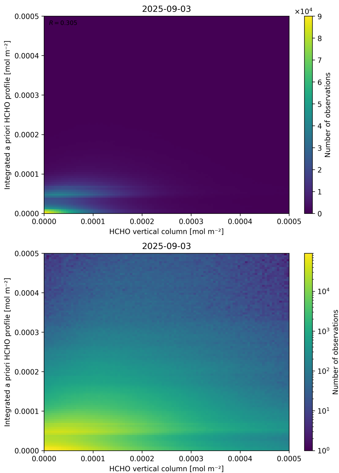
Figure 135: Scatter density plot of “HCHO vertical column” against “Integrated a priori HCHO profile” for 2025-09-02 to 2025-09-04.
