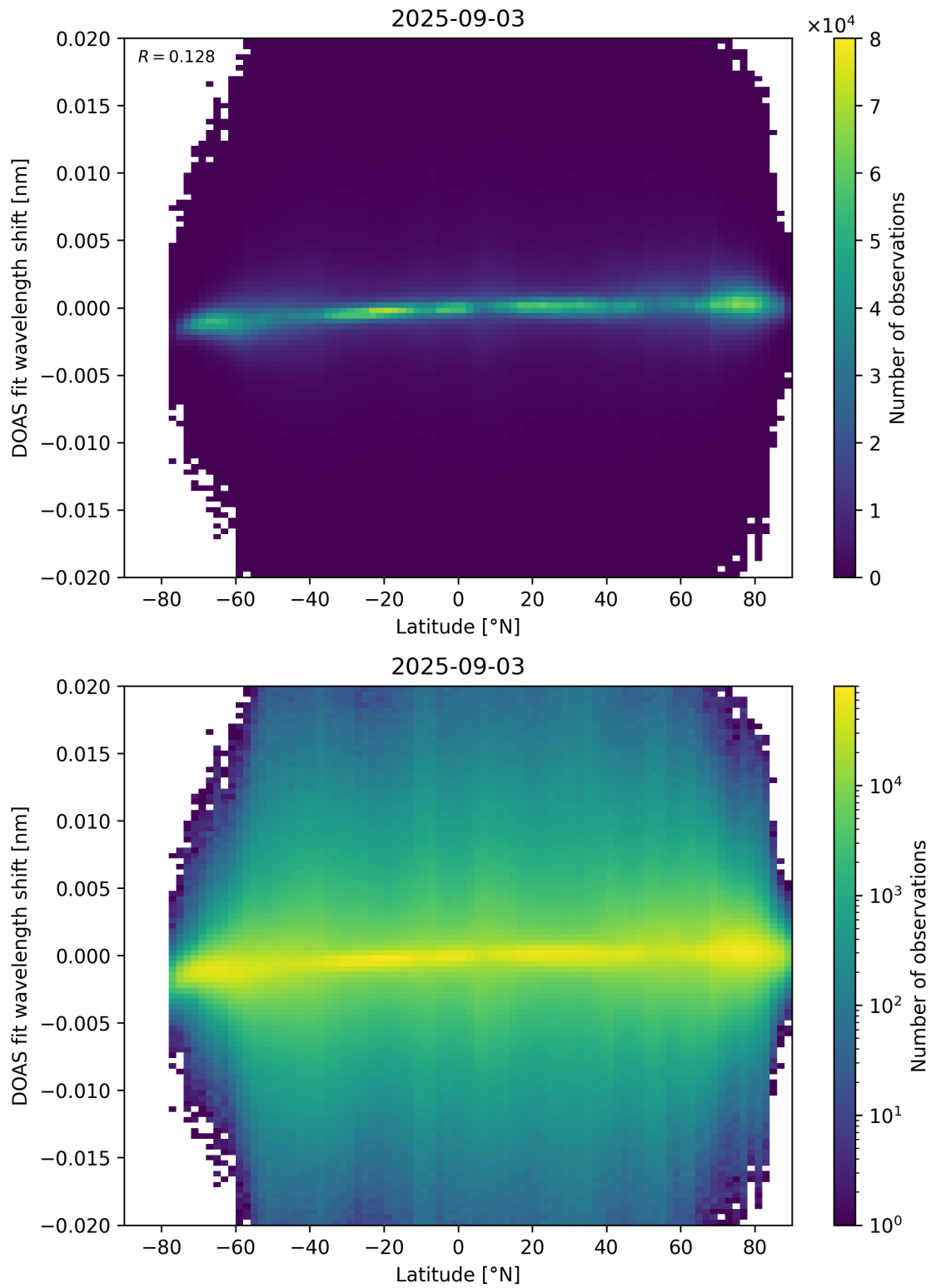
Figure 154: Scatter density plot of “Latitude” against “DOAS fit wavelength shift” for 2025-09-02 to 2025-09-04.
