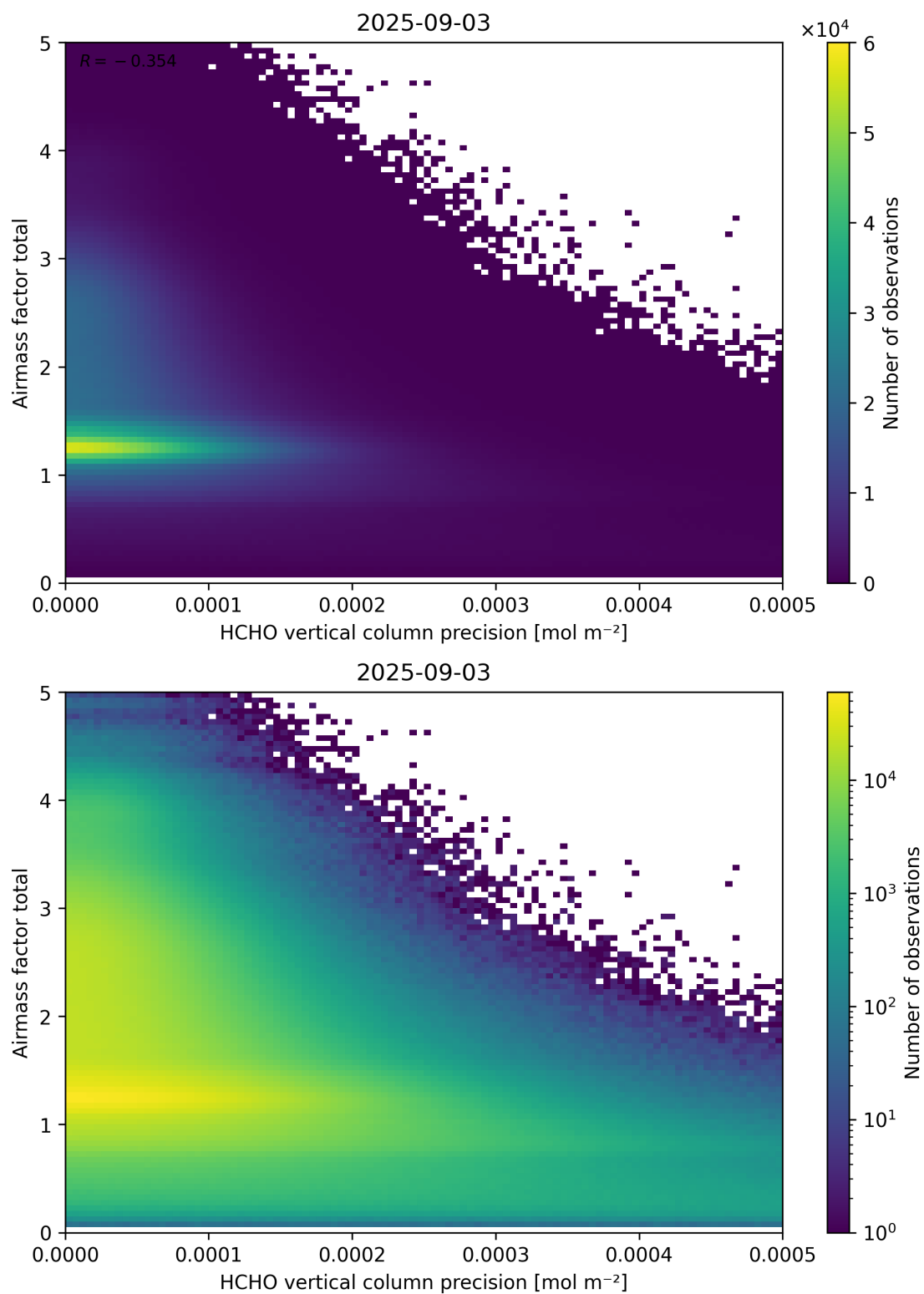
Figure 144: Scatter density plot of “HCHO vertical column precision” against “Airmass factor total” for 2025-09-02 to 2025-09-04.
