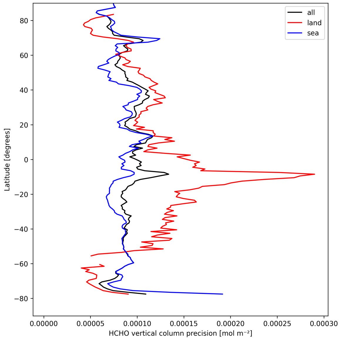
Figure 22: Zonal average of “HCHO vertical column precision” for 2025-09-02 to 2025-09-04.
