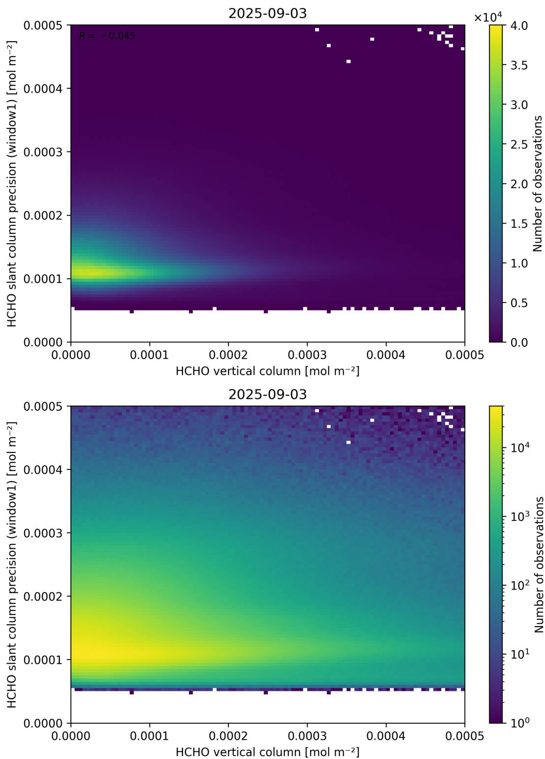
Figure 130: Scatter density plot of “HCHO vertical column” against “HCHO slant column precision (window1)” for 2025-09-02 to 2025-09-04.
