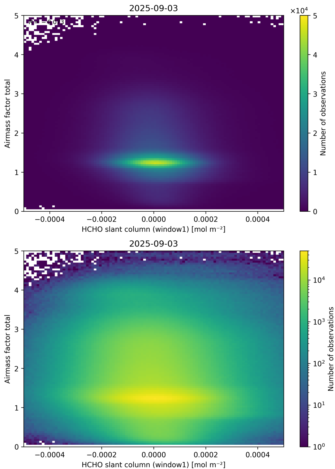
Figure 85: Scatter density plot of “HCHO slant column (window1)” against “Airmass factor total” for 2025-09-02 to 2025-09-04.
