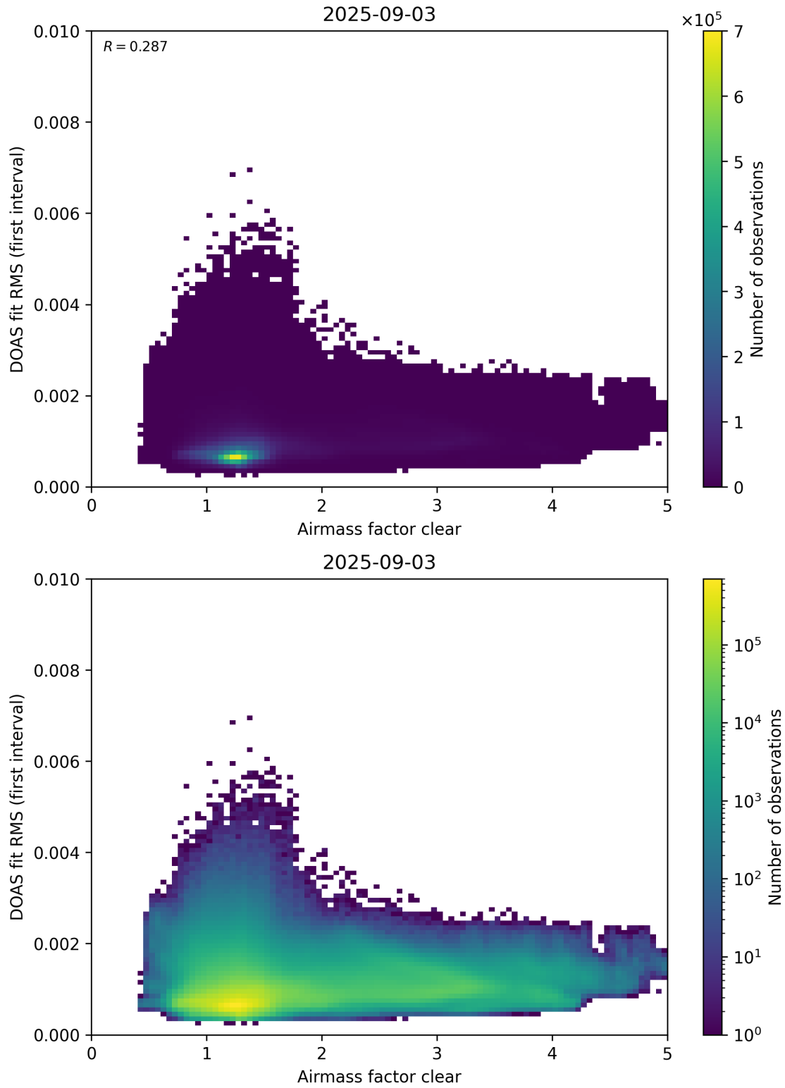
Figure 71: Scatter density plot of “Airmass factor clear” against “DOAS fit RMS (first interval)” for 2025-09-02 to 2025-09-04.
