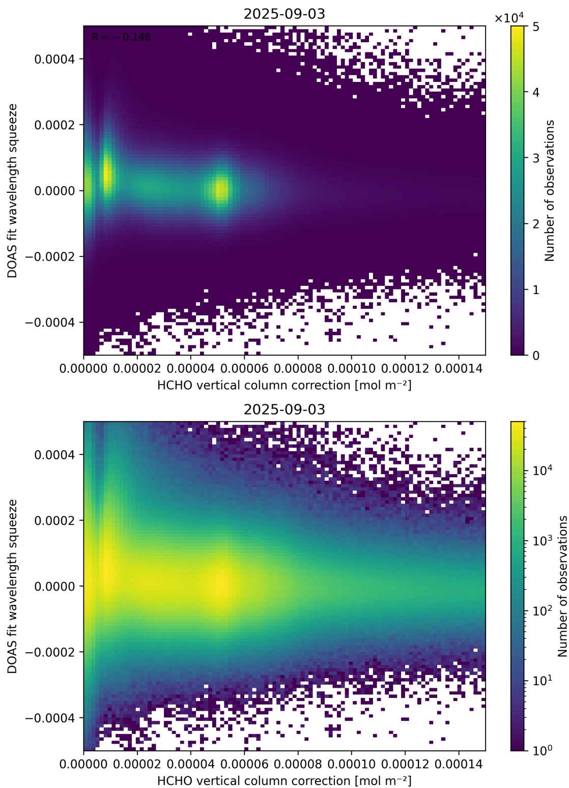
Figure 114: Scatter density plot of “HCHO vertical column correction” against “DOAS fit wavelength squeeze” for 2025-09-02 to 2025-09-04.
