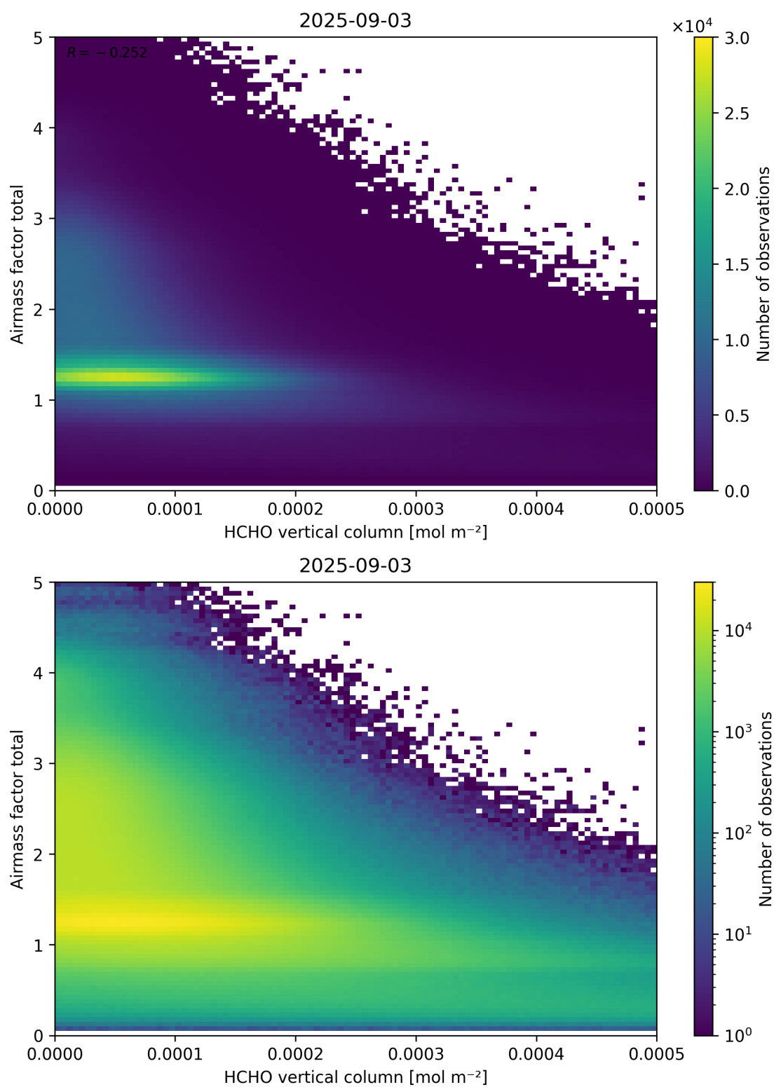
Figure 131: Scatter density plot of “HCHO vertical column” against “Airmass factor total” for 2025-09-02 to 2025-09-04.
