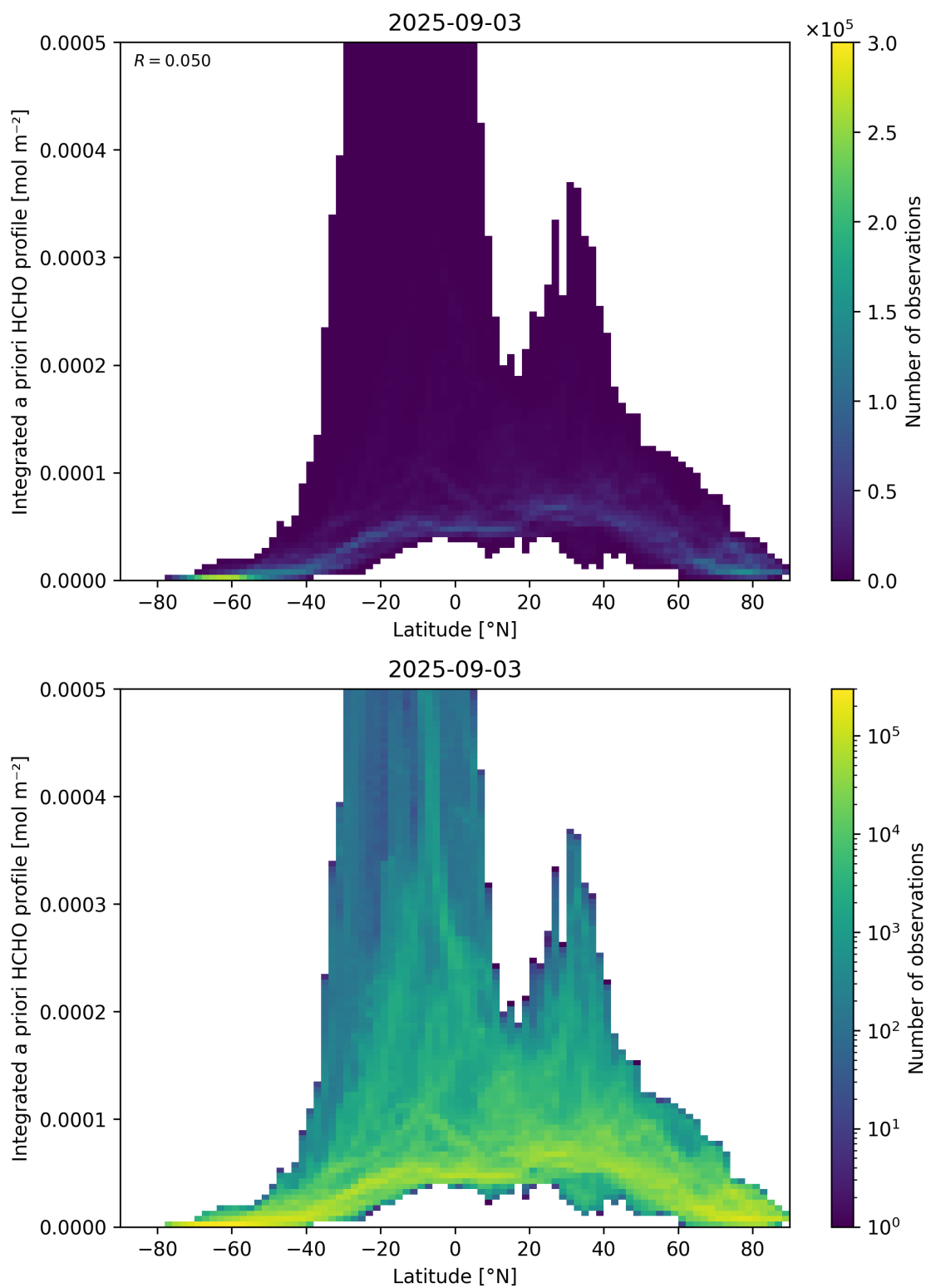
Figure 166: Scatter density plot of “Latitude” against “Integrated a priori HCHO profile” for 2025-09-02 to 2025-09-04.
