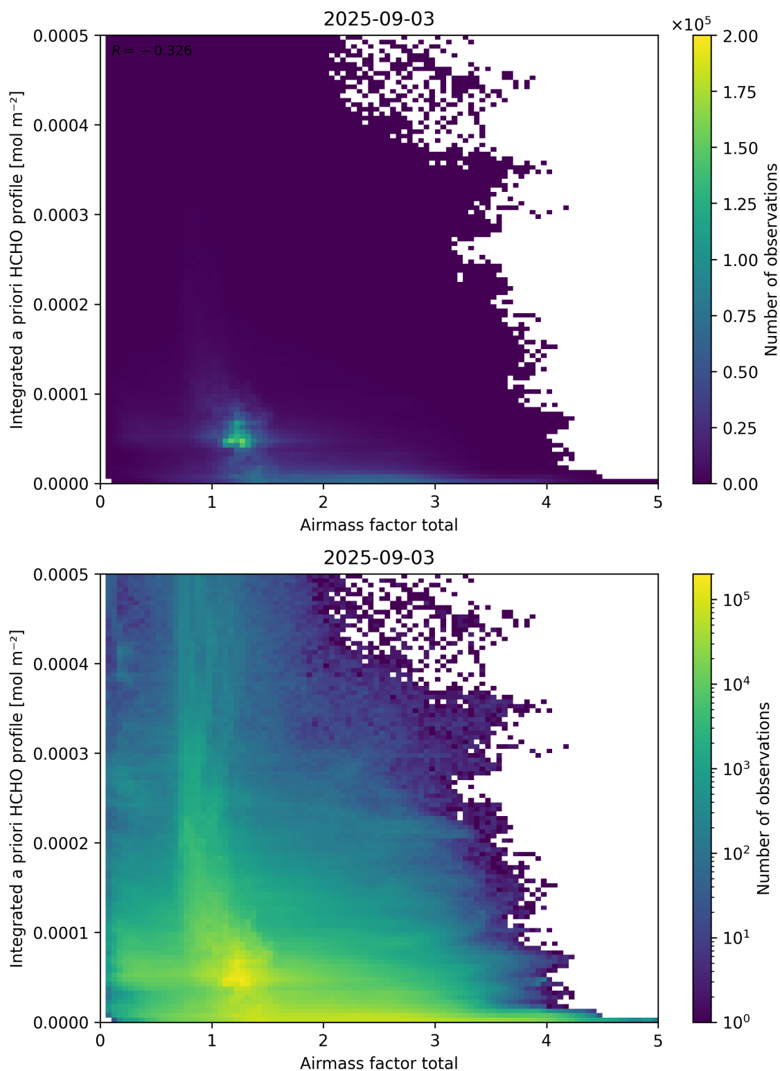
Figure 104: Scatter density plot of “Airmass factor total” against “Integrated a priori HCHO profile” for 2025-09-02 to 2025-09-04.
