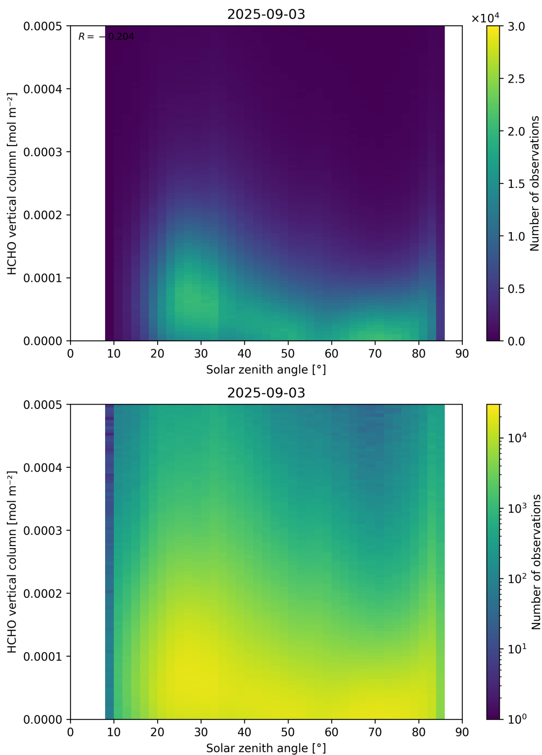
Figure 177: Scatter density plot of “Solar zenith angle” against “HCHO vertical column” for 2025-09-02 to 2025-09-04.
