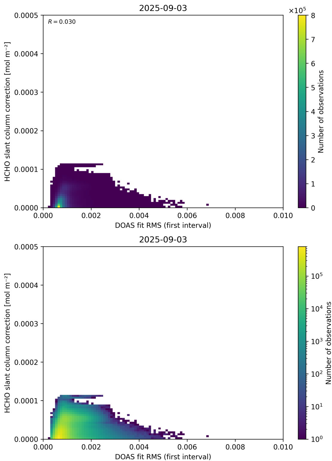
Figure 63: Scatter density plot of “DOAS fit RMS (first interval)” against “HCHO slant column correction” for 2025-09-02 to 2025-09-04.
