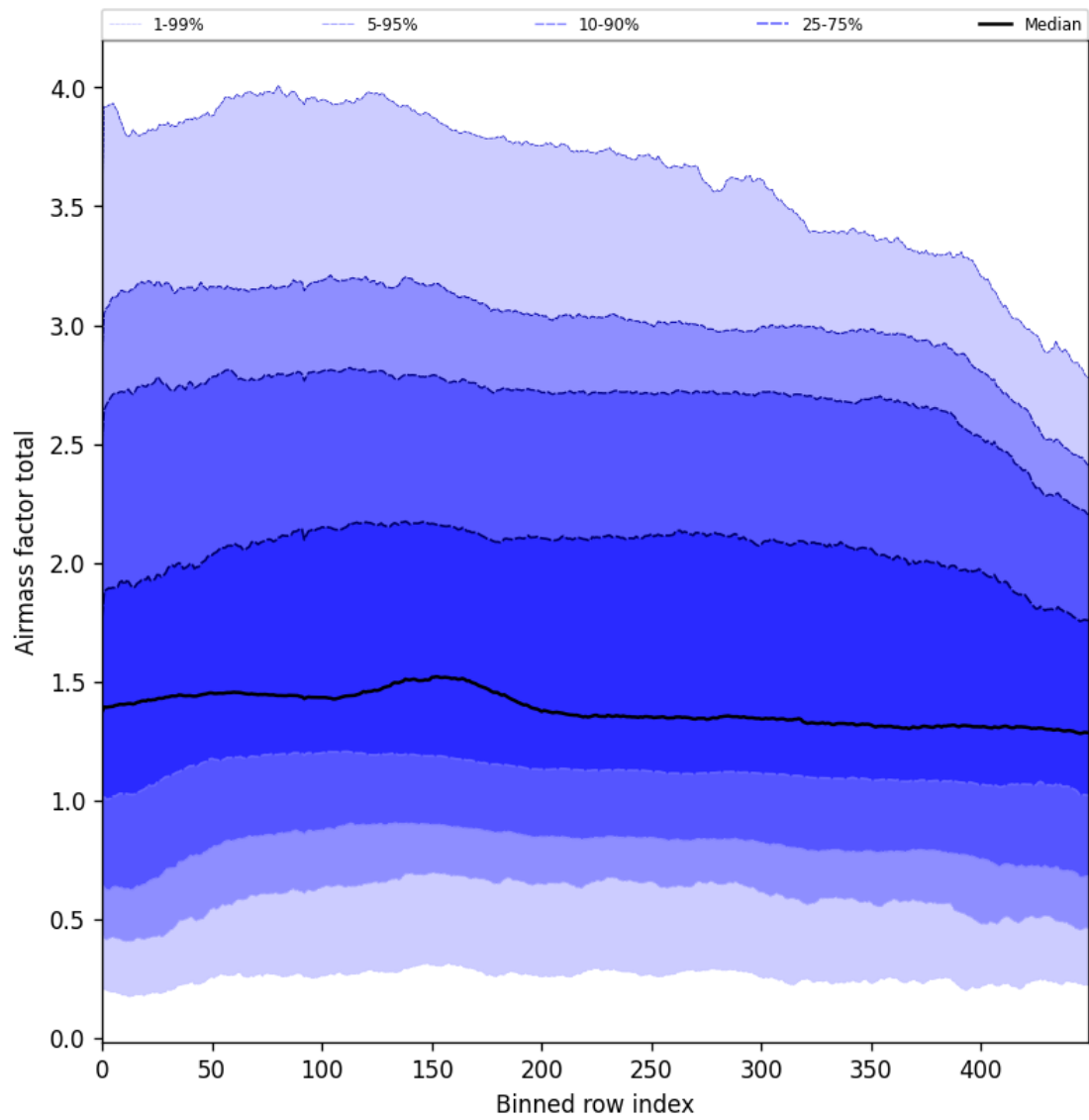
Figure 54: Along track statistics of “Airmass factor total” for 2025-09-02 to 2025-09-04
