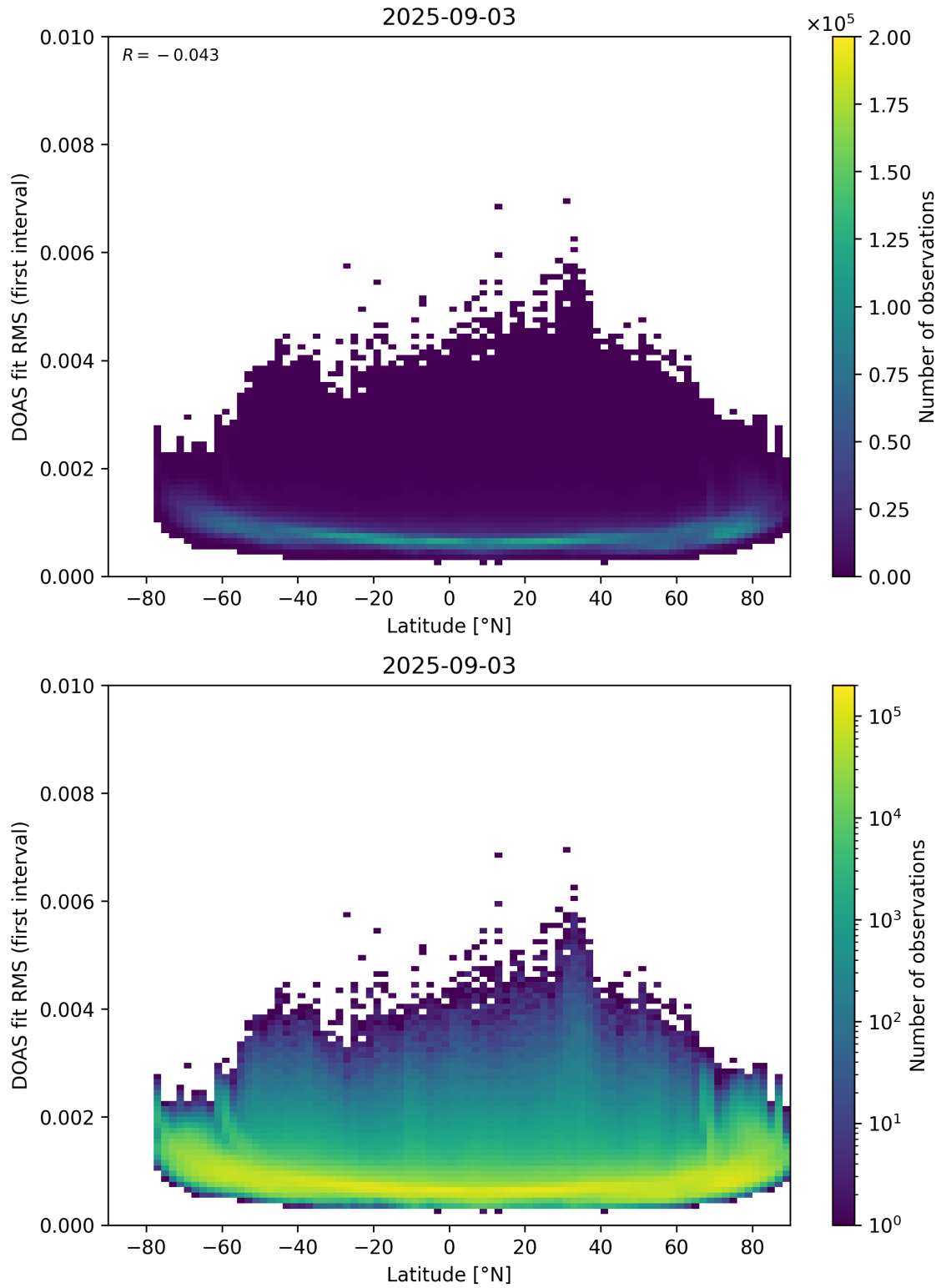
Figure 153: Scatter density plot of “Latitude” against “DOAS fit RMS (first interval)” for 2025-09-02 to 2025-09-04.
