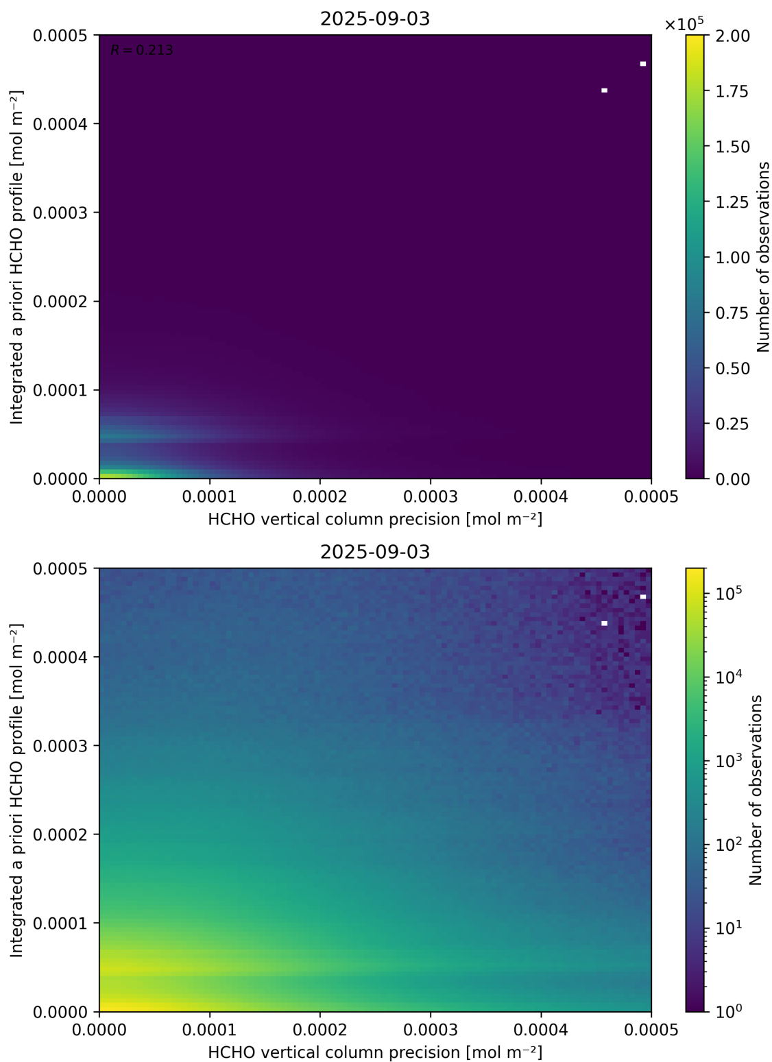
Figure 147: Scatter density plot of “HCHO vertical column precision” against “Integrated a priori HCHO profile” for 2025-09-02 to 2025-09-04.
