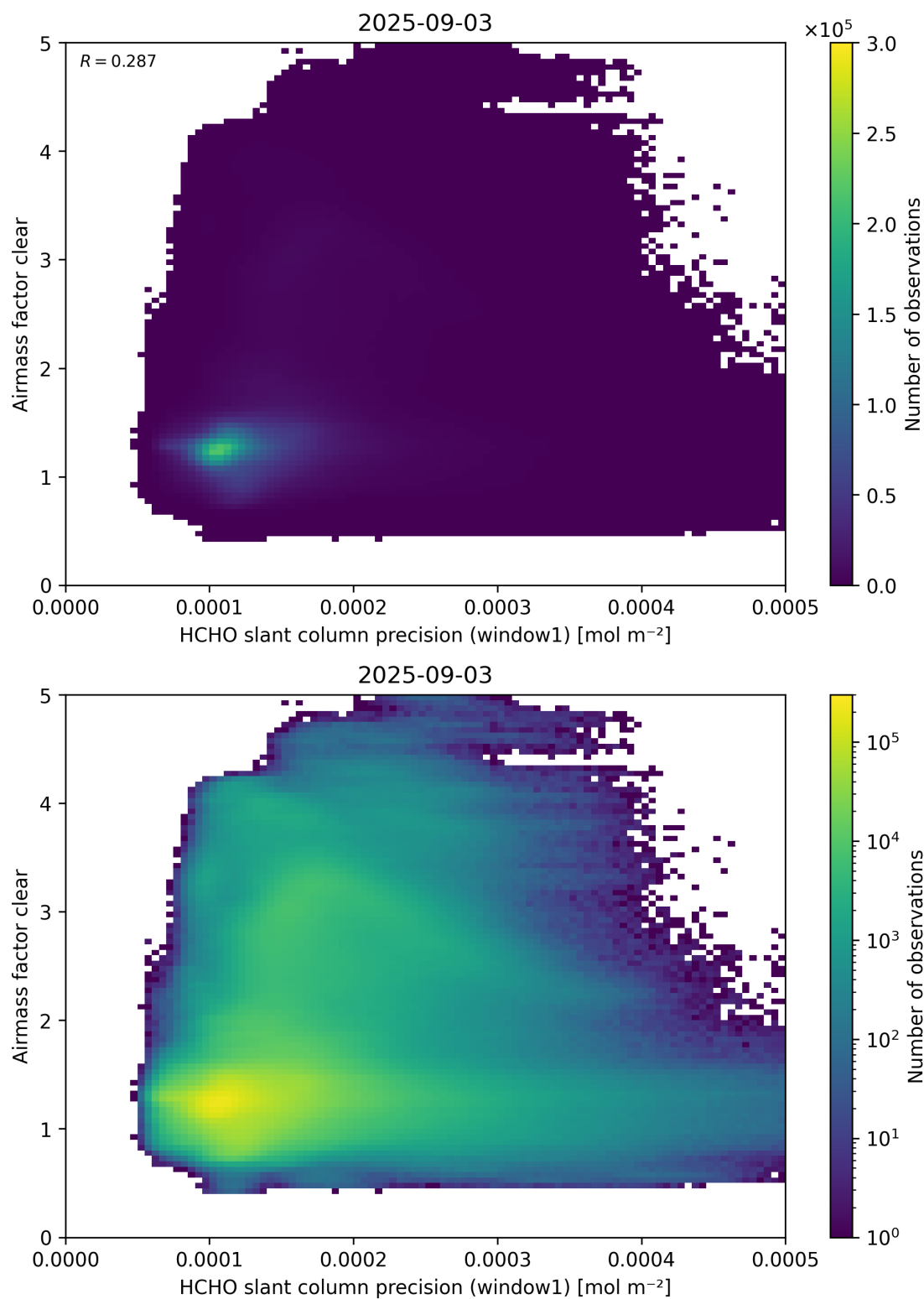
Figure 91: Scatter density plot of “HCHO slant column precision (window1)” against “Airmass factor clear” for 2025-09-02 to 2025-09-04.
