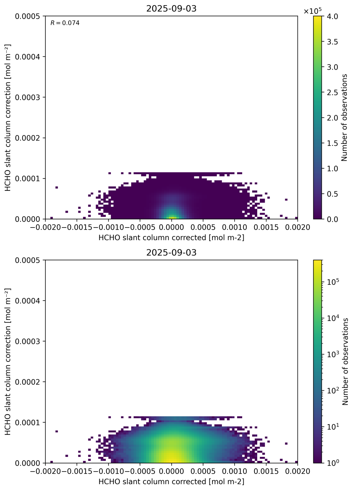
Figure 77: Scatter density plot of “HCHO slant column corrected” against “HCHO slant column correction” for 2025-09-02 to 2025-09-04.
