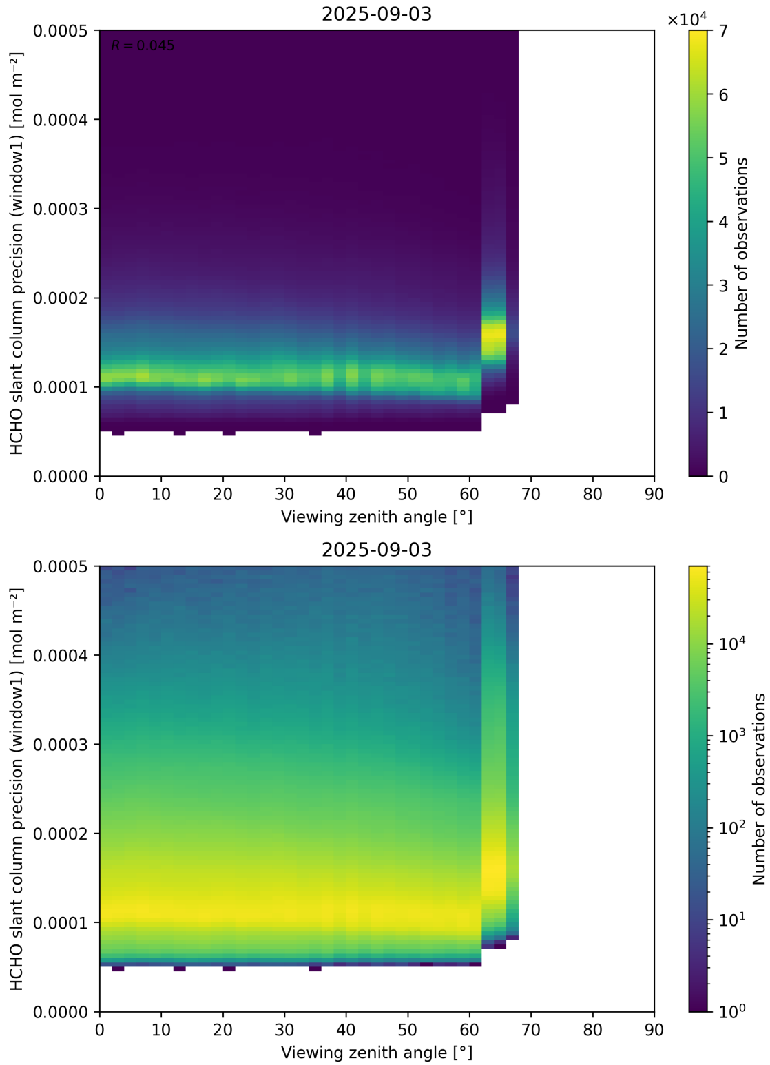
Figure 189: Scatter density plot of “Viewing zenith angle” against “HCHO slant column precision (window1)” for 2025-09-02 to 2025-09-04.
