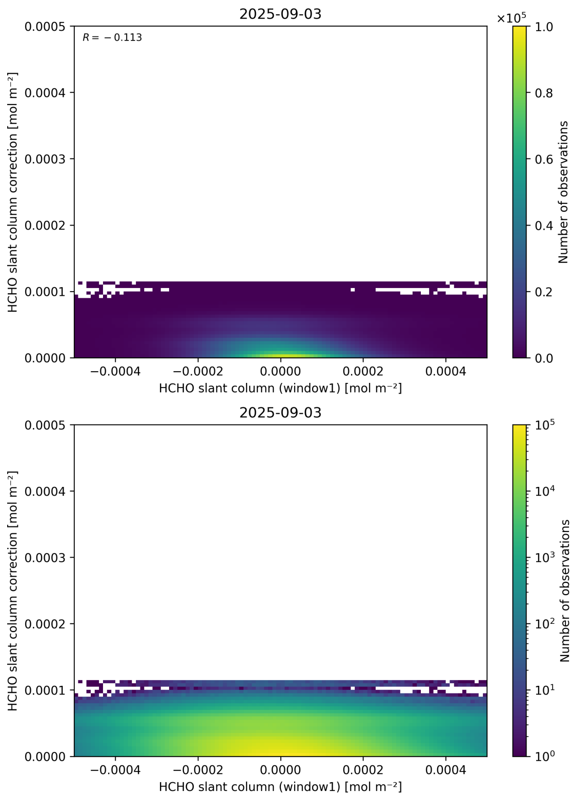
Figure 83: Scatter density plot of “HCHO slant column (window1)” against “HCHO slant column correction” for 2025-09-02 to 2025-09-04.
