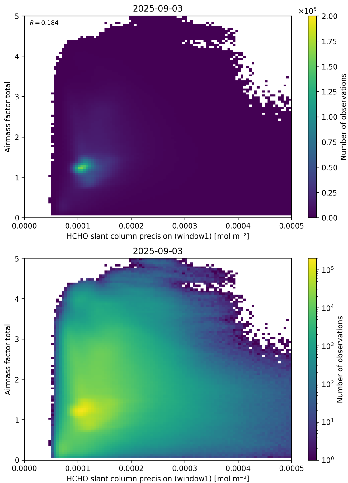
Figure 94: Scatter density plot of “HCHO slant column precision (window1)” against “Airmass factor total” for 2025-09-02 to 2025-09-04.
