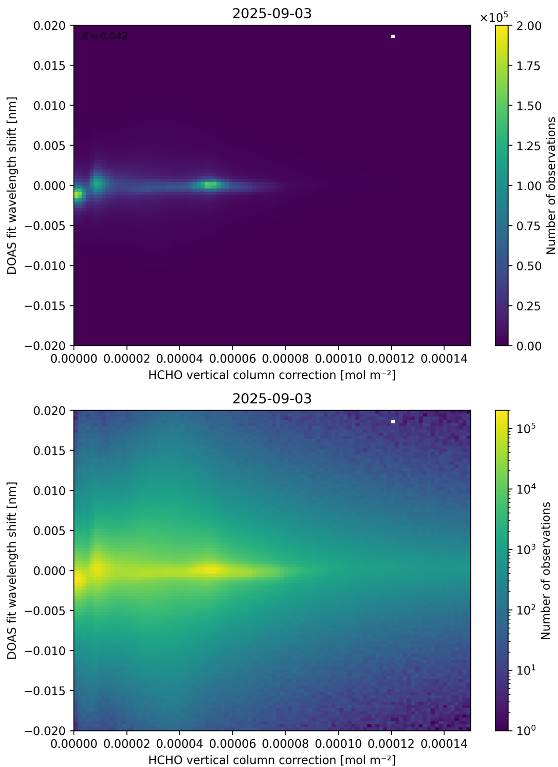
Figure 113: Scatter density plot of “HCHO vertical column correction” against “DOAS fit wavelength shift” for 2025-09-02 to 2025-09-04.
