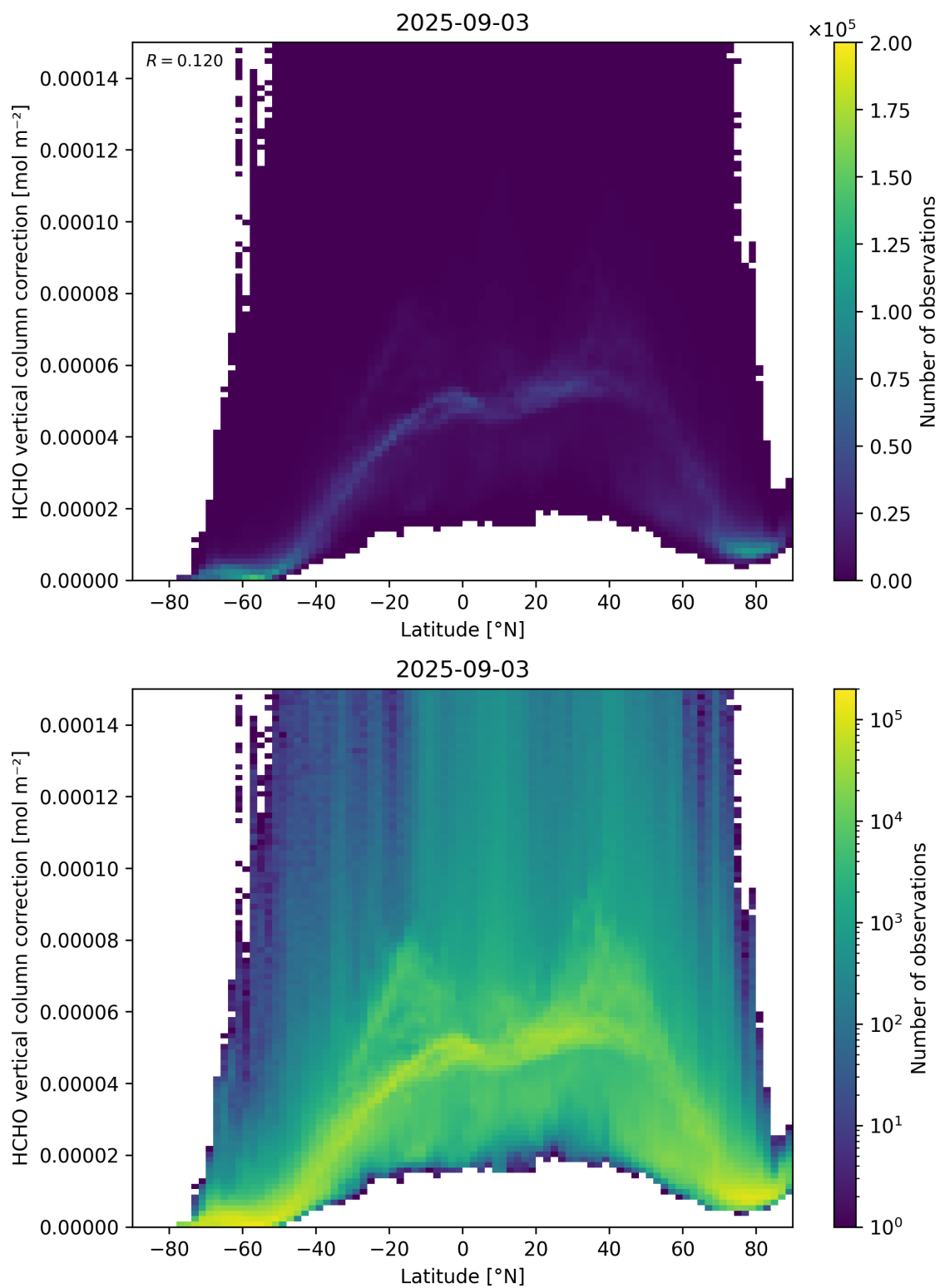
Figure 164: Scatter density plot of “Latitude” against “HCHO vertical column correction” for 2025-09-02 to 2025-09-04.
