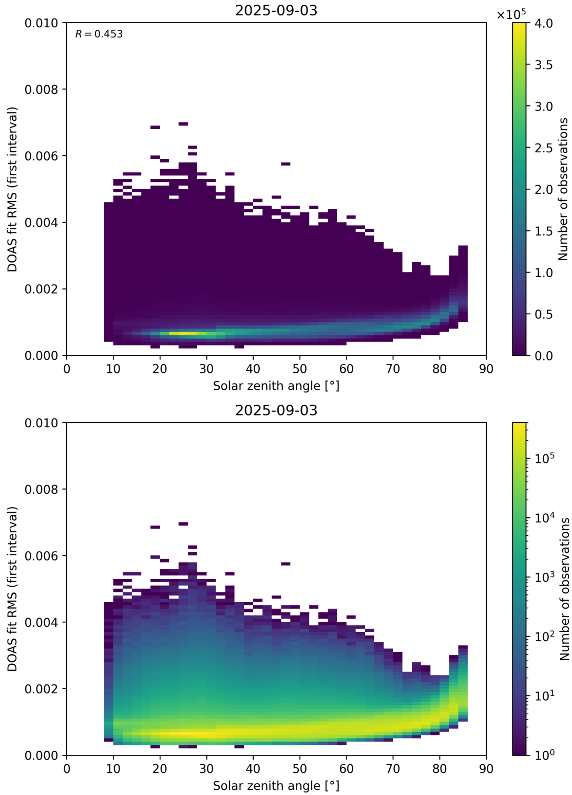
Figure 167: Scatter density plot of “Solar zenith angle” against “DOAS fit RMS (first interval)” for 2025-09-02 to 2025-09-04.
