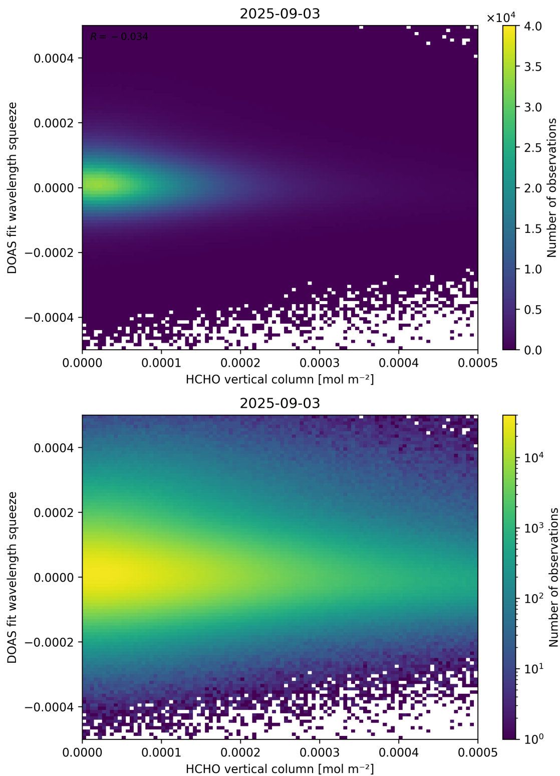
Figure 125: Scatter density plot of “HCHO vertical column” against “DOAS fit wavelength squeeze” for 2025-09-02 to 2025-09-04.
