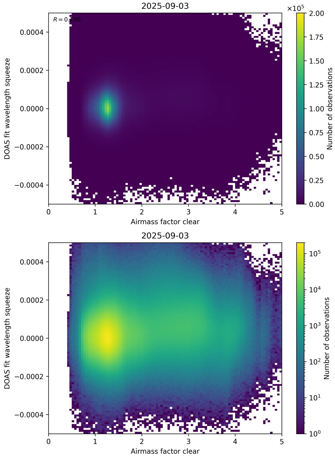
Figure 73: Scatter density plot of “Airmass factor clear” against “DOAS fit wavelength squeeze” for 2025-09-02 to 2025-09-04.
