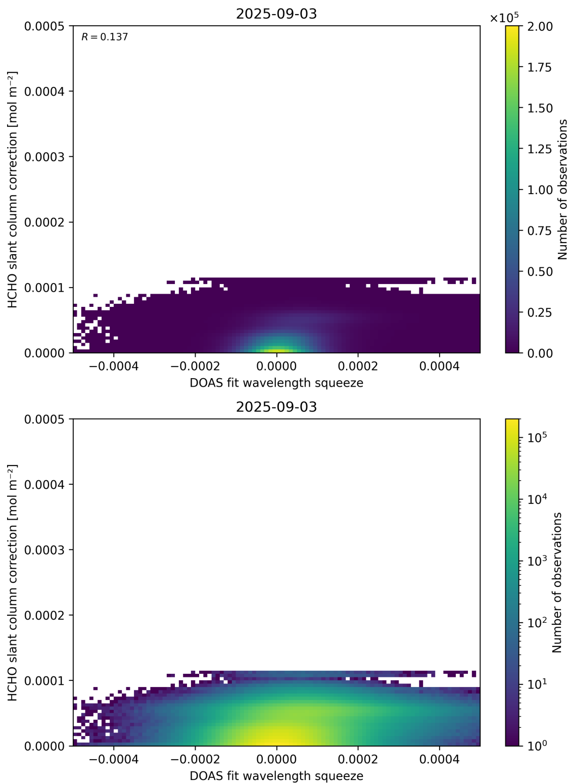
Figure 70: Scatter density plot of “DOAS fit wavelength squeeze” against “HCHO slant column correction” for 2025-09-02 to 2025-09-04.
