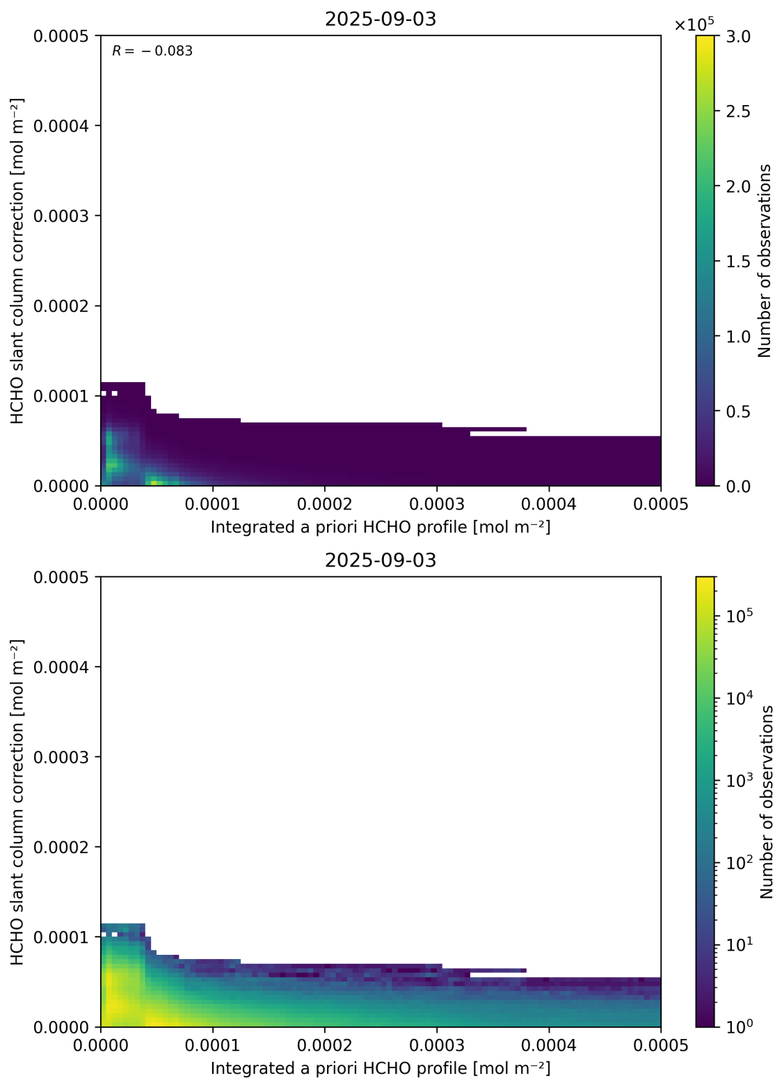
Figure 152: Scatter density plot of “Integrated a priori HCHO profile” against “HCHO slant column correction” for 2025-09-02 to 2025-09-04.
