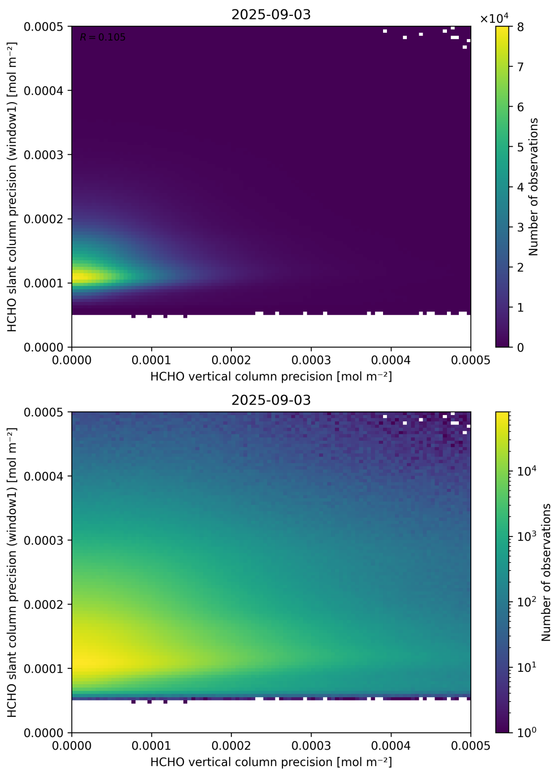
Figure 143: Scatter density plot of “HCHO vertical column precision” against “HCHO slant column precision (window1)” for 2025-09-02 to 2025-09-04.
