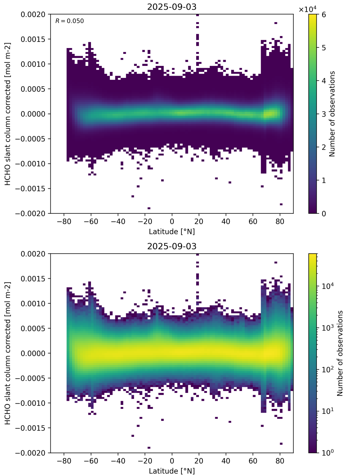
Figure 157: Scatter density plot of “Latitude” against “HCHO slant column corrected” for 2025-09-02 to 2025-09-04.
