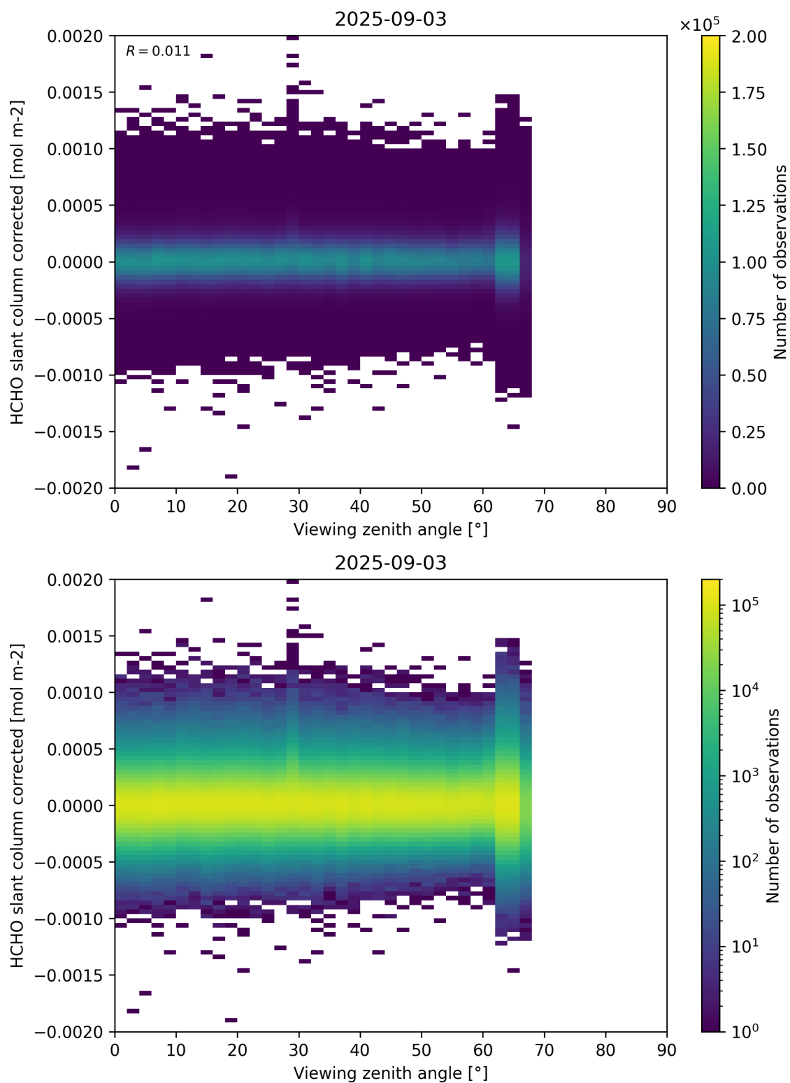
Figure 186: Scatter density plot of “Viewing zenith angle” against “HCHO slant column corrected” for 2025-09-02 to 2025-09-04.
