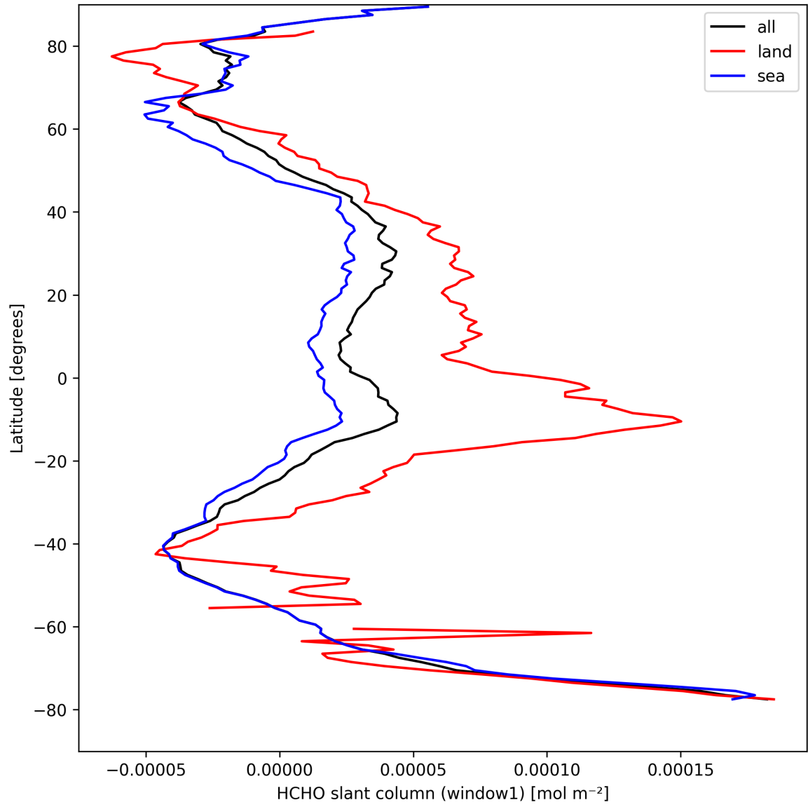
Figure 24: Zonal average of “HCHO slant column (window1)” for 2025-09-02 to 2025-09-04.
