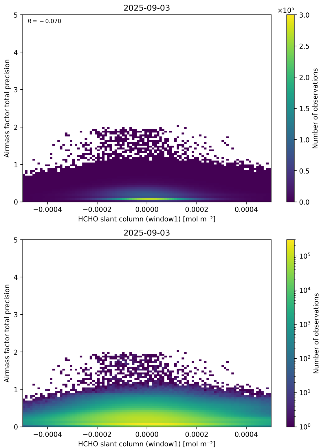
Figure 86: Scatter density plot of “HCHO slant column (window1)” against “Airmass factor total precision” for 2025-09-02 to 2025-09-04.
