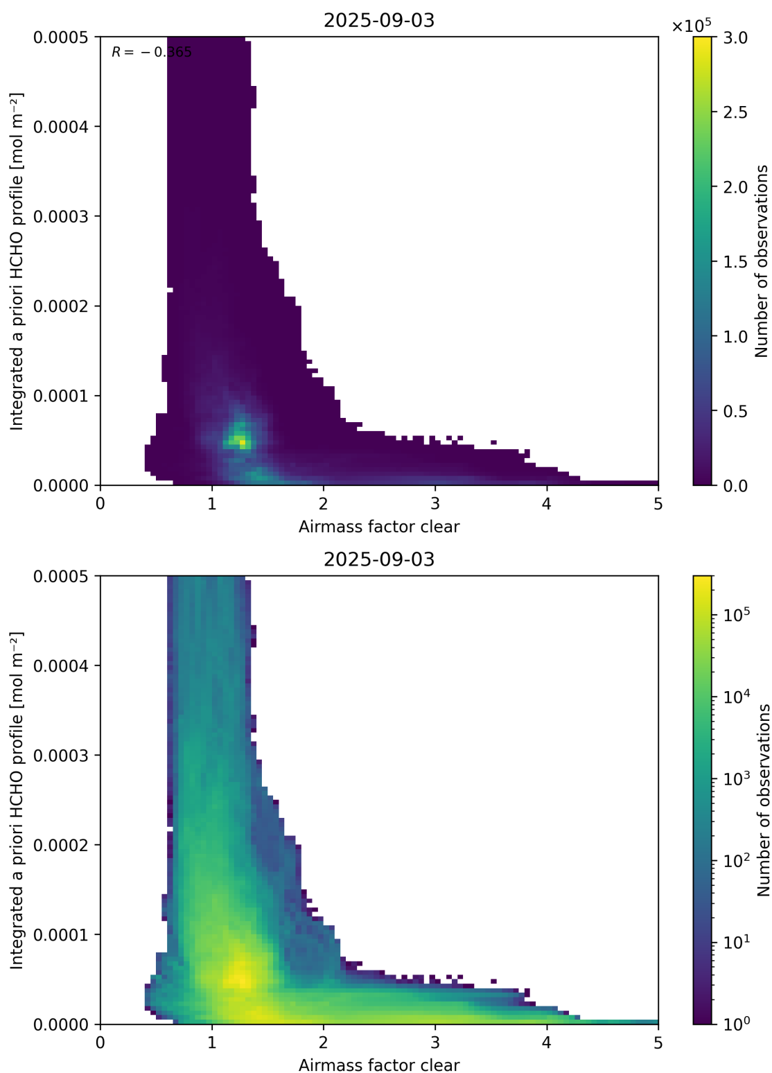
Figure 76: Scatter density plot of “Airmass factor clear” against “Integrated a priori HCHO profile” for 2025-09-02 to 2025-09-04.
