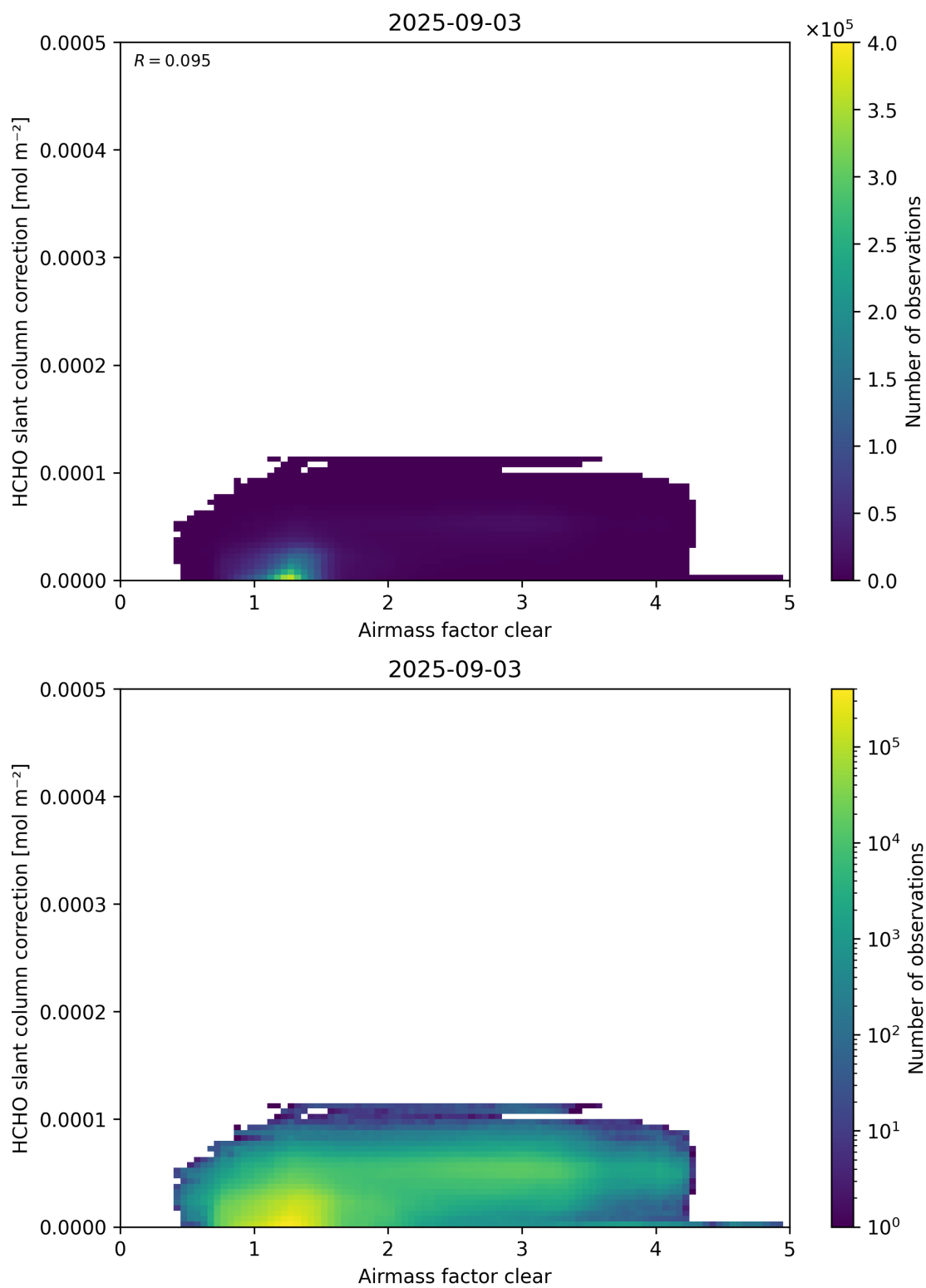
Figure 75: Scatter density plot of “Airmass factor clear” against “HCHO slant column correction” for 2025-09-02 to 2025-09-04.
