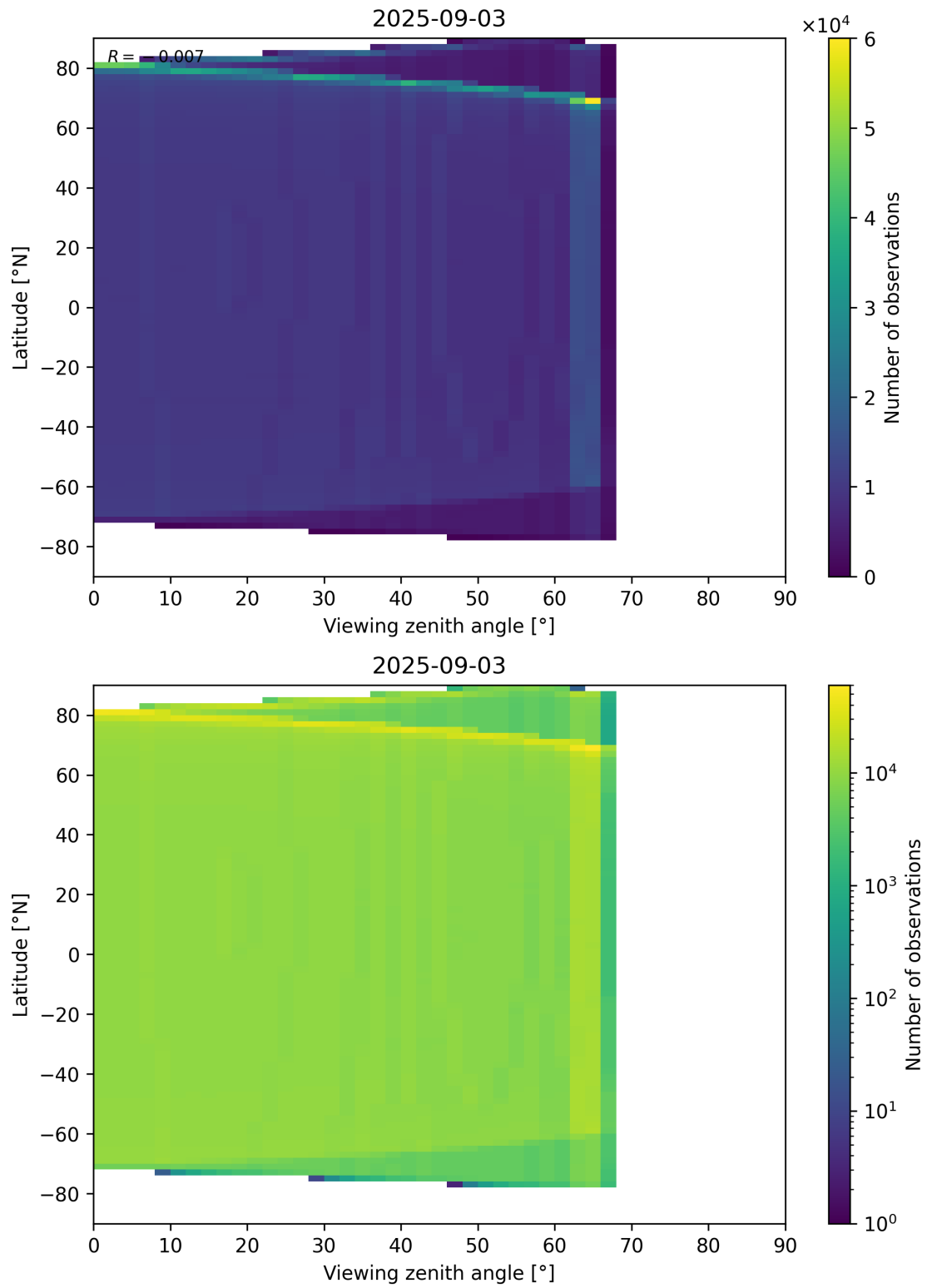
Figure 196: Scatter density plot of “Viewing zenith angle” against “Latitude” for 2025-09-02 to 2025-09-04.
