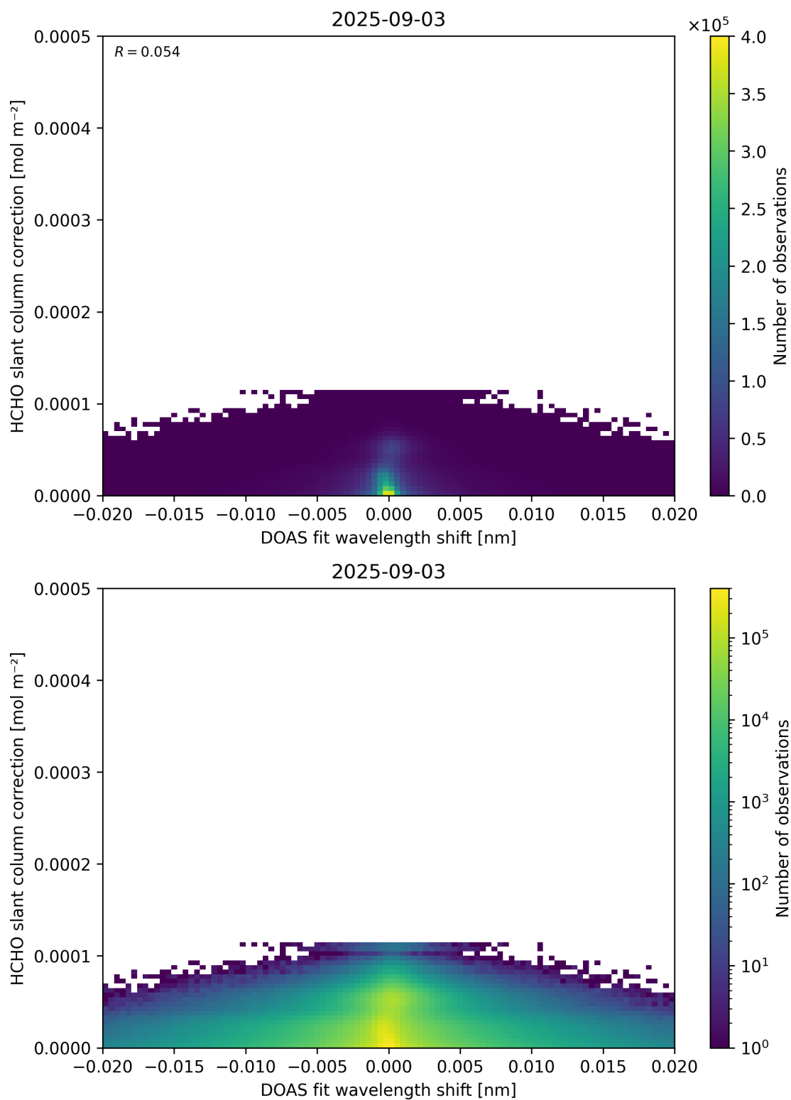
Figure 67: Scatter density plot of “DOAS fit wavelength shift” against “HCHO slant column correction” for 2025-09-02 to 2025-09-04.
