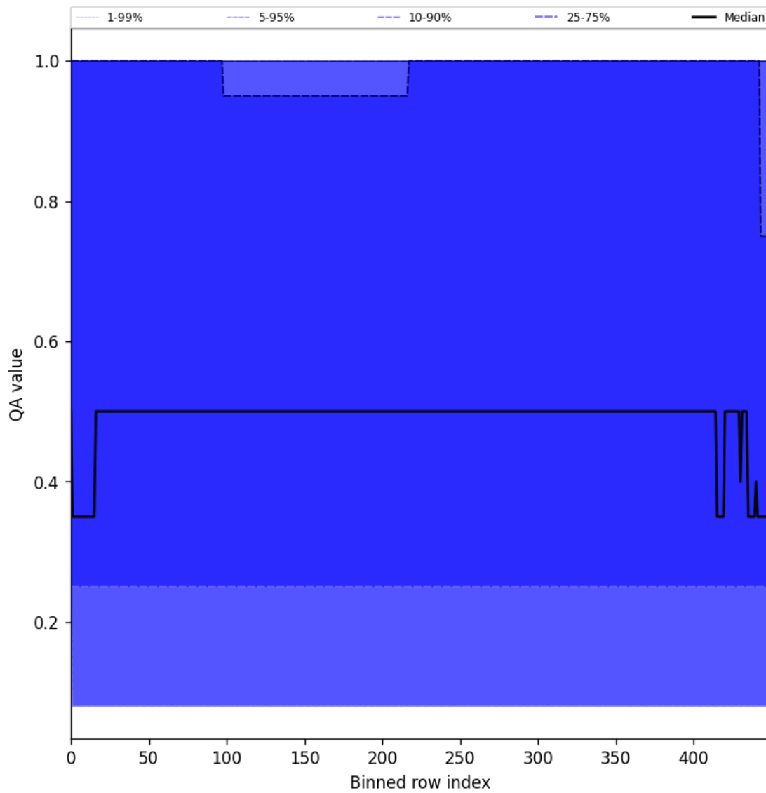
Figure 48: Along track statistics of “QA value” for 2025-09-02 to 2025-09-04
