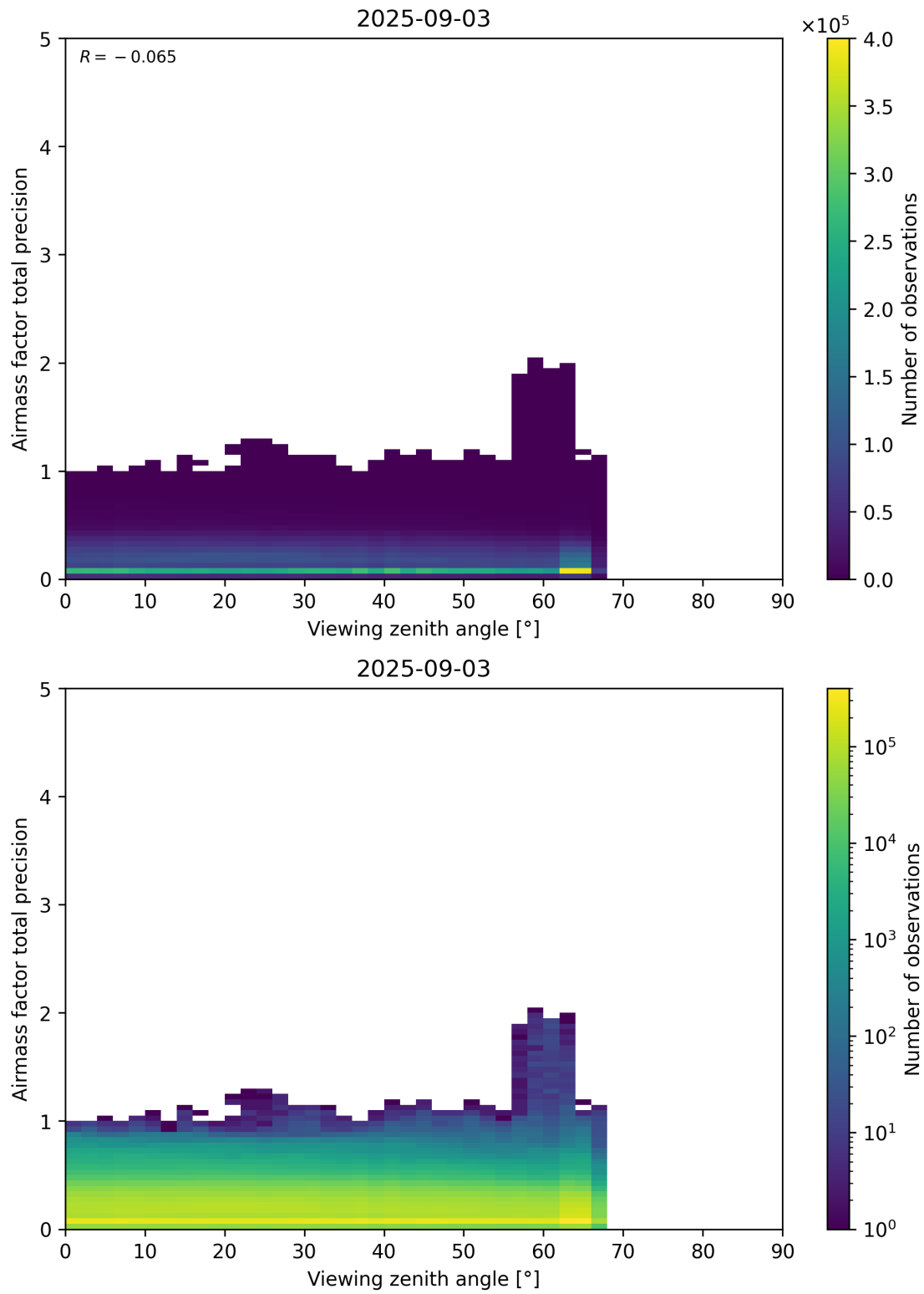
Figure 191: Scatter density plot of “Viewing zenith angle” against “Airmass factor total precision” for 2025-09-02 to 2025-09-04.
