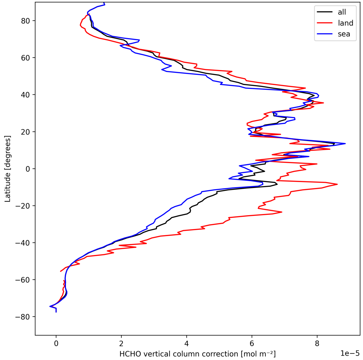
Figure 23: Zonal average of “HCHO vertical column correction” for 2025-09-02 to 2025-09-04.
