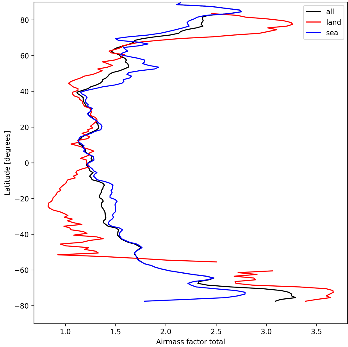
Figure 26: Zonal average of “Airmass factor total” for 2025-09-02 to 2025-09-04.
