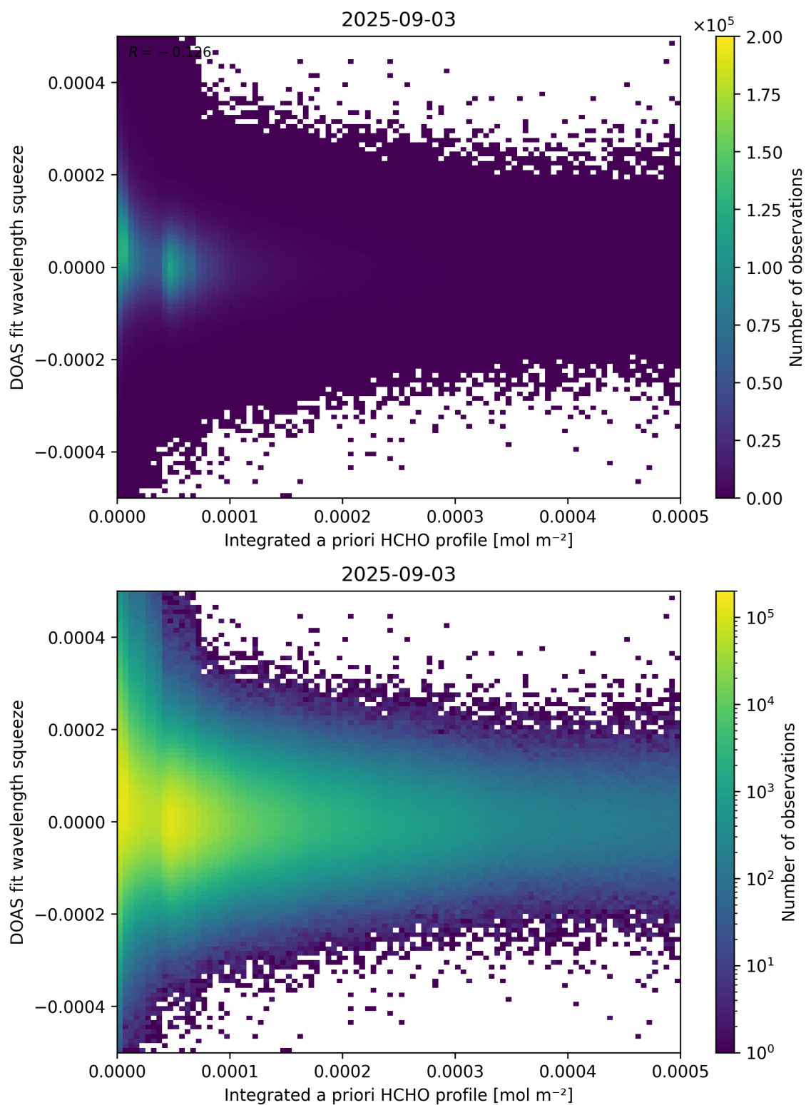
Figure 150: Scatter density plot of “Integrated a priori HCHO profile” against “DOAS fit wavelength squeeze” for 2025-09-02 to 2025-09-04.
