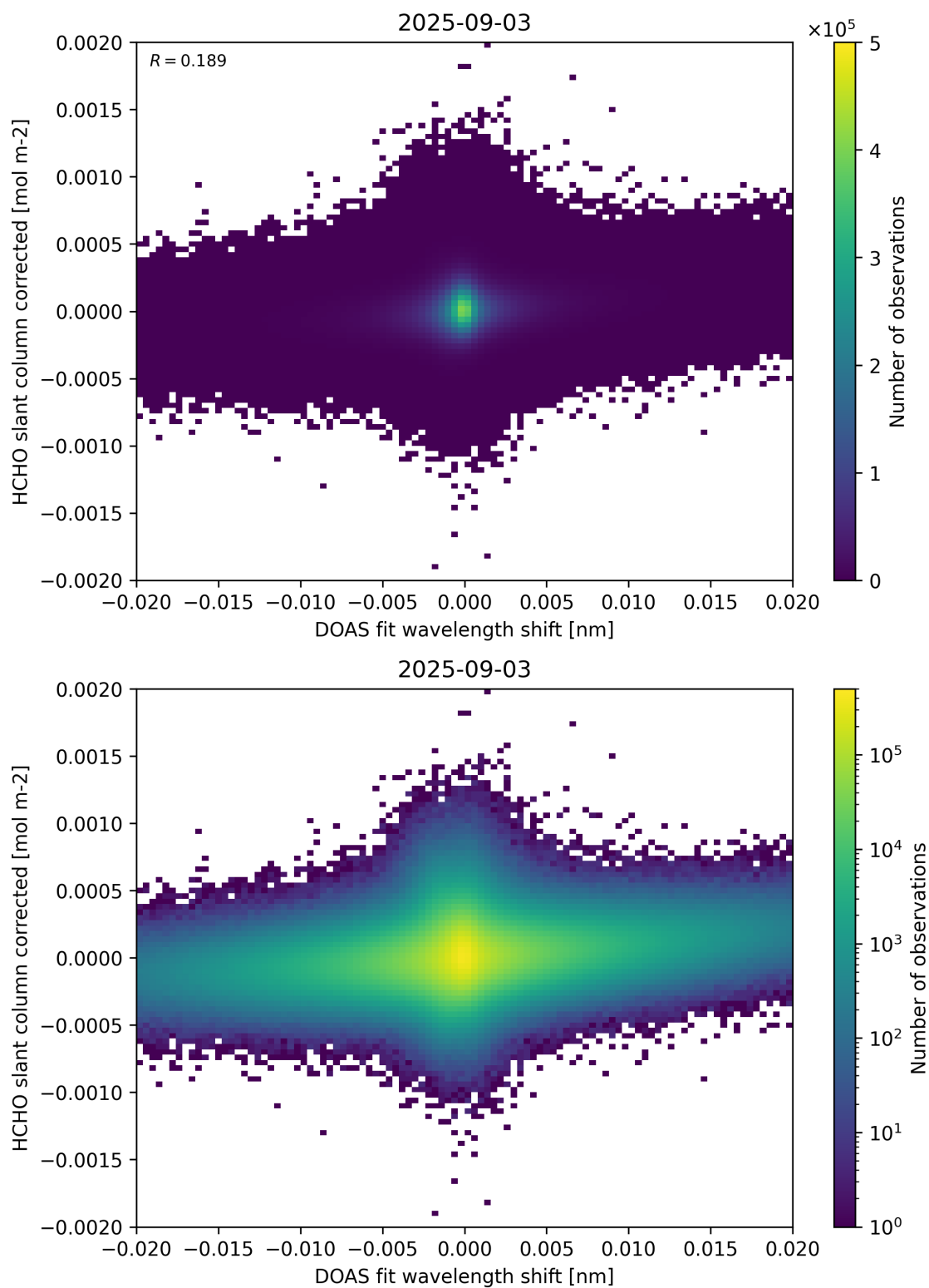
Figure 66: Scatter density plot of “DOAS fit wavelength shift” against “HCHO slant column corrected” for 2025-09-02 to 2025-09-04.
