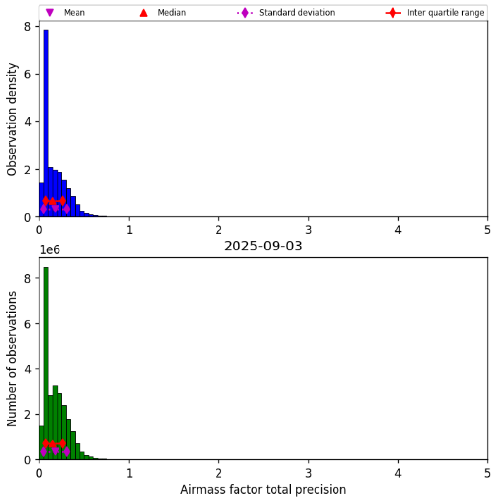
Figure 41: Histogram of “Airmass factor total precision” for 2025-09-02 to 2025-09-04
