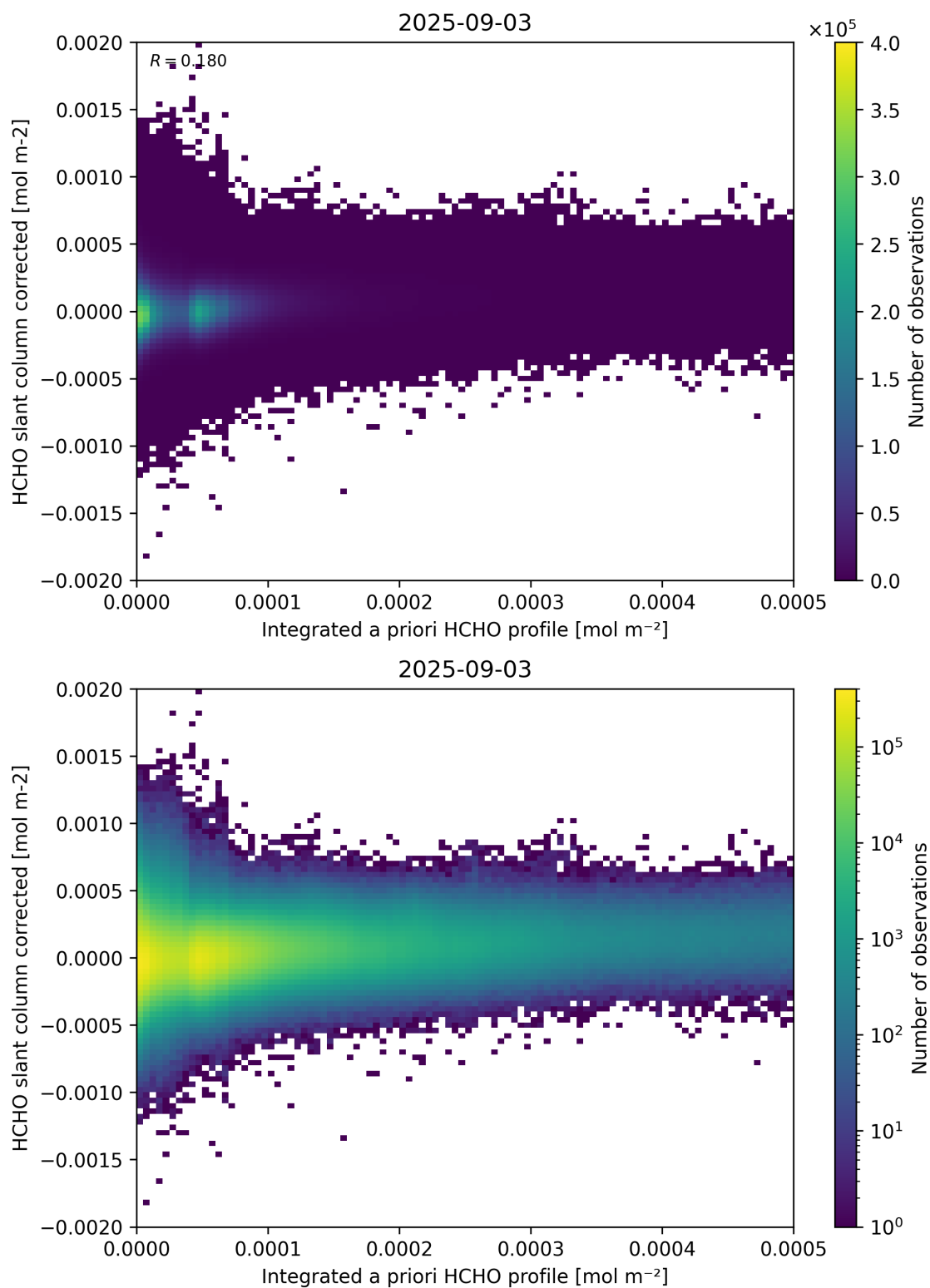
Figure 151: Scatter density plot of “Integrated a priori HCHO profile” against “HCHO slant column corrected” for 2025-09-02 to 2025-09-04.
