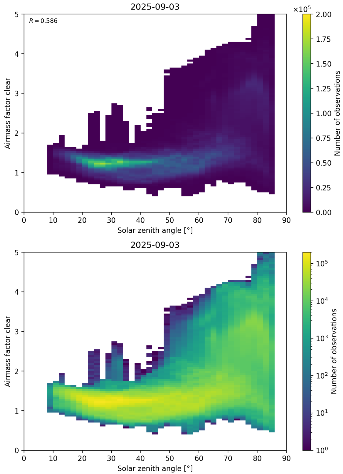
Figure 170: Scatter density plot of “Solar zenith angle” against “Airmass factor clear” for 2025-09-02 to 2025-09-04.
