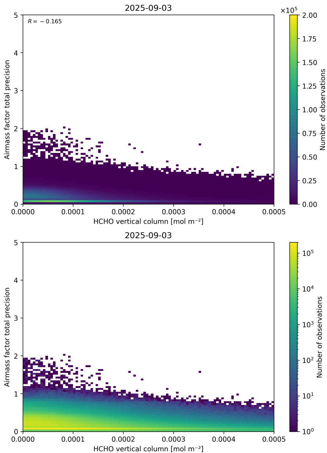
Figure 132: Scatter density plot of “HCHO vertical column” against “Airmass factor total precision” for 2025-09-02 to 2025-09-04.
