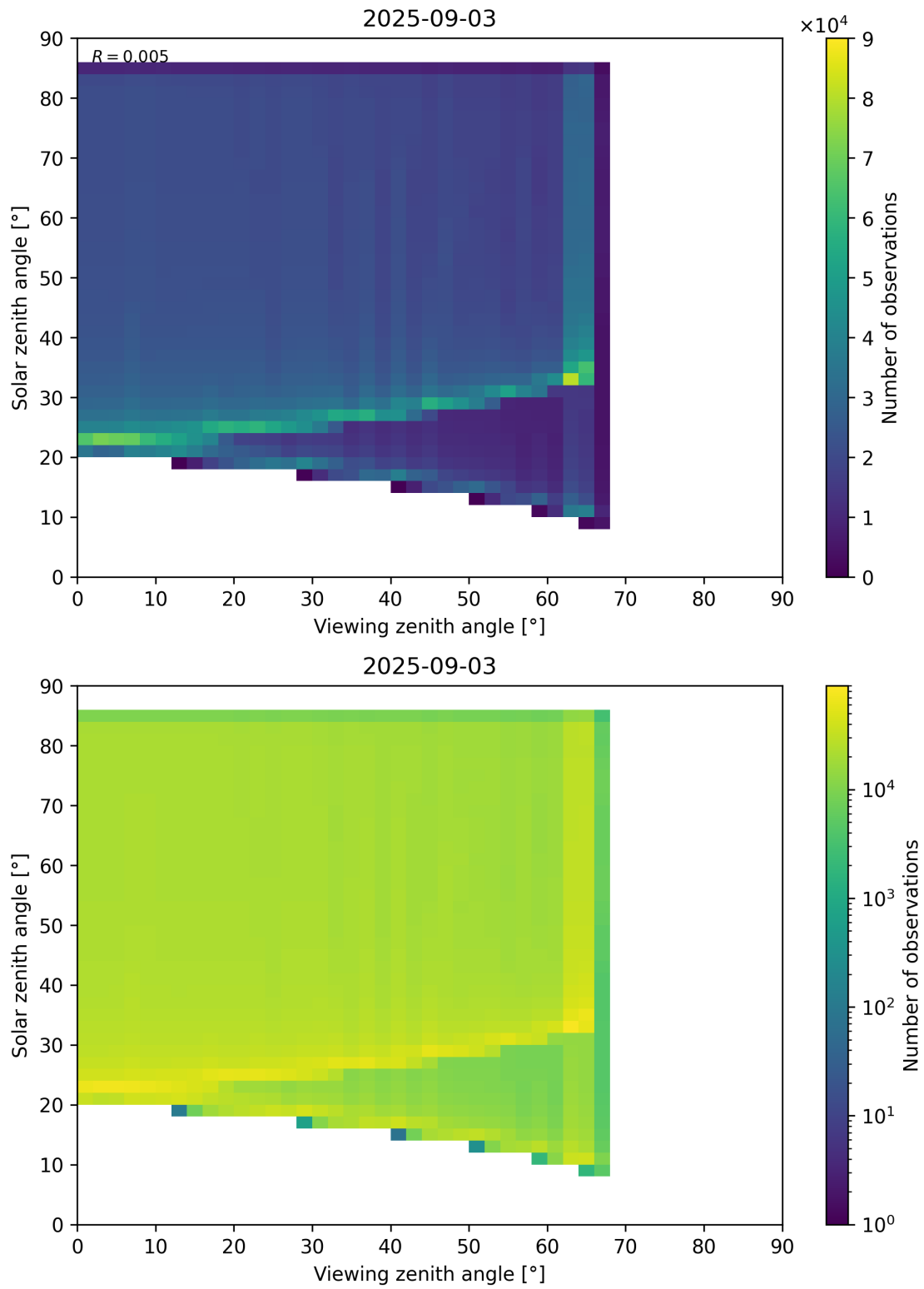
Figure 197: Scatter density plot of “Viewing zenith angle” against “Solar zenith angle” for 2025-09-02 to 2025-09-04.
