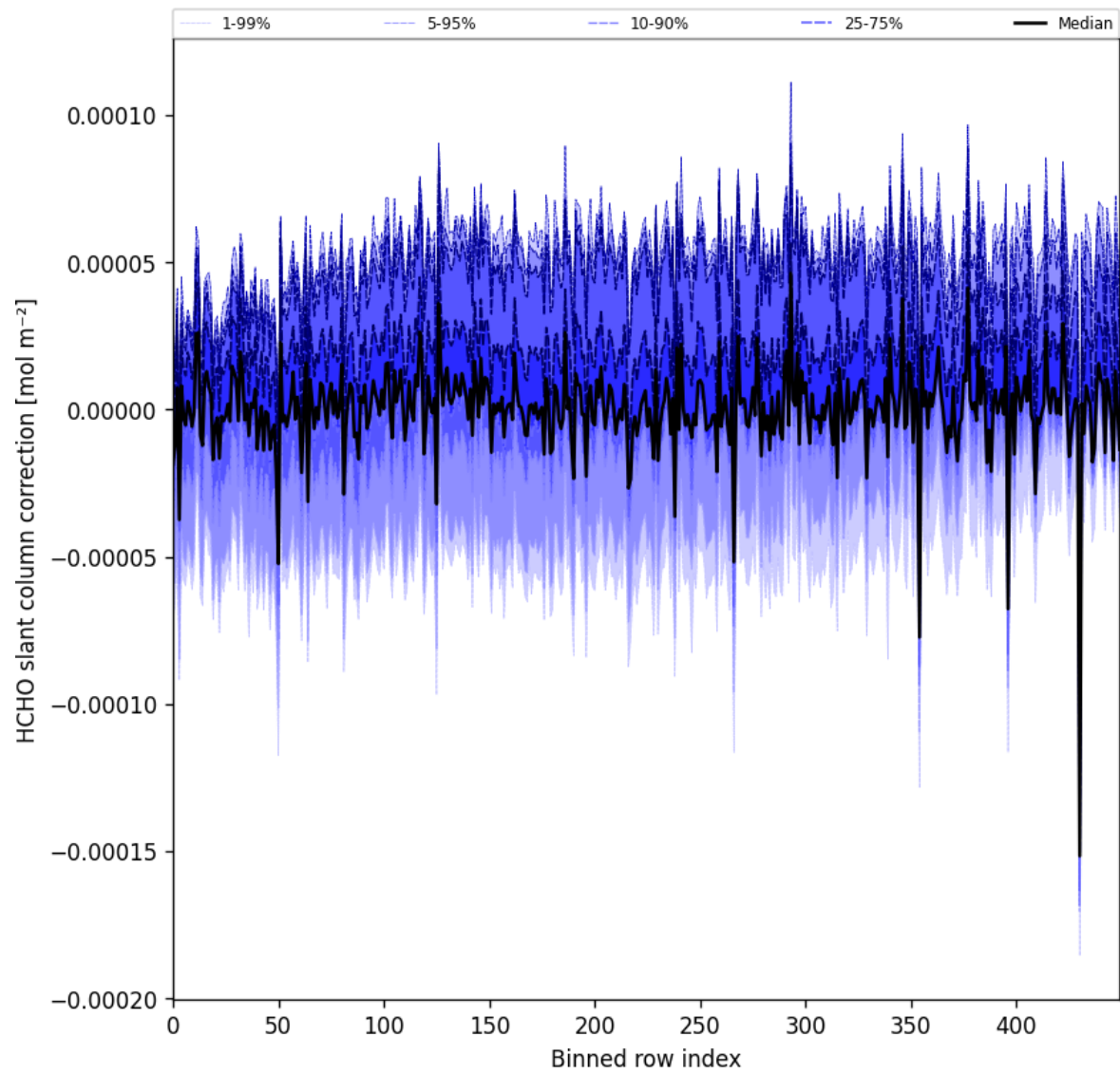
Figure 61: Along track statistics of “HCHO slant column correction” for 2025-09-02 to 2025-09-04
