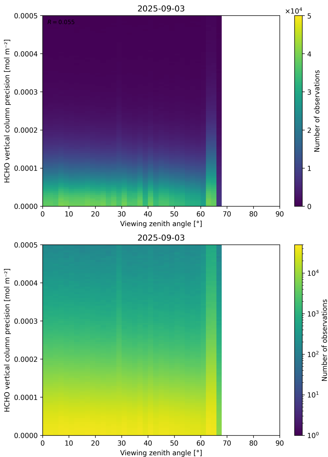
Figure 194: Scatter density plot of “Viewing zenith angle” against “HCHO vertical column precision” for 2025-09-02 to 2025-09-04.
