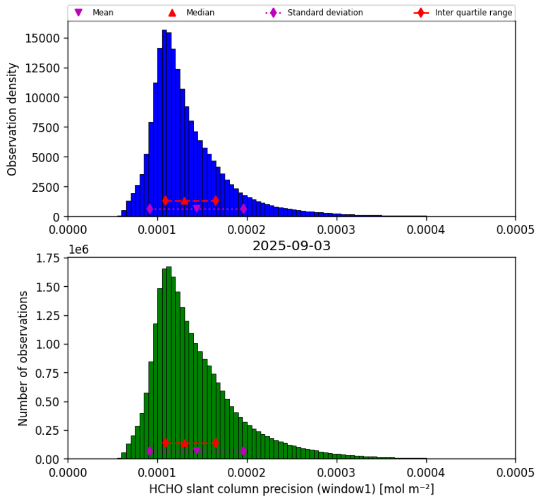
Figure 39: Histogram of “HCHO slant column precision (window1)” for 2025-09-02 to 2025-09-04
