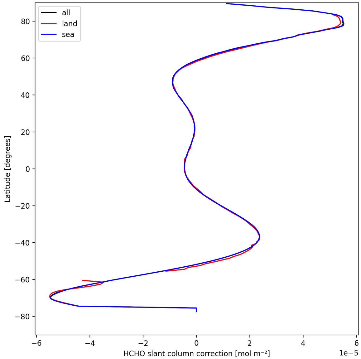
Figure 33: Zonal average of “HCHO slant column correction” for 2025-09-02 to 2025-09-04.
