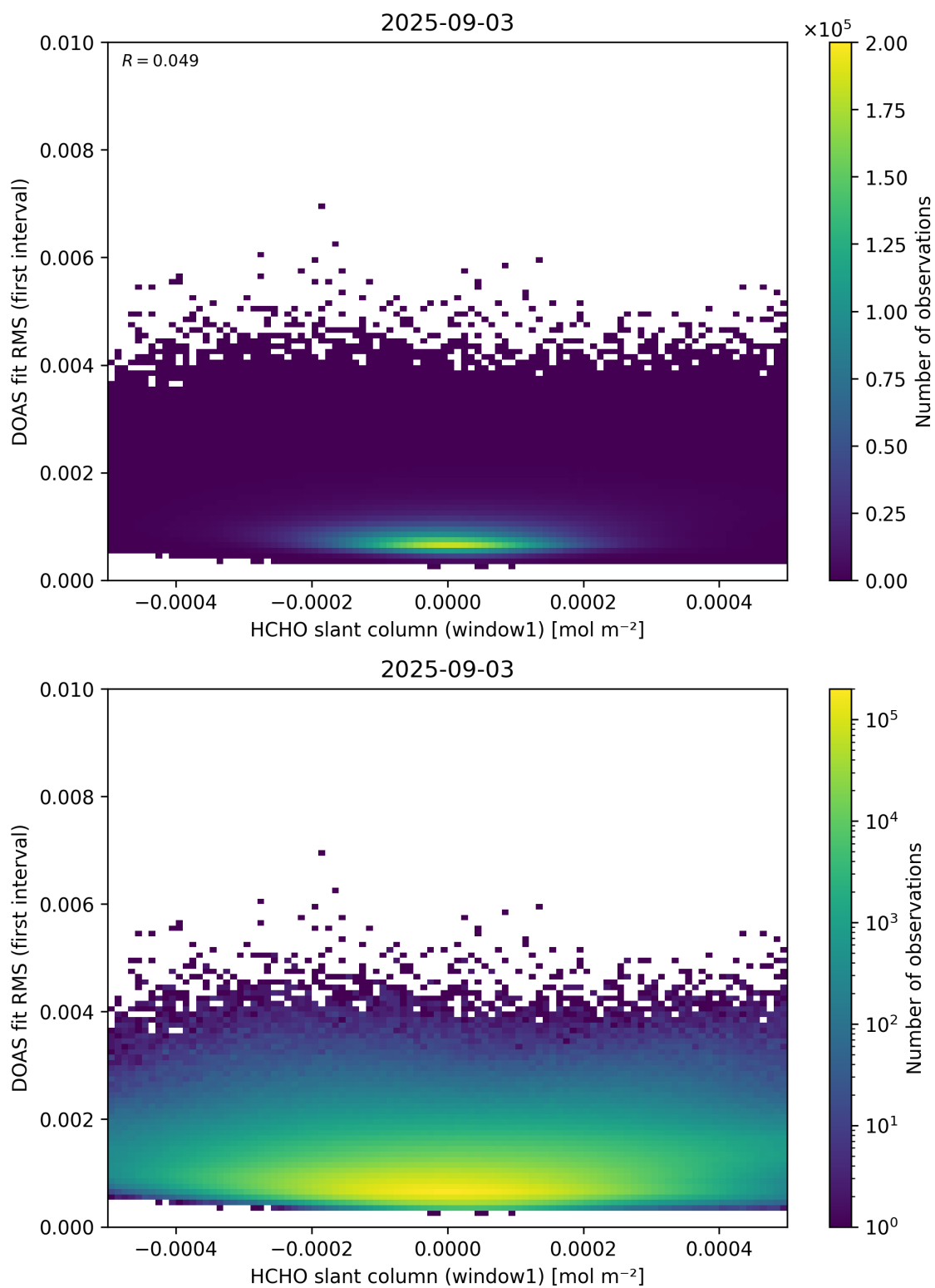
Figure 78: Scatter density plot of “HCHO slant column (window1)” against “DOAS fit RMS (first interval)” for 2025-09-02 to 2025-09-04.
