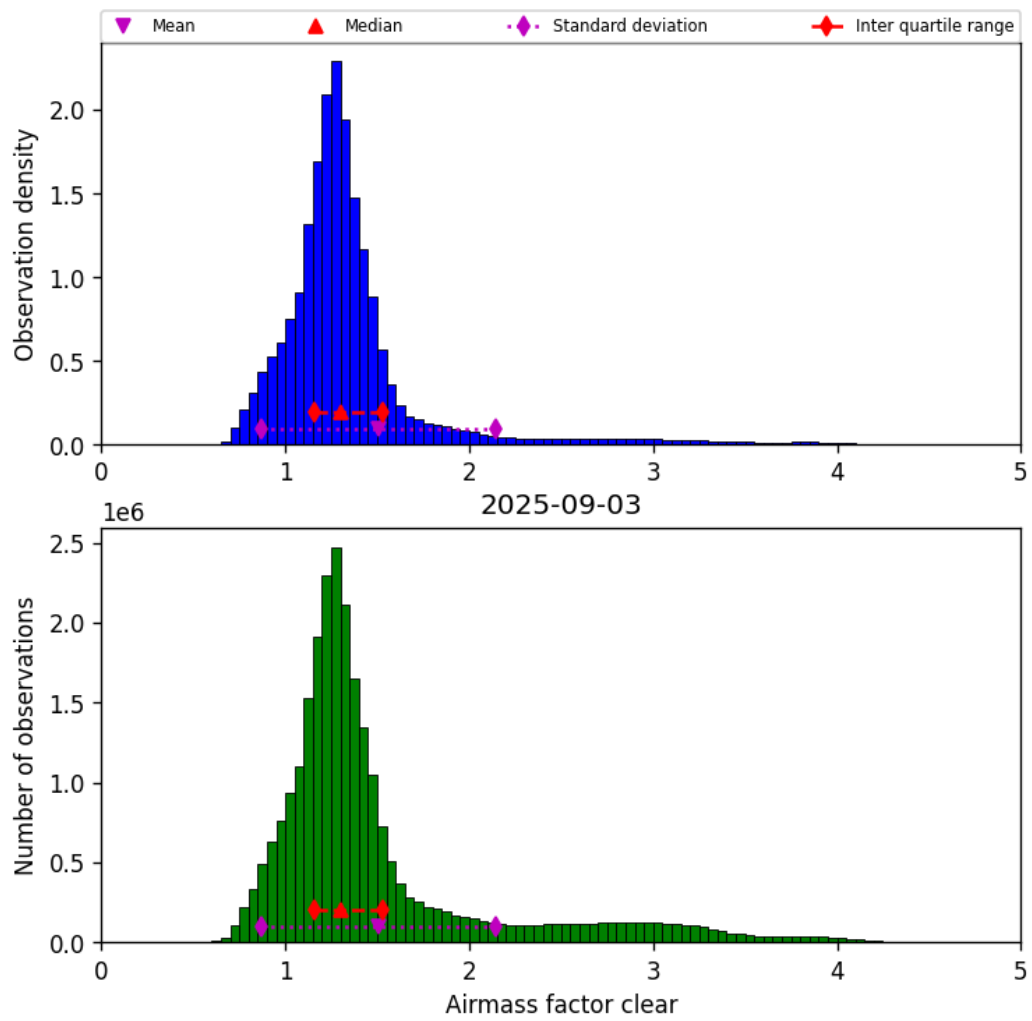
Figure 42: Histogram of “Airmass factor clear” for 2025-09-02 to 2025-09-04
