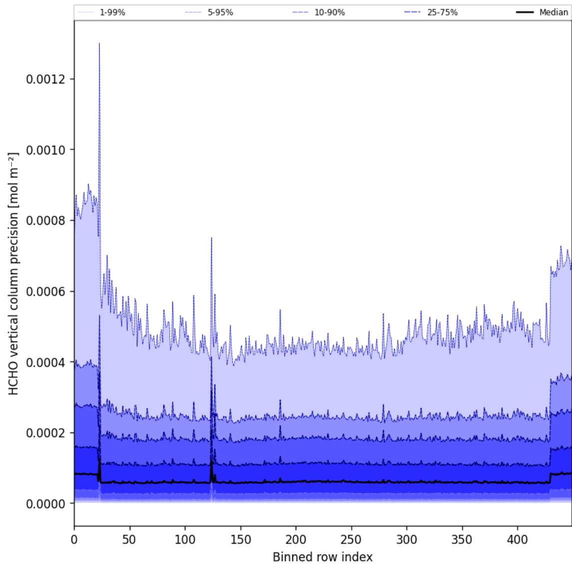
Figure 50: Along track statistics of “HCHO vertical column precision” for 2025-09-02 to 2025-09-04
