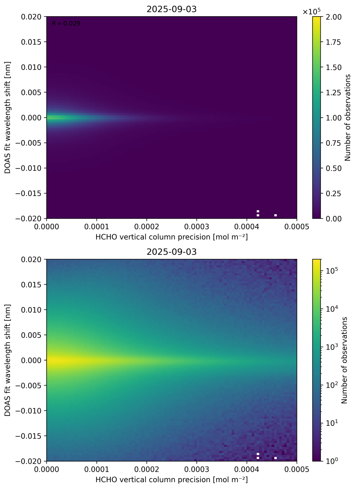
Figure 137: Scatter density plot of “HCHO vertical column precision” against “DOAS fit wavelength shift” for 2025-09-02 to 2025-09-04.
