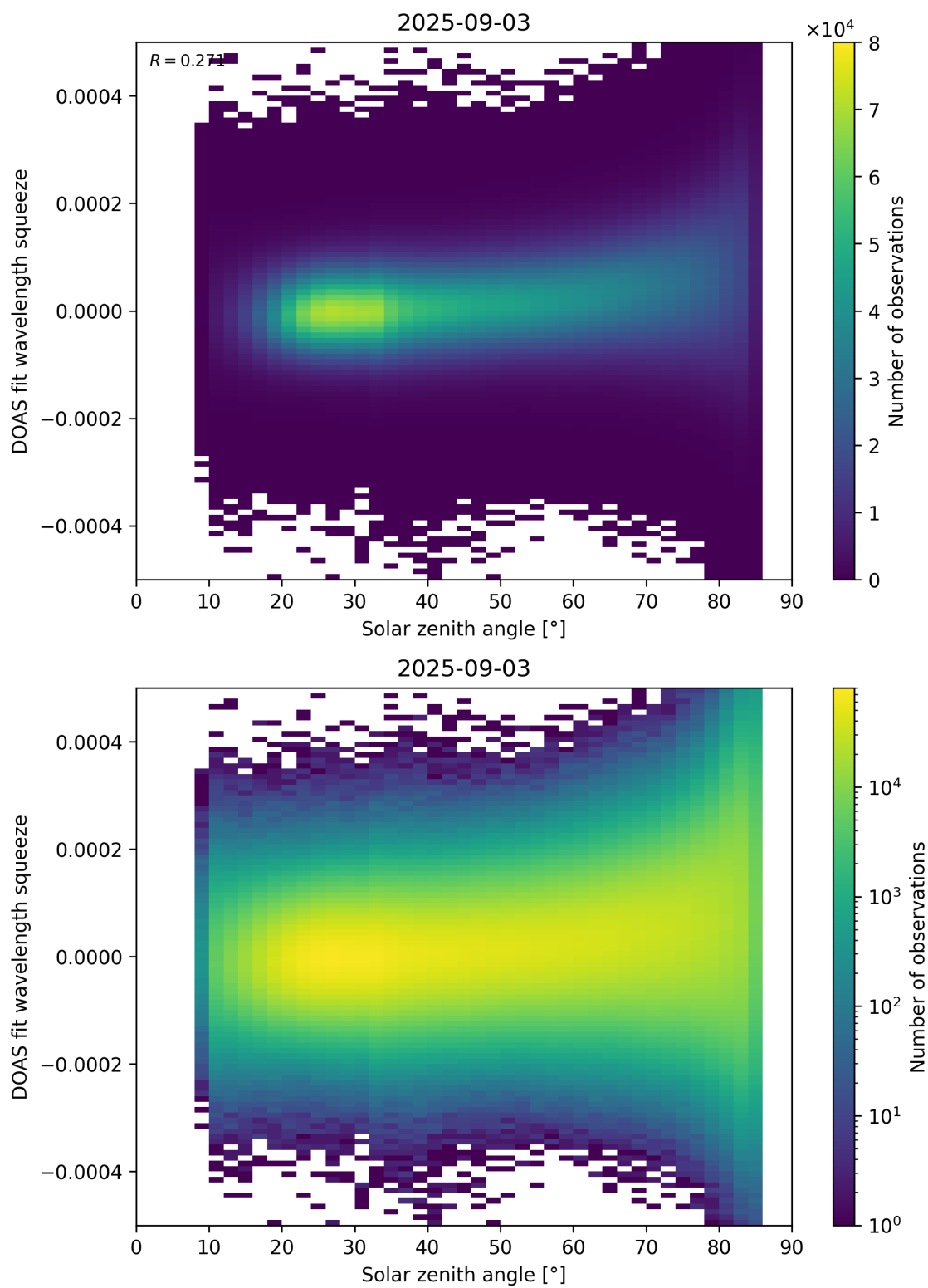
Figure 169: Scatter density plot of “Solar zenith angle” against “DOAS fit wavelength squeeze” for 2025-09-02 to 2025-09-04.
