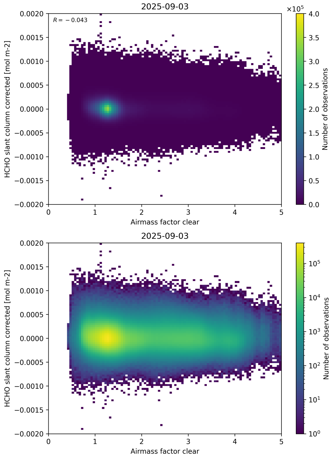
Figure 74: Scatter density plot of “Airmass factor clear” against “HCHO slant column corrected” for 2025-09-02 to 2025-09-04.
