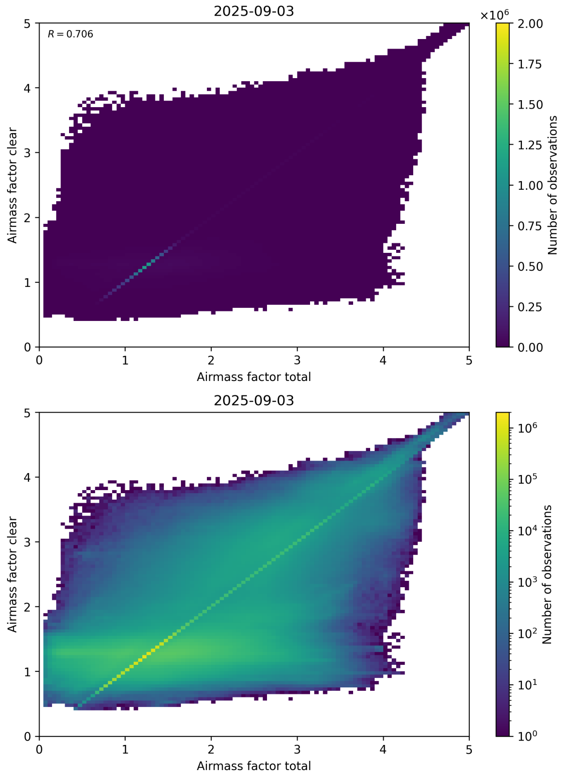
Figure 100: Scatter density plot of “Airmass factor total” against “Airmass factor clear” for 2025-09-02 to 2025-09-04.
