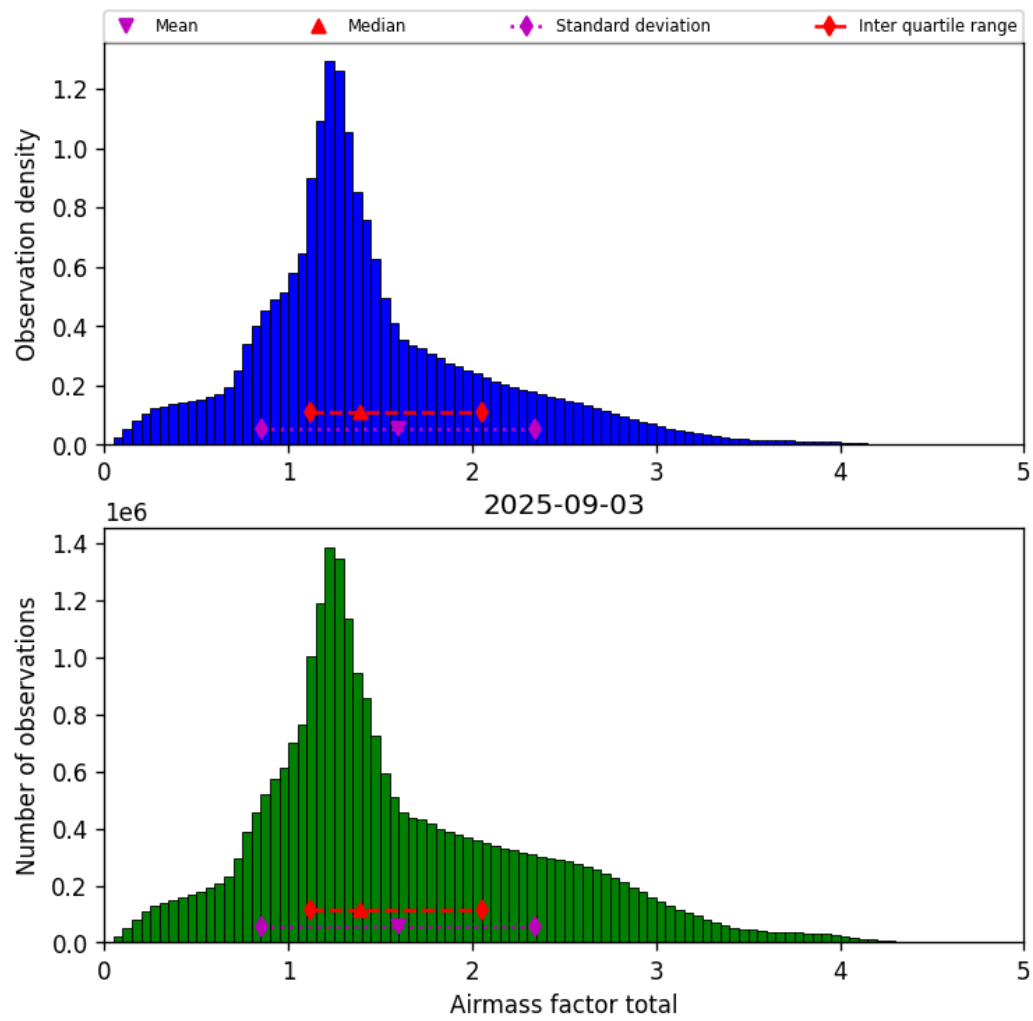
Figure 40: Histogram of “Airmass factor total” for 2025-09-02 to 2025-09-04
