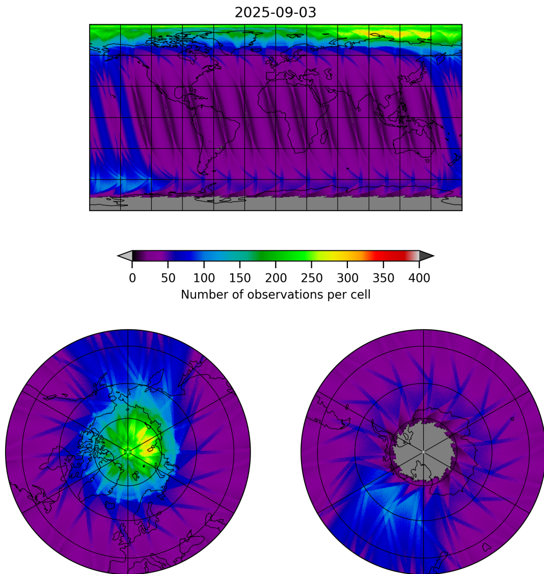
Figure 19: Map of the number of observations for 2025-09-02 to 2025-09-04
