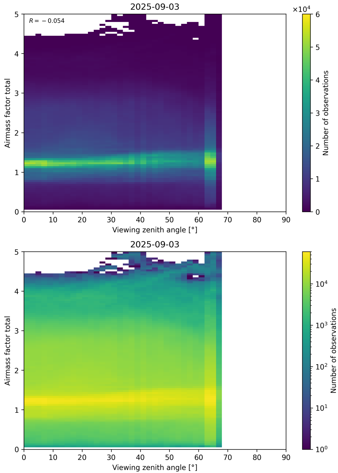
Figure 190: Scatter density plot of “Viewing zenith angle” against “Airmass factor total” for 2025-09-02 to 2025-09-04.
