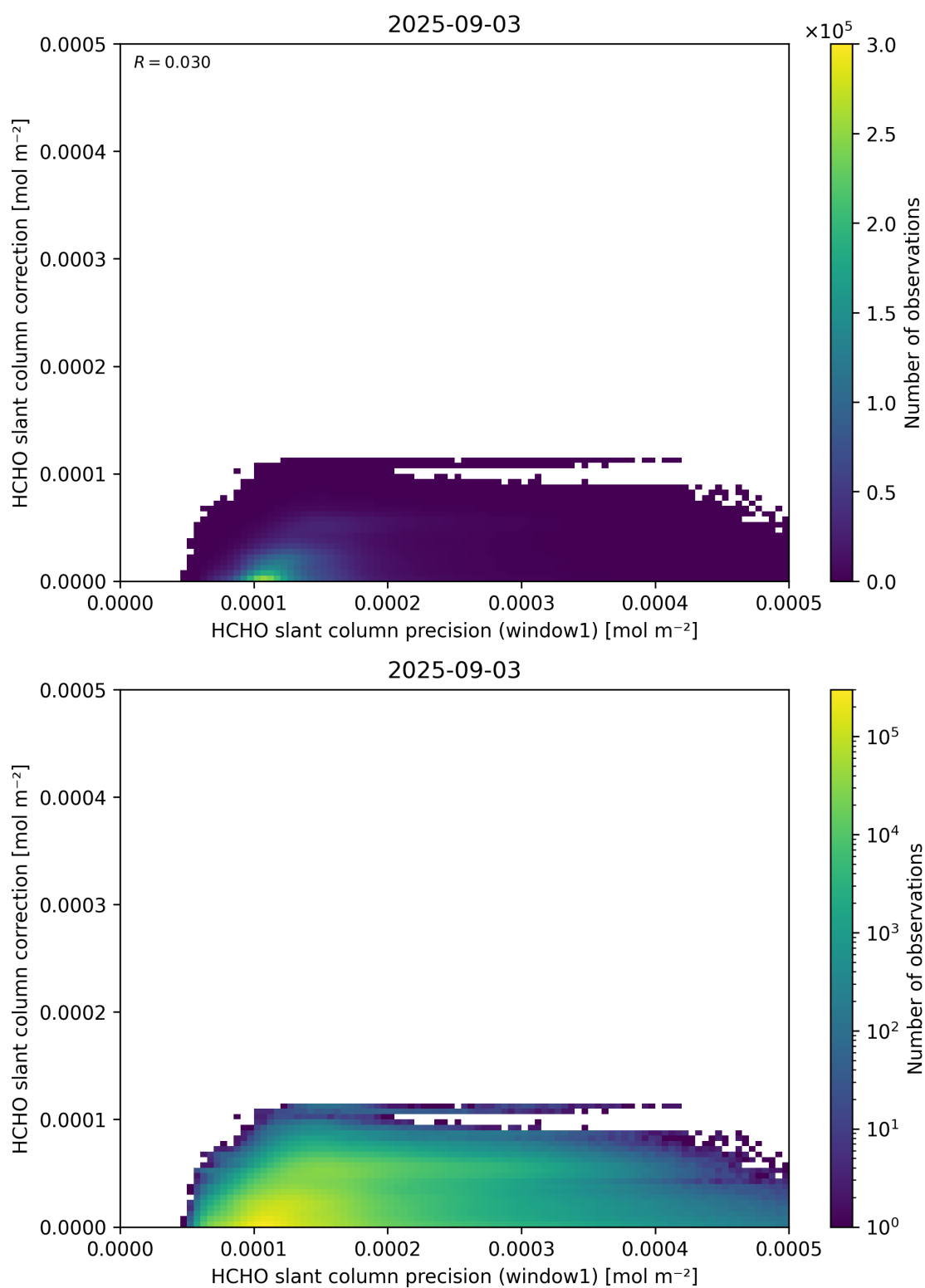
Figure 93: Scatter density plot of “HCHO slant column precision (window1)” against “HCHO slant column correction” for 2025-09-02 to 2025-09-04.
