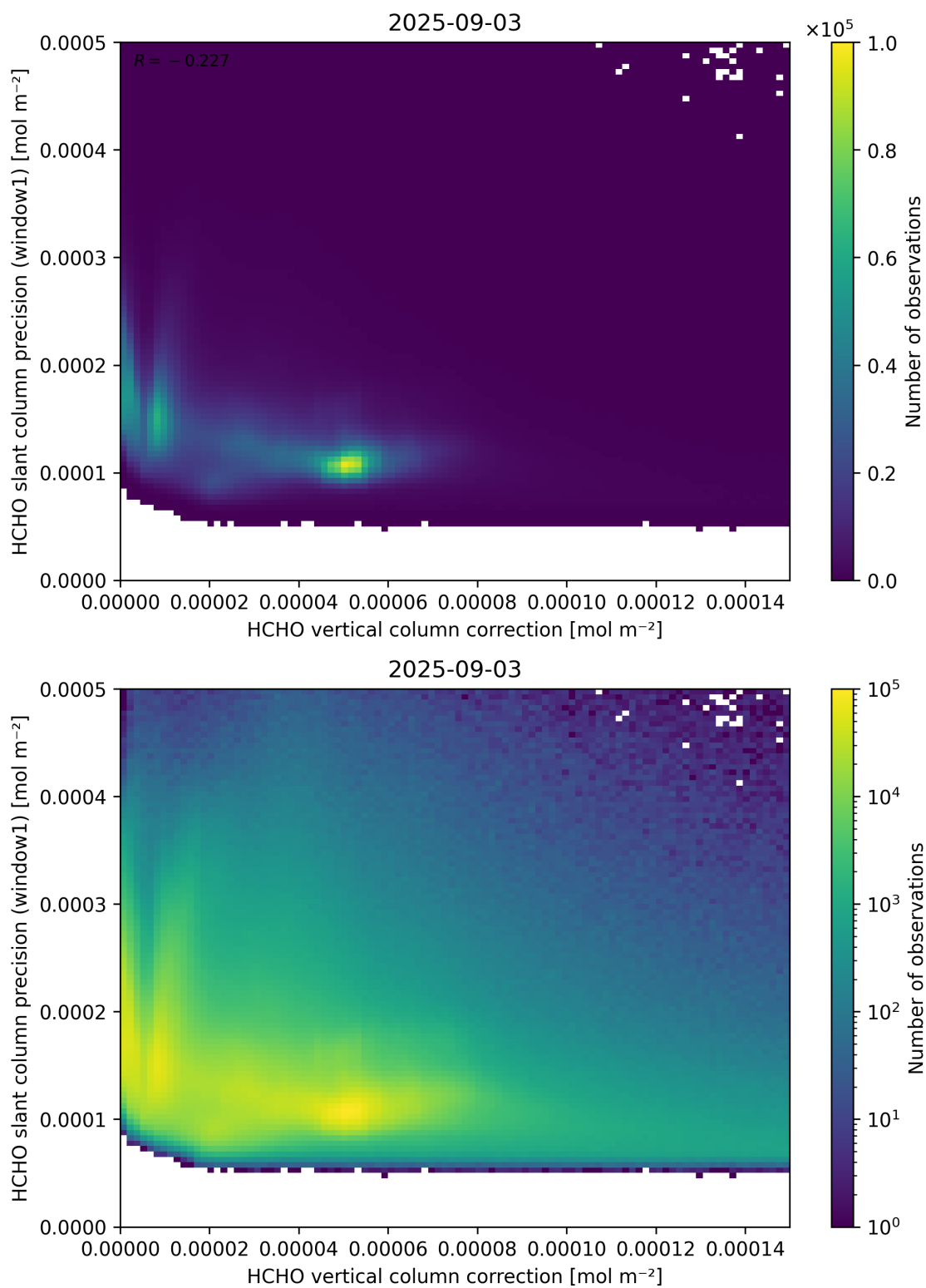
Figure 119: Scatter density plot of “HCHO vertical column correction” against “HCHO slant column precision (window1)” for 2025-09-02 to 2025-09-04.
