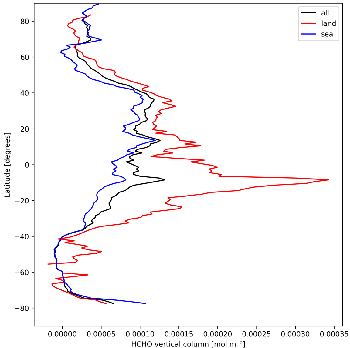
Figure 21: Zonal average of “HCHO vertical column” for 2025-09-02 to 2025-09-04.
