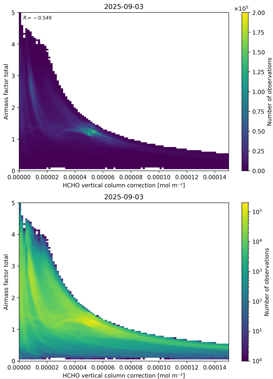
Figure 120: Scatter density plot of “HCHO vertical column correction” against “Airmass factor total” for 2025-09-02 to 2025-09-04.
