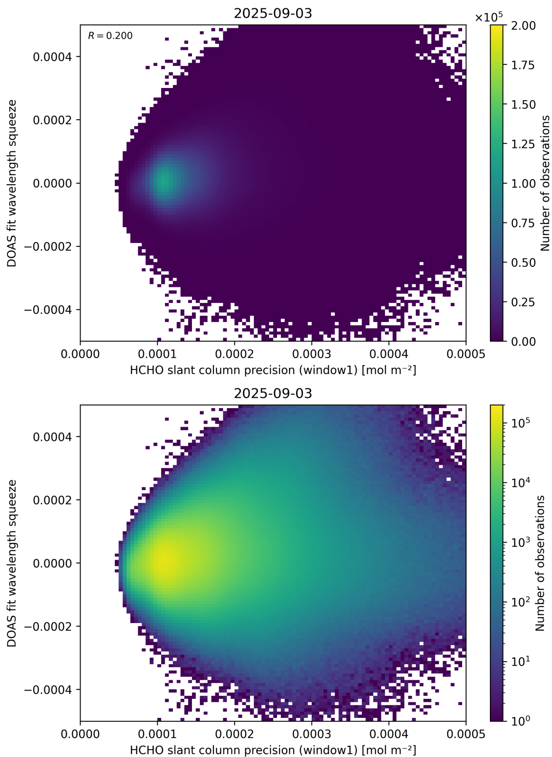
Figure 90: Scatter density plot of “HCHO slant column precision (window1)” against “DOAS fit wavelength squeeze” for 2025-09-02 to 2025-09-04.
