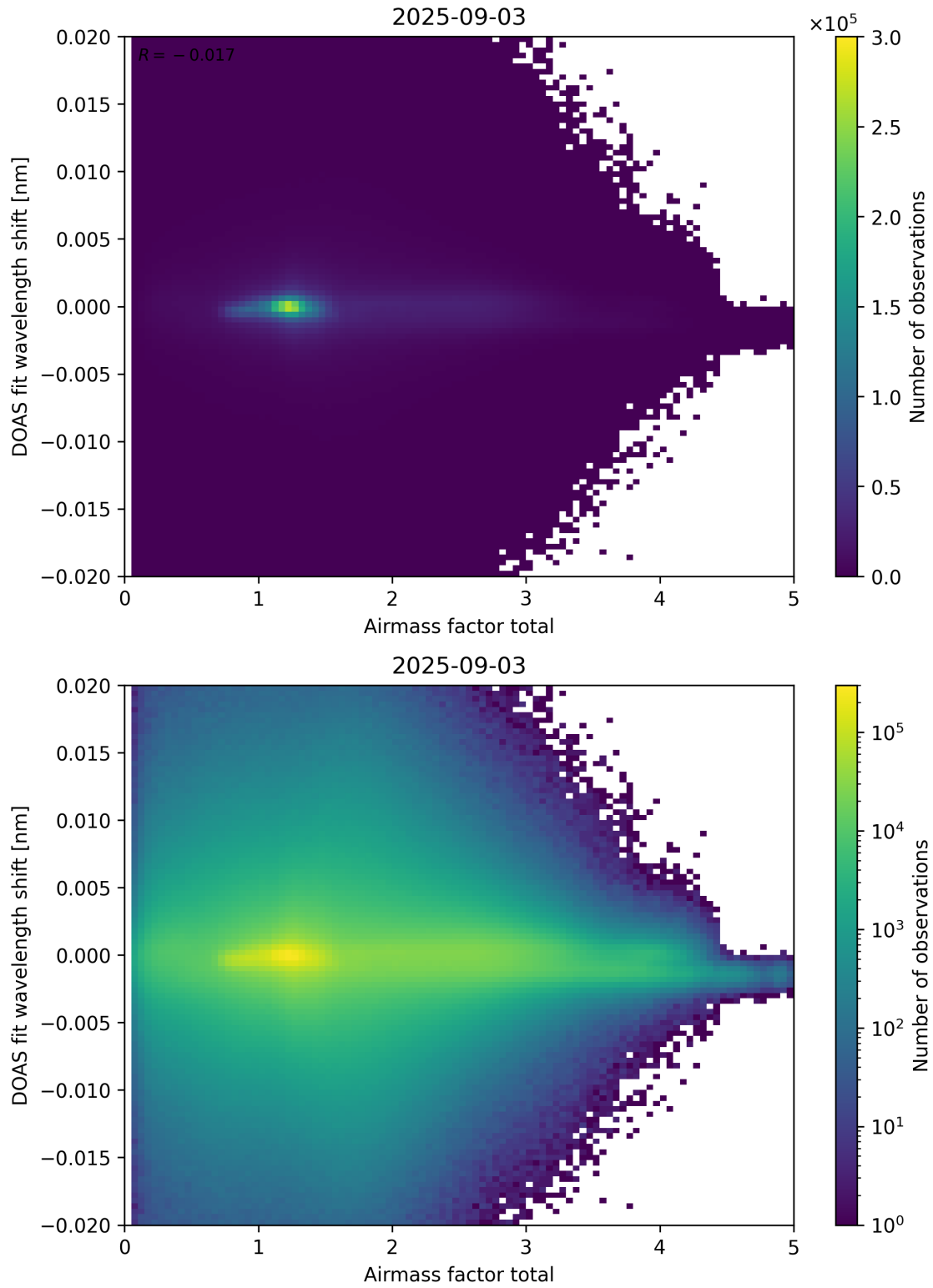
Figure 98: Scatter density plot of “Airmass factor total” against “DOAS fit wavelength shift” for 2025-09-02 to 2025-09-04.
