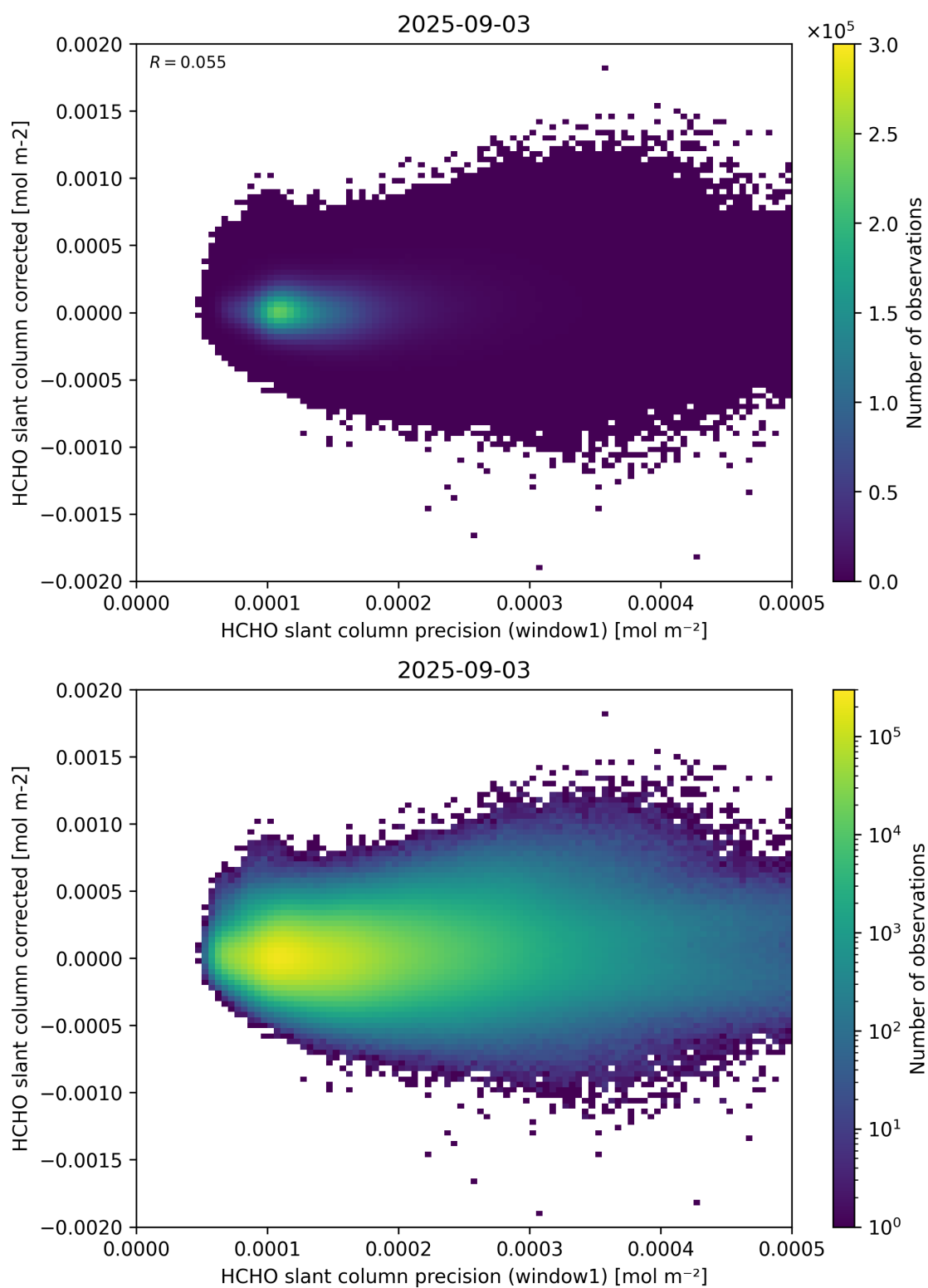
Figure 92: Scatter density plot of “HCHO slant column precision (window1)” against “HCHO slant column corrected” for 2025-09-02 to 2025-09-04.
