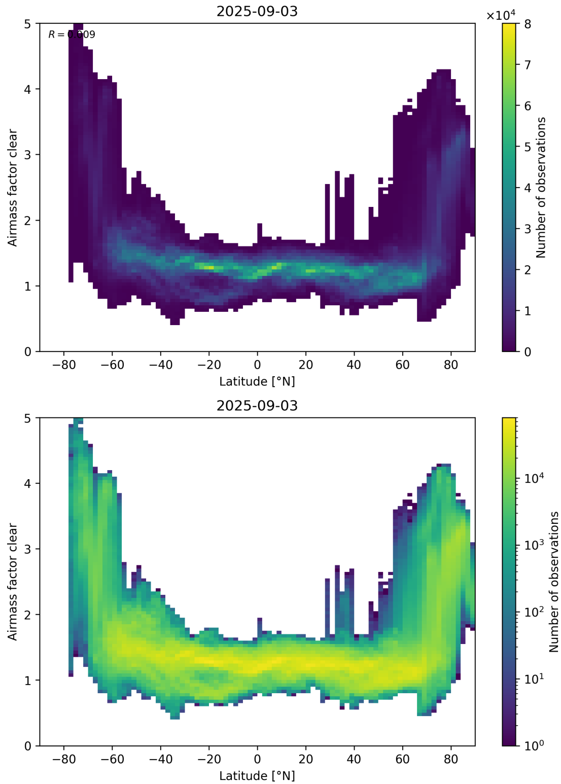
Figure 156: Scatter density plot of “Latitude” against “Airmass factor clear” for 2025-09-02 to 2025-09-04.
