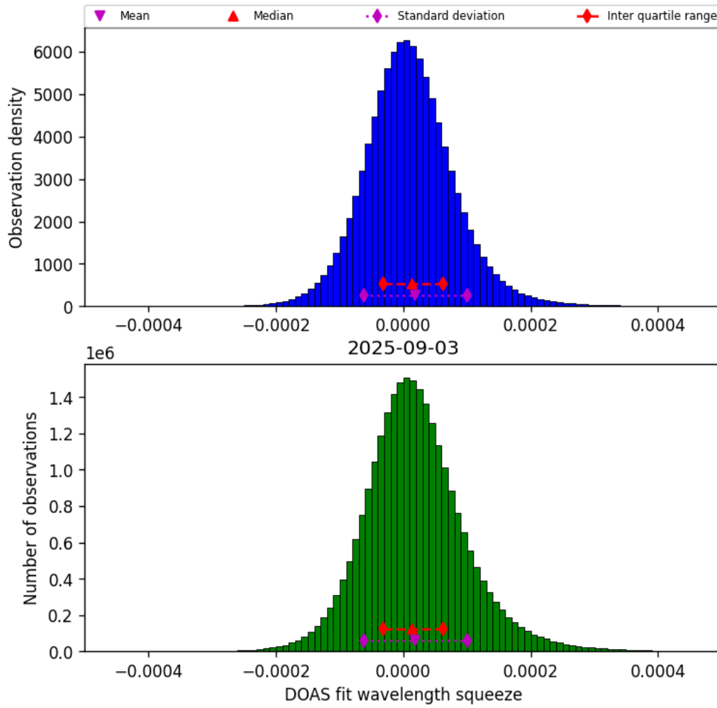
Figure 45: Histogram of “DOAS fit wavelength squeeze” for 2025-09-02 to 2025-09-04
