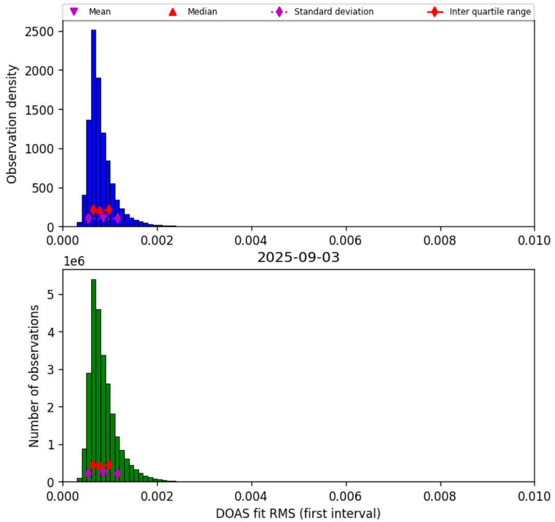
Figure 46: Histogram of “DOAS fit RMS (first interval)” for 2025-09-02 to 2025-09-04
