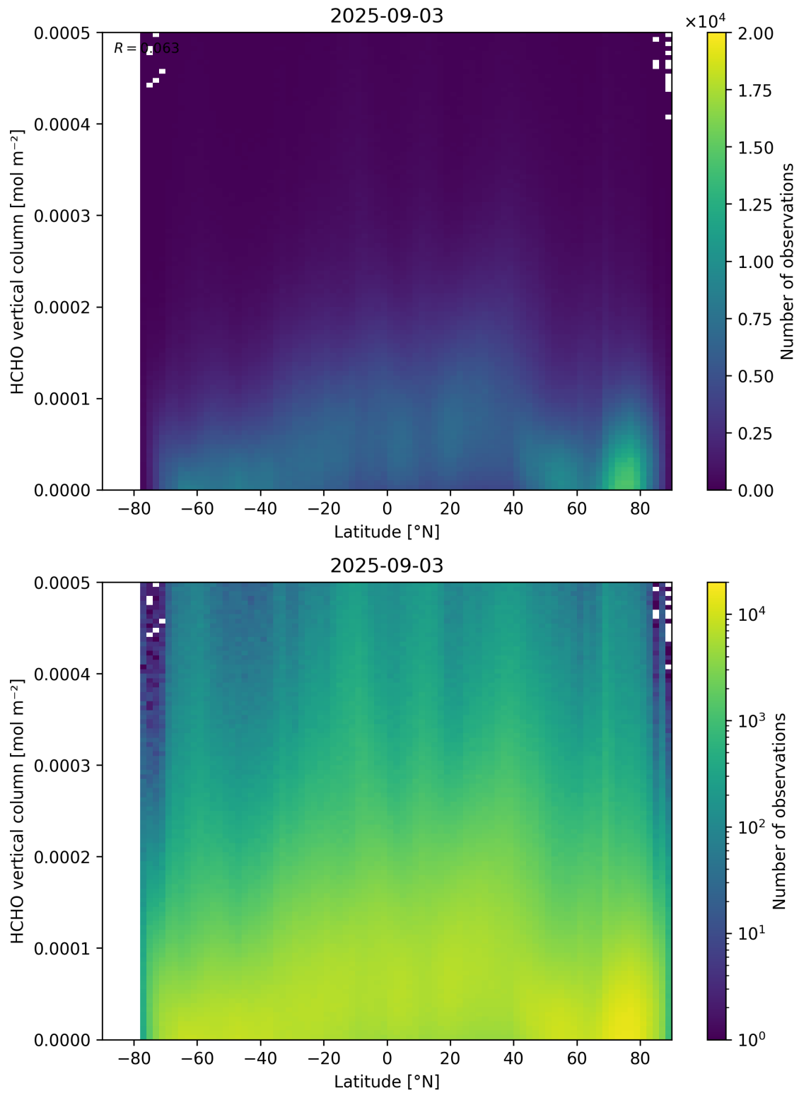
Figure 163: Scatter density plot of “Latitude” against “HCHO vertical column” for 2025-09-02 to 2025-09-04.
