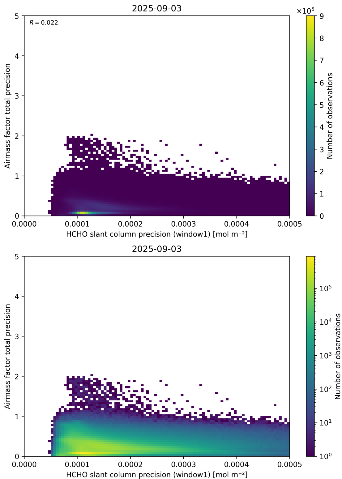
Figure 95: Scatter density plot of “HCHO slant column precision (window1)” against “Airmass factor total precision” for 2025-09-02 to 2025-09-04.
