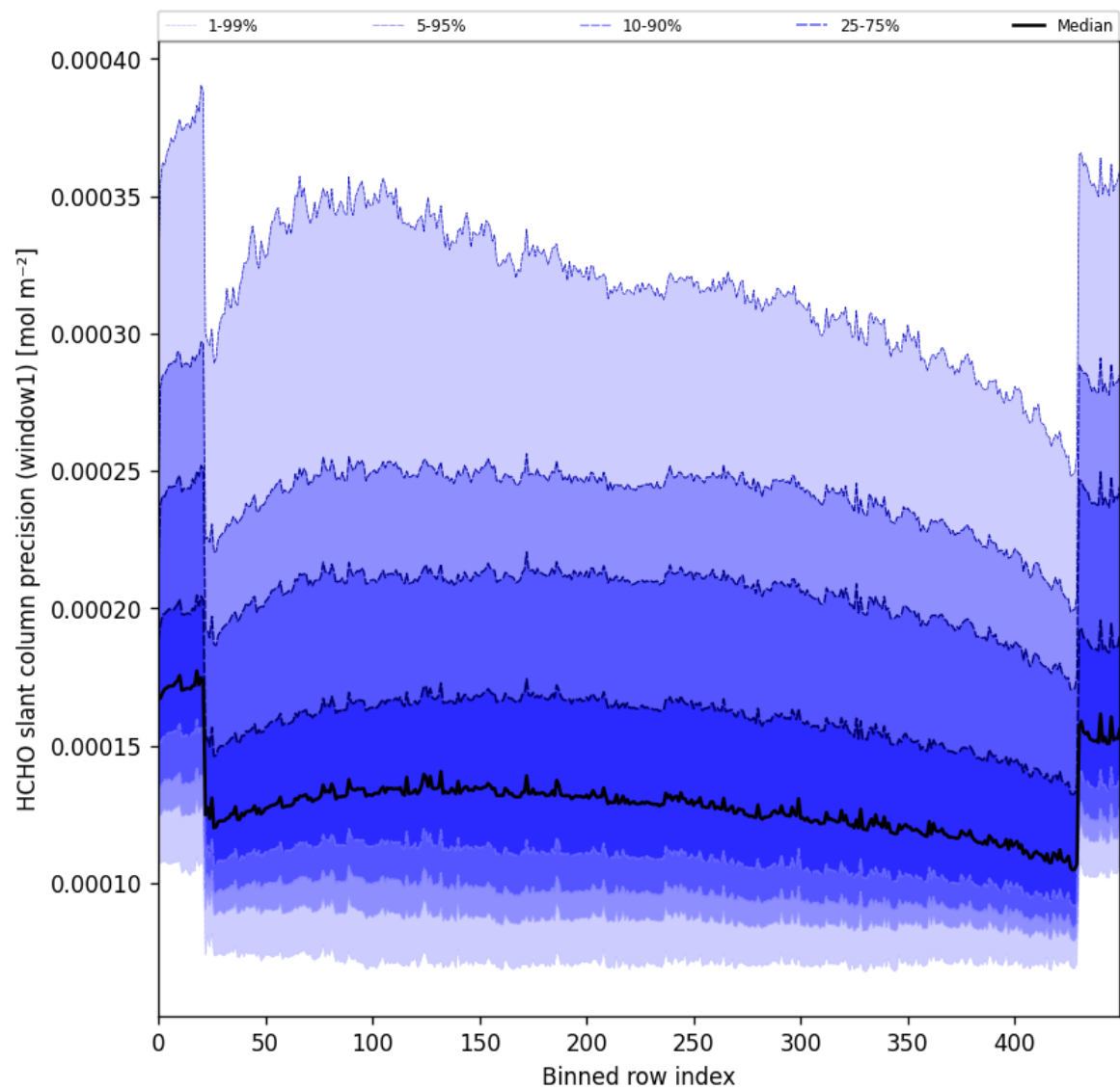
Figure 53: Along track statistics of “HCHO slant column precision (window1)” for 2025-09-02 to 2025-09-04
