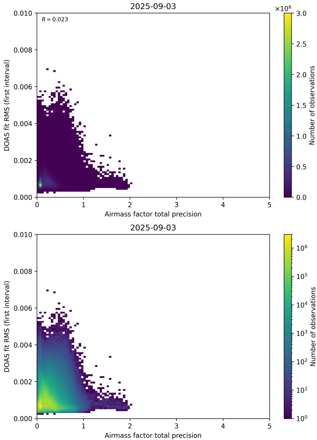
Figure 105: Scatter density plot of “Airmass factor total precision” against “DOAS fit RMS (first interval)” for 2025-09-02 to 2025-09-04.
