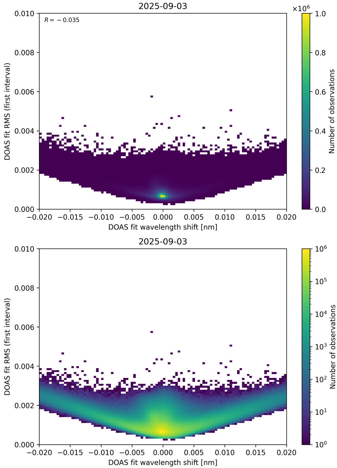
Figure 64: Scatter density plot of “DOAS fit wavelength shift” against “DOAS fit RMS (first interval)” for 2025-09-02 to 2025-09-04.
