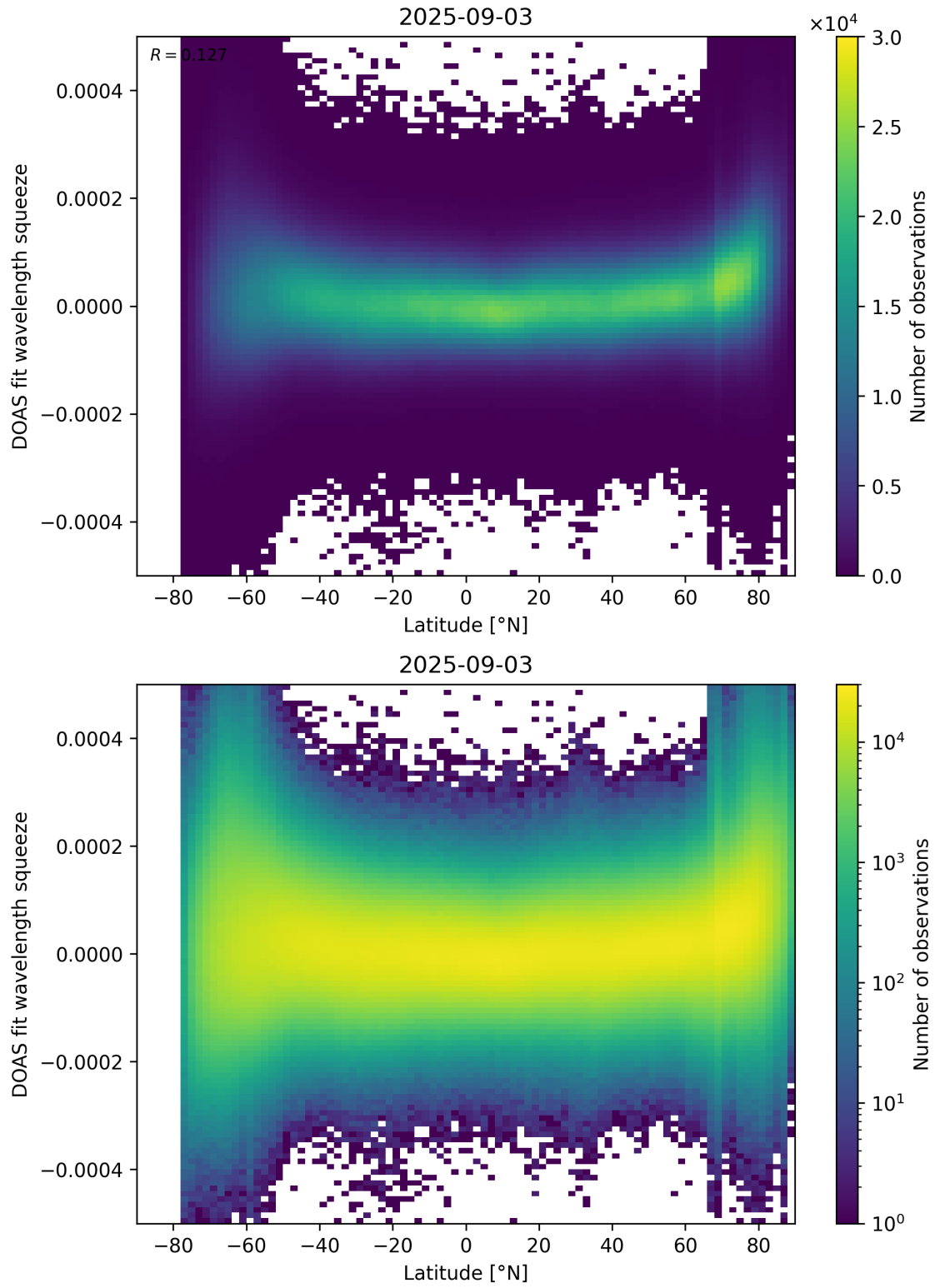
Figure 155: Scatter density plot of “Latitude” against “DOAS fit wavelength squeeze” for 2025-09-02 to 2025-09-04.
