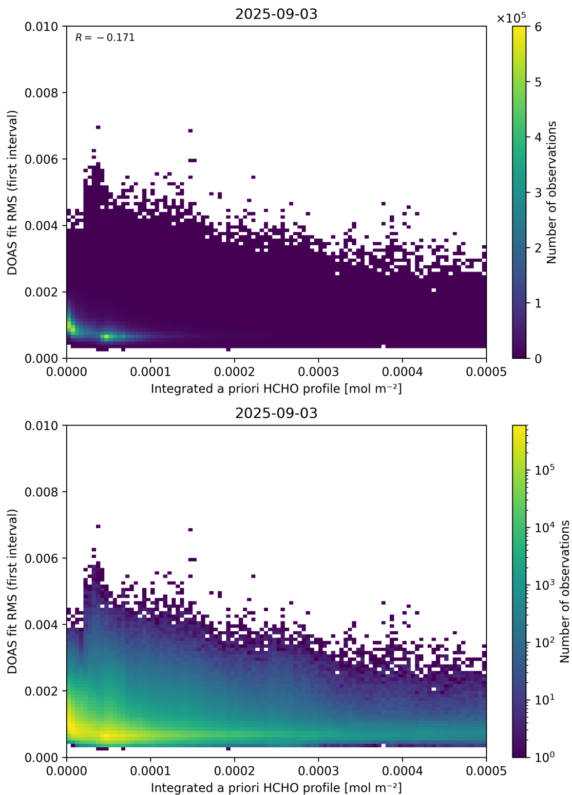
Figure 148: Scatter density plot of “Integrated a priori HCHO profile” against “DOAS fit RMS (first interval)” for 2025-09-02 to 2025-09-04.
