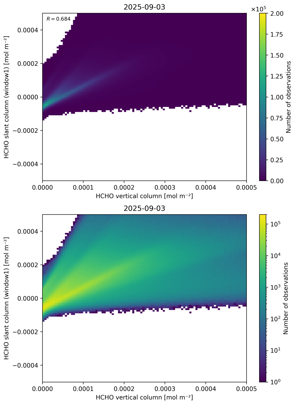
Figure 129: Scatter density plot of “HCHO vertical column” against “HCHO slant column (window1)” for 2025-09-02 to 2025-09-04.
