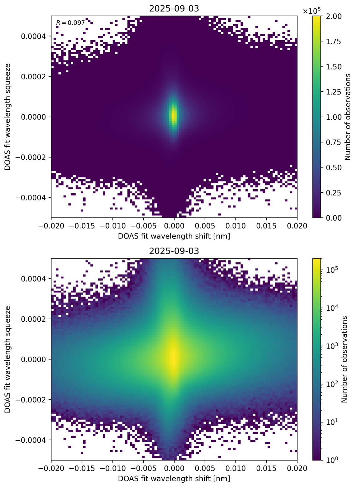
Figure 65: Scatter density plot of “DOAS fit wavelength shift” against “DOAS fit wavelength squeeze” for 2025-09-02 to 2025-09-04.
