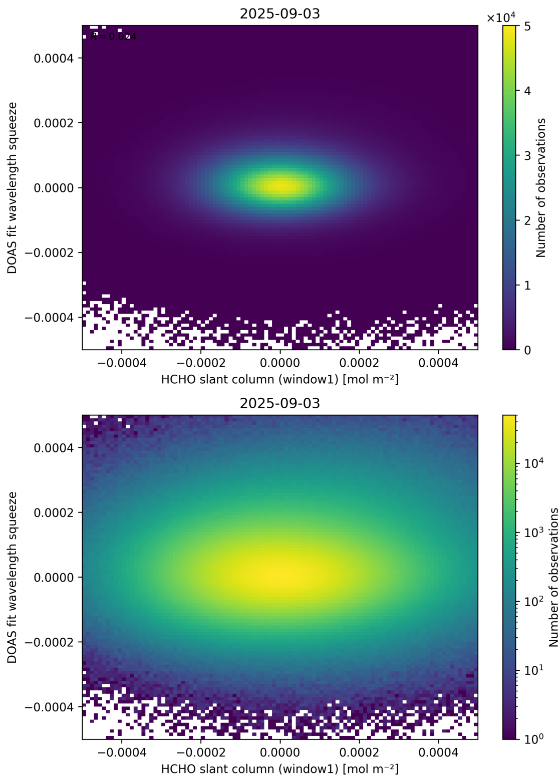
Figure 80: Scatter density plot of “HCHO slant column (window1)” against “DOAS fit wavelength squeeze” for 2025-09-02 to 2025-09-04.
