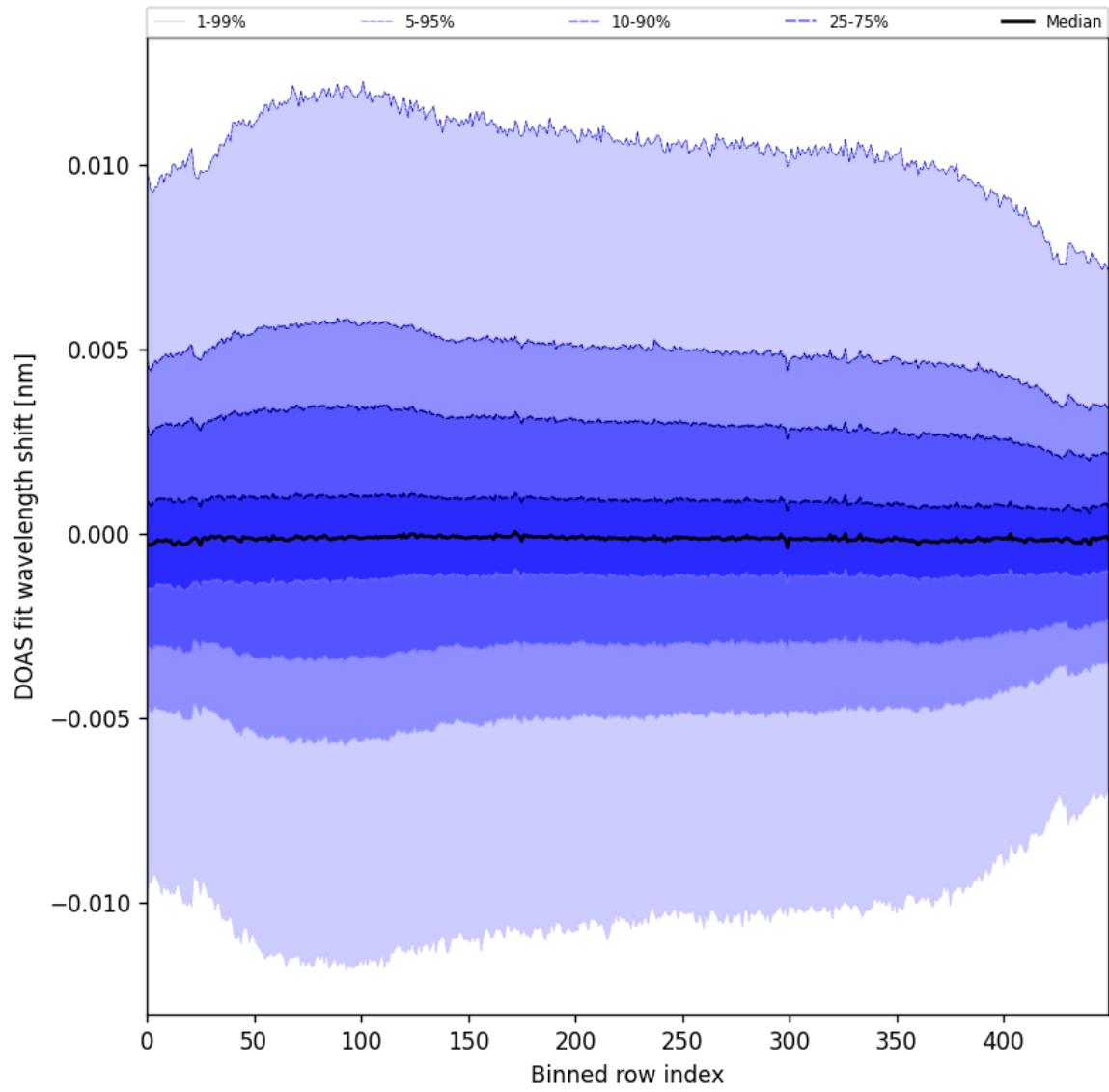
Figure 58: Along track statistics of “DOAS fit wavelength shift” for 2025-09-02 to 2025-09-04
