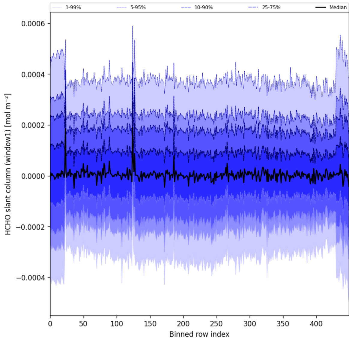
Figure 52: Along track statistics of “HCHO slant column (window1)” for 2025-09-02 to 2025-09-04
