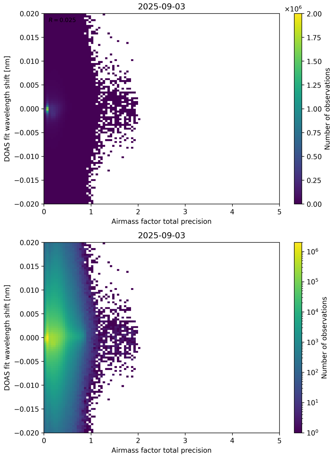
Figure 106: Scatter density plot of “Airmass factor total precision” against “DOAS fit wavelength shift” for 2025-09-02 to 2025-09-04.
