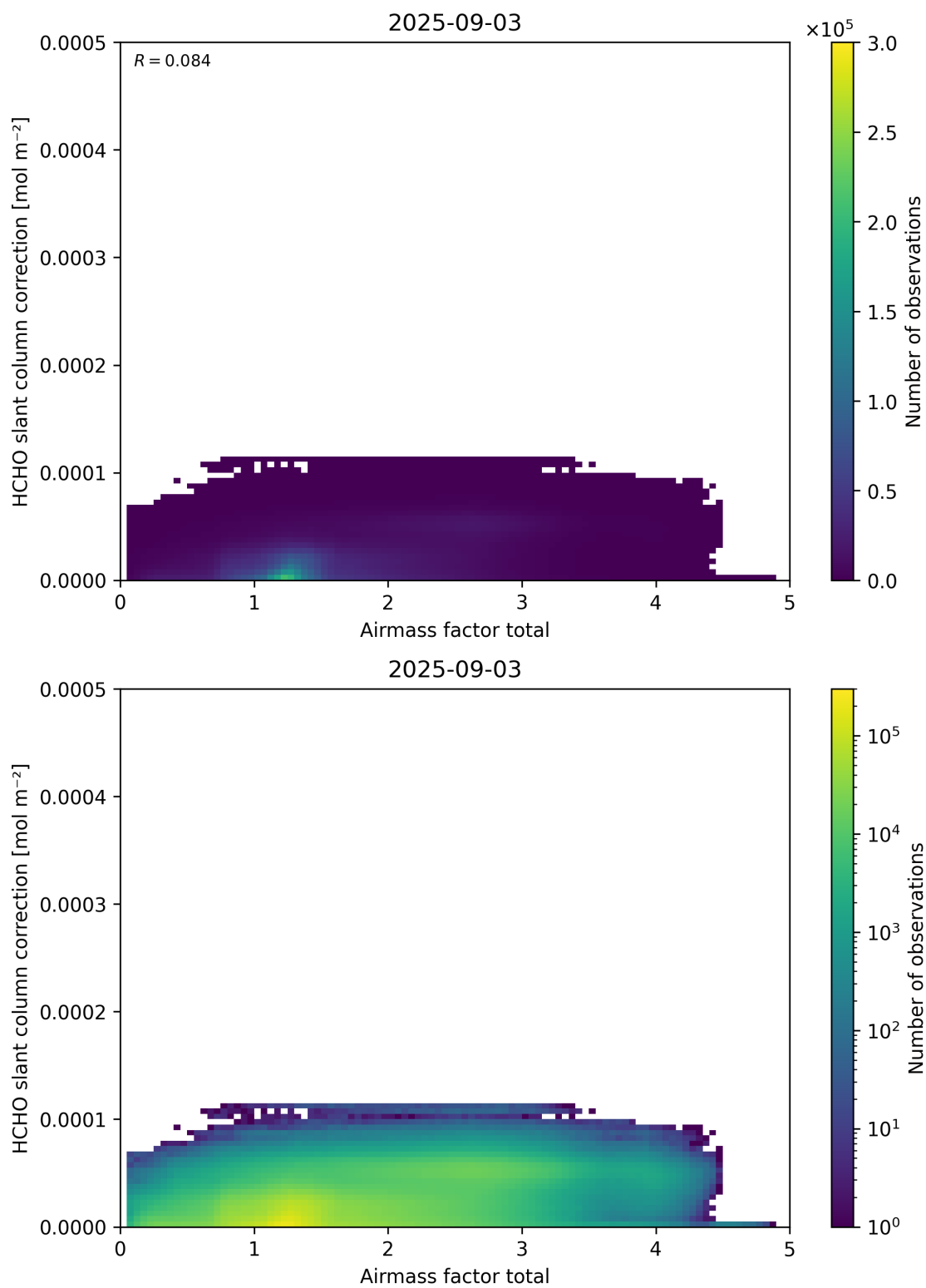
Figure 102: Scatter density plot of “Airmass factor total” against “HCHO slant column correction” for 2025-09-02 to 2025-09-04.
