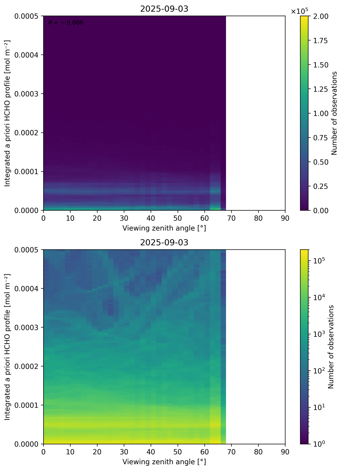
Figure 195: Scatter density plot of “Viewing zenith angle” against “Integrated a priori HCHO profile” for 2025-09-02 to 2025-09-04.
