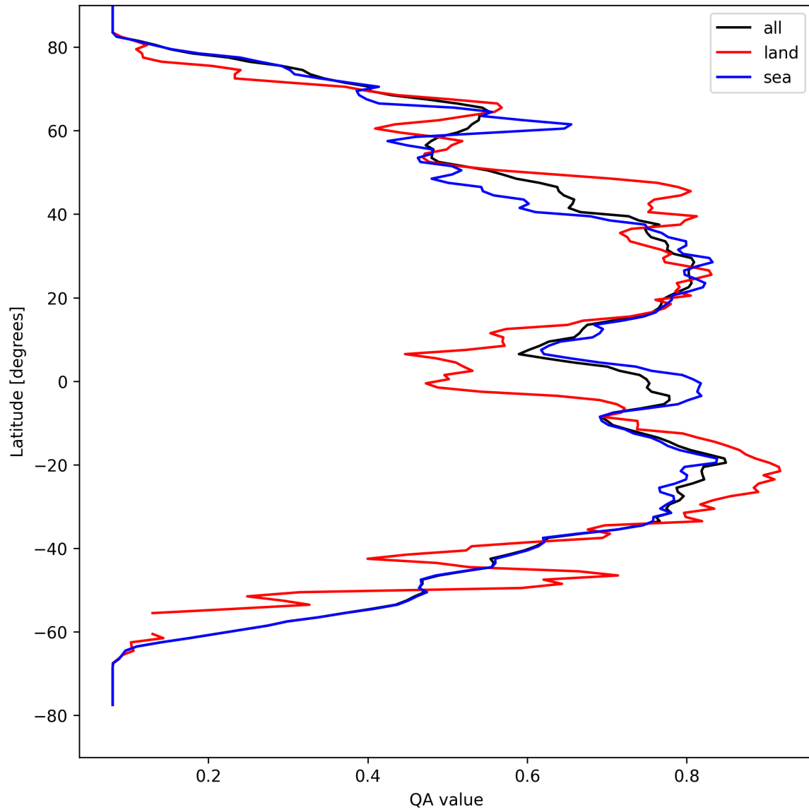
Figure 20: Zonal average of “QA value” for 2025-09-02 to 2025-09-04.
