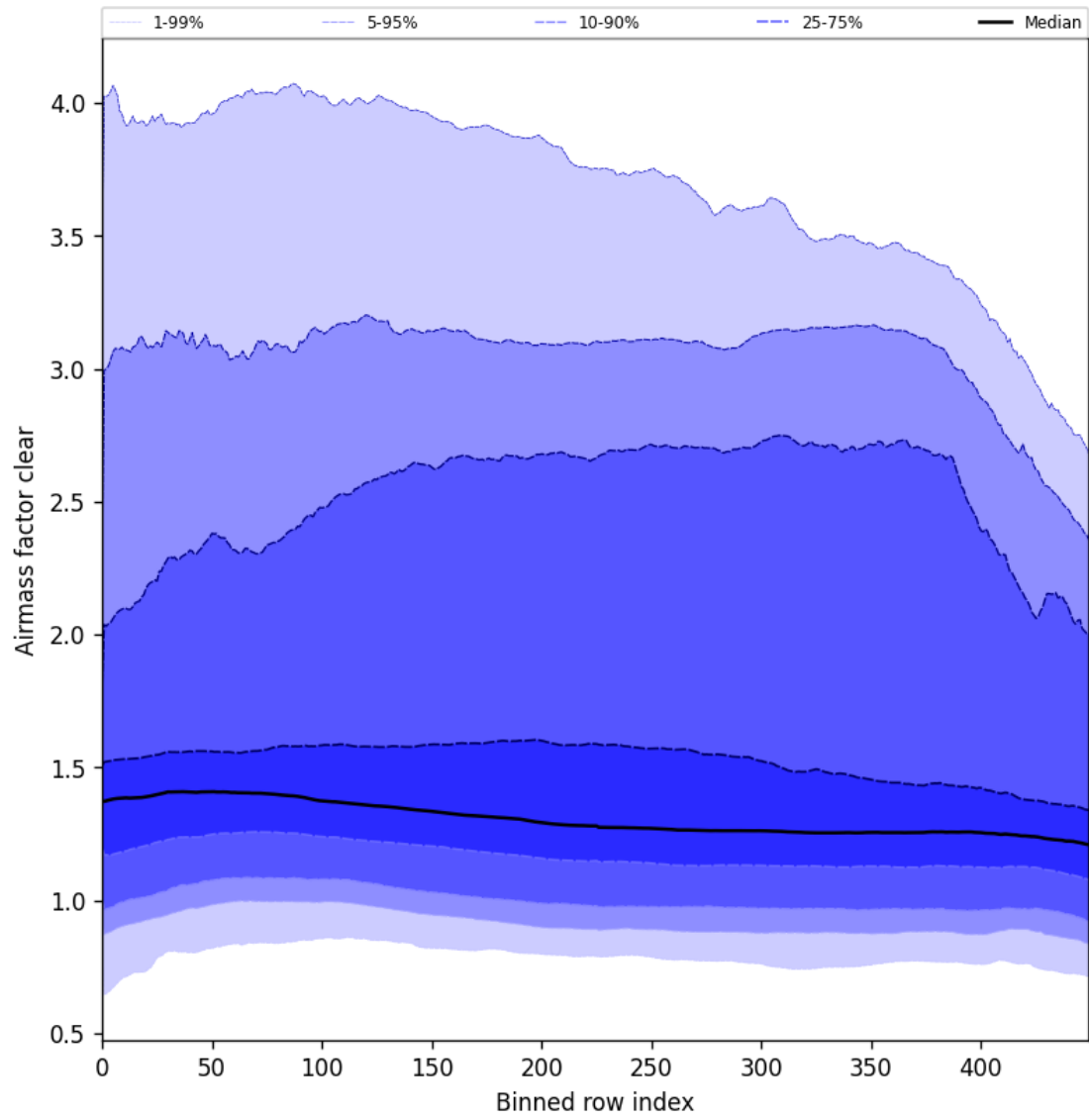
Figure 56: Along track statistics of “Airmass factor clear” for 2025-09-02 to 2025-09-04
