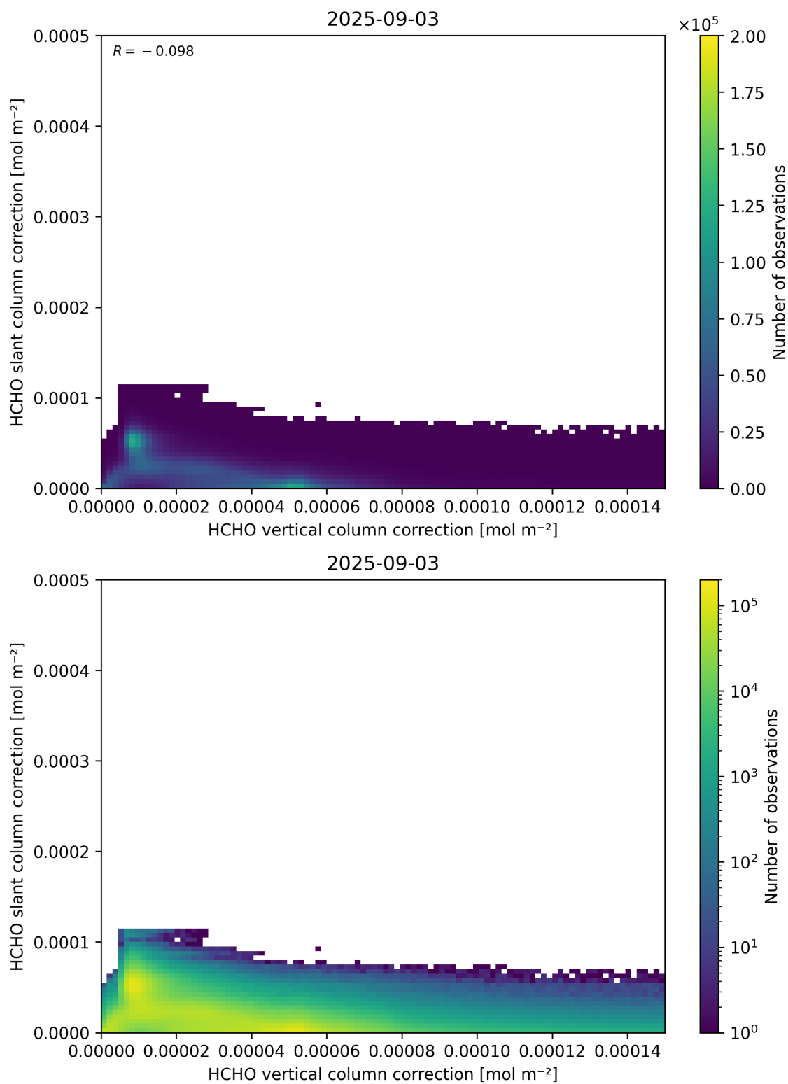
Figure 117: Scatter density plot of “HCHO vertical column correction” against “HCHO slant column correction” for 2025-09-02 to 2025-09-04.
