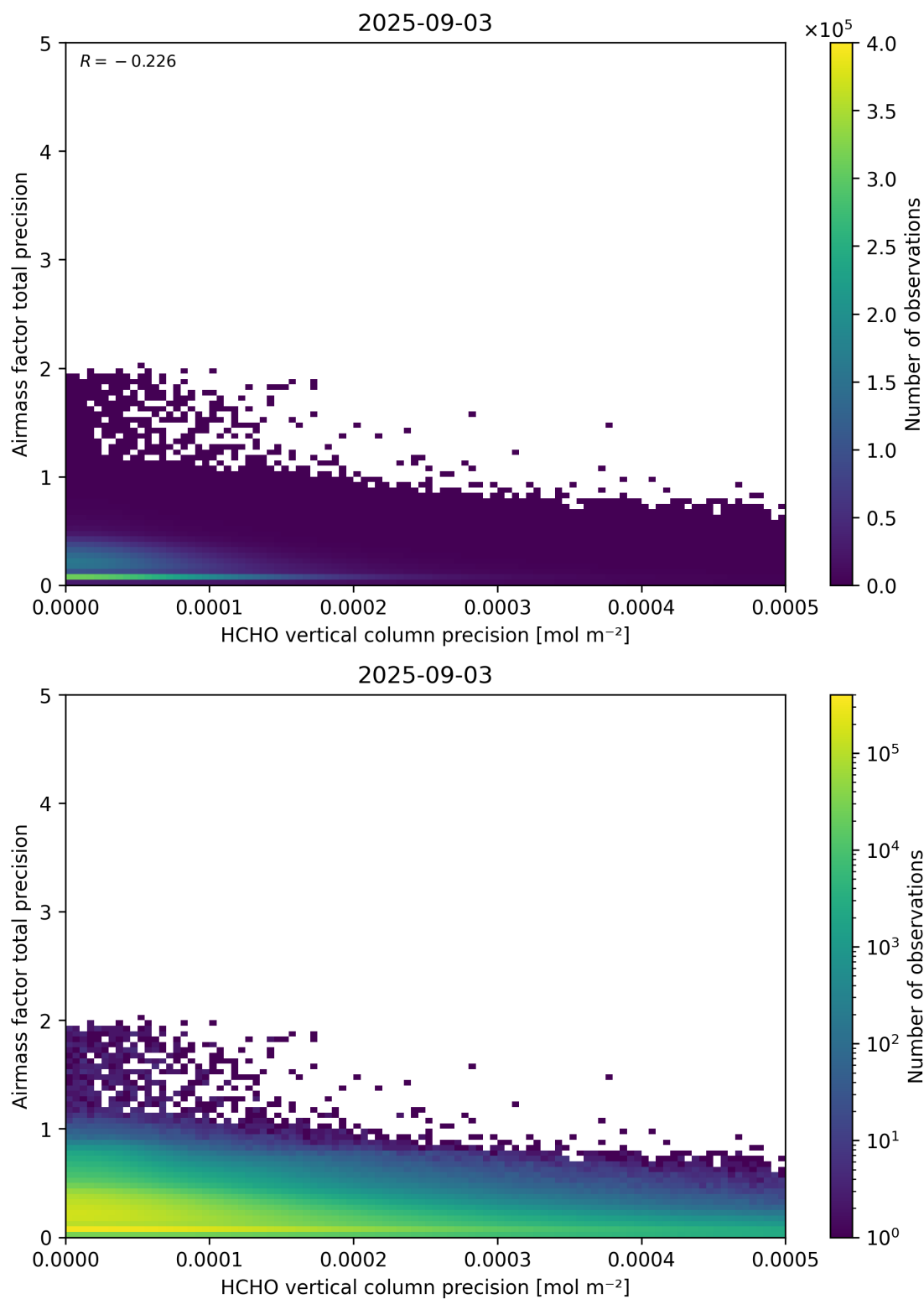
Figure 145: Scatter density plot of “HCHO vertical column precision” against “Airmass factor total precision” for 2025-09-02 to 2025-09-04.
