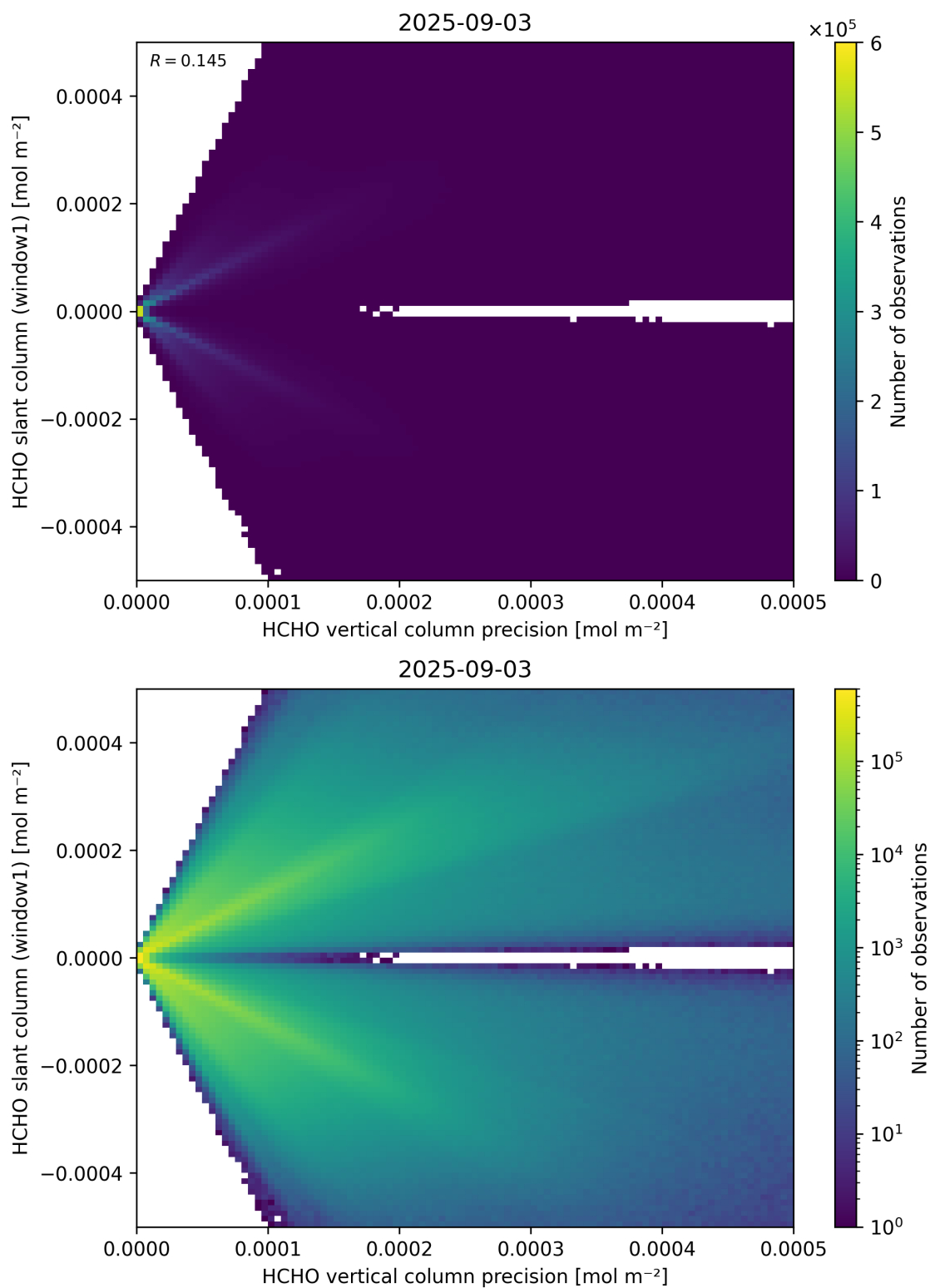
Figure 142: Scatter density plot of “HCHO vertical column precision” against “HCHO slant column (window1)” for 2025-09-02 to 2025-09-04.
