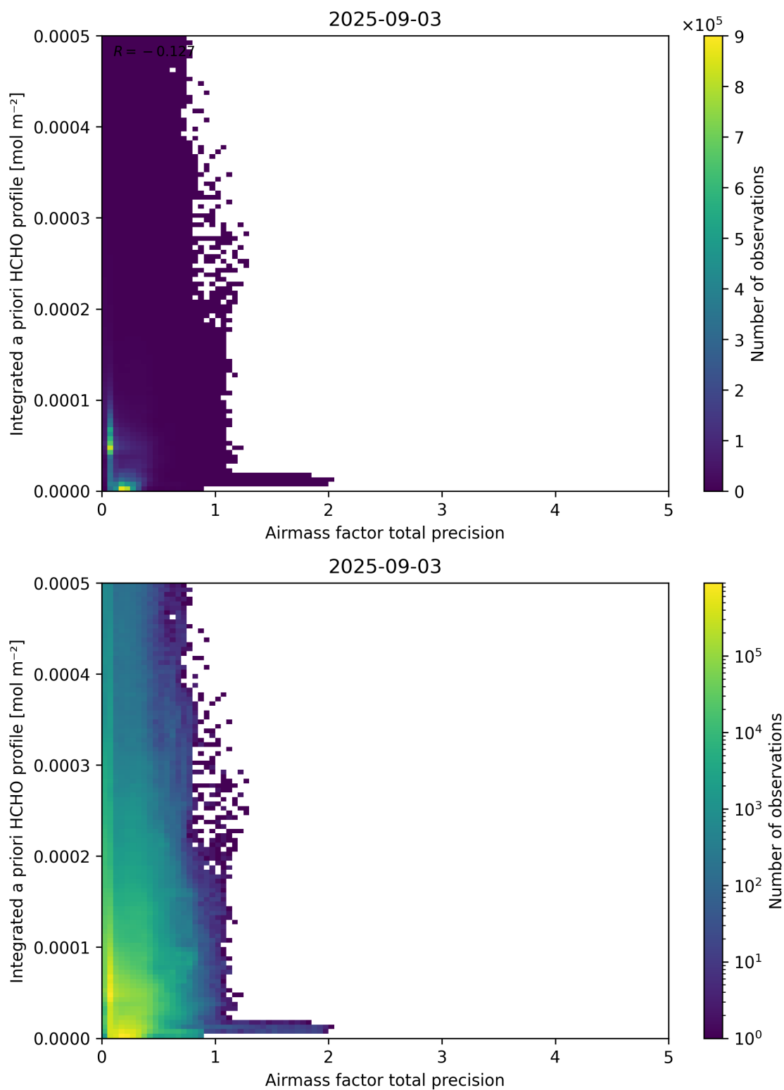
Figure 111: Scatter density plot of “Airmass factor total precision” against “Integrated a priori HCHO profile” for 2025-09-02 to 2025-09-04.
