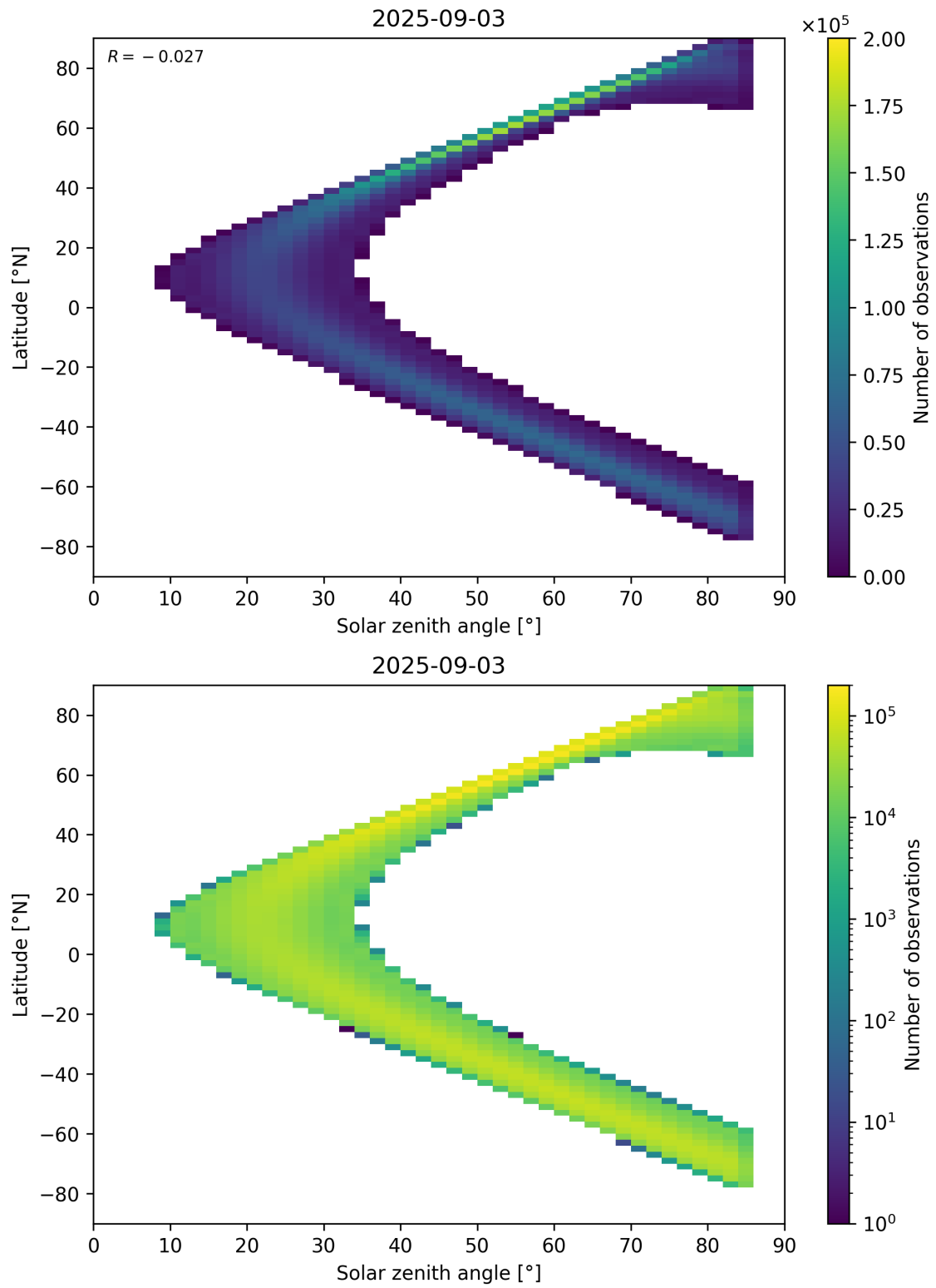
Figure 181: Scatter density plot of “Solar zenith angle” against “Latitude” for 2025-09-02 to 2025-09-04.
