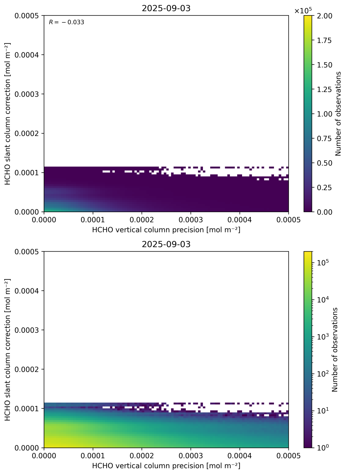
Figure 141: Scatter density plot of “HCHO vertical column precision” against “HCHO slant column correction” for 2025-09-02 to 2025-09-04.
