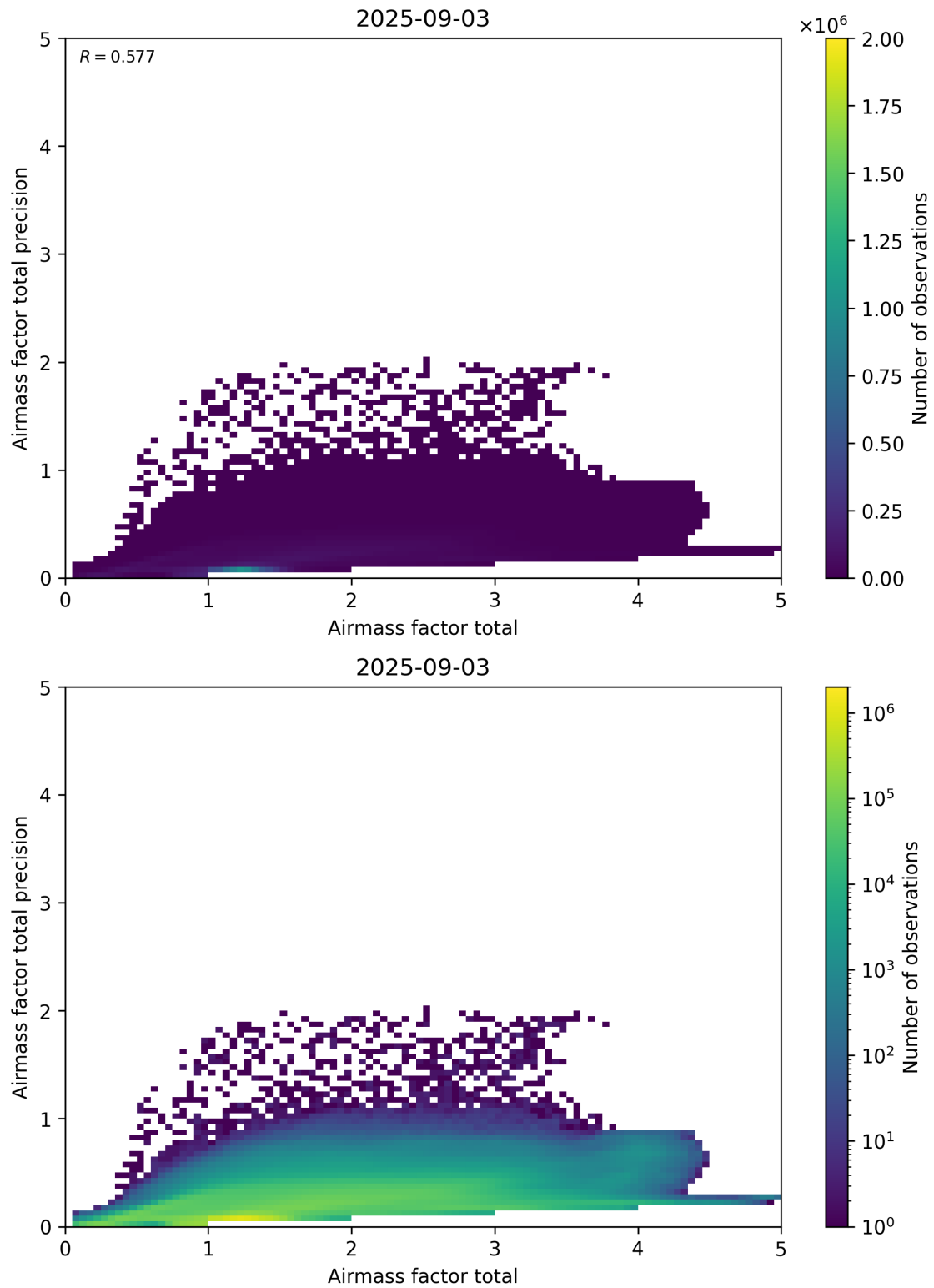
Figure 103: Scatter density plot of “Airmass factor total” against “Airmass factor total precision” for 2025-09-02 to 2025-09-04.
