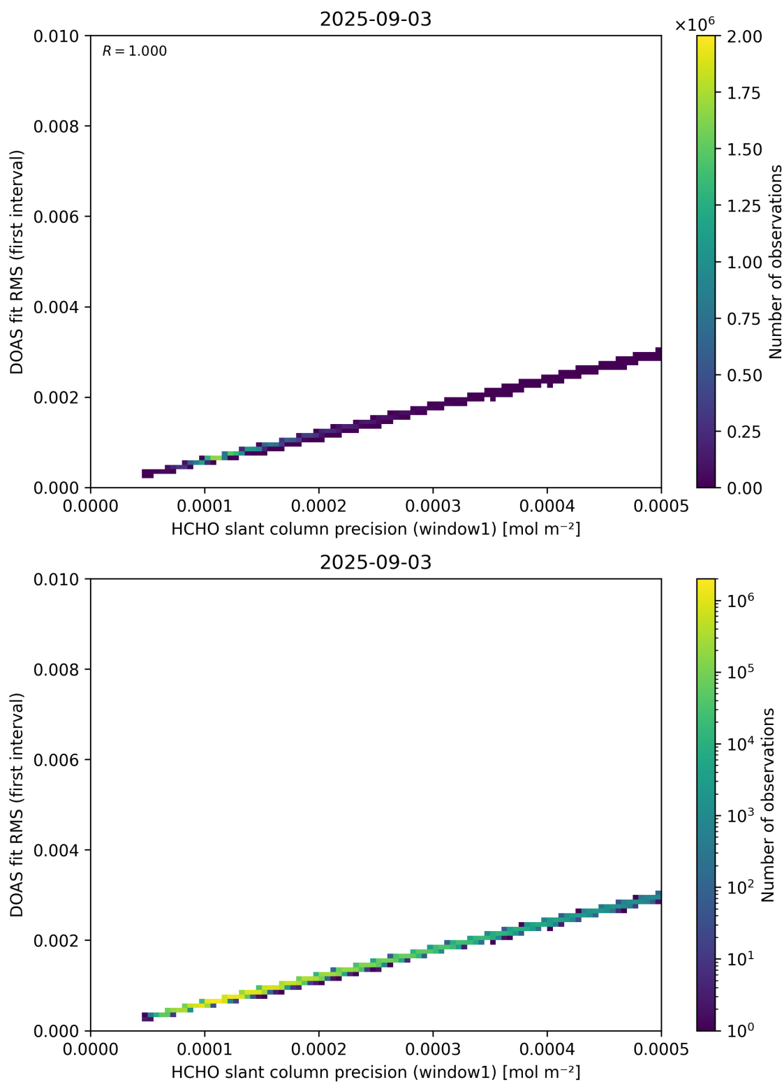
Figure 88: Scatter density plot of “HCHO slant column precision (window1)” against “DOAS fit RMS (first interval)” for 2025-09-02 to 2025-09-04.
