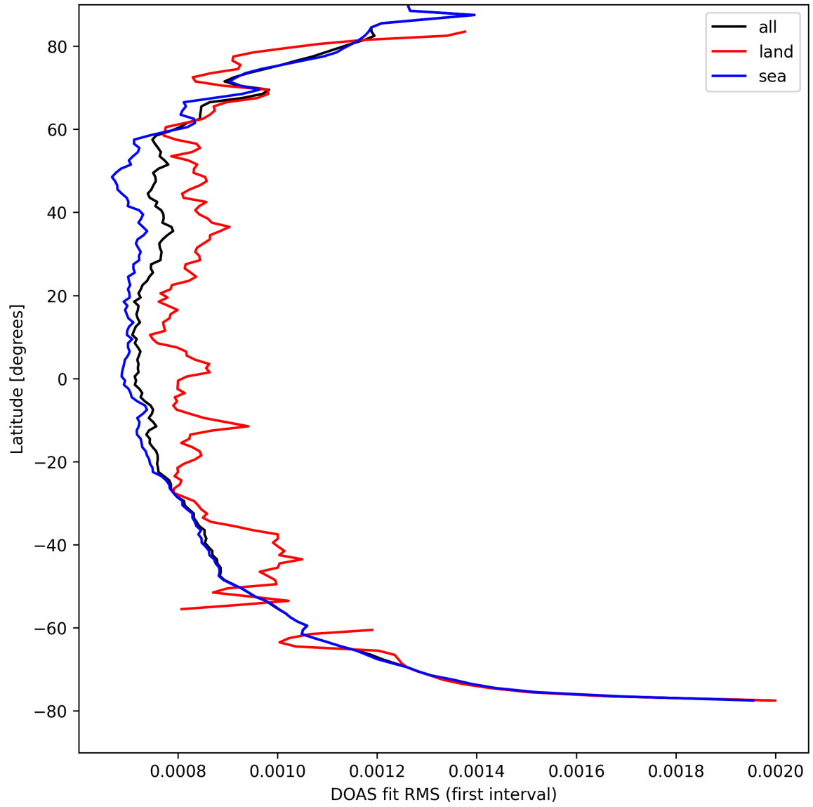
Figure 32: Zonal average of “DOAS fit RMS (first interval)” for 2025-09-02 to 2025-09-04.
