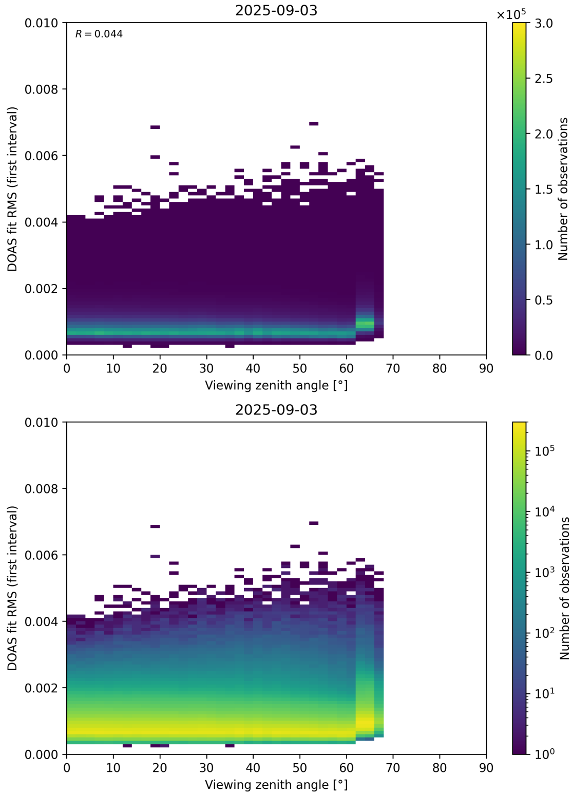
Figure 182: Scatter density plot of “Viewing zenith angle” against “DOAS fit RMS (first interval)” for 2025-09-02 to 2025-09-04.
