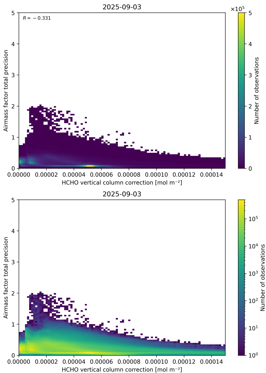
Figure 121: Scatter density plot of “HCHO vertical column correction” against “Airmass factor total precision” for 2025-09-02 to 2025-09-04.
