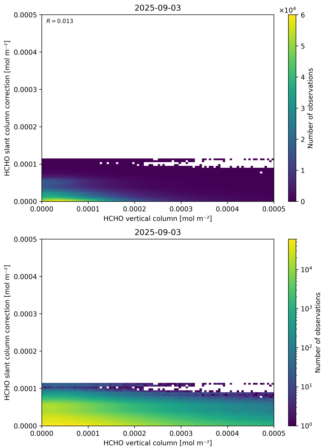
Figure 128: Scatter density plot of “HCHO vertical column” against “HCHO slant column correction” for 2025-09-02 to 2025-09-04.
