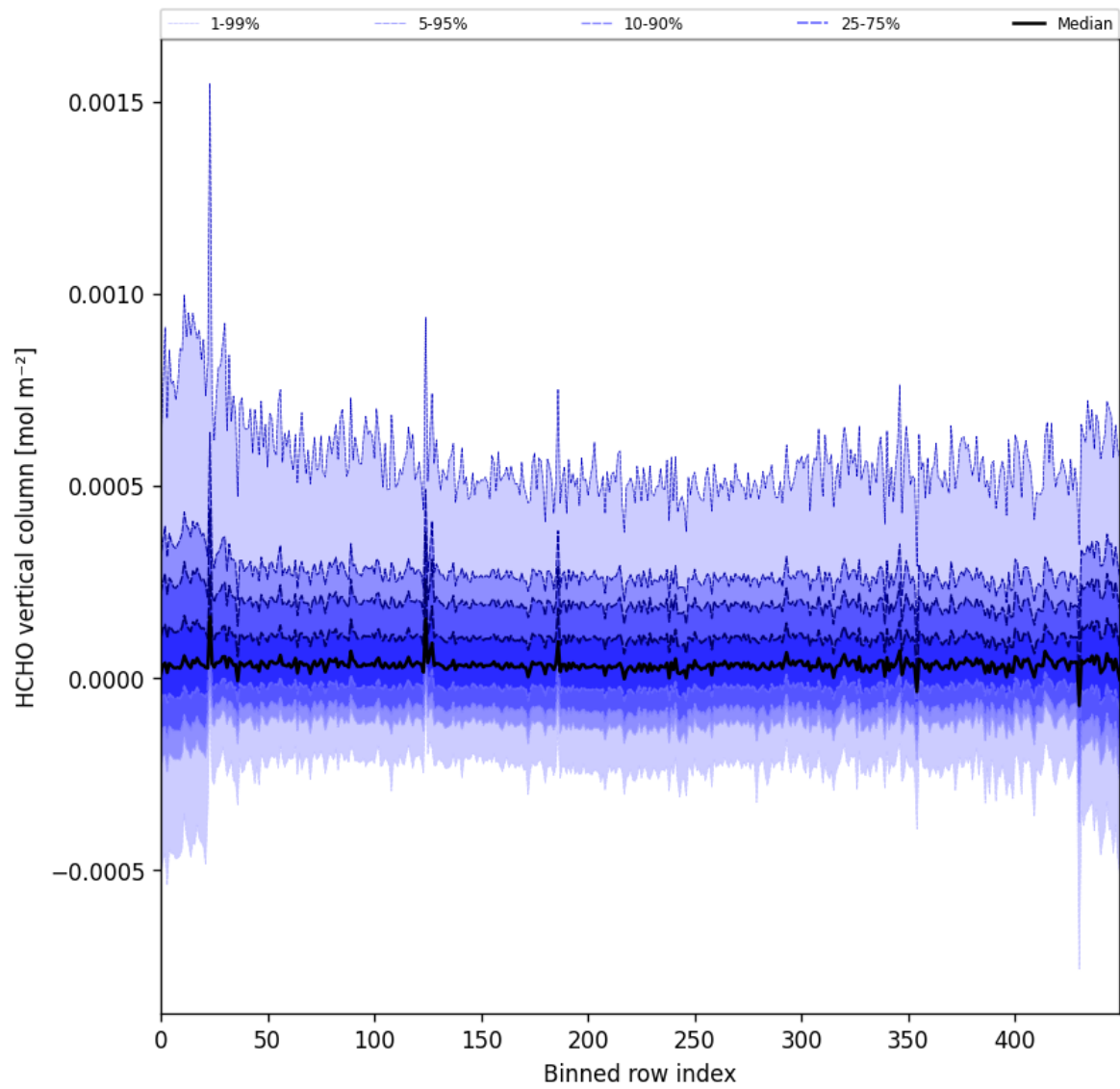
Figure 49: Along track statistics of “HCHO vertical column” for 2025-09-02 to 2025-09-04
