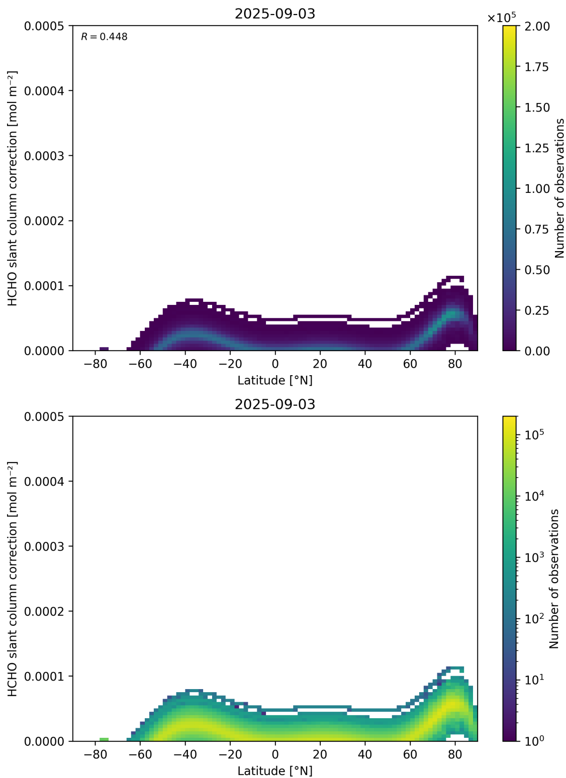
Figure 158: Scatter density plot of “Latitude” against “HCHO slant column correction” for 2025-09-02 to 2025-09-04.
