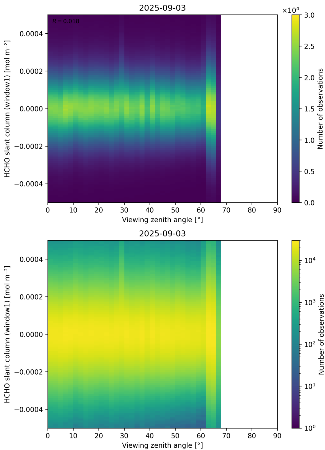
Figure 188: Scatter density plot of “Viewing zenith angle” against “HCHO slant column (window1)” for 2025-09-02 to 2025-09-04.
