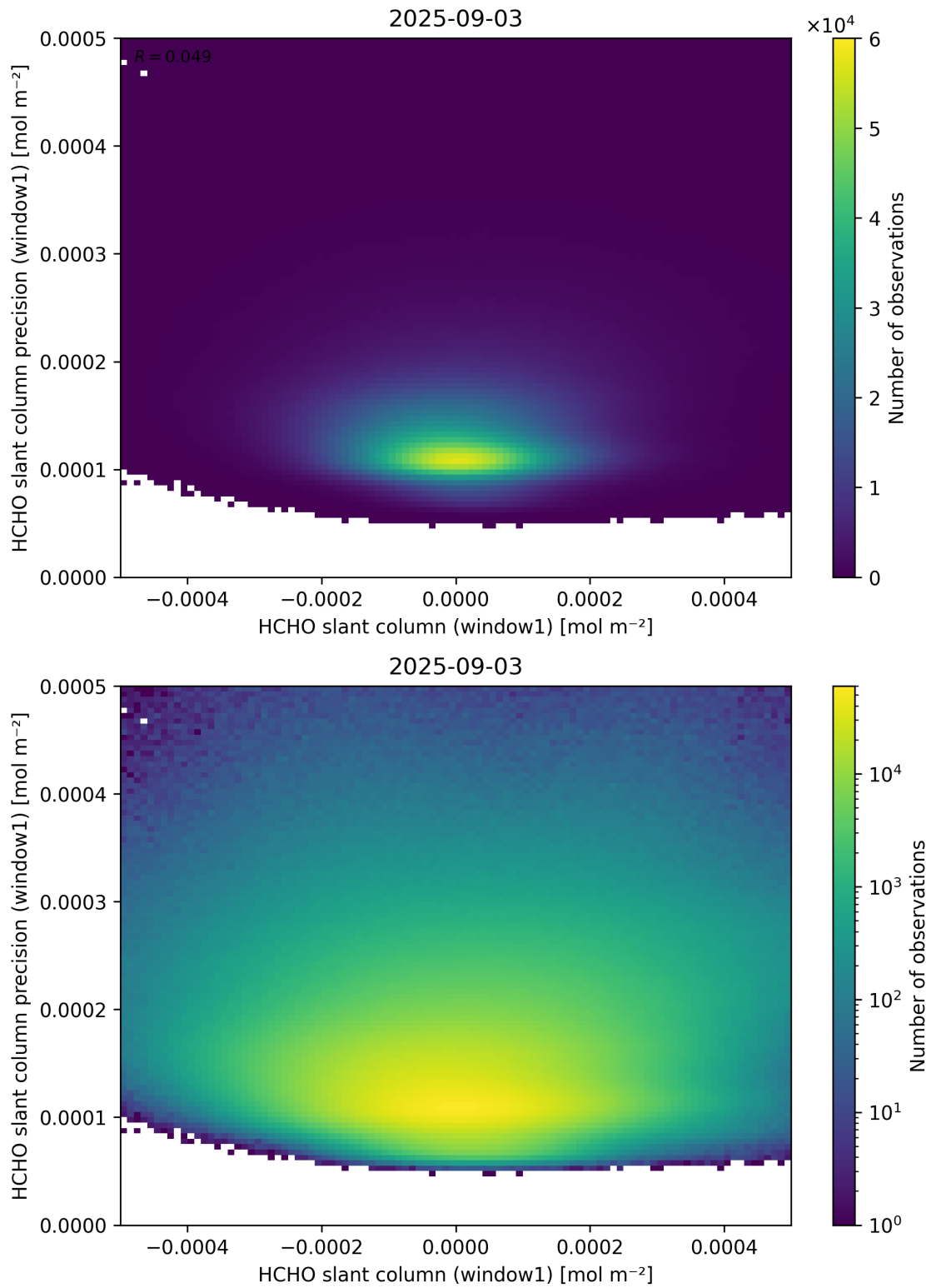
Figure 84: Scatter density plot of “HCHO slant column (window1)” against “HCHO slant column precision (window1)” for 2025-09-02 to 2025-09-04.
