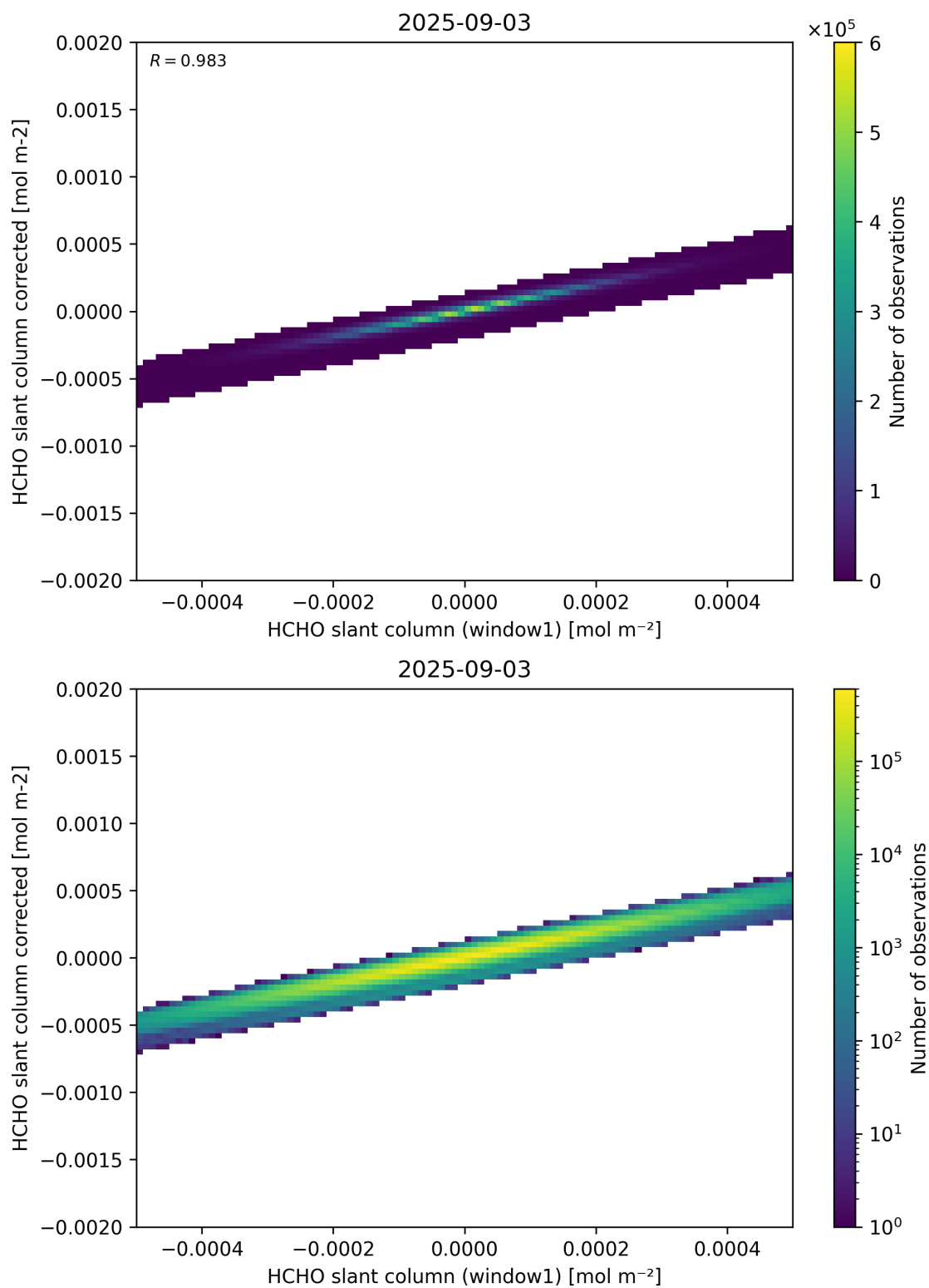
Figure 82: Scatter density plot of “HCHO slant column (window1)” against “HCHO slant column corrected” for 2025-09-02 to 2025-09-04.
