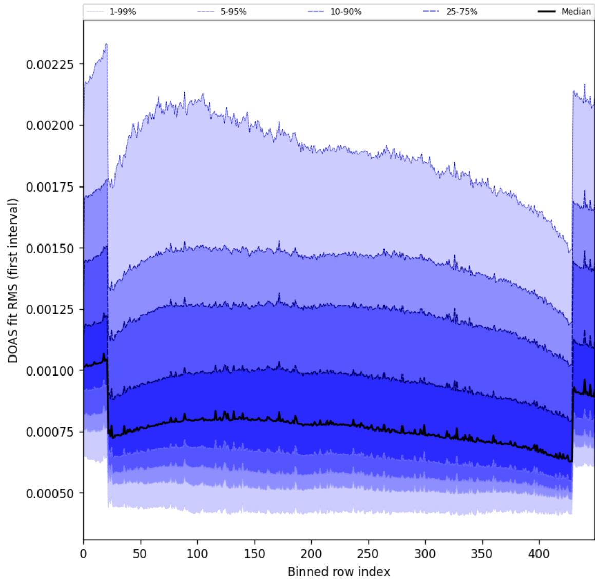
Figure 60: Along track statistics of “DOAS fit RMS (first interval)” for 2025-09-02 to 2025-09-04
