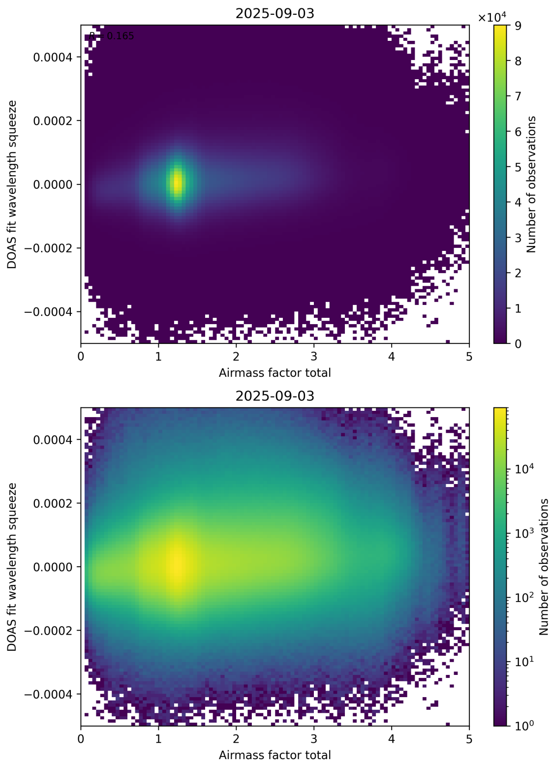
Figure 99: Scatter density plot of “Airmass factor total” against “DOAS fit wavelength squeeze” for 2025-09-02 to 2025-09-04.
