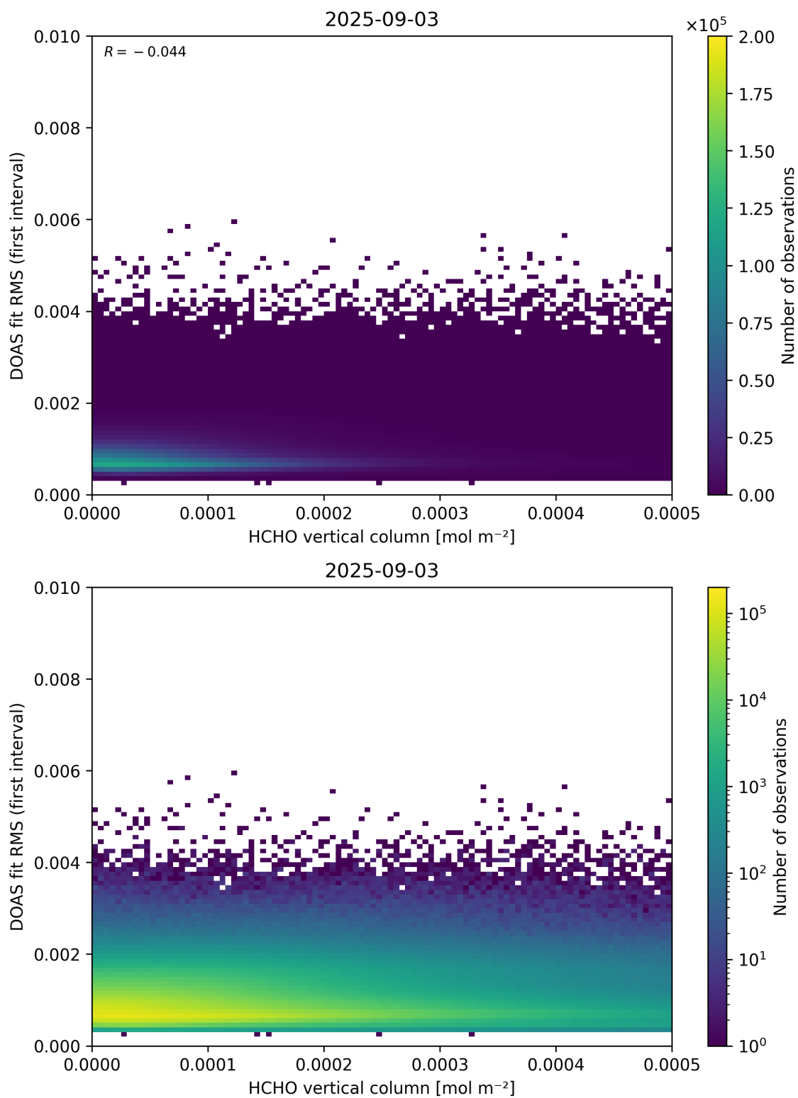
Figure 123: Scatter density plot of “HCHO vertical column” against “DOAS fit RMS (first interval)” for 2025-09-02 to 2025-09-04.
