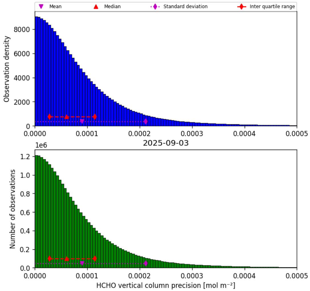
Figure 36: Histogram of “HCHO vertical column precision” for 2025-09-02 to 2025-09-04
