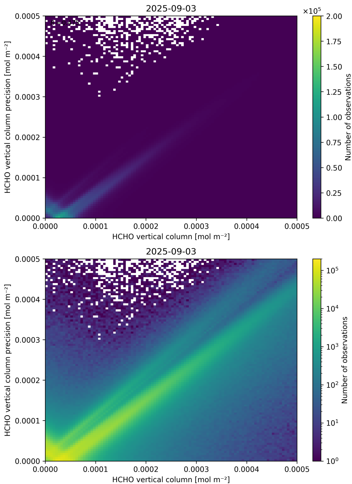
Figure 134: Scatter density plot of “HCHO vertical column” against “HCHO vertical column precision” for 2025-09-02 to 2025-09-04.
