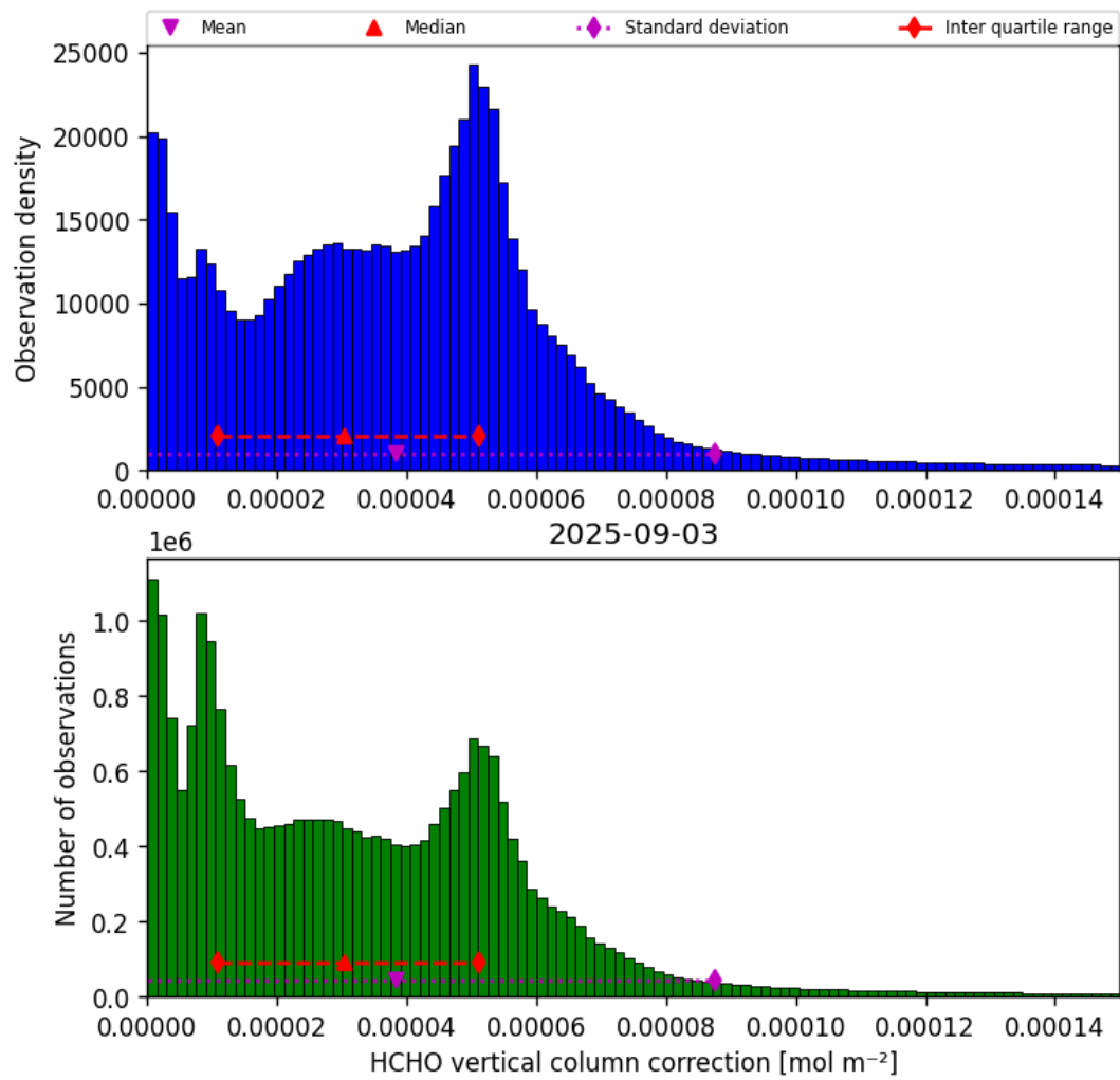
Figure 37: Histogram of “HCHO vertical column correction” for 2025-09-02 to 2025-09-04
