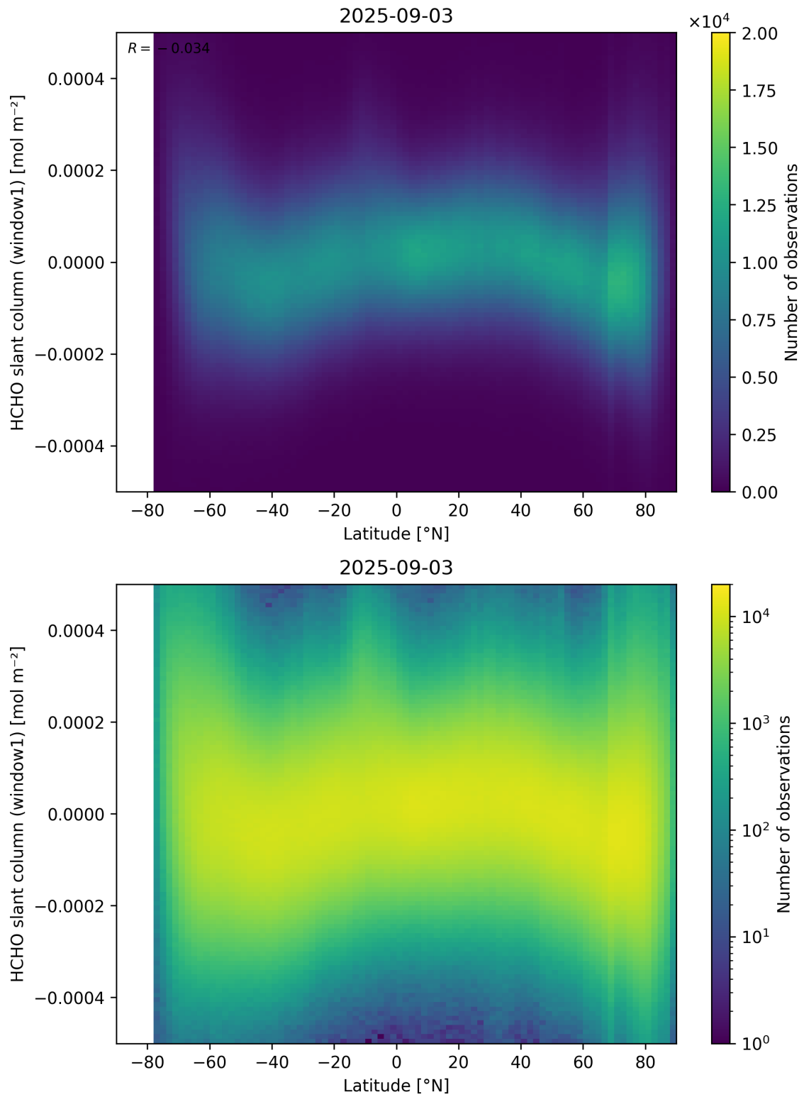
Figure 159: Scatter density plot of “Latitude” against “HCHO slant column (window1)” for 2025-09-02 to 2025-09-04.
