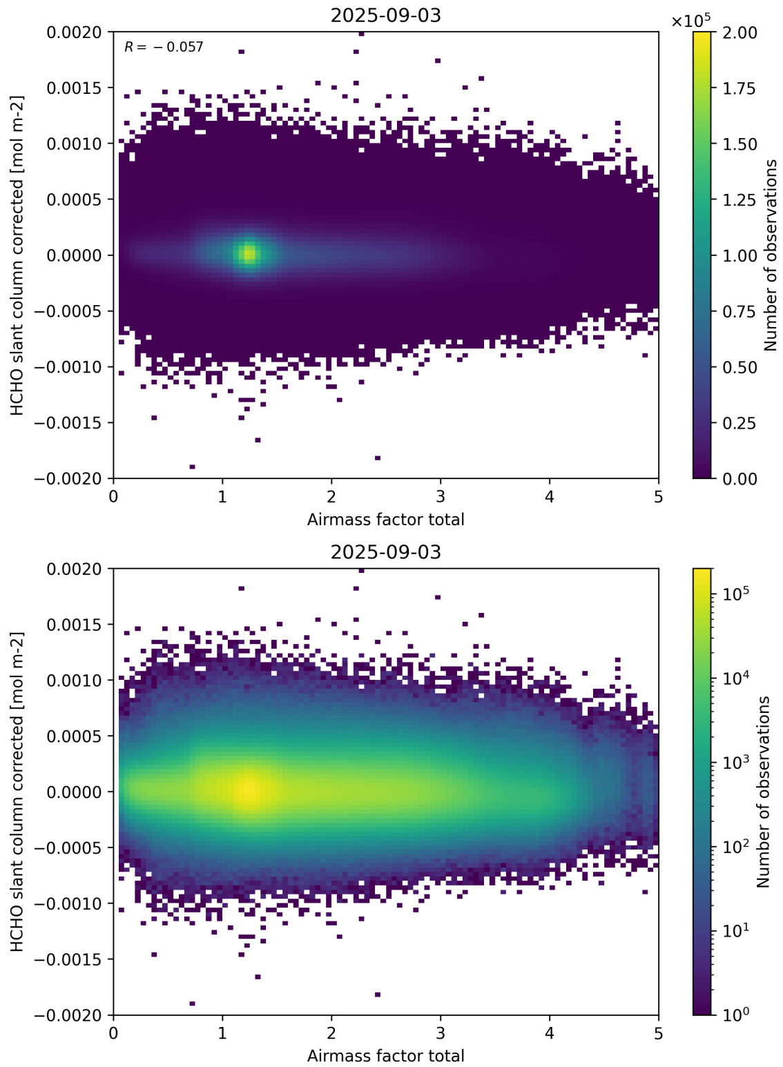
Figure 101: Scatter density plot of “Airmass factor total” against “HCHO slant column corrected” for 2025-09-02 to 2025-09-04.
