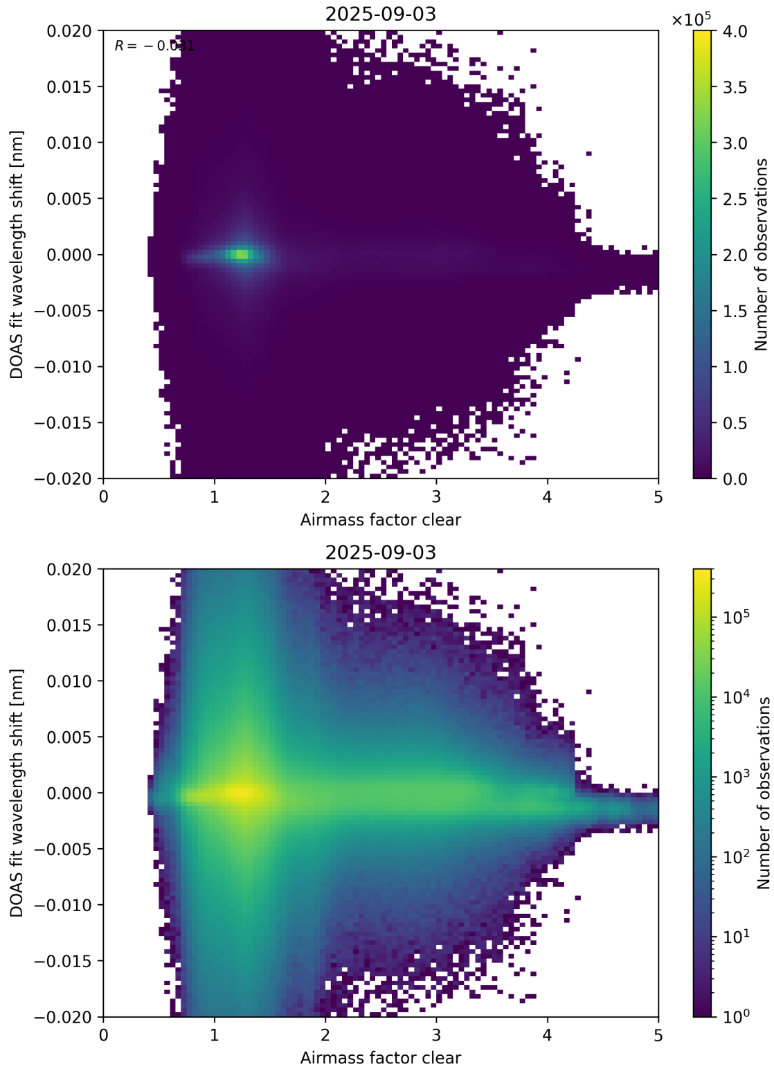
Figure 72: Scatter density plot of “Airmass factor clear” against “DOAS fit wavelength shift” for 2025-09-02 to 2025-09-04.
