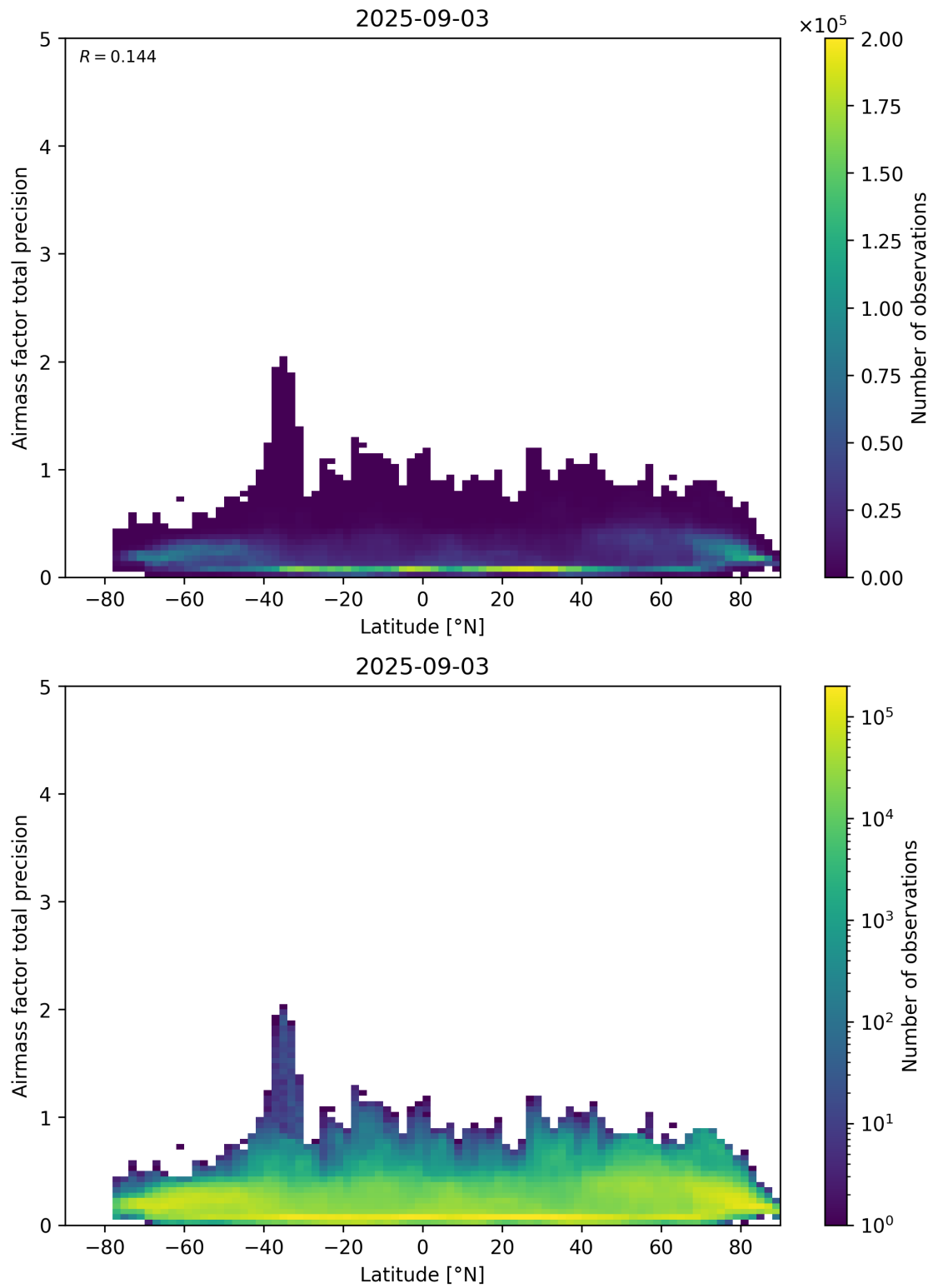
Figure 162: Scatter density plot of “Latitude” against “Airmass factor total precision” for 2025-09-02 to 2025-09-04.
