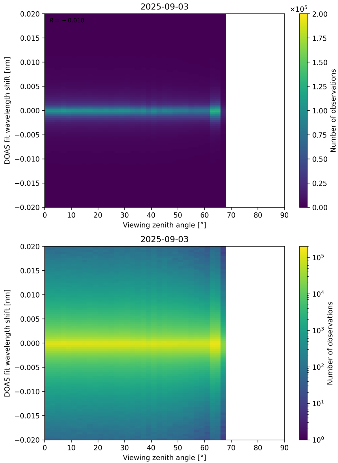
Figure 183: Scatter density plot of “Viewing zenith angle” against “DOAS fit wavelength shift” for 2025-09-02 to 2025-09-04.
