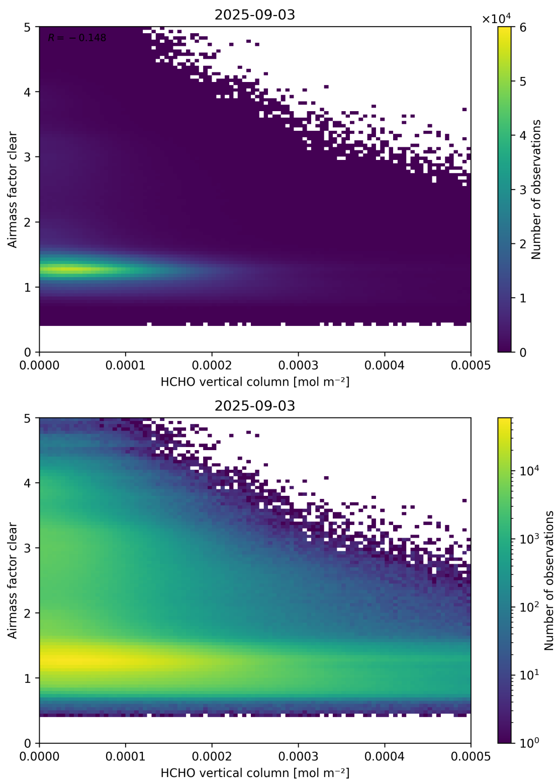
Figure 126: Scatter density plot of “HCHO vertical column” against “Airmass factor clear” for 2025-09-02 to 2025-09-04.
