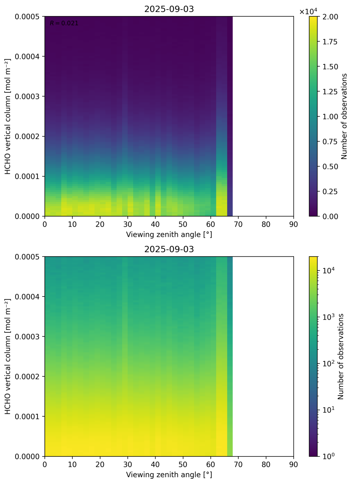
Figure 192: Scatter density plot of “Viewing zenith angle” against “HCHO vertical column” for 2025-09-02 to 2025-09-04.
