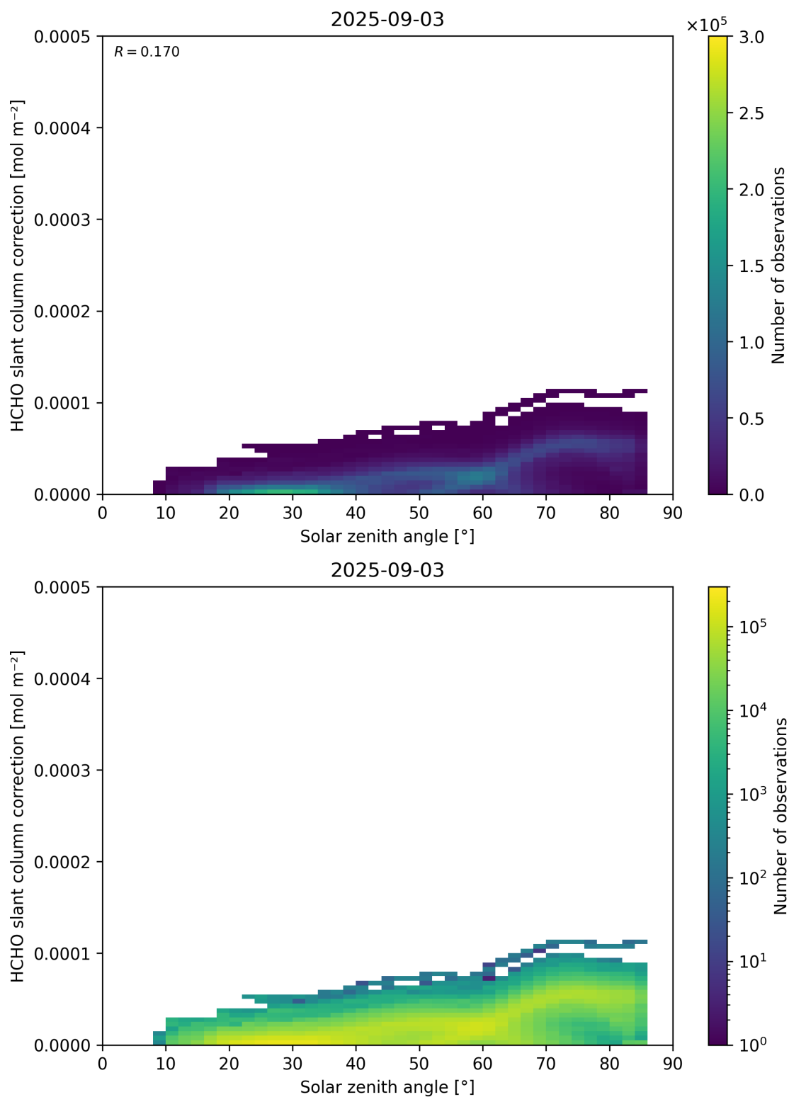
Figure 172: Scatter density plot of “Solar zenith angle” against “HCHO slant column correction” for 2025-09-02 to 2025-09-04.
