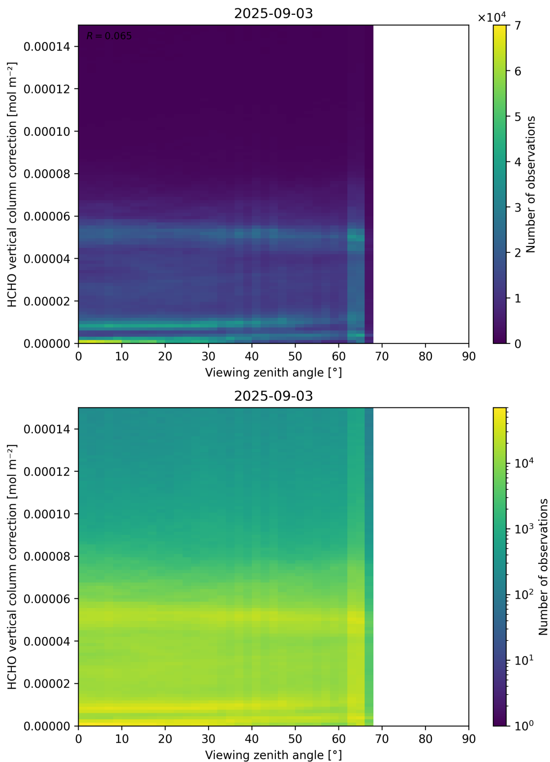
Figure 193: Scatter density plot of “Viewing zenith angle” against “HCHO vertical column correction” for 2025-09-02 to 2025-09-04.
