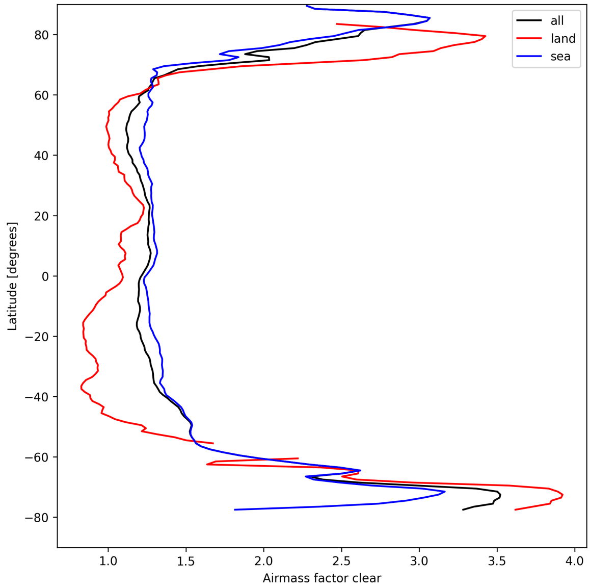
Figure 28: Zonal average of “Airmass factor clear” for 2025-09-02 to 2025-09-04.
