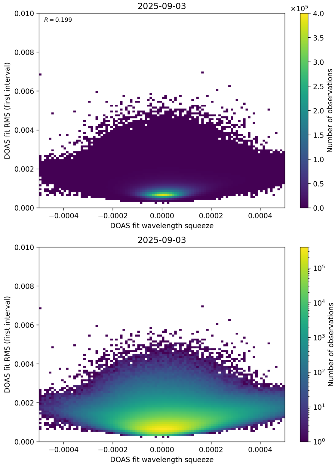
Figure 68: Scatter density plot of “DOAS fit wavelength squeeze” against “DOAS fit RMS (first interval)” for 2025-09-02 to 2025-09-04.
