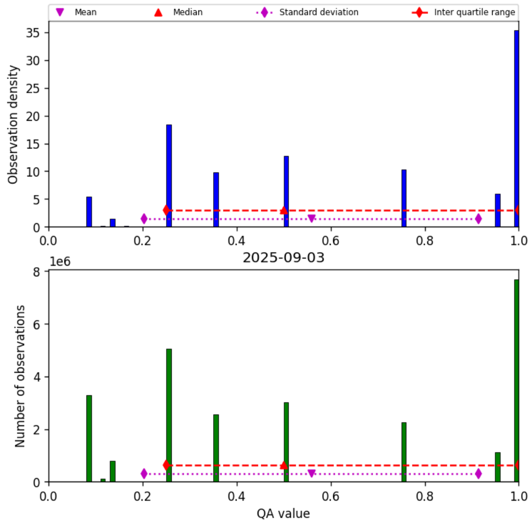
Figure 34: Histogram of “QA value” for 2025-09-02 to 2025-09-04
