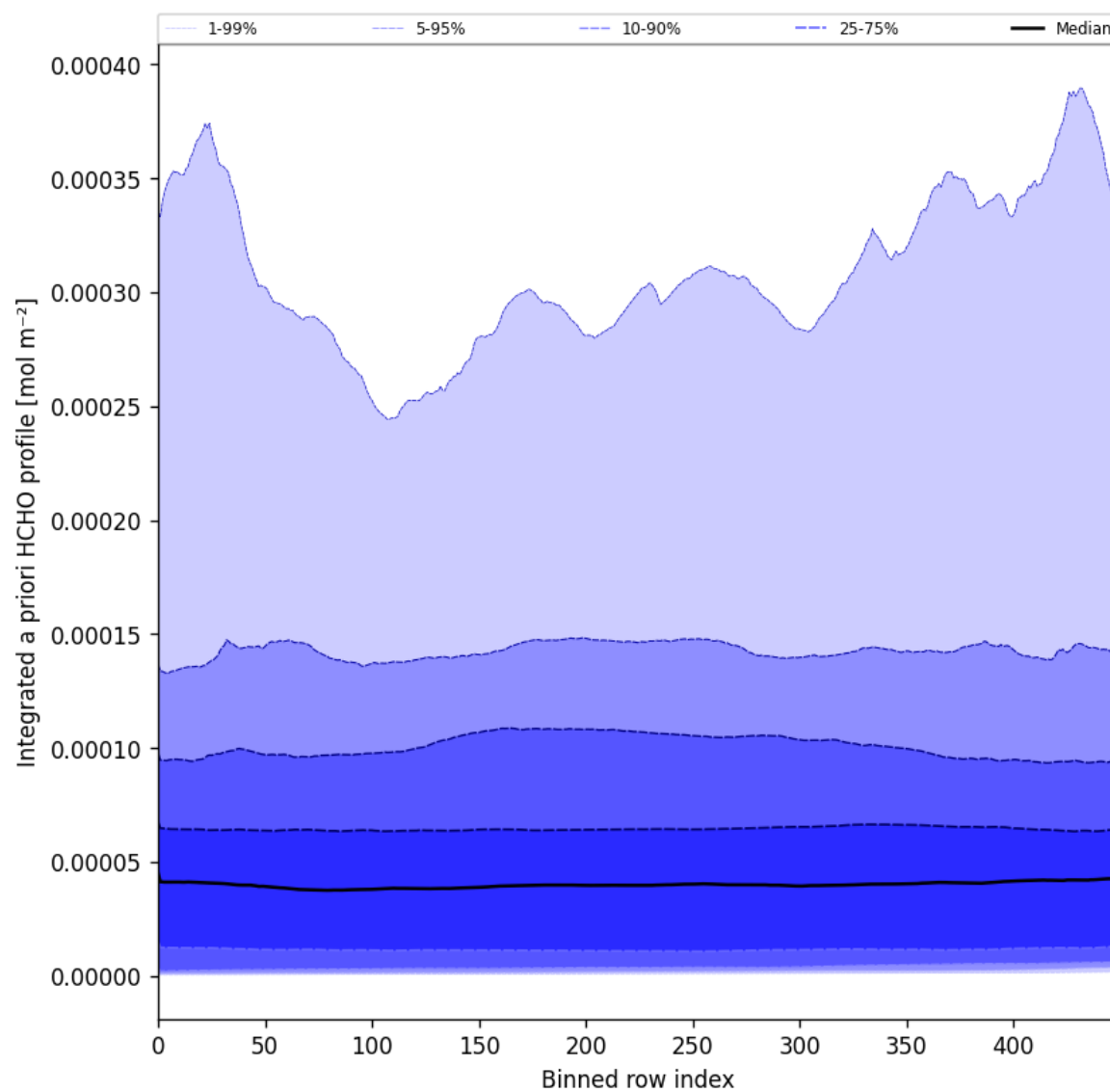
Figure 57: Along track statistics of "Integrated a priori HCHO profile" for 2025-09-02 to 2025-09-04
