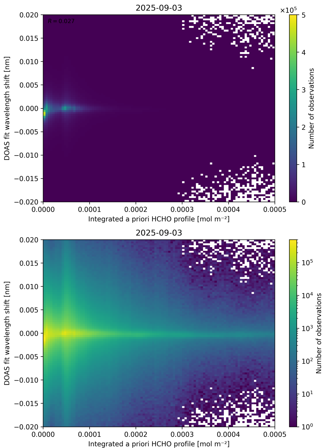
Figure 149: Scatter density plot of “Integrated a priori HCHO profile” against “DOAS fit wavelength shift” for 2025-09-02 to 2025-09-04.
