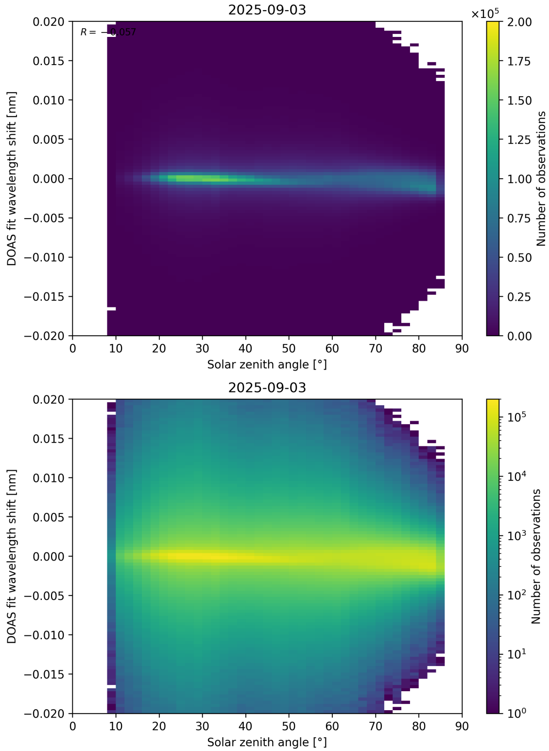
Figure 168: Scatter density plot of “Solar zenith angle” against “DOAS fit wavelength shift” for 2025-09-02 to 2025-09-04.
