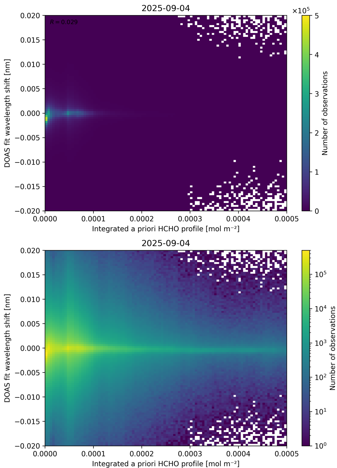
Figure 149: Scatter density plot of “Integrated a priori HCHO profile” against “DOAS fit wavelength shift” for 2025-09-04 to 2025-09-05.
