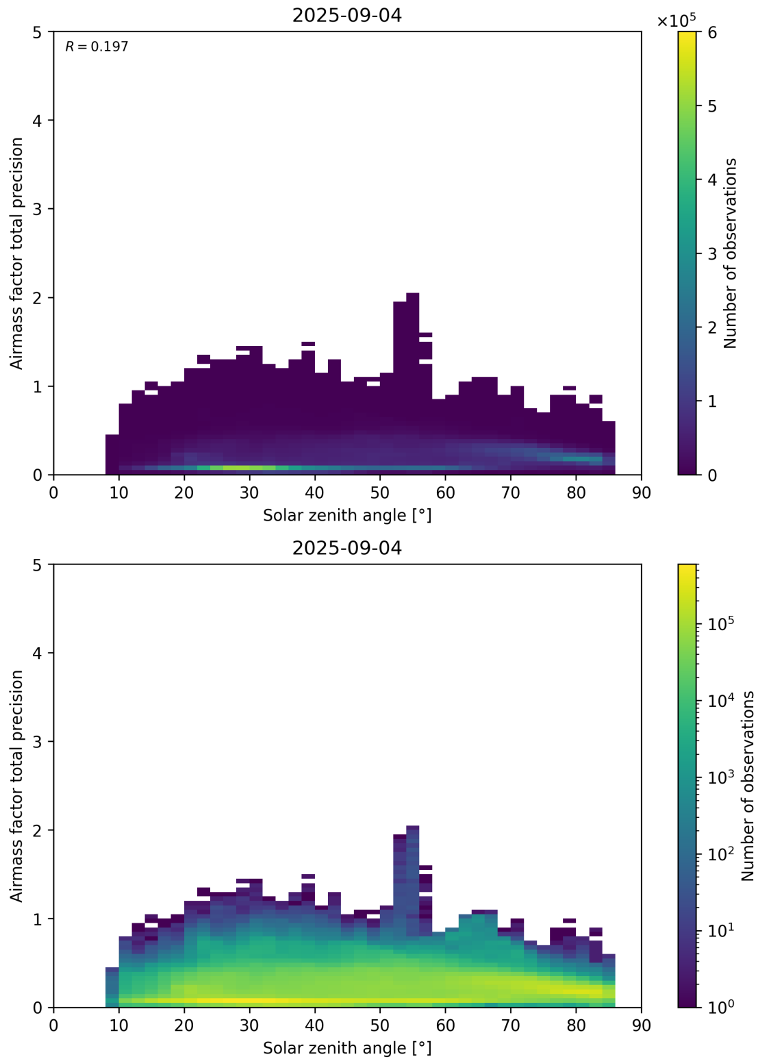
Figure 176: Scatter density plot of “Solar zenith angle” against “Airmass factor total precision” for 2025-09-04 to 2025-09-05.
