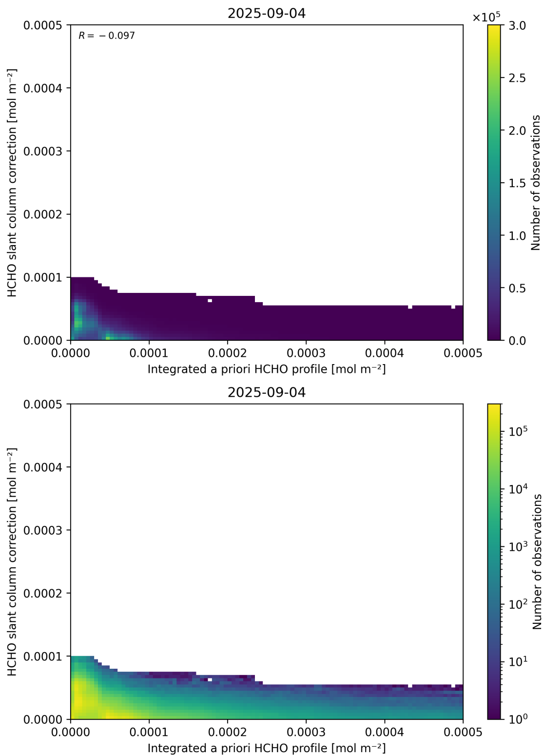
Figure 152: Scatter density plot of “Integrated a priori HCHO profile” against “HCHO slant column correction” for 2025-09-04 to 2025-09-05.
