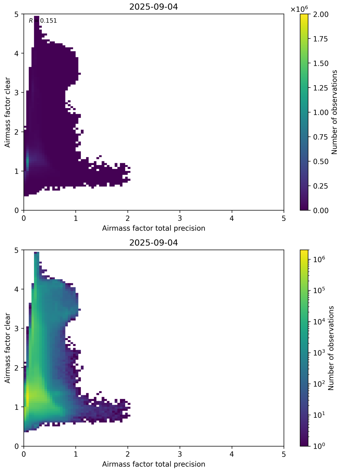
Figure 108: Scatter density plot of “Airmass factor total precision” against “Airmass factor clear” for 2025-09-04 to 2025-09-05.
