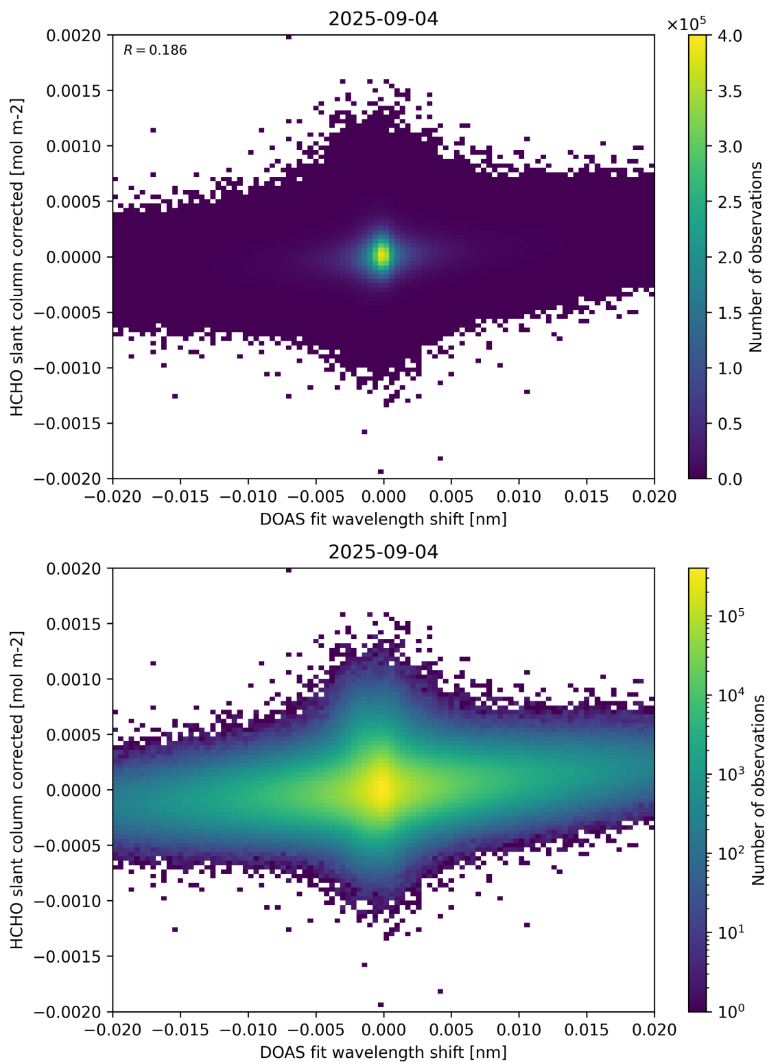
Figure 66: Scatter density plot of “DOAS fit wavelength shift” against “HCHO slant column corrected” for 2025-09-04 to 2025-09-05.
