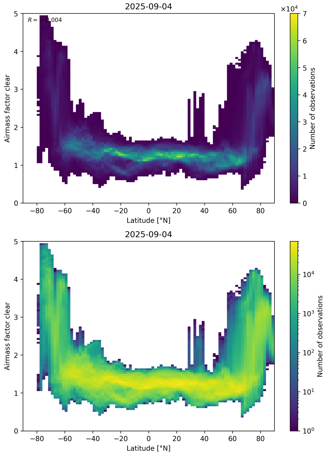
Figure 156: Scatter density plot of “Latitude” against “Airmass factor clear” for 2025-09-04 to 2025-09-05.
