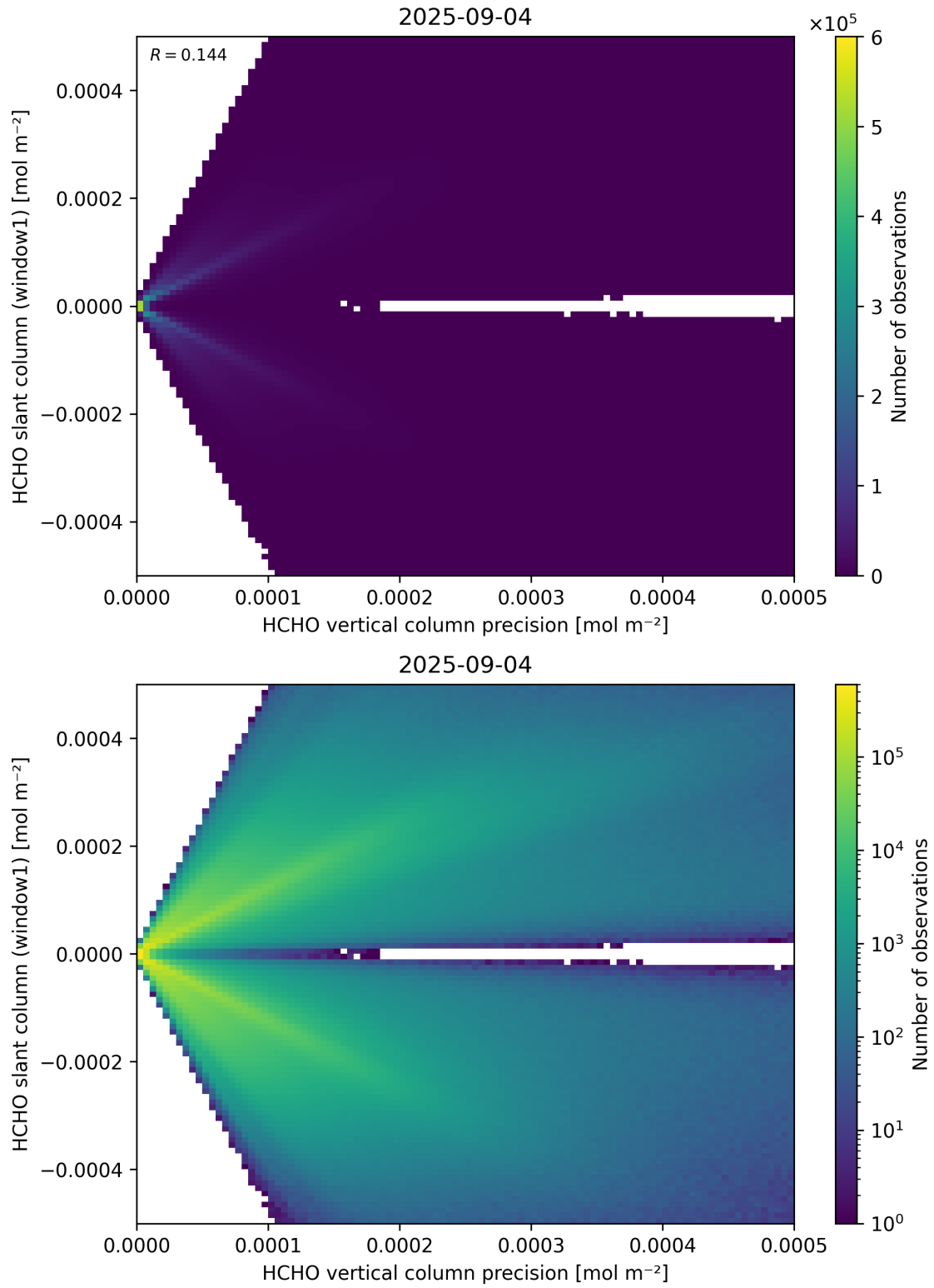
Figure 142: Scatter density plot of “HCHO vertical column precision” against “HCHO slant column (window1)” for 2025-09-04 to 2025-09-05.
