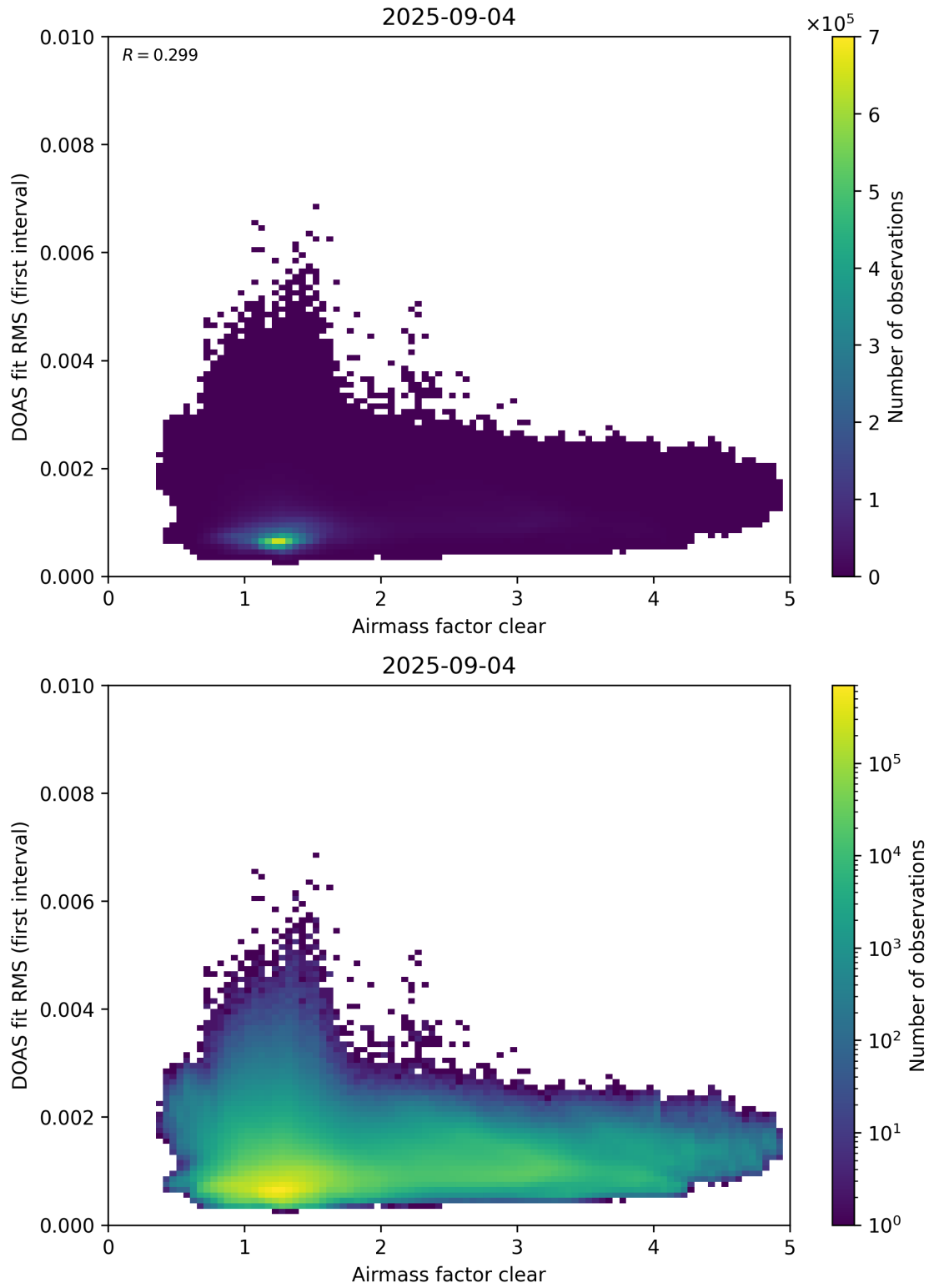
Figure 71: Scatter density plot of “Airmass factor clear” against “DOAS fit RMS (first interval)” for 2025-09-04 to 2025-09-05.
