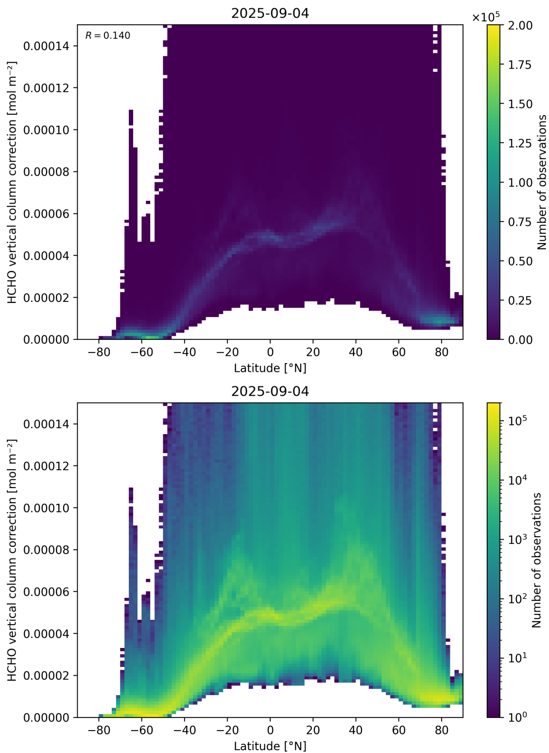
Figure 164: Scatter density plot of “Latitude” against “HCHO vertical column correction” for 2025-09-04 to 2025-09-05.
