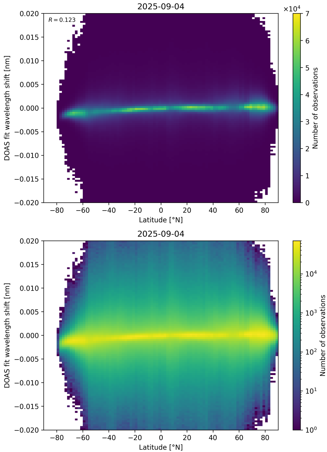
Figure 154: Scatter density plot of “Latitude” against “DOAS fit wavelength shift” for 2025-09-04 to 2025-09-05.
