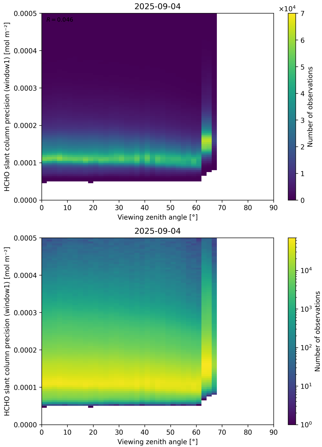
Figure 189: Scatter density plot of “Viewing zenith angle” against “HCHO slant column precision (window1)” for 2025-09-04 to 2025-09-05.
