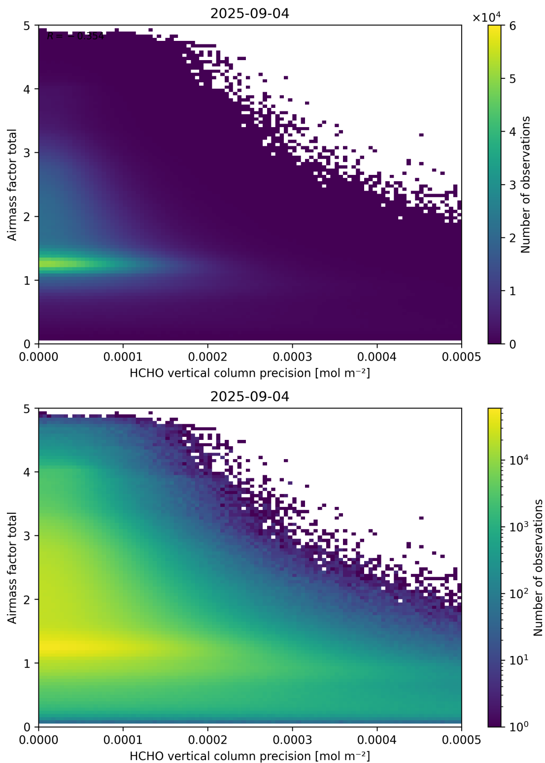
Figure 144: Scatter density plot of “HCHO vertical column precision” against “Airmass factor total” for 2025-09-04 to 2025-09-05.
