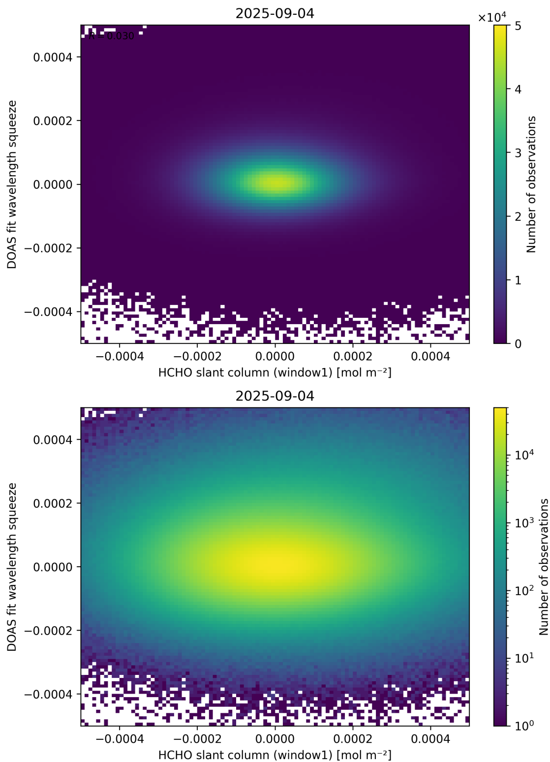
Figure 80: Scatter density plot of “HCHO slant column (window1)” against “DOAS fit wavelength squeeze” for 2025-09-04 to 2025-09-05.
