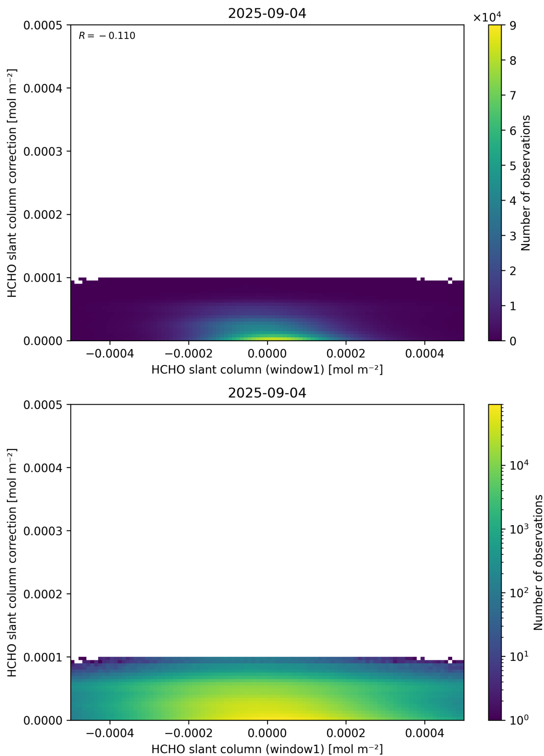
Figure 83: Scatter density plot of “HCHO slant column (window1)” against “HCHO slant column correction” for 2025-09-04 to 2025-09-05.
