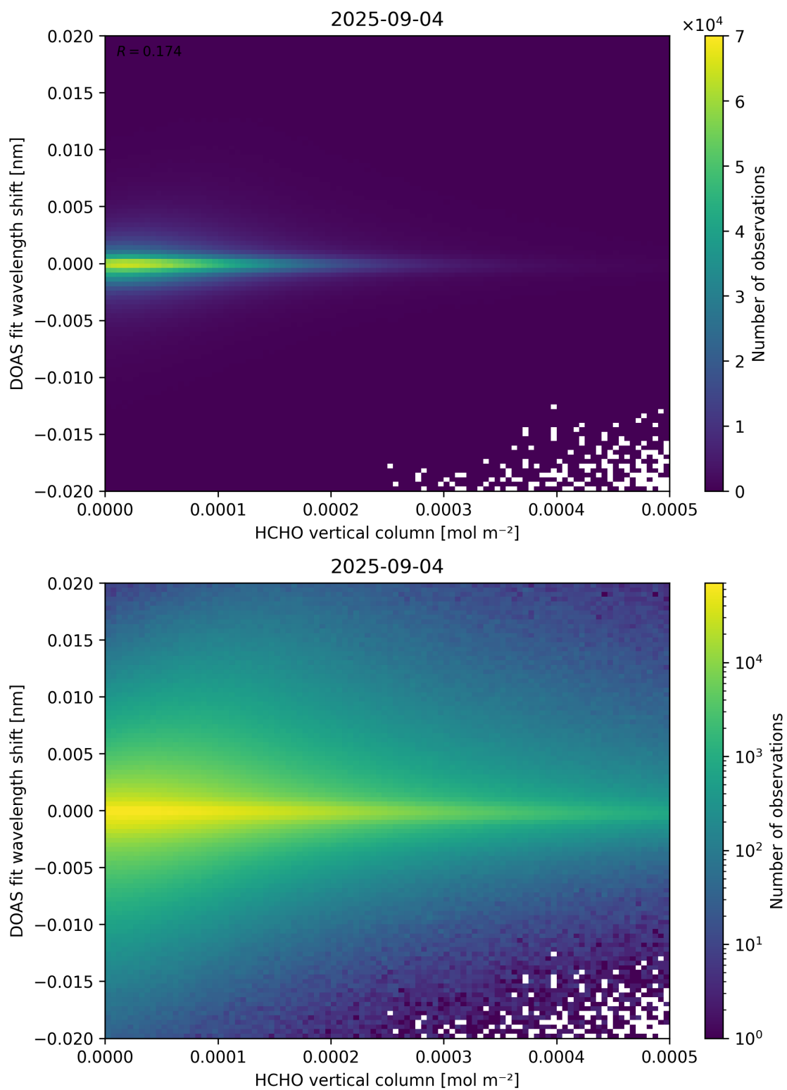
Figure 124: Scatter density plot of “HCHO vertical column” against “DOAS fit wavelength shift” for 2025-09-04 to 2025-09-05.
