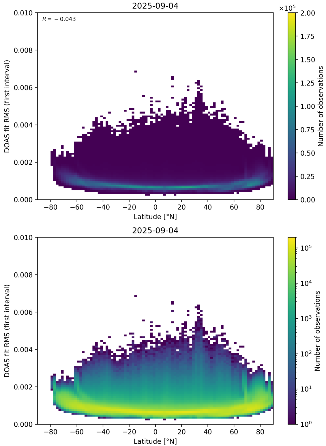
Figure 153: Scatter density plot of “Latitude” against “DOAS fit RMS (first interval)” for 2025-09-04 to 2025-09-05.
