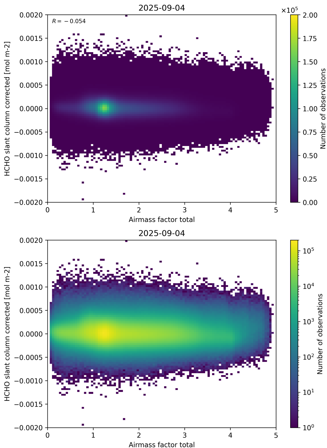
Figure 101: Scatter density plot of “Airmass factor total” against “HCHO slant column corrected” for 2025-09-04 to 2025-09-05.
