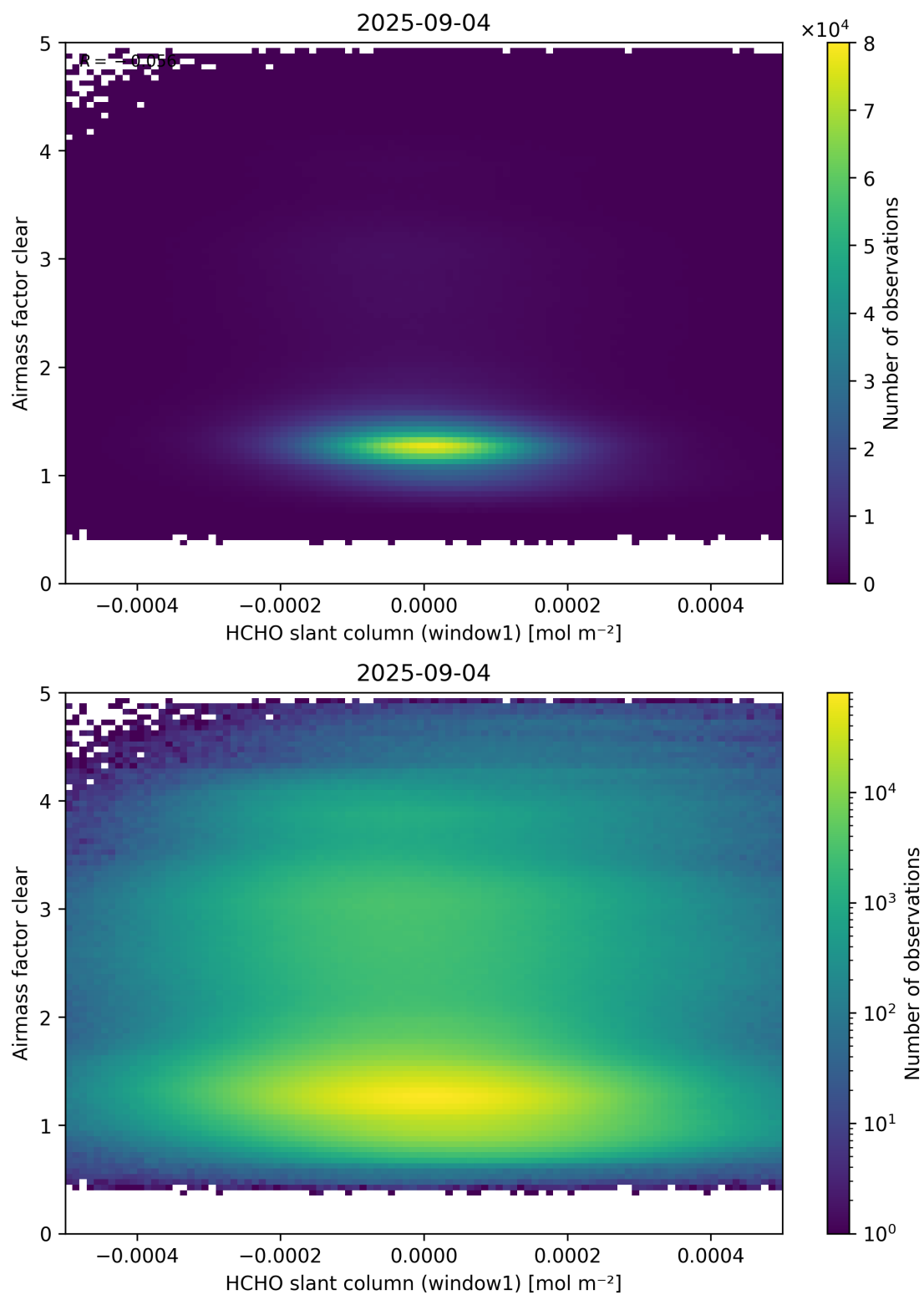
Figure 81: Scatter density plot of “HCHO slant column (window1)” against “Airmass factor clear” for 2025-09-04 to 2025-09-05.
