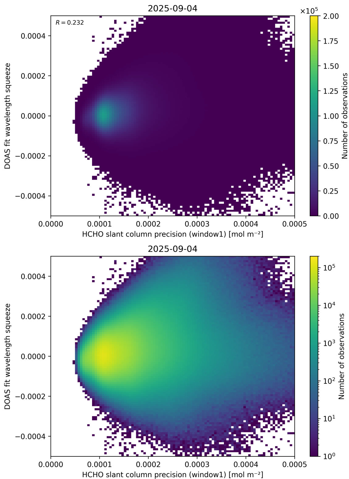
Figure 90: Scatter density plot of “HCHO slant column precision (window1)” against “DOAS fit wavelength squeeze” for 2025-09-04 to 2025-09-05.
