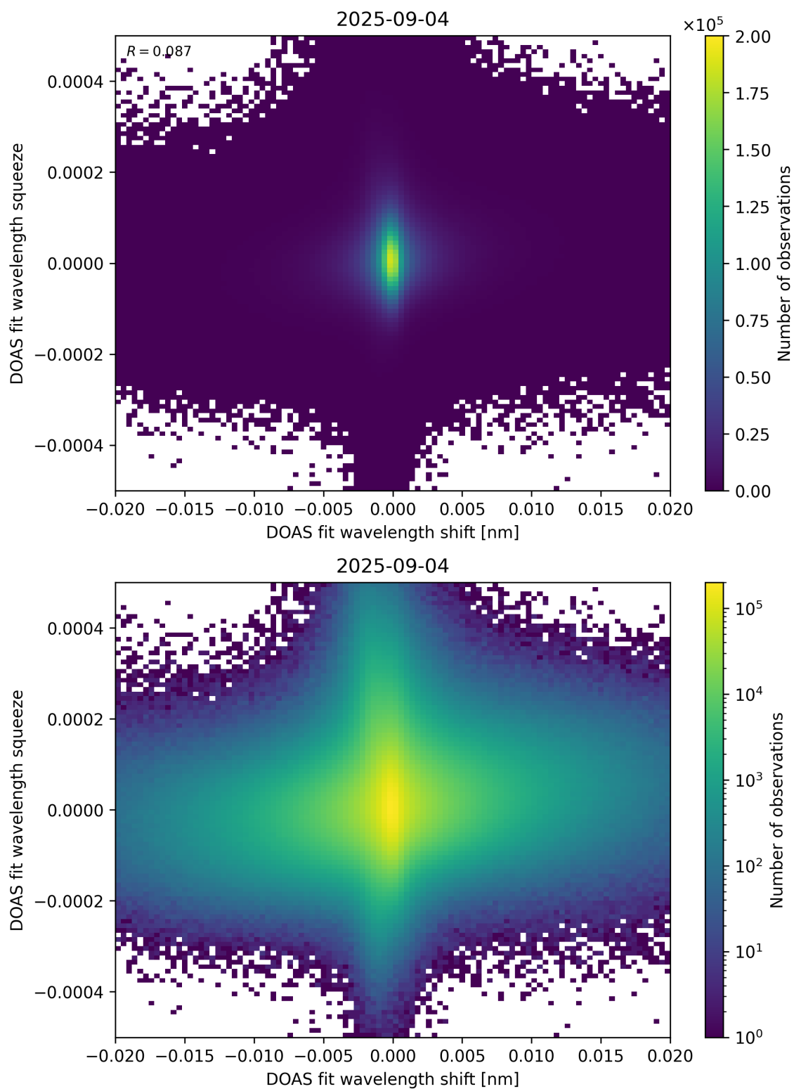
Figure 65: Scatter density plot of “DOAS fit wavelength shift” against “DOAS fit wavelength squeeze” for 2025-09-04 to 2025-09-05.
