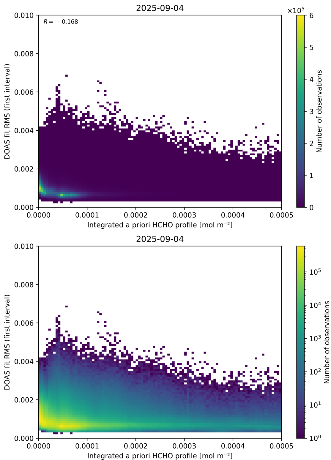
Figure 148: Scatter density plot of “Integrated a priori HCHO profile” against “DOAS fit RMS (first interval)” for 2025-09-04 to 2025-09-05.
