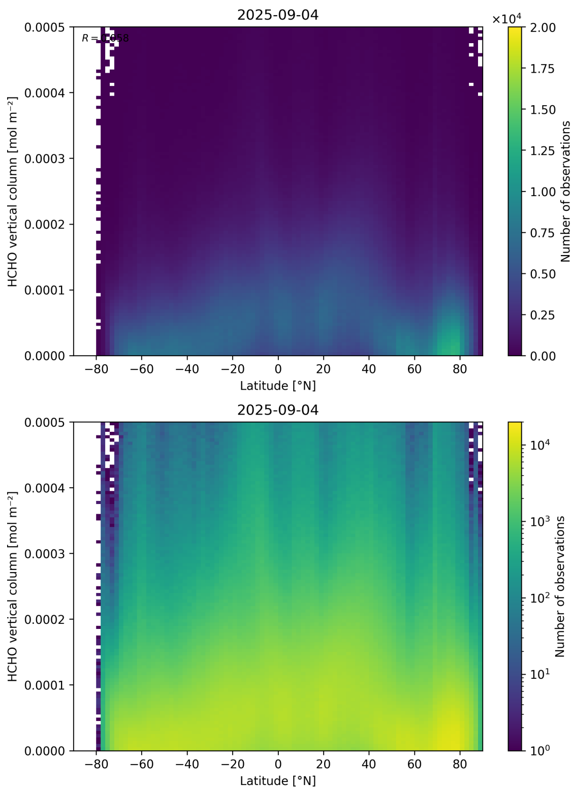
Figure 163: Scatter density plot of “Latitude” against “HCHO vertical column” for 2025-09-04 to 2025-09-05.
