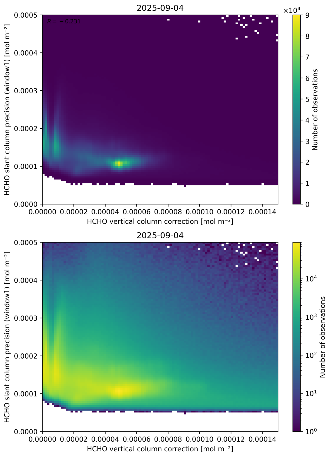
Figure 119: Scatter density plot of “HCHO vertical column correction” against “HCHO slant column precision (window1)” for 2025-09-04 to 2025-09-05.
