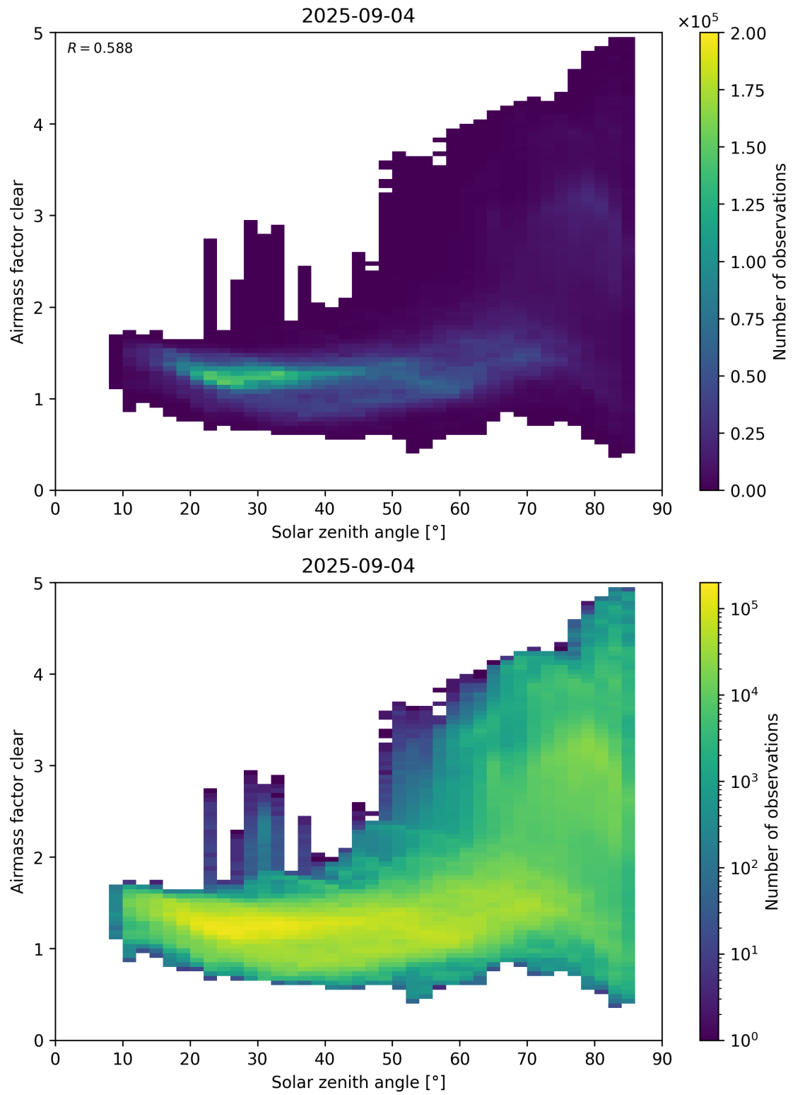
Figure 170: Scatter density plot of “Solar zenith angle” against “Airmass factor clear” for 2025-09-04 to 2025-09-05.
