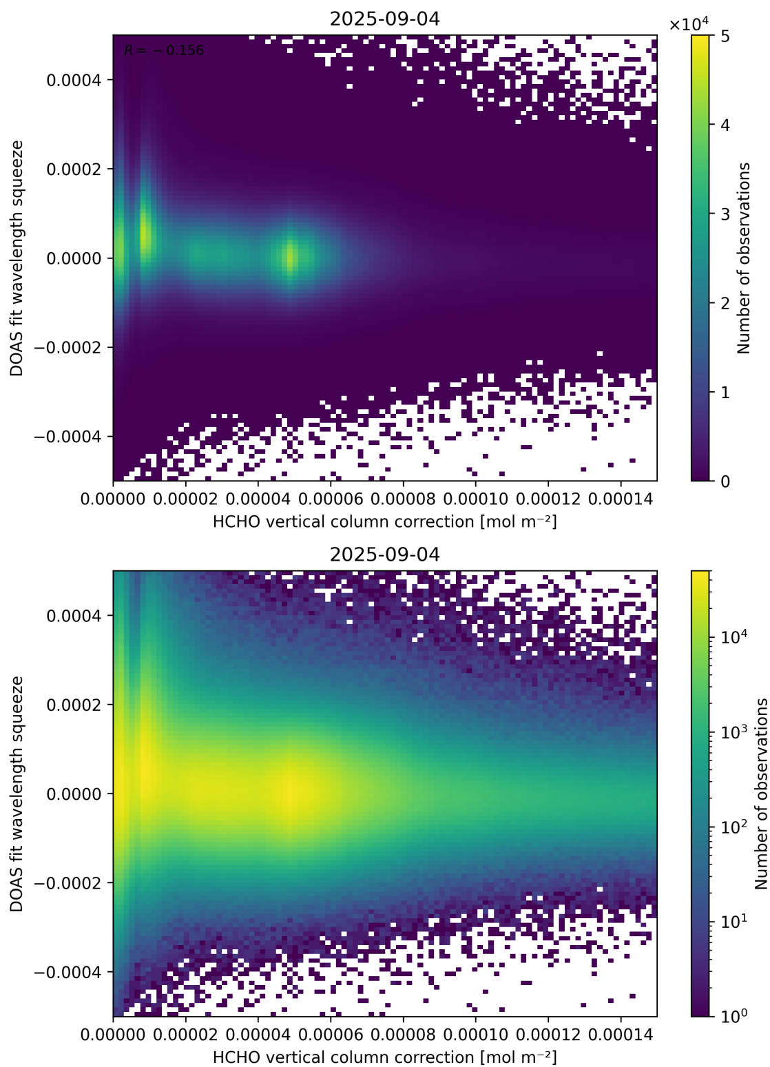
Figure 114: Scatter density plot of “HCHO vertical column correction” against “DOAS fit wavelength squeeze” for 2025-09-04 to 2025-09-05.
