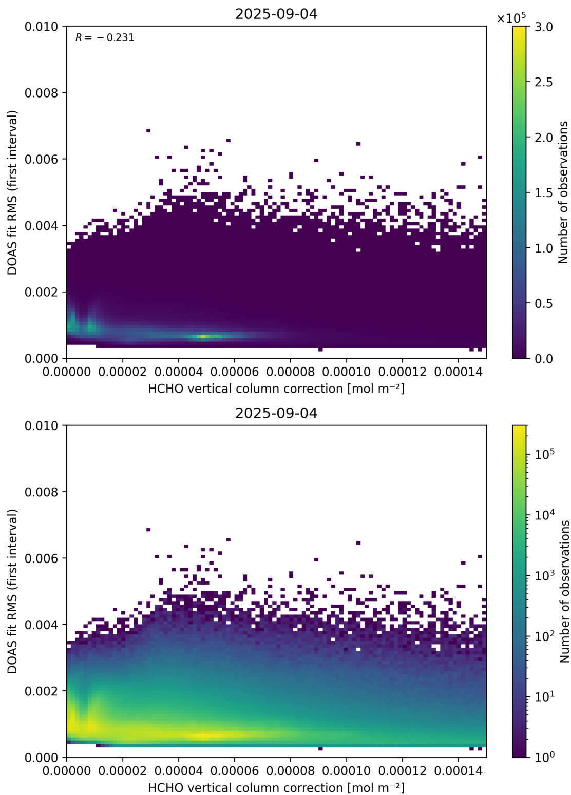
Figure 112: Scatter density plot of “HCHO vertical column correction” against “DOAS fit RMS (first interval)” for 2025-09-04 to 2025-09-05.
