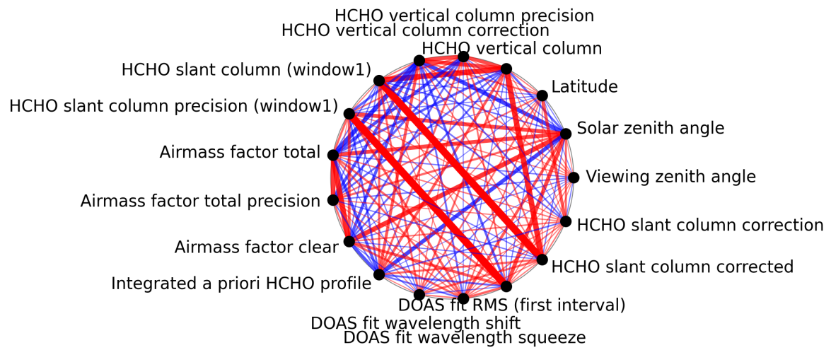
Figure 1: Map of correlation graph for 2025-09-04 to 2025-09-05.
