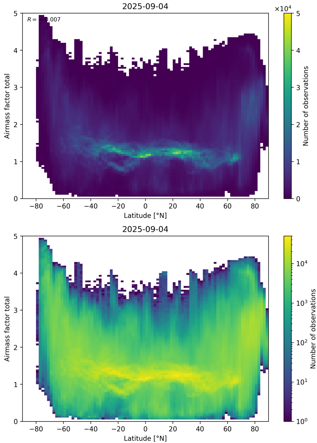
Figure 161: Scatter density plot of “Latitude” against “Airmass factor total” for 2025-09-04 to 2025-09-05.
