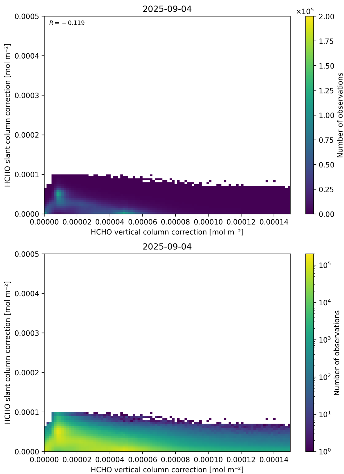
Figure 117: Scatter density plot of “HCHO vertical column correction” against “HCHO slant column correction” for 2025-09-04 to 2025-09-05.
