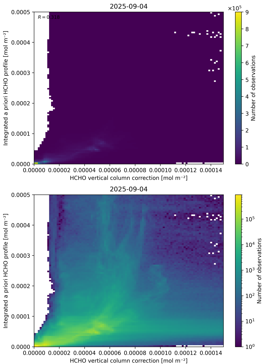
Figure 122: Scatter density plot of “HCHO vertical column correction” against “Integrated a priori HCHO profile” for 2025-09-04 to 2025-09-05.
