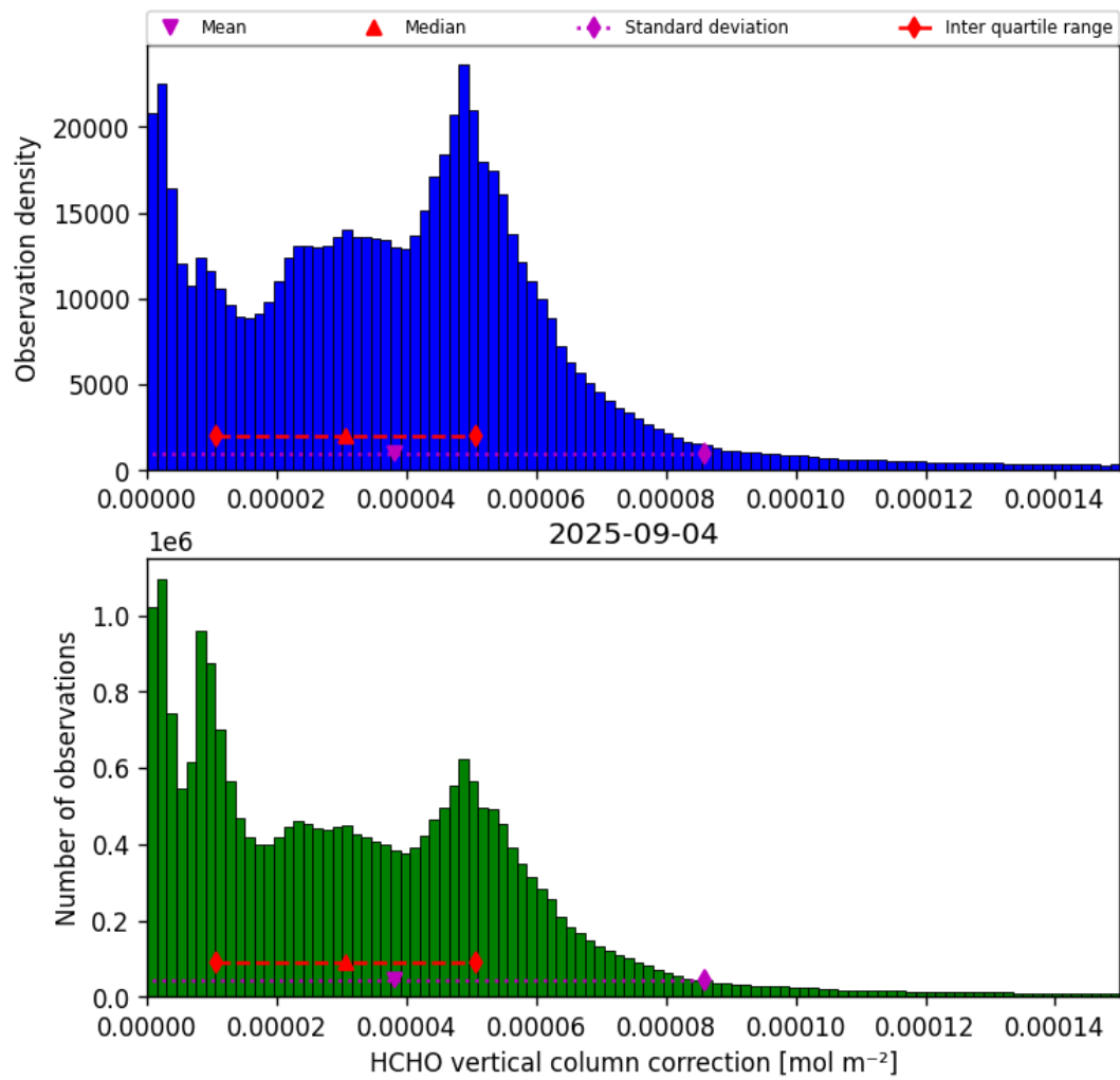
Figure 37: Histogram of “HCHO vertical column correction” for 2025-09-04 to 2025-09-05
