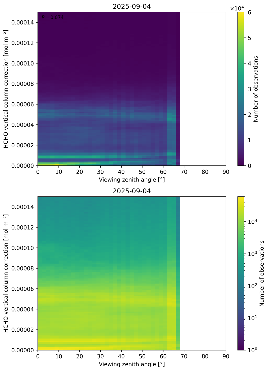
Figure 193: Scatter density plot of “Viewing zenith angle” against “HCHO vertical column correction” for 2025-09-04 to 2025-09-05.
