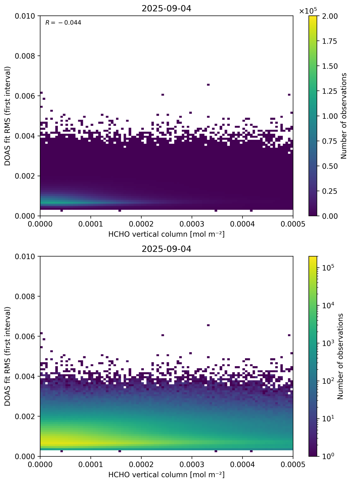
Figure 123: Scatter density plot of “HCHO vertical column” against “DOAS fit RMS (first interval)” for 2025-09-04 to 2025-09-05.
