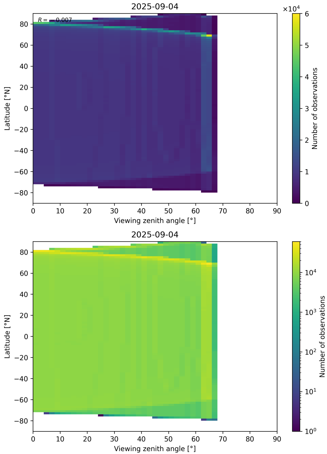
Figure 196: Scatter density plot of “Viewing zenith angle” against “Latitude” for 2025-09-04 to 2025-09-05.
