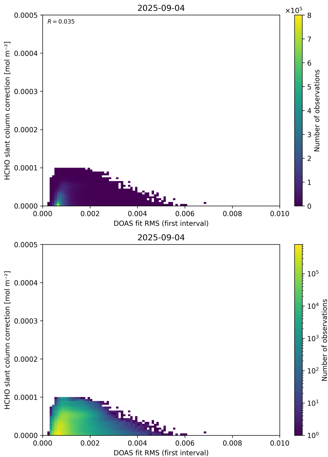
Figure 63: Scatter density plot of “DOAS fit RMS (first interval)” against “HCHO slant column correction” for 2025-09-04 to 2025-09-05.
