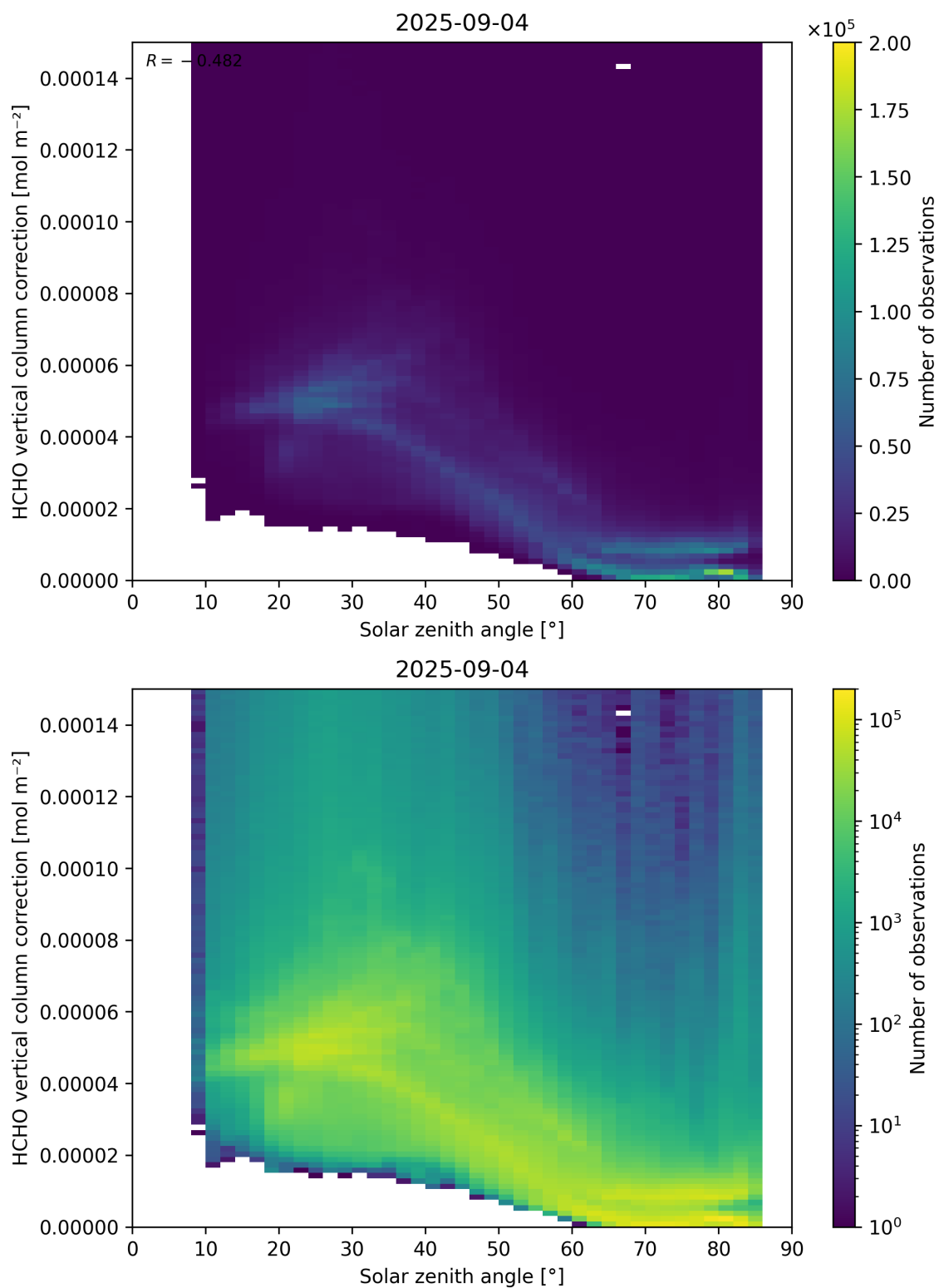
Figure 178: Scatter density plot of “Solar zenith angle” against “HCHO vertical column correction” for 2025-09-04 to 2025-09-05.
