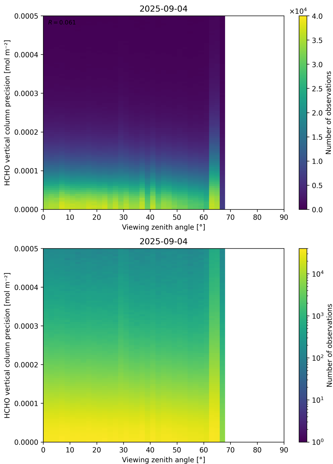
Figure 194: Scatter density plot of “Viewing zenith angle” against “HCHO vertical column precision” for 2025-09-04 to 2025-09-05.
