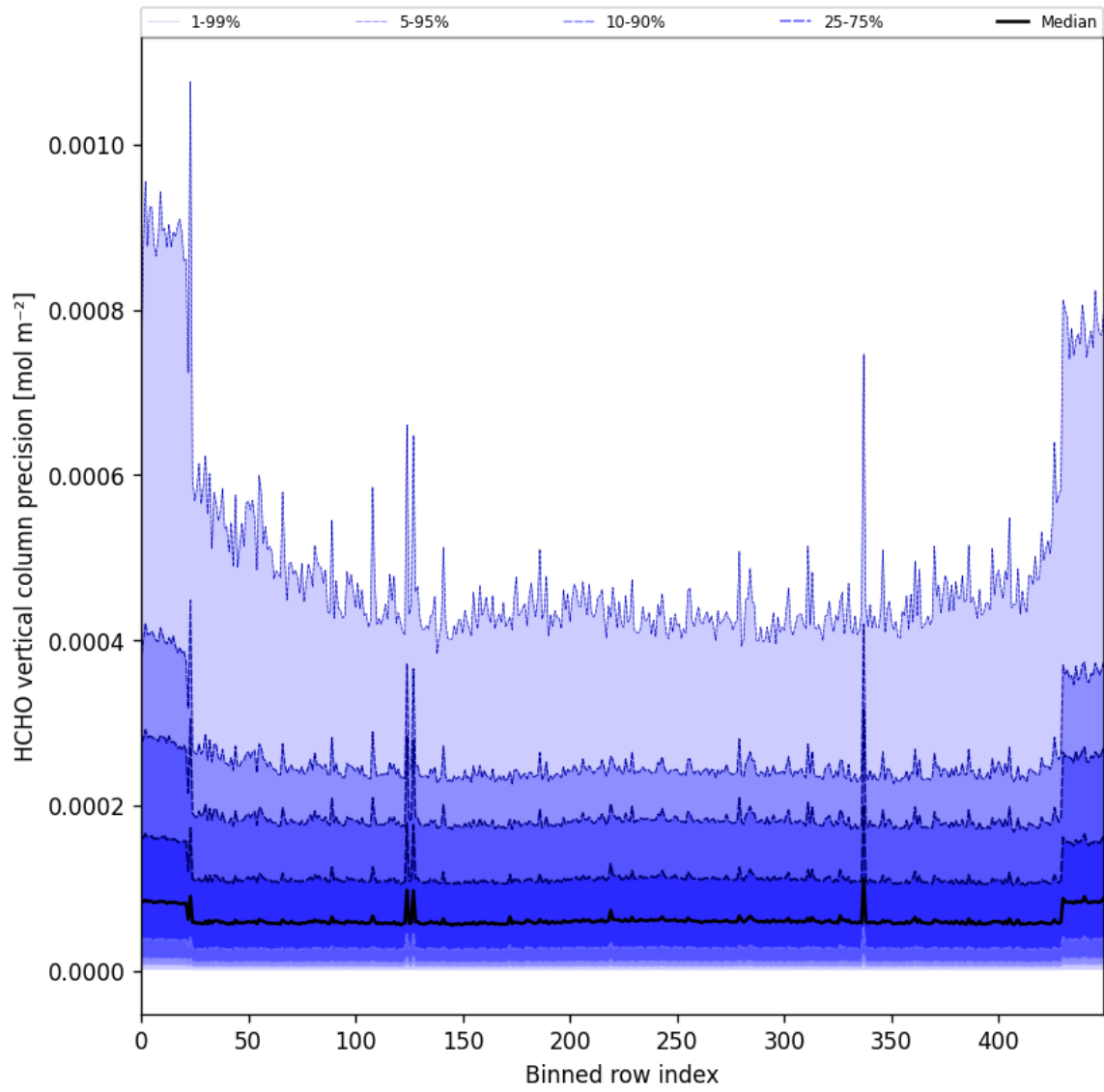
Figure 50: Along track statistics of “HCHO vertical column precision” for 2025-09-04 to 2025-09-05
