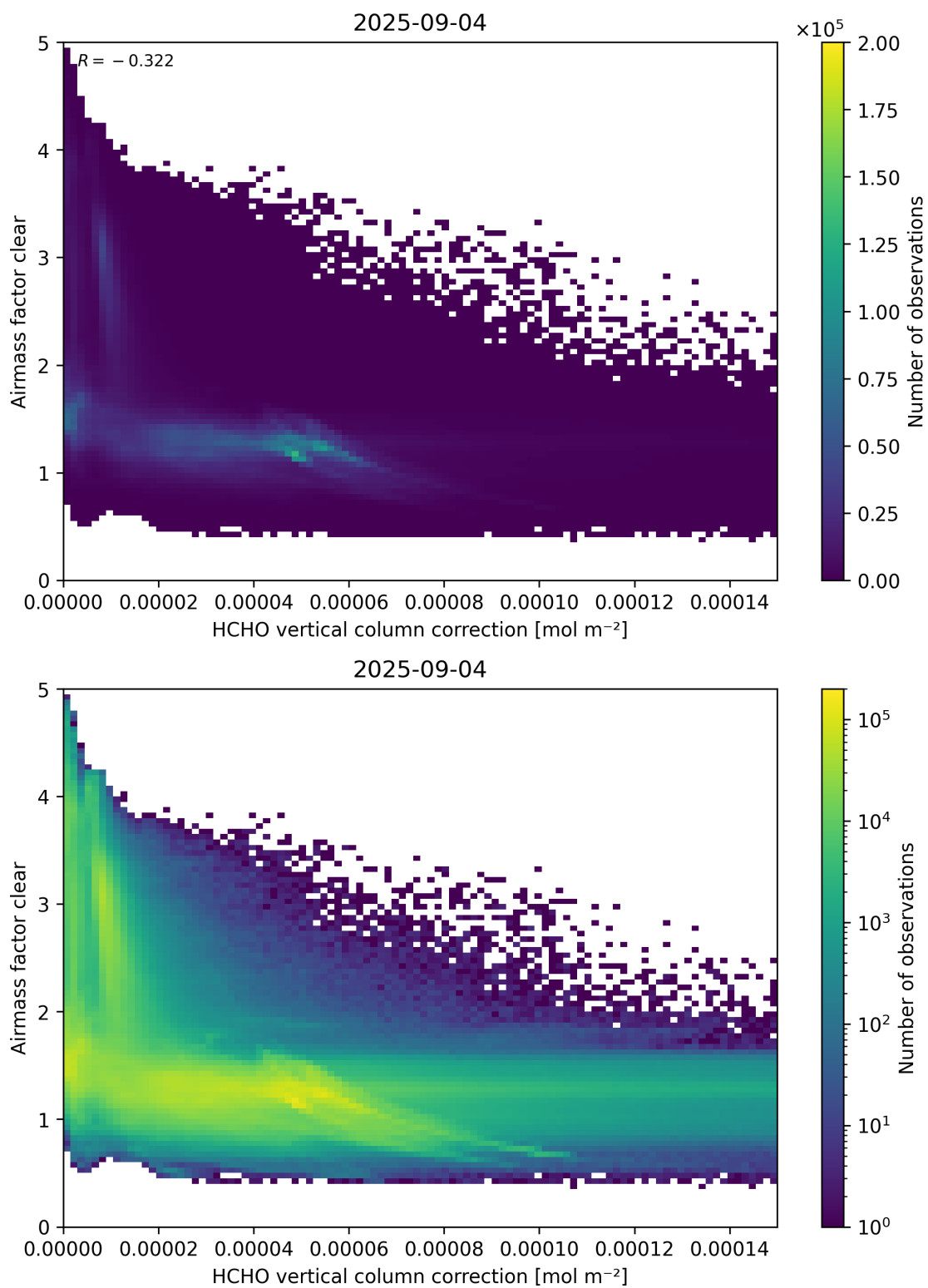
Figure 115: Scatter density plot of “HCHO vertical column correction” against “Airmass factor clear” for 2025-09-04 to 2025-09-05.
