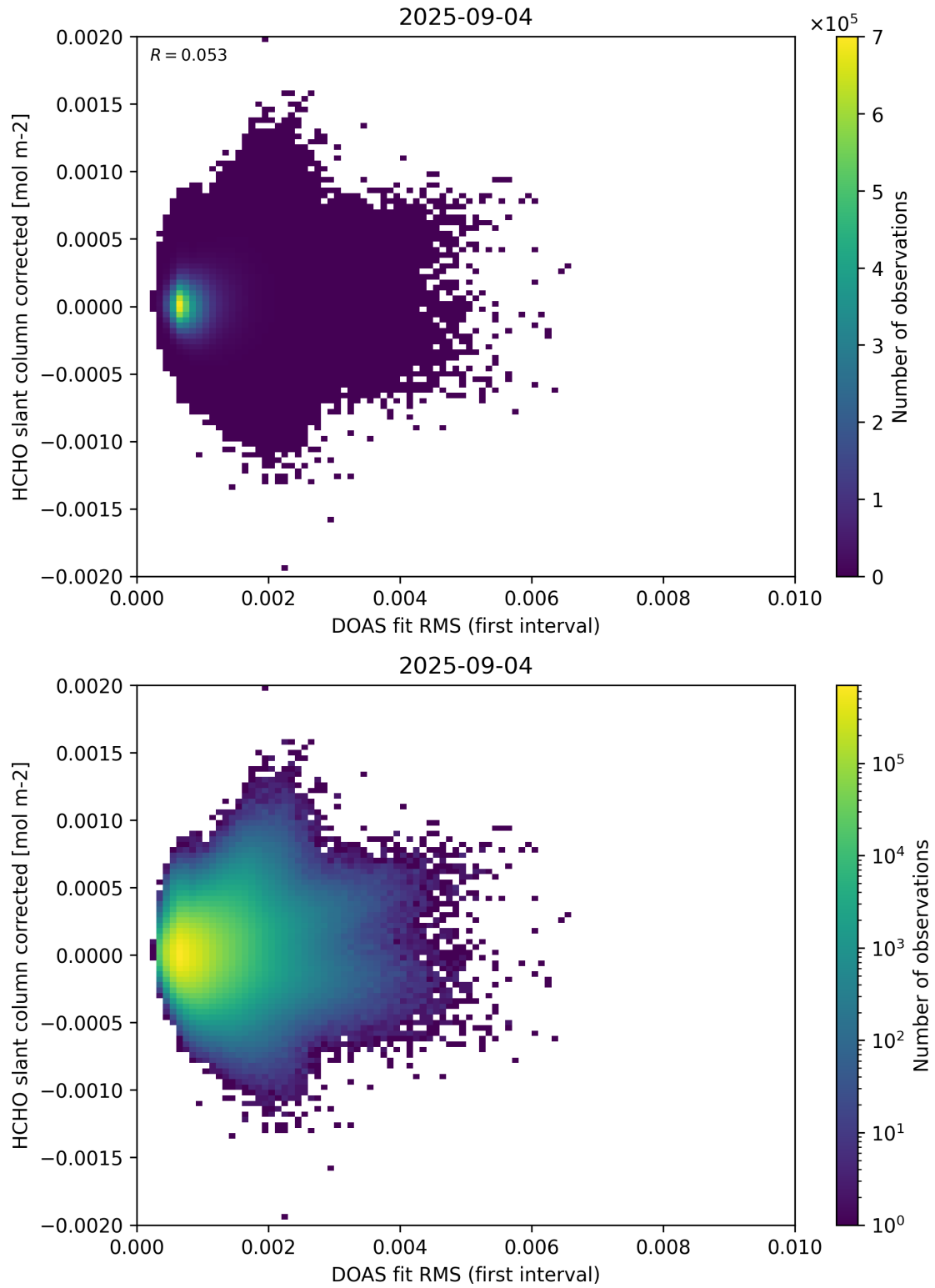
Figure 62: Scatter density plot of “DOAS fit RMS (first interval)” against “HCHO slant column corrected” for 2025-09-04 to 2025-09-05.
