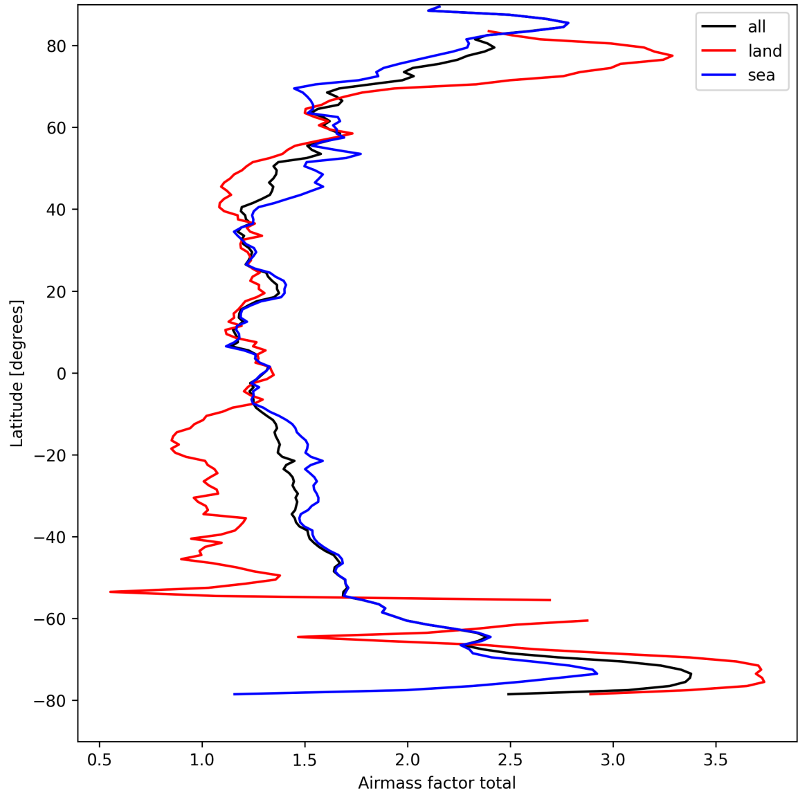
Figure 26: Zonal average of “Airmass factor total” for 2025-09-04 to 2025-09-05.
