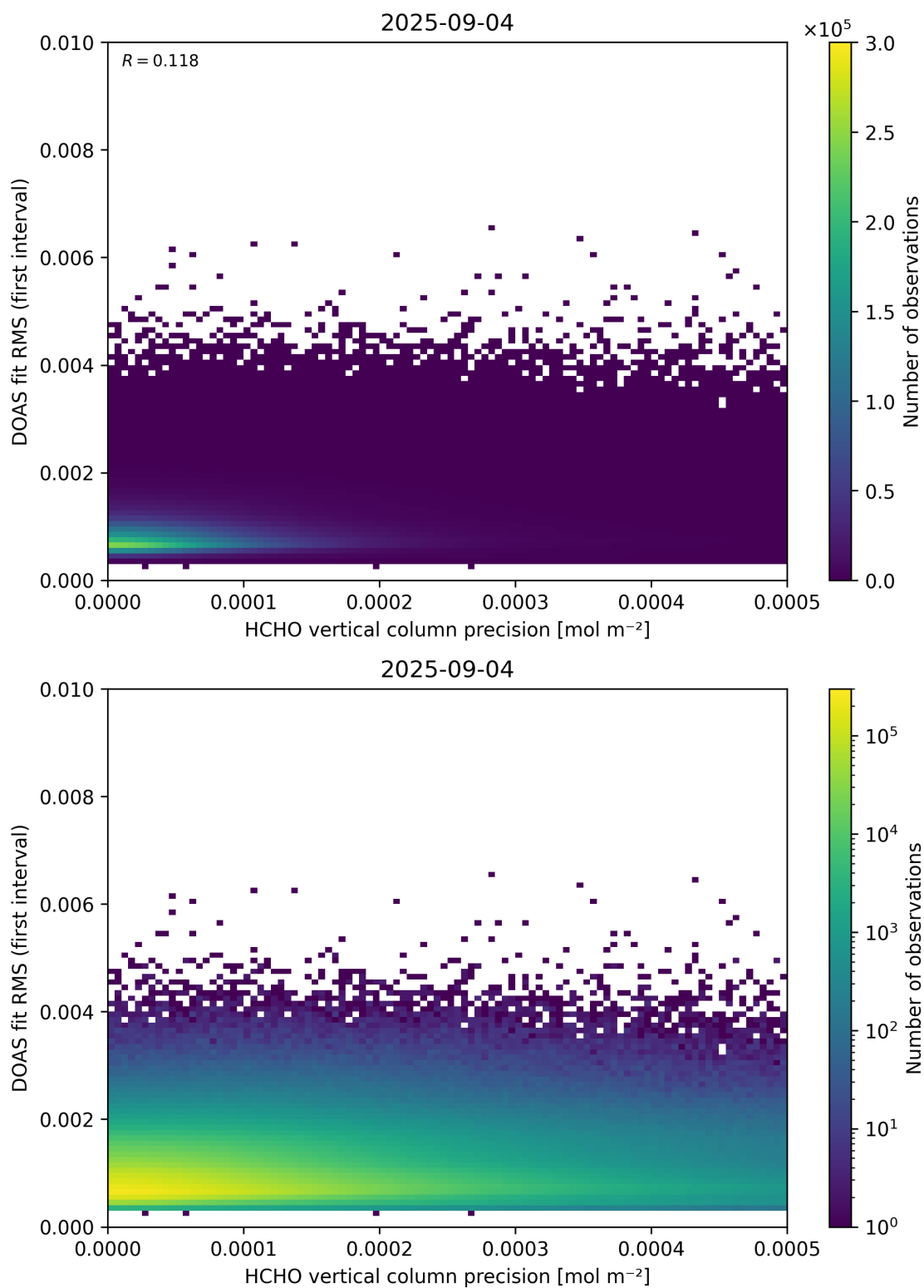
Figure 136: Scatter density plot of “HCHO vertical column precision” against “DOAS fit RMS (first interval)” for 2025-09-04 to 2025-09-05.
