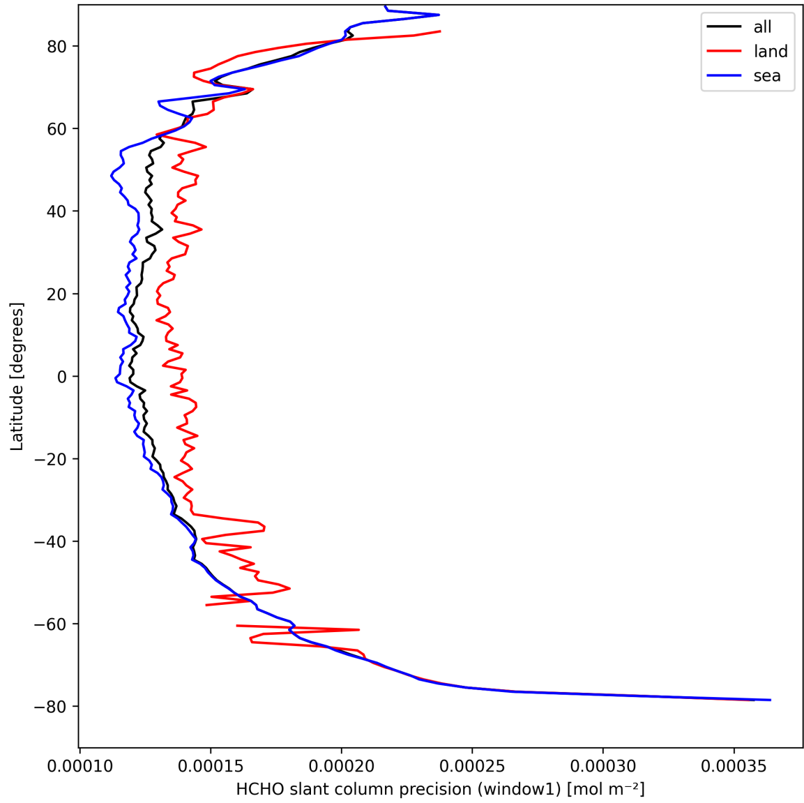
Figure 25: Zonal average of “HCHO slant column precision (window1)” for 2025-09-04 to 2025-09-05.
