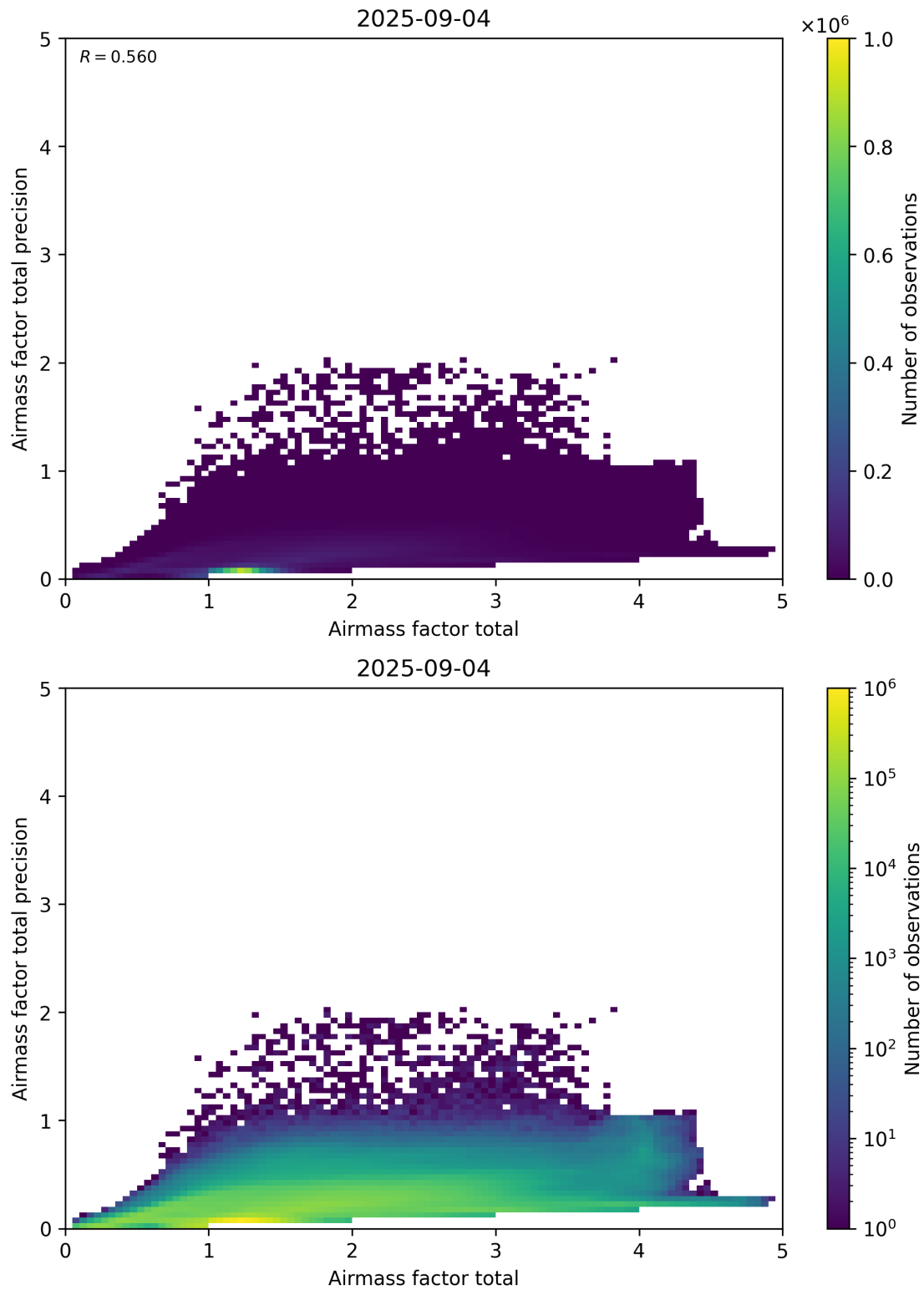
Figure 103: Scatter density plot of “Airmass factor total” against “Airmass factor total precision” for 2025-09-04 to 2025-09-05.
