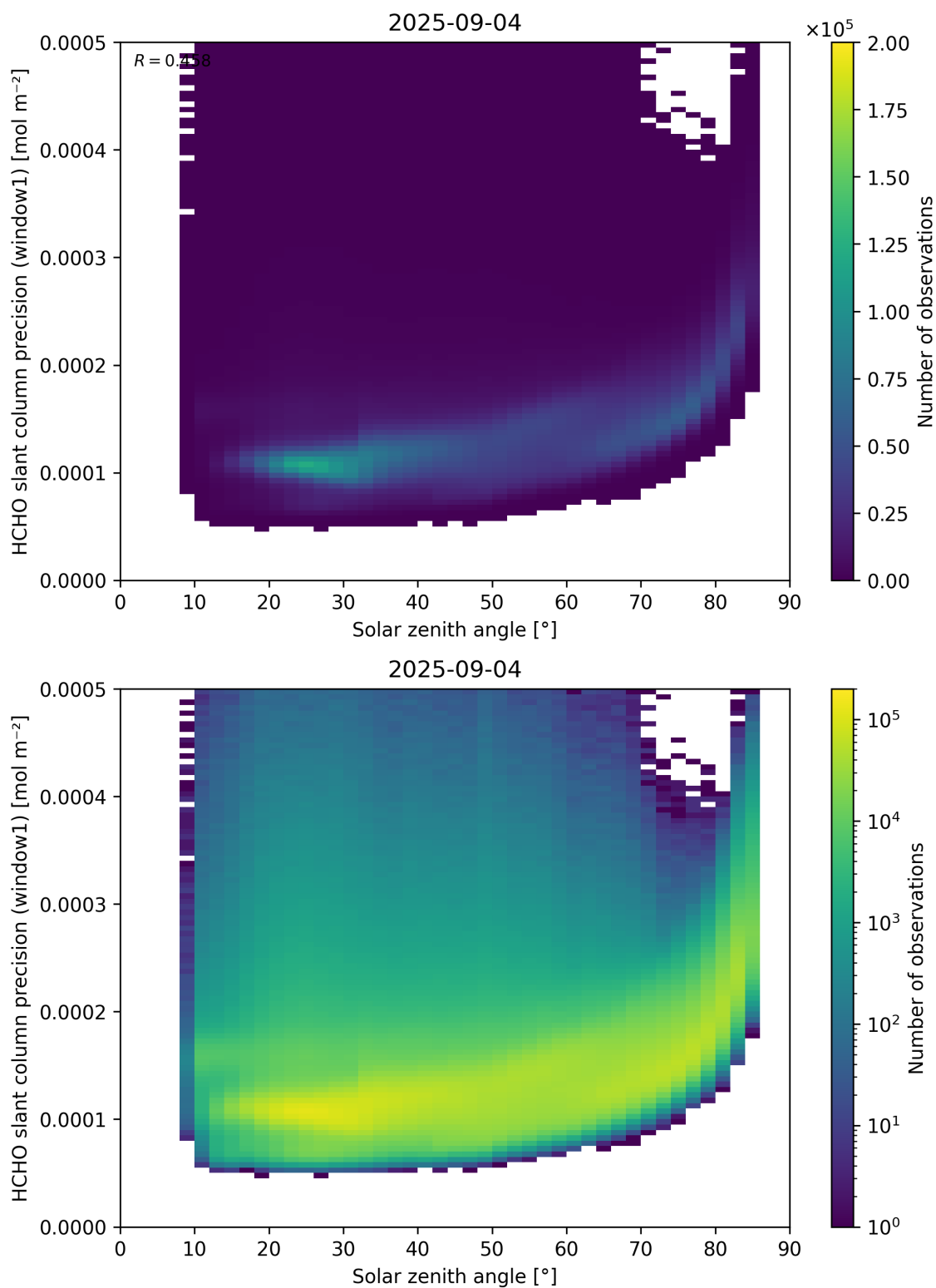
Figure 174: Scatter density plot of “Solar zenith angle” against “HCHO slant column precision (window1)” for 2025-09-04 to 2025-09-05.
