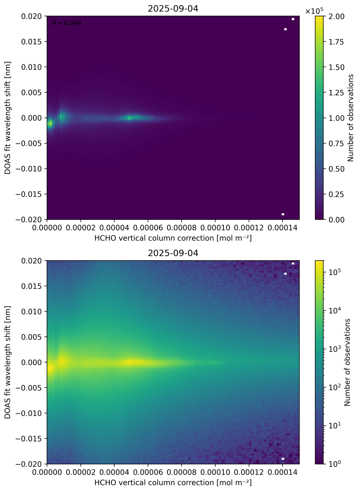
Figure 113: Scatter density plot of “HCHO vertical column correction” against “DOAS fit wavelength shift” for 2025-09-04 to 2025-09-05.
