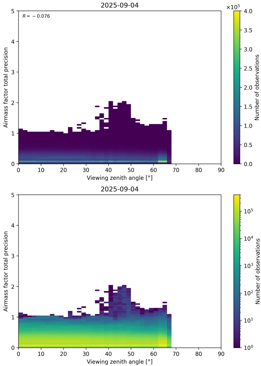
Figure 191: Scatter density plot of “Viewing zenith angle” against “Airmass factor total precision” for 2025-09-04 to 2025-09-05.
