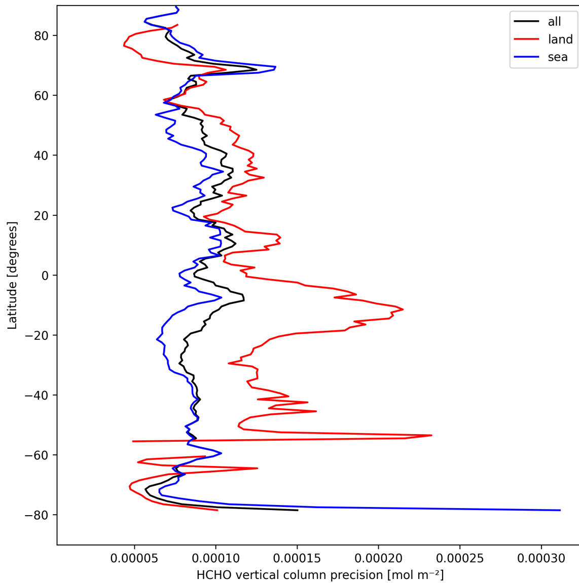
Figure 22: Zonal average of “HCHO vertical column precision” for 2025-09-04 to 2025-09-05.
