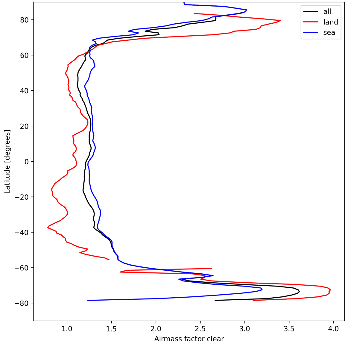
Figure 28: Zonal average of “Airmass factor clear” for 2025-09-04 to 2025-09-05.
