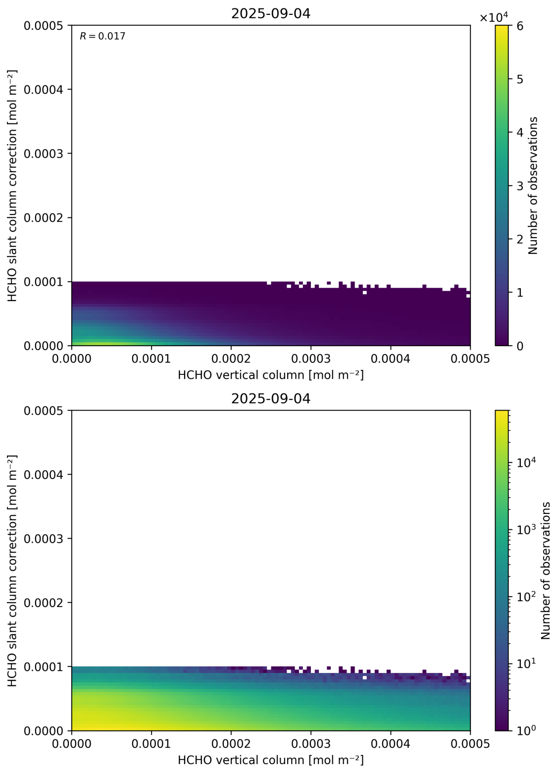
Figure 128: Scatter density plot of “HCHO vertical column” against “HCHO slant column correction” for 2025-09-04 to 2025-09-05.
