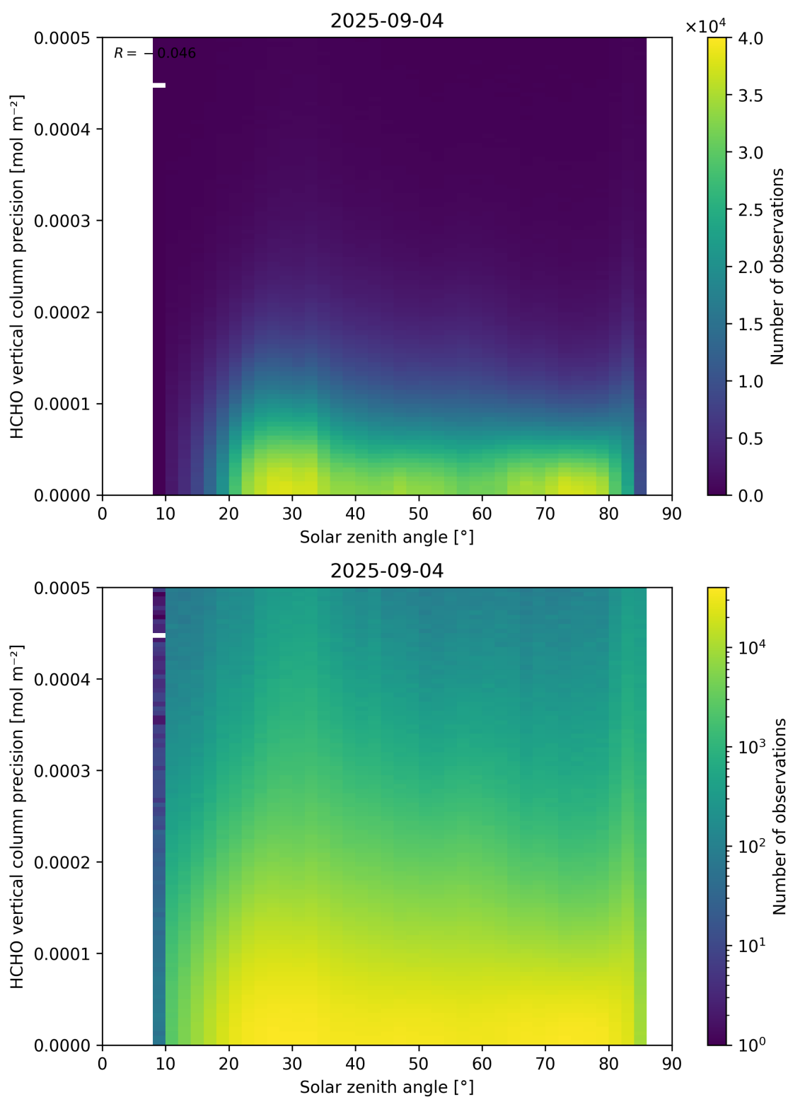
Figure 179: Scatter density plot of “Solar zenith angle” against “HCHO vertical column precision” for 2025-09-04 to 2025-09-05.
