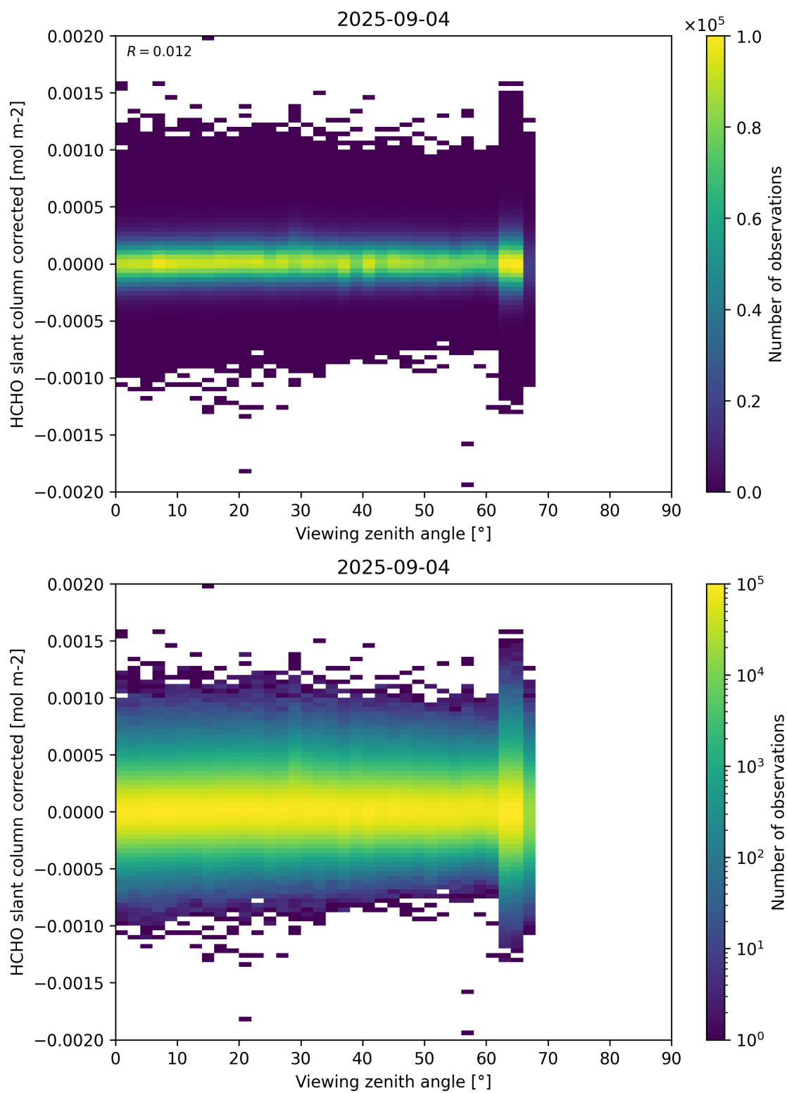
Figure 186: Scatter density plot of “Viewing zenith angle” against “HCHO slant column corrected” for 2025-09-04 to 2025-09-05.
