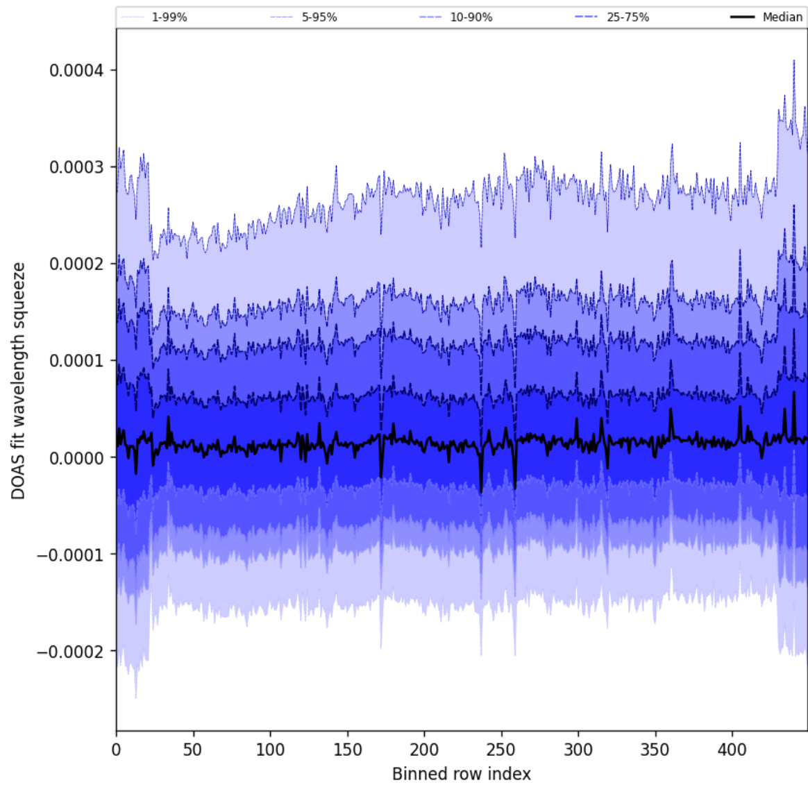
Figure 59: Along track statistics of “DOAS fit wavelength squeeze” for 2025-09-04 to 2025-09-05
