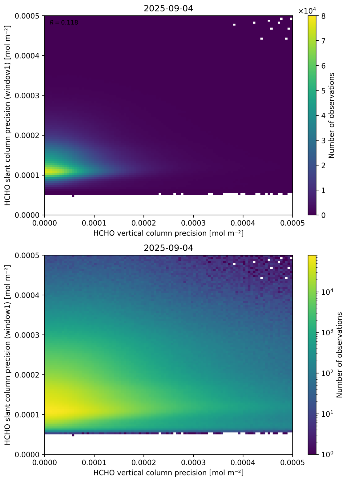
Figure 143: Scatter density plot of “HCHO vertical column precision” against “HCHO slant column precision (window1)” for 2025-09-04 to 2025-09-05.
