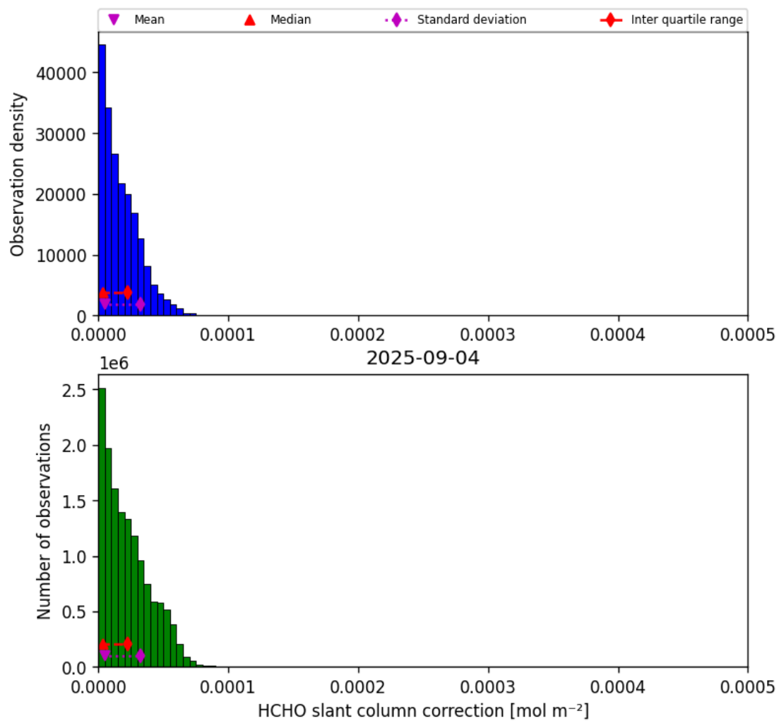
Figure 47: Histogram of “HCHO slant column correction” for 2025-09-04 to 2025-09-05
