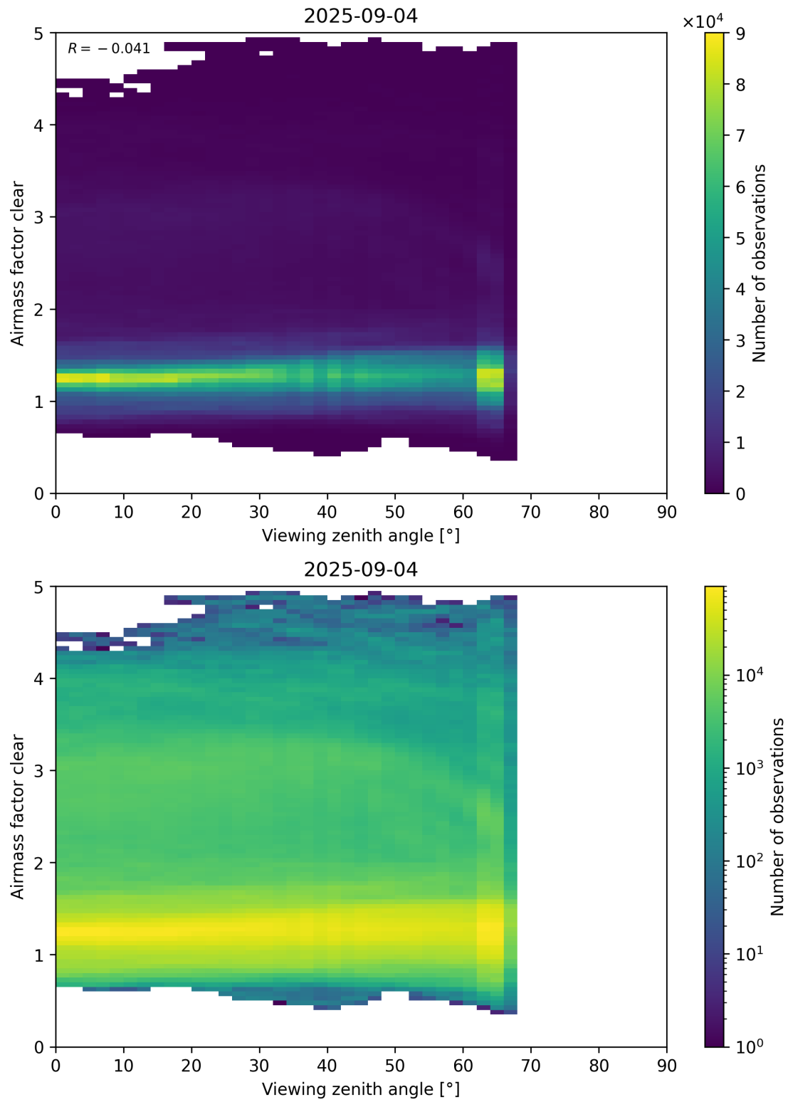
Figure 185: Scatter density plot of “Viewing zenith angle” against “Airmass factor clear” for 2025-09-04 to 2025-09-05.
