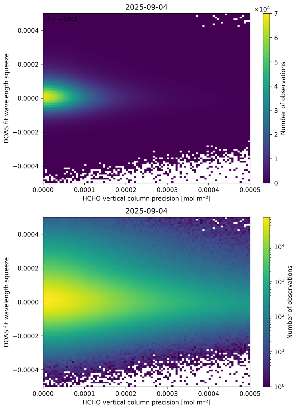
Figure 138: Scatter density plot of “HCHO vertical column precision” against “DOAS fit wavelength squeeze” for 2025-09-04 to 2025-09-05.
