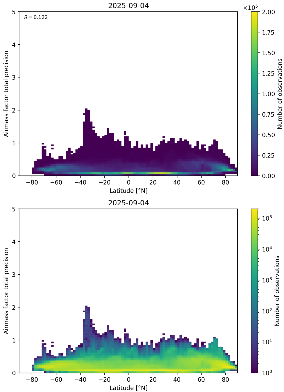
Figure 162: Scatter density plot of “Latitude” against “Airmass factor total precision” for 2025-09-04 to 2025-09-05.
