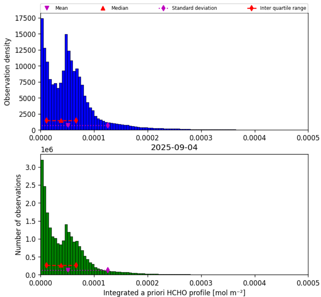
Figure 43: Histogram of “Integrated a priori HCHO profile” for 2025-09-04 to 2025-09-05
