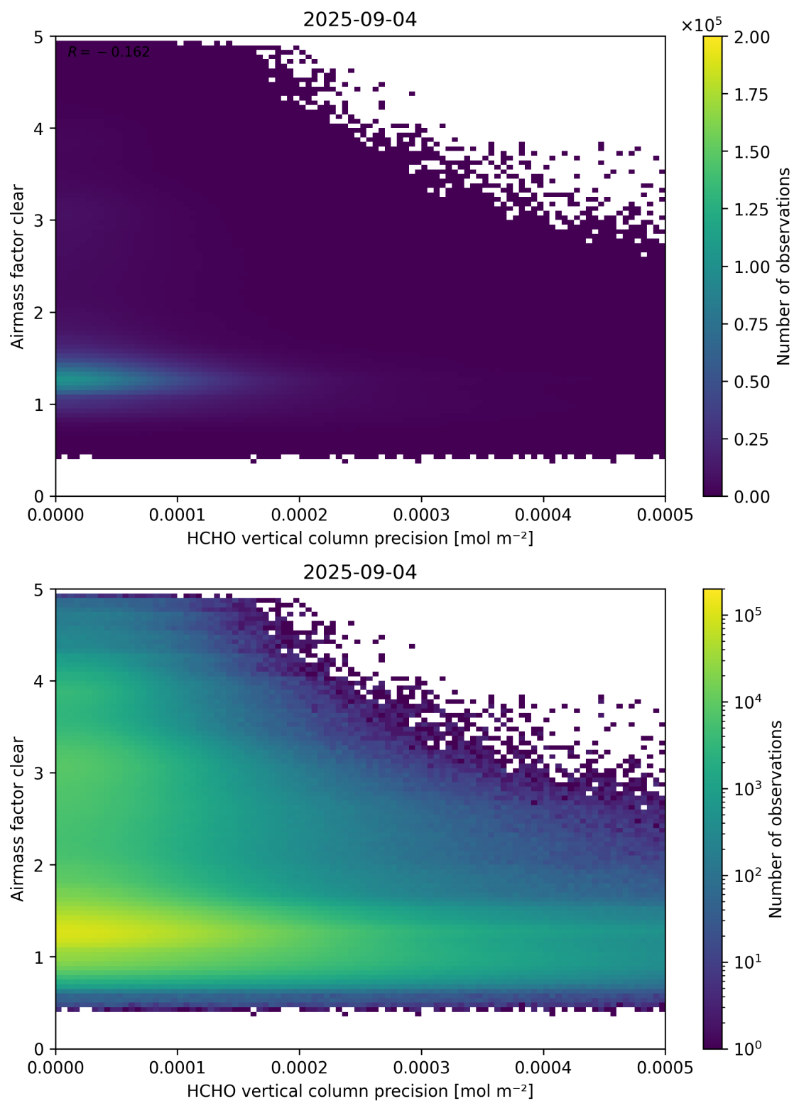
Figure 139: Scatter density plot of “HCHO vertical column precision” against “Airmass factor clear” for 2025-09-04 to 2025-09-05.
