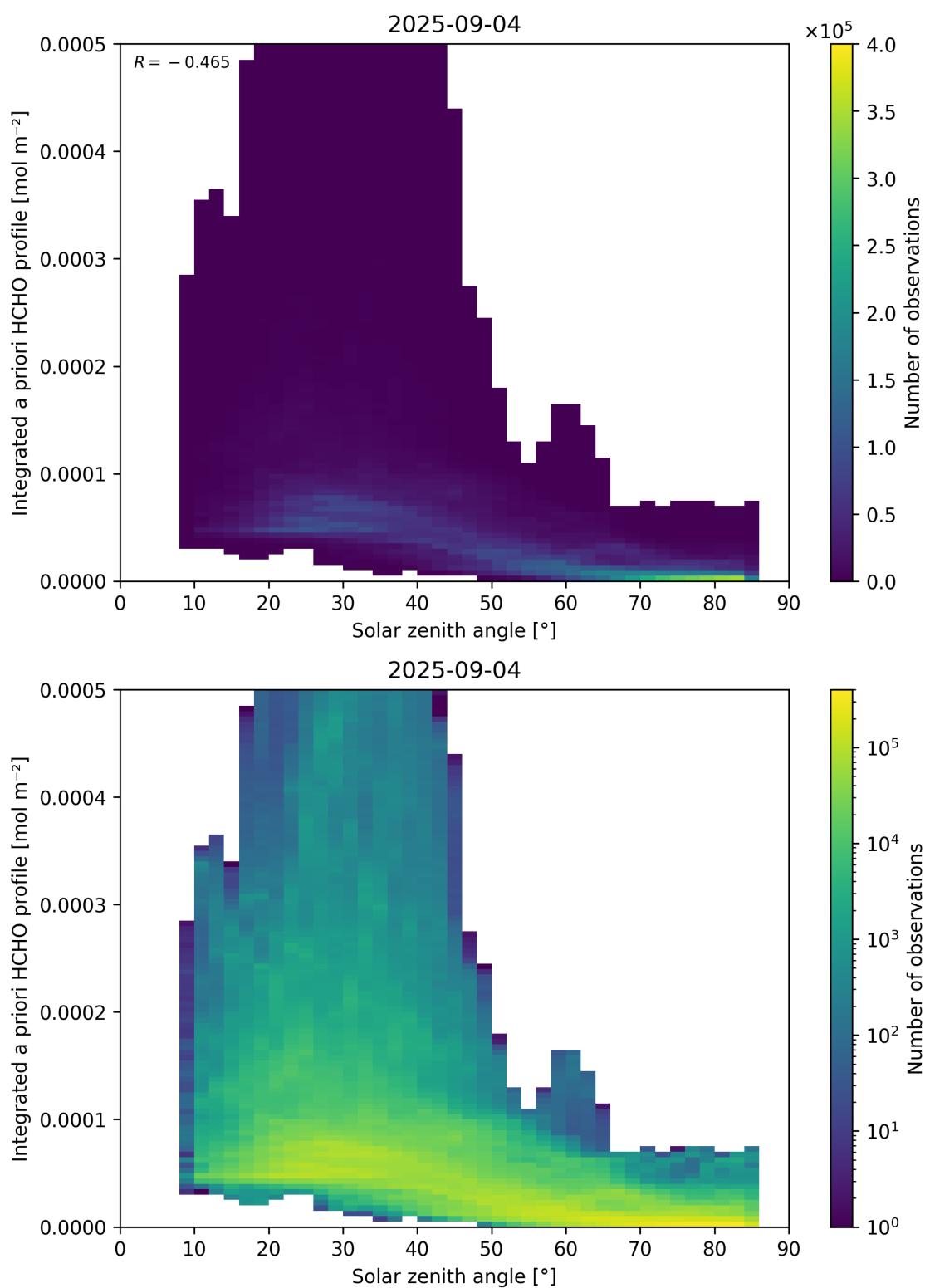
Figure 180: Scatter density plot of “Solar zenith angle” against “Integrated a priori HCHO profile” for 2025-09-04 to 2025-09-05.
