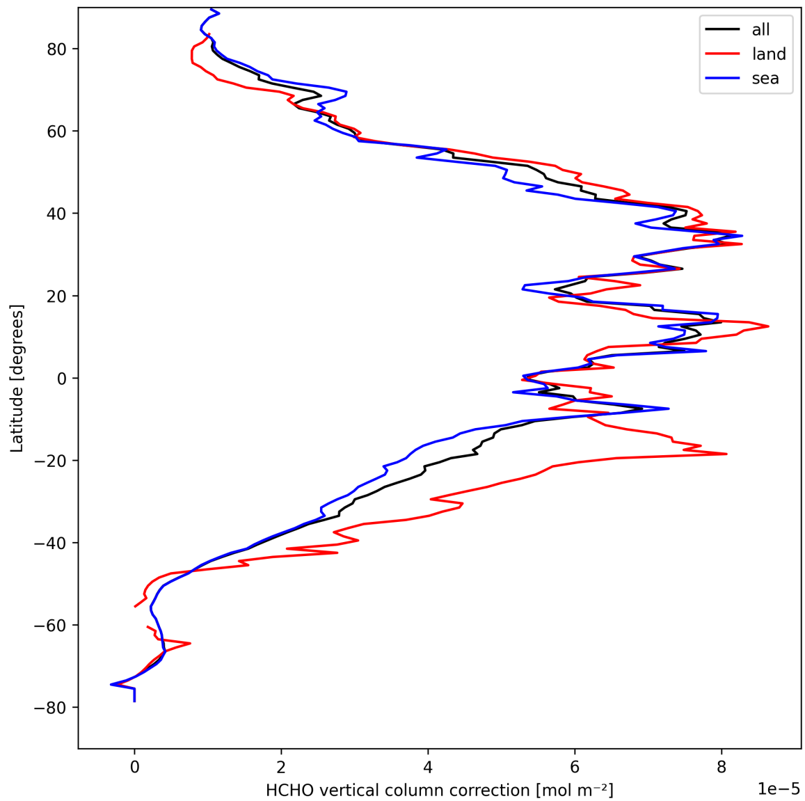
Figure 23: Zonal average of “HCHO vertical column correction” for 2025-09-04 to 2025-09-05.
