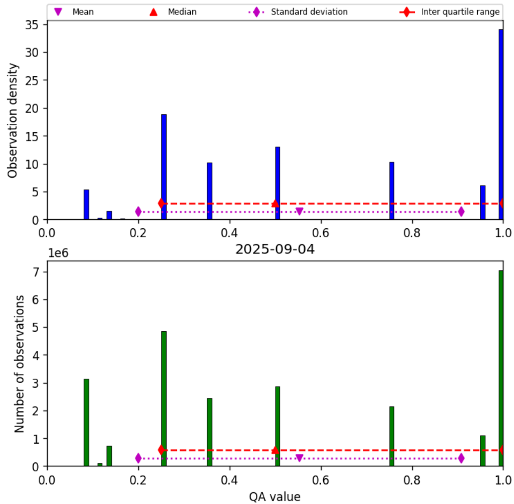
Figure 34: Histogram of “QA value” for 2025-09-04 to 2025-09-05
