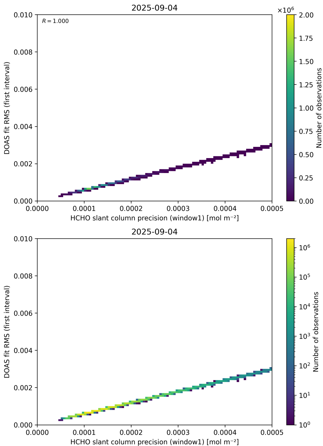
Figure 88: Scatter density plot of “HCHO slant column precision (window1)” against “DOAS fit RMS (first interval)” for 2025-09-04 to 2025-09-05.
