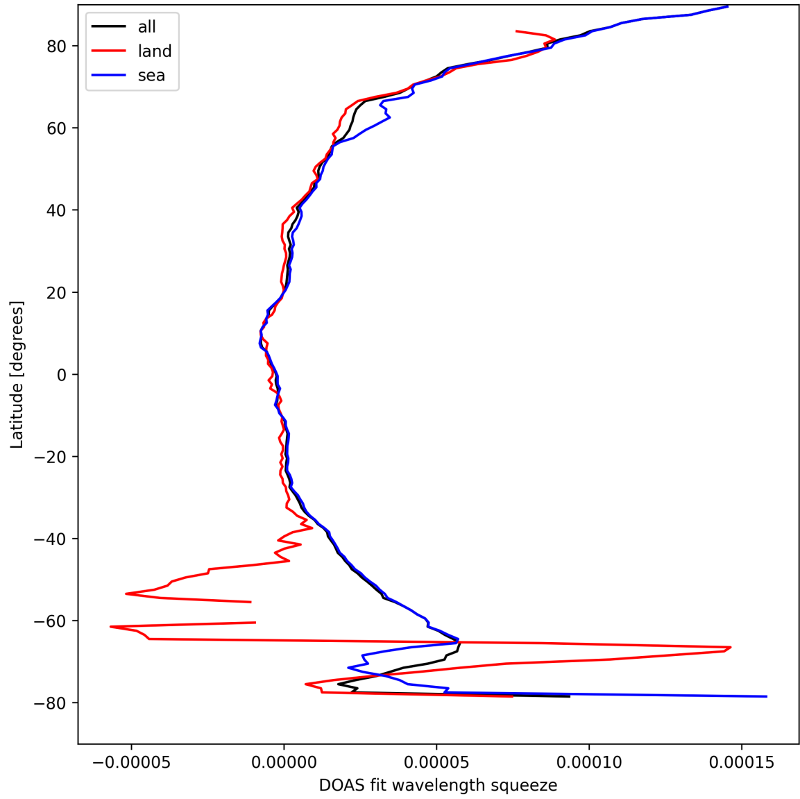
Figure 31: Zonal average of “DOAS fit wavelength squeeze” for 2025-09-04 to 2025-09-05.
