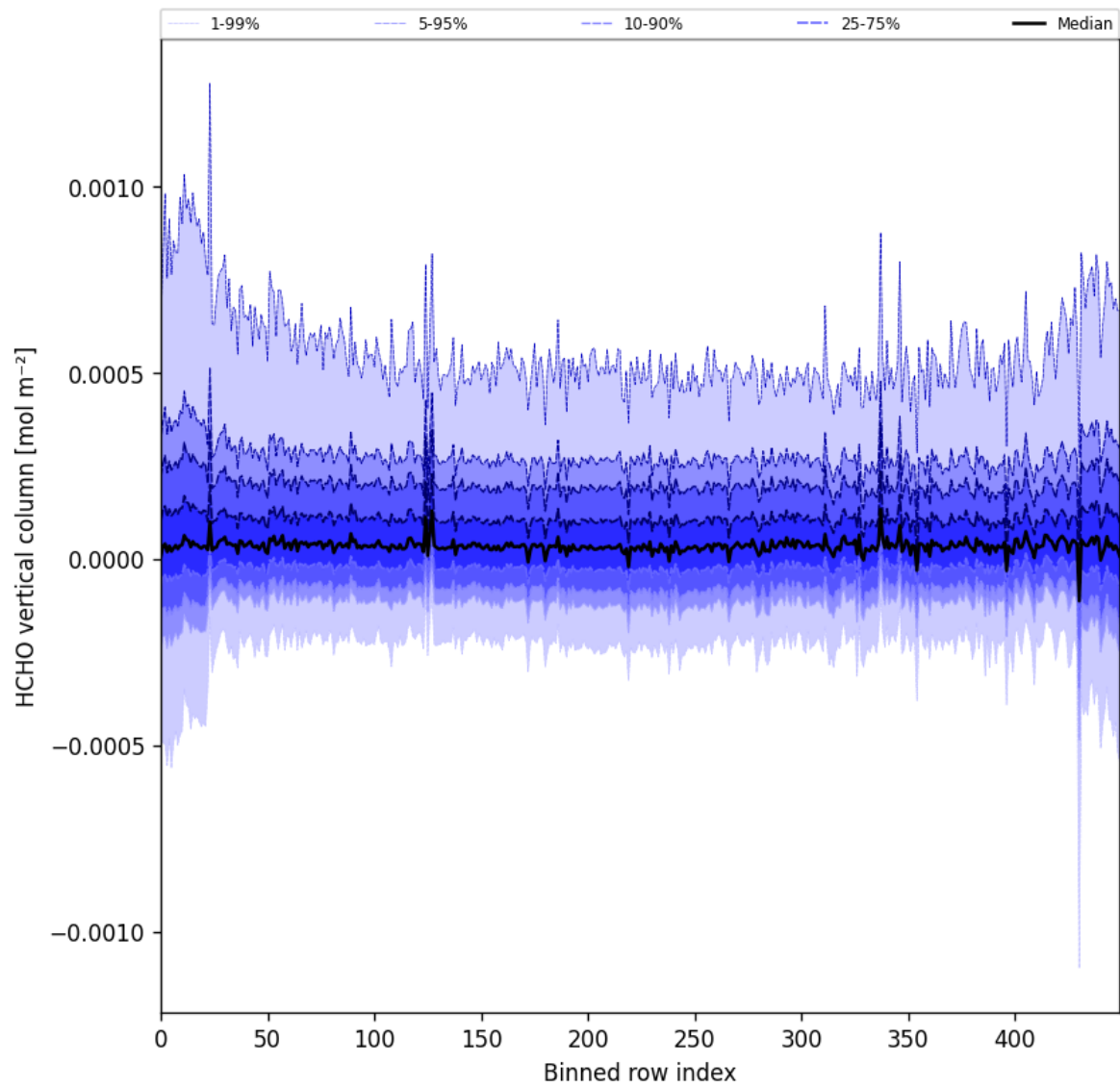
Figure 49: Along track statistics of “HCHO vertical column” for 2025-09-04 to 2025-09-05
