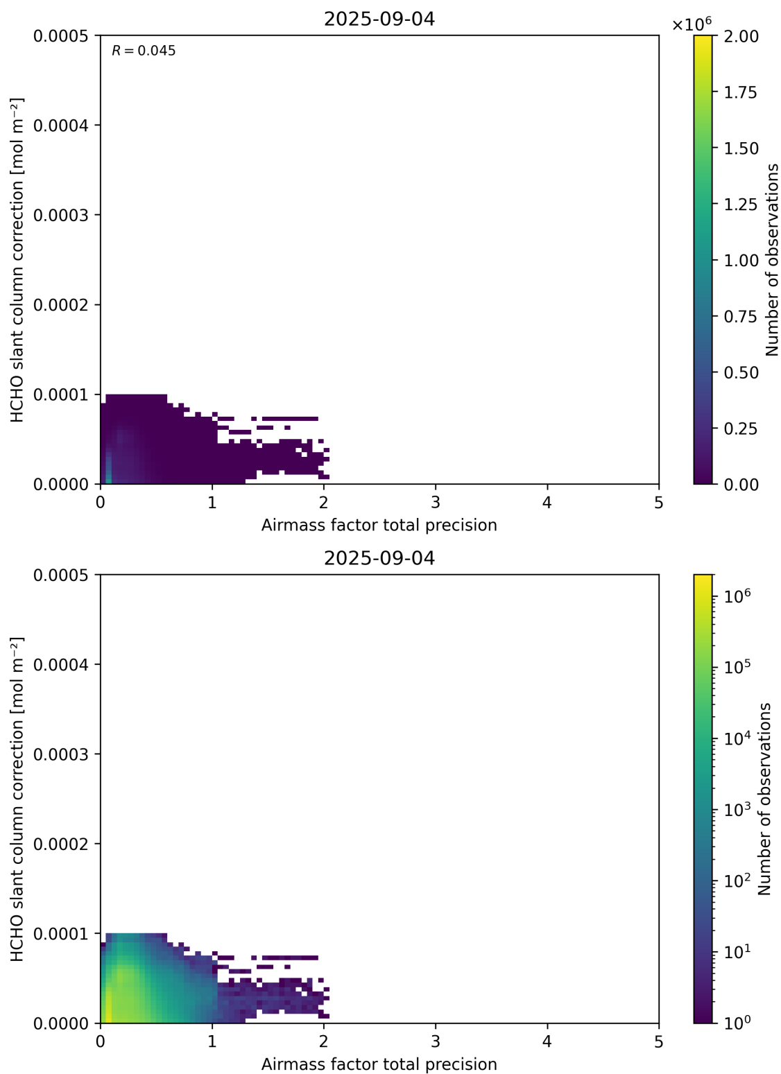
Figure 110: Scatter density plot of “Airmass factor total precision” against “HCHO slant column correction” for 2025-09-04 to 2025-09-05.
