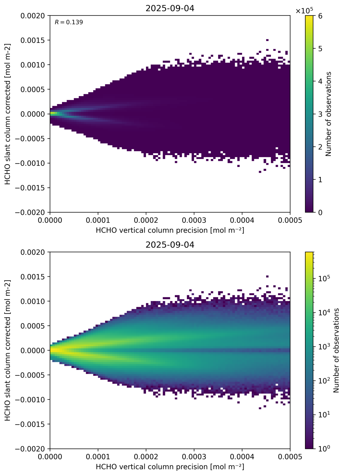
Figure 140: Scatter density plot of “HCHO vertical column precision” against “HCHO slant column corrected” for 2025-09-04 to 2025-09-05.
