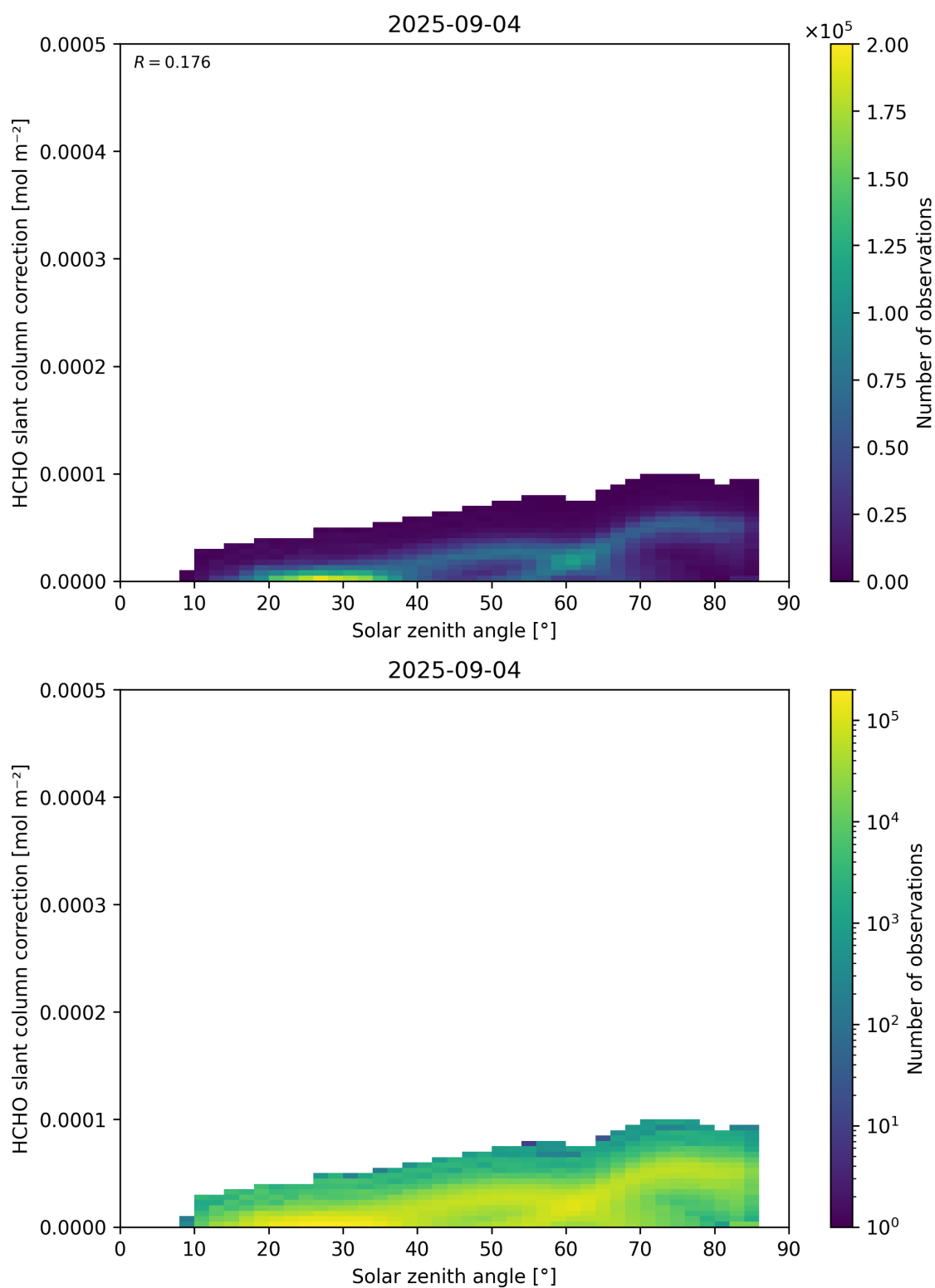
Figure 172: Scatter density plot of “Solar zenith angle” against “HCHO slant column correction” for 2025-09-04 to 2025-09-05.
