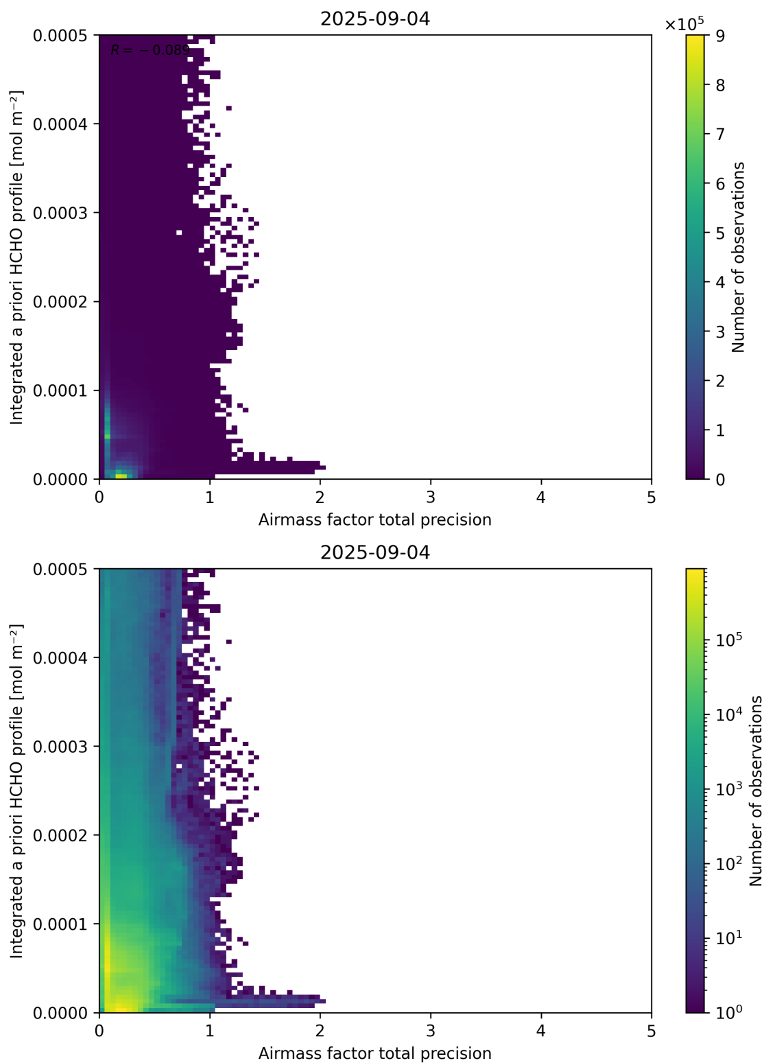
Figure 111: Scatter density plot of “Airmass factor total precision” against “Integrated a priori HCHO profile” for 2025-09-04 to 2025-09-05.
