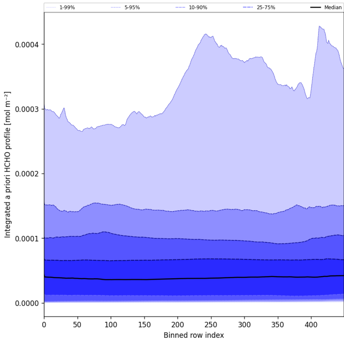
Figure 57: Along track statistics of “Integrated a priori HCHO profile” for 2025-09-04 to 2025-09-05
