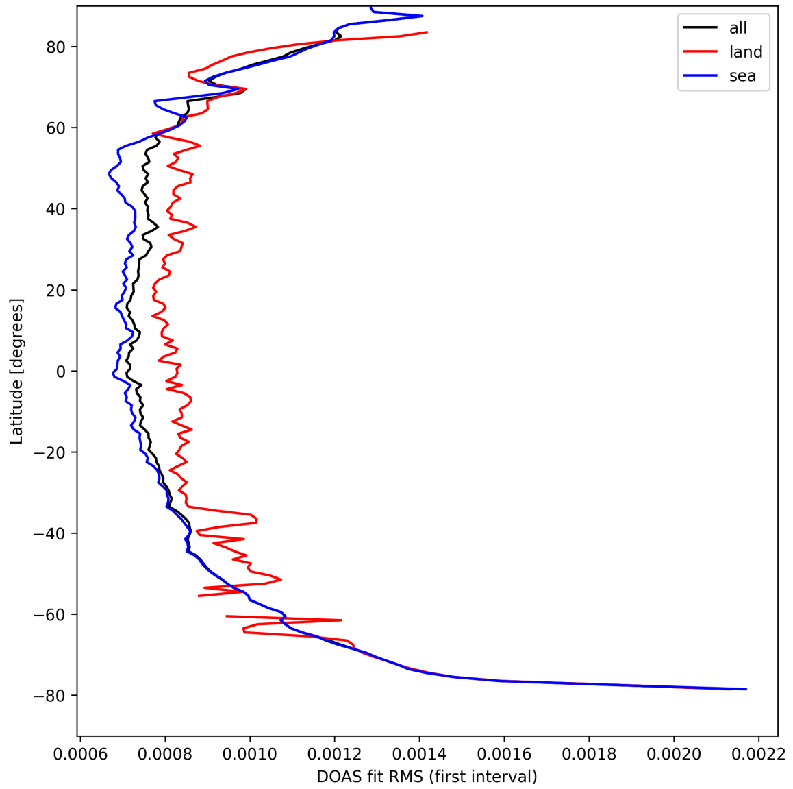
Figure 32: Zonal average of "DOAS fit RMS (first interval)" for 2025-09-04 to 2025-09-05.
