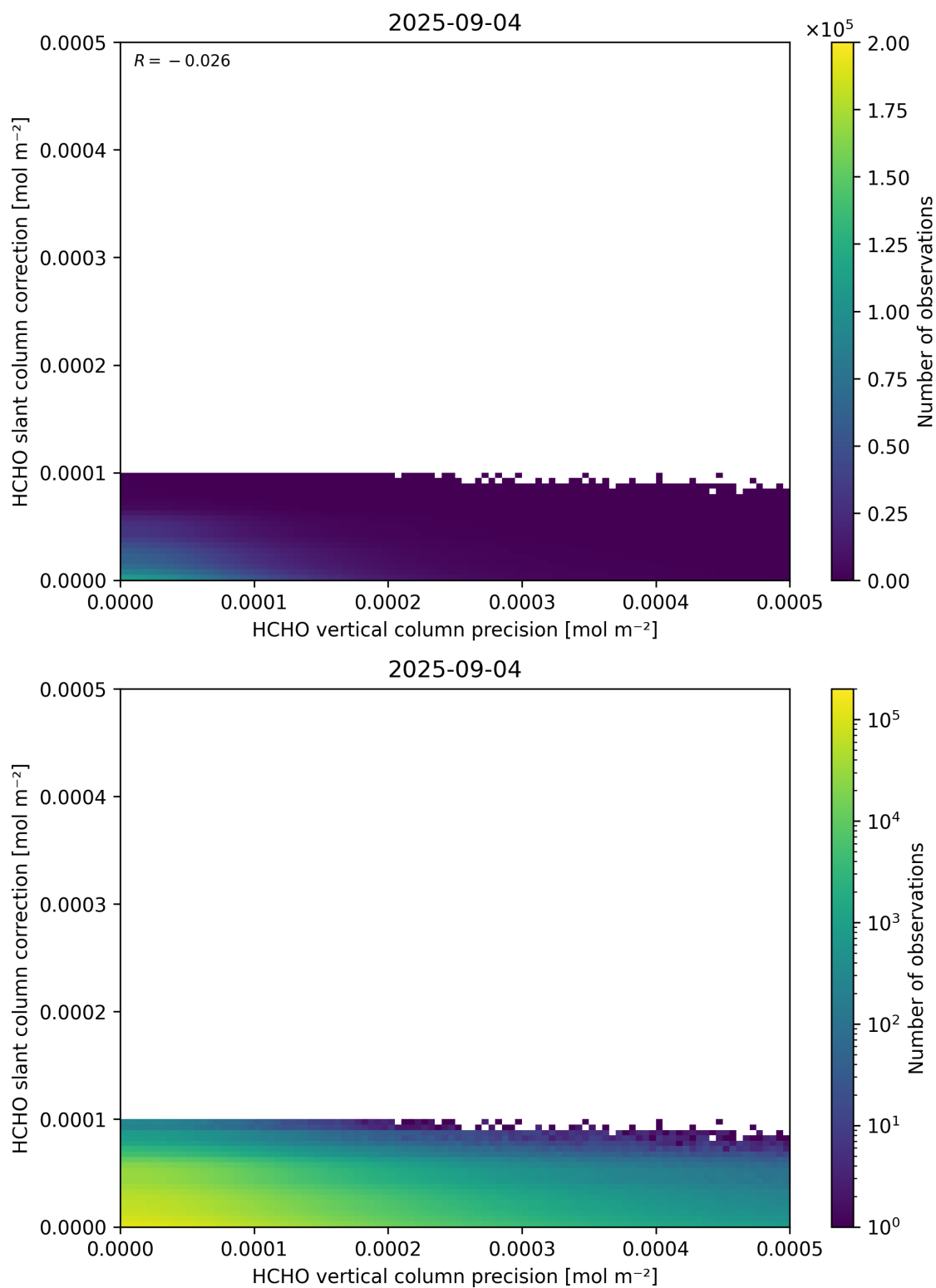
Figure 141: Scatter density plot of “HCHO vertical column precision” against “HCHO slant column correction” for 2025-09-04 to 2025-09-05.
