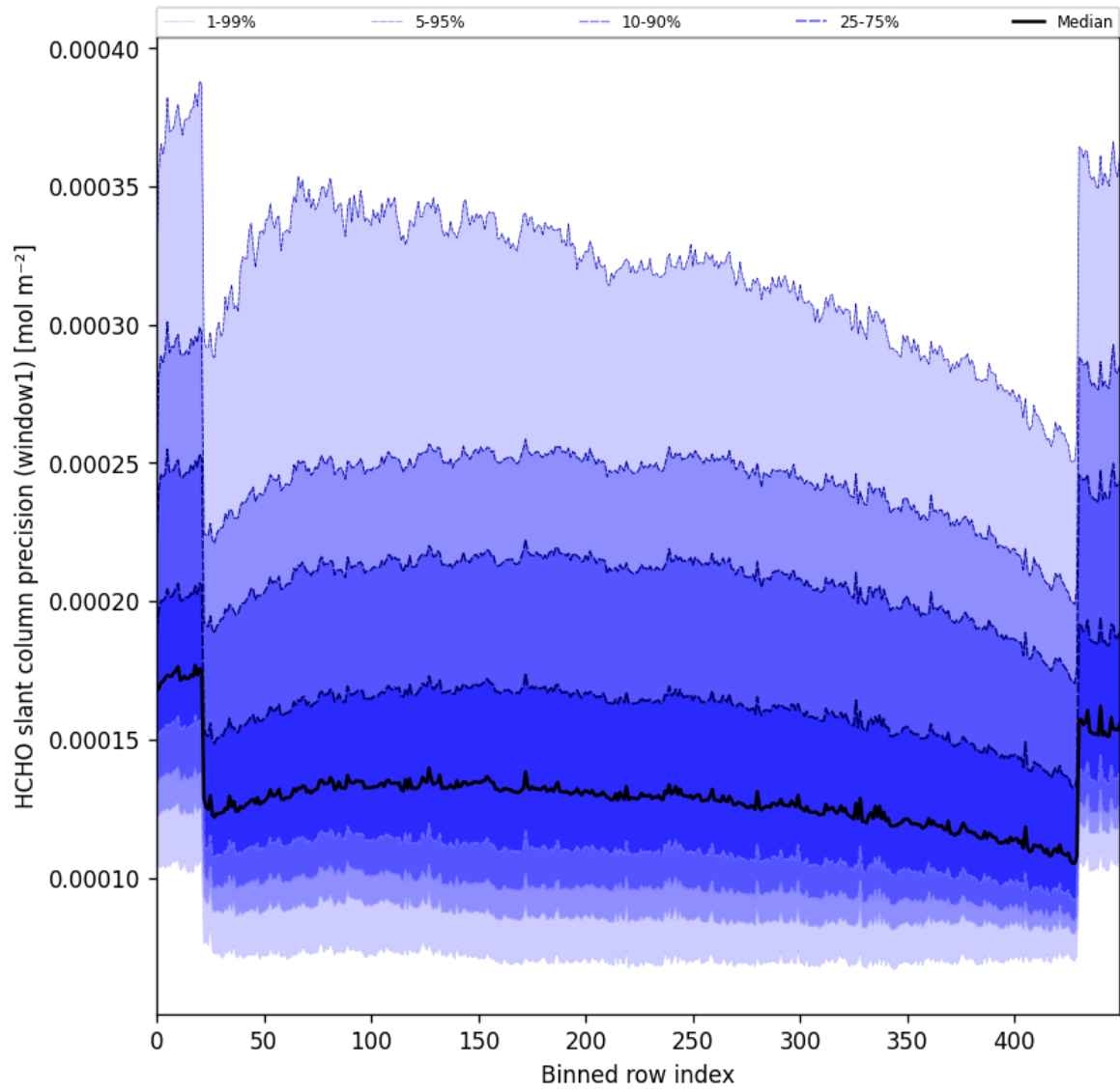
Figure 53: Along track statistics of “HCHO slant column precision (window1)” for 2025-09-04 to 2025-09-05
