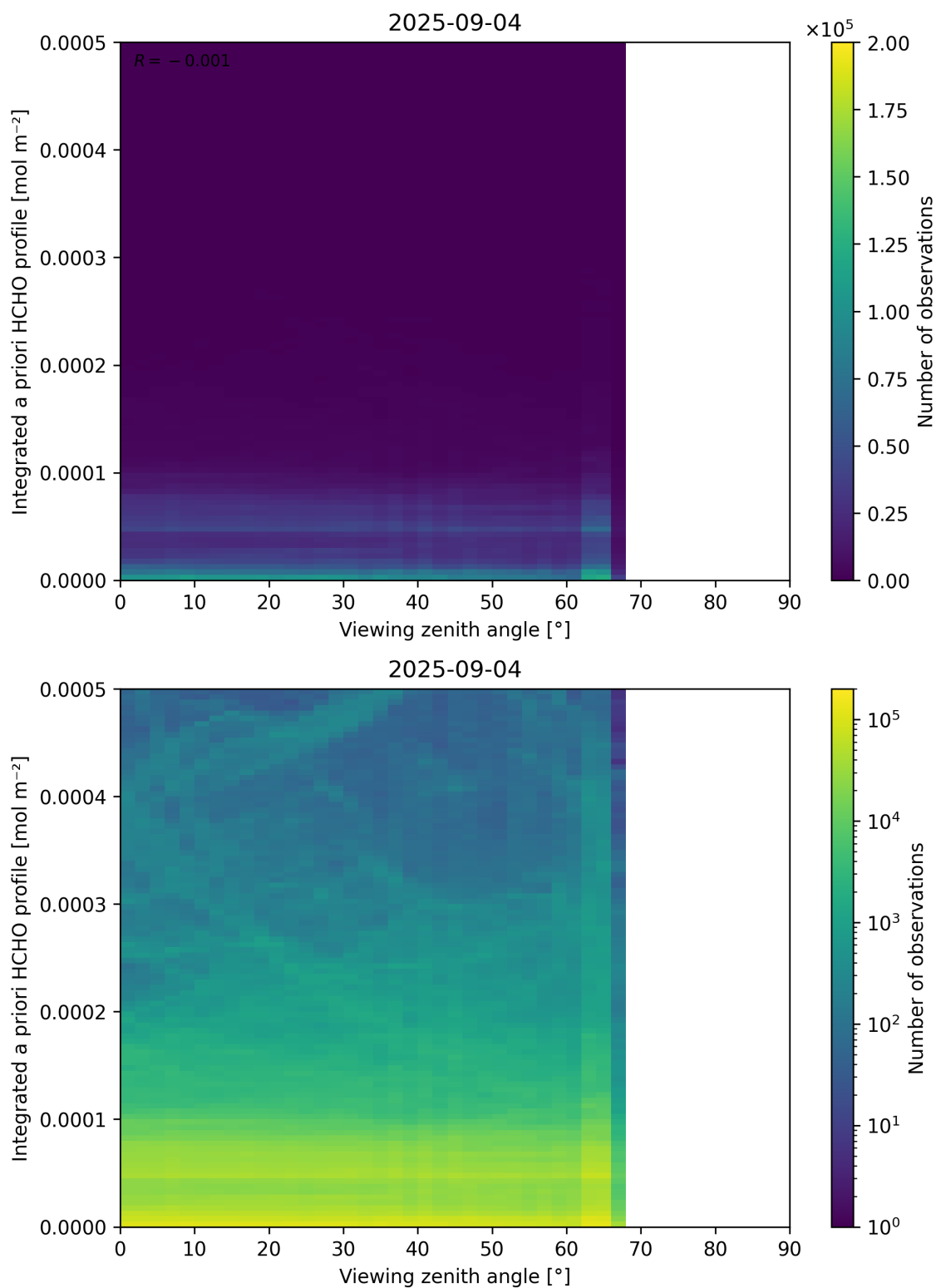
Figure 195: Scatter density plot of “Viewing zenith angle” against “Integrated a priori HCHO profile” for 2025-09-04 to 2025-09-05.
