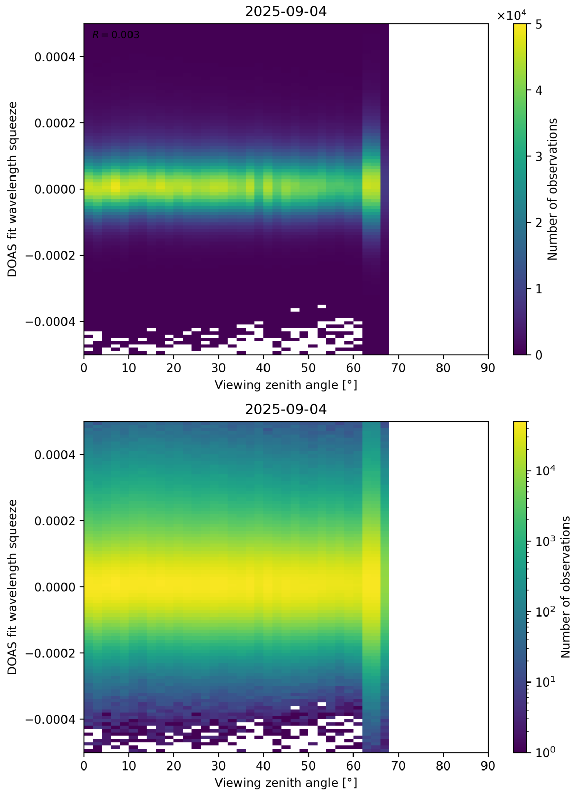
Figure 184: Scatter density plot of “Viewing zenith angle” against “DOAS fit wavelength squeeze” for 2025-09-04 to 2025-09-05.
