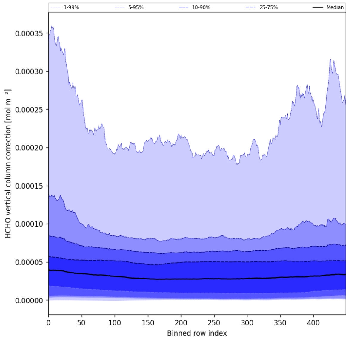
Figure 51: Along track statistics of “HCHO vertical column correction” for 2025-09-04 to 2025-09-05
