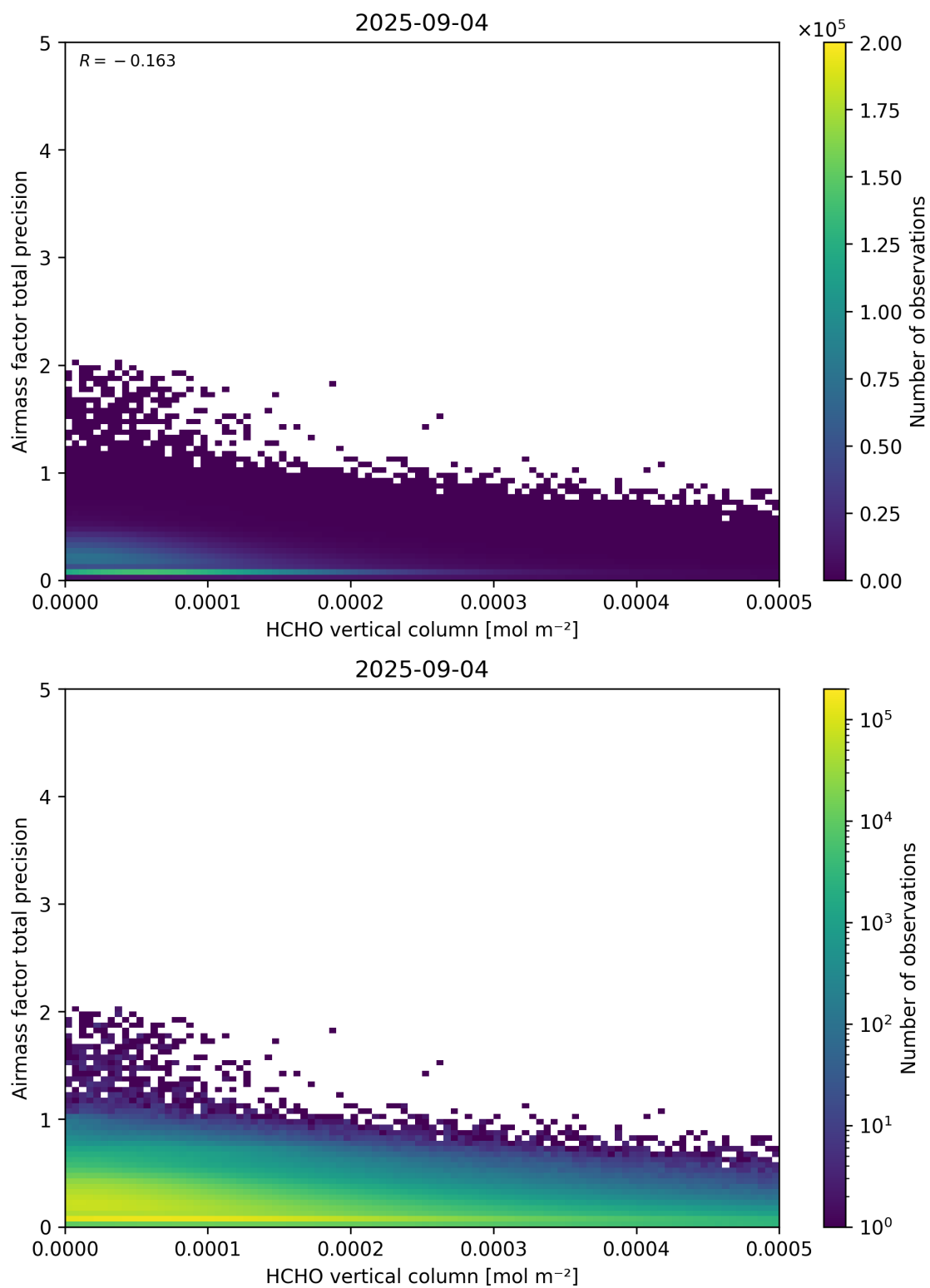
Figure 132: Scatter density plot of “HCHO vertical column” against “Airmass factor total precision” for 2025-09-04 to 2025-09-05.
