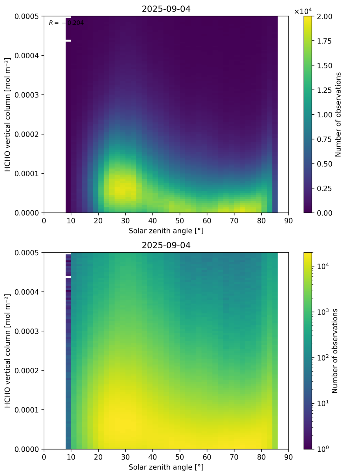
Figure 177: Scatter density plot of “Solar zenith angle” against “HCHO vertical column” for 2025-09-04 to 2025-09-05.
