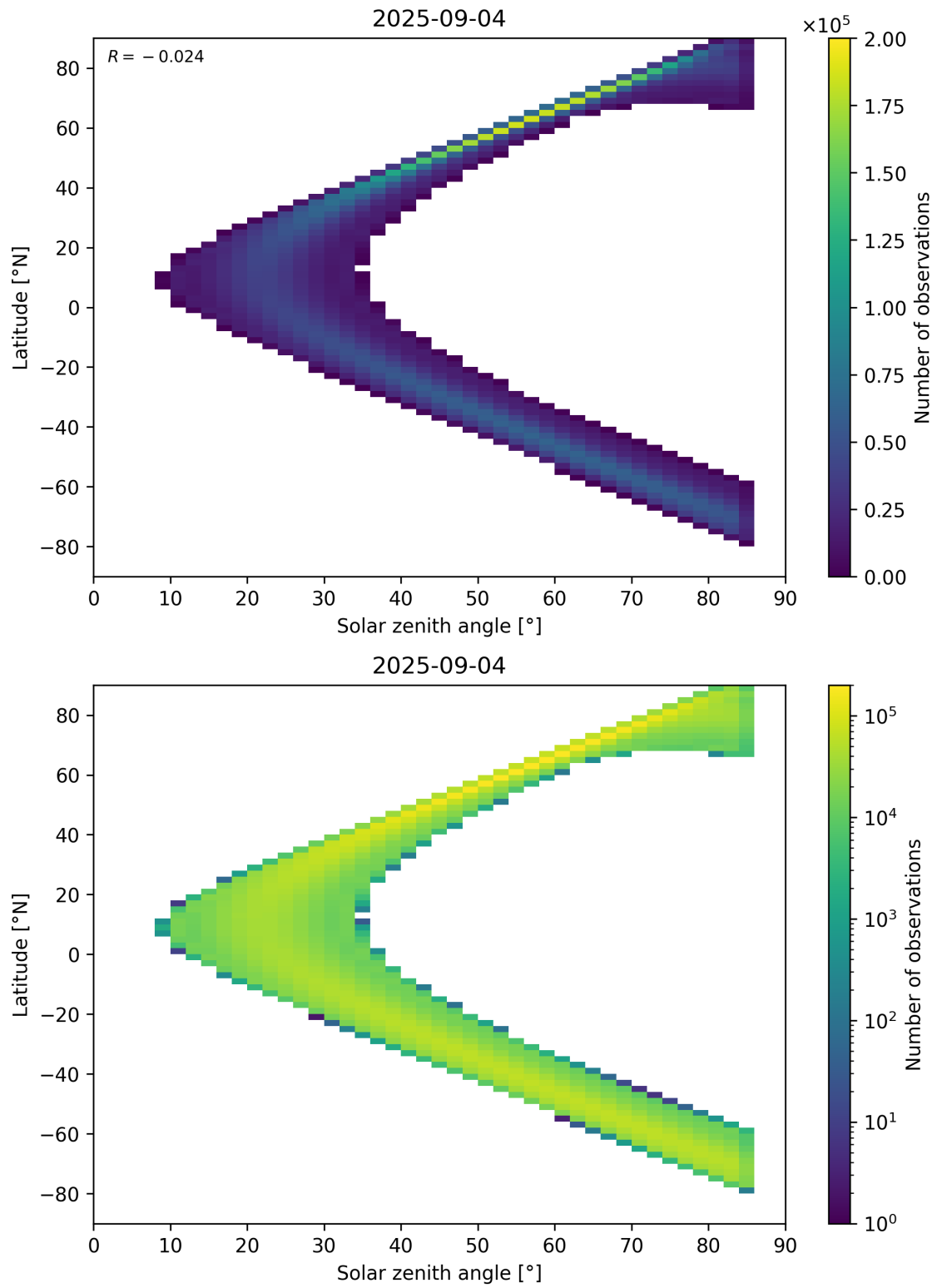
Figure 181: Scatter density plot of “Solar zenith angle” against “Latitude” for 2025-09-04 to 2025-09-05.
