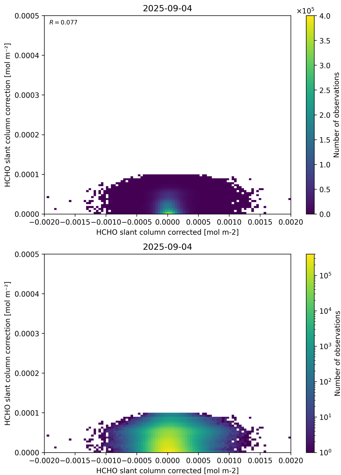
Figure 77: Scatter density plot of “HCHO slant column corrected” against “HCHO slant column correction” for 2025-09-04 to 2025-09-05.
