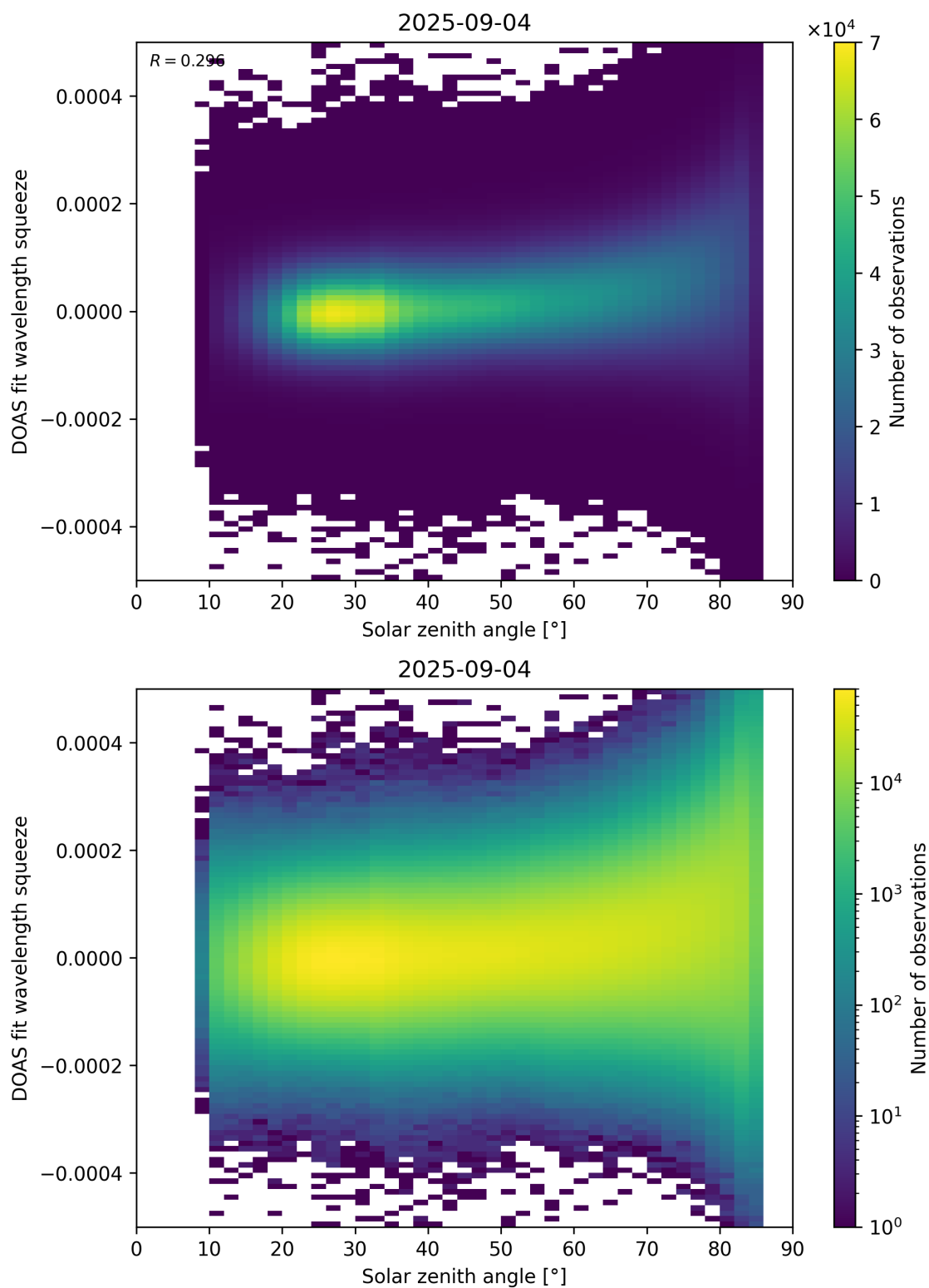
Figure 169: Scatter density plot of “Solar zenith angle” against “DOAS fit wavelength squeeze” for 2025-09-04 to 2025-09-05.
