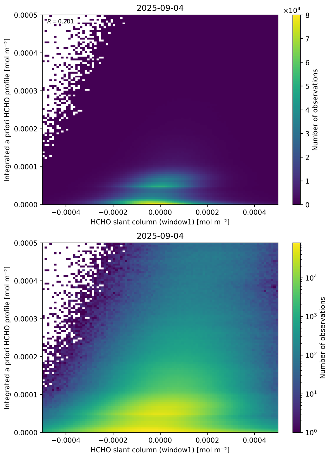
Figure 87: Scatter density plot of “HCHO slant column (window1)” against “Integrated a priori HCHO profile” for 2025-09-04 to 2025-09-05.
