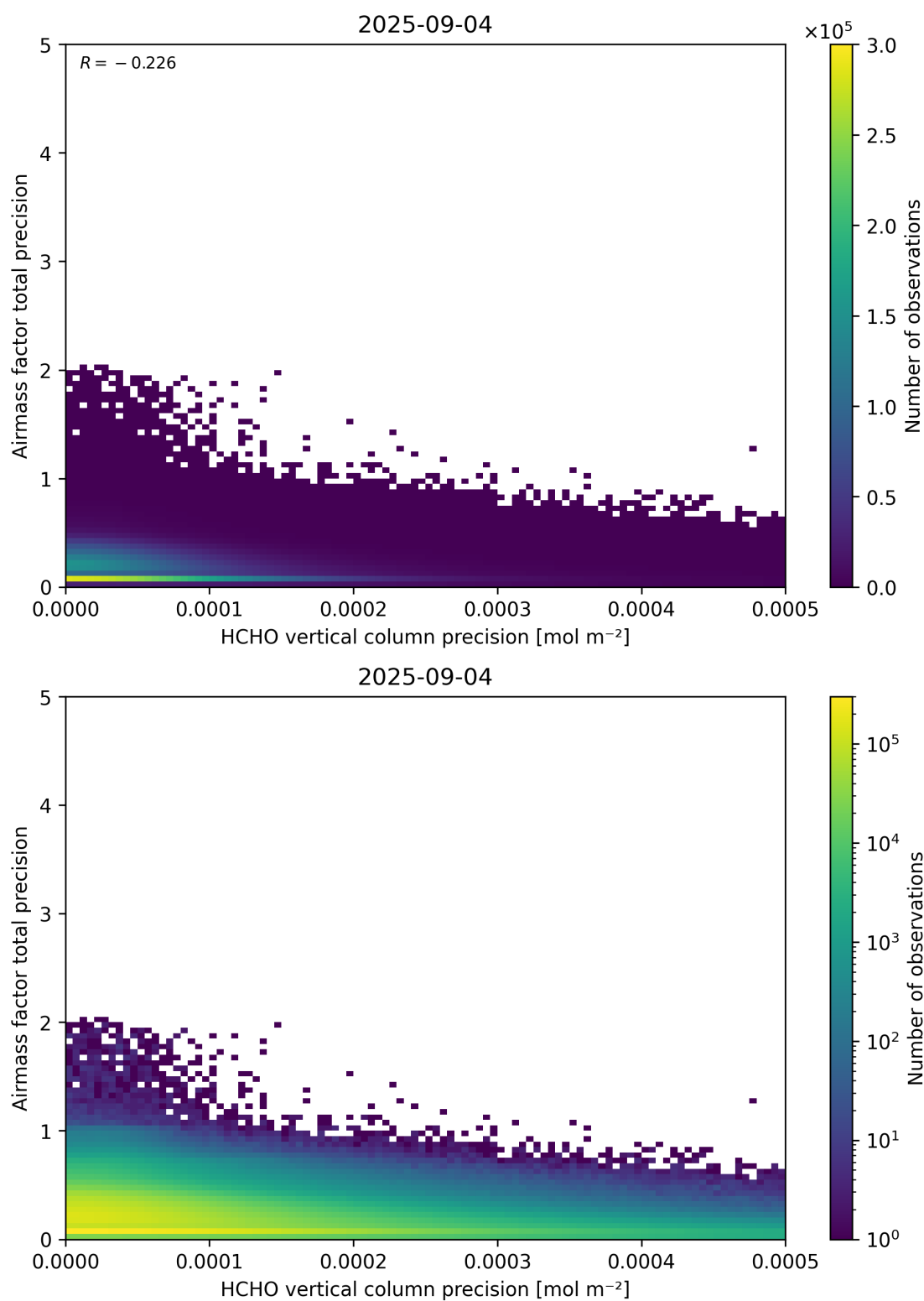
Figure 145: Scatter density plot of “HCHO vertical column precision” against “Airmass factor total precision” for 2025-09-04 to 2025-09-05.
