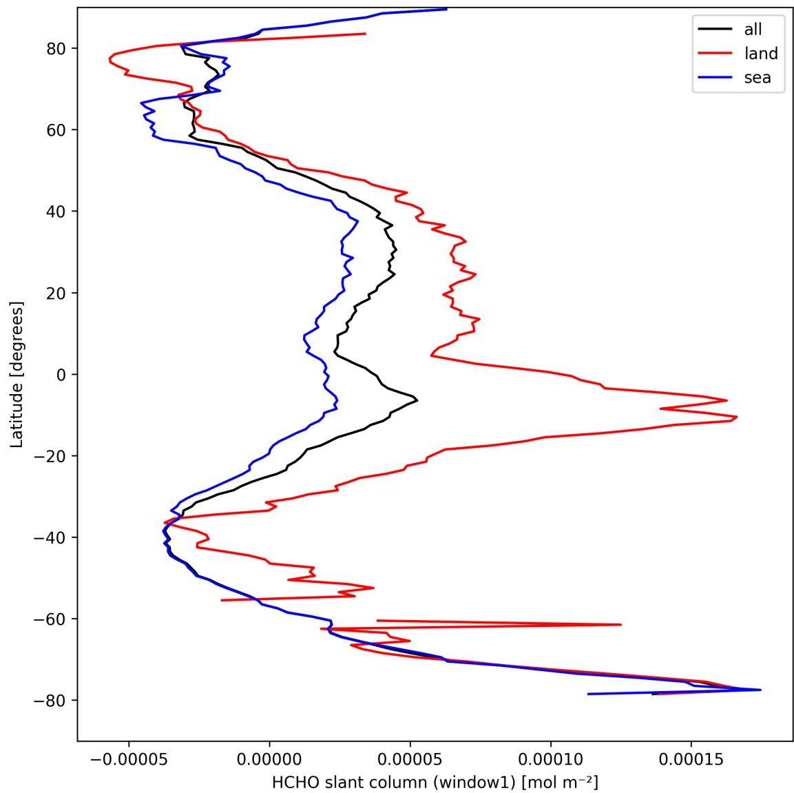
Figure 24: Zonal average of “HCHO slant column (window1)” for 2025-09-04 to 2025-09-05.
