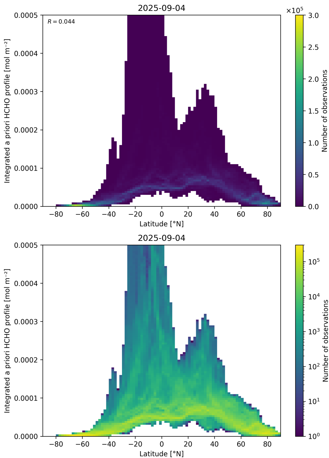
Figure 166: Scatter density plot of “Latitude” against “Integrated a priori HCHO profile” for 2025-09-04 to 2025-09-05.
