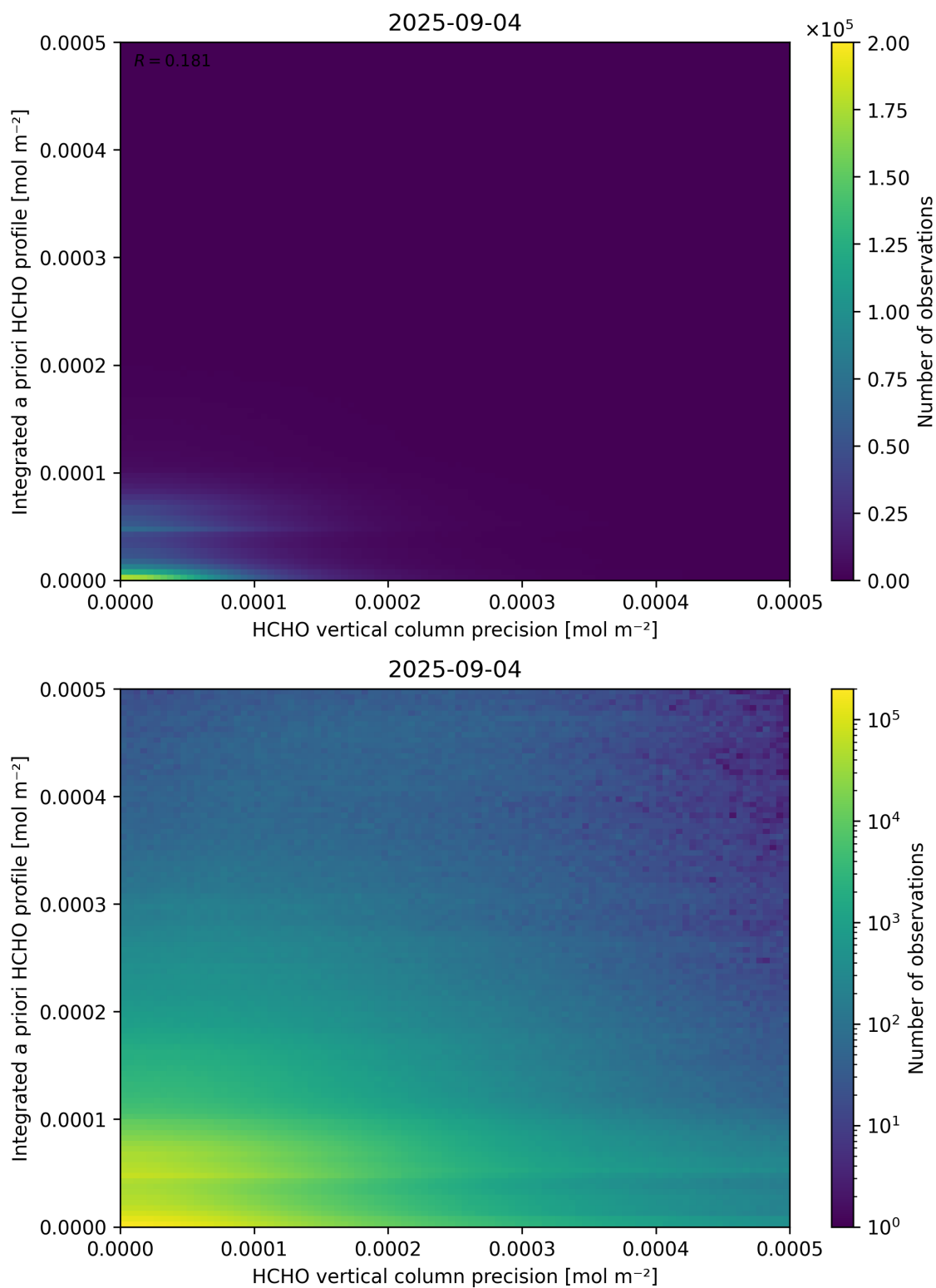
Figure 147: Scatter density plot of “HCHO vertical column precision” against “Integrated a priori HCHO profile” for 2025-09-04 to 2025-09-05.
