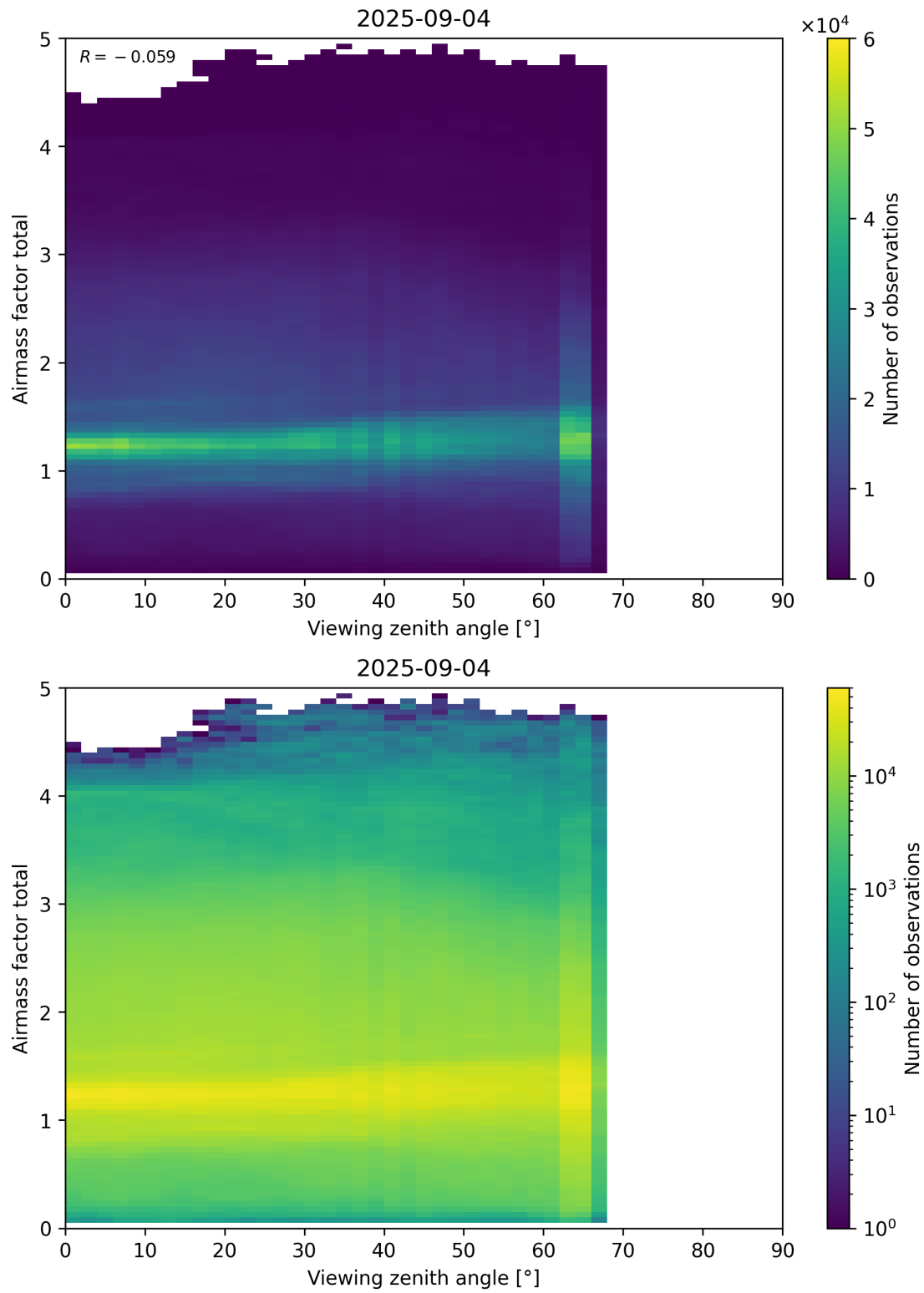
Figure 190: Scatter density plot of “Viewing zenith angle” against “Airmass factor total” for 2025-09-04 to 2025-09-05.
