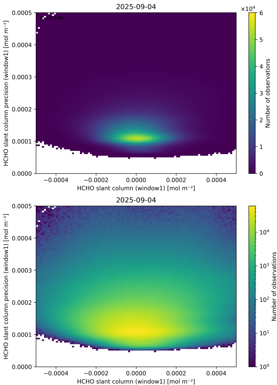
Figure 84: Scatter density plot of “HCHO slant column (window1)” against “HCHO slant column precision (window1)” for 2025-09-04 to 2025-09-05.
