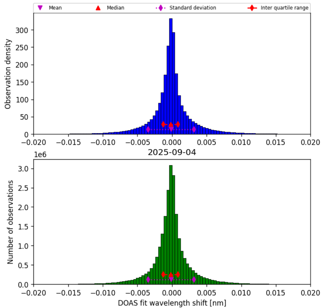
Figure 44: Histogram of “DOAS fit wavelength shift” for 2025-09-04 to 2025-09-05
