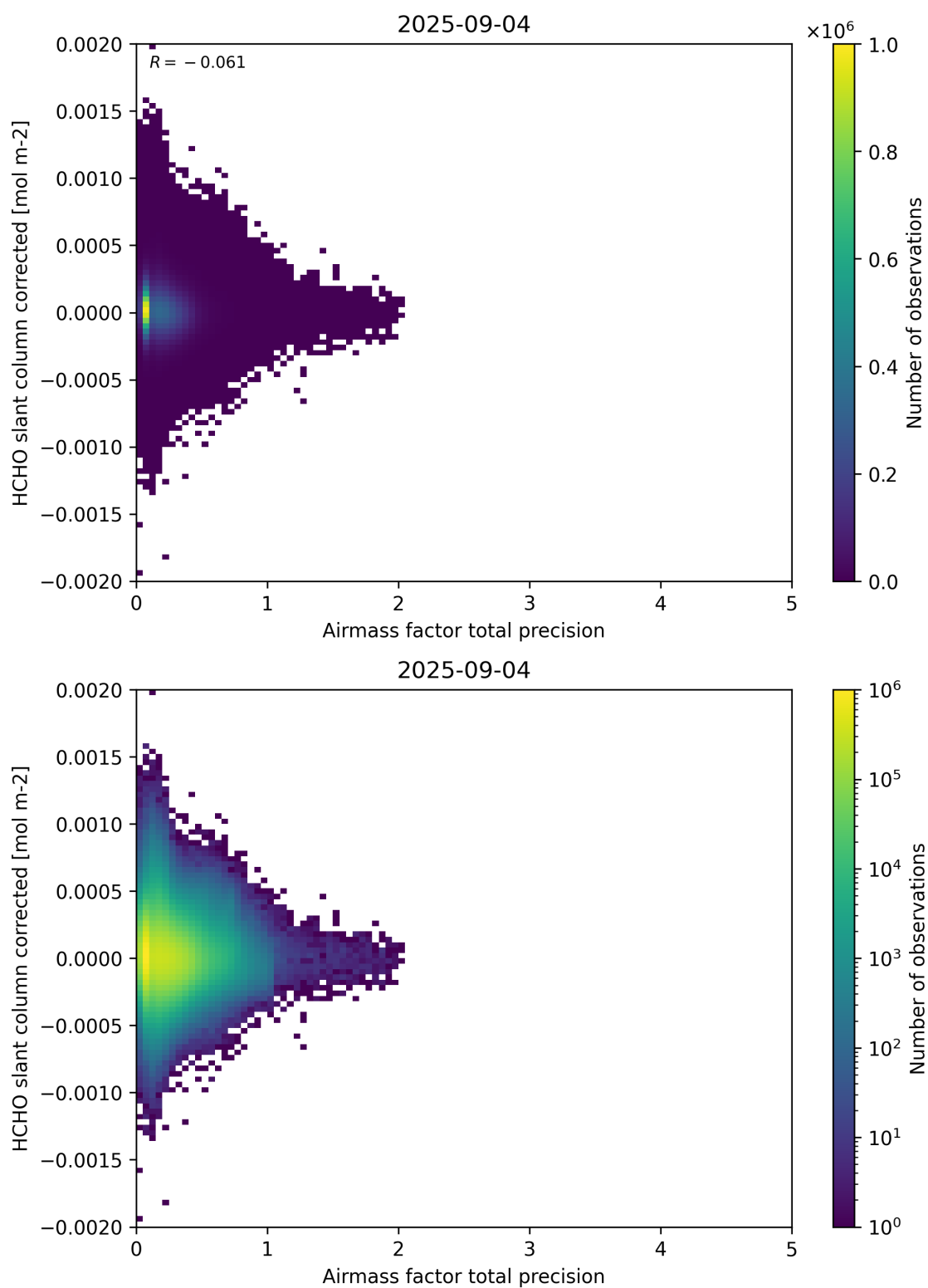
Figure 109: Scatter density plot of “Airmass factor total precision” against “HCHO slant column corrected” for 2025-09-04 to 2025-09-05.
