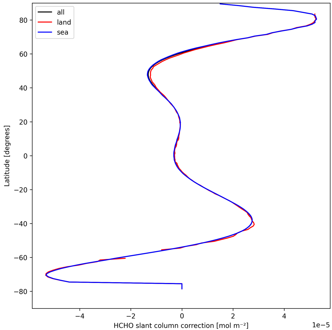
Figure 33: Zonal average of “HCHO slant column correction” for 2025-09-04 to 2025-09-05.
