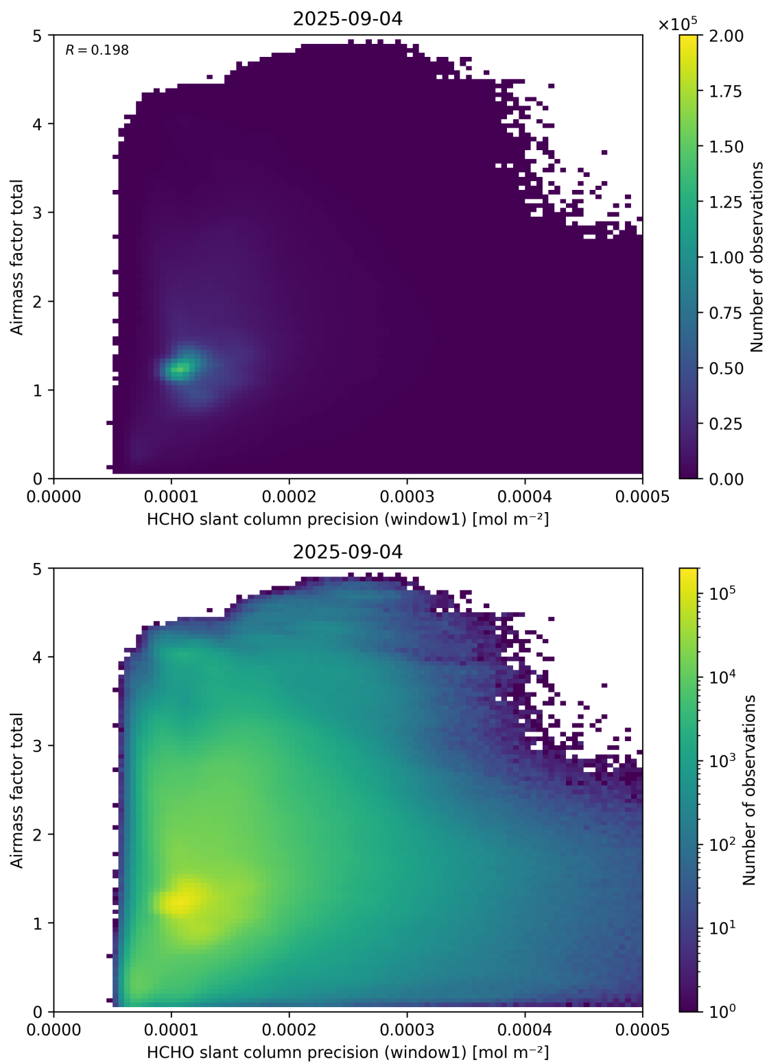
Figure 94: Scatter density plot of “HCHO slant column precision (window1)” against “Airmass factor total” for 2025-09-04 to 2025-09-05.
