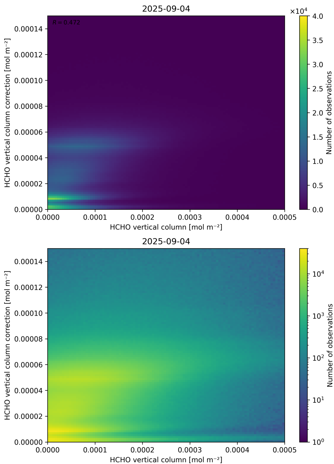
Figure 133: Scatter density plot of “HCHO vertical column” against “HCHO vertical column correction” for 2025-09-04 to 2025-09-05.
