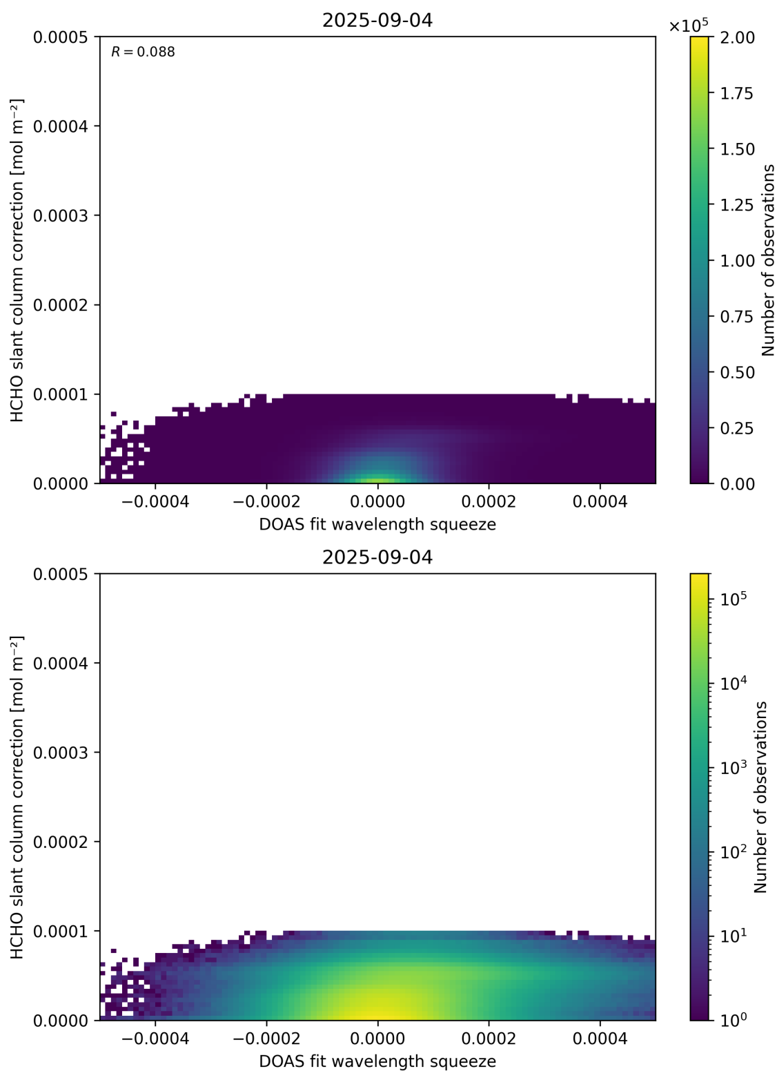
Figure 70: Scatter density plot of “DOAS fit wavelength squeeze” against “HCHO slant column correction” for 2025-09-04 to 2025-09-05.
