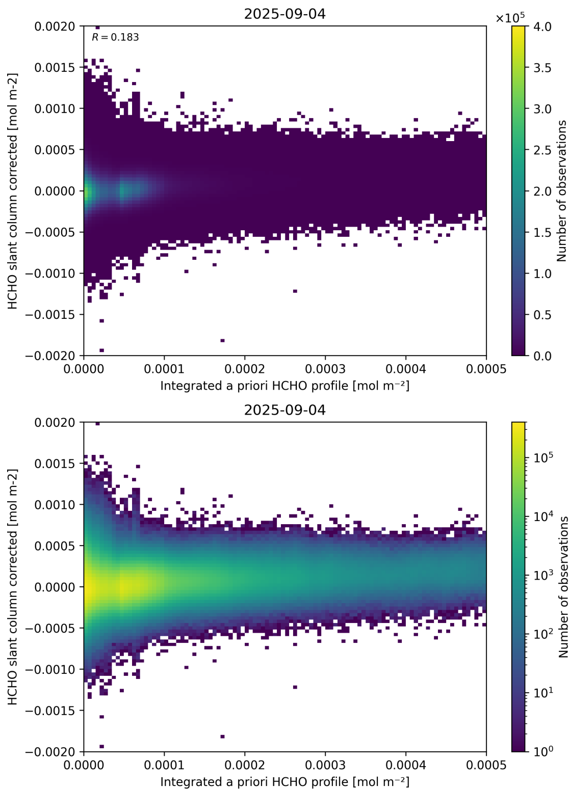
Figure 151: Scatter density plot of “Integrated a priori HCHO profile” against “HCHO slant column corrected” for 2025-09-04 to 2025-09-05.
