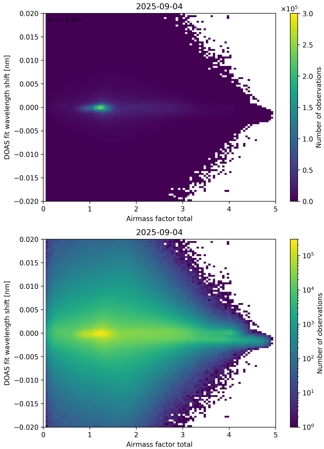
Figure 98: Scatter density plot of “Airmass factor total” against “DOAS fit wavelength shift” for 2025-09-04 to 2025-09-05.
