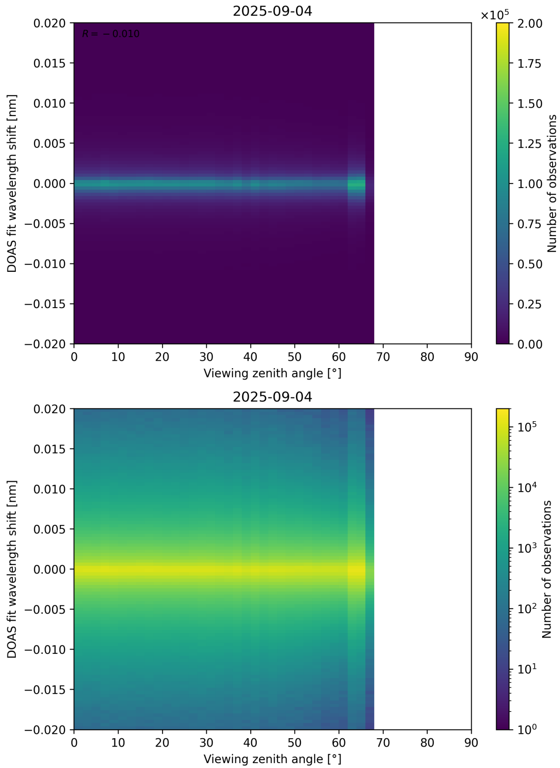
Figure 183: Scatter density plot of “Viewing zenith angle” against “DOAS fit wavelength shift” for 2025-09-04 to 2025-09-05.
