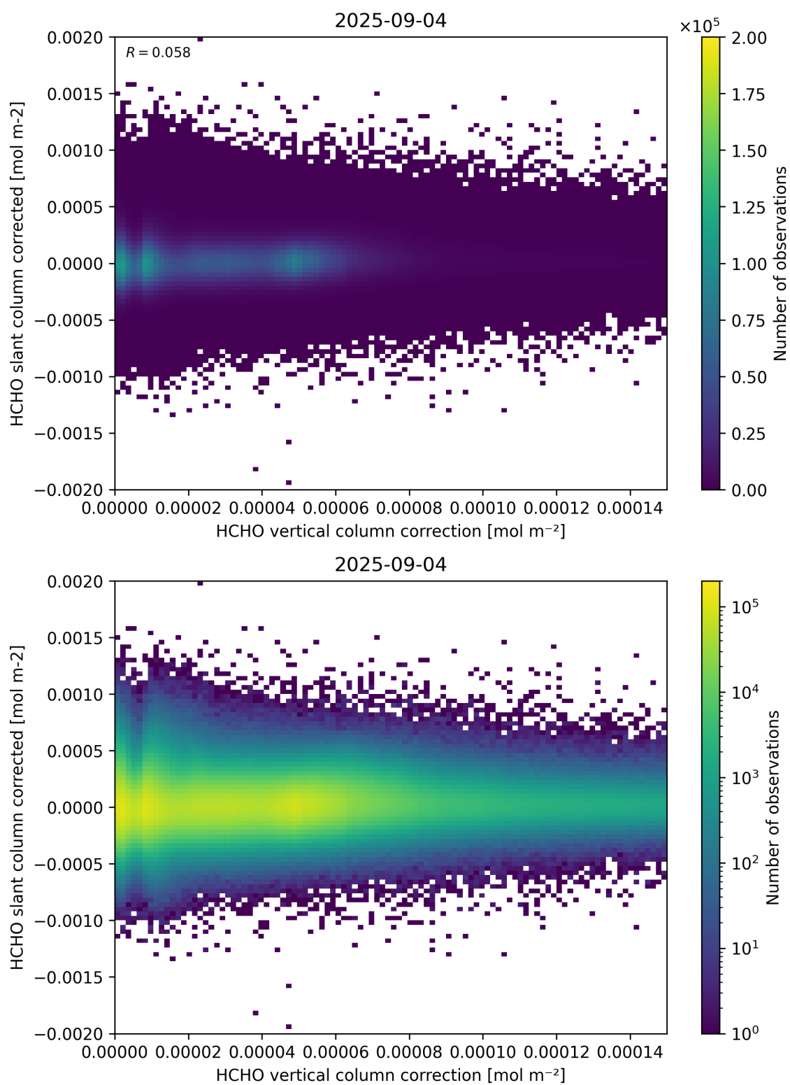
Figure 116: Scatter density plot of “HCHO vertical column correction” against “HCHO slant column corrected” for 2025-09-04 to 2025-09-05.
