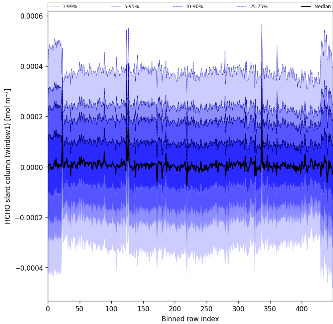
Figure 52: Along track statistics of “HCHO slant column (window1)” for 2025-09-04 to 2025-09-05
