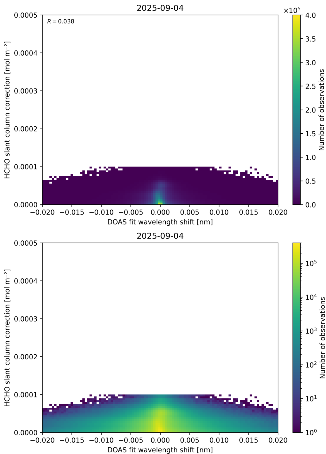
Figure 67: Scatter density plot of “DOAS fit wavelength shift” against “HCHO slant column correction” for 2025-09-04 to 2025-09-05.
