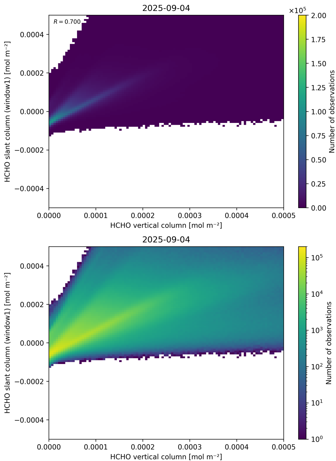
Figure 129: Scatter density plot of “HCHO vertical column” against “HCHO slant column (window1)” for 2025-09-04 to 2025-09-05.
