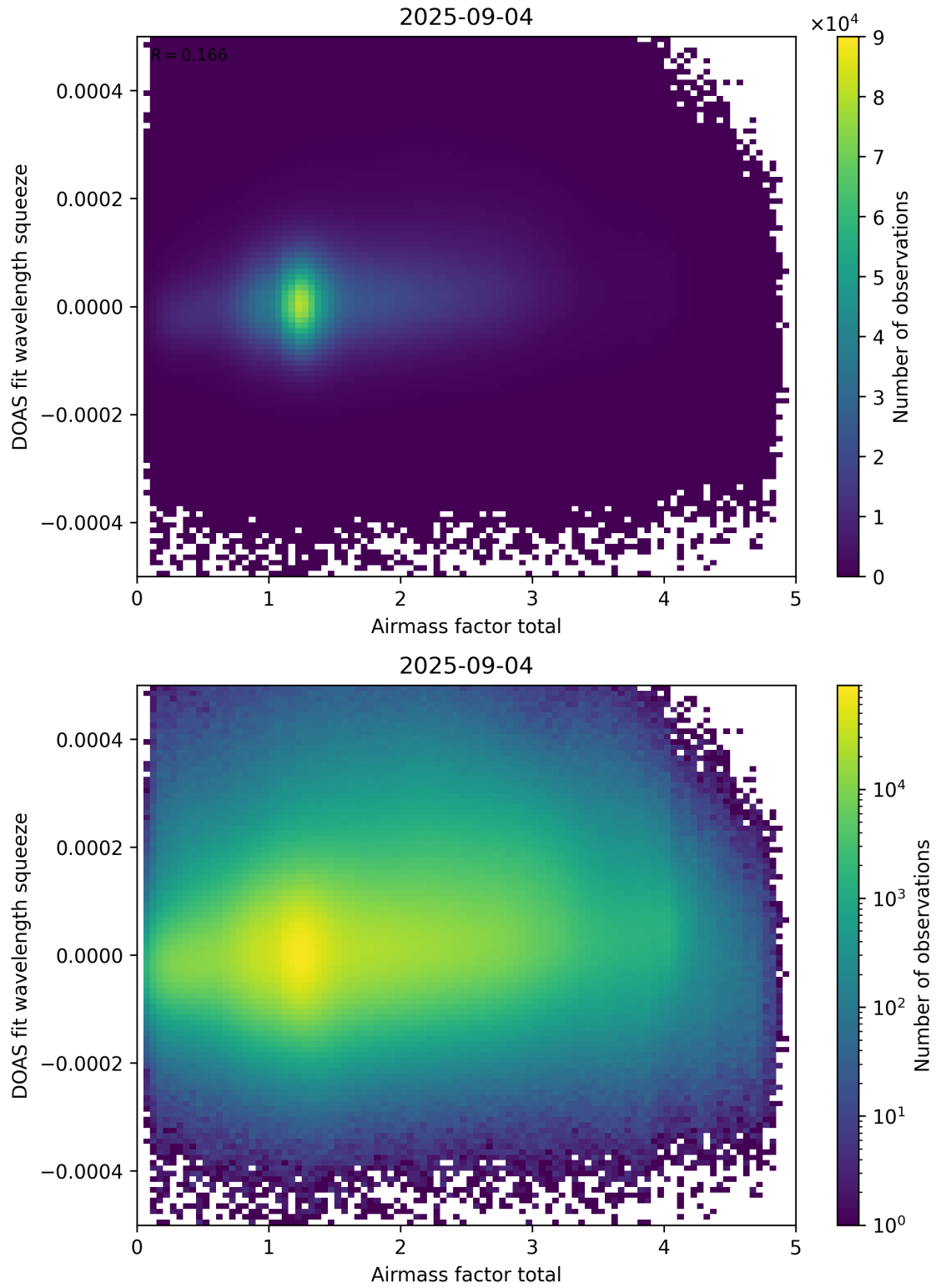
Figure 99: Scatter density plot of “Airmass factor total” against “DOAS fit wavelength squeeze” for 2025-09-04 to 2025-09-05.
