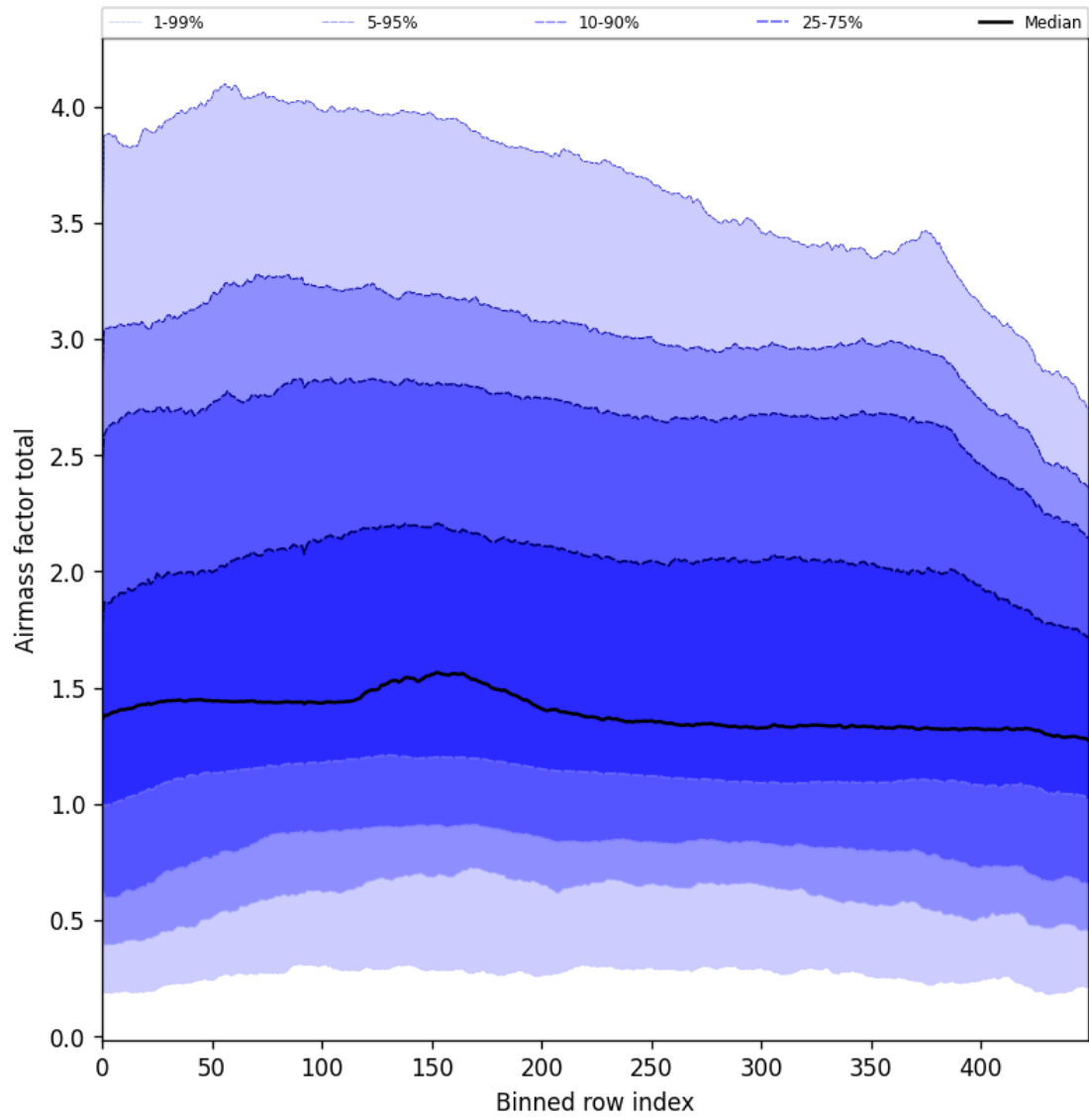
Figure 54: Along track statistics of “Airmass factor total” for 2025-09-04 to 2025-09-05
