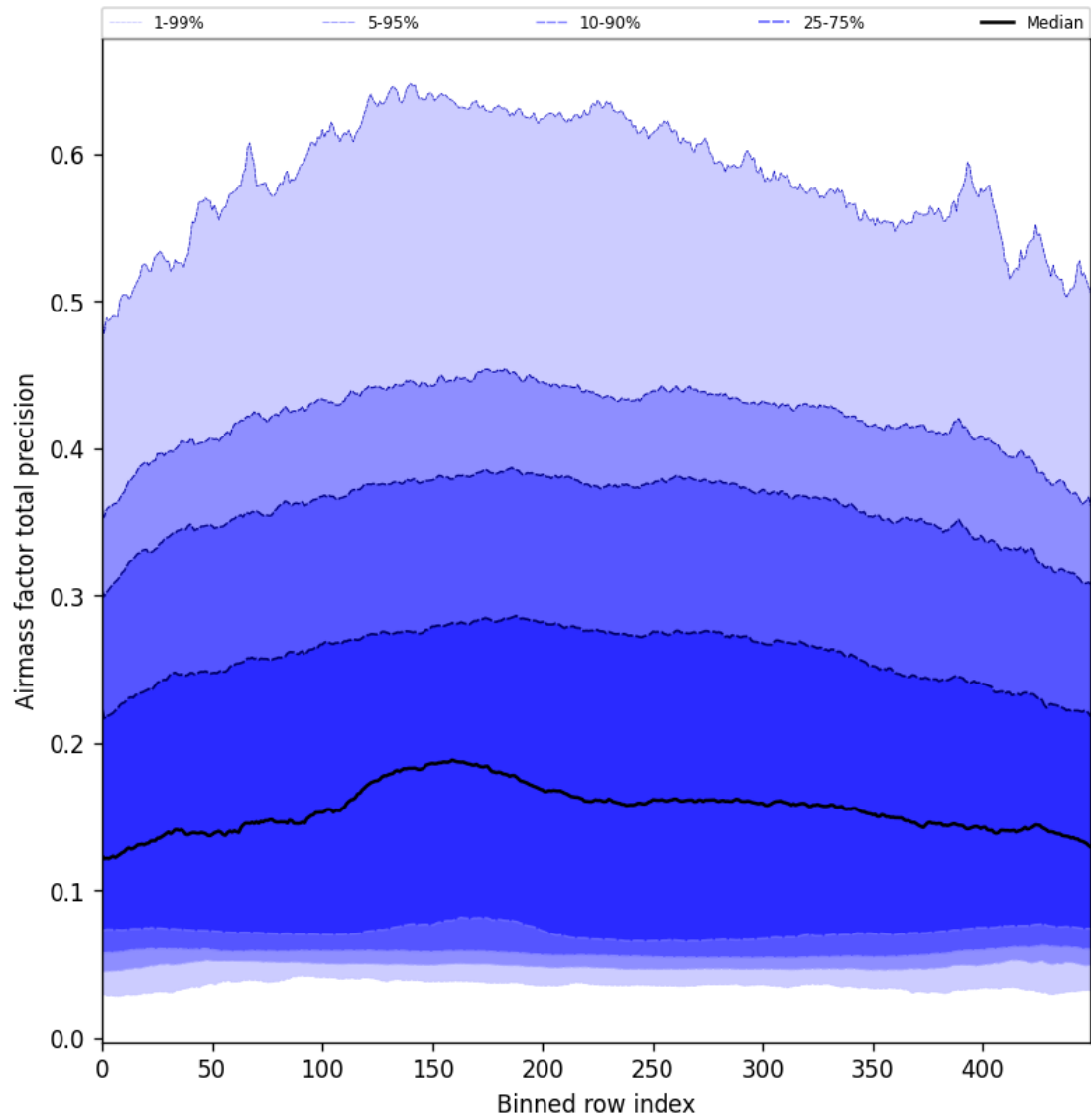
Figure 55: Along track statistics of “Airmass factor total precision” for 2025-09-04 to 2025-09-05
