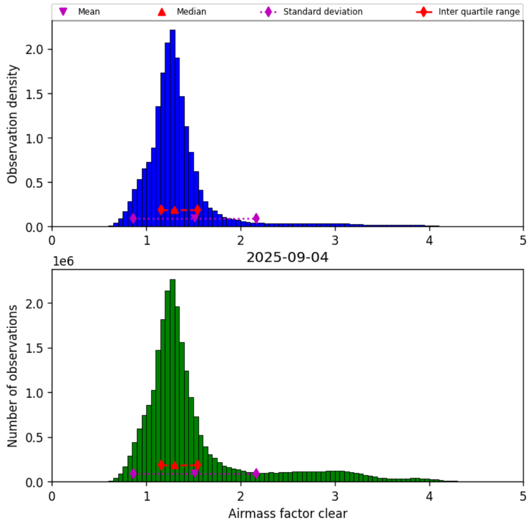
Figure 42: Histogram of “Airmass factor clear” for 2025-09-04 to 2025-09-05
