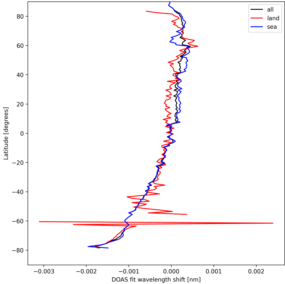
Figure 30: Zonal average of “DOAS fit wavelength shift” for 2025-09-04 to 2025-09-05.
