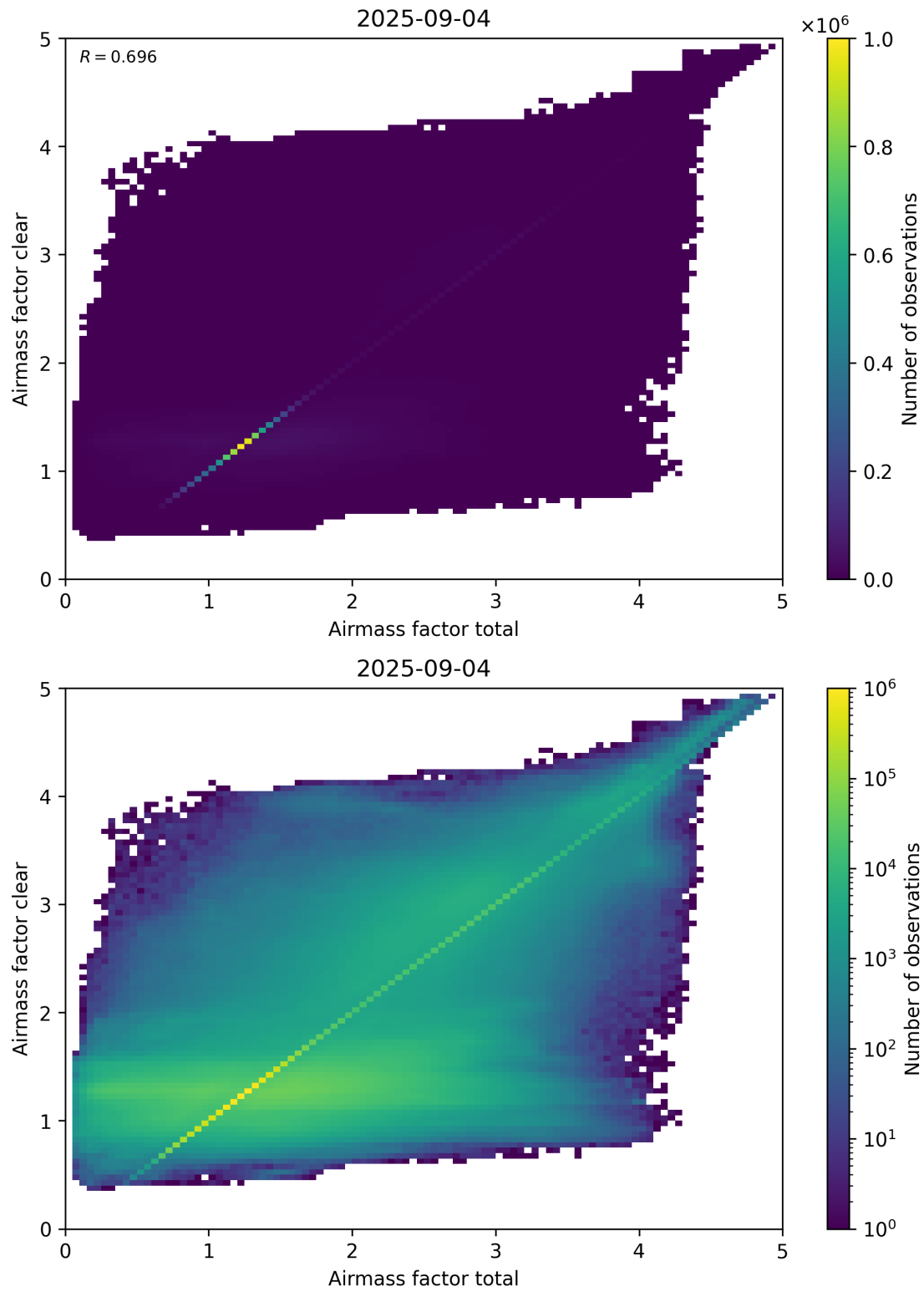
Figure 100: Scatter density plot of “Airmass factor total” against “Airmass factor clear” for 2025-09-04 to 2025-09-05.
