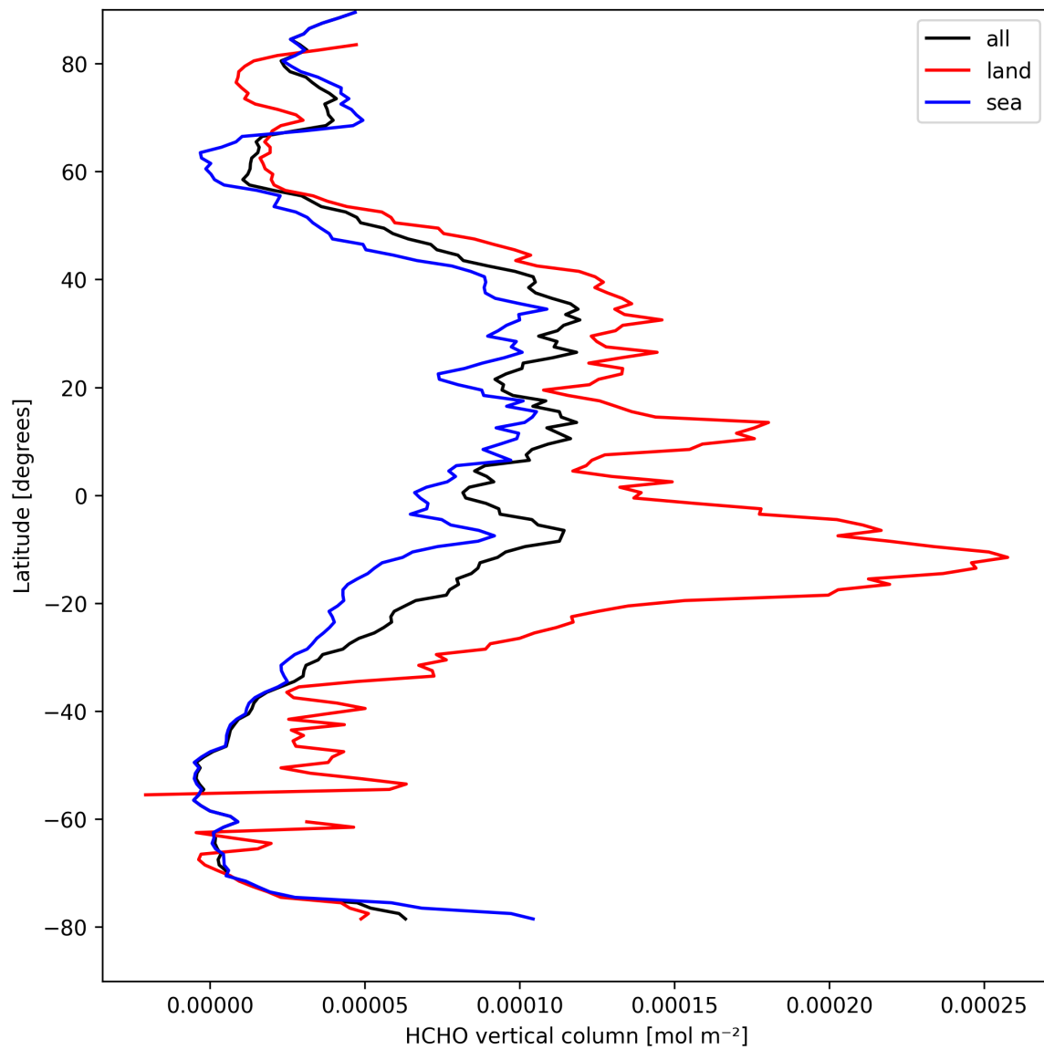
Figure 21: Zonal average of “HCHO vertical column” for 2025-09-04 to 2025-09-05.
