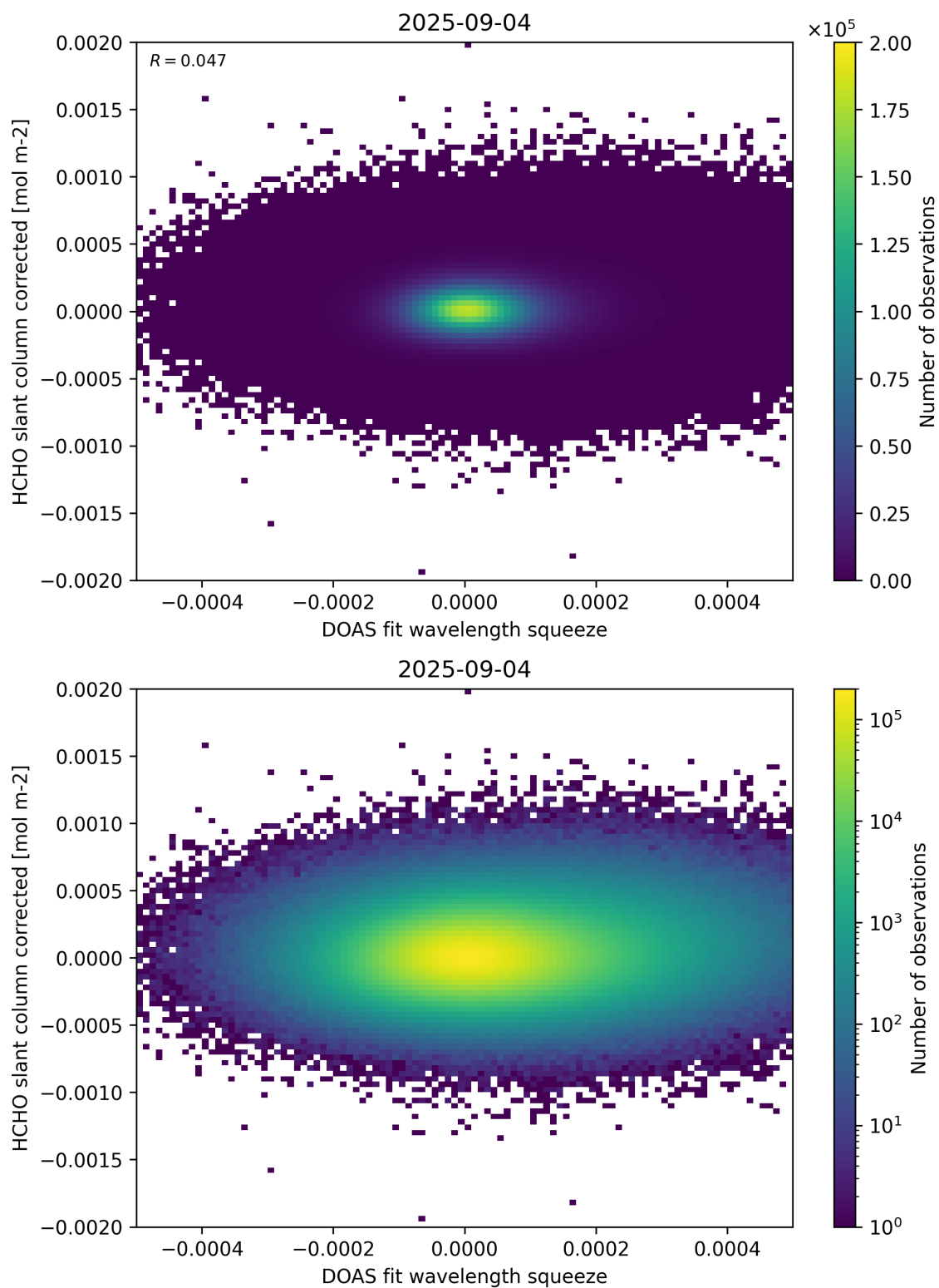
Figure 69: Scatter density plot of “DOAS fit wavelength squeeze” against “HCHO slant column corrected” for 2025-09-04 to 2025-09-05.
