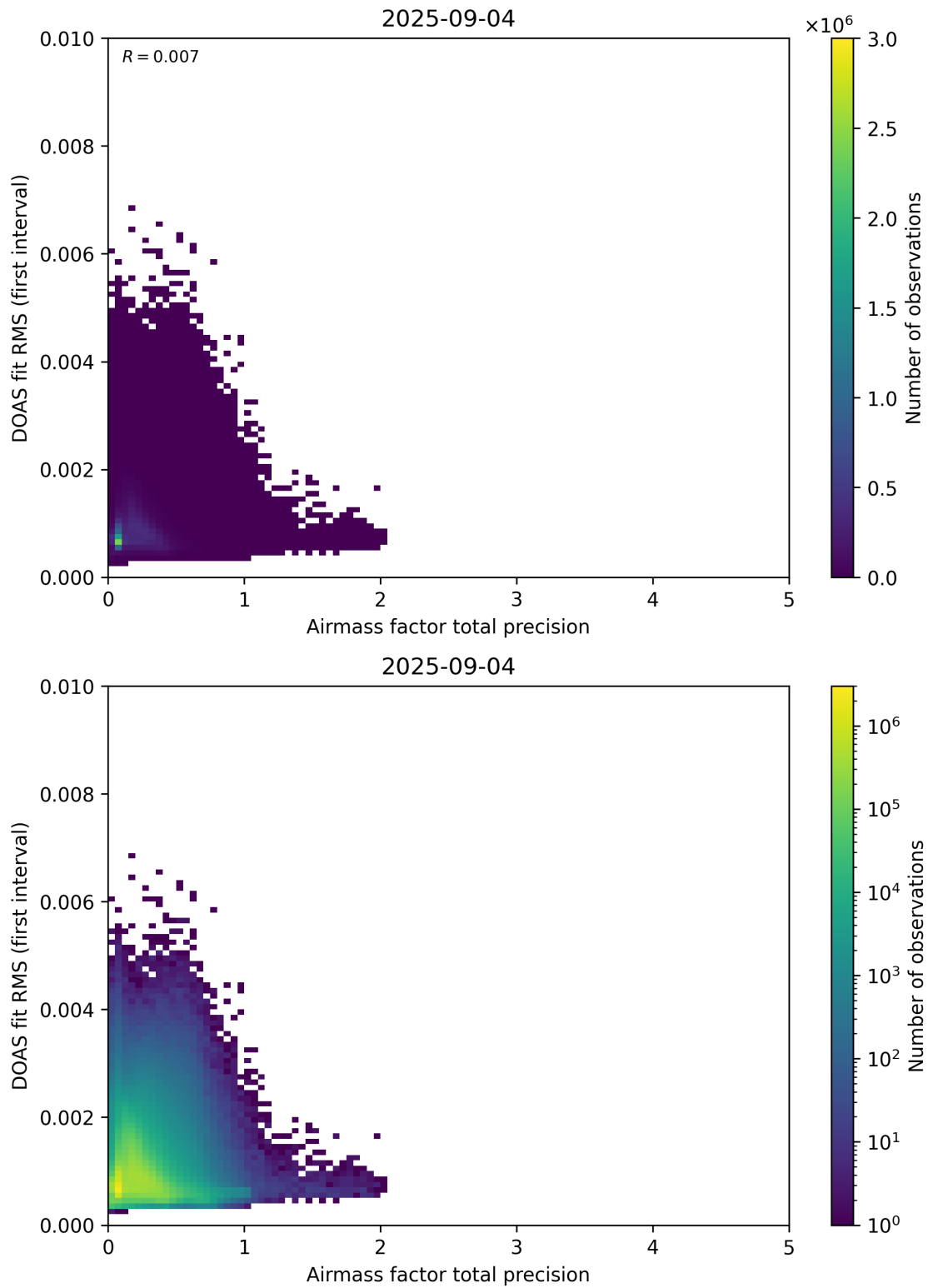
Figure 105: Scatter density plot of “Airmass factor total precision” against “DOAS fit RMS (first interval)” for 2025-09-04 to 2025-09-05.
