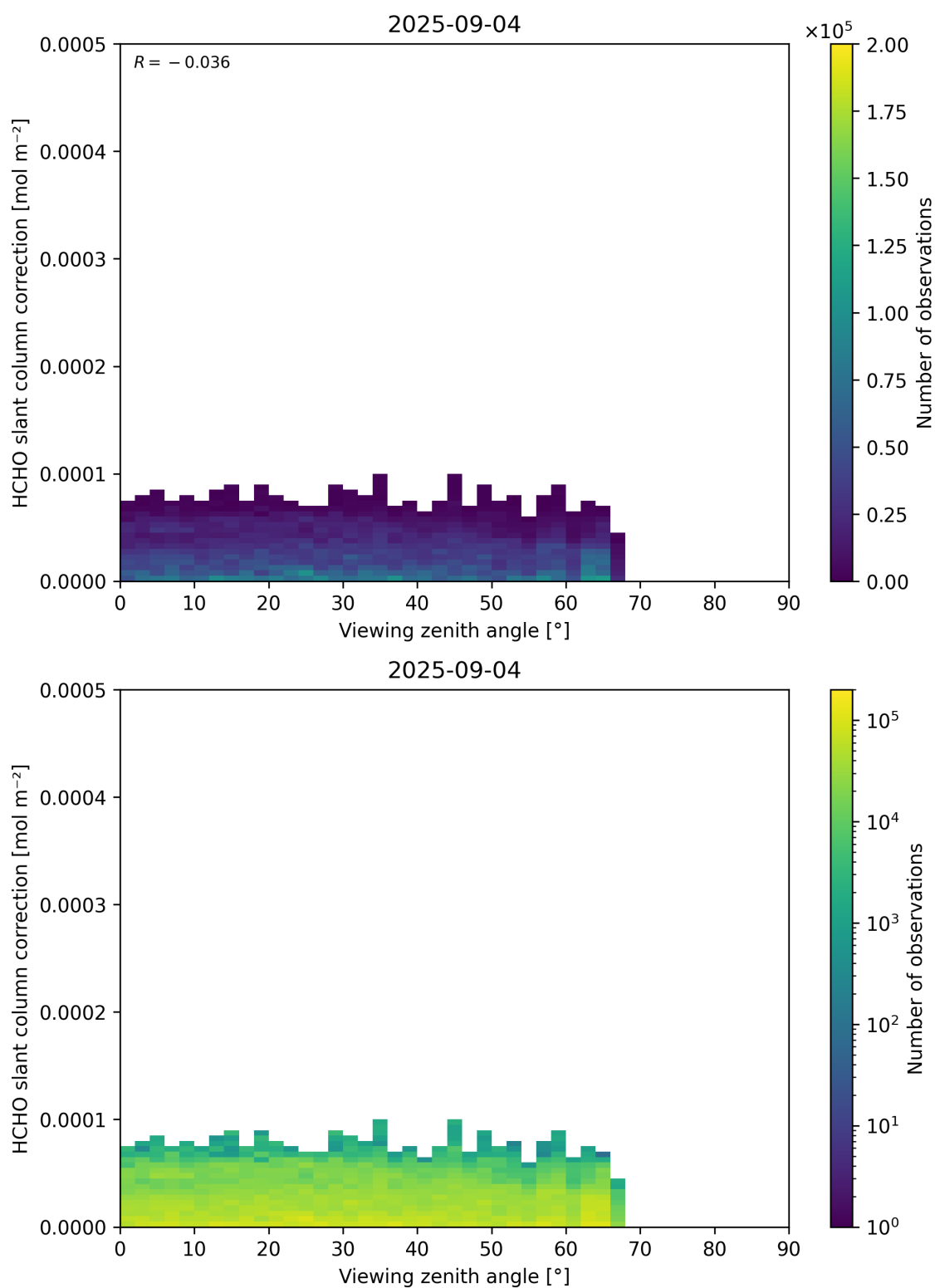
Figure 187: Scatter density plot of “Viewing zenith angle” against “HCHO slant column correction” for 2025-09-04 to 2025-09-05.
