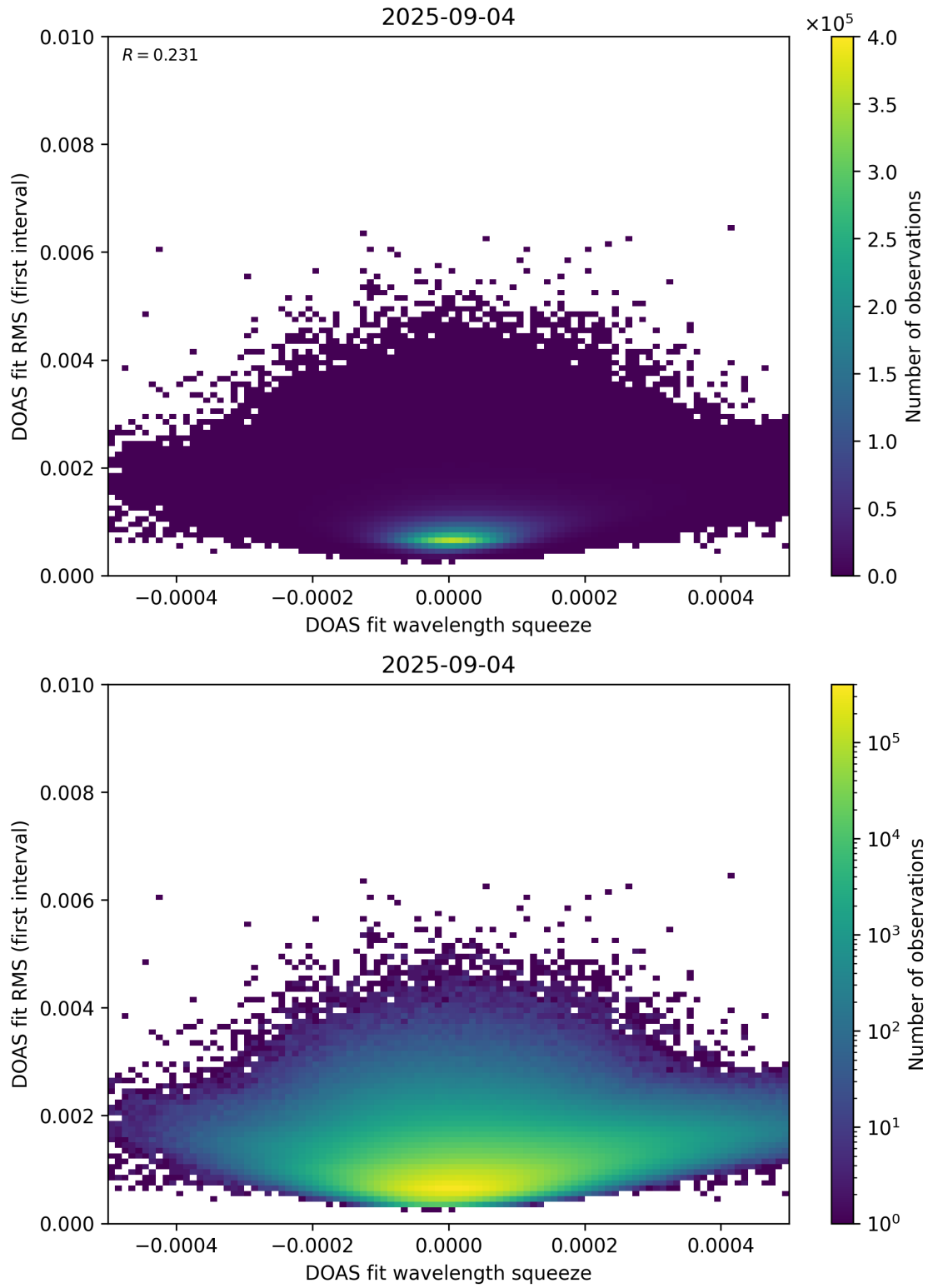
Figure 68: Scatter density plot of “DOAS fit wavelength squeeze” against “DOAS fit RMS (first interval)” for 2025-09-04 to 2025-09-05.
