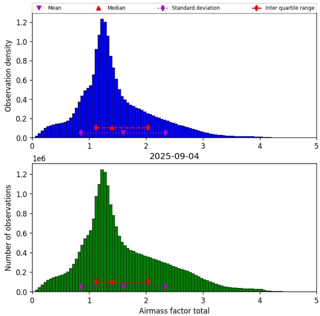
Figure 40: Histogram of “Airmass factor total” for 2025-09-04 to 2025-09-05
