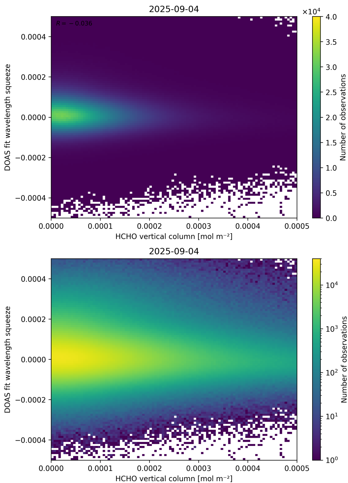
Figure 125: Scatter density plot of “HCHO vertical column” against “DOAS fit wavelength squeeze” for 2025-09-04 to 2025-09-05.
