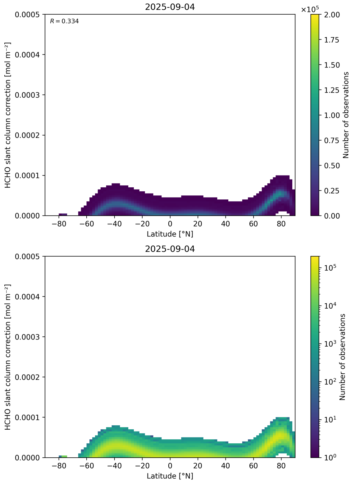
Figure 158: Scatter density plot of “Latitude” against “HCHO slant column correction” for 2025-09-04 to 2025-09-05.
