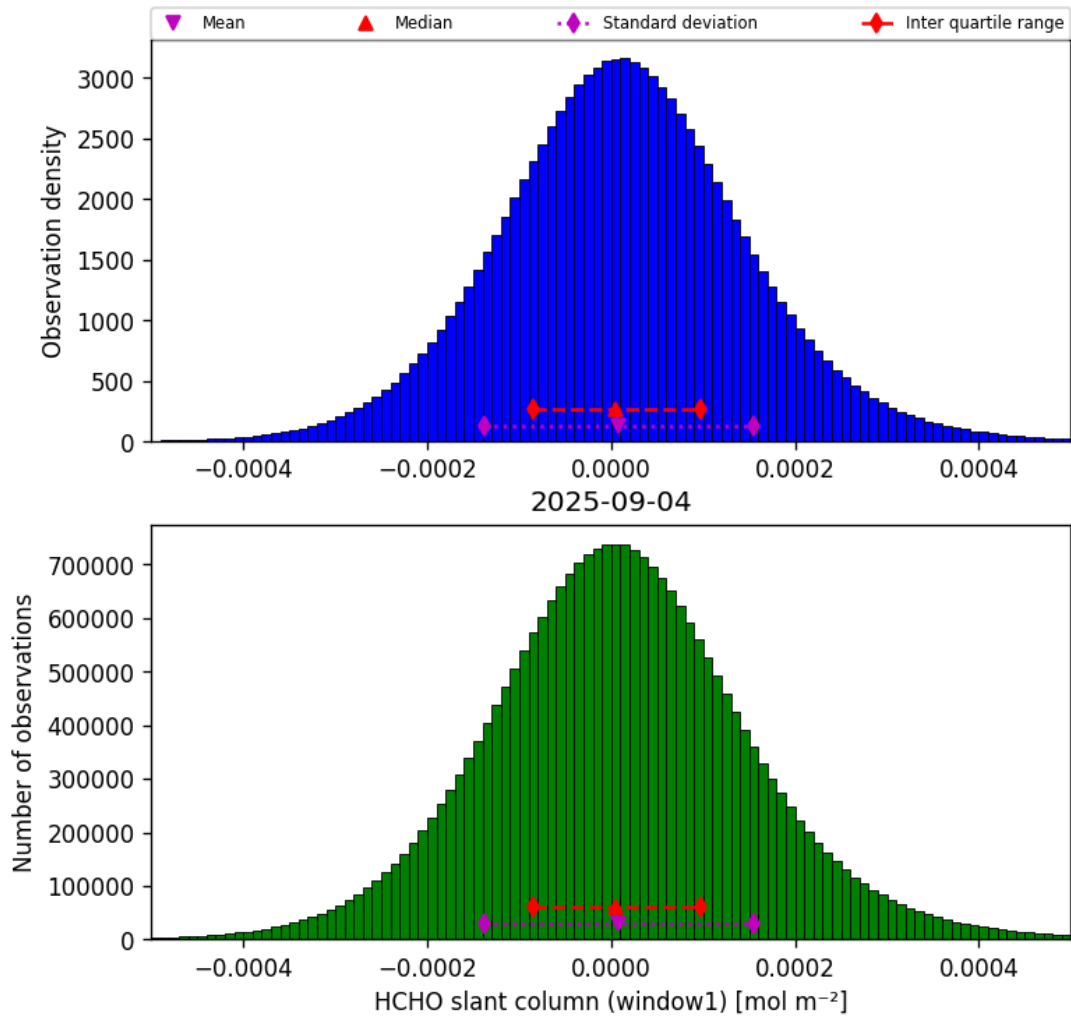
Figure 38: Histogram of “HCHO slant column (window1)” for 2025-09-04 to 2025-09-05
