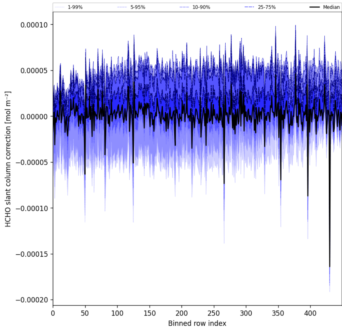
Figure 61: Along track statistics of “HCHO slant column correction” for 2025-09-04 to 2025-09-05
