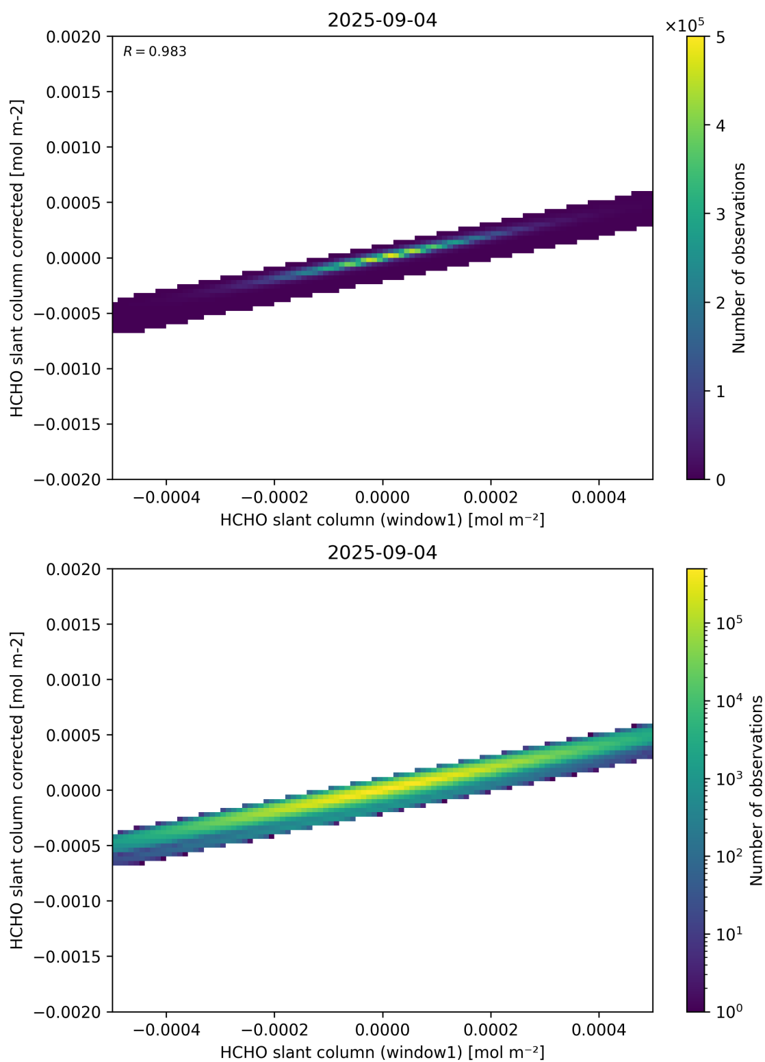
Figure 82: Scatter density plot of “HCHO slant column (window1)” against “HCHO slant column corrected” for 2025-09-04 to 2025-09-05.
