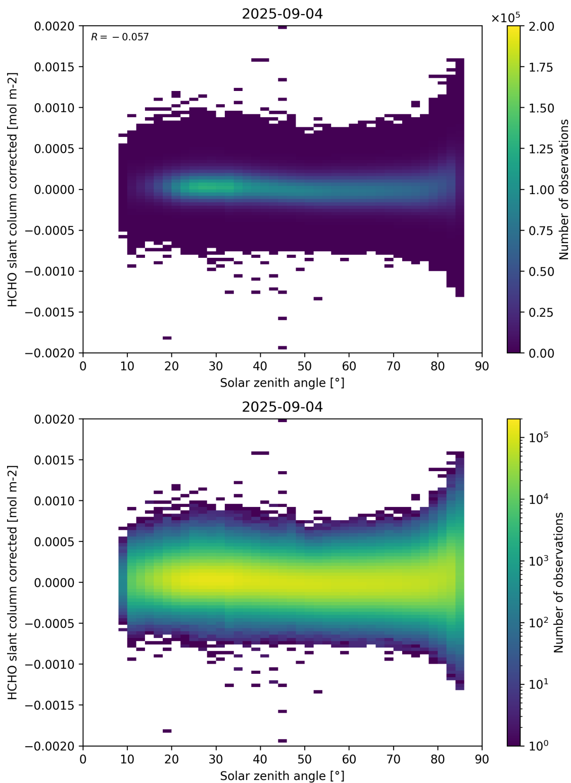
Figure 171: Scatter density plot of “Solar zenith angle” against “HCHO slant column corrected” for 2025-09-04 to 2025-09-05.
