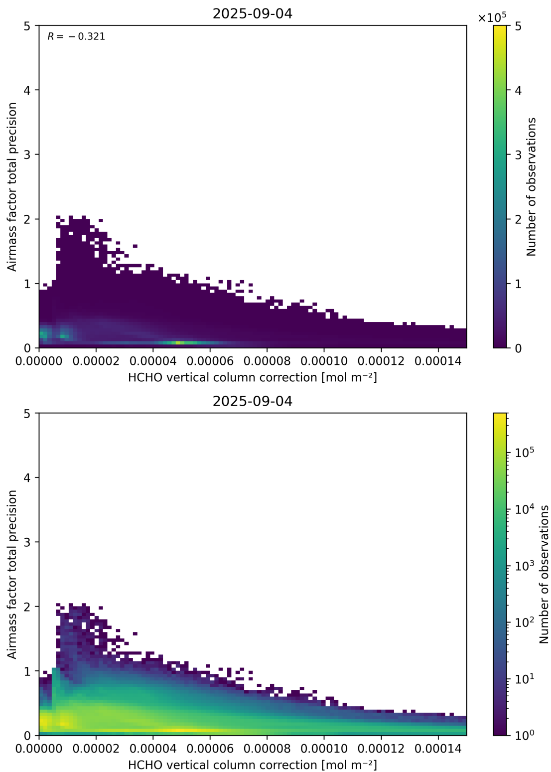
Figure 121: Scatter density plot of “HCHO vertical column correction” against “Airmass factor total precision” for 2025-09-04 to 2025-09-05.
