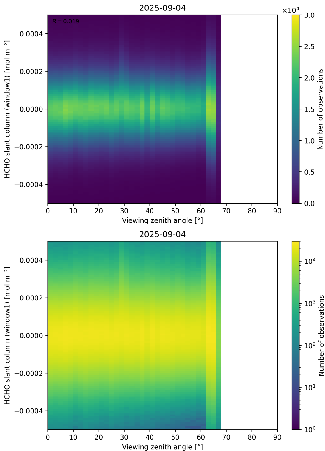
Figure 188: Scatter density plot of “Viewing zenith angle” against “HCHO slant column (window1)” for 2025-09-04 to 2025-09-05.
