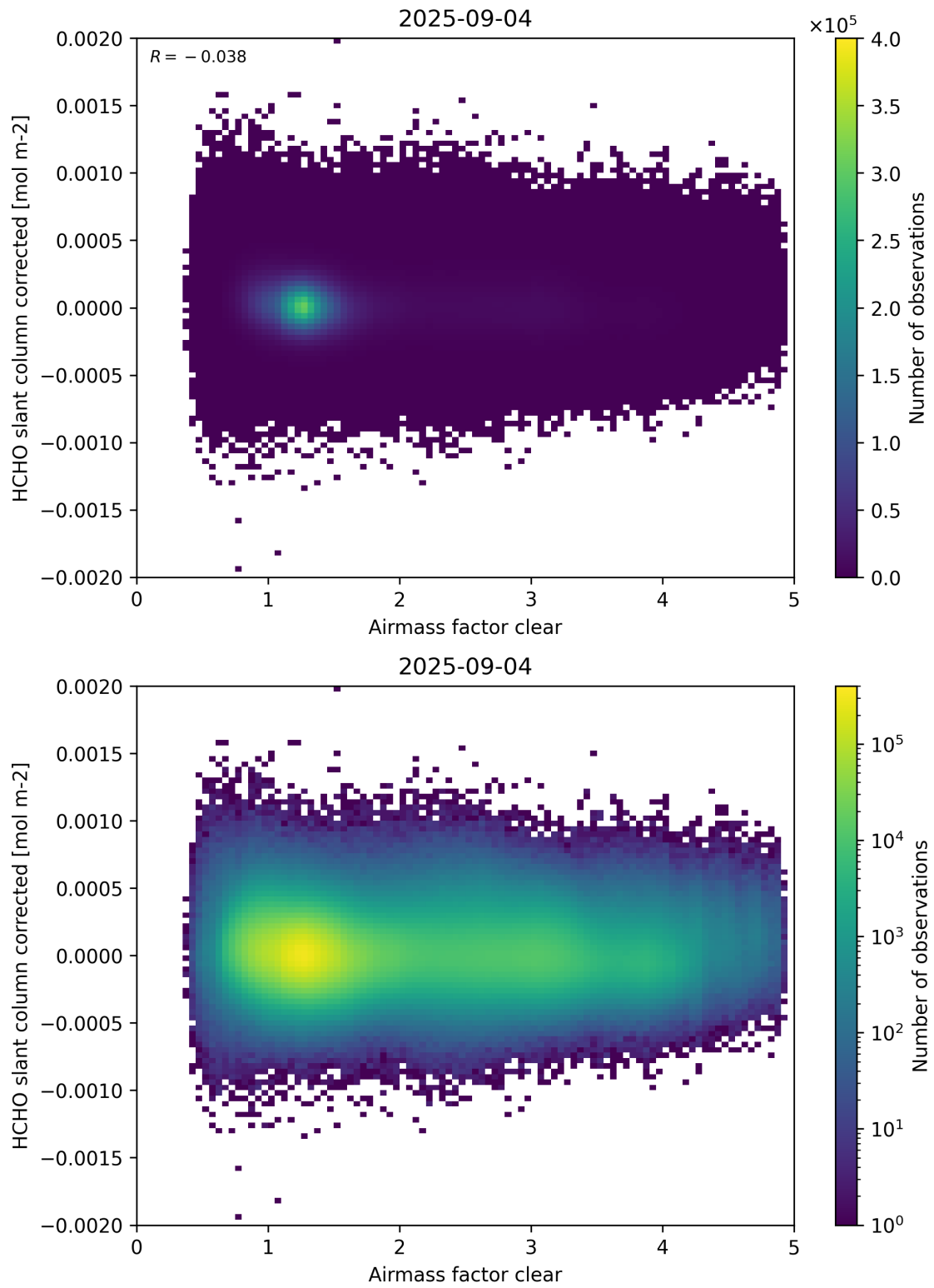
Figure 74: Scatter density plot of “Airmass factor clear” against “HCHO slant column corrected” for 2025-09-04 to 2025-09-05.
