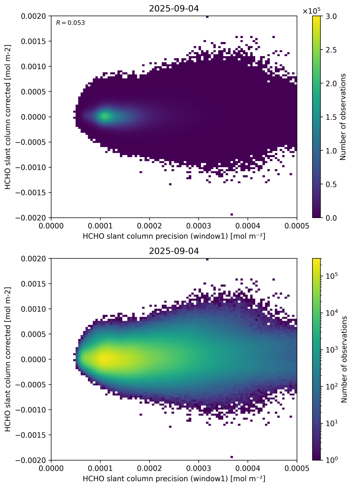
Figure 92: Scatter density plot of “HCHO slant column precision (window1)” against “HCHO slant column corrected” for 2025-09-04 to 2025-09-05.
