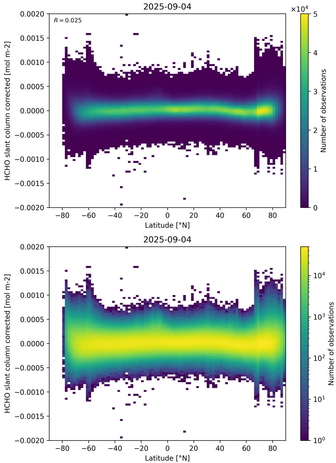
Figure 157: Scatter density plot of “Latitude” against “HCHO slant column corrected” for 2025-09-04 to 2025-09-05.
