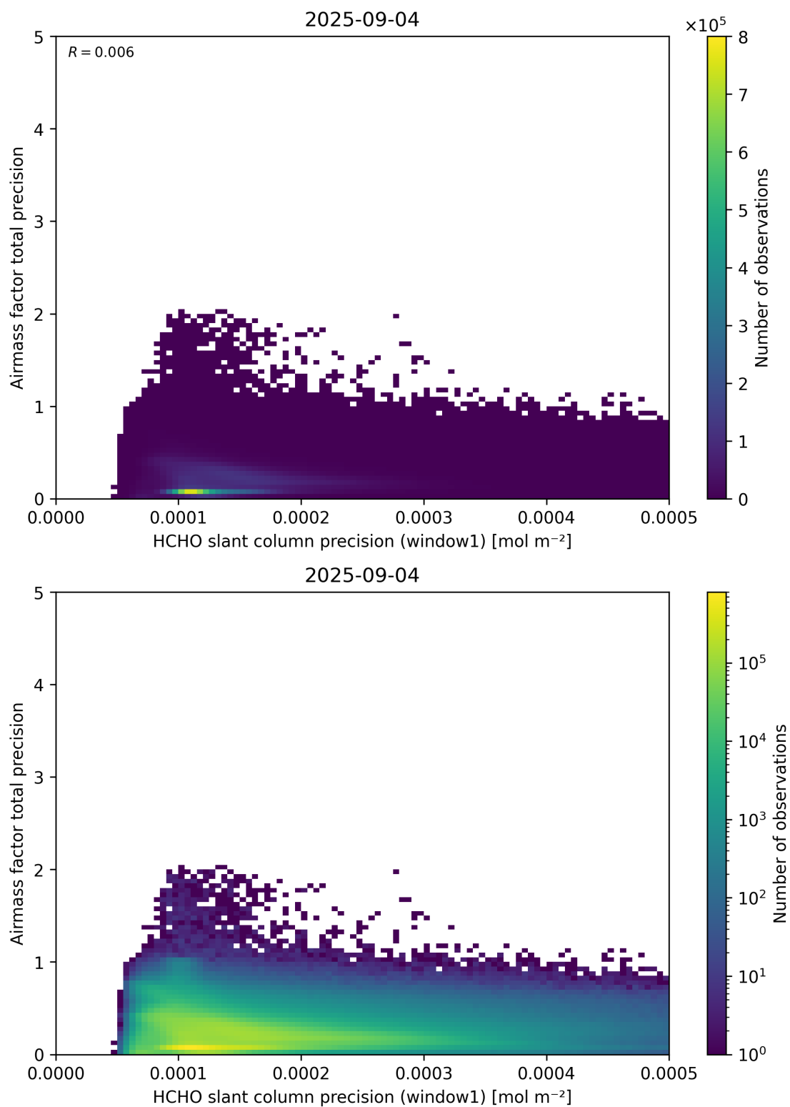
Figure 95: Scatter density plot of “HCHO slant column precision (window1)” against “Airmass factor total precision” for 2025-09-04 to 2025-09-05.
