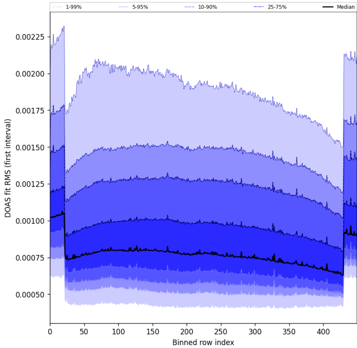
Figure 60: Along track statistics of “DOAS fit RMS (first interval)” for 2025-09-04 to 2025-09-05
