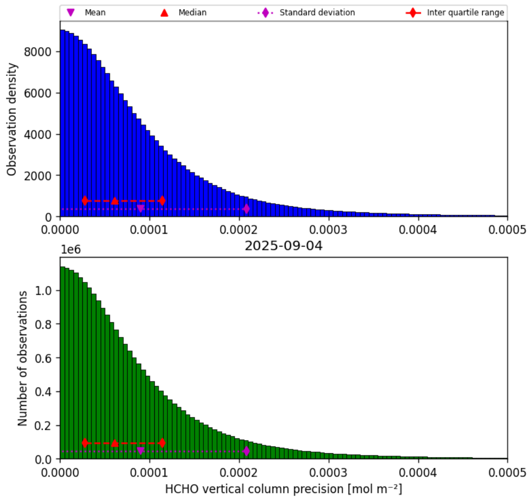
Figure 36: Histogram of “HCHO vertical column precision” for 2025-09-04 to 2025-09-05
