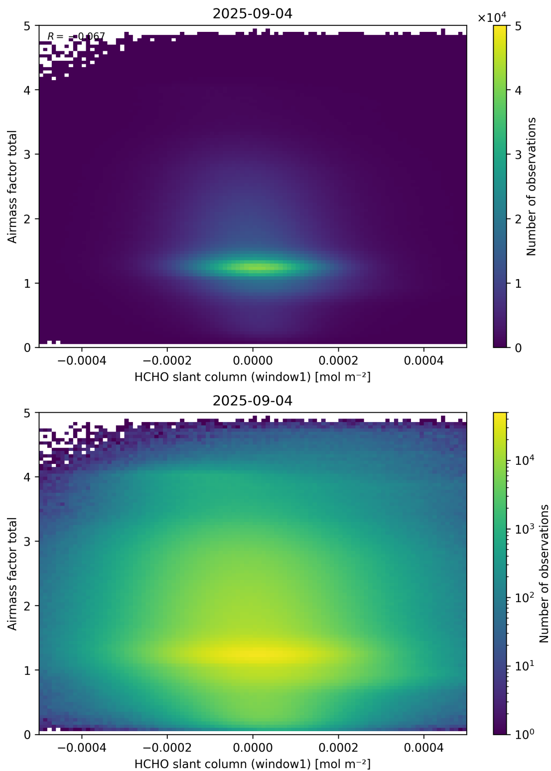
Figure 85: Scatter density plot of “HCHO slant column (window1)” against “Airmass factor total” for 2025-09-04 to 2025-09-05.
