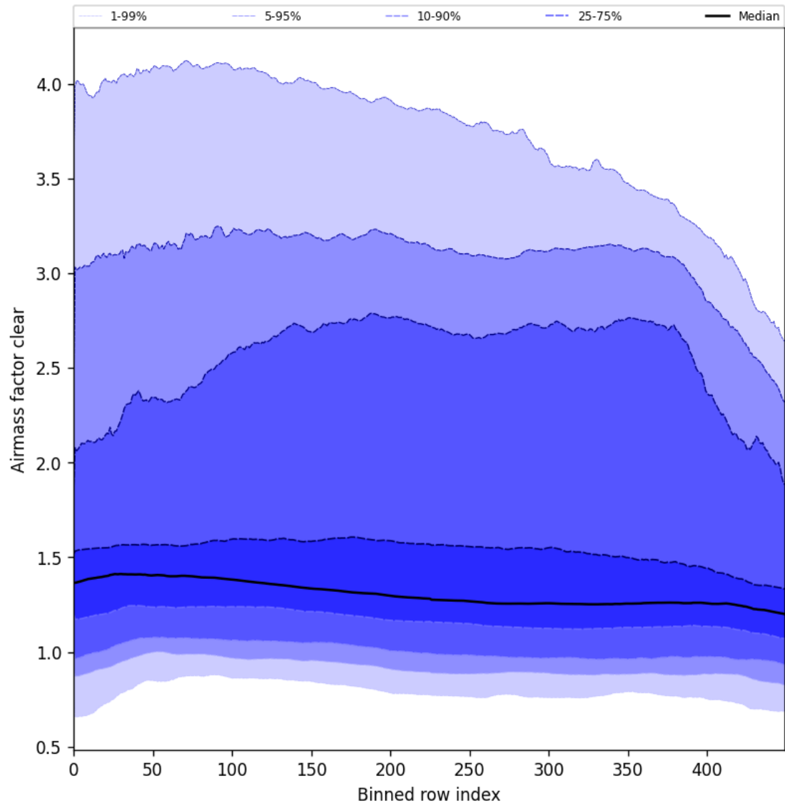
Figure 56: Along track statistics of “Air mass factor clear” for 2025-09-04 to 2025-09-05
