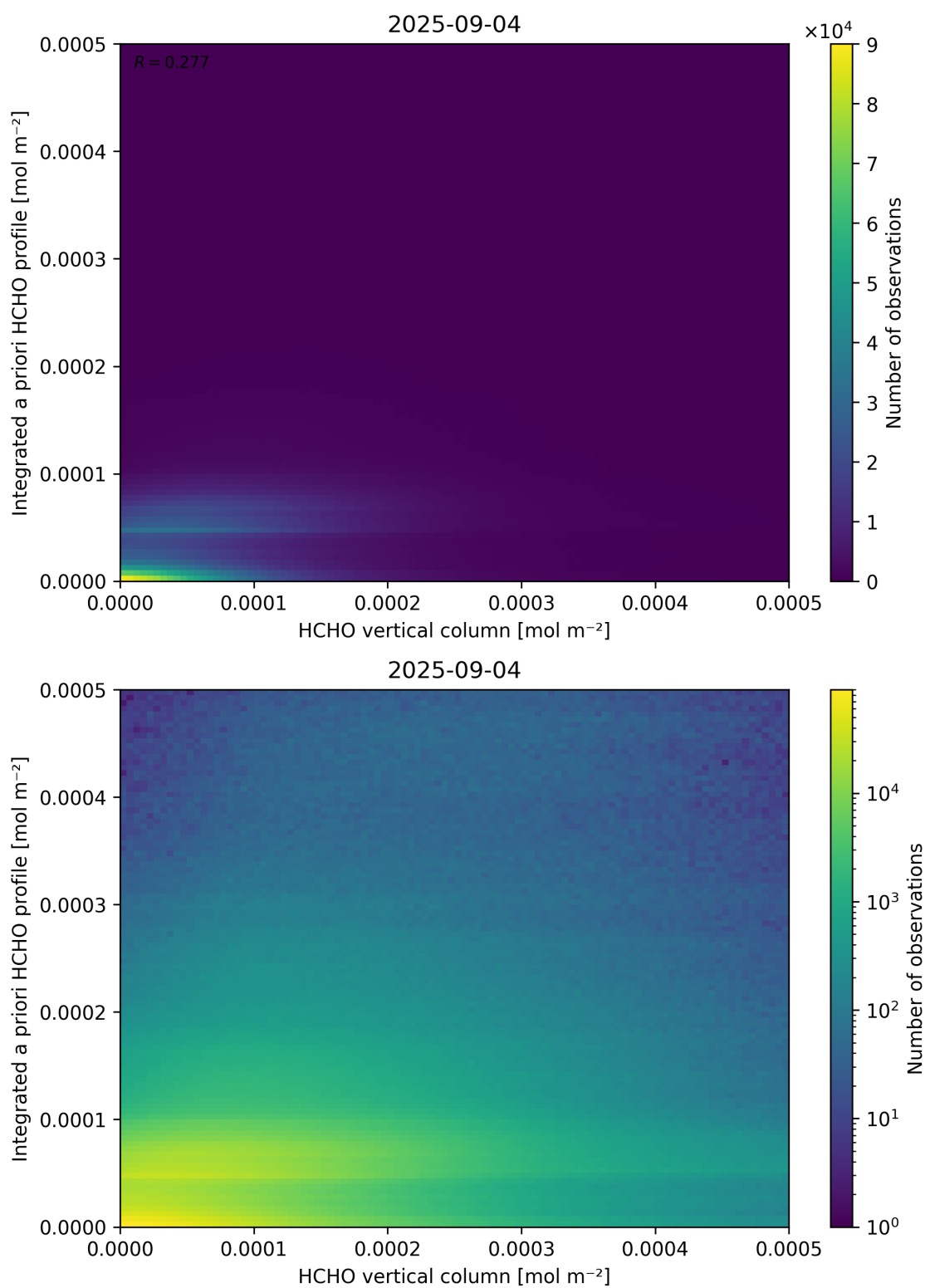
Figure 135: Scatter density plot of “HCHO vertical column” against “Integrated a priori HCHO profile” for 2025-09-04 to 2025-09-05.
