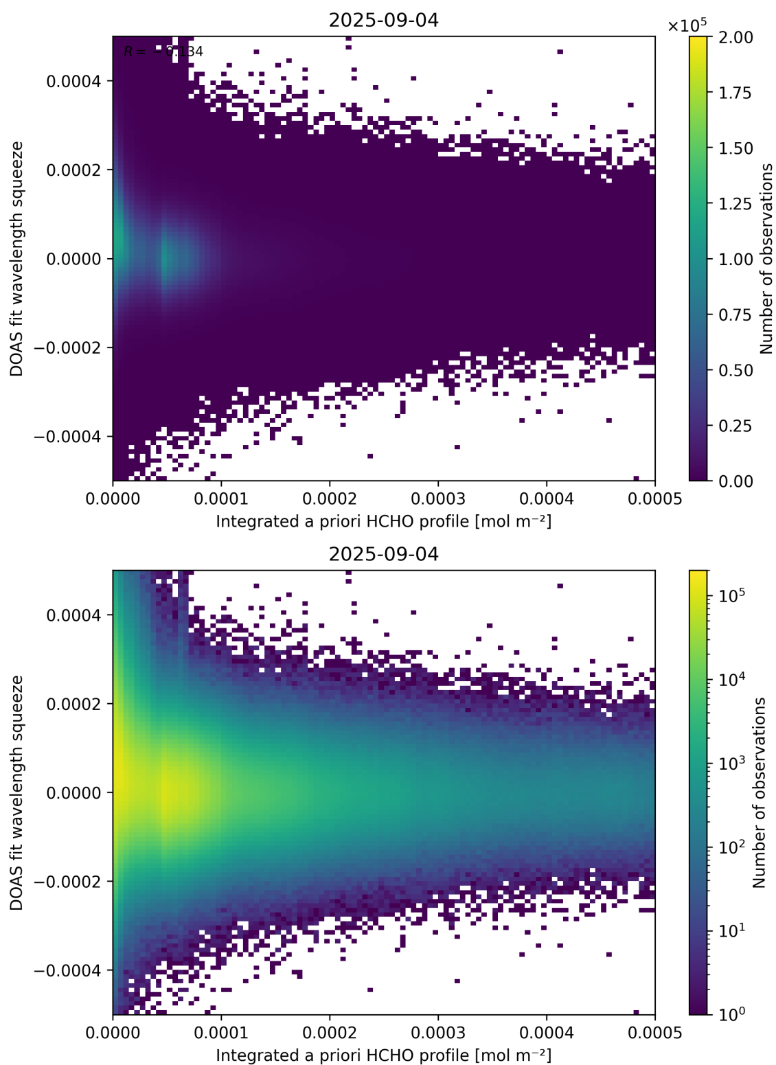
Figure 150: Scatter density plot of “Integrated a priori HCHO profile” against “DOAS fit wavelength squeeze” for 2025-09-04 to 2025-09-05.
