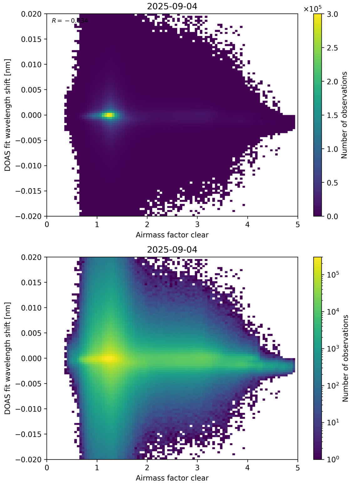
Figure 72: Scatter density plot of “Airmass factor clear” against “DOAS fit wavelength shift” for 2025-09-04 to 2025-09-05.
