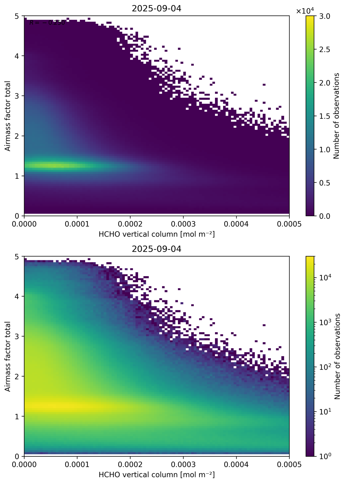
Figure 131: Scatter density plot of “HCHO vertical column” against “Airmass factor total” for 2025-09-04 to 2025-09-05.
