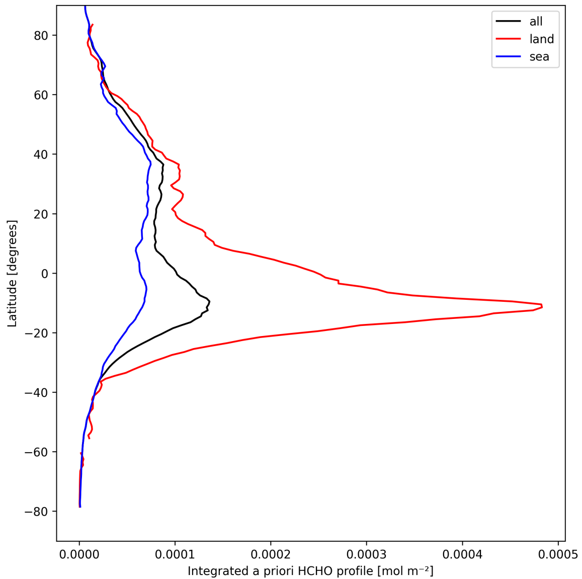
Figure 29: Zonal average of “Integrated a priori HCHO profile” for 2025-09-04 to 2025-09-05.
