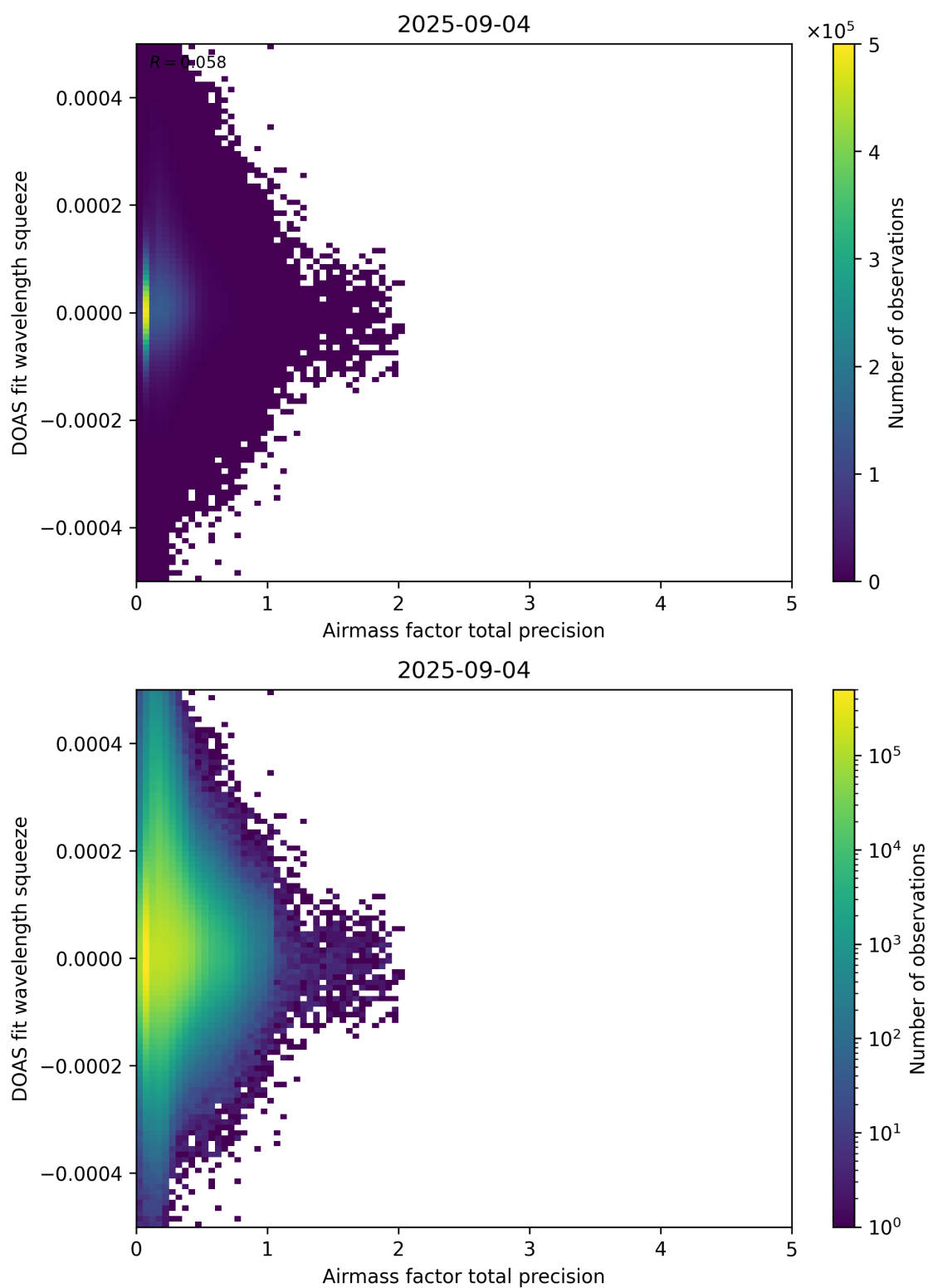
Figure 107: Scatter density plot of “Airmass factor total precision” against “DOAS fit wavelength squeeze” for 2025-09-04 to 2025-09-05.
