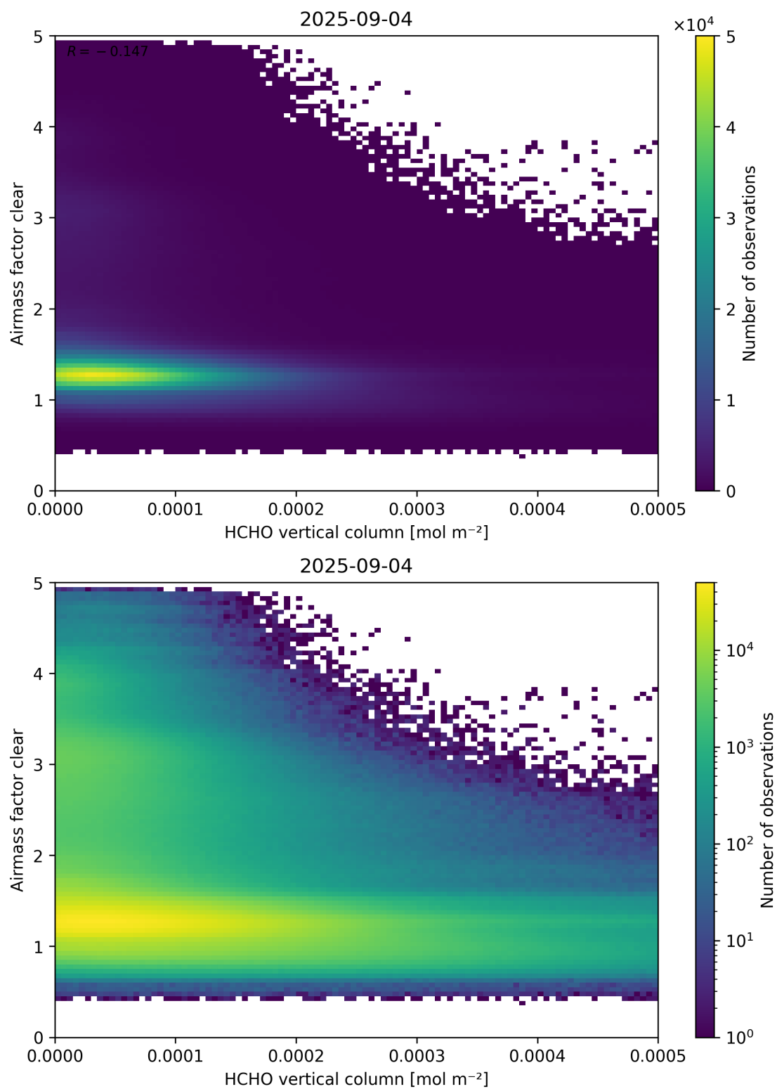
Figure 126: Scatter density plot of “HCHO vertical column” against “Airmass factor clear” for 2025-09-04 to 2025-09-05.
