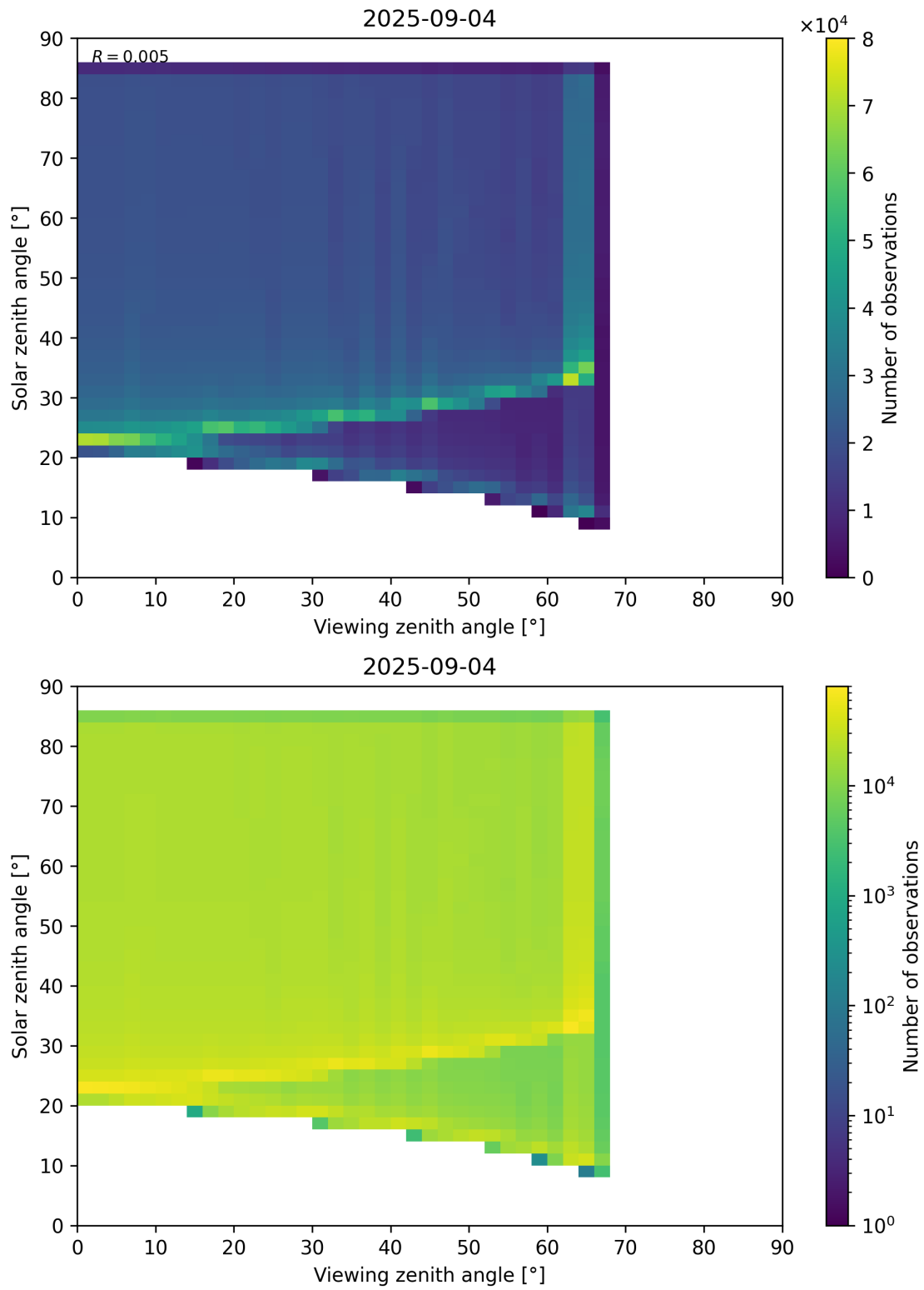
Figure 197: Scatter density plot of “Viewing zenith angle” against “Solar zenith angle” for 2025-09-04 to 2025-09-05.
