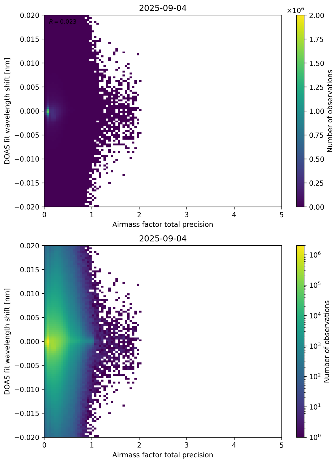
Figure 106: Scatter density plot of “Airmass factor total precision” against “DOAS fit wavelength shift” for 2025-09-04 to 2025-09-05.
