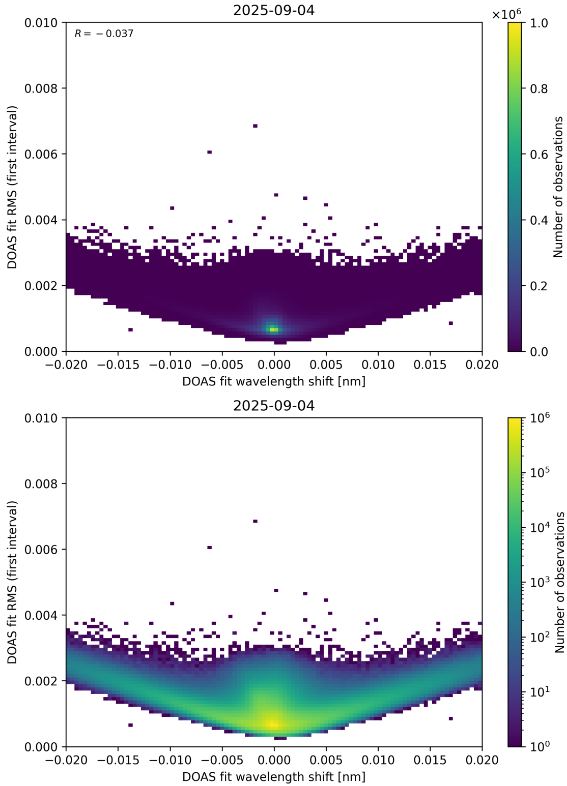
Figure 64: Scatter density plot of “DOAS fit wavelength shift” against “DOAS fit RMS (first interval)” for 2025-09-04 to 2025-09-05.
