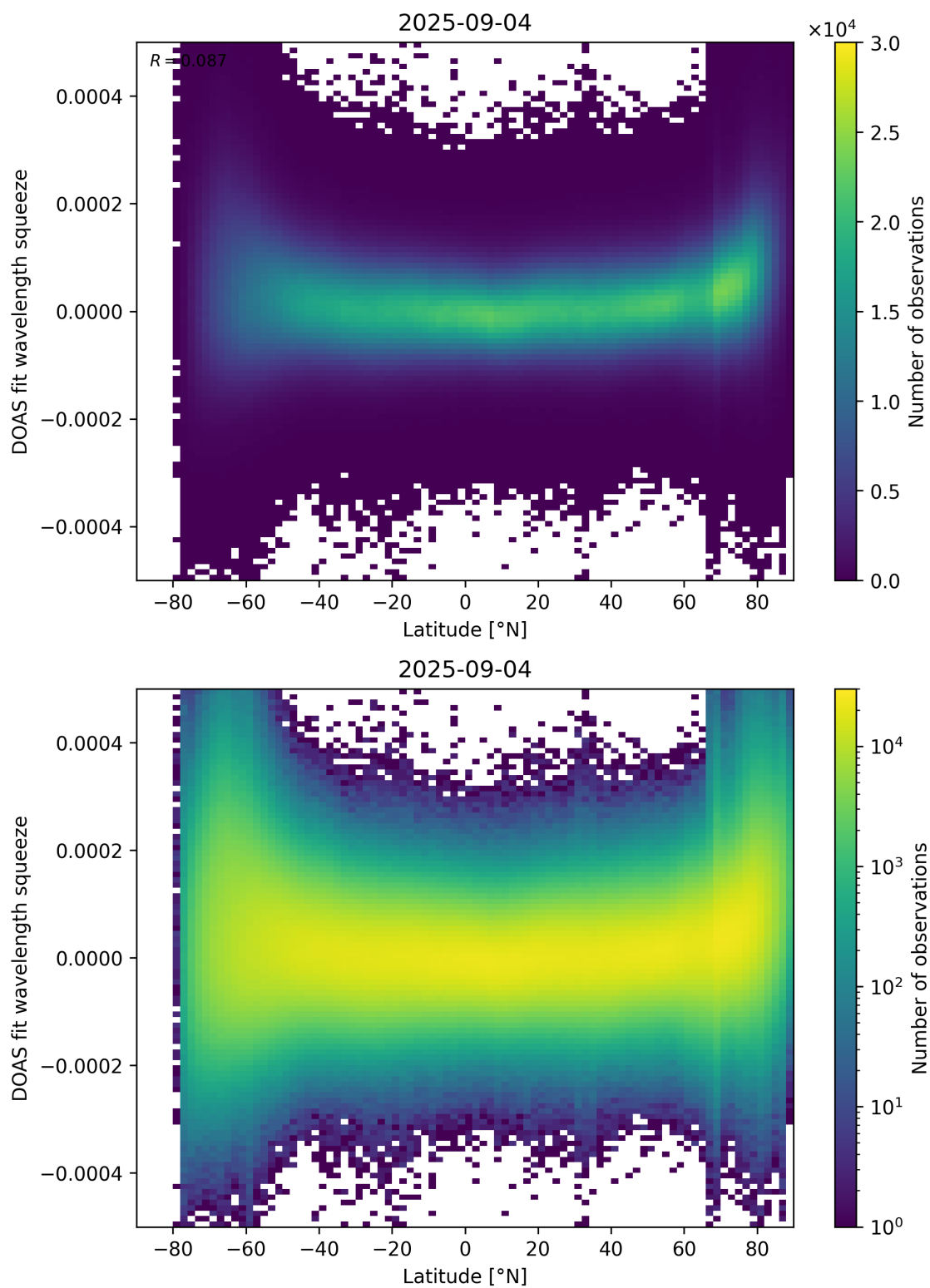
Figure 155: Scatter density plot of “Latitude” against “DOAS fit wavelength squeeze” for 2025-09-04 to 2025-09-05.
