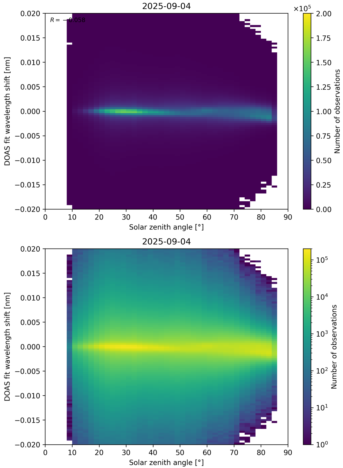
Figure 168: Scatter density plot of “Solar zenith angle” against “DOAS fit wavelength shift” for 2025-09-04 to 2025-09-05.
