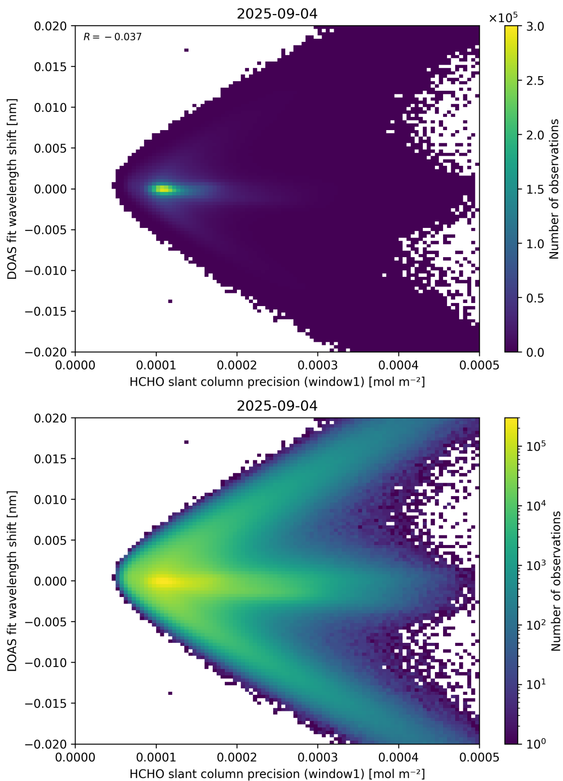
Figure 89: Scatter density plot of “HCHO slant column precision (window1)” against “DOAS fit wavelength shift” for 2025-09-04 to 2025-09-05.
