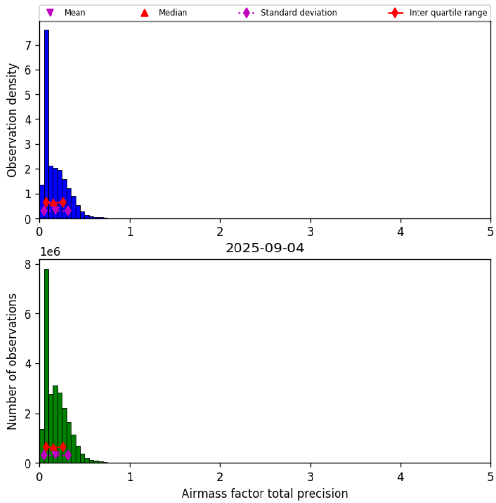
Figure 41: Histogram of “Airmass factor total precision” for 2025-09-04 to 2025-09-05
