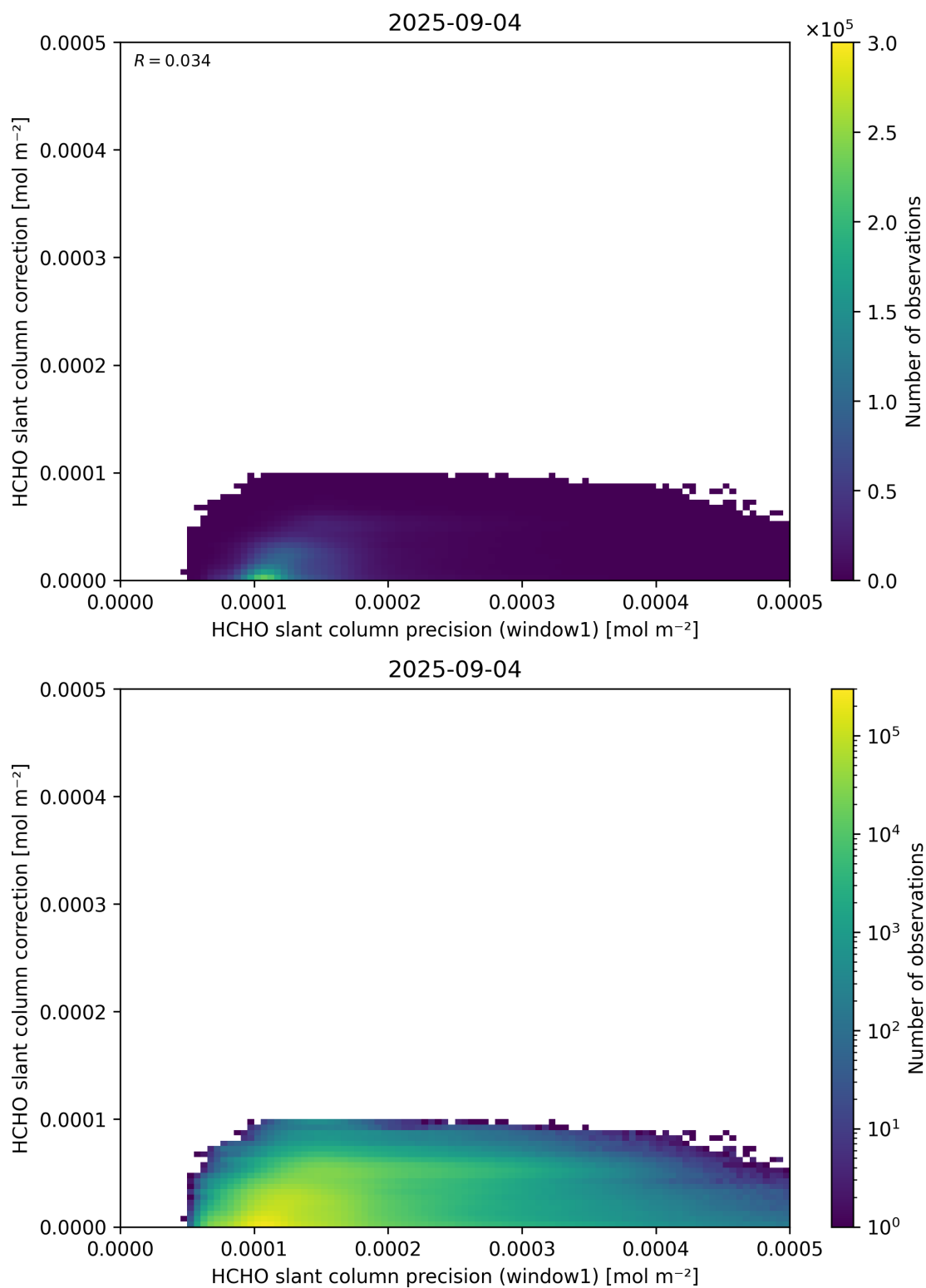
Figure 93: Scatter density plot of “HCHO slant column precision (window1)” against “HCHO slant column correction” for 2025-09-04 to 2025-09-05.
