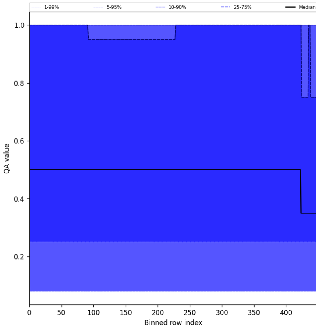
Figure 48: Along track statistics of “QA value” for 2025-09-04 to 2025-09-05
