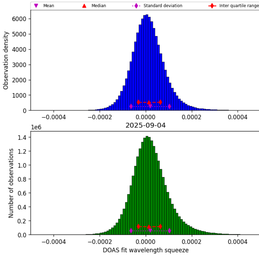
Figure 45: Histogram of “DOAS fit wavelength squeeze” for 2025-09-04 to 2025-09-05
