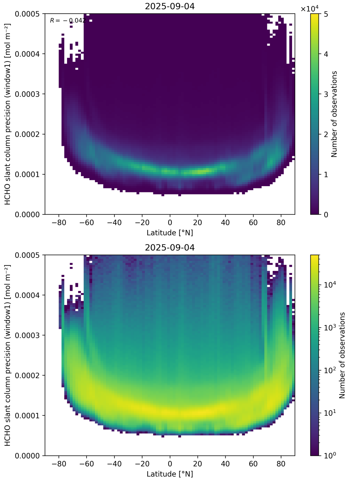
Figure 160: Scatter density plot of “Latitude” against “HCHO slant column precision (window1)” for 2025-09-04 to 2025-09-05.
