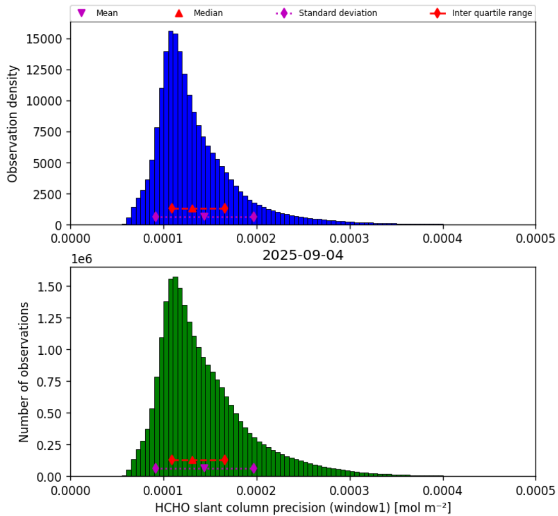
Figure 39: Histogram of “HCHO slant column precision (window1)” for 2025-09-04 to 2025-09-05
