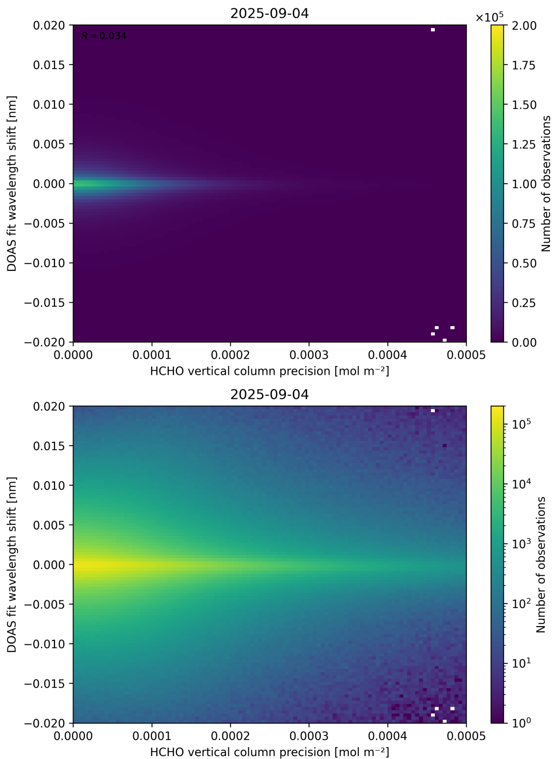
Figure 137: Scatter density plot of “HCHO vertical column precision” against “DOAS fit wavelength shift” for 2025-09-04 to 2025-09-05.
