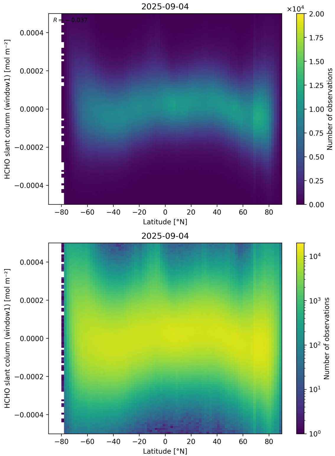
Figure 159: Scatter density plot of “Latitude” against “HCHO slant column (window1)” for 2025-09-04 to 2025-09-05.
