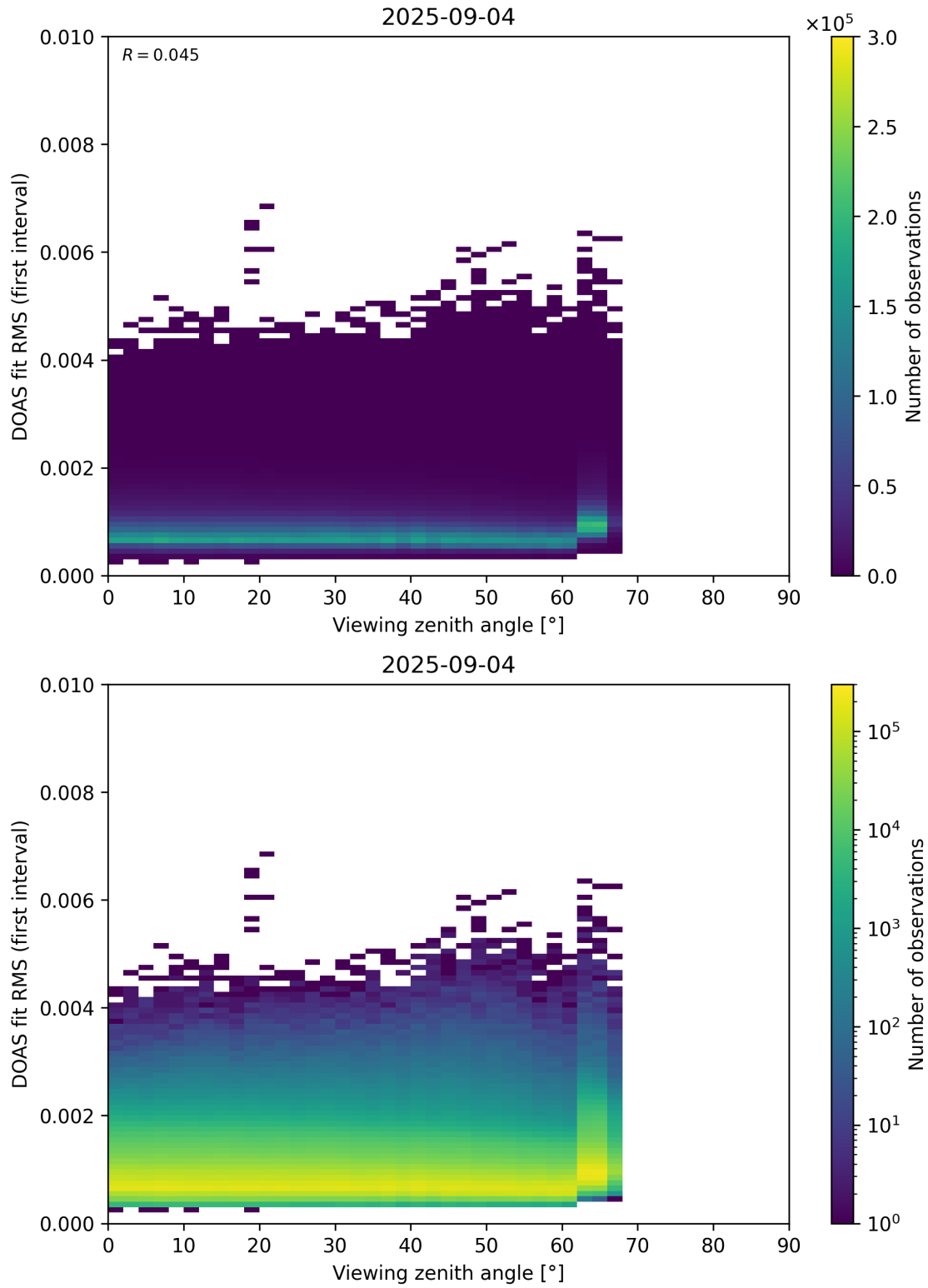
Figure 182: Scatter density plot of “Viewing zenith angle” against “DOAS fit RMS (first interval)” for 2025-09-04 to 2025-09-05.
