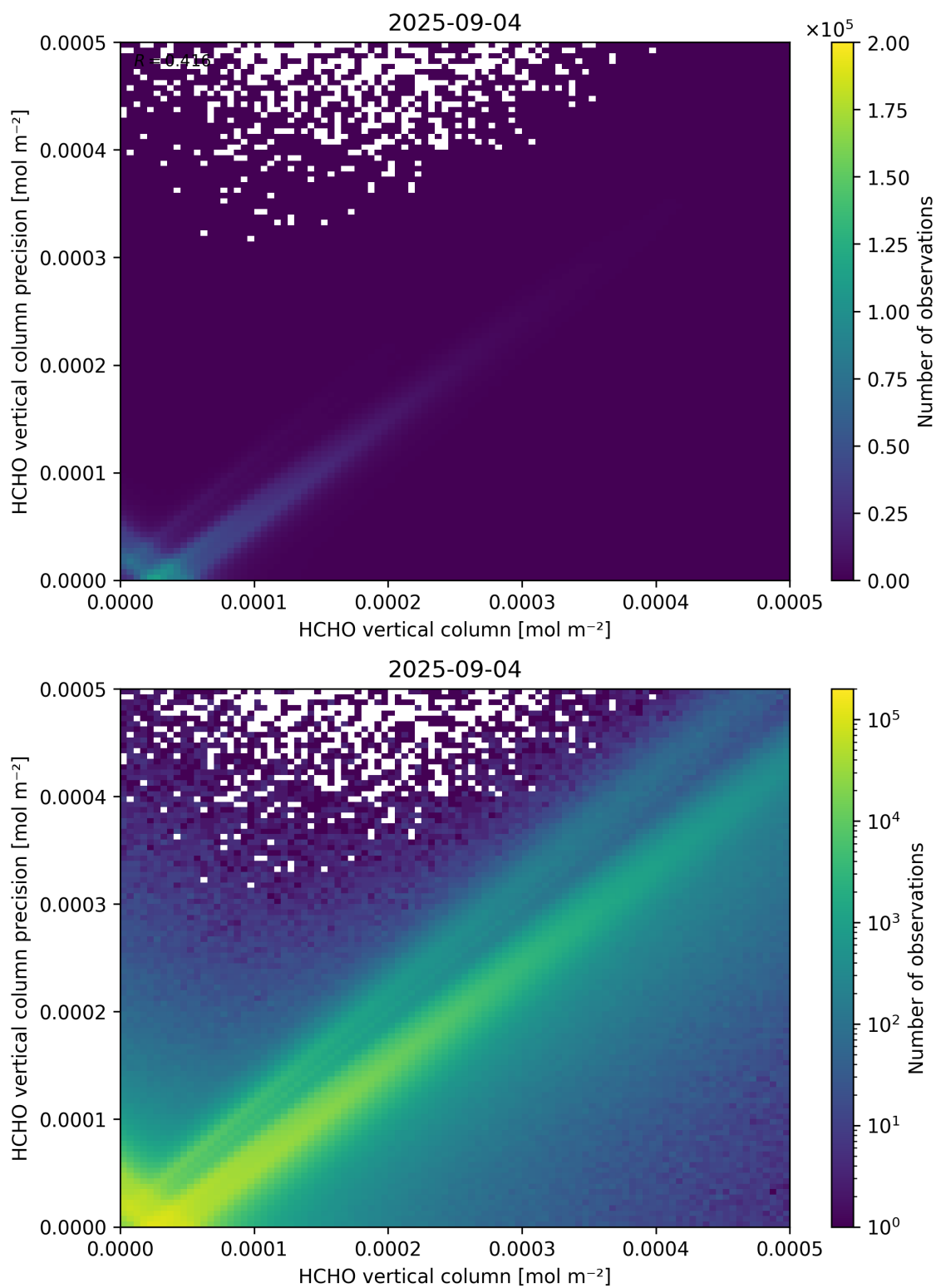
Figure 134: Scatter density plot of “HCHO vertical column” against “HCHO vertical column precision” for 2025-09-04 to 2025-09-05.
