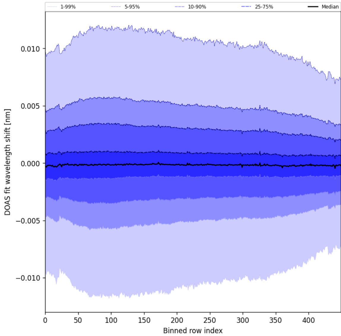
Figure 58: Along track statistics of “DOAS fit wavelength shift” for 2025-09-04 to 2025-09-05
