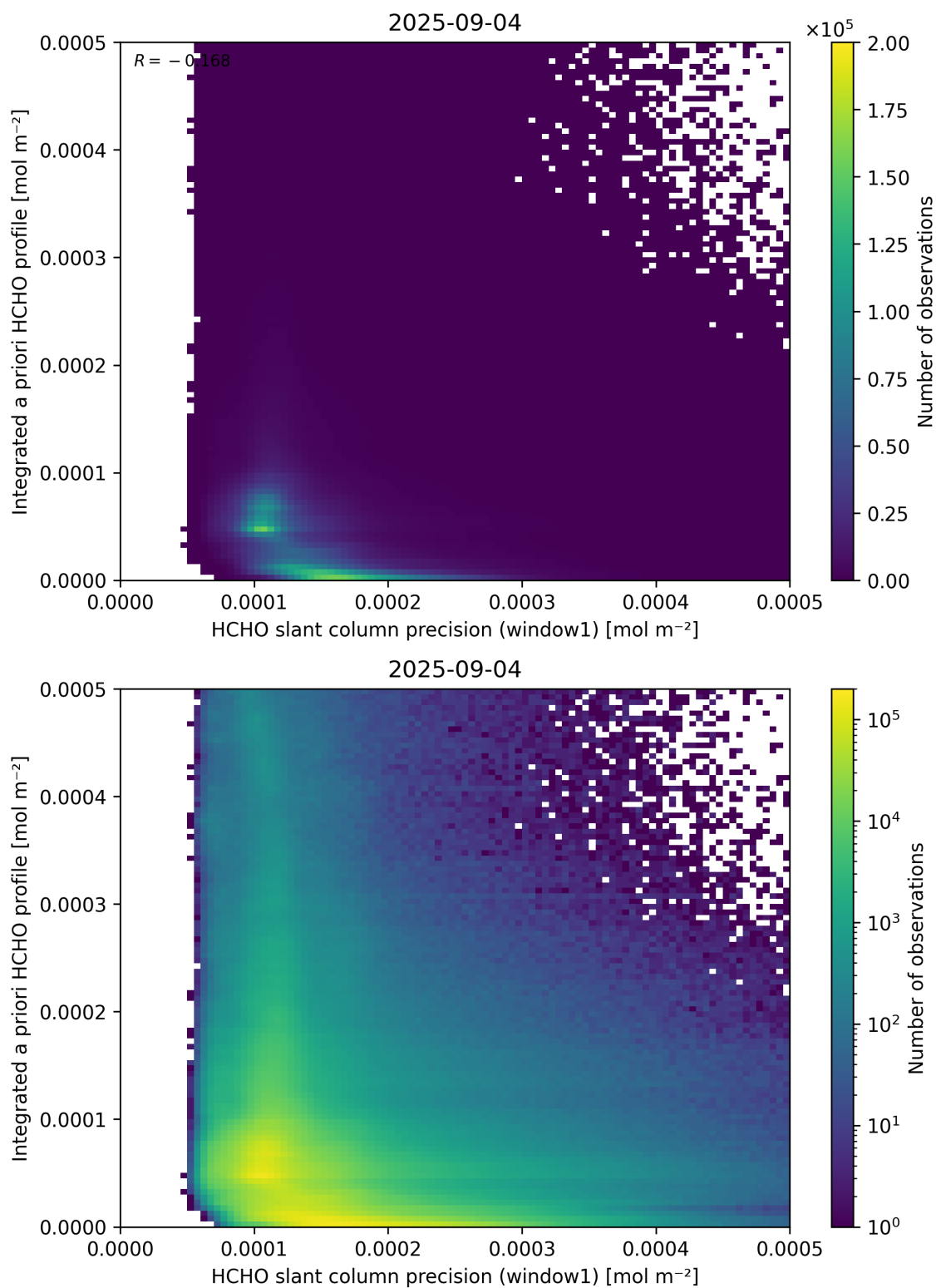
Figure 96: Scatter density plot of “HCHO slant column precision (window1)” against “Integrated a priori HCHO profile” for 2025-09-04 to 2025-09-05.
