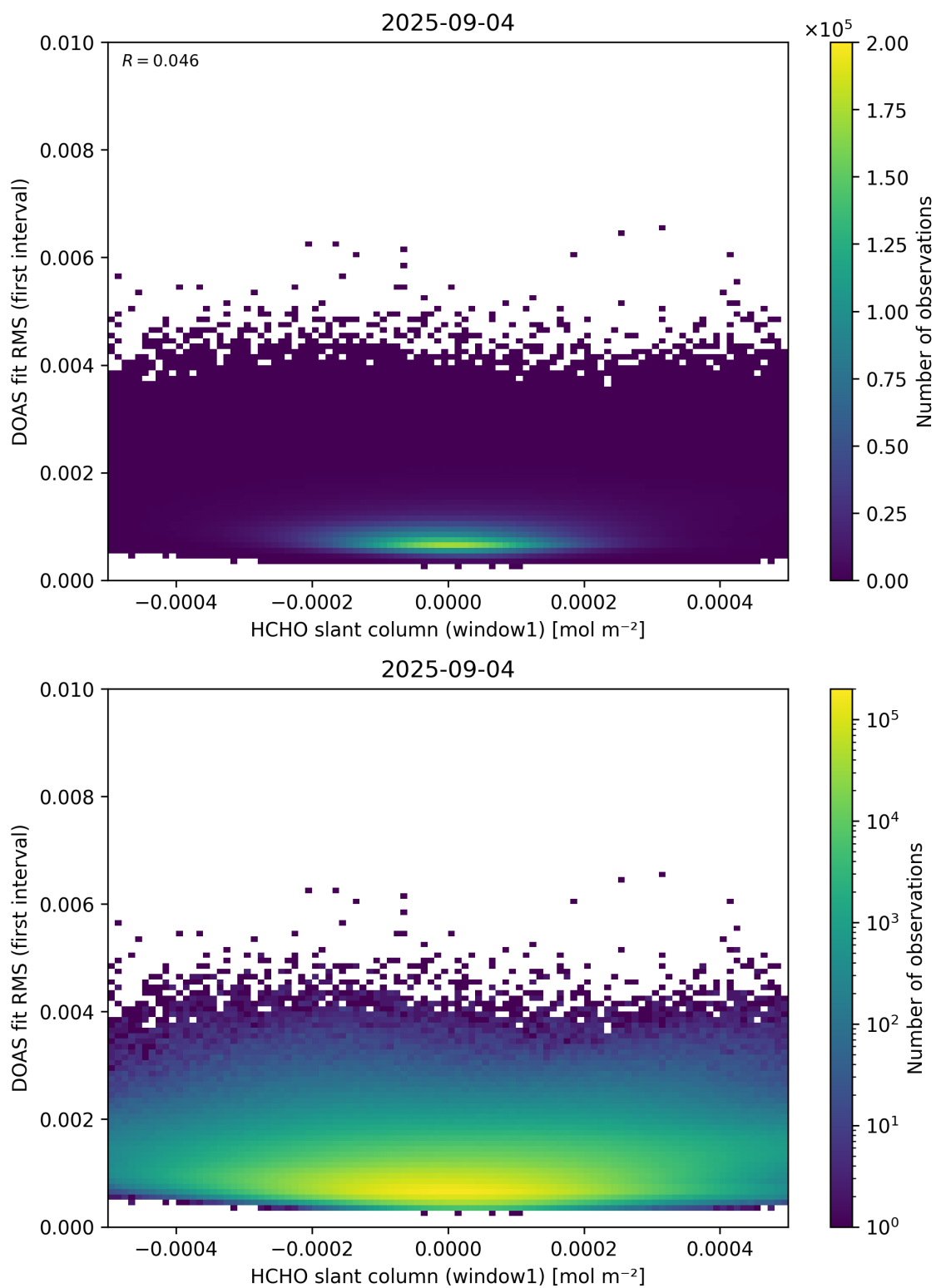
Figure 78: Scatter density plot of “HCHO slant column (window1)” against “DOAS fit RMS (first interval)” for 2025-09-04 to 2025-09-05.
