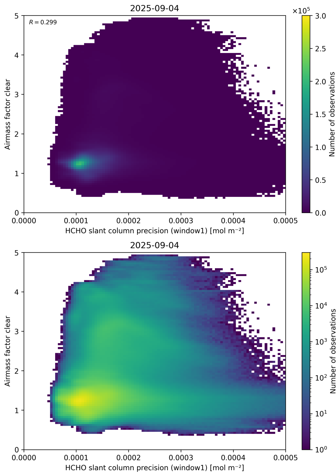
Figure 91: Scatter density plot of “HCHO slant column precision (window1)” against “Airmass factor clear” for 2025-09-04 to 2025-09-05.
