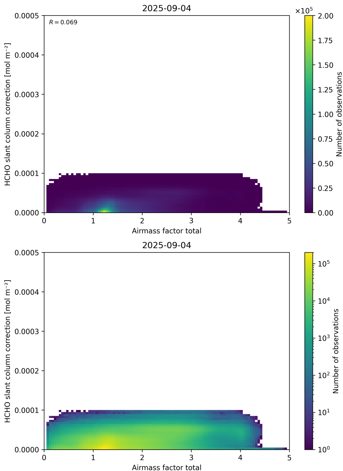
Figure 102: Scatter density plot of “Airmass factor total” against “HCHO slant column correction” for 2025-09-04 to 2025-09-05.
