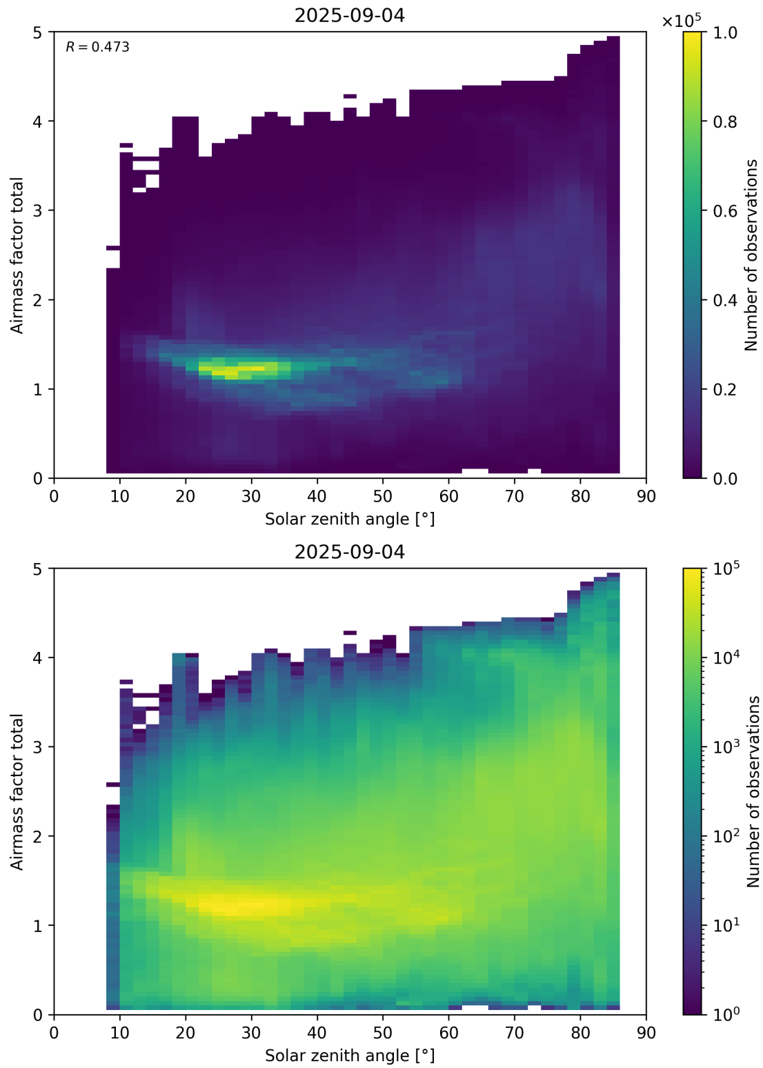
Figure 175: Scatter density plot of “Solar zenith angle” against “Airmass factor total” for 2025-09-04 to 2025-09-05.
