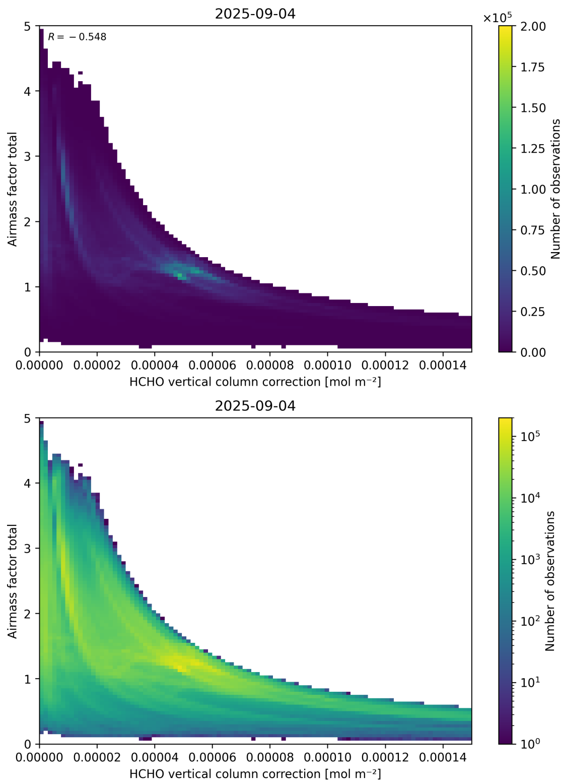
Figure 120: Scatter density plot of “HCHO vertical column correction” against “Airmass factor total” for 2025-09-04 to 2025-09-05.
