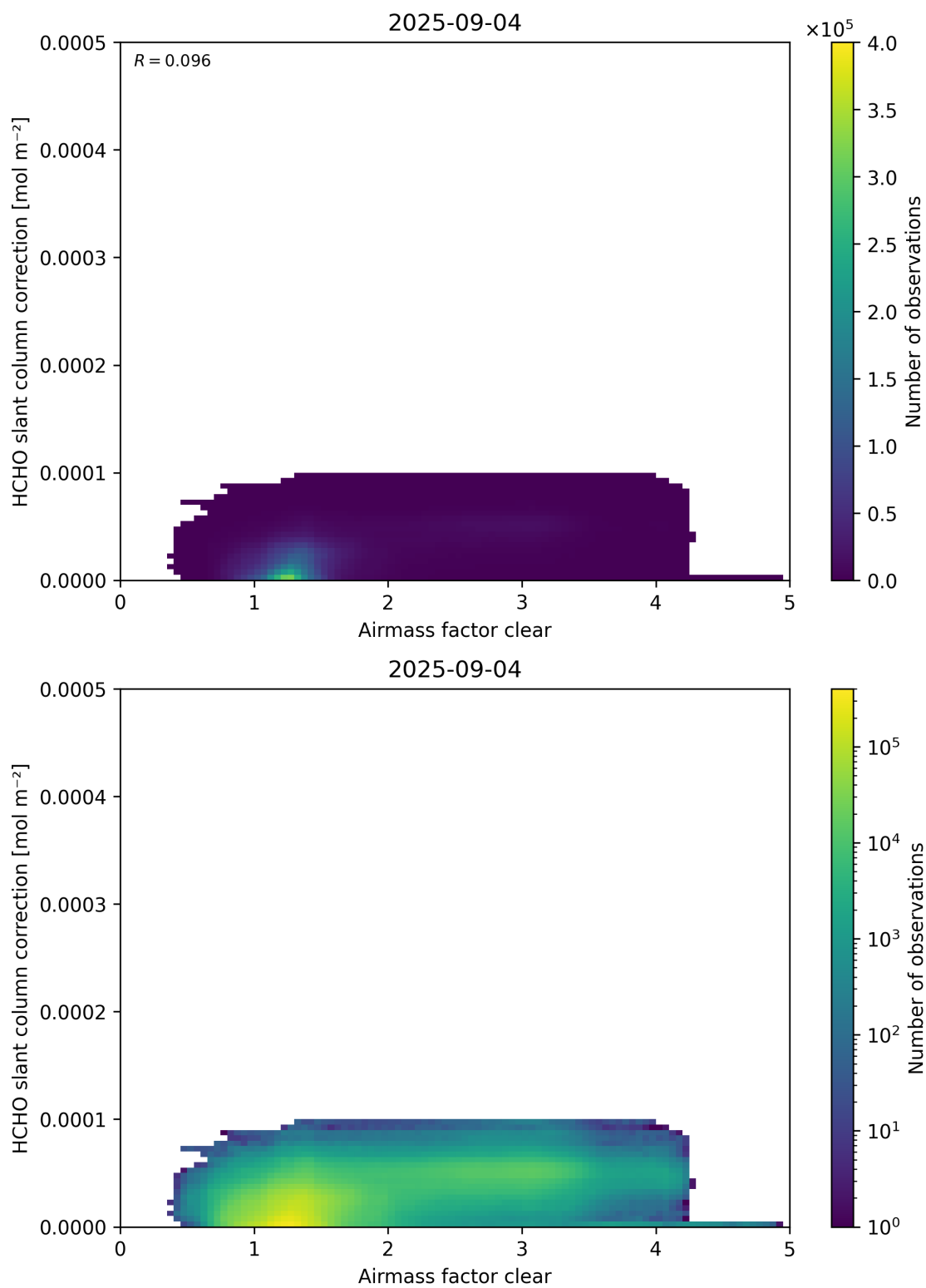
Figure 75: Scatter density plot of “Airmass factor clear” against “HCHO slant column correction” for 2025-09-04 to 2025-09-05.
