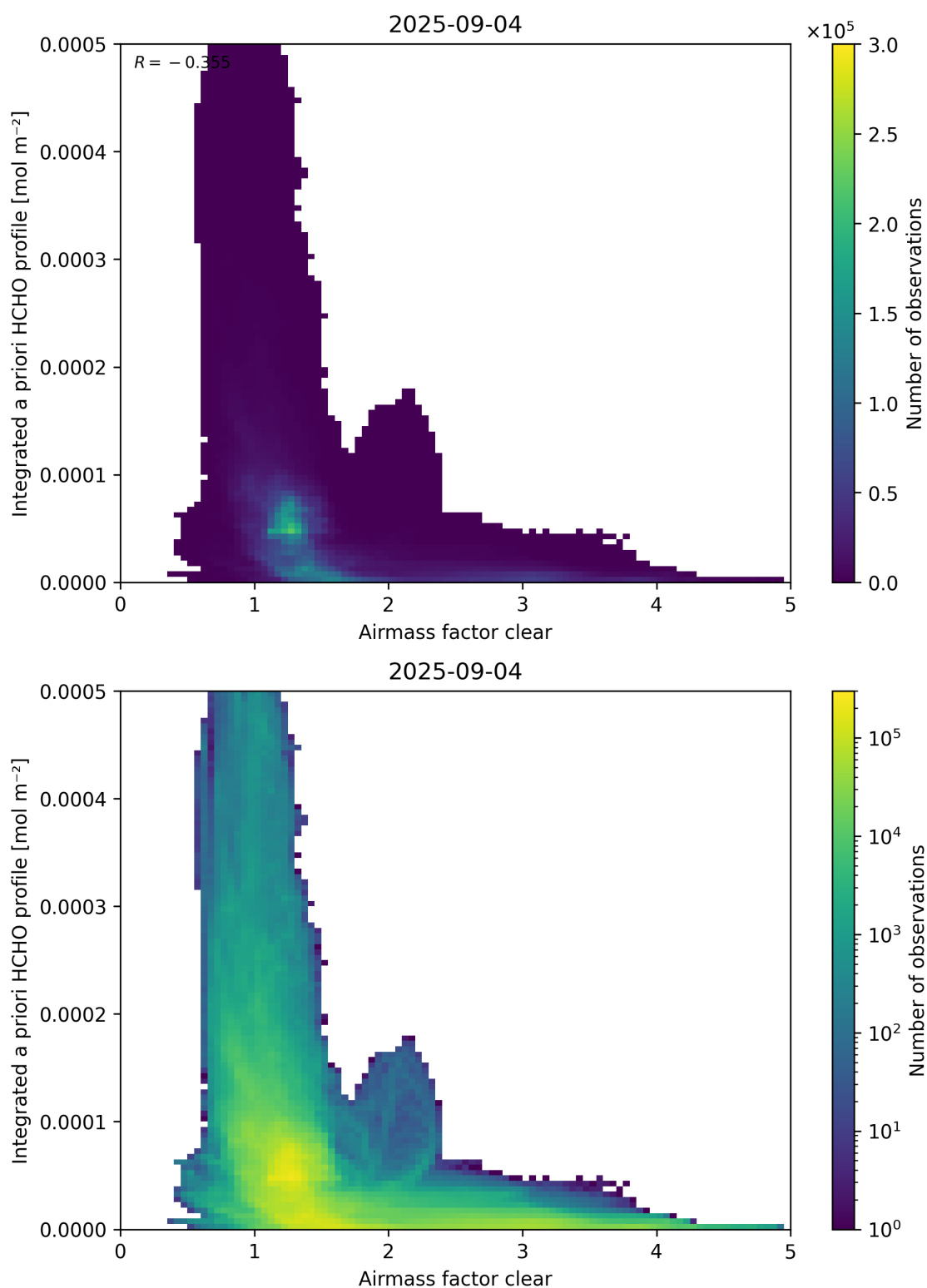
Figure 76: Scatter density plot of “Airmass factor clear” against “Integrated a priori HCHO profile” for 2025-09-04 to 2025-09-05.
