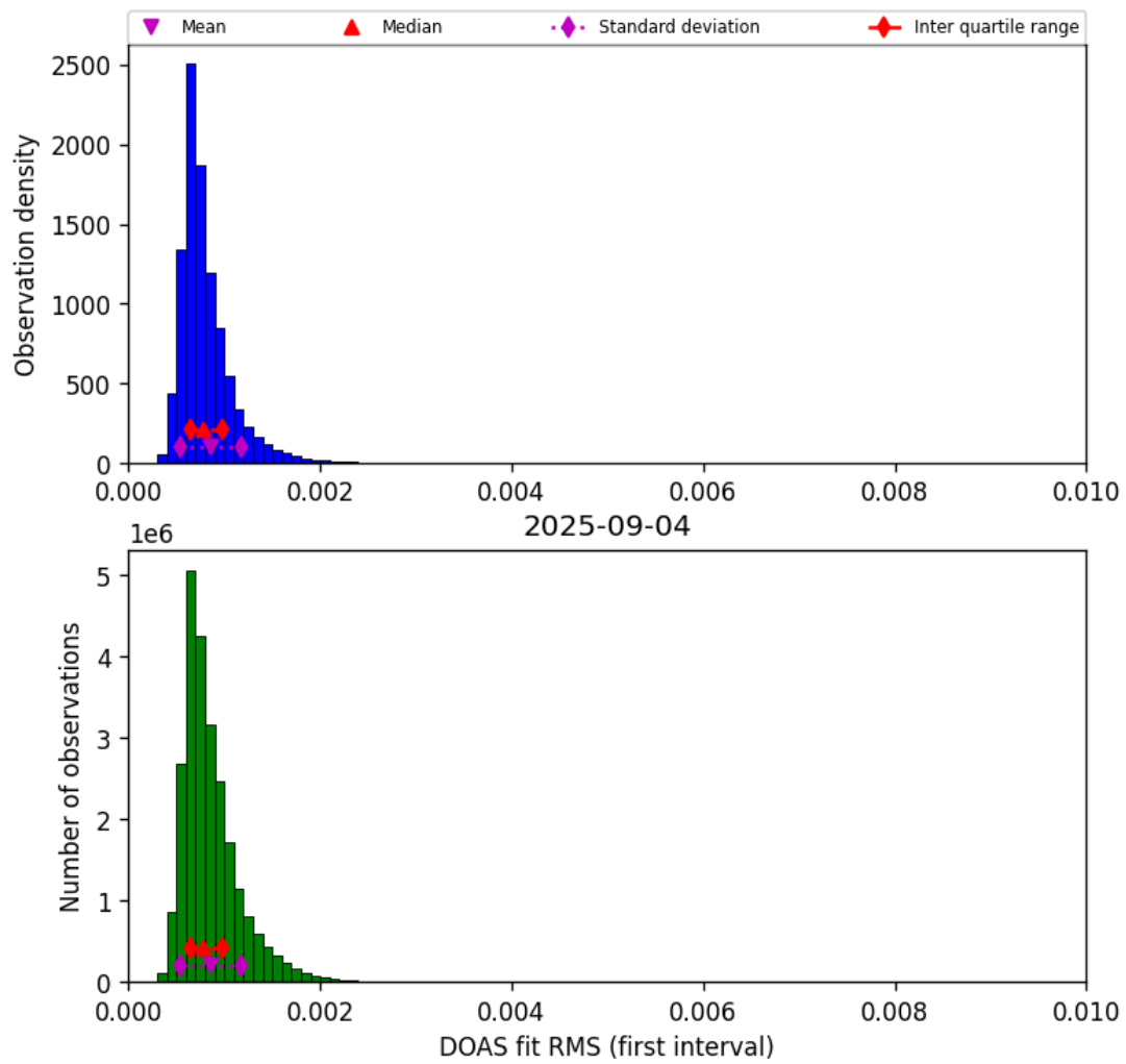
Figure 46: Histogram of “DOAS fit RMS (first interval)” for 2025-09-04 to 2025-09-05
