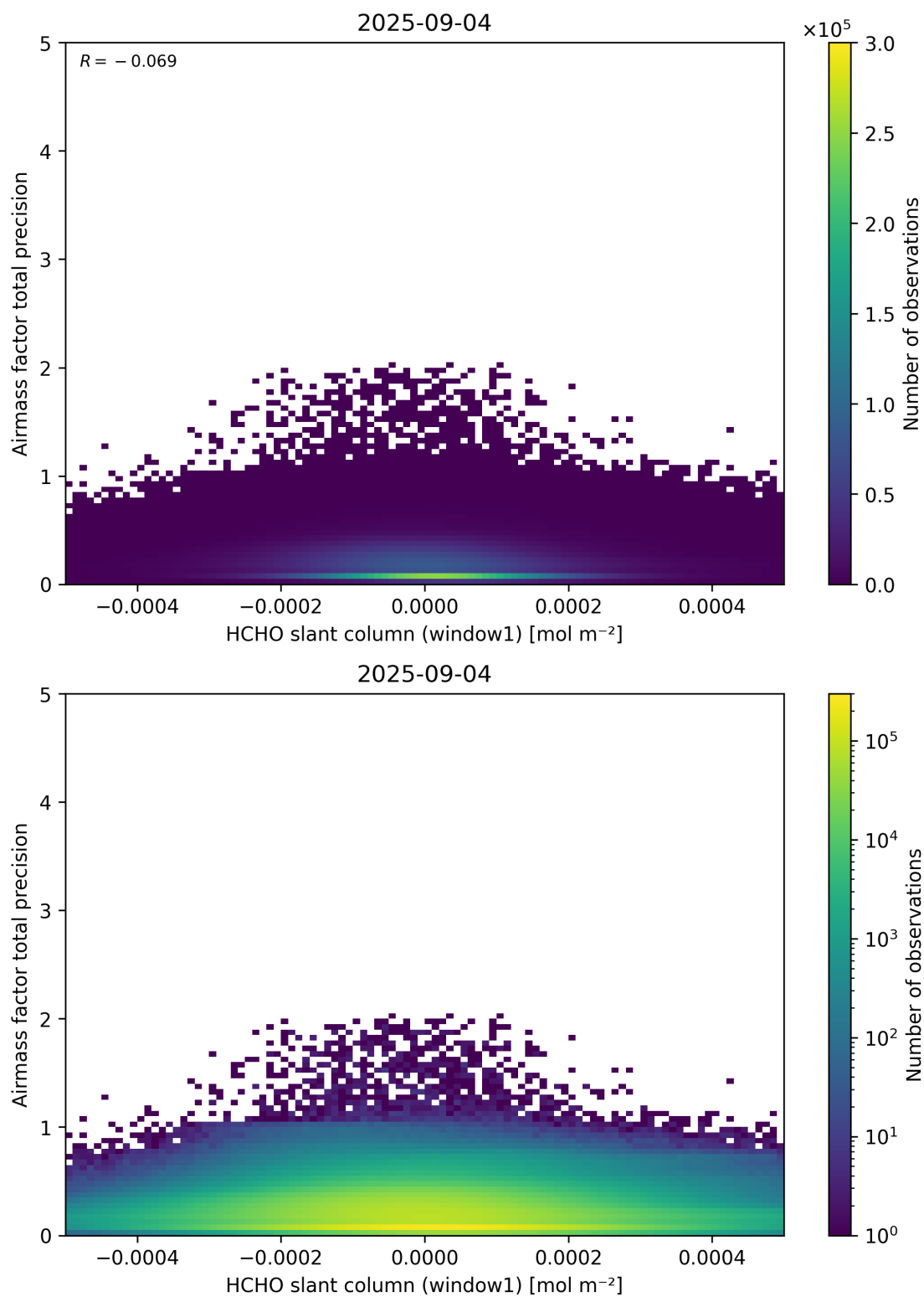
Figure 86: Scatter density plot of “HCHO slant column (window1)” against “Airmass factor total precision” for 2025-09-04 to 2025-09-05.
