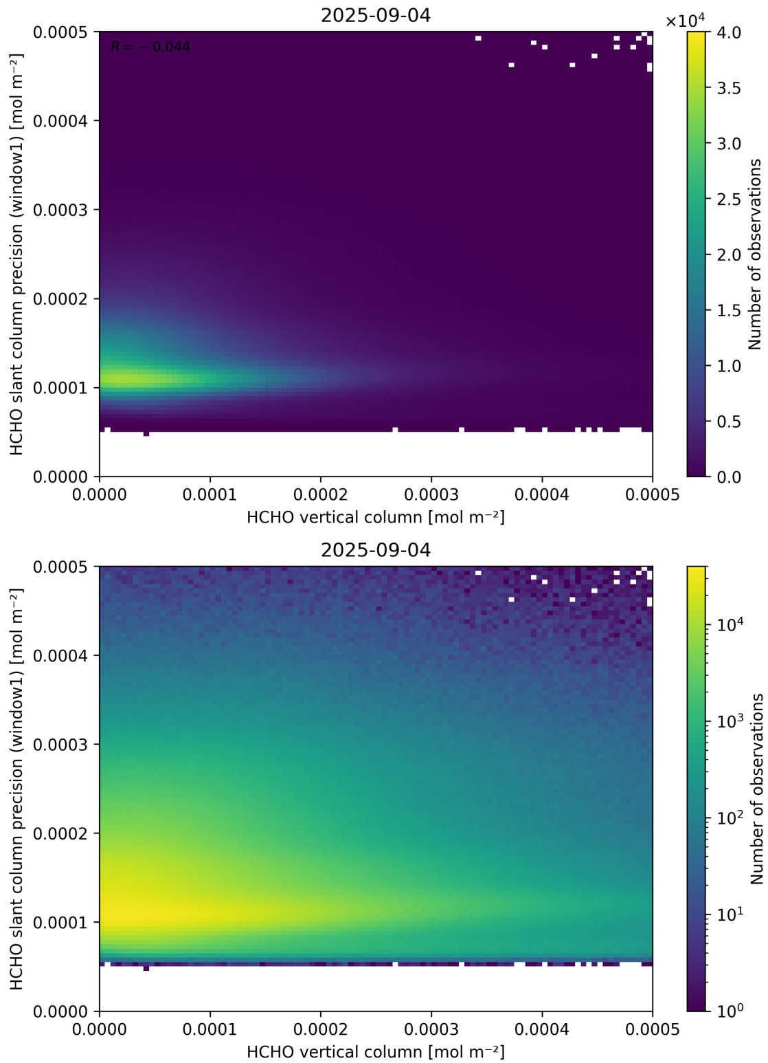
Figure 130: Scatter density plot of “HCHO vertical column” against “HCHO slant column precision (window1)” for 2025-09-04 to 2025-09-05.
