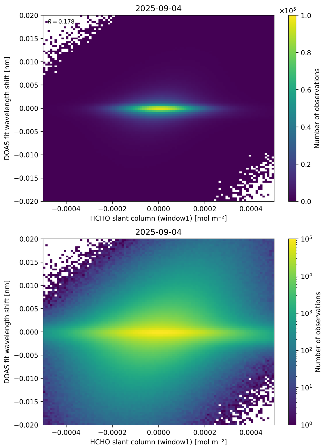
Figure 79: Scatter density plot of “HCHO slant column (window1)” against “DOAS fit wavelength shift” for 2025-09-04 to 2025-09-05.
