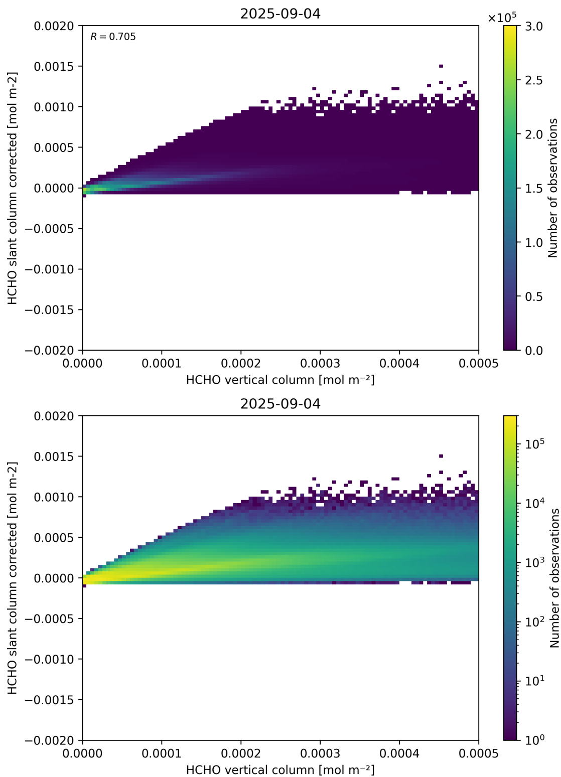
Figure 127: Scatter density plot of “HCHO vertical column” against “HCHO slant column corrected” for 2025-09-04 to 2025-09-05.
