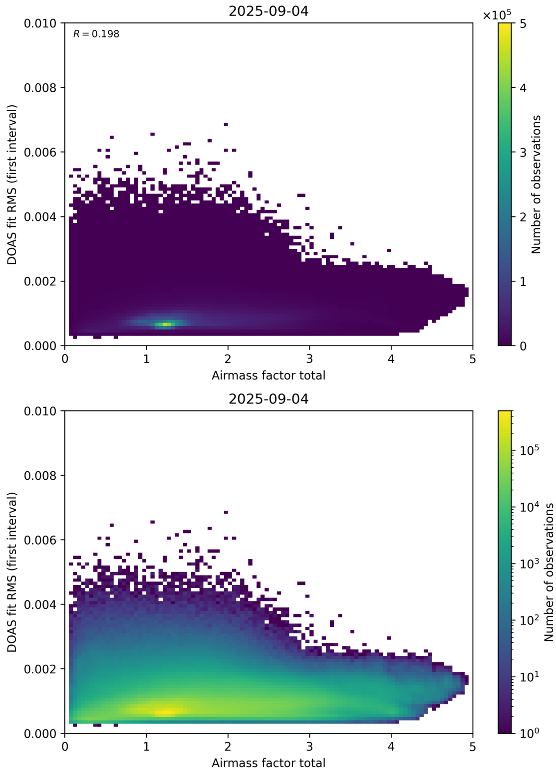
Figure 97: Scatter density plot of “Airmass factor total” against “DOAS fit RMS (first interval)” for 2025-09-04 to 2025-09-05.
