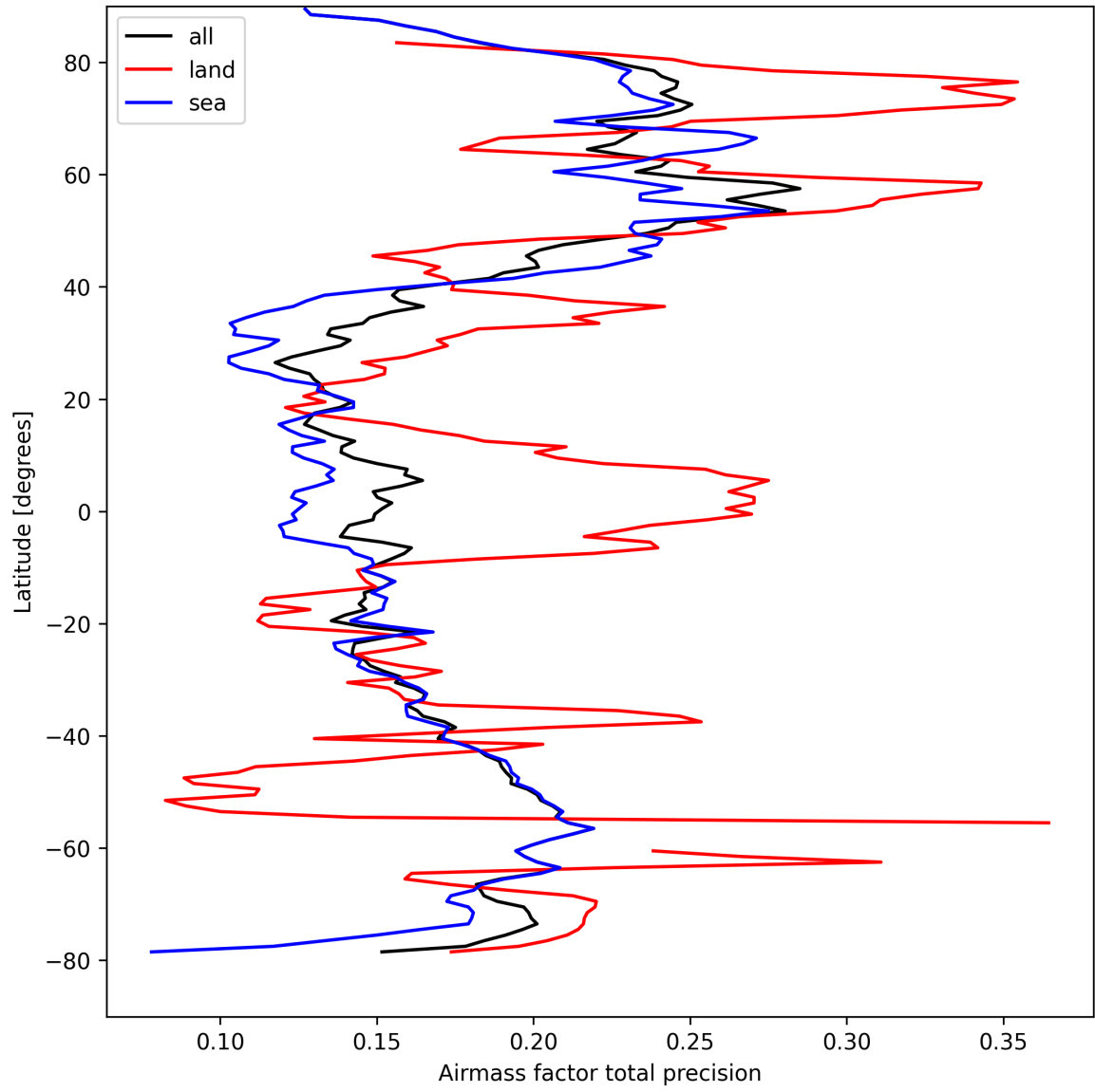
Figure 27: Zonal average of “Airmass factor total precision” for 2025-09-04 to 2025-09-05.
