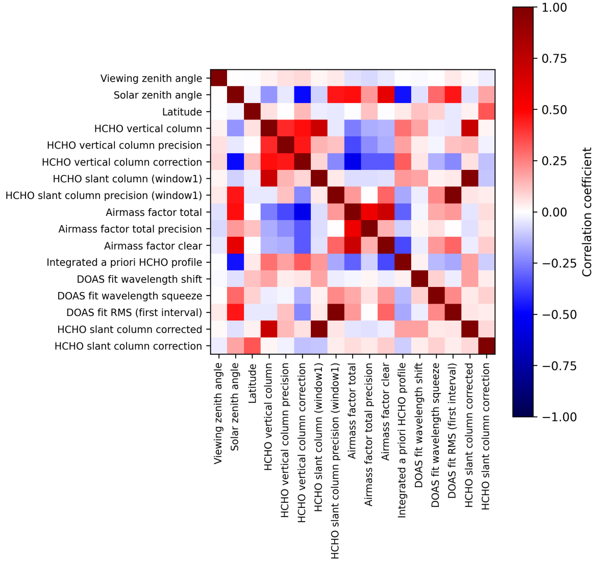
Figure 2: Map of correlation matrix for 2025-09-04 to 2025-09-05.
