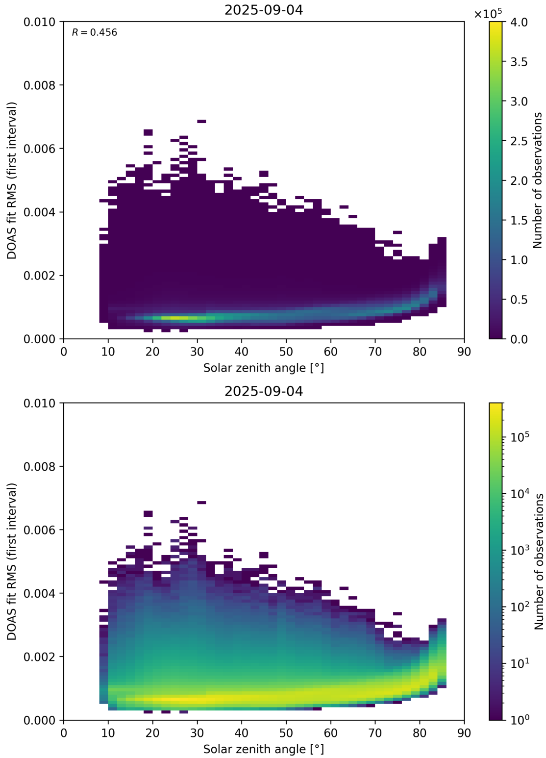
Figure 167: Scatter density plot of “Solar zenith angle” against “DOAS fit RMS (first interval)” for 2025-09-04 to 2025-09-05.
