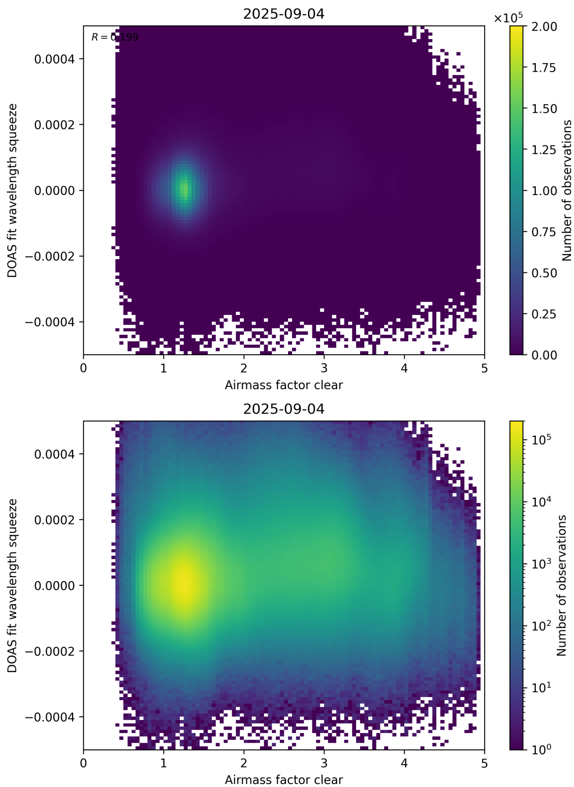
Figure 73: Scatter density plot of “Airmass factor clear” against “DOAS fit wavelength squeeze” for 2025-09-04 to 2025-09-05.
