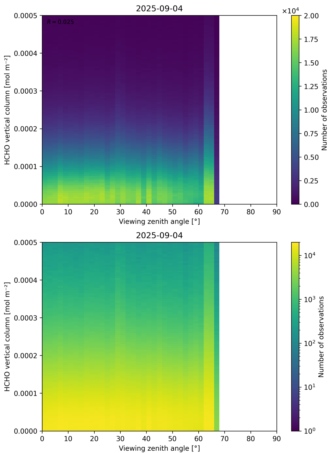
Figure 192: Scatter density plot of “Viewing zenith angle” against “HCHO vertical column” for 2025-09-04 to 2025-09-05.
