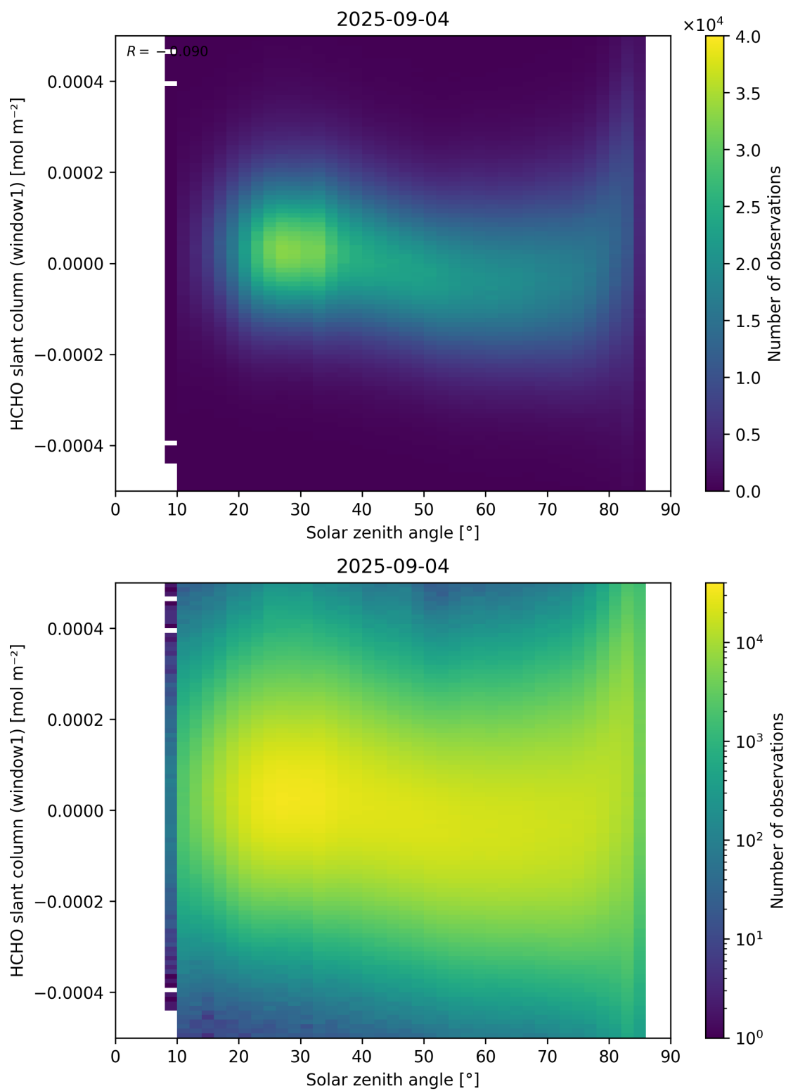
Figure 173: Scatter density plot of “Solar zenith angle” against “HCHO slant column (window1)” for 2025-09-04 to 2025-09-05.
