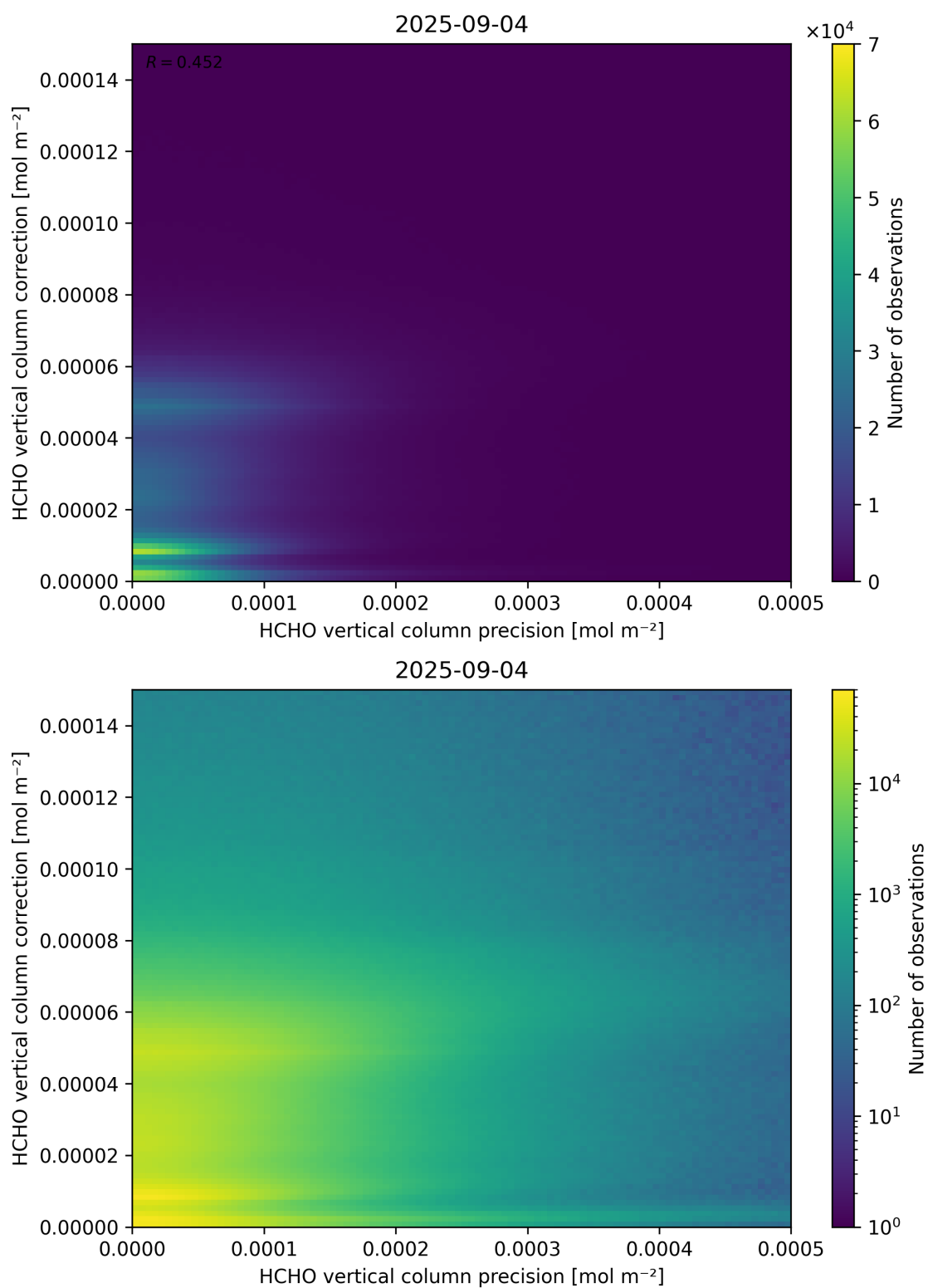
Figure 146: Scatter density plot of “HCHO vertical column precision” against “HCHO vertical column correction” for 2025-09-04 to 2025-09-05.
