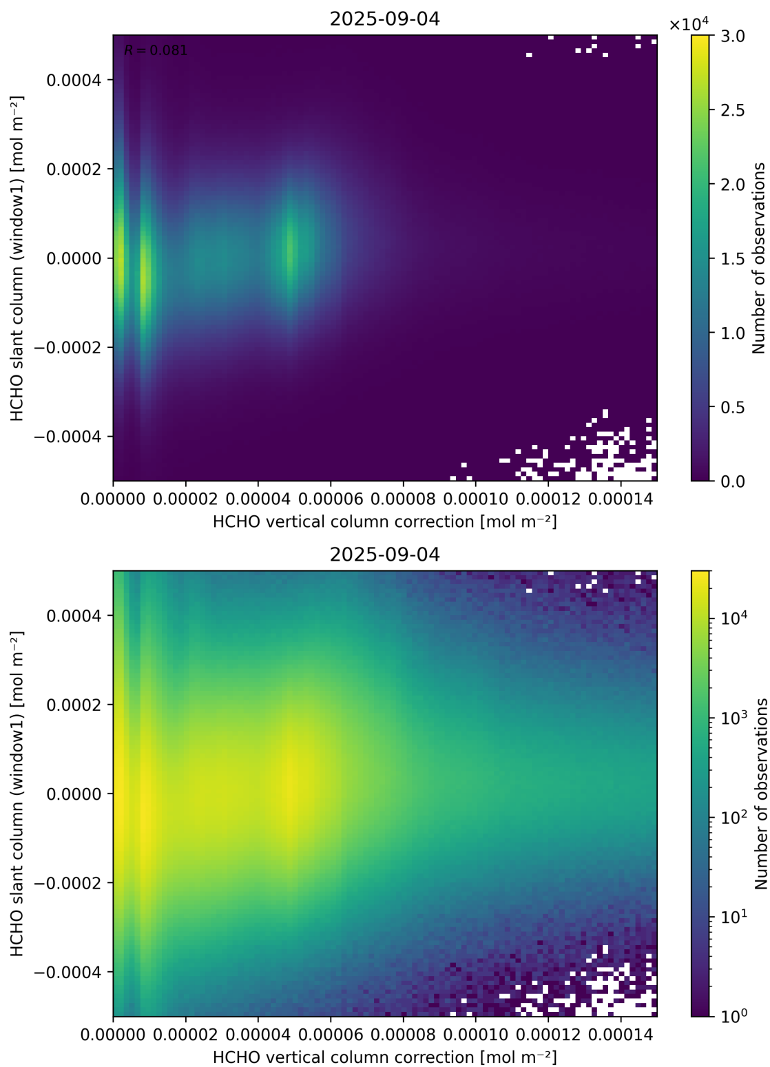
Figure 118: Scatter density plot of “HCHO vertical column correction” against “HCHO slant column (window1)” for 2025-09-04 to 2025-09-05.
