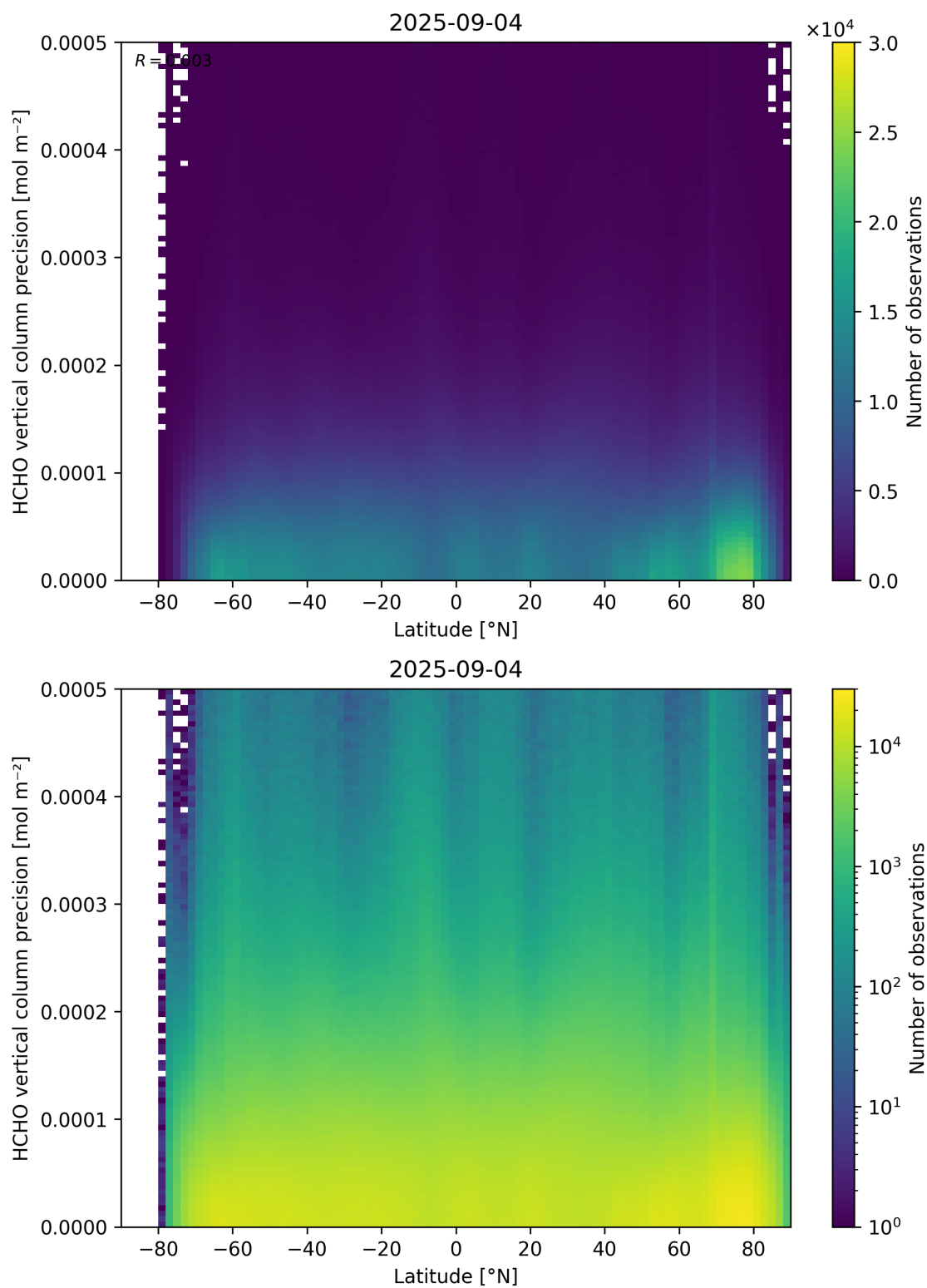
Figure 165: Scatter density plot of “Latitude” against “HCHO vertical column precision” for 2025-09-04 to 2025-09-05.
