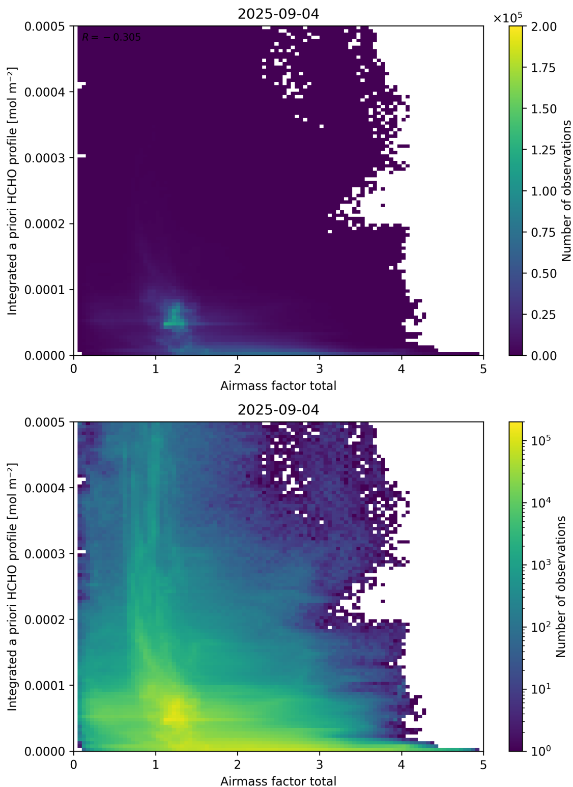
Figure 104: Scatter density plot of “Airmass factor total” against “Integrated a priori HCHO profile” for 2025-09-04 to 2025-09-05.
