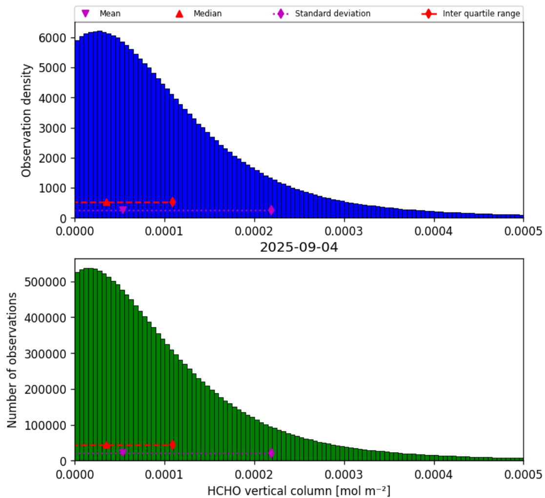
Figure 35: Histogram of “HCHO vertical column” for 2025-09-04 to 2025-09-05
