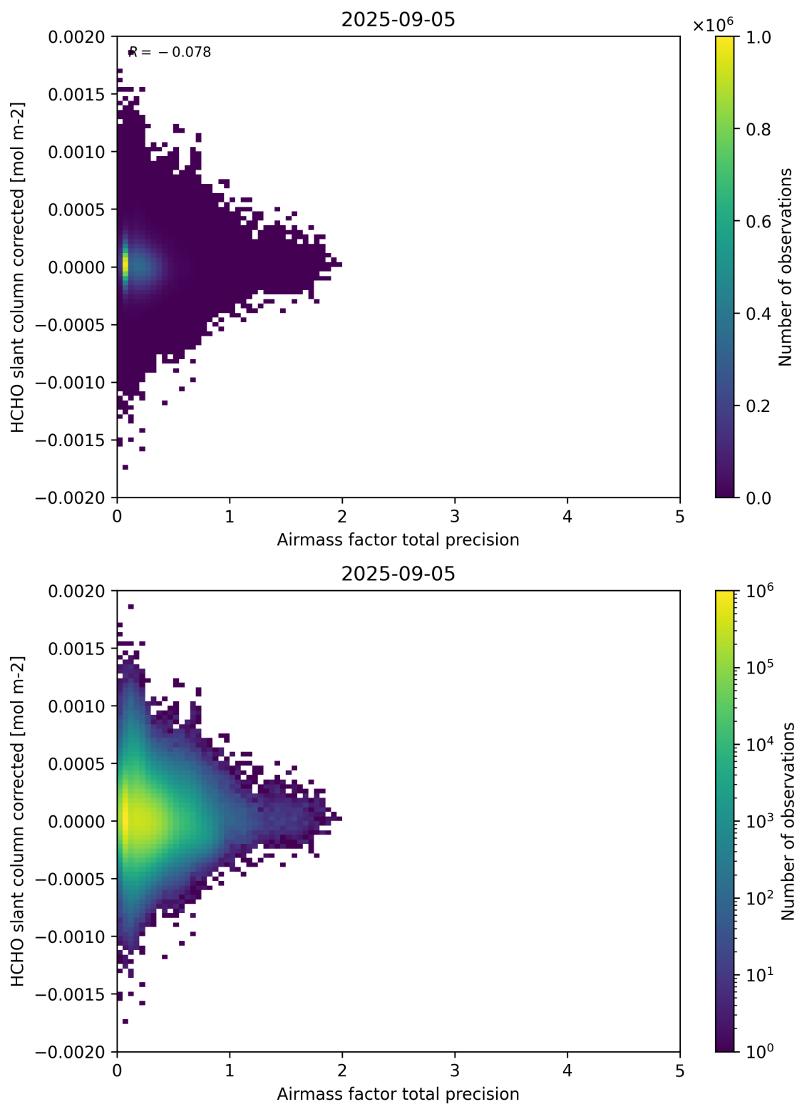
Figure 109: Scatter density plot of “Airmass factor total precision” against “HCHO slant column corrected” for 2025-09-04 to 2025-09-06.
