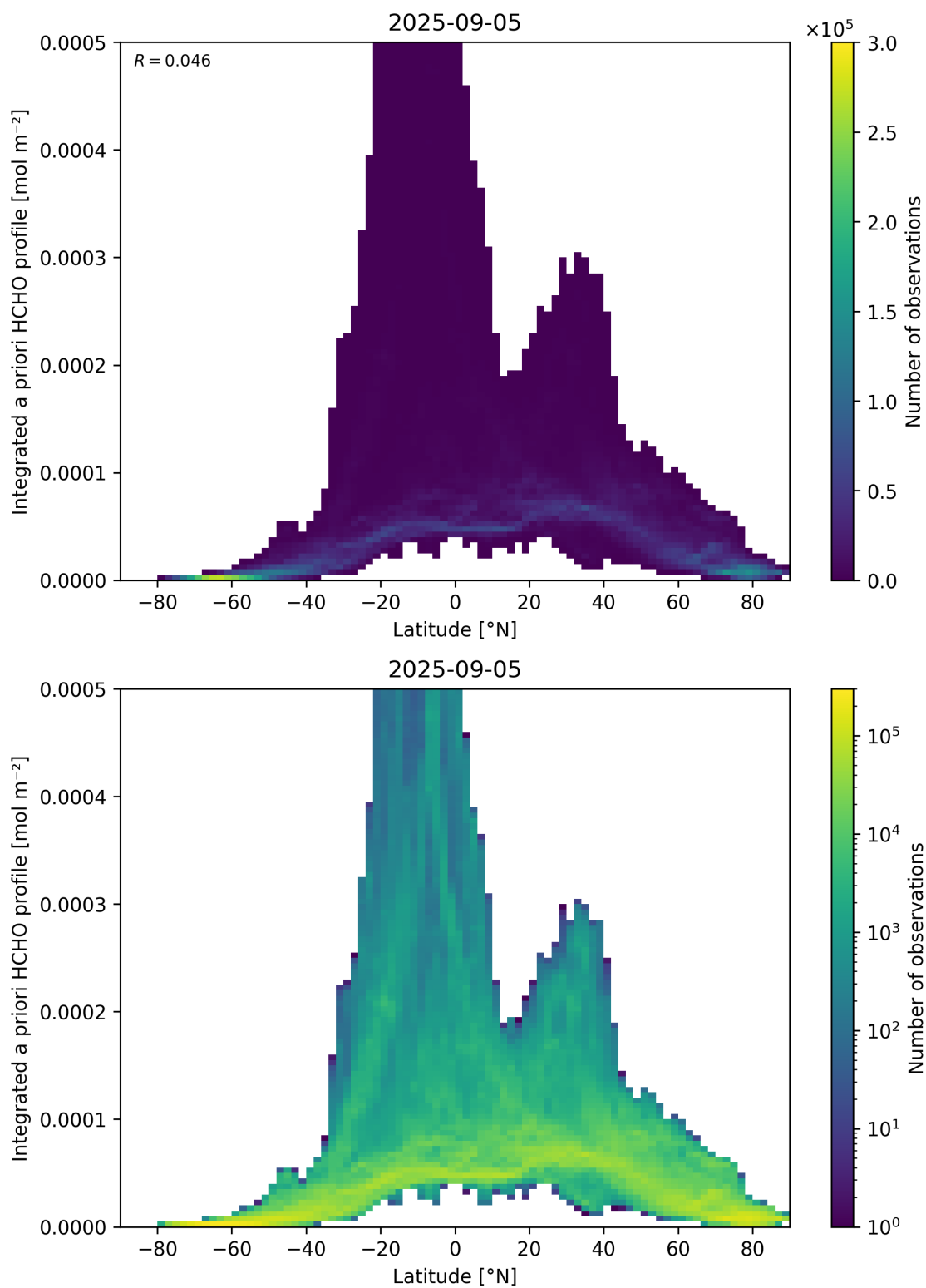
Figure 166: Scatter density plot of “Latitude” against “Integrated a priori HCHO profile” for 2025-09-04 to 2025-09-06.
