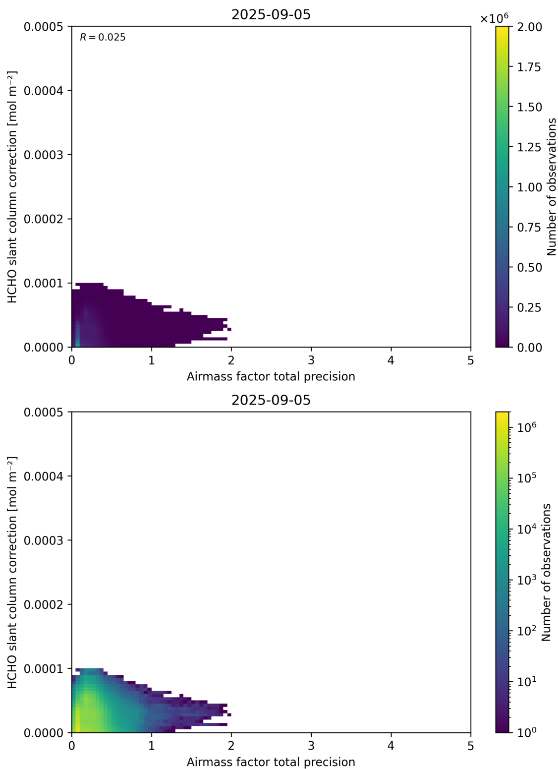
Figure 110: Scatter density plot of “Airmass factor total precision” against “HCHO slant column correction” for 2025-09-04 to 2025-09-06.
