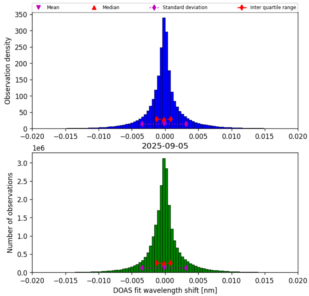
Figure 44: Histogram of “DOAS fit wavelength shift” for 2025-09-04 to 2025-09-06
