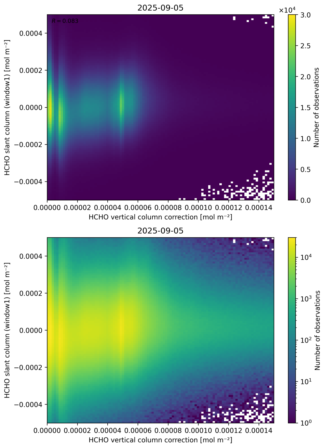
Figure 118: Scatter density plot of “HCHO vertical column correction” against “HCHO slant column (window1)” for 2025-09-04 to 2025-09-06.
