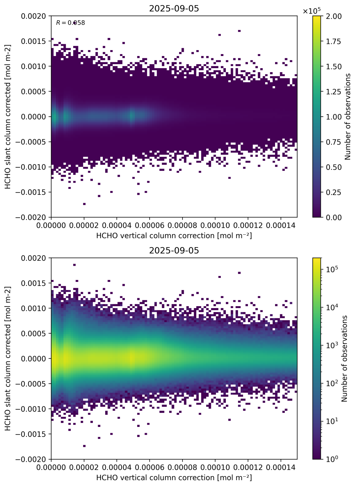
Figure 116: Scatter density plot of “HCHO vertical column correction” against “HCHO slant column corrected” for 2025-09-04 to 2025-09-06.
