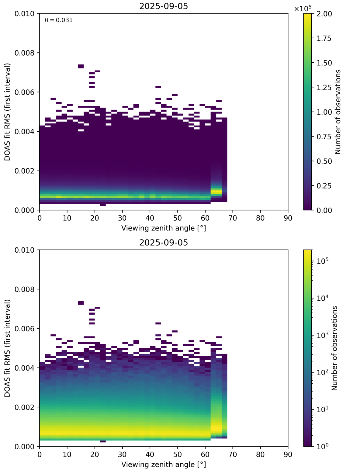
Figure 182: Scatter density plot of “Viewing zenith angle” against “DOAS fit RMS (first interval)” for 2025-09-04 to 2025-09-06.
