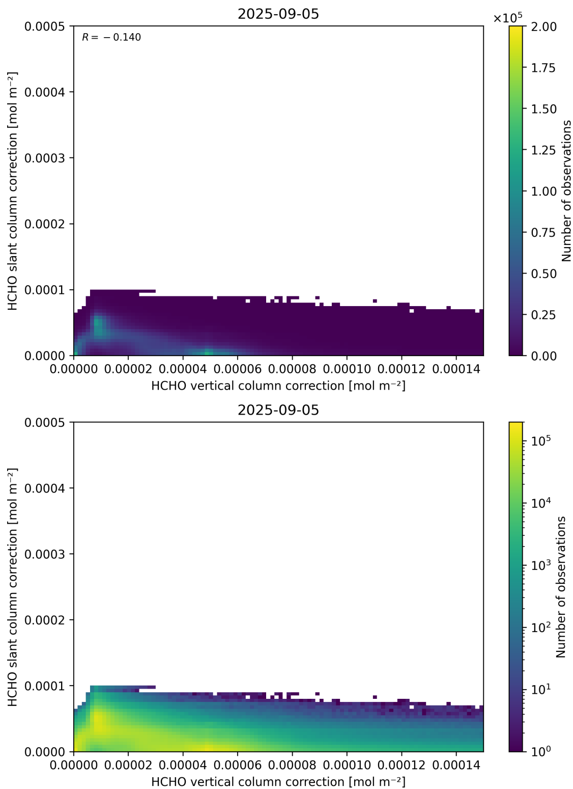
Figure 117: Scatter density plot of “HCHO vertical column correction” against “HCHO slant column correction” for 2025-09-04 to 2025-09-06.
