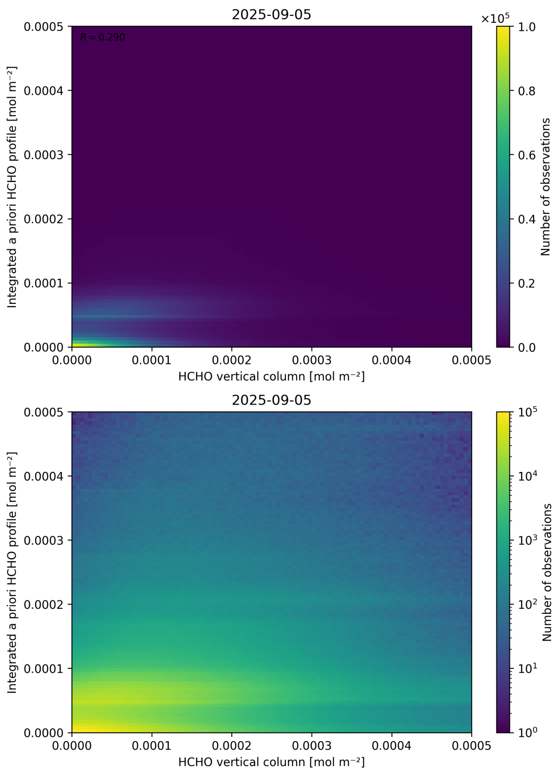
Figure 135: Scatter density plot of “HCHO vertical column” against “Integrated a priori HCHO profile” for 2025-09-04 to 2025-09-06.
