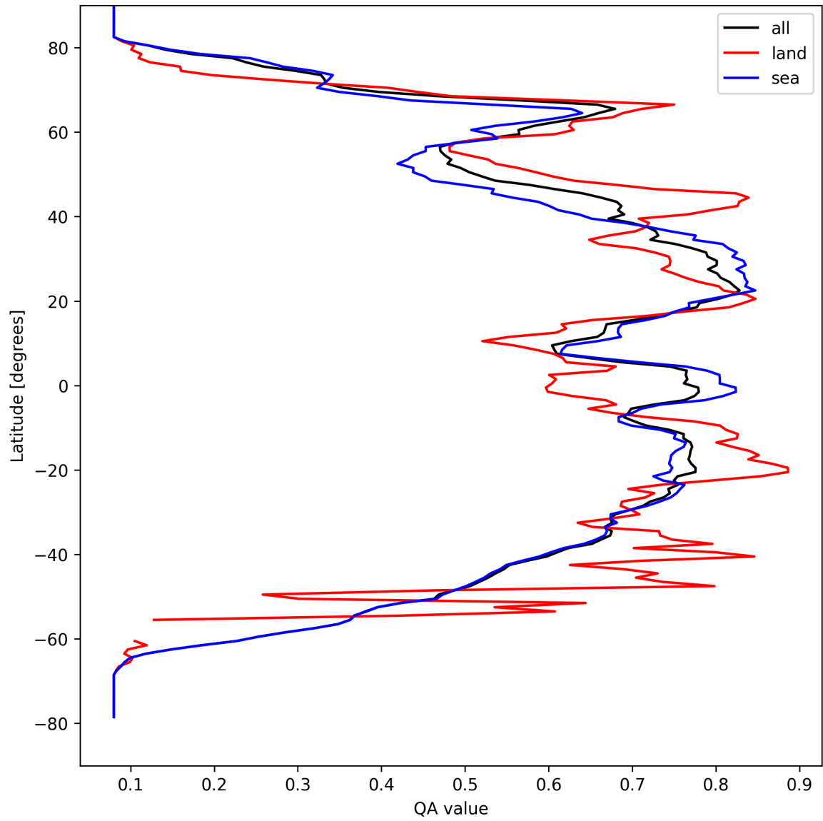
Figure 20: Zonal average of "QA value" for 2025-09-04 to 2025-09-06.
