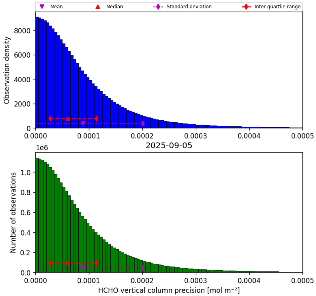
Figure 36: Histogram of “HCHO vertical column precision” for 2025-09-04 to 2025-09-06
