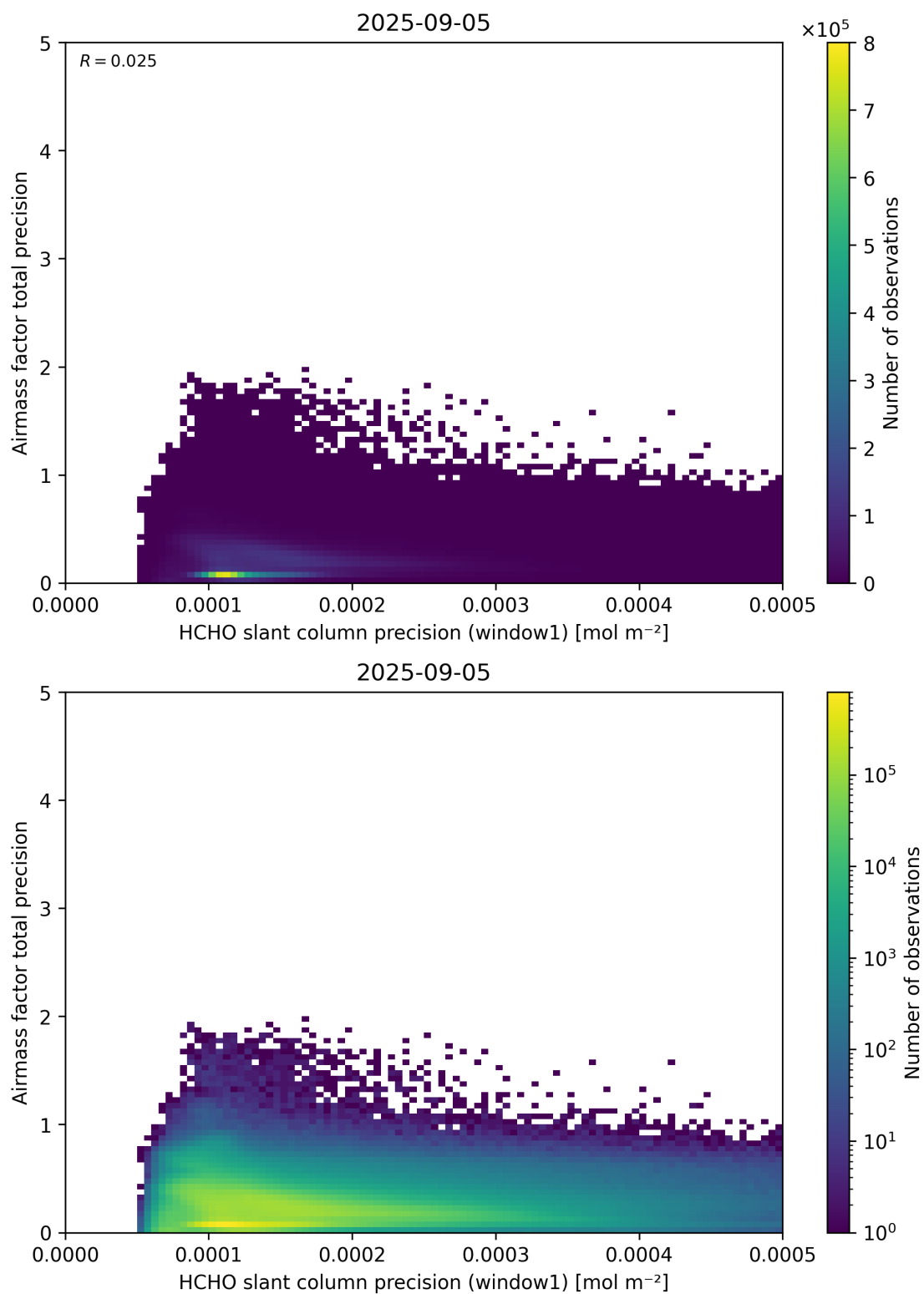
Figure 95: Scatter density plot of “HCHO slant column precision (window1)” against “Airmass factor total precision” for 2025-09-04 to 2025-09-06.
