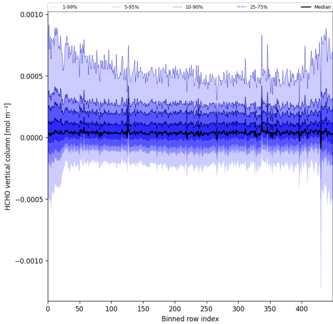
Figure 49: Along track statistics of “HCHO vertical column” for 2025-09-04 to 2025-09-06
