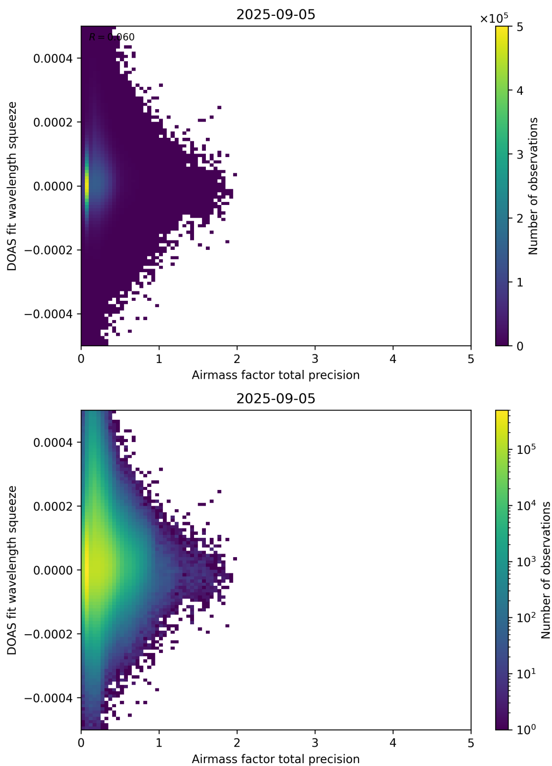
Figure 107: Scatter density plot of “Airmass factor total precision” against “DOAS fit wavelength squeeze” for 2025-09-04 to 2025-09-06.
