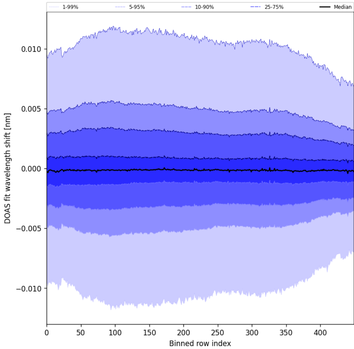
Figure 58: Along track statistics of “DOAS fit wavelength shift” for 2025-09-04 to 2025-09-06
