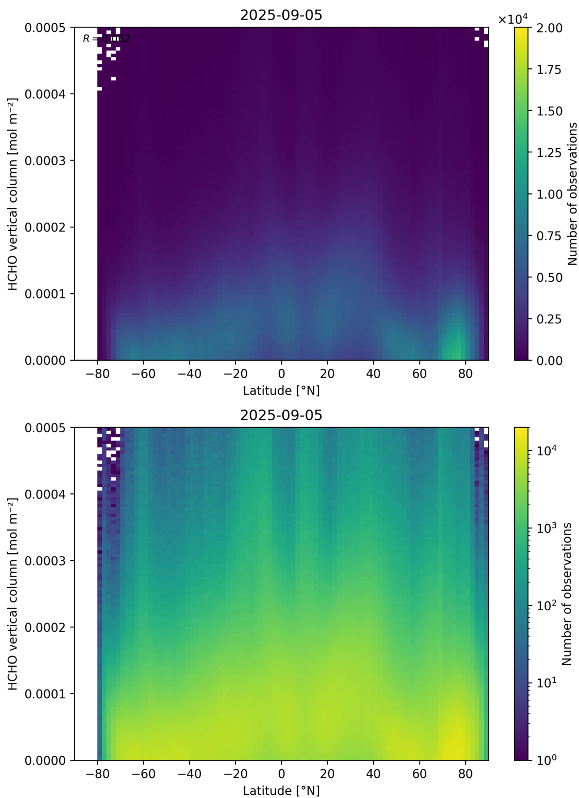
Figure 163: Scatter density plot of “Latitude” against “HCHO vertical column” for 2025-09-04 to 2025-09-06.
