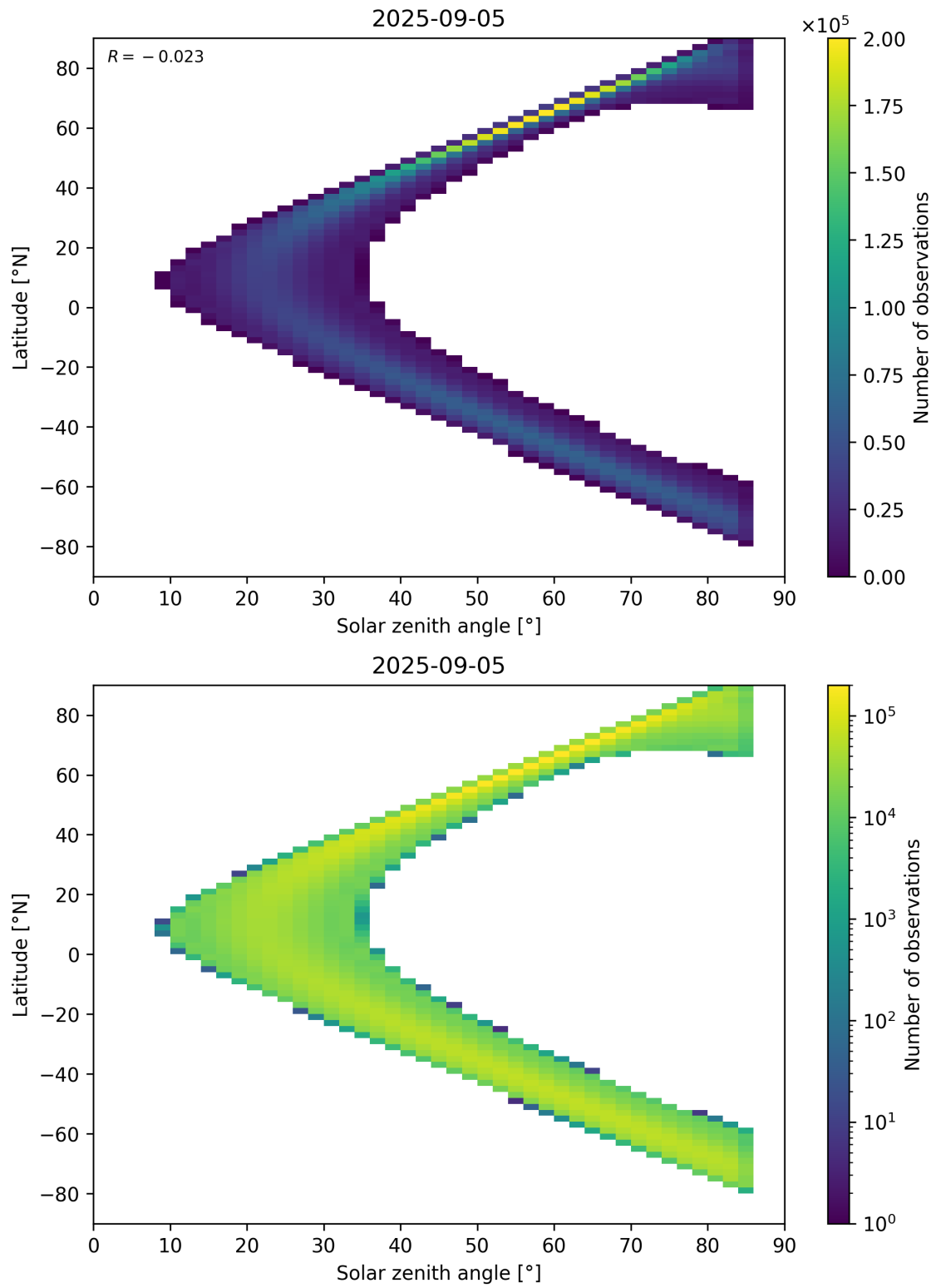
Figure 181: Scatter density plot of “Solar zenith angle” against “Latitude” for 2025-09-04 to 2025-09-06.
