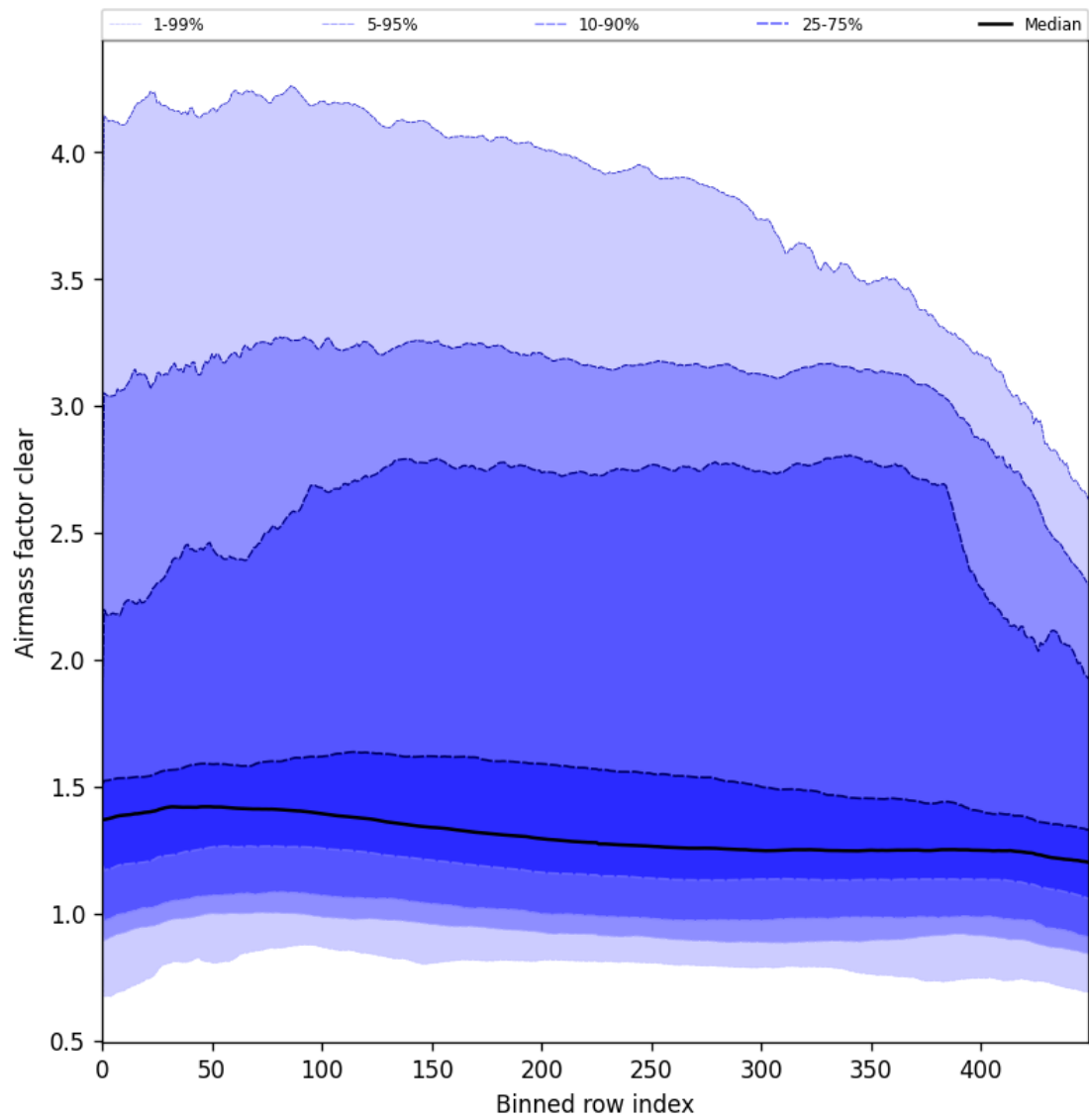
Figure 56: Along track statistics of “Airmass factor clear” for 2025-09-04 to 2025-09-06
