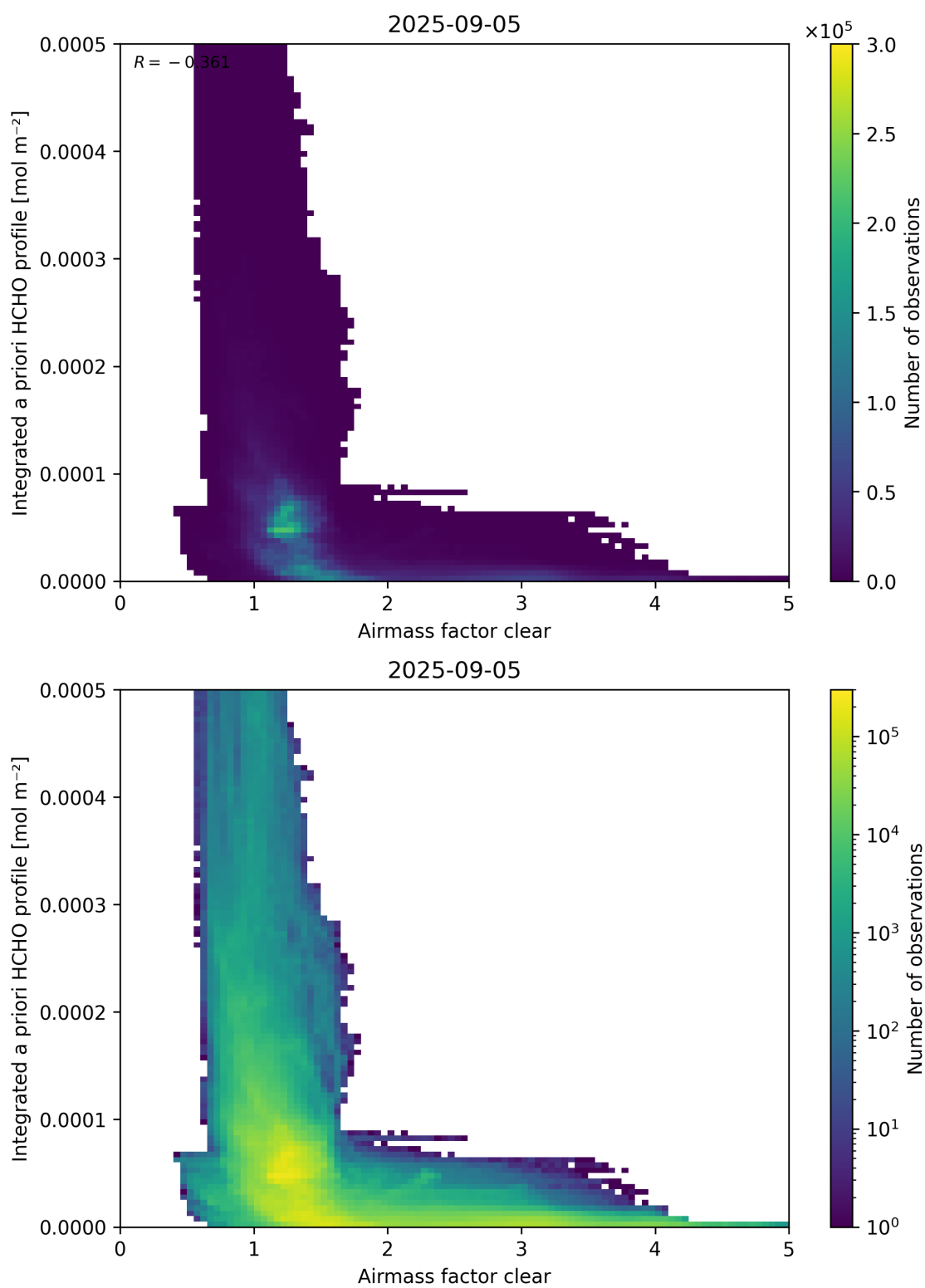
Figure 76: Scatter density plot of “Airmass factor clear” against “Integrated a priori HCHO profile” for 2025-09-04 to 2025-09-06.
