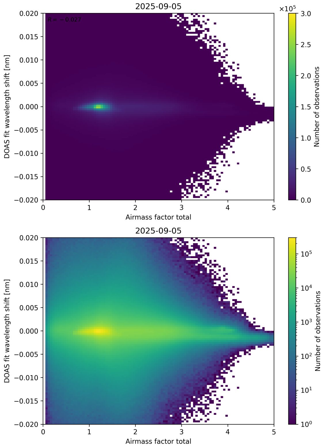
Figure 98: Scatter density plot of “Airmass factor total” against “DOAS fit wavelength shift” for 2025-09-04 to 2025-09-06.
