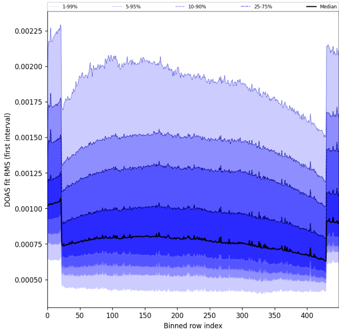
Figure 60: Along track statistics of “DOAS fit RMS (first interval)” for 2025-09-04 to 2025-09-06
