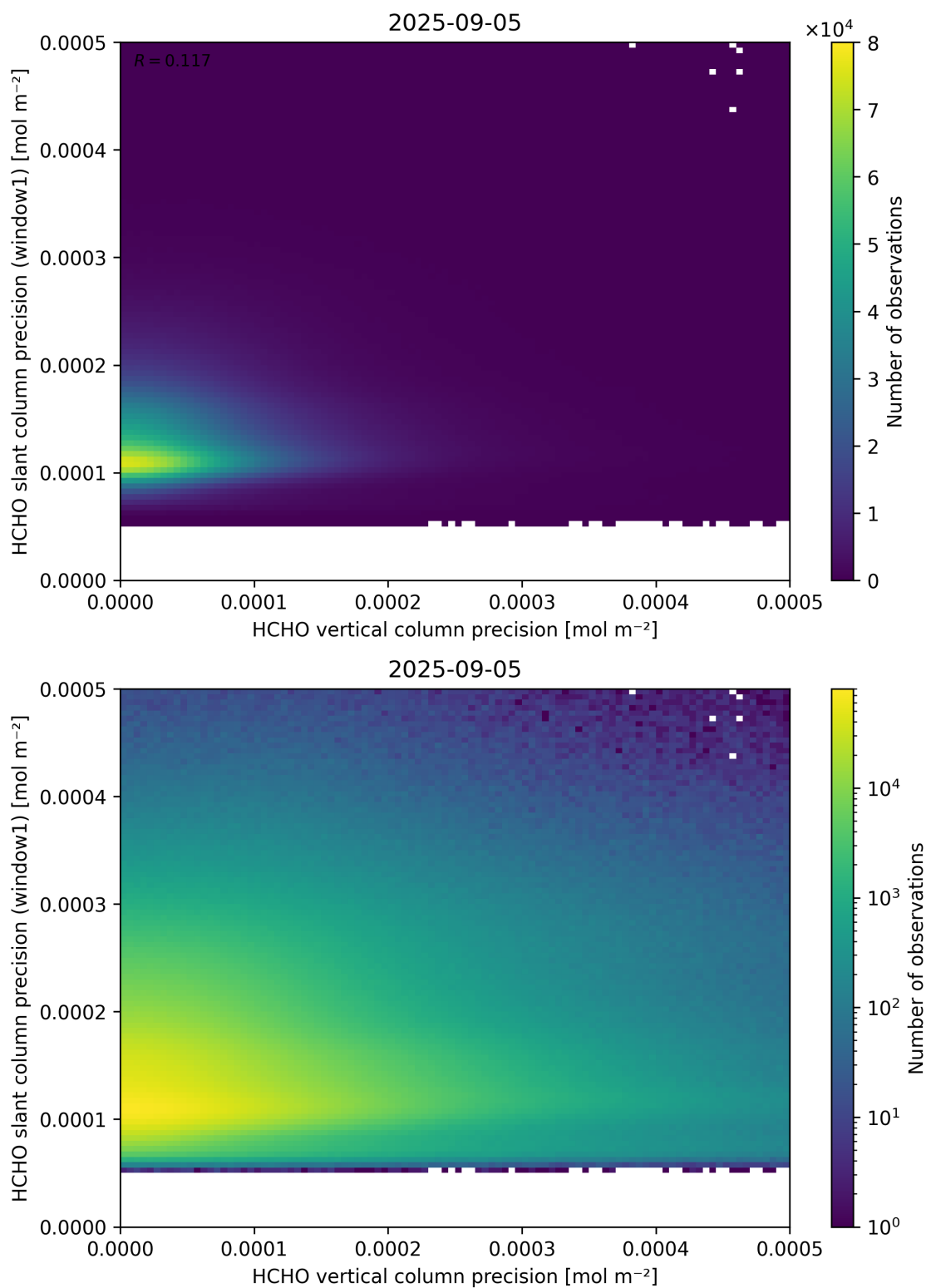
Figure 143: Scatter density plot of “HCHO vertical column precision” against “HCHO slant column precision (window1)” for 2025-09-04 to 2025-09-06.
