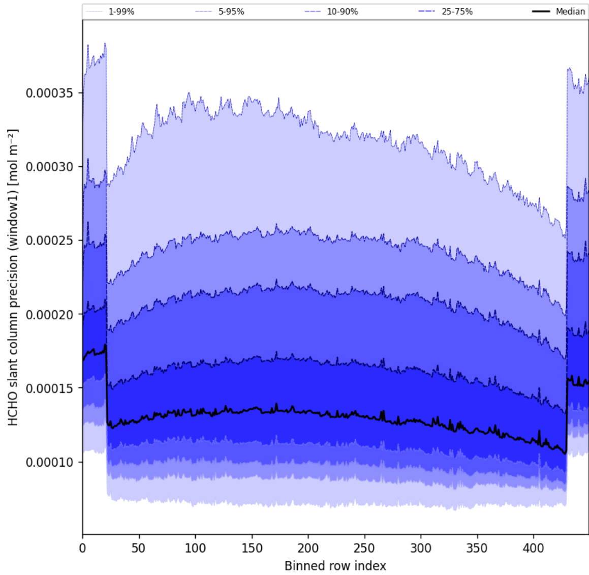
Figure 53: Along track statistics of “HCHO slant column precision (window1)” for 2025-09-04 to 2025-09-06
