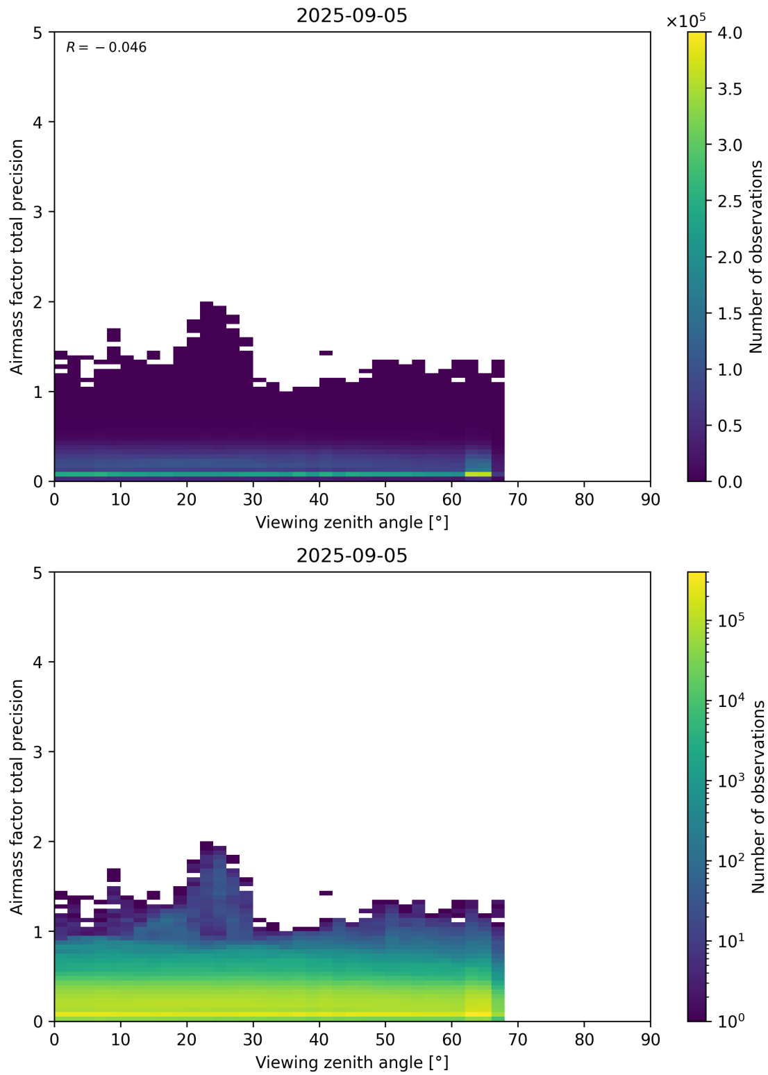
Figure 191: Scatter density plot of “Viewing zenith angle” against “Airmass factor total precision” for 2025-09-04 to 2025-09-06.
