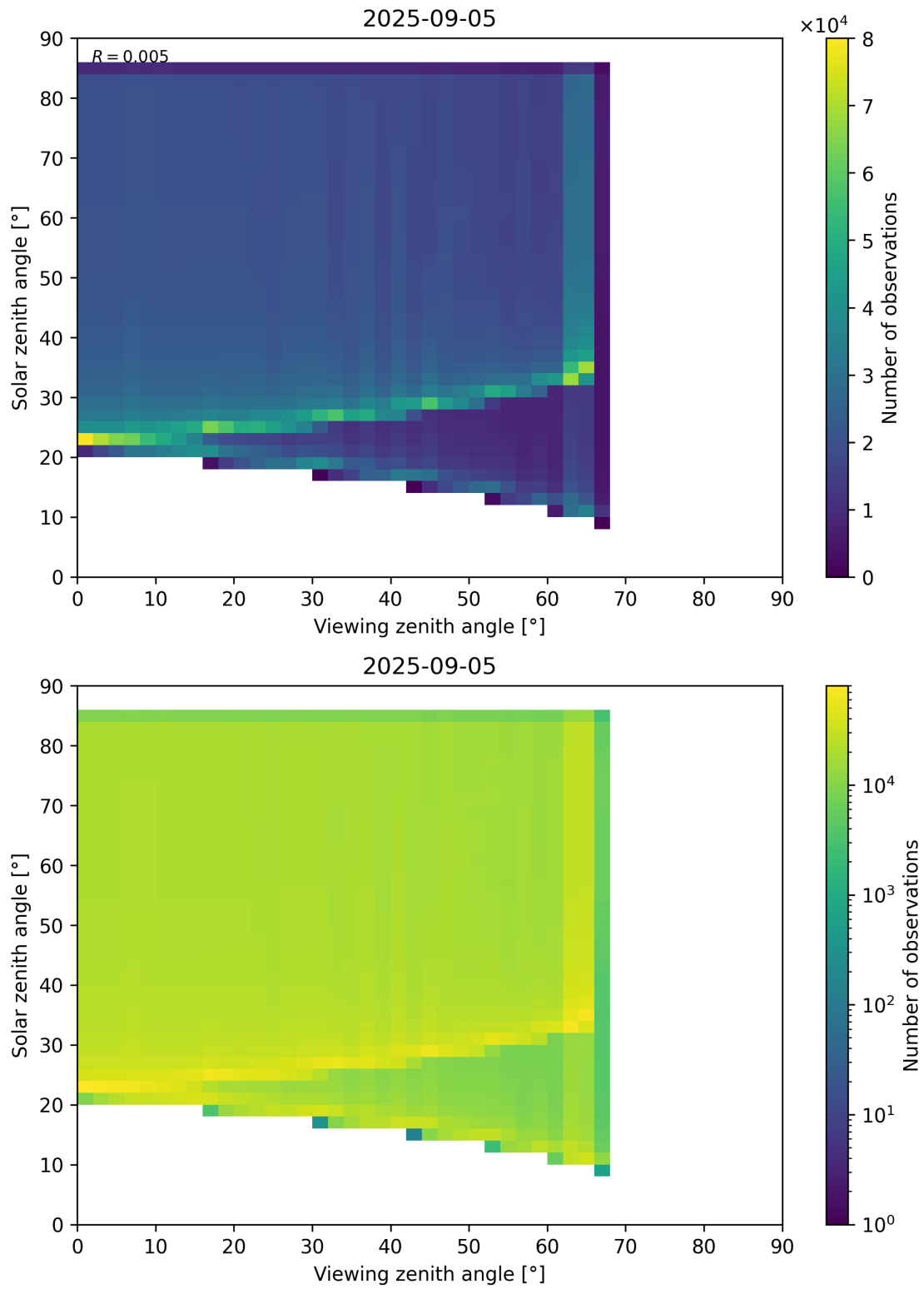
Figure 197: Scatter density plot of “Viewing zenith angle” against “Solar zenith angle” for 2025-09-04 to 2025-09-06.
