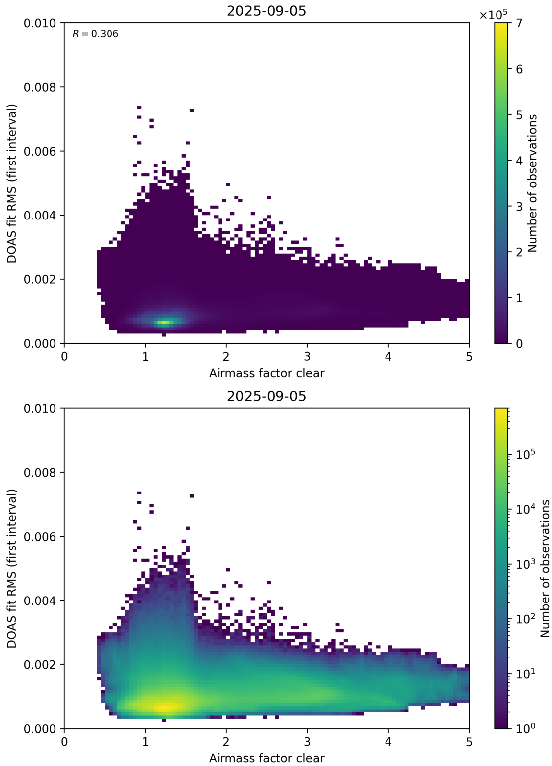
Figure 71: Scatter density plot of “Airmass factor clear” against “DOAS fit RMS (first interval)” for 2025-09-04 to 2025-09-06.
