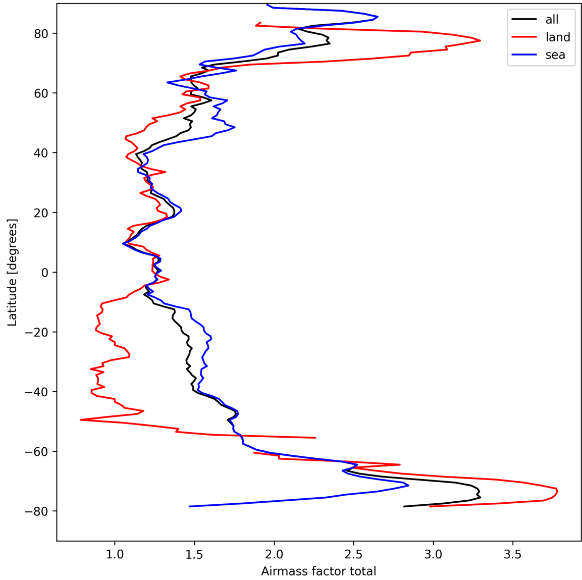
Figure 26: Zonal average of "Airmass factor total" for 2025-09-04 to 2025-09-06.
