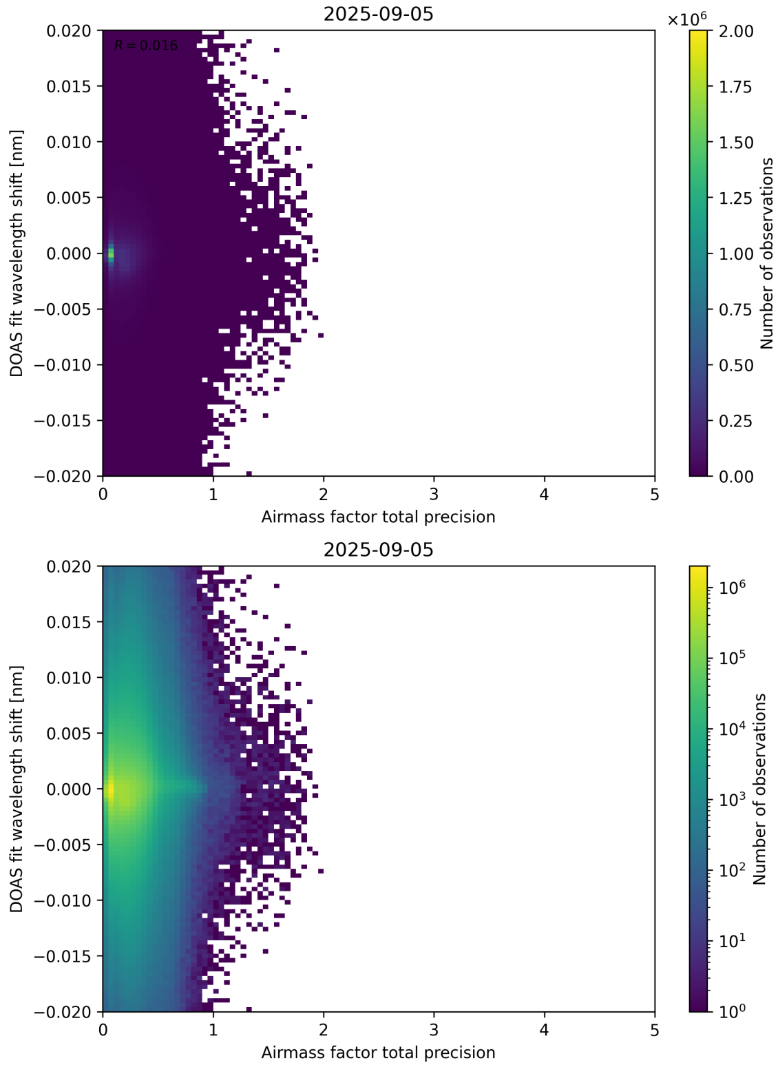
Figure 106: Scatter density plot of “Airmass factor total precision” against “DOAS fit wavelength shift” for 2025-09-04 to 2025-09-06.
