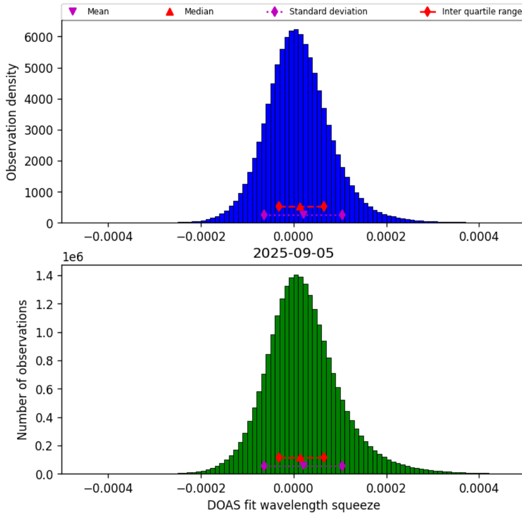
Figure 45: Histogram of “DOAS fit wavelength squeeze” for 2025-09-04 to 2025-09-06
