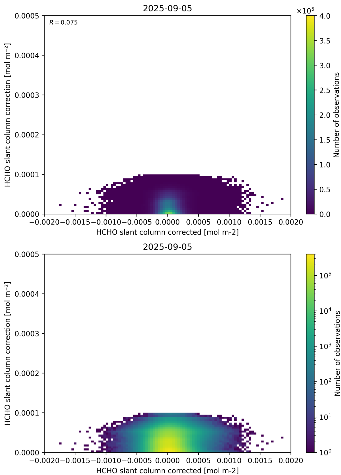
Figure 77: Scatter density plot of “HCHO slant column corrected” against “HCHO slant column correction” for 2025-09-04 to 2025-09-06.
