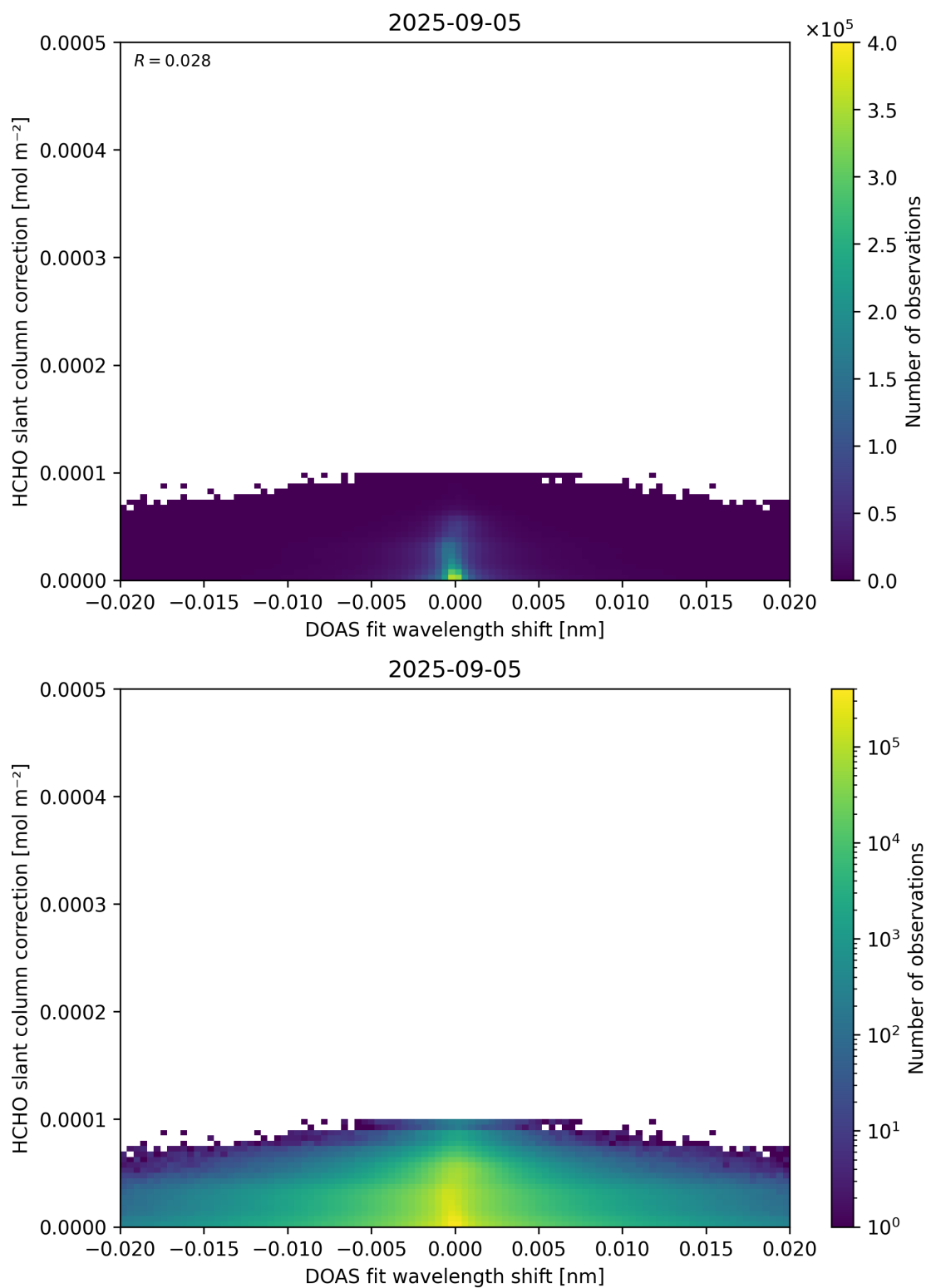
Figure 67: Scatter density plot of “DOAS fit wavelength shift” against “HCHO slant column correction” for 2025-09-04 to 2025-09-06.
