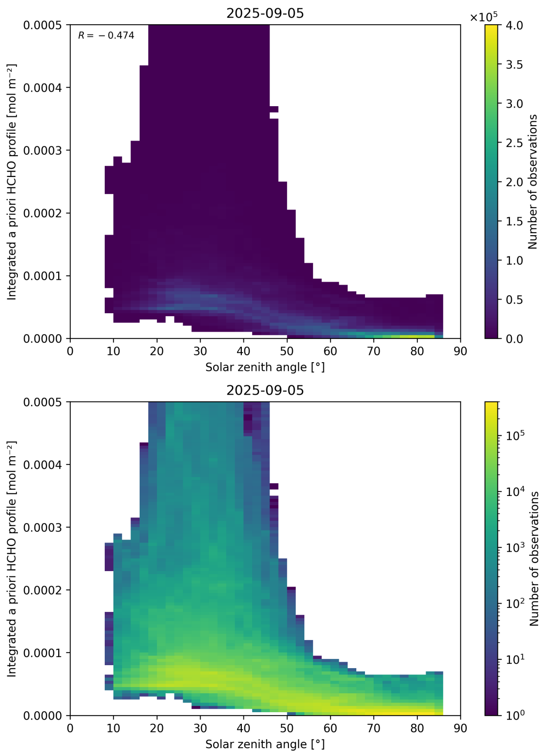
Figure 180: Scatter density plot of “Solar zenith angle” against “Integrated a priori HCHO profile” for 2025-09-04 to 2025-09-06.
