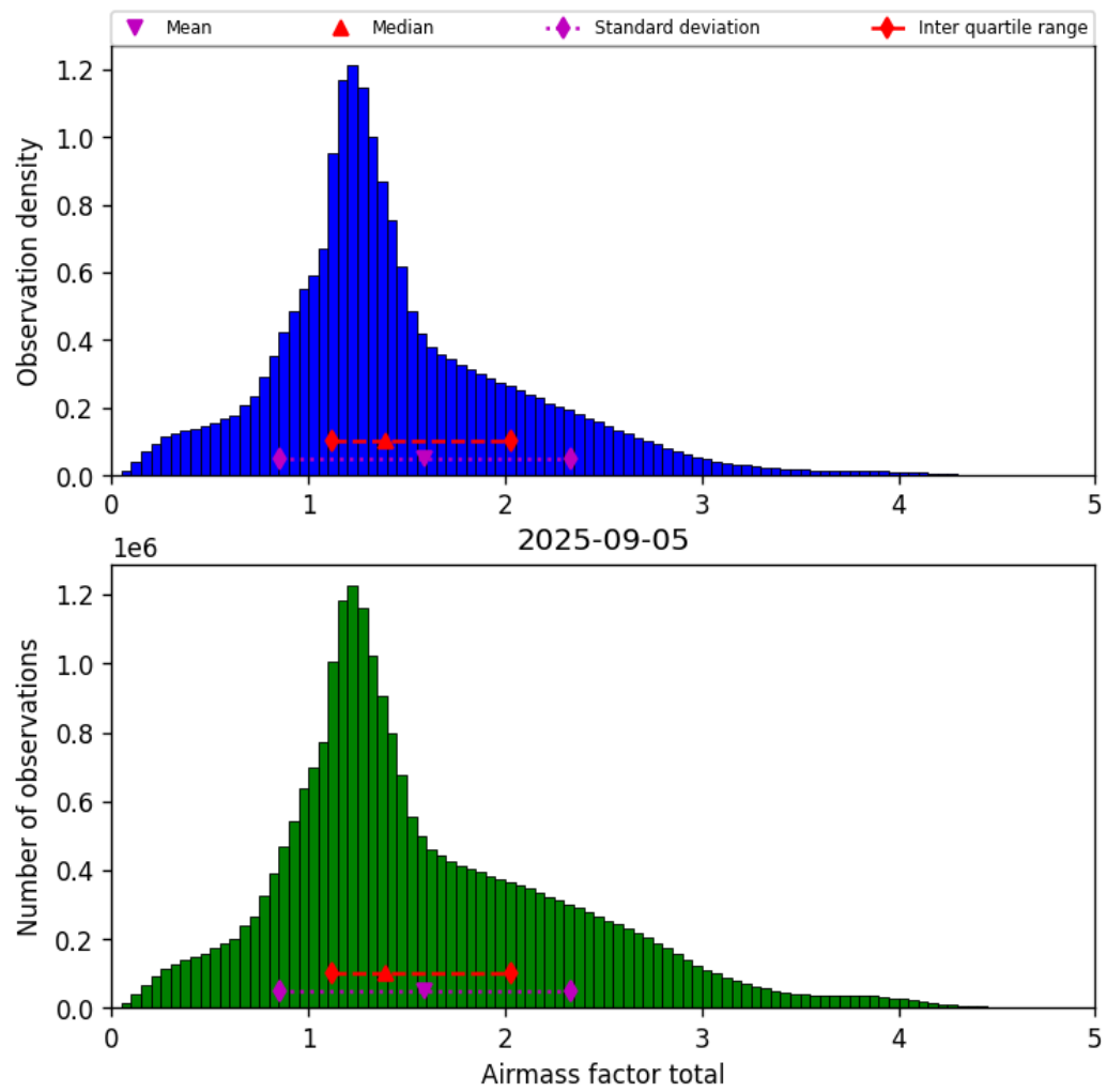
Figure 40: Histogram of “Airmass factor total” for 2025-09-04 to 2025-09-06
