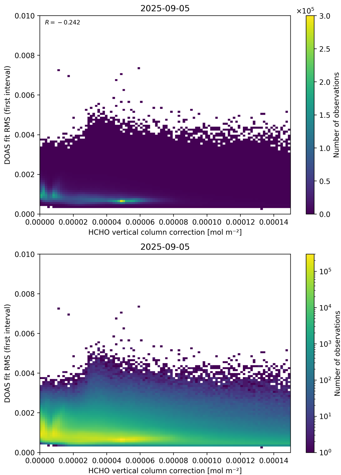
Figure 112: Scatter density plot of “HCHO vertical column correction” against “DOAS fit RMS (first interval)” for 2025-09-04 to 2025-09-06.
