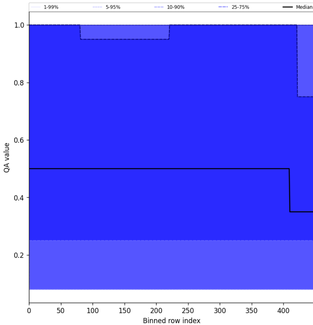
Figure 48: Along track statistics of “QA value” for 2025-09-04 to 2025-09-06
