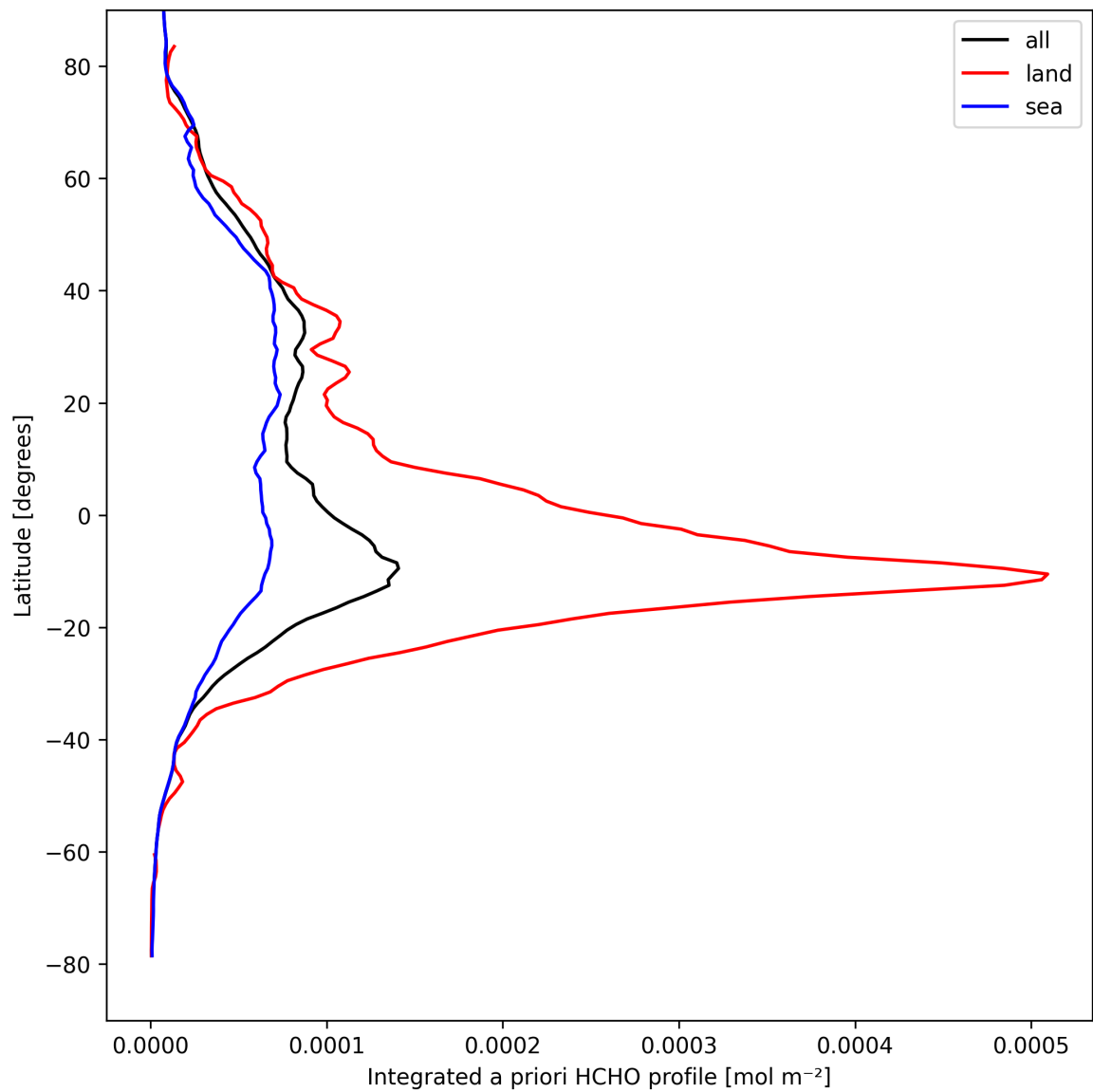
Figure 29: Zonal average of “Integrated a priori HCHO profile” for 2025-09-04 to 2025-09-06.
