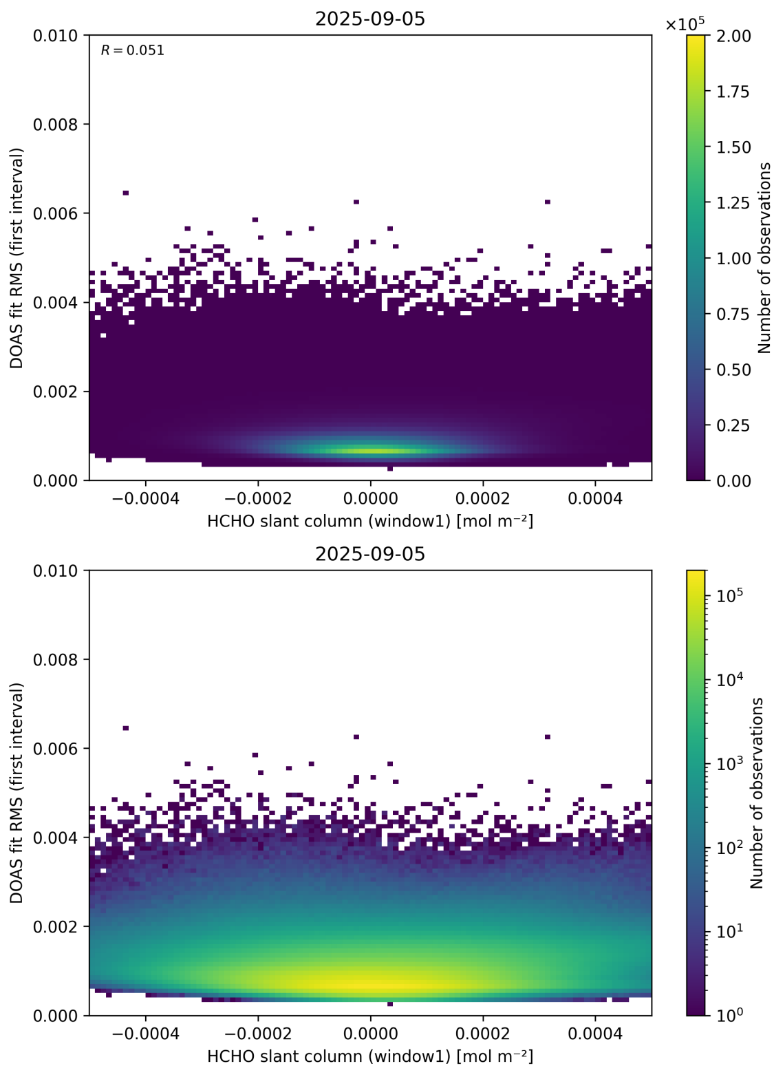
Figure 78: Scatter density plot of “HCHO slant column (window1)” against “DOAS fit RMS (first interval)” for 2025-09-04 to 2025-09-06.
