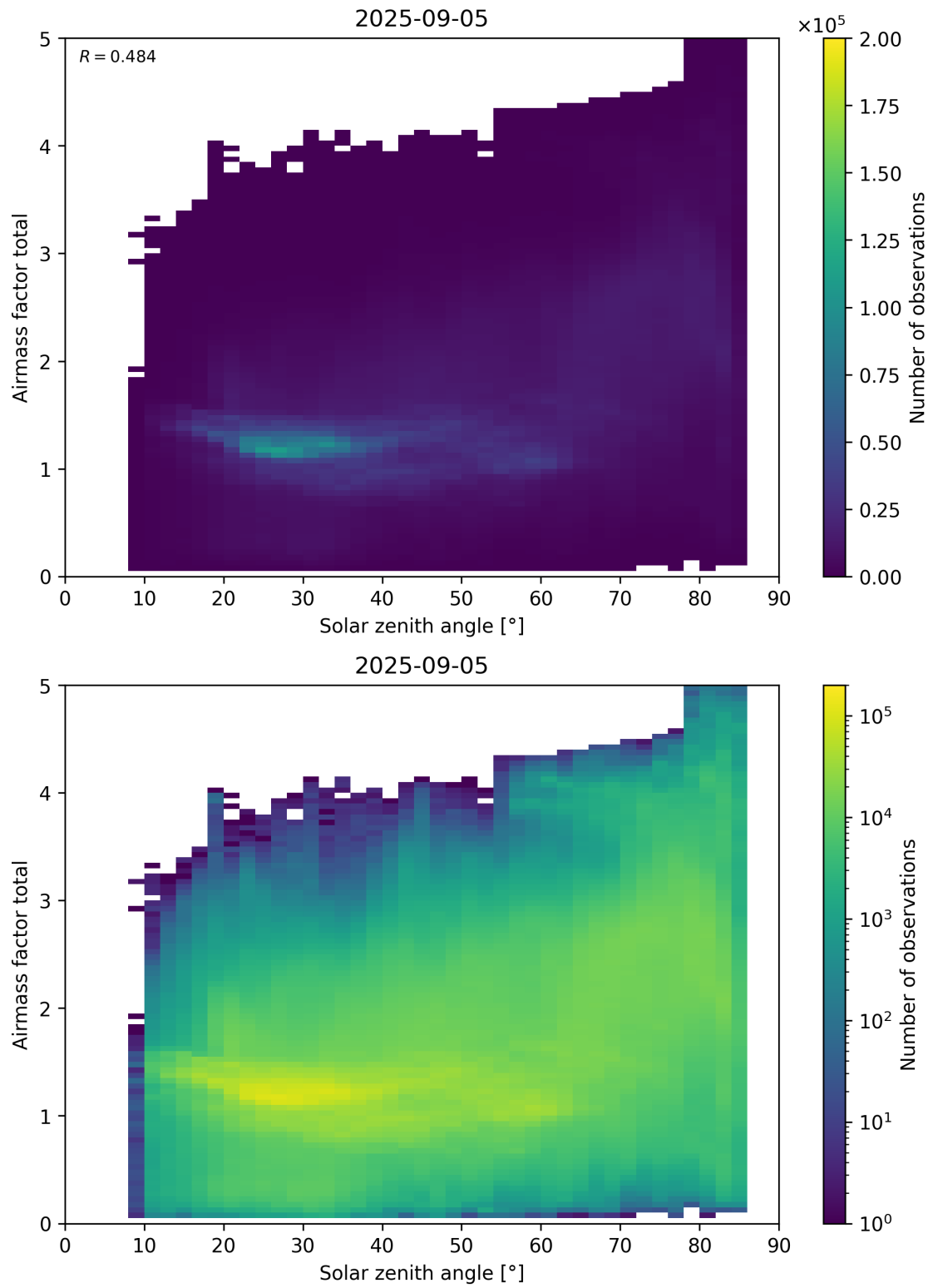
Figure 175: Scatter density plot of “Solar zenith angle” against “Airmass factor total” for 2025-09-04 to 2025-09-06.
