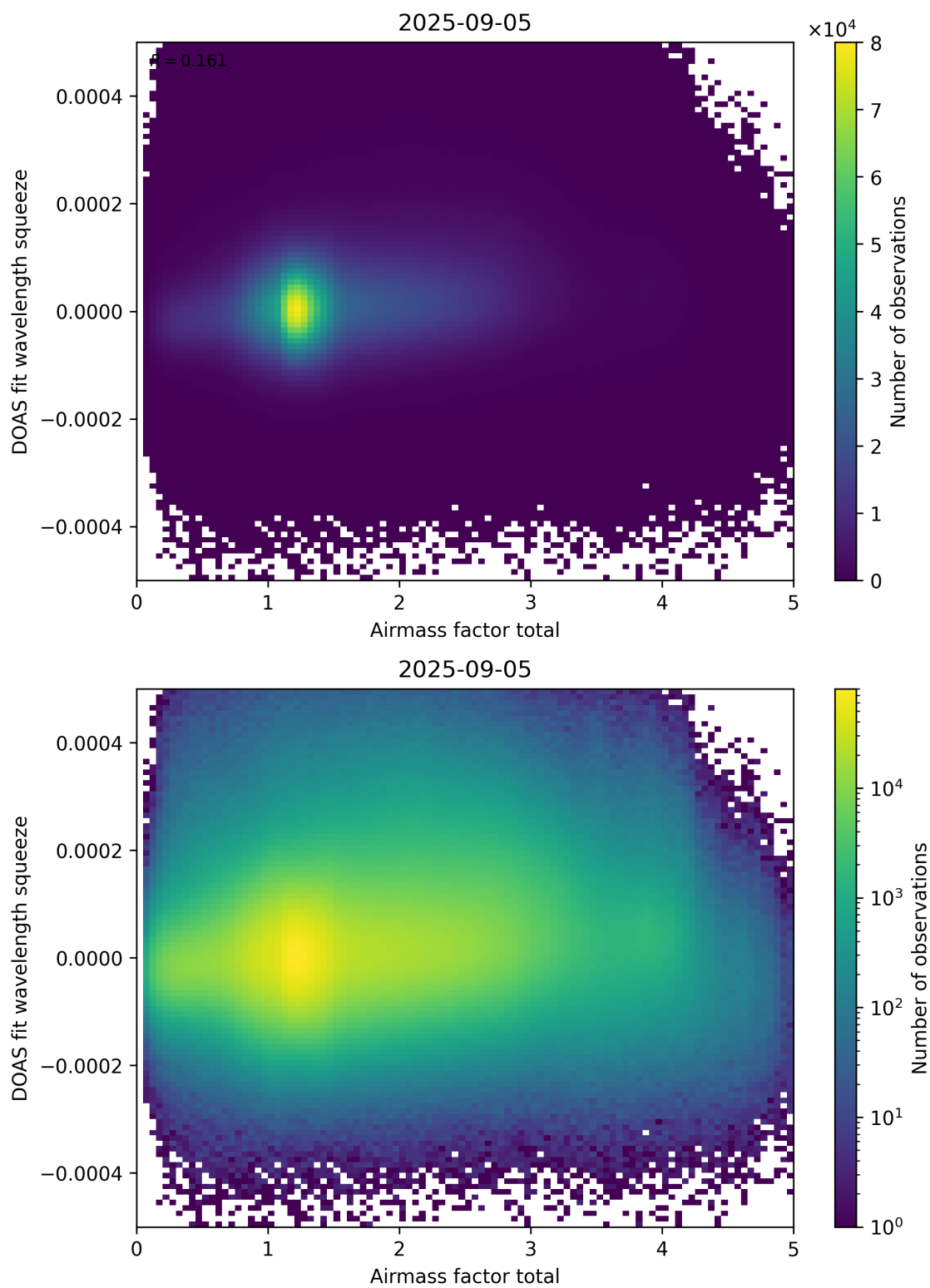
Figure 99: Scatter density plot of “Airmass factor total” against “DOAS fit wavelength squeeze” for 2025-09-04 to 2025-09-06.
