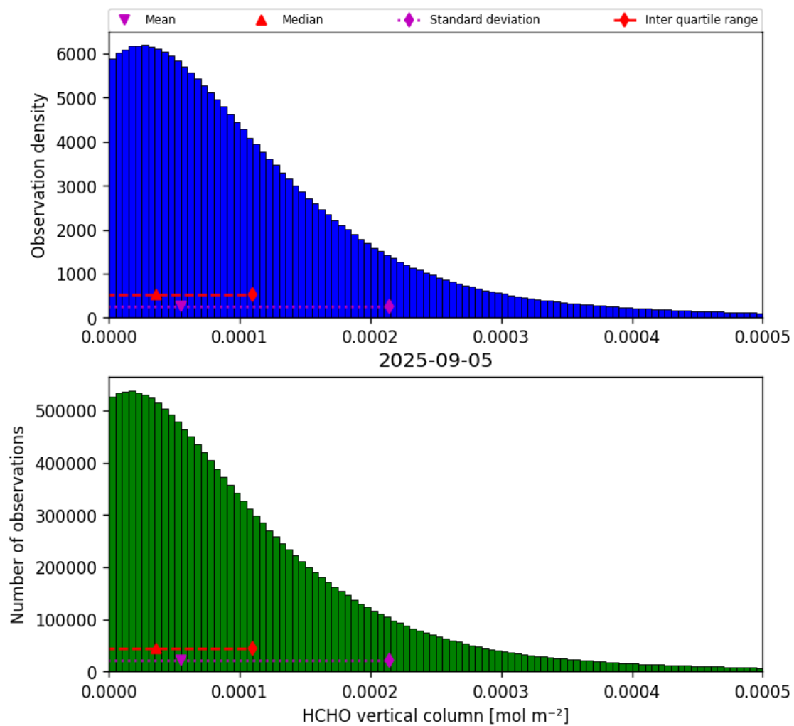
Figure 35: Histogram of “HCHO vertical column” for 2025-09-04 to 2025-09-06
