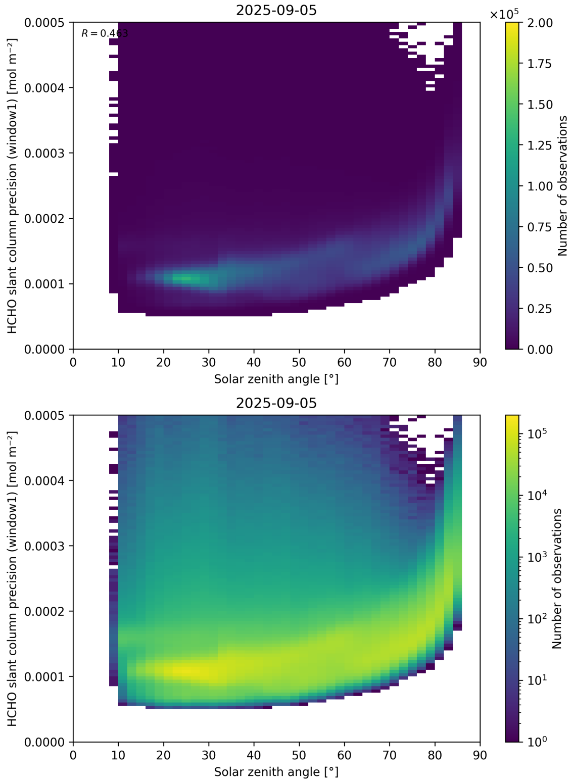
Figure 174: Scatter density plot of “Solar zenith angle” against “HCHO slant column precision (window1)” for 2025-09-04 to 2025-09-06.
