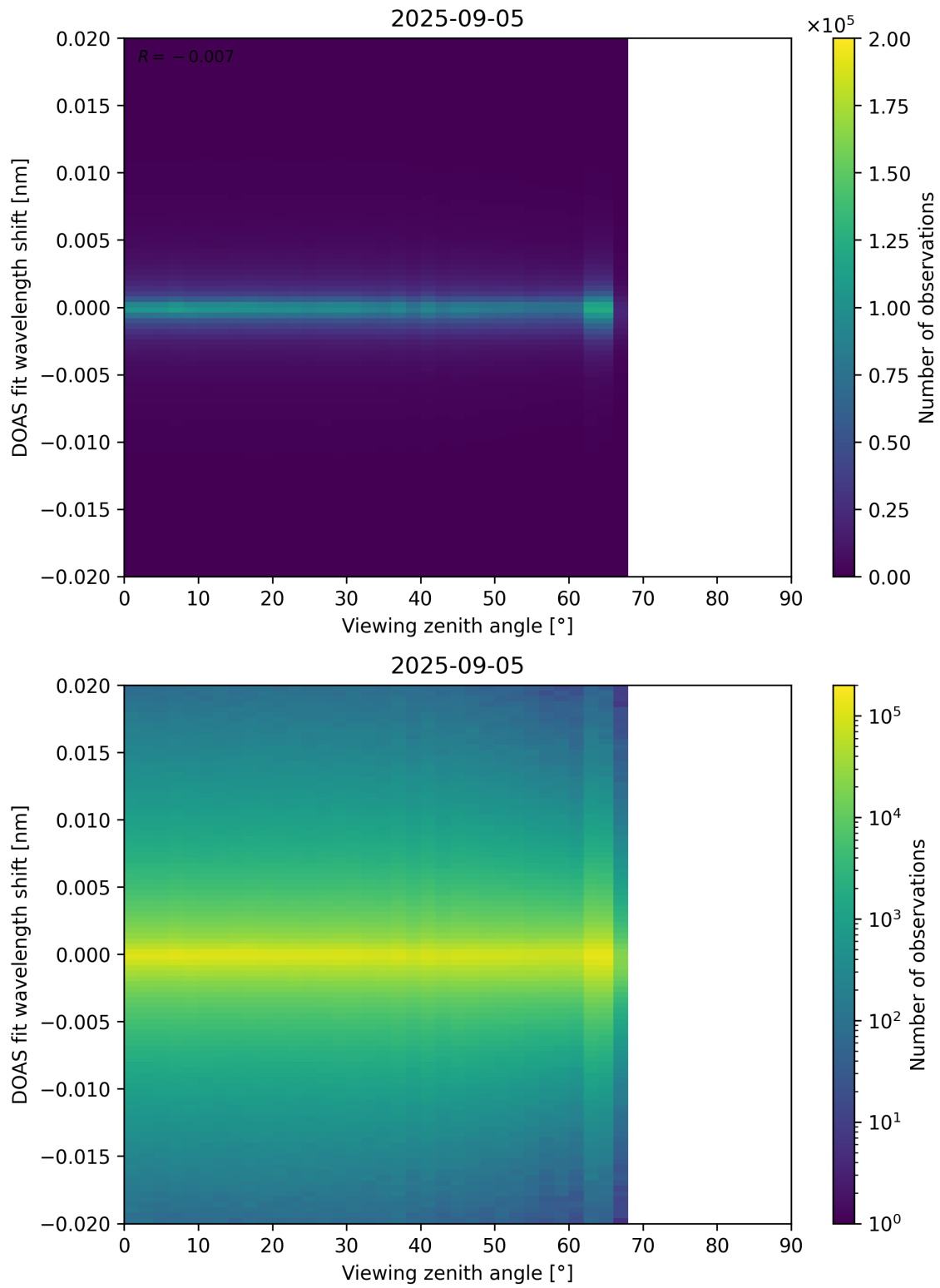
Figure 183: Scatter density plot of “Viewing zenith angle” against “DOAS fit wavelength shift” for 2025-09-04 to 2025-09-06.
