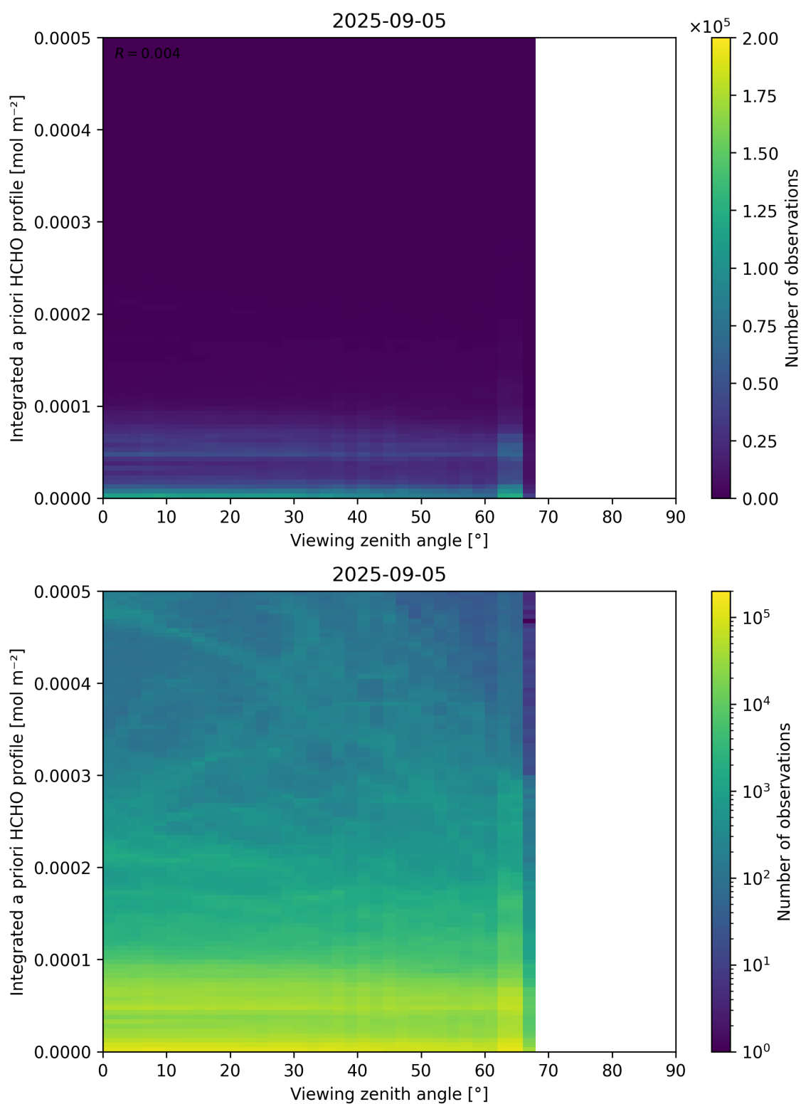
Figure 195: Scatter density plot of “Viewing zenith angle” against “Integrated a priori HCHO profile” for 2025-09-04 to 2025-09-06.
