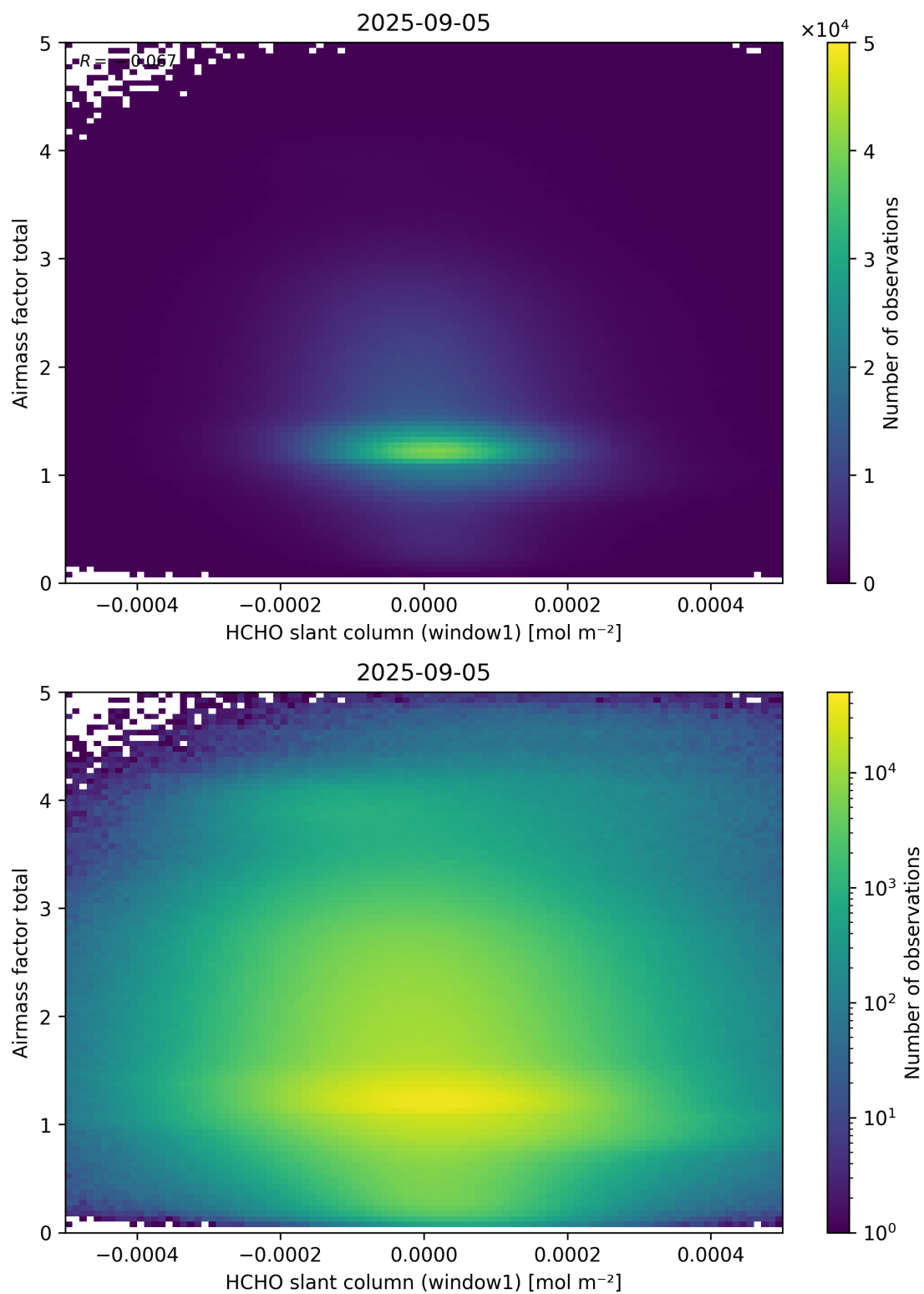
Figure 85: Scatter density plot of “HCHO slant column (window1)” against “Airmass factor total” for 2025-09-04 to 2025-09-06.
