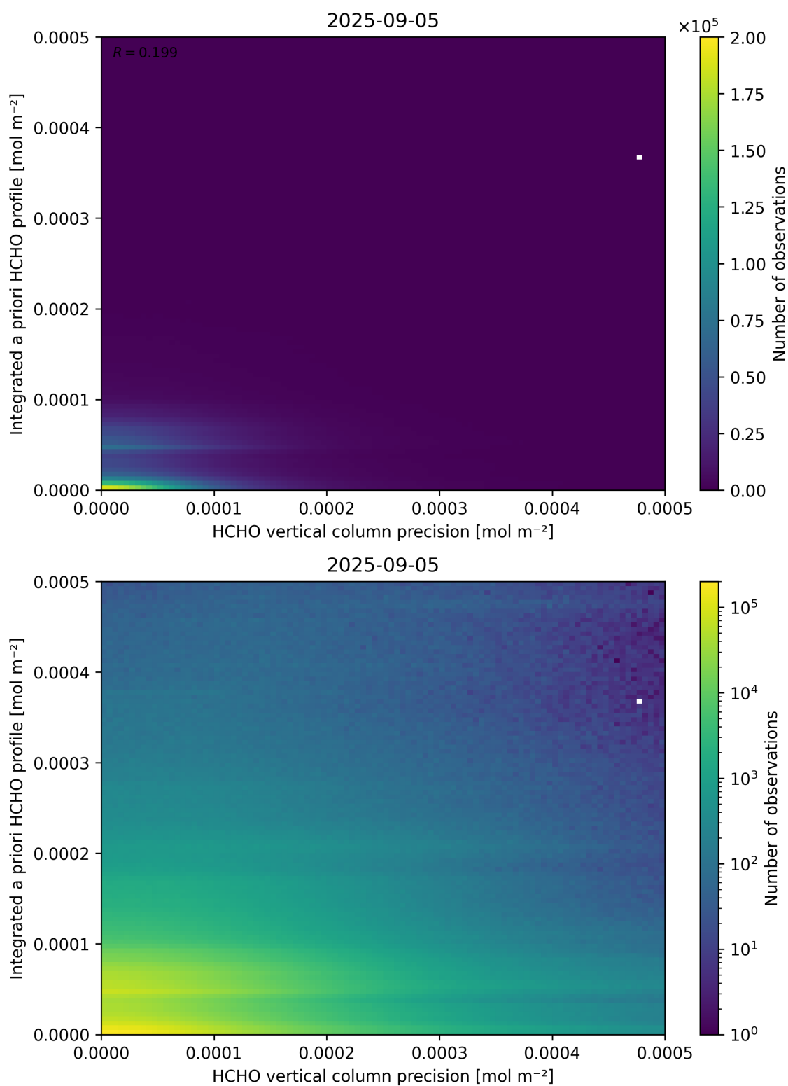
Figure 147: Scatter density plot of “HCHO vertical column precision” against “Integrated a priori HCHO profile” for 2025-09-04 to 2025-09-06.
