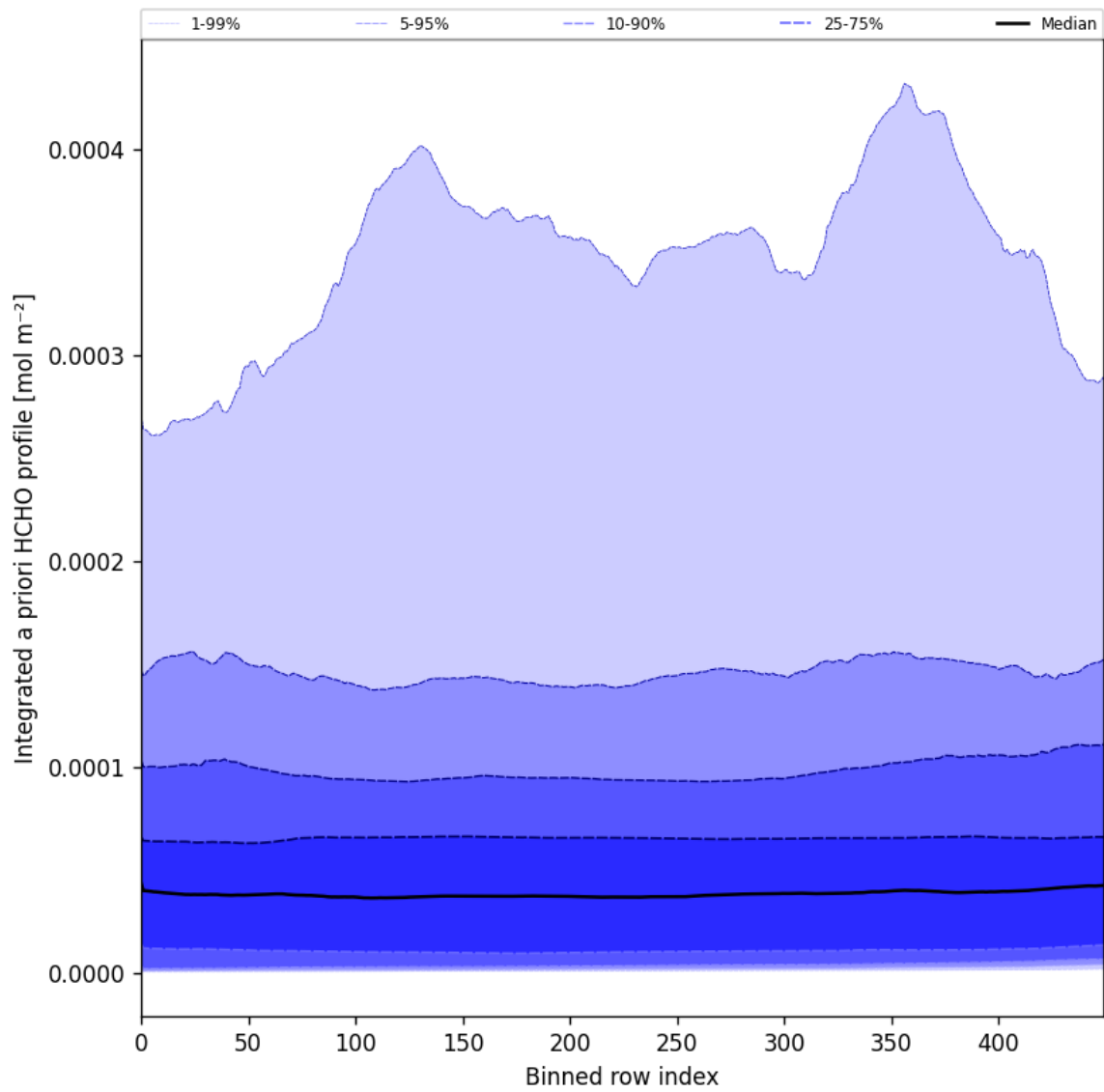
Figure 57: Along track statistics of “Integrated a priori HCHO profile” for 2025-09-04 to 2025-09-06
