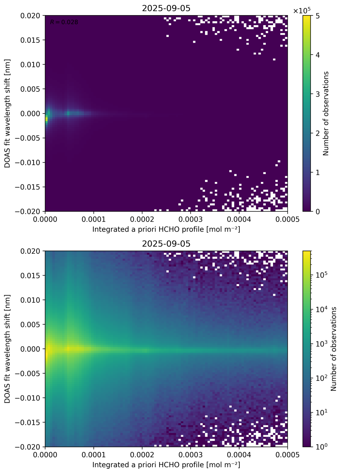
Figure 149: Scatter density plot of “Integrated a priori HCHO profile” against “DOAS fit wavelength shift” for 2025-09-04 to 2025-09-06.
