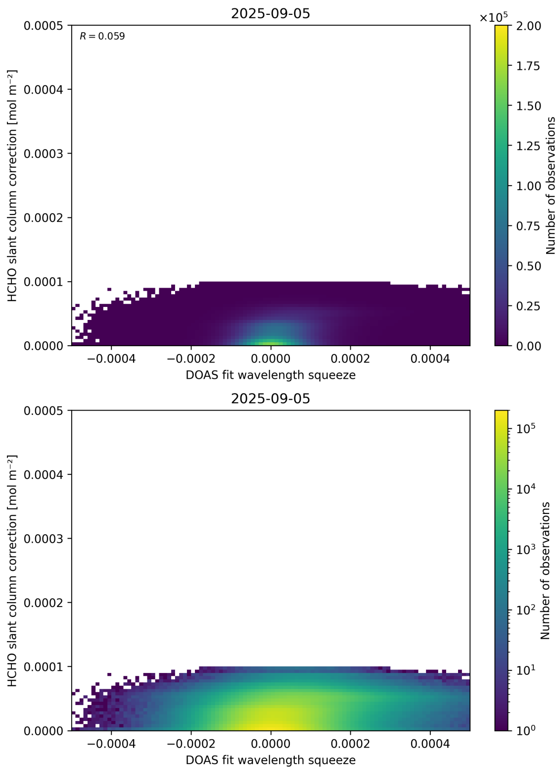
Figure 70: Scatter density plot of “DOAS fit wavelength squeeze” against “HCHO slant column correction” for 2025-09-04 to 2025-09-06.
