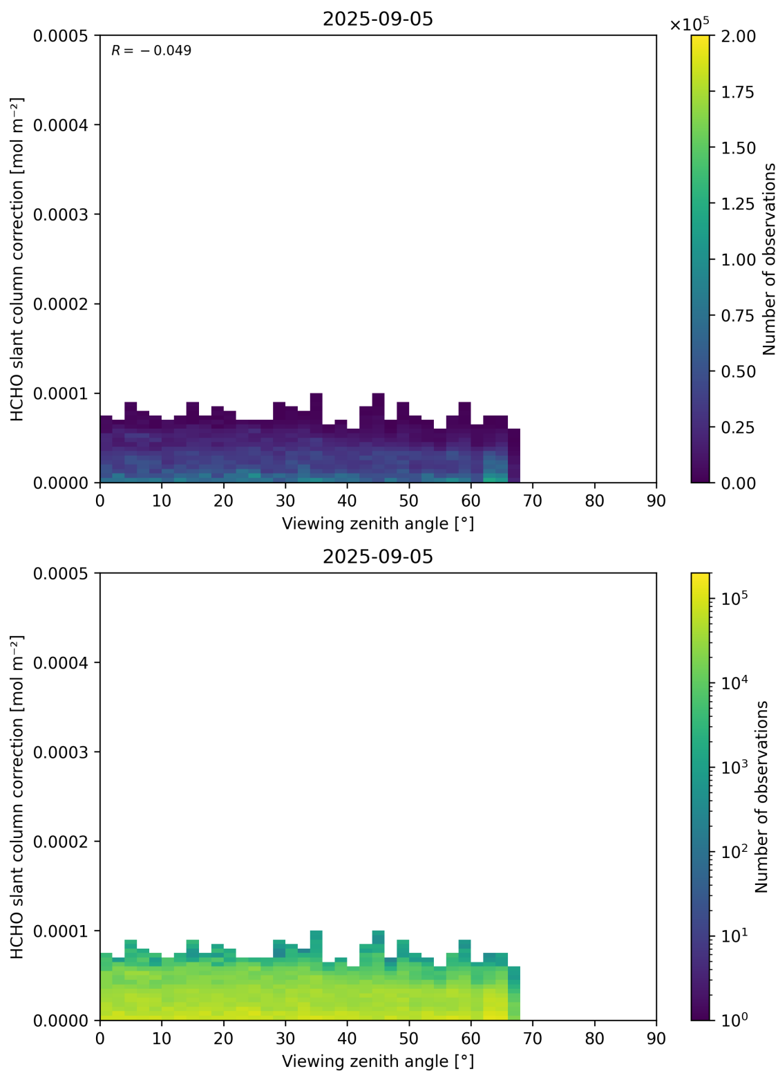
Figure 187: Scatter density plot of “Viewing zenith angle” against “HCHO slant column correction” for 2025-09-04 to 2025-09-06.
