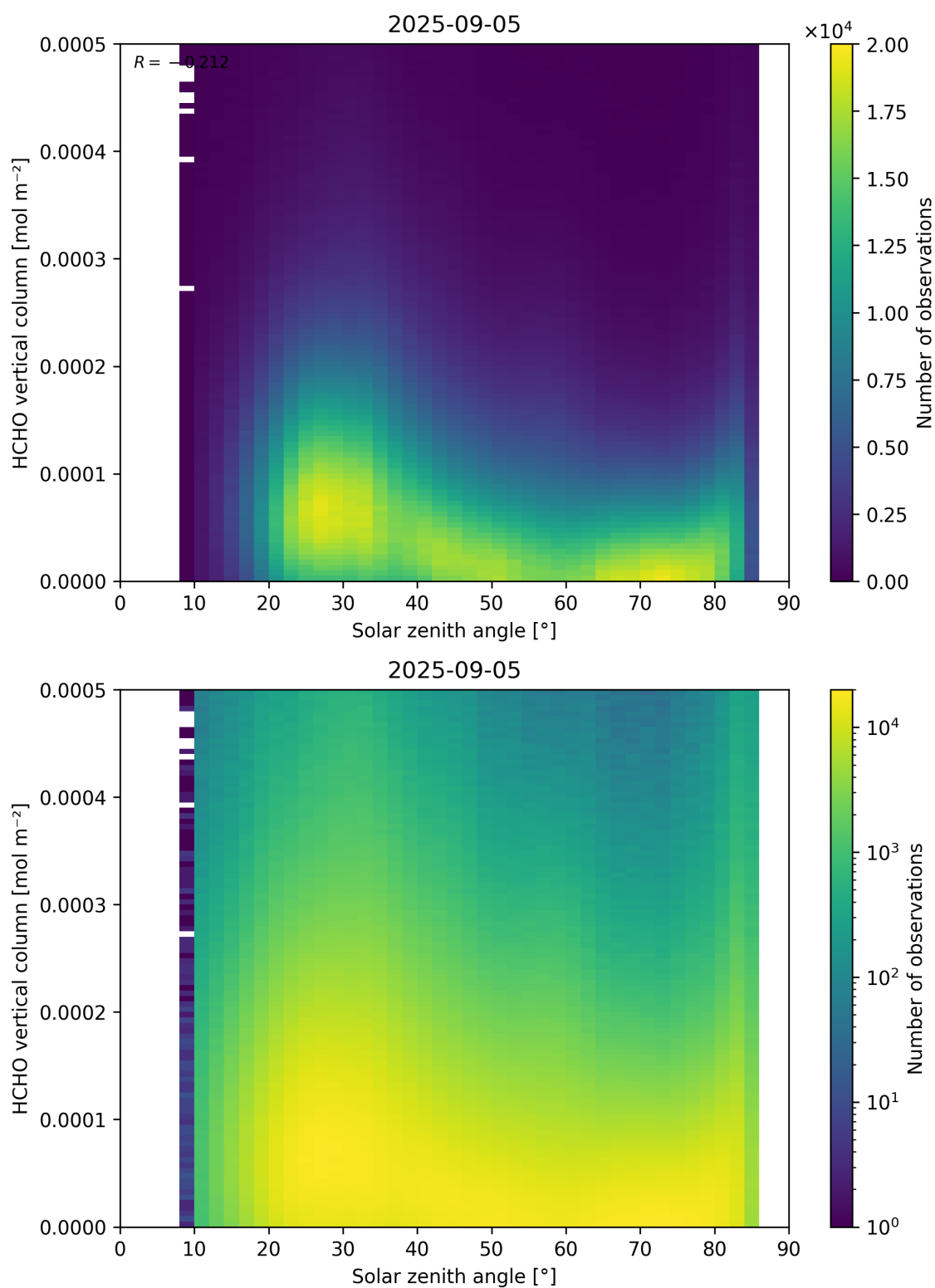
Figure 177: Scatter density plot of “Solar zenith angle” against “HCHO vertical column” for 2025-09-04 to 2025-09-06.
