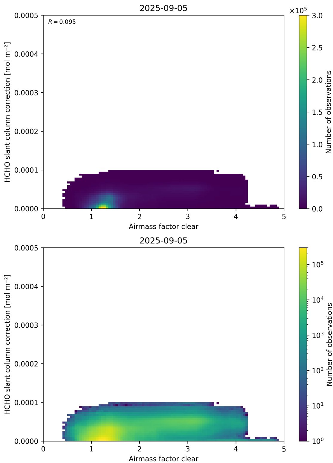
Figure 75: Scatter density plot of “Airmass factor clear” against “HCHO slant column correction” for 2025-09-04 to 2025-09-06.
