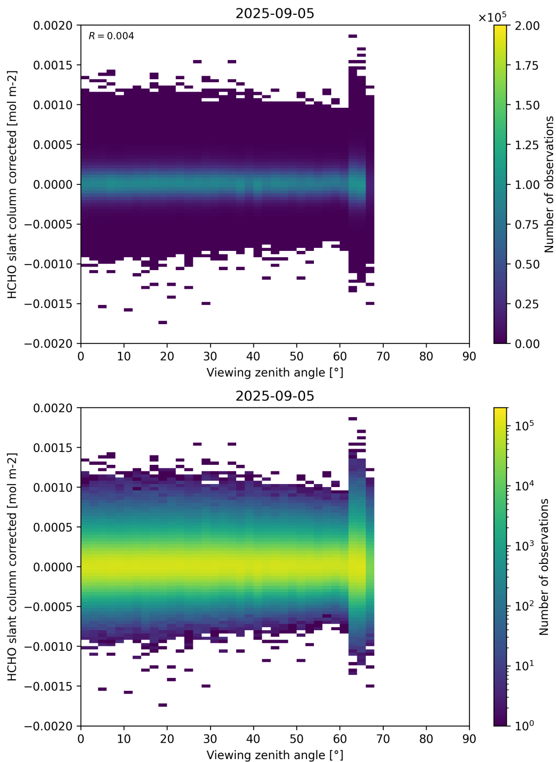
Figure 186: Scatter density plot of “Viewing zenith angle” against “HCHO slant column corrected” for 2025-09-04 to 2025-09-06.
