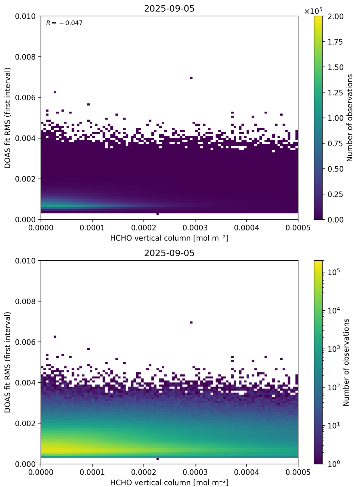
Figure 123: Scatter density plot of “HCHO vertical column” against “DOAS fit RMS (first interval)” for 2025-09-04 to 2025-09-06.
