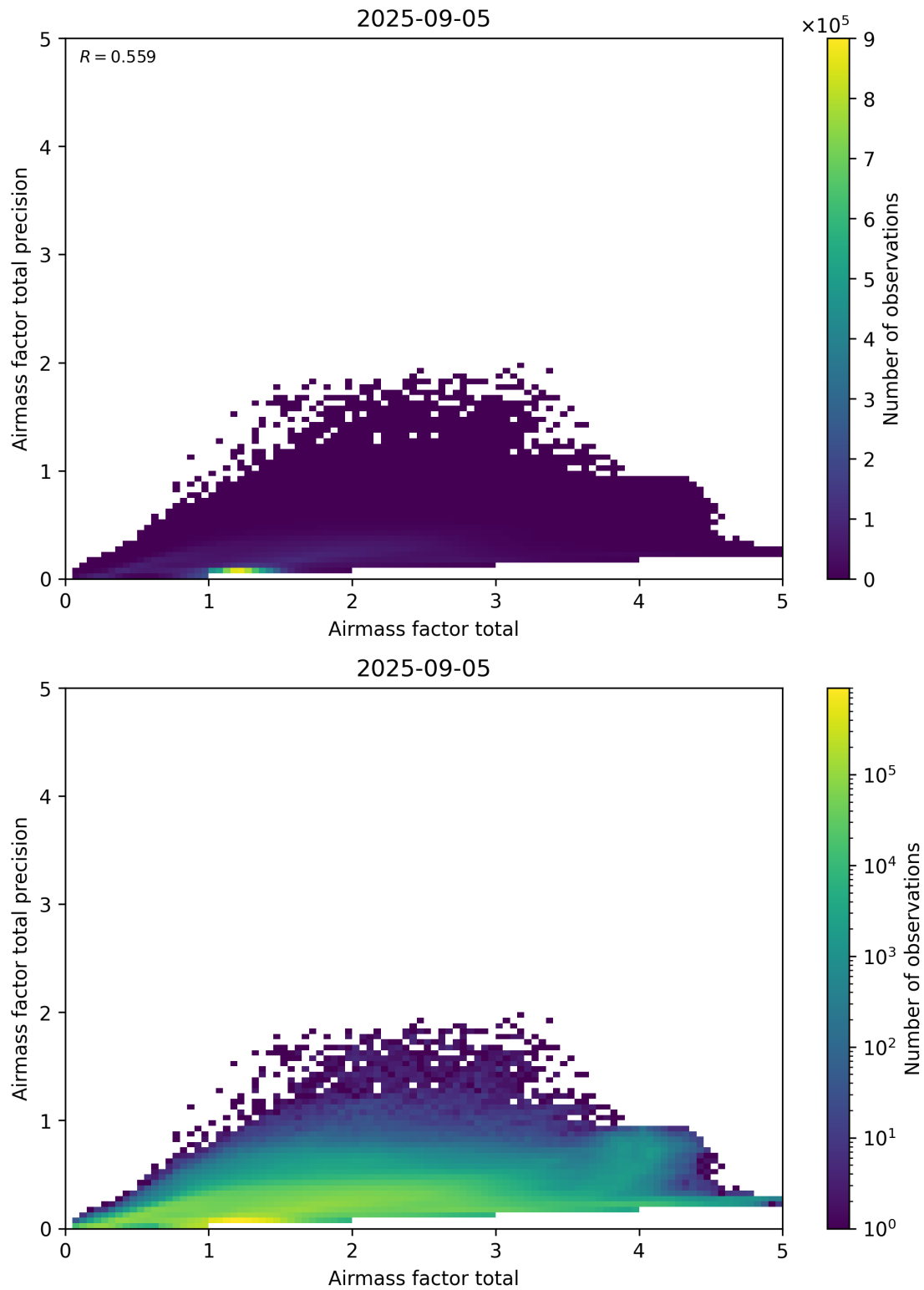
Figure 103: Scatter density plot of “Airmass factor total” against “Airmass factor total precision” for 2025-09-04 to 2025-09-06.
