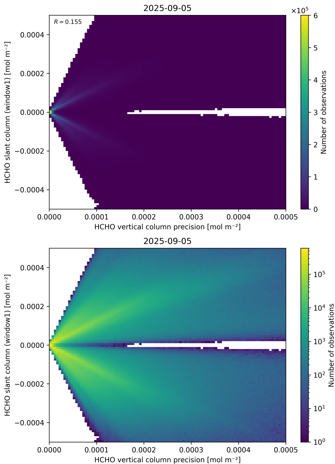
Figure 142: Scatter density plot of “HCHO vertical column precision” against “HCHO slant column (window1)” for 2025-09-04 to 2025-09-06.
