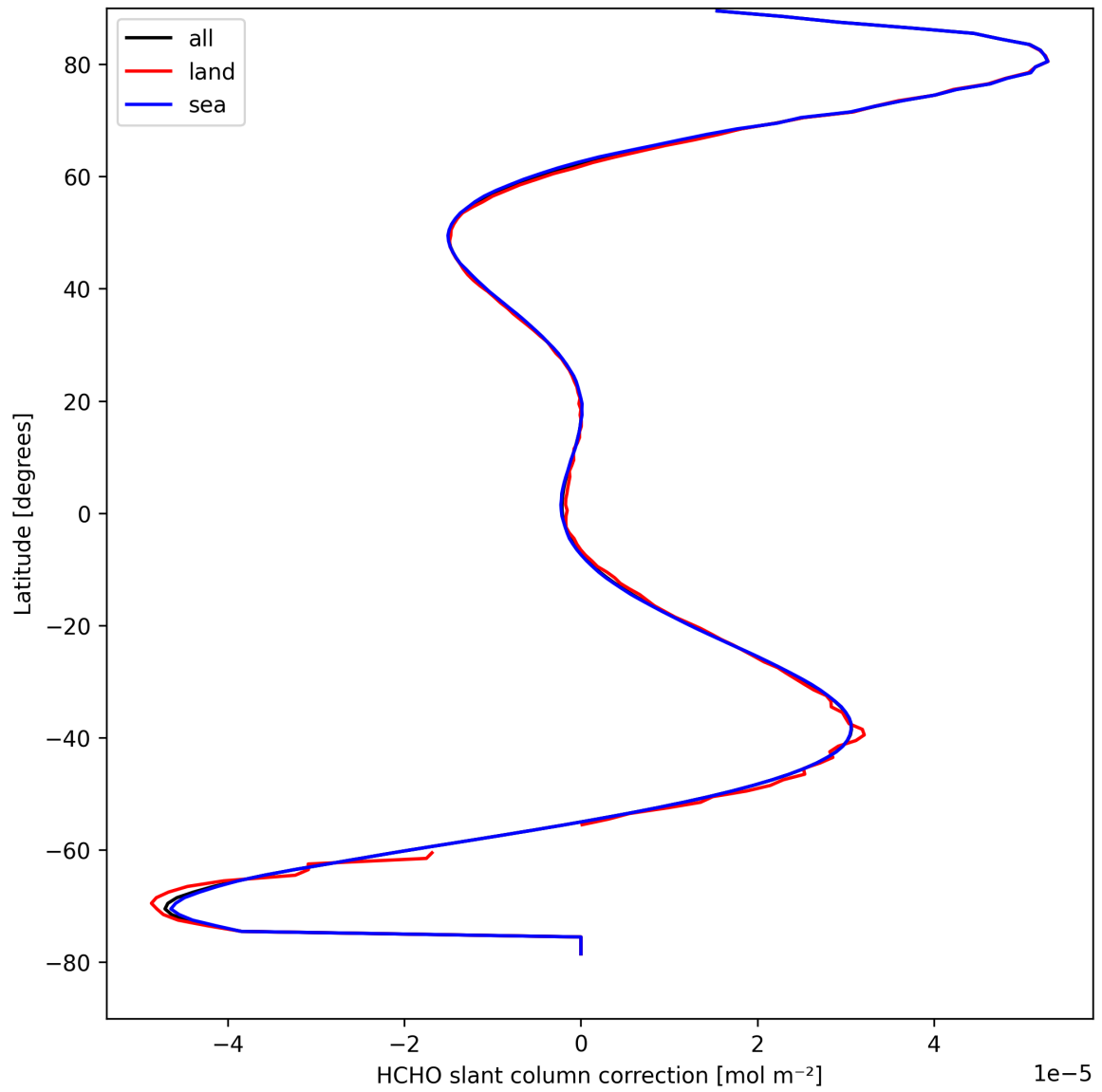
Figure 33: Zonal average of “HCHO slant column correction” for 2025-09-04 to 2025-09-06.
