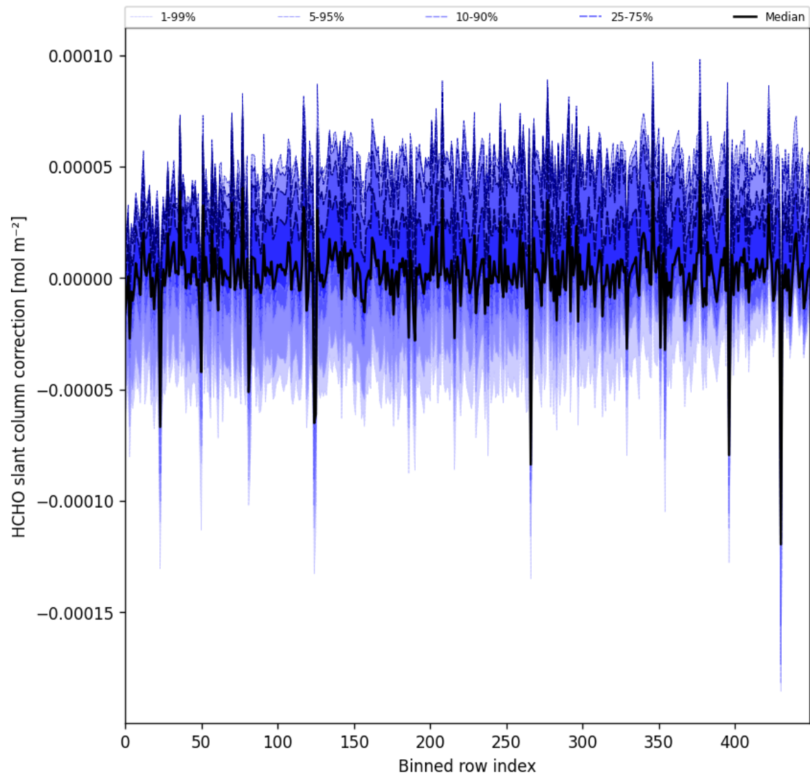
Figure 61: Along track statistics of “HCHO slant column correction” for 2025-09-04 to 2025-09-06
