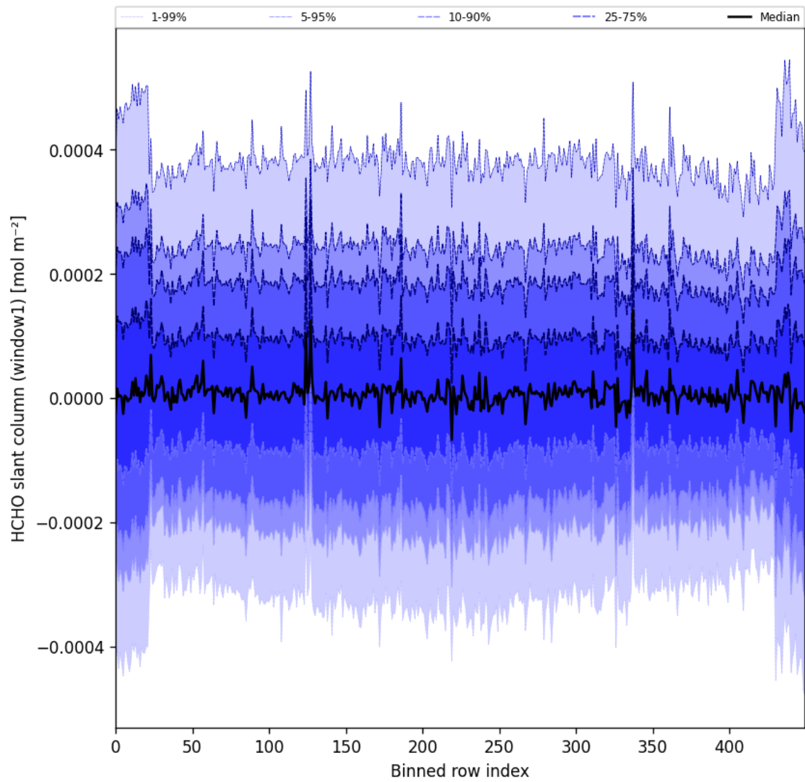
Figure 52: Along track statistics of “HCHO slant column (window1)” for 2025-09-04 to 2025-09-06
