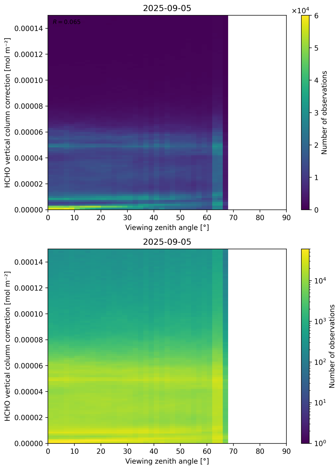
Figure 193: Scatter density plot of “Viewing zenith angle” against “HCHO vertical column correction” for 2025-09-04 to 2025-09-06.
