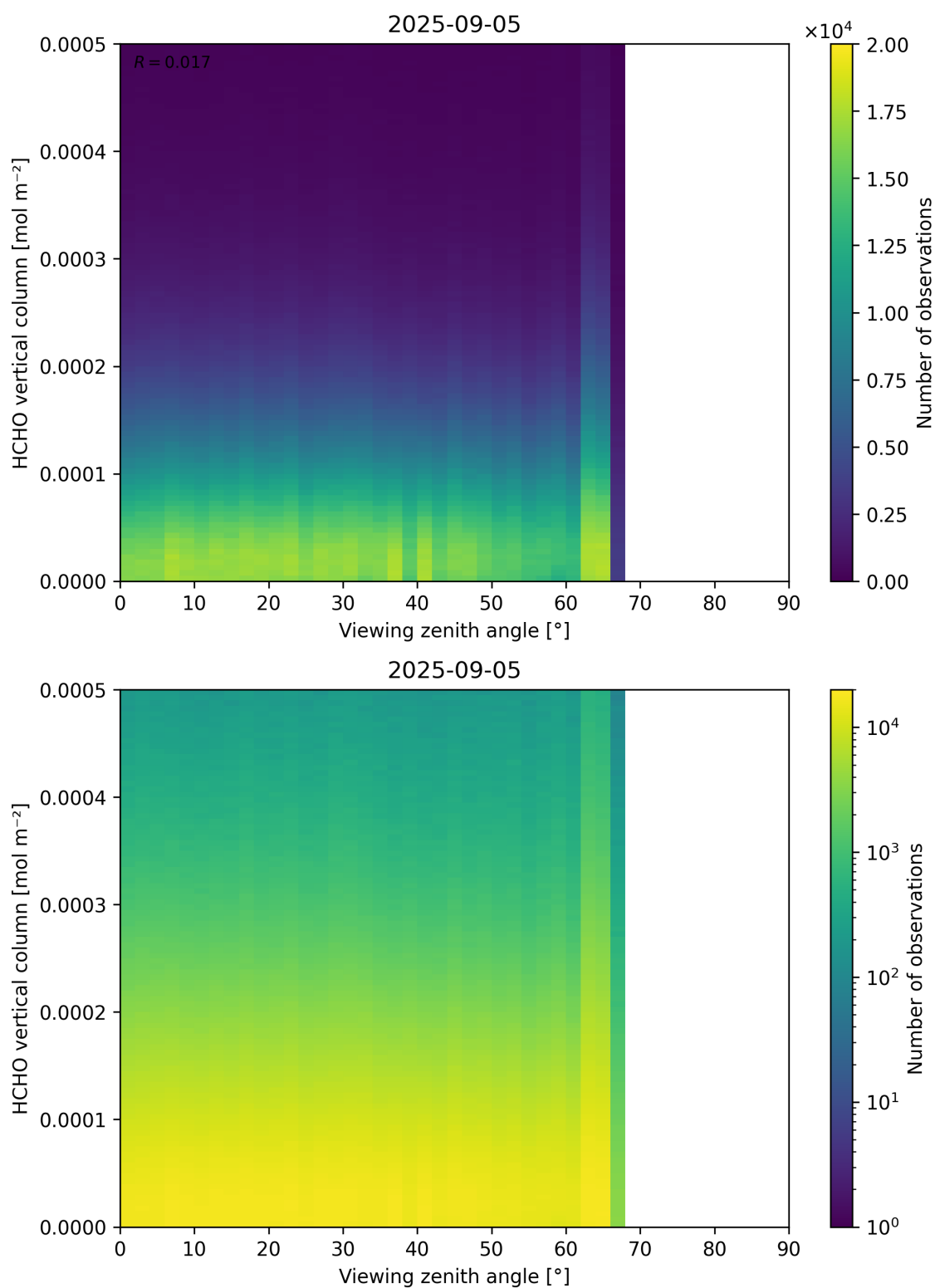
Figure 192: Scatter density plot of “Viewing zenith angle” against “HCHO vertical column” for 2025-09-04 to 2025-09-06.
