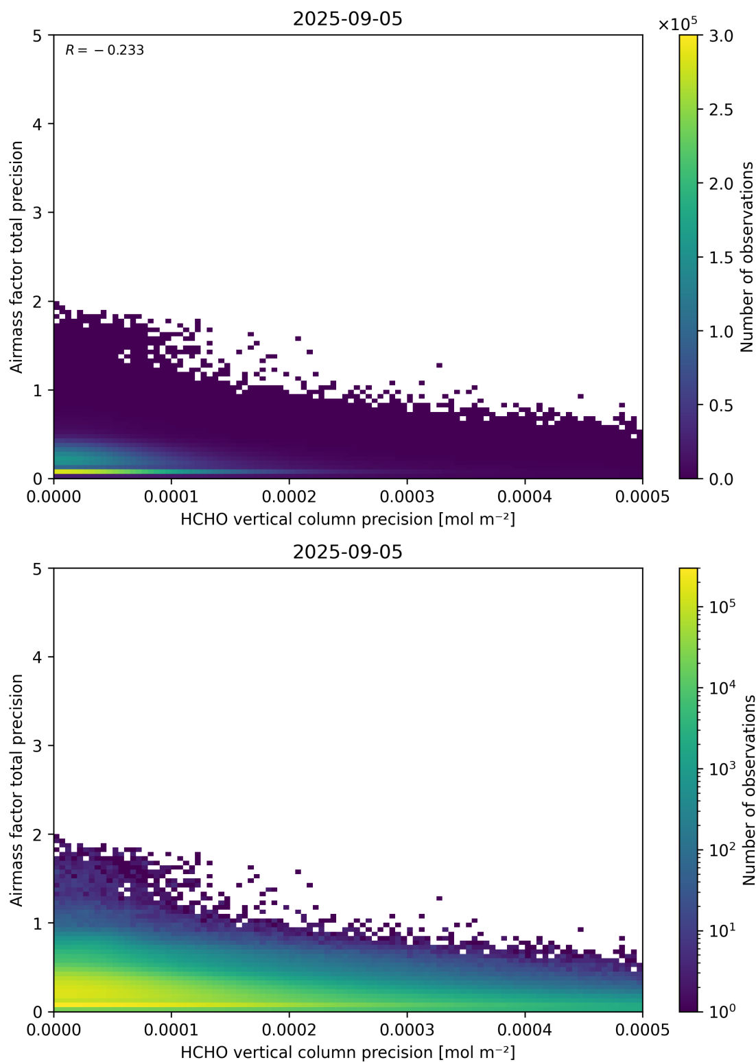
Figure 145: Scatter density plot of “HCHO vertical column precision” against “Airmass factor total precision” for 2025-09-04 to 2025-09-06.
