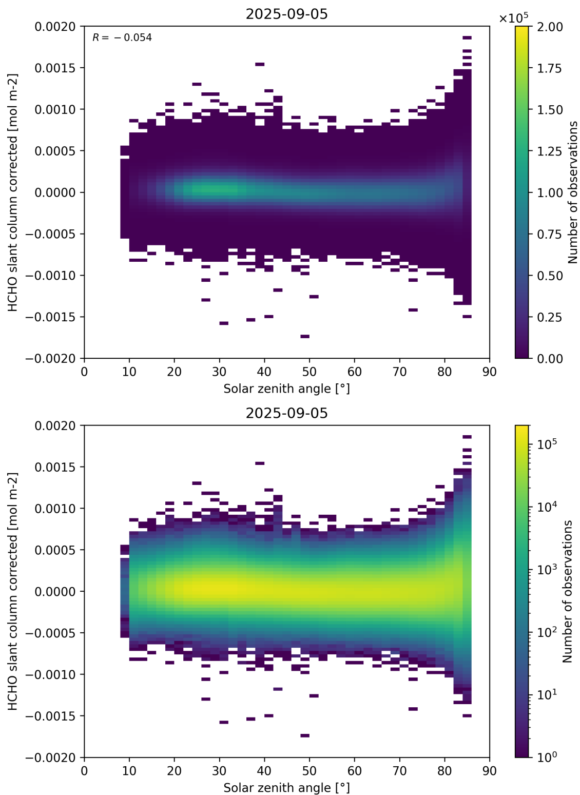
Figure 171: Scatter density plot of “Solar zenith angle” against “HCHO slant column corrected” for 2025-09-04 to 2025-09-06.
