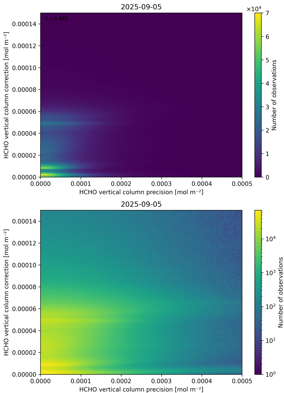
Figure 146: Scatter density plot of “HCHO vertical column precision” against “HCHO vertical column correction” for 2025-09-04 to 2025-09-06.
