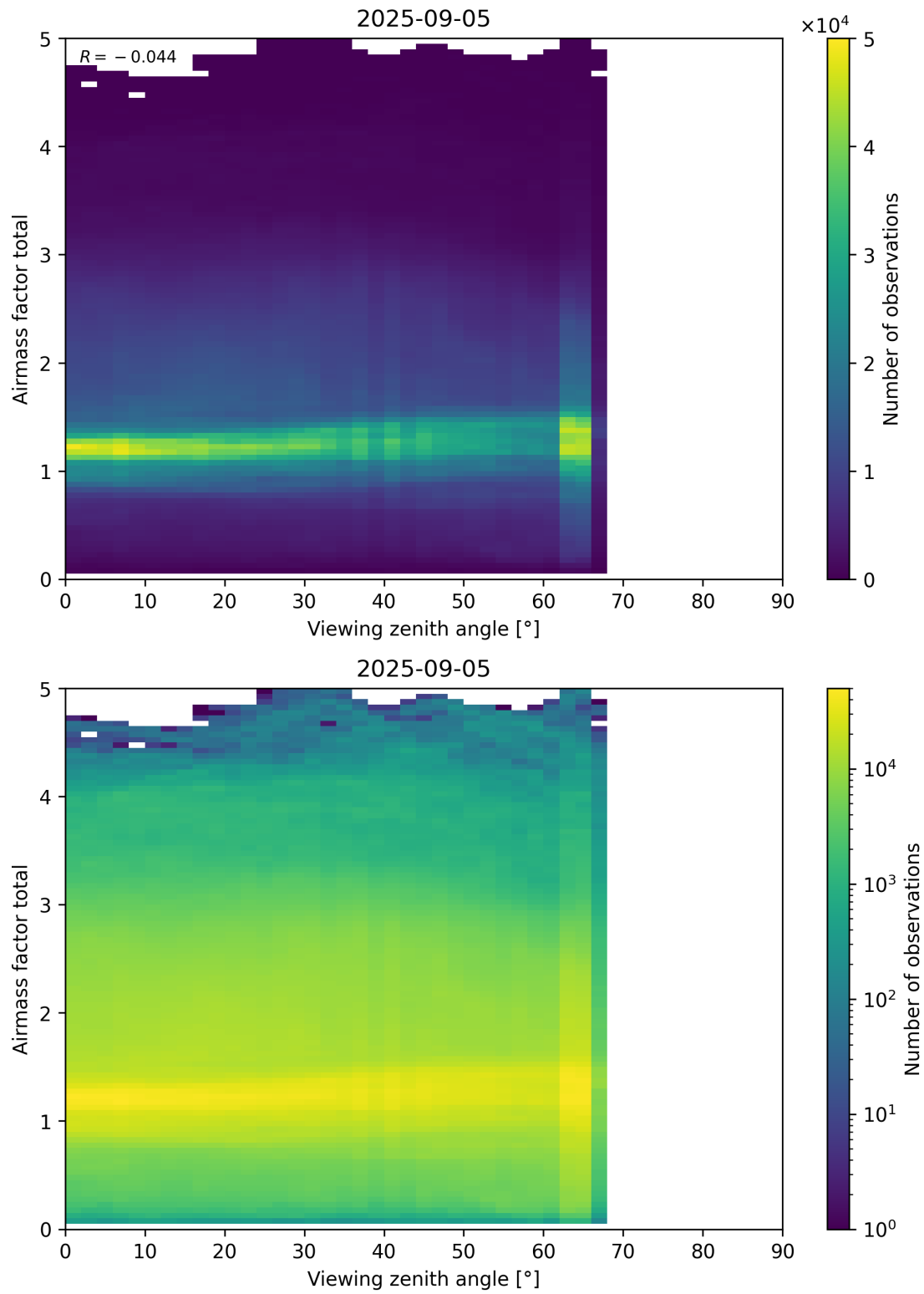
Figure 190: Scatter density plot of “Viewing zenith angle” against “Airmass factor total” for 2025-09-04 to 2025-09-06.
