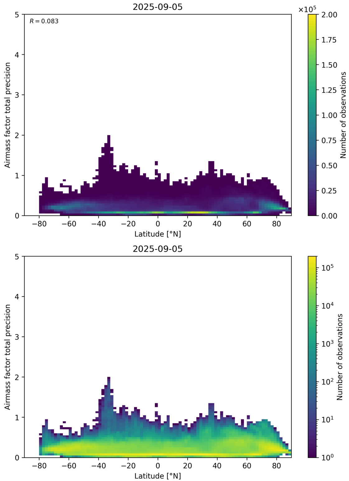
Figure 162: Scatter density plot of “Latitude” against “Airmass factor total precision” for 2025-09-04 to 2025-09-06.
