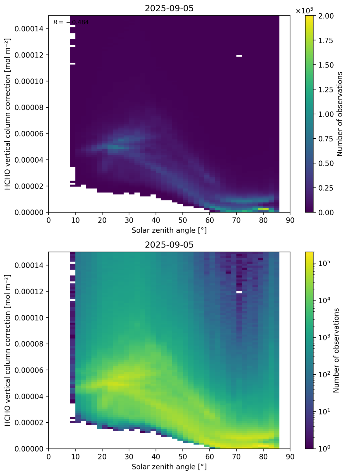
Figure 178: Scatter density plot of “Solar zenith angle” against “HCHO vertical column correction” for 2025-09-04 to 2025-09-06.
