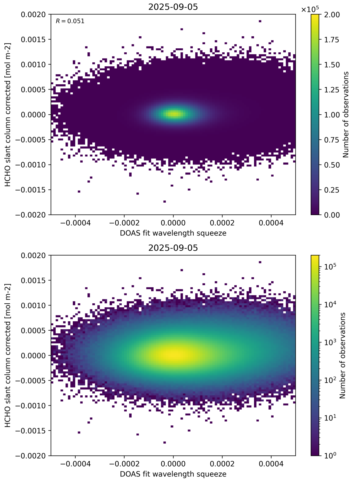
Figure 69: Scatter density plot of “DOAS fit wavelength squeeze” against “HCHO slant column corrected” for 2025-09-04 to 2025-09-06.
