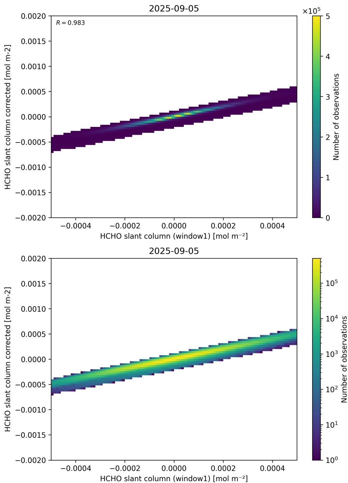
Figure 82: Scatter density plot of “HCHO slant column (window1)” against “HCHO slant column corrected” for 2025-09-04 to 2025-09-06.
