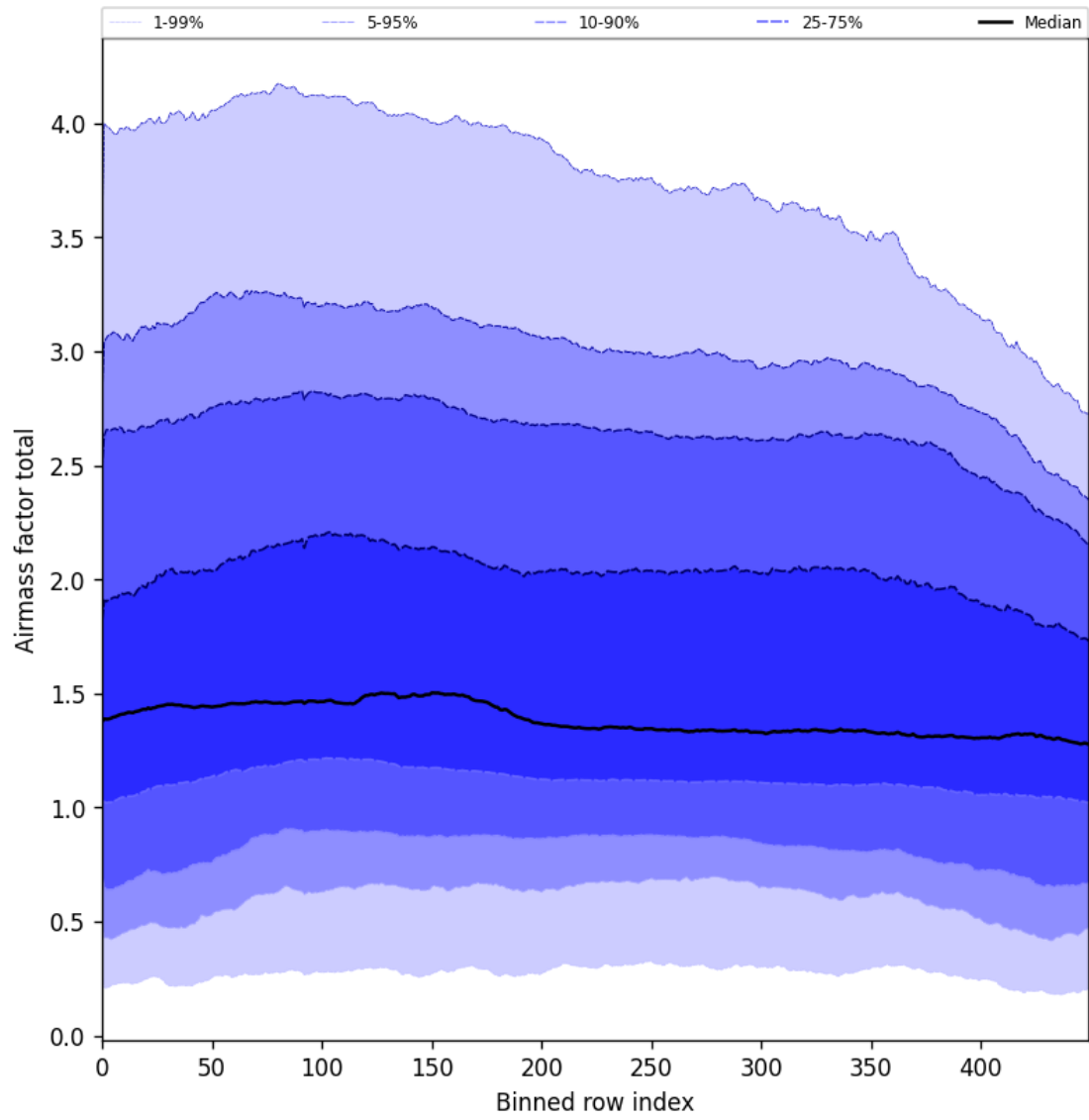
Figure 54: Along track statistics of “Airmass factor total” for 2025-09-04 to 2025-09-06
