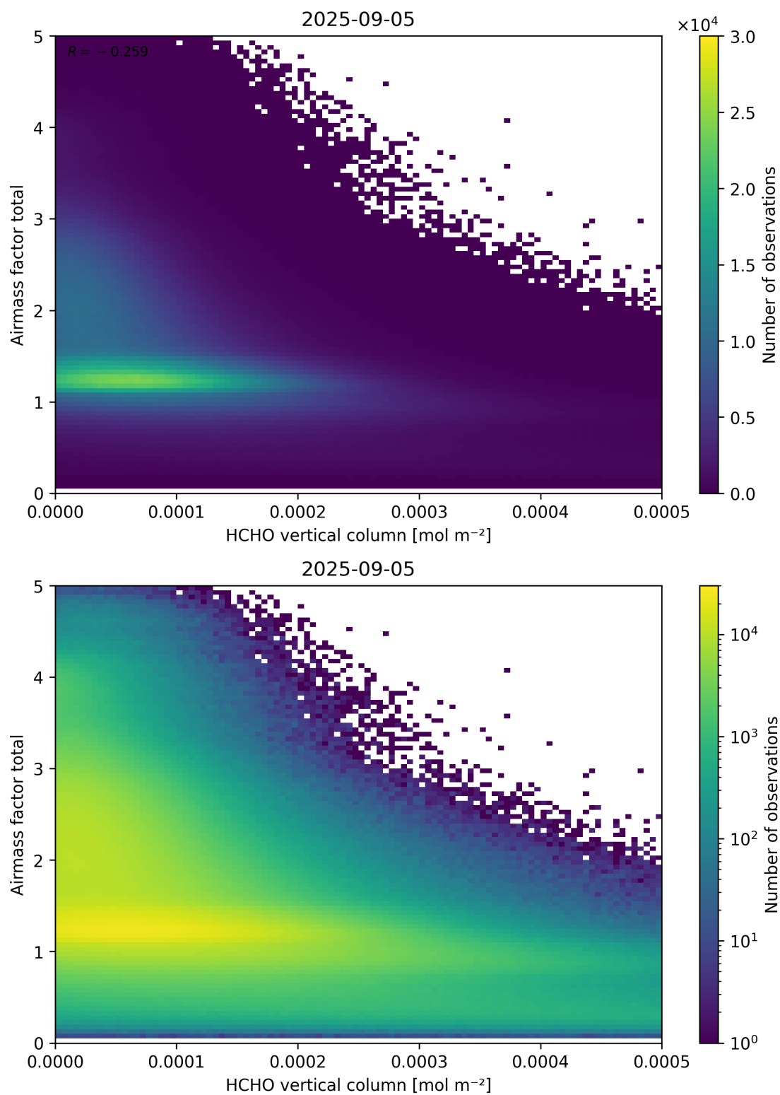
Figure 131: Scatter density plot of “HCHO vertical column” against “Airmass factor total” for 2025-09-04 to 2025-09-06.
