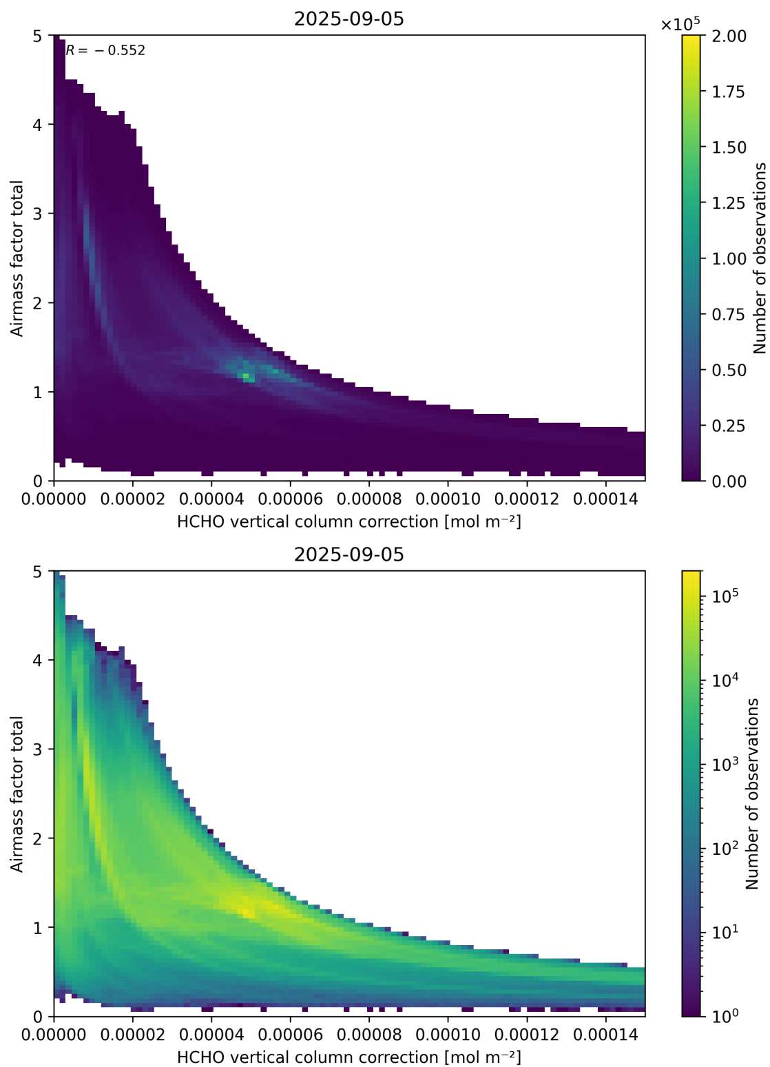
Figure 120: Scatter density plot of “HCHO vertical column correction” against “Airmass factor total” for 2025-09-04 to 2025-09-06.
