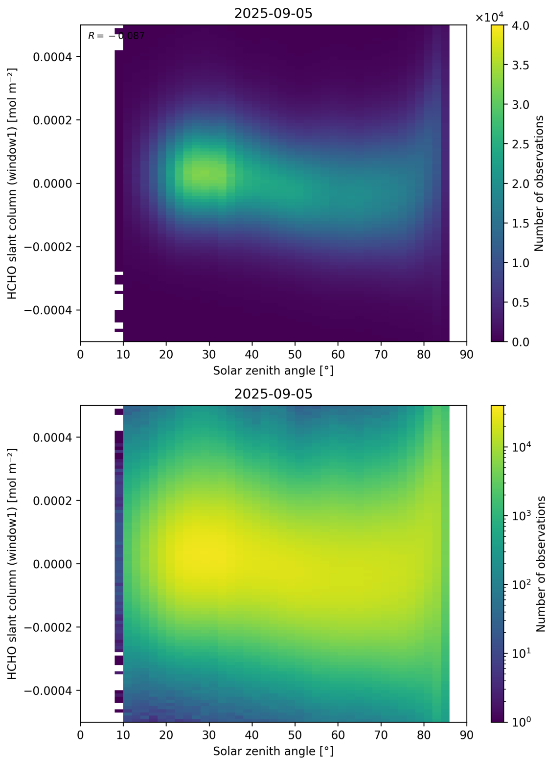
Figure 173: Scatter density plot of “Solar zenith angle” against “HCHO slant column (window1)” for 2025-09-04 to 2025-09-06.
