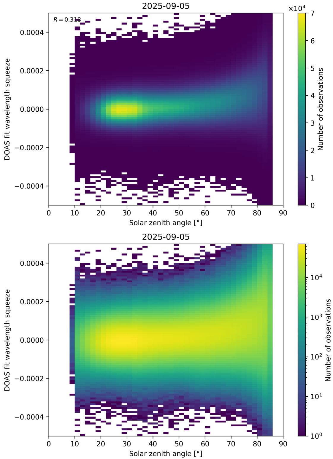
Figure 169: Scatter density plot of “Solar zenith angle” against “DOAS fit wavelength squeeze” for 2025-09-04 to 2025-09-06.
