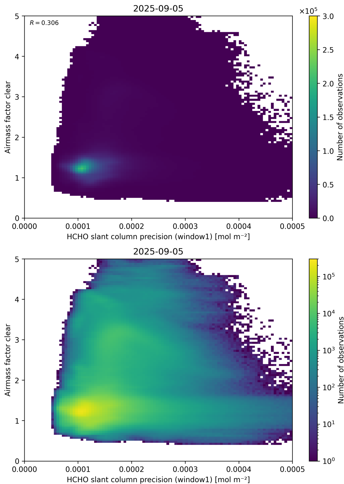
Figure 91: Scatter density plot of “HCHO slant column precision (window1)” against “Airmass factor clear” for 2025-09-04 to 2025-09-06.
