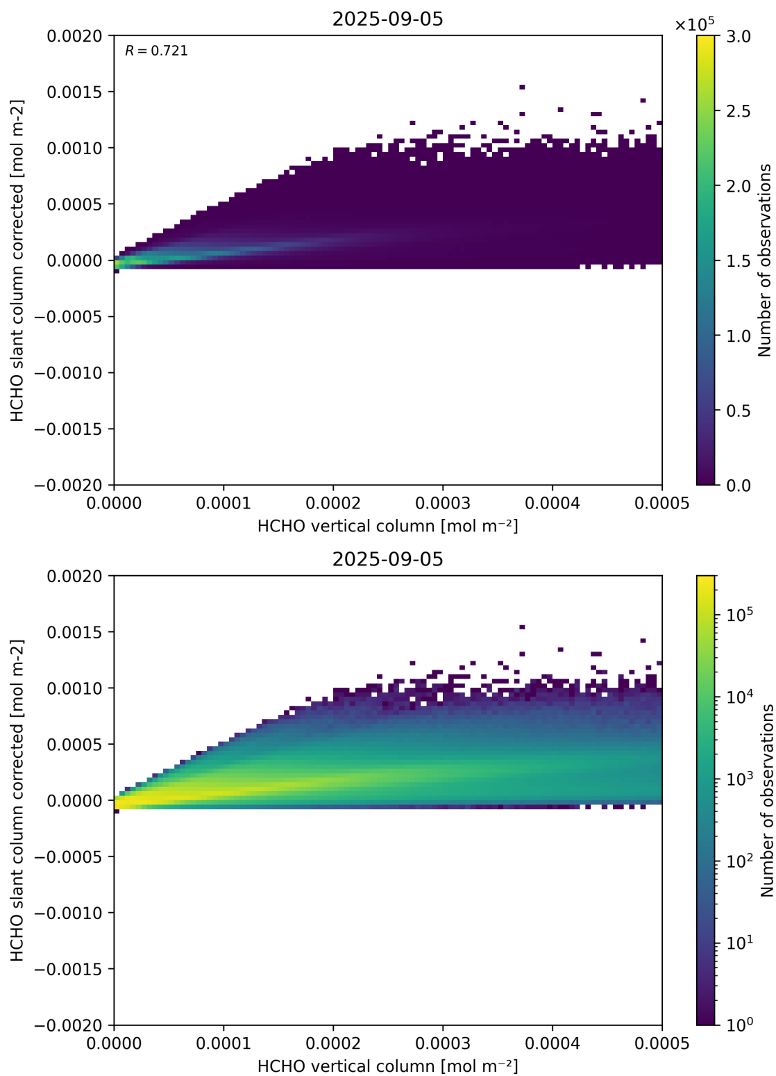
Figure 127: Scatter density plot of “HCHO vertical column” against “HCHO slant column corrected” for 2025-09-04 to 2025-09-06.
