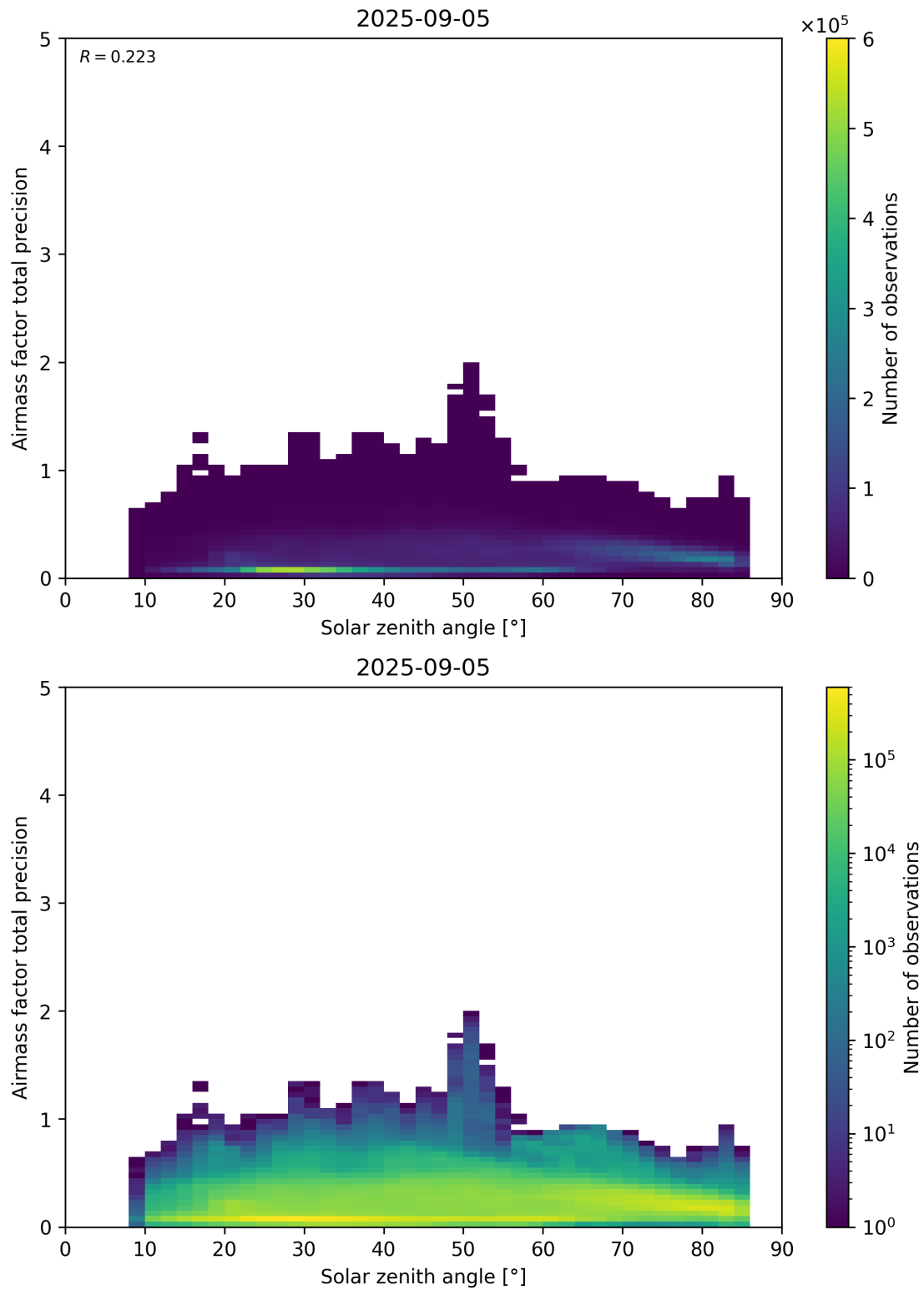
Figure 176: Scatter density plot of “Solar zenith angle” against “Airmass factor total precision” for 2025-09-04 to 2025-09-06.
