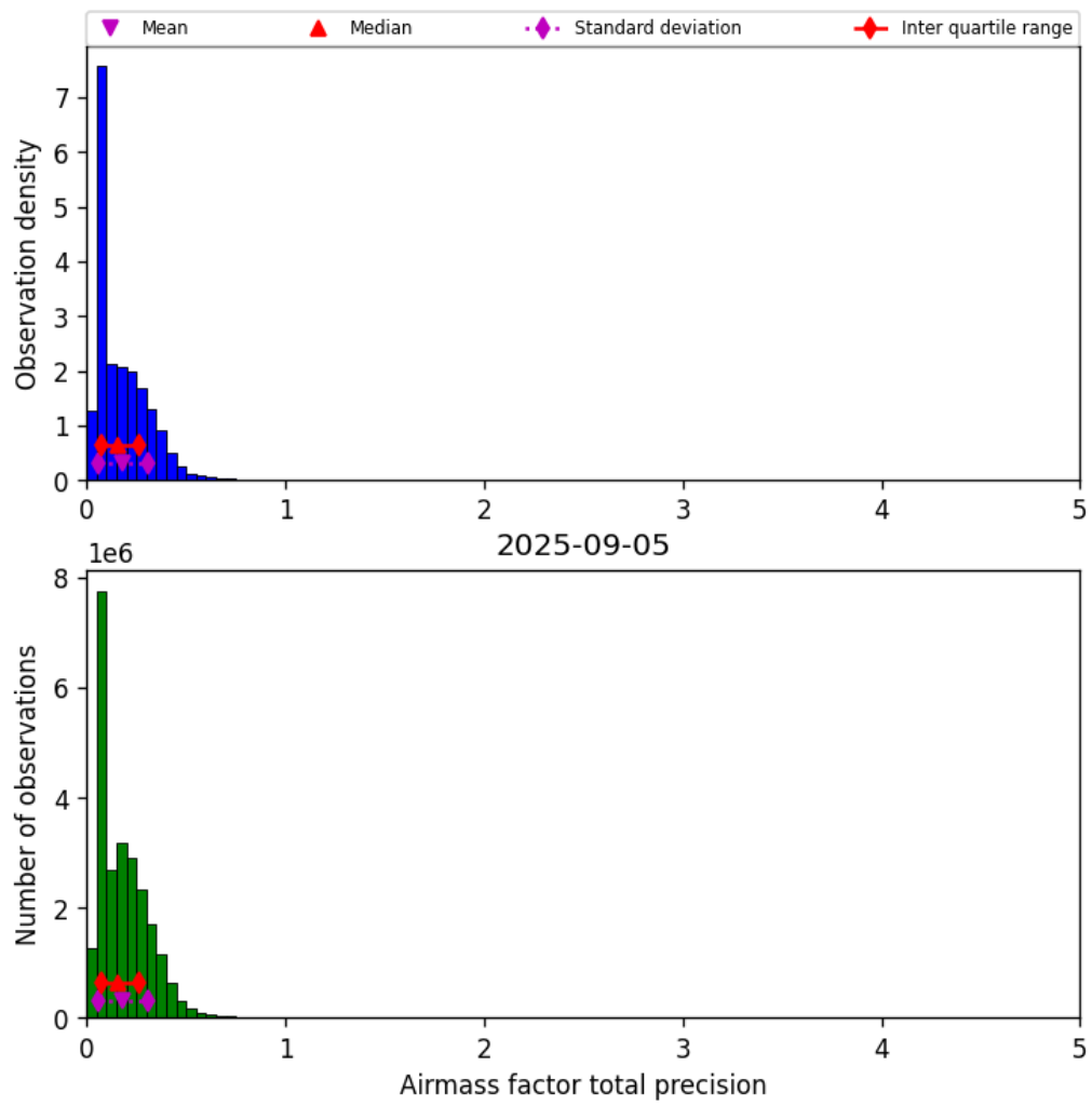
Figure 41: Histogram of “Airmass factor total precision” for 2025-09-04 to 2025-09-06
