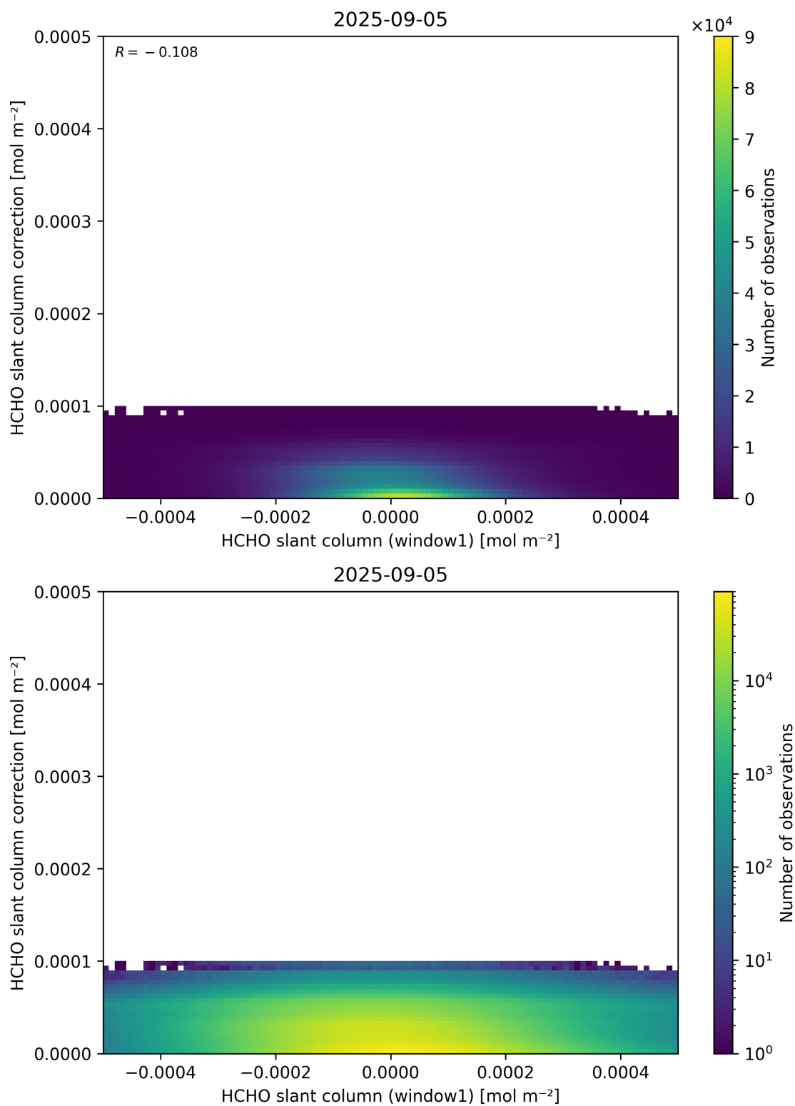
Figure 83: Scatter density plot of “HCHO slant column (window1)” against “HCHO slant column correction” for 2025-09-04 to 2025-09-06.
