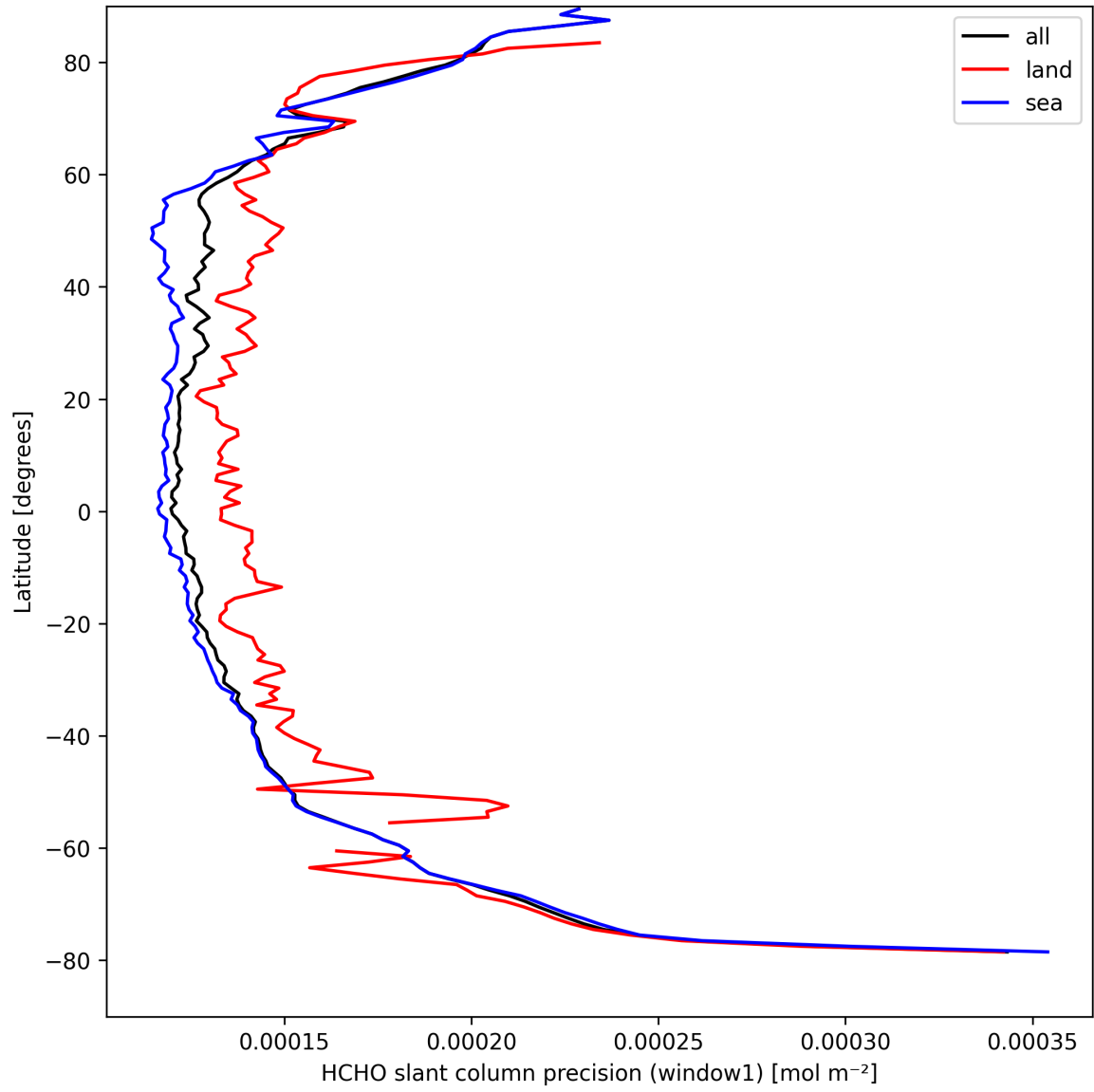
Figure 25: Zonal average of “HCHO slant column precision (window1)” for 2025-09-04 to 2025-09-06.
