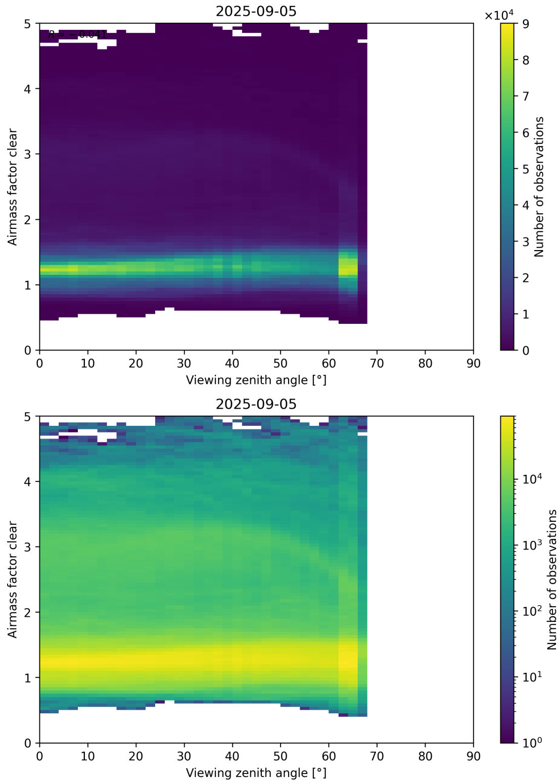
Figure 185: Scatter density plot of “Viewing zenith angle” against “Airmass factor clear” for 2025-09-04 to 2025-09-06.
