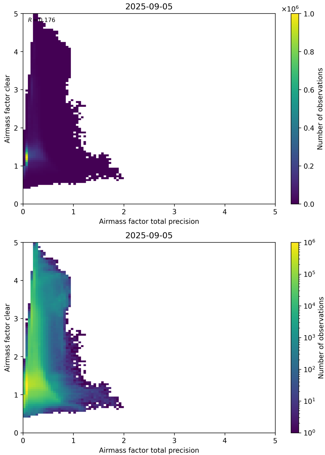
Figure 108: Scatter density plot of “Airmass factor total precision” against “Airmass factor clear” for 2025-09-04 to 2025-09-06.
