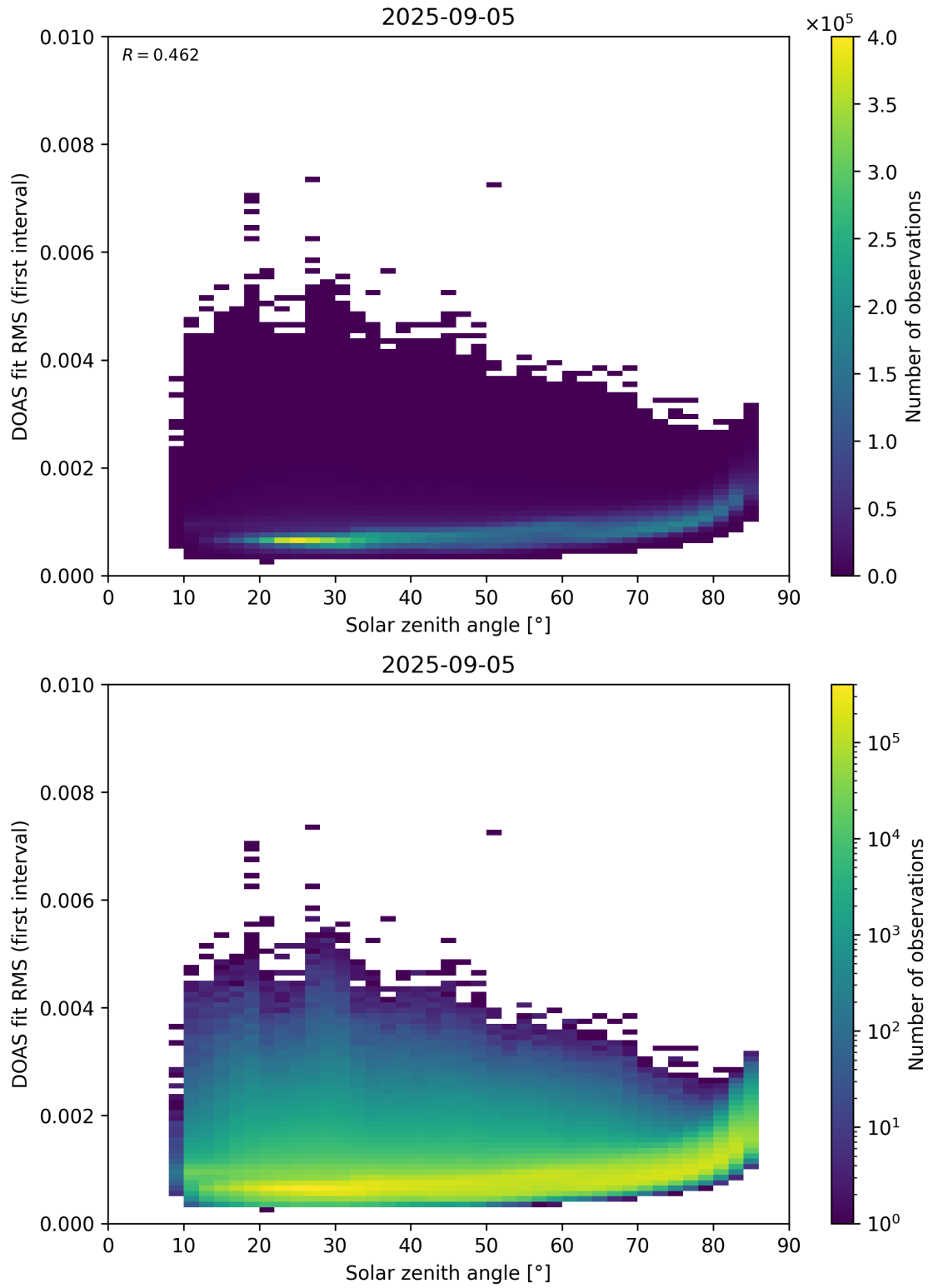
Figure 167: Scatter density plot of “Solar zenith angle” against “DOAS fit RMS (first interval)” for 2025-09-04 to 2025-09-06.
