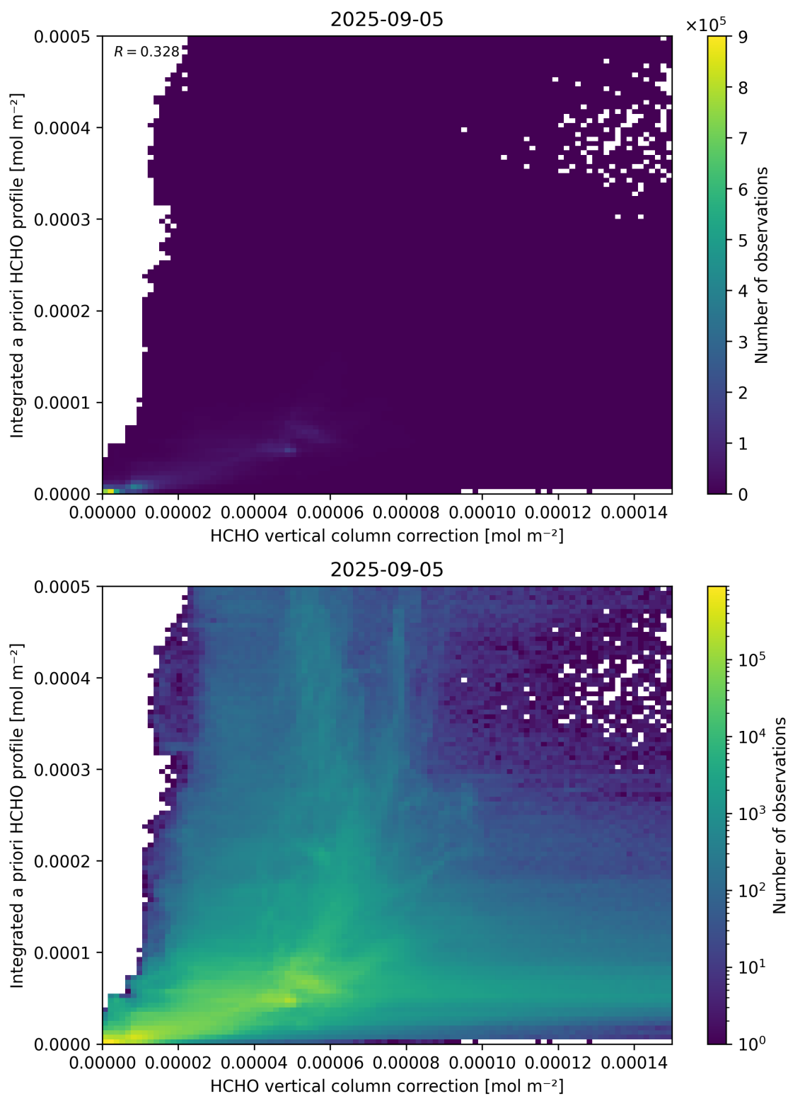
Figure 122: Scatter density plot of “HCHO vertical column correction” against “Integrated a priori HCHO profile” for 2025-09-04 to 2025-09-06.
