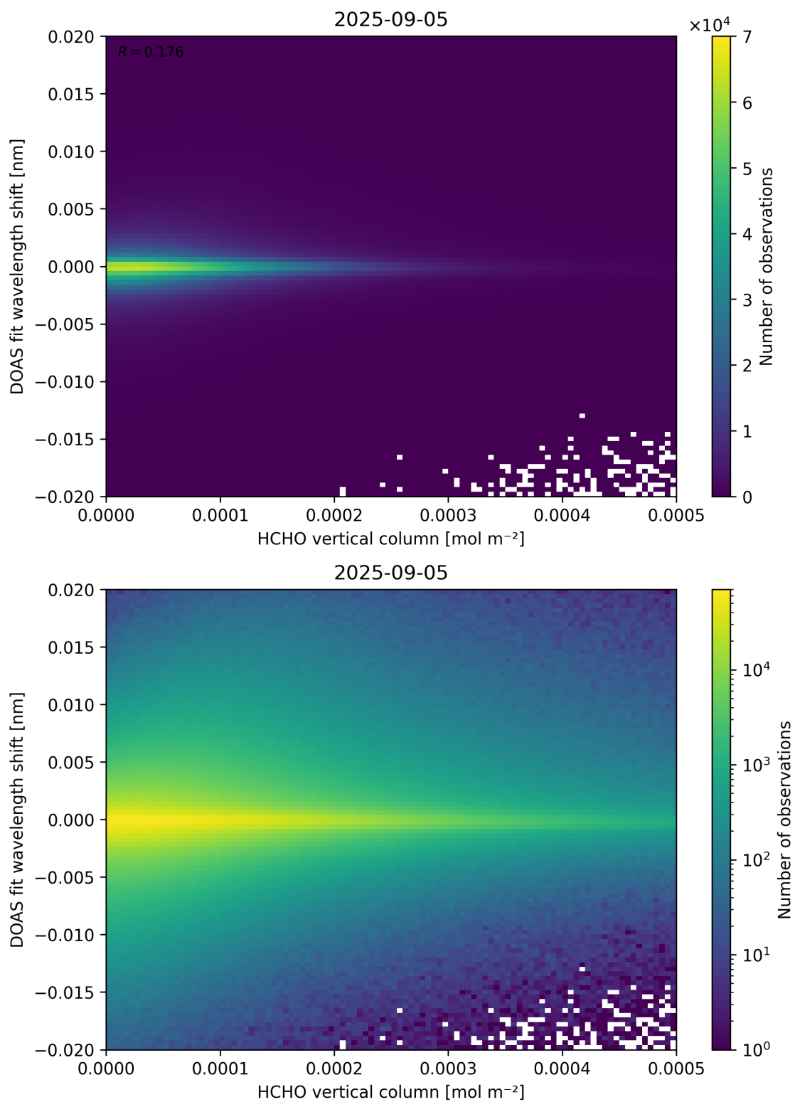
Figure 124: Scatter density plot of “HCHO vertical column” against “DOAS fit wavelength shift” for 2025-09-04 to 2025-09-06.
