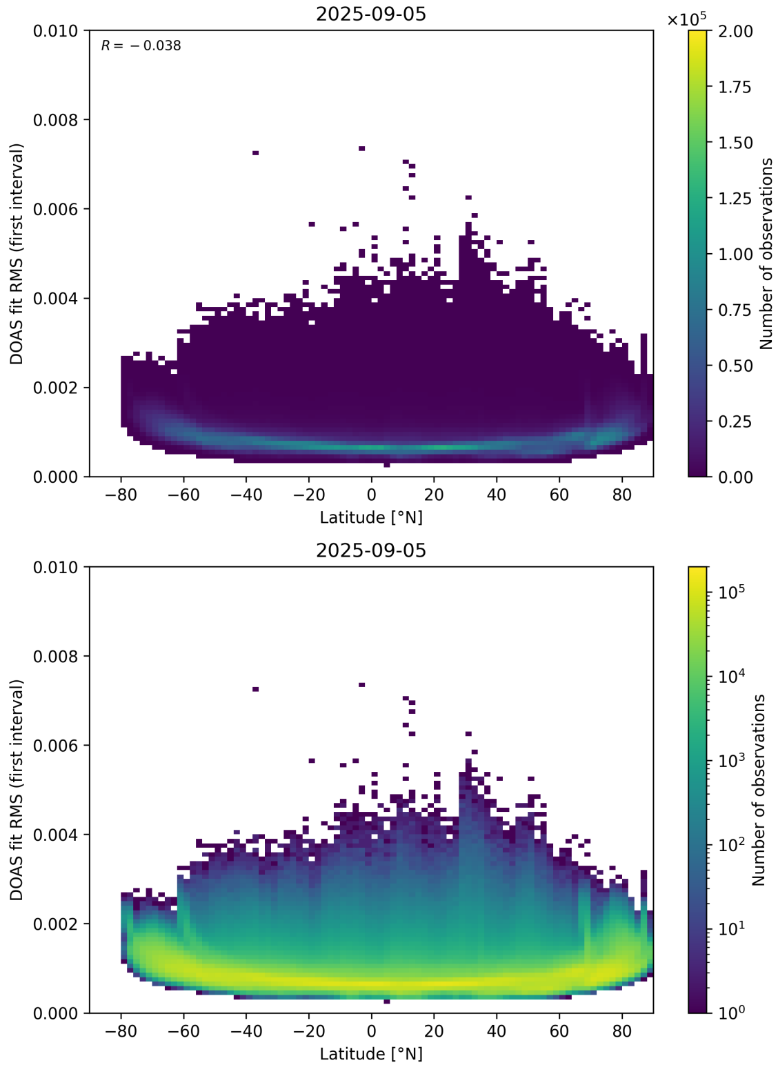
Figure 153: Scatter density plot of “Latitude” against “DOAS fit RMS (first interval)” for 2025-09-04 to 2025-09-06.
