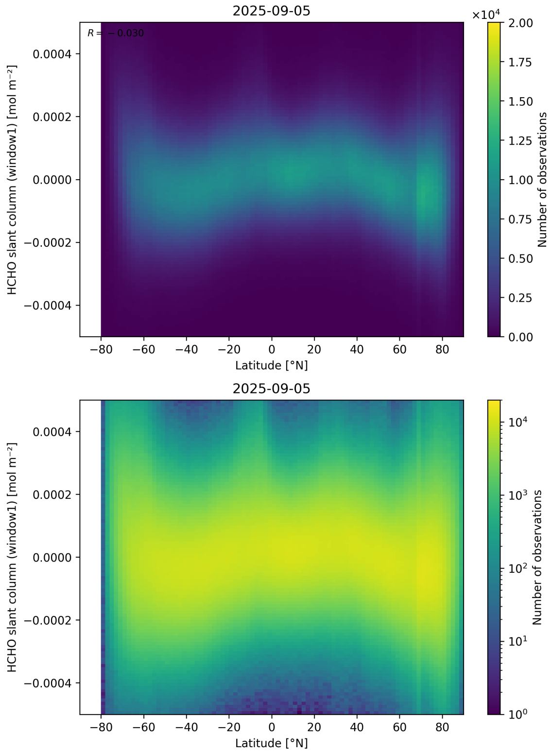
Figure 159: Scatter density plot of “Latitude” against “HCHO slant column (window1)” for 2025-09-04 to 2025-09-06.
