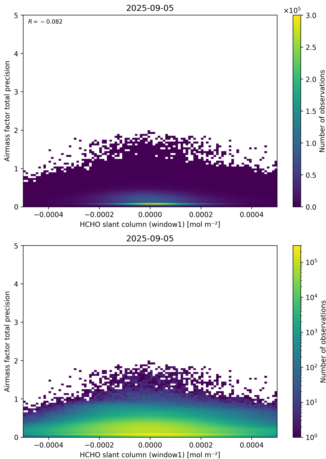
Figure 86: Scatter density plot of “HCHO slant column (window1)” against “Airmass factor total precision” for 2025-09-04 to 2025-09-06.
