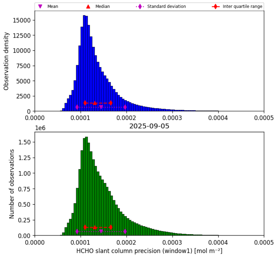
Figure 39: Histogram of “HCHO slant column precision (window1)” for 2025-09-04 to 2025-09-06
