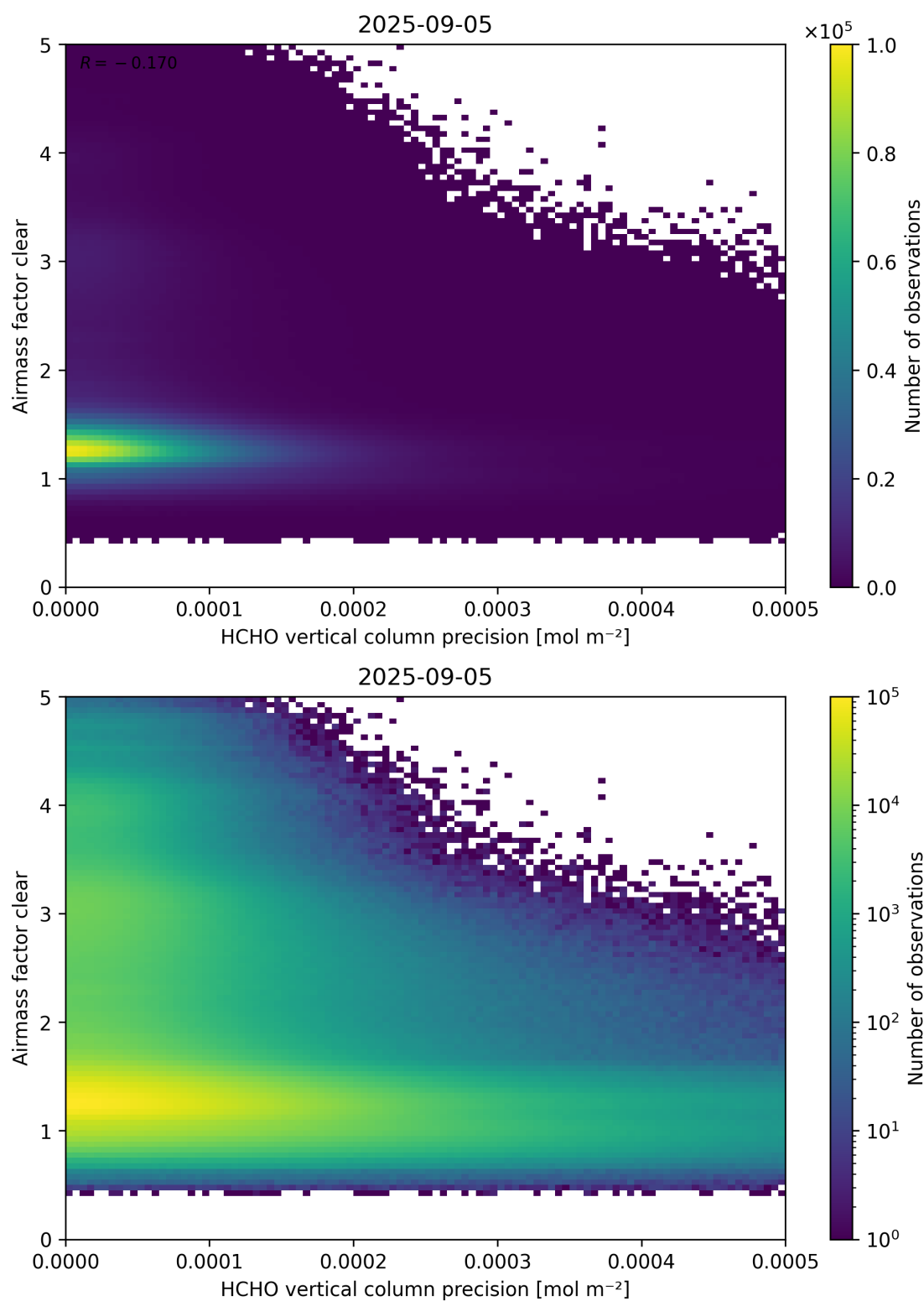
Figure 139: Scatter density plot of “HCHO vertical column precision” against “Airmass factor clear” for 2025-09-04 to 2025-09-06.
