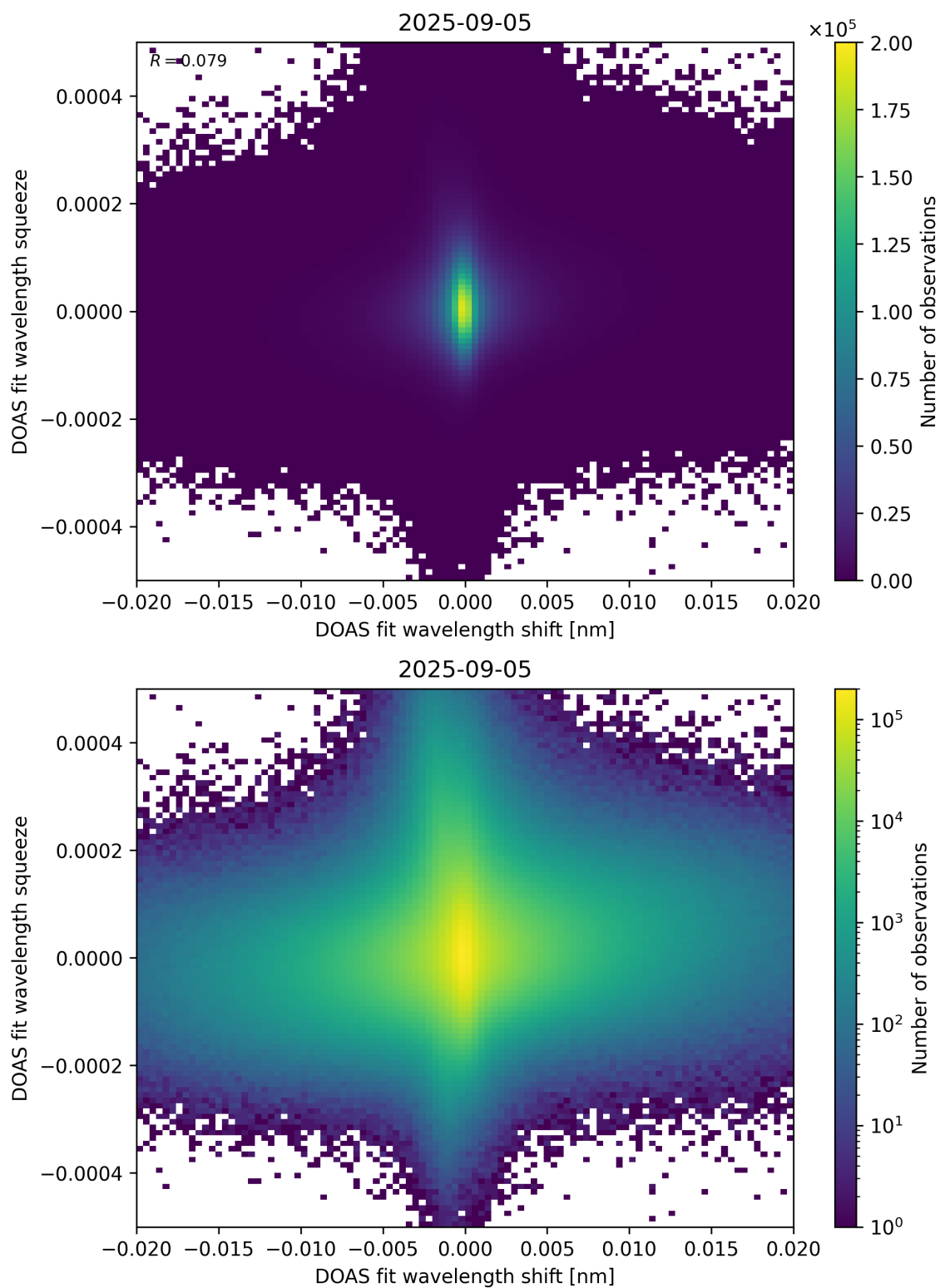
Figure 65: Scatter density plot of “DOAS fit wavelength shift” against “DOAS fit wavelength squeeze” for 2025-09-04 to 2025-09-06.
