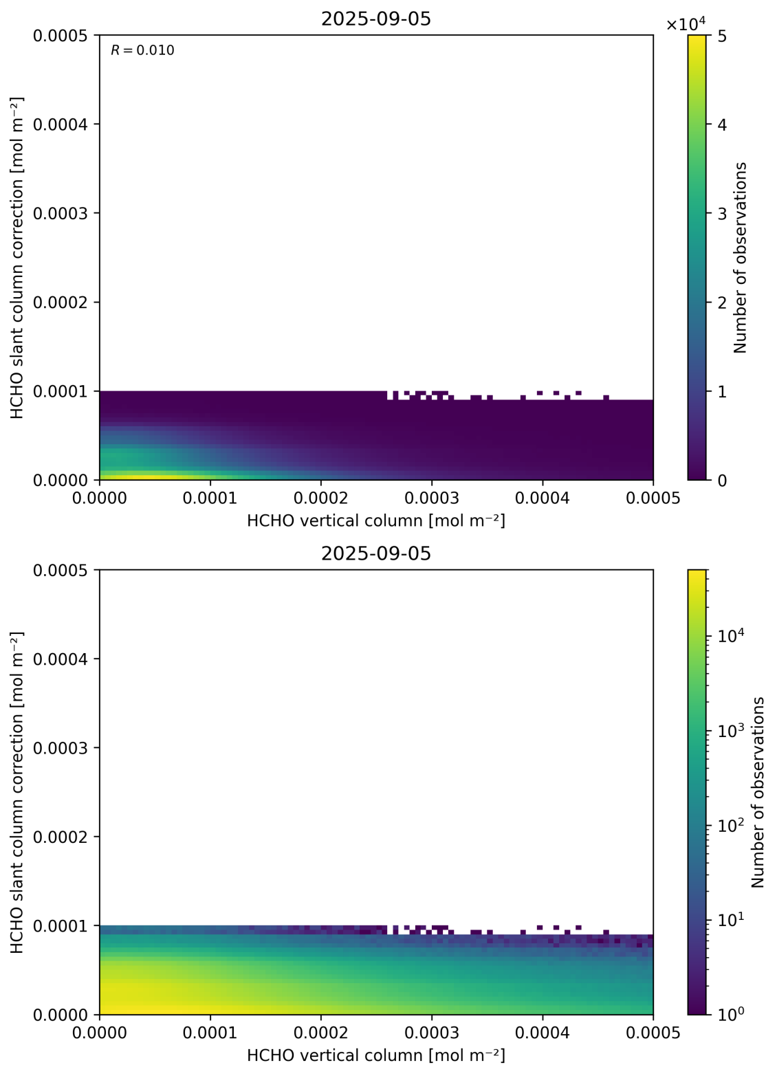
Figure 128: Scatter density plot of “HCHO vertical column” against “HCHO slant column correction” for 2025-09-04 to 2025-09-06.
