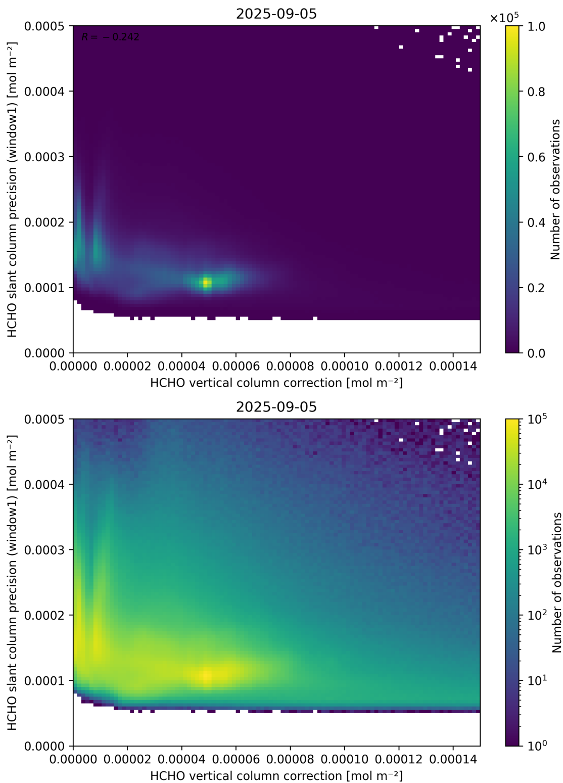
Figure 119: Scatter density plot of “HCHO vertical column correction” against “HCHO slant column precision (window1)” for 2025-09-04 to 2025-09-06.
