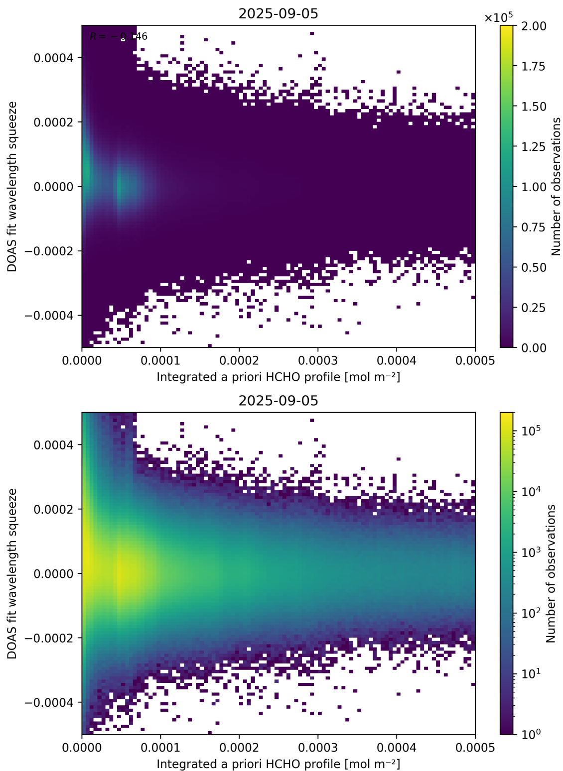
Figure 150: Scatter density plot of “Integrated a priori HCHO profile” against “DOAS fit wavelength squeeze” for 2025-09-04 to 2025-09-06.
