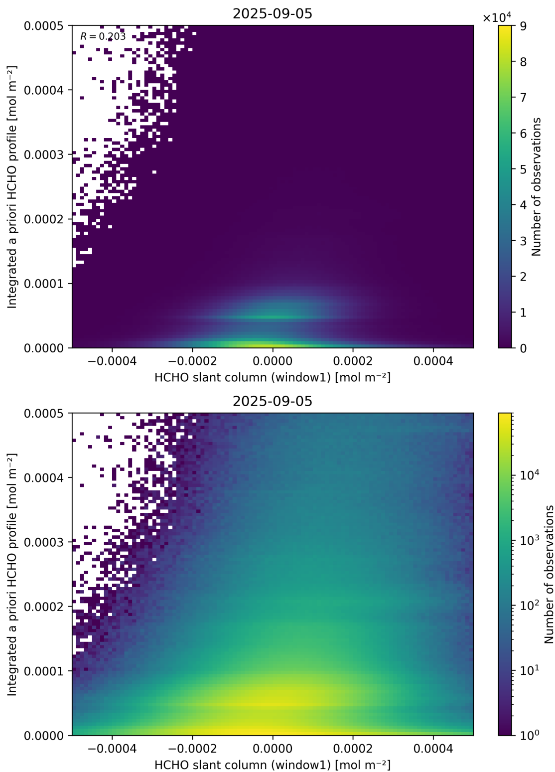
Figure 87: Scatter density plot of “HCHO slant column (window1)” against “Integrated a priori HCHO profile” for 2025-09-04 to 2025-09-06.
