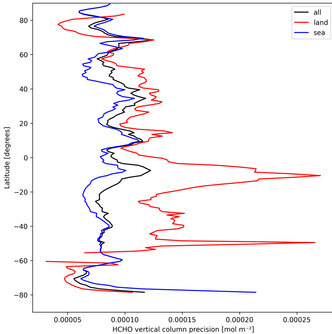
Figure 22: Zonal average of “HCHO vertical column precision” for 2025-09-04 to 2025-09-06.
