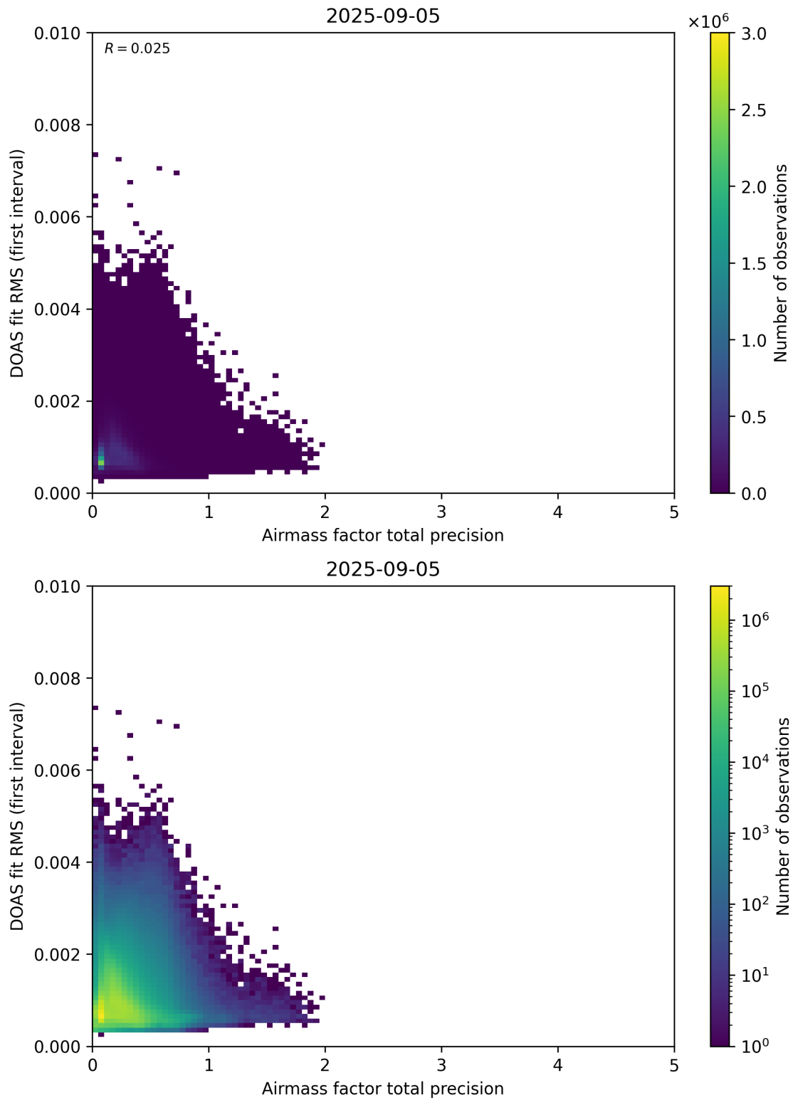
Figure 105: Scatter density plot of “Airmass factor total precision” against “DOAS fit RMS (first interval)” for 2025-09-04 to 2025-09-06.
