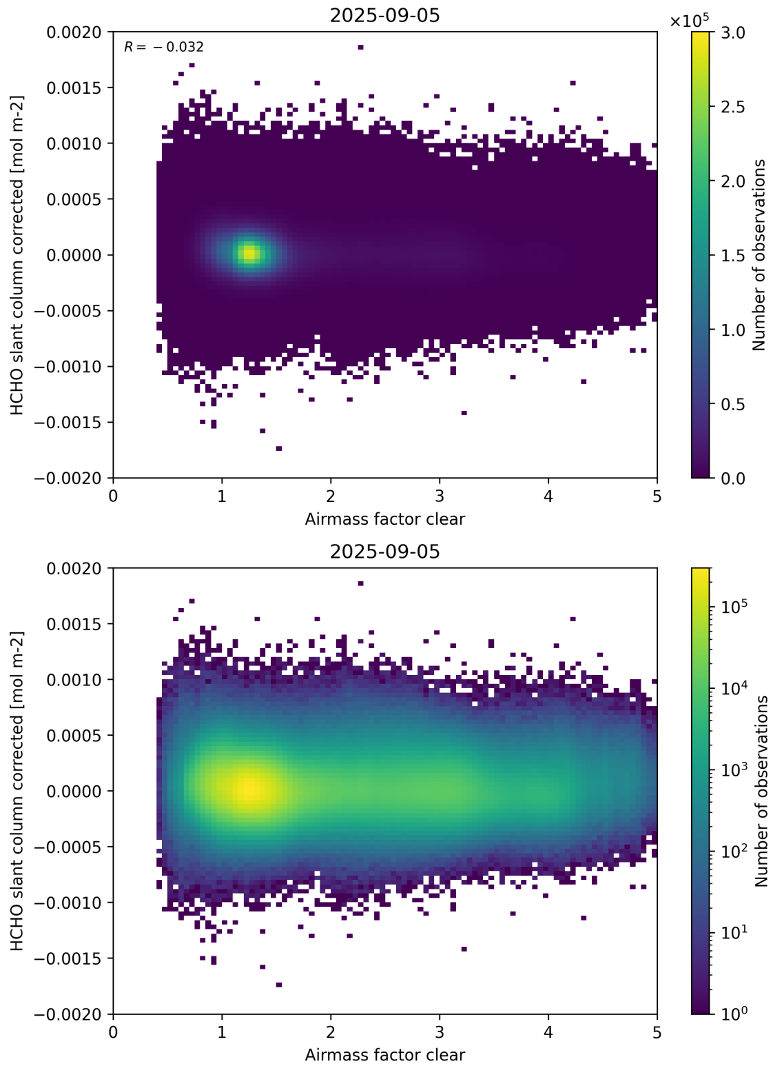
Figure 74: Scatter density plot of “Airmass factor clear” against “HCHO slant column corrected” for 2025-09-04 to 2025-09-06.
