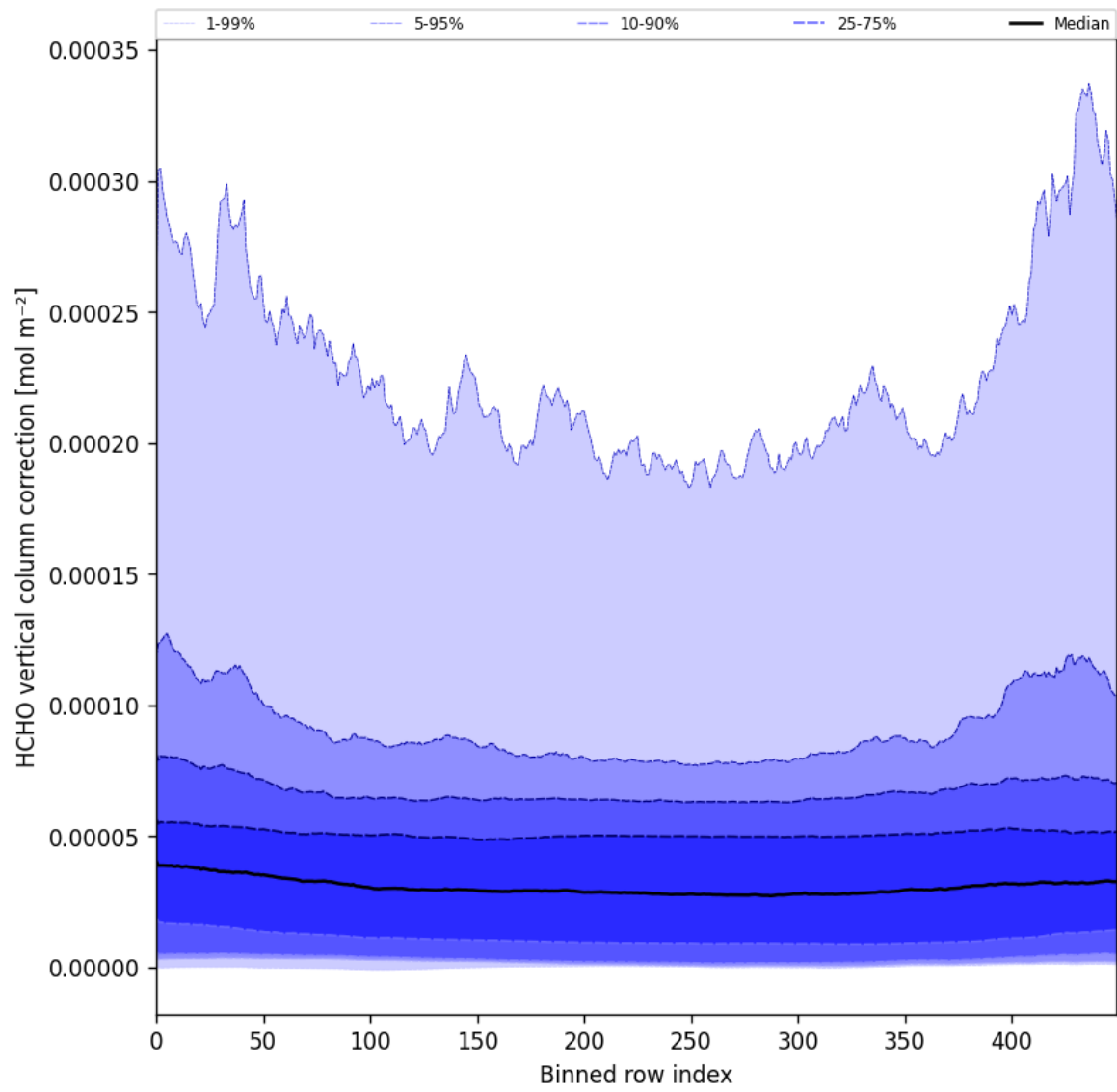
Figure 51: Along track statistics of “HCHO vertical column correction” for 2025-09-04 to 2025-09-06
