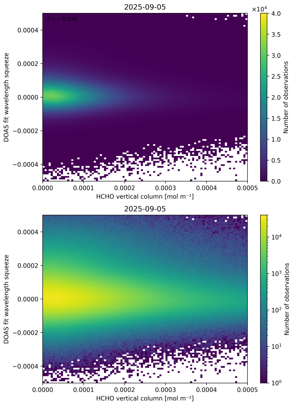
Figure 125: Scatter density plot of “HCHO vertical column” against “DOAS fit wavelength squeeze” for 2025-09-04 to 2025-09-06.
