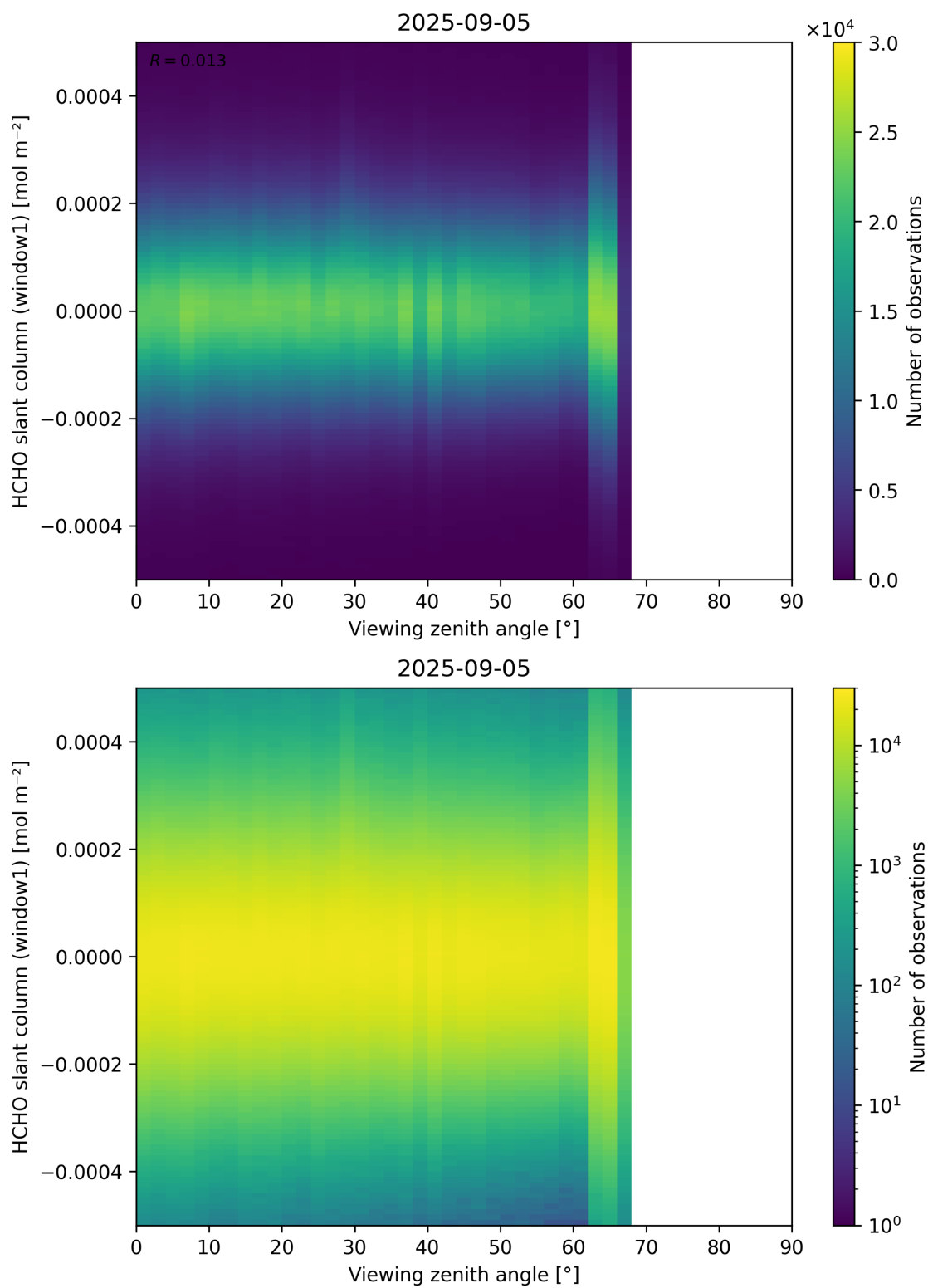
Figure 188: Scatter density plot of “Viewing zenith angle” against “HCHO slant column (window1)” for 2025-09-04 to 2025-09-06.
