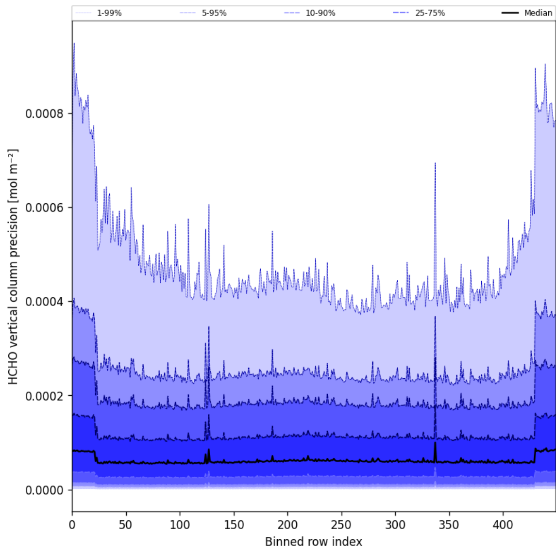
Figure 50: Along track statistics of "HCHO vertical column precision" for 2025-09-04 to 2025-09-06
