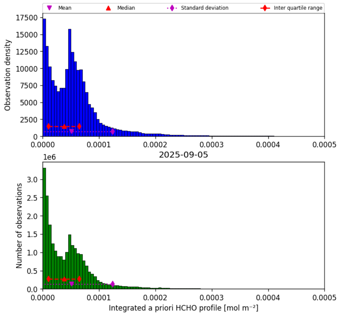
Figure 43: Histogram of “Integrated a priori HCHO profile” for 2025-09-04 to 2025-09-06
