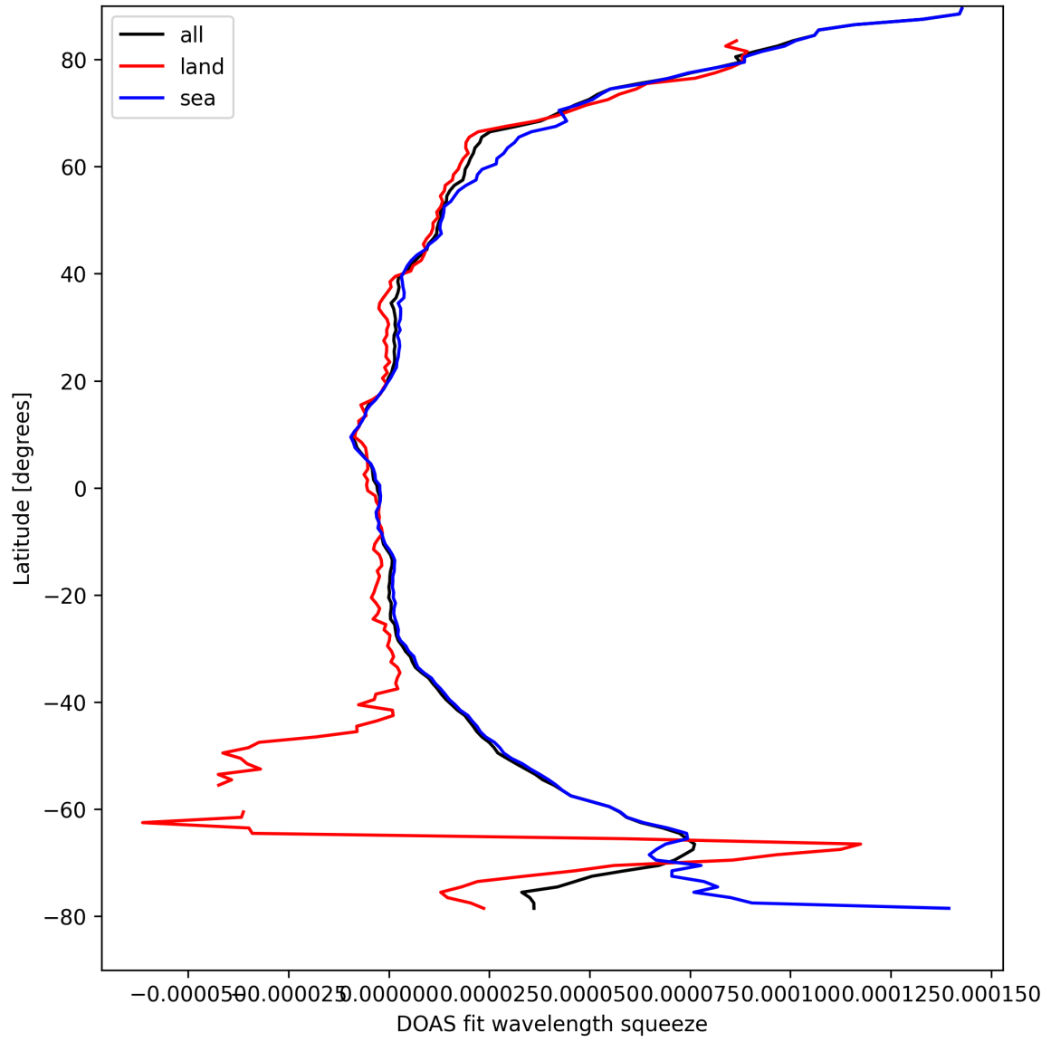
Figure 31: Zonal average of “DOAS fit wavelength squeeze” for 2025-09-04 to 2025-09-06.
