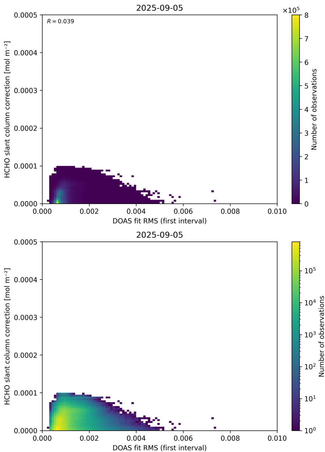
Figure 63: Scatter density plot of “DOAS fit RMS (first interval)” against “HCHO slant column correction” for 2025-09-04 to 2025-09-06.
