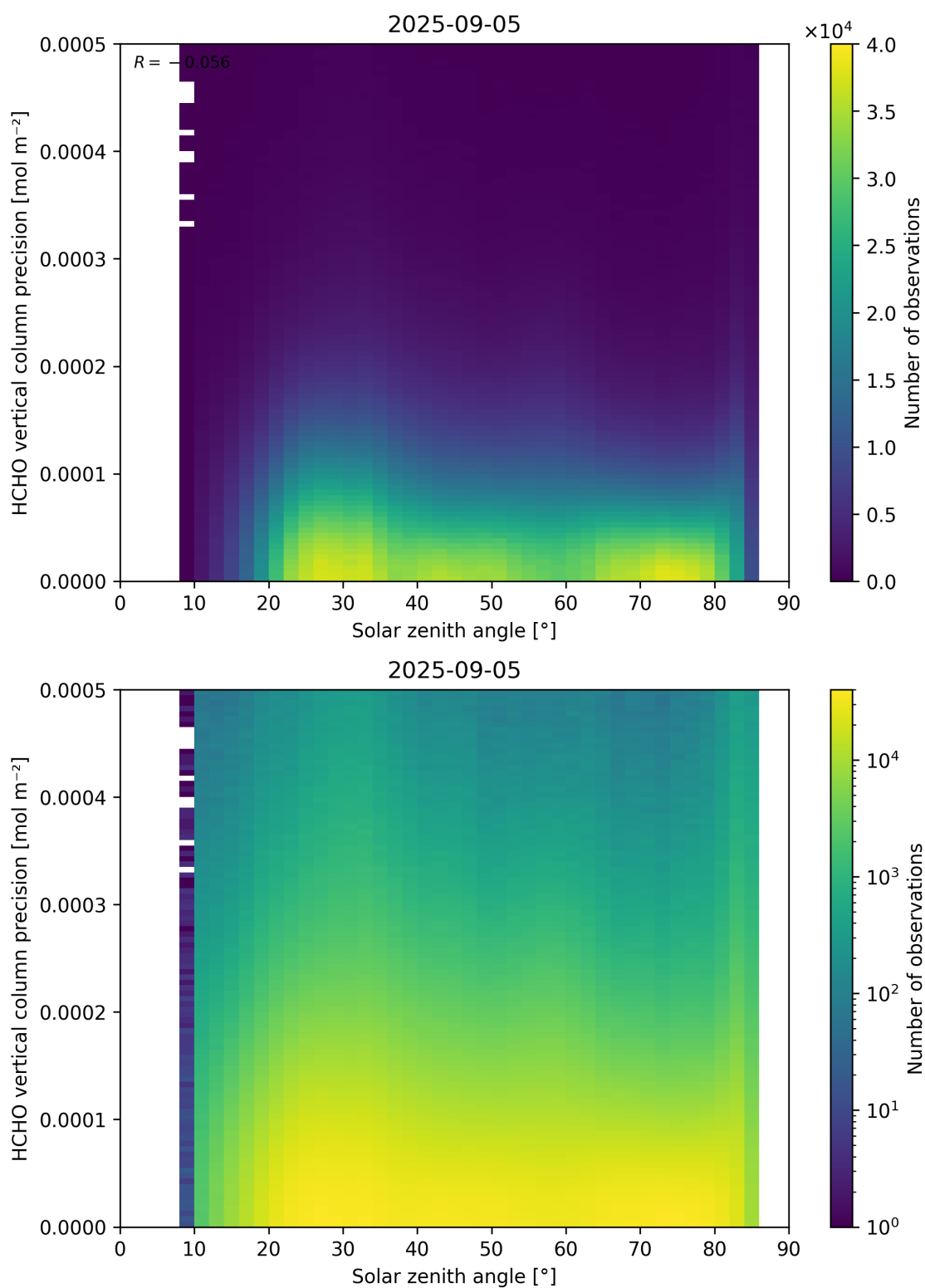
Figure 179: Scatter density plot of “Solar zenith angle” against “HCHO vertical column precision” for 2025-09-04 to 2025-09-06.
