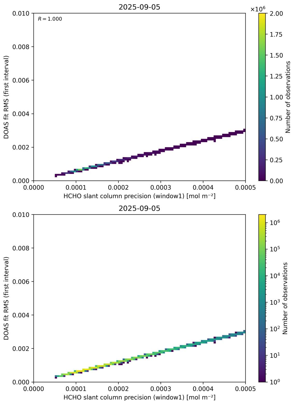
Figure 88: Scatter density plot of “HCHO slant column precision (window1)” against “DOAS fit RMS (first interval)” for 2025-09-04 to 2025-09-06.
