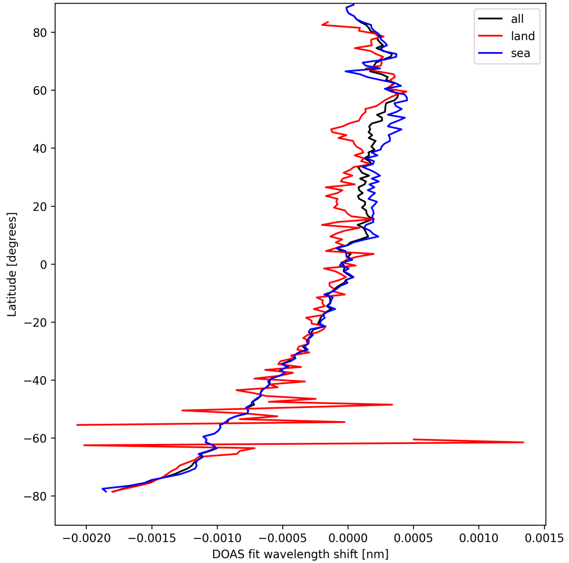
Figure 30: Zonal average of “DOAS fit wavelength shift” for 2025-09-04 to 2025-09-06.
