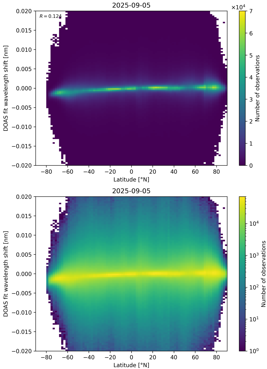
Figure 154: Scatter density plot of “Latitude” against “DOAS fit wavelength shift” for 2025-09-04 to 2025-09-06.
