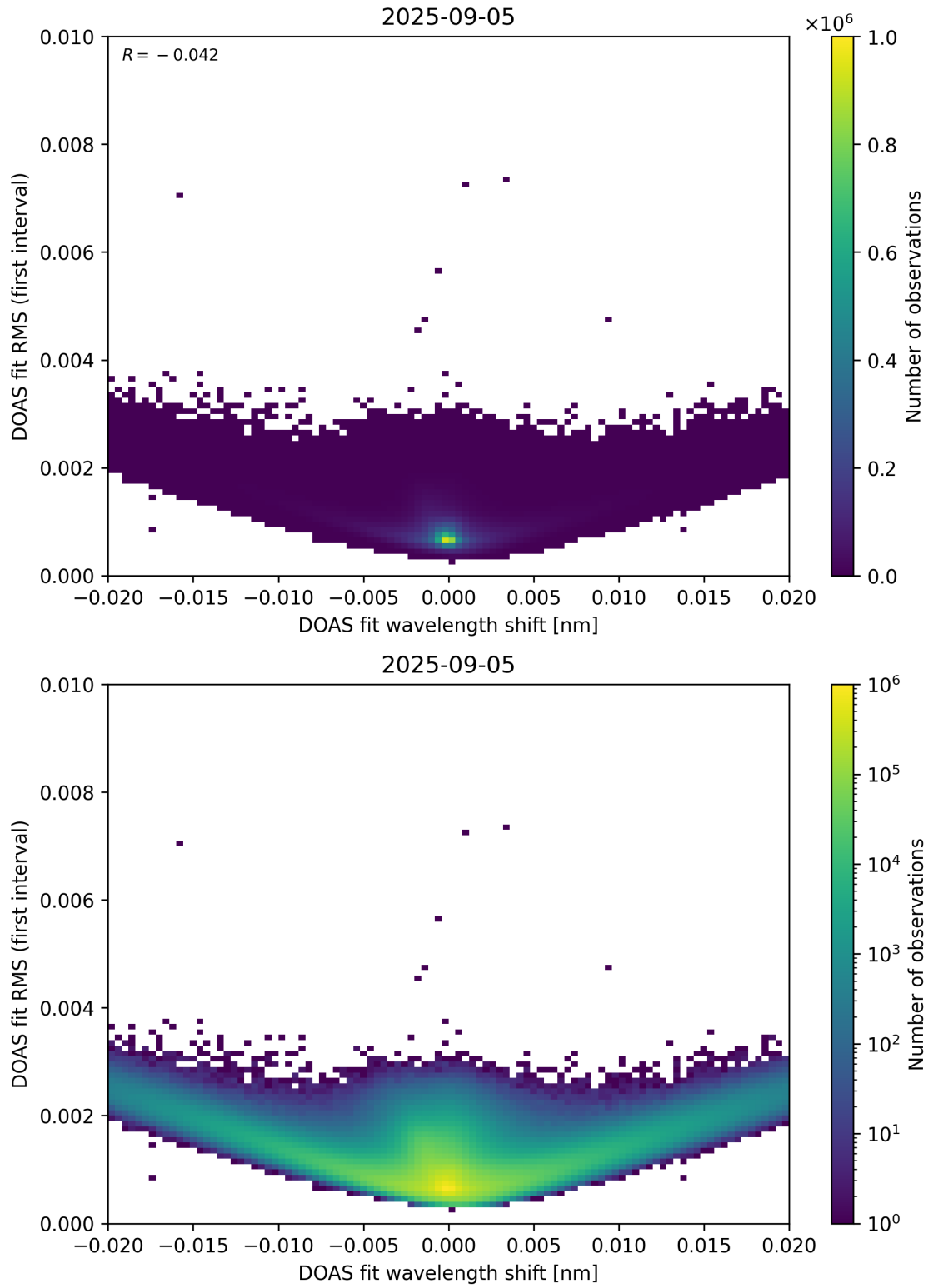
Figure 64: Scatter density plot of “DOAS fit wavelength shift” against “DOAS fit RMS (first interval)” for 2025-09-04 to 2025-09-06.
