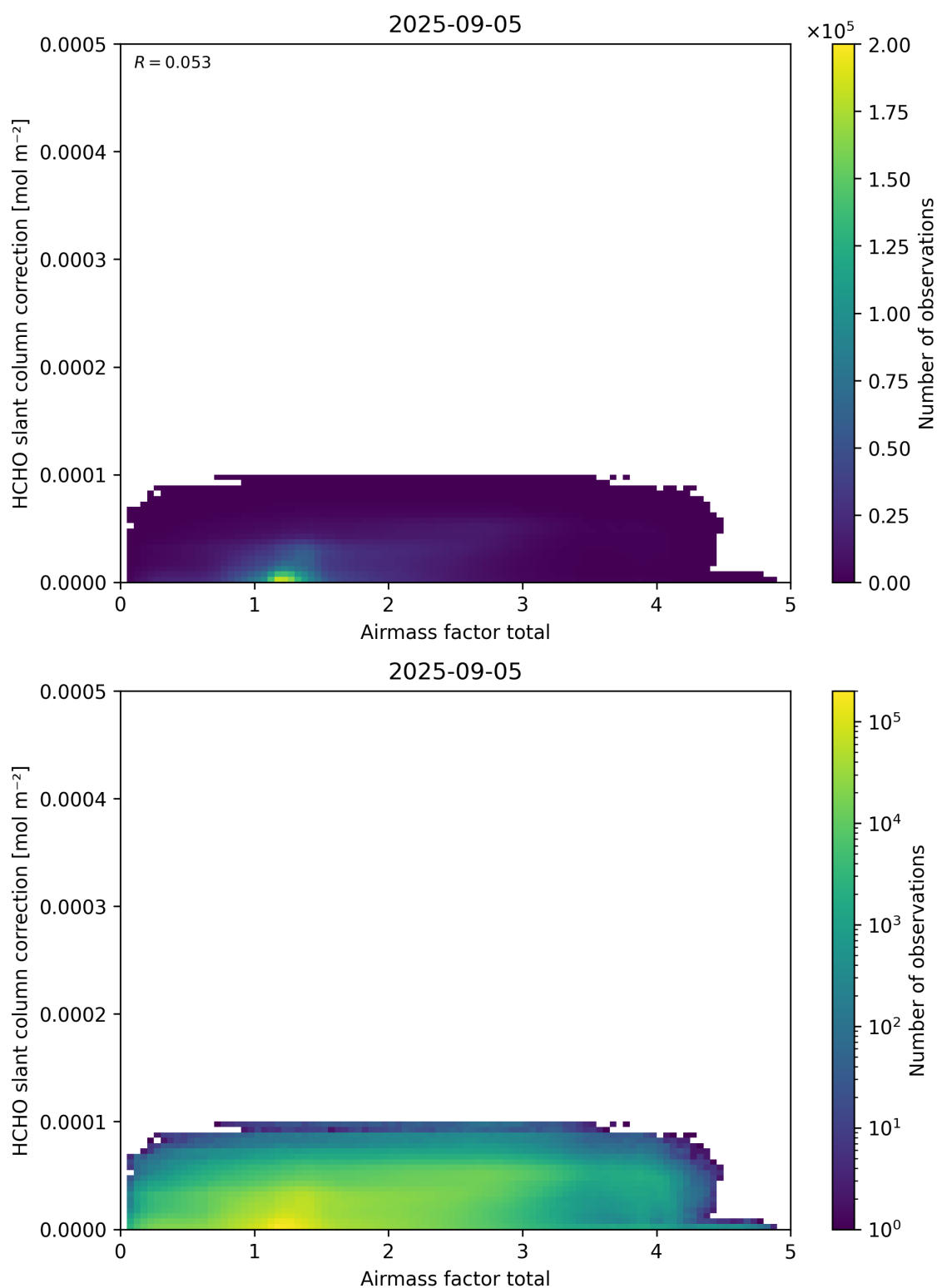
Figure 102: Scatter density plot of “Airmass factor total” against “HCHO slant column correction” for 2025-09-04 to 2025-09-06.
