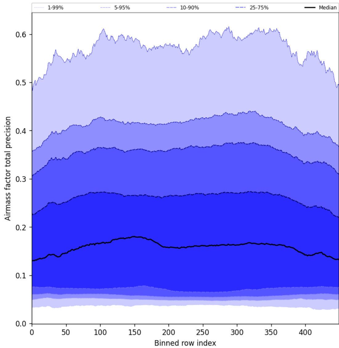
Figure 55: Along track statistics of “Airmass factor total precision” for 2025-09-04 to 2025-09-06
