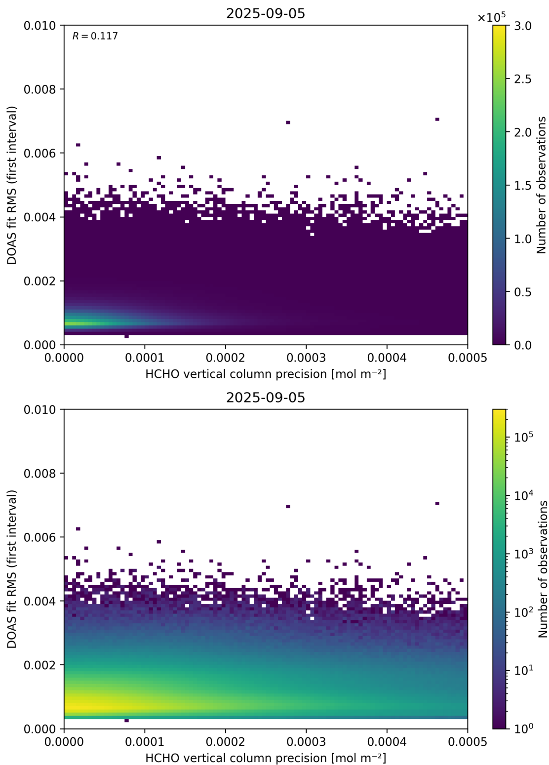
Figure 136: Scatter density plot of “HCHO vertical column precision” against “DOAS fit RMS (first interval)” for 2025-09-04 to 2025-09-06.
