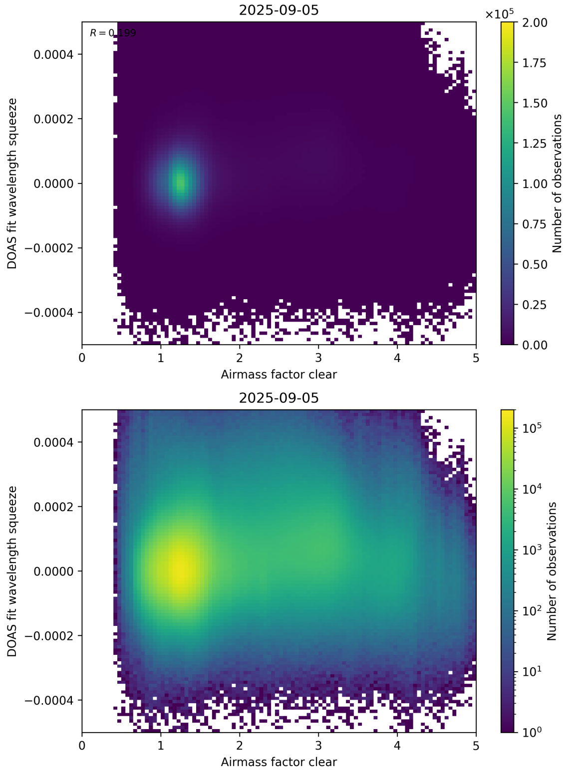
Figure 73: Scatter density plot of “Airmass factor clear” against “DOAS fit wavelength squeeze” for 2025-09-04 to 2025-09-06.
