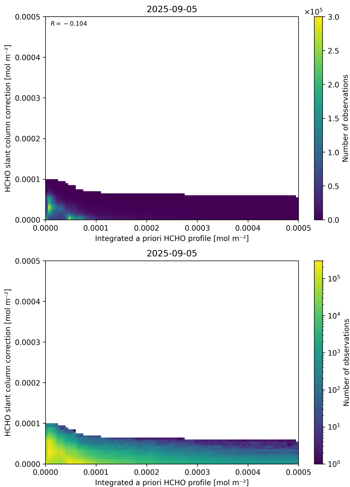
Figure 152: Scatter density plot of “Integrated a priori HCHO profile” against “HCHO slant column correction” for 2025-09-04 to 2025-09-06.
