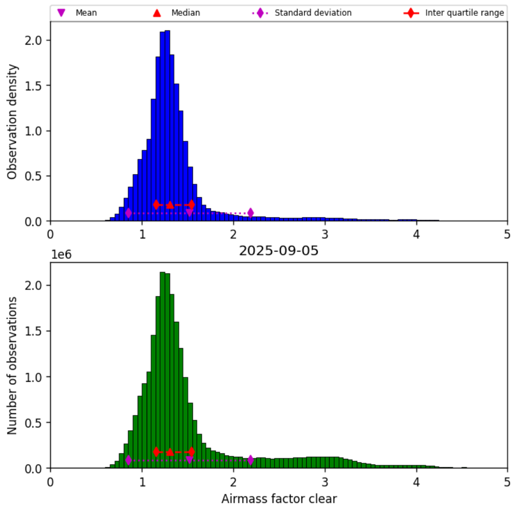
Figure 42: Histogram of “Airmass factor clear” for 2025-09-04 to 2025-09-06
