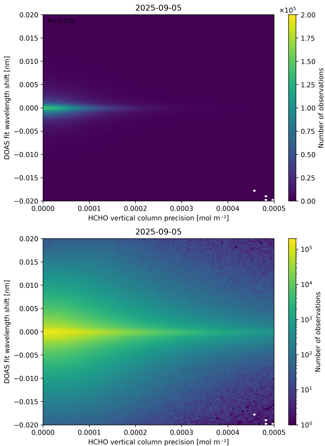
Figure 137: Scatter density plot of “HCHO vertical column precision” against “DOAS fit wavelength shift” for 2025-09-04 to 2025-09-06.
