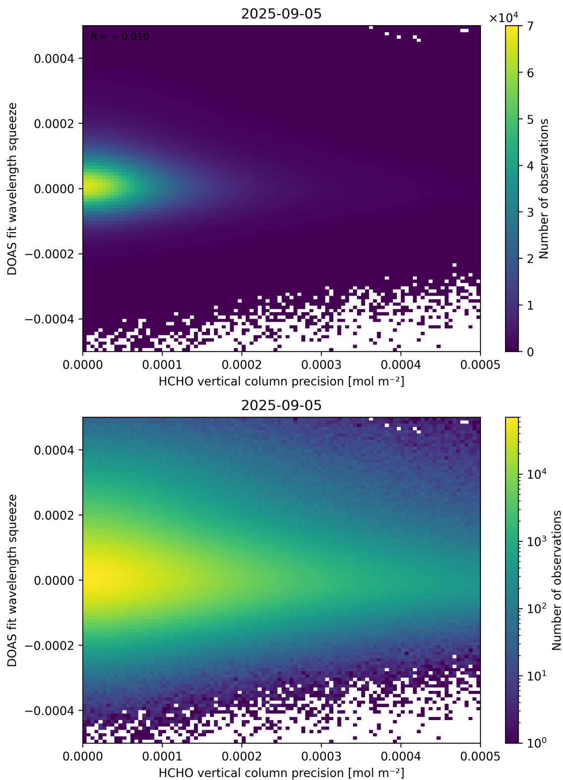
Figure 138: Scatter density plot of “HCHO vertical column precision” against “DOAS fit wavelength squeeze” for 2025-09-04 to 2025-09-06.
