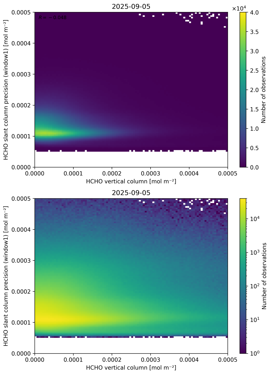
Figure 130: Scatter density plot of “HCHO vertical column” against “HCHO slant column precision (window1)” for 2025-09-04 to 2025-09-06.
