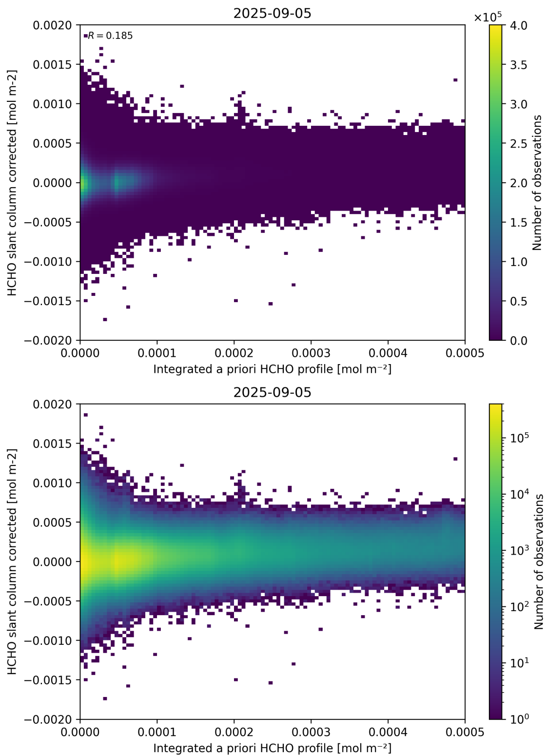
Figure 151: Scatter density plot of “Integrated a priori HCHO profile” against “HCHO slant column corrected” for 2025-09-04 to 2025-09-06.
