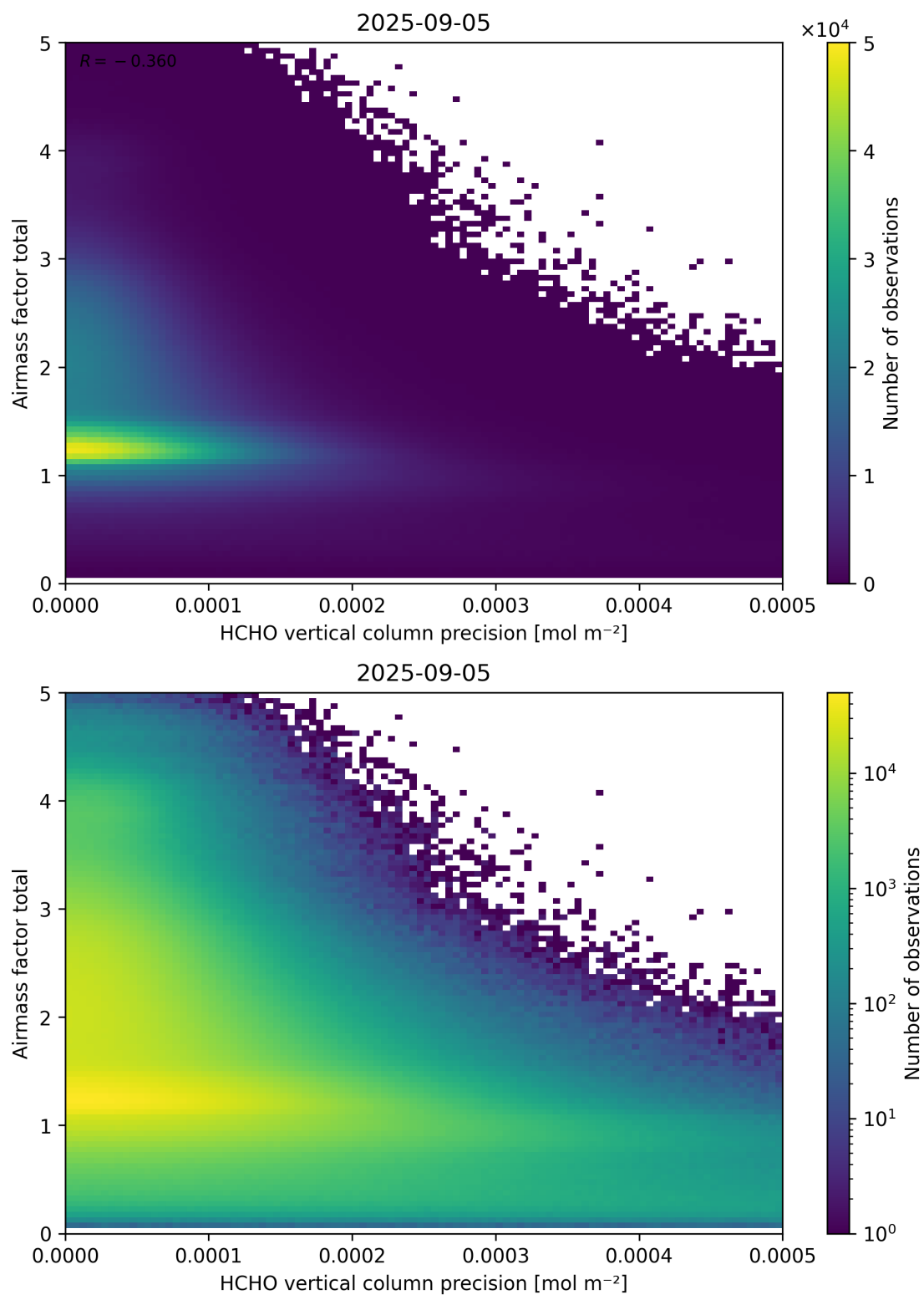
Figure 144: Scatter density plot of “HCHO vertical column precision” against “Airmass factor total” for 2025-09-04 to 2025-09-06.
