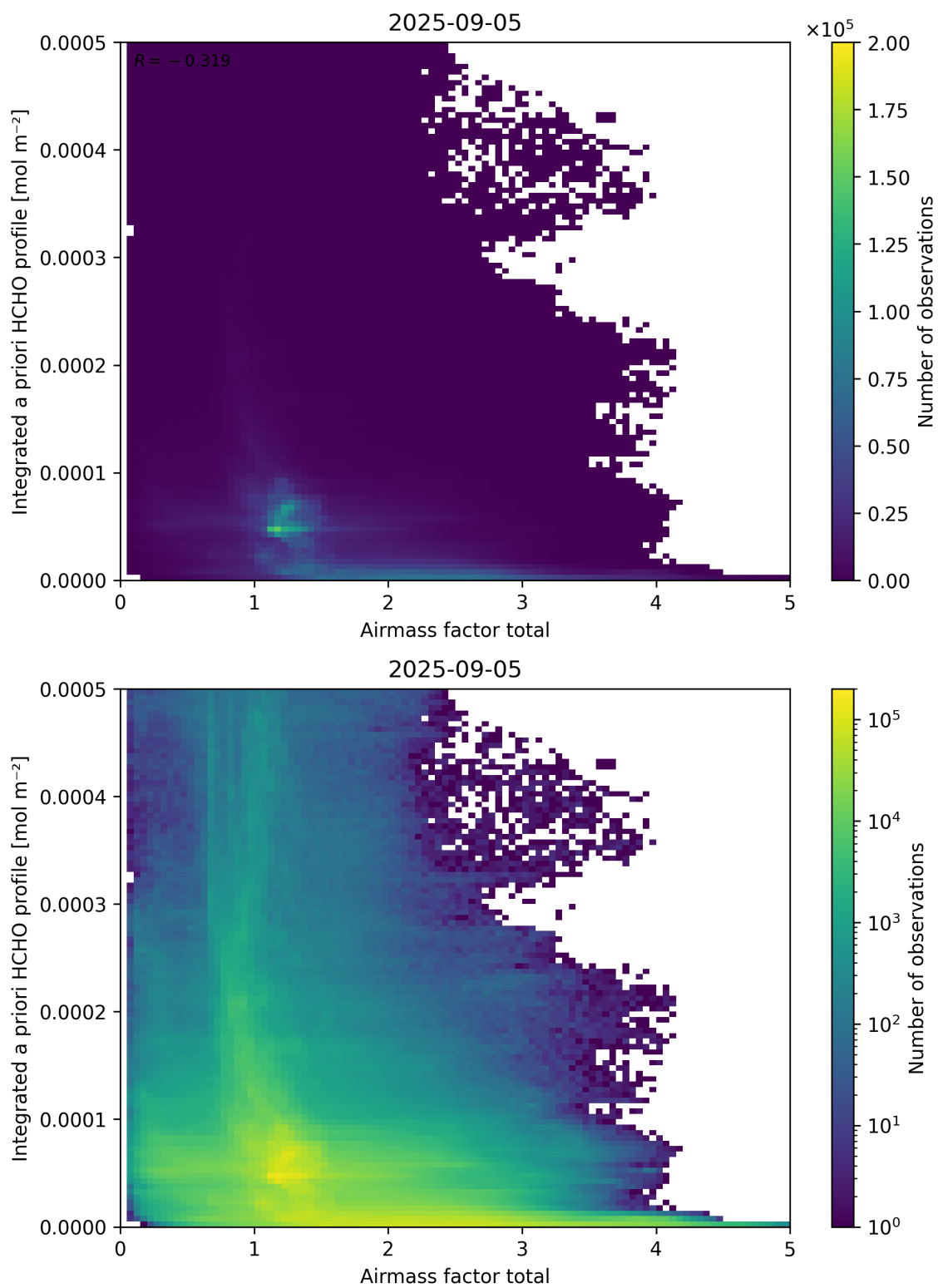
Figure 104: Scatter density plot of “Airmass factor total” against “Integrated a priori HCHO profile” for 2025-09-04 to 2025-09-06.
