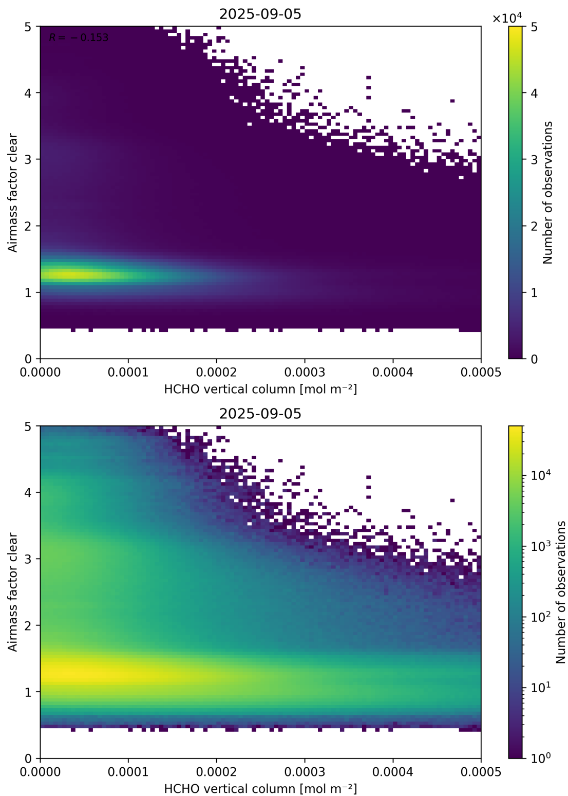
Figure 126: Scatter density plot of “HCHO vertical column” against “Airmass factor clear” for 2025-09-04 to 2025-09-06.
