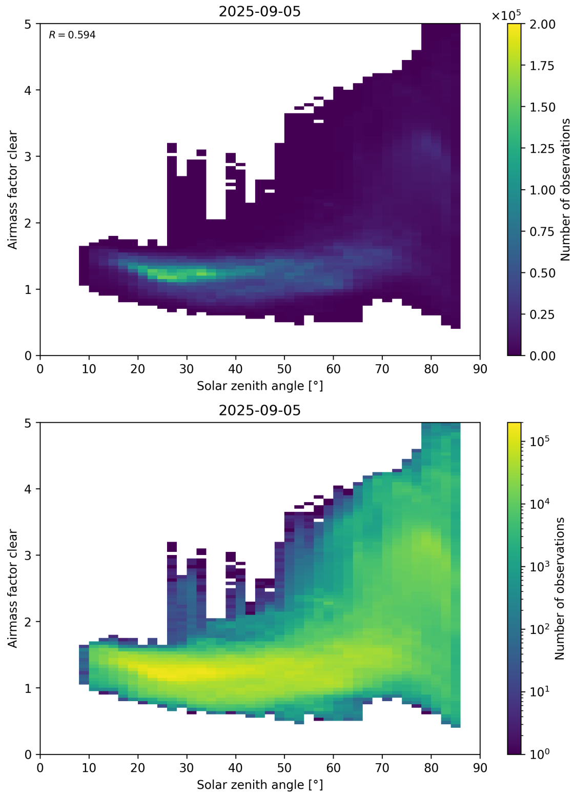
Figure 170: Scatter density plot of “Solar zenith angle” against “Airmass factor clear” for 2025-09-04 to 2025-09-06.
