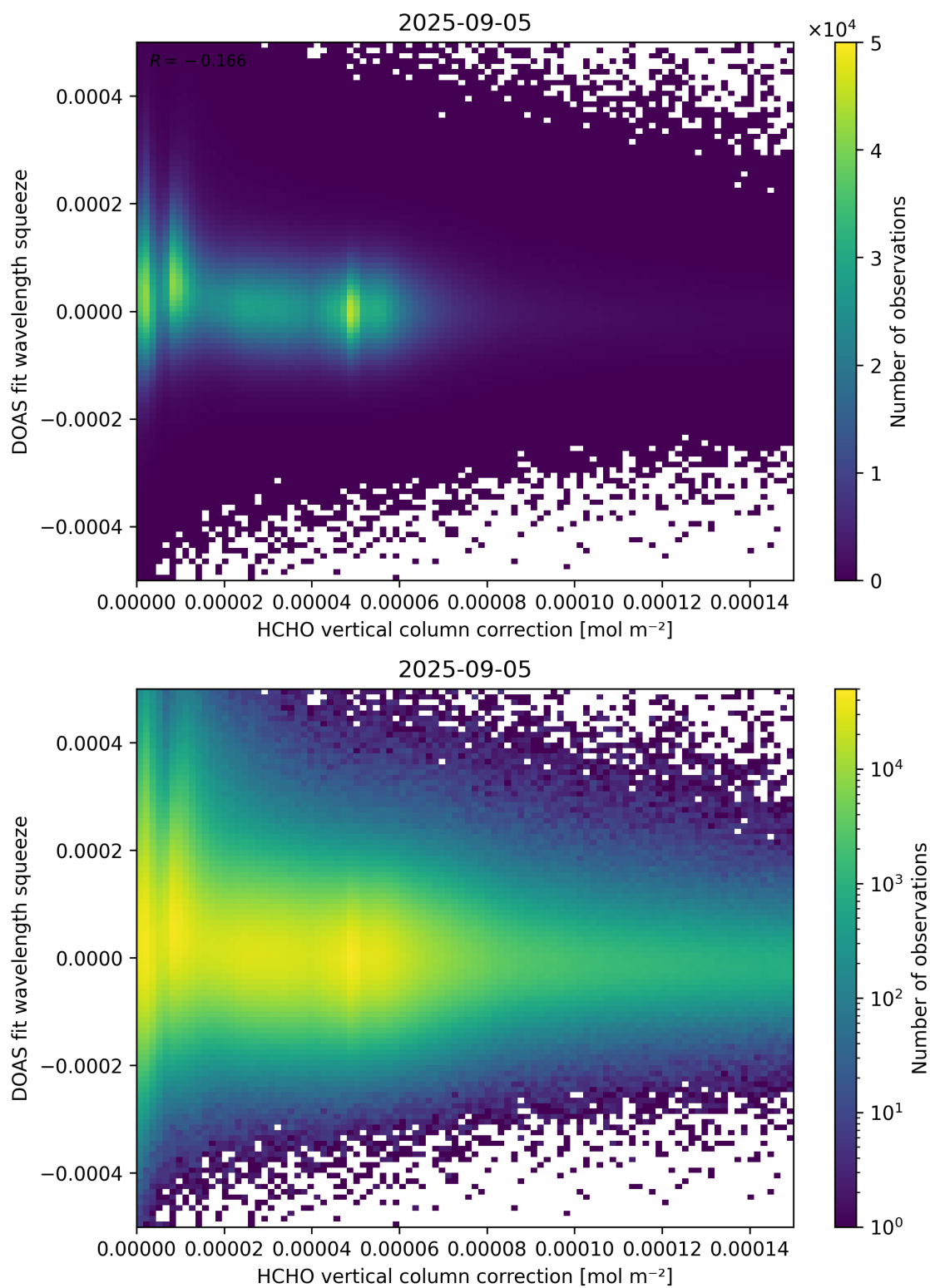
Figure 114: Scatter density plot of “HCHO vertical column correction” against “DOAS fit wavelength squeeze” for 2025-09-04 to 2025-09-06.
