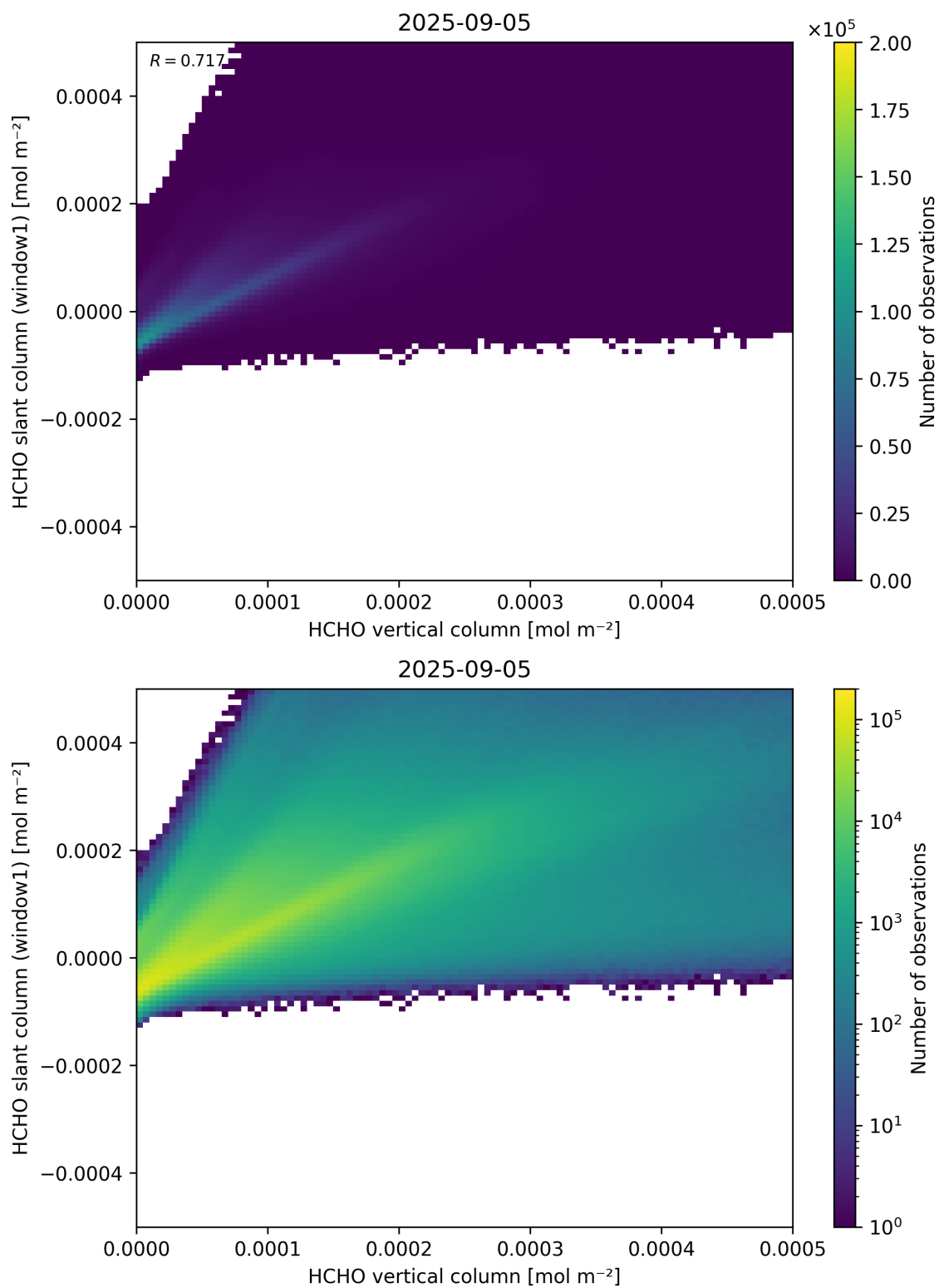
Figure 129: Scatter density plot of “HCHO vertical column” against “HCHO slant column (window1)” for 2025-09-04 to 2025-09-06.
