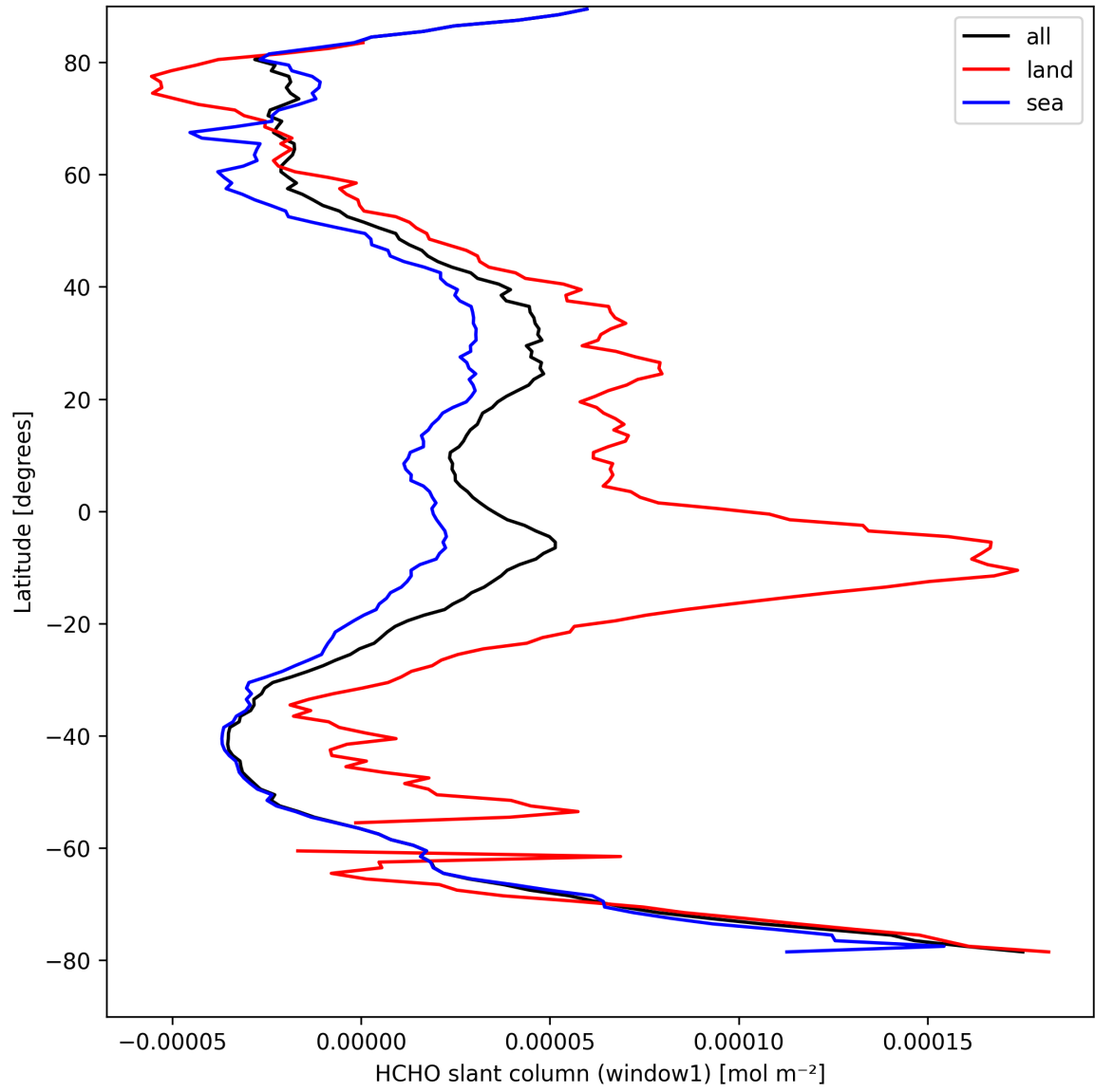
Figure 24: Zonal average of “HCHO slant column (window1)” for 2025-09-04 to 2025-09-06.
