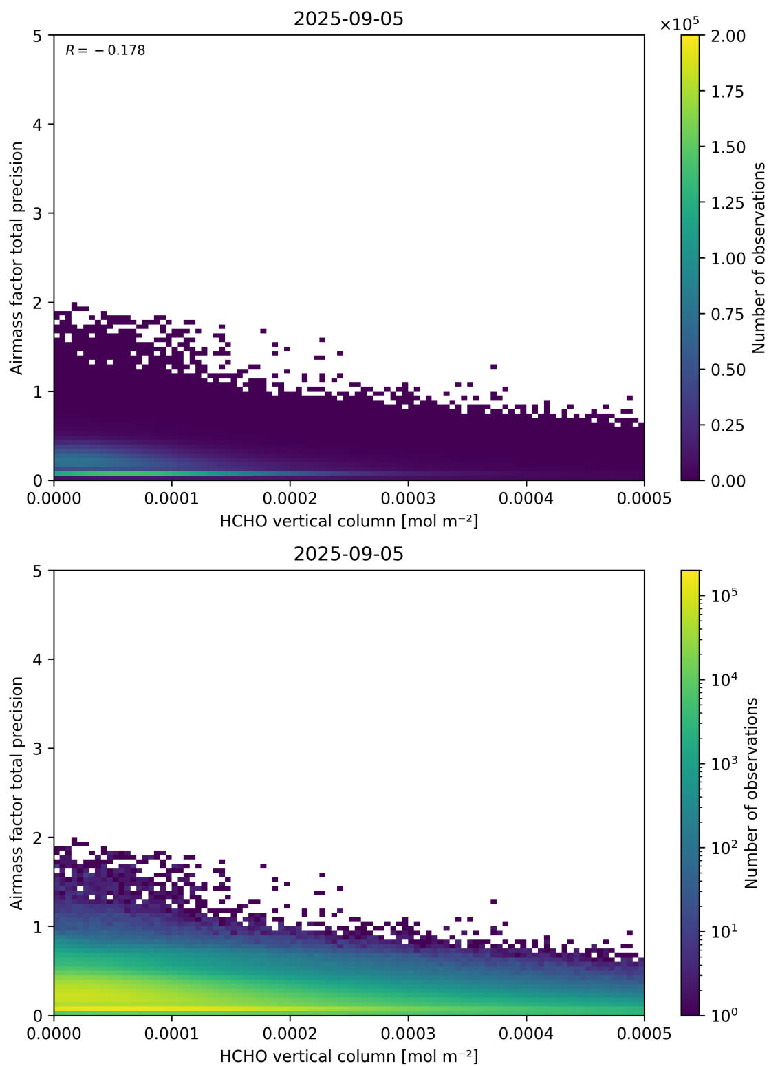
Figure 132: Scatter density plot of “HCHO vertical column” against “Airmass factor total precision” for 2025-09-04 to 2025-09-06.
