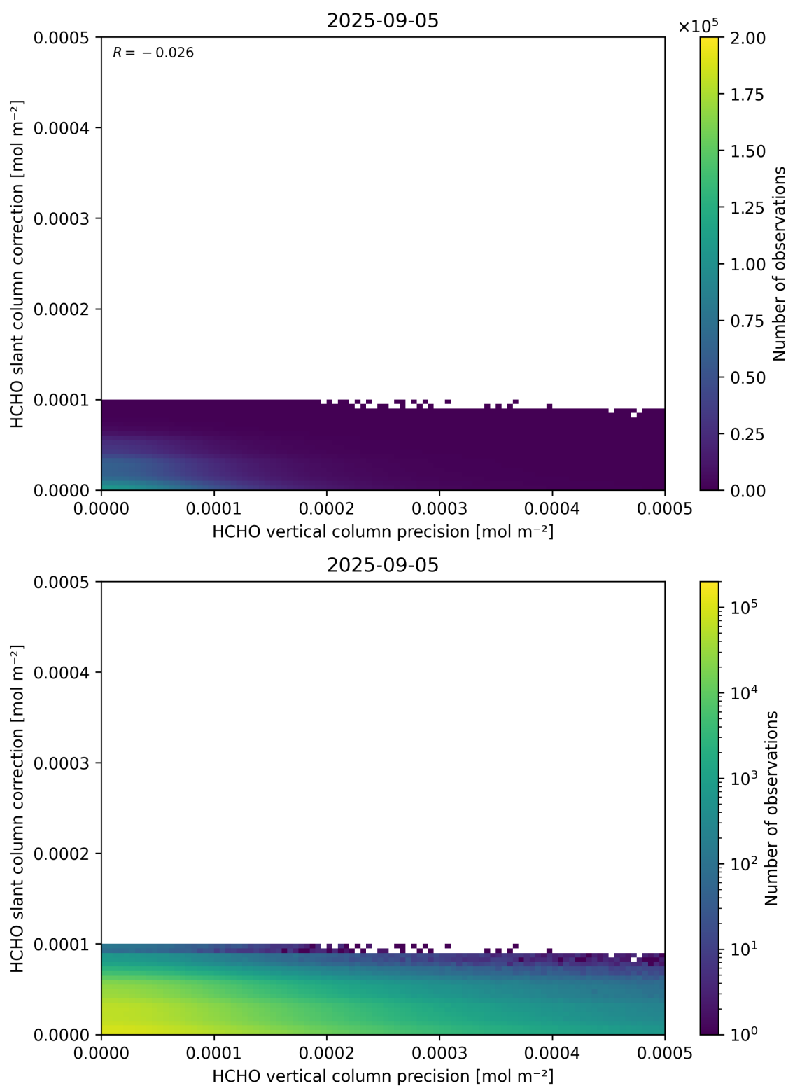
Figure 141: Scatter density plot of “HCHO vertical column precision” against “HCHO slant column correction” for 2025-09-04 to 2025-09-06.
