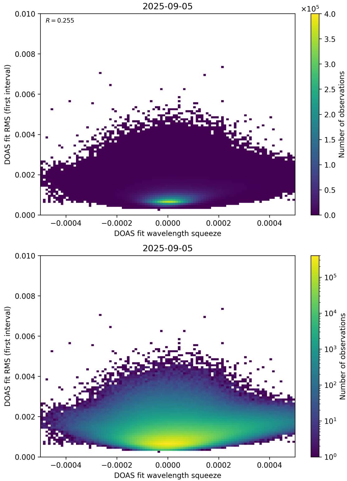
Figure 68: Scatter density plot of “DOAS fit wavelength squeeze” against “DOAS fit RMS (first interval)” for 2025-09-04 to 2025-09-06.
