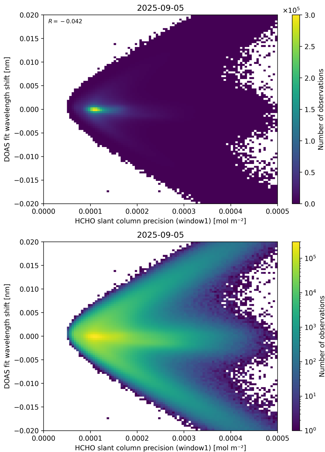
Figure 89: Scatter density plot of “HCHO slant column precision (window1)” against “DOAS fit wavelength shift” for 2025-09-04 to 2025-09-06.
