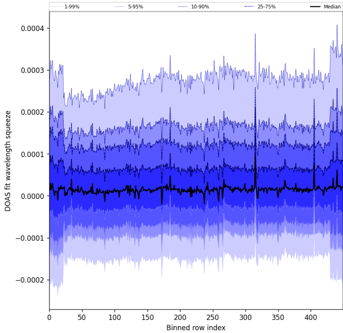
Figure 59: Along track statistics of “DOAS fit wavelength squeeze” for 2025-09-04 to 2025-09-06
