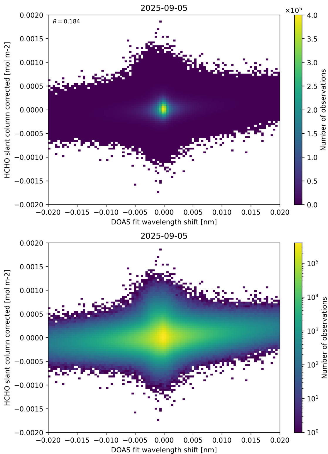
Figure 66: Scatter density plot of “DOAS fit wavelength shift” against “HCHO slant column corrected” for 2025-09-04 to 2025-09-06.
