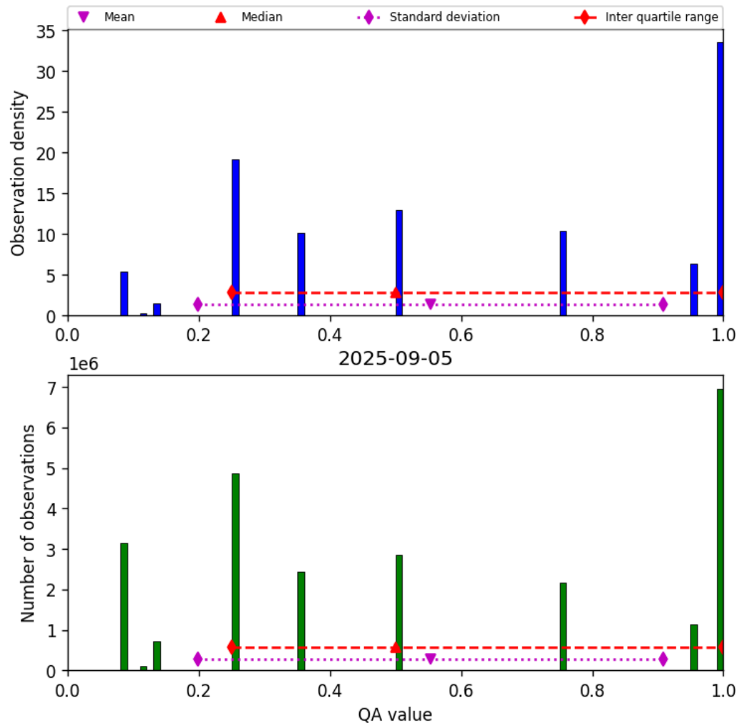
Figure 34: Histogram of “QA value” for 2025-09-04 to 2025-09-06
