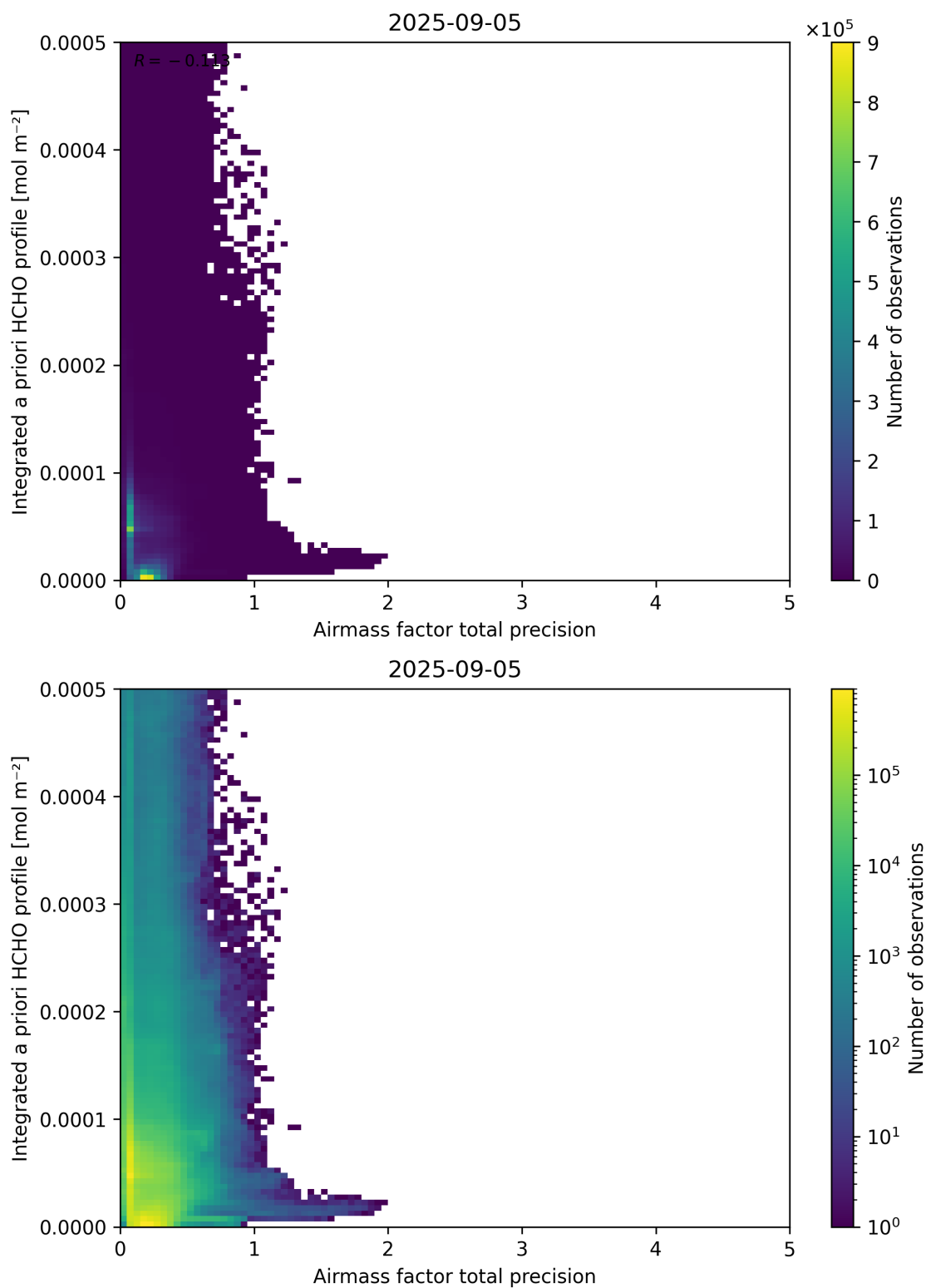
Figure 111: Scatter density plot of “Airmass factor total precision” against “Integrated a priori HCHO profile” for 2025-09-04 to 2025-09-06.
