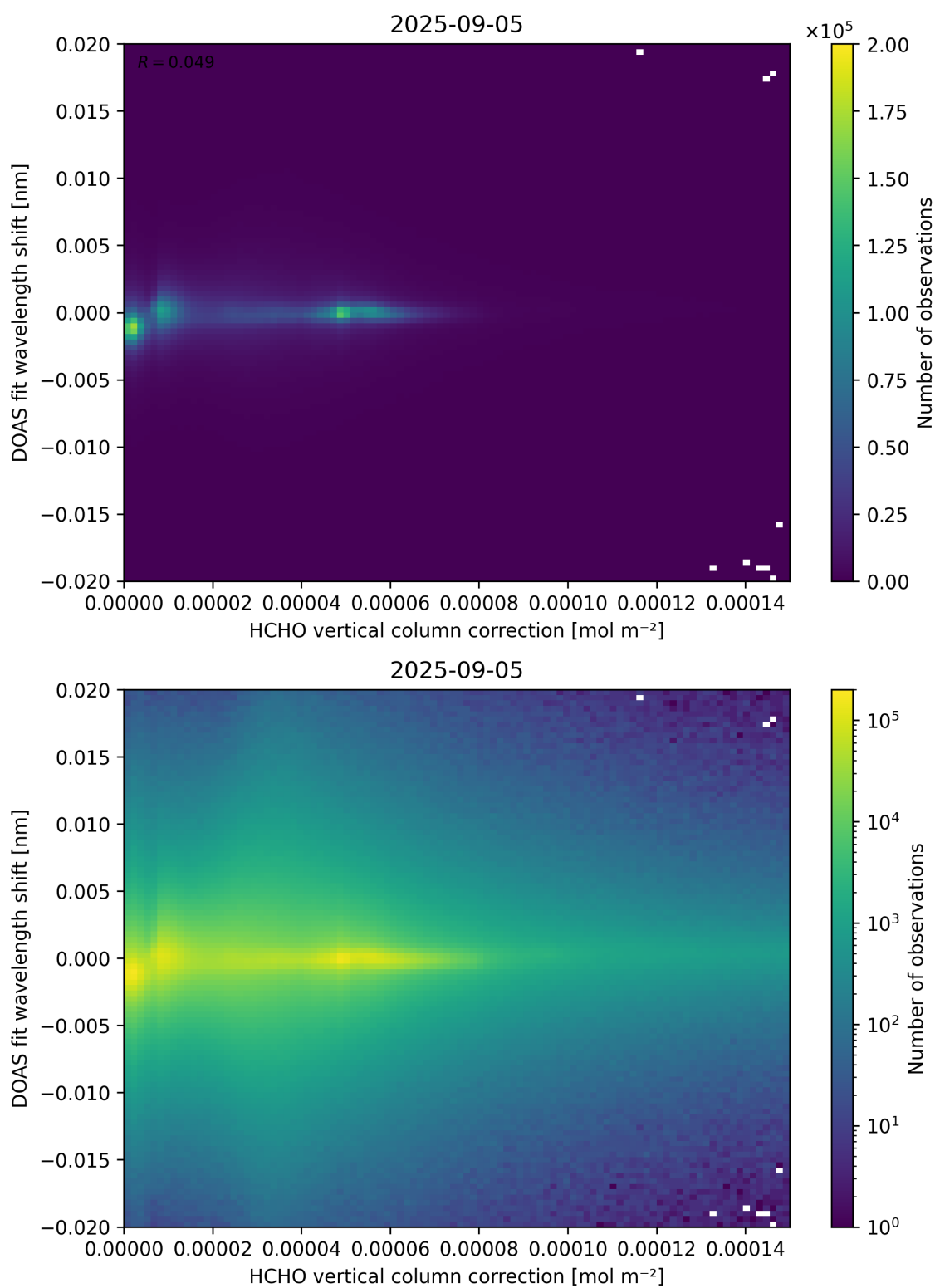
Figure 113: Scatter density plot of “HCHO vertical column correction” against “DOAS fit wavelength shift” for 2025-09-04 to 2025-09-06.
