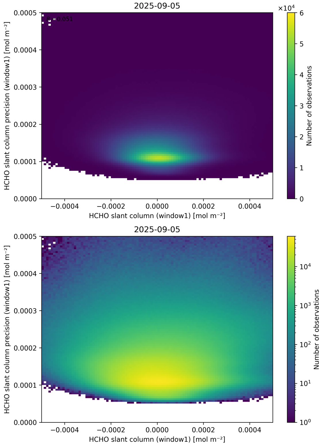
Figure 84: Scatter density plot of “HCHO slant column (window1)” against “HCHO slant column precision (window1)” for 2025-09-04 to 2025-09-06.
