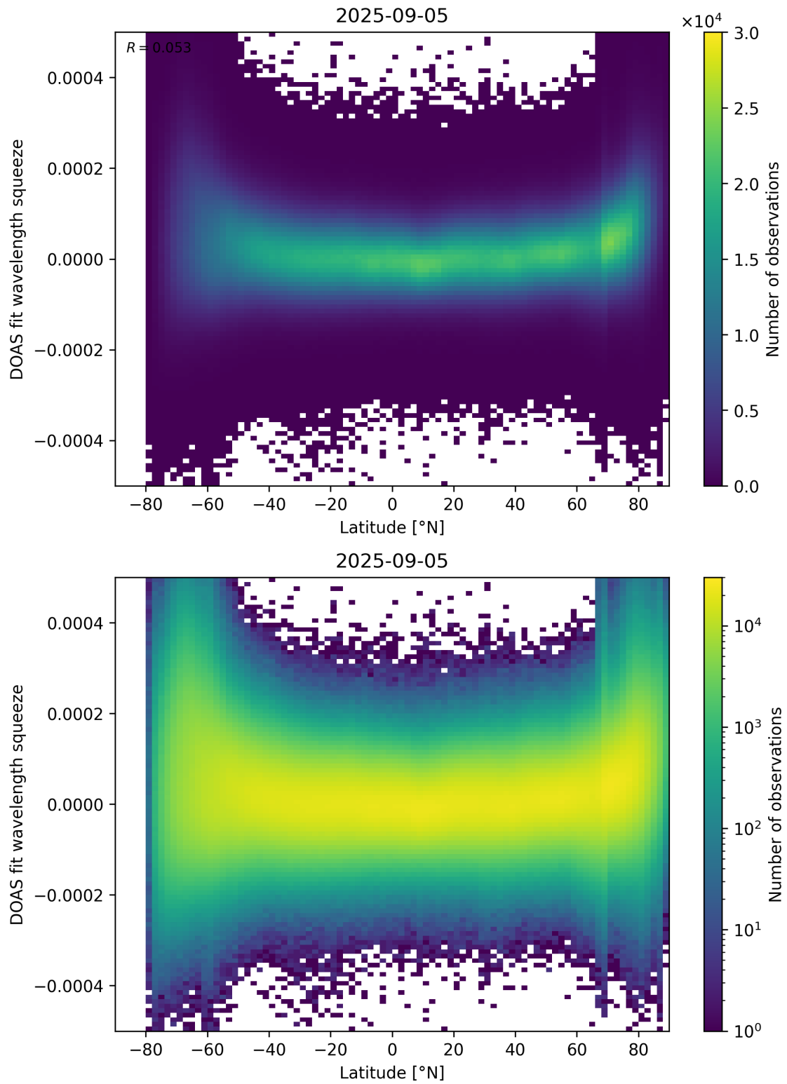
Figure 155: Scatter density plot of “Latitude” against “DOAS fit wavelength squeeze” for 2025-09-04 to 2025-09-06.
