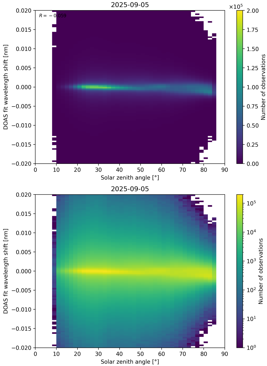
Figure 168: Scatter density plot of “Solar zenith angle” against “DOAS fit wavelength shift” for 2025-09-04 to 2025-09-06.
