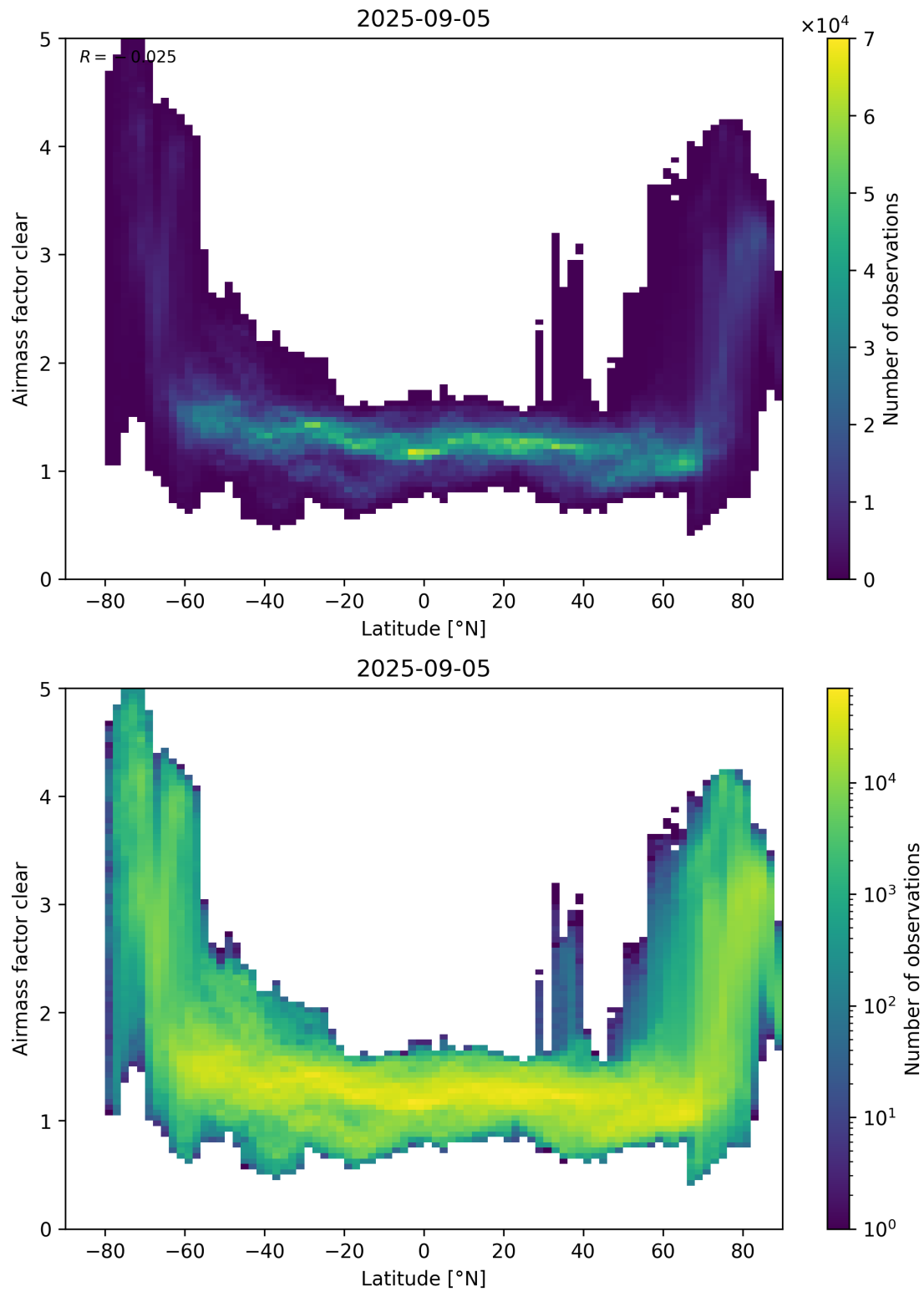
Figure 156: Scatter density plot of “Latitude” against “Airmass factor clear” for 2025-09-04 to 2025-09-06.
