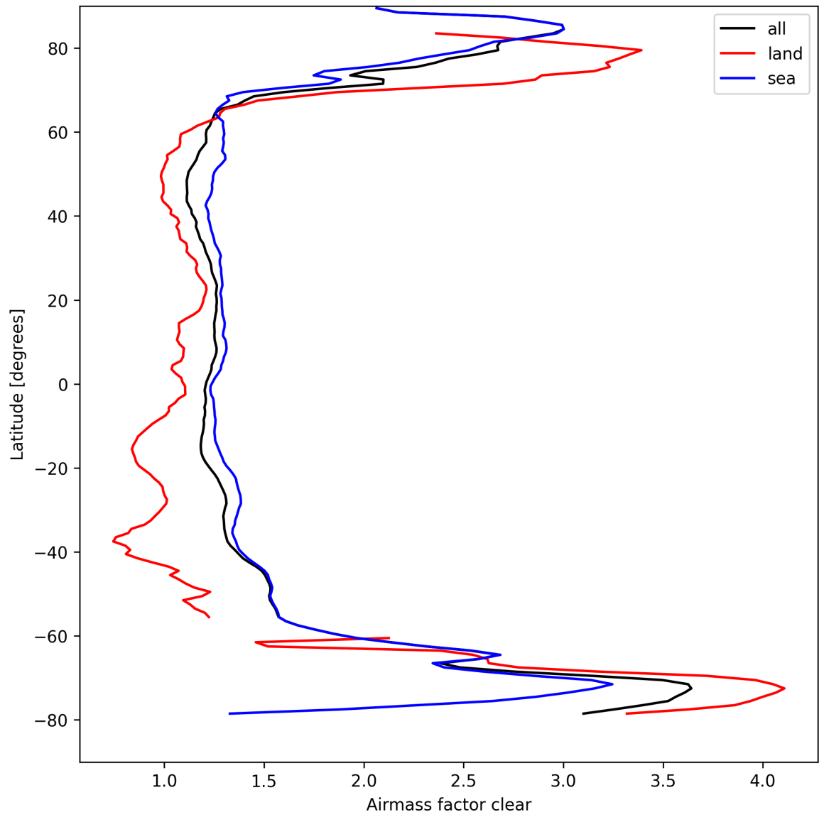
Figure 28: Zonal average of “Airmass factor clear” for 2025-09-04 to 2025-09-06.
