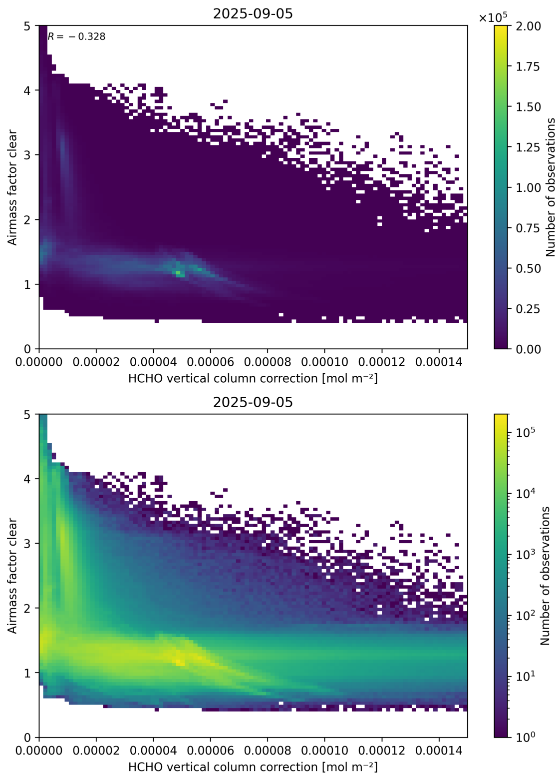
Figure 115: Scatter density plot of “HCHO vertical column correction” against “Airmass factor clear” for 2025-09-04 to 2025-09-06.
