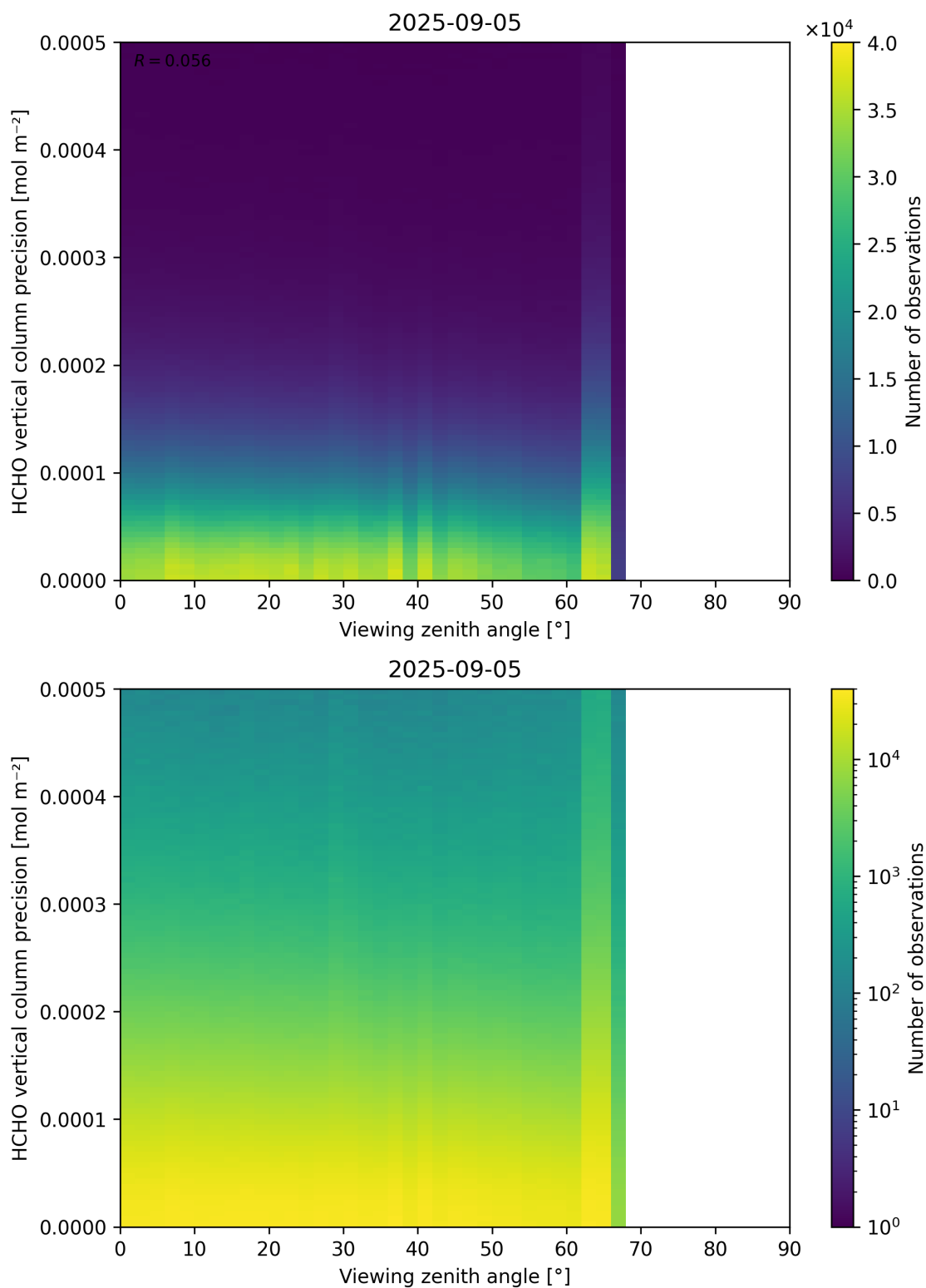
Figure 194: Scatter density plot of “Viewing zenith angle” against “HCHO vertical column precision” for 2025-09-04 to 2025-09-06.
