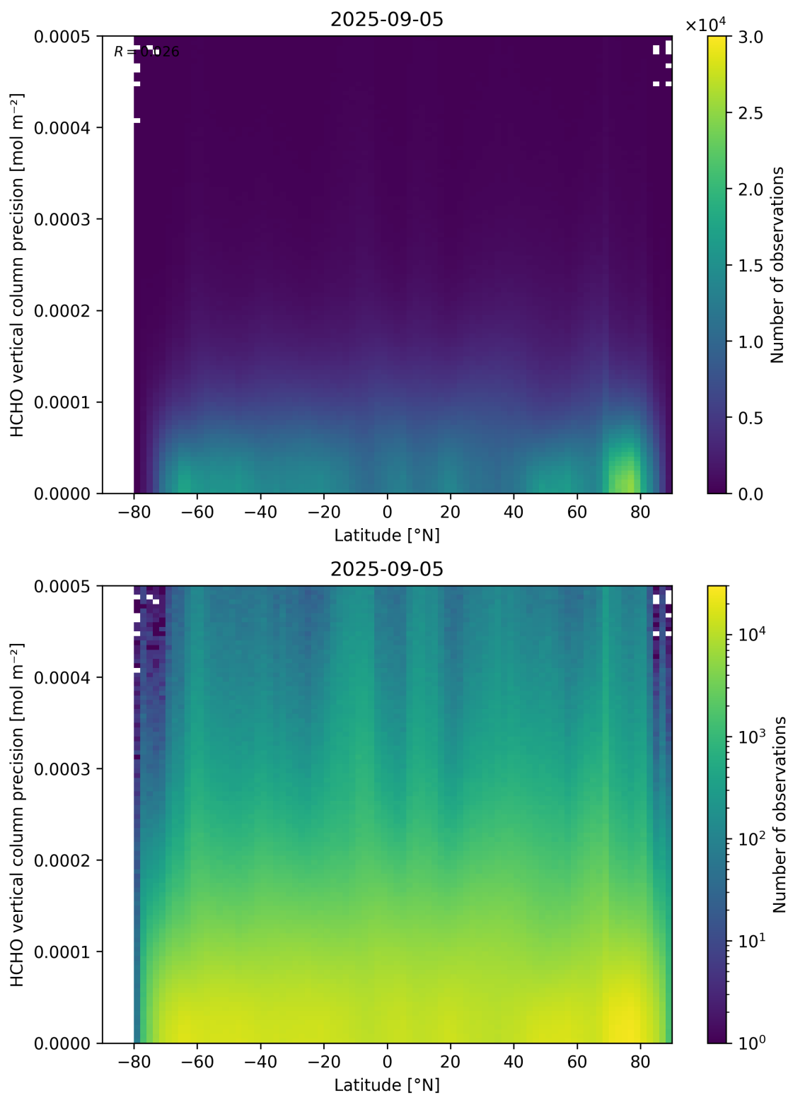
Figure 165: Scatter density plot of “Latitude” against “HCHO vertical column precision” for 2025-09-04 to 2025-09-06.
