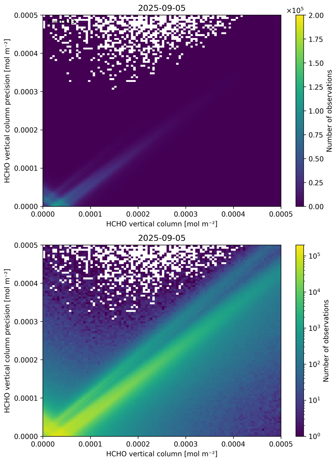
Figure 134: Scatter density plot of “HCHO vertical column” against “HCHO vertical column precision” for 2025-09-04 to 2025-09-06.
