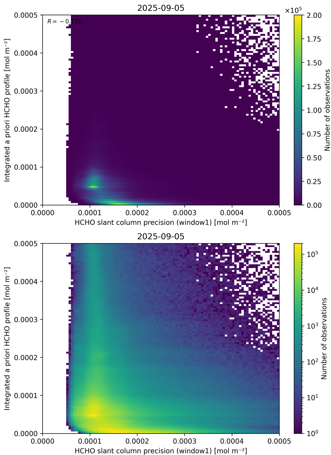
Figure 96: Scatter density plot of “HCHO slant column precision (window1)” against “Integrated a priori HCHO profile” for 2025-09-04 to 2025-09-06.
