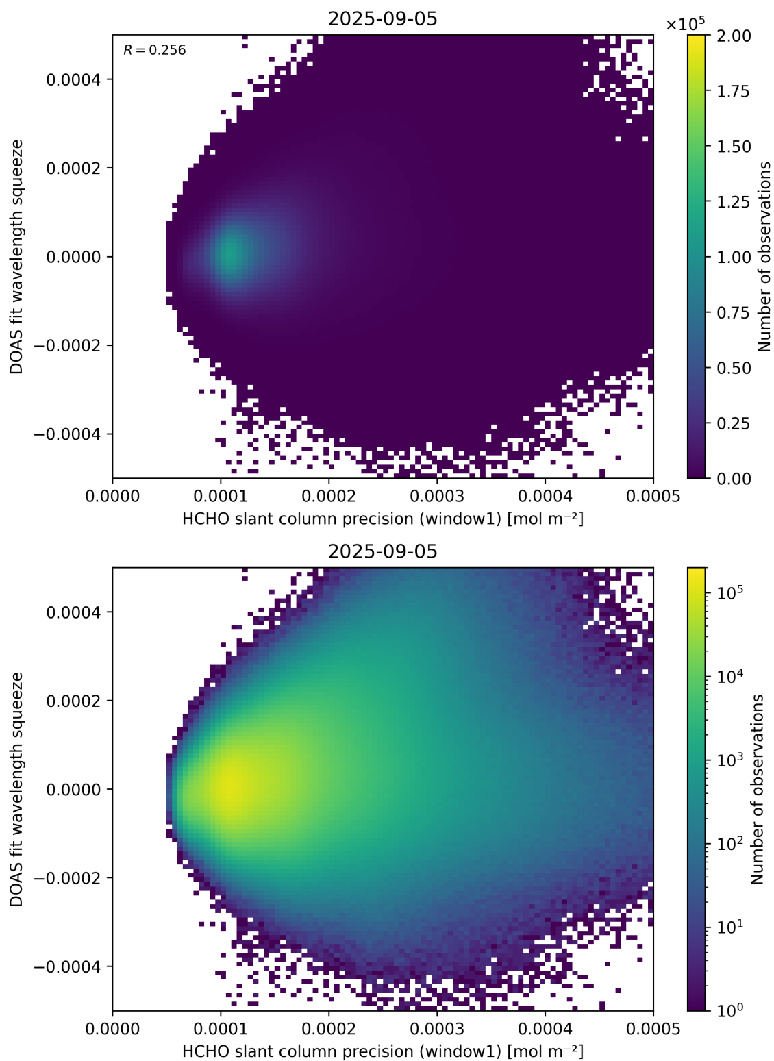
Figure 90: Scatter density plot of “HCHO slant column precision (window1)” against “DOAS fit wavelength squeeze” for 2025-09-04 to 2025-09-06.
