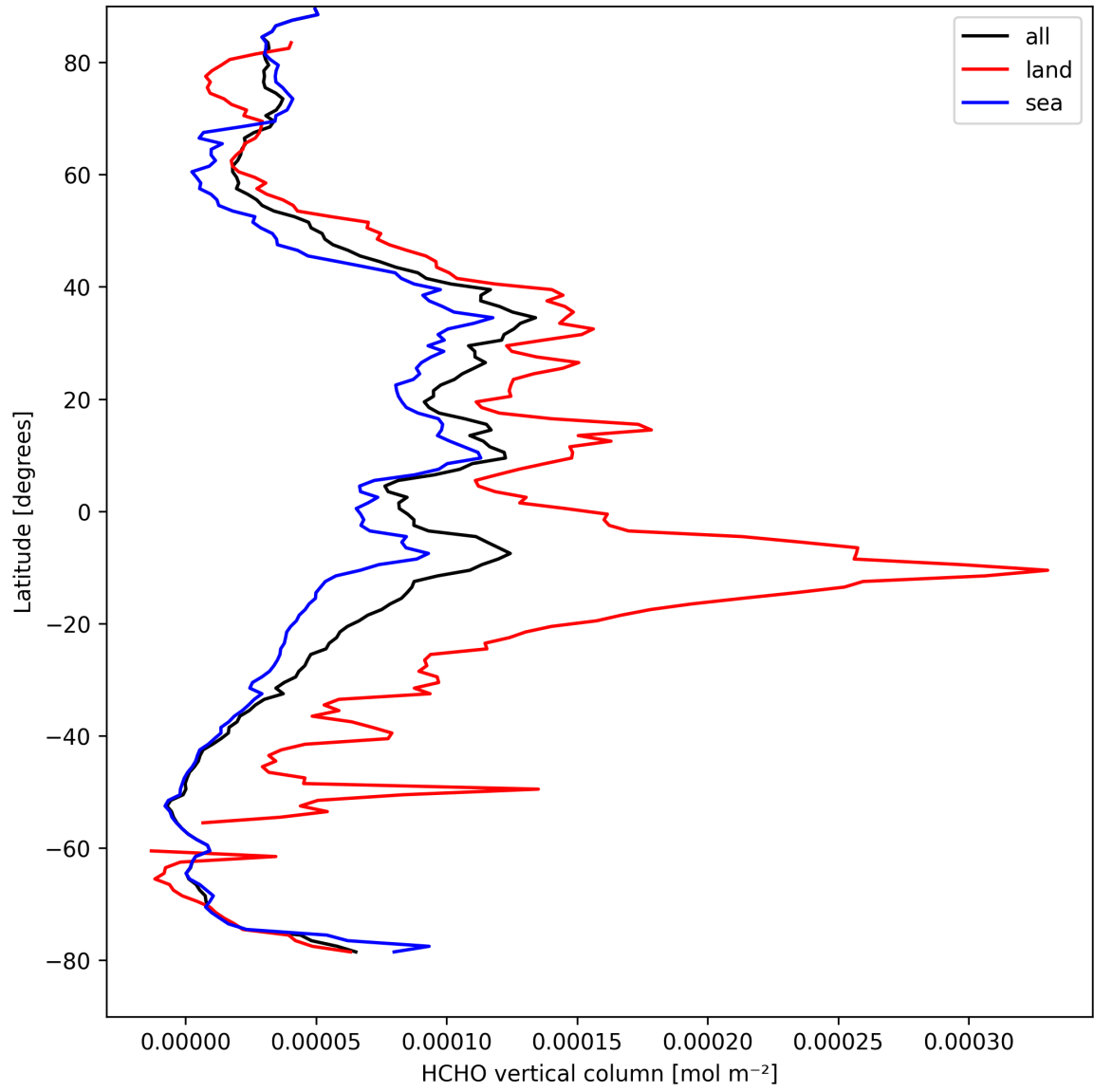
Figure 21: Zonal average of “HCHO vertical column” for 2025-09-04 to 2025-09-06.
