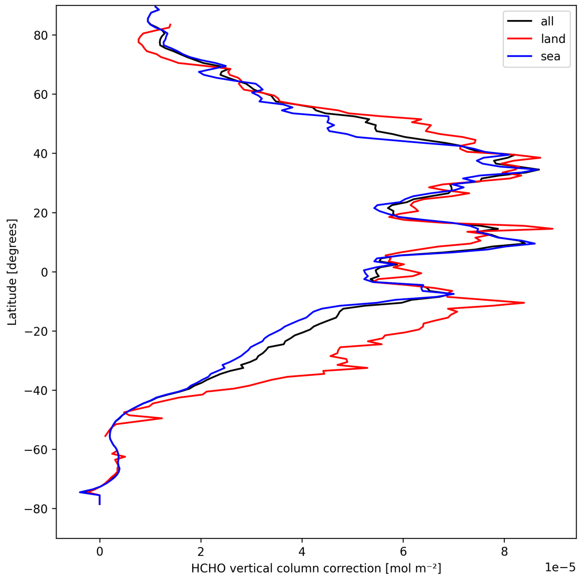
Figure 23: Zonal average of “HCHO vertical column correction” for 2025-09-04 to 2025-09-06.
