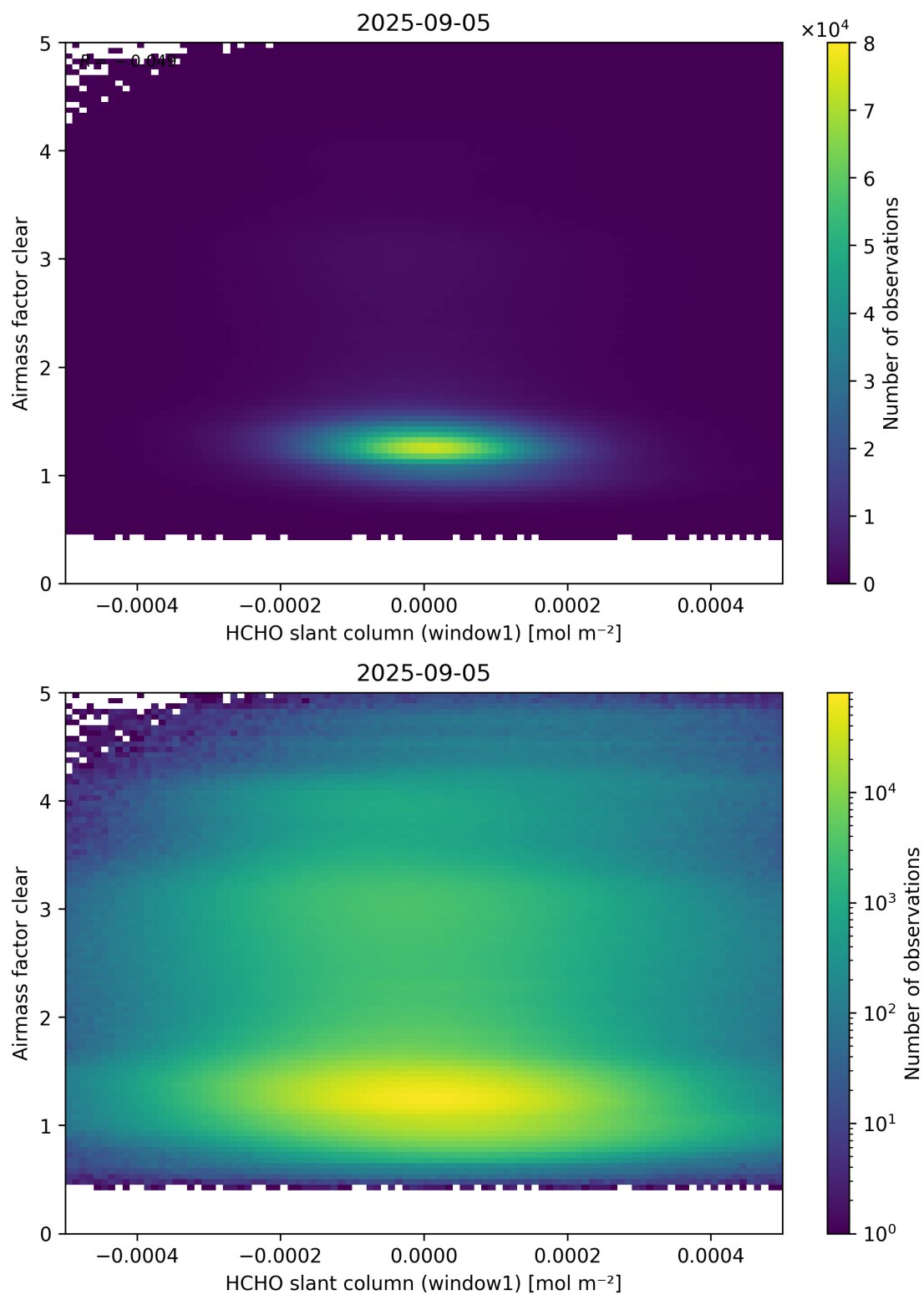
Figure 81: Scatter density plot of “HCHO slant column (window1)” against “Airmass factor clear” for 2025-09-04 to 2025-09-06.
