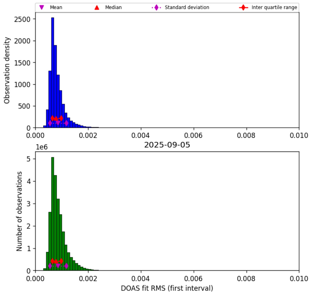
Figure 46: Histogram of “DOAS fit RMS (first interval)” for 2025-09-04 to 2025-09-06
