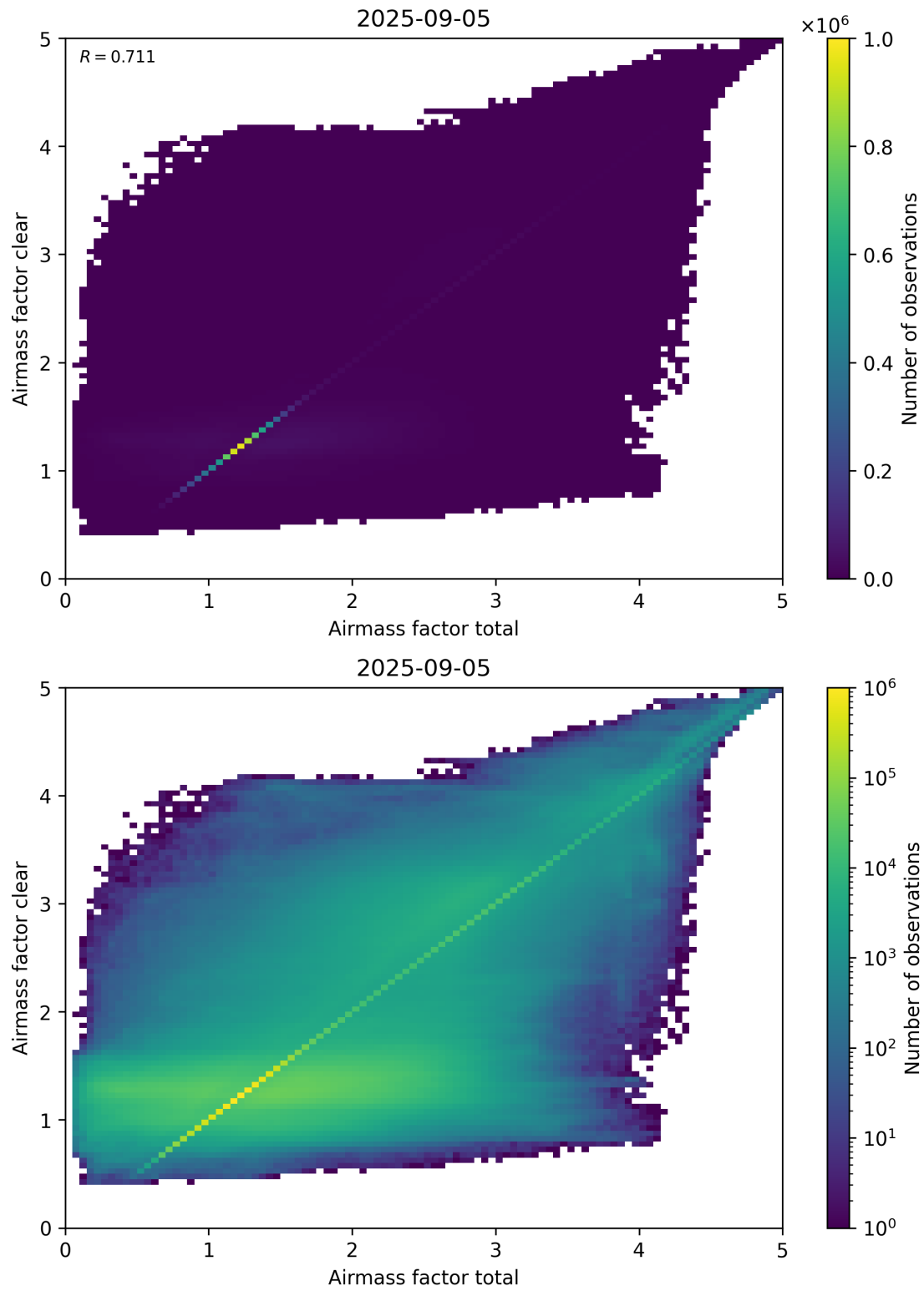
Figure 100: Scatter density plot of “Airmass factor total” against “Airmass factor clear” for 2025-09-04 to 2025-09-06.
