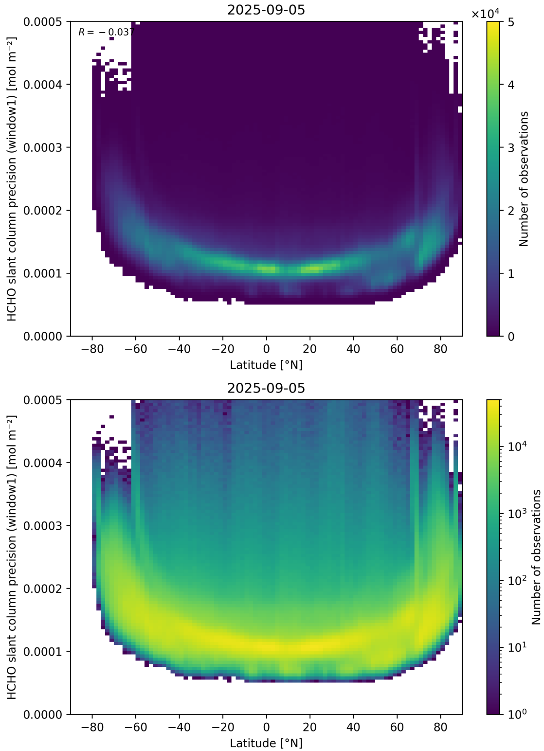
Figure 160: Scatter density plot of “Latitude” against “HCHO slant column precision (window1)” for 2025-09-04 to 2025-09-06.
