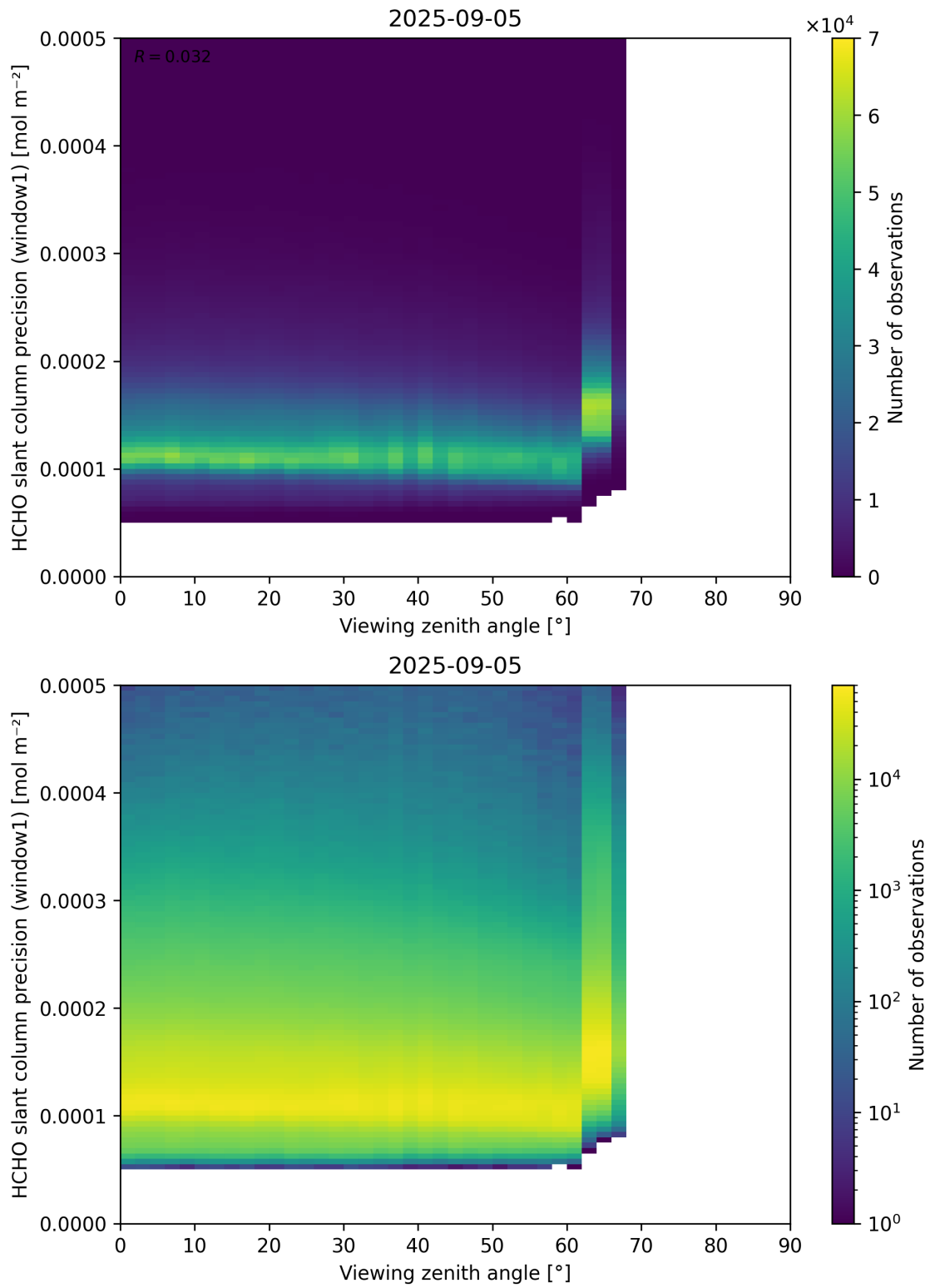
Figure 189: Scatter density plot of “Viewing zenith angle” against “HCHO slant column precision (window1)” for 2025-09-04 to 2025-09-06.
