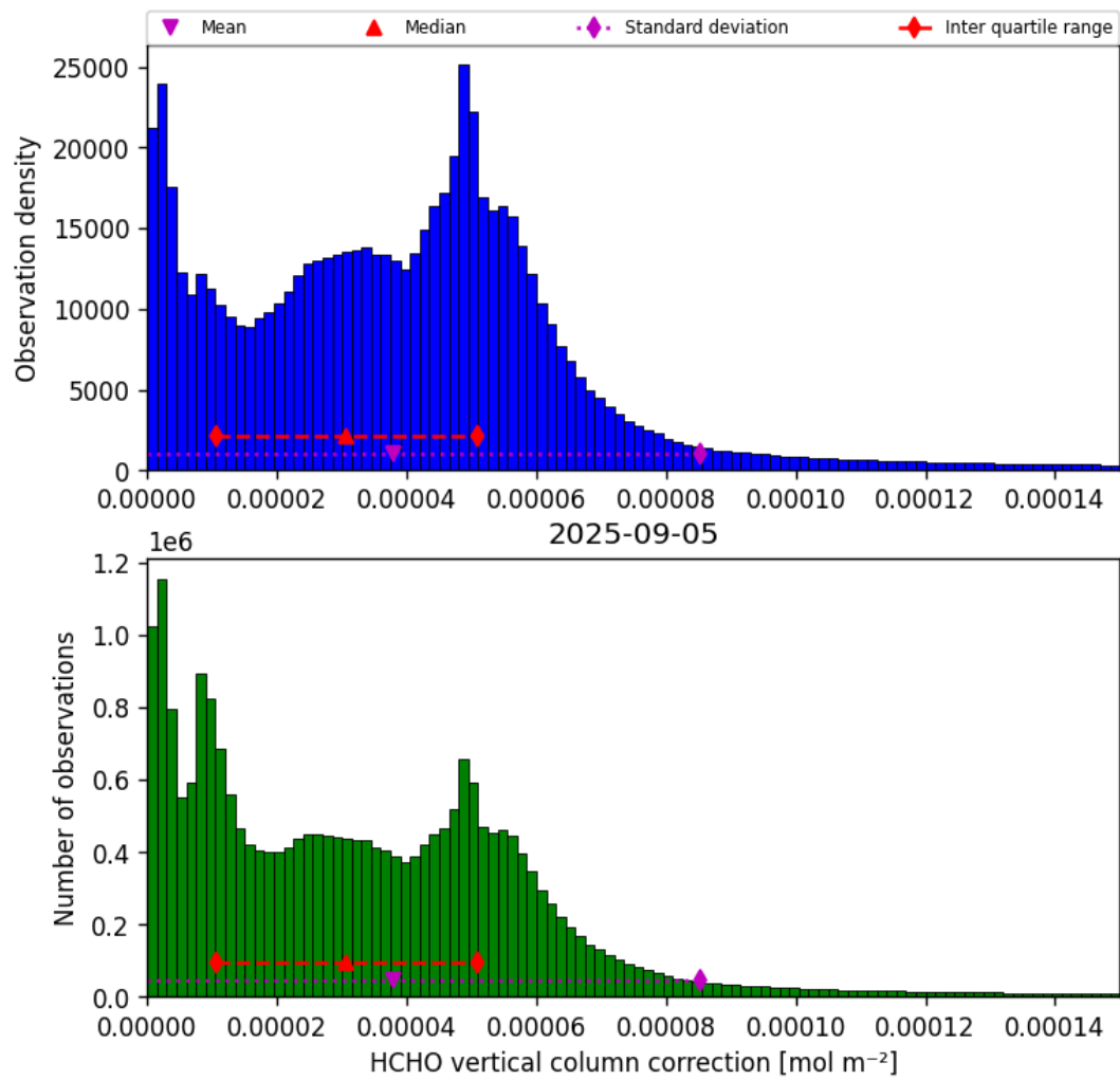
Figure 37: Histogram of “HCHO vertical column correction” for 2025-09-04 to 2025-09-06
