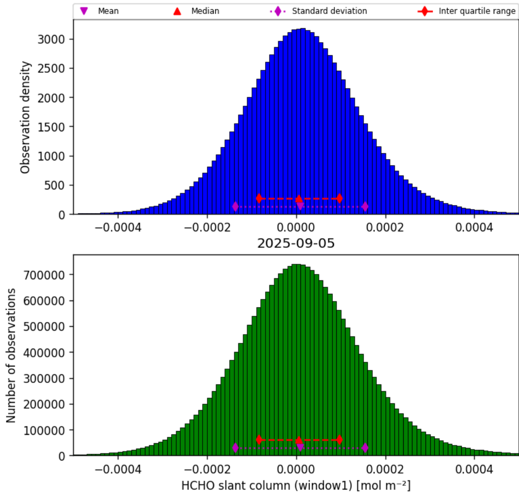
Figure 38: Histogram of “HCHO slant column (window1)” for 2025-09-04 to 2025-09-06
