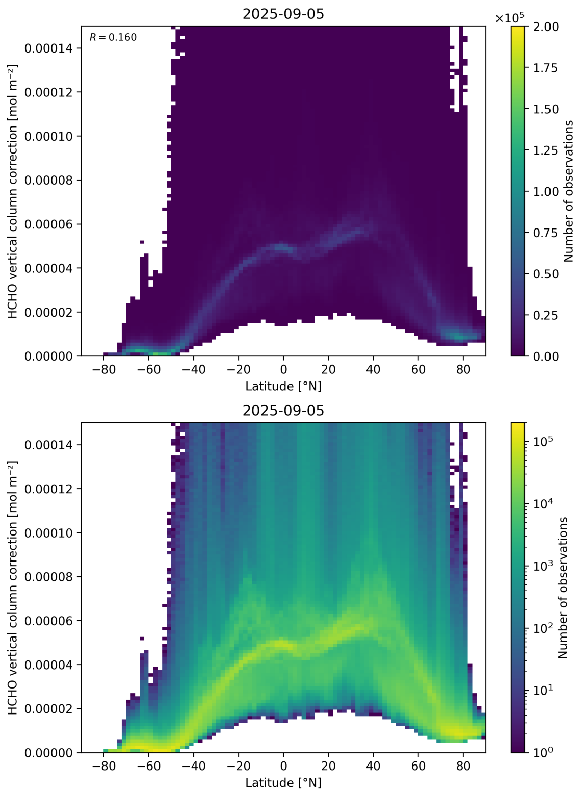
Figure 164: Scatter density plot of “Latitude” against “HCHO vertical column correction” for 2025-09-04 to 2025-09-06.
