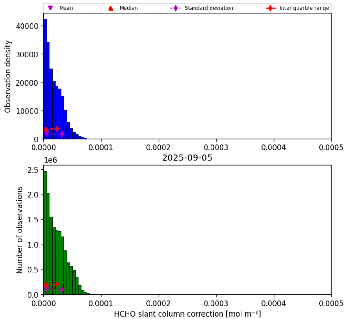
Figure 47: Histogram of “HCHO slant column correction” for 2025-09-04 to 2025-09-06
