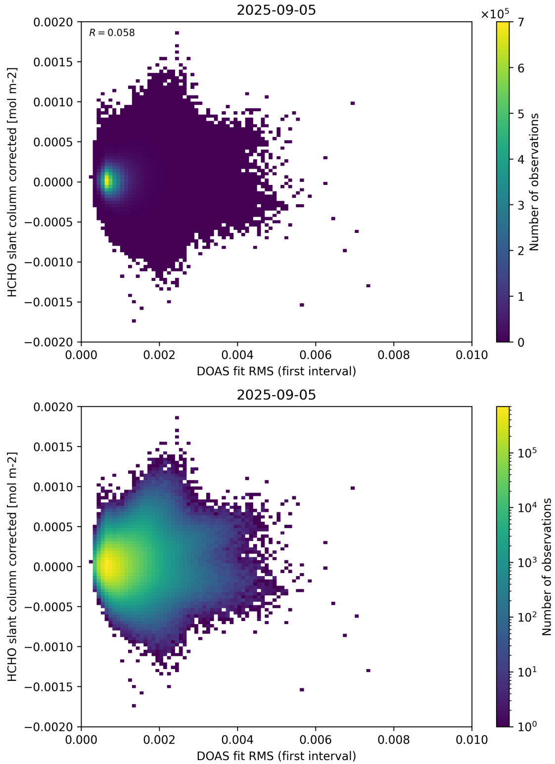
Figure 62: Scatter density plot of “DOAS fit RMS (first interval)” against “HCHO slant column corrected” for 2025-09-04 to 2025-09-06.
