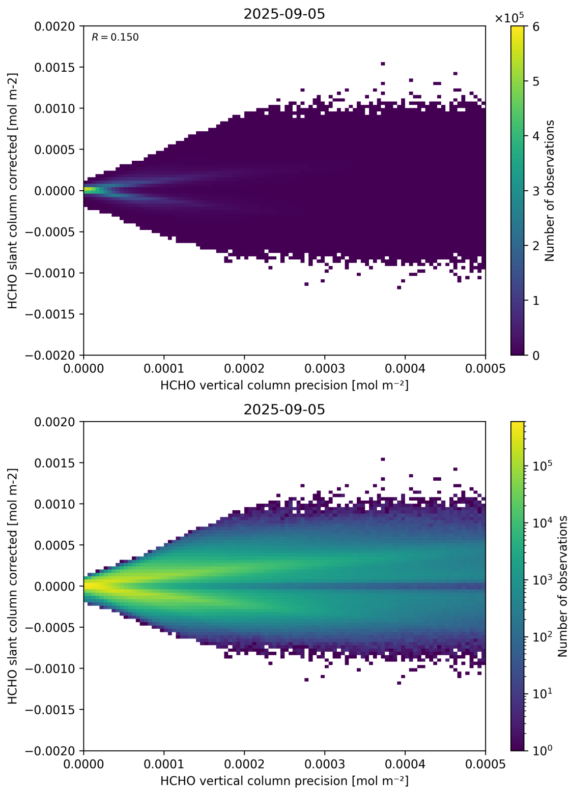
Figure 140: Scatter density plot of “HCHO vertical column precision” against “HCHO slant column corrected” for 2025-09-04 to 2025-09-06.
