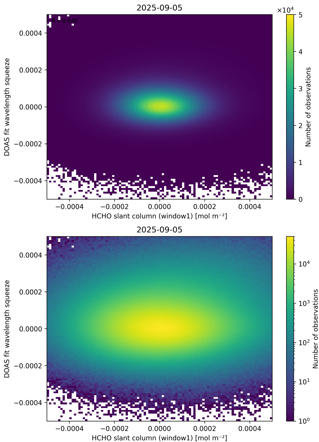
Figure 80: Scatter density plot of “HCHO slant column (window1)” against “DOAS fit wavelength squeeze” for 2025-09-04 to 2025-09-06.
