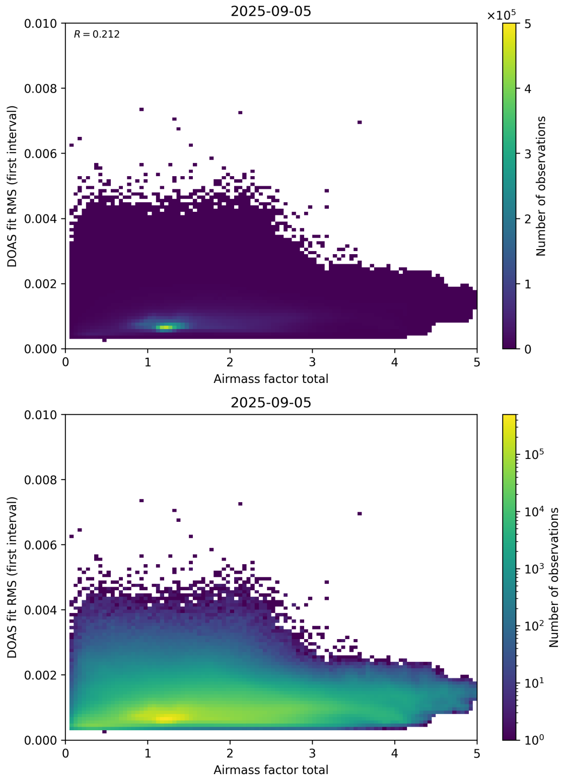
Figure 97: Scatter density plot of “Airmass factor total” against “DOAS fit RMS (first interval)” for 2025-09-04 to 2025-09-06.
