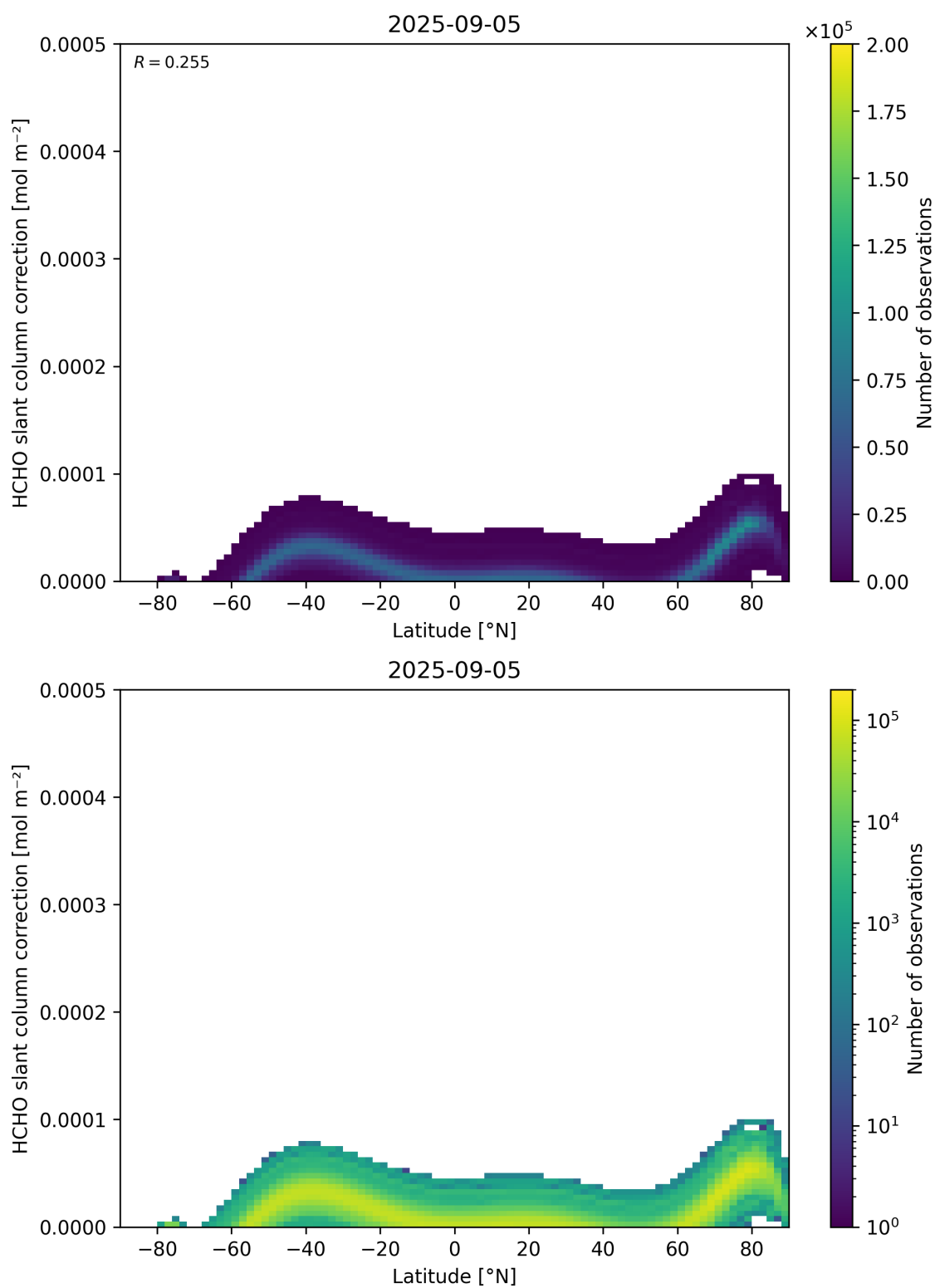
Figure 158: Scatter density plot of “Latitude” against “HCHO slant column correction” for 2025-09-04 to 2025-09-06.
