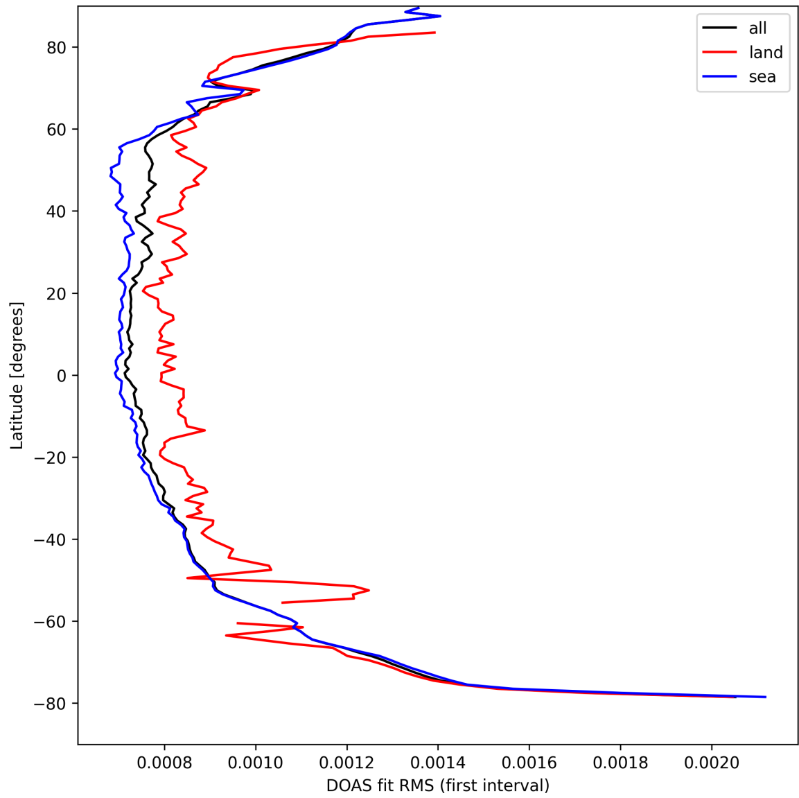
Figure 32: Zonal average of “DOAS fit RMS (first interval)” for 2025-09-04 to 2025-09-06.
