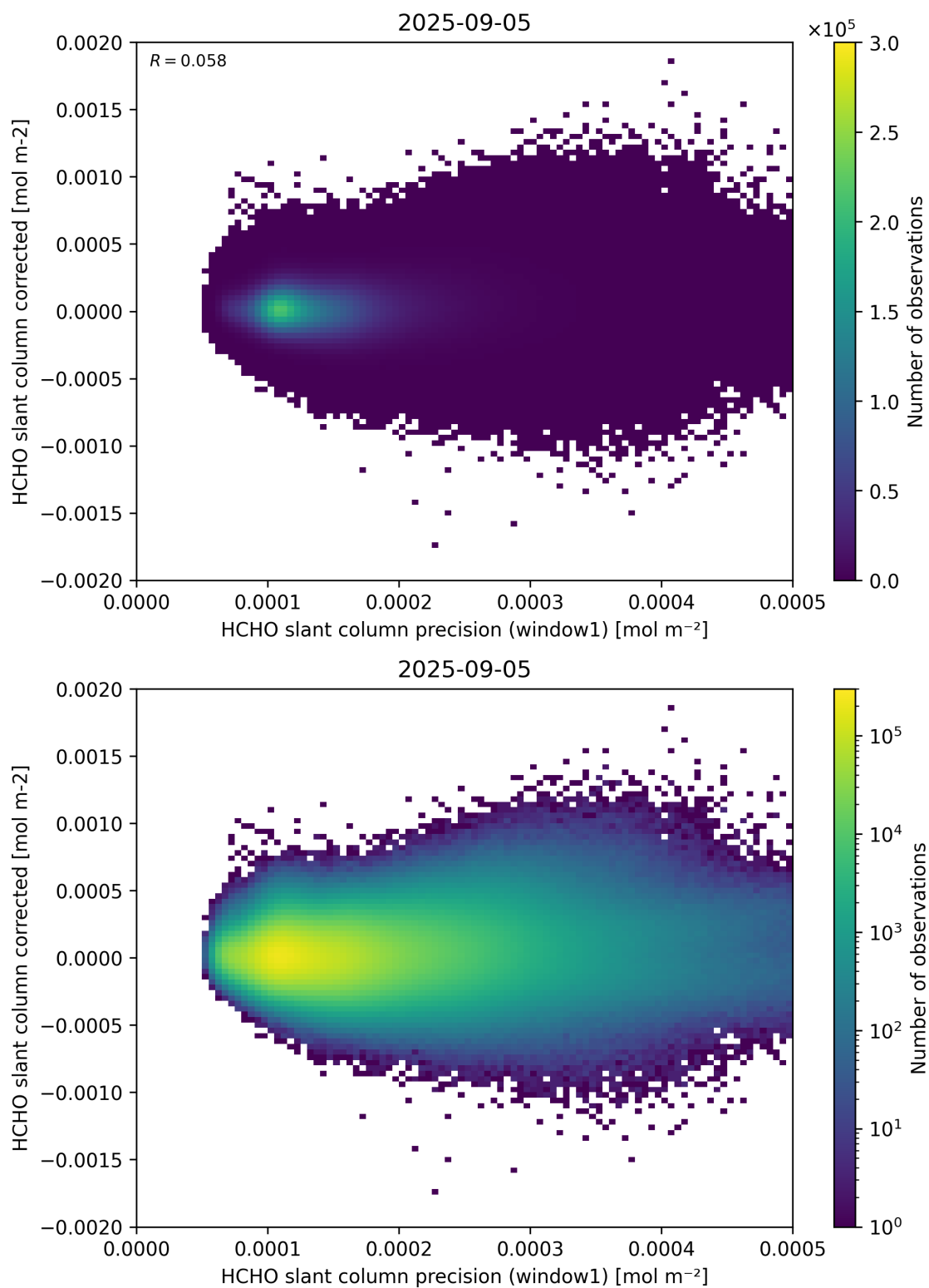
Figure 92: Scatter density plot of “HCHO slant column precision (window1)” against “HCHO slant column corrected” for 2025-09-04 to 2025-09-06.
