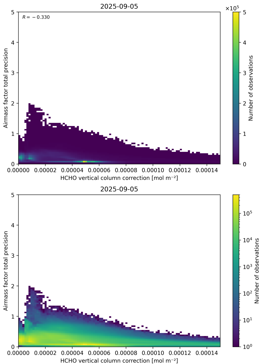
Figure 121: Scatter density plot of “HCHO vertical column correction” against “Airmass factor total precision” for 2025-09-04 to 2025-09-06.
