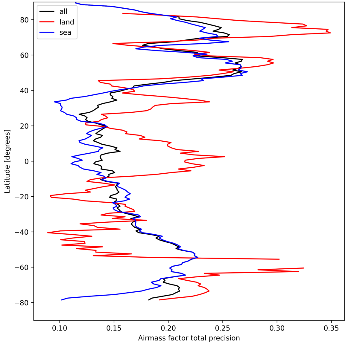
Figure 27: Zonal average of “Airmass factor total precision” for 2025-09-04 to 2025-09-06.
