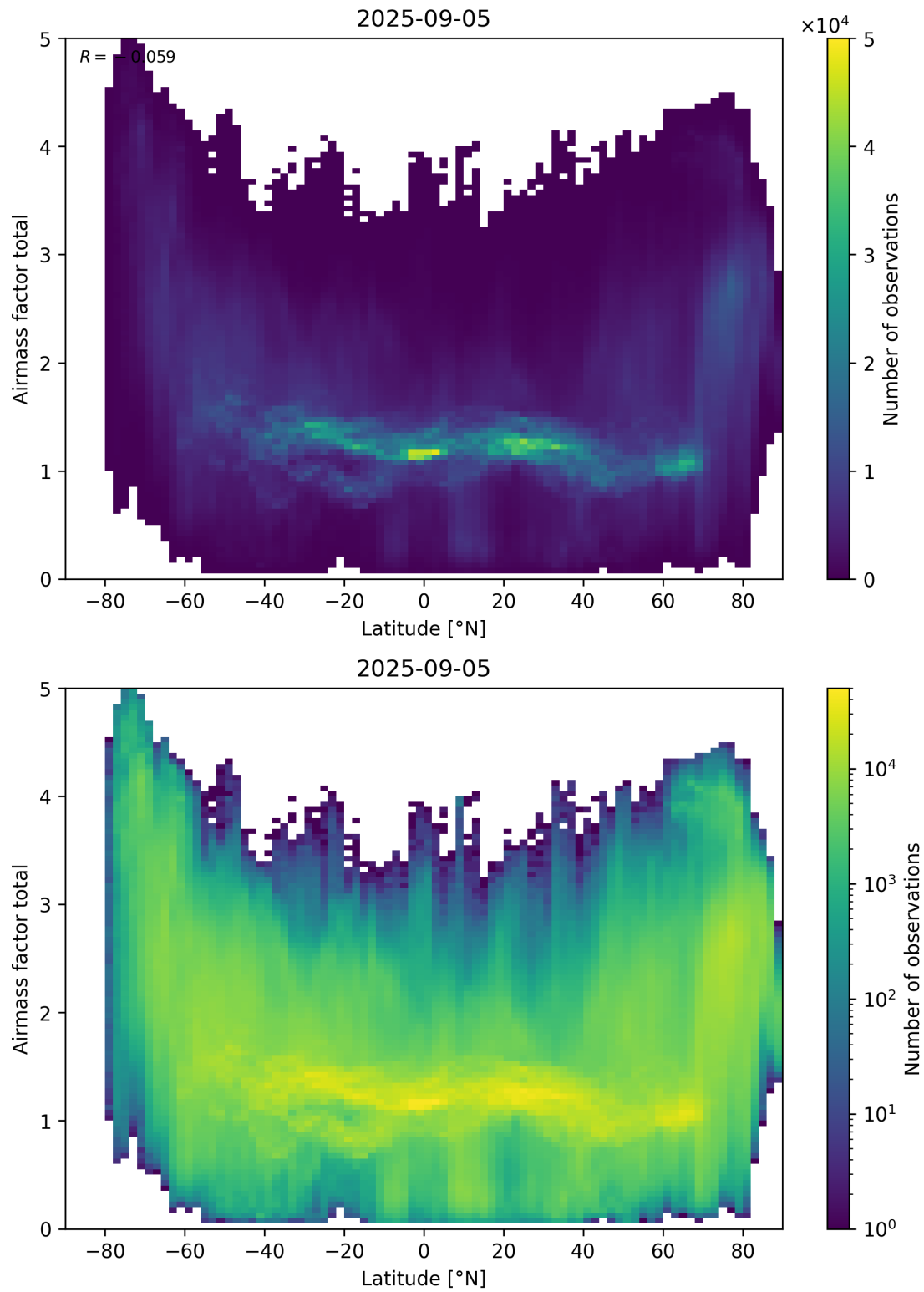
Figure 161: Scatter density plot of “Latitude” against “Airmass factor total” for 2025-09-04 to 2025-09-06.
