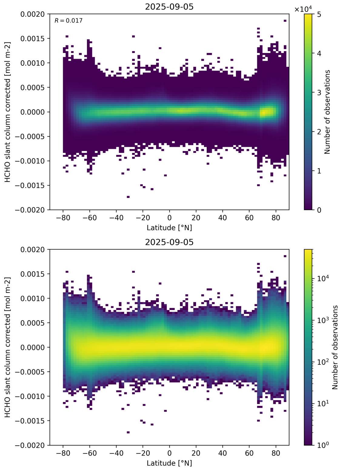
Figure 157: Scatter density plot of “Latitude” against “HCHO slant column corrected” for 2025-09-04 to 2025-09-06.
