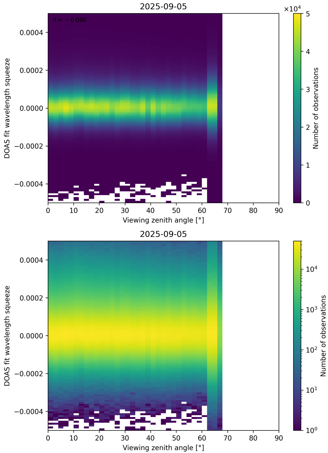
Figure 184: Scatter density plot of “Viewing zenith angle” against “DOAS fit wavelength squeeze” for 2025-09-04 to 2025-09-06.
