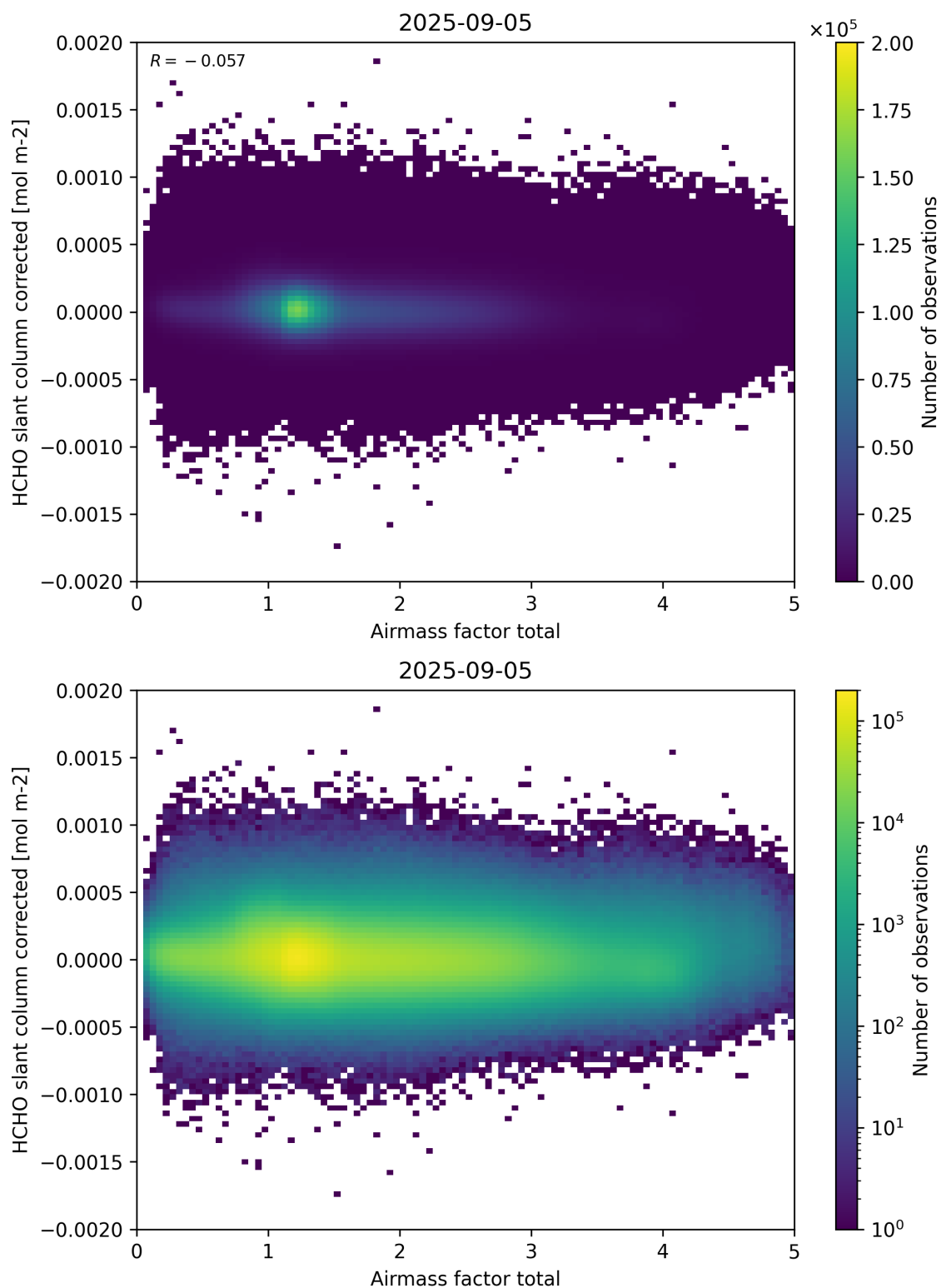
Figure 101: Scatter density plot of “Airmass factor total” against “HCHO slant column corrected” for 2025-09-04 to 2025-09-06.
