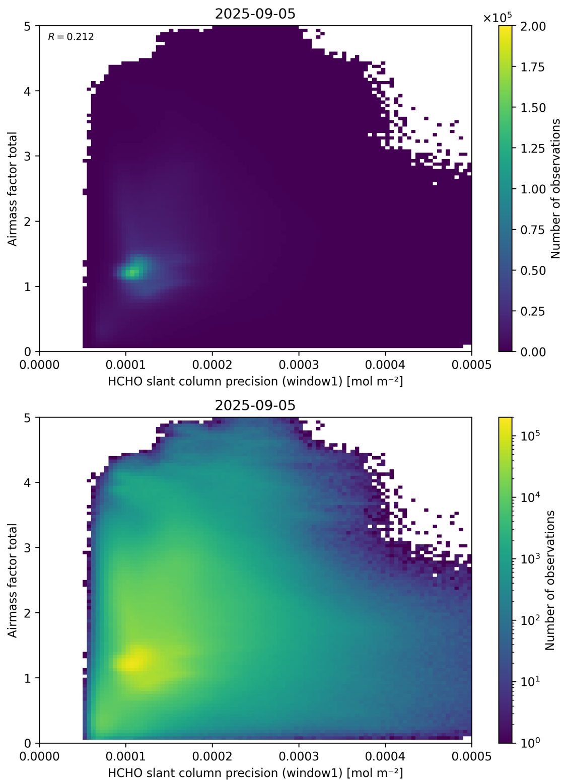
Figure 94: Scatter density plot of “HCHO slant column precision (window1)” against “Airmass factor total” for 2025-09-04 to 2025-09-06.
