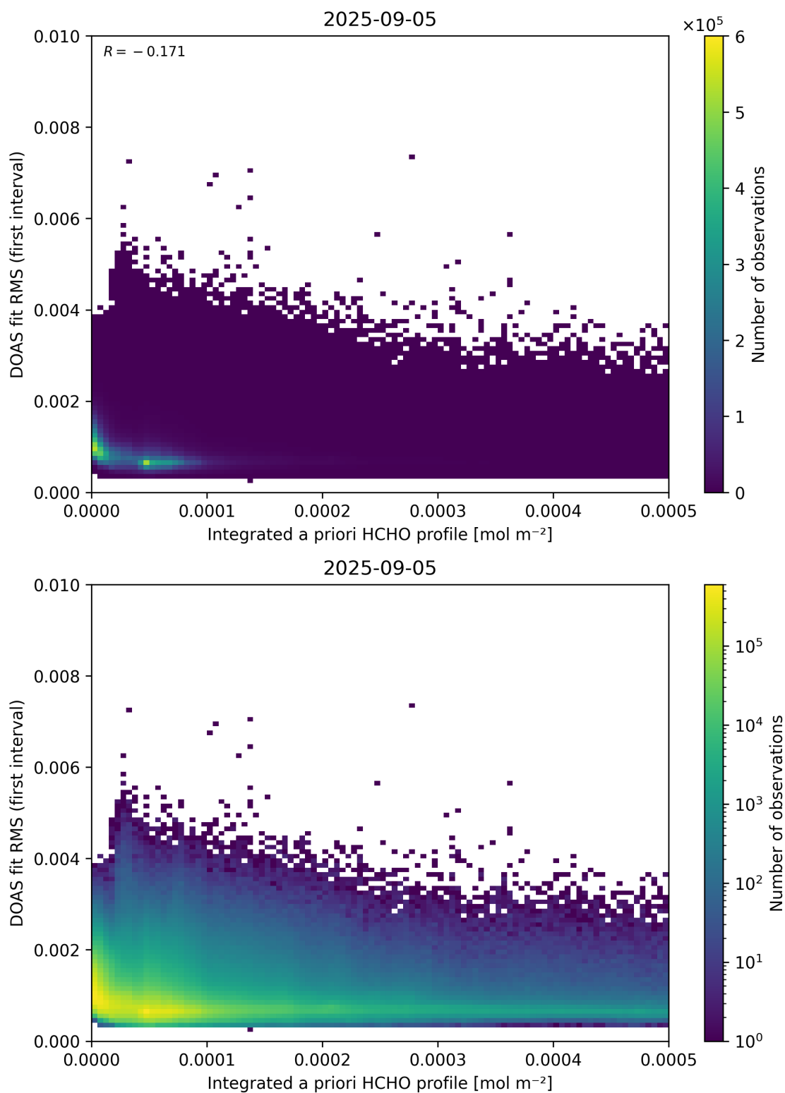
Figure 148: Scatter density plot of “Integrated a priori HCHO profile” against “DOAS fit RMS (first interval)” for 2025-09-04 to 2025-09-06.
