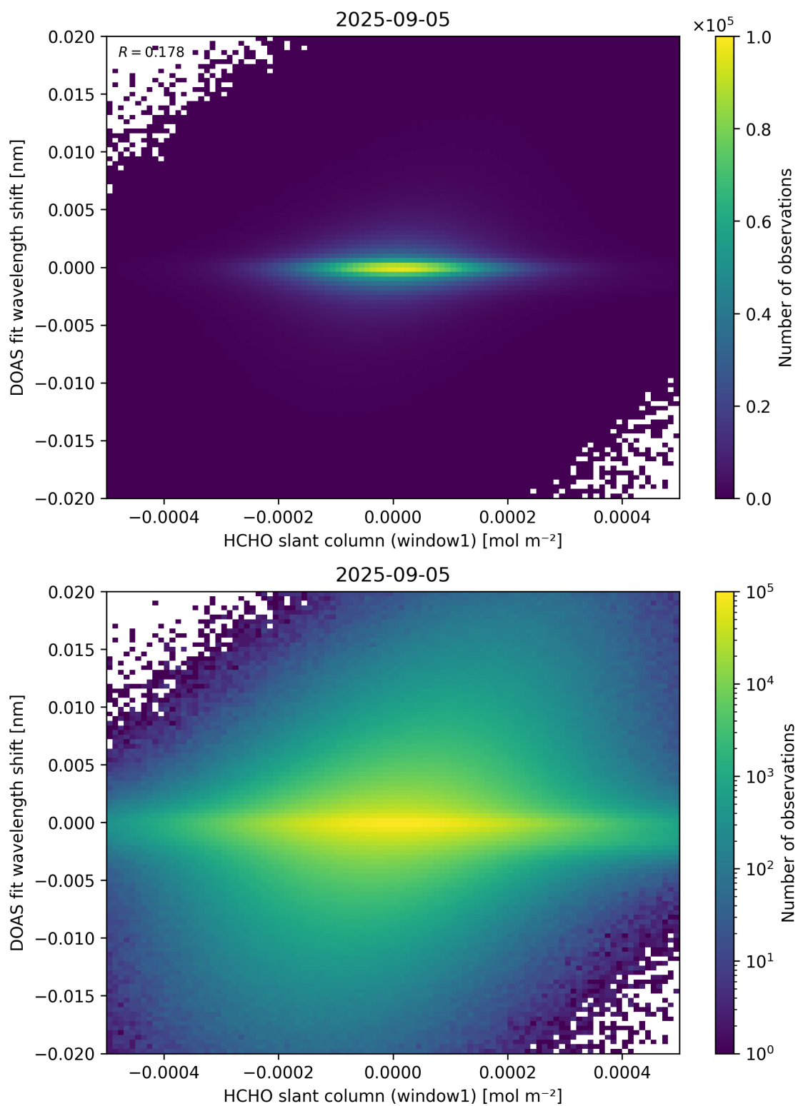
Figure 79: Scatter density plot of “HCHO slant column (window1)” against “DOAS fit wavelength shift” for 2025-09-04 to 2025-09-06.
