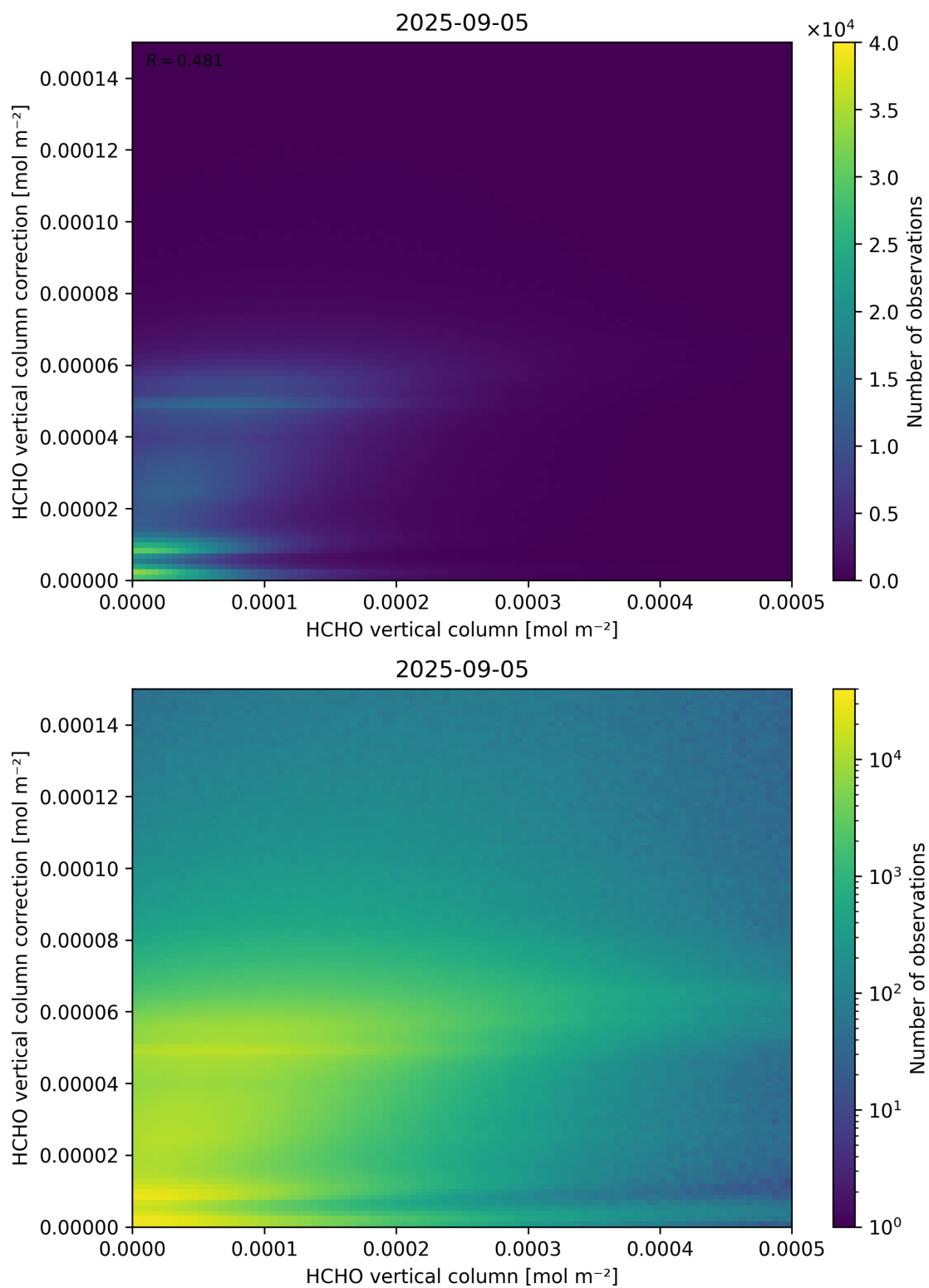
Figure 133: Scatter density plot of “HCHO vertical column” against “HCHO vertical column correction” for 2025-09-04 to 2025-09-06.
