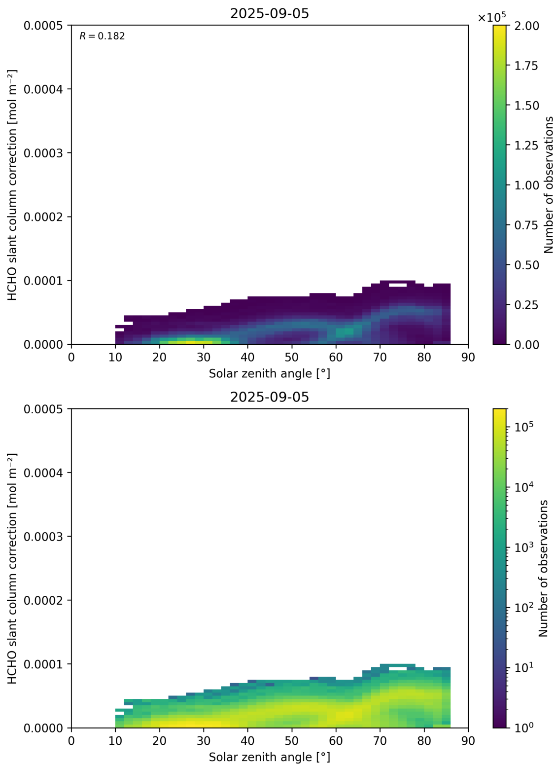
Figure 172: Scatter density plot of “Solar zenith angle” against “HCHO slant column correction” for 2025-09-04 to 2025-09-06.
