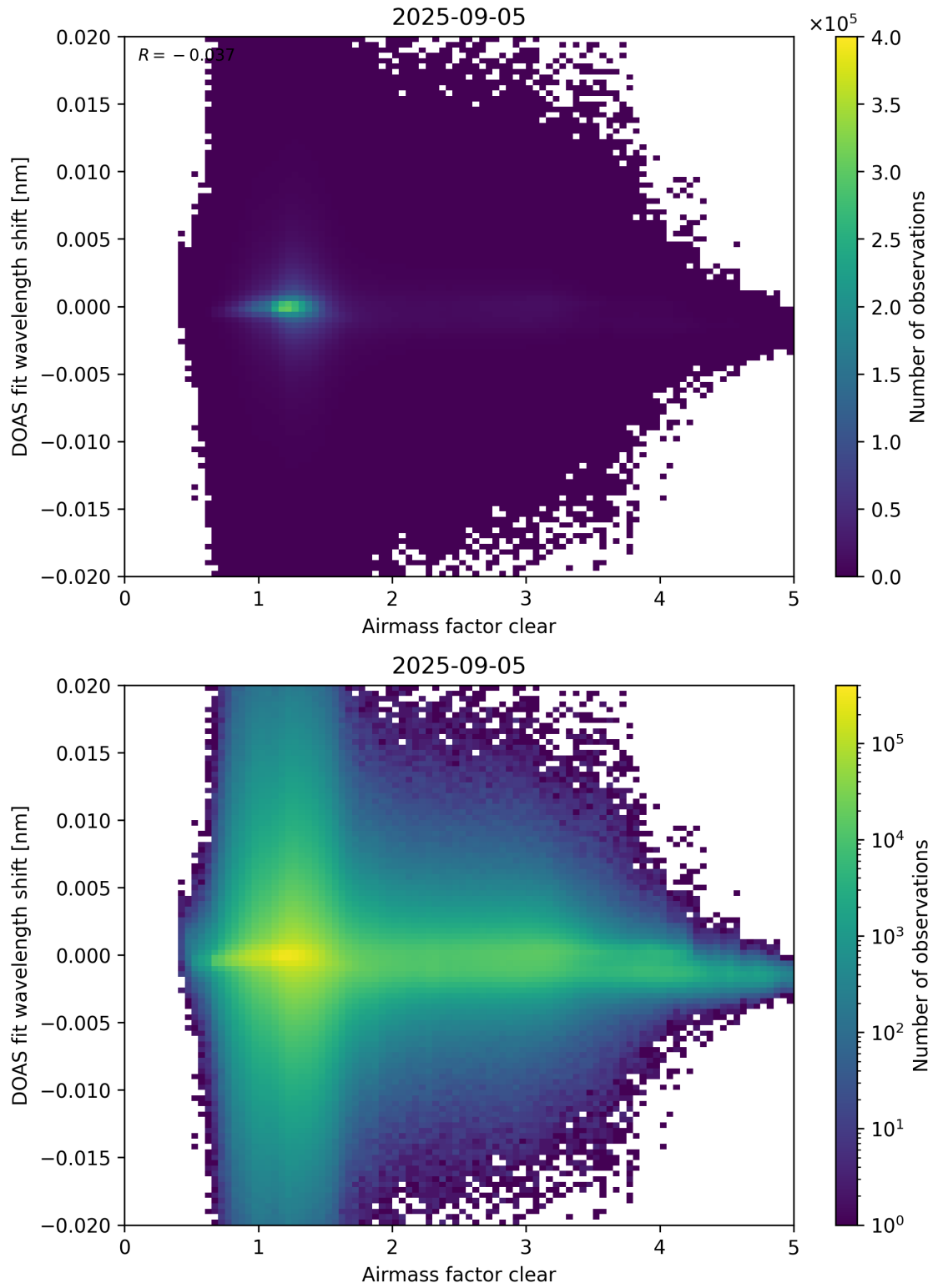
Figure 72: Scatter density plot of “Airmass factor clear” against “DOAS fit wavelength shift” for 2025-09-04 to 2025-09-06.
