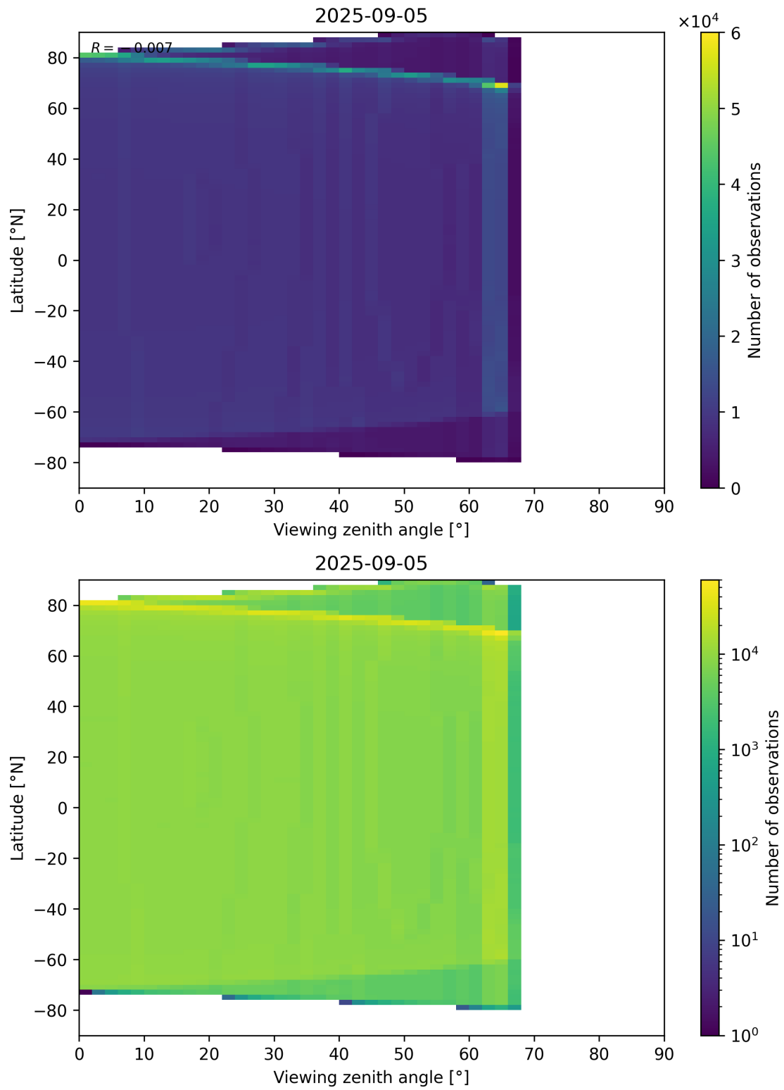
Figure 196: Scatter density plot of “Viewing zenith angle” against “Latitude” for 2025-09-04 to 2025-09-06.
