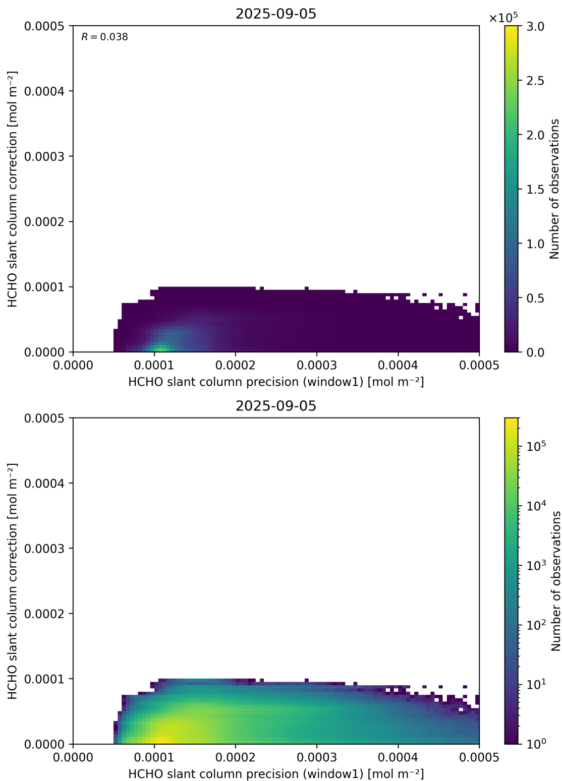
Figure 93: Scatter density plot of “HCHO slant column precision (window1)” against “HCHO slant column correction” for 2025-09-04 to 2025-09-06.
