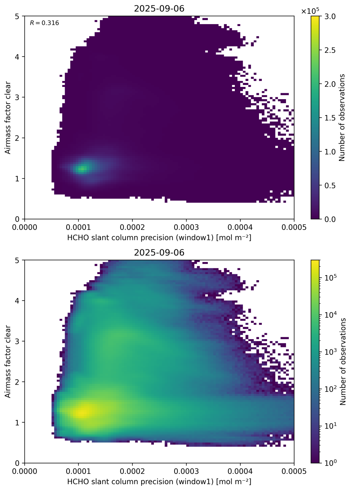
Figure 91: Scatter density plot of “HCHO slant column precision (window1)” against “Airmass factor clear” for 2025-09-05 to 2025-09-07.
