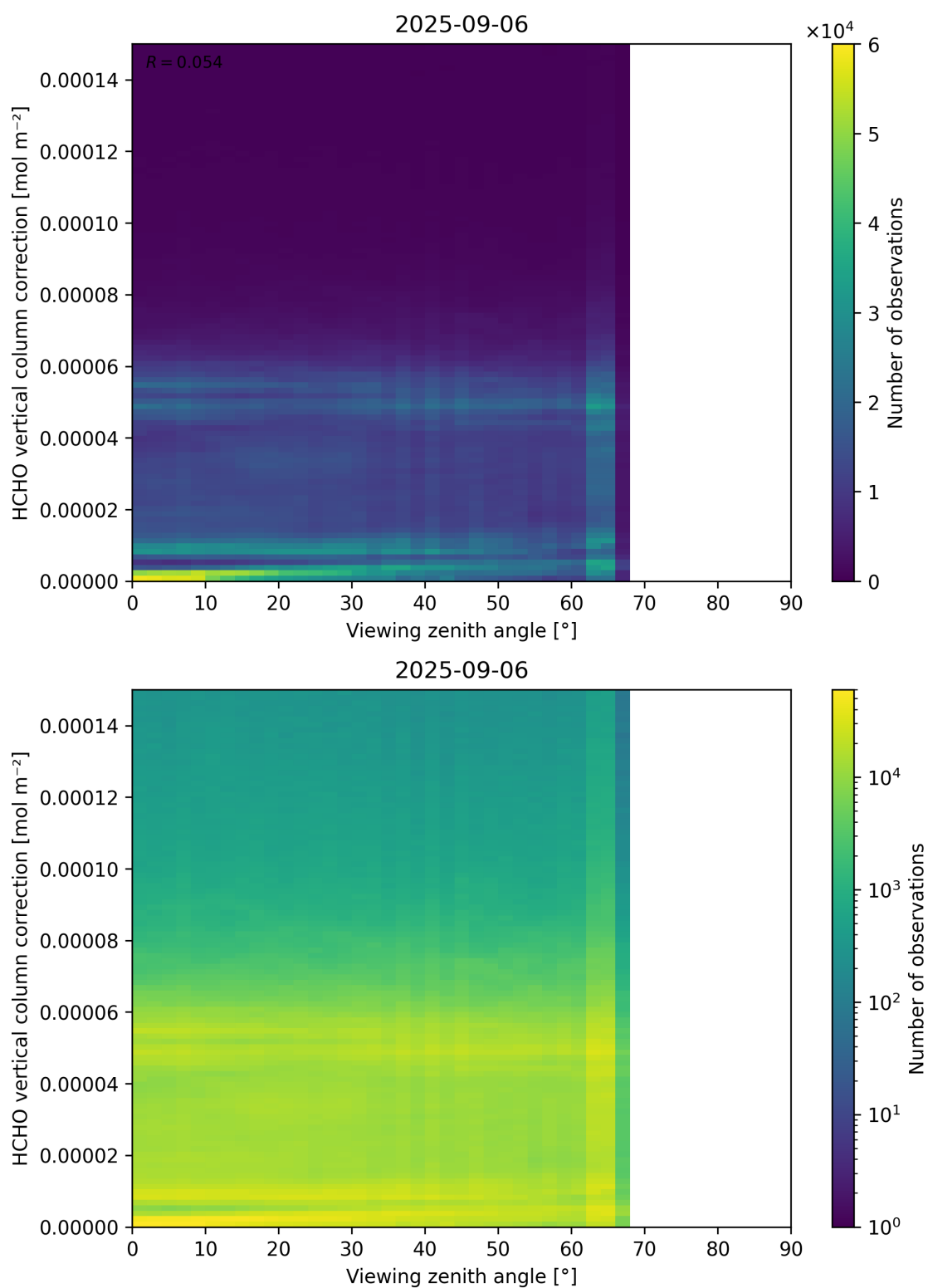
Figure 193: Scatter density plot of “Viewing zenith angle” against “HCHO vertical column correction” for 2025-09-05 to 2025-09-07.
