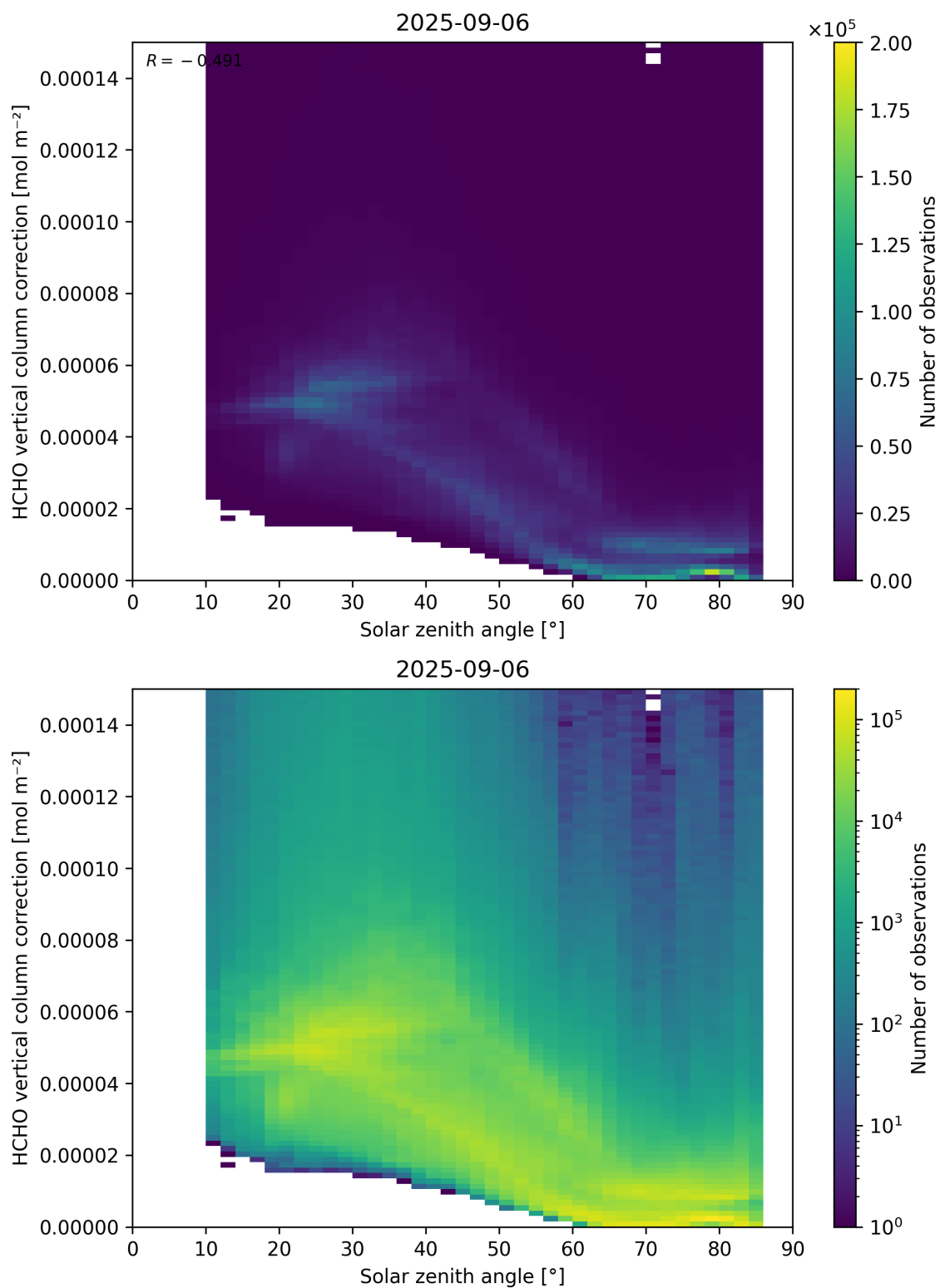
Figure 178: Scatter density plot of “Solar zenith angle” against “HCHO vertical column correction” for 2025-09-05 to 2025-09-07.
