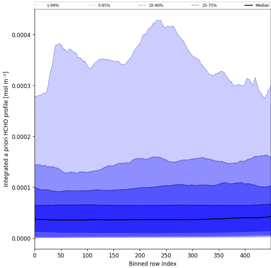
Figure 57: Along track statistics of "Integrated a priori HCHO profile" for 2025-09-05 to 2025-09-07
