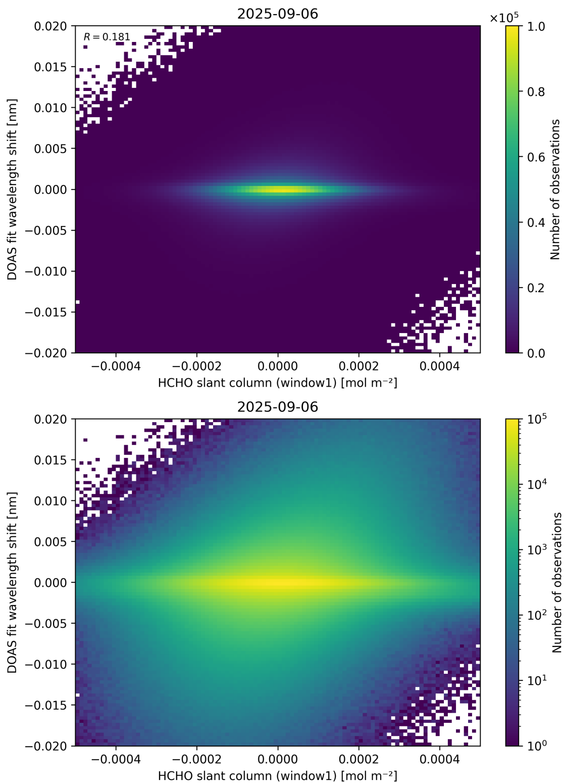
Figure 79: Scatter density plot of “HCHO slant column (window1)” against “DOAS fit wavelength shift” for 2025-09-05 to 2025-09-07.
