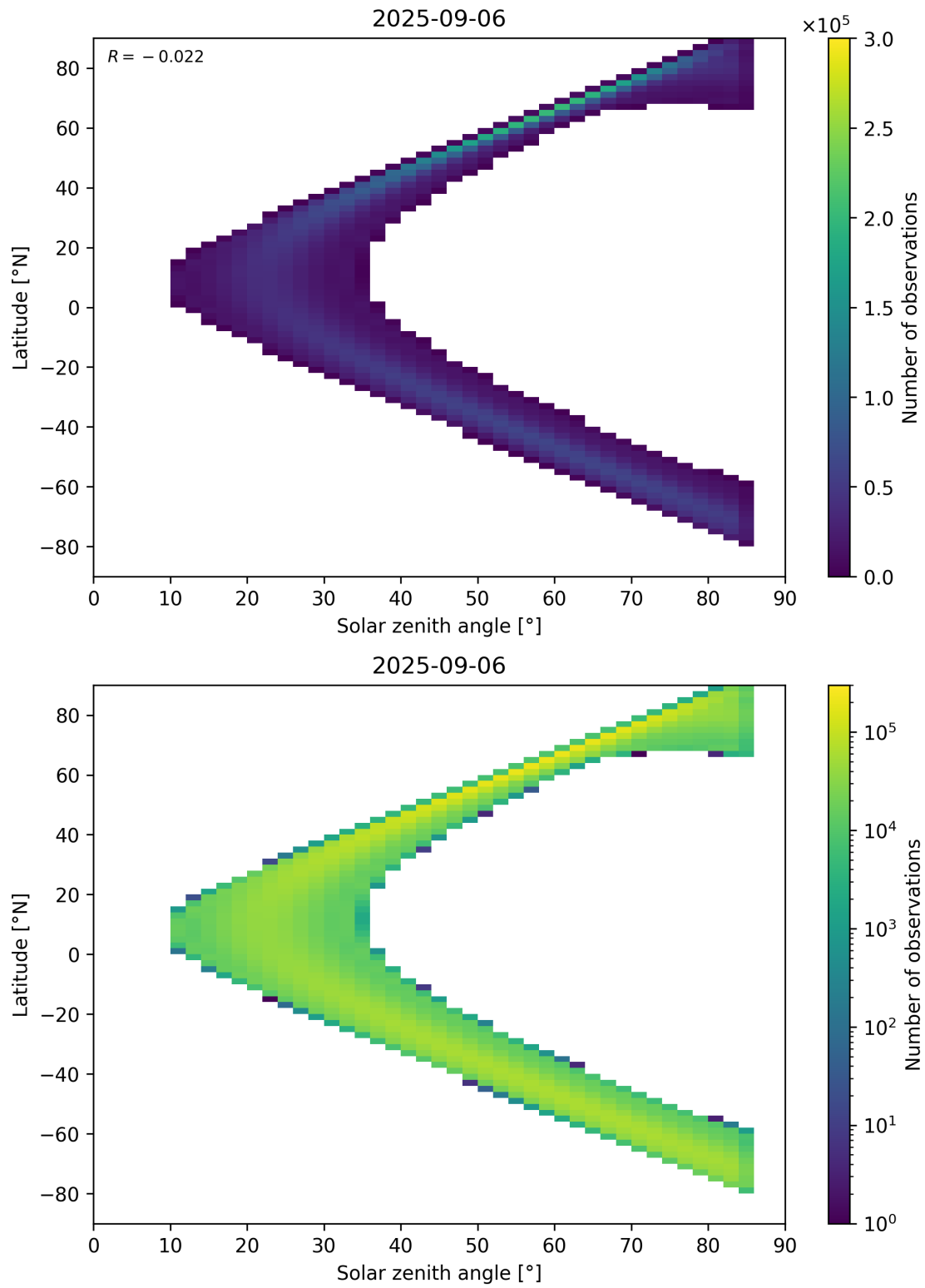
Figure 181: Scatter density plot of “Solar zenith angle” against “Latitude” for 2025-09-05 to 2025-09-07.
