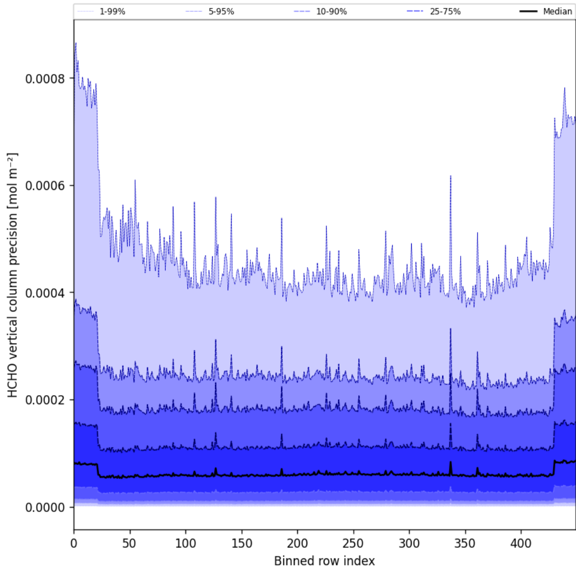
Figure 50: Along track statistics of “HCHO vertical column precision” for 2025-09-05 to 2025-09-07
