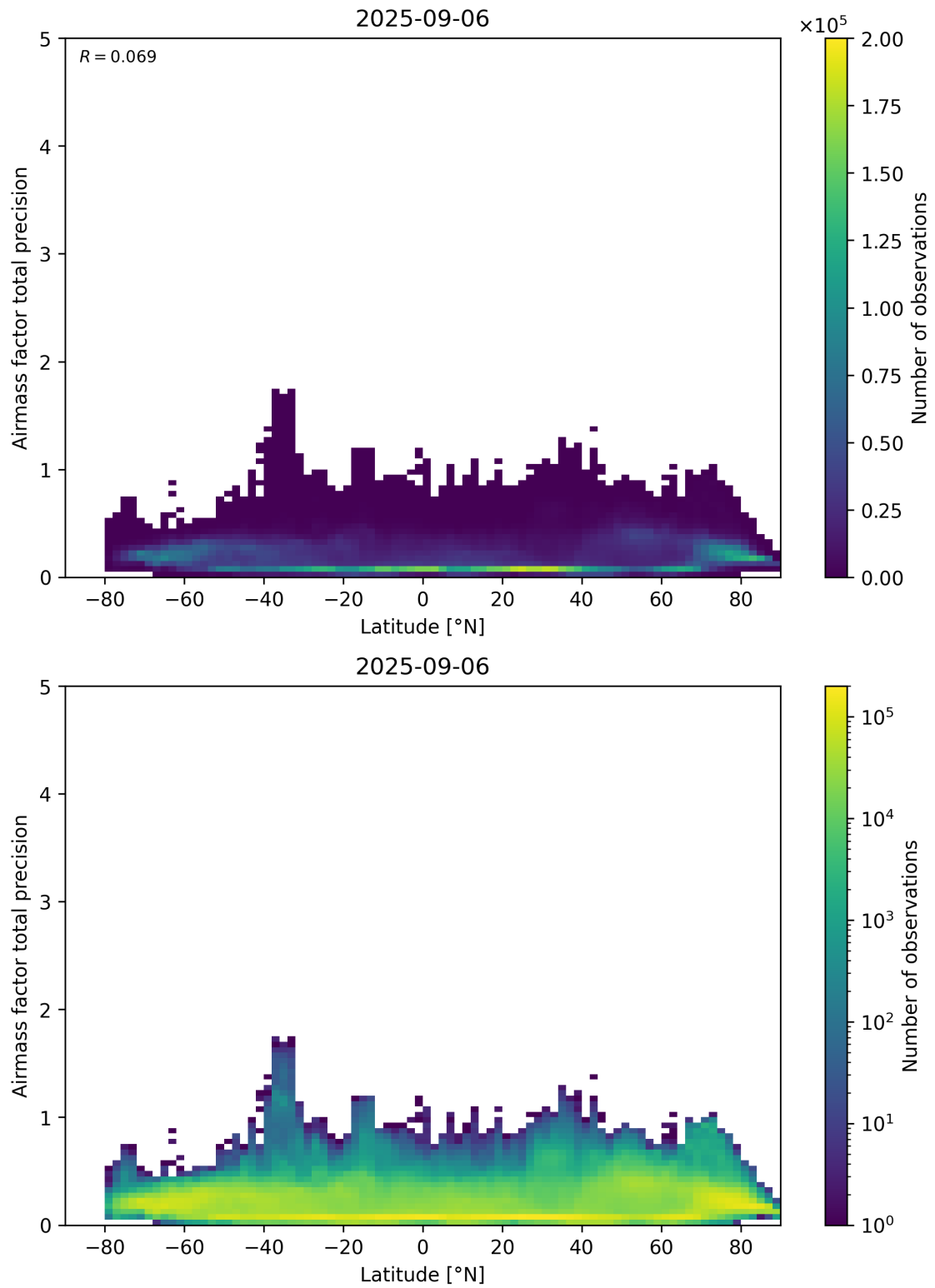
Figure 162: Scatter density plot of “Latitude” against “Airmass factor total precision” for 2025-09-05 to 2025-09-07.
