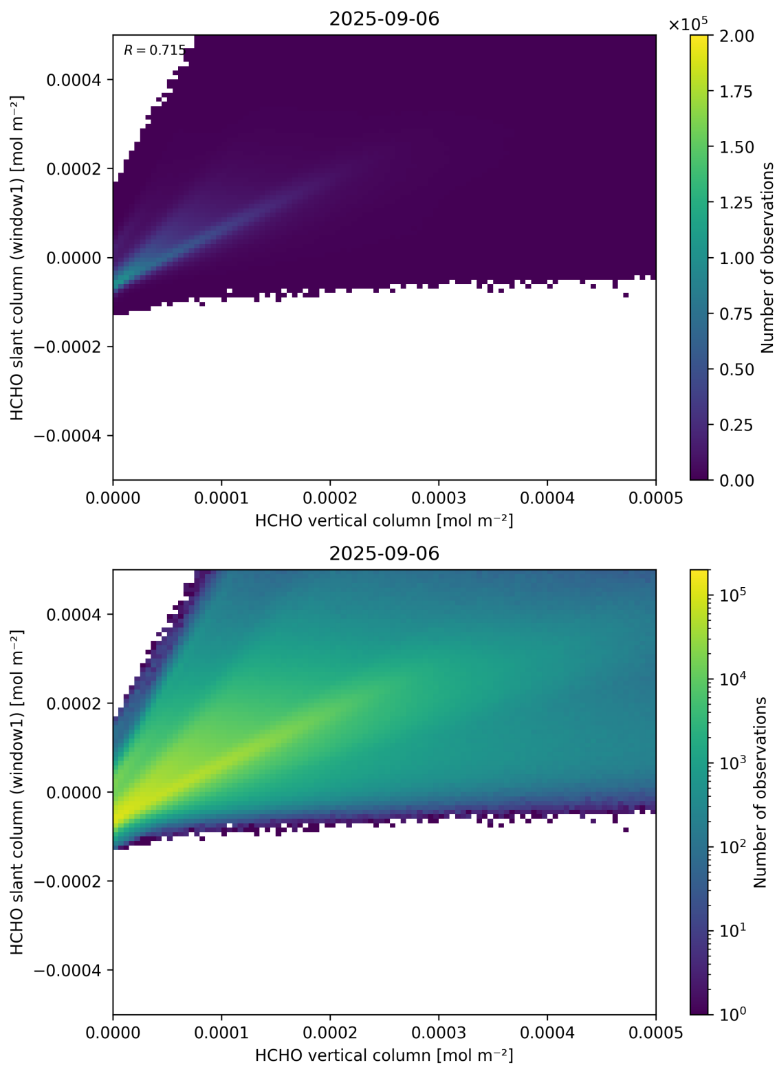
Figure 129: Scatter density plot of “HCHO vertical column” against “HCHO slant column (window1)” for 2025-09-05 to 2025-09-07.
