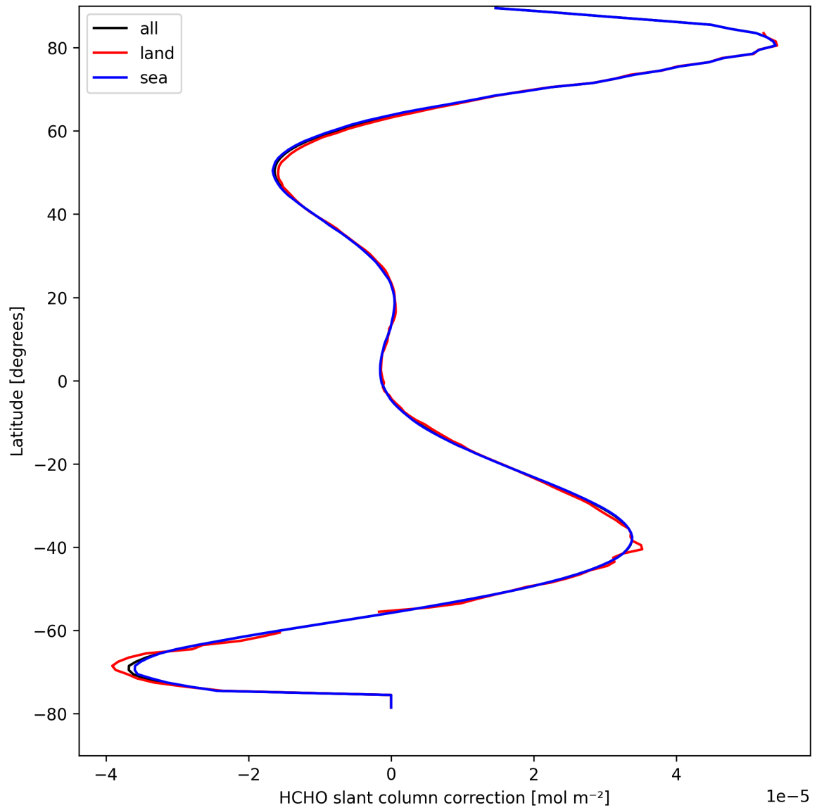
Figure 33: Zonal average of “HCHO slant column correction” for 2025-09-05 to 2025-09-07.
