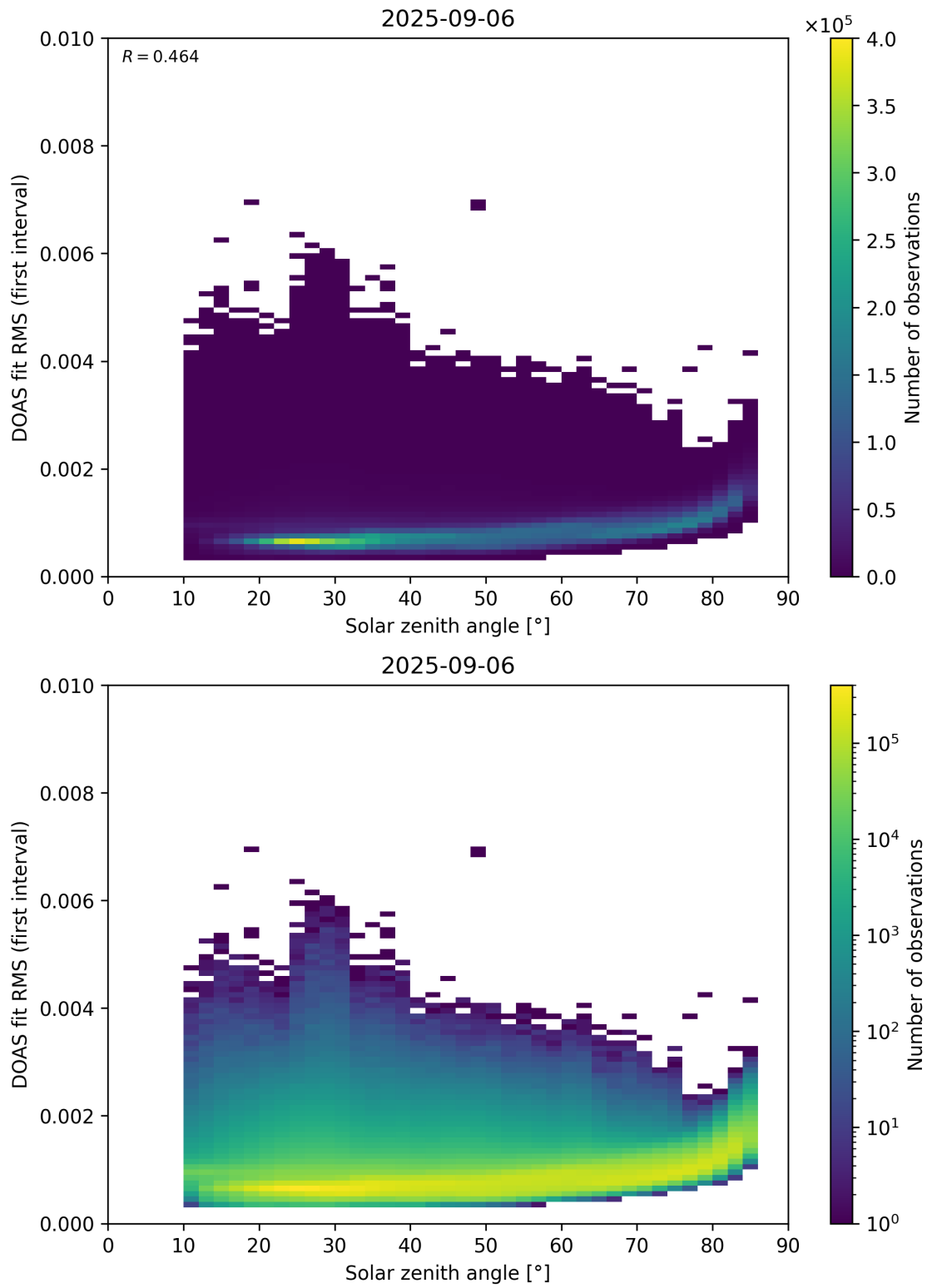
Figure 167: Scatter density plot of “Solar zenith angle” against “DOAS fit RMS (first interval)” for 2025-09-05 to 2025-09-07.
