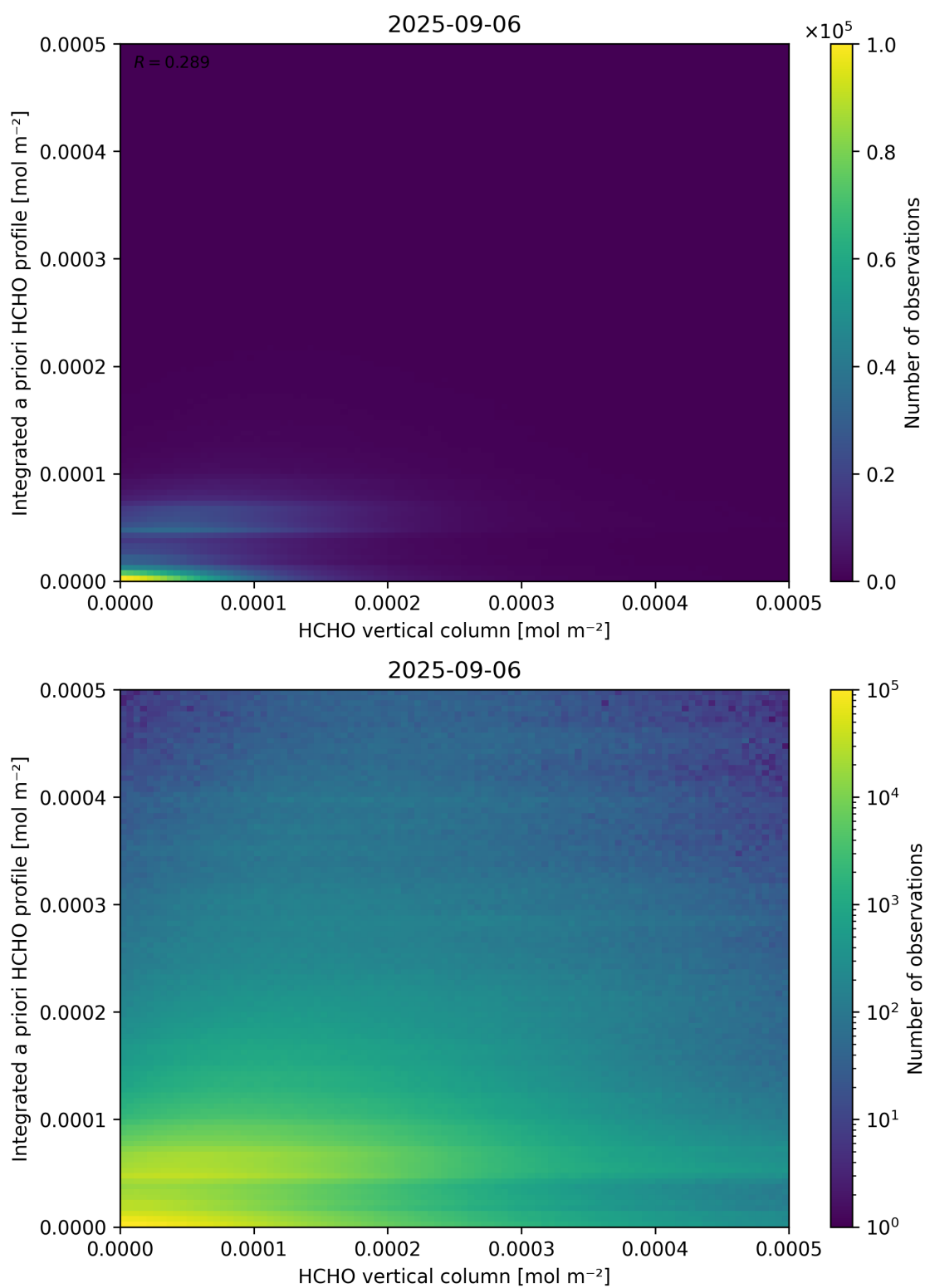
Figure 135: Scatter density plot of “HCHO vertical column” against “Integrated a priori HCHO profile” for 2025-09-05 to 2025-09-07.
