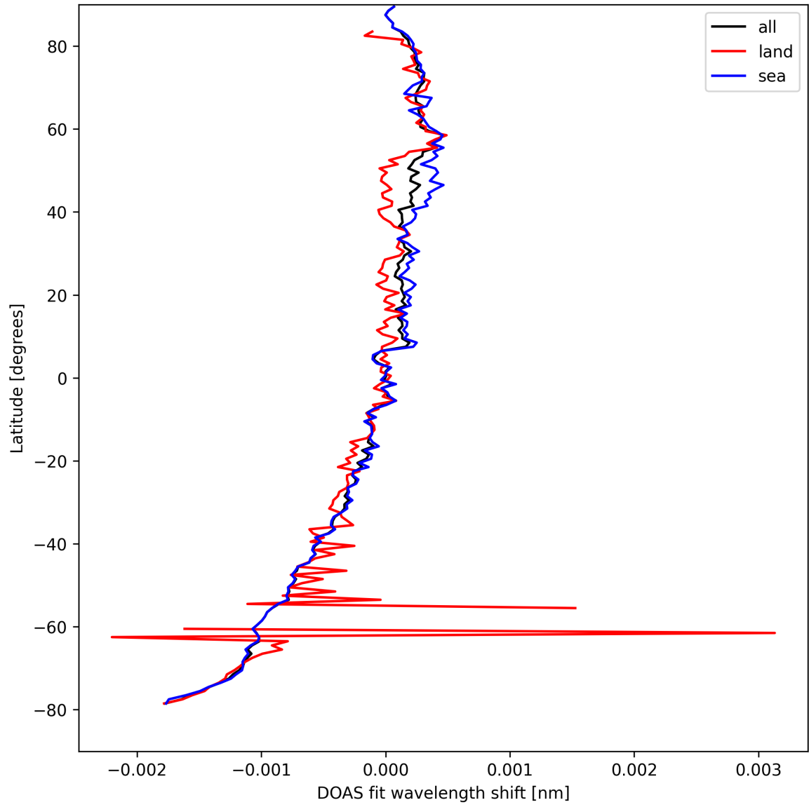
Figure 30: Zonal average of "DOAS fit wavelength shift" for 2025-09-05 to 2025-09-07.
