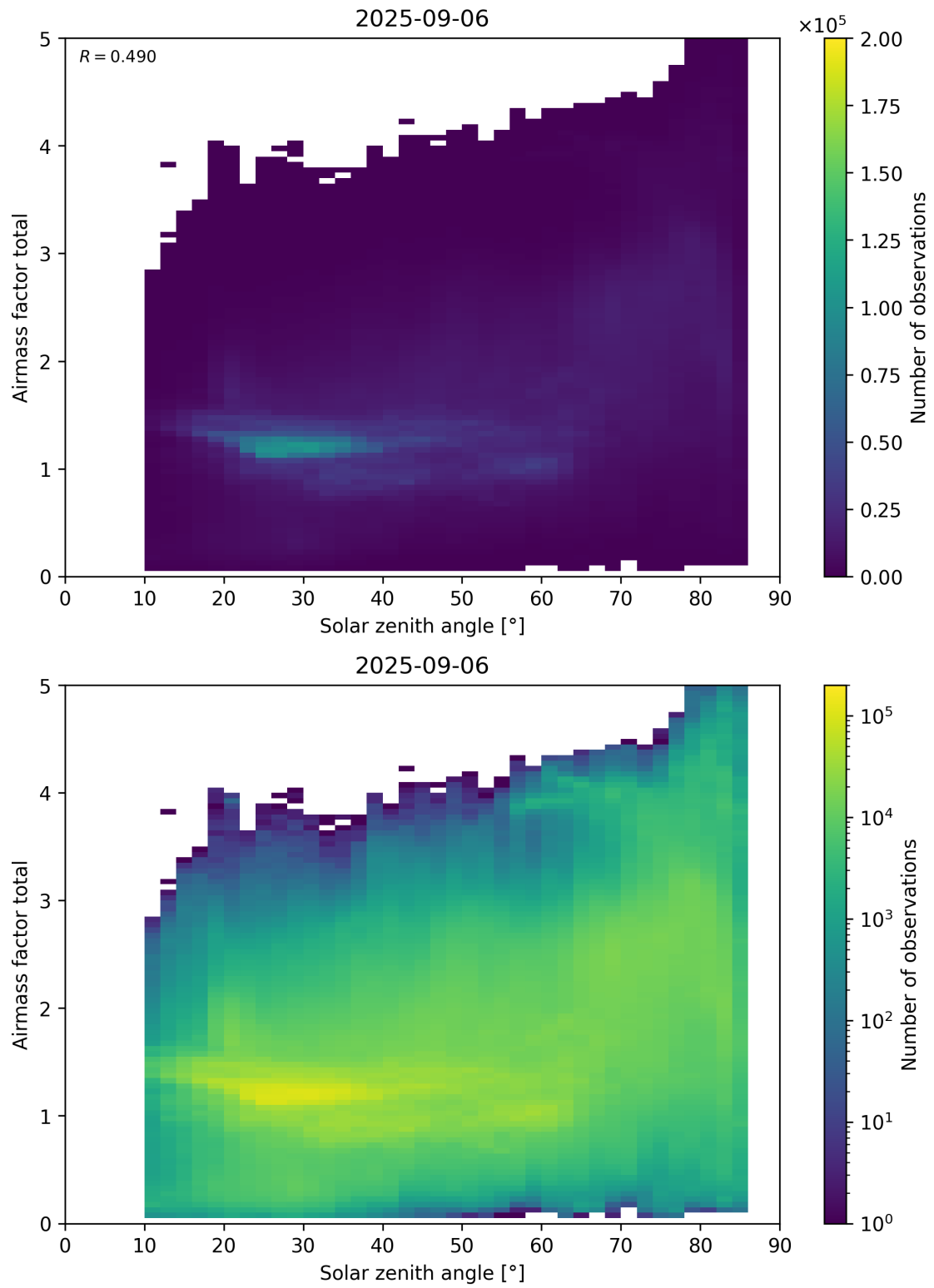
Figure 175: Scatter density plot of “Solar zenith angle” against “Airmass factor total” for 2025-09-05 to 2025-09-07.
