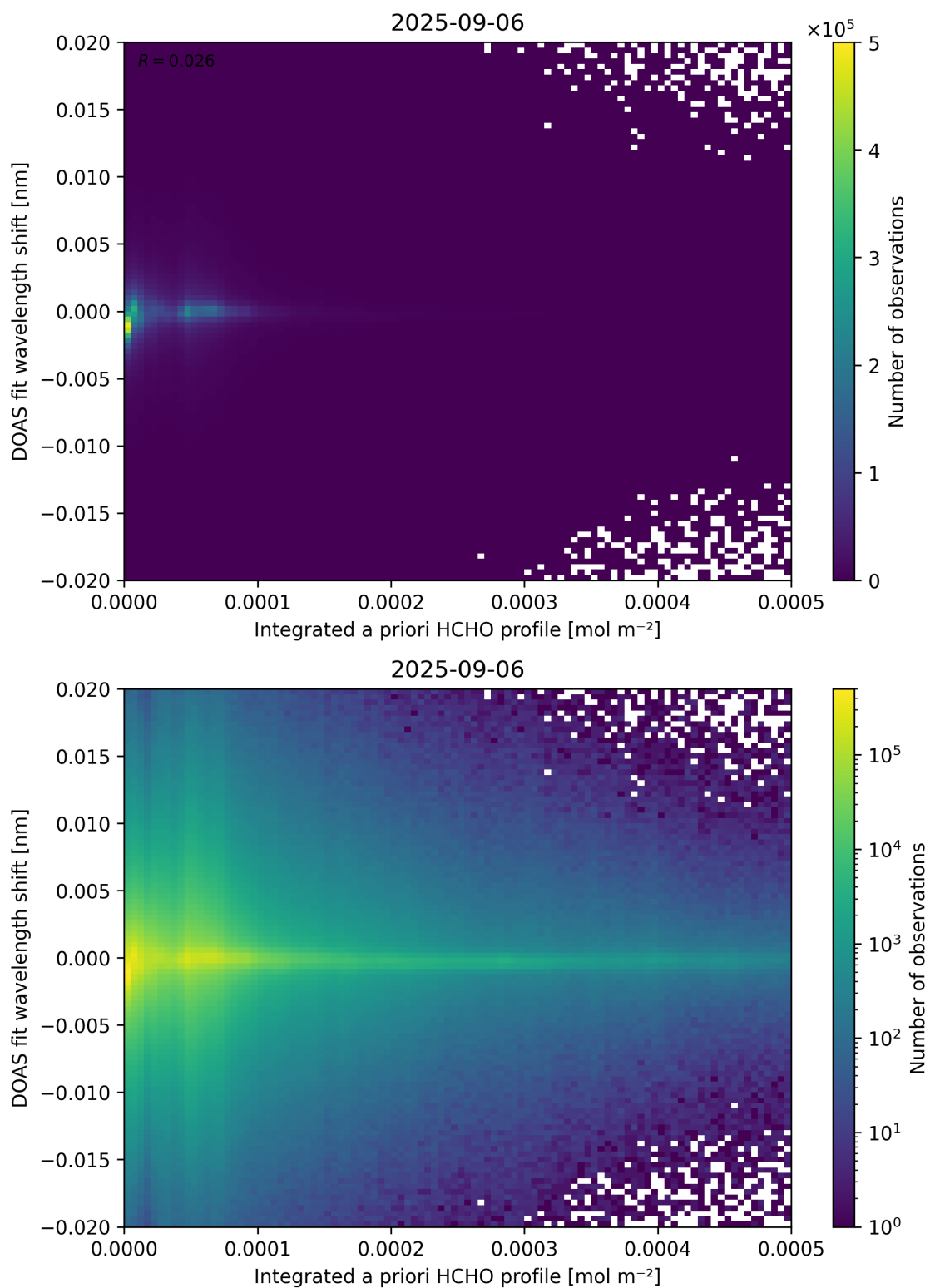
Figure 149: Scatter density plot of “Integrated a priori HCHO profile” against “DOAS fit wavelength shift” for 2025-09-05 to 2025-09-07.
