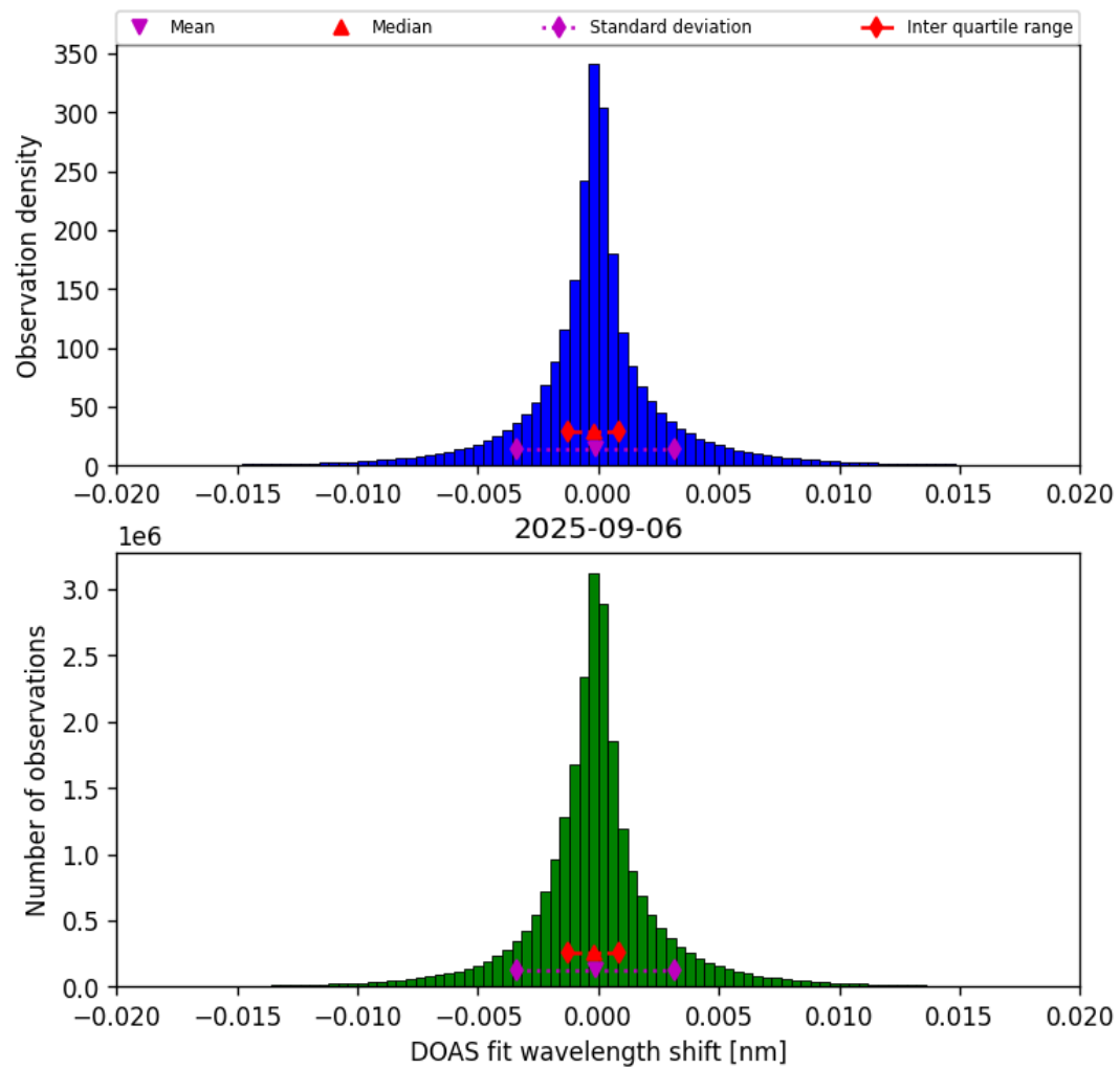
Figure 44: Histogram of “DOAS fit wavelength shift” for 2025-09-05 to 2025-09-07
