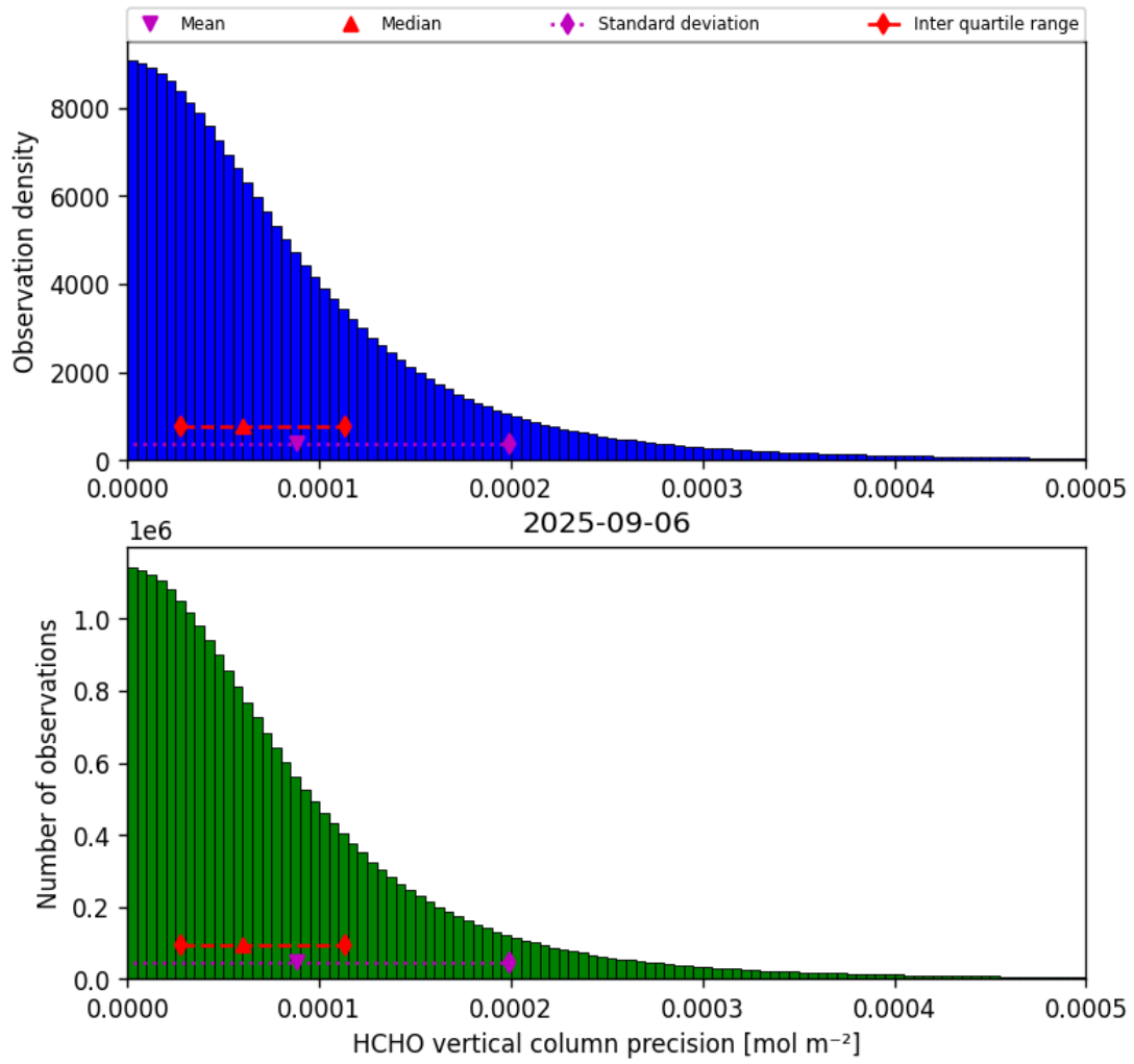
Figure 36: Histogram of “HCHO vertical column precision” for 2025-09-05 to 2025-09-07
