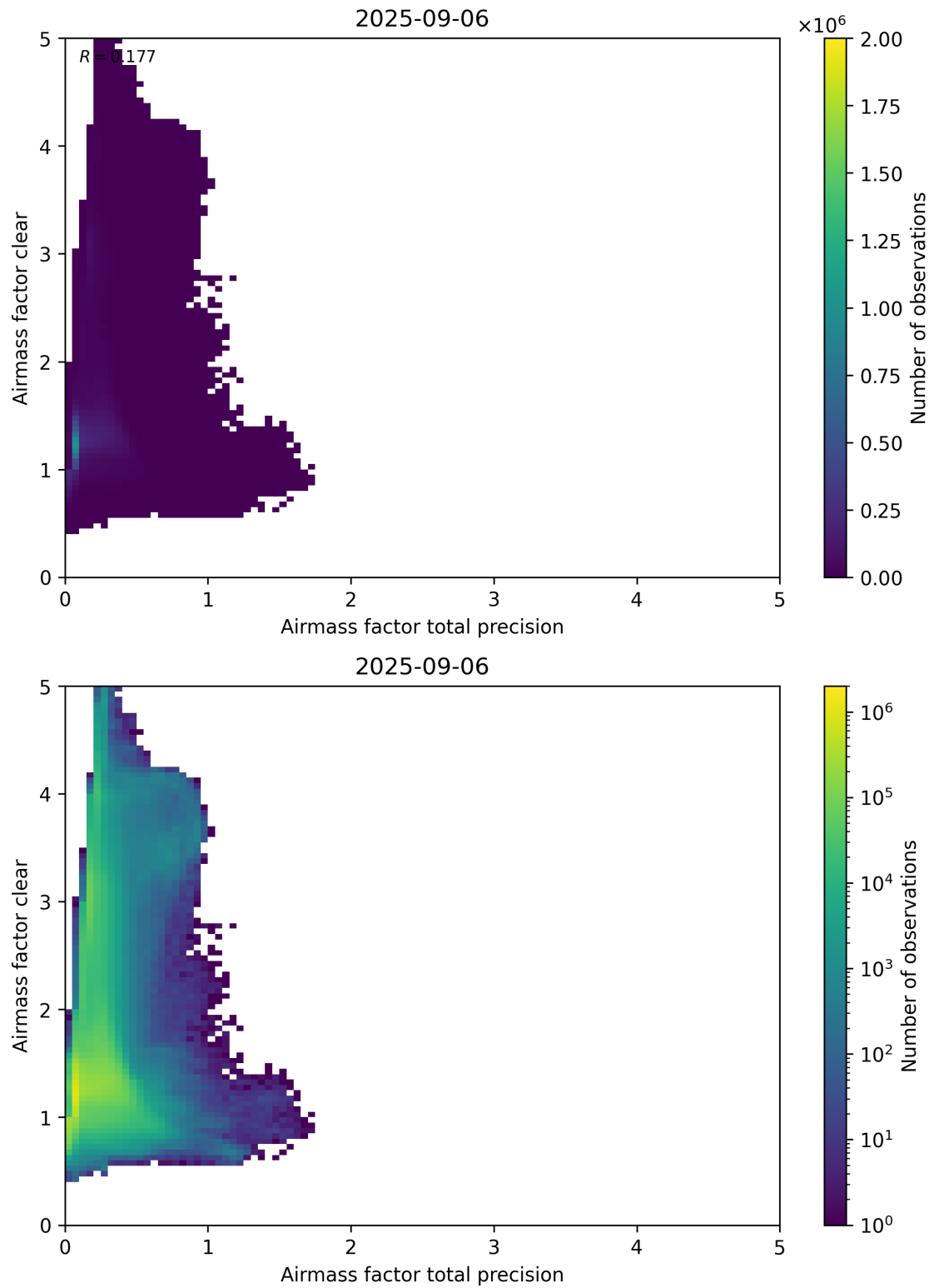
Figure 108: Scatter density plot of “Airmass factor total precision” against “Airmass factor clear” for 2025-09-05 to 2025-09-07.
