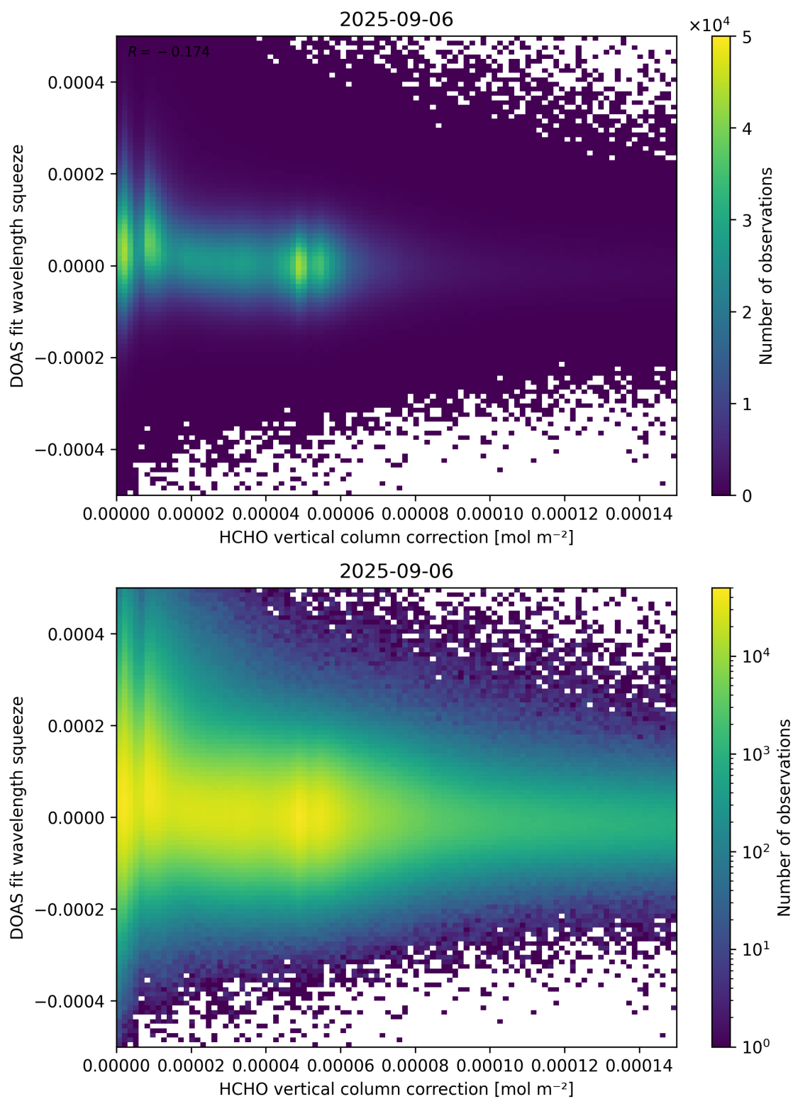
Figure 114: Scatter density plot of “HCHO vertical column correction” against “DOAS fit wavelength squeeze” for 2025-09-05 to 2025-09-07.
