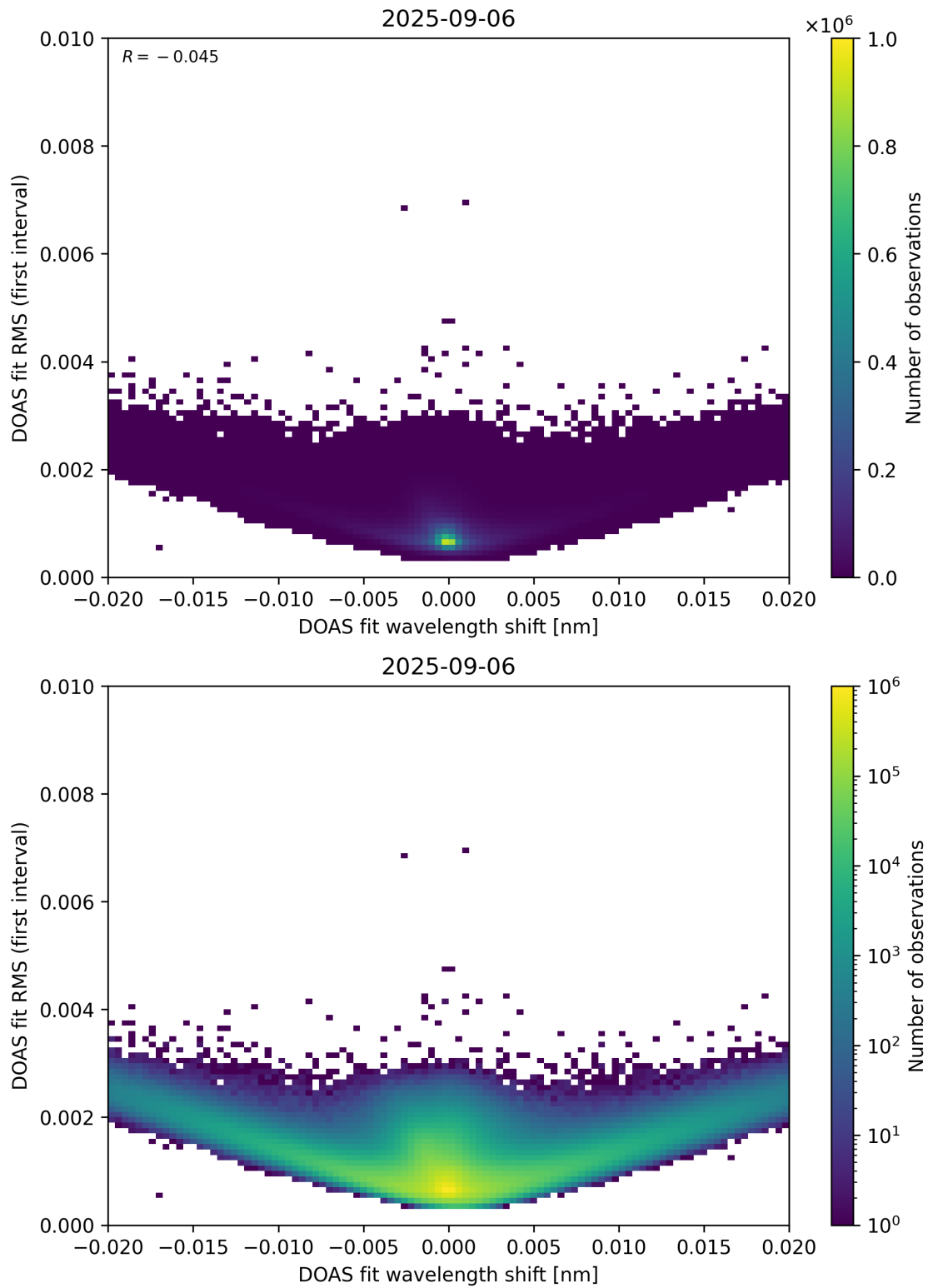
Figure 64: Scatter density plot of “DOAS fit wavelength shift” against “DOAS fit RMS (first interval)” for 2025-09-05 to 2025-09-07.
