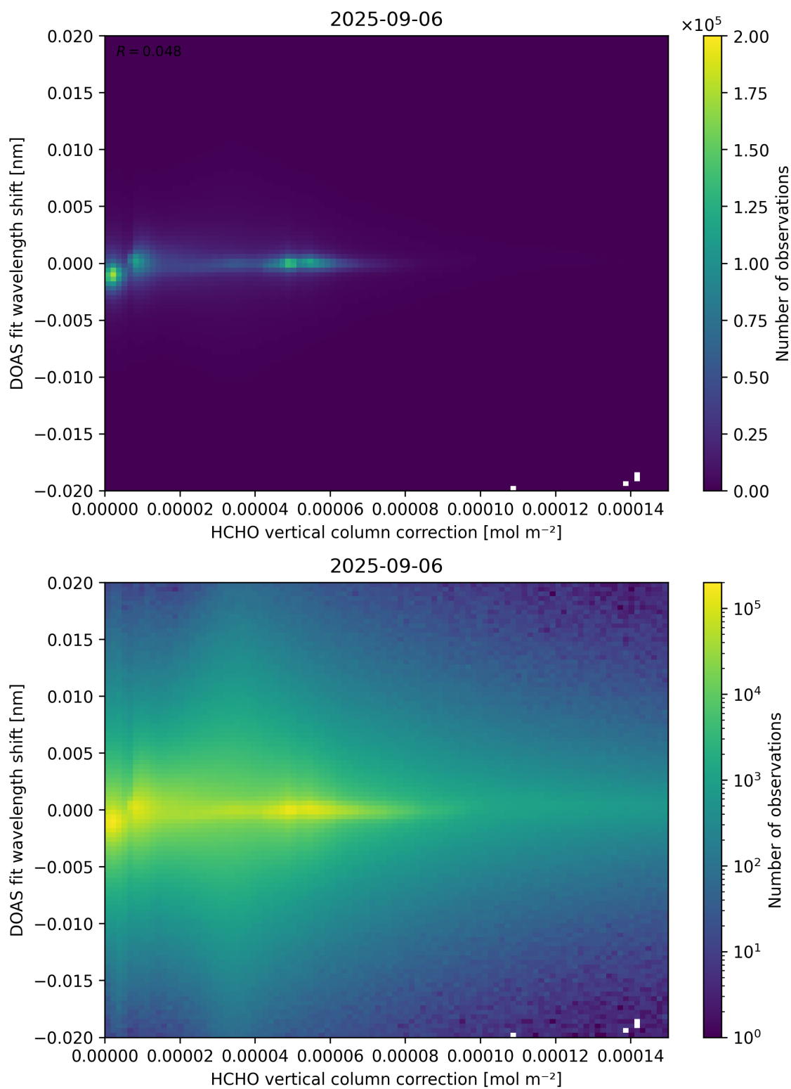
Figure 113: Scatter density plot of “HCHO vertical column correction” against “DOAS fit wavelength shift” for 2025-09-05 to 2025-09-07.
