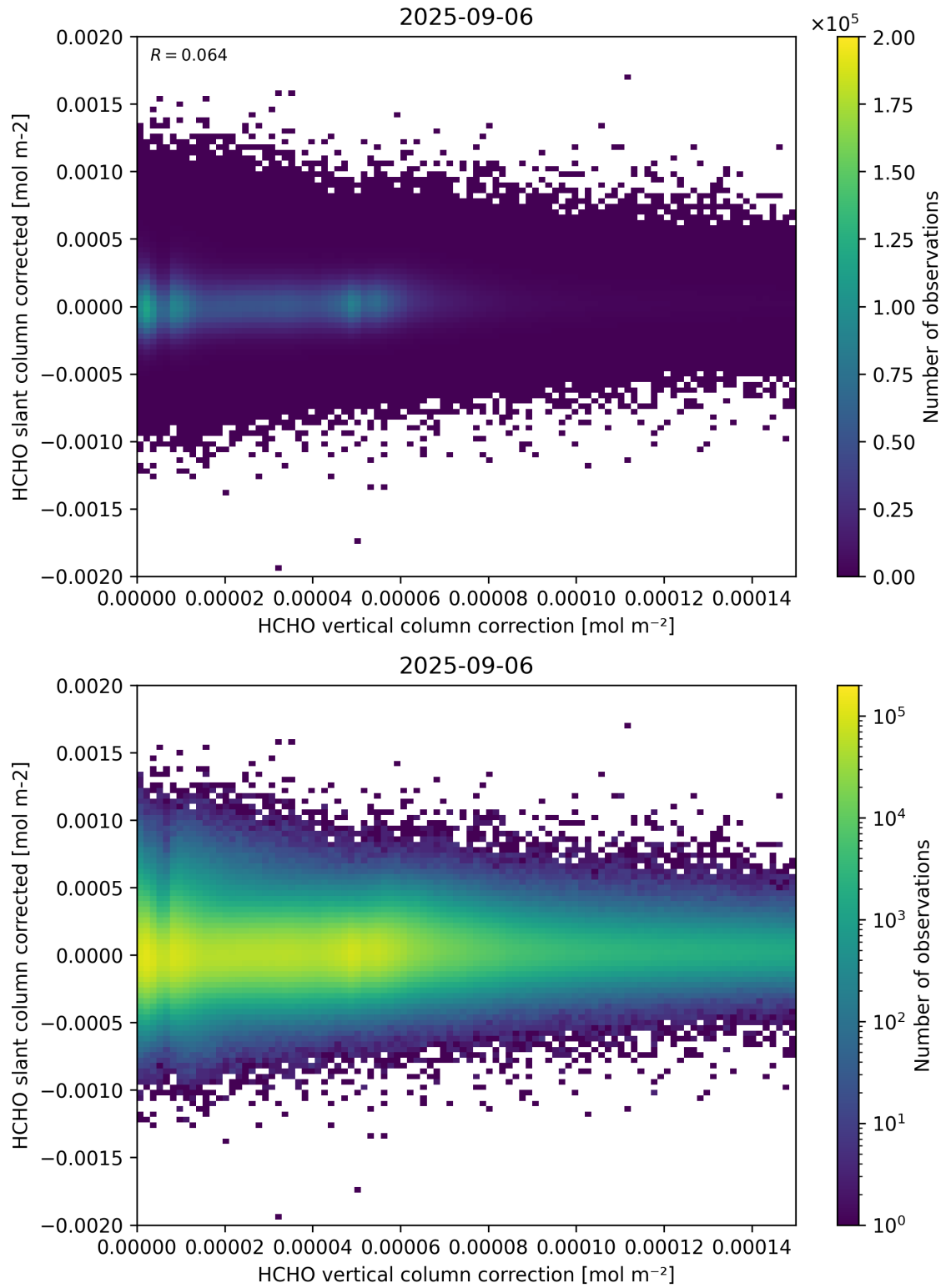
Figure 116: Scatter density plot of “HCHO vertical column correction” against “HCHO slant column corrected” for 2025-09-05 to 2025-09-07.
