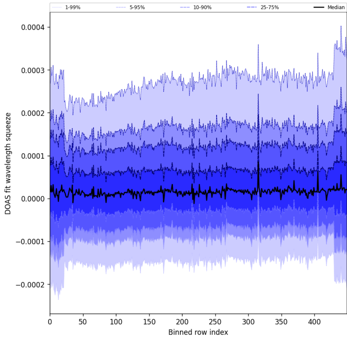
Figure 59: Along track statistics of “DOAS fit wavelength squeeze” for 2025-09-05 to 2025-09-07
