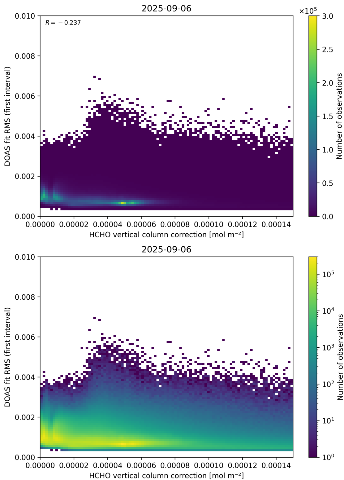
Figure 112: Scatter density plot of “HCHO vertical column correction” against “DOAS fit RMS (first interval)” for 2025-09-05 to 2025-09-07.
