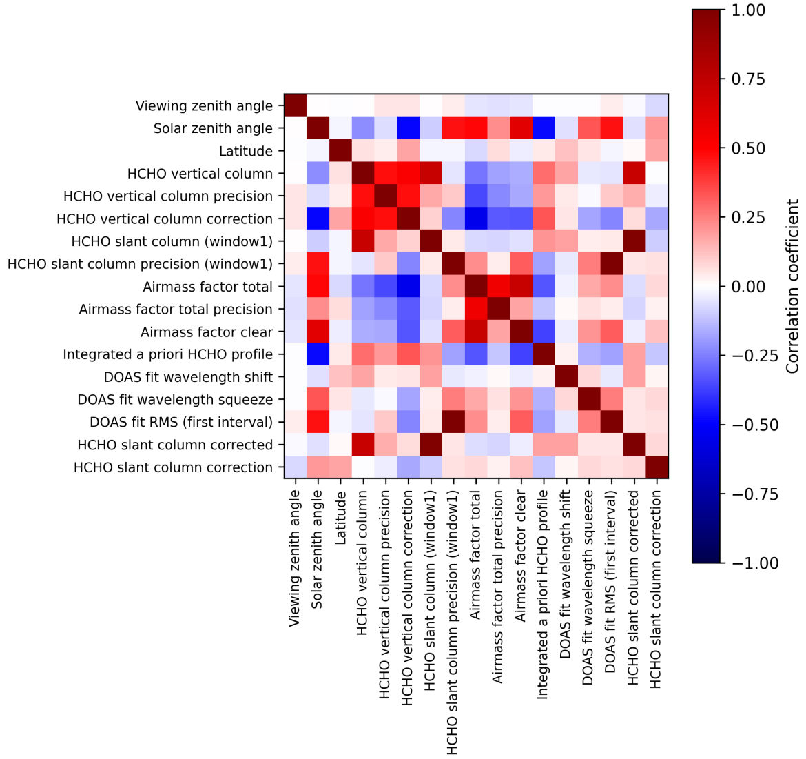
Figure 2: Map of correlation matrix for 2025-09-05 to 2025-09-07.
