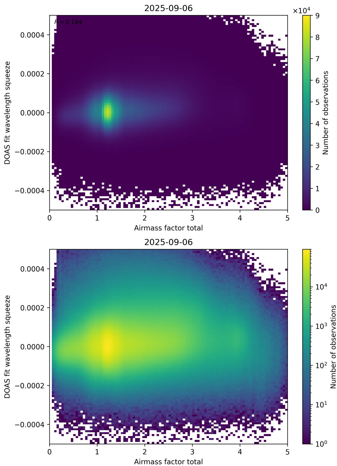
Figure 99: Scatter density plot of “Airmass factor total” against “DOAS fit wavelength squeeze” for 2025-09-05 to 2025-09-07.
