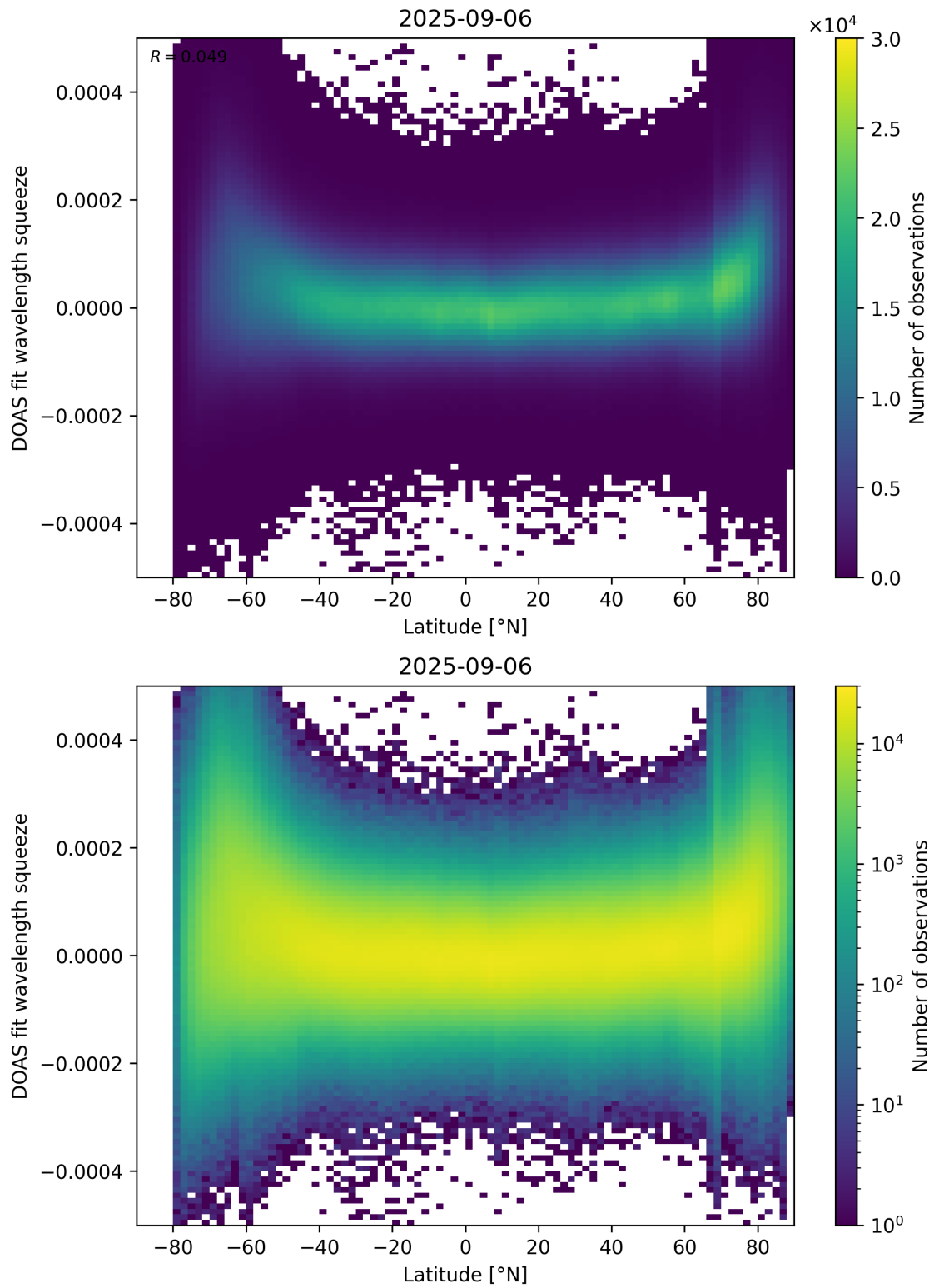
Figure 155: Scatter density plot of “Latitude” against “DOAS fit wavelength squeeze” for 2025-09-05 to 2025-09-07.
