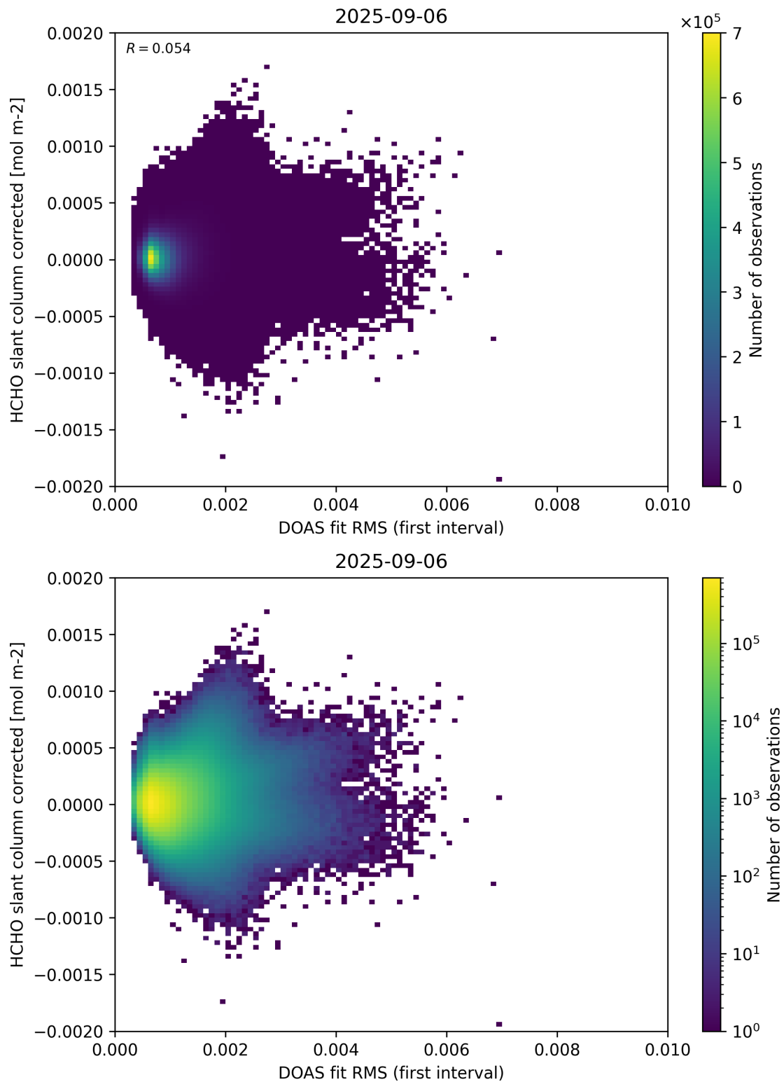
Figure 62: Scatter density plot of “DOAS fit RMS (first interval)” against “HCHO slant column corrected” for 2025-09-05 to 2025-09-07.
