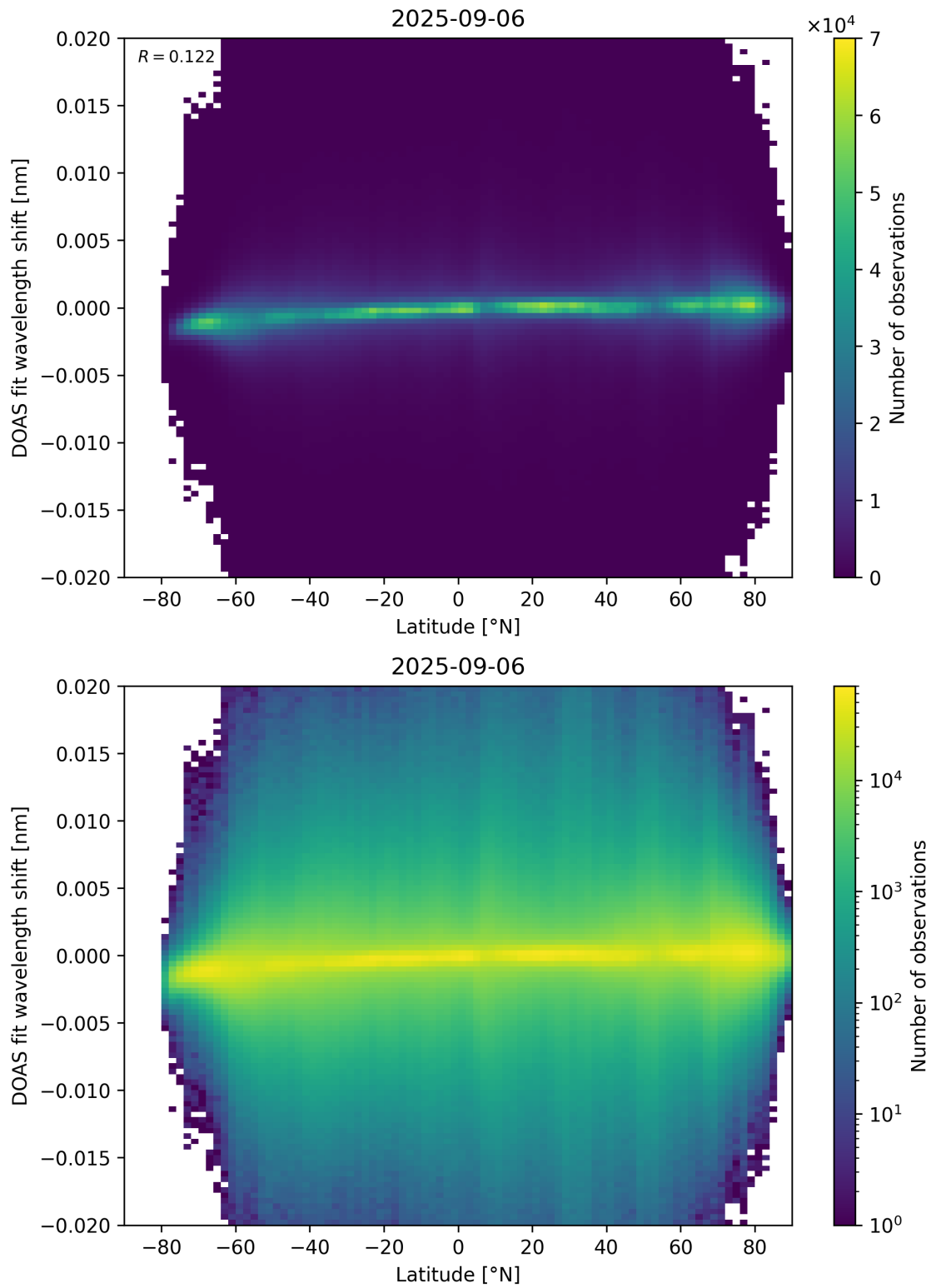
Figure 154: Scatter density plot of “Latitude” against “DOAS fit wavelength shift” for 2025-09-05 to 2025-09-07.
