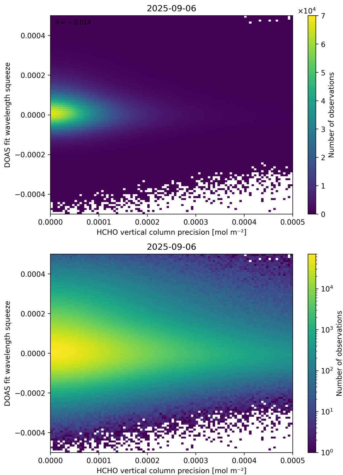
Figure 138: Scatter density plot of “HCHO vertical column precision” against “DOAS fit wavelength squeeze” for 2025-09-05 to 2025-09-07.
