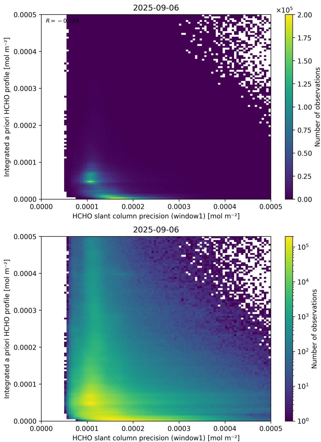
Figure 96: Scatter density plot of “HCHO slant column precision (window1)” against “Integrated a priori HCHO profile” for 2025-09-05 to 2025-09-07.
