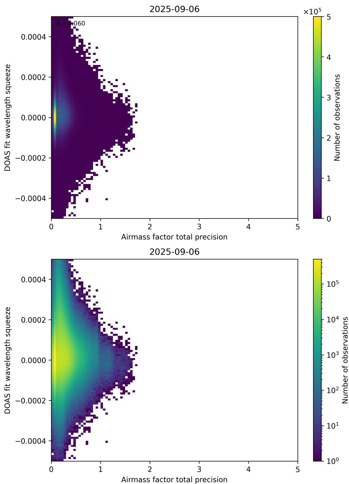
Figure 107: Scatter density plot of “Airmass factor total precision” against “DOAS fit wavelength squeeze” for 2025-09-05 to 2025-09-07.
