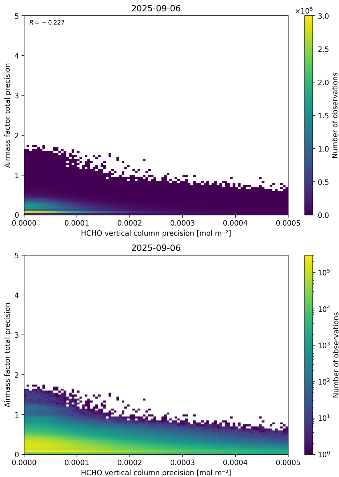
Figure 145: Scatter density plot of “HCHO vertical column precision” against “Airmass factor total precision” for 2025-09-05 to 2025-09-07.
