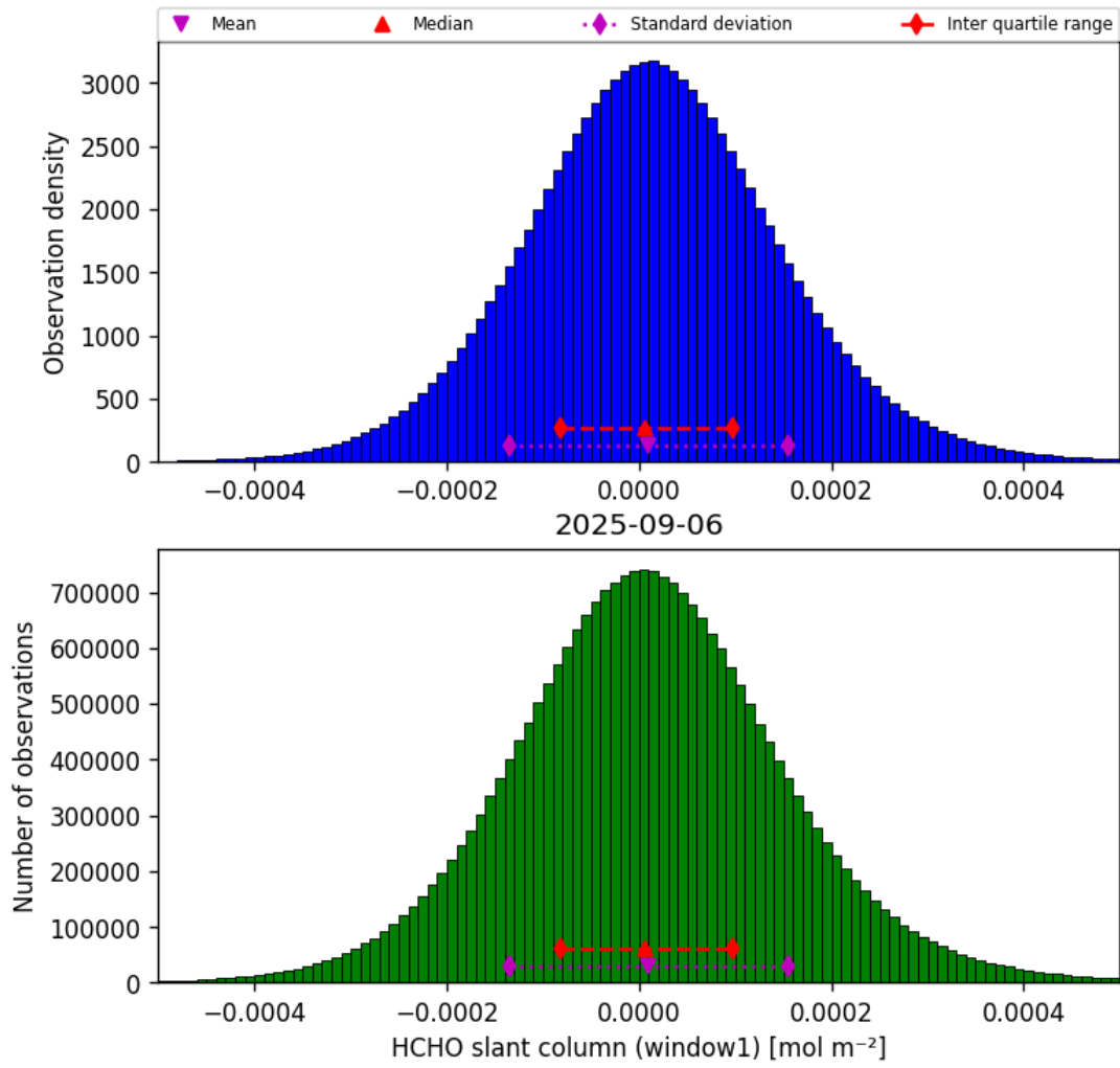
Figure 38: Histogram of “HCHO slant column (window1)” for 2025-09-05 to 2025-09-07
