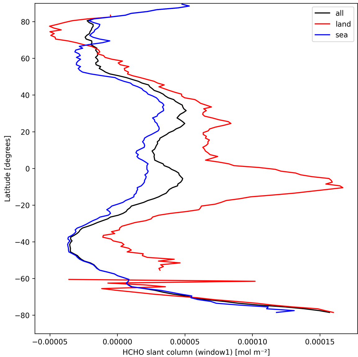
Figure 24: Zonal average of “HCHO slant column (window1)” for 2025-09-05 to 2025-09-07.
