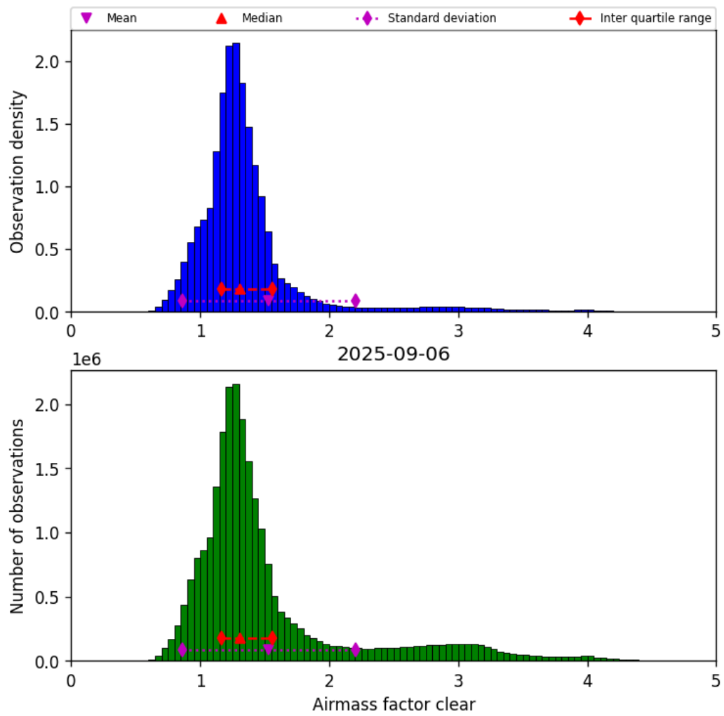
Figure 42: Histogram of “Airmass factor clear” for 2025-09-05 to 2025-09-07
