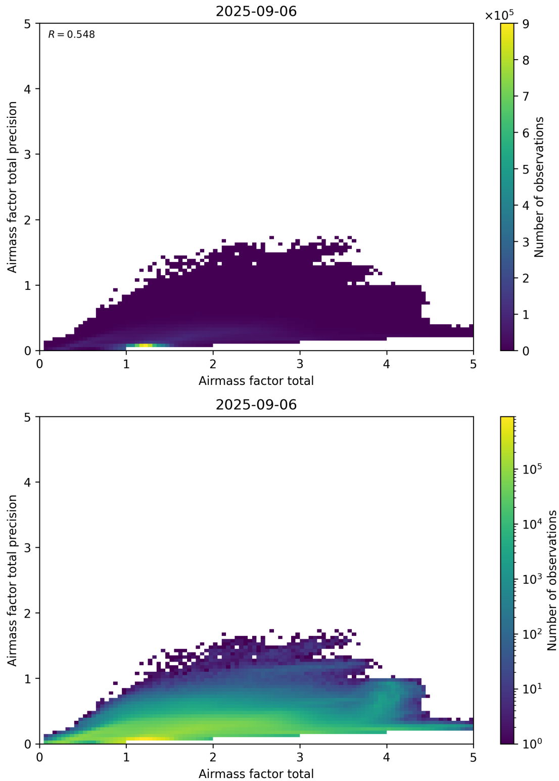
Figure 103: Scatter density plot of “Airmass factor total” against “Airmass factor total precision” for 2025-09-05 to 2025-09-07.
