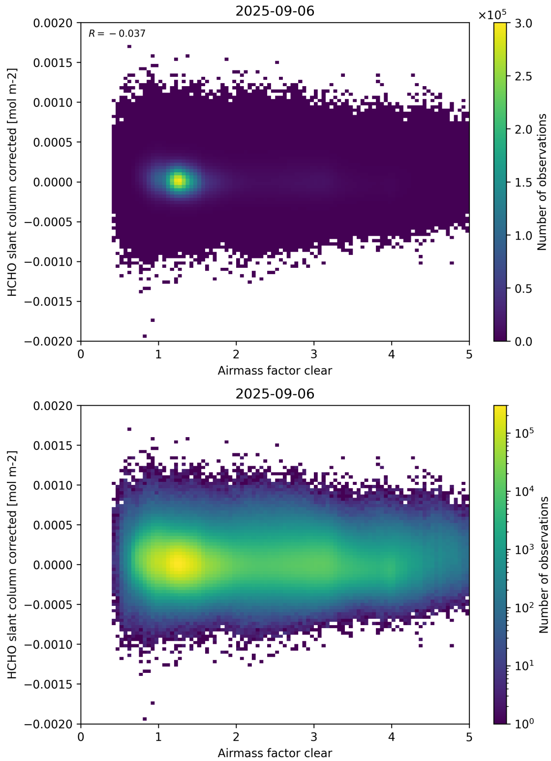
Figure 74: Scatter density plot of “Airmass factor clear” against “HCHO slant column corrected” for 2025-09-05 to 2025-09-07.
