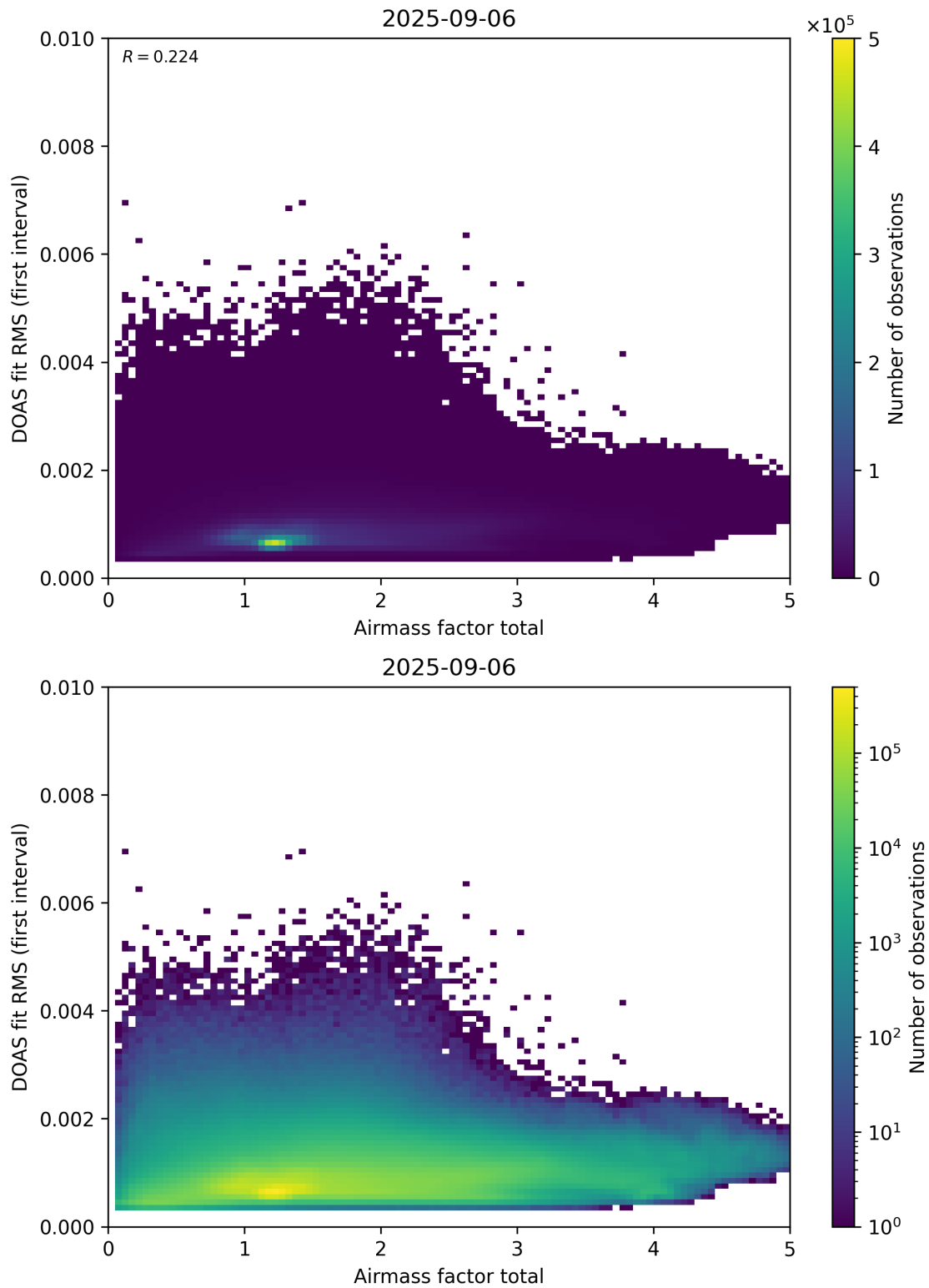
Figure 97: Scatter density plot of “Airmass factor total” against “DOAS fit RMS (first interval)” for 2025-09-05 to 2025-09-07.
