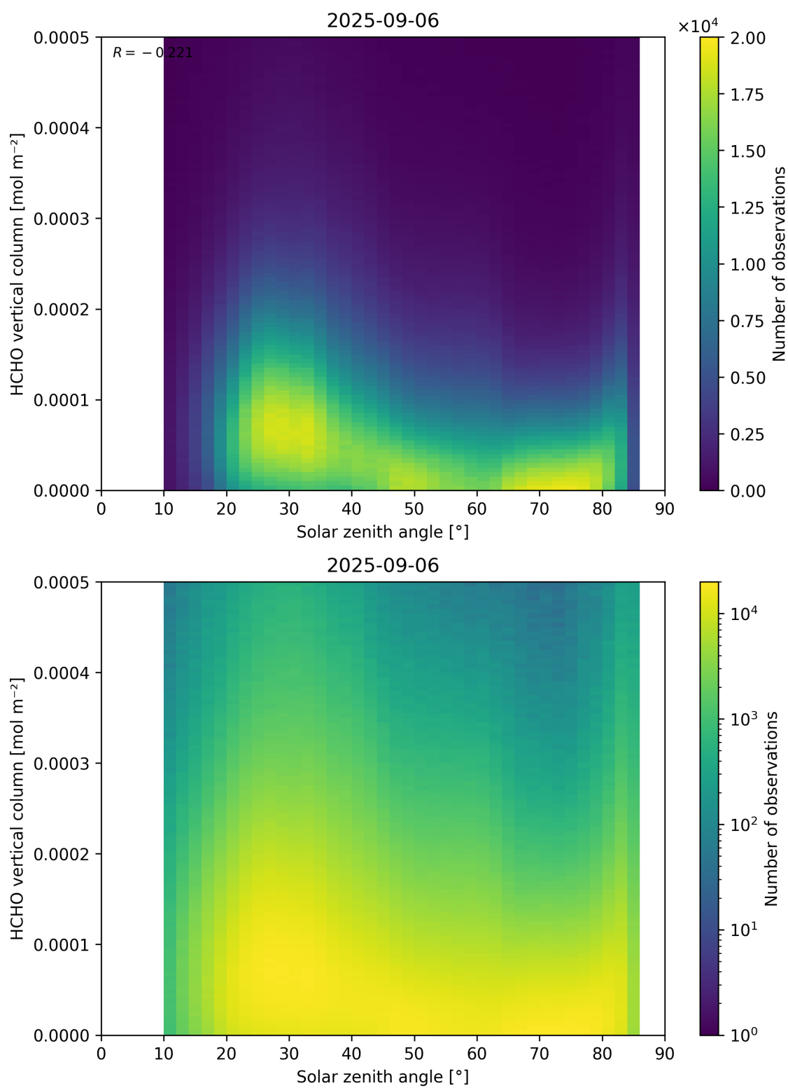
Figure 177: Scatter density plot of “Solar zenith angle” against “HCHO vertical column” for 2025-09-05 to 2025-09-07.
