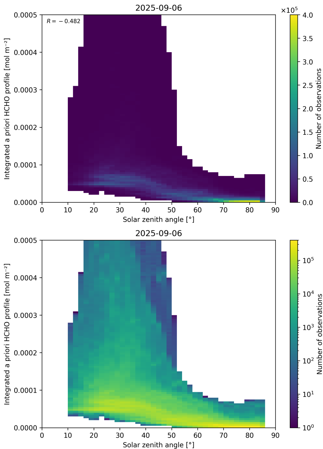
Figure 180: Scatter density plot of “Solar zenith angle” against “Integrated a priori HCHO profile” for 2025-09-05 to 2025-09-07.
