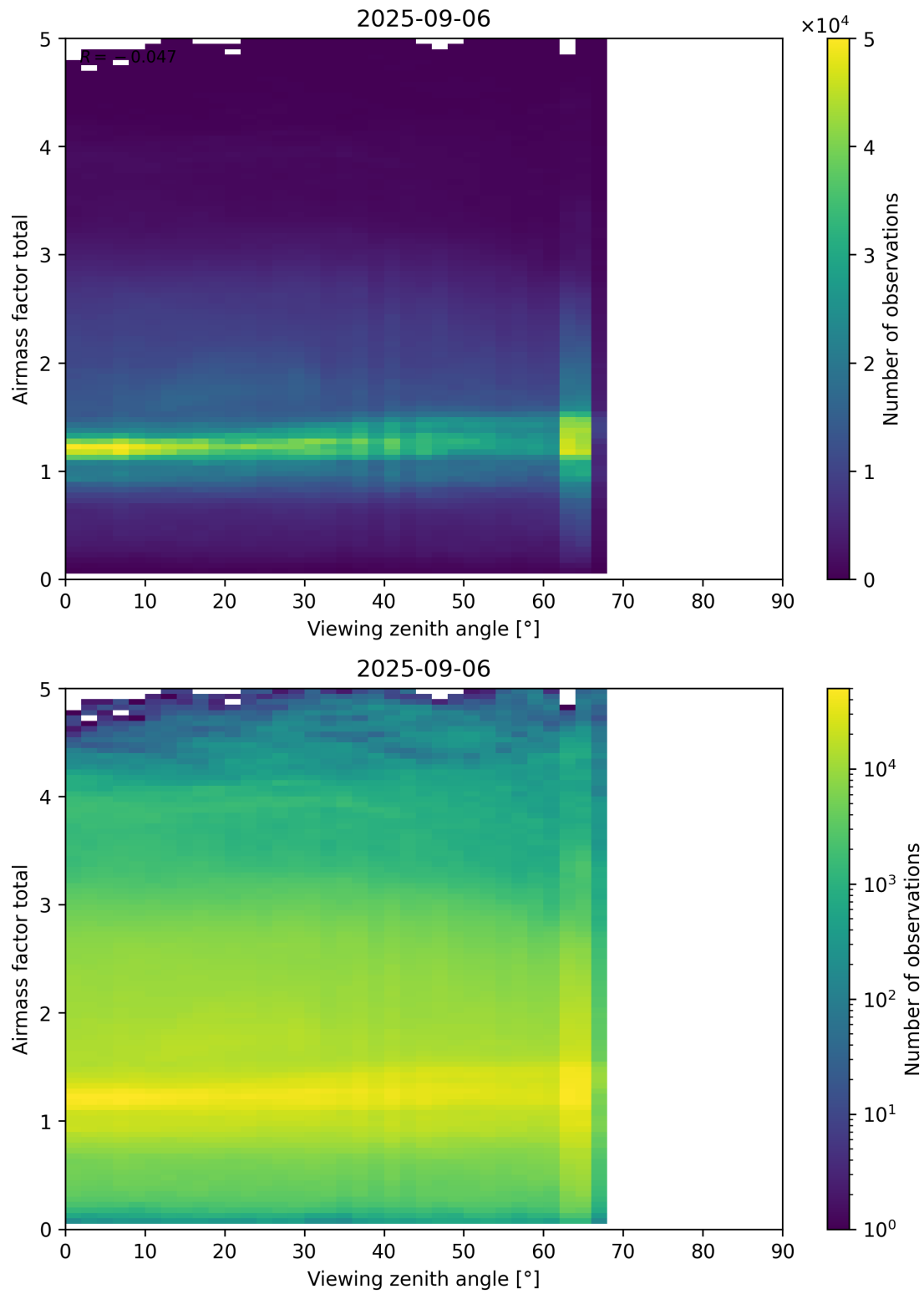
Figure 190: Scatter density plot of “Viewing zenith angle” against “Airmass factor total” for 2025-09-05 to 2025-09-07.
