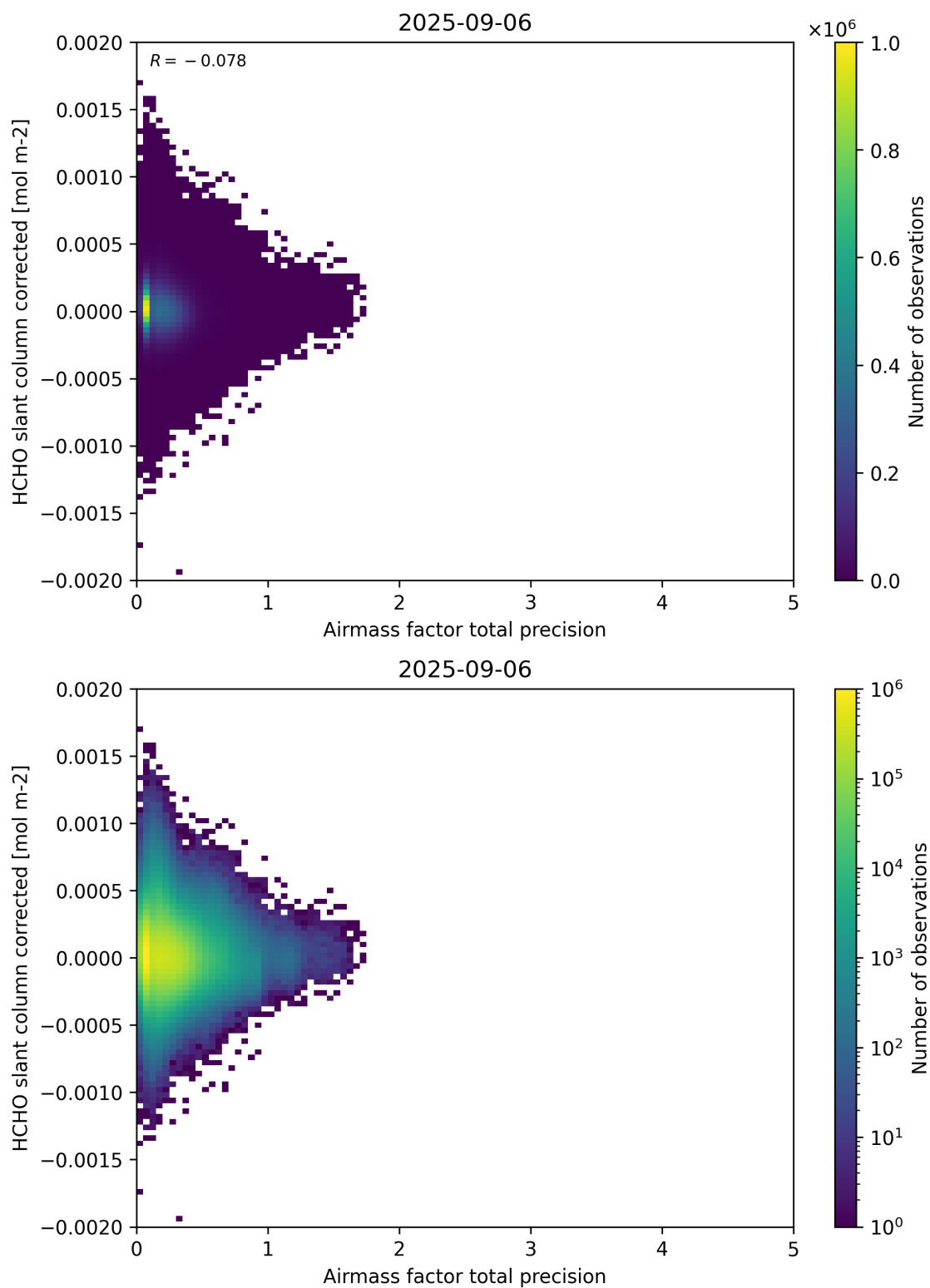
Figure 109: Scatter density plot of “Airmass factor total precision” against “HCHO slant column corrected” for 2025-09-05 to 2025-09-07.
