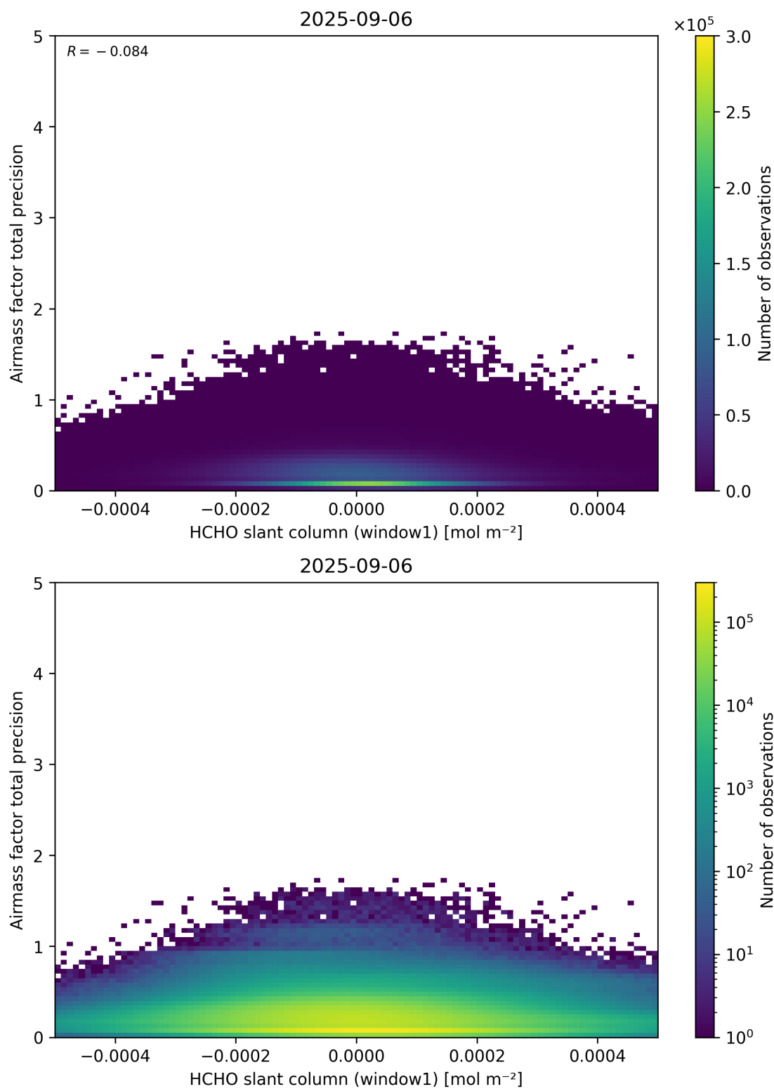
Figure 86: Scatter density plot of “HCHO slant column (window1)” against “Airmass factor total precision” for 2025-09-05 to 2025-09-07.
