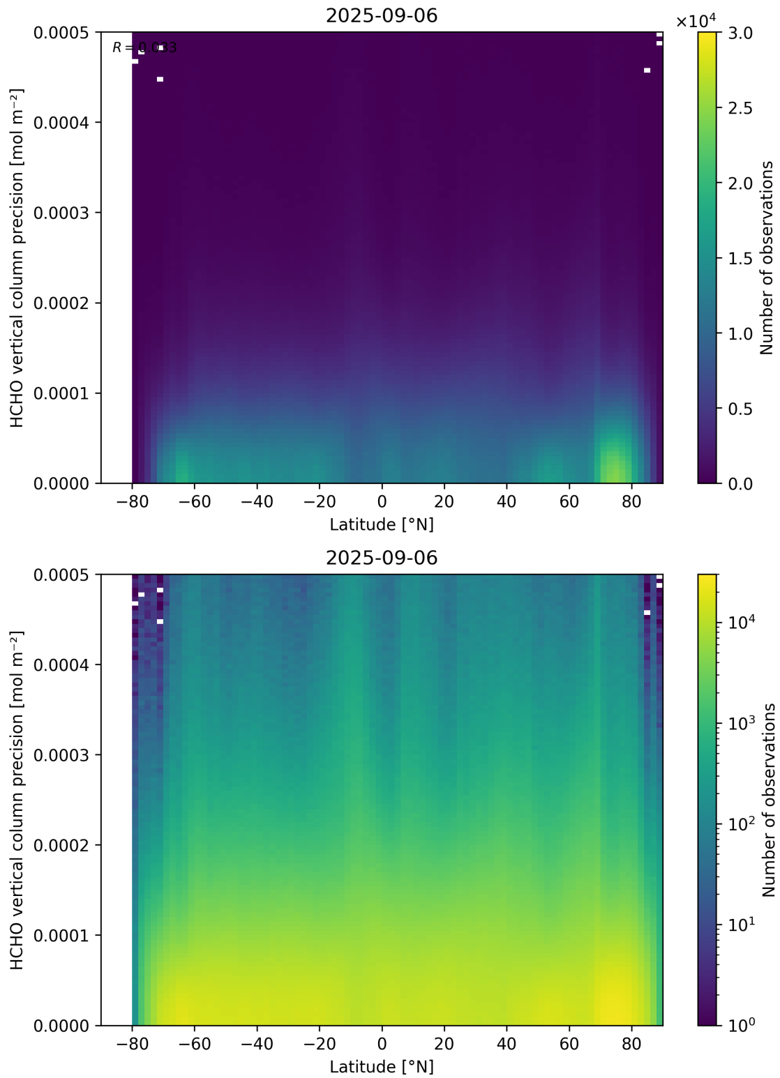
Figure 165: Scatter density plot of “Latitude” against “HCHO vertical column precision” for 2025-09-05 to 2025-09-07.
