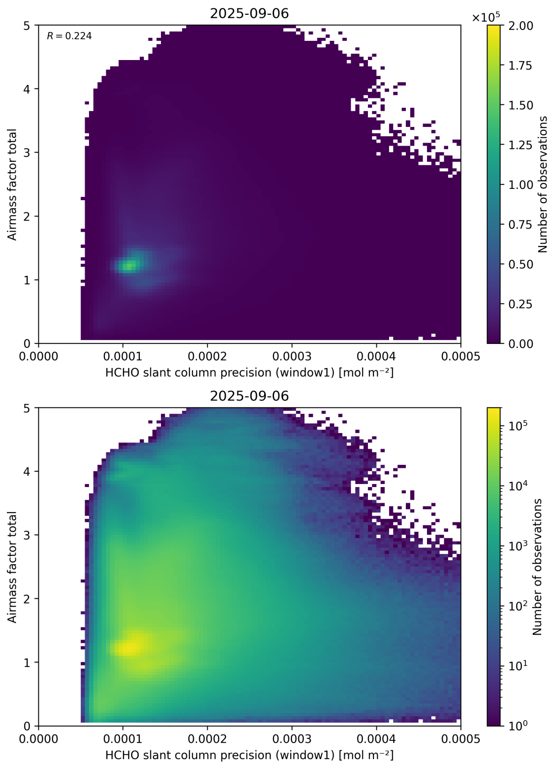
Figure 94: Scatter density plot of “HCHO slant column precision (window1)” against “Airmass factor total” for 2025-09-05 to 2025-09-07.
