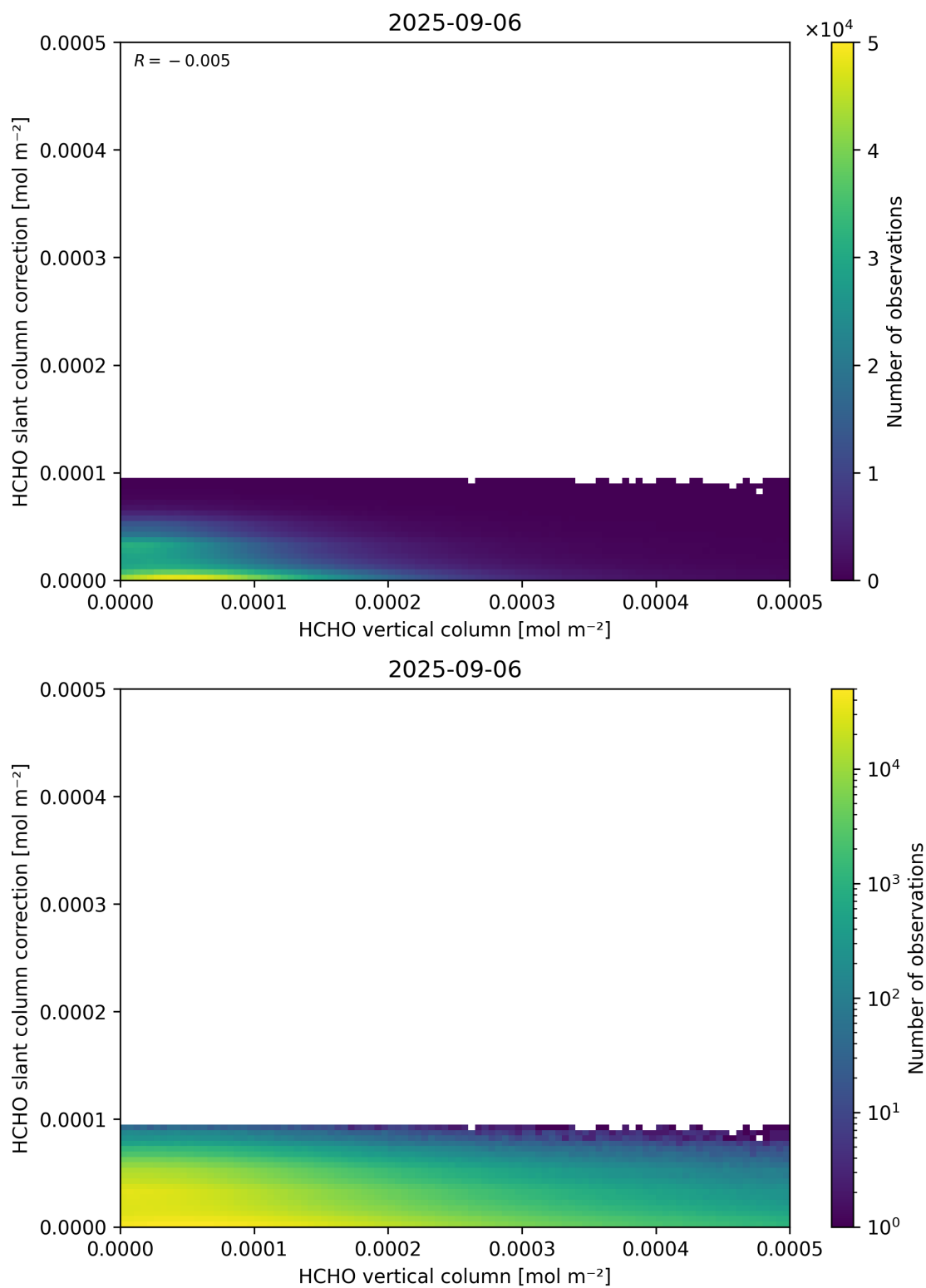
Figure 128: Scatter density plot of “HCHO vertical column” against “HCHO slant column correction” for 2025-09-05 to 2025-09-07.
