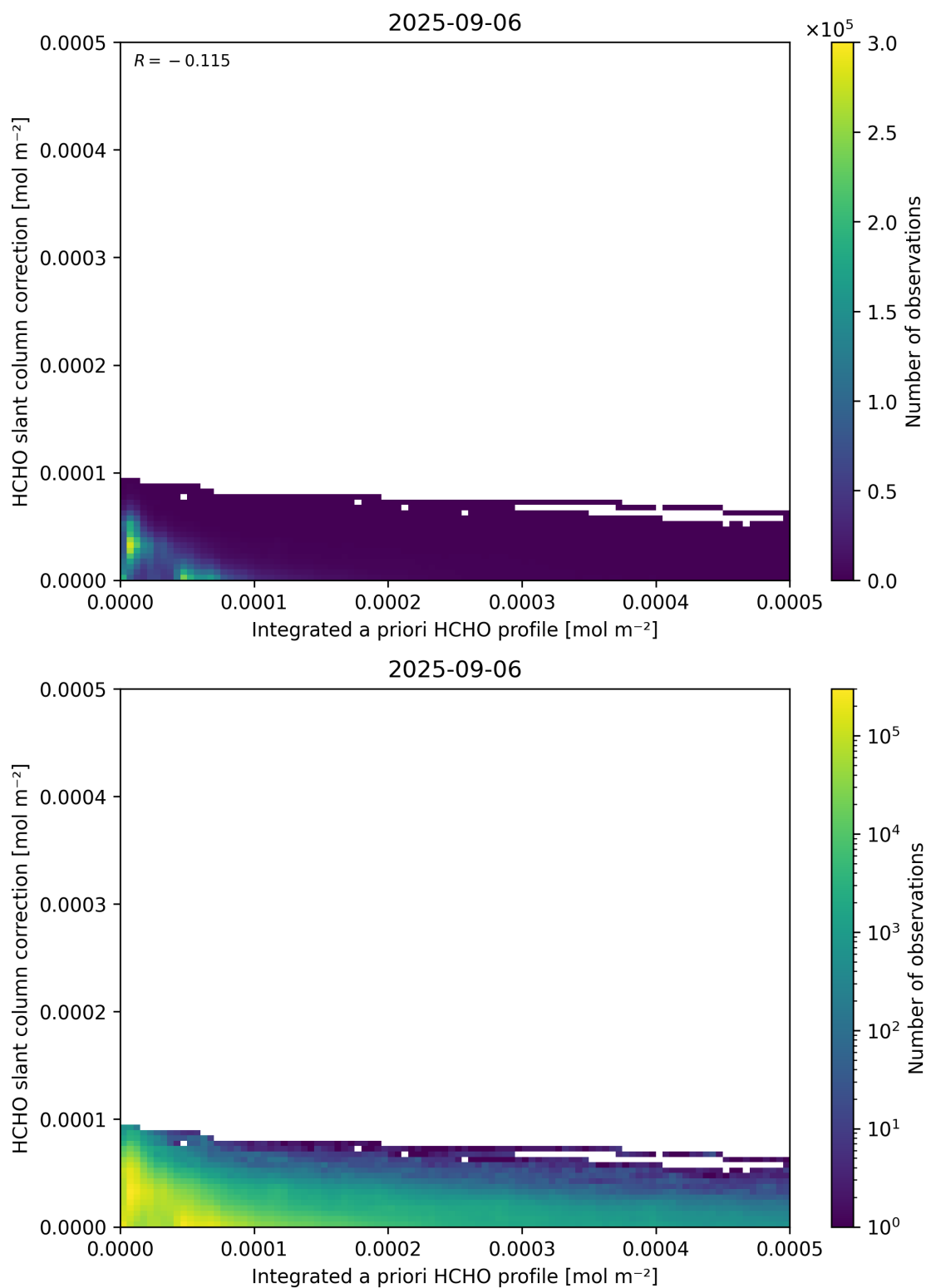
Figure 152: Scatter density plot of “Integrated a priori HCHO profile” against “HCHO slant column correction” for 2025-09-05 to 2025-09-07.
