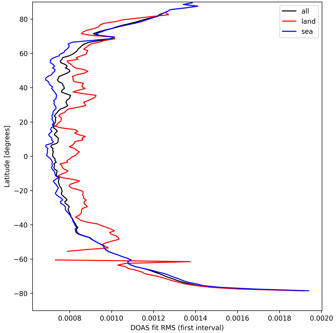
Figure 32: Zonal average of “DOAS fit RMS (first interval)” for 2025-09-05 to 2025-09-07.
