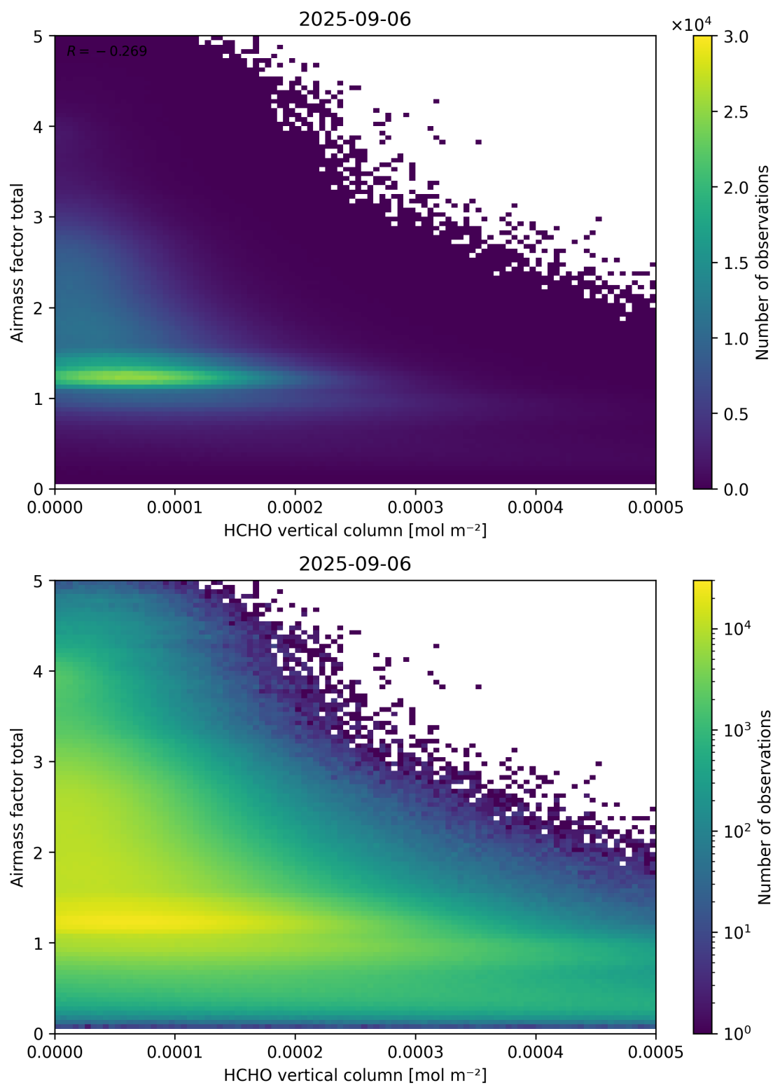
Figure 131: Scatter density plot of “HCHO vertical column” against “Airmass factor total” for 2025-09-05 to 2025-09-07.
