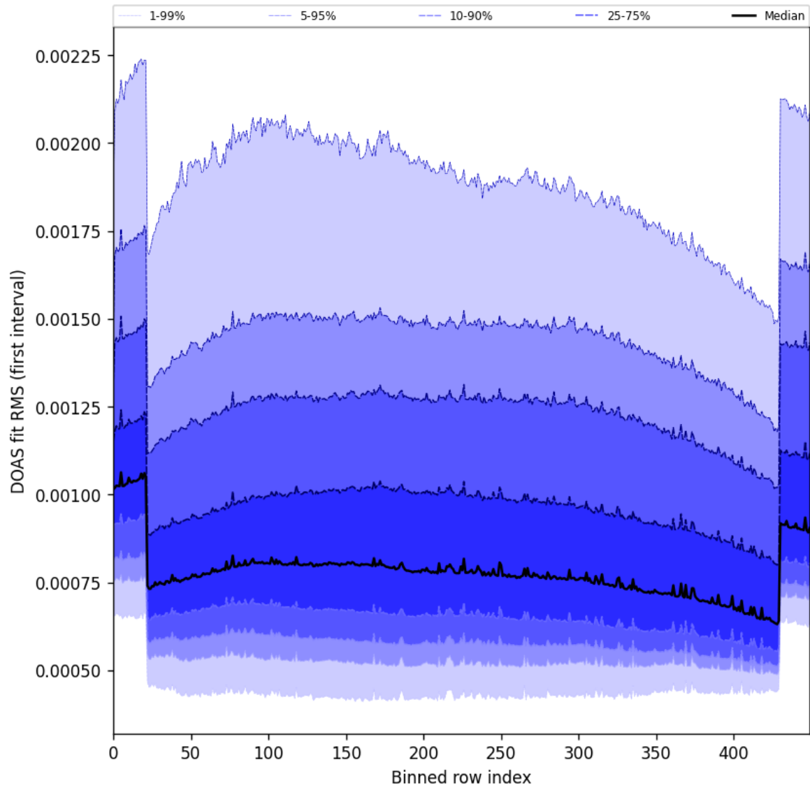
Figure 60: Along track statistics of “DOAS fit RMS (first interval)” for 2025-09-05 to 2025-09-07
