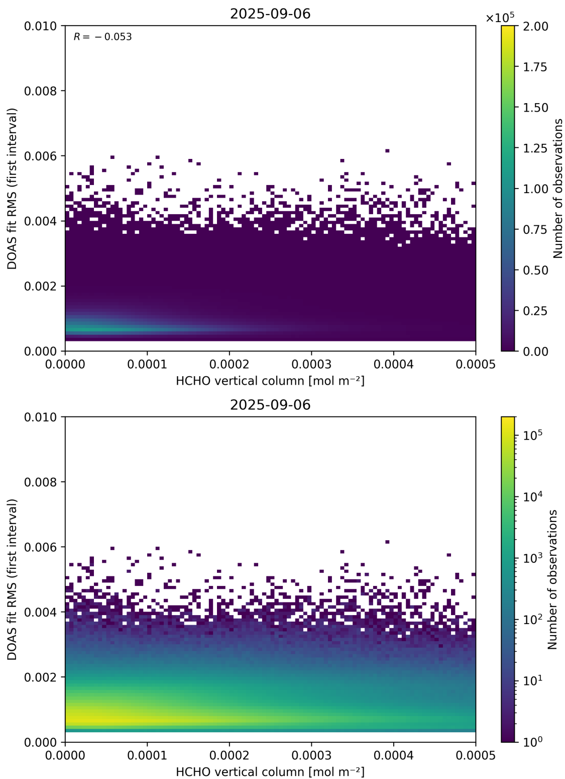
Figure 123: Scatter density plot of “HCHO vertical column” against “DOAS fit RMS (first interval)” for 2025-09-05 to 2025-09-07.
