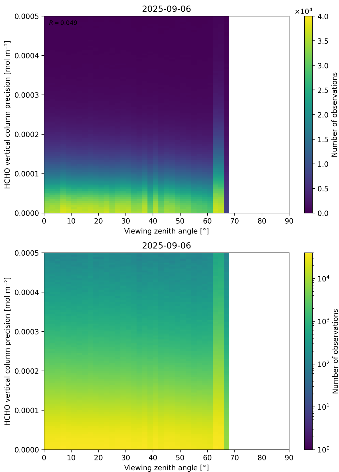
Figure 194: Scatter density plot of “Viewing zenith angle” against “HCHO vertical column precision” for 2025-09-05 to 2025-09-07.
