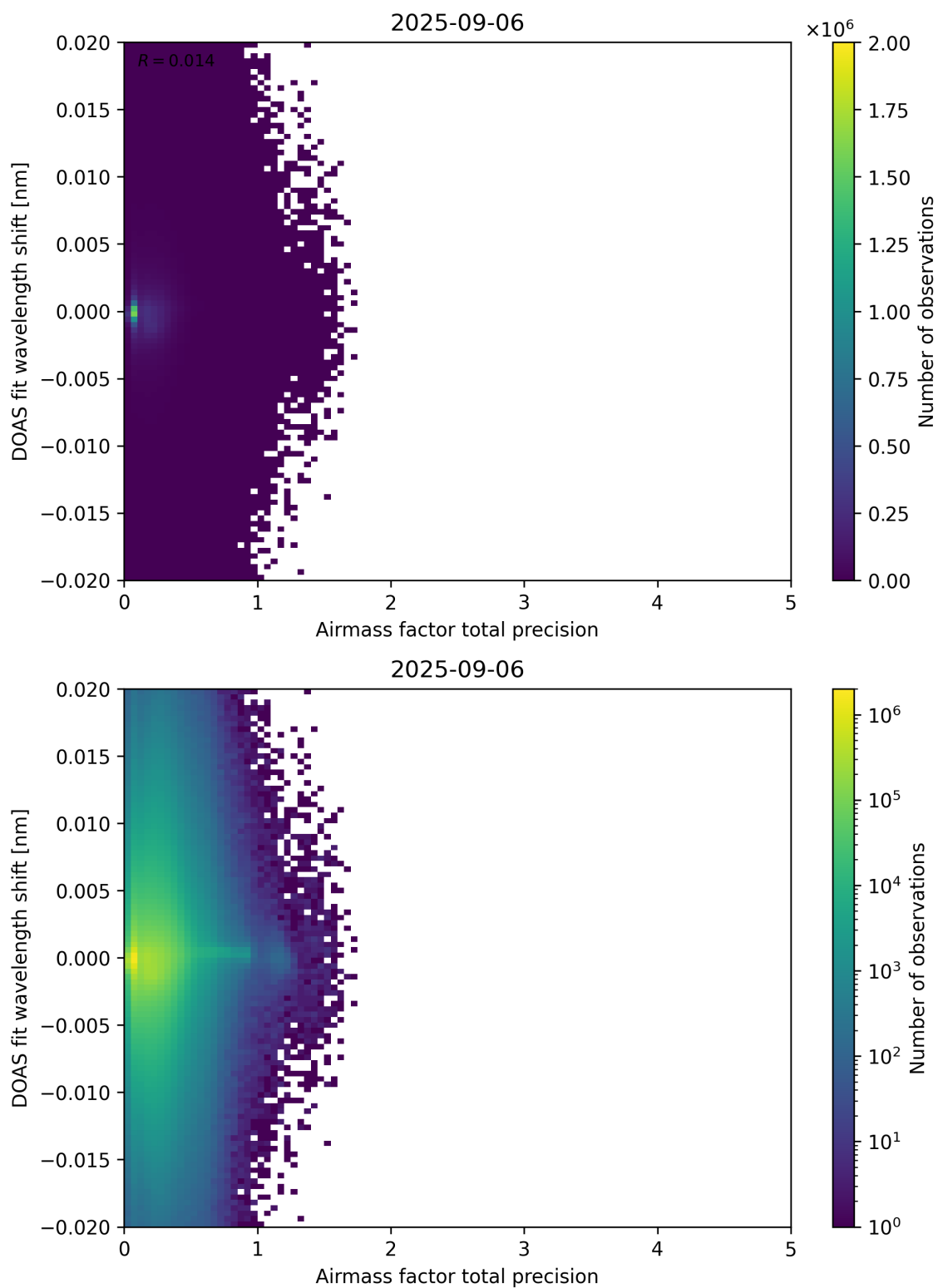
Figure 106: Scatter density plot of “Airmass factor total precision” against “DOAS fit wavelength shift” for 2025-09-05 to 2025-09-07.
