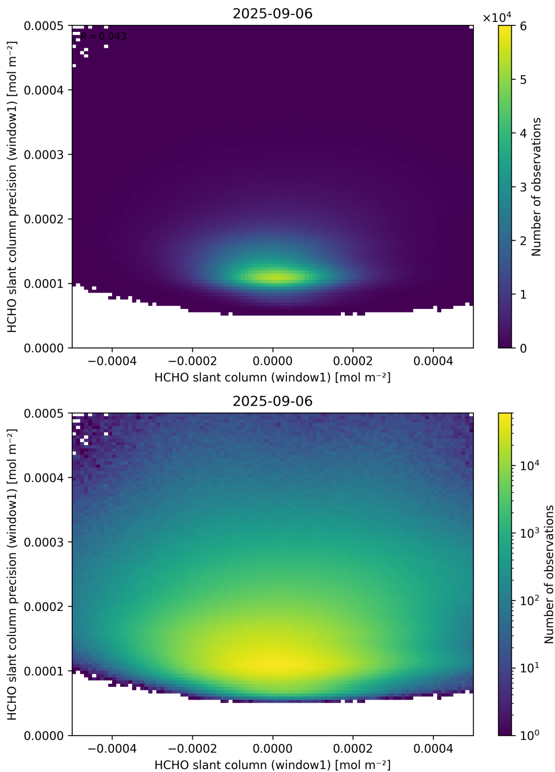
Figure 84: Scatter density plot of “HCHO slant column (window1)” against “HCHO slant column precision (window1)” for 2025-09-05 to 2025-09-07.
