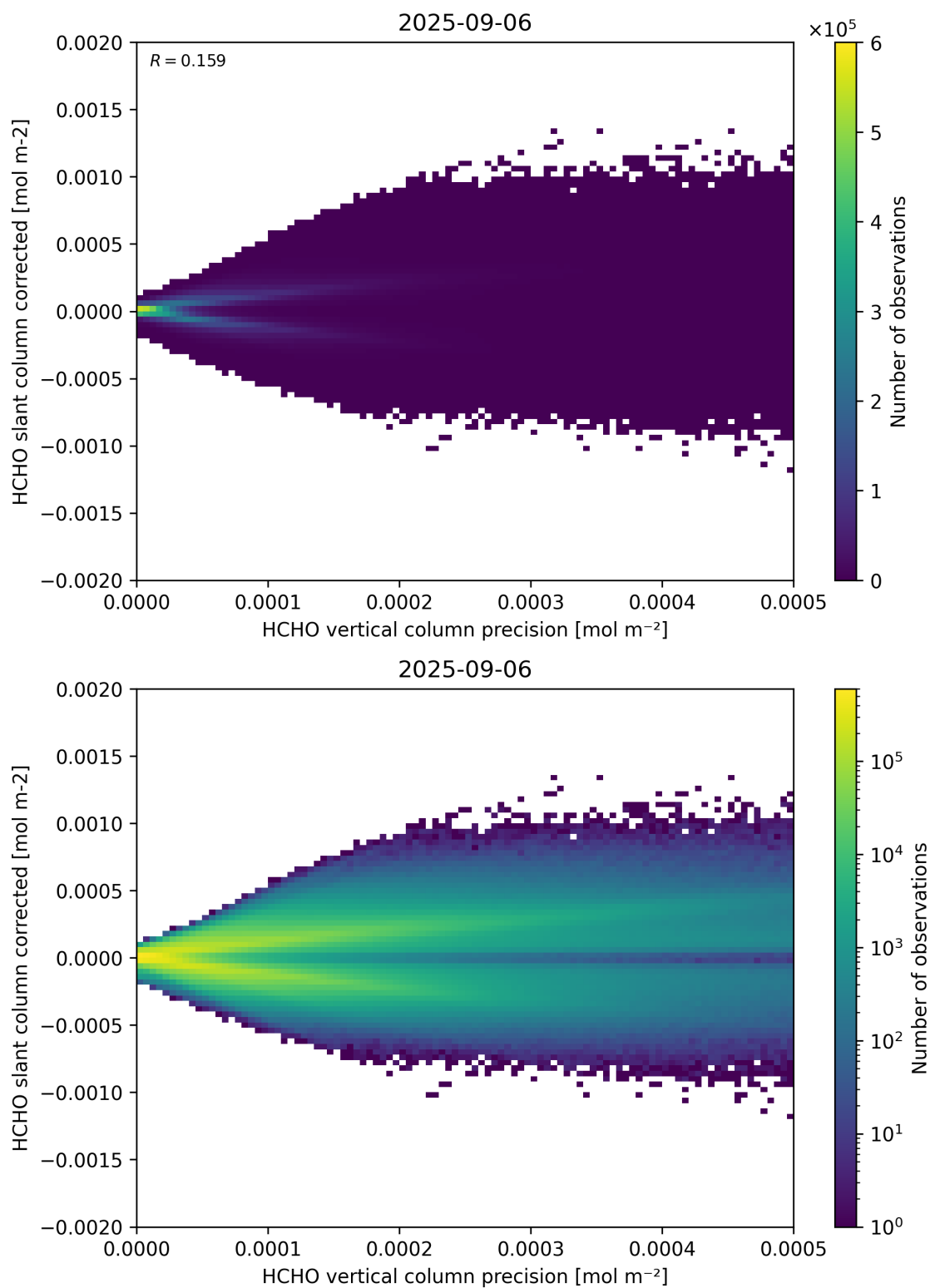
Figure 140: Scatter density plot of “HCHO vertical column precision” against “HCHO slant column corrected” for 2025-09-05 to 2025-09-07.
