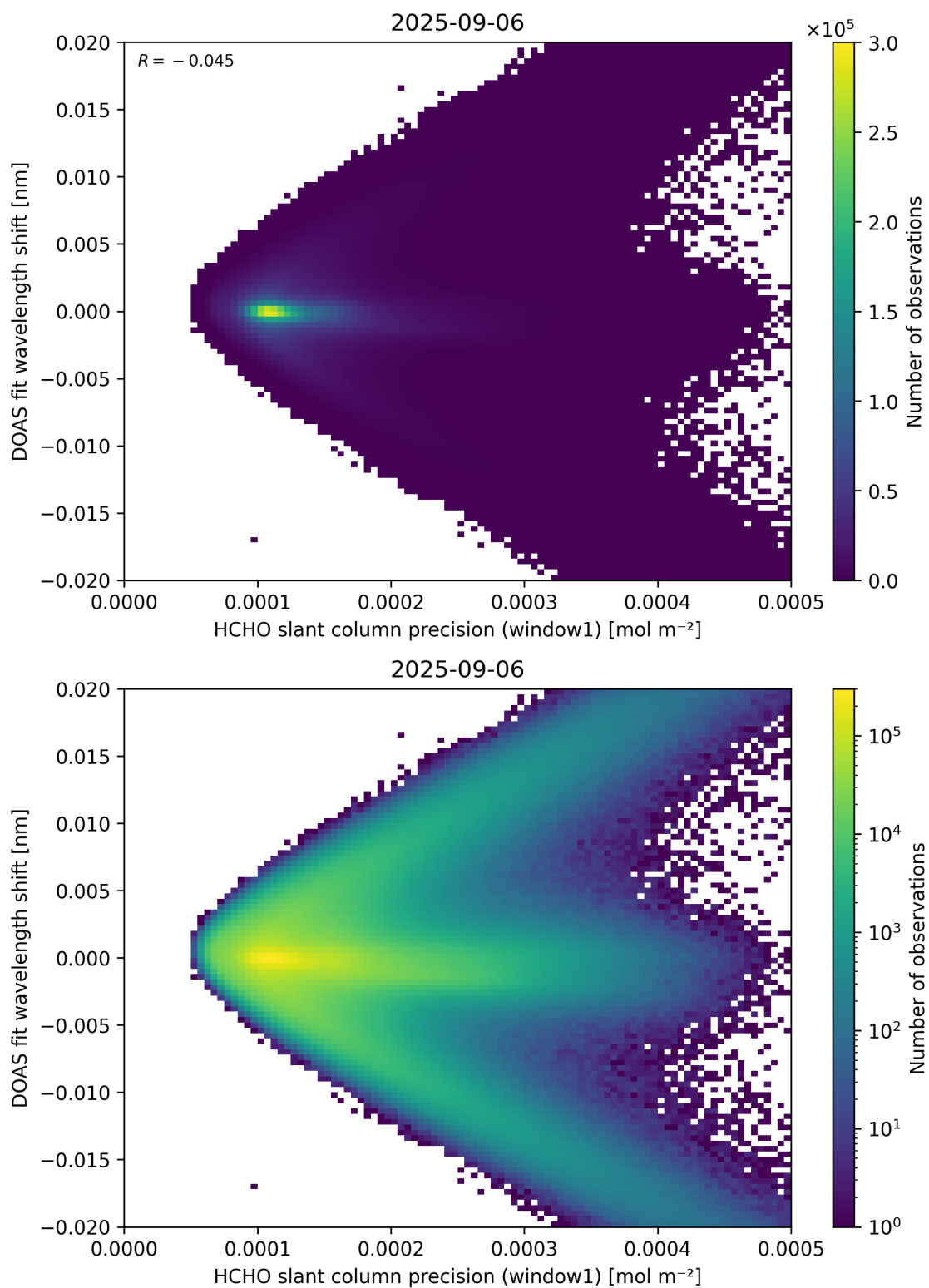
Figure 89: Scatter density plot of “HCHO slant column precision (window1)” against “DOAS fit wavelength shift” for 2025-09-05 to 2025-09-07.
