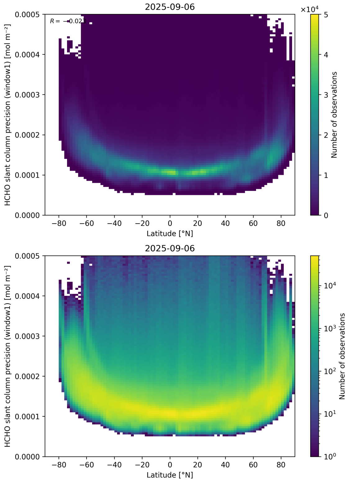
Figure 160: Scatter density plot of “Latitude” against “HCHO slant column precision (window1)” for 2025-09-05 to 2025-09-07.
