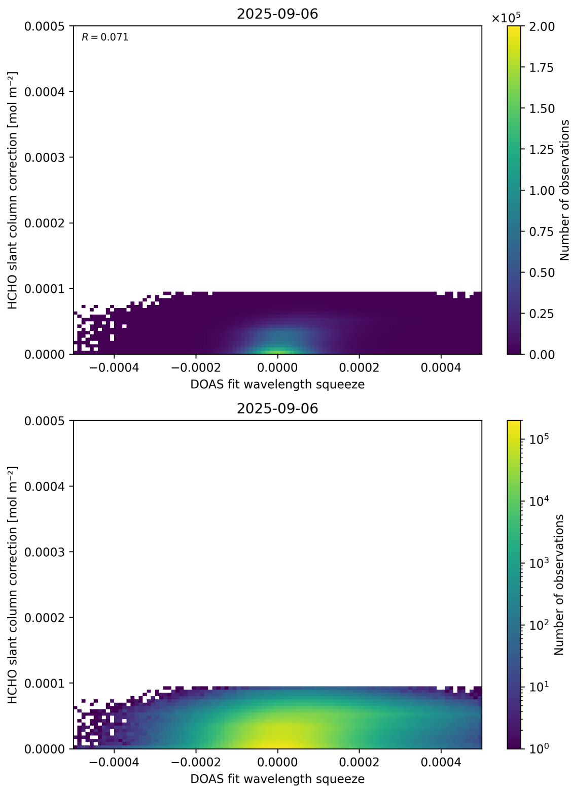
Figure 70: Scatter density plot of “DOAS fit wavelength squeeze” against “HCHO slant column correction” for 2025-09-05 to 2025-09-07.
