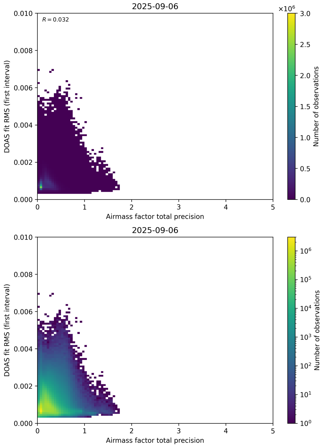
Figure 105: Scatter density plot of “Airmass factor total precision” against “DOAS fit RMS (first interval)” for 2025-09-05 to 2025-09-07.
