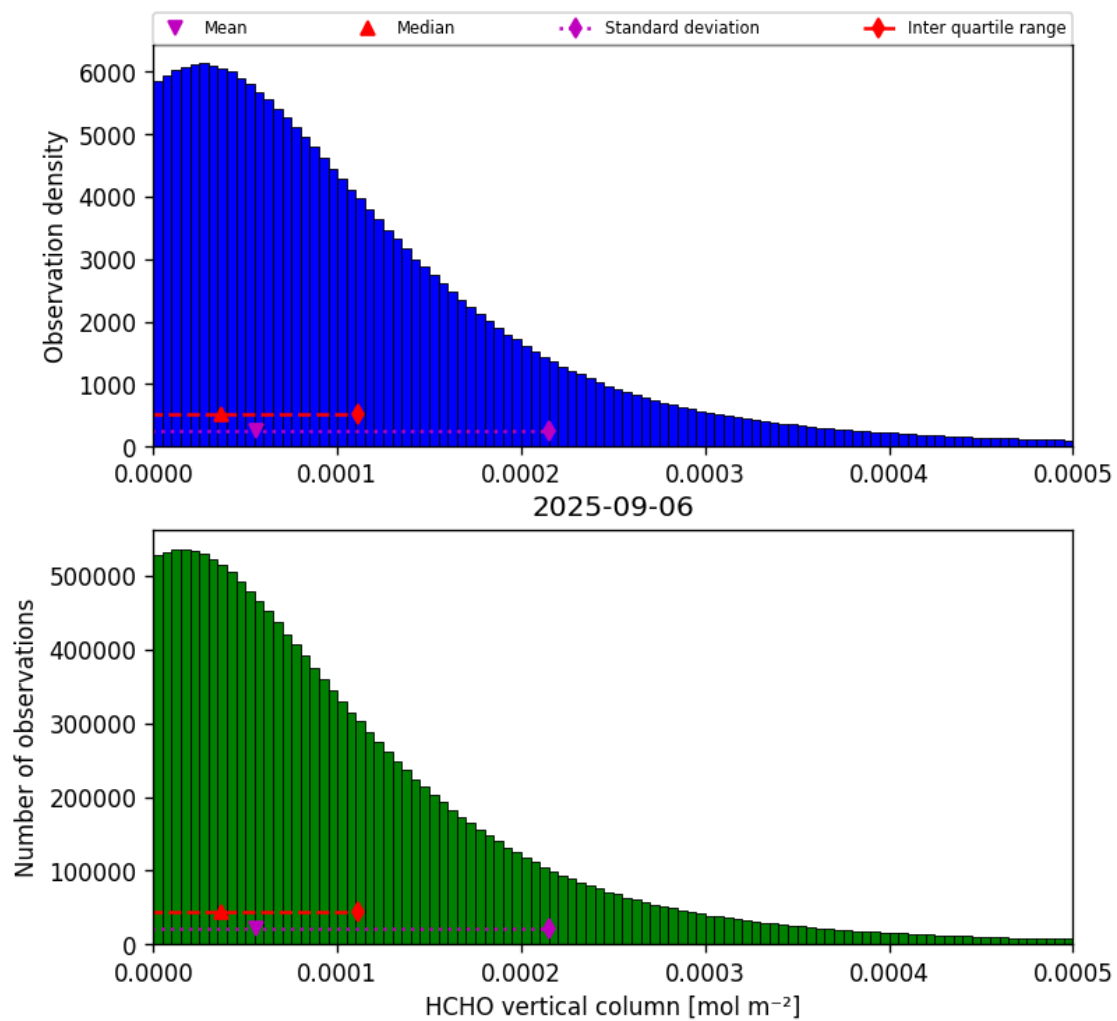
Figure 35: Histogram of “HCHO vertical column” for 2025-09-05 to 2025-09-07
