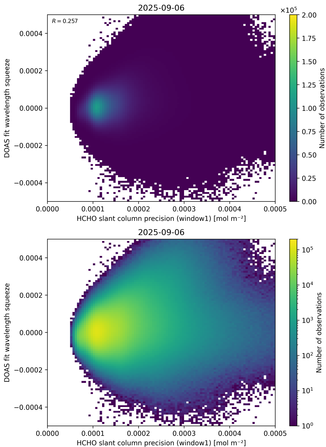
Figure 90: Scatter density plot of “HCHO slant column precision (window1)” against “DOAS fit wavelength squeeze” for 2025-09-05 to 2025-09-07.
