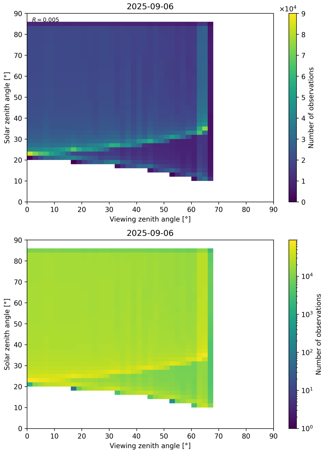
Figure 197: Scatter density plot of “Viewing zenith angle” against “Solar zenith angle” for 2025-09-05 to 2025-09-07.
