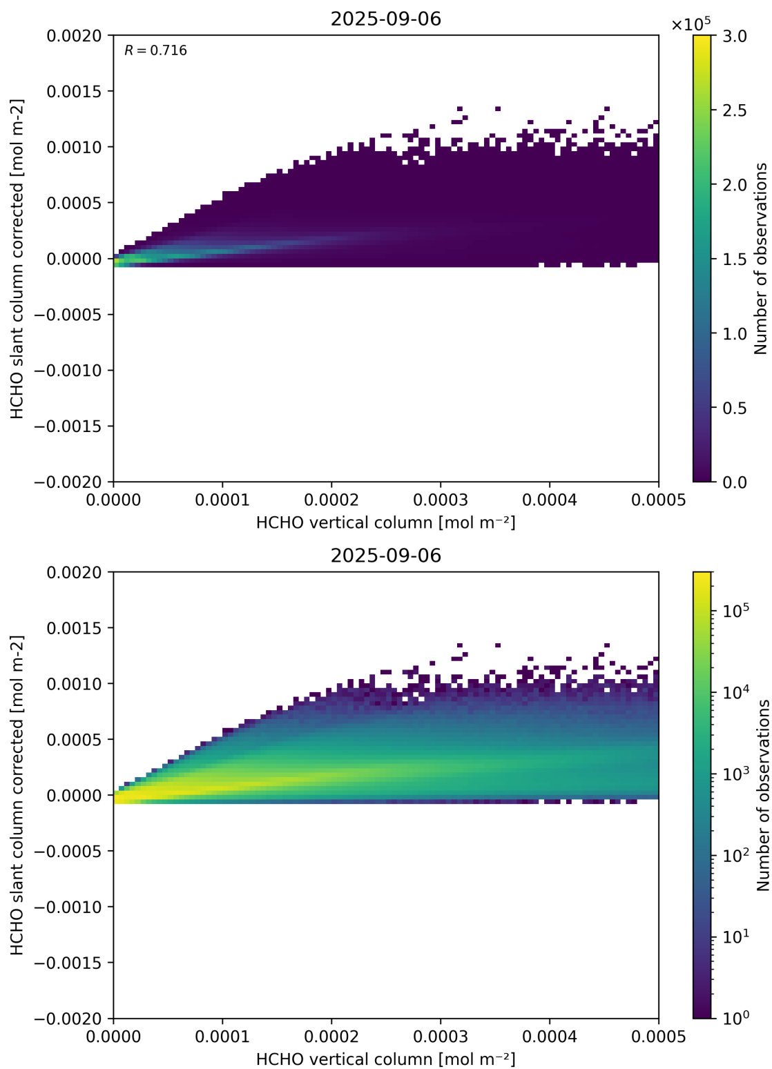
Figure 127: Scatter density plot of “HCHO vertical column” against “HCHO slant column corrected” for 2025-09-05 to 2025-09-07.
