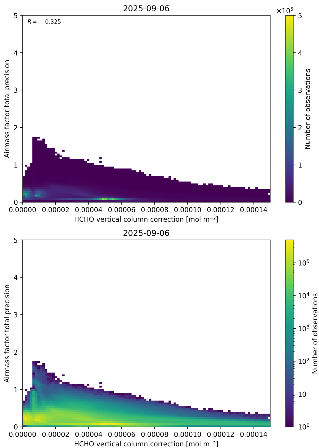
Figure 121: Scatter density plot of “HCHO vertical column correction” against “Airmass factor total precision” for 2025-09-05 to 2025-09-07.
