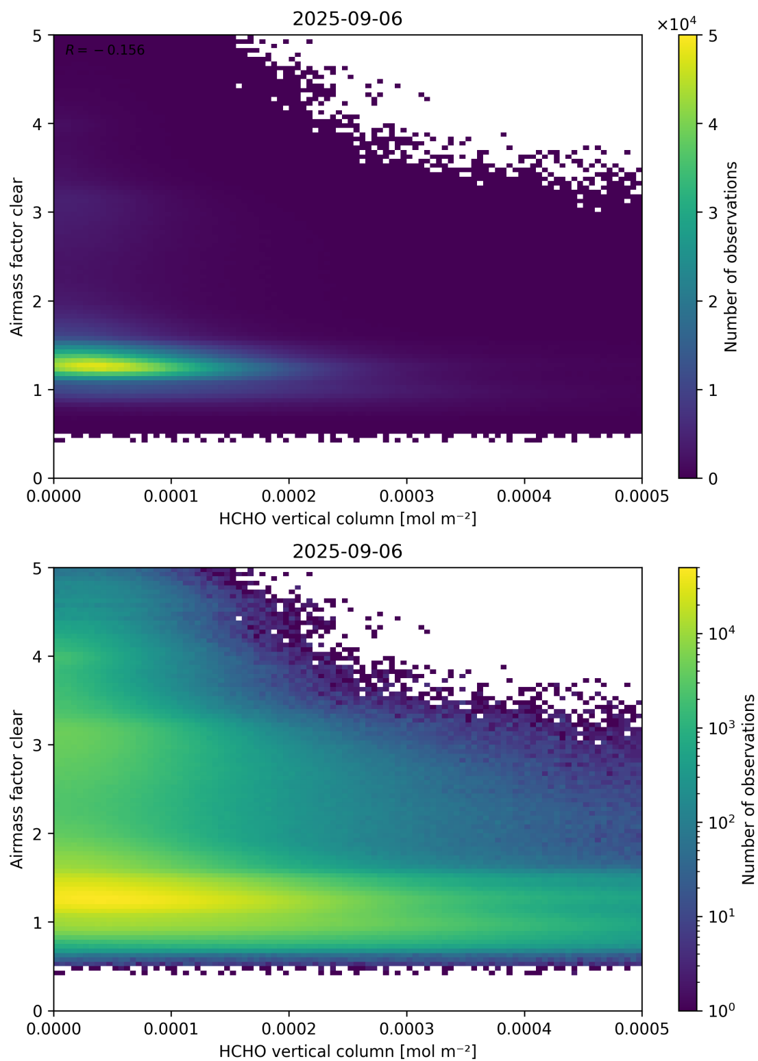
Figure 126: Scatter density plot of “HCHO vertical column” against “Airmass factor clear” for 2025-09-05 to 2025-09-07.
