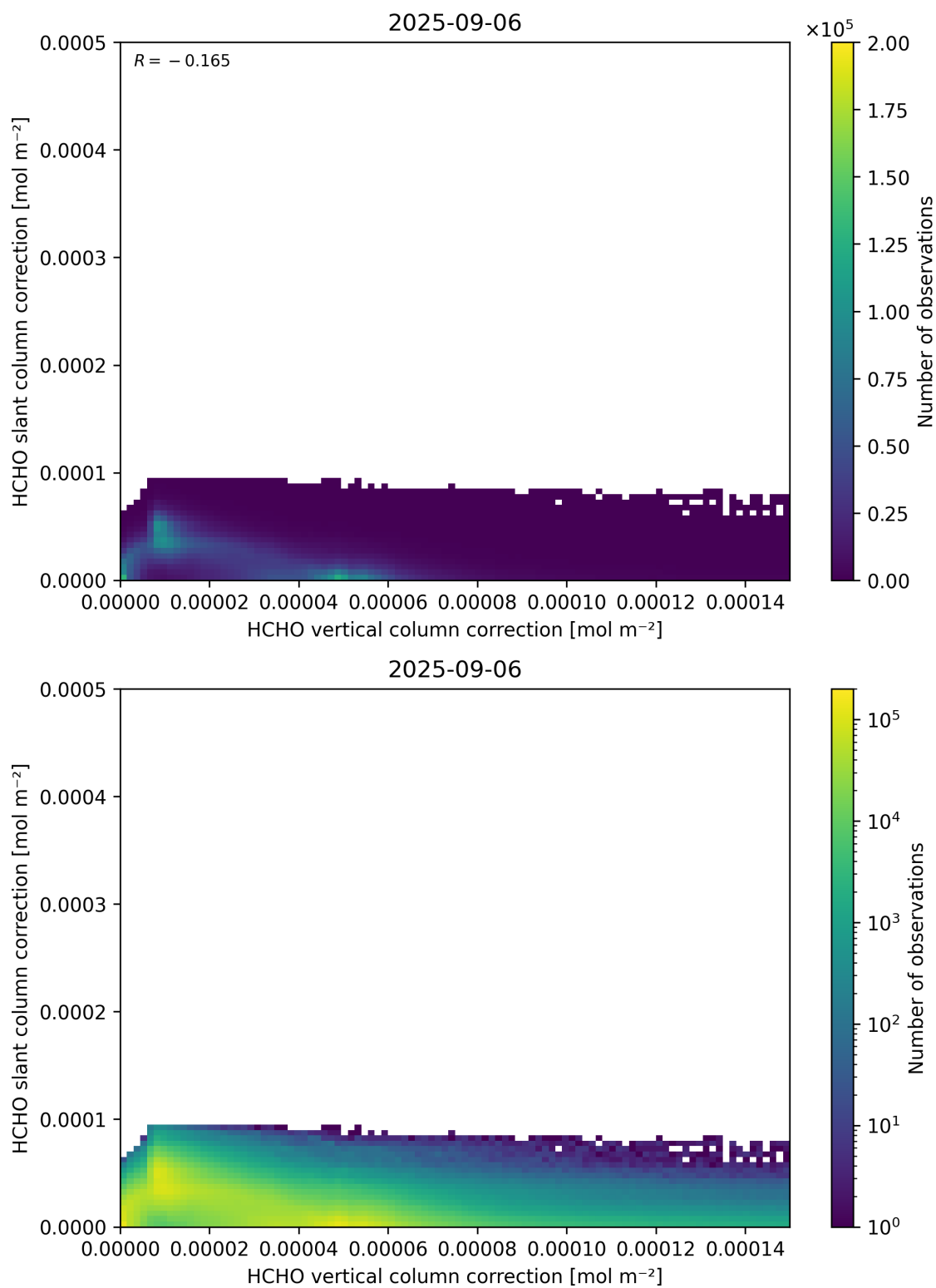
Figure 117: Scatter density plot of “HCHO vertical column correction” against “HCHO slant column correction” for 2025-09-05 to 2025-09-07.
