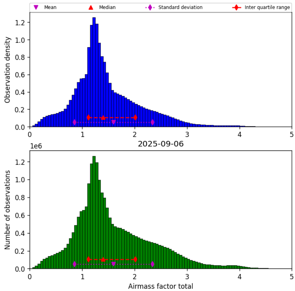
Figure 40: Histogram of “Airmass factor total” for 2025-09-05 to 2025-09-07
