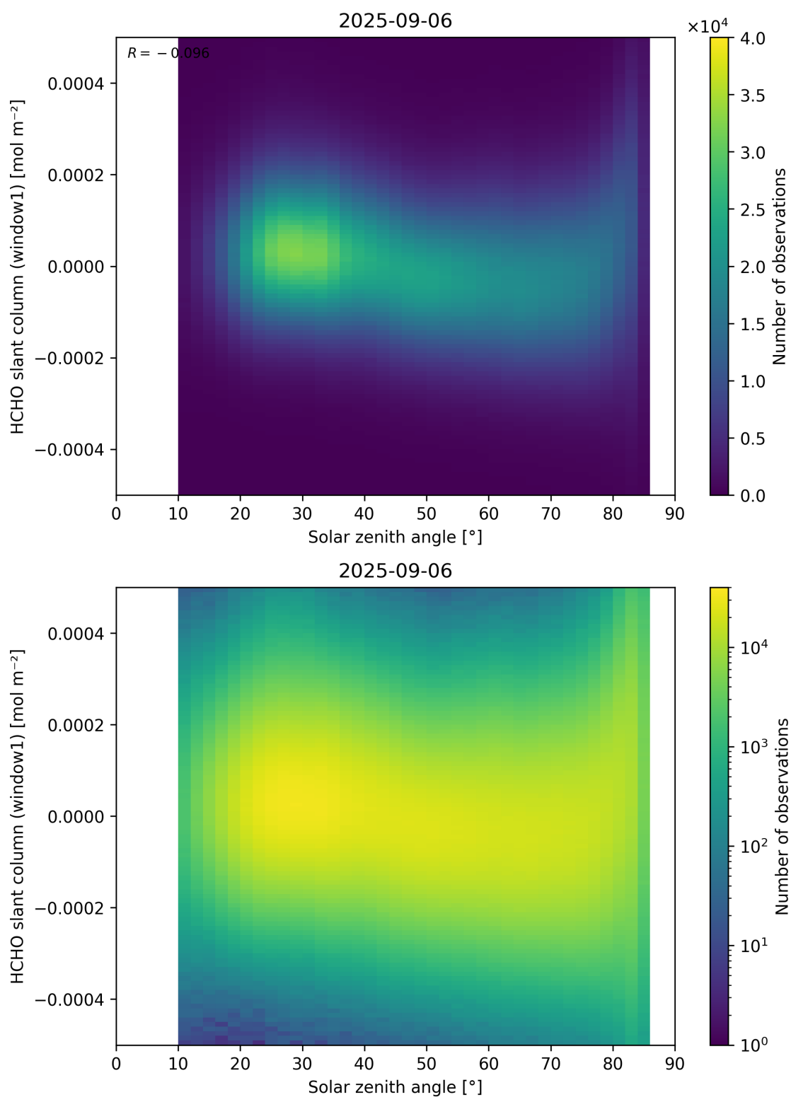
Figure 173: Scatter density plot of “Solar zenith angle” against “HCHO slant column (window1)” for 2025-09-05 to 2025-09-07.
