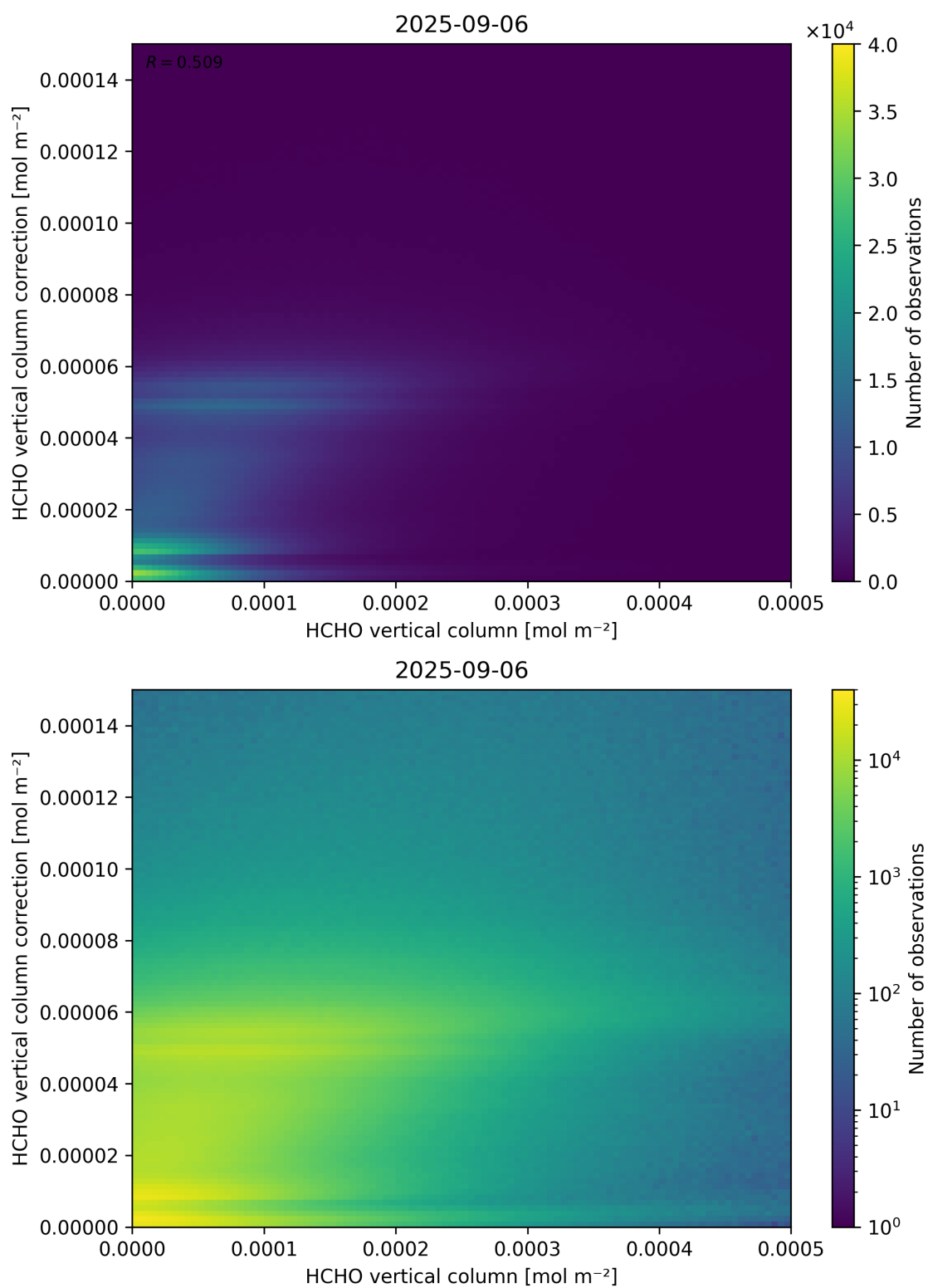
Figure 133: Scatter density plot of “HCHO vertical column” against “HCHO vertical column correction” for 2025-09-05 to 2025-09-07.
