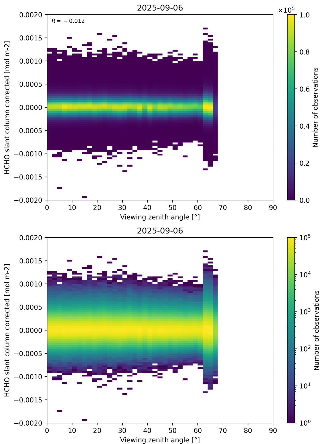
Figure 186: Scatter density plot of “Viewing zenith angle” against “HCHO slant column corrected” for 2025-09-05 to 2025-09-07.
