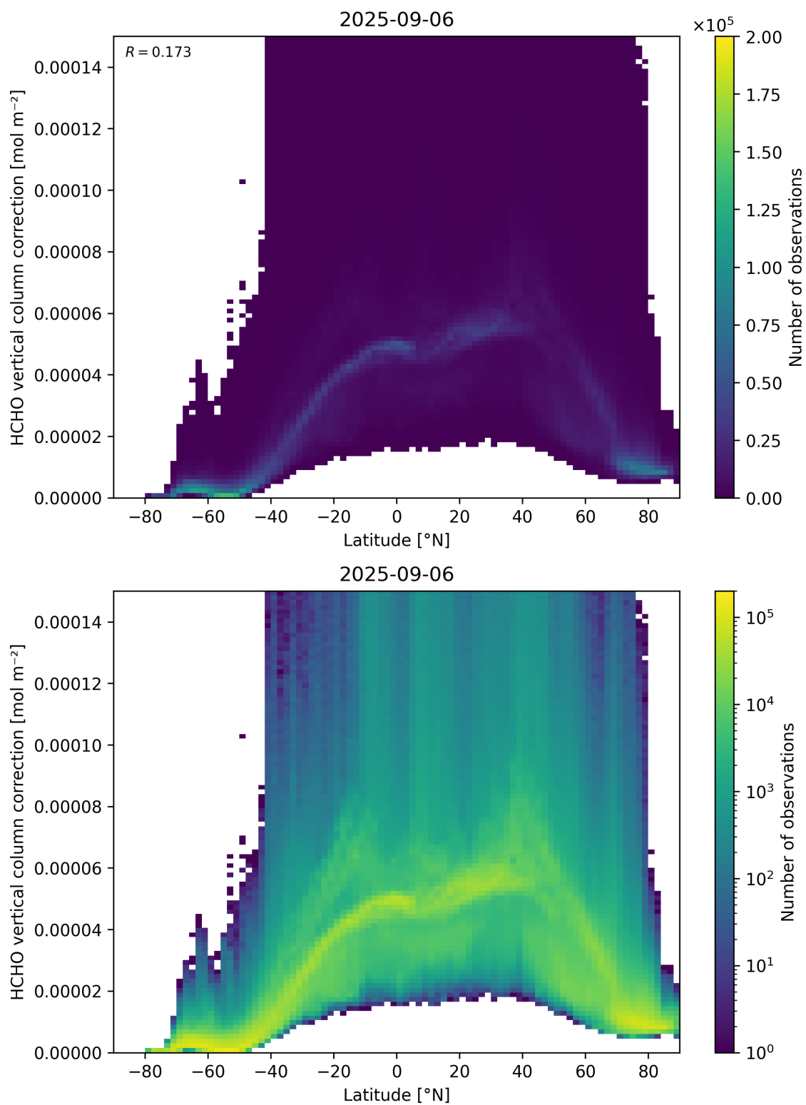
Figure 164: Scatter density plot of “Latitude” against “HCHO vertical column correction” for 2025-09-05 to 2025-09-07.
