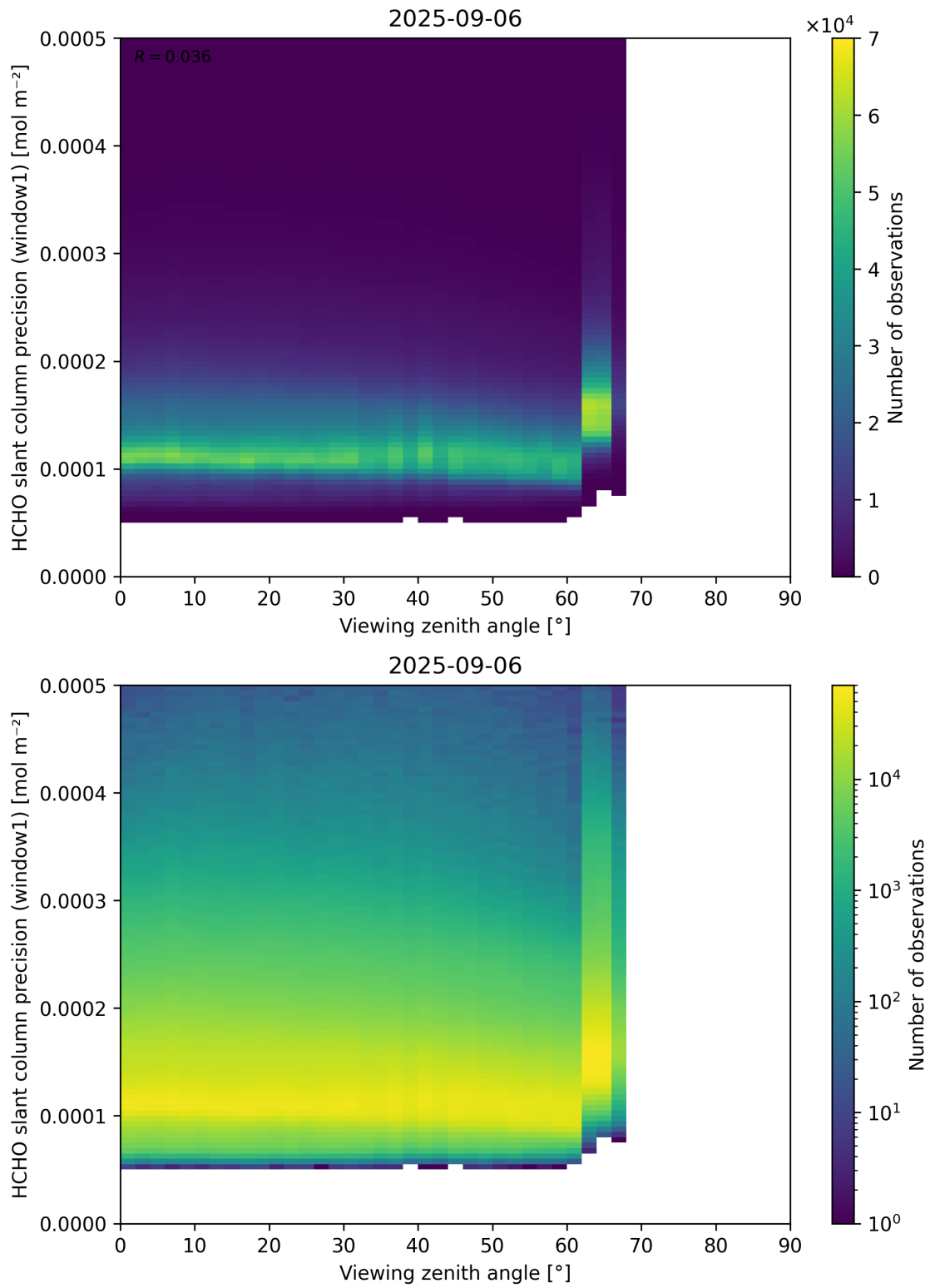
Figure 189: Scatter density plot of “Viewing zenith angle” against “HCHO slant column precision (window1)” for 2025-09-05 to 2025-09-07.
