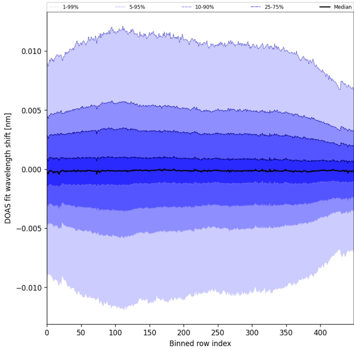
Figure 58: Along track statistics of “DOAS fit wavelength shift” for 2025-09-05 to 2025-09-07
