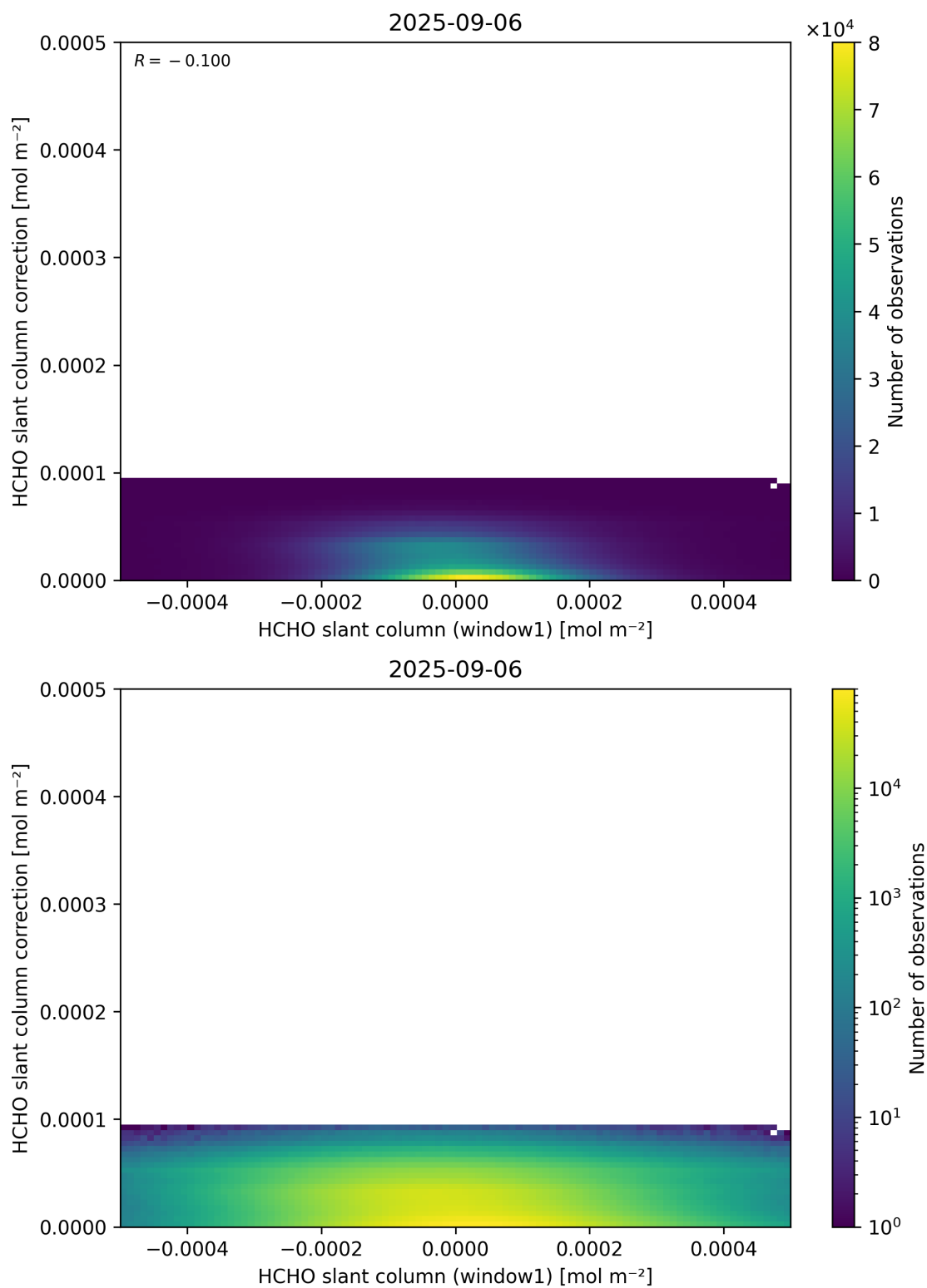
Figure 83: Scatter density plot of “HCHO slant column (window1)” against “HCHO slant column correction” for 2025-09-05 to 2025-09-07.
