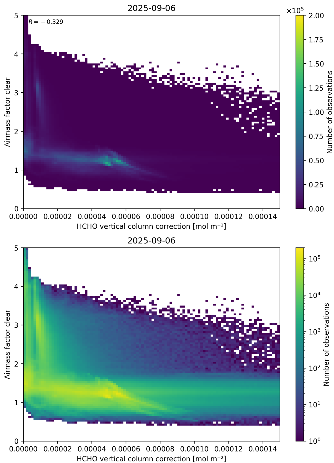
Figure 115: Scatter density plot of “HCHO vertical column correction” against “Airmass factor clear” for 2025-09-05 to 2025-09-07.
