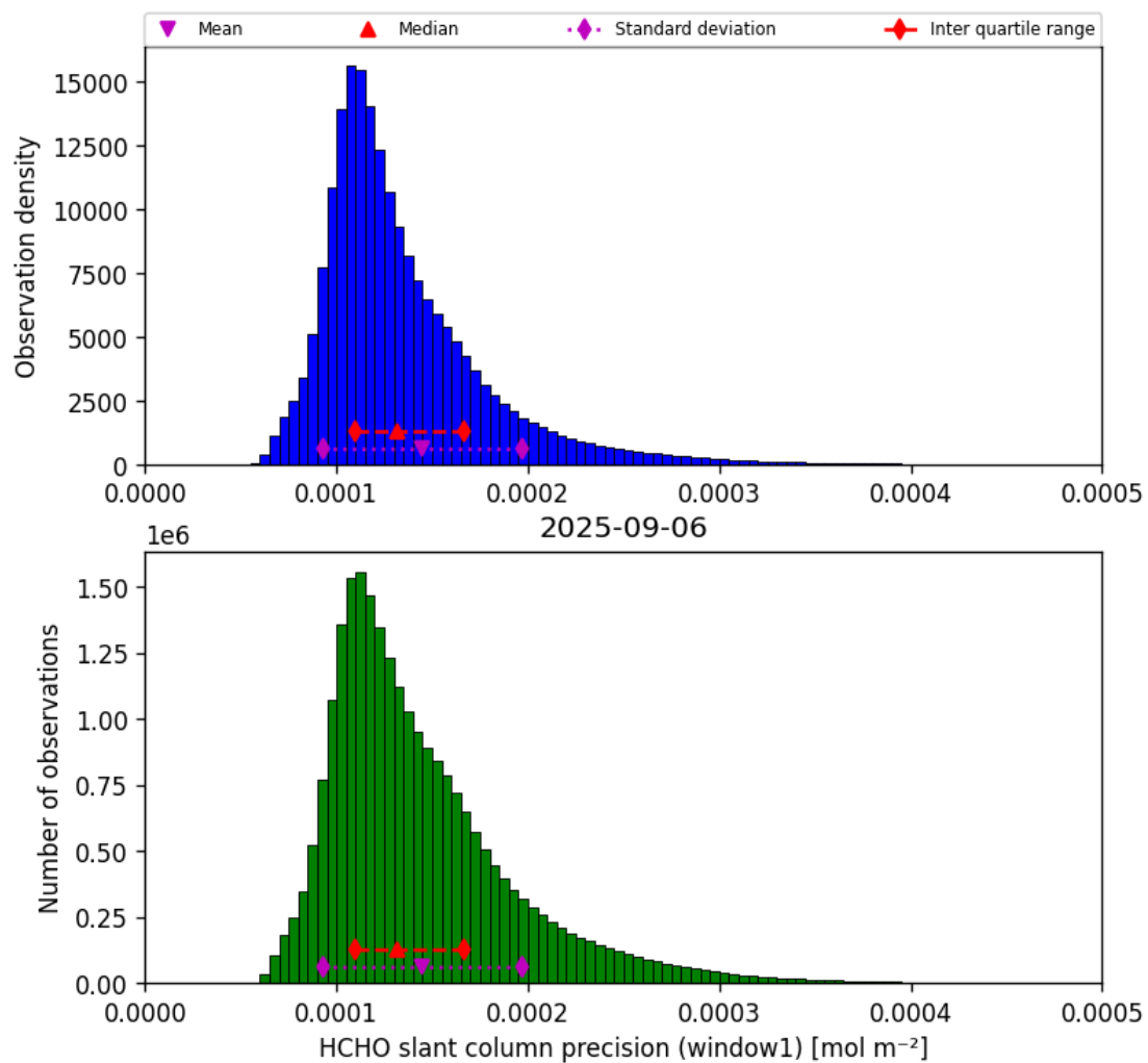
Figure 39: Histogram of “HCHO slant column precision (window1)” for 2025-09-05 to 2025-09-07
