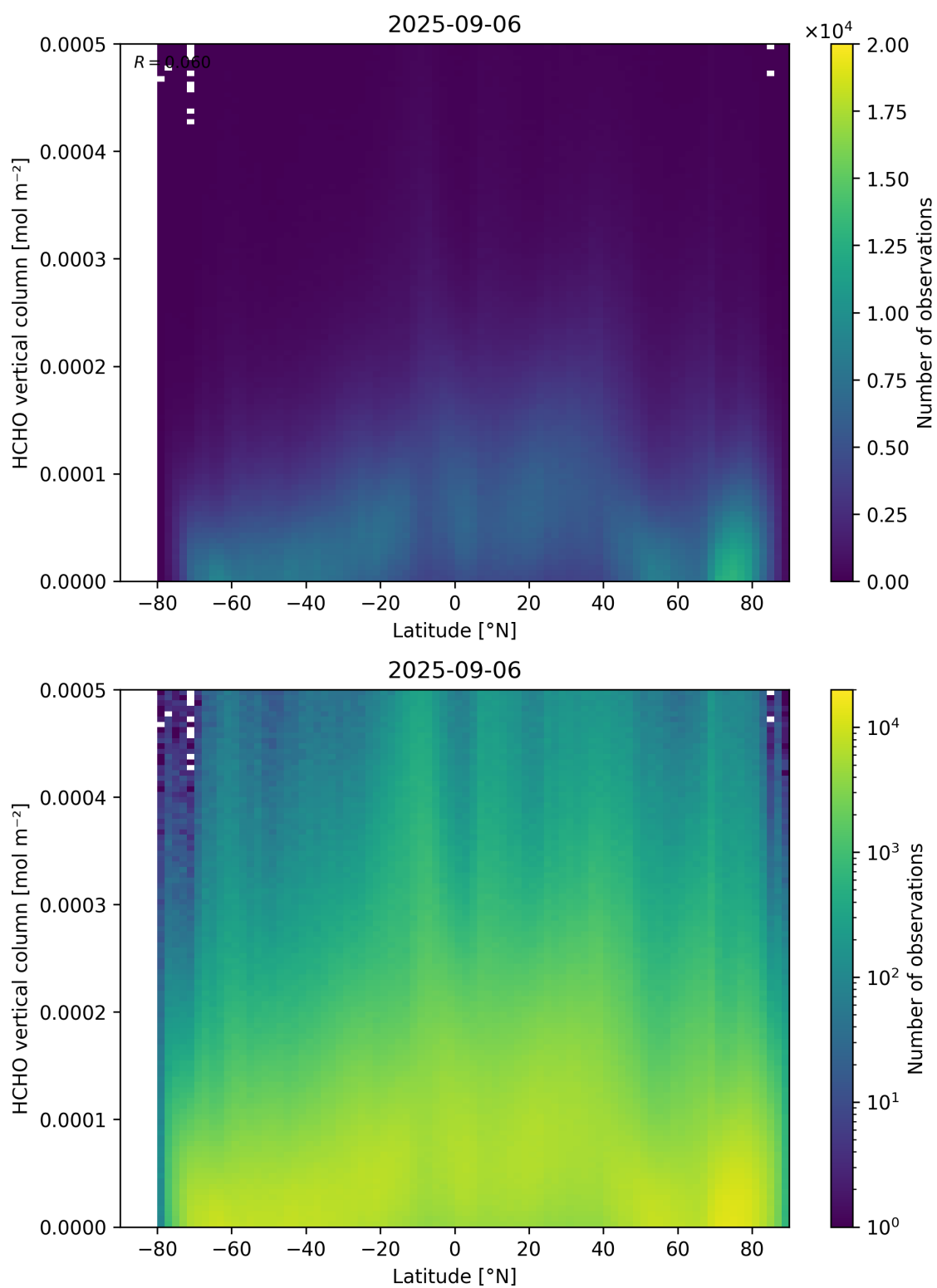
Figure 163: Scatter density plot of “Latitude” against “HCHO vertical column” for 2025-09-05 to 2025-09-07.
