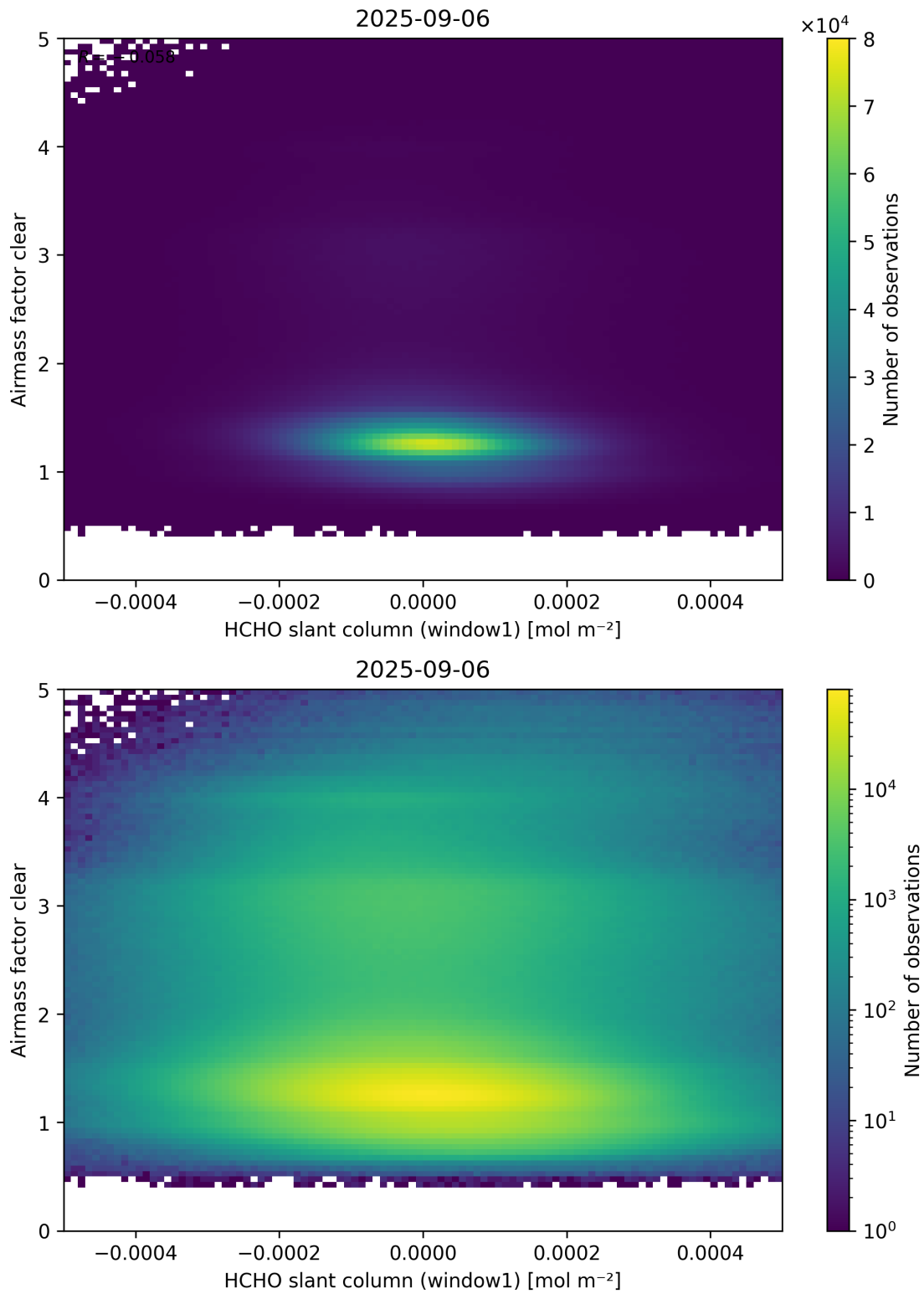
Figure 81: Scatter density plot of “HCHO slant column (window1)” against “Airmass factor clear” for 2025-09-05 to 2025-09-07.
