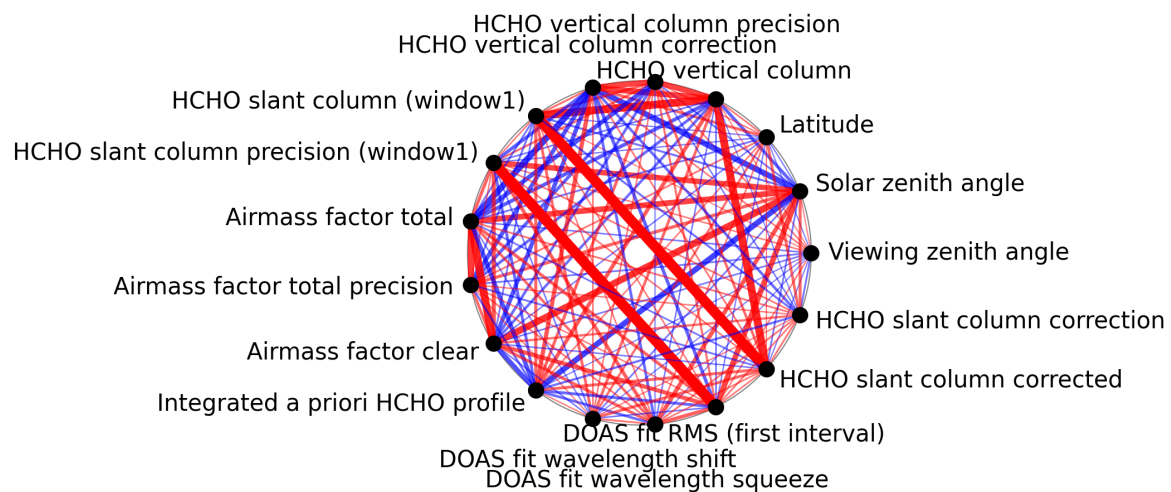
Figure 1: Map of correlation graph for 2025-09-05 to 2025-09-07.
