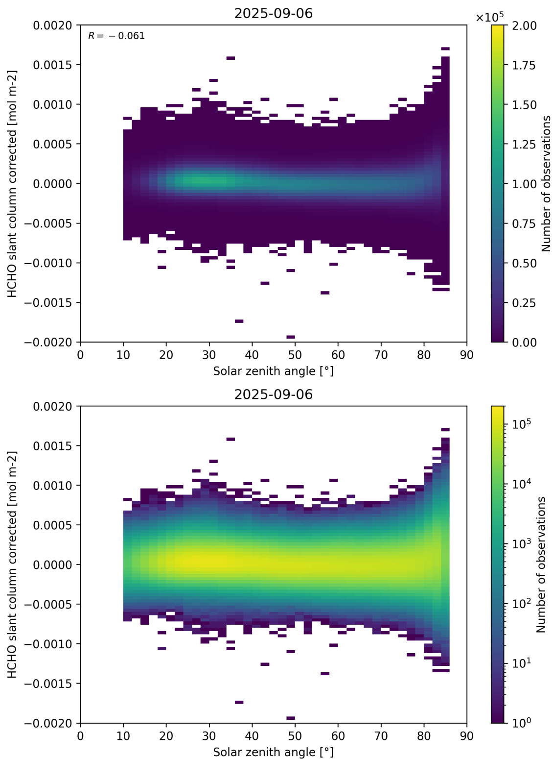
Figure 171: Scatter density plot of “Solar zenith angle” against “HCHO slant column corrected” for 2025-09-05 to 2025-09-07.
