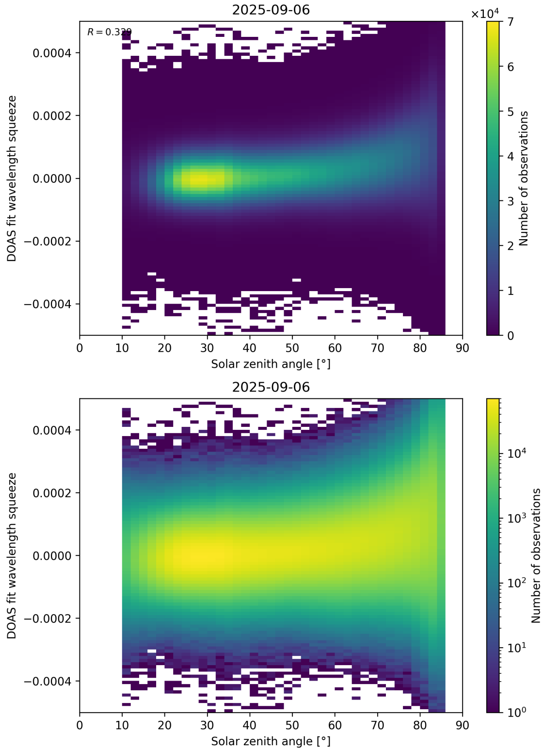
Figure 169: Scatter density plot of “Solar zenith angle” against “DOAS fit wavelength squeeze” for 2025-09-05 to 2025-09-07.
