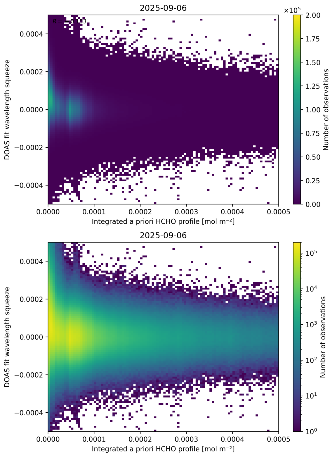
Figure 150: Scatter density plot of “Integrated a priori HCHO profile” against “DOAS fit wavelength squeeze” for 2025-09-05 to 2025-09-07.
