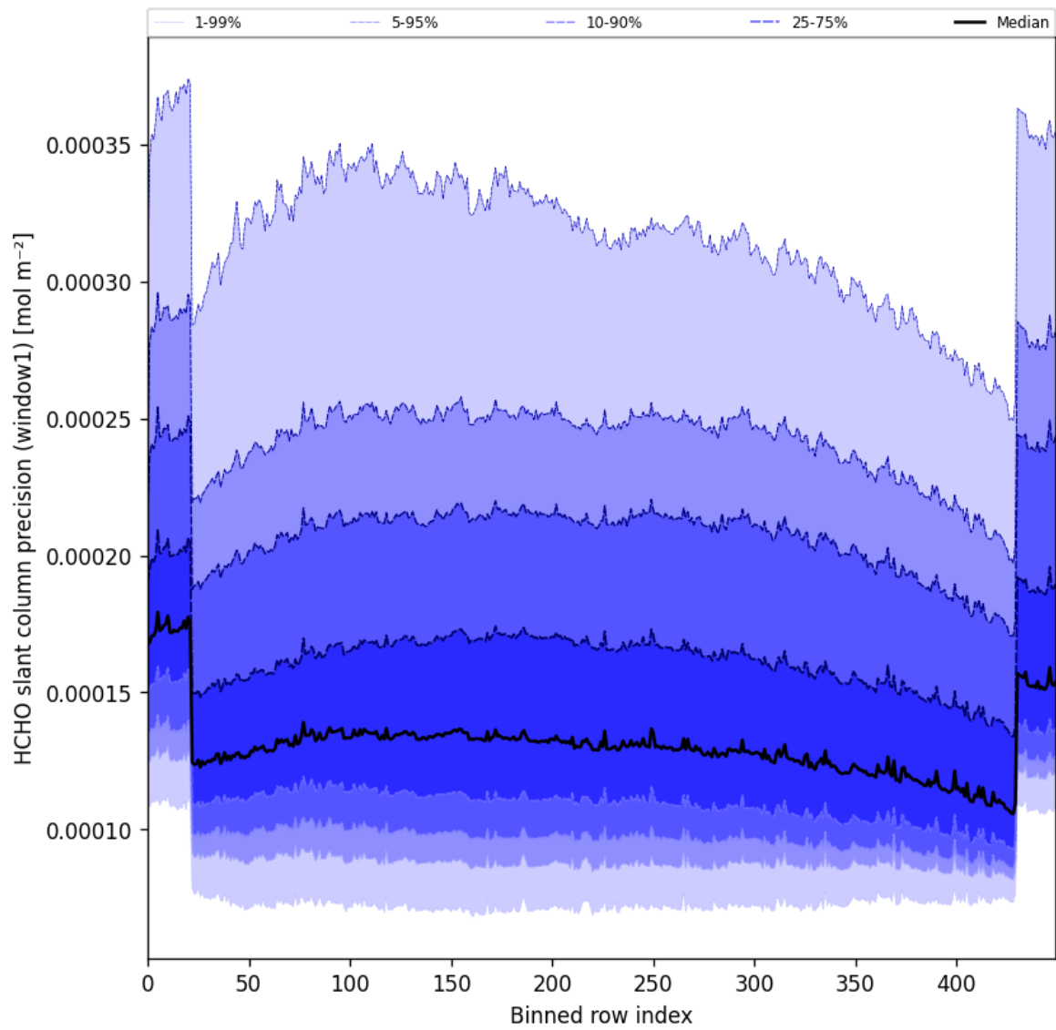
Figure 53: Along track statistics of “HCHO slant column precision (window1)” for 2025-09-05 to 2025-09-07
