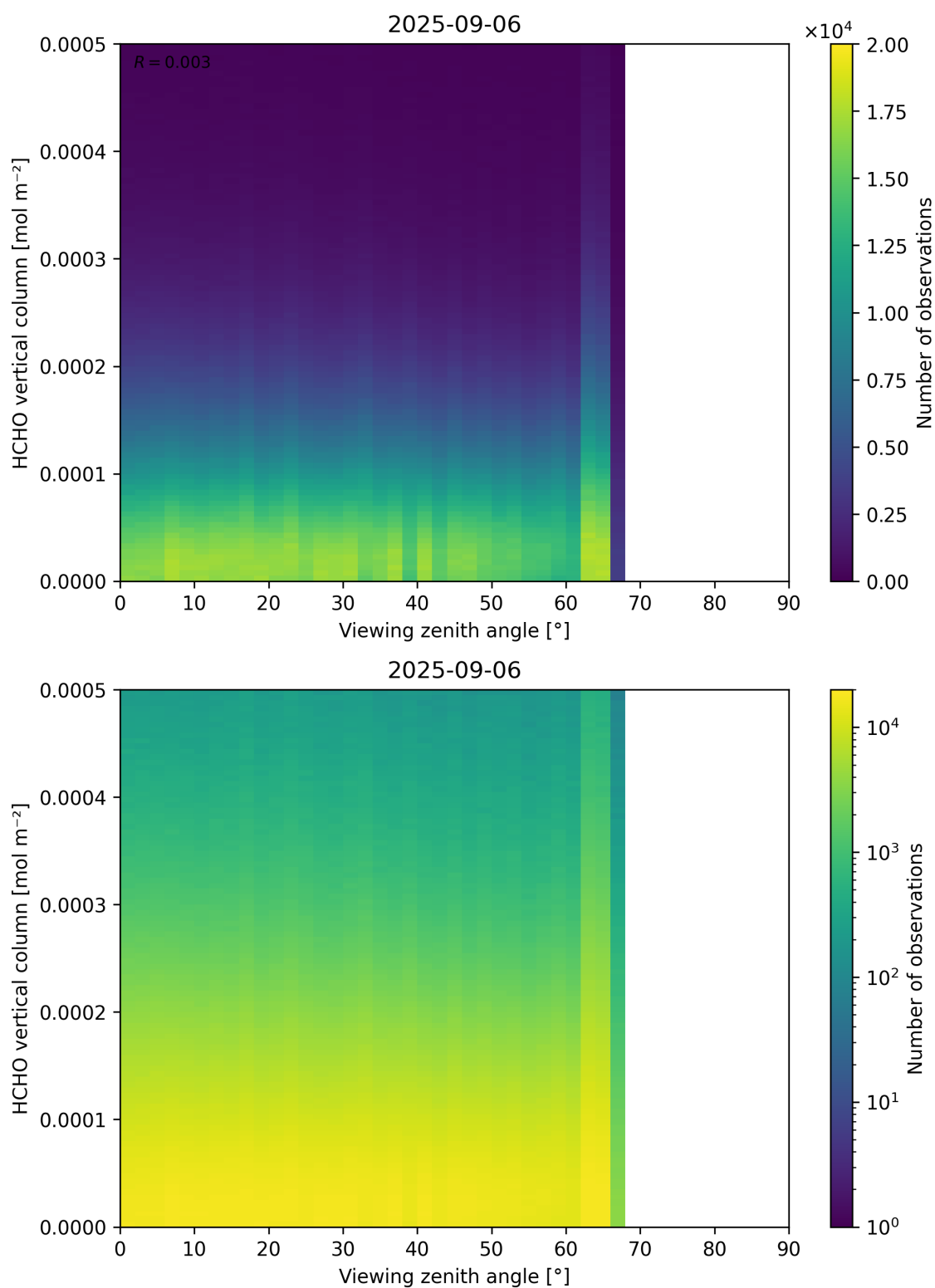
Figure 192: Scatter density plot of “Viewing zenith angle” against “HCHO vertical column” for 2025-09-05 to 2025-09-07.
