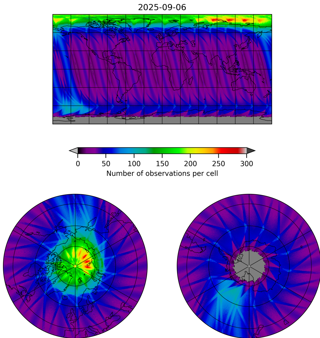
Figure 19: Map of the number of observations for 2025-09-05 to 2025-09-07
