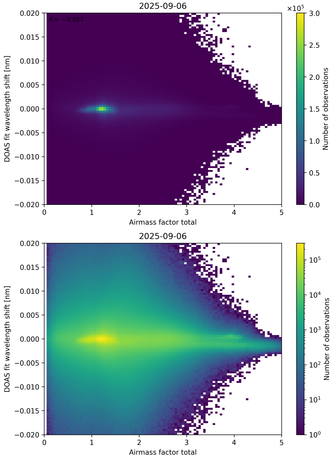
Figure 98: Scatter density plot of “Airmass factor total” against “DOAS fit wavelength shift” for 2025-09-05 to 2025-09-07.
