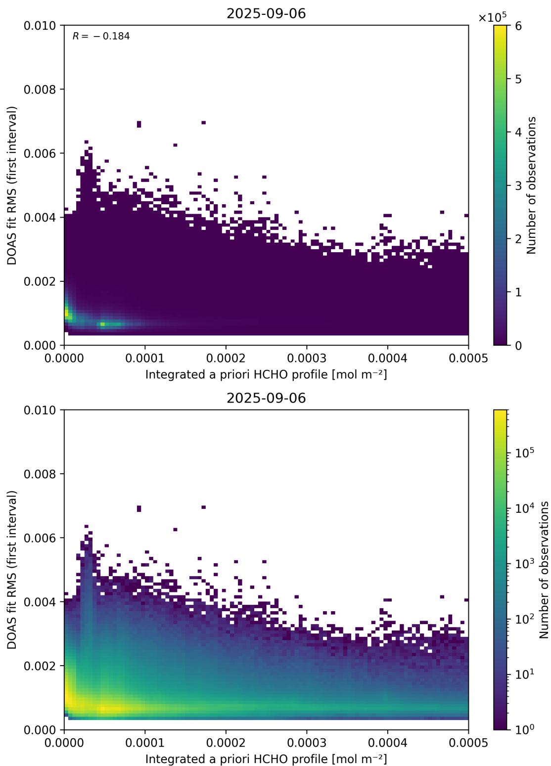
Figure 148: Scatter density plot of “Integrated a priori HCHO profile” against “DOAS fit RMS (first interval)” for 2025-09-05 to 2025-09-07.
