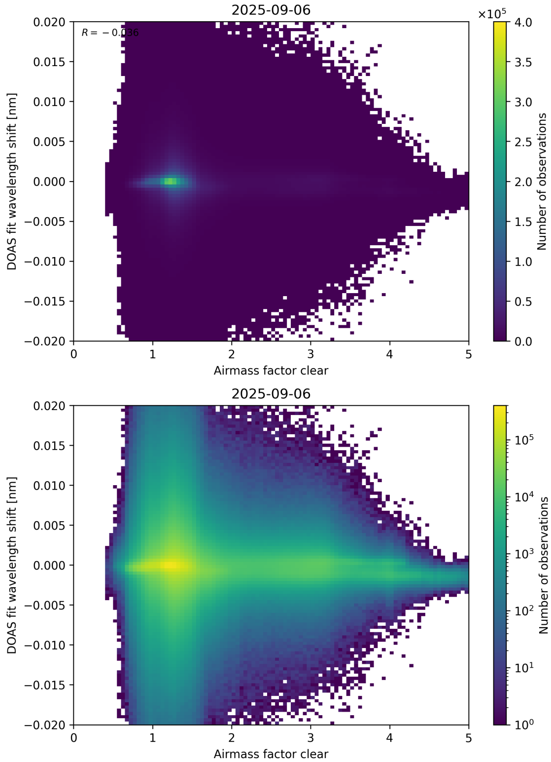
Figure 72: Scatter density plot of “Airmass factor clear” against “DOAS fit wavelength shift” for 2025-09-05 to 2025-09-07.
