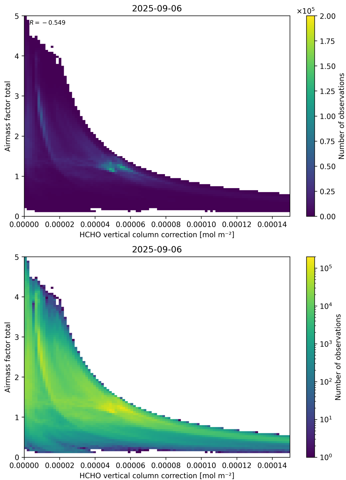
Figure 120: Scatter density plot of “HCHO vertical column correction” against “Airmass factor total” for 2025-09-05 to 2025-09-07.
