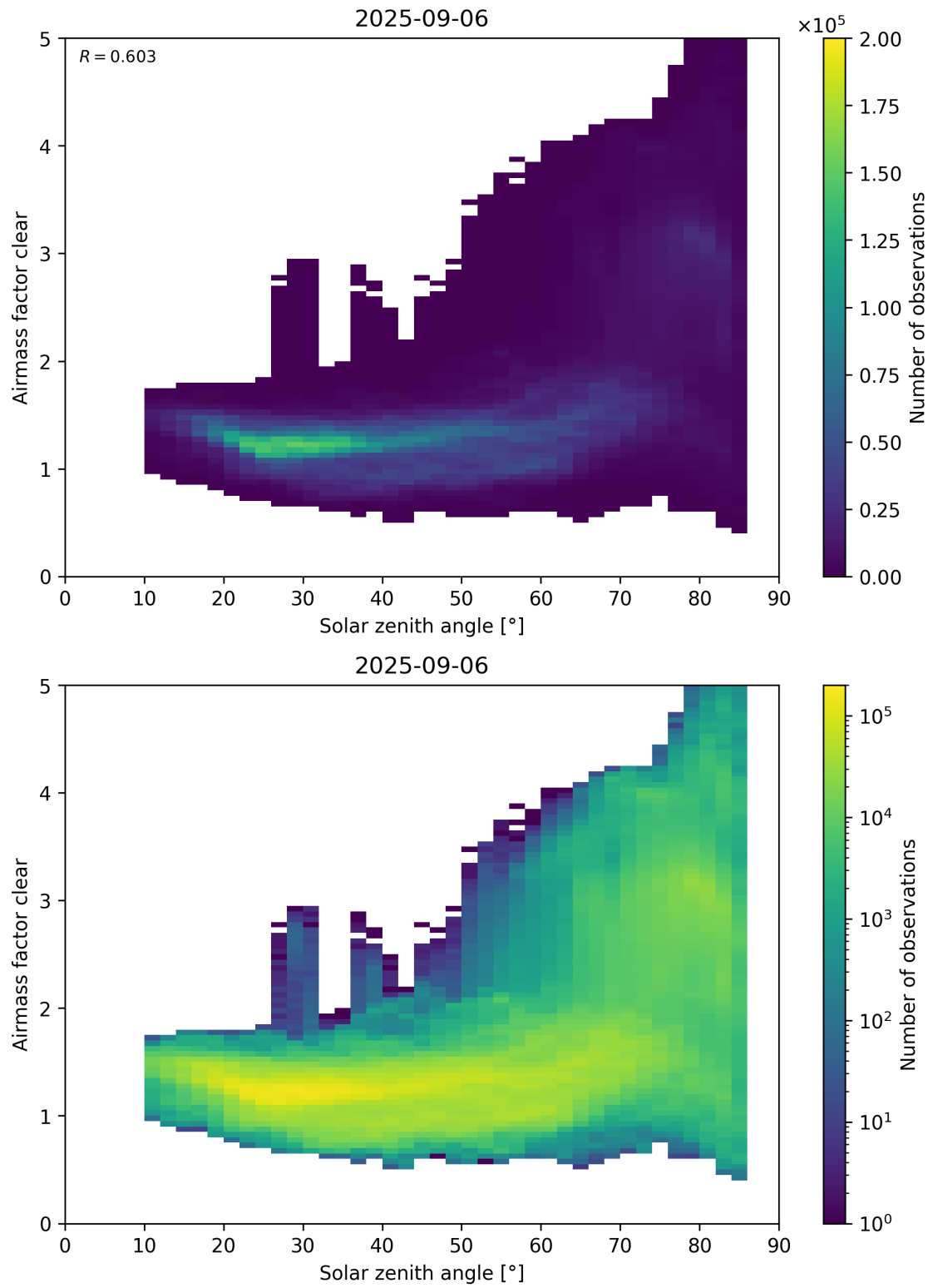
Figure 170: Scatter density plot of “Solar zenith angle” against “Airmass factor clear” for 2025-09-05 to 2025-09-07.
