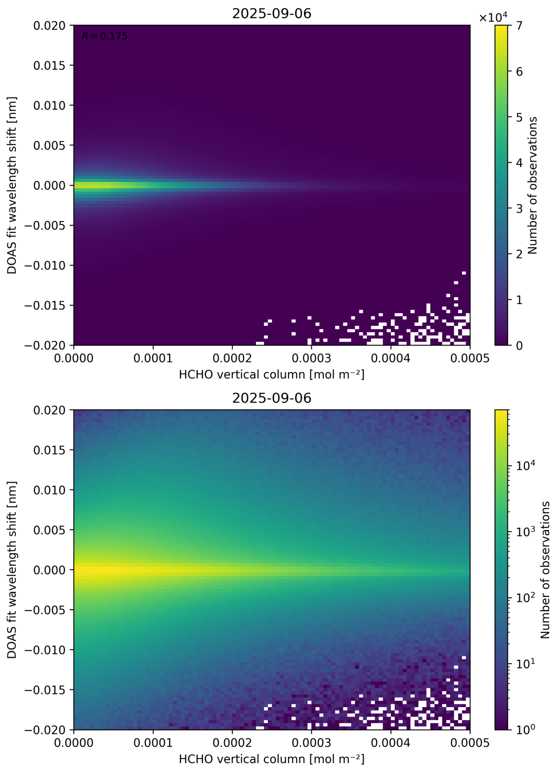
Figure 124: Scatter density plot of “HCHO vertical column” against “DOAS fit wavelength shift” for 2025-09-05 to 2025-09-07.
