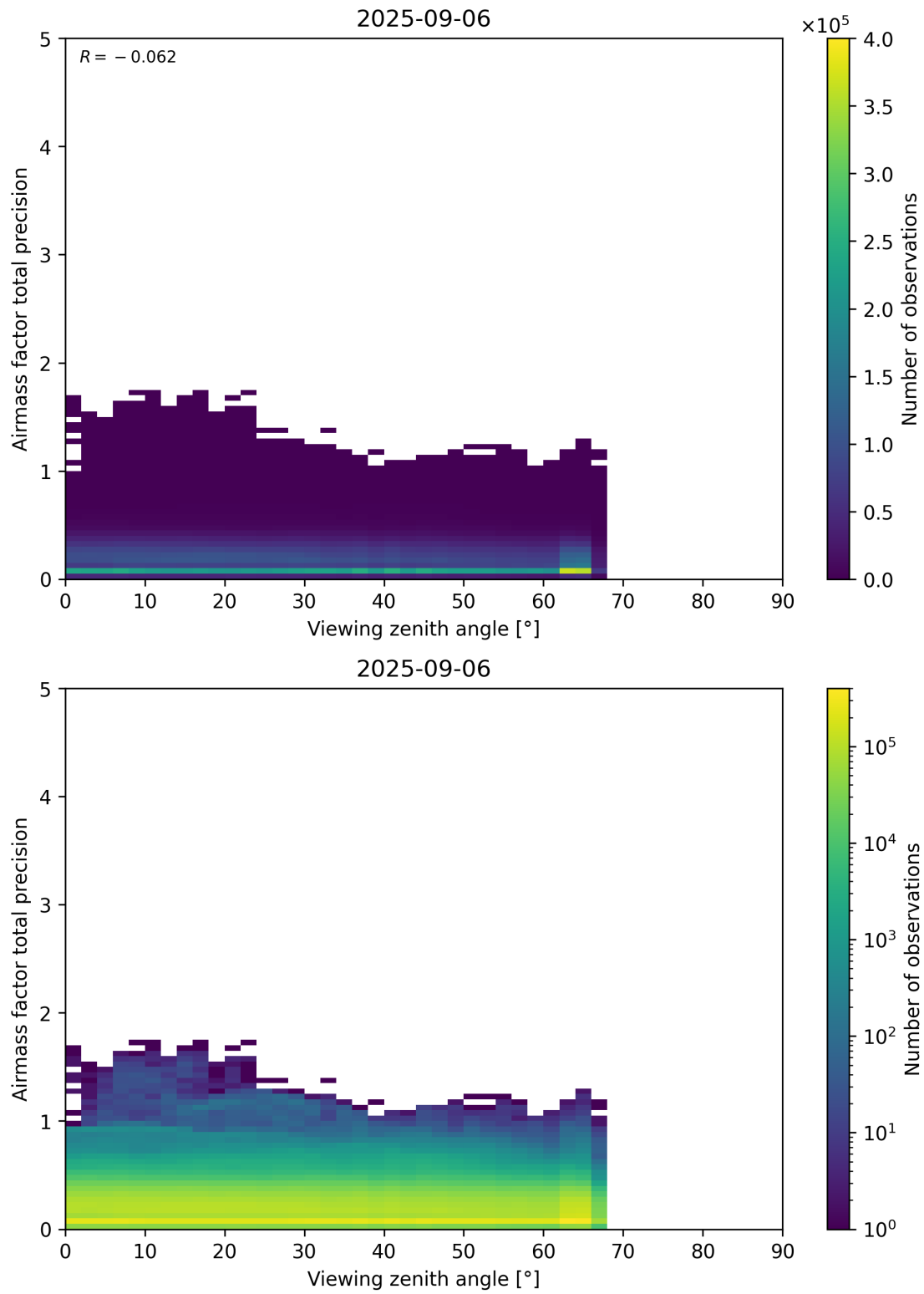
Figure 191: Scatter density plot of “Viewing zenith angle” against “Airmass factor total precision” for 2025-09-05 to 2025-09-07.
