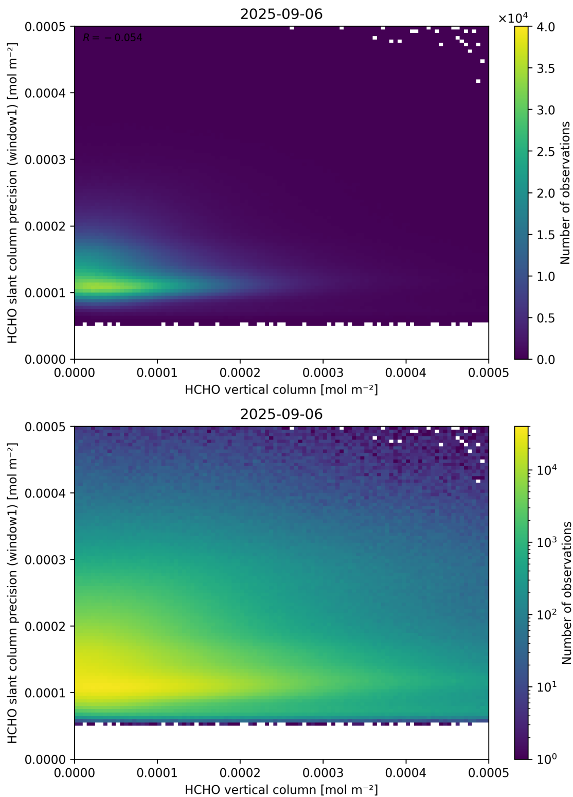
Figure 130: Scatter density plot of “HCHO vertical column” against “HCHO slant column precision (window1)” for 2025-09-05 to 2025-09-07.
