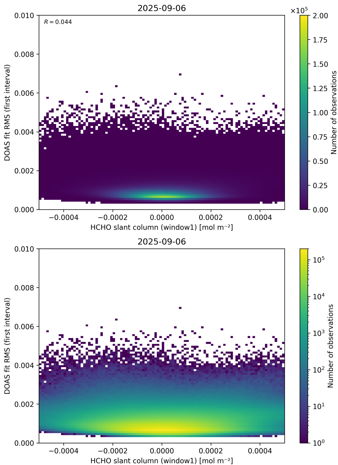
Figure 78: Scatter density plot of “HCHO slant column (window1)” against “DOAS fit RMS (first interval)” for 2025-09-05 to 2025-09-07.
