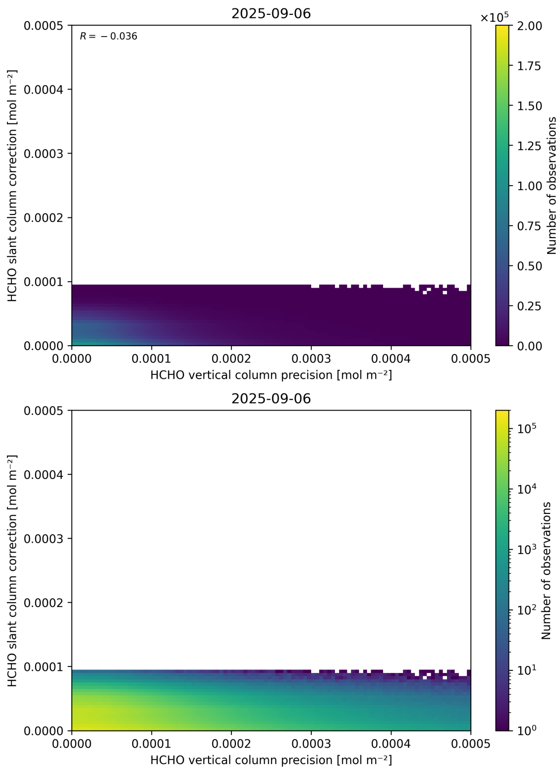
Figure 141: Scatter density plot of “HCHO vertical column precision” against “HCHO slant column correction” for 2025-09-05 to 2025-09-07.
