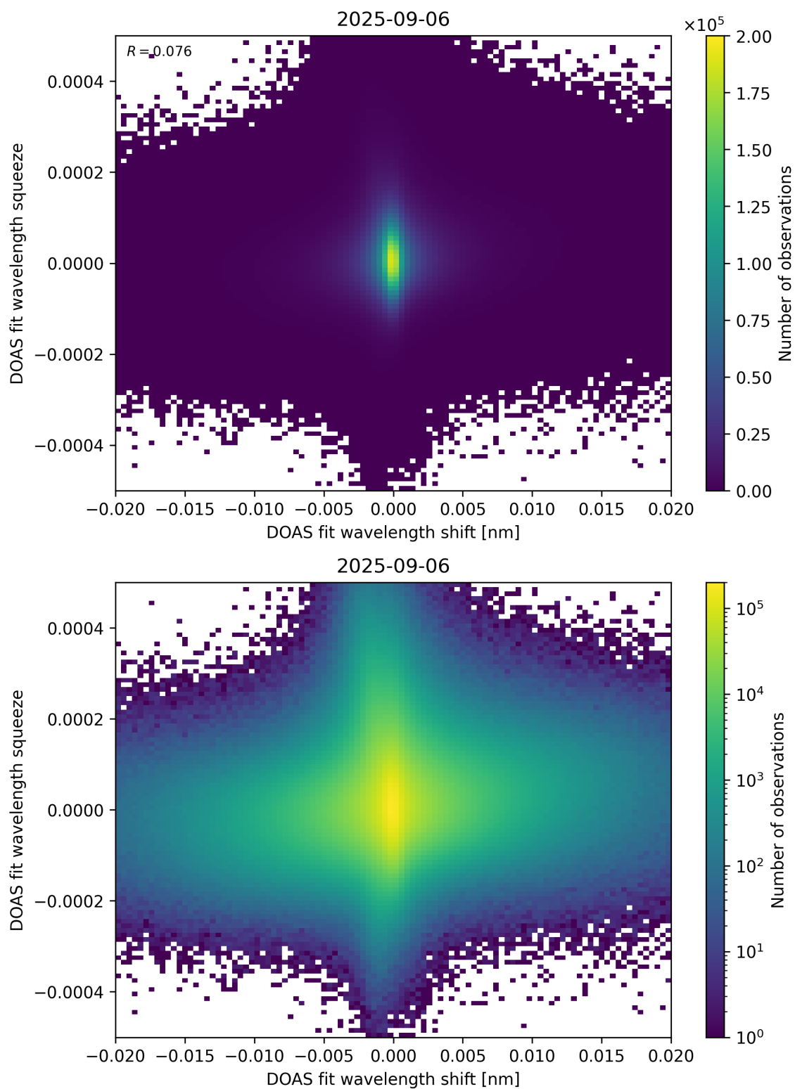
Figure 65: Scatter density plot of “DOAS fit wavelength shift” against “DOAS fit wavelength squeeze” for 2025-09-05 to 2025-09-07.
