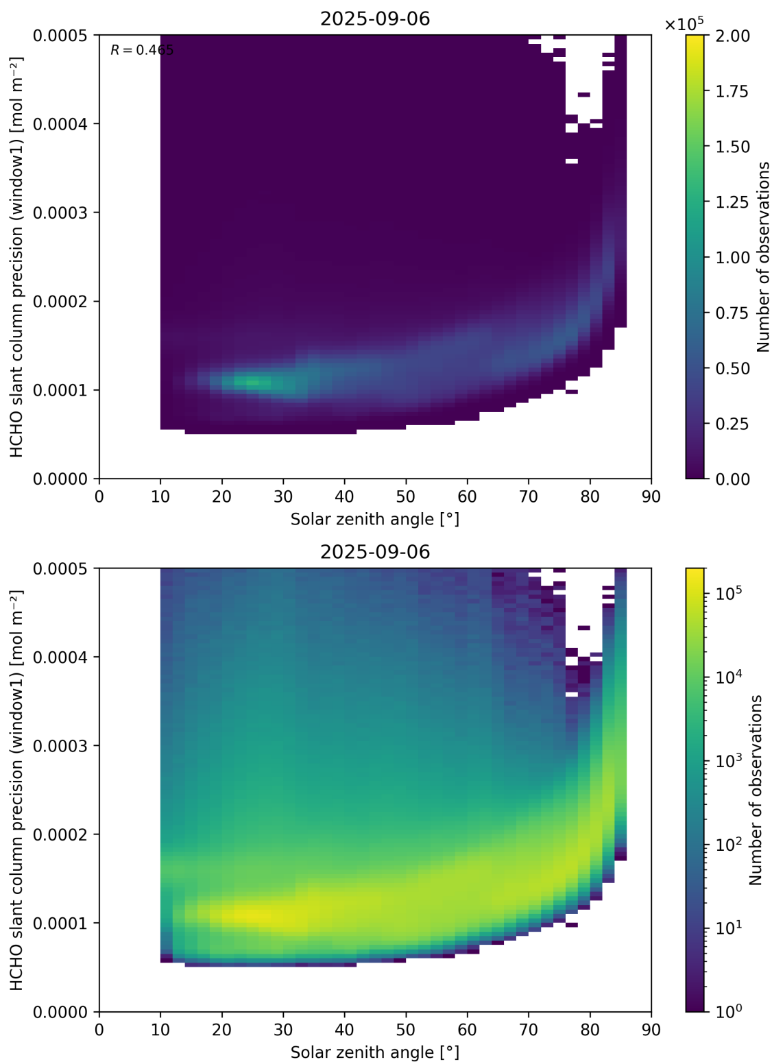
Figure 174: Scatter density plot of “Solar zenith angle” against “HCHO slant column precision (window1)” for 2025-09-05 to 2025-09-07.
