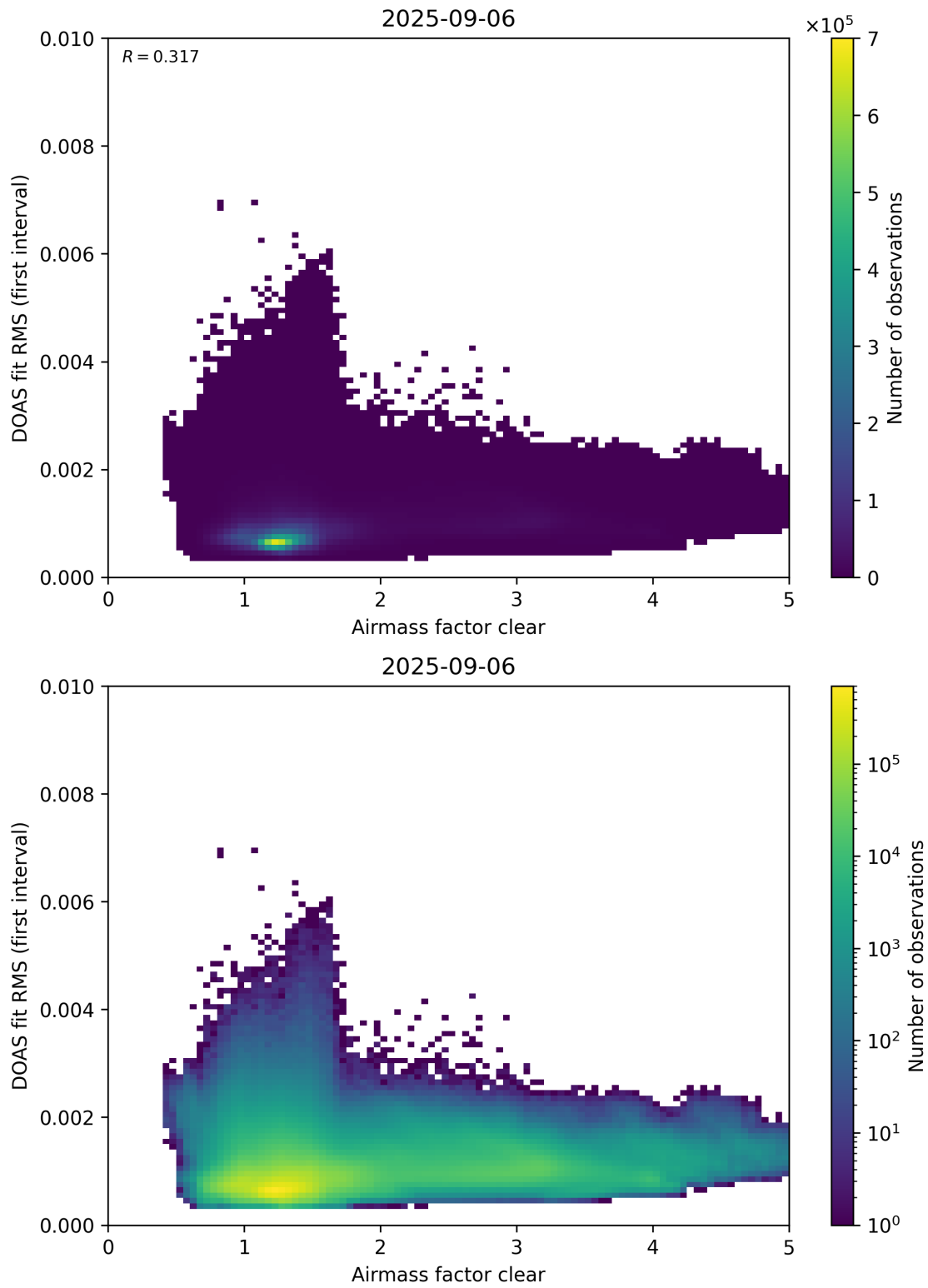
Figure 71: Scatter density plot of “Airmass factor clear” against “DOAS fit RMS (first interval)” for 2025-09-05 to 2025-09-07.
