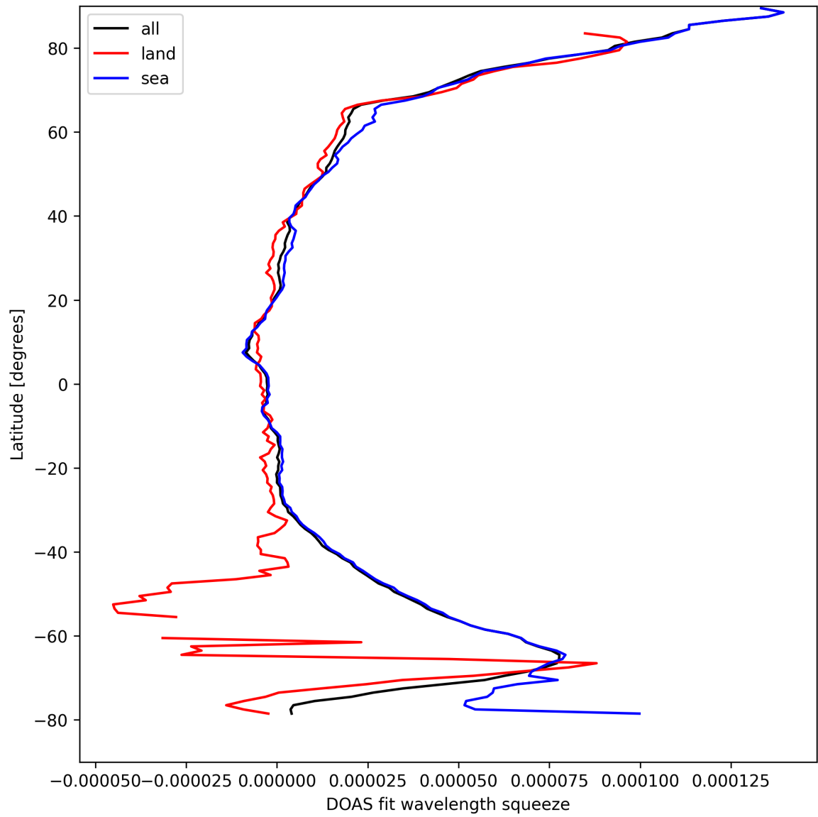
Figure 31: Zonal average of “DOAS fit wavelength squeeze” for 2025-09-05 to 2025-09-07.
