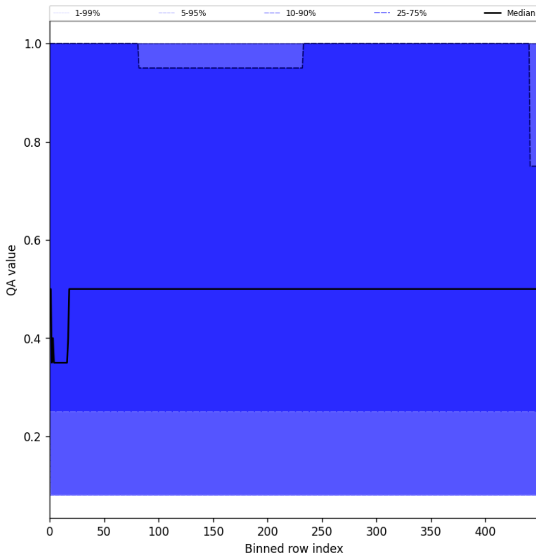
Figure 48: Along track statistics of “QA value” for 2025-09-05 to 2025-09-07
