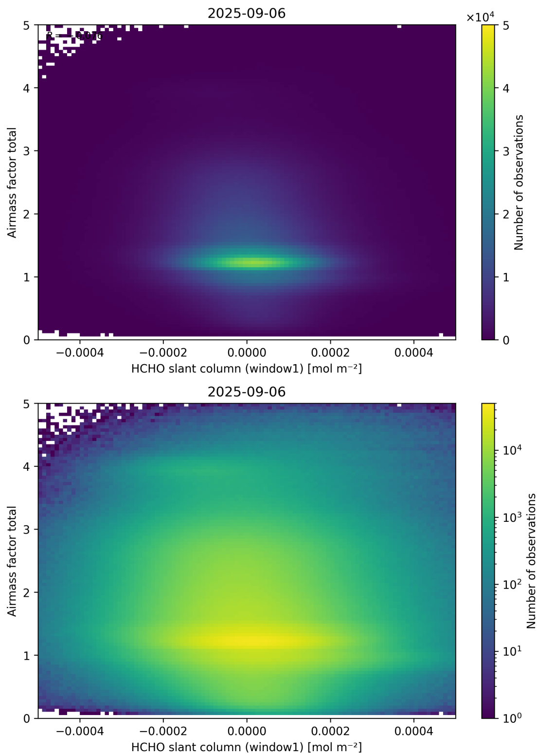
Figure 85: Scatter density plot of “HCHO slant column (window1)” against “Airmass factor total” for 2025-09-05 to 2025-09-07.
