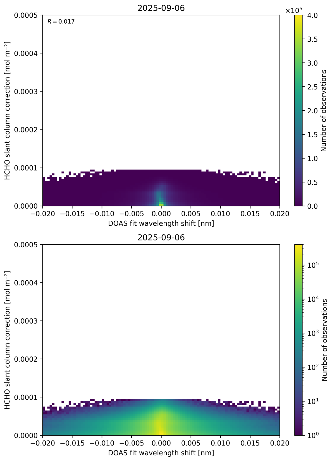
Figure 67: Scatter density plot of “DOAS fit wavelength shift” against “HCHO slant column correction” for 2025-09-05 to 2025-09-07.
