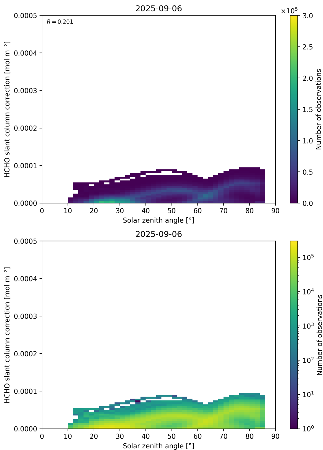
Figure 172: Scatter density plot of “Solar zenith angle” against “HCHO slant column correction” for 2025-09-05 to 2025-09-07.
