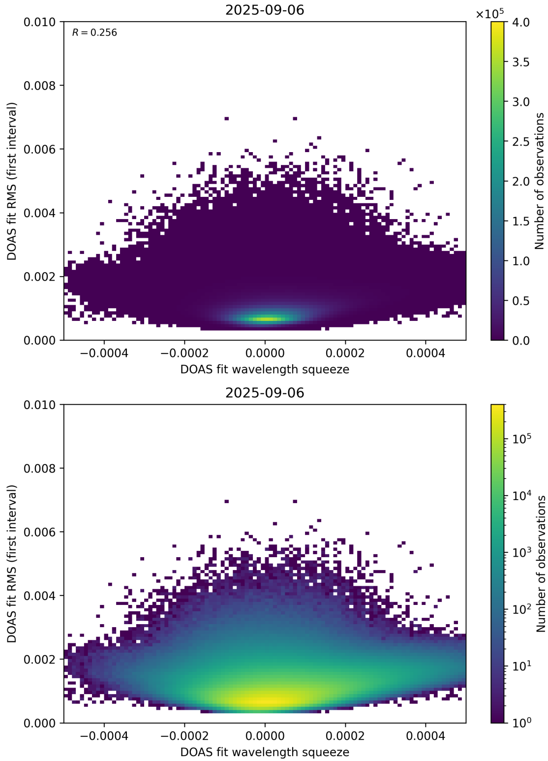
Figure 68: Scatter density plot of “DOAS fit wavelength squeeze” against “DOAS fit RMS (first interval)” for 2025-09-05 to 2025-09-07.
