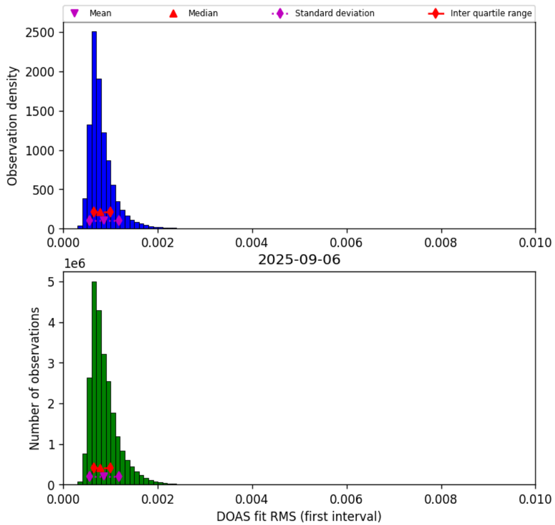
Figure 46: Histogram of “DOAS fit RMS (first interval)” for 2025-09-05 to 2025-09-07
