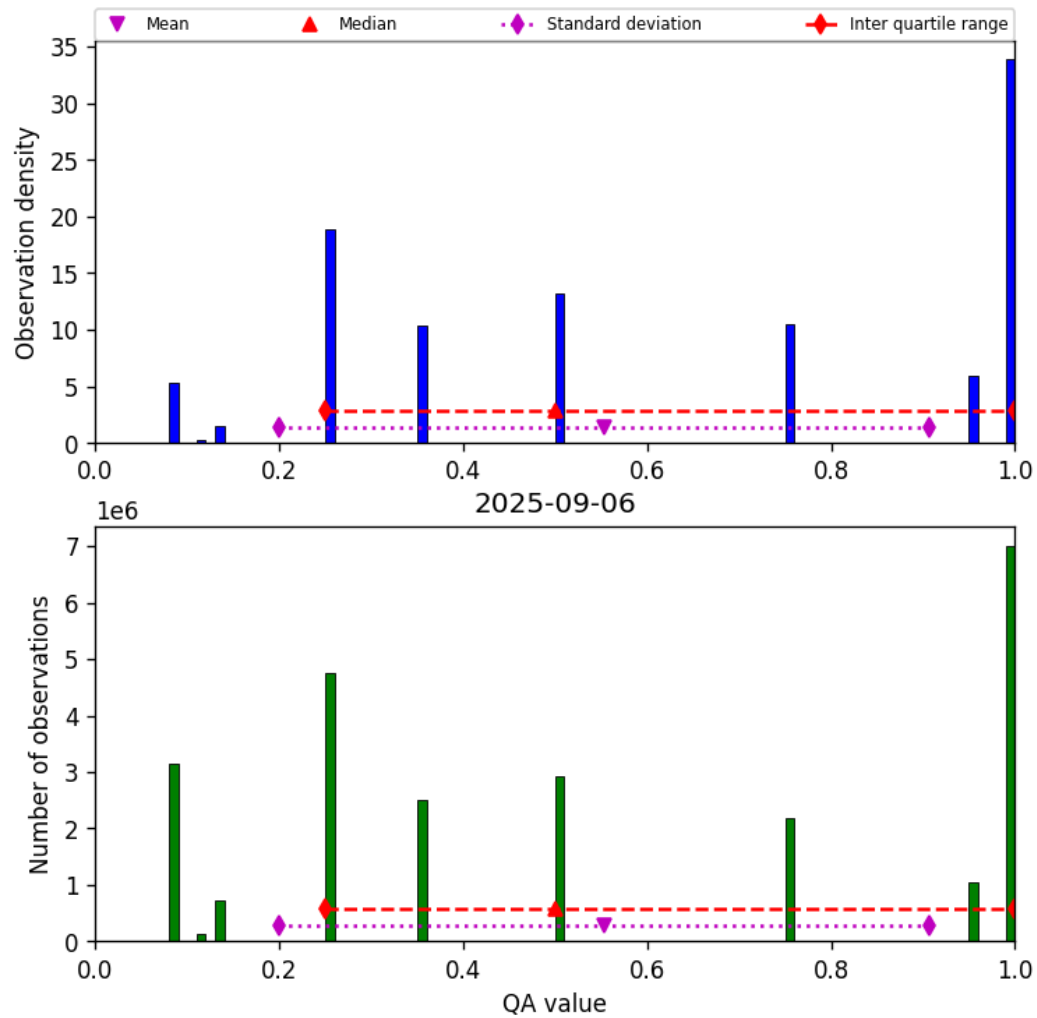
Figure 34: Histogram of “QA value” for 2025-09-05 to 2025-09-07
