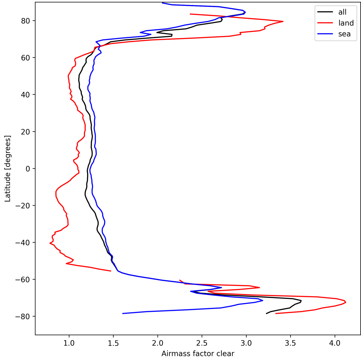
Figure 28: Zonal average of “Airmass factor clear” for 2025-09-05 to 2025-09-07.
