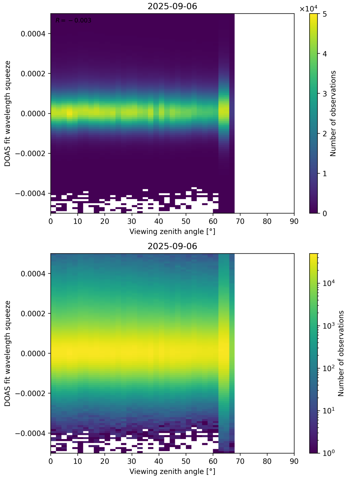
Figure 184: Scatter density plot of “Viewing zenith angle” against “DOAS fit wavelength squeeze” for 2025-09-05 to 2025-09-07.
