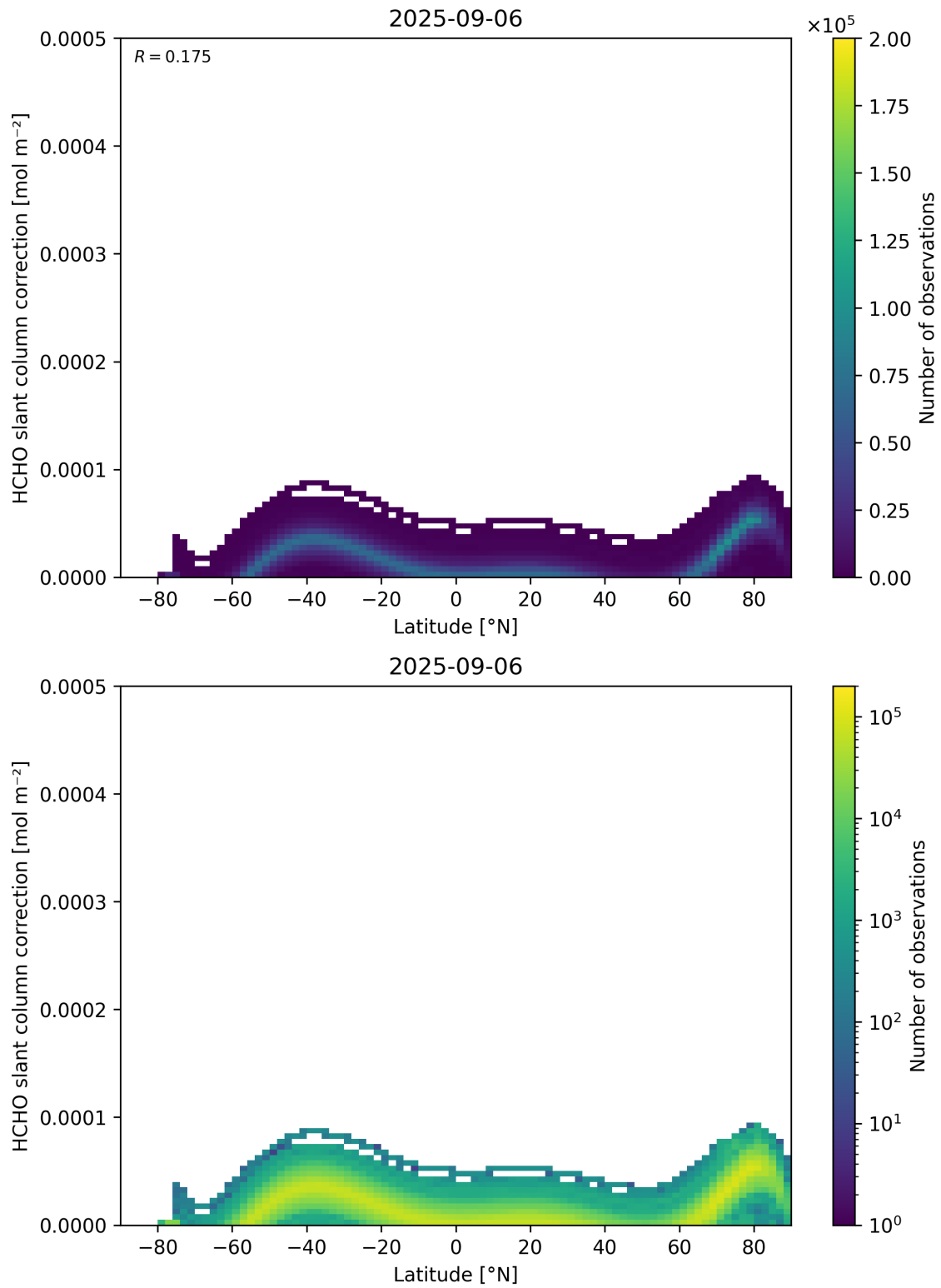
Figure 158: Scatter density plot of “Latitude” against “HCHO slant column correction” for 2025-09-05 to 2025-09-07.
