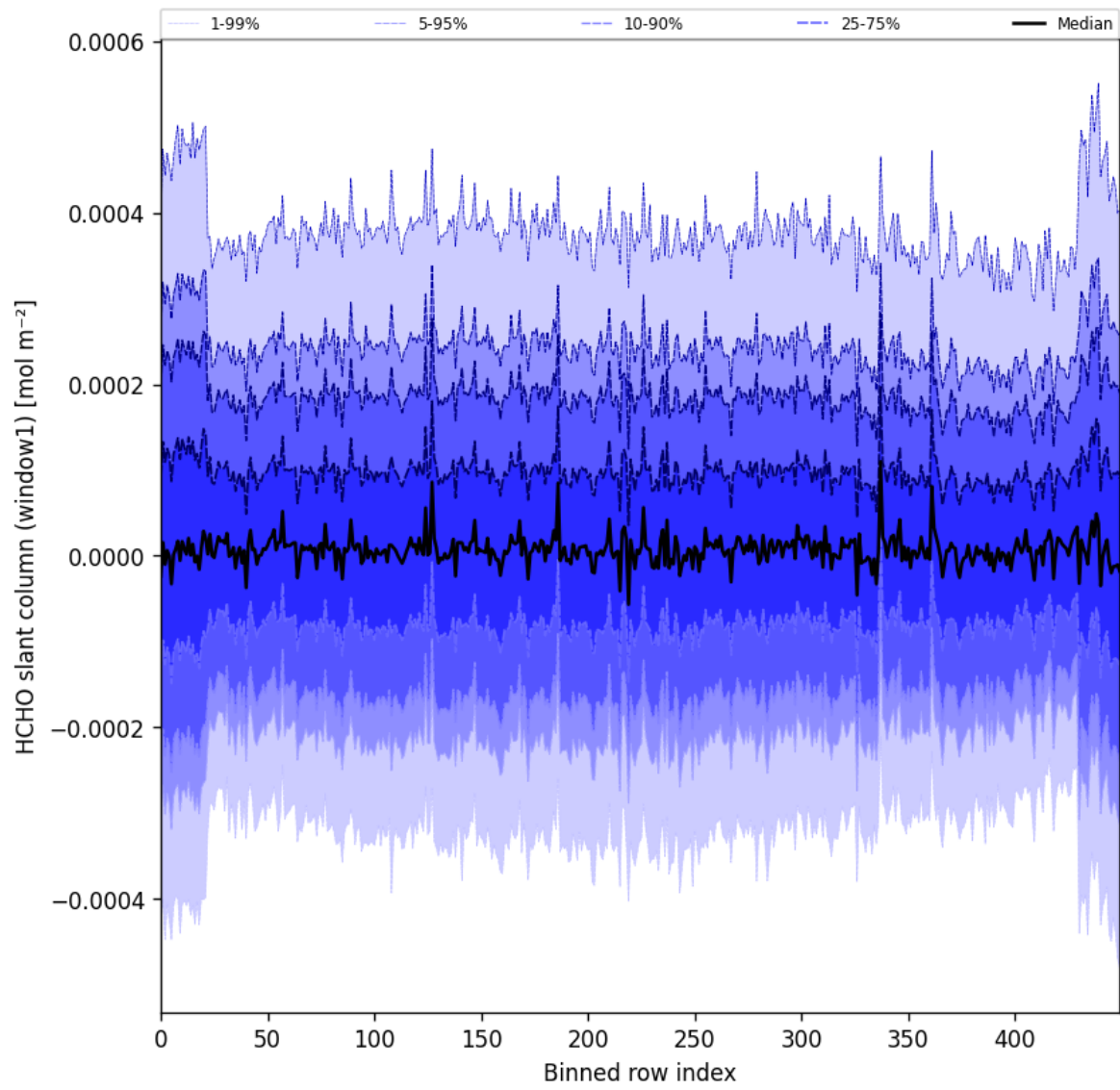
Figure 52: Along track statistics of “HCHO slant column (window1)” for 2025-09-05 to 2025-09-07
