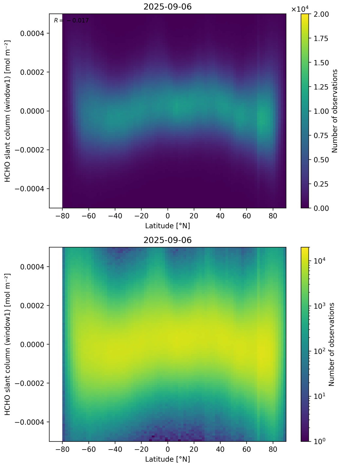
Figure 159: Scatter density plot of “Latitude” against “HCHO slant column (window1)” for 2025-09-05 to 2025-09-07.
