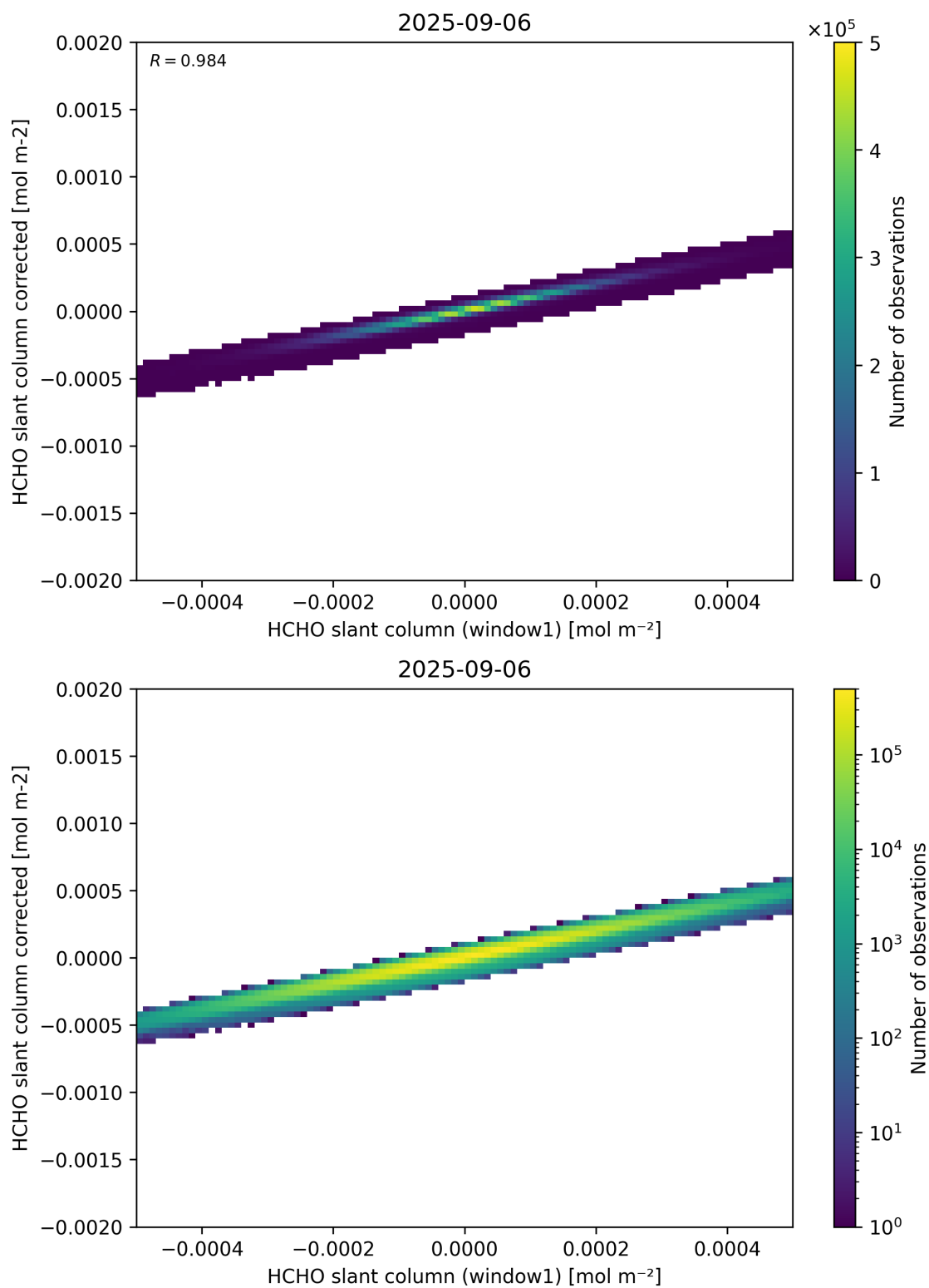
Figure 82: Scatter density plot of “HCHO slant column (window1)” against “HCHO slant column corrected” for 2025-09-05 to 2025-09-07.
