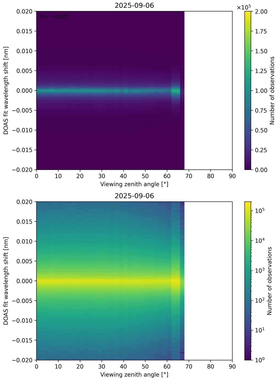
Figure 183: Scatter density plot of “Viewing zenith angle” against “DOAS fit wavelength shift” for 2025-09-05 to 2025-09-07.
