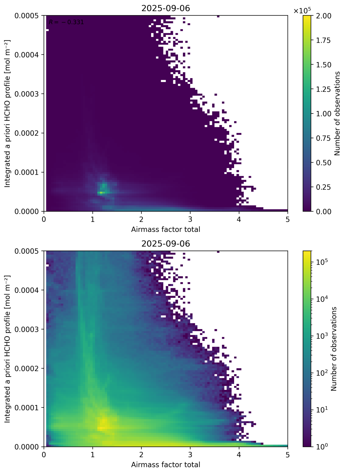
Figure 104: Scatter density plot of “Airmass factor total” against “Integrated a priori HCHO profile” for 2025-09-05 to 2025-09-07.
