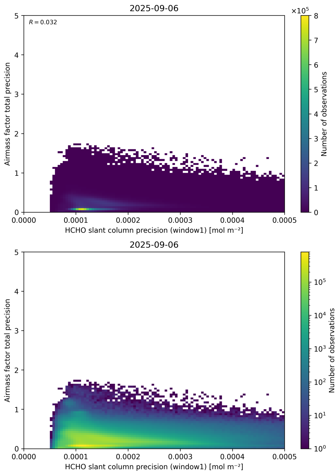
Figure 95: Scatter density plot of “HCHO slant column precision (window1)” against “Airmass factor total precision” for 2025-09-05 to 2025-09-07.
