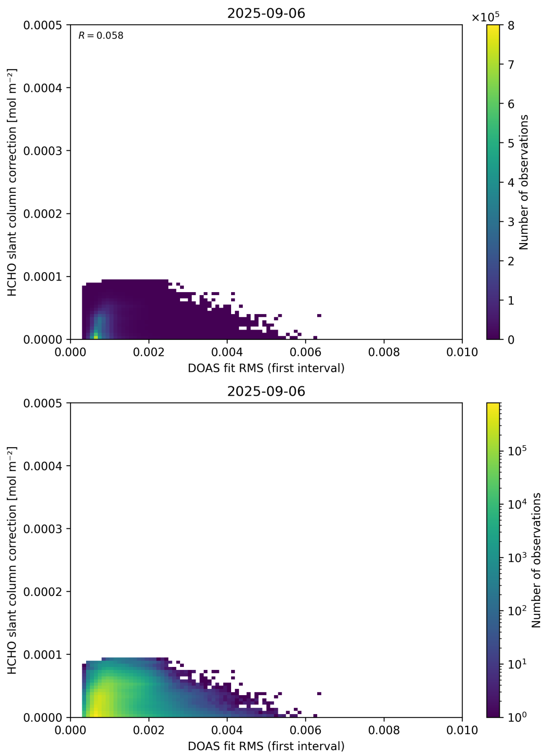
Figure 63: Scatter density plot of “DOAS fit RMS (first interval)” against “HCHO slant column correction” for 2025-09-05 to 2025-09-07.
