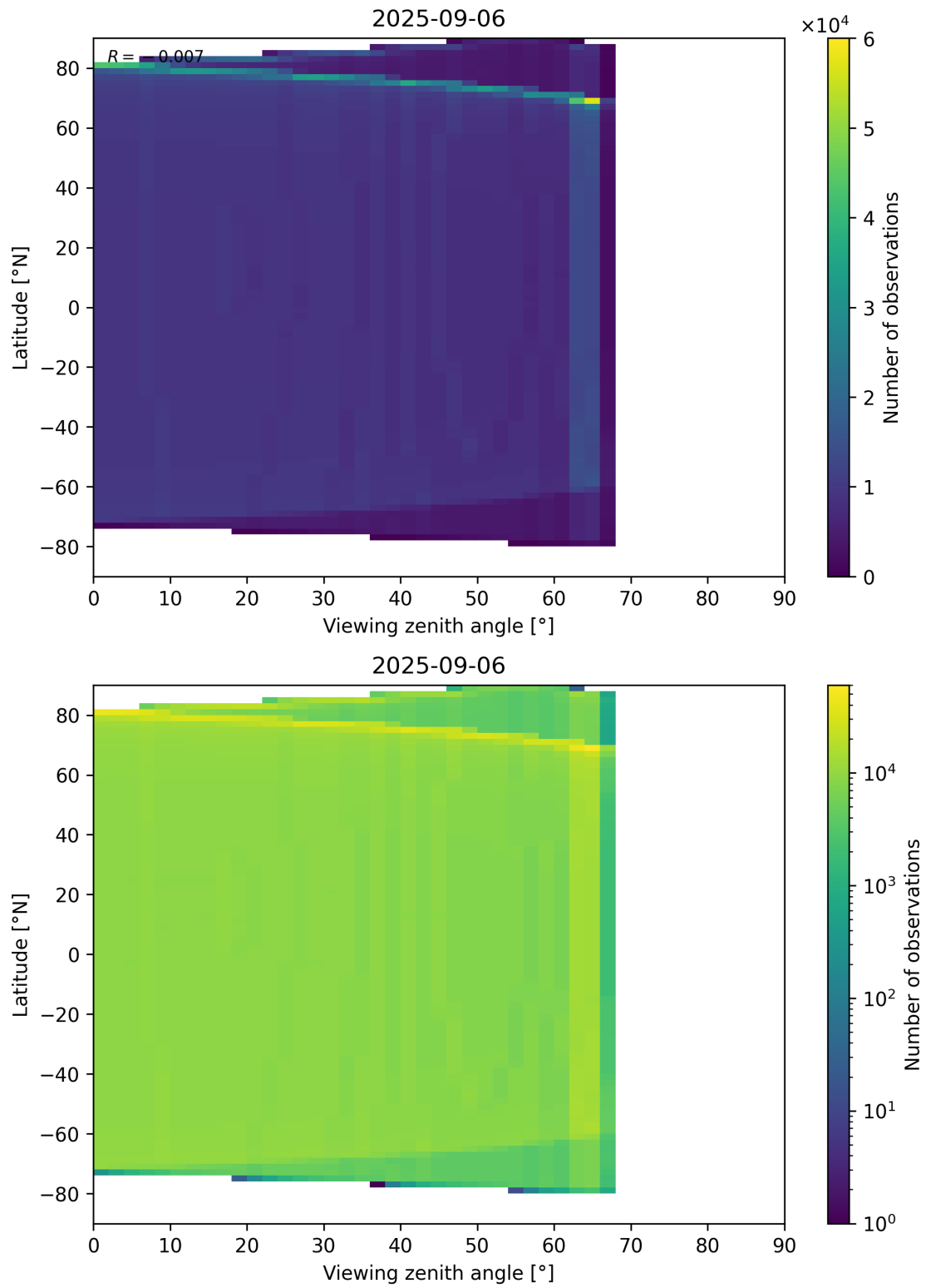
Figure 196: Scatter density plot of “Viewing zenith angle” against “Latitude” for 2025-09-05 to 2025-09-07.
