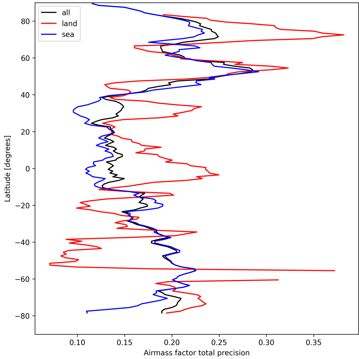
Figure 27: Zonal average of “Airmass factor total precision” for 2025-09-05 to 2025-09-07.
