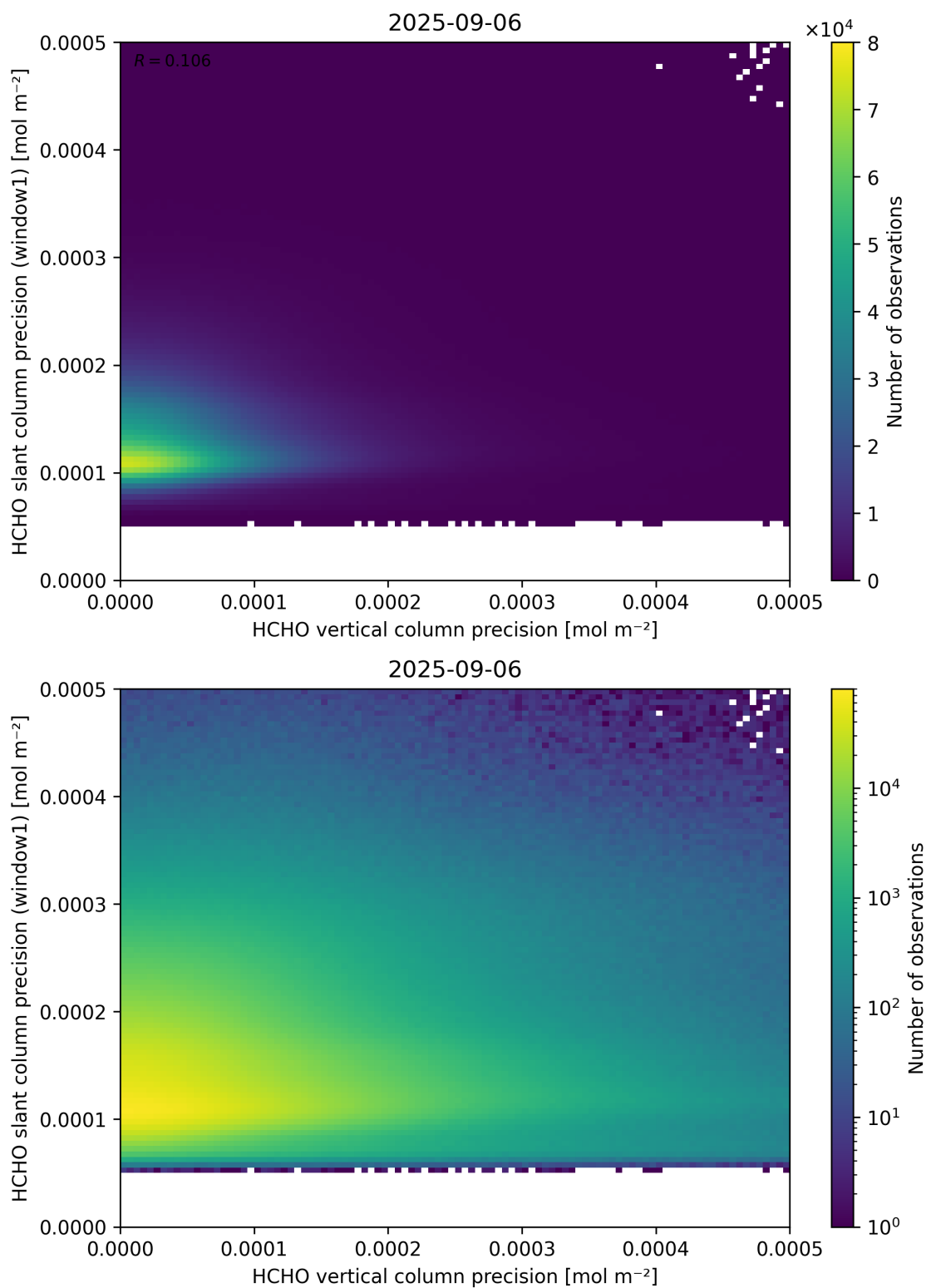
Figure 143: Scatter density plot of “HCHO vertical column precision” against “HCHO slant column precision (window1)” for 2025-09-05 to 2025-09-07.
