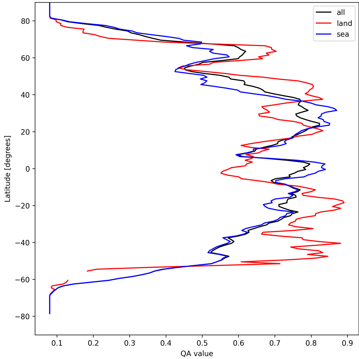
Figure 20: Zonal average of “QA value” for 2025-09-05 to 2025-09-07.
