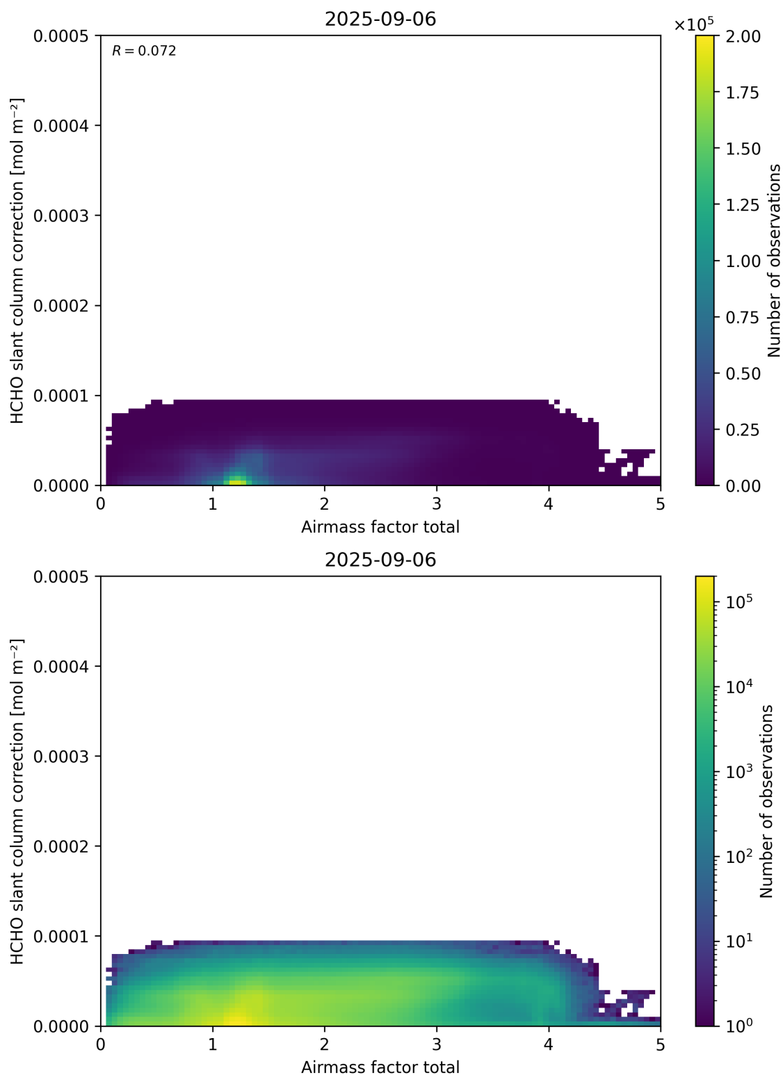
Figure 102: Scatter density plot of “Airmass factor total” against “HCHO slant column correction” for 2025-09-05 to 2025-09-07.
