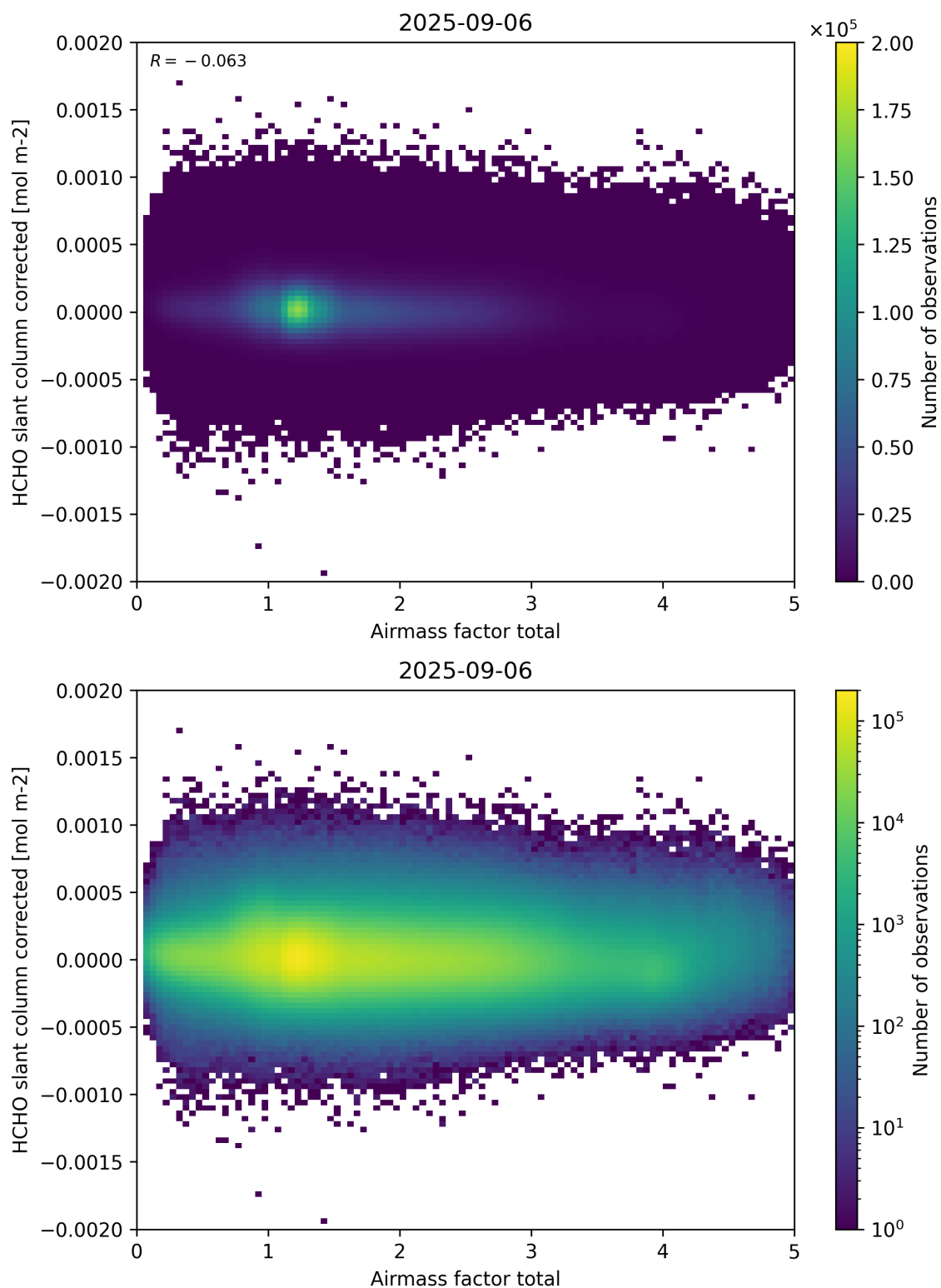
Figure 101: Scatter density plot of “Airmass factor total” against “HCHO slant column corrected” for 2025-09-05 to 2025-09-07.
