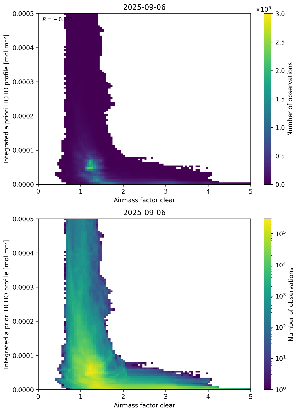
Figure 76: Scatter density plot of “Airmass factor clear” against “Integrated a priori HCHO profile” for 2025-09-05 to 2025-09-07.
