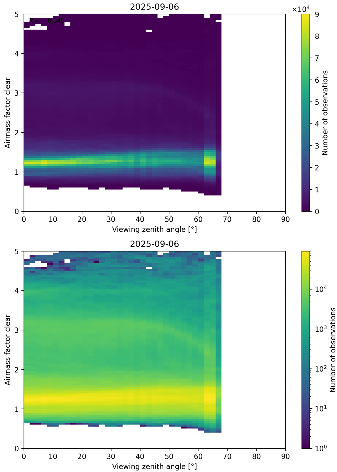
Figure 185: Scatter density plot of “Viewing zenith angle” against “Airmass factor clear” for 2025-09-05 to 2025-09-07.
