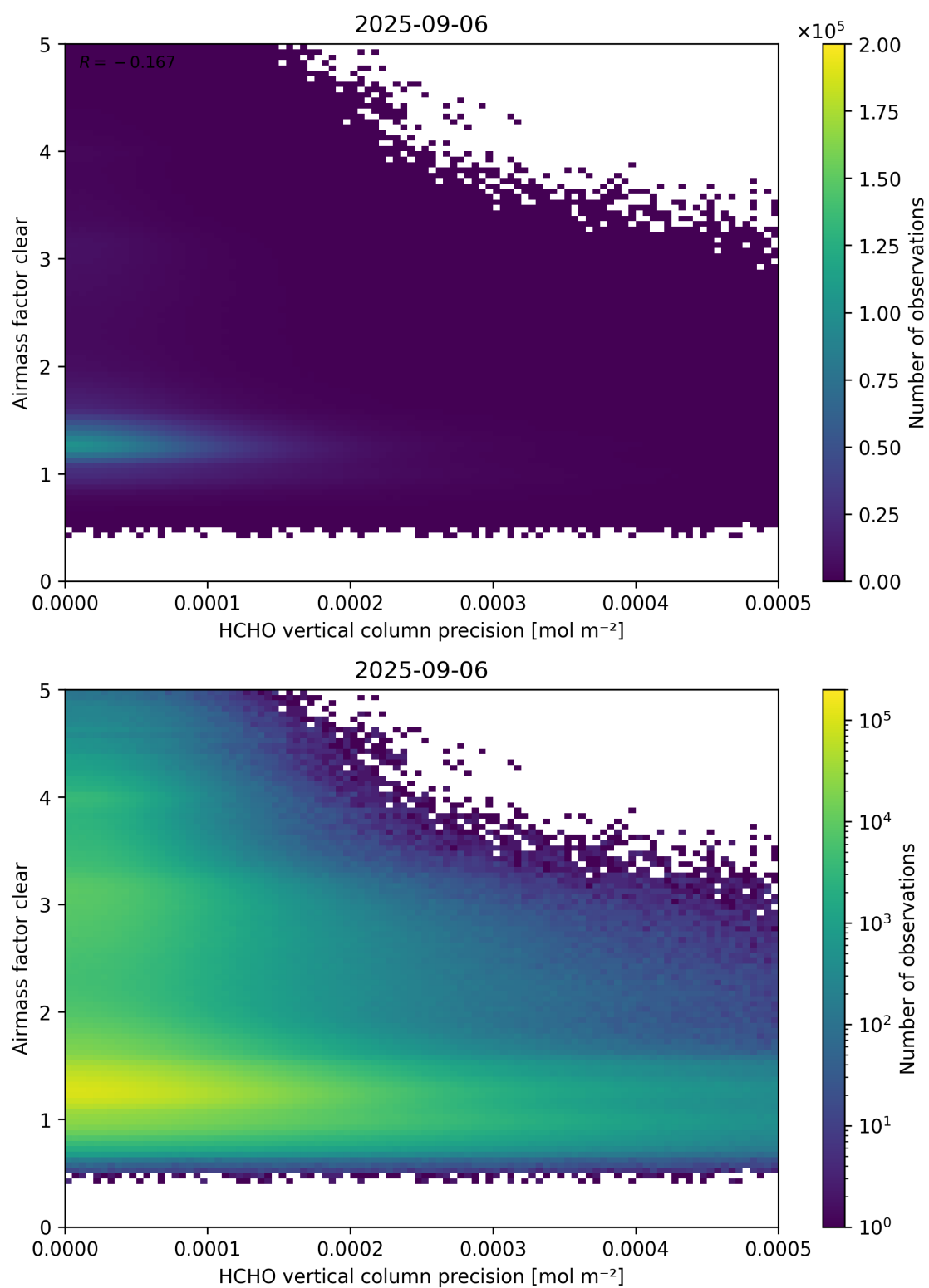
Figure 139: Scatter density plot of “HCHO vertical column precision” against “Airmass factor clear” for 2025-09-05 to 2025-09-07.
