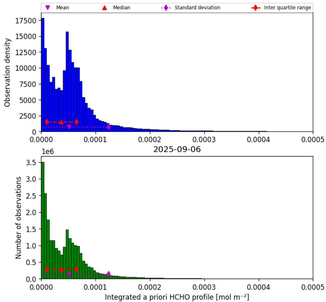
Figure 43: Histogram of “Integrated a priori HCHO profile” for 2025-09-05 to 2025-09-07
