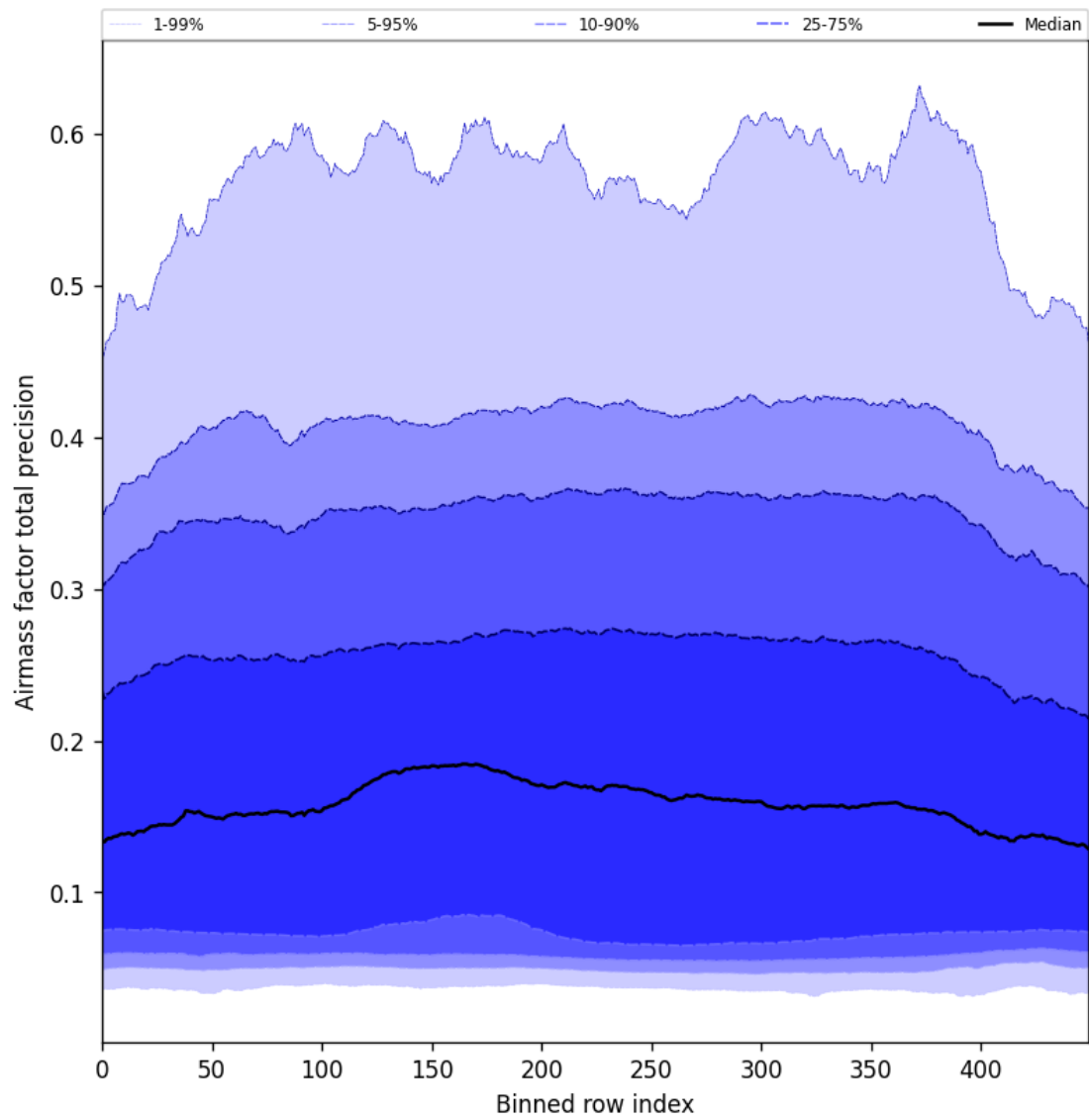
Figure 55: Along track statistics of “Airmass factor total precision” for 2025-09-05 to 2025-09-07
