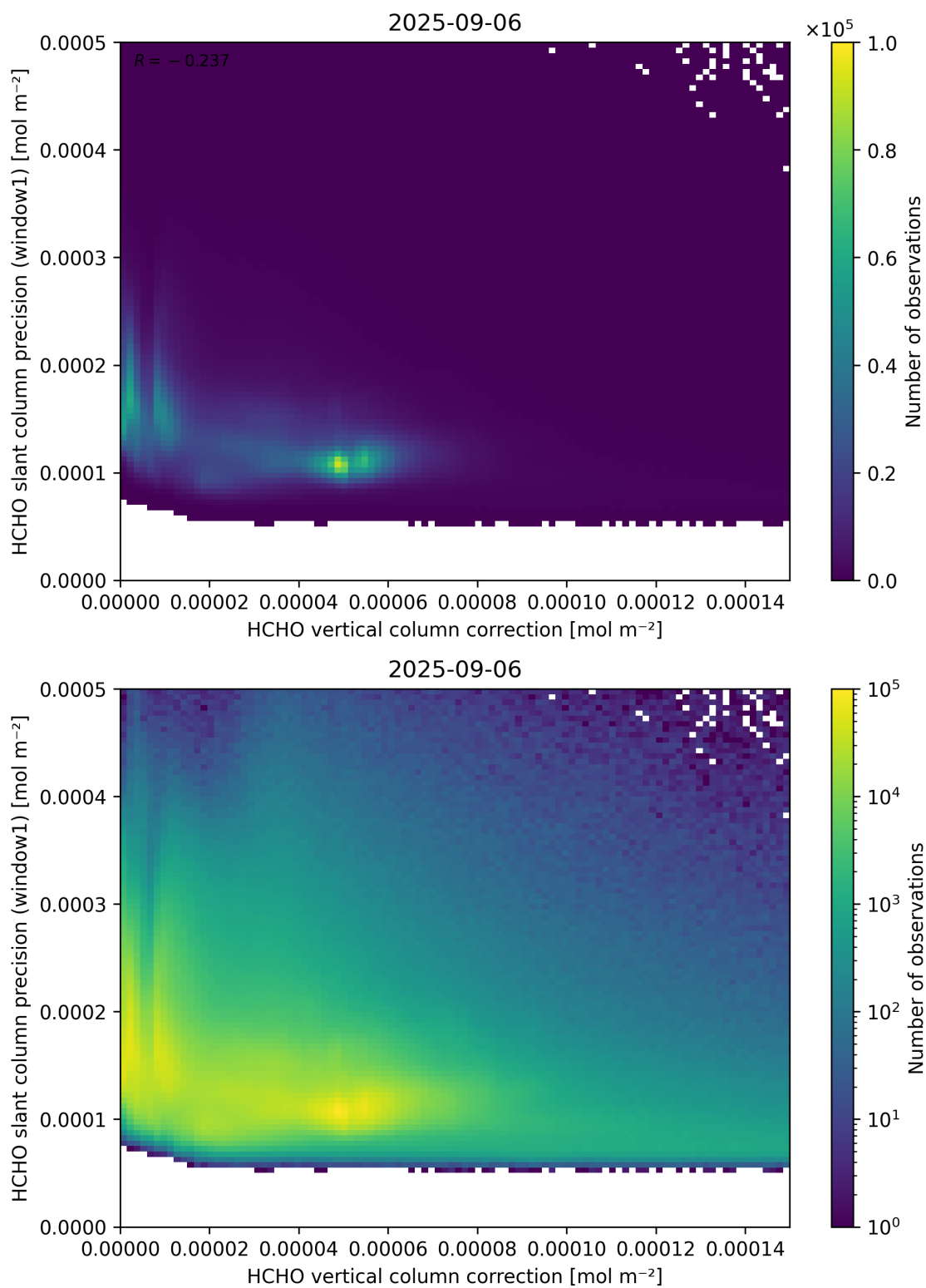
Figure 119: Scatter density plot of “HCHO vertical column correction” against “HCHO slant column precision (window1)” for 2025-09-05 to 2025-09-07.
