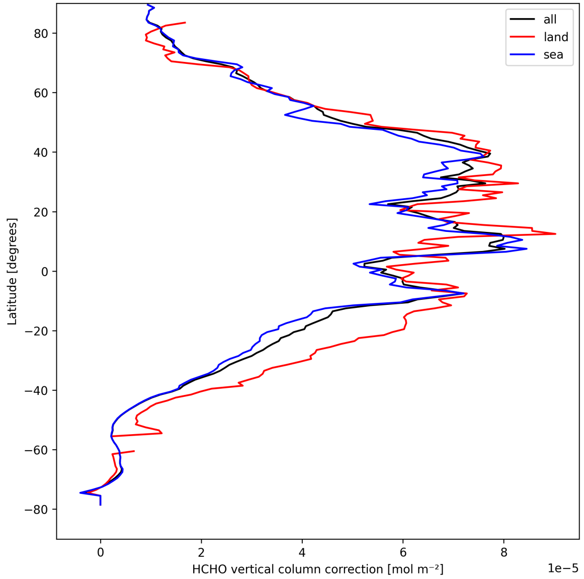
Figure 23: Zonal average of “HCHO vertical column correction” for 2025-09-05 to 2025-09-07.
