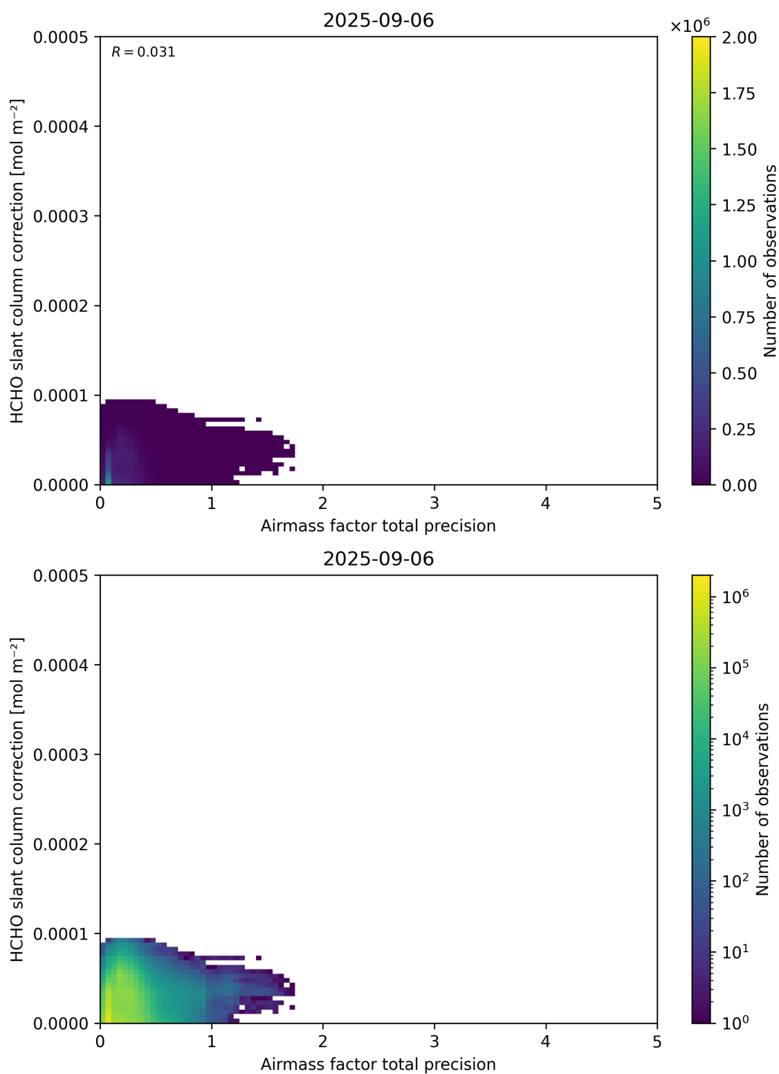
Figure 110: Scatter density plot of “Airmass factor total precision” against “HCHO slant column correction” for 2025-09-05 to 2025-09-07.
