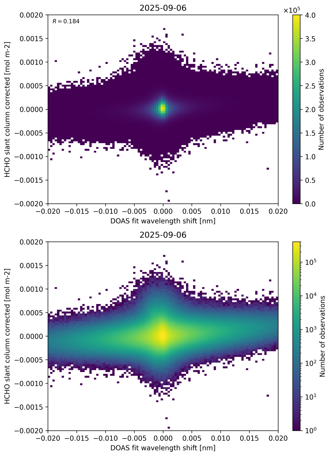
Figure 66: Scatter density plot of “DOAS fit wavelength shift” against “HCHO slant column corrected” for 2025-09-05 to 2025-09-07.
