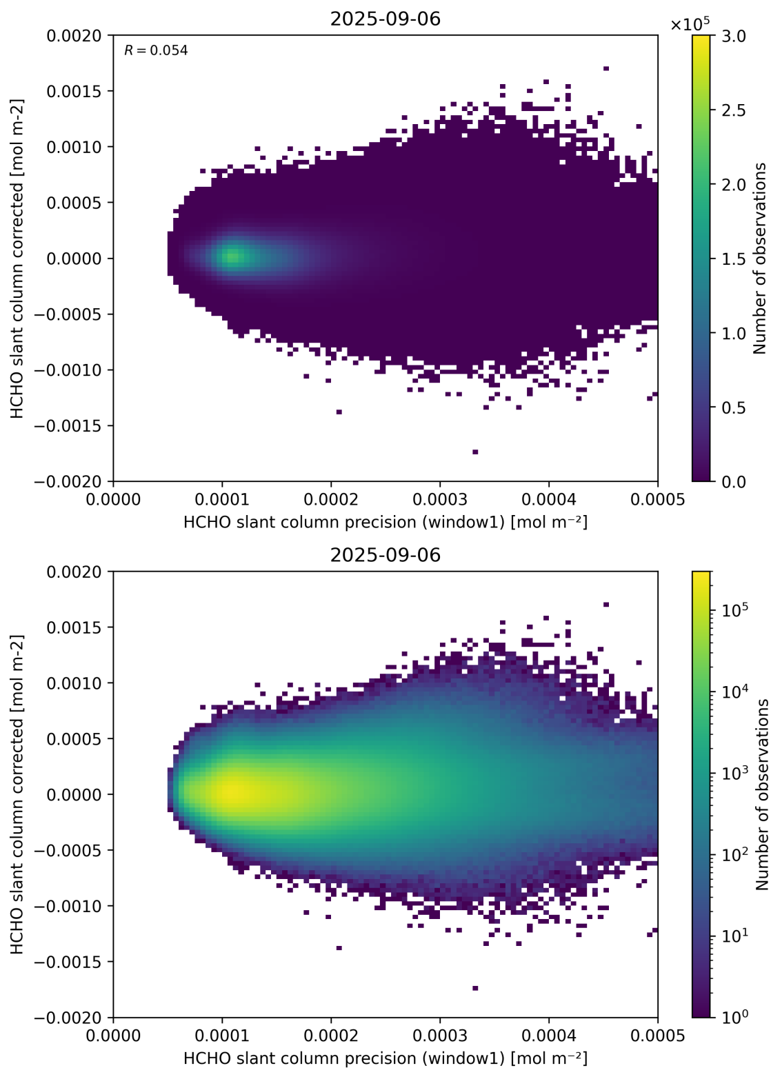
Figure 92: Scatter density plot of “HCHO slant column precision (window1)” against “HCHO slant column corrected” for 2025-09-05 to 2025-09-07.
