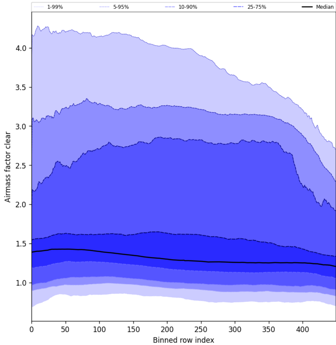
Figure 56: Along track statistics of “Airmass factor clear” for 2025-09-05 to 2025-09-07
