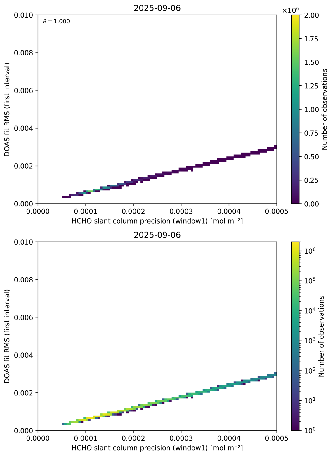
Figure 88: Scatter density plot of “HCHO slant column precision (window1)” against “DOAS fit RMS (first interval)” for 2025-09-05 to 2025-09-07.
