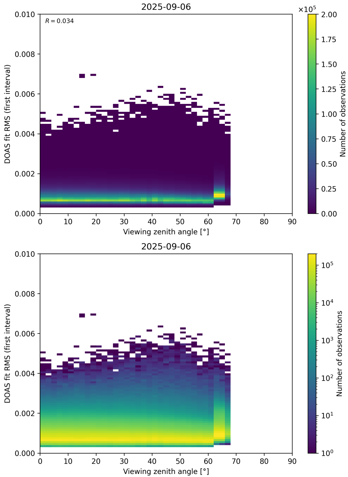
Figure 182: Scatter density plot of “Viewing zenith angle” against “DOAS fit RMS (first interval)” for 2025-09-05 to 2025-09-07.
