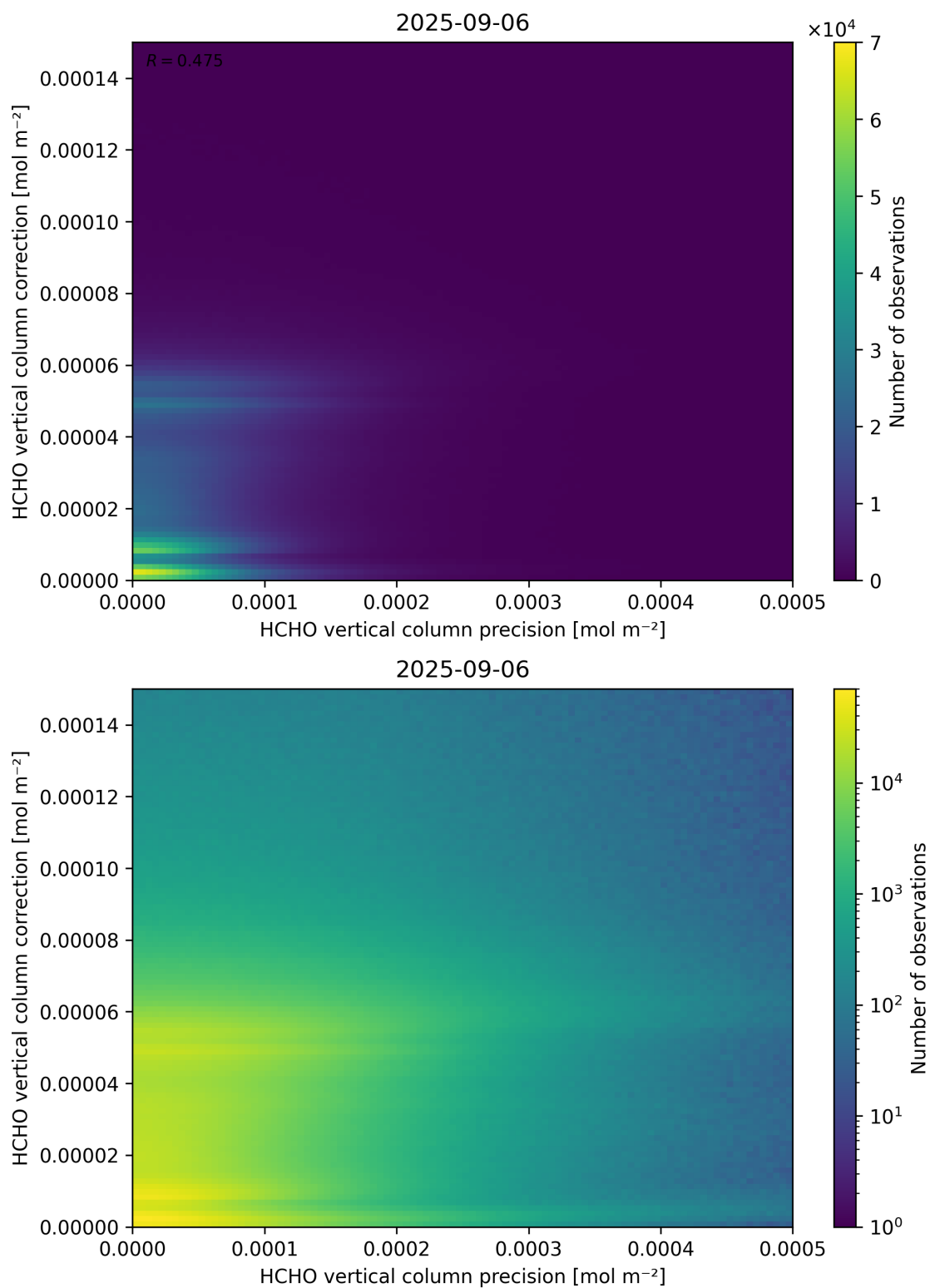
Figure 146: Scatter density plot of “HCHO vertical column precision” against “HCHO vertical column correction” for 2025-09-05 to 2025-09-07.
