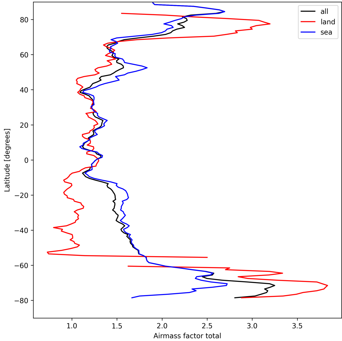
Figure 26: Zonal average of “Airmass factor total” for 2025-09-05 to 2025-09-07.
