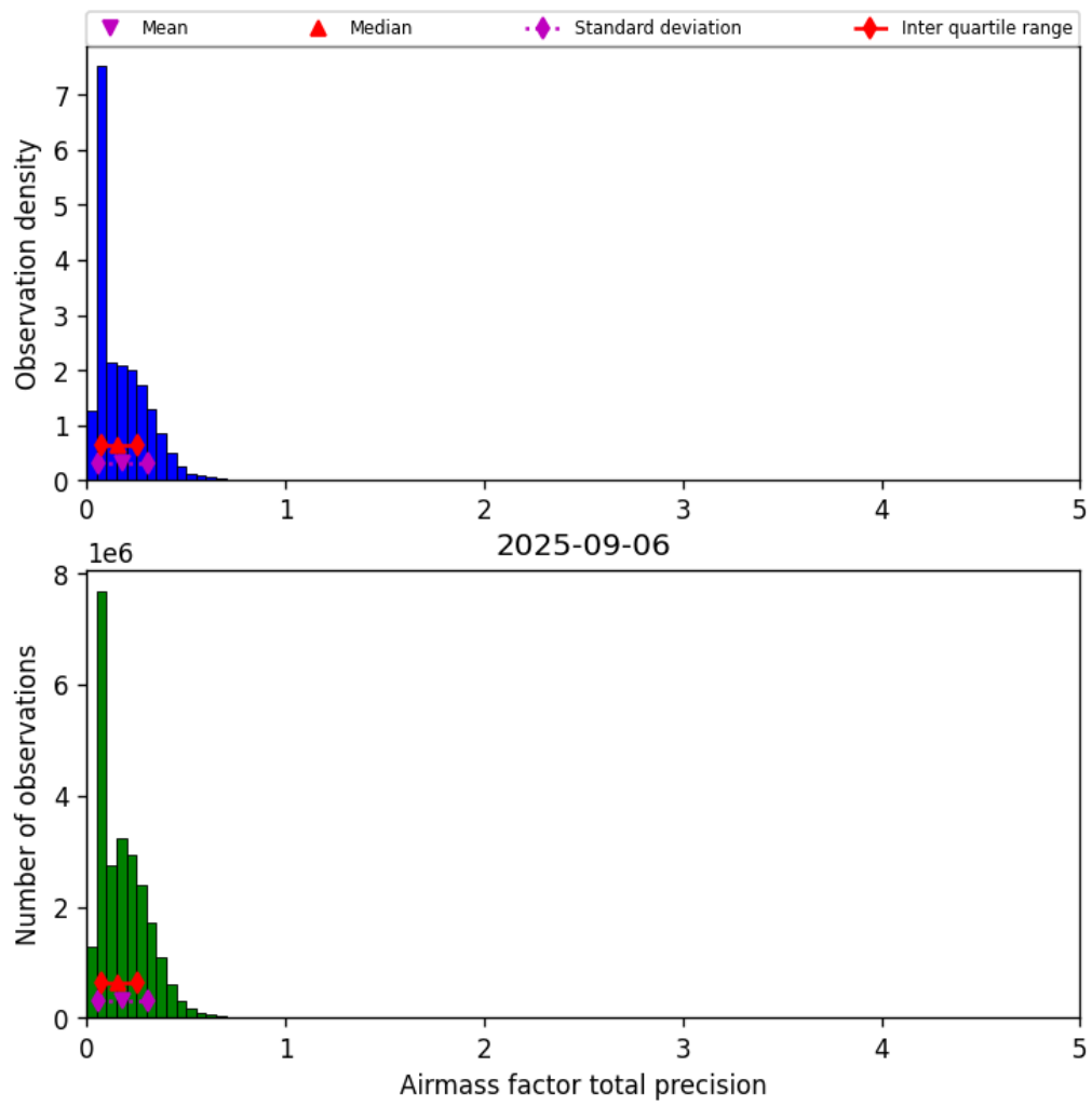
Figure 41: Histogram of “Airmass factor total precision” for 2025-09-05 to 2025-09-07
