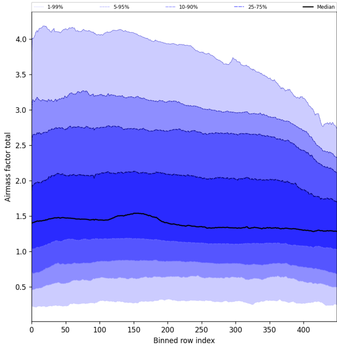
Figure 54: Along track statistics of “Airmass factor total” for 2025-09-05 to 2025-09-07
