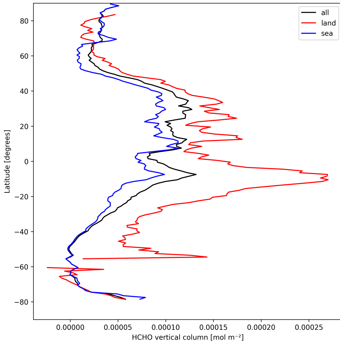
Figure 21: Zonal average of “HCHO vertical column” for 2025-09-05 to 2025-09-07.
