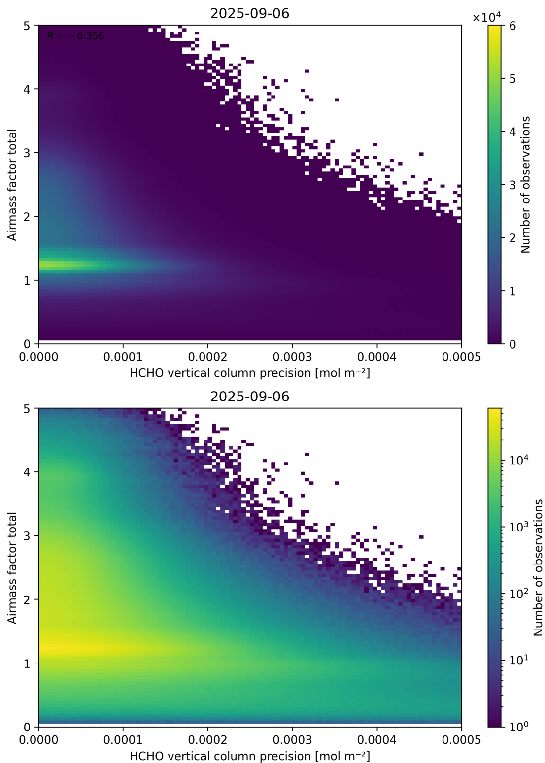
Figure 144: Scatter density plot of “HCHO vertical column precision” against “Airmass factor total” for 2025-09-05 to 2025-09-07.
