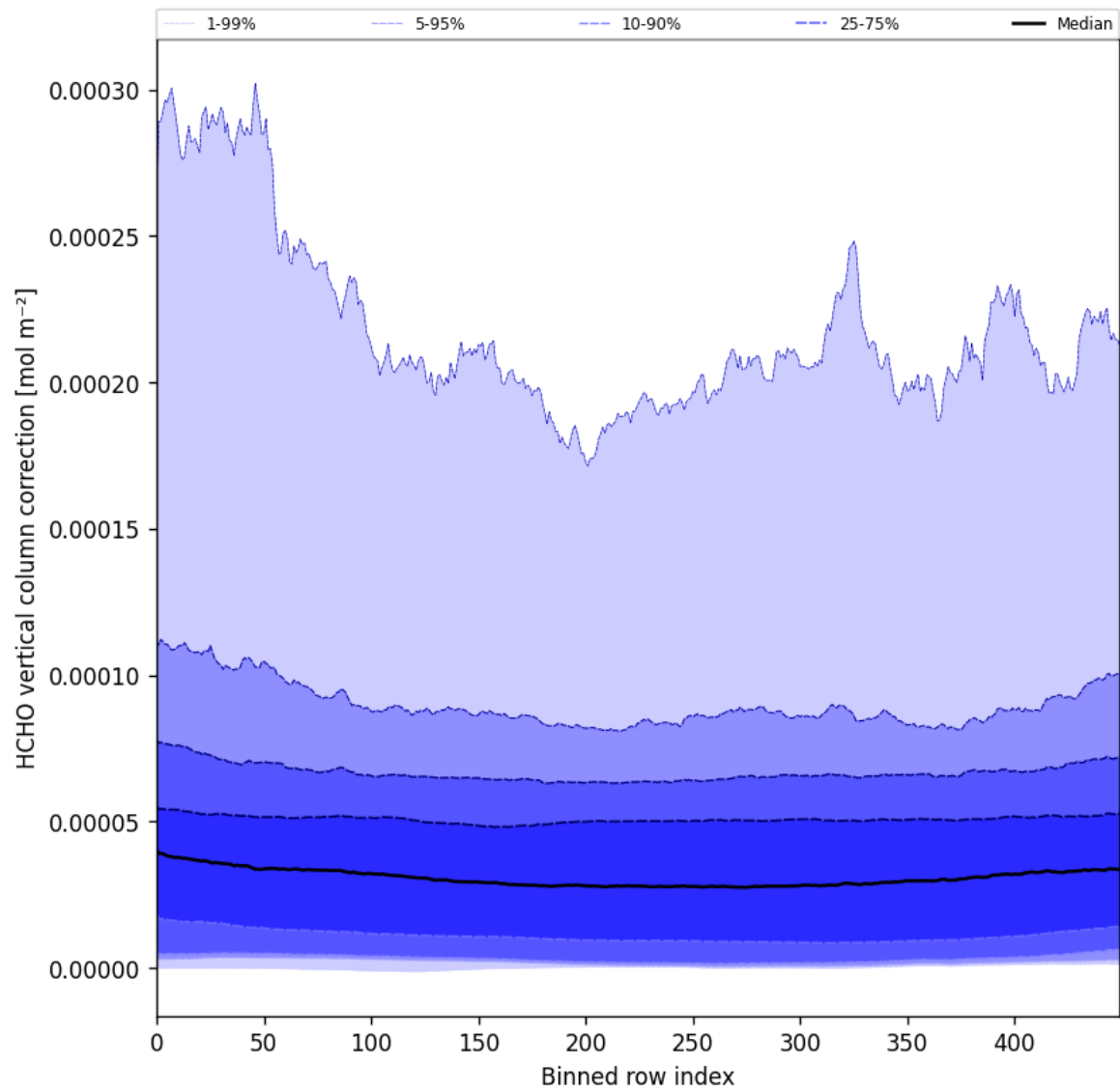
Figure 51: Along track statistics of “HCHO vertical column correction” for 2025-09-05 to 2025-09-07
