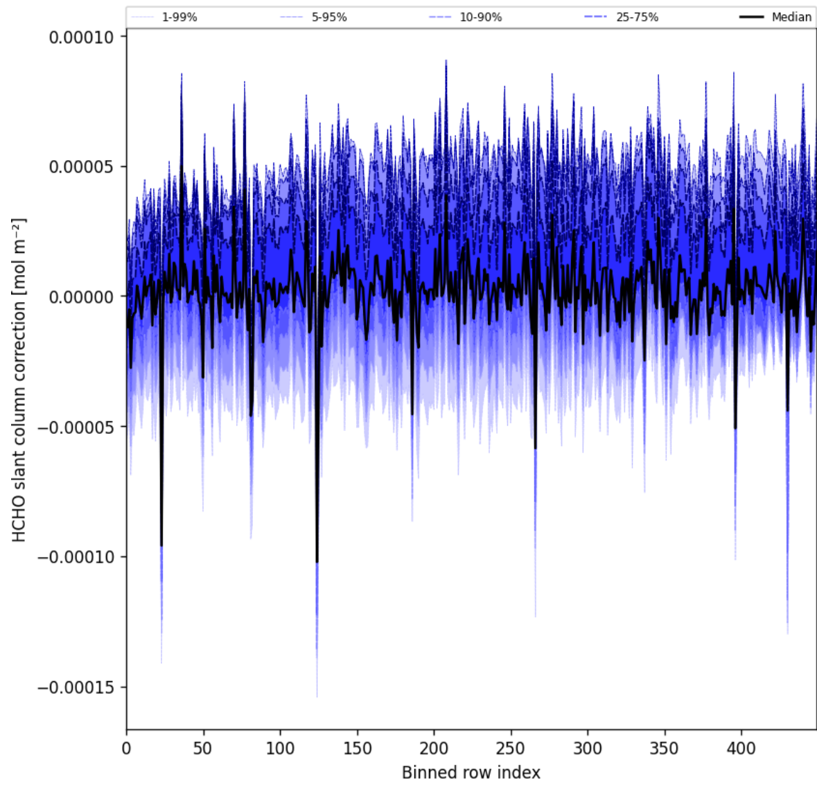
Figure 61: Along track statistics of “HCHO slant column correction” for 2025-09-05 to 2025-09-07
