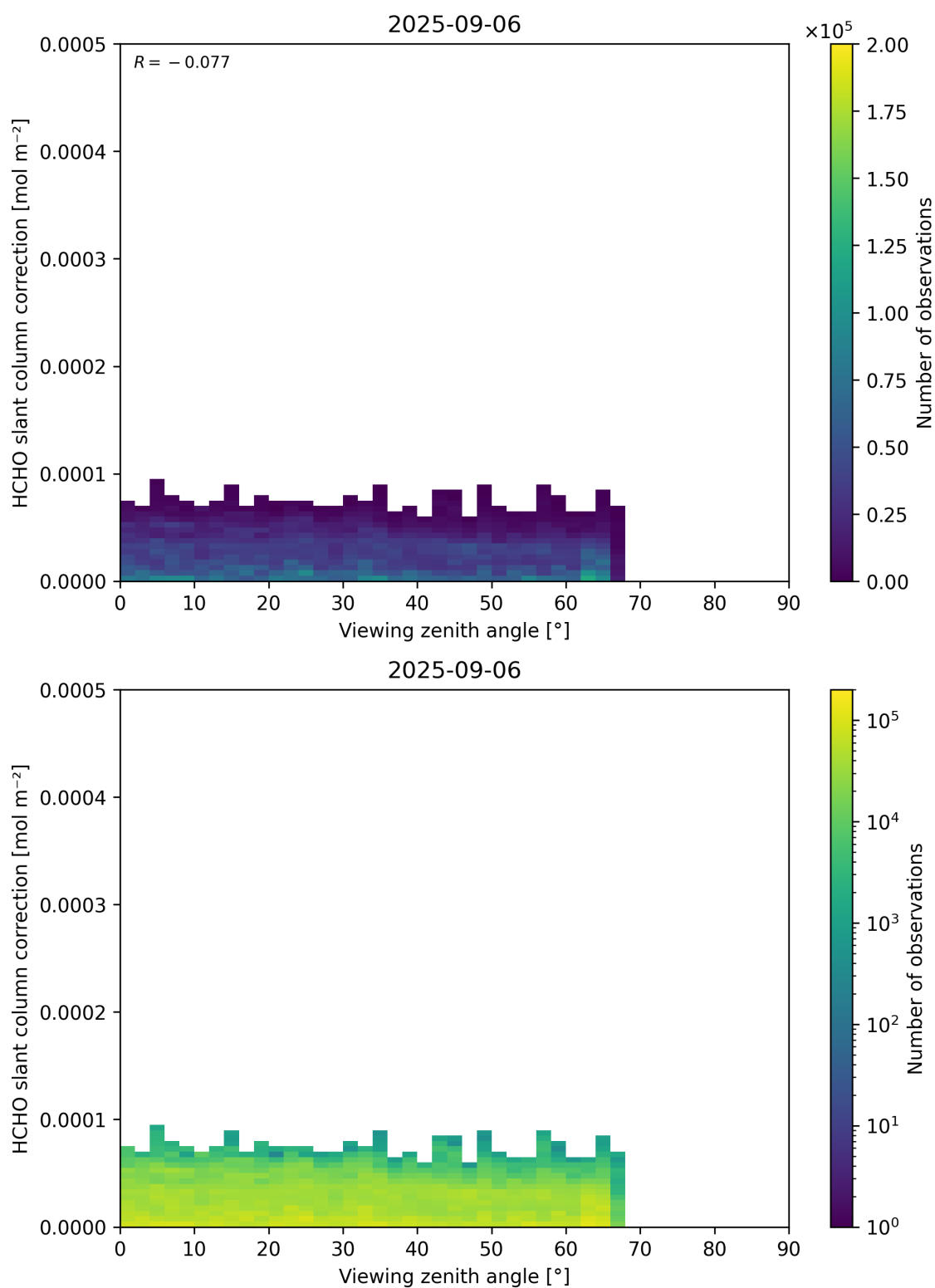
Figure 187: Scatter density plot of “Viewing zenith angle” against “HCHO slant column correction” for 2025-09-05 to 2025-09-07.
