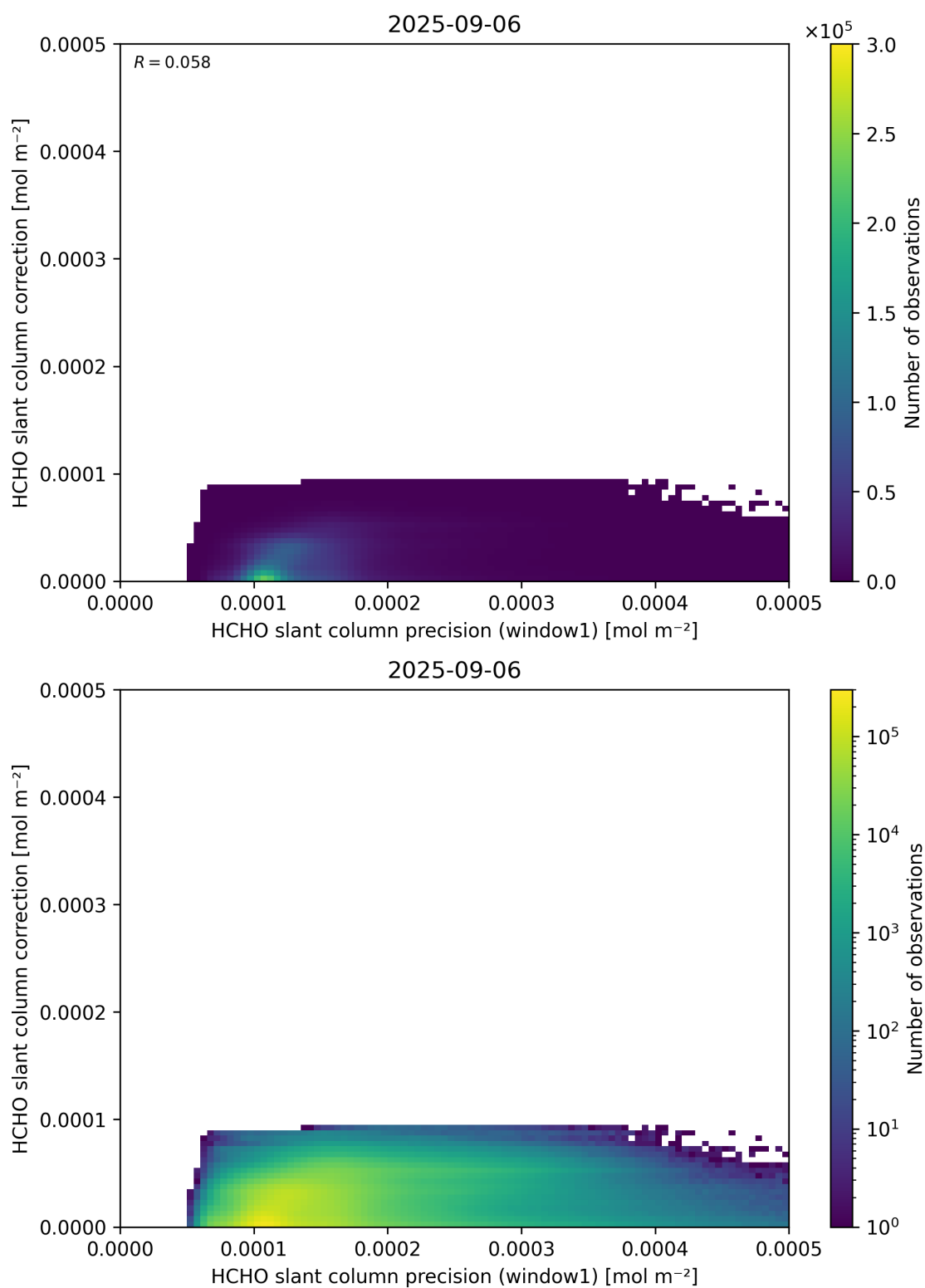
Figure 93: Scatter density plot of “HCHO slant column precision (window1)” against “HCHO slant column correction” for 2025-09-05 to 2025-09-07.
