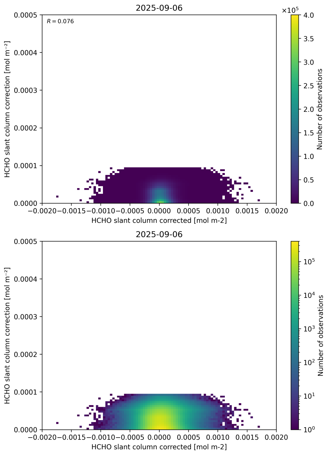
Figure 77: Scatter density plot of “HCHO slant column corrected” against “HCHO slant column correction” for 2025-09-05 to 2025-09-07.
