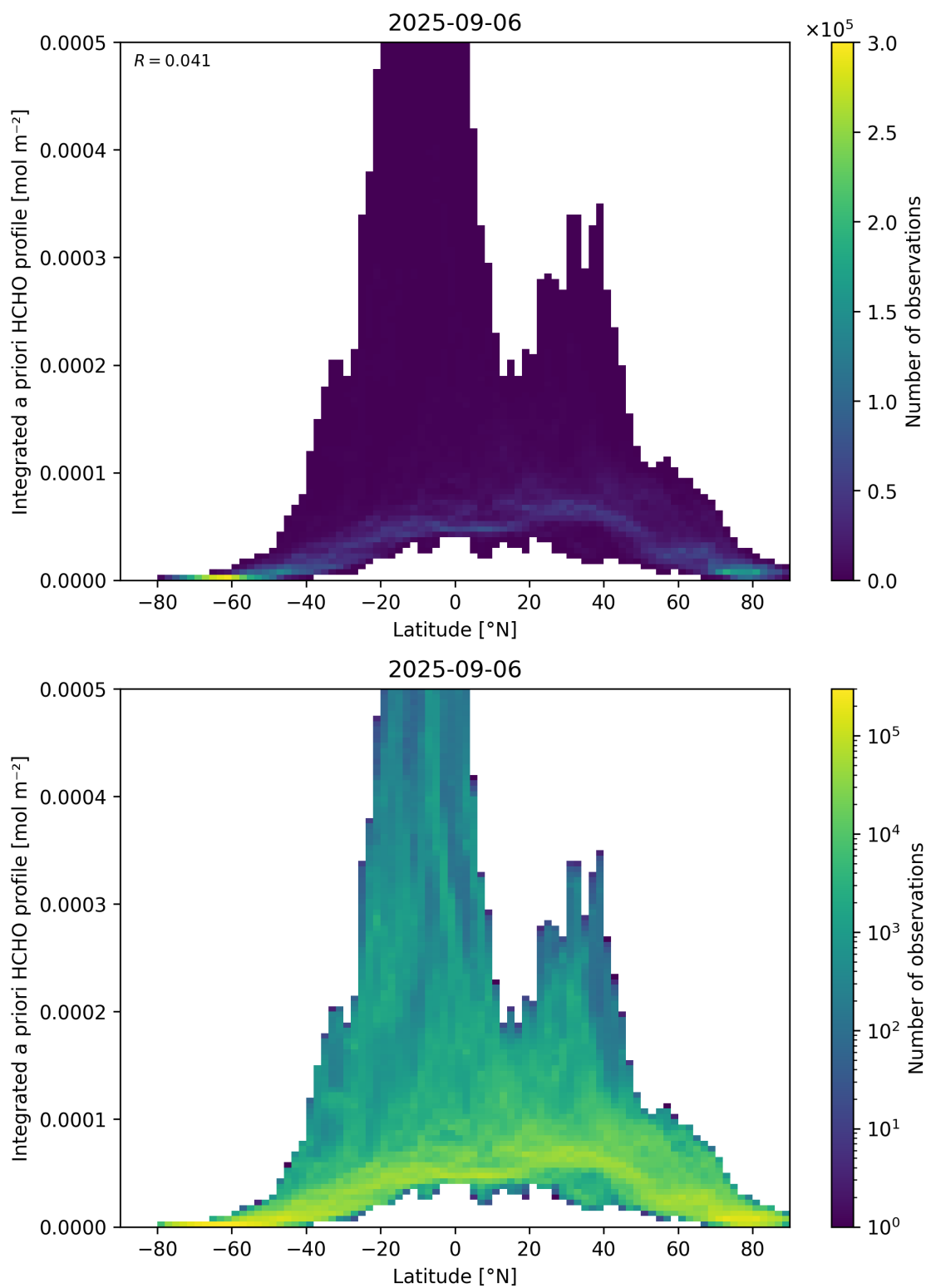
Figure 166: Scatter density plot of “Latitude” against “Integrated a priori HCHO profile” for 2025-09-05 to 2025-09-07.
