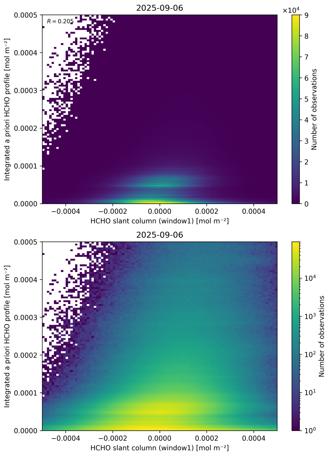
Figure 87: Scatter density plot of “HCHO slant column (window1)” against “Integrated a priori HCHO profile” for 2025-09-05 to 2025-09-07.
