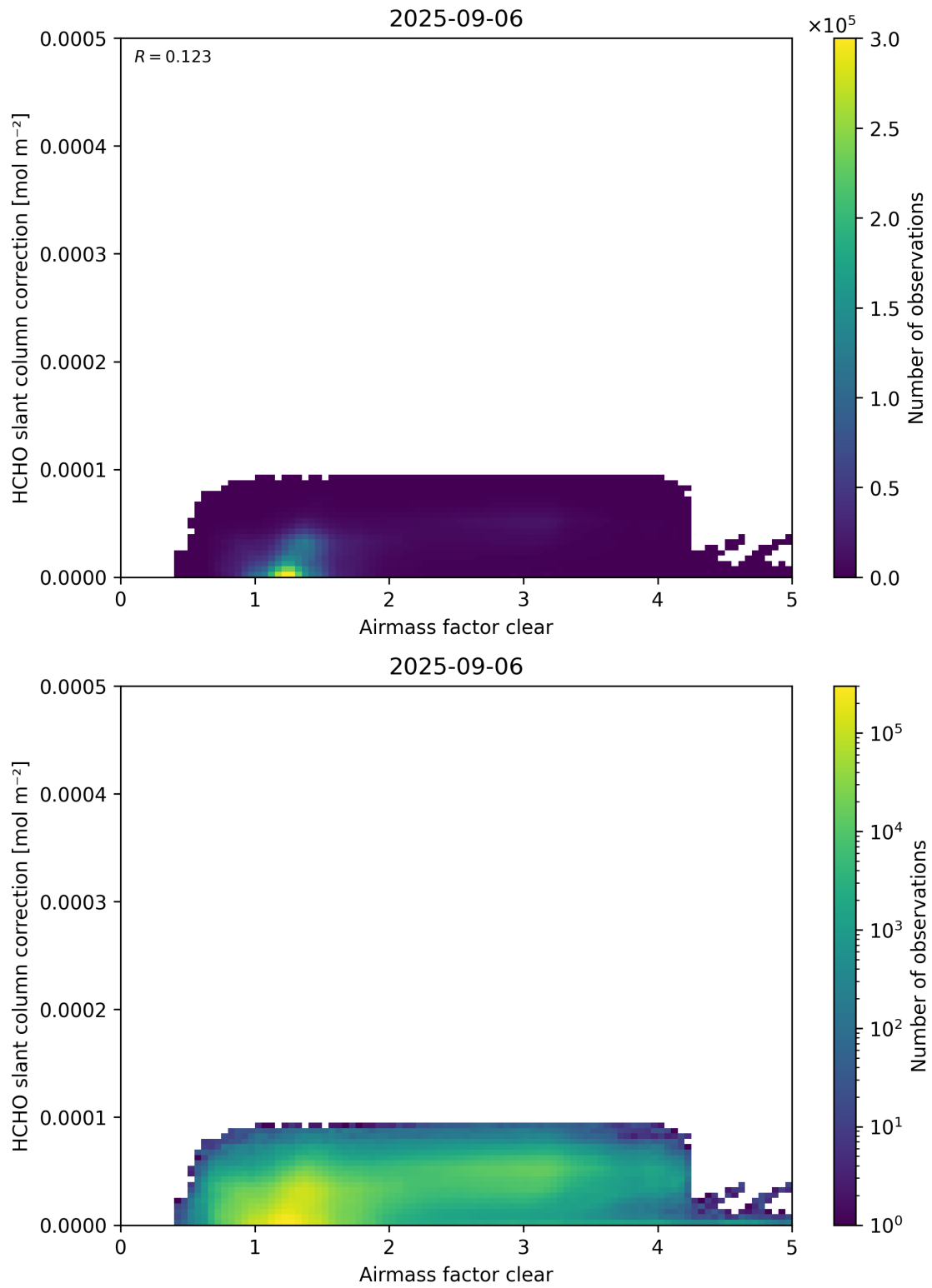
Figure 75: Scatter density plot of “Airmass factor clear” against “HCHO slant column correction” for 2025-09-05 to 2025-09-07.
