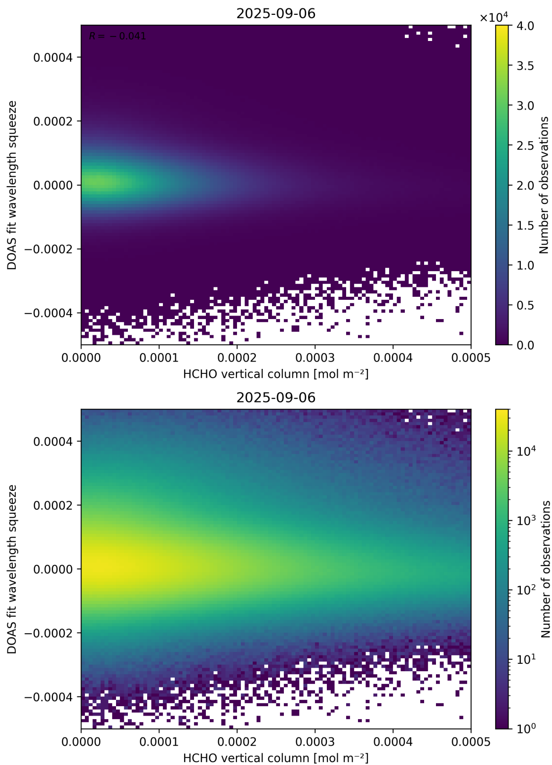
Figure 125: Scatter density plot of “HCHO vertical column” against “DOAS fit wavelength squeeze” for 2025-09-05 to 2025-09-07.
