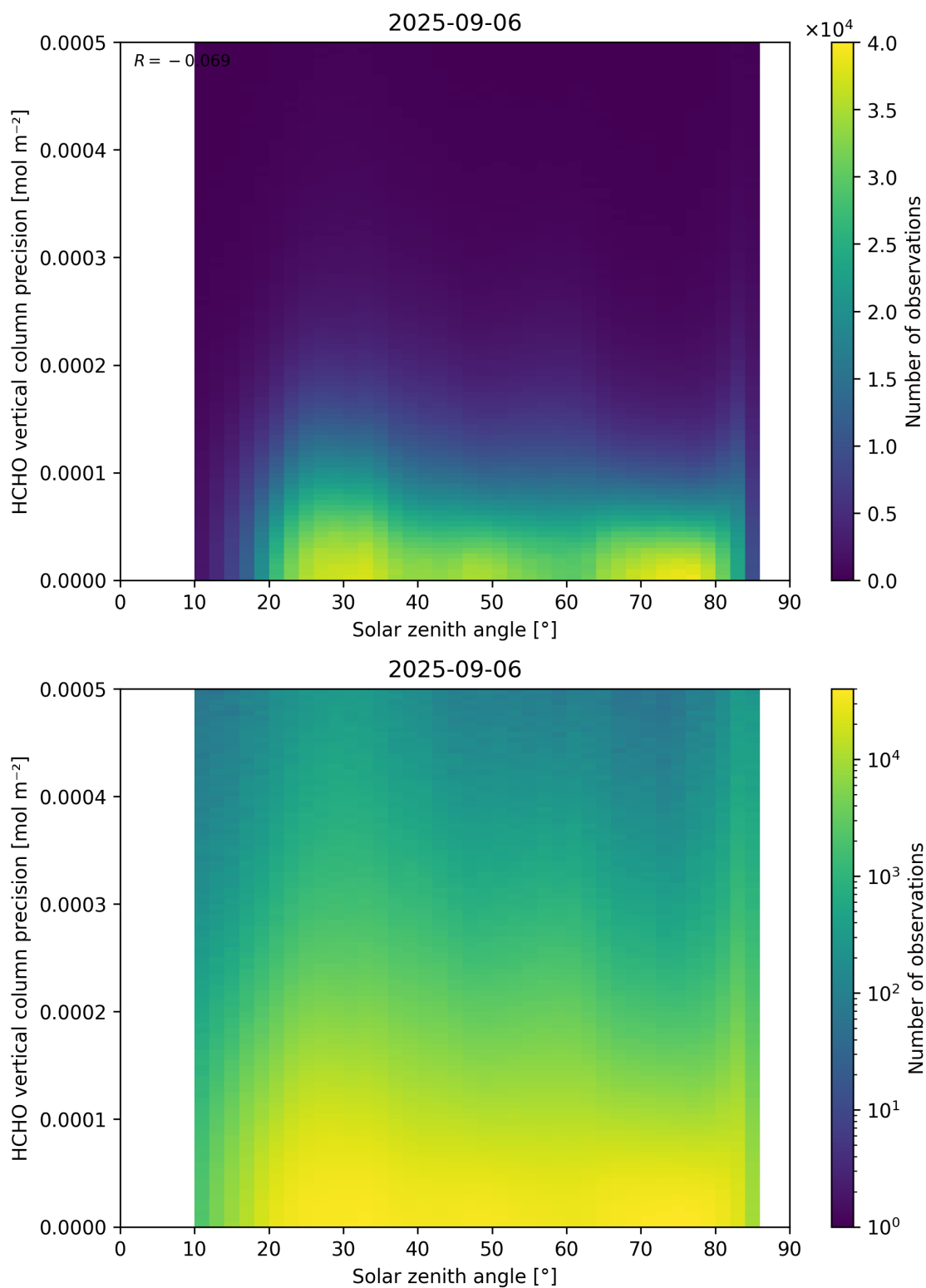
Figure 179: Scatter density plot of “Solar zenith angle” against “HCHO vertical column precision” for 2025-09-05 to 2025-09-07.
