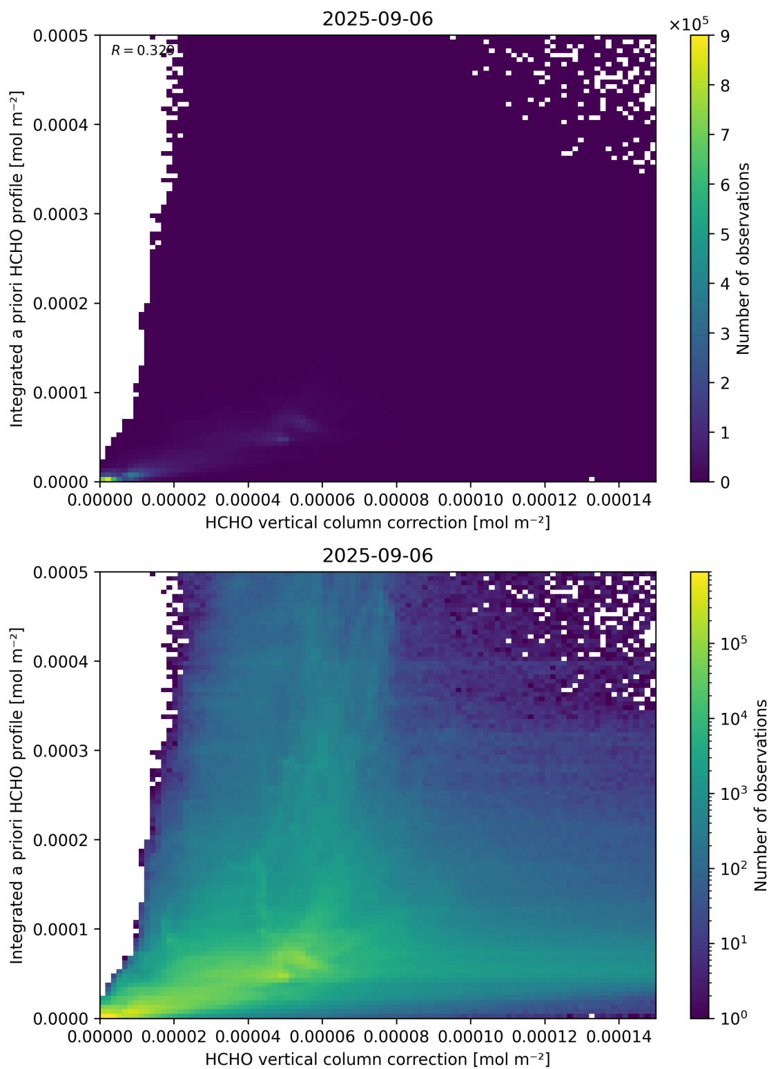
Figure 122: Scatter density plot of “HCHO vertical column correction” against “Integrated a priori HCHO profile” for 2025-09-05 to 2025-09-07.
