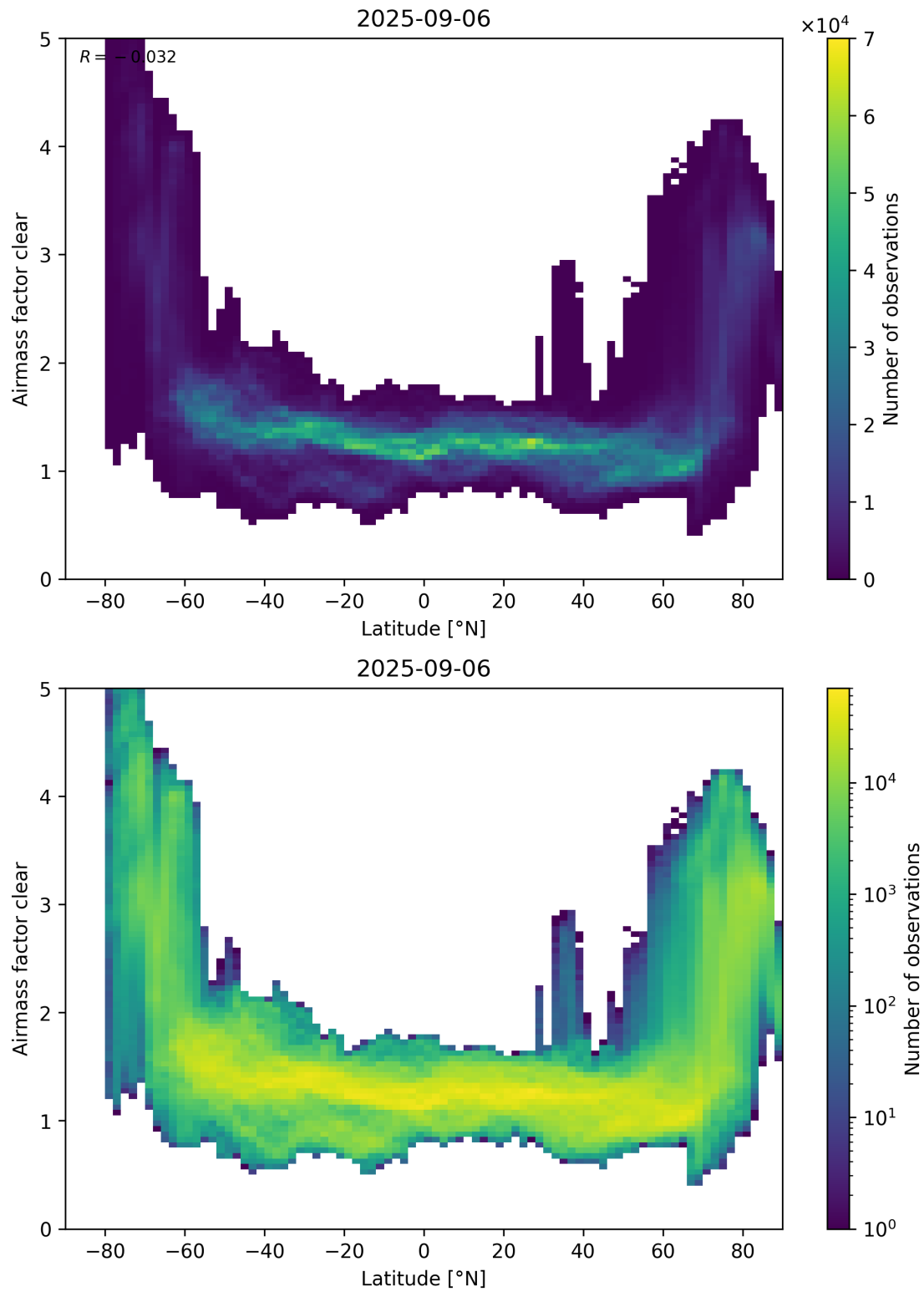
Figure 156: Scatter density plot of “Latitude” against “Airmass factor clear” for 2025-09-05 to 2025-09-07.
