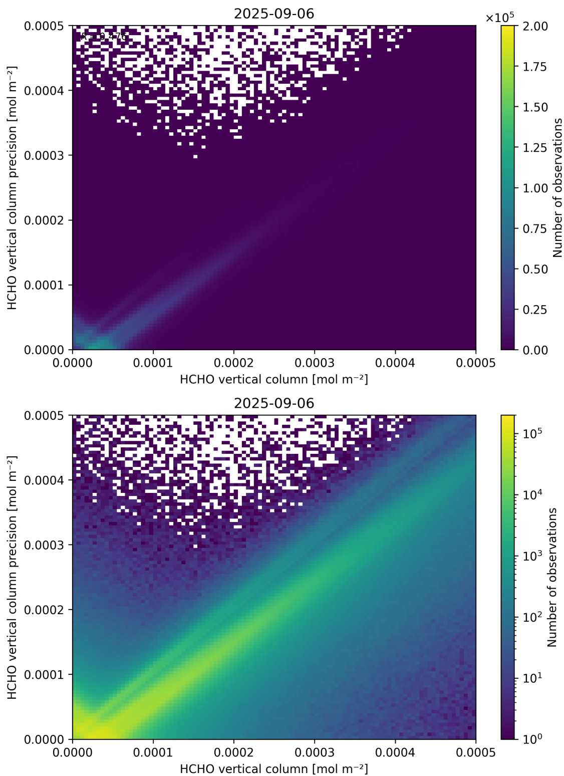
Figure 134: Scatter density plot of “HCHO vertical column” against “HCHO vertical column precision” for 2025-09-05 to 2025-09-07.
