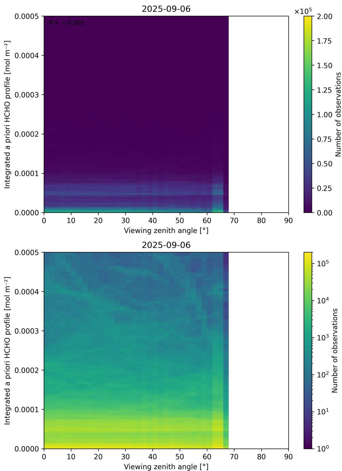
Figure 195: Scatter density plot of “Viewing zenith angle” against “Integrated a priori HCHO profile” for 2025-09-05 to 2025-09-07.
