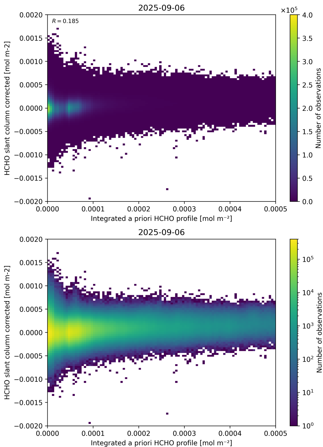
Figure 151: Scatter density plot of “Integrated a priori HCHO profile” against “HCHO slant column corrected” for 2025-09-05 to 2025-09-07.
