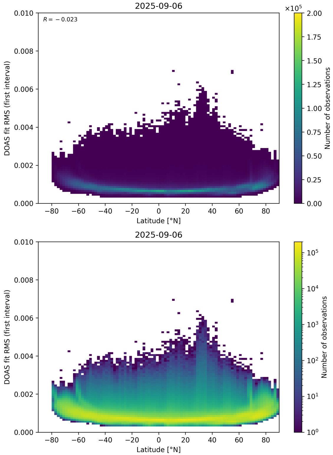
Figure 153: Scatter density plot of “Latitude” against “DOAS fit RMS (first interval)” for 2025-09-05 to 2025-09-07.
