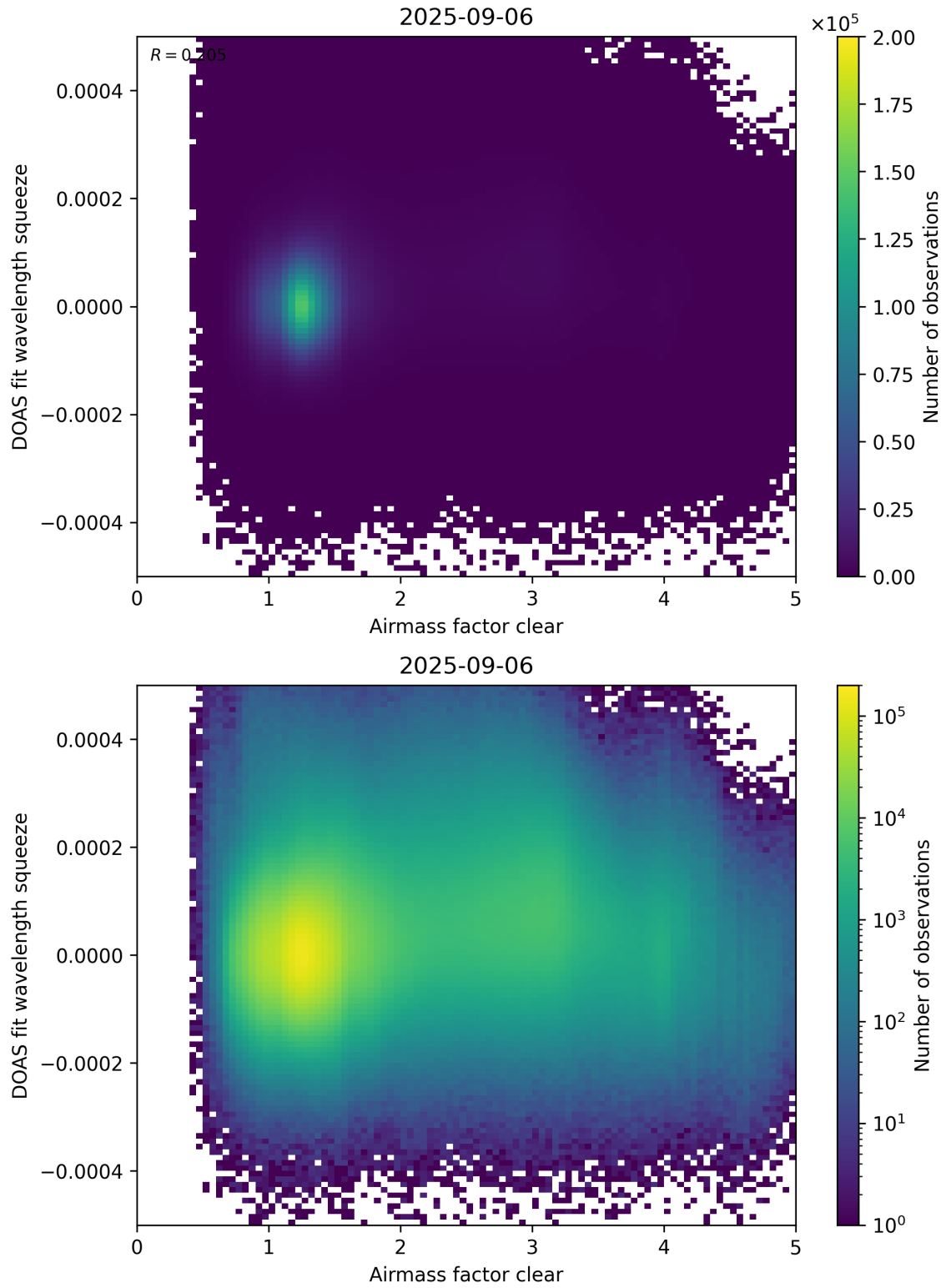
Figure 73: Scatter density plot of “Airmass factor clear” against “DOAS fit wavelength squeeze” for 2025-09-05 to 2025-09-07.
