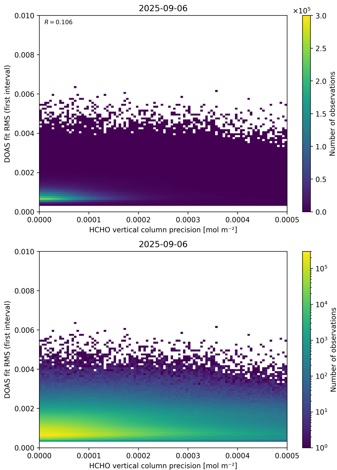
Figure 136: Scatter density plot of “HCHO vertical column precision” against “DOAS fit RMS (first interval)” for 2025-09-05 to 2025-09-07.
