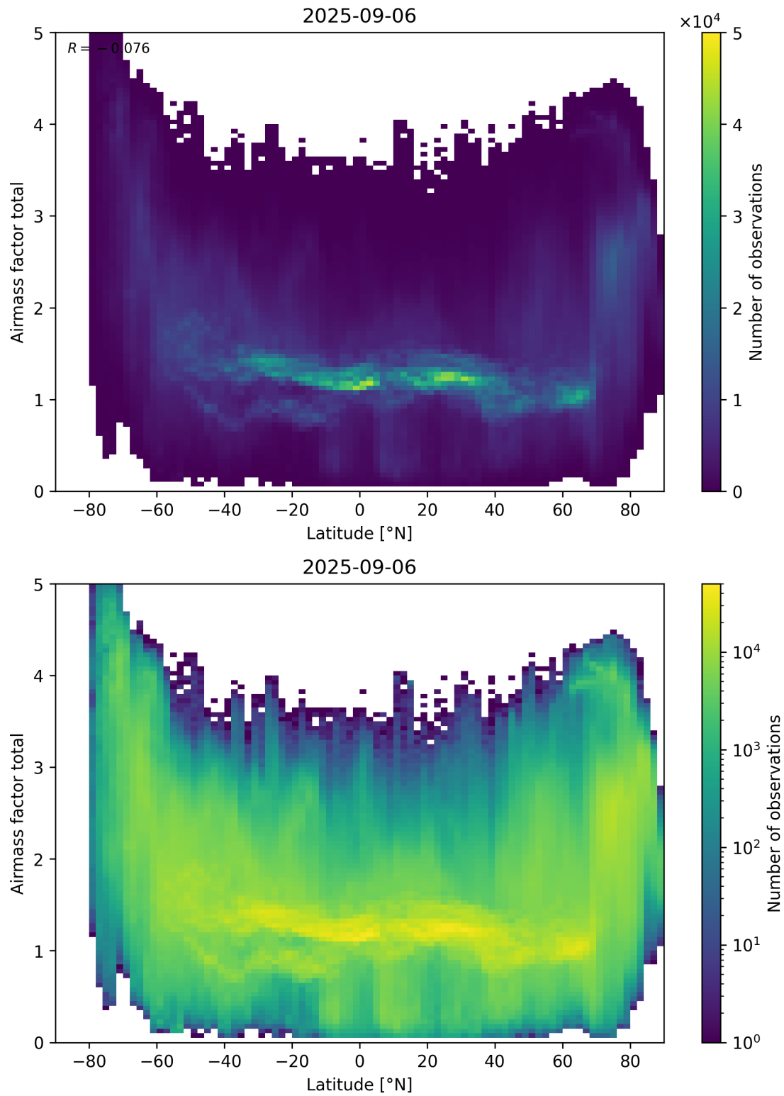
Figure 161: Scatter density plot of “Latitude” against “Airmass factor total” for 2025-09-05 to 2025-09-07.
