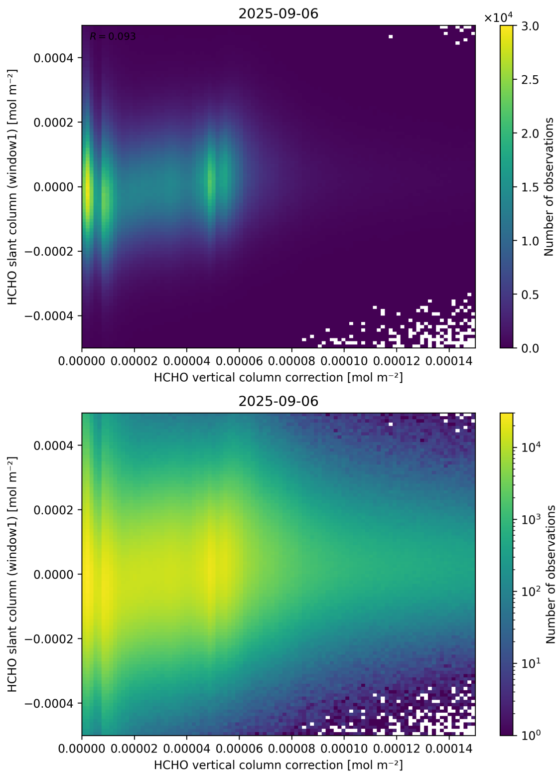
Figure 118: Scatter density plot of “HCHO vertical column correction” against “HCHO slant column (window1)” for 2025-09-05 to 2025-09-07.
