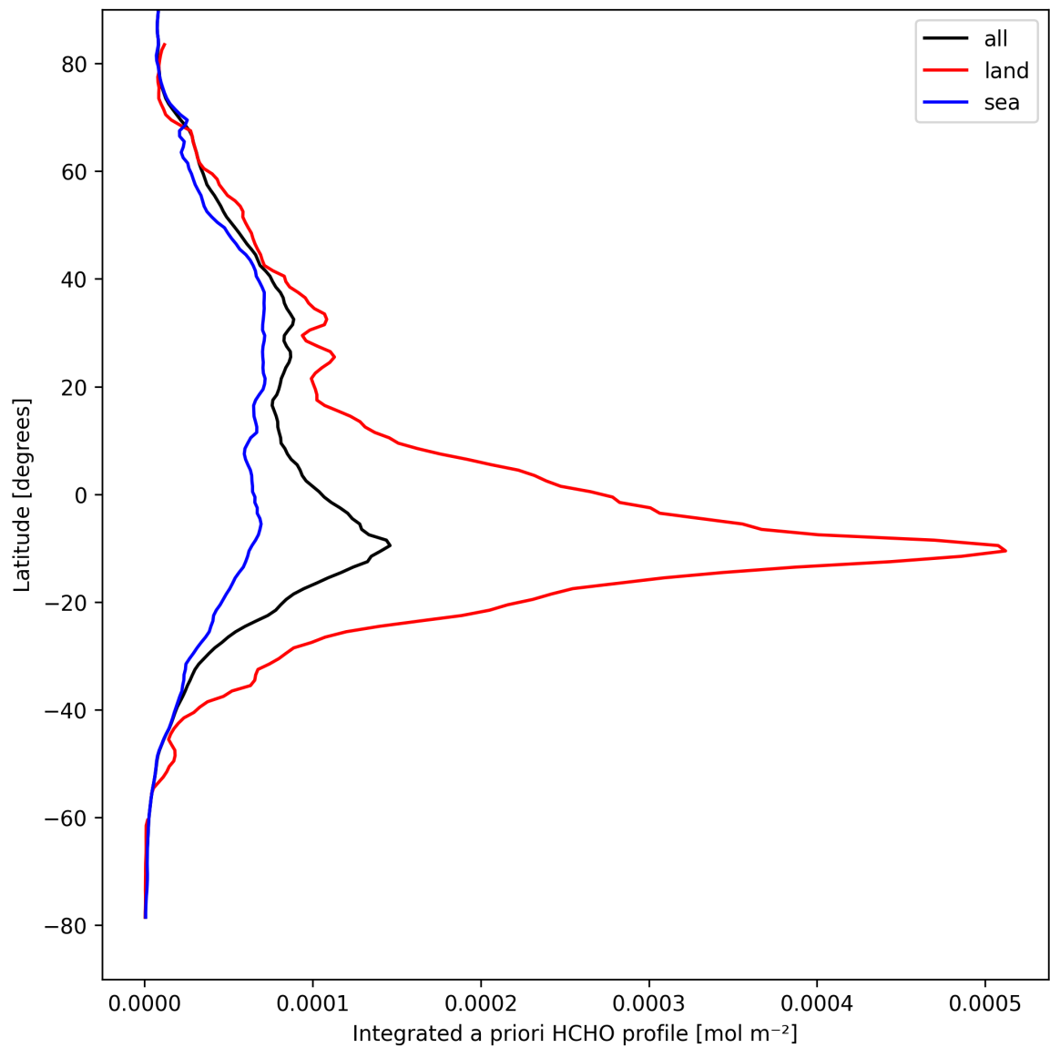
Figure 29: Zonal average of “Integrated a priori HCHO profile” for 2025-09-05 to 2025-09-07.
