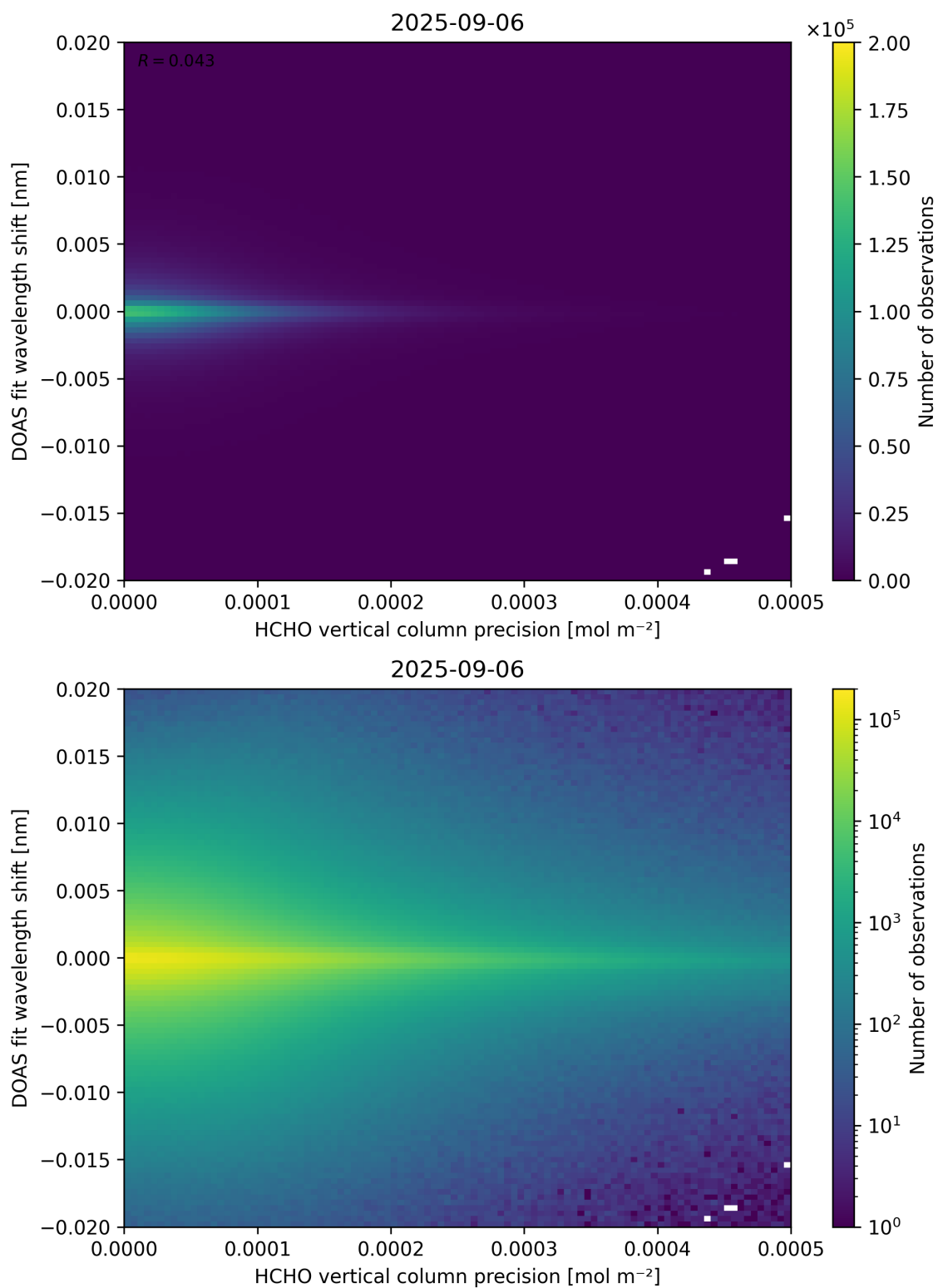
Figure 137: Scatter density plot of “HCHO vertical column precision” against “DOAS fit wavelength shift” for 2025-09-05 to 2025-09-07.
