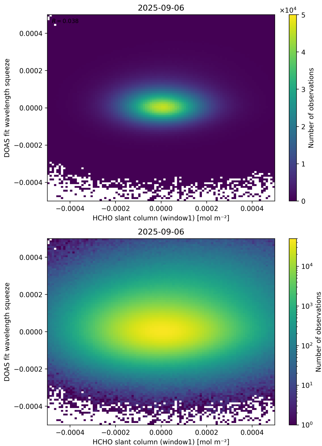
Figure 80: Scatter density plot of “HCHO slant column (window1)” against “DOAS fit wavelength squeeze” for 2025-09-05 to 2025-09-07.
