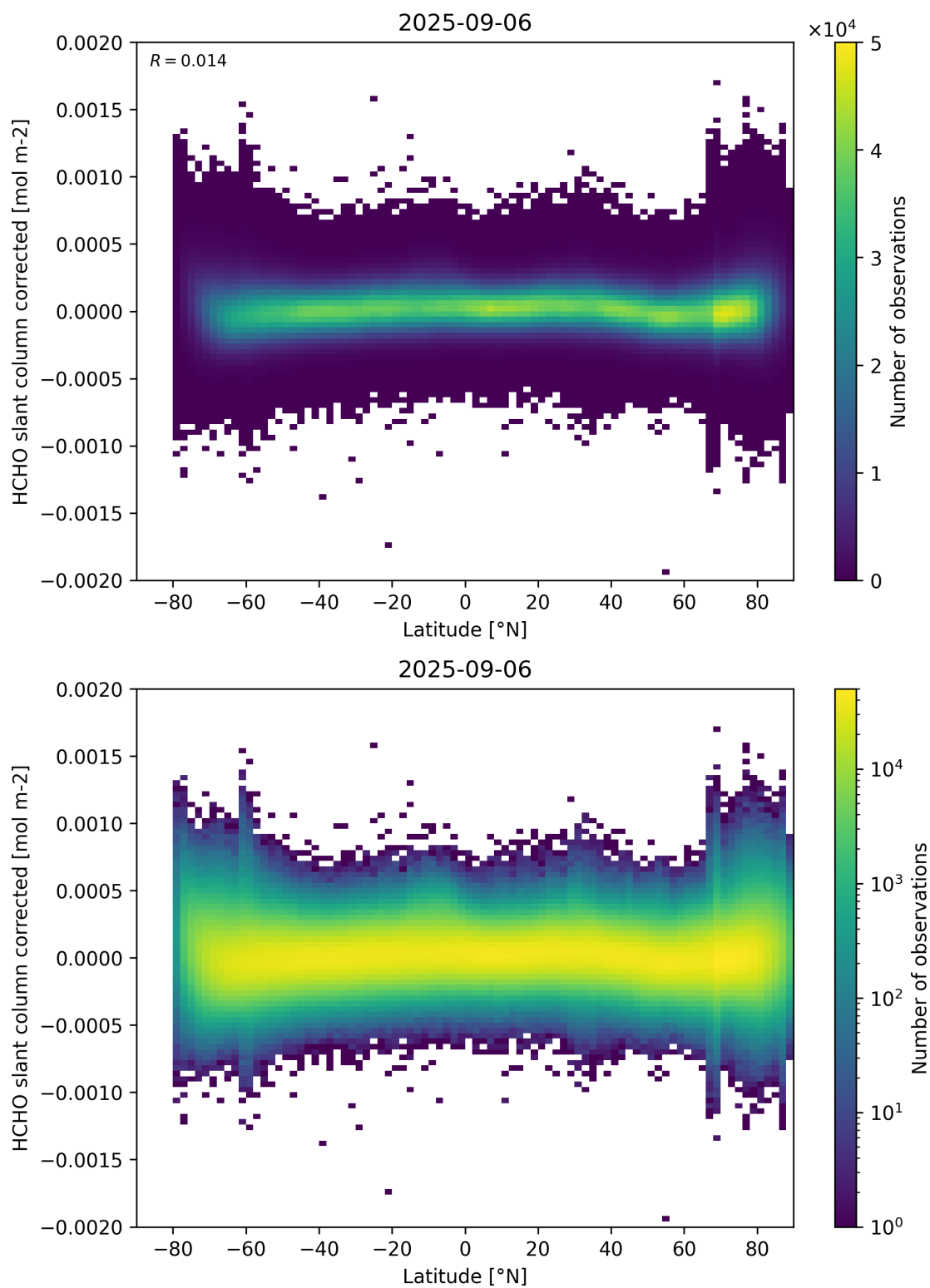
Figure 157: Scatter density plot of “Latitude” against “HCHO slant column corrected” for 2025-09-05 to 2025-09-07.
