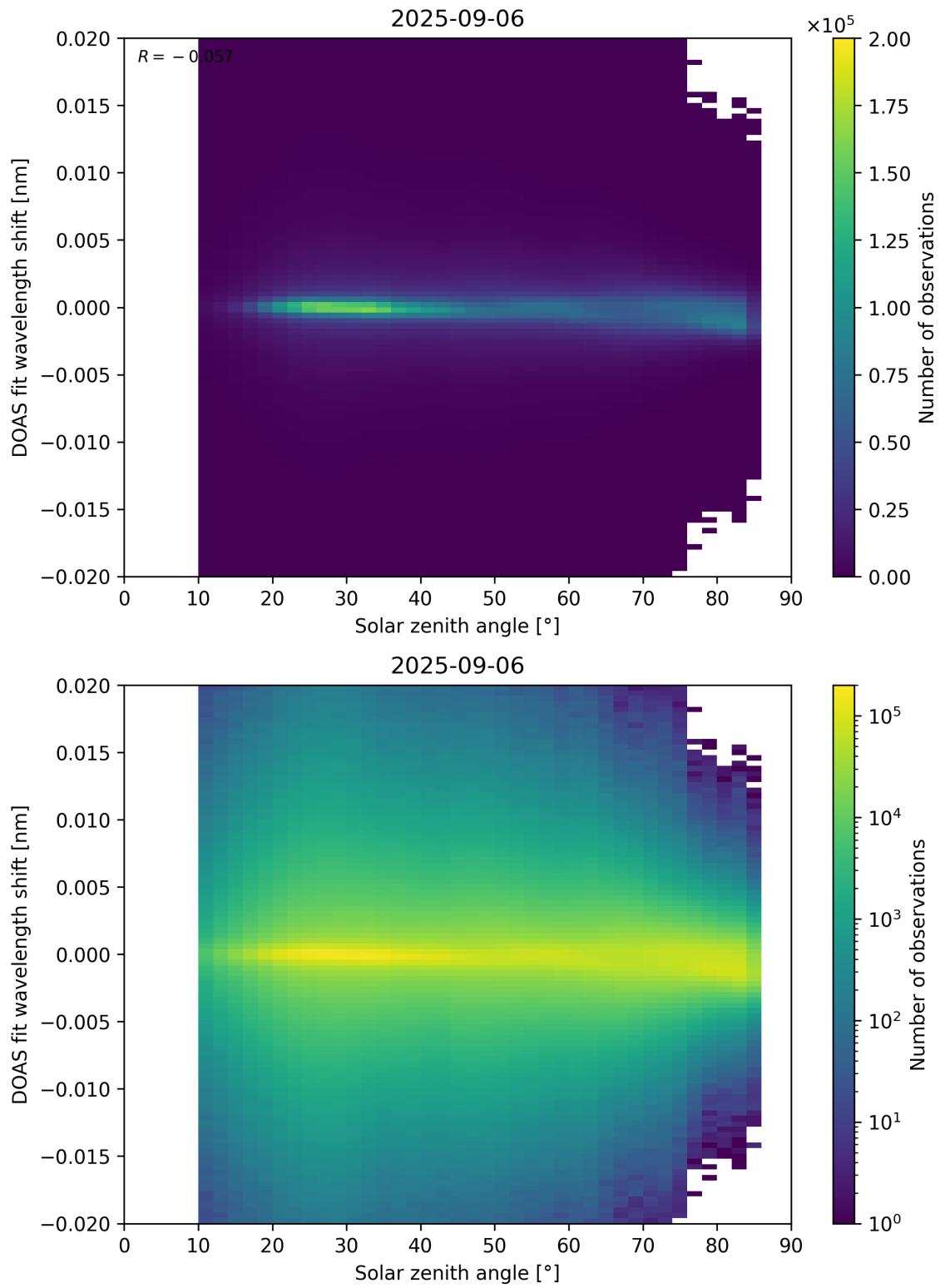
Figure 168: Scatter density plot of “Solar zenith angle” against “DOAS fit wavelength shift” for 2025-09-05 to 2025-09-07.
