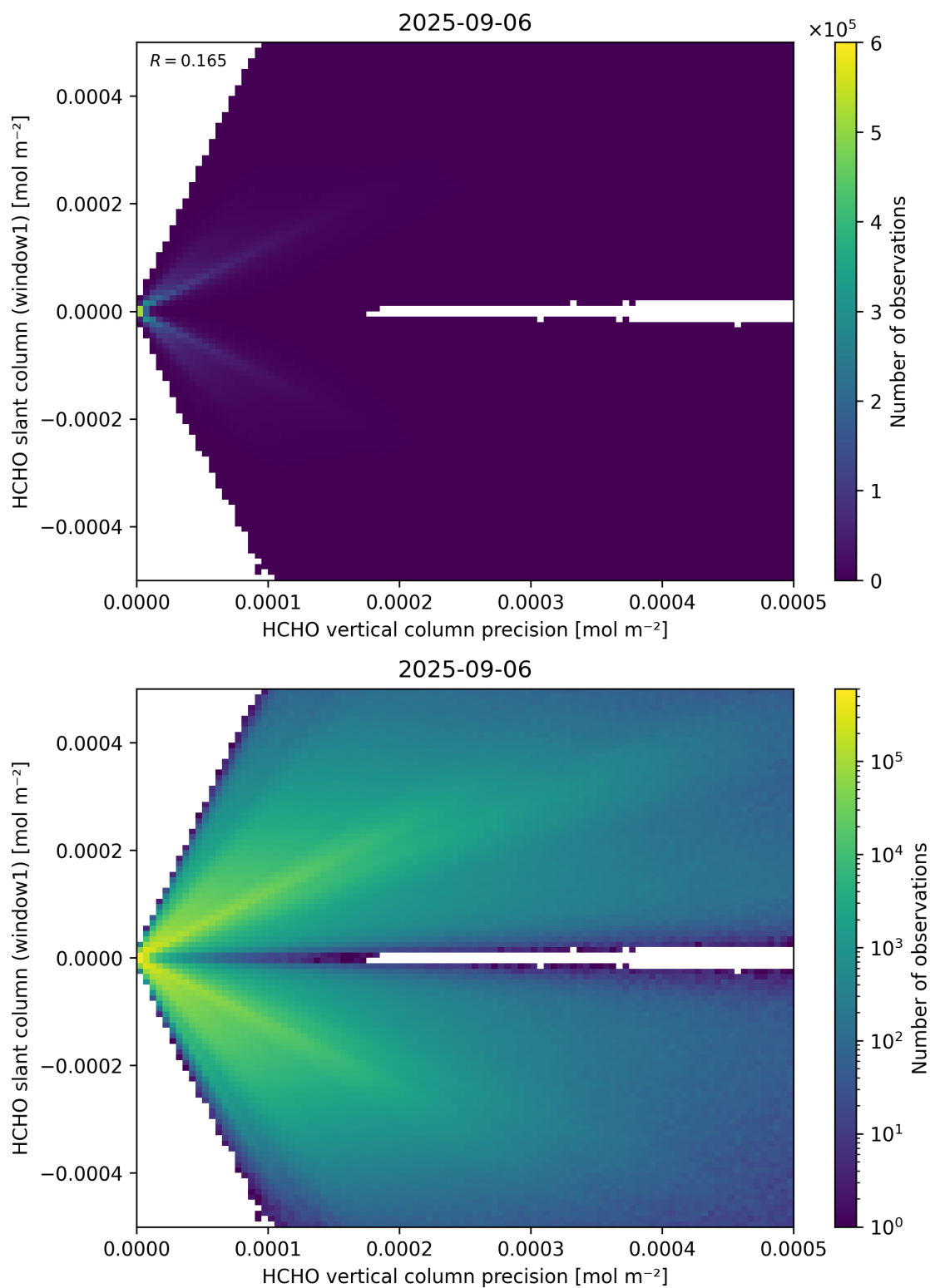
Figure 142: Scatter density plot of “HCHO vertical column precision” against “HCHO slant column (window1)” for 2025-09-05 to 2025-09-07.
