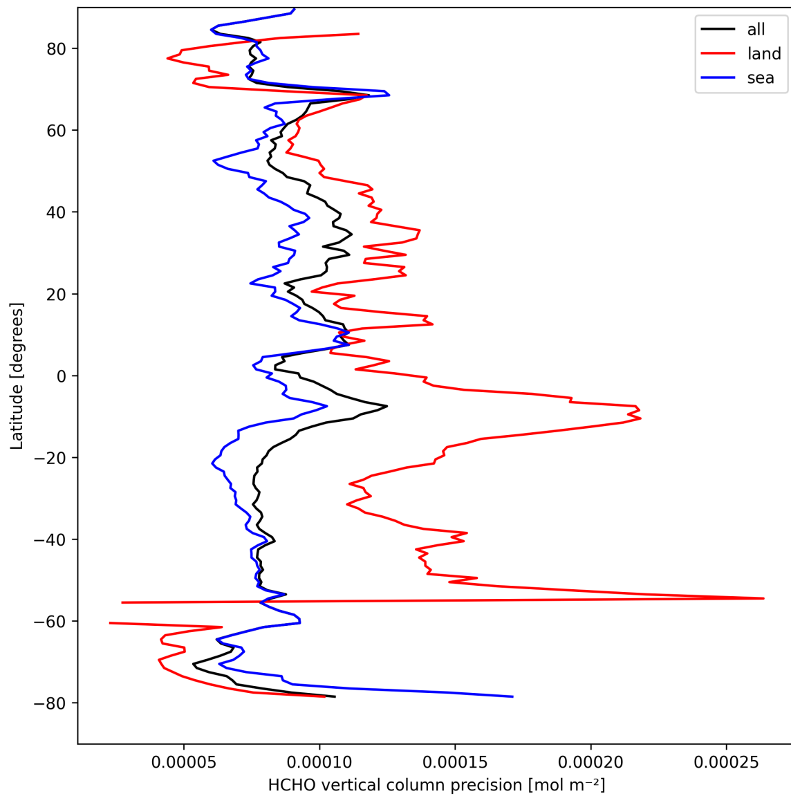
Figure 22: Zonal average of “HCHO vertical column precision” for 2025-09-05 to 2025-09-07.
