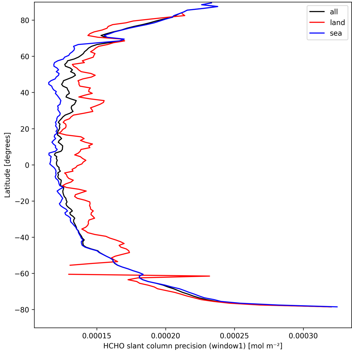
Figure 25: Zonal average of “HCHO slant column precision (window1)” for 2025-09-05 to 2025-09-07.
