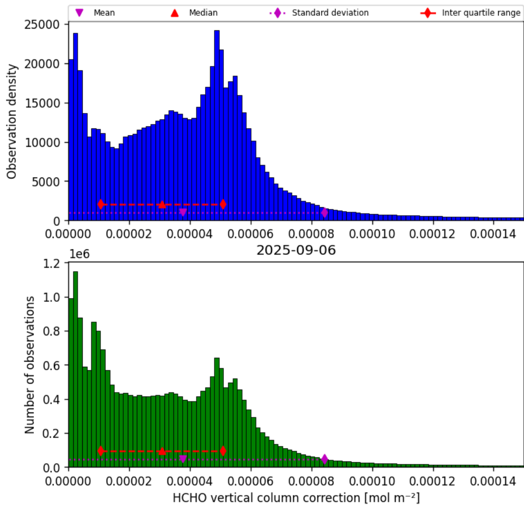
Figure 37: Histogram of “HCHO vertical column correction” for 2025-09-05 to 2025-09-07
