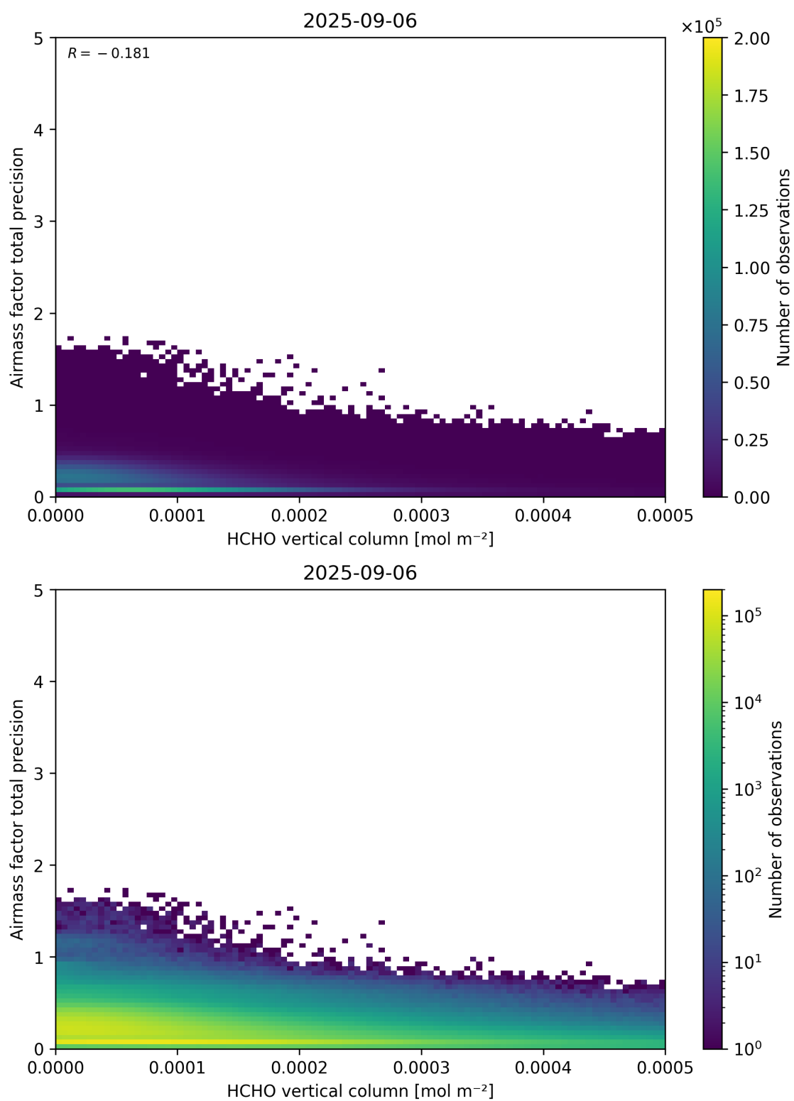
Figure 132: Scatter density plot of “HCHO vertical column” against “Airmass factor total precision” for 2025-09-05 to 2025-09-07.
