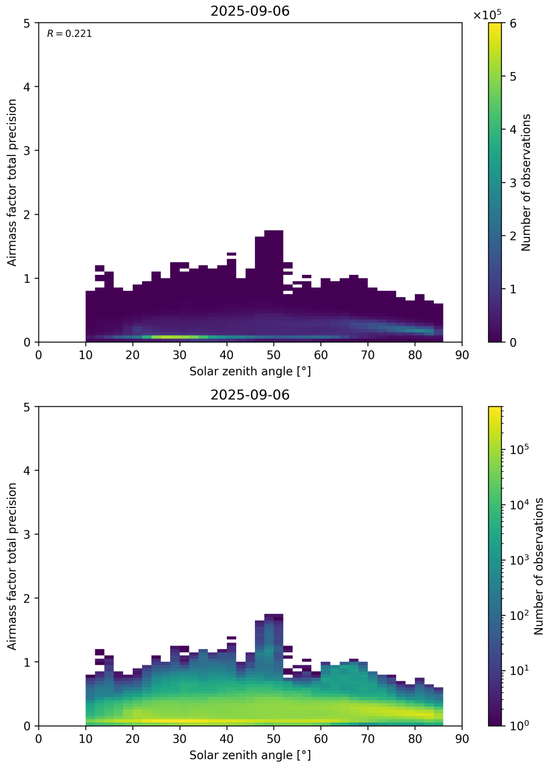
Figure 176: Scatter density plot of “Solar zenith angle” against “Airmass factor total precision” for 2025-09-05 to 2025-09-07.
