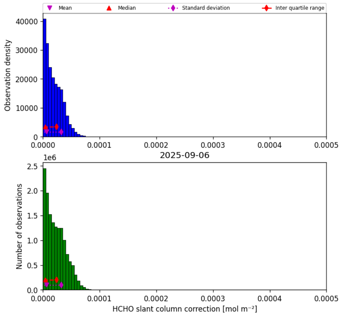
Figure 47: Histogram of “HCHO slant column correction” for 2025-09-05 to 2025-09-07
