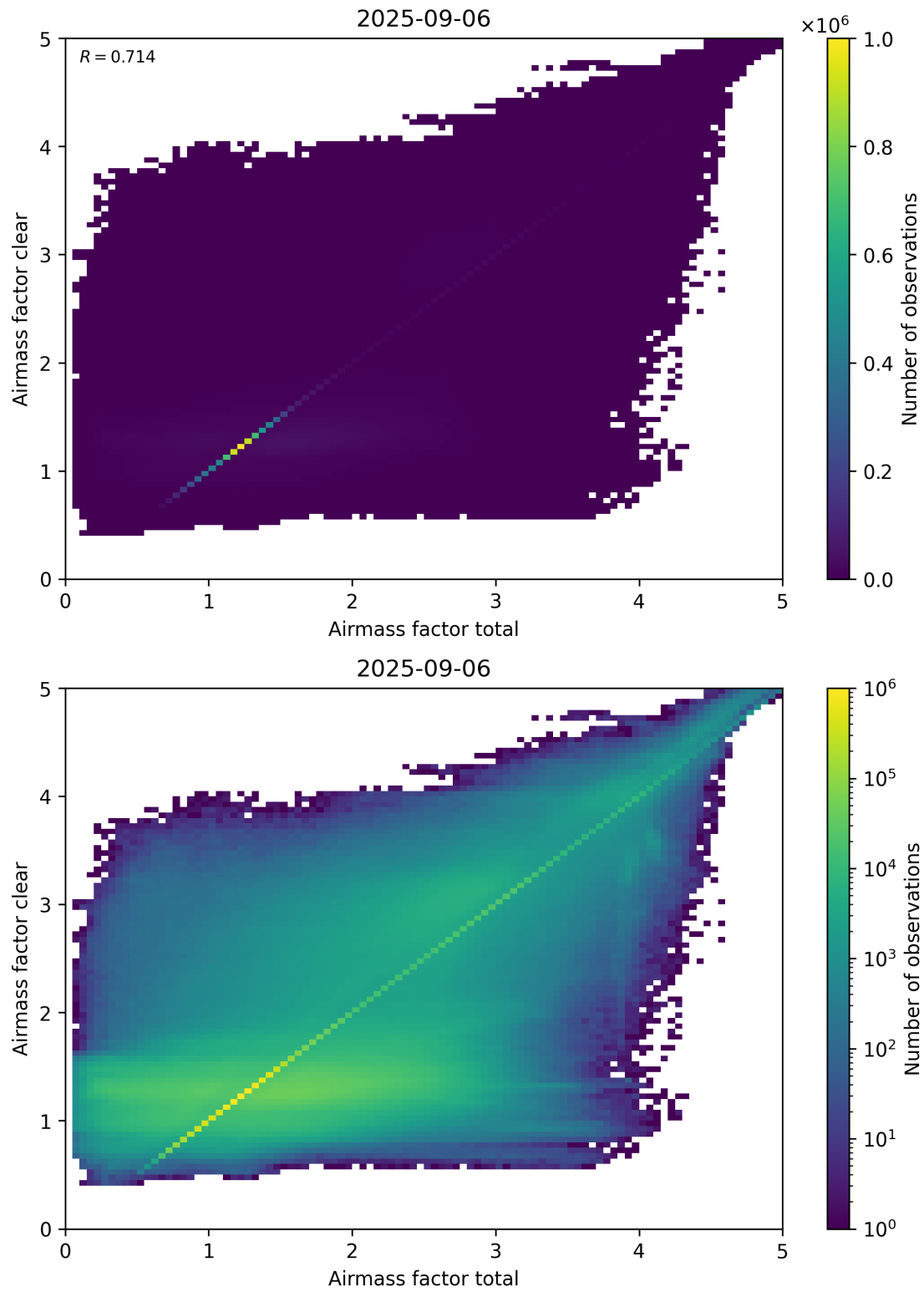
Figure 100: Scatter density plot of “Airmass factor total” against “Airmass factor clear” for 2025-09-05 to 2025-09-07.
