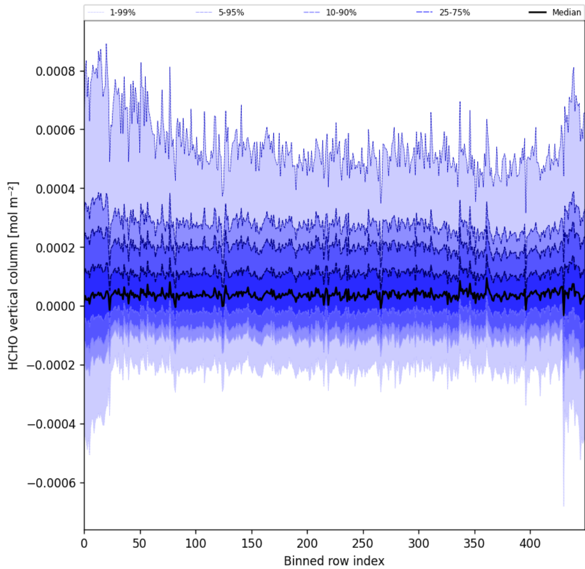
Figure 49: Along track statistics of “HCHO vertical column” for 2025-09-05 to 2025-09-07
