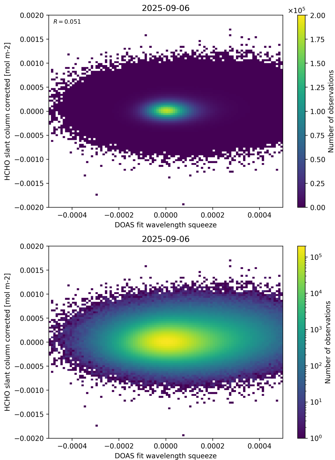
Figure 69: Scatter density plot of “DOAS fit wavelength squeeze” against “HCHO slant column corrected” for 2025-09-05 to 2025-09-07.
