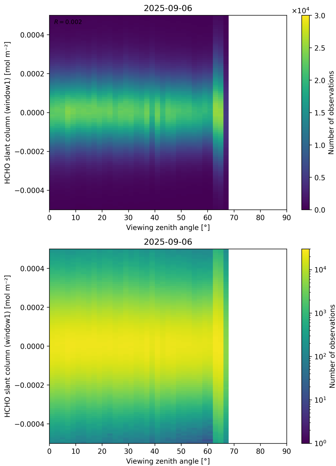
Figure 188: Scatter density plot of “Viewing zenith angle” against “HCHO slant column (window1)” for 2025-09-05 to 2025-09-07.
