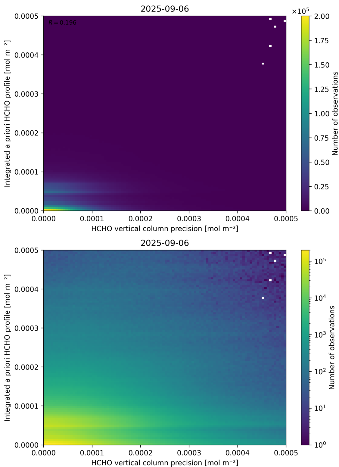
Figure 147: Scatter density plot of “HCHO vertical column precision” against “Integrated a priori HCHO profile” for 2025-09-05 to 2025-09-07.
