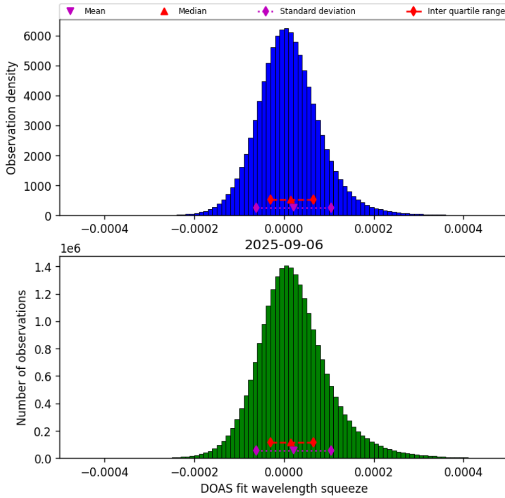
Figure 45: Histogram of “DOAS fit wavelength squeeze” for 2025-09-05 to 2025-09-07
