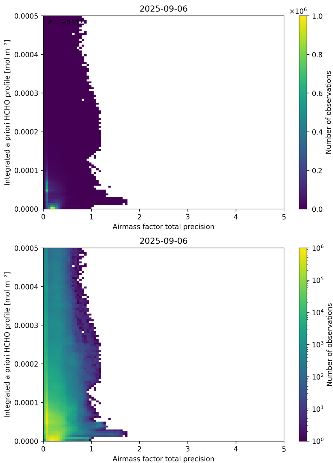
Figure 111: Scatter density plot of “Airmass factor total precision” against “Integrated a priori HCHO profile” for 2025-09-05 to 2025-09-07.
