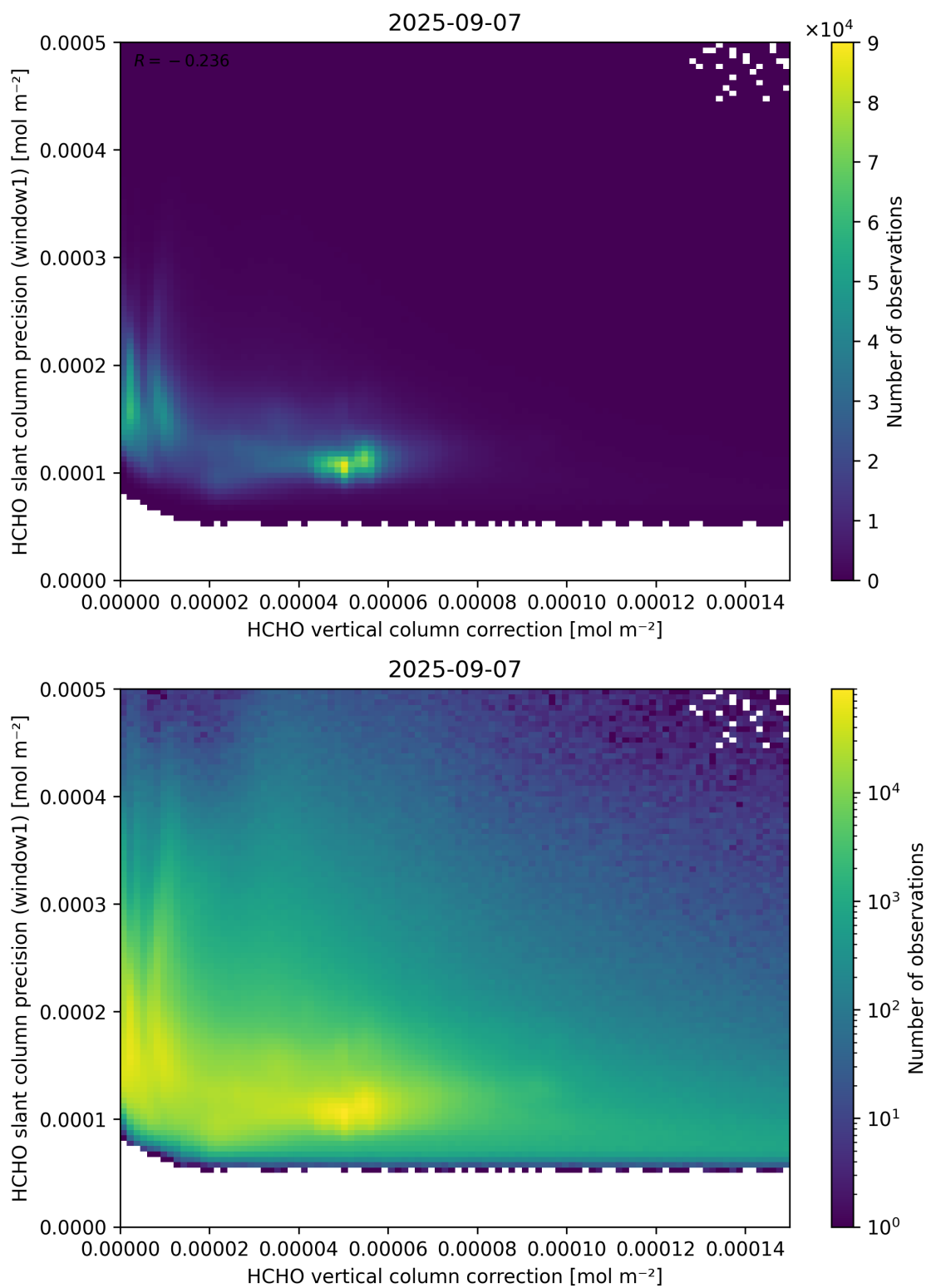
Figure 119: Scatter density plot of “HCHO vertical column correction” against “HCHO slant column precision (window1)” for 2025-09-06 to 2025-09-08.
