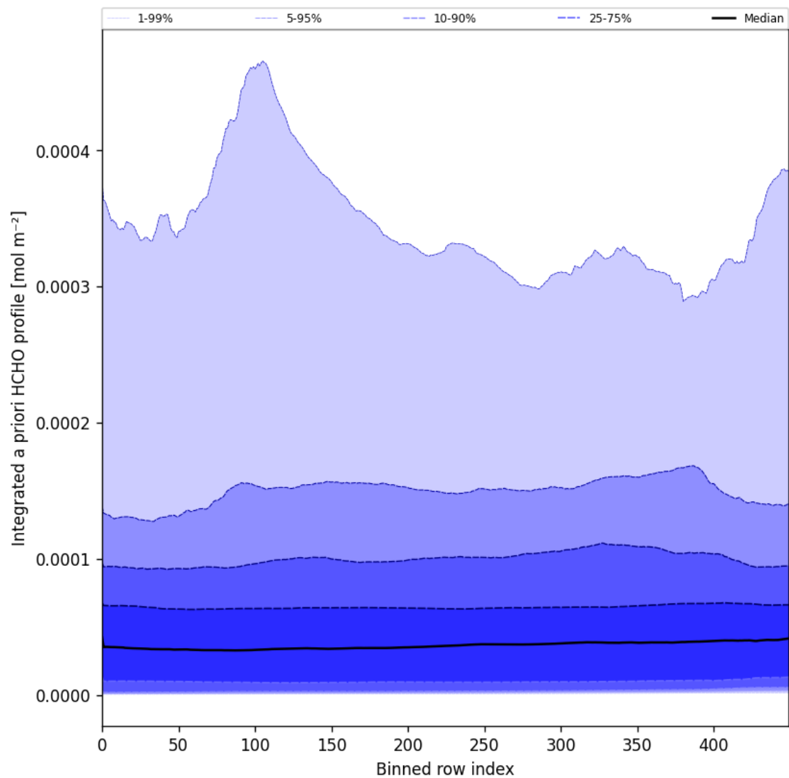
Figure 57: Along track statistics of “Integrated a priori HCHO profile” for 2025-09-06 to 2025-09-08
