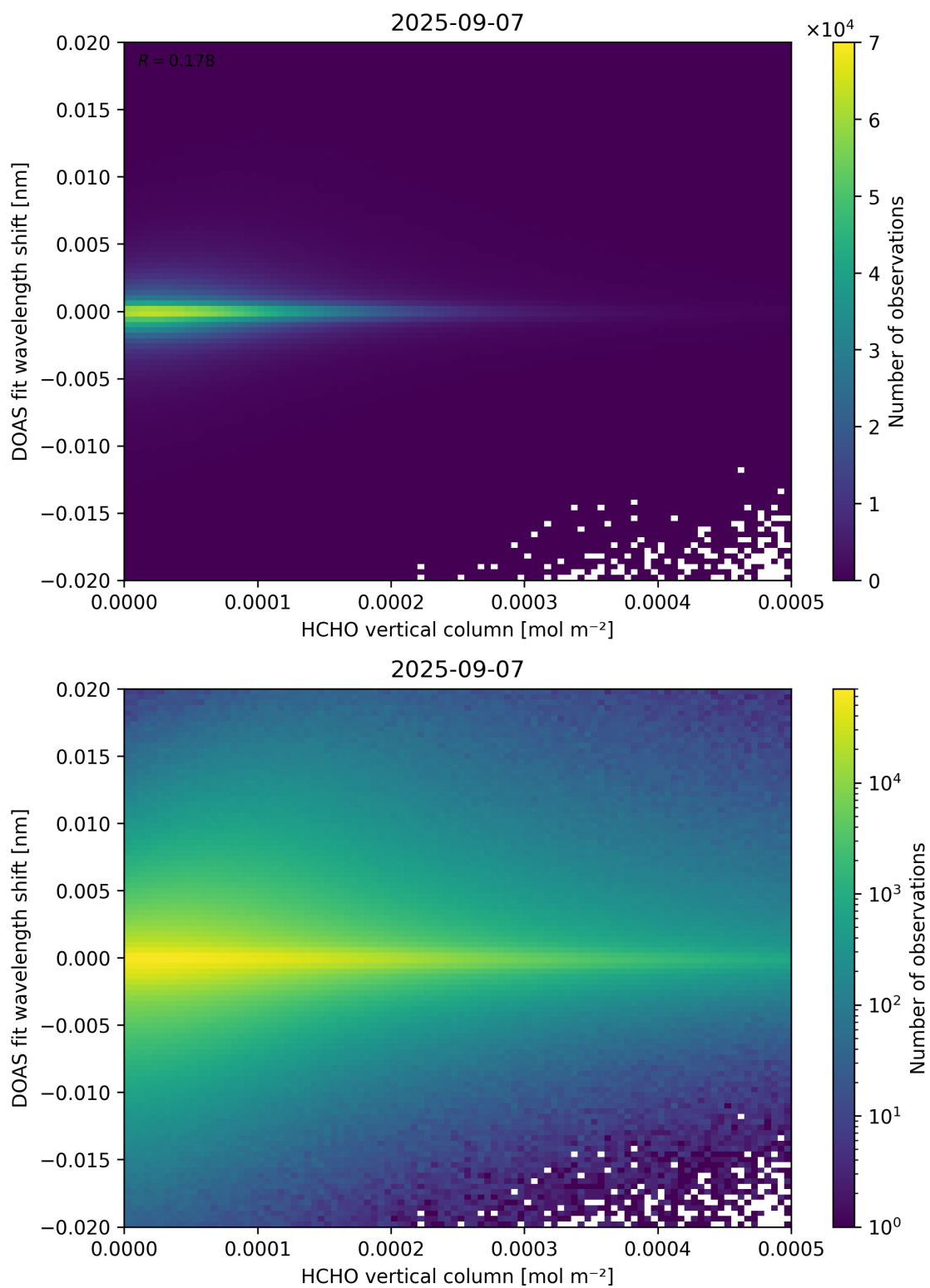
Figure 124: Scatter density plot of “HCHO vertical column” against “DOAS fit wavelength shift” for 2025-09-06 to 2025-09-08.
