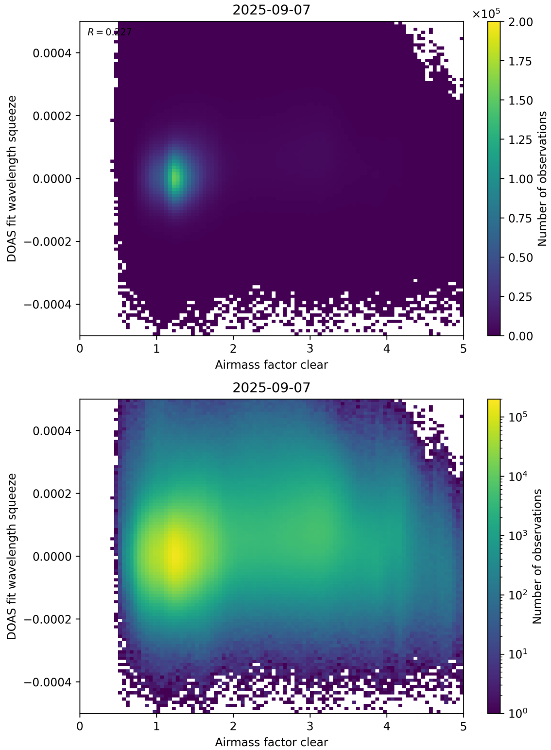
Figure 73: Scatter density plot of “Airmass factor clear” against “DOAS fit wavelength squeeze” for 2025-09-06 to 2025-09-08.
