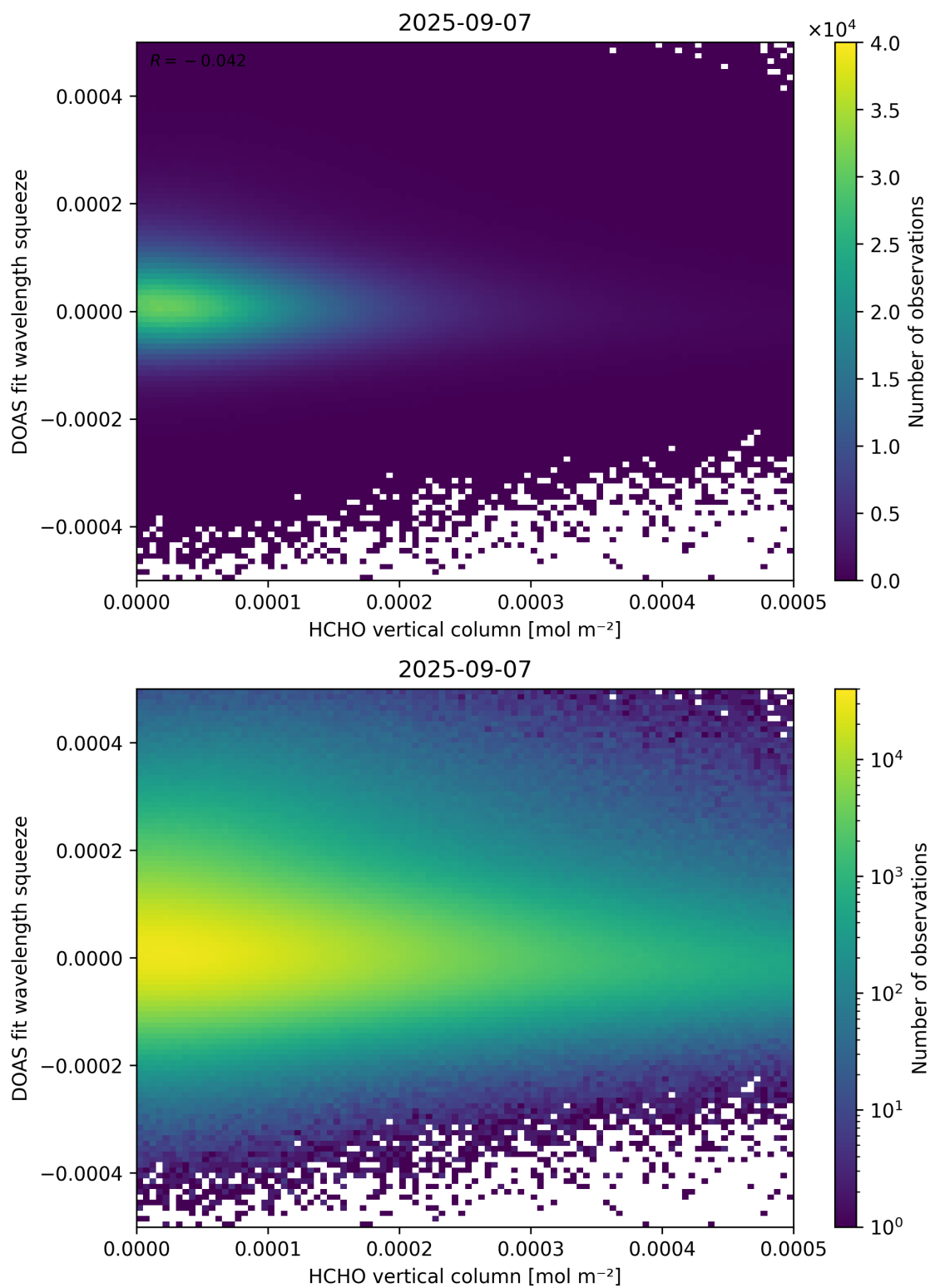
Figure 125: Scatter density plot of “HCHO vertical column” against “DOAS fit wavelength squeeze” for 2025-09-06 to 2025-09-08.
