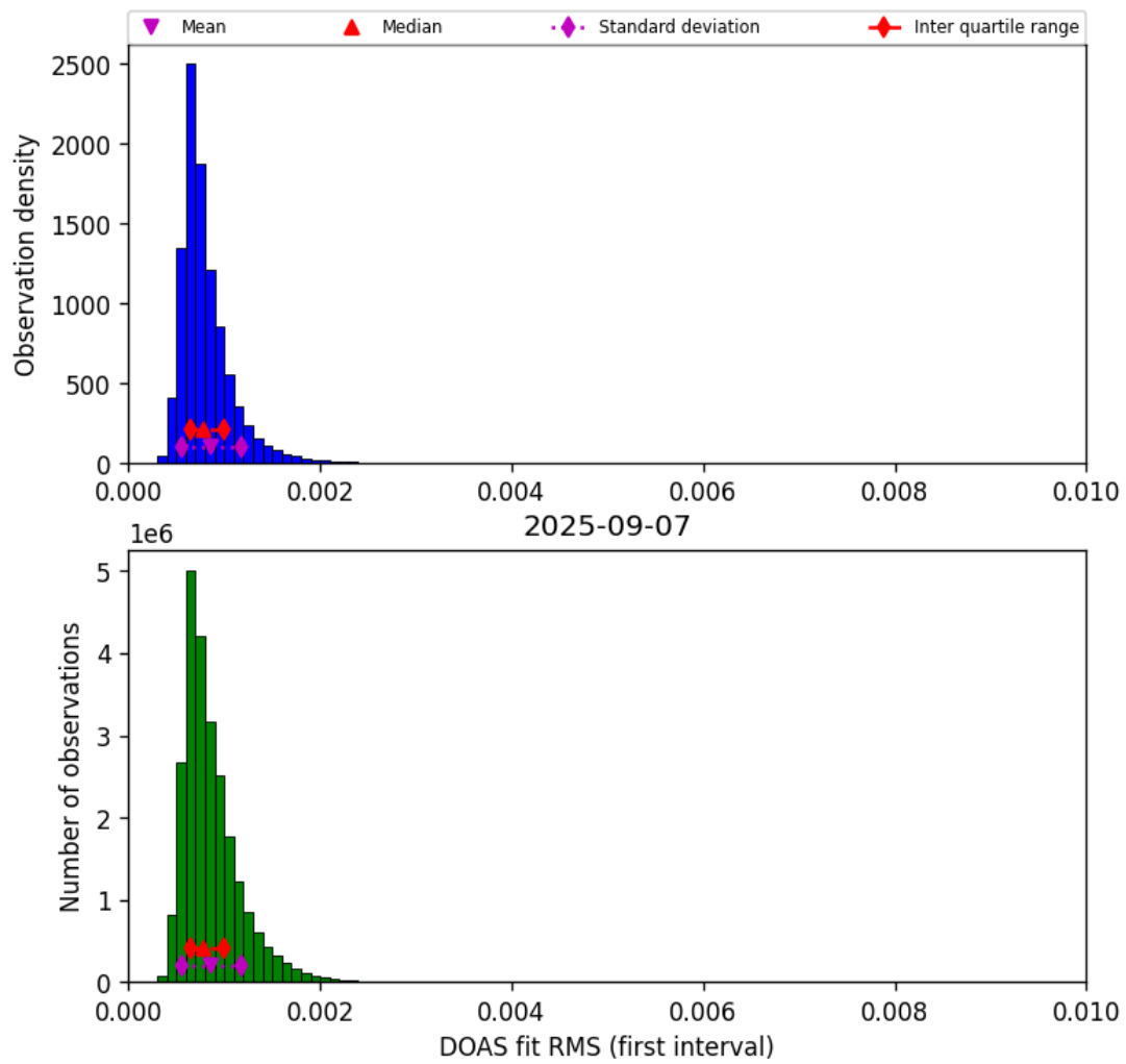
Figure 46: Histogram of “DOAS fit RMS (first interval)” for 2025-09-06 to 2025-09-08
