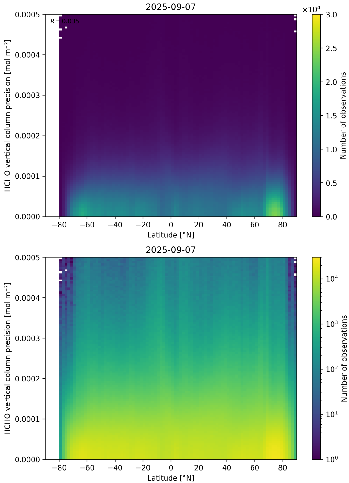
Figure 165: Scatter density plot of “Latitude” against “HCHO vertical column precision” for 2025-09-06 to 2025-09-08.
