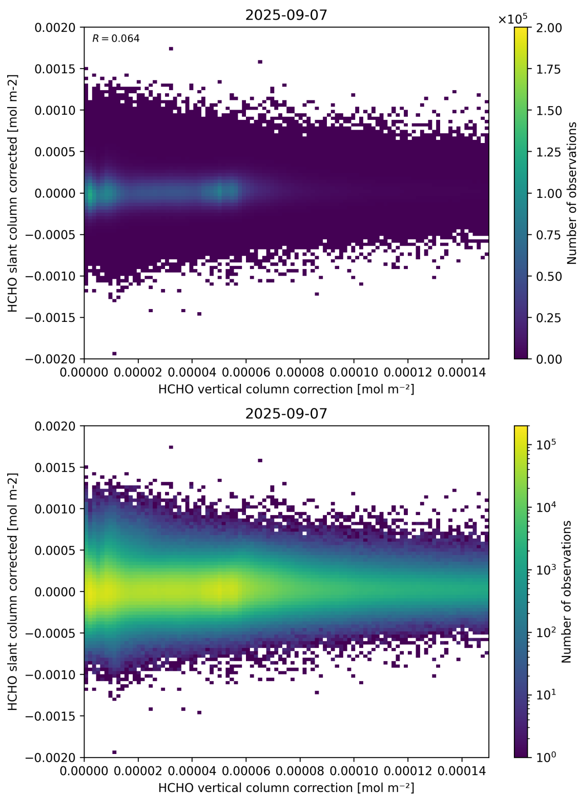
Figure 116: Scatter density plot of “HCHO vertical column correction” against “HCHO slant column corrected” for 2025-09-06 to 2025-09-08.
