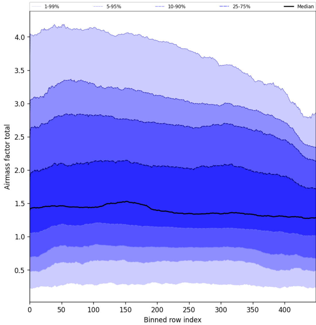
Figure 54: Along track statistics of “Airmass factor total” for 2025-09-06 to 2025-09-08
