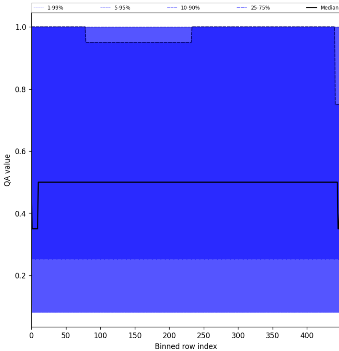
Figure 48: Along track statistics of “QA value” for 2025-09-06 to 2025-09-08
