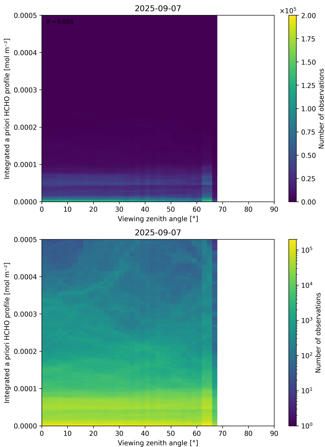
Figure 195: Scatter density plot of “Viewing zenith angle” against “Integrated a priori HCHO profile” for 2025-09-06 to 2025-09-08.
