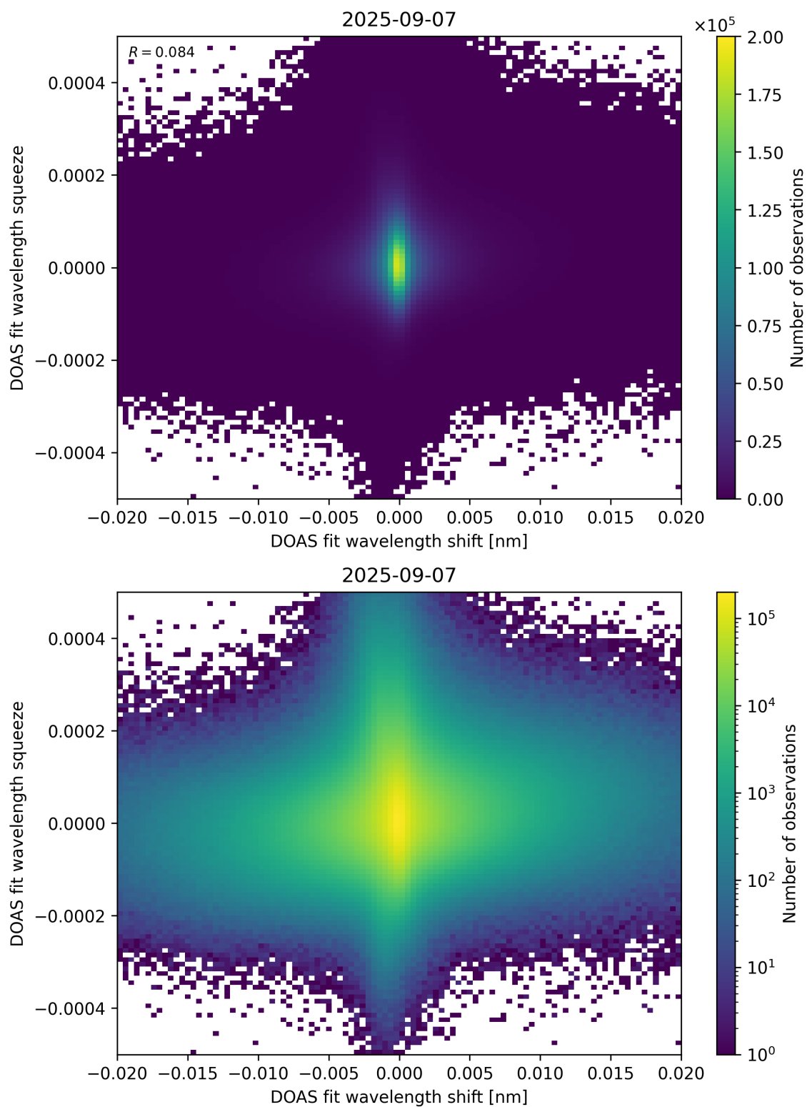
Figure 65: Scatter density plot of “DOAS fit wavelength shift” against “DOAS fit wavelength squeeze” for 2025-09-06 to 2025-09-08.
