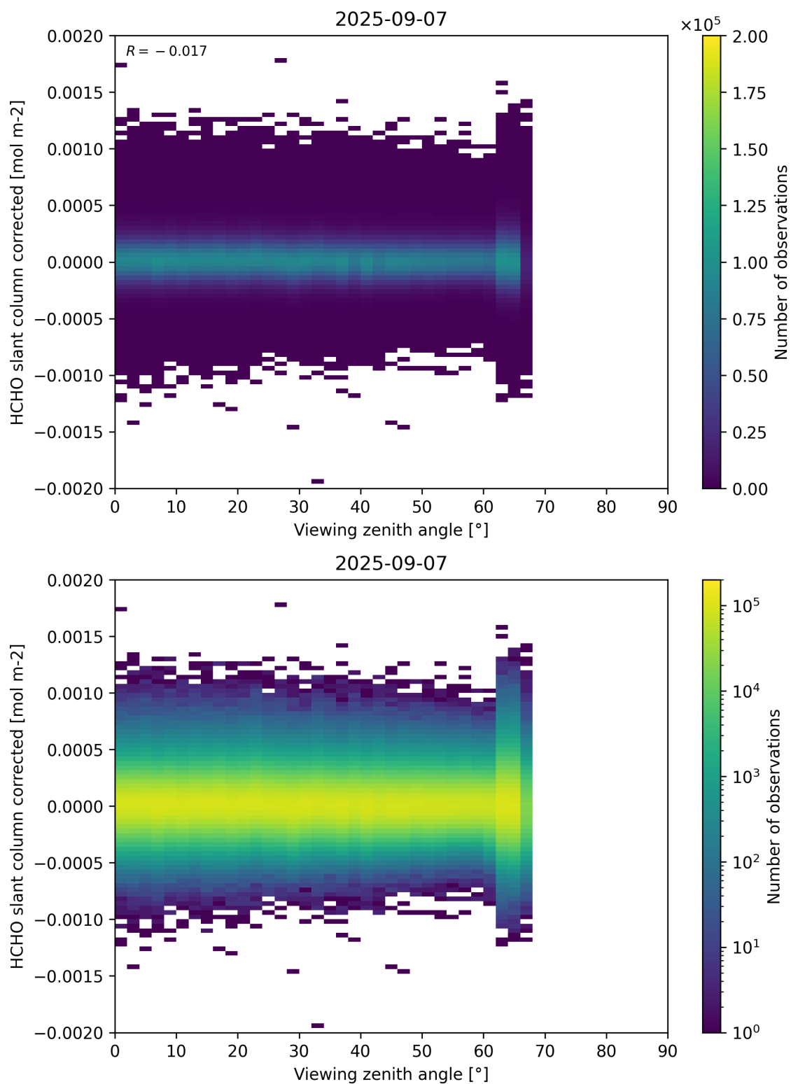
Figure 186: Scatter density plot of “Viewing zenith angle” against “HCHO slant column corrected” for 2025-09-06 to 2025-09-08.
