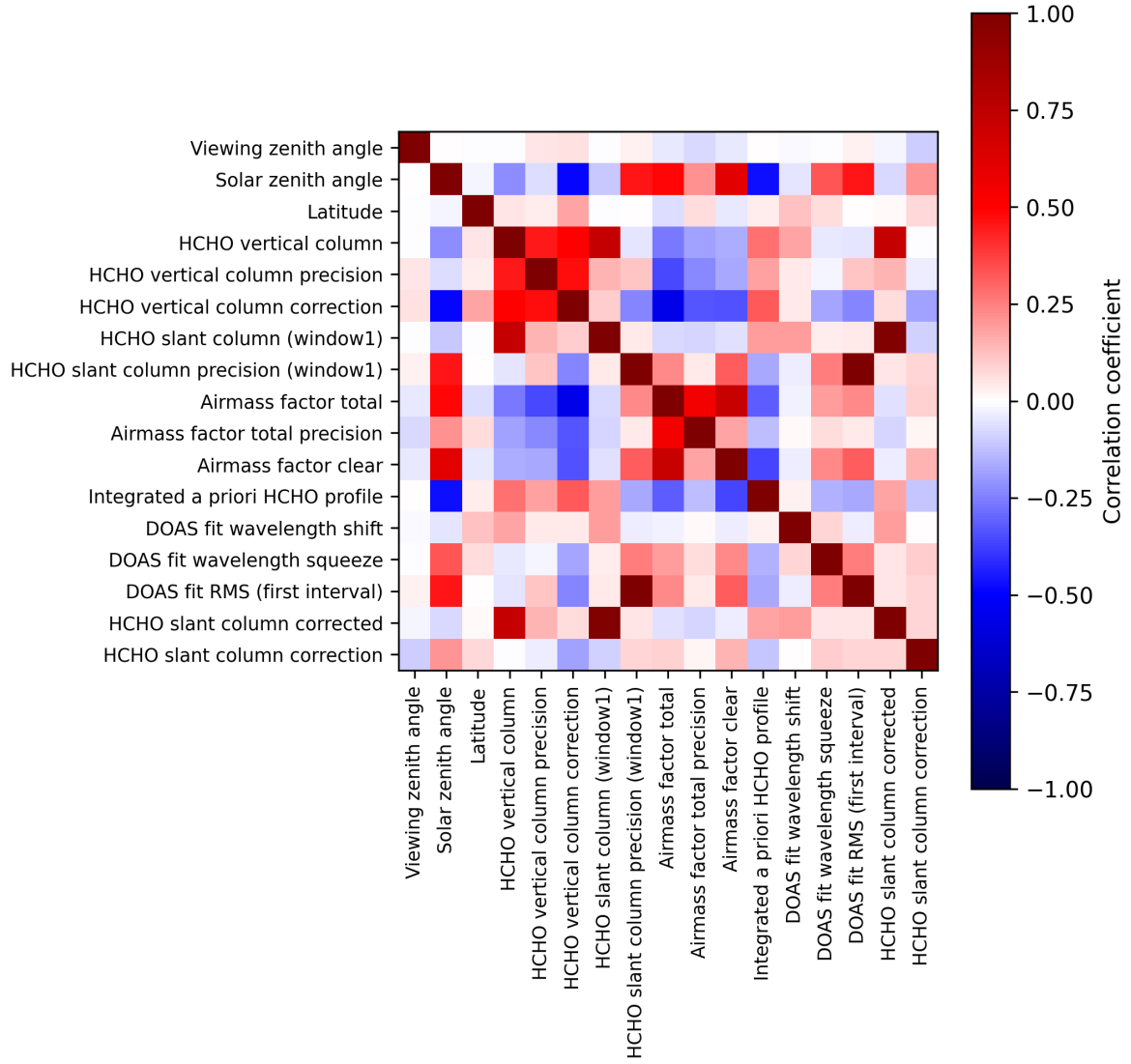
Figure 2: Map of correlation matrix for 2025-09-06 to 2025-09-08.
