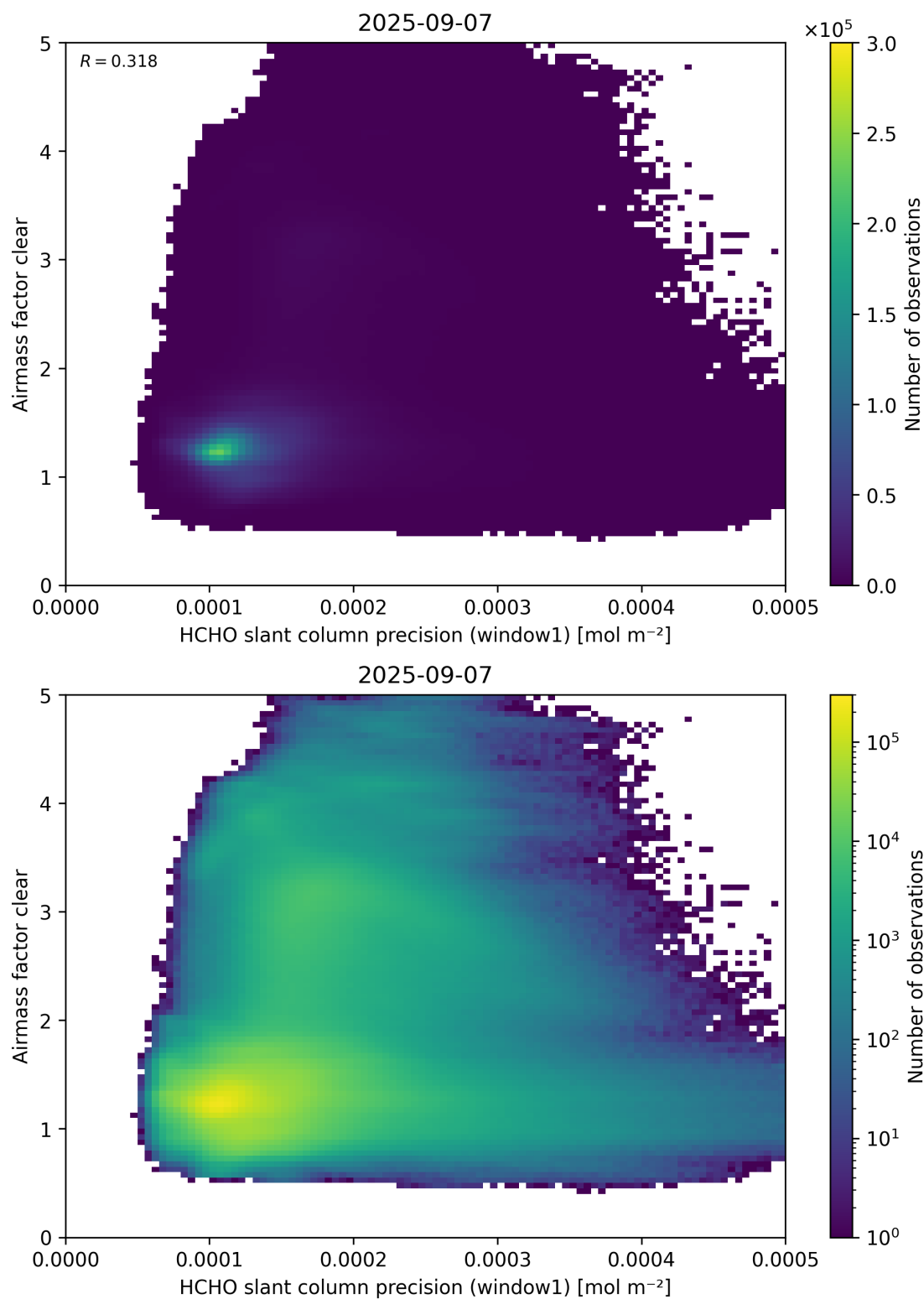
Figure 91: Scatter density plot of “HCHO slant column precision (window1)” against “Airmass factor clear” for 2025-09-06 to 2025-09-08.
