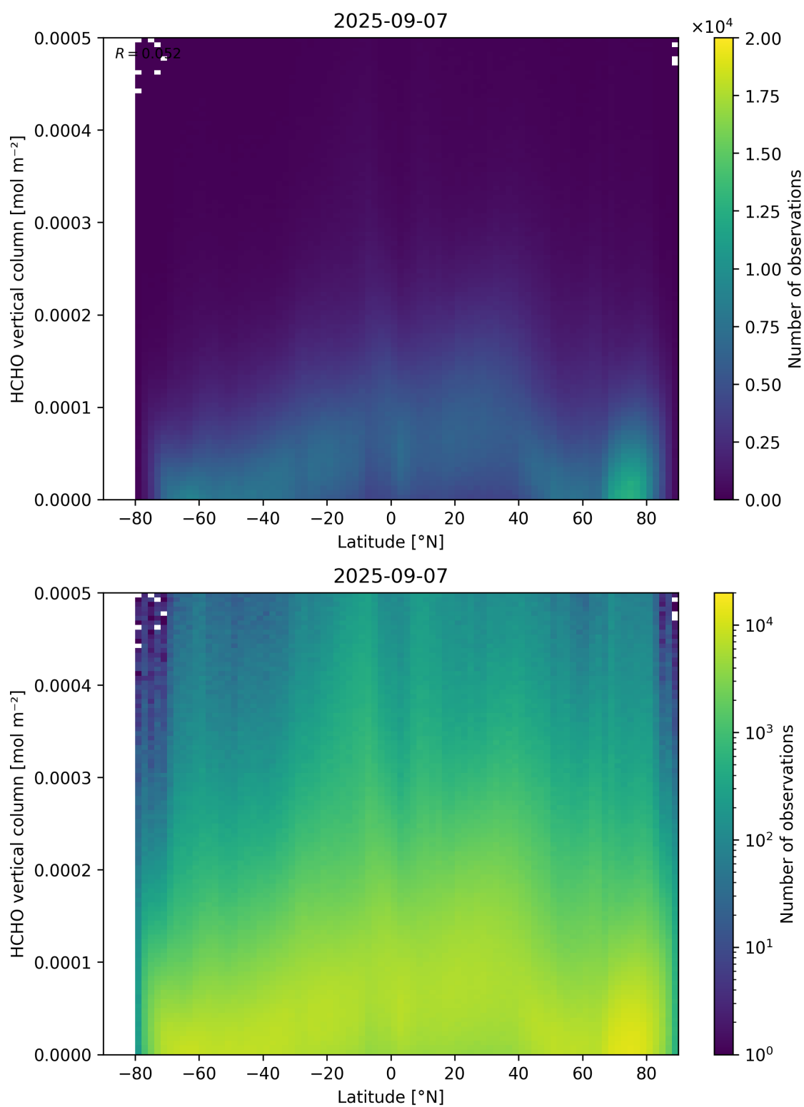
Figure 163: Scatter density plot of “Latitude” against “HCHO vertical column” for 2025-09-06 to 2025-09-08.
