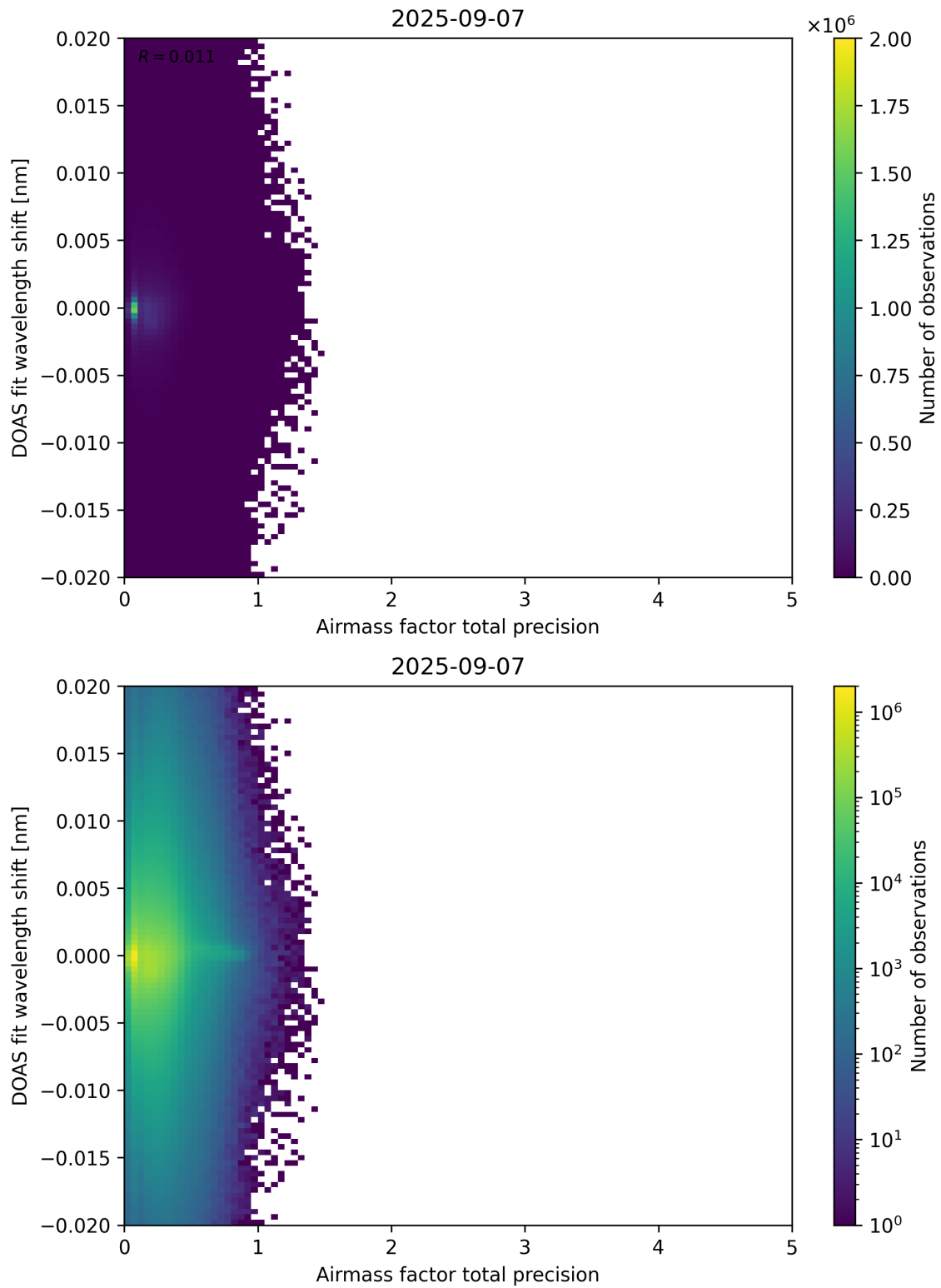
Figure 106: Scatter density plot of “Airmass factor total precision” against “DOAS fit wavelength shift” for 2025-09-06 to 2025-09-08.
