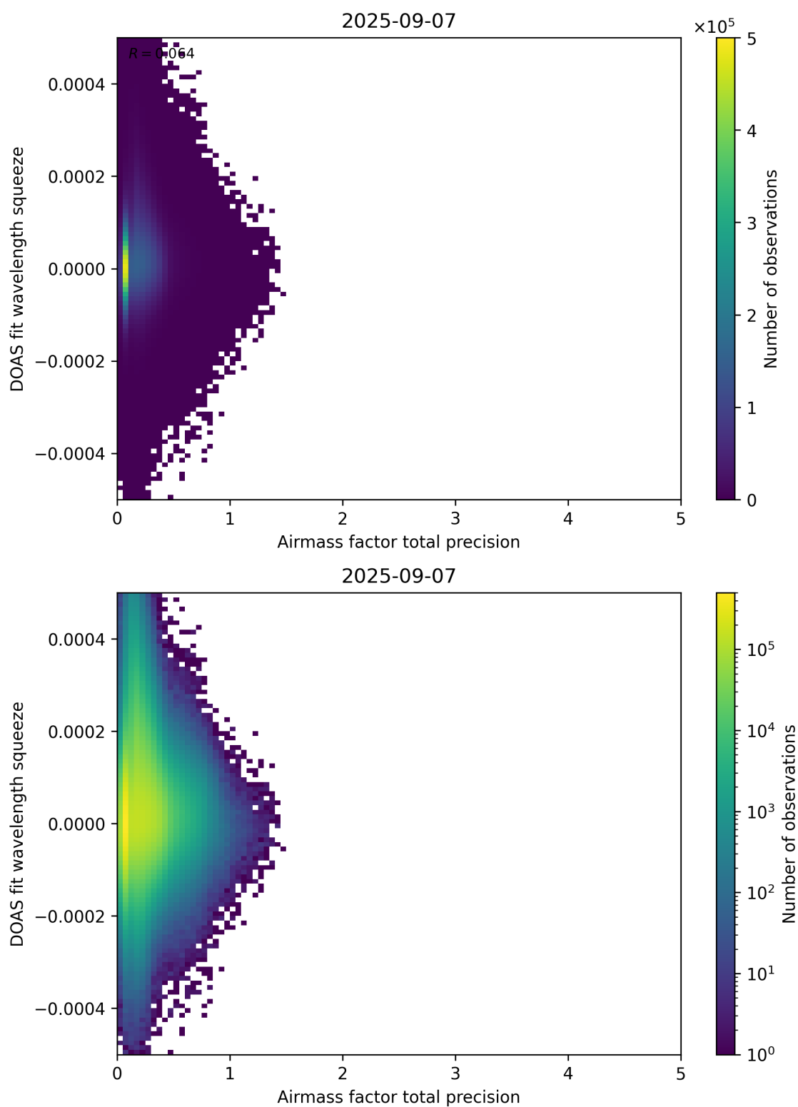
Figure 107: Scatter density plot of “Airmass factor total precision” against “DOAS fit wavelength squeeze” for 2025-09-06 to 2025-09-08.
