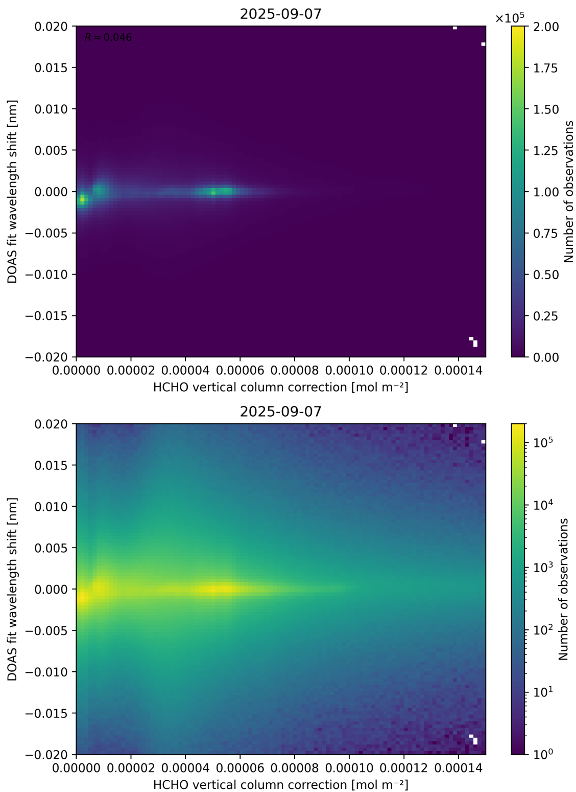
Figure 113: Scatter density plot of “HCHO vertical column correction” against “DOAS fit wavelength shift” for 2025-09-06 to 2025-09-08.
