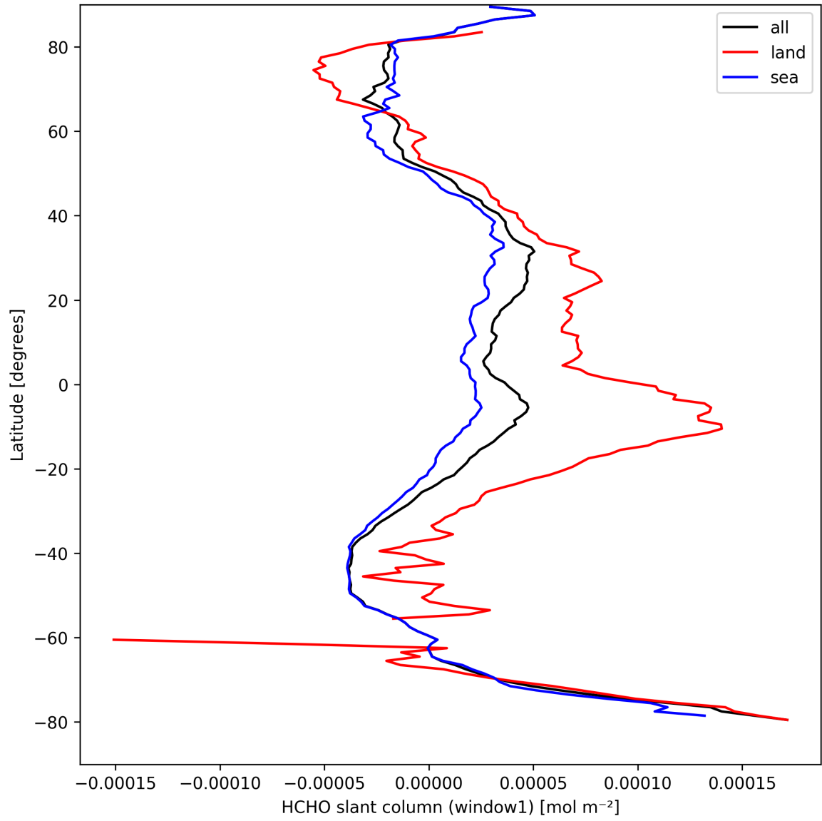
Figure 24: Zonal average of “HCHO slant column (window1)” for 2025-09-06 to 2025-09-08.
