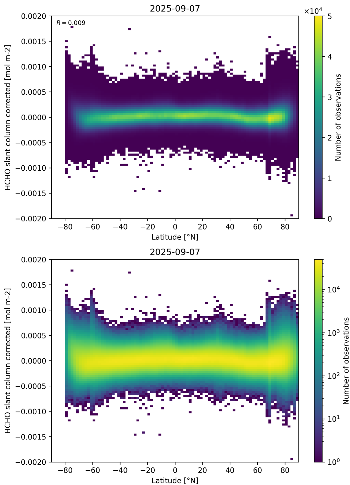
Figure 157: Scatter density plot of “Latitude” against “HCHO slant column corrected” for 2025-09-06 to 2025-09-08.
