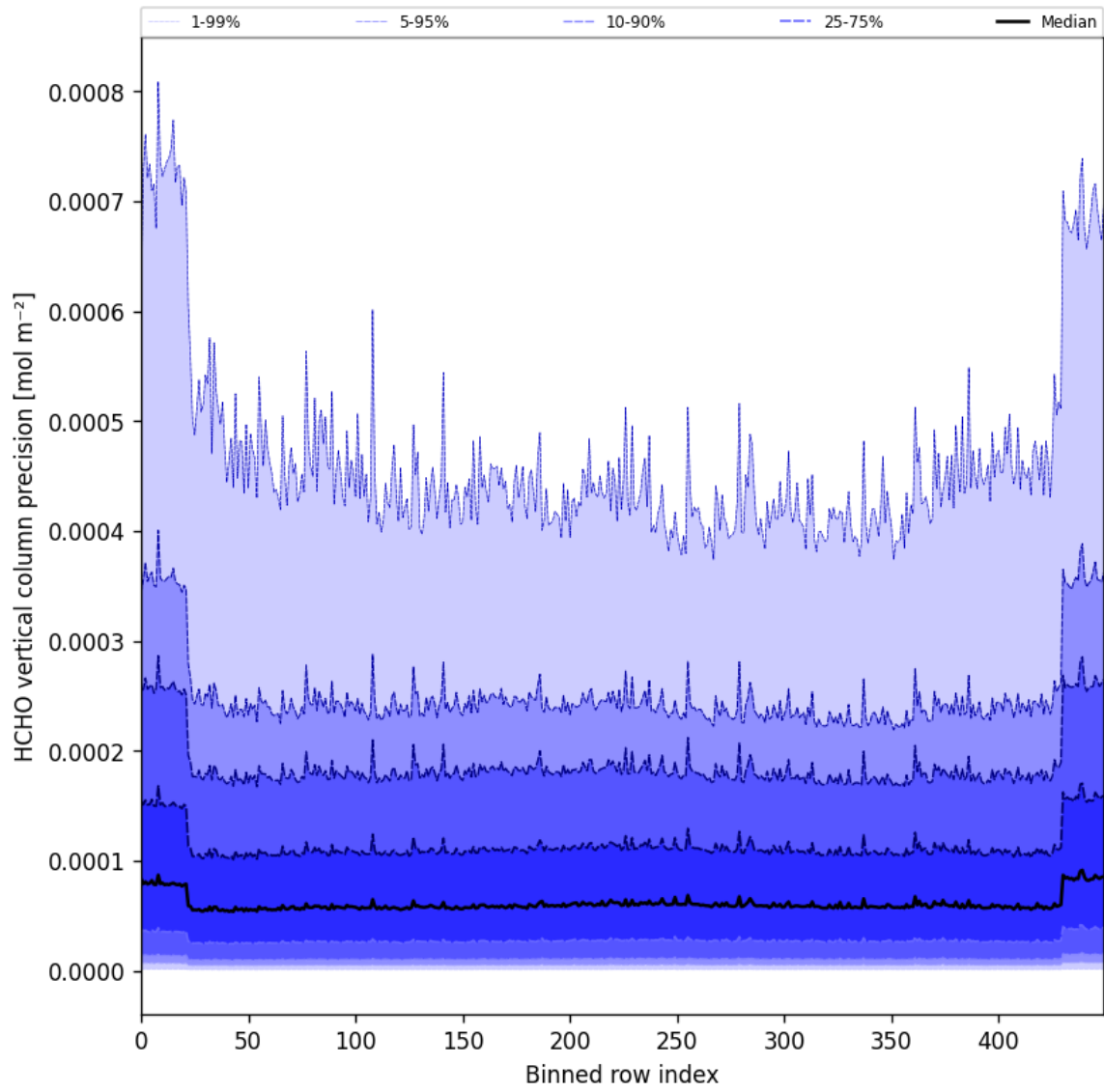
Figure 50: Along track statistics of “HCHO vertical column precision” for 2025-09-06 to 2025-09-08
