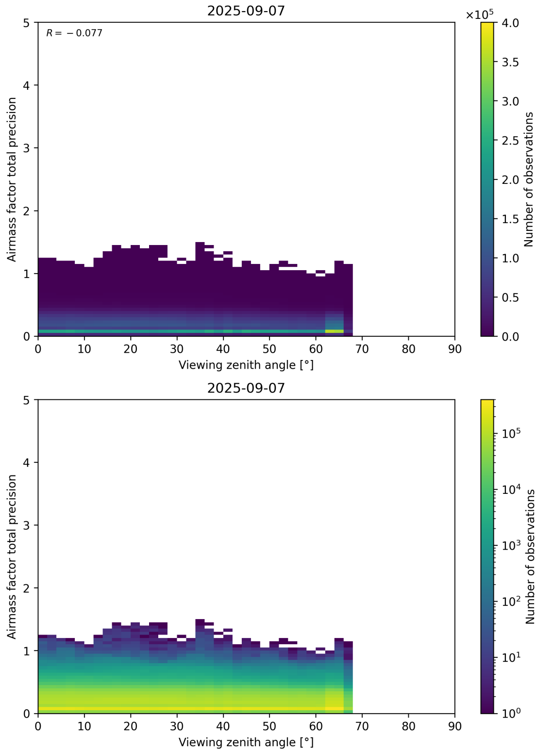
Figure 191: Scatter density plot of “Viewing zenith angle” against “Airmass factor total precision” for 2025-09-06 to 2025-09-08.
