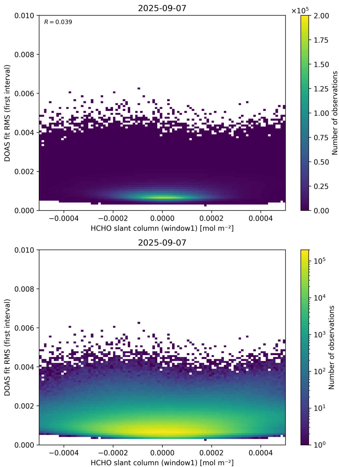
Figure 78: Scatter density plot of “HCHO slant column (window1)” against “DOAS fit RMS (first interval)” for 2025-09-06 to 2025-09-08.
