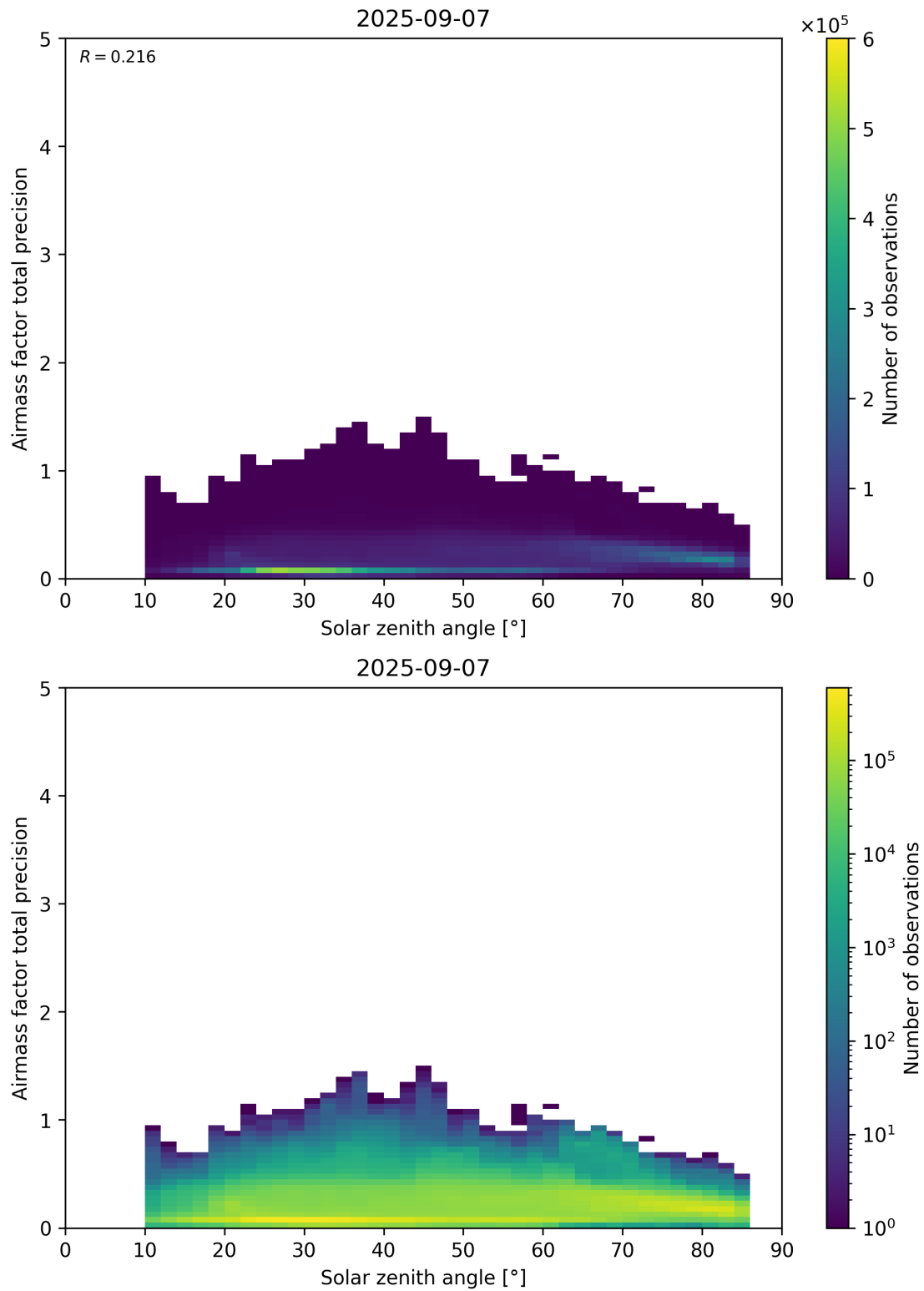
Figure 176: Scatter density plot of “Solar zenith angle” against “Airmass factor total precision” for 2025-09-06 to 2025-09-08.
