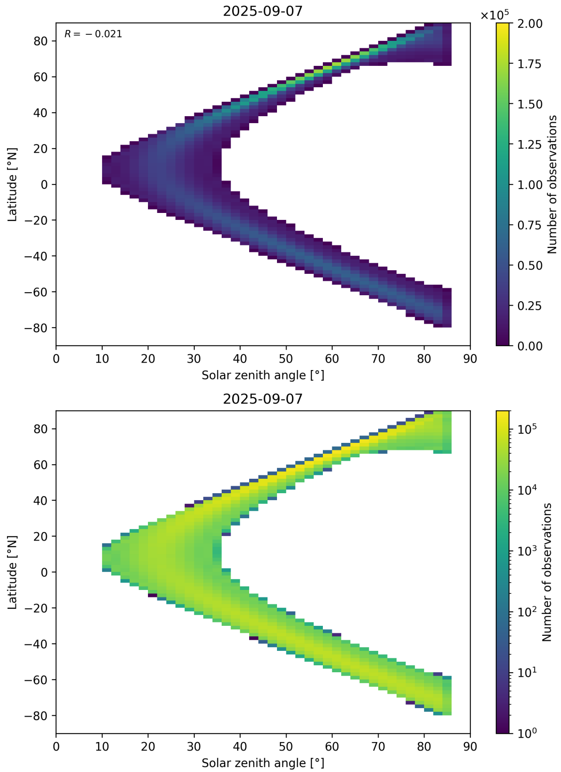
Figure 181: Scatter density plot of “Solar zenith angle” against “Latitude” for 2025-09-06 to 2025-09-08.
