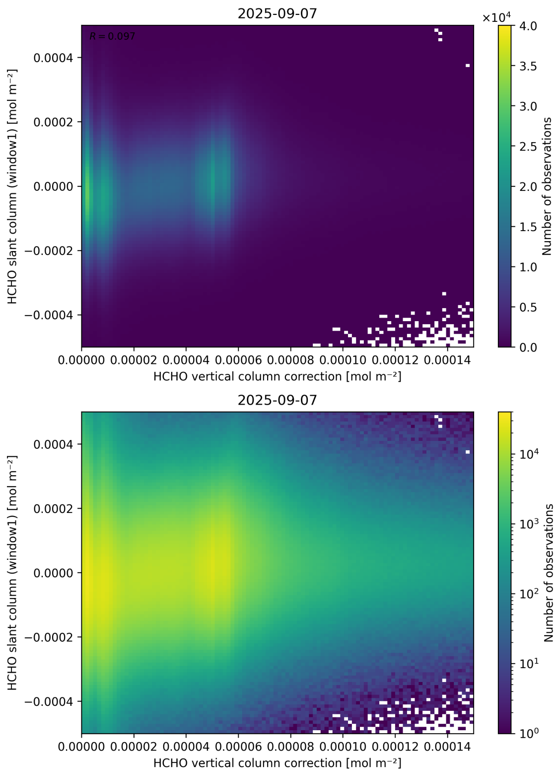
Figure 118: Scatter density plot of “HCHO vertical column correction” against “HCHO slant column (window1)” for 2025-09-06 to 2025-09-08.
