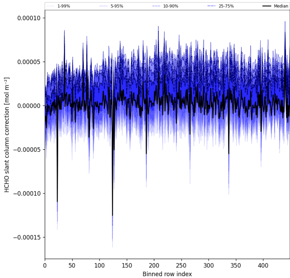
Figure 61: Along track statistics of “HCHO slant column correction” for 2025-09-06 to 2025-09-08
