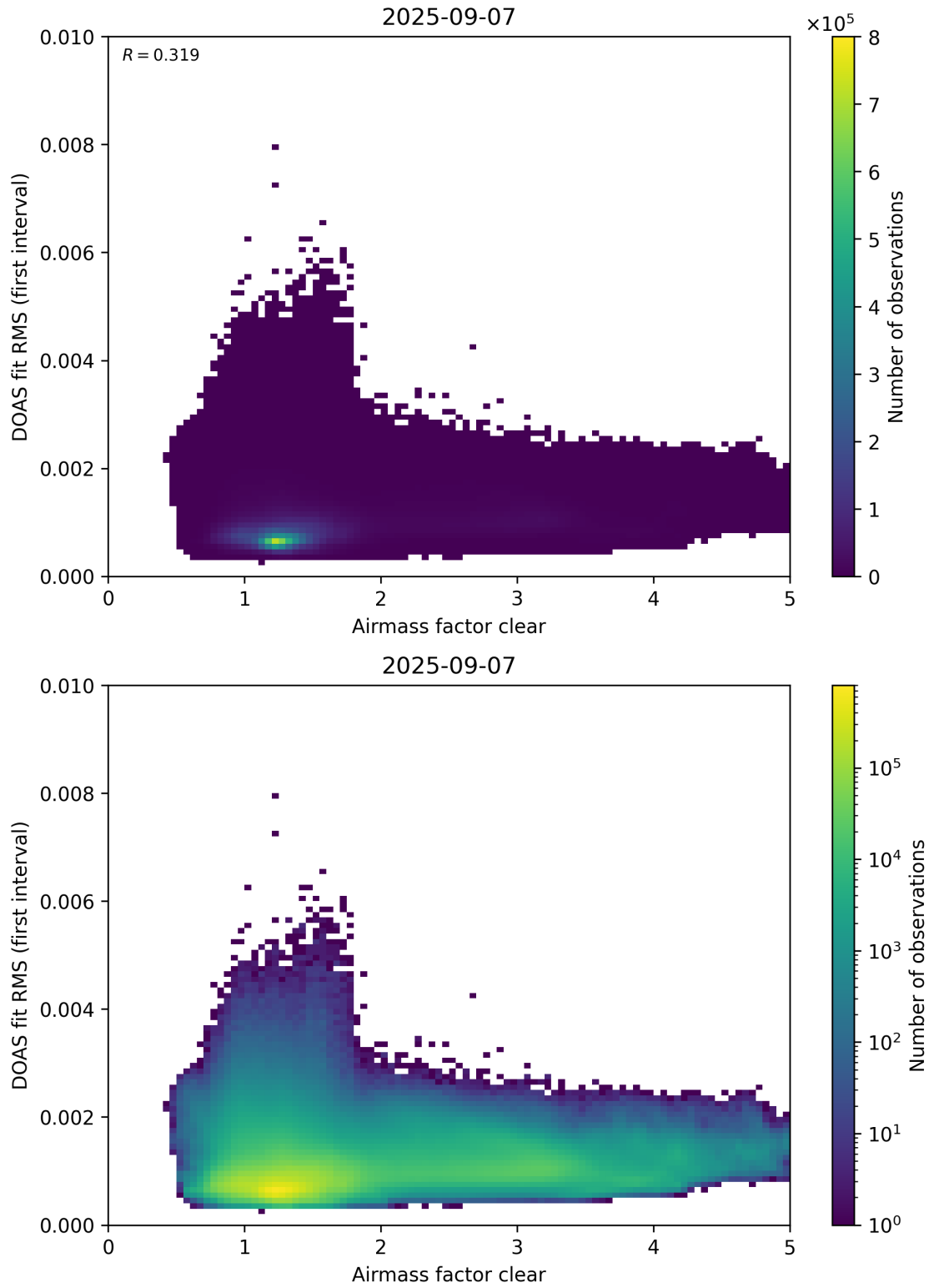
Figure 71: Scatter density plot of “Airmass factor clear” against “DOAS fit RMS (first interval)” for 2025-09-06 to 2025-09-08.
