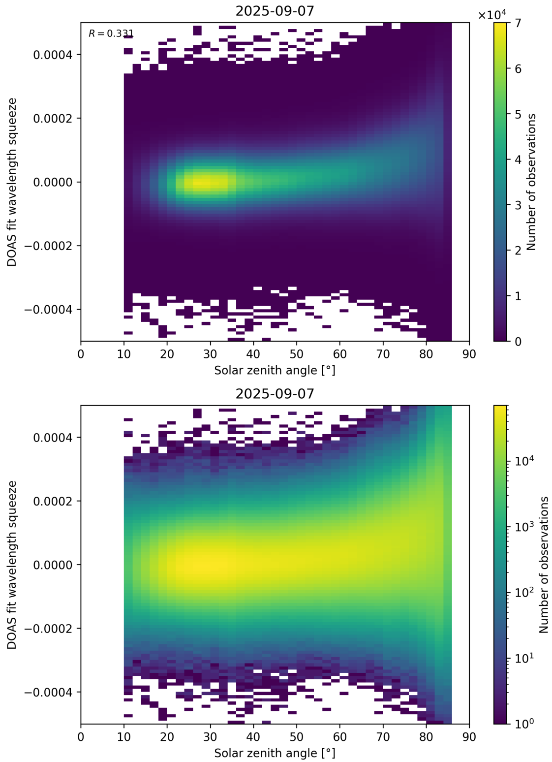
Figure 169: Scatter density plot of “Solar zenith angle” against “DOAS fit wavelength squeeze” for 2025-09-06 to 2025-09-08.
