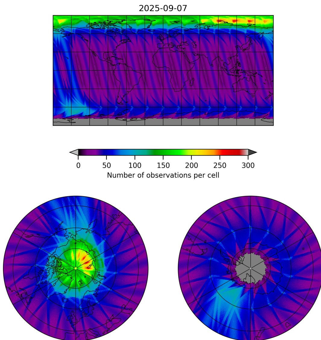
Figure 19: Map of the number of observations for 2025-09-06 to 2025-09-08
