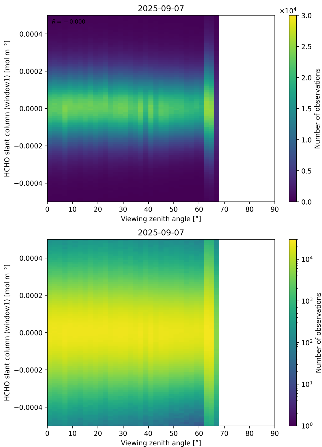
Figure 188: Scatter density plot of “Viewing zenith angle” against “HCHO slant column (window1)” for 2025-09-06 to 2025-09-08.
