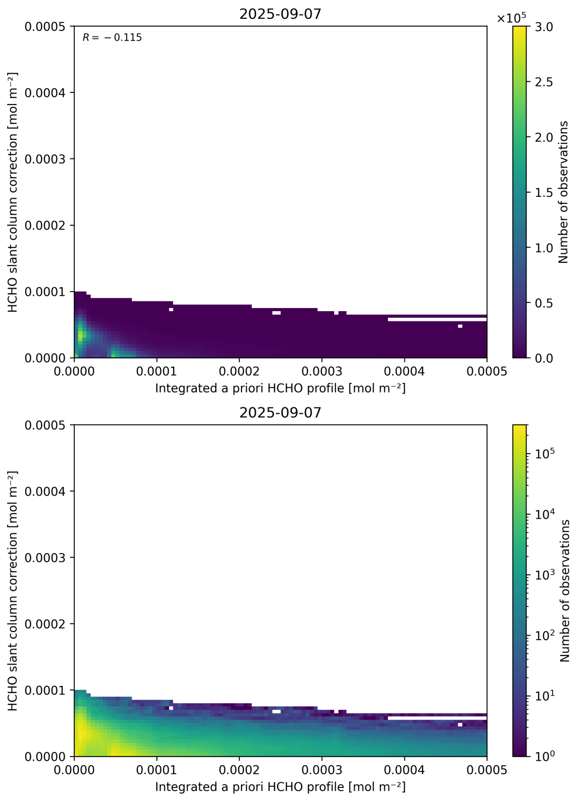
Figure 152: Scatter density plot of “Integrated a priori HCHO profile” against “HCHO slant column correction” for 2025-09-06 to 2025-09-08.
