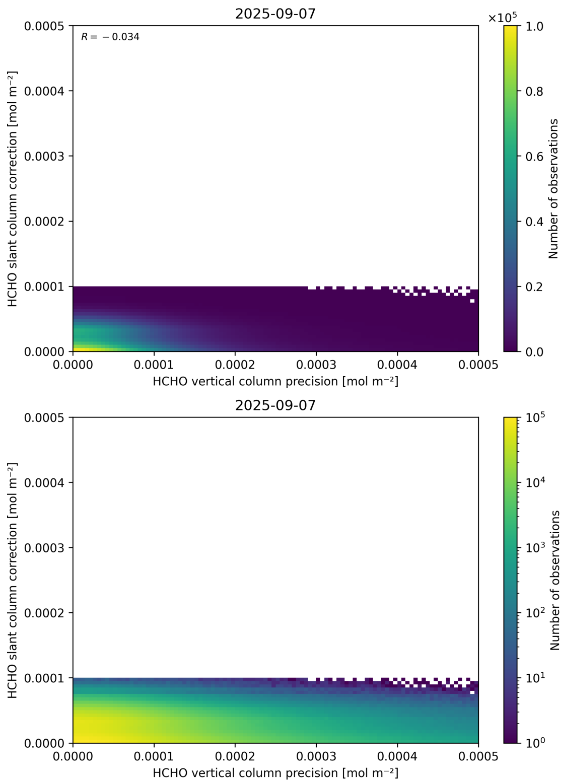
Figure 141: Scatter density plot of “HCHO vertical column precision” against “HCHO slant column correction” for 2025-09-06 to 2025-09-08.
