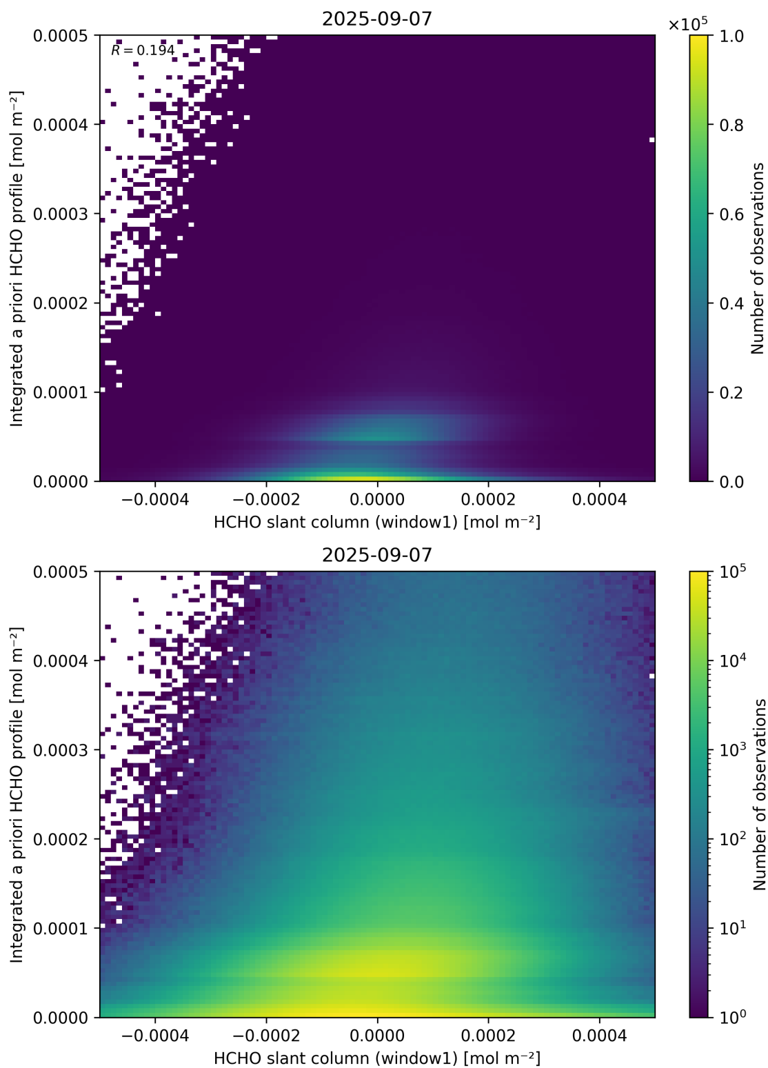
Figure 87: Scatter density plot of “HCHO slant column (window1)” against “Integrated a priori HCHO profile” for 2025-09-06 to 2025-09-08.
