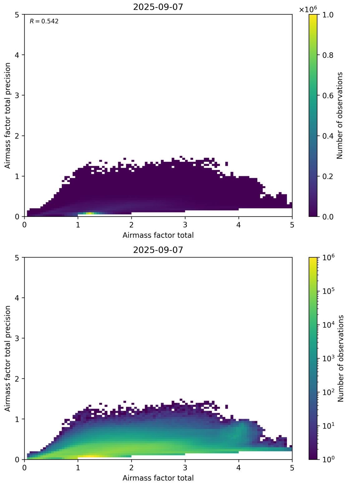
Figure 103: Scatter density plot of “Airmass factor total” against “Airmass factor total precision” for 2025-09-06 to 2025-09-08.
