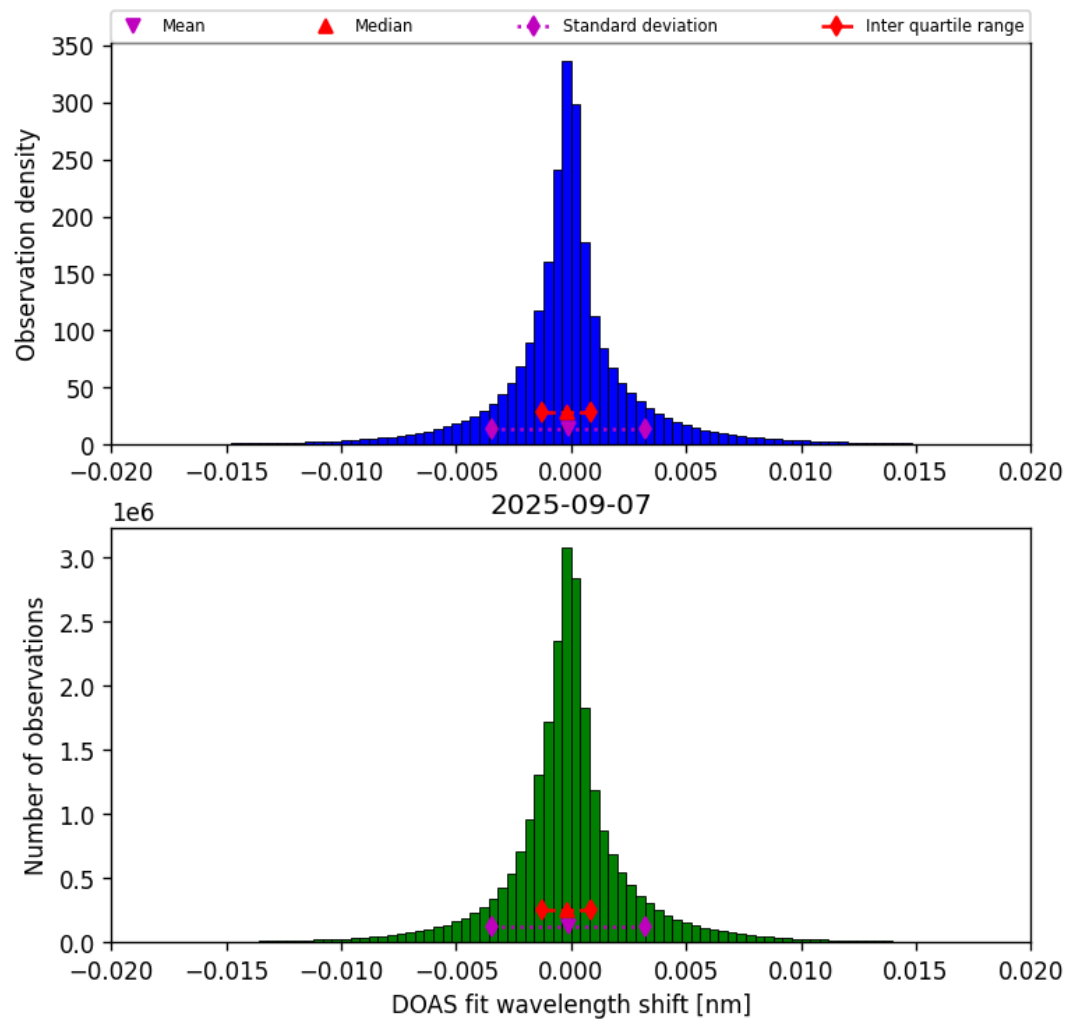
Figure 44: Histogram of “DOAS fit wavelength shift” for 2025-09-06 to 2025-09-08
