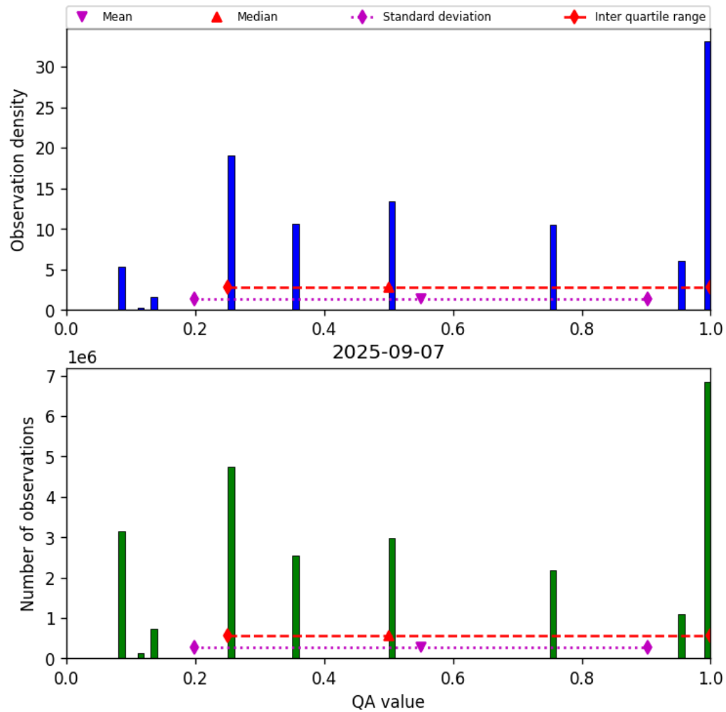
Figure 34: Histogram of “QA value” for 2025-09-06 to 2025-09-08
