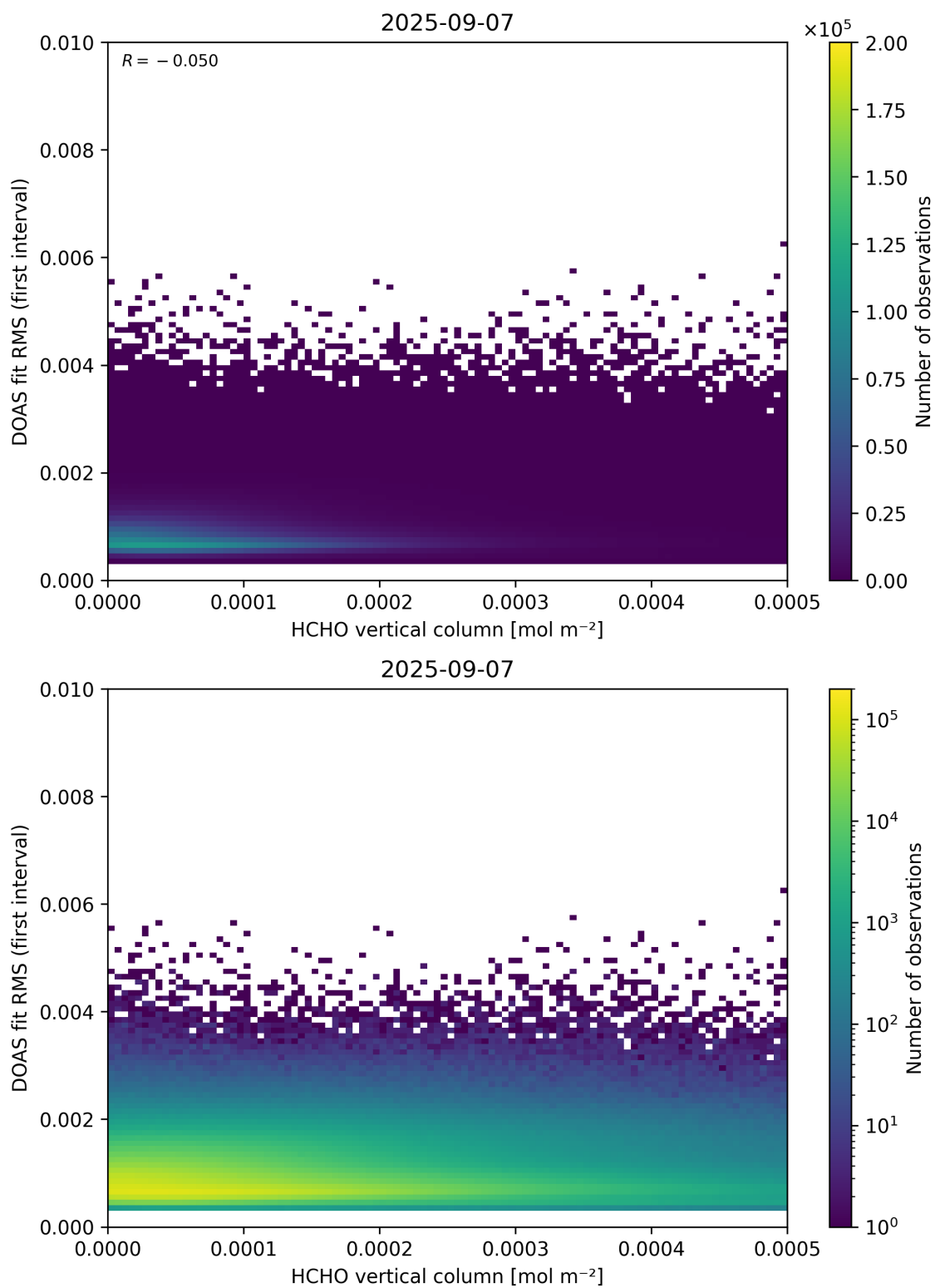
Figure 123: Scatter density plot of “HCHO vertical column” against “DOAS fit RMS (first interval)” for 2025-09-06 to 2025-09-08.
