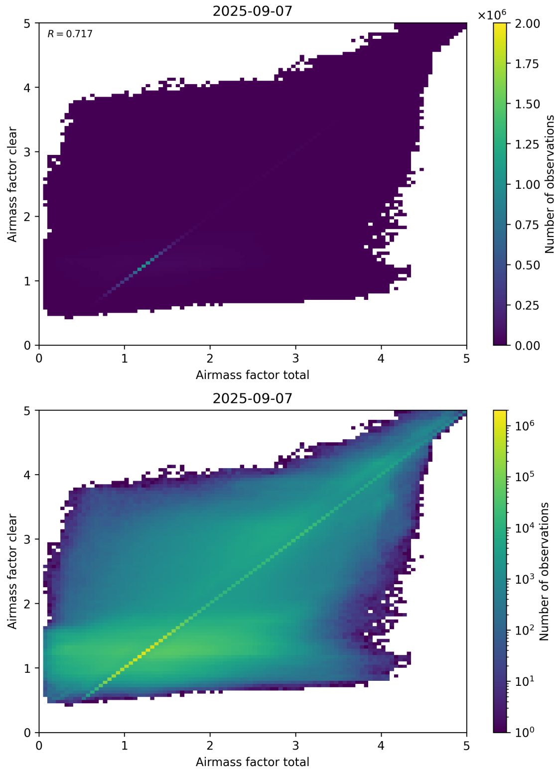
Figure 100: Scatter density plot of “Airmass factor total” against “Airmass factor clear” for 2025-09-06 to 2025-09-08.
