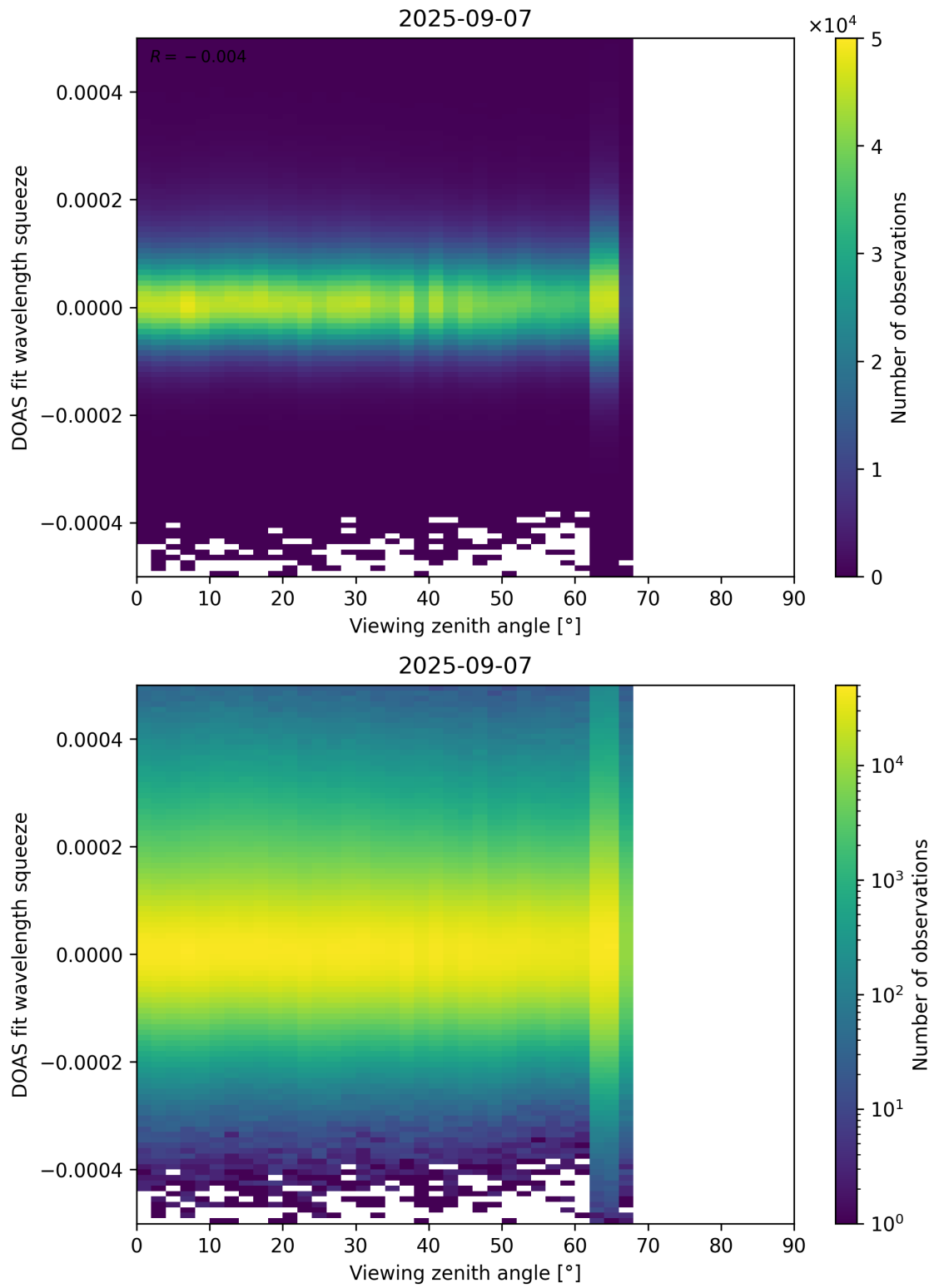
Figure 184: Scatter density plot of “Viewing zenith angle” against “DOAS fit wavelength squeeze” for 2025-09-06 to 2025-09-08.
