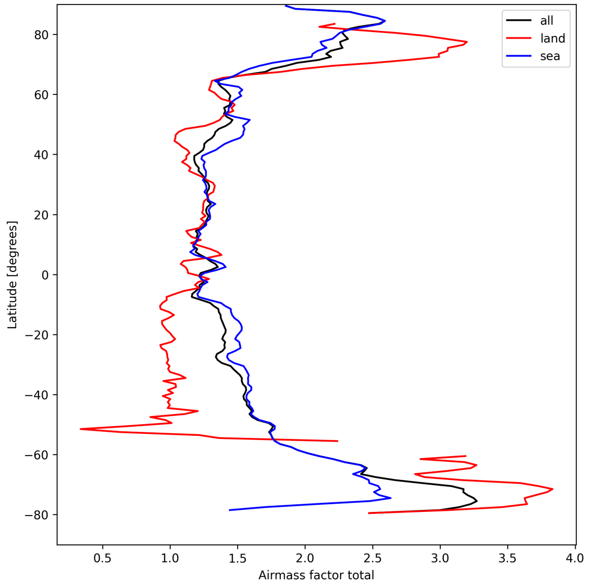
Figure 26: Zonal average of “Airmass factor total” for 2025-09-06 to 2025-09-08.
