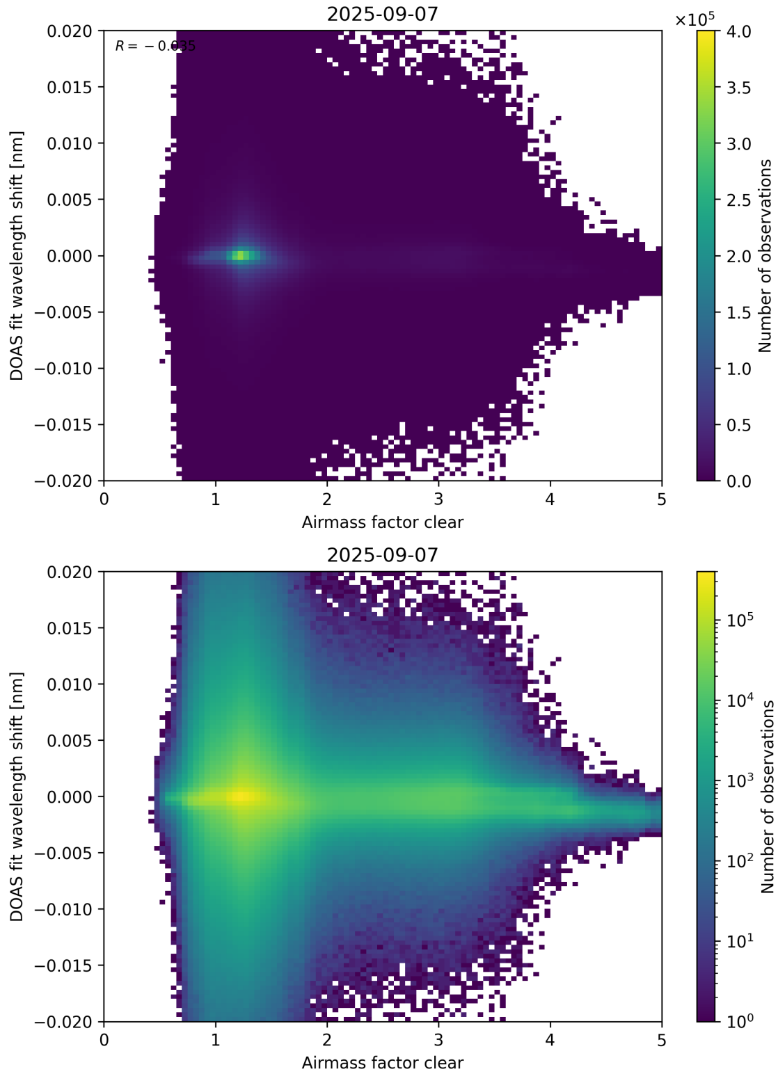
Figure 72: Scatter density plot of “Airmass factor clear” against “DOAS fit wavelength shift” for 2025-09-06 to 2025-09-08.
