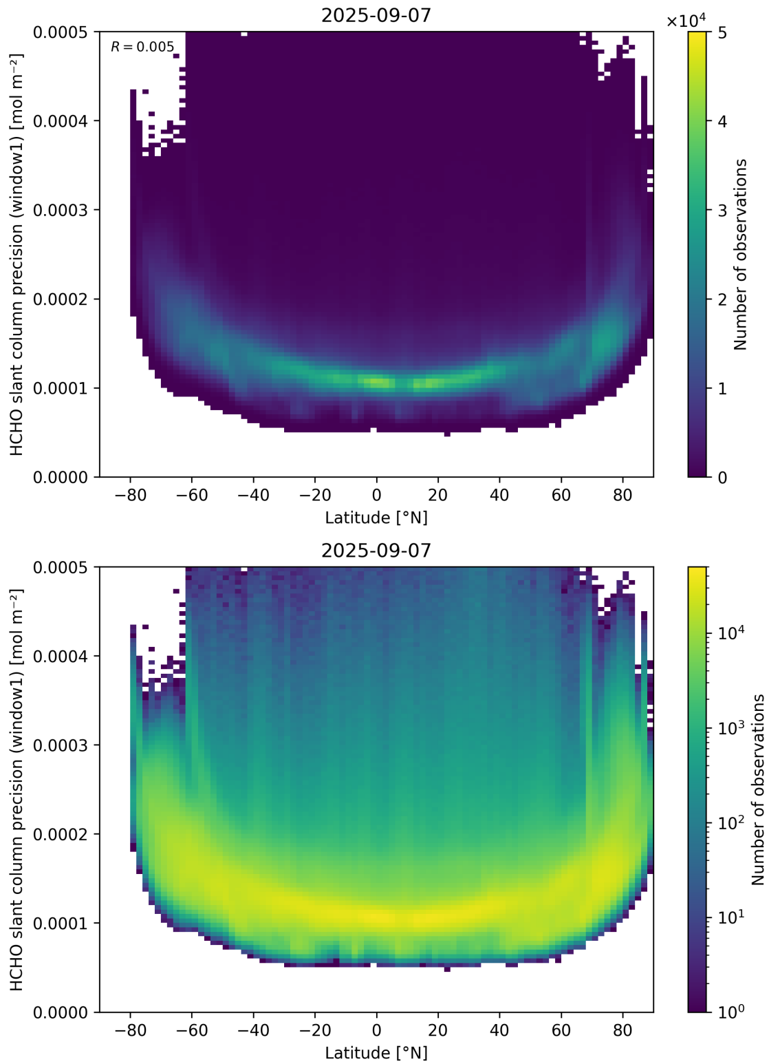
Figure 160: Scatter density plot of “Latitude” against “HCHO slant column precision (window1)” for 2025-09-06 to 2025-09-08.
