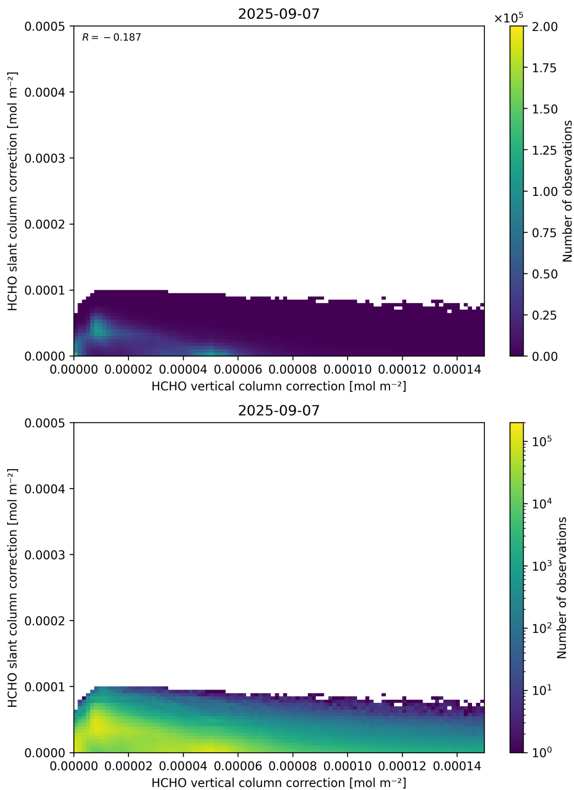
Figure 117: Scatter density plot of “HCHO vertical column correction” against “HCHO slant column correction” for 2025-09-06 to 2025-09-08.
