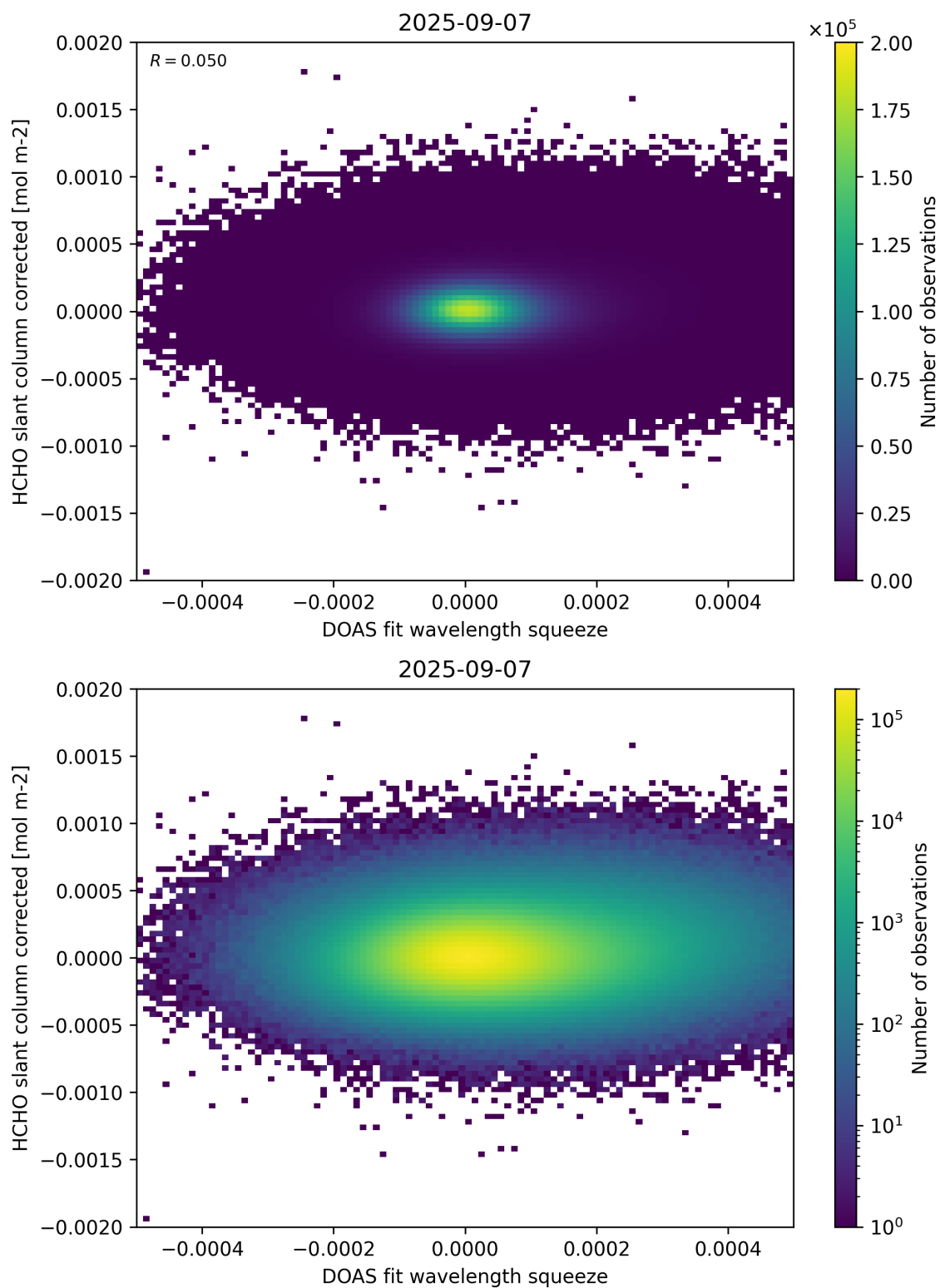
Figure 69: Scatter density plot of “DOAS fit wavelength squeeze” against “HCHO slant column corrected” for 2025-09-06 to 2025-09-08.
