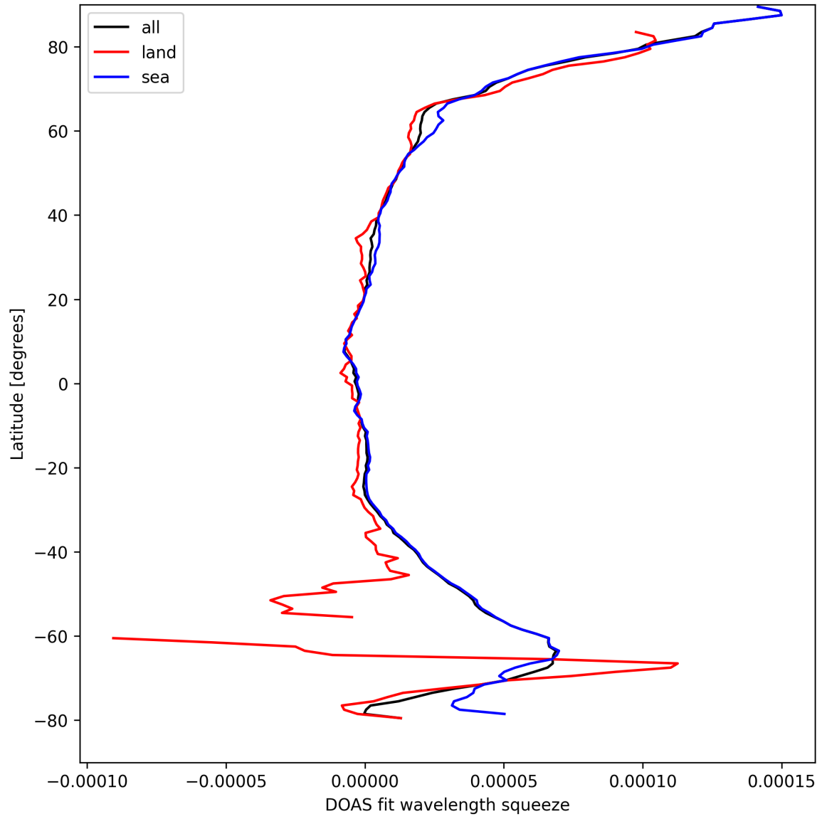
Figure 31: Zonal average of “DOAS fit wavelength squeeze” for 2025-09-06 to 2025-09-08.
