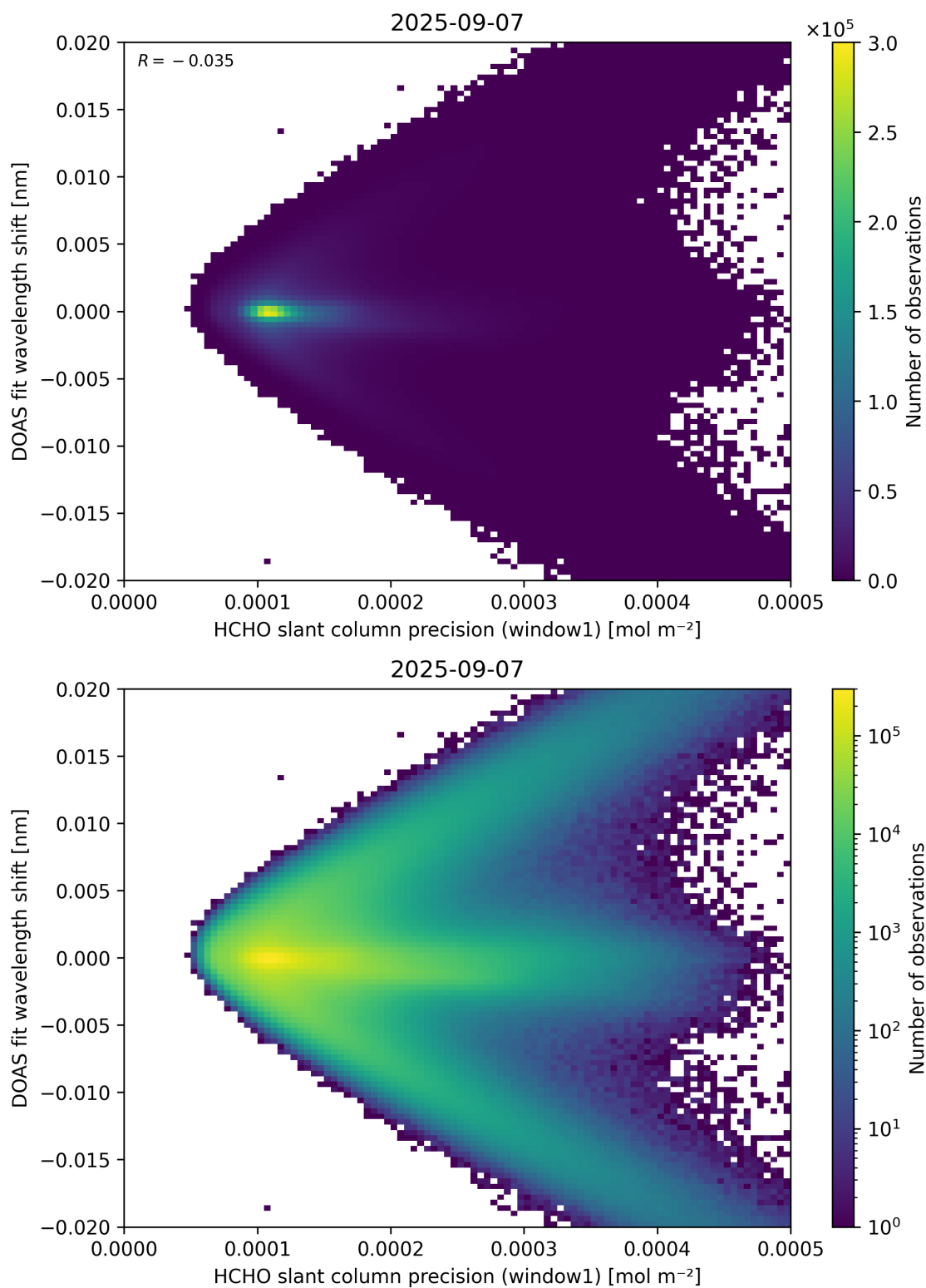
Figure 89: Scatter density plot of “HCHO slant column precision (window1)” against “DOAS fit wavelength shift” for 2025-09-06 to 2025-09-08.
