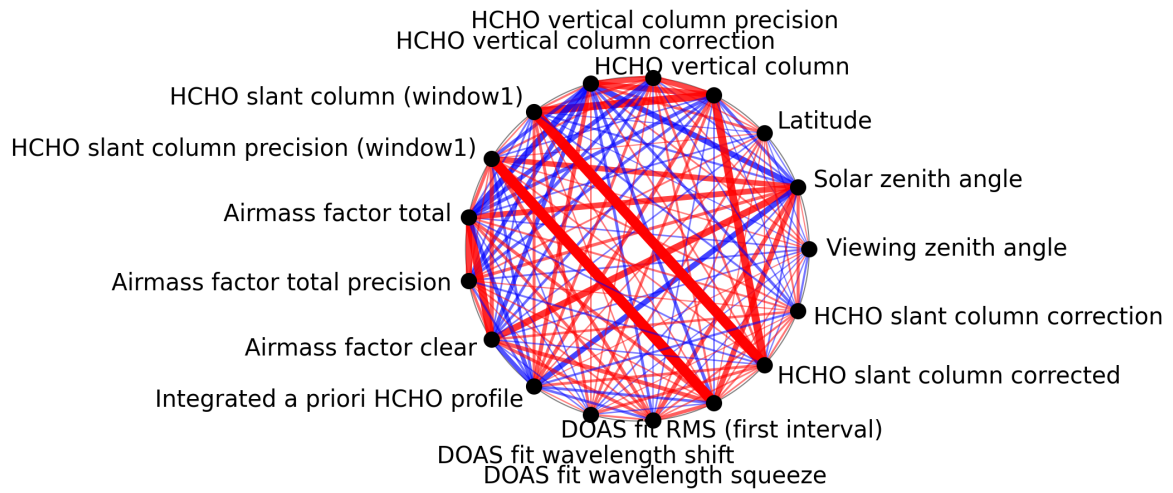
Figure 1: Map of correlation graph for 2025-09-06 to 2025-09-08.
