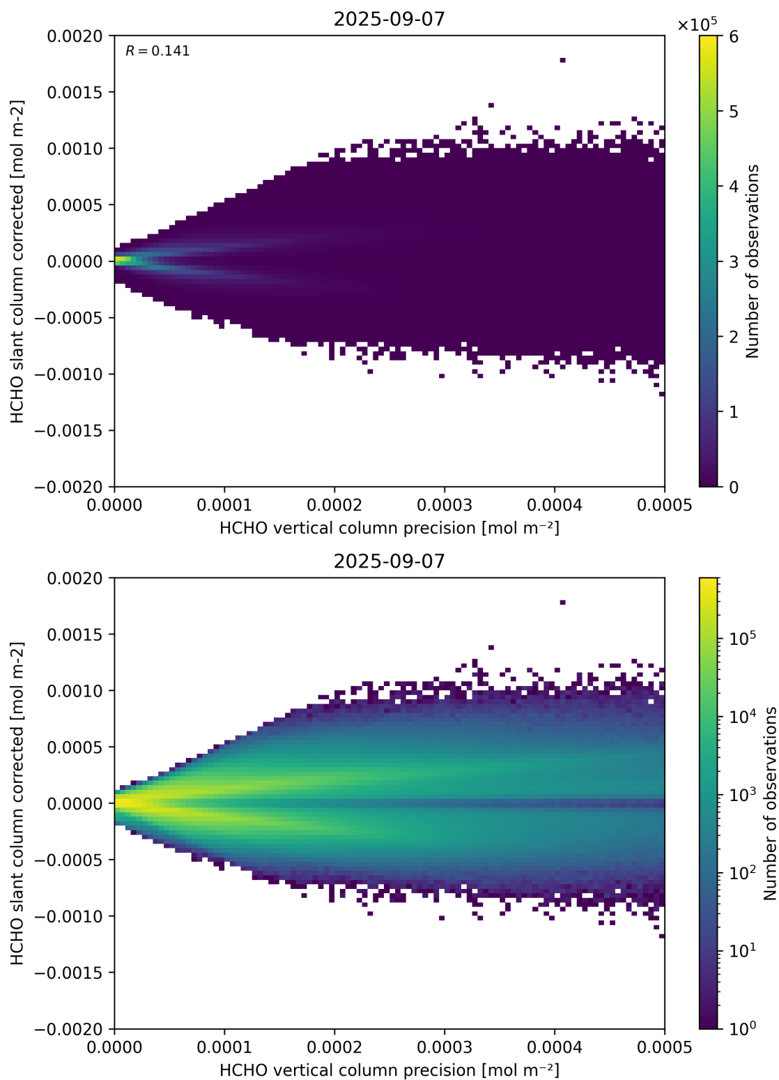
Figure 140: Scatter density plot of “HCHO vertical column precision” against “HCHO slant column corrected” for 2025-09-06 to 2025-09-08.
