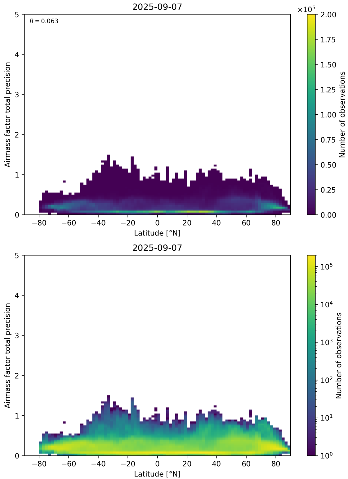
Figure 162: Scatter density plot of “Latitude” against “Airmass factor total precision” for 2025-09-06 to 2025-09-08.
