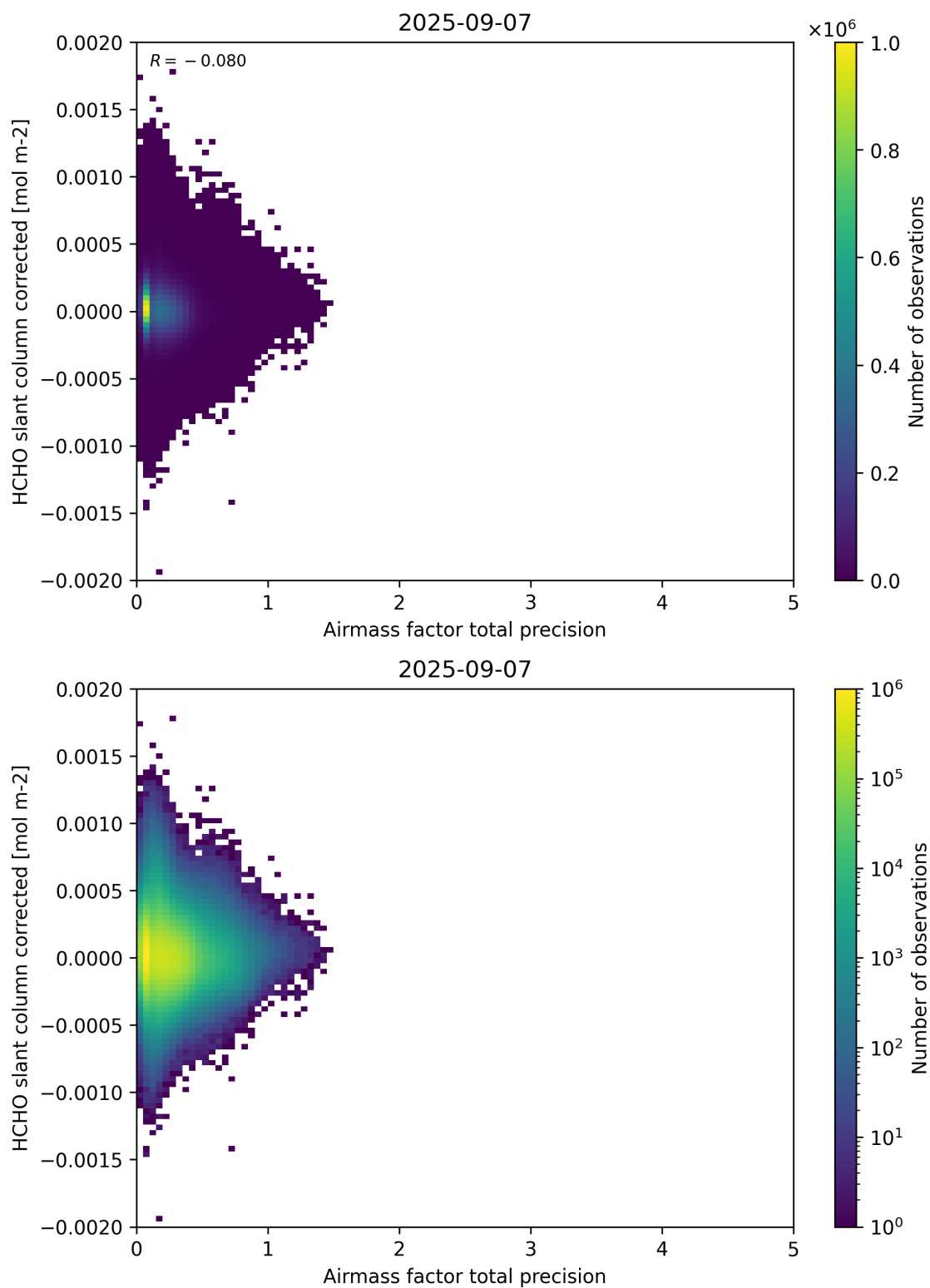
Figure 109: Scatter density plot of “Airmass factor total precision” against “HCHO slant column corrected” for 2025-09-06 to 2025-09-08.
