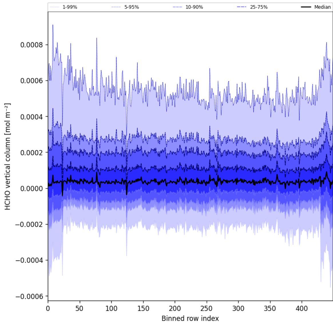
Figure 49: Along track statistics of “HCHO vertical column” for 2025-09-06 to 2025-09-08
