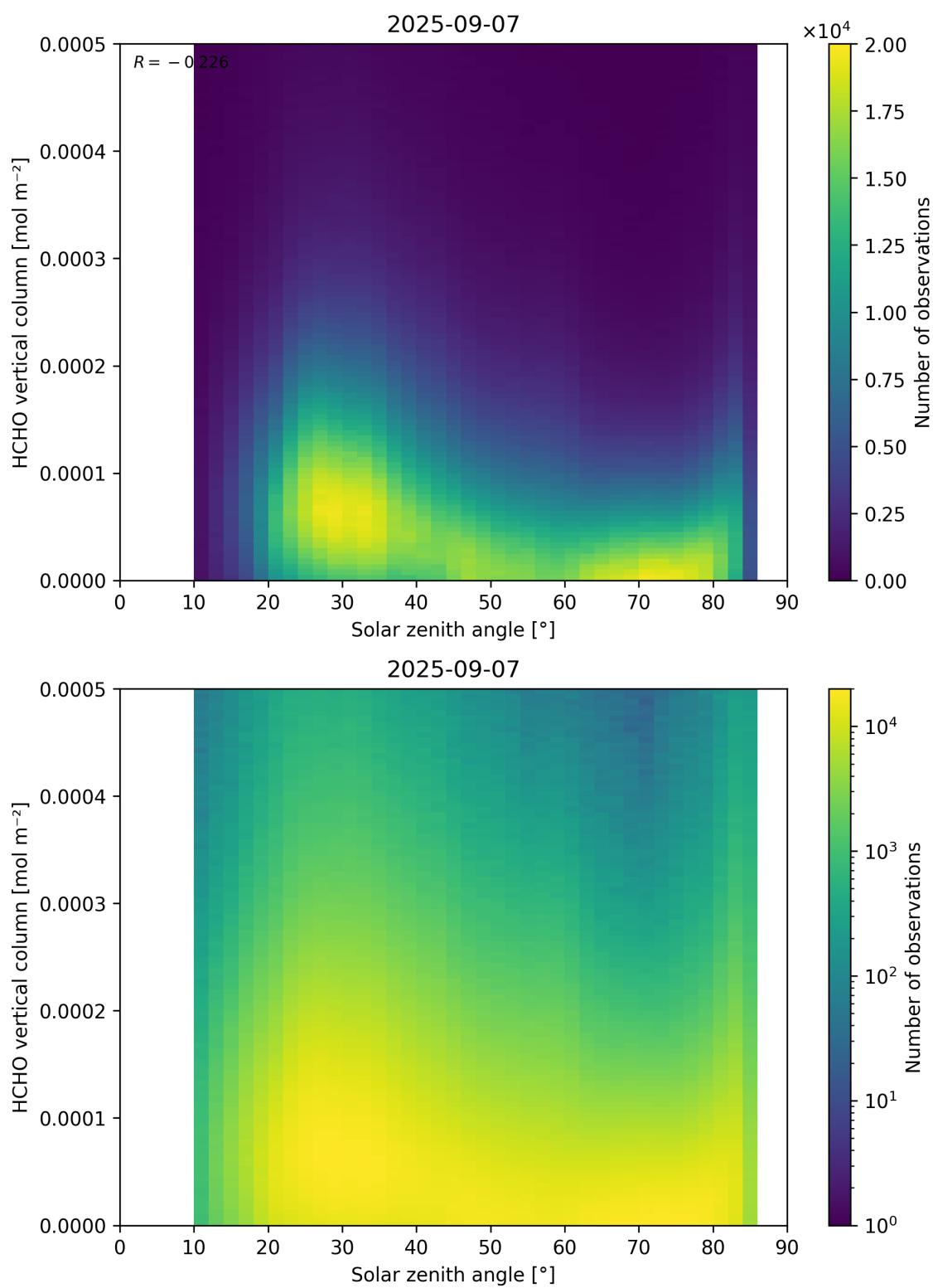
Figure 177: Scatter density plot of “Solar zenith angle” against “HCHO vertical column” for 2025-09-06 to 2025-09-08.
