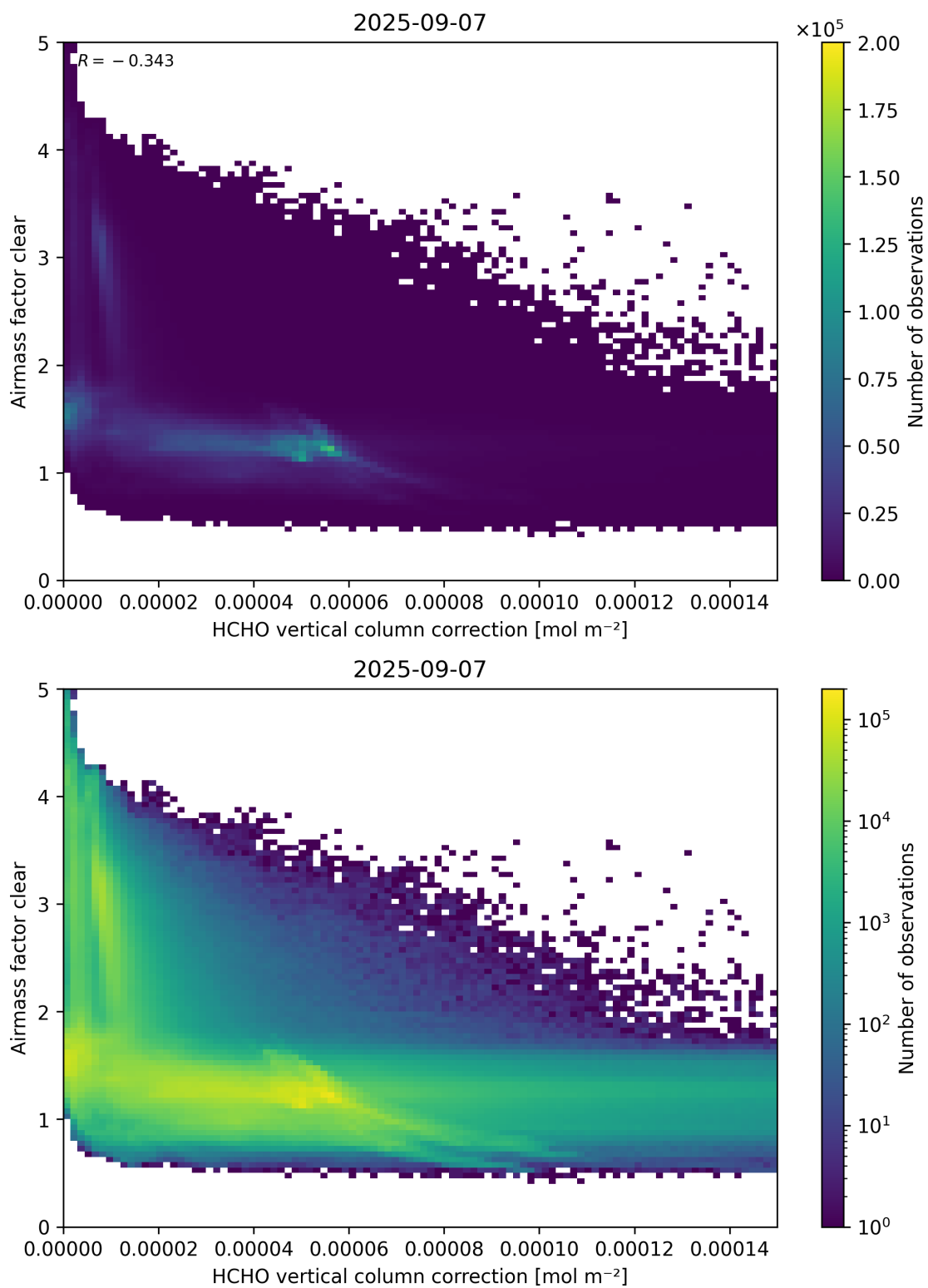
Figure 115: Scatter density plot of “HCHO vertical column correction” against “Airmass factor clear” for 2025-09-06 to 2025-09-08.
