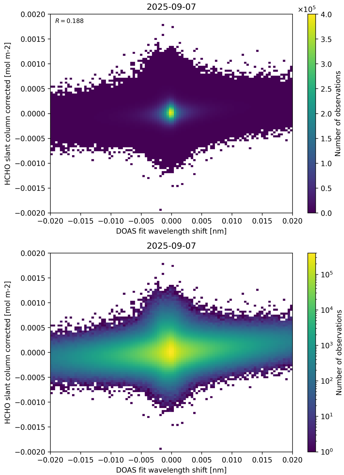
Figure 66: Scatter density plot of “DOAS fit wavelength shift” against “HCHO slant column corrected” for 2025-09-06 to 2025-09-08.
