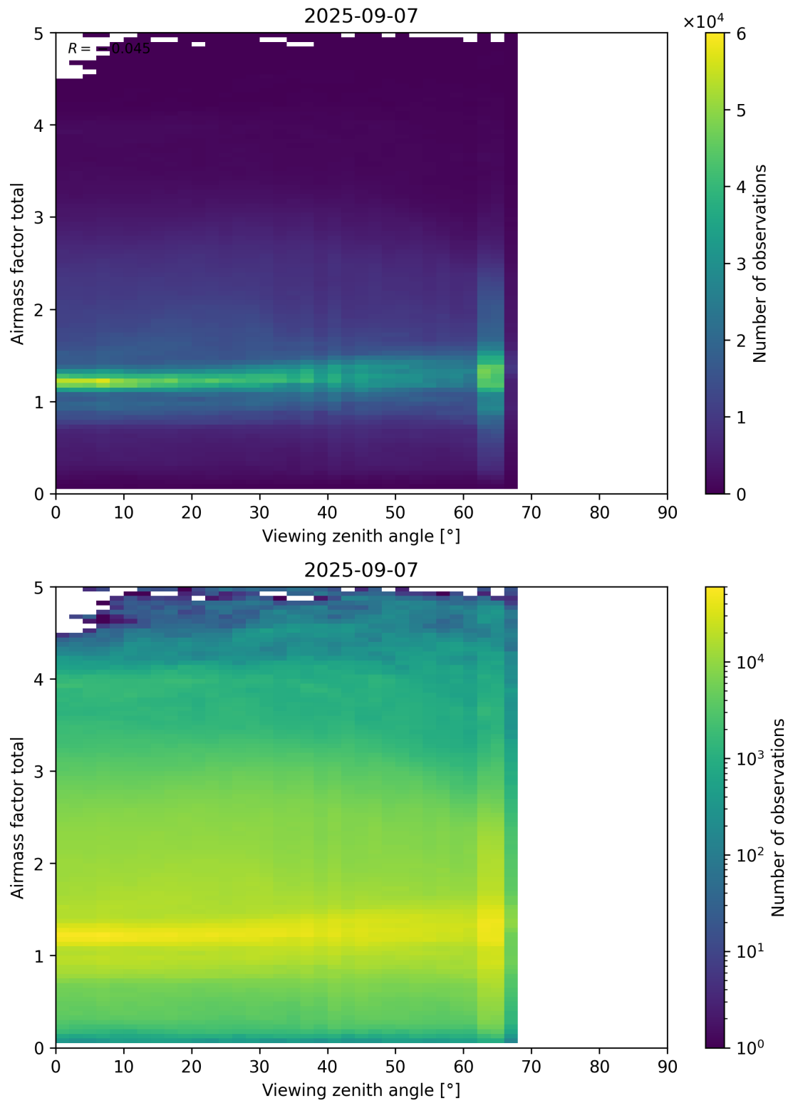
Figure 190: Scatter density plot of “Viewing zenith angle” against “Airmass factor total” for 2025-09-06 to 2025-09-08.
