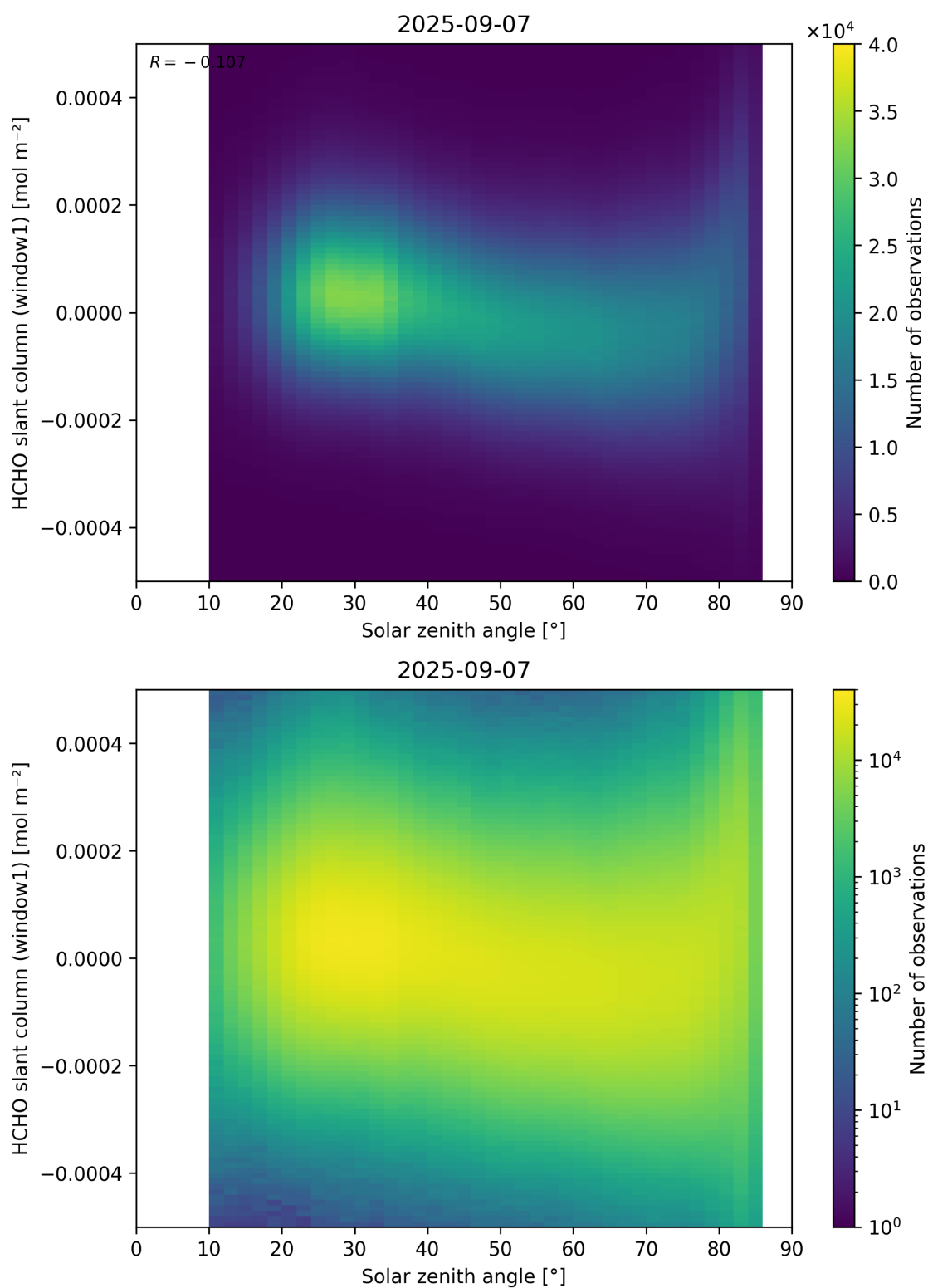
Figure 173: Scatter density plot of “Solar zenith angle” against “HCHO slant column (window1)” for 2025-09-06 to 2025-09-08.
