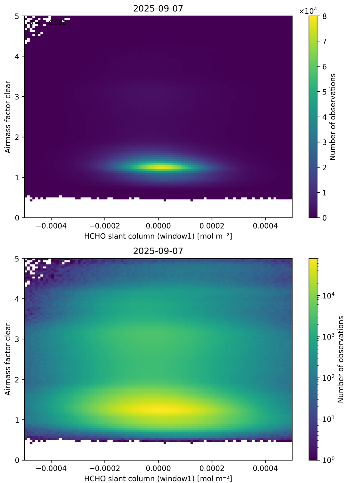
Figure 81: Scatter density plot of “HCHO slant column (window1)” against “Airmass factor clear” for 2025-09-06 to 2025-09-08.
