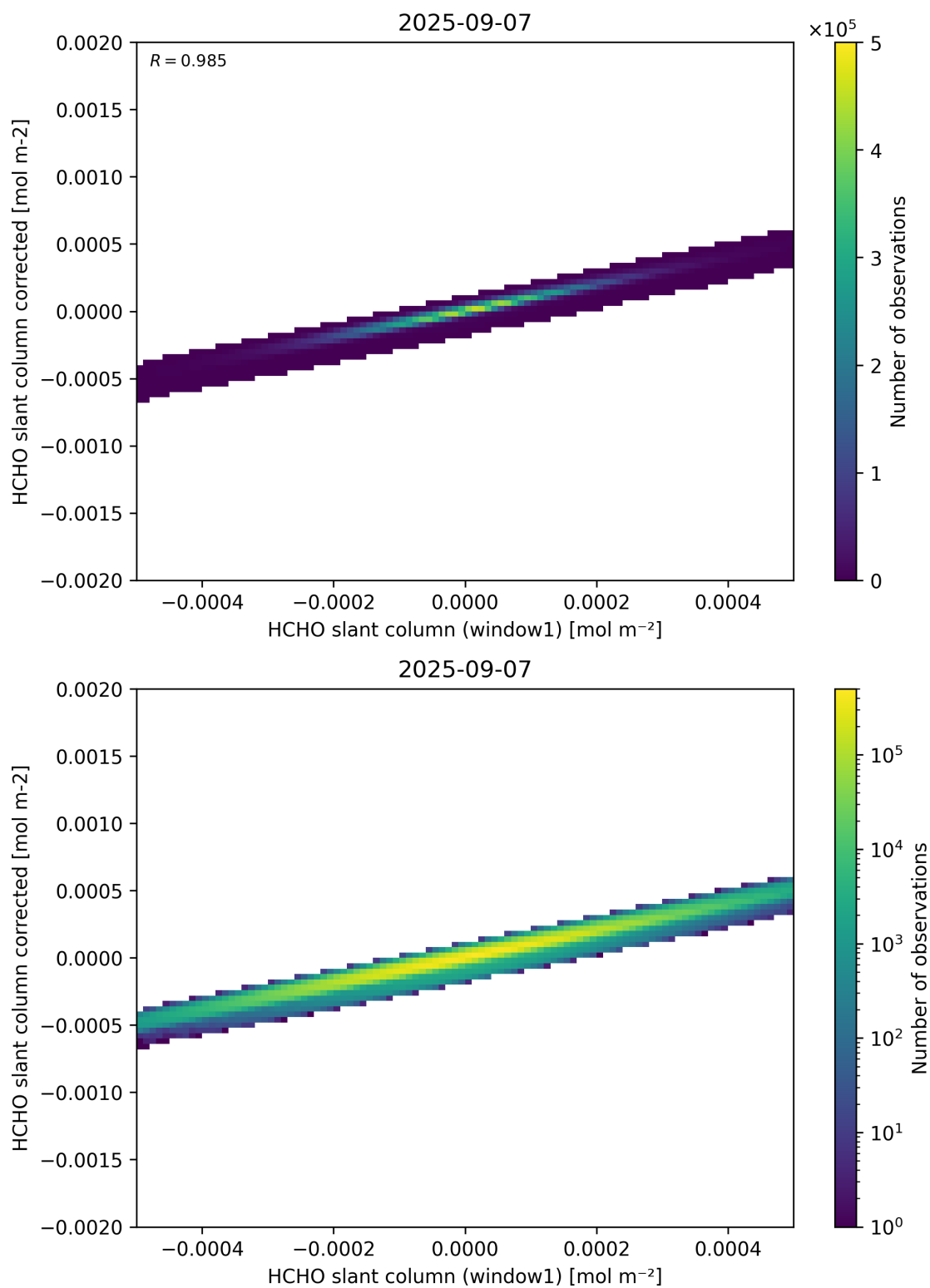
Figure 82: Scatter density plot of “HCHO slant column (window1)” against “HCHO slant column corrected” for 2025-09-06 to 2025-09-08.
