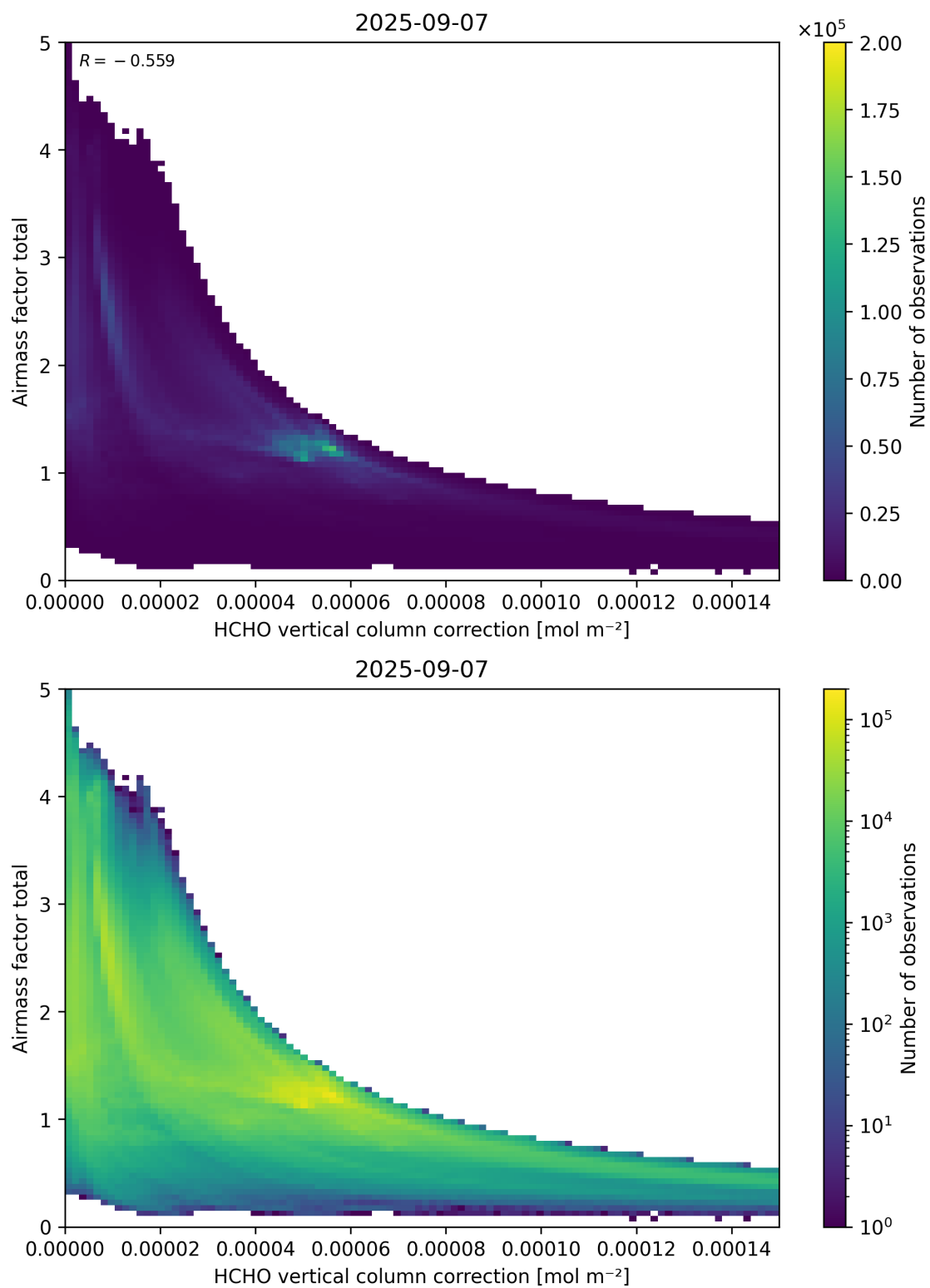
Figure 120: Scatter density plot of “HCHO vertical column correction” against “Airmass factor total” for 2025-09-06 to 2025-09-08.
