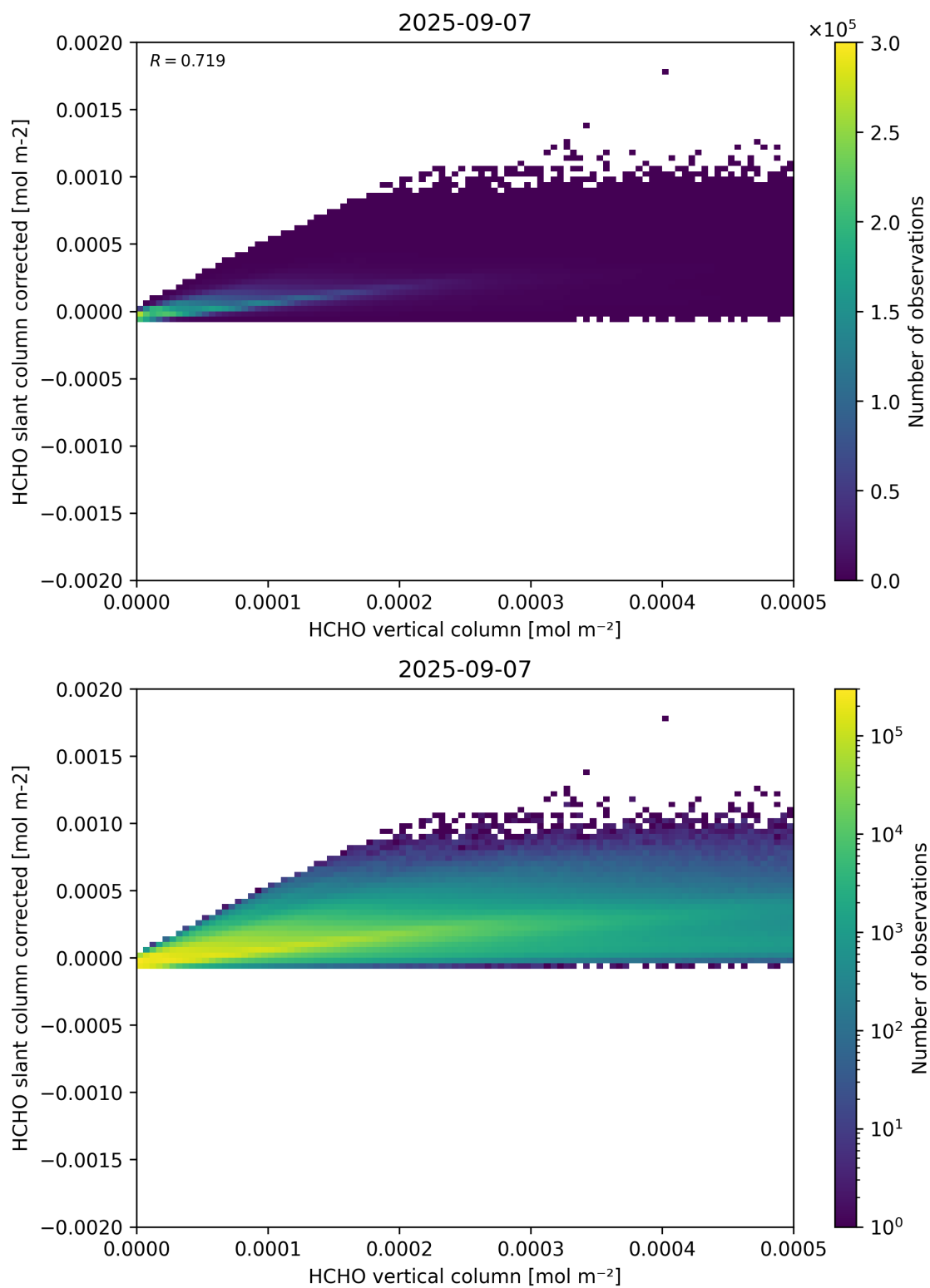
Figure 127: Scatter density plot of “HCHO vertical column” against “HCHO slant column corrected” for 2025-09-06 to 2025-09-08.
