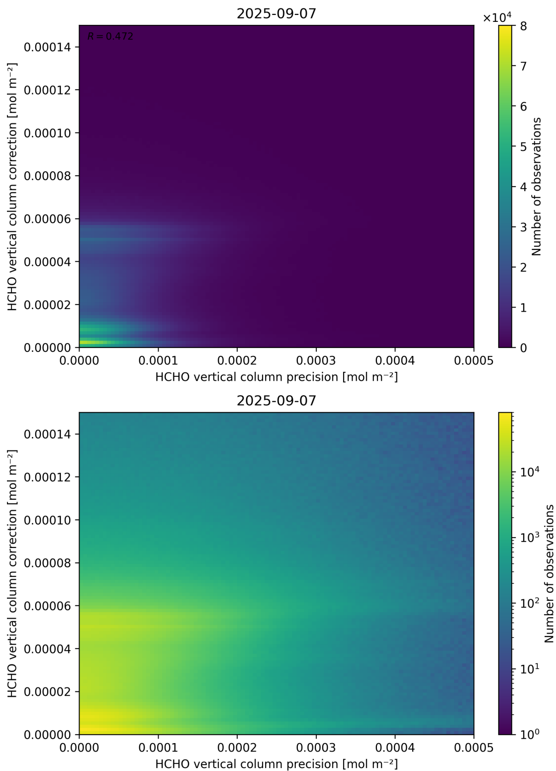
Figure 146: Scatter density plot of “HCHO vertical column precision” against “HCHO vertical column correction” for 2025-09-06 to 2025-09-08.
