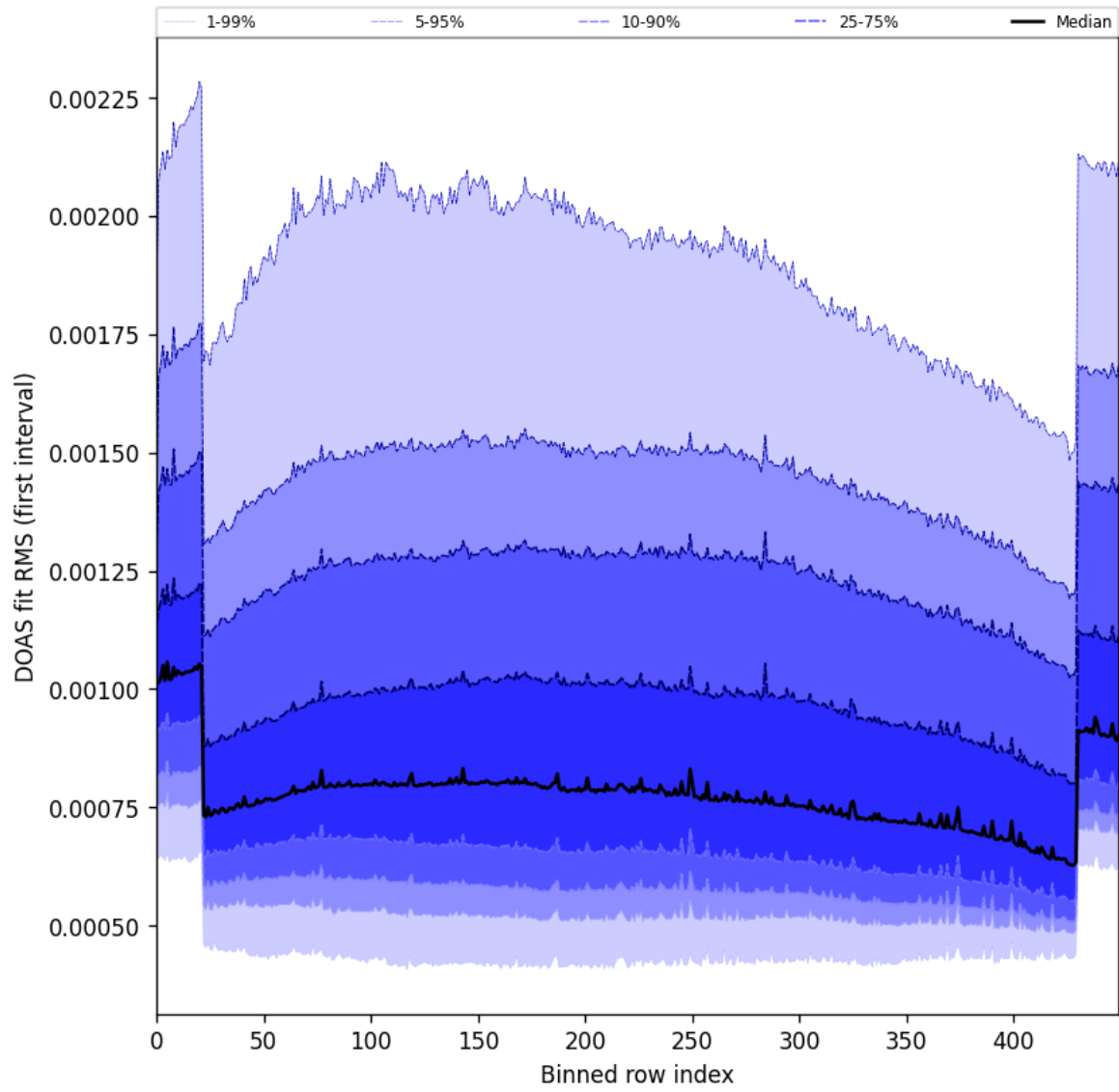
Figure 60: Along track statistics of “DOAS fit RMS (first interval)” for 2025-09-06 to 2025-09-08
