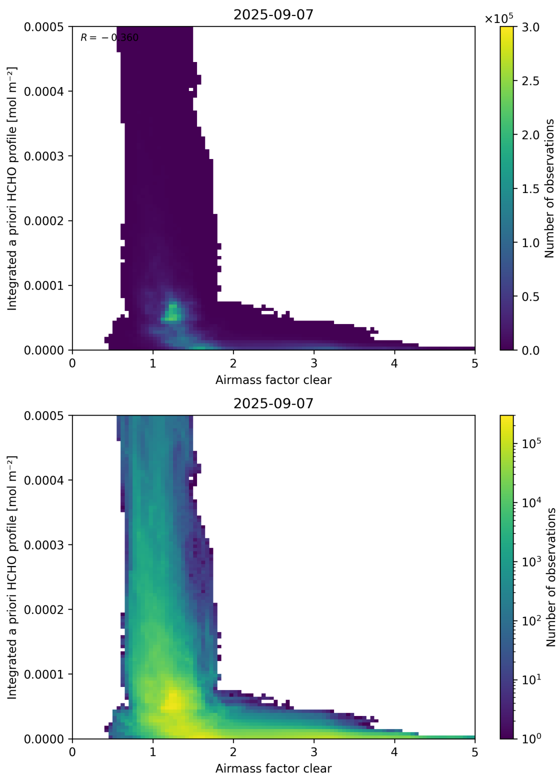
Figure 76: Scatter density plot of “Airmass factor clear” against “Integrated a priori HCHO profile” for 2025-09-06 to 2025-09-08.
