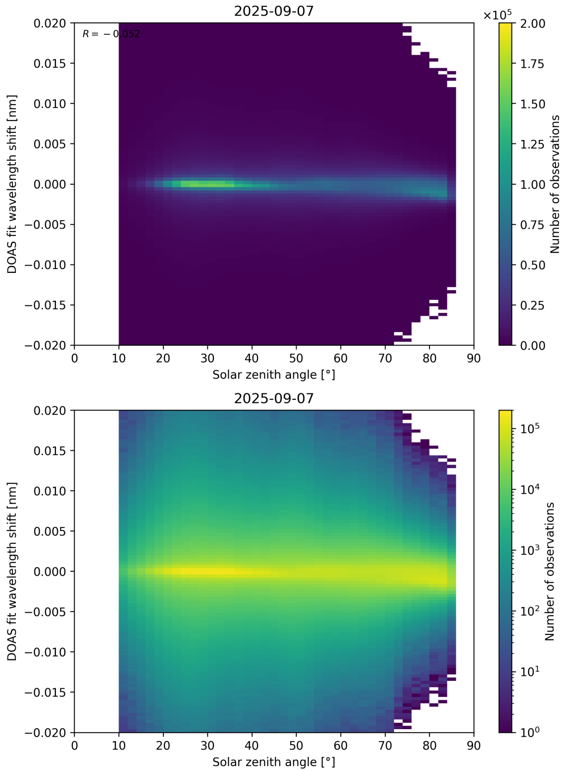
Figure 168: Scatter density plot of “Solar zenith angle” against “DOAS fit wavelength shift” for 2025-09-06 to 2025-09-08.
