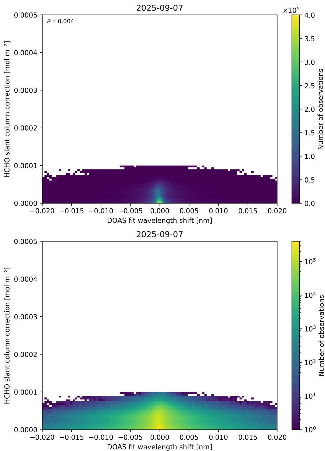
Figure 67: Scatter density plot of “DOAS fit wavelength shift” against “HCHO slant column correction” for 2025-09-06 to 2025-09-08.
