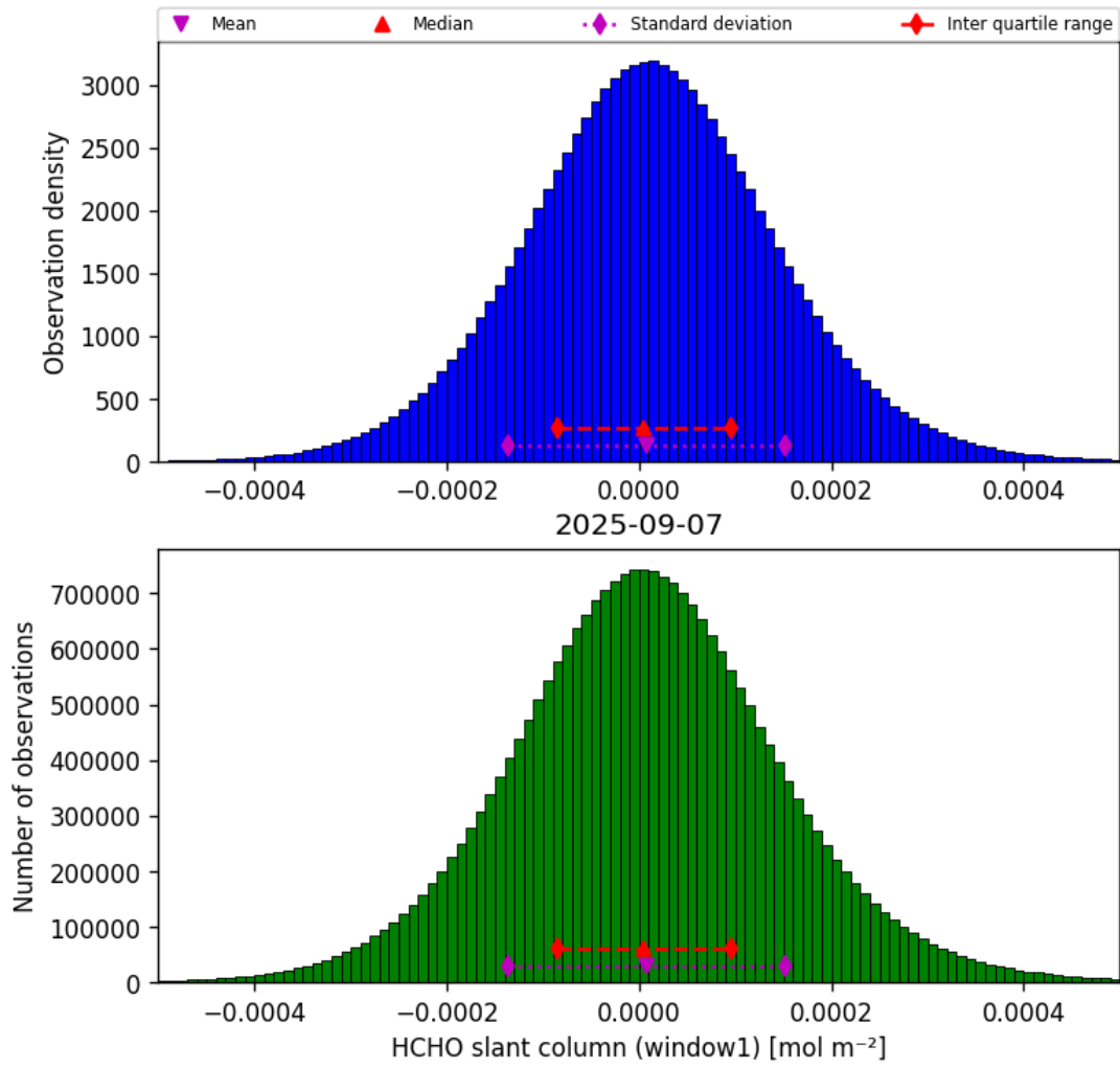
Figure 38: Histogram of “HCHO slant column (window1)” for 2025-09-06 to 2025-09-08
