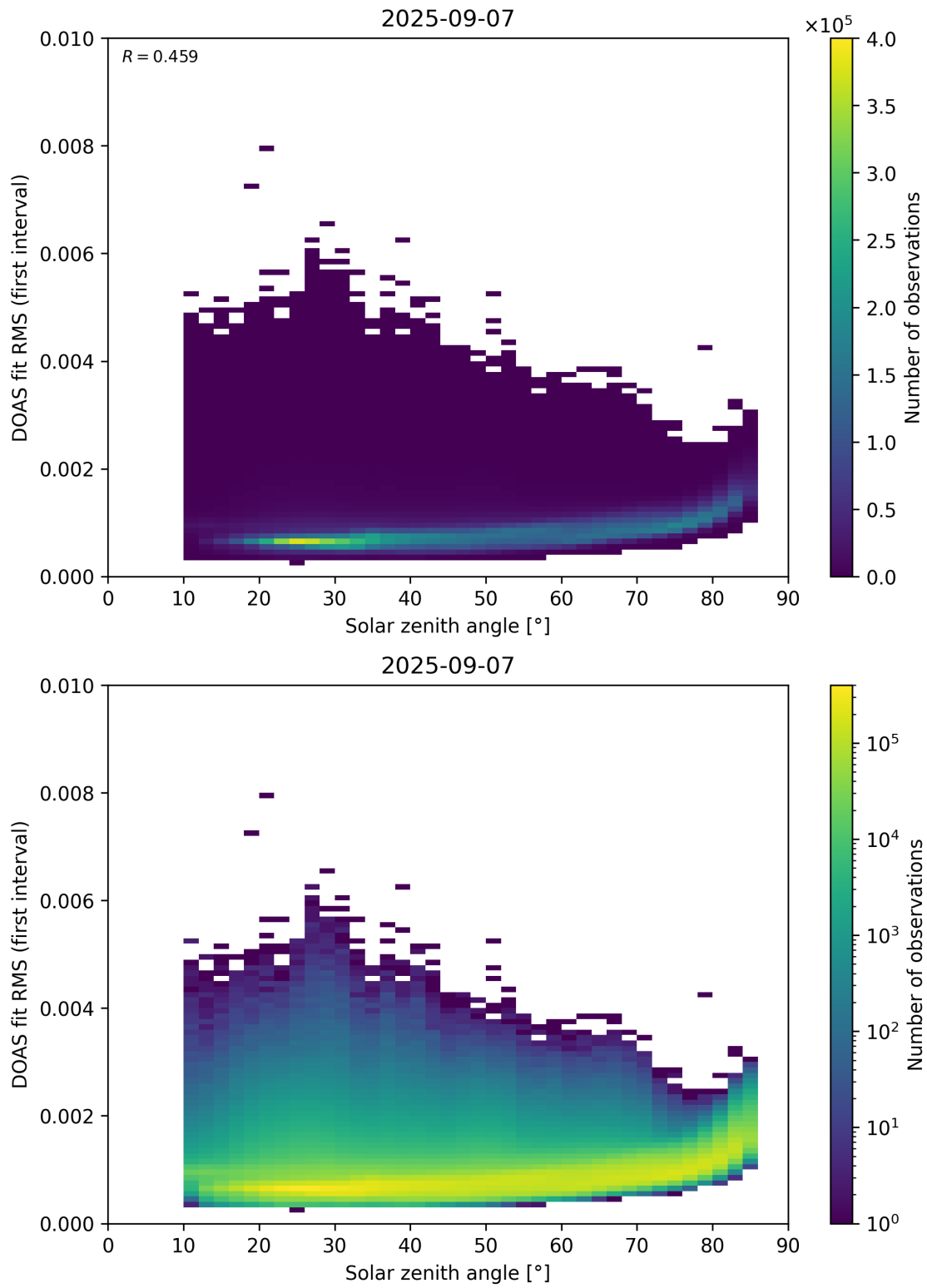
Figure 167: Scatter density plot of “Solar zenith angle” against “DOAS fit RMS (first interval)” for 2025-09-06 to 2025-09-08.
