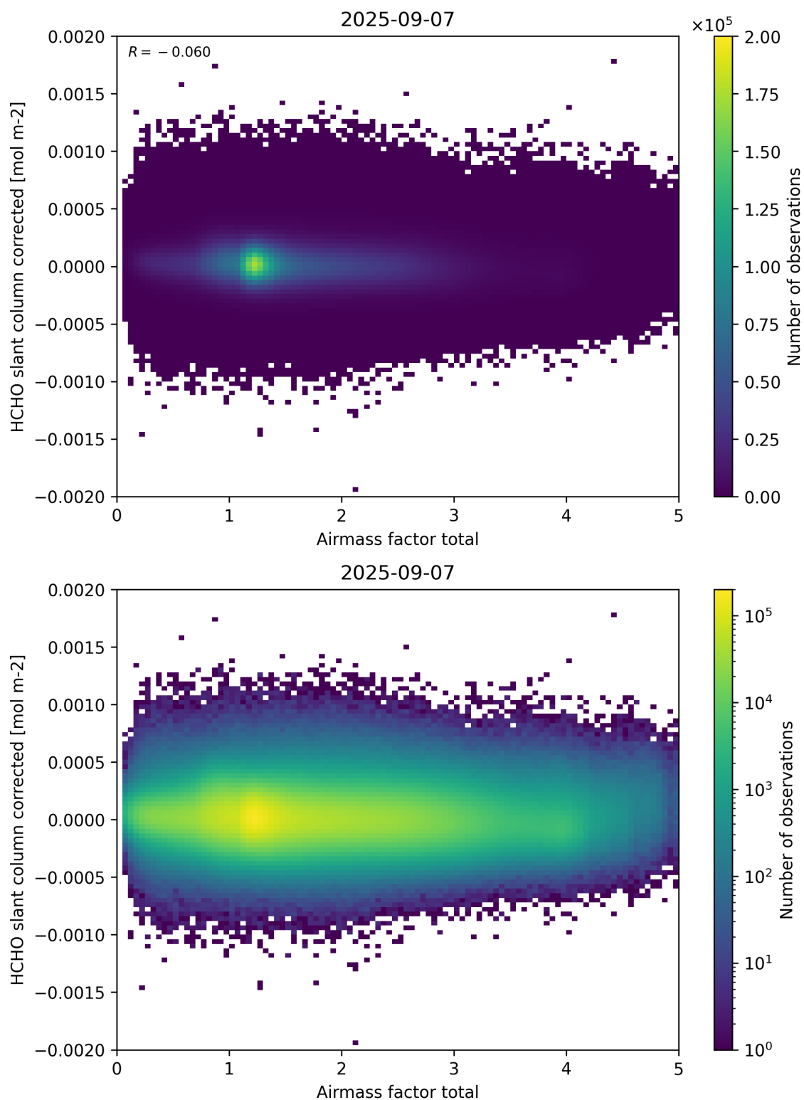
Figure 101: Scatter density plot of “Airmass factor total” against “HCHO slant column corrected” for 2025-09-06 to 2025-09-08.
