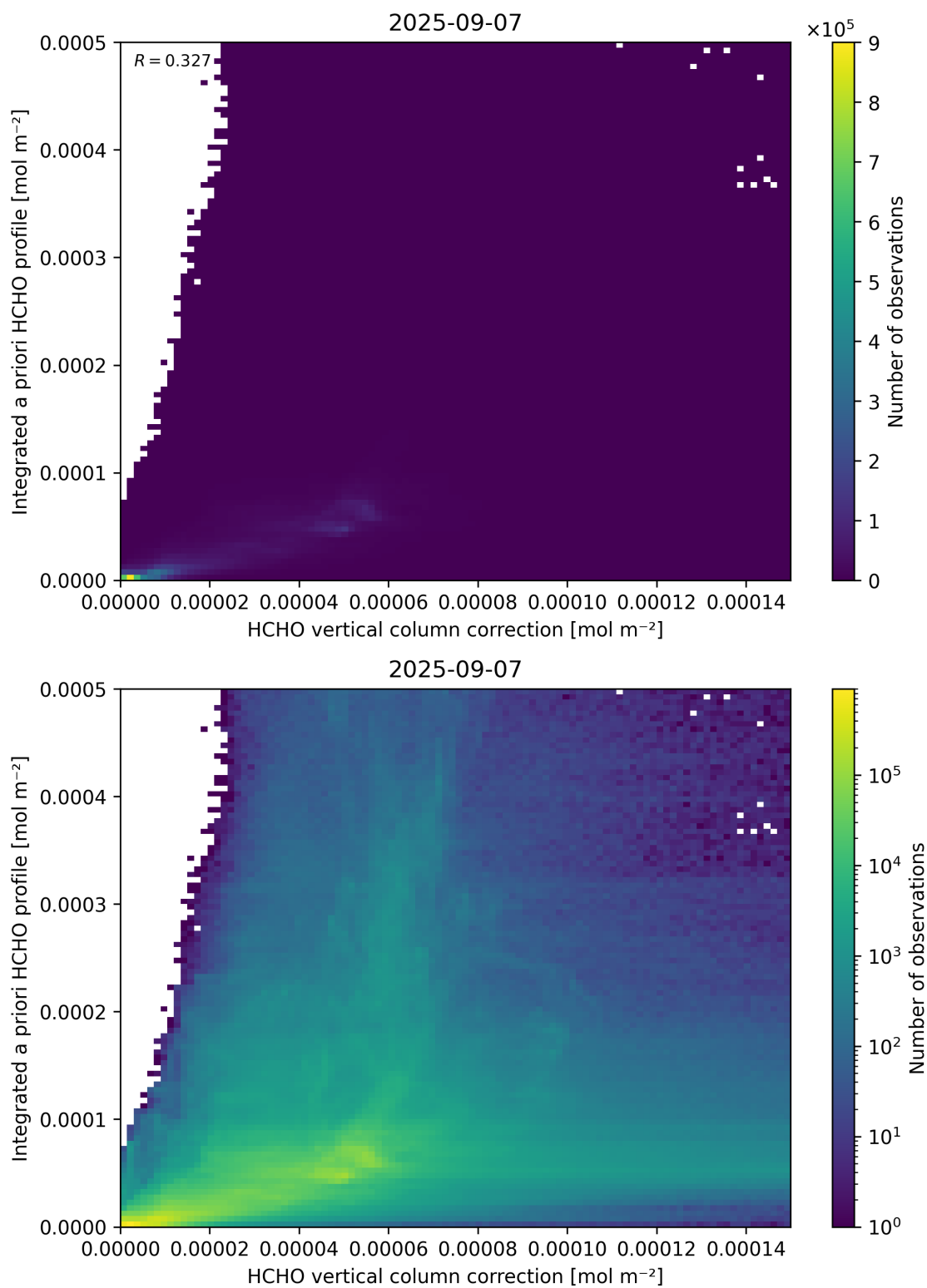
Figure 122: Scatter density plot of “HCHO vertical column correction” against “Integrated a priori HCHO profile” for 2025-09-06 to 2025-09-08.
