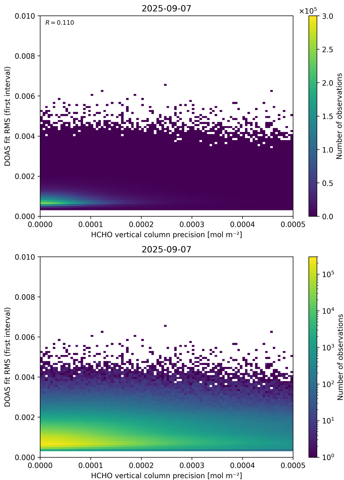
Figure 136: Scatter density plot of “HCHO vertical column precision” against “DOAS fit RMS (first interval)” for 2025-09-06 to 2025-09-08.
