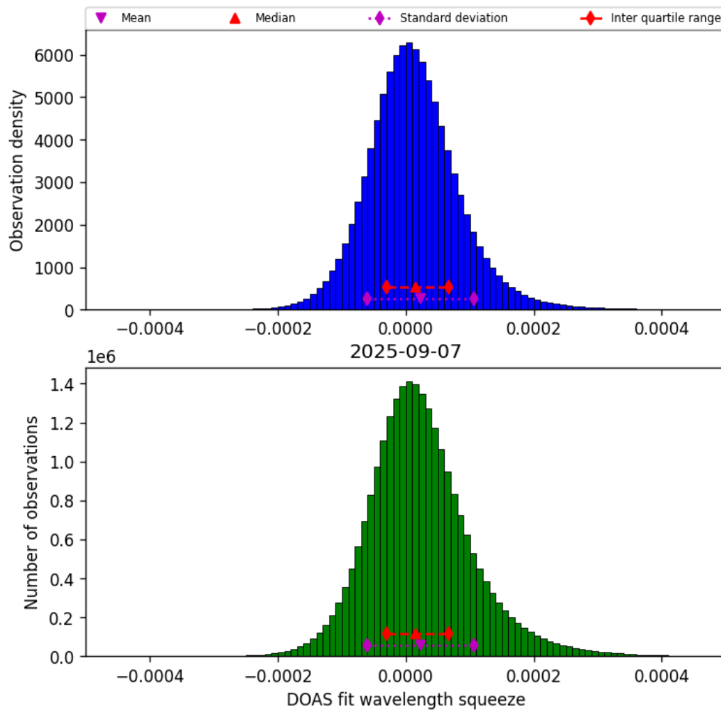
Figure 45: Histogram of “DOAS fit wavelength squeeze” for 2025-09-06 to 2025-09-08
