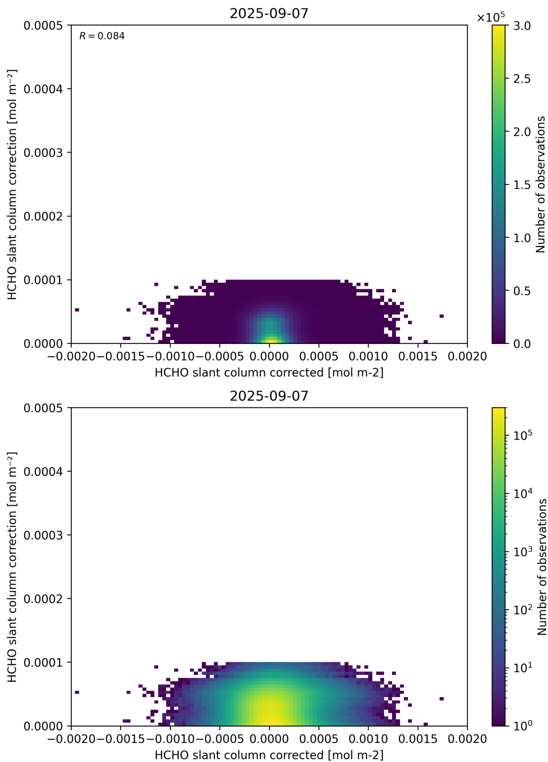
Figure 77: Scatter density plot of “HCHO slant column corrected” against “HCHO slant column correction” for 2025-09-06 to 2025-09-08.
