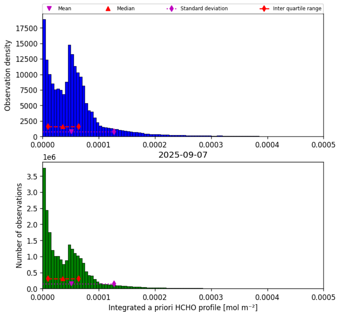
Figure 43: Histogram of “Integrated a priori HCHO profile” for 2025-09-06 to 2025-09-08
