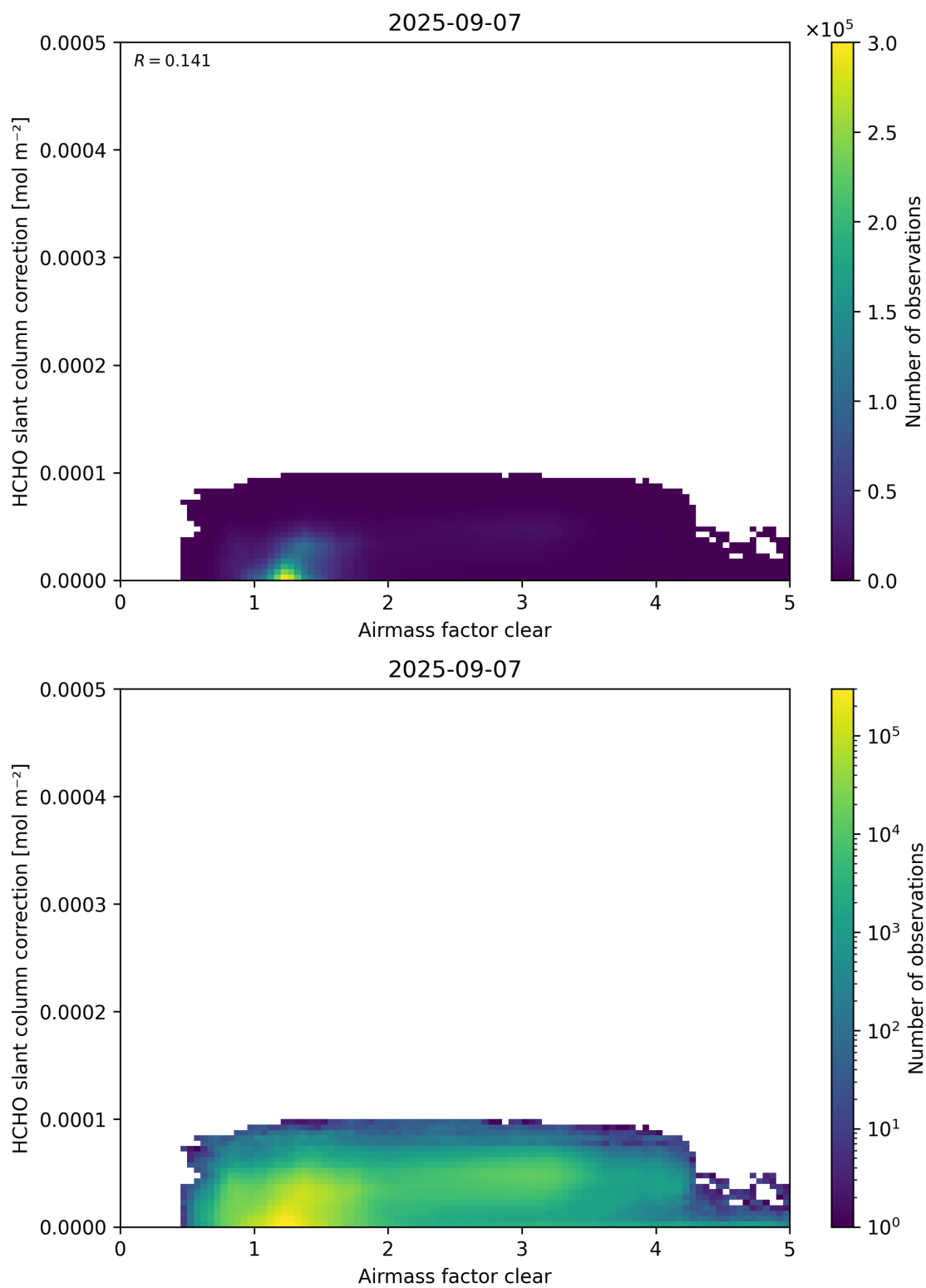
Figure 75: Scatter density plot of “Airmass factor clear” against “HCHO slant column correction” for 2025-09-06 to 2025-09-08.
