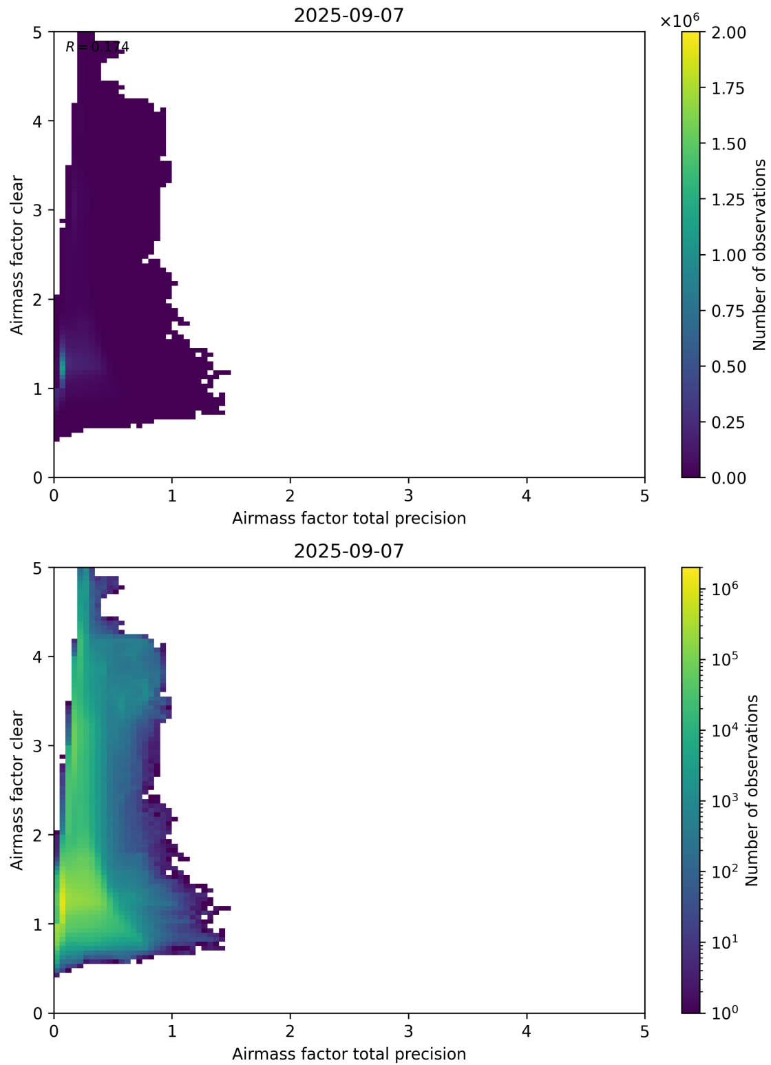
Figure 108: Scatter density plot of “Airmass factor total precision” against “Airmass factor clear” for 2025-09-06 to 2025-09-08.
