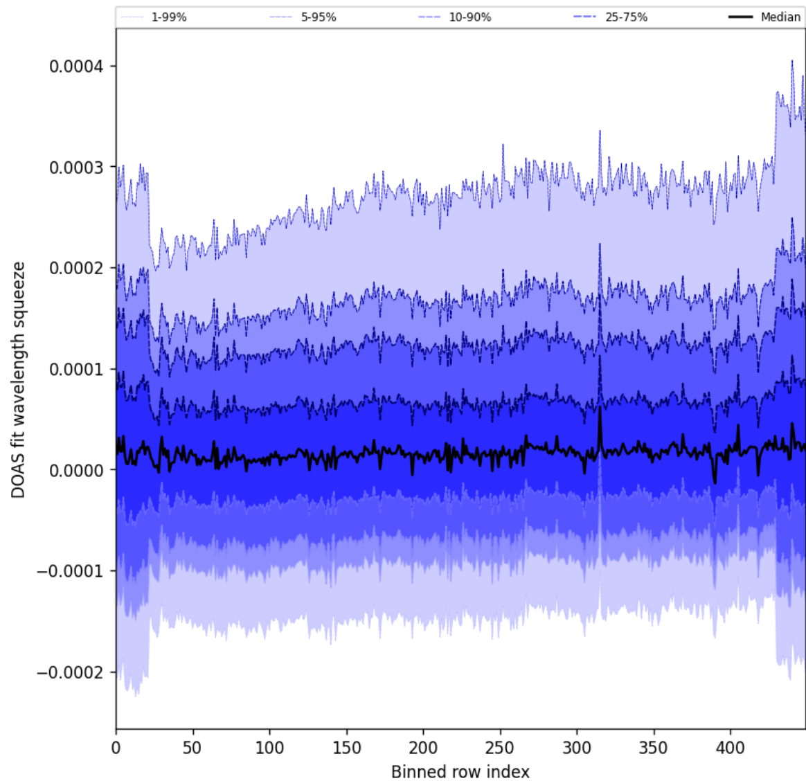
Figure 59: Along track statistics of “DOAS fit wavelength squeeze” for 2025-09-06 to 2025-09-08
