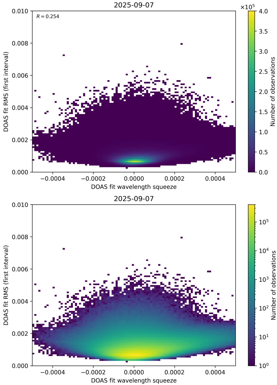
Figure 68: Scatter density plot of “DOAS fit wavelength squeeze” against “DOAS fit RMS (first interval)” for 2025-09-06 to 2025-09-08.
