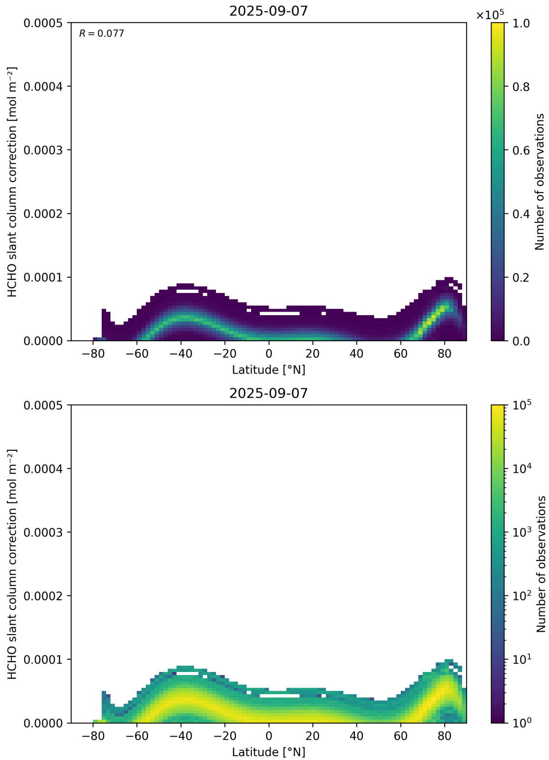
Figure 158: Scatter density plot of “Latitude” against “HCHO slant column correction” for 2025-09-06 to 2025-09-08.
