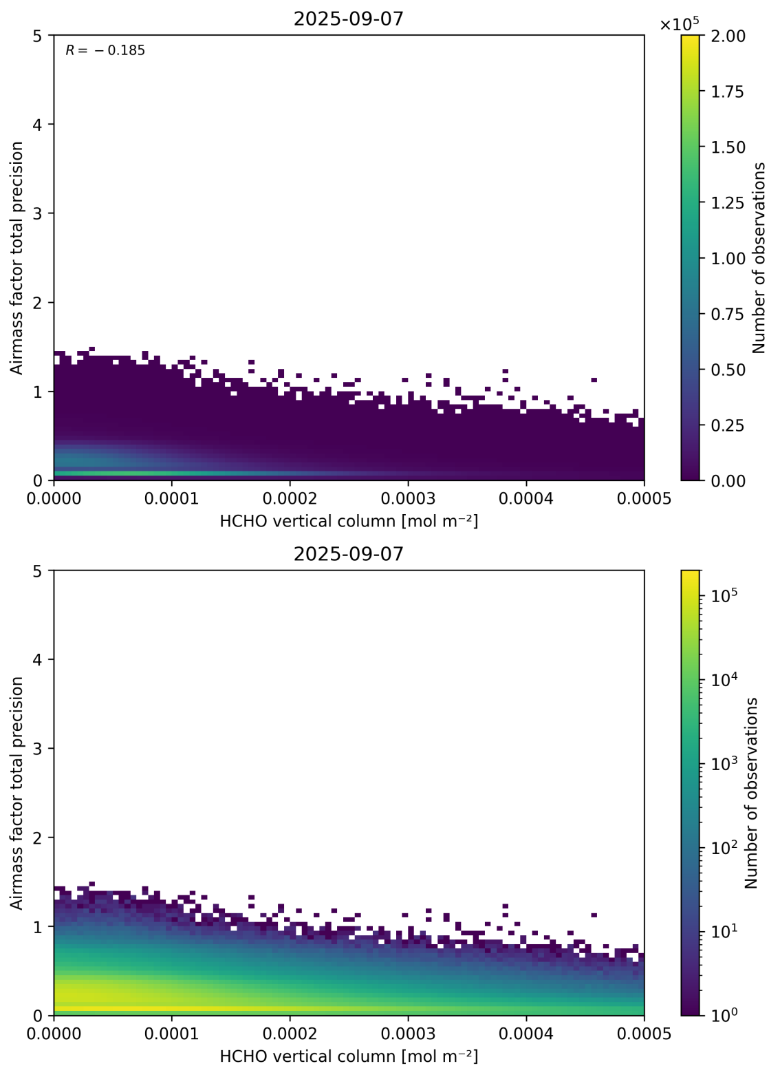
Figure 132: Scatter density plot of “HCHO vertical column” against “Airmass factor total precision” for 2025-09-06 to 2025-09-08.
