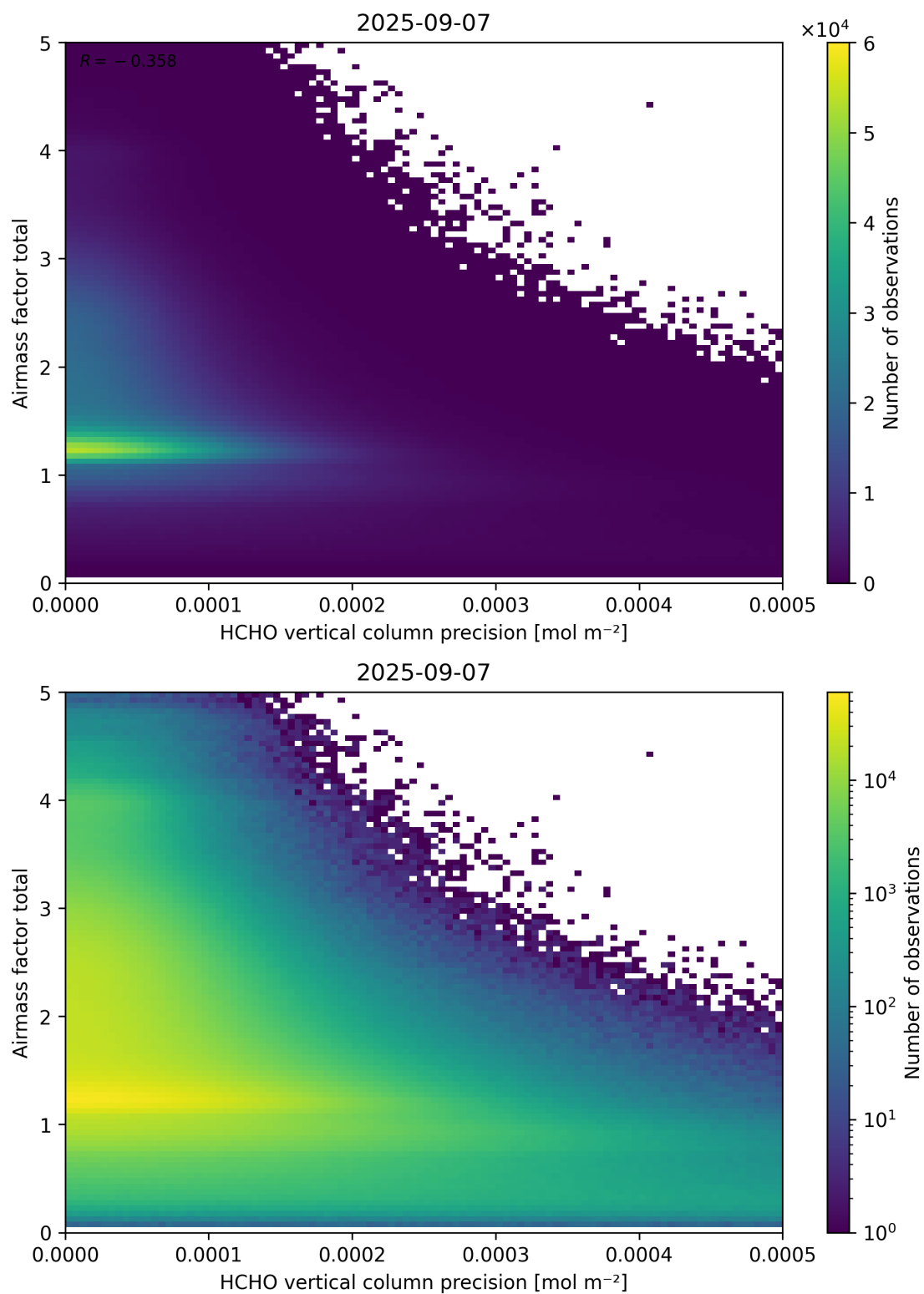
Figure 144: Scatter density plot of “HCHO vertical column precision” against “Airmass factor total” for 2025-09-06 to 2025-09-08.
