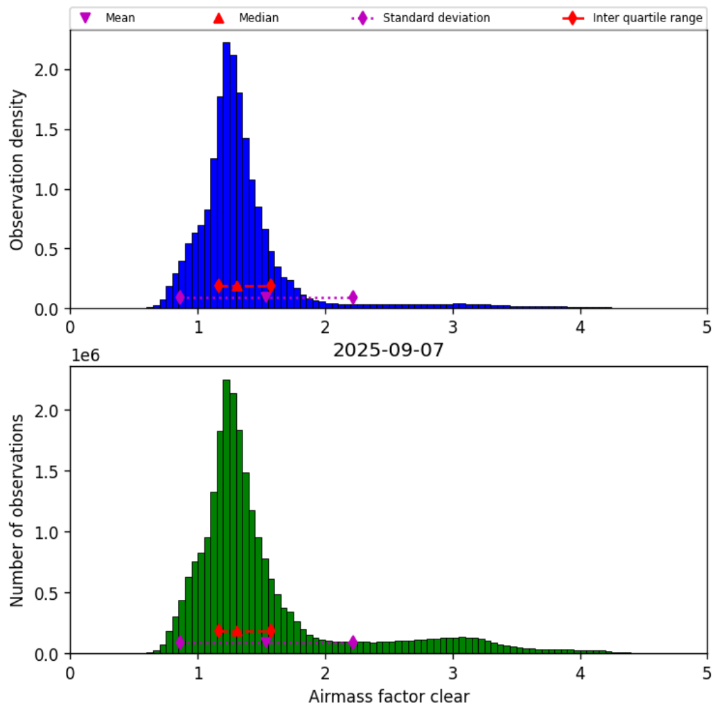
Figure 42: Histogram of “Airmass factor clear” for 2025-09-06 to 2025-09-08
