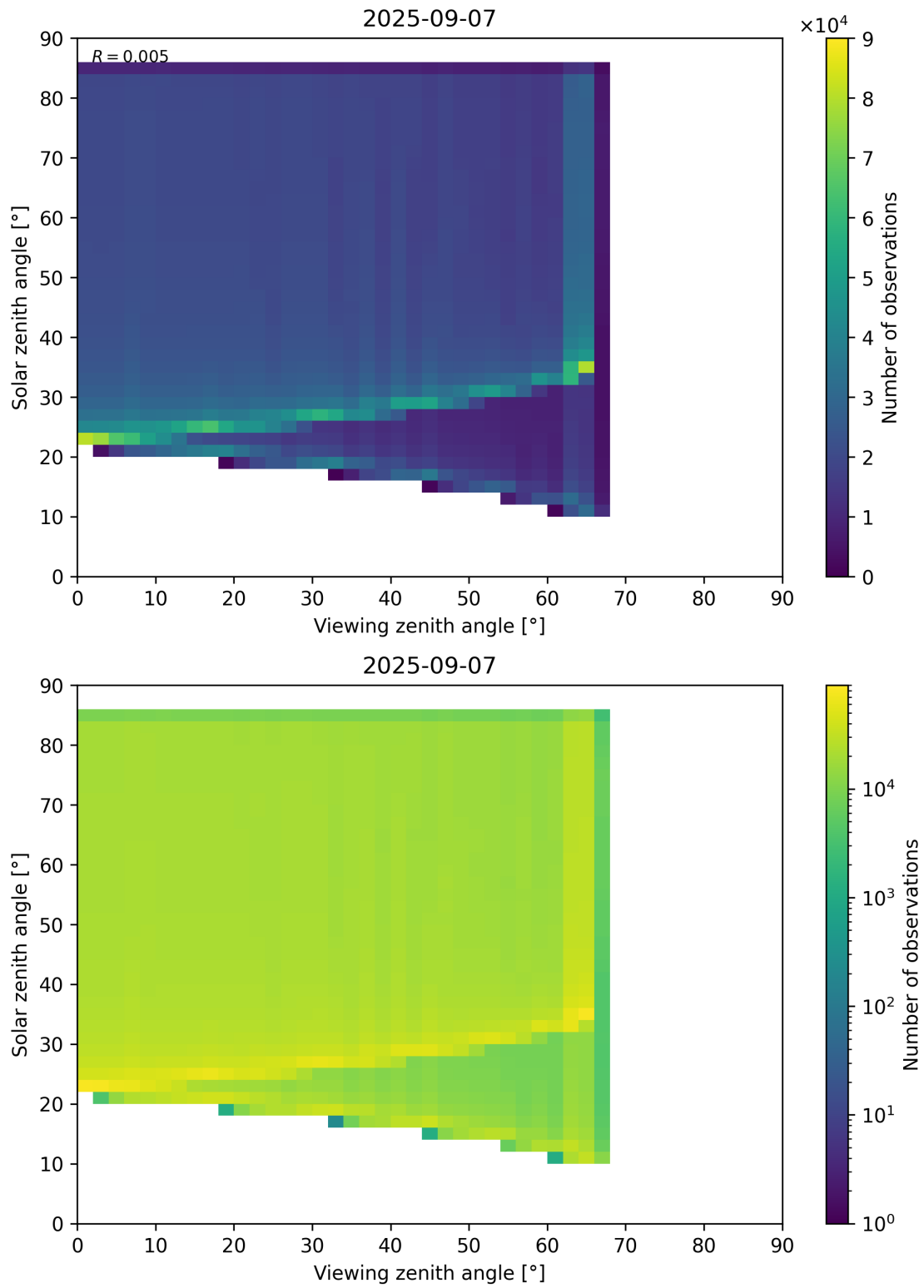
Figure 197: Scatter density plot of “Viewing zenith angle” against “Solar zenith angle” for 2025-09-06 to 2025-09-08.
