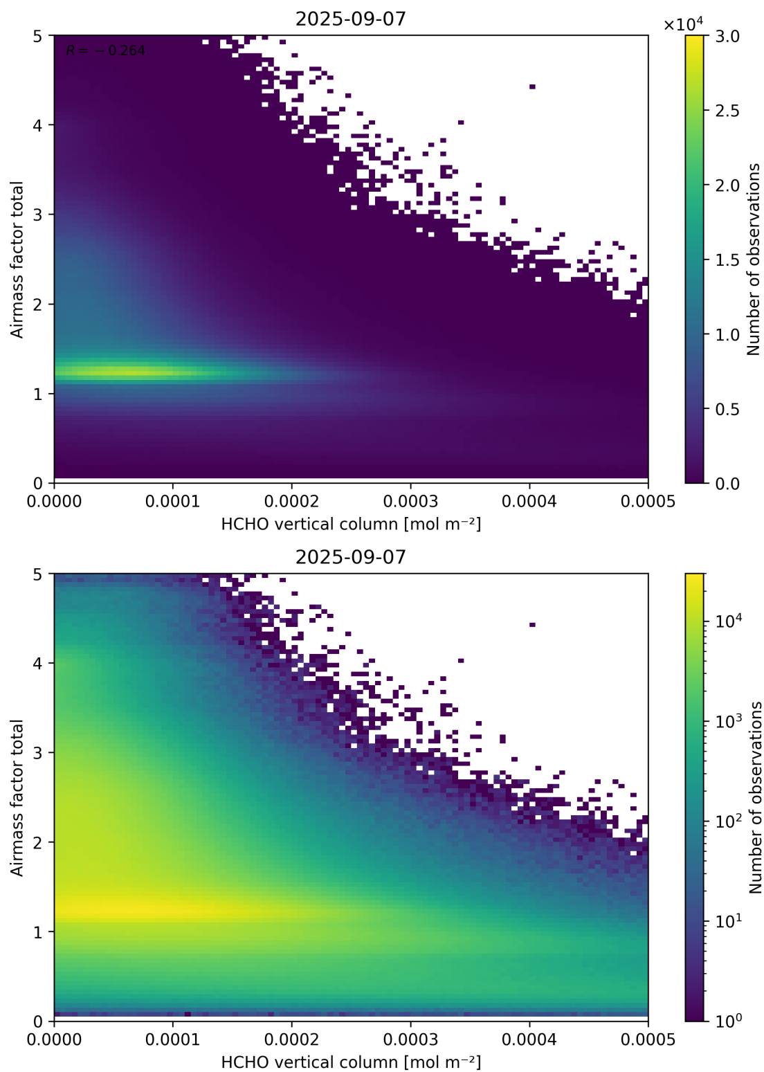
Figure 131: Scatter density plot of “HCHO vertical column” against “Airmass factor total” for 2025-09-06 to 2025-09-08.
