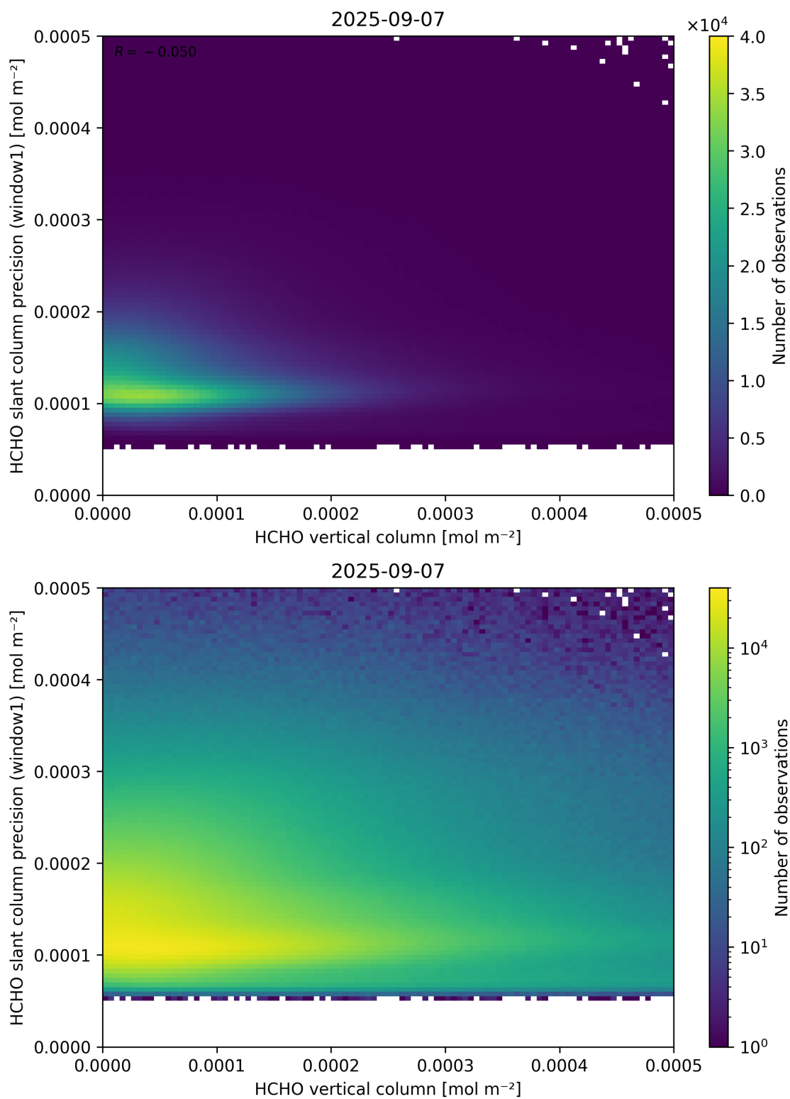
Figure 130: Scatter density plot of “HCHO vertical column” against “HCHO slant column precision (window1)” for 2025-09-06 to 2025-09-08.
