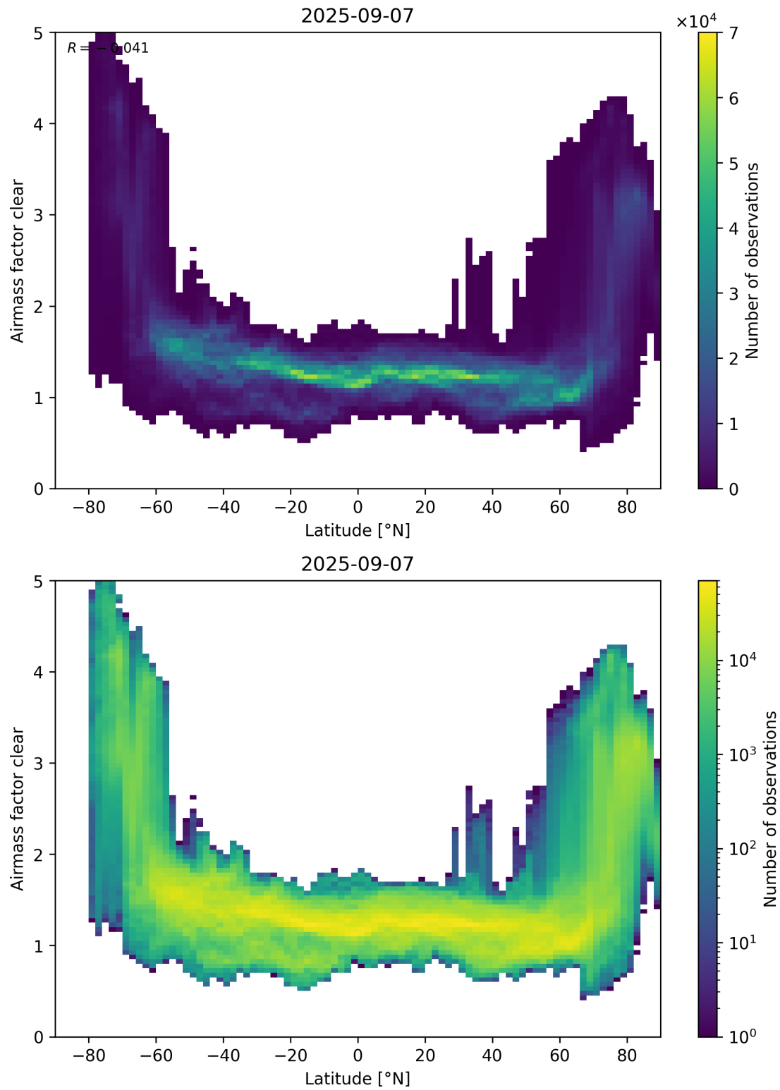
Figure 156: Scatter density plot of “Latitude” against “Airmass factor clear” for 2025-09-06 to 2025-09-08.
