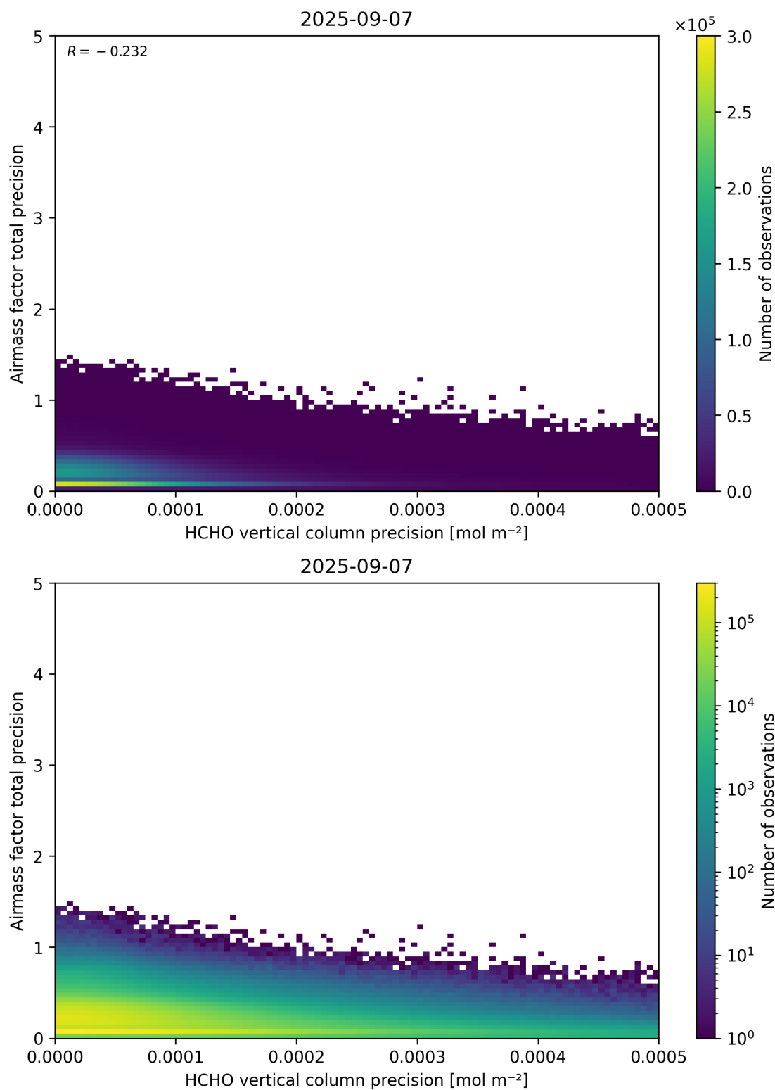
Figure 145: Scatter density plot of “HCHO vertical column precision” against “Airmass factor total precision” for 2025-09-06 to 2025-09-08.
