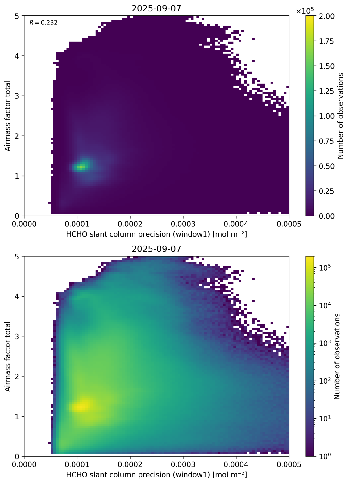
Figure 94: Scatter density plot of “HCHO slant column precision (window1)” against “Airmass factor total” for 2025-09-06 to 2025-09-08.
