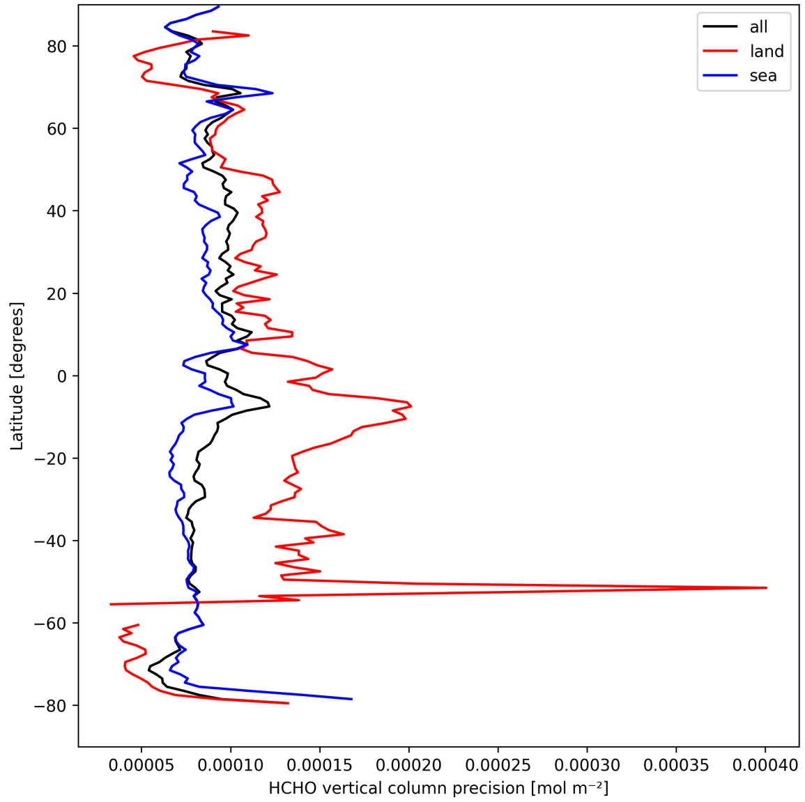
Figure 22: Zonal average of “HCHO vertical column precision” for 2025-09-06 to 2025-09-08.
