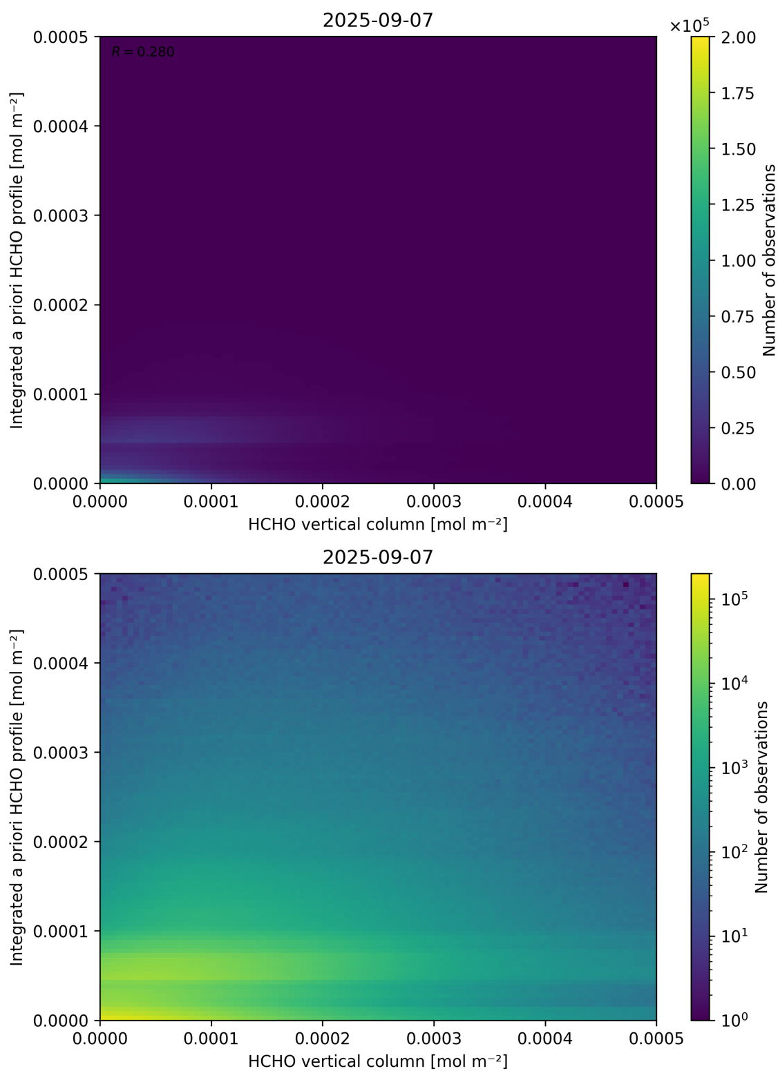
Figure 135: Scatter density plot of “HCHO vertical column” against “Integrated a priori HCHO profile” for 2025-09-06 to 2025-09-08.
