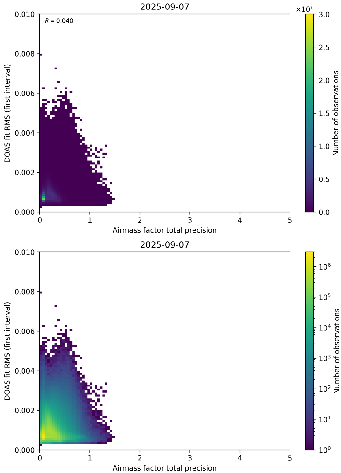
Figure 105: Scatter density plot of “Airmass factor total precision” against “DOAS fit RMS (first interval)” for 2025-09-06 to 2025-09-08.
