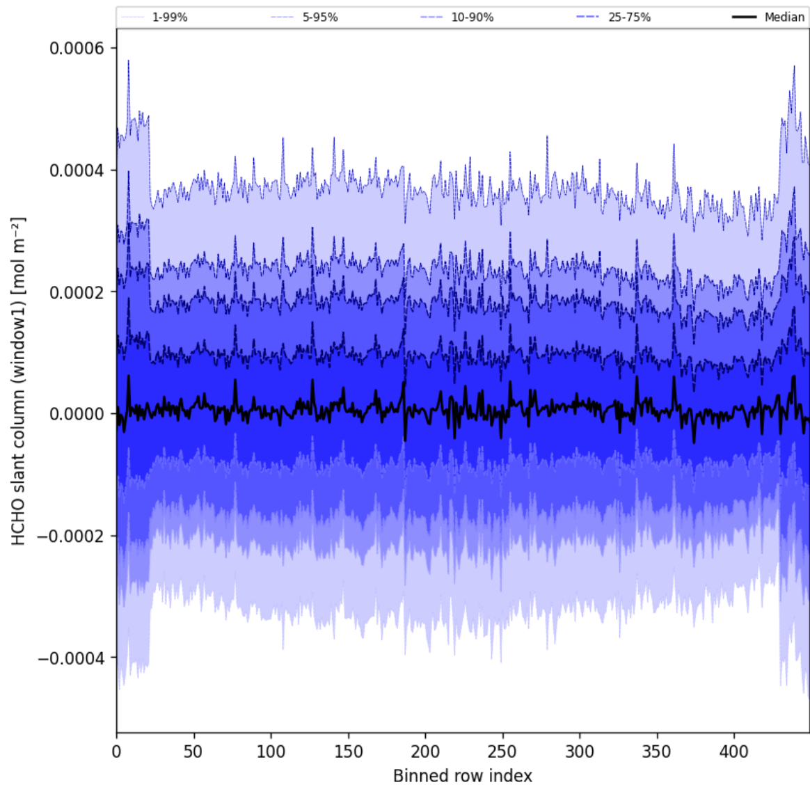
Figure 52: Along track statistics of “HCHO slant column (window1)” for 2025-09-06 to 2025-09-08
