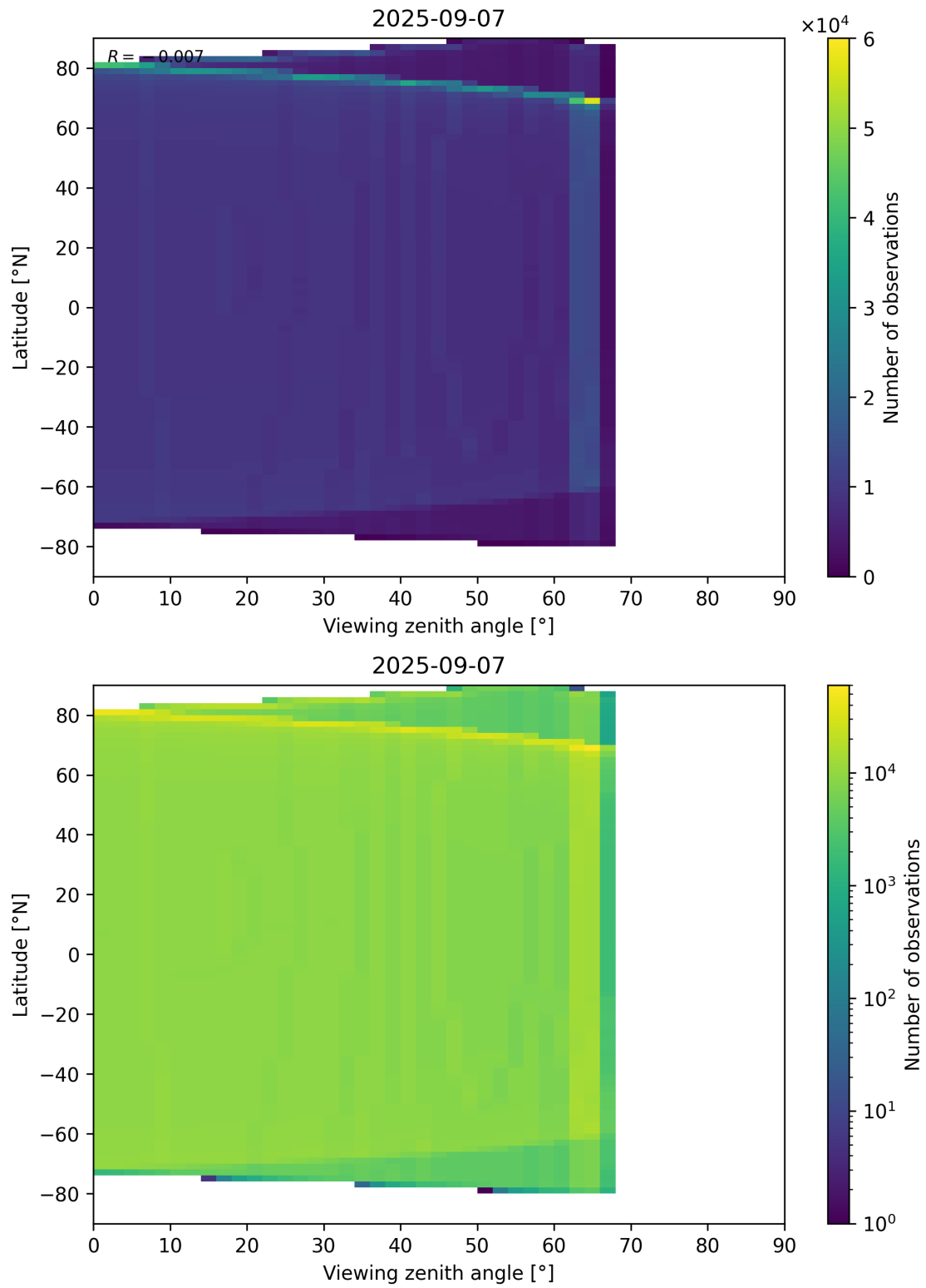
Figure 196: Scatter density plot of “Viewing zenith angle” against “Latitude” for 2025-09-06 to 2025-09-08.
