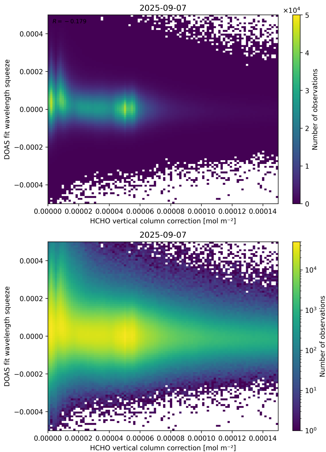
Figure 114: Scatter density plot of “HCHO vertical column correction” against “DOAS fit wavelength squeeze” for 2025-09-06 to 2025-09-08.
