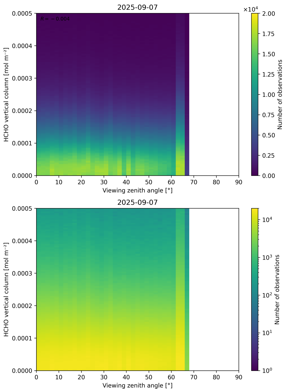
Figure 192: Scatter density plot of “Viewing zenith angle” against “HCHO vertical column” for 2025-09-06 to 2025-09-08.
