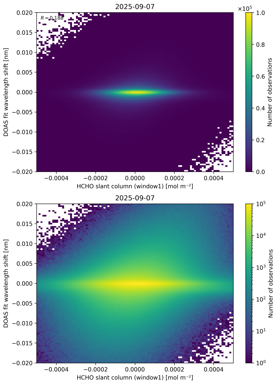
Figure 79: Scatter density plot of “HCHO slant column (window1)” against “DOAS fit wavelength shift” for 2025-09-06 to 2025-09-08.
