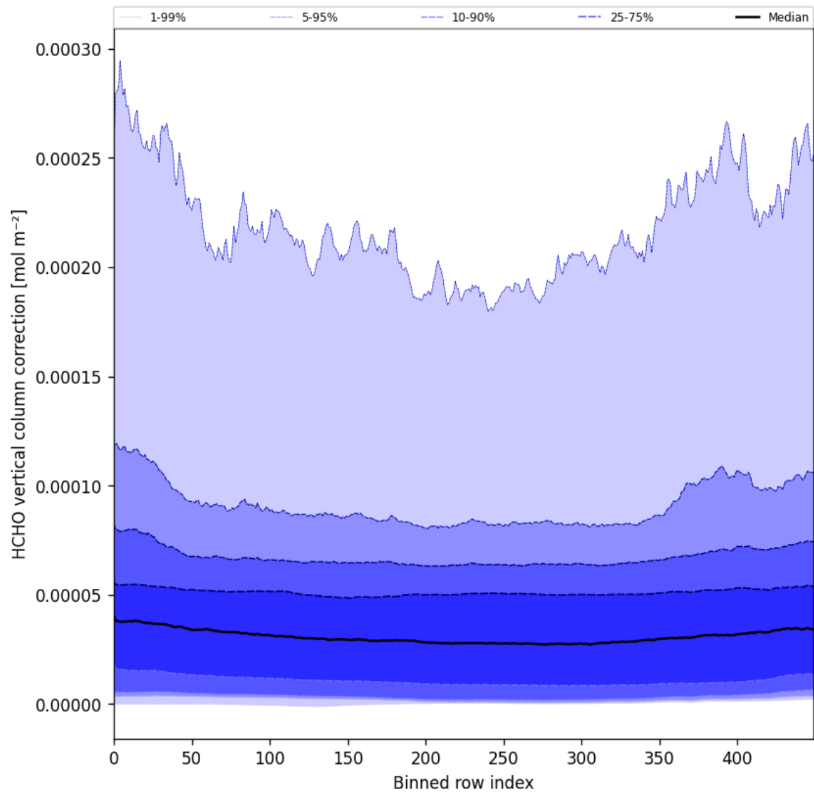
Figure 51: Along track statistics of “HCHO vertical column correction” for 2025-09-06 to 2025-09-08
