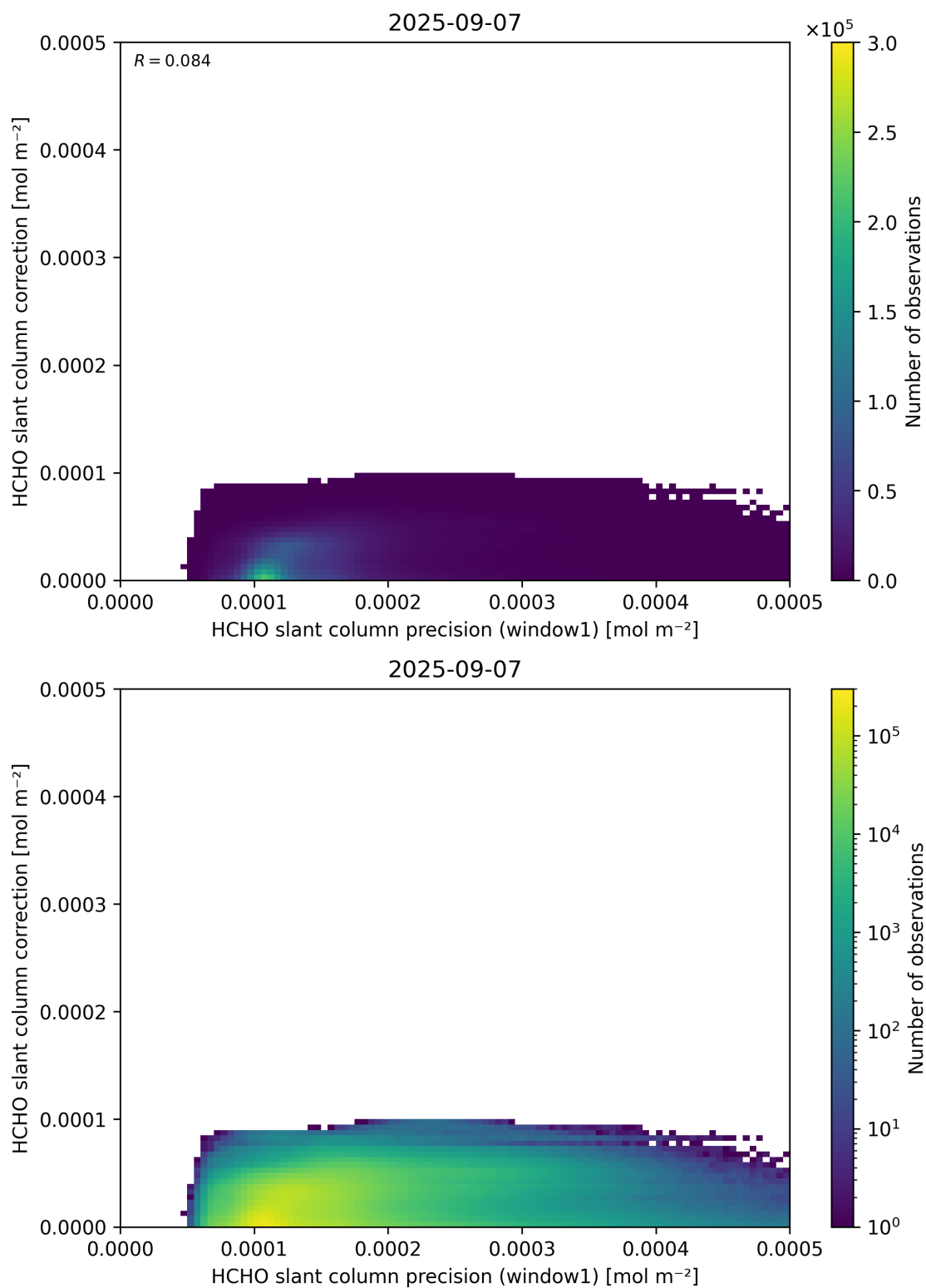
Figure 93: Scatter density plot of “HCHO slant column precision (window1)” against “HCHO slant column correction” for 2025-09-06 to 2025-09-08.
