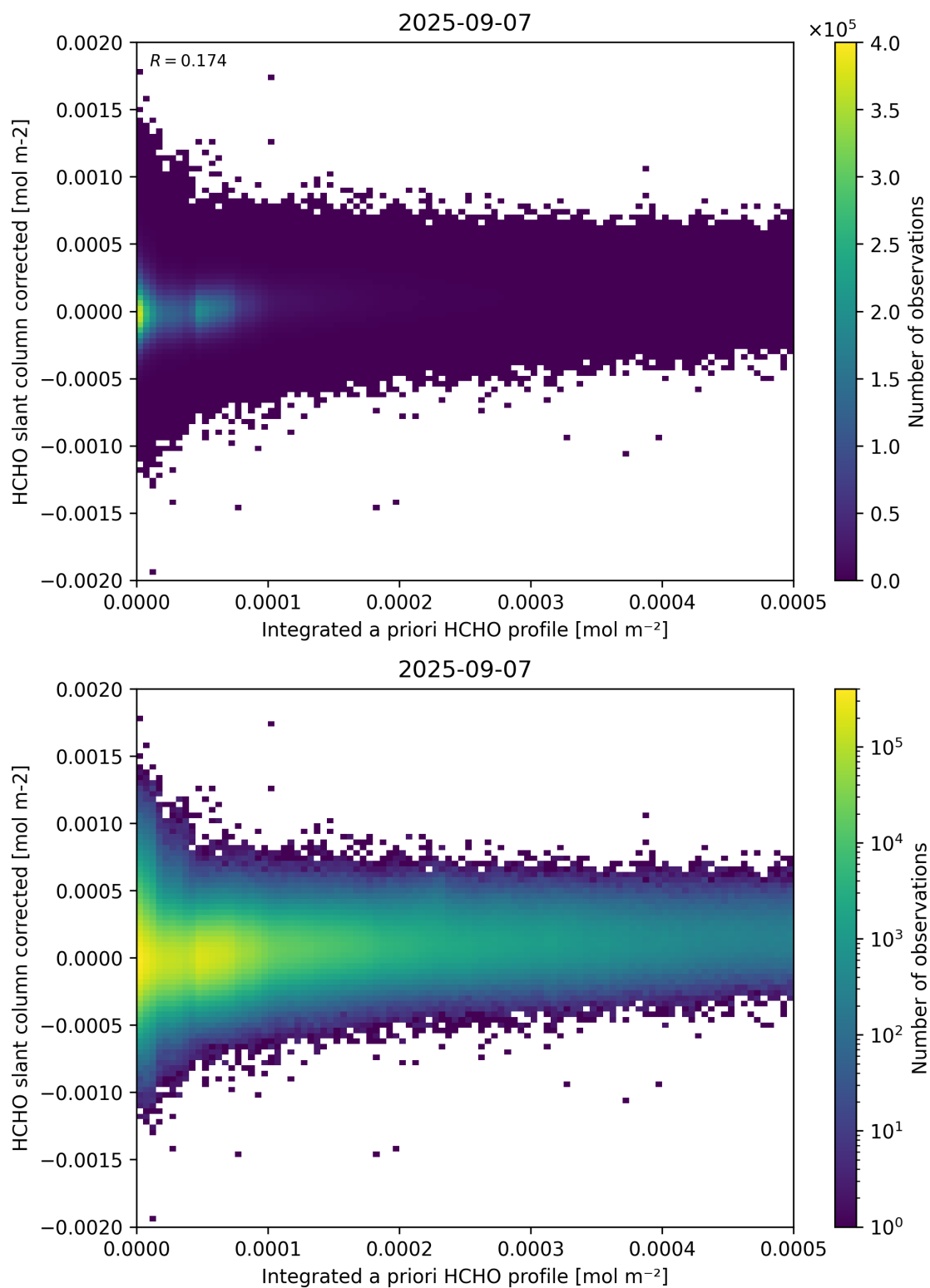
Figure 151: Scatter density plot of “Integrated a priori HCHO profile” against “HCHO slant column corrected” for 2025-09-06 to 2025-09-08.
