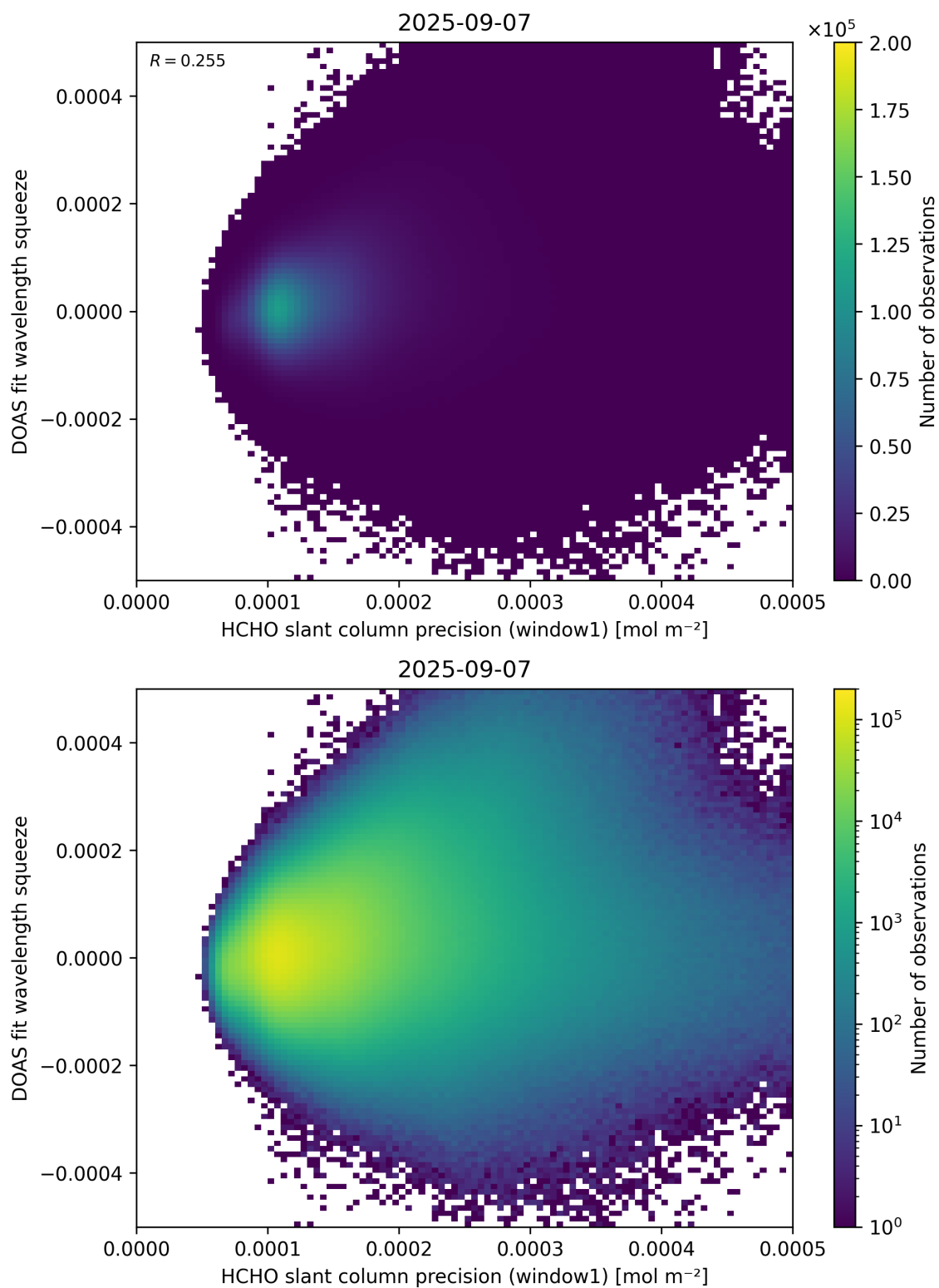
Figure 90: Scatter density plot of “HCHO slant column precision (window1)” against “DOAS fit wavelength squeeze” for 2025-09-06 to 2025-09-08.
