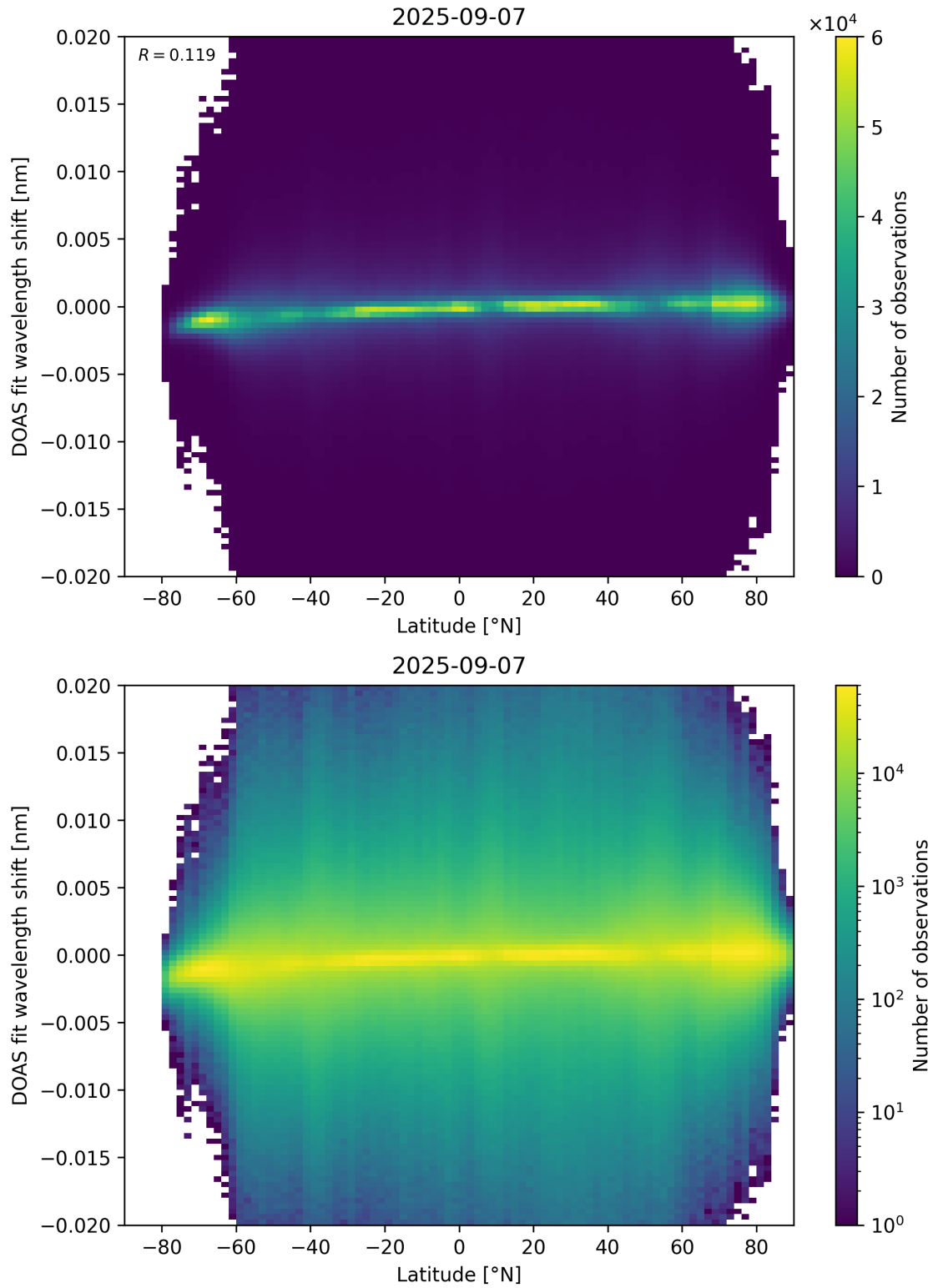
Figure 154: Scatter density plot of “Latitude” against “DOAS fit wavelength shift” for 2025-09-06 to 2025-09-08.
