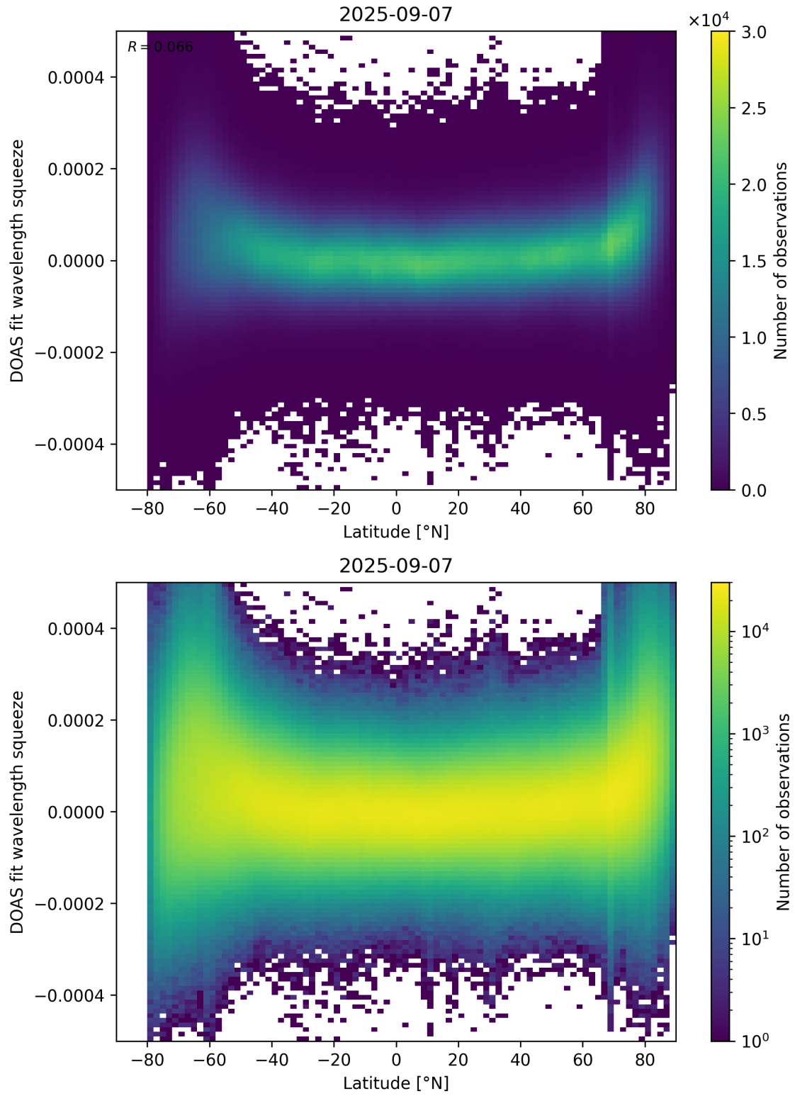
Figure 155: Scatter density plot of “Latitude” against “DOAS fit wavelength squeeze” for 2025-09-06 to 2025-09-08.
