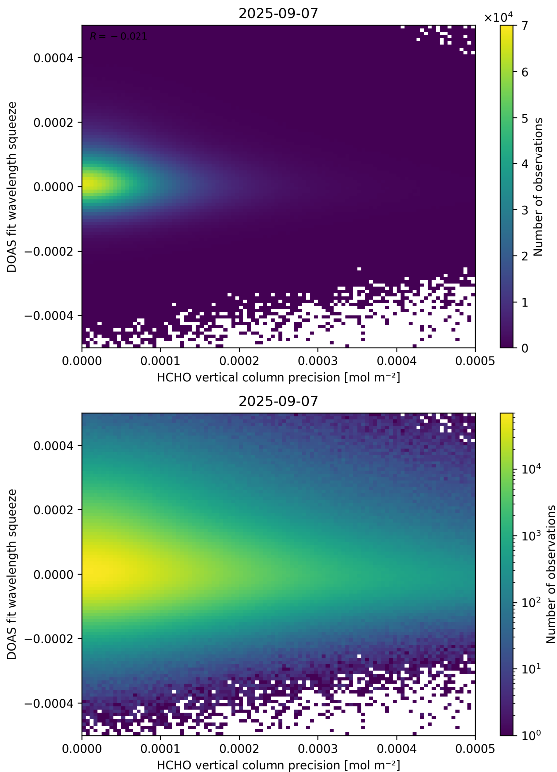
Figure 138: Scatter density plot of “HCHO vertical column precision” against “DOAS fit wavelength squeeze” for 2025-09-06 to 2025-09-08.
