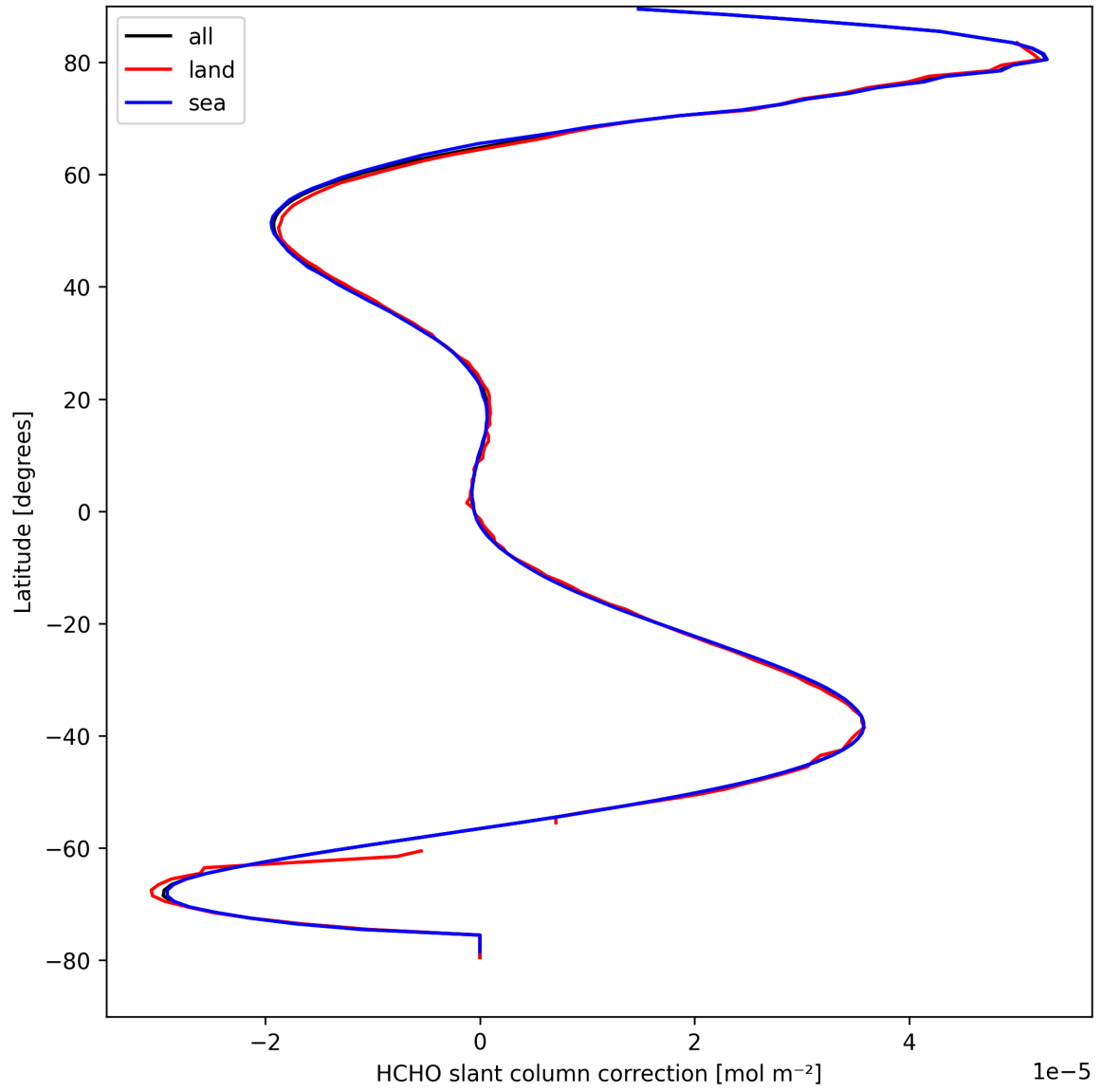
Figure 33: Zonal average of “HCHO slant column correction” for 2025-09-06 to 2025-09-08.
