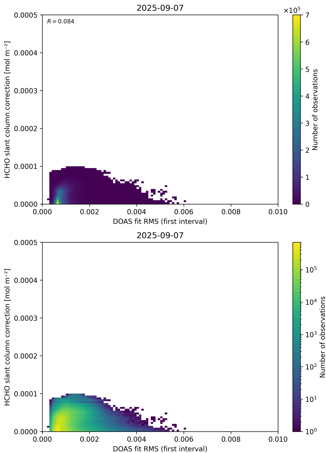
Figure 63: Scatter density plot of “DOAS fit RMS (first interval)” against “HCHO slant column correction” for 2025-09-06 to 2025-09-08.
