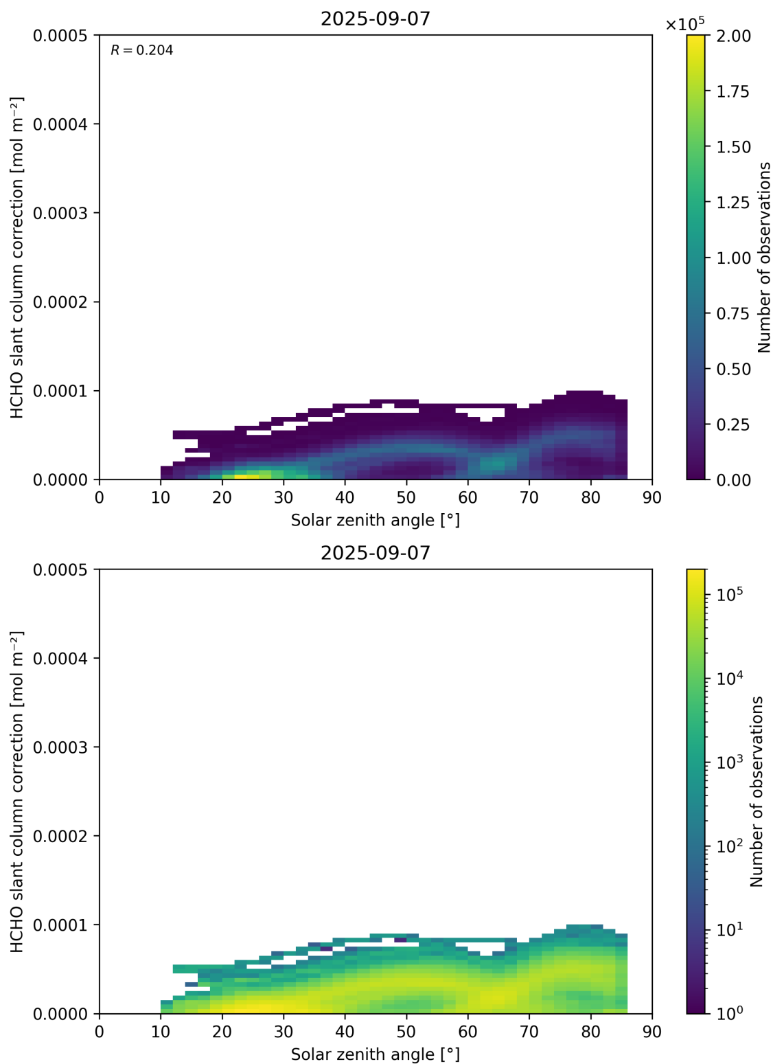
Figure 172: Scatter density plot of “Solar zenith angle” against “HCHO slant column correction” for 2025-09-06 to 2025-09-08.
