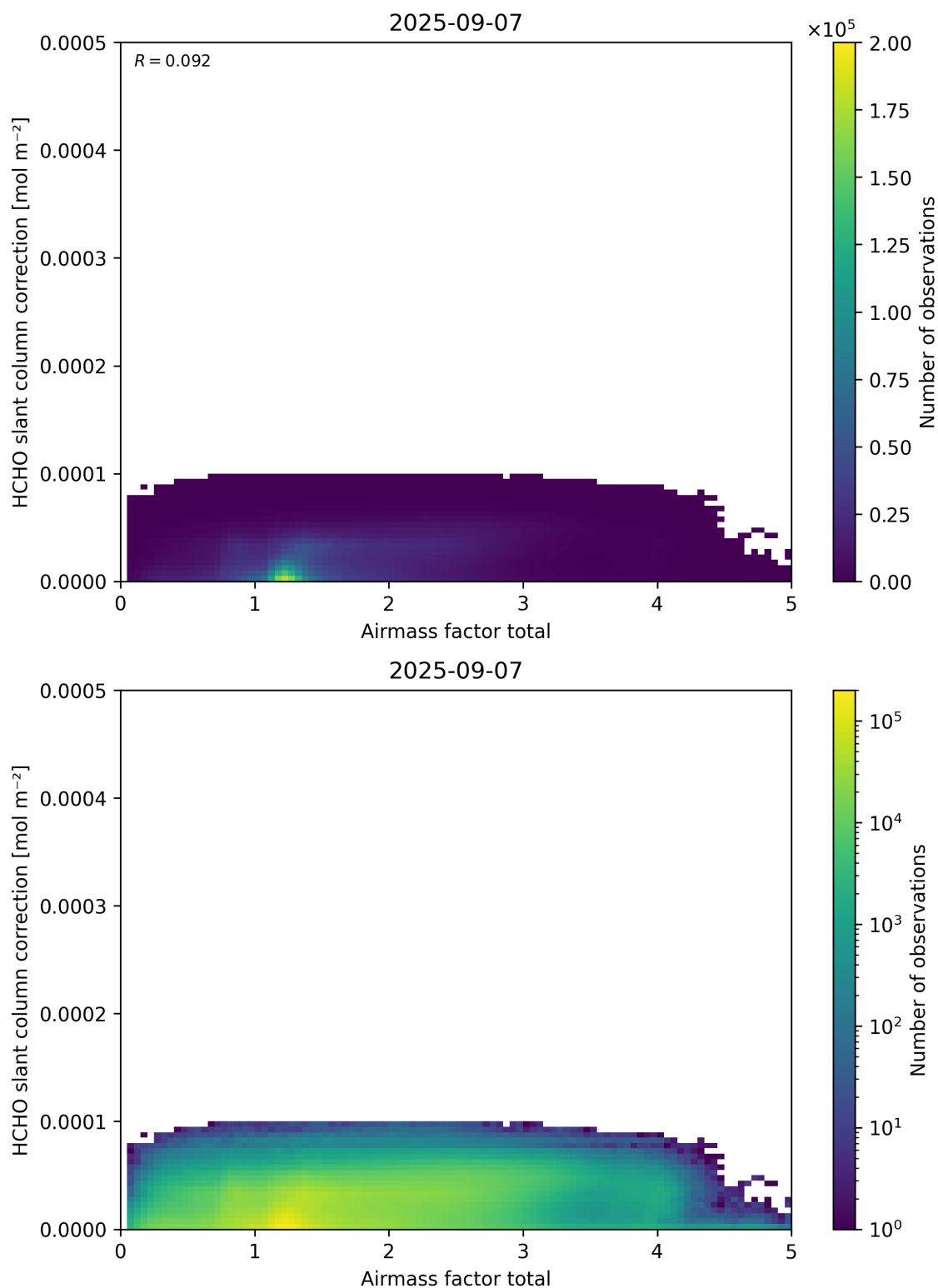
Figure 102: Scatter density plot of “Airmass factor total” against “HCHO slant column correction” for 2025-09-06 to 2025-09-08.
