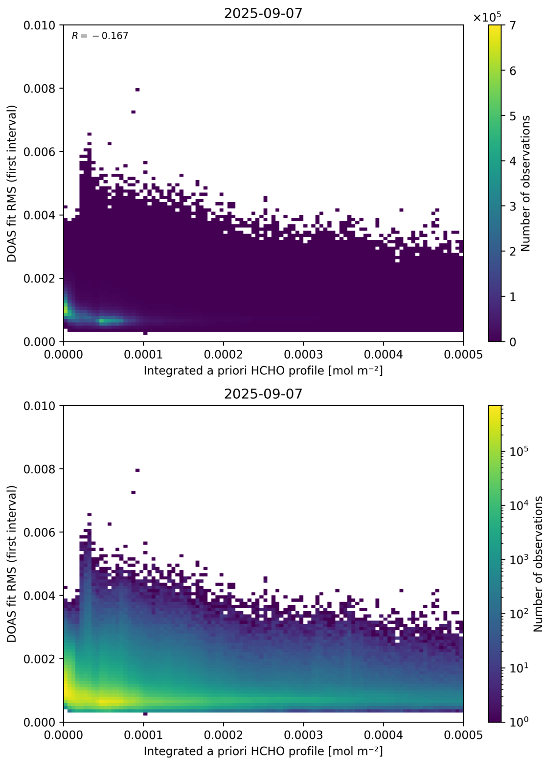
Figure 148: Scatter density plot of “Integrated a priori HCHO profile” against “DOAS fit RMS (first interval)” for 2025-09-06 to 2025-09-08.
