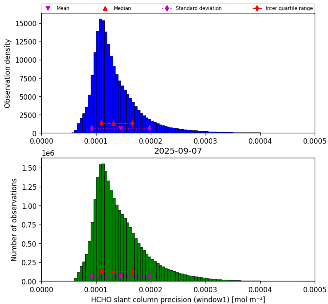
Figure 39: Histogram of “HCHO slant column precision (window1)” for 2025-09-06 to 2025-09-08
