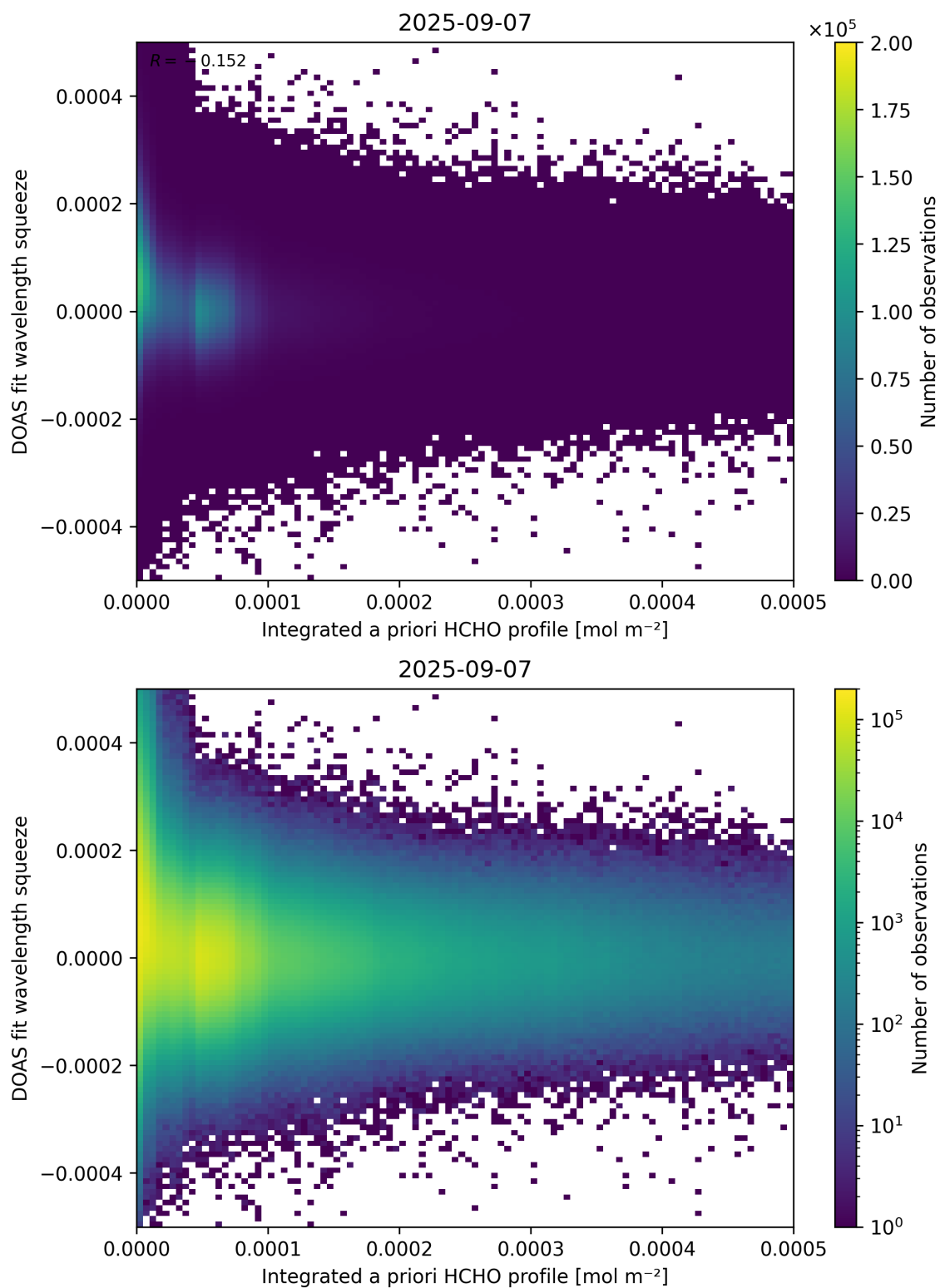
Figure 150: Scatter density plot of “Integrated a priori HCHO profile” against “DOAS fit wavelength squeeze” for 2025-09-06 to 2025-09-08.
