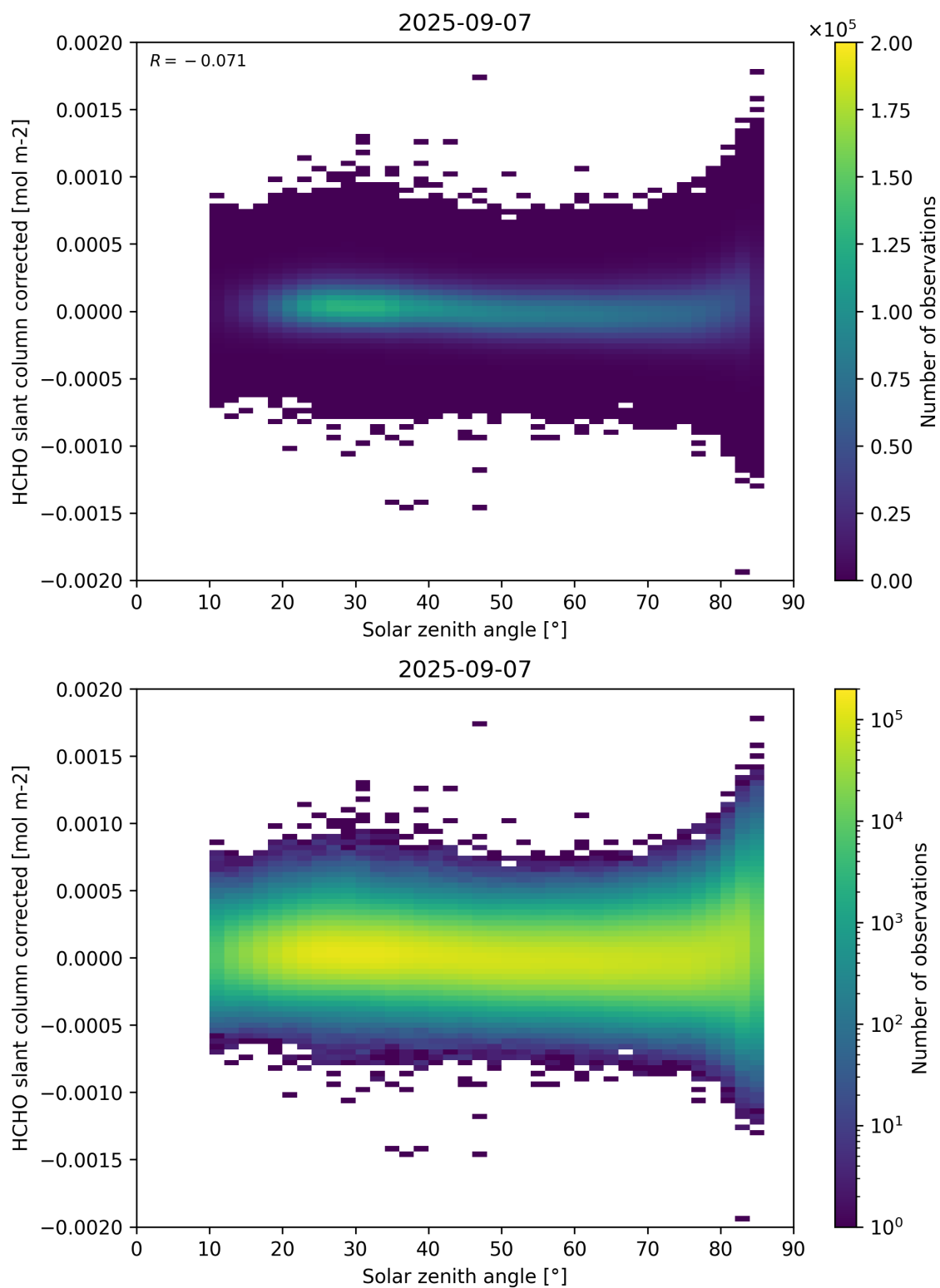
Figure 171: Scatter density plot of “Solar zenith angle” against “HCHO slant column corrected” for 2025-09-06 to 2025-09-08.
