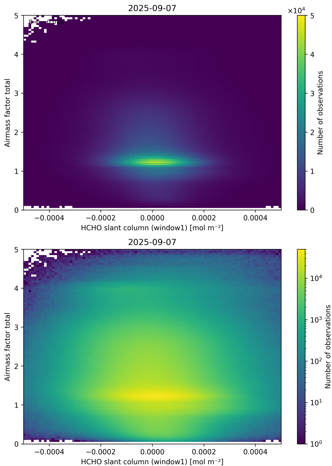
Figure 85: Scatter density plot of “HCHO slant column (window1)” against “Airmass factor total” for 2025-09-06 to 2025-09-08.
