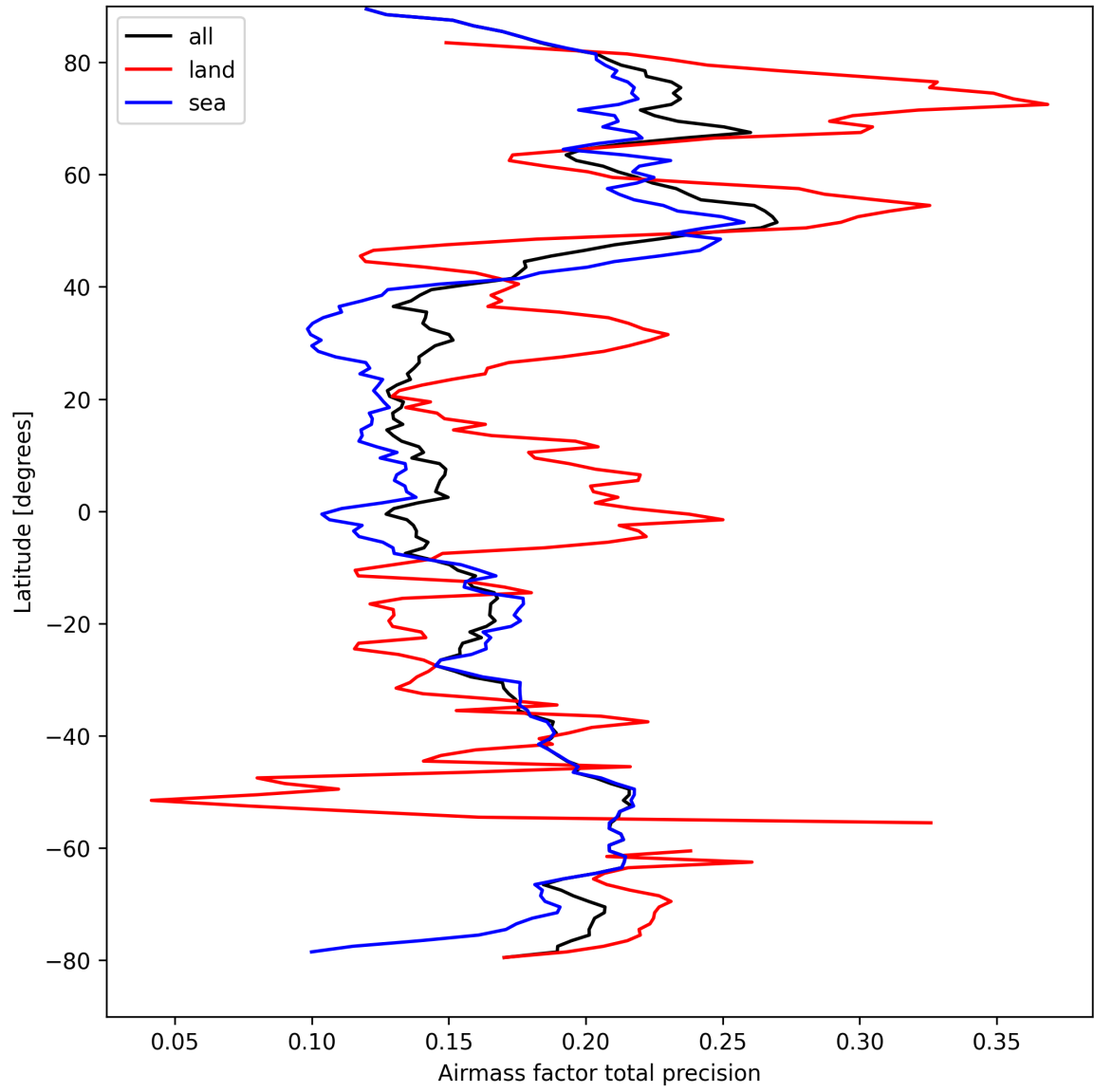
Figure 27: Zonal average of “Airmass factor total precision” for 2025-09-06 to 2025-09-08.
