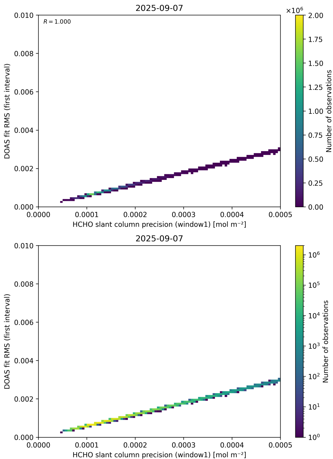
Figure 88: Scatter density plot of “HCHO slant column precision (window1)” against “DOAS fit RMS (first interval)” for 2025-09-06 to 2025-09-08.
