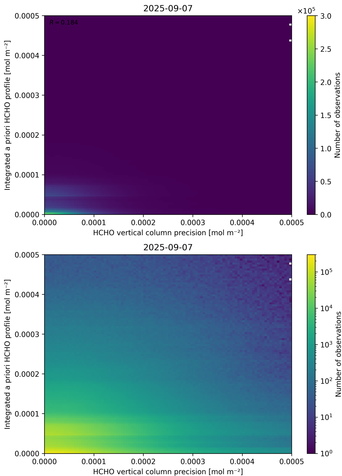
Figure 147: Scatter density plot of “HCHO vertical column precision” against “Integrated a priori HCHO profile” for 2025-09-06 to 2025-09-08.
