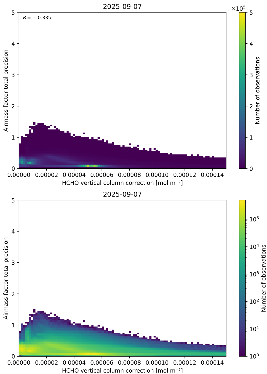
Figure 121: Scatter density plot of “HCHO vertical column correction” against “Airmass factor total precision” for 2025-09-06 to 2025-09-08.
