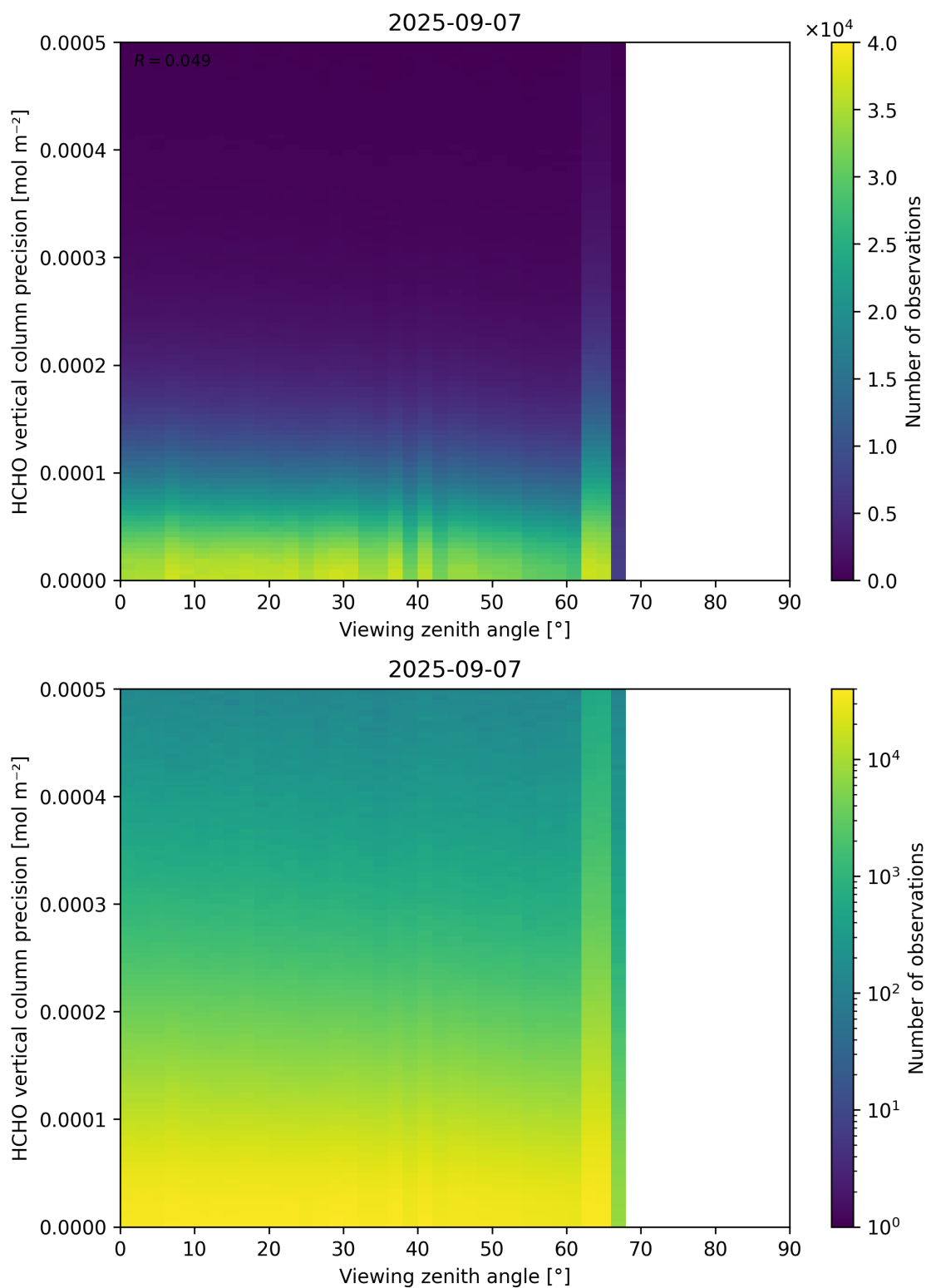
Figure 194: Scatter density plot of “Viewing zenith angle” against “HCHO vertical column precision” for 2025-09-06 to 2025-09-08.
