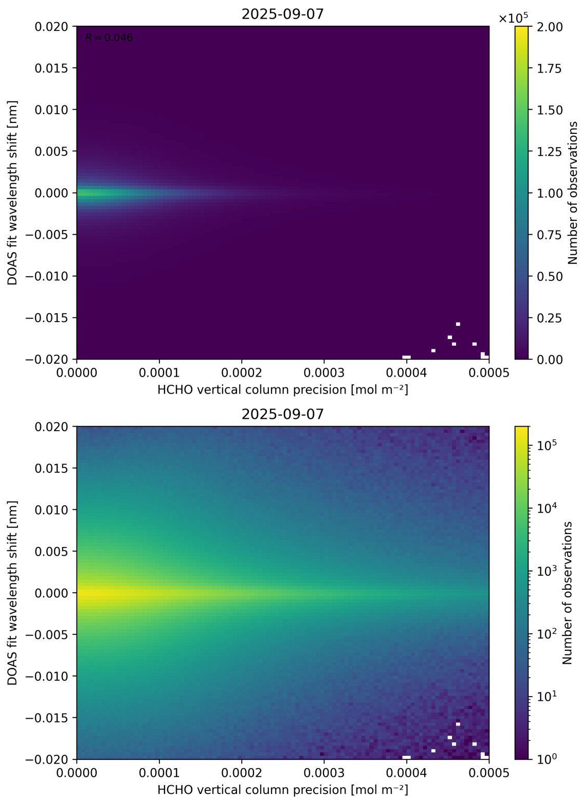
Figure 137: Scatter density plot of “HCHO vertical column precision” against “DOAS fit wavelength shift” for 2025-09-06 to 2025-09-08.
