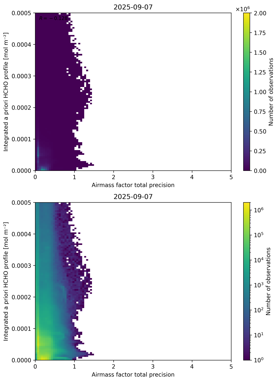
Figure 111: Scatter density plot of “Airmass factor total precision” against “Integrated a priori HCHO profile” for 2025-09-06 to 2025-09-08.
