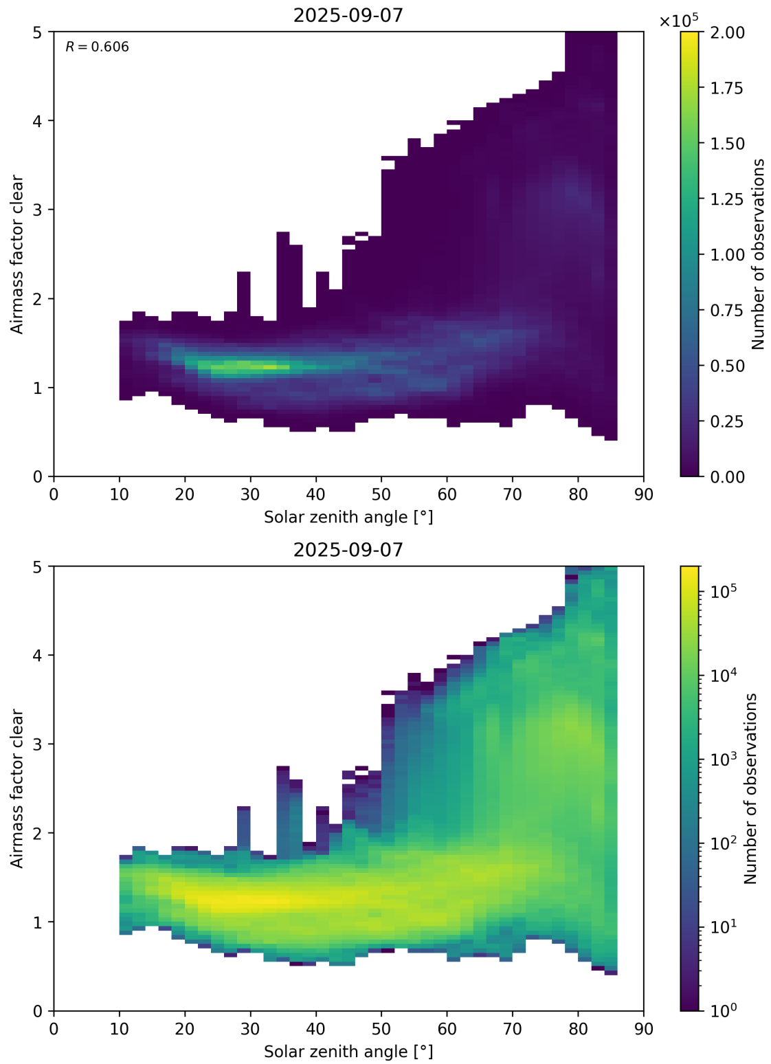
Figure 170: Scatter density plot of “Solar zenith angle” against “Airmass factor clear” for 2025-09-06 to 2025-09-08.
