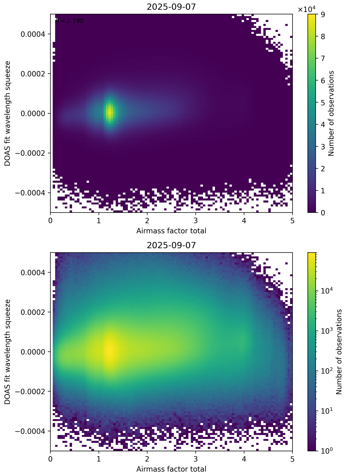
Figure 99: Scatter density plot of “Airmass factor total” against “DOAS fit wavelength squeeze” for 2025-09-06 to 2025-09-08.
