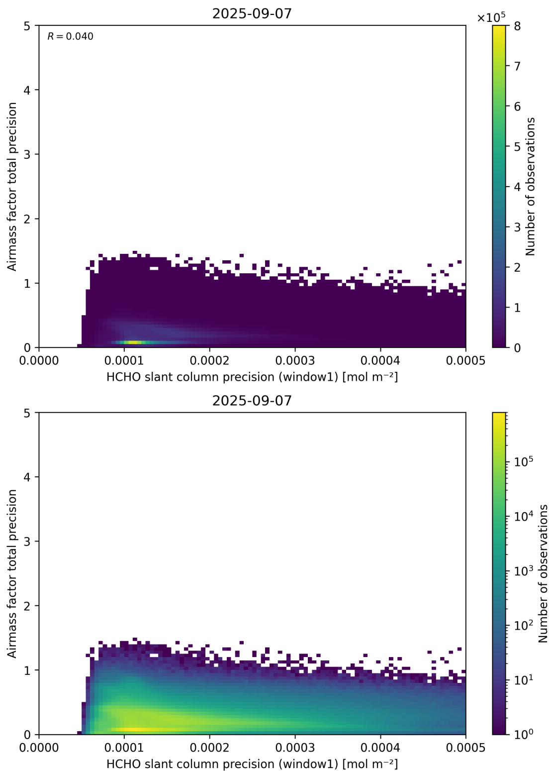
Figure 95: Scatter density plot of “HCHO slant column precision (window1)” against “Airmass factor total precision” for 2025-09-06 to 2025-09-08.
