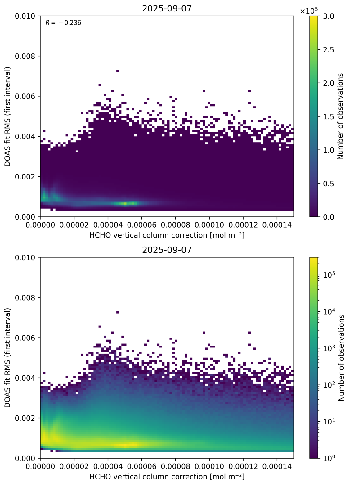
Figure 112: Scatter density plot of “HCHO vertical column correction” against “DOAS fit RMS (first interval)” for 2025-09-06 to 2025-09-08.
