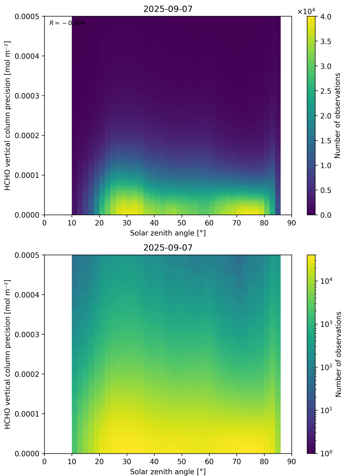
Figure 179: Scatter density plot of “Solar zenith angle” against “HCHO vertical column precision” for 2025-09-06 to 2025-09-08.
