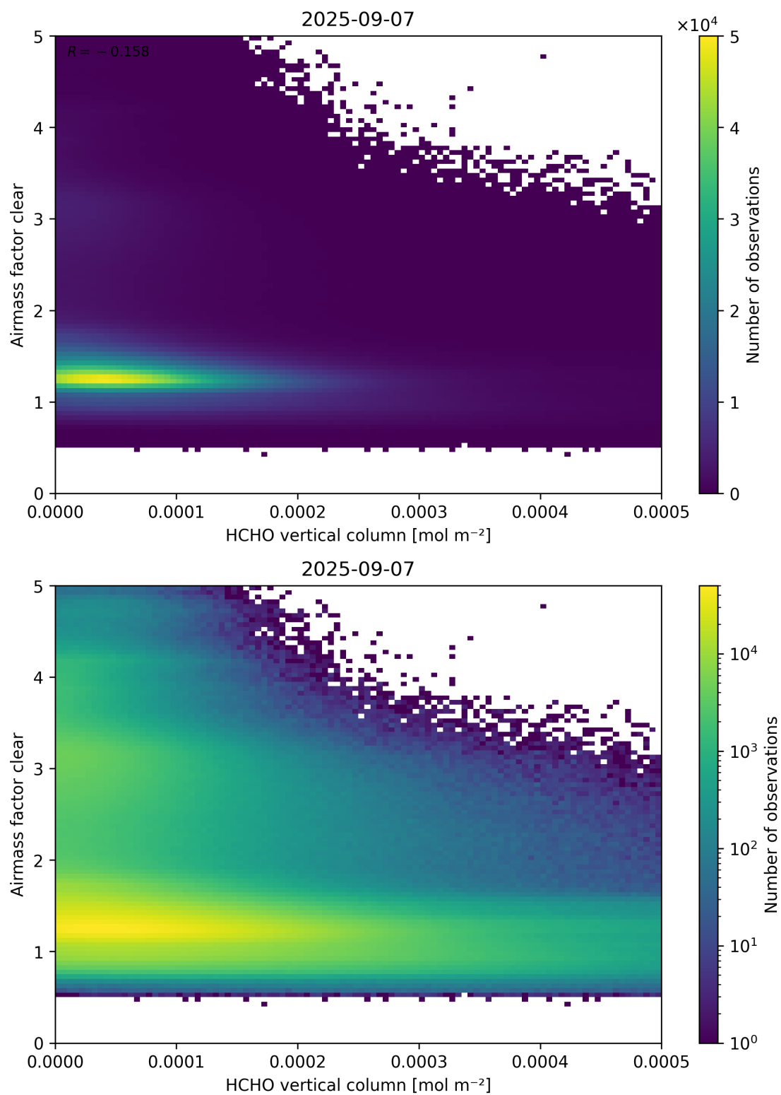
Figure 126: Scatter density plot of “HCHO vertical column” against “Airmass factor clear” for 2025-09-06 to 2025-09-08.
