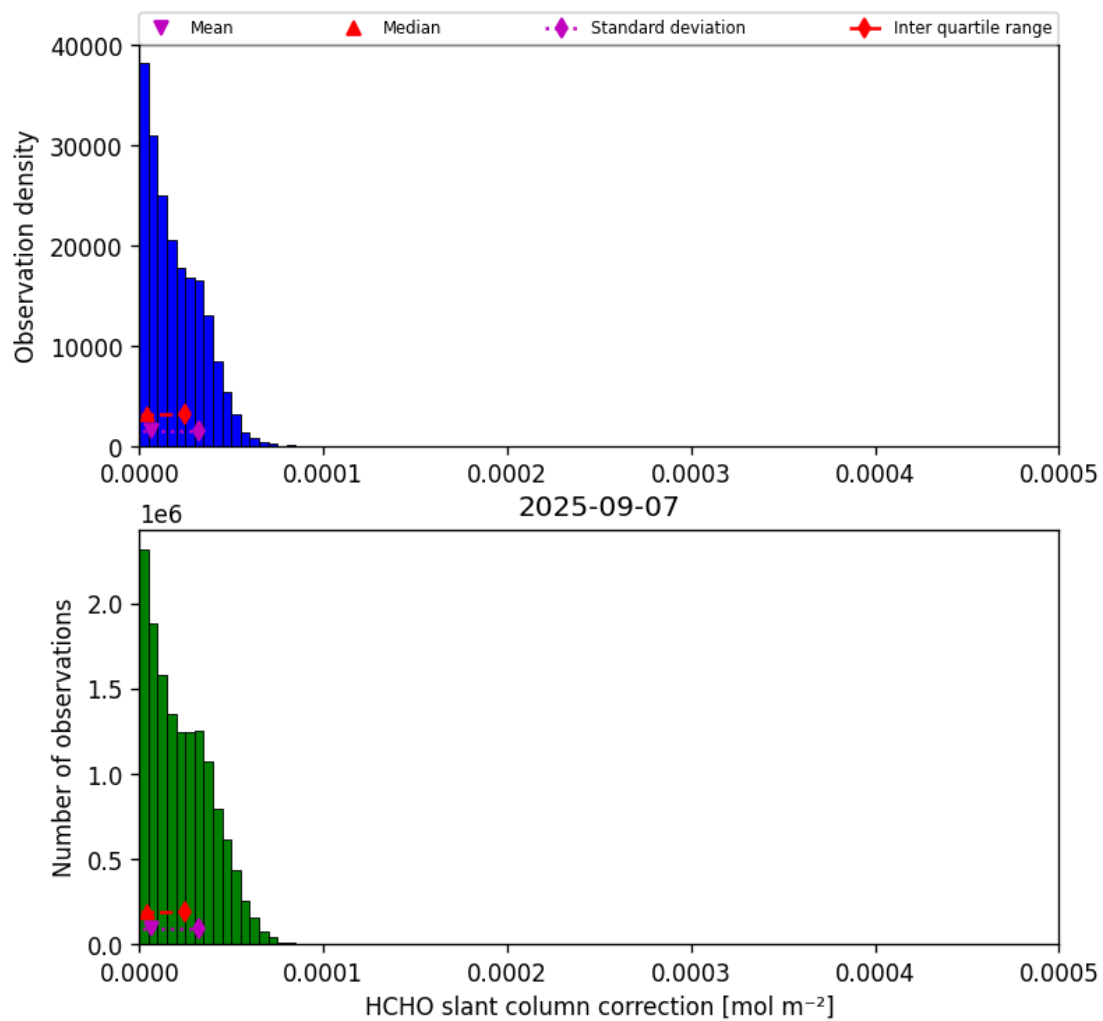
Figure 47: Histogram of “HCHO slant column correction” for 2025-09-06 to 2025-09-08
