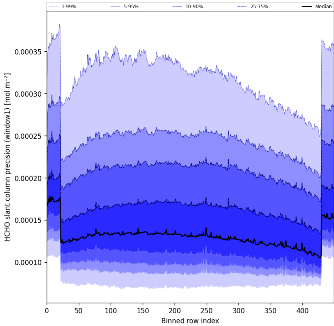
Figure 53: Along track statistics of “HCHO slant column precision (window1)” for 2025-09-06 to 2025-09-08
