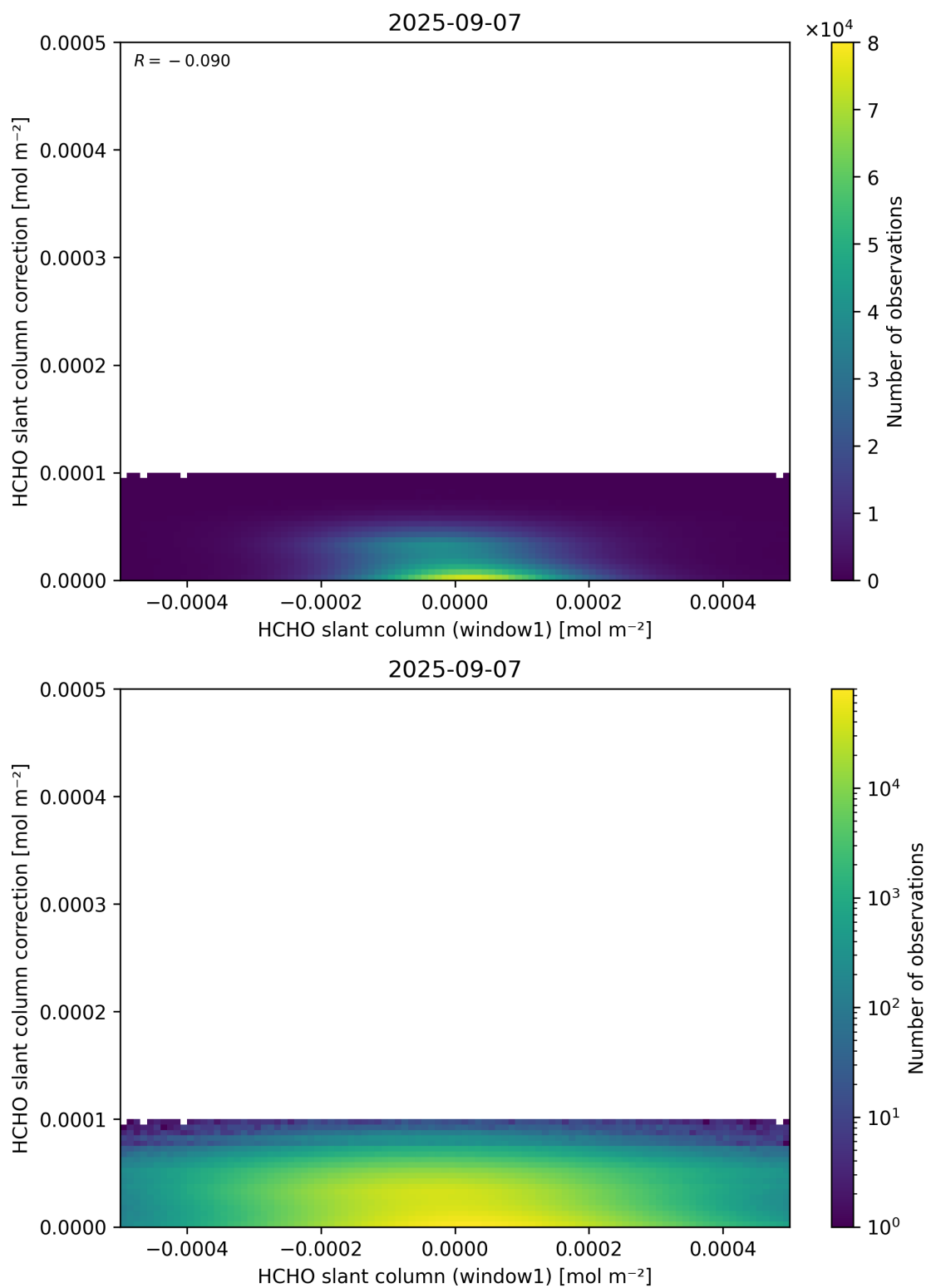
Figure 83: Scatter density plot of “HCHO slant column (window1)” against “HCHO slant column correction” for 2025-09-06 to 2025-09-08.
