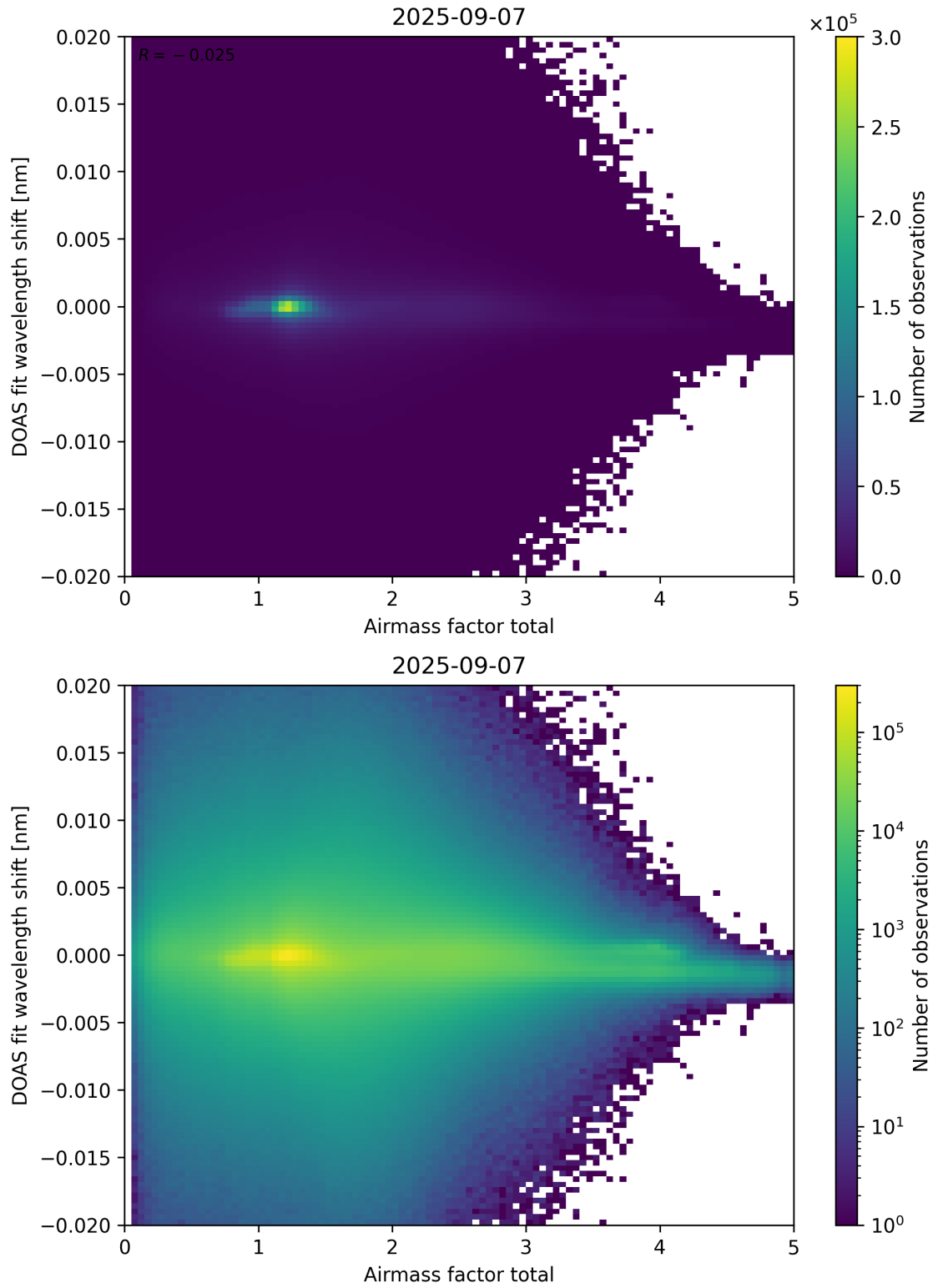
Figure 98: Scatter density plot of “Airmass factor total” against “DOAS fit wavelength shift” for 2025-09-06 to 2025-09-08.
