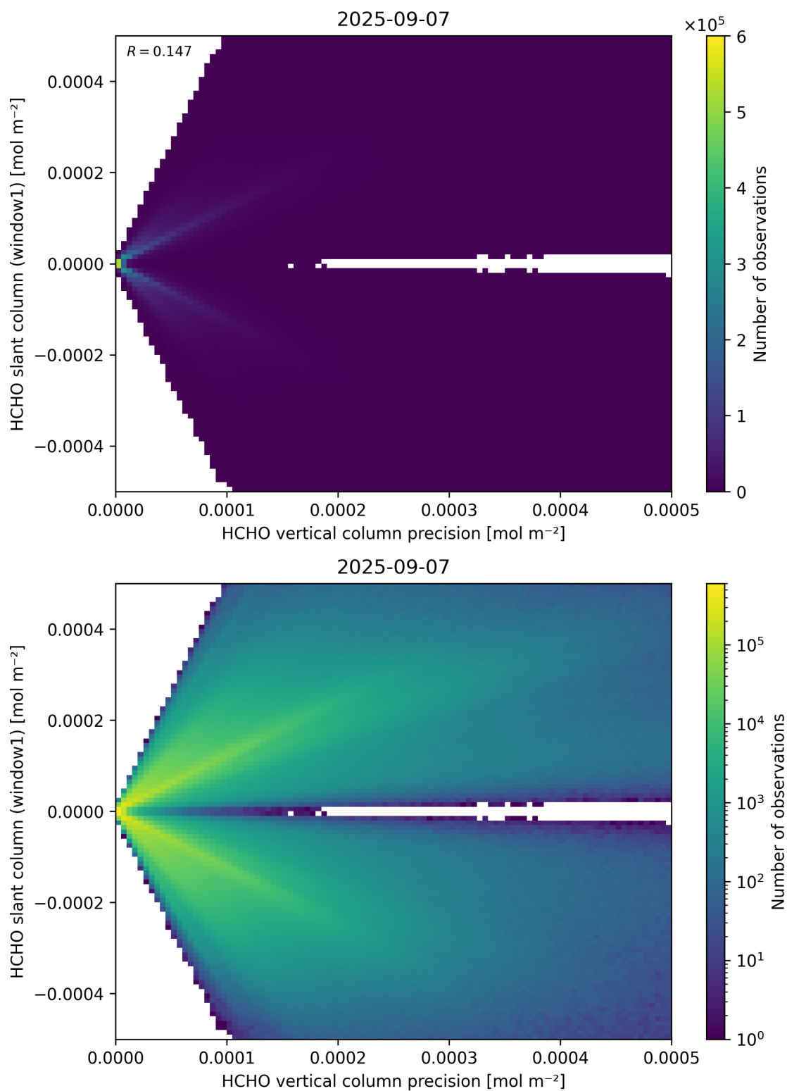
Figure 142: Scatter density plot of “HCHO vertical column precision” against “HCHO slant column (window1)” for 2025-09-06 to 2025-09-08.
