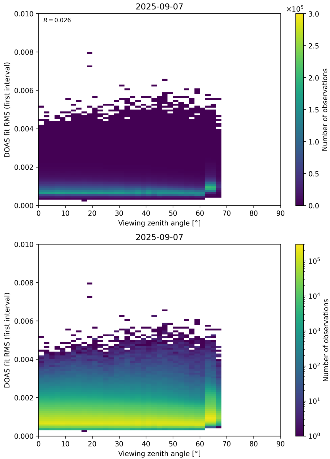
Figure 182: Scatter density plot of “Viewing zenith angle” against “DOAS fit RMS (first interval)” for 2025-09-06 to 2025-09-08.
