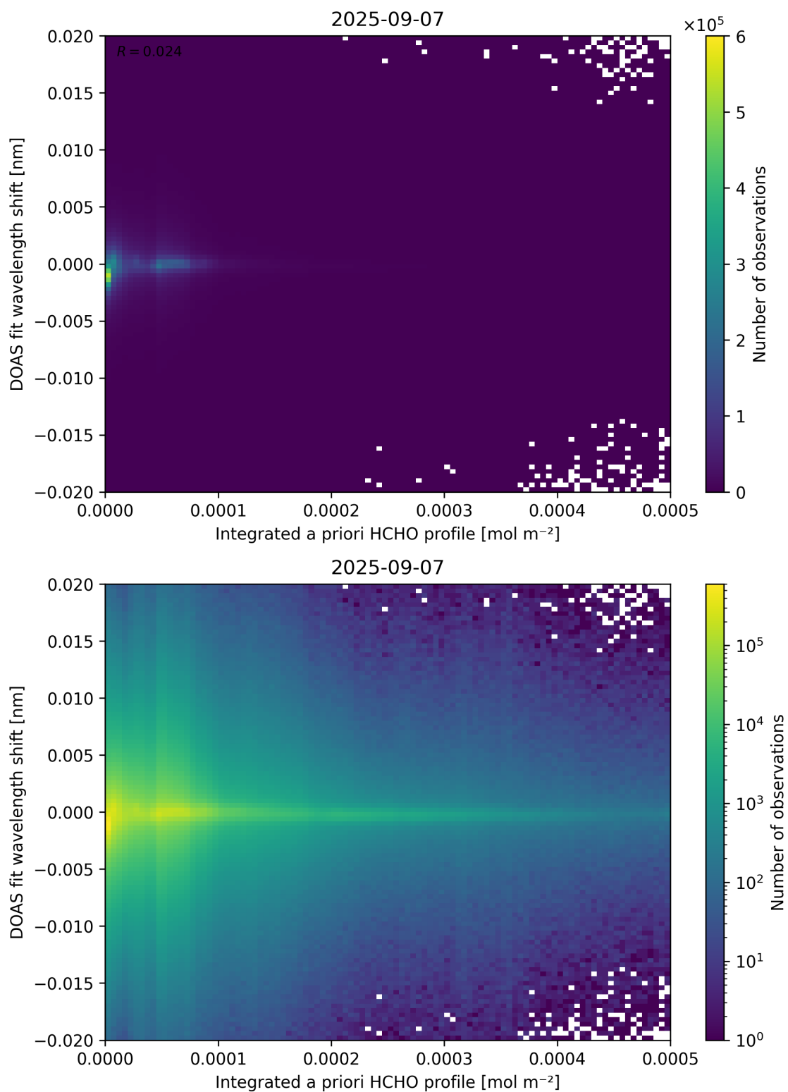
Figure 149: Scatter density plot of “Integrated a priori HCHO profile” against “DOAS fit wavelength shift” for 2025-09-06 to 2025-09-08.
