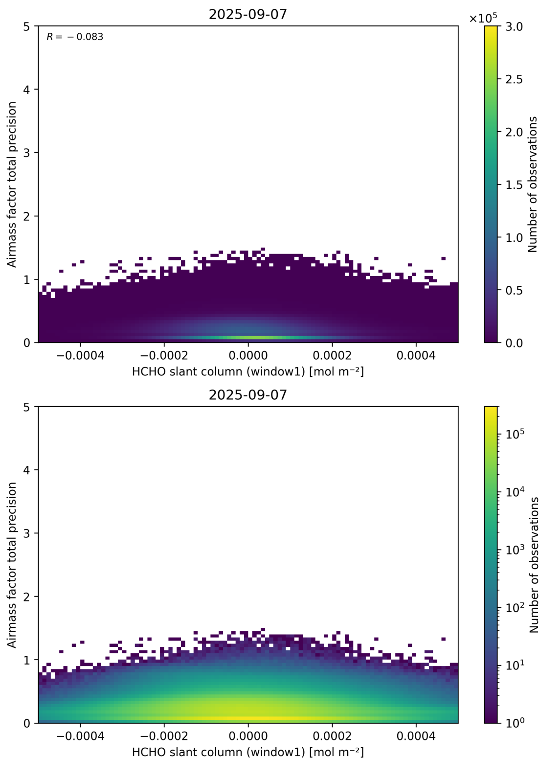
Figure 86: Scatter density plot of “HCHO slant column (window1)” against “Airmass factor total precision” for 2025-09-06 to 2025-09-08.
