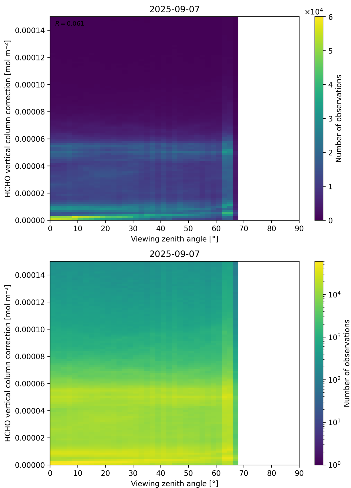
Figure 193: Scatter density plot of “Viewing zenith angle” against “HCHO vertical column correction” for 2025-09-06 to 2025-09-08.
