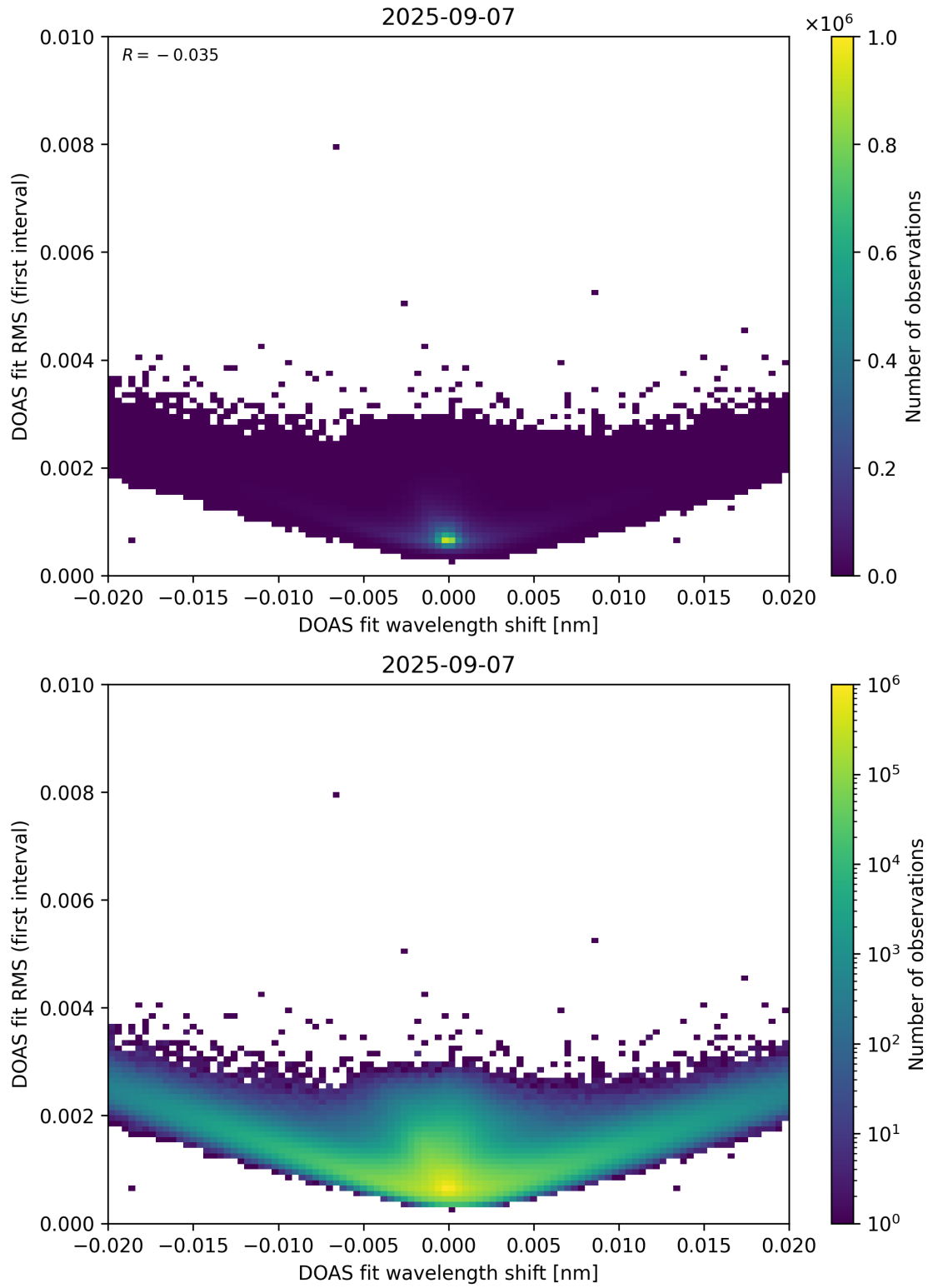
Figure 64: Scatter density plot of “DOAS fit wavelength shift” against “DOAS fit RMS (first interval)” for 2025-09-06 to 2025-09-08.
