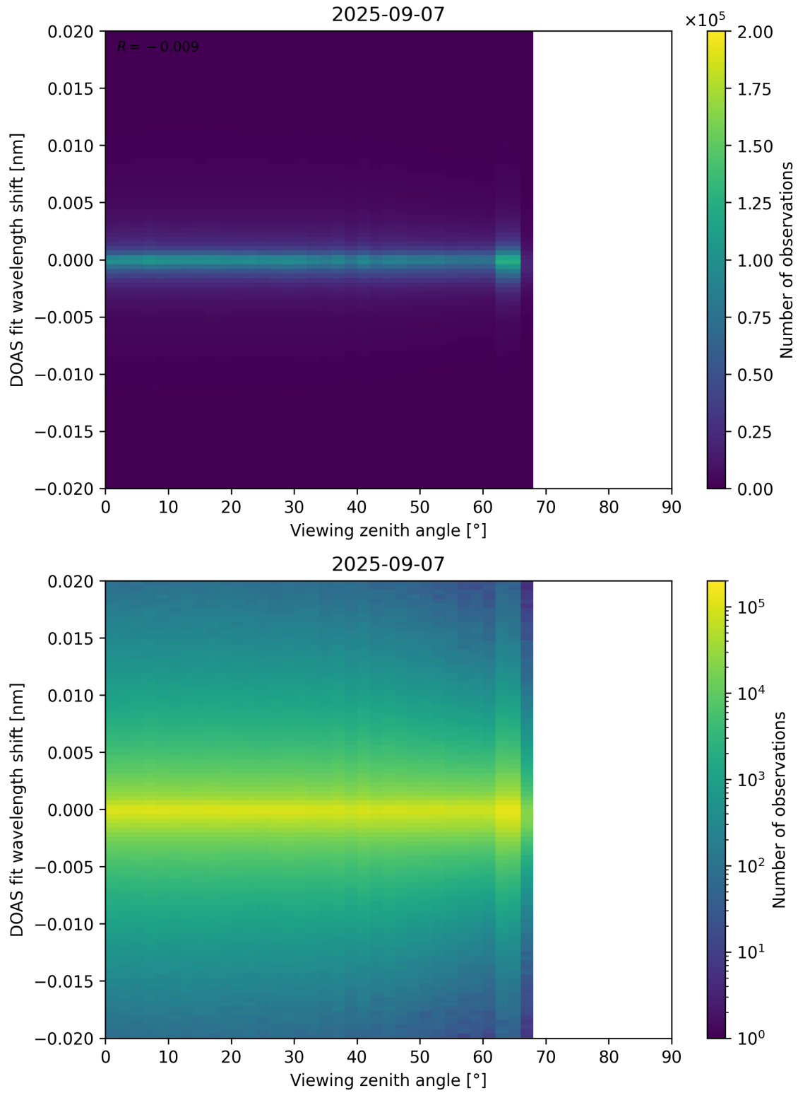
Figure 183: Scatter density plot of “Viewing zenith angle” against “DOAS fit wavelength shift” for 2025-09-06 to 2025-09-08.
