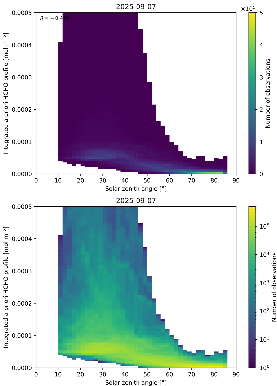
Figure 180: Scatter density plot of “Solar zenith angle” against “Integrated a priori HCHO profile” for 2025-09-06 to 2025-09-08.
