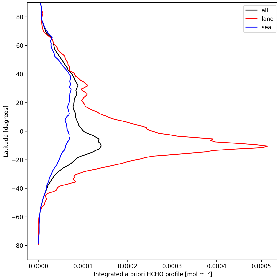
Figure 29: Zonal average of “Integrated a priori HCHO profile” for 2025-09-06 to 2025-09-08.
