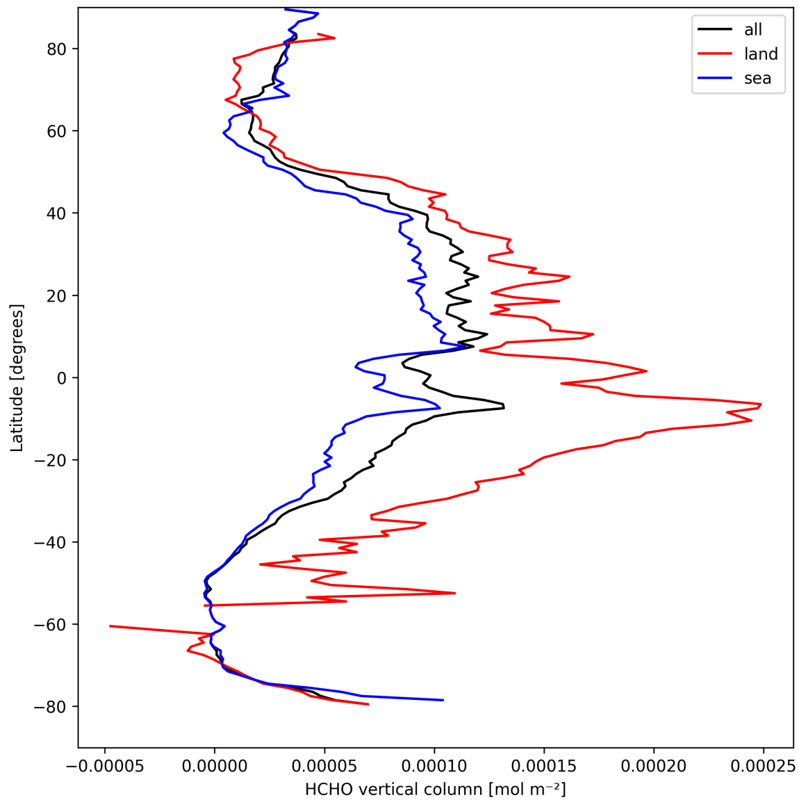
Figure 21: Zonal average of “HCHO vertical column” for 2025-09-06 to 2025-09-08.
