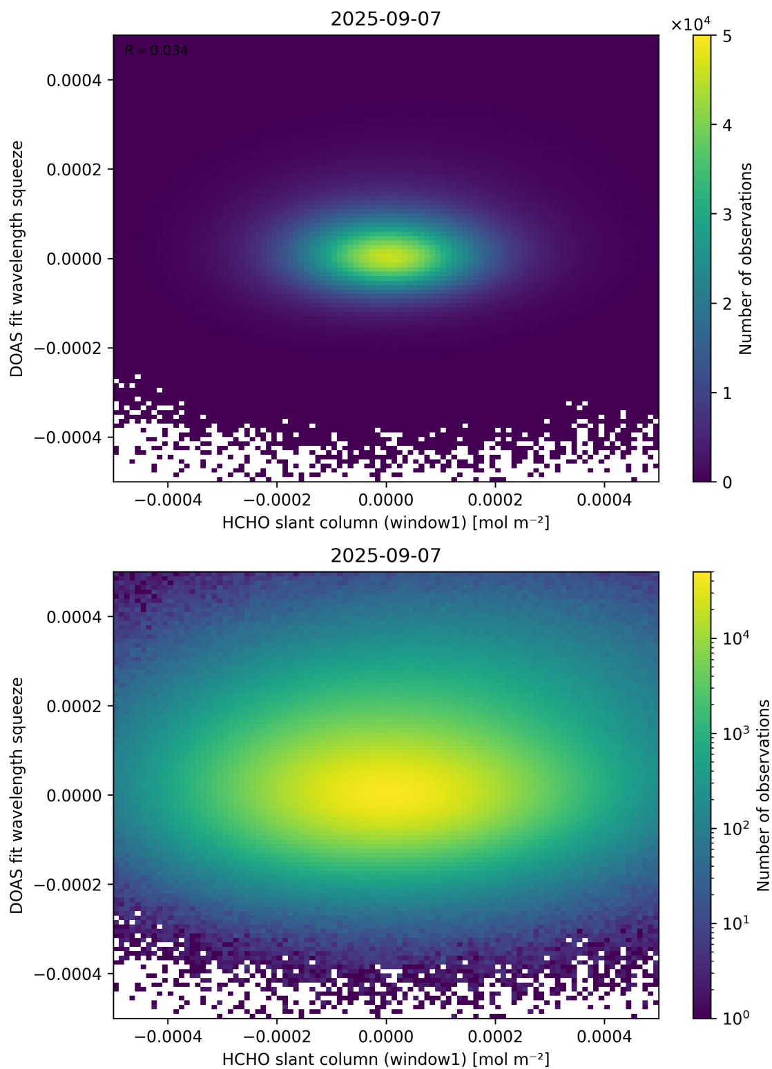
Figure 80: Scatter density plot of “HCHO slant column (window1)” against “DOAS fit wavelength squeeze” for 2025-09-06 to 2025-09-08.
