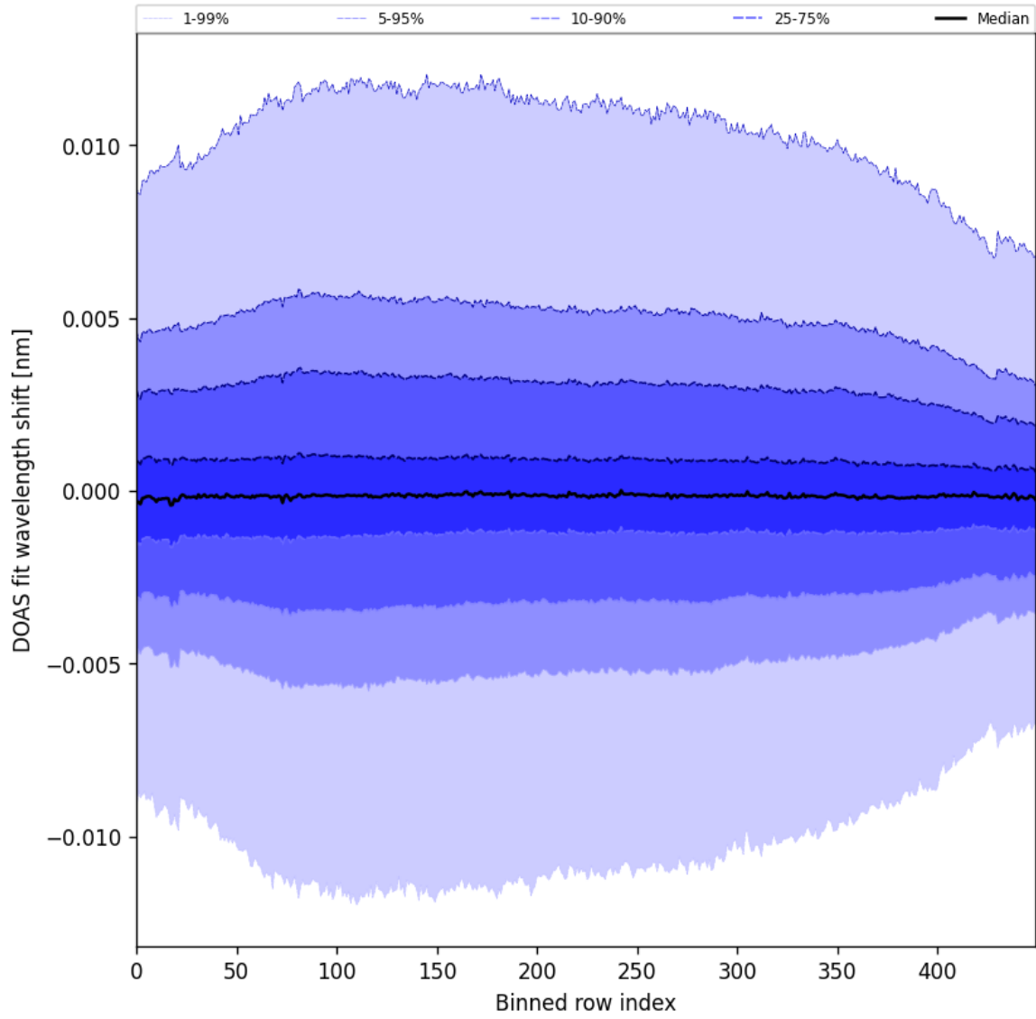
Figure 58: Along track statistics of “DOAS fit wavelength shift” for 2025-09-06 to 2025-09-08
