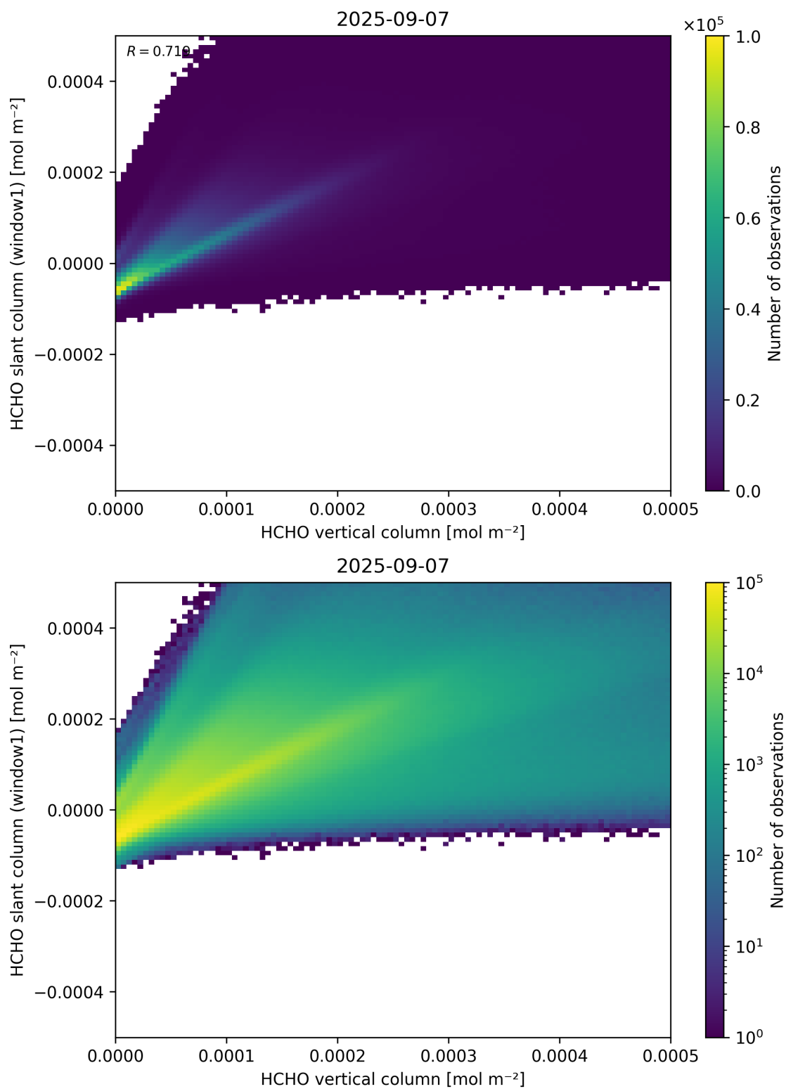
Figure 129: Scatter density plot of “HCHO vertical column” against “HCHO slant column (window1)” for 2025-09-06 to 2025-09-08.
