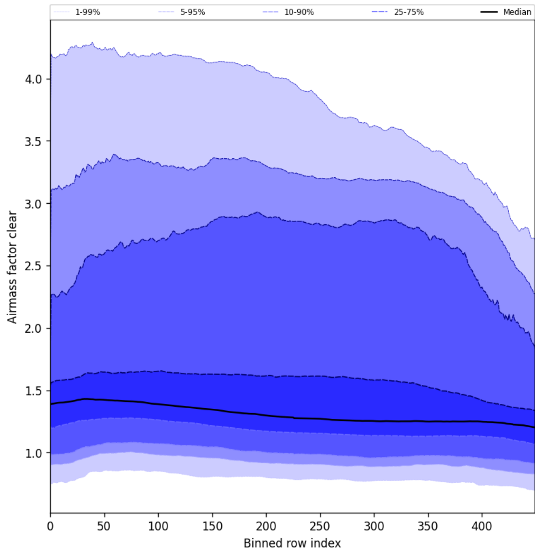
Figure 56: Along track statistics of “Air mass factor clear” for 2025-09-06 to 2025-09-08
