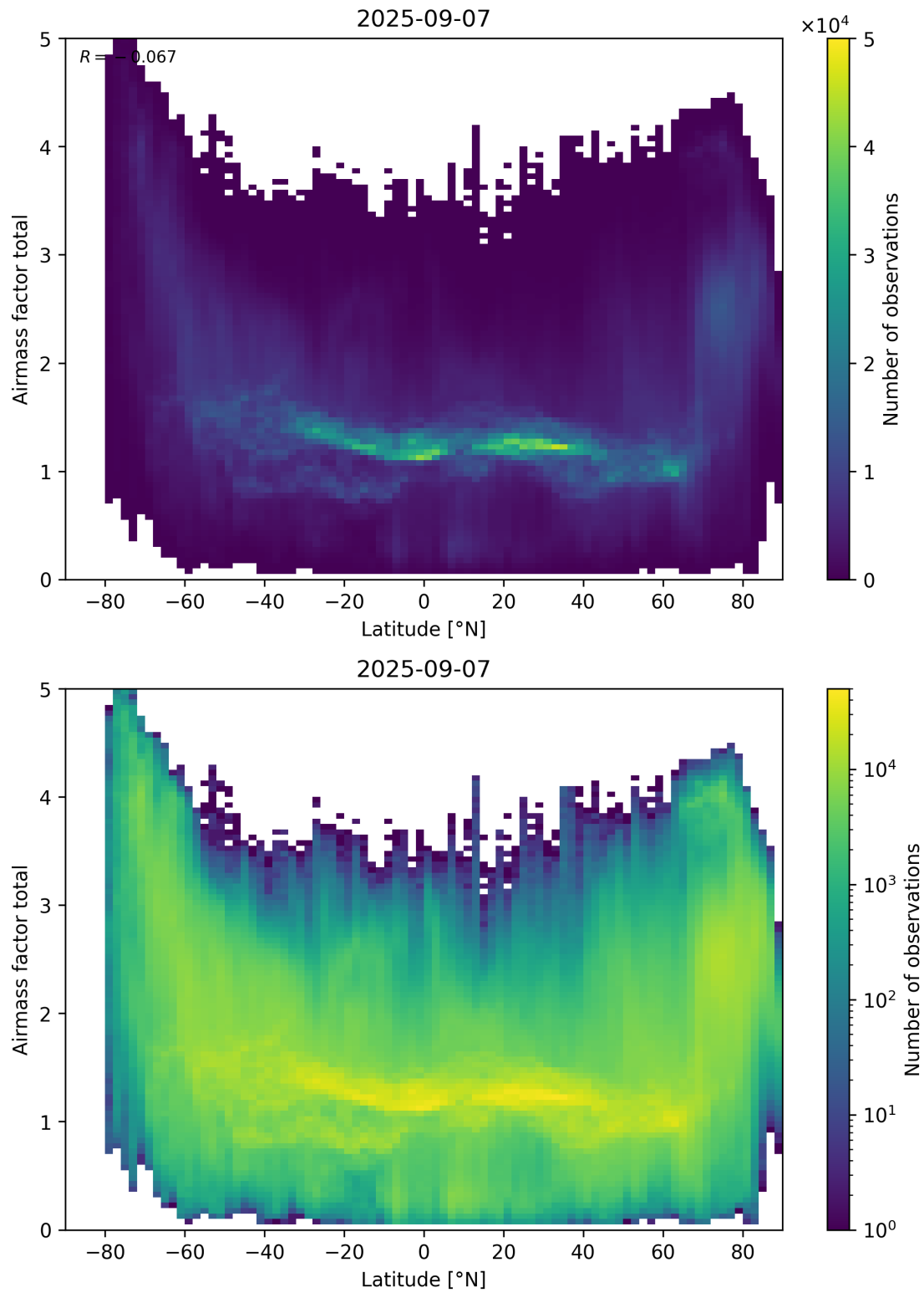
Figure 161: Scatter density plot of “Latitude” against “Airmass factor total” for 2025-09-06 to 2025-09-08.
