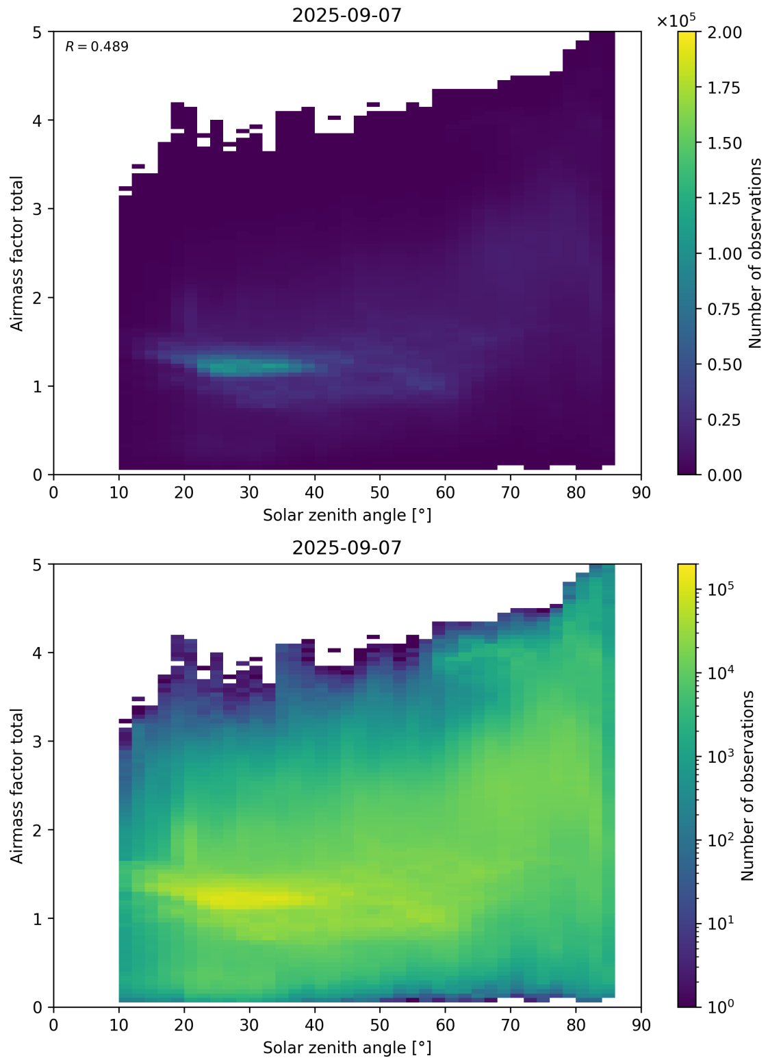
Figure 175: Scatter density plot of “Solar zenith angle” against “Airmass factor total” for 2025-09-06 to 2025-09-08.
