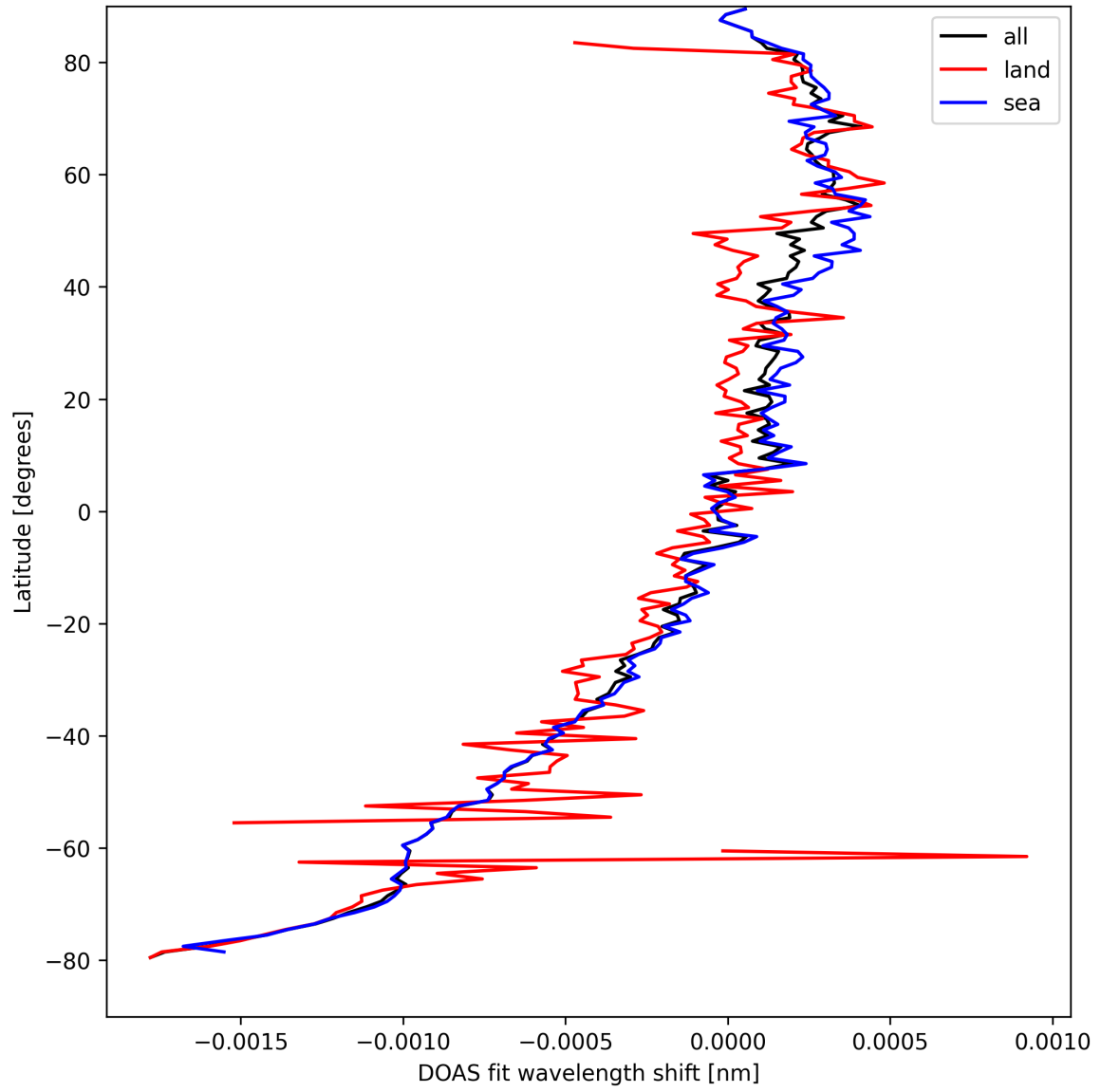
Figure 30: Zonal average of “DOAS fit wavelength shift” for 2025-09-06 to 2025-09-08.
