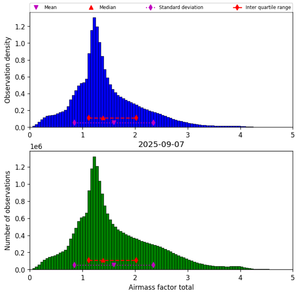
Figure 40: Histogram of “Airmass factor total” for 2025-09-06 to 2025-09-08
