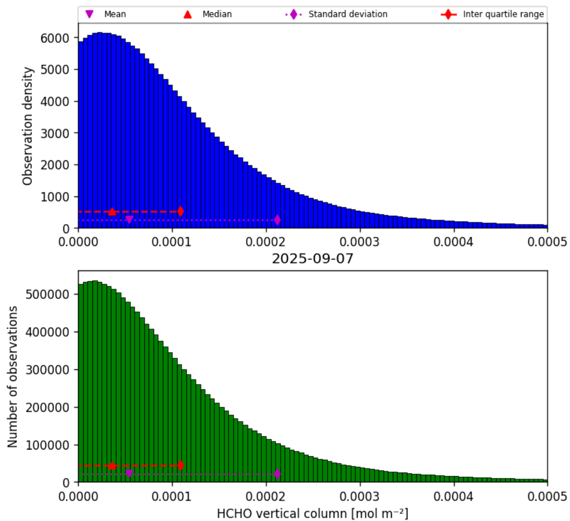
Figure 35: Histogram of “HCHO vertical column” for 2025-09-06 to 2025-09-08
