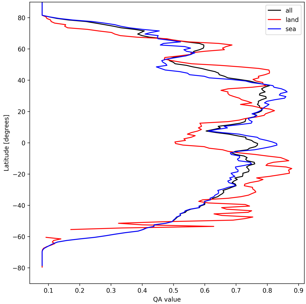
Figure 20: Zonal average of “QA value” for 2025-09-06 to 2025-09-08.
