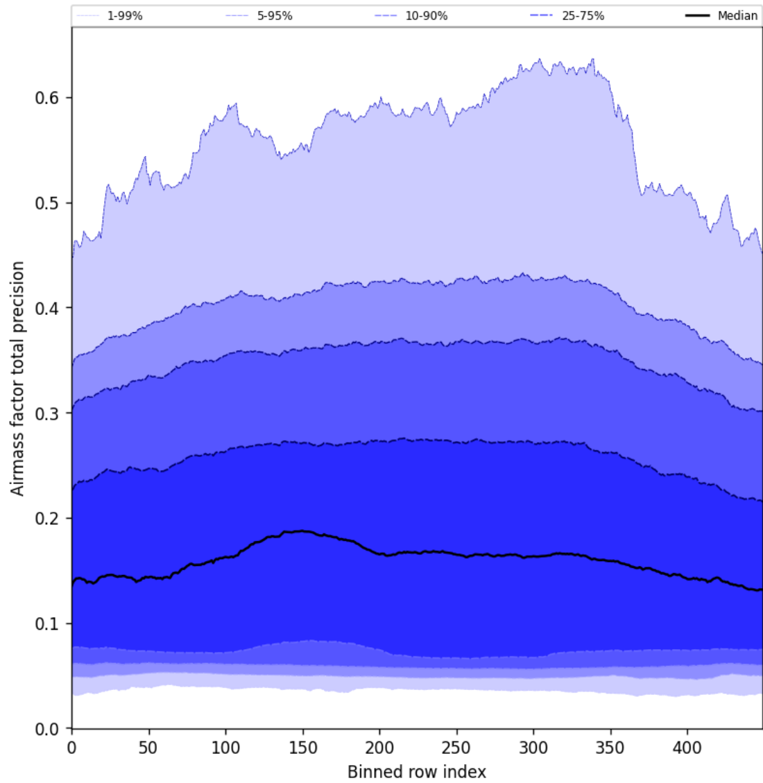
Figure 55: Along track statistics of “Airmass factor total precision” for 2025-09-06 to 2025-09-08
