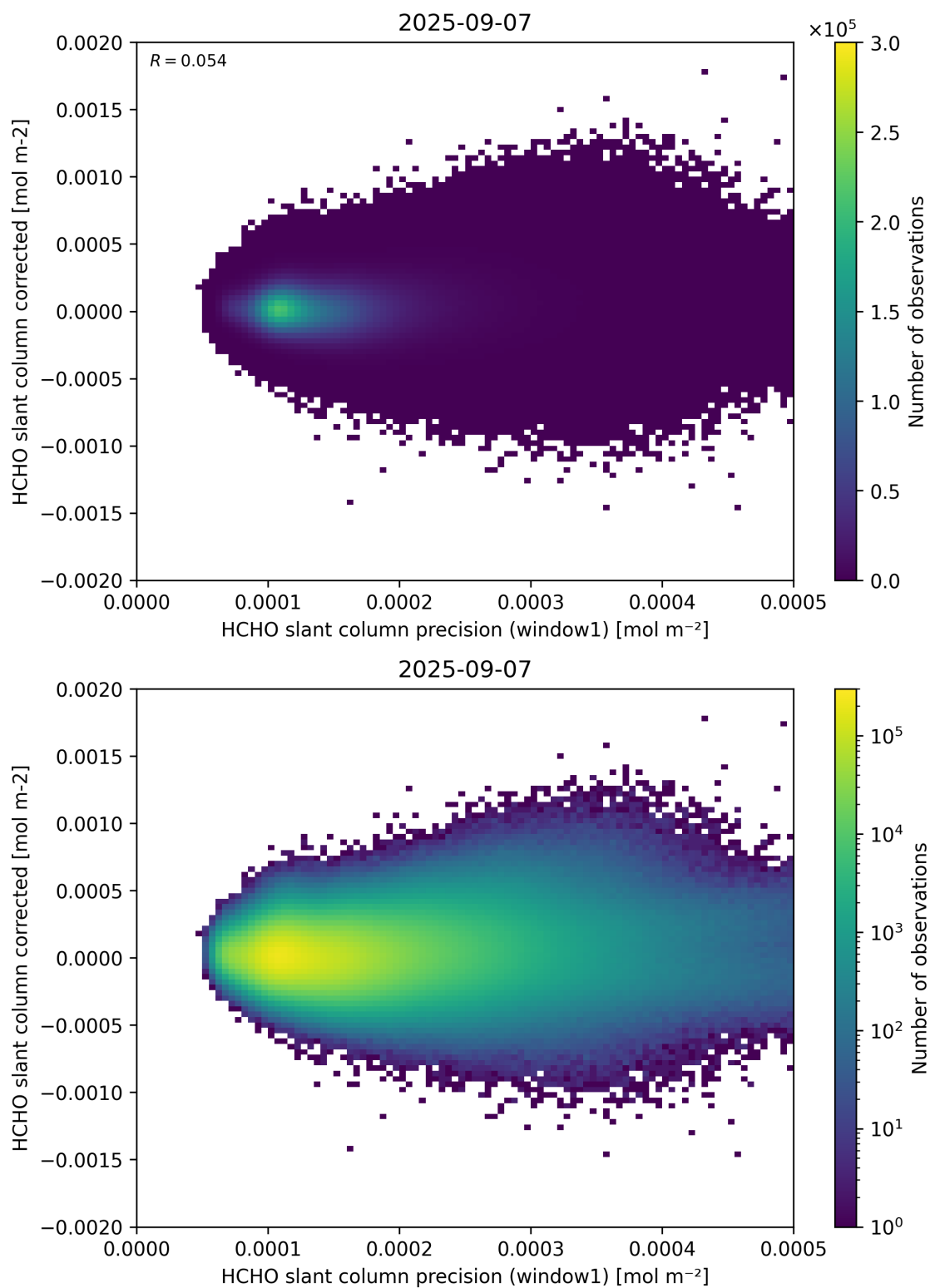
Figure 92: Scatter density plot of “HCHO slant column precision (window1)” against “HCHO slant column corrected” for 2025-09-06 to 2025-09-08.
