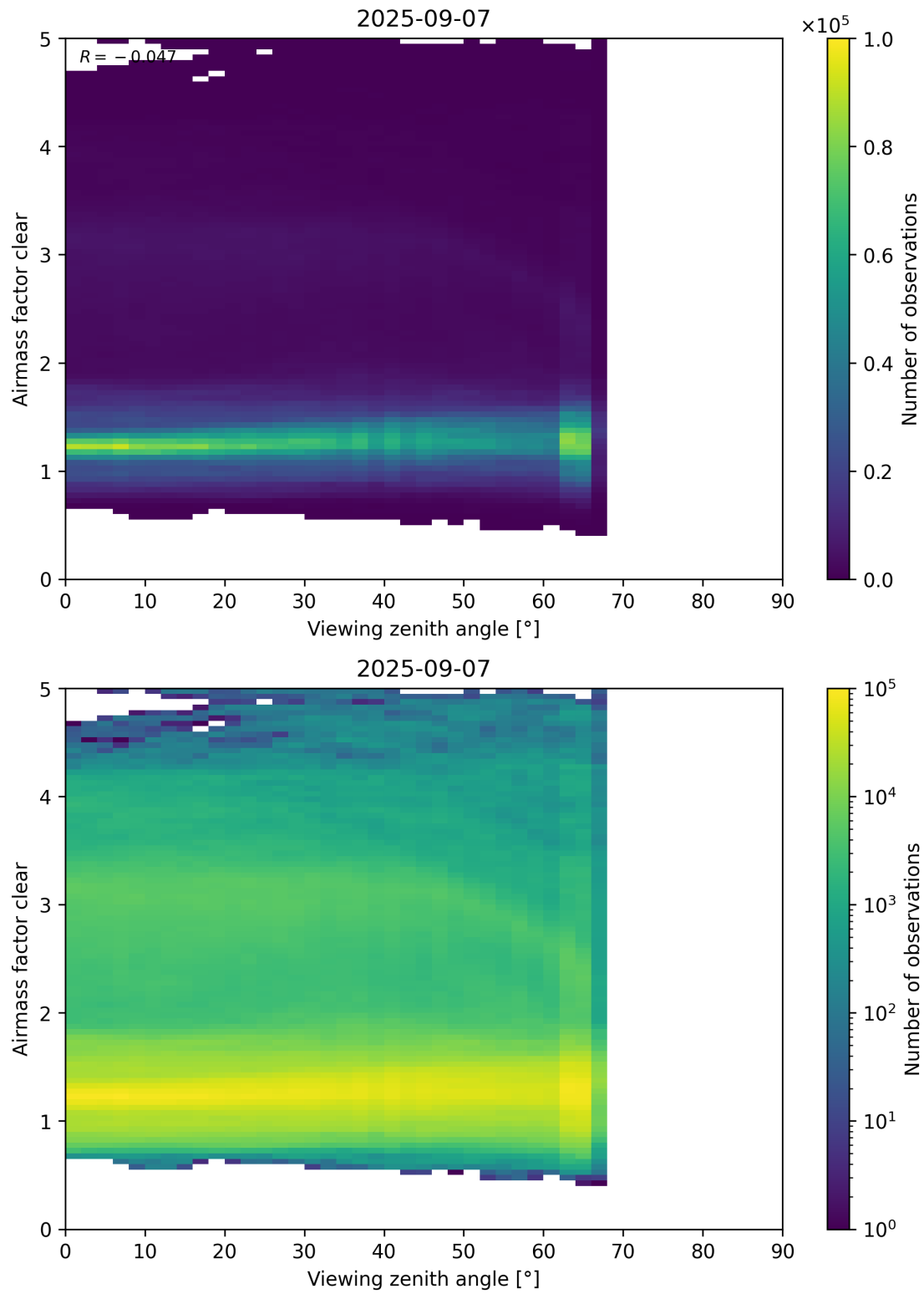
Figure 185: Scatter density plot of “Viewing zenith angle” against “Airmass factor clear” for 2025-09-06 to 2025-09-08.
