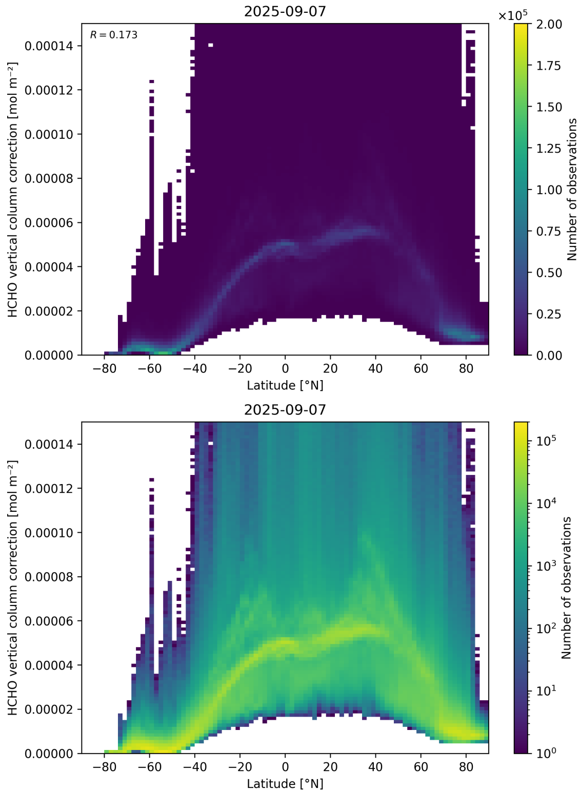
Figure 164: Scatter density plot of “Latitude” against “HCHO vertical column correction” for 2025-09-06 to 2025-09-08.
