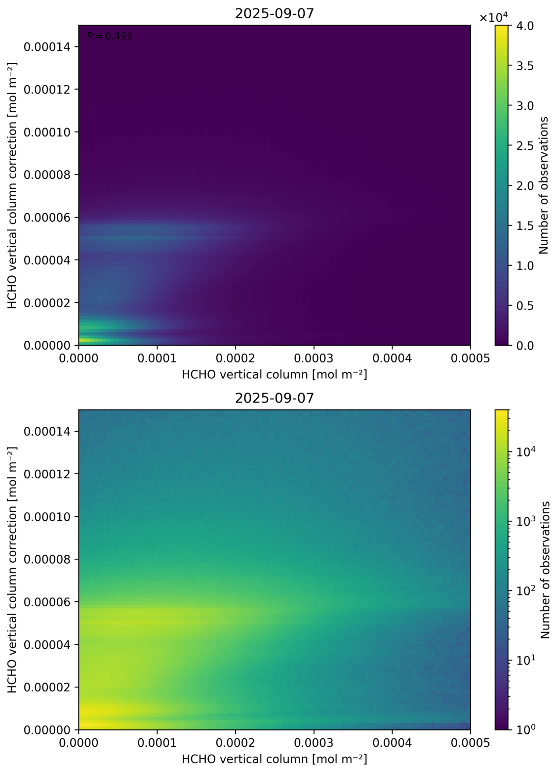
Figure 133: Scatter density plot of “HCHO vertical column” against “HCHO vertical column correction” for 2025-09-06 to 2025-09-08.
