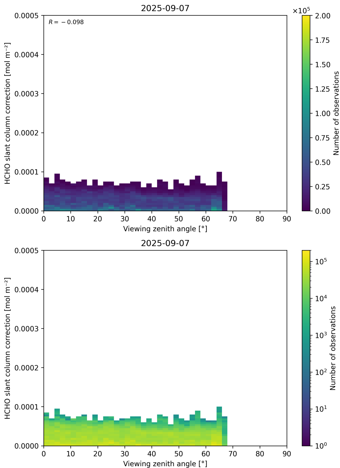
Figure 187: Scatter density plot of “Viewing zenith angle” against “HCHO slant column correction” for 2025-09-06 to 2025-09-08.
