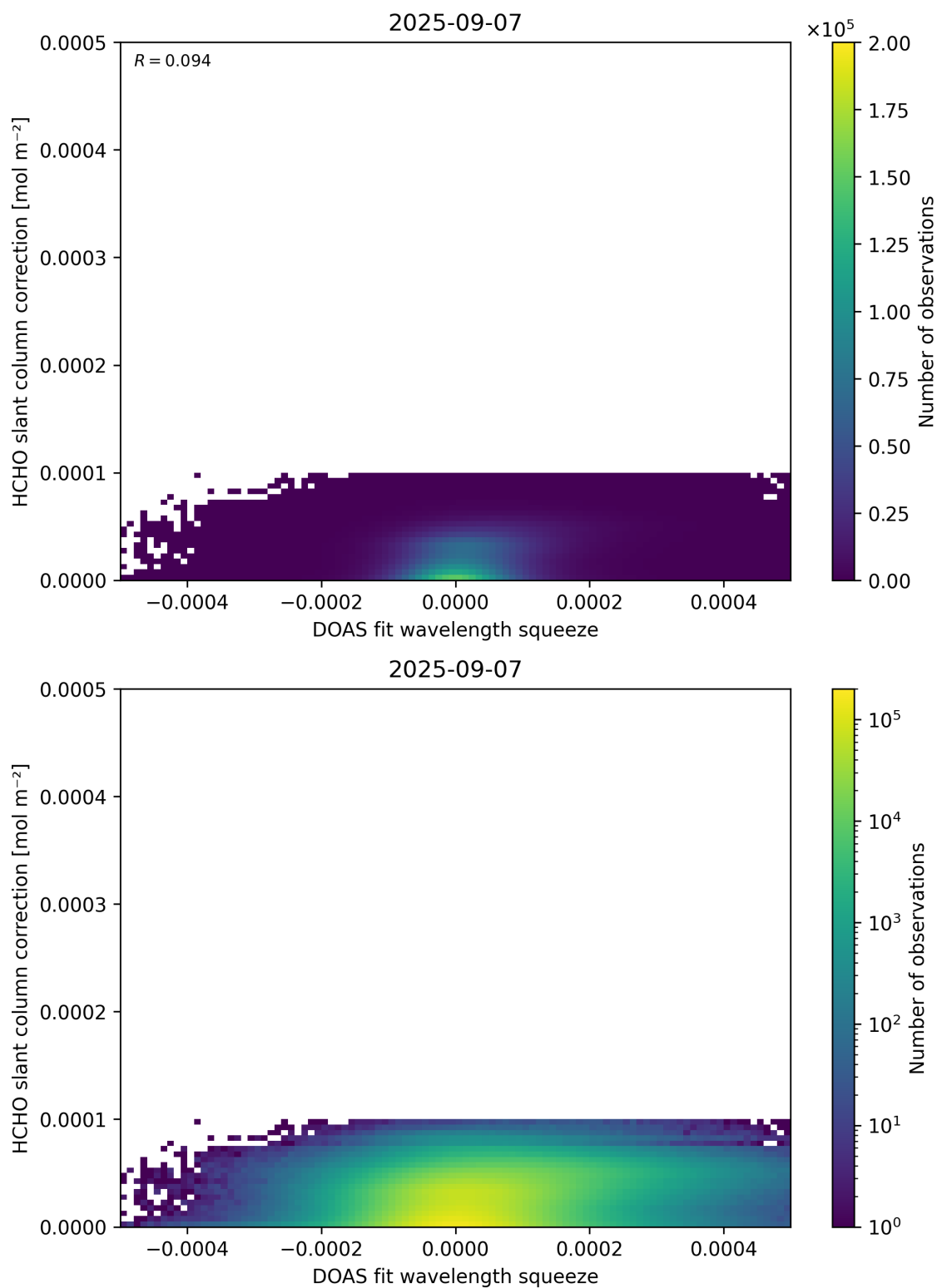
Figure 70: Scatter density plot of “DOAS fit wavelength squeeze” against “HCHO slant column correction” for 2025-09-06 to 2025-09-08.
