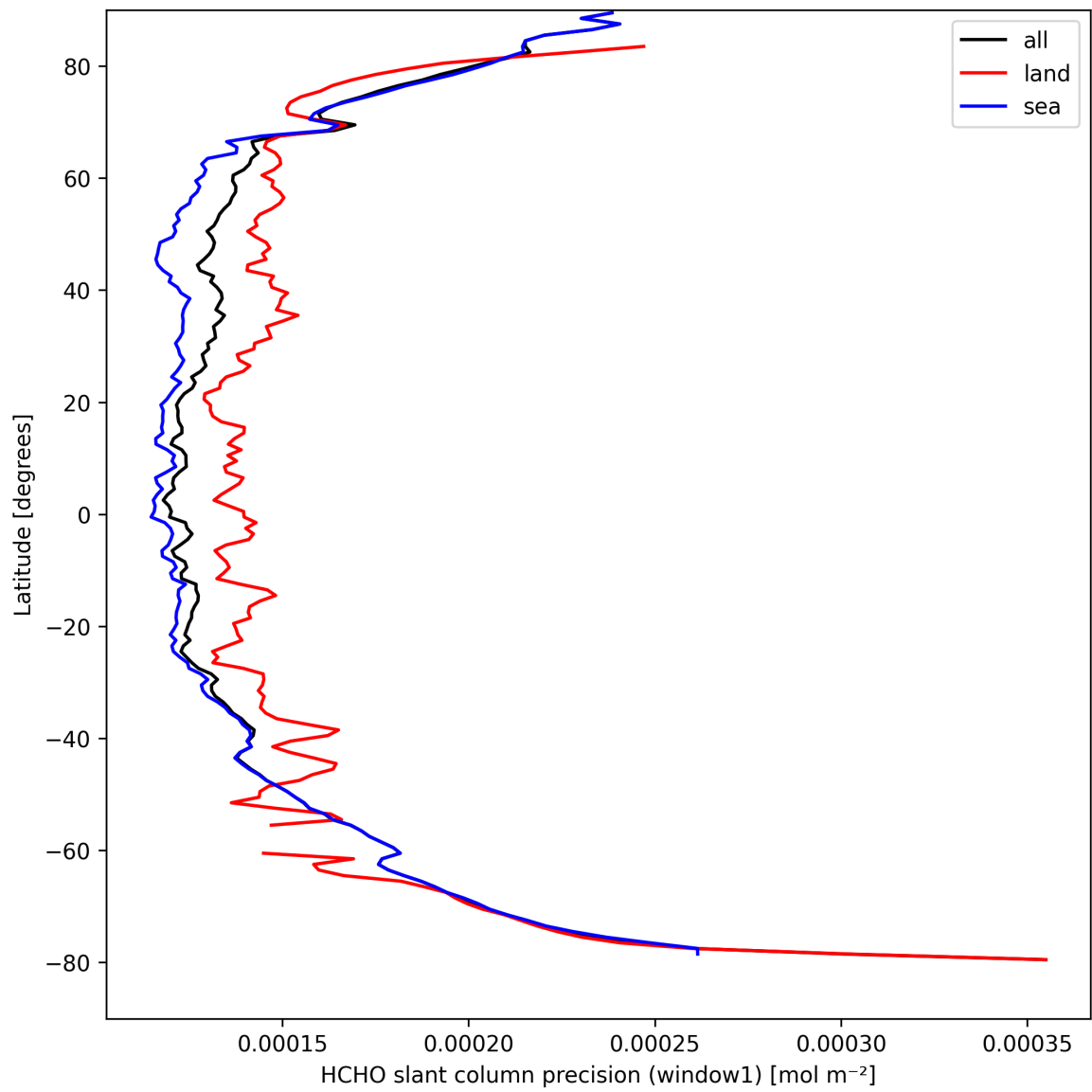
Figure 25: Zonal average of “HCHO slant column precision (window1)” for 2025-09-06 to 2025-09-08.
