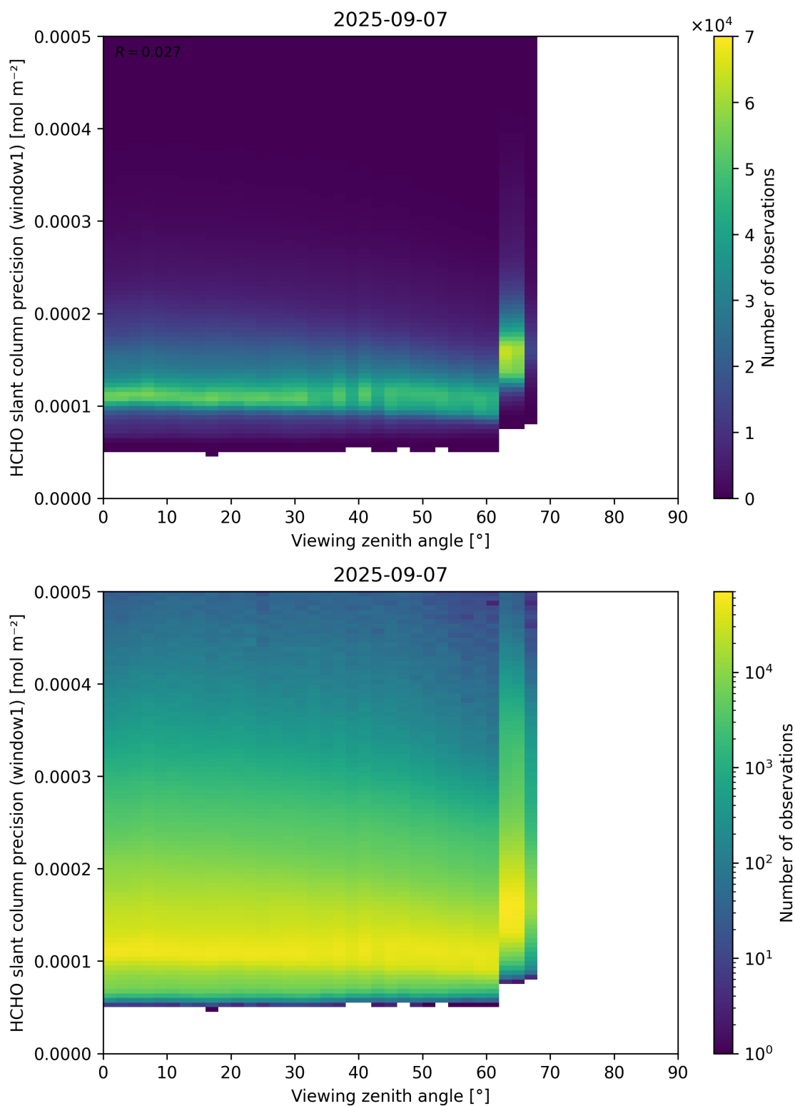
Figure 189: Scatter density plot of “Viewing zenith angle” against “HCHO slant column precision (window1)” for 2025-09-06 to 2025-09-08.
