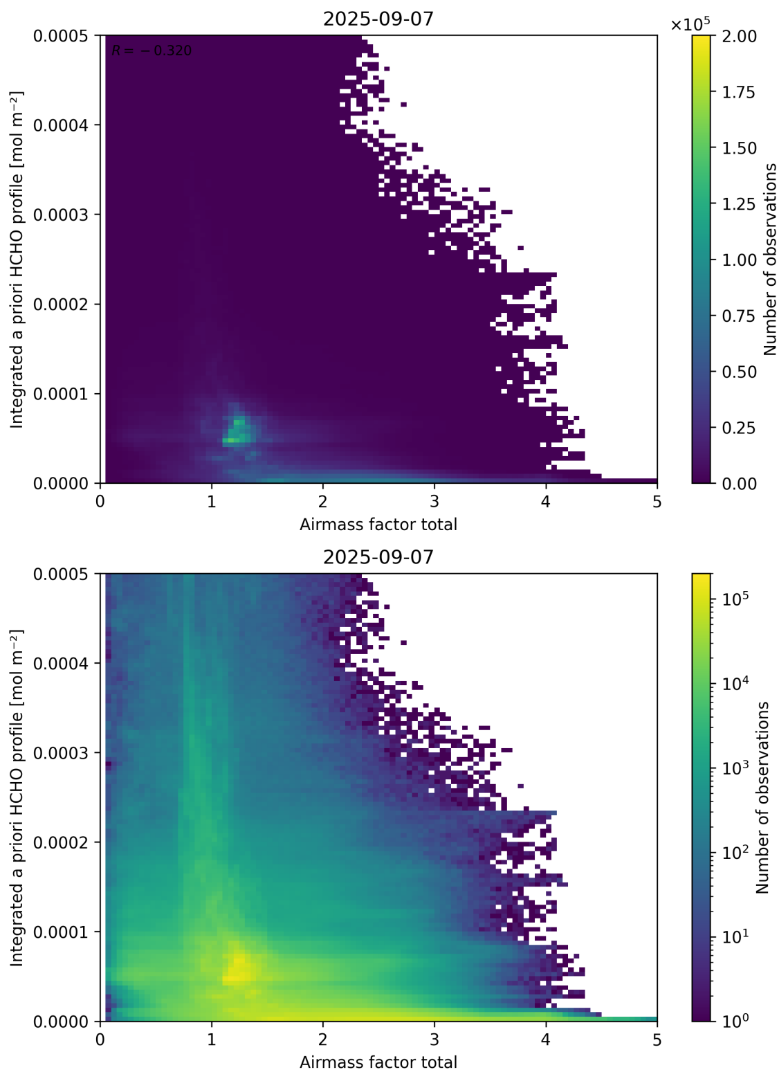
Figure 104: Scatter density plot of “Airmass factor total” against “Integrated a priori HCHO profile” for 2025-09-06 to 2025-09-08.
