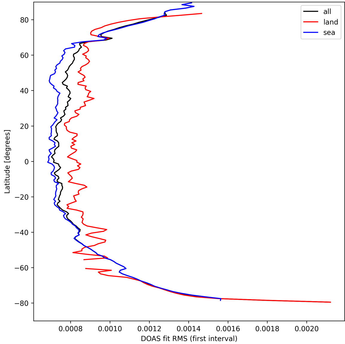
Figure 32: Zonal average of “DOAS fit RMS (first interval)” for 2025-09-06 to 2025-09-08.
