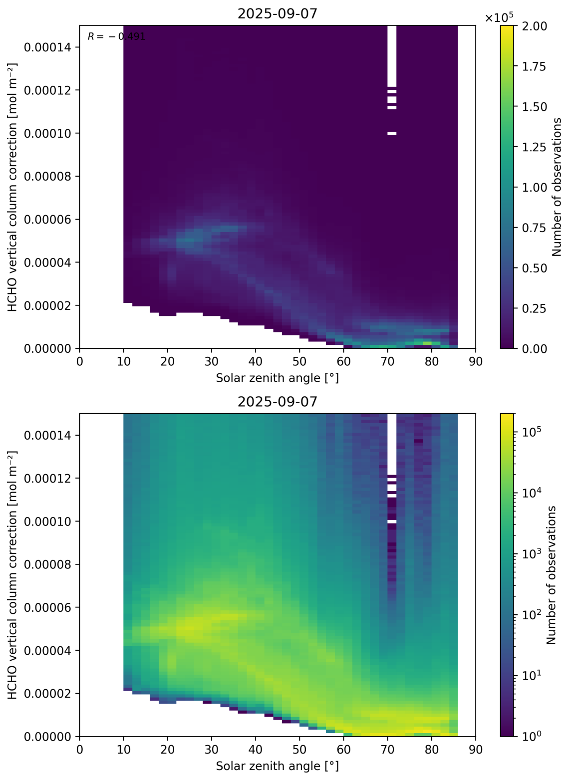
Figure 178: Scatter density plot of “Solar zenith angle” against “HCHO vertical column correction” for 2025-09-06 to 2025-09-08.
