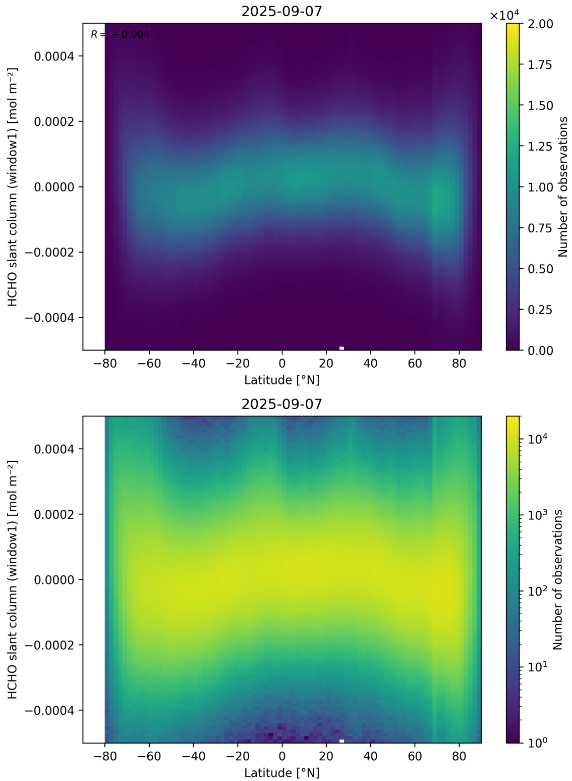
Figure 159: Scatter density plot of “Latitude” against “HCHO slant column (window1)” for 2025-09-06 to 2025-09-08.
