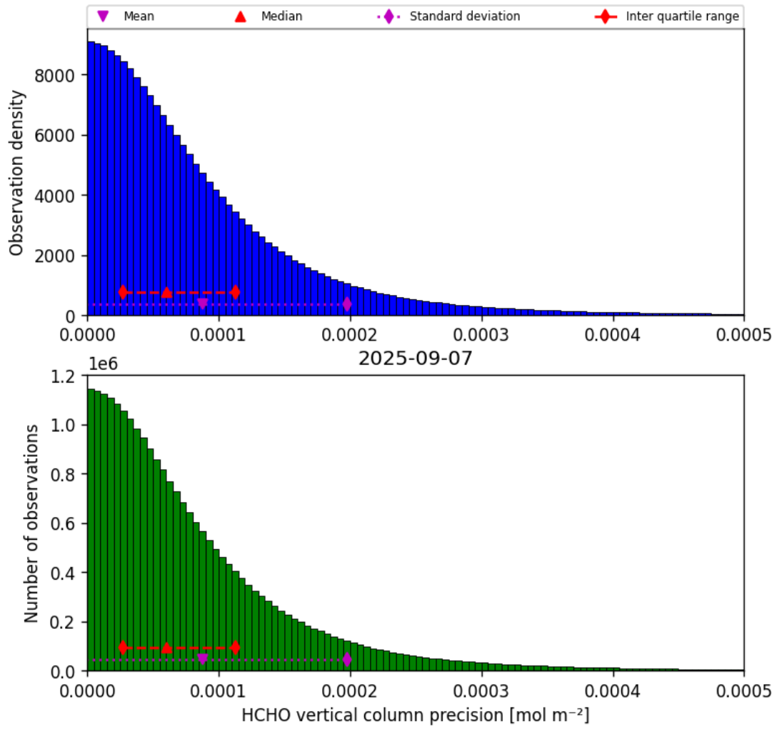
Figure 36: Histogram of “HCHO vertical column precision” for 2025-09-06 to 2025-09-08
