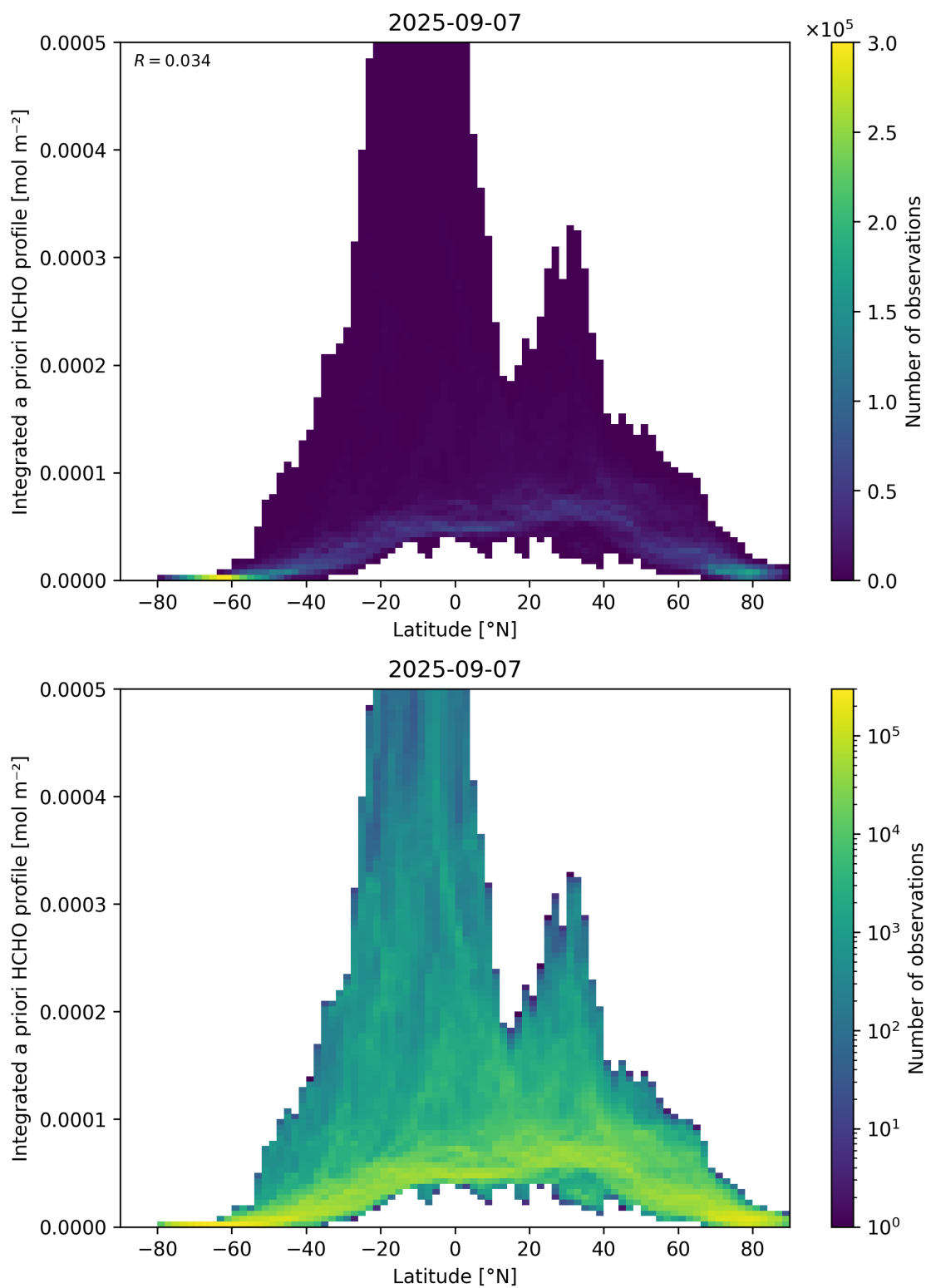
Figure 166: Scatter density plot of “Latitude” against “Integrated a priori HCHO profile” for 2025-09-06 to 2025-09-08.
