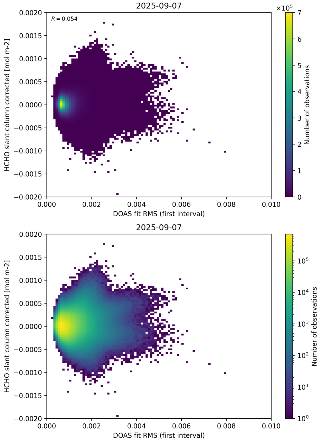
Figure 62: Scatter density plot of “DOAS fit RMS (first interval)” against “HCHO slant column corrected” for 2025-09-06 to 2025-09-08.
