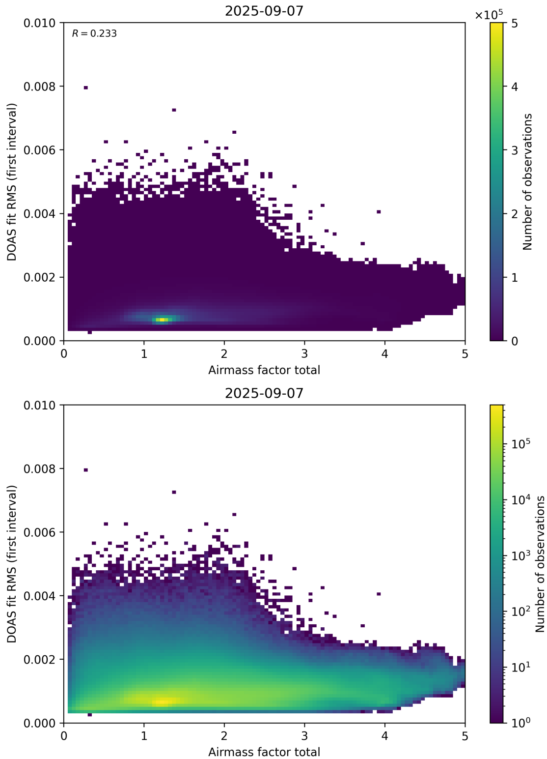
Figure 97: Scatter density plot of “Airmass factor total” against “DOAS fit RMS (first interval)” for 2025-09-06 to 2025-09-08.
