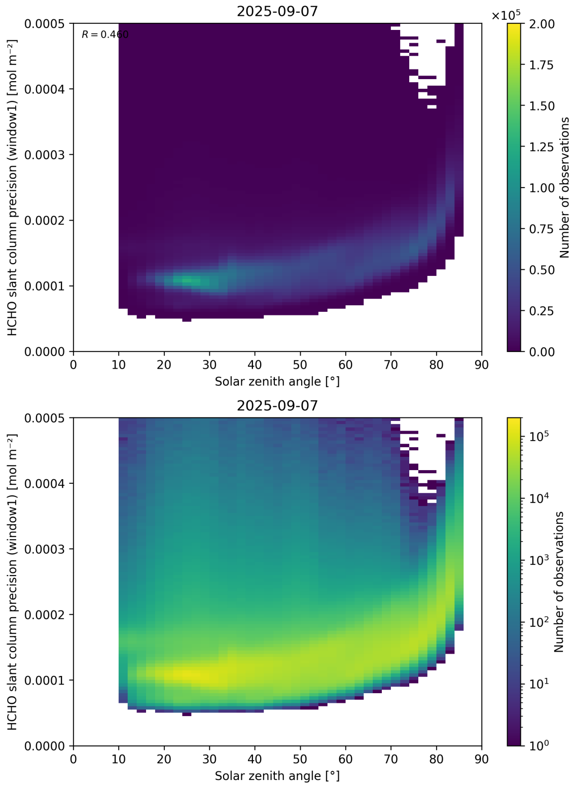
Figure 174: Scatter density plot of “Solar zenith angle” against “HCHO slant column precision (window1)” for 2025-09-06 to 2025-09-08.
