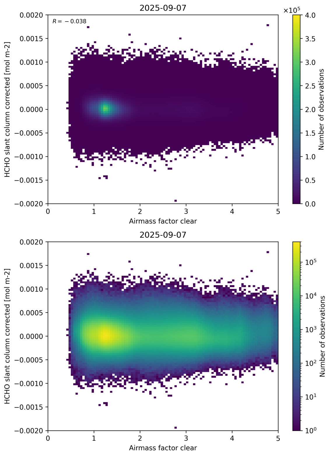
Figure 74: Scatter density plot of “Airmass factor clear” against “HCHO slant column corrected” for 2025-09-06 to 2025-09-08.
