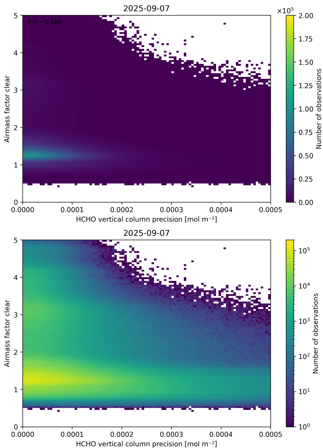
Figure 139: Scatter density plot of “HCHO vertical column precision” against “Airmass factor clear” for 2025-09-06 to 2025-09-08.
