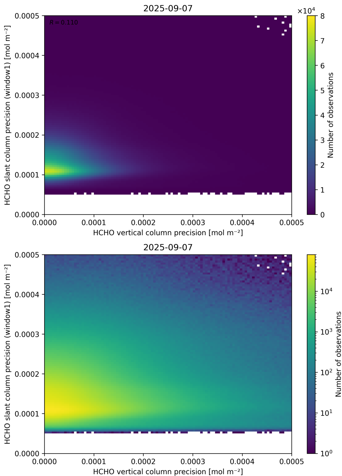
Figure 143: Scatter density plot of “HCHO vertical column precision” against “HCHO slant column precision (window1)” for 2025-09-06 to 2025-09-08.
