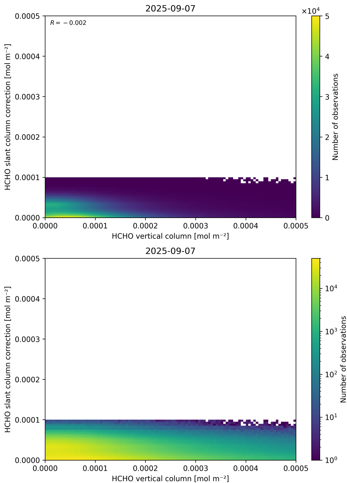
Figure 128: Scatter density plot of “HCHO vertical column” against “HCHO slant column correction” for 2025-09-06 to 2025-09-08.
