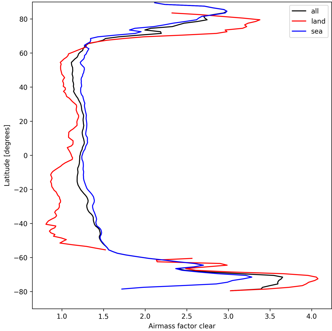
Figure 28: Zonal average of “Airmass factor clear” for 2025-09-06 to 2025-09-08.
