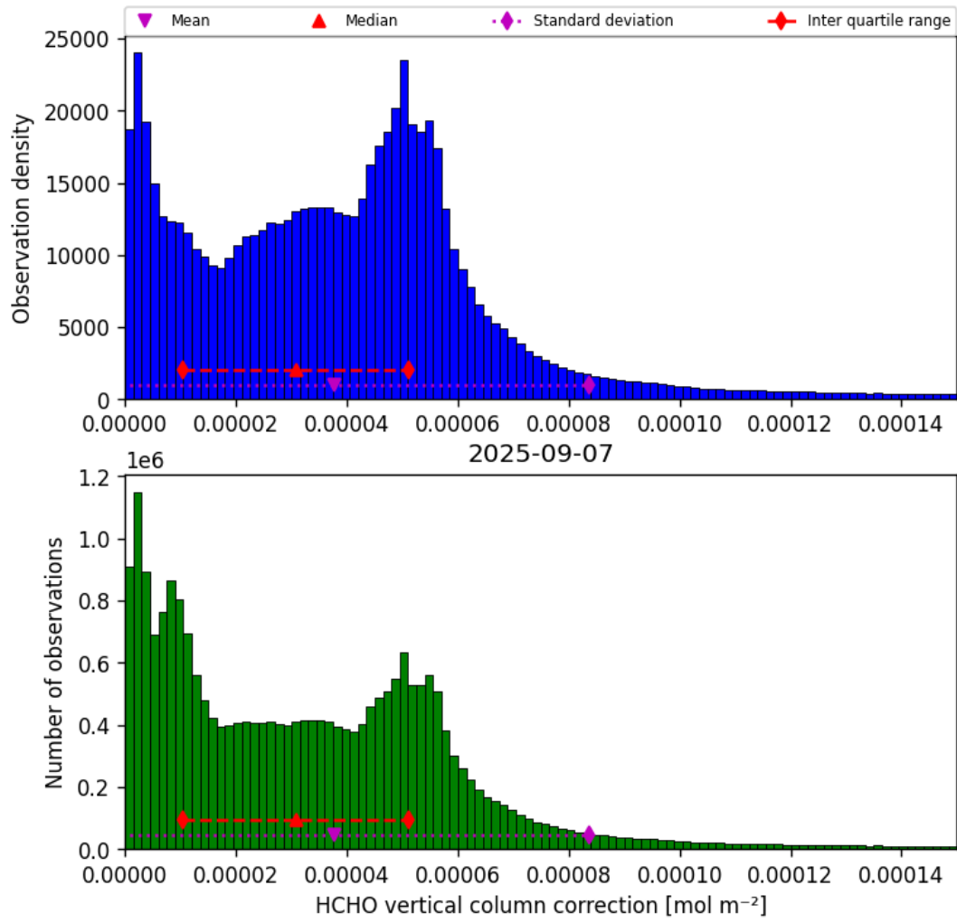
Figure 37: Histogram of “HCHO vertical column correction” for 2025-09-06 to 2025-09-08
