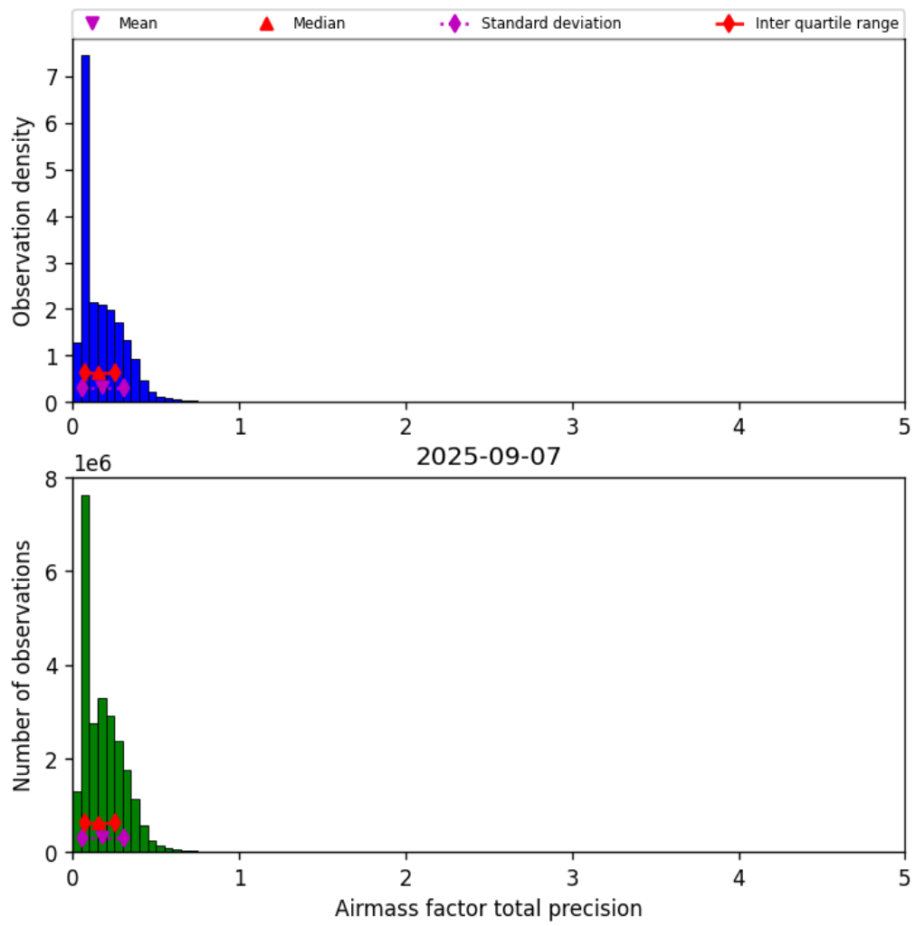
Figure 41: Histogram of “Airmass factor total precision” for 2025-09-06 to 2025-09-08
