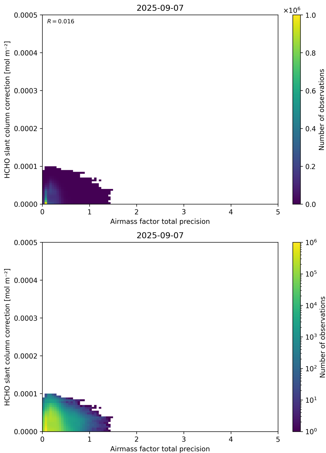
Figure 110: Scatter density plot of “Airmass factor total precision” against “HCHO slant column correction” for 2025-09-06 to 2025-09-08.
