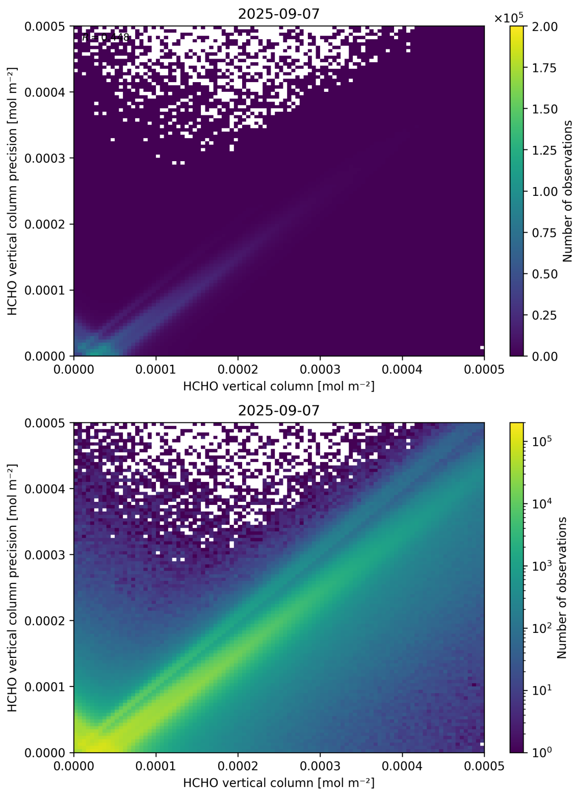
Figure 134: Scatter density plot of “HCHO vertical column” against “HCHO vertical column precision” for 2025-09-06 to 2025-09-08.
