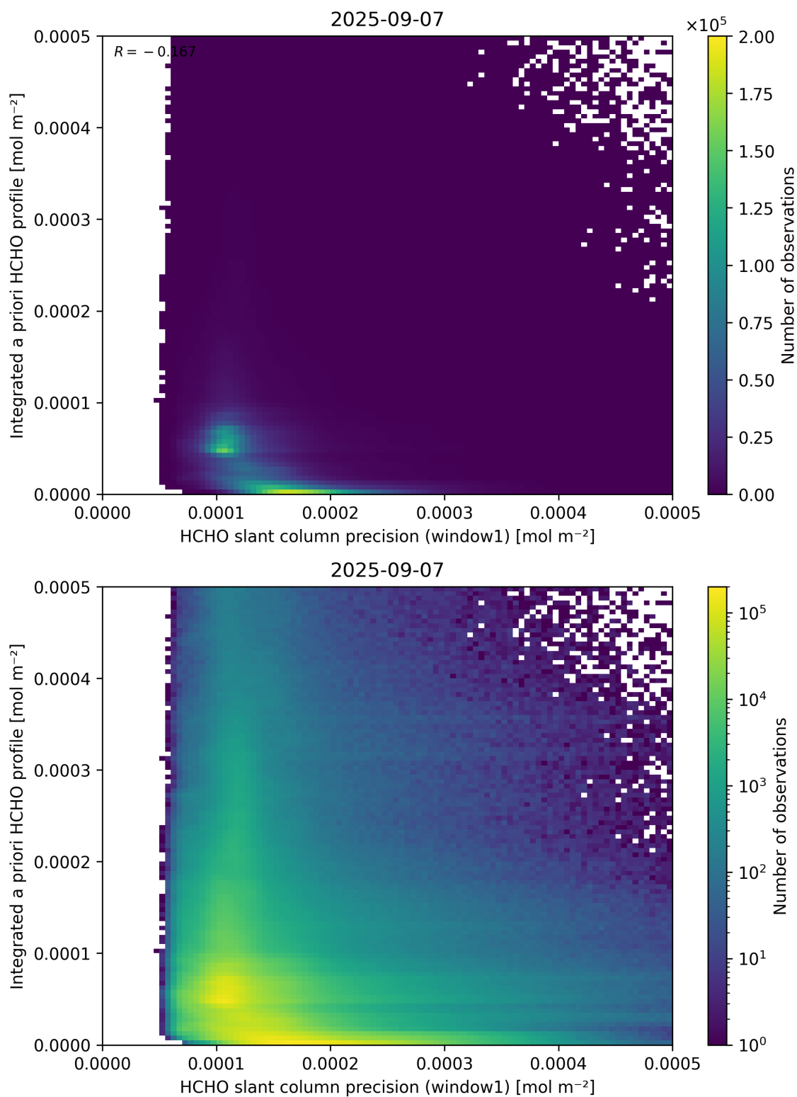
Figure 96: Scatter density plot of “HCHO slant column precision (window1)” against “Integrated a priori HCHO profile” for 2025-09-06 to 2025-09-08.
