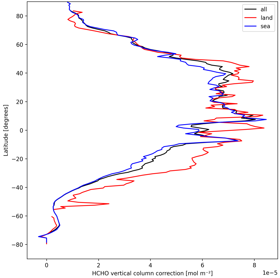
Figure 23: Zonal average of “HCHO vertical column correction” for 2025-09-06 to 2025-09-08.
