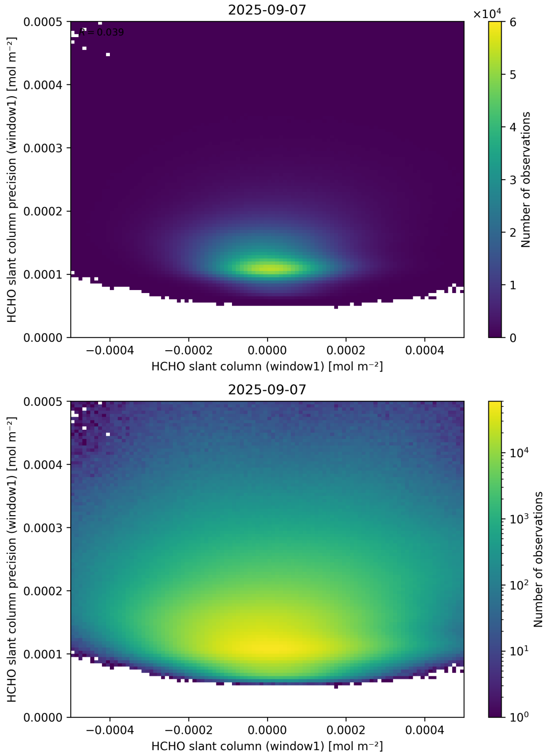
Figure 84: Scatter density plot of “HCHO slant column (window1)” against “HCHO slant column precision (window1)” for 2025-09-06 to 2025-09-08.
