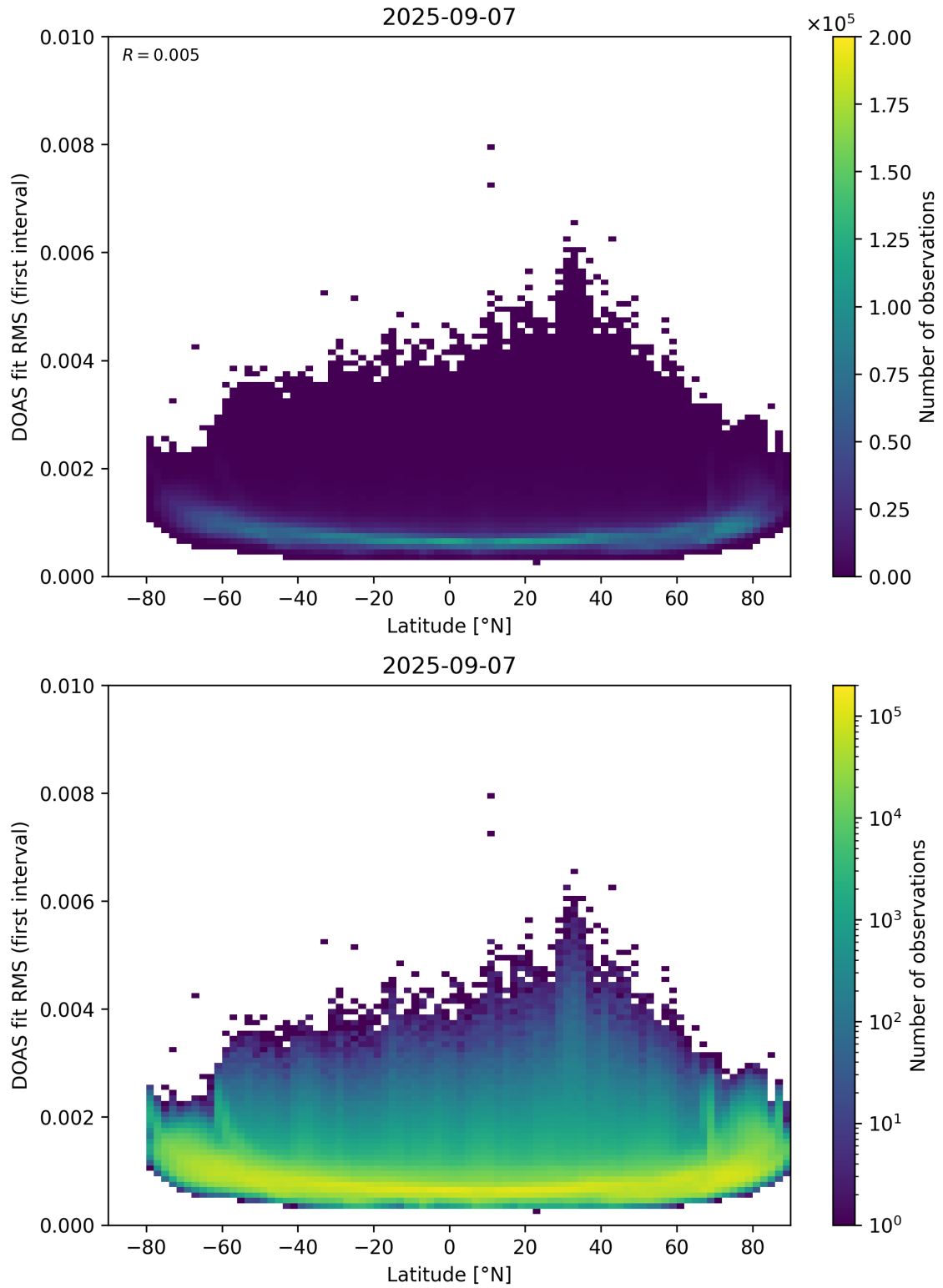
Figure 153: Scatter density plot of “Latitude” against “DOAS fit RMS (first interval)” for 2025-09-06 to 2025-09-08.
