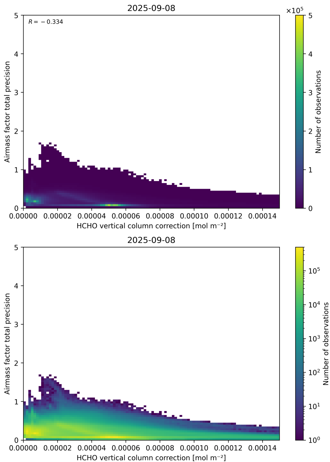
Figure 121: Scatter density plot of “HCHO vertical column correction” against “Airmass factor total precision” for 2025-09-07 to 2025-09-09.
