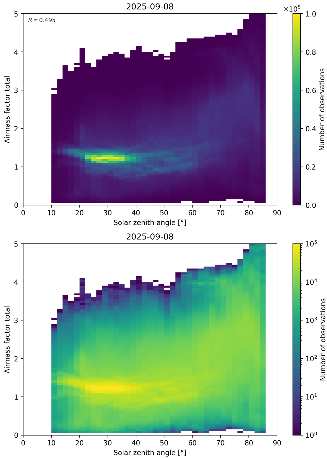
Figure 175: Scatter density plot of “Solar zenith angle” against “Airmass factor total” for 2025-09-07 to 2025-09-09.
