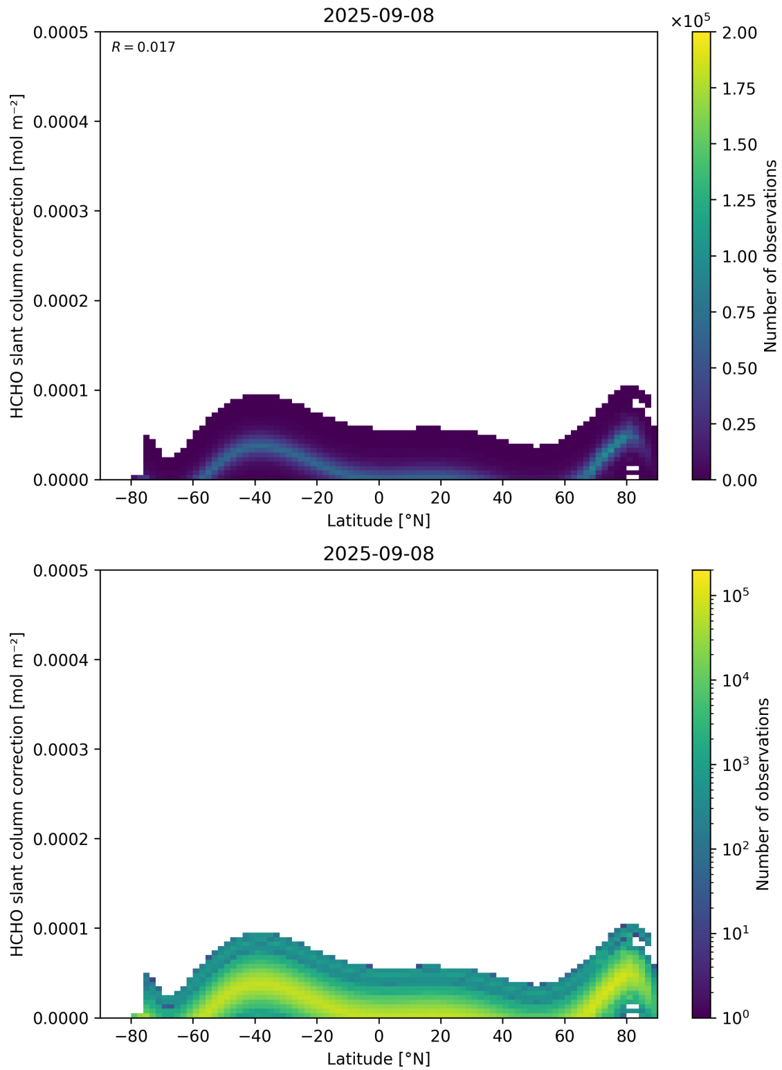
Figure 158: Scatter density plot of “Latitude” against “HCHO slant column correction” for 2025-09-07 to 2025-09-09.
