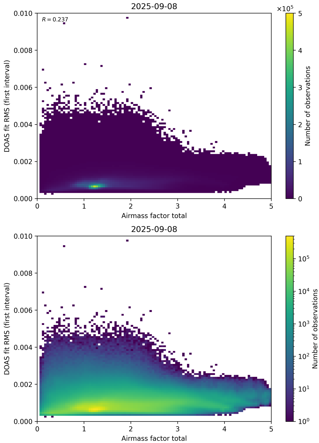
Figure 97: Scatter density plot of “Airmass factor total” against “DOAS fit RMS (first interval)” for 2025-09-07 to 2025-09-09.
