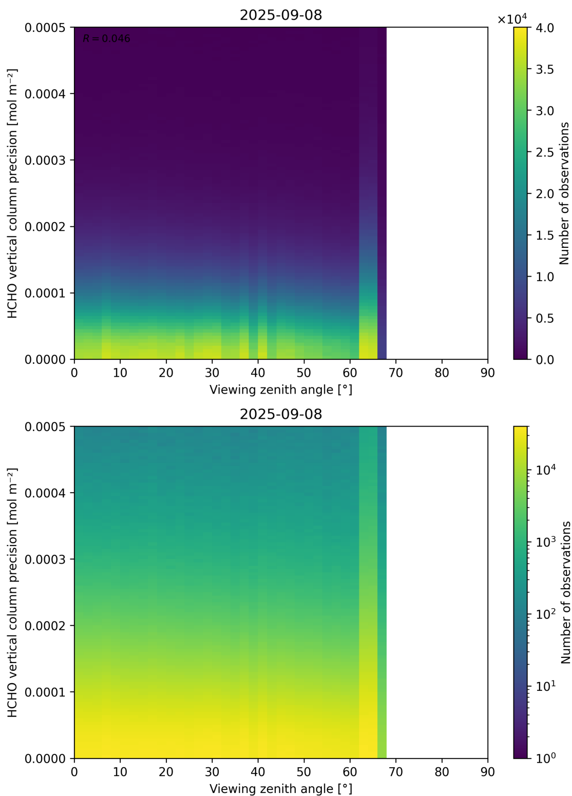
Figure 194: Scatter density plot of “Viewing zenith angle” against “HCHO vertical column precision” for 2025-09-07 to 2025-09-09.
