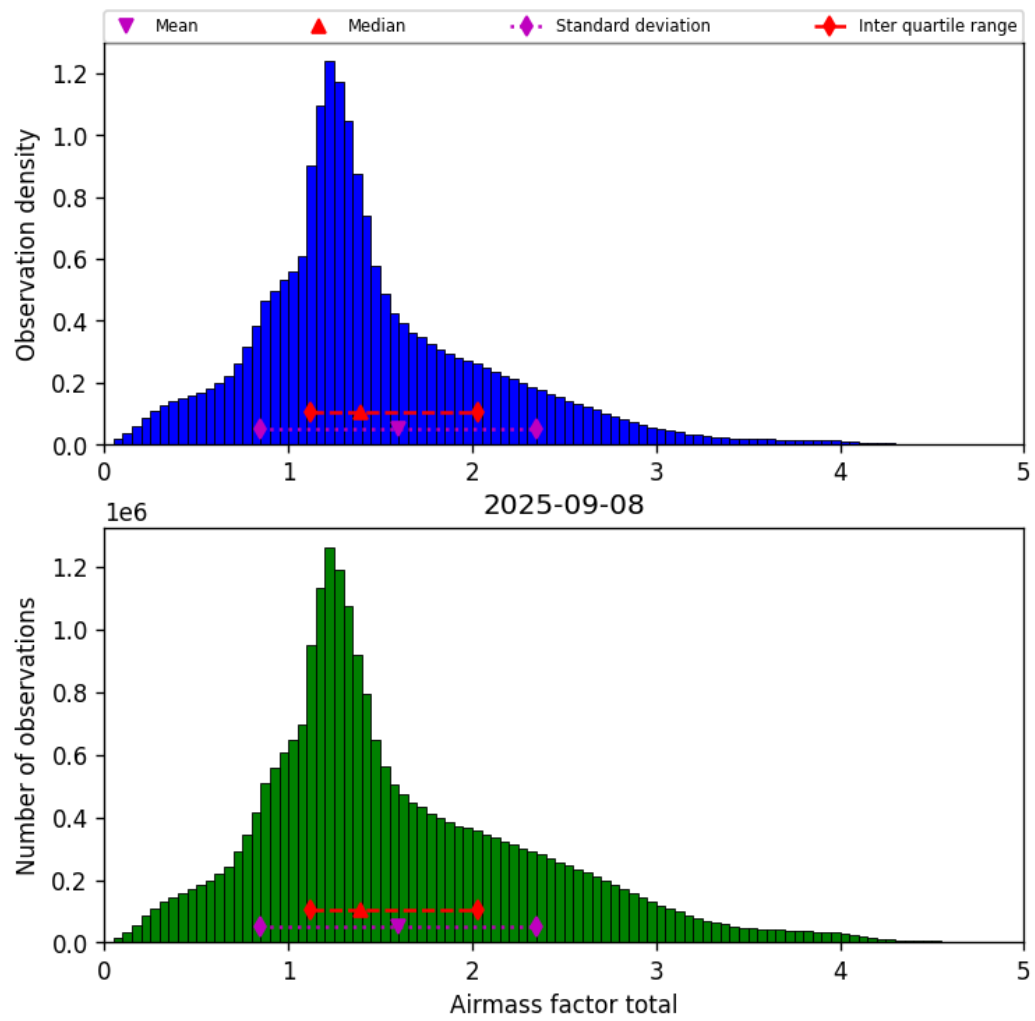
Figure 40: Histogram of “Airmass factor total” for 2025-09-07 to 2025-09-09
