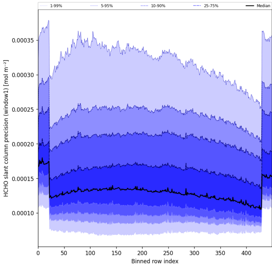
Figure 53: Along track statistics of “HCHO slant column precision (window1)” for 2025-09-07 to 2025-09-09
