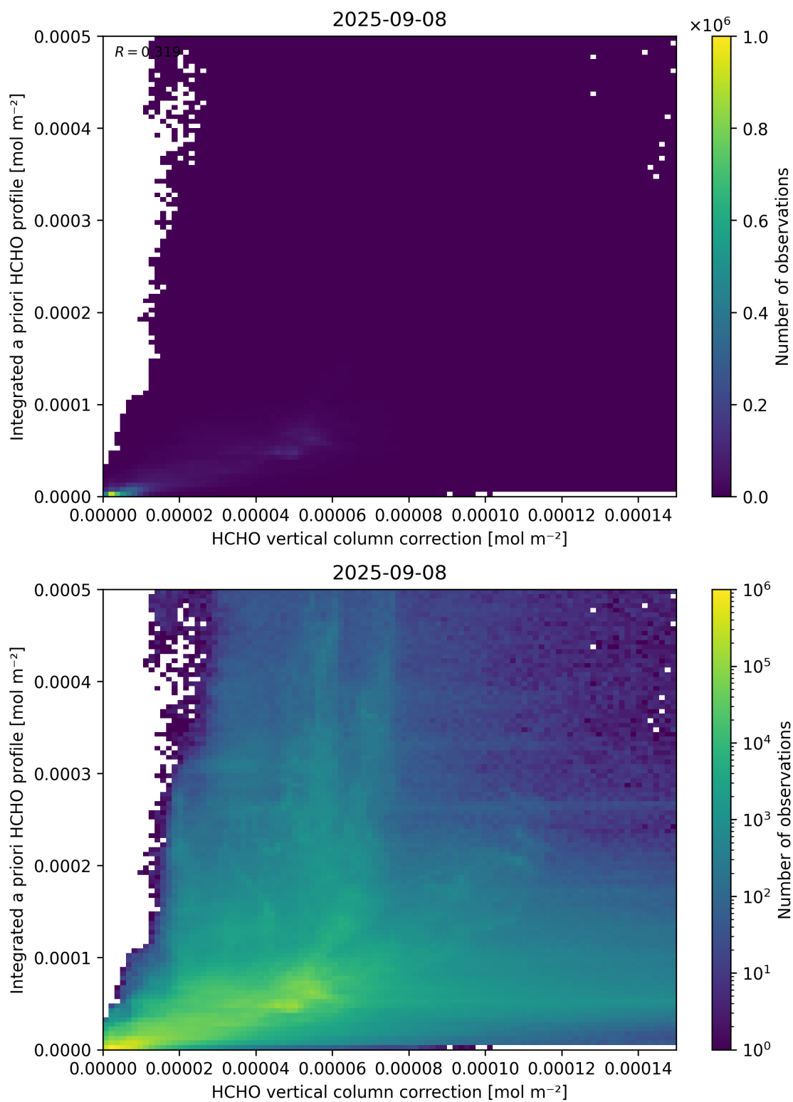
Figure 122: Scatter density plot of “HCHO vertical column correction” against “Integrated a priori HCHO profile” for 2025-09-07 to 2025-09-09.
