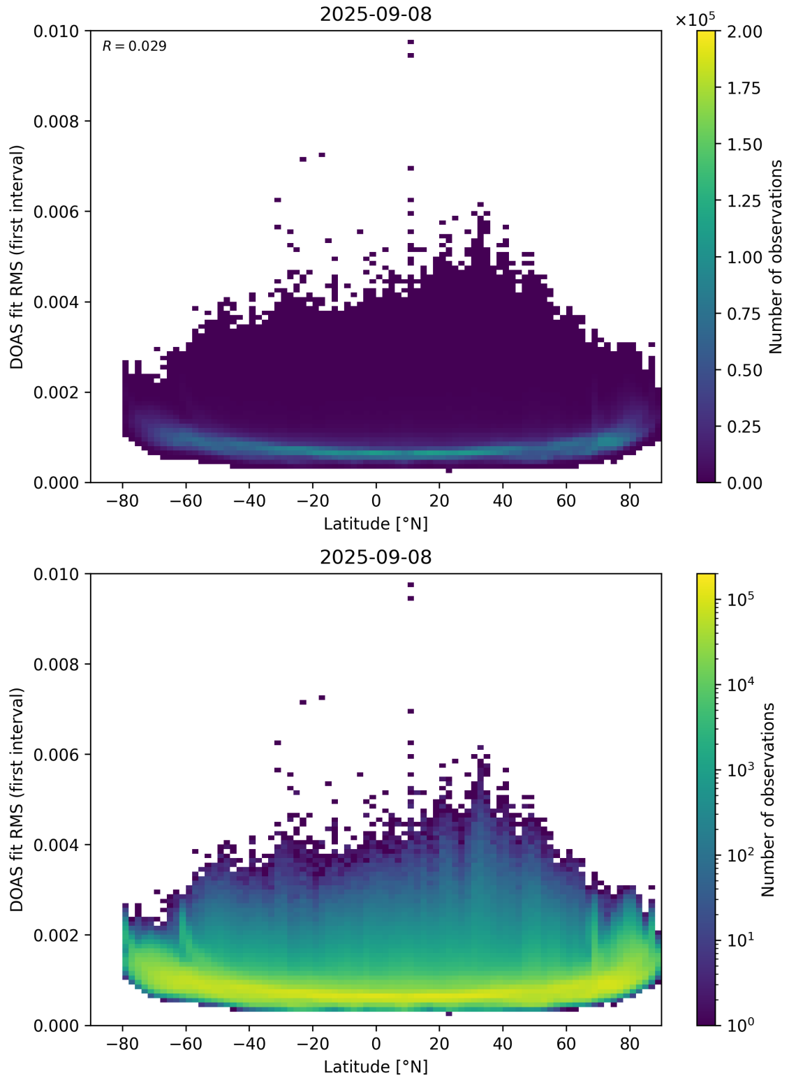
Figure 153: Scatter density plot of “Latitude” against “DOAS fit RMS (first interval)” for 2025-09-07 to 2025-09-09.
