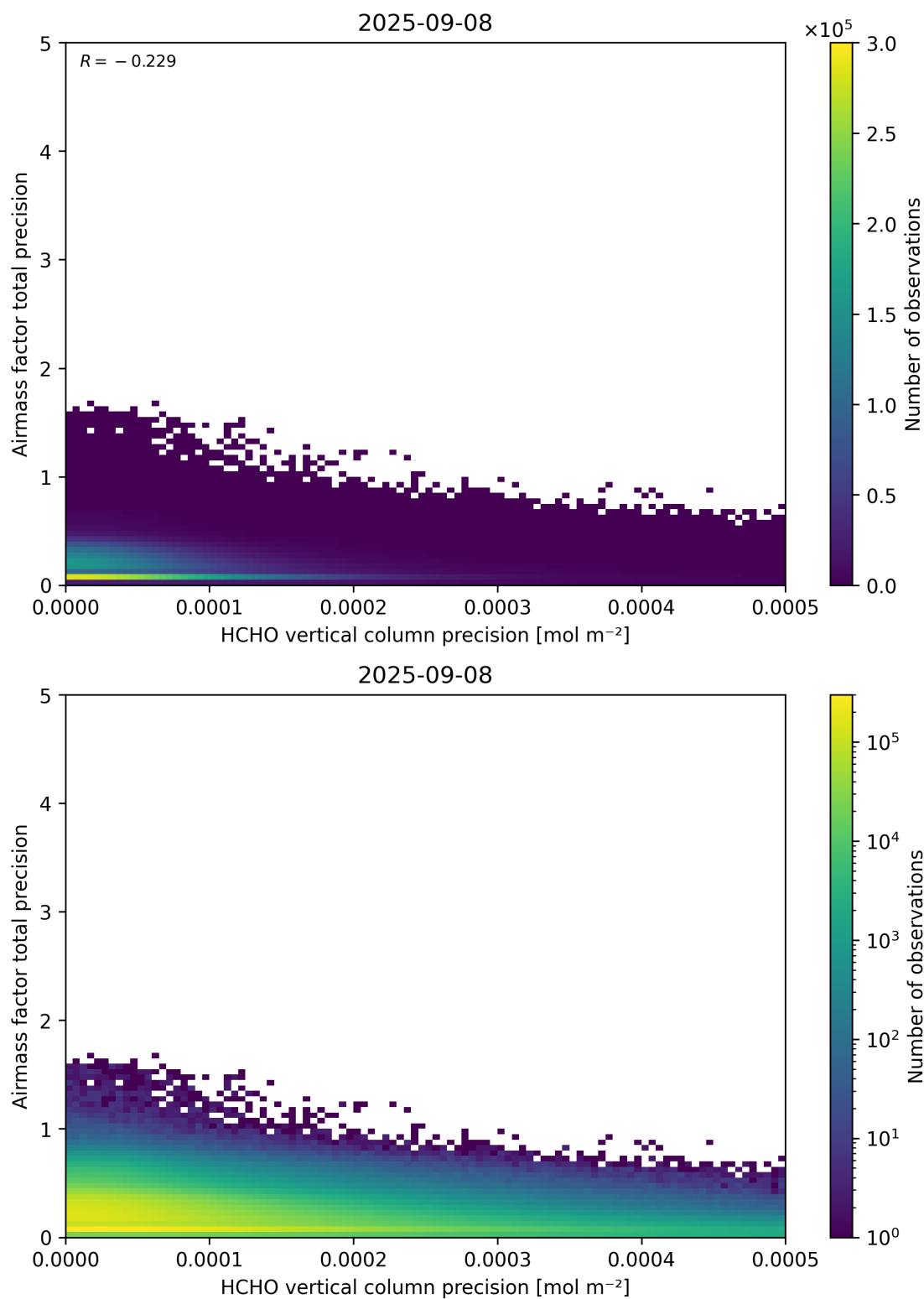
Figure 145: Scatter density plot of “HCHO vertical column precision” against “Airmass factor total precision” for 2025-09-07 to 2025-09-09.
