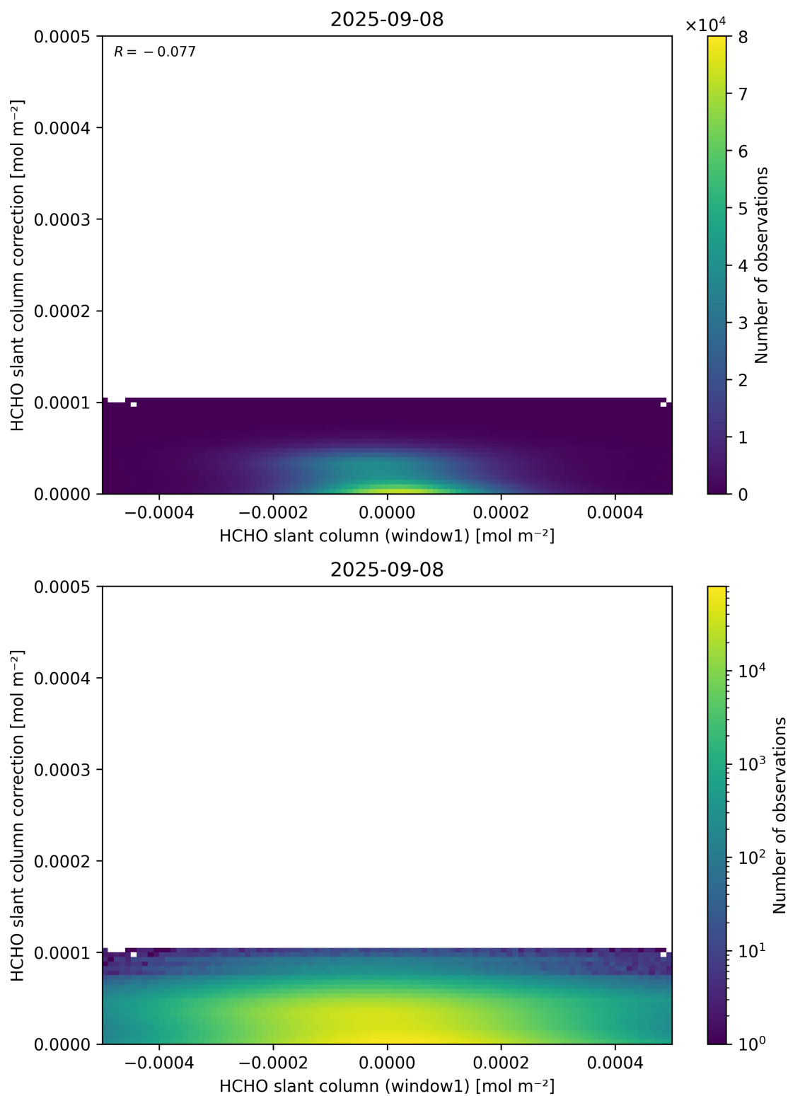
Figure 83: Scatter density plot of “HCHO slant column (window1)” against “HCHO slant column correction” for 2025-09-07 to 2025-09-09.
