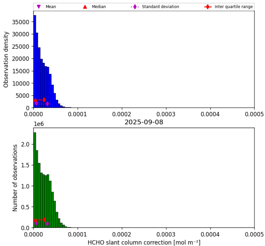
Figure 47: Histogram of “HCHO slant column correction” for 2025-09-07 to 2025-09-09
