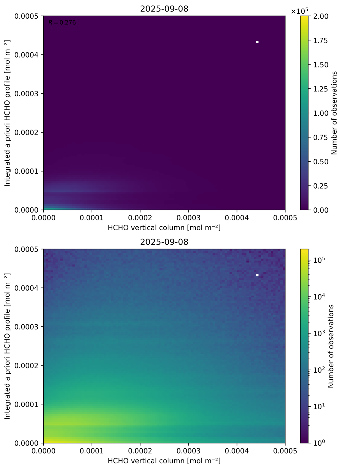
Figure 135: Scatter density plot of “HCHO vertical column” against “Integrated a priori HCHO profile” for 2025-09-07 to 2025-09-09.
