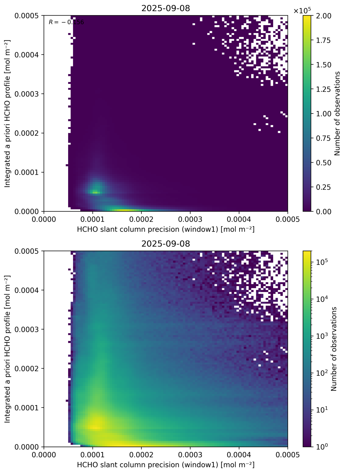
Figure 96: Scatter density plot of “HCHO slant column precision (window1)” against “Integrated a priori HCHO profile” for 2025-09-07 to 2025-09-09.
