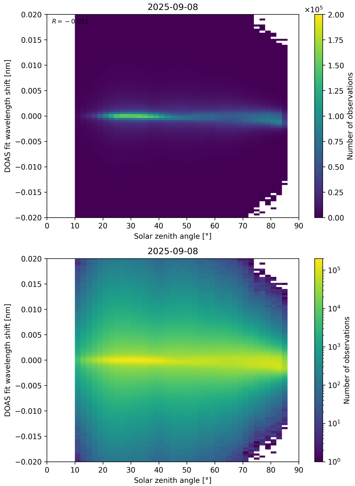
Figure 168: Scatter density plot of “Solar zenith angle” against “DOAS fit wavelength shift” for 2025-09-07 to 2025-09-09.
