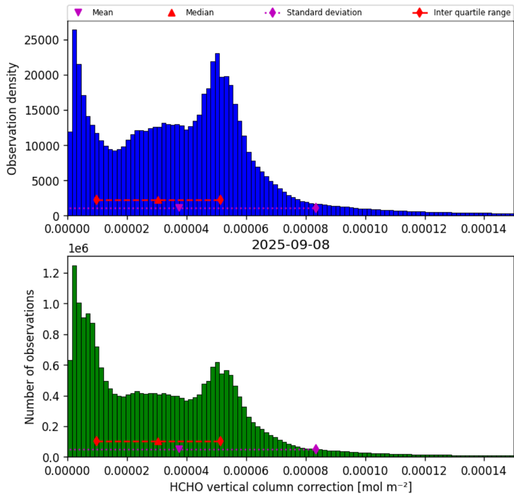
Figure 37: Histogram of “HCHO vertical column correction” for 2025-09-07 to 2025-09-09
