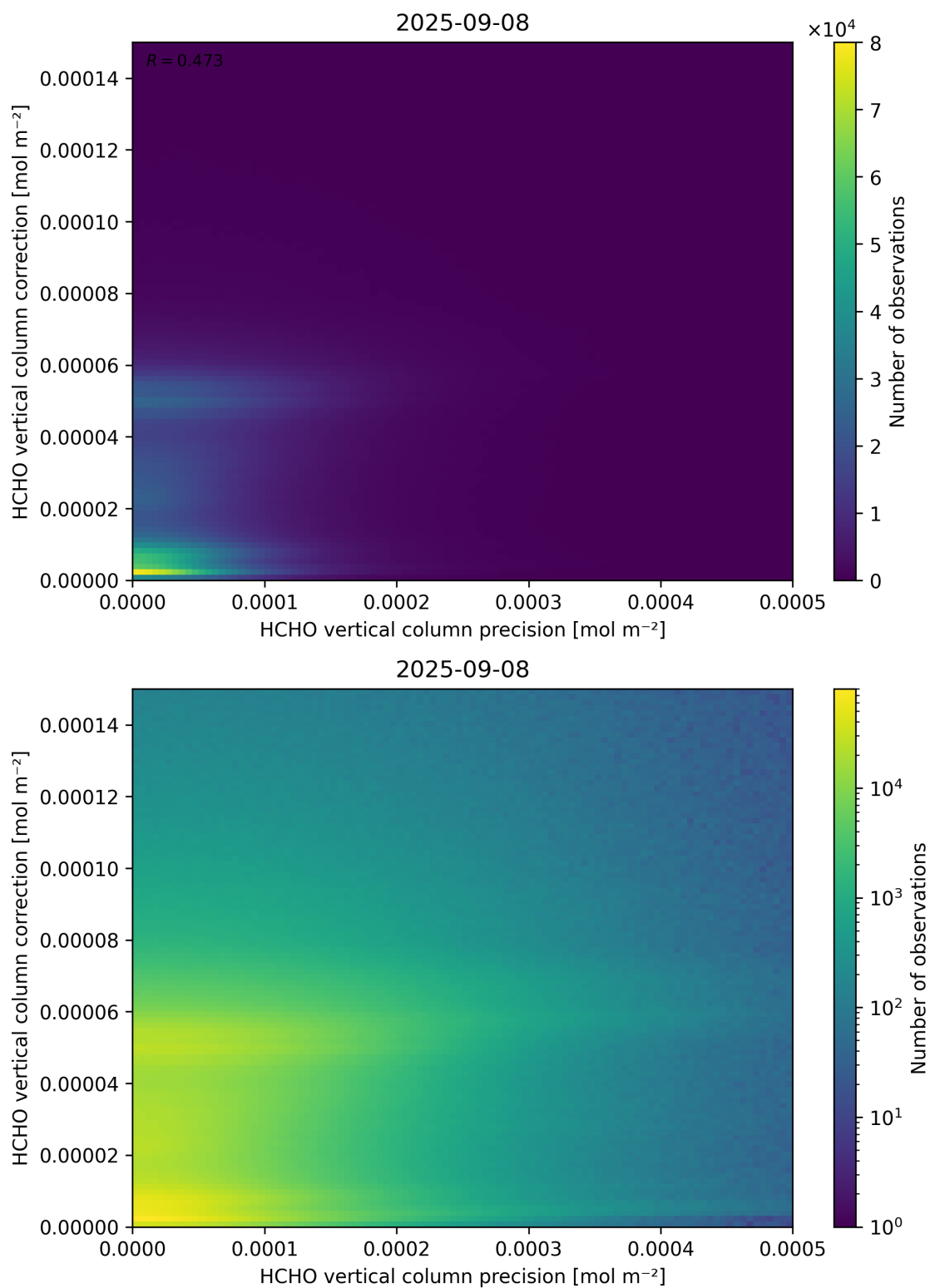
Figure 146: Scatter density plot of “HCHO vertical column precision” against “HCHO vertical column correction” for 2025-09-07 to 2025-09-09.
