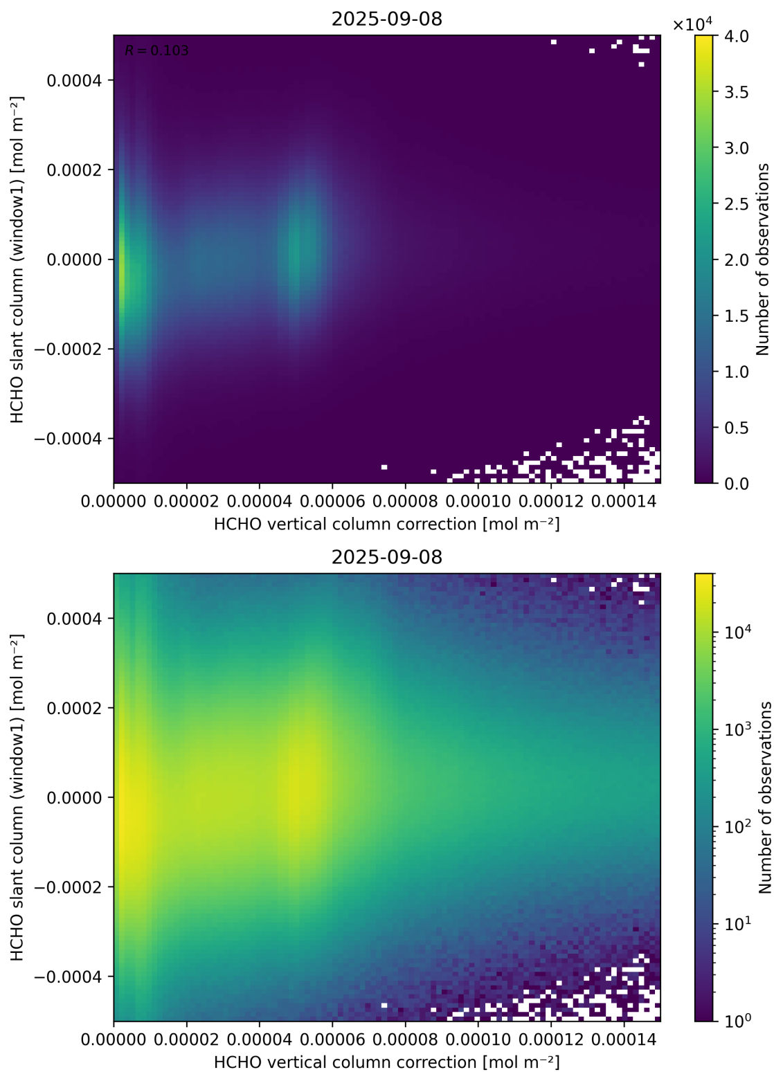
Figure 118: Scatter density plot of “HCHO vertical column correction” against “HCHO slant column (window1)” for 2025-09-07 to 2025-09-09.
