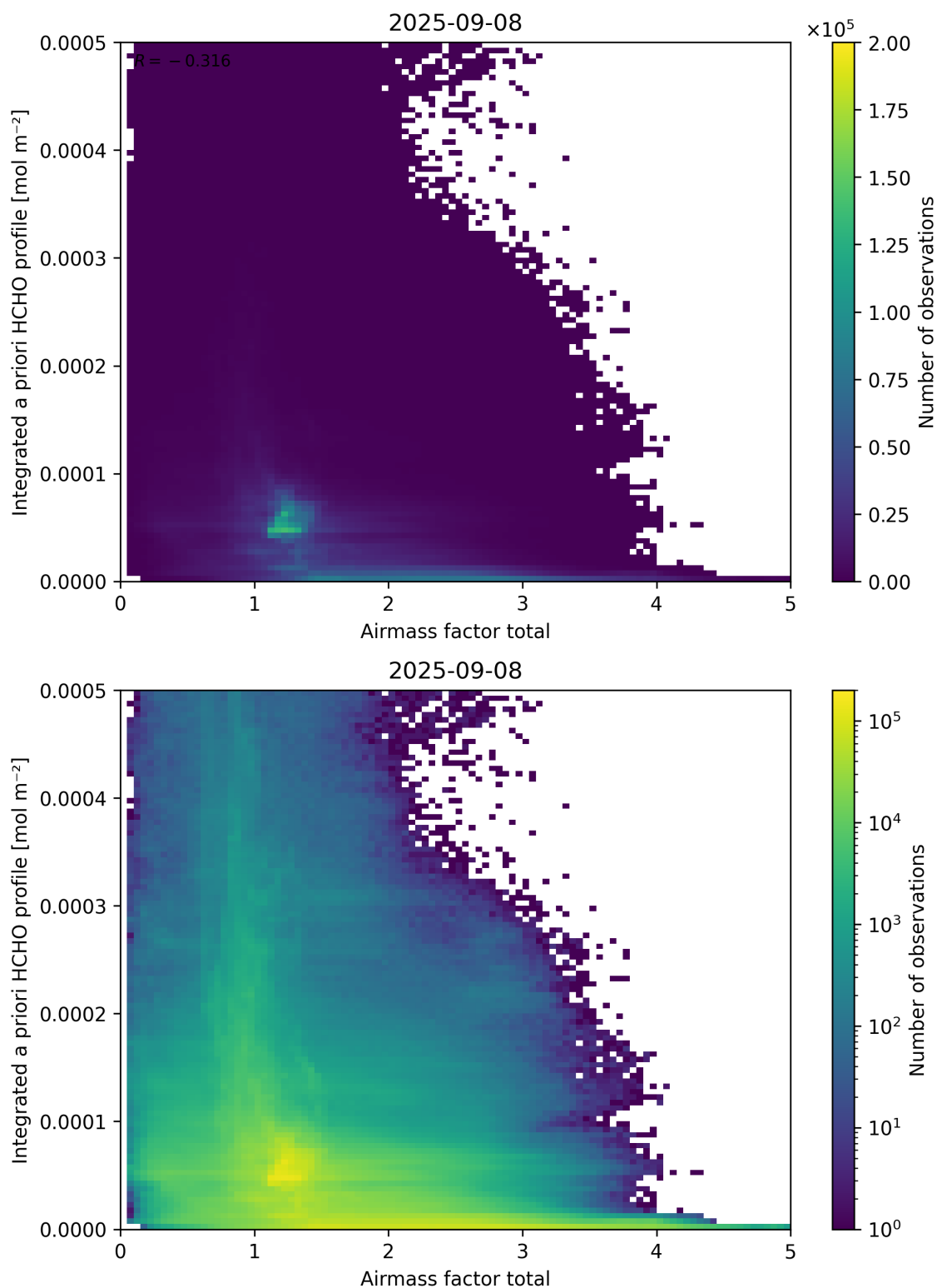
Figure 104: Scatter density plot of “Airmass factor total” against “Integrated a priori HCHO profile” for 2025-09-07 to 2025-09-09.
