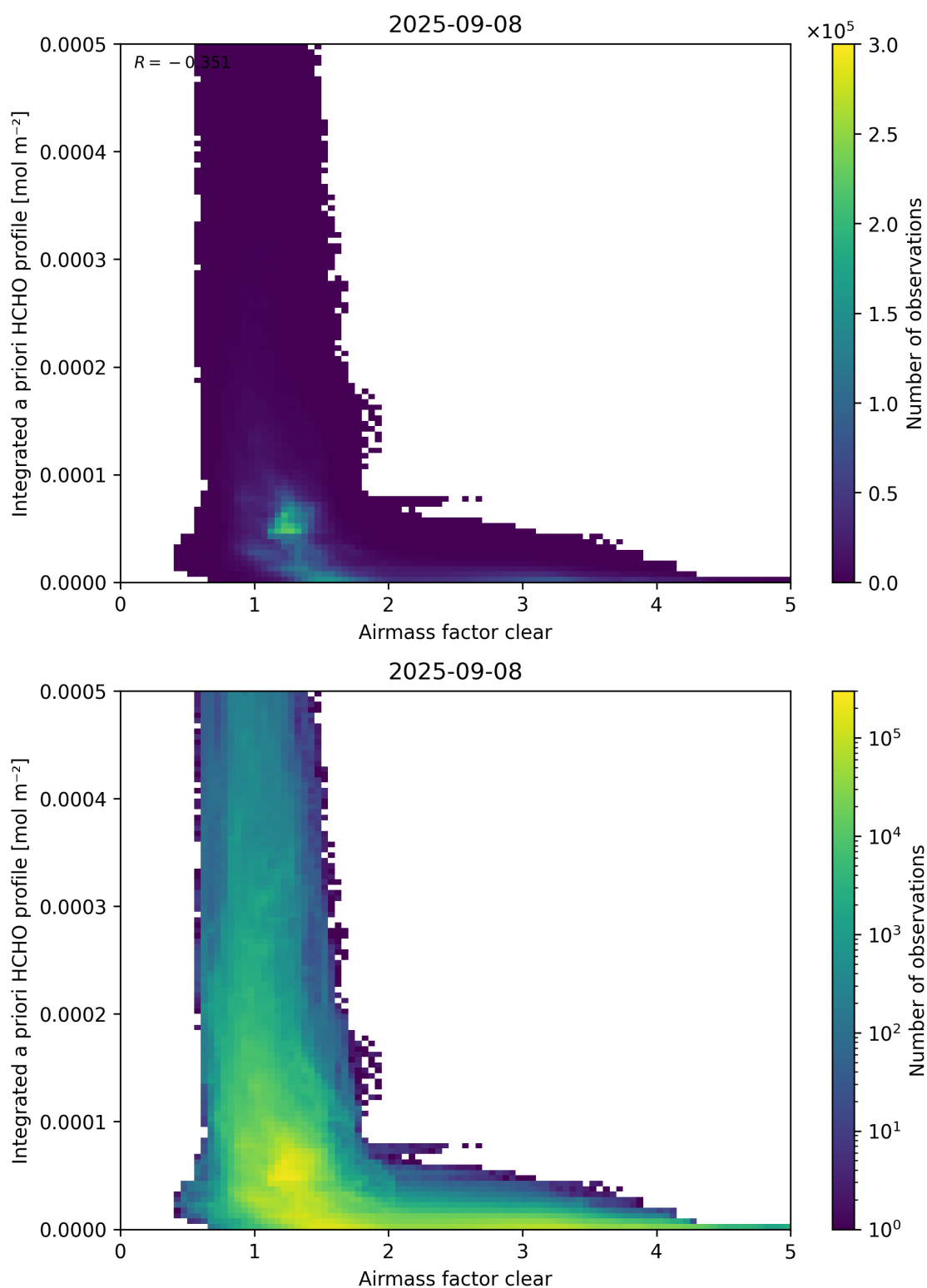
Figure 76: Scatter density plot of “Airmass factor clear” against “Integrated a priori HCHO profile” for 2025-09-07 to 2025-09-09.
