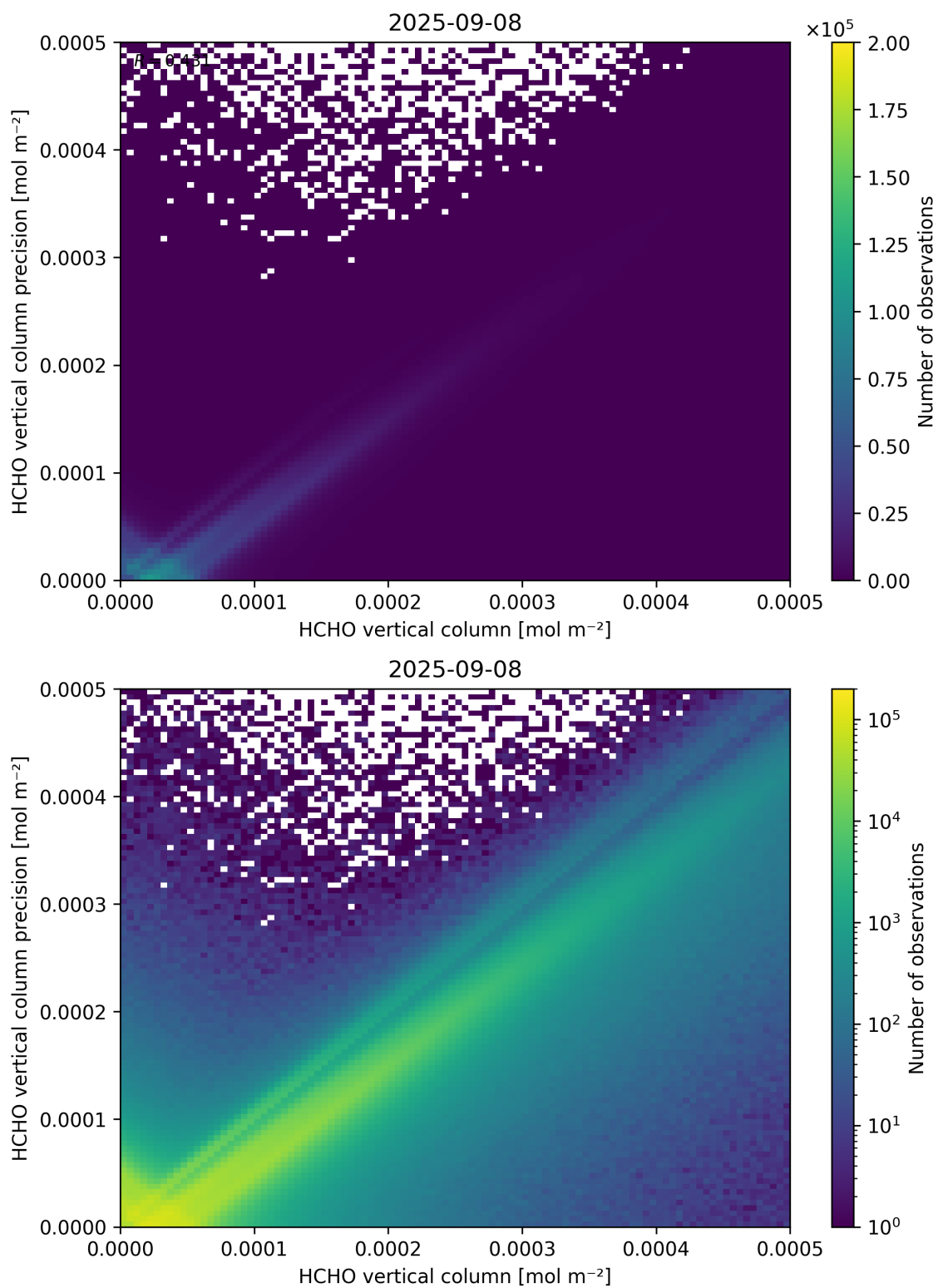
Figure 134: Scatter density plot of “HCHO vertical column” against “HCHO vertical column precision” for 2025-09-07 to 2025-09-09.
