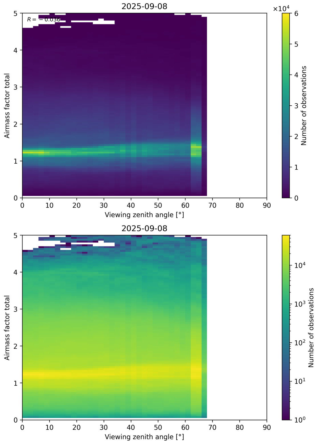
Figure 190: Scatter density plot of “Viewing zenith angle” against “Airmass factor total” for 2025-09-07 to 2025-09-09.
