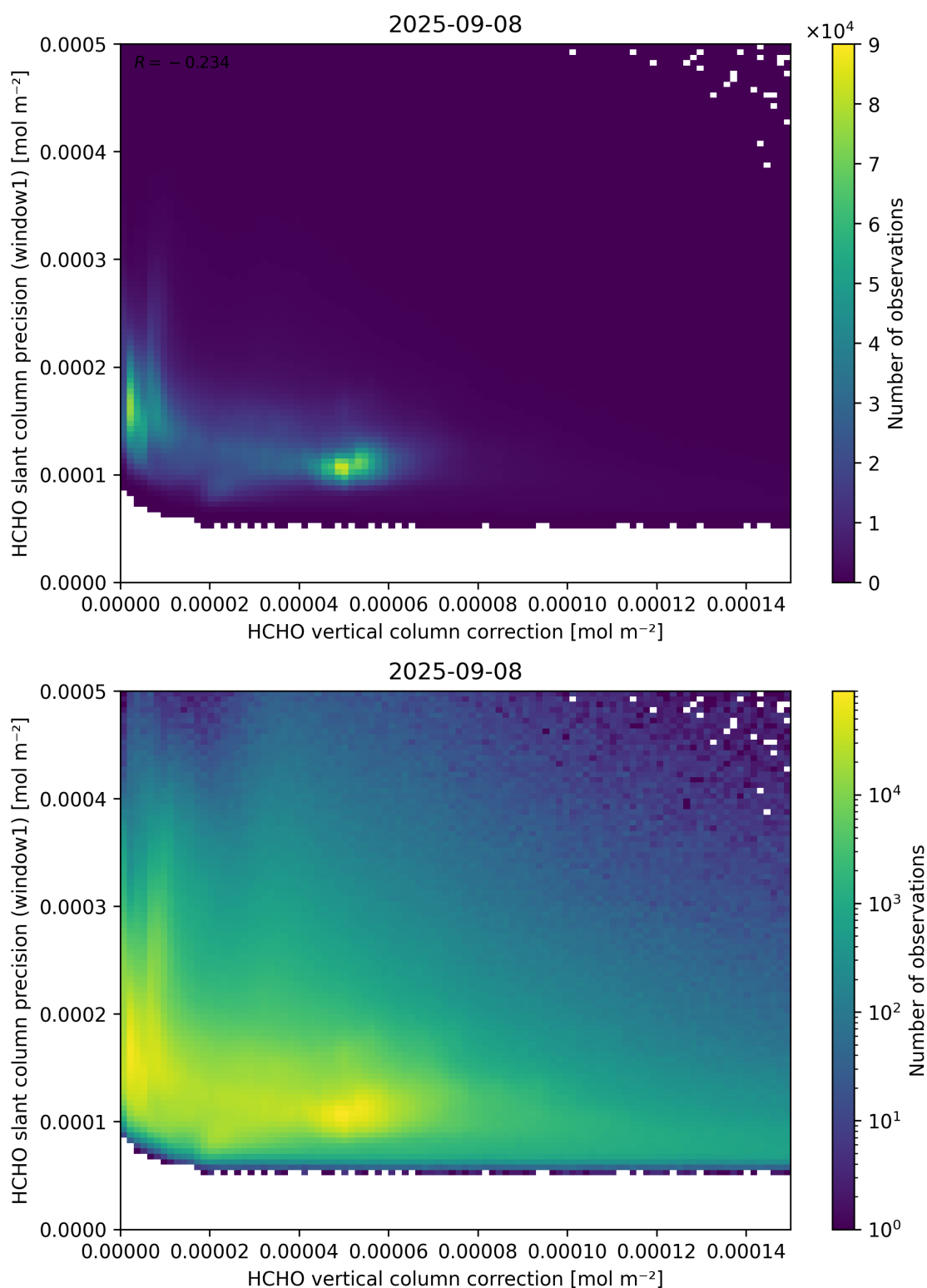
Figure 119: Scatter density plot of “HCHO vertical column correction” against “HCHO slant column precision (window1)” for 2025-09-07 to 2025-09-09.
