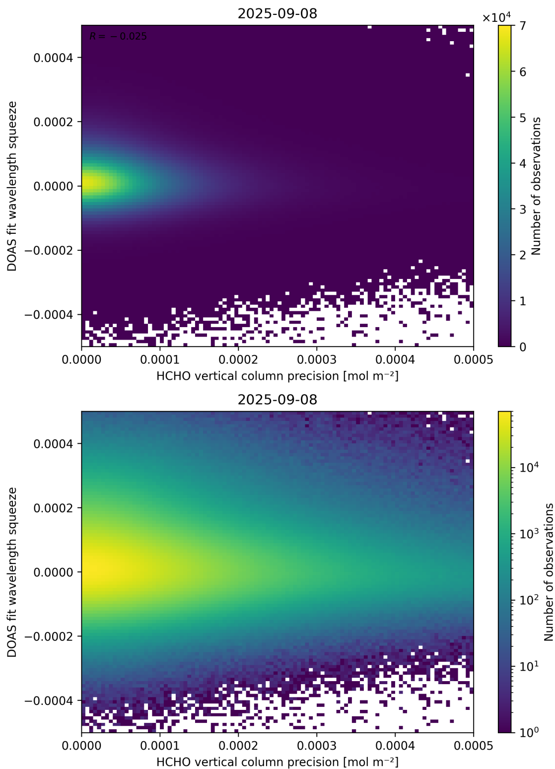
Figure 138: Scatter density plot of “HCHO vertical column precision” against “DOAS fit wavelength squeeze” for 2025-09-07 to 2025-09-09.
