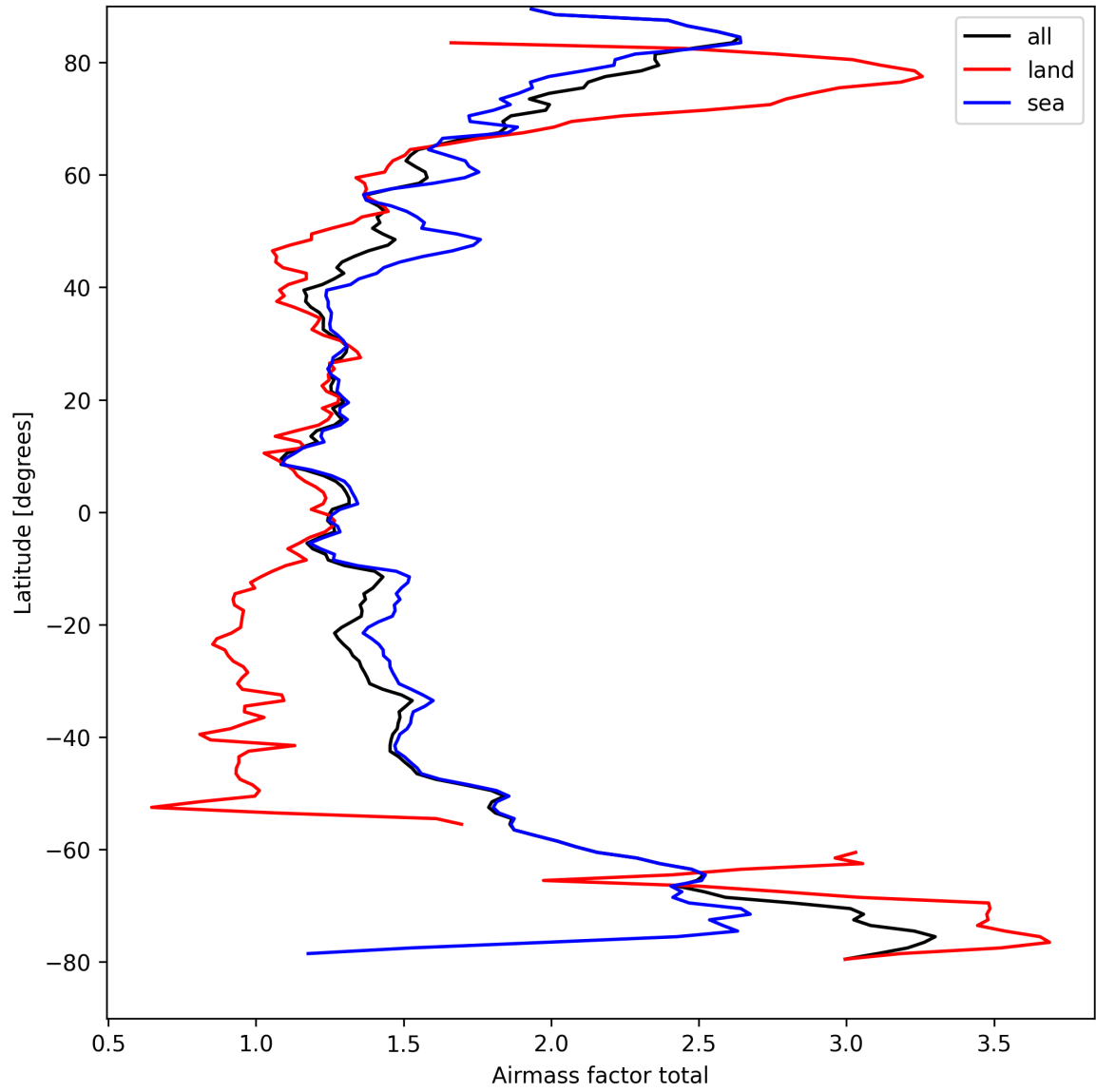
Figure 26: Zonal average of “Airmass factor total” for 2025-09-07 to 2025-09-09.
