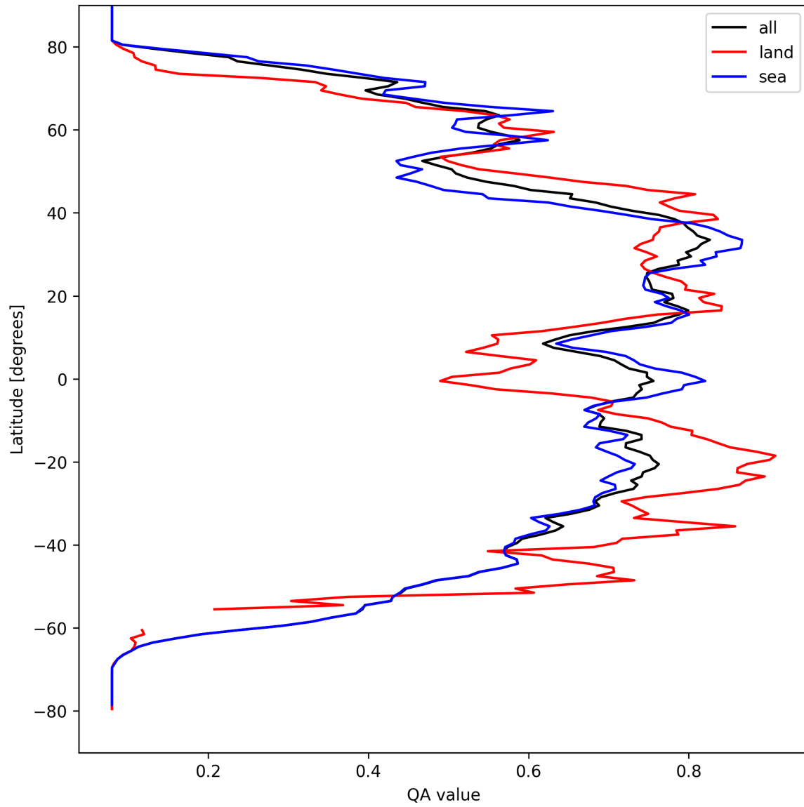
Figure 20: Zonal average of “QA value” for 2025-09-07 to 2025-09-09.
