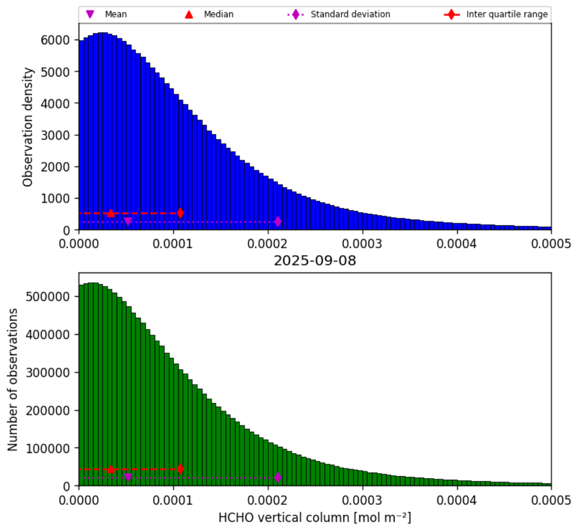
Figure 35: Histogram of “HCHO vertical column” for 2025-09-07 to 2025-09-09
