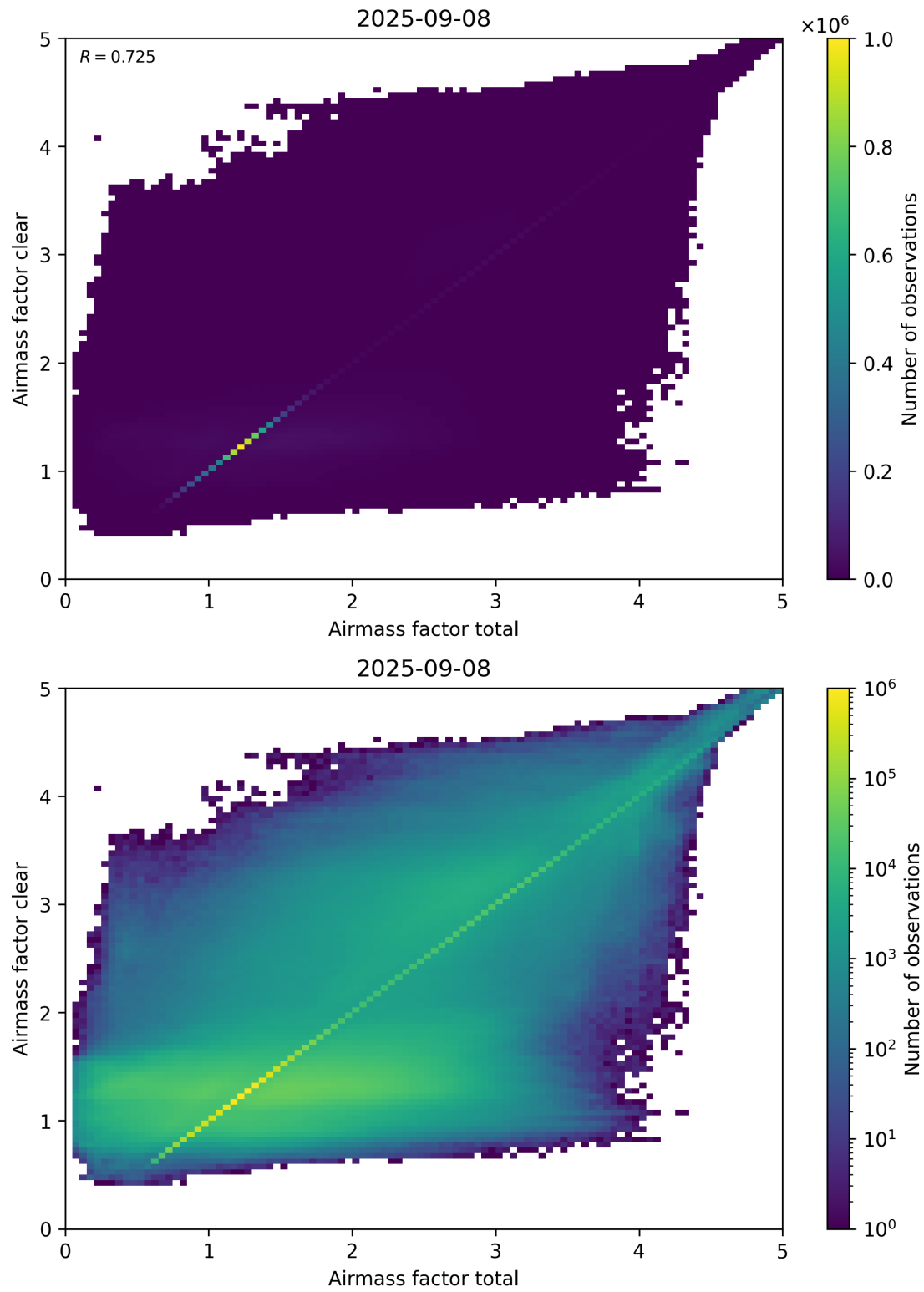
Figure 100: Scatter density plot of “Airmass factor total” against “Airmass factor clear” for 2025-09-07 to 2025-09-09.
