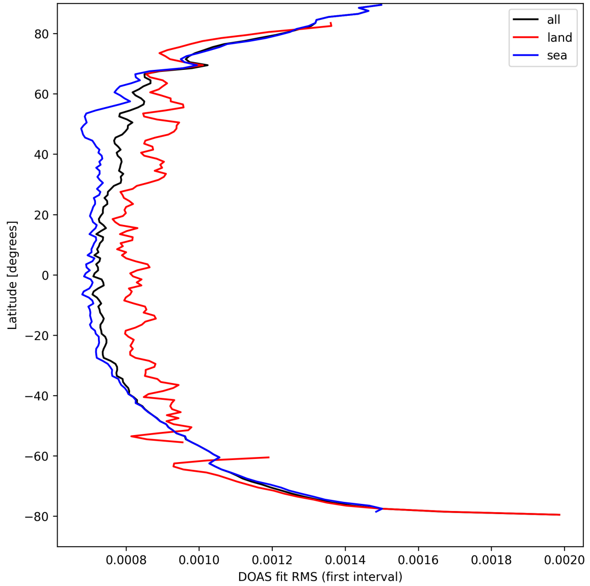
Figure 32: Zonal average of "DOAS fit RMS (first interval)" for 2025-09-07 to 2025-09-09.
