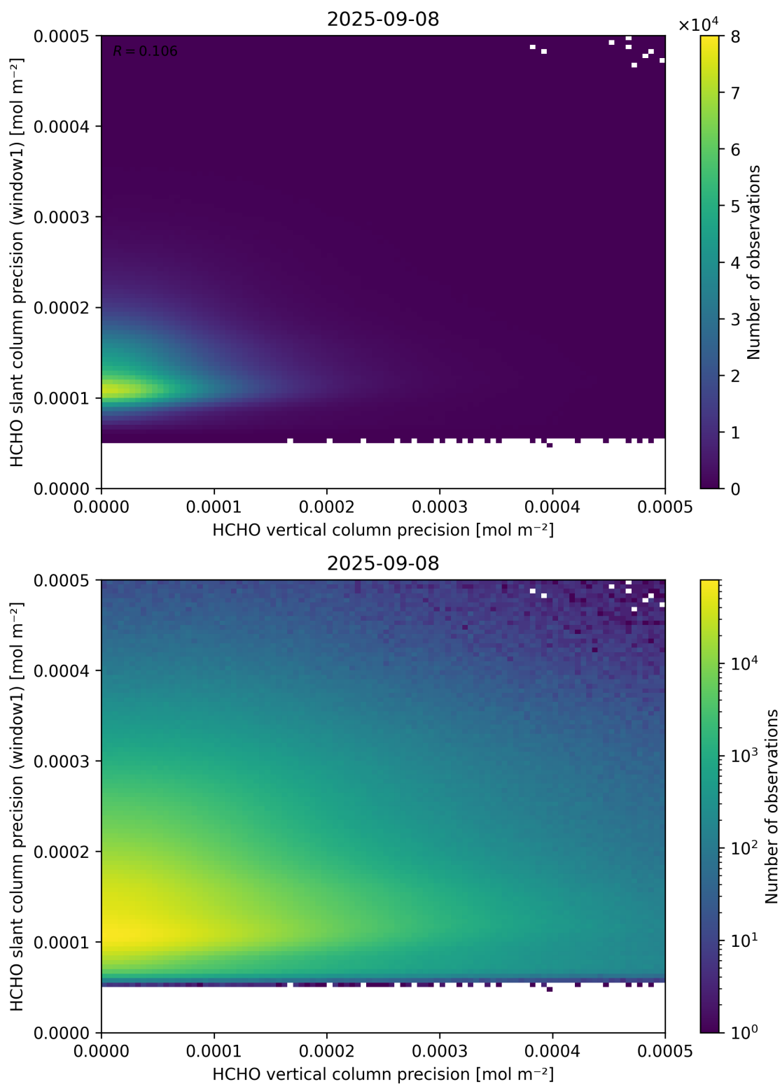
Figure 143: Scatter density plot of “HCHO vertical column precision” against “HCHO slant column precision (window1)” for 2025-09-07 to 2025-09-09.
