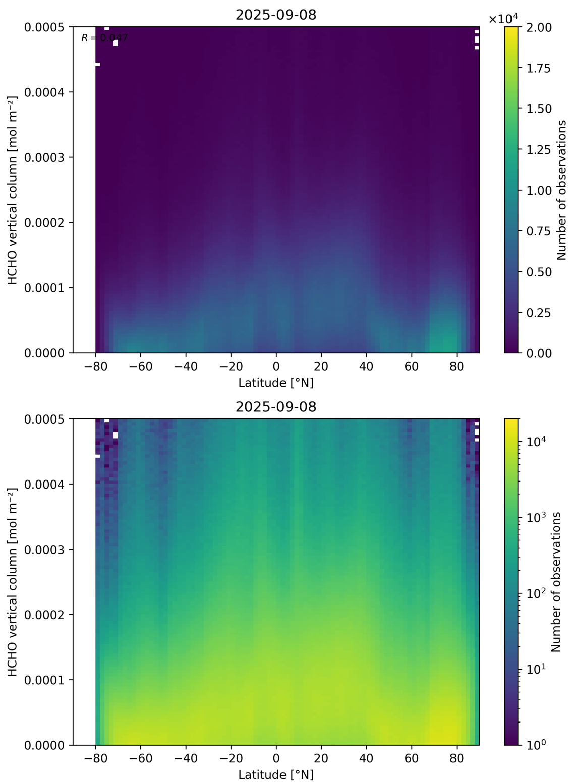
Figure 163: Scatter density plot of “Latitude” against “HCHO vertical column” for 2025-09-07 to 2025-09-09.
