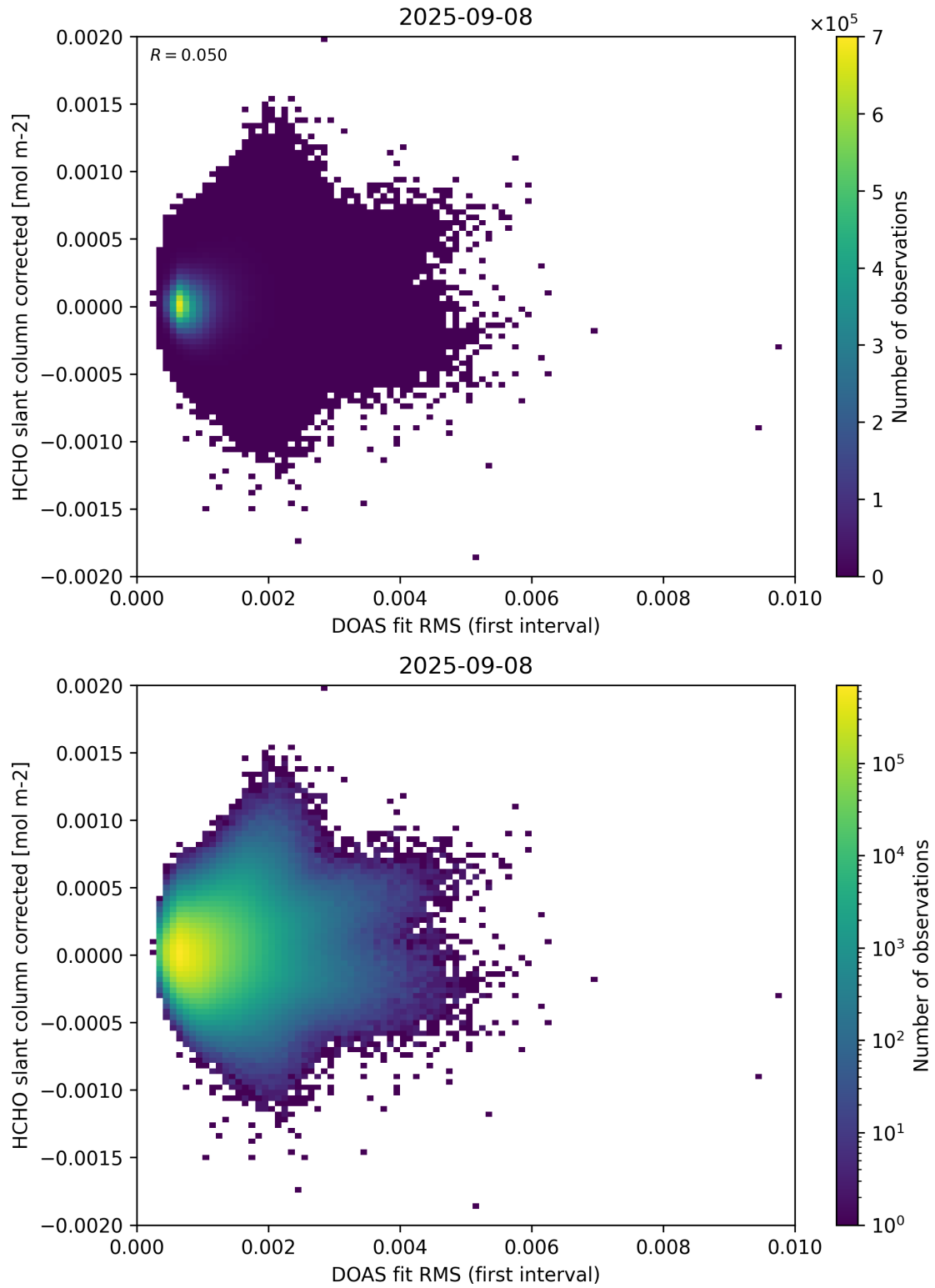
Figure 62: Scatter density plot of “DOAS fit RMS (first interval)” against “HCHO slant column corrected” for 2025-09-07 to 2025-09-09.
