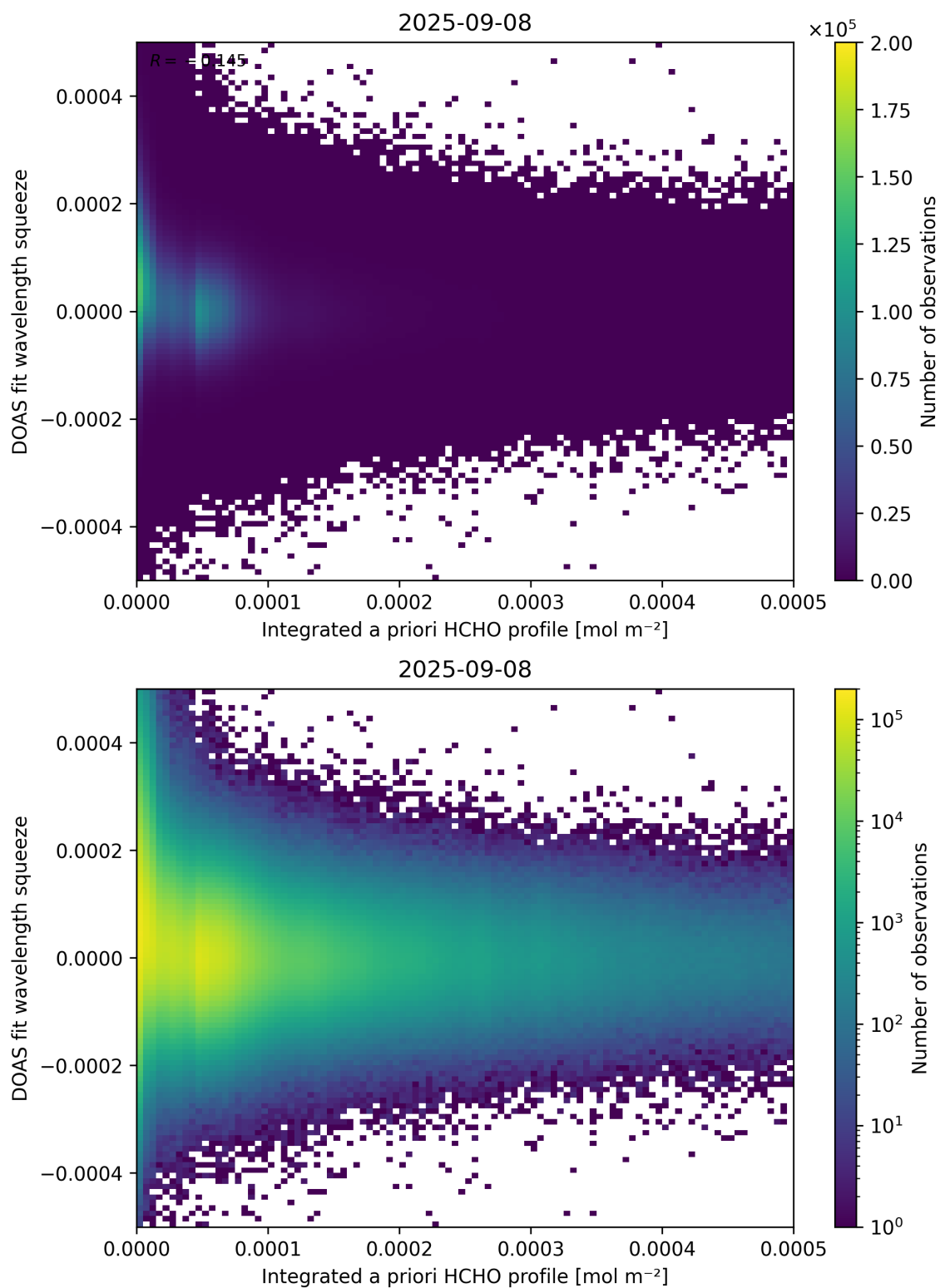
Figure 150: Scatter density plot of “Integrated a priori HCHO profile” against “DOAS fit wavelength squeeze” for 2025-09-07 to 2025-09-09.
