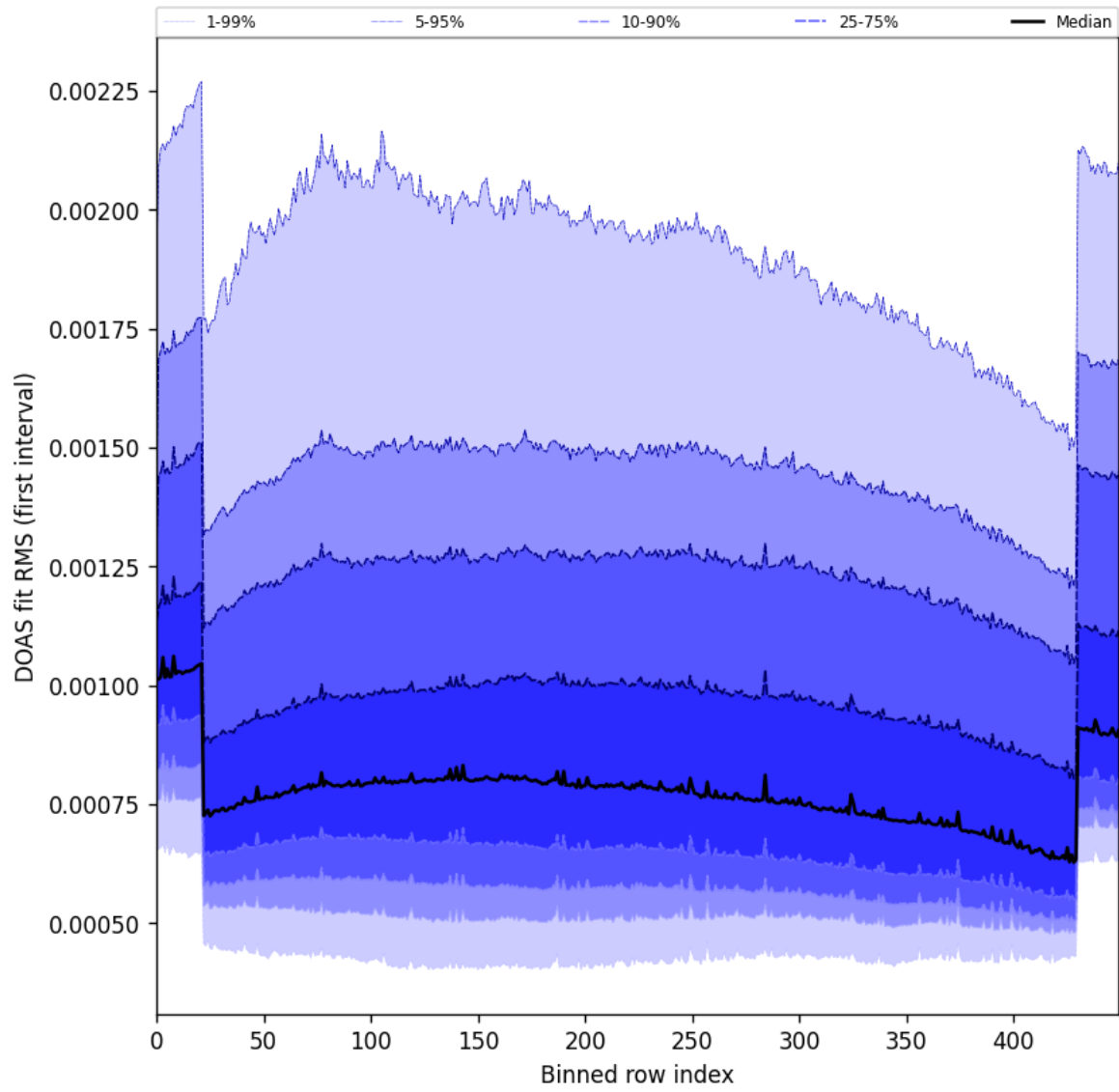
Figure 60: Along track statistics of “DOAS fit RMS (first interval)” for 2025-09-07 to 2025-09-09
