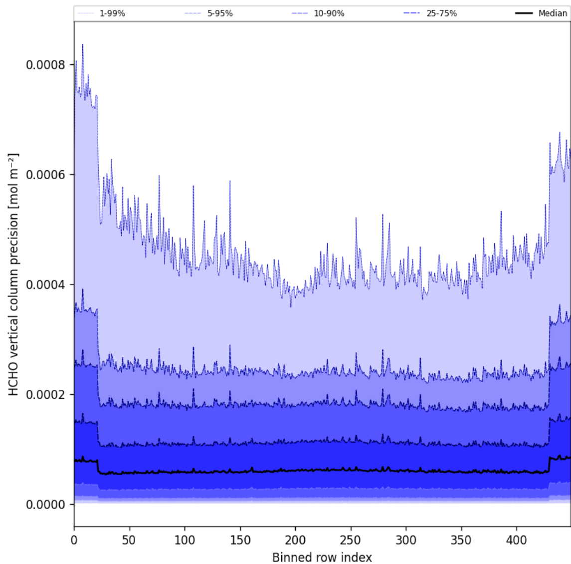
Figure 50: Along track statistics of “HCHO vertical column precision” for 2025-09-07 to 2025-09-09
