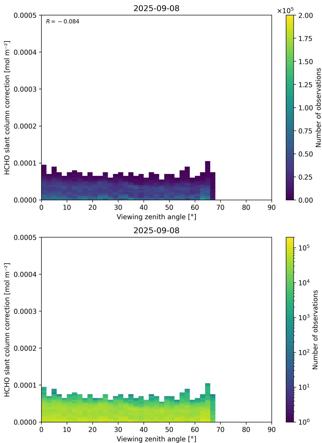
Figure 187: Scatter density plot of “Viewing zenith angle” against “HCHO slant column correction” for 2025-09-07 to 2025-09-09.
