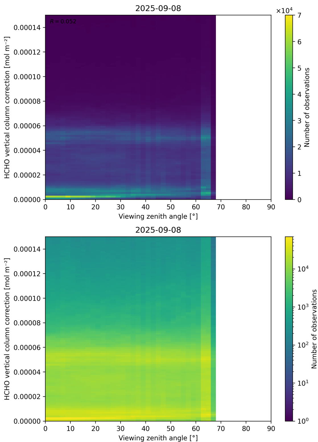
Figure 193: Scatter density plot of “Viewing zenith angle” against “HCHO vertical column correction” for 2025-09-07 to 2025-09-09.
