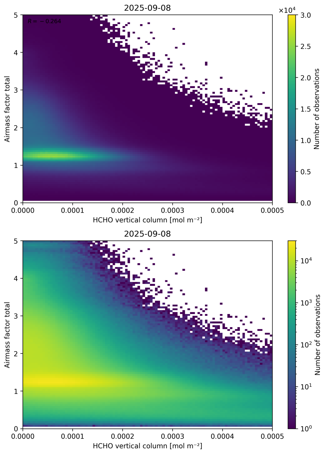
Figure 131: Scatter density plot of “HCHO vertical column” against “Airmass factor total” for 2025-09-07 to 2025-09-09.
