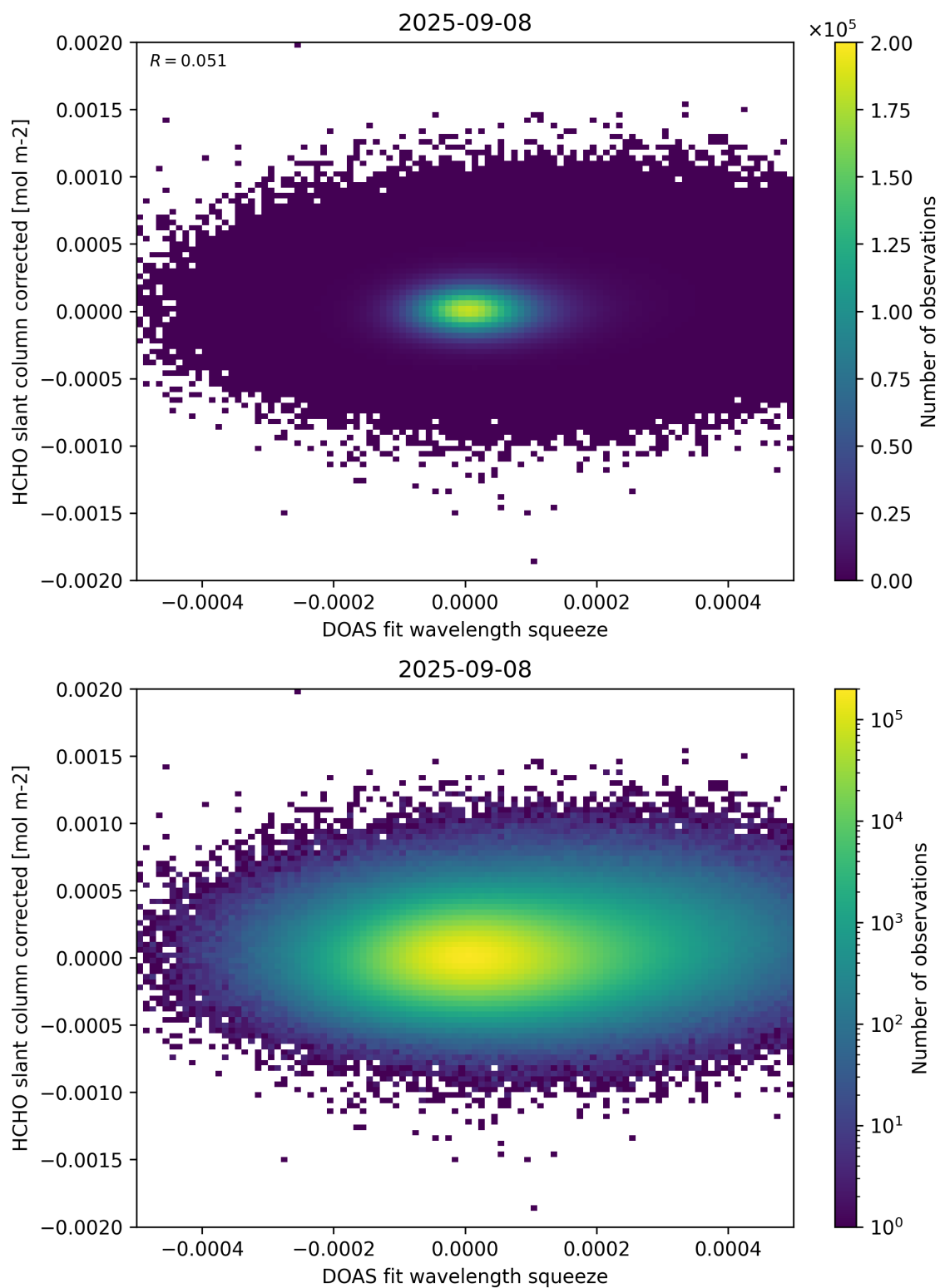
Figure 69: Scatter density plot of “DOAS fit wavelength squeeze” against “HCHO slant column corrected” for 2025-09-07 to 2025-09-09.
