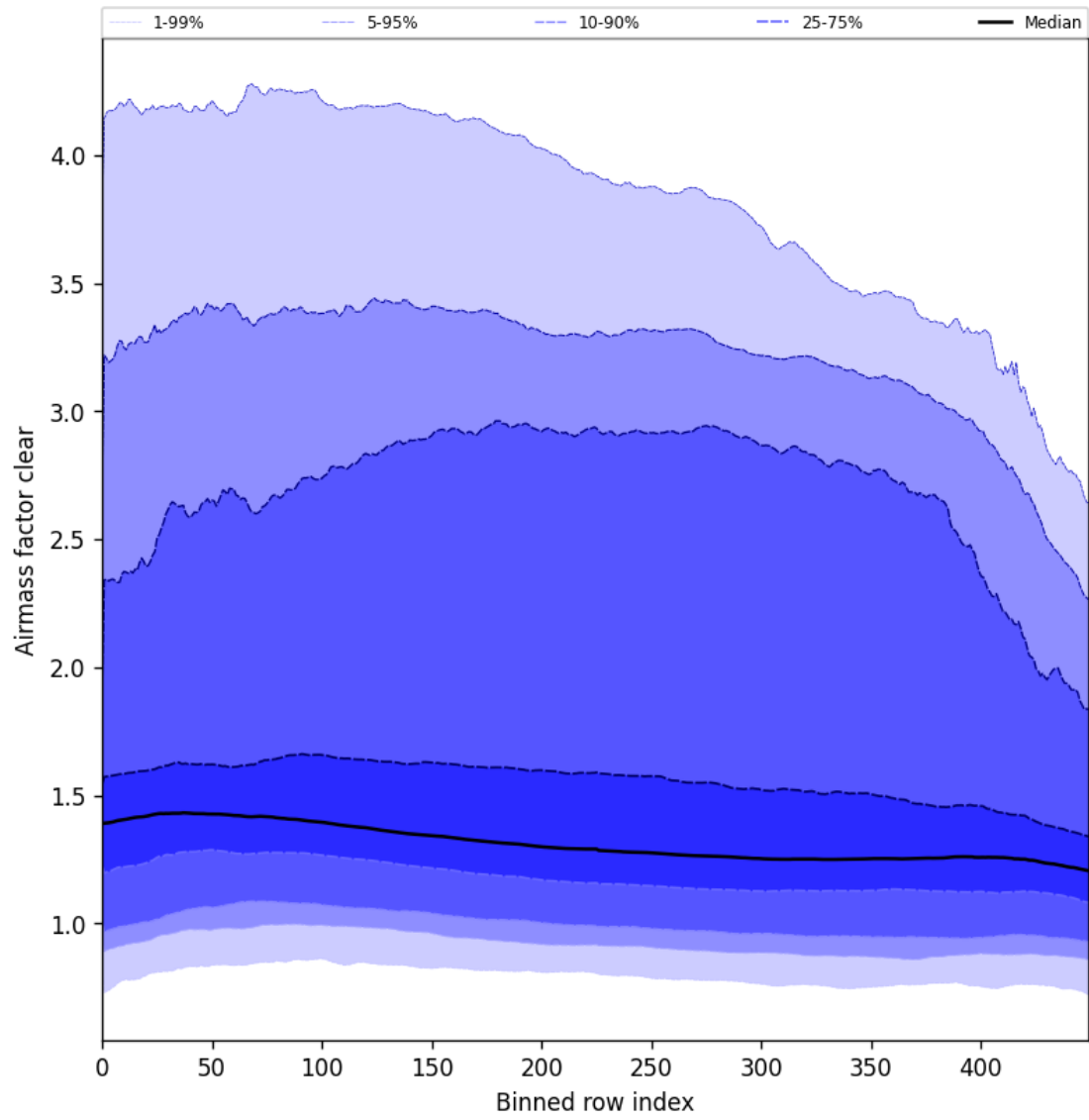
Figure 56: Along track statistics of “Airmass factor clear” for 2025-09-07 to 2025-09-09
