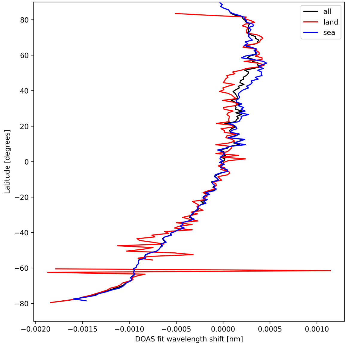
Figure 30: Zonal average of “DOAS fit wavelength shift” for 2025-09-07 to 2025-09-09.
