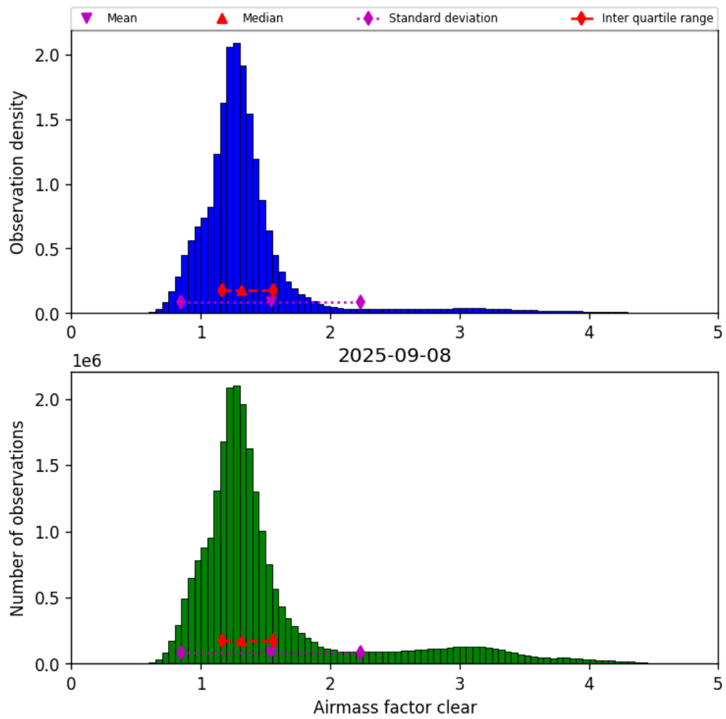
Figure 42: Histogram of “Airmass factor clear” for 2025-09-07 to 2025-09-09
