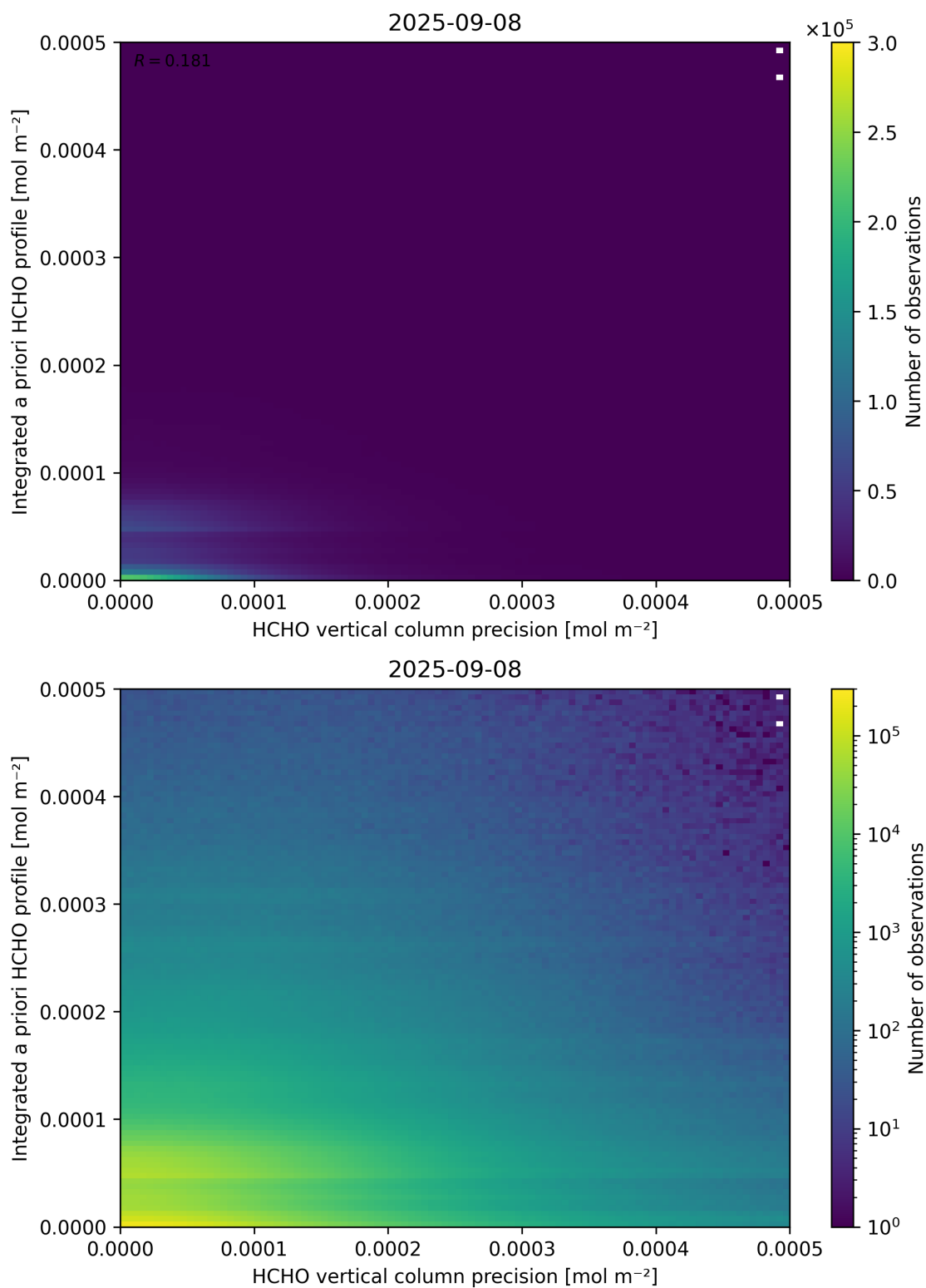
Figure 147: Scatter density plot of “HCHO vertical column precision” against “Integrated a priori HCHO profile” for 2025-09-07 to 2025-09-09.
