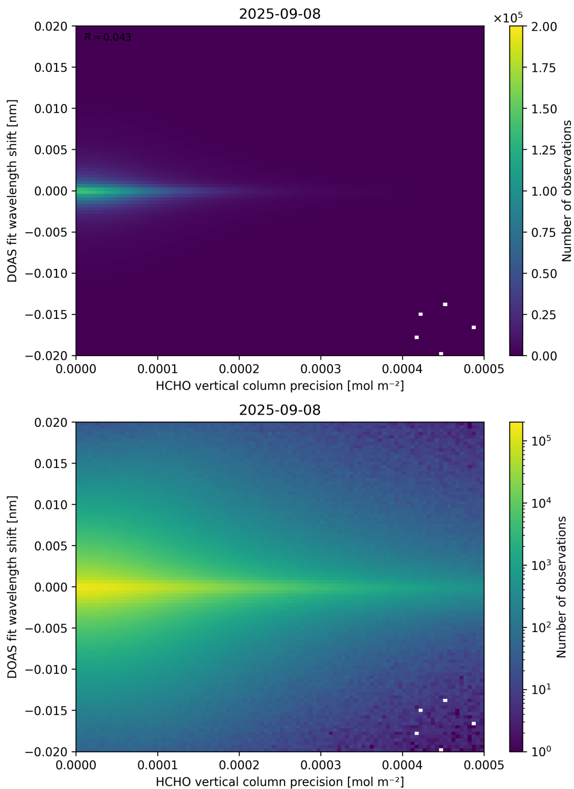
Figure 137: Scatter density plot of “HCHO vertical column precision” against “DOAS fit wavelength shift” for 2025-09-07 to 2025-09-09.
