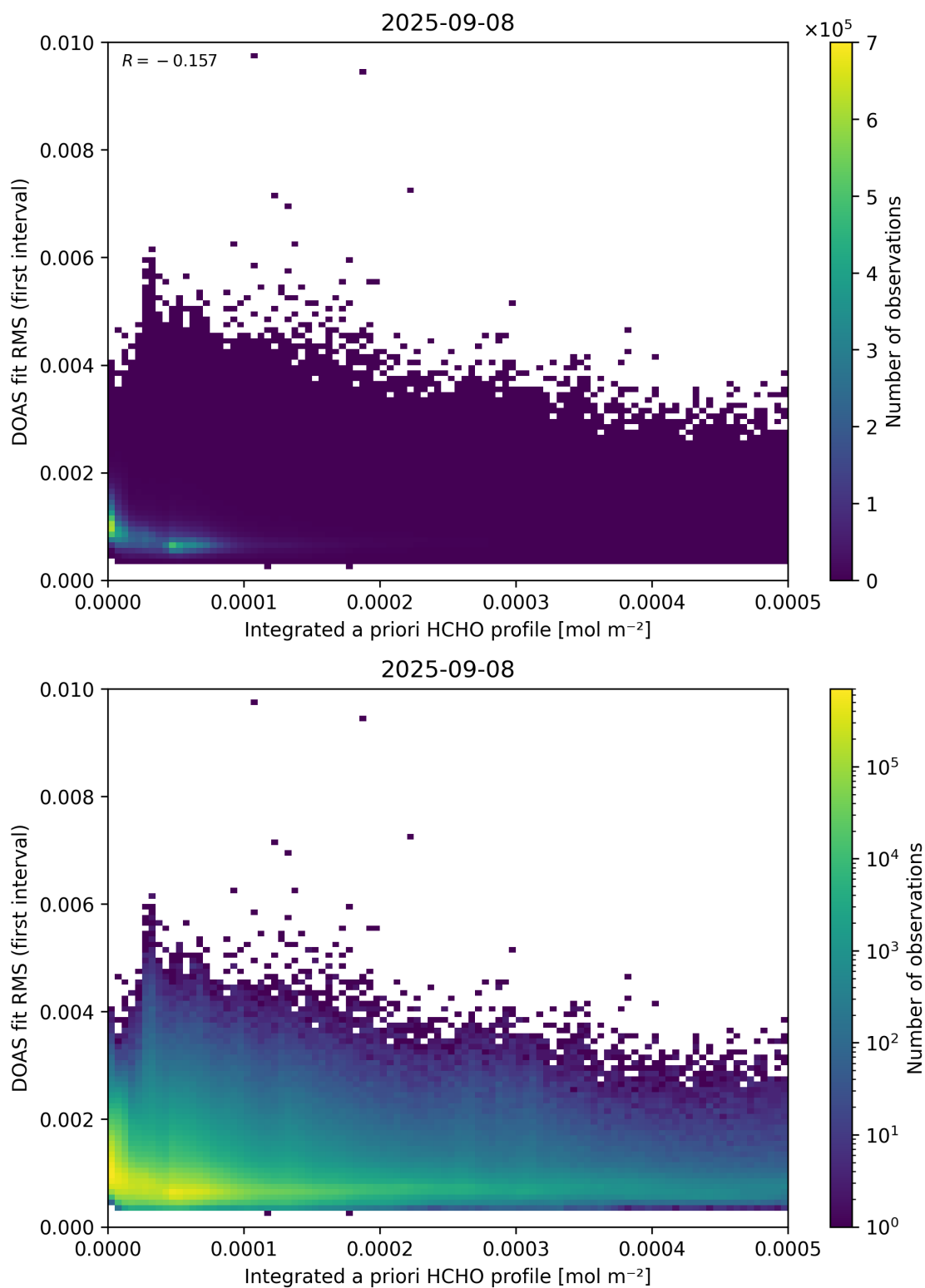
Figure 148: Scatter density plot of “Integrated a priori HCHO profile” against “DOAS fit RMS (first interval)” for 2025-09-07 to 2025-09-09.
