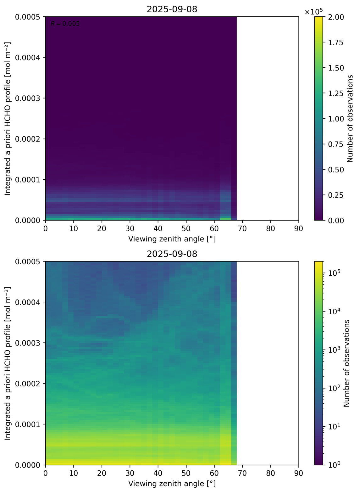
Figure 195: Scatter density plot of “Viewing zenith angle” against “Integrated a priori HCHO profile” for 2025-09-07 to 2025-09-09.
