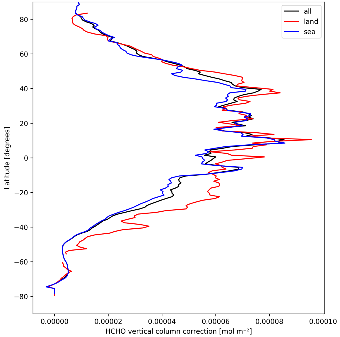
Figure 23: Zonal average of “HCHO vertical column correction” for 2025-09-07 to 2025-09-09.
