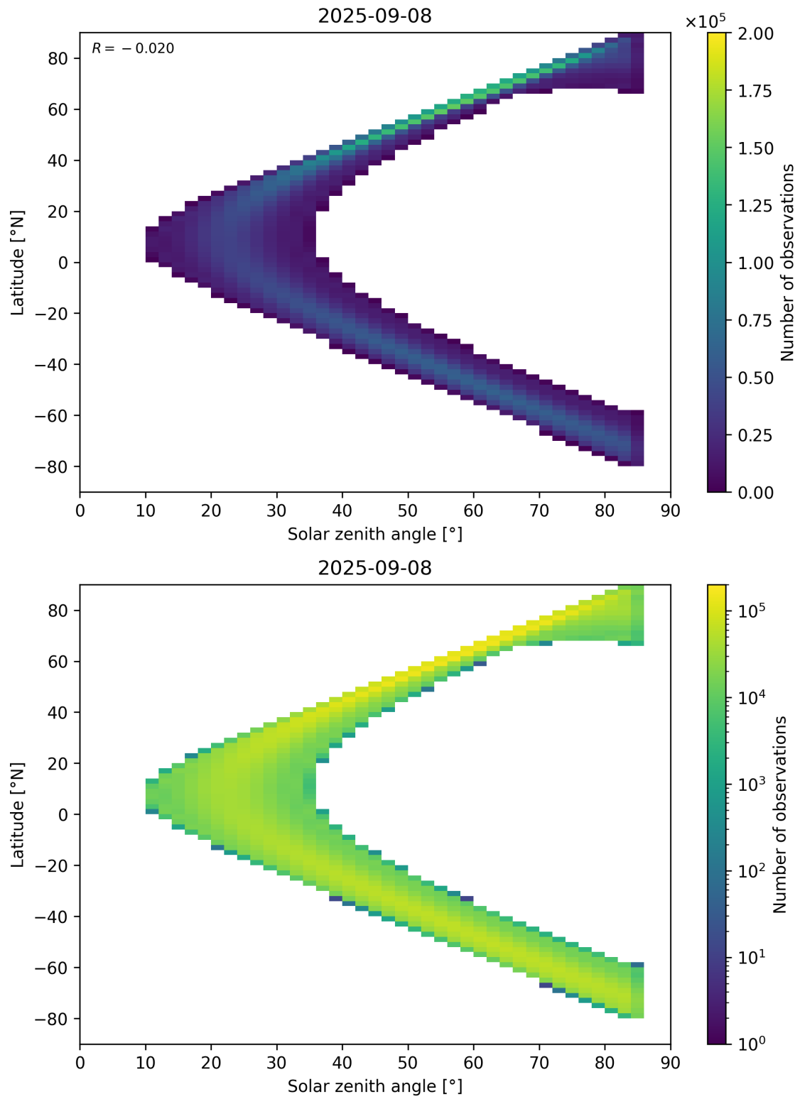
Figure 181: Scatter density plot of “Solar zenith angle” against “Latitude” for 2025-09-07 to 2025-09-09.
