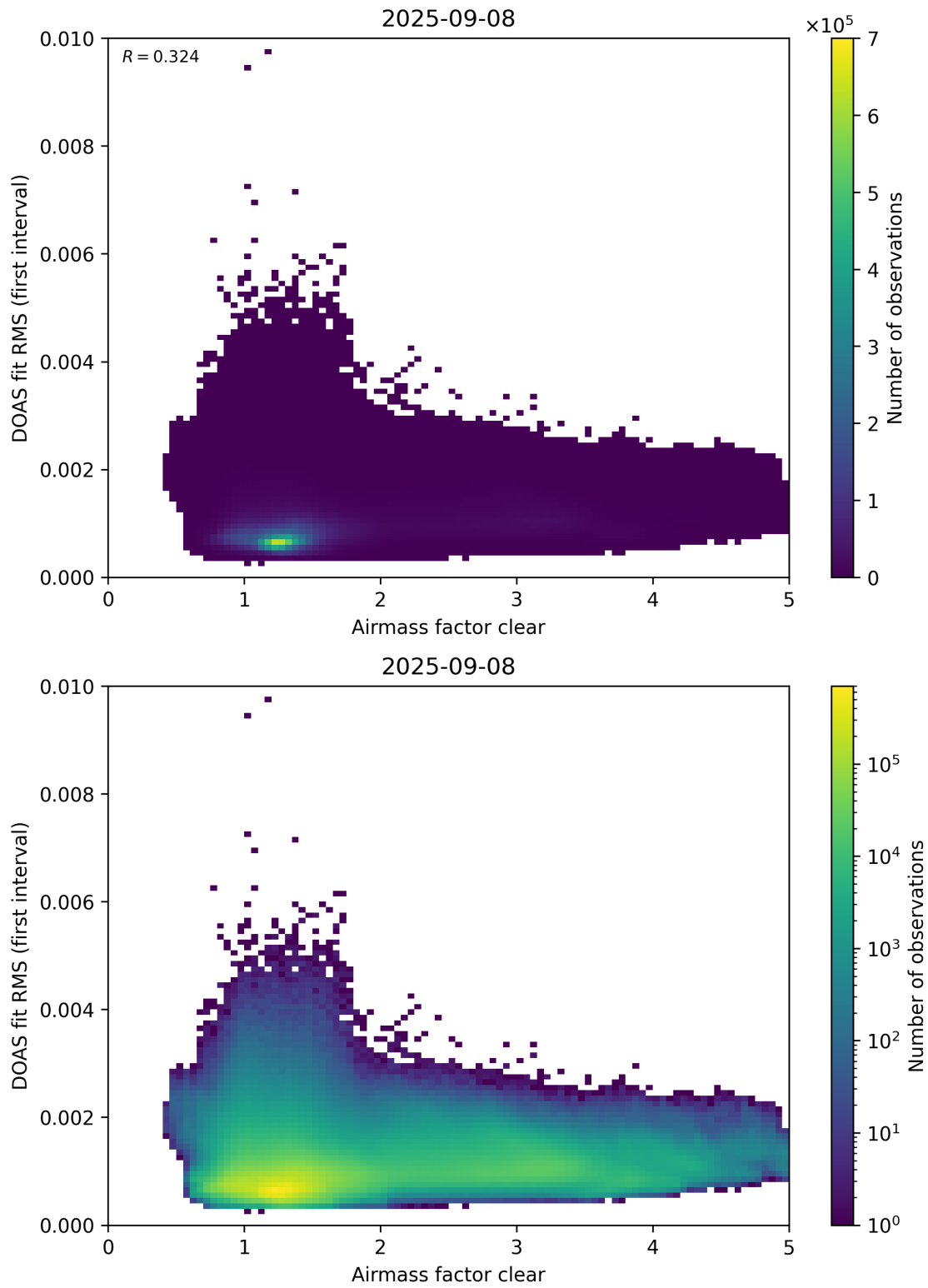
Figure 71: Scatter density plot of “Airmass factor clear” against “DOAS fit RMS (first interval)” for 2025-09-07 to 2025-09-09.
