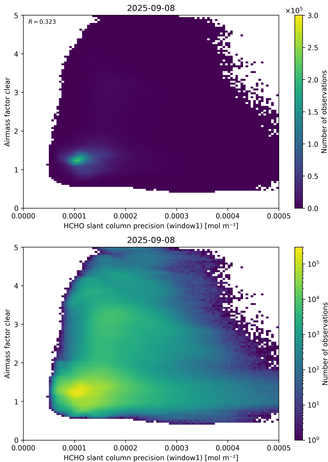
Figure 91: Scatter density plot of “HCHO slant column precision (window1)” against “Airmass factor clear” for 2025-09-07 to 2025-09-09.
