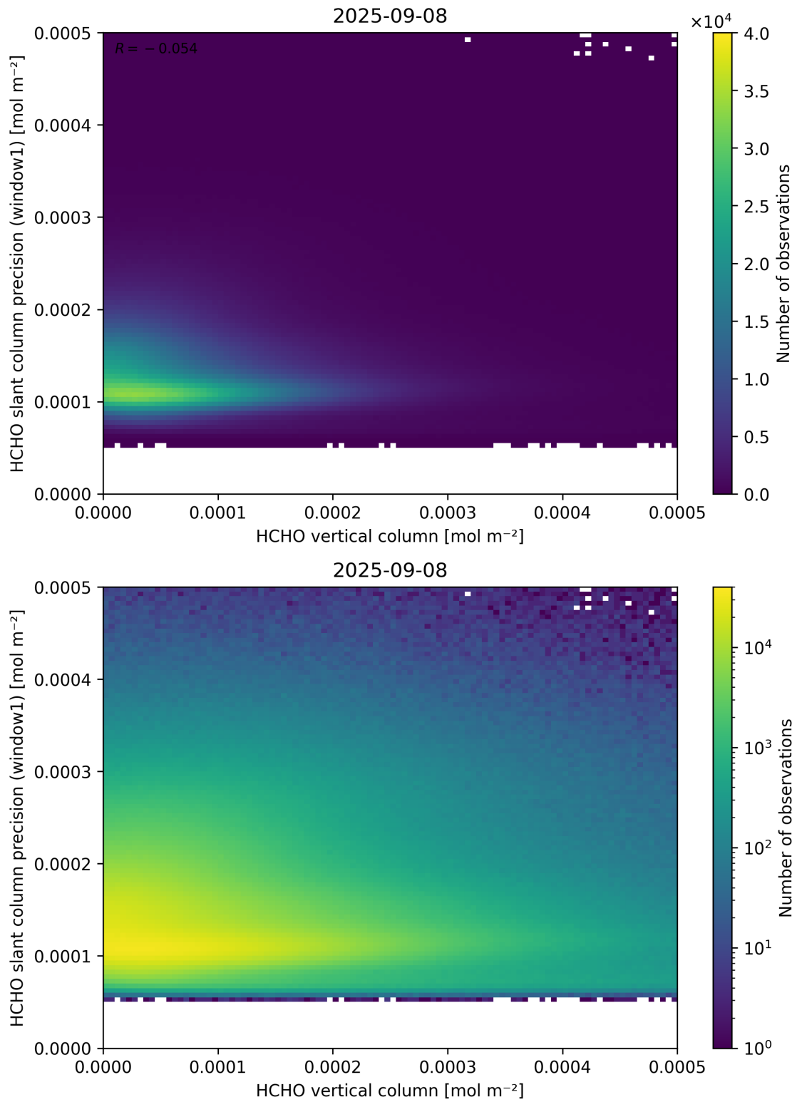
Figure 130: Scatter density plot of “HCHO vertical column” against “HCHO slant column precision (window1)” for 2025-09-07 to 2025-09-09.
