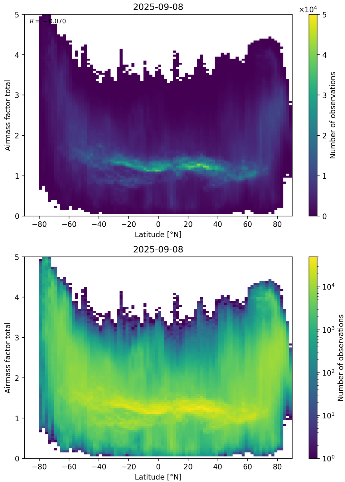
Figure 161: Scatter density plot of “Latitude” against “Airmass factor total” for 2025-09-07 to 2025-09-09.
