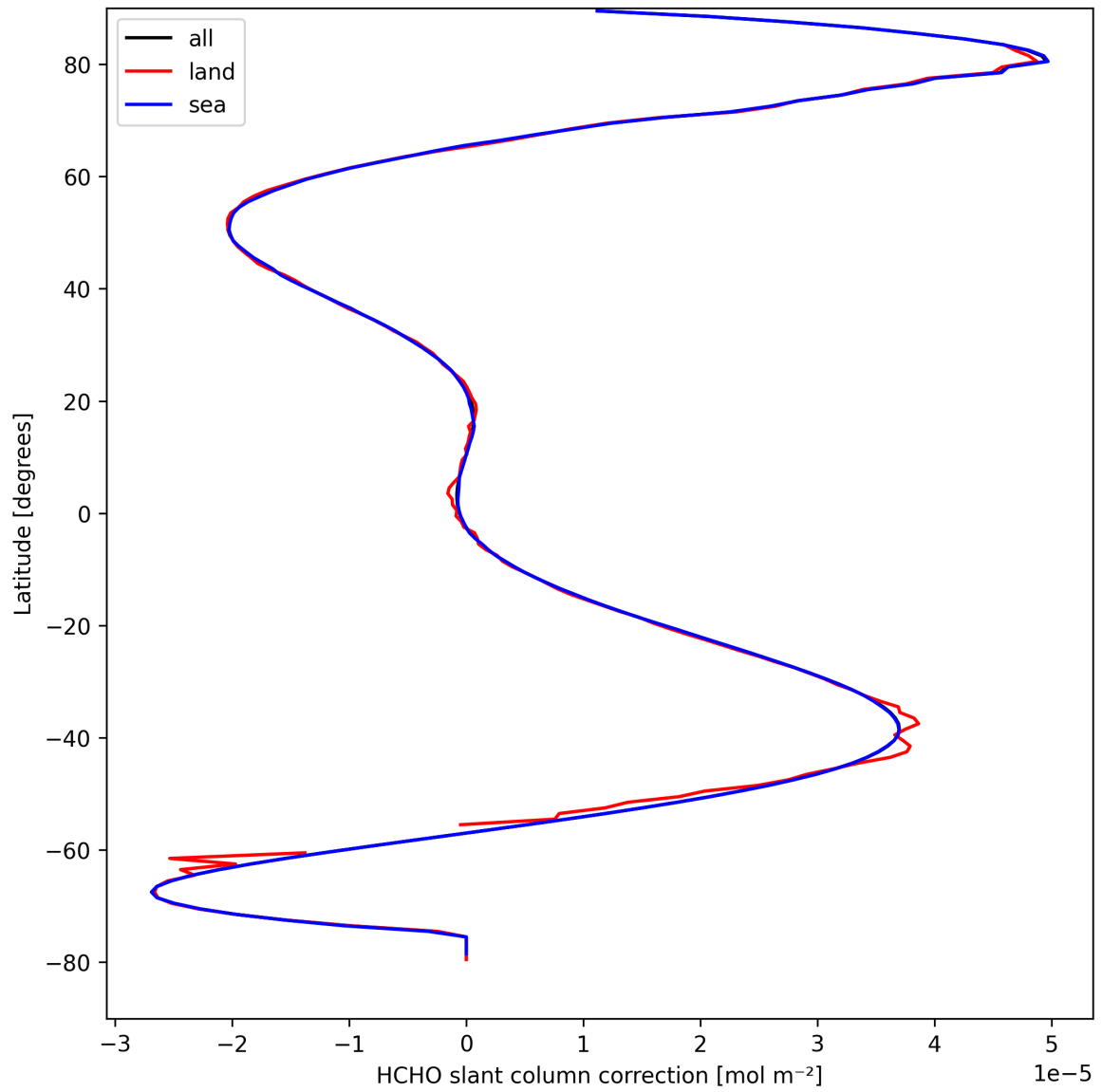
Figure 33: Zonal average of “HCHO slant column correction” for 2025-09-07 to 2025-09-09.
