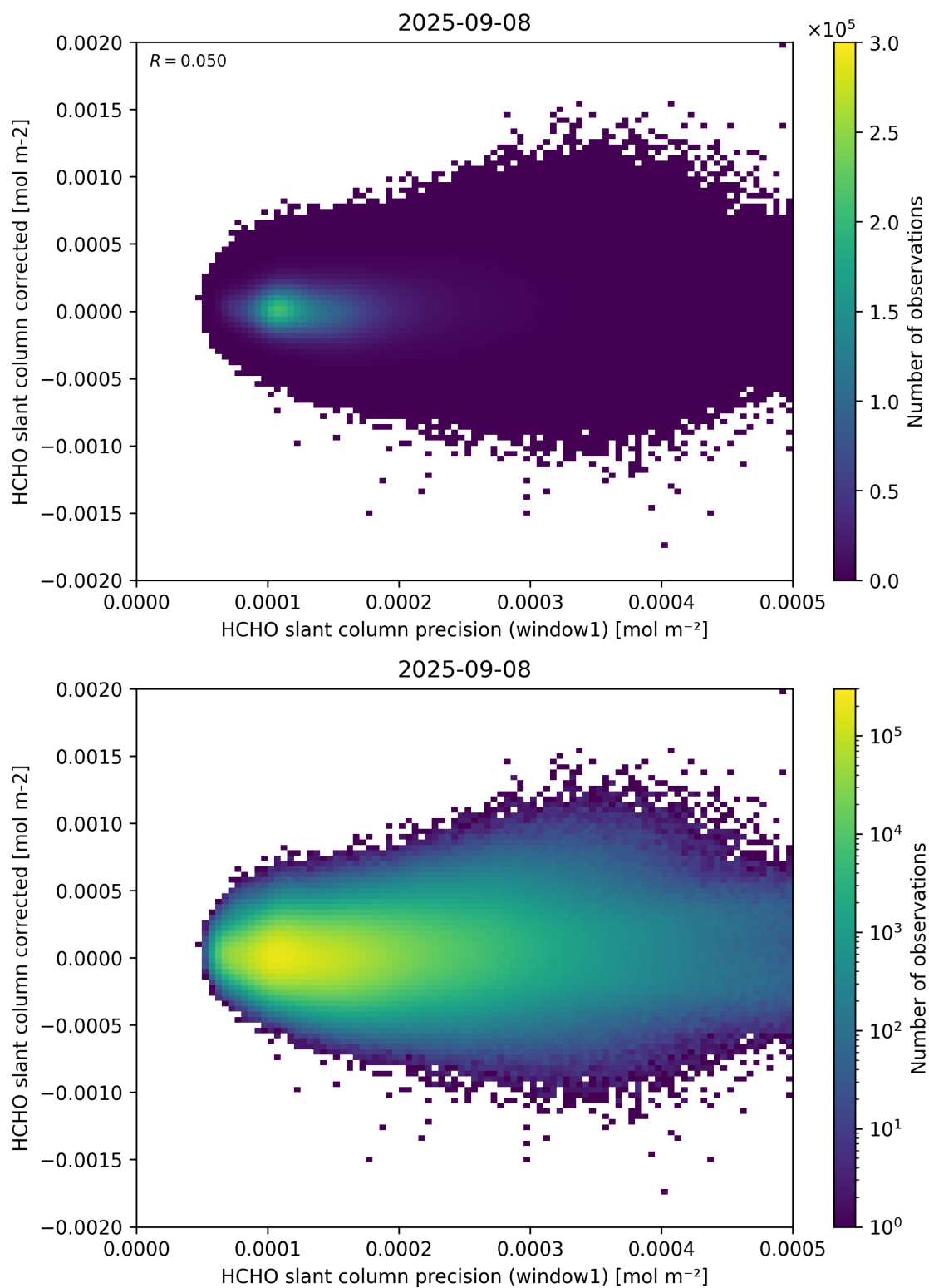
Figure 92: Scatter density plot of “HCHO slant column precision (window1)” against “HCHO slant column corrected” for 2025-09-07 to 2025-09-09.
