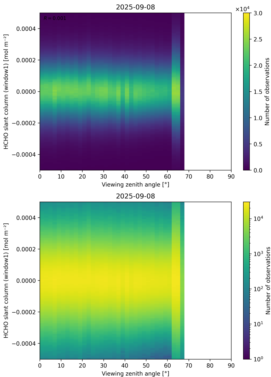
Figure 188: Scatter density plot of “Viewing zenith angle” against “HCHO slant column (window1)” for 2025-09-07 to 2025-09-09.
