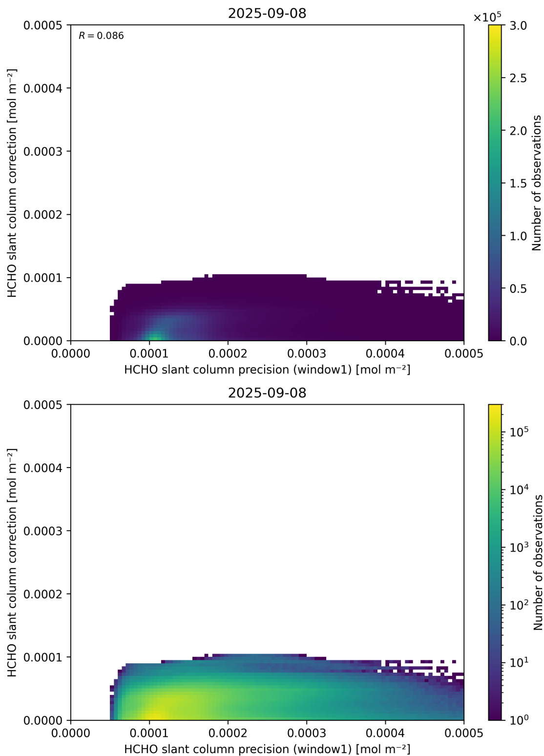
Figure 93: Scatter density plot of “HCHO slant column precision (window1)” against “HCHO slant column correction” for 2025-09-07 to 2025-09-09.
