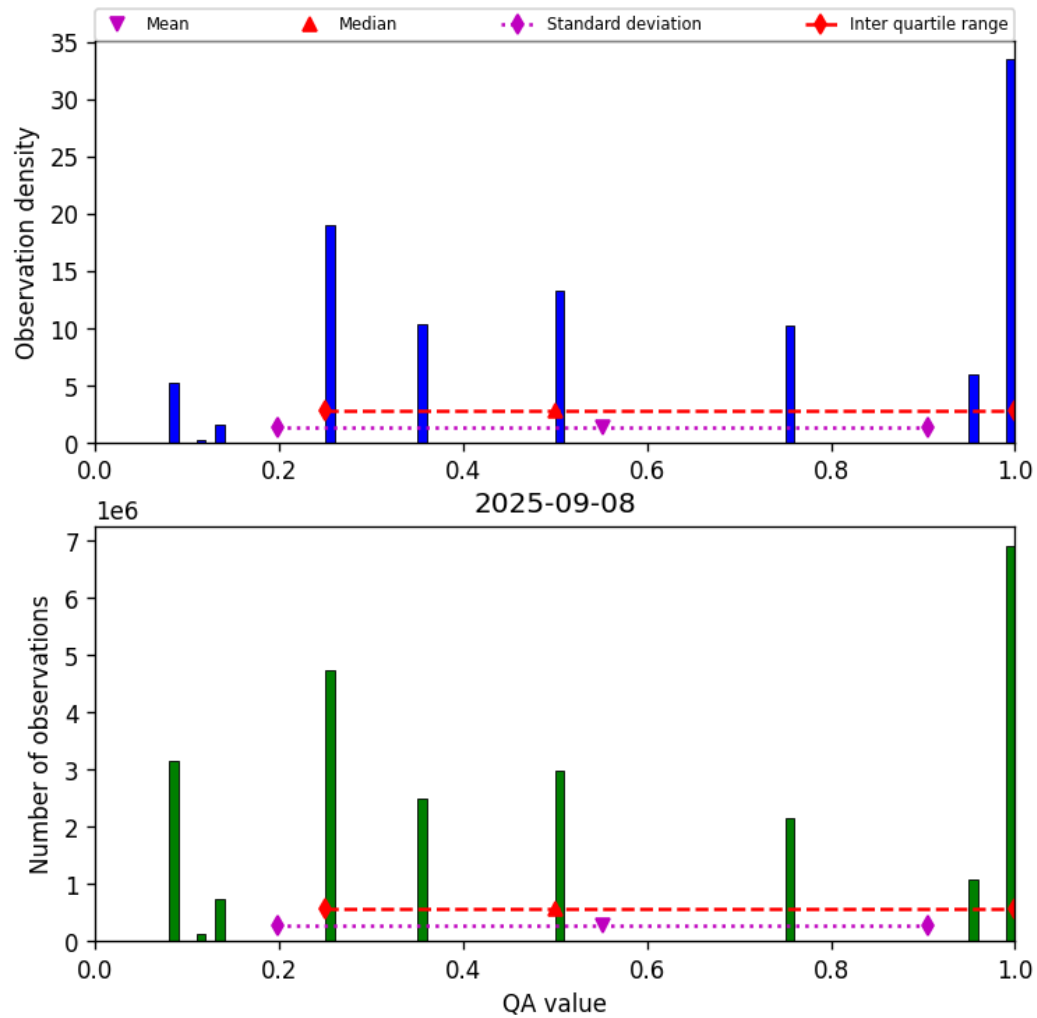
Figure 34: Histogram of “QA value” for 2025-09-07 to 2025-09-09
