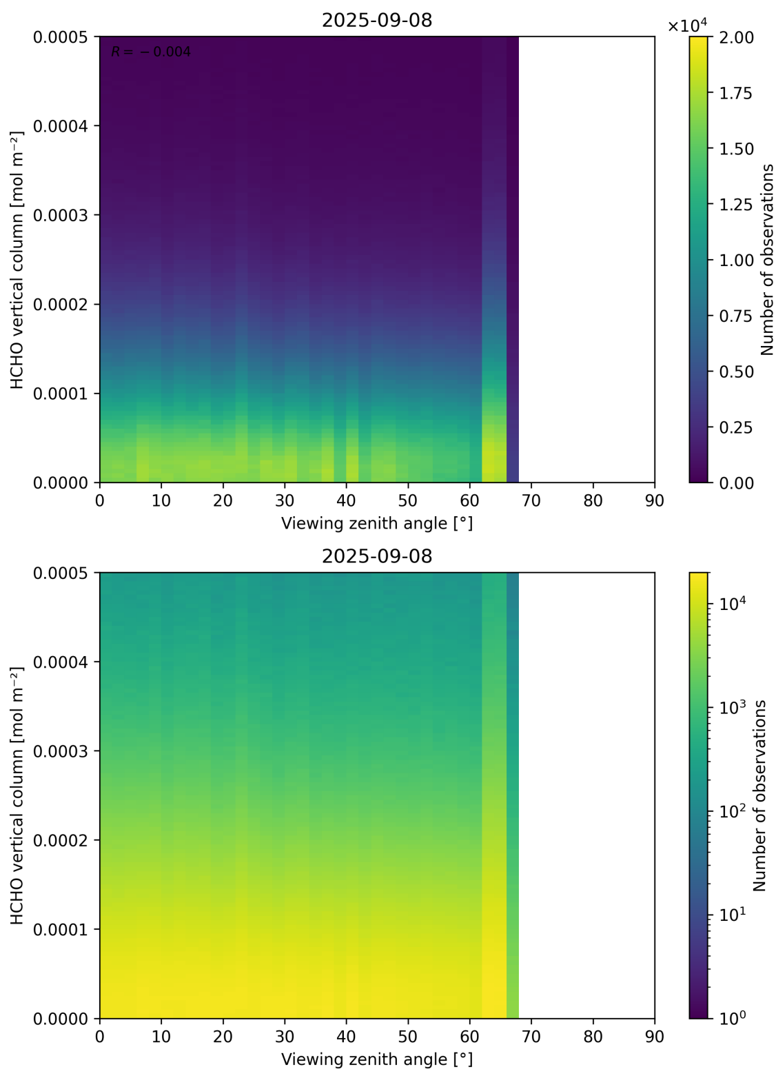
Figure 192: Scatter density plot of “Viewing zenith angle” against “HCHO vertical column” for 2025-09-07 to 2025-09-09.
