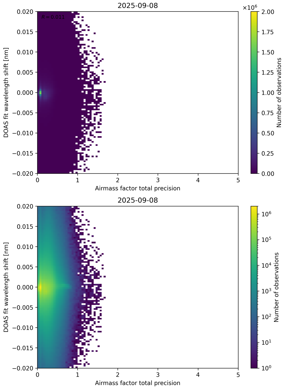
Figure 106: Scatter density plot of “Airmass factor total precision” against “DOAS fit wavelength shift” for 2025-09-07 to 2025-09-09.
