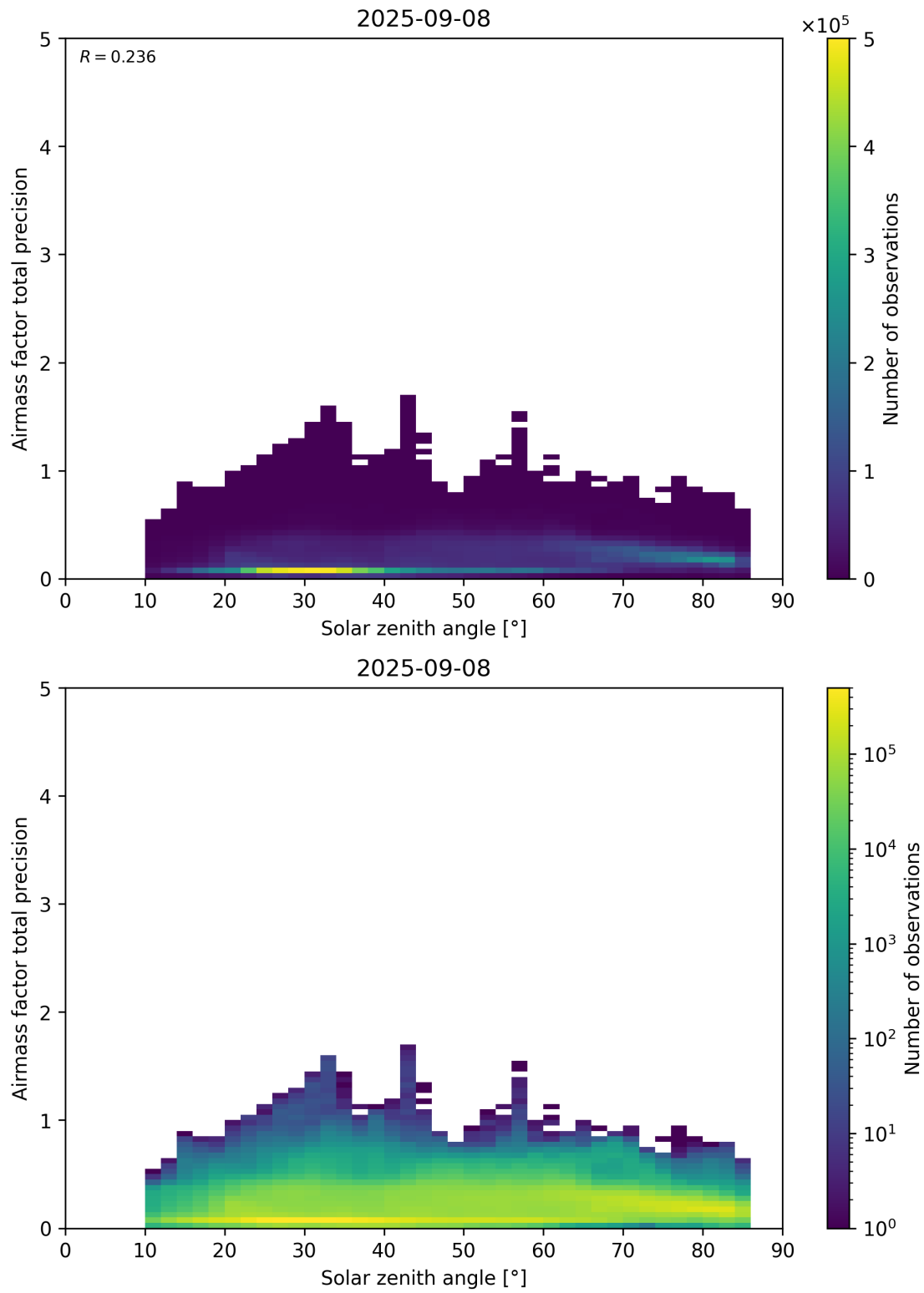
Figure 176: Scatter density plot of “Solar zenith angle” against “Airmass factor total precision” for 2025-09-07 to 2025-09-09.
