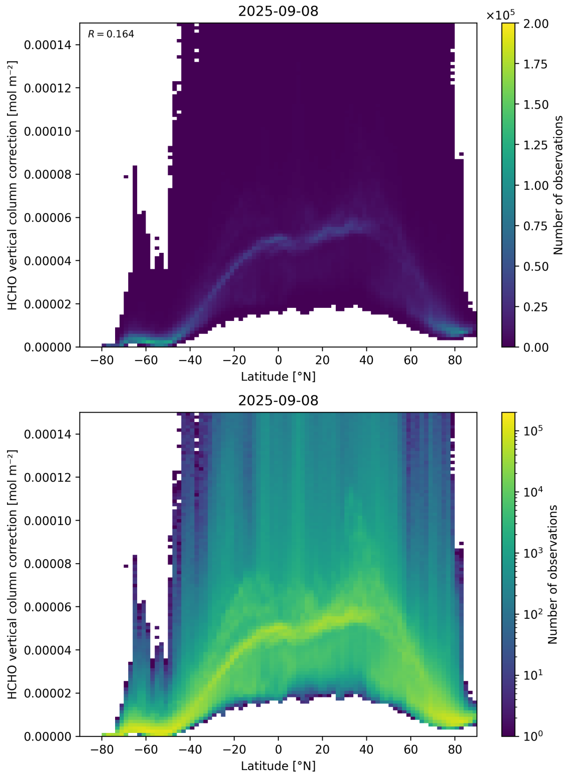
Figure 164: Scatter density plot of “Latitude” against “HCHO vertical column correction” for 2025-09-07 to 2025-09-09.
