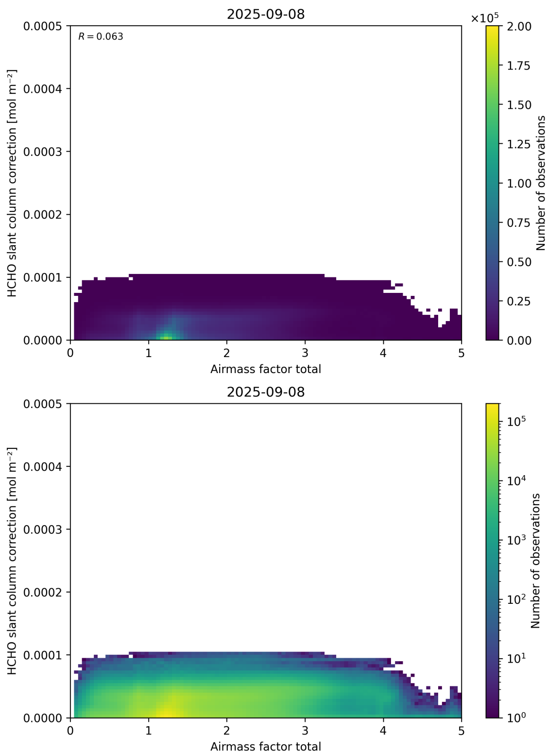
Figure 102: Scatter density plot of “Airmass factor total” against “HCHO slant column correction” for 2025-09-07 to 2025-09-09.
