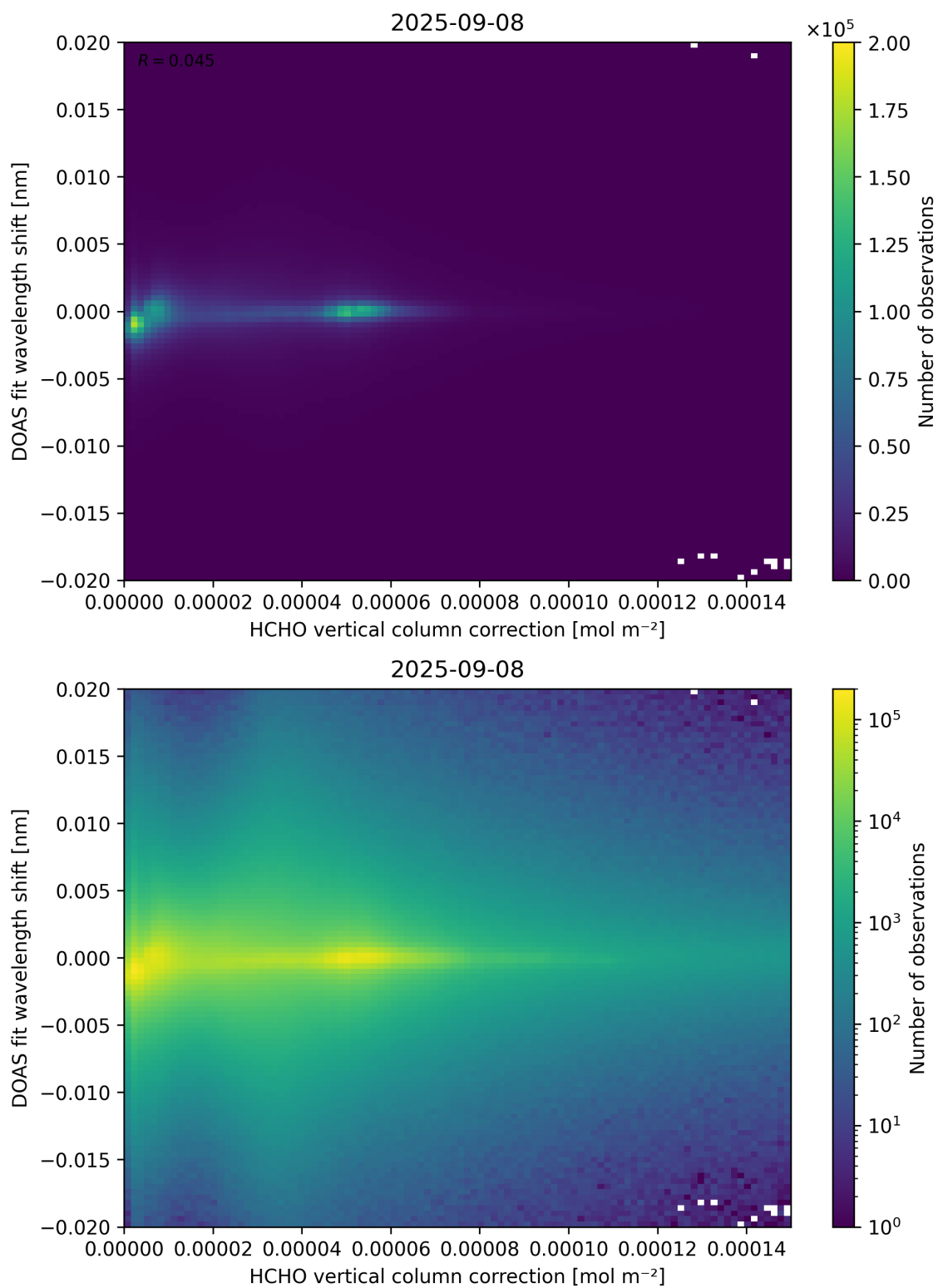
Figure 113: Scatter density plot of “HCHO vertical column correction” against “DOAS fit wavelength shift” for 2025-09-07 to 2025-09-09.
