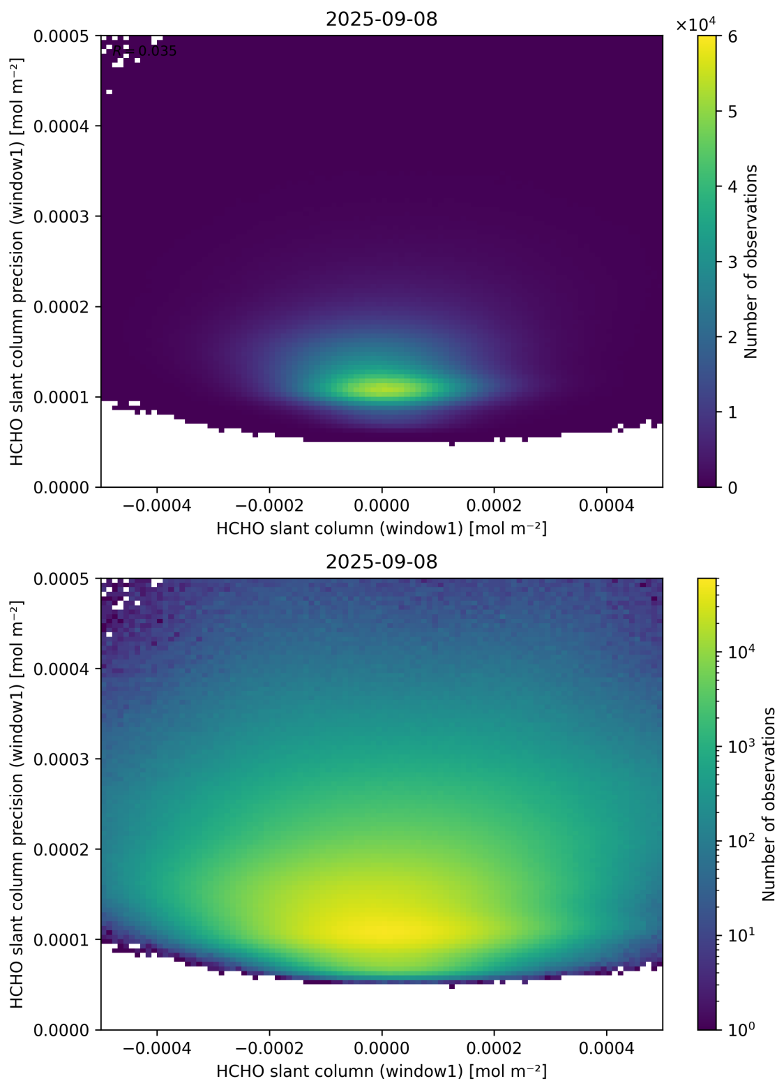
Figure 84: Scatter density plot of “HCHO slant column (window1)” against “HCHO slant column precision (window1)” for 2025-09-07 to 2025-09-09.
