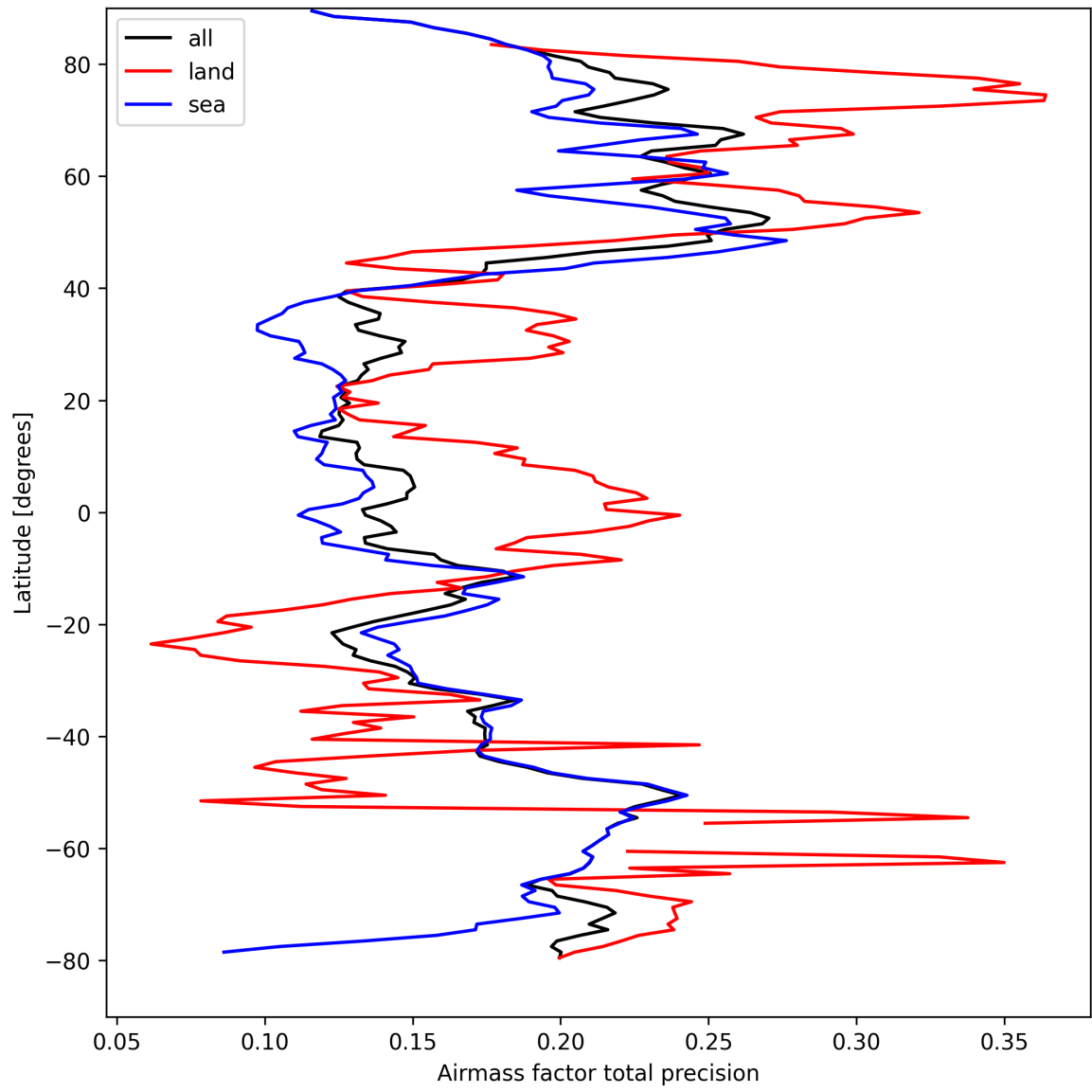
Figure 27: Zonal average of “Airmass factor total precision” for 2025-09-07 to 2025-09-09.
