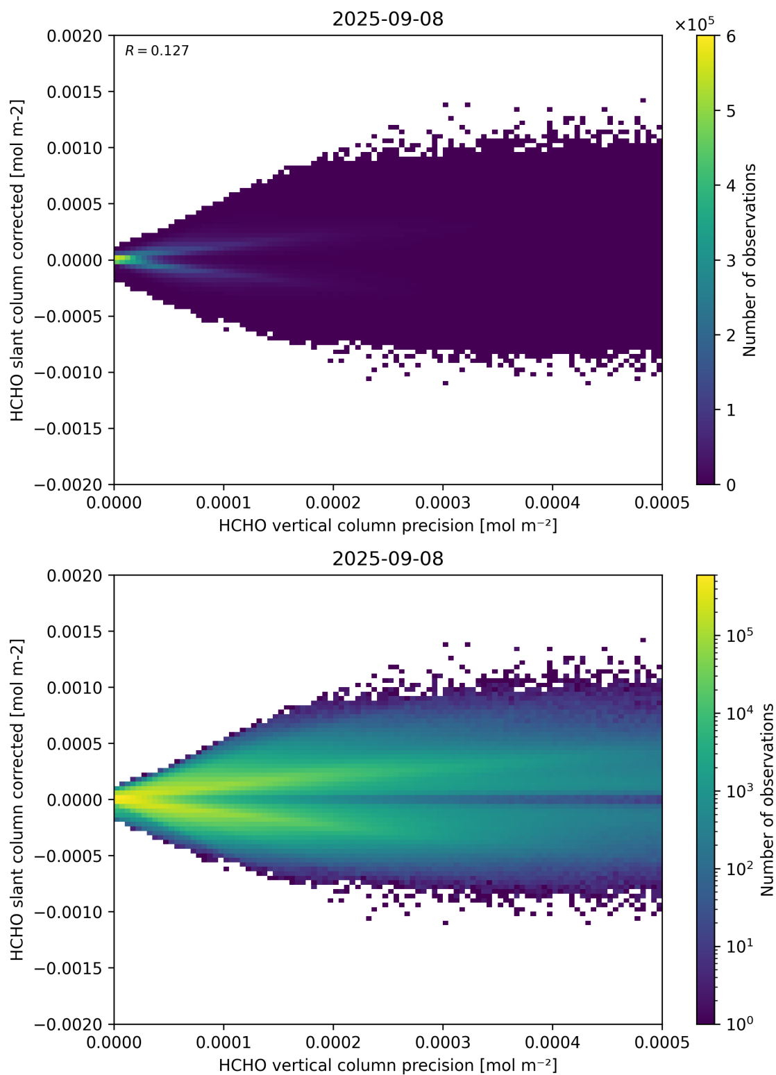
Figure 140: Scatter density plot of “HCHO vertical column precision” against “HCHO slant column corrected” for 2025-09-07 to 2025-09-09.
