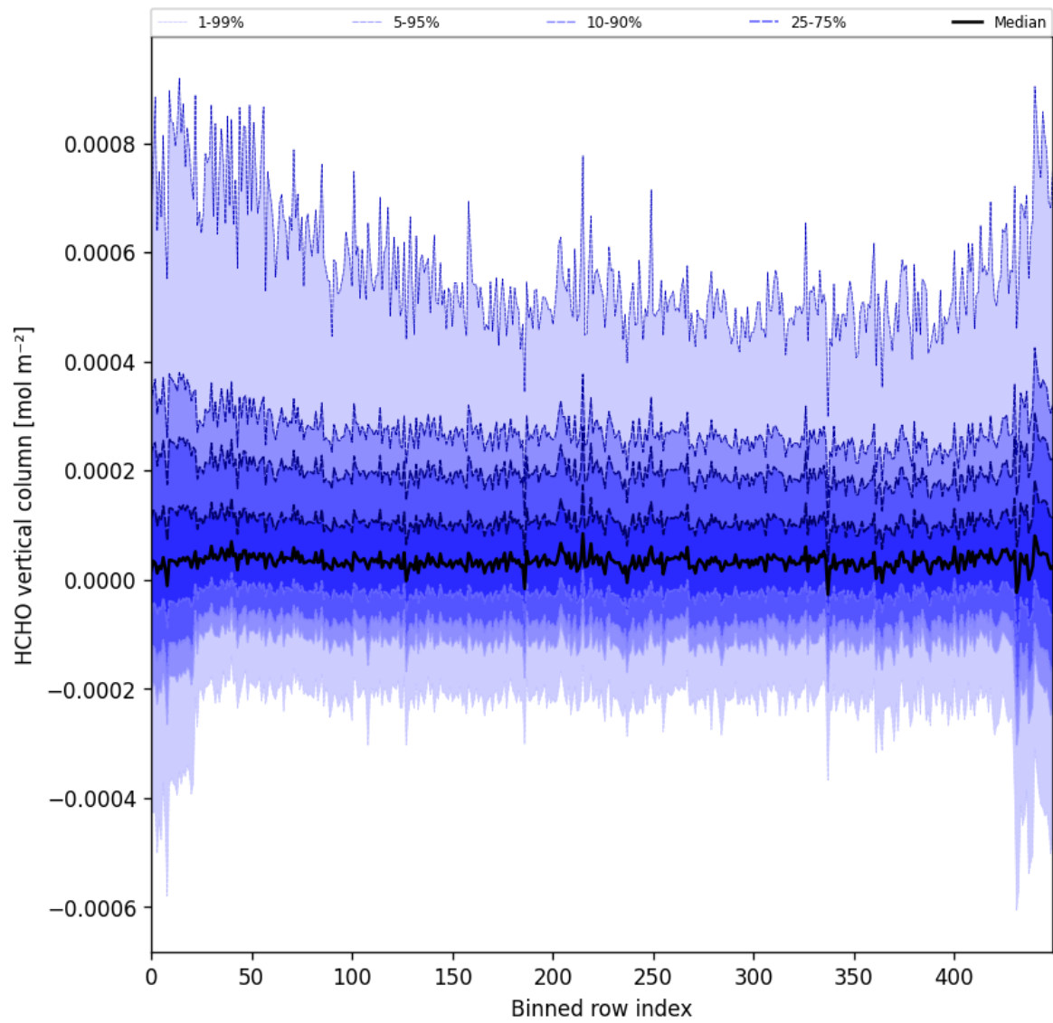
Figure 49: Along track statistics of “HCHO vertical column” for 2025-09-10 to 2025-09-12
