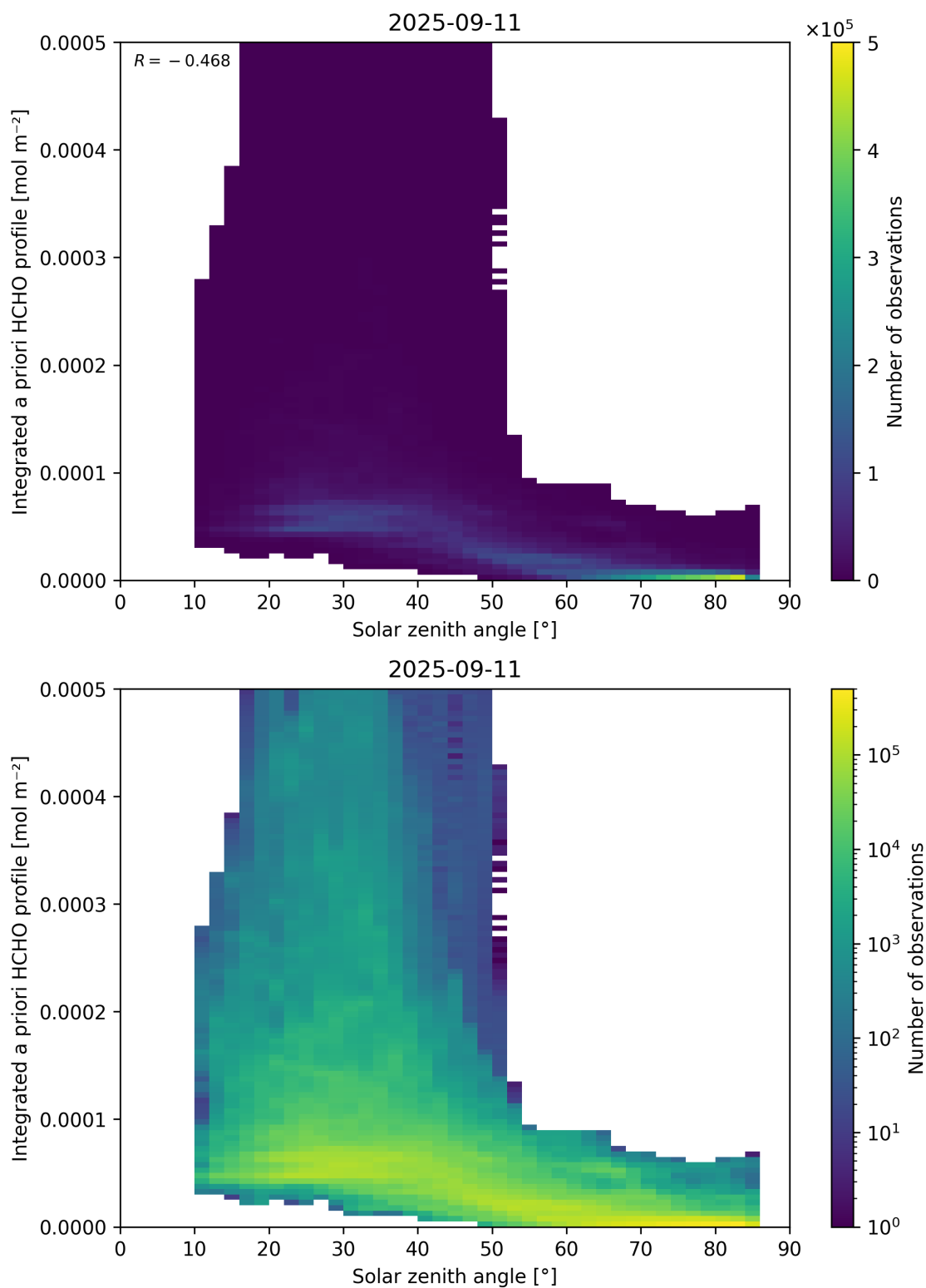
Figure 180: Scatter density plot of “Solar zenith angle” against “Integrated a priori HCHO profile” for 2025-09-10 to 2025-09-12.
