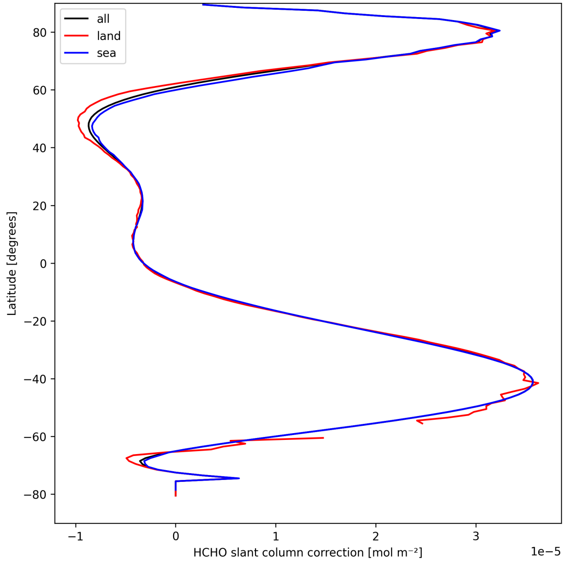
Figure 33: Zonal average of "HCHO slant column correction" for 2025-09-10 to 2025-09-12.
