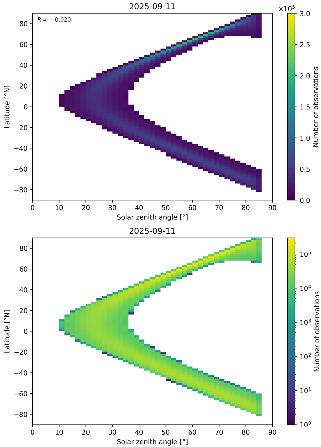
Figure 181: Scatter density plot of “Solar zenith angle” against “Latitude” for 2025-09-10 to 2025-09-12.
