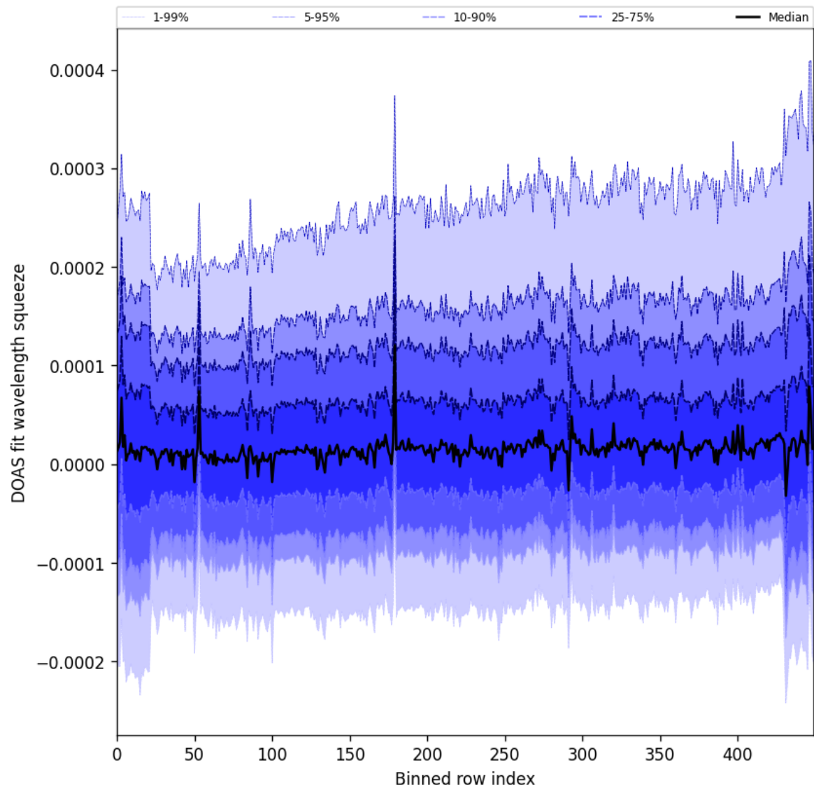
Figure 59: Along track statistics of “DOAS fit wavelength squeeze” for 2025-09-10 to 2025-09-12
