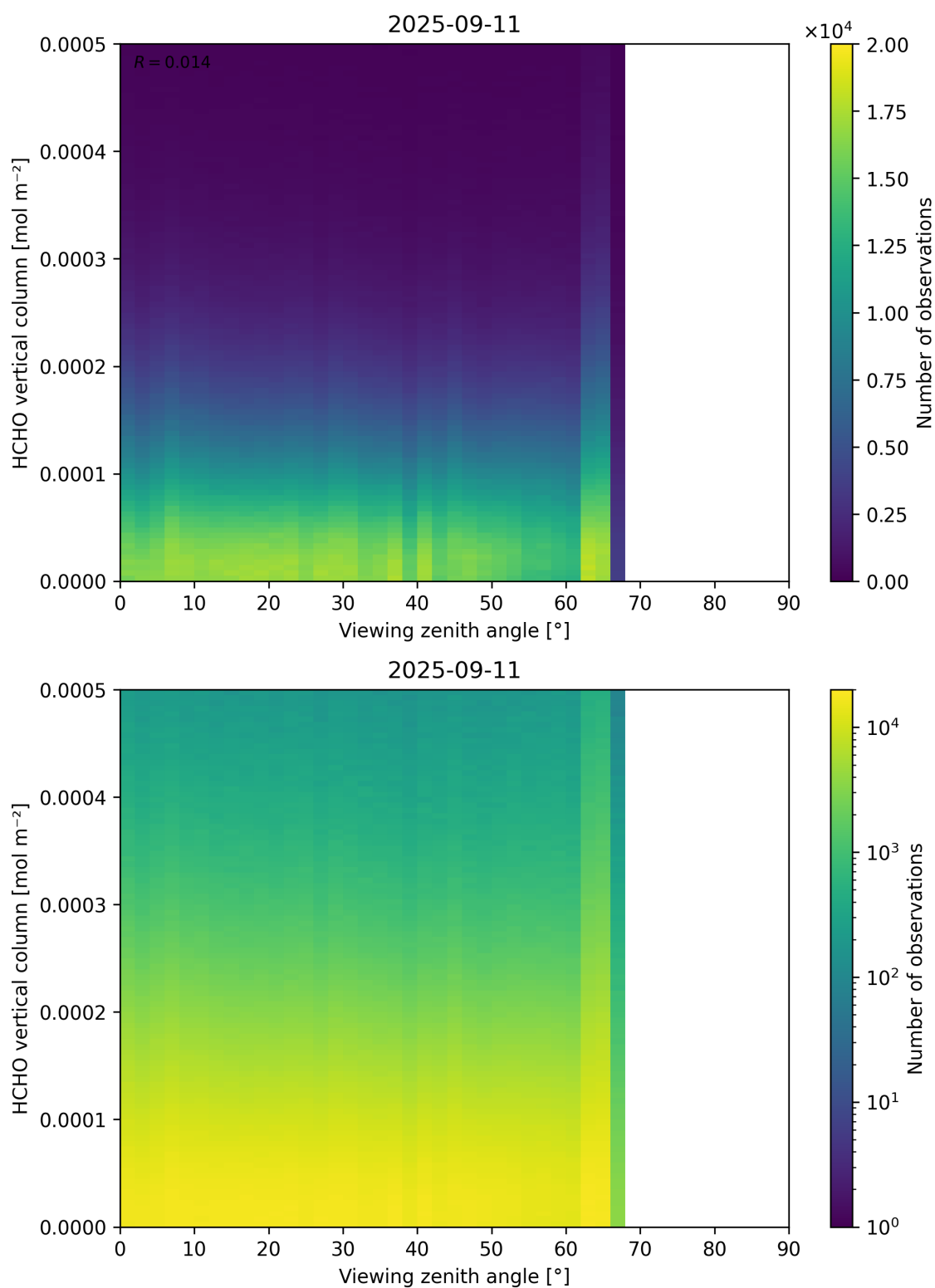
Figure 192: Scatter density plot of “Viewing zenith angle” against “HCHO vertical column” for 2025-09-10 to 2025-09-12.
