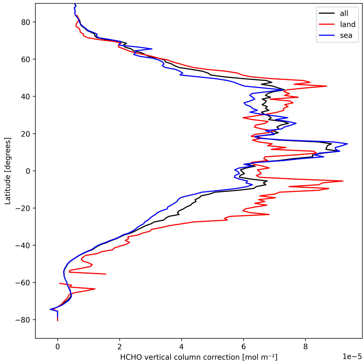
Figure 23: Zonal average of “HCHO vertical column correction” for 2025-09-10 to 2025-09-12.
