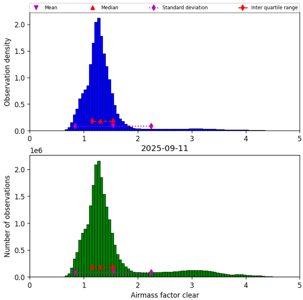
Figure 42: Histogram of “Airmass factor clear” for 2025-09-10 to 2025-09-12
