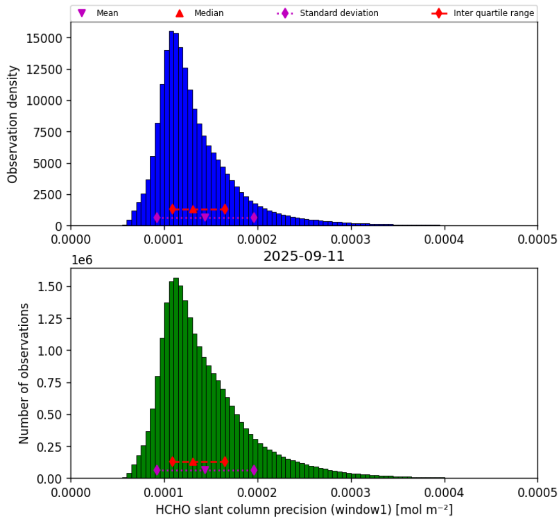
Figure 39: Histogram of “HCHO slant column precision (window1)” for 2025-09-10 to 2025-09-12
