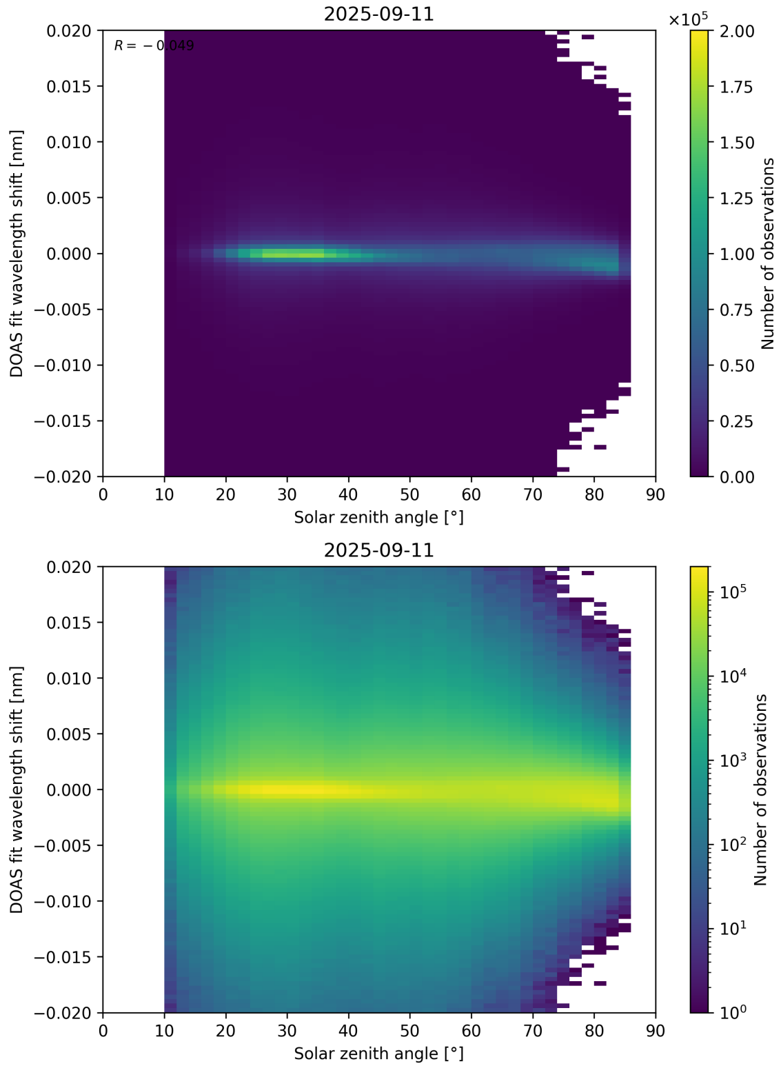
Figure 168: Scatter density plot of “Solar zenith angle” against “DOAS fit wavelength shift” for 2025-09-10 to 2025-09-12.
