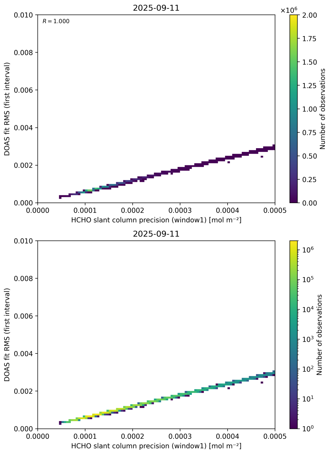
Figure 88: Scatter density plot of “HCHO slant column precision (window1)” against “DOAS fit RMS (first interval)” for 2025-09-10 to 2025-09-12.
