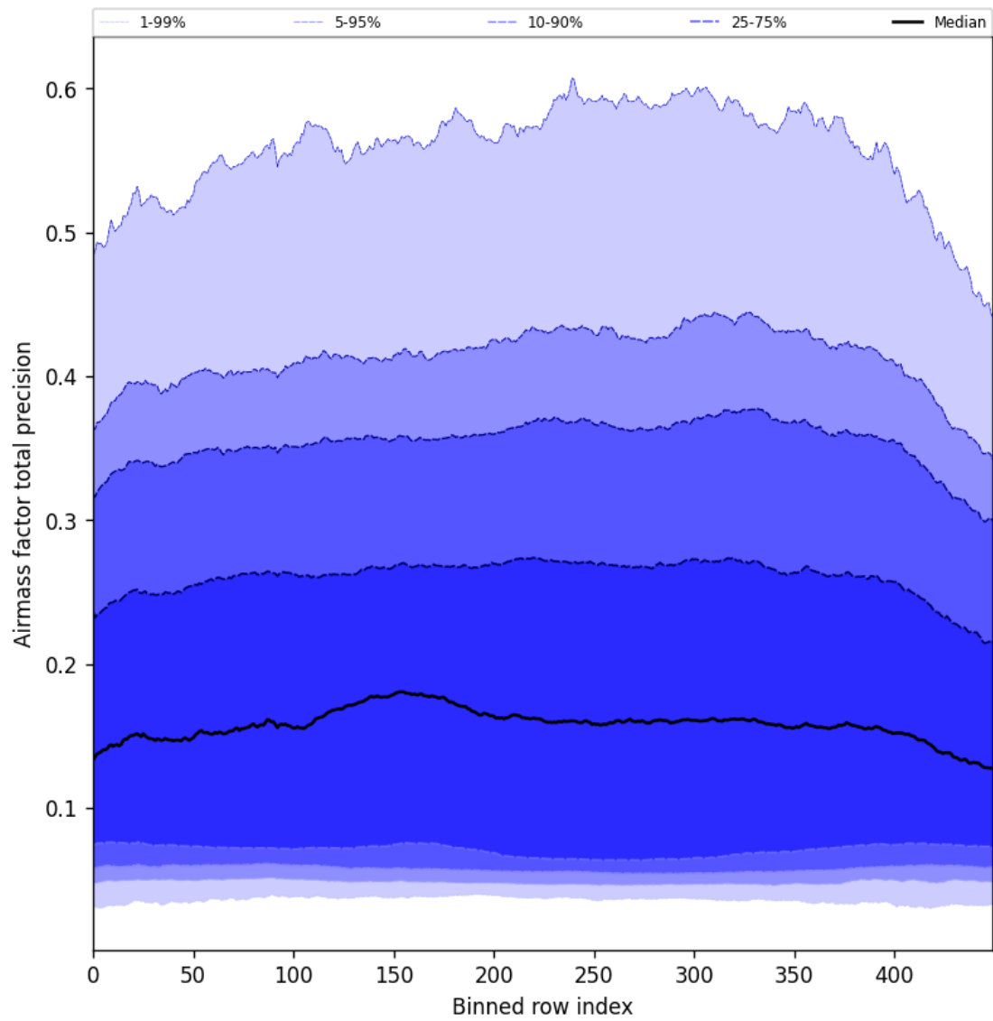
Figure 55: Along track statistics of “Airmass factor total precision” for 2025-09-10 to 2025-09-12
