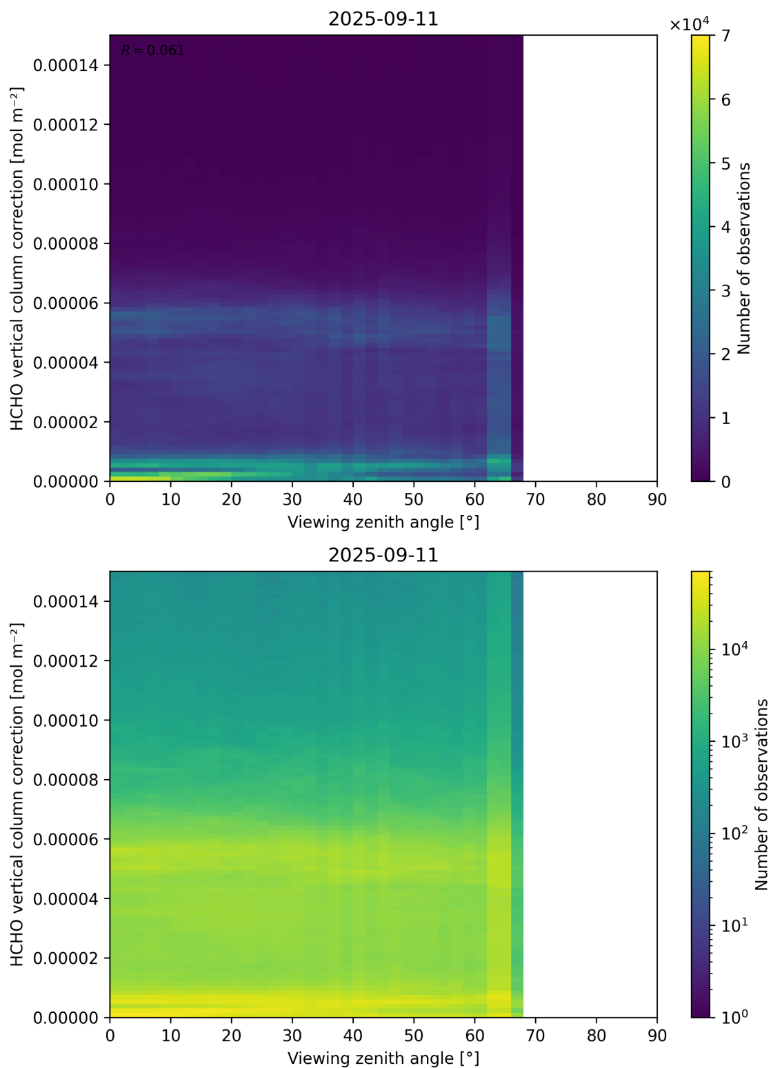
Figure 193: Scatter density plot of “Viewing zenith angle” against “HCHO vertical column correction” for 2025-09-10 to 2025-09-12.
