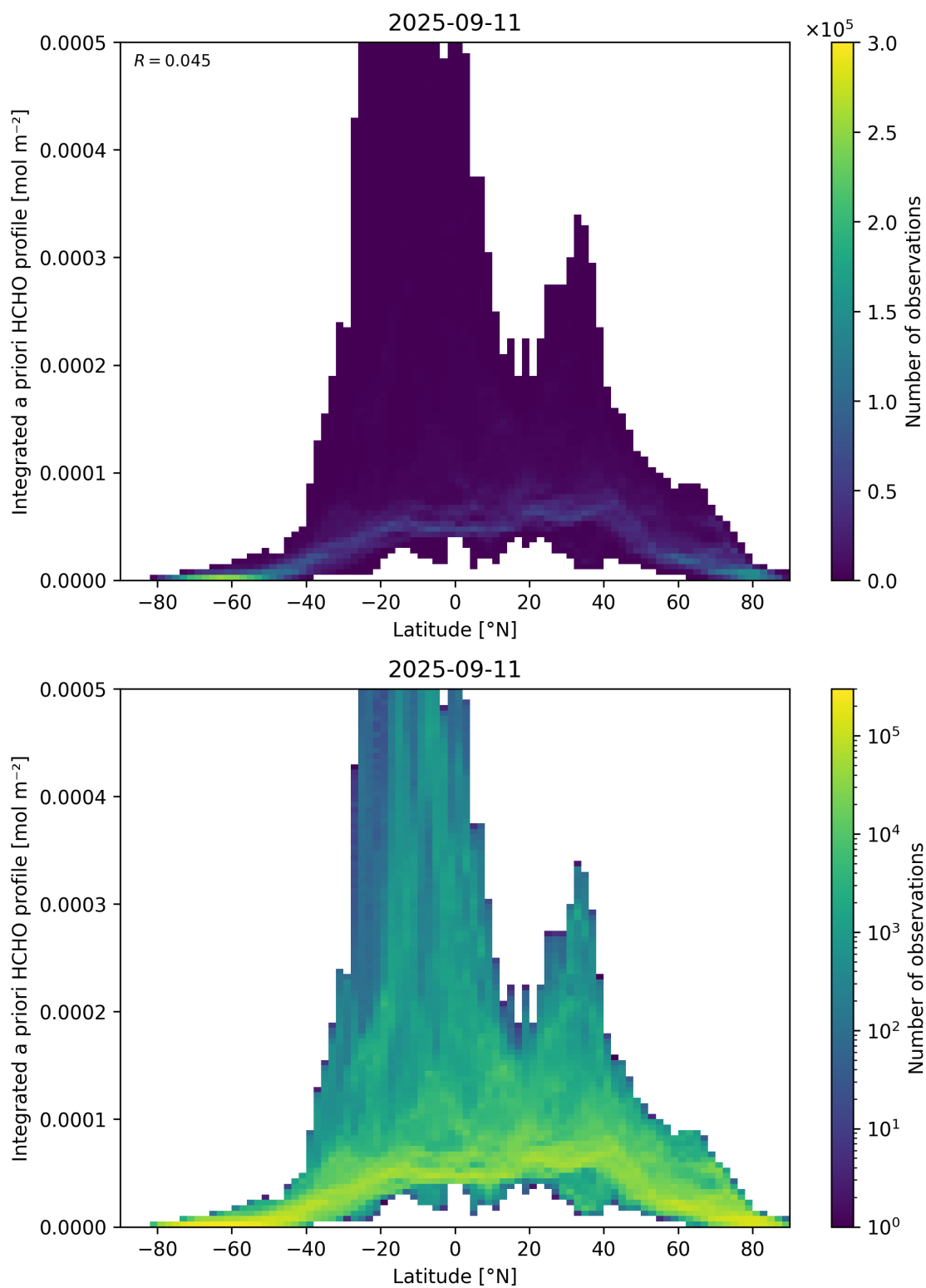
Figure 166: Scatter density plot of “Latitude” against “Integrated a priori HCHO profile” for 2025-09-10 to 2025-09-12.
