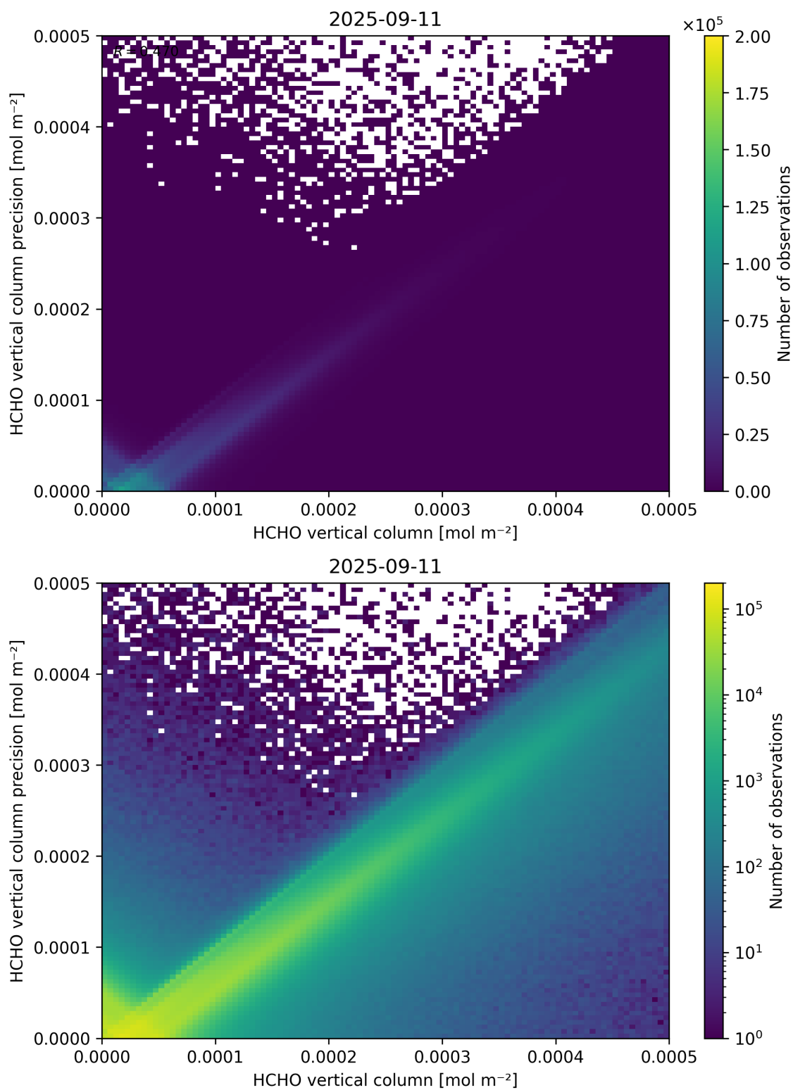
Figure 134: Scatter density plot of “HCHO vertical column” against “HCHO vertical column precision” for 2025-09-10 to 2025-09-12.
