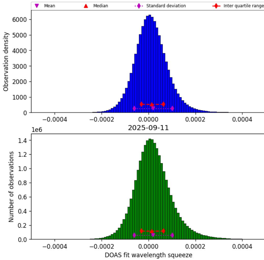
Figure 45: Histogram of “DOAS fit wavelength squeeze” for 2025-09-10 to 2025-09-12
