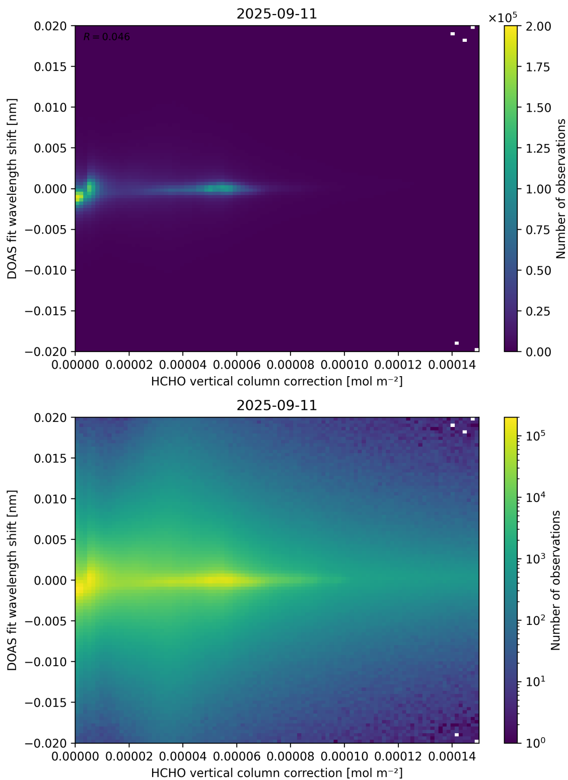
Figure 113: Scatter density plot of “HCHO vertical column correction” against “DOAS fit wavelength shift” for 2025-09-10 to 2025-09-12.
