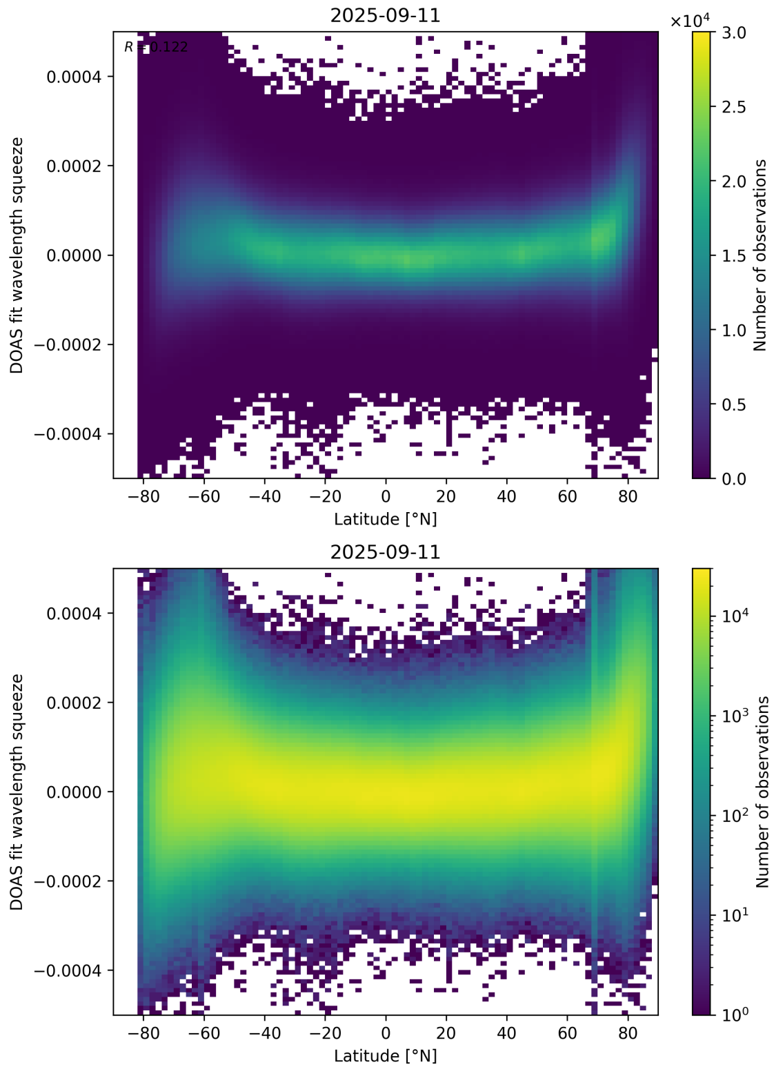
Figure 155: Scatter density plot of “Latitude” against “DOAS fit wavelength squeeze” for 2025-09-10 to 2025-09-12.
