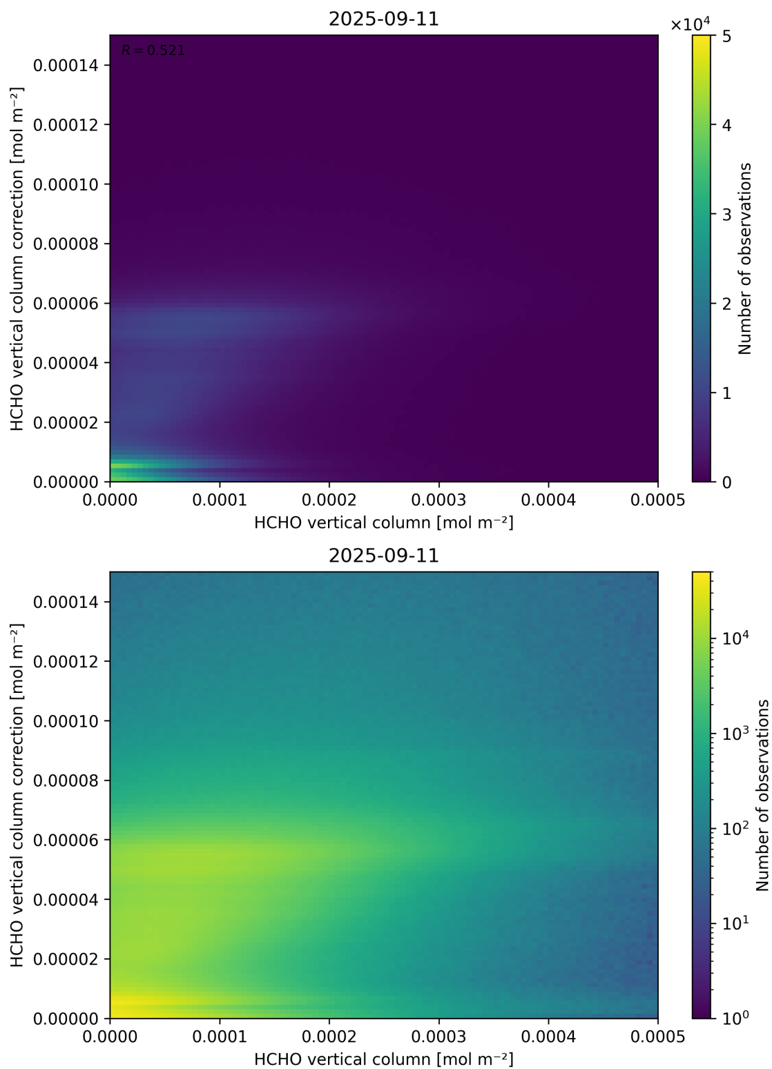
Figure 133: Scatter density plot of “HCHO vertical column” against “HCHO vertical column correction” for 2025-09-10 to 2025-09-12.
