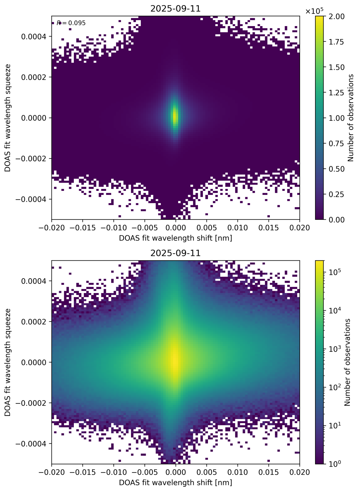
Figure 65: Scatter density plot of “DOAS fit wavelength shift” against “DOAS fit wavelength squeeze” for 2025-09-10 to 2025-09-12.
