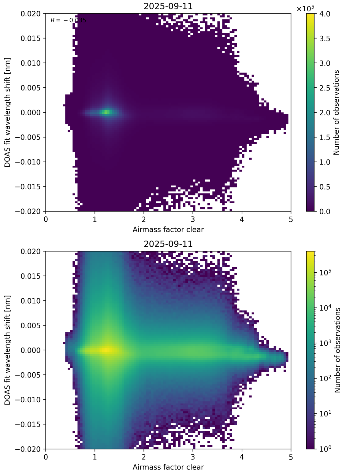
Figure 72: Scatter density plot of “Airmass factor clear” against “DOAS fit wavelength shift” for 2025-09-10 to 2025-09-12.
