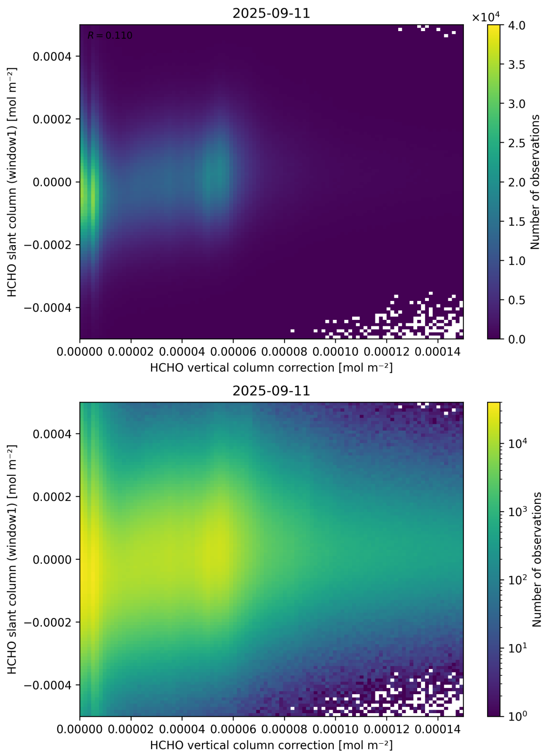
Figure 118: Scatter density plot of “HCHO vertical column correction” against “HCHO slant column (window1)” for 2025-09-10 to 2025-09-12.
