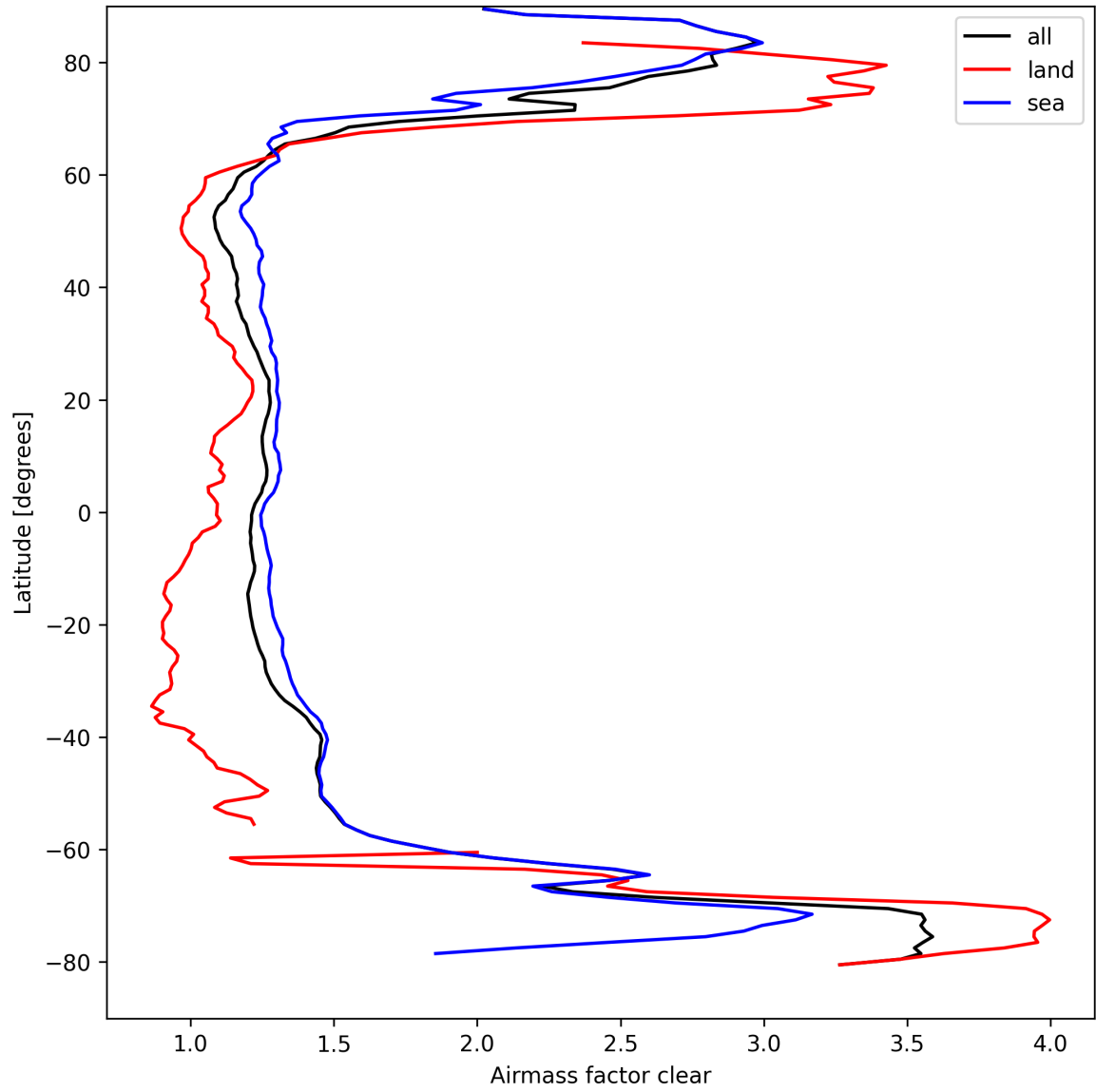
Figure 28: Zonal average of “Airmass factor clear” for 2025-09-10 to 2025-09-12.
