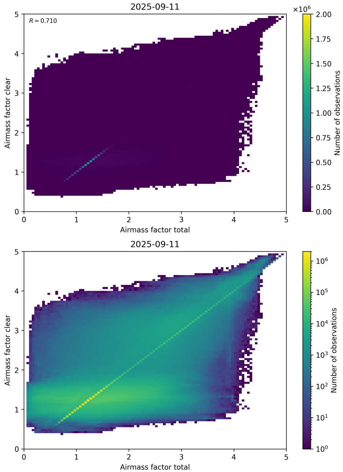
Figure 100: Scatter density plot of “Airmass factor total” against “Airmass factor clear” for 2025-09-10 to 2025-09-12.
