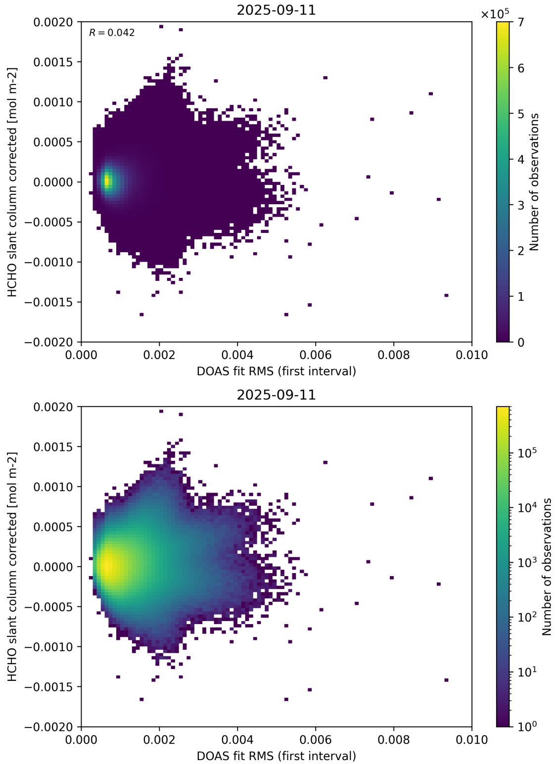
Figure 62: Scatter density plot of “DOAS fit RMS (first interval)” against “HCHO slant column corrected” for 2025-09-10 to 2025-09-12.
