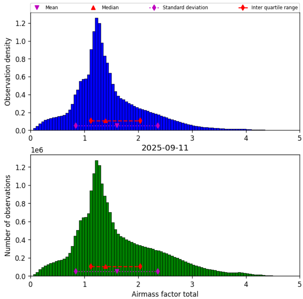
Figure 40: Histogram of “Airmass factor total” for 2025-09-10 to 2025-09-12
