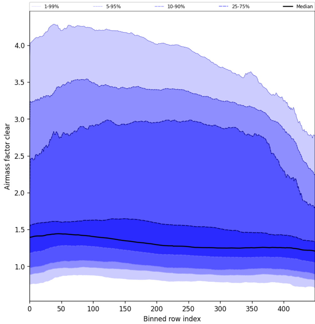
Figure 56: Along track statistics of “Air mass factor clear” for 2025-09-10 to 2025-09-12
