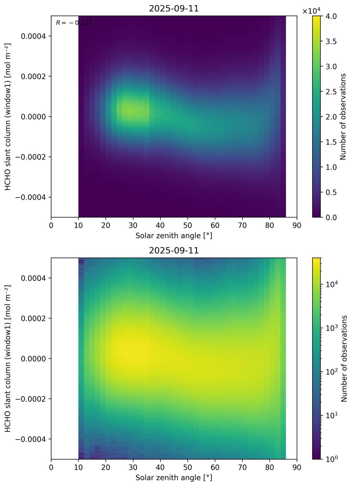
Figure 173: Scatter density plot of “Solar zenith angle” against “HCHO slant column (window1)” for 2025-09-10 to 2025-09-12.
