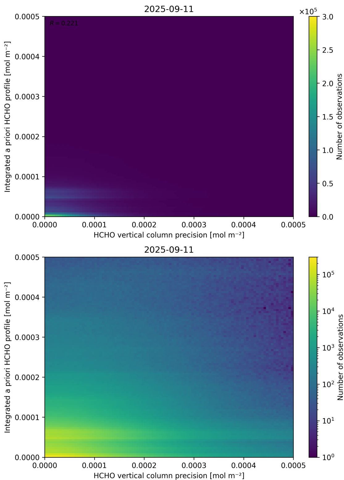
Figure 147: Scatter density plot of “HCHO vertical column precision” against “Integrated a priori HCHO profile” for 2025-09-10 to 2025-09-12.
