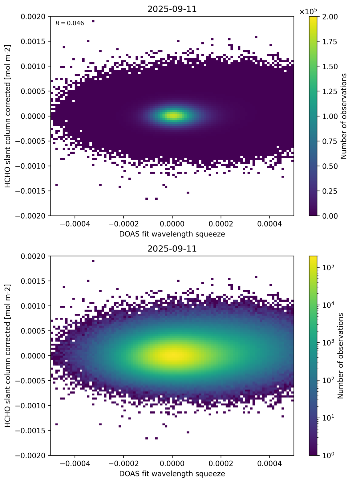
Figure 69: Scatter density plot of “DOAS fit wavelength squeeze” against “HCHO slant column corrected” for 2025-09-10 to 2025-09-12.
