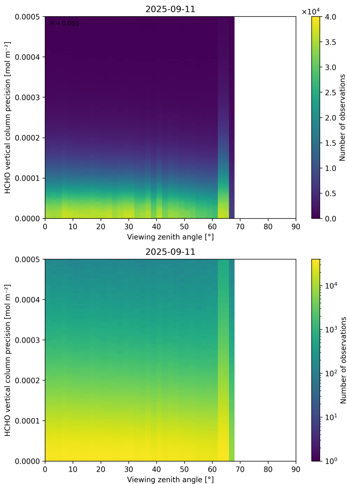
Figure 194: Scatter density plot of “Viewing zenith angle” against “HCHO vertical column precision” for 2025-09-10 to 2025-09-12.
