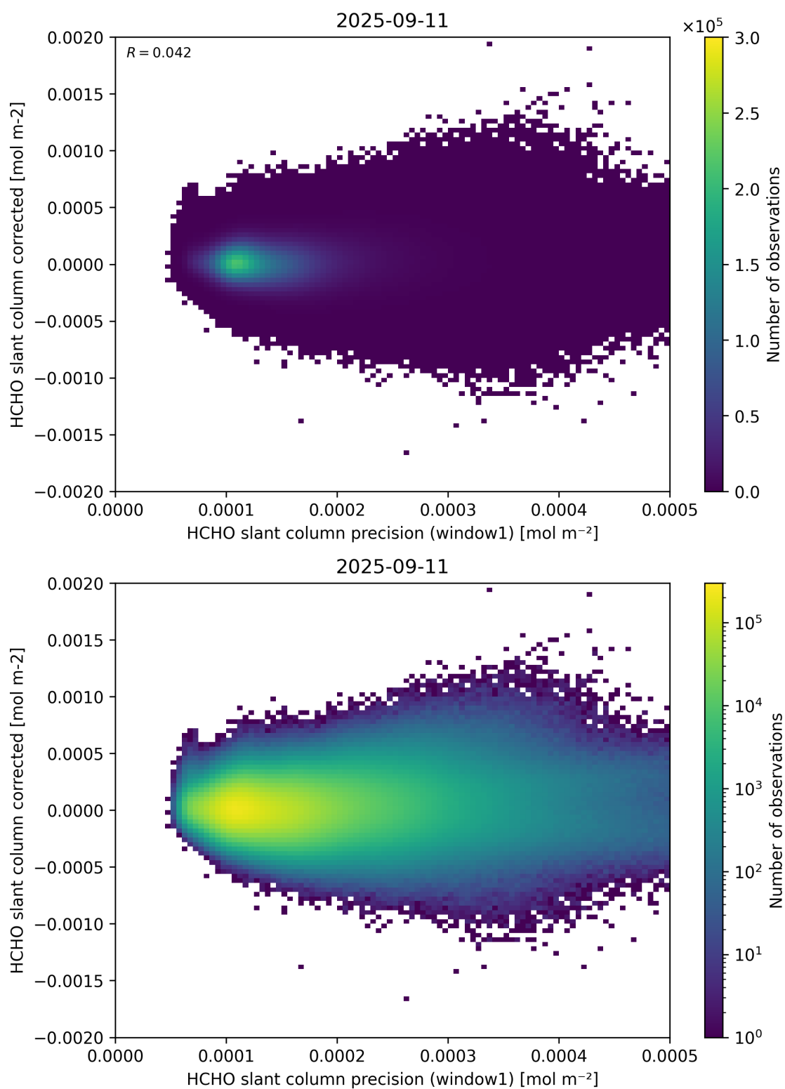
Figure 92: Scatter density plot of “HCHO slant column precision (window1)” against “HCHO slant column corrected” for 2025-09-10 to 2025-09-12.
