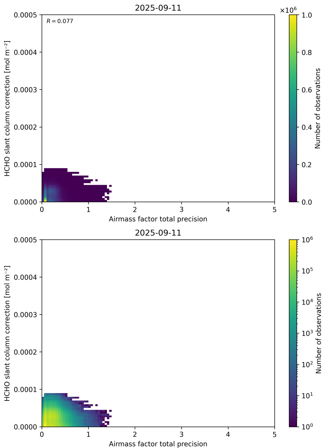
Figure 110: Scatter density plot of “Airmass factor total precision” against “HCHO slant column correction” for 2025-09-10 to 2025-09-12.
