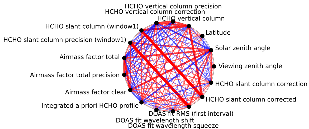
Figure 1: Map of correlation graph for 2025-09-10 to 2025-09-12.
