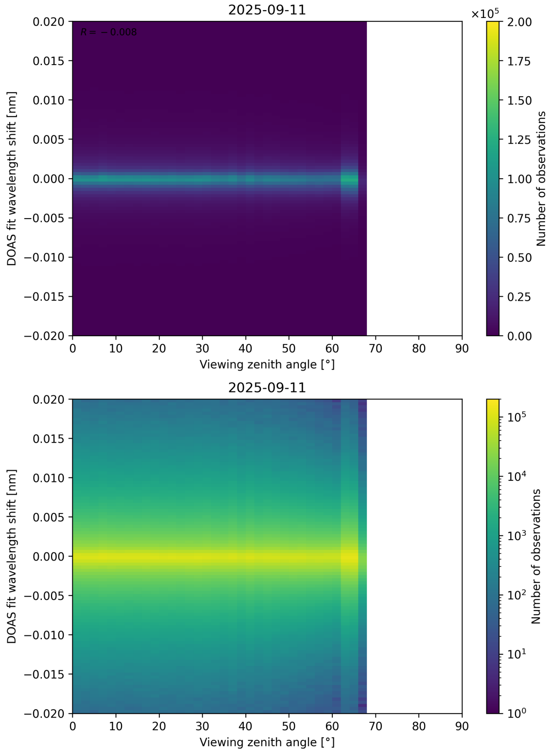
Figure 183: Scatter density plot of “Viewing zenith angle” against “DOAS fit wavelength shift” for 2025-09-10 to 2025-09-12.
