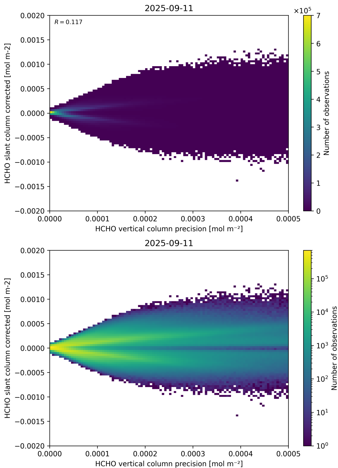
Figure 140: Scatter density plot of “HCHO vertical column precision” against “HCHO slant column corrected” for 2025-09-10 to 2025-09-12.
