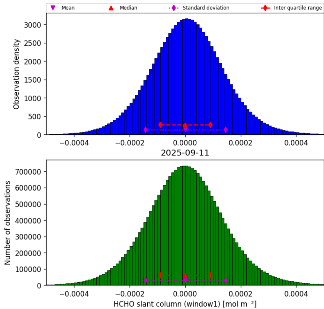
Figure 38: Histogram of “HCHO slant column (window1)” for 2025-09-10 to 2025-09-12
