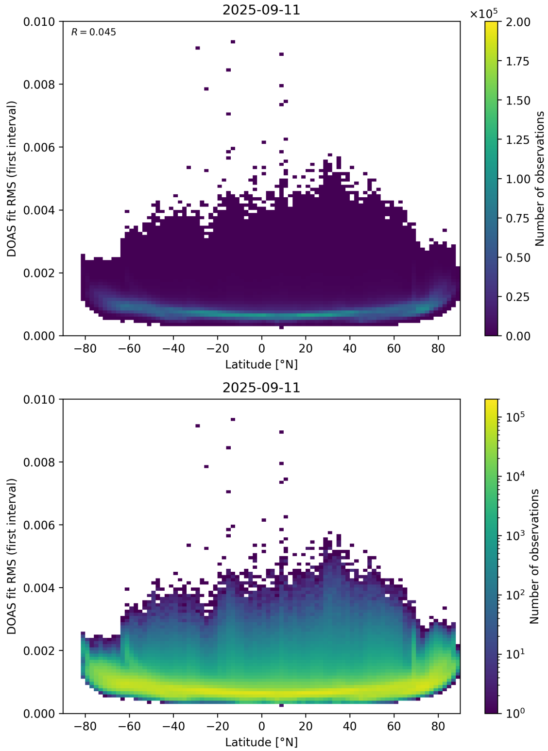
Figure 153: Scatter density plot of “Latitude” against “DOAS fit RMS (first interval)” for 2025-09-10 to 2025-09-12.
