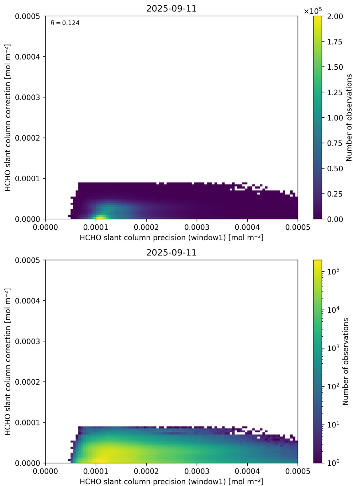
Figure 93: Scatter density plot of “HCHO slant column precision (window1)” against “HCHO slant column correction” for 2025-09-10 to 2025-09-12.
