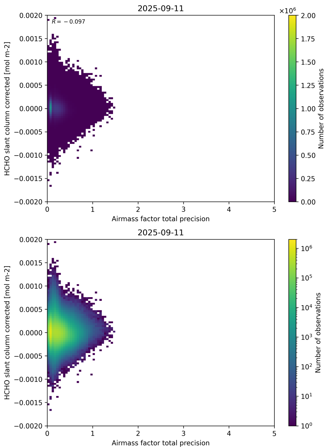
Figure 109: Scatter density plot of “Airmass factor total precision” against “HCHO slant column corrected” for 2025-09-10 to 2025-09-12.
