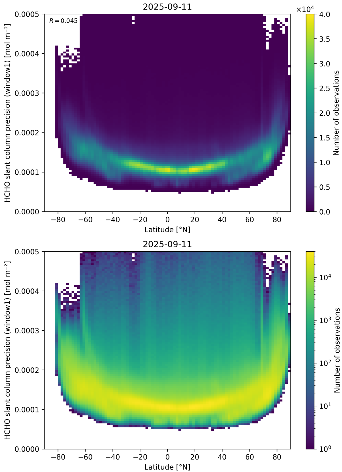
Figure 160: Scatter density plot of “Latitude” against “HCHO slant column precision (window1)” for 2025-09-10 to 2025-09-12.
