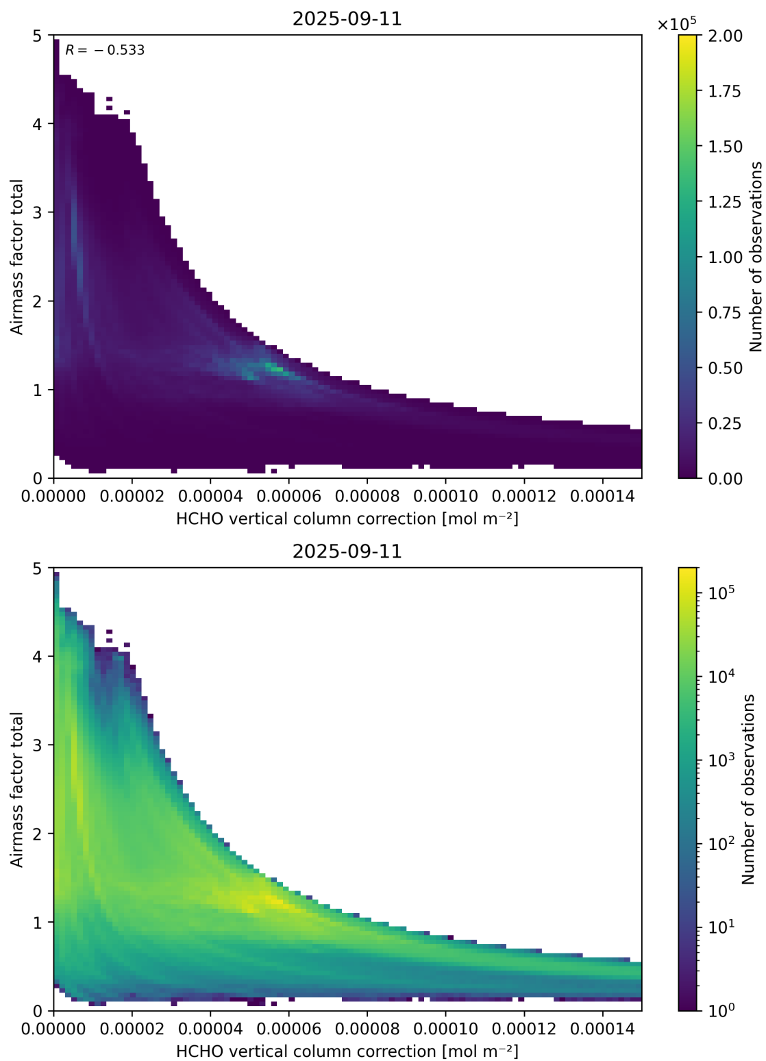
Figure 120: Scatter density plot of “HCHO vertical column correction” against “Airmass factor total” for 2025-09-10 to 2025-09-12.
