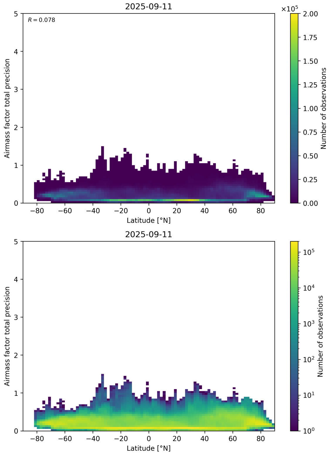
Figure 162: Scatter density plot of “Latitude” against “Airmass factor total precision” for 2025-09-10 to 2025-09-12.
