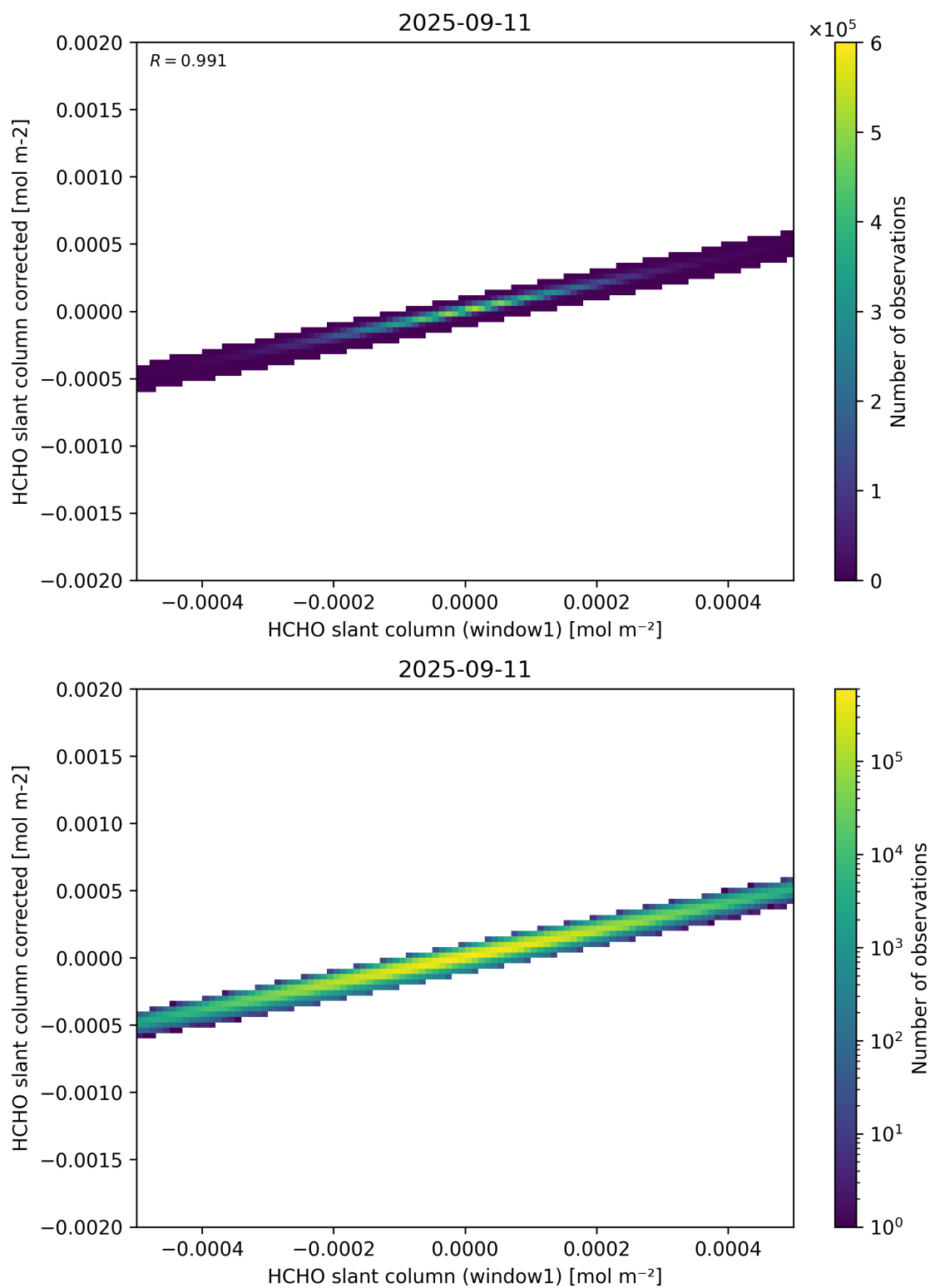
Figure 82: Scatter density plot of “HCHO slant column (window1)” against “HCHO slant column corrected” for 2025-09-10 to 2025-09-12.
