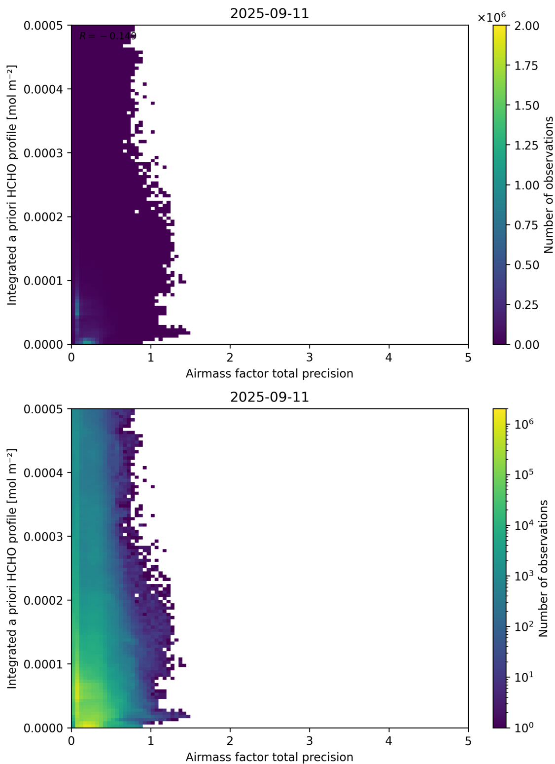
Figure 111: Scatter density plot of “Airmass factor total precision” against “Integrated a priori HCHO profile” for 2025-09-10 to 2025-09-12.
