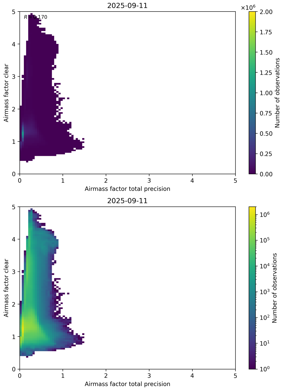
Figure 108: Scatter density plot of “Airmass factor total precision” against “Airmass factor clear” for 2025-09-10 to 2025-09-12.
