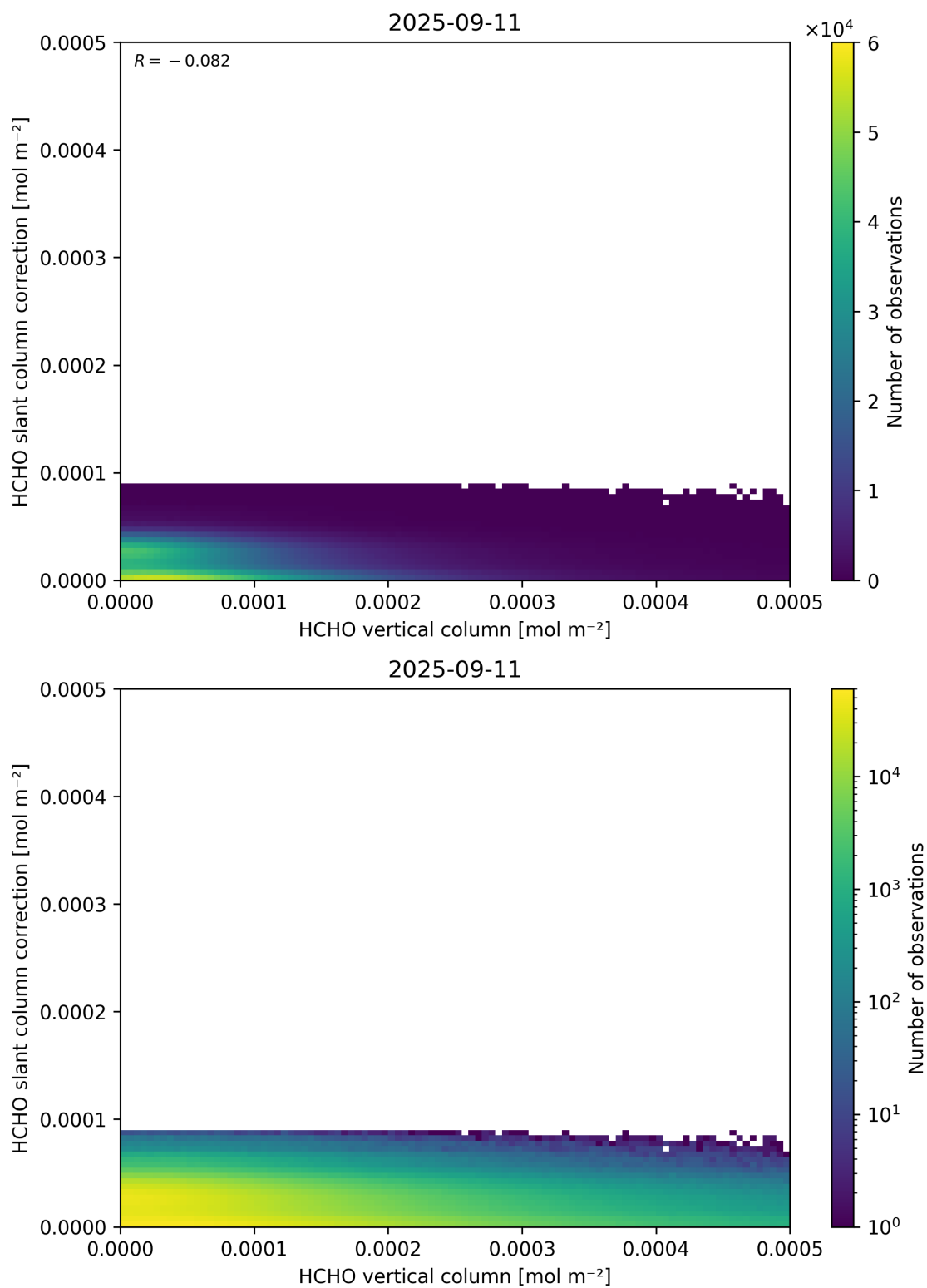
Figure 128: Scatter density plot of “HCHO vertical column” against “HCHO slant column correction” for 2025-09-10 to 2025-09-12.
