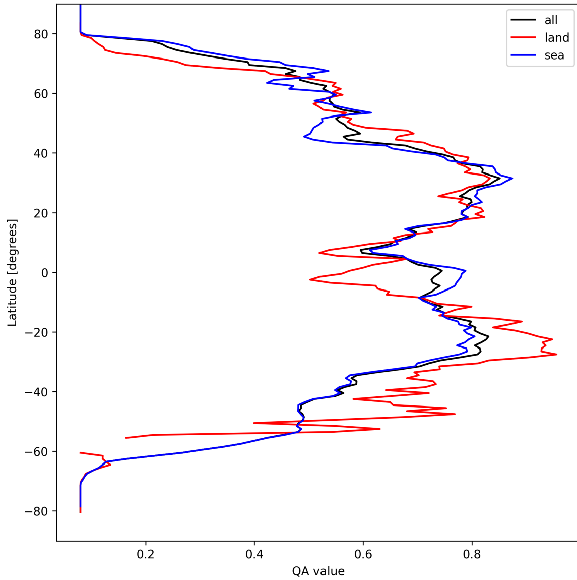
Figure 20: Zonal average of “QA value” for 2025-09-10 to 2025-09-12.
