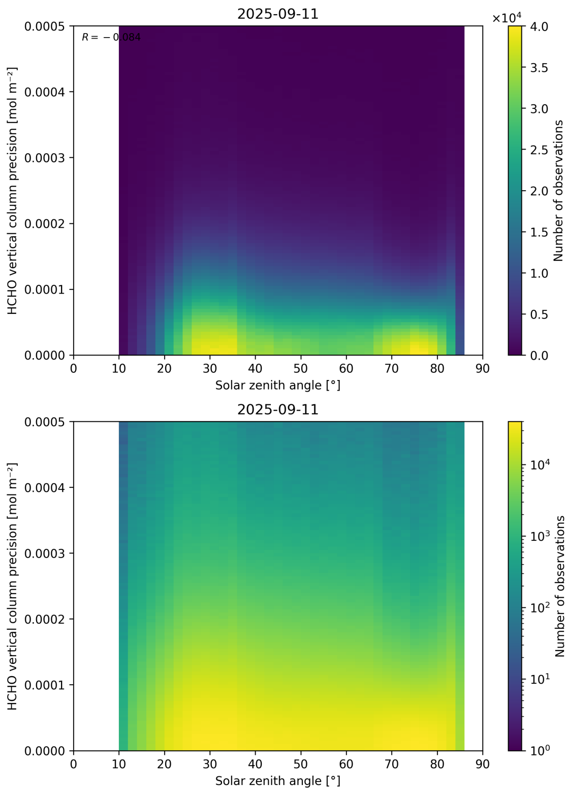
Figure 179: Scatter density plot of “Solar zenith angle” against “HCHO vertical column precision” for 2025-09-10 to 2025-09-12.
