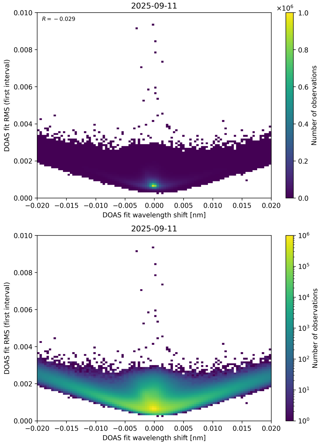
Figure 64: Scatter density plot of “DOAS fit wavelength shift” against “DOAS fit RMS (first interval)” for 2025-09-10 to 2025-09-12.
