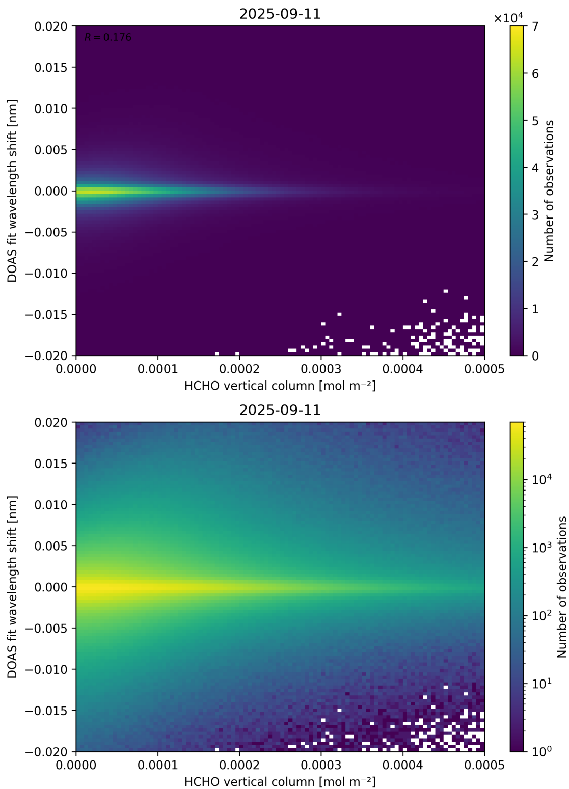
Figure 124: Scatter density plot of “HCHO vertical column” against “DOAS fit wavelength shift” for 2025-09-10 to 2025-09-12.
