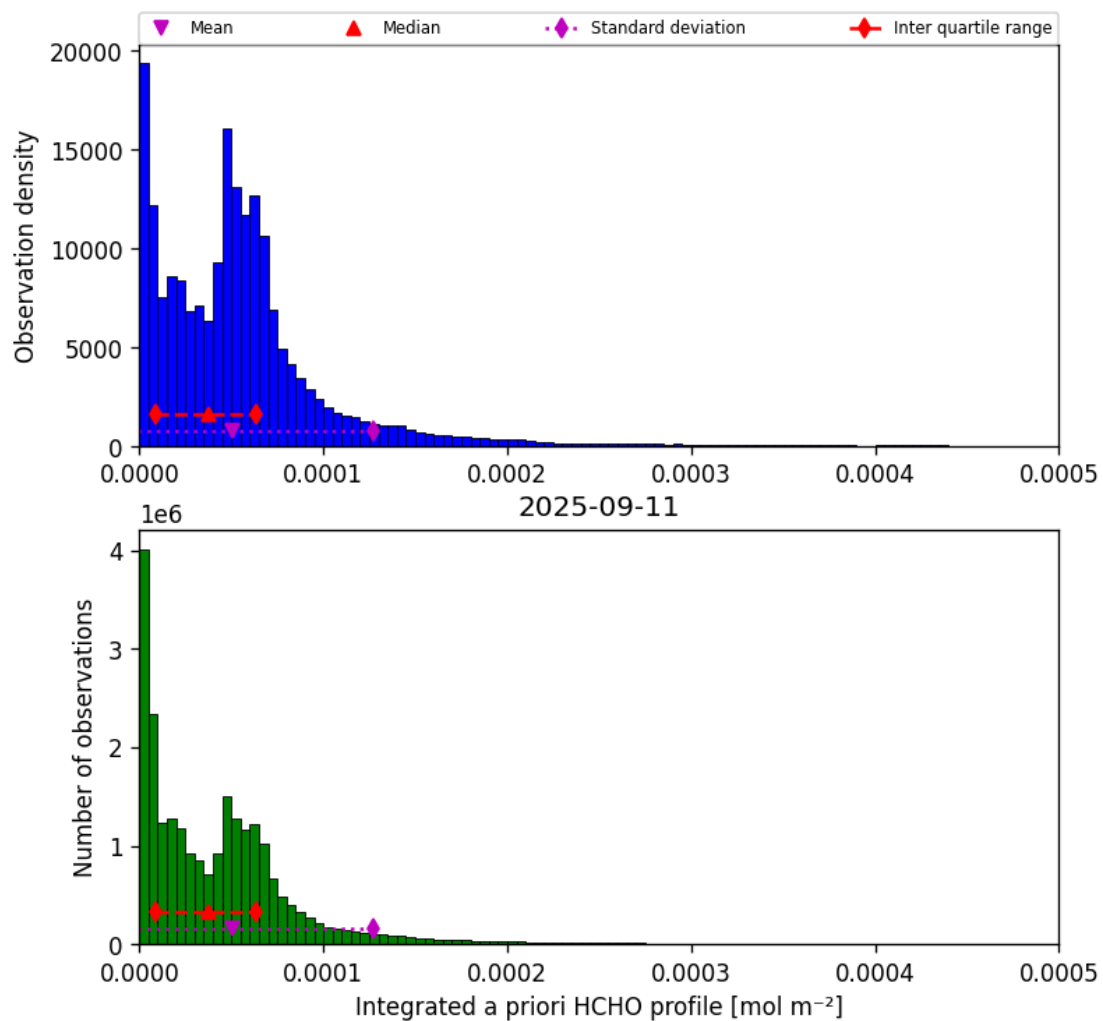
Figure 43: Histogram of “Integrated a priori HCHO profile” for 2025-09-10 to 2025-09-12
