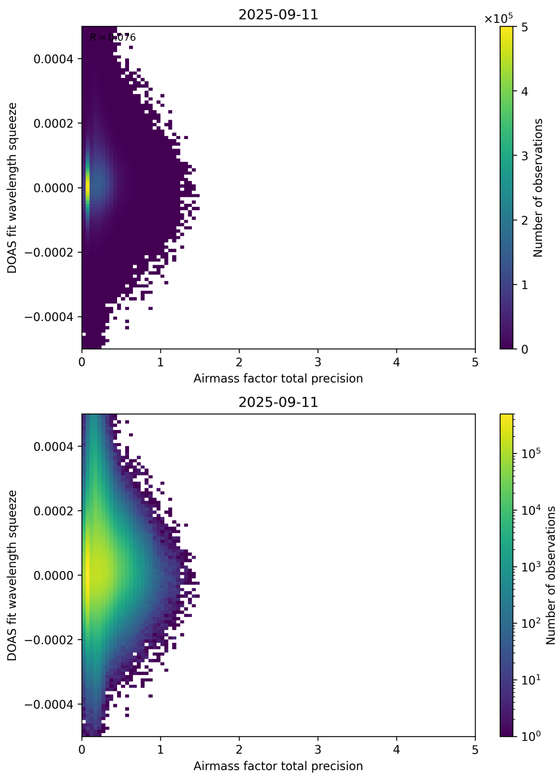
Figure 107: Scatter density plot of “Airmass factor total precision” against “DOAS fit wavelength squeeze” for 2025-09-10 to 2025-09-12.
