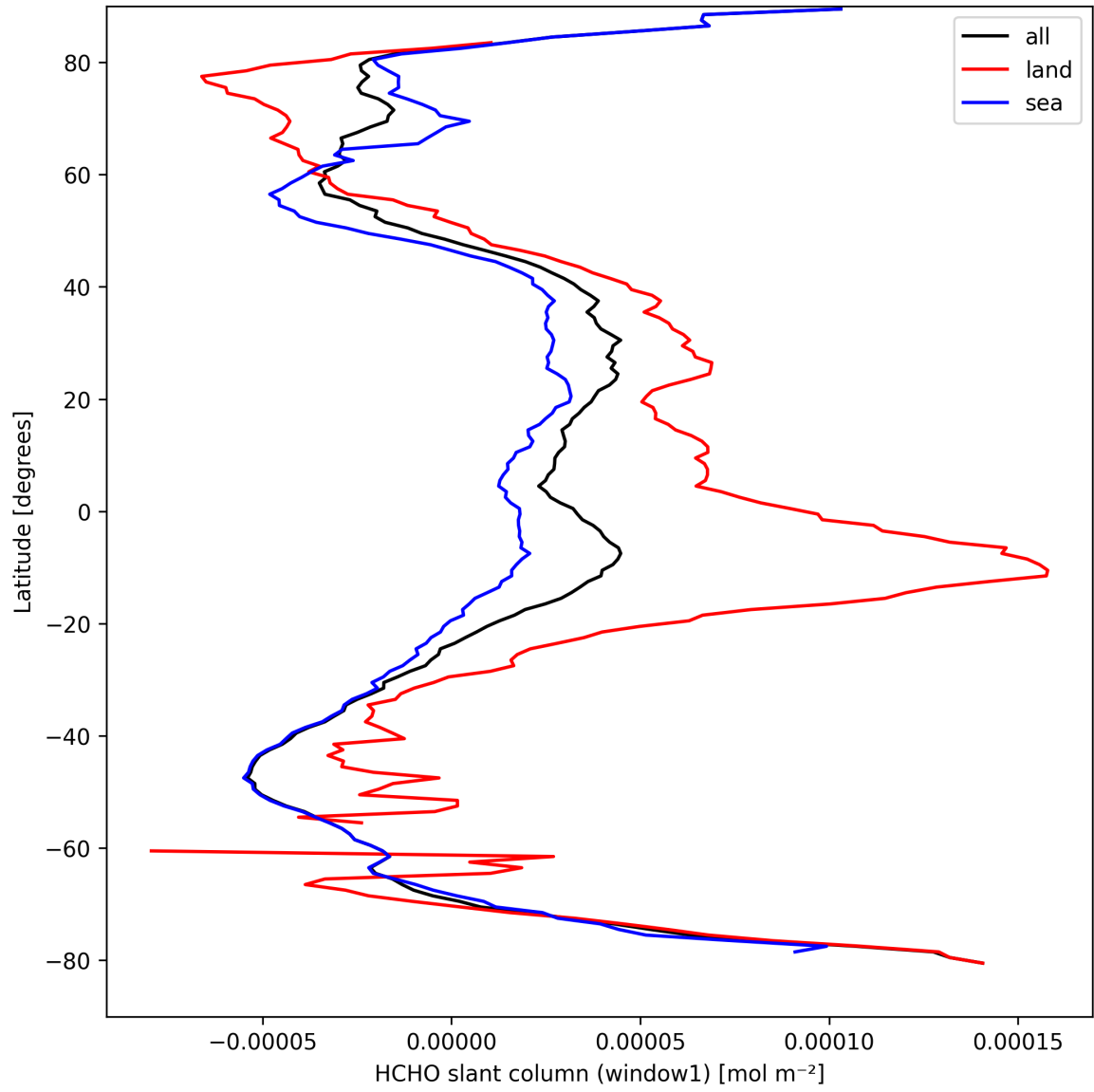
Figure 24: Zonal average of “HCHO slant column (window1)” for 2025-09-10 to 2025-09-12.
