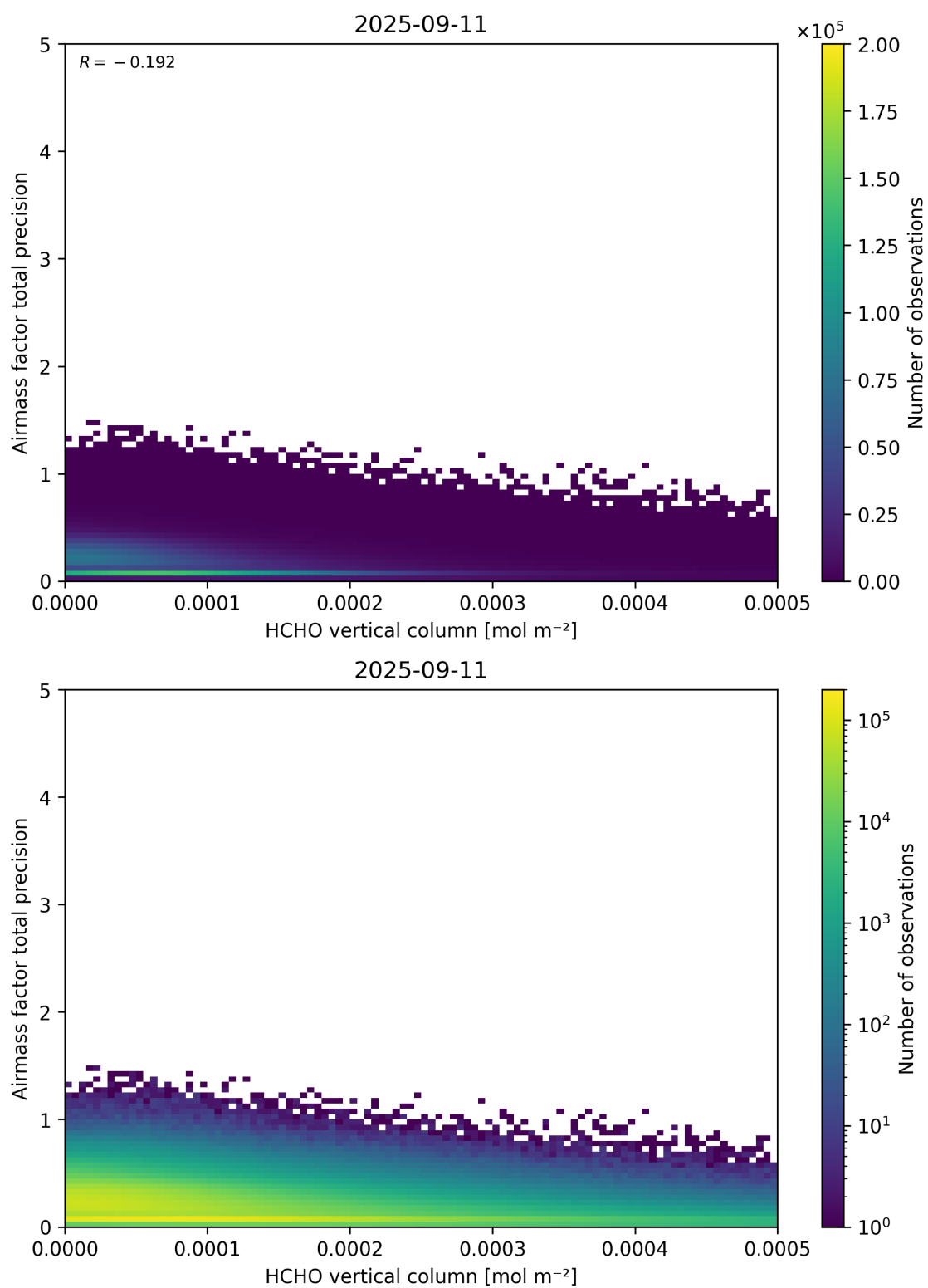
Figure 132: Scatter density plot of “HCHO vertical column” against “Airmass factor total precision” for 2025-09-10 to 2025-09-12.
