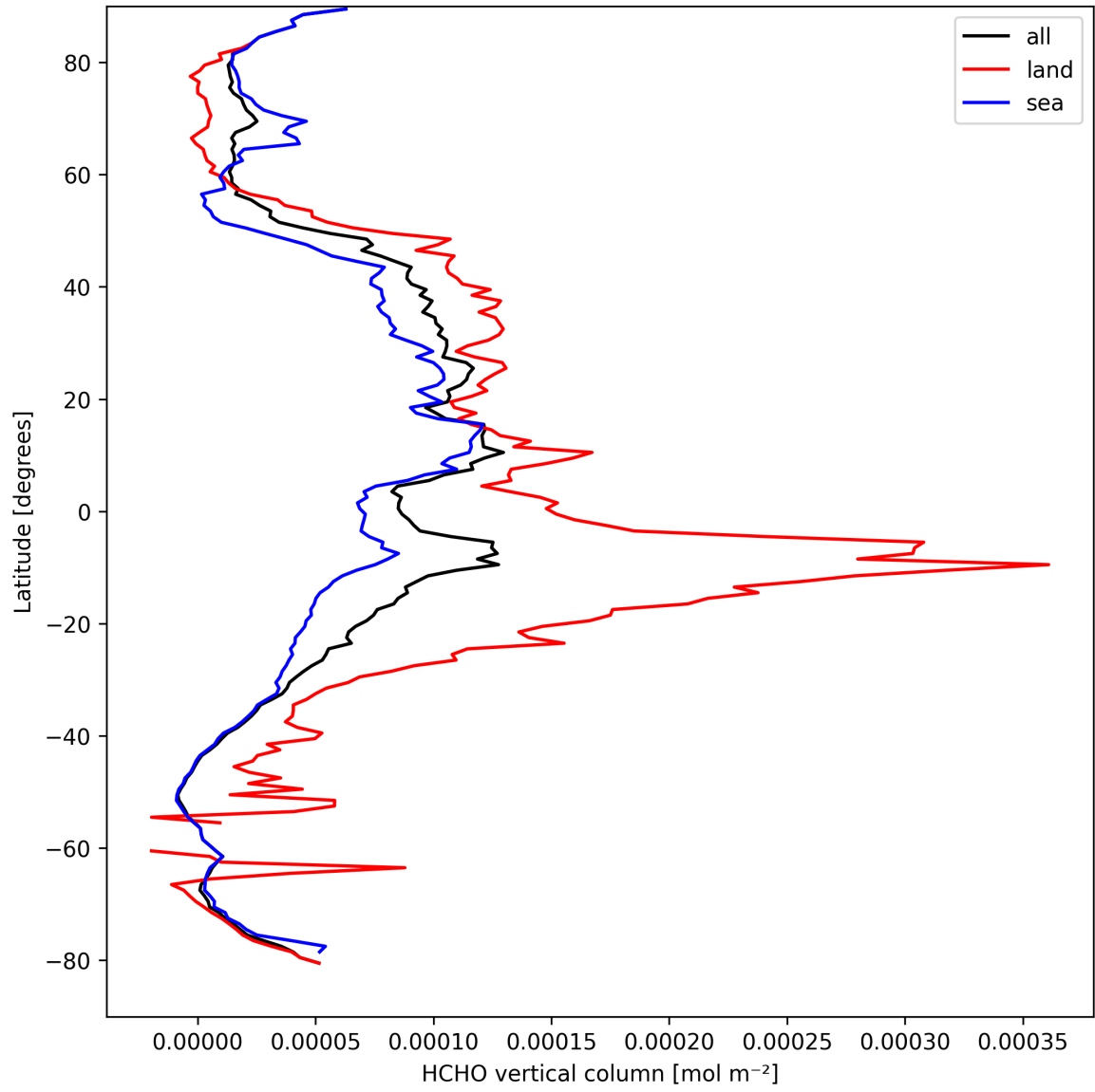
Figure 21: Zonal average of “HCHO vertical column” for 2025-09-10 to 2025-09-12.
