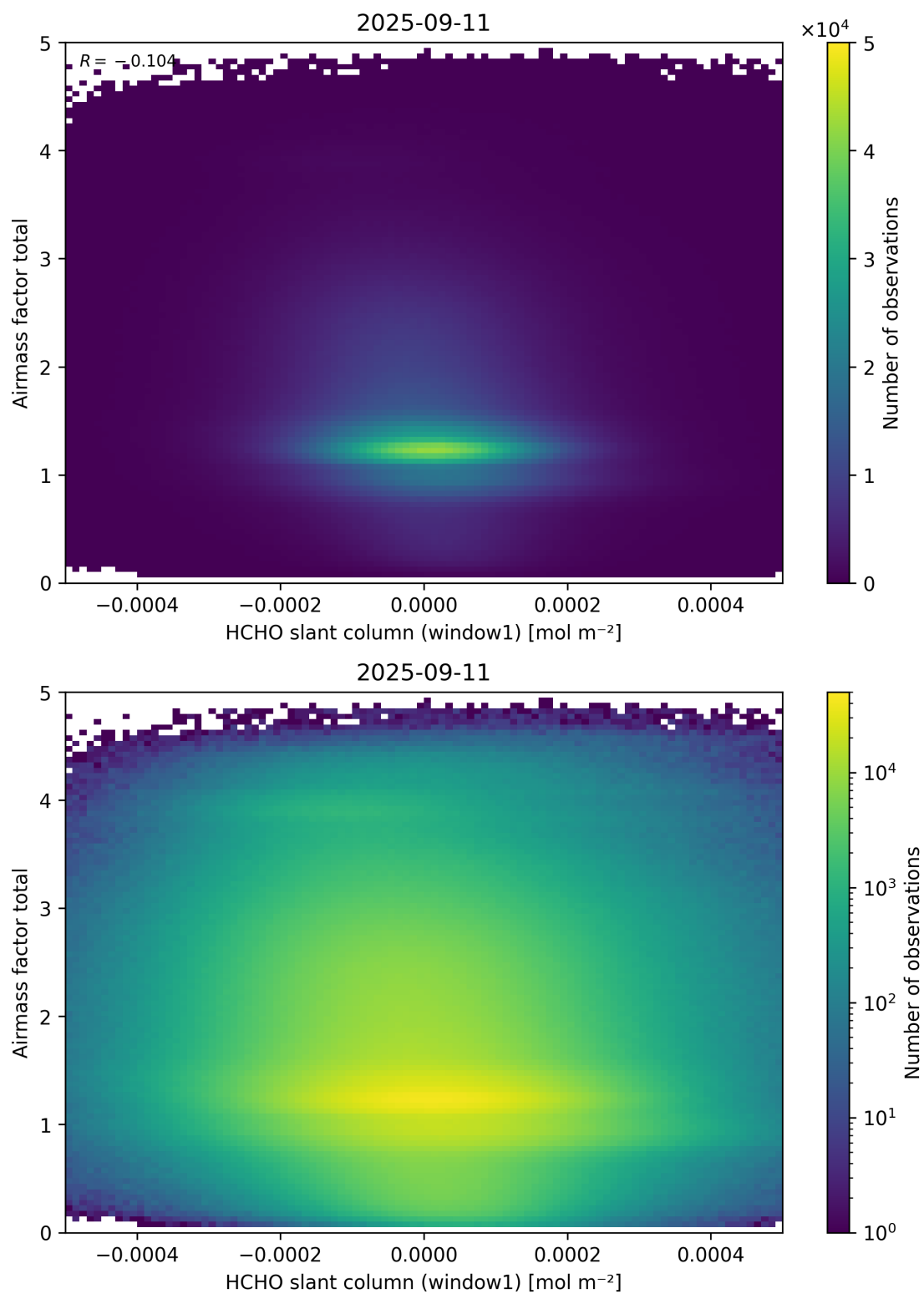
Figure 85: Scatter density plot of “HCHO slant column (window1)” against “Airmass factor total” for 2025-09-10 to 2025-09-12.
