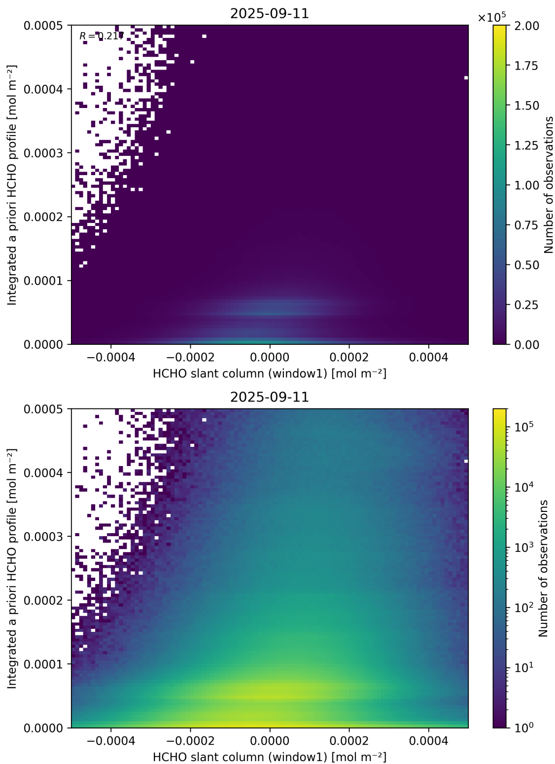
Figure 87: Scatter density plot of “HCHO slant column (window1)” against “Integrated a priori HCHO profile” for 2025-09-10 to 2025-09-12.
