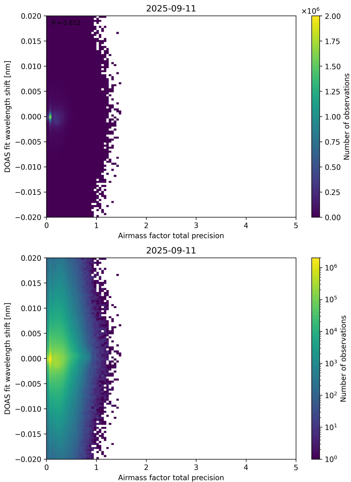
Figure 106: Scatter density plot of “Airmass factor total precision” against “DOAS fit wavelength shift” for 2025-09-10 to 2025-09-12.
