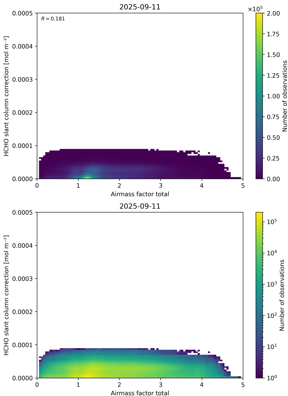
Figure 102: Scatter density plot of “Airmass factor total” against “HCHO slant column correction” for 2025-09-10 to 2025-09-12.
