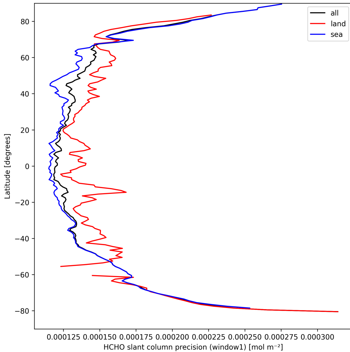
Figure 25: Zonal average of “HCHO slant column precision (window1)” for 2025-09-10 to 2025-09-12.
