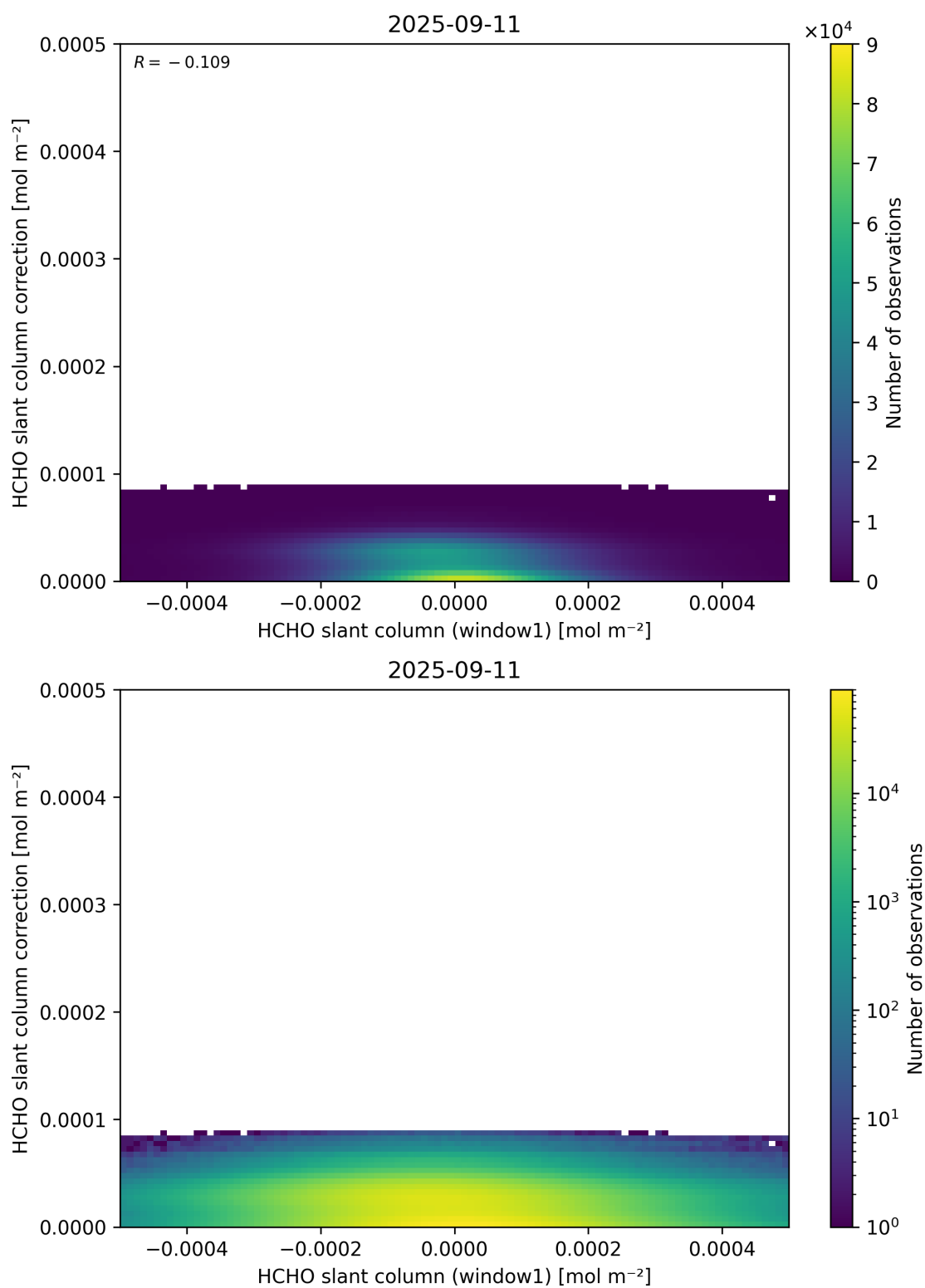
Figure 83: Scatter density plot of “HCHO slant column (window1)” against “HCHO slant column correction” for 2025-09-10 to 2025-09-12.
