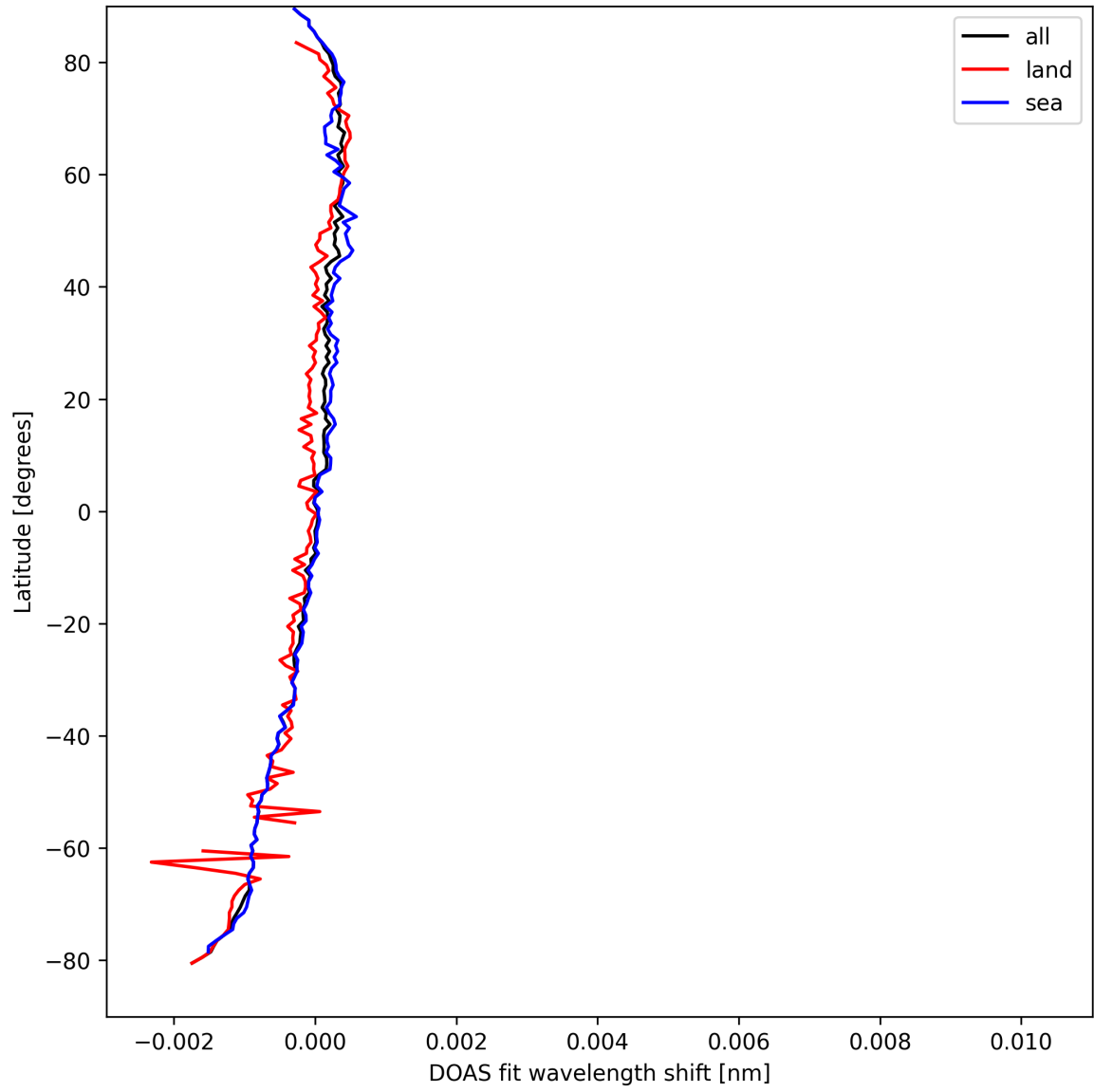
Figure 30: Zonal average of "DOAS fit wavelength shift" for 2025-09-10 to 2025-09-12.
