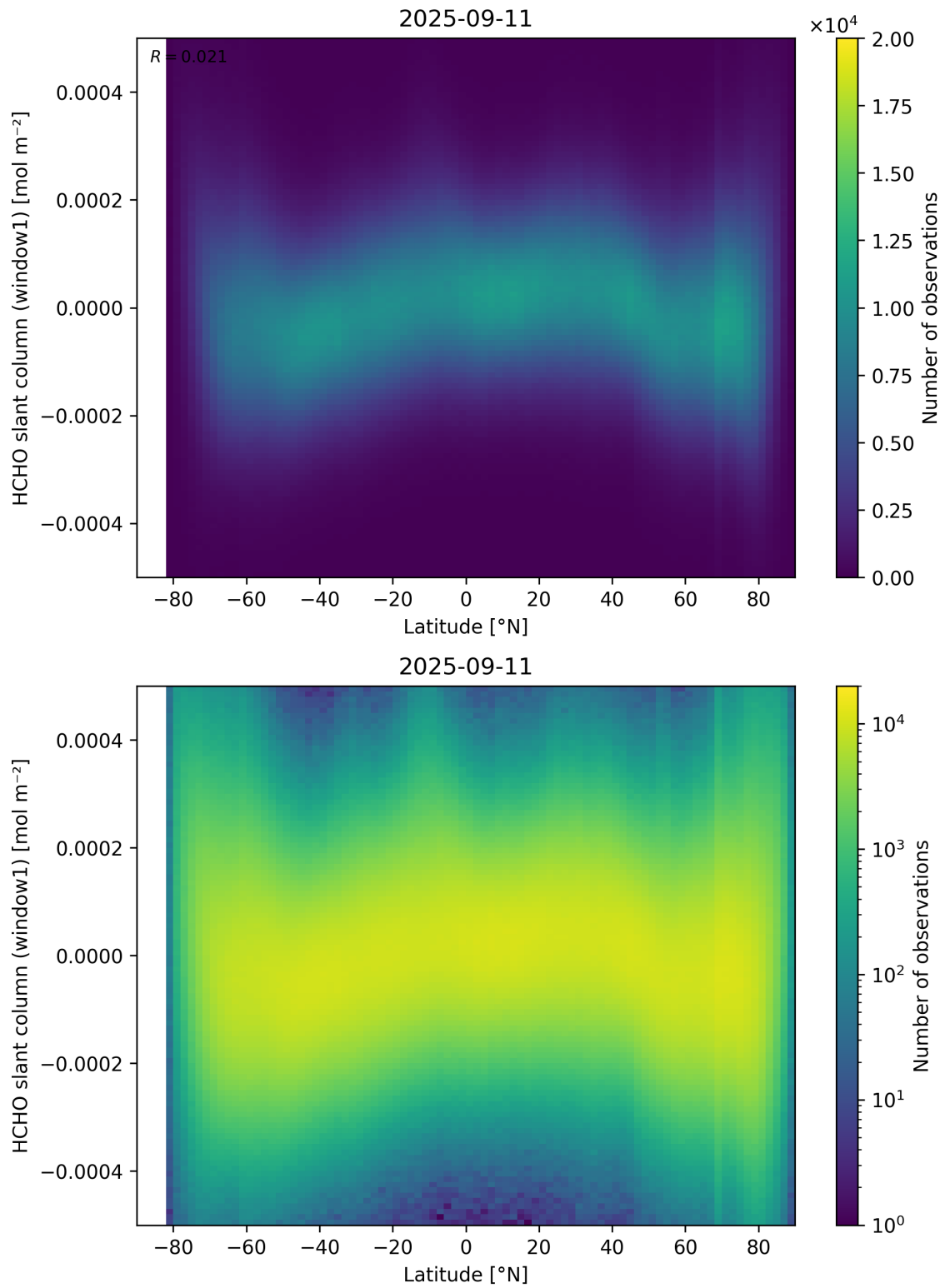
Figure 159: Scatter density plot of “Latitude” against “HCHO slant column (window1)” for 2025-09-10 to 2025-09-12.
