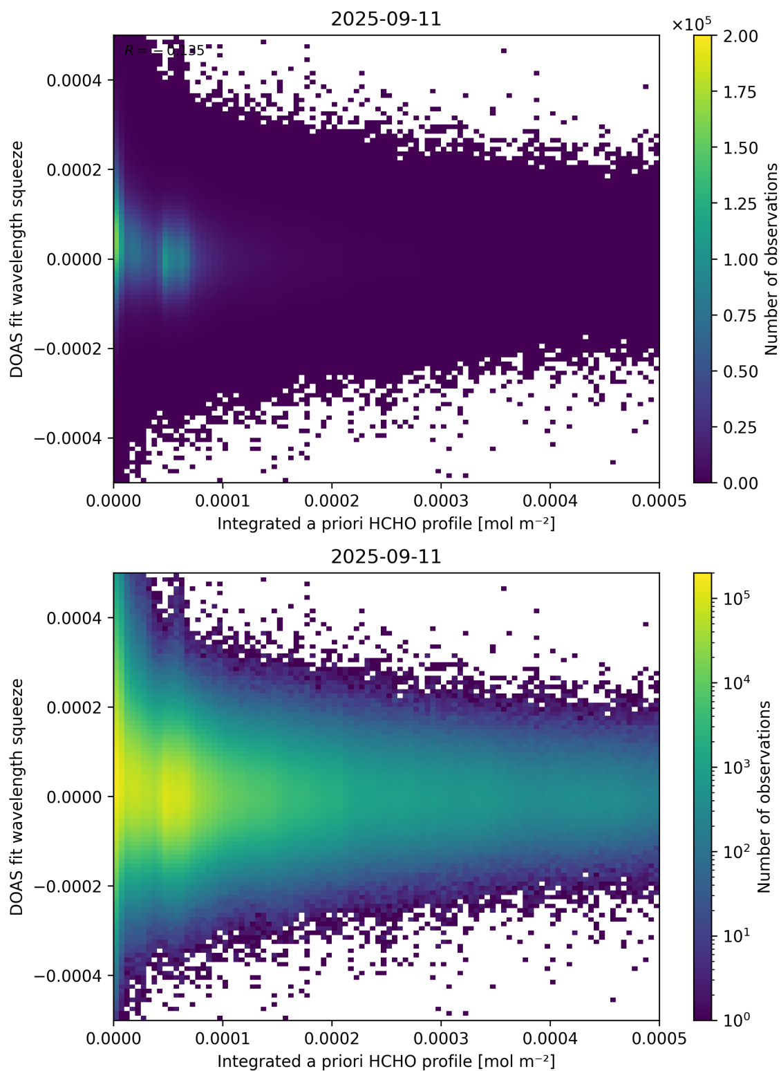
Figure 150: Scatter density plot of “Integrated a priori HCHO profile” against “DOAS fit wavelength squeeze” for 2025-09-10 to 2025-09-12.
