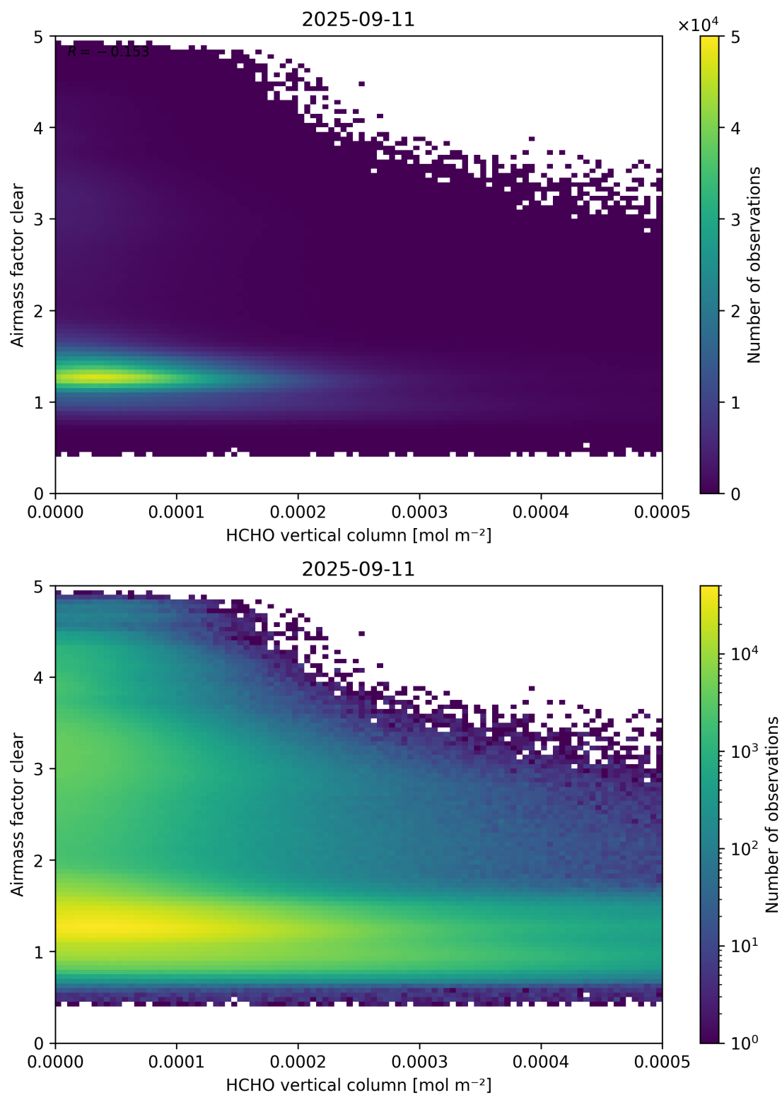
Figure 126: Scatter density plot of “HCHO vertical column” against “Airmass factor clear” for 2025-09-10 to 2025-09-12.
