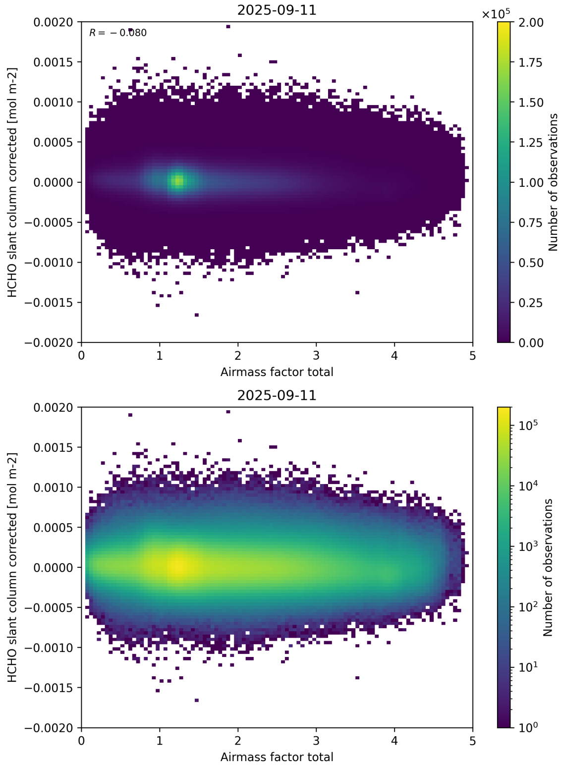
Figure 101: Scatter density plot of “Airmass factor total” against “HCHO slant column corrected” for 2025-09-10 to 2025-09-12.
