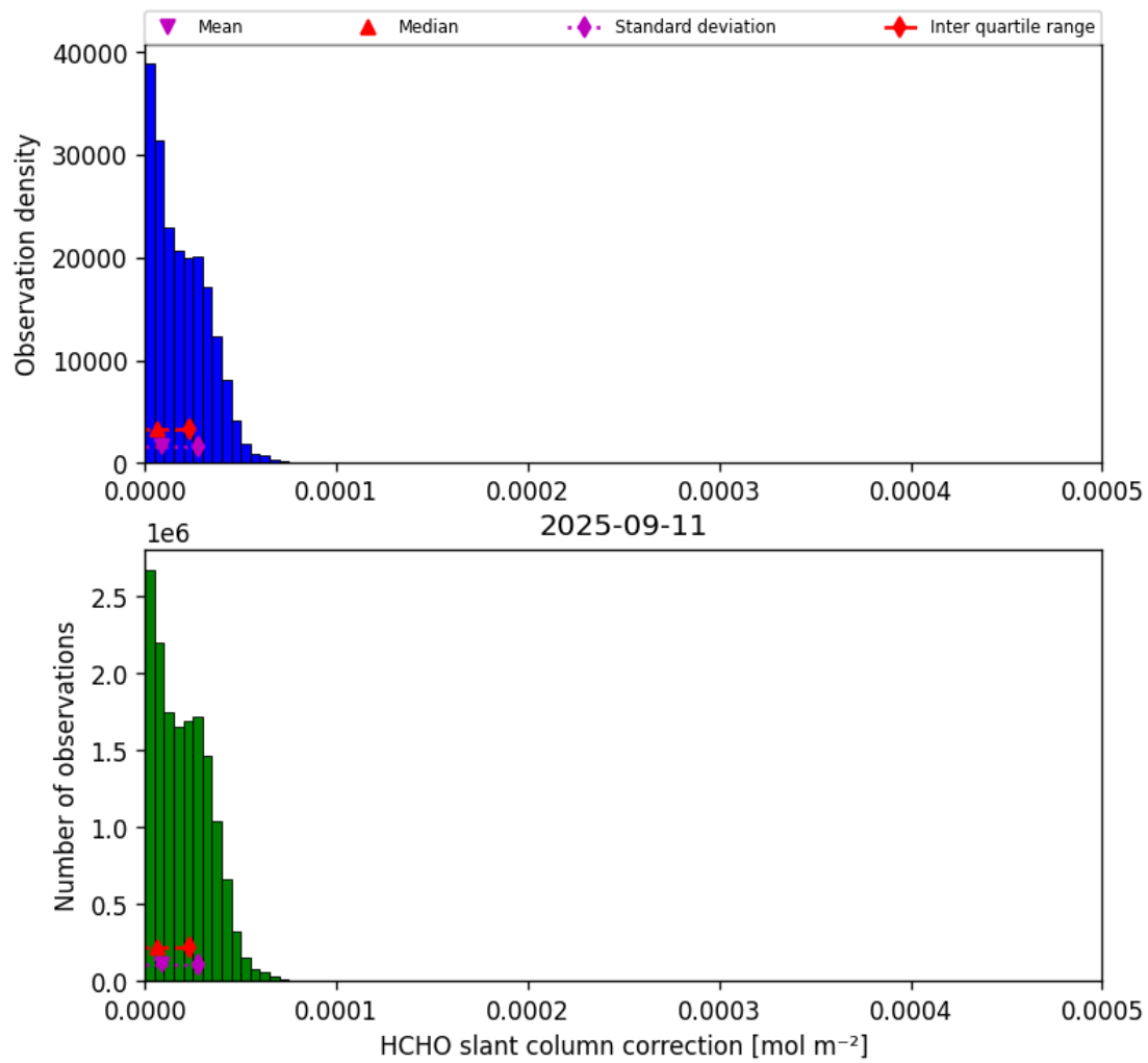
Figure 47: Histogram of “HCHO slant column correction” for 2025-09-10 to 2025-09-12
