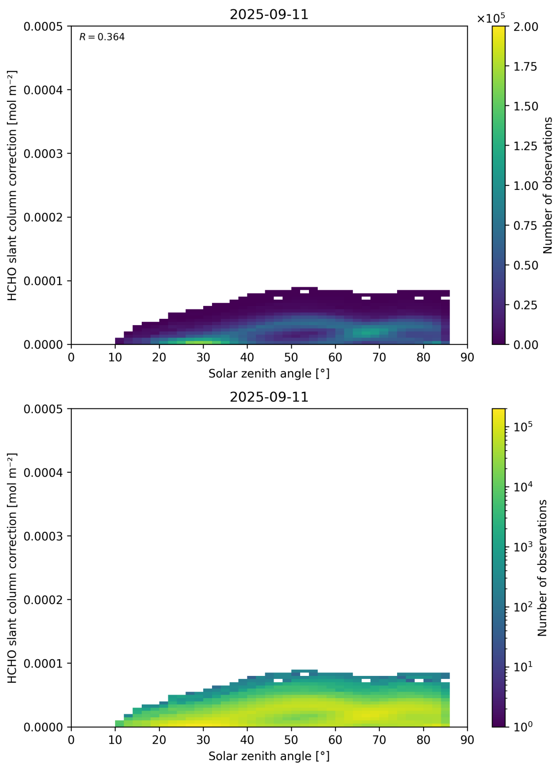
Figure 172: Scatter density plot of “Solar zenith angle” against “HCHO slant column correction” for 2025-09-10 to 2025-09-12.
