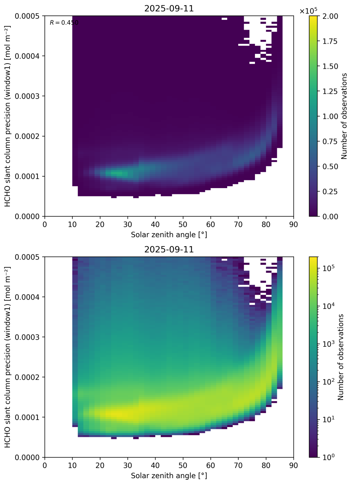
Figure 174: Scatter density plot of “Solar zenith angle” against “HCHO slant column precision (window1)” for 2025-09-10 to 2025-09-12.
