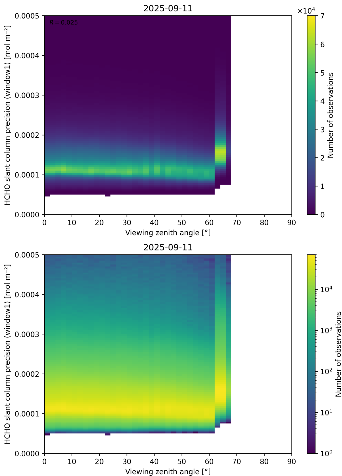
Figure 189: Scatter density plot of “Viewing zenith angle” against “HCHO slant column precision (window1)” for 2025-09-10 to 2025-09-12.
