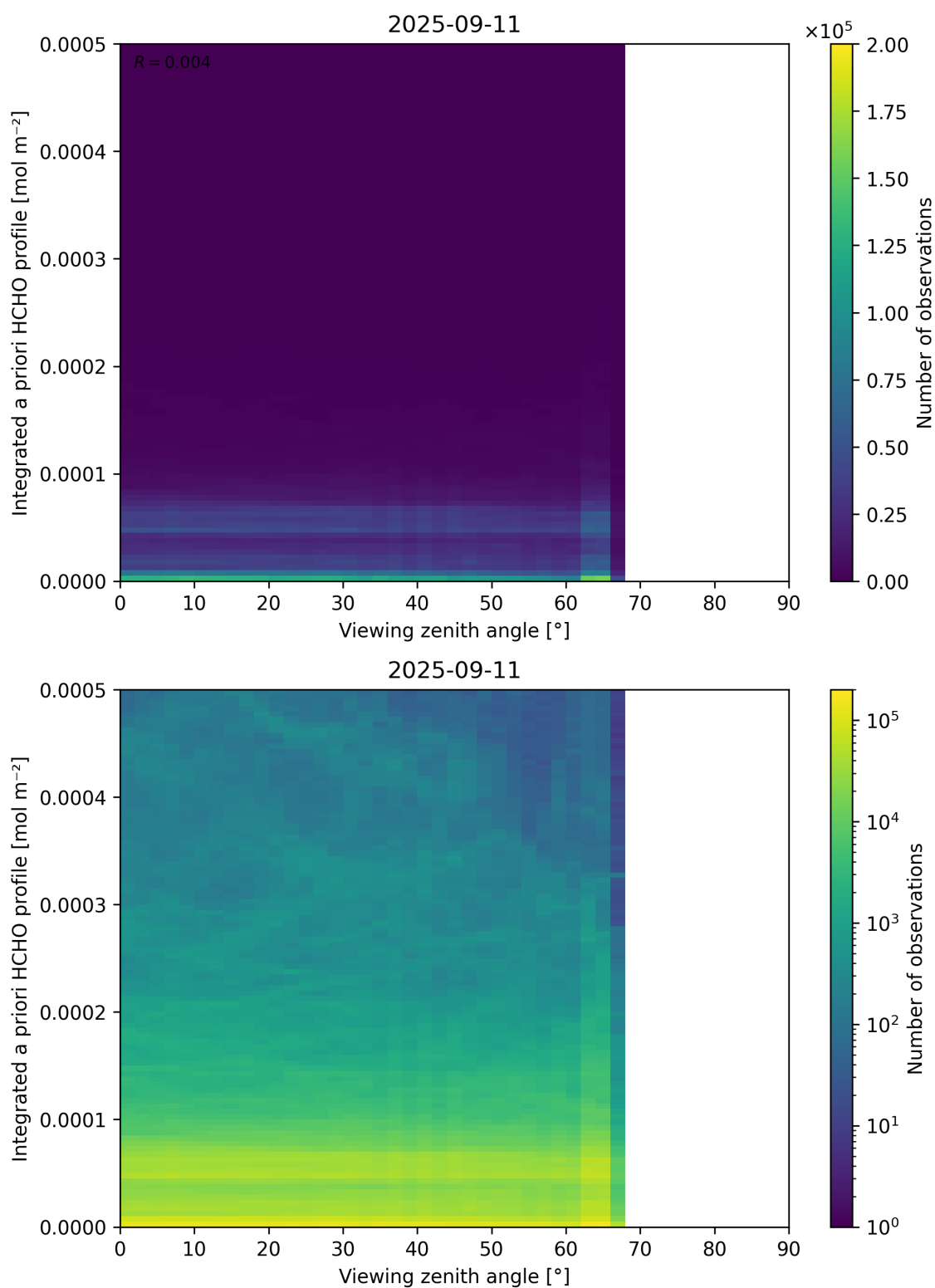
Figure 195: Scatter density plot of “Viewing zenith angle” against “Integrated a priori HCHO profile” for 2025-09-10 to 2025-09-12.
