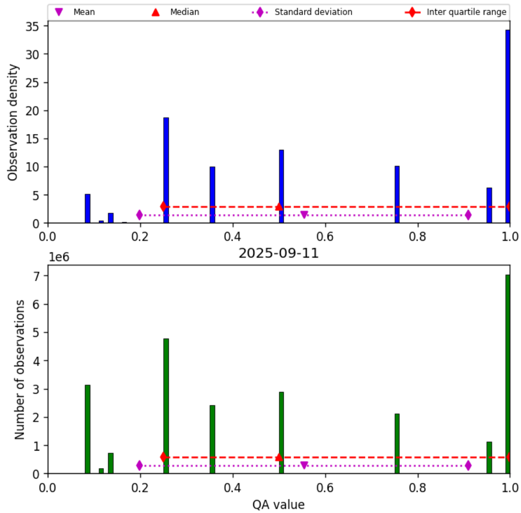
Figure 34: Histogram of “QA value” for 2025-09-10 to 2025-09-12
