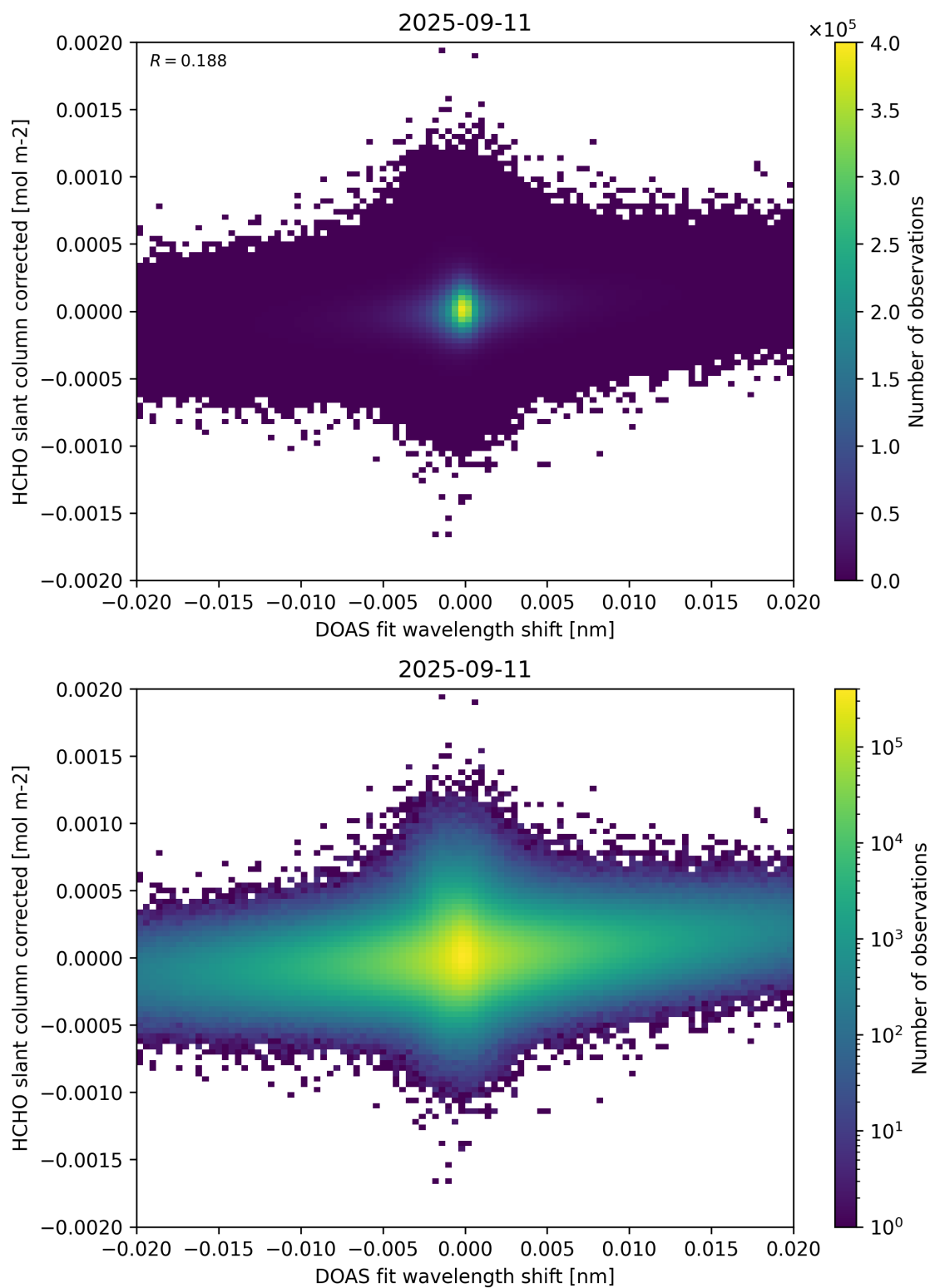
Figure 66: Scatter density plot of “DOAS fit wavelength shift” against “HCHO slant column corrected” for 2025-09-10 to 2025-09-12.
