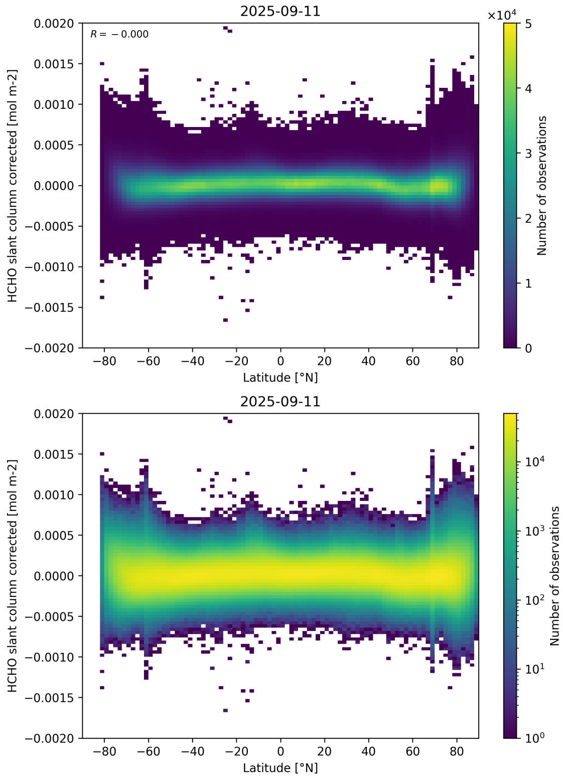
Figure 157: Scatter density plot of "Latitude" against "HCHO slant column corrected" for 2025-09-10 to 2025-09-12.
