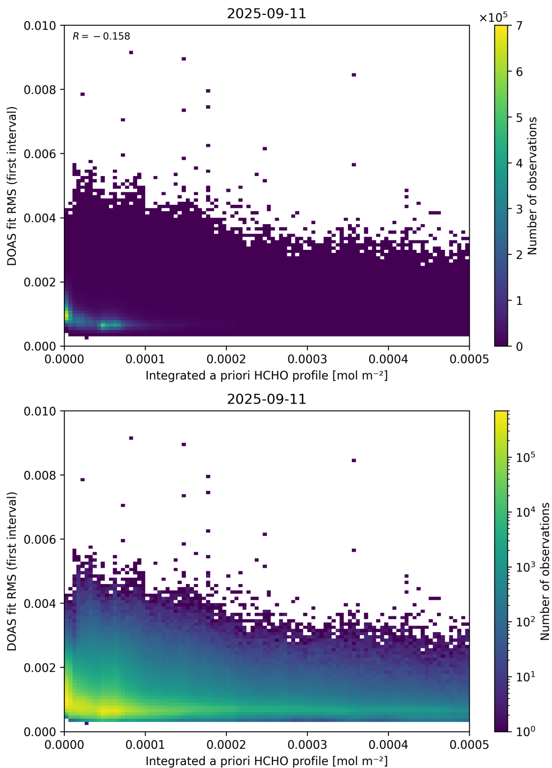
Figure 148: Scatter density plot of “Integrated a priori HCHO profile” against “DOAS fit RMS (first interval)” for 2025-09-10 to 2025-09-12.
