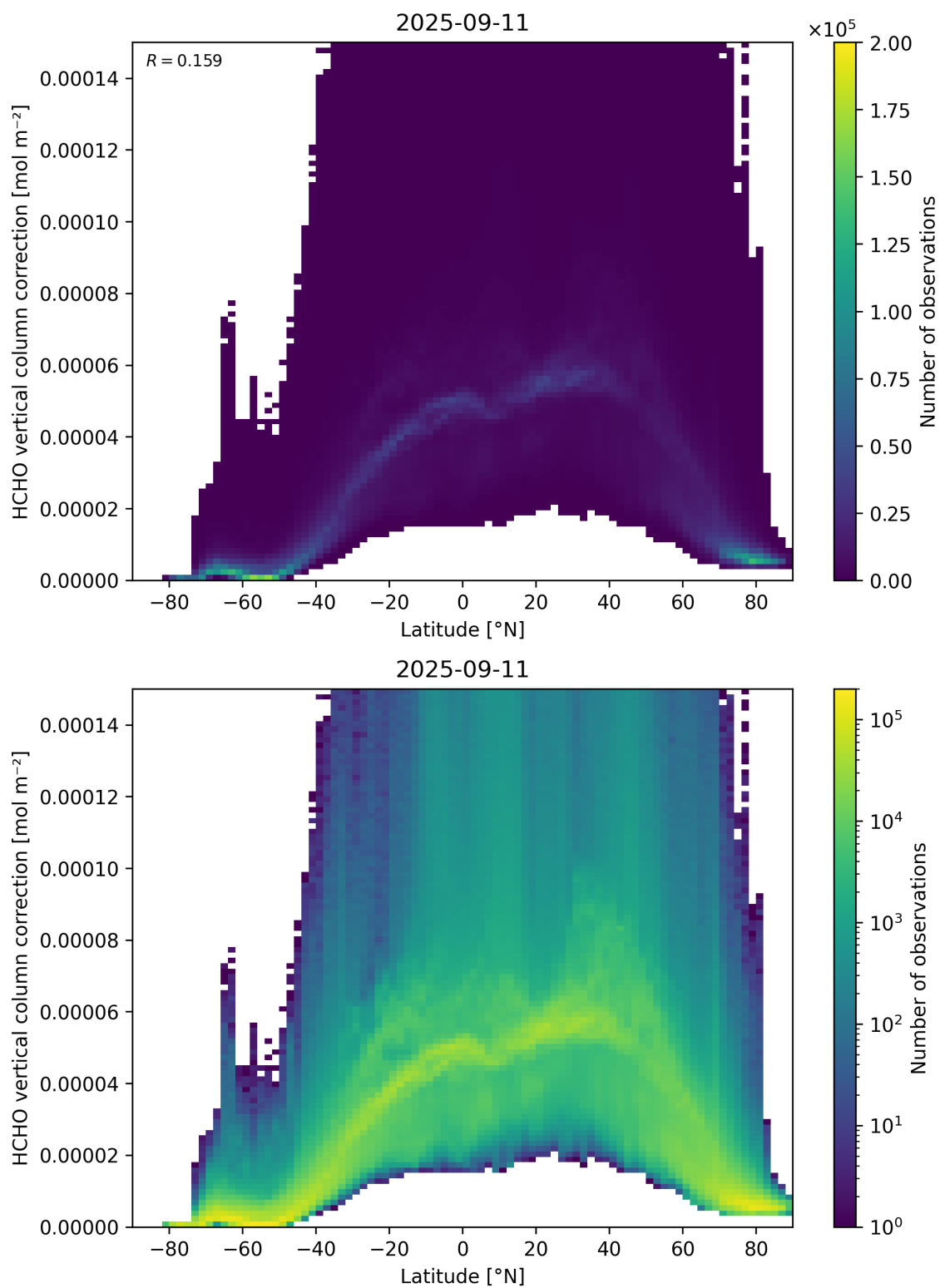
Figure 164: Scatter density plot of “Latitude” against “HCHO vertical column correction” for 2025-09-10 to 2025-09-12.
