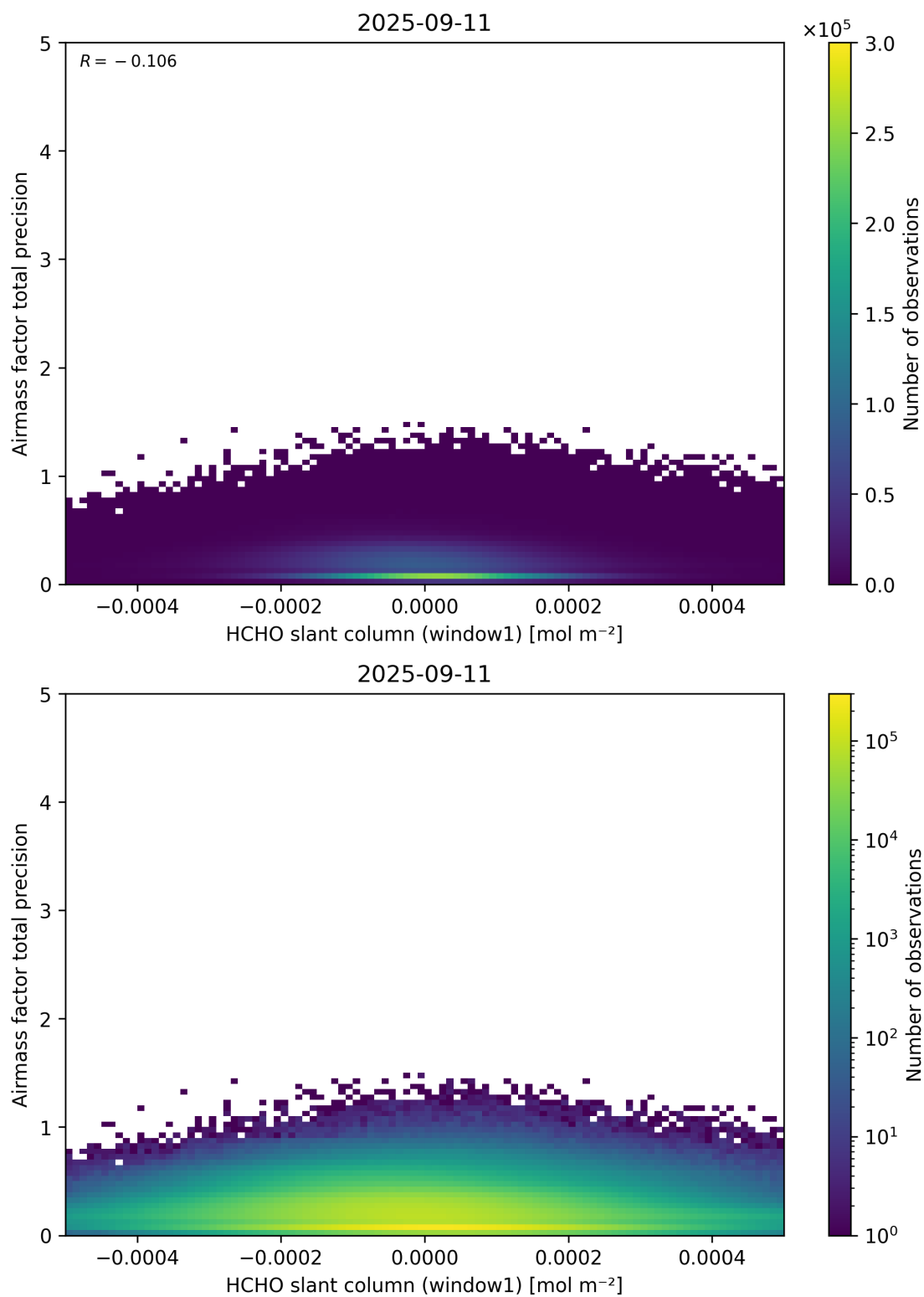
Figure 86: Scatter density plot of “HCHO slant column (window1)” against “Airmass factor total precision” for 2025-09-10 to 2025-09-12.
