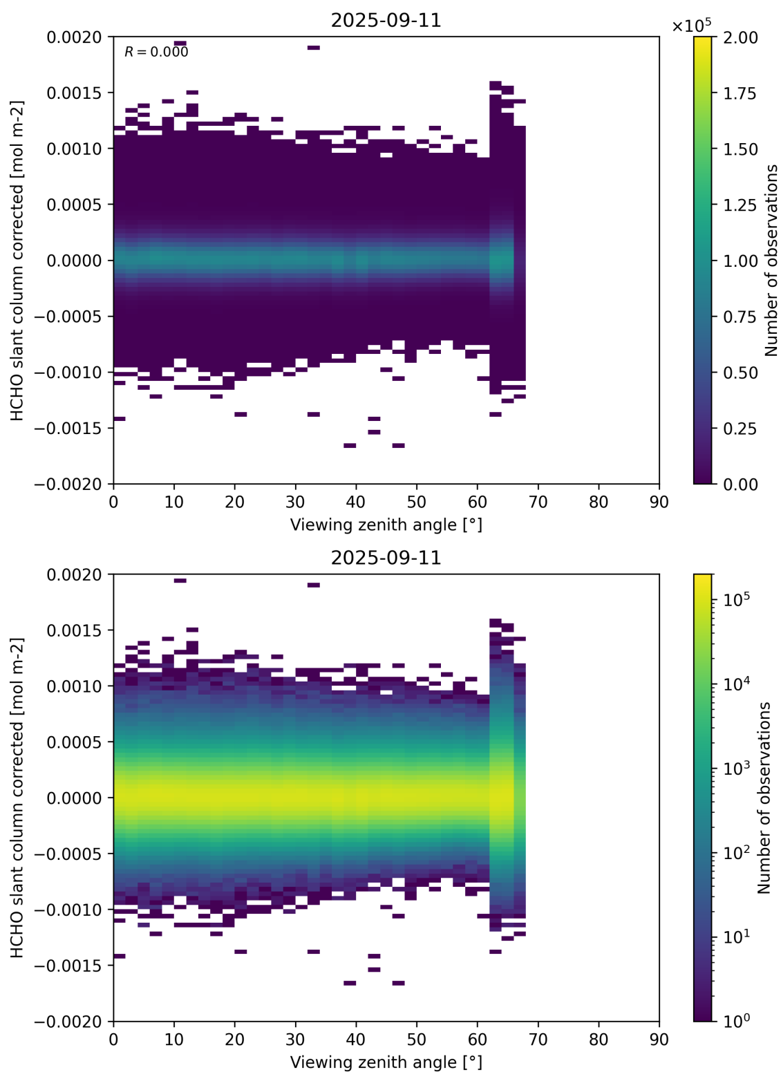
Figure 186: Scatter density plot of “Viewing zenith angle” against “HCHO slant column corrected” for 2025-09-10 to 2025-09-12.
