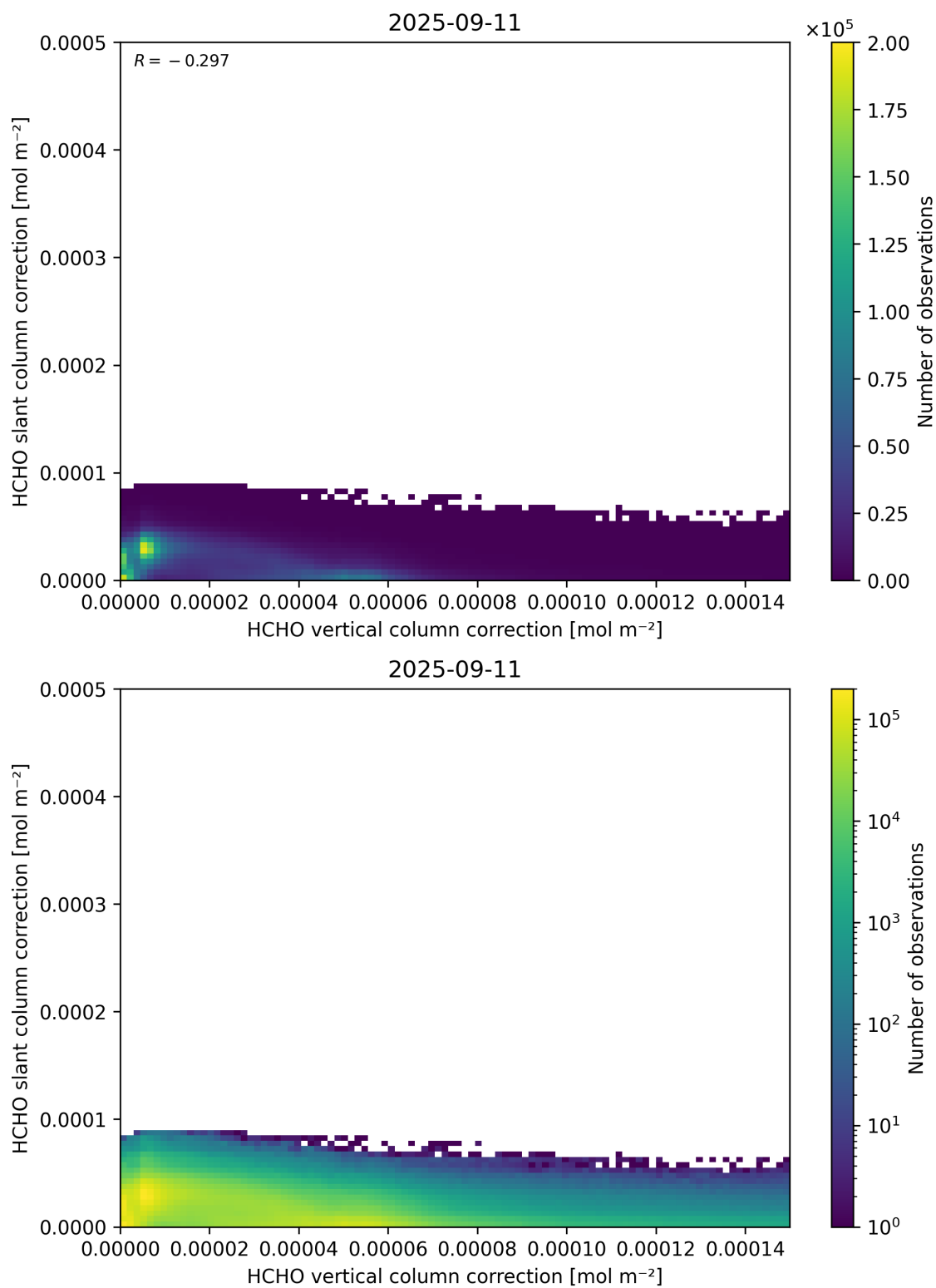
Figure 117: Scatter density plot of “HCHO vertical column correction” against “HCHO slant column correction” for 2025-09-10 to 2025-09-12.
