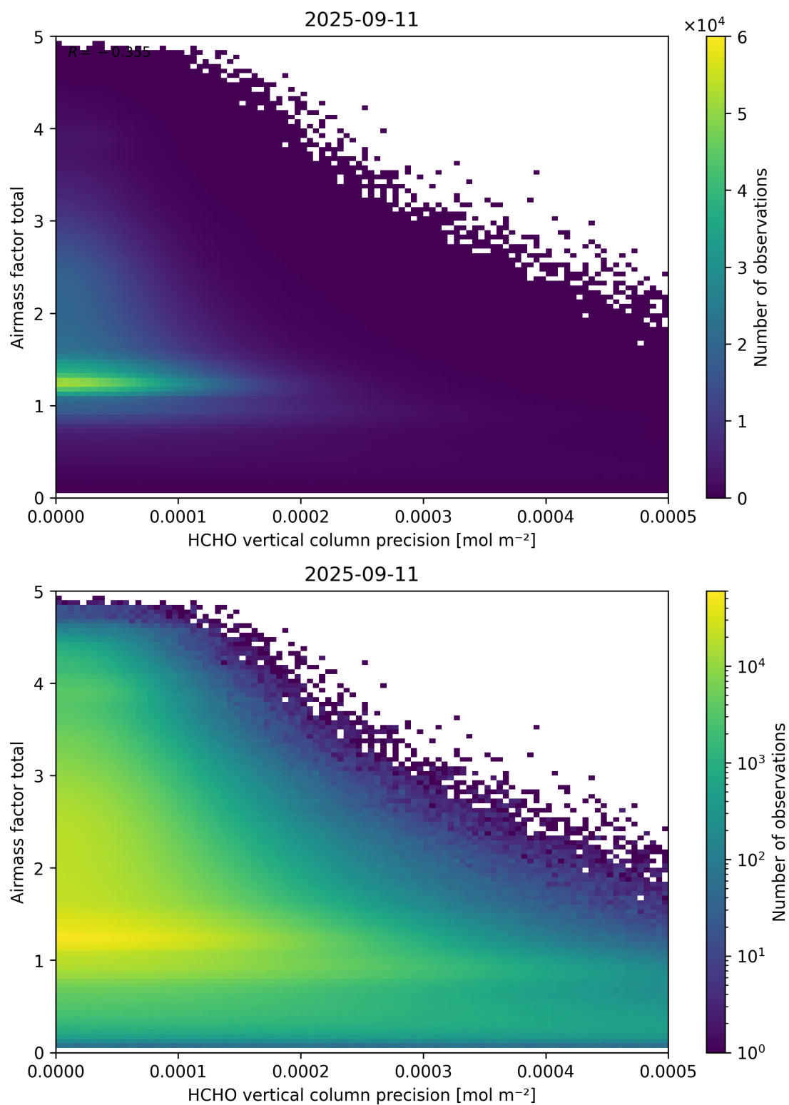
Figure 144: Scatter density plot of “HCHO vertical column precision” against “Airmass factor total” for 2025-09-10 to 2025-09-12.
