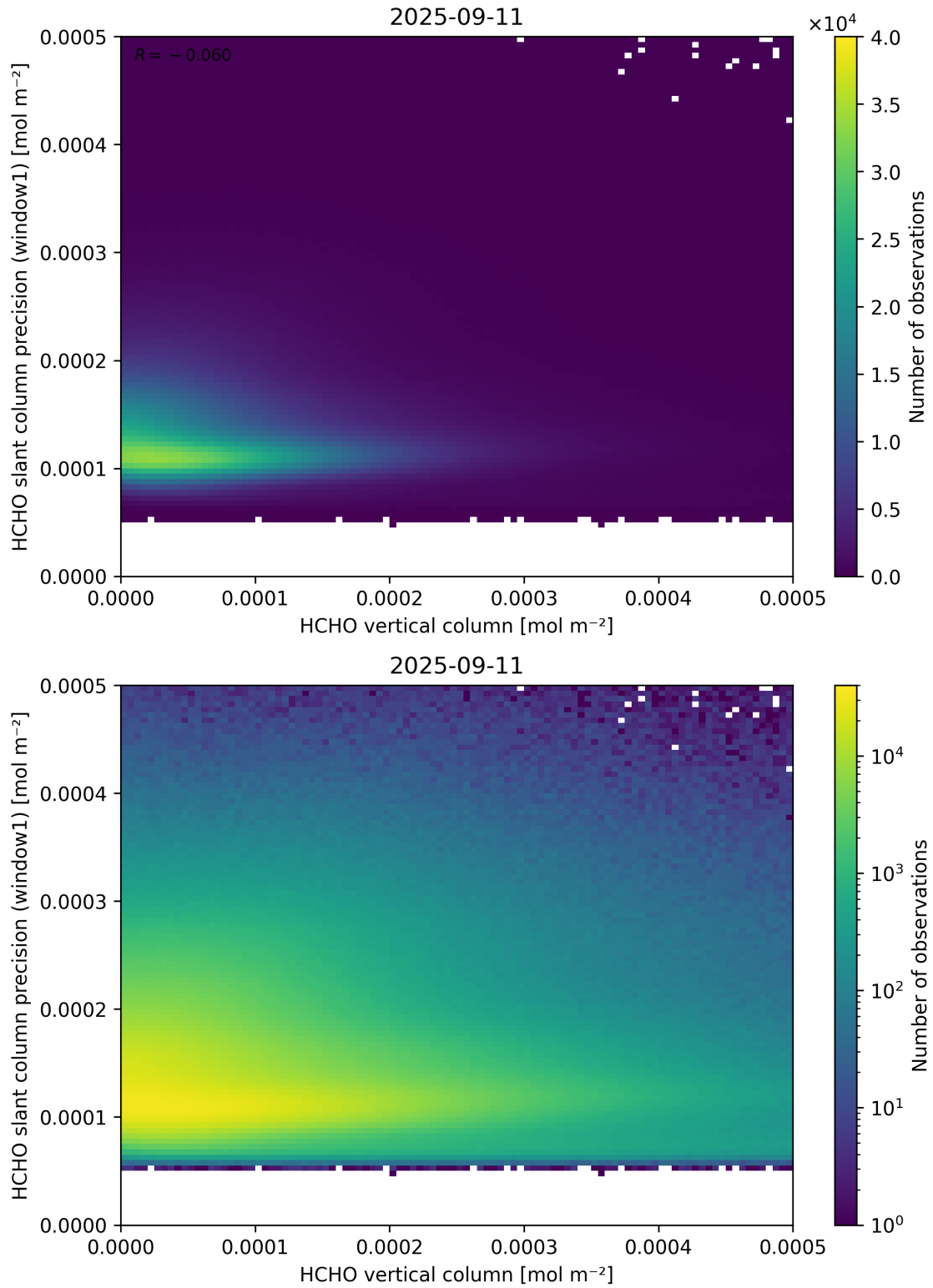
Figure 130: Scatter density plot of “HCHO vertical column” against “HCHO slant column precision (window1)” for 2025-09-10 to 2025-09-12.
