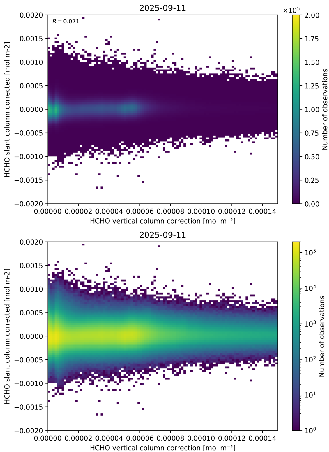
Figure 116: Scatter density plot of “HCHO vertical column correction” against “HCHO slant column corrected” for 2025-09-10 to 2025-09-12.
