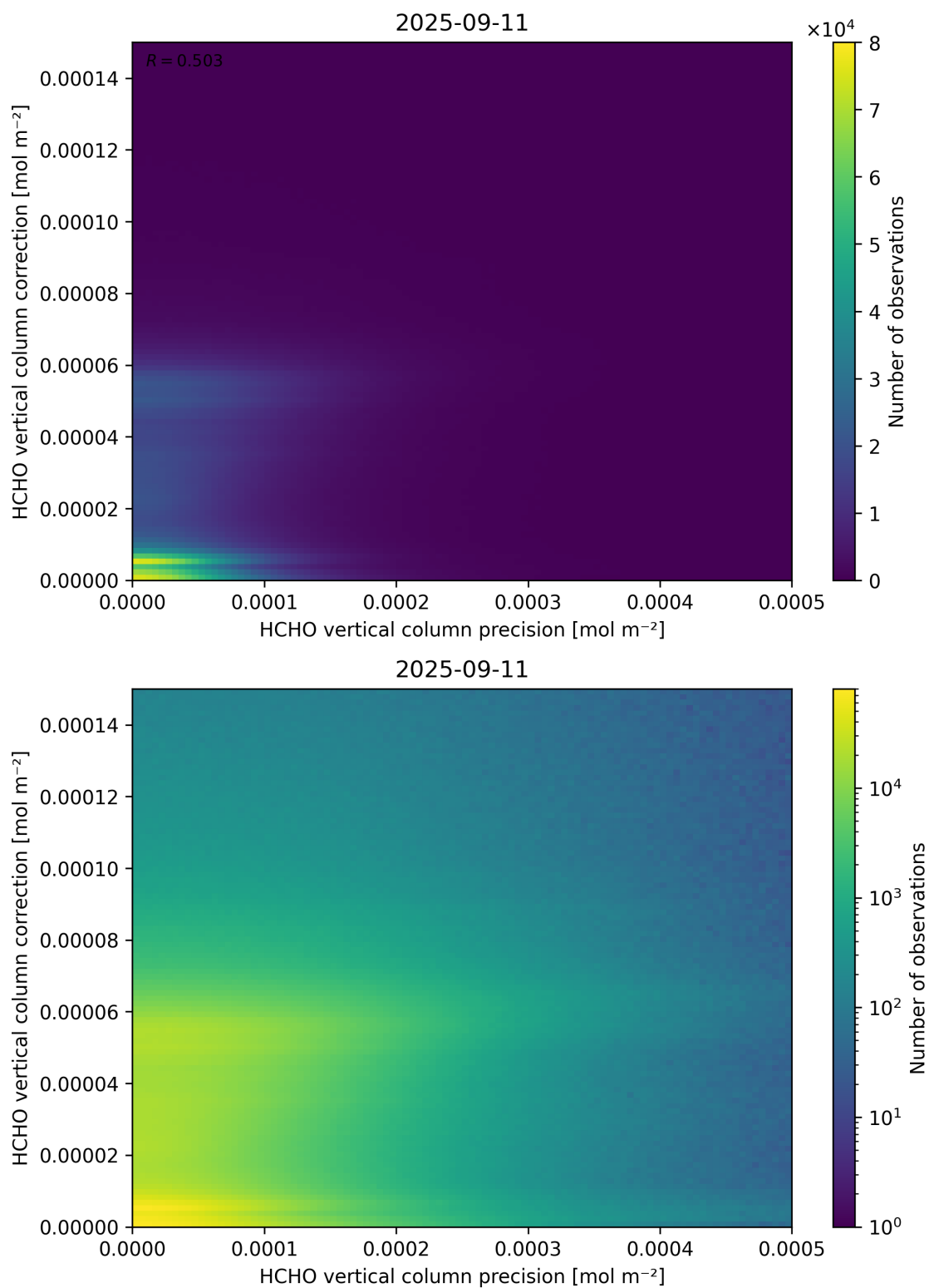
Figure 146: Scatter density plot of “HCHO vertical column precision” against “HCHO vertical column correction” for 2025-09-10 to 2025-09-12.
