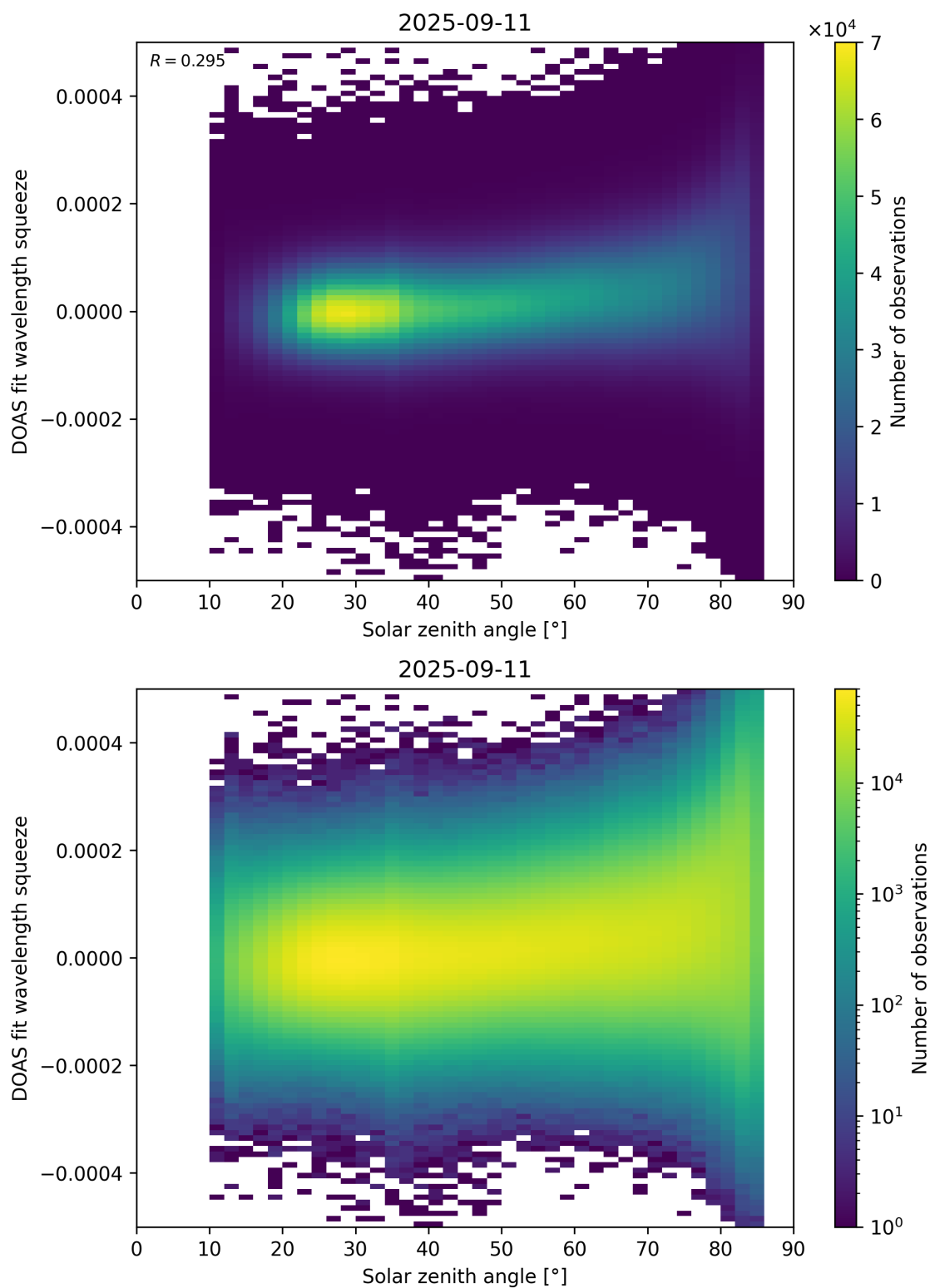
Figure 169: Scatter density plot of “Solar zenith angle” against “DOAS fit wavelength squeeze” for 2025-09-10 to 2025-09-12.
