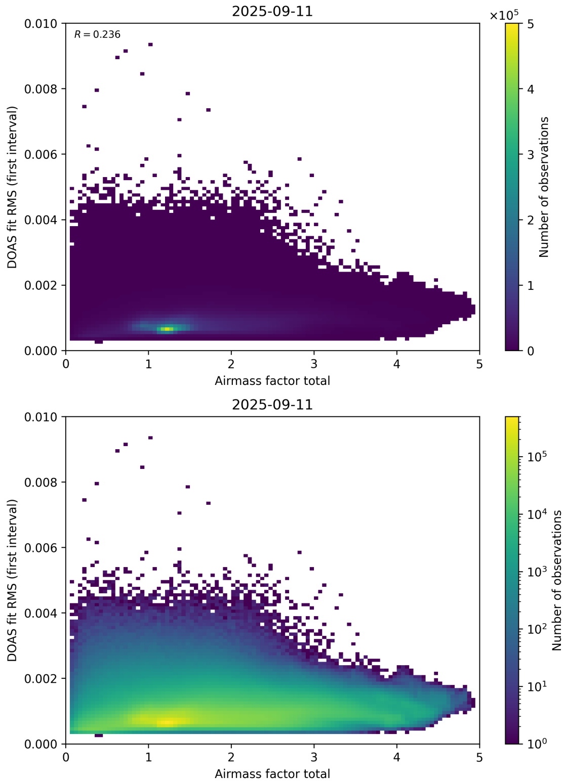
Figure 97: Scatter density plot of “Airmass factor total” against “DOAS fit RMS (first interval)” for 2025-09-10 to 2025-09-12.
