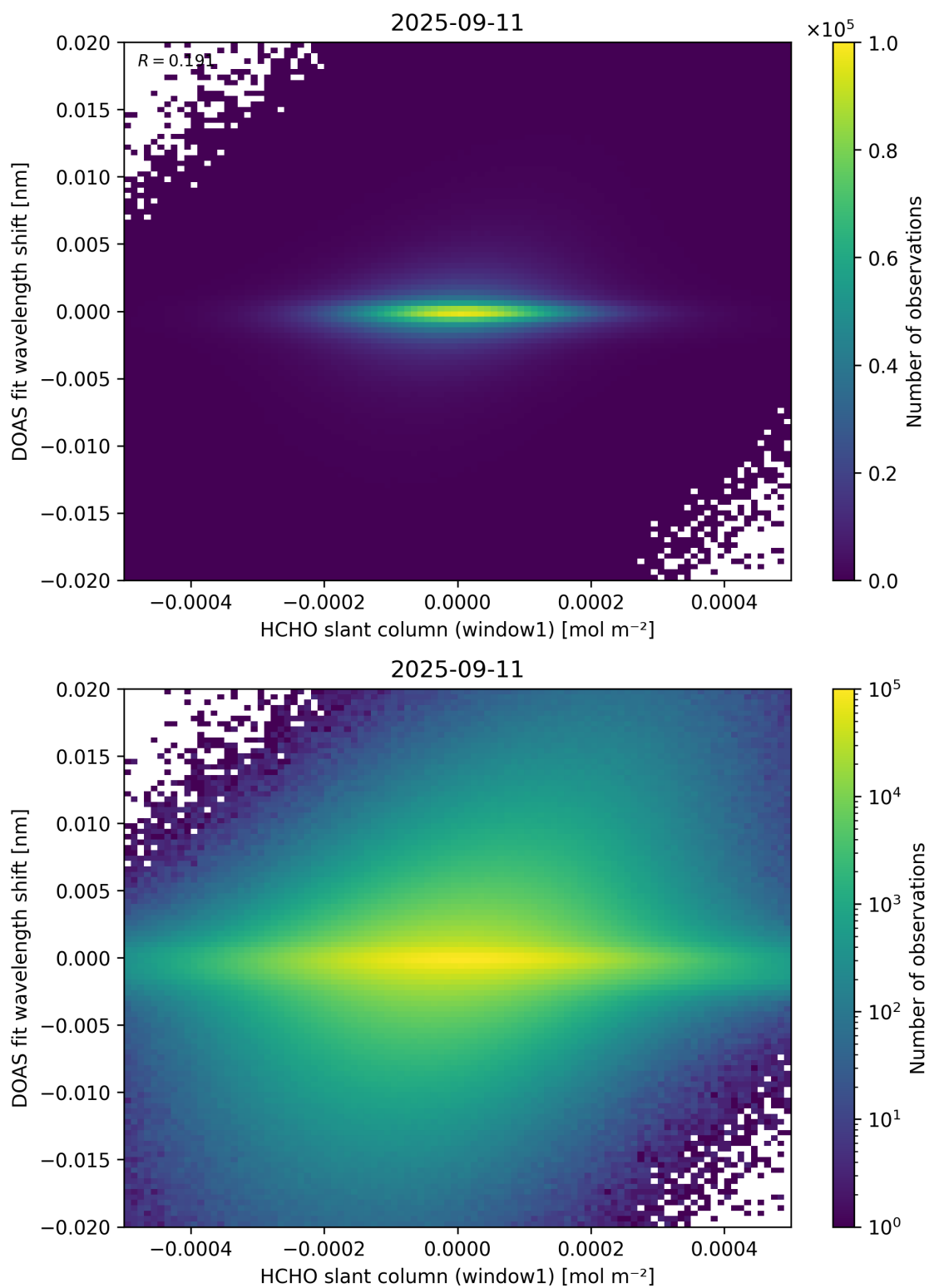
Figure 79: Scatter density plot of “HCHO slant column (window1)” against “DOAS fit wavelength shift” for 2025-09-10 to 2025-09-12.
