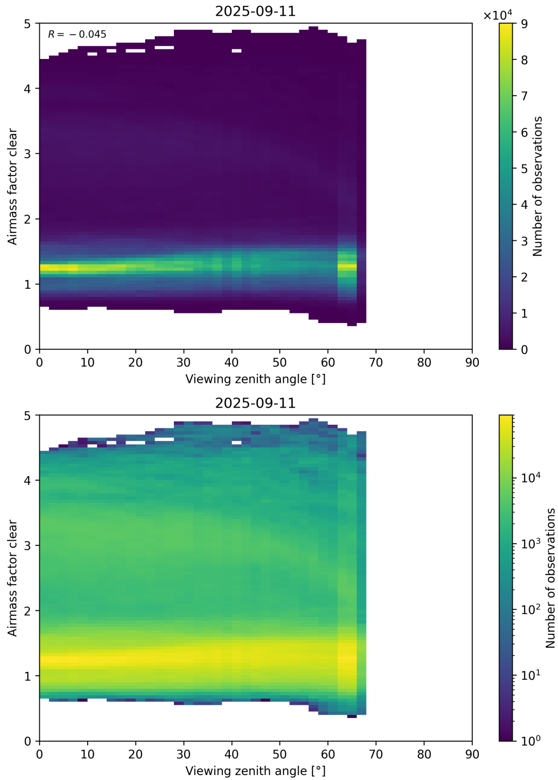
Figure 185: Scatter density plot of “Viewing zenith angle” against “Airmass factor clear” for 2025-09-10 to 2025-09-12.
