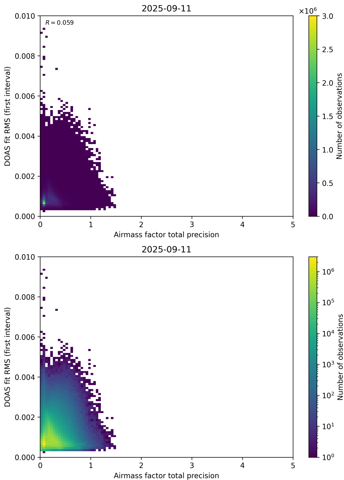
Figure 105: Scatter density plot of “Airmass factor total precision” against “DOAS fit RMS (first interval)” for 2025-09-10 to 2025-09-12.
