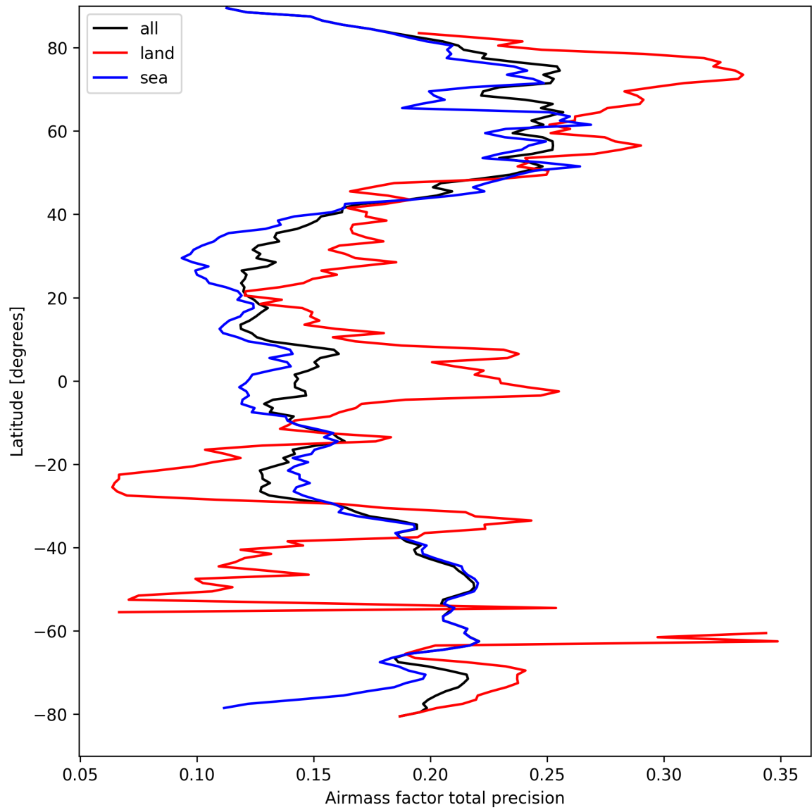
Figure 27: Zonal average of “Airmass factor total precision” for 2025-09-10 to 2025-09-12.
