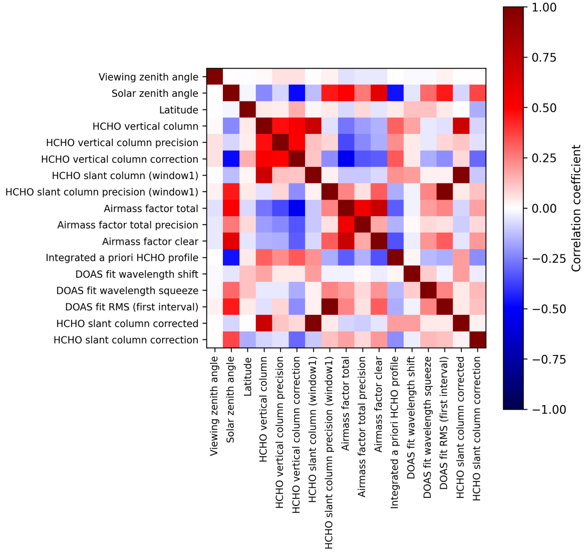
Figure 2: Map of correlation matrix for 2025-09-10 to 2025-09-12.
