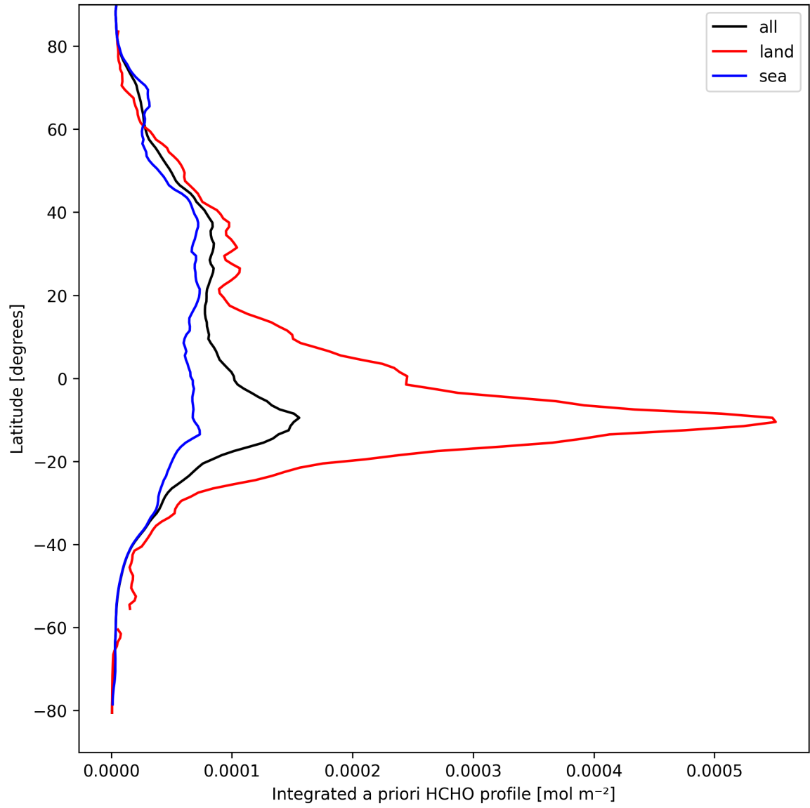
Figure 29: Zonal average of “Integrated a priori HCHO profile” for 2025-09-10 to 2025-09-12.
