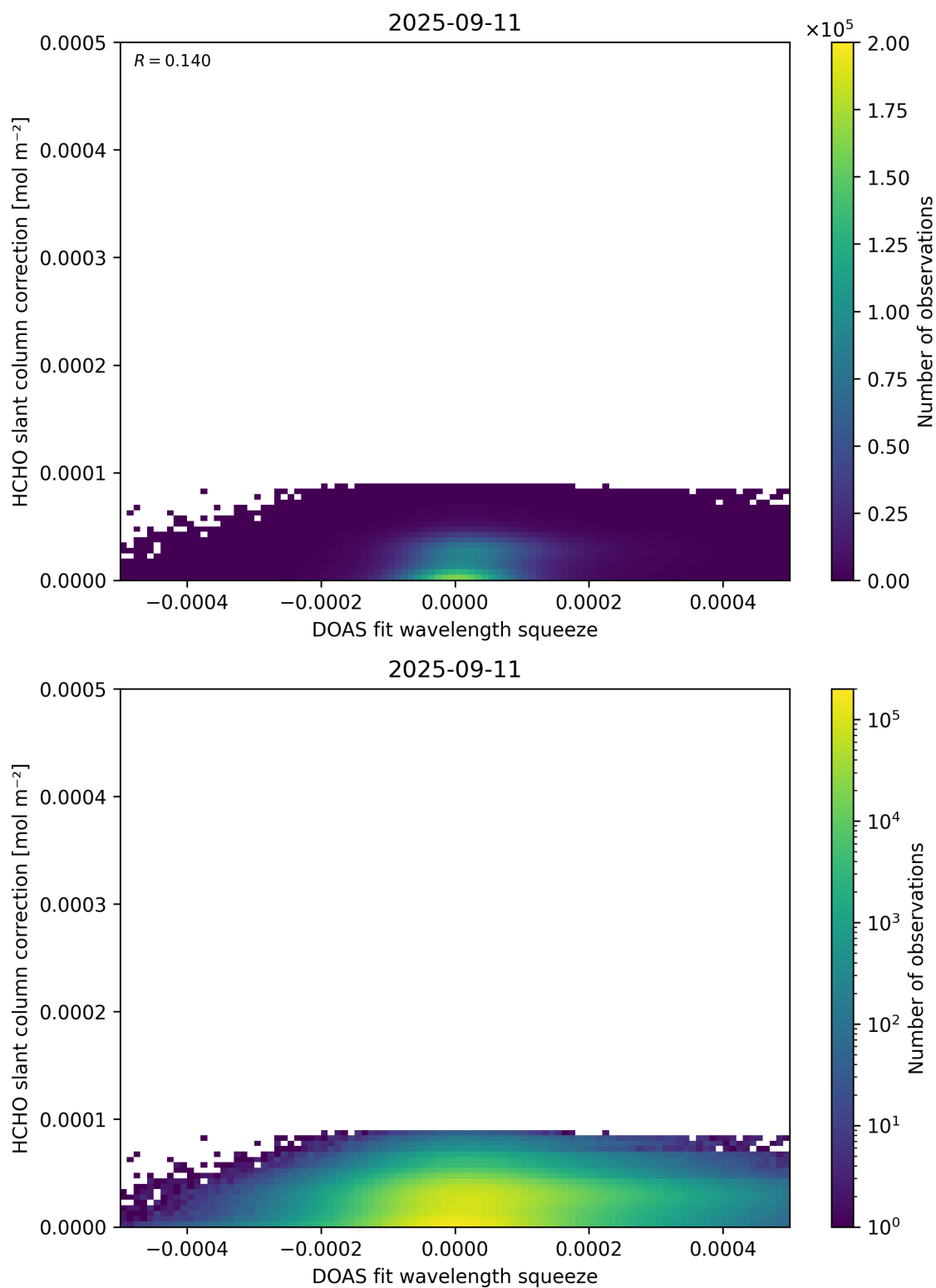
Figure 70: Scatter density plot of “DOAS fit wavelength squeeze” against “HCHO slant column correction” for 2025-09-10 to 2025-09-12.
