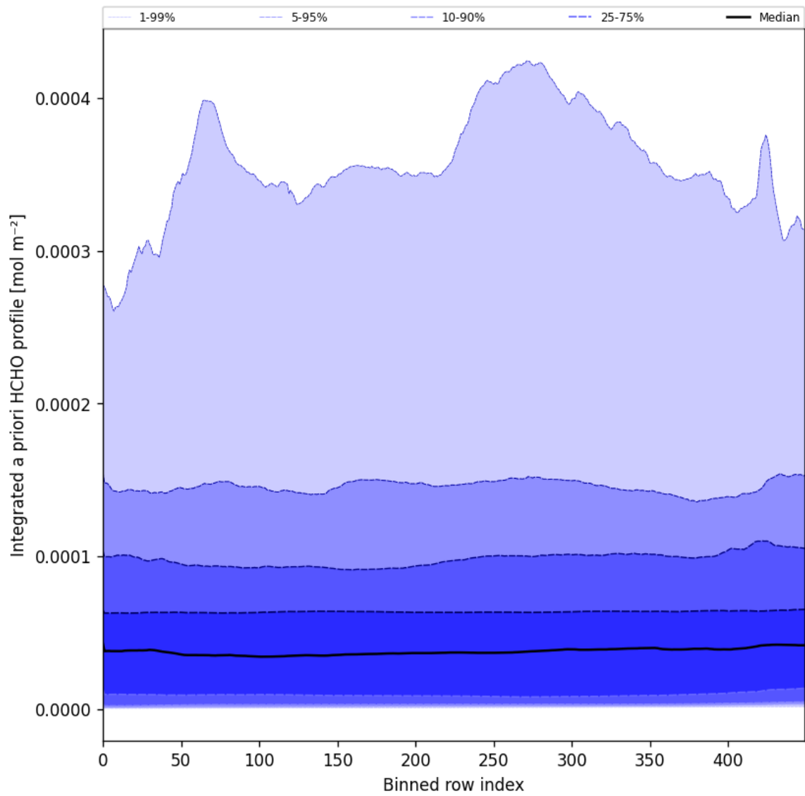
Figure 57: Along track statistics of “Integrated a priori HCHO profile” for 2025-09-10 to 2025-09-12
