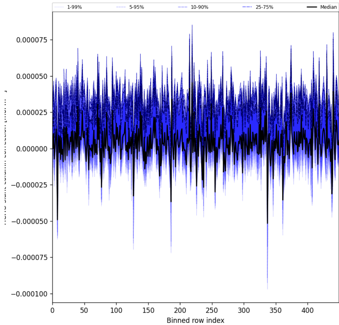
Figure 61: Along track statistics of “HCHO slant column correction” for 2025-09-10 to 2025-09-12
