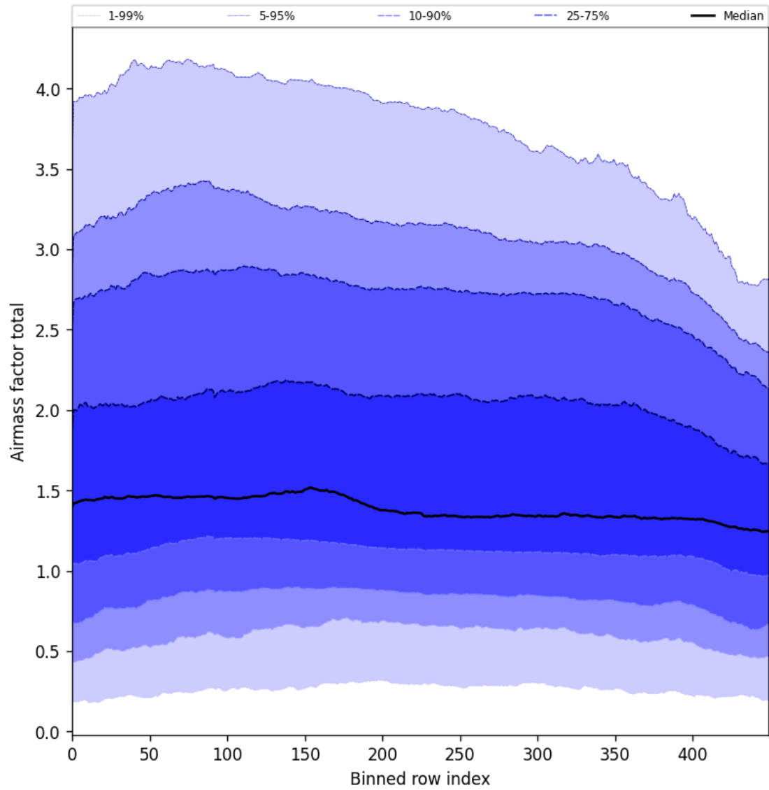
Figure 54: Along track statistics of “Airmass factor total” for 2025-09-10 to 2025-09-12
