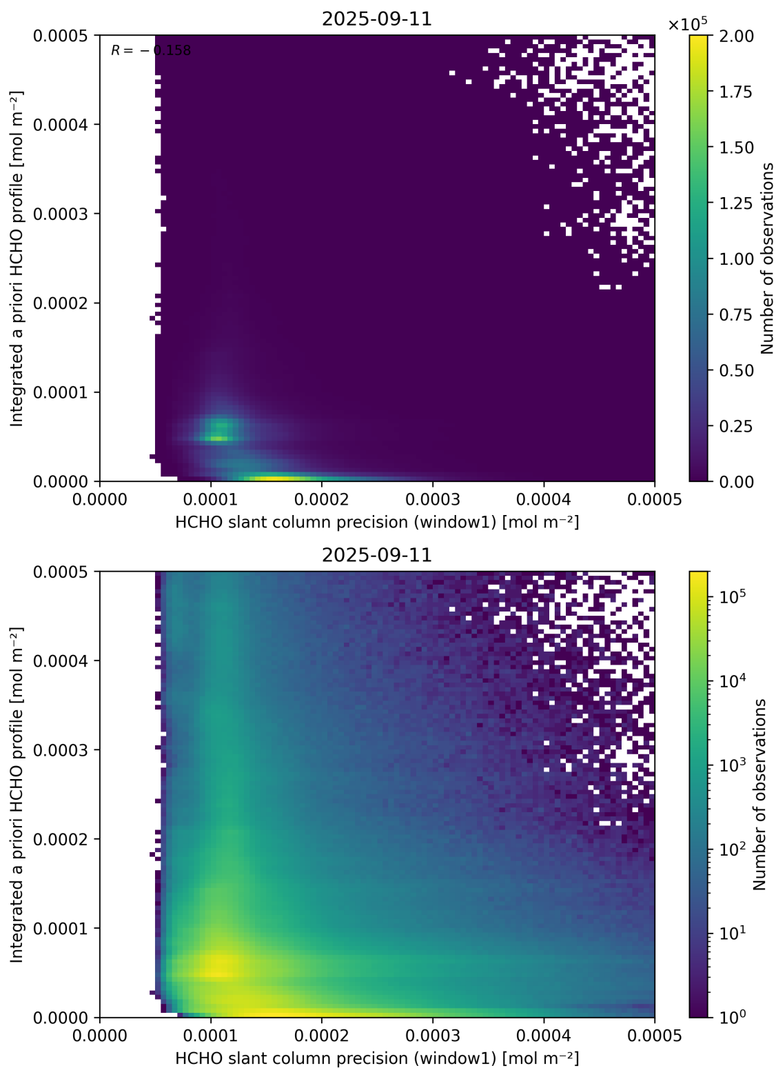
Figure 96: Scatter density plot of “HCHO slant column precision (window1)” against “Integrated a priori HCHO profile” for 2025-09-10 to 2025-09-12.
