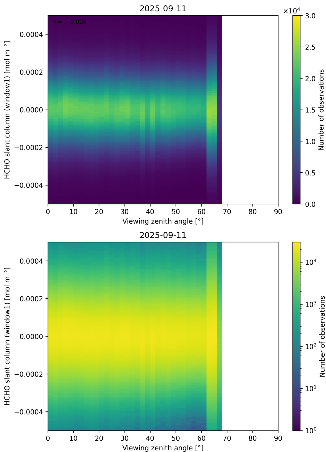
Figure 188: Scatter density plot of “Viewing zenith angle” against “HCHO slant column (window1)” for 2025-09-10 to 2025-09-12.
