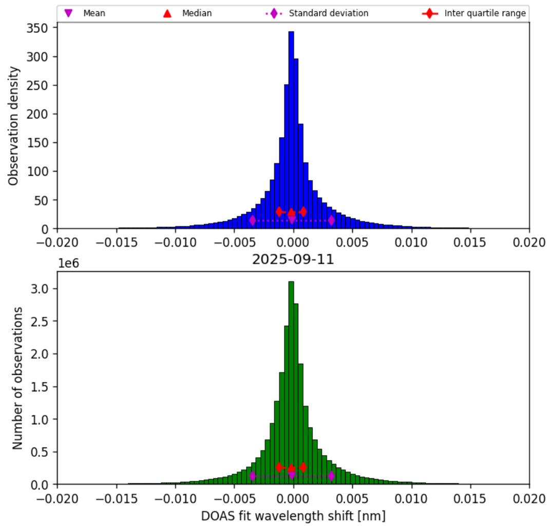
Figure 44: Histogram of “DOAS fit wavelength shift” for 2025-09-10 to 2025-09-12
