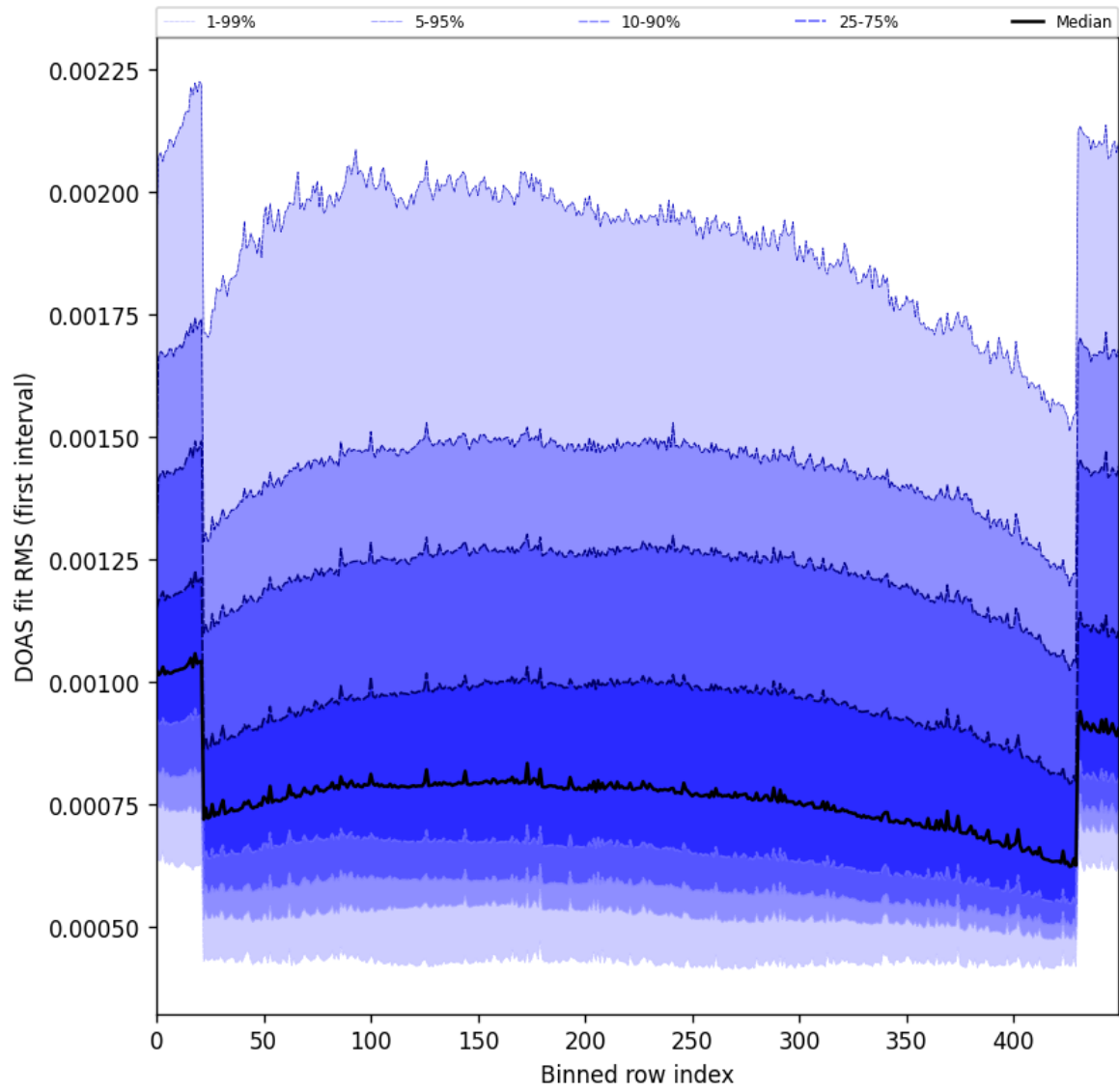
Figure 60: Along track statistics of “DOAS fit RMS (first interval)” for 2025-09-10 to 2025-09-12
