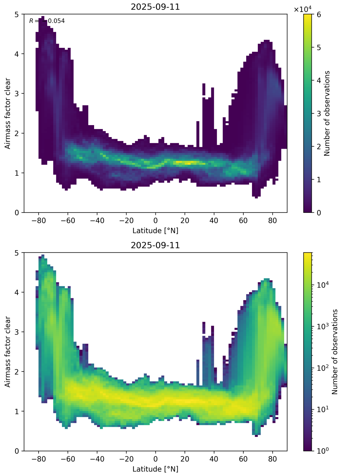
Figure 156: Scatter density plot of “Latitude” against “Airmass factor clear” for 2025-09-10 to 2025-09-12.
