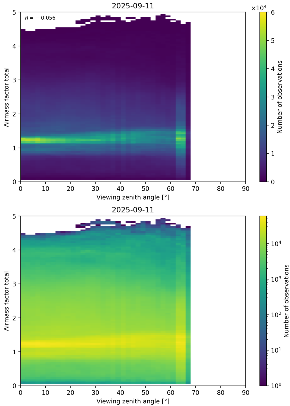
Figure 190: Scatter density plot of “Viewing zenith angle” against “Airmass factor total” for 2025-09-10 to 2025-09-12.
