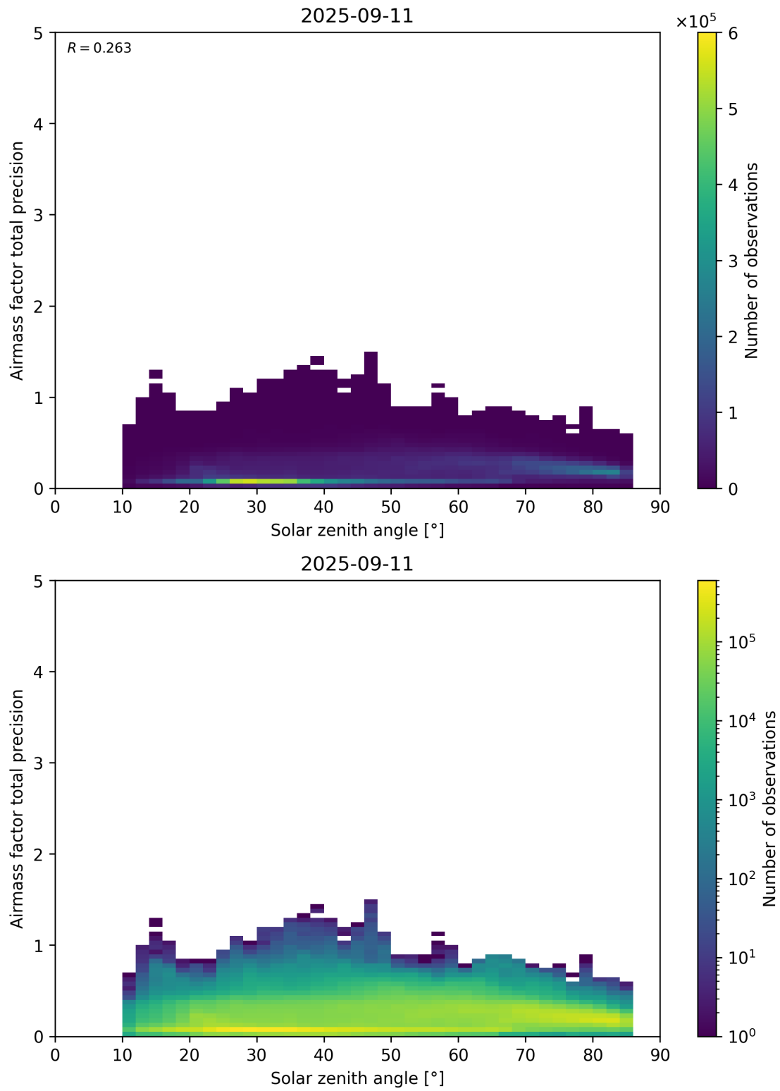
Figure 176: Scatter density plot of “Solar zenith angle” against “Airmass factor total precision” for 2025-09-10 to 2025-09-12.
