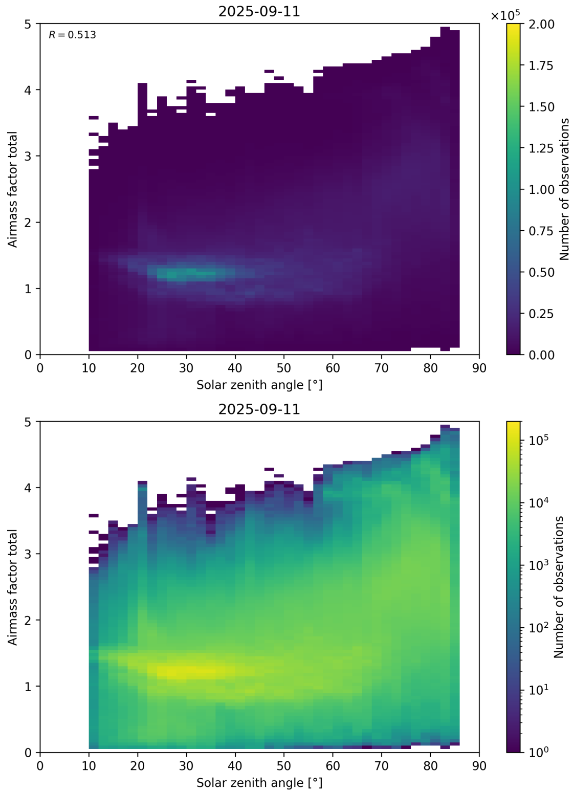
Figure 175: Scatter density plot of “Solar zenith angle” against “Airmass factor total” for 2025-09-10 to 2025-09-12.
