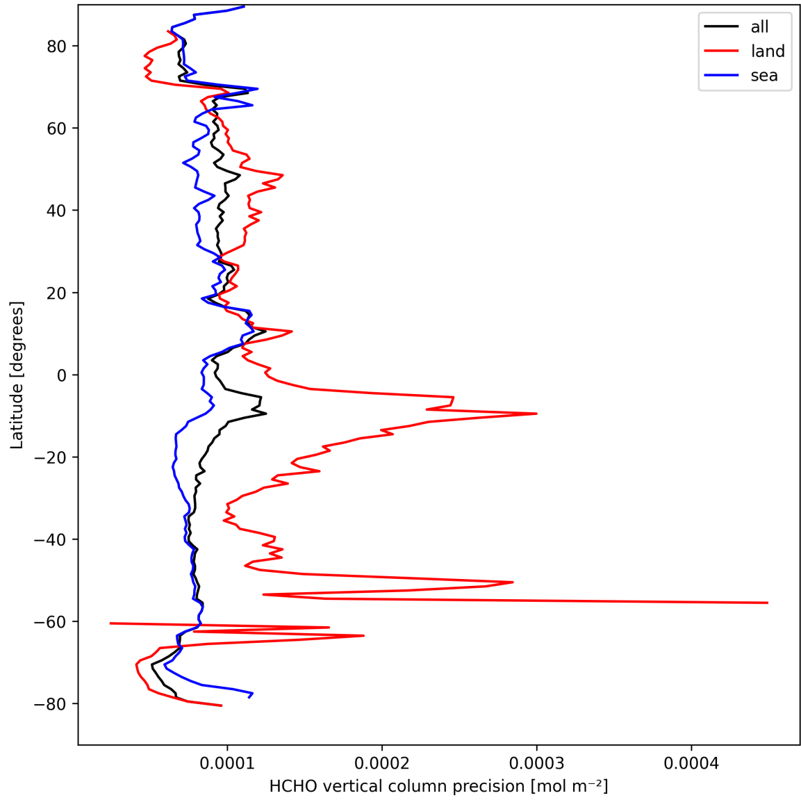
Figure 22: Zonal average of “HCHO vertical column precision” for 2025-09-10 to 2025-09-12.
