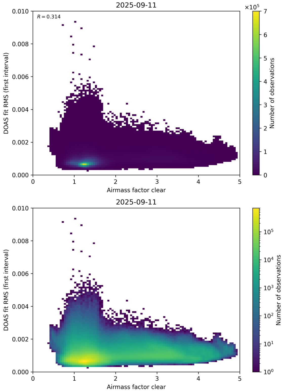
Figure 71: Scatter density plot of “Airmass factor clear” against “DOAS fit RMS (first interval)” for 2025-09-10 to 2025-09-12.
