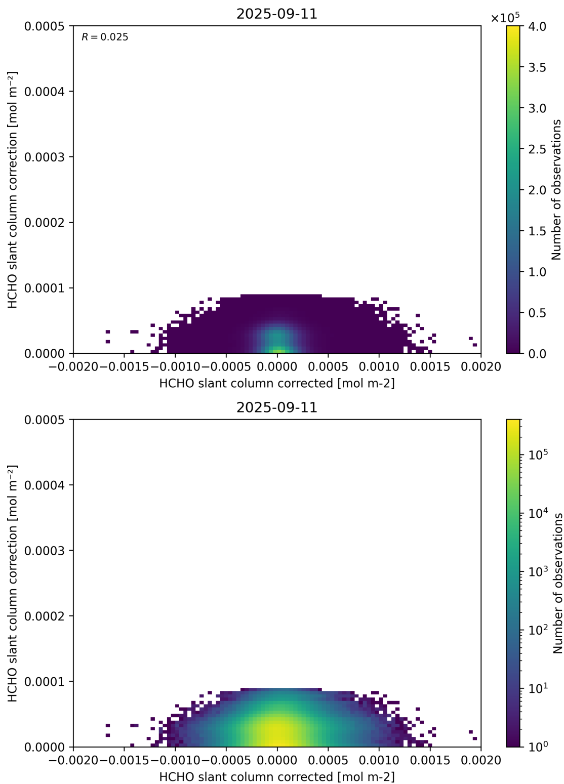
Figure 77: Scatter density plot of “HCHO slant column corrected” against “HCHO slant column correction” for 2025-09-10 to 2025-09-12.
