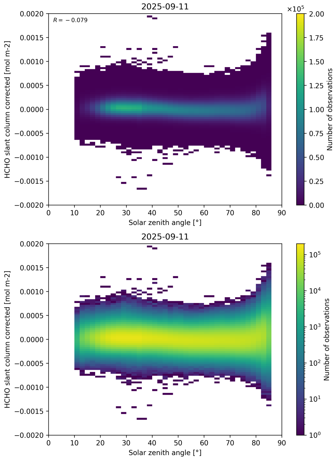
Figure 171: Scatter density plot of “Solar zenith angle” against “HCHO slant column corrected” for 2025-09-10 to 2025-09-12.
