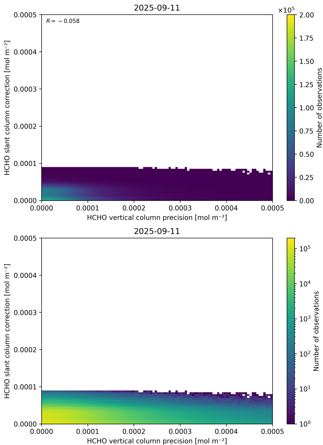
Figure 141: Scatter density plot of “HCHO vertical column precision” against “HCHO slant column correction” for 2025-09-10 to 2025-09-12.
