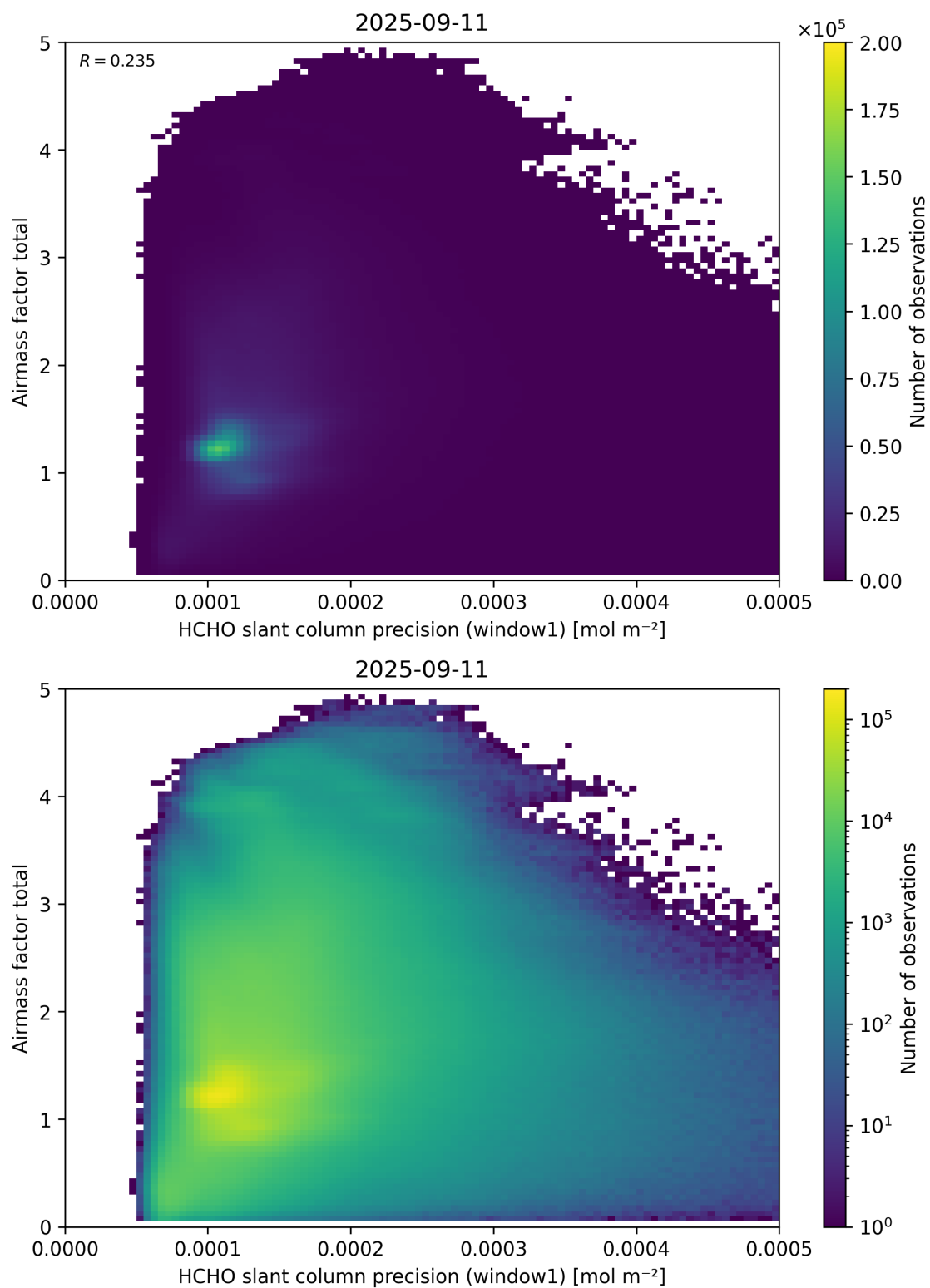
Figure 94: Scatter density plot of “HCHO slant column precision (window1)” against “Airmass factor total” for 2025-09-10 to 2025-09-12.
