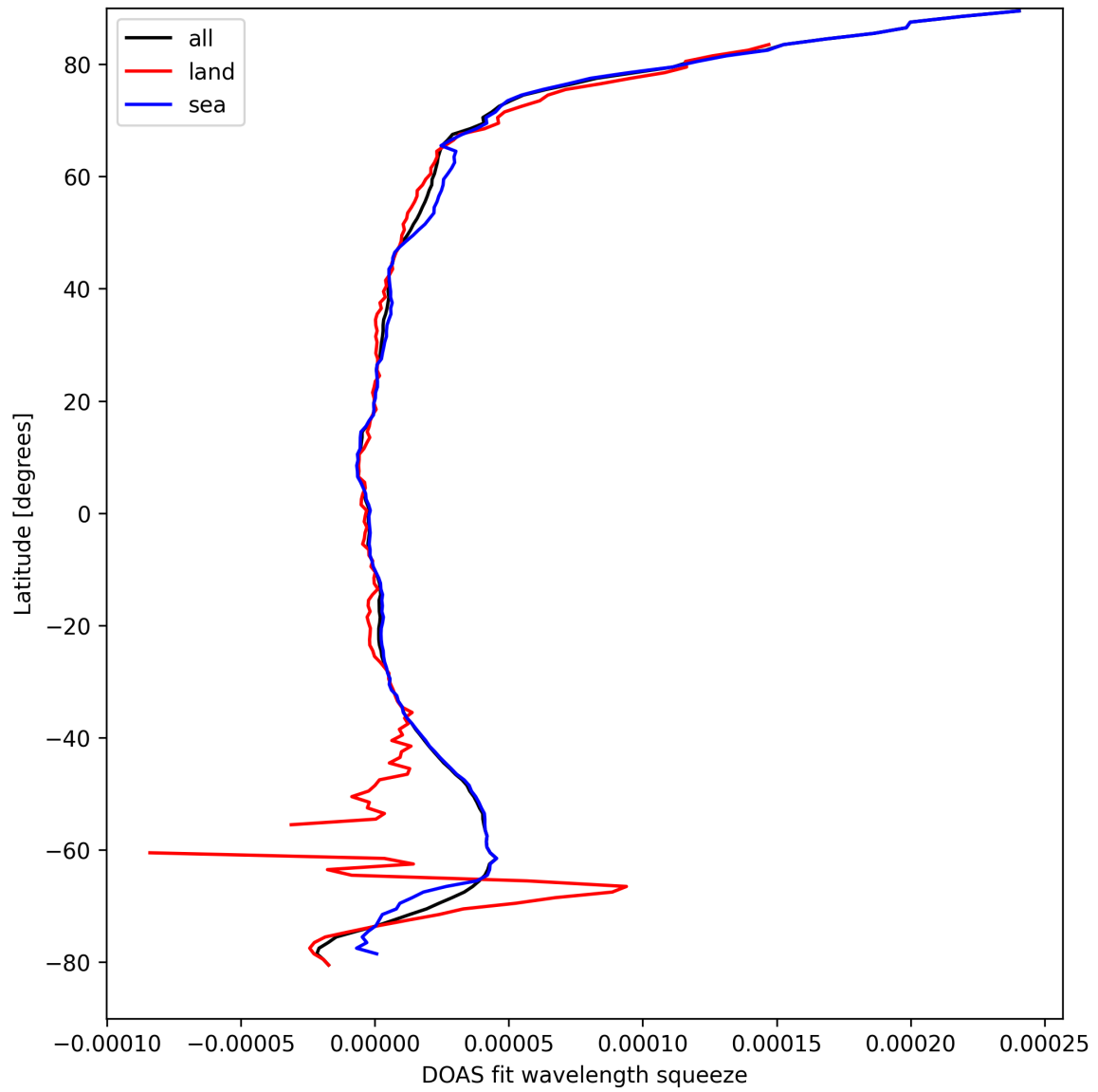
Figure 31: Zonal average of “DOAS fit wavelength squeeze” for 2025-09-10 to 2025-09-12.
