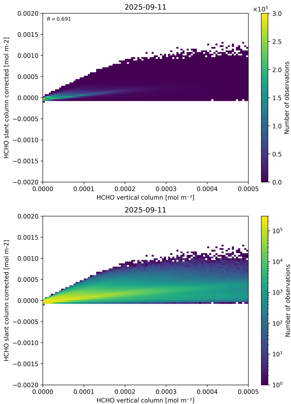
Figure 127: Scatter density plot of “HCHO vertical column” against “HCHO slant column corrected” for 2025-09-10 to 2025-09-12.
