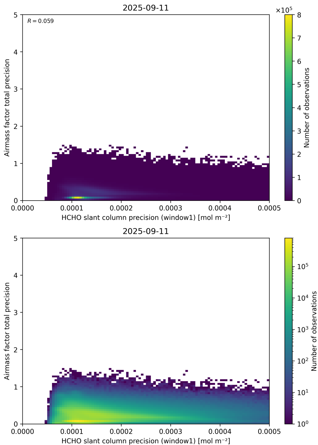
Figure 95: Scatter density plot of “HCHO slant column precision (window1)” against “Airmass factor total precision” for 2025-09-10 to 2025-09-12.
