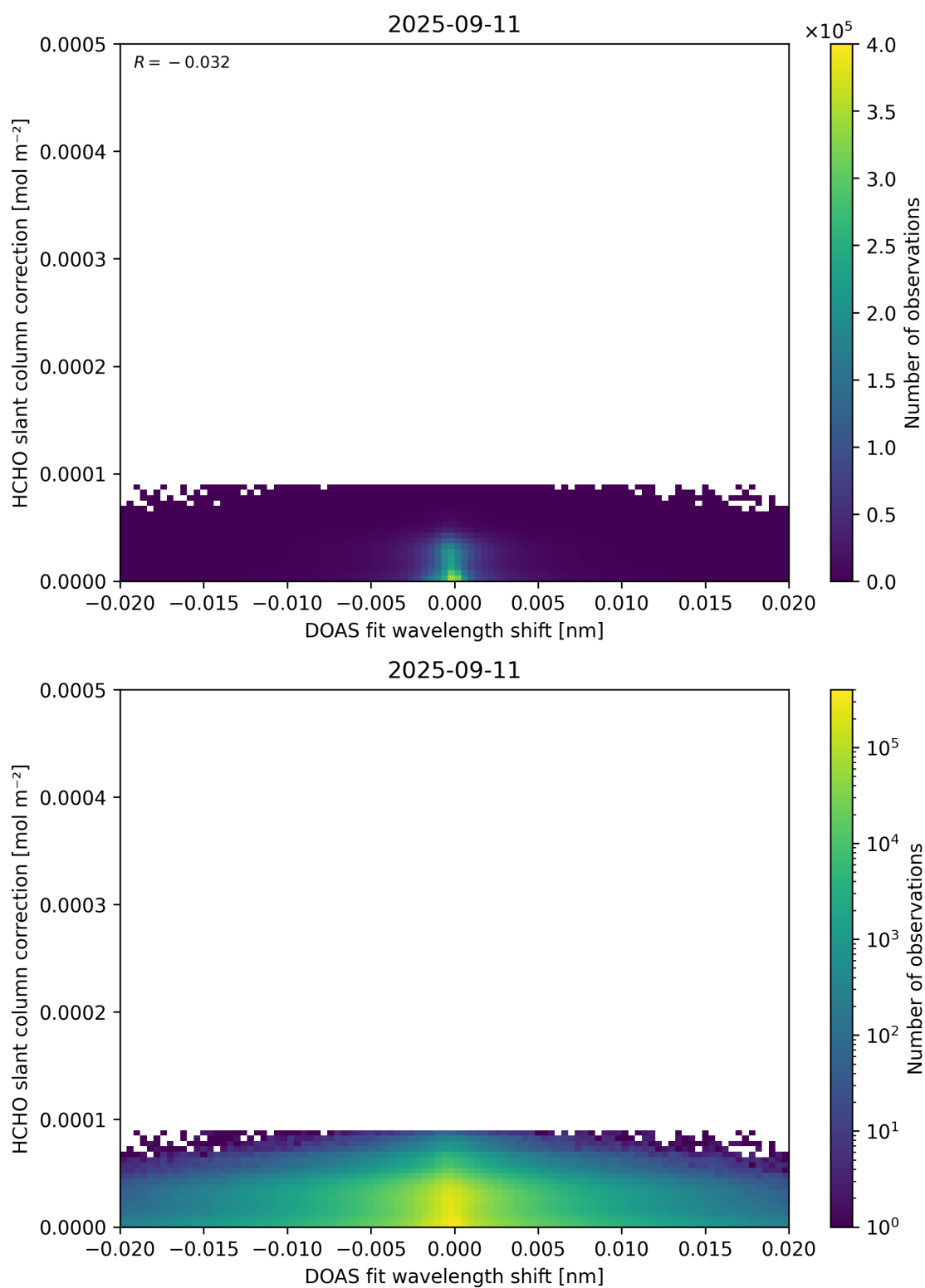
Figure 67: Scatter density plot of “DOAS fit wavelength shift” against “HCHO slant column correction” for 2025-09-10 to 2025-09-12.
