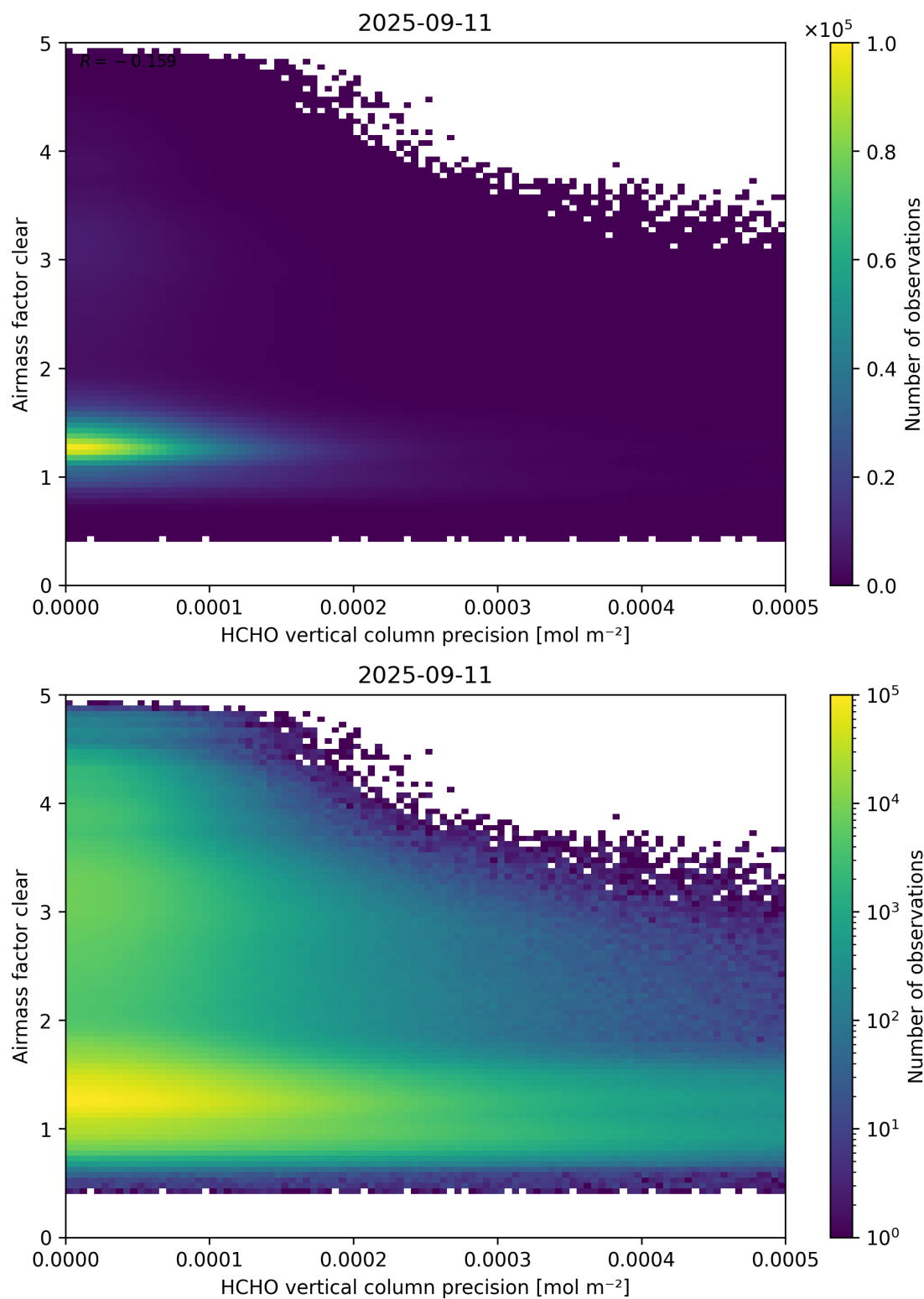
Figure 139: Scatter density plot of “HCHO vertical column precision” against “Airmass factor clear” for 2025-09-10 to 2025-09-12.
