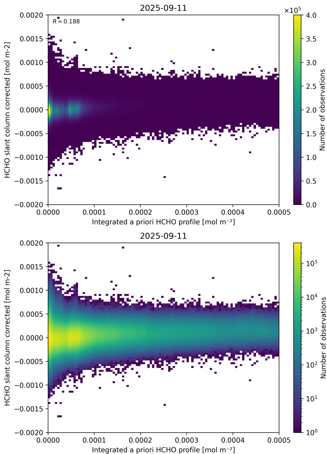
Figure 151: Scatter density plot of “Integrated a priori HCHO profile” against “HCHO slant column corrected” for 2025-09-10 to 2025-09-12.
