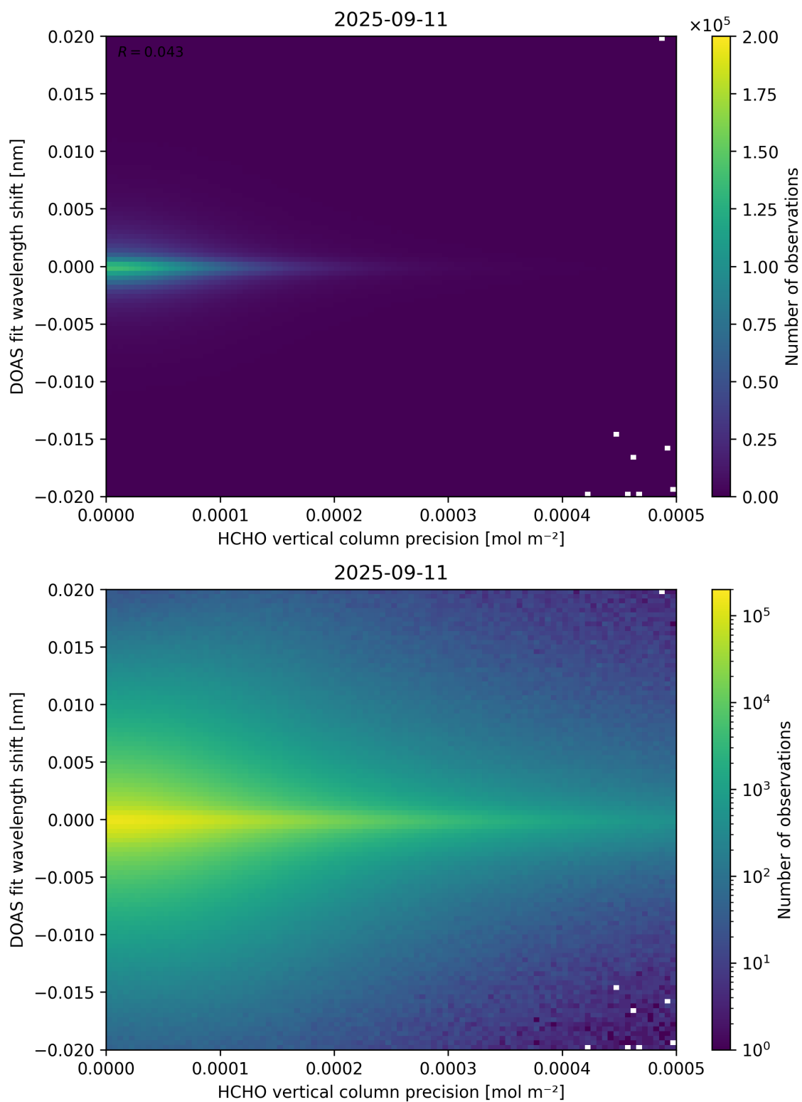
Figure 137: Scatter density plot of “HCHO vertical column precision” against “DOAS fit wavelength shift” for 2025-09-10 to 2025-09-12.
