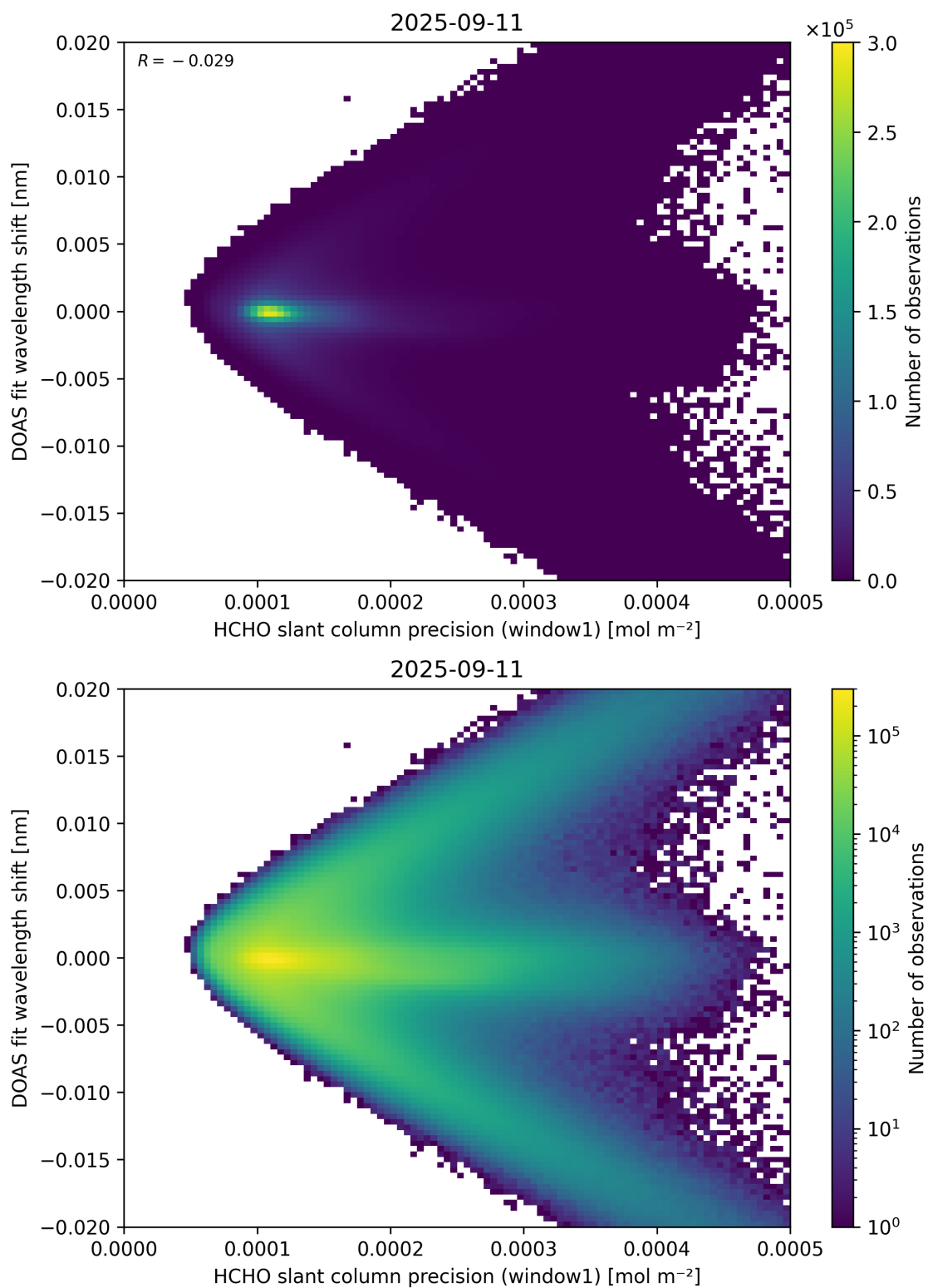
Figure 89: Scatter density plot of “HCHO slant column precision (window1)” against “DOAS fit wavelength shift” for 2025-09-10 to 2025-09-12.
