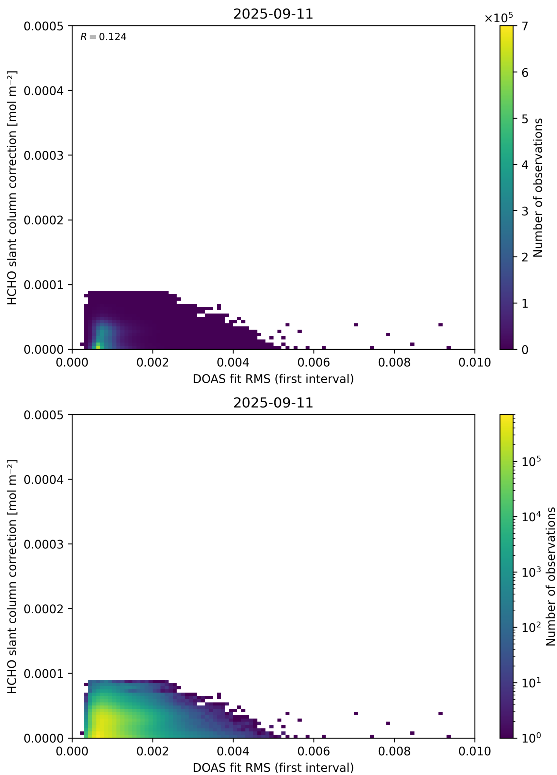
Figure 63: Scatter density plot of “DOAS fit RMS (first interval)” against “HCHO slant column correction” for 2025-09-10 to 2025-09-12.
