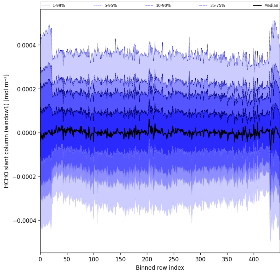
Figure 52: Along track statistics of “HCHO slant column (window1)” for 2025-09-10 to 2025-09-12
