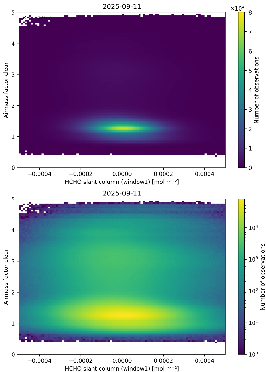
Figure 81: Scatter density plot of “HCHO slant column (window1)” against “Airmass factor clear” for 2025-09-10 to 2025-09-12.
