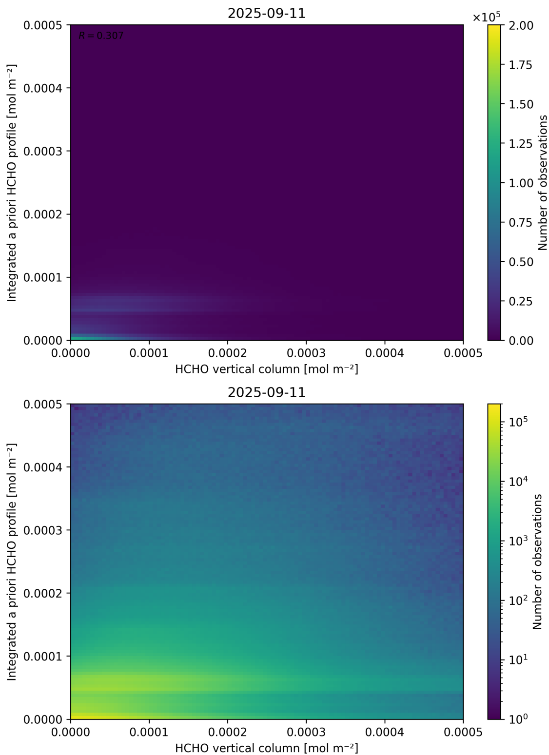
Figure 135: Scatter density plot of “HCHO vertical column” against “Integrated a priori HCHO profile” for 2025-09-10 to 2025-09-12.
