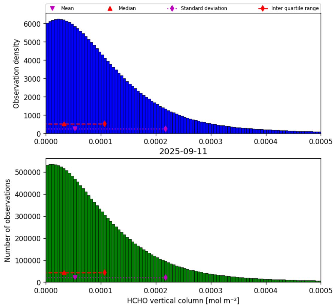
Figure 35: Histogram of “HCHO vertical column” for 2025-09-10 to 2025-09-12
