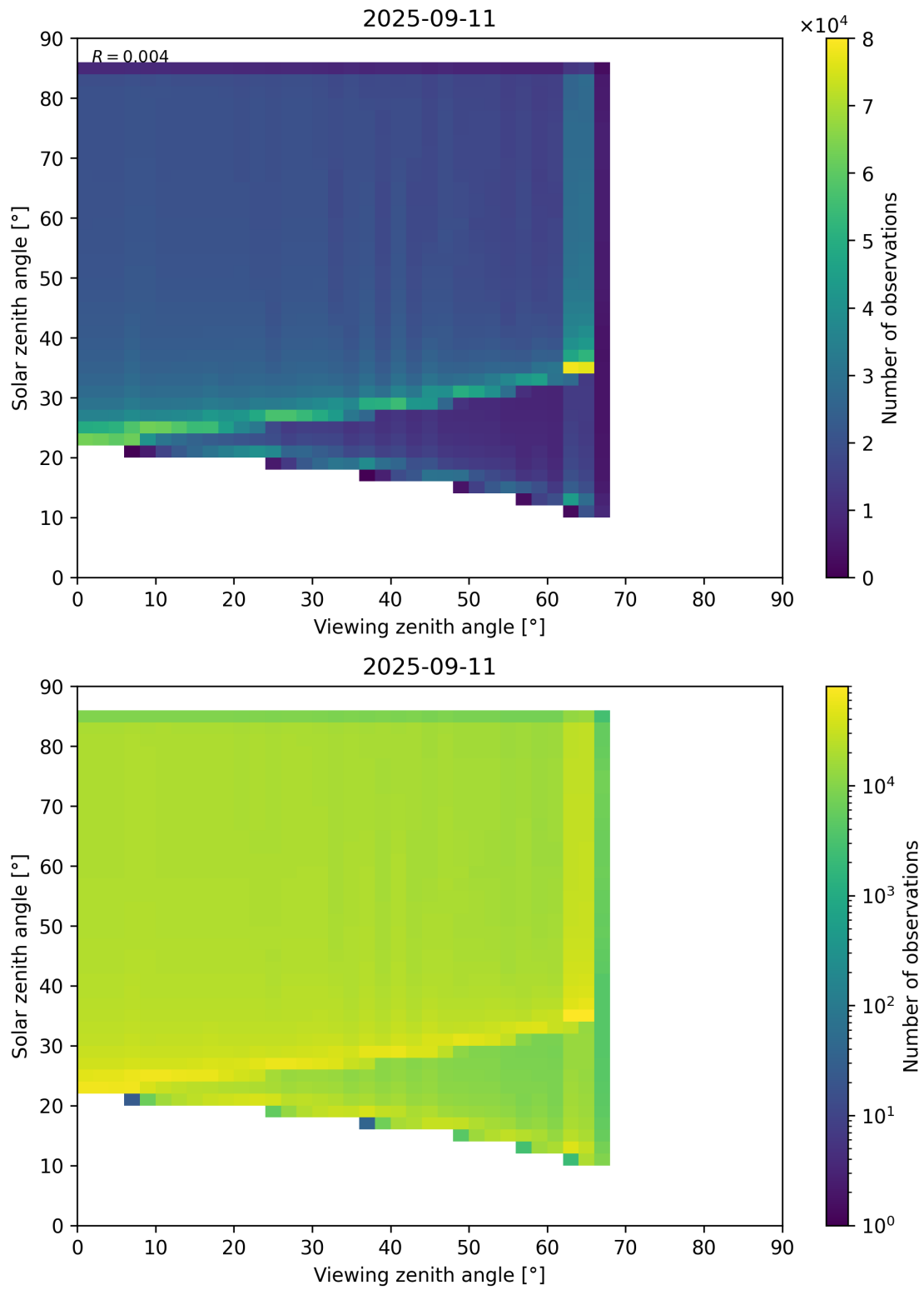
Figure 197: Scatter density plot of “Viewing zenith angle” against “Solar zenith angle” for 2025-09-10 to 2025-09-12.
