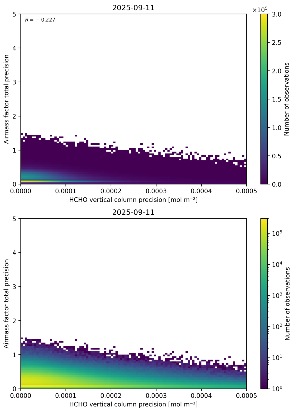
Figure 145: Scatter density plot of “HCHO vertical column precision” against “Airmass factor total precision” for 2025-09-10 to 2025-09-12.
