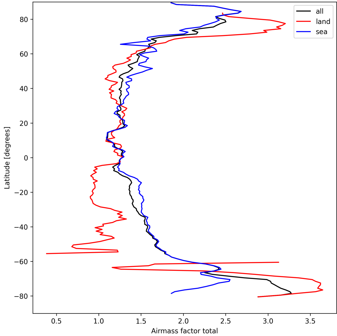
Figure 26: Zonal average of “Airmass factor total” for 2025-09-10 to 2025-09-12.
