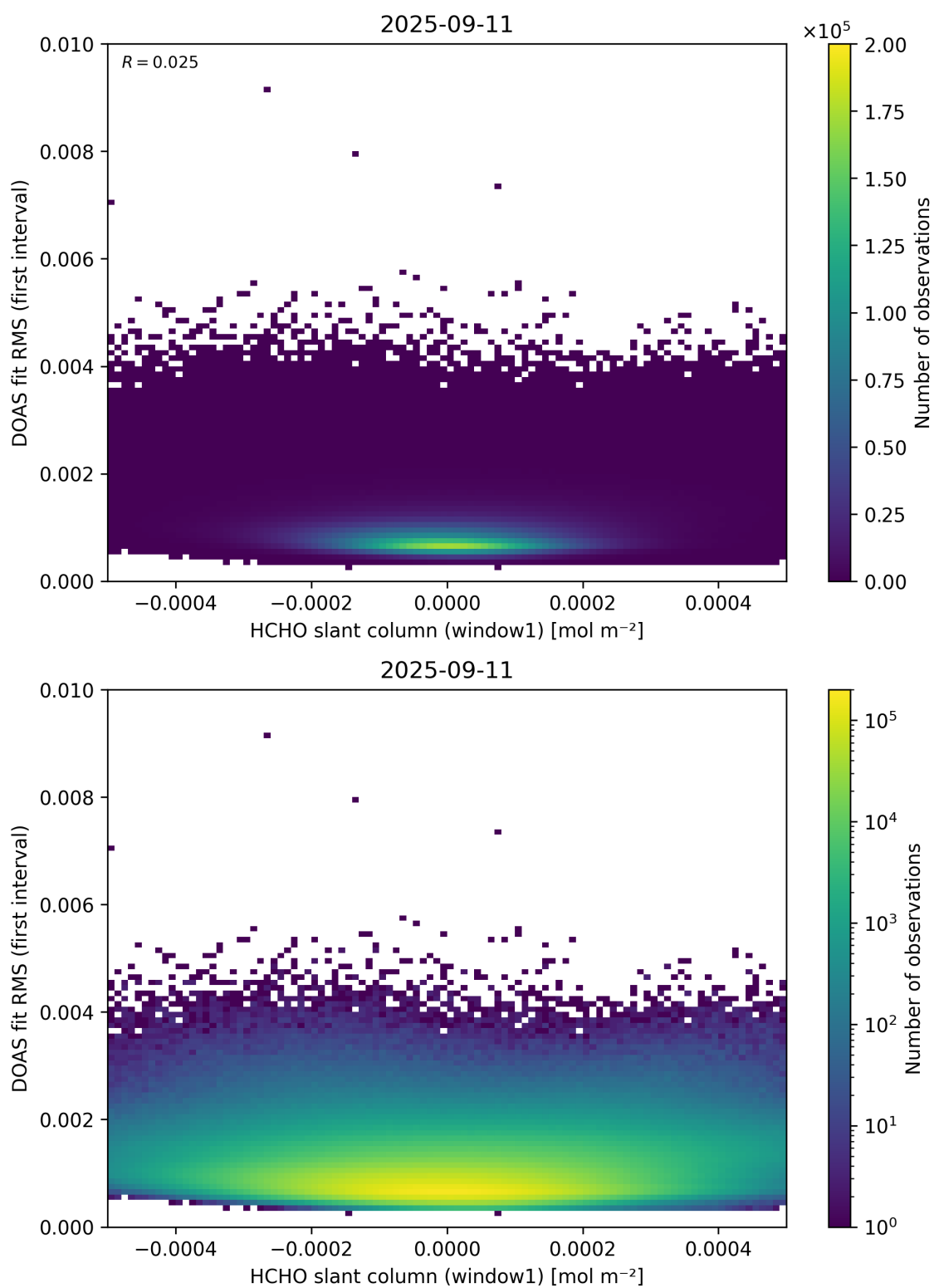
Figure 78: Scatter density plot of “HCHO slant column (window1)” against “DOAS fit RMS (first interval)” for 2025-09-10 to 2025-09-12.
