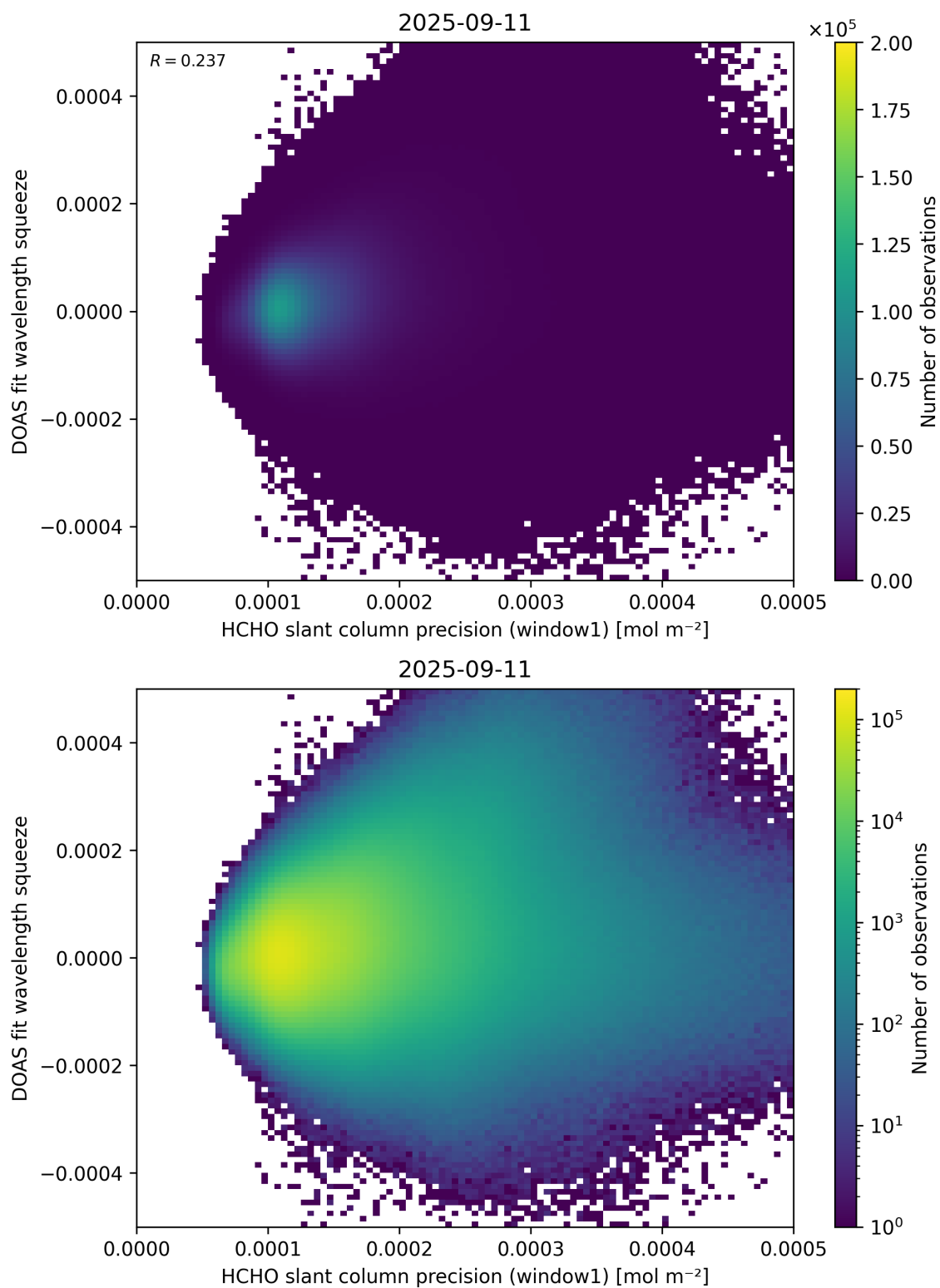
Figure 90: Scatter density plot of “HCHO slant column precision (window1)” against “DOAS fit wavelength squeeze” for 2025-09-10 to 2025-09-12.
