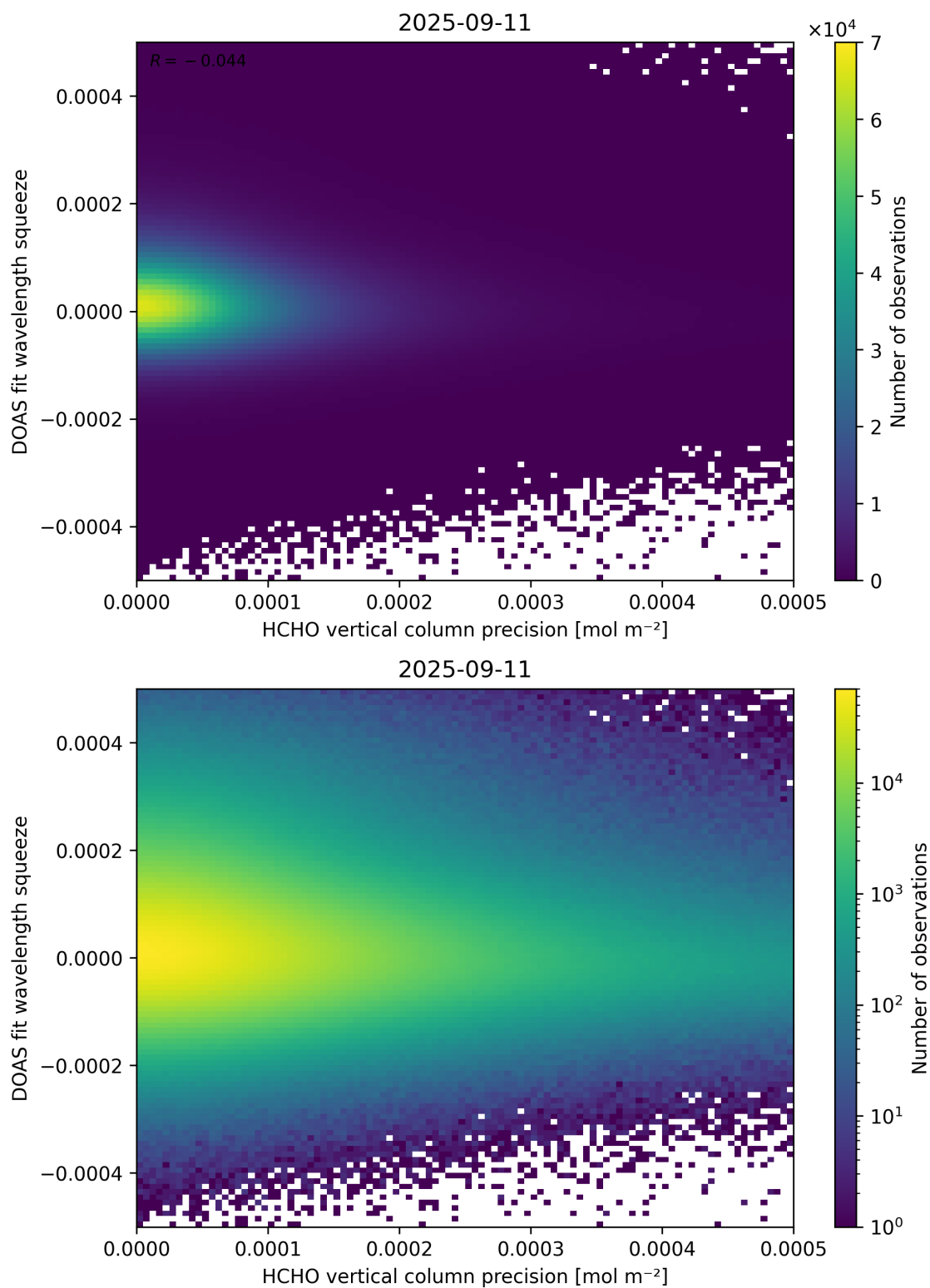
Figure 138: Scatter density plot of “HCHO vertical column precision” against “DOAS fit wavelength squeeze” for 2025-09-10 to 2025-09-12.
