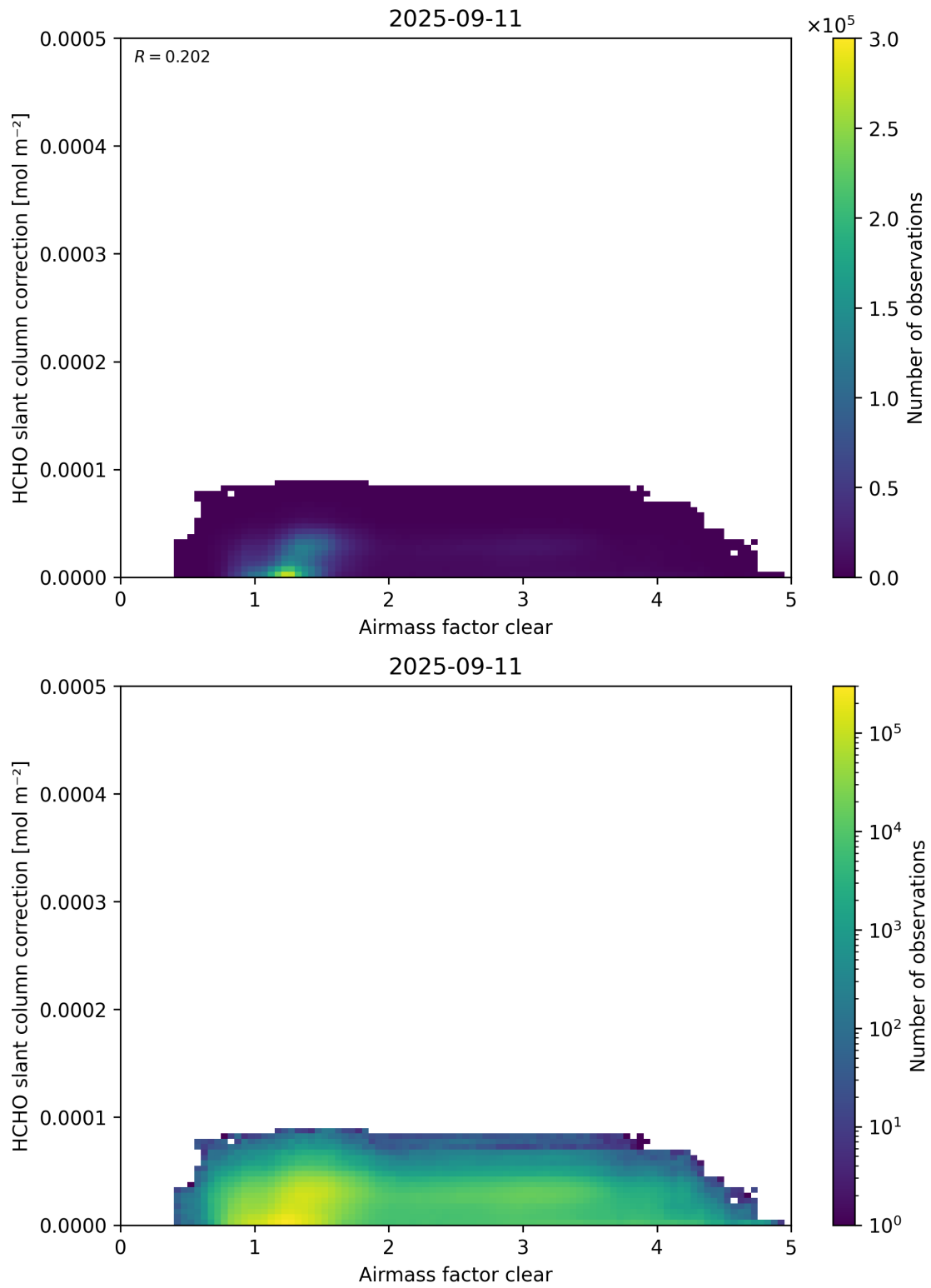
Figure 75: Scatter density plot of “Airmass factor clear” against “HCHO slant column correction” for 2025-09-10 to 2025-09-12.
