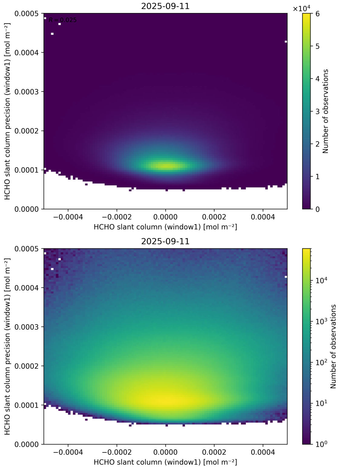
Figure 84: Scatter density plot of “HCHO slant column (window1)” against “HCHO slant column precision (window1)” for 2025-09-10 to 2025-09-12.
