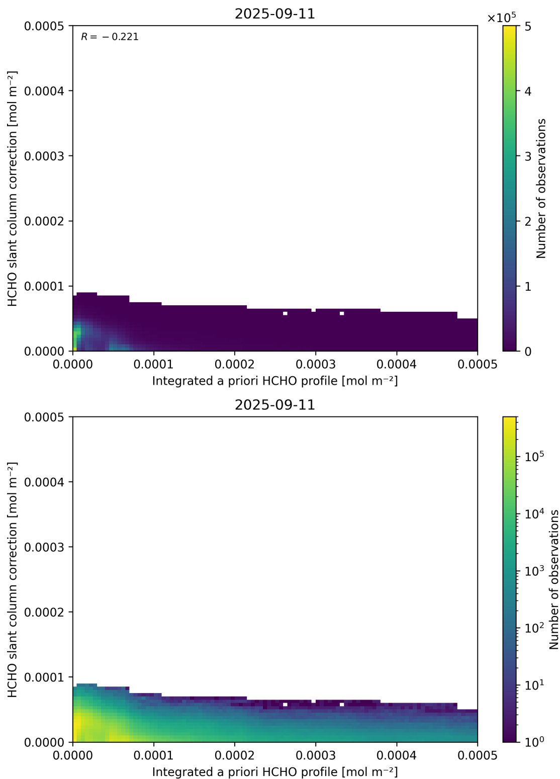
Figure 152: Scatter density plot of “Integrated a priori HCHO profile” against “HCHO slant column correction” for 2025-09-10 to 2025-09-12.
