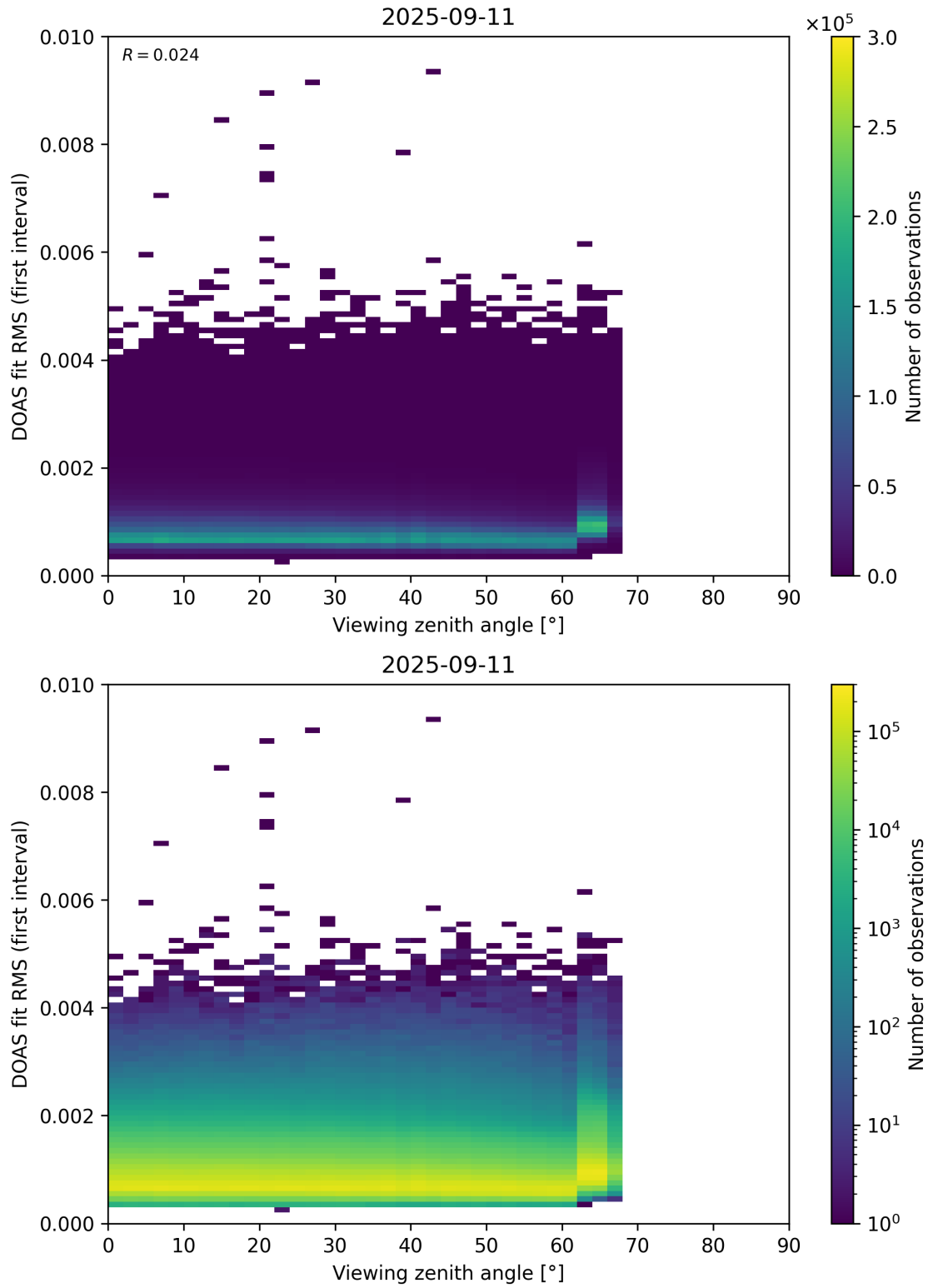
Figure 182: Scatter density plot of “Viewing zenith angle” against “DOAS fit RMS (first interval)” for 2025-09-10 to 2025-09-12.
