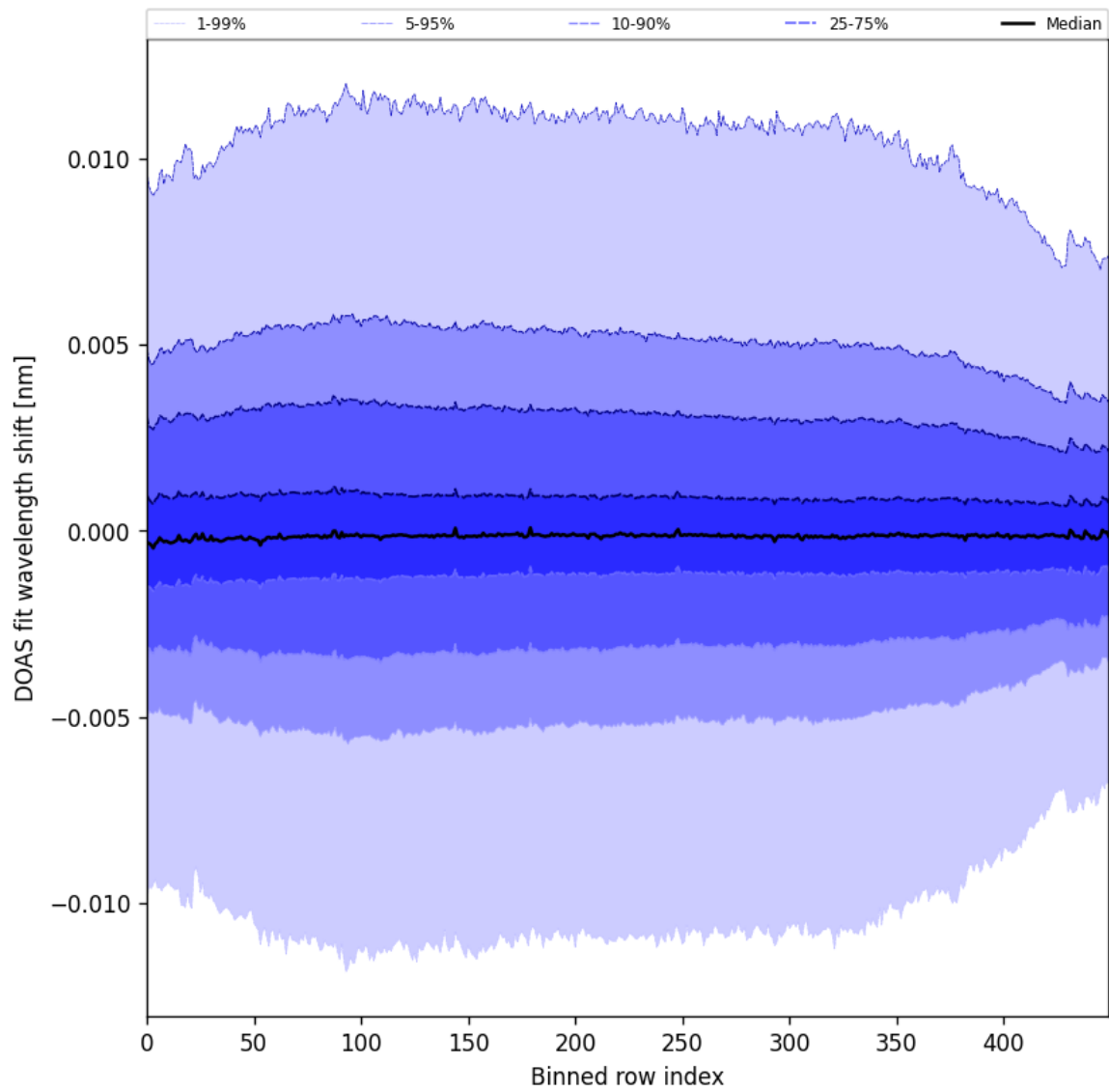
Figure 58: Along track statistics of “DOAS fit wavelength shift” for 2025-09-10 to 2025-09-12
