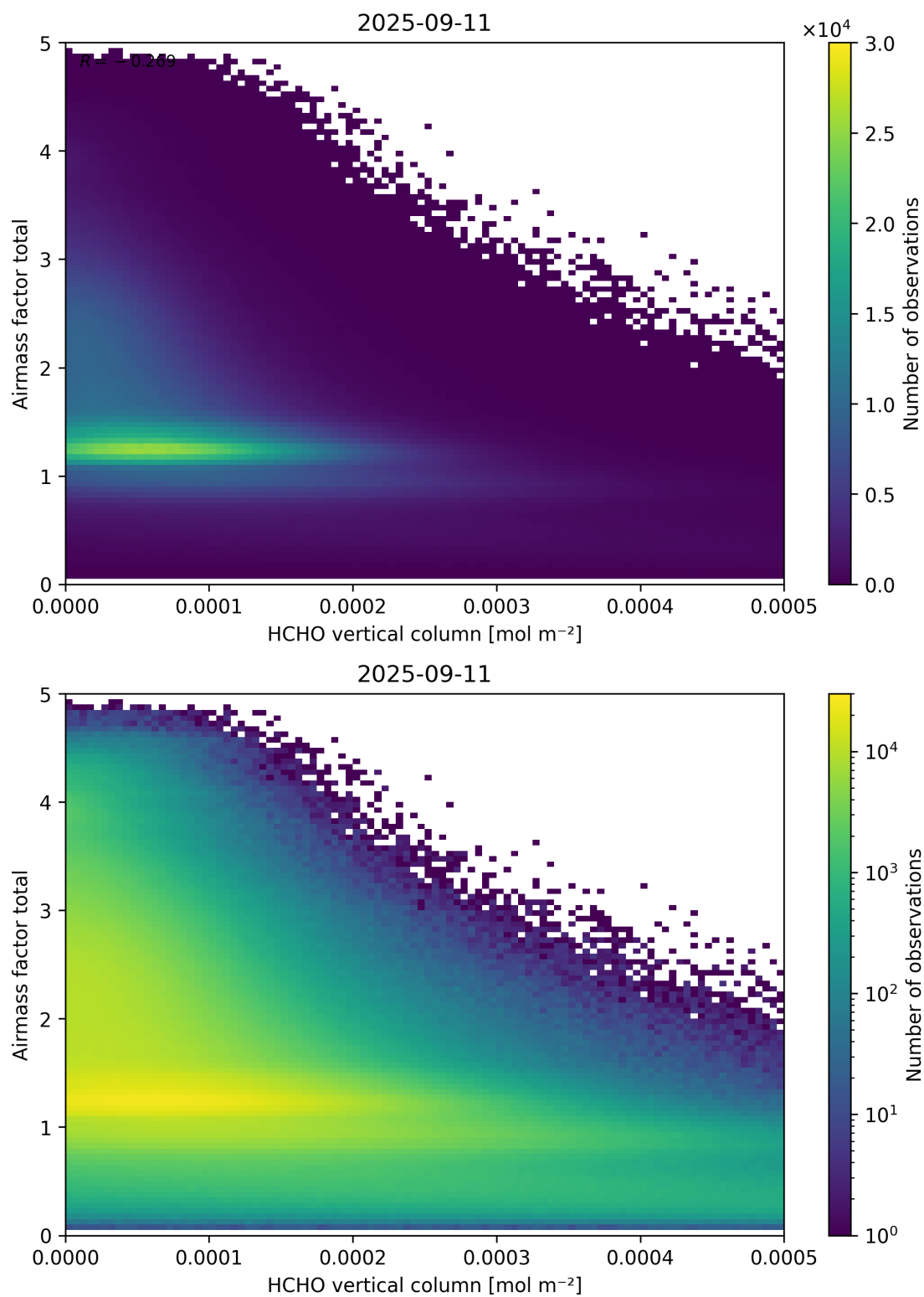
Figure 131: Scatter density plot of “HCHO vertical column” against “Airmass factor total” for 2025-09-10 to 2025-09-12.
