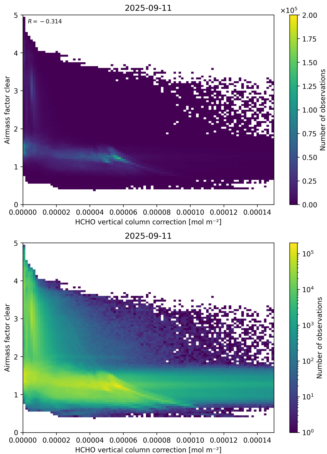
Figure 115: Scatter density plot of “HCHO vertical column correction” against “Airmass factor clear” for 2025-09-10 to 2025-09-12.
