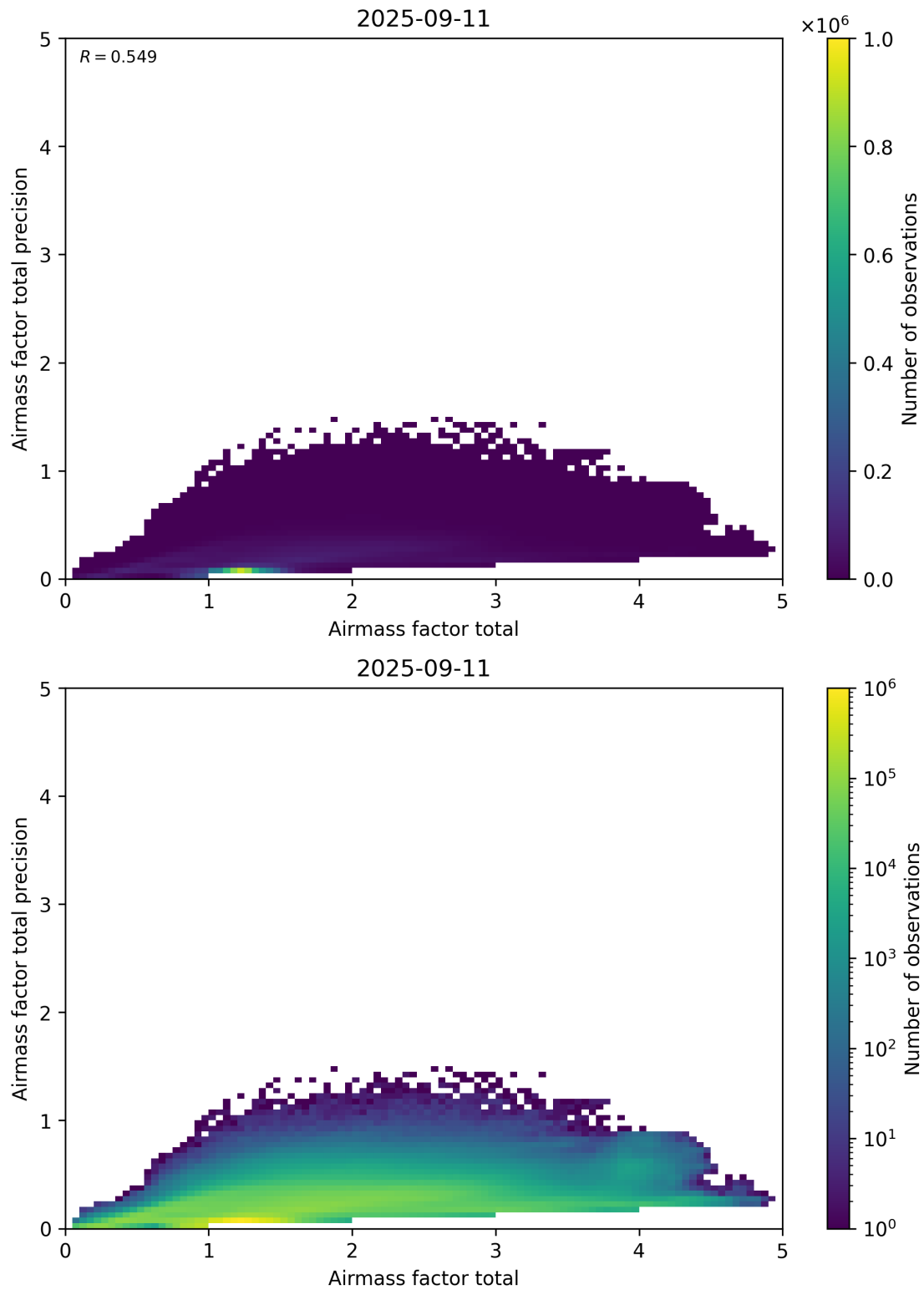
Figure 103: Scatter density plot of “Airmass factor total” against “Airmass factor total precision” for 2025-09-10 to 2025-09-12.
