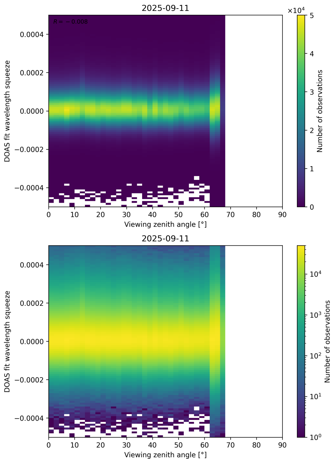
Figure 184: Scatter density plot of “Viewing zenith angle” against “DOAS fit wavelength squeeze” for 2025-09-10 to 2025-09-12.
