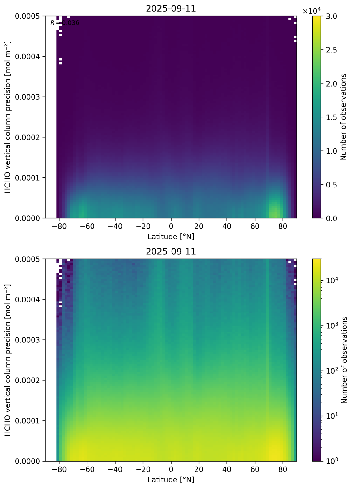
Figure 165: Scatter density plot of “Latitude” against “HCHO vertical column precision” for 2025-09-10 to 2025-09-12.
