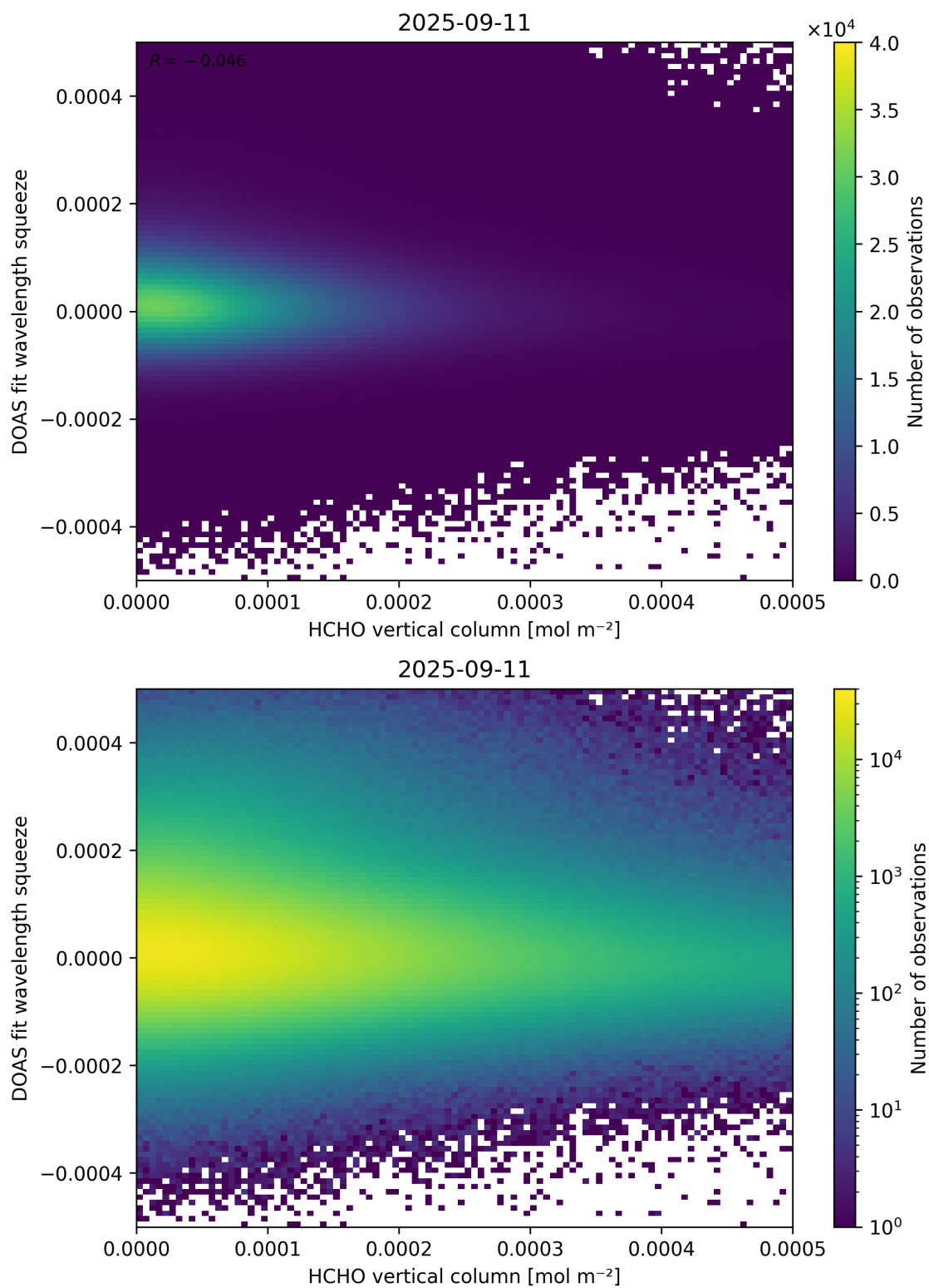
Figure 125: Scatter density plot of “HCHO vertical column” against “DOAS fit wavelength squeeze” for 2025-09-10 to 2025-09-12.
