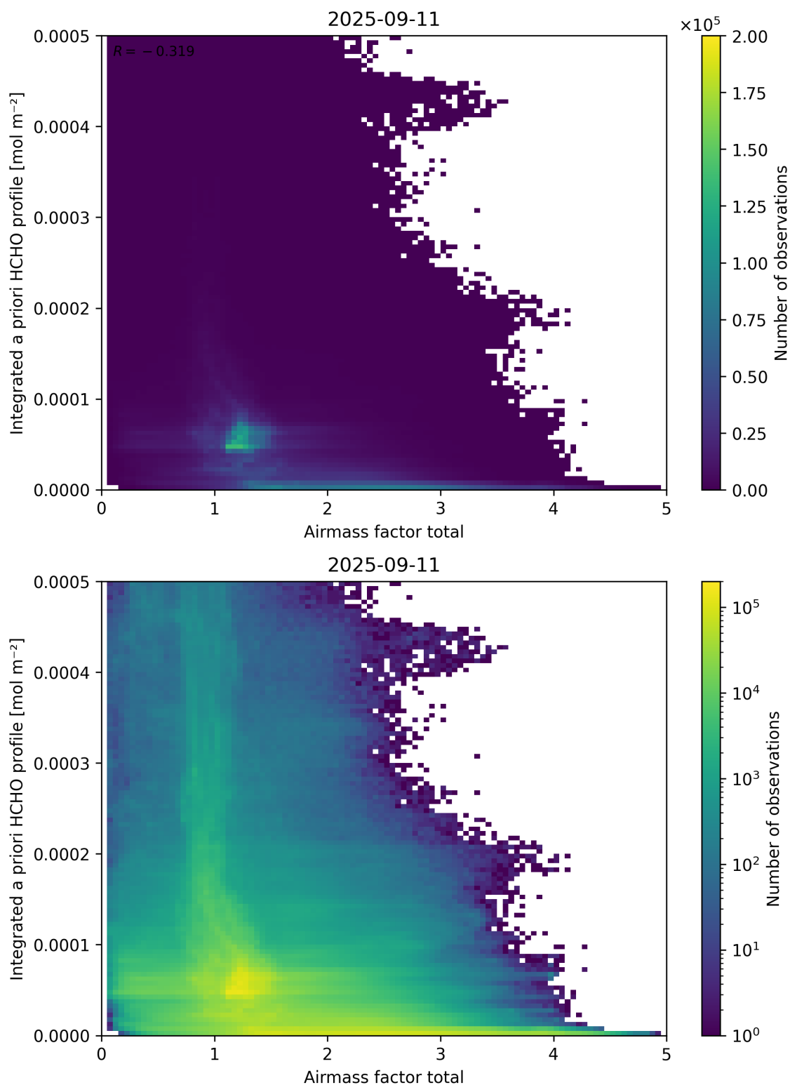
Figure 104: Scatter density plot of “Airmass factor total” against “Integrated a priori HCHO profile” for 2025-09-10 to 2025-09-12.
