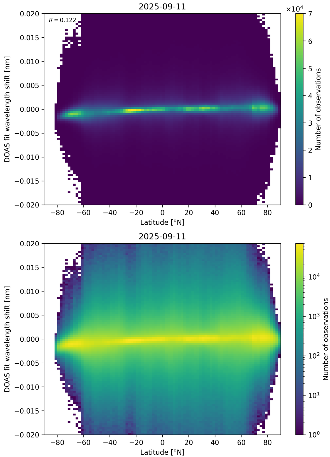
Figure 154: Scatter density plot of “Latitude” against “DOAS fit wavelength shift” for 2025-09-10 to 2025-09-12.
