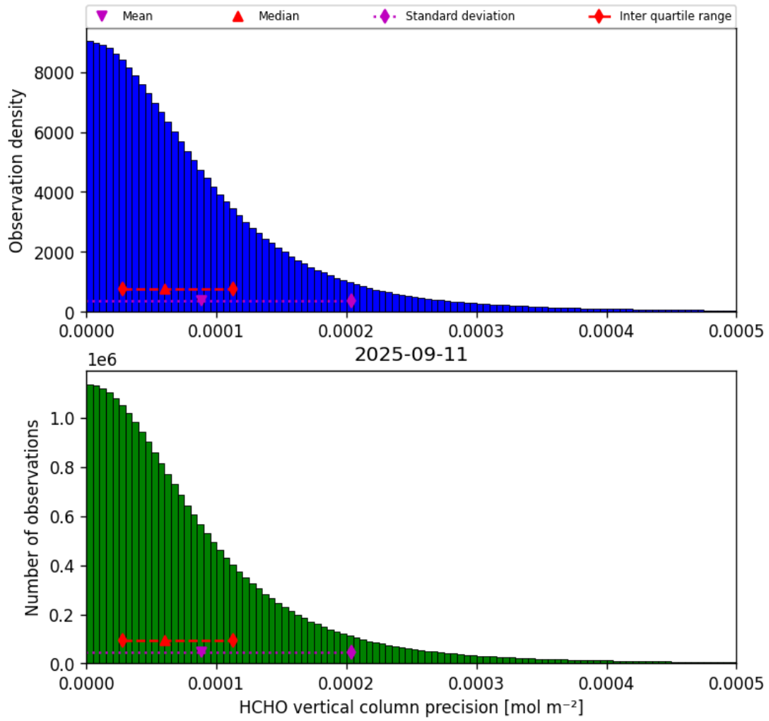
Figure 36: Histogram of “HCHO vertical column precision” for 2025-09-10 to 2025-09-12
