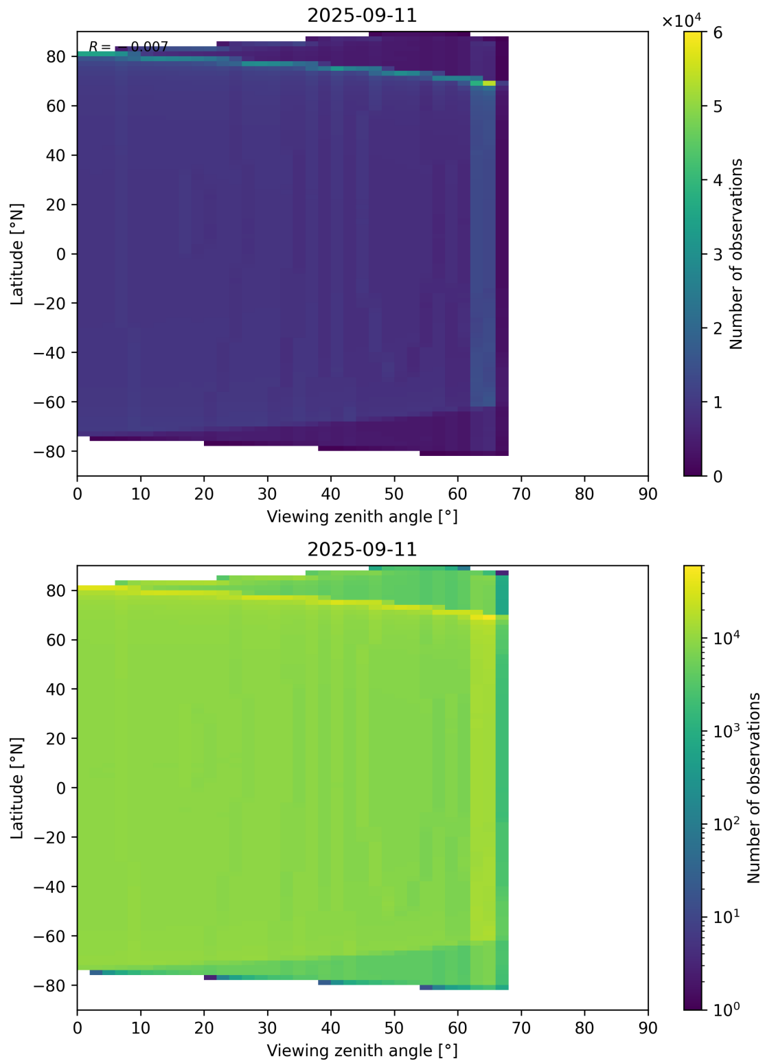
Figure 196: Scatter density plot of “Viewing zenith angle” against “Latitude” for 2025-09-10 to 2025-09-12.
