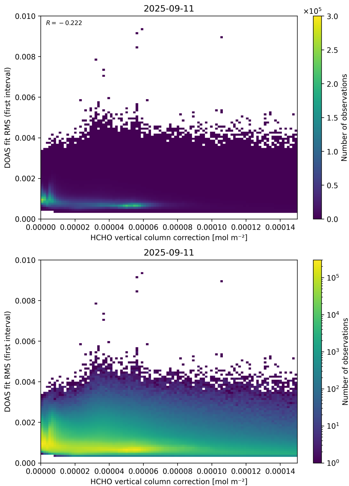
Figure 112: Scatter density plot of “HCHO vertical column correction” against “DOAS fit RMS (first interval)” for 2025-09-10 to 2025-09-12.
