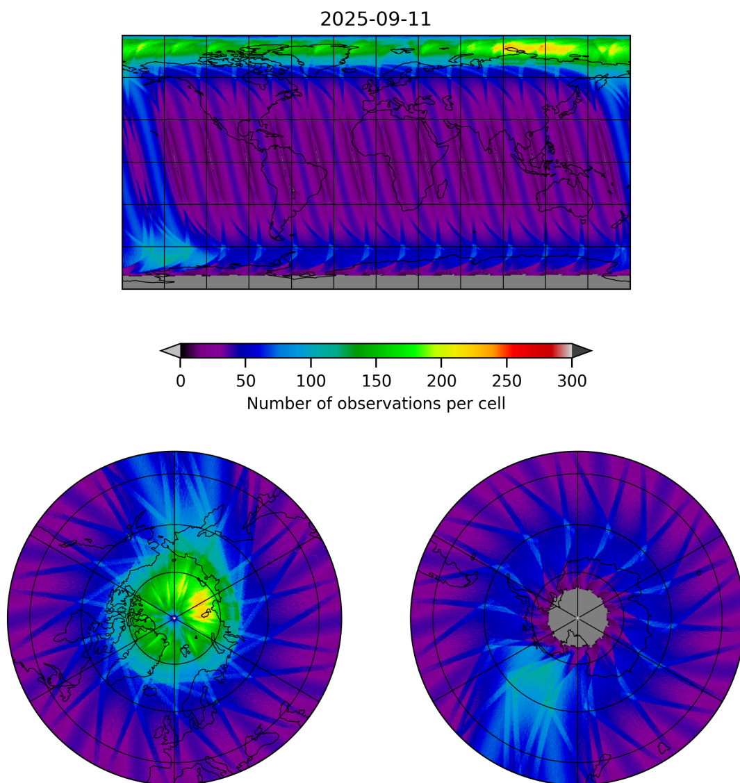
Figure 19: Map of the number of observations for 2025-09-10 to 2025-09-12
