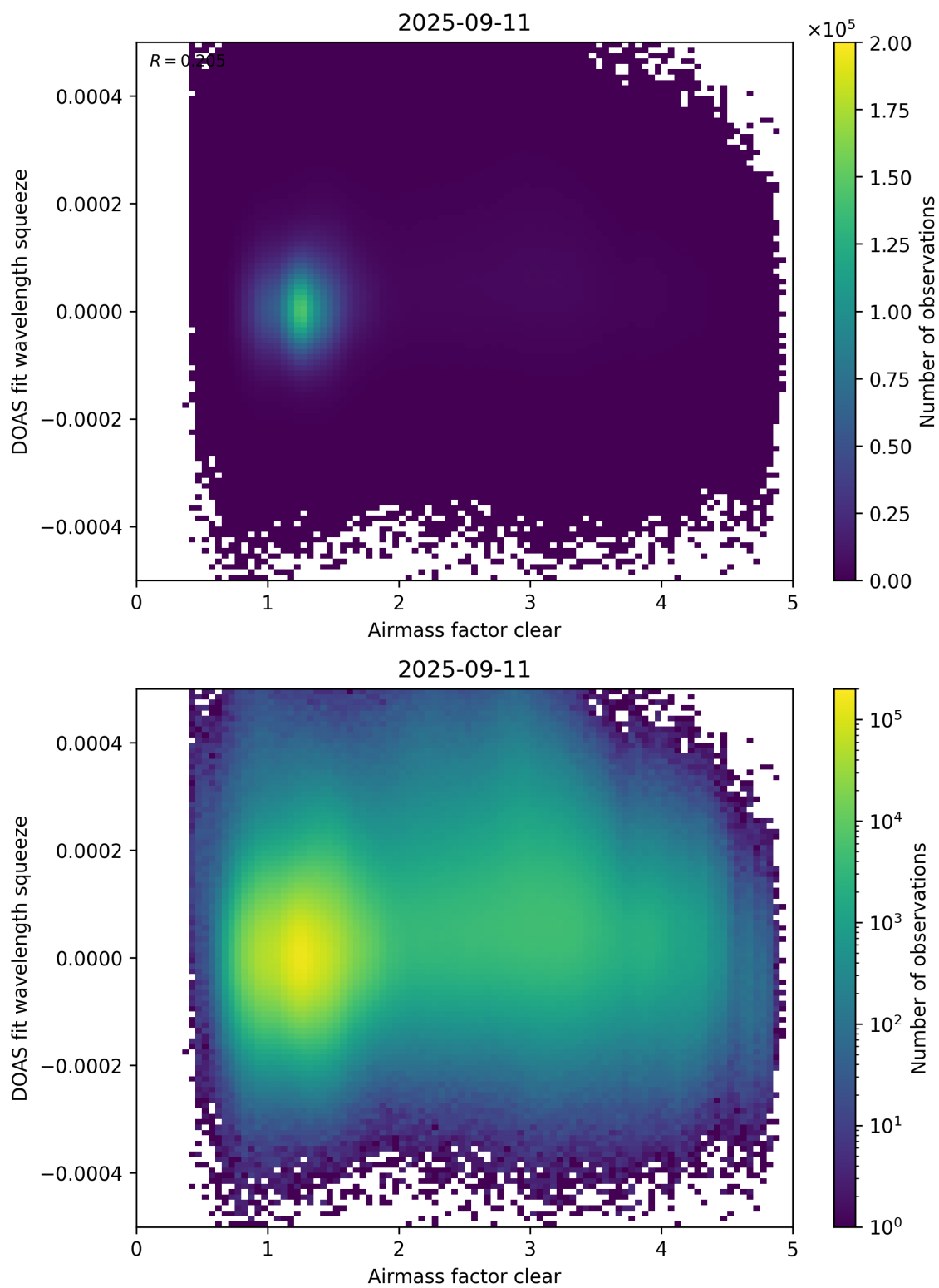
Figure 73: Scatter density plot of “Airmass factor clear” against “DOAS fit wavelength squeeze” for 2025-09-10 to 2025-09-12.
