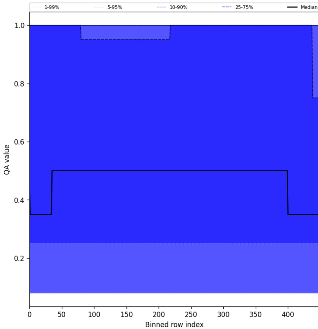
Figure 48: Along track statistics of “QA value” for 2025-09-10 to 2025-09-12
