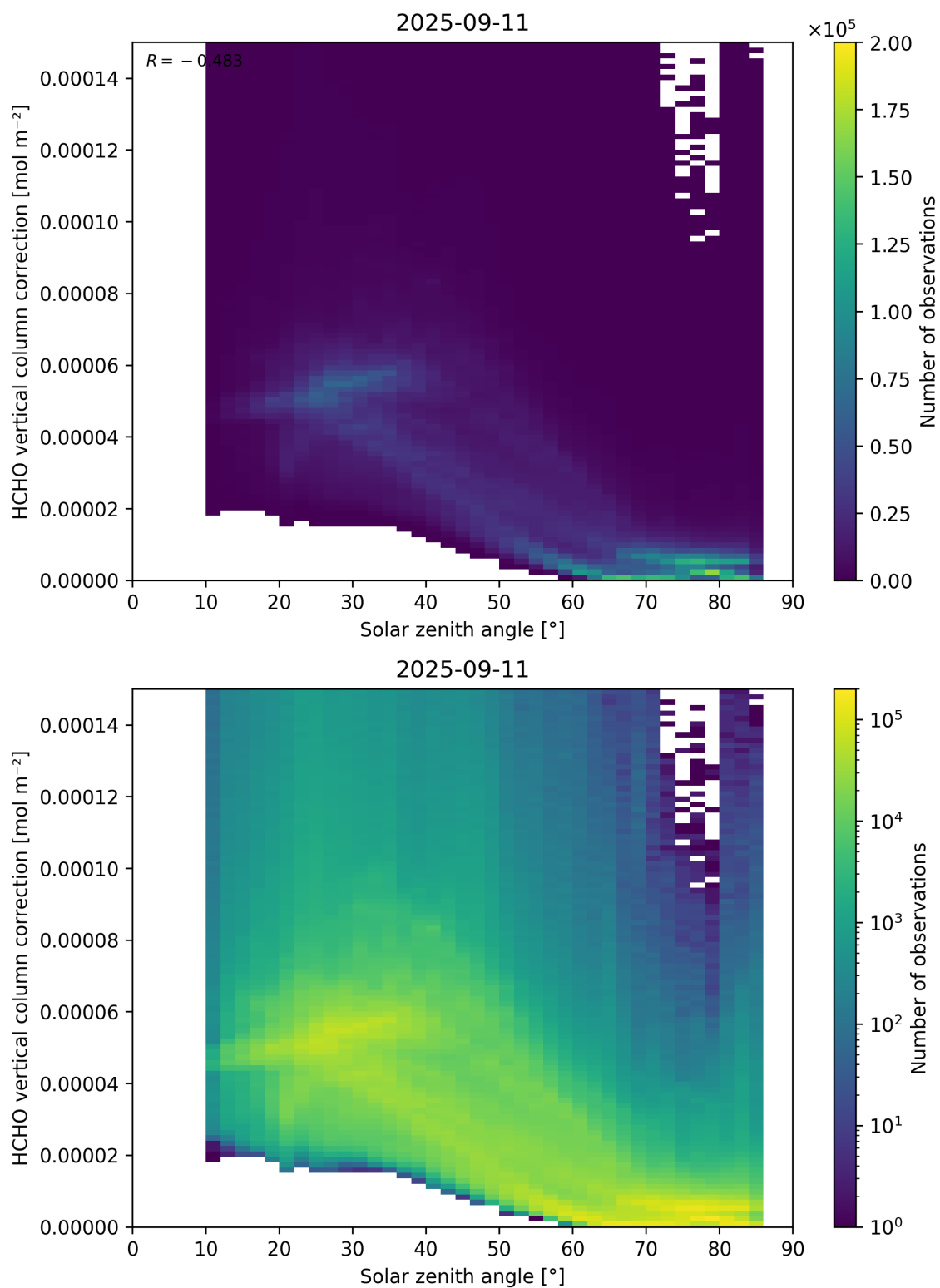
Figure 178: Scatter density plot of “Solar zenith angle” against “HCHO vertical column correction” for 2025-09-10 to 2025-09-12.
