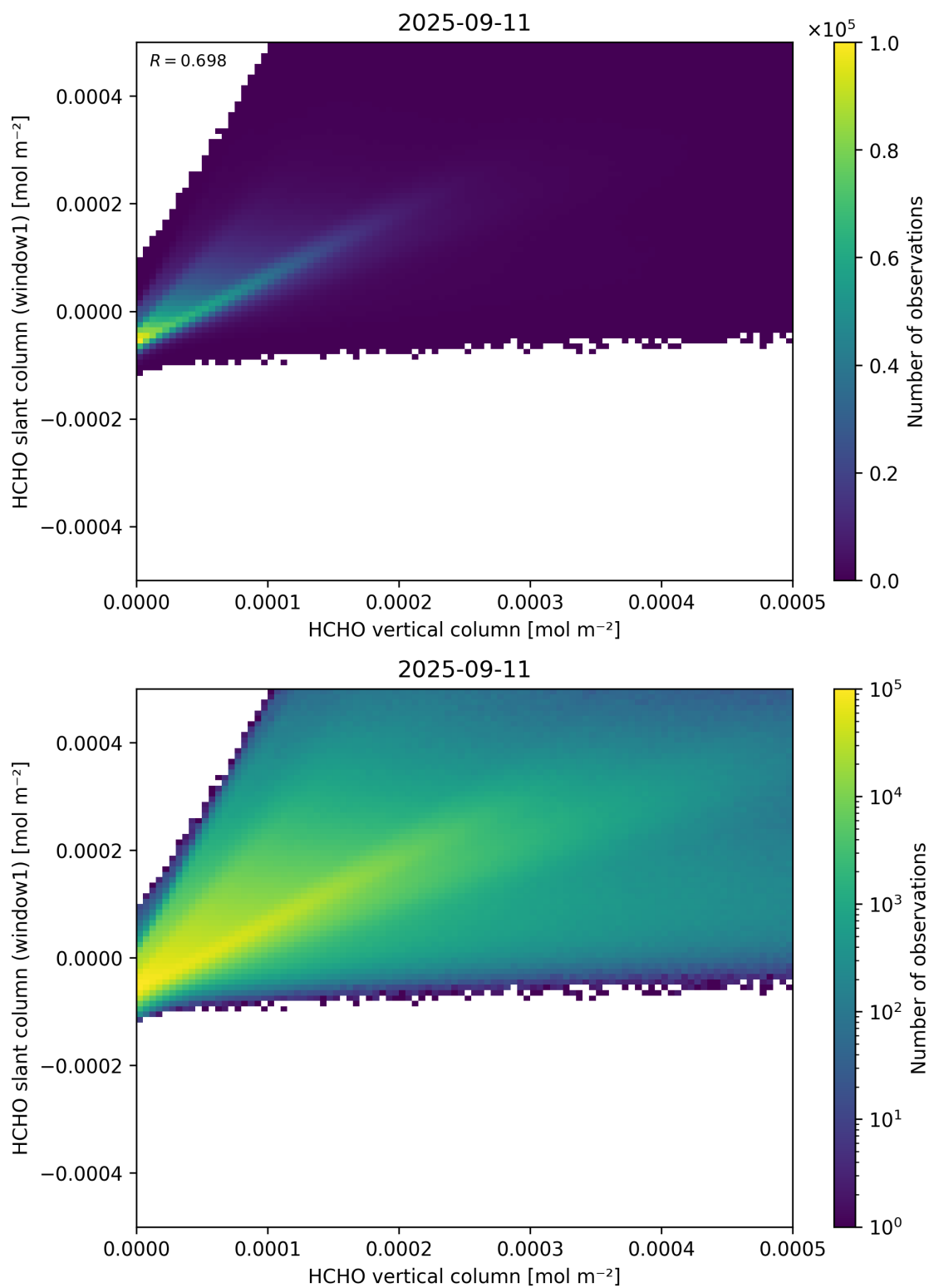
Figure 129: Scatter density plot of “HCHO vertical column” against “HCHO slant column (window1)” for 2025-09-10 to 2025-09-12.
