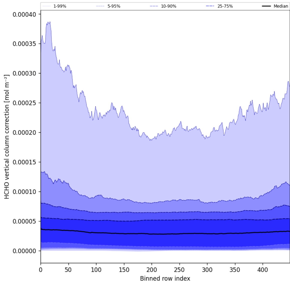
Figure 51: Along track statistics of “HCHO vertical column correction” for 2025-09-10 to 2025-09-12
