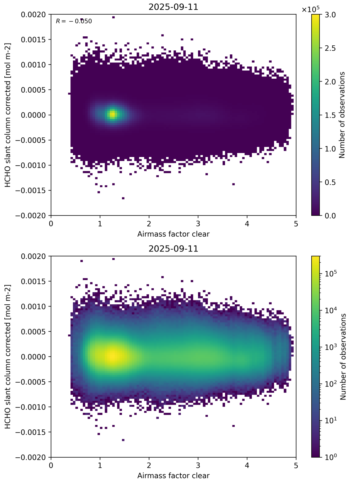
Figure 74: Scatter density plot of “Airmass factor clear” against “HCHO slant column corrected” for 2025-09-10 to 2025-09-12.
