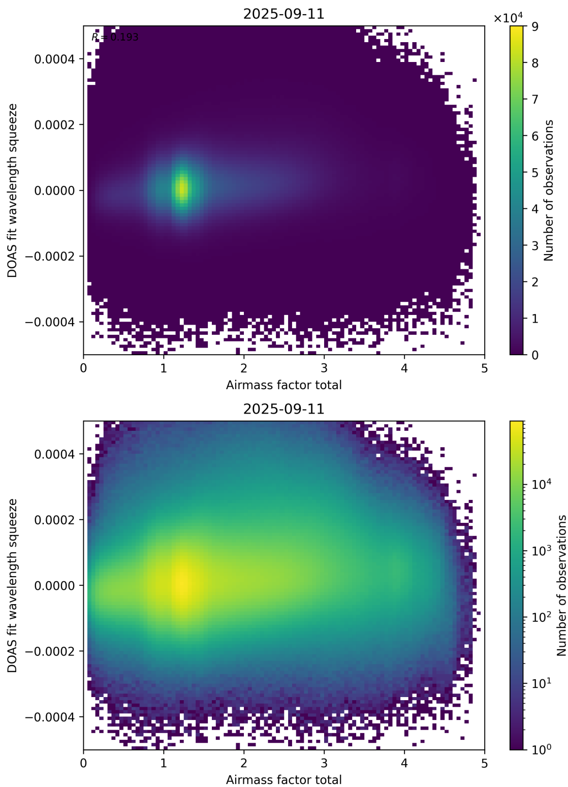
Figure 99: Scatter density plot of “Airmass factor total” against “DOAS fit wavelength squeeze” for 2025-09-10 to 2025-09-12.
