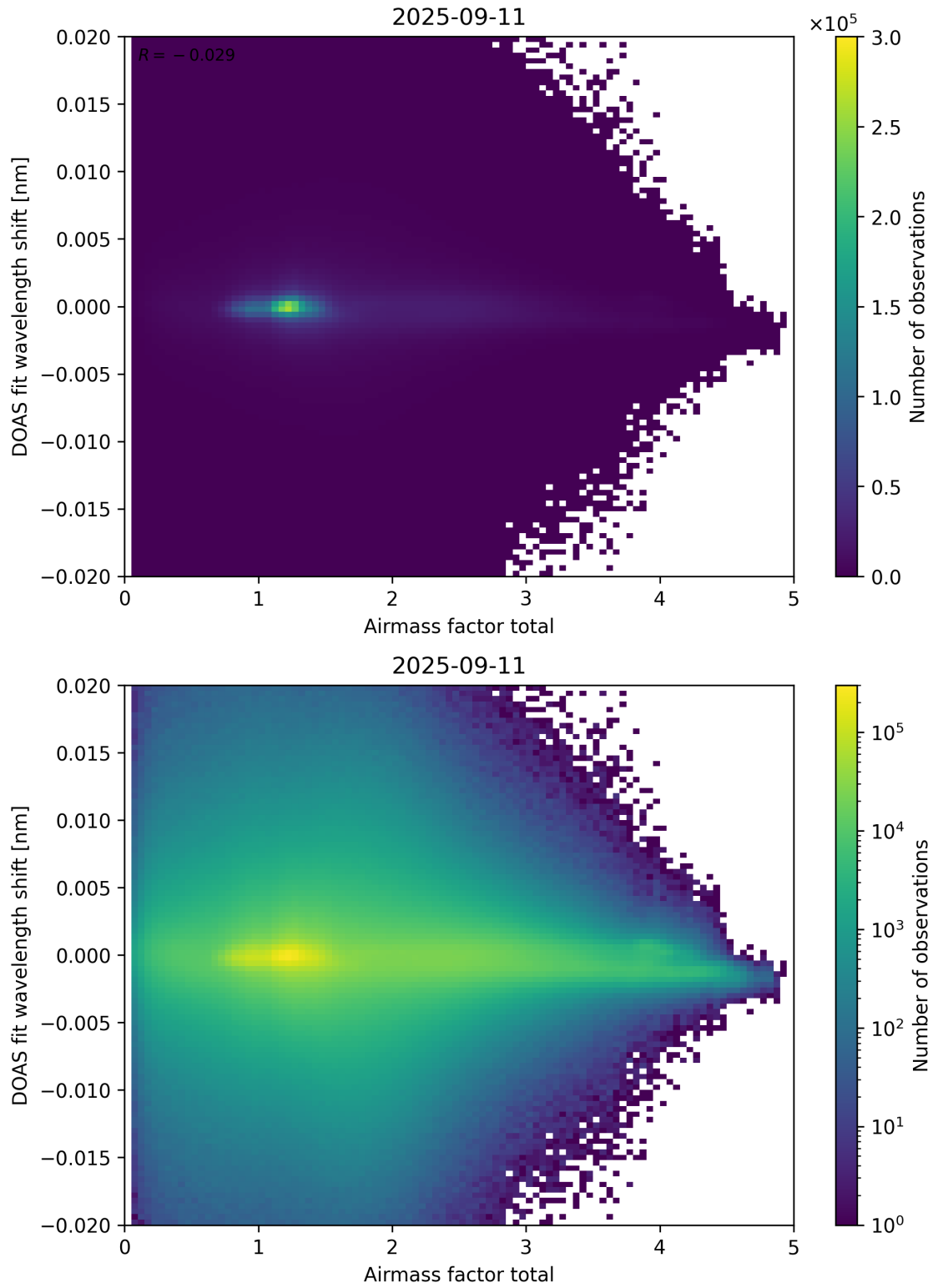
Figure 98: Scatter density plot of “Airmass factor total” against “DOAS fit wavelength shift” for 2025-09-10 to 2025-09-12.
