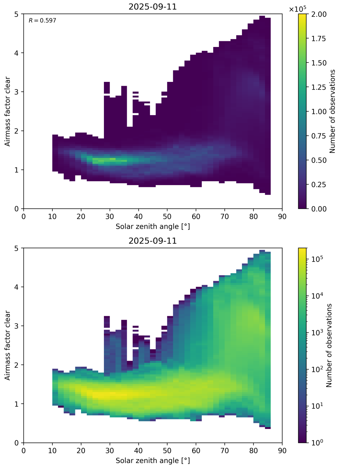
Figure 170: Scatter density plot of “Solar zenith angle” against “Airmass factor clear” for 2025-09-10 to 2025-09-12.
