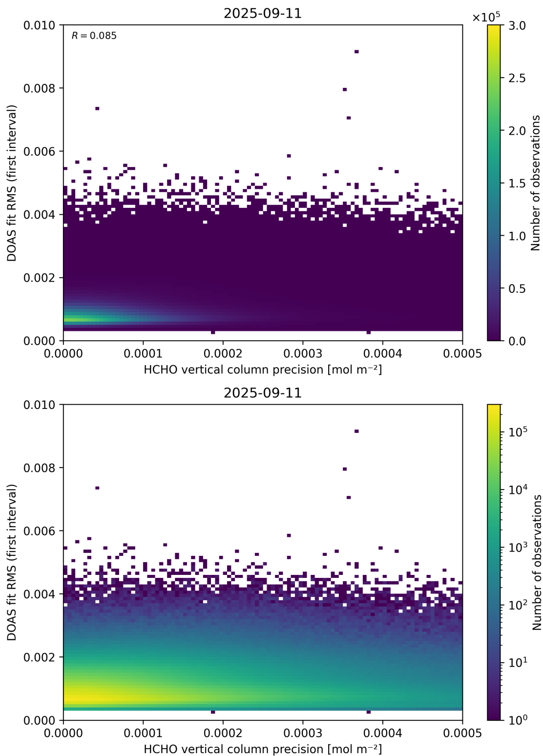
Figure 136: Scatter density plot of “HCHO vertical column precision” against “DOAS fit RMS (first interval)” for 2025-09-10 to 2025-09-12.
