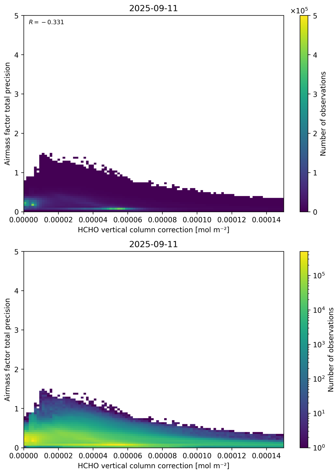
Figure 121: Scatter density plot of “HCHO vertical column correction” against “Airmass factor total precision” for 2025-09-10 to 2025-09-12.
