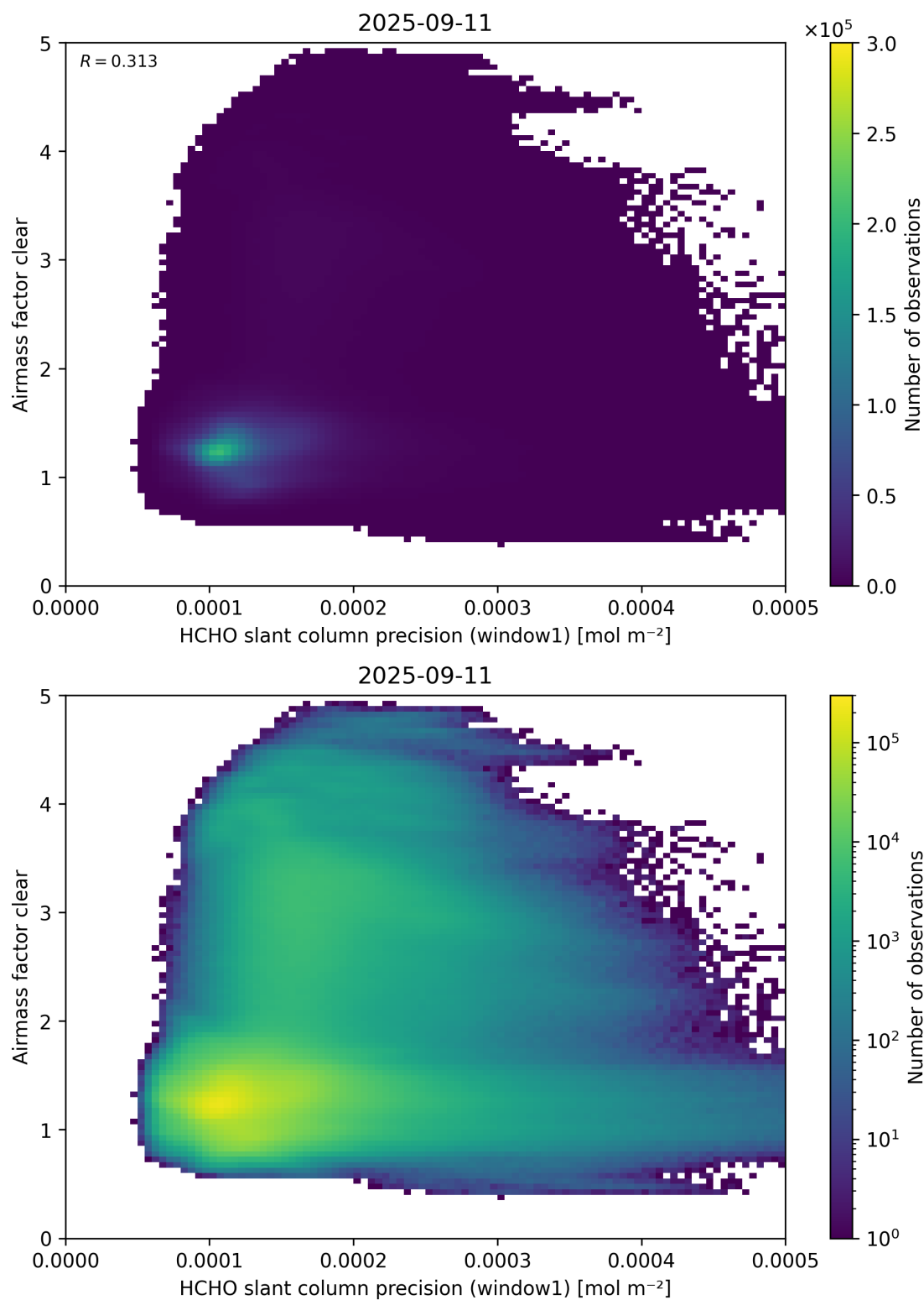
Figure 91: Scatter density plot of “HCHO slant column precision (window1)” against “Airmass factor clear” for 2025-09-10 to 2025-09-12.
