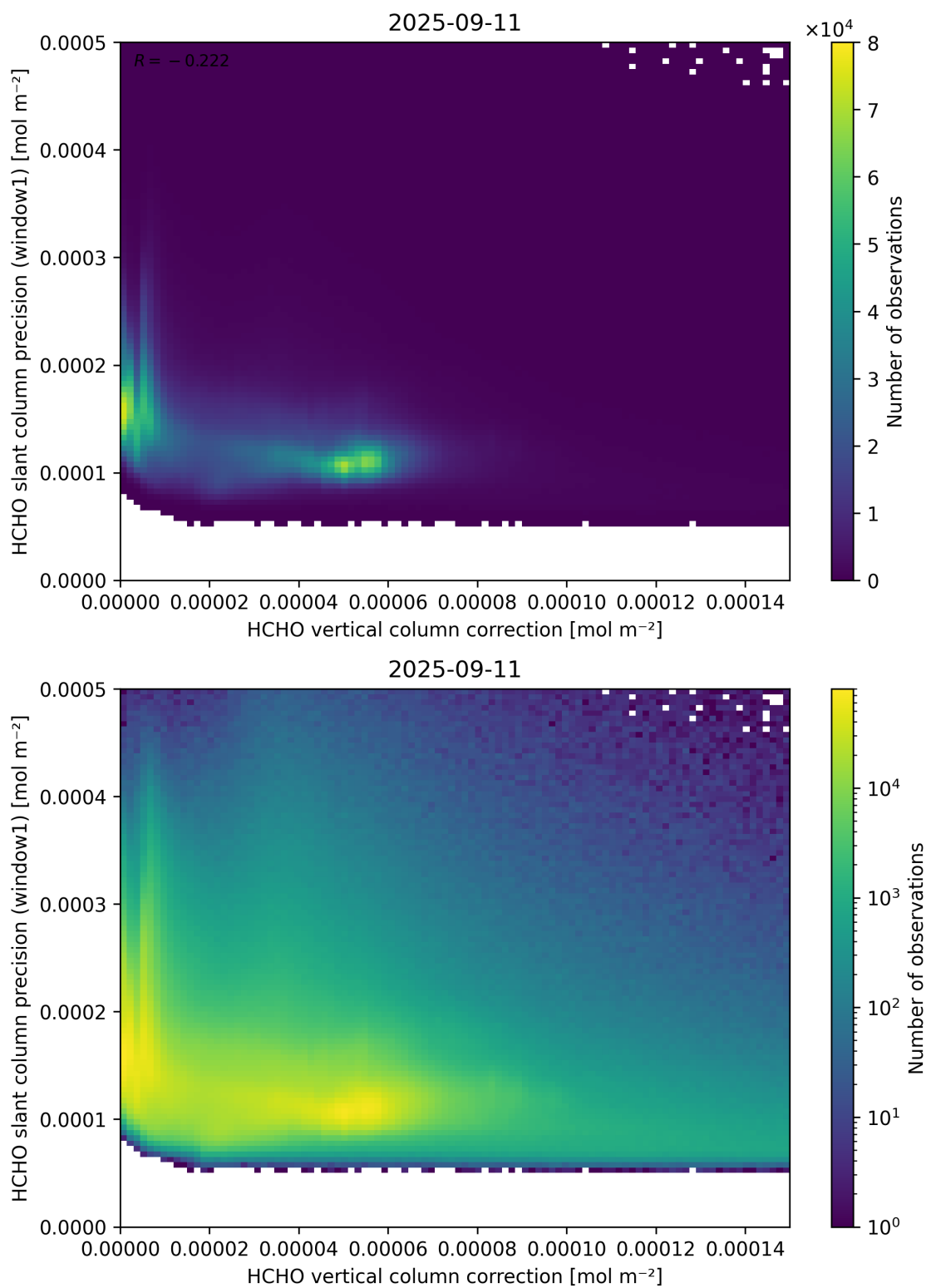
Figure 119: Scatter density plot of “HCHO vertical column correction” against “HCHO slant column precision (window1)” for 2025-09-10 to 2025-09-12.
