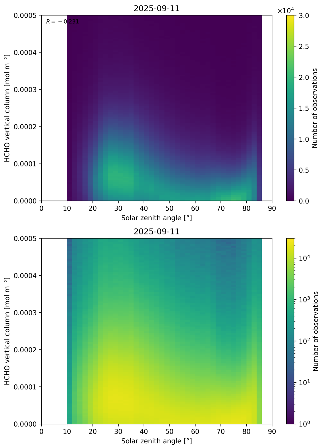
Figure 177: Scatter density plot of “Solar zenith angle” against “HCHO vertical column” for 2025-09-10 to 2025-09-12.
