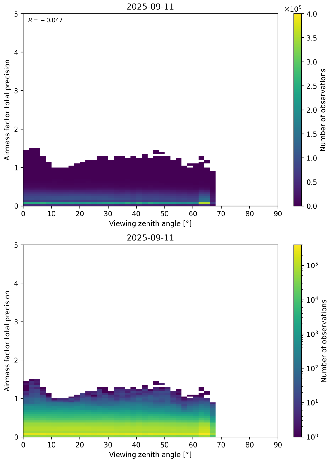
Figure 191: Scatter density plot of “Viewing zenith angle” against “Airmass factor total precision” for 2025-09-10 to 2025-09-12.
