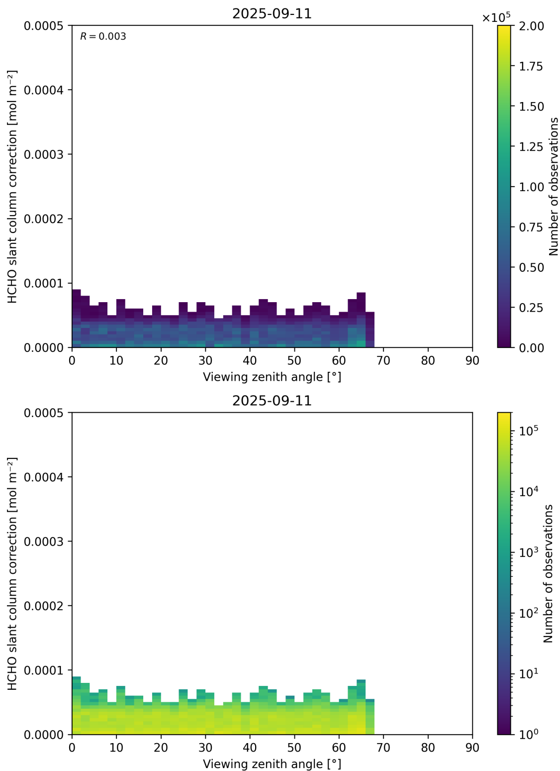
Figure 187: Scatter density plot of “Viewing zenith angle” against “HCHO slant column correction” for 2025-09-10 to 2025-09-12.
