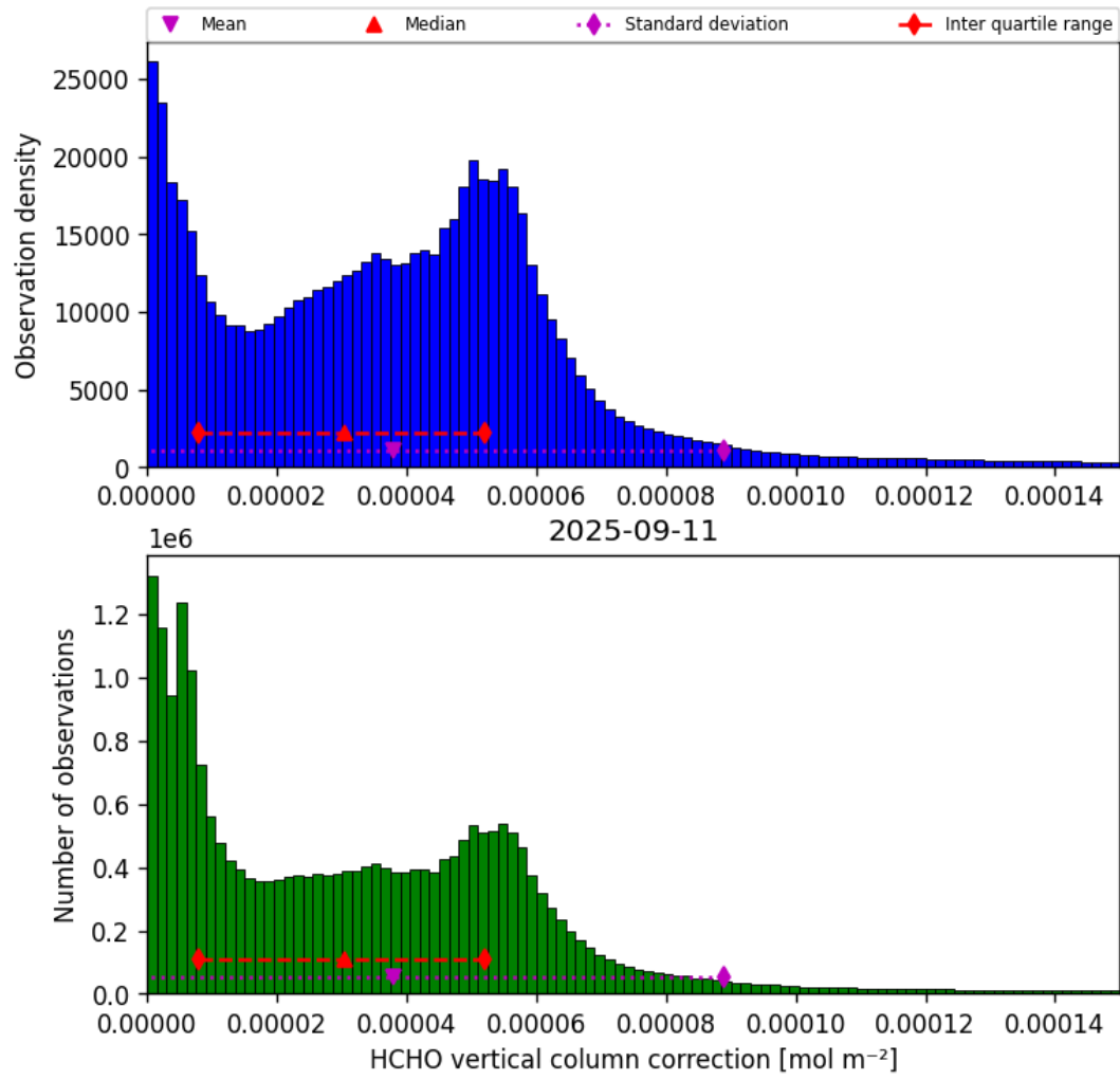
Figure 37: Histogram of “HCHO vertical column correction” for 2025-09-10 to 2025-09-12
