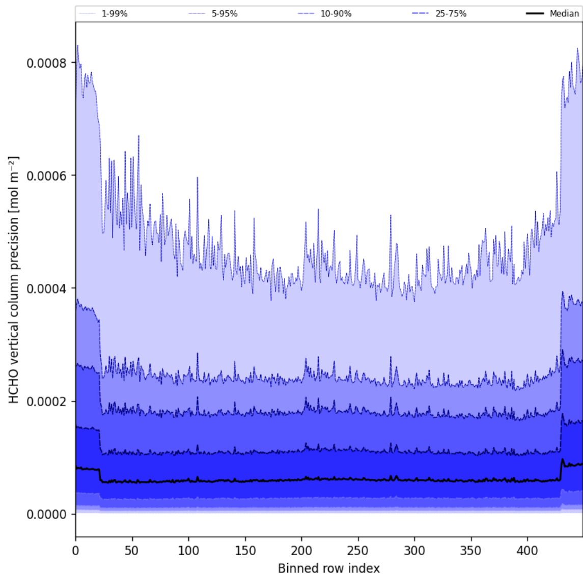
Figure 50: Along track statistics of “HCHO vertical column precision” for 2025-09-10 to 2025-09-12
