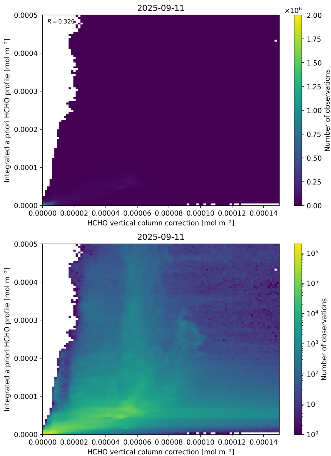
Figure 122: Scatter density plot of “HCHO vertical column correction” against “Integrated a priori HCHO profile” for 2025-09-10 to 2025-09-12.
