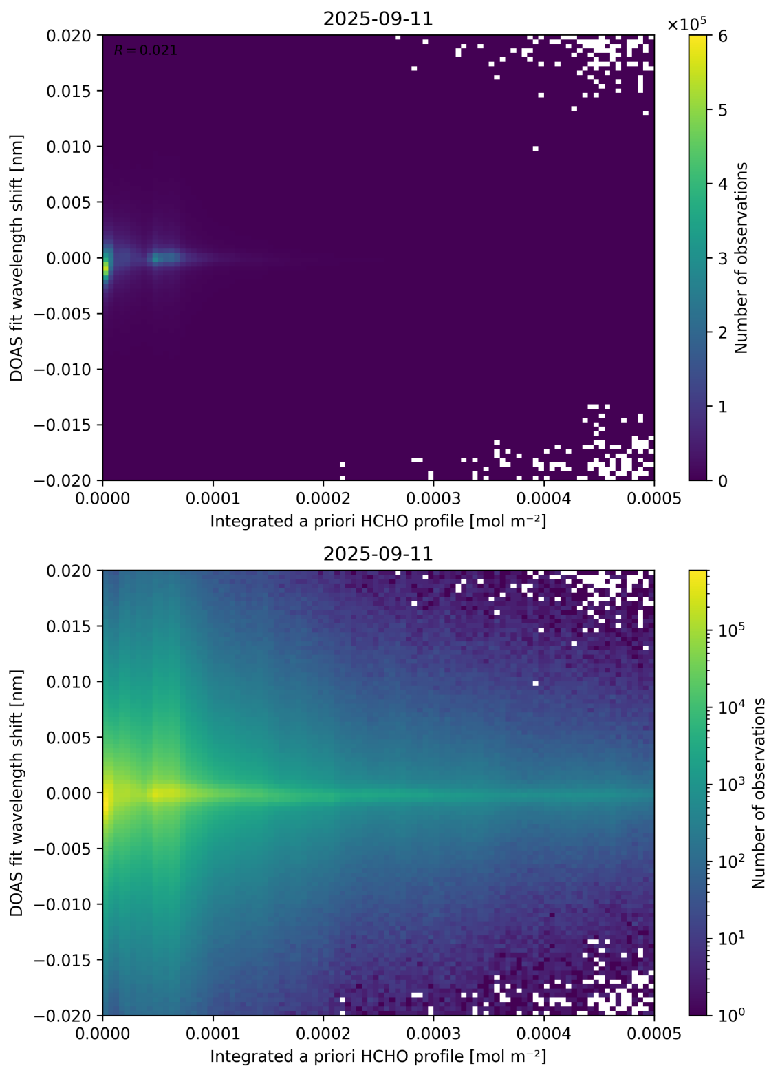
Figure 149: Scatter density plot of “Integrated a priori HCHO profile” against “DOAS fit wavelength shift” for 2025-09-10 to 2025-09-12.
