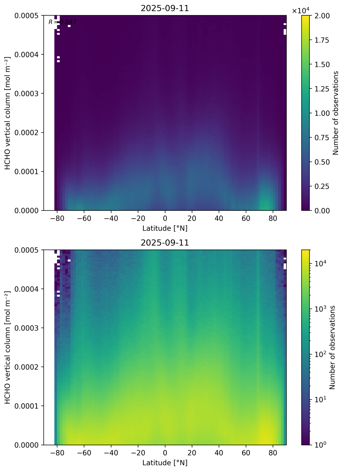
Figure 163: Scatter density plot of “Latitude” against “HCHO vertical column” for 2025-09-10 to 2025-09-12.
