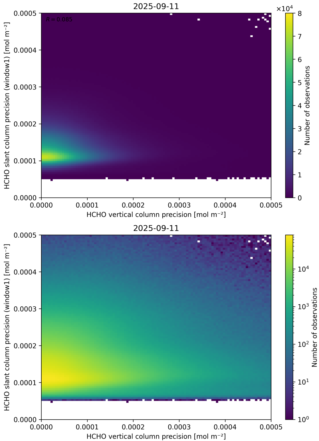
Figure 143: Scatter density plot of “HCHO vertical column precision” against “HCHO slant column precision (window1)” for 2025-09-10 to 2025-09-12.
