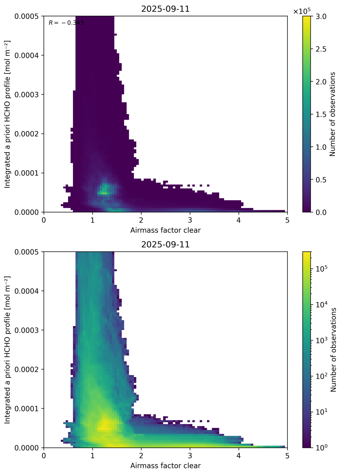
Figure 76: Scatter density plot of “Airmass factor clear” against “Integrated a priori HCHO profile” for 2025-09-10 to 2025-09-12.
