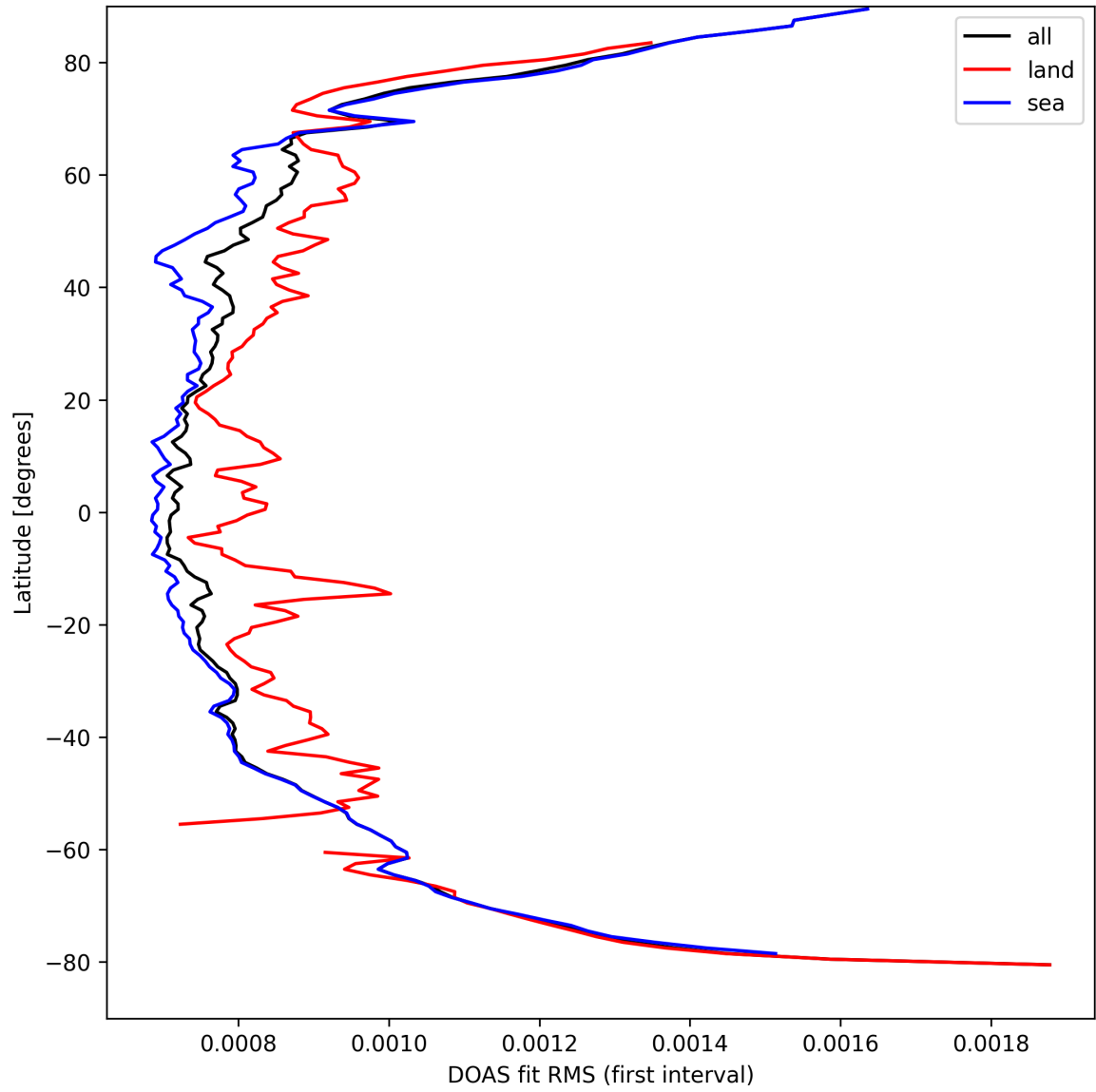
Figure 32: Zonal average of "DOAS fit RMS (first interval)" for 2025-09-10 to 2025-09-12.
