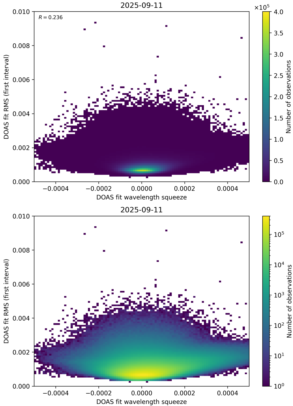
Figure 68: Scatter density plot of “DOAS fit wavelength squeeze” against “DOAS fit RMS (first interval)” for 2025-09-10 to 2025-09-12.
