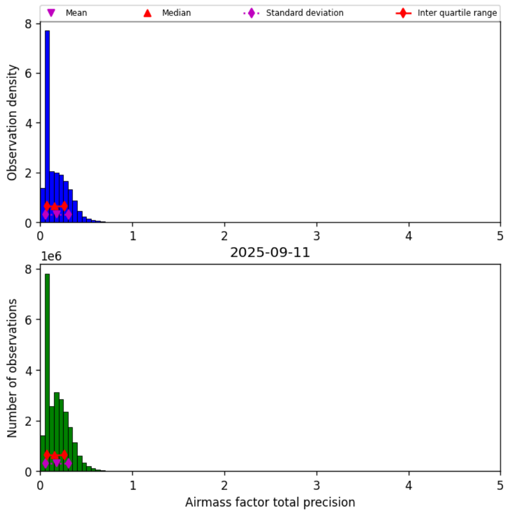
Figure 41: Histogram of “Airmass factor total precision” for 2025-09-10 to 2025-09-12
