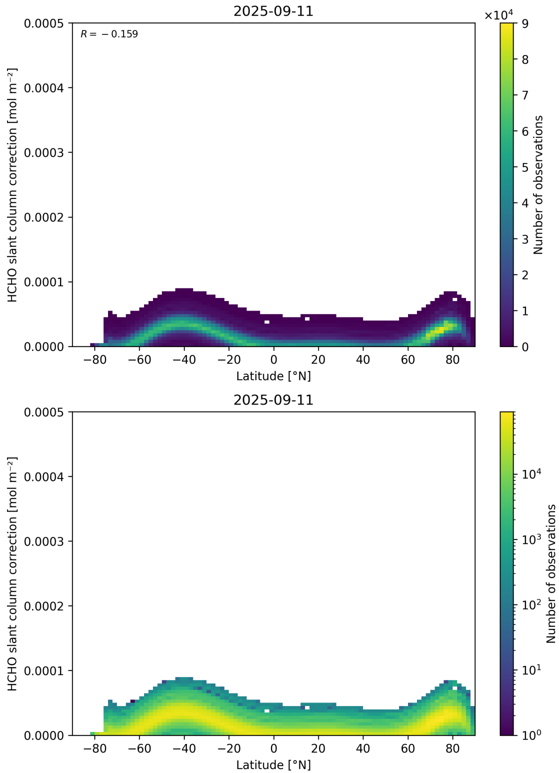
Figure 158: Scatter density plot of “Latitude” against “HCHO slant column correction” for 2025-09-10 to 2025-09-12.
