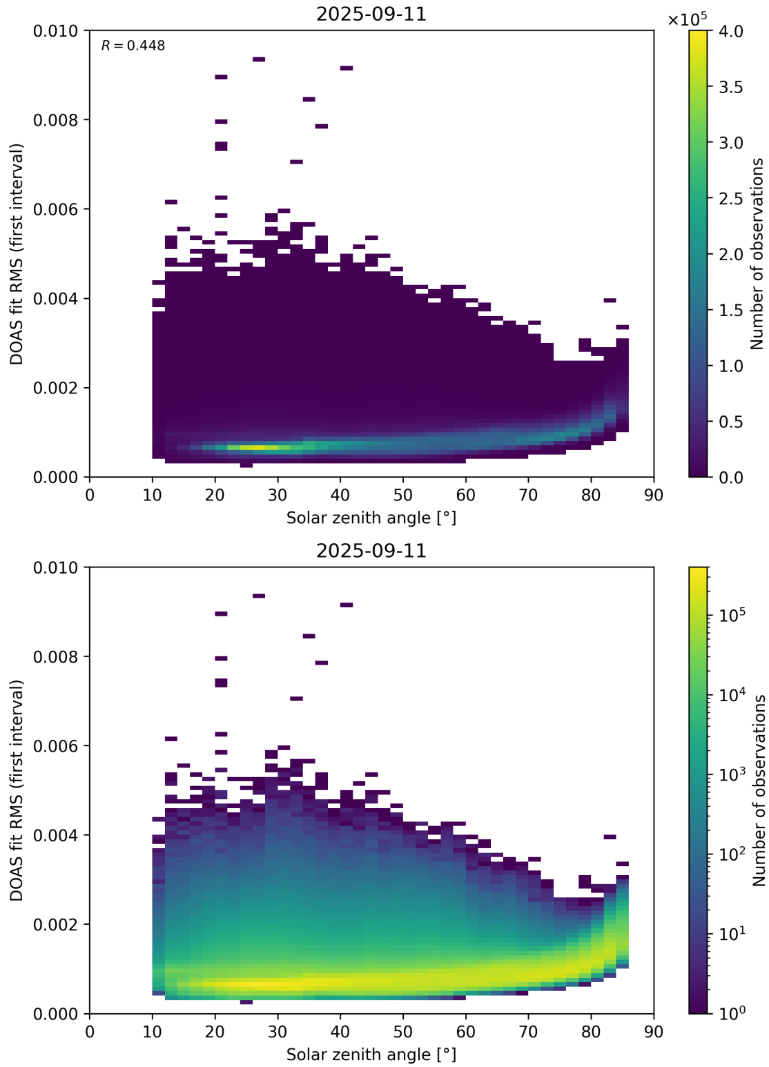
Figure 167: Scatter density plot of “Solar zenith angle” against “DOAS fit RMS (first interval)” for 2025-09-10 to 2025-09-12.
