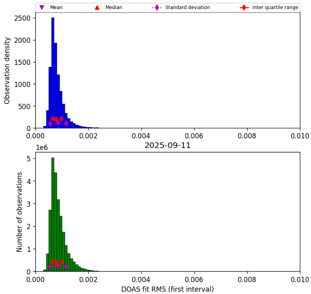
Figure 46: Histogram of “DOAS fit RMS (first interval)” for 2025-09-10 to 2025-09-12
