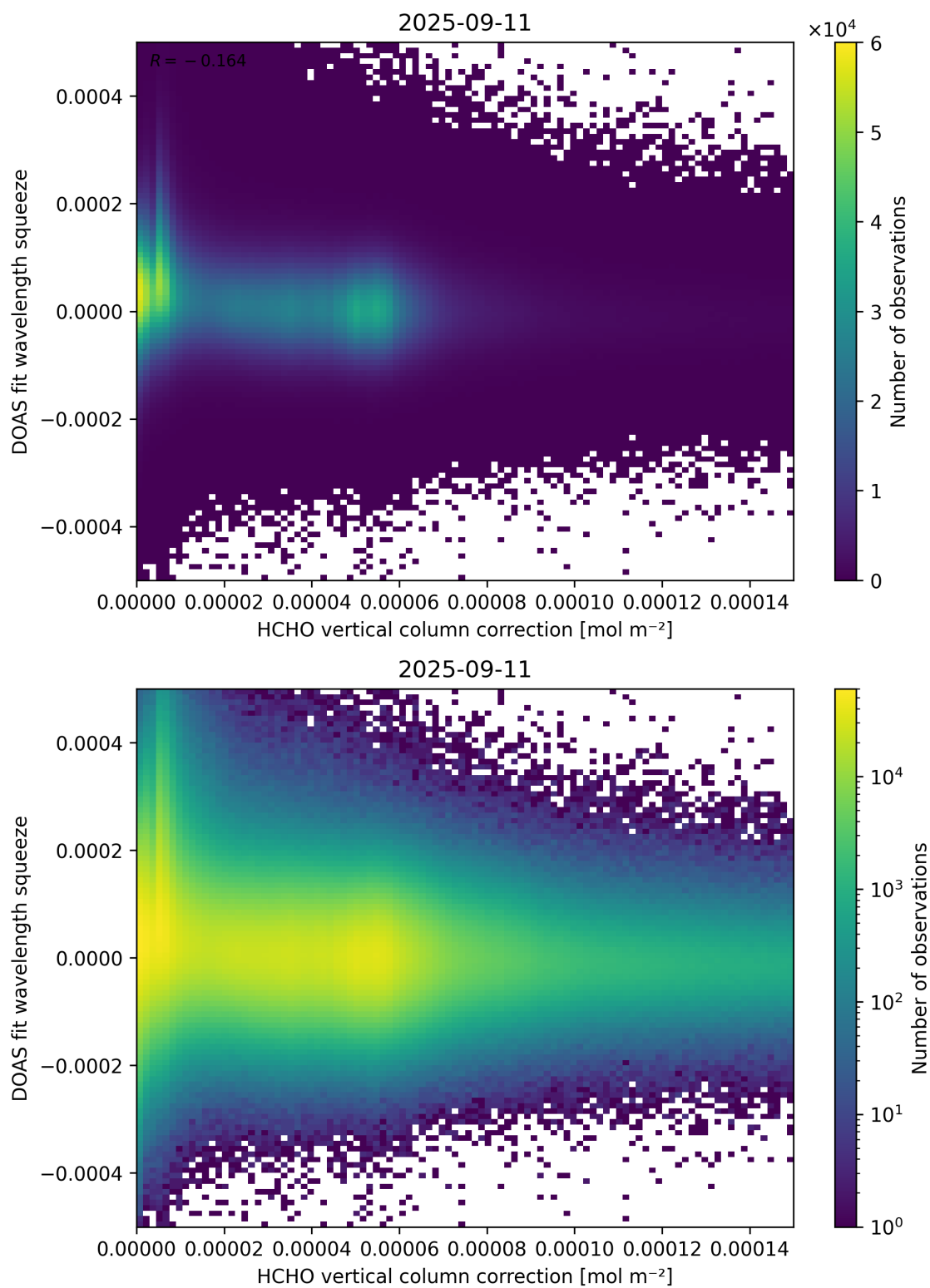
Figure 114: Scatter density plot of “HCHO vertical column correction” against “DOAS fit wavelength squeeze” for 2025-09-10 to 2025-09-12.
