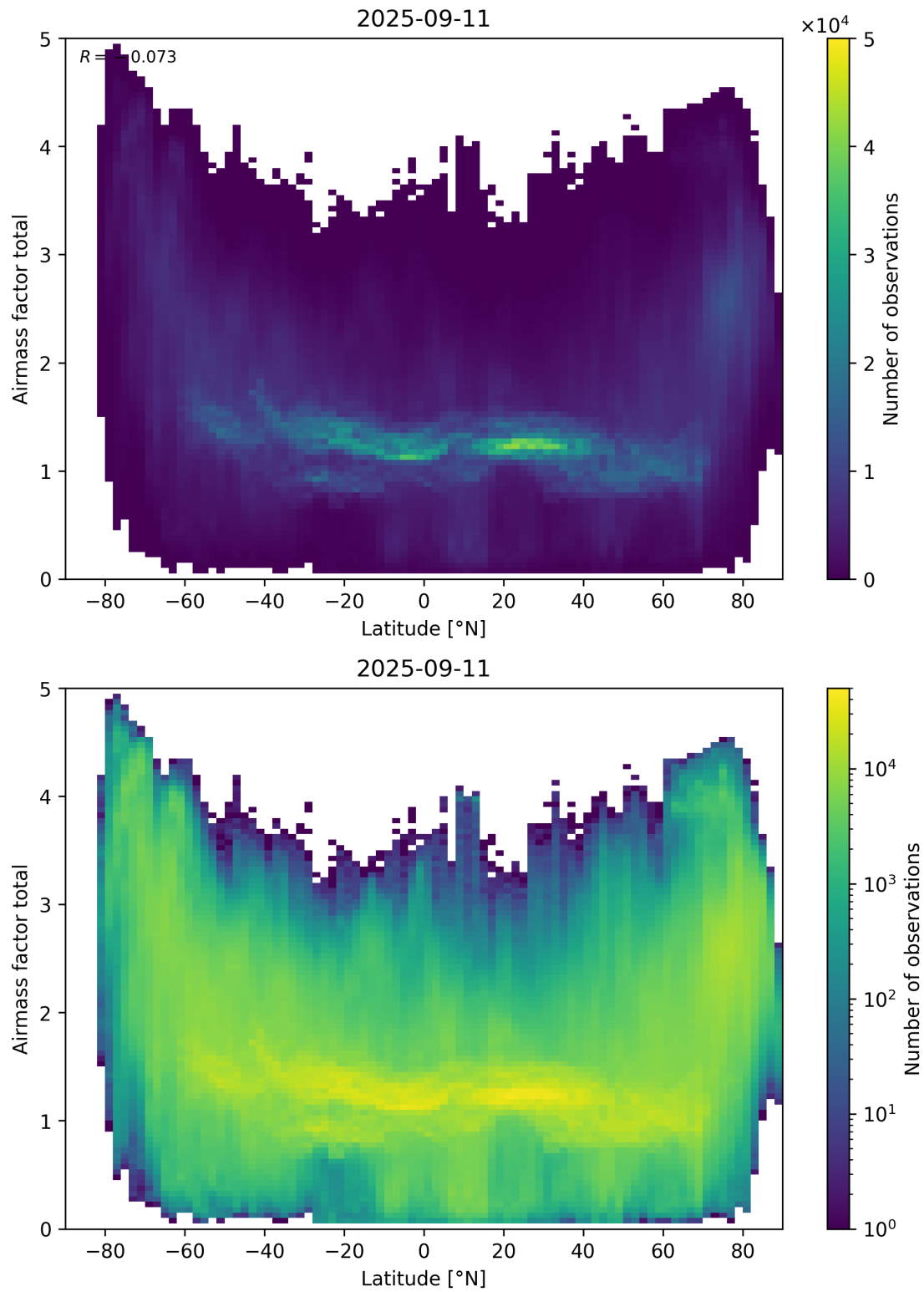
Figure 161: Scatter density plot of “Latitude” against “Airmass factor total” for 2025-09-10 to 2025-09-12.
