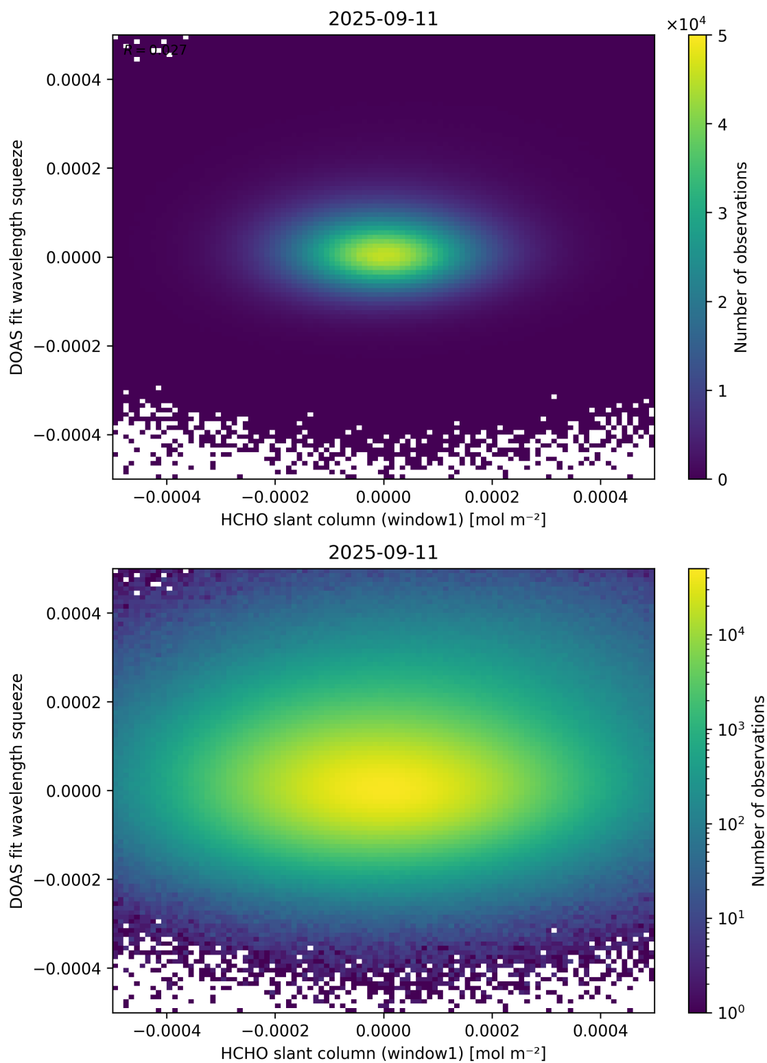
Figure 80: Scatter density plot of “HCHO slant column (window1)” against “DOAS fit wavelength squeeze” for 2025-09-10 to 2025-09-12.
