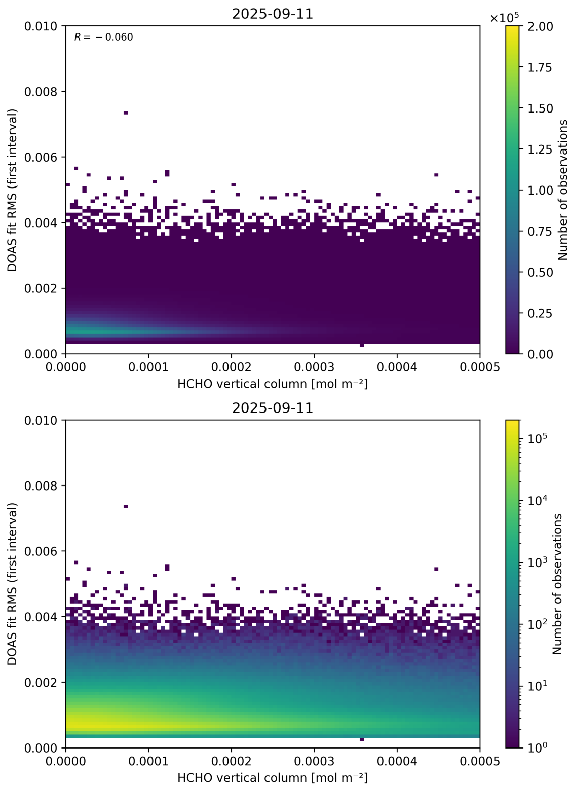
Figure 123: Scatter density plot of “HCHO vertical column” against “DOAS fit RMS (first interval)” for 2025-09-10 to 2025-09-12.
