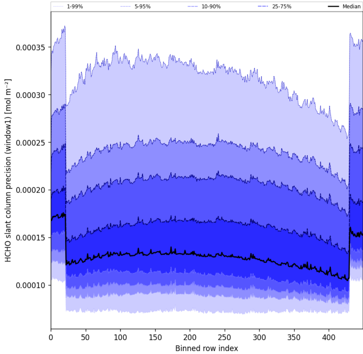
Figure 53: Along track statistics of “HCHO slant column precision (window1)” for 2025-09-10 to 2025-09-12
