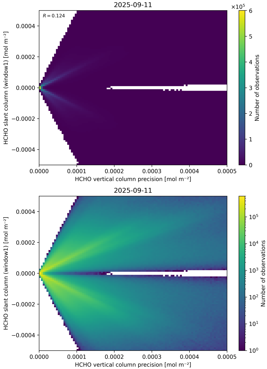
Figure 142: Scatter density plot of “HCHO vertical column precision” against “HCHO slant column (window1)” for 2025-09-10 to 2025-09-12.
