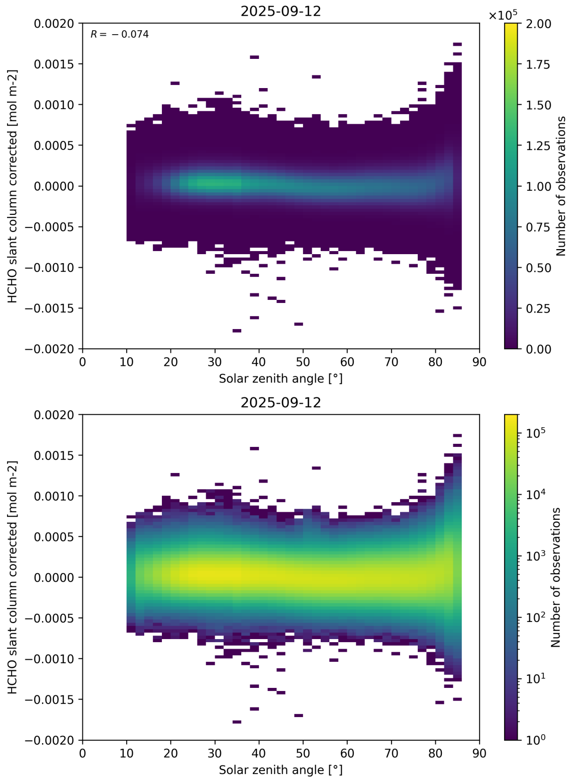
Figure 171: Scatter density plot of “Solar zenith angle” against “HCHO slant column corrected” for 2025-09-11 to 2025-09-13.
