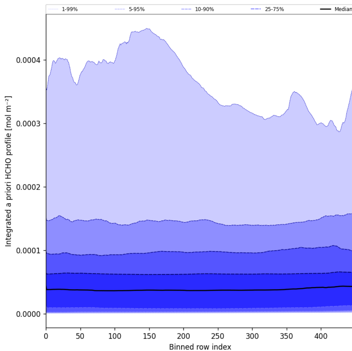
Figure 57: Along track statistics of “Integrated a priori HCHO profile” for 2025-09-11 to 2025-09-13
