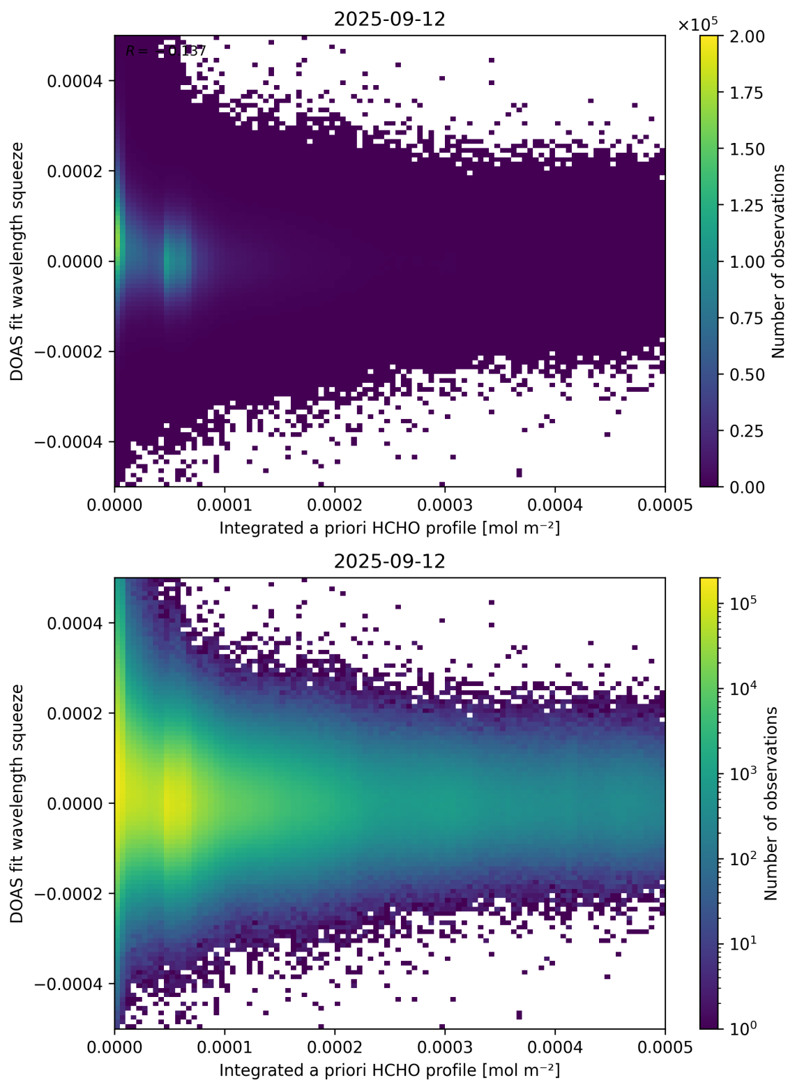
Figure 150: Scatter density plot of “Integrated a priori HCHO profile” against “DOAS fit wavelength squeeze” for 2025-09-11 to 2025-09-13.
