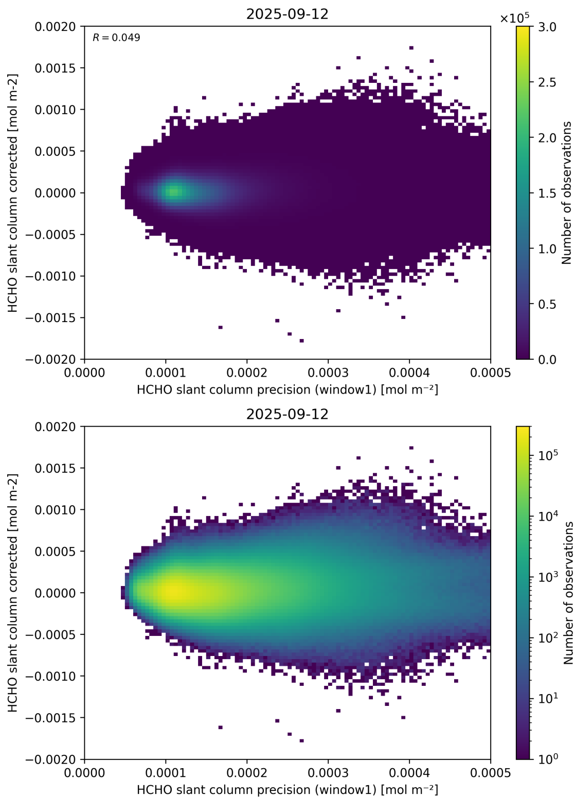
Figure 92: Scatter density plot of “HCHO slant column precision (window1)” against “HCHO slant column corrected” for 2025-09-11 to 2025-09-13.
