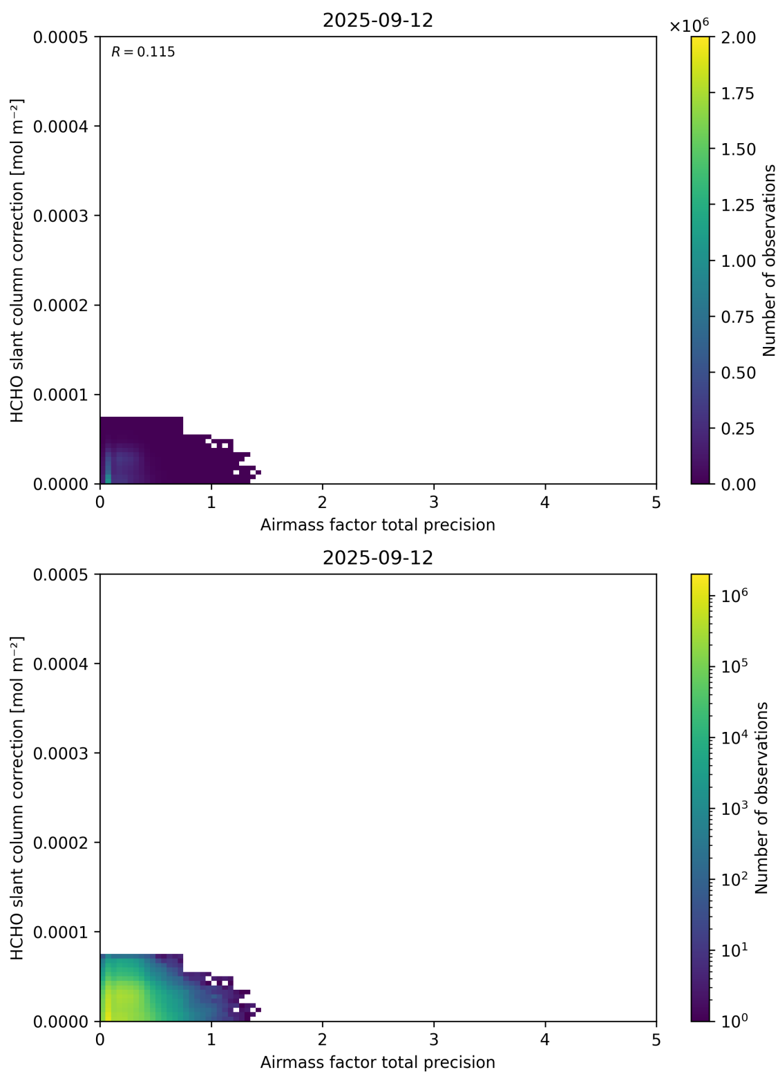
Figure 110: Scatter density plot of “Airmass factor total precision” against “HCHO slant column correction” for 2025-09-11 to 2025-09-13.
