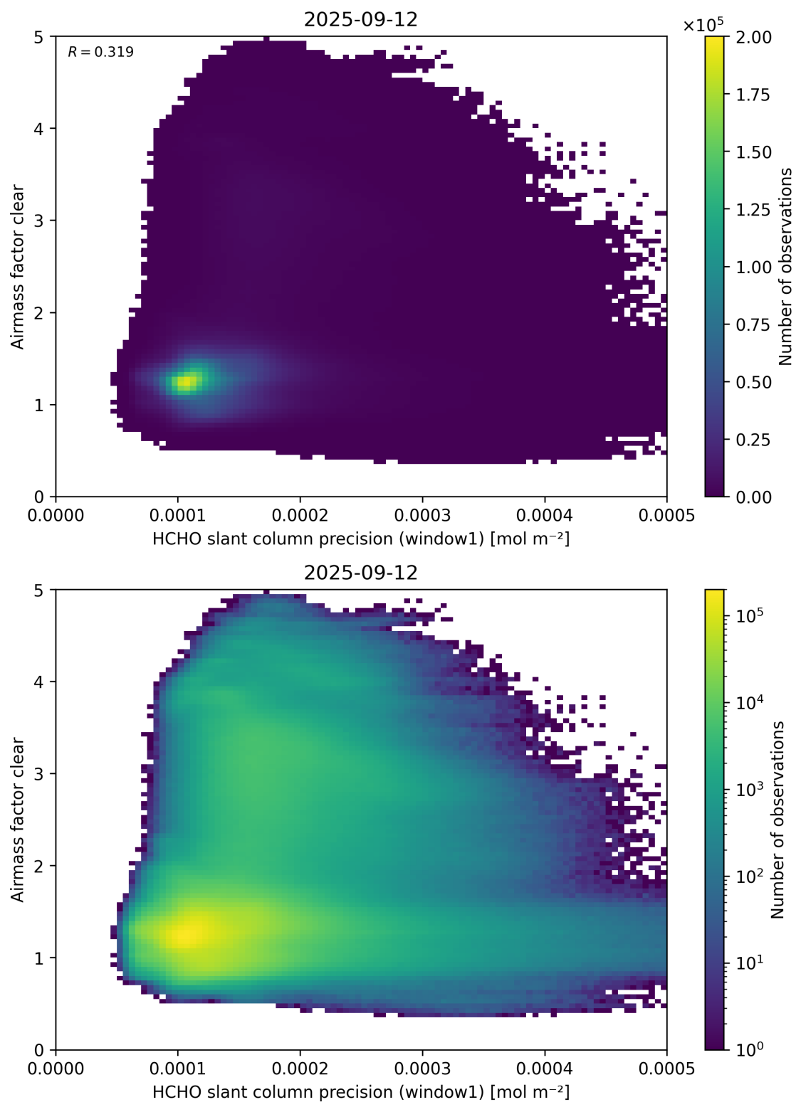
Figure 91: Scatter density plot of “HCHO slant column precision (window1)” against “Airmass factor clear” for 2025-09-11 to 2025-09-13.
