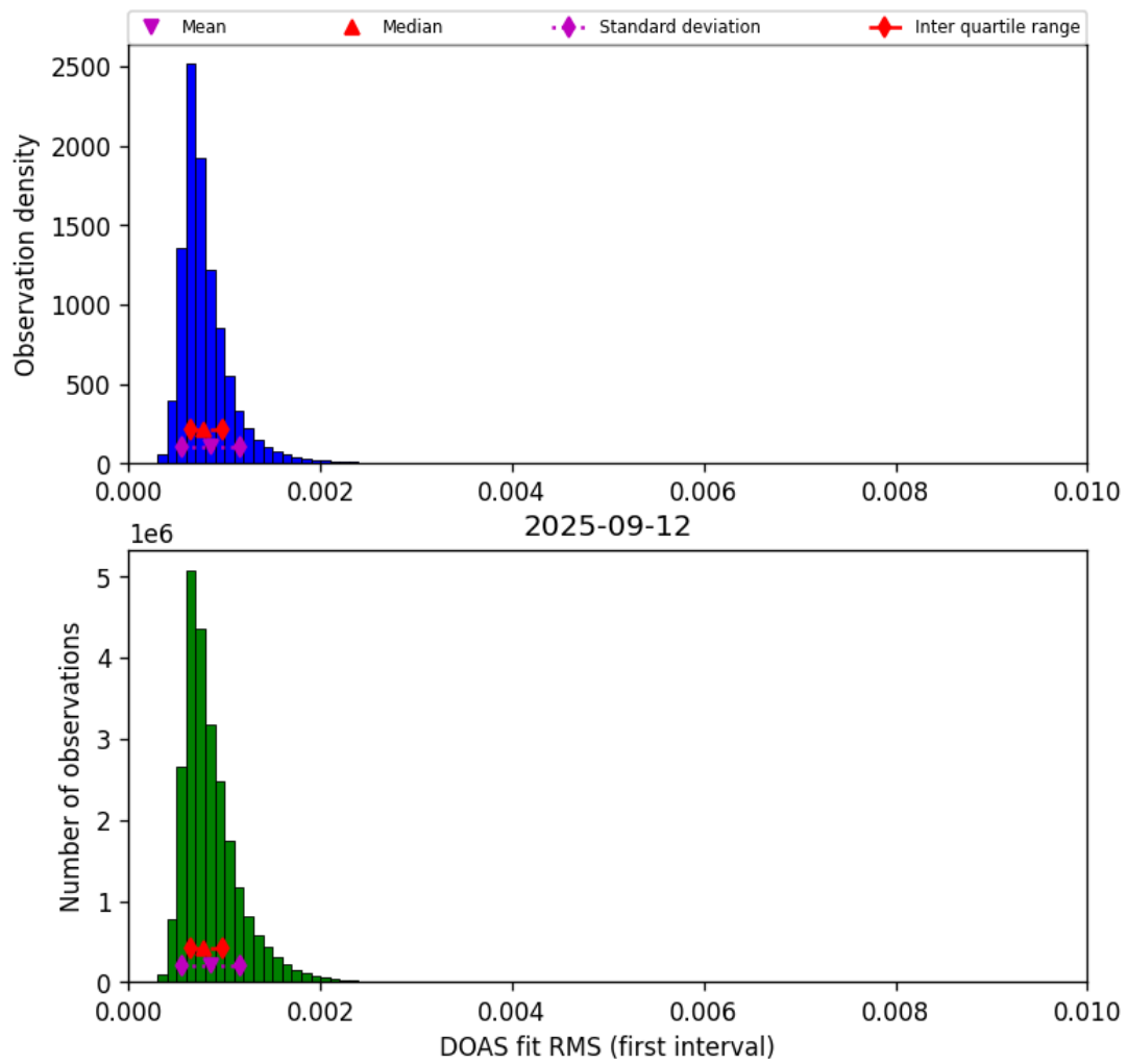
Figure 46: Histogram of “DOAS fit RMS (first interval)” for 2025-09-11 to 2025-09-13
