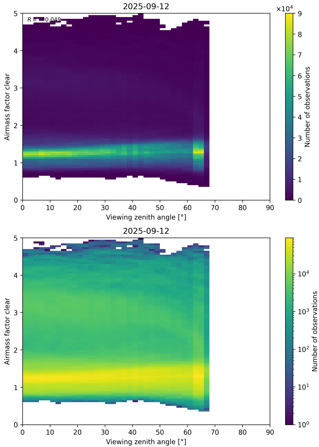
Figure 185: Scatter density plot of “Viewing zenith angle” against “Airmass factor clear” for 2025-09-11 to 2025-09-13.
