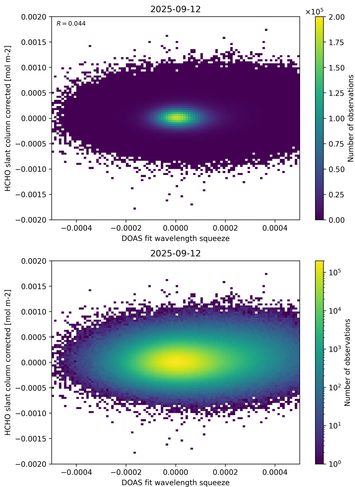
Figure 69: Scatter density plot of “DOAS fit wavelength squeeze” against “HCHO slant column corrected” for 2025-09-11 to 2025-09-13.
