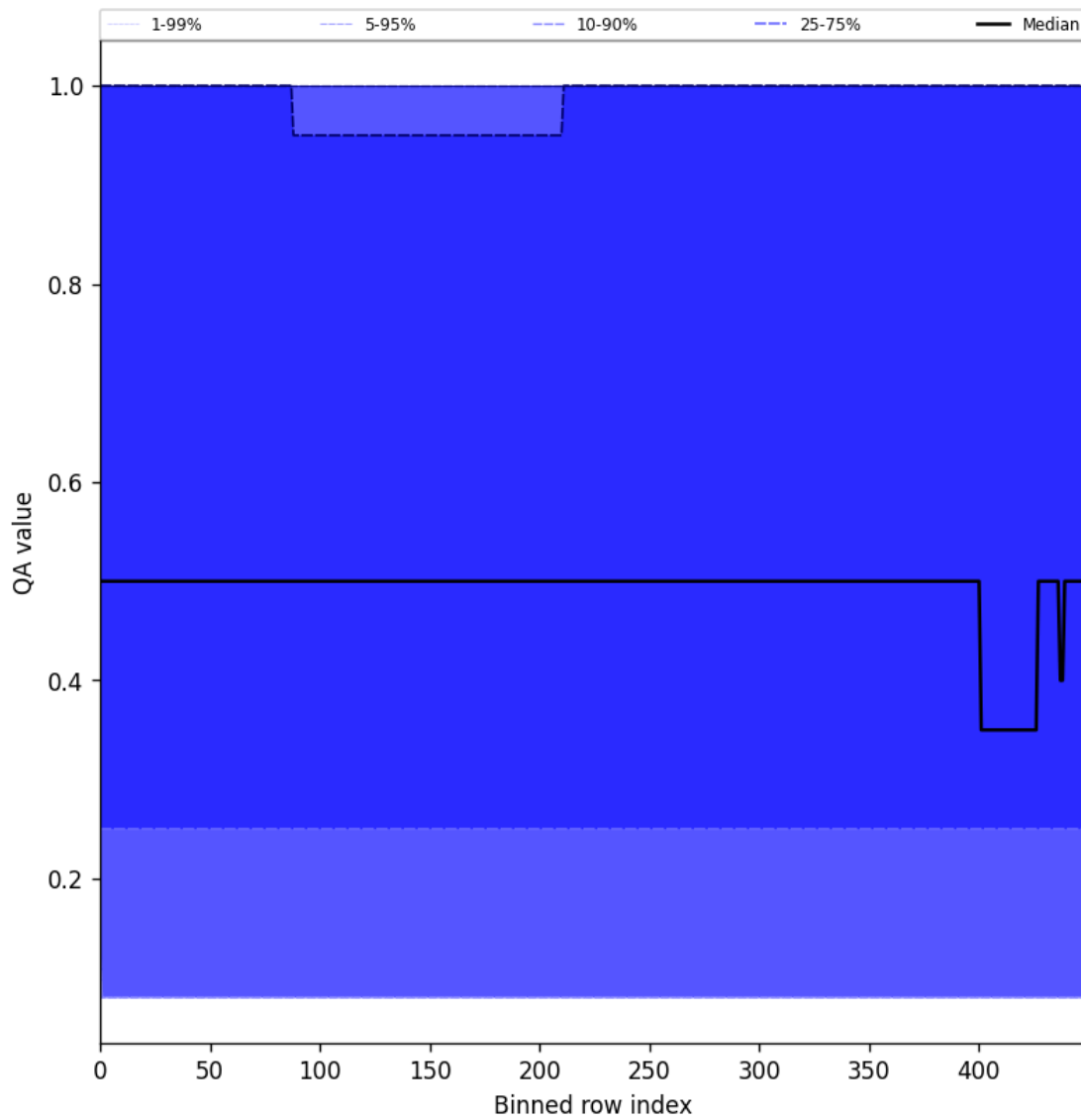
Figure 48: Along track statistics of “QA value” for 2025-09-11 to 2025-09-13
