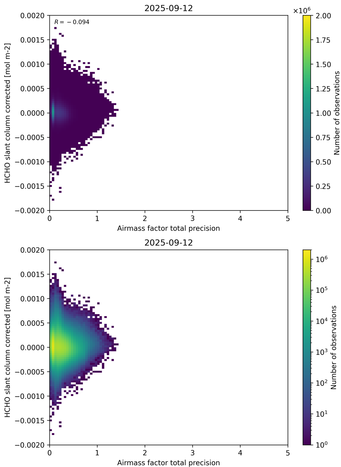
Figure 109: Scatter density plot of “Airmass factor total precision” against “HCHO slant column corrected” for 2025-09-11 to 2025-09-13.
