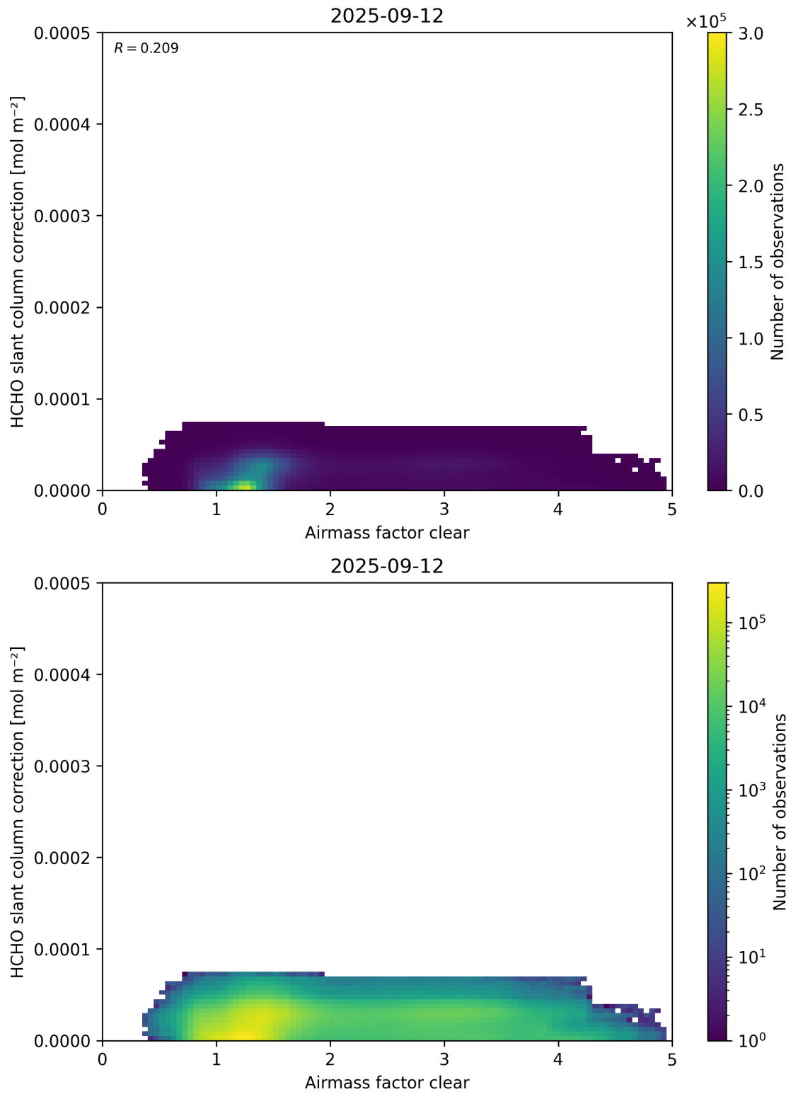
Figure 75: Scatter density plot of “Airmass factor clear” against “HCHO slant column correction” for 2025-09-11 to 2025-09-13.
