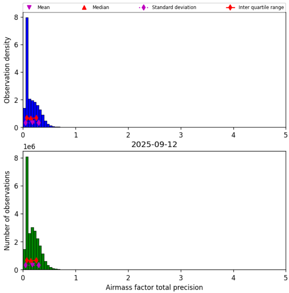
Figure 41: Histogram of “Airmass factor total precision” for 2025-09-11 to 2025-09-13
