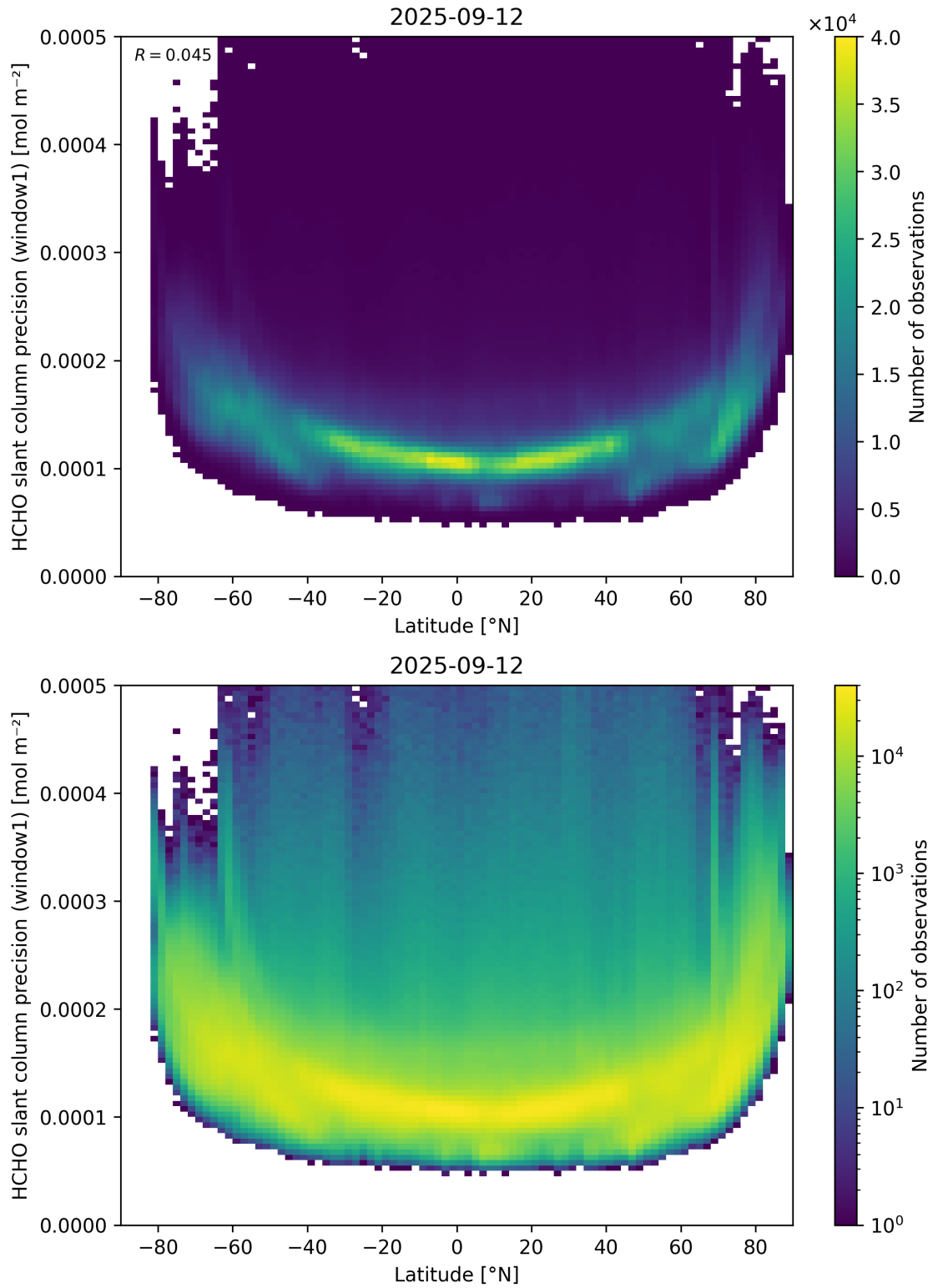
Figure 160: Scatter density plot of “Latitude” against “HCHO slant column precision (window1)” for 2025-09-11 to 2025-09-13.
