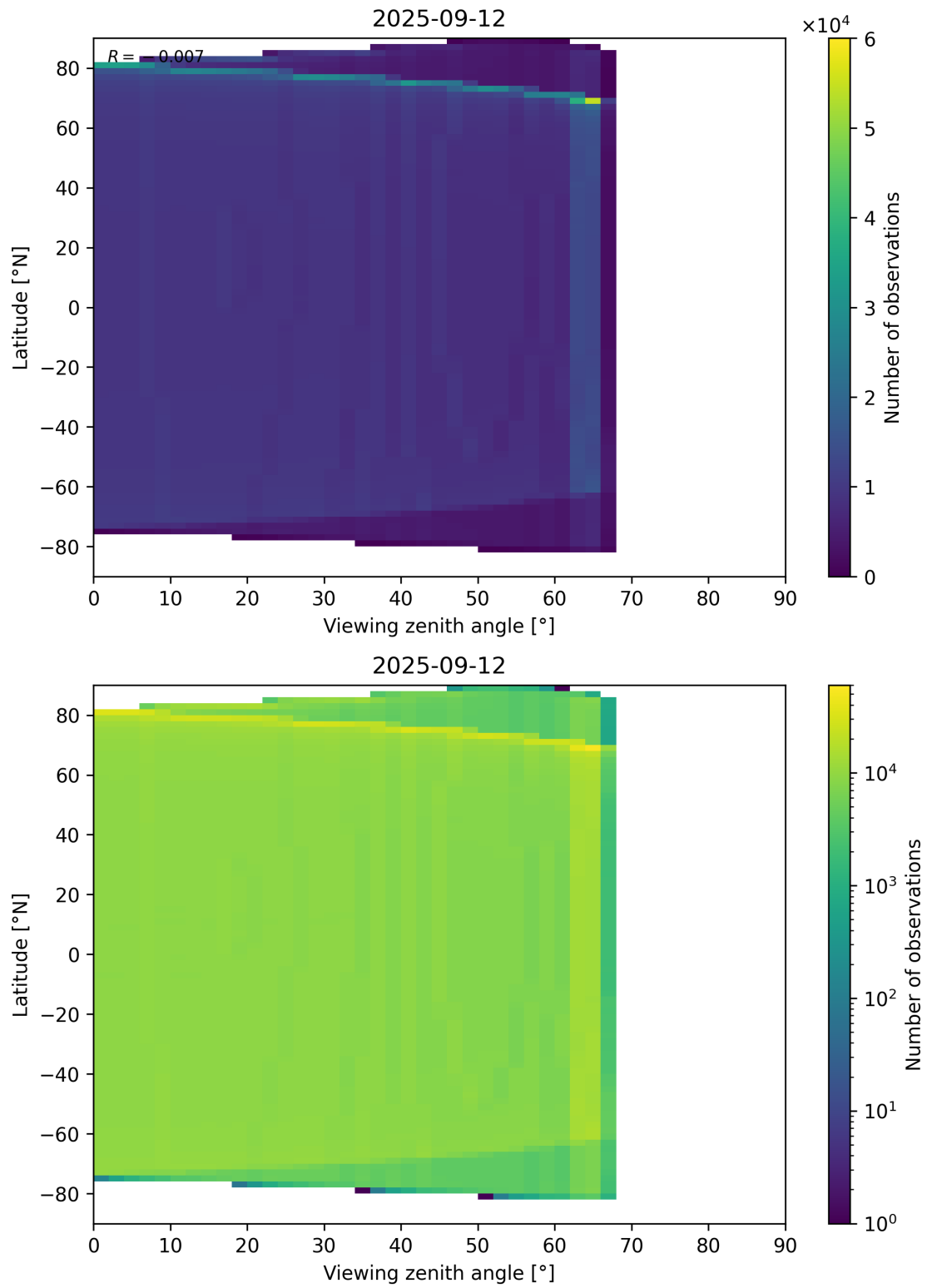
Figure 196: Scatter density plot of “Viewing zenith angle” against “Latitude” for 2025-09-11 to 2025-09-13.
