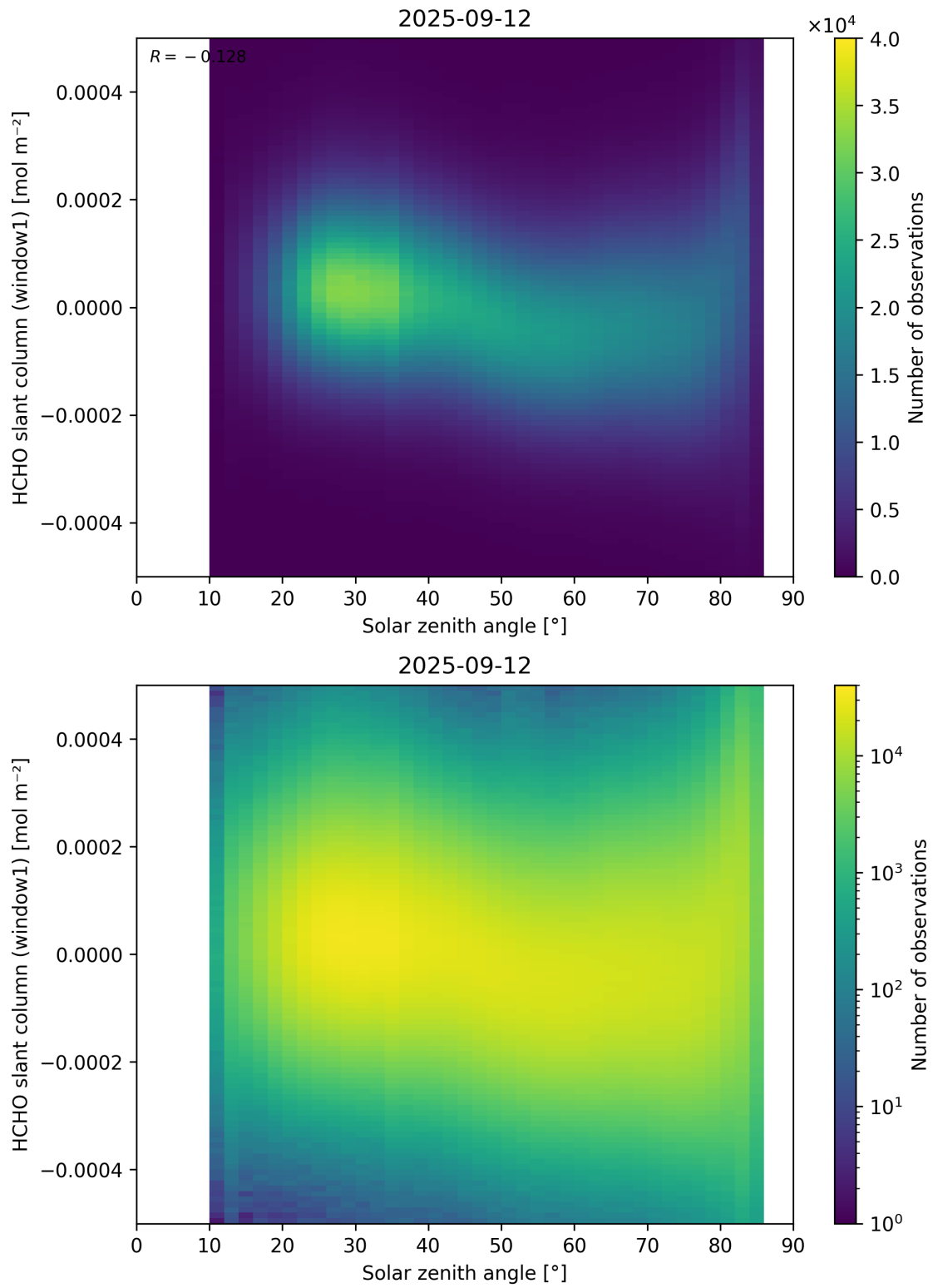
Figure 173: Scatter density plot of “Solar zenith angle” against “HCHO slant column (window1)” for 2025-09-11 to 2025-09-13.
