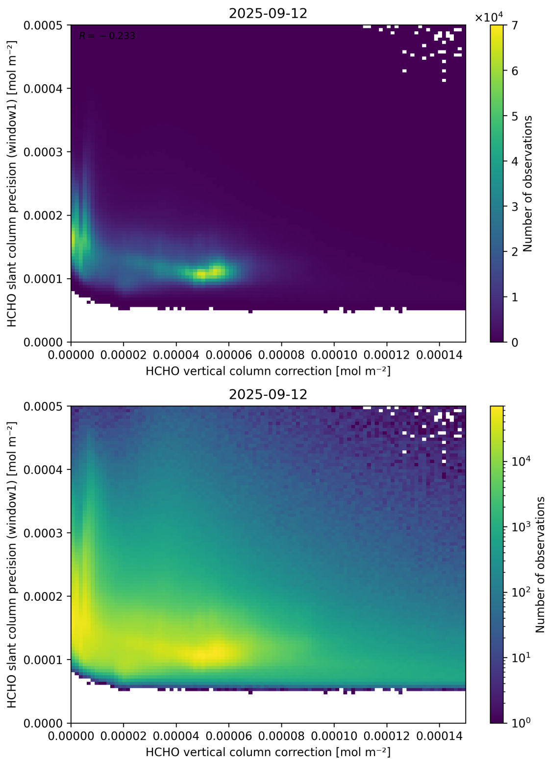
Figure 119: Scatter density plot of “HCHO vertical column correction” against “HCHO slant column precision (window1)” for 2025-09-11 to 2025-09-13.
