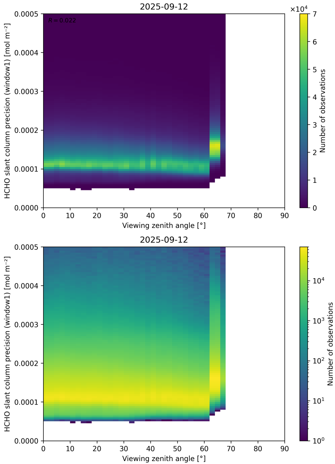
Figure 189: Scatter density plot of “Viewing zenith angle” against “HCHO slant column precision (window1)” for 2025-09-11 to 2025-09-13.
