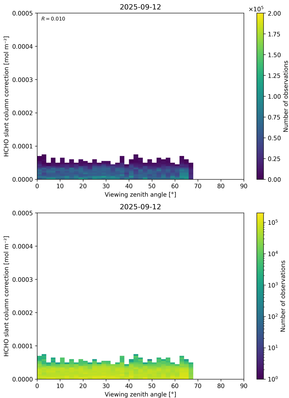
Figure 187: Scatter density plot of “Viewing zenith angle” against “HCHO slant column correction” for 2025-09-11 to 2025-09-13.
