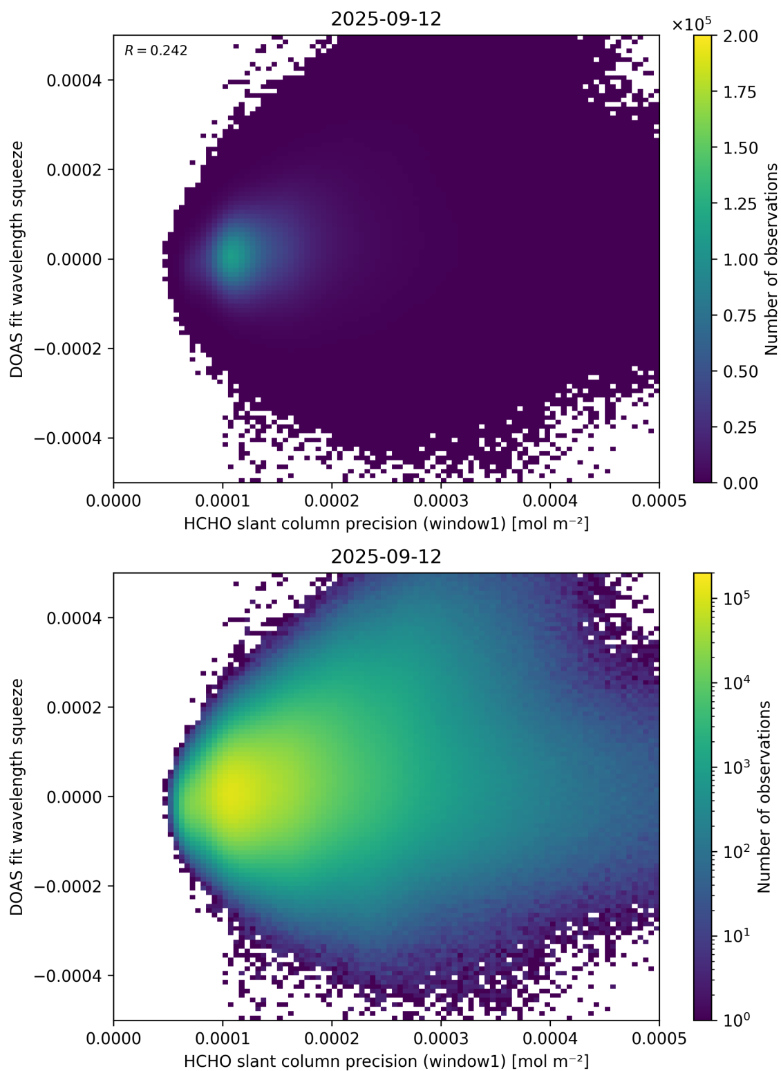
Figure 90: Scatter density plot of “HCHO slant column precision (window1)” against “DOAS fit wavelength squeeze” for 2025-09-11 to 2025-09-13.
