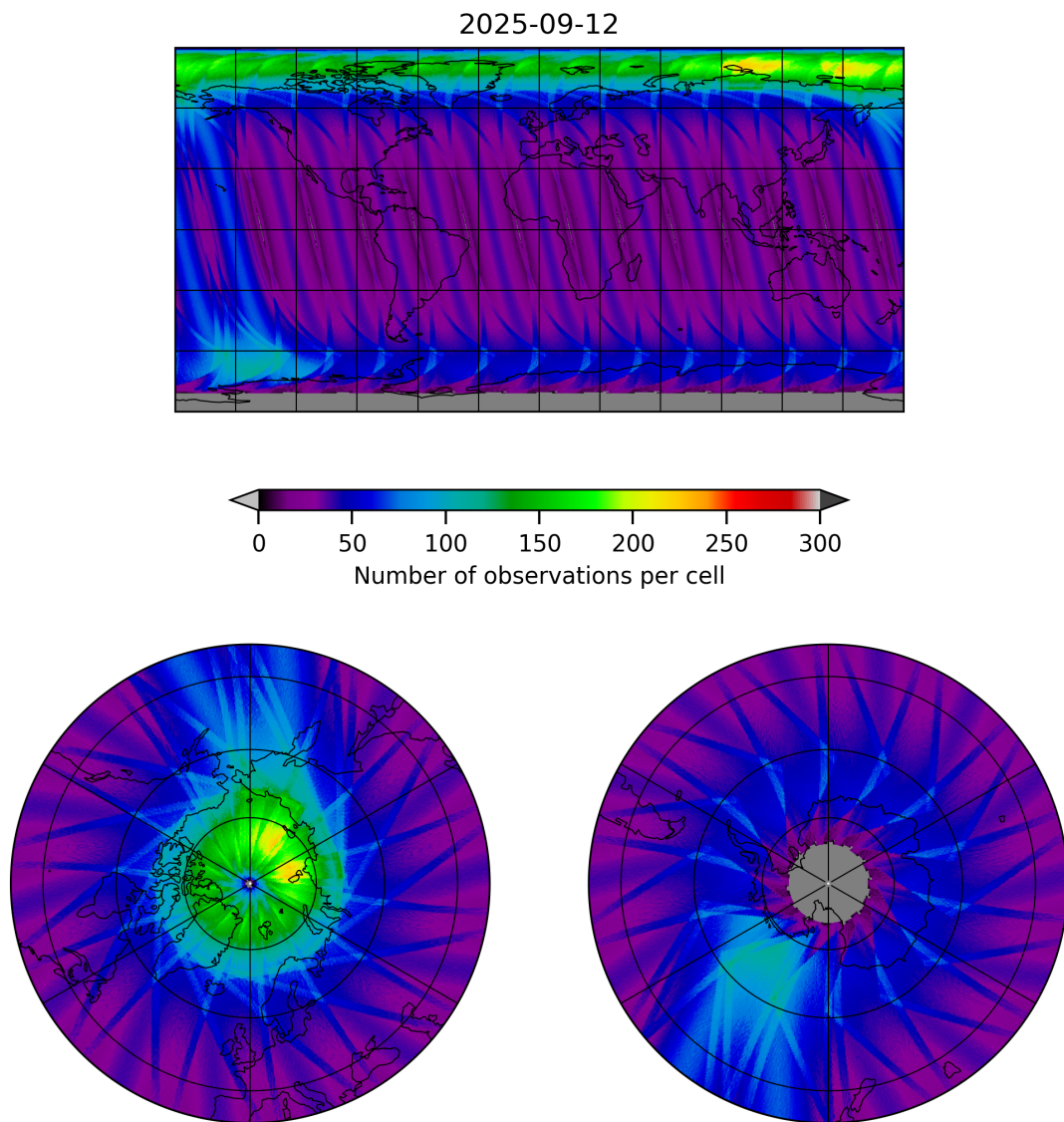
Figure 19: Map of the number of observations for 2025-09-11 to 2025-09-13
