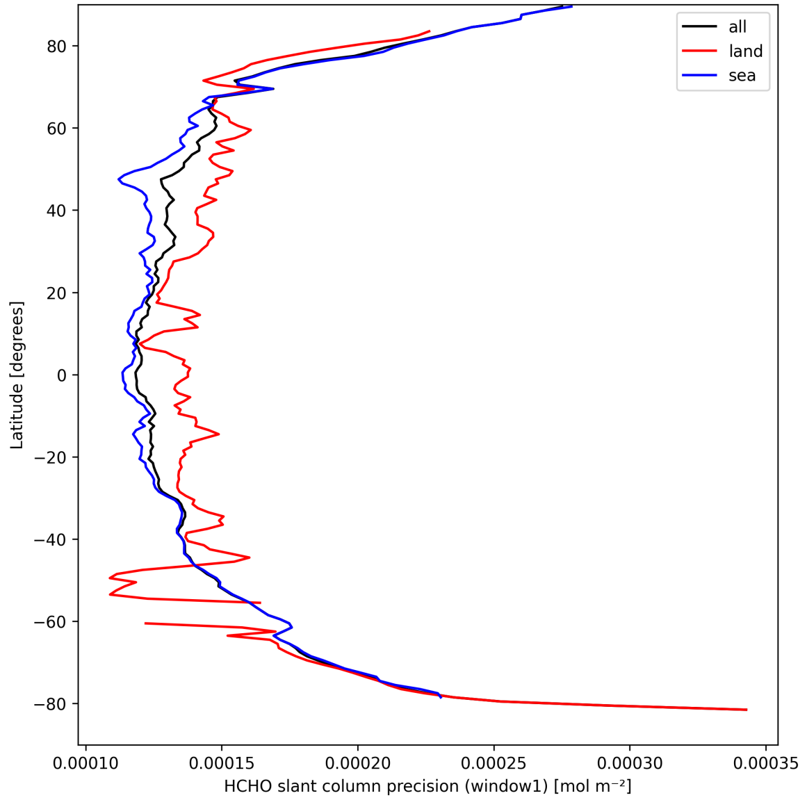
Figure 25: Zonal average of “HCHO slant column precision (window1)” for 2025-09-11 to 2025-09-13.
