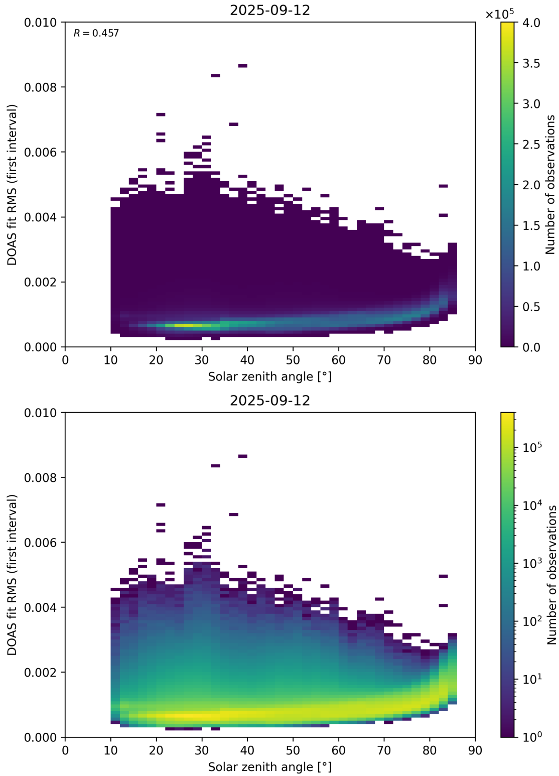
Figure 167: Scatter density plot of “Solar zenith angle” against “DOAS fit RMS (first interval)” for 2025-09-11 to 2025-09-13.
