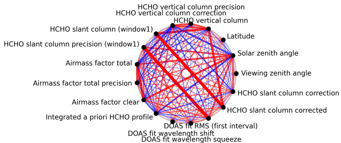
Figure 1: Map of correlation graph for 2025-09-11 to 2025-09-13.
