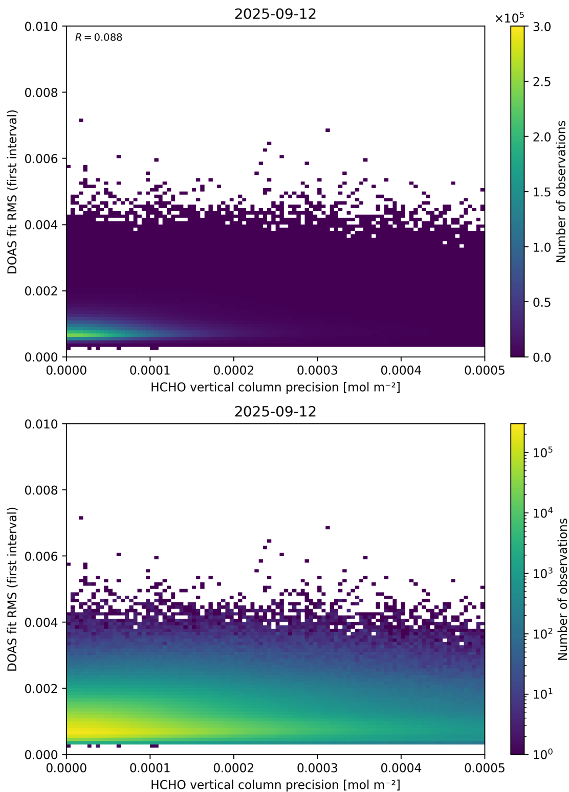
Figure 136: Scatter density plot of “HCHO vertical column precision” against “DOAS fit RMS (first interval)” for 2025-09-11 to 2025-09-13.
