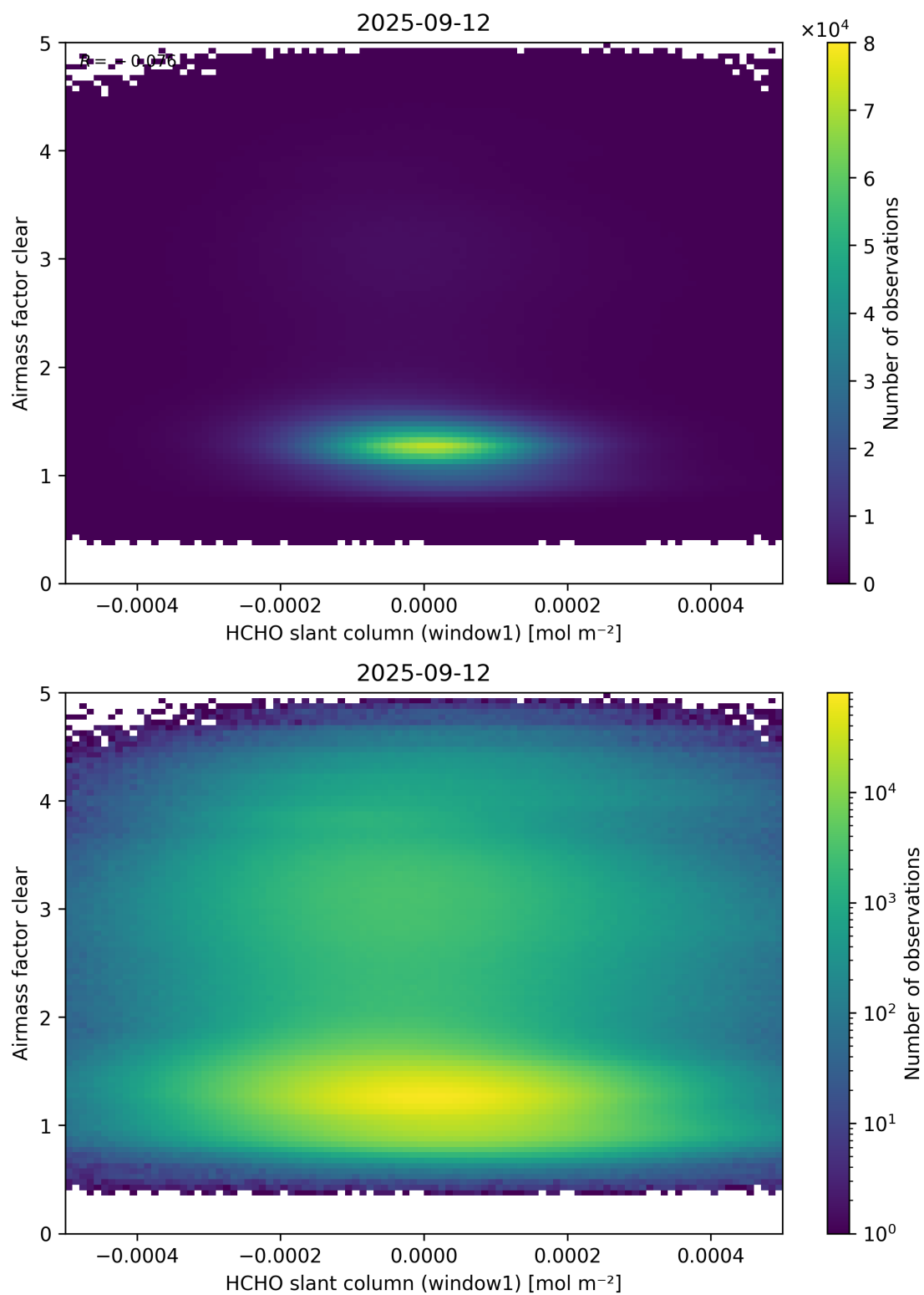
Figure 81: Scatter density plot of “HCHO slant column (window1)” against “Airmass factor clear” for 2025-09-11 to 2025-09-13.
