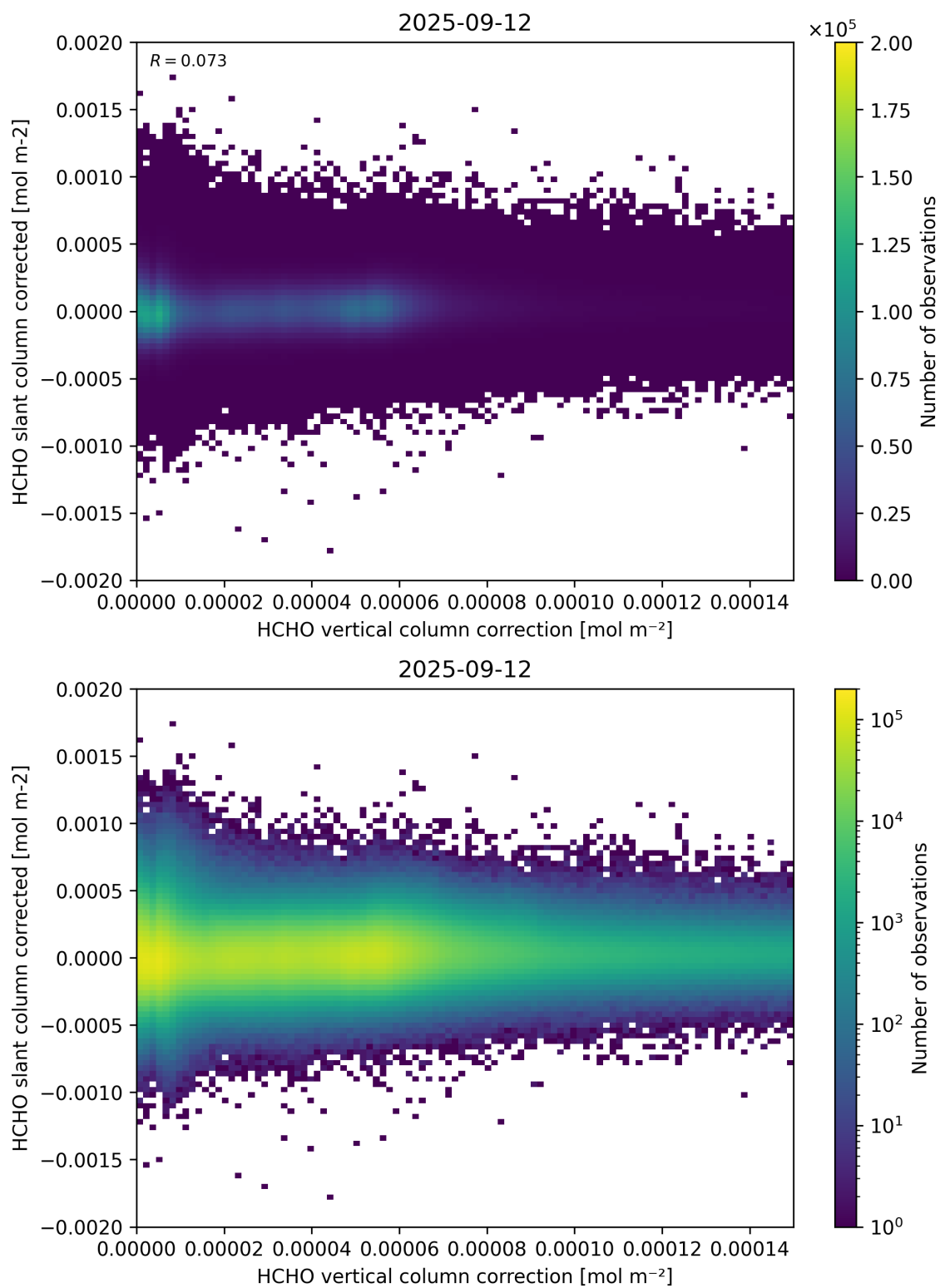
Figure 116: Scatter density plot of “HCHO vertical column correction” against “HCHO slant column corrected” for 2025-09-11 to 2025-09-13.
