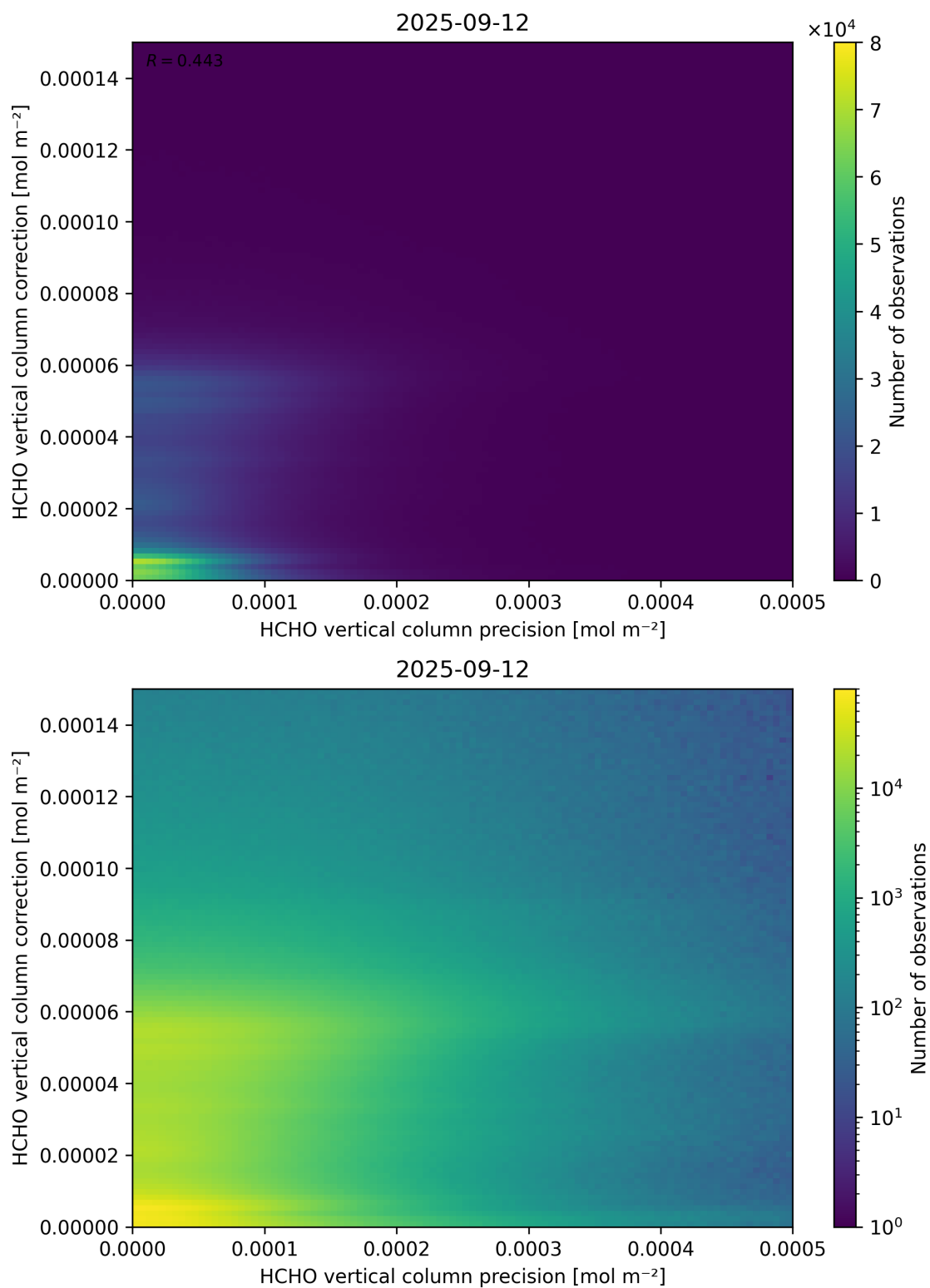
Figure 146: Scatter density plot of “HCHO vertical column precision” against “HCHO vertical column correction” for 2025-09-11 to 2025-09-13.
