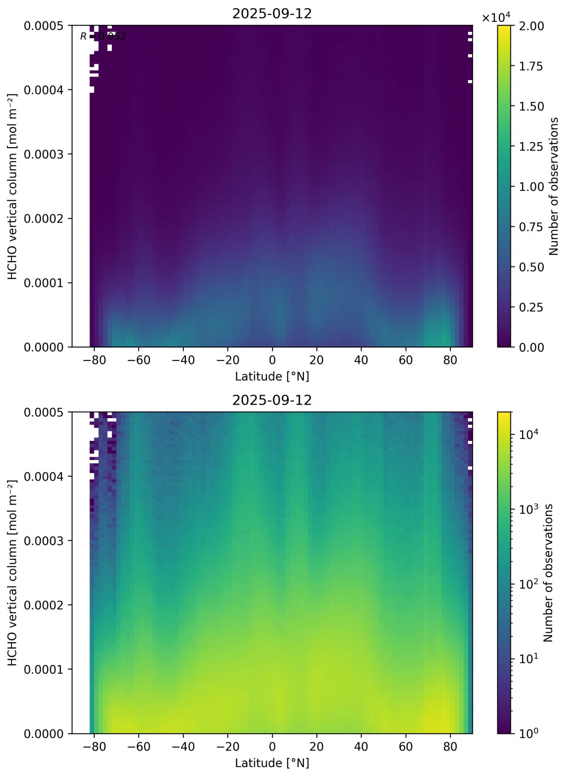
Figure 163: Scatter density plot of “Latitude” against “HCHO vertical column” for 2025-09-11 to 2025-09-13.
