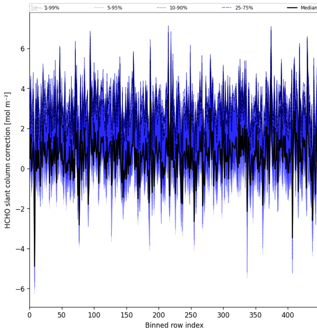
Figure 61: Along track statistics of “HCHO slant column correction” for 2025-09-11 to 2025-09-13
