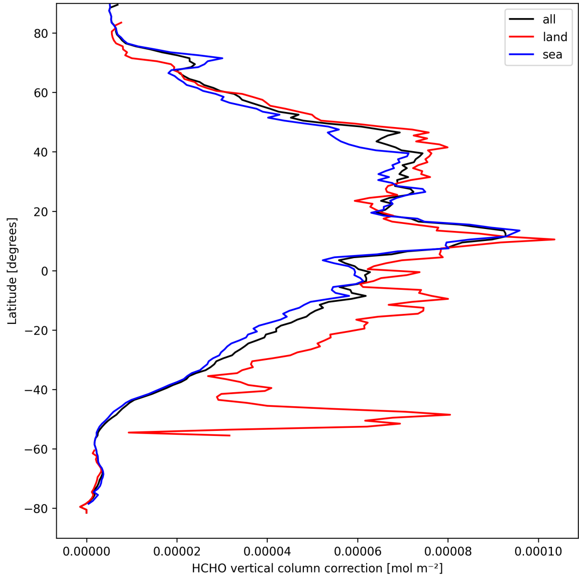
Figure 23: Zonal average of “HCHO vertical column correction” for 2025-09-11 to 2025-09-13.
