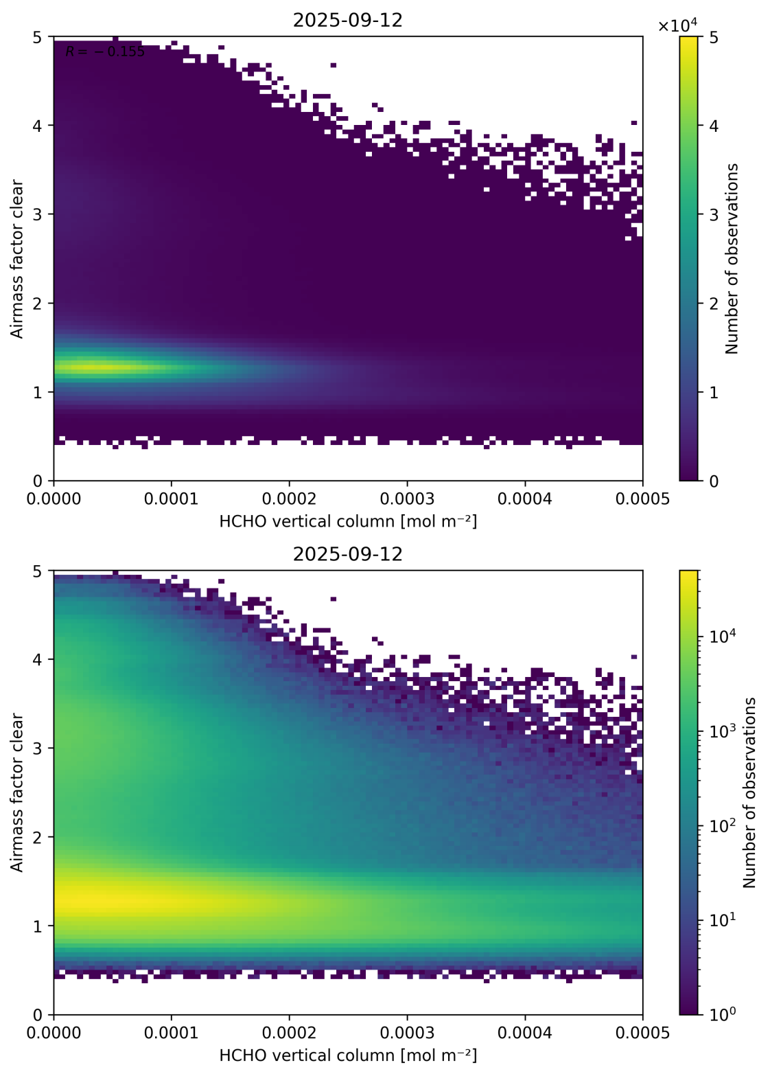
Figure 126: Scatter density plot of “HCHO vertical column” against “Airmass factor clear” for 2025-09-11 to 2025-09-13.
