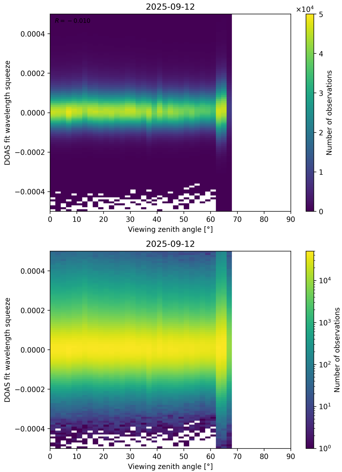
Figure 184: Scatter density plot of “Viewing zenith angle” against “DOAS fit wavelength squeeze” for 2025-09-11 to 2025-09-13.
