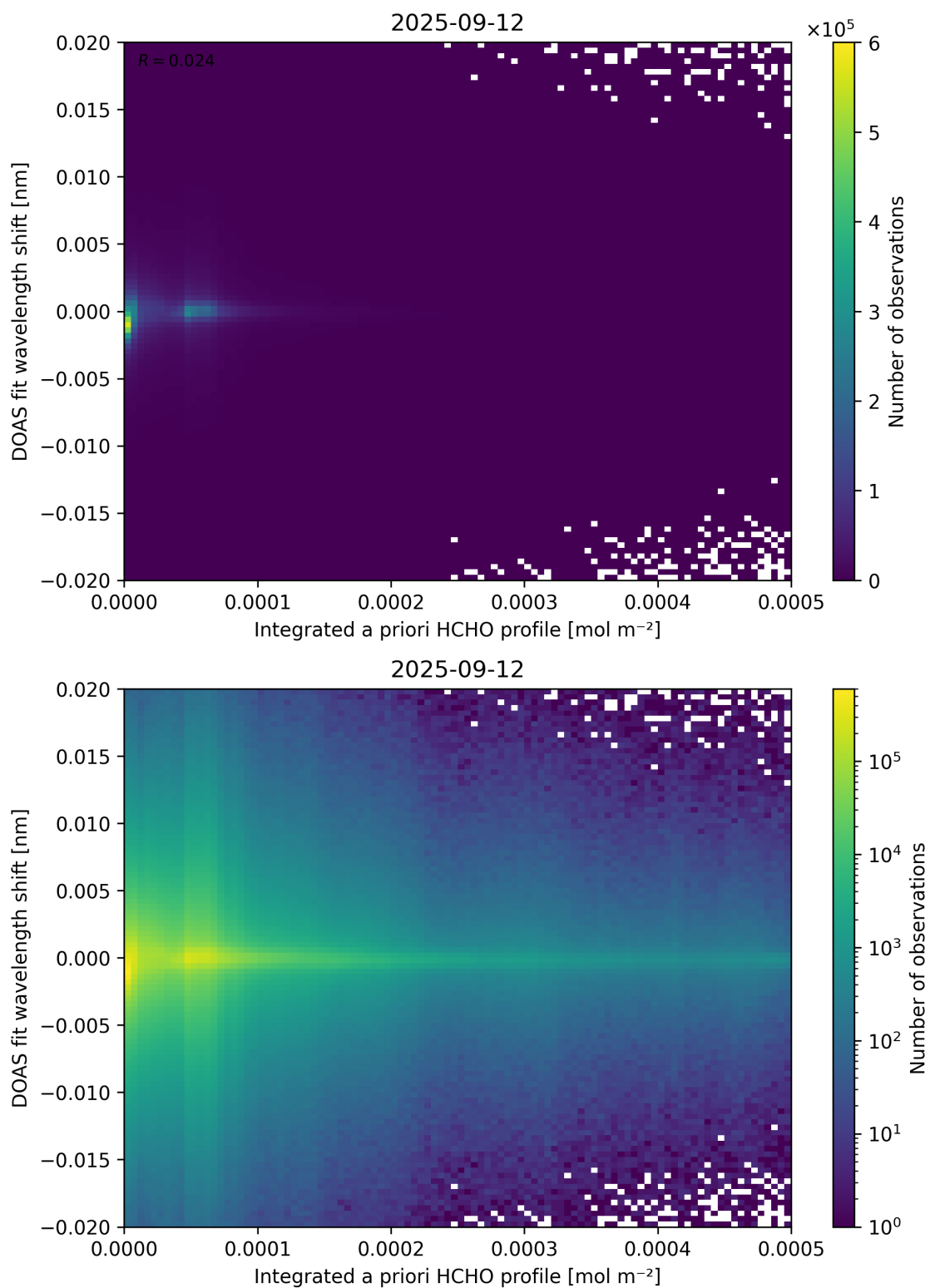
Figure 149: Scatter density plot of “Integrated a priori HCHO profile” against “DOAS fit wavelength shift” for 2025-09-11 to 2025-09-13.
