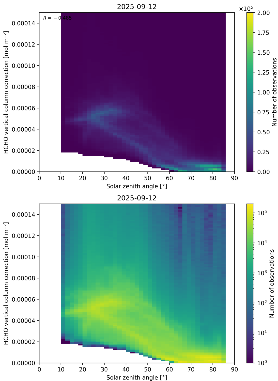
Figure 178: Scatter density plot of “Solar zenith angle” against “HCHO vertical column correction” for 2025-09-11 to 2025-09-13.
