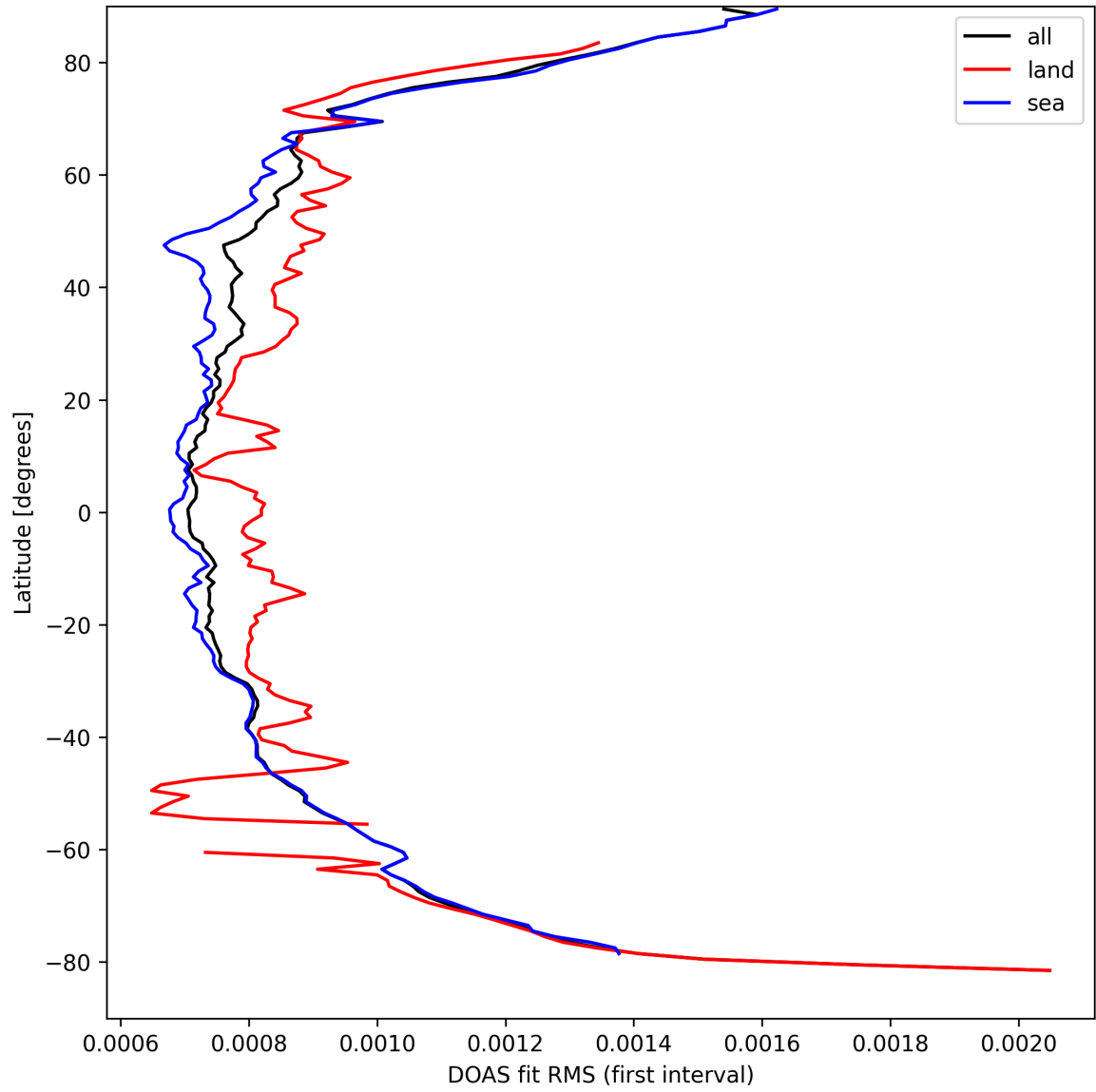
Figure 32: Zonal average of “DOAS fit RMS (first interval)” for 2025-09-11 to 2025-09-13.
