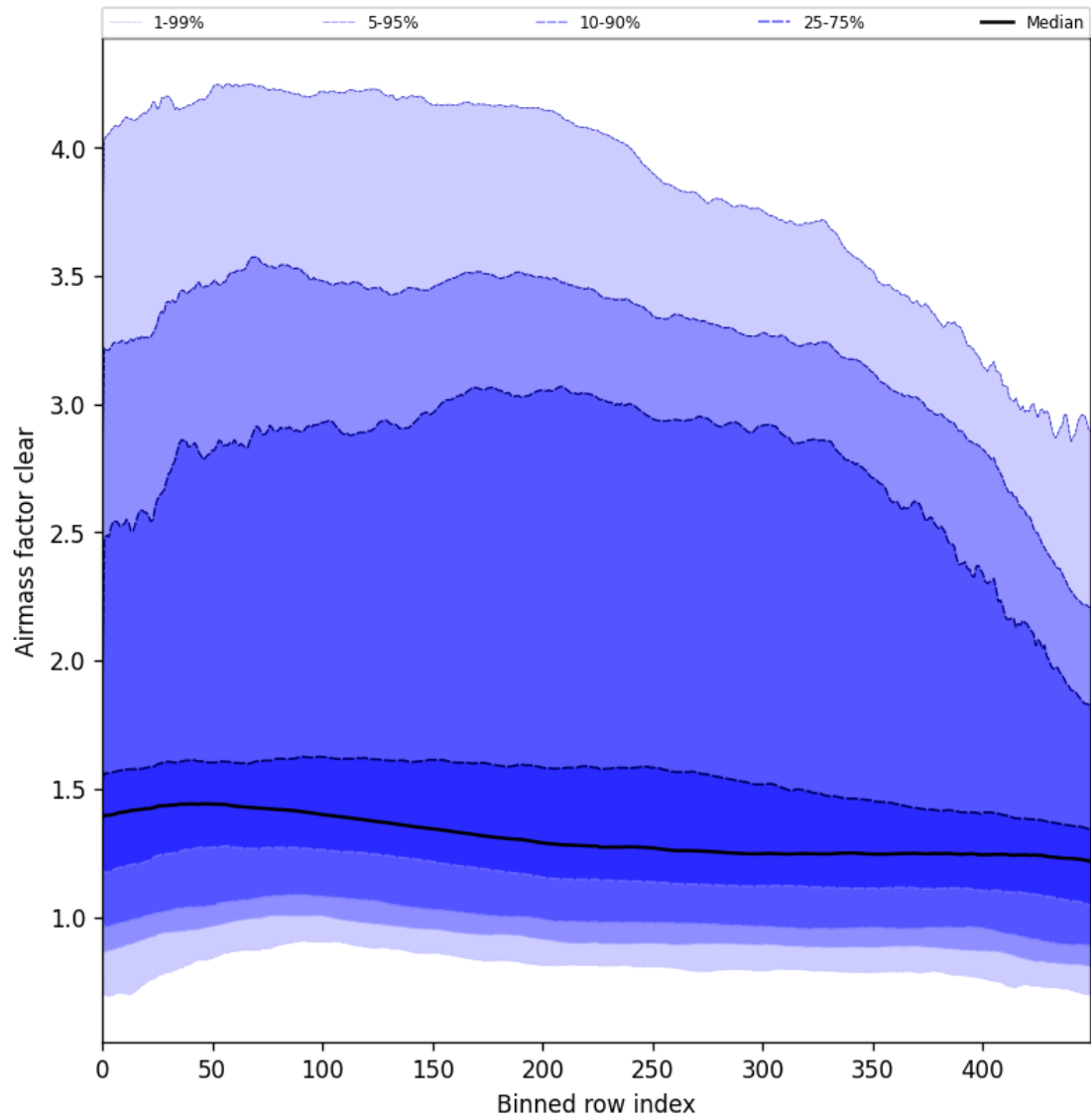
Figure 56: Along track statistics of “Air mass factor clear” for 2025-09-11 to 2025-09-13
