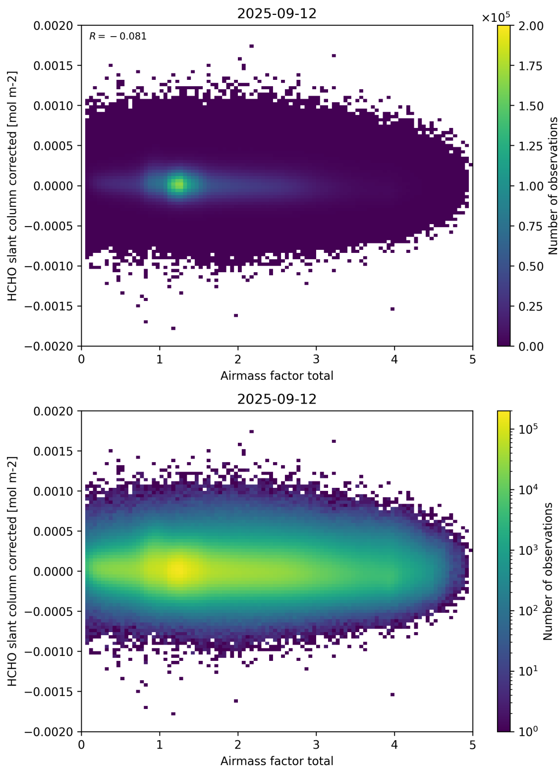
Figure 101: Scatter density plot of “Airmass factor total” against “HCHO slant column corrected” for 2025-09-11 to 2025-09-13.
