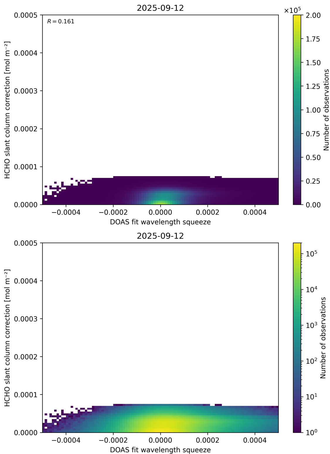
Figure 70: Scatter density plot of “DOAS fit wavelength squeeze” against “HCHO slant column correction” for 2025-09-11 to 2025-09-13.
