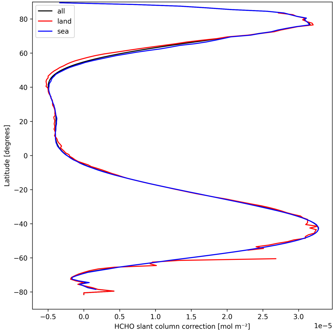
Figure 33: Zonal average of “HCHO slant column correction” for 2025-09-11 to 2025-09-13.
