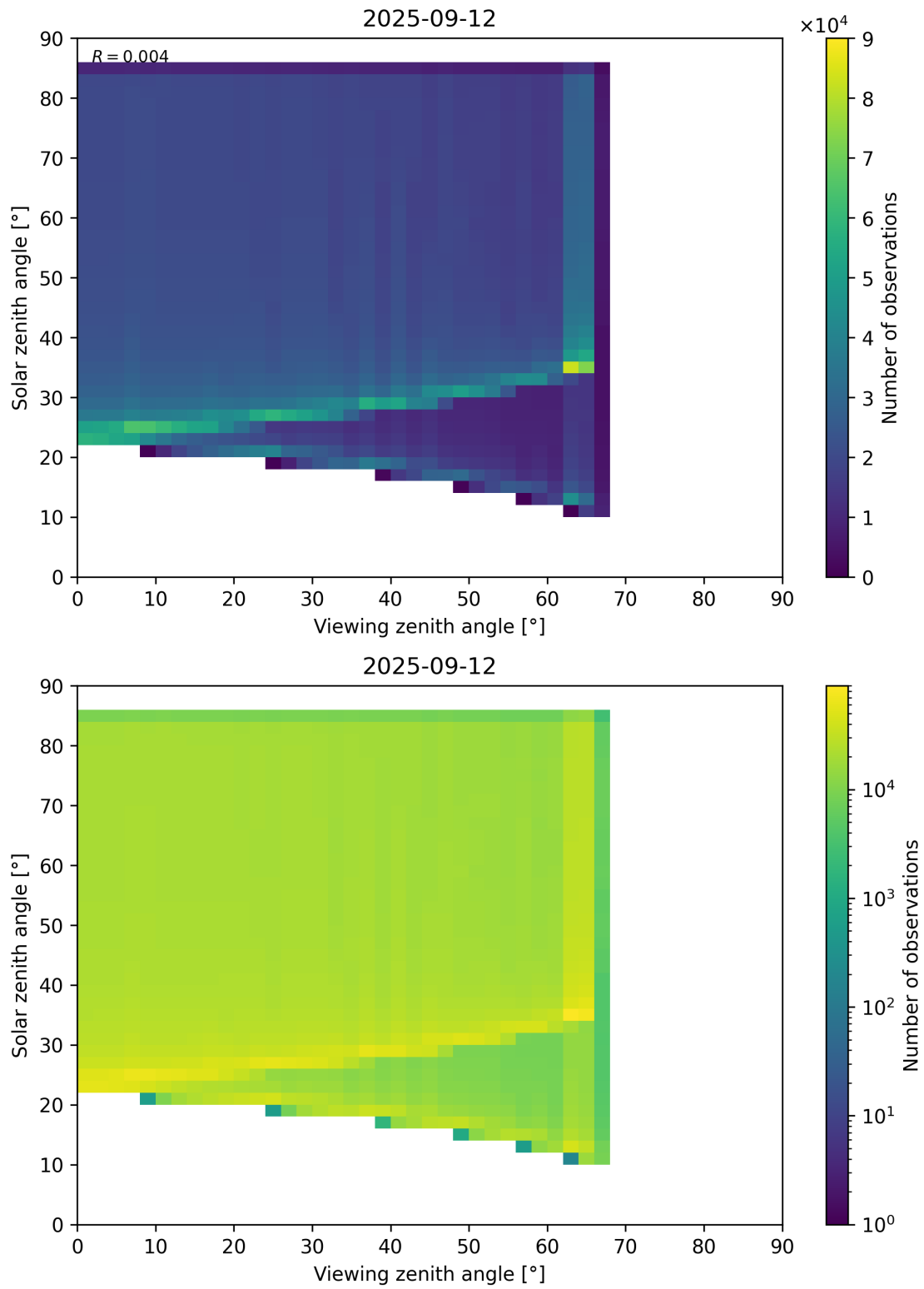
Figure 197: Scatter density plot of “Viewing zenith angle” against “Solar zenith angle” for 2025-09-11 to 2025-09-13.
