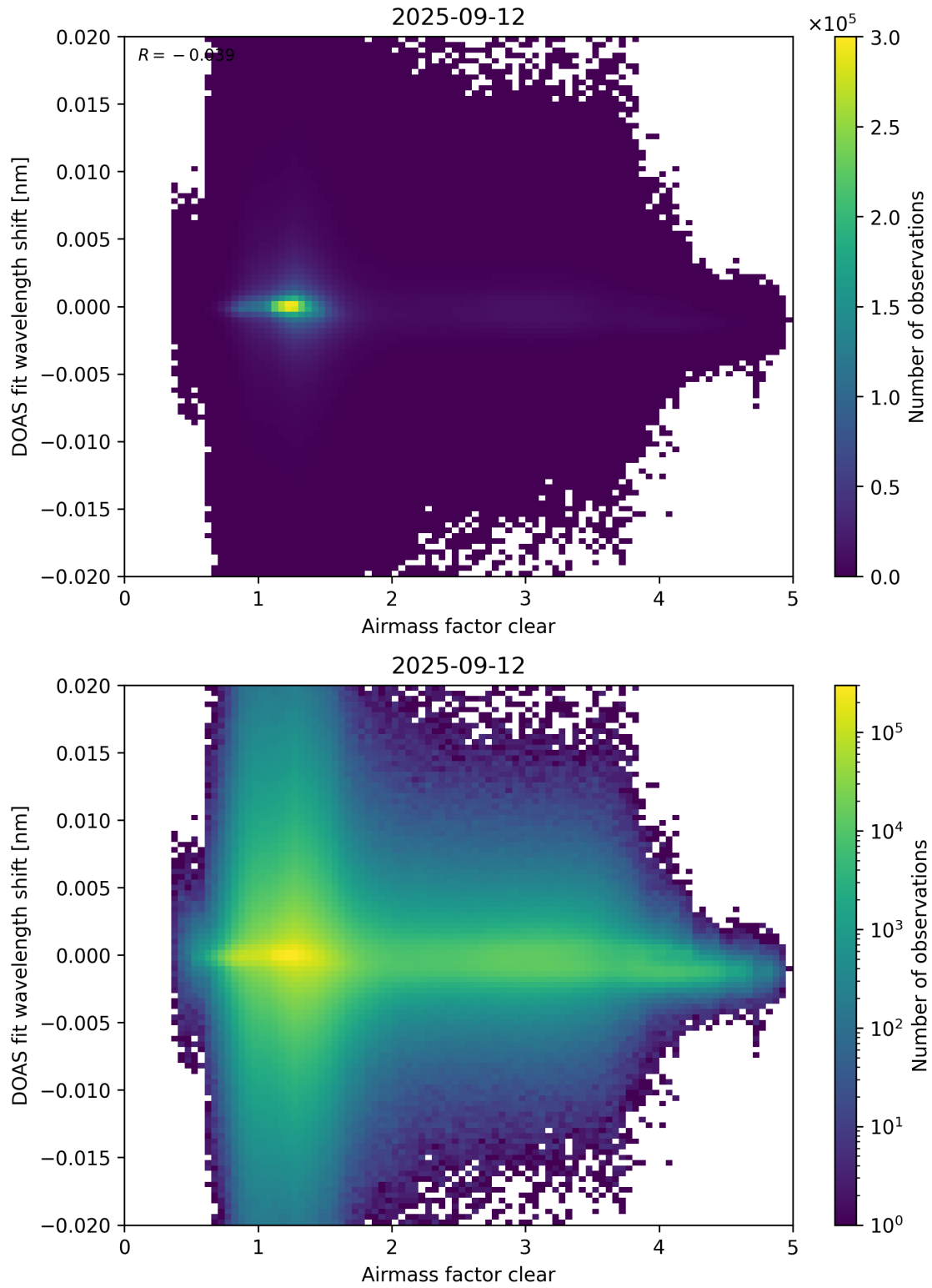
Figure 72: Scatter density plot of “Airmass factor clear” against “DOAS fit wavelength shift” for 2025-09-11 to 2025-09-13.
