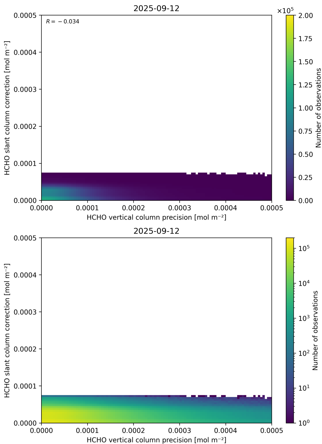
Figure 141: Scatter density plot of “HCHO vertical column precision” against “HCHO slant column correction” for 2025-09-11 to 2025-09-13.
