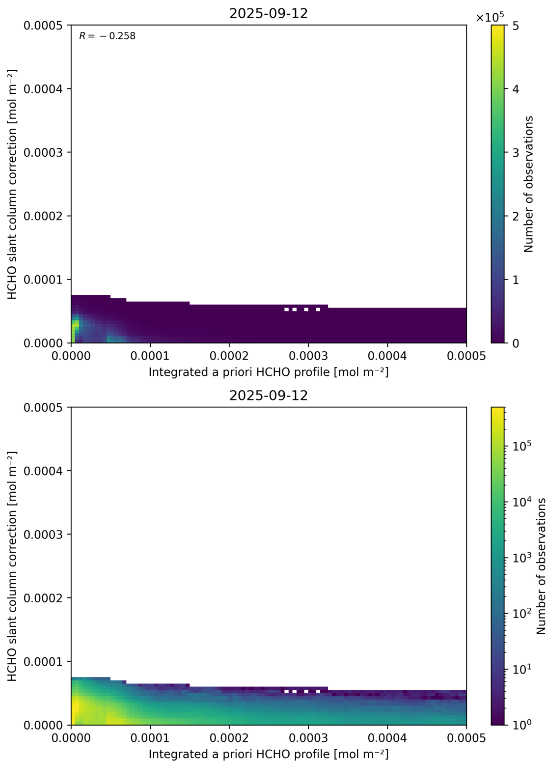
Figure 152: Scatter density plot of “Integrated a priori HCHO profile” against “HCHO slant column correction” for 2025-09-11 to 2025-09-13.
