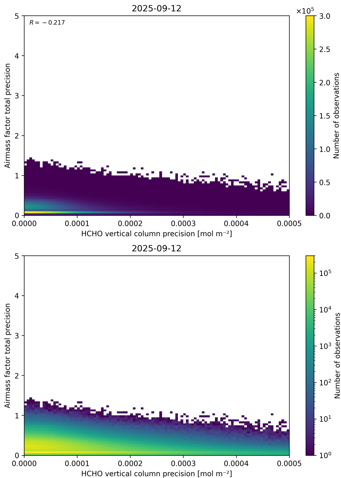
Figure 145: Scatter density plot of “HCHO vertical column precision” against “Airmass factor total precision” for 2025-09-11 to 2025-09-13.
