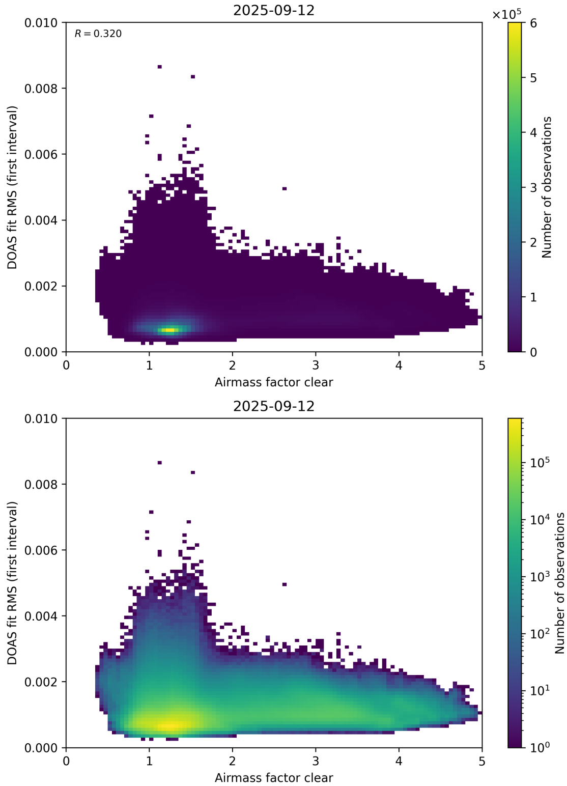
Figure 71: Scatter density plot of “Airmass factor clear” against “DOAS fit RMS (first interval)” for 2025-09-11 to 2025-09-13.
