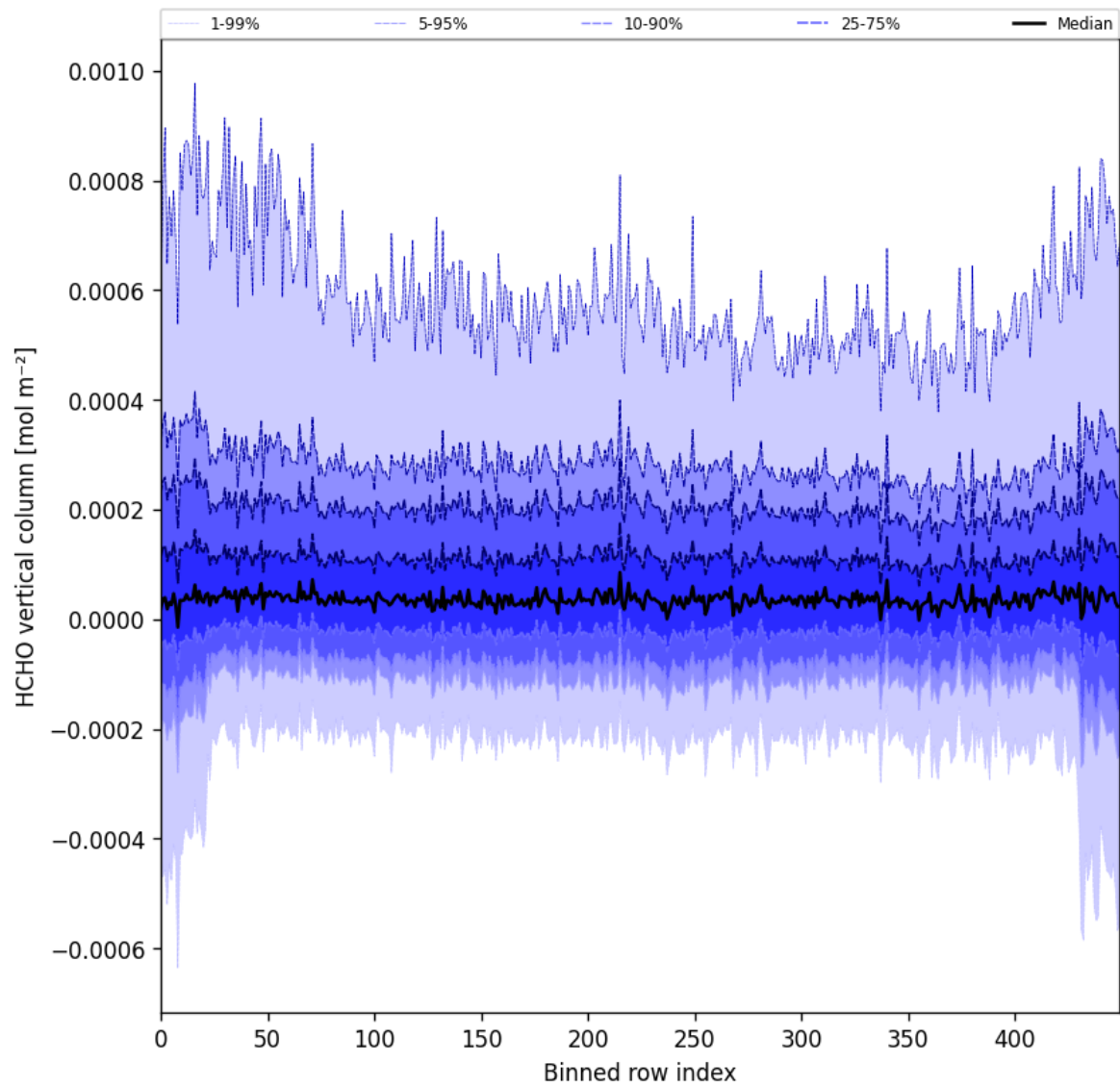
Figure 49: Along track statistics of “HCHO vertical column” for 2025-09-11 to 2025-09-13
