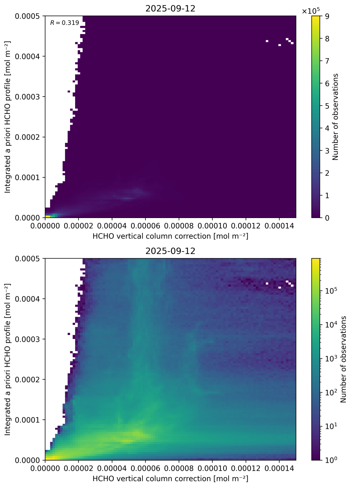
Figure 122: Scatter density plot of “HCHO vertical column correction” against “Integrated a priori HCHO profile” for 2025-09-11 to 2025-09-13.
