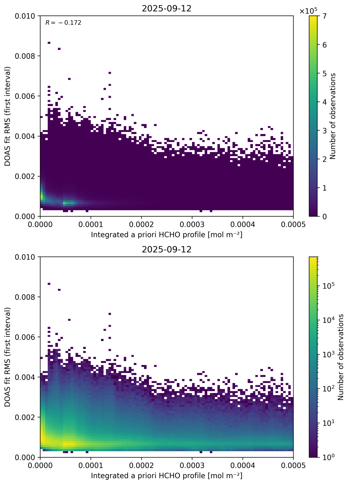
Figure 148: Scatter density plot of “Integrated a priori HCHO profile” against “DOAS fit RMS (first interval)” for 2025-09-11 to 2025-09-13.
