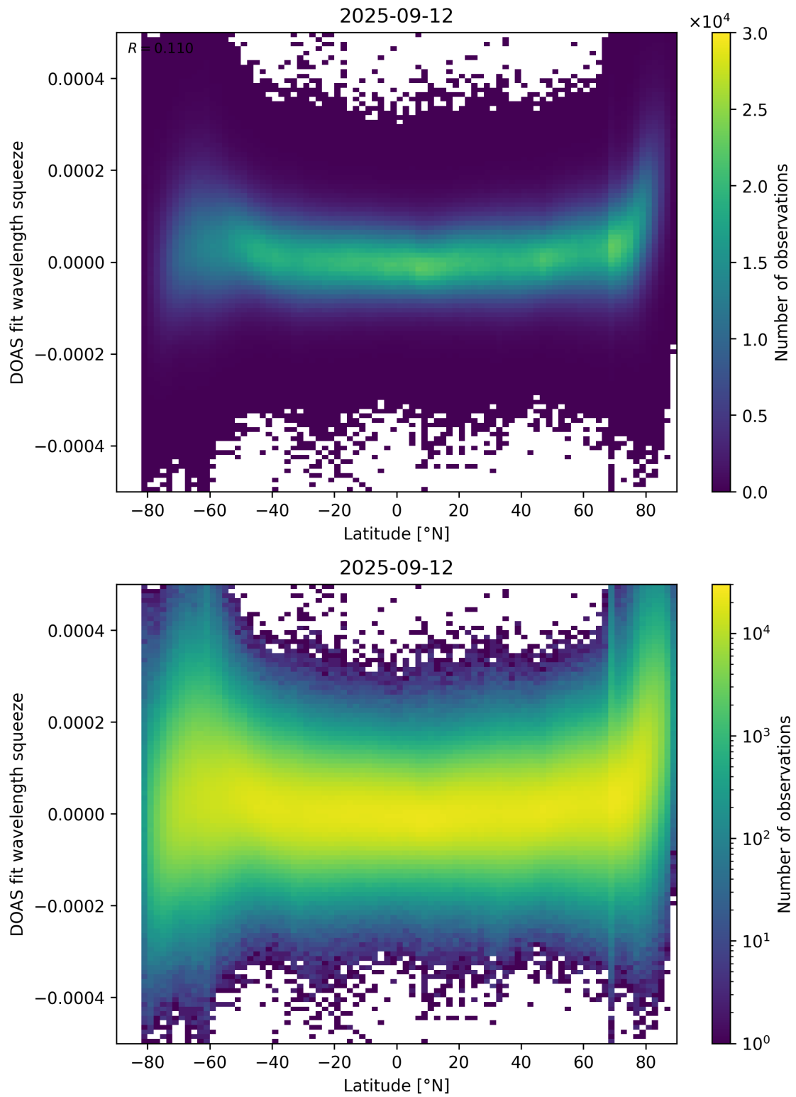
Figure 155: Scatter density plot of “Latitude” against “DOAS fit wavelength squeeze” for 2025-09-11 to 2025-09-13.
