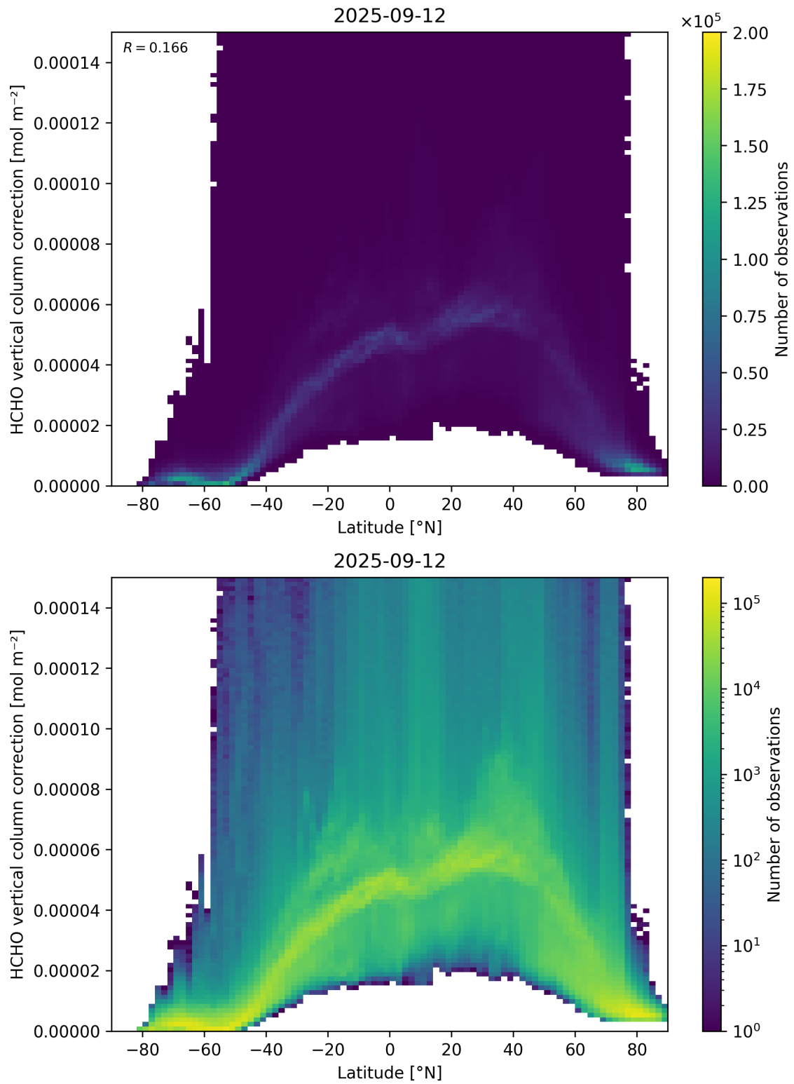
Figure 164: Scatter density plot of “Latitude” against “HCHO vertical column correction” for 2025-09-11 to 2025-09-13.
