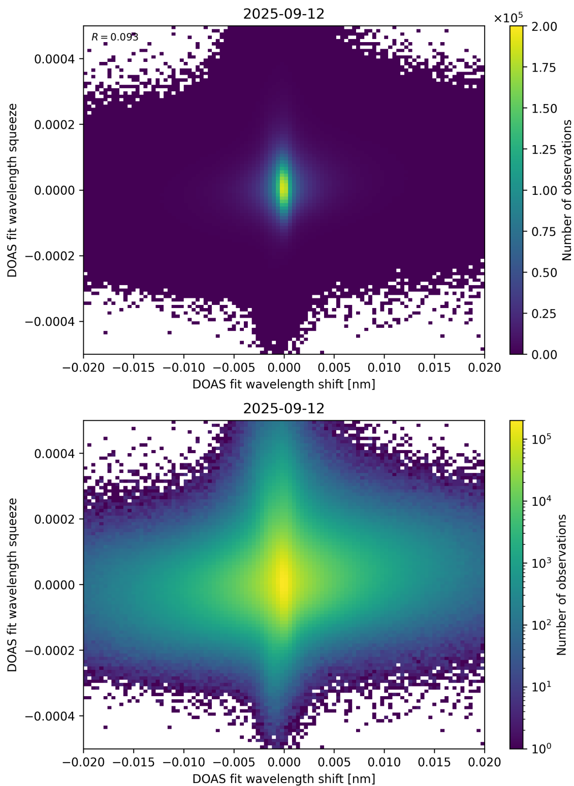
Figure 65: Scatter density plot of “DOAS fit wavelength shift” against “DOAS fit wavelength squeeze” for 2025-09-11 to 2025-09-13.
