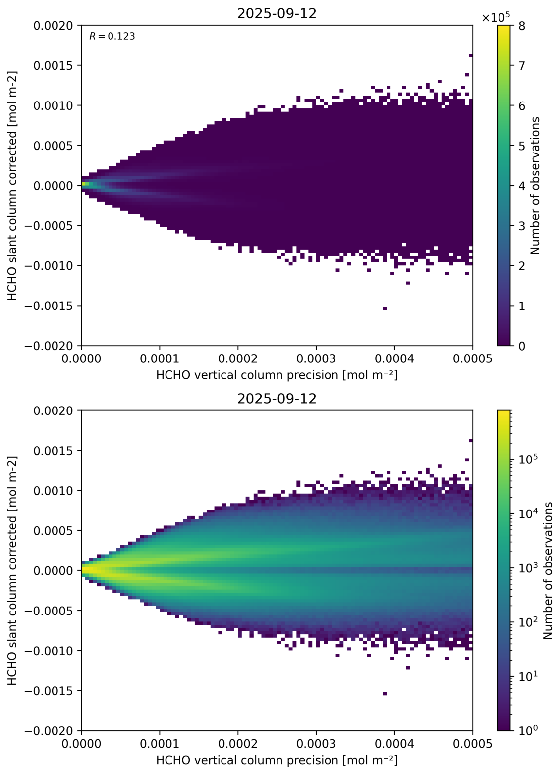
Figure 140: Scatter density plot of “HCHO vertical column precision” against “HCHO slant column corrected” for 2025-09-11 to 2025-09-13.
