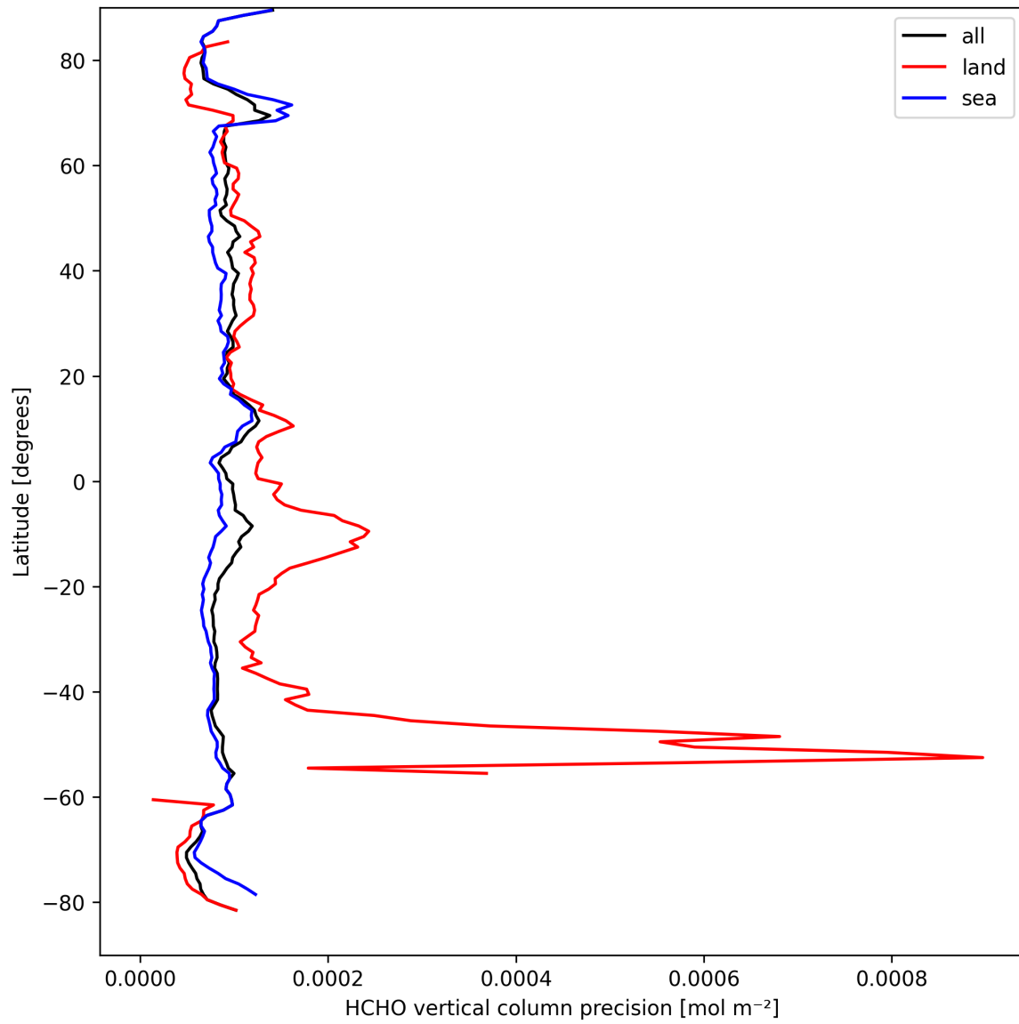
Figure 22: Zonal average of “HCHO vertical column precision” for 2025-09-11 to 2025-09-13.
