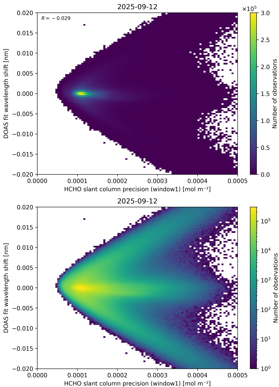
Figure 89: Scatter density plot of “HCHO slant column precision (window1)” against “DOAS fit wavelength shift” for 2025-09-11 to 2025-09-13.
