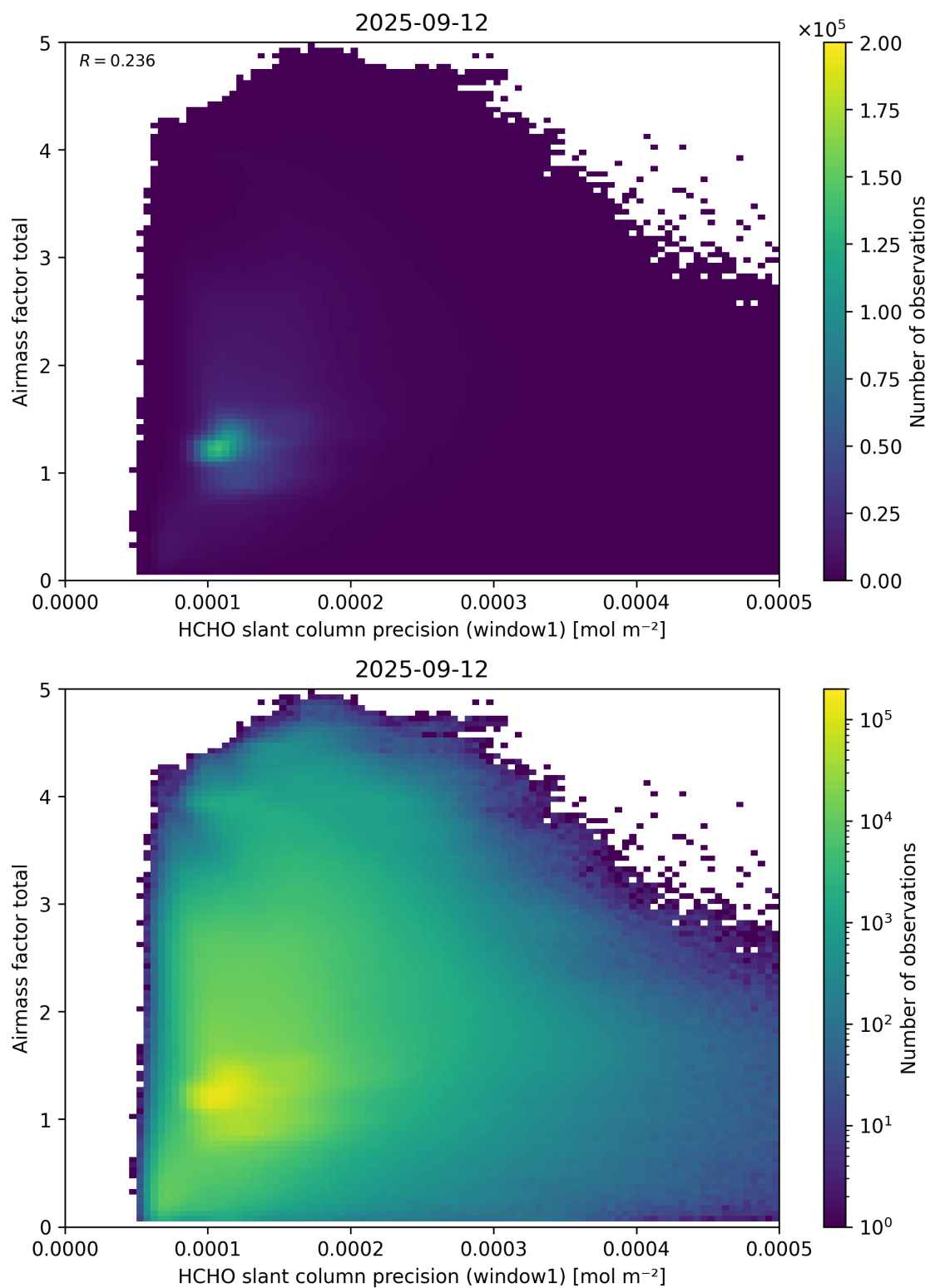
Figure 94: Scatter density plot of “HCHO slant column precision (window1)” against “Airmass factor total” for 2025-09-11 to 2025-09-13.
