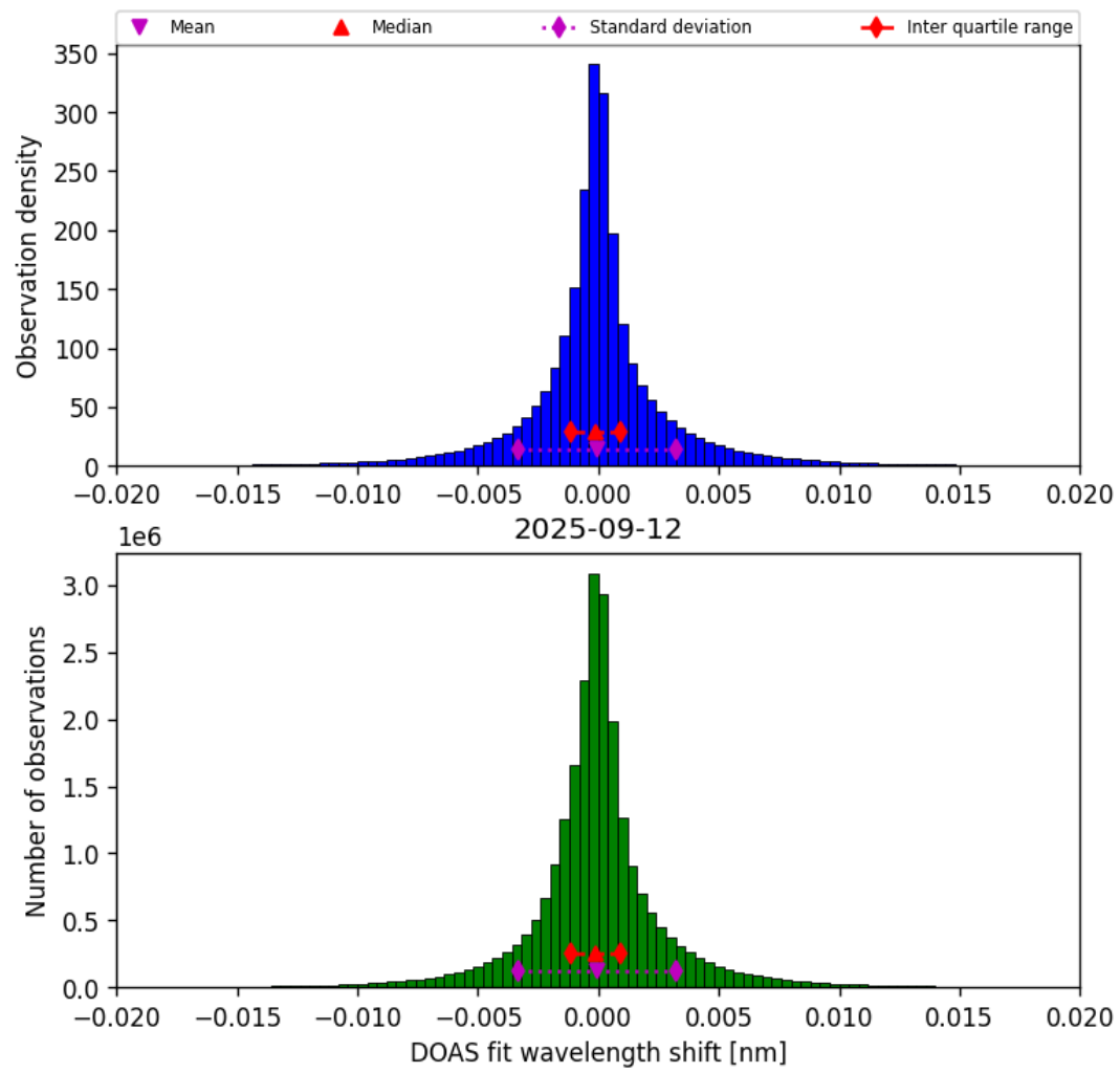
Figure 44: Histogram of “DOAS fit wavelength shift” for 2025-09-11 to 2025-09-13
