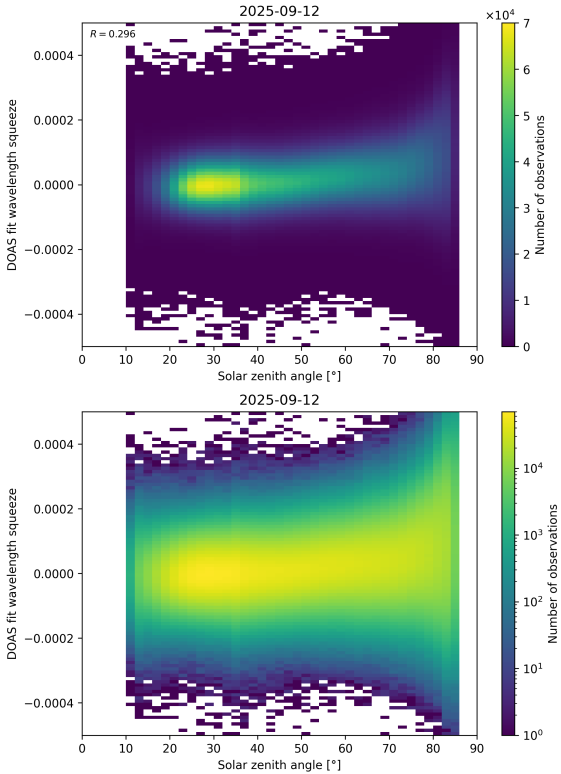
Figure 169: Scatter density plot of “Solar zenith angle” against “DOAS fit wavelength squeeze” for 2025-09-11 to 2025-09-13.
