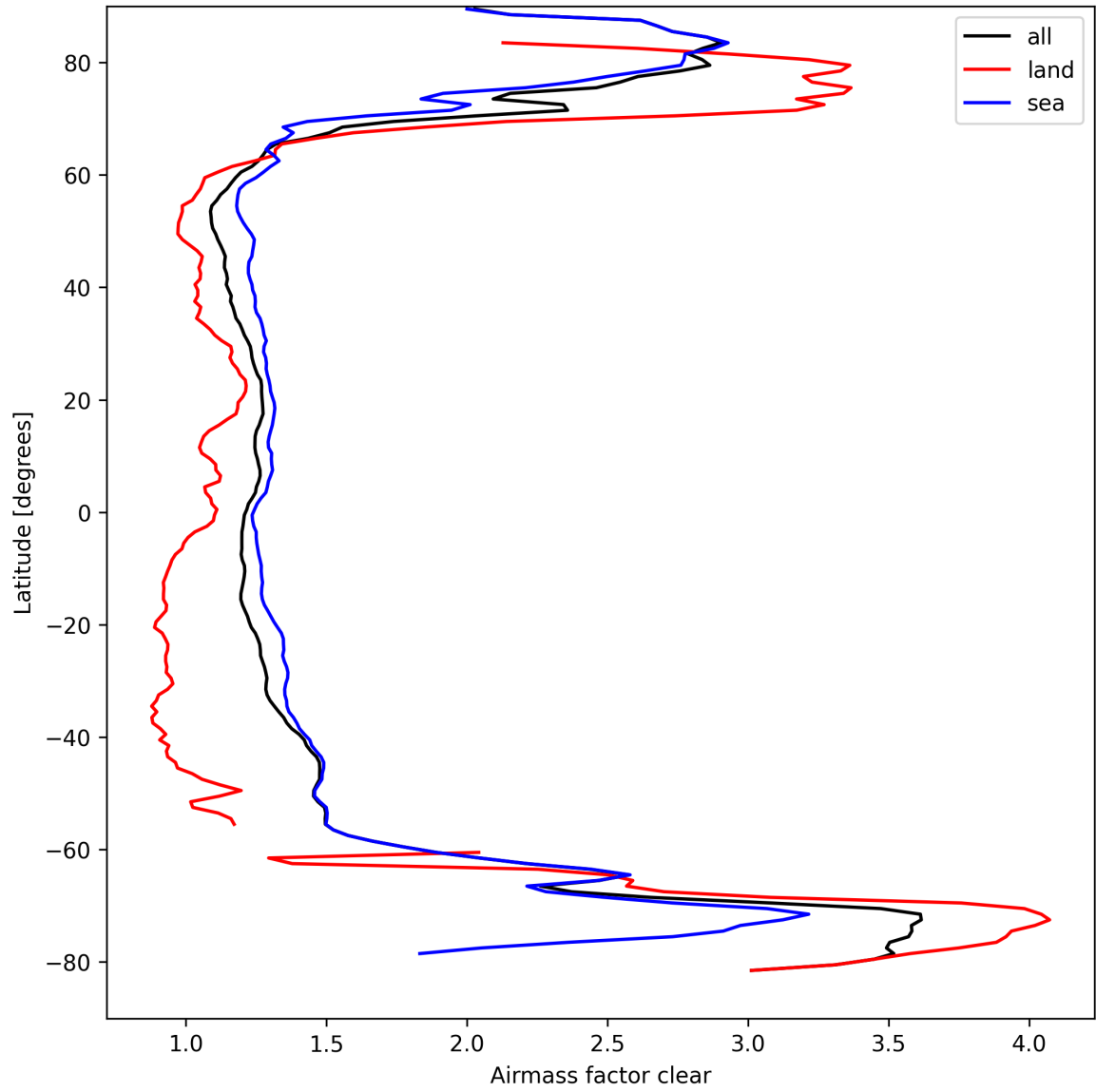
Figure 28: Zonal average of “Airmass factor clear” for 2025-09-11 to 2025-09-13.
