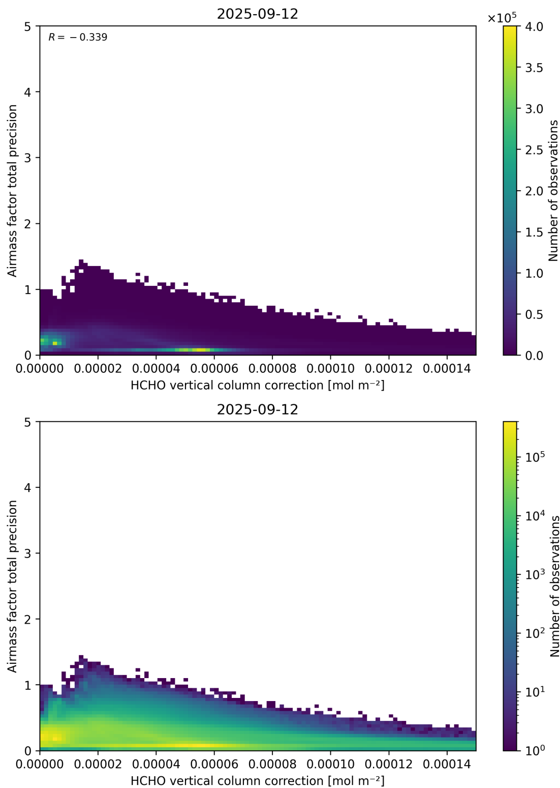
Figure 121: Scatter density plot of “HCHO vertical column correction” against “Airmass factor total precision” for 2025-09-11 to 2025-09-13.
