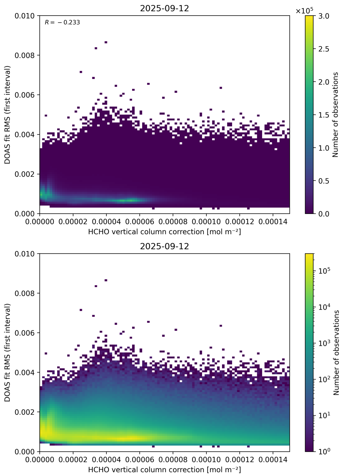
Figure 112: Scatter density plot of “HCHO vertical column correction” against “DOAS fit RMS (first interval)” for 2025-09-11 to 2025-09-13.
