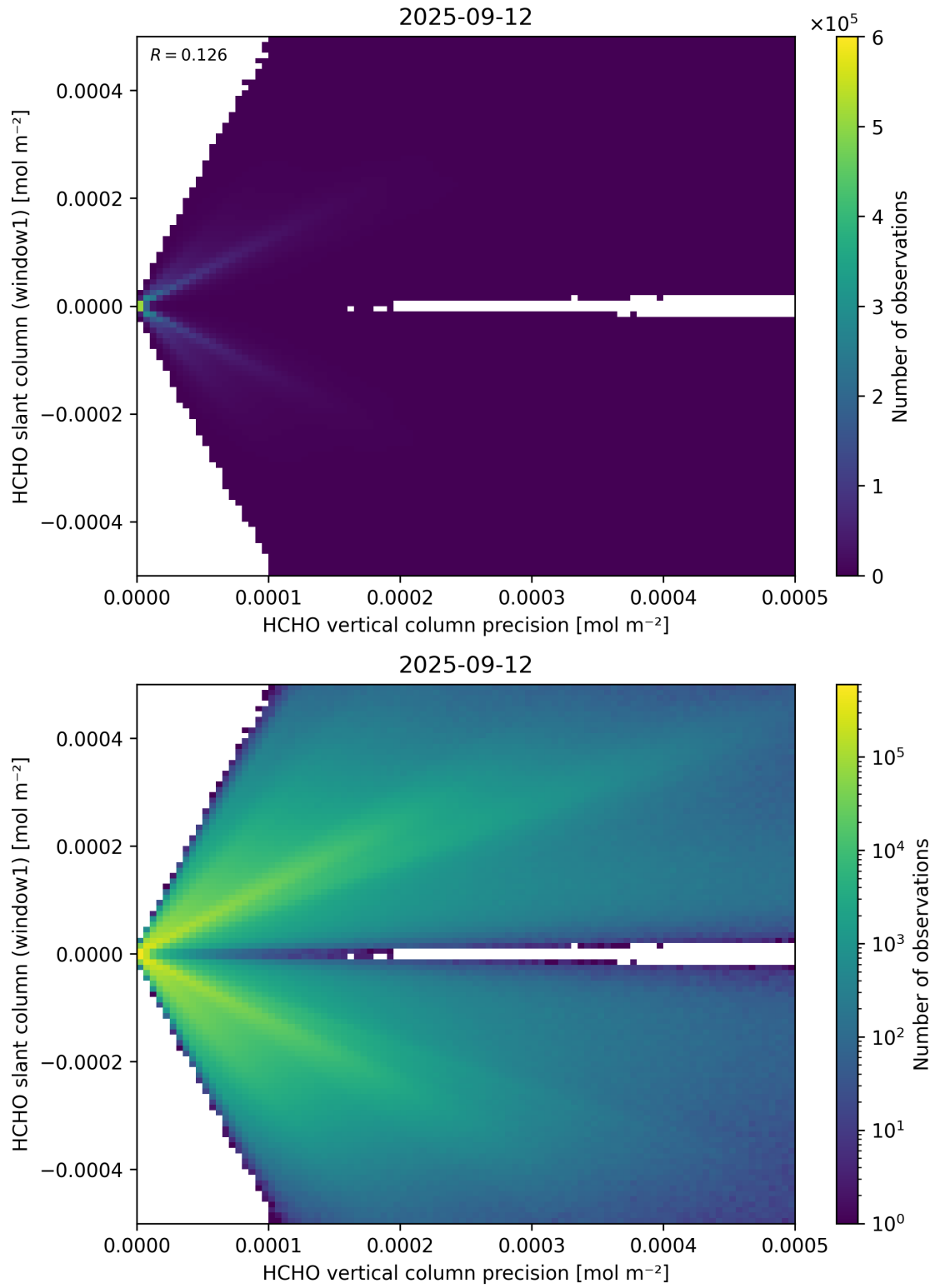
Figure 142: Scatter density plot of “HCHO vertical column precision” against “HCHO slant column (window1)” for 2025-09-11 to 2025-09-13.
