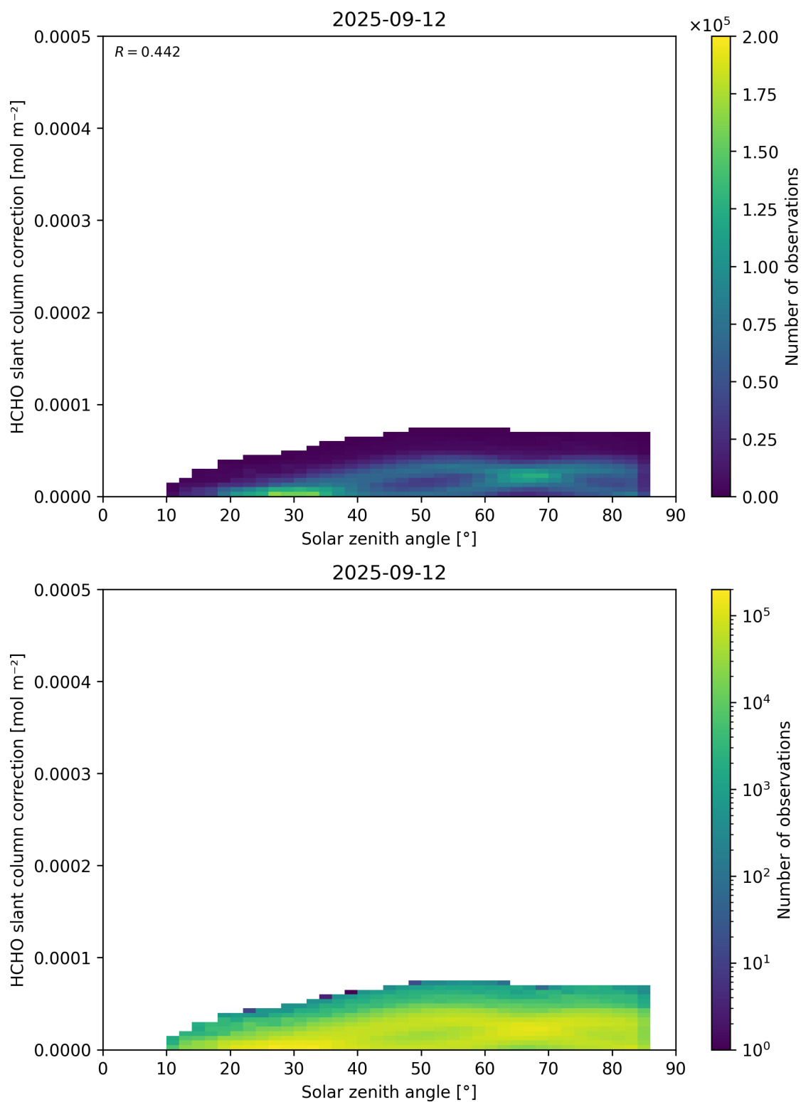
Figure 172: Scatter density plot of “Solar zenith angle” against “HCHO slant column correction” for 2025-09-11 to 2025-09-13.
