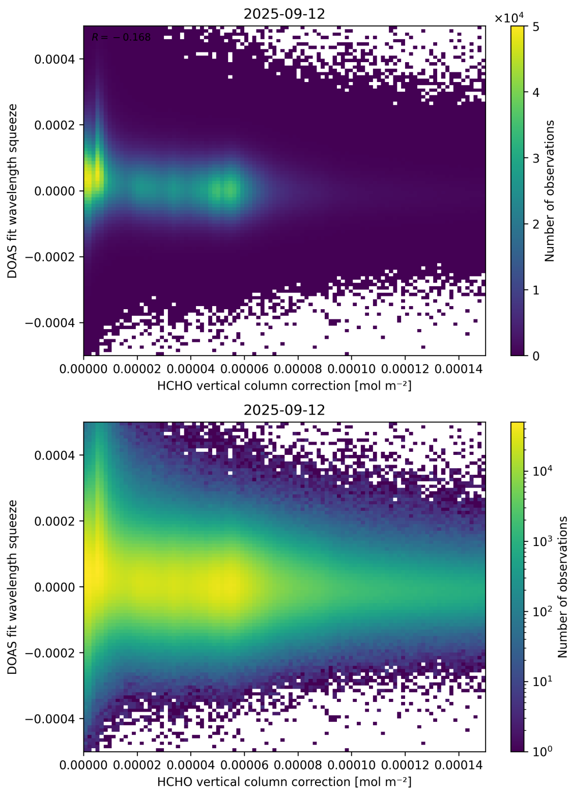
Figure 114: Scatter density plot of “HCHO vertical column correction” against “DOAS fit wavelength squeeze” for 2025-09-11 to 2025-09-13.
