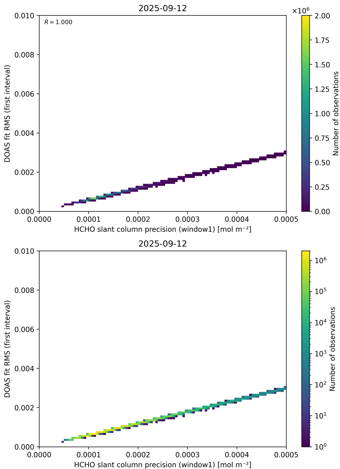
Figure 88: Scatter density plot of “HCHO slant column precision (window1)” against “DOAS fit RMS (first interval)” for 2025-09-11 to 2025-09-13.
