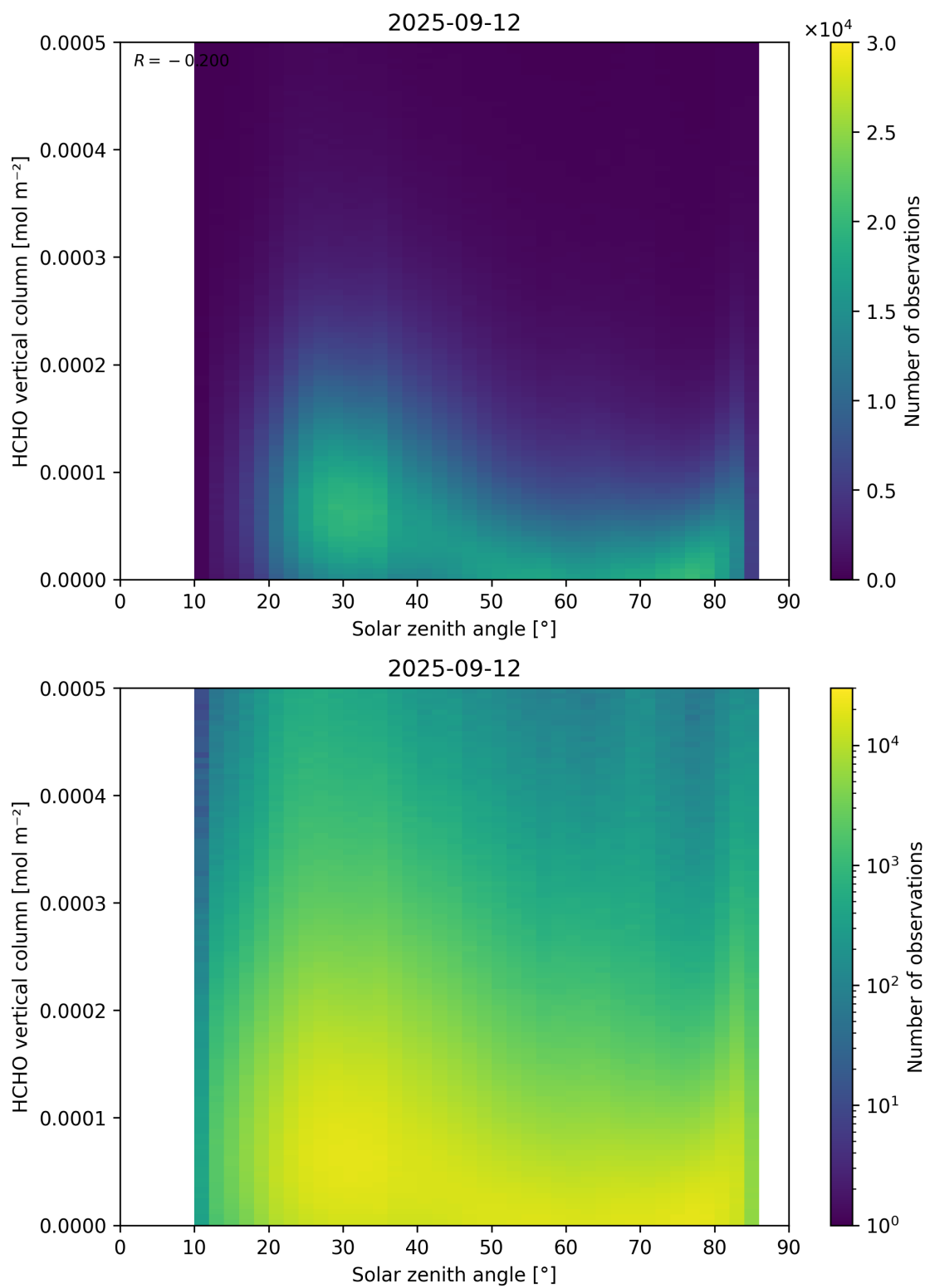
Figure 177: Scatter density plot of “Solar zenith angle” against “HCHO vertical column” for 2025-09-11 to 2025-09-13.
