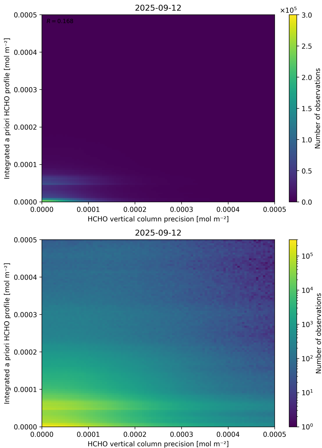
Figure 147: Scatter density plot of “HCHO vertical column precision” against “Integrated a priori HCHO profile” for 2025-09-11 to 2025-09-13.
