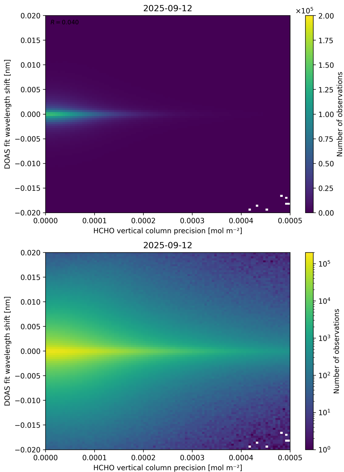
Figure 137: Scatter density plot of “HCHO vertical column precision” against “DOAS fit wavelength shift” for 2025-09-11 to 2025-09-13.
