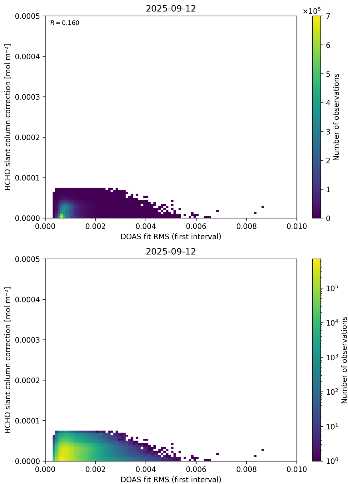
Figure 63: Scatter density plot of “DOAS fit RMS (first interval)” against “HCHO slant column correction” for 2025-09-11 to 2025-09-13.
