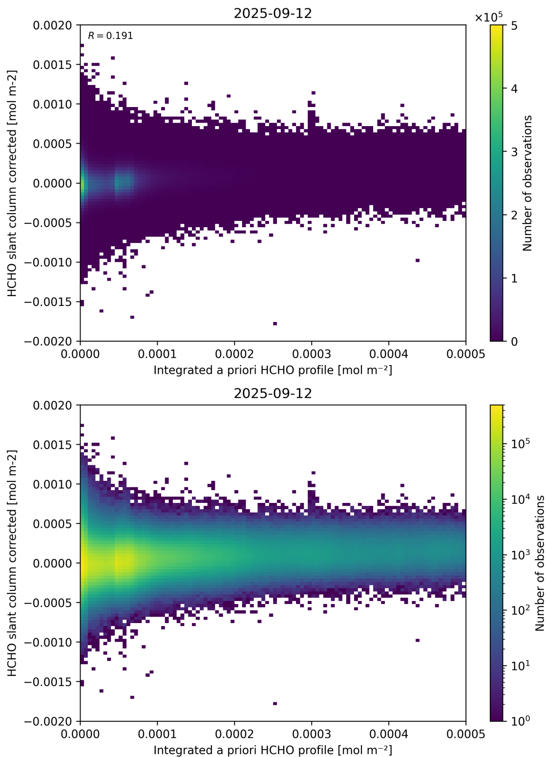
Figure 151: Scatter density plot of “Integrated a priori HCHO profile” against “HCHO slant column corrected” for 2025-09-11 to 2025-09-13.
