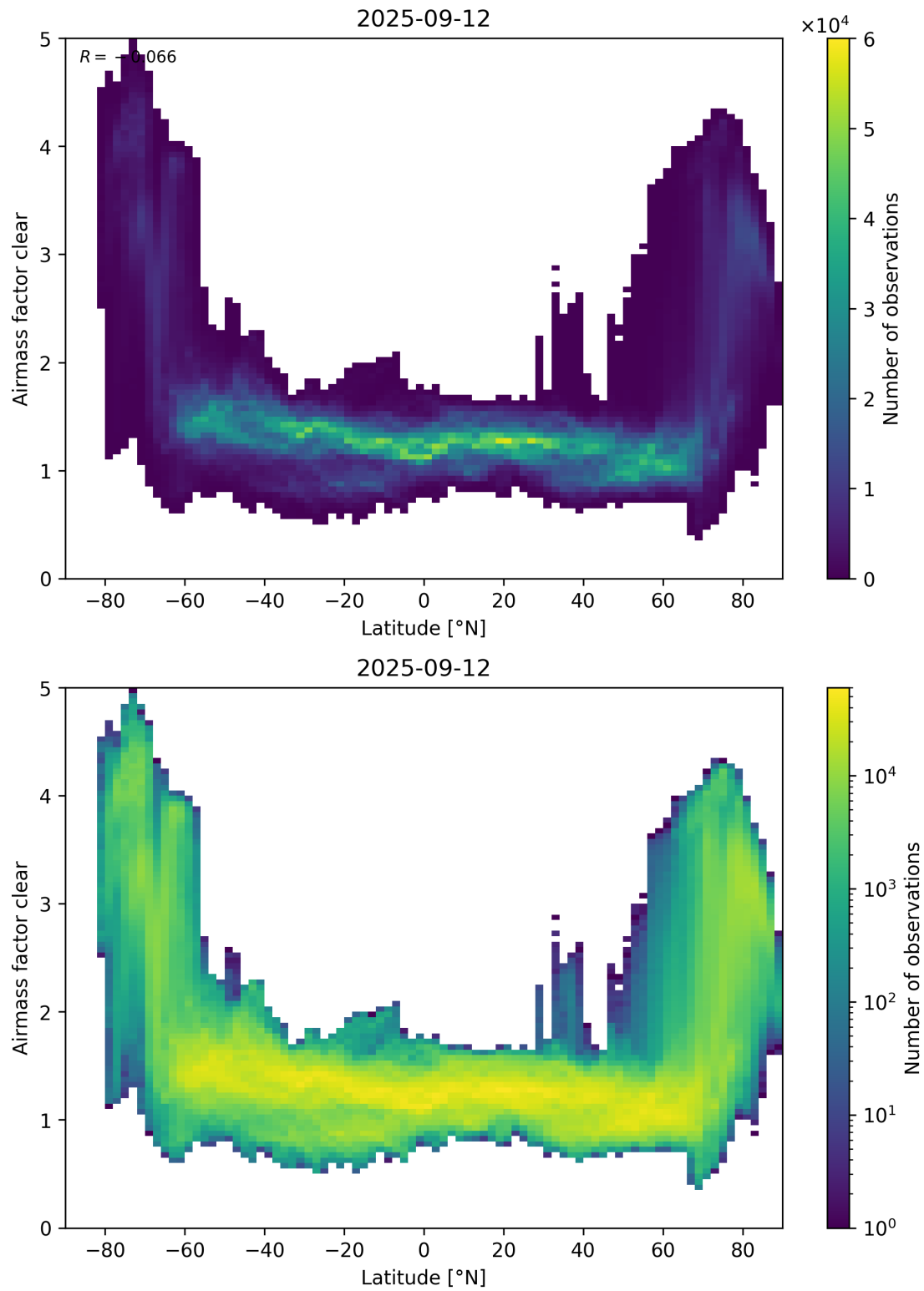
Figure 156: Scatter density plot of “Latitude” against “Airmass factor clear” for 2025-09-11 to 2025-09-13.
