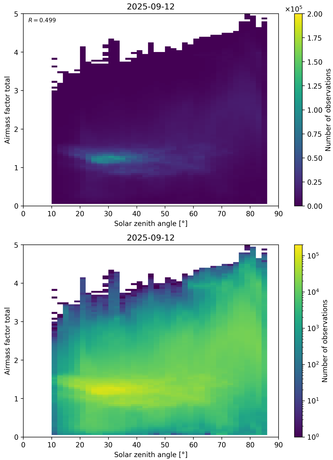
Figure 175: Scatter density plot of “Solar zenith angle” against “Airmass factor total” for 2025-09-11 to 2025-09-13.
