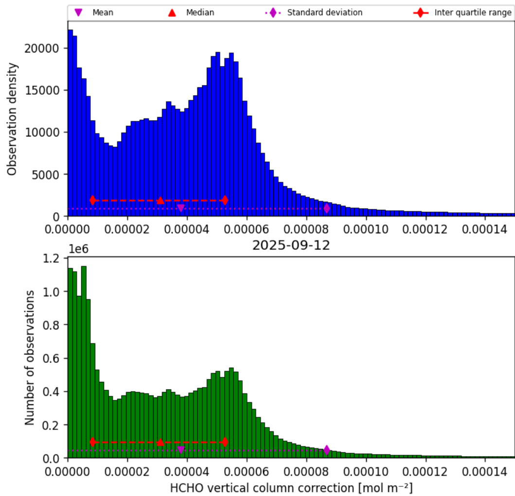
Figure 37: Histogram of “HCHO vertical column correction” for 2025-09-11 to 2025-09-13
