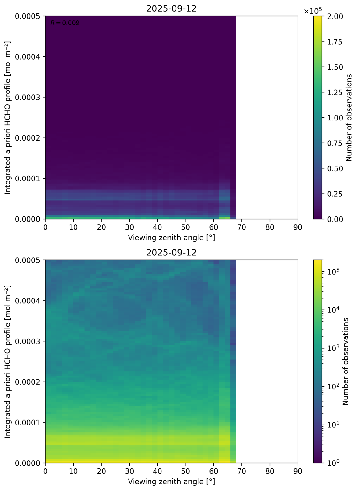
Figure 195: Scatter density plot of “Viewing zenith angle” against “Integrated a priori HCHO profile” for 2025-09-11 to 2025-09-13.
