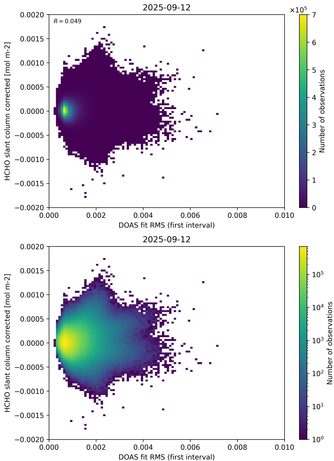
Figure 62: Scatter density plot of “DOAS fit RMS (first interval)” against “HCHO slant column corrected” for 2025-09-11 to 2025-09-13.
