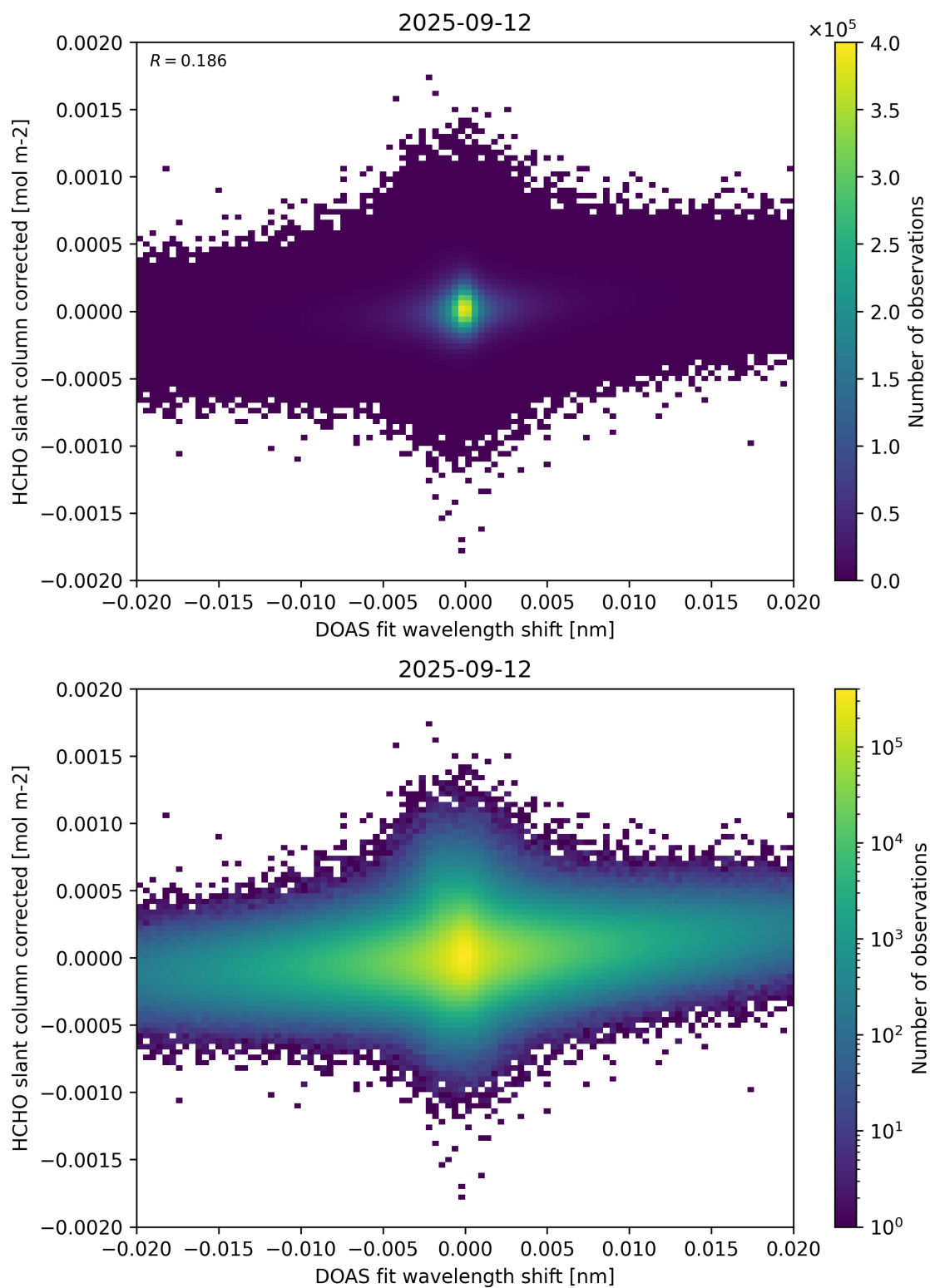
Figure 66: Scatter density plot of “DOAS fit wavelength shift” against “HCHO slant column corrected” for 2025-09-11 to 2025-09-13.
