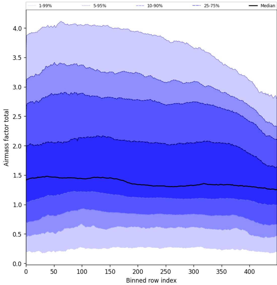
Figure 54: Along track statistics of “Airmass factor total” for 2025-09-11 to 2025-09-13
