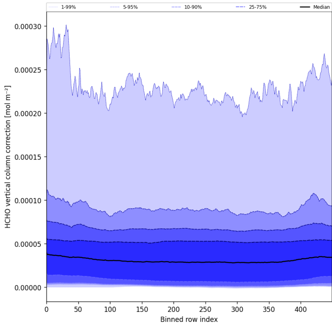
Figure 51: Along track statistics of “HCHO vertical column correction” for 2025-09-11 to 2025-09-13
