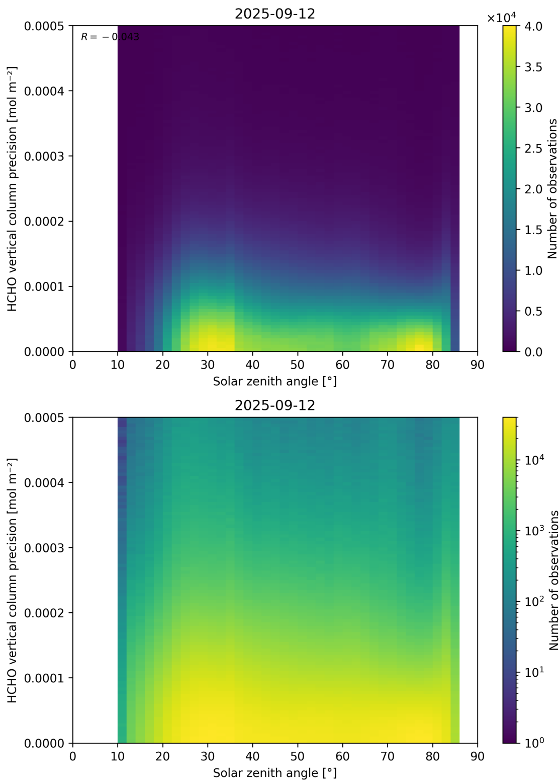
Figure 179: Scatter density plot of “Solar zenith angle” against “HCHO vertical column precision” for 2025-09-11 to 2025-09-13.
