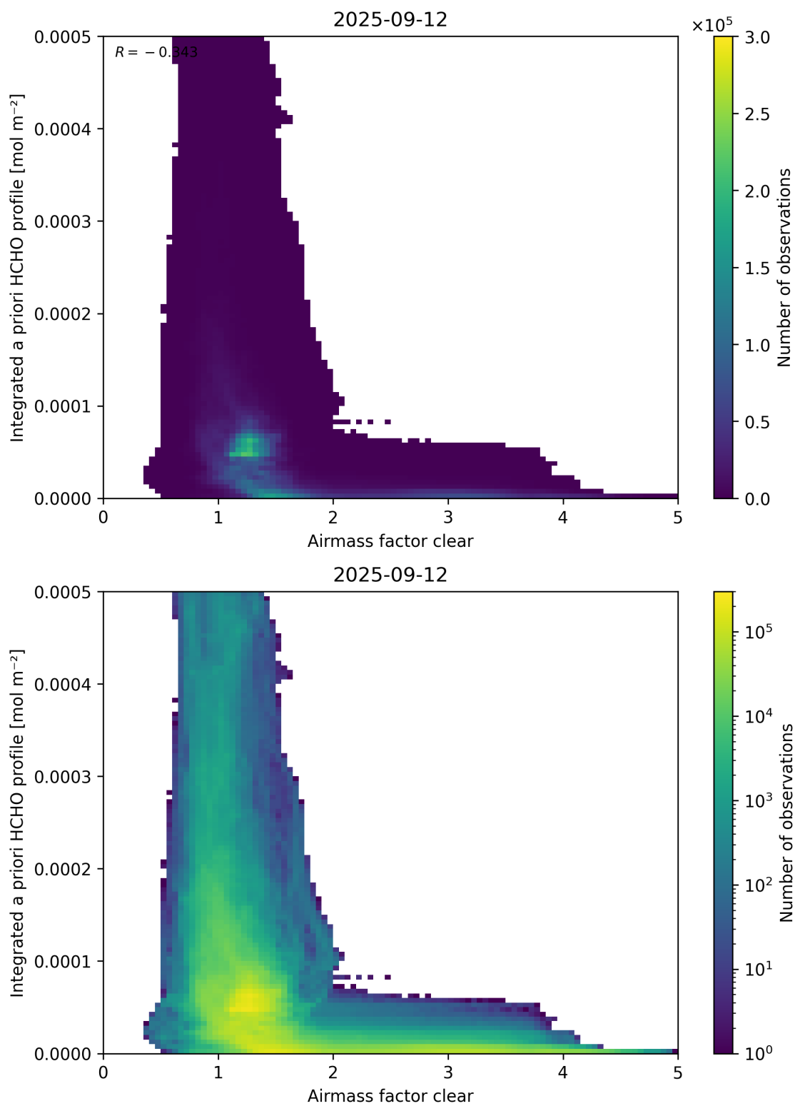
Figure 76: Scatter density plot of “Airmass factor clear” against “Integrated a priori HCHO profile” for 2025-09-11 to 2025-09-13.
