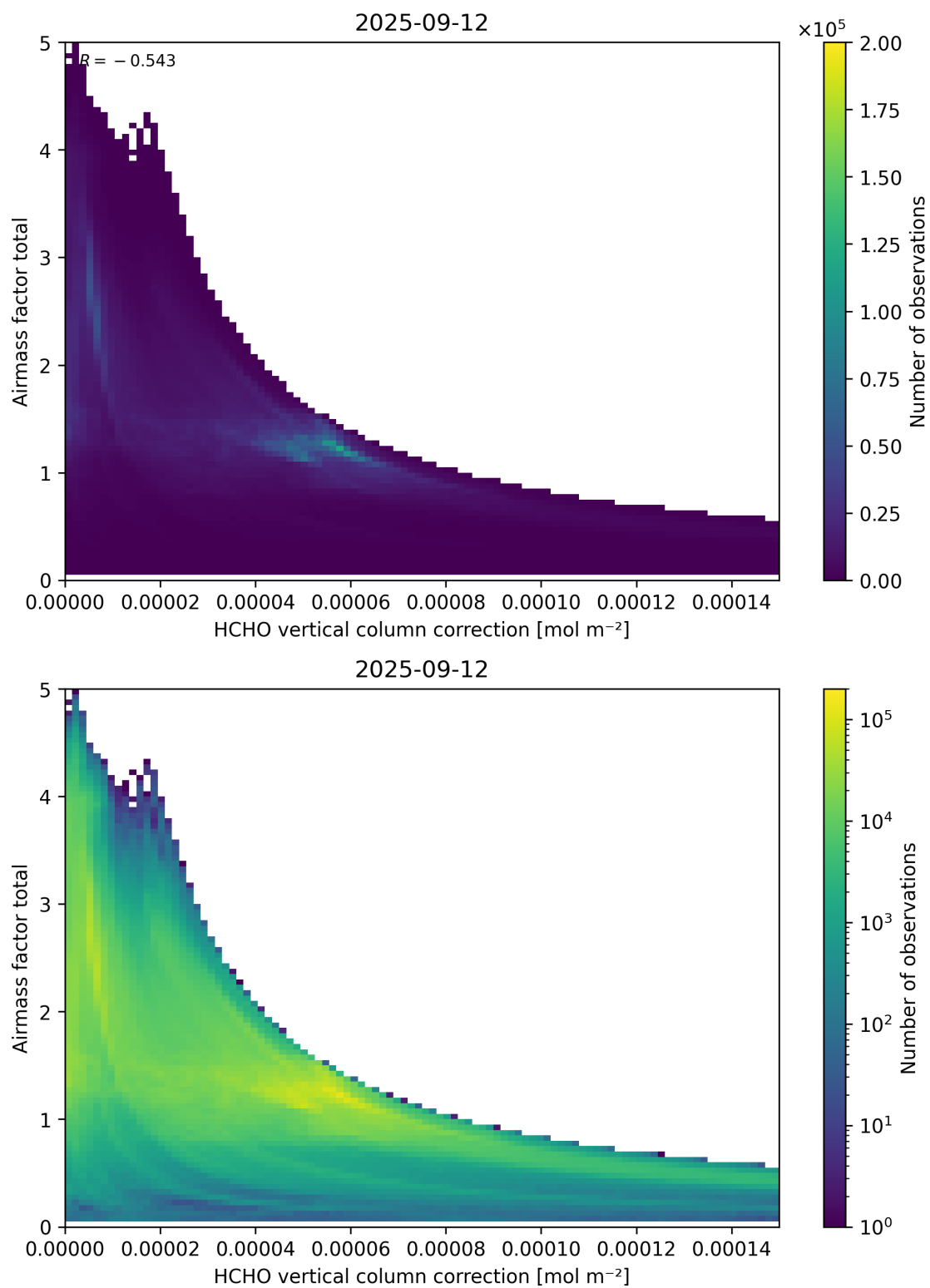
Figure 120: Scatter density plot of “HCHO vertical column correction” against “Airmass factor total” for 2025-09-11 to 2025-09-13.
