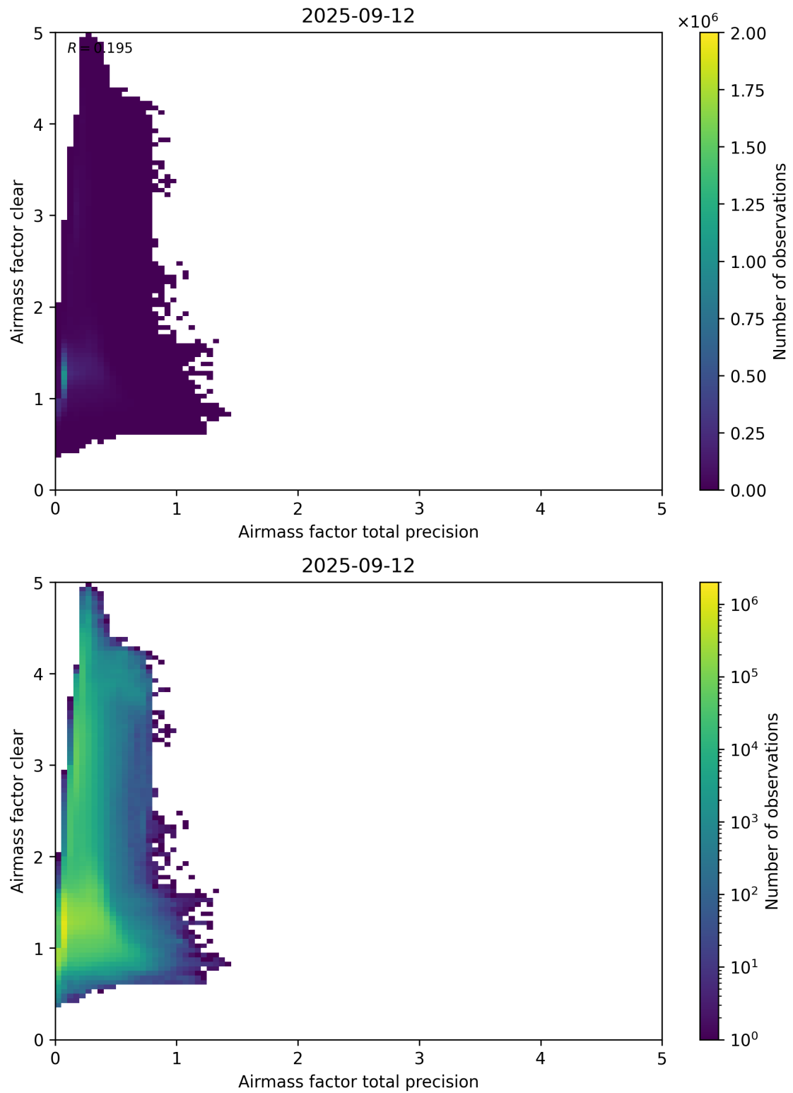
Figure 108: Scatter density plot of “Airmass factor total precision” against “Airmass factor clear” for 2025-09-11 to 2025-09-13.
