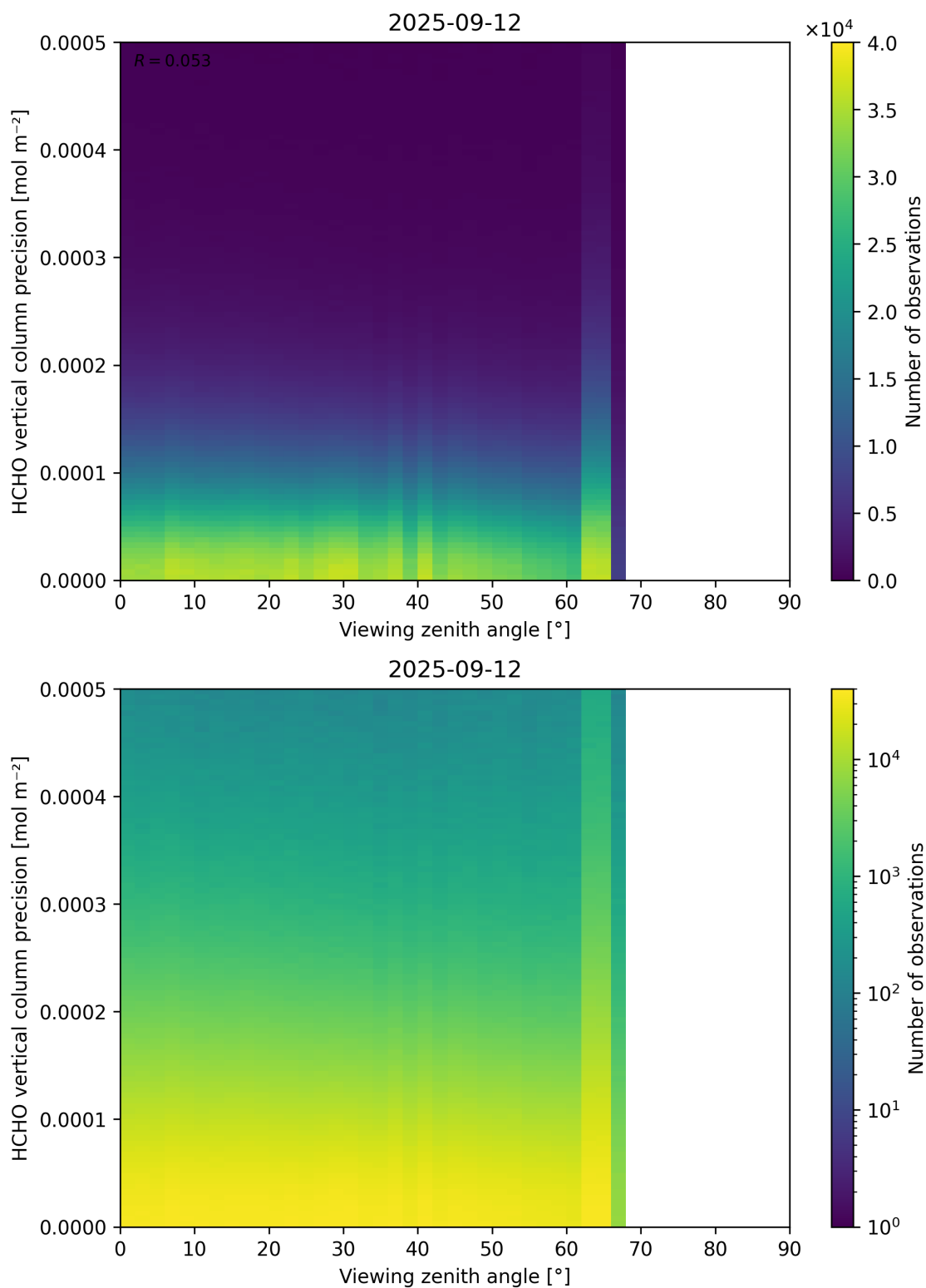
Figure 194: Scatter density plot of “Viewing zenith angle” against “HCHO vertical column precision” for 2025-09-11 to 2025-09-13.
