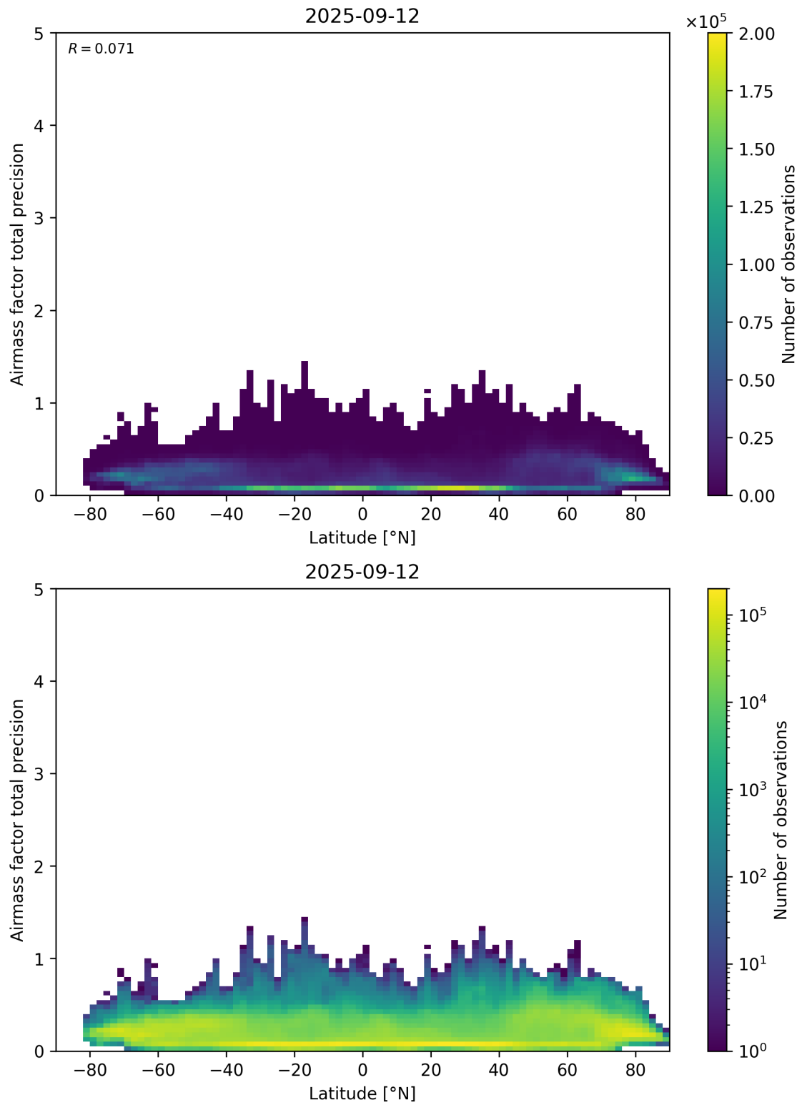
Figure 162: Scatter density plot of “Latitude” against “Airmass factor total precision” for 2025-09-11 to 2025-09-13.
