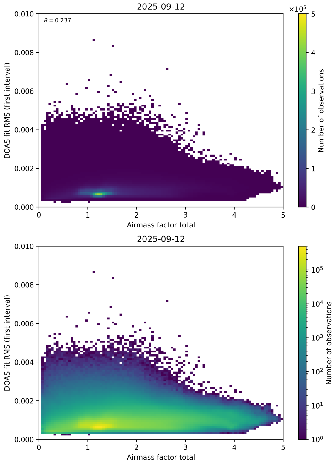
Figure 97: Scatter density plot of “Airmass factor total” against “DOAS fit RMS (first interval)” for 2025-09-11 to 2025-09-13.
