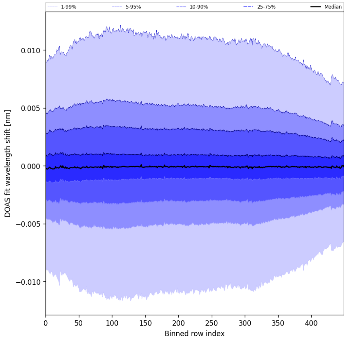
Figure 58: Along track statistics of “DOAS fit wavelength shift” for 2025-09-11 to 2025-09-13
