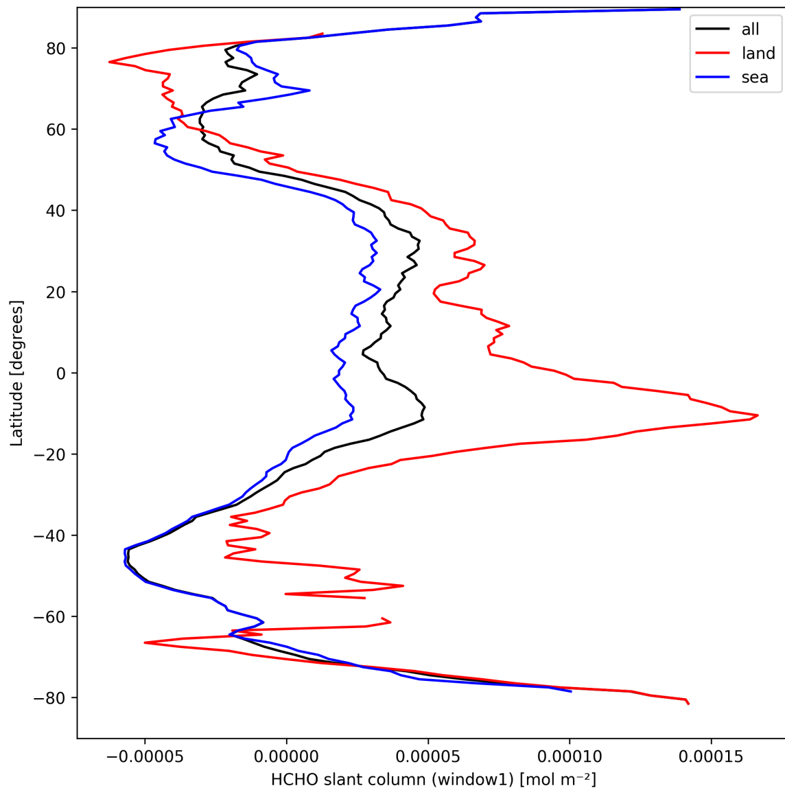
Figure 24: Zonal average of “HCHO slant column (window1)” for 2025-09-11 to 2025-09-13.
