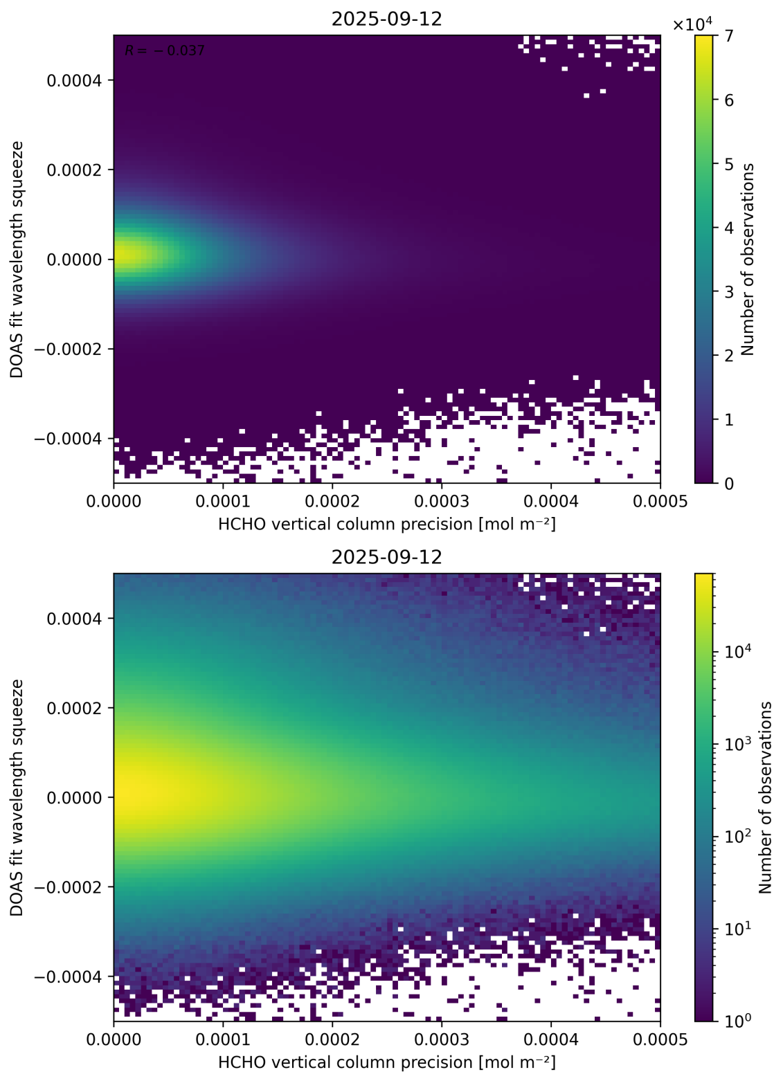
Figure 138: Scatter density plot of “HCHO vertical column precision” against “DOAS fit wavelength squeeze” for 2025-09-11 to 2025-09-13.
