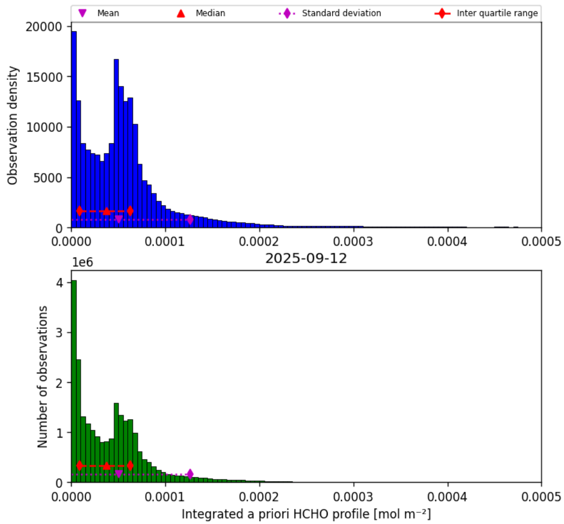
Figure 43: Histogram of “Integrated a priori HCHO profile” for 2025-09-11 to 2025-09-13
