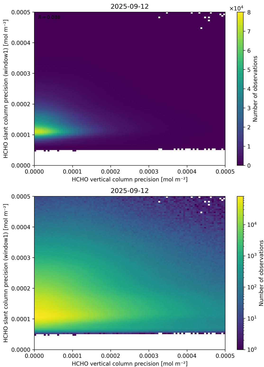
Figure 143: Scatter density plot of “HCHO vertical column precision” against “HCHO slant column precision (window1)” for 2025-09-11 to 2025-09-13.
