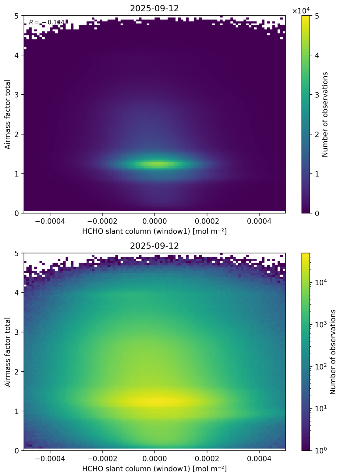
Figure 85: Scatter density plot of “HCHO slant column (window1)” against “Airmass factor total” for 2025-09-11 to 2025-09-13.
