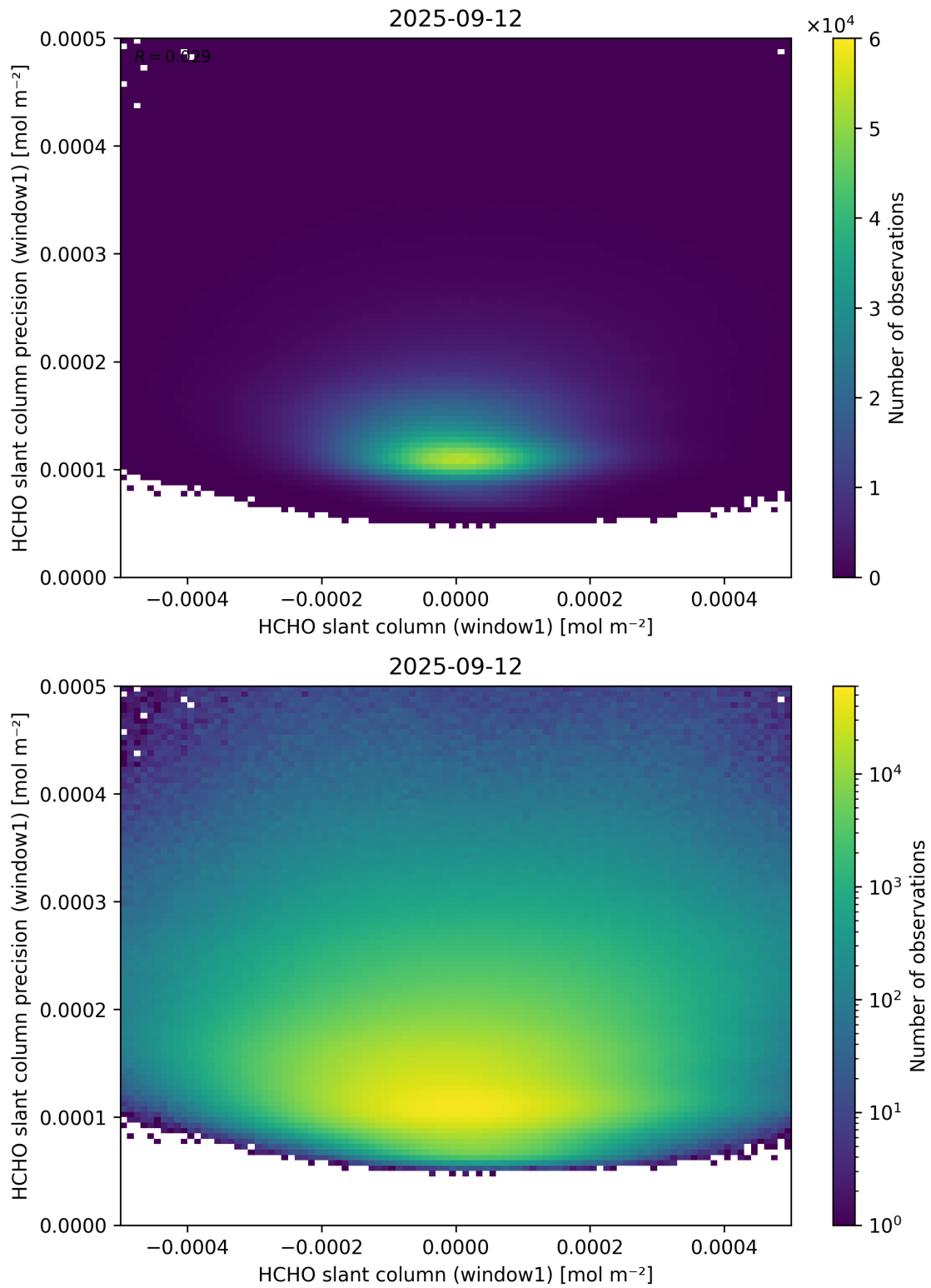
Figure 84: Scatter density plot of “HCHO slant column (window1)” against “HCHO slant column precision (window1)” for 2025-09-11 to 2025-09-13.
