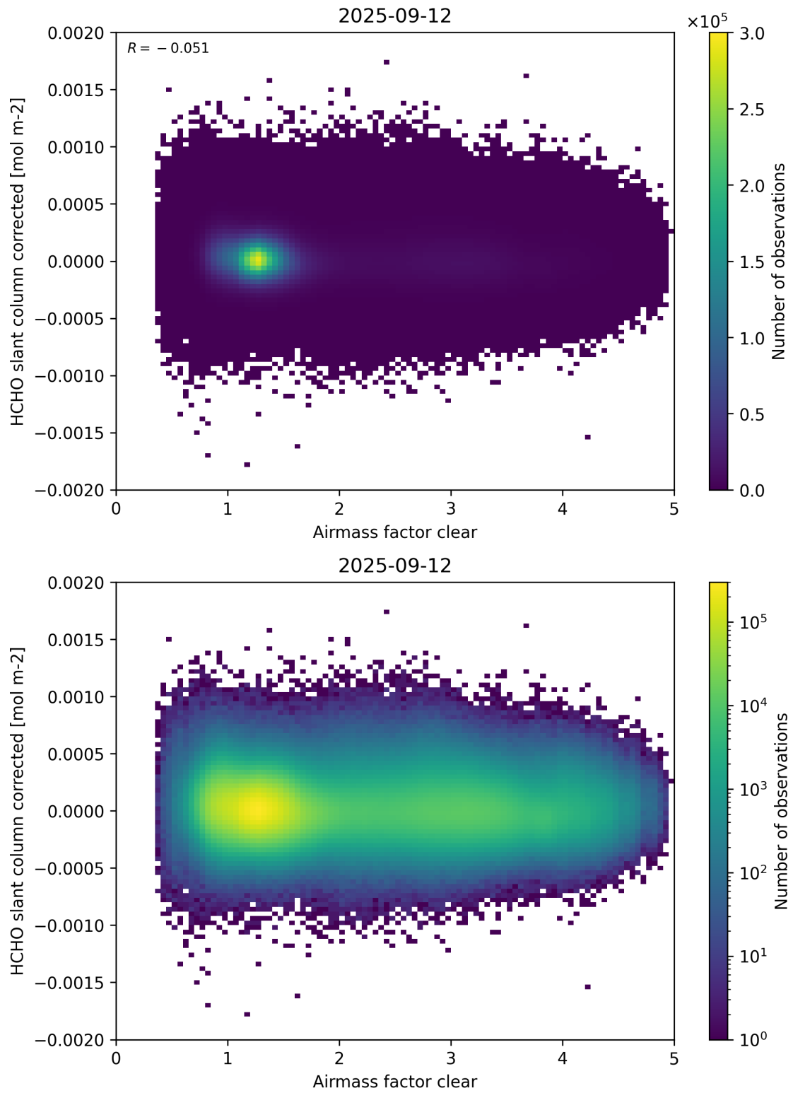
Figure 74: Scatter density plot of “Airmass factor clear” against “HCHO slant column corrected” for 2025-09-11 to 2025-09-13.
