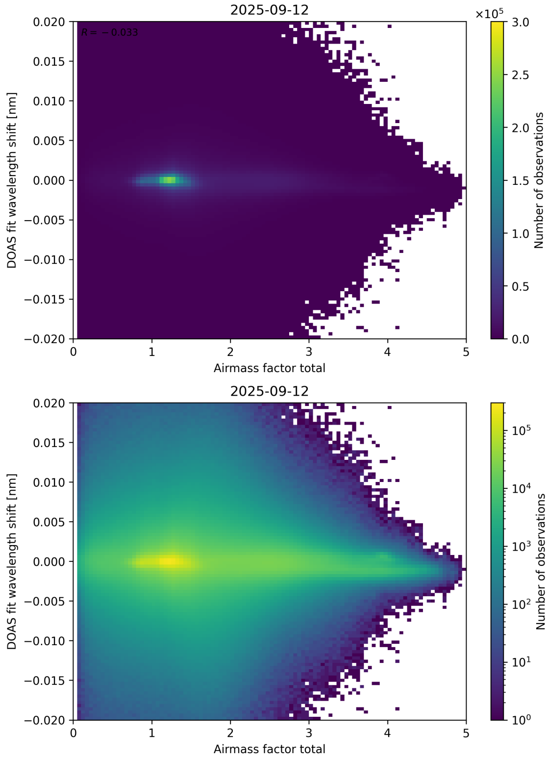
Figure 98: Scatter density plot of “Airmass factor total” against “DOAS fit wavelength shift” for 2025-09-11 to 2025-09-13.
