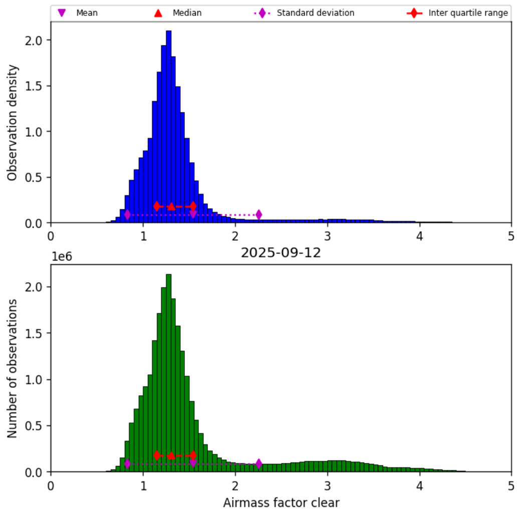
Figure 42: Histogram of “Airmass factor clear” for 2025-09-11 to 2025-09-13
