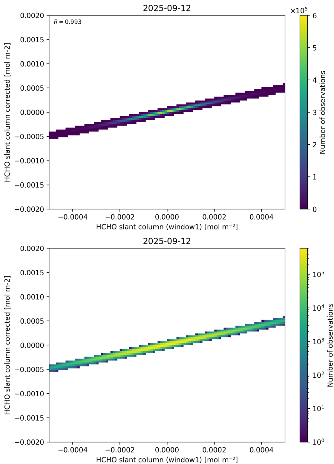
Figure 82: Scatter density plot of “HCHO slant column (window1)” against “HCHO slant column corrected” for 2025-09-11 to 2025-09-13.
