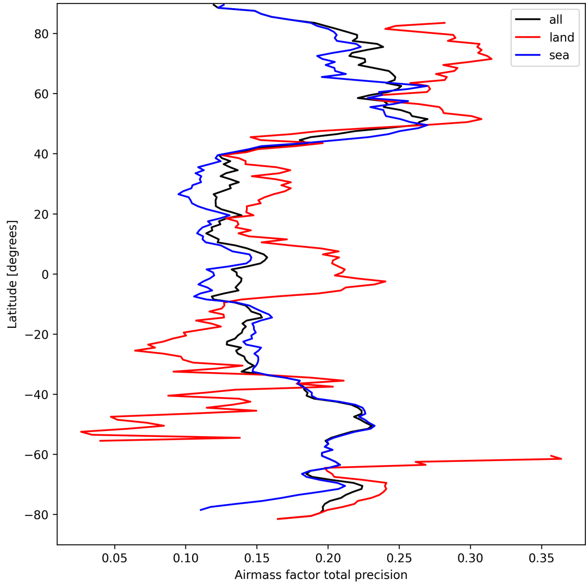
Figure 27: Zonal average of “Airmass factor total precision” for 2025-09-11 to 2025-09-13.
