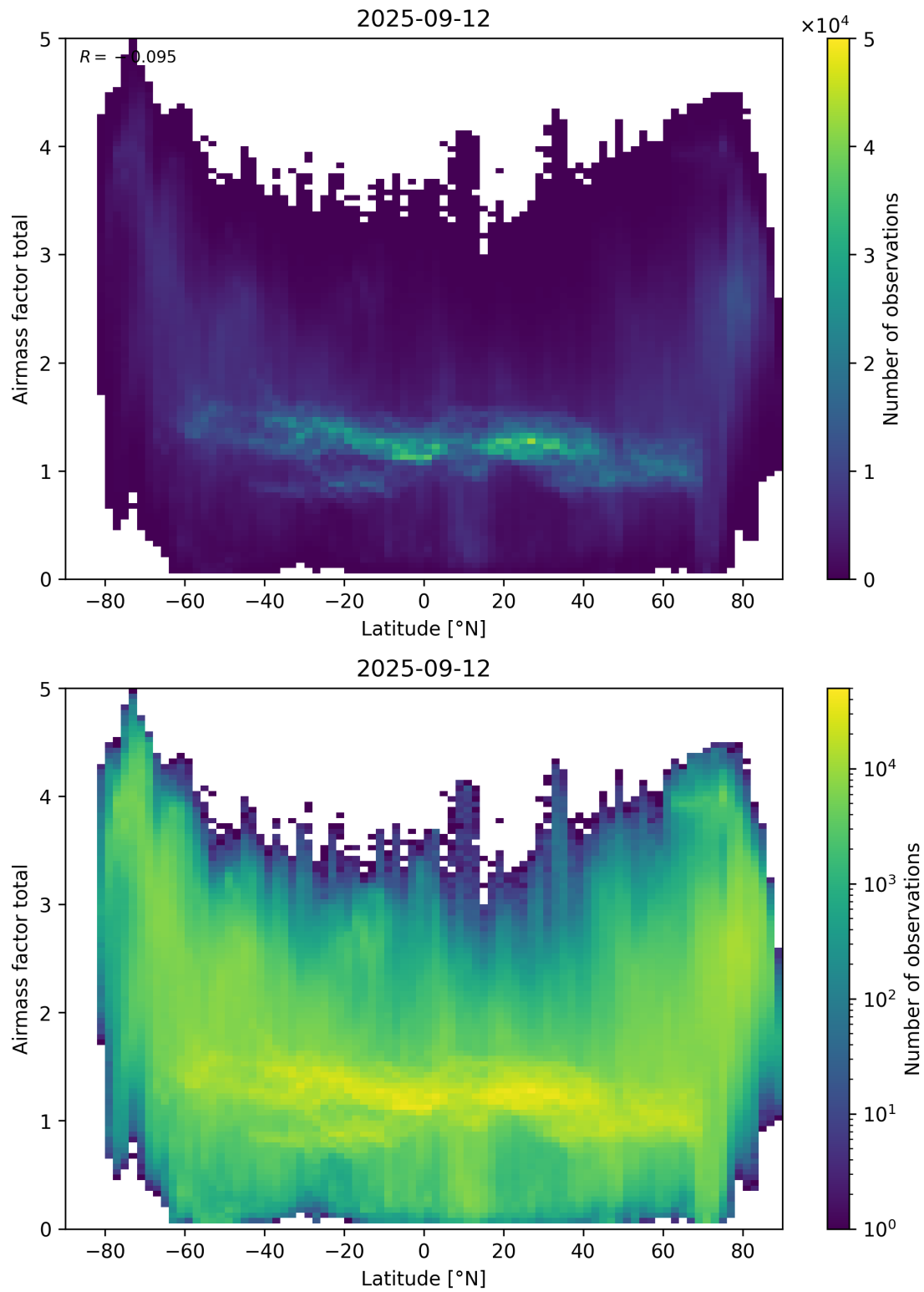
Figure 161: Scatter density plot of “Latitude” against “Airmass factor total” for 2025-09-11 to 2025-09-13.
