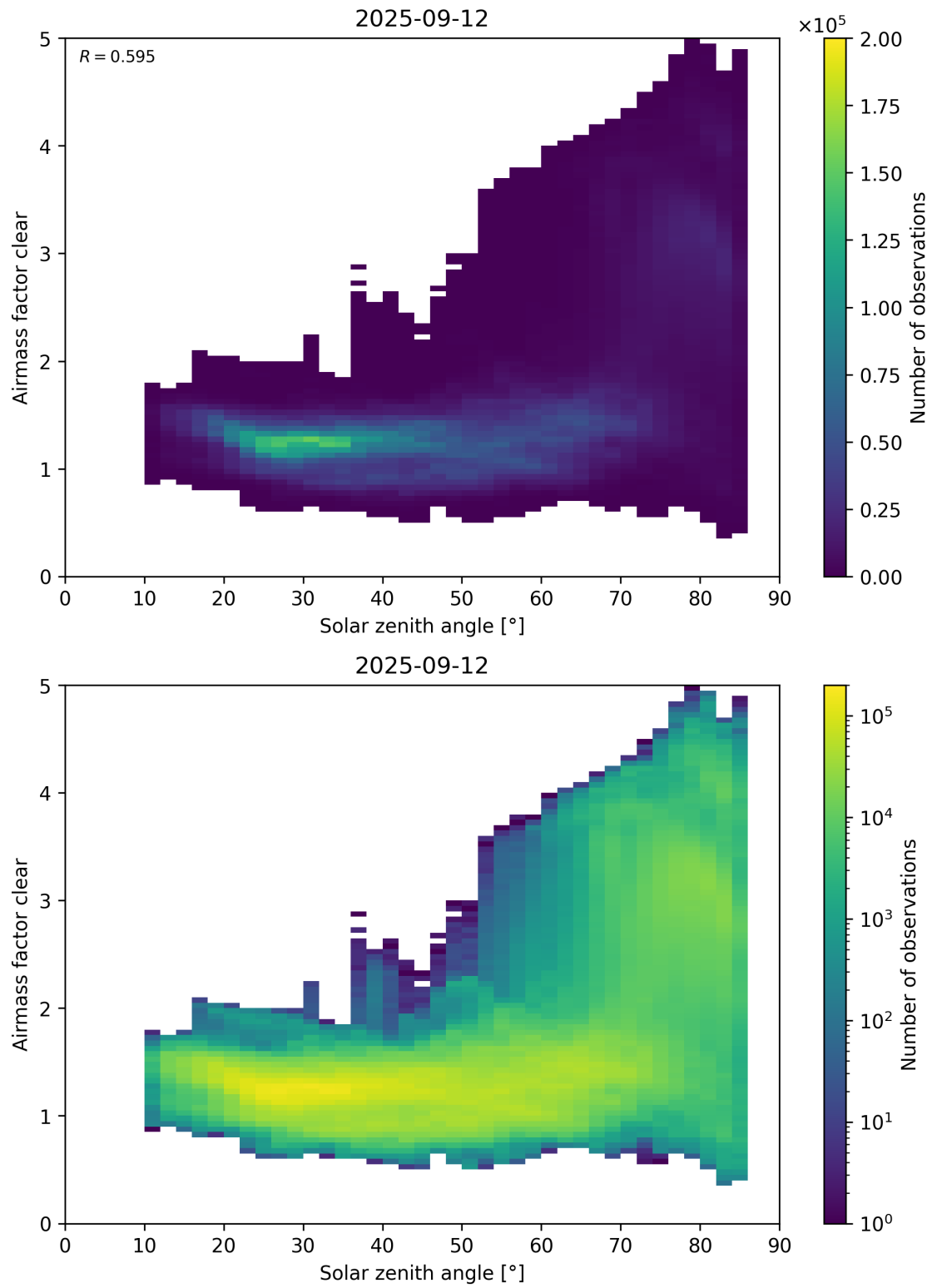
Figure 170: Scatter density plot of “Solar zenith angle” against “Airmass factor clear” for 2025-09-11 to 2025-09-13.
