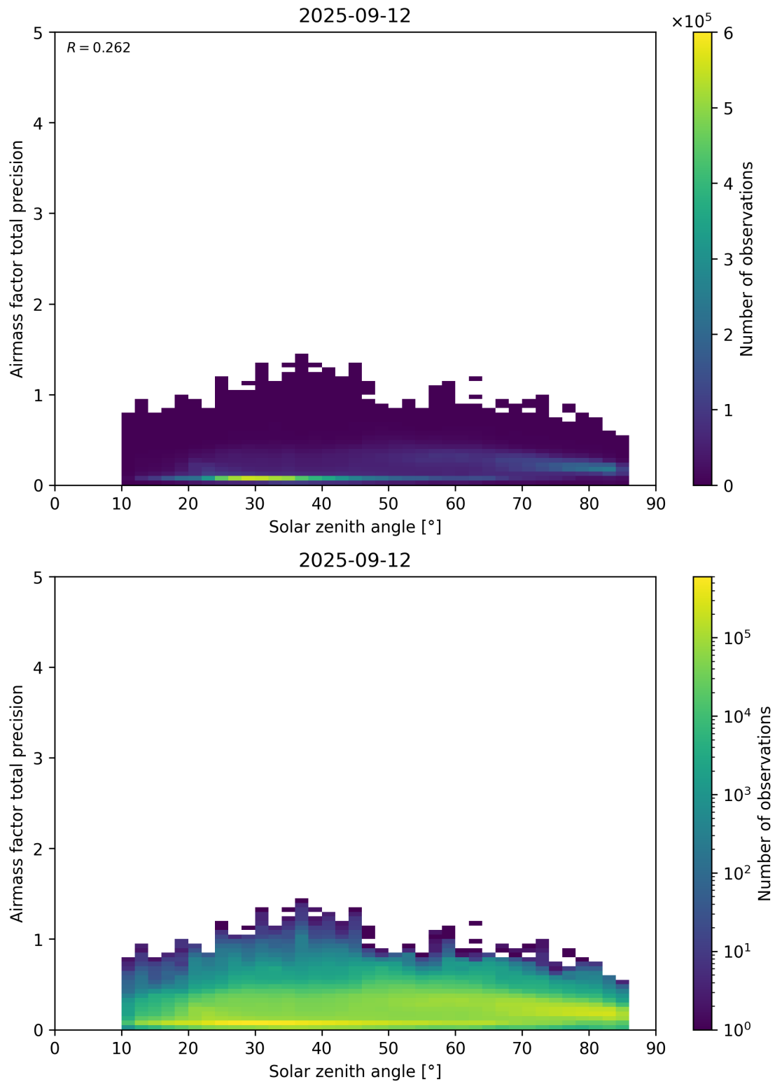
Figure 176: Scatter density plot of “Solar zenith angle” against “Airmass factor total precision” for 2025-09-11 to 2025-09-13.
