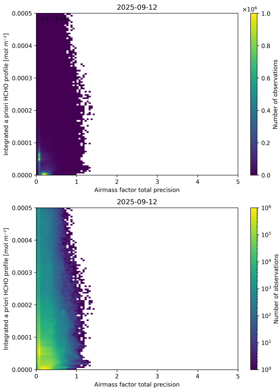
Figure 111: Scatter density plot of “Airmass factor total precision” against “Integrated a priori HCHO profile” for 2025-09-11 to 2025-09-13.
