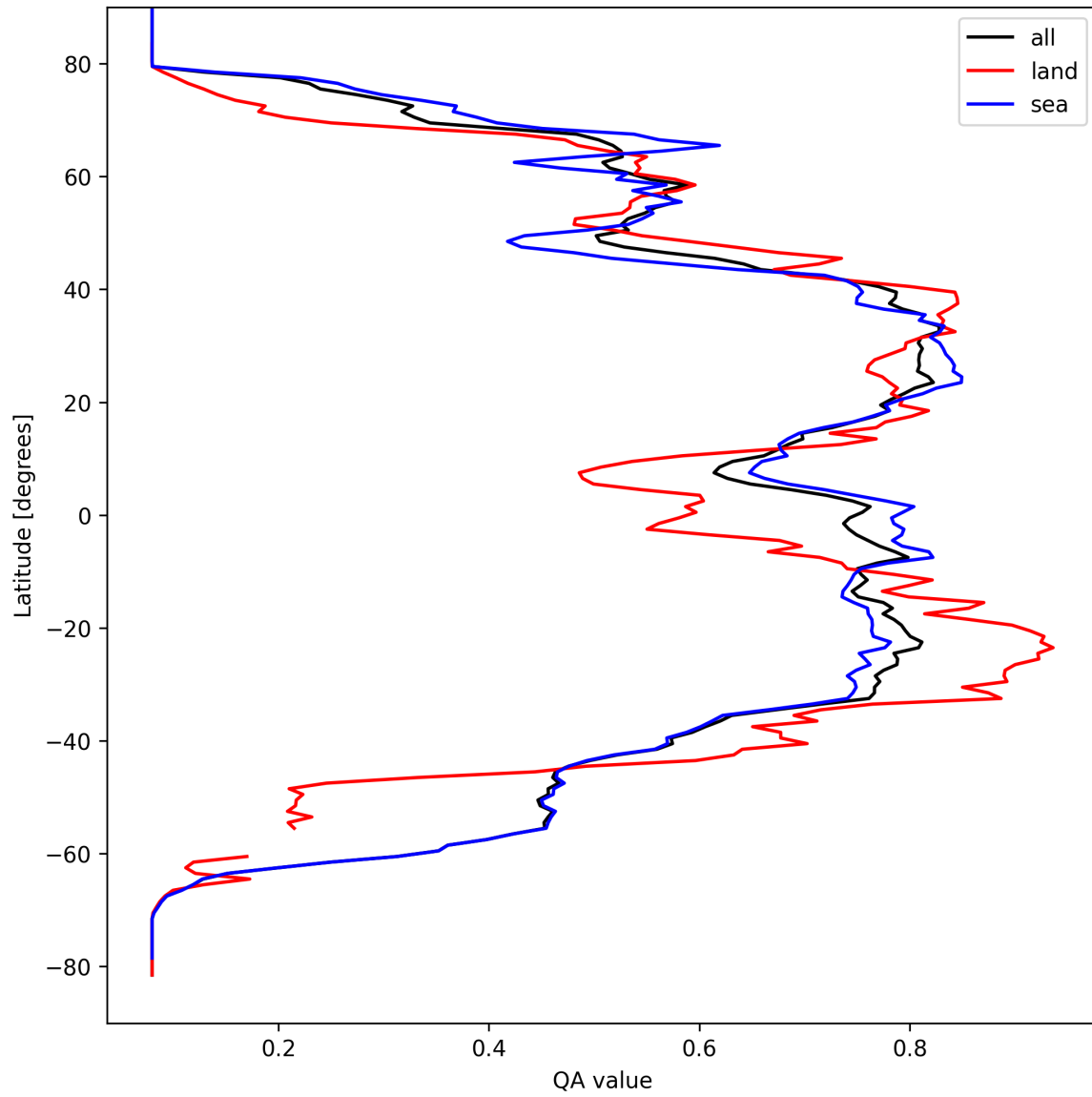
Figure 20: Zonal average of “QA value” for 2025-09-11 to 2025-09-13.
