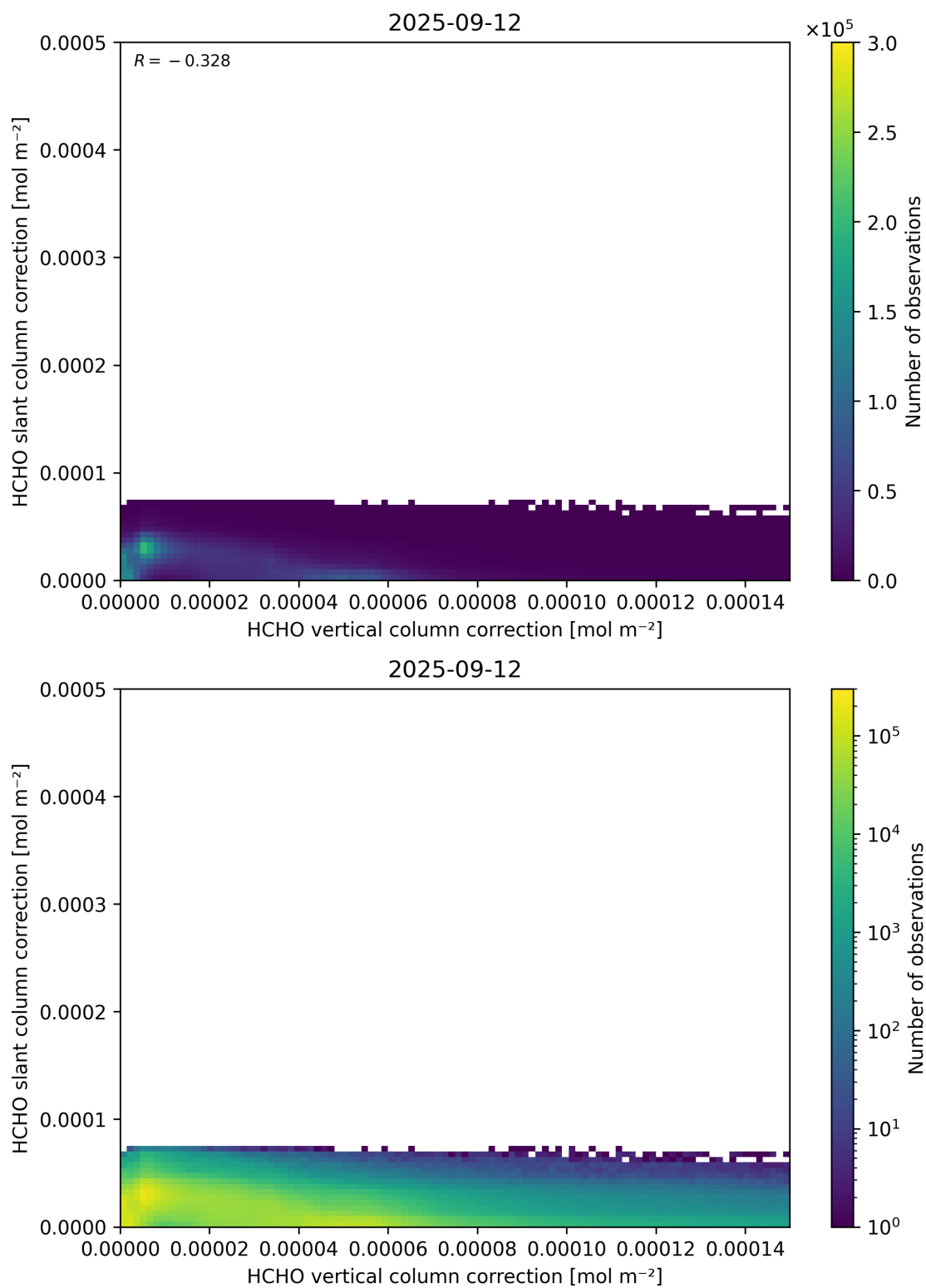
Figure 117: Scatter density plot of “HCHO vertical column correction” against “HCHO slant column correction” for 2025-09-11 to 2025-09-13.
