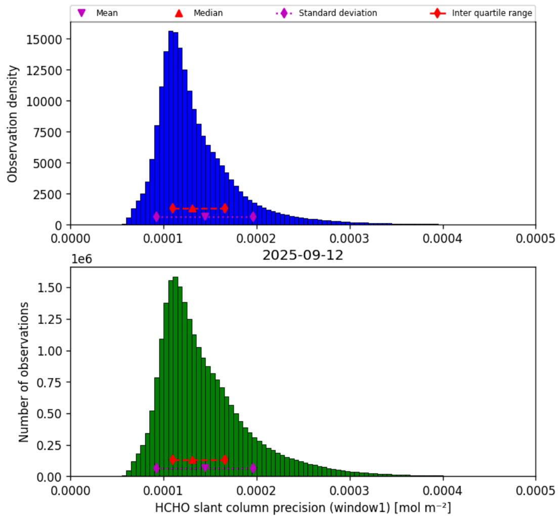
Figure 39: Histogram of “HCHO slant column precision (window1)” for 2025-09-11 to 2025-09-13
