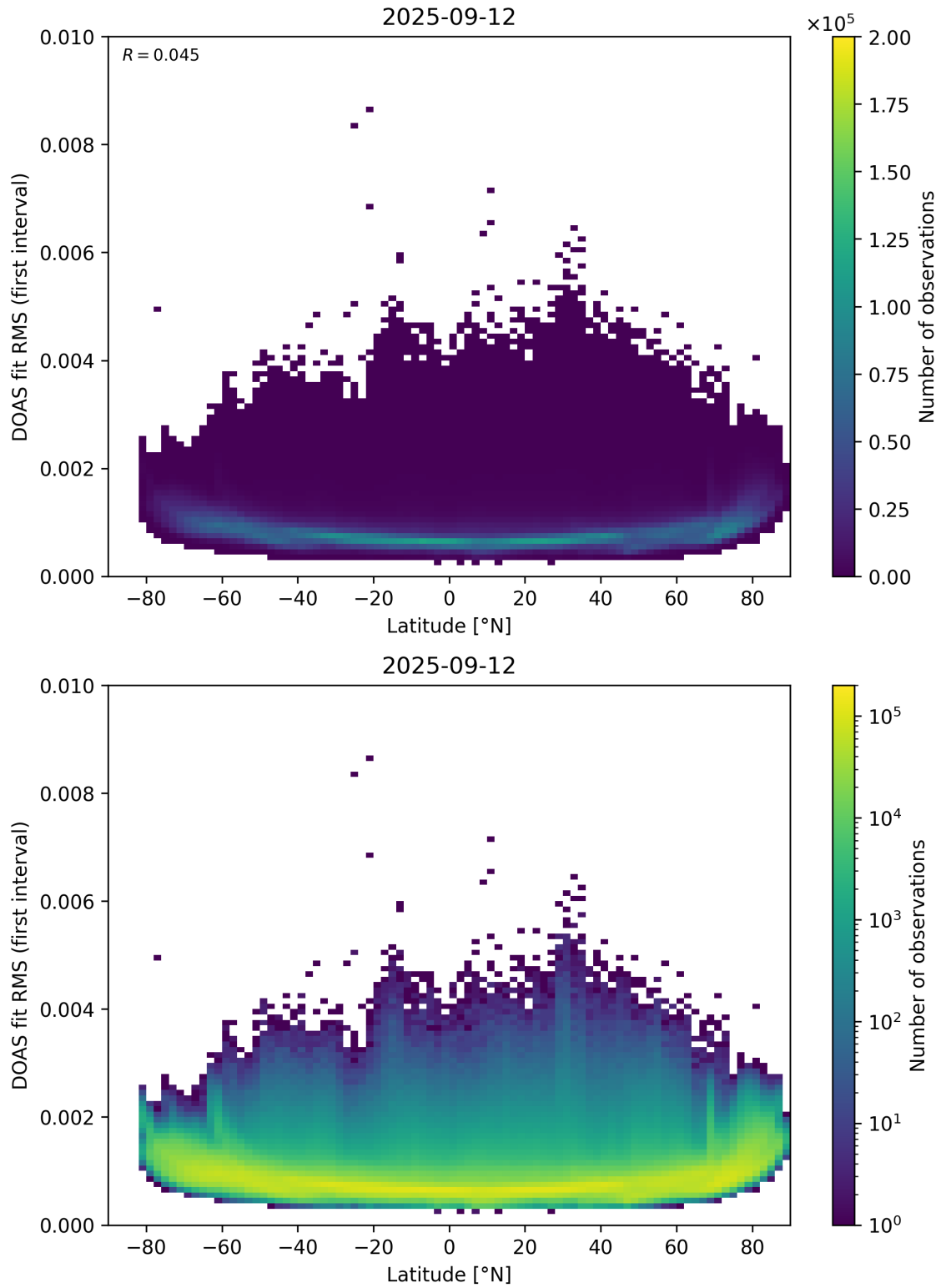
Figure 153: Scatter density plot of “Latitude” against “DOAS fit RMS (first interval)” for 2025-09-11 to 2025-09-13.
