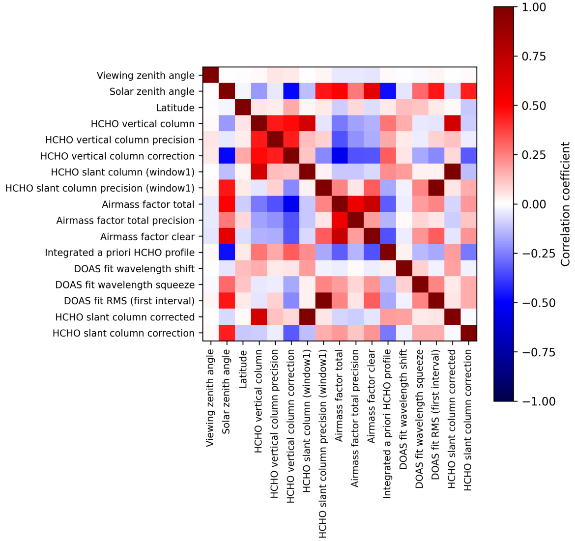
Figure 2: Map of correlation matrix for 2025-09-11 to 2025-09-13.
