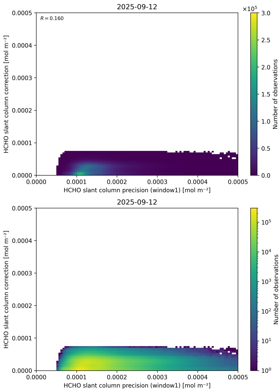
Figure 93: Scatter density plot of “HCHO slant column precision (window1)” against “HCHO slant column correction” for 2025-09-11 to 2025-09-13.
