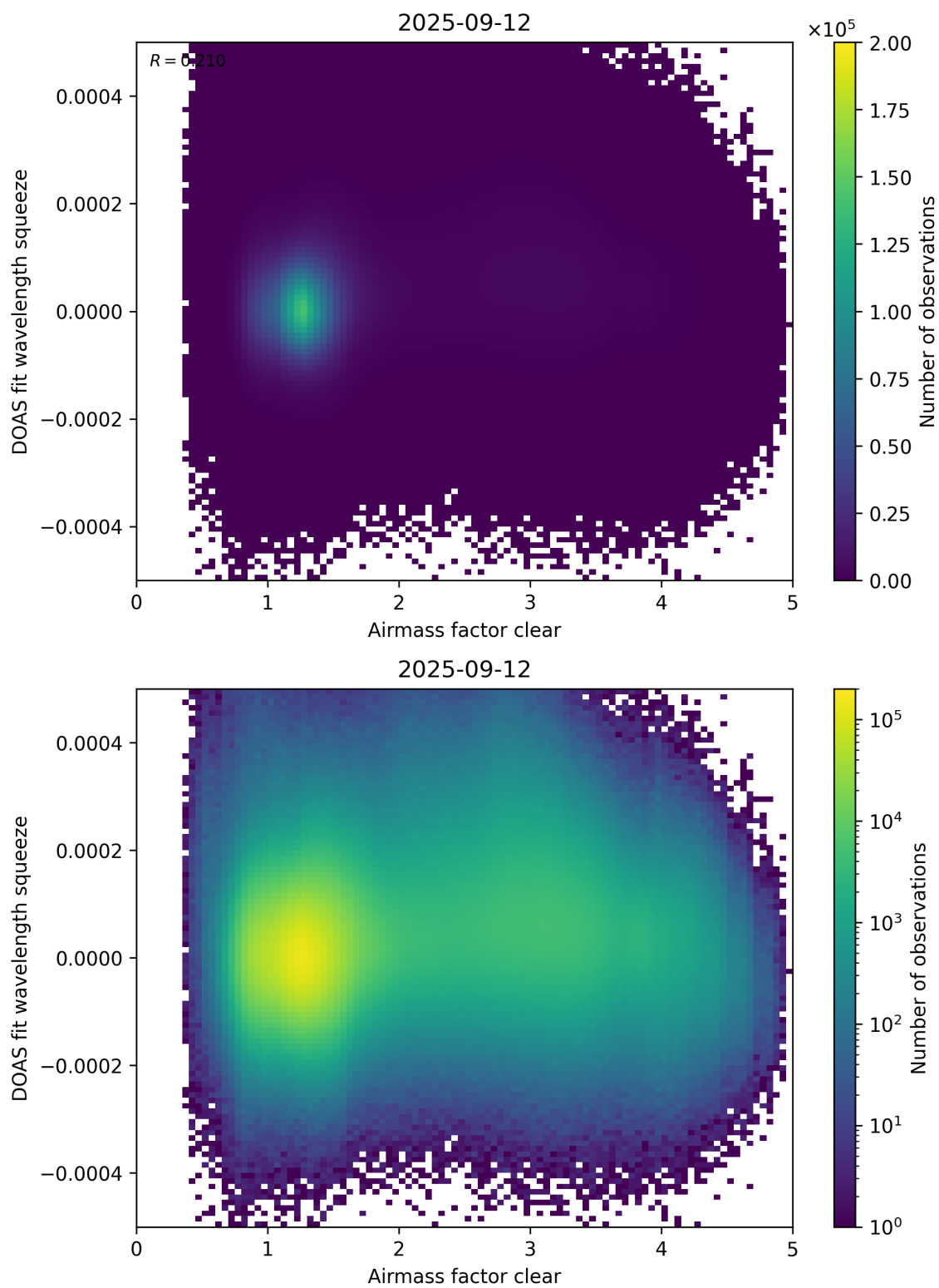
Figure 73: Scatter density plot of “Airmass factor clear” against “DOAS fit wavelength squeeze” for 2025-09-11 to 2025-09-13.
