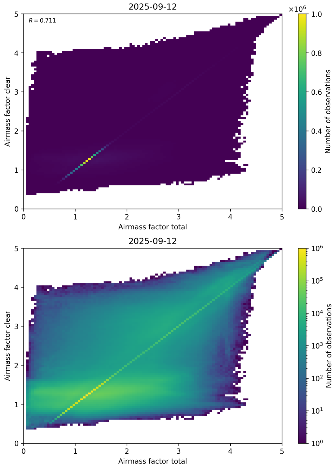
Figure 100: Scatter density plot of “Airmass factor total” against “Airmass factor clear” for 2025-09-11 to 2025-09-13.
