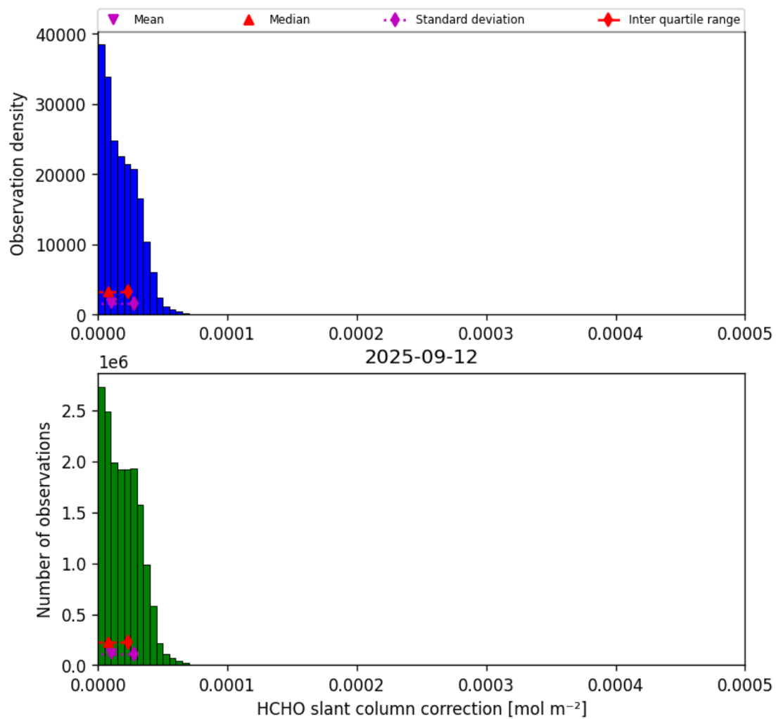
Figure 47: Histogram of “HCHO slant column correction” for 2025-09-11 to 2025-09-13
