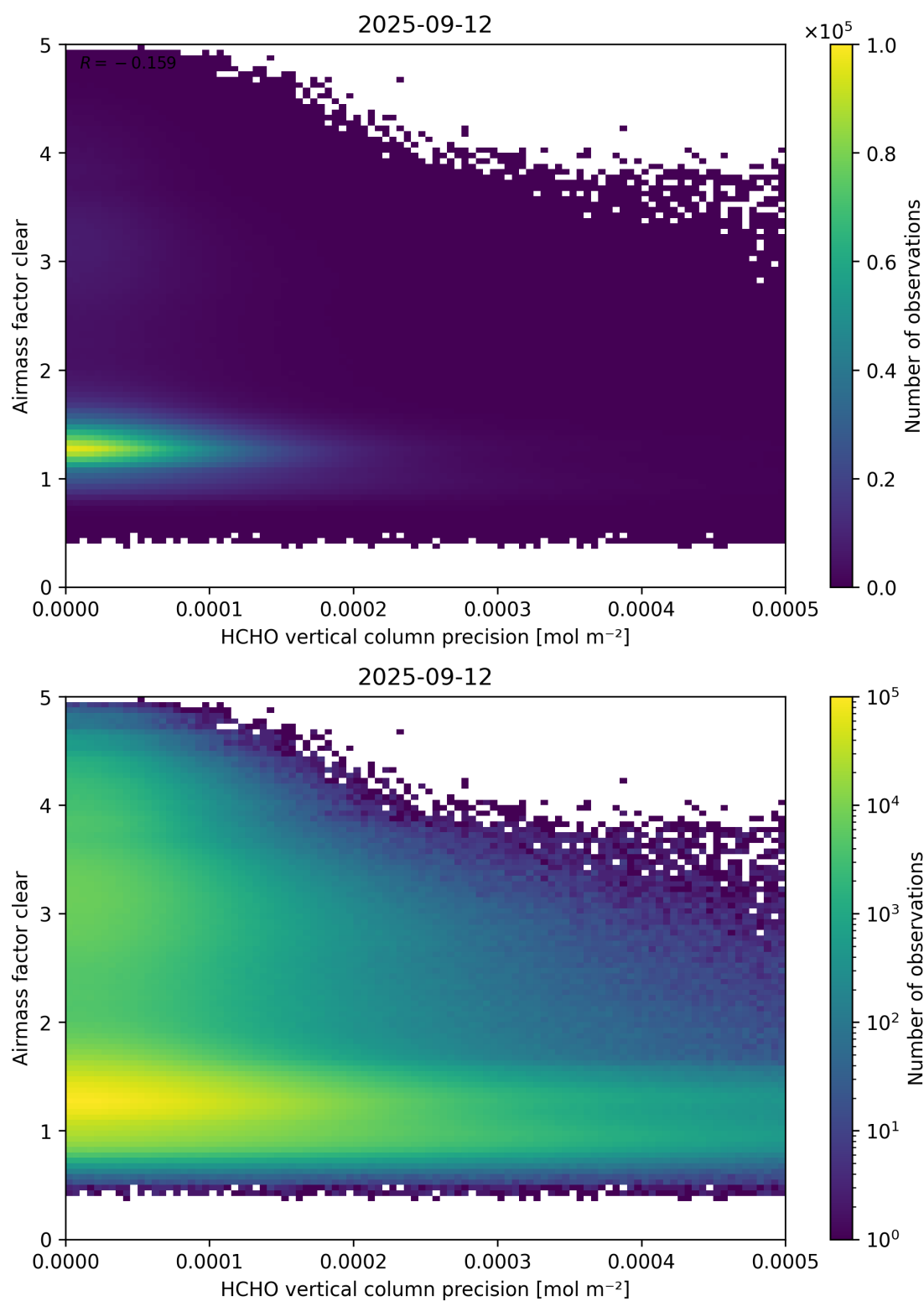
Figure 139: Scatter density plot of “HCHO vertical column precision” against “Airmass factor clear” for 2025-09-11 to 2025-09-13.
