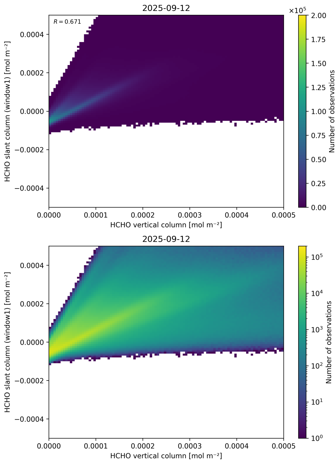
Figure 129: Scatter density plot of “HCHO vertical column” against “HCHO slant column (window1)” for 2025-09-11 to 2025-09-13.
