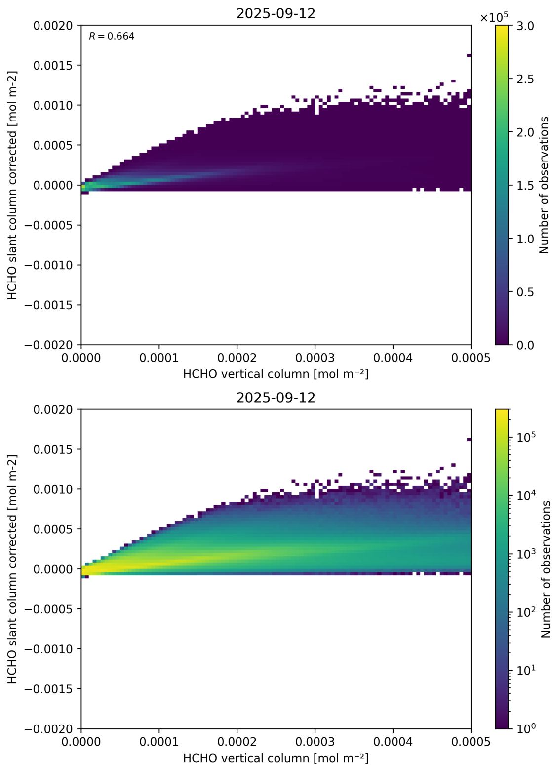
Figure 127: Scatter density plot of “HCHO vertical column” against “HCHO slant column corrected” for 2025-09-11 to 2025-09-13.
