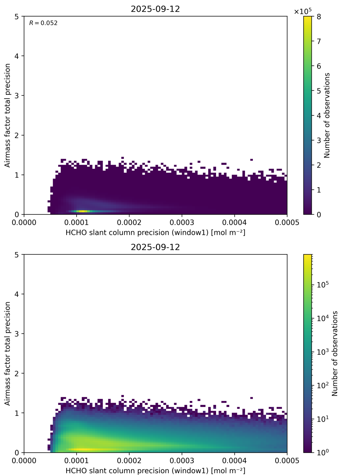
Figure 95: Scatter density plot of “HCHO slant column precision (window1)” against “Airmass factor total precision” for 2025-09-11 to 2025-09-13.
