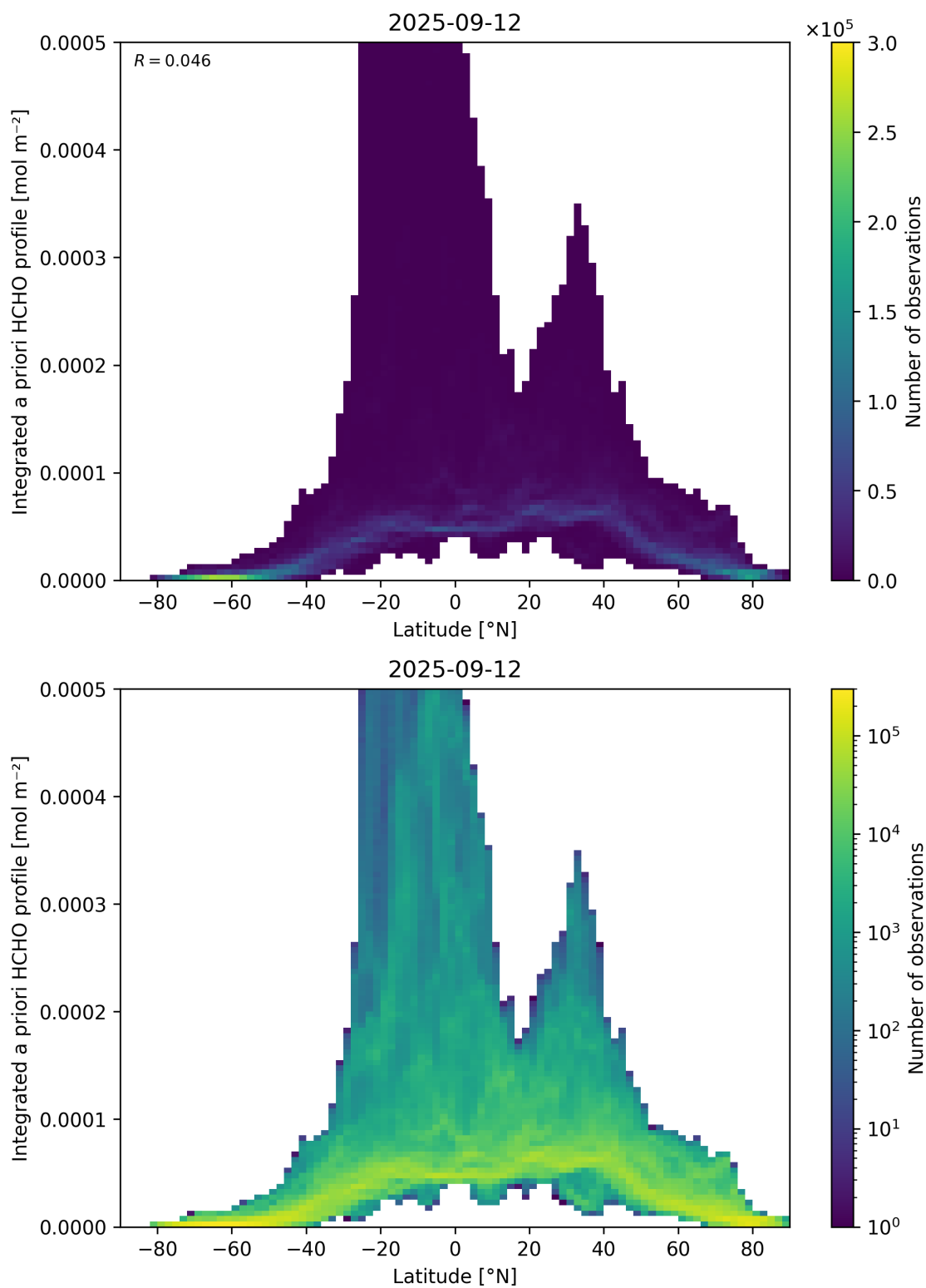
Figure 166: Scatter density plot of “Latitude” against “Integrated a priori HCHO profile” for 2025-09-11 to 2025-09-13.
