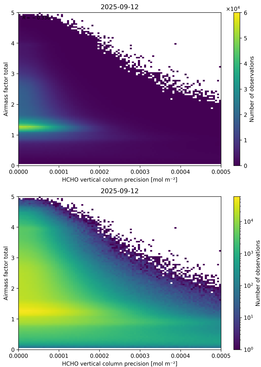
Figure 144: Scatter density plot of “HCHO vertical column precision” against “Airmass factor total” for 2025-09-11 to 2025-09-13.
