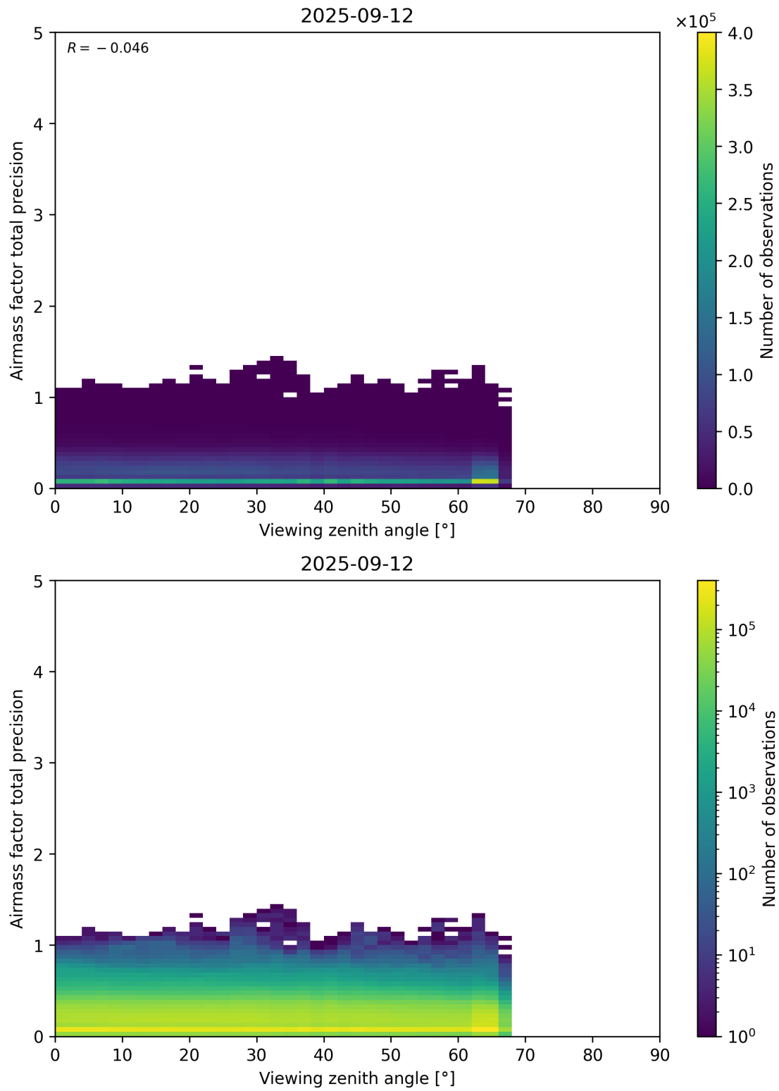
Figure 191: Scatter density plot of “Viewing zenith angle” against “Airmass factor total precision” for 2025-09-11 to 2025-09-13.
