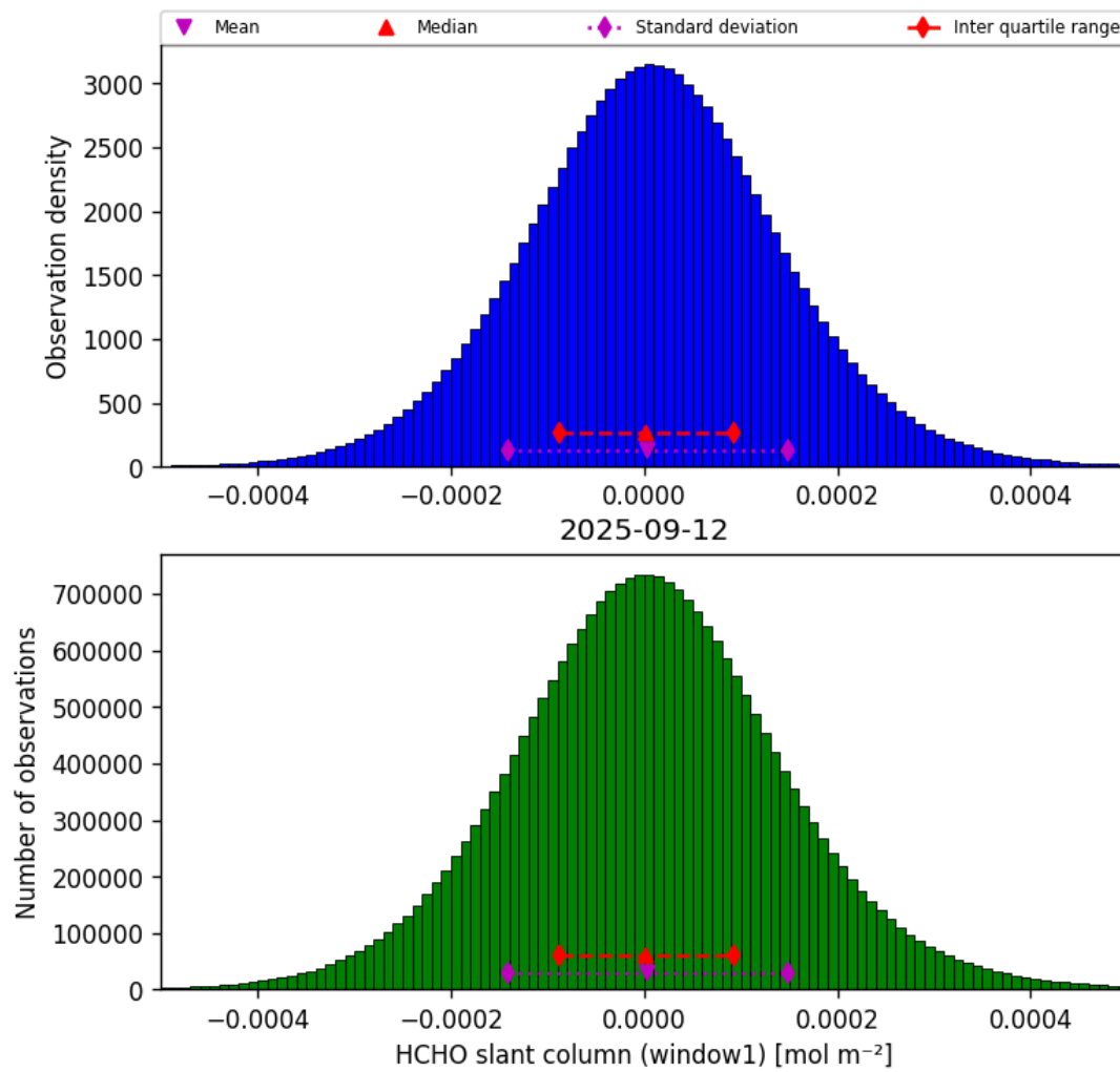
Figure 38: Histogram of “HCHO slant column (window1)” for 2025-09-11 to 2025-09-13
