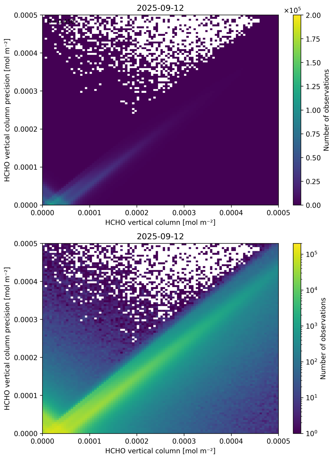
Figure 134: Scatter density plot of “HCHO vertical column” against “HCHO vertical column precision” for 2025-09-11 to 2025-09-13.
