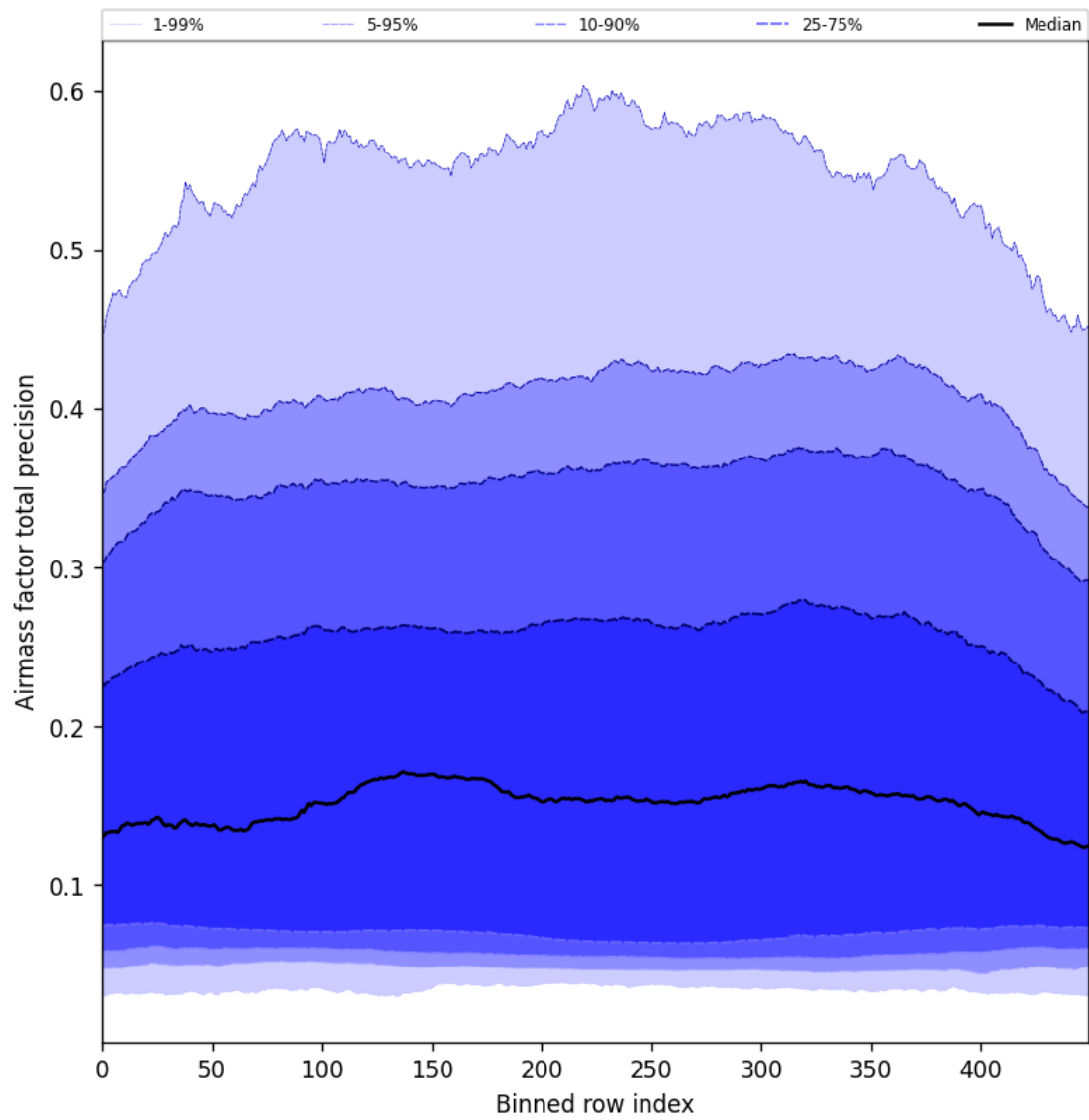
Figure 55: Along track statistics of “Airmass factor total precision” for 2025-09-11 to 2025-09-13
