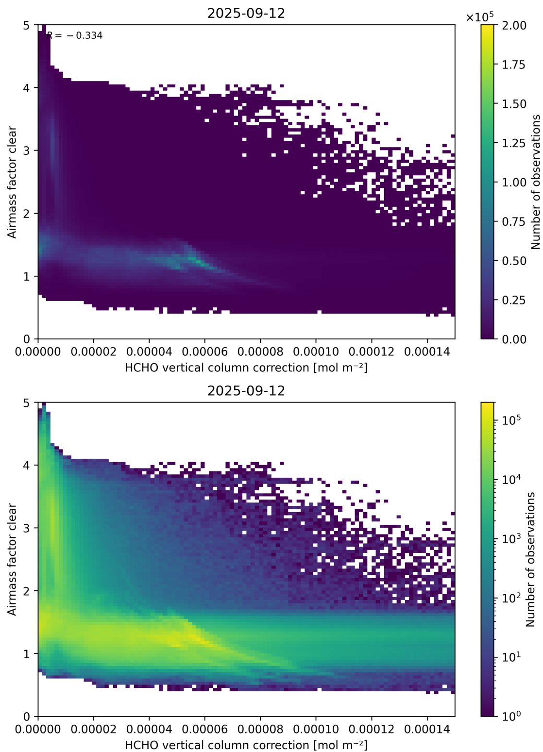
Figure 115: Scatter density plot of “HCHO vertical column correction” against “Air mass factor clear” for 2025-09-11 to 2025-09-13.
