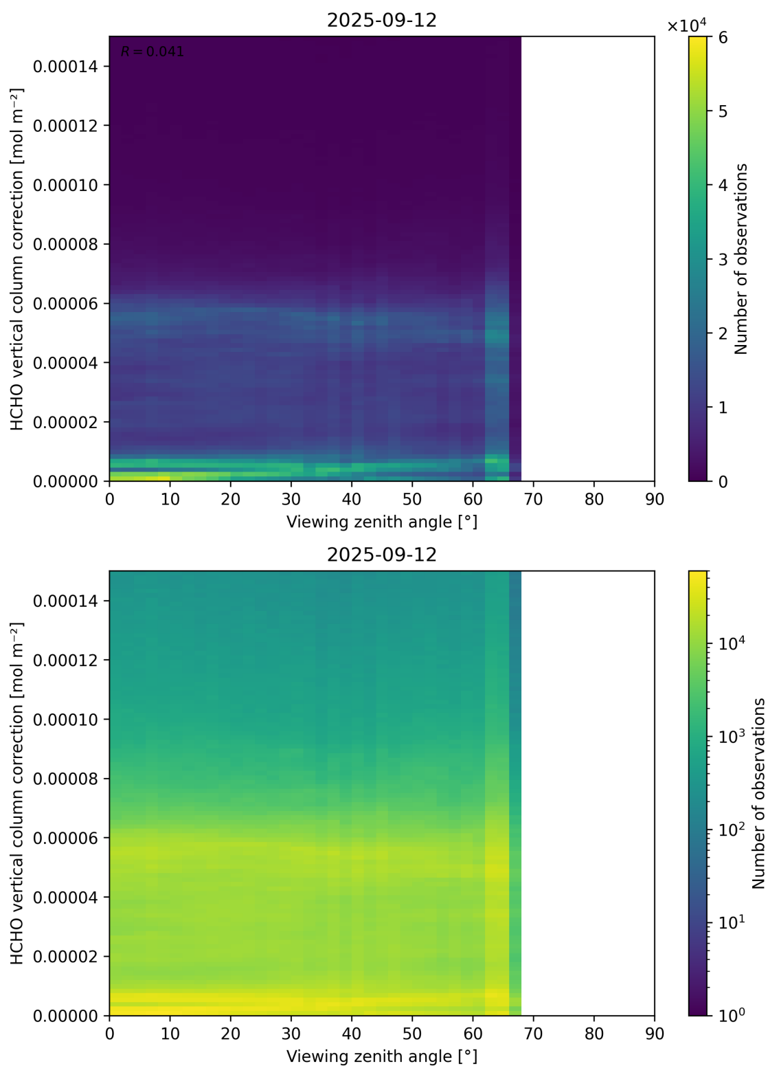
Figure 193: Scatter density plot of “Viewing zenith angle” against “HCHO vertical column correction” for 2025-09-11 to 2025-09-13.
