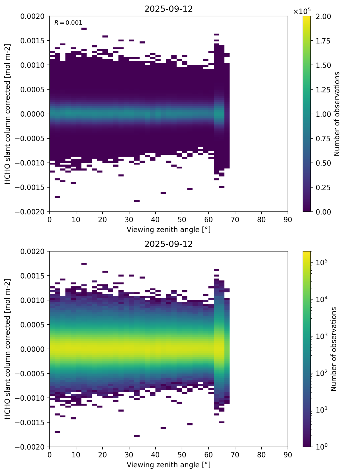
Figure 186: Scatter density plot of “Viewing zenith angle” against “HCHO slant column corrected” for 2025-09-11 to 2025-09-13.
