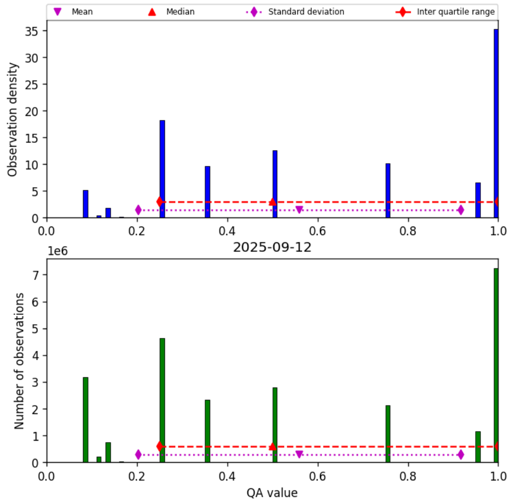
Figure 34: Histogram of “QA value” for 2025-09-11 to 2025-09-13
