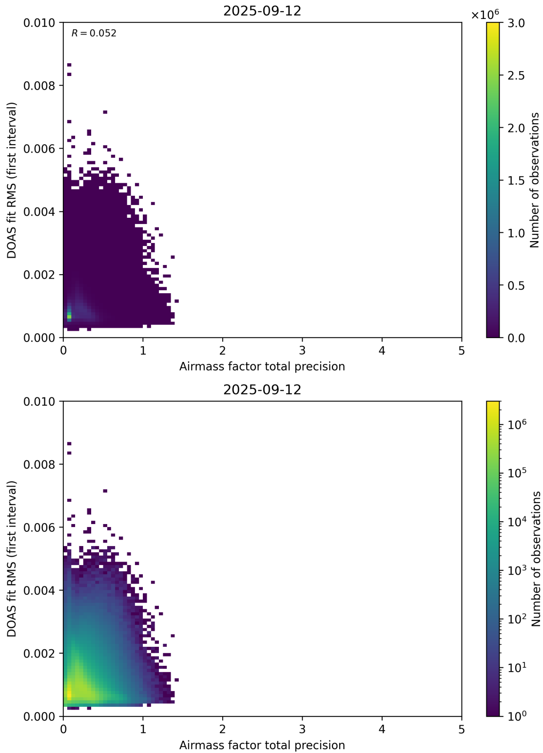
Figure 105: Scatter density plot of “Airmass factor total precision” against “DOAS fit RMS (first interval)” for 2025-09-11 to 2025-09-13.
