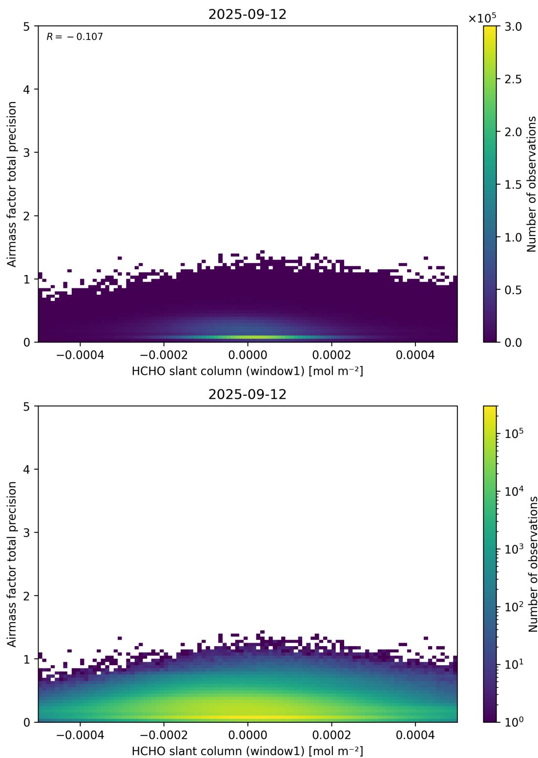
Figure 86: Scatter density plot of “HCHO slant column (window1)” against “Airmass factor total precision” for 2025-09-11 to 2025-09-13.
