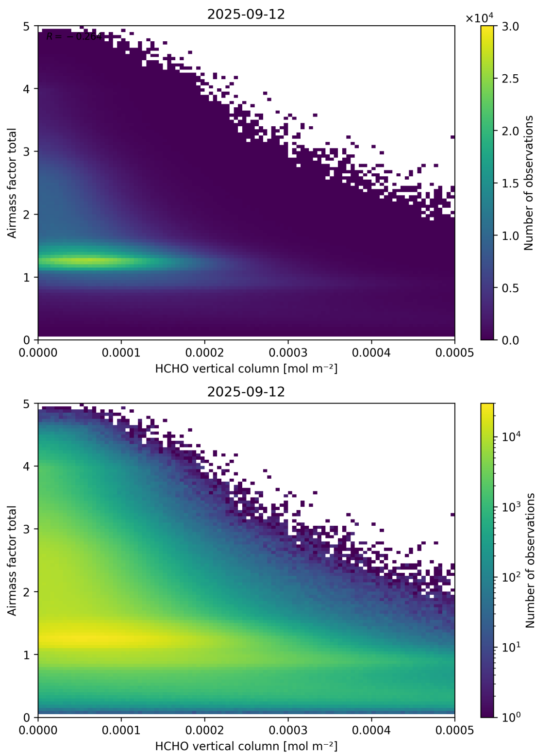
Figure 131: Scatter density plot of “HCHO vertical column” against “Airmass factor total” for 2025-09-11 to 2025-09-13.
