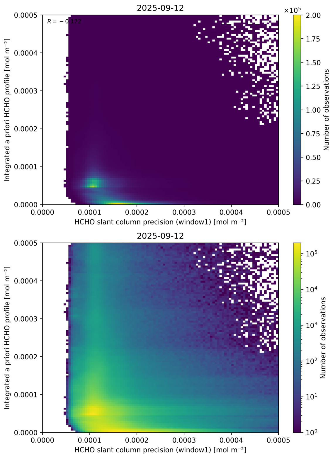
Figure 96: Scatter density plot of “HCHO slant column precision (window1)” against “Integrated a priori HCHO profile” for 2025-09-11 to 2025-09-13.
