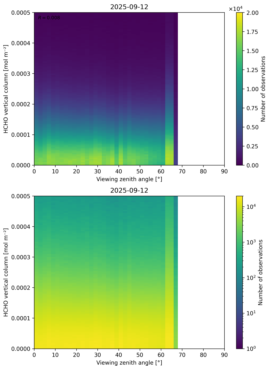
Figure 192: Scatter density plot of “Viewing zenith angle” against “HCHO vertical column” for 2025-09-11 to 2025-09-13.
