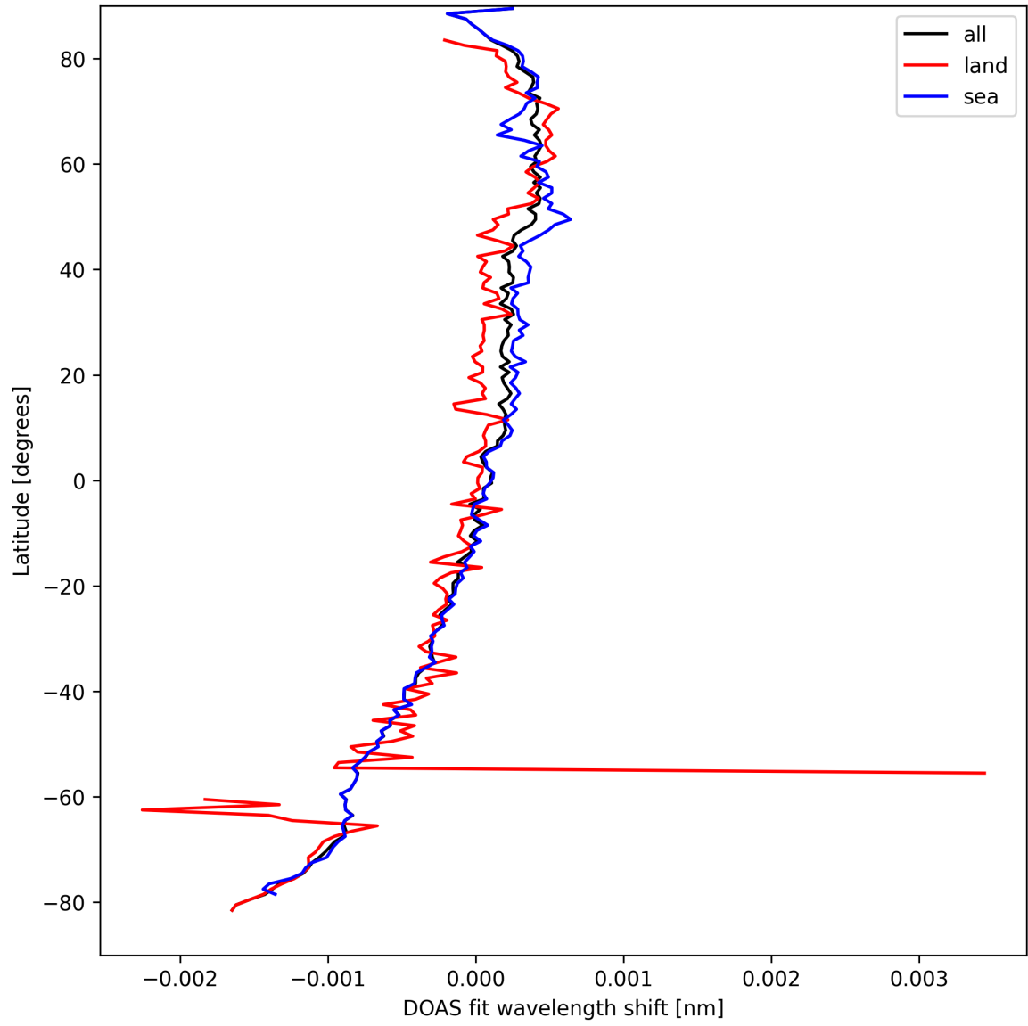
Figure 30: Zonal average of "DOAS fit wavelength shift" for 2025-09-11 to 2025-09-13.
