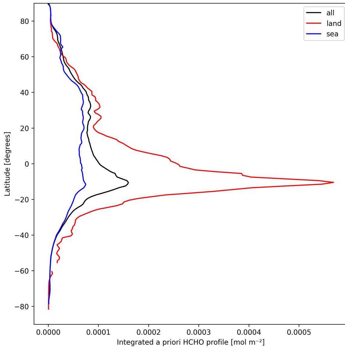
Figure 29: Zonal average of “Integrated a priori HCHO profile” for 2025-09-11 to 2025-09-13.
