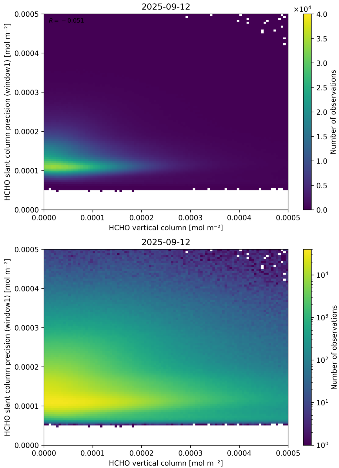
Figure 130: Scatter density plot of “HCHO vertical column” against “HCHO slant column precision (window1)” for 2025-09-11 to 2025-09-13.
