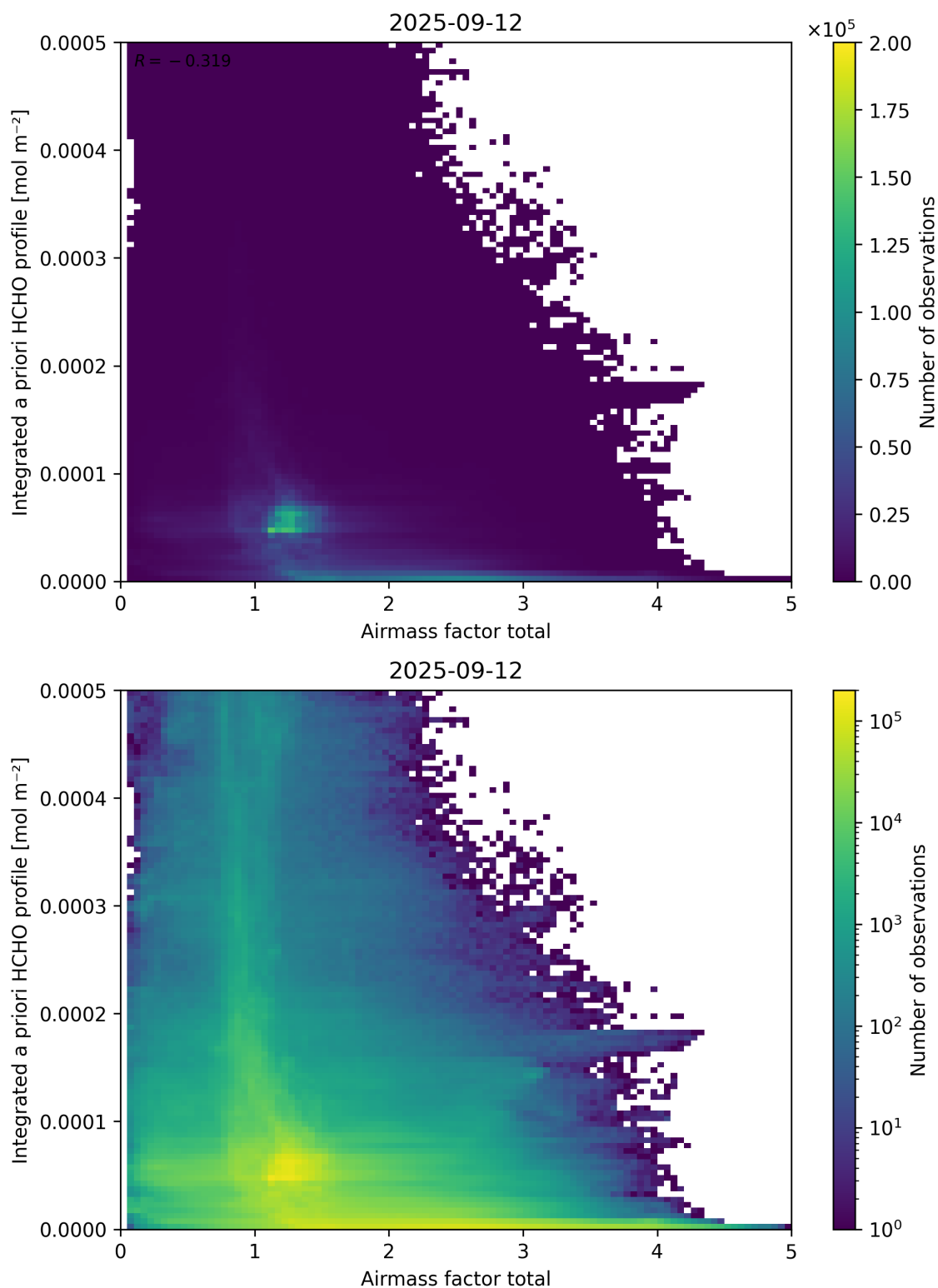
Figure 104: Scatter density plot of “Airmass factor total” against “Integrated a priori HCHO profile” for 2025-09-11 to 2025-09-13.
