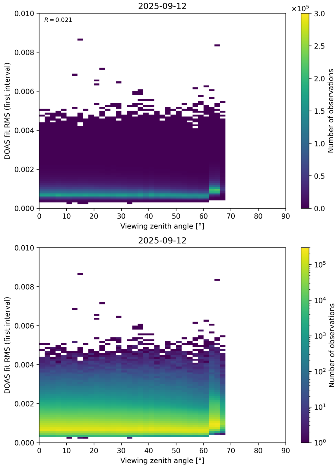
Figure 182: Scatter density plot of “Viewing zenith angle” against “DOAS fit RMS (first interval)” for 2025-09-11 to 2025-09-13.
