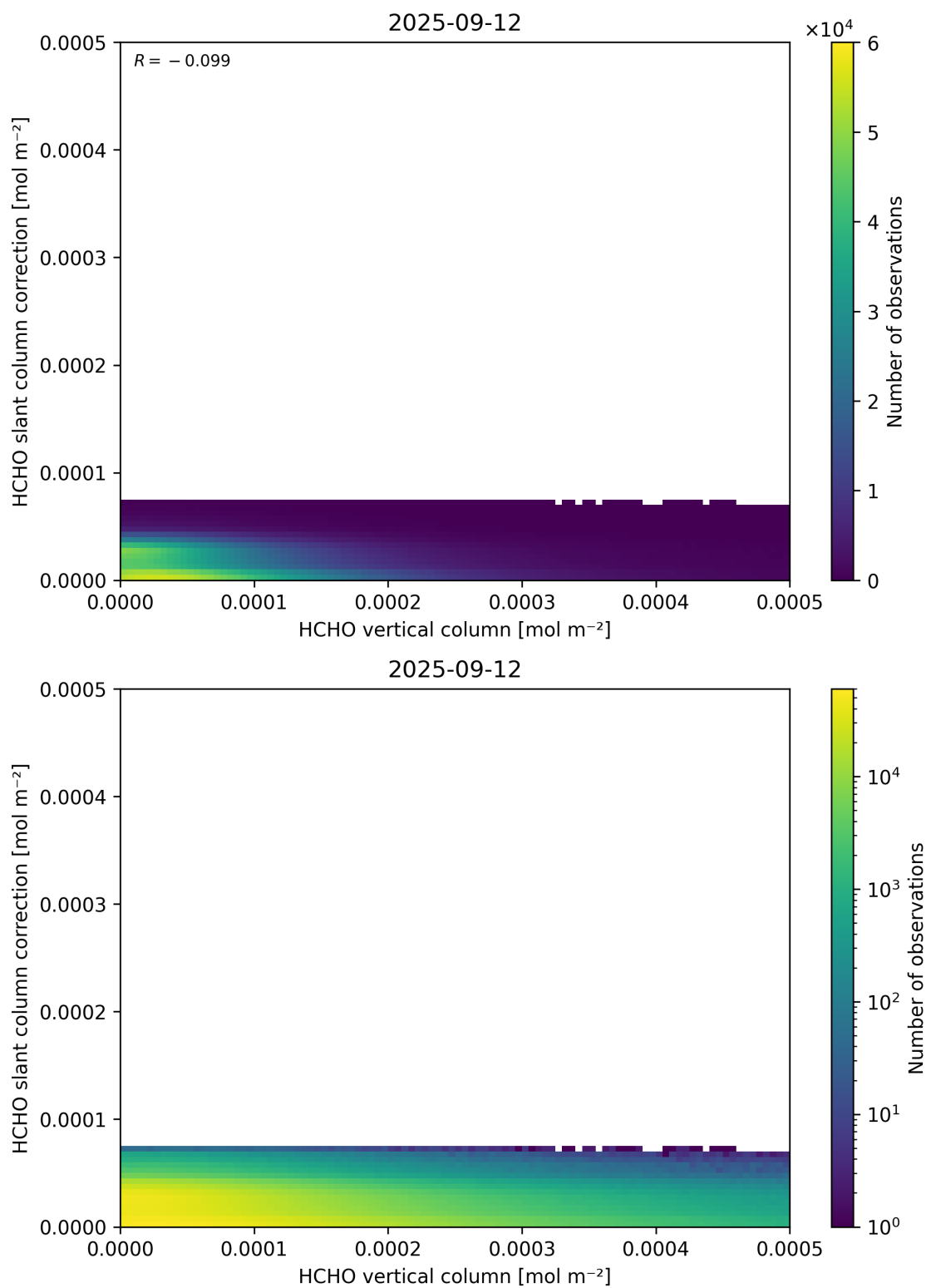
Figure 128: Scatter density plot of “HCHO vertical column” against “HCHO slant column correction” for 2025-09-11 to 2025-09-13.
