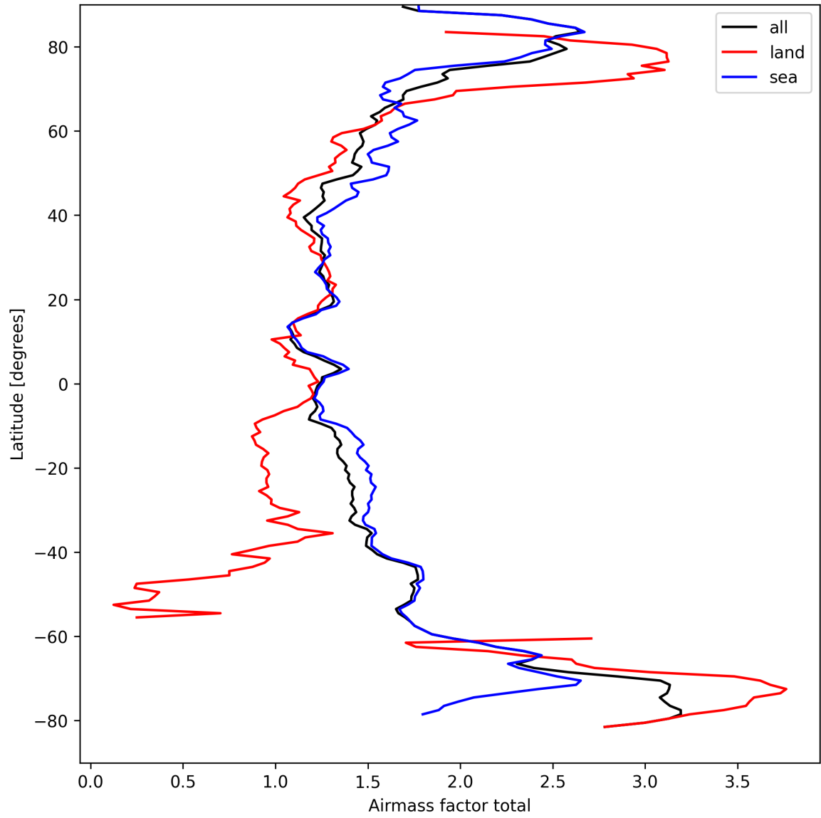
Figure 26: Zonal average of “Airmass factor total” for 2025-09-11 to 2025-09-13.
