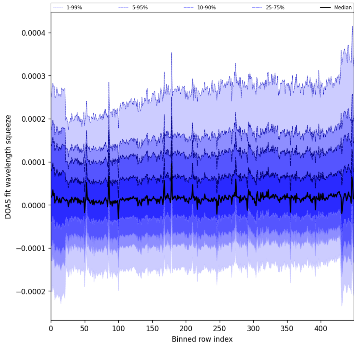
Figure 59: Along track statistics of “DOAS fit wavelength squeeze” for 2025-09-11 to 2025-09-13
