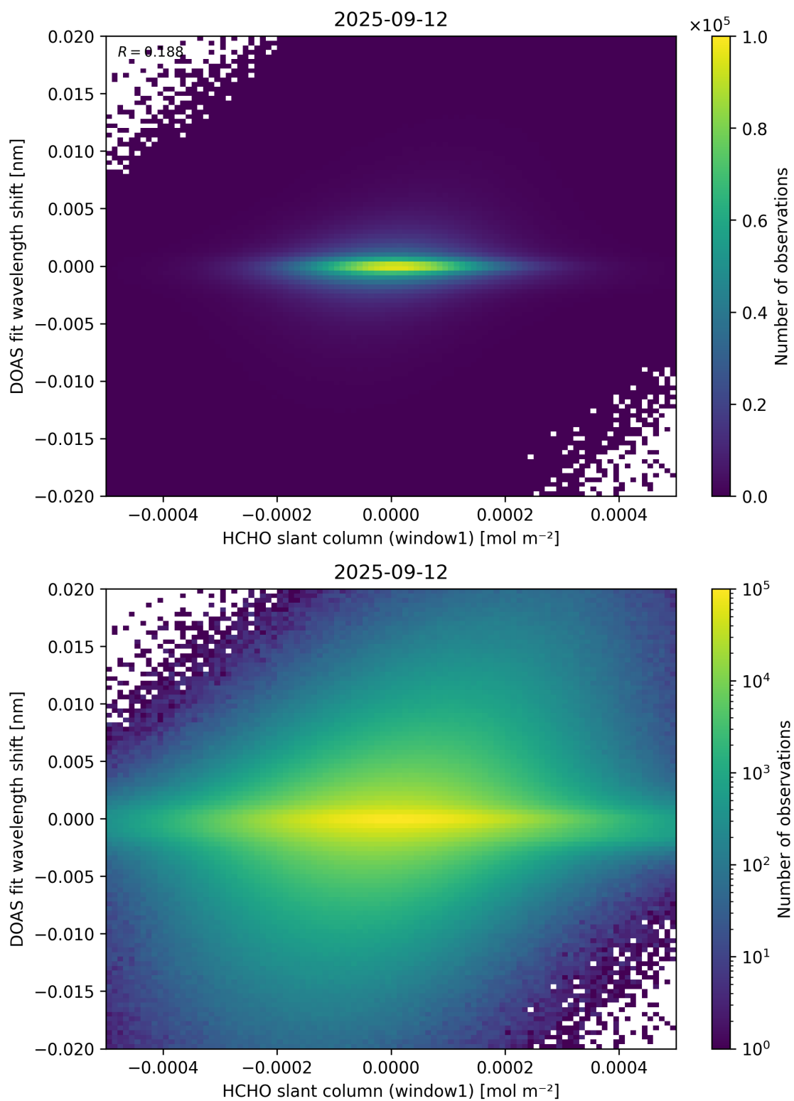
Figure 79: Scatter density plot of “HCHO slant column (window1)” against “DOAS fit wavelength shift” for 2025-09-11 to 2025-09-13.
