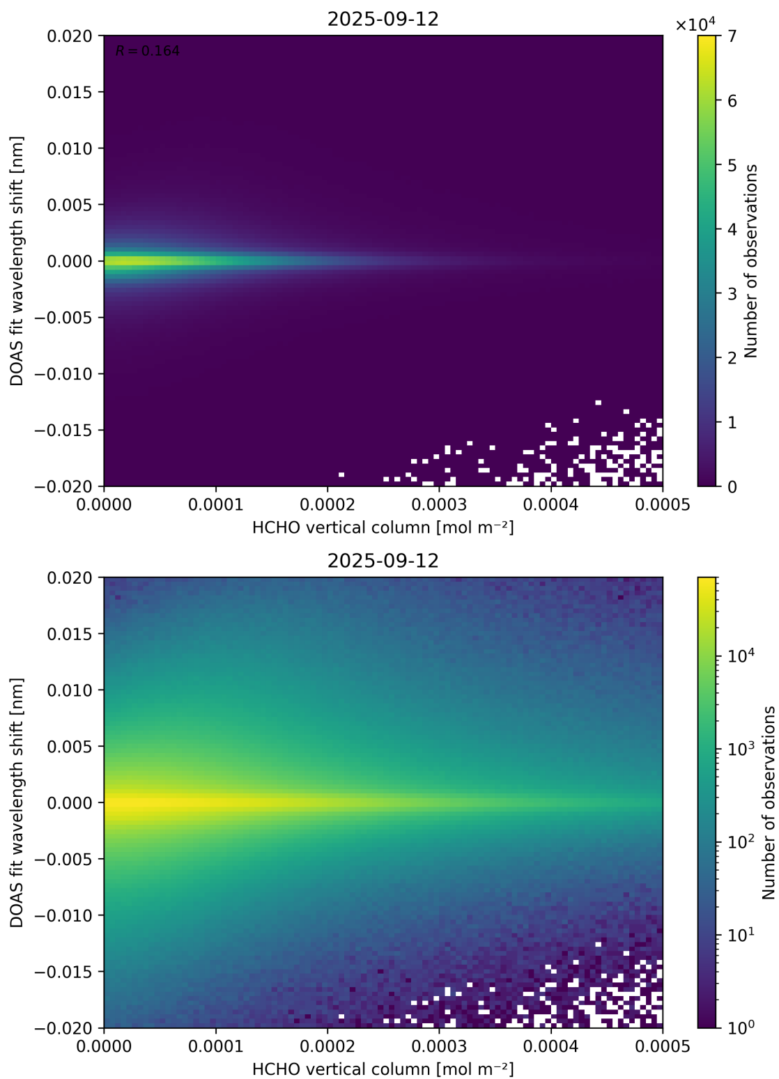
Figure 124: Scatter density plot of “HCHO vertical column” against “DOAS fit wavelength shift” for 2025-09-11 to 2025-09-13.
