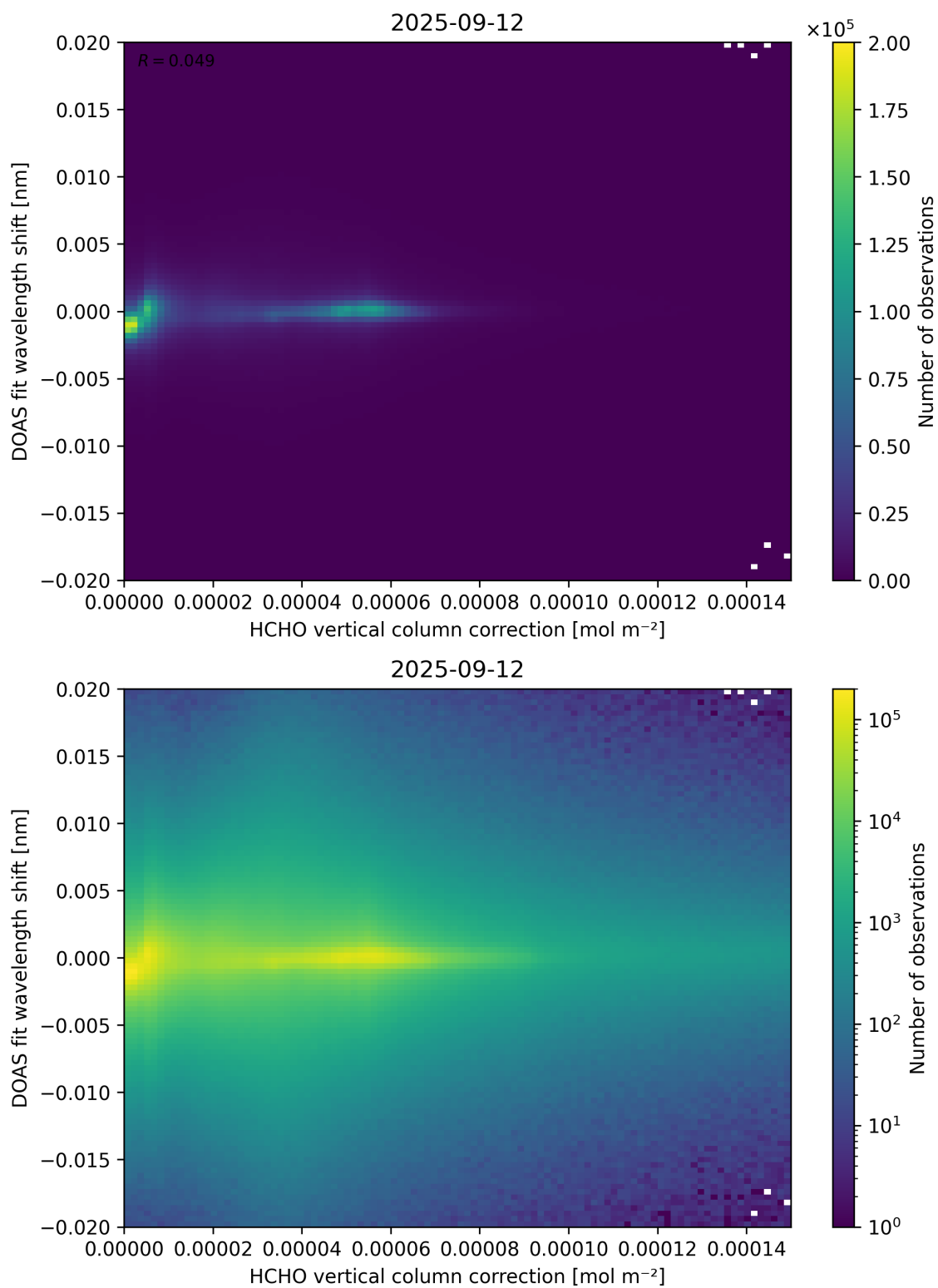
Figure 113: Scatter density plot of “HCHO vertical column correction” against “DOAS fit wavelength shift” for 2025-09-11 to 2025-09-13.
