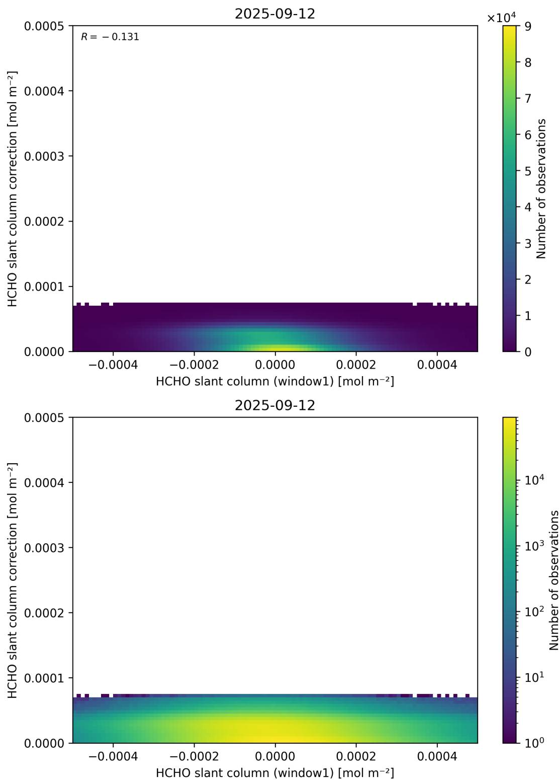
Figure 83: Scatter density plot of “HCHO slant column (window1)” against “HCHO slant column correction” for 2025-09-11 to 2025-09-13.
