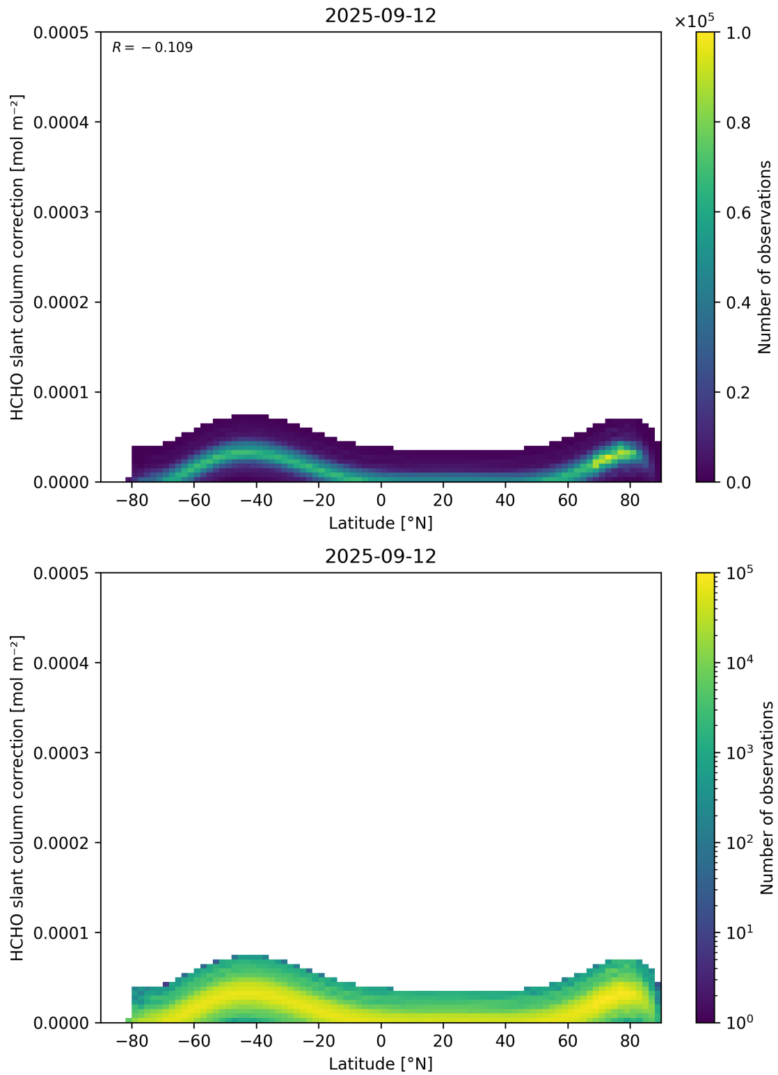
Figure 158: Scatter density plot of “Latitude” against “HCHO slant column correction” for 2025-09-11 to 2025-09-13.
