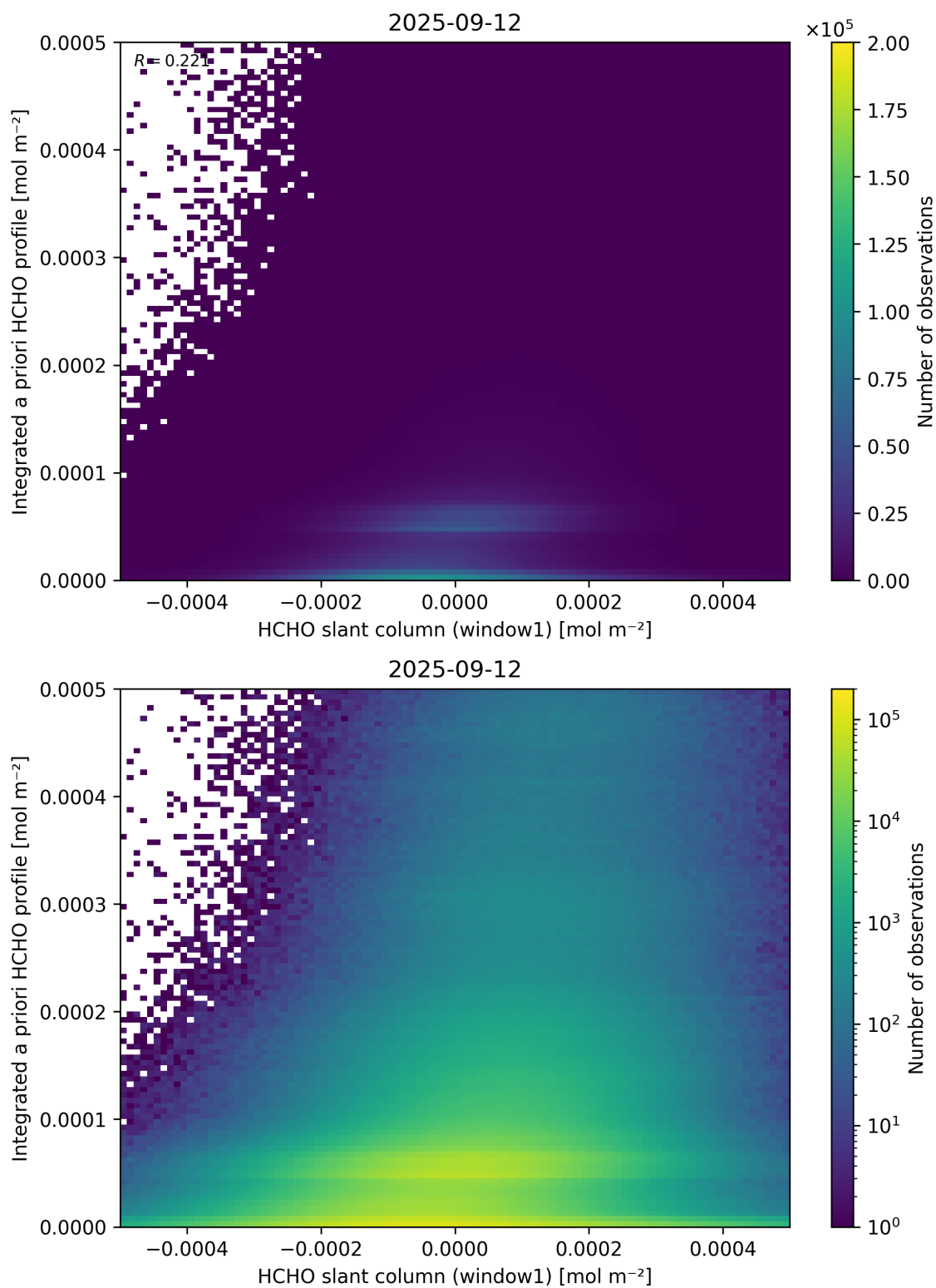
Figure 87: Scatter density plot of “HCHO slant column (window1)” against “Integrated a priori HCHO profile” for 2025-09-11 to 2025-09-13.
