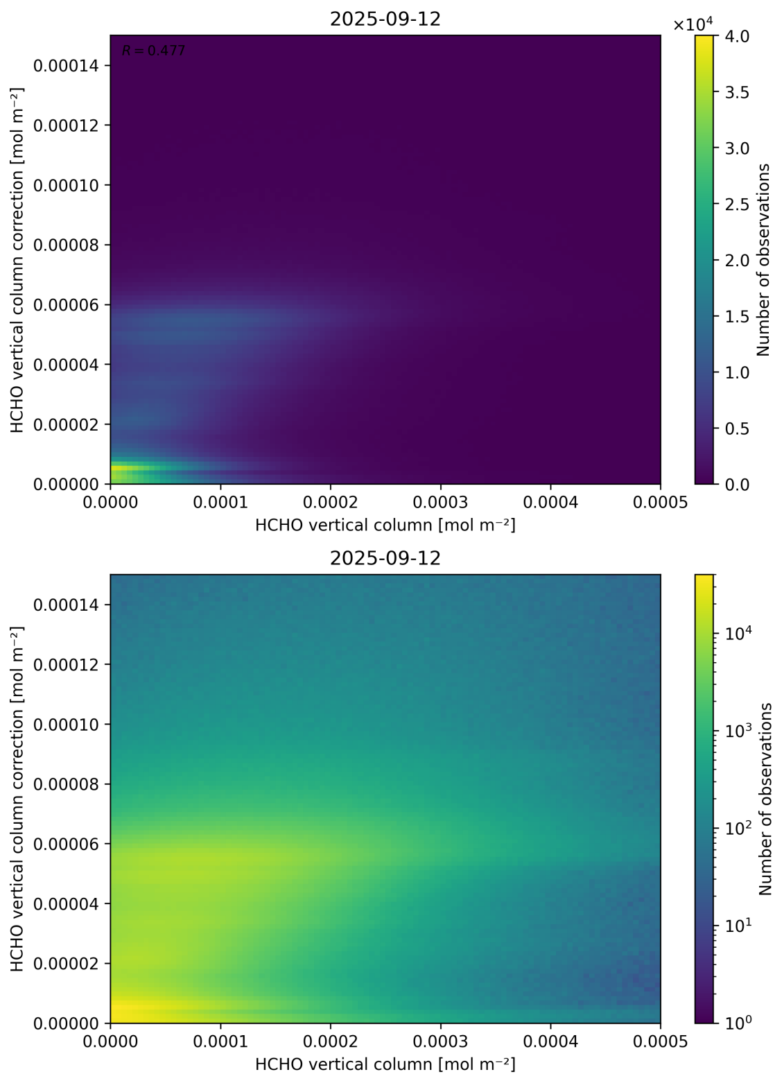
Figure 133: Scatter density plot of “HCHO vertical column” against “HCHO vertical column correction” for 2025-09-11 to 2025-09-13.
