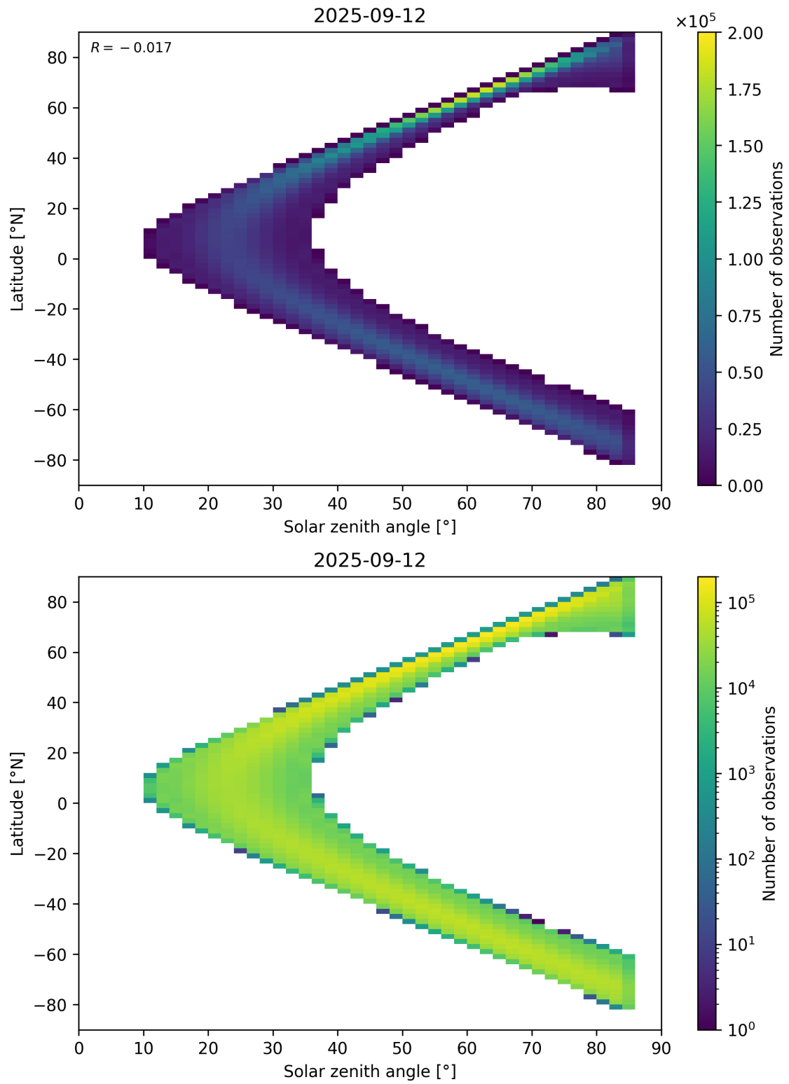
Figure 181: Scatter density plot of “Solar zenith angle” against “Latitude” for 2025-09-11 to 2025-09-13.
