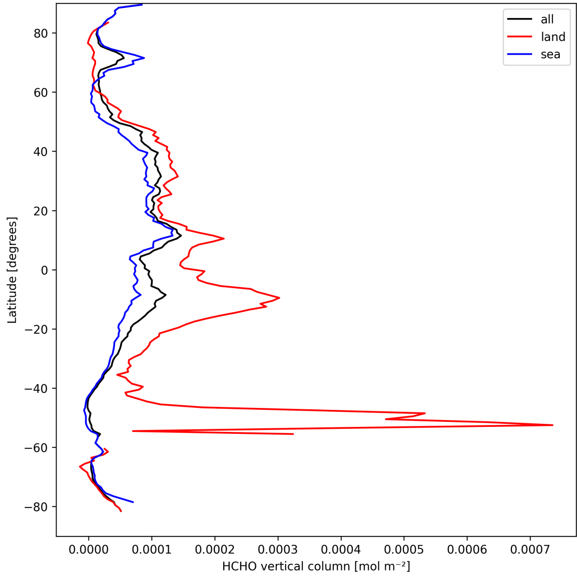
Figure 21: Zonal average of “HCHO vertical column” for 2025-09-11 to 2025-09-13.
