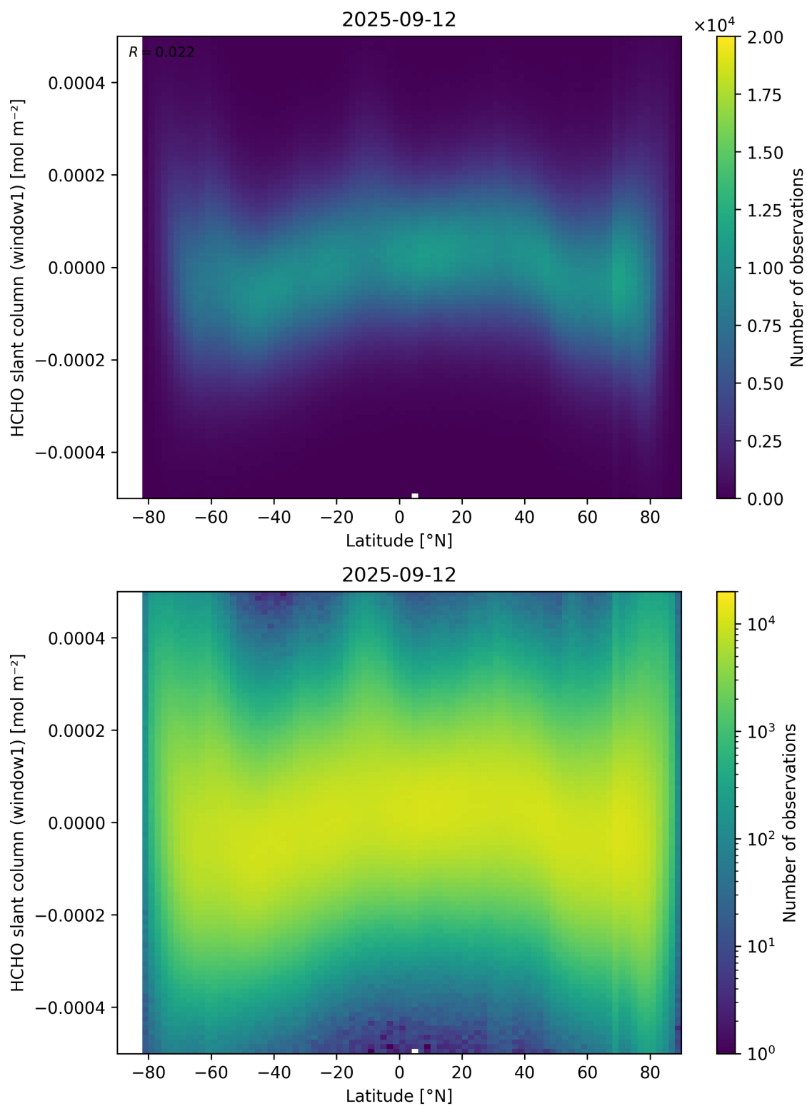
Figure 159: Scatter density plot of “Latitude” against “HCHO slant column (window1)” for 2025-09-11 to 2025-09-13.
