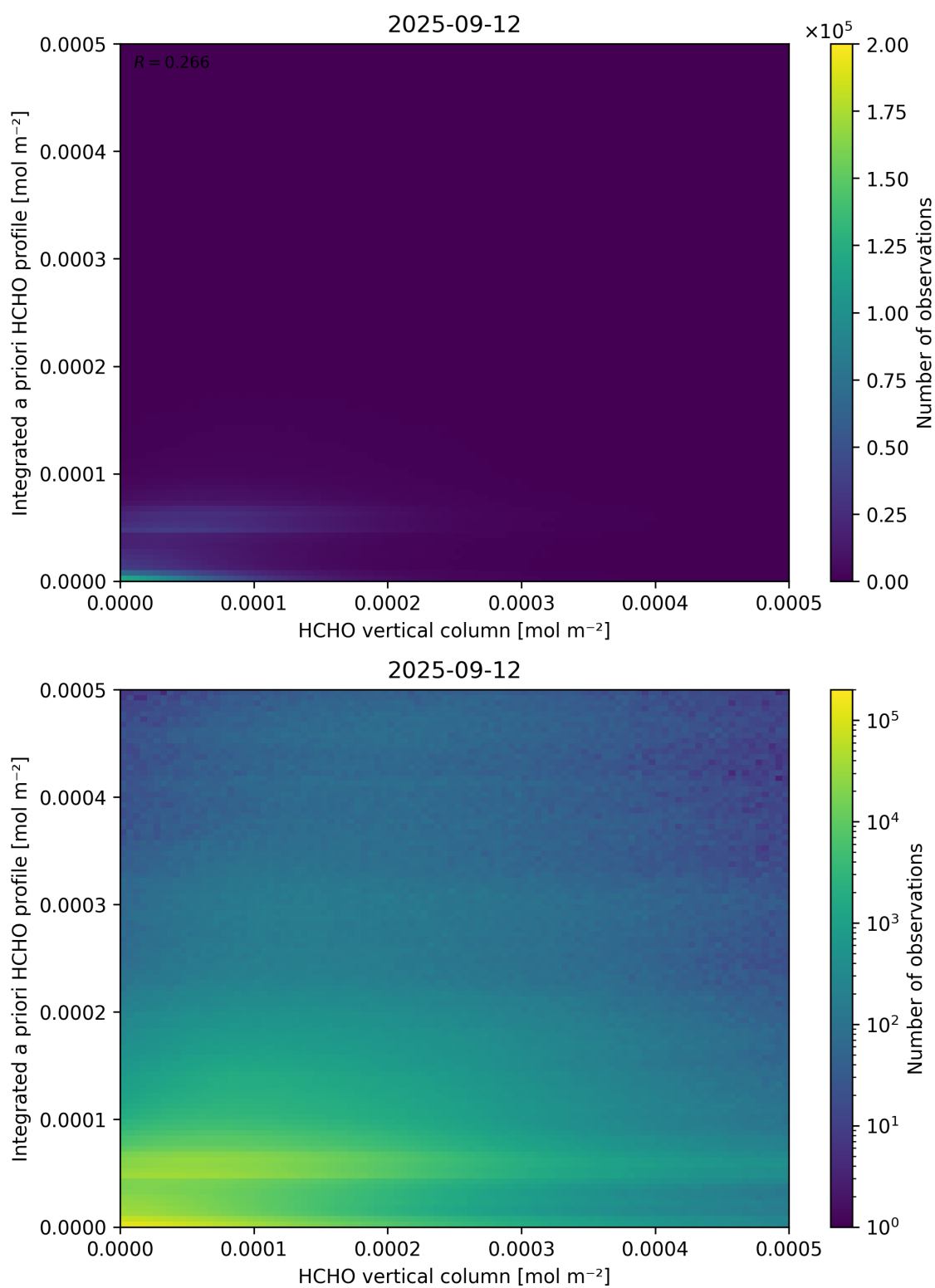
Figure 135: Scatter density plot of “HCHO vertical column” against “Integrated a priori HCHO profile” for 2025-09-11 to 2025-09-13.
