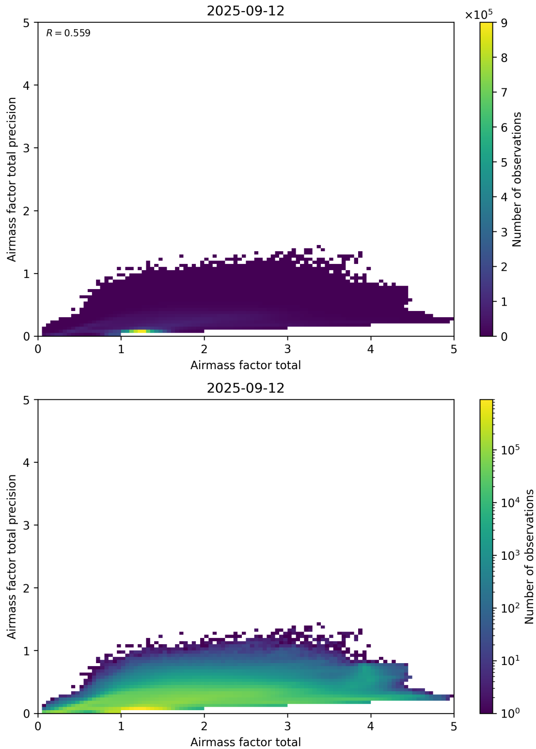
Figure 103: Scatter density plot of “Airmass factor total” against “Airmass factor total precision” for 2025-09-11 to 2025-09-13.
