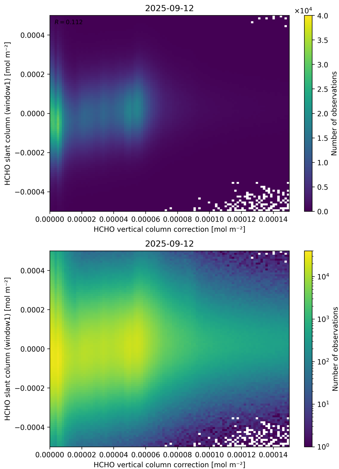
Figure 118: Scatter density plot of “HCHO vertical column correction” against “HCHO slant column (window1)” for 2025-09-11 to 2025-09-13.
