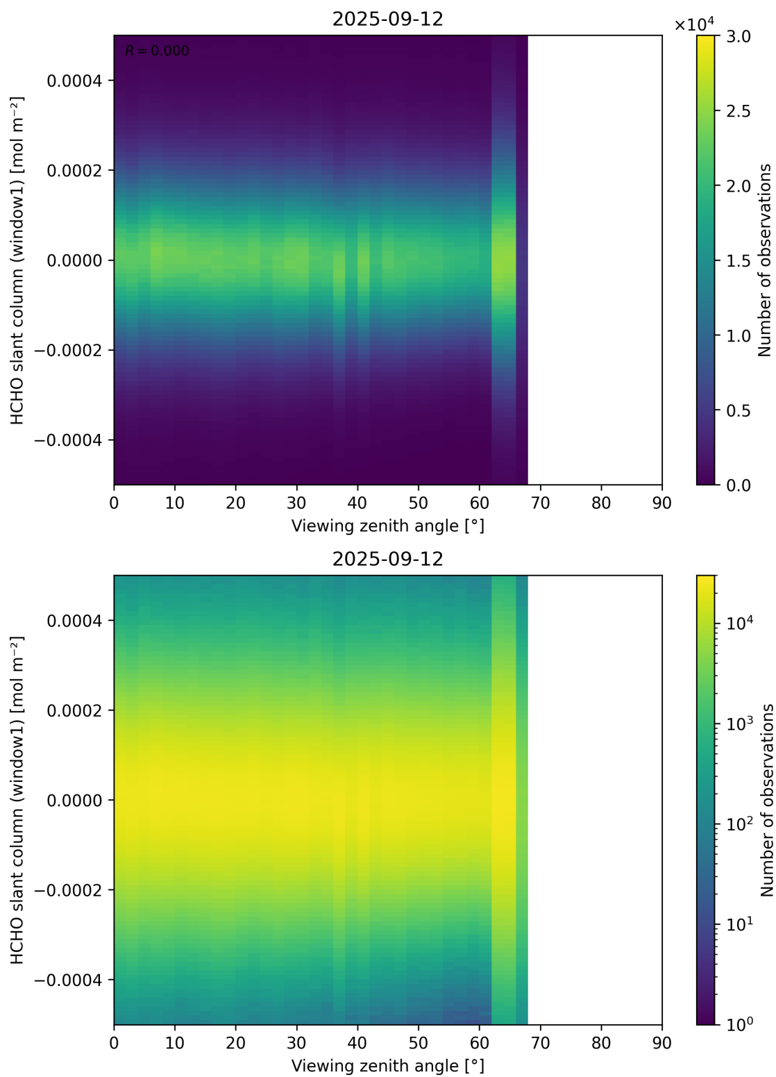
Figure 188: Scatter density plot of “Viewing zenith angle” against “HCHO slant column (window1)” for 2025-09-11 to 2025-09-13.
