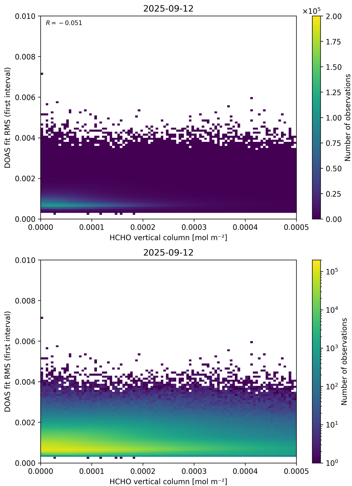
Figure 123: Scatter density plot of “HCHO vertical column” against “DOAS fit RMS (first interval)” for 2025-09-11 to 2025-09-13.
