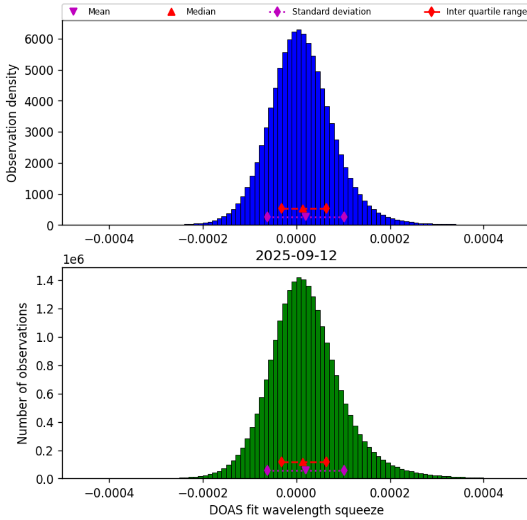
Figure 45: Histogram of “DOAS fit wavelength squeeze” for 2025-09-11 to 2025-09-13
