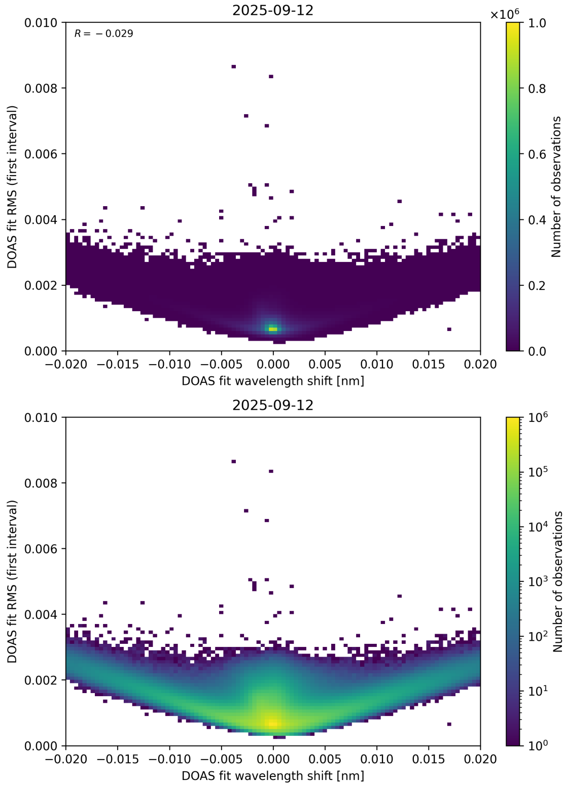
Figure 64: Scatter density plot of “DOAS fit wavelength shift” against “DOAS fit RMS (first interval)” for 2025-09-11 to 2025-09-13.
