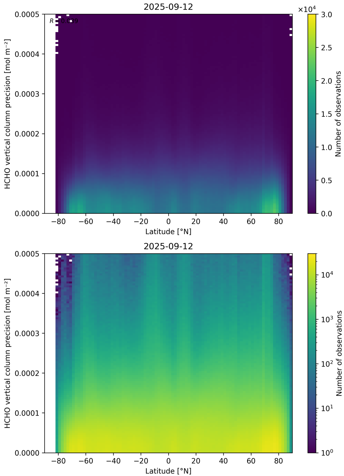
Figure 165: Scatter density plot of “Latitude” against “HCHO vertical column precision” for 2025-09-11 to 2025-09-13.
