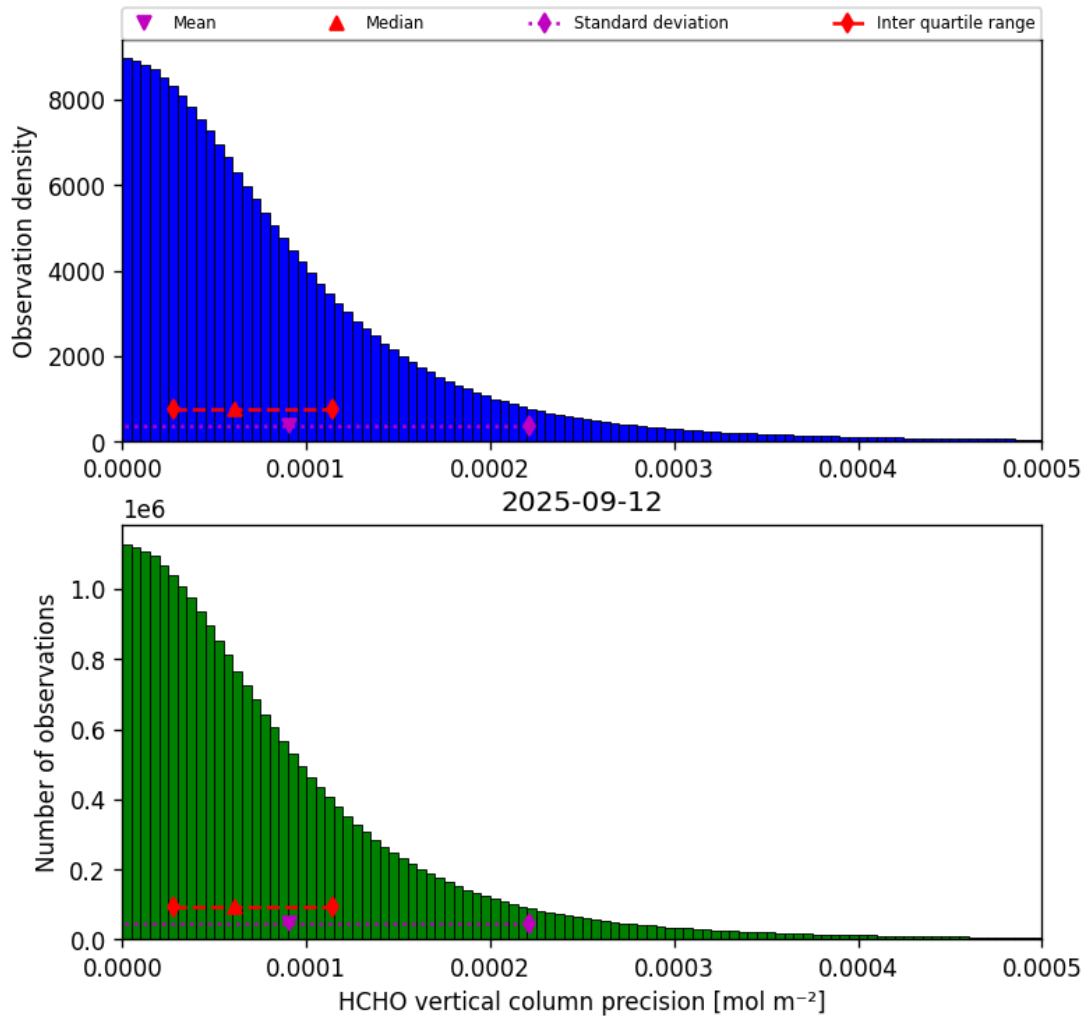
Figure 36: Histogram of “HCHO vertical column precision” for 2025-09-11 to 2025-09-13
