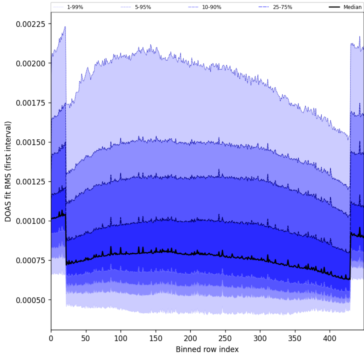
Figure 60: Along track statistics of “DOAS fit RMS (first interval)” for 2025-09-11 to 2025-09-13
