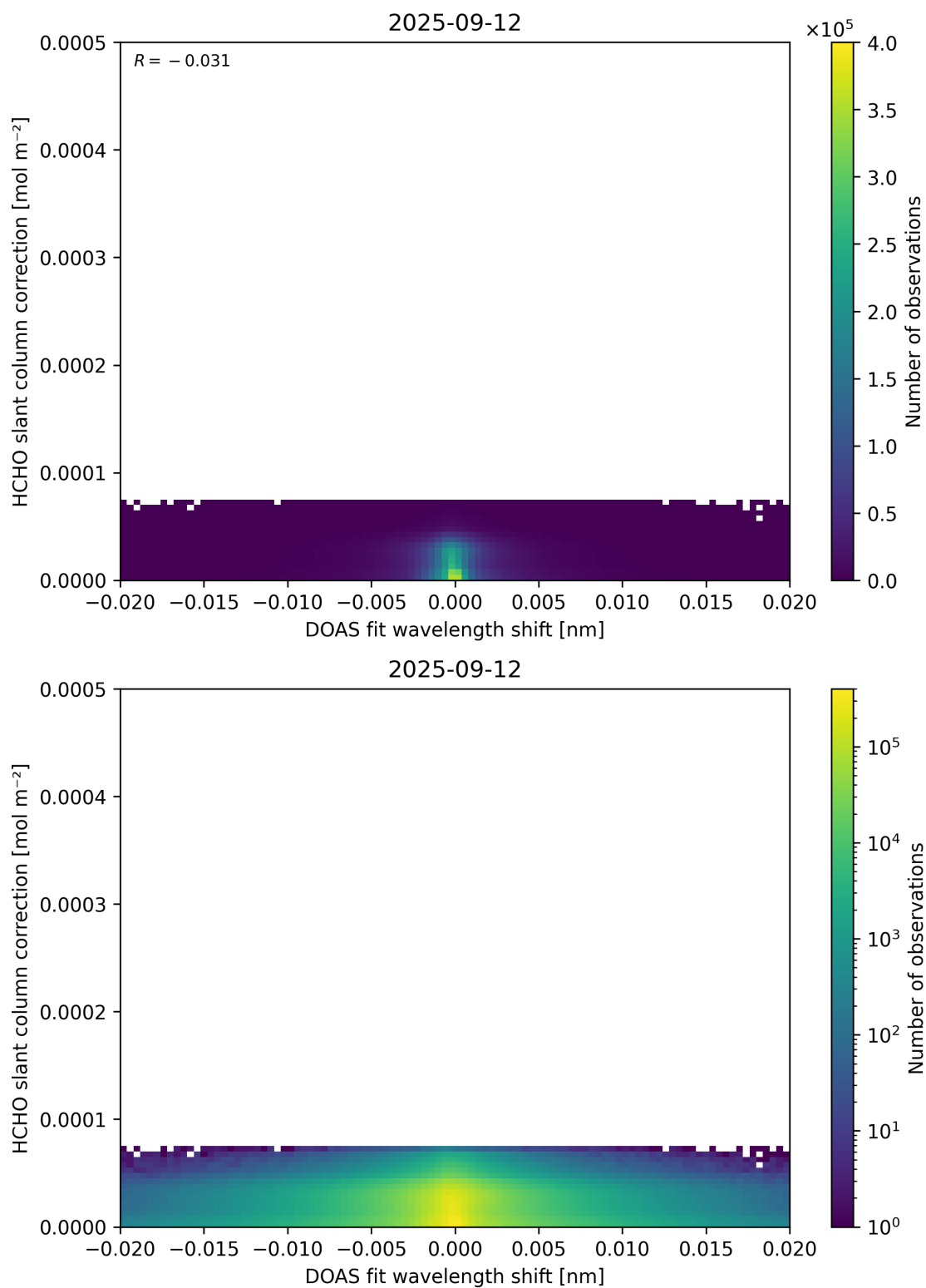
Figure 67: Scatter density plot of “DOAS fit wavelength shift” against “HCHO slant column correction” for 2025-09-11 to 2025-09-13.
