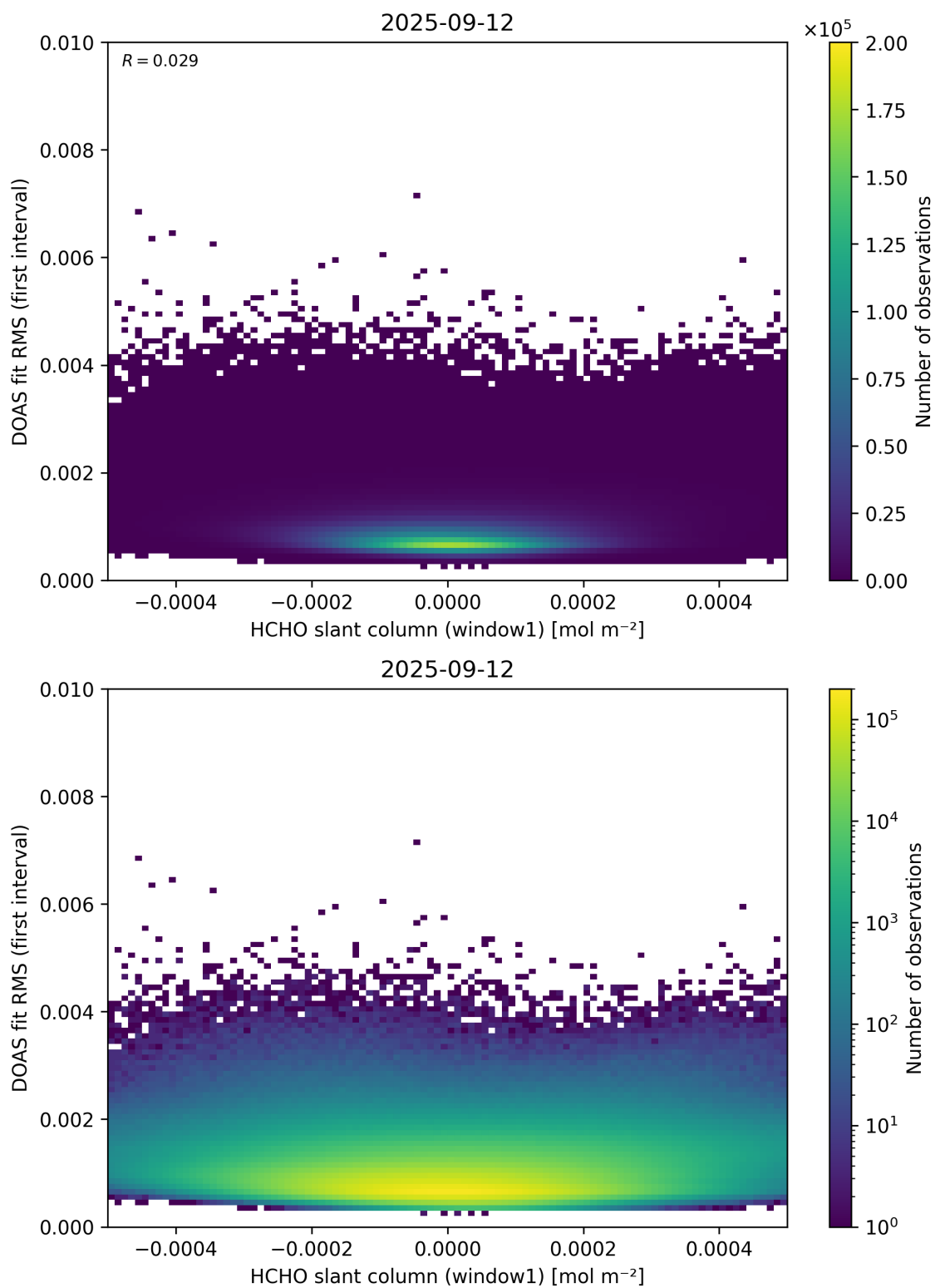
Figure 78: Scatter density plot of “HCHO slant column (window1)” against “DOAS fit RMS (first interval)” for 2025-09-11 to 2025-09-13.
