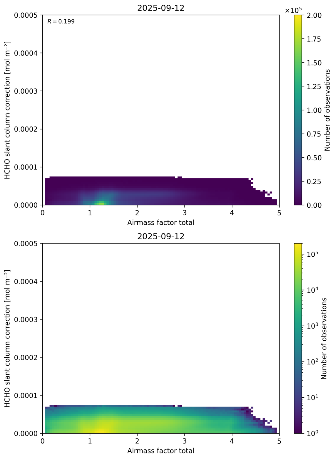
Figure 102: Scatter density plot of “Airmass factor total” against “HCHO slant column correction” for 2025-09-11 to 2025-09-13.
