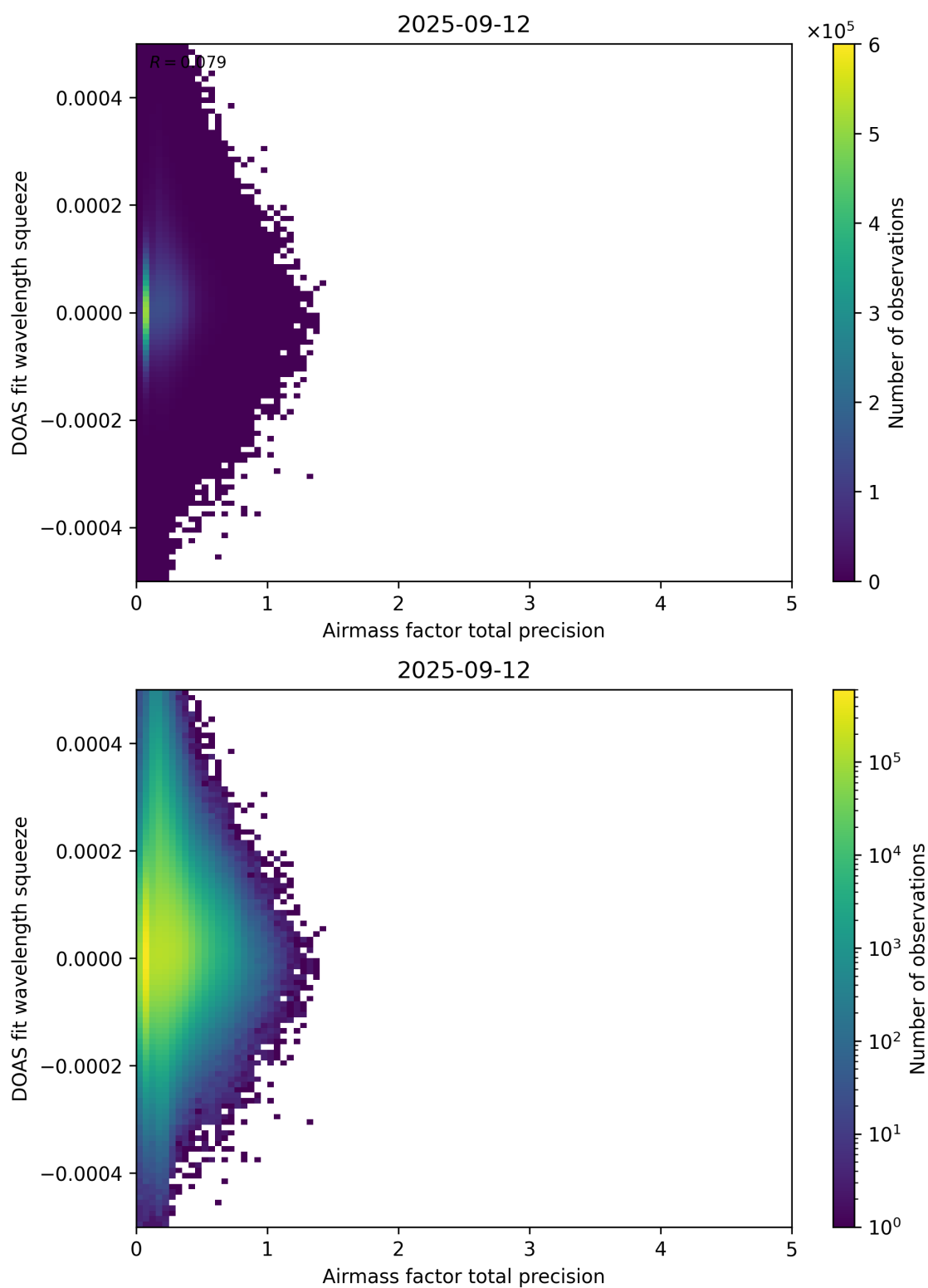
Figure 107: Scatter density plot of “Airmass factor total precision” against “DOAS fit wavelength squeeze” for 2025-09-11 to 2025-09-13.
