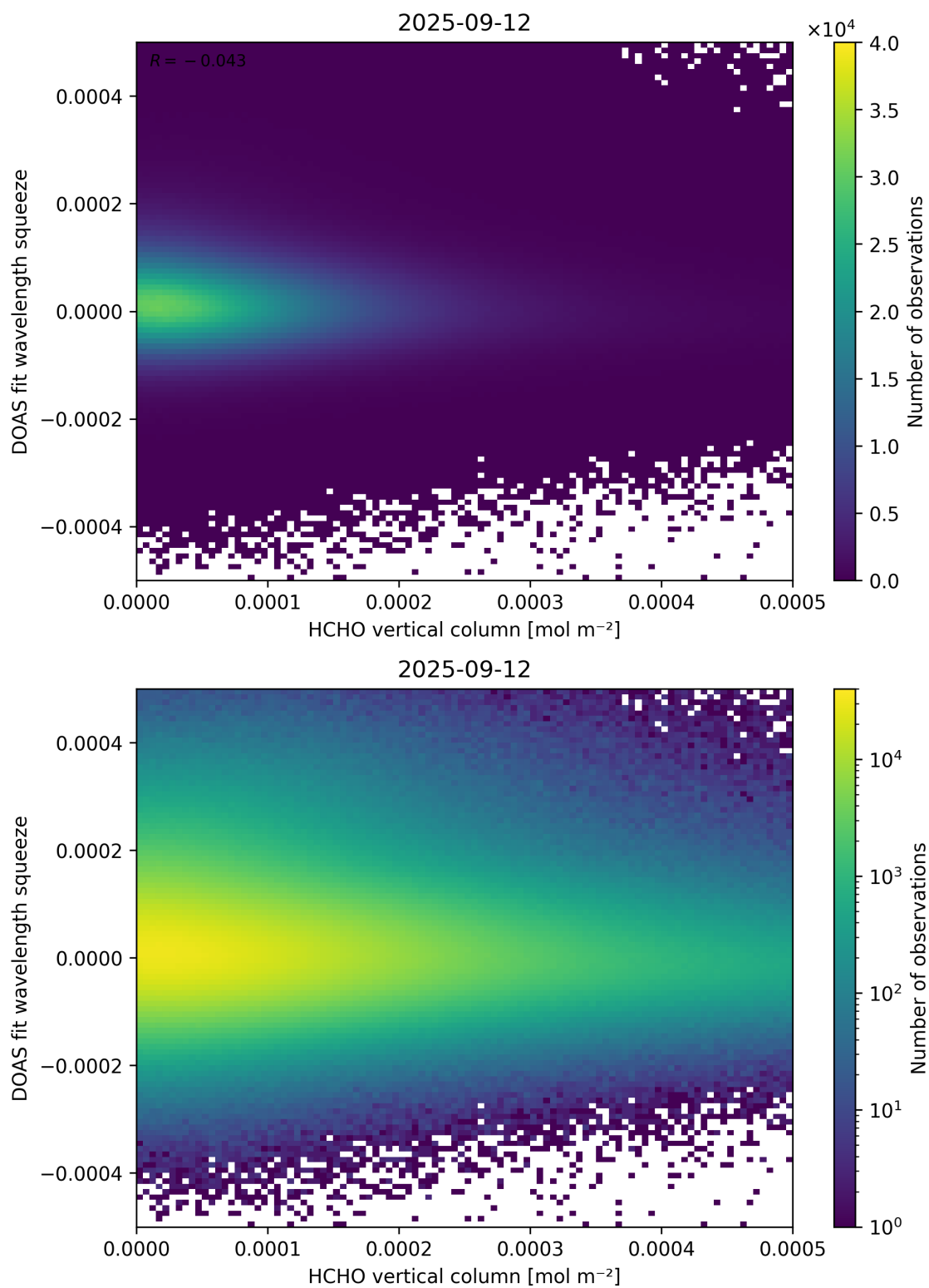
Figure 125: Scatter density plot of “HCHO vertical column” against “DOAS fit wavelength squeeze” for 2025-09-11 to 2025-09-13.
