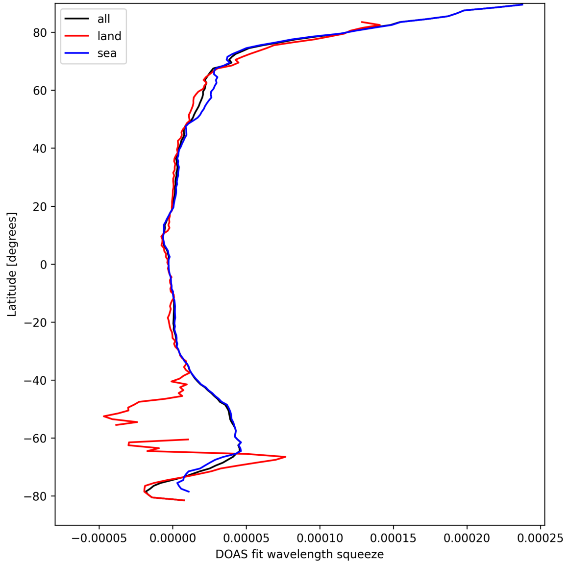
Figure 31: Zonal average of “DOAS fit wavelength squeeze” for 2025-09-11 to 2025-09-13.
