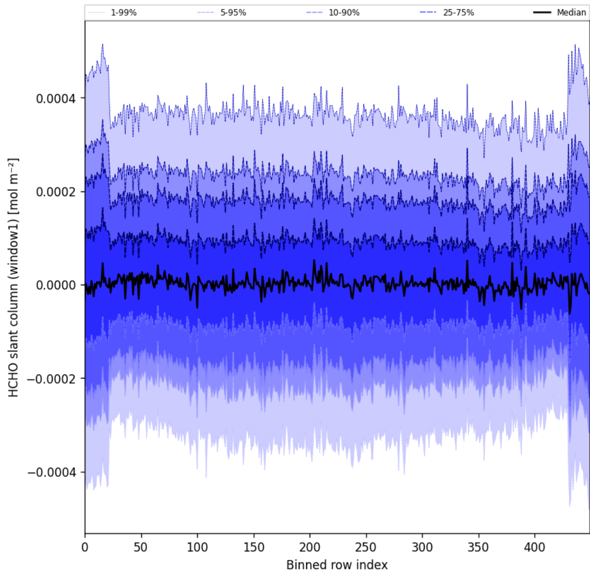
Figure 52: Along track statistics of “HCHO slant column (window1)” for 2025-09-11 to 2025-09-13
