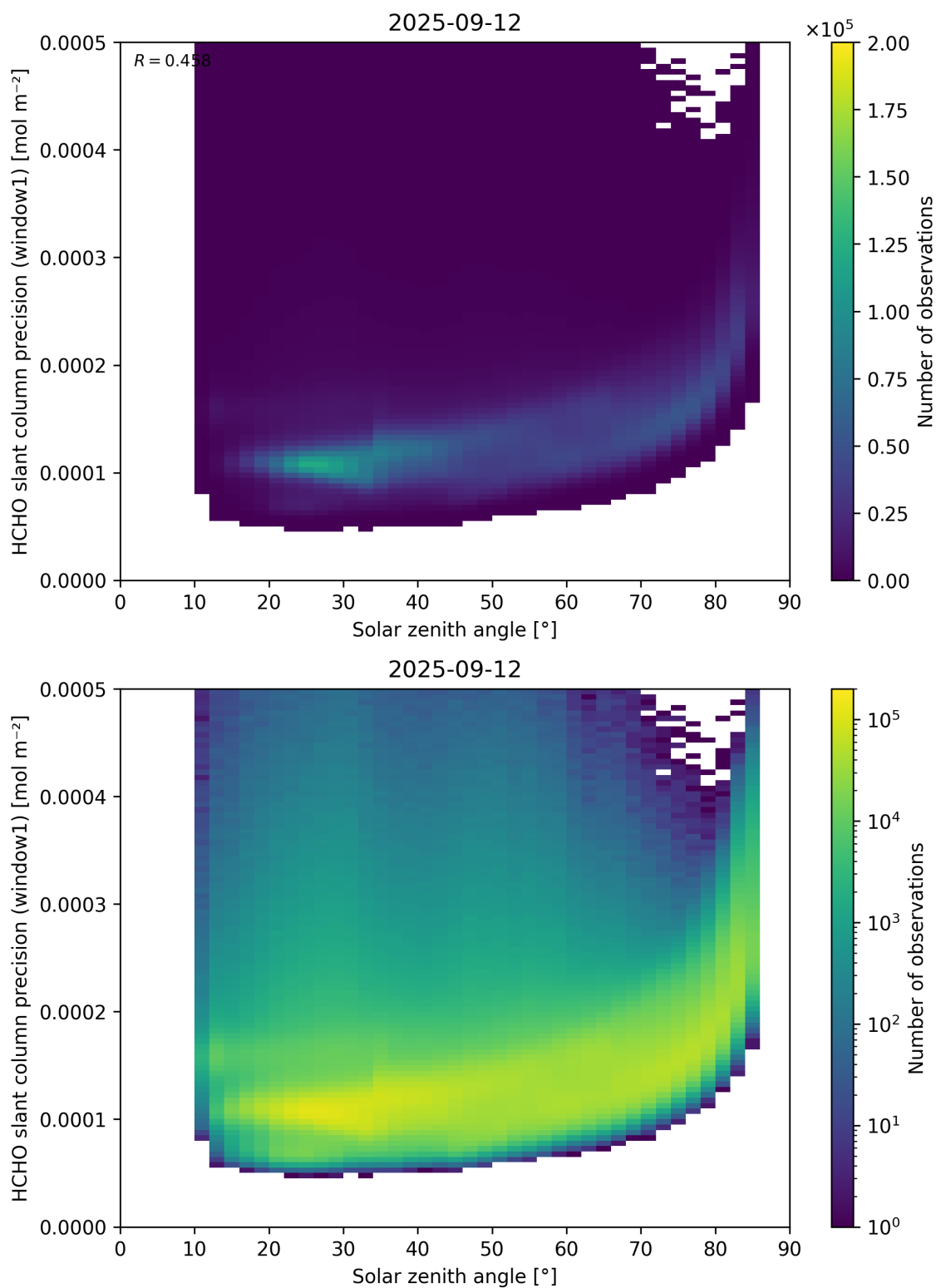
Figure 174: Scatter density plot of “Solar zenith angle” against “HCHO slant column precision (window1)” for 2025-09-11 to 2025-09-13.
