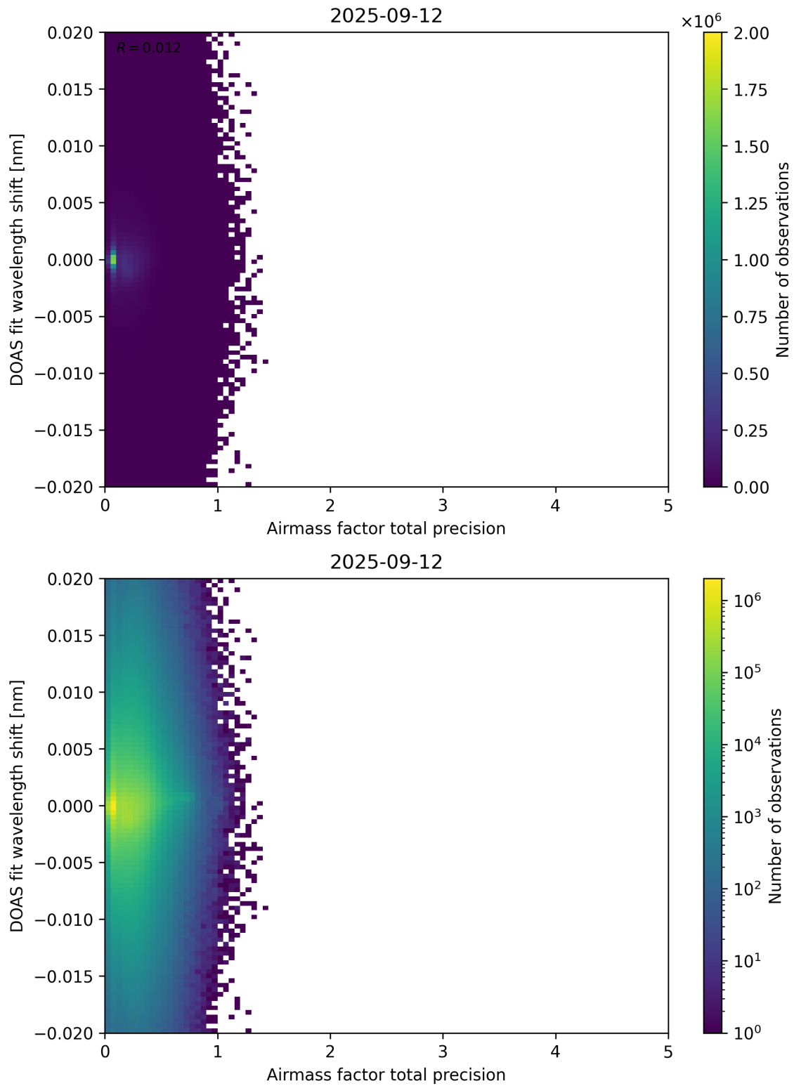
Figure 106: Scatter density plot of “Airmass factor total precision” against “DOAS fit wavelength shift” for 2025-09-11 to 2025-09-13.
