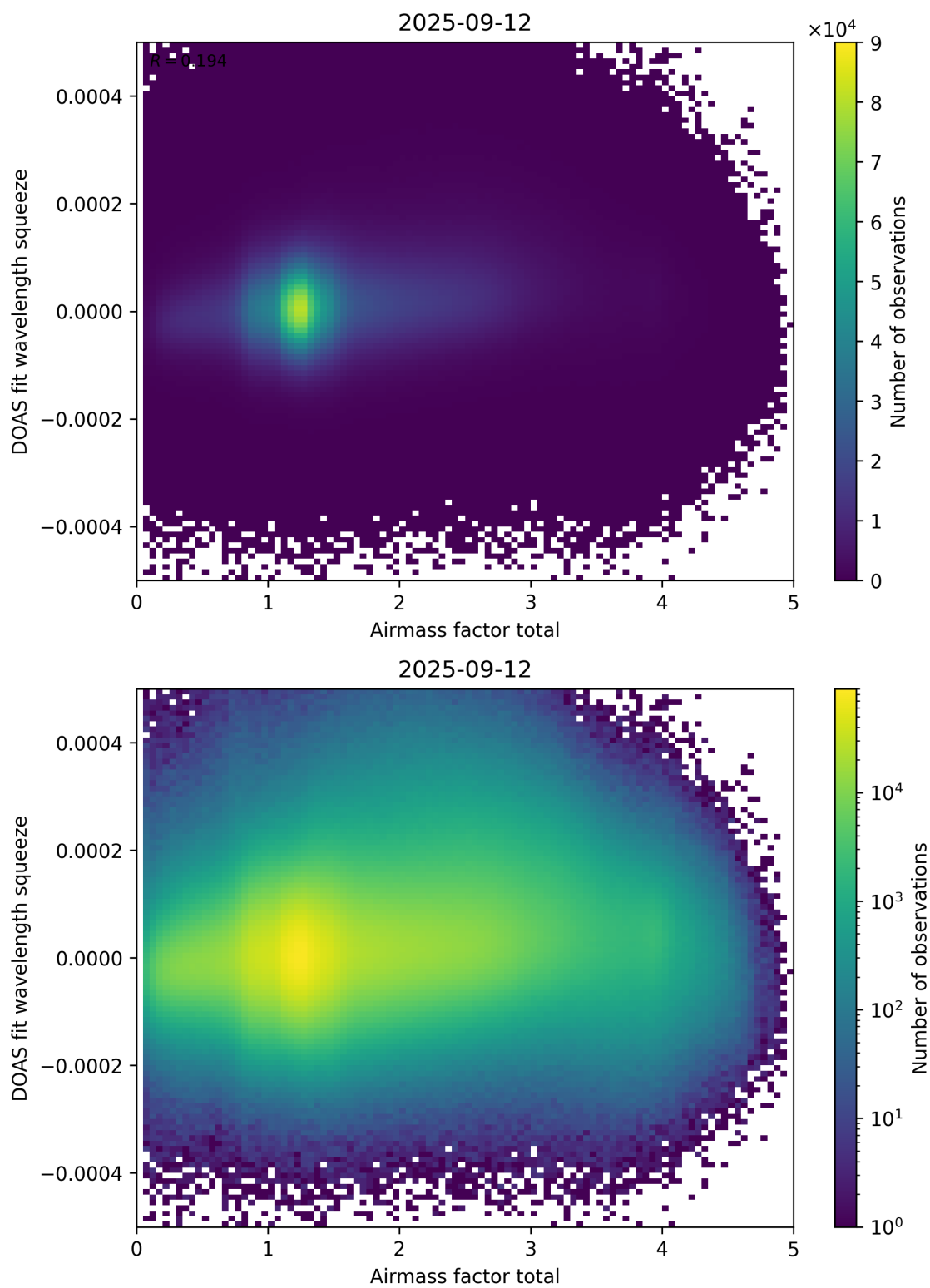
Figure 99: Scatter density plot of “Airmass factor total” against “DOAS fit wavelength squeeze” for 2025-09-11 to 2025-09-13.
