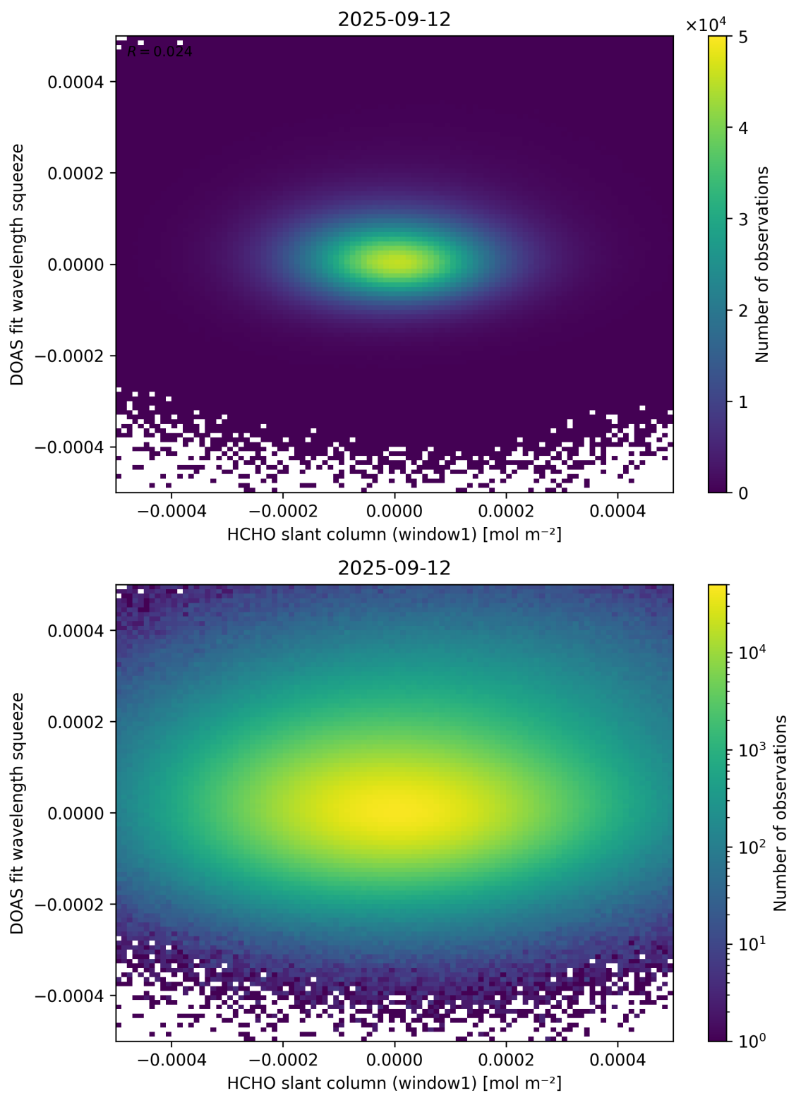
Figure 80: Scatter density plot of “HCHO slant column (window1)” against “DOAS fit wavelength squeeze” for 2025-09-11 to 2025-09-13.
