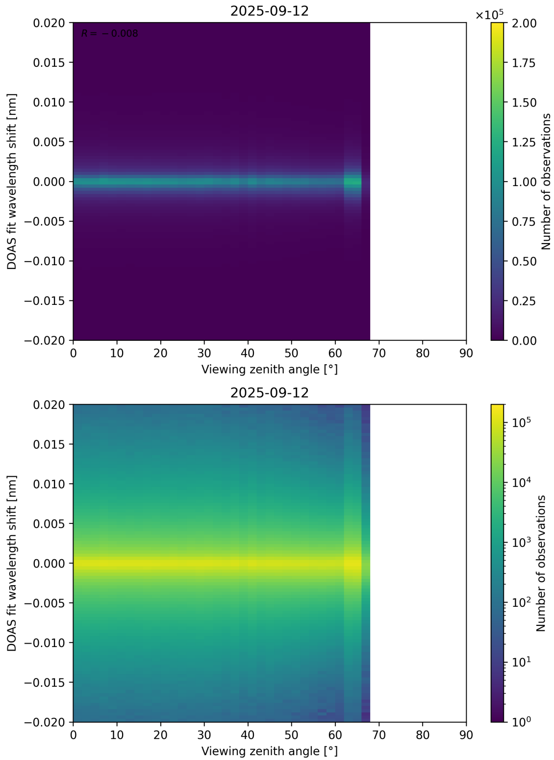
Figure 183: Scatter density plot of “Viewing zenith angle” against “DOAS fit wavelength shift” for 2025-09-11 to 2025-09-13.
