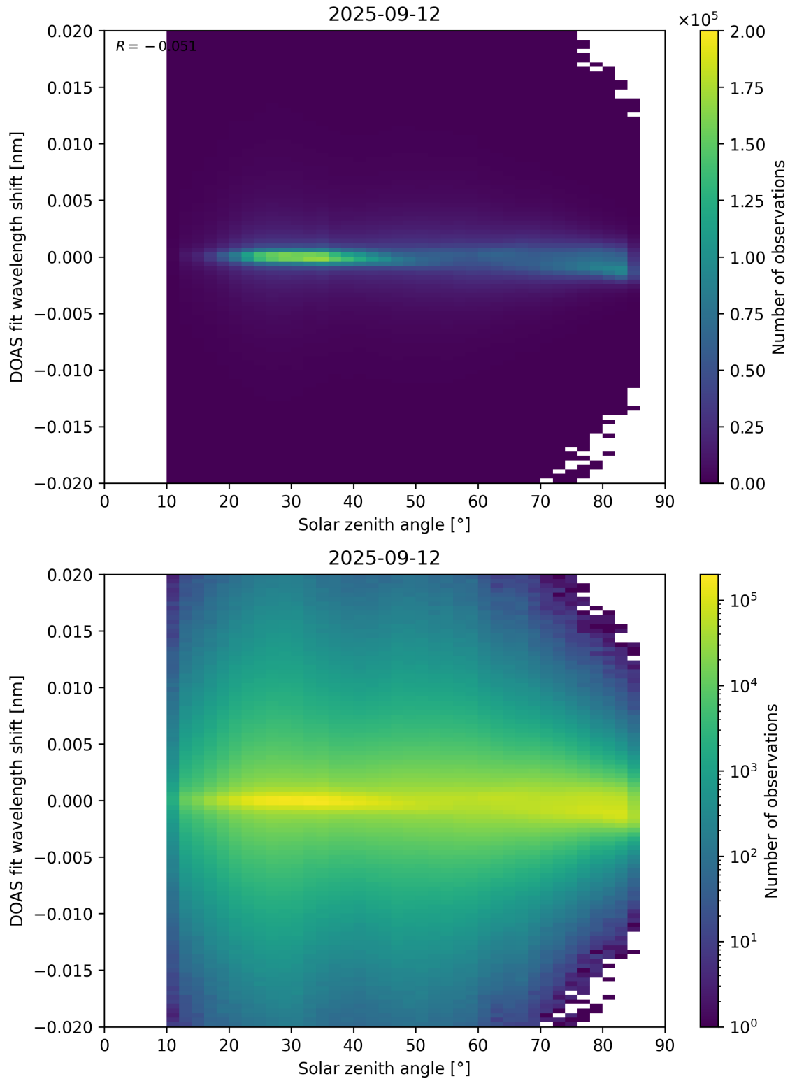
Figure 168: Scatter density plot of “Solar zenith angle” against “DOAS fit wavelength shift” for 2025-09-11 to 2025-09-13.
