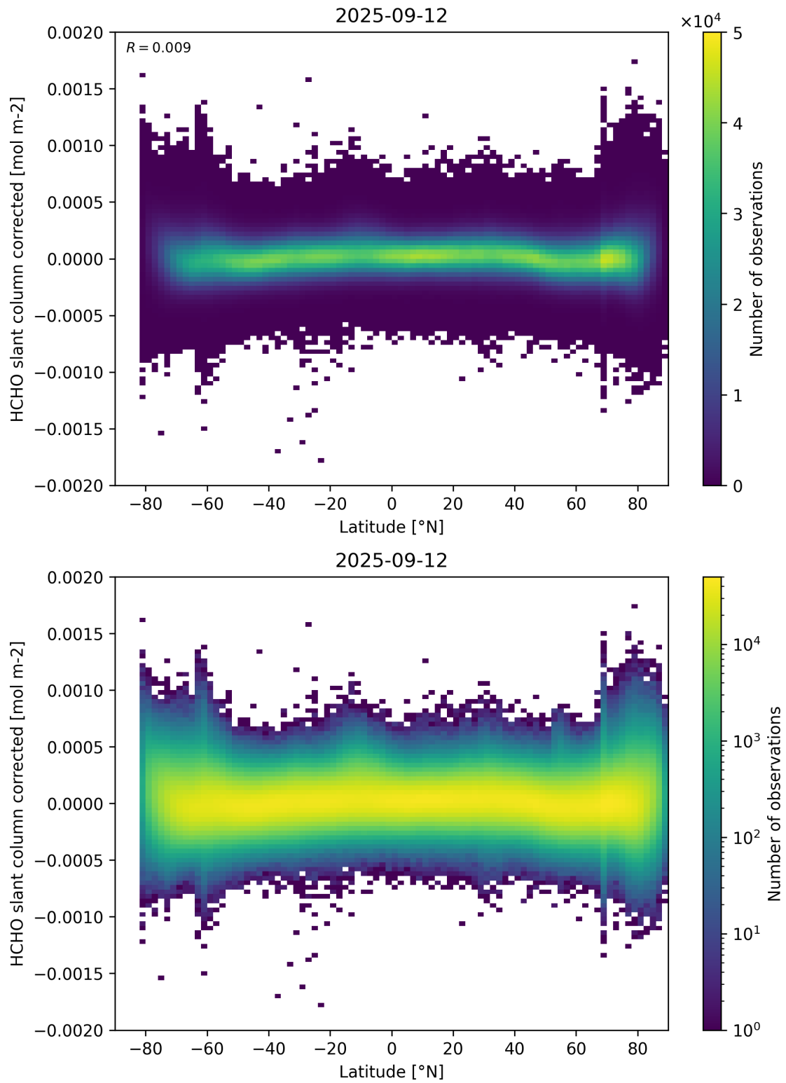
Figure 157: Scatter density plot of “Latitude” against “HCHO slant column corrected” for 2025-09-11 to 2025-09-13.
