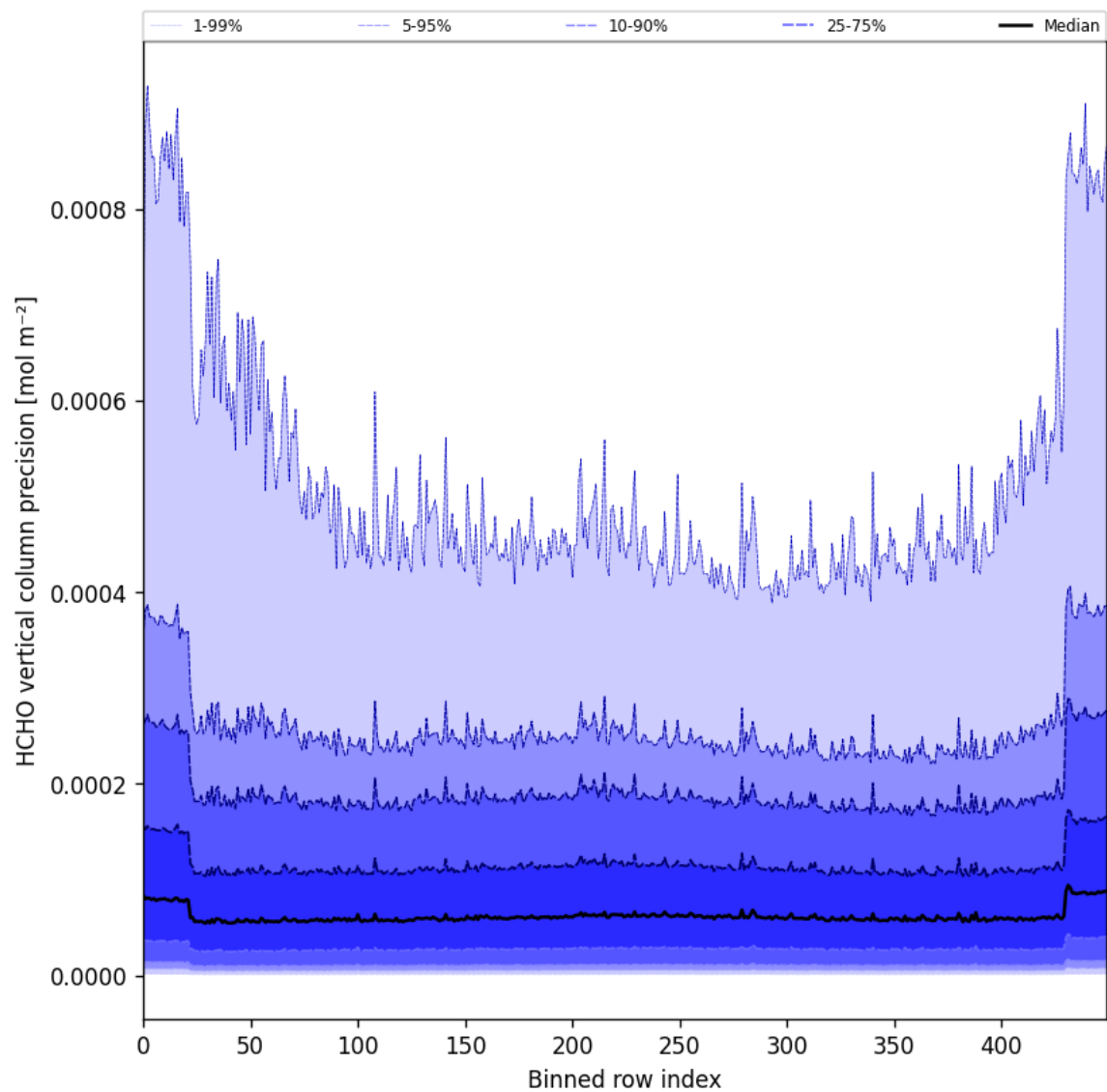
Figure 50: Along track statistics of “HCHO vertical column precision” for 2025-09-11 to 2025-09-13
