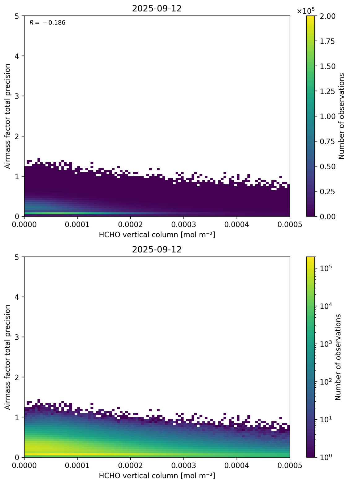
Figure 132: Scatter density plot of “HCHO vertical column” against “Airmass factor total precision” for 2025-09-11 to 2025-09-13.
