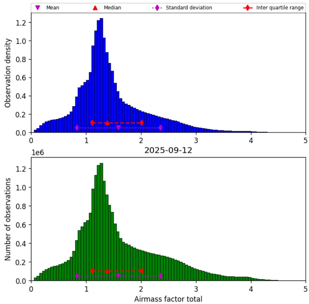
Figure 40: Histogram of “Airmass factor total” for 2025-09-11 to 2025-09-13
