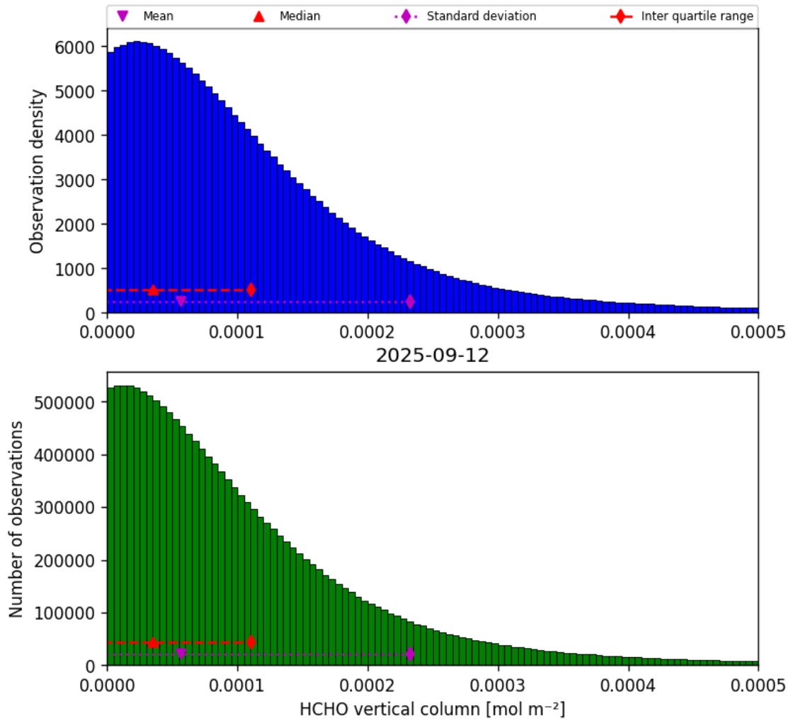
Figure 35: Histogram of “HCHO vertical column” for 2025-09-11 to 2025-09-13
