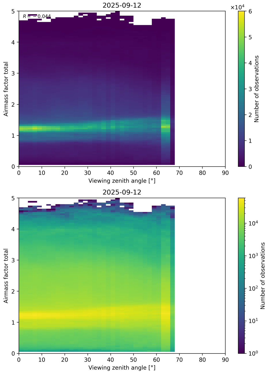
Figure 190: Scatter density plot of “Viewing zenith angle” against “Airmass factor total” for 2025-09-11 to 2025-09-13.
