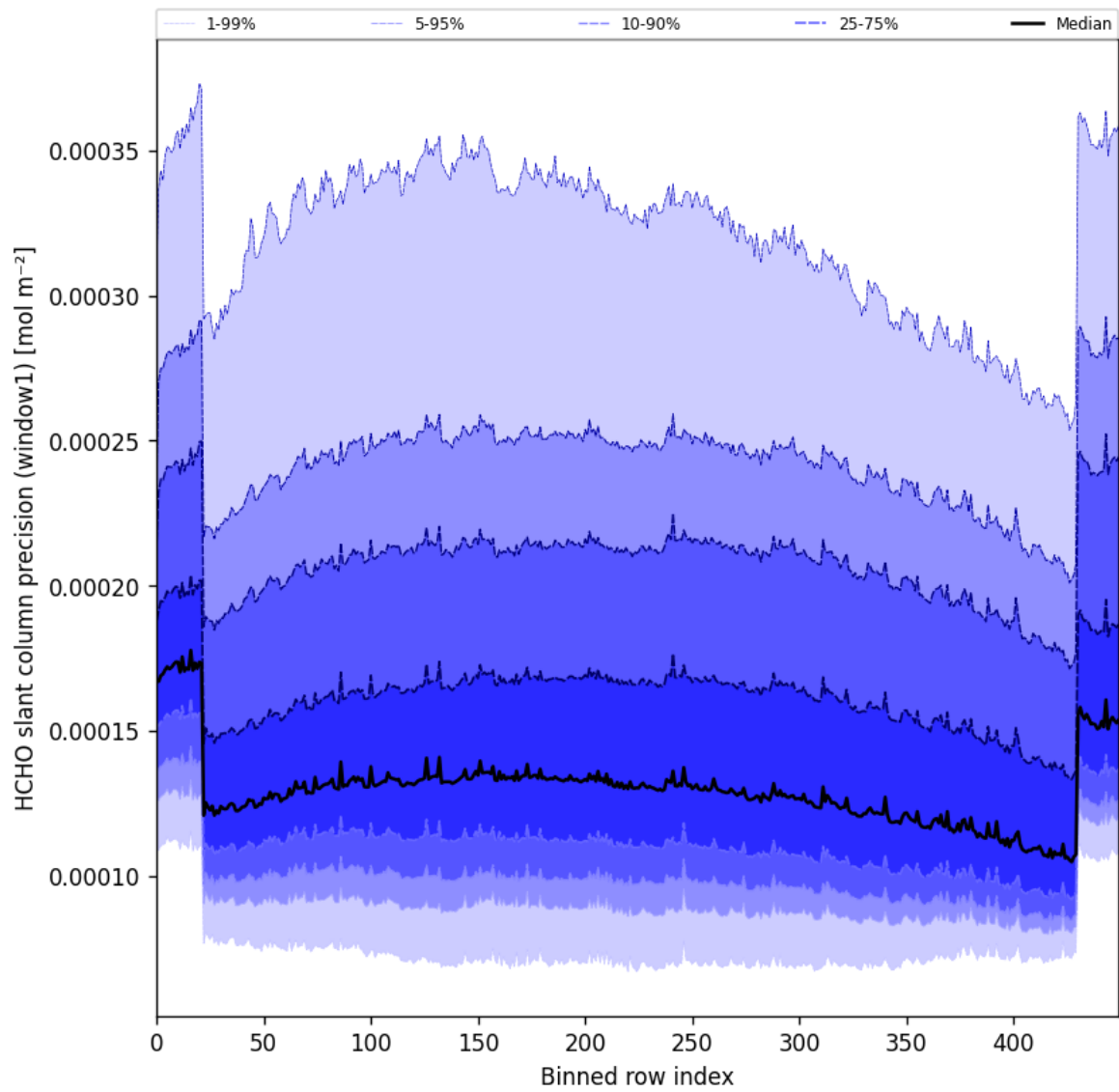
Figure 53: Along track statistics of “HCHO slant column precision (window1)” for 2025-09-11 to 2025-09-13
