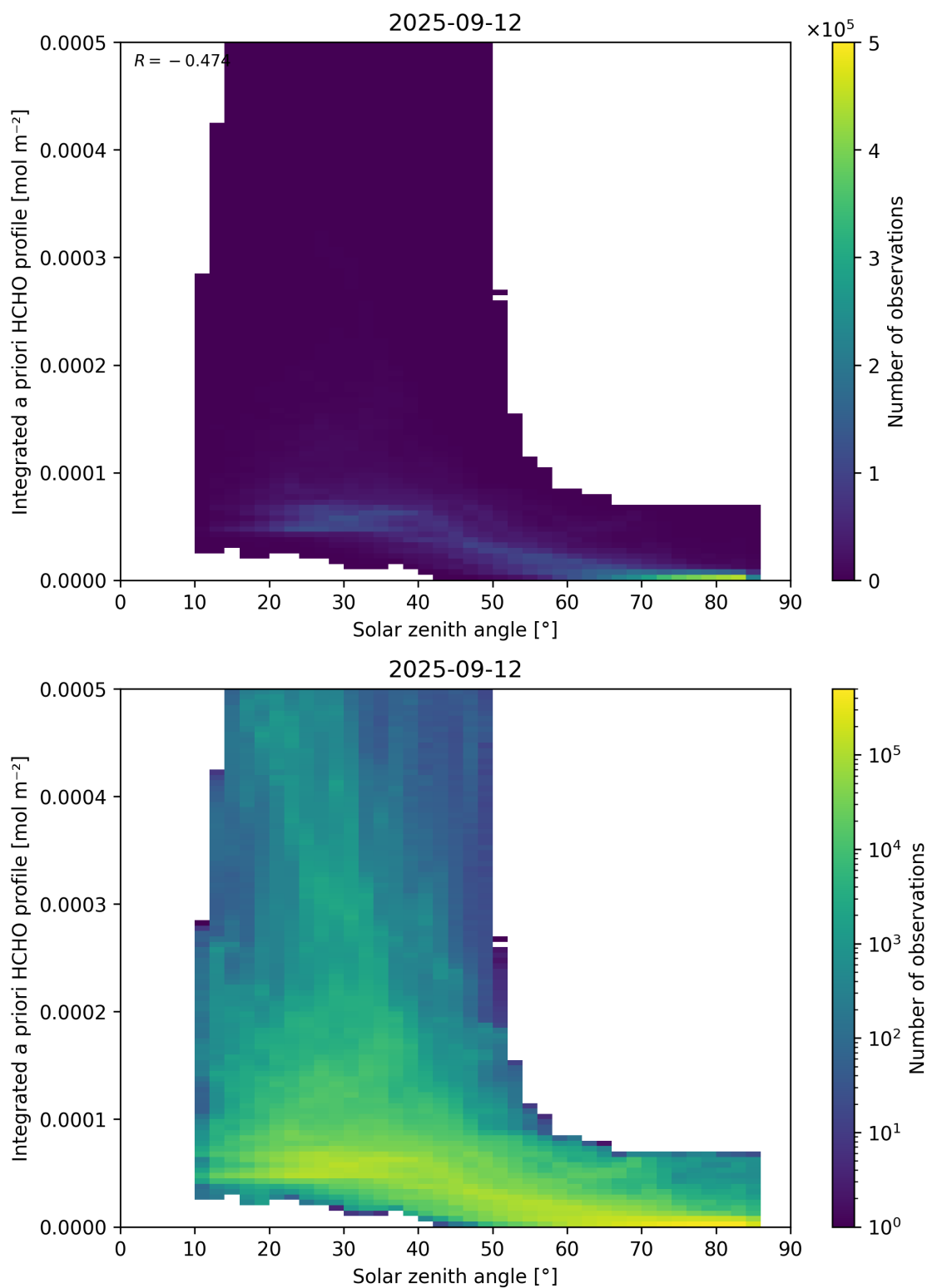
Figure 180: Scatter density plot of “Solar zenith angle” against “Integrated a priori HCHO profile” for 2025-09-11 to 2025-09-13.
