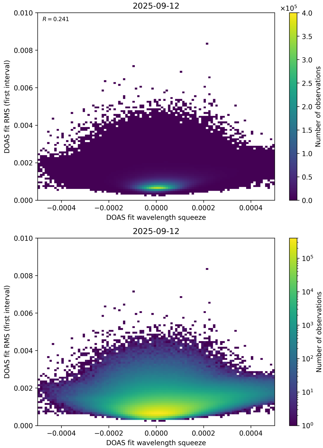
Figure 68: Scatter density plot of “DOAS fit wavelength squeeze” against “DOAS fit RMS (first interval)” for 2025-09-11 to 2025-09-13.
