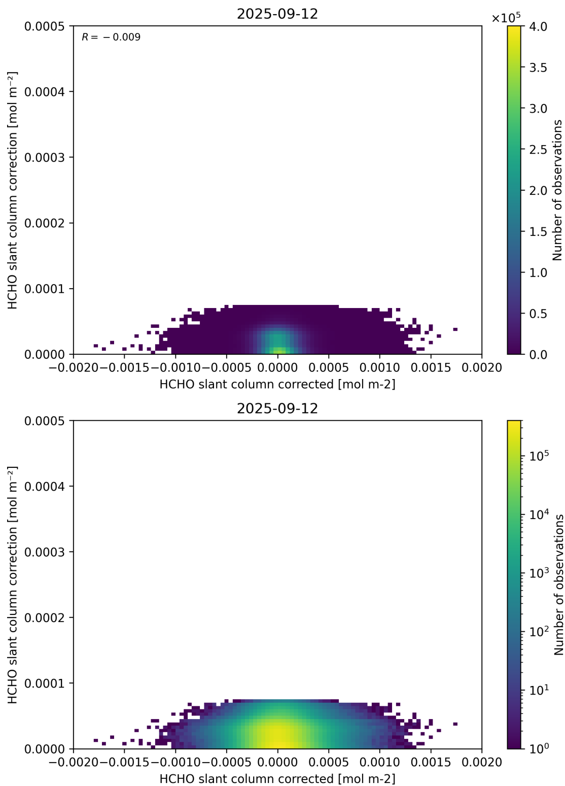
Figure 77: Scatter density plot of “HCHO slant column corrected” against “HCHO slant column correction” for 2025-09-11 to 2025-09-13.
