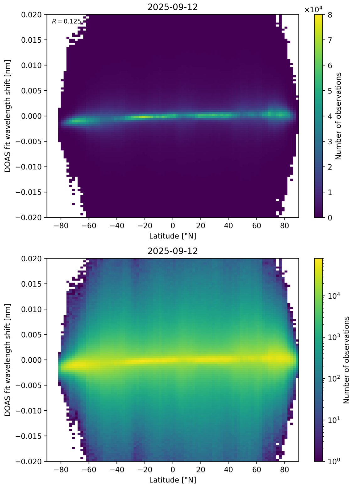
Figure 154: Scatter density plot of “Latitude” against “DOAS fit wavelength shift” for 2025-09-11 to 2025-09-13.
