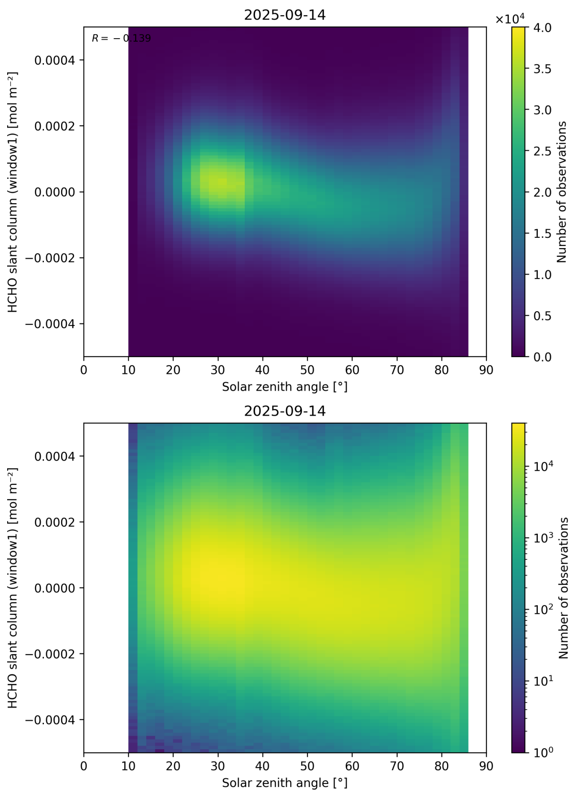
Figure 173: Scatter density plot of “Solar zenith angle” against “HCHO slant column (window1)” for 2025-09-13 to 2025-09-15.
