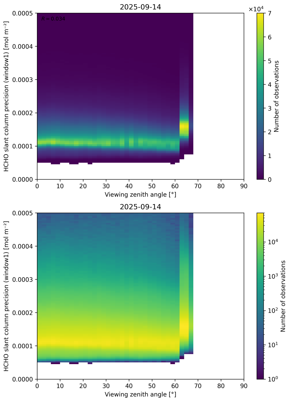
Figure 189: Scatter density plot of “Viewing zenith angle” against “HCHO slant column precision (window1)” for 2025-09-13 to 2025-09-15.
