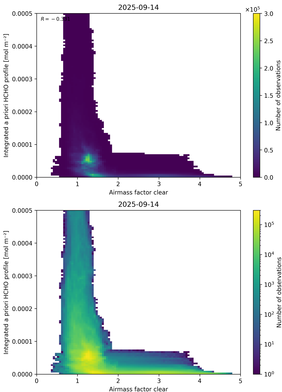
Figure 76: Scatter density plot of “Airmass factor clear” against “Integrated a priori HCHO profile” for 2025-09-13 to 2025-09-15.
