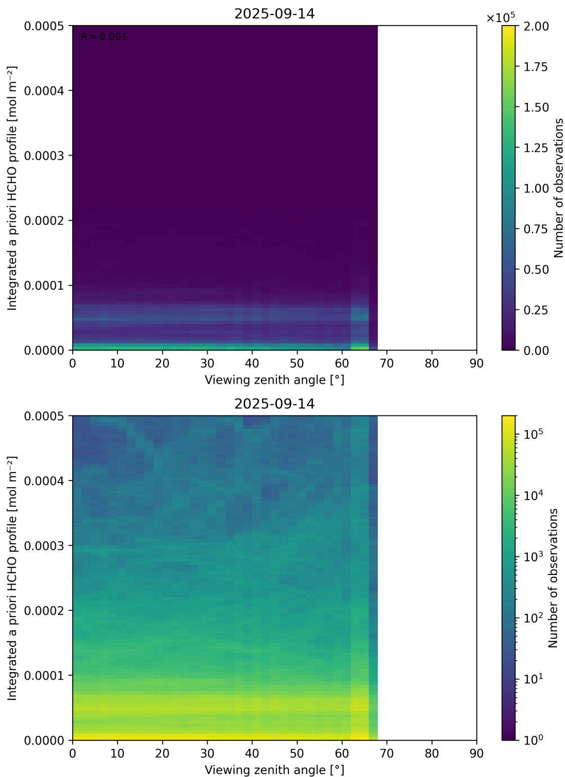
Figure 195: Scatter density plot of “Viewing zenith angle” against “Integrated a priori HCHO profile” for 2025-09-13 to 2025-09-15.
