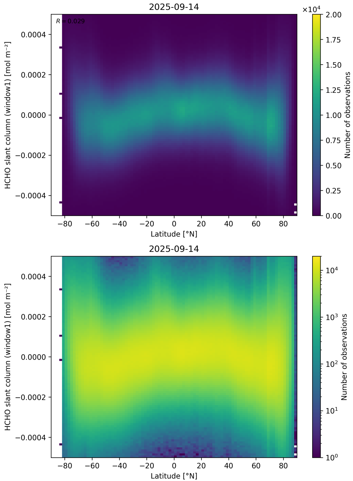
Figure 159: Scatter density plot of “Latitude” against “HCHO slant column (window1)” for 2025-09-13 to 2025-09-15.
