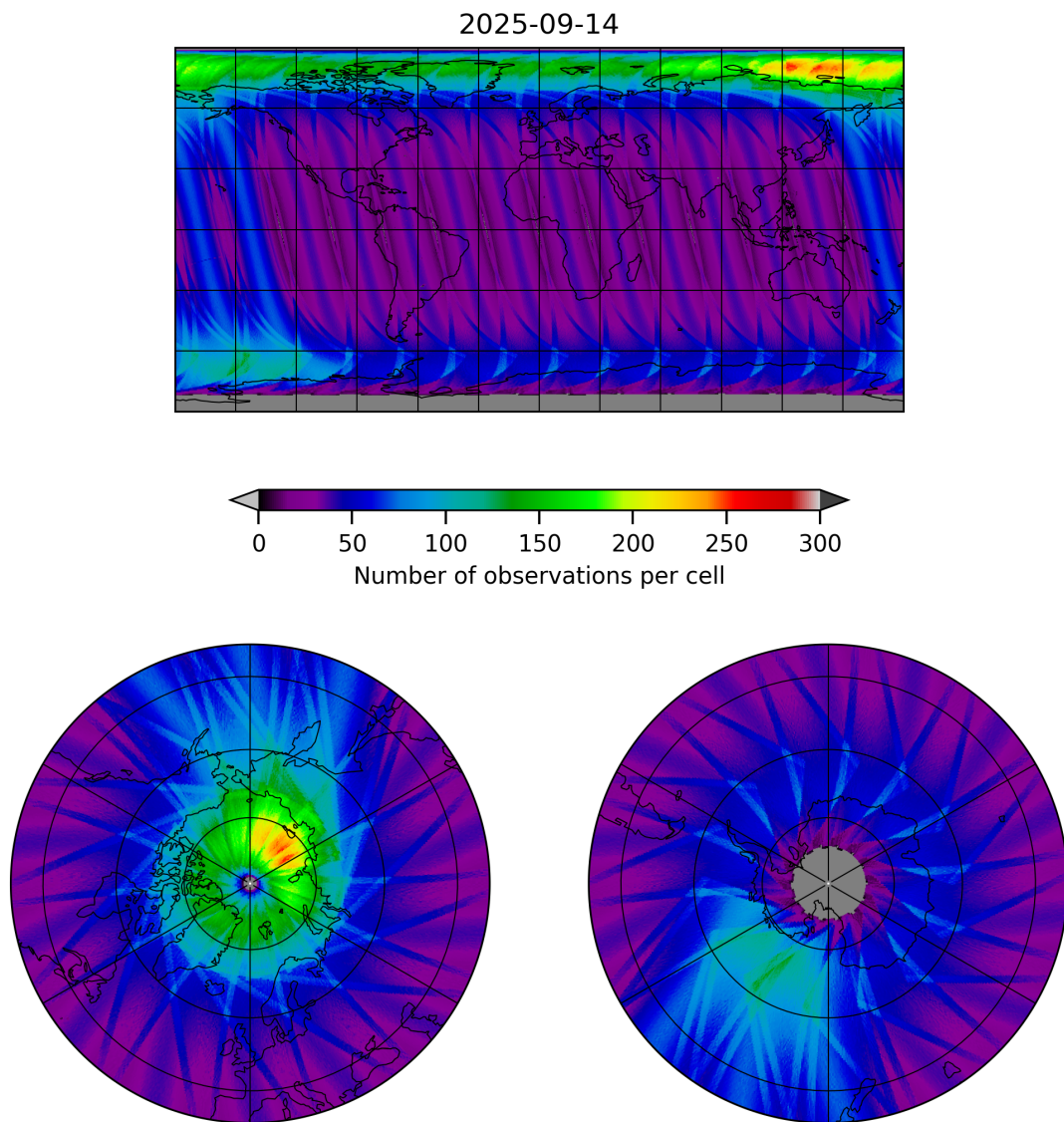
Figure 19: Map of the number of observations for 2025-09-13 to 2025-09-15
