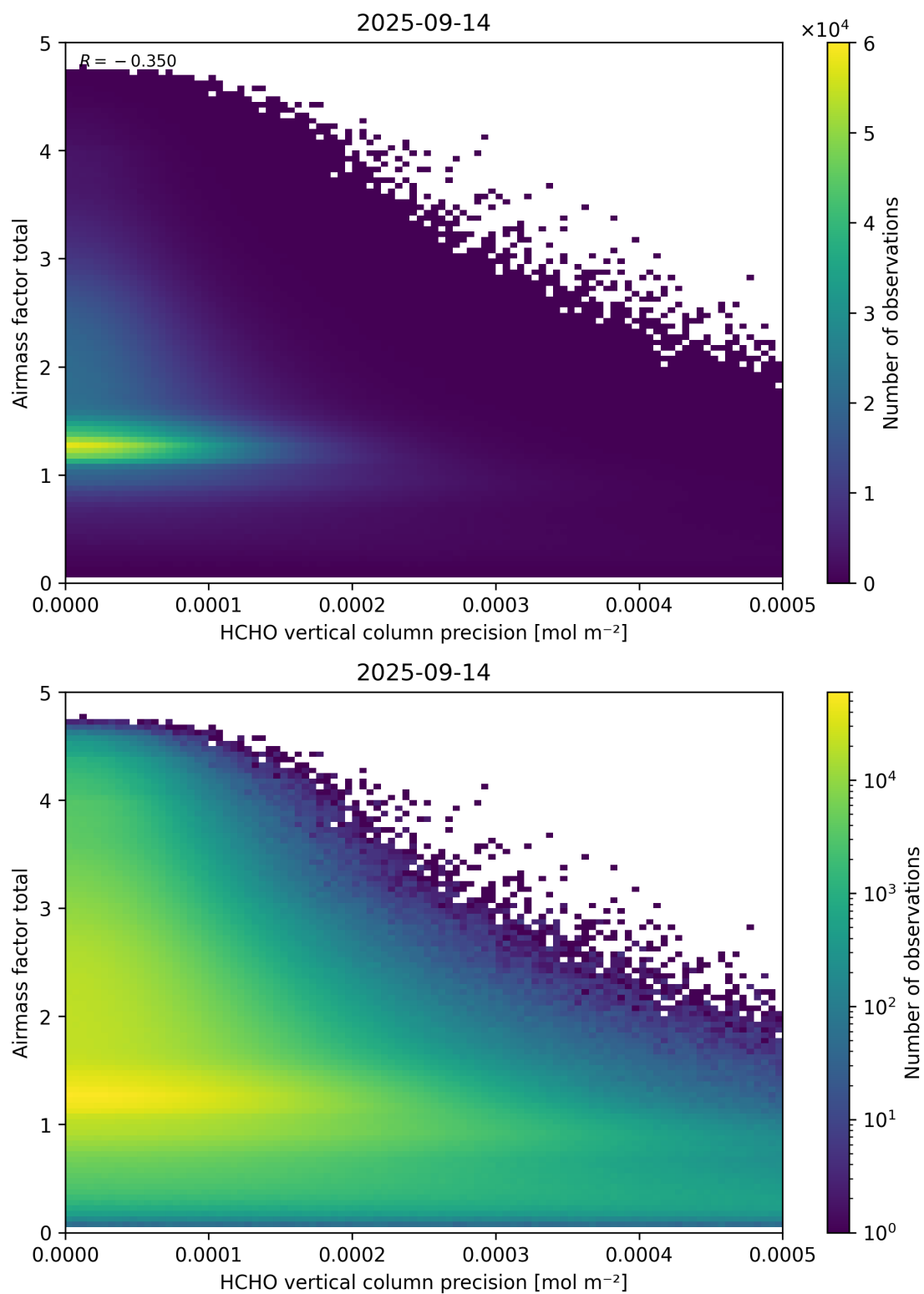
Figure 144: Scatter density plot of “HCHO vertical column precision” against “Airmass factor total” for 2025-09-13 to 2025-09-15.
