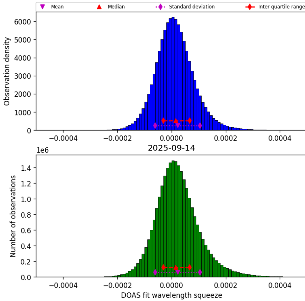
Figure 45: Histogram of “DOAS fit wavelength squeeze” for 2025-09-13 to 2025-09-15
