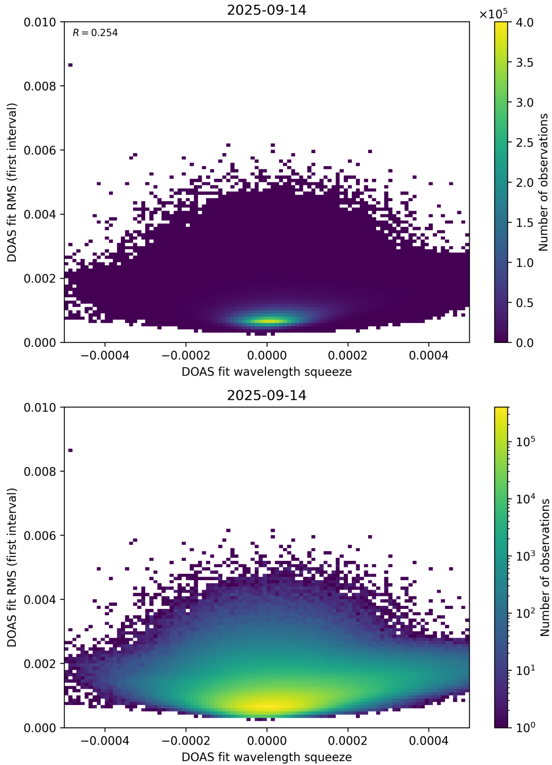
Figure 68: Scatter density plot of “DOAS fit wavelength squeeze” against “DOAS fit RMS (first interval)” for 2025-09-13 to 2025-09-15.
