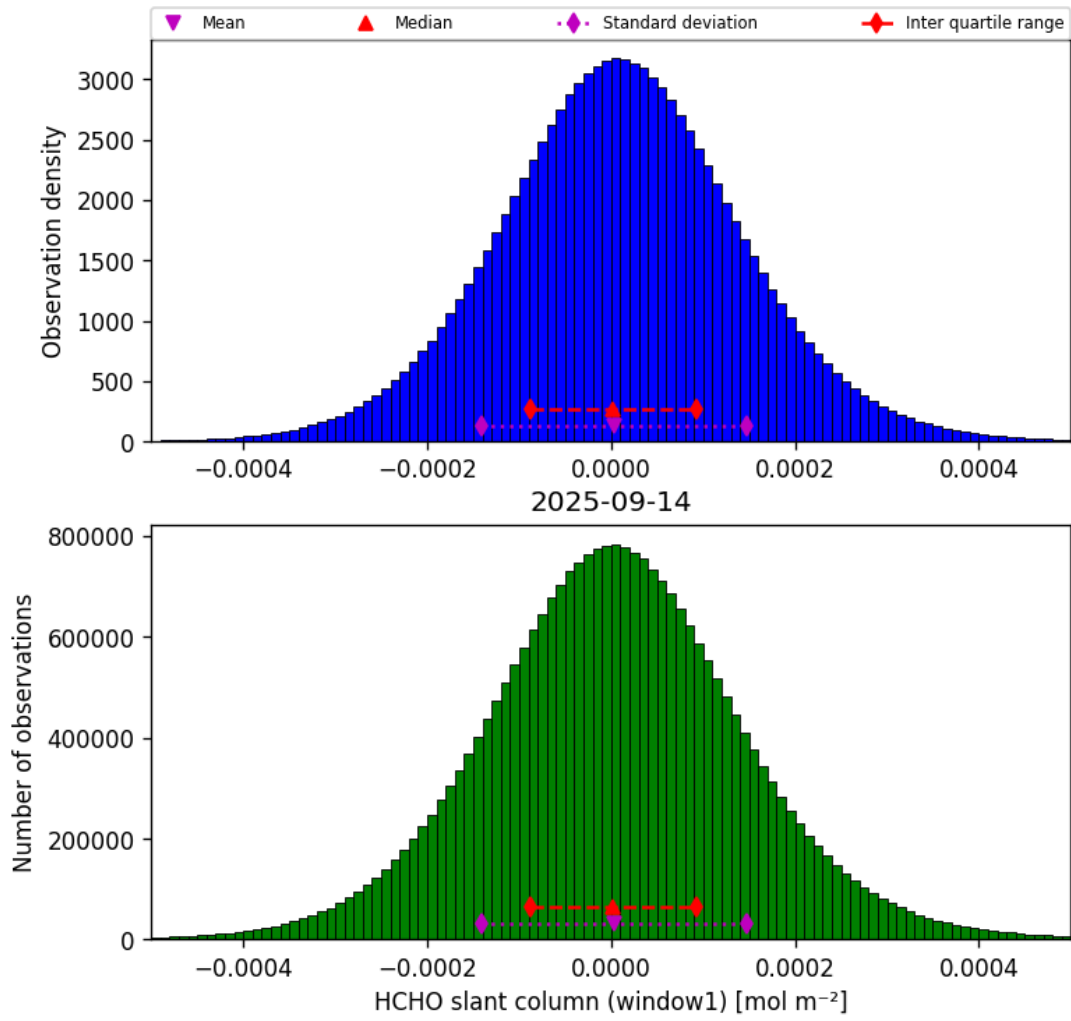
Figure 38: Histogram of “HCHO slant column (window1)” for 2025-09-13 to 2025-09-15
