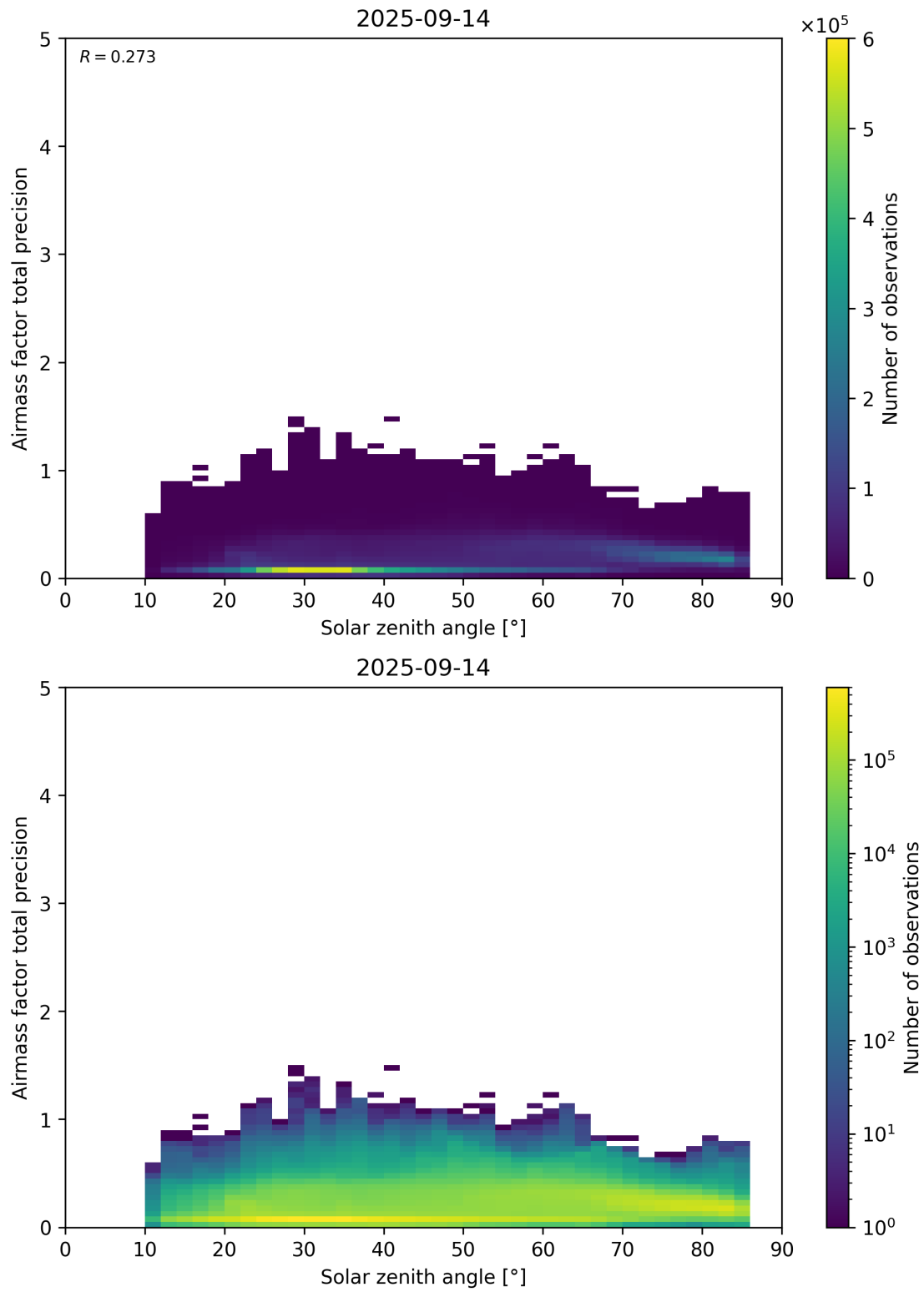
Figure 176: Scatter density plot of “Solar zenith angle” against “Airmass factor total precision” for 2025-09-13 to 2025-09-15.
