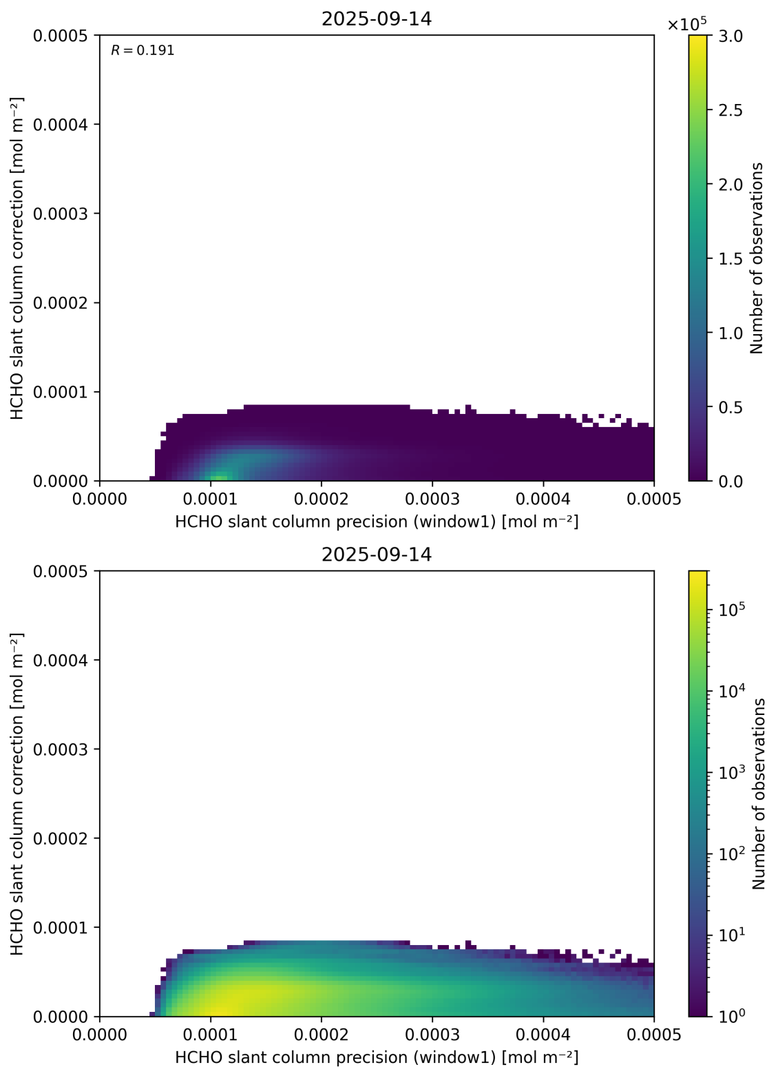
Figure 93: Scatter density plot of “HCHO slant column precision (window1)” against “HCHO slant column correction” for 2025-09-13 to 2025-09-15.
