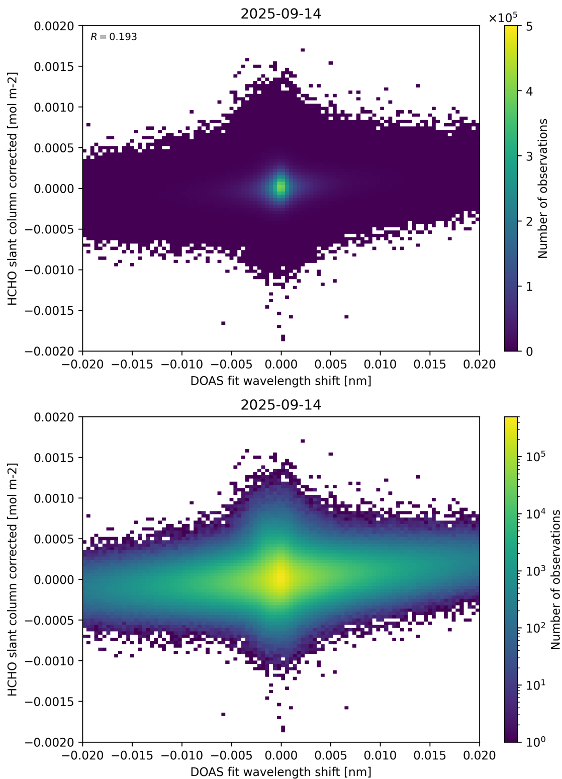
Figure 66: Scatter density plot of “DOAS fit wavelength shift” against “HCHO slant column corrected” for 2025-09-13 to 2025-09-15.
