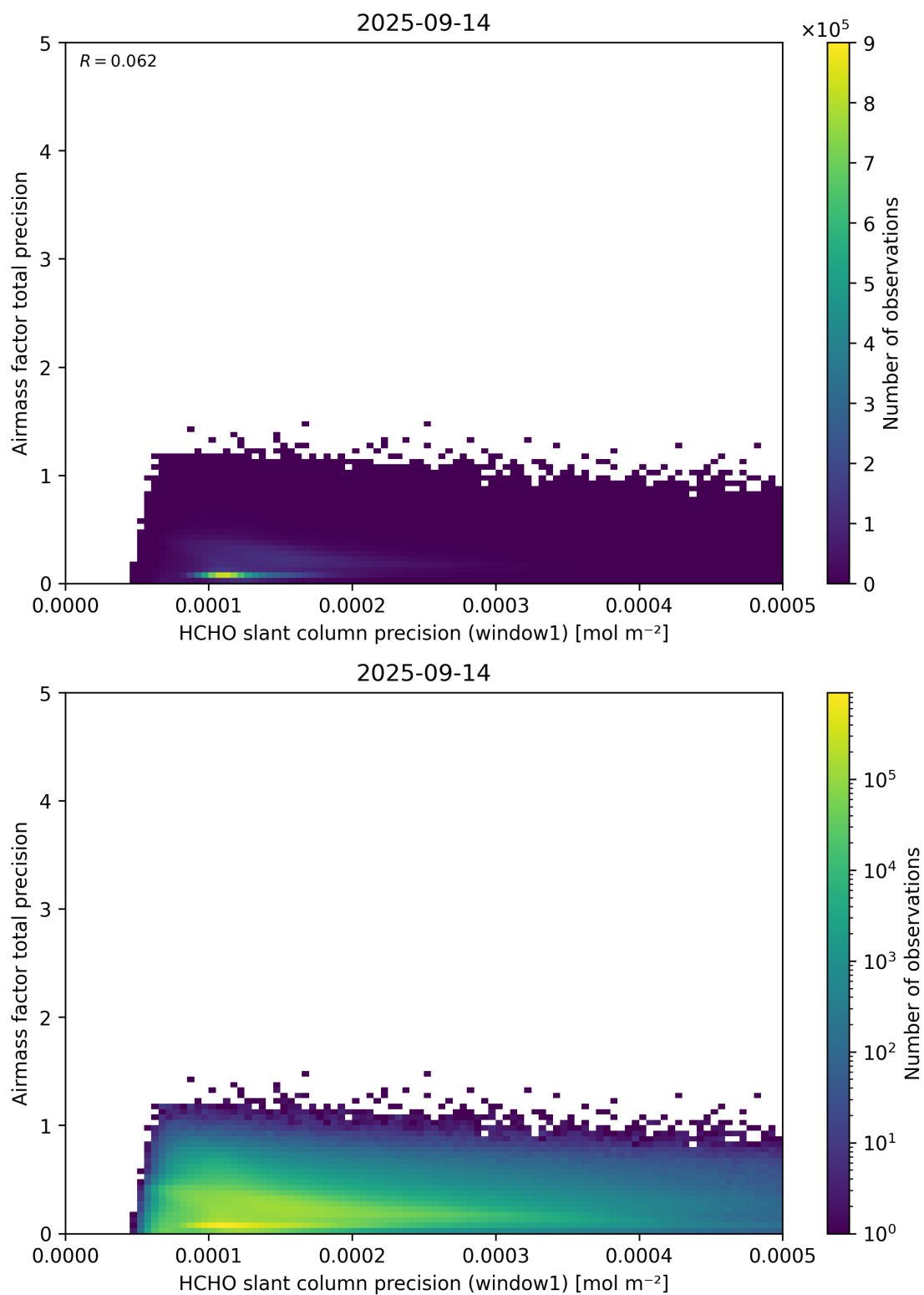
Figure 95: Scatter density plot of “HCHO slant column precision (window1)” against “Airmass factor total precision” for 2025-09-13 to 2025-09-15.
