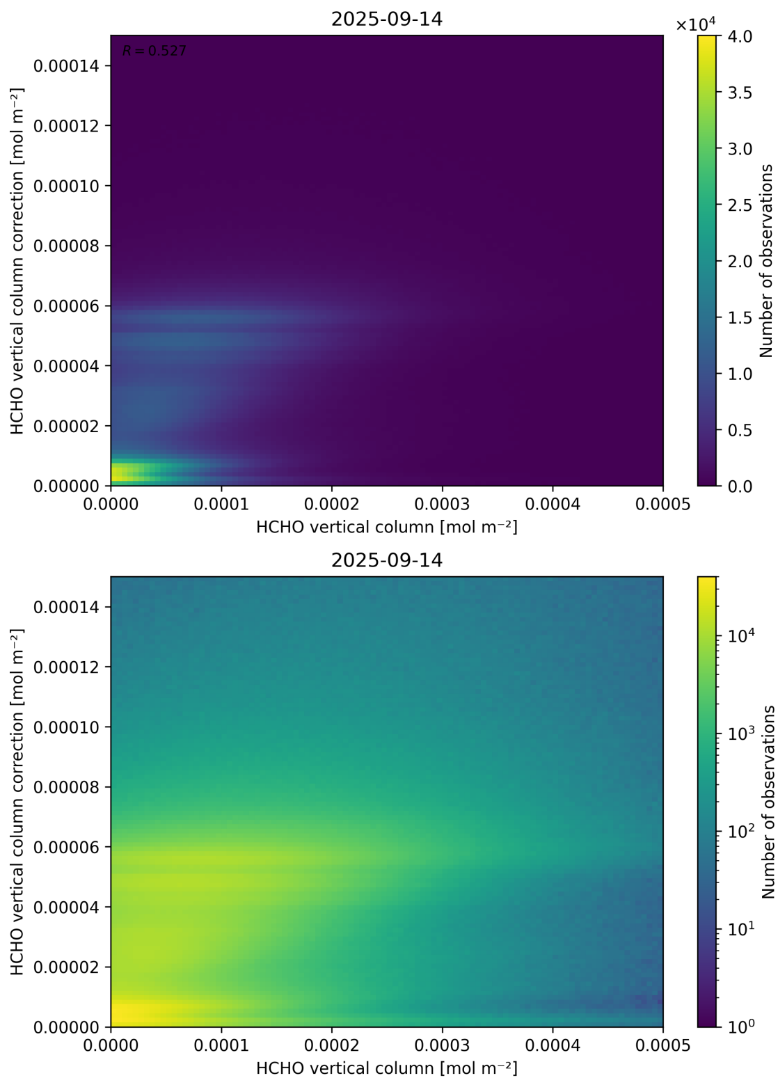
Figure 133: Scatter density plot of “HCHO vertical column” against “HCHO vertical column correction” for 2025-09-13 to 2025-09-15.
