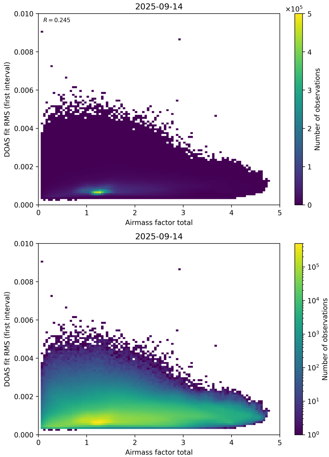
Figure 97: Scatter density plot of “Airmass factor total” against “DOAS fit RMS (first interval)” for 2025-09-13 to 2025-09-15.
