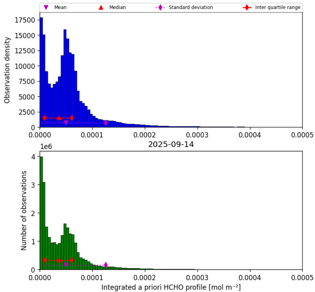
Figure 43: Histogram of “Integrated a priori HCHO profile” for 2025-09-13 to 2025-09-15
