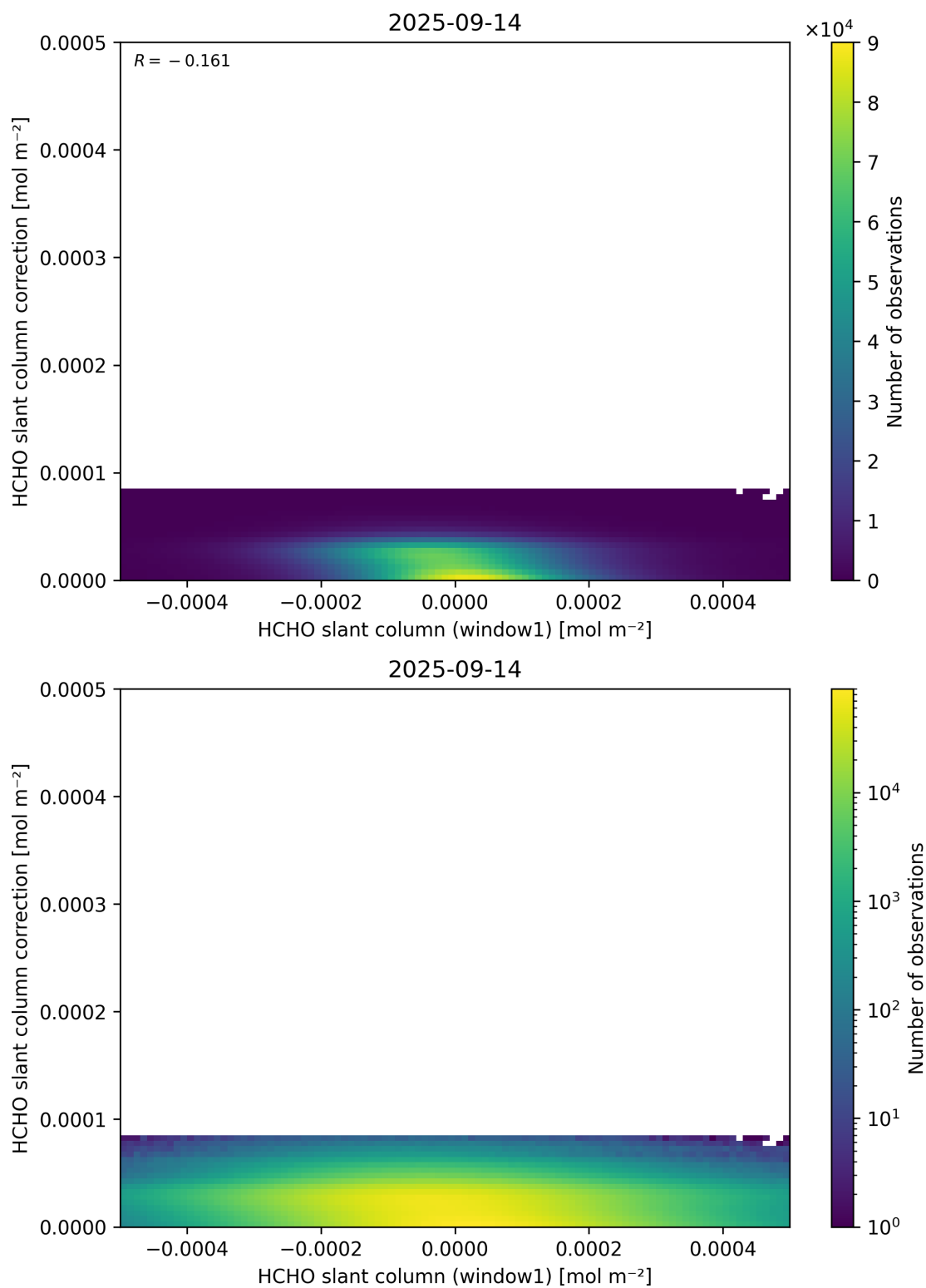
Figure 83: Scatter density plot of “HCHO slant column (window1)” against “HCHO slant column correction” for 2025-09-13 to 2025-09-15.
