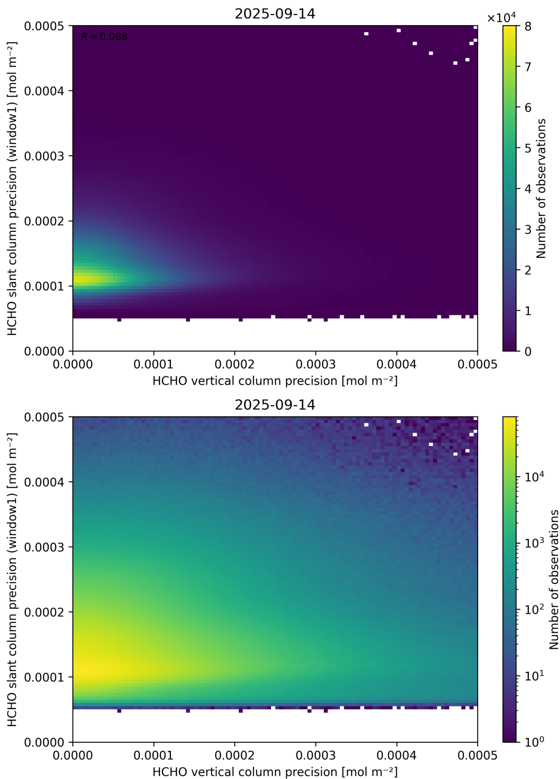
Figure 143: Scatter density plot of “HCHO vertical column precision” against “HCHO slant column precision (window1)” for 2025-09-13 to 2025-09-15.
