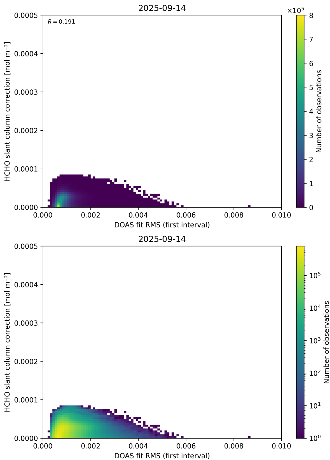
Figure 63: Scatter density plot of “DOAS fit RMS (first interval)” against “HCHO slant column correction” for 2025-09-13 to 2025-09-15.
