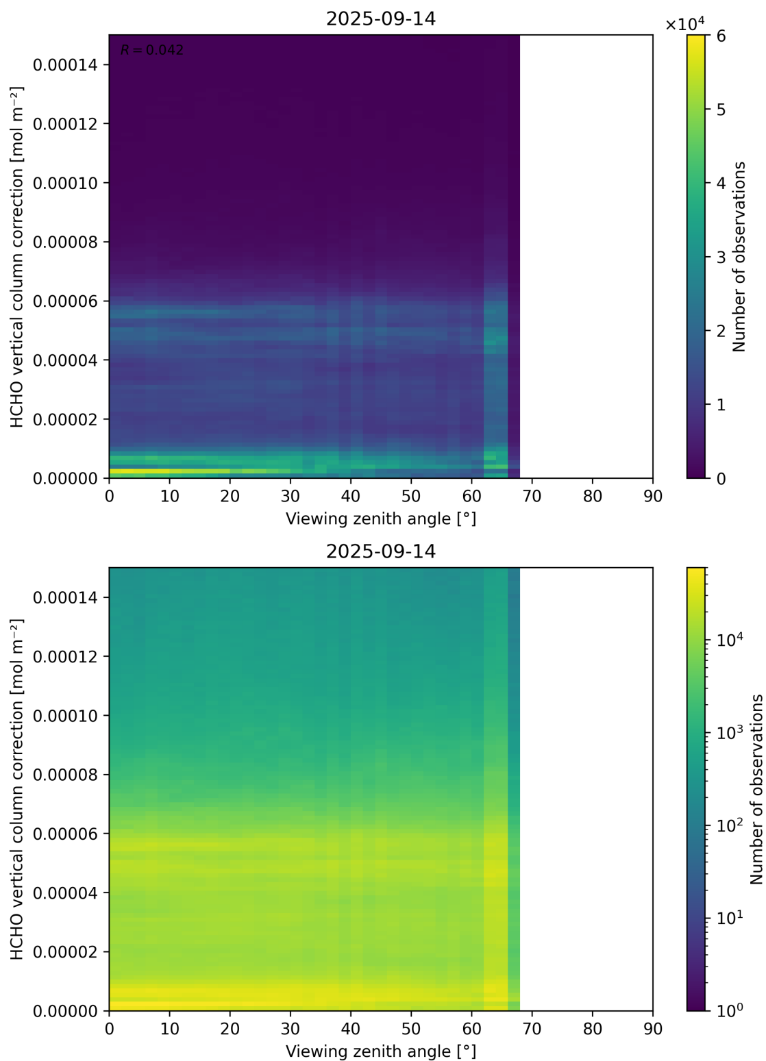
Figure 193: Scatter density plot of “Viewing zenith angle” against “HCHO vertical column correction” for 2025-09-13 to 2025-09-15.
