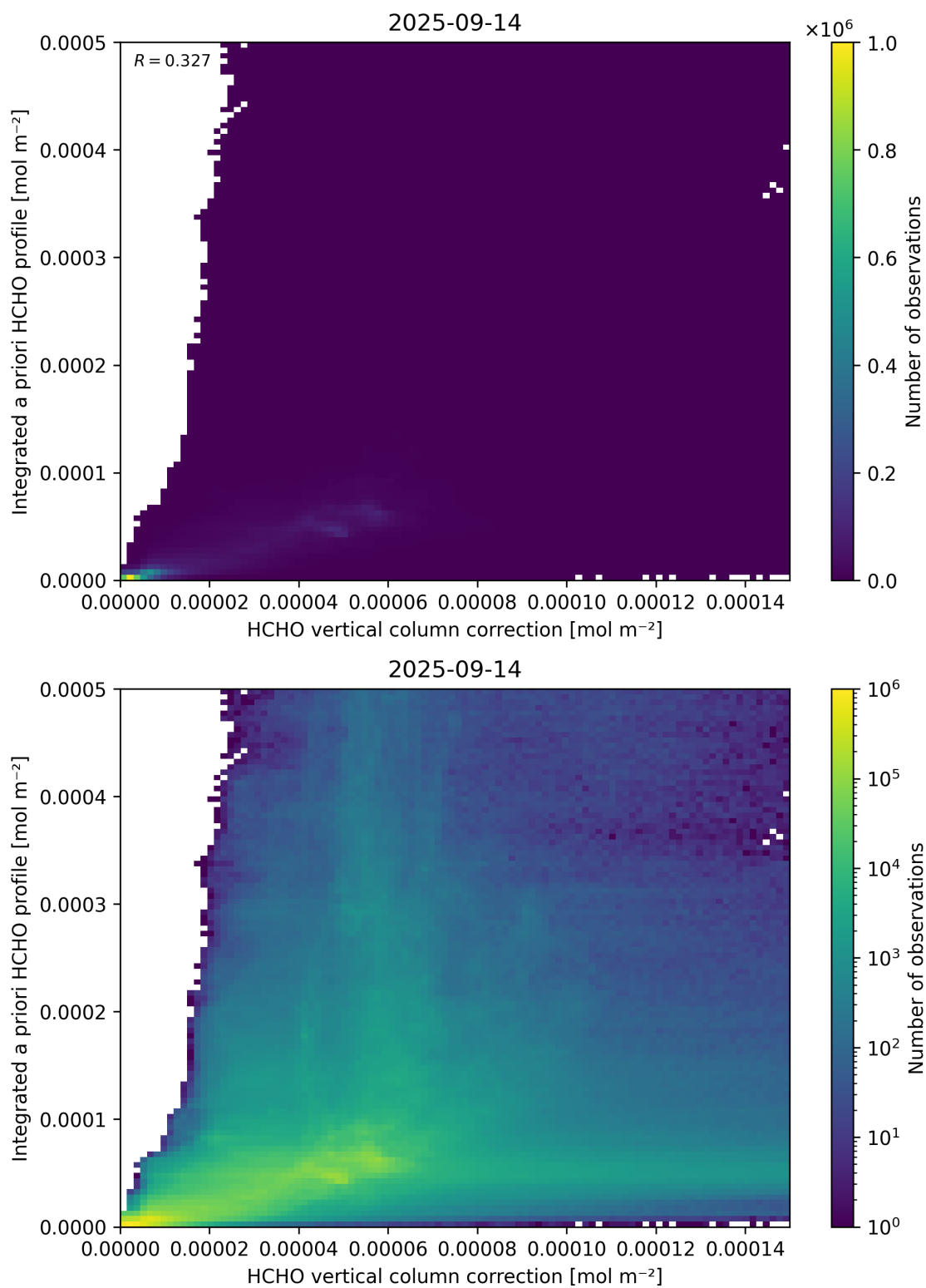
Figure 122: Scatter density plot of “HCHO vertical column correction” against “Integrated a priori HCHO profile” for 2025-09-13 to 2025-09-15.
