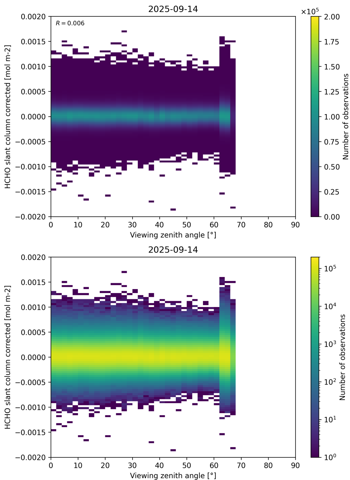
Figure 186: Scatter density plot of “Viewing zenith angle” against “HCHO slant column corrected” for 2025-09-13 to 2025-09-15.
