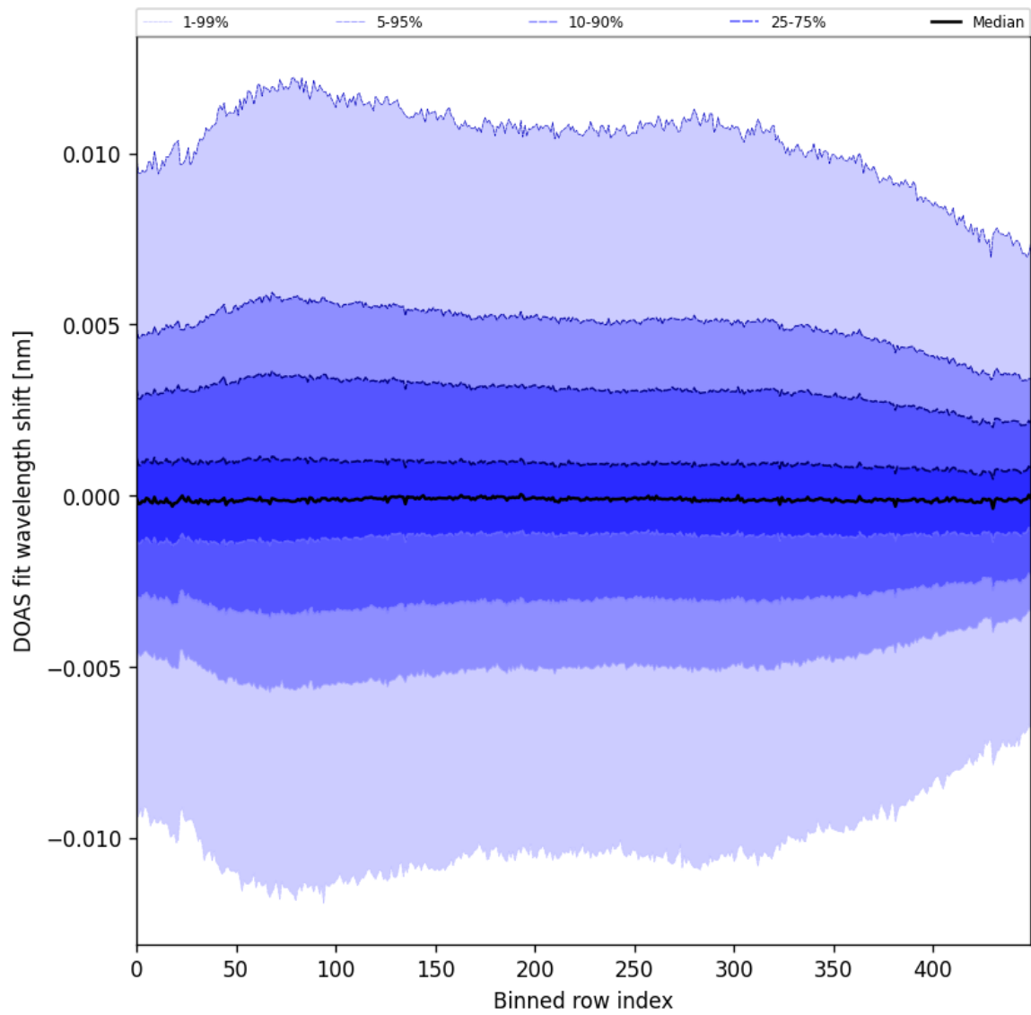
Figure 58: Along track statistics of “DOAS fit wavelength shift” for 2025-09-13 to 2025-09-15
