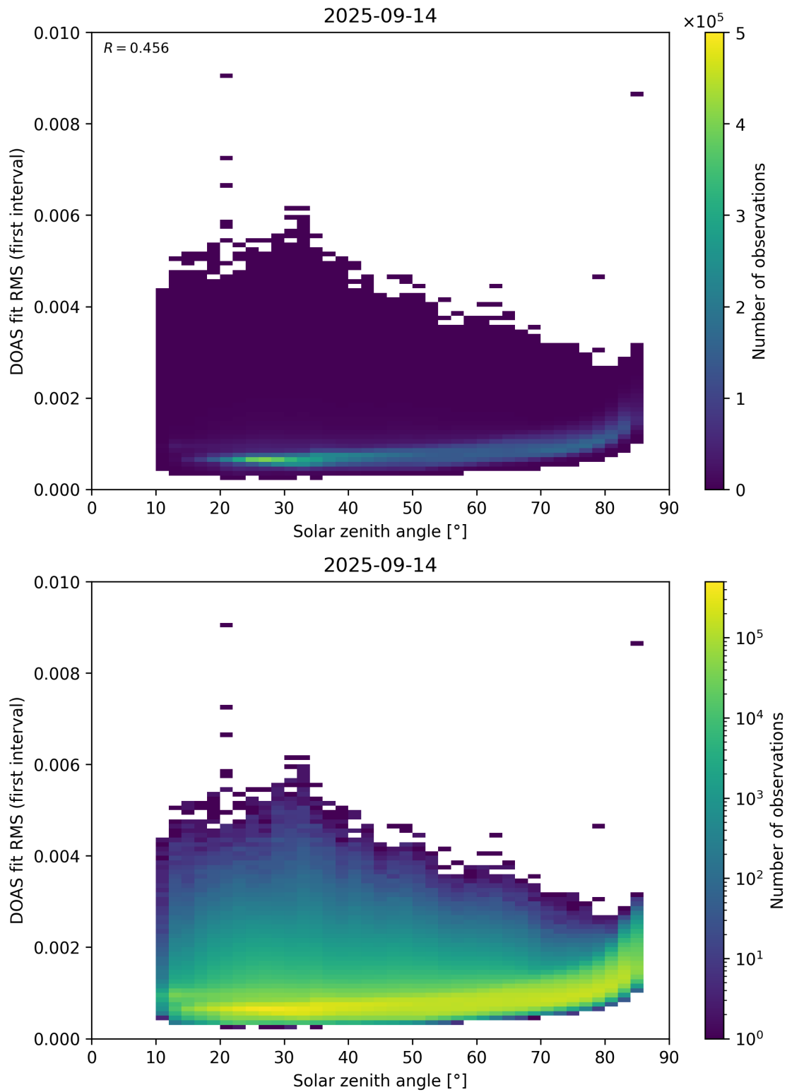
Figure 167: Scatter density plot of “Solar zenith angle” against “DOAS fit RMS (first interval)” for 2025-09-13 to 2025-09-15.
