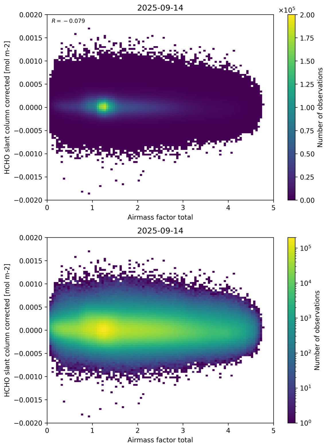
Figure 101: Scatter density plot of “Airmass factor total” against “HCHO slant column corrected” for 2025-09-13 to 2025-09-15.
