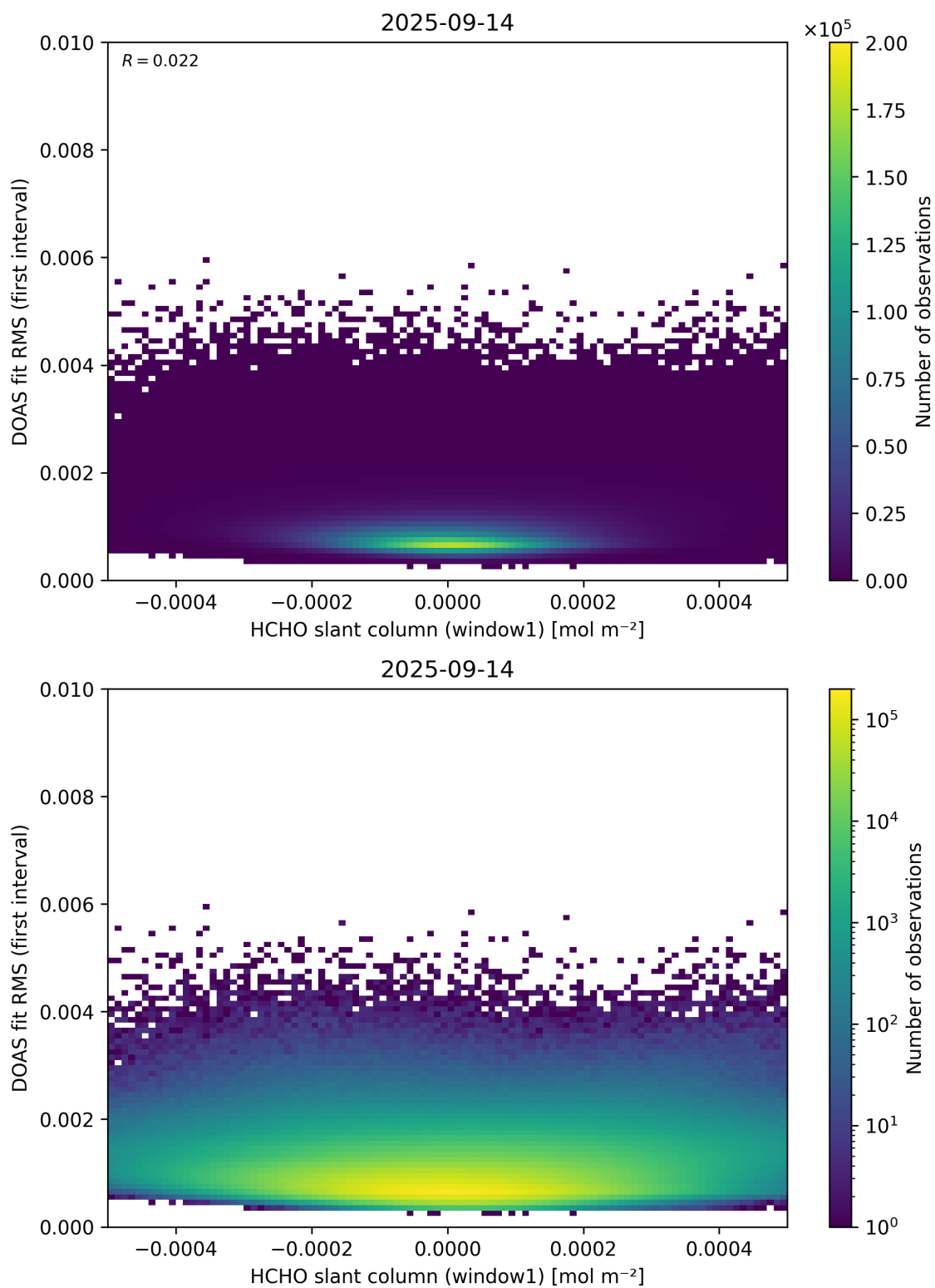
Figure 78: Scatter density plot of “HCHO slant column (window1)” against “DOAS fit RMS (first interval)” for 2025-09-13 to 2025-09-15.
