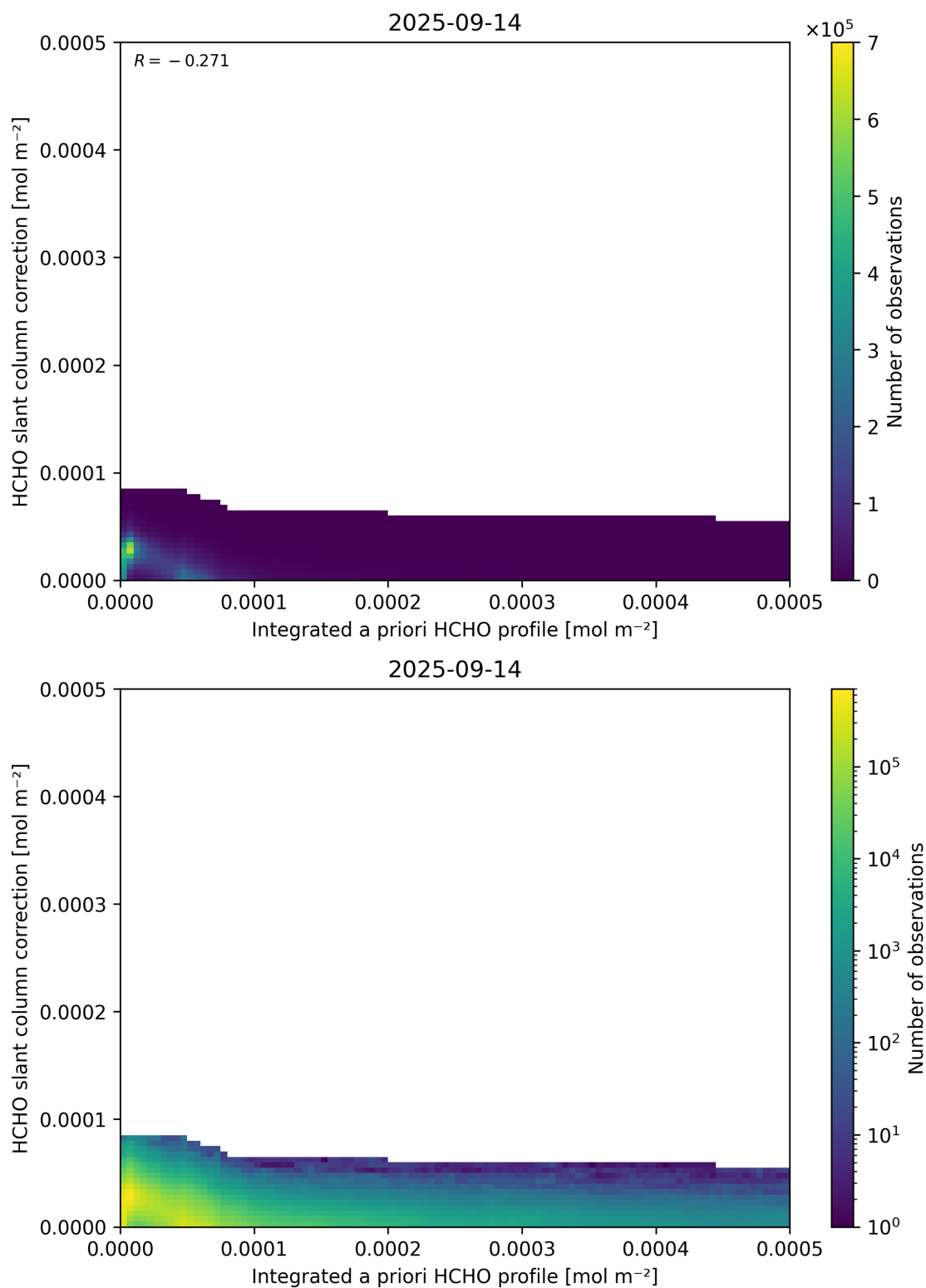
Figure 152: Scatter density plot of “Integrated a priori HCHO profile” against “HCHO slant column correction” for 2025-09-13 to 2025-09-15.
