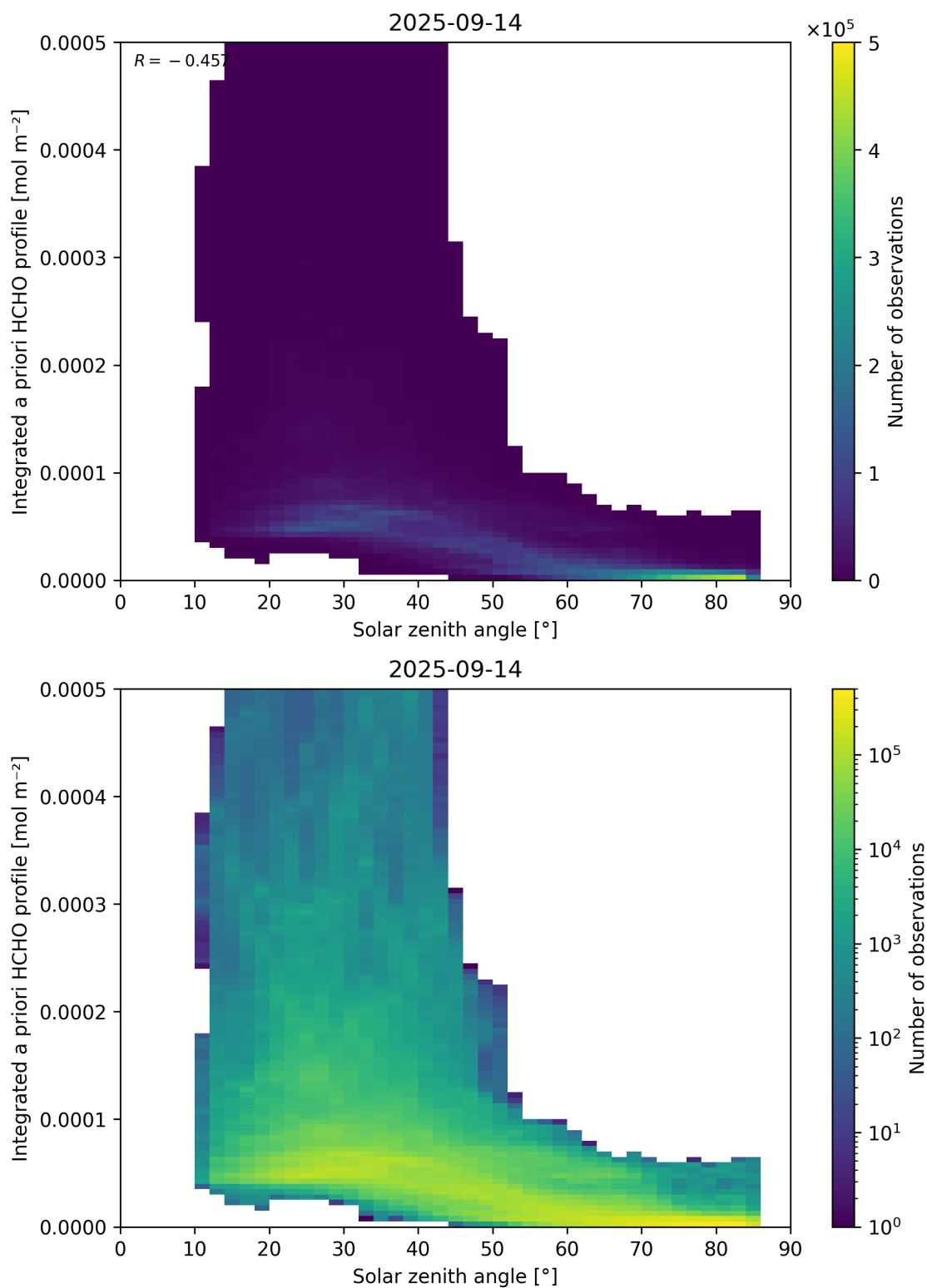
Figure 180: Scatter density plot of “Solar zenith angle” against “Integrated a priori HCHO profile” for 2025-09-13 to 2025-09-15.
