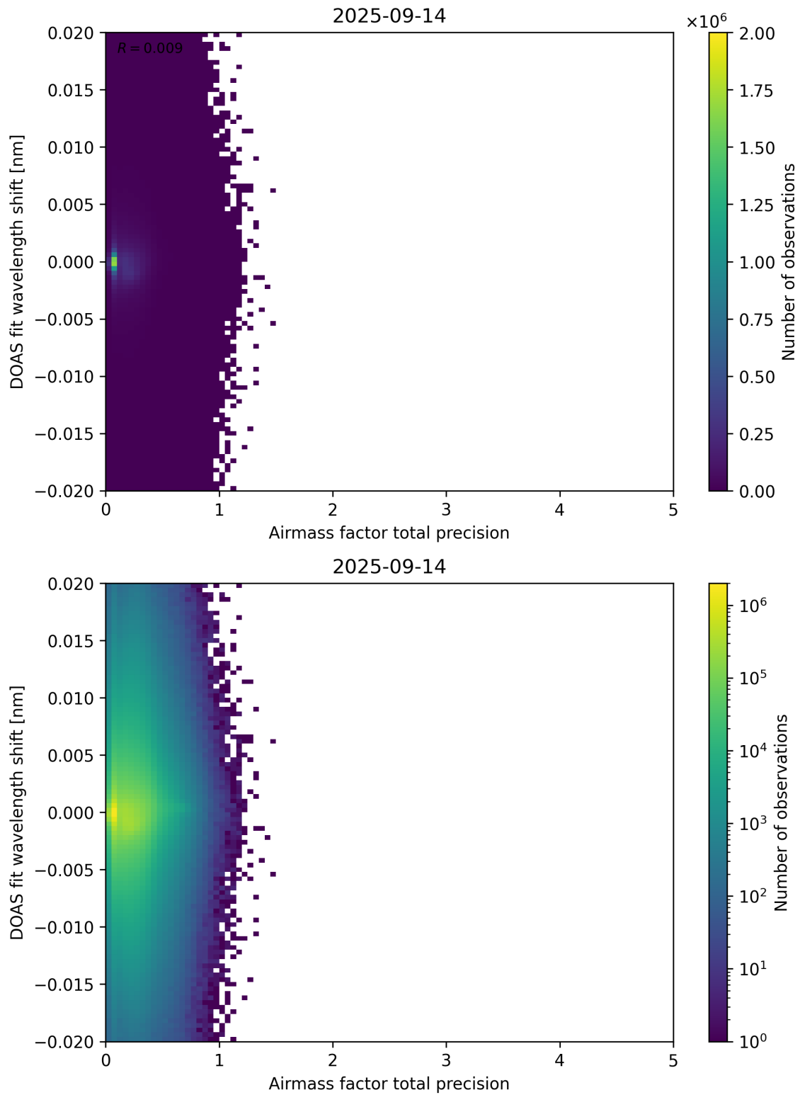
Figure 106: Scatter density plot of “Airmass factor total precision” against “DOAS fit wavelength shift” for 2025-09-13 to 2025-09-15.
