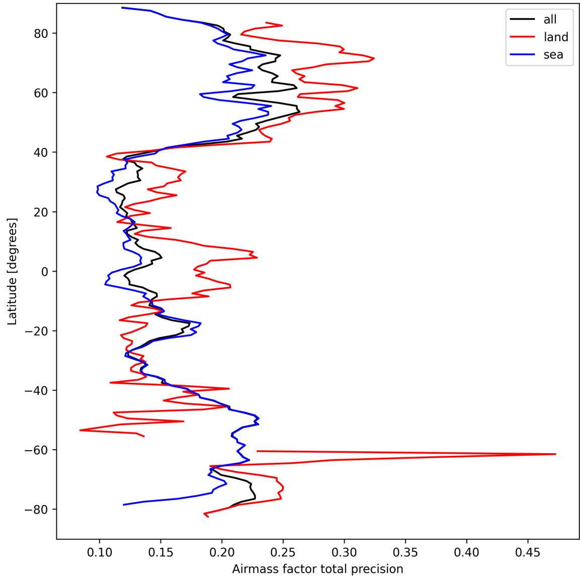
Figure 27: Zonal average of “Airmass factor total precision” for 2025-09-13 to 2025-09-15.
