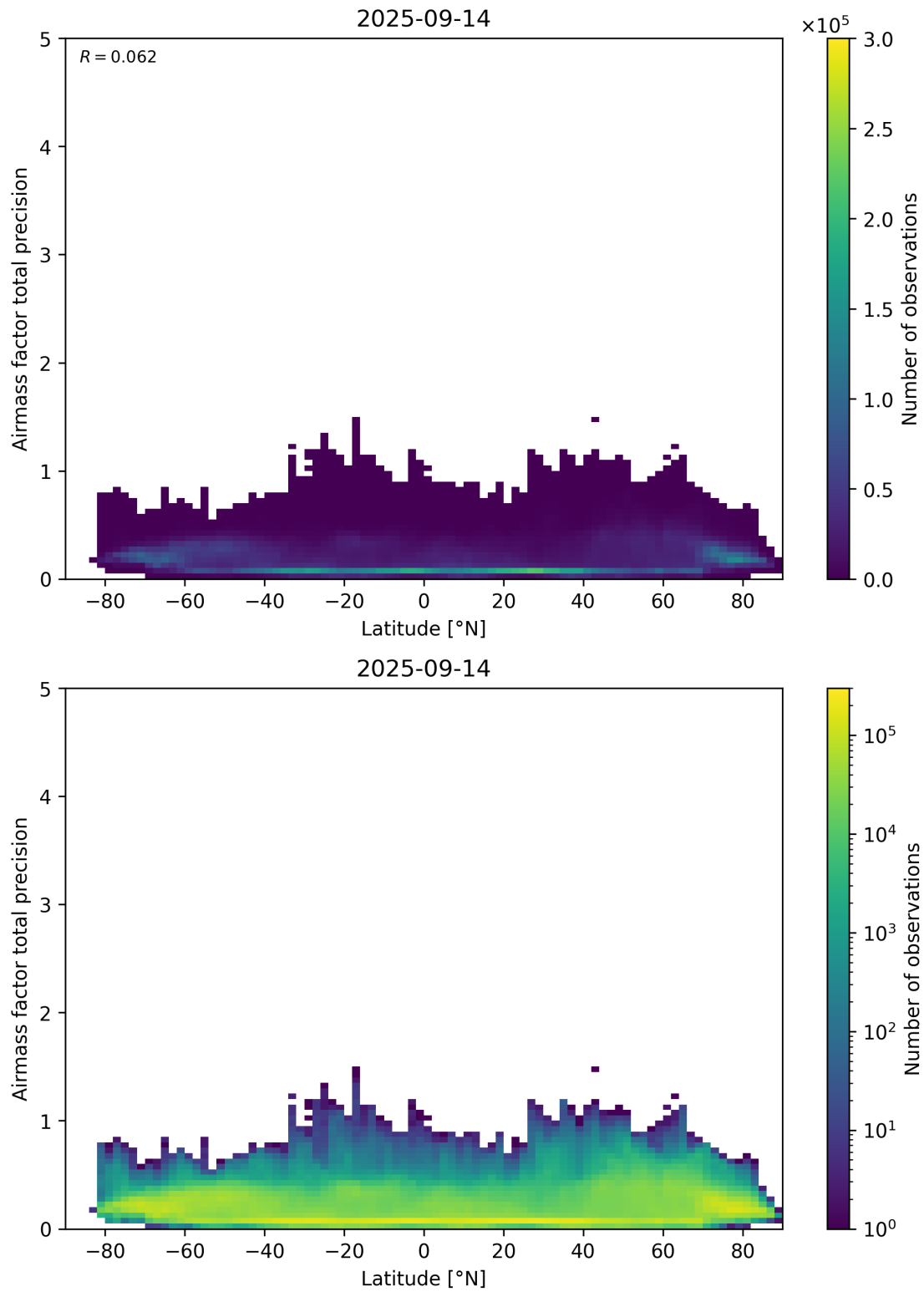
Figure 162: Scatter density plot of “Latitude” against “Airmass factor total precision” for 2025-09-13 to 2025-09-15.
