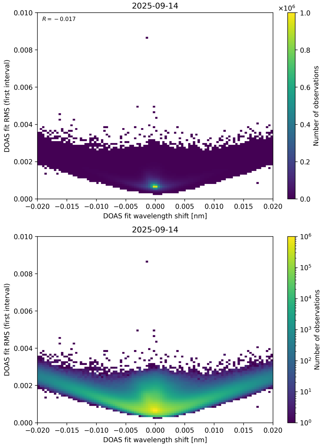
Figure 64: Scatter density plot of “DOAS fit wavelength shift” against “DOAS fit RMS (first interval)” for 2025-09-13 to 2025-09-15.
