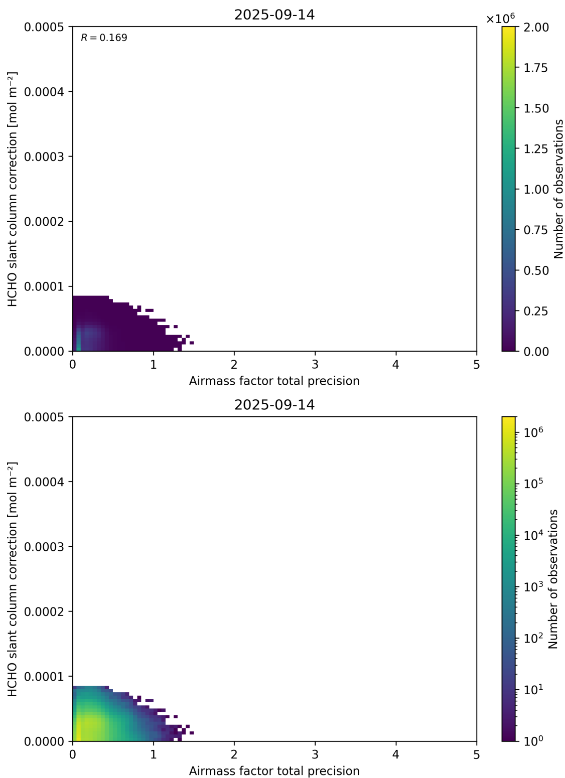
Figure 110: Scatter density plot of “Airmass factor total precision” against “HCHO slant column correction” for 2025-09-13 to 2025-09-15.
