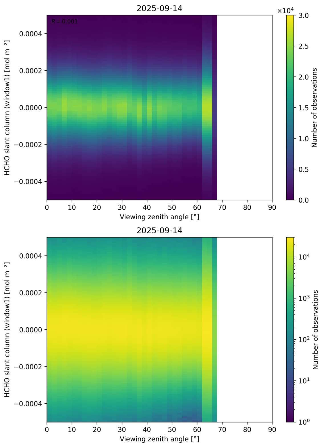
Figure 188: Scatter density plot of “Viewing zenith angle” against “HCHO slant column (window1)” for 2025-09-13 to 2025-09-15.
