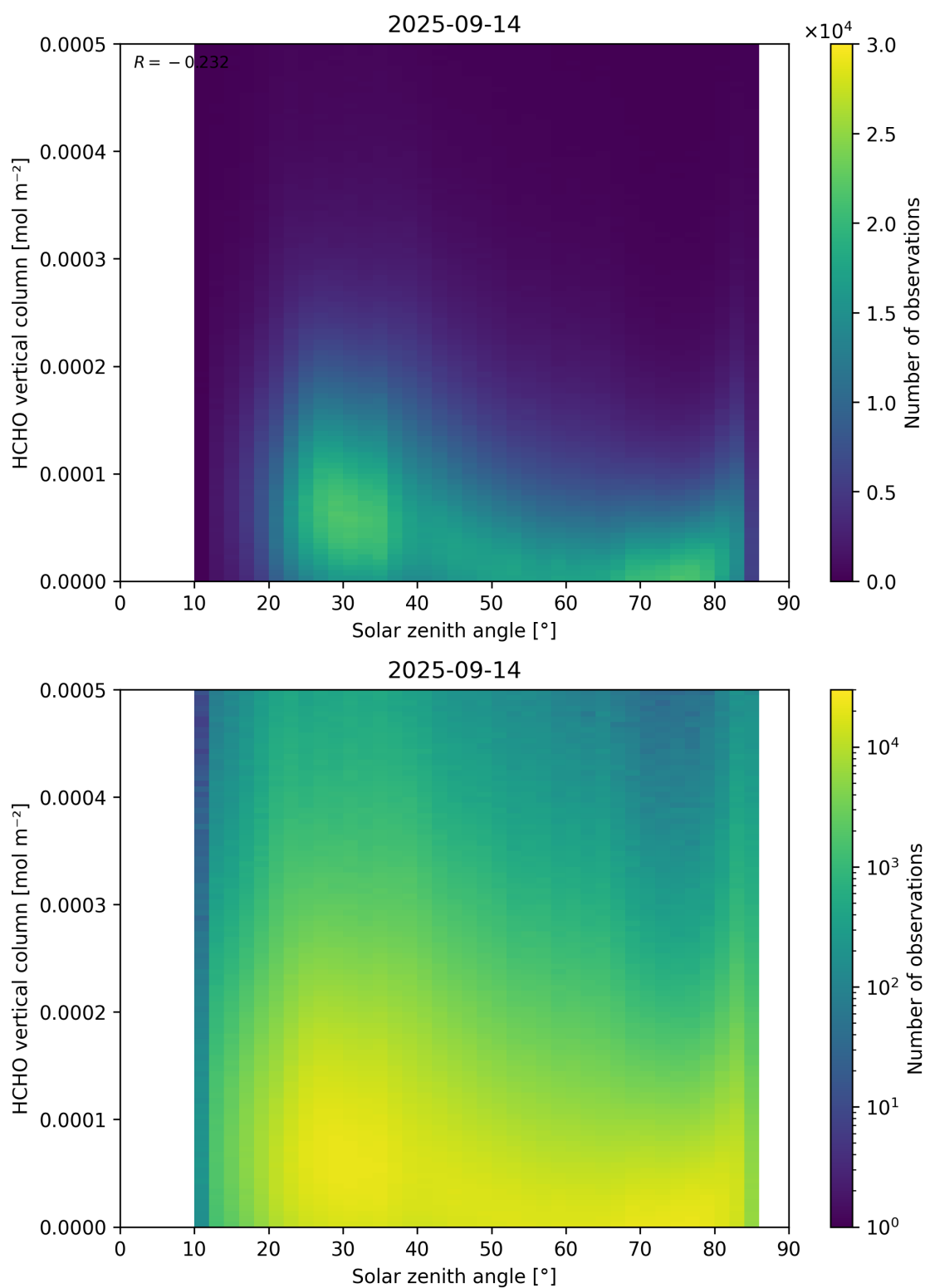
Figure 177: Scatter density plot of “Solar zenith angle” against “HCHO vertical column” for 2025-09-13 to 2025-09-15.
