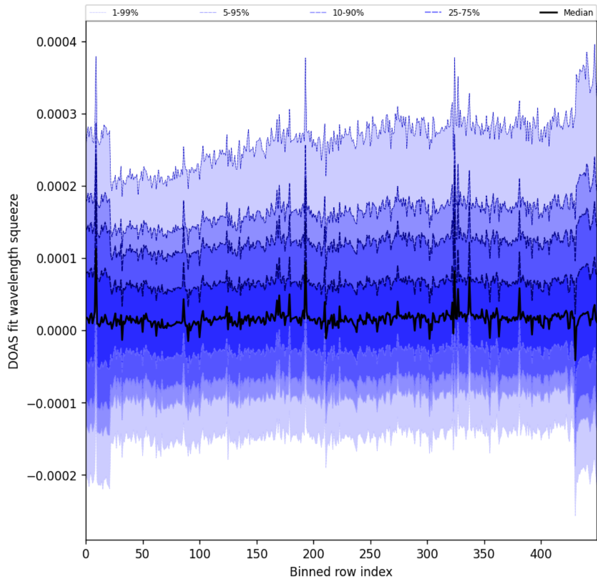
Figure 59: Along track statistics of “DOAS fit wavelength squeeze” for 2025-09-13 to 2025-09-15
