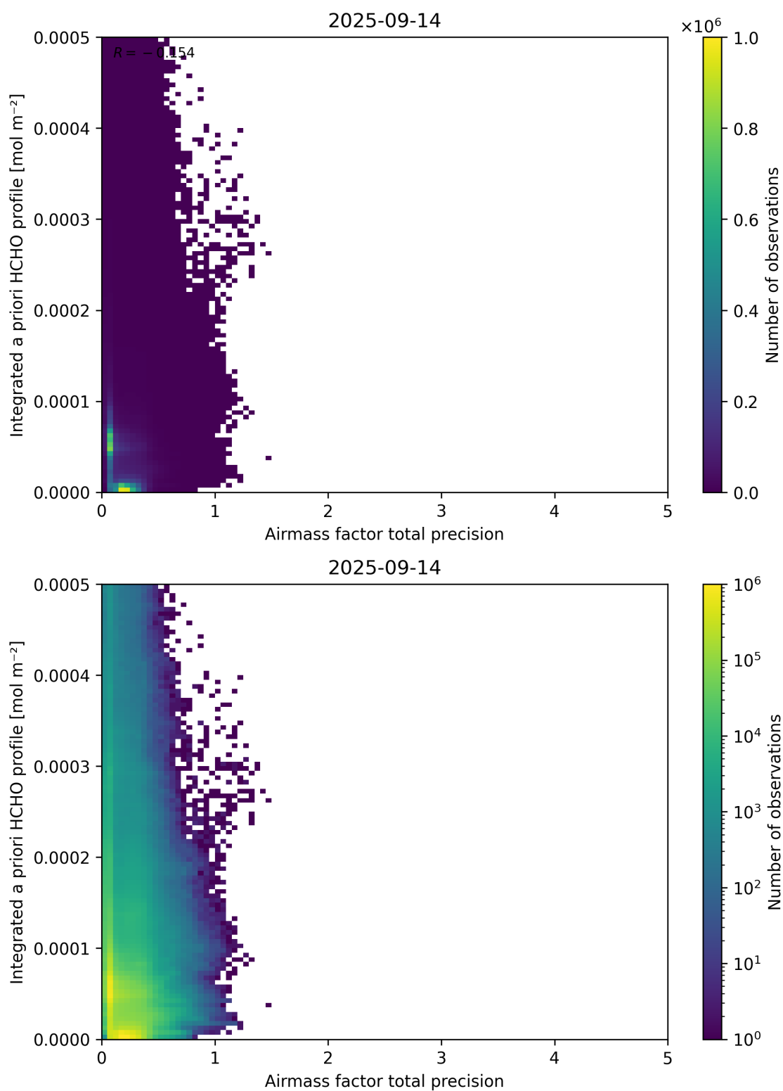
Figure 111: Scatter density plot of “Airmass factor total precision” against “Integrated a priori HCHO profile” for 2025-09-13 to 2025-09-15.
