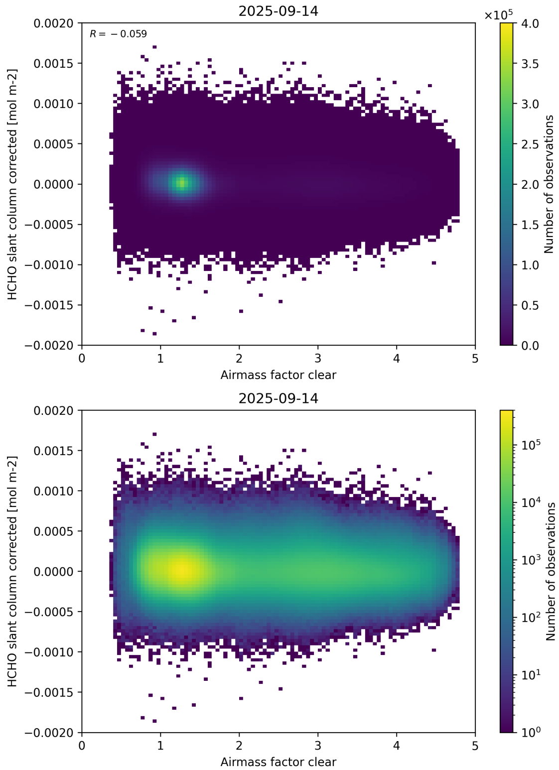
Figure 74: Scatter density plot of “Airmass factor clear” against “HCHO slant column corrected” for 2025-09-13 to 2025-09-15.
