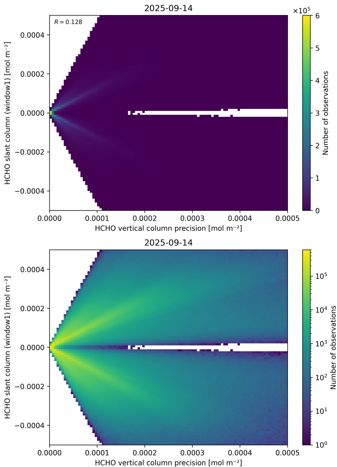
Figure 142: Scatter density plot of “HCHO vertical column precision” against “HCHO slant column (window1)” for 2025-09-13 to 2025-09-15.
