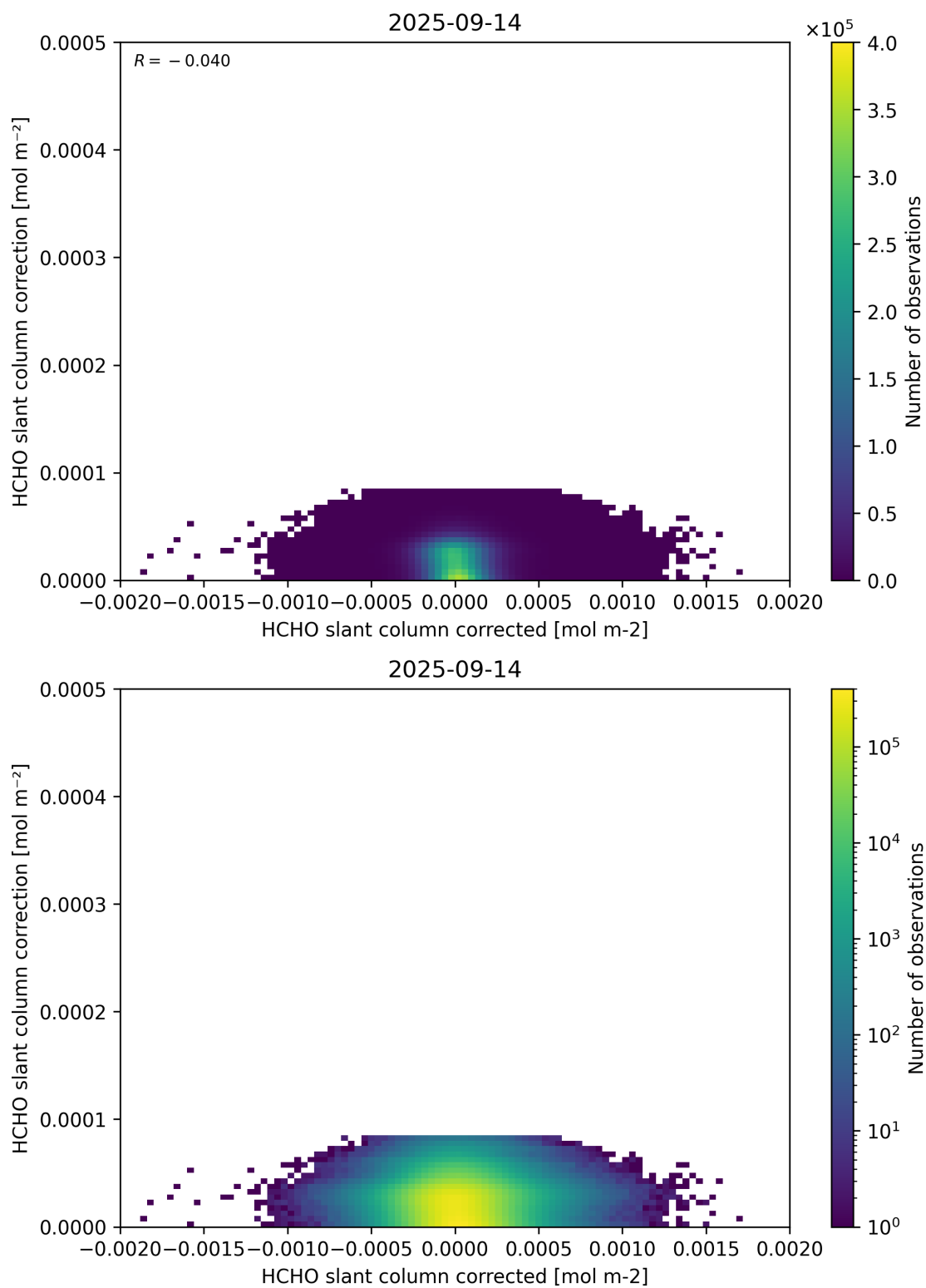
Figure 77: Scatter density plot of “HCHO slant column corrected” against “HCHO slant column correction” for 2025-09-13 to 2025-09-15.
