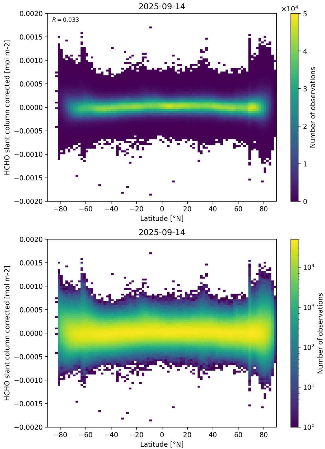
Figure 157: Scatter density plot of “Latitude” against “HCHO slant column corrected” for 2025-09-13 to 2025-09-15.
