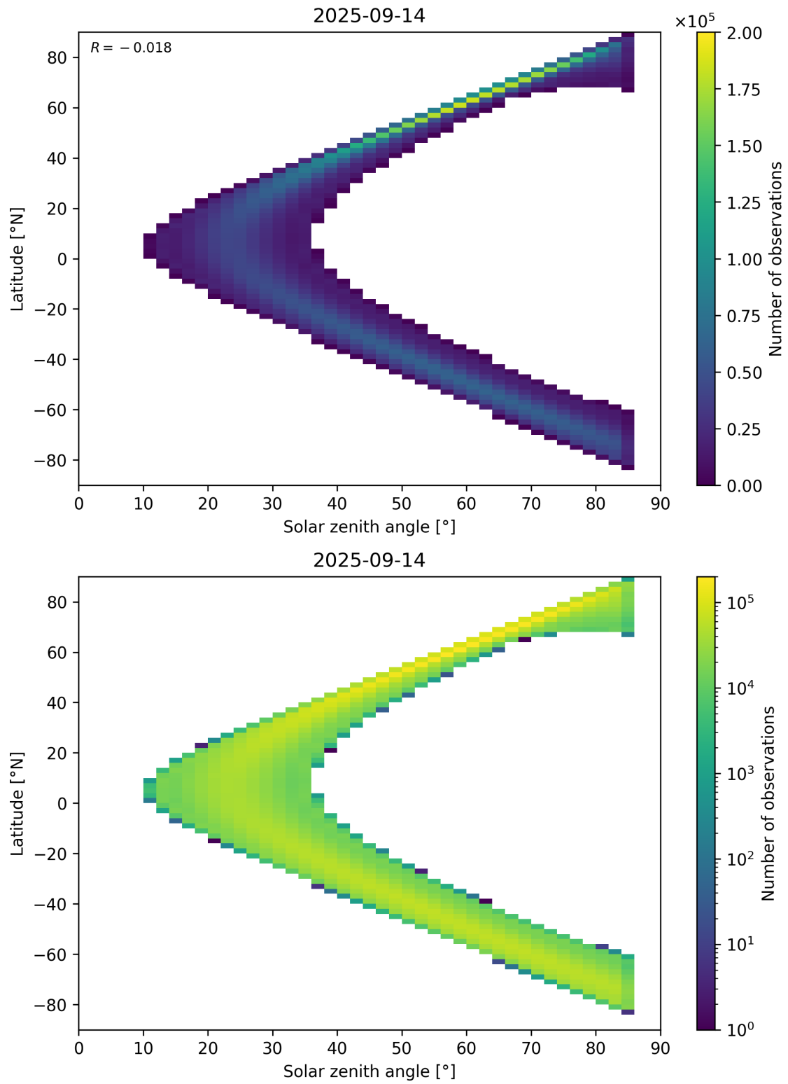
Figure 181: Scatter density plot of “Solar zenith angle” against “Latitude” for 2025-09-13 to 2025-09-15.
