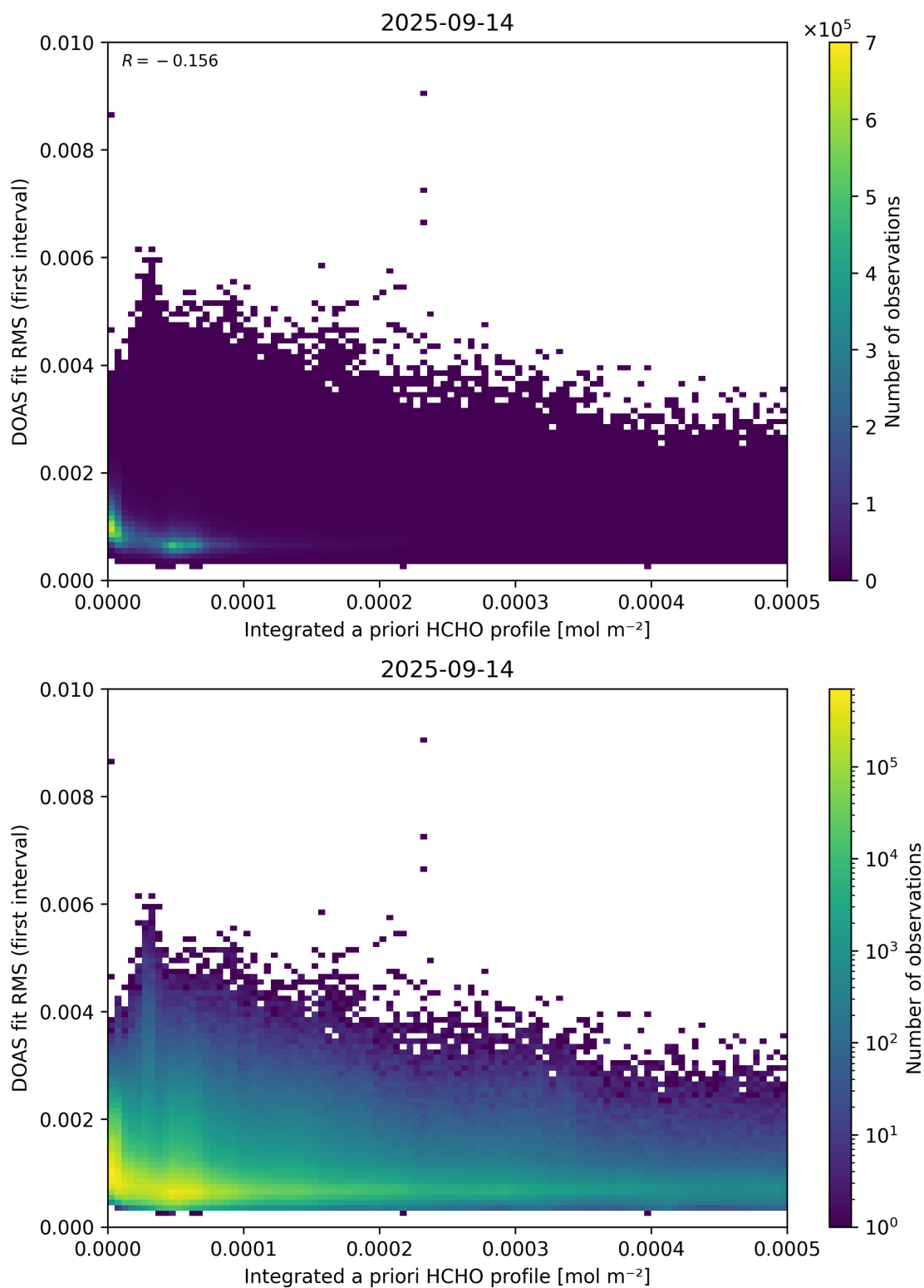
Figure 148: Scatter density plot of “Integrated a priori HCHO profile” against “DOAS fit RMS (first interval)” for 2025-09-13 to 2025-09-15.
