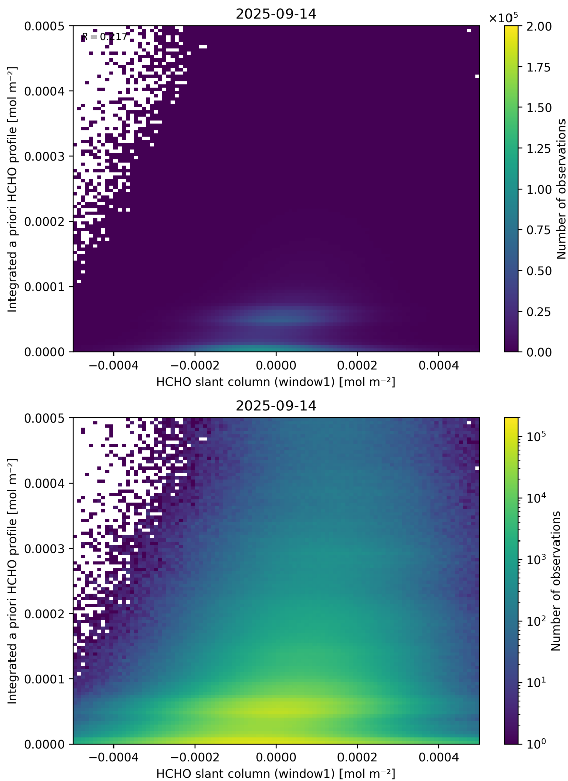
Figure 87: Scatter density plot of “HCHO slant column (window1)” against “Integrated a priori HCHO profile” for 2025-09-13 to 2025-09-15.
