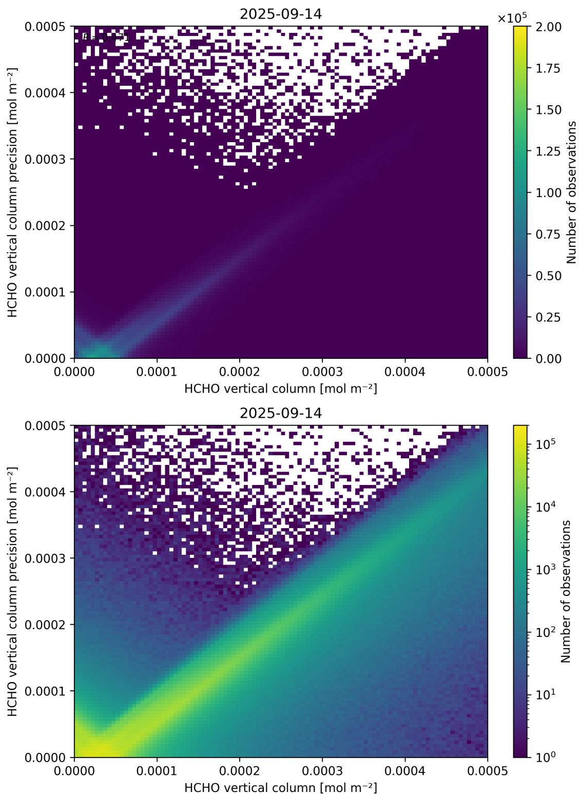
Figure 134: Scatter density plot of “HCHO vertical column” against “HCHO vertical column precision” for 2025-09-13 to 2025-09-15.
