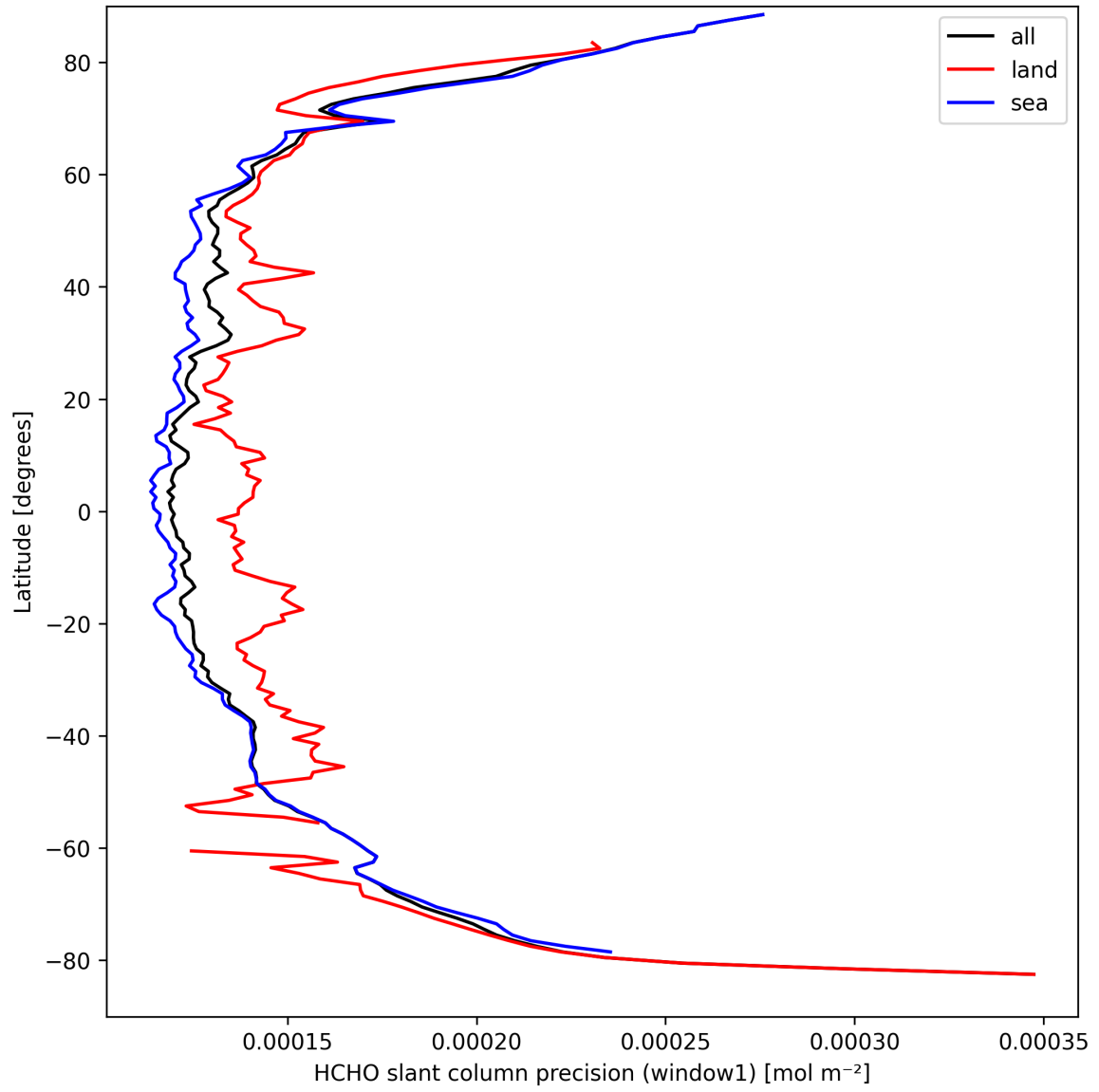
Figure 25: Zonal average of “HCHO slant column precision (window1)” for 2025-09-13 to 2025-09-15.
