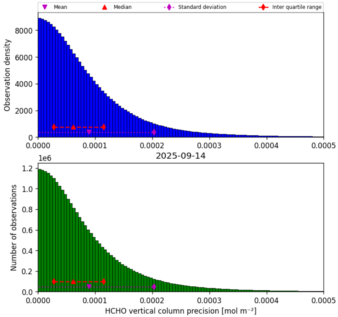
Figure 36: Histogram of “HCHO vertical column precision” for 2025-09-13 to 2025-09-15
