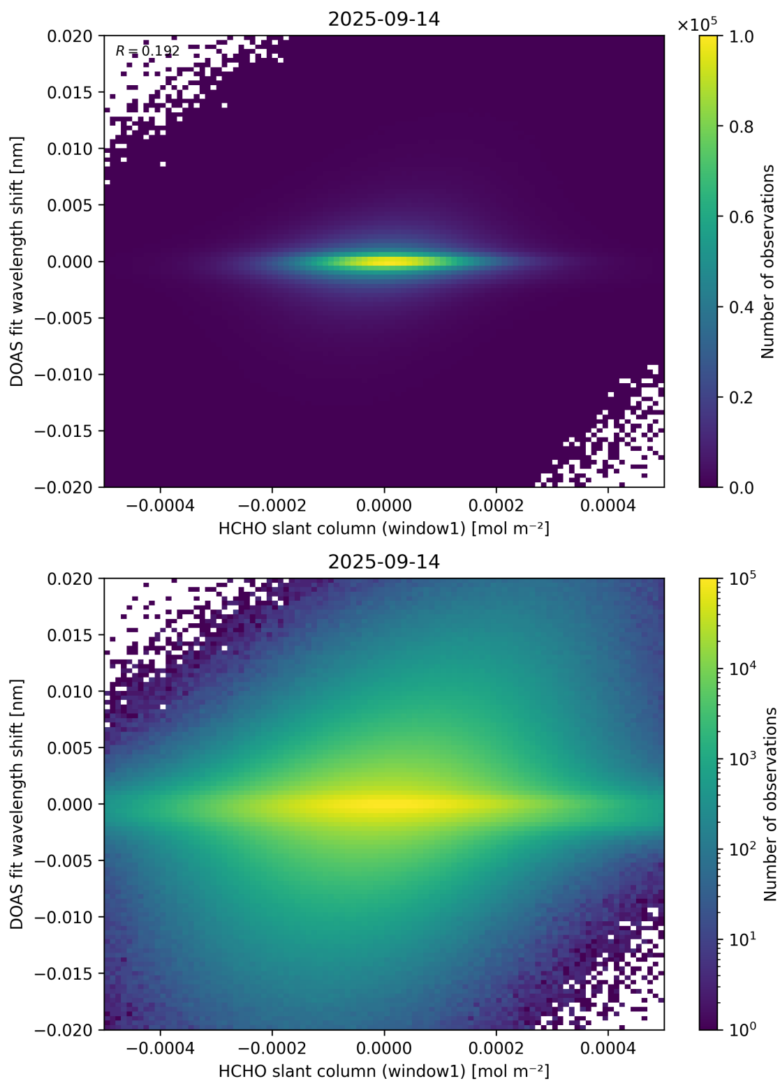
Figure 79: Scatter density plot of “HCHO slant column (window1)” against “DOAS fit wavelength shift” for 2025-09-13 to 2025-09-15.
