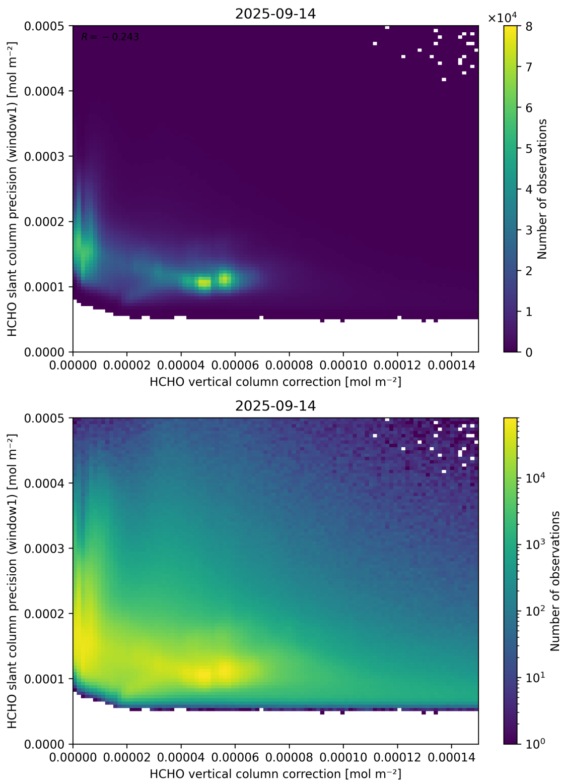
Figure 119: Scatter density plot of “HCHO vertical column correction” against “HCHO slant column precision (window1)” for 2025-09-13 to 2025-09-15.
