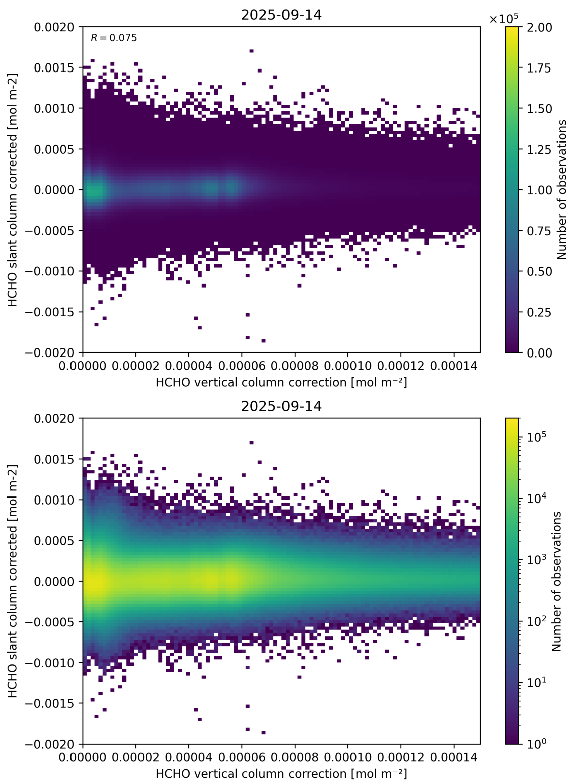
Figure 116: Scatter density plot of “HCHO vertical column correction” against “HCHO slant column corrected” for 2025-09-13 to 2025-09-15.
