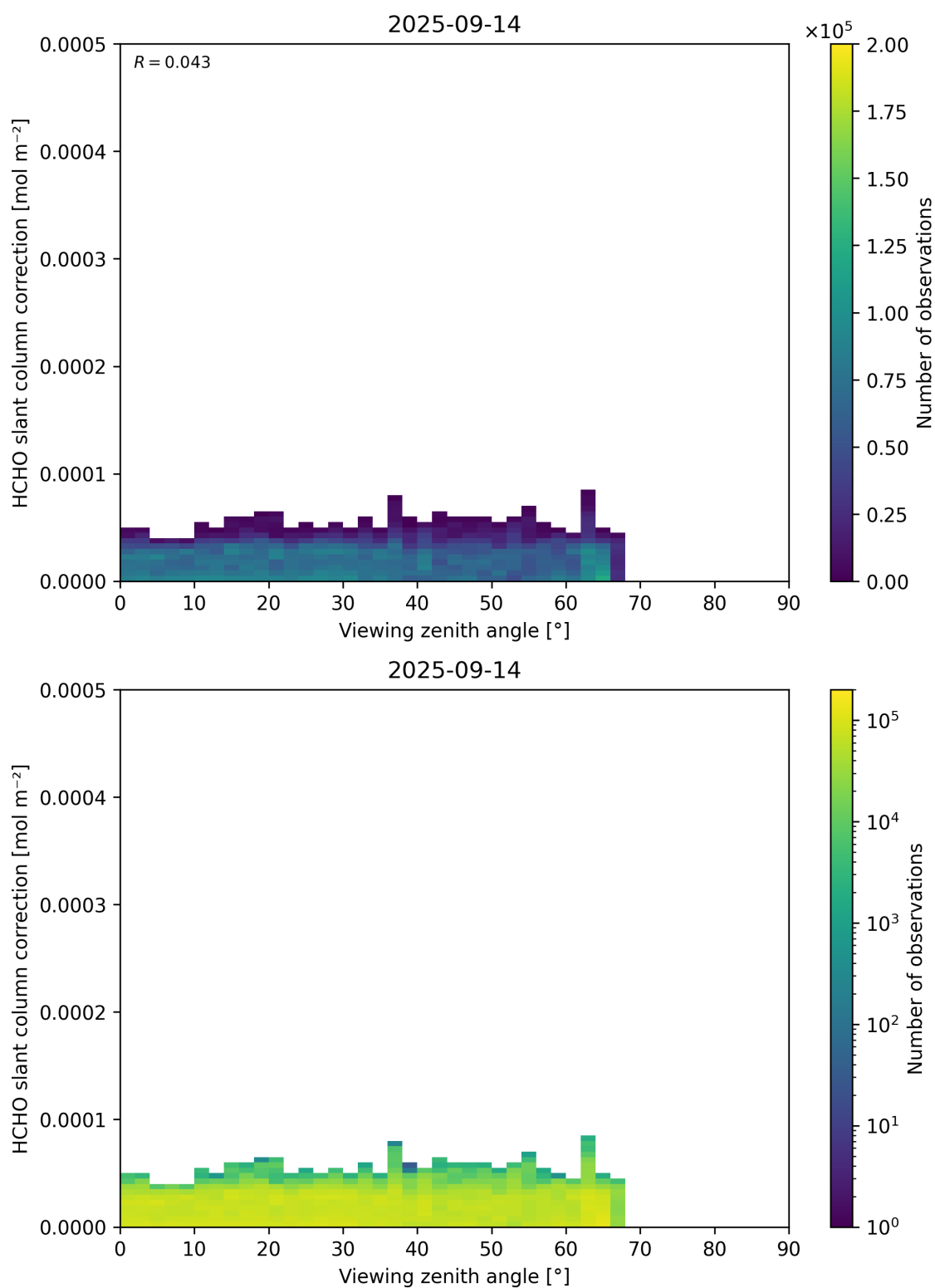
Figure 187: Scatter density plot of “Viewing zenith angle” against “HCHO slant column correction” for 2025-09-13 to 2025-09-15.
