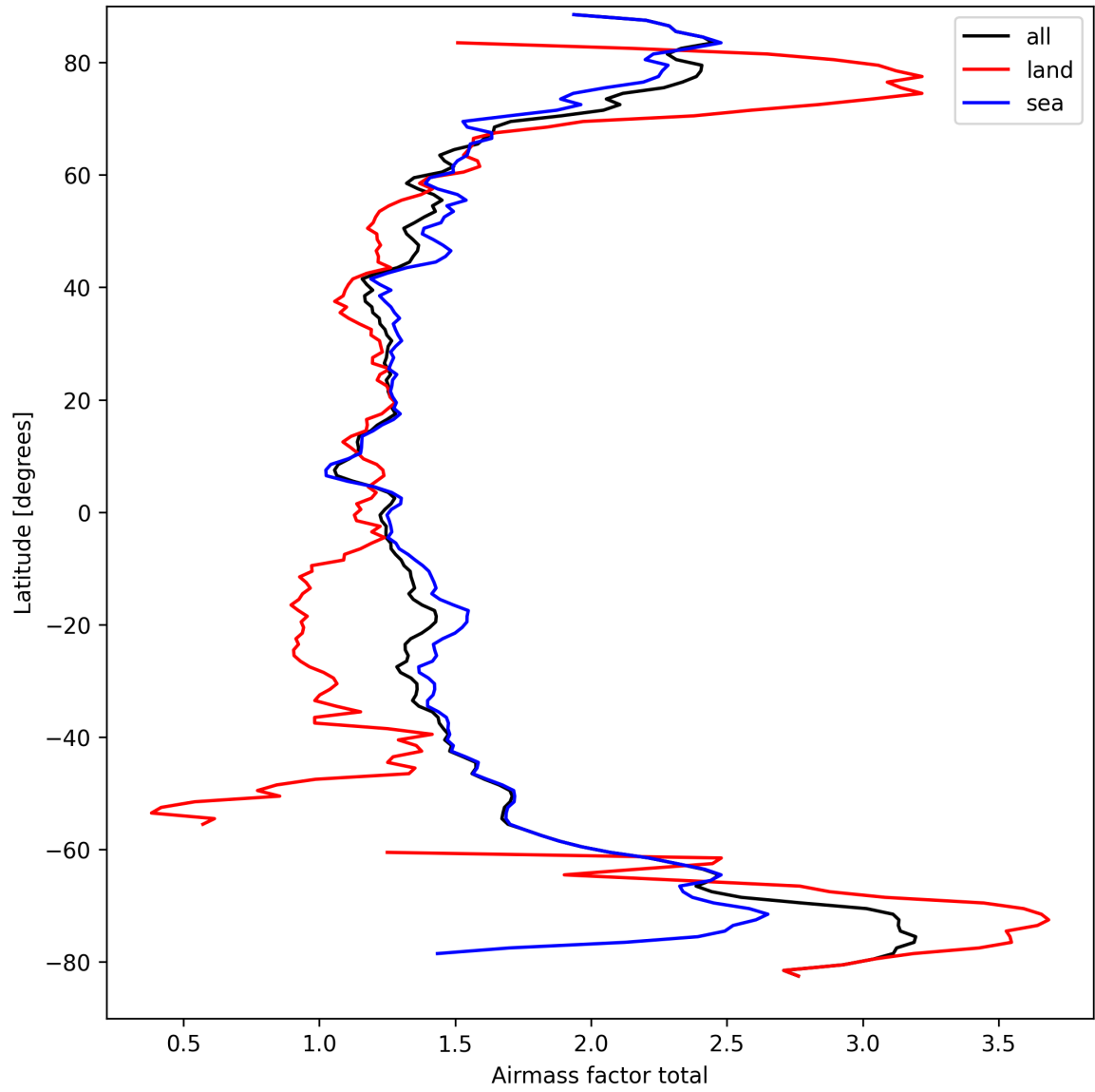
Figure 26: Zonal average of “Airmass factor total” for 2025-09-13 to 2025-09-15.
