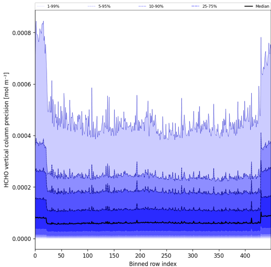
Figure 50: Along track statistics of “HCHO vertical column precision” for 2025-09-13 to 2025-09-15
