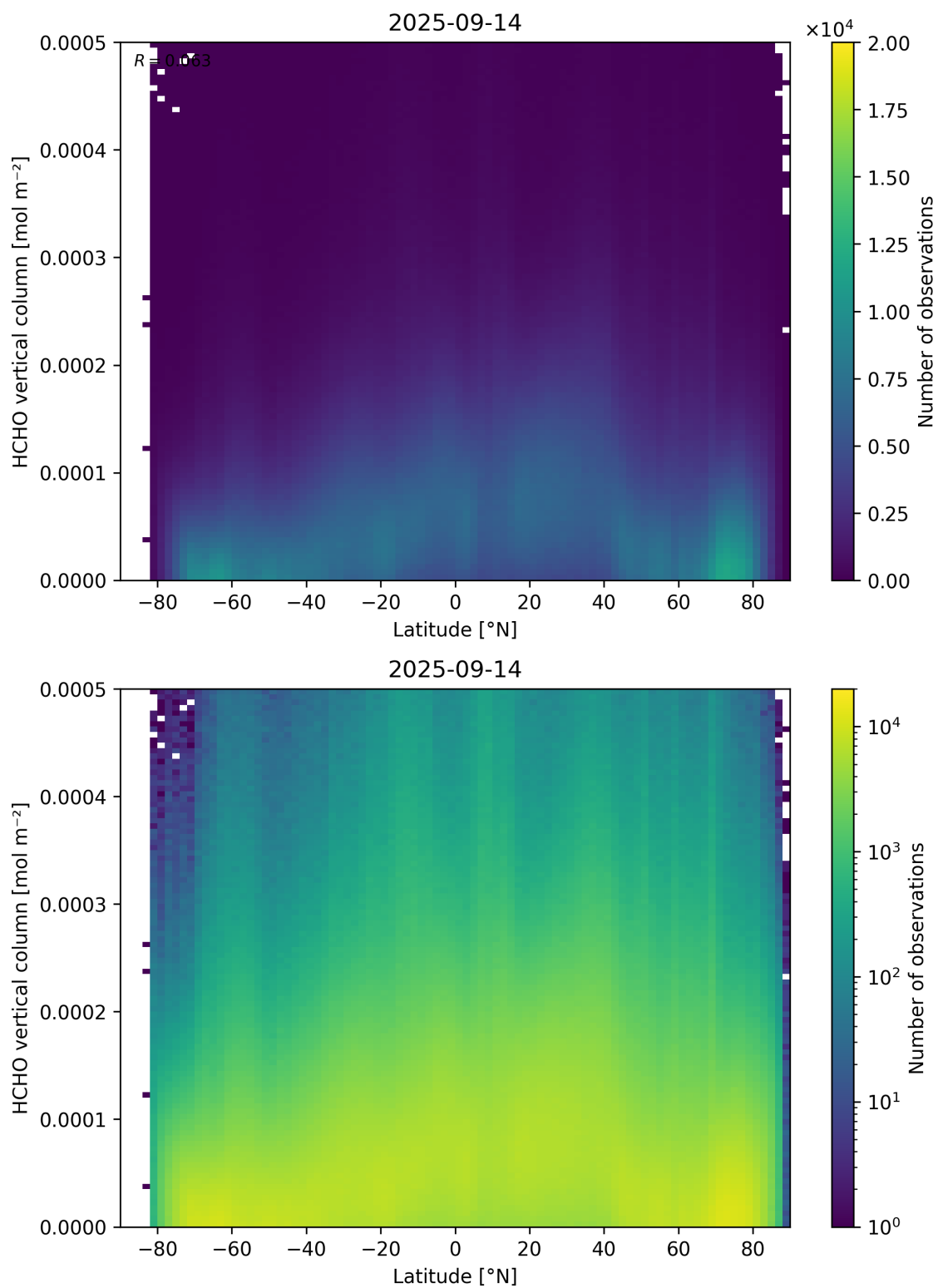
Figure 163: Scatter density plot of “Latitude” against “HCHO vertical column” for 2025-09-13 to 2025-09-15.
