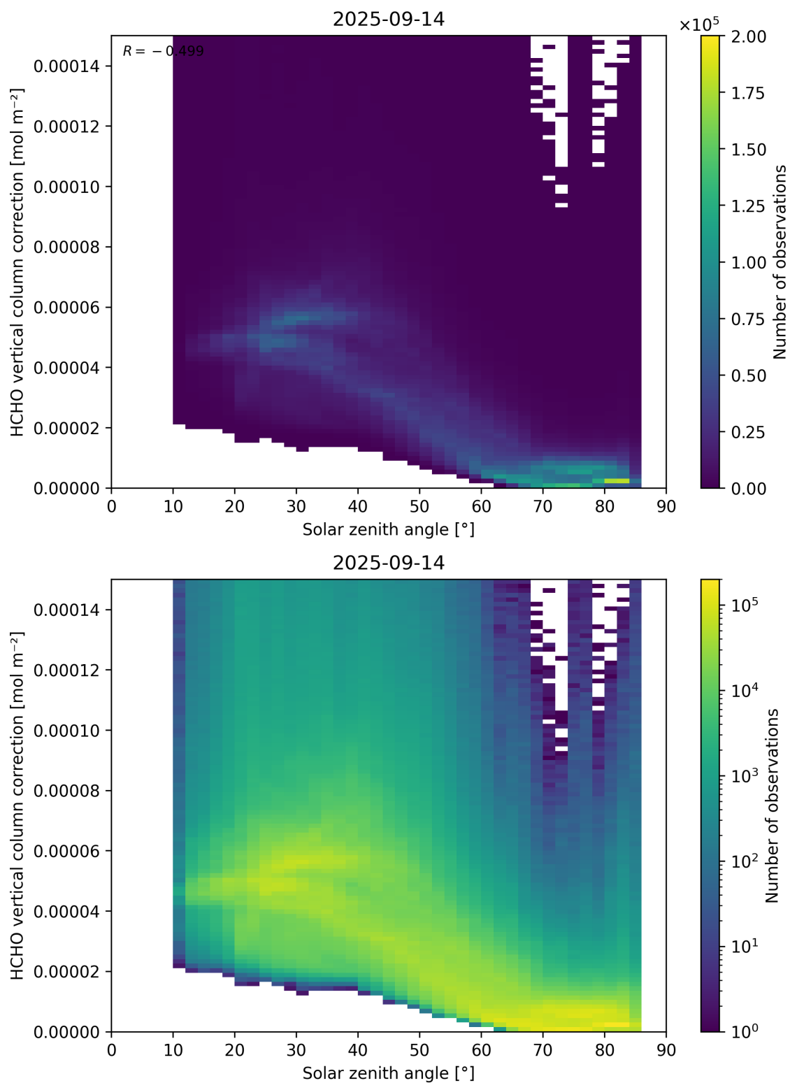
Figure 178: Scatter density plot of “Solar zenith angle” against “HCHO vertical column correction” for 2025-09-13 to 2025-09-15.
