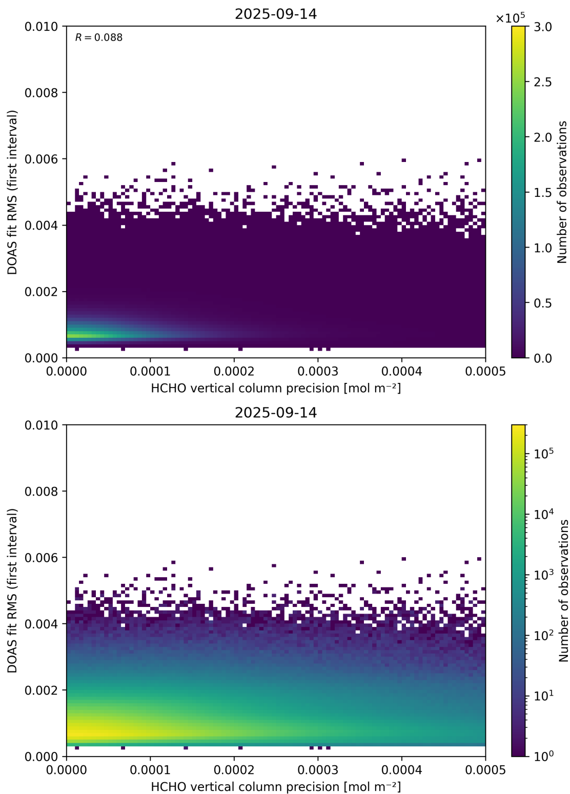
Figure 136: Scatter density plot of “HCHO vertical column precision” against “DOAS fit RMS (first interval)” for 2025-09-13 to 2025-09-15.
