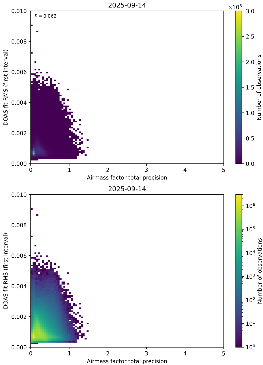
Figure 105: Scatter density plot of “Airmass factor total precision” against “DOAS fit RMS (first interval)” for 2025-09-13 to 2025-09-15.
