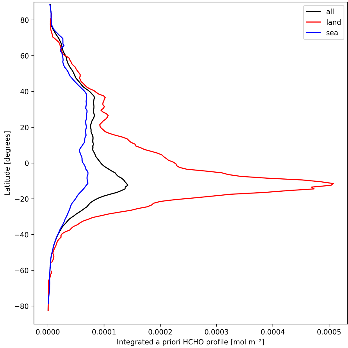
Figure 29: Zonal average of “Integrated a priori HCHO profile” for 2025-09-13 to 2025-09-15.
