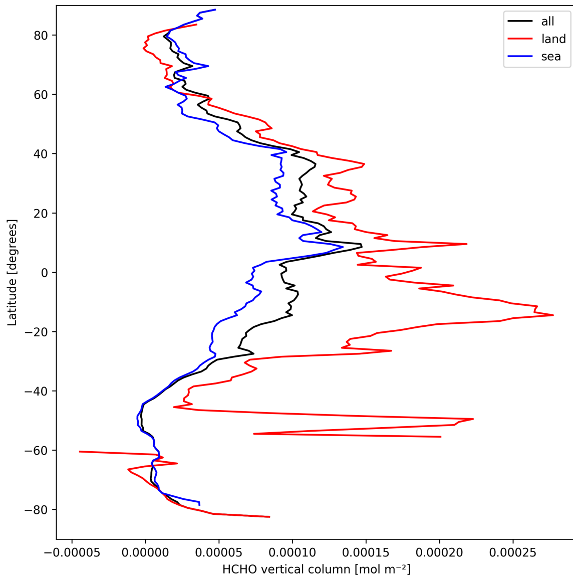
Figure 21: Zonal average of “HCHO vertical column” for 2025-09-13 to 2025-09-15.
