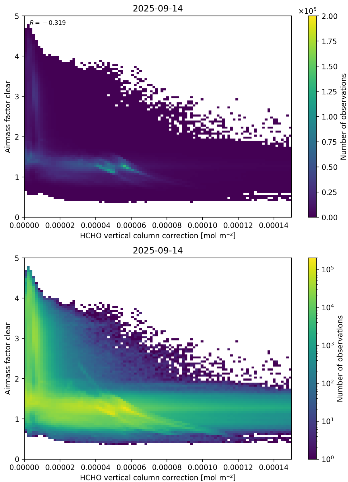
Figure 115: Scatter density plot of “HCHO vertical column correction” against “Airmass factor clear” for 2025-09-13 to 2025-09-15.
