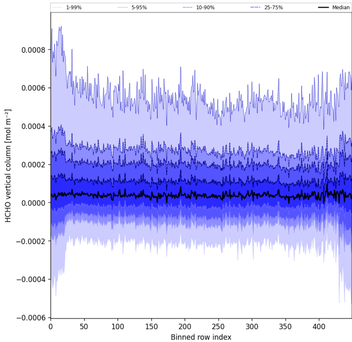
Figure 49: Along track statistics of “HCHO vertical column” for 2025-09-13 to 2025-09-15
