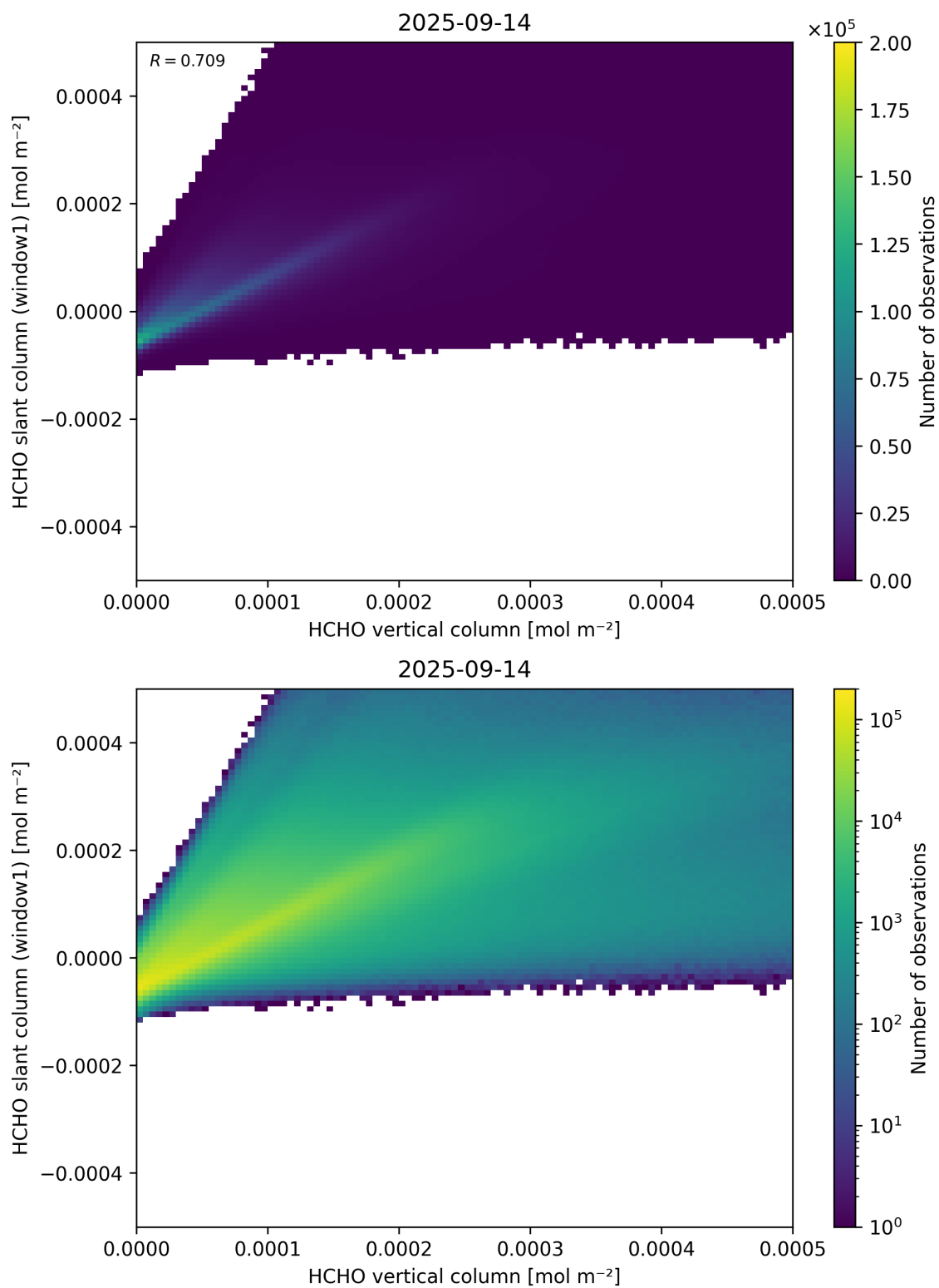
Figure 129: Scatter density plot of “HCHO vertical column” against “HCHO slant column (window1)” for 2025-09-13 to 2025-09-15.
