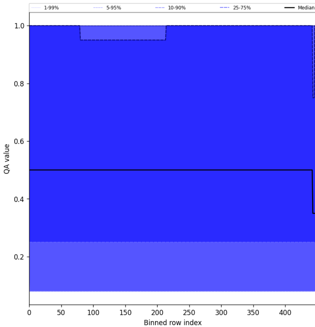
Figure 48: Along track statistics of “QA value” for 2025-09-13 to 2025-09-15
