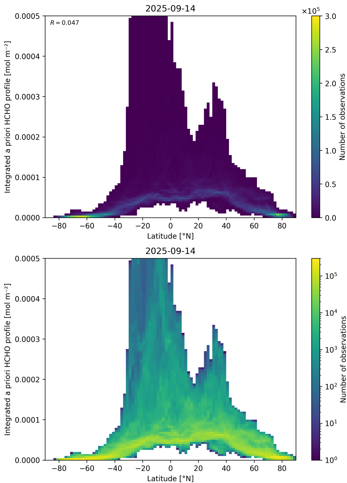
Figure 166: Scatter density plot of “Latitude” against “Integrated a priori HCHO profile” for 2025-09-13 to 2025-09-15.
