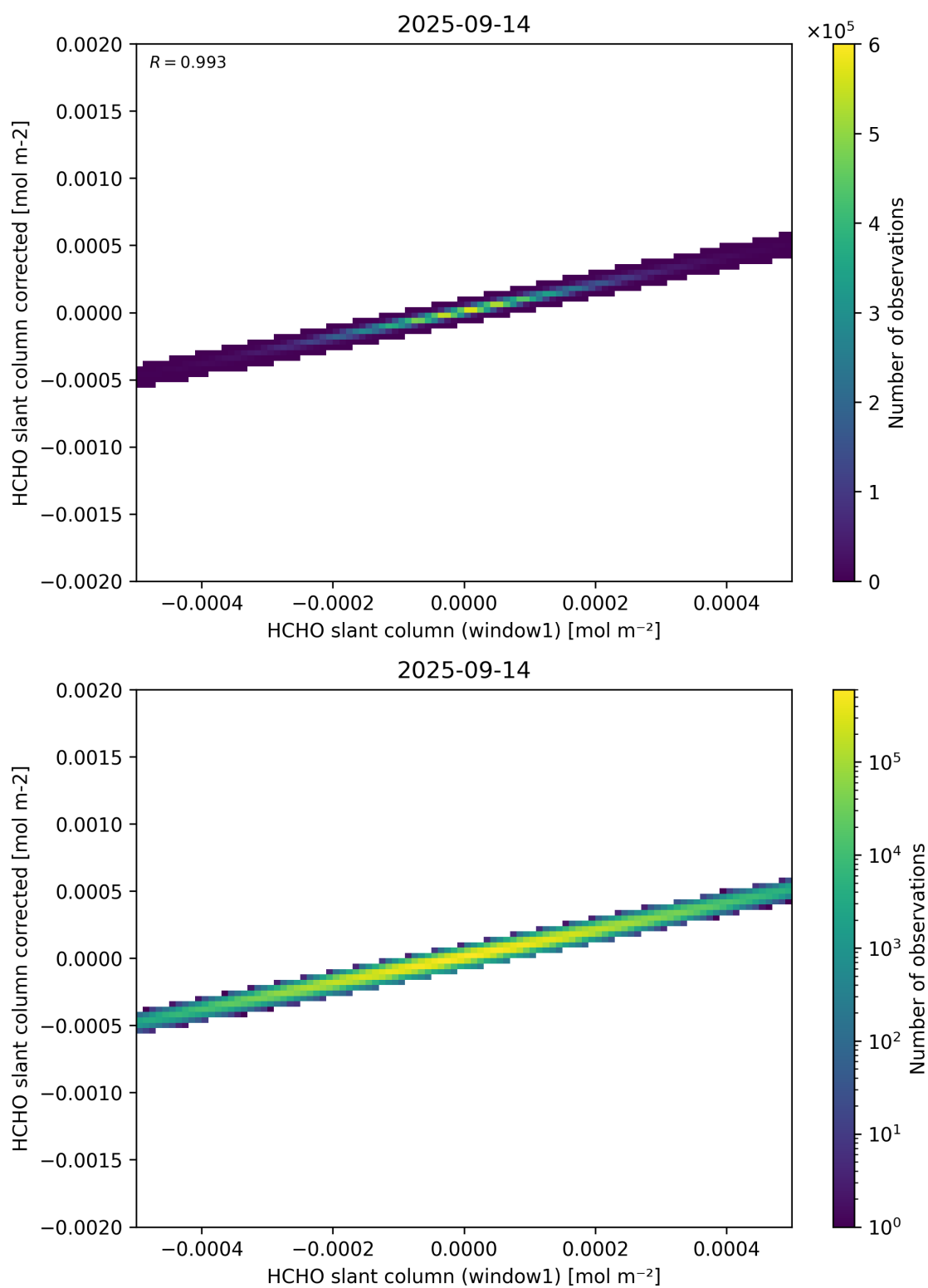
Figure 82: Scatter density plot of “HCHO slant column (window1)” against “HCHO slant column corrected” for 2025-09-13 to 2025-09-15.
