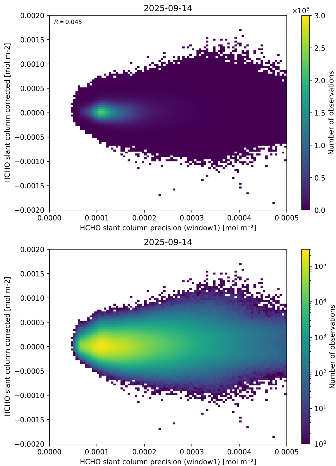
Figure 92: Scatter density plot of “HCHO slant column precision (window1)” against “HCHO slant column corrected” for 2025-09-13 to 2025-09-15.
