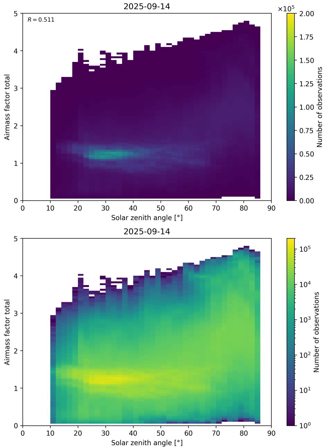
Figure 175: Scatter density plot of “Solar zenith angle” against “Airmass factor total” for 2025-09-13 to 2025-09-15.
