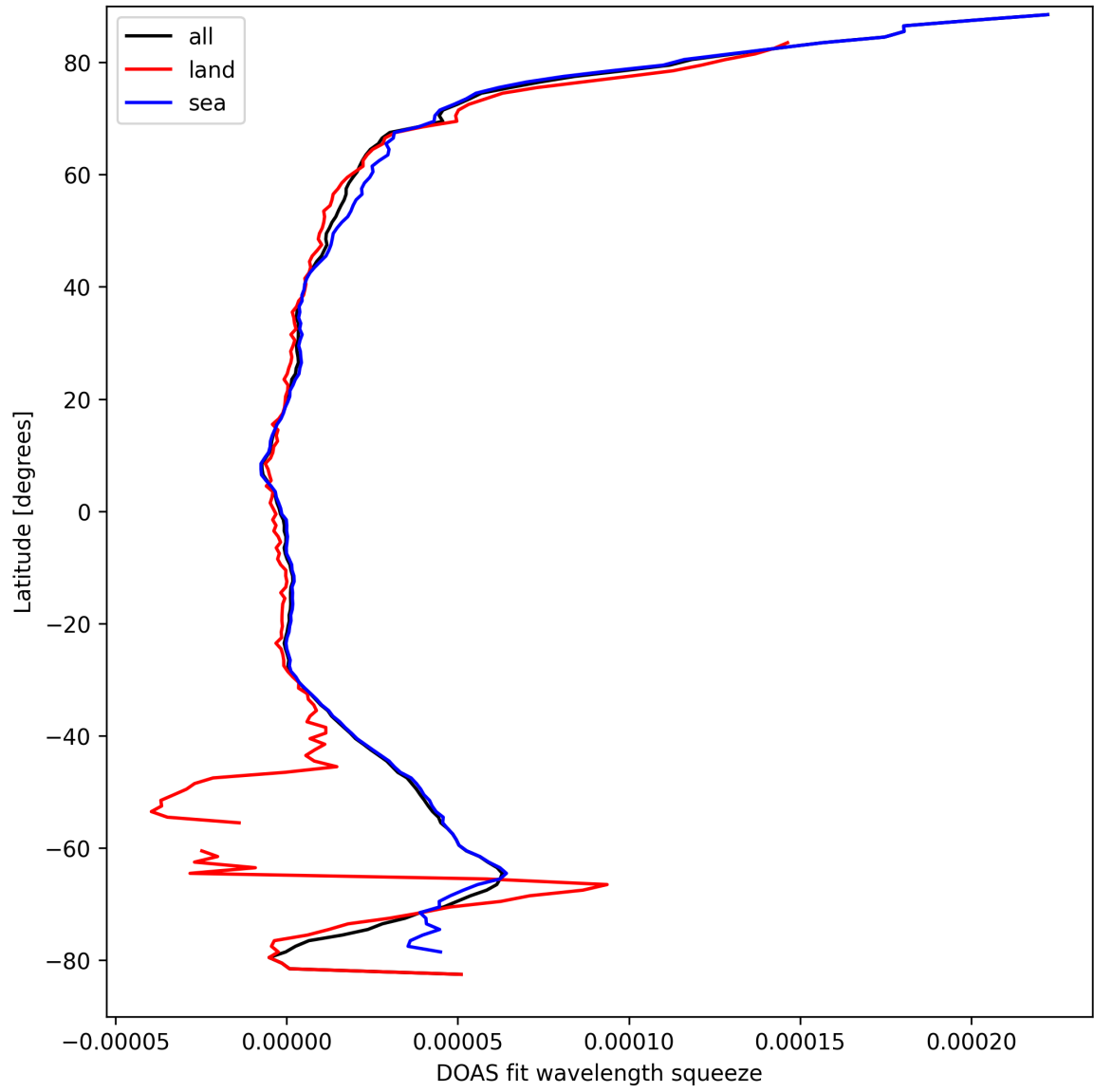
Figure 31: Zonal average of “DOAS fit wavelength squeeze” for 2025-09-13 to 2025-09-15.
