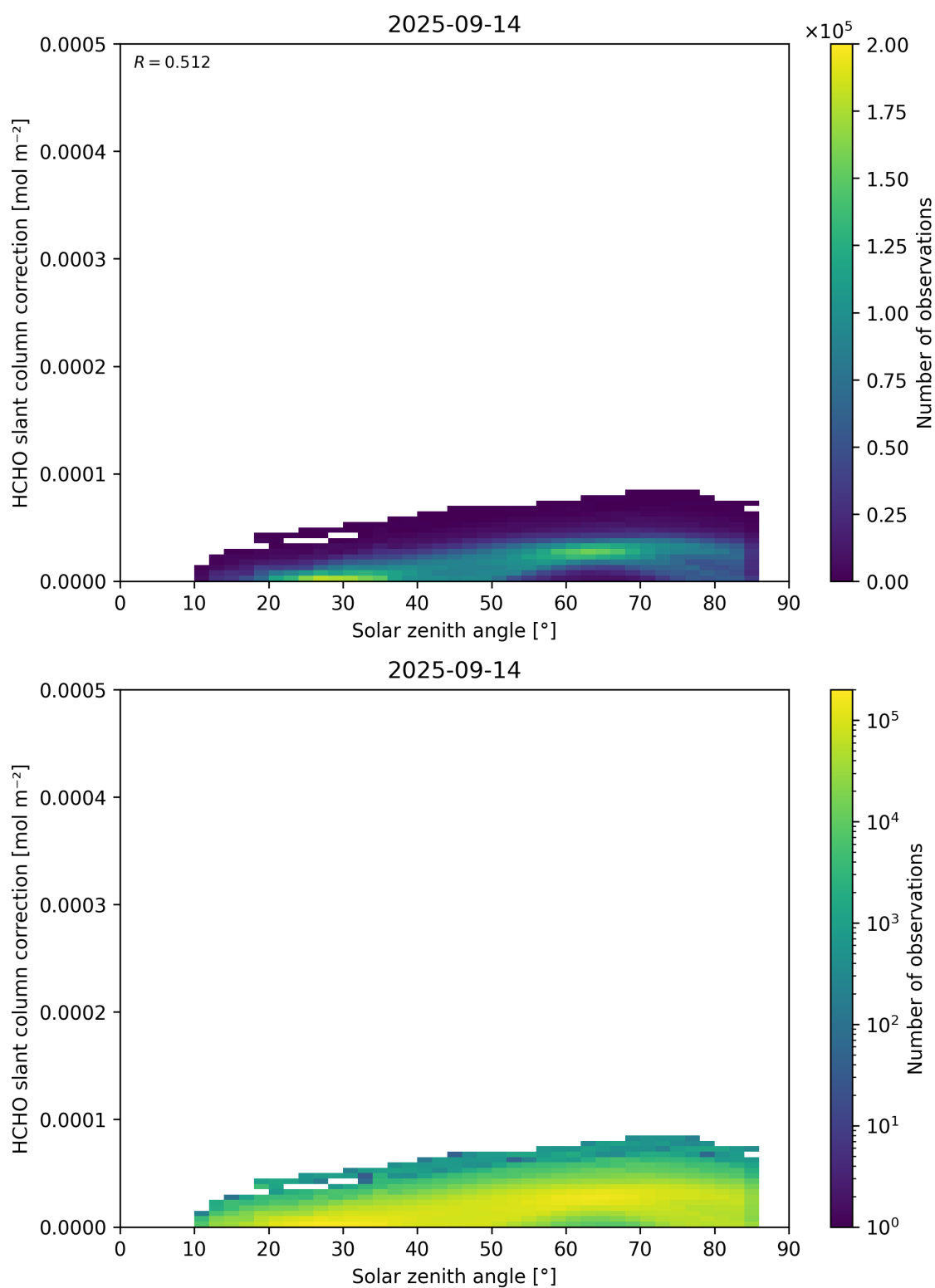
Figure 172: Scatter density plot of “Solar zenith angle” against “HCHO slant column correction” for 2025-09-13 to 2025-09-15.
