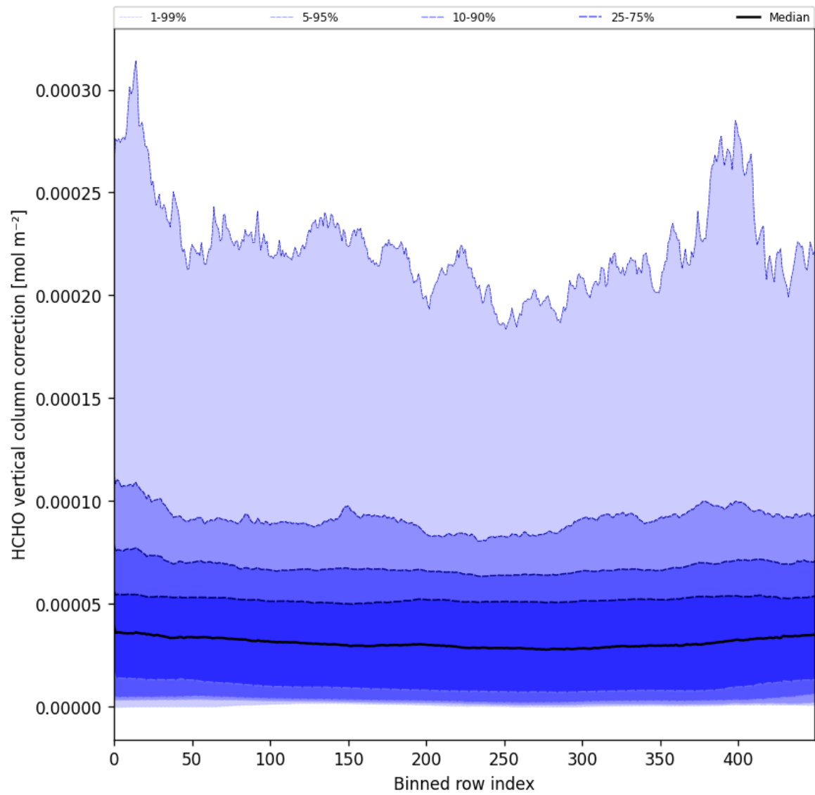
Figure 51: Along track statistics of “HCHO vertical column correction” for 2025-09-13 to 2025-09-15
