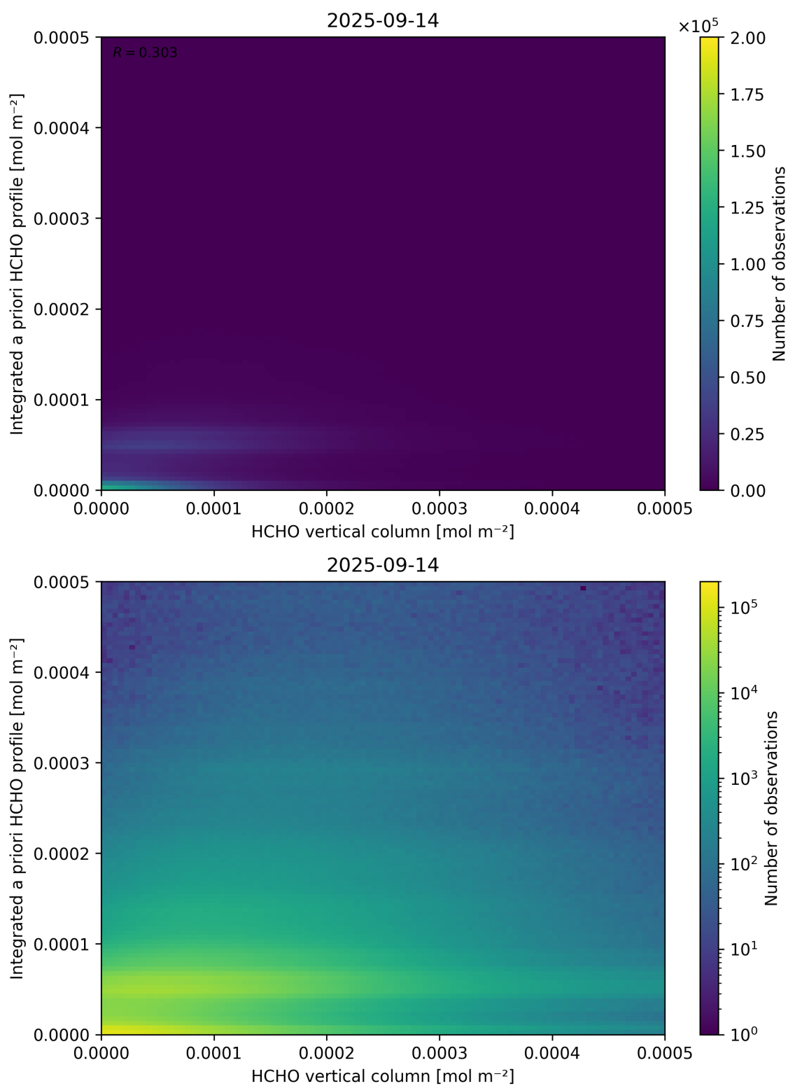
Figure 135: Scatter density plot of “HCHO vertical column” against “Integrated a priori HCHO profile” for 2025-09-13 to 2025-09-15.
