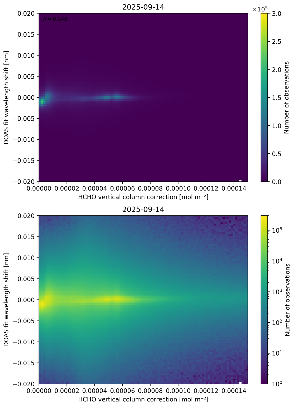
Figure 113: Scatter density plot of “HCHO vertical column correction” against “DOAS fit wavelength shift” for 2025-09-13 to 2025-09-15.
