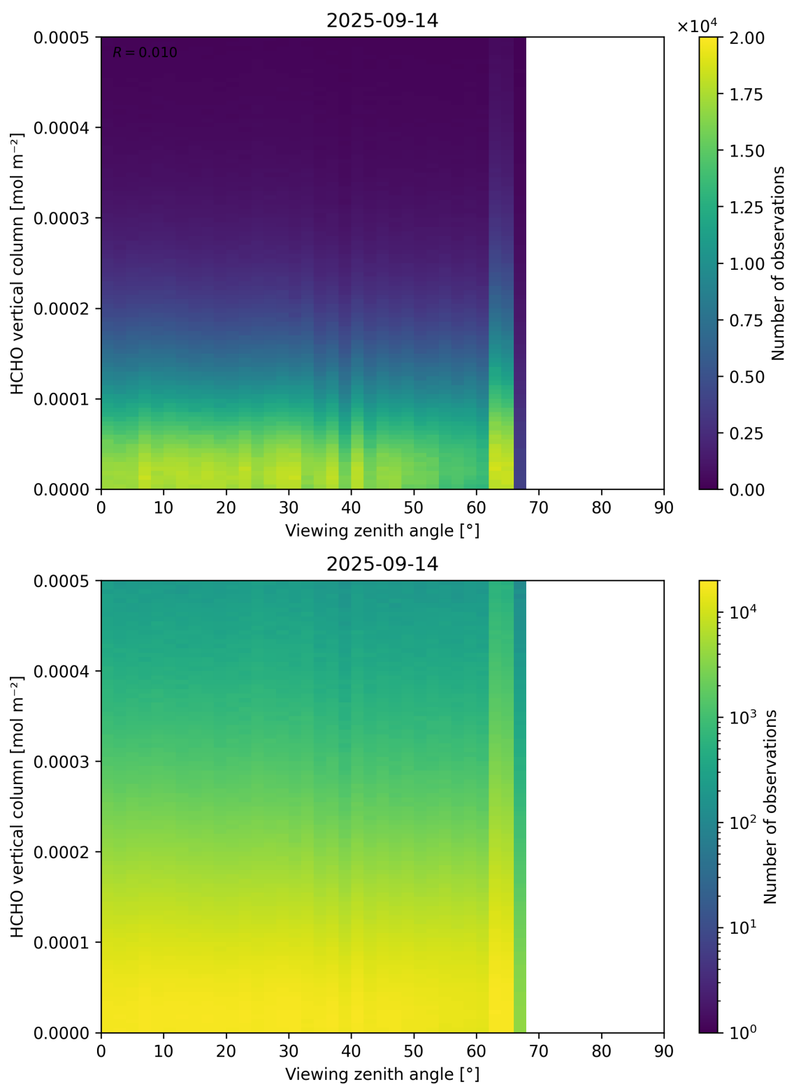
Figure 192: Scatter density plot of “Viewing zenith angle” against “HCHO vertical column” for 2025-09-13 to 2025-09-15.
