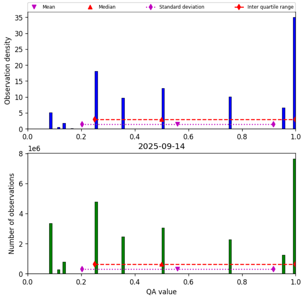
Figure 34: Histogram of “QA value” for 2025-09-13 to 2025-09-15
