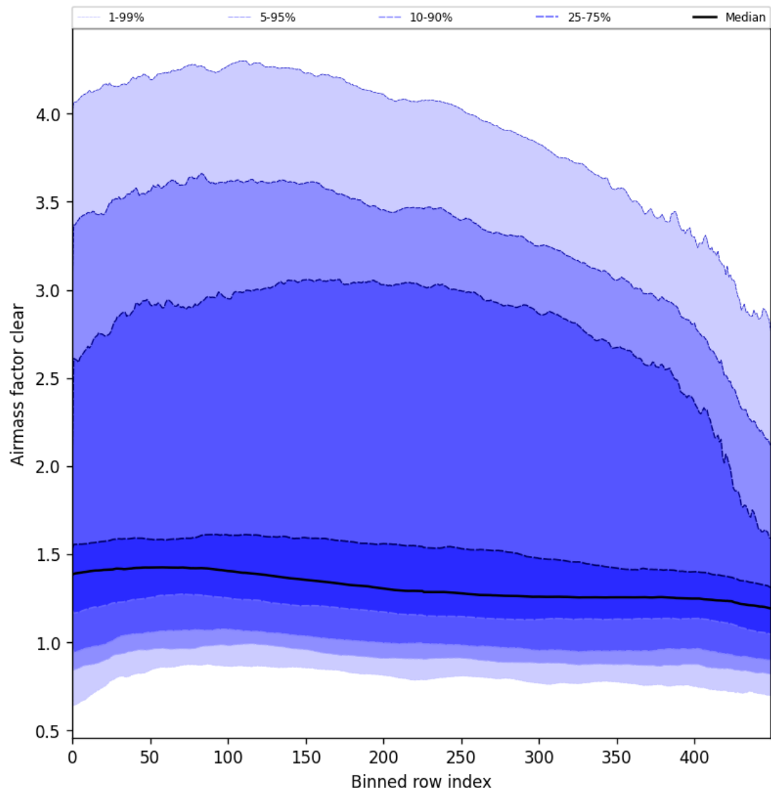
Figure 56: Along track statistics of “Air mass factor clear” for 2025-09-13 to 2025-09-15
