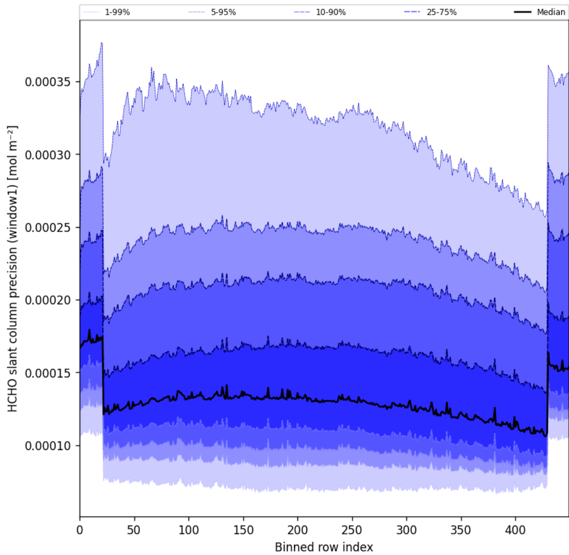
Figure 53: Along track statistics of “HCHO slant column precision (window1)” for 2025-09-13 to 2025-09-15
