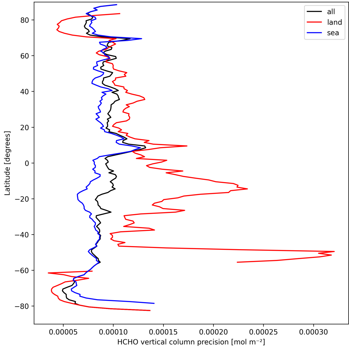
Figure 22: Zonal average of “HCHO vertical column precision” for 2025-09-13 to 2025-09-15.
