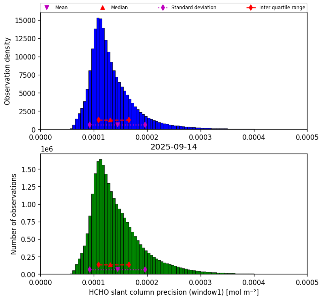
Figure 39: Histogram of “HCHO slant column precision (window1)” for 2025-09-13 to 2025-09-15
