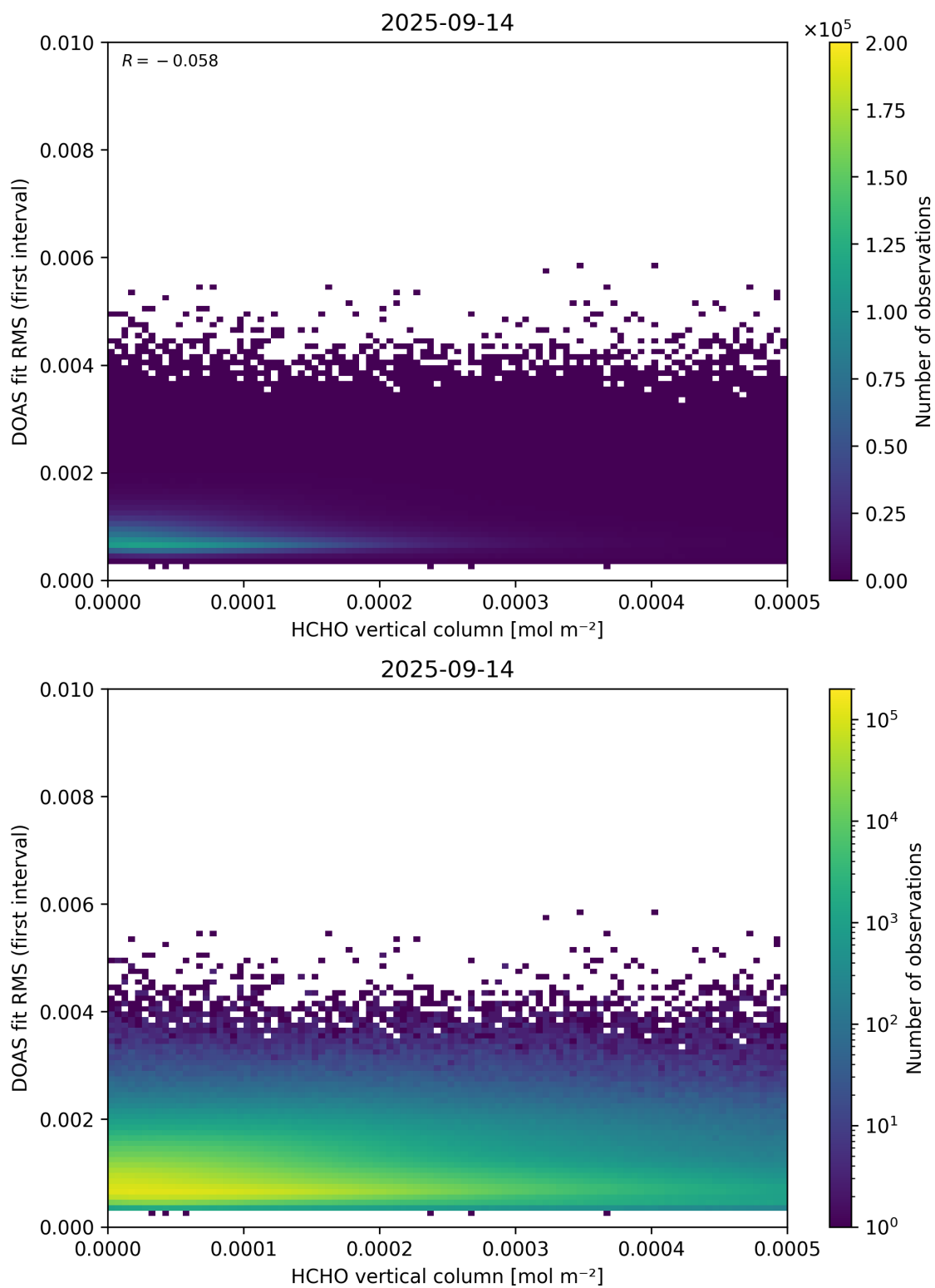
Figure 123: Scatter density plot of “HCHO vertical column” against “DOAS fit RMS (first interval)” for 2025-09-13 to 2025-09-15.
