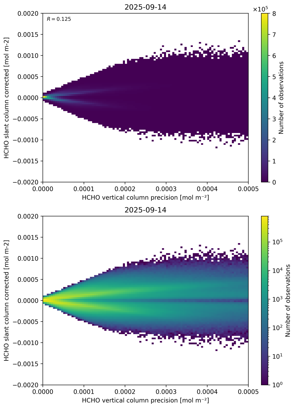
Figure 140: Scatter density plot of “HCHO vertical column precision” against “HCHO slant column corrected” for 2025-09-13 to 2025-09-15.
