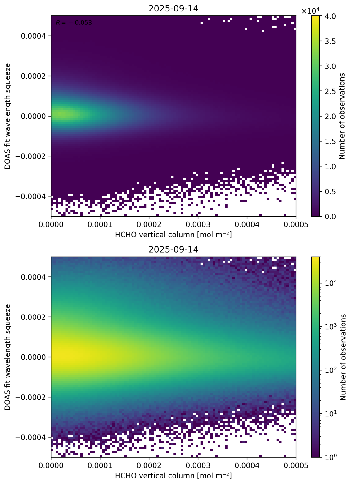
Figure 125: Scatter density plot of “HCHO vertical column” against “DOAS fit wavelength squeeze” for 2025-09-13 to 2025-09-15.
