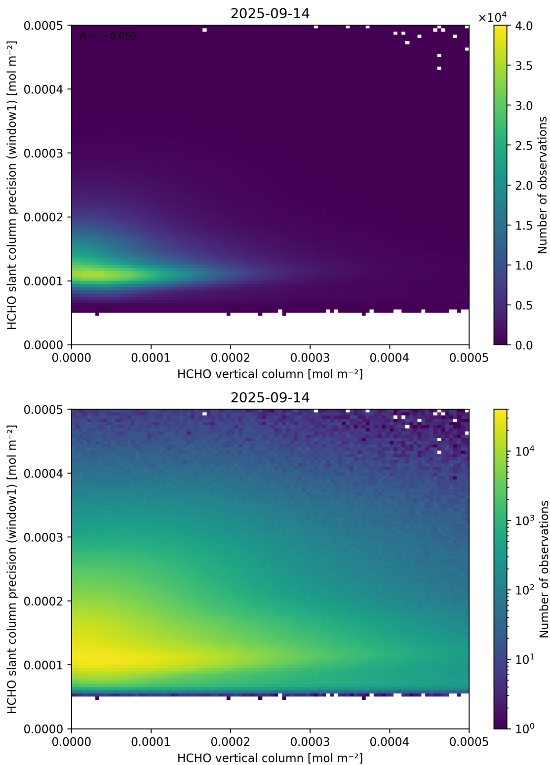
Figure 130: Scatter density plot of “HCHO vertical column” against “HCHO slant column precision (window1)” for 2025-09-13 to 2025-09-15.
