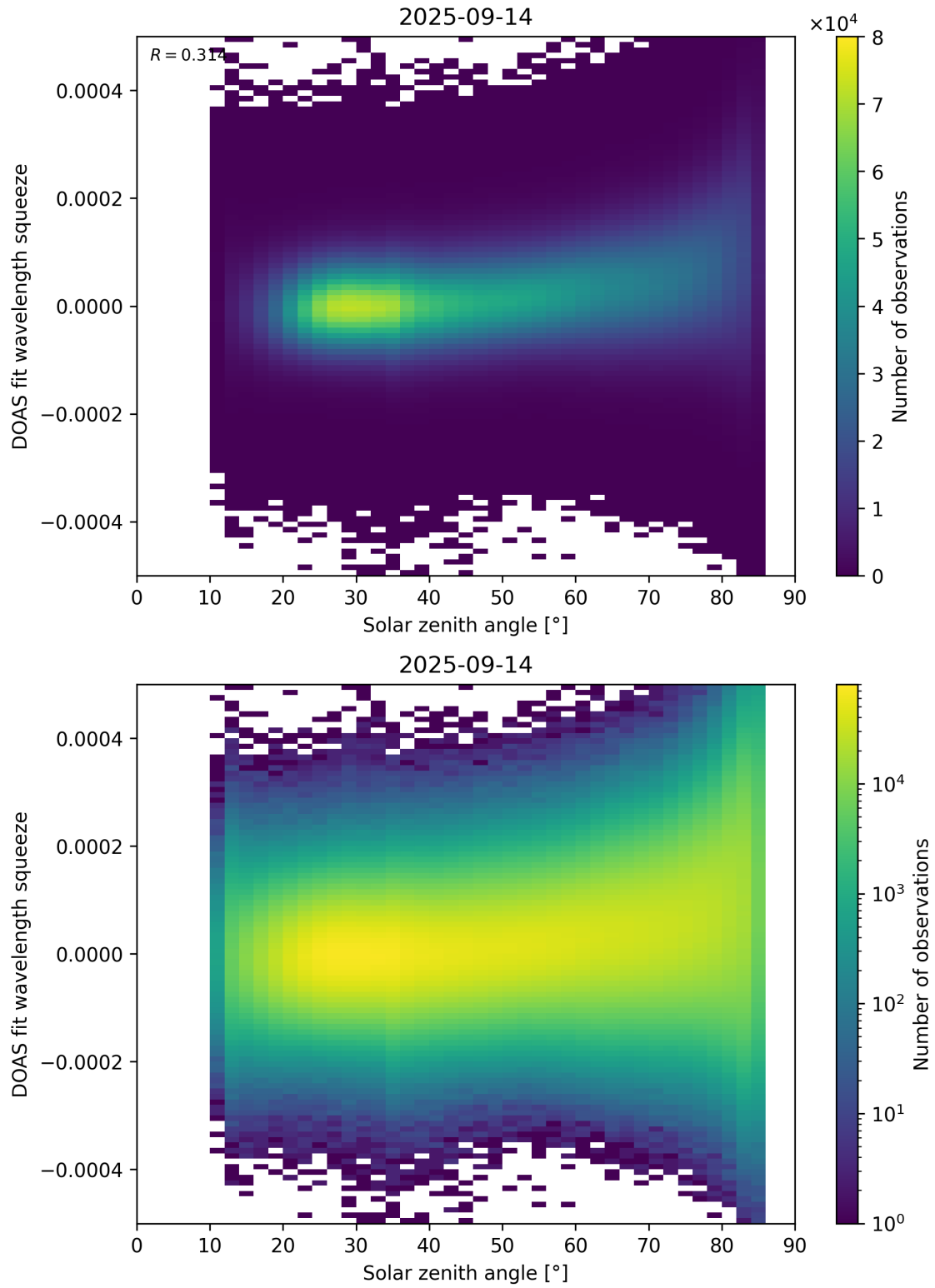
Figure 169: Scatter density plot of “Solar zenith angle” against “DOAS fit wavelength squeeze” for 2025-09-13 to 2025-09-15.
