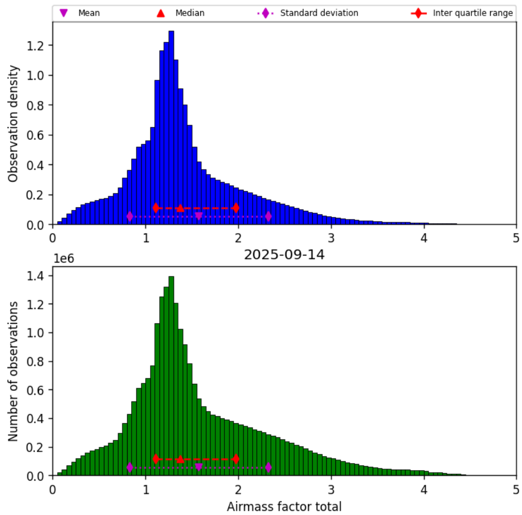
Figure 40: Histogram of “Airmass factor total” for 2025-09-13 to 2025-09-15
