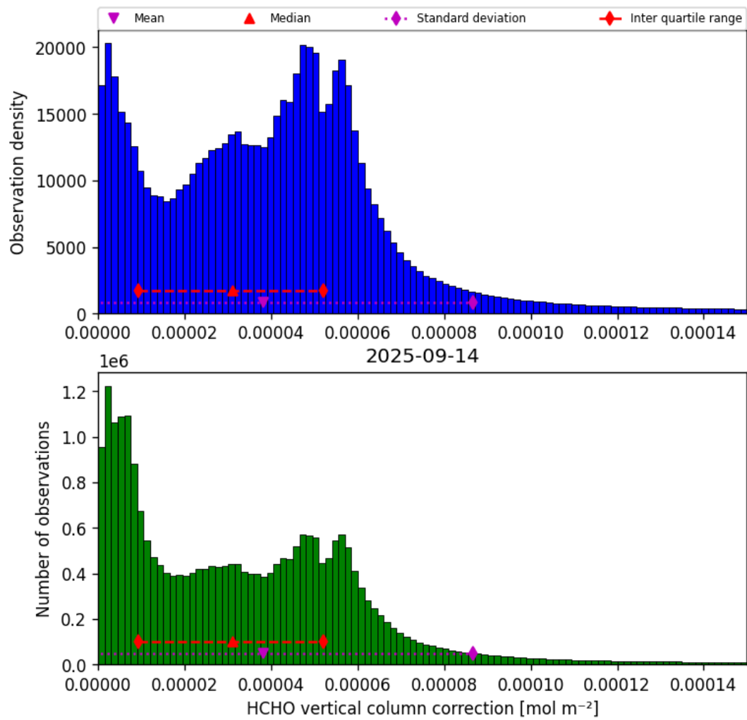
Figure 37: Histogram of “HCHO vertical column correction” for 2025-09-13 to 2025-09-15
