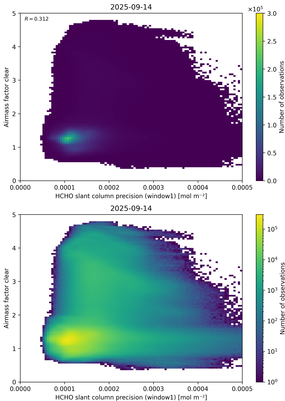
Figure 91: Scatter density plot of “HCHO slant column precision (window1)” against “Airmass factor clear” for 2025-09-13 to 2025-09-15.
