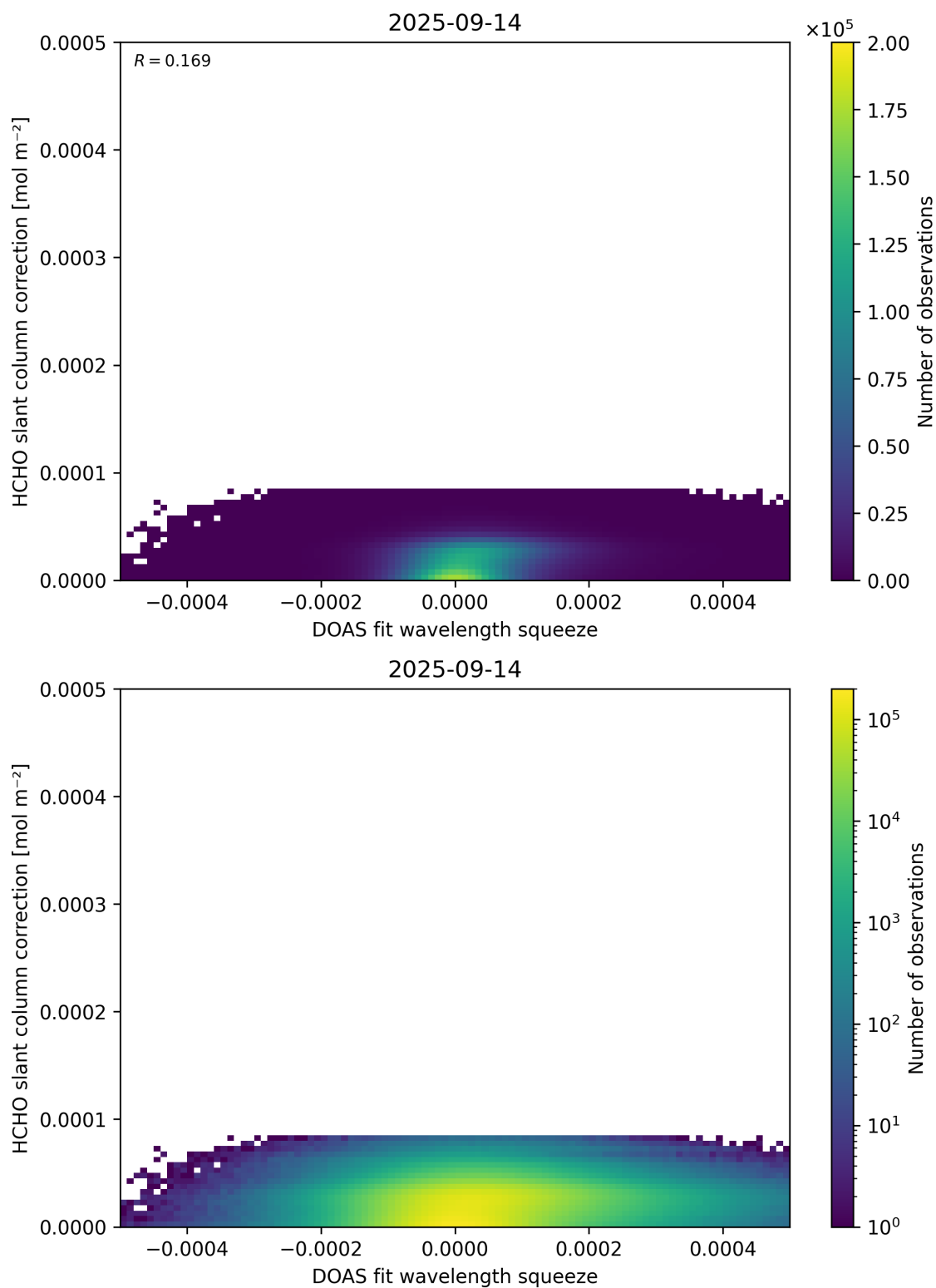
Figure 70: Scatter density plot of “DOAS fit wavelength squeeze” against “HCHO slant column correction” for 2025-09-13 to 2025-09-15.
