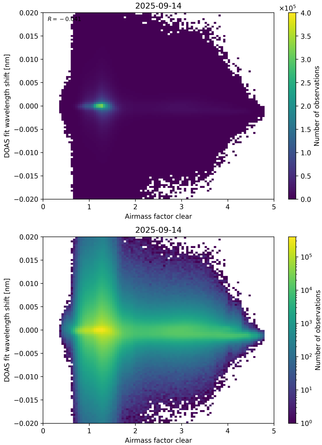
Figure 72: Scatter density plot of “Airmass factor clear” against “DOAS fit wavelength shift” for 2025-09-13 to 2025-09-15.
