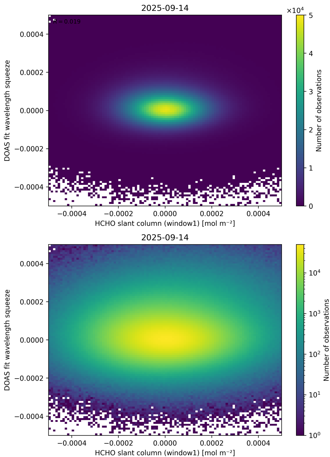
Figure 80: Scatter density plot of “HCHO slant column (window1)” against “DOAS fit wavelength squeeze” for 2025-09-13 to 2025-09-15.
