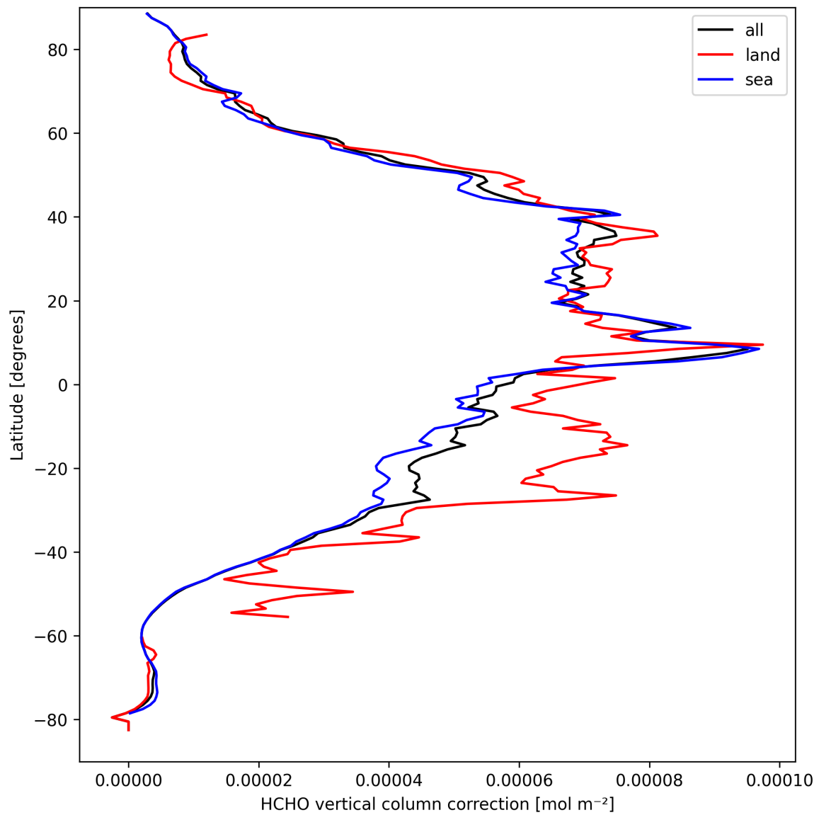
Figure 23: Zonal average of “HCHO vertical column correction” for 2025-09-13 to 2025-09-15.
