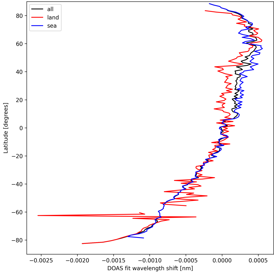
Figure 30: Zonal average of "DOAS fit wavelength shift" for 2025-09-13 to 2025-09-15.
