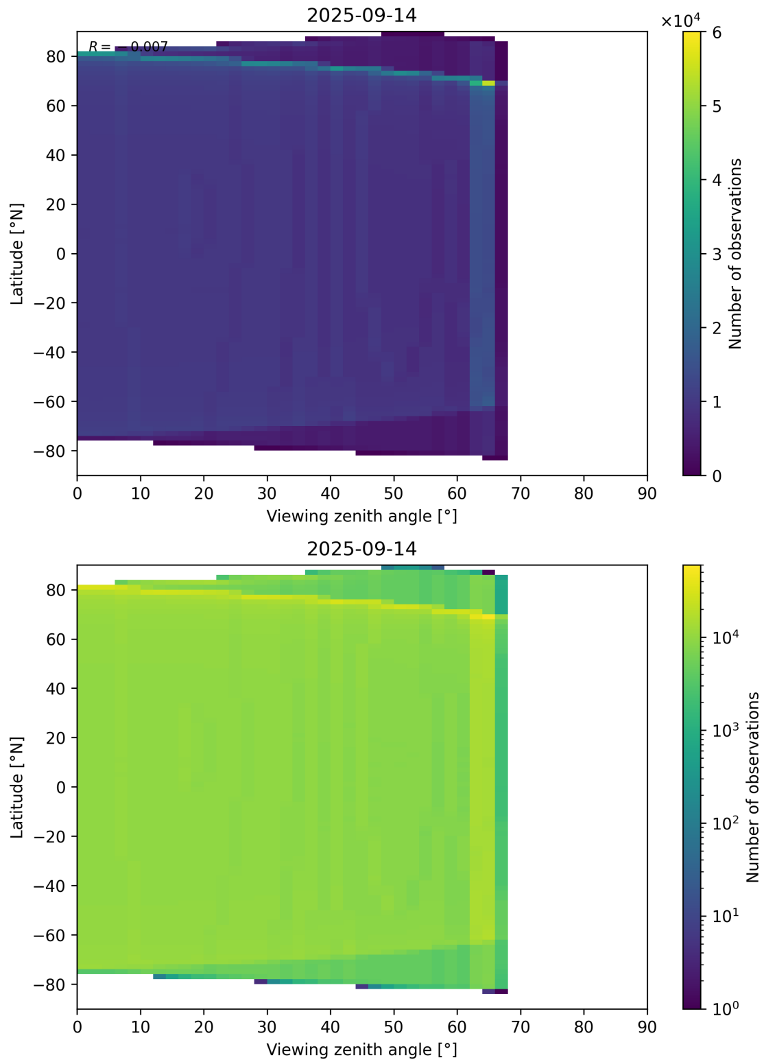
Figure 196: Scatter density plot of “Viewing zenith angle” against “Latitude” for 2025-09-13 to 2025-09-15.
