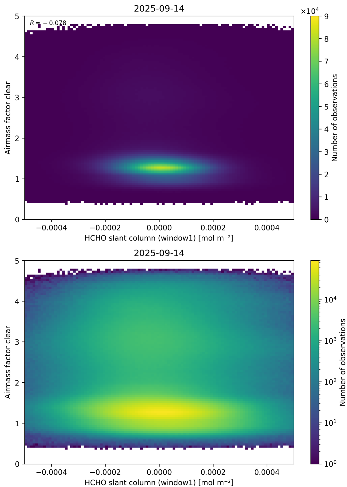
Figure 81: Scatter density plot of “HCHO slant column (window1)” against “Airmass factor clear” for 2025-09-13 to 2025-09-15.
