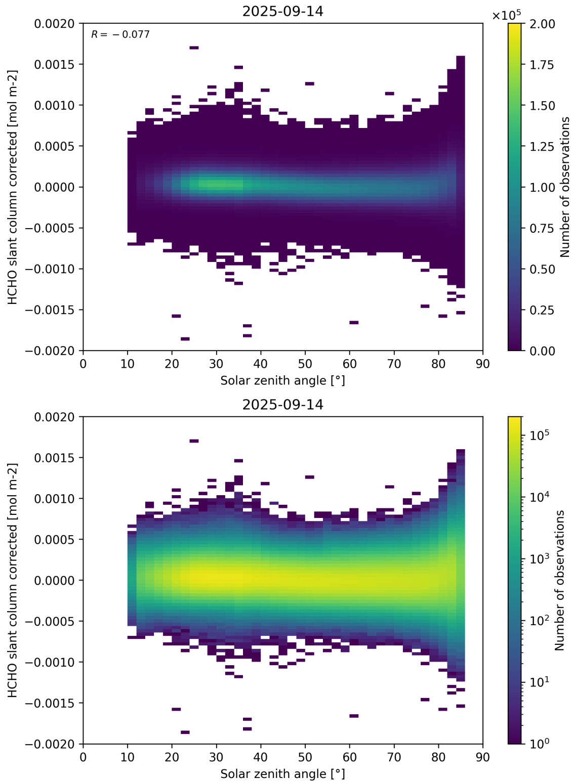
Figure 171: Scatter density plot of “Solar zenith angle” against “HCHO slant column corrected” for 2025-09-13 to 2025-09-15.
