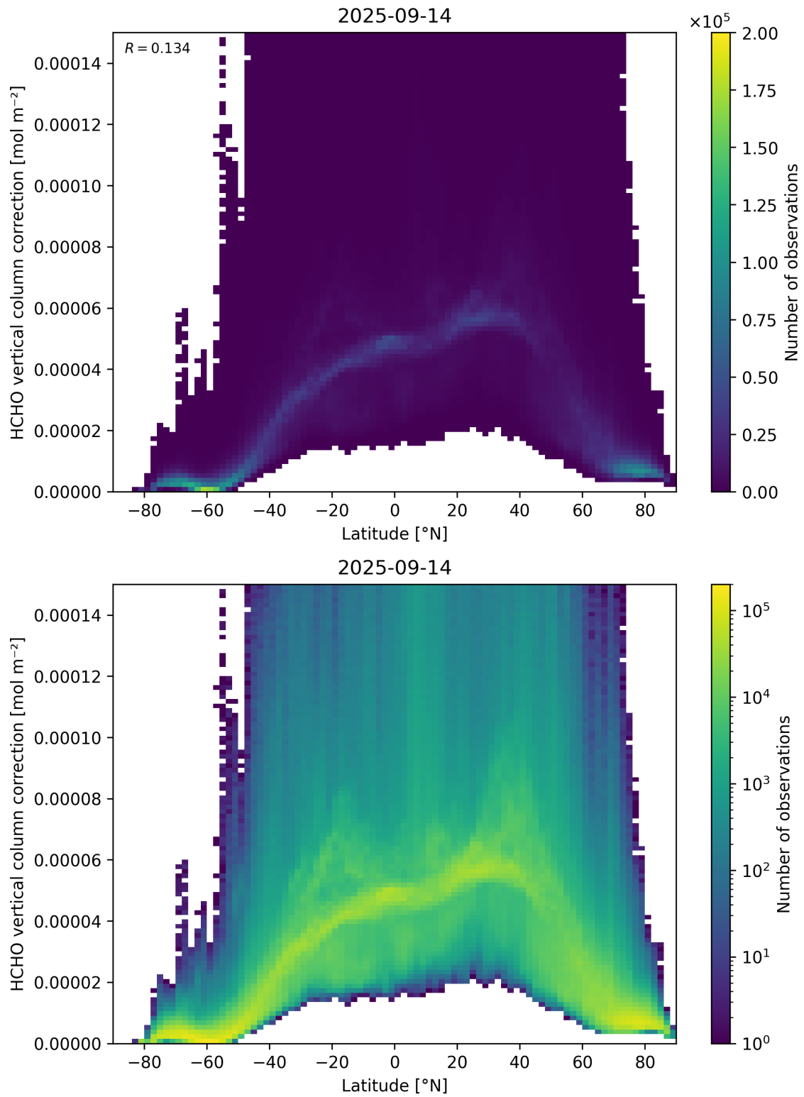
Figure 164: Scatter density plot of “Latitude” against “HCHO vertical column correction” for 2025-09-13 to 2025-09-15.
