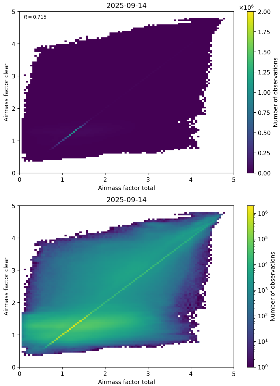
Figure 100: Scatter density plot of “Airmass factor total” against “Airmass factor clear” for 2025-09-13 to 2025-09-15.
