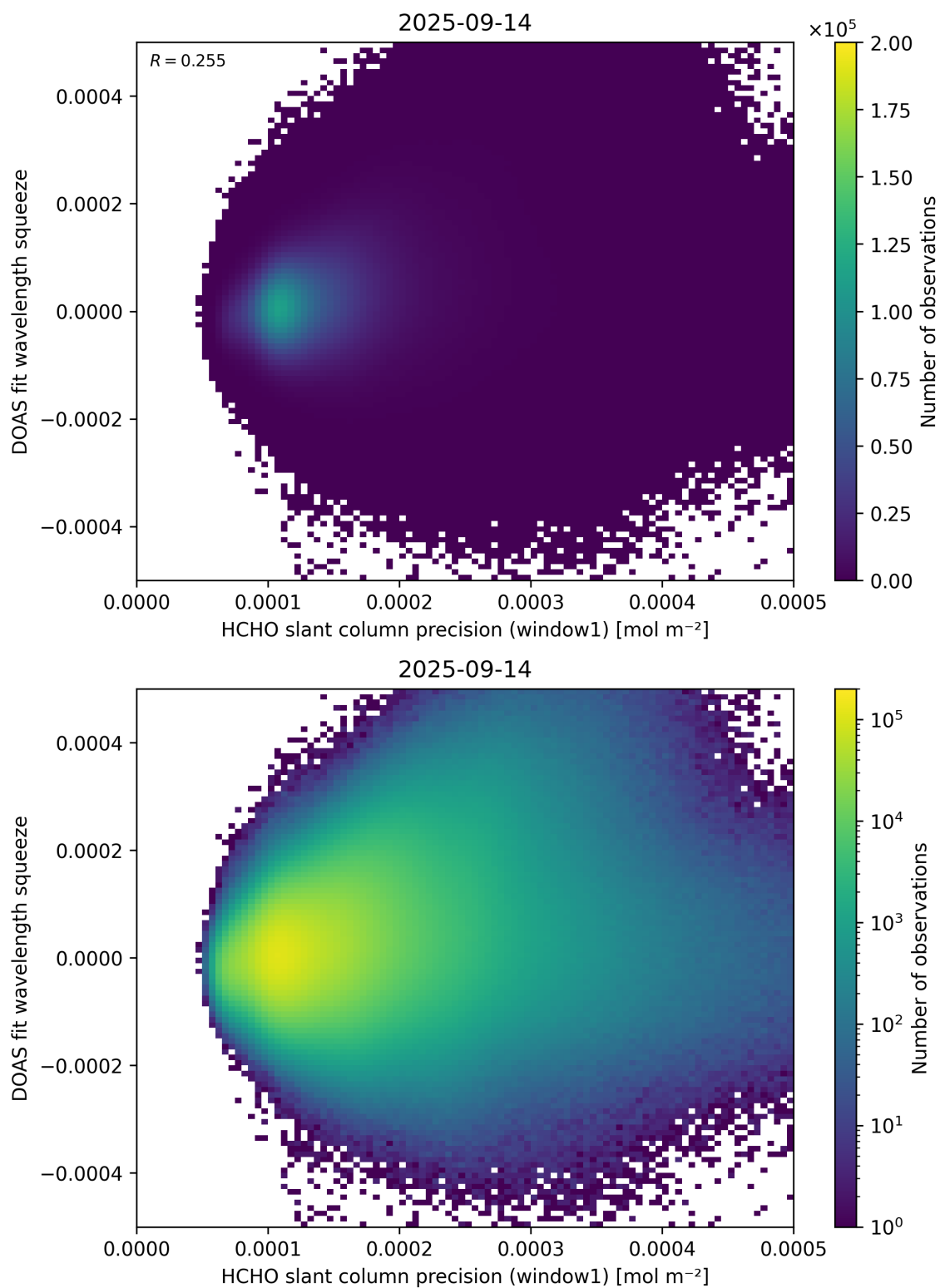
Figure 90: Scatter density plot of “HCHO slant column precision (window1)” against “DOAS fit wavelength squeeze” for 2025-09-13 to 2025-09-15.
