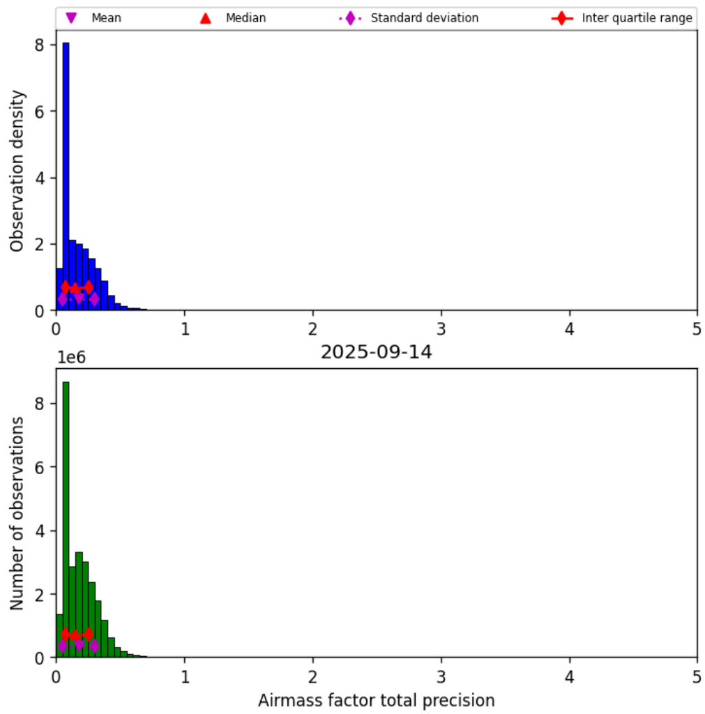
Figure 41: Histogram of “Airmass factor total precision” for 2025-09-13 to 2025-09-15
