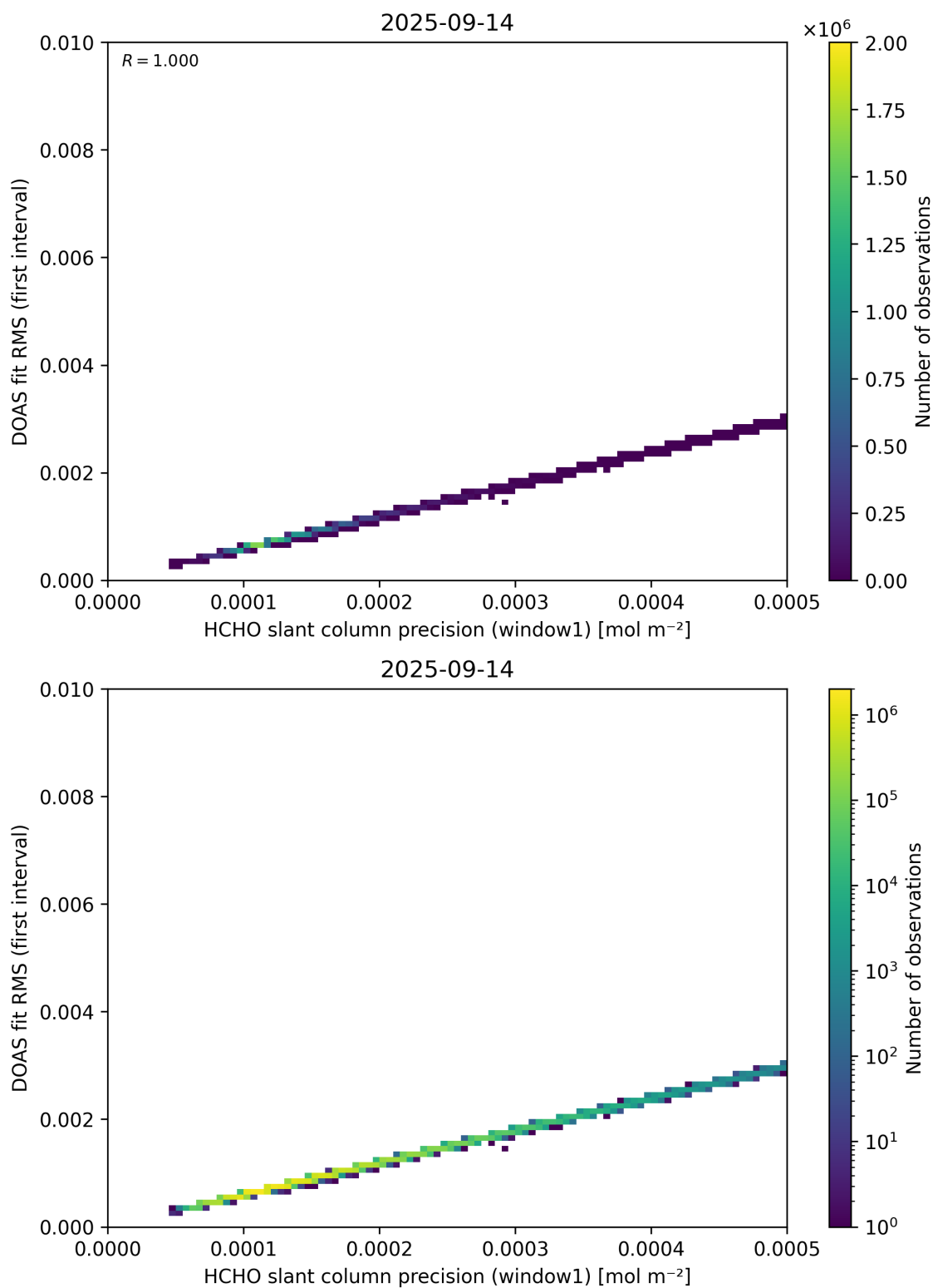
Figure 88: Scatter density plot of “HCHO slant column precision (window1)” against “DOAS fit RMS (first interval)” for 2025-09-13 to 2025-09-15.
