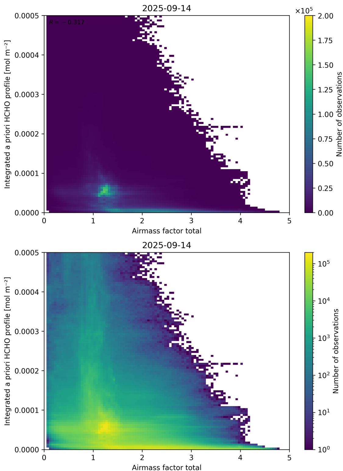
Figure 104: Scatter density plot of “Airmass factor total” against “Integrated a priori HCHO profile” for 2025-09-13 to 2025-09-15.
