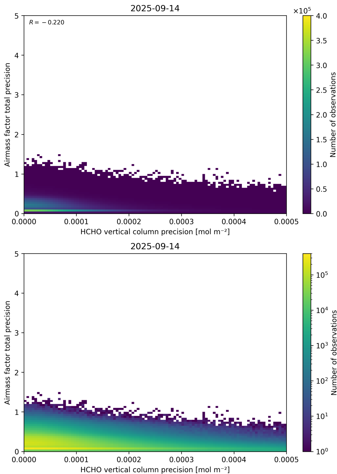
Figure 145: Scatter density plot of “HCHO vertical column precision” against “Airmass factor total precision” for 2025-09-13 to 2025-09-15.
