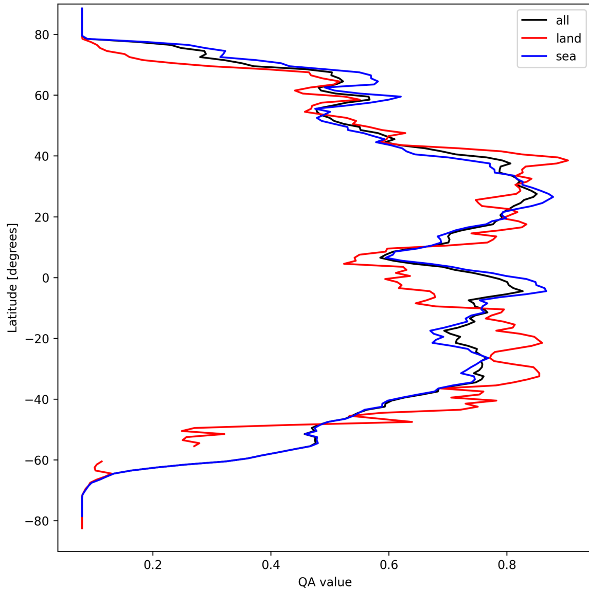
Figure 20: Zonal average of “QA value” for 2025-09-13 to 2025-09-15.
