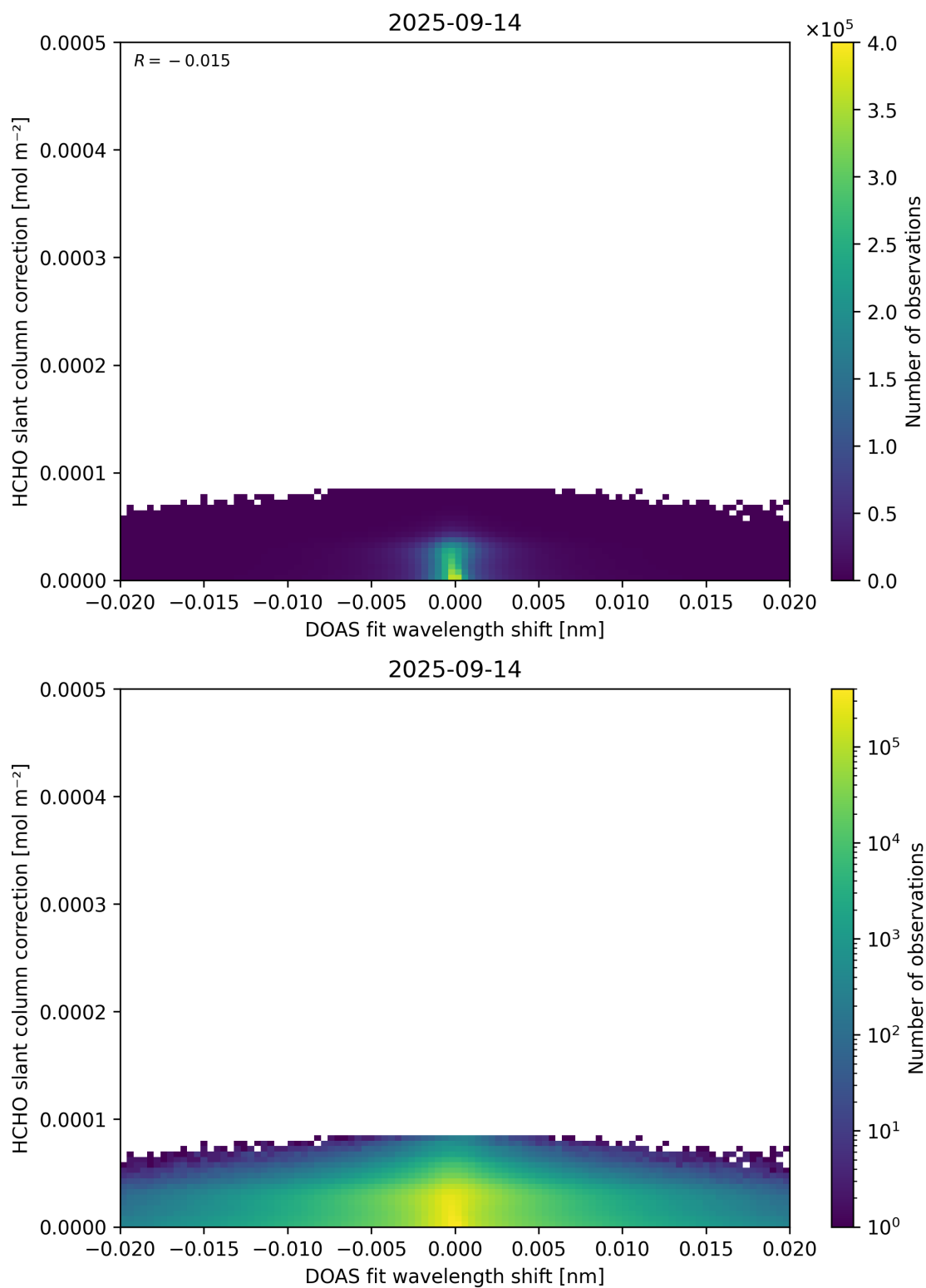
Figure 67: Scatter density plot of “DOAS fit wavelength shift” against “HCHO slant column correction” for 2025-09-13 to 2025-09-15.
