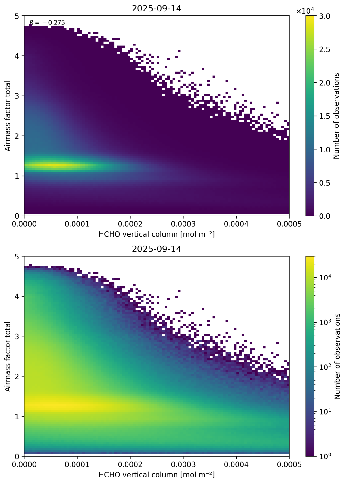
Figure 131: Scatter density plot of “HCHO vertical column” against “Airmass factor total” for 2025-09-13 to 2025-09-15.
