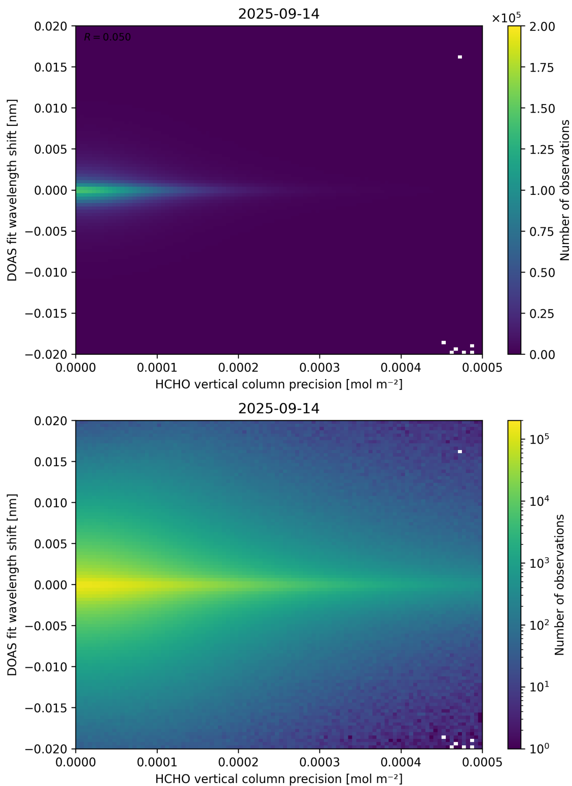
Figure 137: Scatter density plot of “HCHO vertical column precision” against “DOAS fit wavelength shift” for 2025-09-13 to 2025-09-15.
