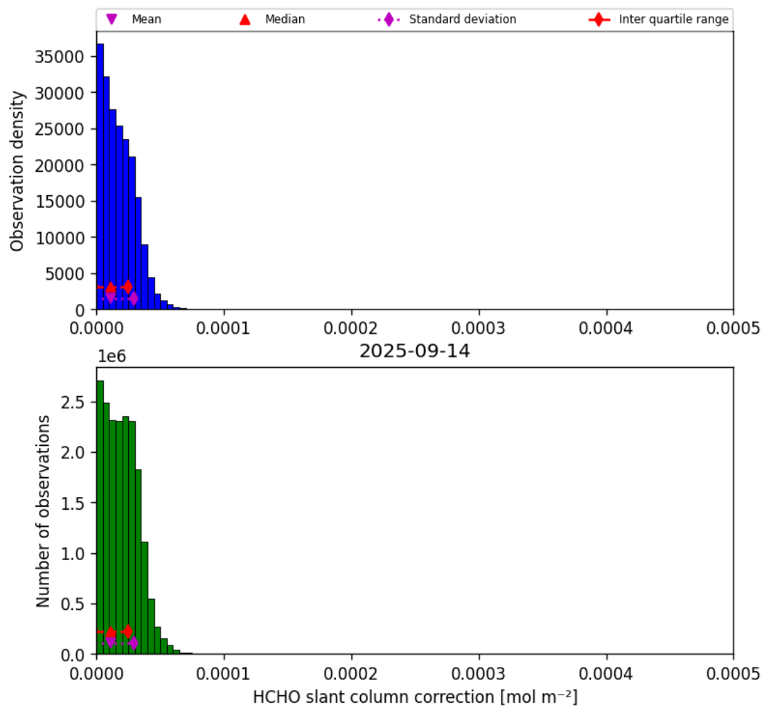
Figure 47: Histogram of “HCHO slant column correction” for 2025-09-13 to 2025-09-15
