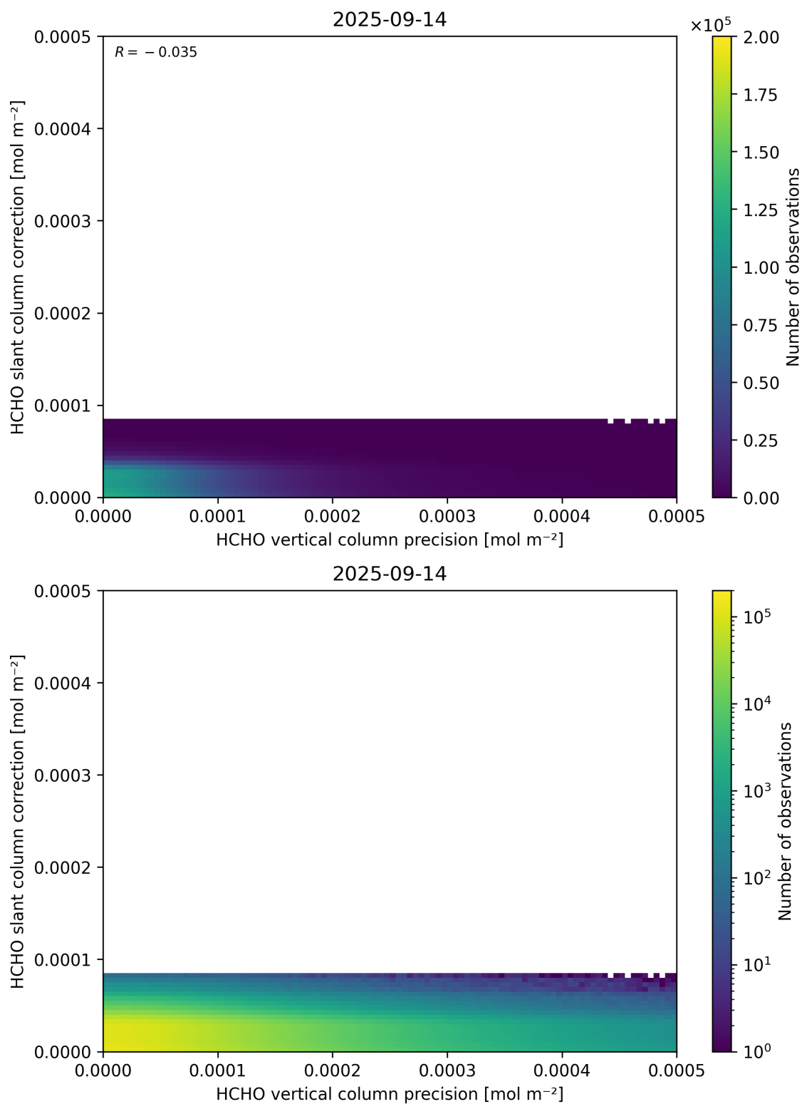
Figure 141: Scatter density plot of “HCHO vertical column precision” against “HCHO slant column correction” for 2025-09-13 to 2025-09-15.
