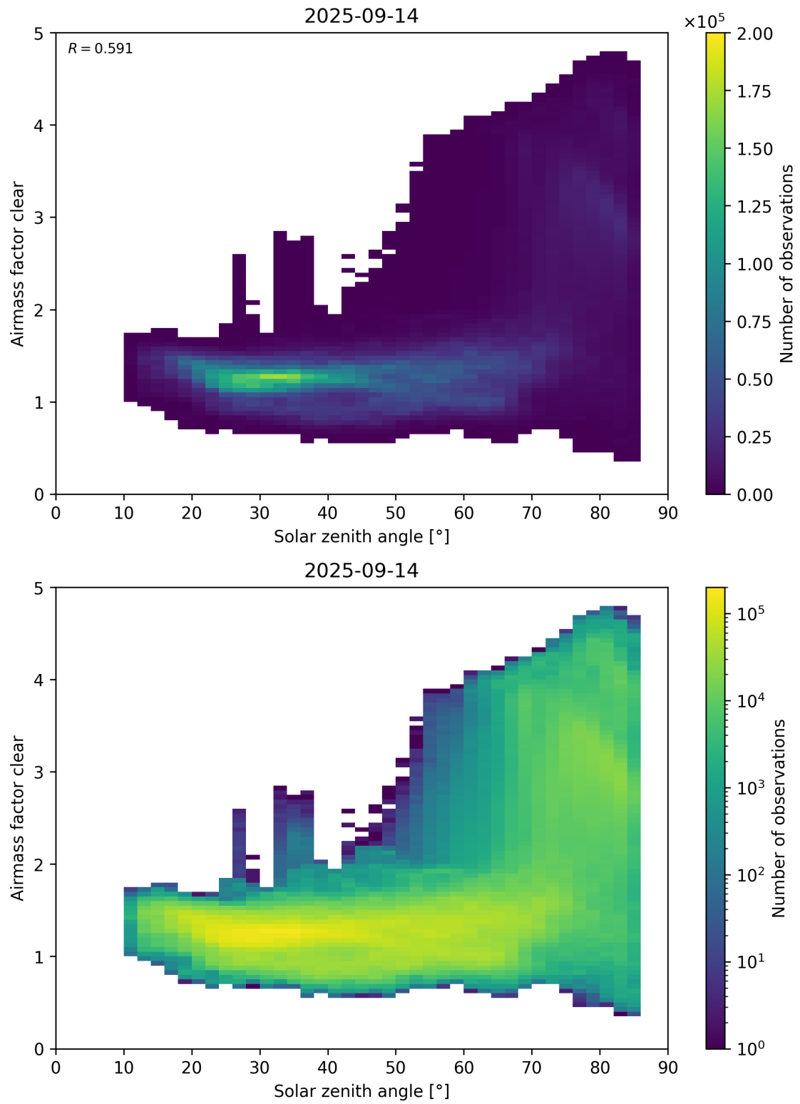
Figure 170: Scatter density plot of “Solar zenith angle” against “Airmass factor clear” for 2025-09-13 to 2025-09-15.
