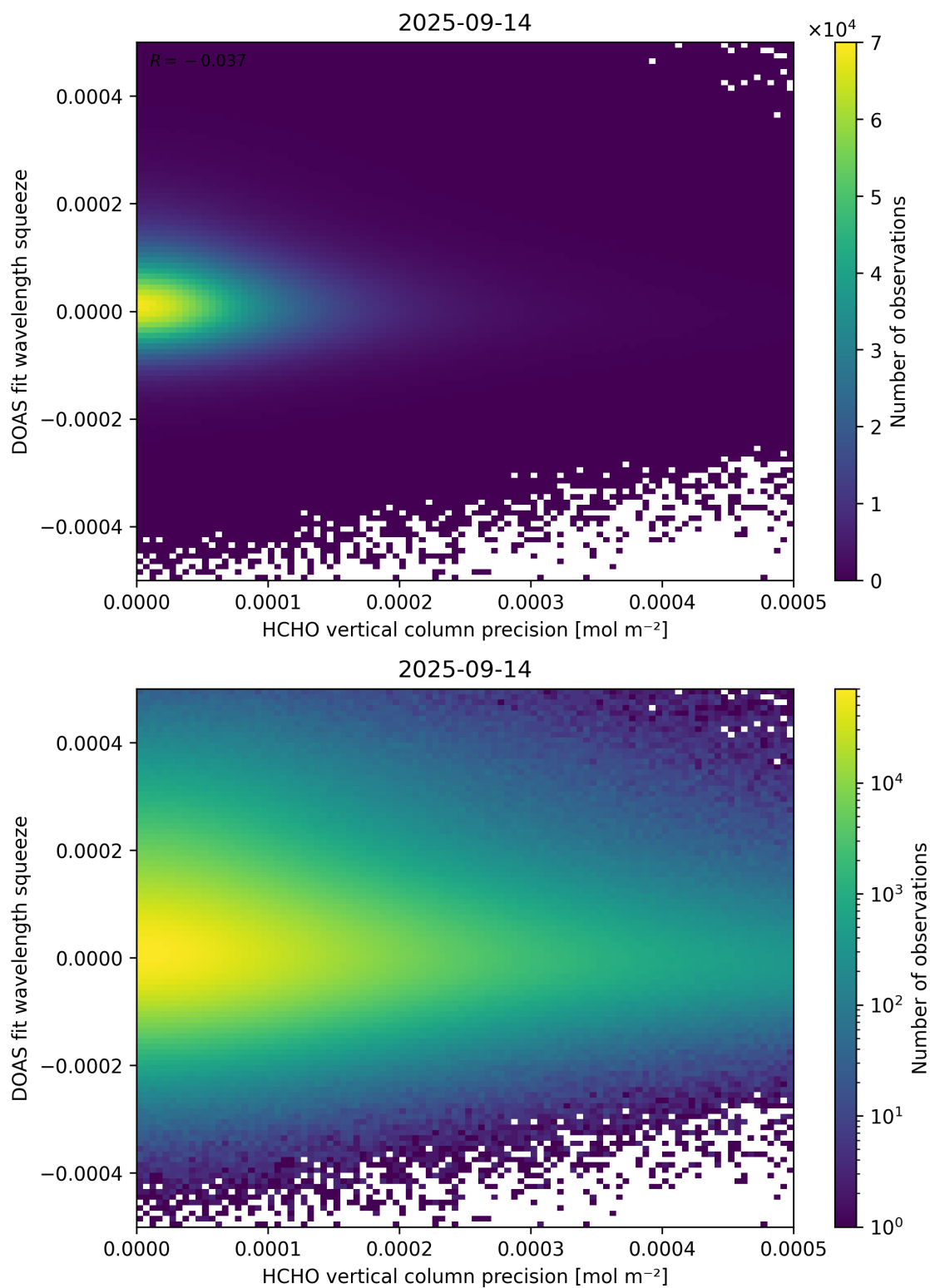
Figure 138: Scatter density plot of “HCHO vertical column precision” against “DOAS fit wavelength squeeze” for 2025-09-13 to 2025-09-15.
