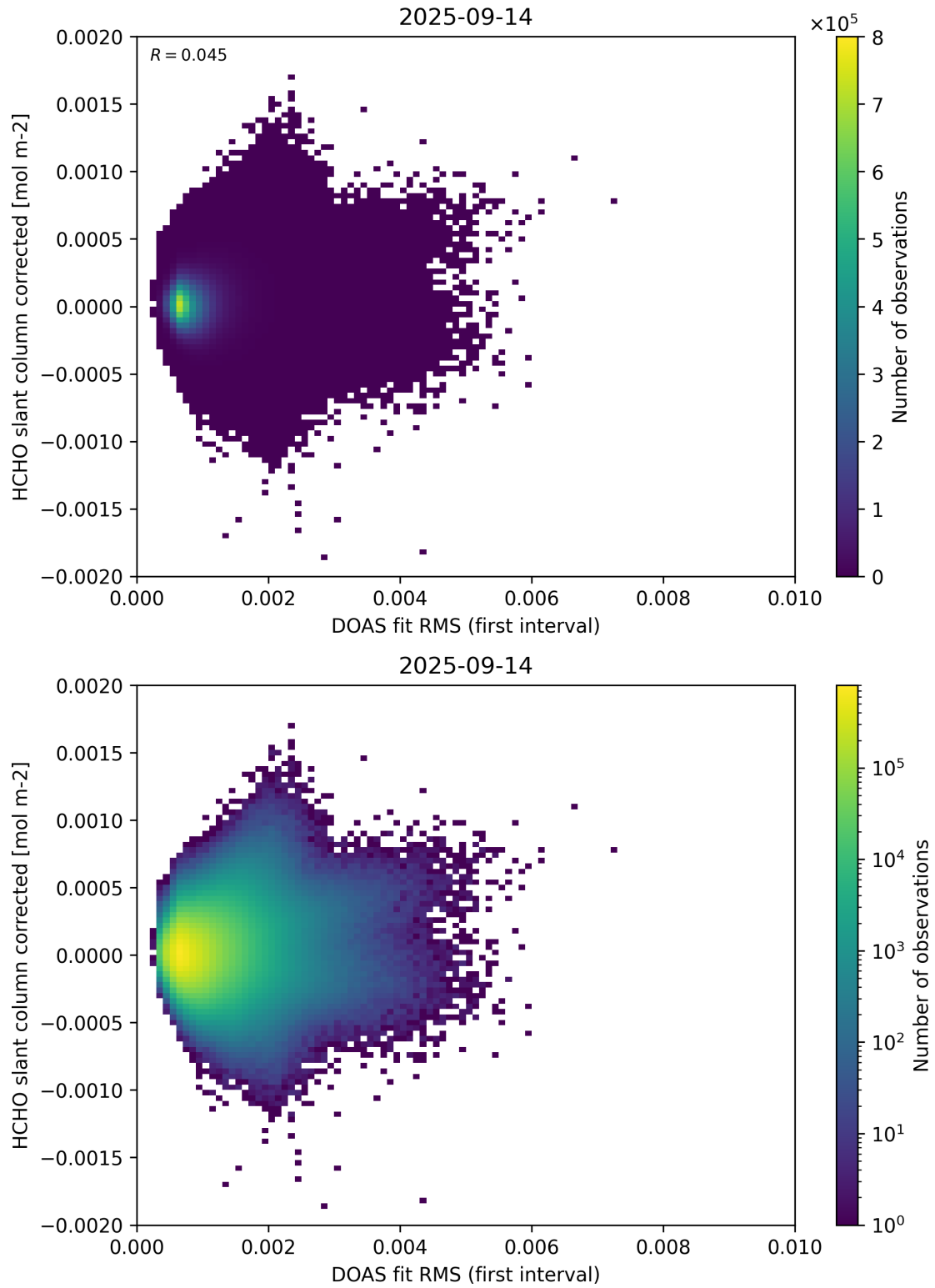
Figure 62: Scatter density plot of “DOAS fit RMS (first interval)” against “HCHO slant column corrected” for 2025-09-13 to 2025-09-15.
