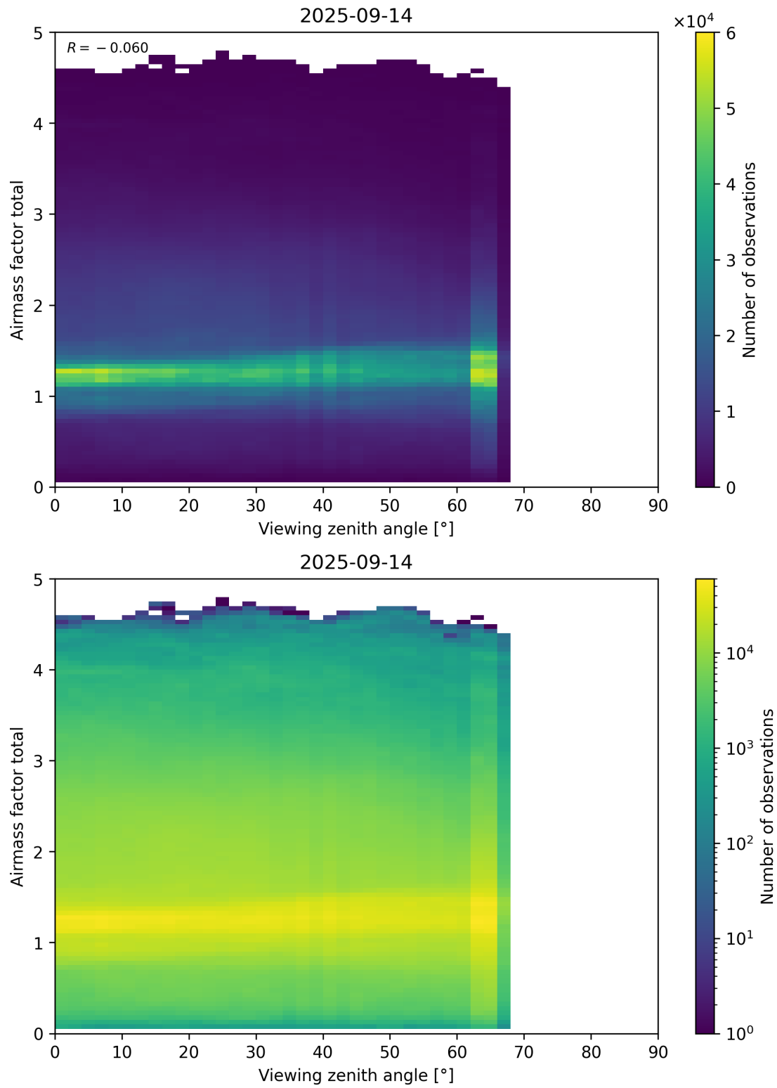
Figure 190: Scatter density plot of “Viewing zenith angle” against “Airmass factor total” for 2025-09-13 to 2025-09-15.
