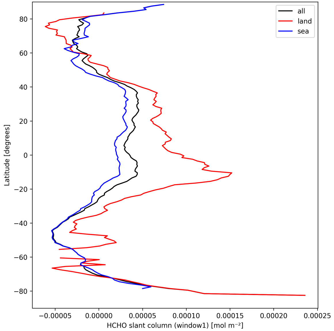
Figure 24: Zonal average of “HCHO slant column (window1)” for 2025-09-13 to 2025-09-15.
