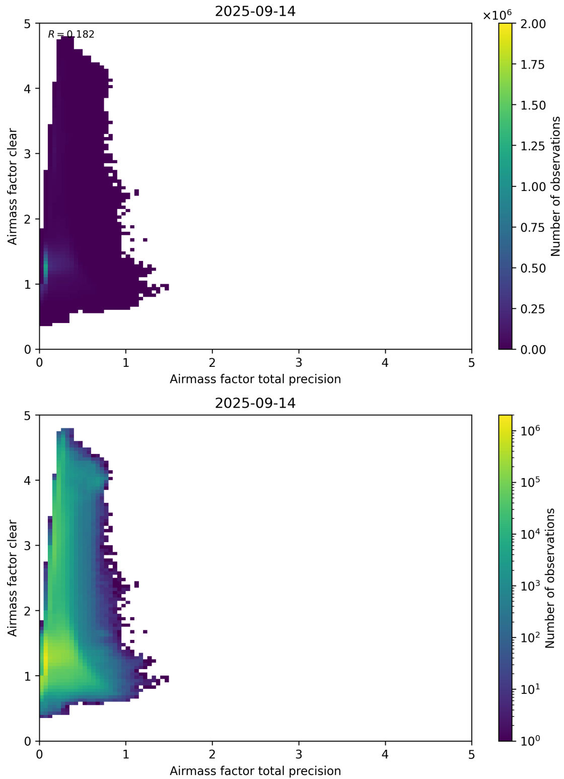
Figure 108: Scatter density plot of “Airmass factor total precision” against “Airmass factor clear” for 2025-09-13 to 2025-09-15.
