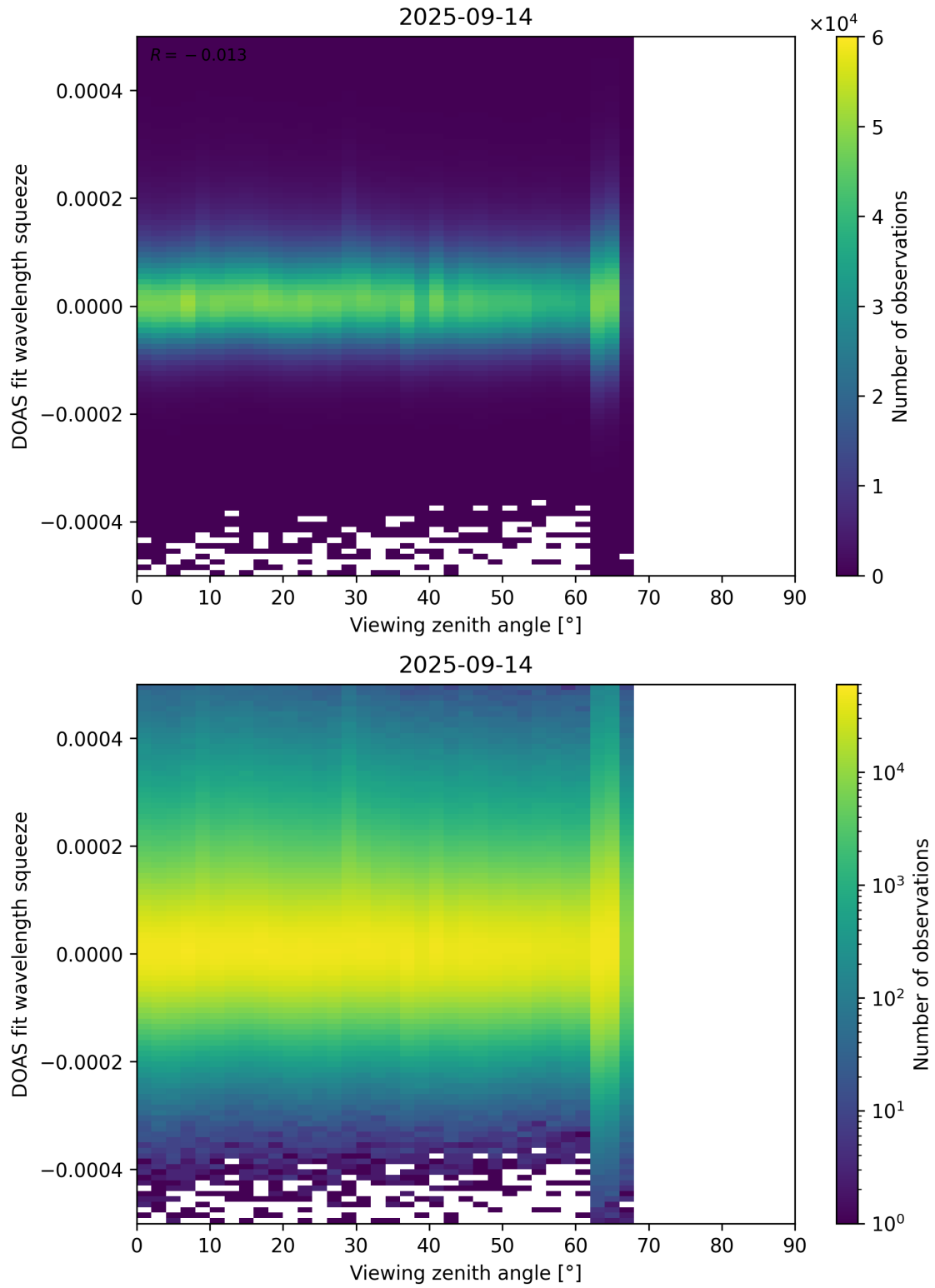
Figure 184: Scatter density plot of “Viewing zenith angle” against “DOAS fit wavelength squeeze” for 2025-09-13 to 2025-09-15.
