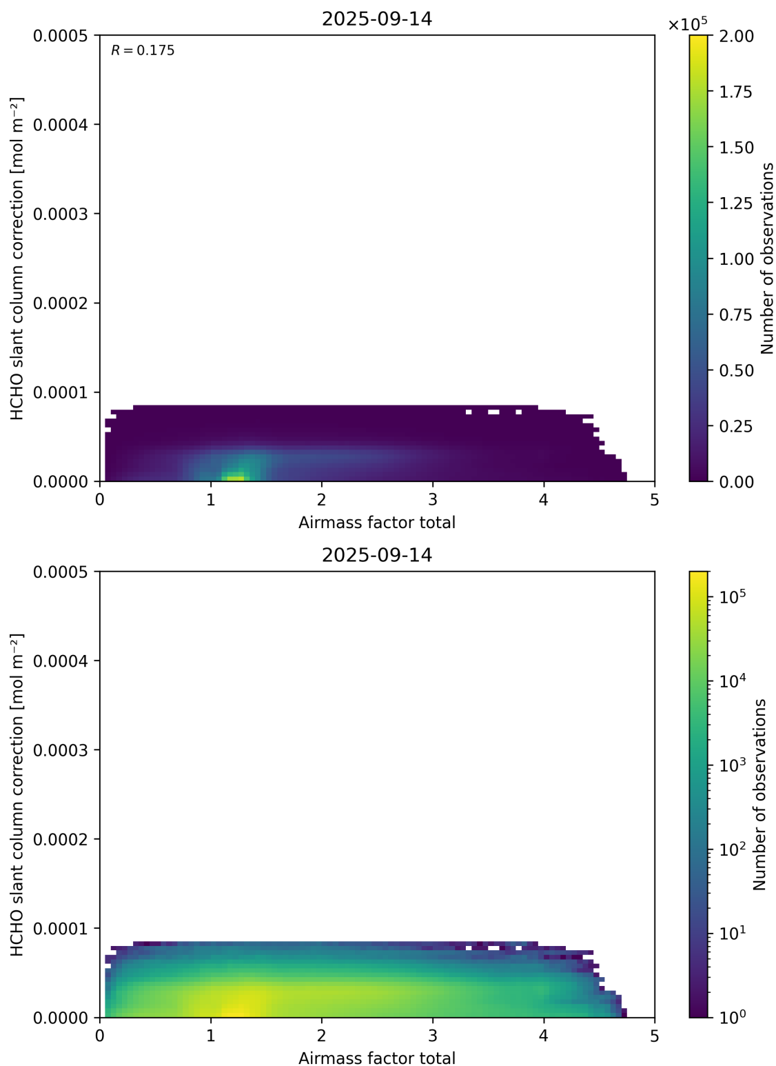
Figure 102: Scatter density plot of “Airmass factor total” against “HCHO slant column correction” for 2025-09-13 to 2025-09-15.
