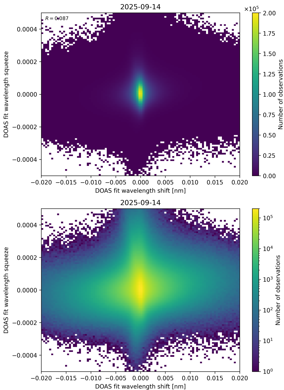
Figure 65: Scatter density plot of “DOAS fit wavelength shift” against “DOAS fit wavelength squeeze” for 2025-09-13 to 2025-09-15.
