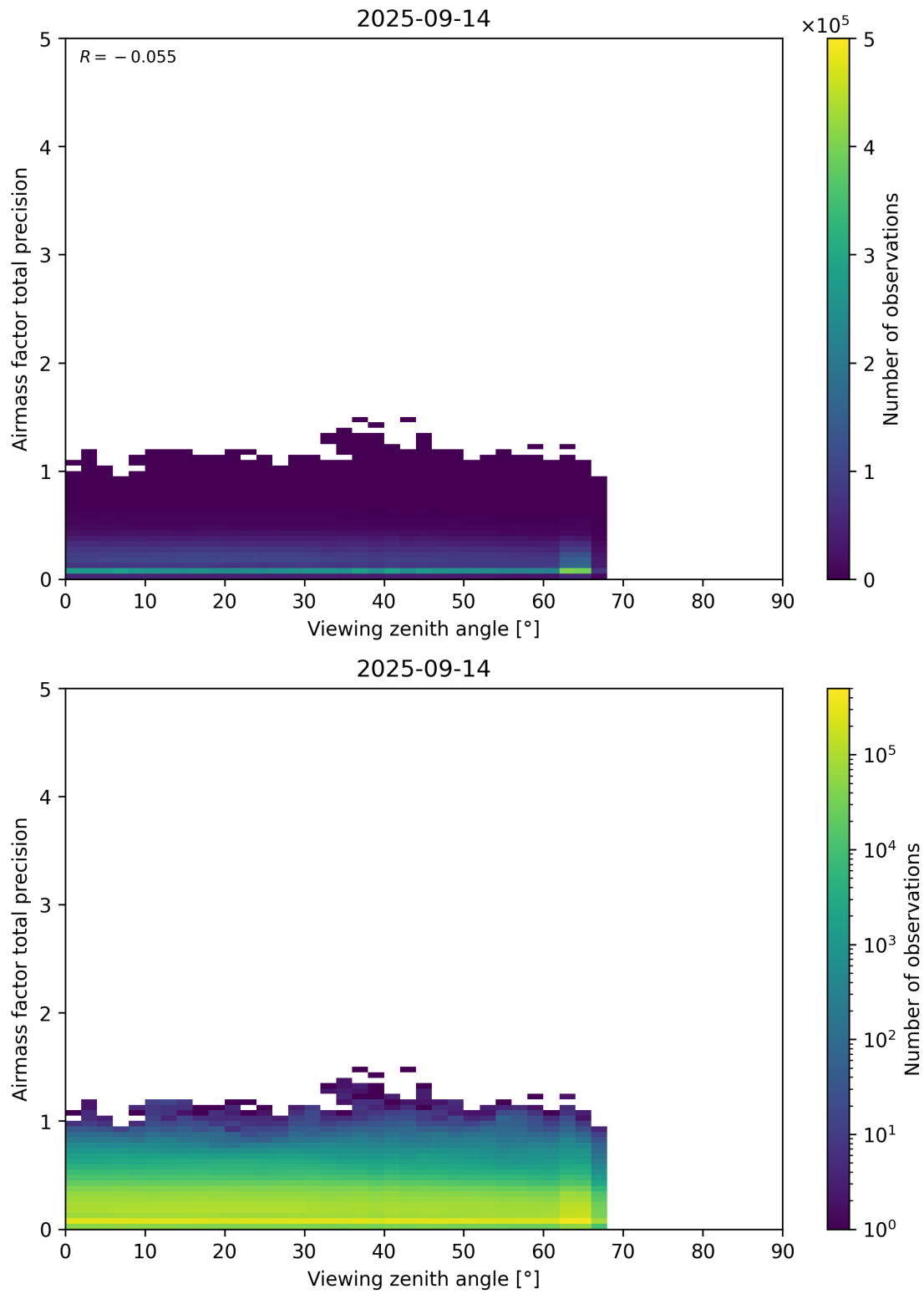
Figure 191: Scatter density plot of “Viewing zenith angle” against “Airmass factor total precision” for 2025-09-13 to 2025-09-15.
