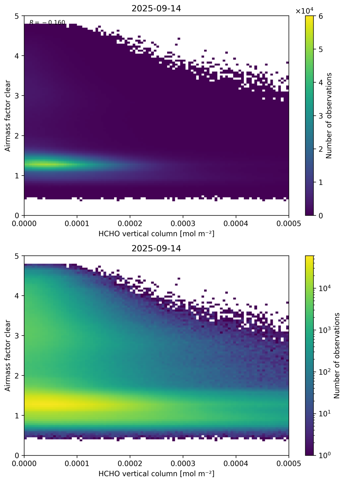
Figure 126: Scatter density plot of “HCHO vertical column” against “Airmass factor clear” for 2025-09-13 to 2025-09-15.
