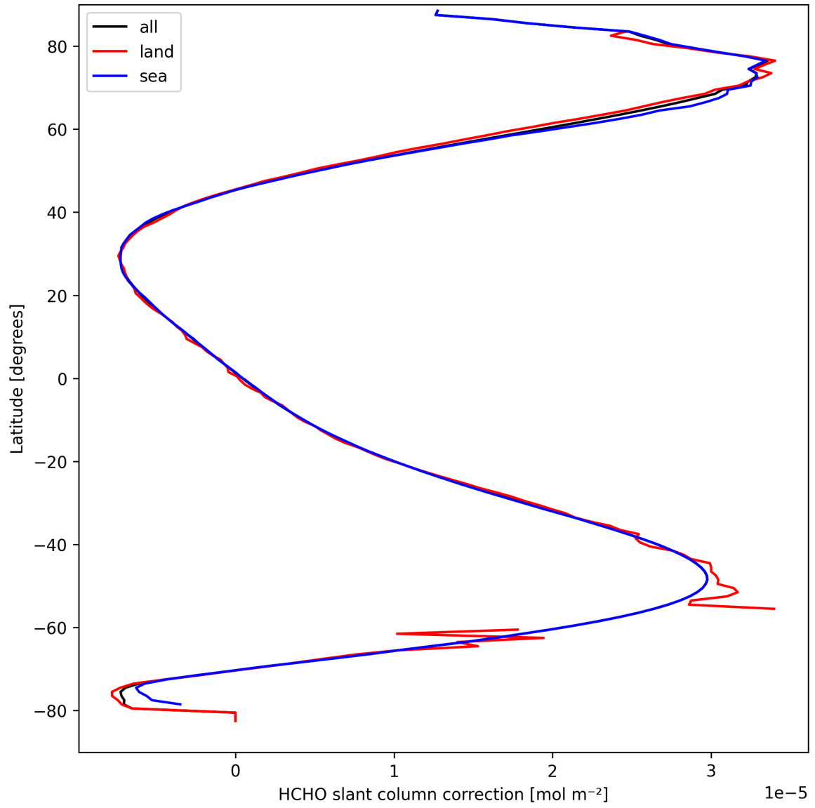
Figure 33: Zonal average of "HCHO slant column correction" for 2025-09-13 to 2025-09-15.
