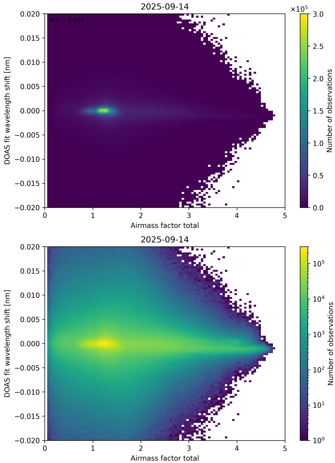
Figure 98: Scatter density plot of “Airmass factor total” against “DOAS fit wavelength shift” for 2025-09-13 to 2025-09-15.
