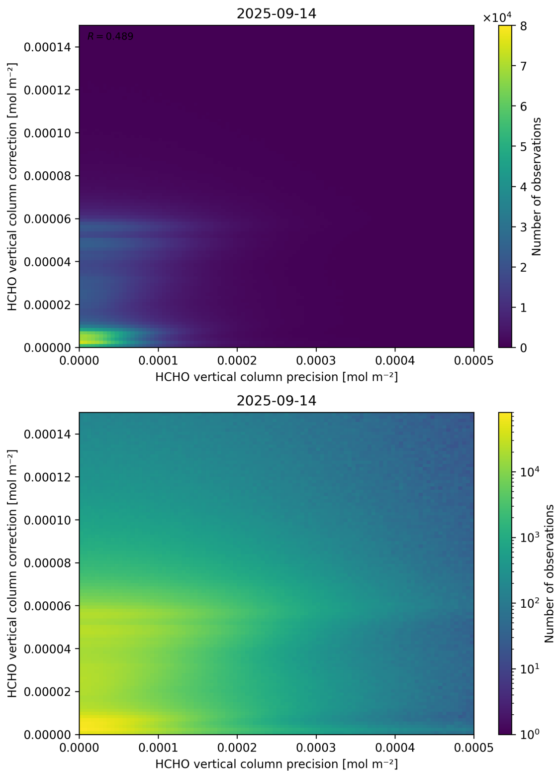
Figure 146: Scatter density plot of “HCHO vertical column precision” against “HCHO vertical column correction” for 2025-09-13 to 2025-09-15.
