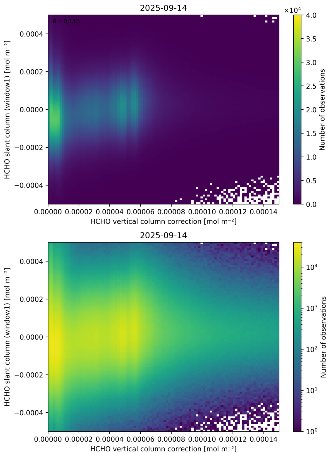
Figure 118: Scatter density plot of “HCHO vertical column correction” against “HCHO slant column (window1)” for 2025-09-13 to 2025-09-15.
