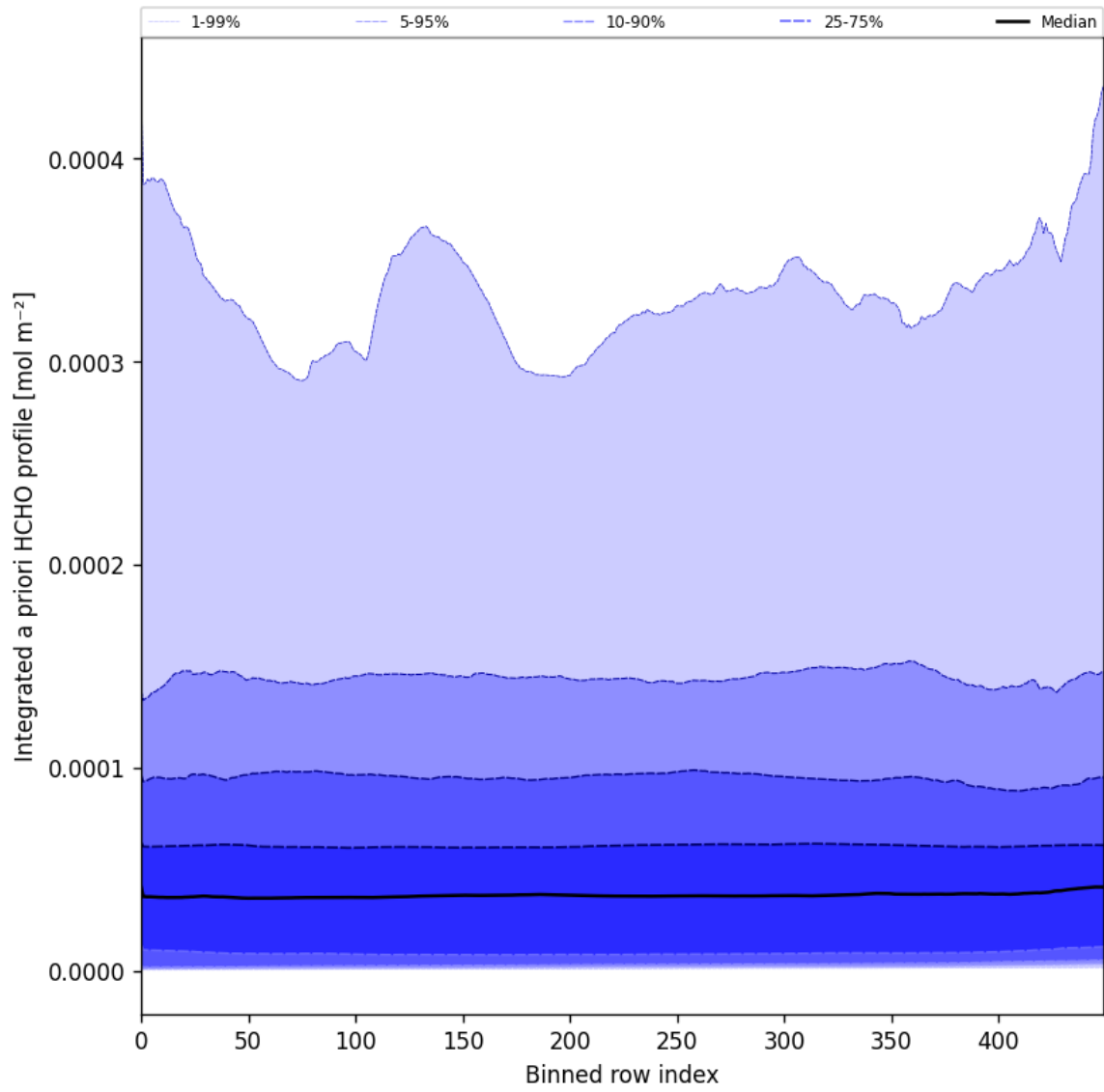
Figure 57: Along track statistics of “Integrated a priori HCHO profile” for 2025-09-13 to 2025-09-15
