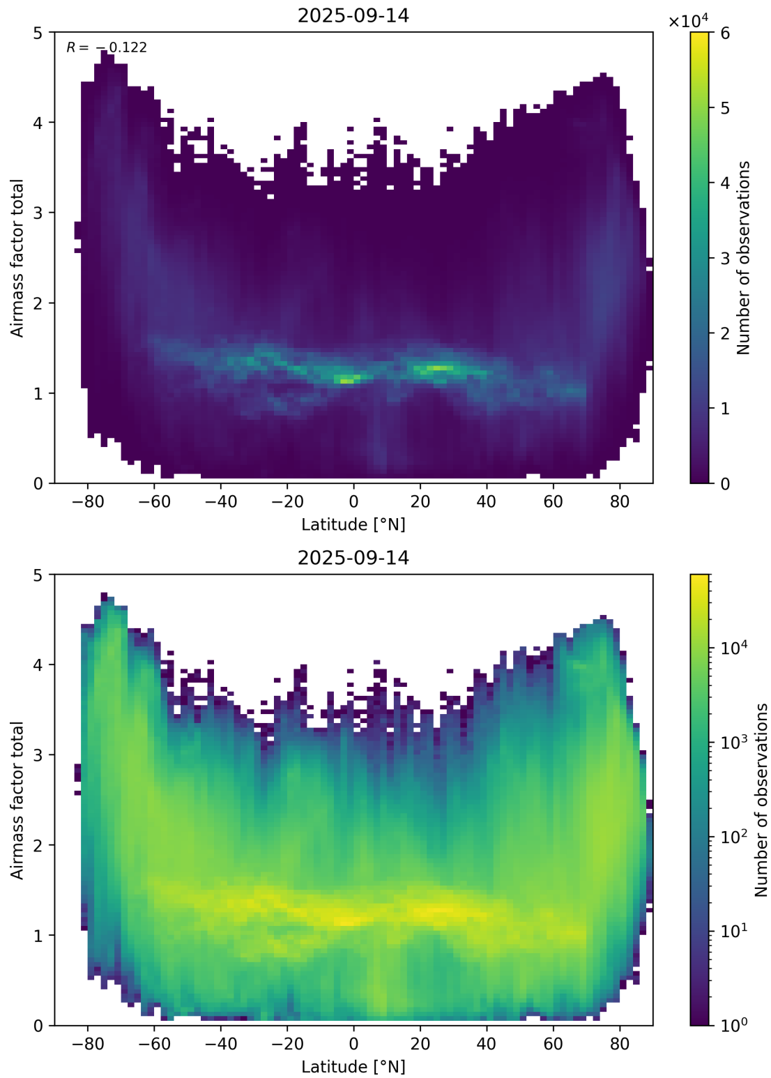
Figure 161: Scatter density plot of “Latitude” against “Airmass factor total” for 2025-09-13 to 2025-09-15.
