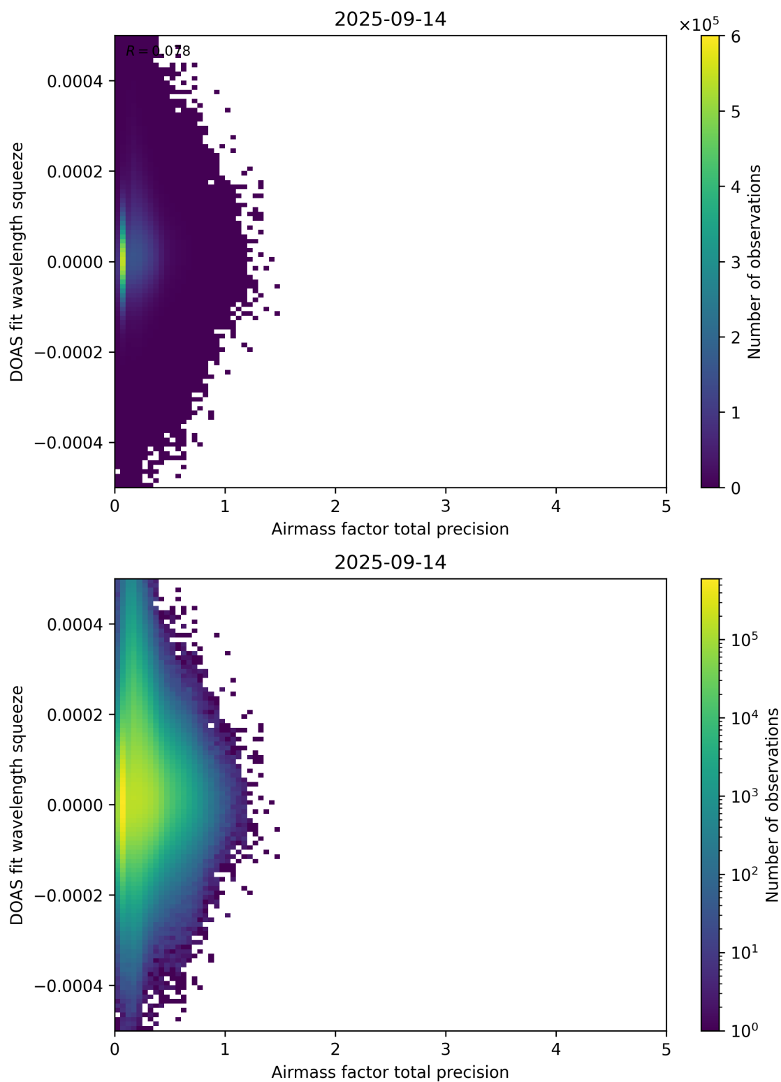
Figure 107: Scatter density plot of “Airmass factor total precision” against “DOAS fit wavelength squeeze” for 2025-09-13 to 2025-09-15.
