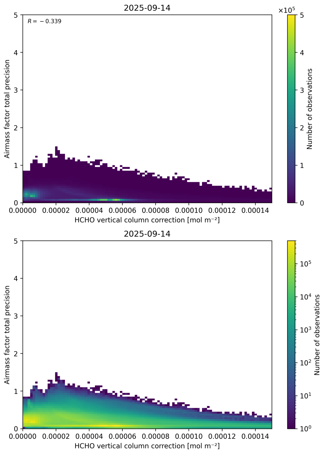
Figure 121: Scatter density plot of “HCHO vertical column correction” against “Airmass factor total precision” for 2025-09-13 to 2025-09-15.
