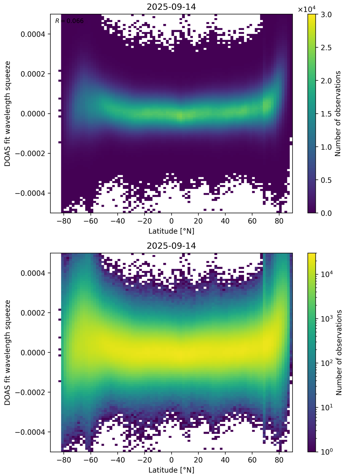
Figure 155: Scatter density plot of “Latitude” against “DOAS fit wavelength squeeze” for 2025-09-13 to 2025-09-15.
