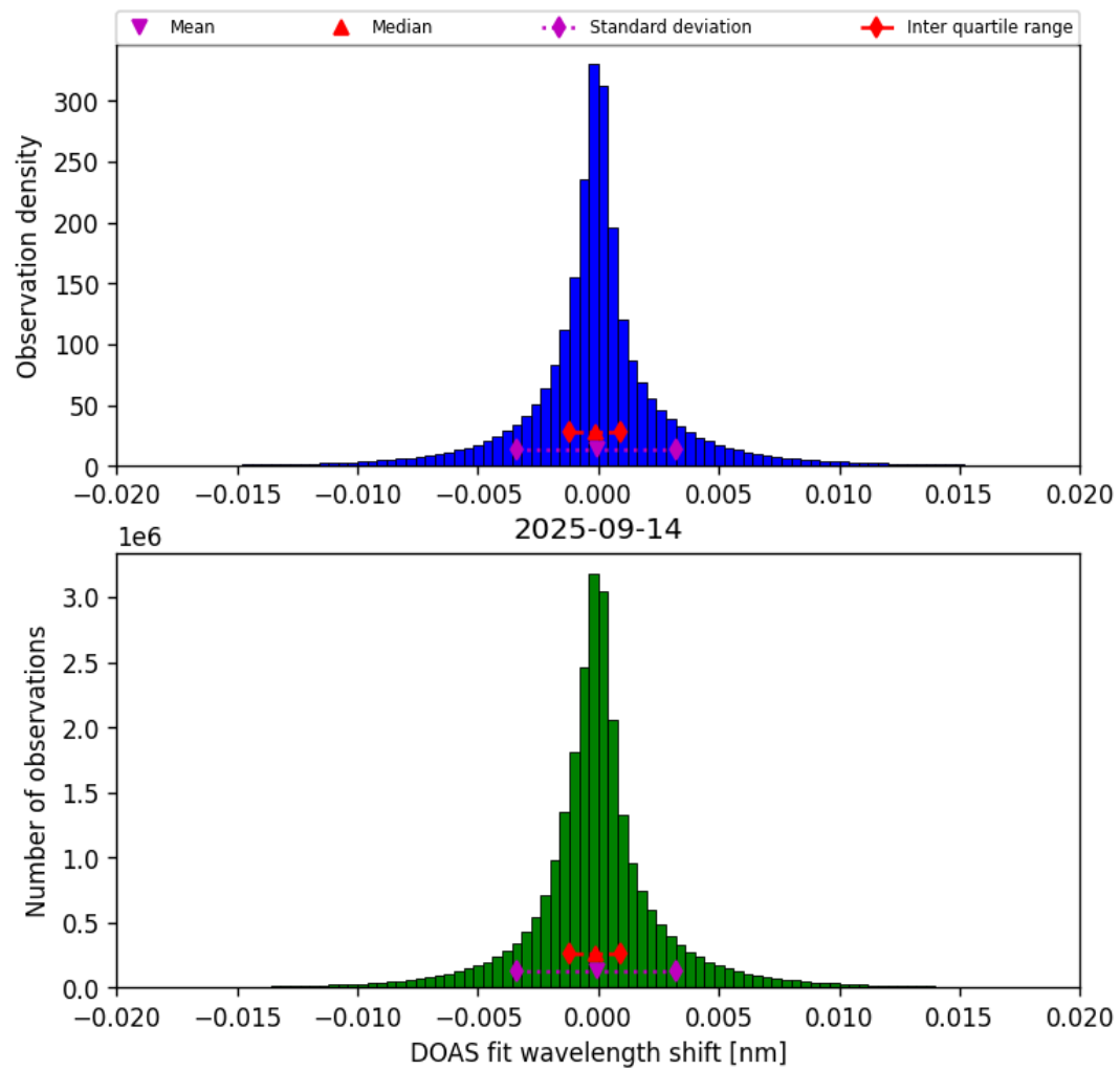
Figure 44: Histogram of “DOAS fit wavelength shift” for 2025-09-13 to 2025-09-15
