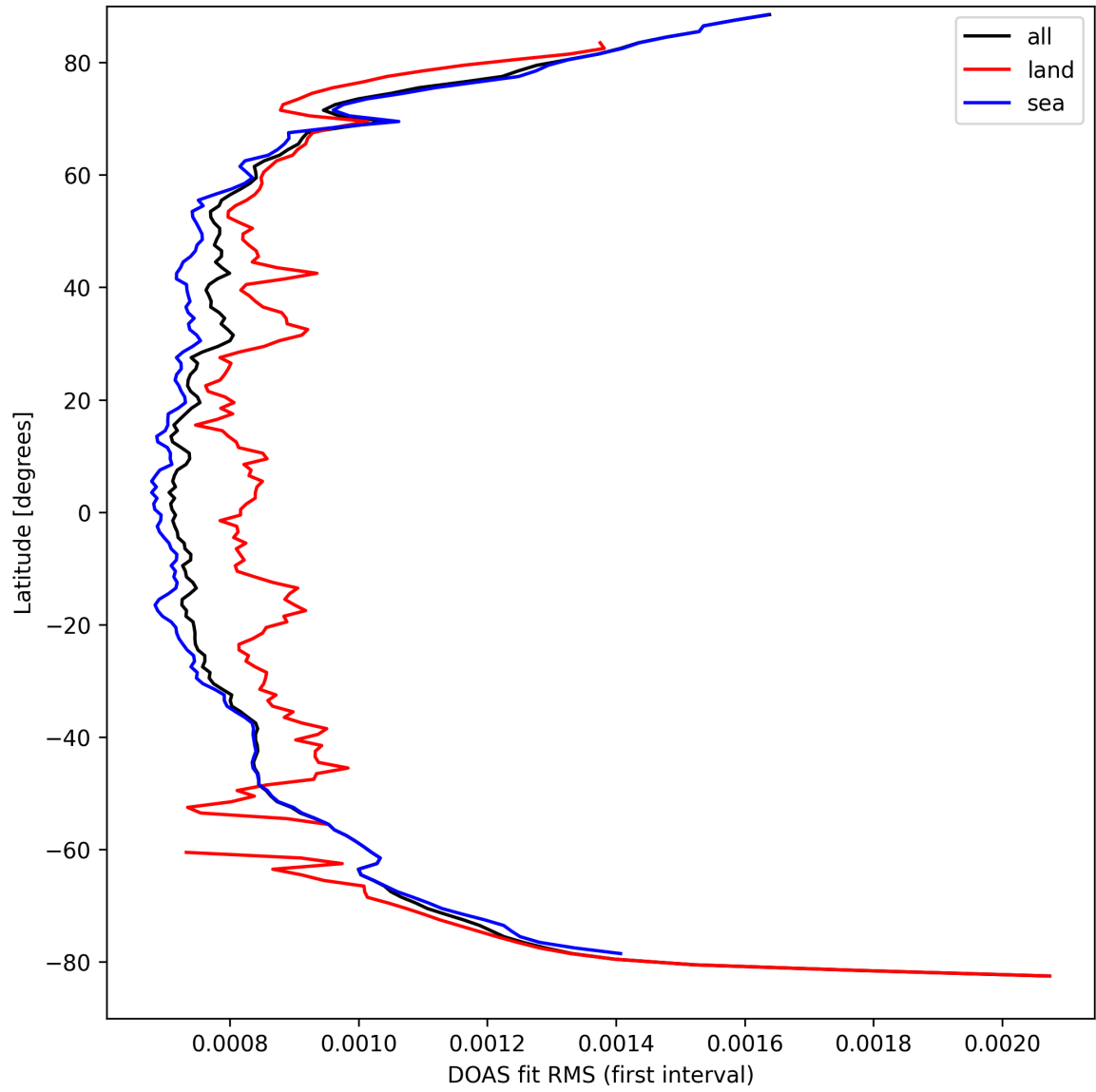
Figure 32: Zonal average of “DOAS fit RMS (first interval)” for 2025-09-13 to 2025-09-15.
