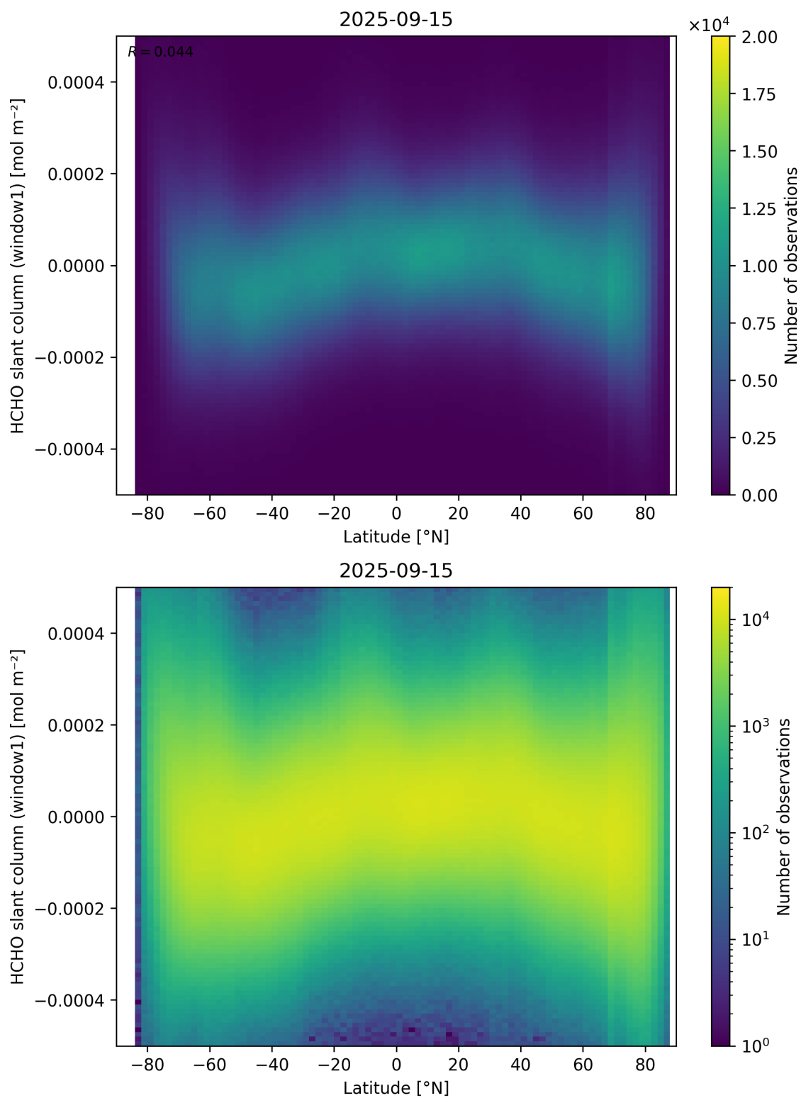
Figure 159: Scatter density plot of “Latitude” against “HCHO slant column (window1)” for 2025-09-15 to 2025-09-16.
