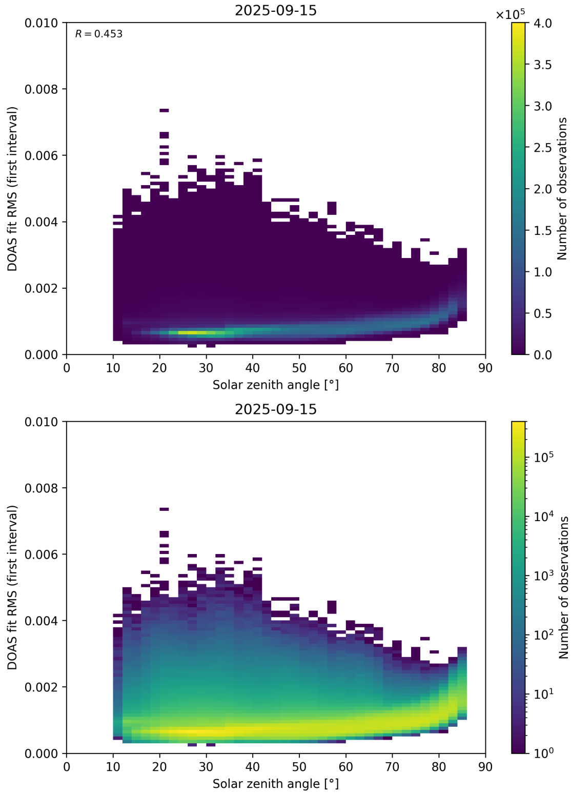
Figure 167: Scatter density plot of “Solar zenith angle” against “DOAS fit RMS (first interval)” for 2025-09-15 to 2025-09-16.
