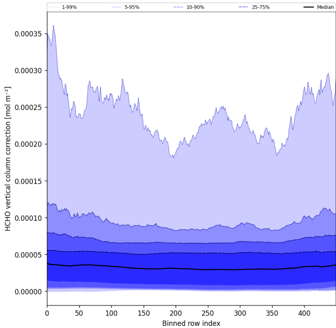
Figure 51: Along track statistics of “HCHO vertical column correction” for 2025-09-15 to 2025-09-16
