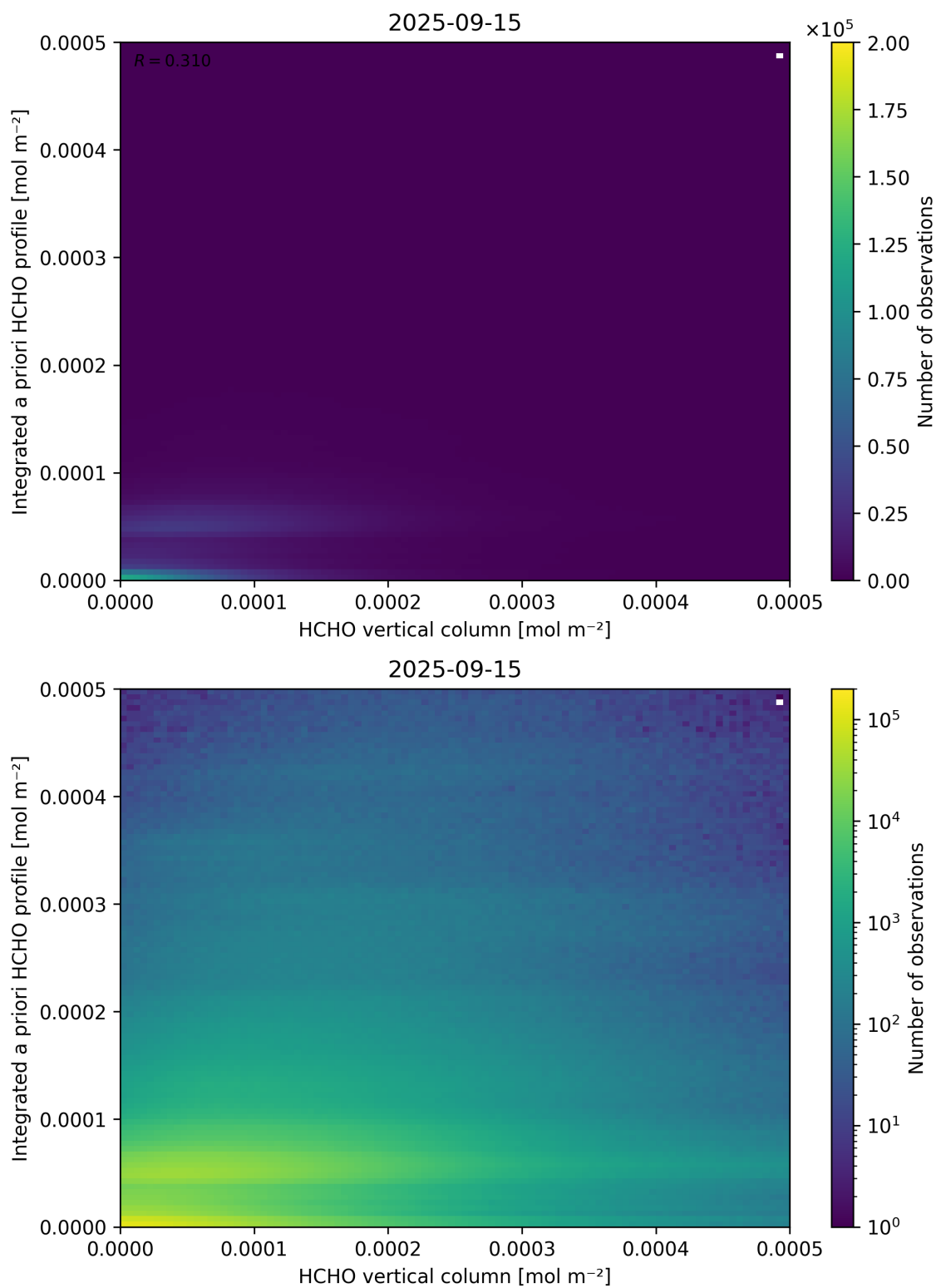
Figure 135: Scatter density plot of “HCHO vertical column” against “Integrated a priori HCHO profile” for 2025-09-15 to 2025-09-16.
