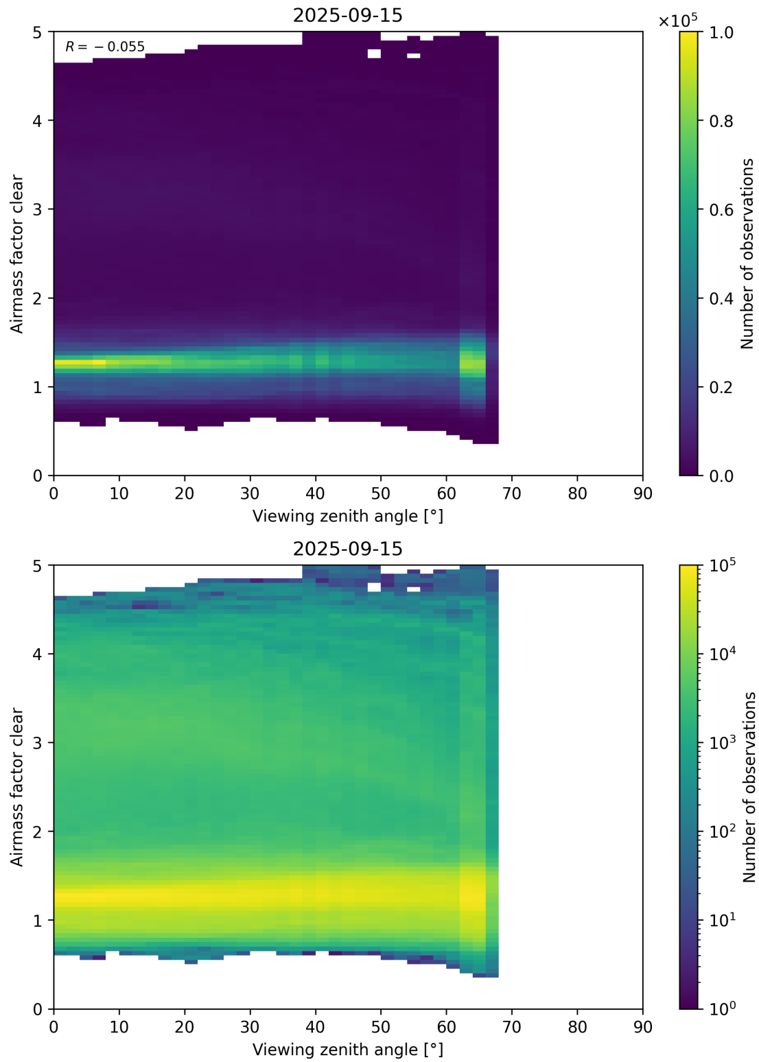
Figure 185: Scatter density plot of “Viewing zenith angle” against “Airmass factor clear” for 2025-09-15 to 2025-09-16.
