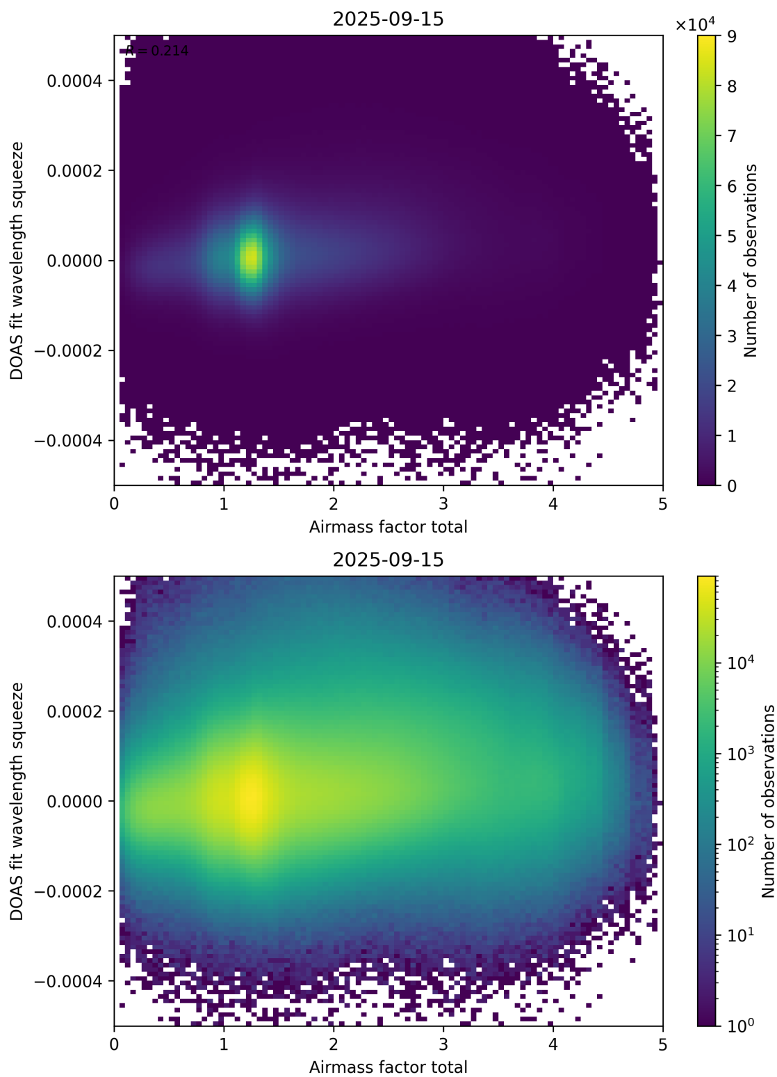
Figure 99: Scatter density plot of “Airmass factor total” against “DOAS fit wavelength squeeze” for 2025-09-15 to 2025-09-16.
