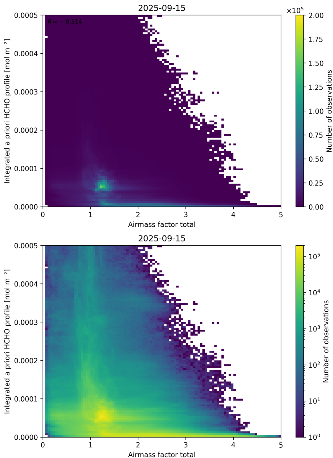
Figure 104: Scatter density plot of “Airmass factor total” against “Integrated a priori HCHO profile” for 2025-09-15 to 2025-09-16.
