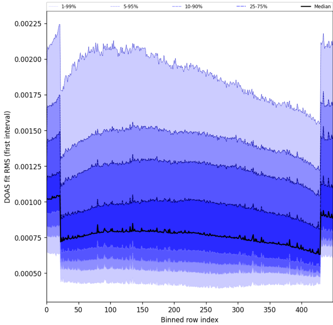
Figure 60: Along track statistics of “DOAS fit RMS (first interval)” for 2025-09-15 to 2025-09-16
