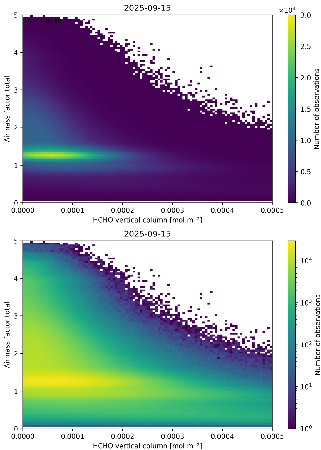
Figure 131: Scatter density plot of “HCHO vertical column” against “Airmass factor total” for 2025-09-15 to 2025-09-16.
