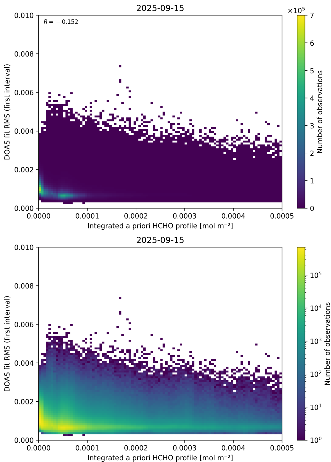
Figure 148: Scatter density plot of “Integrated a priori HCHO profile” against “DOAS fit RMS (first interval)” for 2025-09-15 to 2025-09-16.
