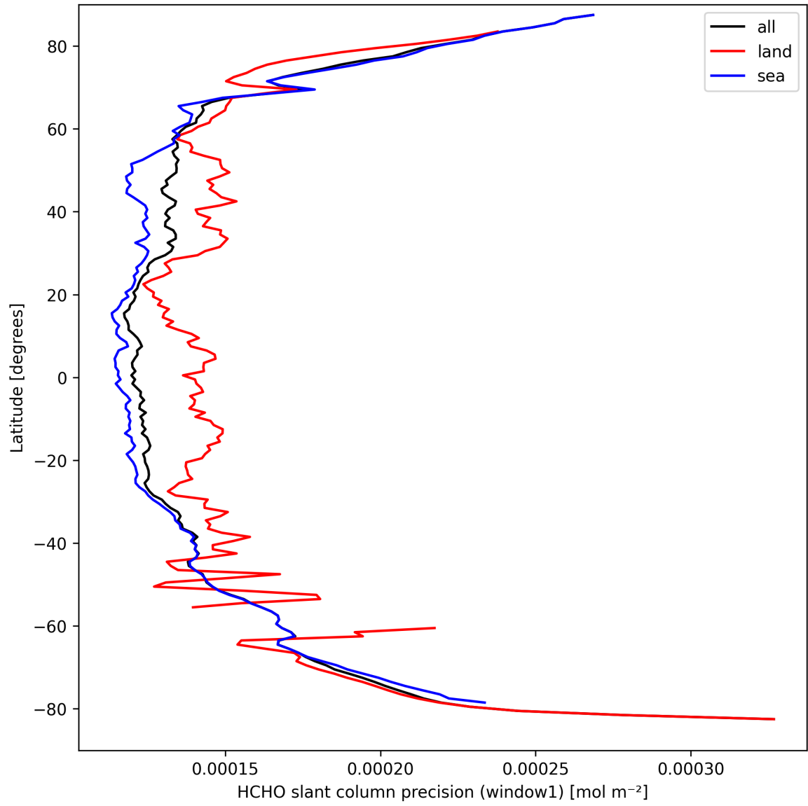
Figure 25: Zonal average of “HCHO slant column precision (window1)” for 2025-09-15 to 2025-09-16.
