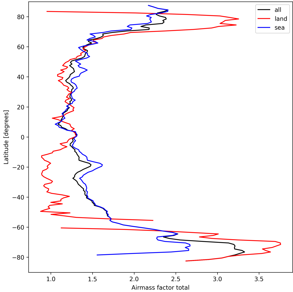
Figure 26: Zonal average of “Airmass factor total” for 2025-09-15 to 2025-09-16.
