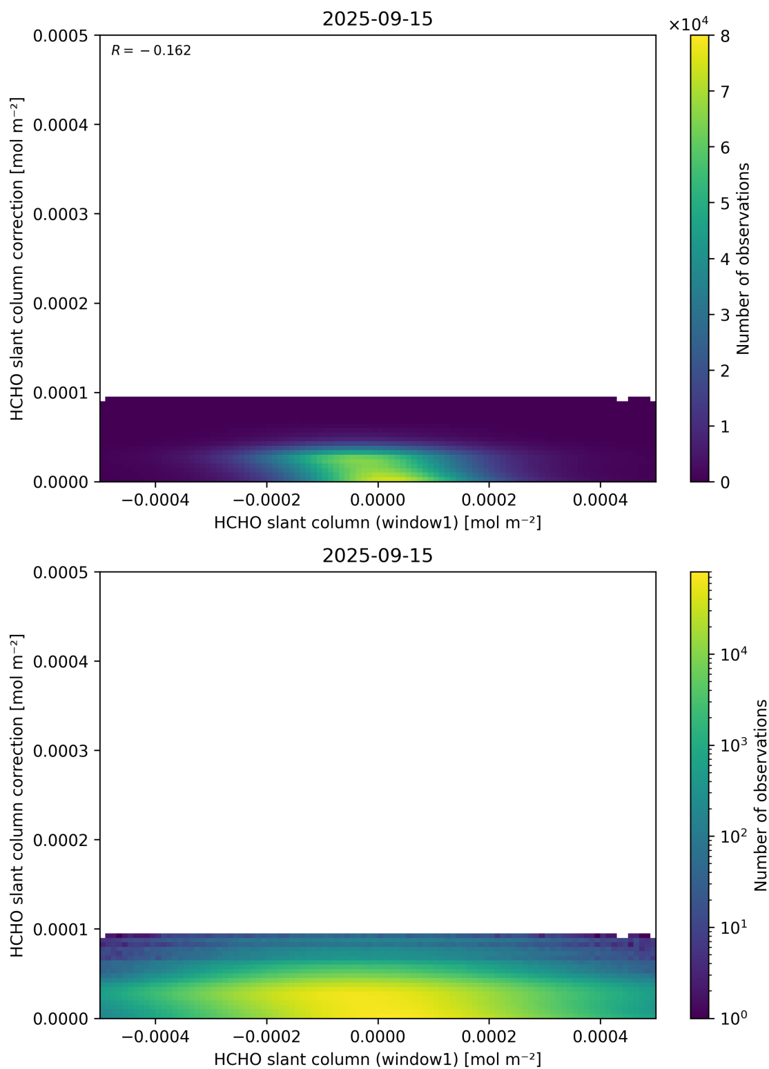
Figure 83: Scatter density plot of “HCHO slant column (window1)” against “HCHO slant column correction” for 2025-09-15 to 2025-09-16.
