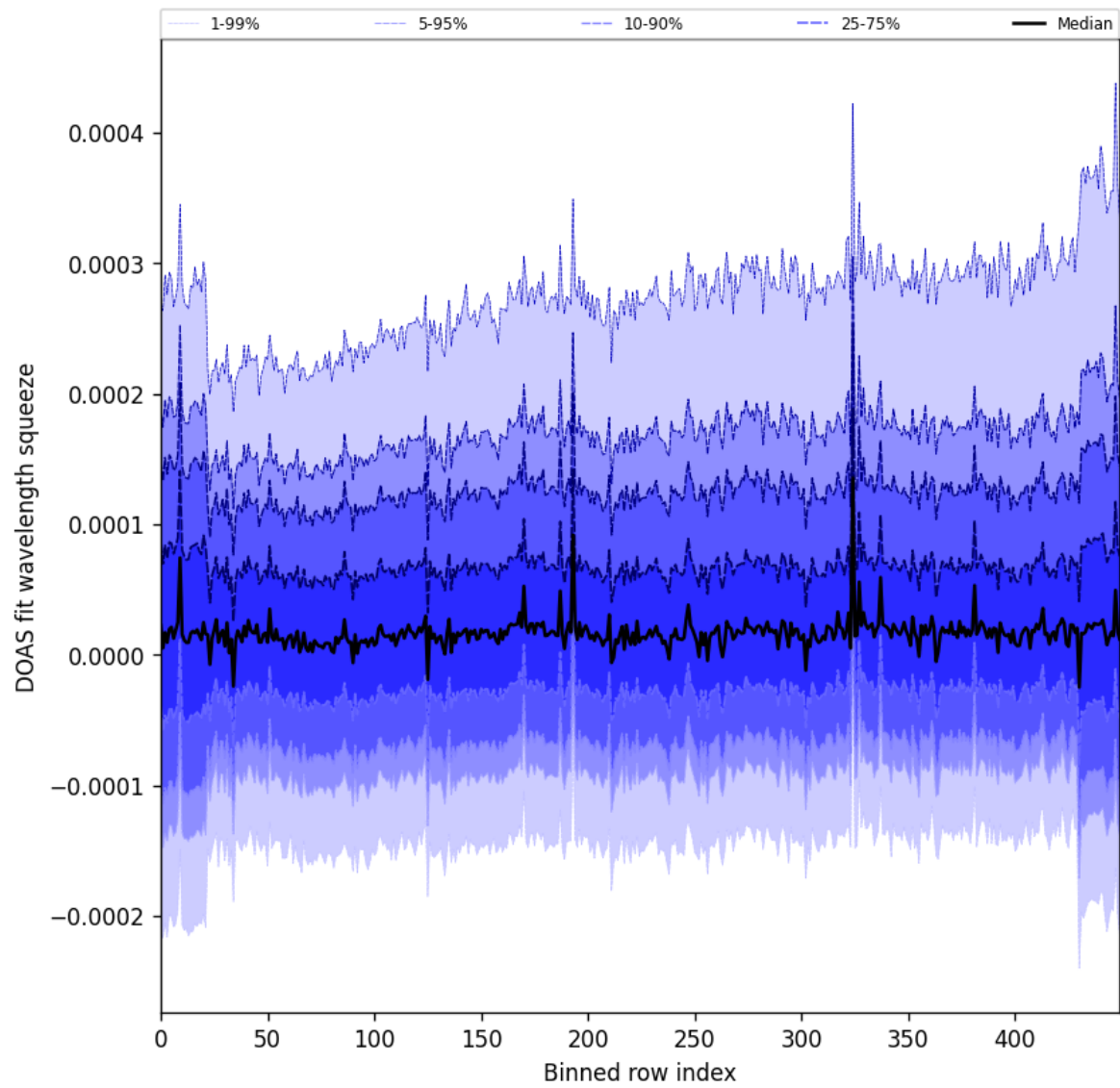
Figure 59: Along track statistics of “DOAS fit wavelength squeeze” for 2025-09-15 to 2025-09-16
