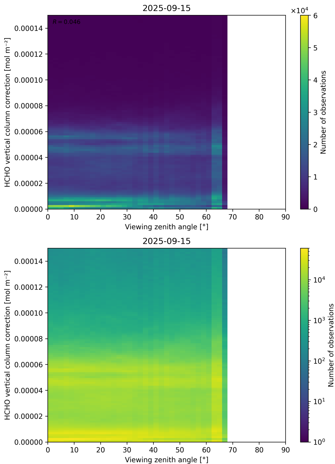
Figure 193: Scatter density plot of “Viewing zenith angle” against “HCHO vertical column correction” for 2025-09-15 to 2025-09-16.
