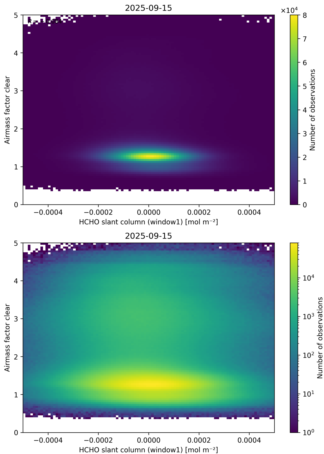
Figure 81: Scatter density plot of “HCHO slant column (window1)” against “Airmass factor clear” for 2025-09-15 to 2025-09-16.
