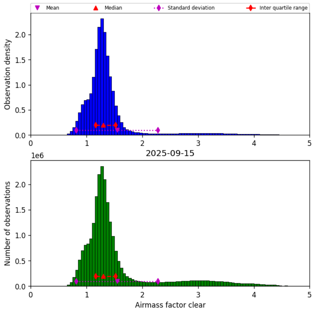
Figure 42: Histogram of “Airmass factor clear” for 2025-09-15 to 2025-09-16
