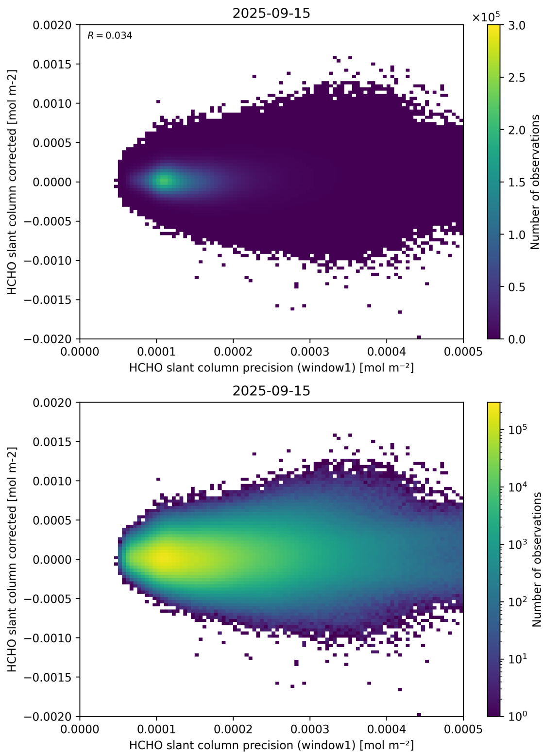
Figure 92: Scatter density plot of “HCHO slant column precision (window1)” against “HCHO slant column corrected” for 2025-09-15 to 2025-09-16.
