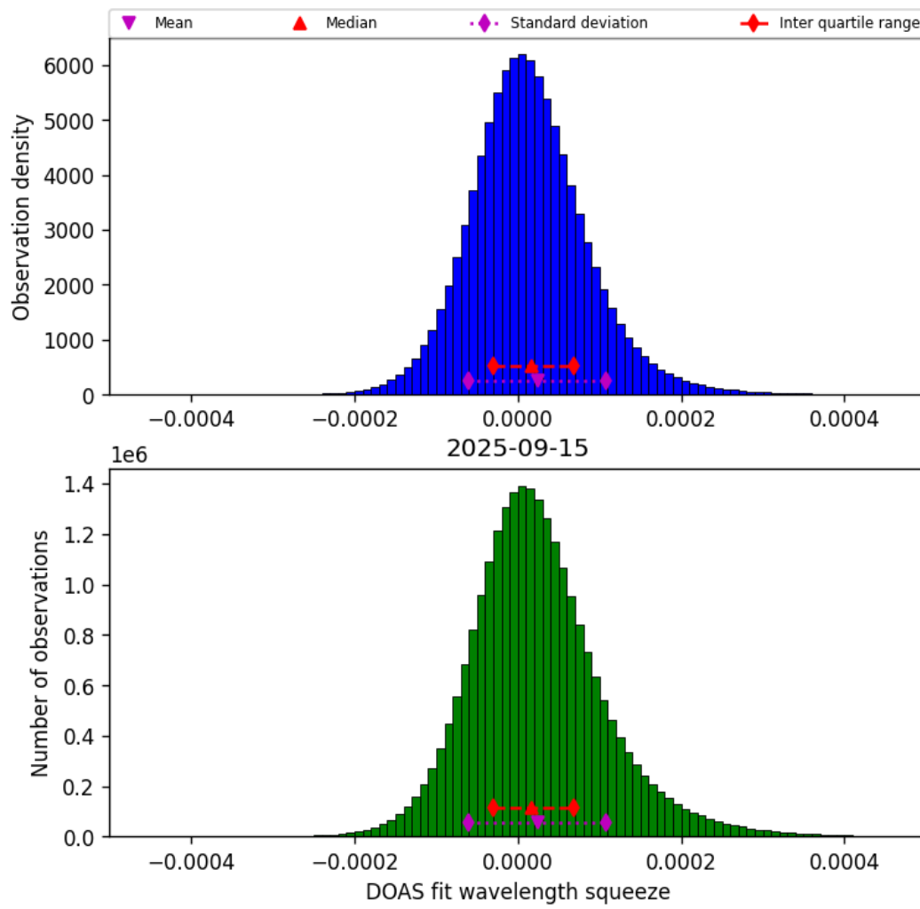
Figure 45: Histogram of “DOAS fit wavelength squeeze” for 2025-09-15 to 2025-09-16
