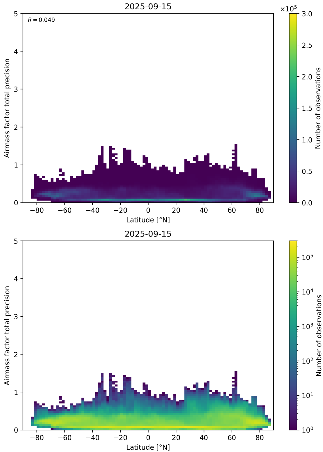
Figure 162: Scatter density plot of “Latitude” against “Airmass factor total precision” for 2025-09-15 to 2025-09-16.
