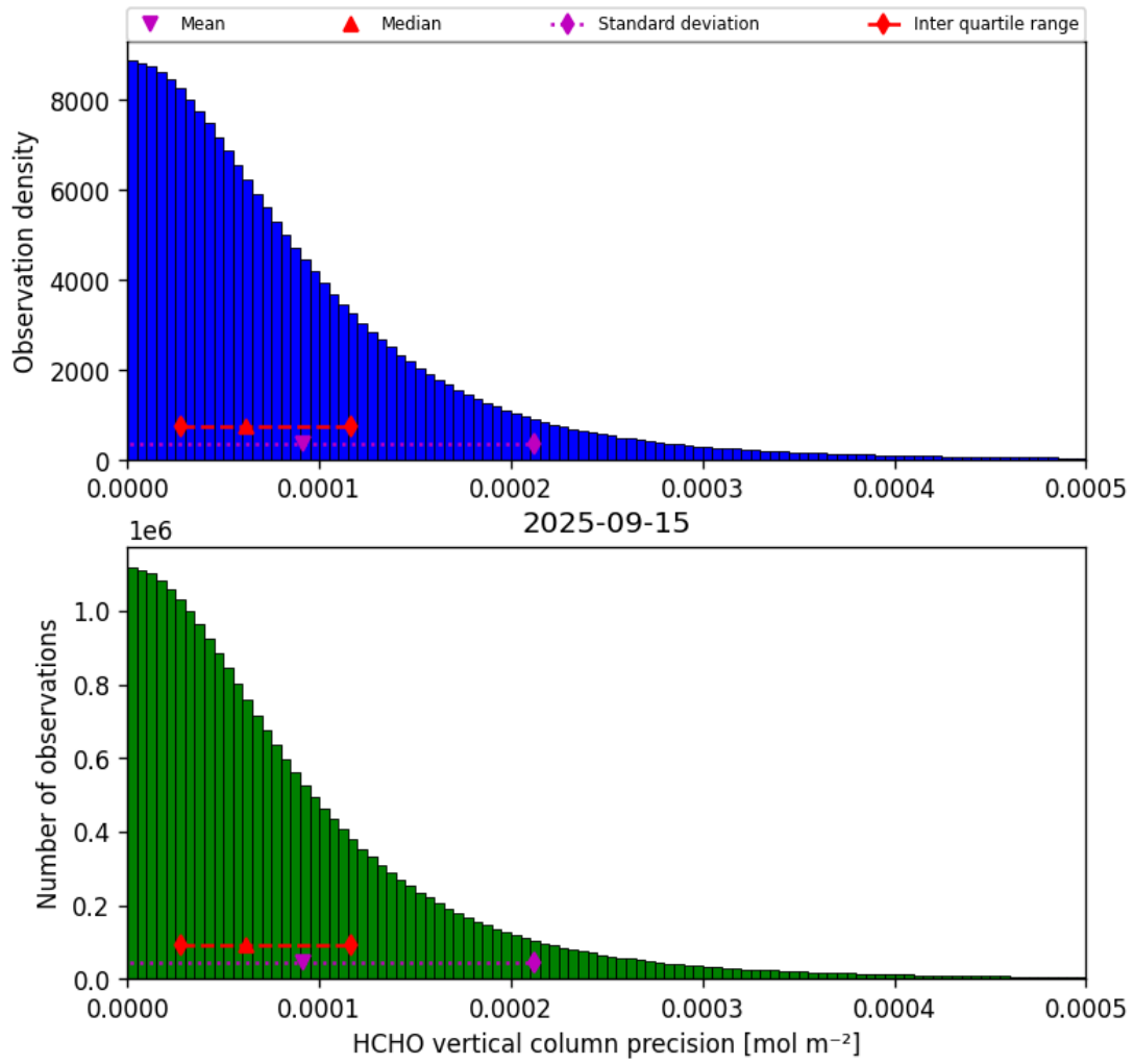
Figure 36: Histogram of “HCHO vertical column precision” for 2025-09-15 to 2025-09-16
