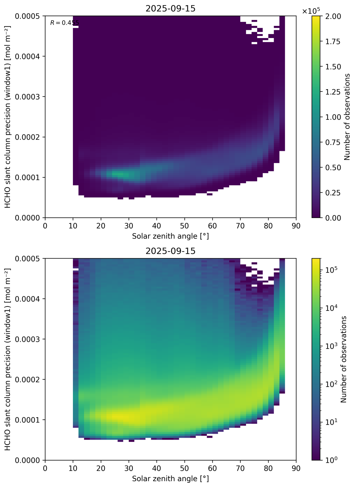
Figure 174: Scatter density plot of “Solar zenith angle” against “HCHO slant column precision (window1)” for 2025-09-15 to 2025-09-16.
