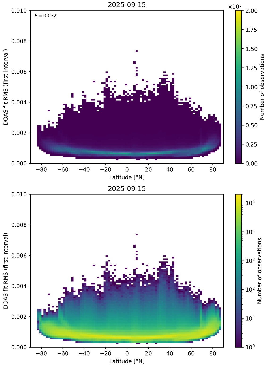
Figure 153: Scatter density plot of “Latitude” against “DOAS fit RMS (first interval)” for 2025-09-15 to 2025-09-16.
