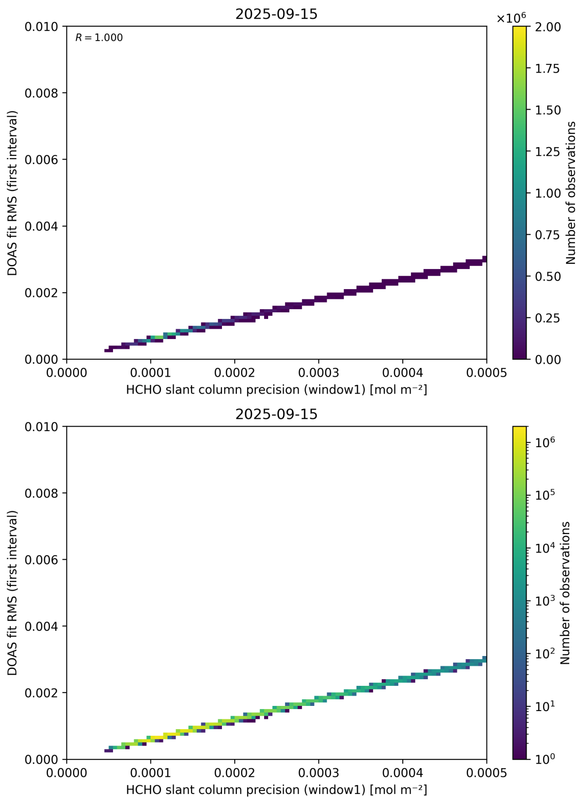
Figure 88: Scatter density plot of “HCHO slant column precision (window1)” against “DOAS fit RMS (first interval)” for 2025-09-15 to 2025-09-16.
