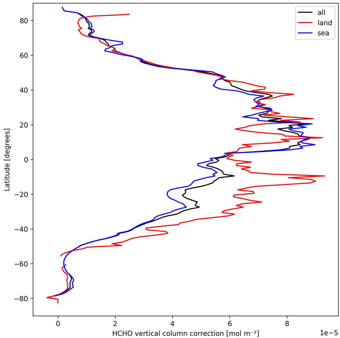
Figure 23: Zonal average of “HCHO vertical column correction” for 2025-09-15 to 2025-09-16.
