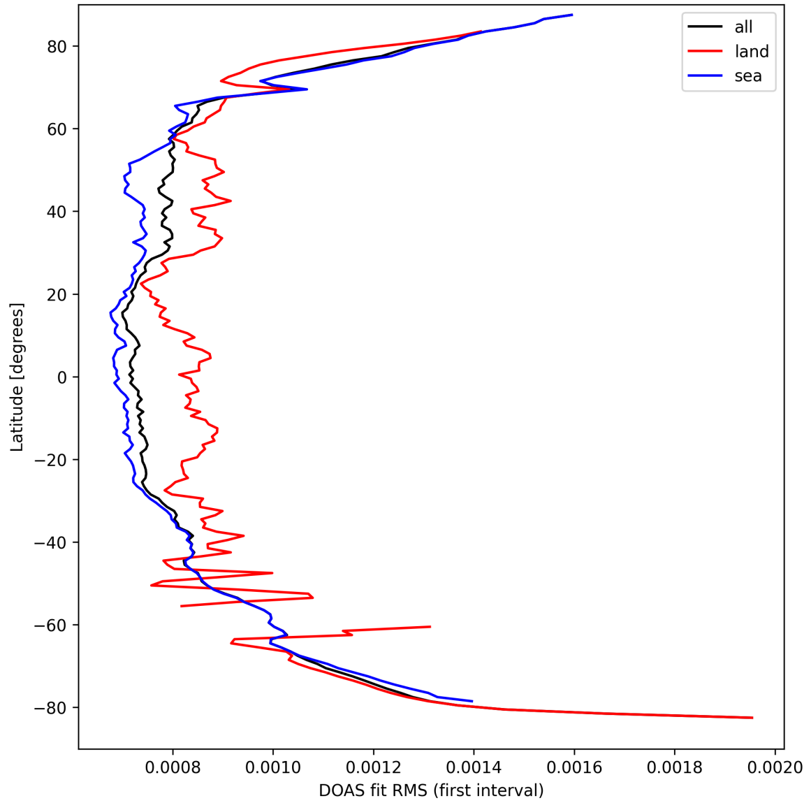
Figure 32: Zonal average of “DOAS fit RMS (first interval)” for 2025-09-15 to 2025-09-16.
