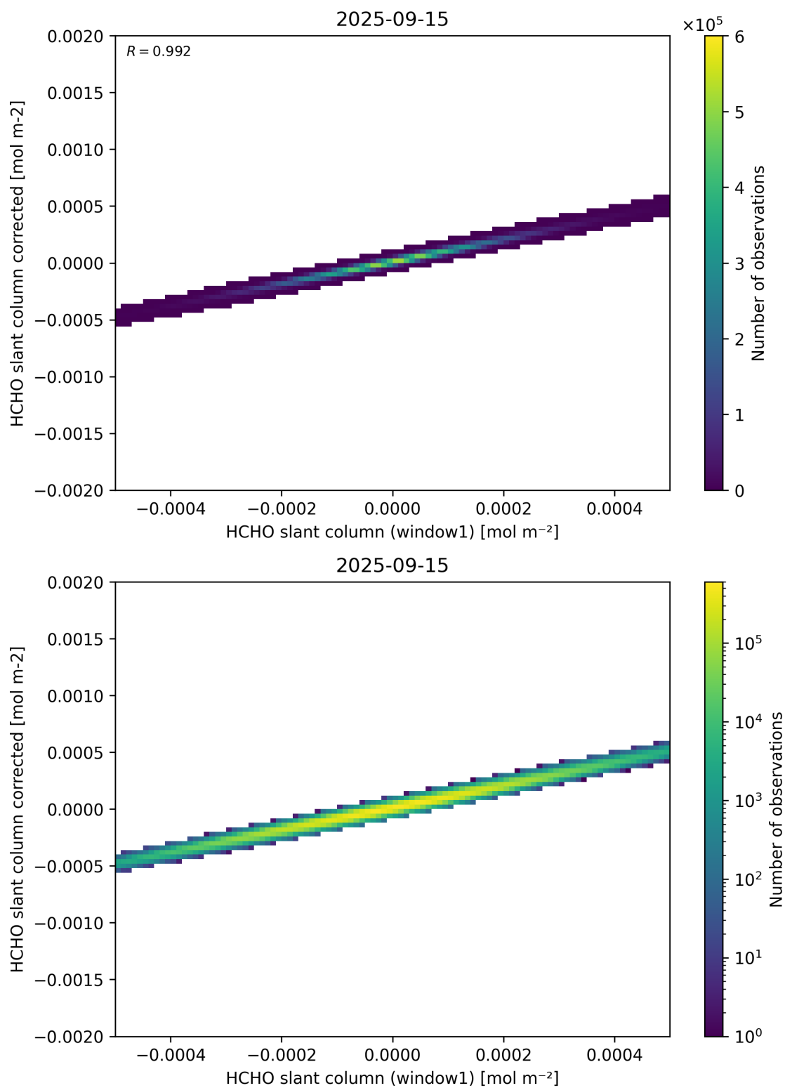
Figure 82: Scatter density plot of “HCHO slant column (window1)” against “HCHO slant column corrected” for 2025-09-15 to 2025-09-16.
