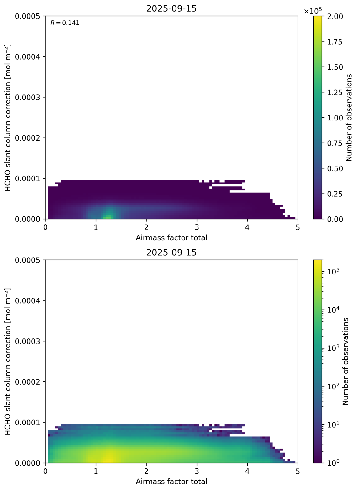
Figure 102: Scatter density plot of “Airmass factor total” against “HCHO slant column correction” for 2025-09-15 to 2025-09-16.
