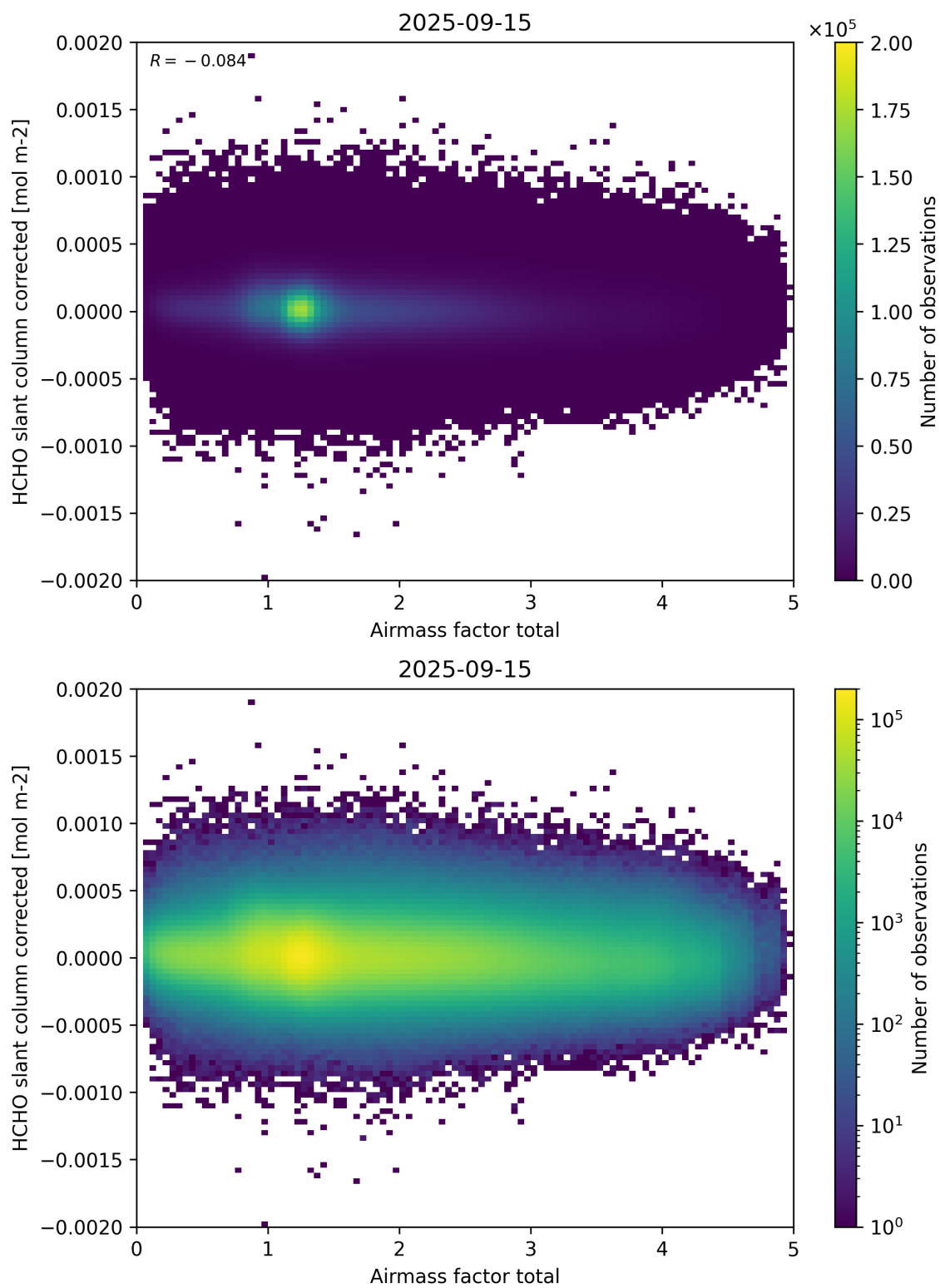
Figure 101: Scatter density plot of “Airmass factor total” against “HCHO slant column corrected” for 2025-09-15 to 2025-09-16.
