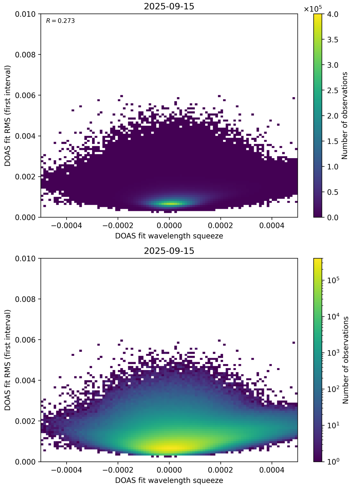
Figure 68: Scatter density plot of “DOAS fit wavelength squeeze” against “DOAS fit RMS (first interval)” for 2025-09-15 to 2025-09-16.
