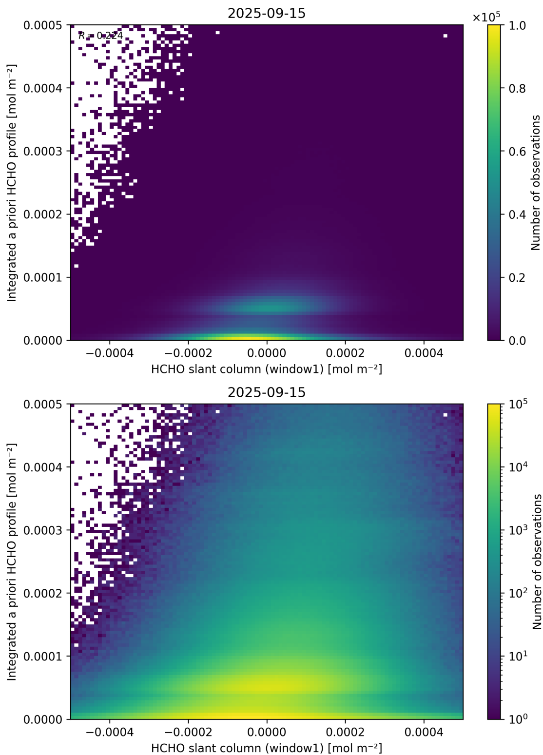
Figure 87: Scatter density plot of “HCHO slant column (window1)” against “Integrated a priori HCHO profile” for 2025-09-15 to 2025-09-16.
