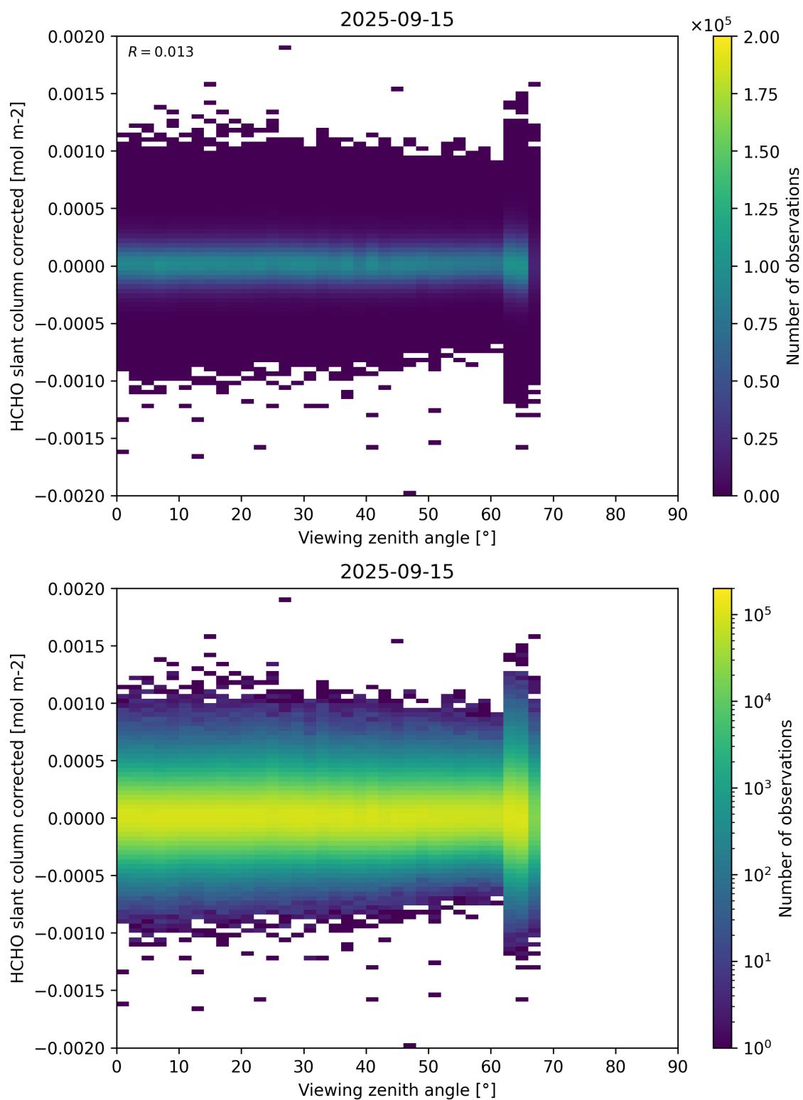
Figure 186: Scatter density plot of “Viewing zenith angle” against “HCHO slant column corrected” for 2025-09-15 to 2025-09-16.
