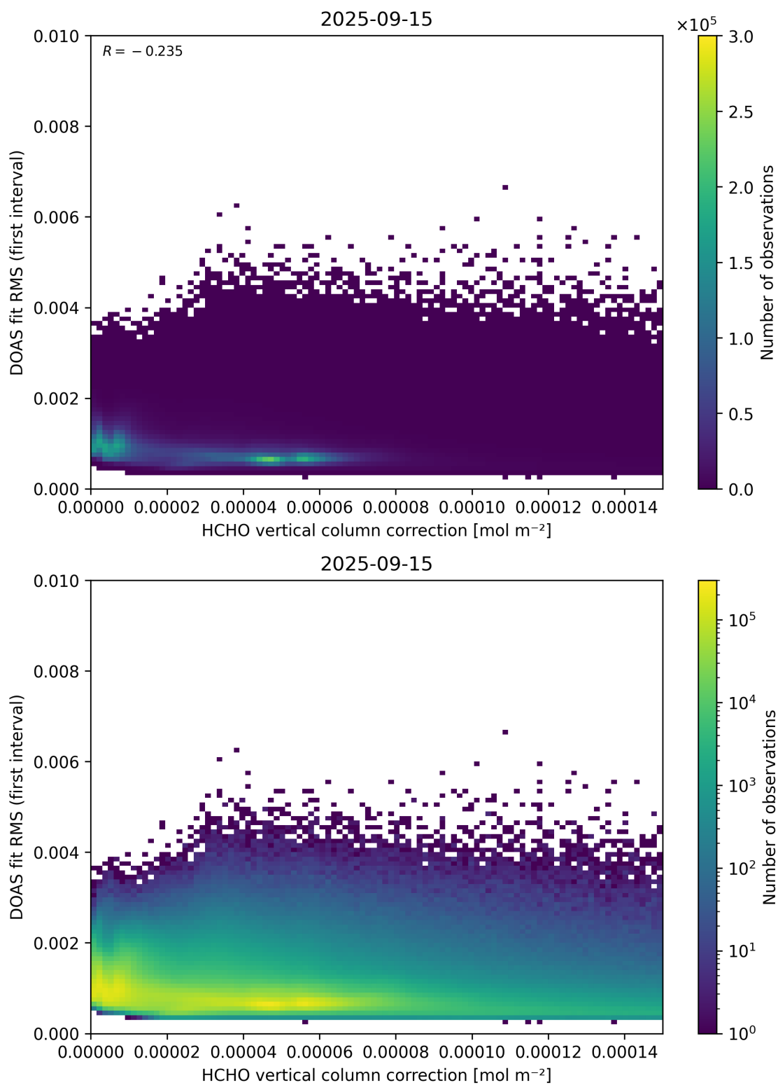
Figure 112: Scatter density plot of “HCHO vertical column correction” against “DOAS fit RMS (first interval)” for 2025-09-15 to 2025-09-16.
