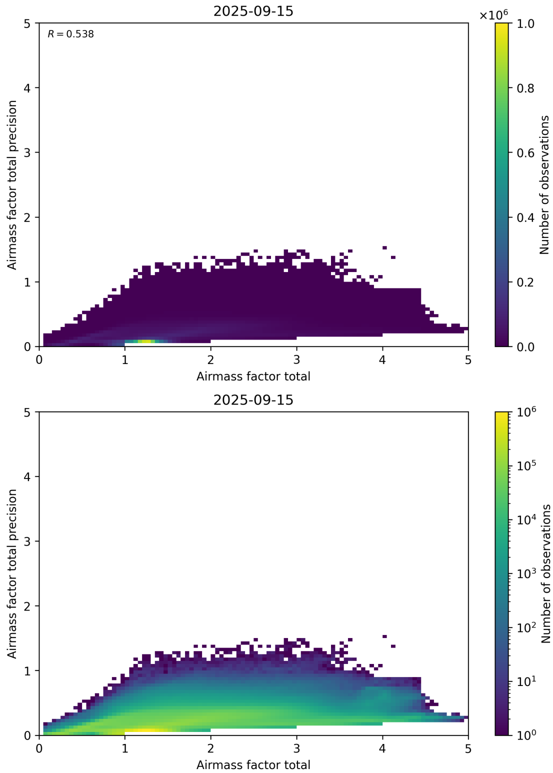
Figure 103: Scatter density plot of “Airmass factor total” against “Airmass factor total precision” for 2025-09-15 to 2025-09-16.
