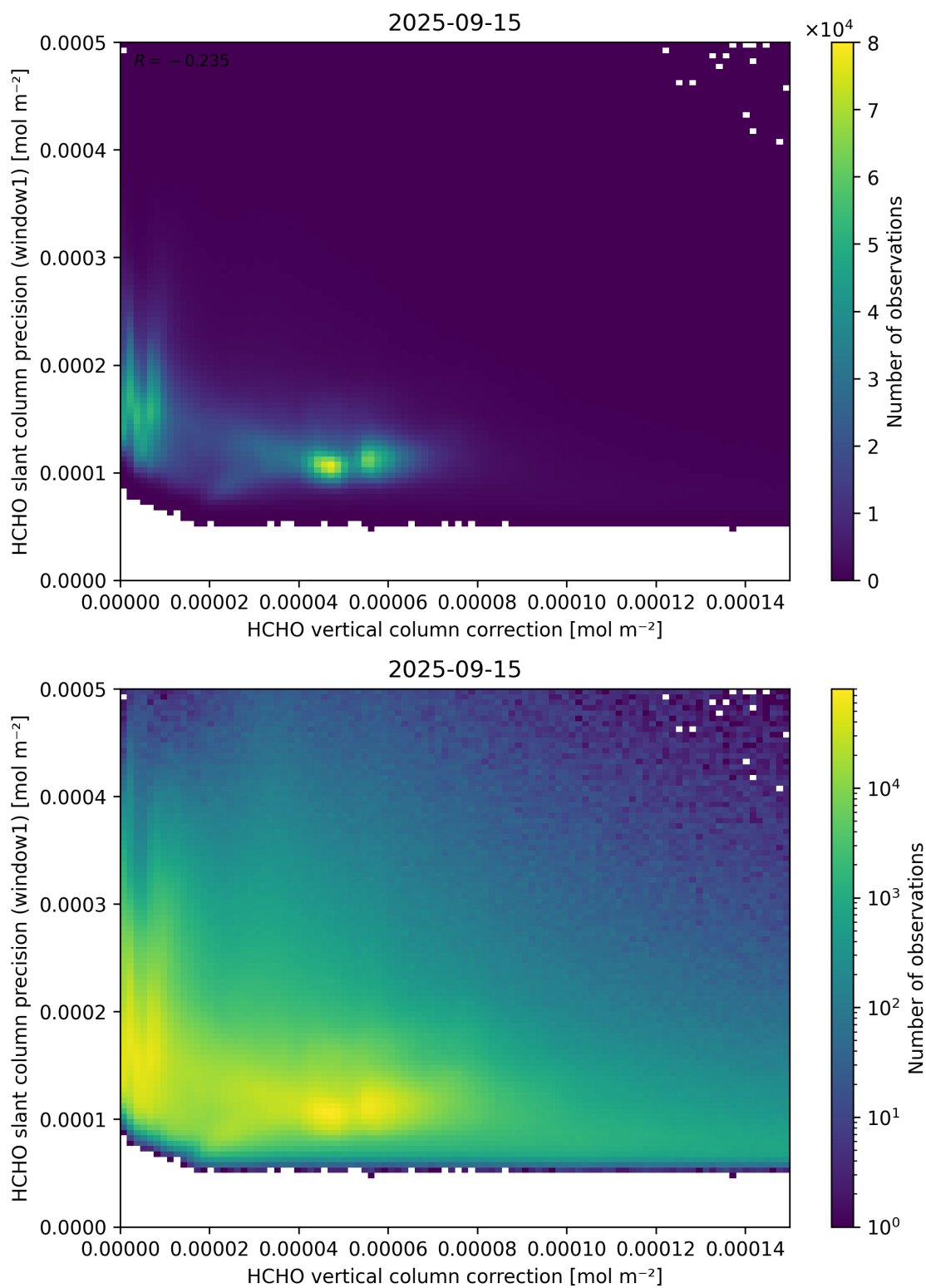
Figure 119: Scatter density plot of “HCHO vertical column correction” against “HCHO slant column precision (window1)” for 2025-09-15 to 2025-09-16.
