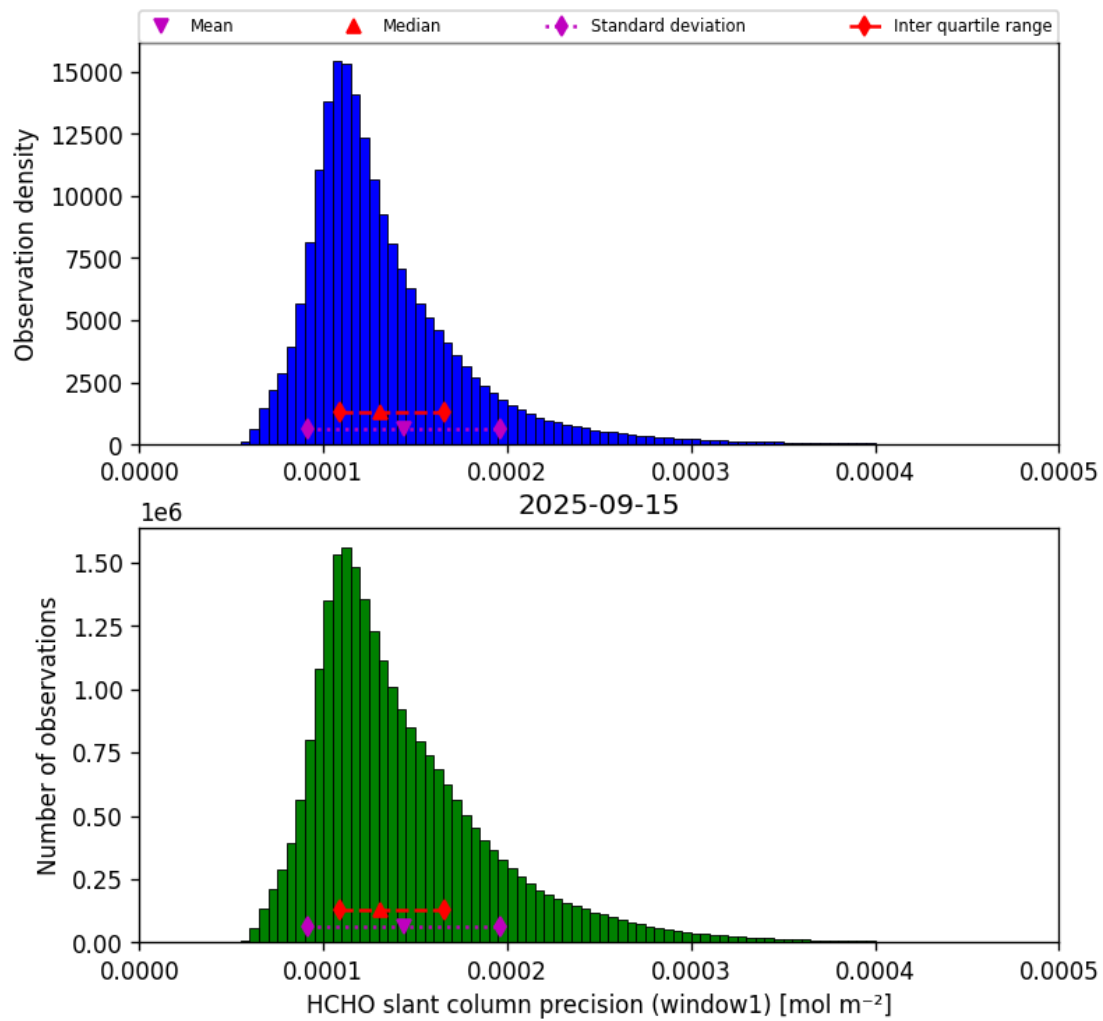
Figure 39: Histogram of “HCHO slant column precision (window1)” for 2025-09-15 to 2025-09-16
