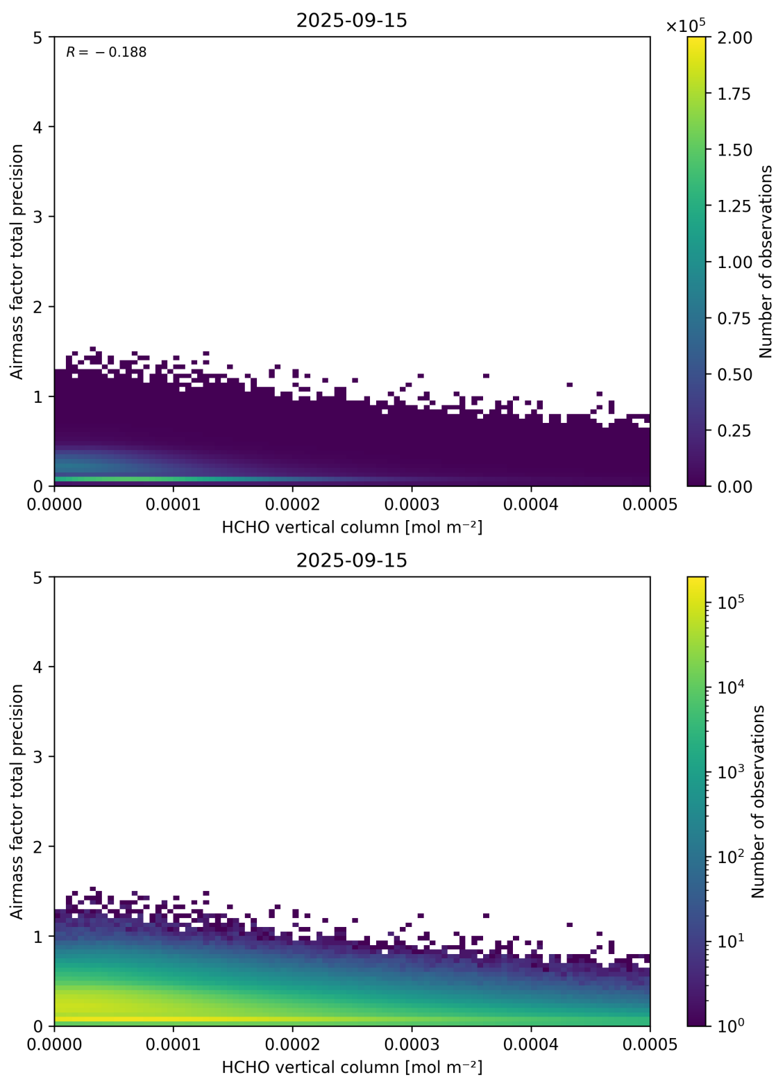
Figure 132: Scatter density plot of “HCHO vertical column” against “Airmass factor total precision” for 2025-09-15 to 2025-09-16.
