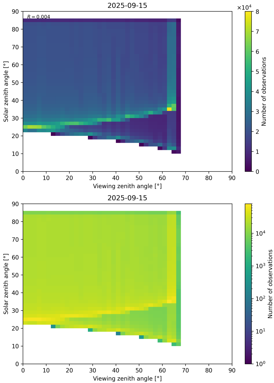
Figure 197: Scatter density plot of “Viewing zenith angle” against “Solar zenith angle” for 2025-09-15 to 2025-09-16.
