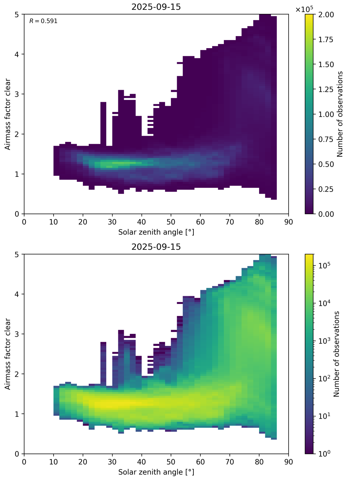
Figure 170: Scatter density plot of “Solar zenith angle” against “Airmass factor clear” for 2025-09-15 to 2025-09-16.
