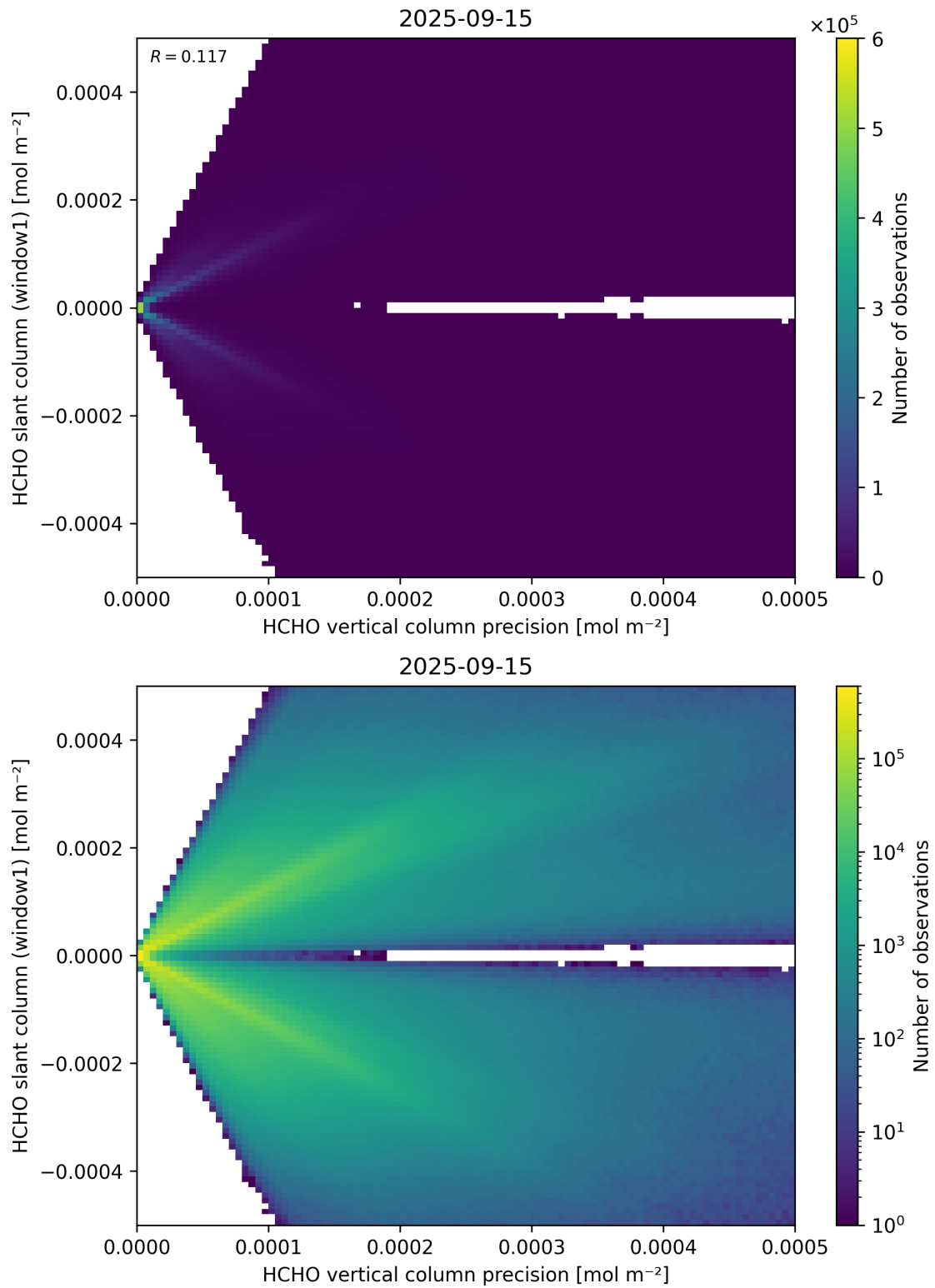
Figure 142: Scatter density plot of “HCHO vertical column precision” against “HCHO slant column (window1)” for 2025-09-15 to 2025-09-16.
