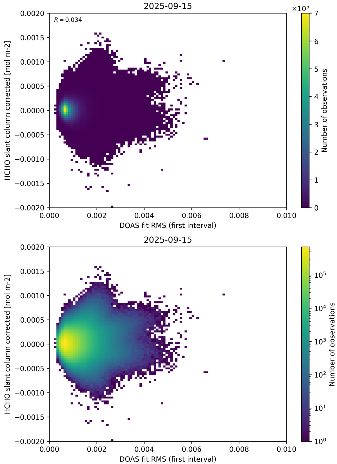
Figure 62: Scatter density plot of “DOAS fit RMS (first interval)” against “HCHO slant column corrected” for 2025-09-15 to 2025-09-16.
