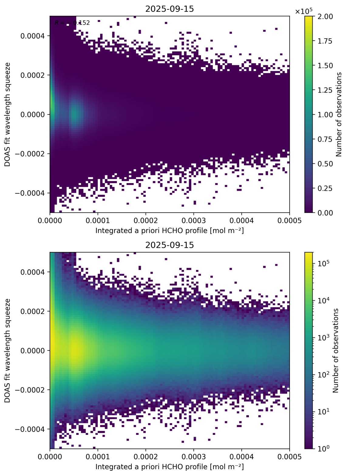
Figure 150: Scatter density plot of “Integrated a priori HCHO profile” against “DOAS fit wavelength squeeze” for 2025-09-15 to 2025-09-16.
