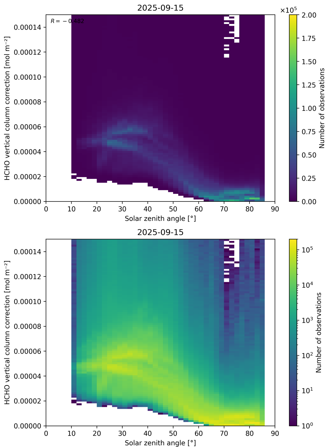
Figure 178: Scatter density plot of “Solar zenith angle” against “HCHO vertical column correction” for 2025-09-15 to 2025-09-16.
