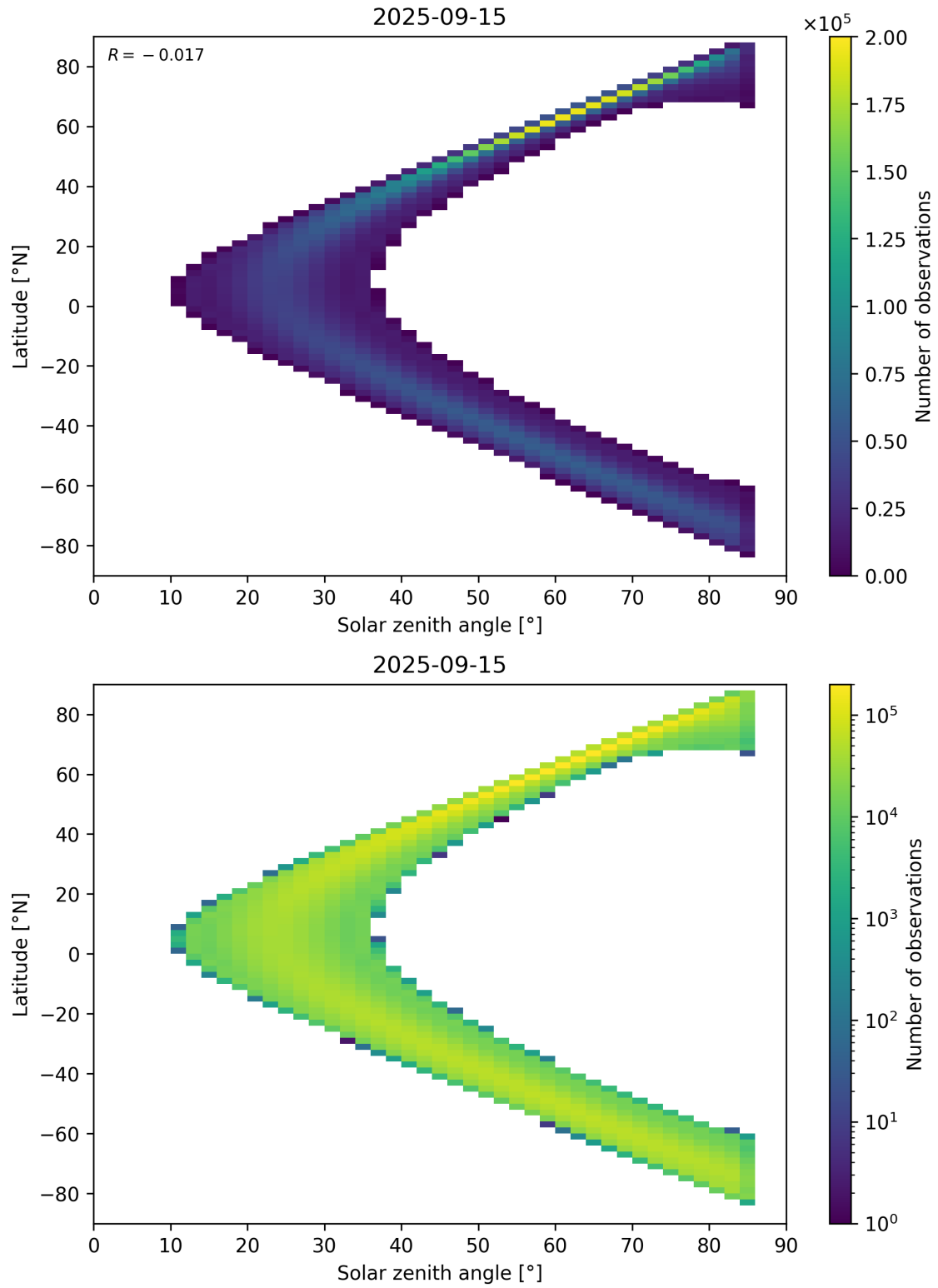
Figure 181: Scatter density plot of “Solar zenith angle” against “Latitude” for 2025-09-15 to 2025-09-16.
