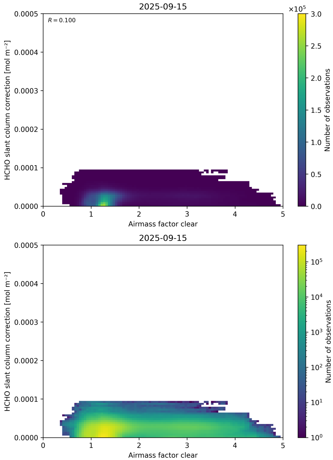
Figure 75: Scatter density plot of “Airmass factor clear” against “HCHO slant column correction” for 2025-09-15 to 2025-09-16.
