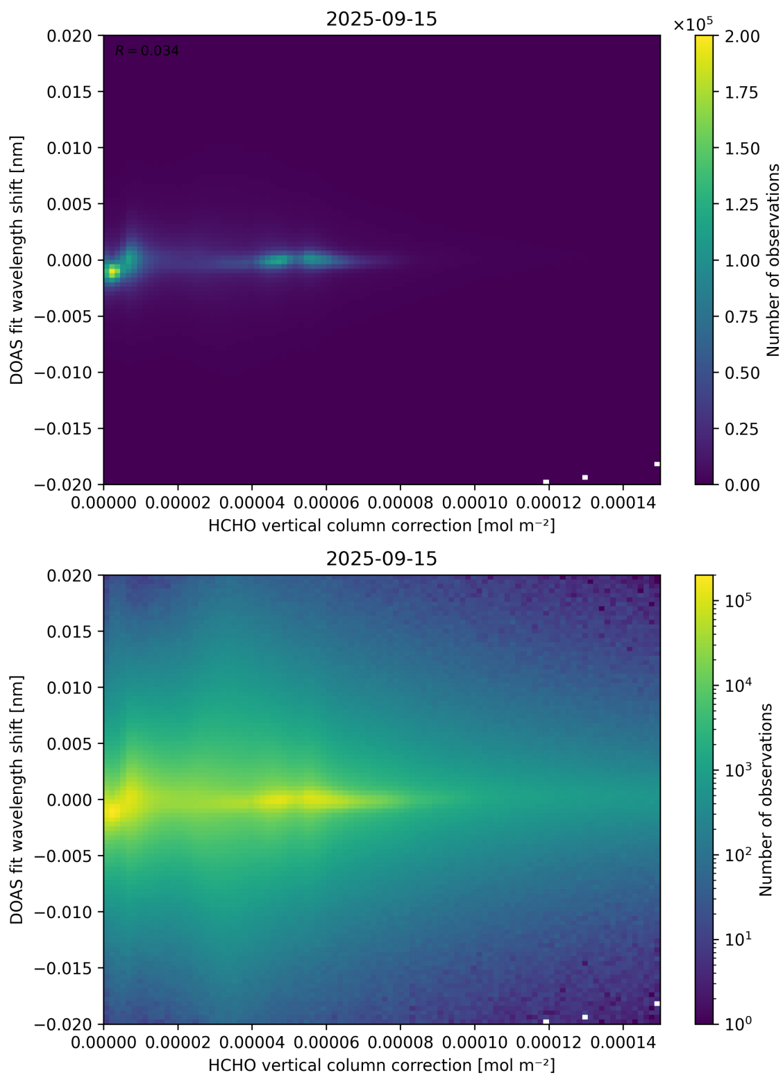
Figure 113: Scatter density plot of “HCHO vertical column correction” against “DOAS fit wavelength shift” for 2025-09-15 to 2025-09-16.
