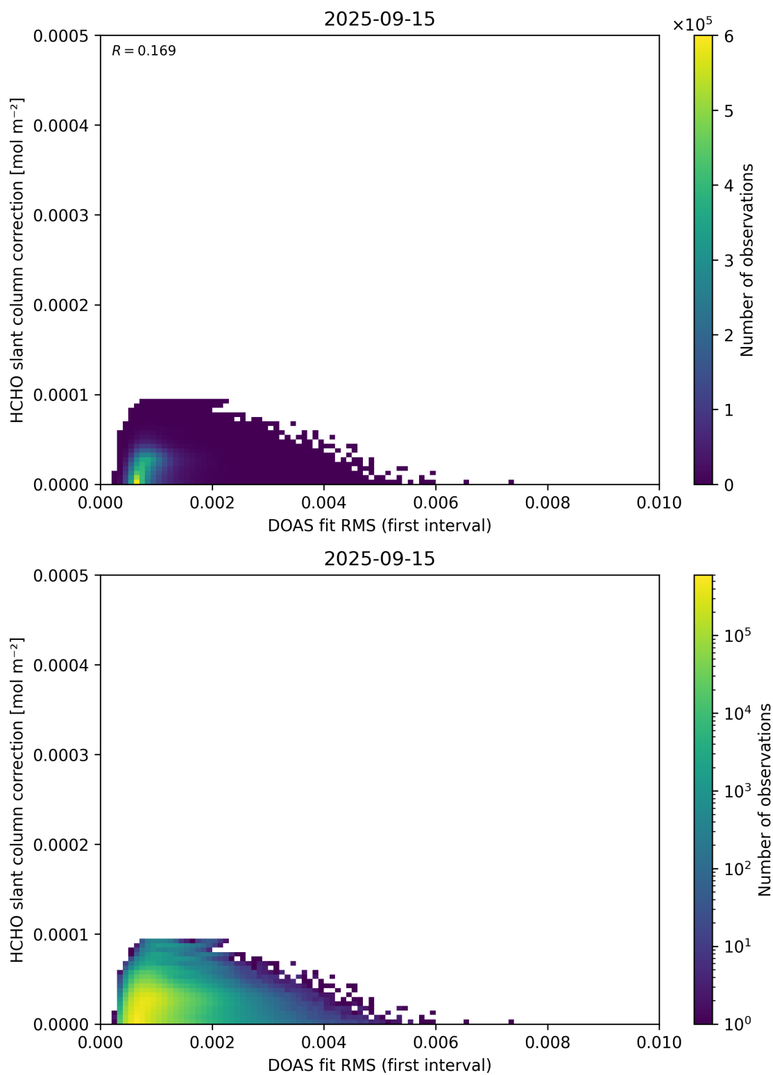
Figure 63: Scatter density plot of “DOAS fit RMS (first interval)” against “HCHO slant column correction” for 2025-09-15 to 2025-09-16.
