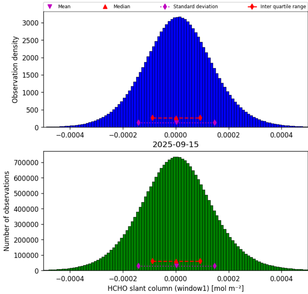
Figure 38: Histogram of “HCHO slant column (window1)” for 2025-09-15 to 2025-09-16
