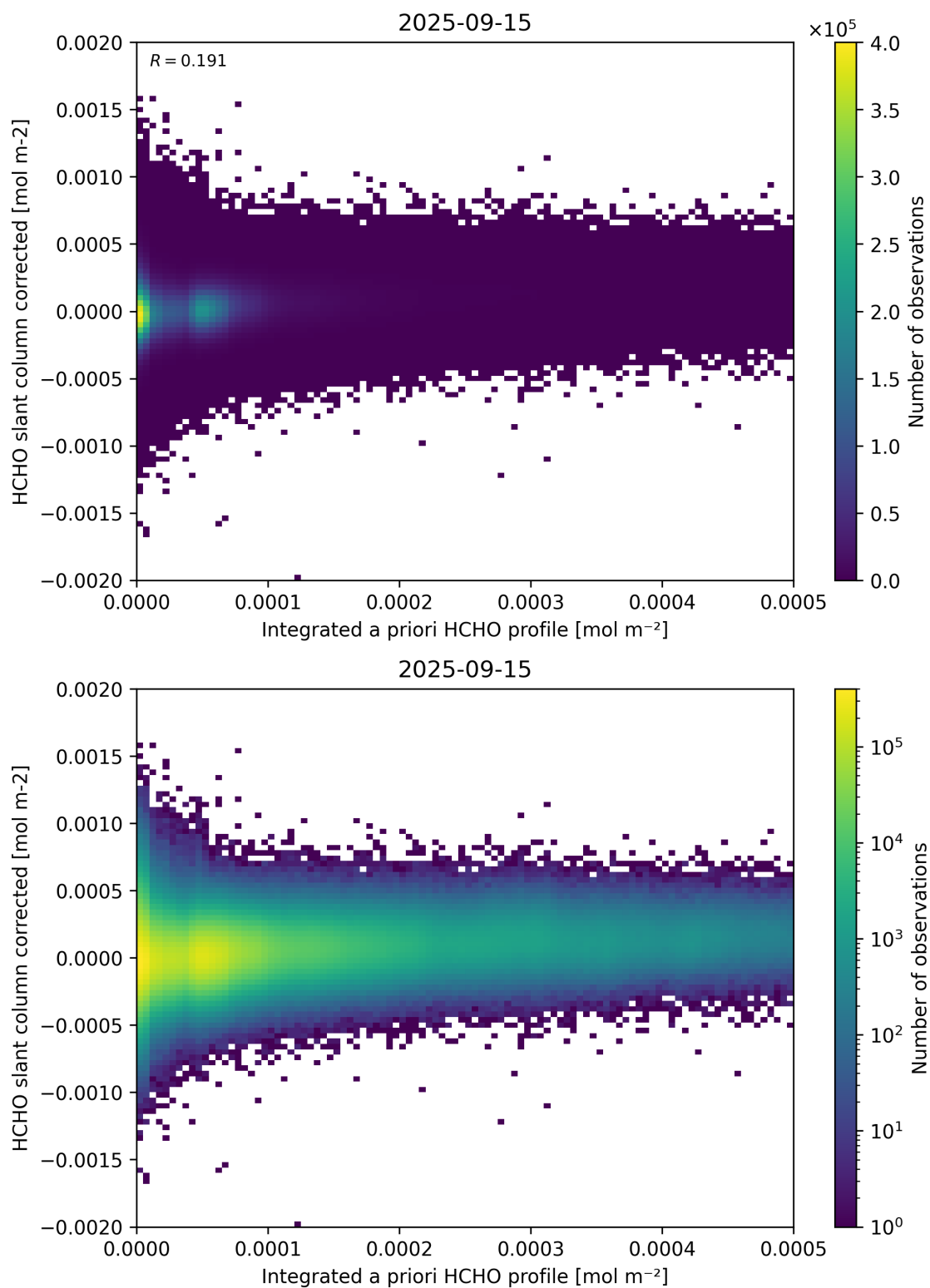
Figure 151: Scatter density plot of “Integrated a priori HCHO profile” against “HCHO slant column corrected” for 2025-09-15 to 2025-09-16.
