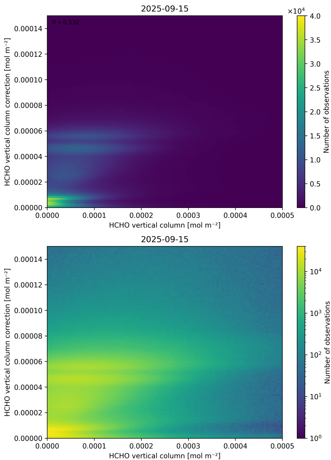
Figure 133: Scatter density plot of “HCHO vertical column” against “HCHO vertical column correction” for 2025-09-15 to 2025-09-16.
