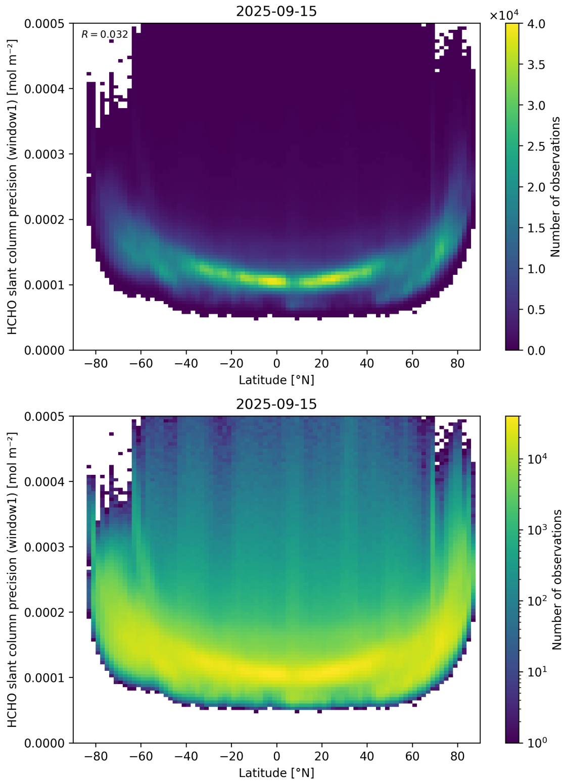
Figure 160: Scatter density plot of “Latitude” against “HCHO slant column precision (window1)” for 2025-09-15 to 2025-09-16.
