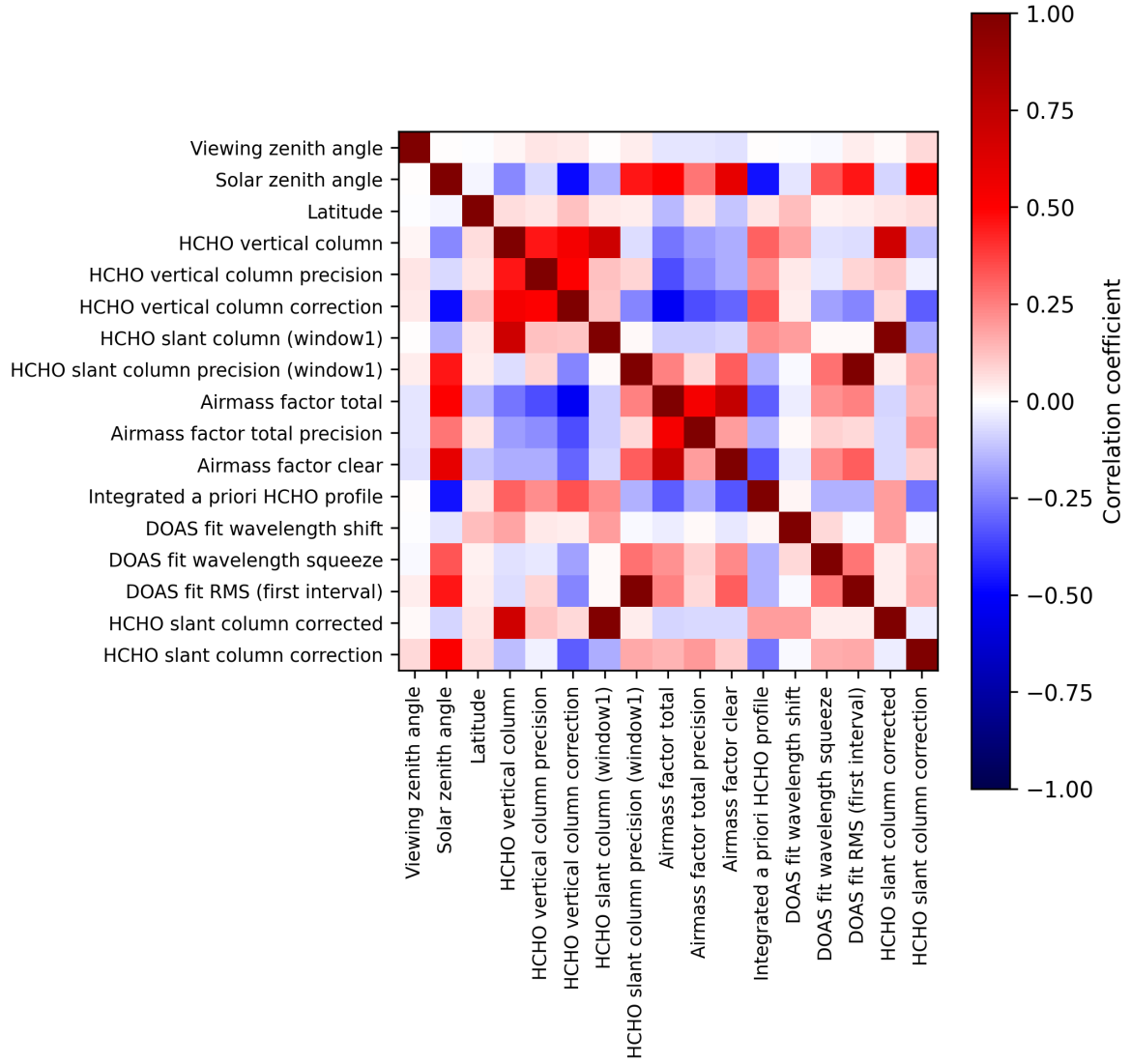
Figure 2: Map of correlation matrix for 2025-09-15 to 2025-09-16.
