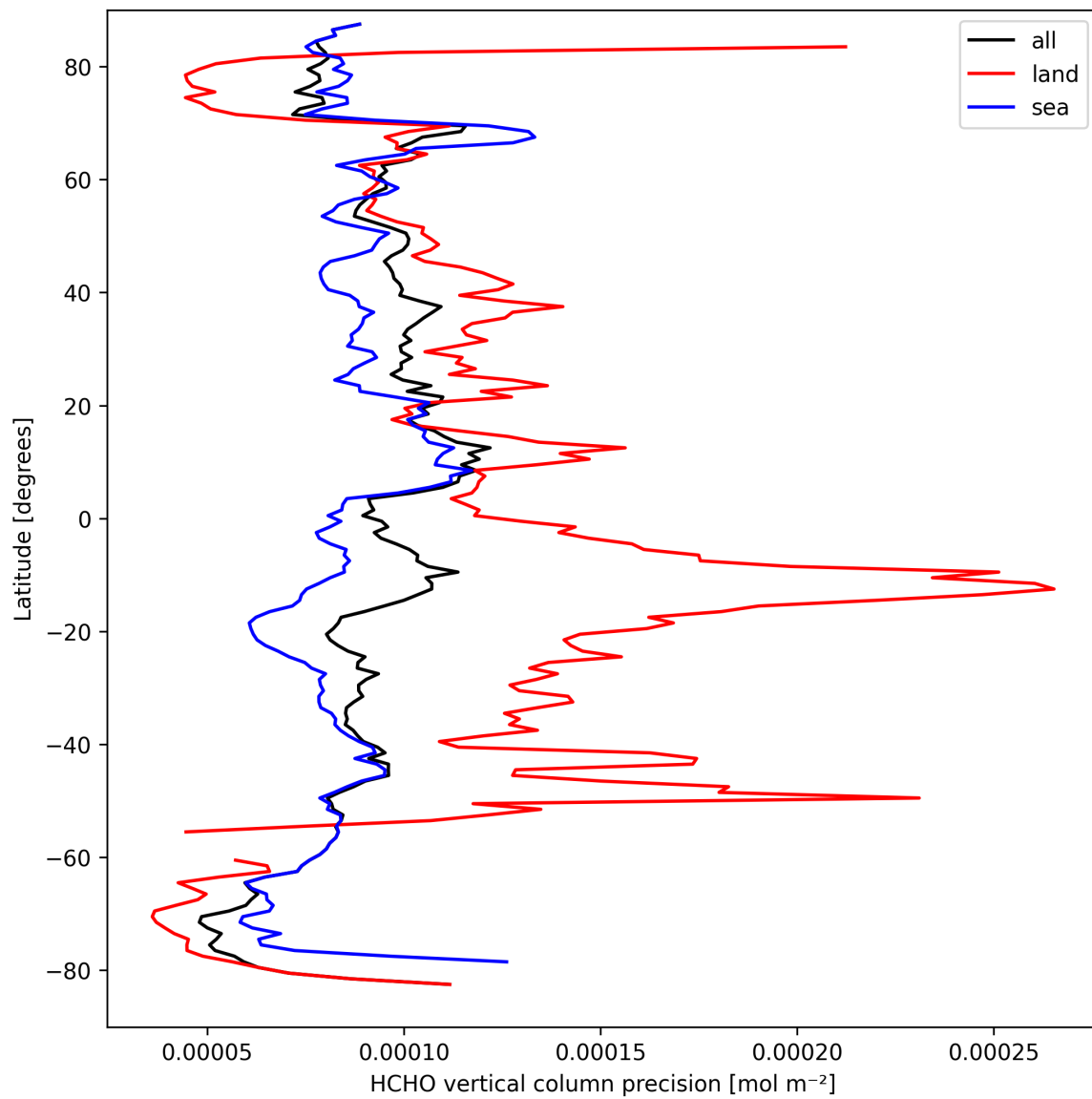
Figure 22: Zonal average of “HCHO vertical column precision” for 2025-09-15 to 2025-09-16.
