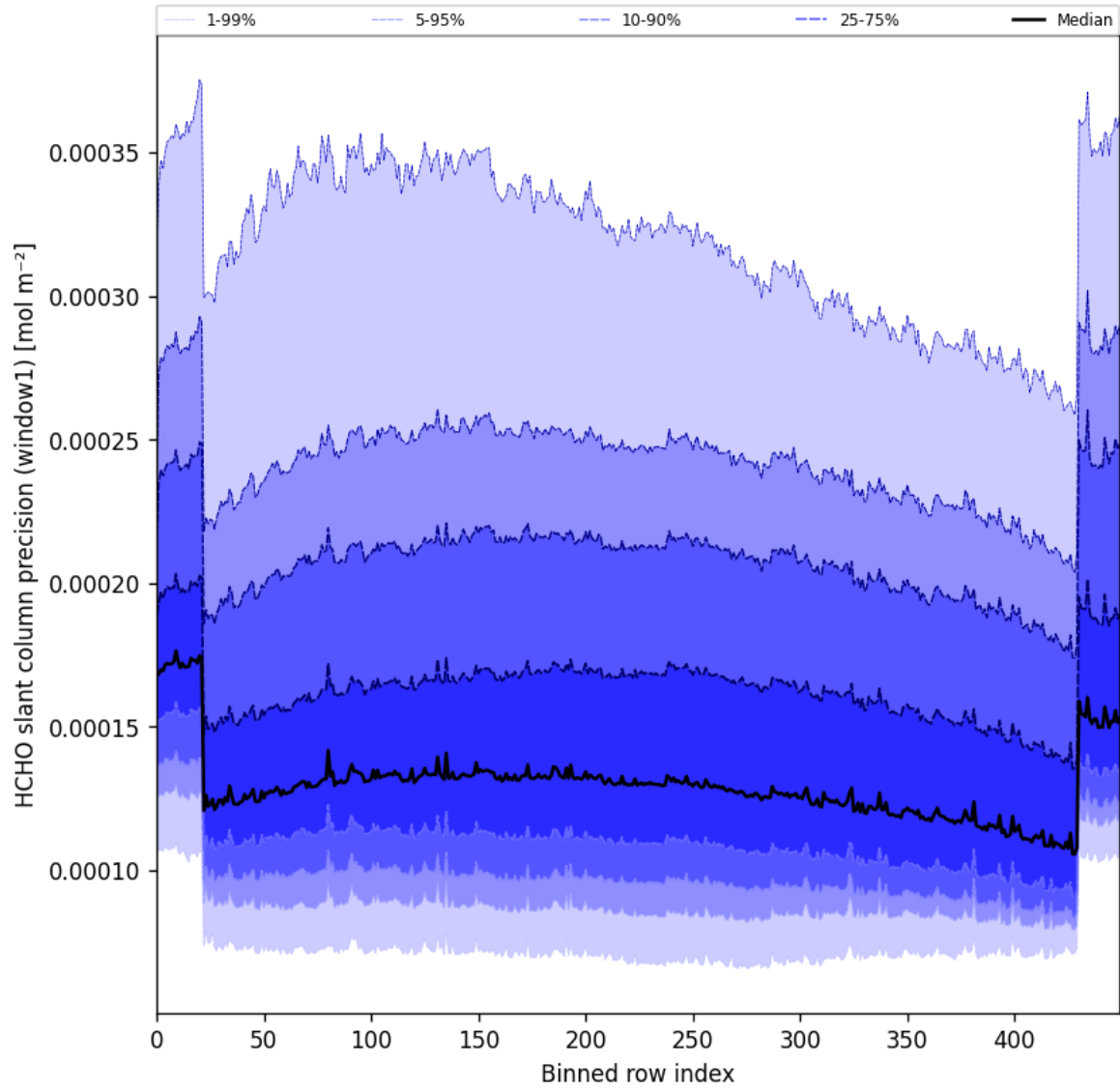
Figure 53: Along track statistics of “HCHO slant column precision (window1)” for 2025-09-15 to 2025-09-16
