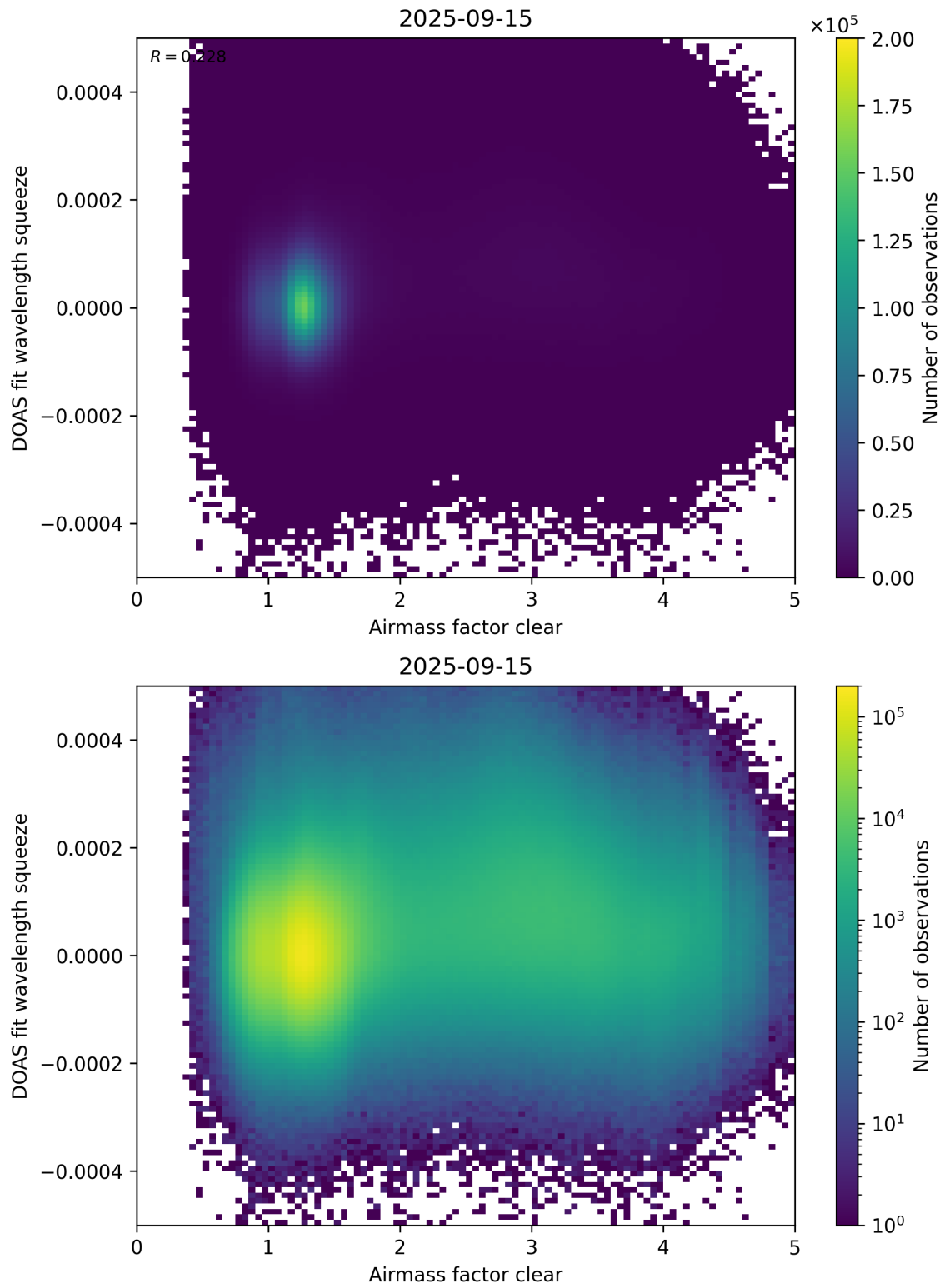
Figure 73: Scatter density plot of “Airmass factor clear” against “DOAS fit wavelength squeeze” for 2025-09-15 to 2025-09-16.
