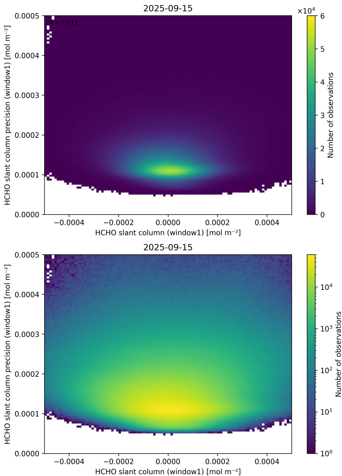
Figure 84: Scatter density plot of “HCHO slant column (window1)” against “HCHO slant column precision (window1)” for 2025-09-15 to 2025-09-16.
