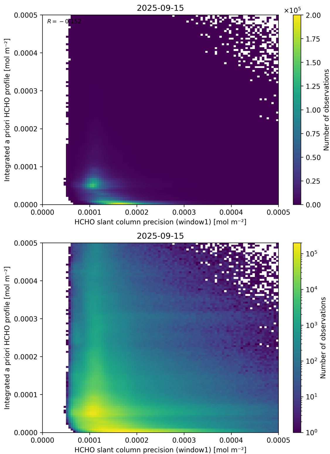
Figure 96: Scatter density plot of “HCHO slant column precision (window1)” against “Integrated a priori HCHO profile” for 2025-09-15 to 2025-09-16.
