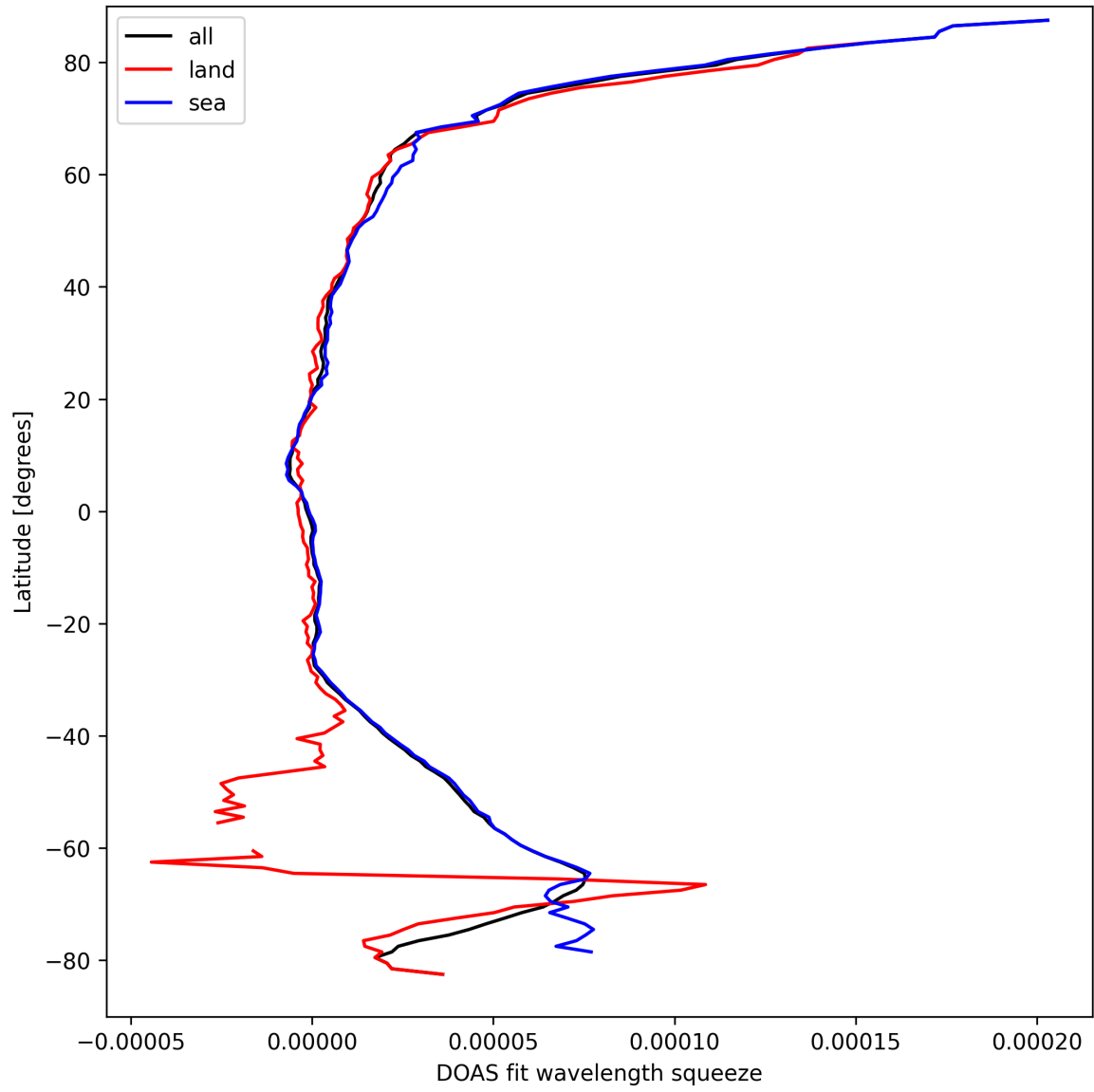
Figure 31: Zonal average of “DOAS fit wavelength squeeze” for 2025-09-15 to 2025-09-16.
