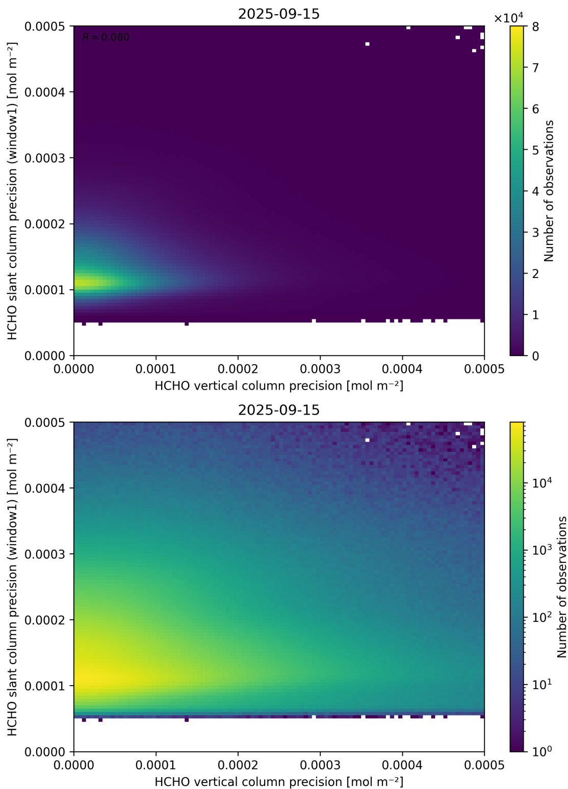
Figure 143: Scatter density plot of “HCHO vertical column precision” against “HCHO slant column precision (window1)” for 2025-09-15 to 2025-09-16.
