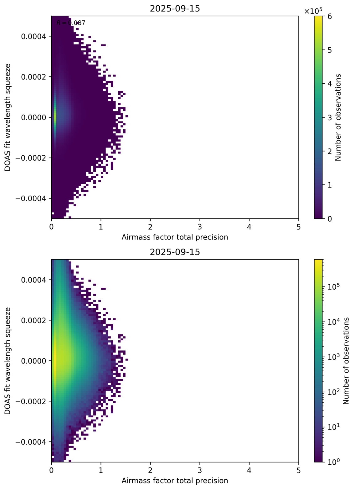
Figure 107: Scatter density plot of “Airmass factor total precision” against “DOAS fit wavelength squeeze” for 2025-09-15 to 2025-09-16.
