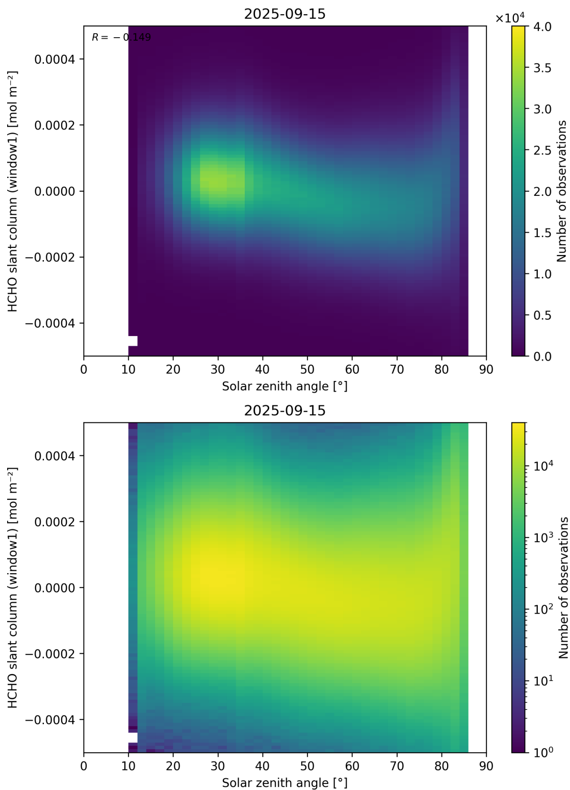
Figure 173: Scatter density plot of “Solar zenith angle” against “HCHO slant column (window1)” for 2025-09-15 to 2025-09-16.
