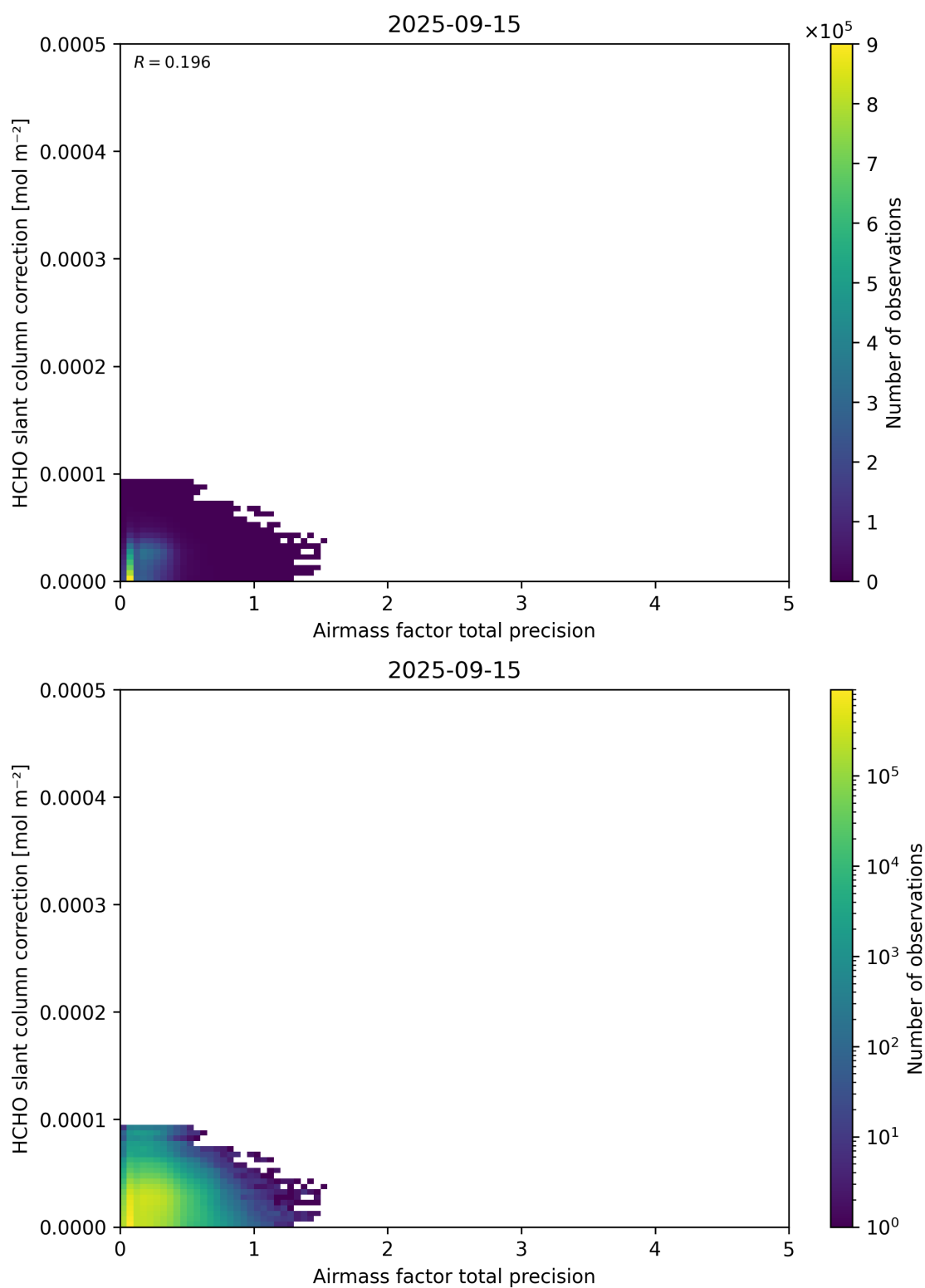
Figure 110: Scatter density plot of “Airmass factor total precision” against “HCHO slant column correction” for 2025-09-15 to 2025-09-16.
