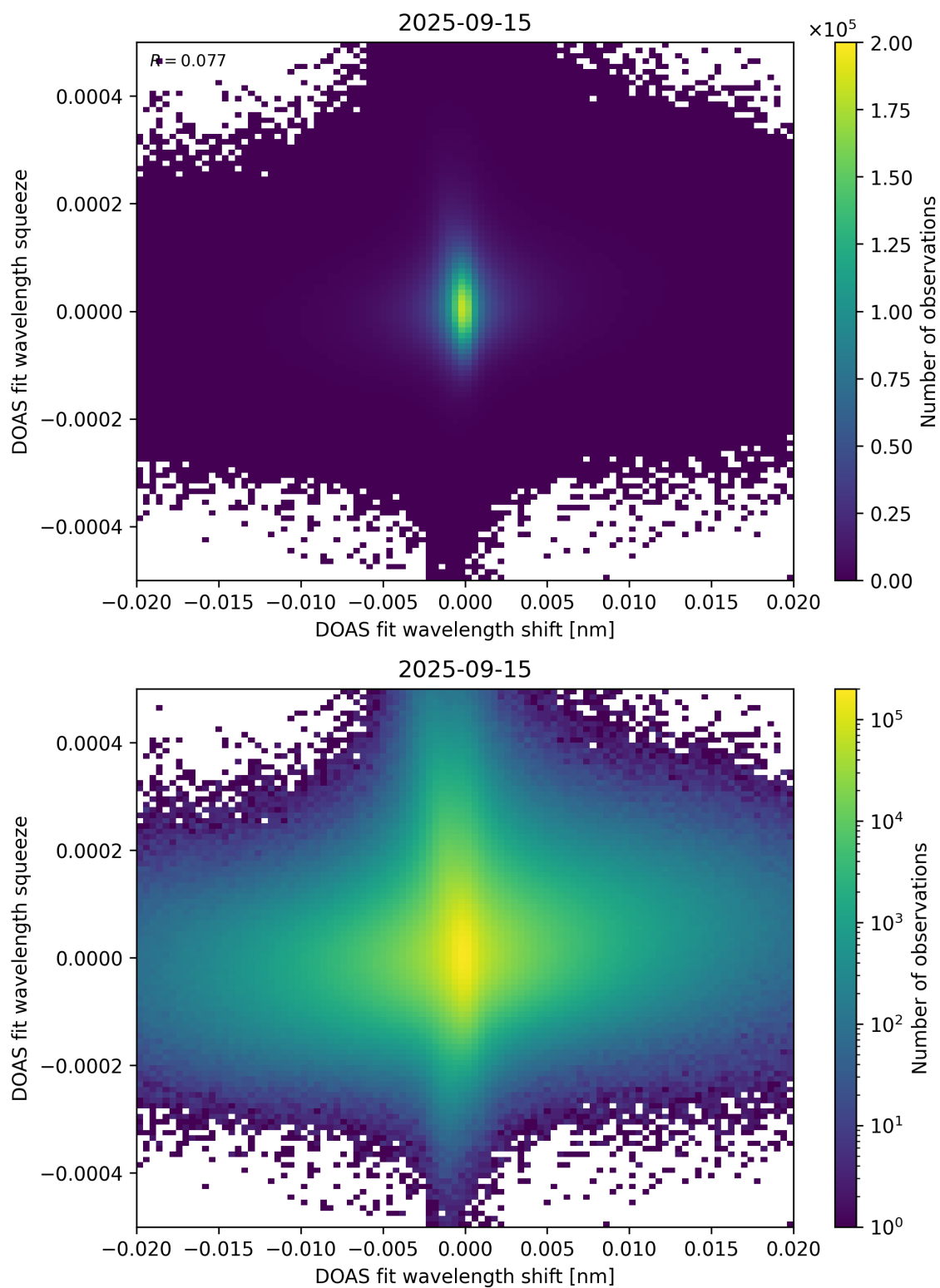
Figure 65: Scatter density plot of “DOAS fit wavelength shift” against “DOAS fit wavelength squeeze” for 2025-09-15 to 2025-09-16.
