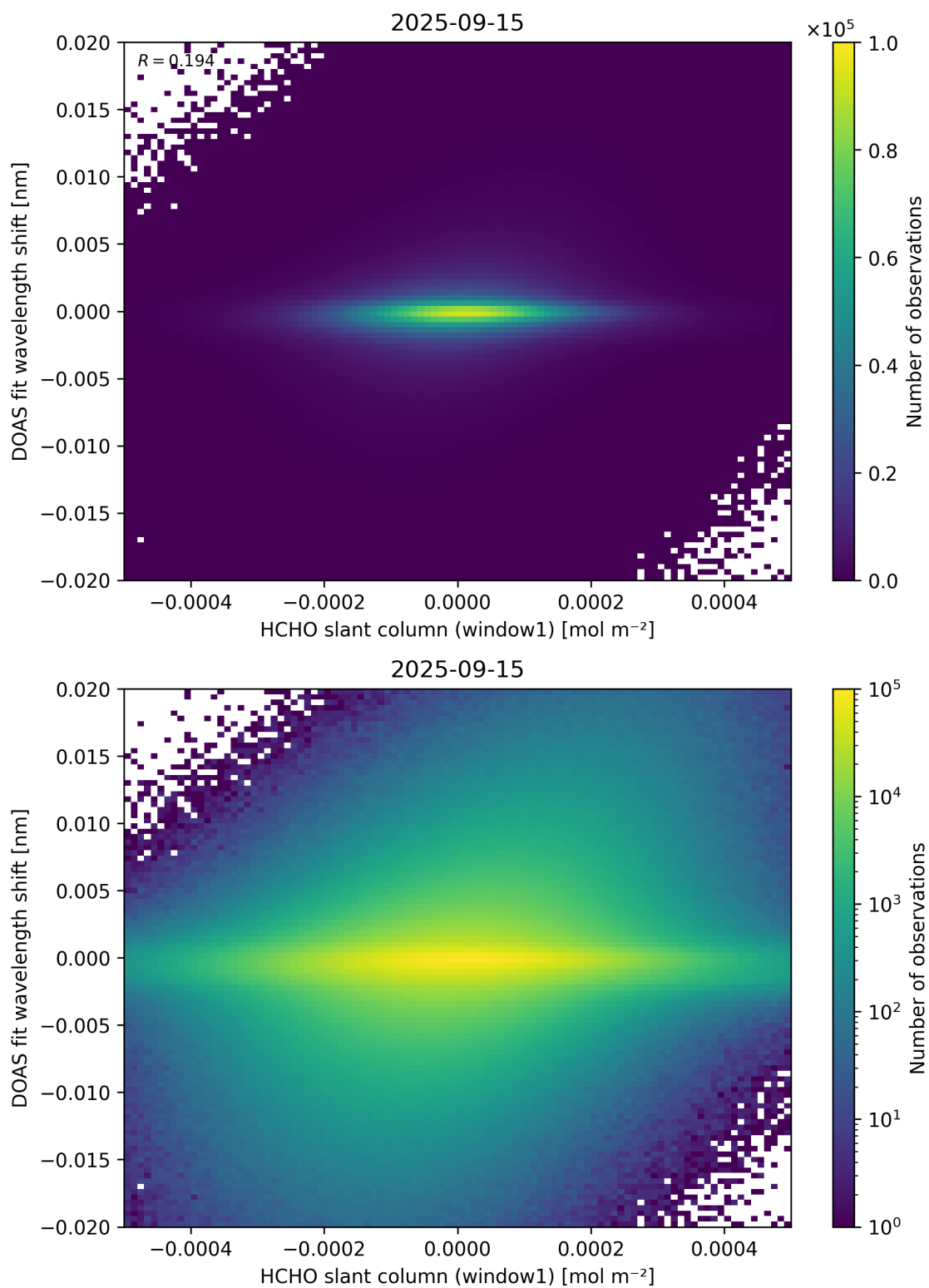
Figure 79: Scatter density plot of “HCHO slant column (window1)” against “DOAS fit wavelength shift” for 2025-09-15 to 2025-09-16.
