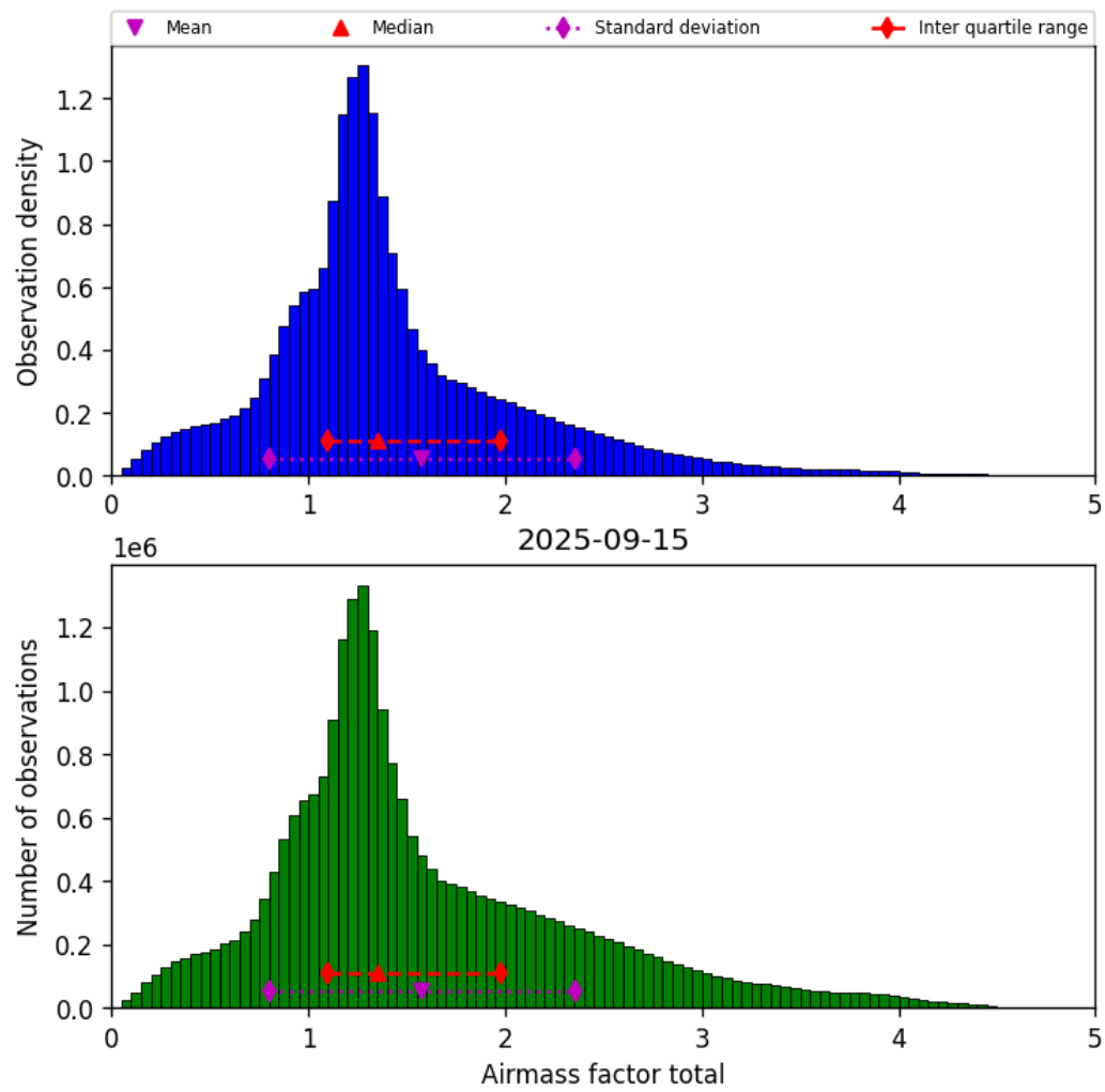
Figure 40: Histogram of “Airmass factor total” for 2025-09-15 to 2025-09-16
