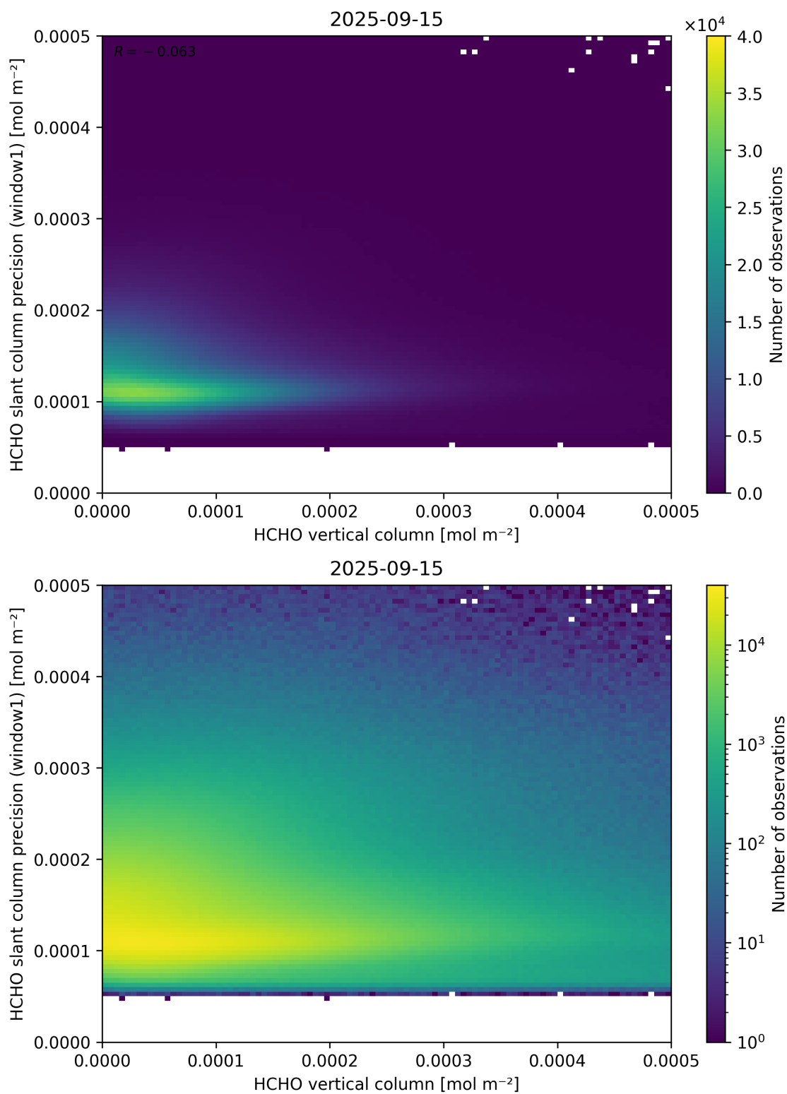
Figure 130: Scatter density plot of “HCHO vertical column” against “HCHO slant column precision (window1)” for 2025-09-15 to 2025-09-16.
