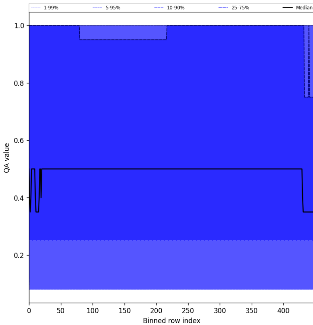
Figure 48: Along track statistics of “QA value” for 2025-09-15 to 2025-09-16
