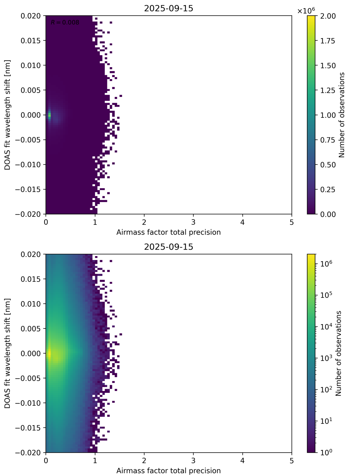
Figure 106: Scatter density plot of “Airmass factor total precision” against “DOAS fit wavelength shift” for 2025-09-15 to 2025-09-16.
