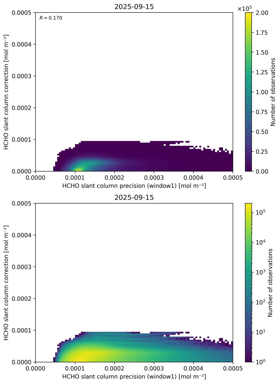
Figure 93: Scatter density plot of “HCHO slant column precision (window1)” against “HCHO slant column correction” for 2025-09-15 to 2025-09-16.
