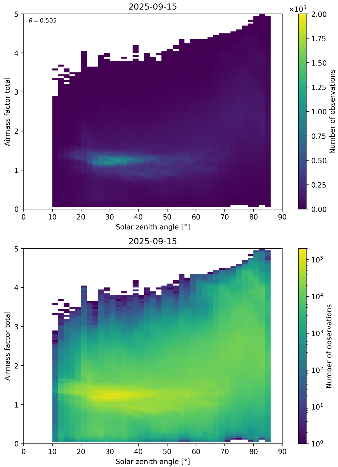
Figure 175: Scatter density plot of “Solar zenith angle” against “Airmass factor total” for 2025-09-15 to 2025-09-16.
