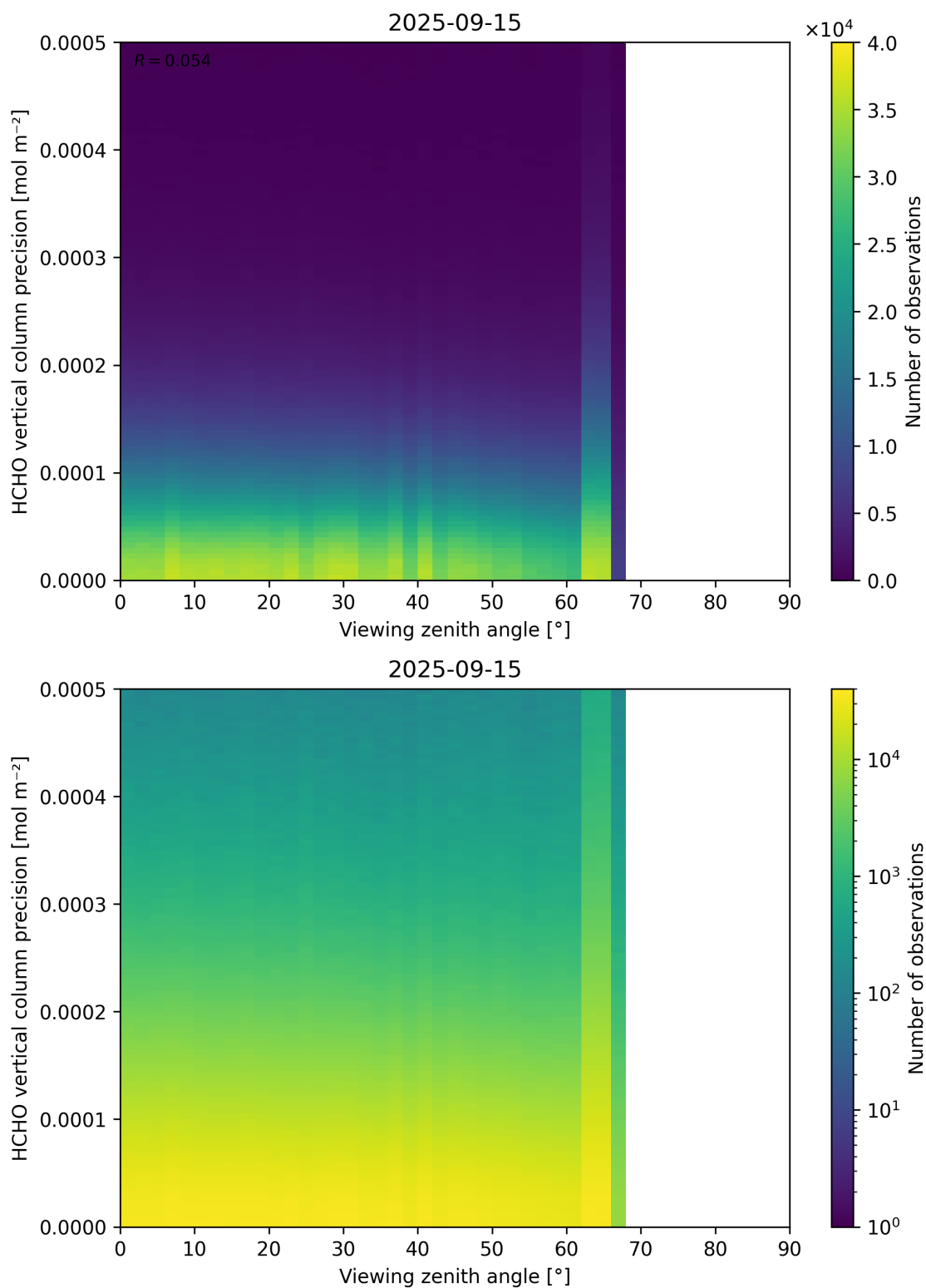
Figure 194: Scatter density plot of “Viewing zenith angle” against “HCHO vertical column precision” for 2025-09-15 to 2025-09-16.
