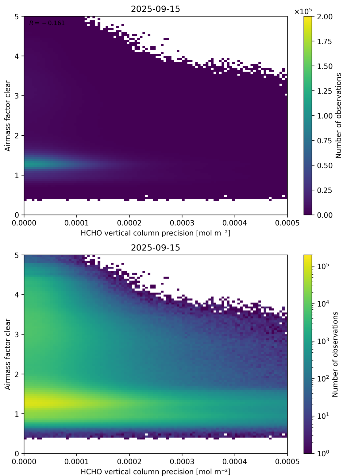
Figure 139: Scatter density plot of “HCHO vertical column precision” against “Airmass factor clear” for 2025-09-15 to 2025-09-16.
