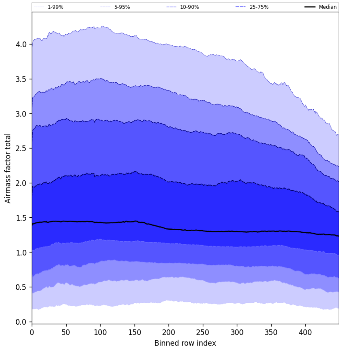
Figure 54: Along track statistics of “Airmass factor total” for 2025-09-15 to 2025-09-16
