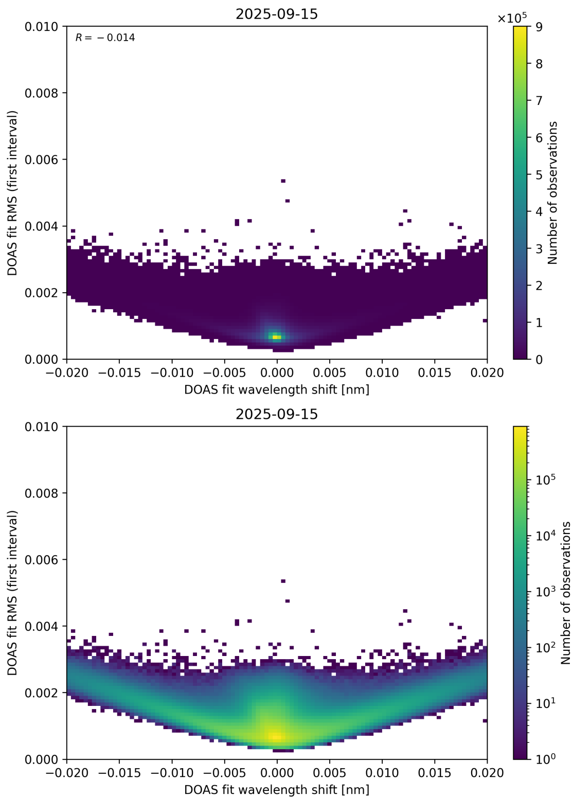
Figure 64: Scatter density plot of “DOAS fit wavelength shift” against “DOAS fit RMS (first interval)” for 2025-09-15 to 2025-09-16.
