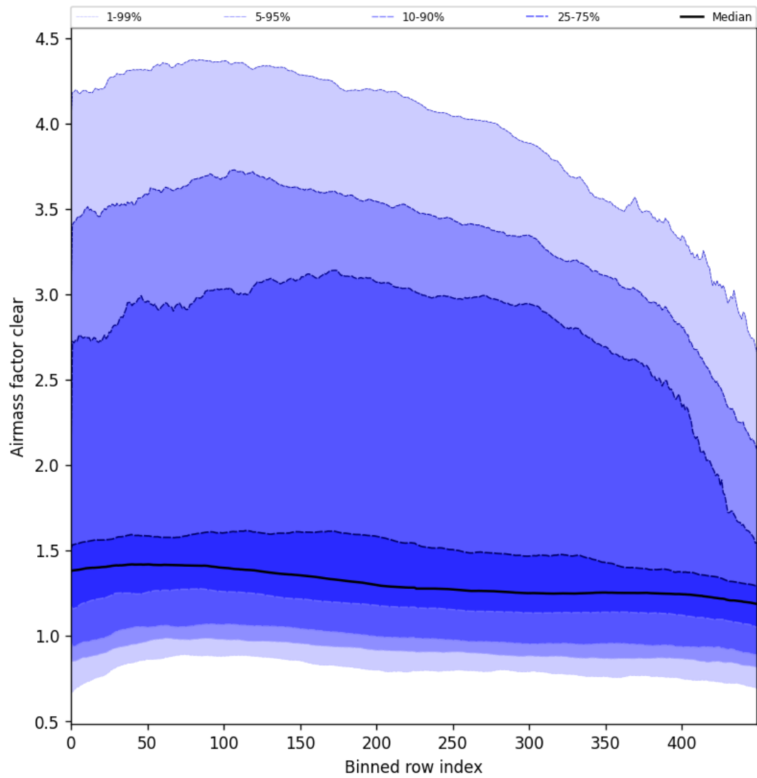
Figure 56: Along track statistics of “Air mass factor clear” for 2025-09-15 to 2025-09-16
