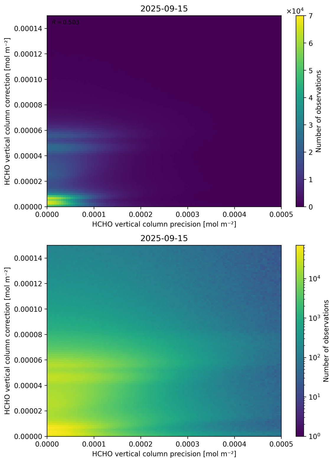
Figure 146: Scatter density plot of “HCHO vertical column precision” against “HCHO vertical column correction” for 2025-09-15 to 2025-09-16.
