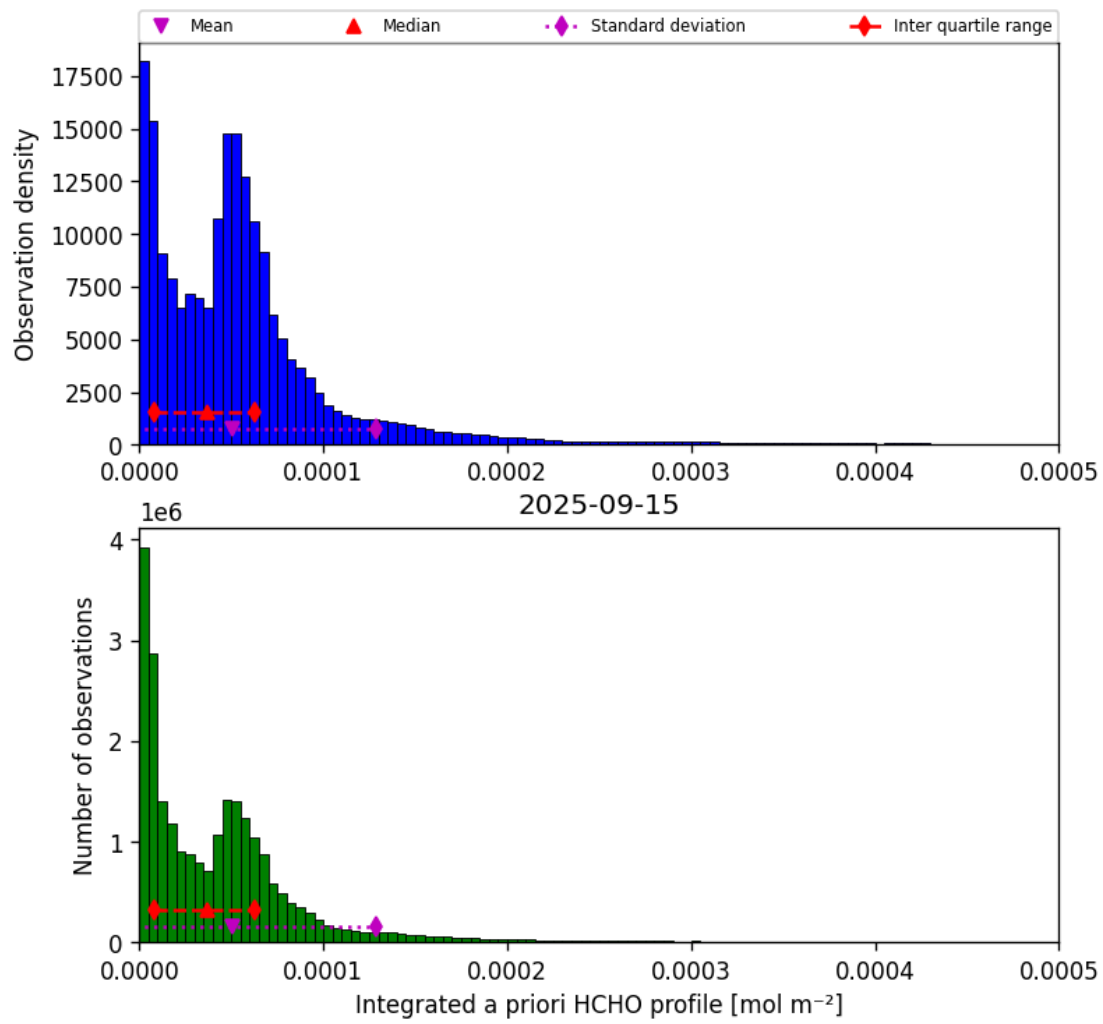
Figure 43: Histogram of “Integrated a priori HCHO profile” for 2025-09-15 to 2025-09-16
