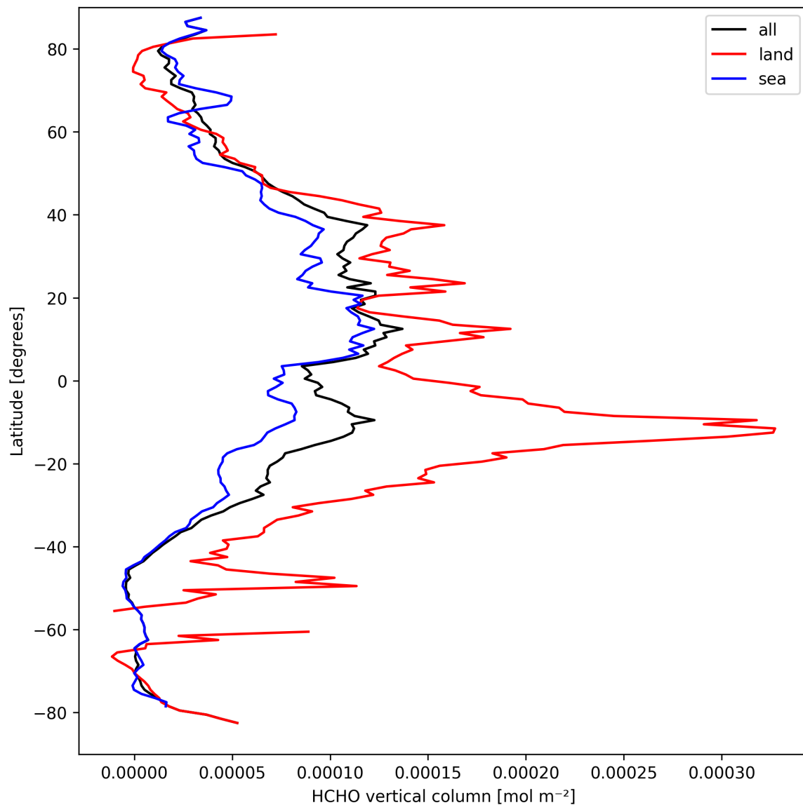
Figure 21: Zonal average of “HCHO vertical column” for 2025-09-15 to 2025-09-16.
