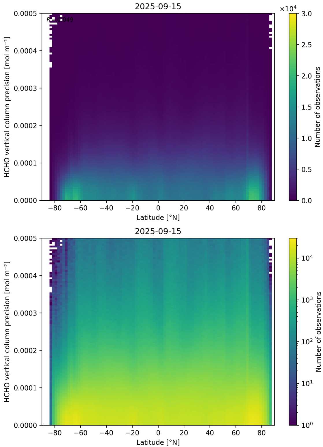
Figure 165: Scatter density plot of “Latitude” against “HCHO vertical column precision” for 2025-09-15 to 2025-09-16.
