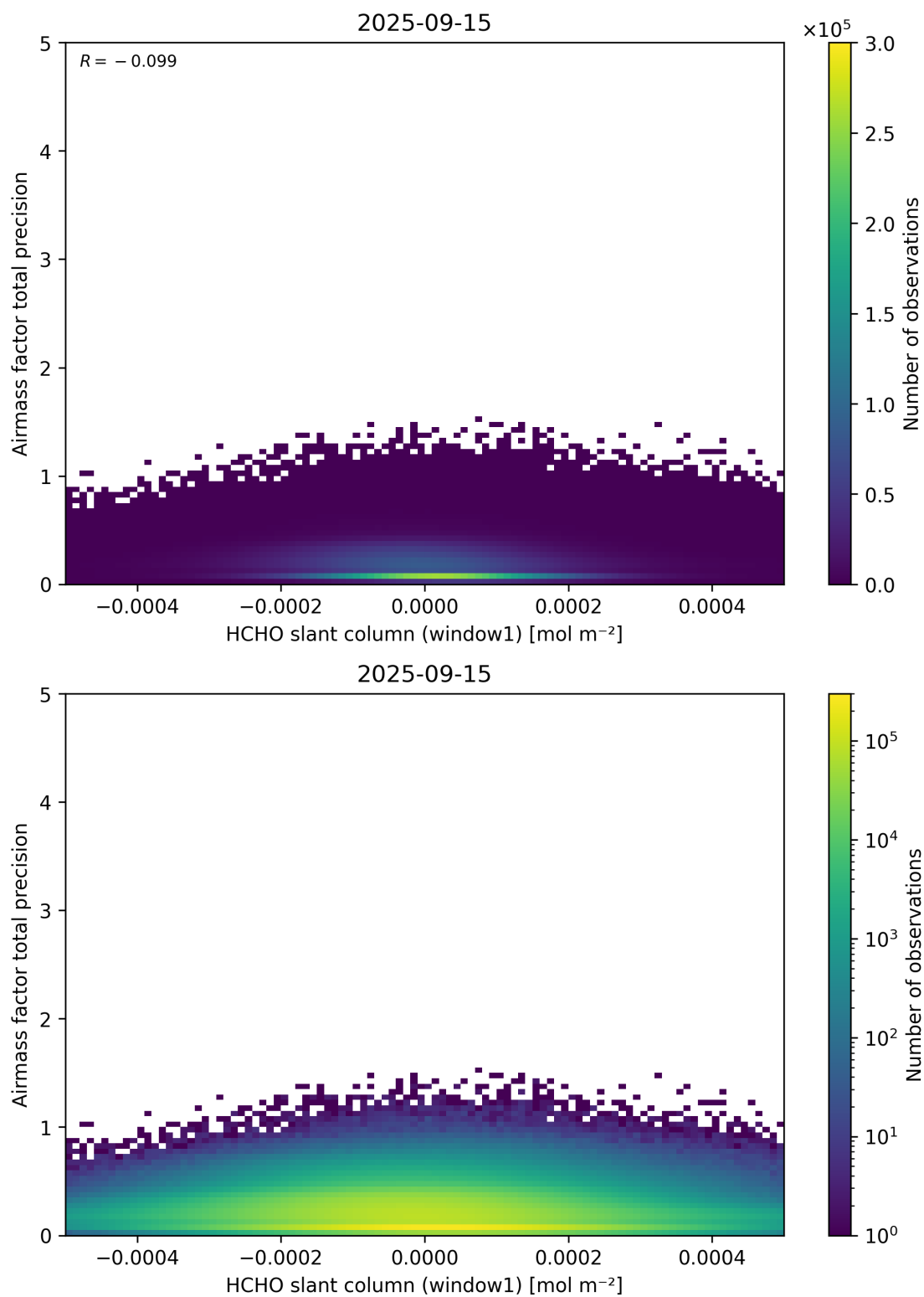
Figure 86: Scatter density plot of “HCHO slant column (window1)” against “Airmass factor total precision” for 2025-09-15 to 2025-09-16.
