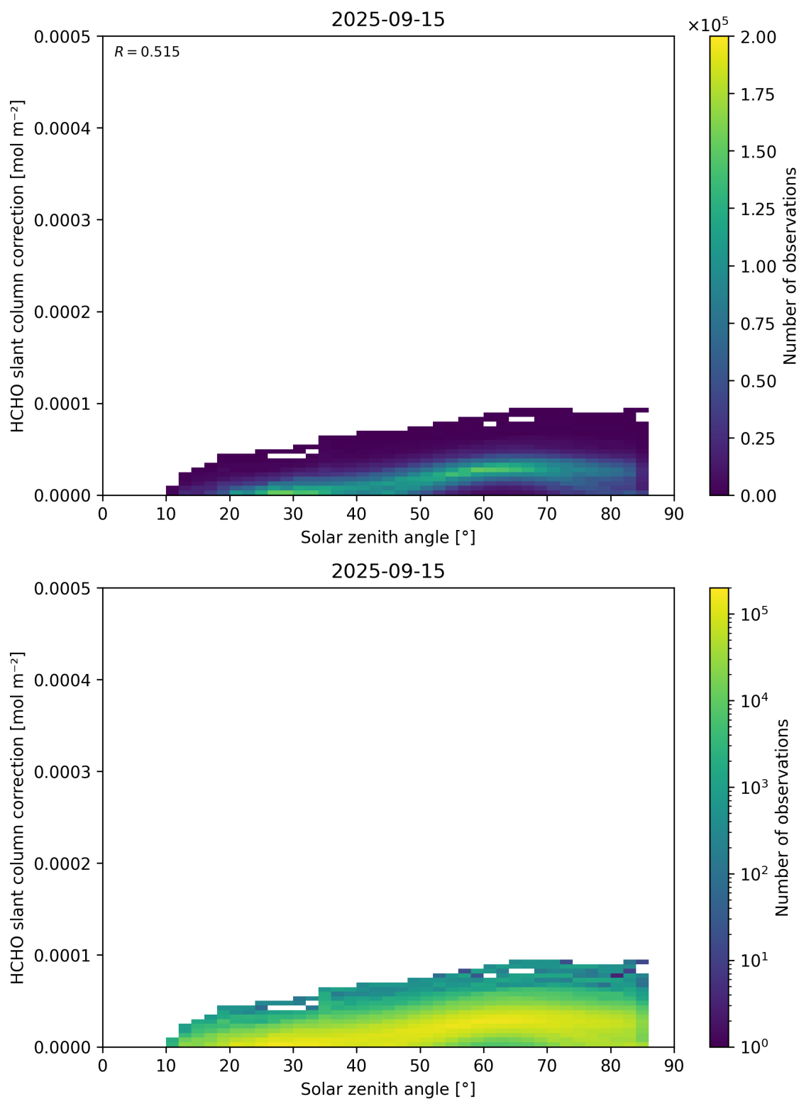
Figure 172: Scatter density plot of “Solar zenith angle” against “HCHO slant column correction” for 2025-09-15 to 2025-09-16.
