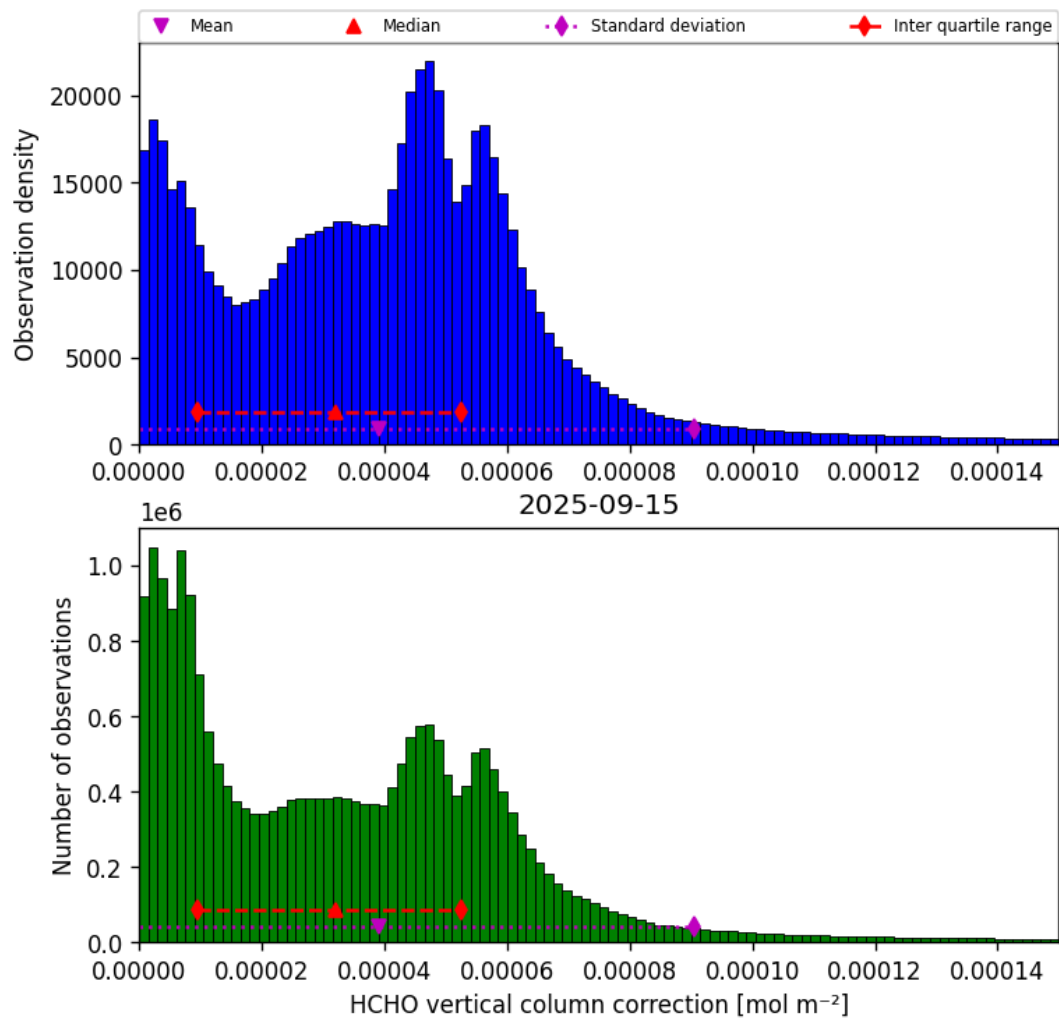
Figure 37: Histogram of “HCHO vertical column correction” for 2025-09-15 to 2025-09-16
