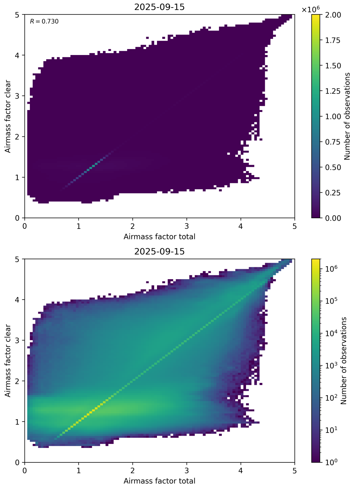
Figure 100: Scatter density plot of “Airmass factor total” against “Airmass factor clear” for 2025-09-15 to 2025-09-16.
