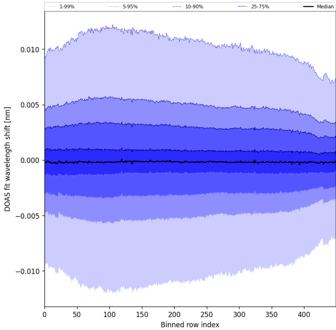
Figure 58: Along track statistics of “DOAS fit wavelength shift” for 2025-09-15 to 2025-09-16
