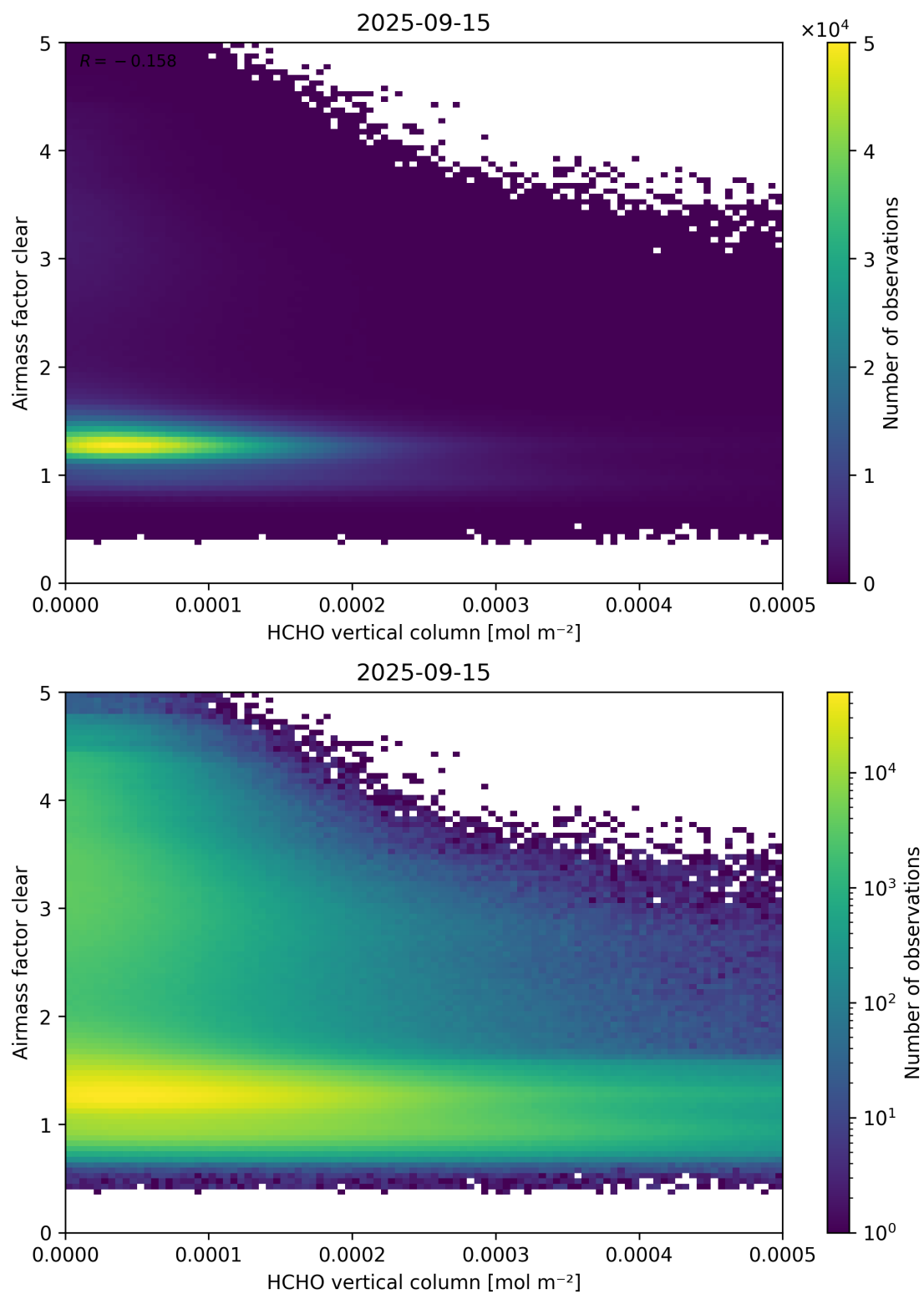
Figure 126: Scatter density plot of “HCHO vertical column” against “Airmass factor clear” for 2025-09-15 to 2025-09-16.
