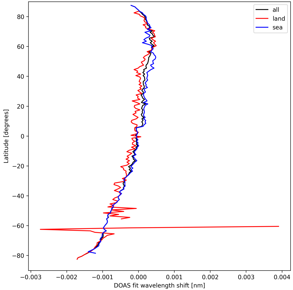
Figure 30: Zonal average of "DOAS fit wavelength shift" for 2025-09-15 to 2025-09-16.
