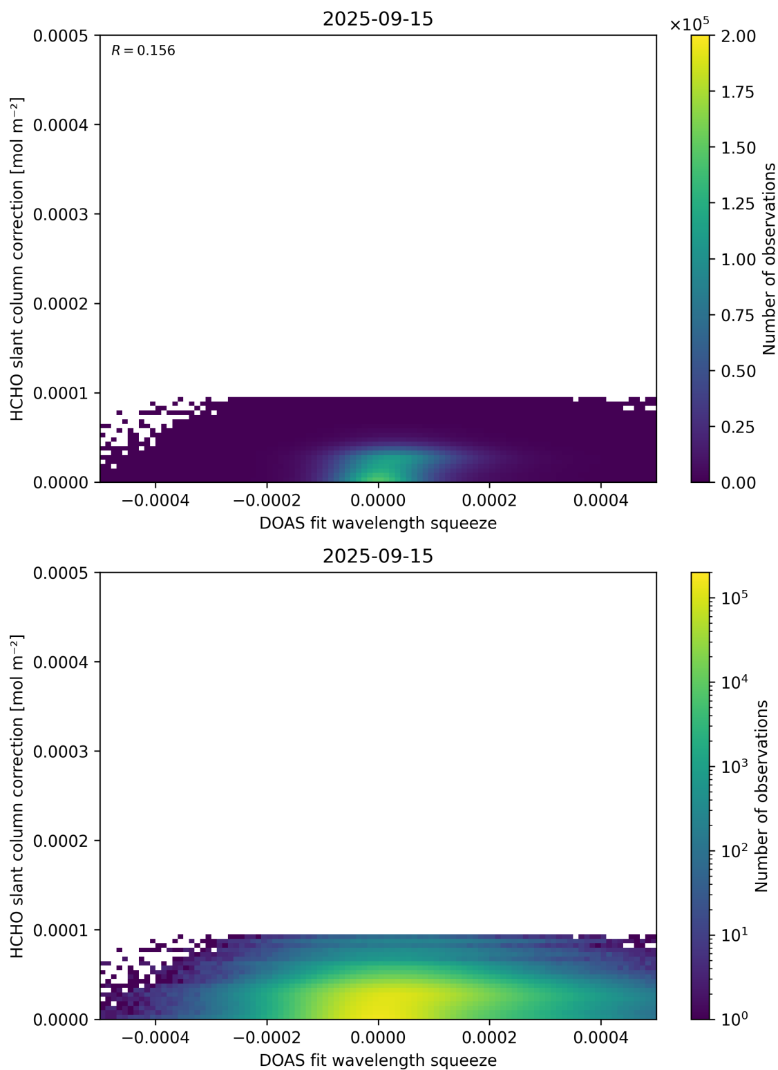
Figure 70: Scatter density plot of “DOAS fit wavelength squeeze” against “HCHO slant column correction” for 2025-09-15 to 2025-09-16.
