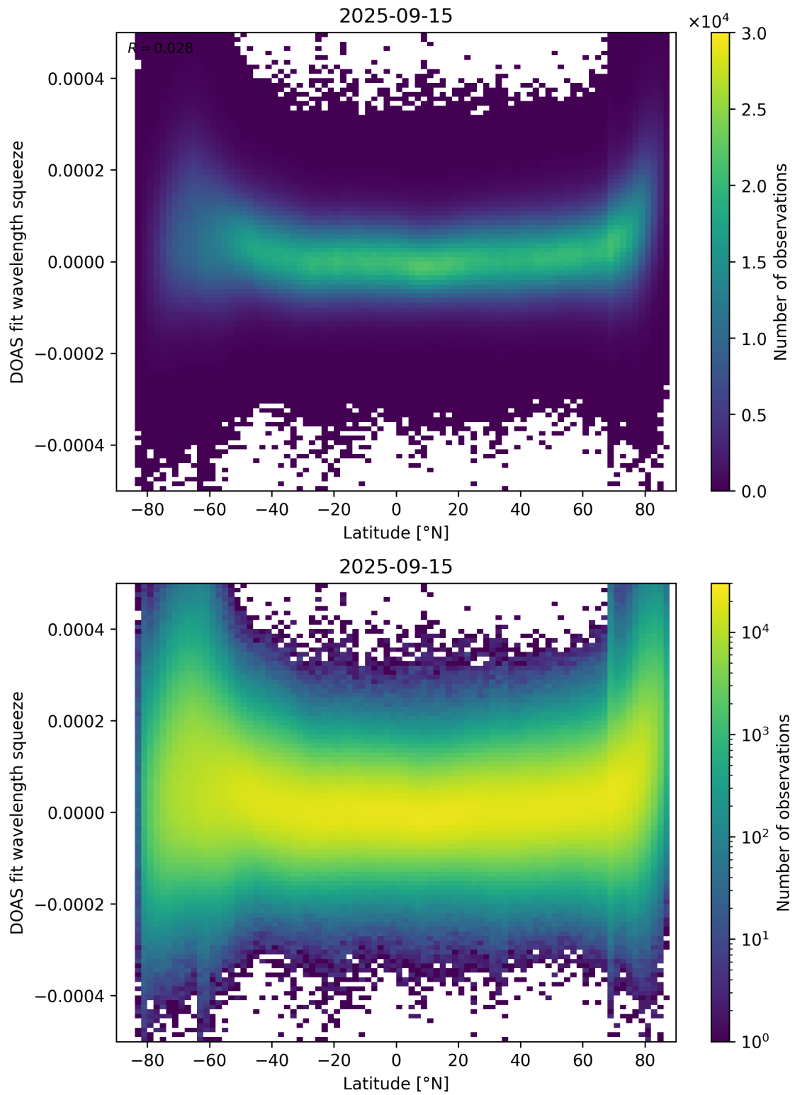
Figure 155: Scatter density plot of “Latitude” against “DOAS fit wavelength squeeze” for 2025-09-15 to 2025-09-16.
