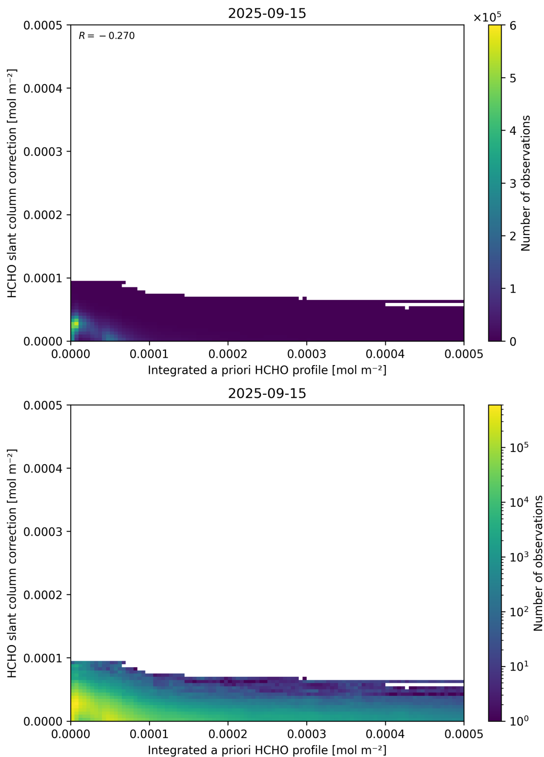
Figure 152: Scatter density plot of “Integrated a priori HCHO profile” against “HCHO slant column correction” for 2025-09-15 to 2025-09-16.
