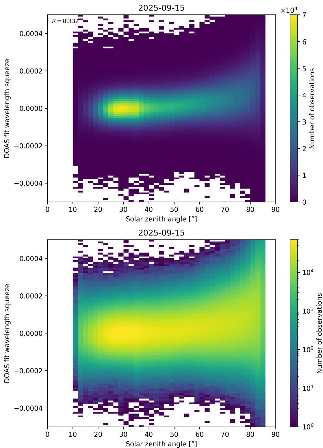
Figure 169: Scatter density plot of “Solar zenith angle” against “DOAS fit wavelength squeeze” for 2025-09-15 to 2025-09-16.
