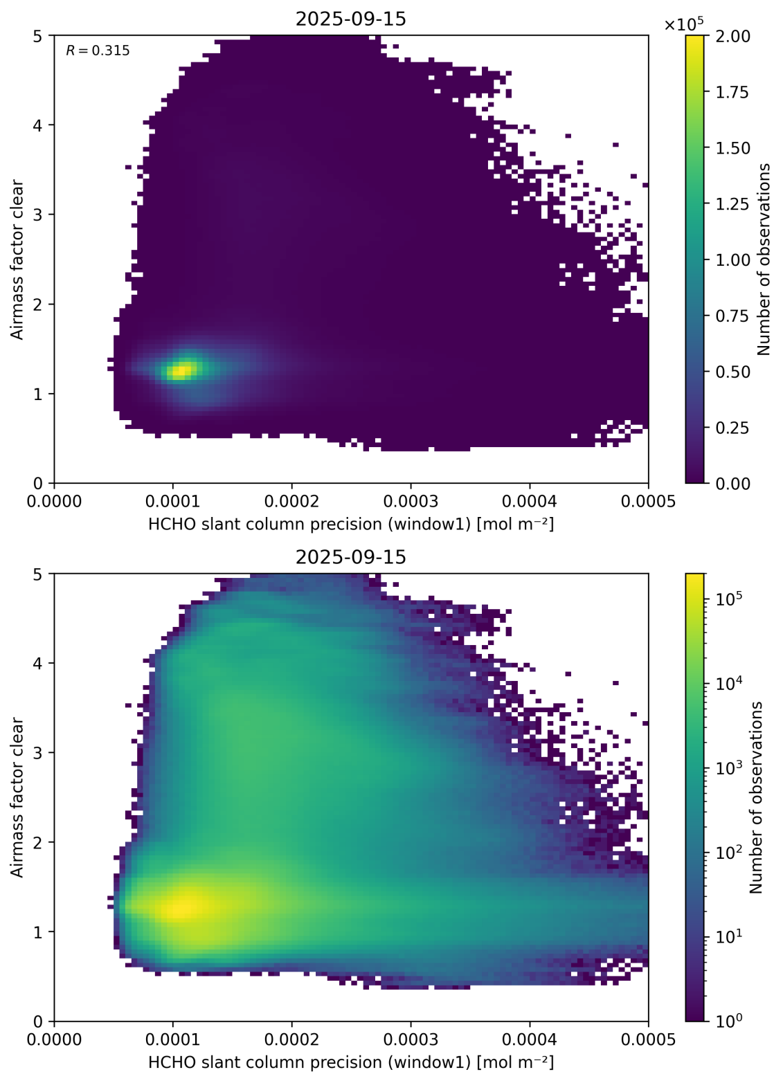
Figure 91: Scatter density plot of “HCHO slant column precision (window1)” against “Airmass factor clear” for 2025-09-15 to 2025-09-16.
