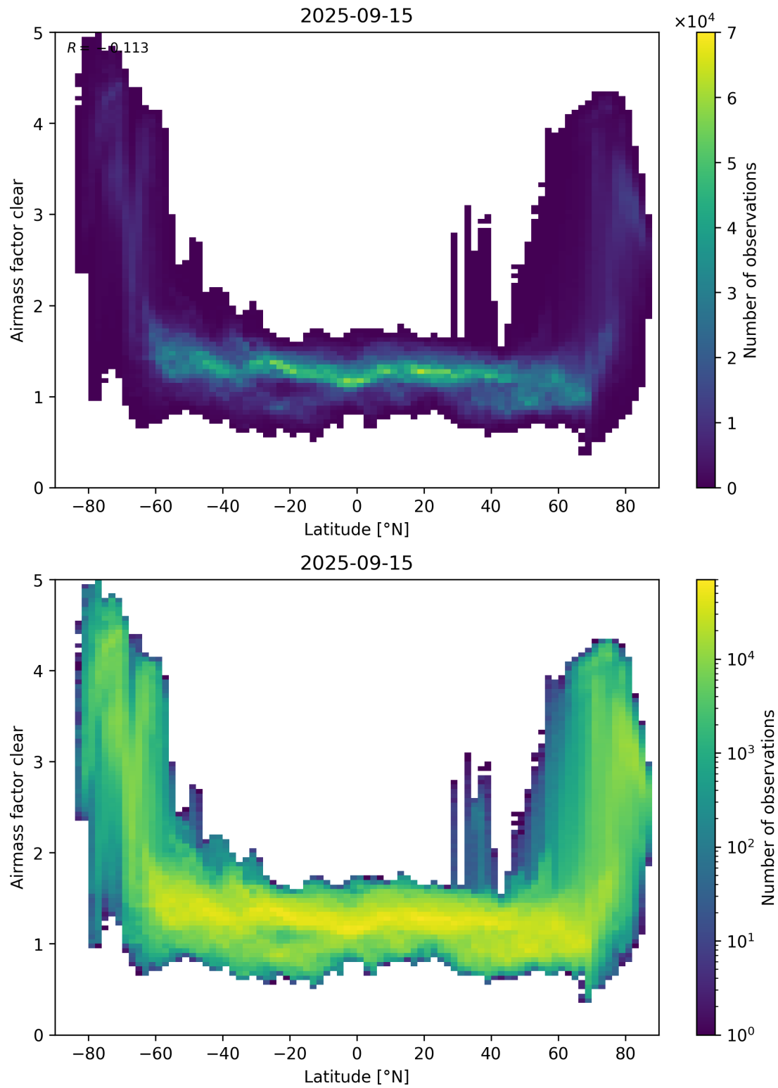
Figure 156: Scatter density plot of “Latitude” against “Airmass factor clear” for 2025-09-15 to 2025-09-16.
