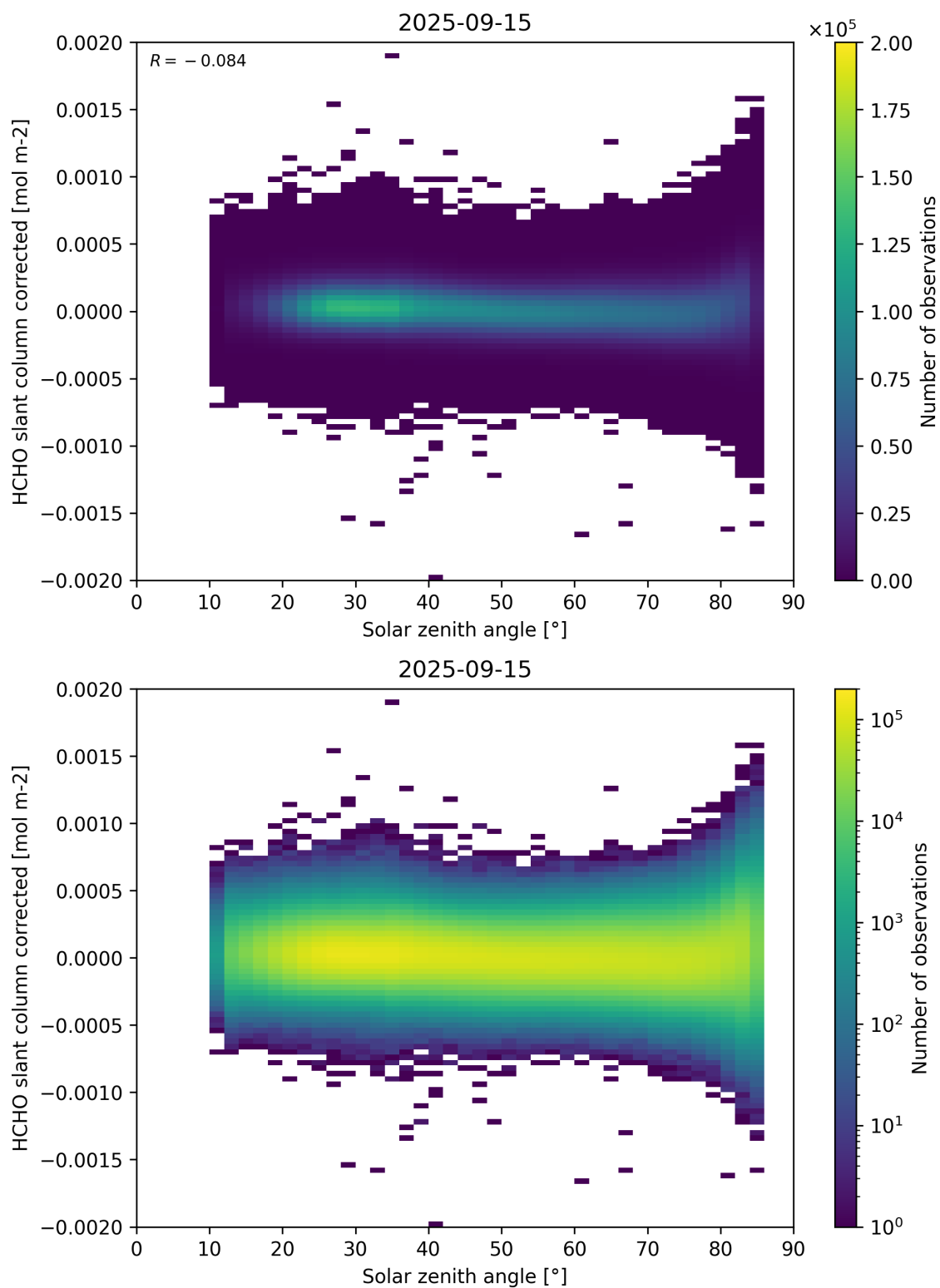
Figure 171: Scatter density plot of “Solar zenith angle” against “HCHO slant column corrected” for 2025-09-15 to 2025-09-16.
