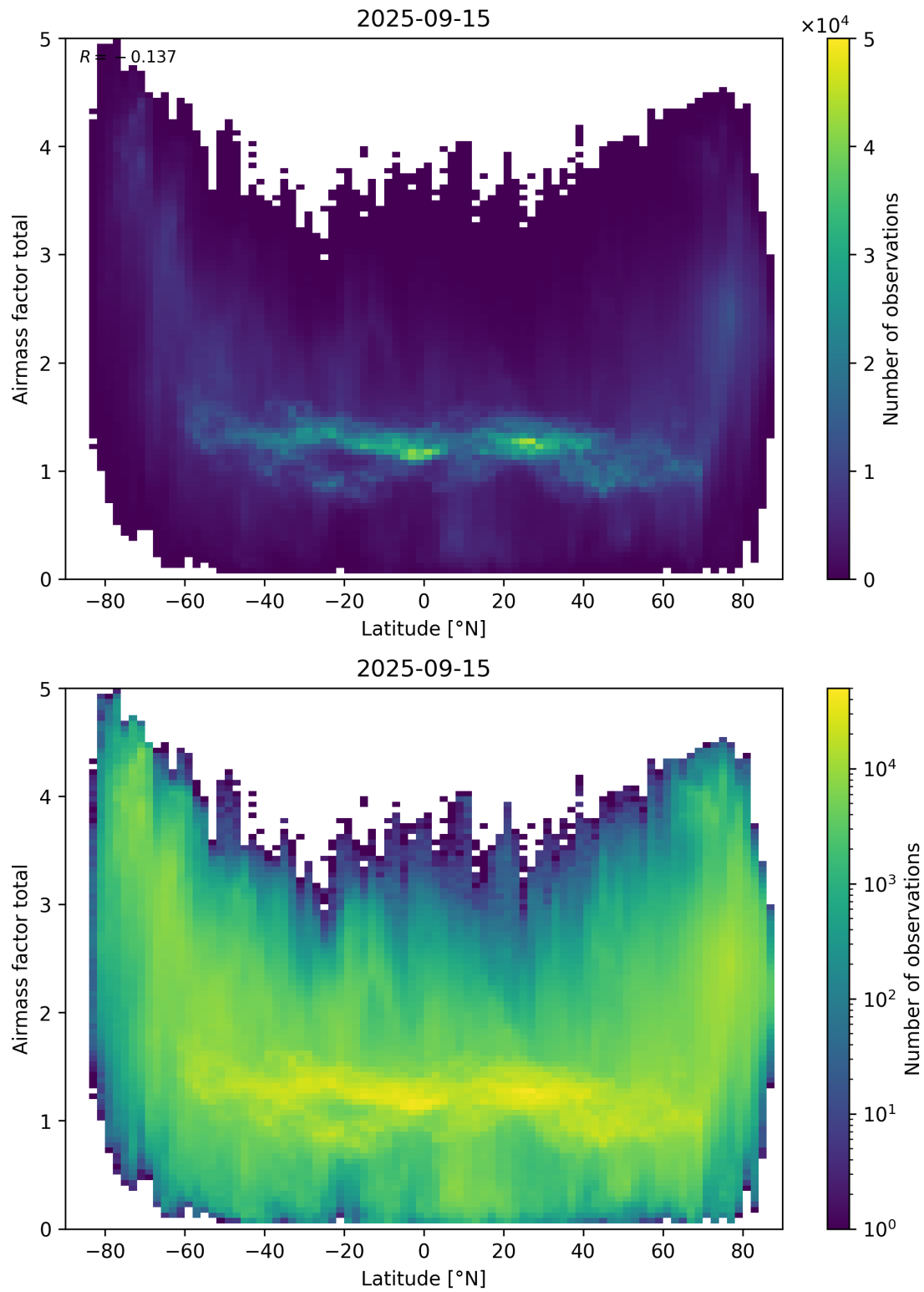
Figure 161: Scatter density plot of “Latitude” against “Airmass factor total” for 2025-09-15 to 2025-09-16.
