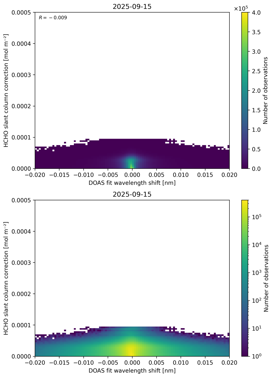
Figure 67: Scatter density plot of “DOAS fit wavelength shift” against “HCHO slant column correction” for 2025-09-15 to 2025-09-16.
