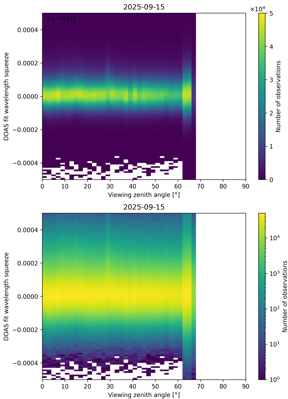
Figure 184: Scatter density plot of “Viewing zenith angle” against “DOAS fit wavelength squeeze” for 2025-09-15 to 2025-09-16.
