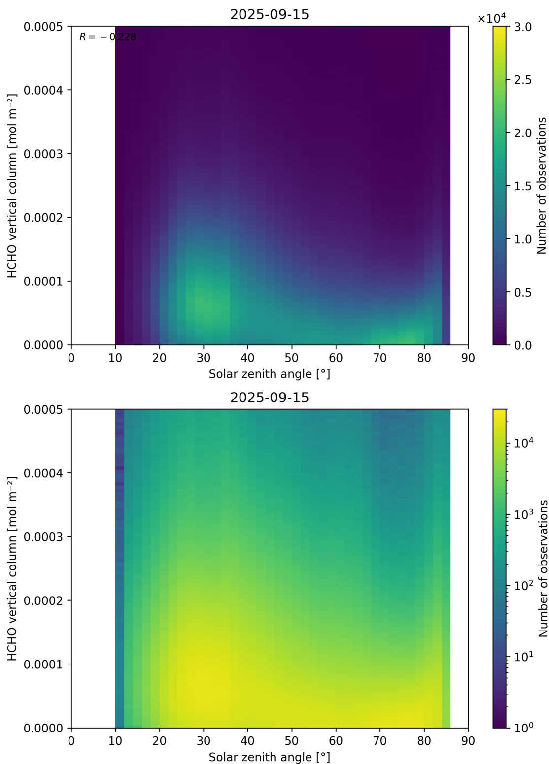
Figure 177: Scatter density plot of “Solar zenith angle” against “HCHO vertical column” for 2025-09-15 to 2025-09-16.
