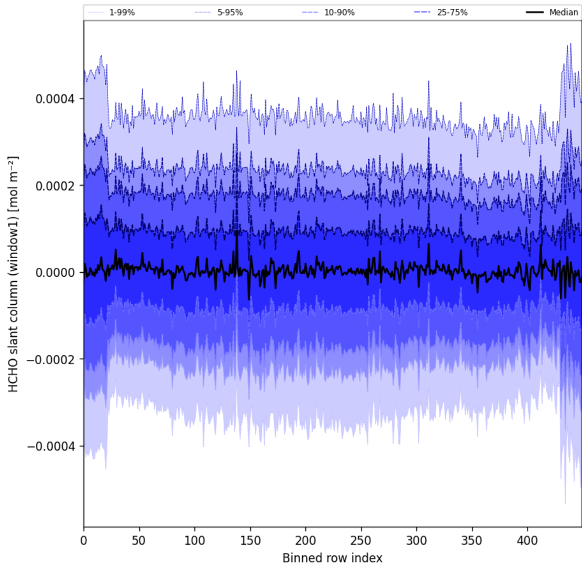
Figure 52: Along track statistics of “HCHO slant column (window1)” for 2025-09-15 to 2025-09-16
