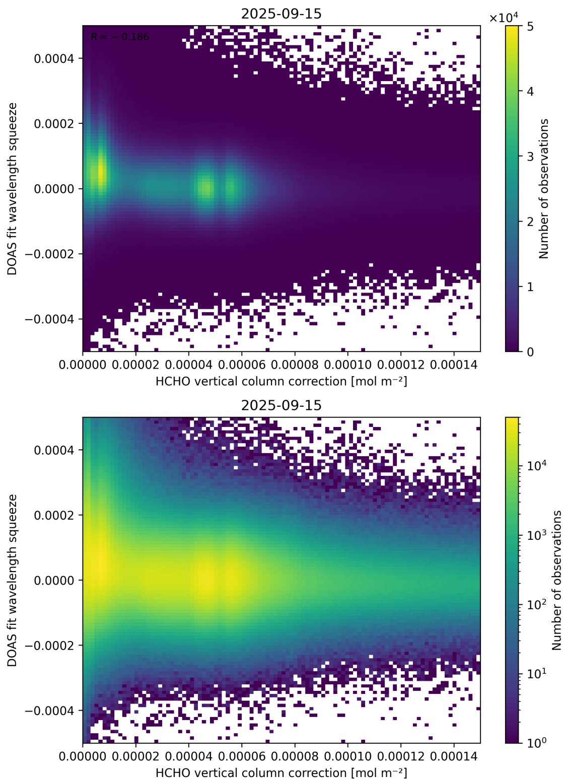
Figure 114: Scatter density plot of “HCHO vertical column correction” against “DOAS fit wavelength squeeze” for 2025-09-15 to 2025-09-16.
