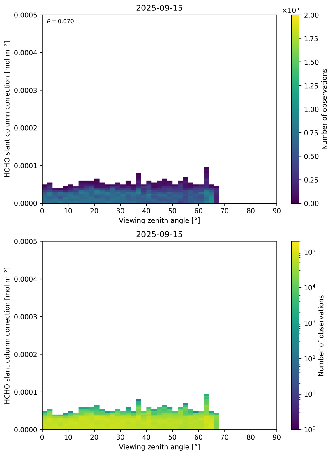
Figure 187: Scatter density plot of “Viewing zenith angle” against “HCHO slant column correction” for 2025-09-15 to 2025-09-16.
