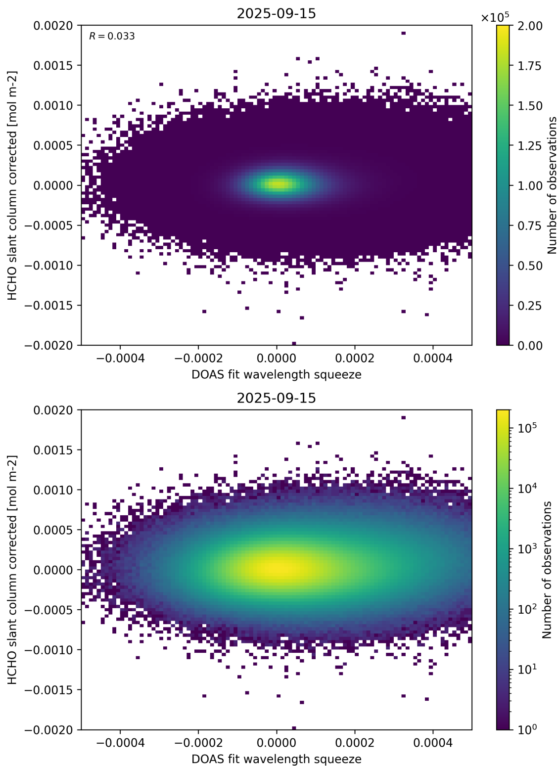
Figure 69: Scatter density plot of “DOAS fit wavelength squeeze” against “HCHO slant column corrected” for 2025-09-15 to 2025-09-16.
