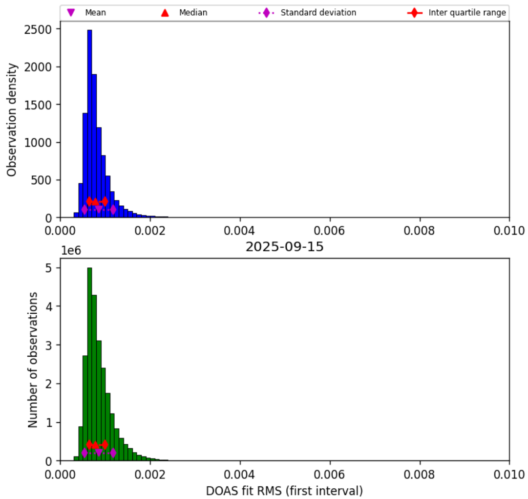
Figure 46: Histogram of “DOAS fit RMS (first interval)” for 2025-09-15 to 2025-09-16
