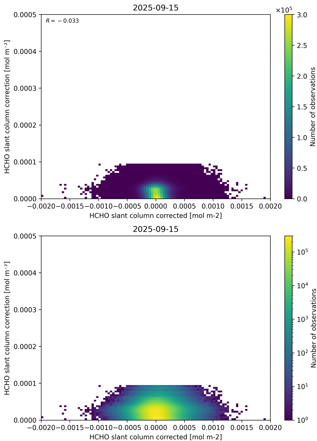
Figure 77: Scatter density plot of “HCHO slant column corrected” against “HCHO slant column correction” for 2025-09-15 to 2025-09-16.
