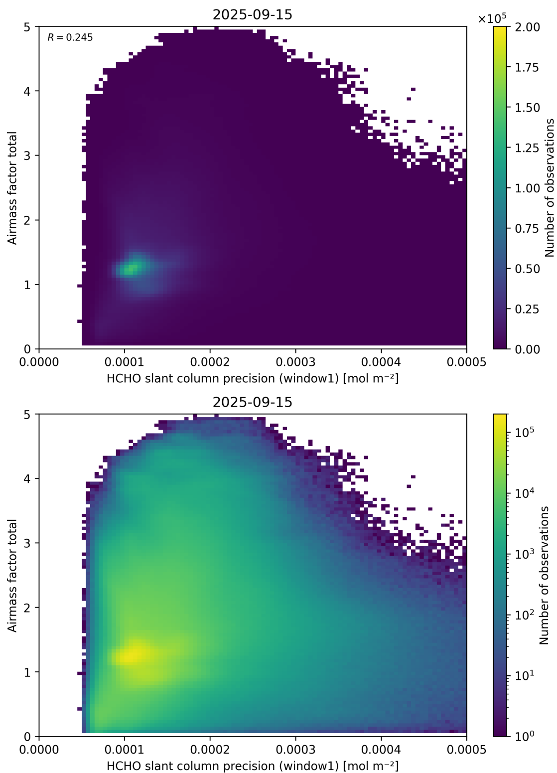
Figure 94: Scatter density plot of “HCHO slant column precision (window1)” against “Airmass factor total” for 2025-09-15 to 2025-09-16.
