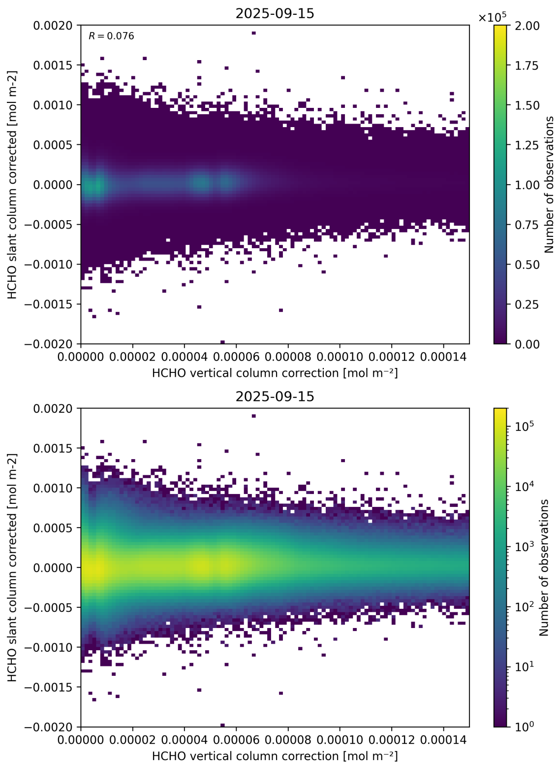
Figure 116: Scatter density plot of “HCHO vertical column correction” against “HCHO slant column corrected” for 2025-09-15 to 2025-09-16.
