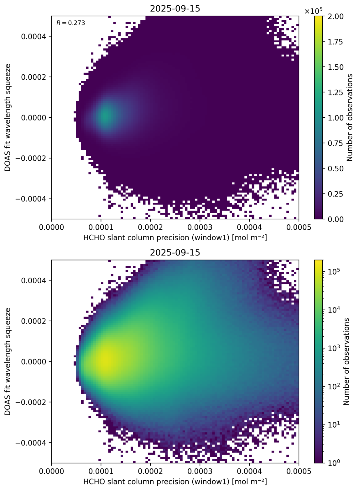
Figure 90: Scatter density plot of “HCHO slant column precision (window1)” against “DOAS fit wavelength squeeze” for 2025-09-15 to 2025-09-16.
