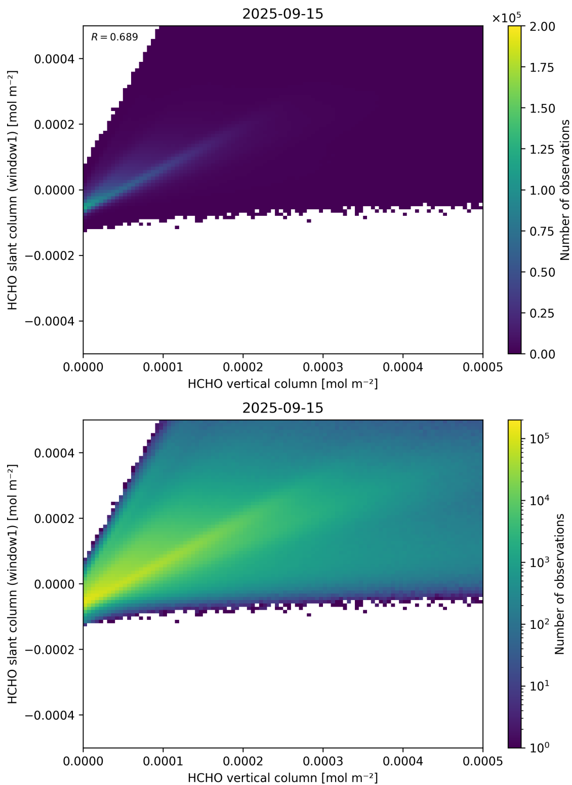
Figure 129: Scatter density plot of “HCHO vertical column” against “HCHO slant column (window1)” for 2025-09-15 to 2025-09-16.
