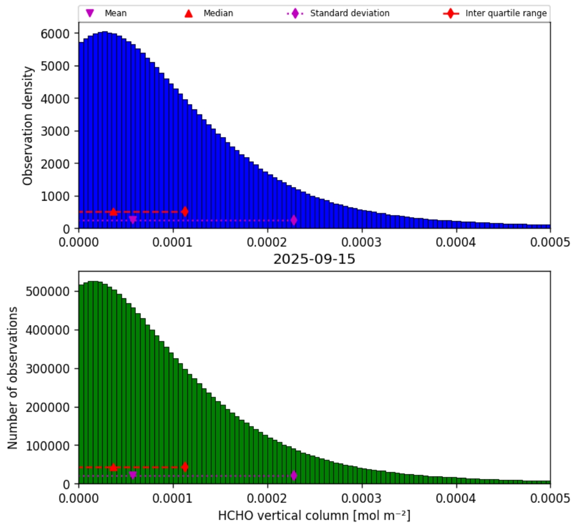
Figure 35: Histogram of “HCHO vertical column” for 2025-09-15 to 2025-09-16
