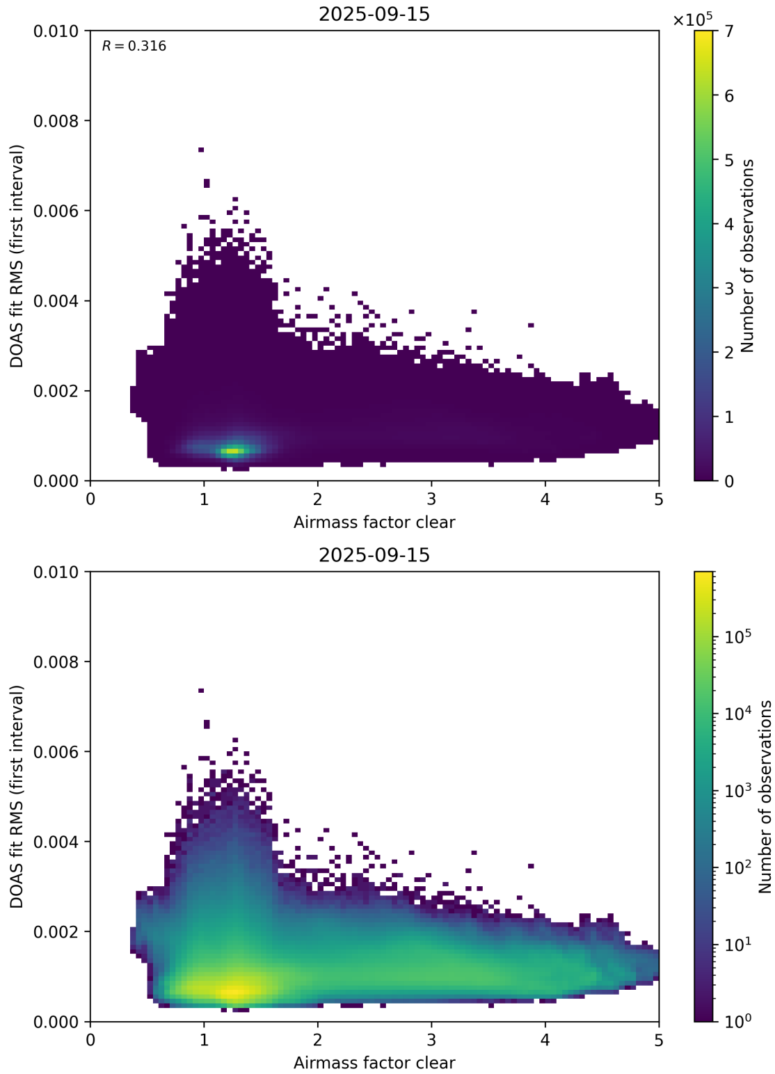
Figure 71: Scatter density plot of “Airmass factor clear” against “DOAS fit RMS (first interval)” for 2025-09-15 to 2025-09-16.
