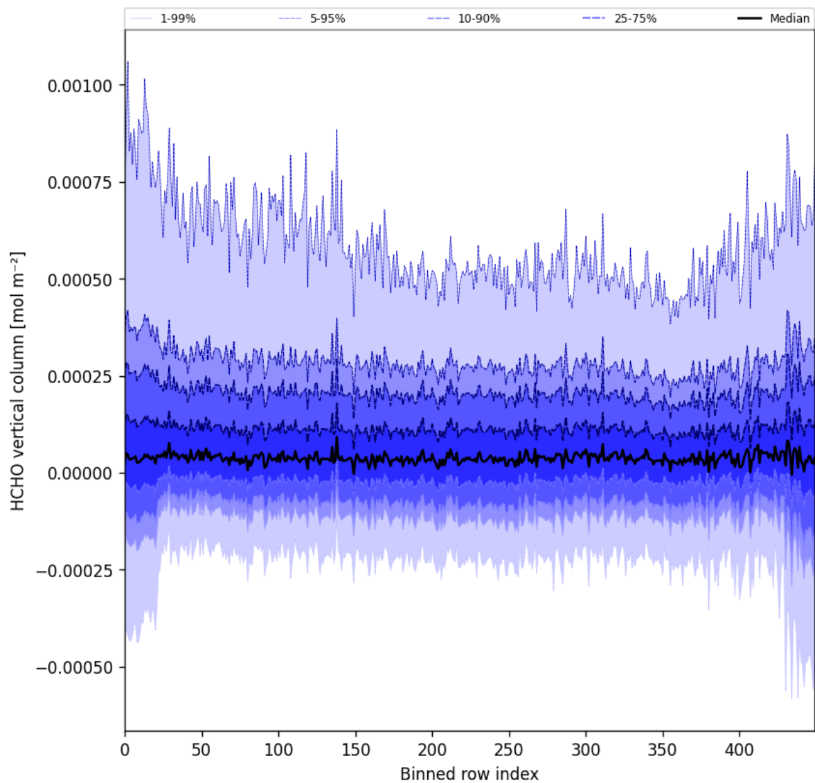
Figure 49: Along track statistics of “HCHO vertical column” for 2025-09-15 to 2025-09-16
