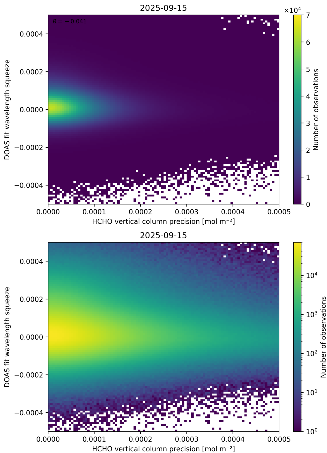
Figure 138: Scatter density plot of “HCHO vertical column precision” against “DOAS fit wavelength squeeze” for 2025-09-15 to 2025-09-16.
