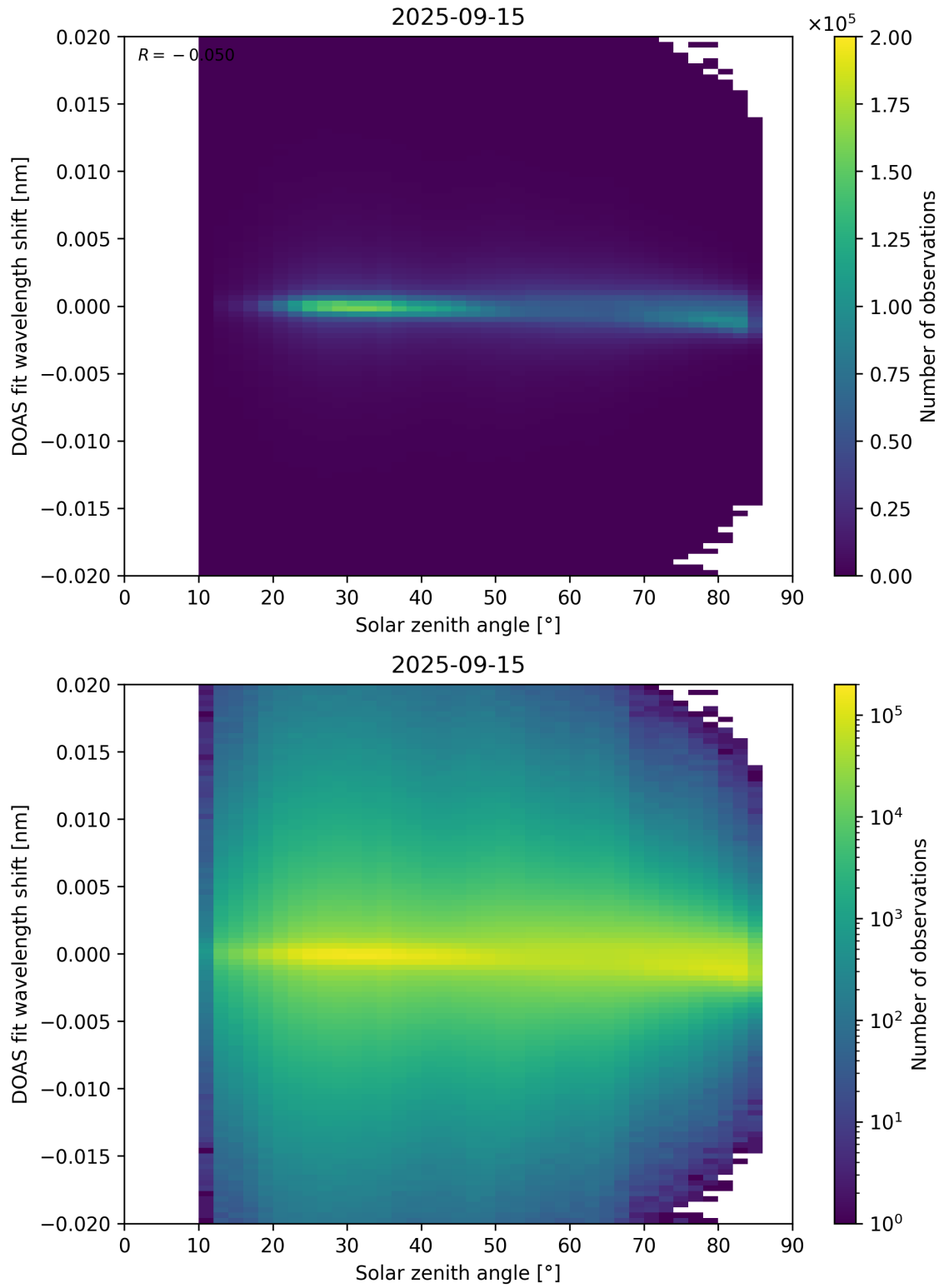
Figure 168: Scatter density plot of “Solar zenith angle” against “DOAS fit wavelength shift” for 2025-09-15 to 2025-09-16.
