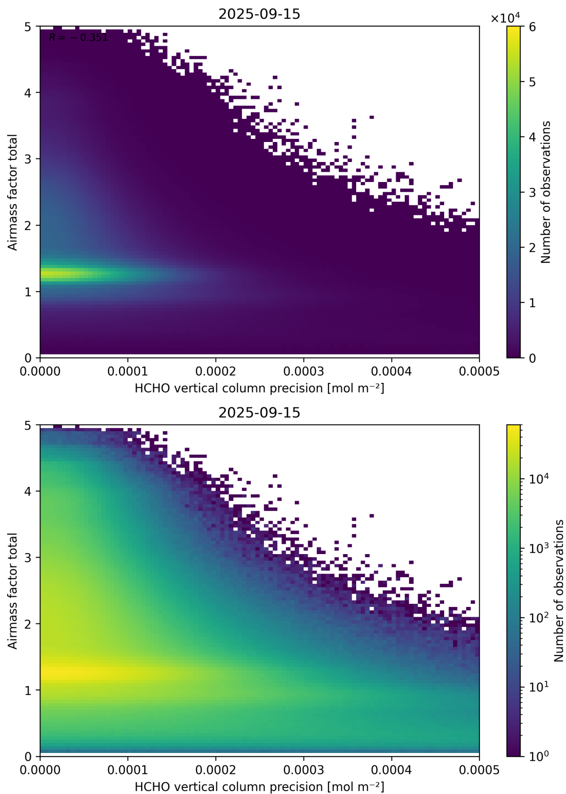
Figure 144: Scatter density plot of “HCHO vertical column precision” against “Airmass factor total” for 2025-09-15 to 2025-09-16.
