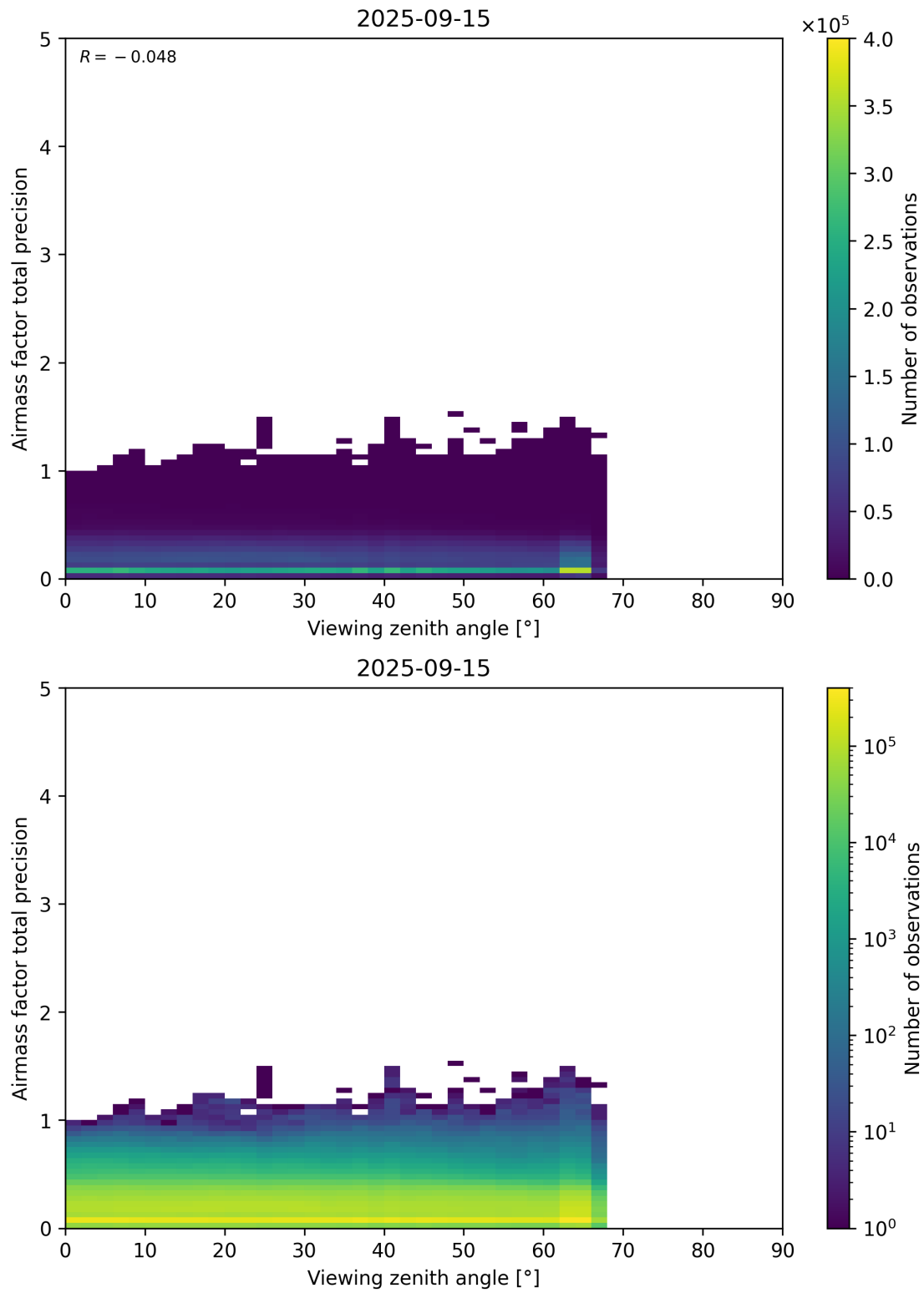
Figure 191: Scatter density plot of “Viewing zenith angle” against “Airmass factor total precision” for 2025-09-15 to 2025-09-16.
