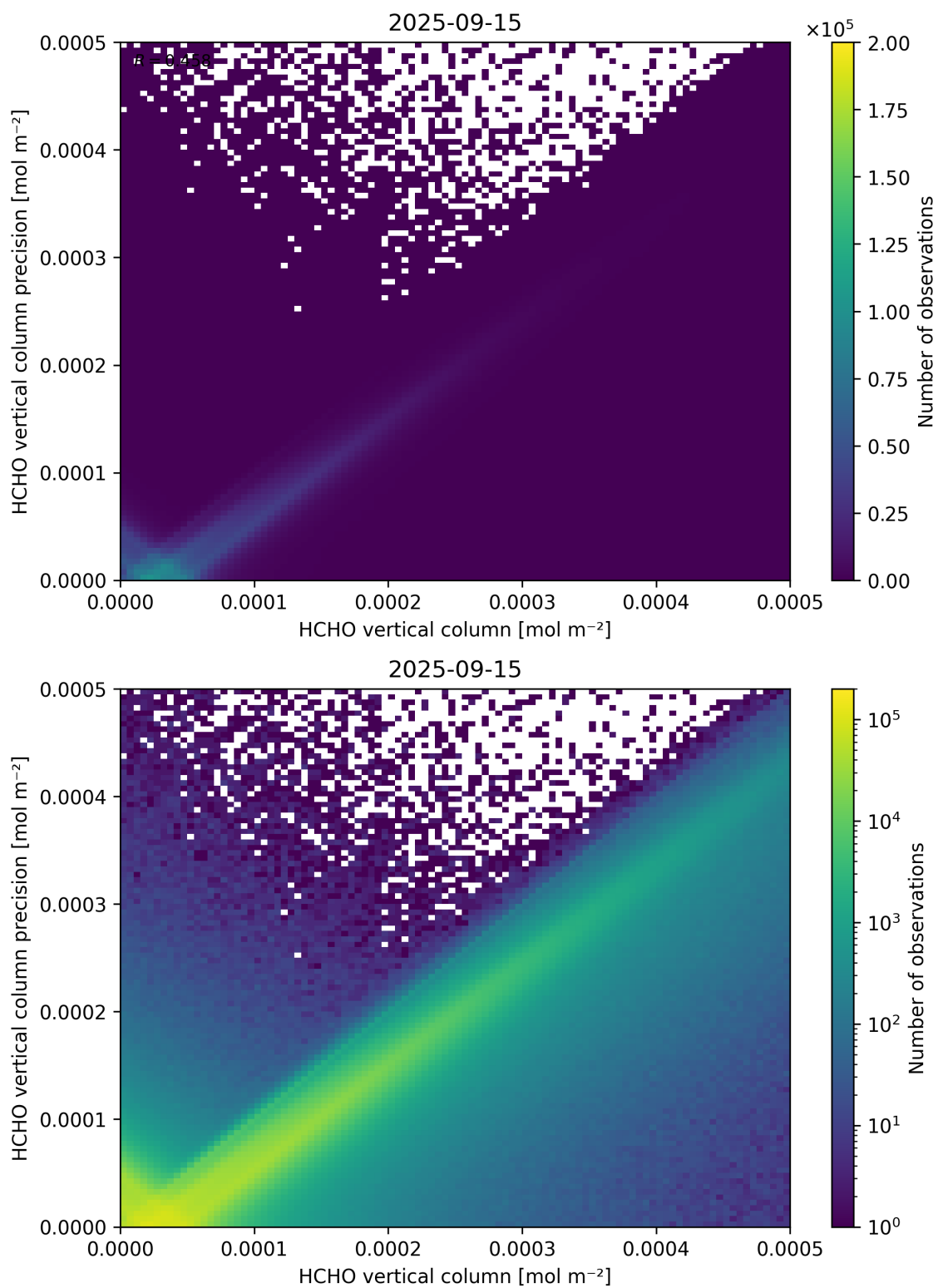
Figure 134: Scatter density plot of “HCHO vertical column” against “HCHO vertical column precision” for 2025-09-15 to 2025-09-16.
