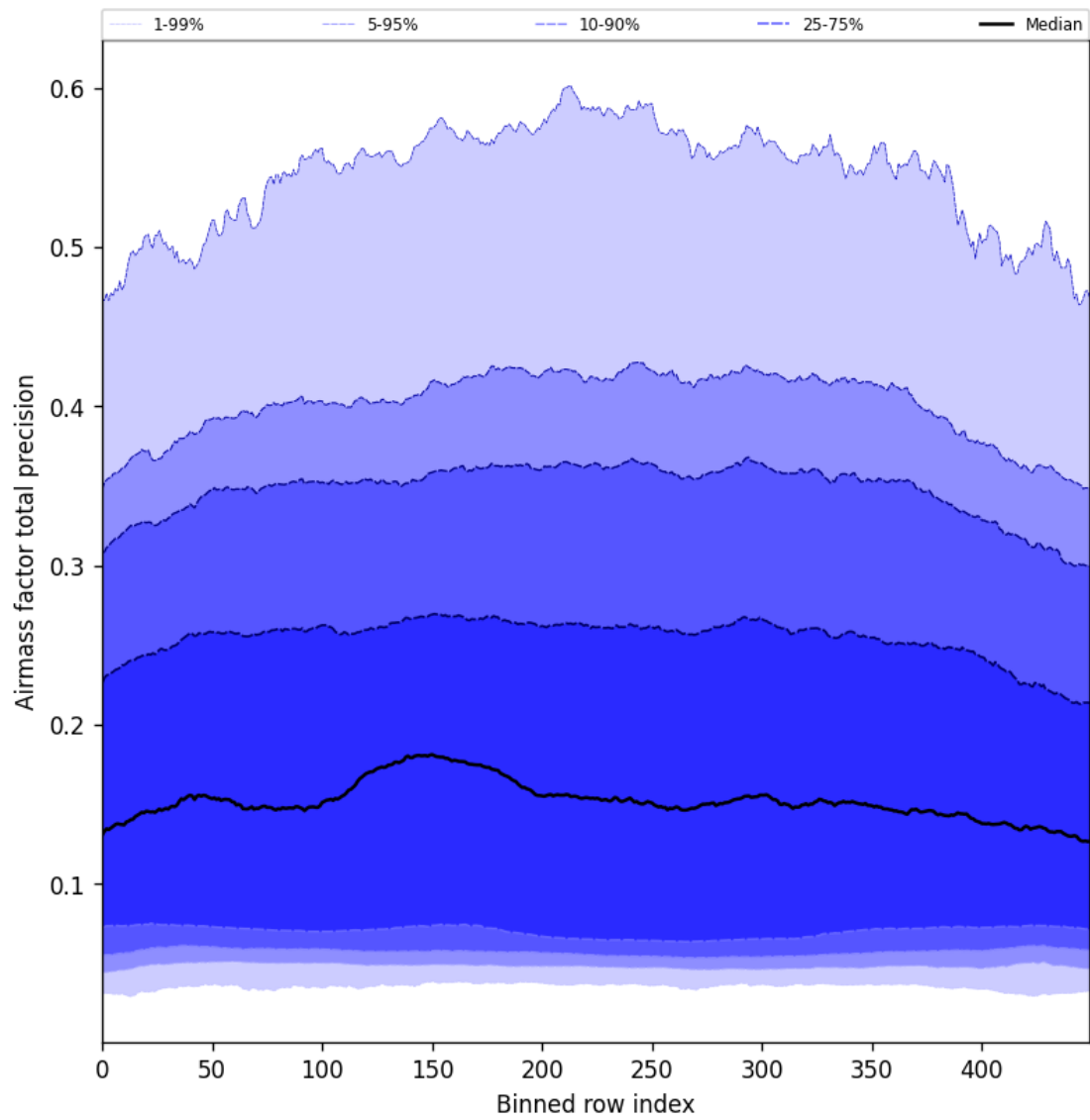
Figure 55: Along track statistics of “Airmass factor total precision” for 2025-09-15 to 2025-09-16
