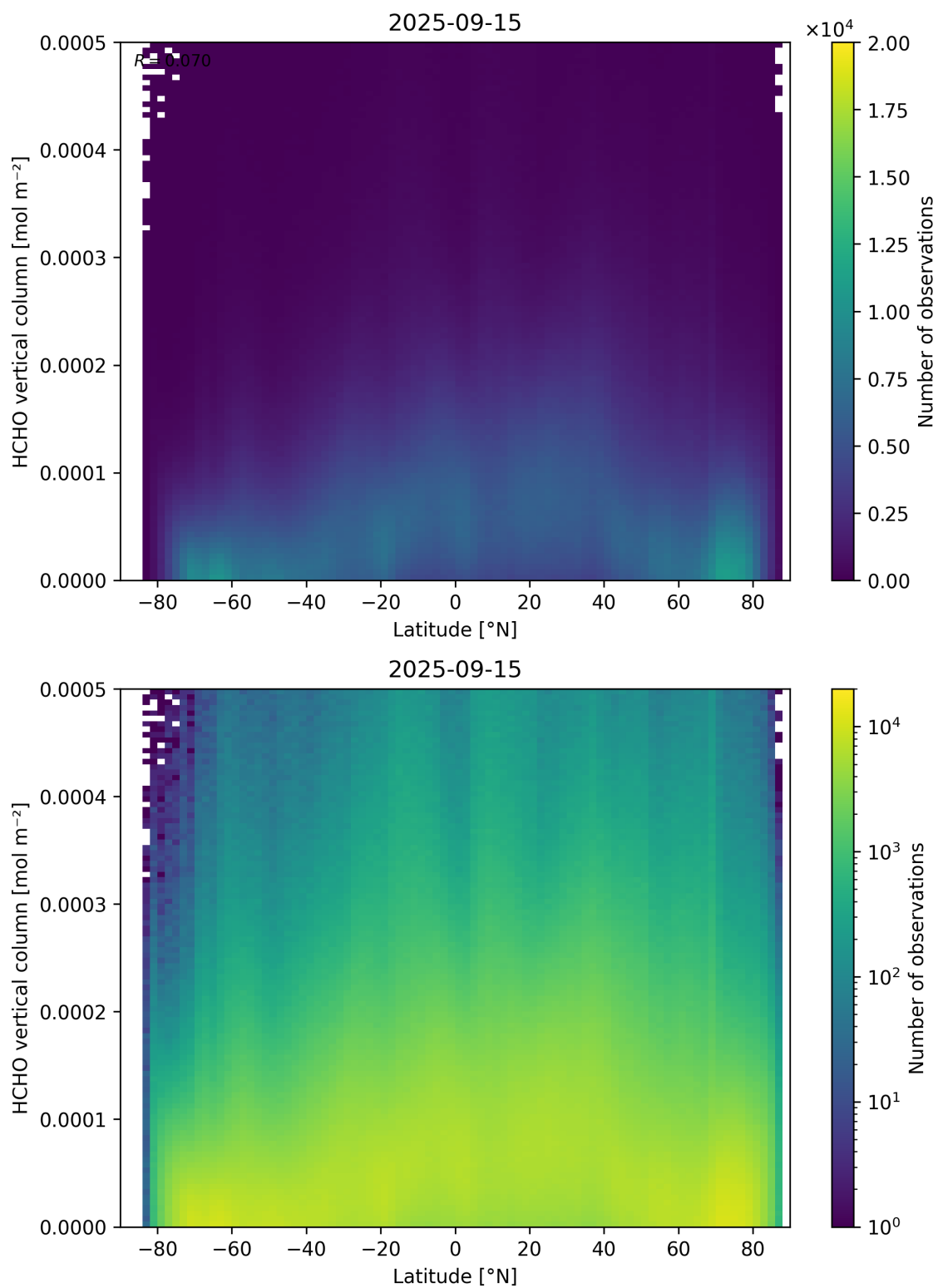
Figure 163: Scatter density plot of “Latitude” against “HCHO vertical column” for 2025-09-15 to 2025-09-16.
