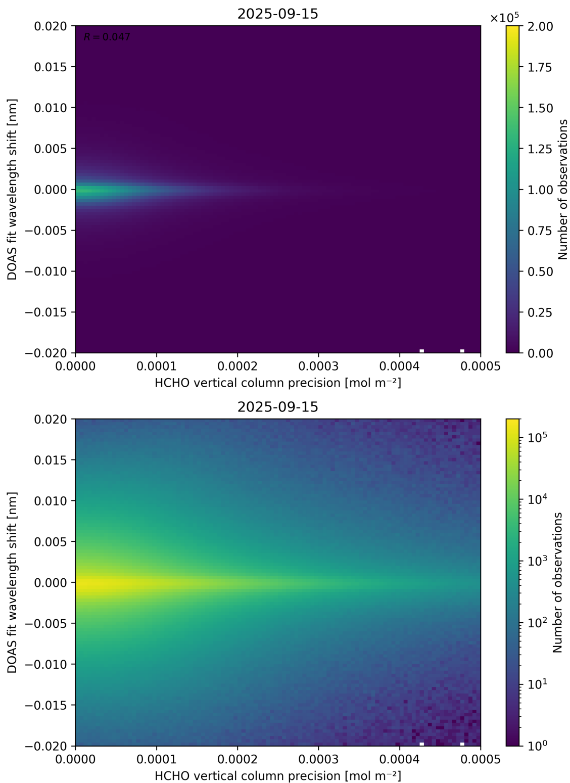
Figure 137: Scatter density plot of “HCHO vertical column precision” against “DOAS fit wavelength shift” for 2025-09-15 to 2025-09-16.
