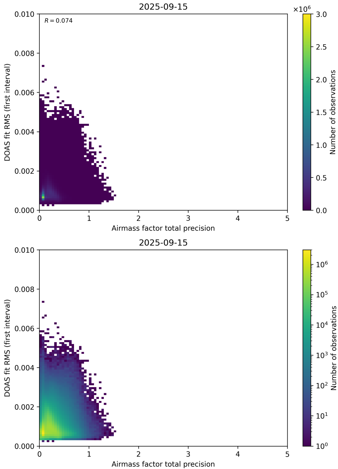
Figure 105: Scatter density plot of “Airmass factor total precision” against “DOAS fit RMS (first interval)” for 2025-09-15 to 2025-09-16.
