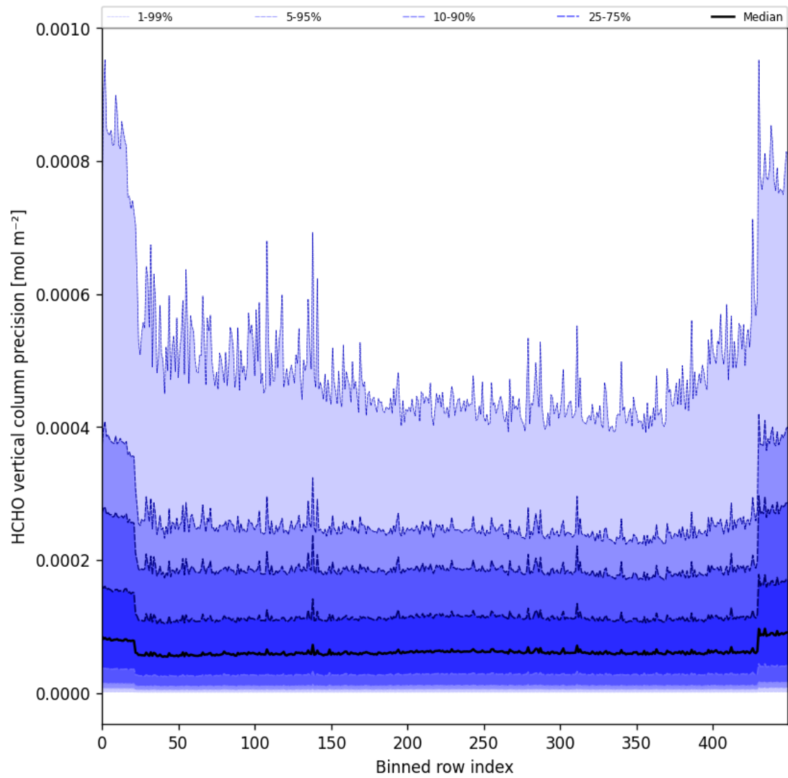
Figure 50: Along track statistics of “HCHO vertical column precision” for 2025-09-15 to 2025-09-16
