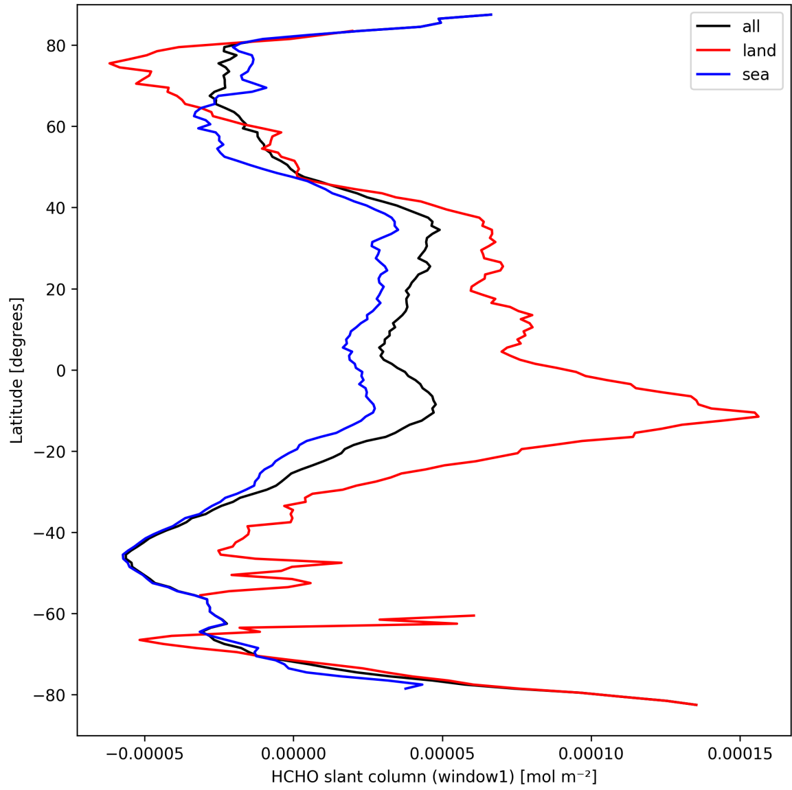
Figure 24: Zonal average of “HCHO slant column (window1)” for 2025-09-15 to 2025-09-16.
