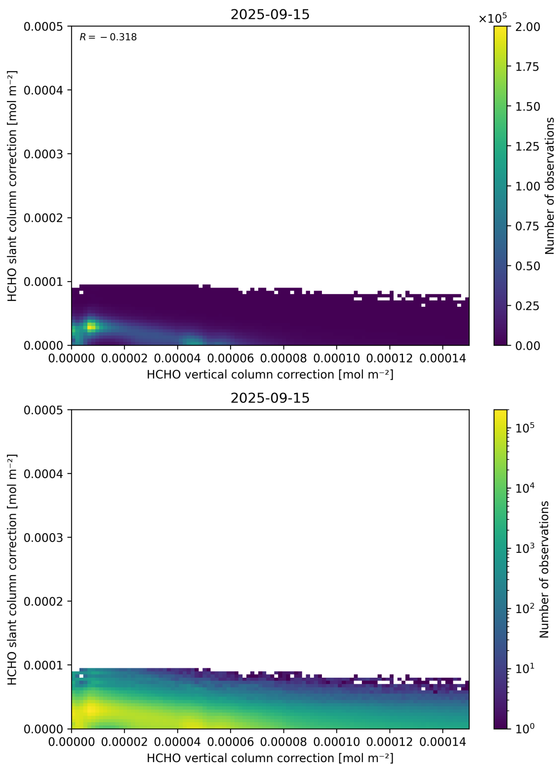
Figure 117: Scatter density plot of “HCHO vertical column correction” against “HCHO slant column correction” for 2025-09-15 to 2025-09-16.
