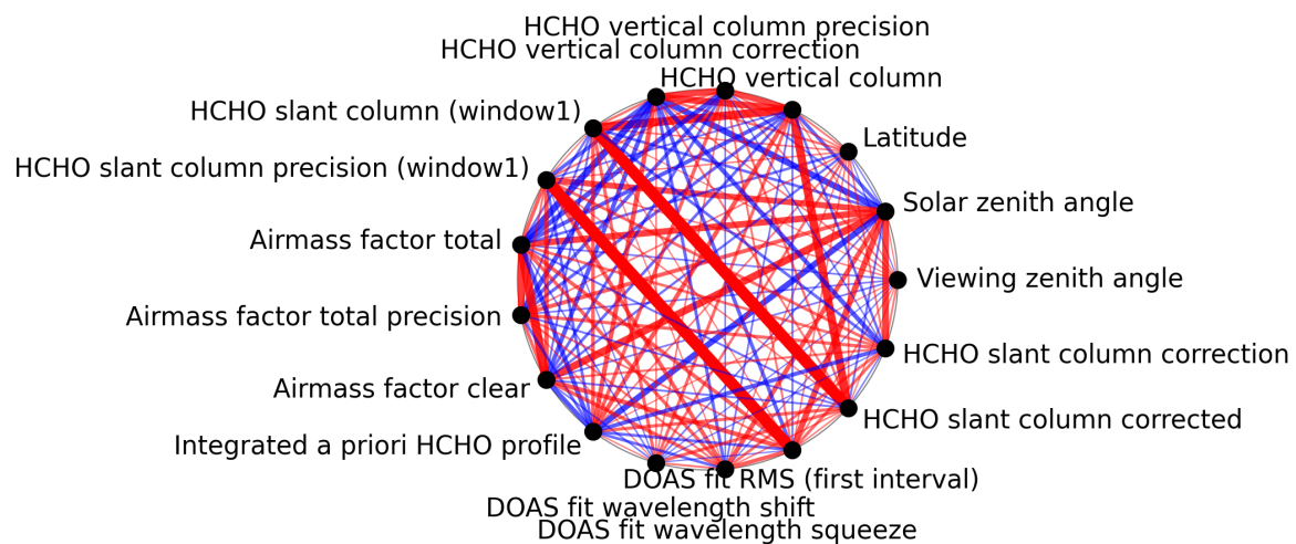
Figure 1: Map of correlation graph for 2025-09-15 to 2025-09-16.
