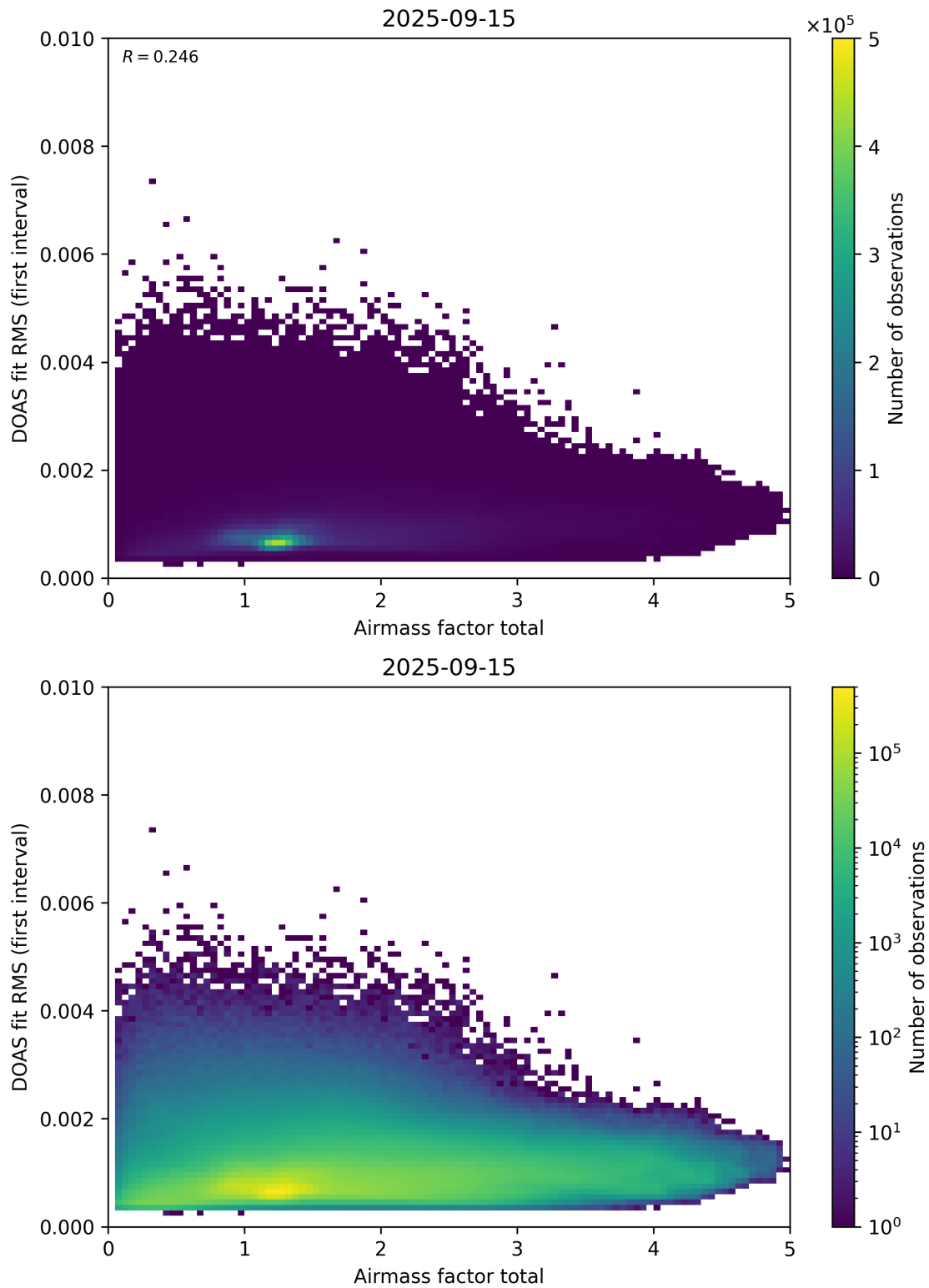
Figure 97: Scatter density plot of “Airmass factor total” against “DOAS fit RMS (first interval)” for 2025-09-15 to 2025-09-16.
