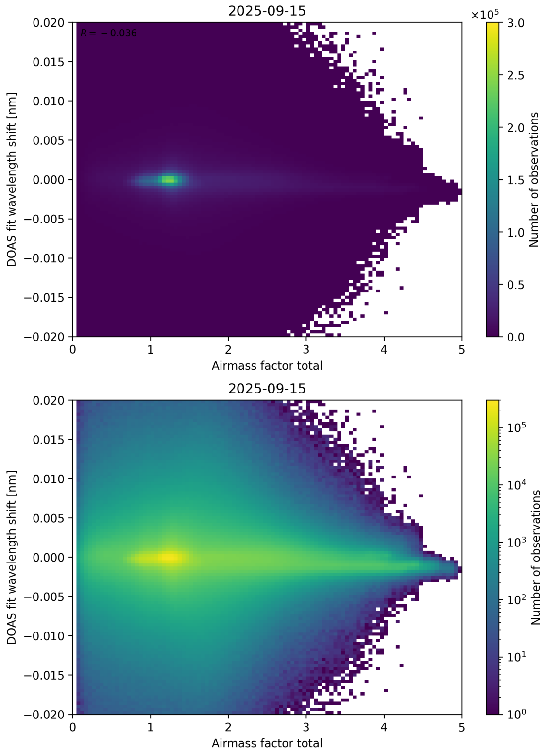
Figure 98: Scatter density plot of “Airmass factor total” against “DOAS fit wavelength shift” for 2025-09-15 to 2025-09-16.
