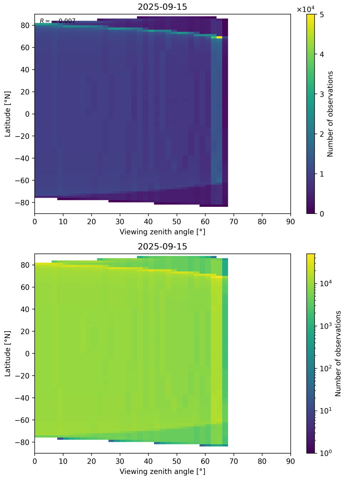
Figure 196: Scatter density plot of “Viewing zenith angle” against “Latitude” for 2025-09-15 to 2025-09-16.
