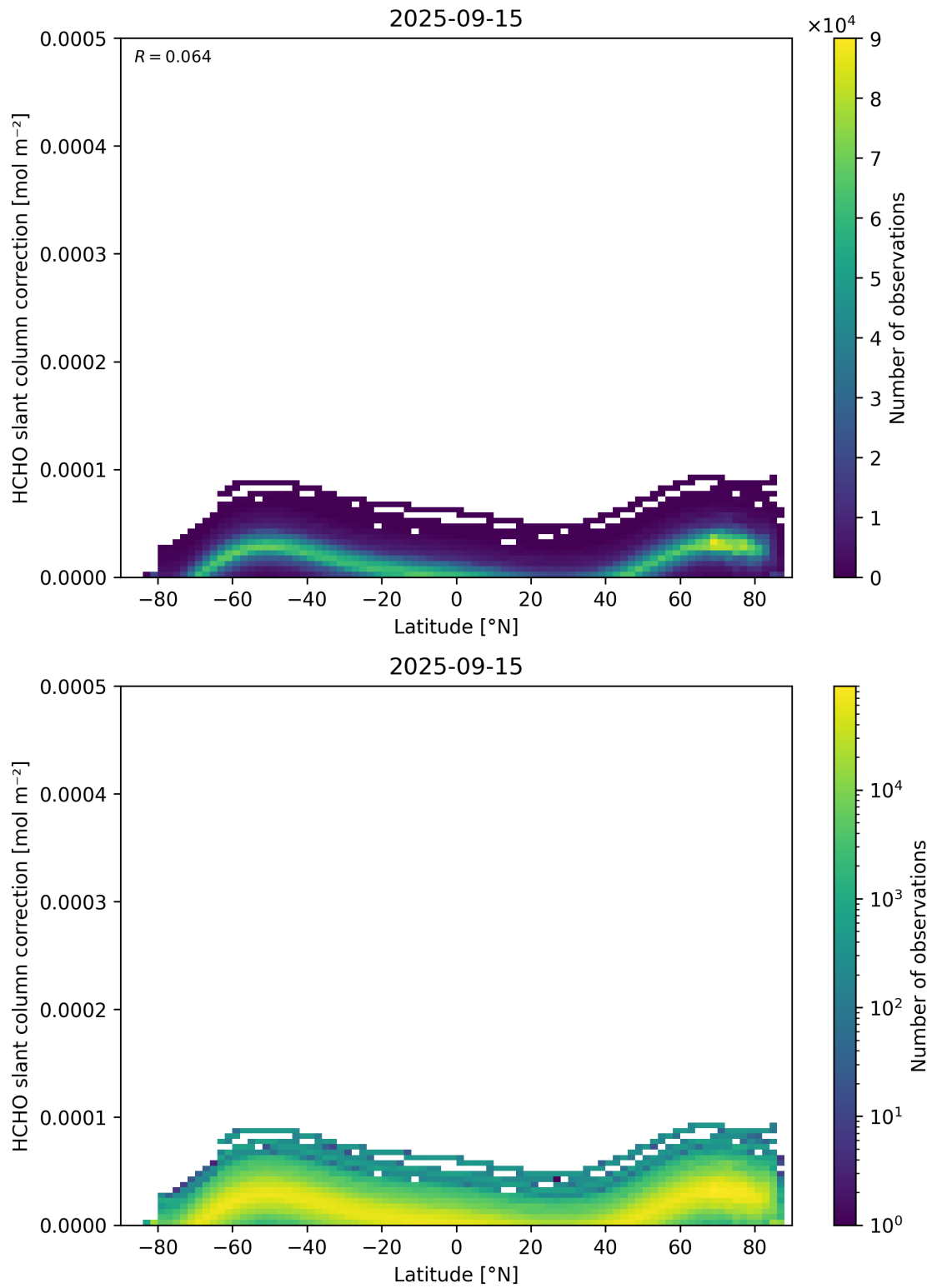
Figure 158: Scatter density plot of “Latitude” against “HCHO slant column correction” for 2025-09-15 to 2025-09-16.
