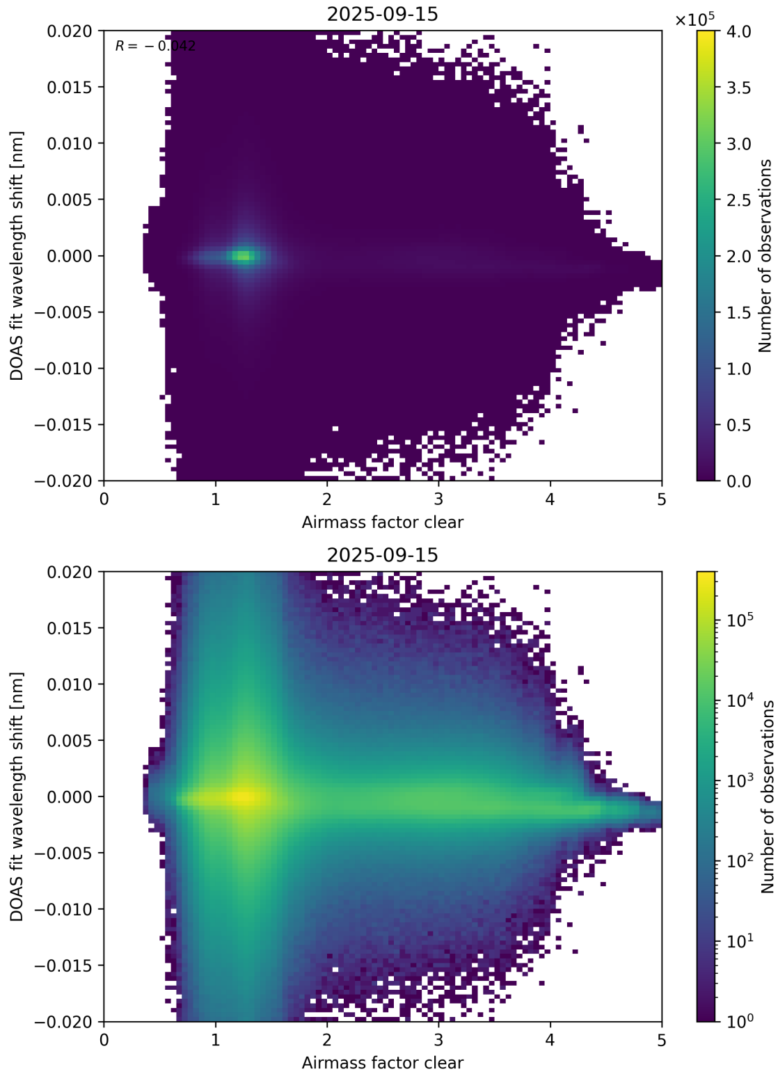
Figure 72: Scatter density plot of “Airmass factor clear” against “DOAS fit wavelength shift” for 2025-09-15 to 2025-09-16.
