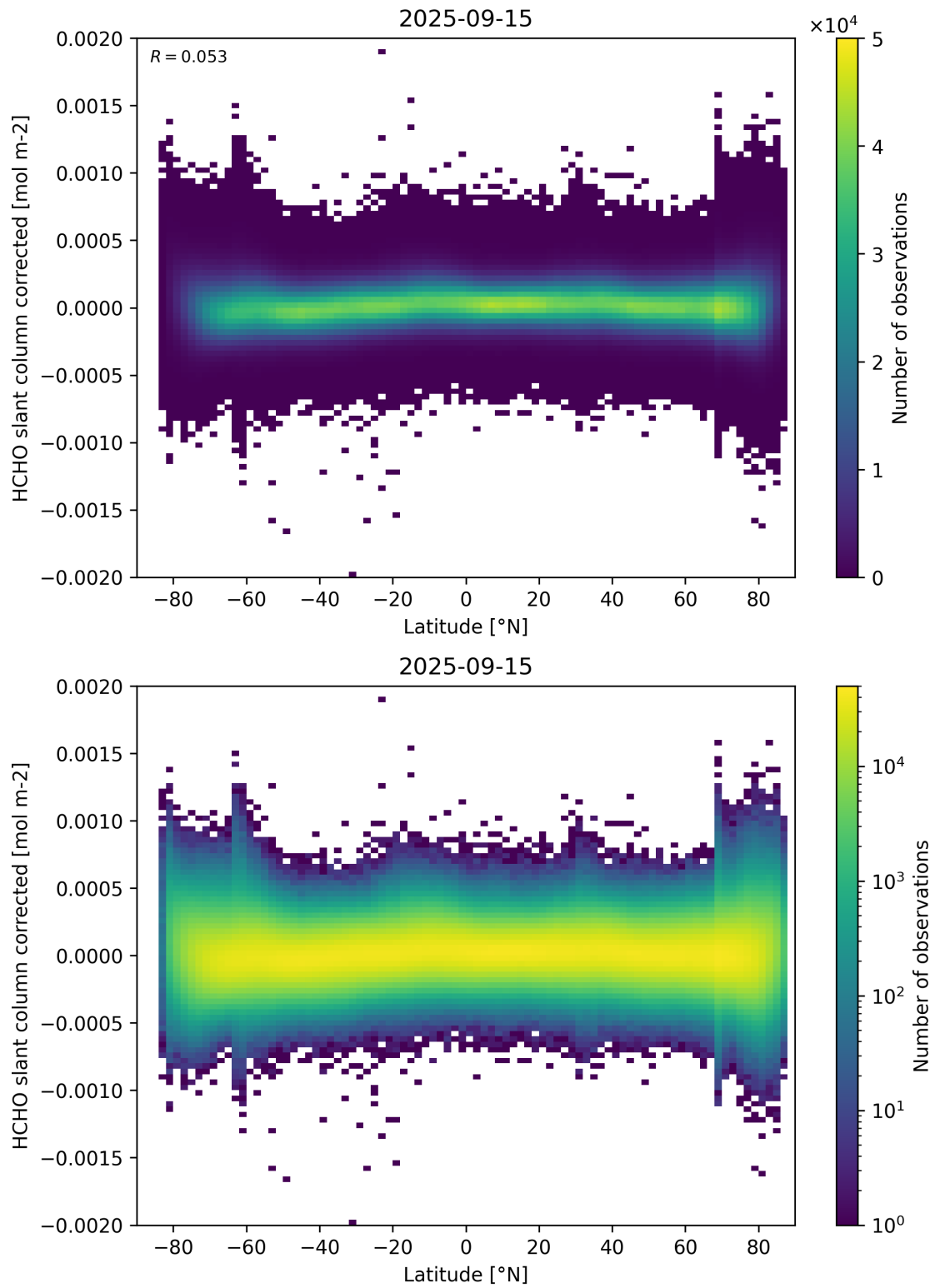
Figure 157: Scatter density plot of “Latitude” against “HCHO slant column corrected” for 2025-09-15 to 2025-09-16.
