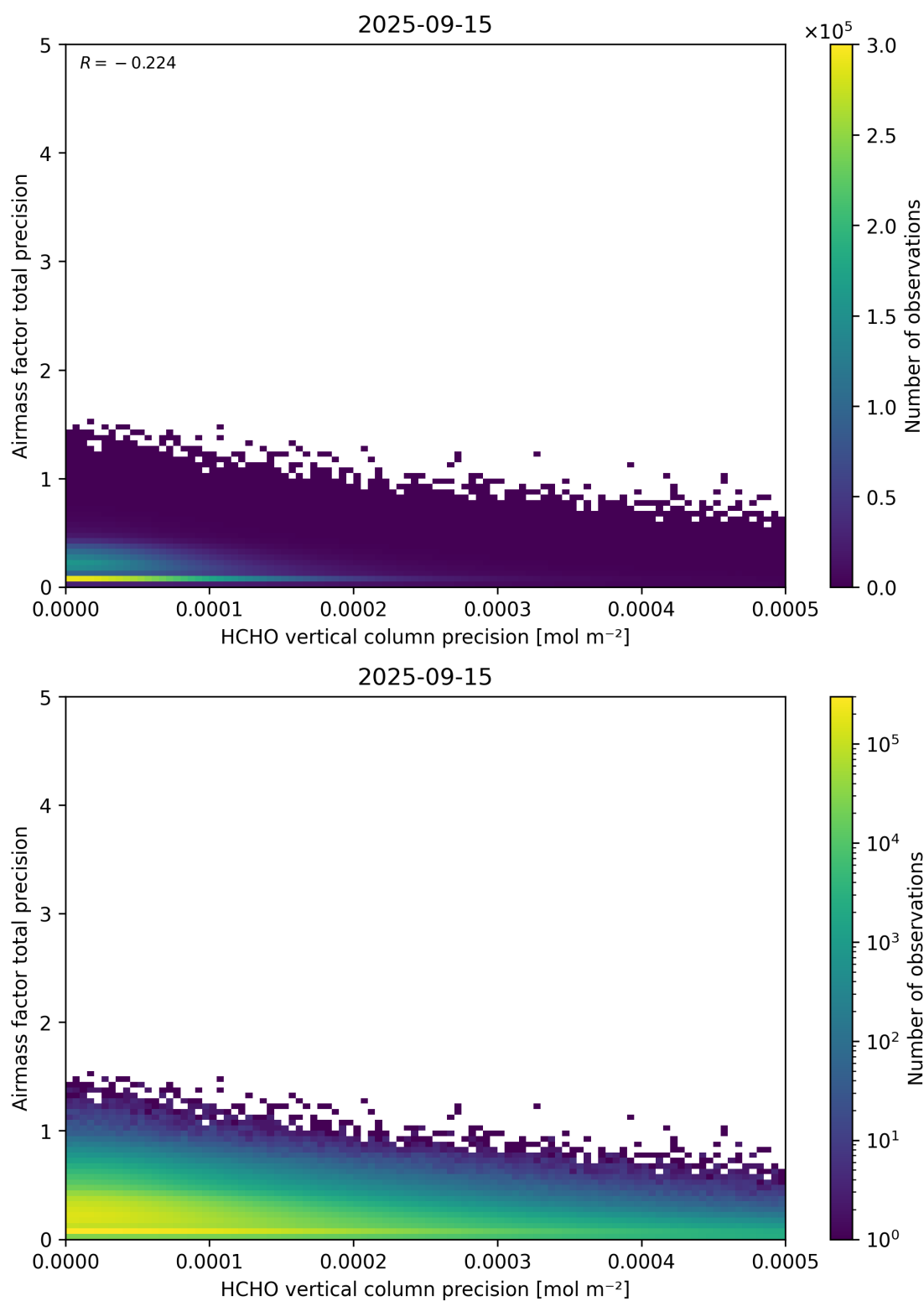
Figure 145: Scatter density plot of “HCHO vertical column precision” against “Airmass factor total precision” for 2025-09-15 to 2025-09-16.
