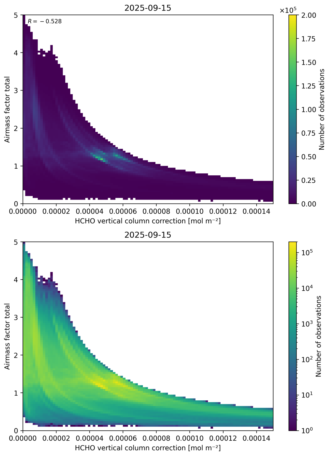
Figure 120: Scatter density plot of “HCHO vertical column correction” against “Airmass factor total” for 2025-09-15 to 2025-09-16.
