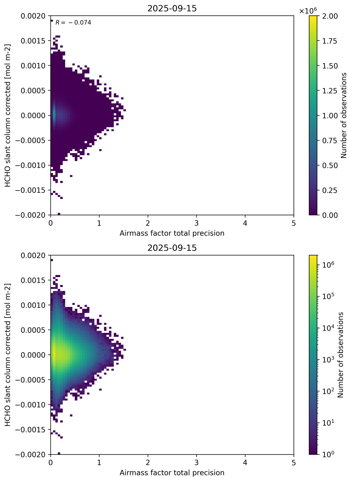
Figure 109: Scatter density plot of “Airmass factor total precision” against “HCHO slant column corrected” for 2025-09-15 to 2025-09-16.
