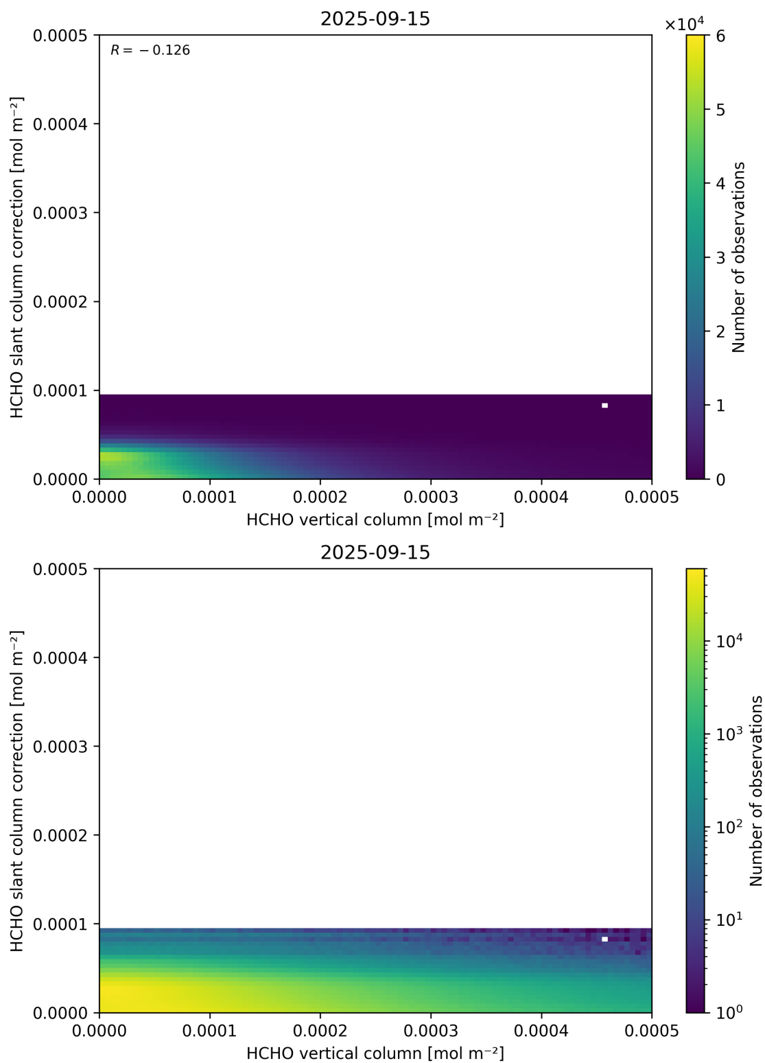
Figure 128: Scatter density plot of “HCHO vertical column” against “HCHO slant column correction” for 2025-09-15 to 2025-09-16.
