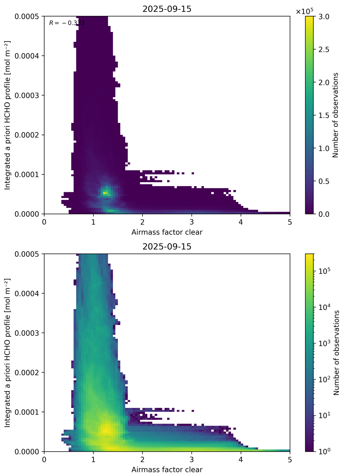
Figure 76: Scatter density plot of “Airmass factor clear” against “Integrated a priori HCHO profile” for 2025-09-15 to 2025-09-16.
