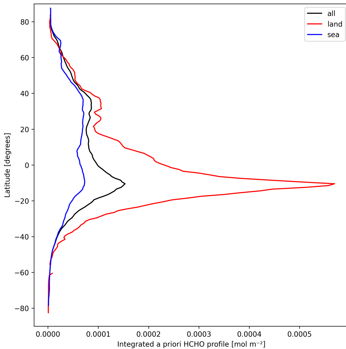
Figure 29: Zonal average of “Integrated a priori HCHO profile” for 2025-09-15 to 2025-09-16.
