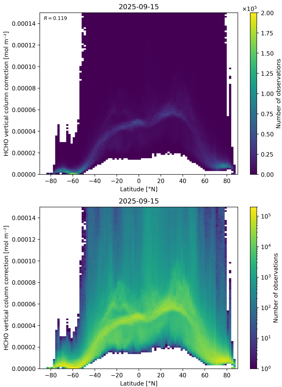
Figure 164: Scatter density plot of “Latitude” against “HCHO vertical column correction” for 2025-09-15 to 2025-09-16.
