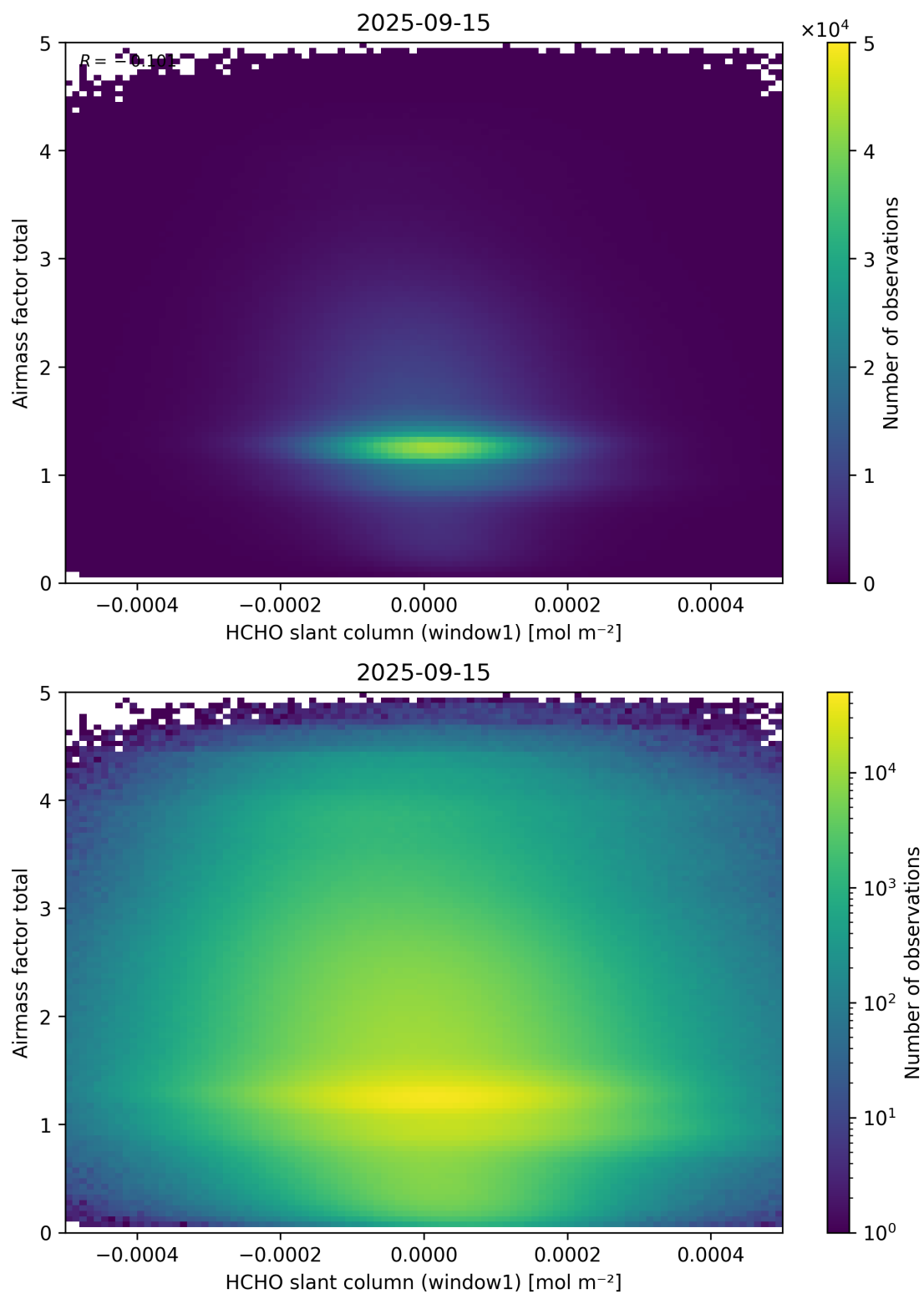
Figure 85: Scatter density plot of “HCHO slant column (window1)” against “Airmass factor total” for 2025-09-15 to 2025-09-16.
