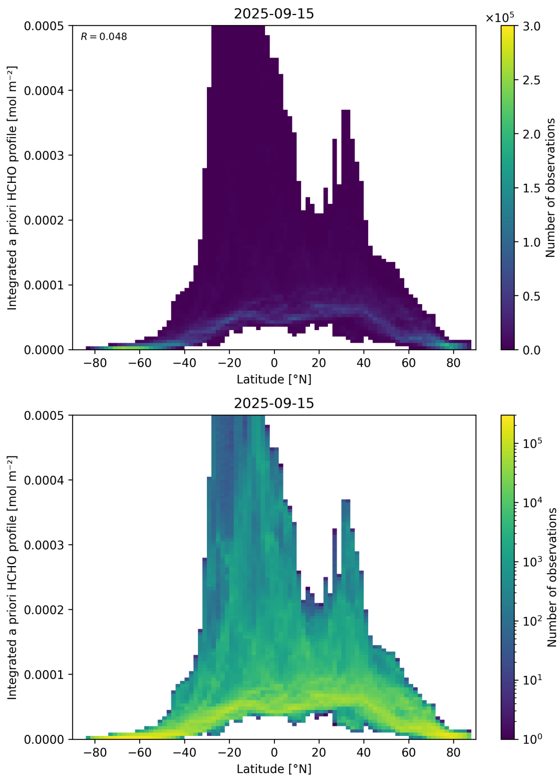
Figure 166: Scatter density plot of “Latitude” against “Integrated a priori HCHO profile” for 2025-09-15 to 2025-09-16.
