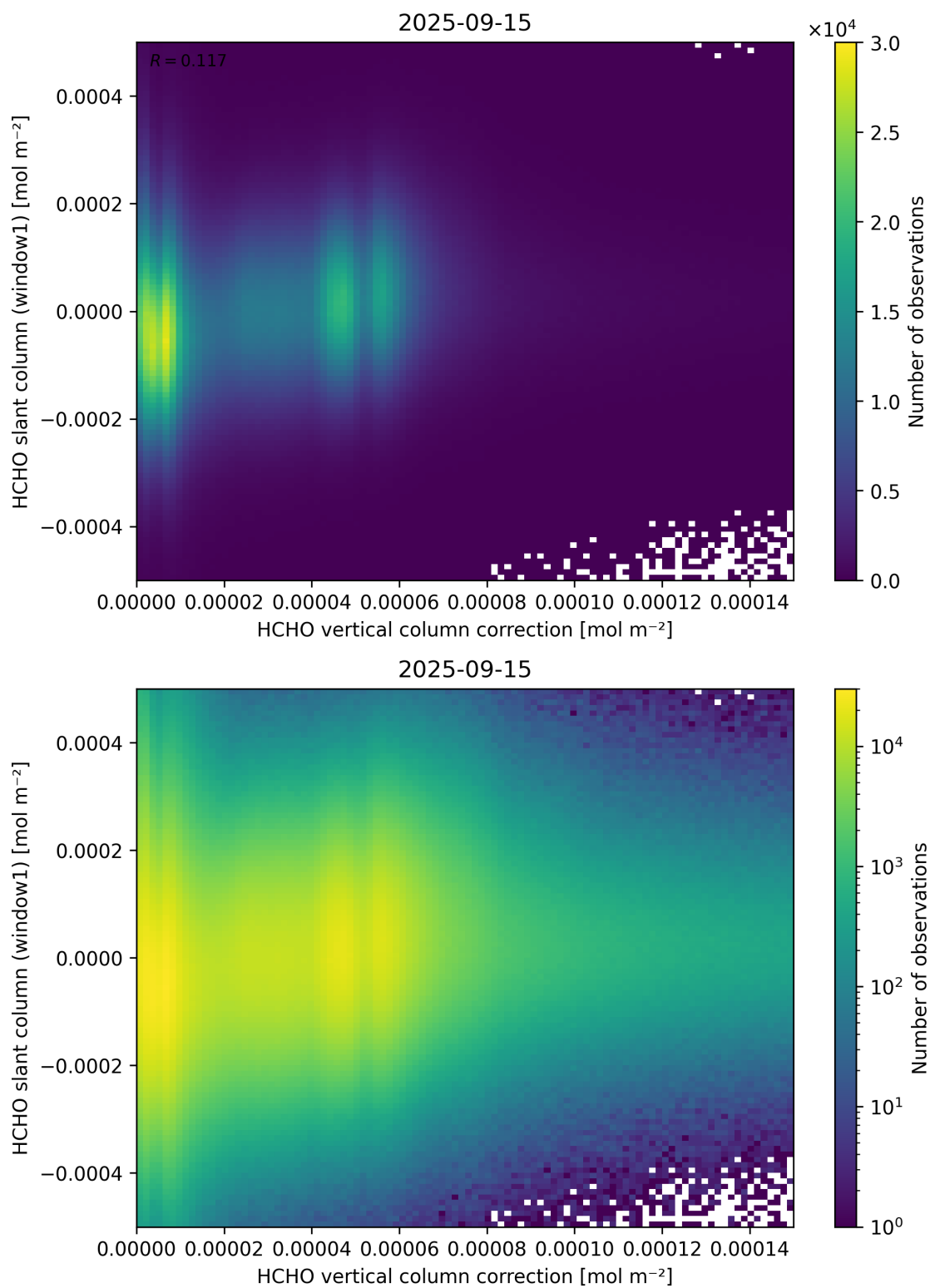
Figure 118: Scatter density plot of “HCHO vertical column correction” against “HCHO slant column (window1)” for 2025-09-15 to 2025-09-16.
