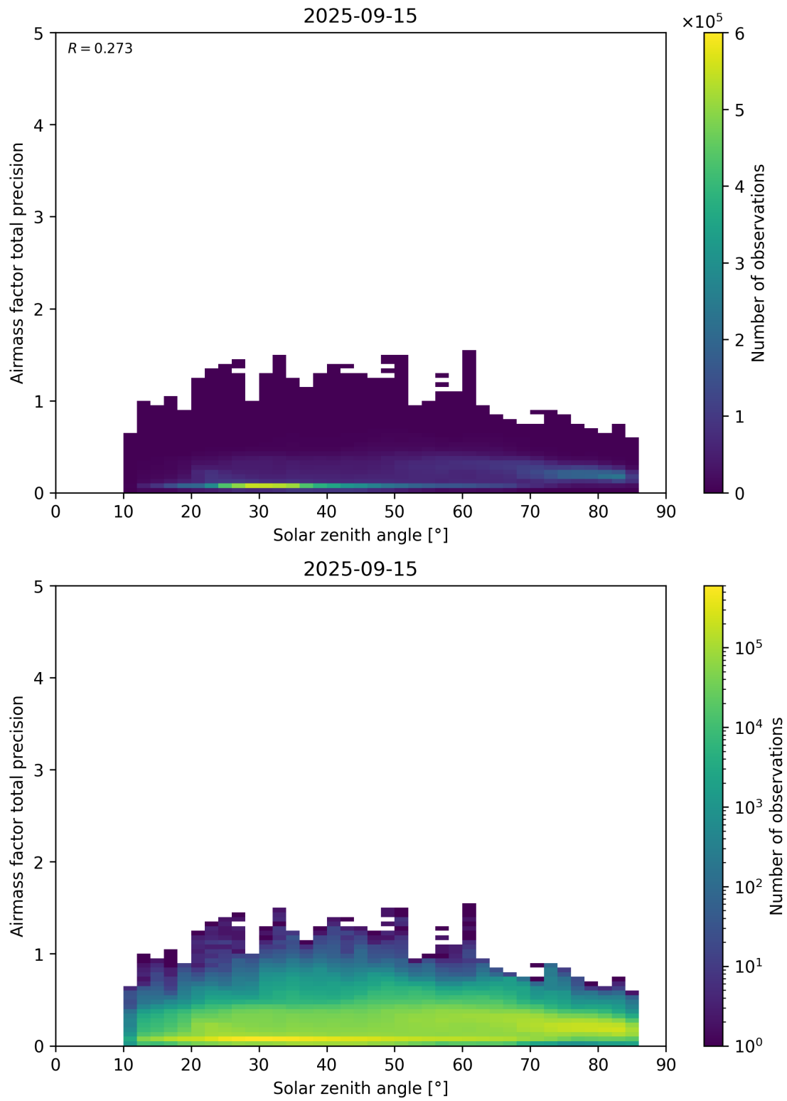
Figure 176: Scatter density plot of “Solar zenith angle” against “Airmass factor total precision” for 2025-09-15 to 2025-09-16.
