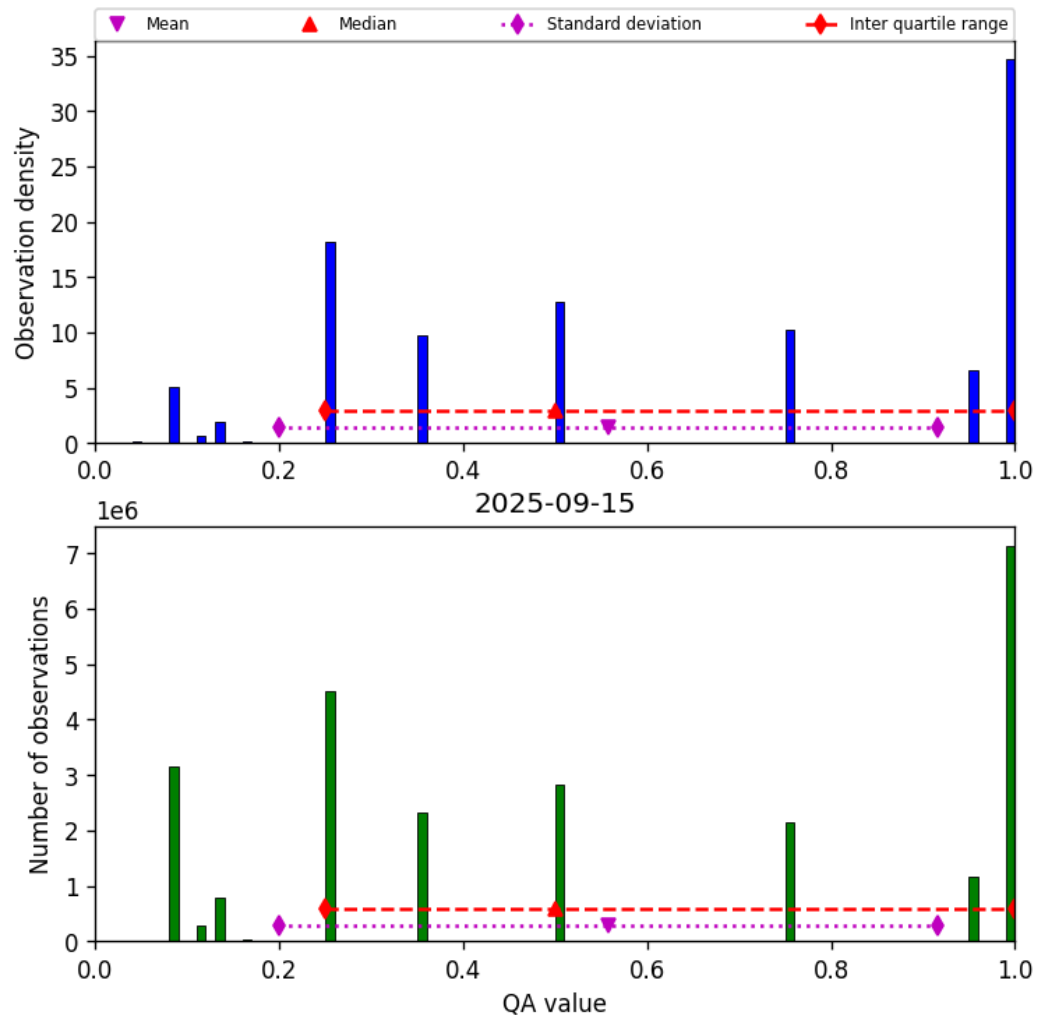
Figure 34: Histogram of “QA value” for 2025-09-15 to 2025-09-16
