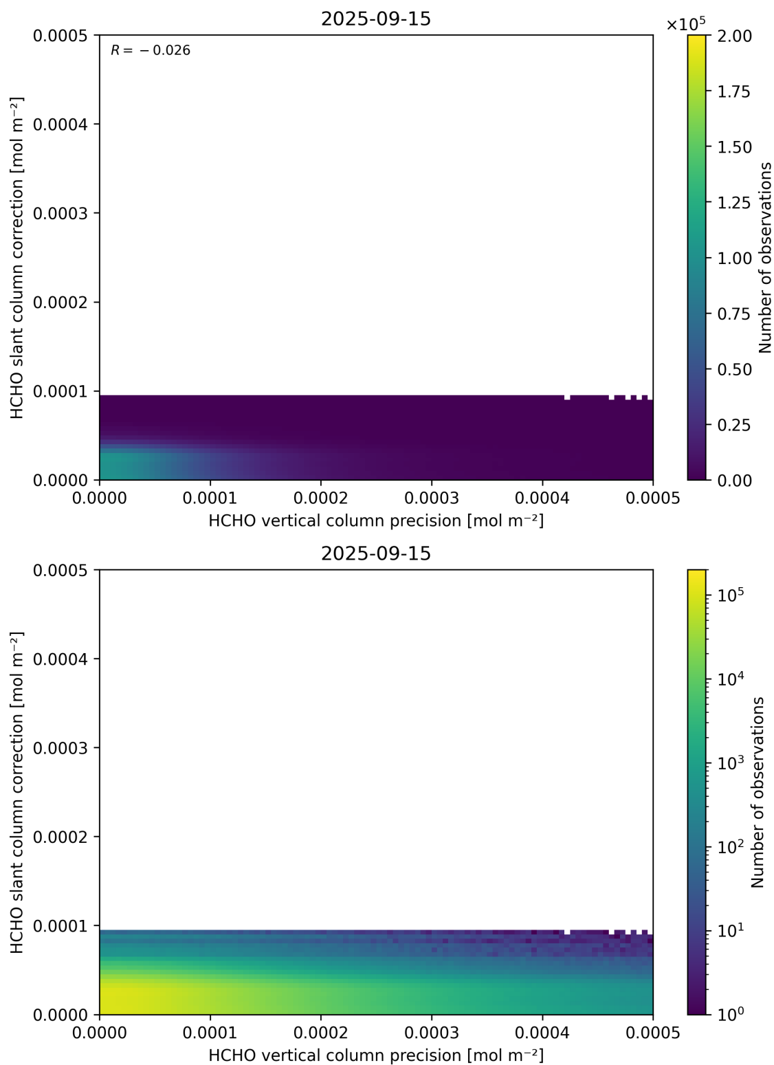
Figure 141: Scatter density plot of “HCHO vertical column precision” against “HCHO slant column correction” for 2025-09-15 to 2025-09-16.
