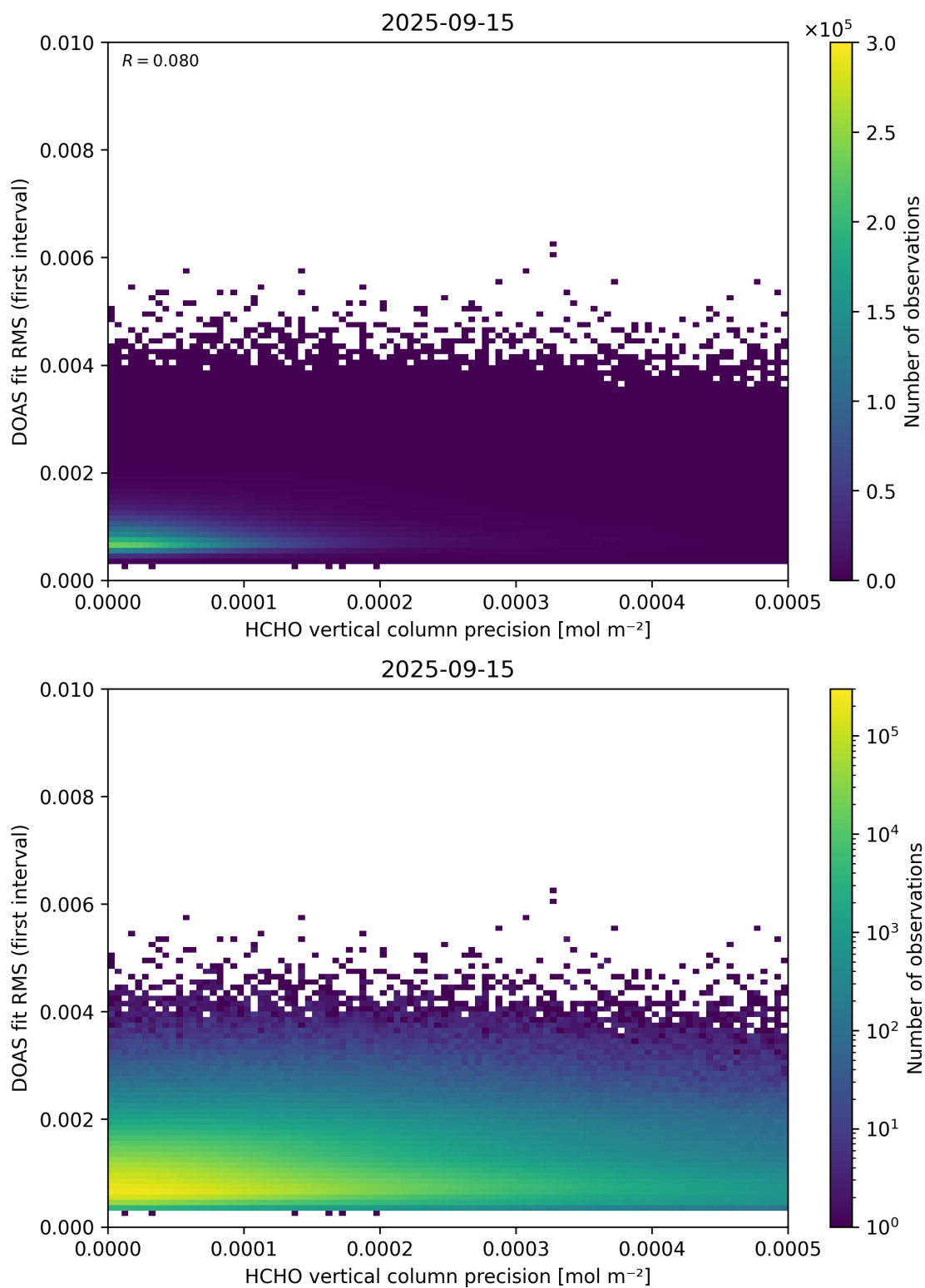
Figure 136: Scatter density plot of “HCHO vertical column precision” against “DOAS fit RMS (first interval)” for 2025-09-15 to 2025-09-16.
