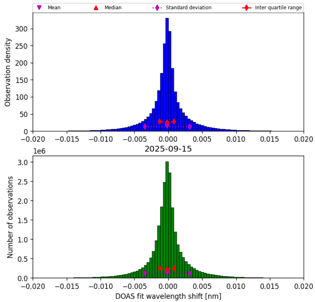
Figure 44: Histogram of “DOAS fit wavelength shift” for 2025-09-15 to 2025-09-16
