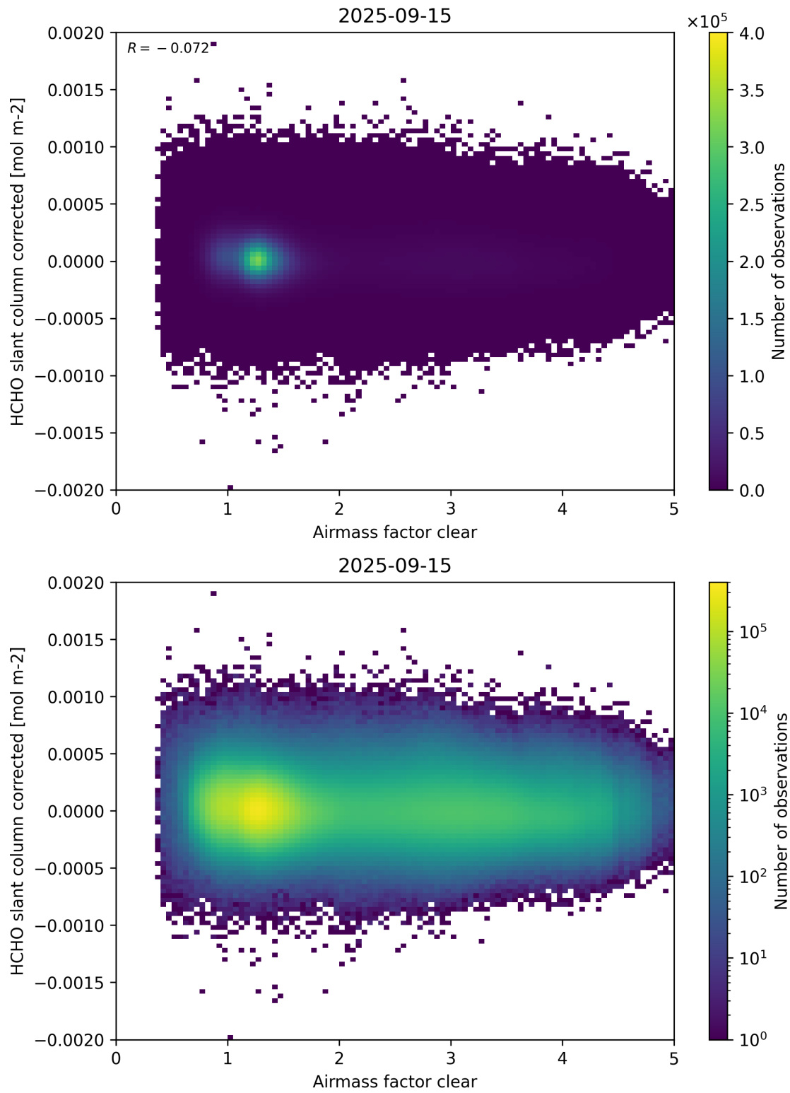
Figure 74: Scatter density plot of “Airmass factor clear” against “HCHO slant column corrected” for 2025-09-15 to 2025-09-16.
