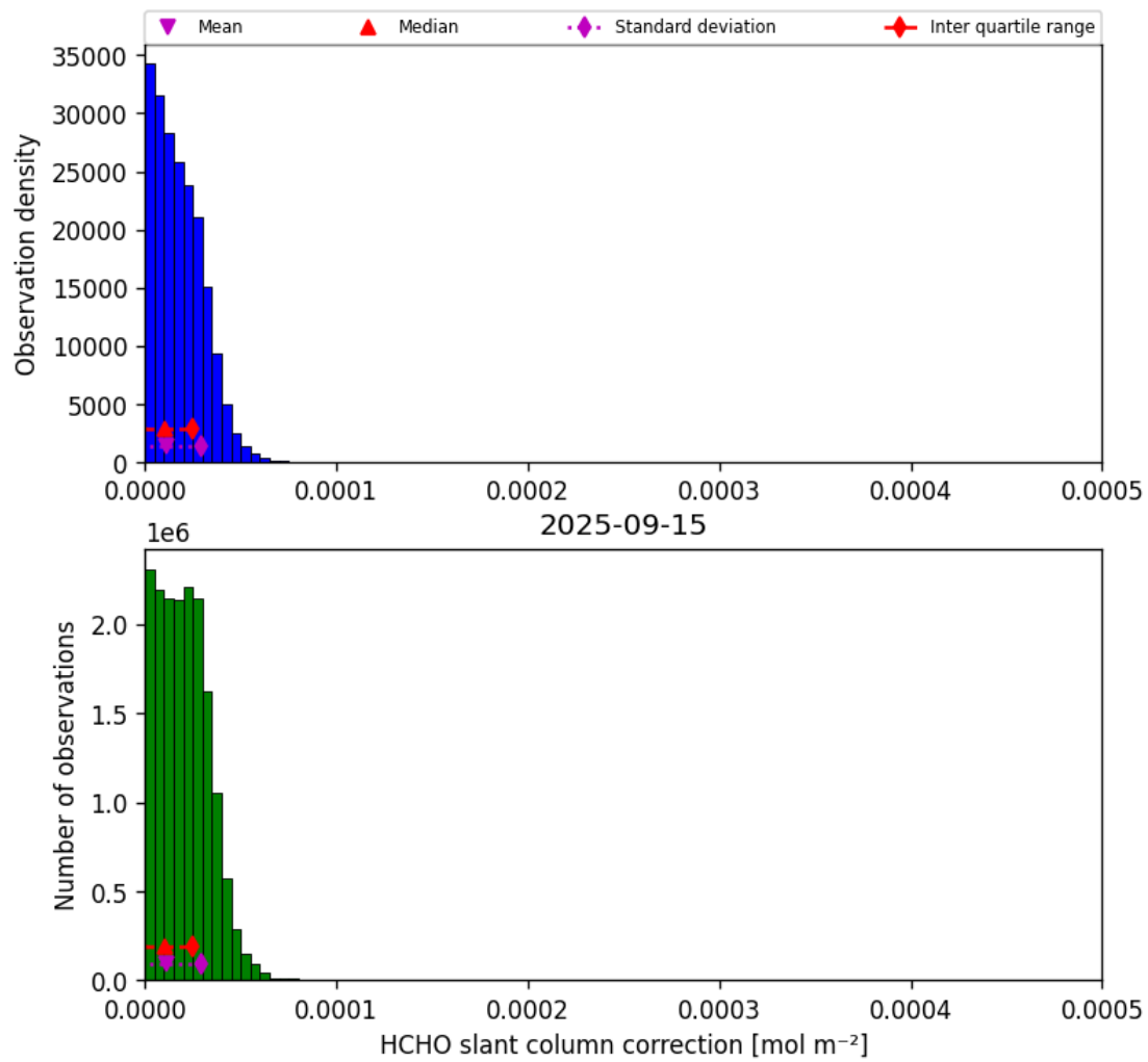
Figure 47: Histogram of “HCHO slant column correction” for 2025-09-15 to 2025-09-16
