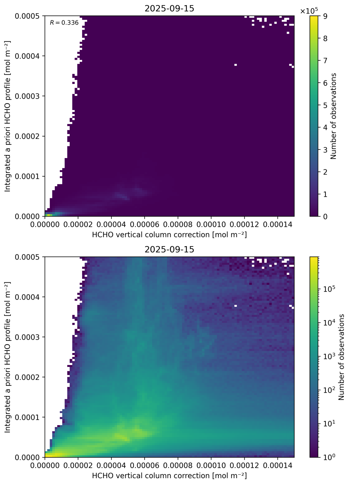
Figure 122: Scatter density plot of “HCHO vertical column correction” against “Integrated a priori HCHO profile” for 2025-09-15 to 2025-09-16.
