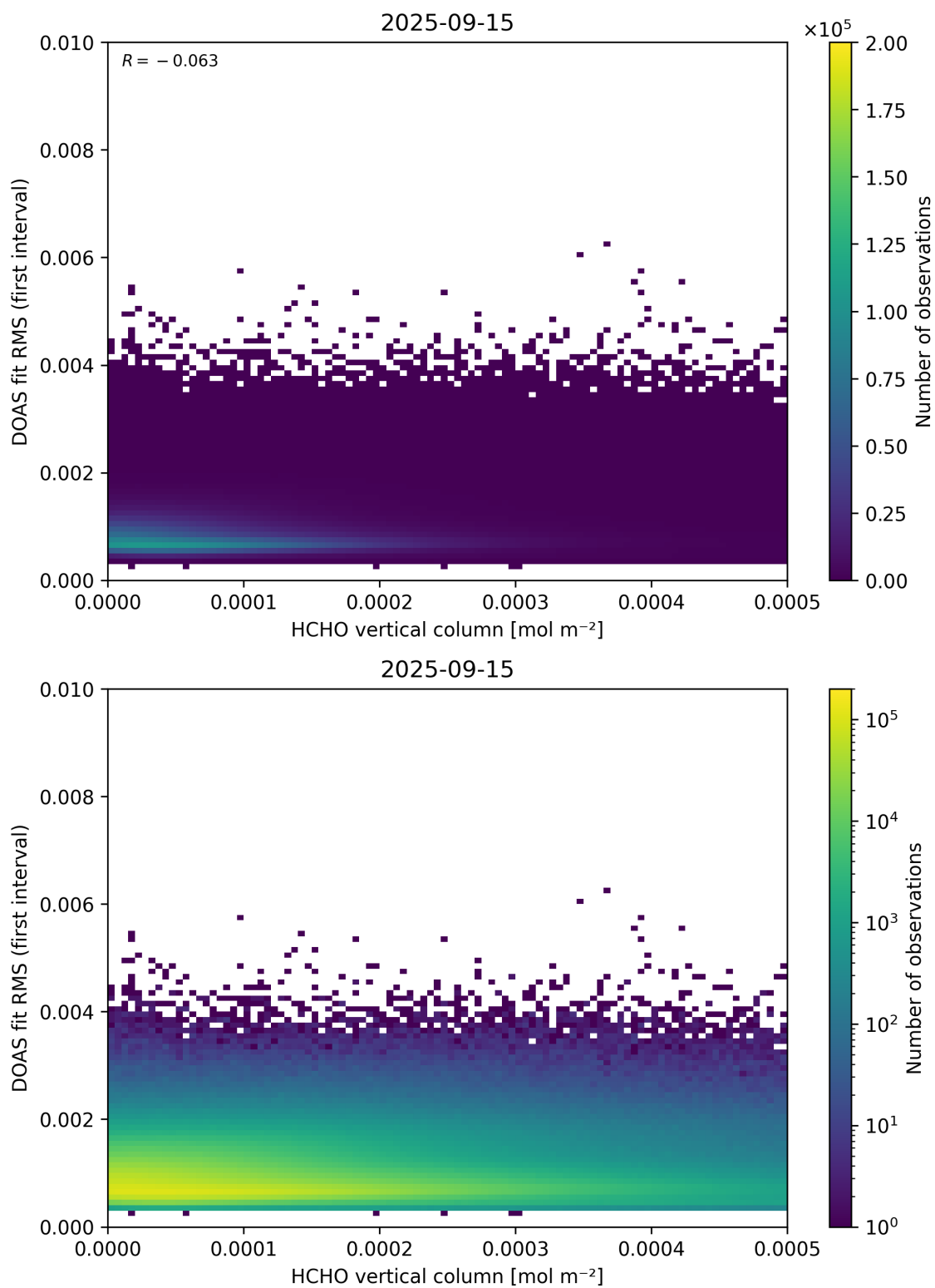
Figure 123: Scatter density plot of “HCHO vertical column” against “DOAS fit RMS (first interval)” for 2025-09-15 to 2025-09-16.
