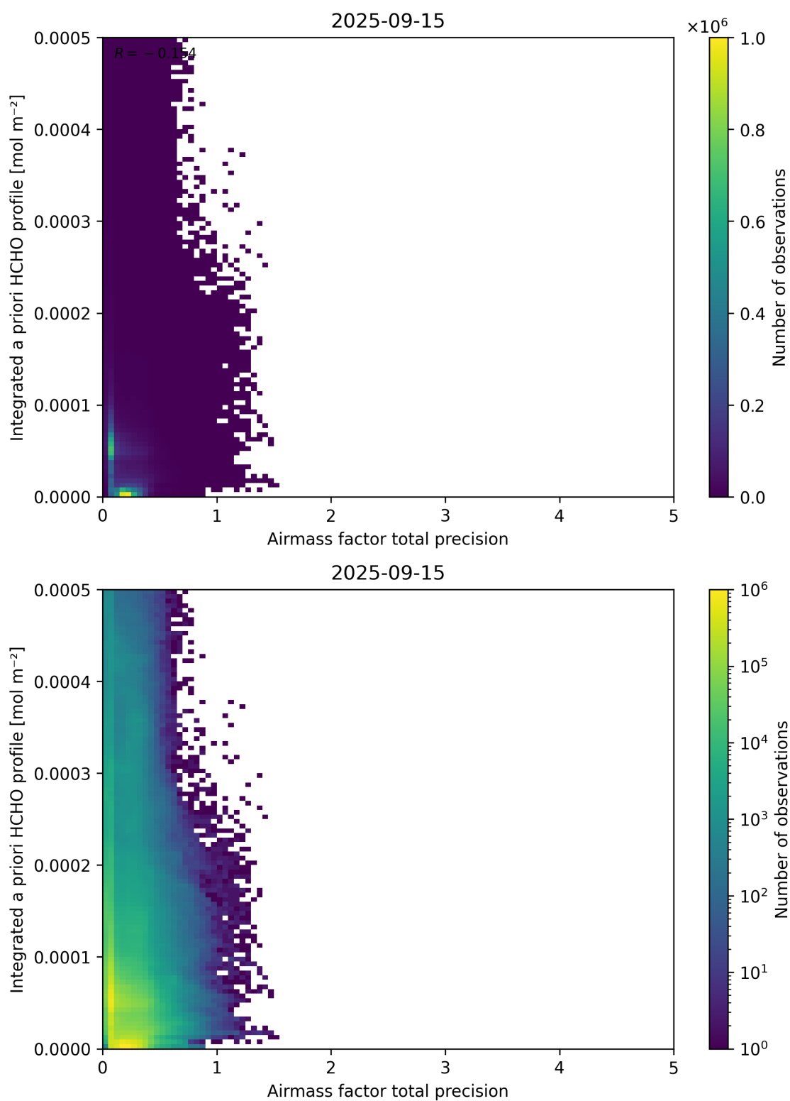
Figure 111: Scatter density plot of “Airmass factor total precision” against “Integrated a priori HCHO profile” for 2025-09-15 to 2025-09-16.
