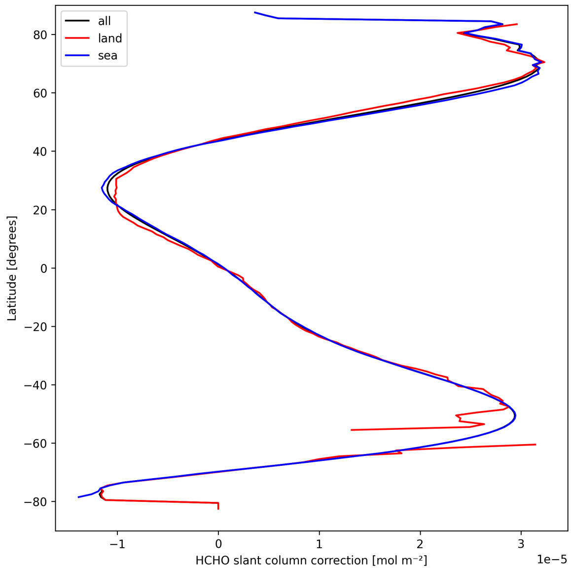
Figure 33: Zonal average of “HCHO slant column correction” for 2025-09-15 to 2025-09-16.
