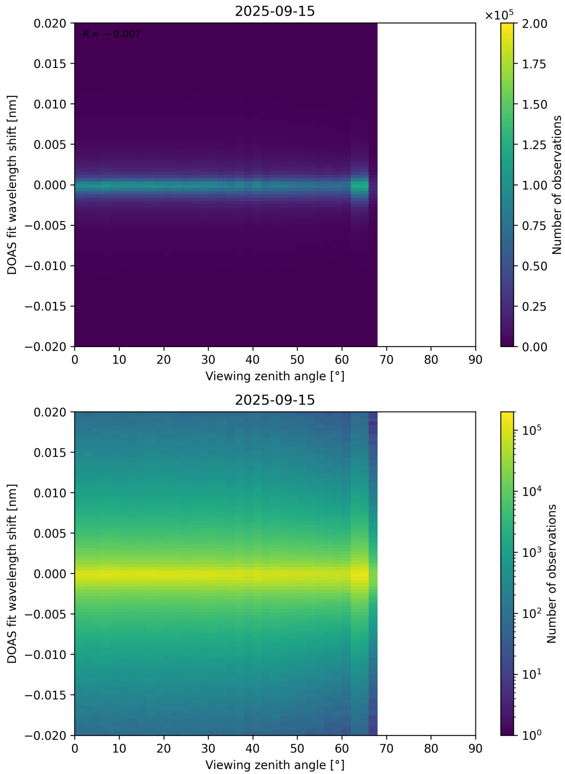
Figure 183: Scatter density plot of “Viewing zenith angle” against “DOAS fit wavelength shift” for 2025-09-15 to 2025-09-16.
