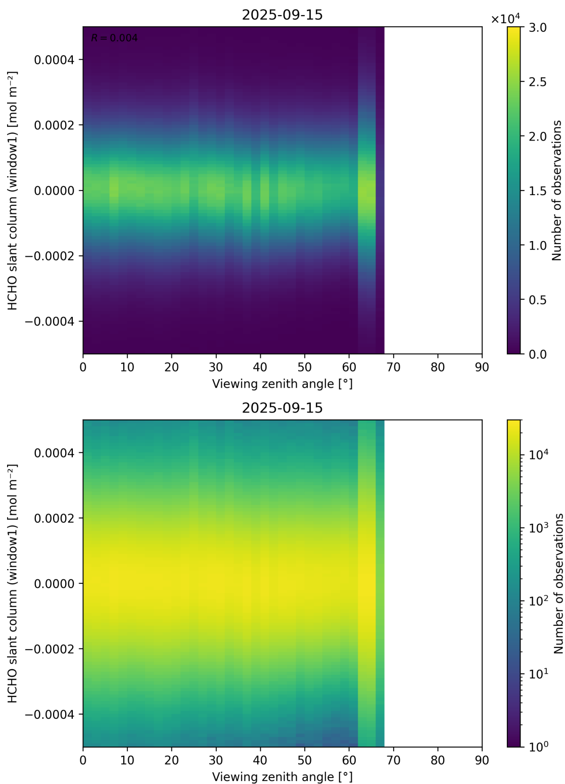
Figure 188: Scatter density plot of “Viewing zenith angle” against “HCHO slant column (window1)” for 2025-09-15 to 2025-09-16.
