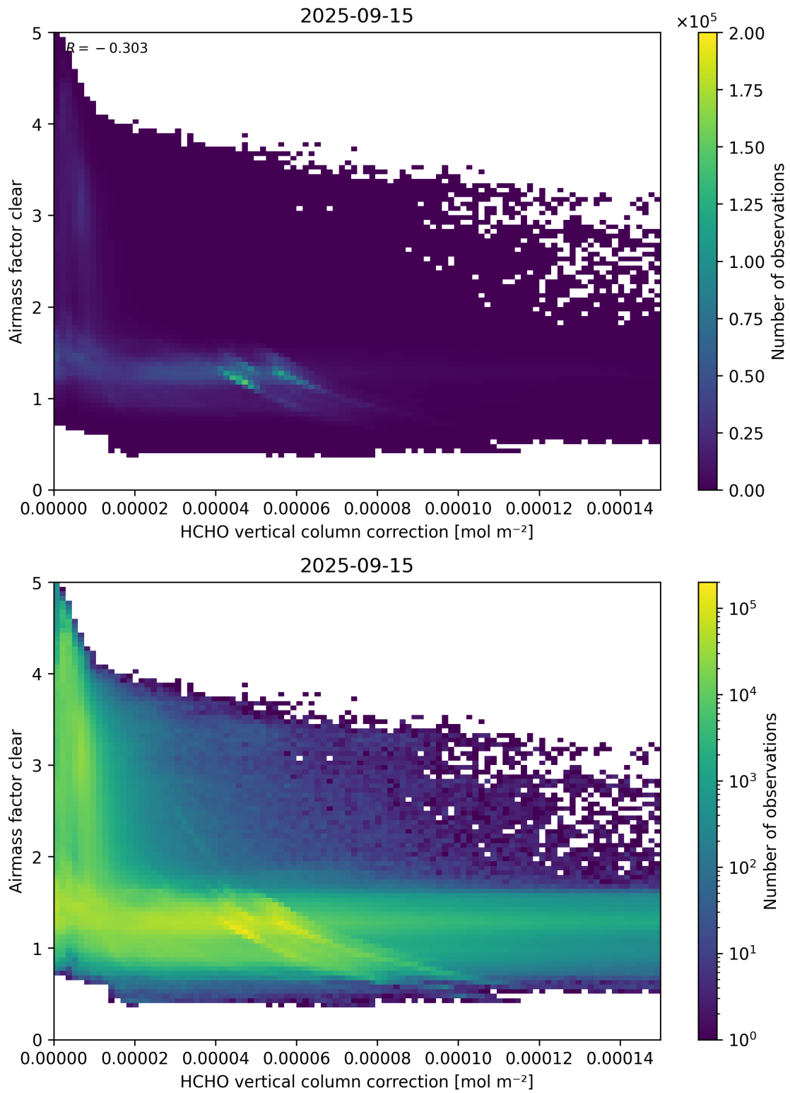
Figure 115: Scatter density plot of “HCHO vertical column correction” against “Airmass factor clear” for 2025-09-15 to 2025-09-16.
