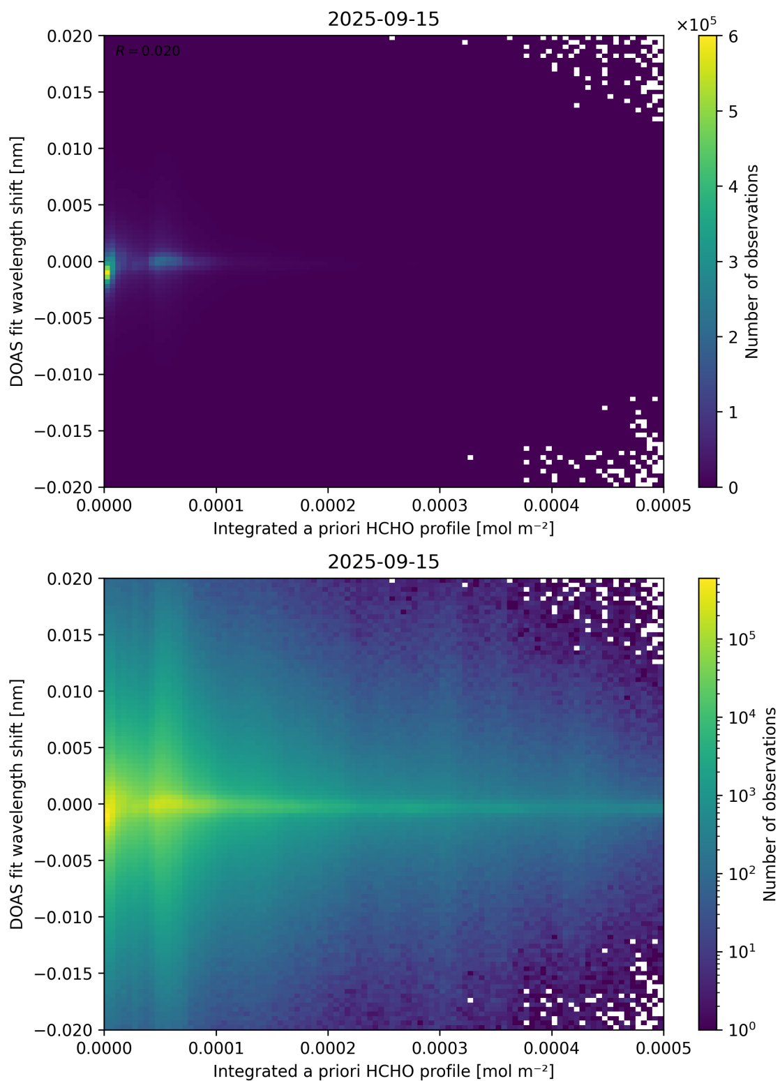
Figure 149: Scatter density plot of “Integrated a priori HCHO profile” against “DOAS fit wavelength shift” for 2025-09-15 to 2025-09-16.
