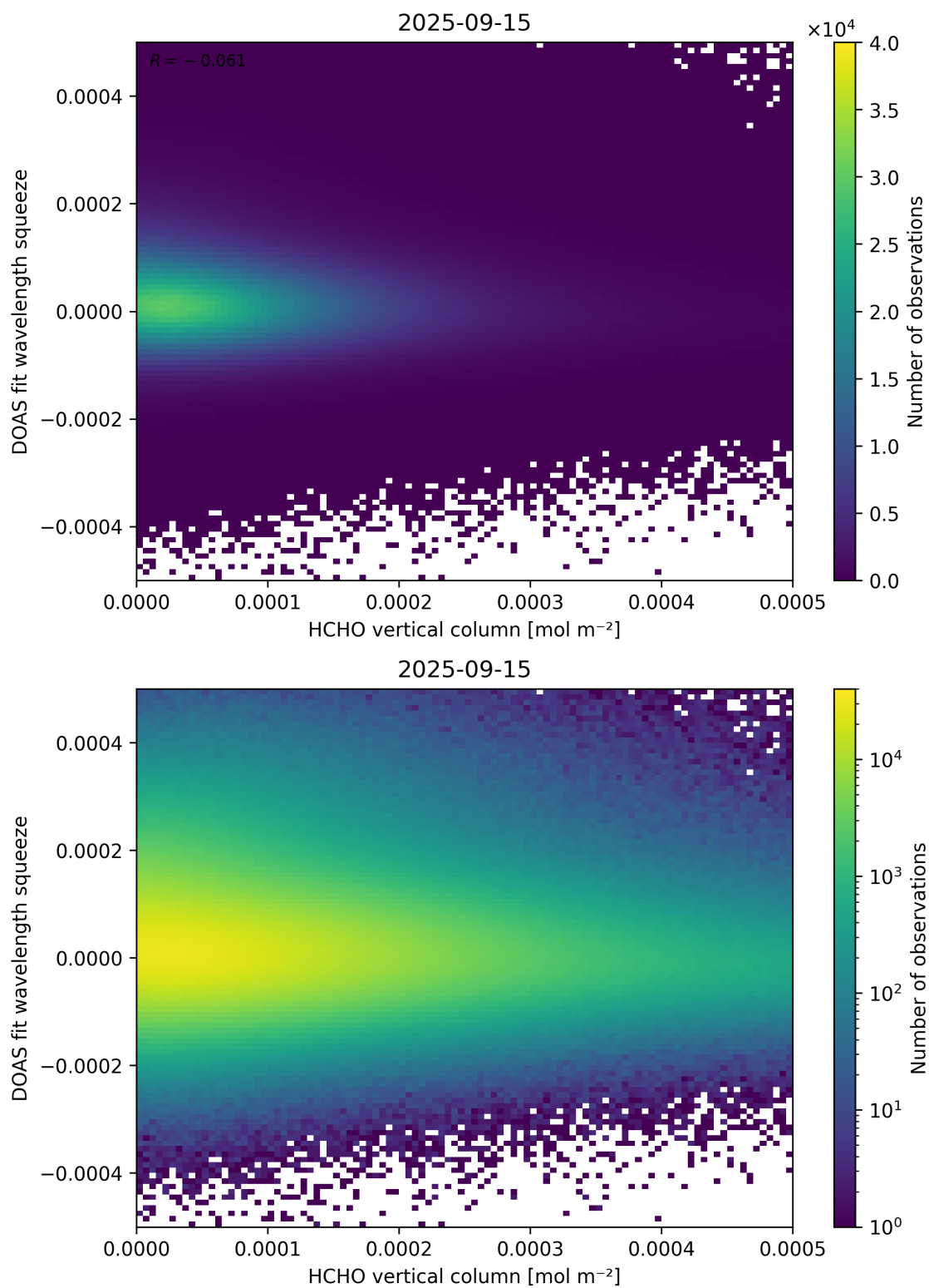
Figure 125: Scatter density plot of “HCHO vertical column” against “DOAS fit wavelength squeeze” for 2025-09-15 to 2025-09-16.
