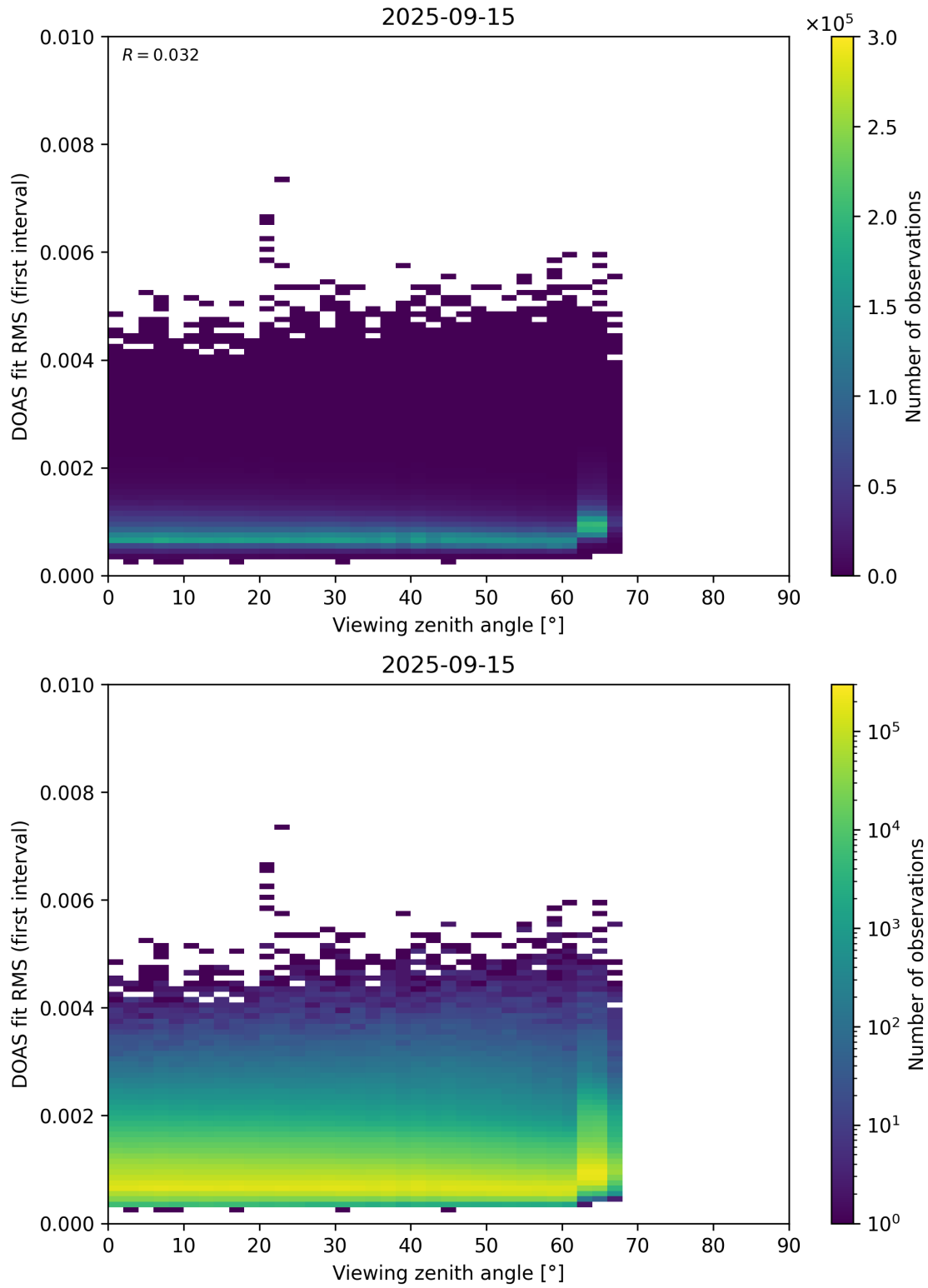
Figure 182: Scatter density plot of “Viewing zenith angle” against “DOAS fit RMS (first interval)” for 2025-09-15 to 2025-09-16.
