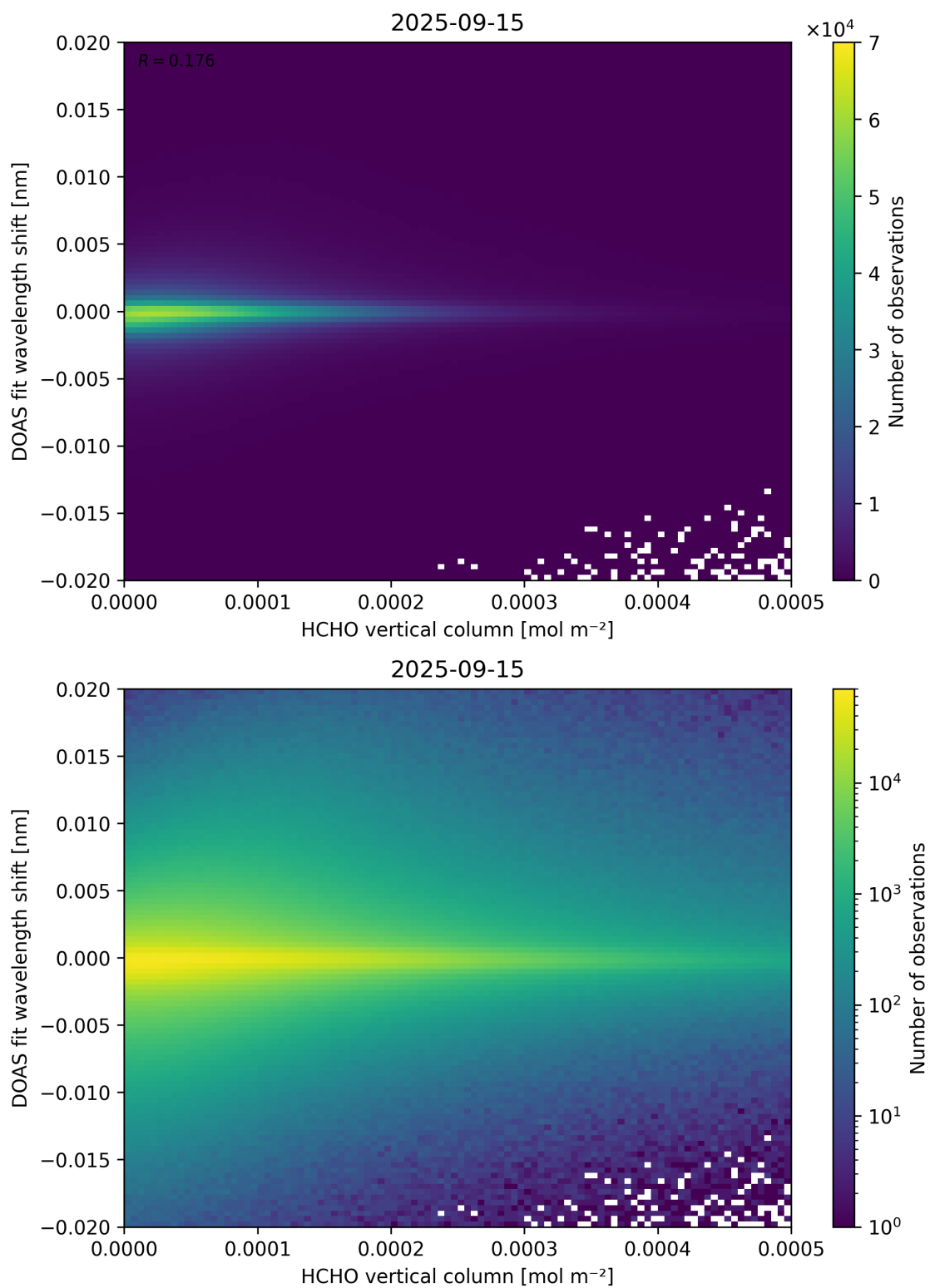
Figure 124: Scatter density plot of “HCHO vertical column” against “DOAS fit wavelength shift” for 2025-09-15 to 2025-09-16.
