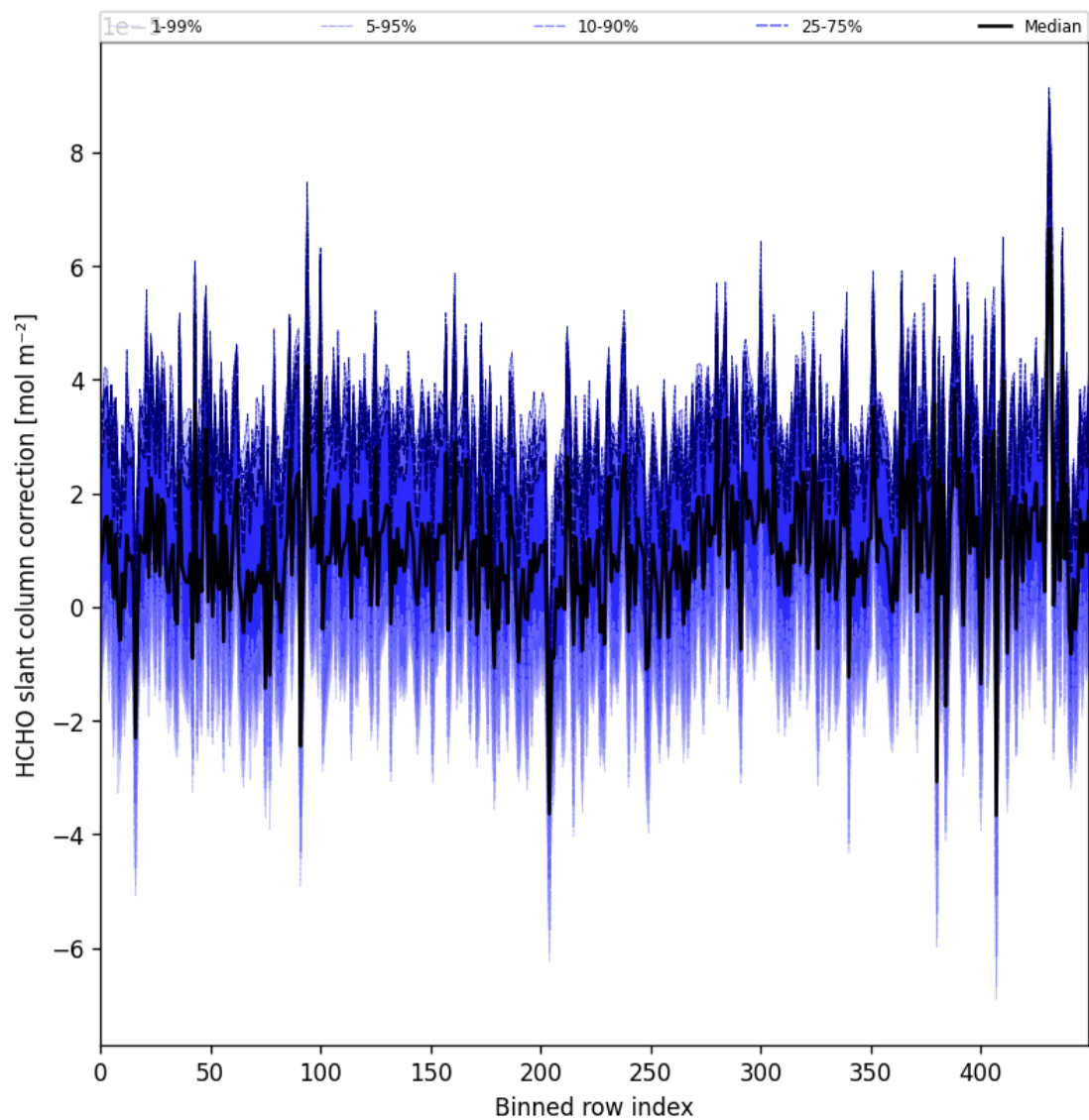
Figure 61: Along track statistics of “HCHO slant column correction” for 2025-09-15 to 2025-09-16
