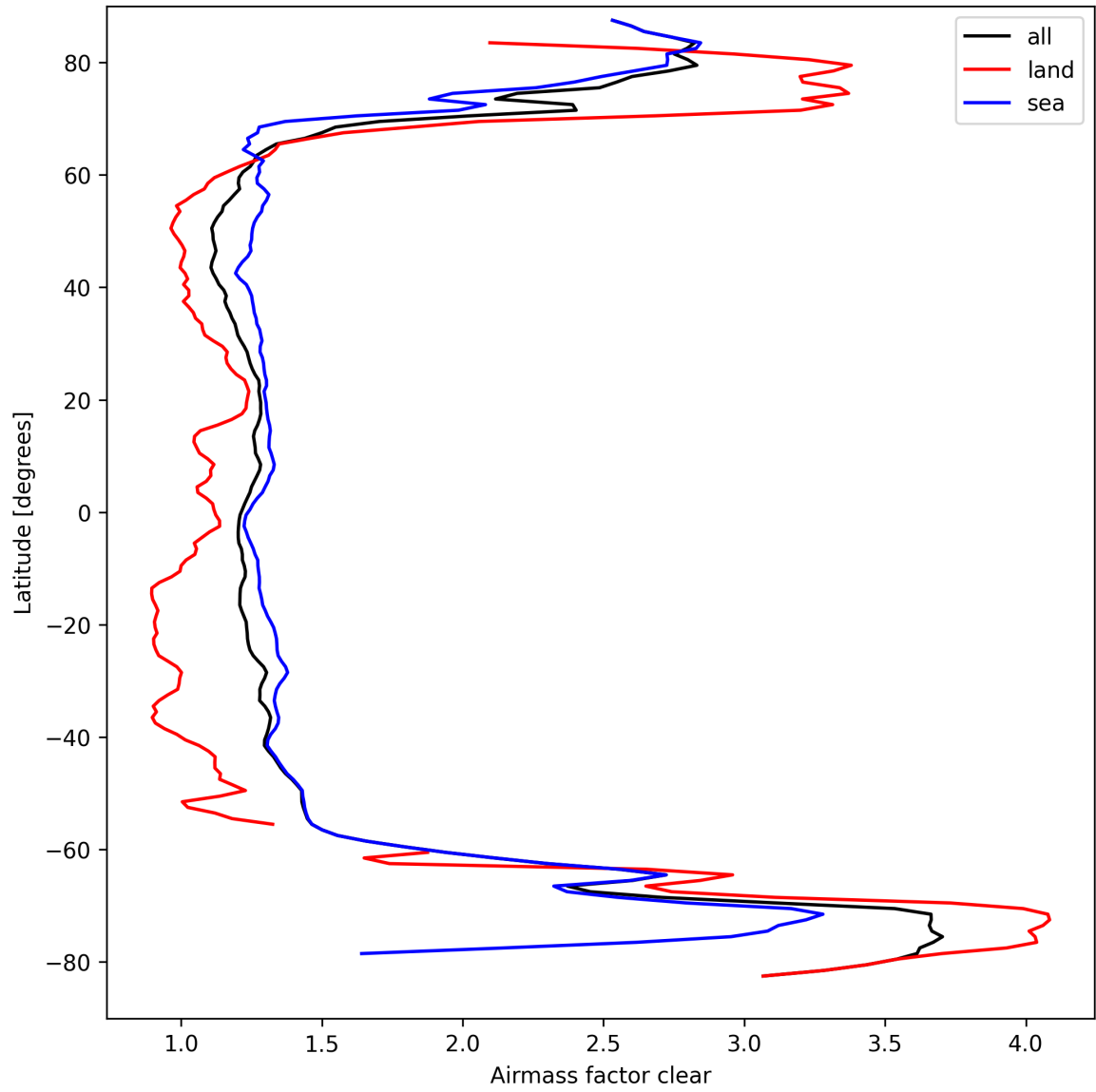
Figure 28: Zonal average of “Airmass factor clear” for 2025-09-15 to 2025-09-16.
