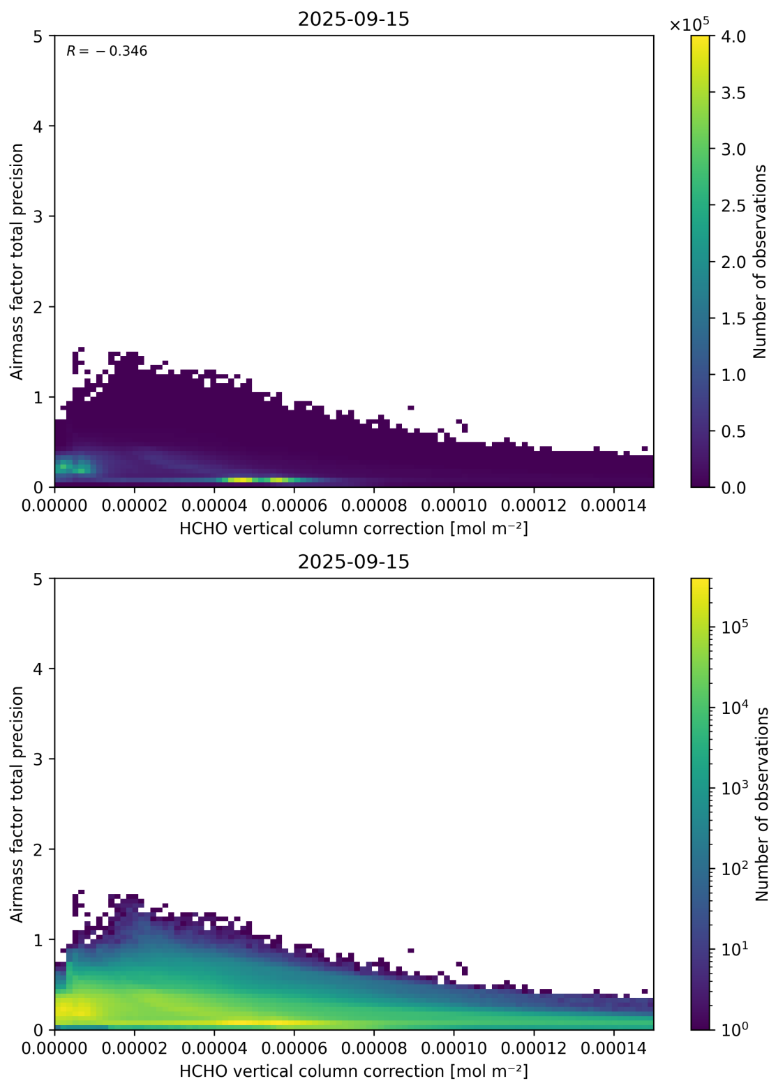
Figure 121: Scatter density plot of “HCHO vertical column correction” against “Airmass factor total precision” for 2025-09-15 to 2025-09-16.
