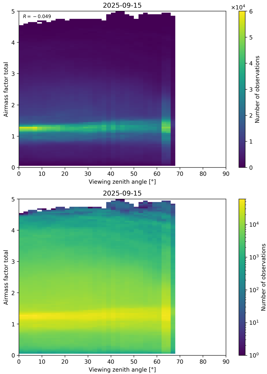
Figure 190: Scatter density plot of “Viewing zenith angle” against “Airmass factor total” for 2025-09-15 to 2025-09-16.
