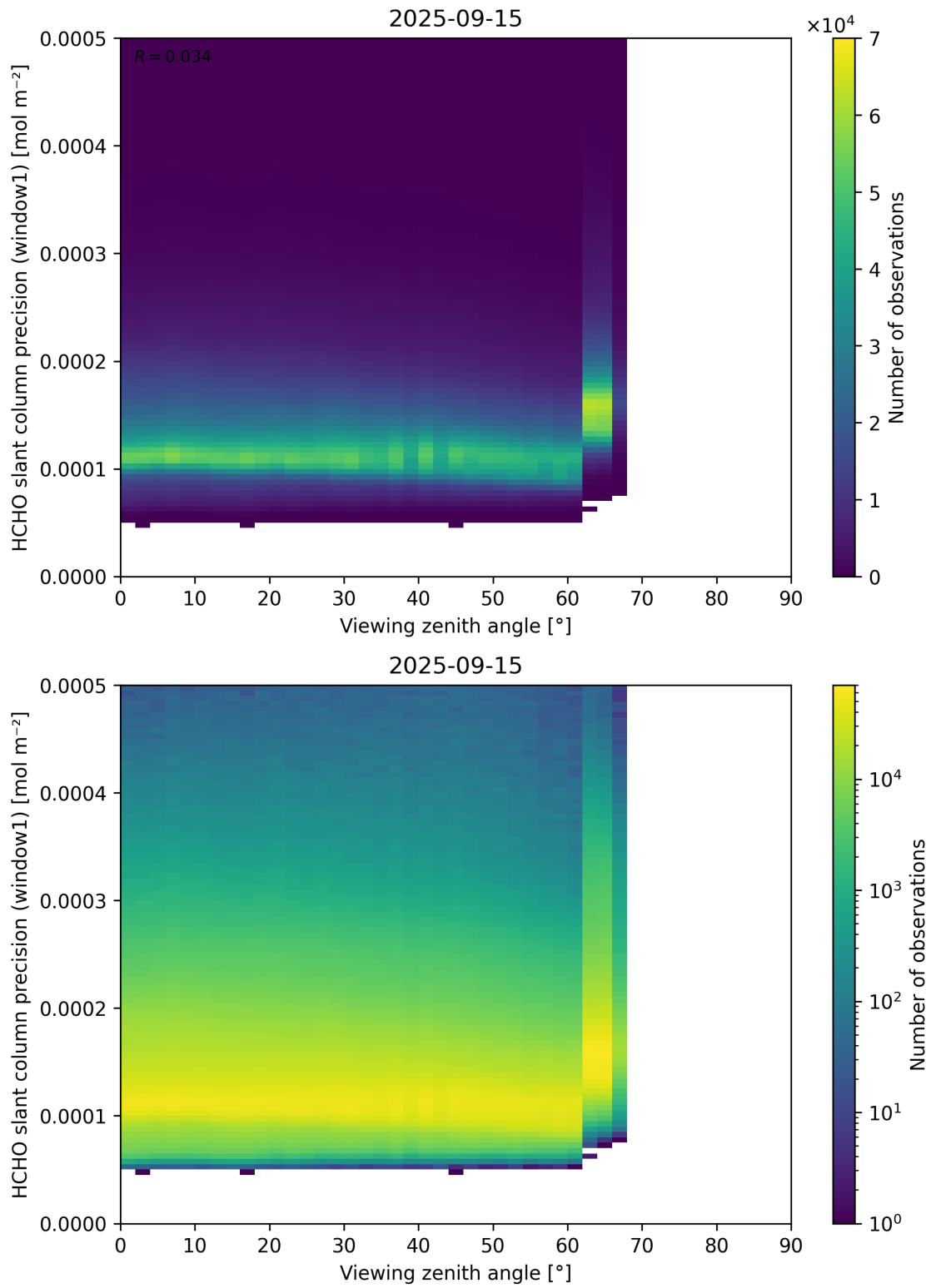
Figure 189: Scatter density plot of “Viewing zenith angle” against “HCHO slant column precision (window1)” for 2025-09-15 to 2025-09-16.
