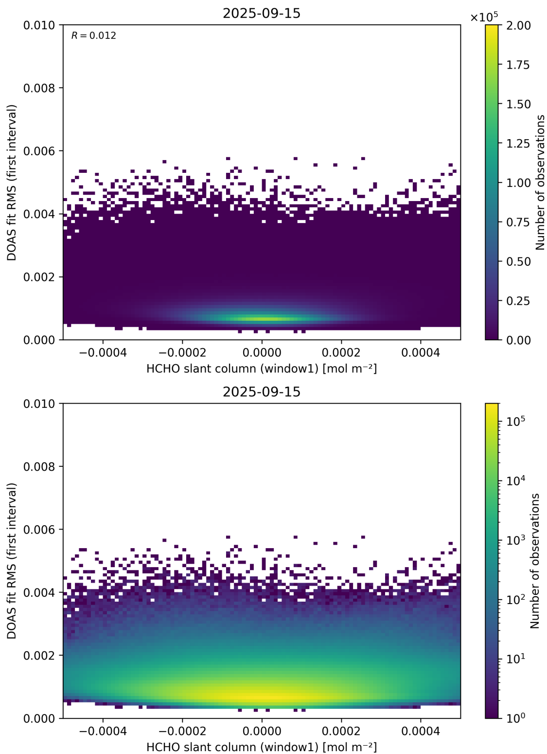
Figure 78: Scatter density plot of “HCHO slant column (window1)” against “DOAS fit RMS (first interval)” for 2025-09-15 to 2025-09-16.
