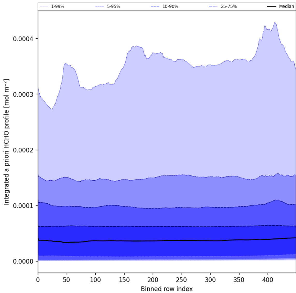
Figure 57: Along track statistics of “Integrated a priori HCHO profile” for 2025-09-15 to 2025-09-16
