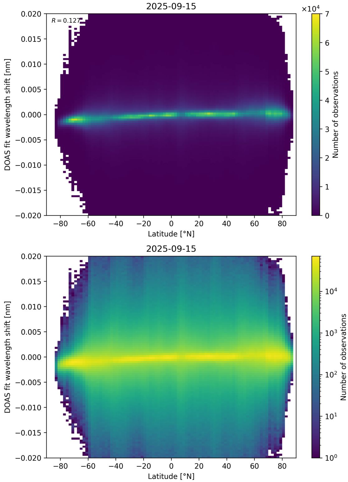
Figure 154: Scatter density plot of “Latitude” against “DOAS fit wavelength shift” for 2025-09-15 to 2025-09-16.
