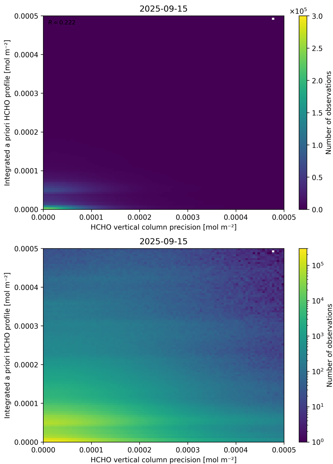
Figure 147: Scatter density plot of “HCHO vertical column precision” against “Integrated a priori HCHO profile” for 2025-09-15 to 2025-09-16.
