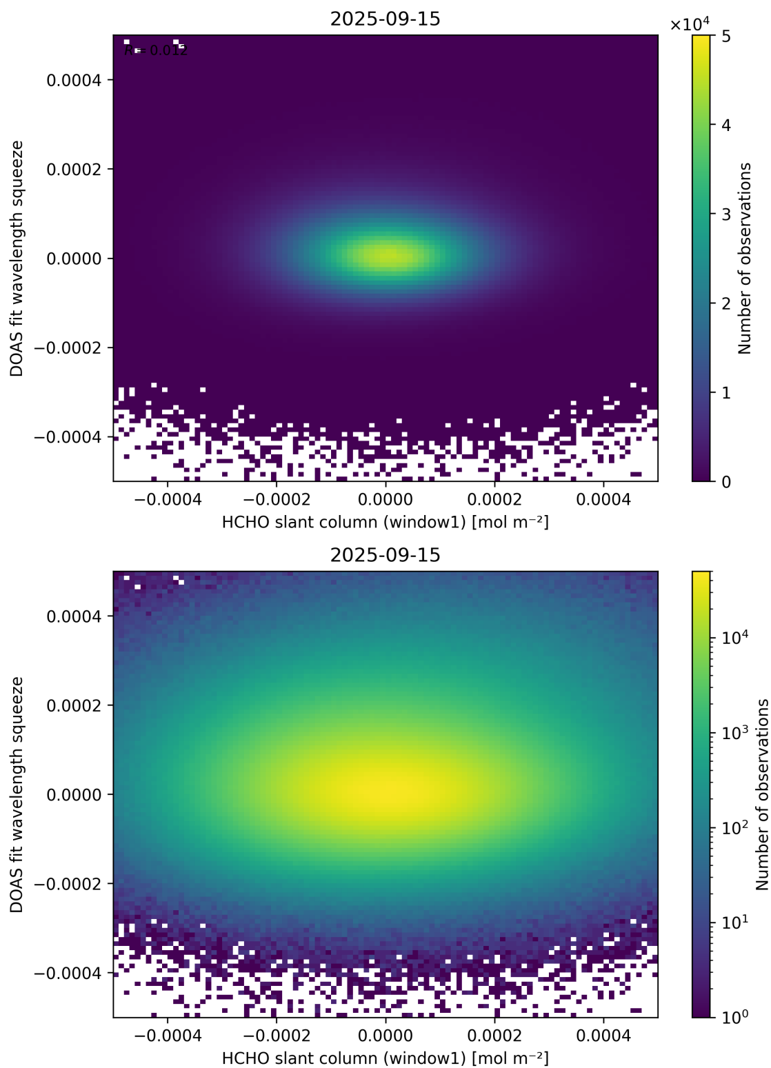
Figure 80: Scatter density plot of “HCHO slant column (window1)” against “DOAS fit wavelength squeeze” for 2025-09-15 to 2025-09-16.
