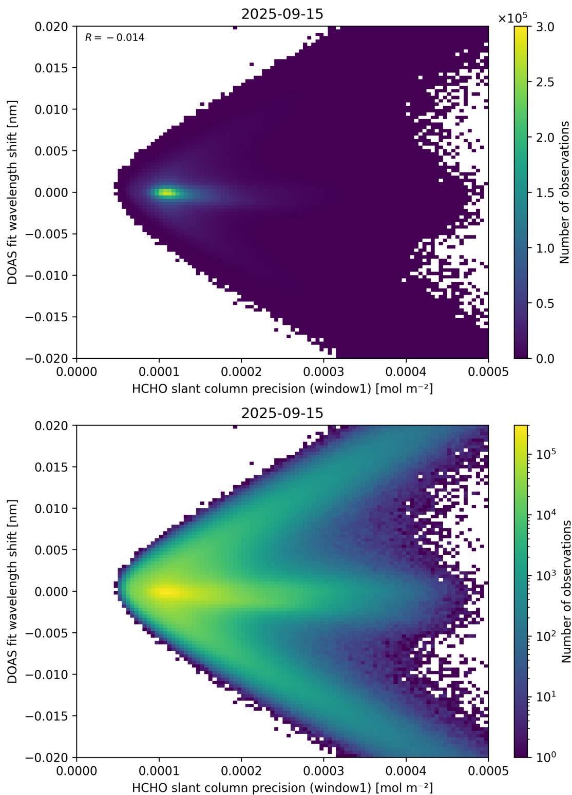
Figure 89: Scatter density plot of “HCHO slant column precision (window1)” against “DOAS fit wavelength shift” for 2025-09-15 to 2025-09-16.
