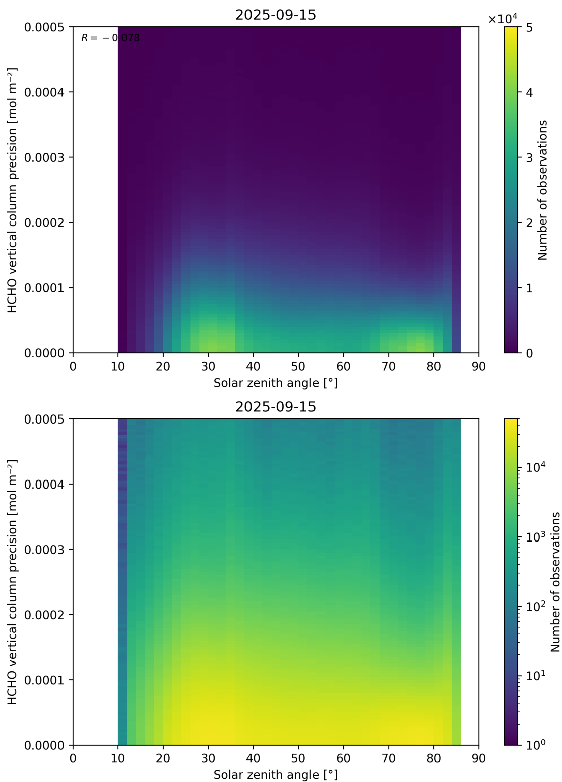
Figure 179: Scatter density plot of “Solar zenith angle” against “HCHO vertical column precision” for 2025-09-15 to 2025-09-16.
