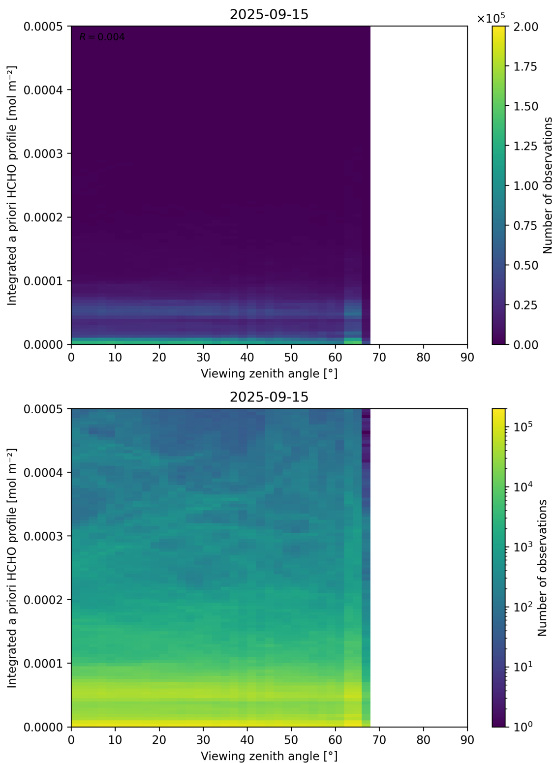
Figure 195: Scatter density plot of “Viewing zenith angle” against “Integrated a priori HCHO profile” for 2025-09-15 to 2025-09-16.
