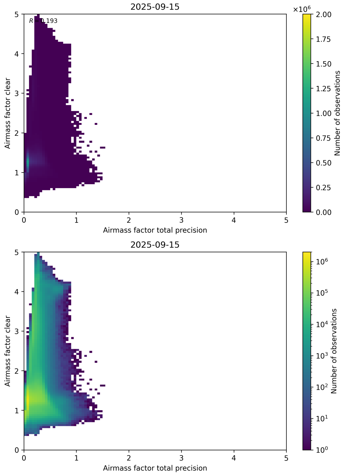
Figure 108: Scatter density plot of “Airmass factor total precision” against “Airmass factor clear” for 2025-09-15 to 2025-09-16.
