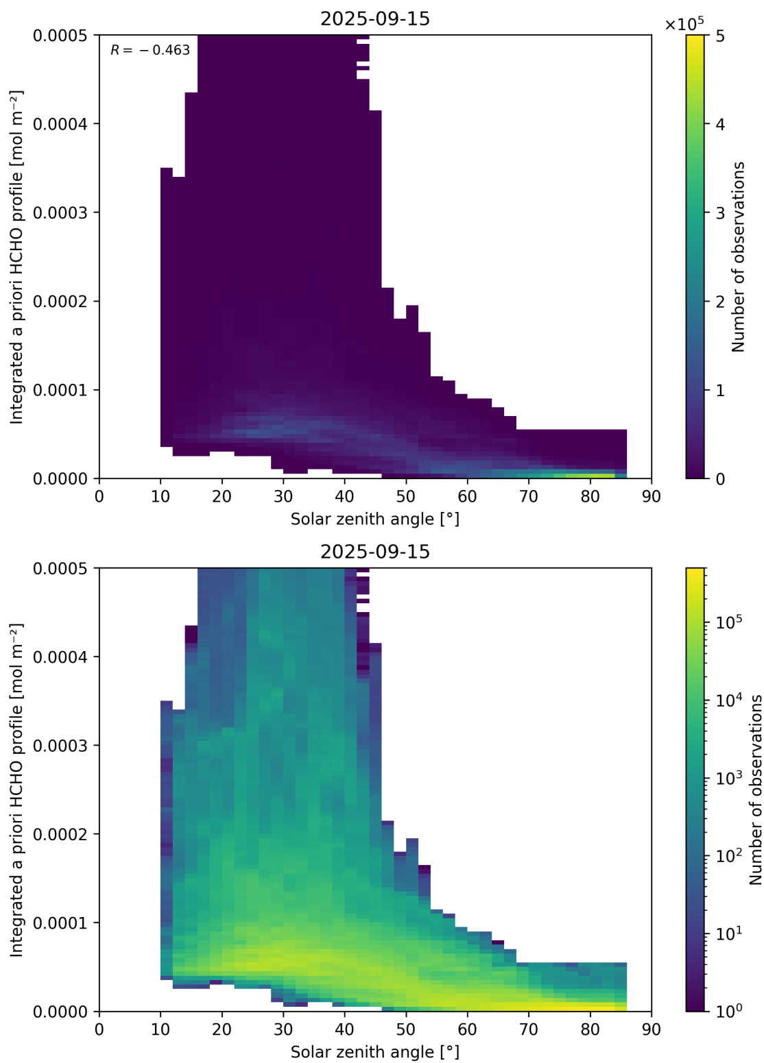
Figure 180: Scatter density plot of “Solar zenith angle” against “Integrated a priori HCHO profile” for 2025-09-15 to 2025-09-16.
