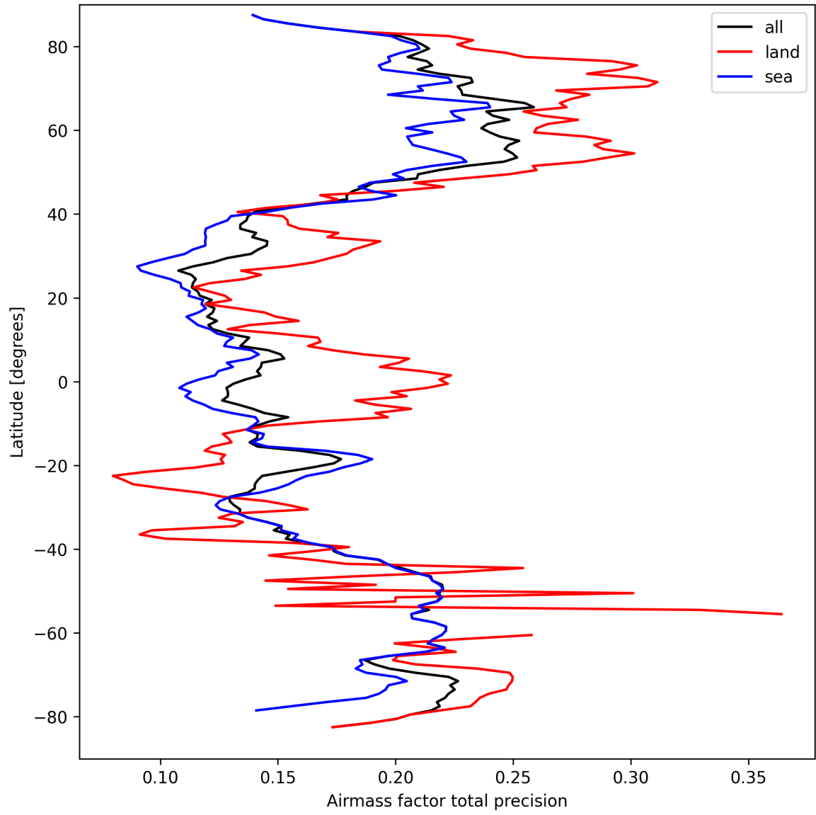
Figure 27: Zonal average of “Airmass factor total precision” for 2025-09-15 to 2025-09-16.
