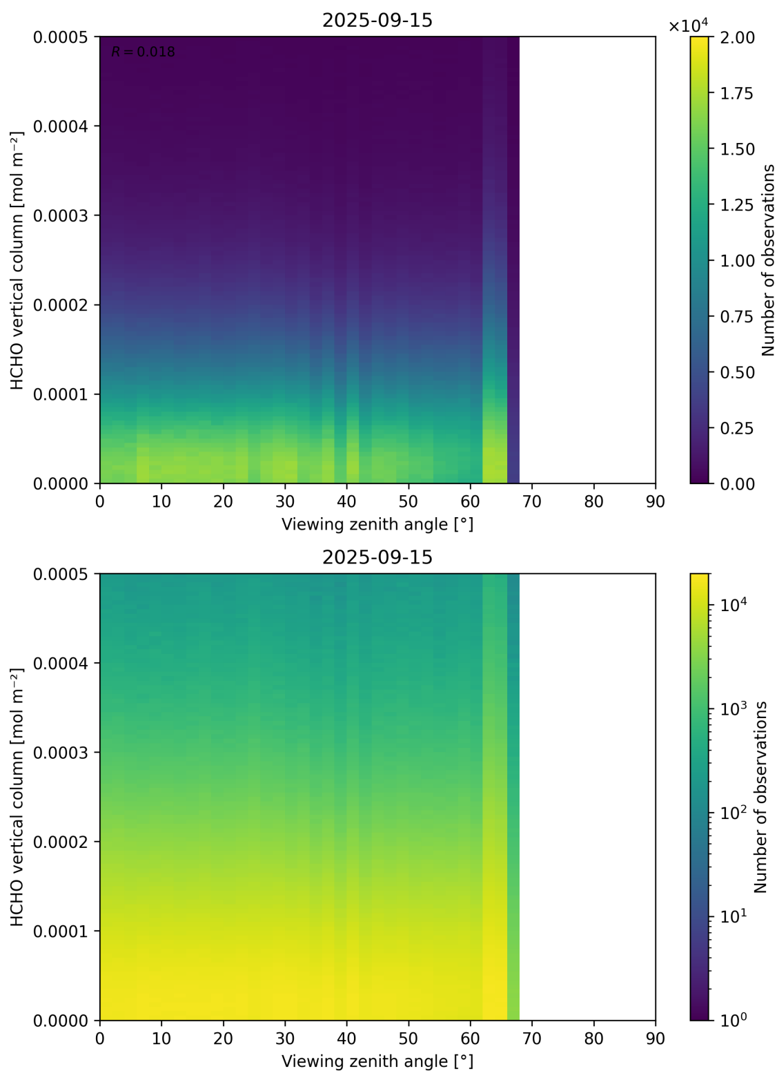
Figure 192: Scatter density plot of “Viewing zenith angle” against “HCHO vertical column” for 2025-09-15 to 2025-09-16.
