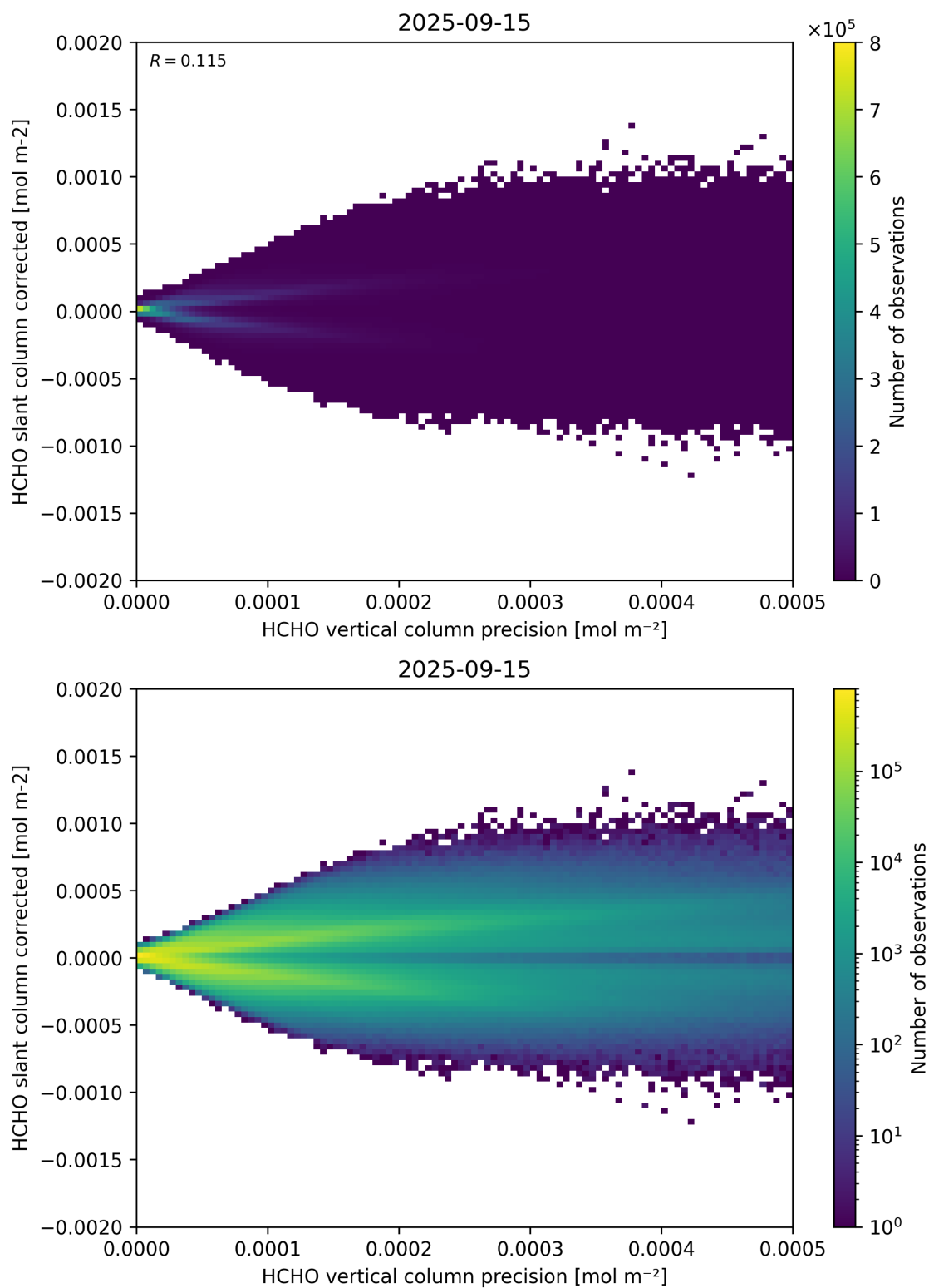
Figure 140: Scatter density plot of “HCHO vertical column precision” against “HCHO slant column corrected” for 2025-09-15 to 2025-09-16.
