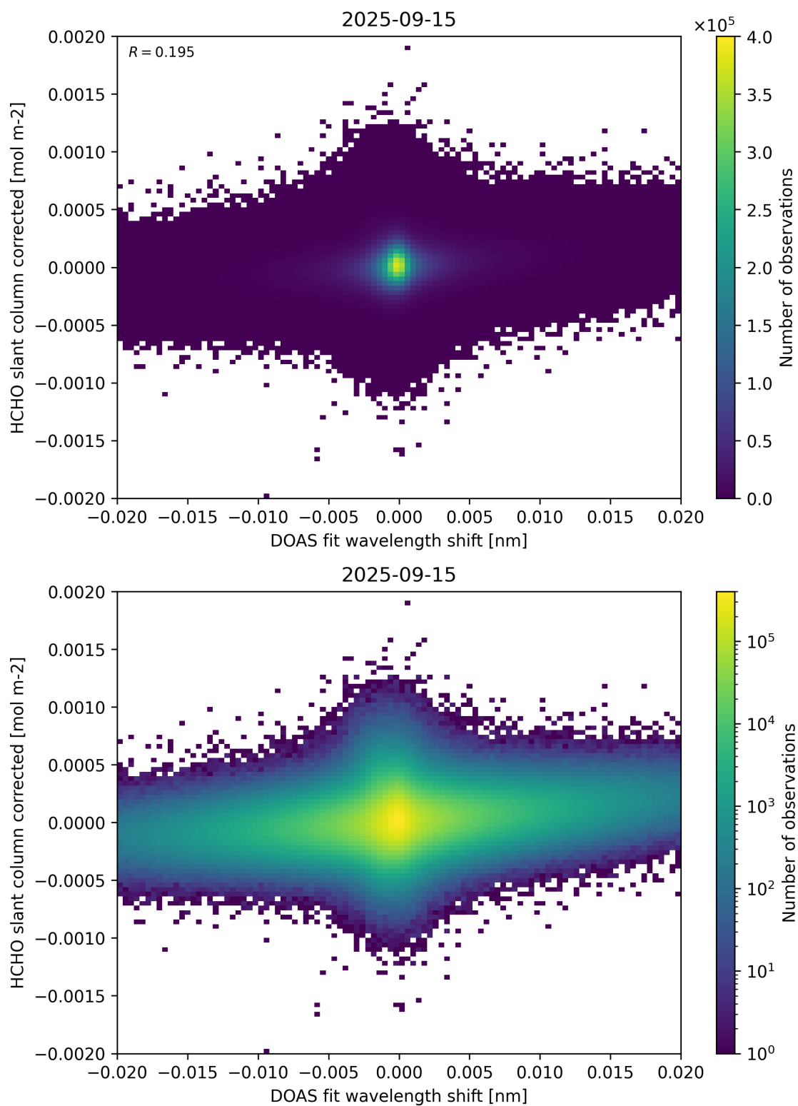
Figure 66: Scatter density plot of “DOAS fit wavelength shift” against “HCHO slant column corrected” for 2025-09-15 to 2025-09-16.
