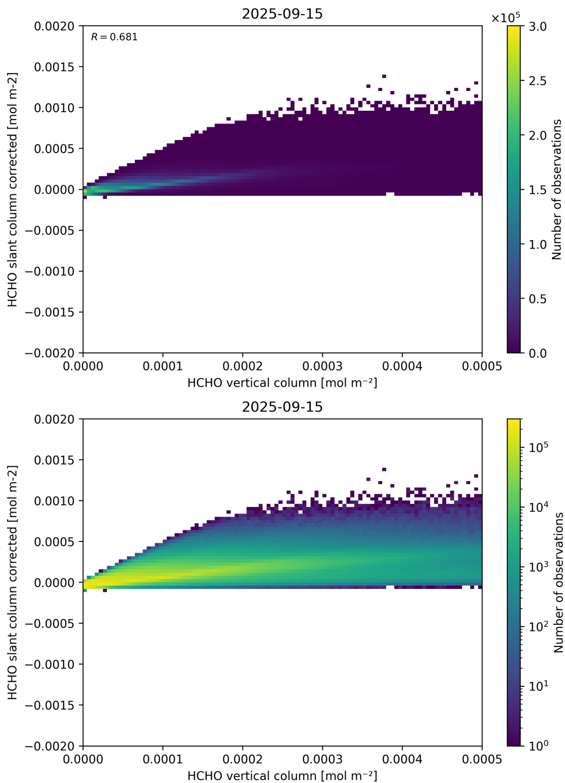
Figure 127: Scatter density plot of “HCHO vertical column” against “HCHO slant column corrected” for 2025-09-15 to 2025-09-16.
