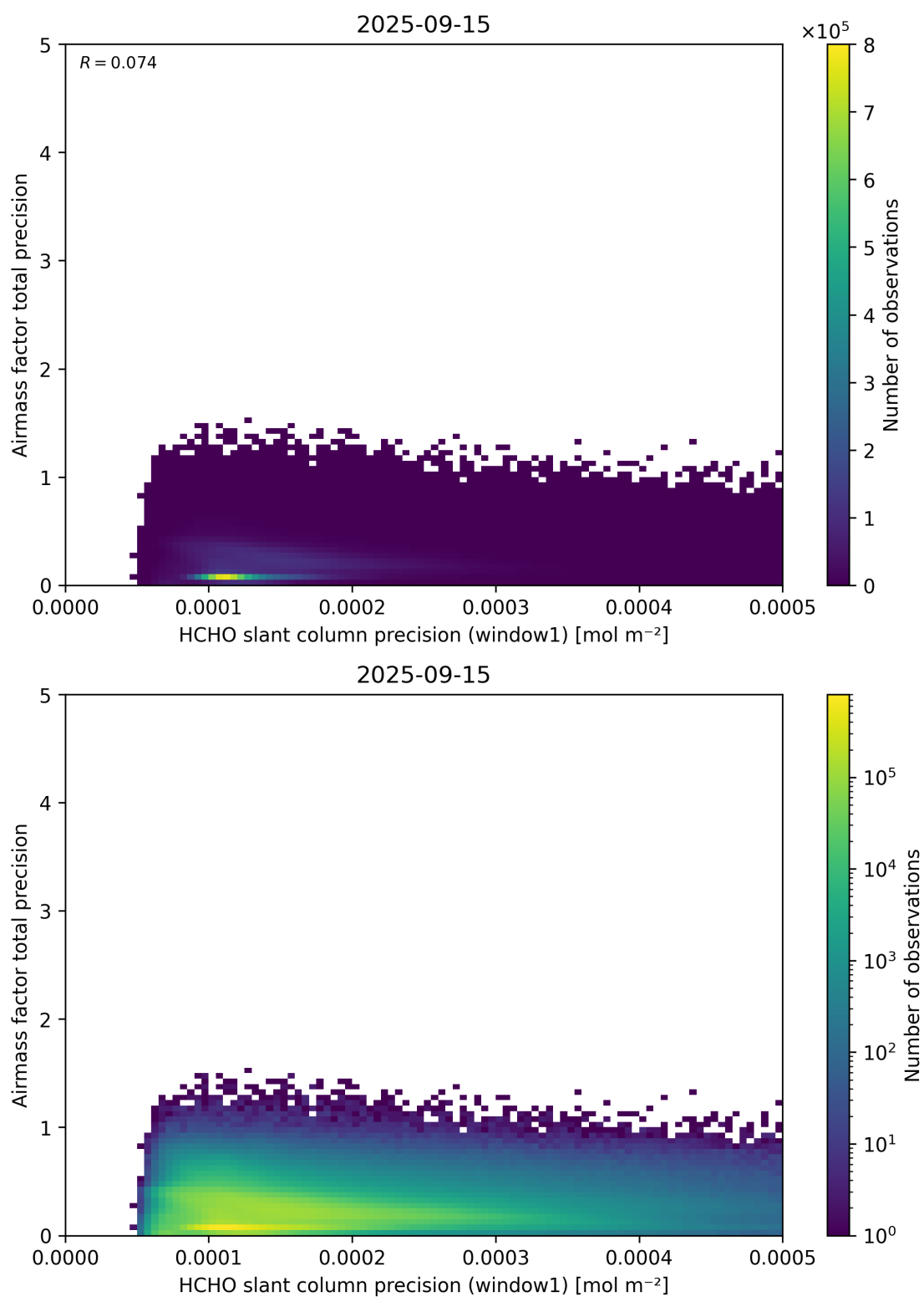
Figure 95: Scatter density plot of “HCHO slant column precision (window1)” against “Airmass factor total precision” for 2025-09-15 to 2025-09-16.
