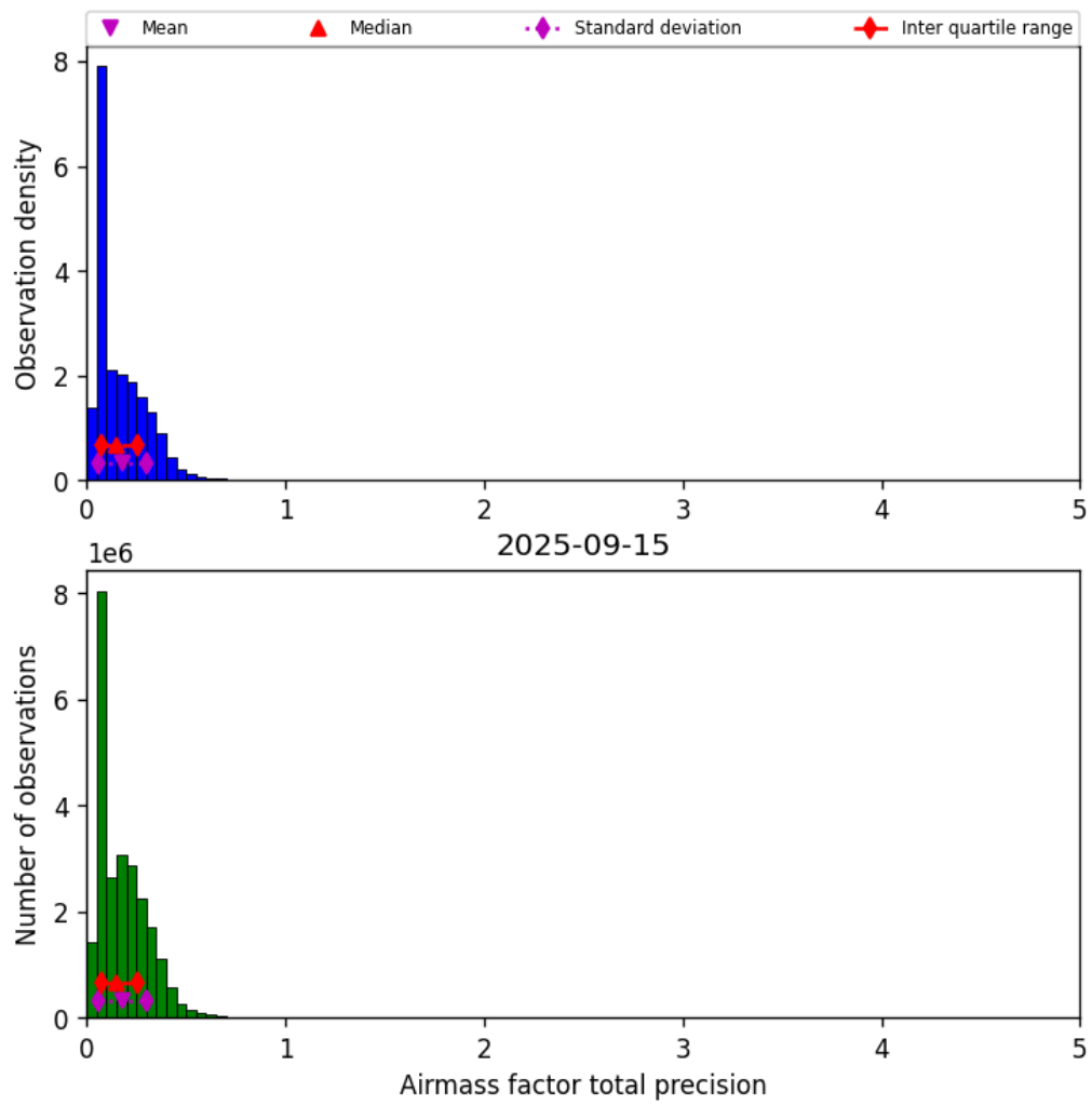
Figure 41: Histogram of “Airmass factor total precision” for 2025-09-15 to 2025-09-16
