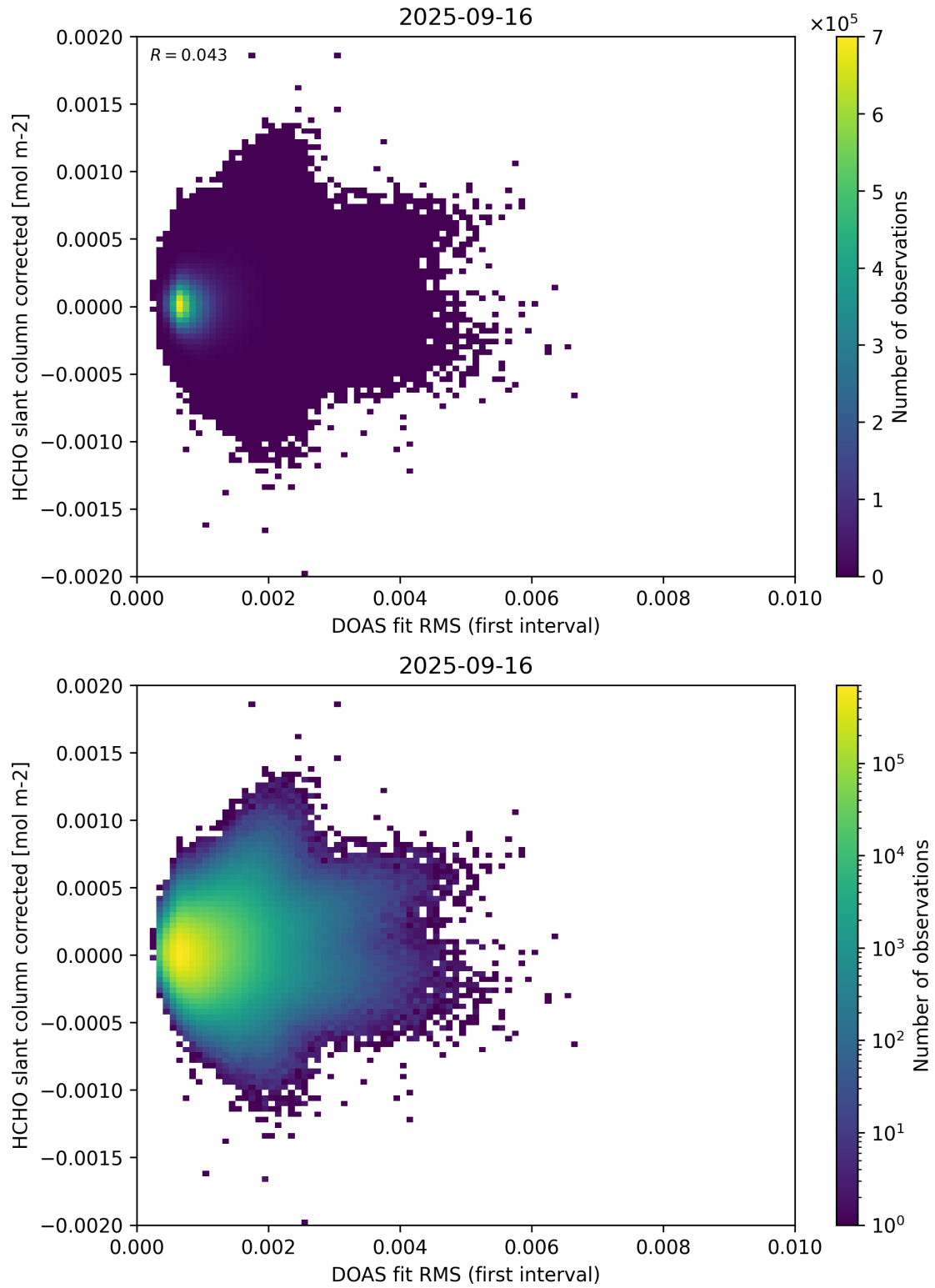
Figure 62: Scatter density plot of “DOAS fit RMS (first interval)” against “HCHO slant column corrected” for 2025-09-15 to 2025-09-17.
