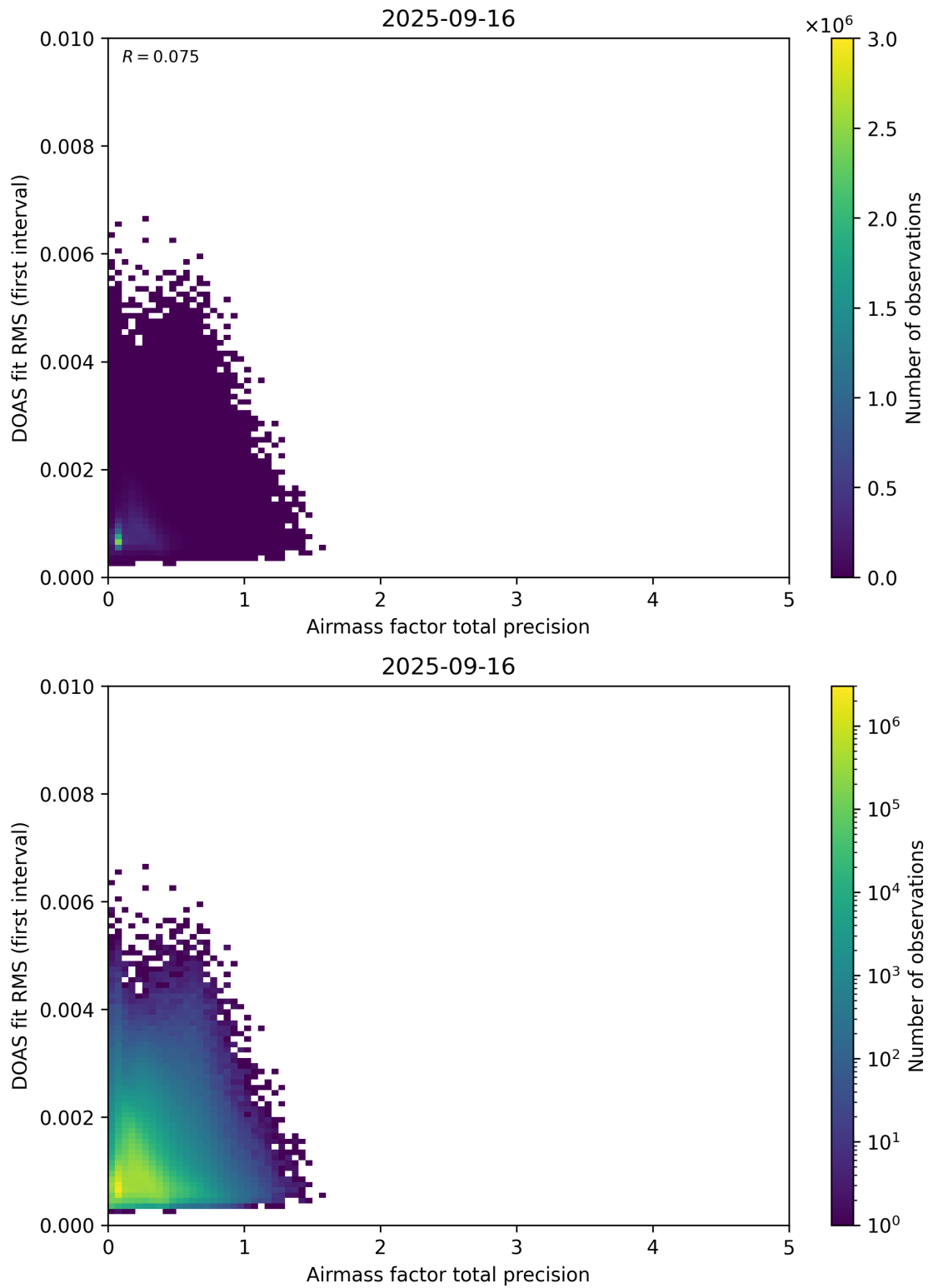
Figure 105: Scatter density plot of “Airmass factor total precision” against “DOAS fit RMS (first interval)” for 2025-09-15 to 2025-09-17.
