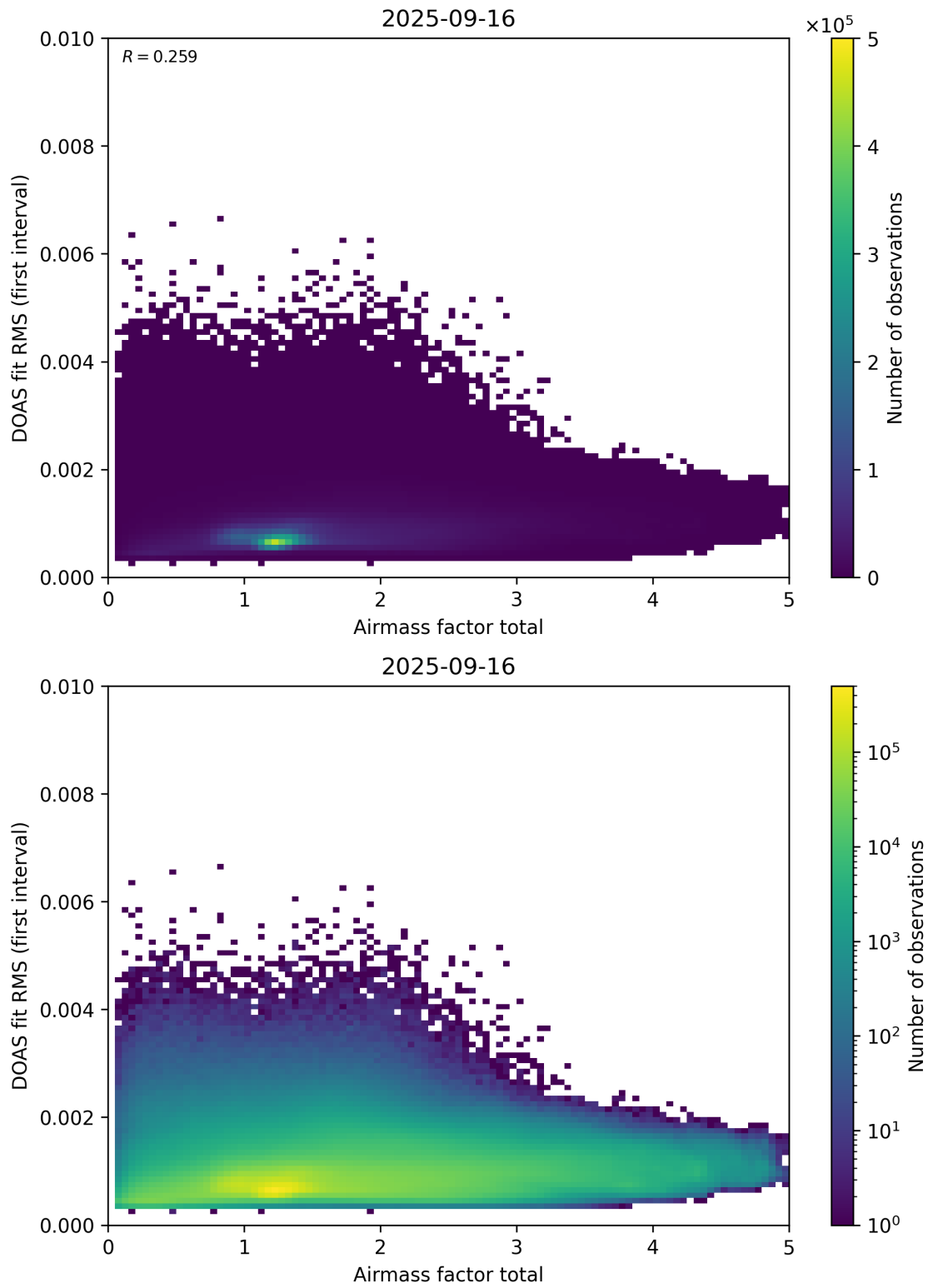
Figure 97: Scatter density plot of “Airmass factor total” against “DOAS fit RMS (first interval)” for 2025-09-15 to 2025-09-17.
