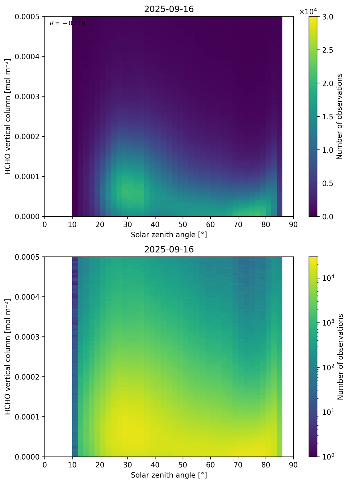
Figure 177: Scatter density plot of “Solar zenith angle” against “HCHO vertical column” for 2025-09-15 to 2025-09-17.
