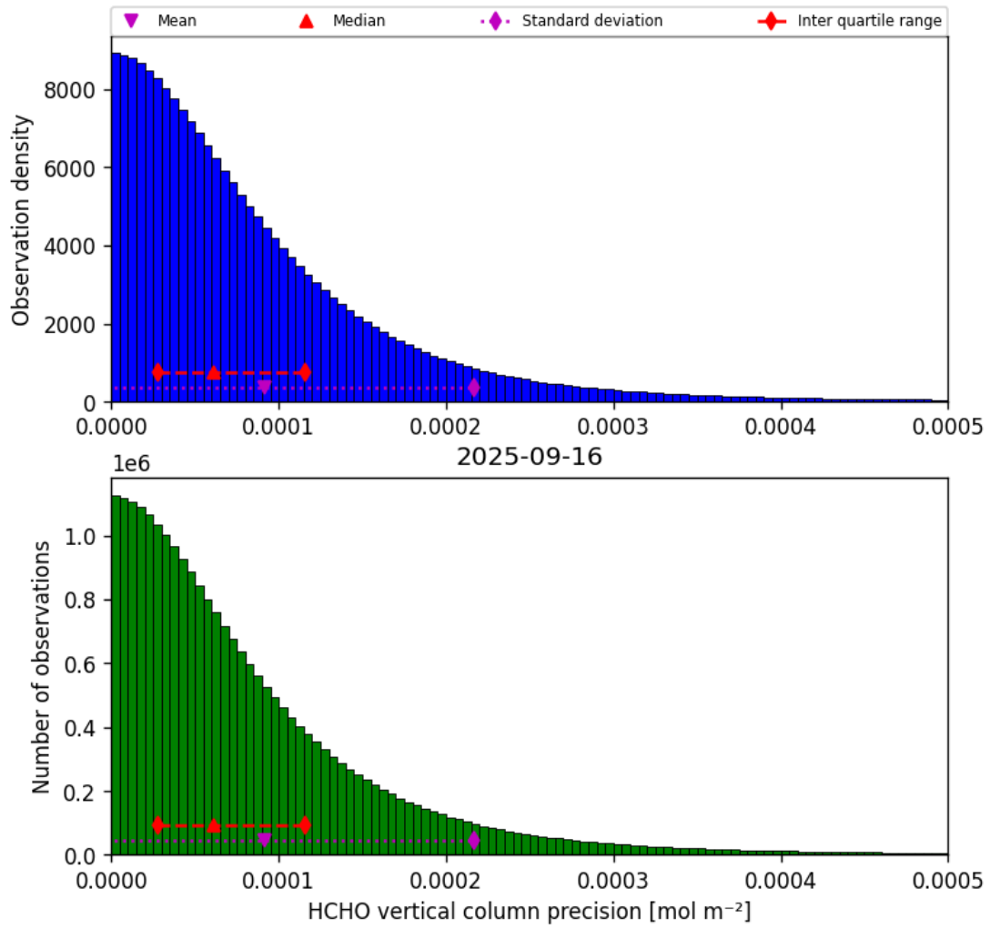
Figure 36: Histogram of “HCHO vertical column precision” for 2025-09-15 to 2025-09-17
