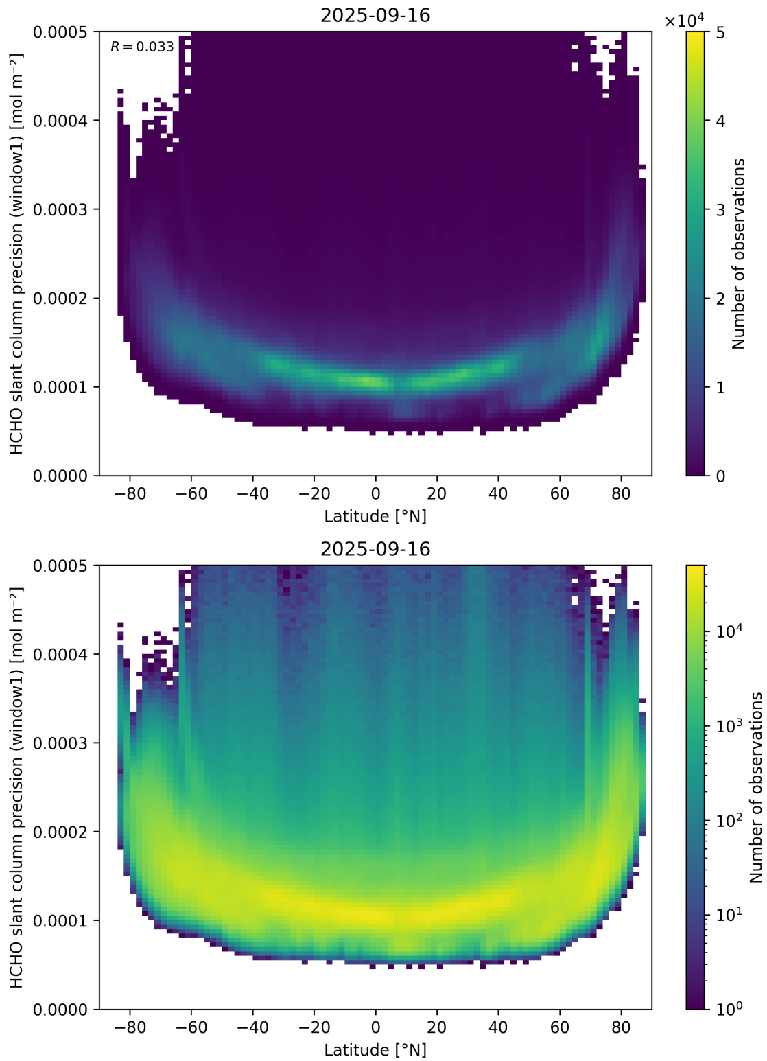
Figure 160: Scatter density plot of “Latitude” against “HCHO slant column precision (window1)” for 2025-09-15 to 2025-09-17.
