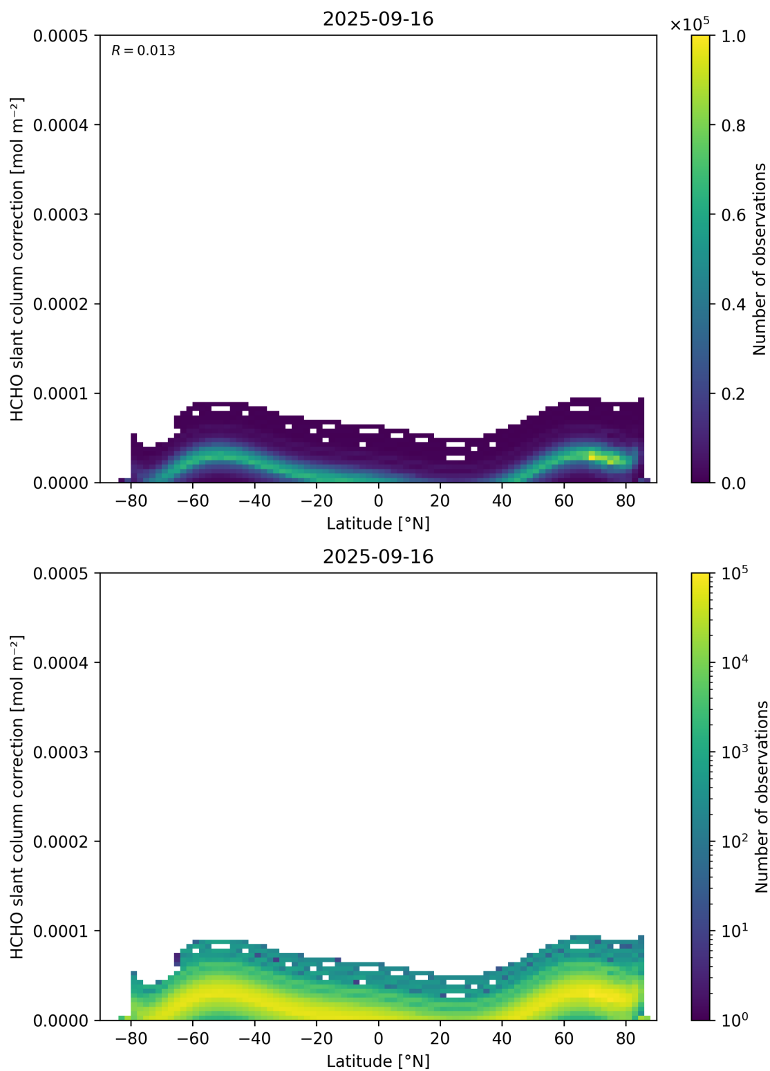
Figure 158: Scatter density plot of “Latitude” against “HCHO slant column correction” for 2025-09-15 to 2025-09-17.
