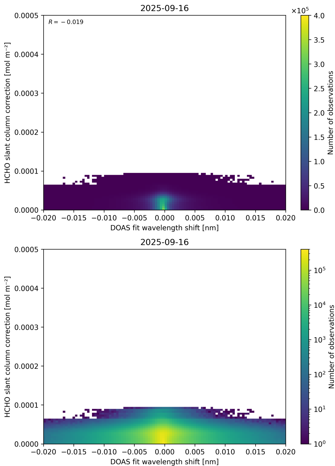
Figure 67: Scatter density plot of “DOAS fit wavelength shift” against “HCHO slant column correction” for 2025-09-15 to 2025-09-17.
