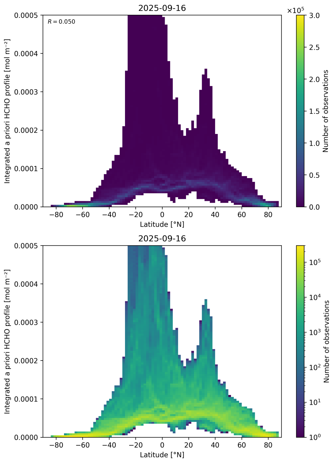
Figure 166: Scatter density plot of “Latitude” against “Integrated a priori HCHO profile” for 2025-09-15 to 2025-09-17.
