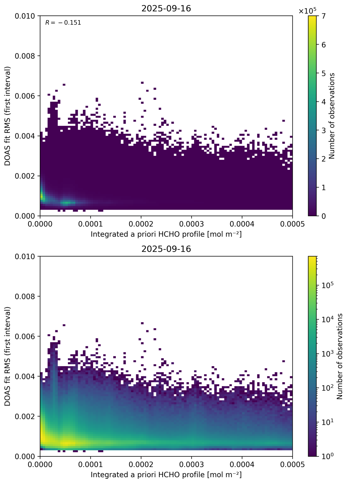
Figure 148: Scatter density plot of “Integrated a priori HCHO profile” against “DOAS fit RMS (first interval)” for 2025-09-15 to 2025-09-17.
