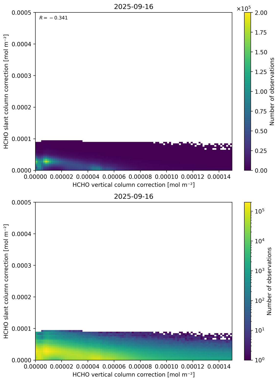
Figure 117: Scatter density plot of “HCHO vertical column correction” against “HCHO slant column correction” for 2025-09-15 to 2025-09-17.
