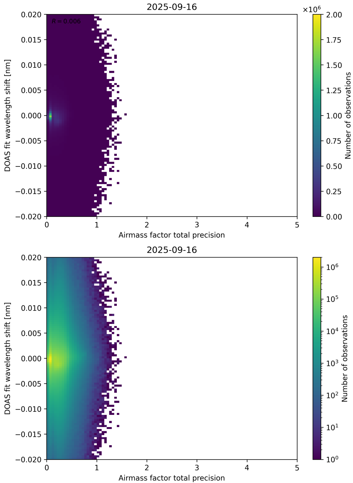
Figure 106: Scatter density plot of “Airmass factor total precision” against “DOAS fit wavelength shift” for 2025-09-15 to 2025-09-17.
