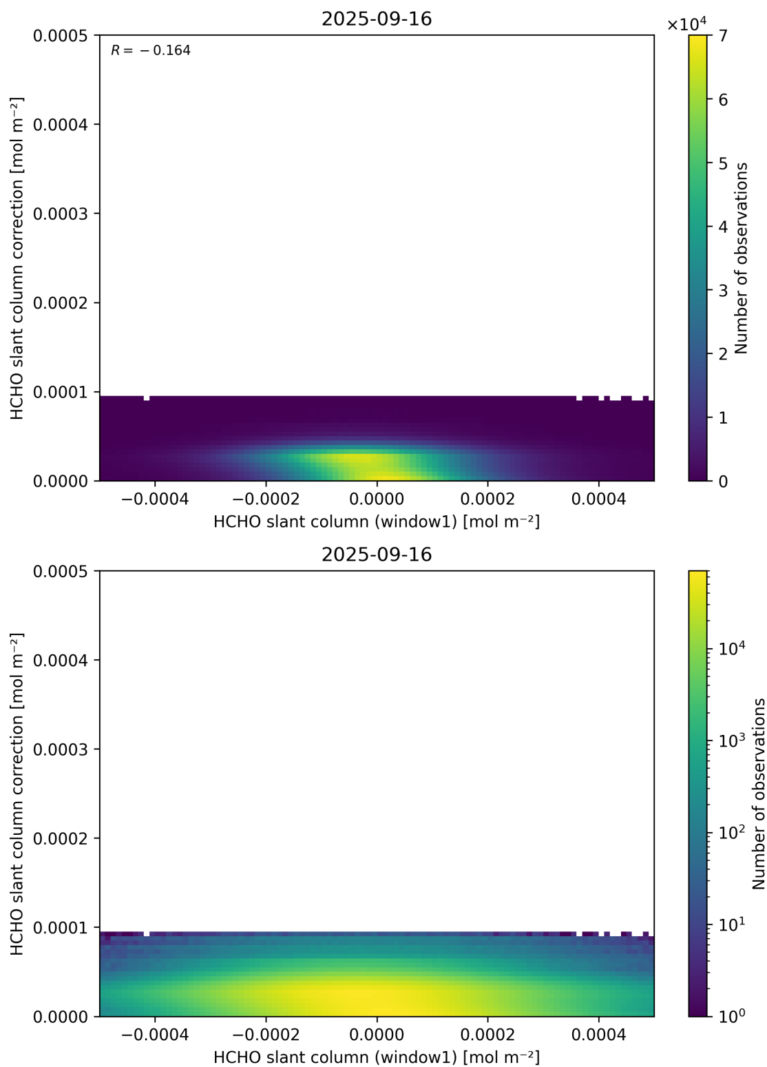
Figure 83: Scatter density plot of “HCHO slant column (window1)” against “HCHO slant column correction” for 2025-09-15 to 2025-09-17.
