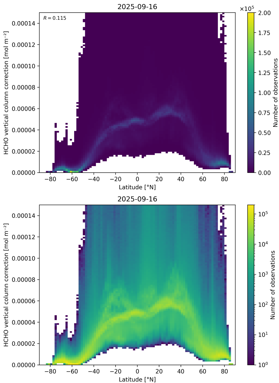
Figure 164: Scatter density plot of “Latitude” against “HCHO vertical column correction” for 2025-09-15 to 2025-09-17.
