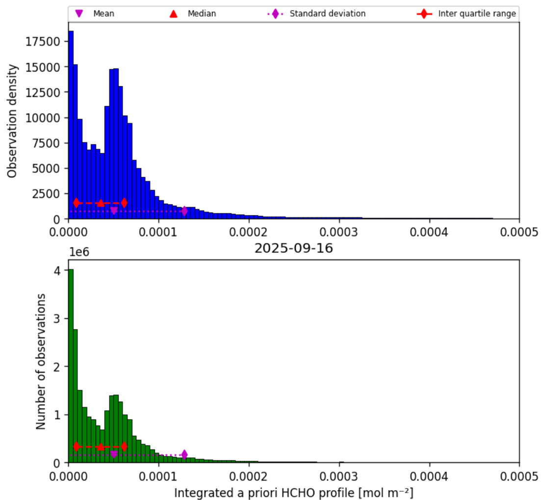
Figure 43: Histogram of “Integrated a priori HCHO profile” for 2025-09-15 to 2025-09-17
