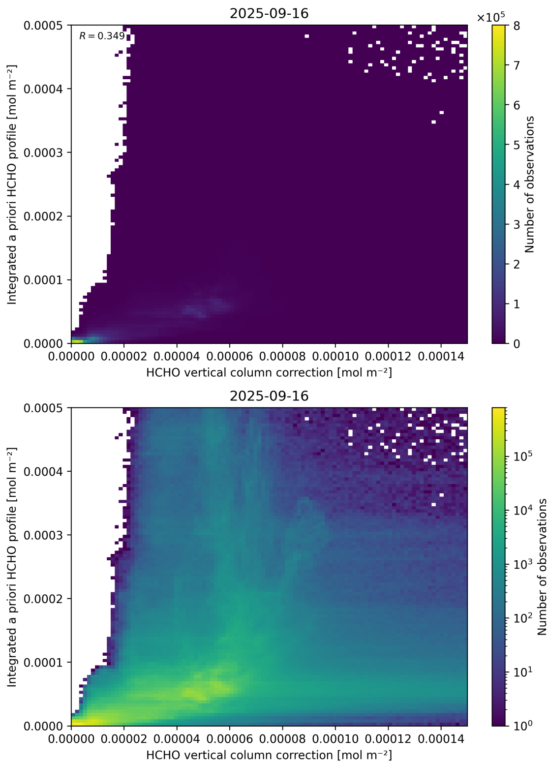
Figure 122: Scatter density plot of “HCHO vertical column correction” against “Integrated a priori HCHO profile” for 2025-09-15 to 2025-09-17.
