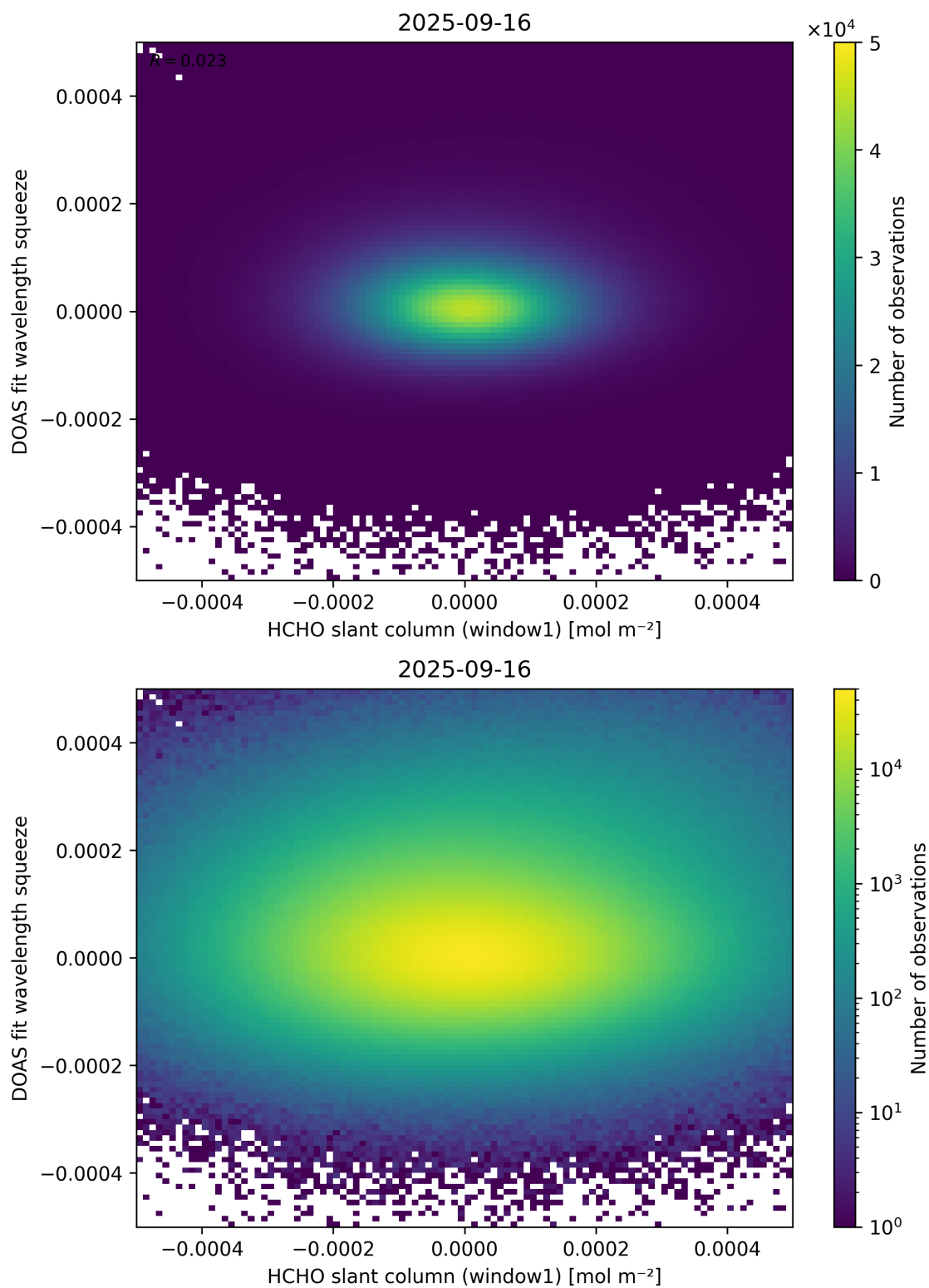
Figure 80: Scatter density plot of “HCHO slant column (window1)” against “DOAS fit wavelength squeeze” for 2025-09-15 to 2025-09-17.
