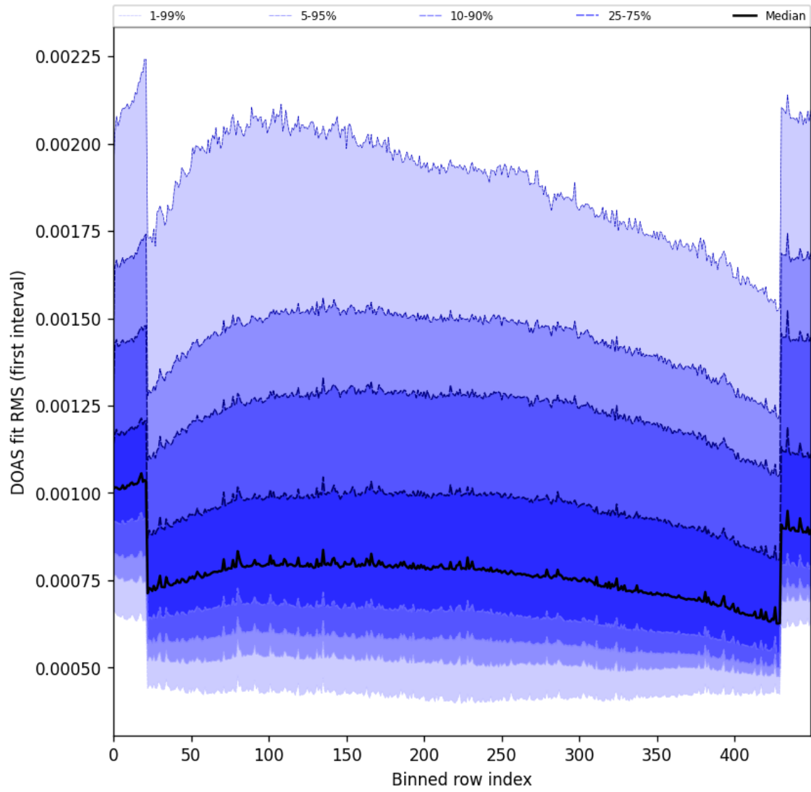
Figure 60: Along track statistics of “DOAS fit RMS (first interval)” for 2025-09-15 to 2025-09-17
