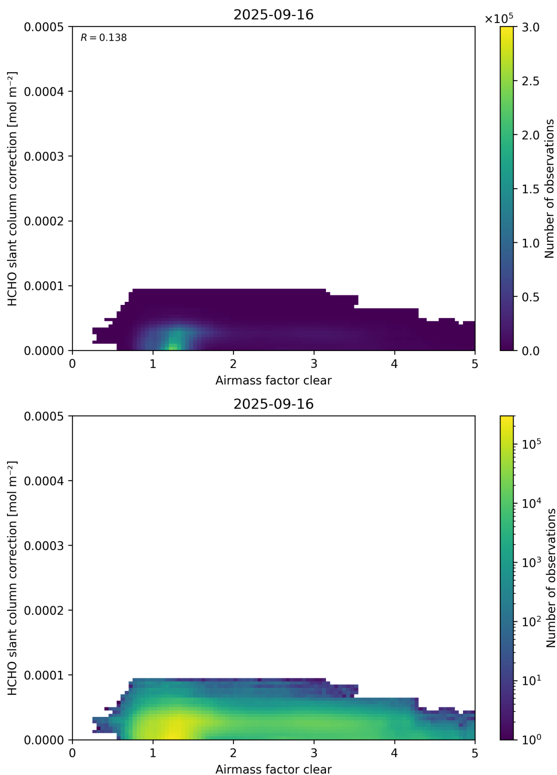
Figure 75: Scatter density plot of “Airmass factor clear” against “HCHO slant column correction” for 2025-09-15 to 2025-09-17.
