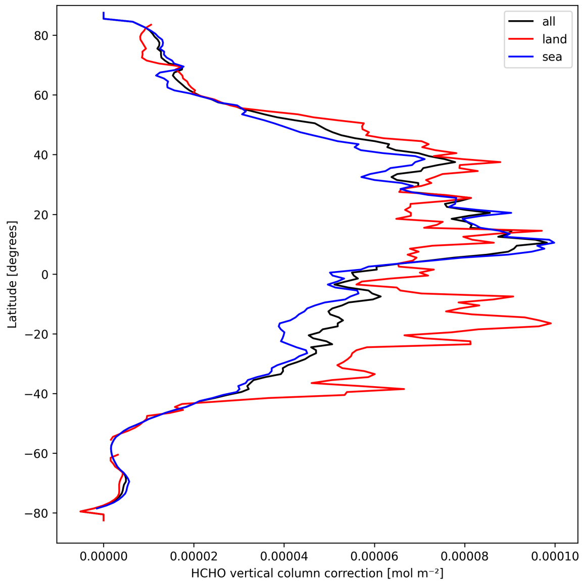
Figure 23: Zonal average of “HCHO vertical column correction” for 2025-09-15 to 2025-09-17.
