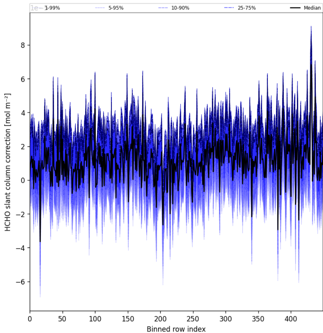
Figure 61: Along track statistics of "HCHO slant column correction" for 2025-09-15 to 2025-09-17
