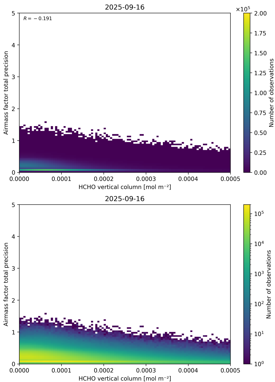
Figure 132: Scatter density plot of “HCHO vertical column” against “Airmass factor total precision” for 2025-09-15 to 2025-09-17.
