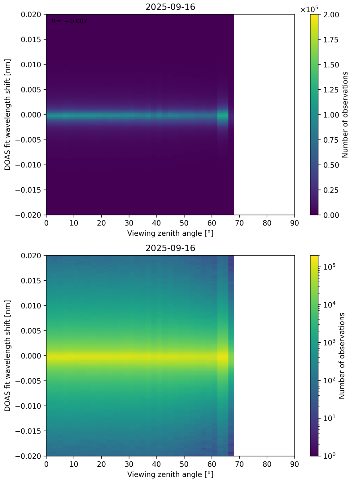
Figure 183: Scatter density plot of “Viewing zenith angle” against “DOAS fit wavelength shift” for 2025-09-15 to 2025-09-17.
