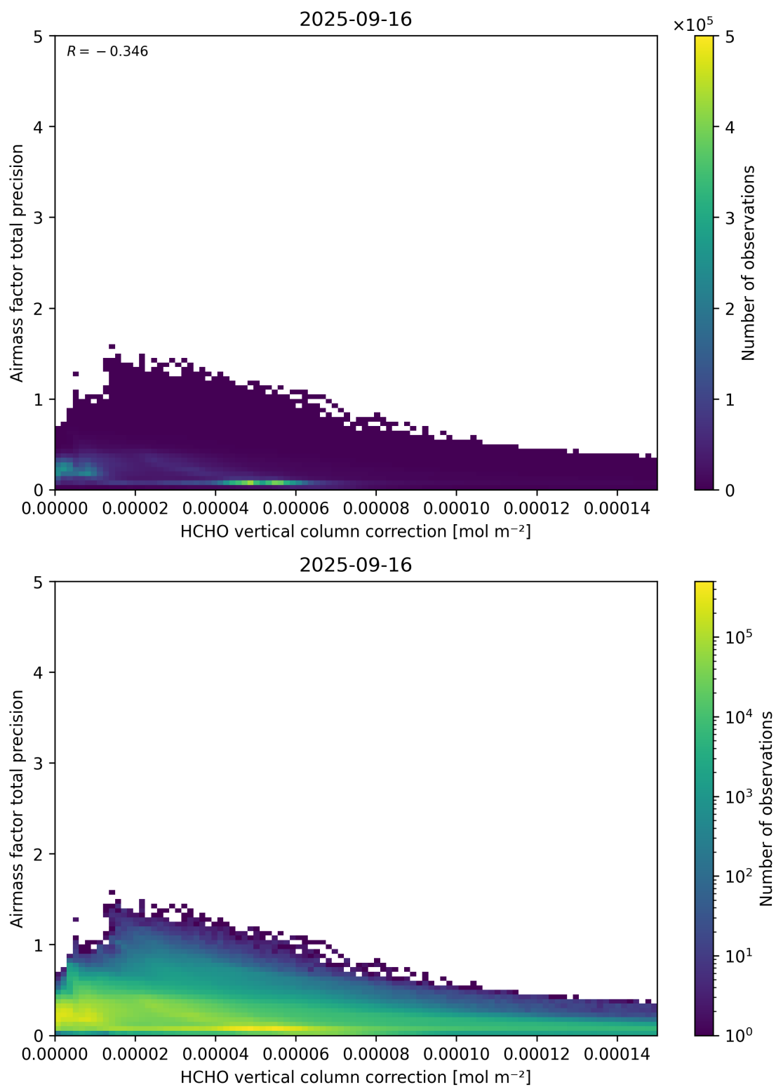
Figure 121: Scatter density plot of “HCHO vertical column correction” against “Airmass factor total precision” for 2025-09-15 to 2025-09-17.
