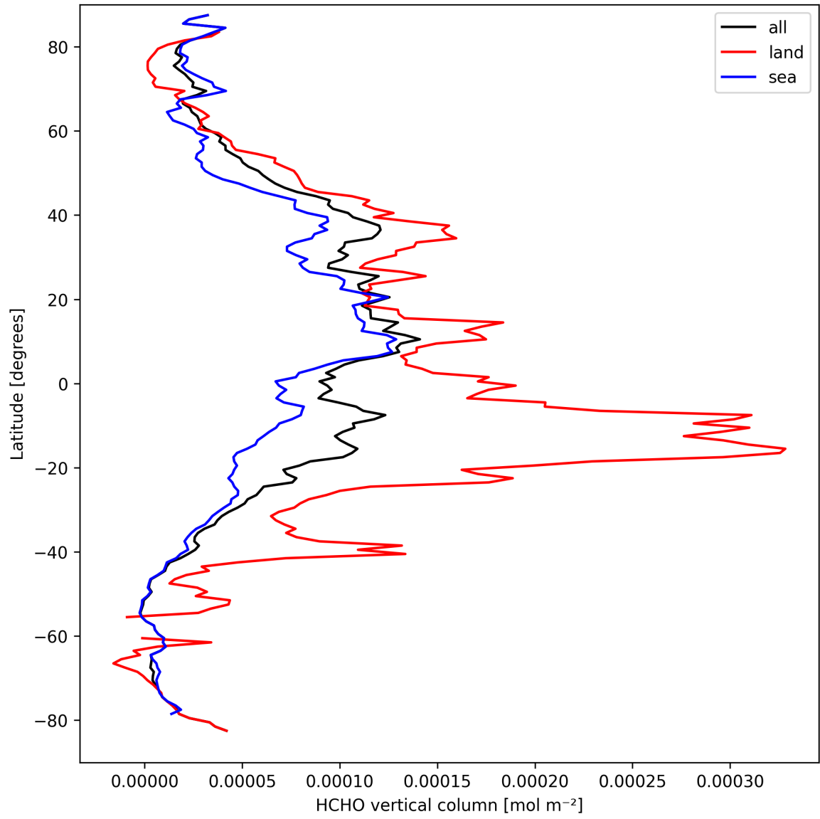
Figure 21: Zonal average of “HCHO vertical column” for 2025-09-15 to 2025-09-17.
