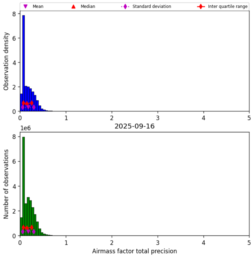
Figure 41: Histogram of “Airmass factor total precision” for 2025-09-15 to 2025-09-17
