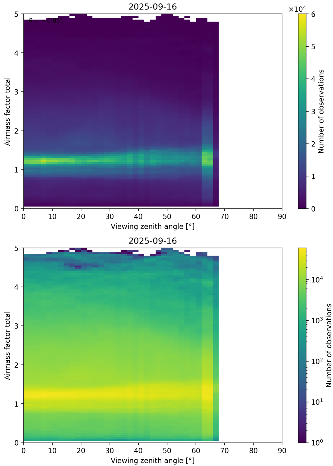
Figure 190: Scatter density plot of “Viewing zenith angle” against “Airmass factor total” for 2025-09-15 to 2025-09-17.
