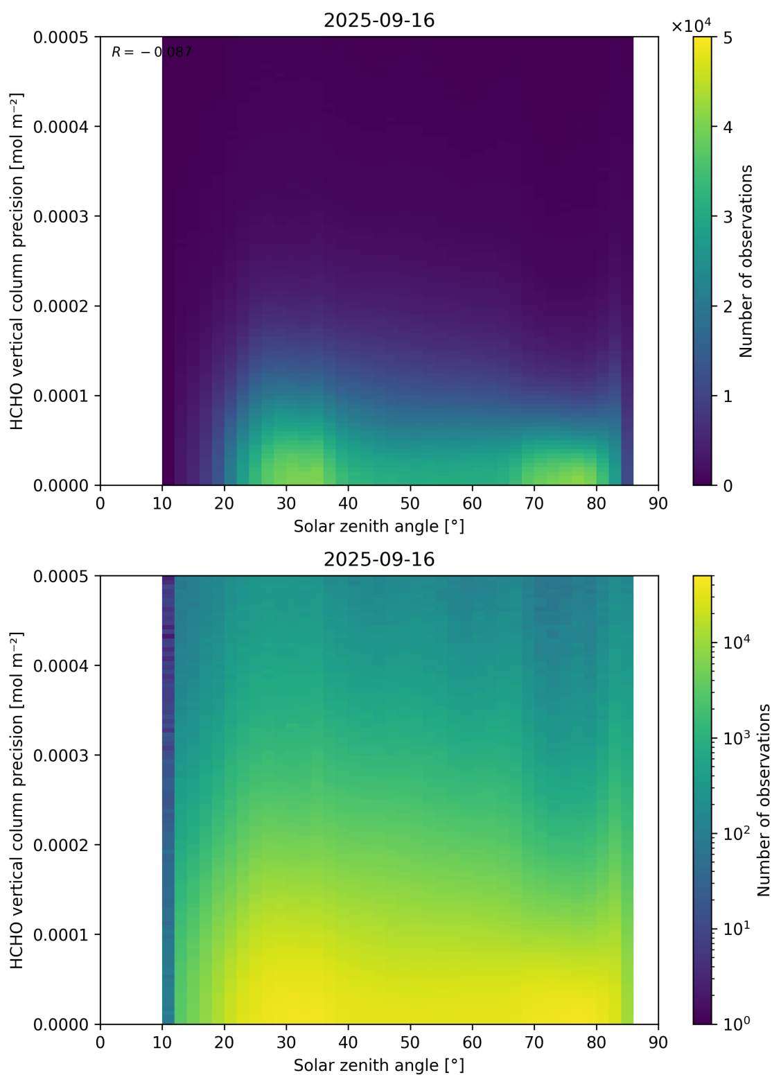
Figure 179: Scatter density plot of “Solar zenith angle” against “HCHO vertical column precision” for 2025-09-15 to 2025-09-17.
