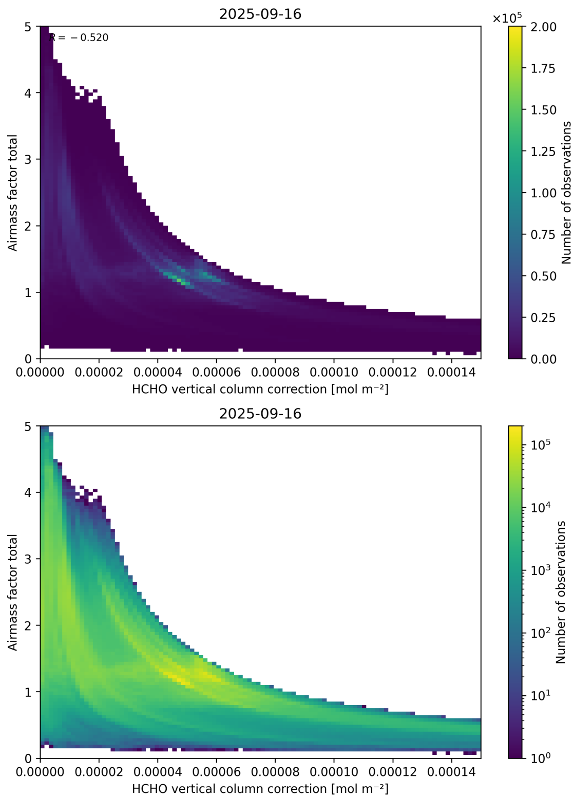
Figure 120: Scatter density plot of “HCHO vertical column correction” against “Airmass factor total” for 2025-09-15 to 2025-09-17.
