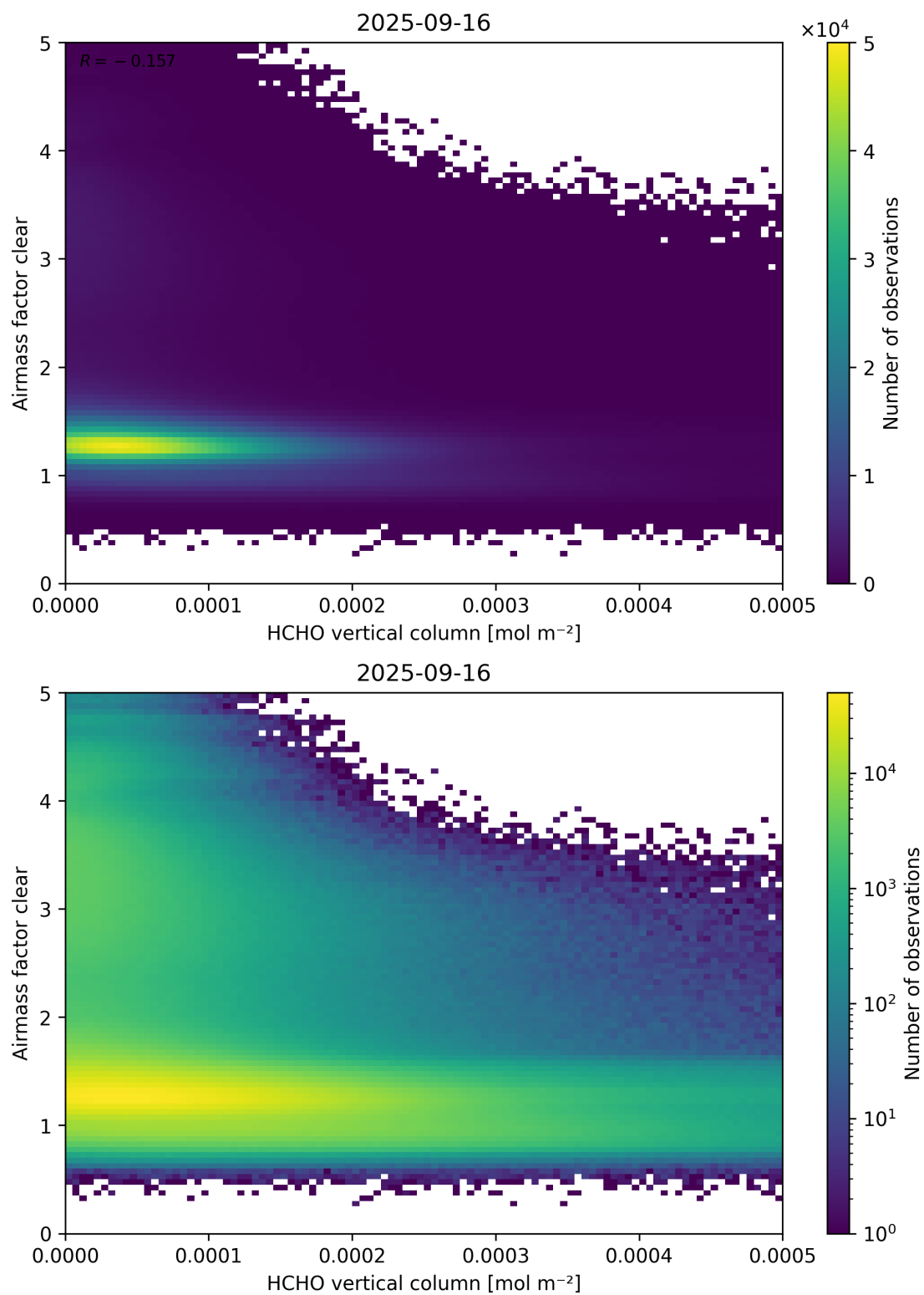
Figure 126: Scatter density plot of “HCHO vertical column” against “Airmass factor clear” for 2025-09-15 to 2025-09-17.
