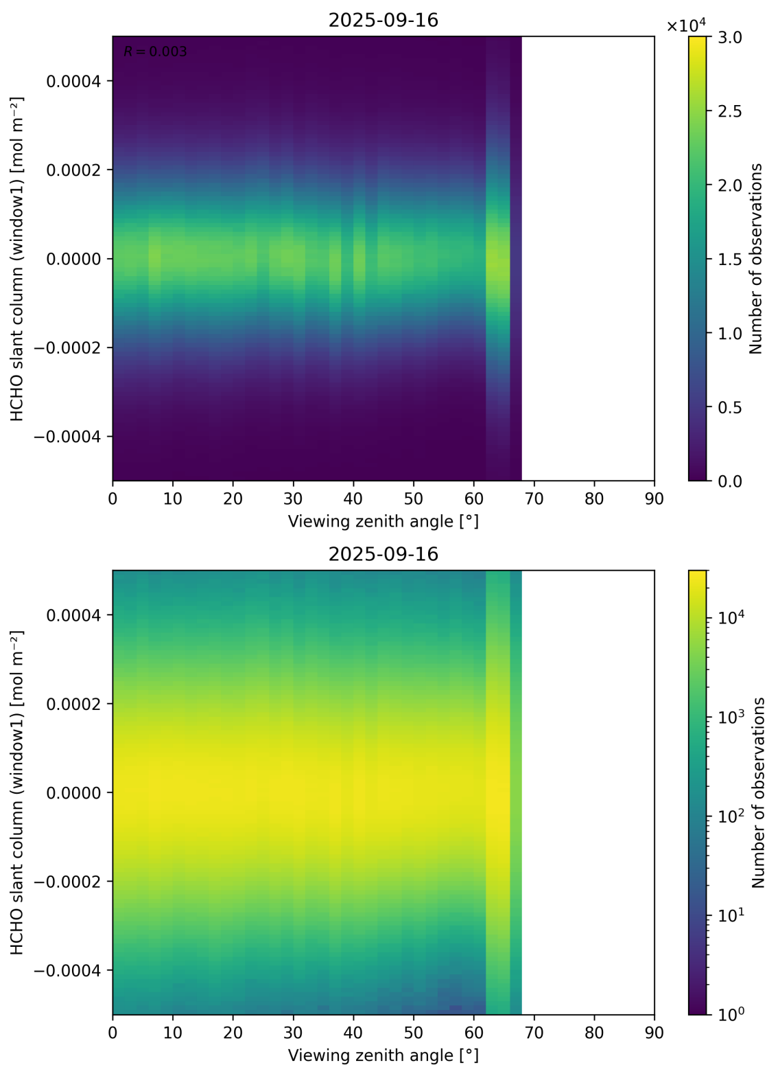
Figure 188: Scatter density plot of “Viewing zenith angle” against “HCHO slant column (window1)” for 2025-09-15 to 2025-09-17.
