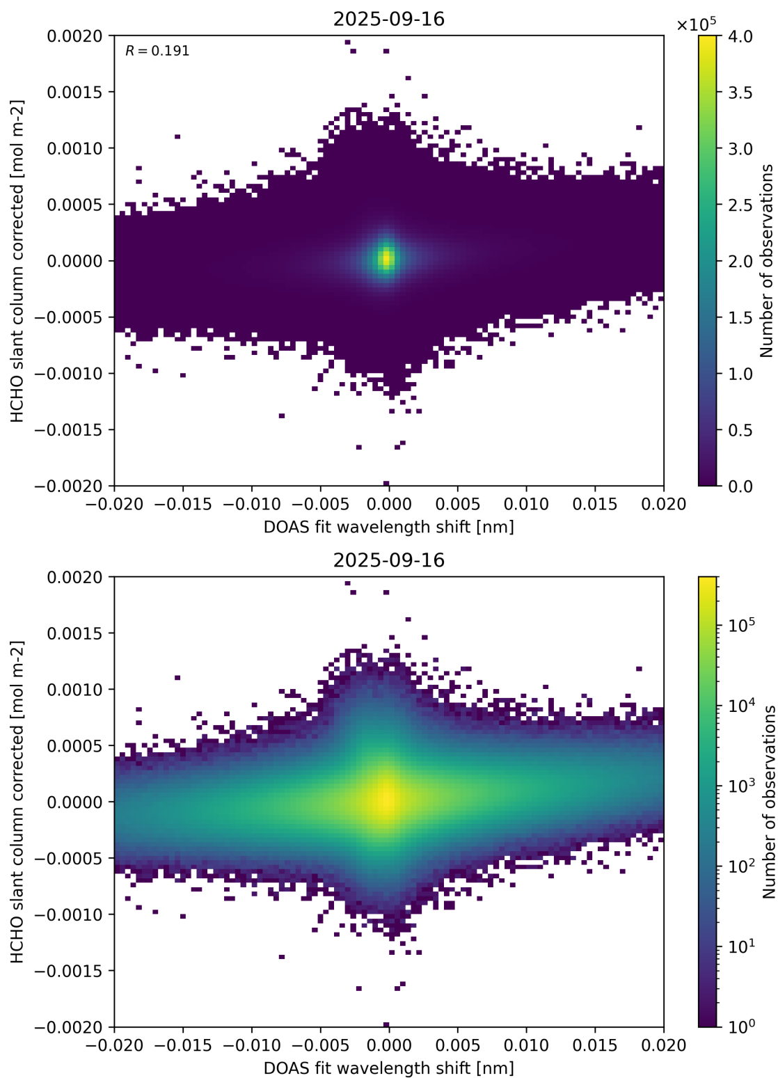
Figure 66: Scatter density plot of “DOAS fit wavelength shift” against “HCHO slant column corrected” for 2025-09-15 to 2025-09-17.
