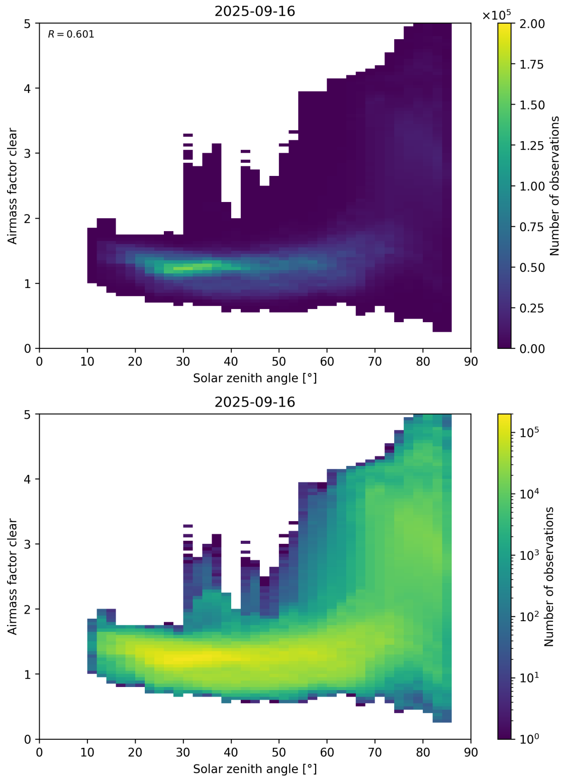
Figure 170: Scatter density plot of “Solar zenith angle” against “Airmass factor clear” for 2025-09-15 to 2025-09-17.
