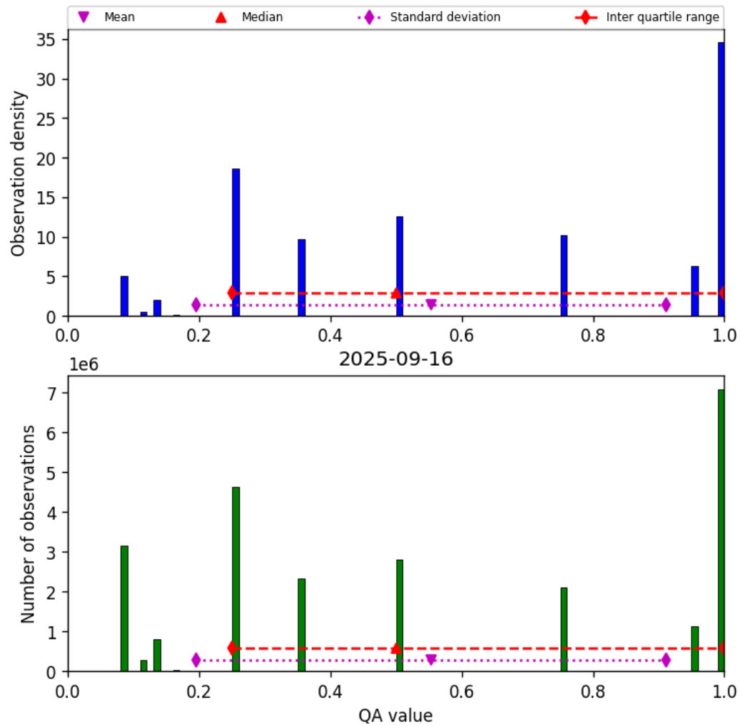
Figure 34: Histogram of “QA value” for 2025-09-15 to 2025-09-17
