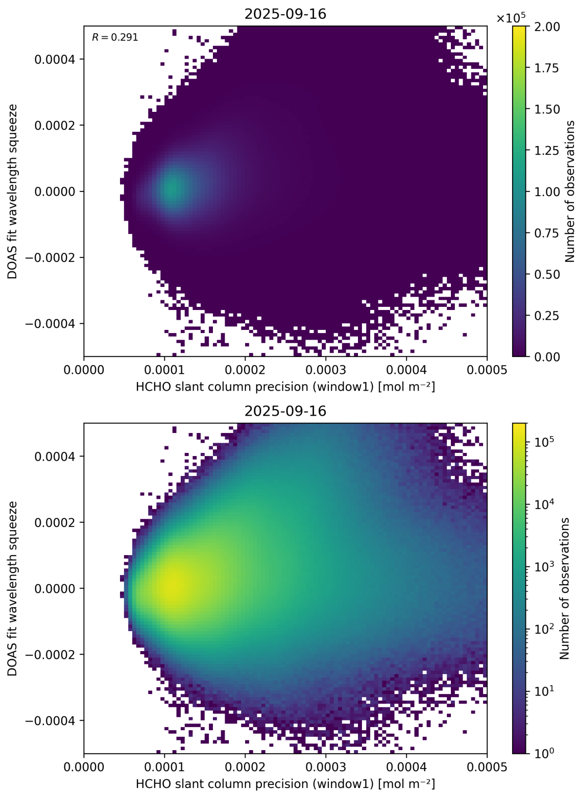
Figure 90: Scatter density plot of “HCHO slant column precision (window1)” against “DOAS fit wavelength squeeze” for 2025-09-15 to 2025-09-17.
