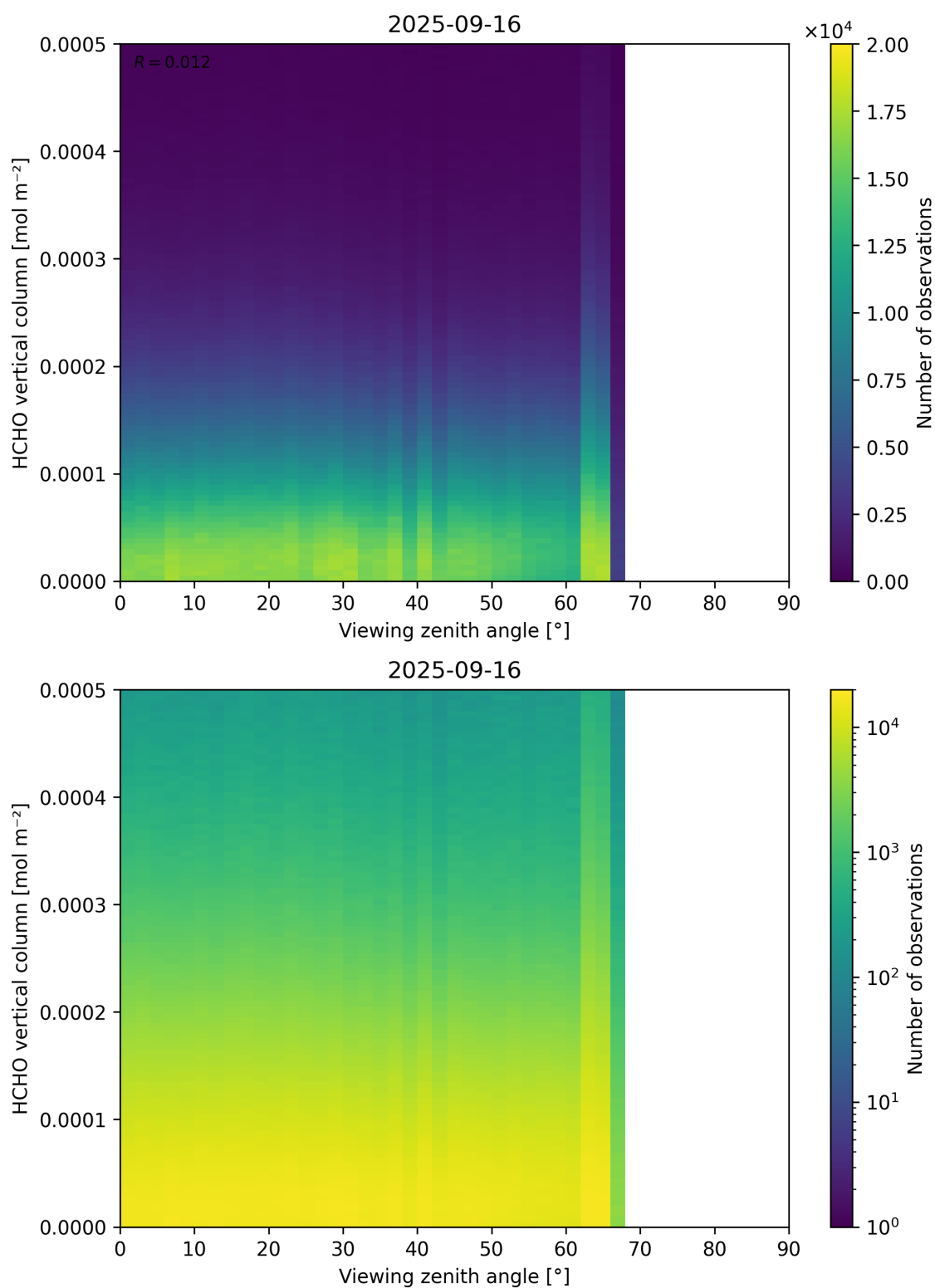
Figure 192: Scatter density plot of “Viewing zenith angle” against “HCHO vertical column” for 2025-09-15 to 2025-09-17.
