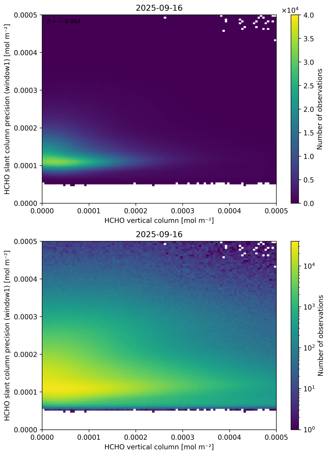
Figure 130: Scatter density plot of “HCHO vertical column” against “HCHO slant column precision (window1)” for 2025-09-15 to 2025-09-17.
