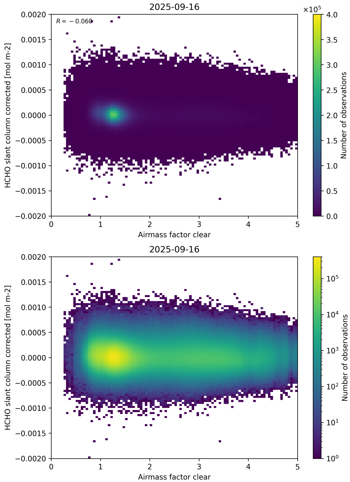
Figure 74: Scatter density plot of “Airmass factor clear” against “HCHO slant column corrected” for 2025-09-15 to 2025-09-17.
