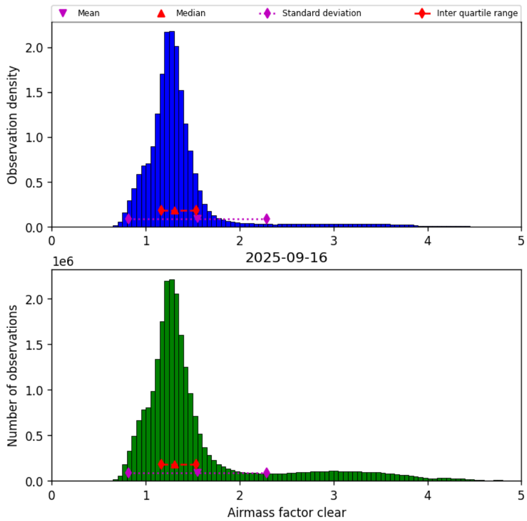
Figure 42: Histogram of “Airmass factor clear” for 2025-09-15 to 2025-09-17
