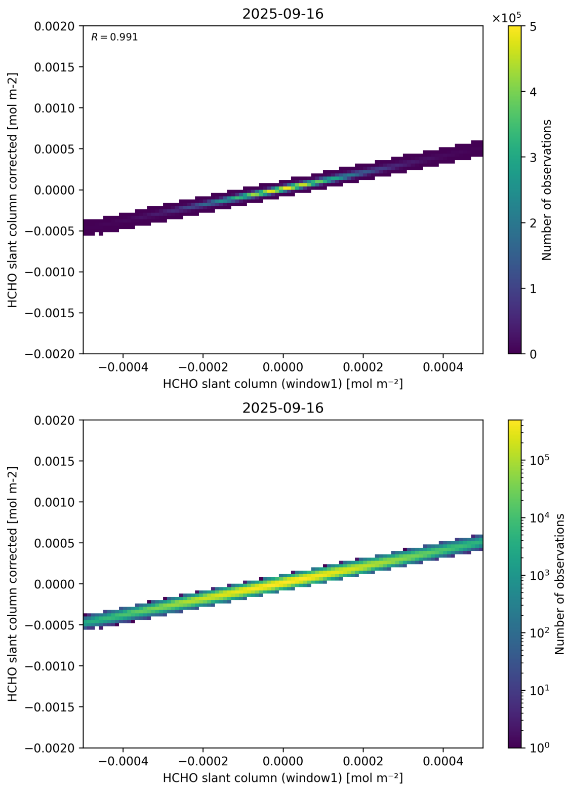
Figure 82: Scatter density plot of “HCHO slant column (window1)” against “HCHO slant column corrected” for 2025-09-15 to 2025-09-17.
