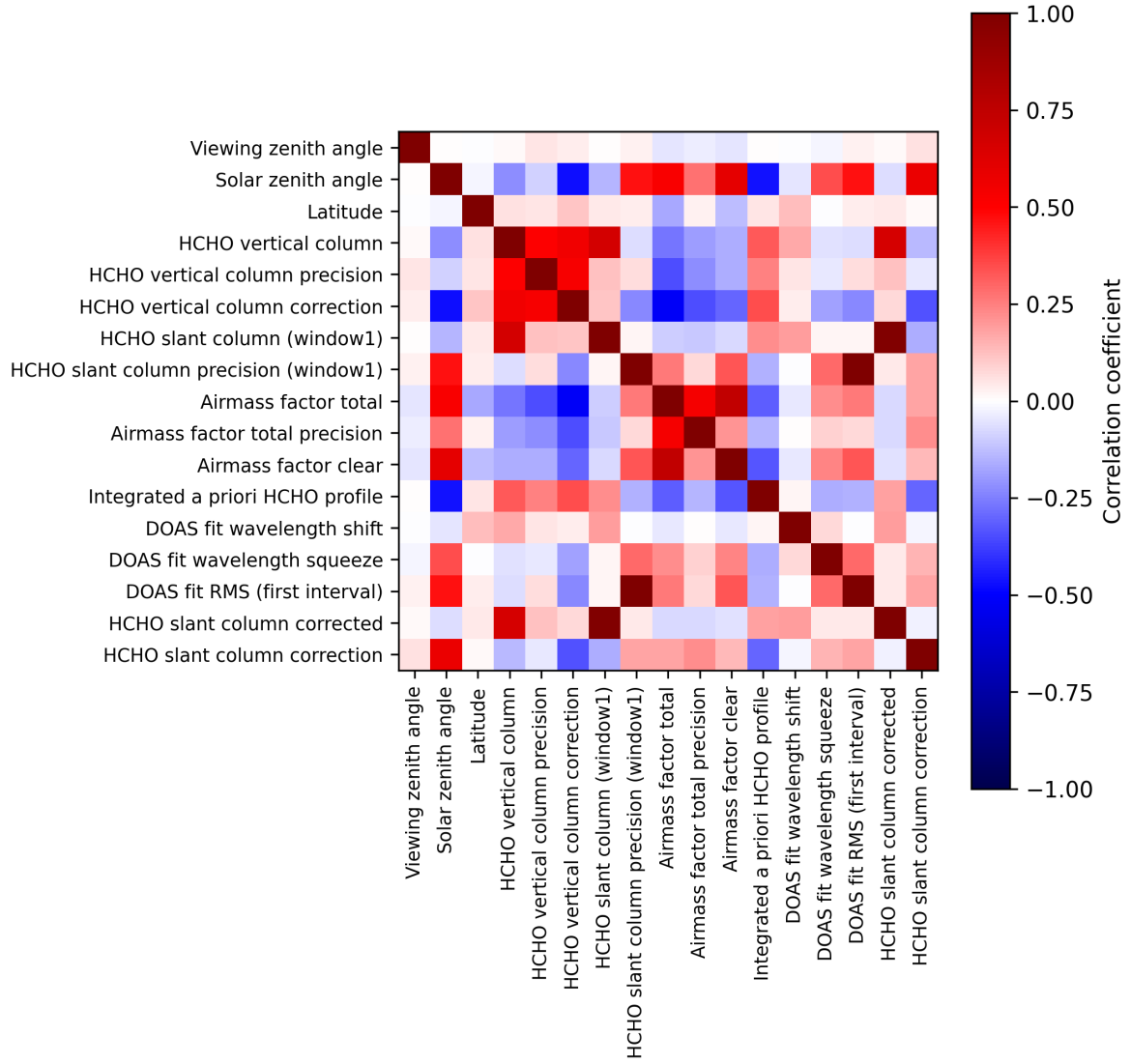
Figure 2: Map of correlation matrix for 2025-09-15 to 2025-09-17.
