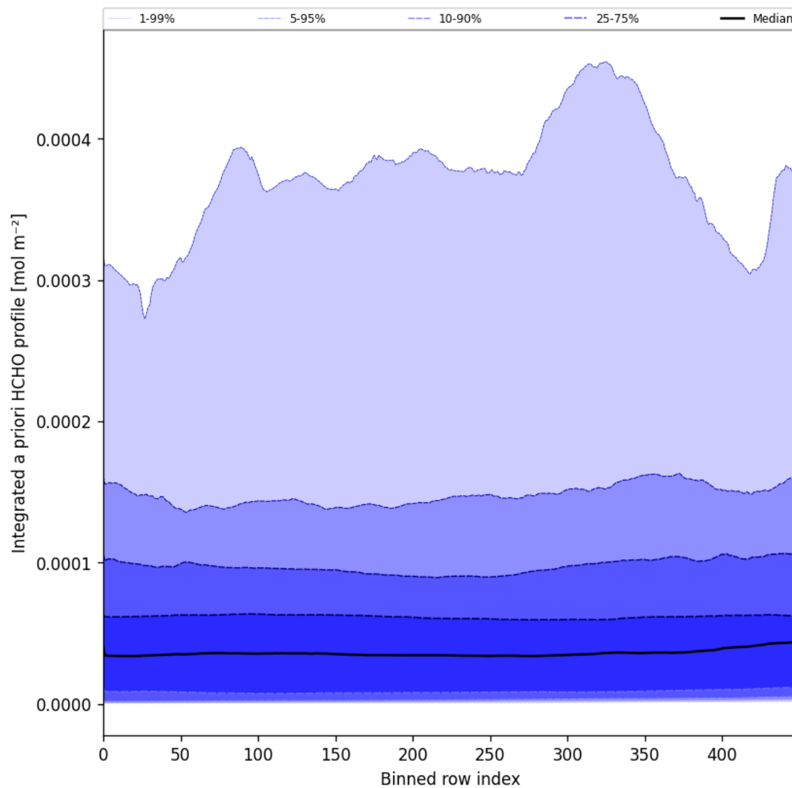
Figure 57: Along track statistics of “Integrated a priori HCHO profile” for 2025-09-15 to 2025-09-17
