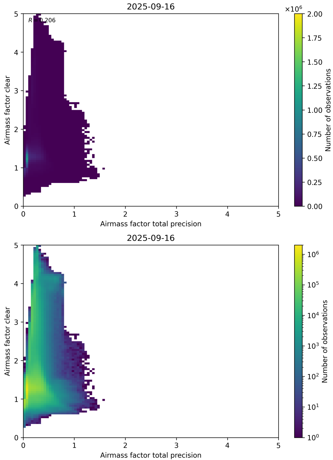
Figure 108: Scatter density plot of “Airmass factor total precision” against “Airmass factor clear” for 2025-09-15 to 2025-09-17.
