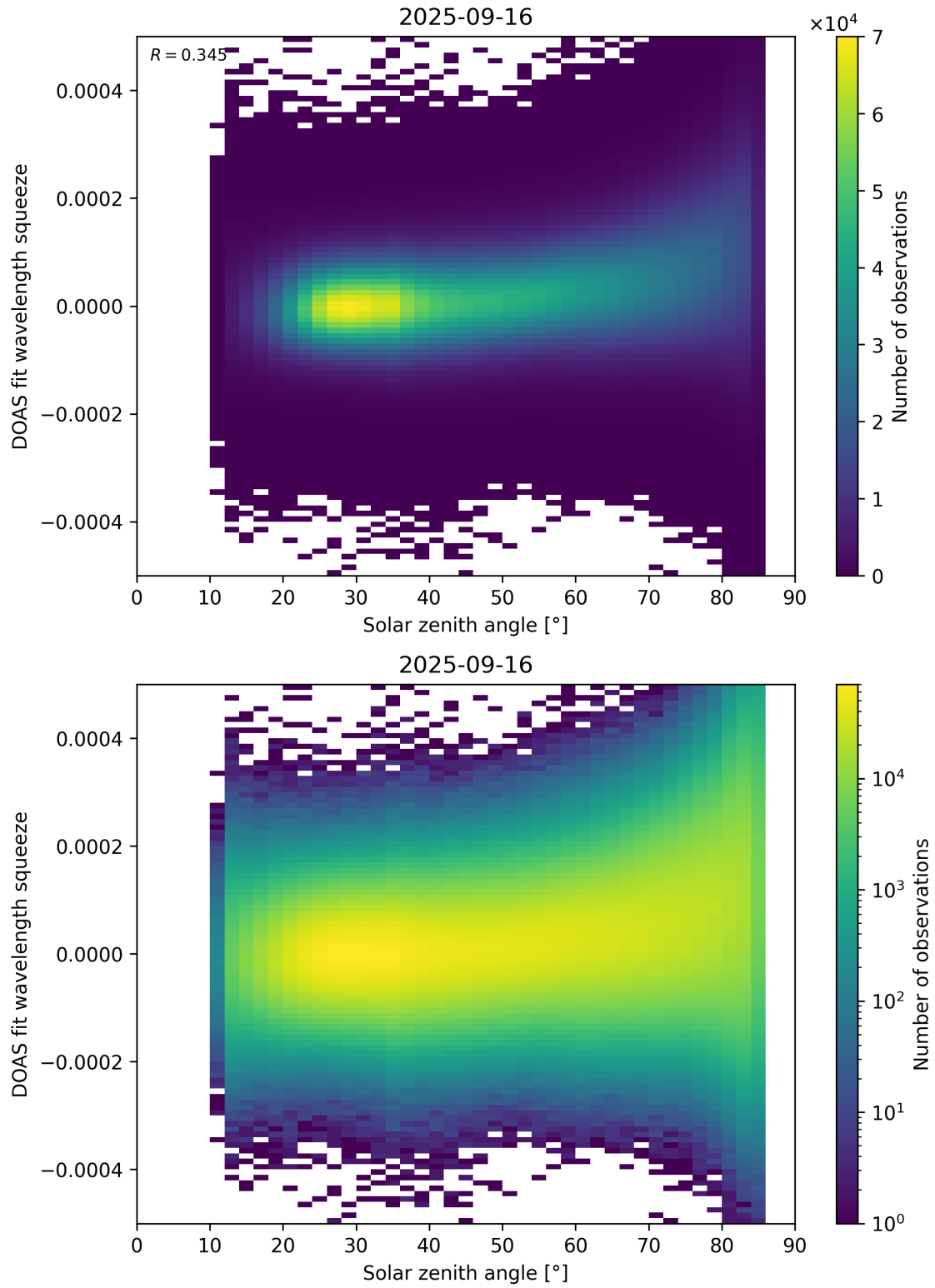
Figure 169: Scatter density plot of “Solar zenith angle” against “DOAS fit wavelength squeeze” for 2025-09-15 to 2025-09-17.
