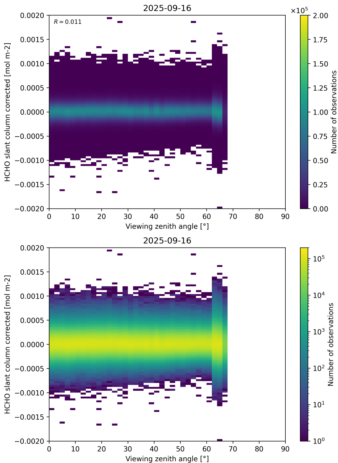
Figure 186: Scatter density plot of “Viewing zenith angle” against “HCHO slant column corrected” for 2025-09-15 to 2025-09-17.
