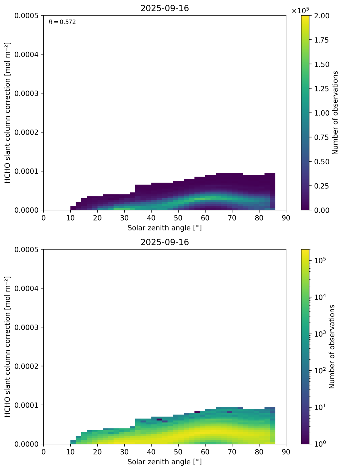
Figure 172: Scatter density plot of “Solar zenith angle” against “HCHO slant column correction” for 2025-09-15 to 2025-09-17.
