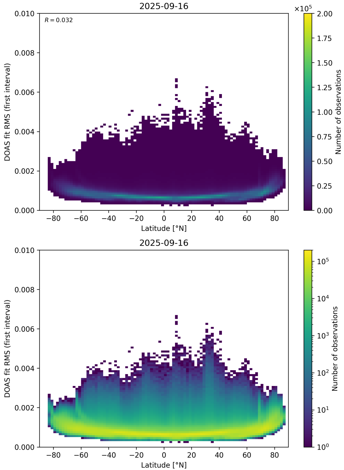
Figure 153: Scatter density plot of “Latitude” against “DOAS fit RMS (first interval)” for 2025-09-15 to 2025-09-17.
