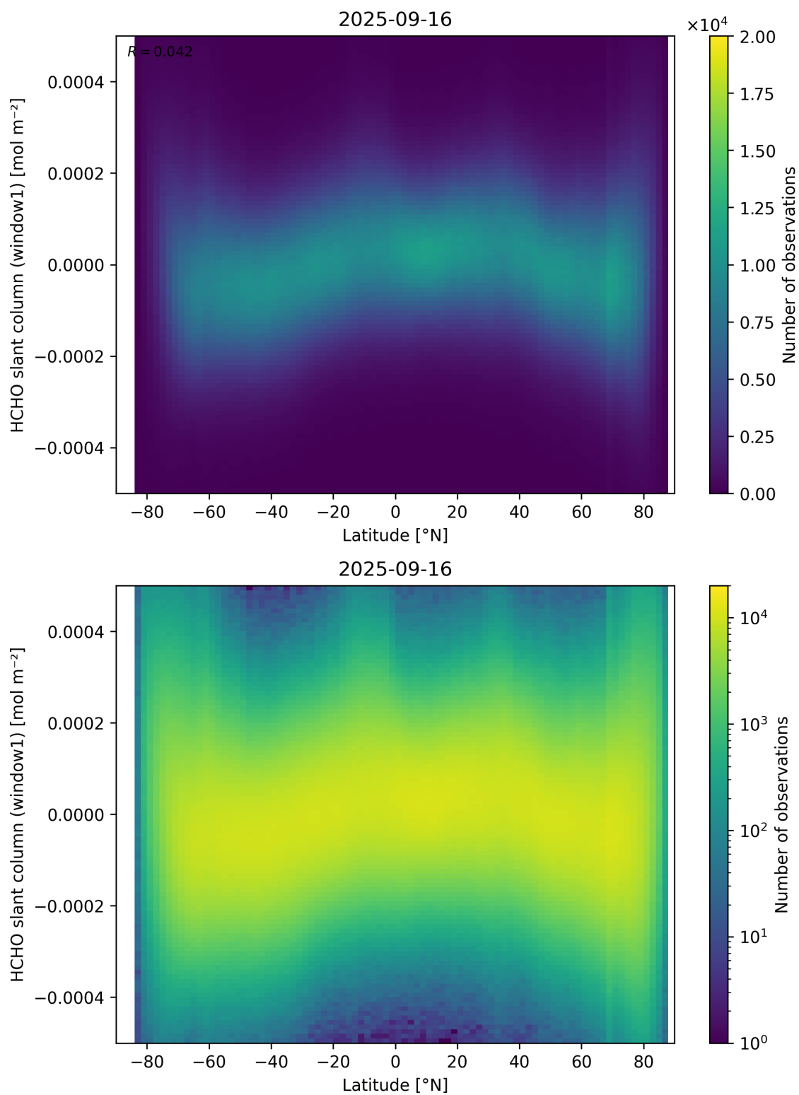
Figure 159: Scatter density plot of “Latitude” against “HCHO slant column (window1)” for 2025-09-15 to 2025-09-17.
