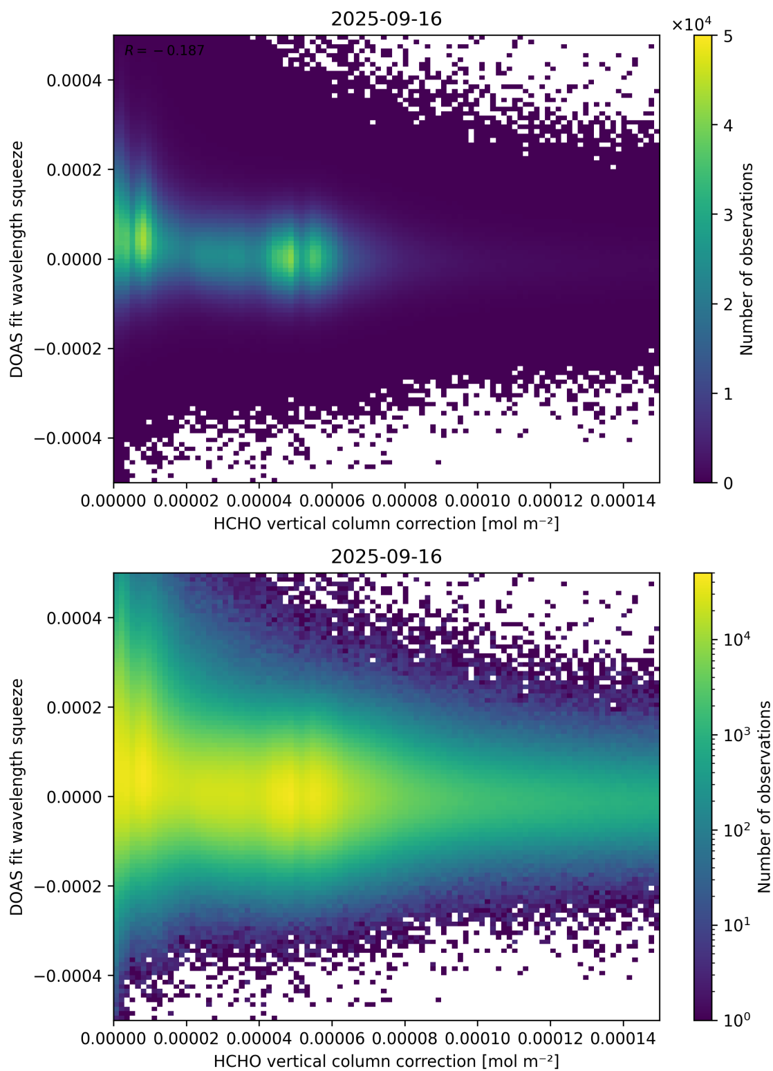
Figure 114: Scatter density plot of “HCHO vertical column correction” against “DOAS fit wavelength squeeze” for 2025-09-15 to 2025-09-17.
