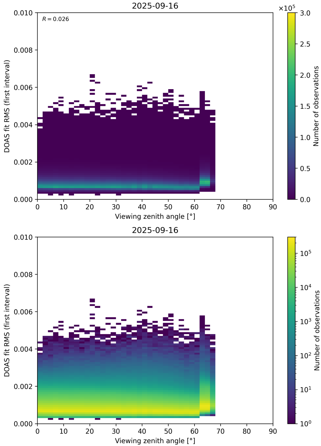
Figure 182: Scatter density plot of “Viewing zenith angle” against “DOAS fit RMS (first interval)” for 2025-09-15 to 2025-09-17.
