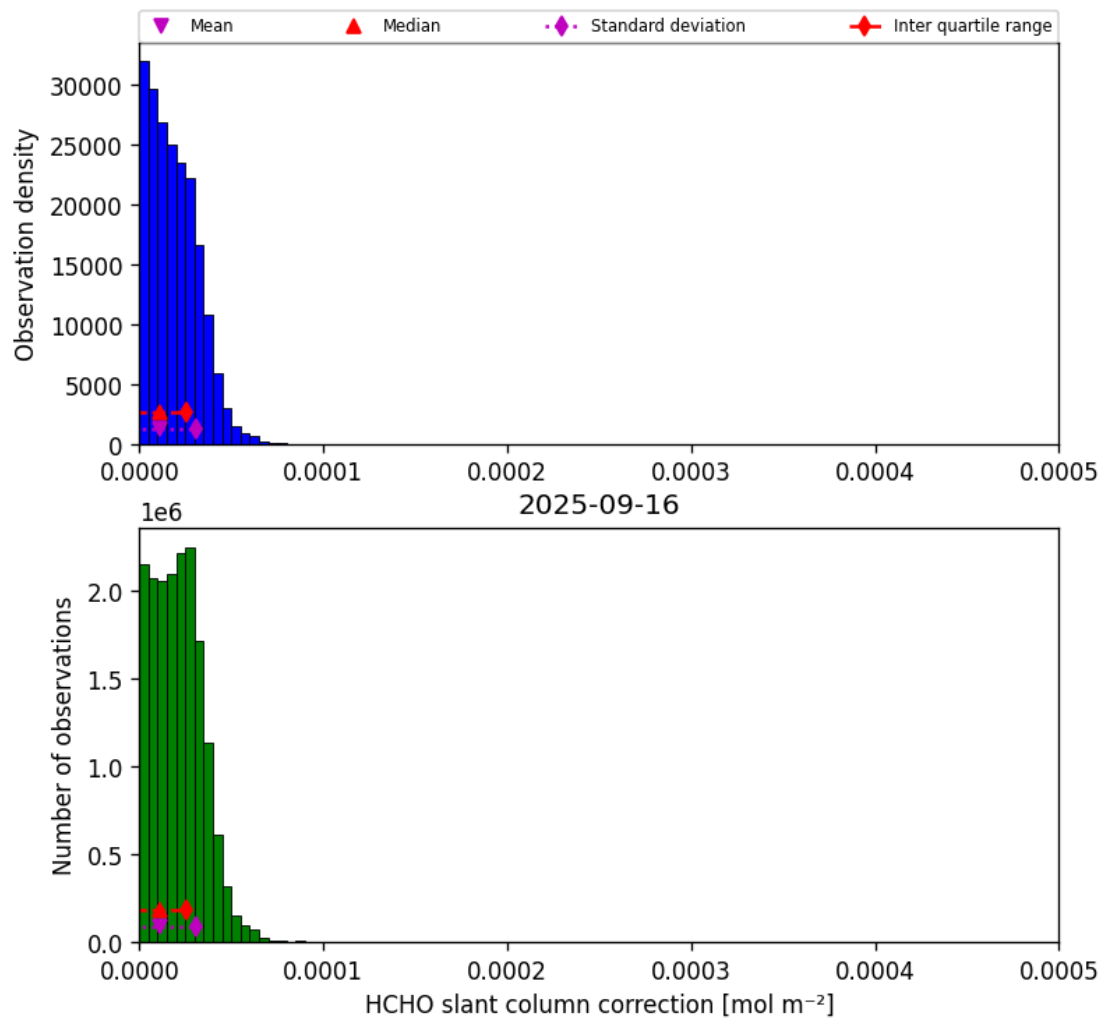
Figure 47: Histogram of “HCHO slant column correction” for 2025-09-15 to 2025-09-17
