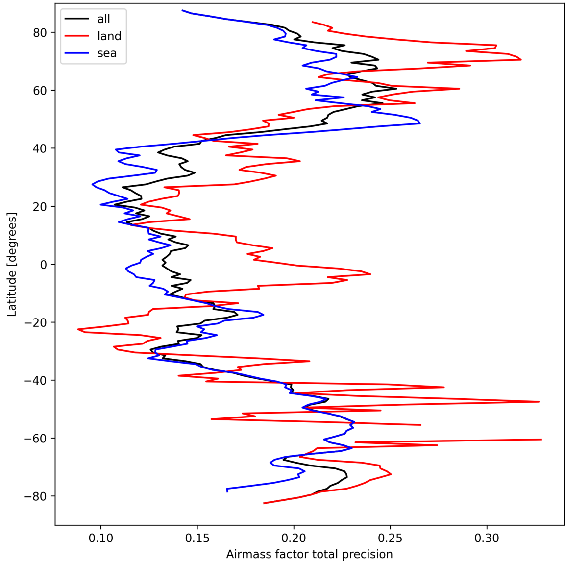
Figure 27: Zonal average of “Airmass factor total precision” for 2025-09-15 to 2025-09-17.
