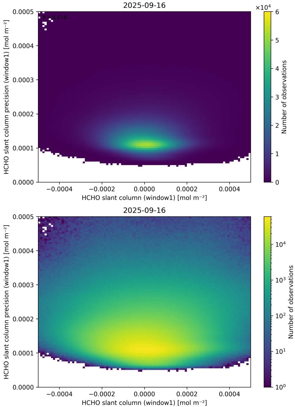
Figure 84: Scatter density plot of “HCHO slant column (window1)” against “HCHO slant column precision (window1)” for 2025-09-15 to 2025-09-17.
