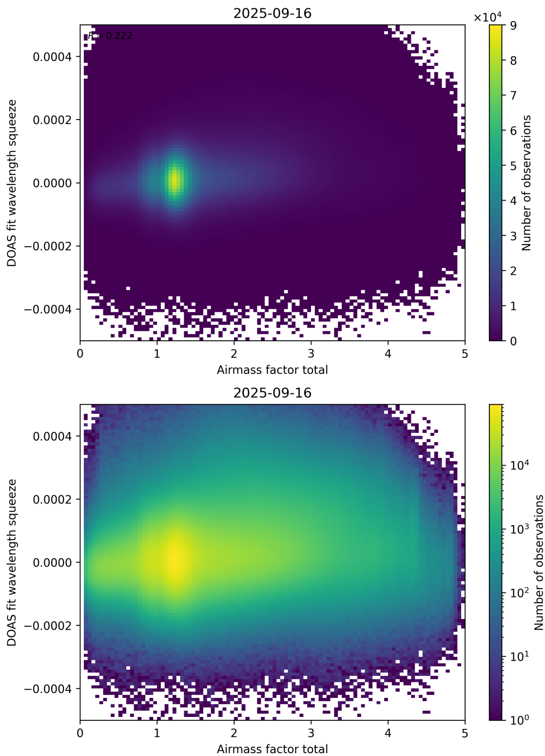
Figure 99: Scatter density plot of “Airmass factor total” against “DOAS fit wavelength squeeze” for 2025-09-15 to 2025-09-17.
