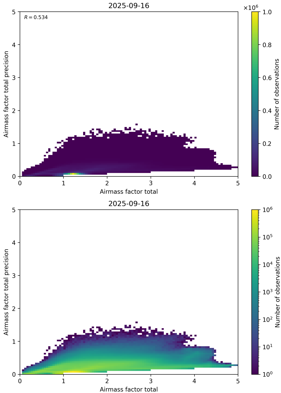
Figure 103: Scatter density plot of “Airmass factor total” against “Airmass factor total precision” for 2025-09-15 to 2025-09-17.
