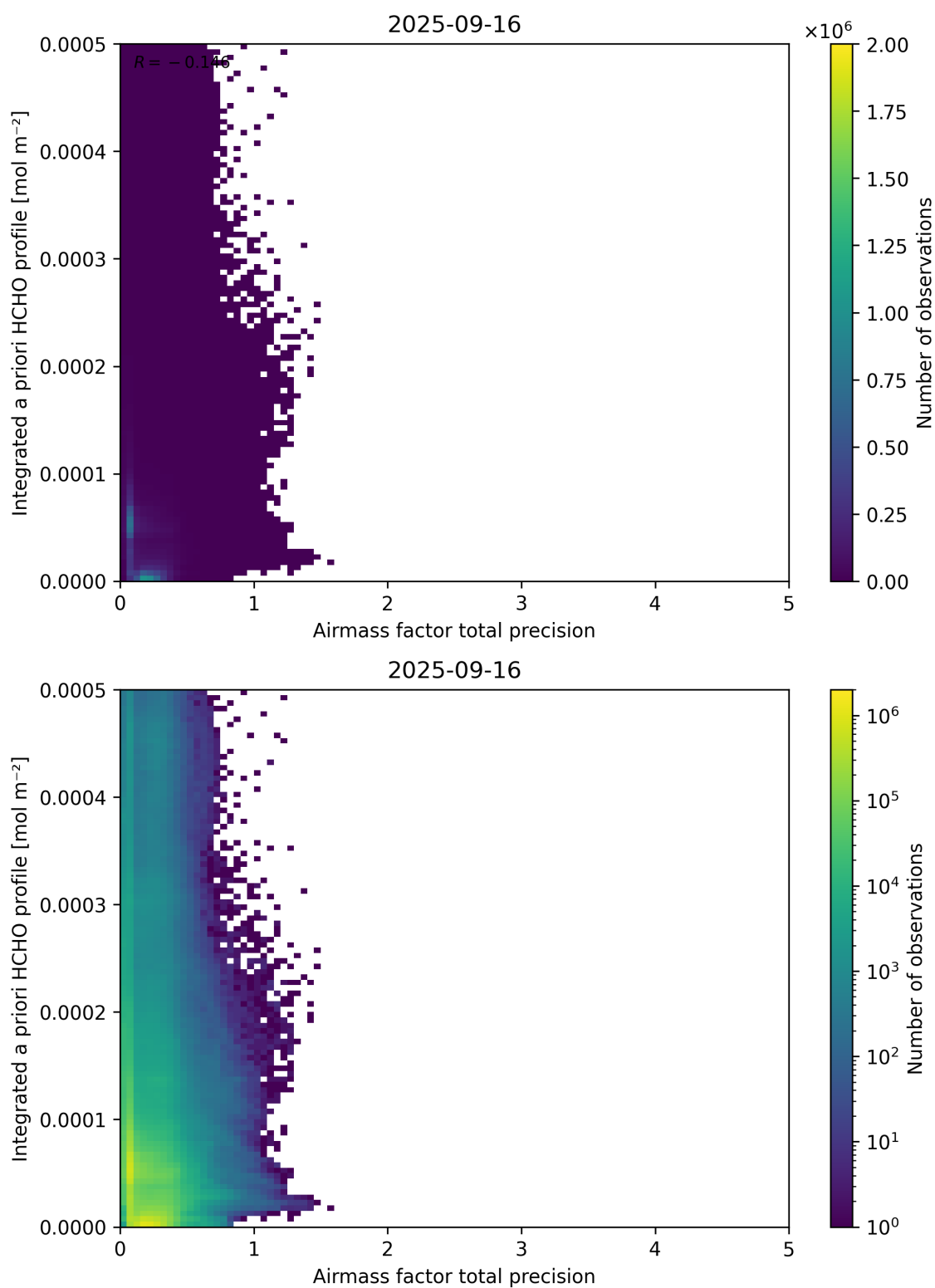
Figure 111: Scatter density plot of “Airmass factor total precision” against “Integrated a priori HCHO profile” for 2025-09-15 to 2025-09-17.
