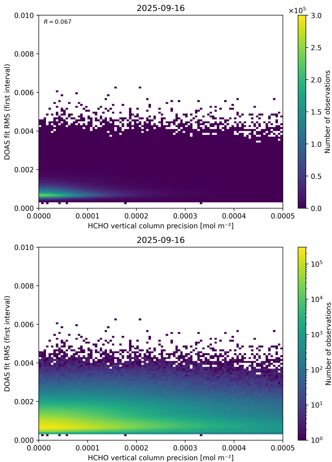
Figure 136: Scatter density plot of “HCHO vertical column precision” against “DOAS fit RMS (first interval)” for 2025-09-15 to 2025-09-17.
