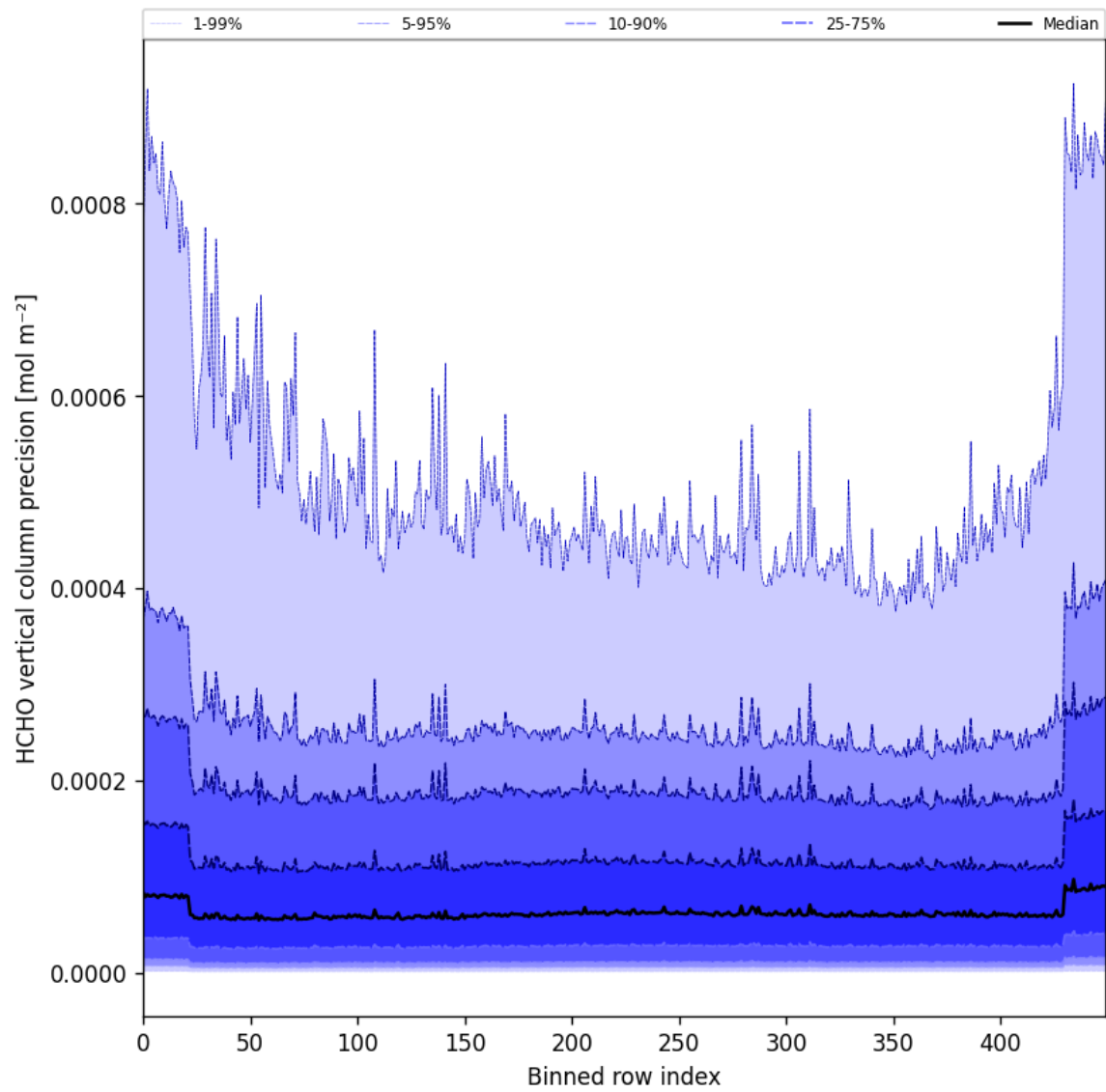
Figure 50: Along track statistics of “HCHO vertical column precision” for 2025-09-15 to 2025-09-17
