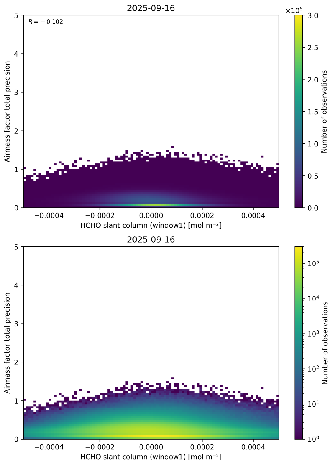
Figure 86: Scatter density plot of “HCHO slant column (window1)” against “Airmass factor total precision” for 2025-09-15 to 2025-09-17.
