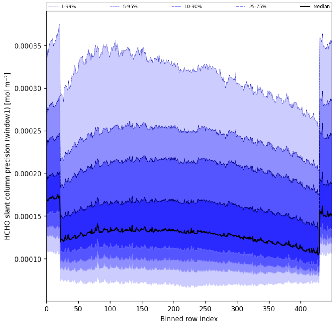
Figure 53: Along track statistics of "HCHO slant column precision (window1)" for 2025-09-15 to 2025-09-17
