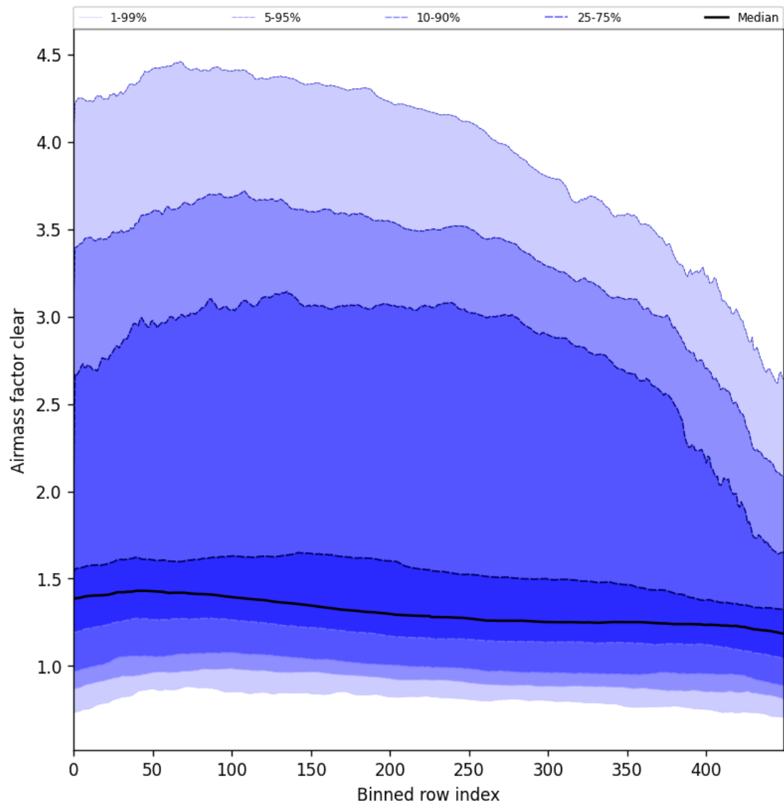
Figure 56: Along track statistics of “Air mass factor clear” for 2025-09-15 to 2025-09-17
