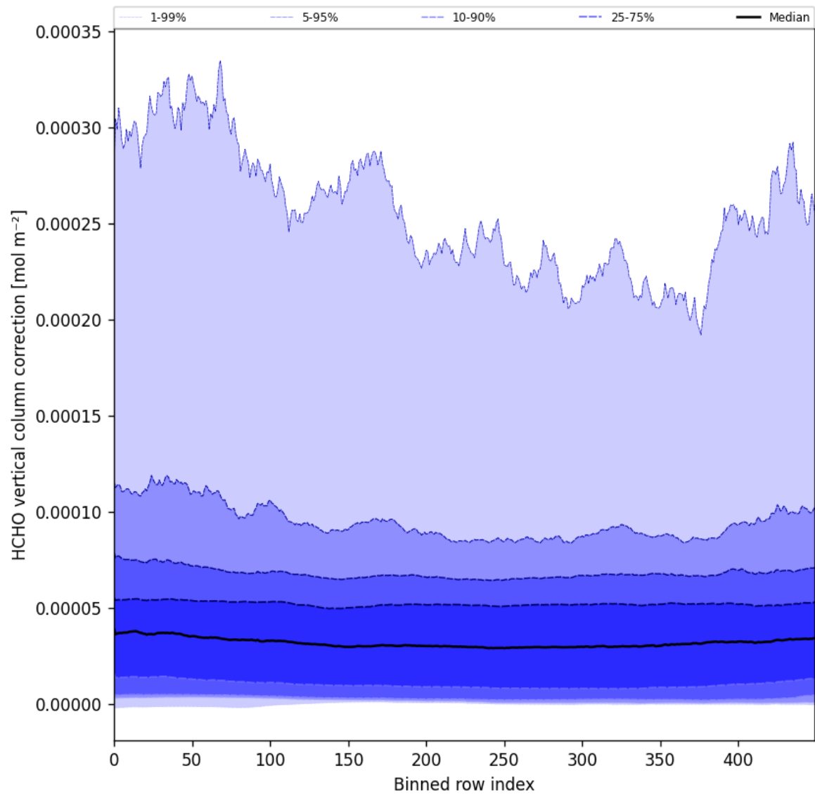
Figure 51: Along track statistics of “HCHO vertical column correction” for 2025-09-15 to 2025-09-17
