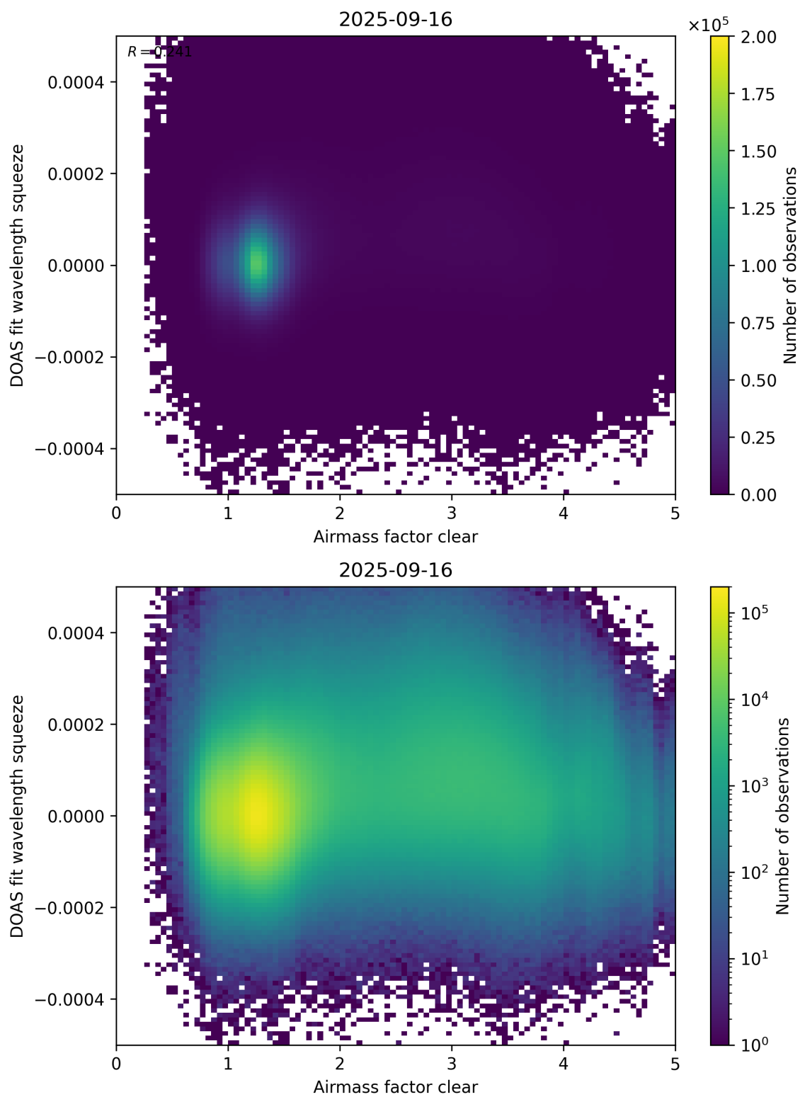
Figure 73: Scatter density plot of “Airmass factor clear” against “DOAS fit wavelength squeeze” for 2025-09-15 to 2025-09-17.
