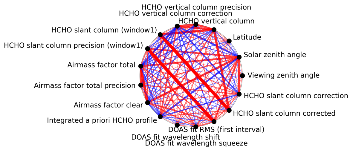
Figure 1: Map of correlation graph for 2025-09-15 to 2025-09-17.
