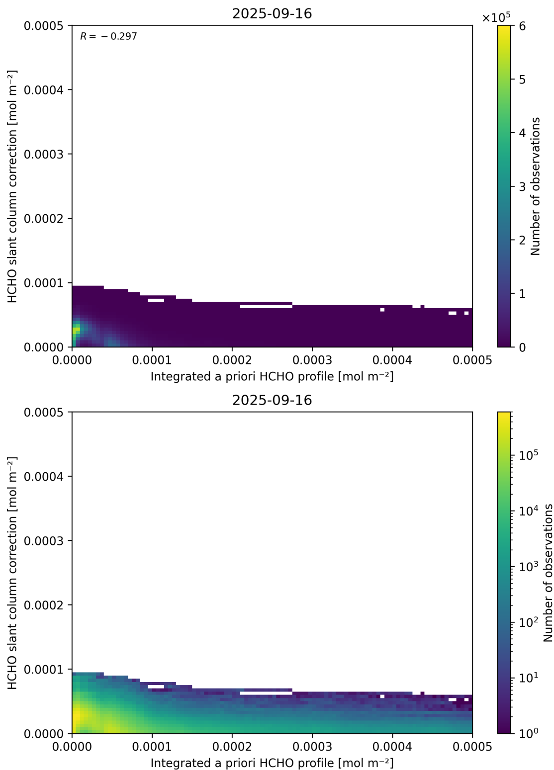
Figure 152: Scatter density plot of “Integrated a priori HCHO profile” against “HCHO slant column correction” for 2025-09-15 to 2025-09-17.
