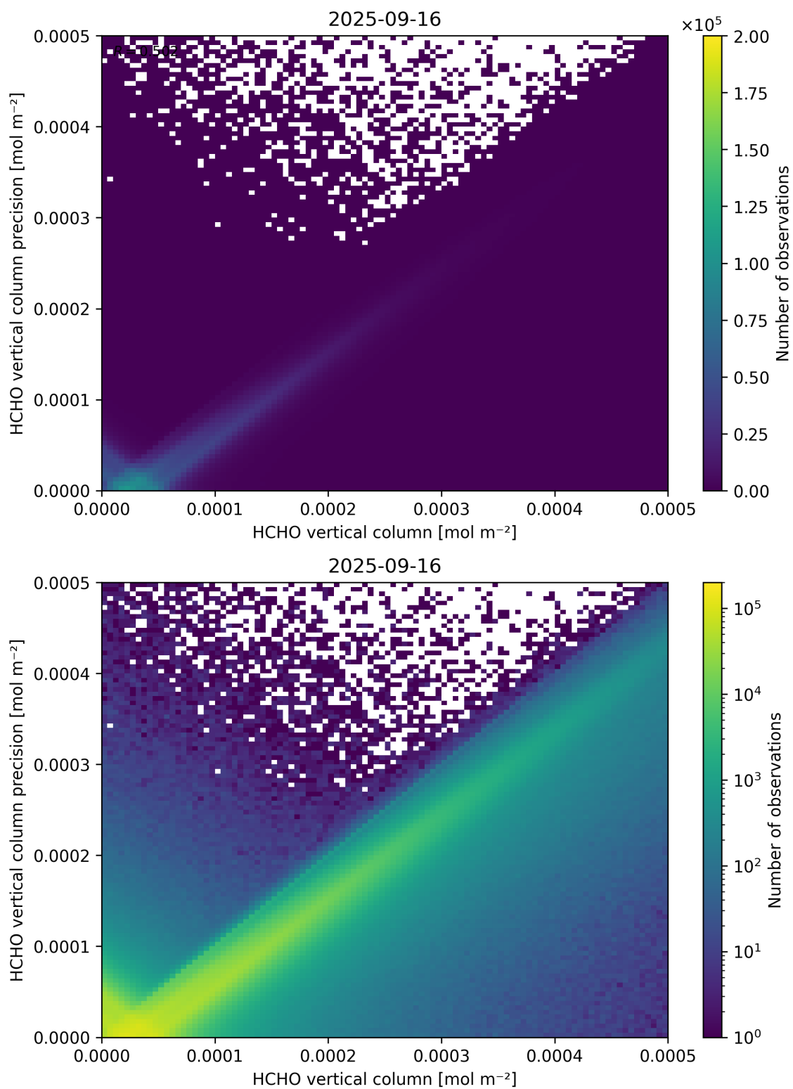
Figure 134: Scatter density plot of “HCHO vertical column” against “HCHO vertical column precision” for 2025-09-15 to 2025-09-17.
