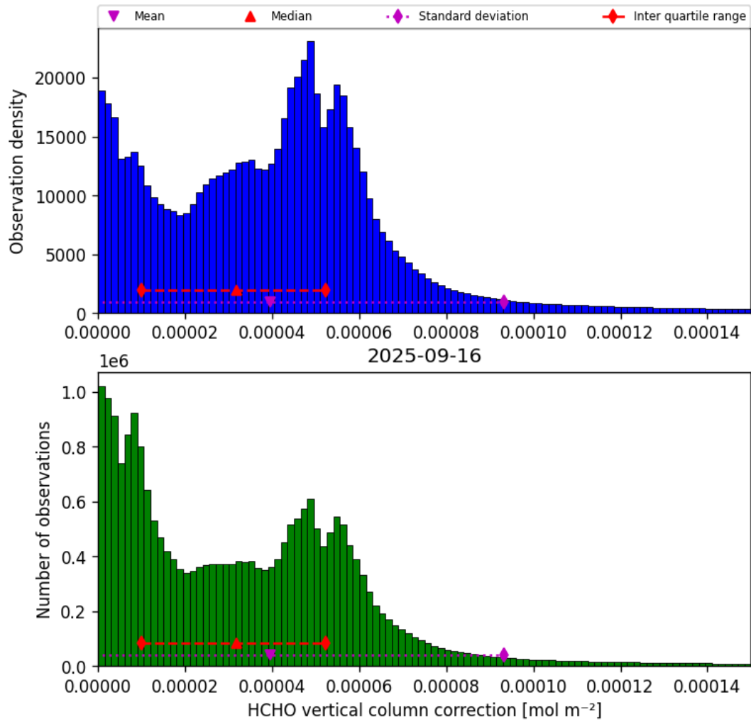
Figure 37: Histogram of “HCHO vertical column correction” for 2025-09-15 to 2025-09-17
