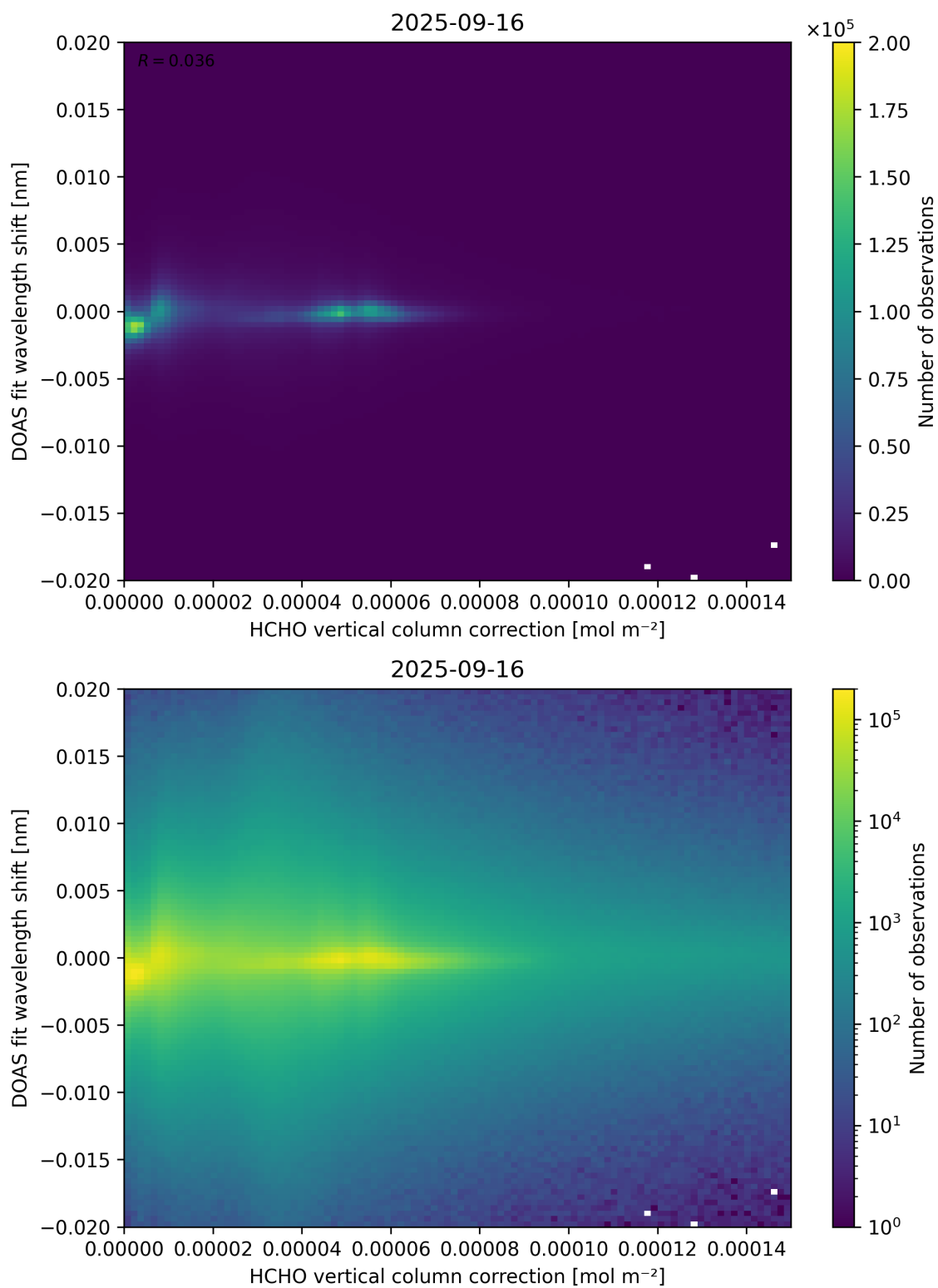
Figure 113: Scatter density plot of “HCHO vertical column correction” against “DOAS fit wavelength shift” for 2025-09-15 to 2025-09-17.
