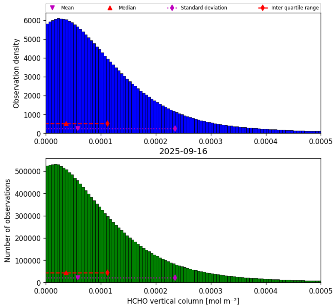
Figure 35: Histogram of “HCHO vertical column” for 2025-09-15 to 2025-09-17
