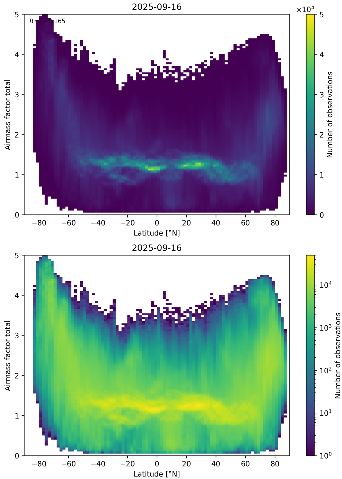
Figure 161: Scatter density plot of “Latitude” against “Airmass factor total” for 2025-09-15 to 2025-09-17.
