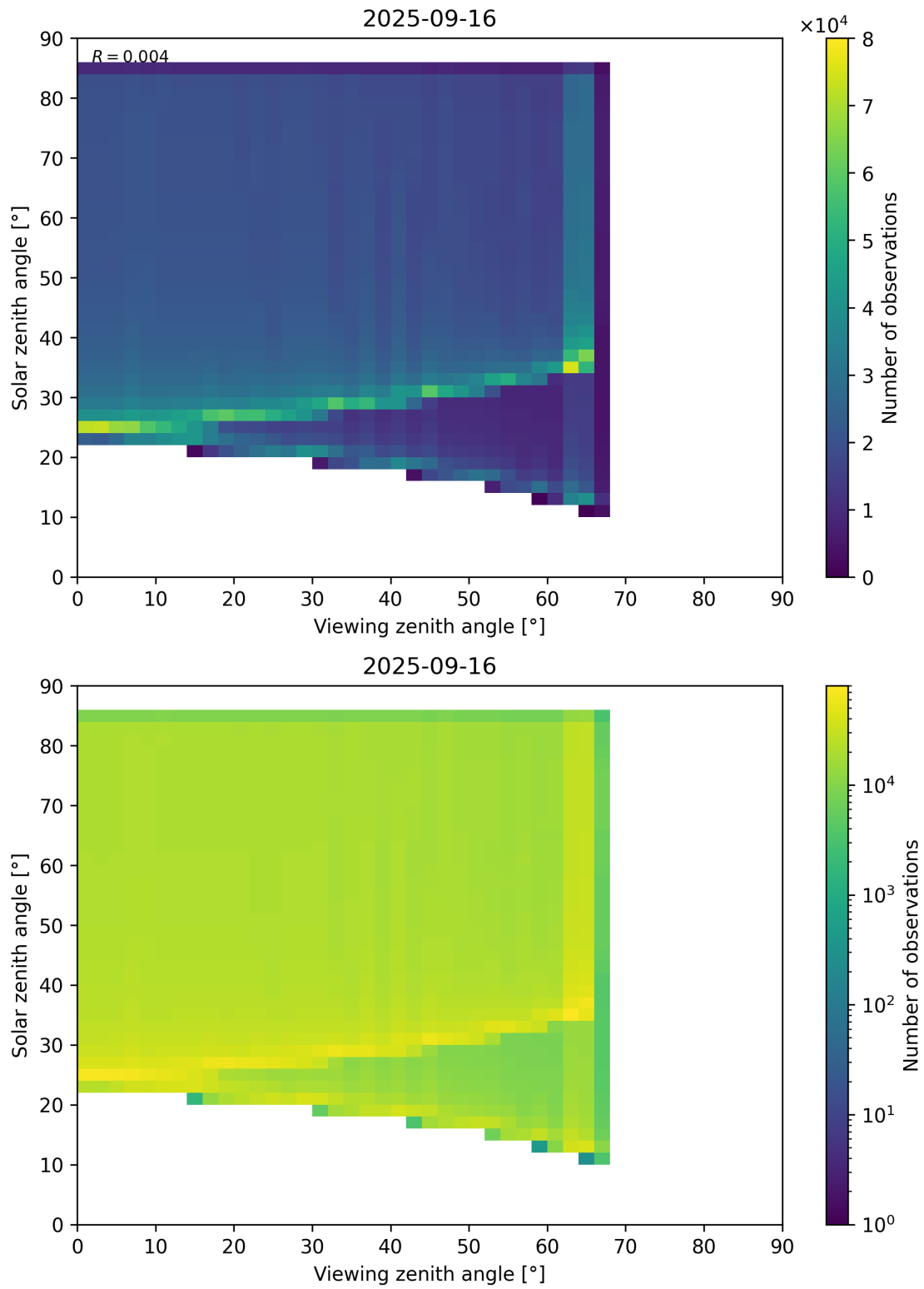
Figure 197: Scatter density plot of “Viewing zenith angle” against “Solar zenith angle” for 2025-09-15 to 2025-09-17.
