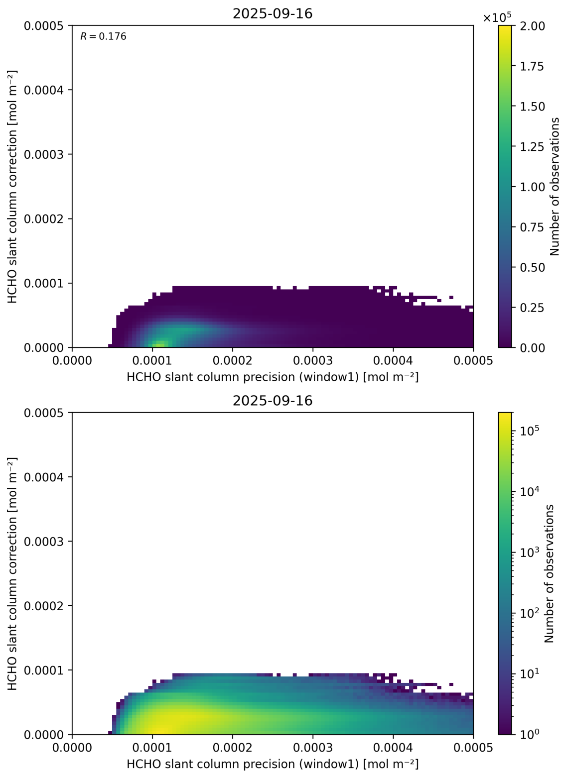
Figure 93: Scatter density plot of “HCHO slant column precision (window1)” against “HCHO slant column correction” for 2025-09-15 to 2025-09-17.
