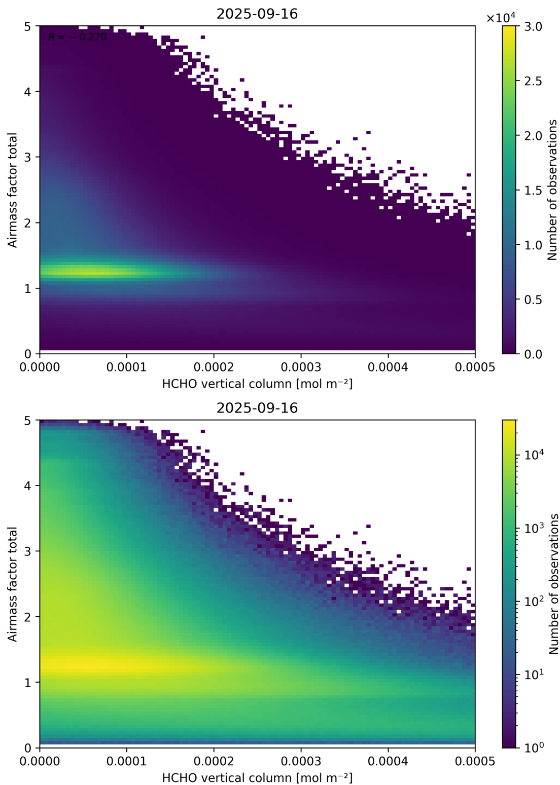
Figure 131: Scatter density plot of “HCHO vertical column” against “Airmass factor total” for 2025-09-15 to 2025-09-17.
