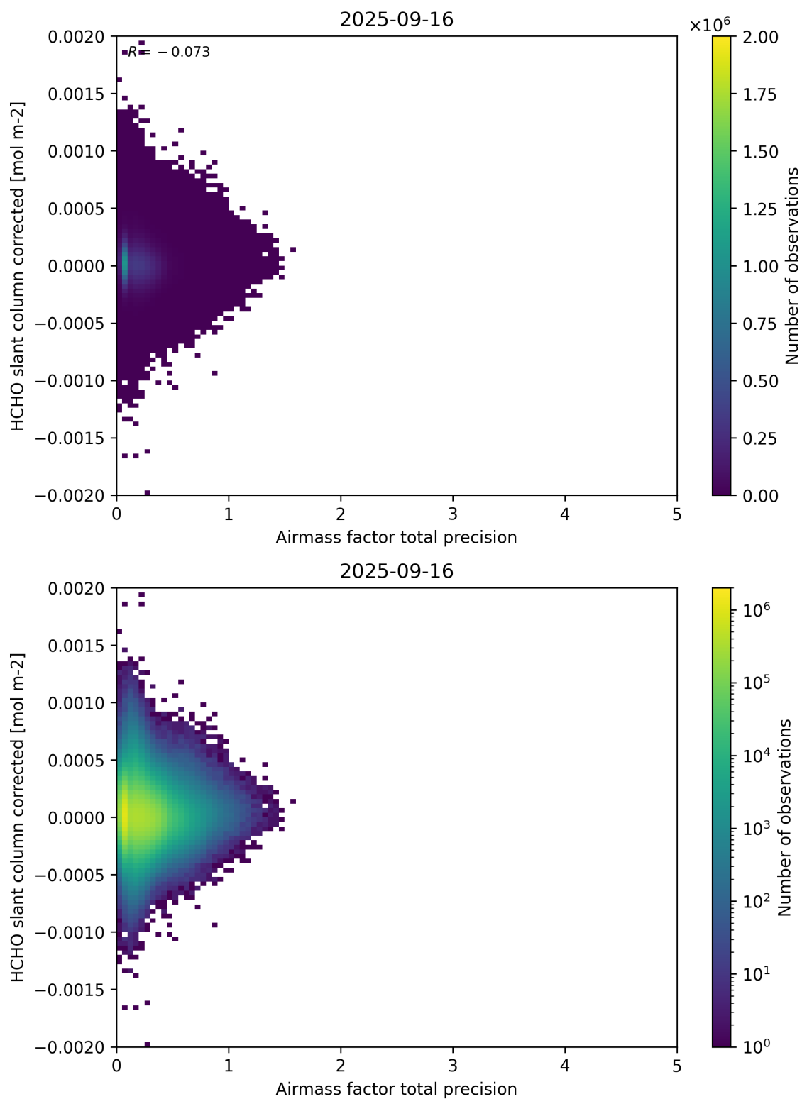
Figure 109: Scatter density plot of “Airmass factor total precision” against “HCHO slant column corrected” for 2025-09-15 to 2025-09-17.
