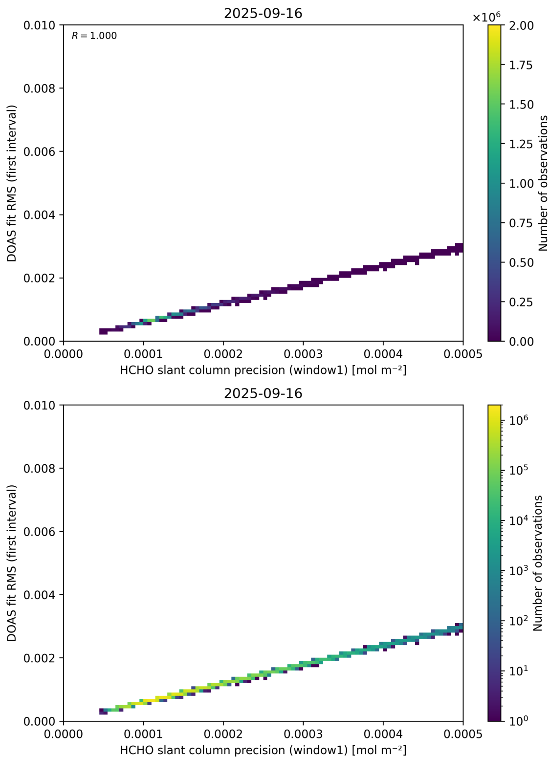
Figure 88: Scatter density plot of “HCHO slant column precision (window1)” against “DOAS fit RMS (first interval)” for 2025-09-15 to 2025-09-17.
