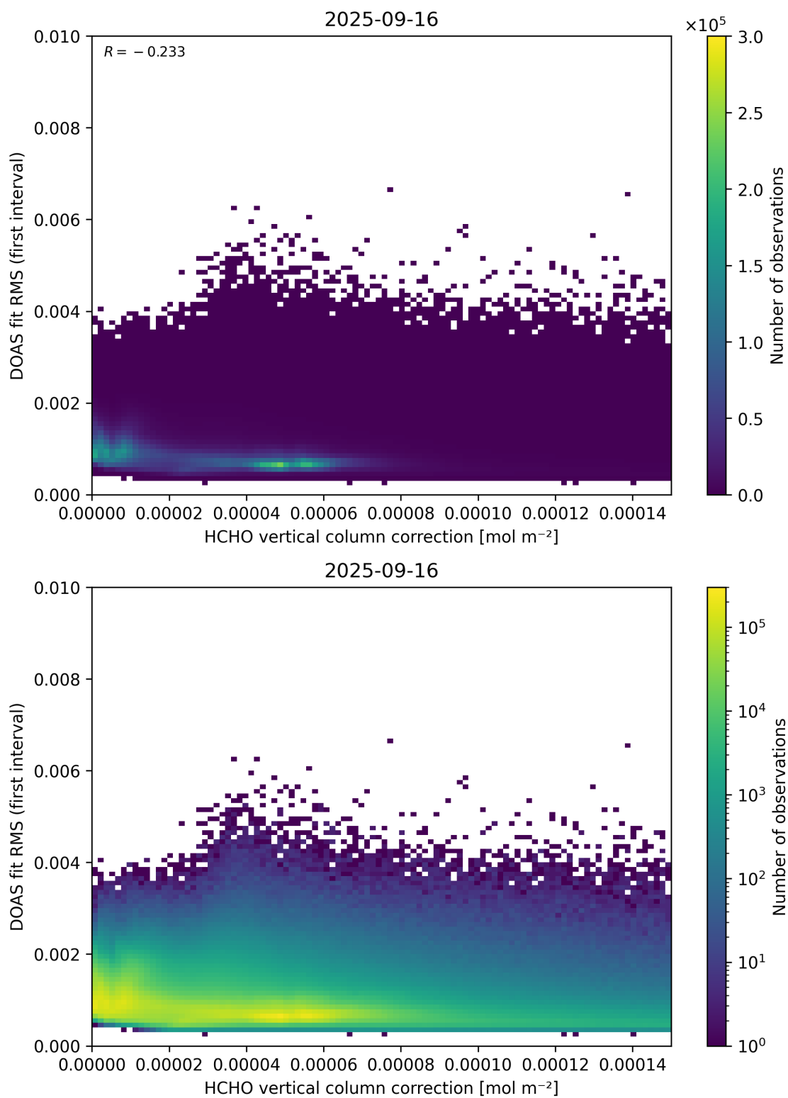
Figure 112: Scatter density plot of “HCHO vertical column correction” against “DOAS fit RMS (first interval)” for 2025-09-15 to 2025-09-17.
