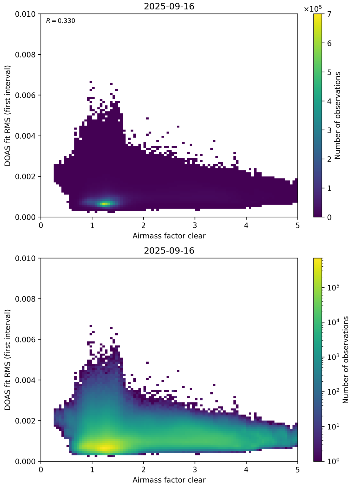
Figure 71: Scatter density plot of “Airmass factor clear” against “DOAS fit RMS (first interval)” for 2025-09-15 to 2025-09-17.
