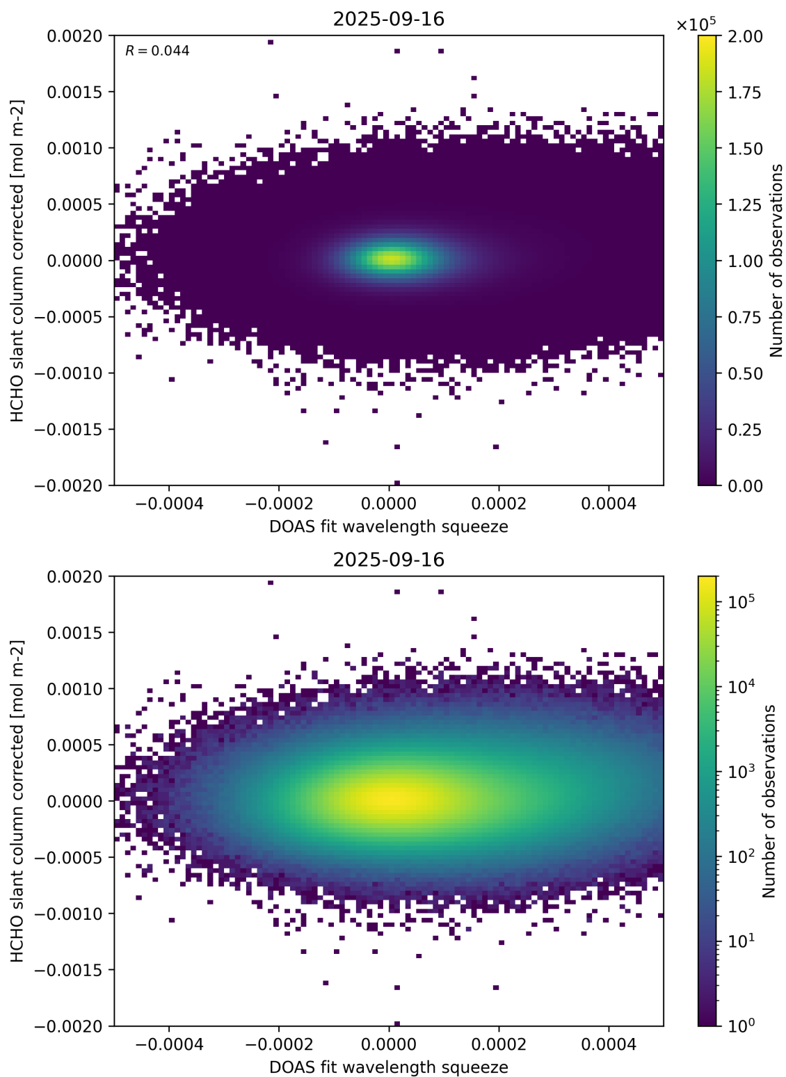
Figure 69: Scatter density plot of “DOAS fit wavelength squeeze” against “HCHO slant column corrected” for 2025-09-15 to 2025-09-17.
