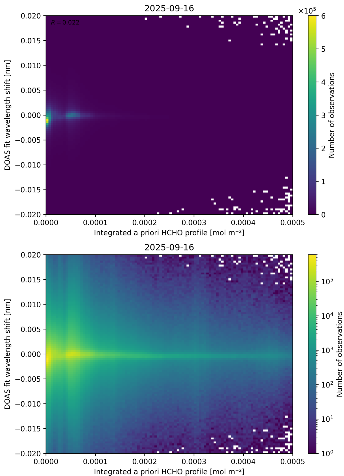
Figure 149: Scatter density plot of “Integrated a priori HCHO profile” against “DOAS fit wavelength shift” for 2025-09-15 to 2025-09-17.
