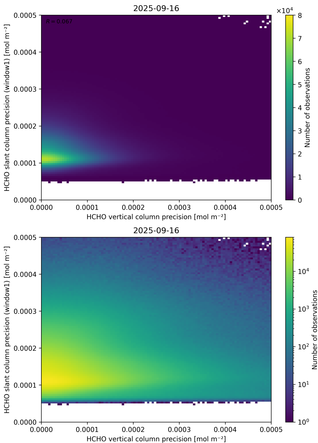
Figure 143: Scatter density plot of “HCHO vertical column precision” against “HCHO slant column precision (window1)” for 2025-09-15 to 2025-09-17.
