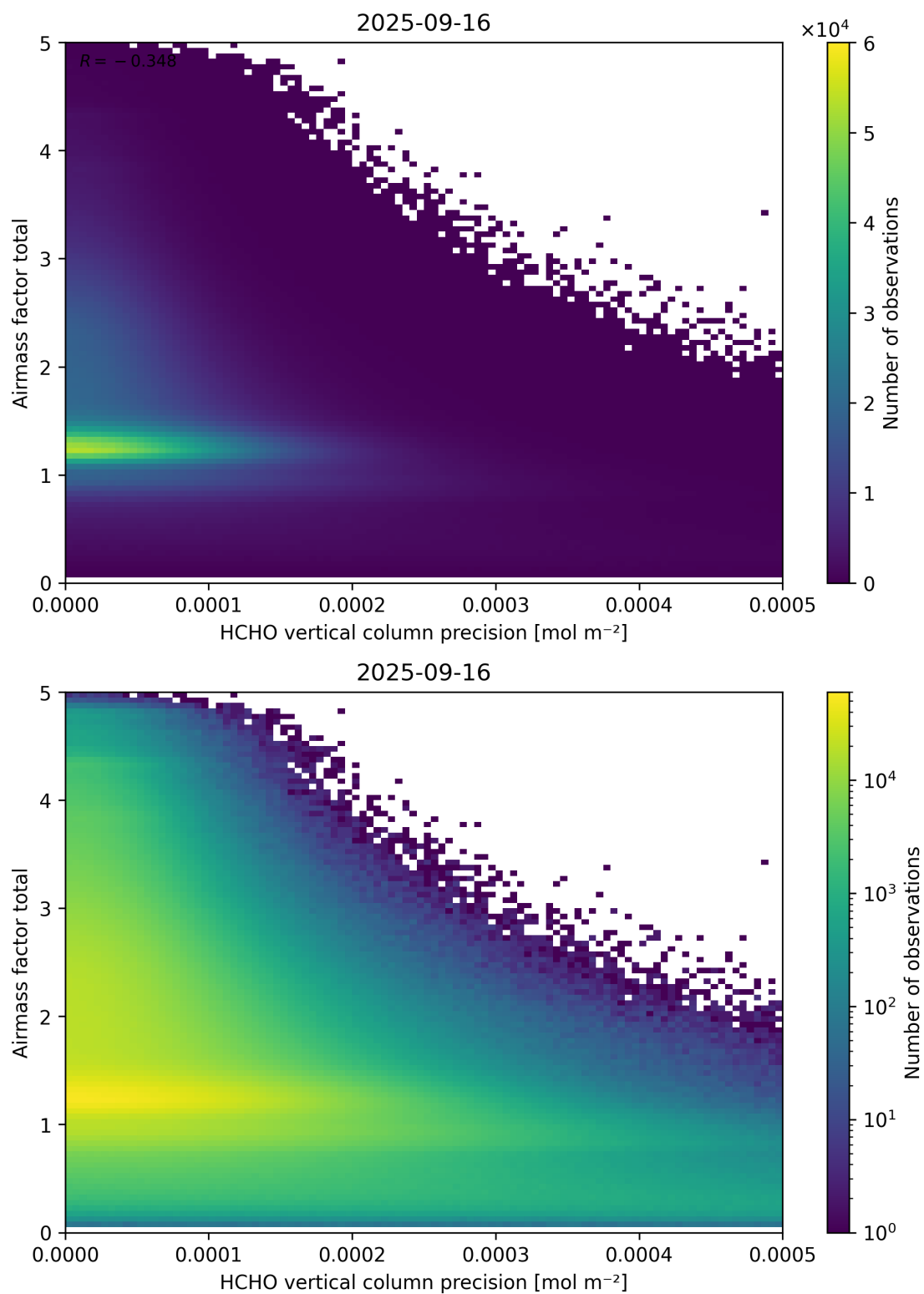
Figure 144: Scatter density plot of “HCHO vertical column precision” against “Airmass factor total” for 2025-09-15 to 2025-09-17.
