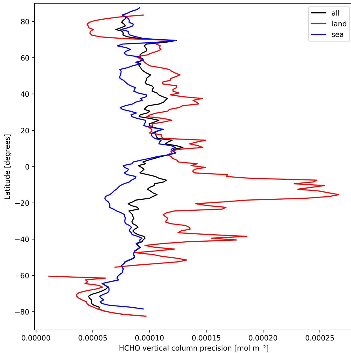
Figure 22: Zonal average of “HCHO vertical column precision” for 2025-09-15 to 2025-09-17.
