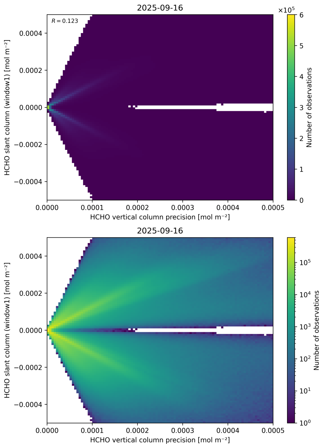
Figure 142: Scatter density plot of “HCHO vertical column precision” against “HCHO slant column (window1)” for 2025-09-15 to 2025-09-17.
