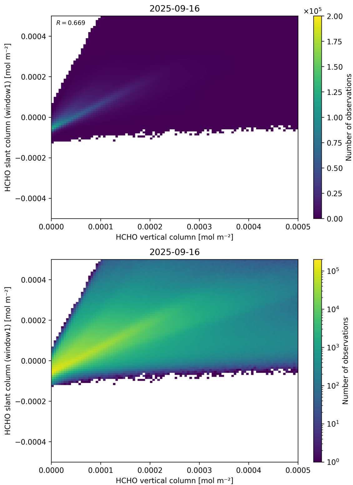
Figure 129: Scatter density plot of “HCHO vertical column” against “HCHO slant column (window1)” for 2025-09-15 to 2025-09-17.
