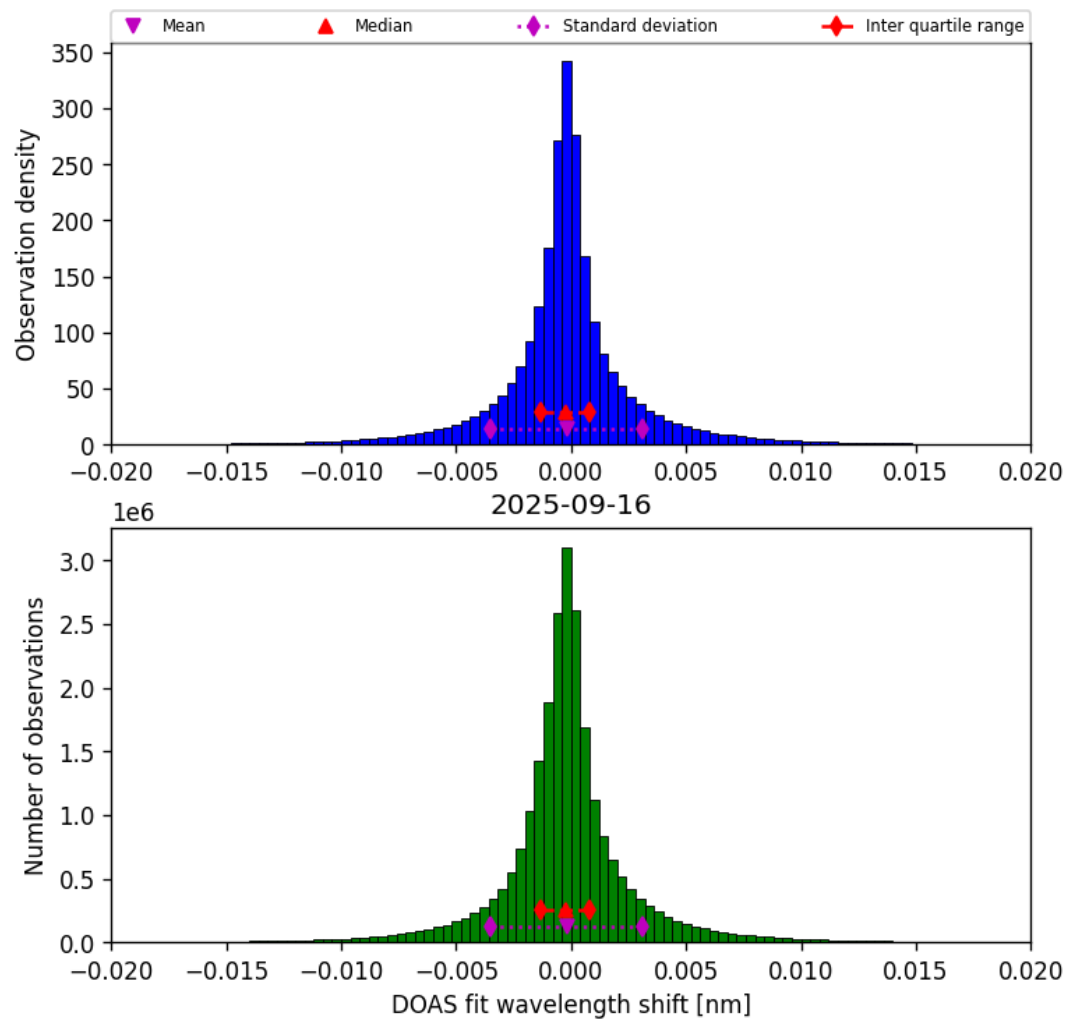
Figure 44: Histogram of “DOAS fit wavelength shift” for 2025-09-15 to 2025-09-17
