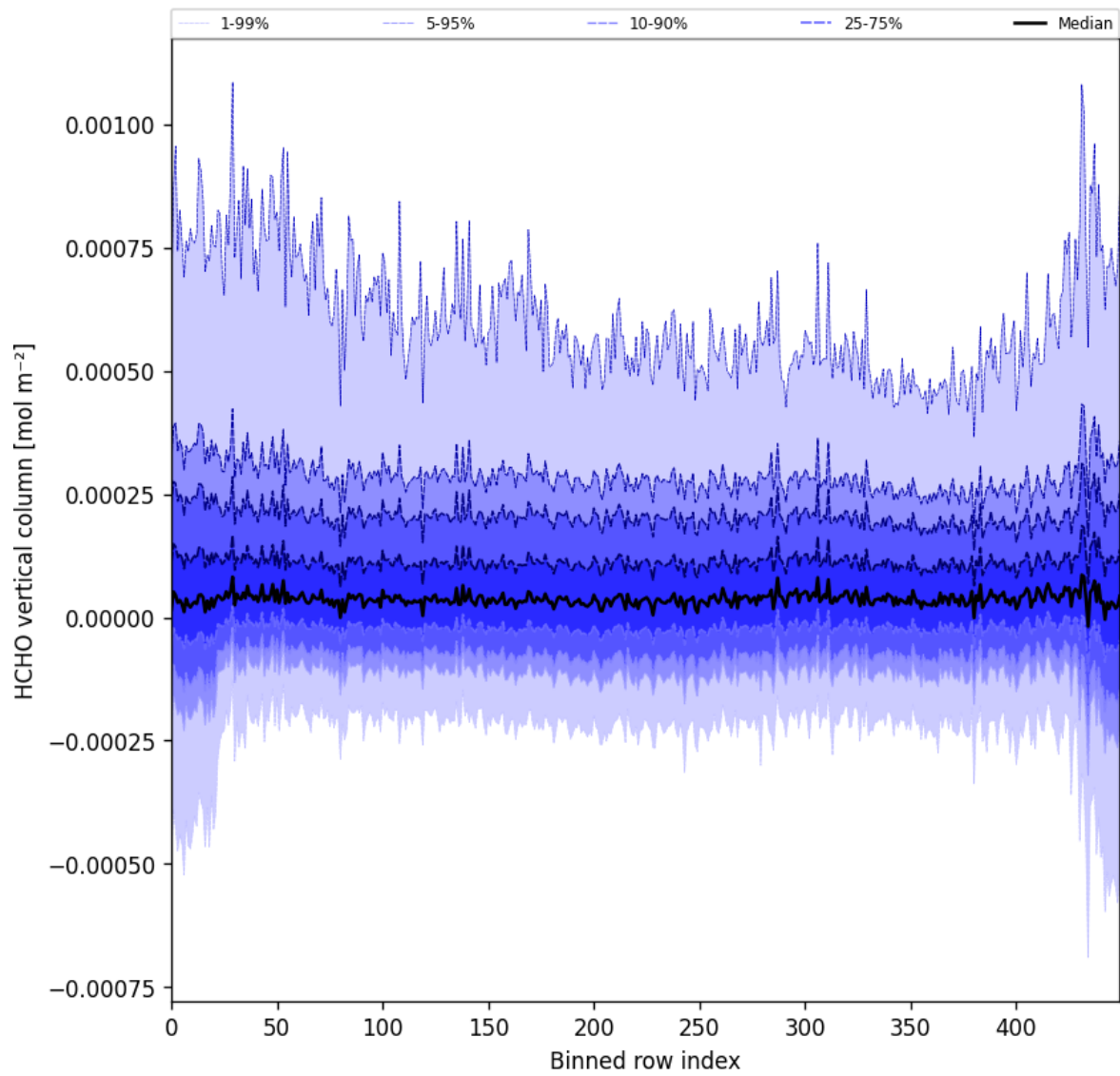
Figure 49: Along track statistics of “HCHO vertical column” for 2025-09-15 to 2025-09-17
