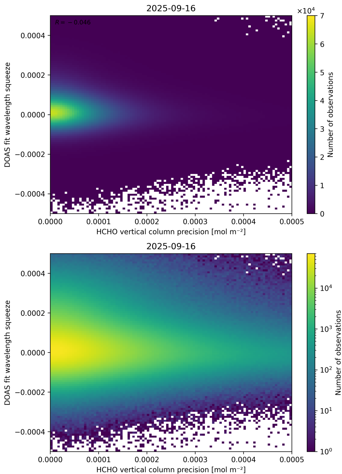
Figure 138: Scatter density plot of “HCHO vertical column precision” against “DOAS fit wavelength squeeze” for 2025-09-15 to 2025-09-17.
