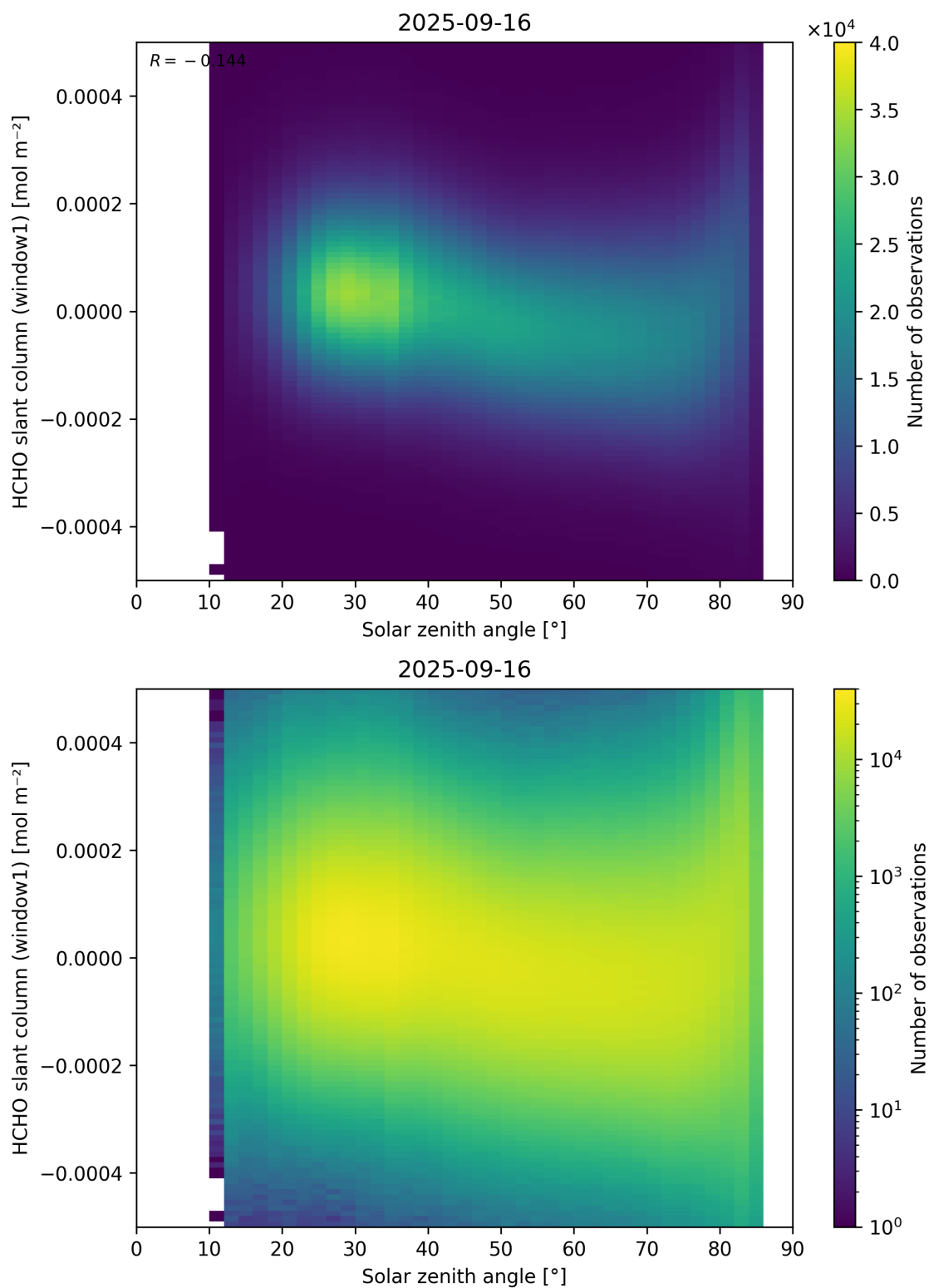
Figure 173: Scatter density plot of “Solar zenith angle” against “HCHO slant column (window1)” for 2025-09-15 to 2025-09-17.
