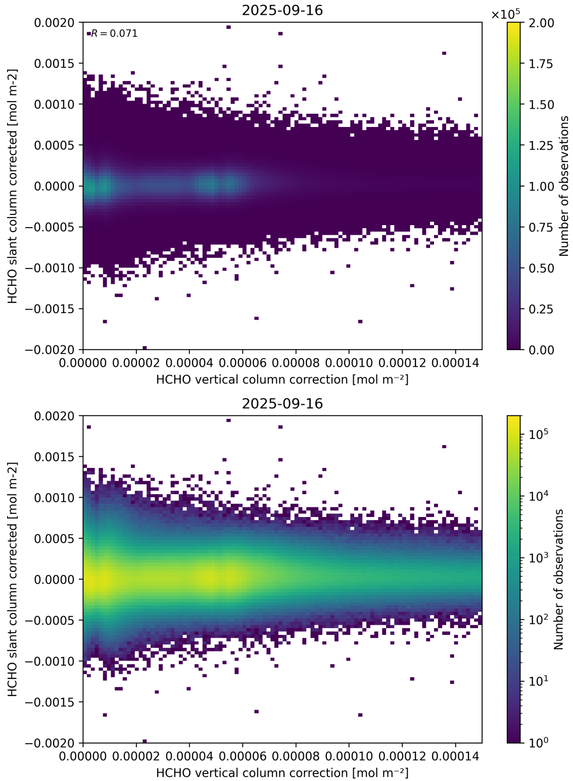
Figure 116: Scatter density plot of “HCHO vertical column correction” against “HCHO slant column corrected” for 2025-09-15 to 2025-09-17.
