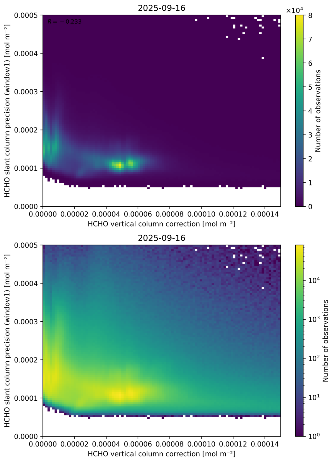
Figure 119: Scatter density plot of “HCHO vertical column correction” against “HCHO slant column precision (window1)” for 2025-09-15 to 2025-09-17.
