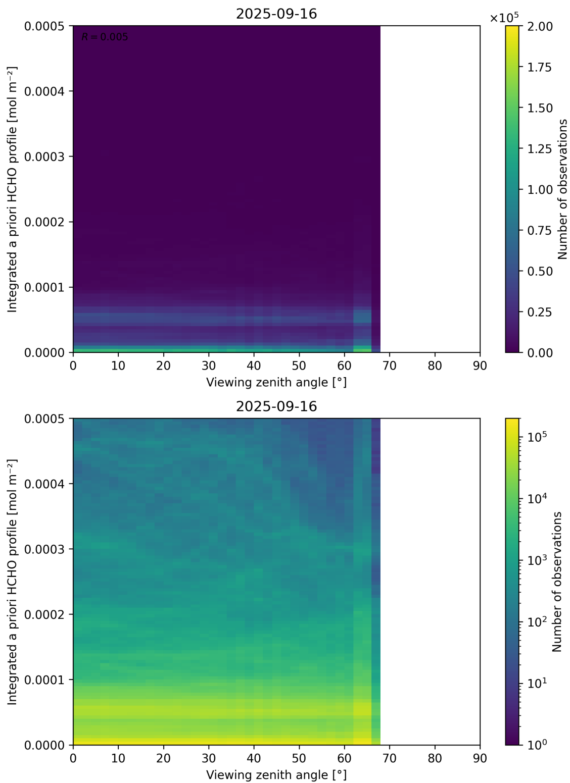
Figure 195: Scatter density plot of “Viewing zenith angle” against “Integrated a priori HCHO profile” for 2025-09-15 to 2025-09-17.
