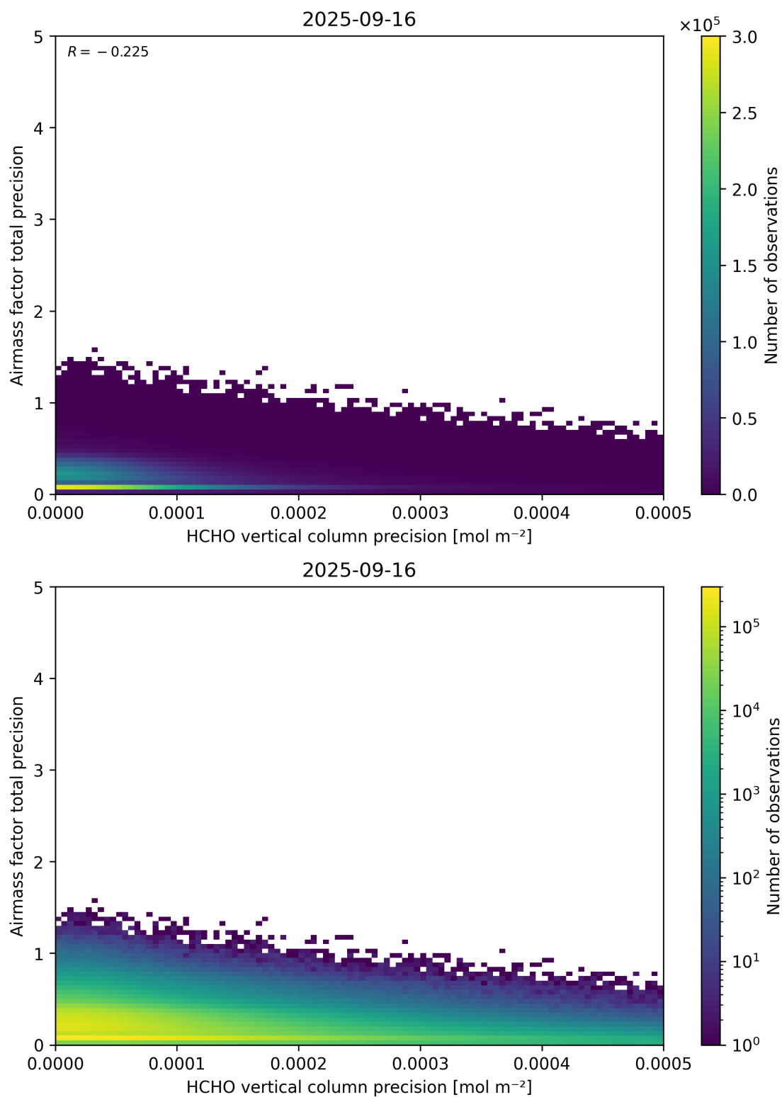
Figure 145: Scatter density plot of “HCHO vertical column precision” against “Airmass factor total precision” for 2025-09-15 to 2025-09-17.
