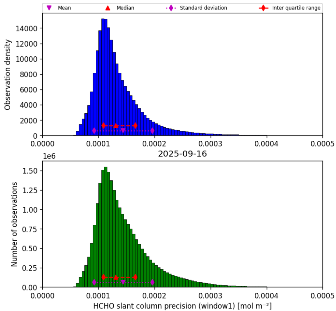
Figure 39: Histogram of “HCHO slant column precision (window1)” for 2025-09-15 to 2025-09-17
