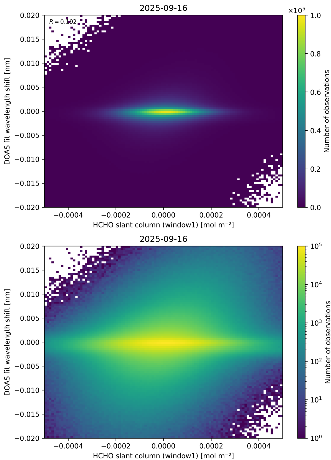
Figure 79: Scatter density plot of “HCHO slant column (window1)” against “DOAS fit wavelength shift” for 2025-09-15 to 2025-09-17.
