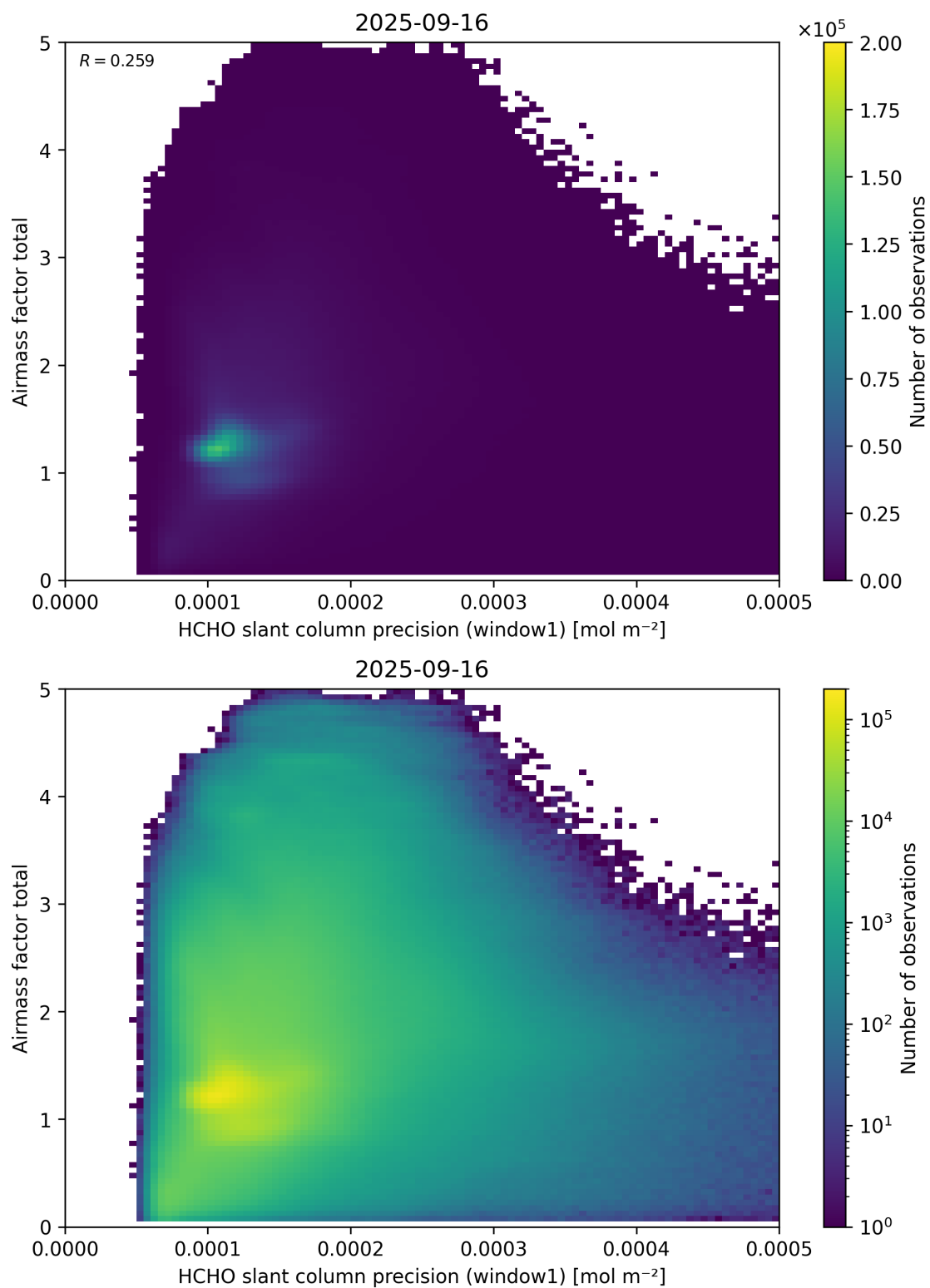
Figure 94: Scatter density plot of “HCHO slant column precision (window1)” against “Airmass factor total” for 2025-09-15 to 2025-09-17.
