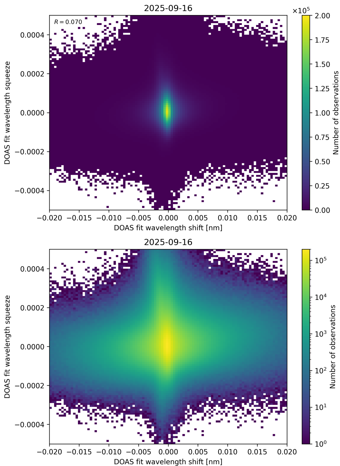
Figure 65: Scatter density plot of “DOAS fit wavelength shift” against “DOAS fit wavelength squeeze” for 2025-09-15 to 2025-09-17.
