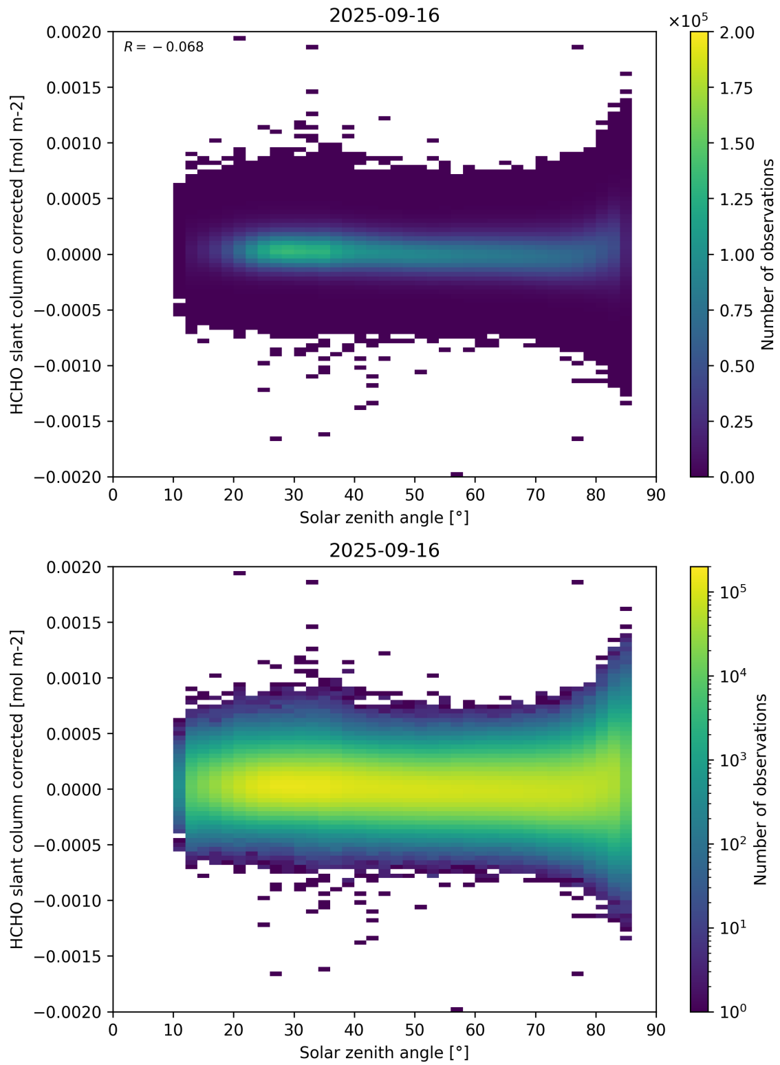
Figure 171: Scatter density plot of “Solar zenith angle” against “HCHO slant column corrected” for 2025-09-15 to 2025-09-17.
