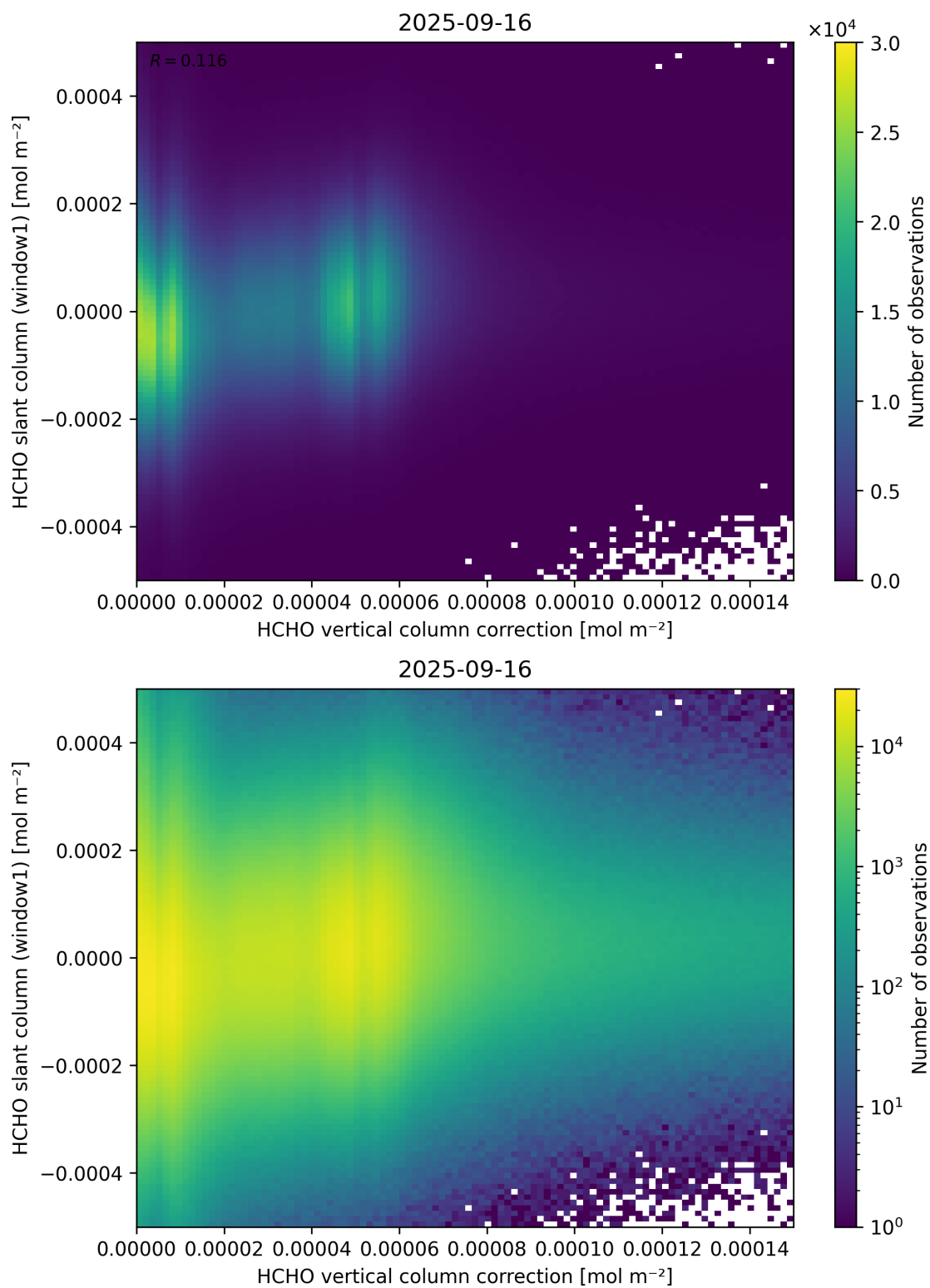
Figure 118: Scatter density plot of “HCHO vertical column correction” against “HCHO slant column (window1)” for 2025-09-15 to 2025-09-17.
