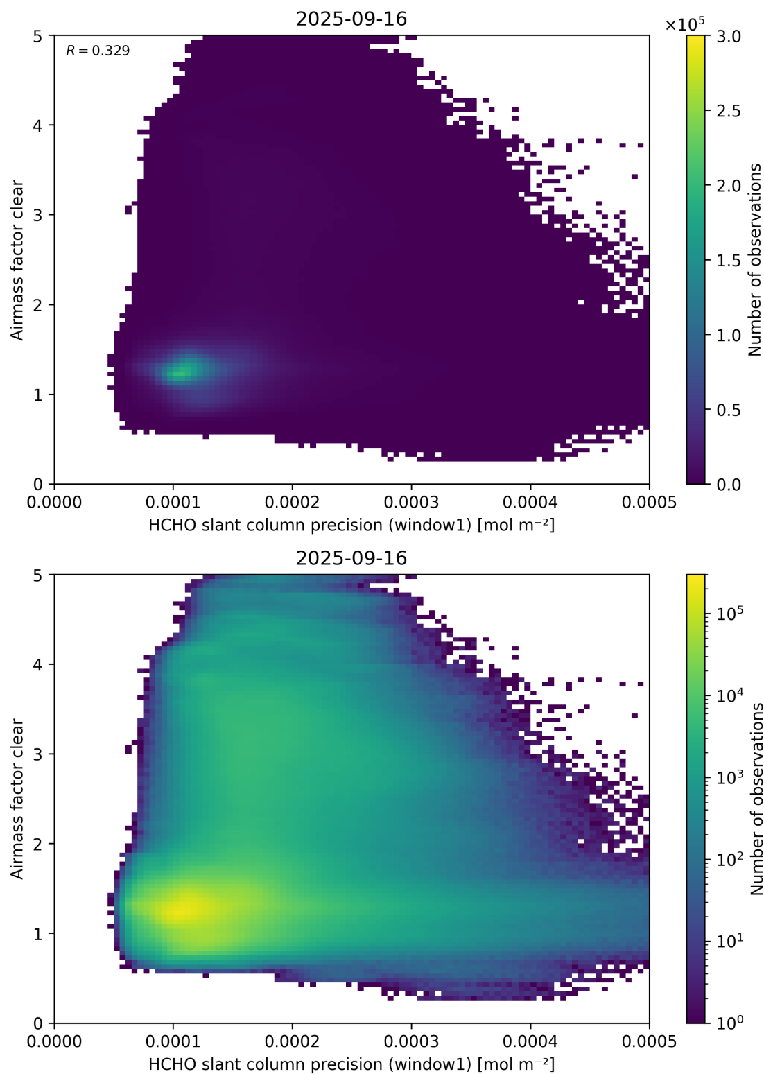
Figure 91: Scatter density plot of “HCHO slant column precision (window1)” against “Airmass factor clear” for 2025-09-15 to 2025-09-17.
