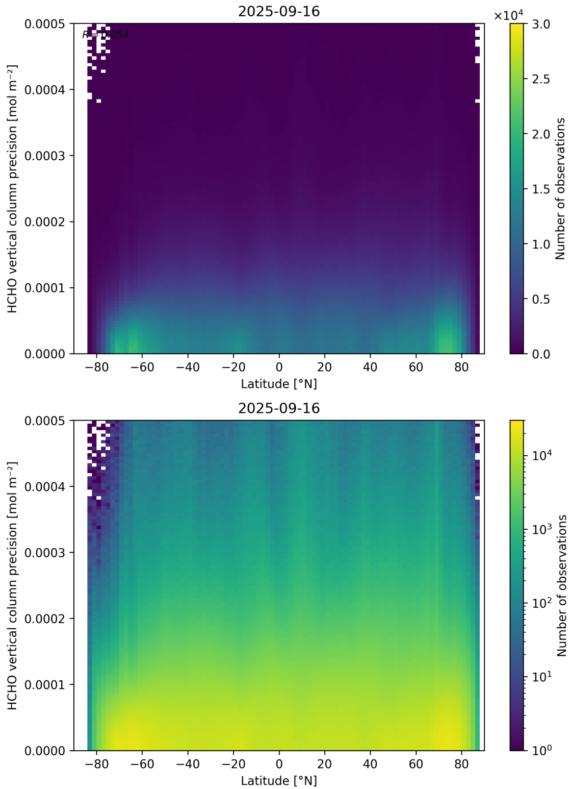
Figure 165: Scatter density plot of “Latitude” against “HCHO vertical column precision” for 2025-09-15 to 2025-09-17.
