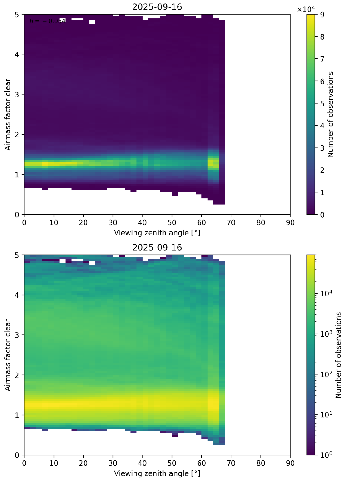
Figure 185: Scatter density plot of “Viewing zenith angle” against “Airmass factor clear” for 2025-09-15 to 2025-09-17.
