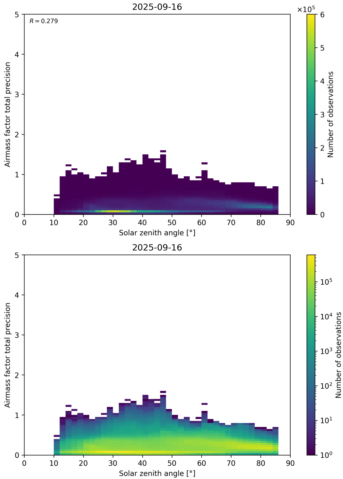
Figure 176: Scatter density plot of “Solar zenith angle” against “Airmass factor total precision” for 2025-09-15 to 2025-09-17.
