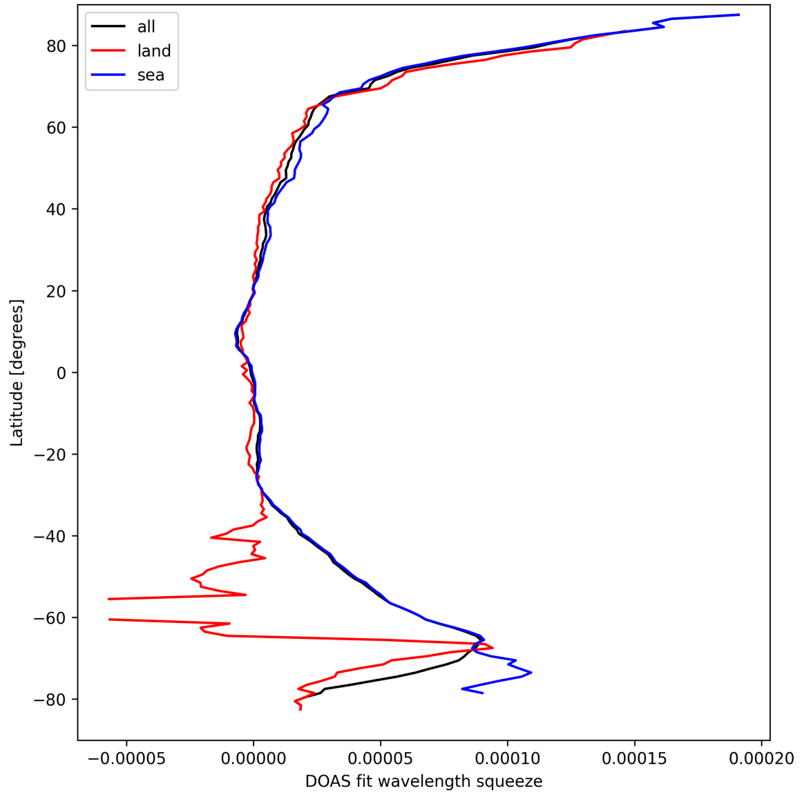
Figure 31: Zonal average of “DOAS fit wavelength squeeze” for 2025-09-15 to 2025-09-17.
