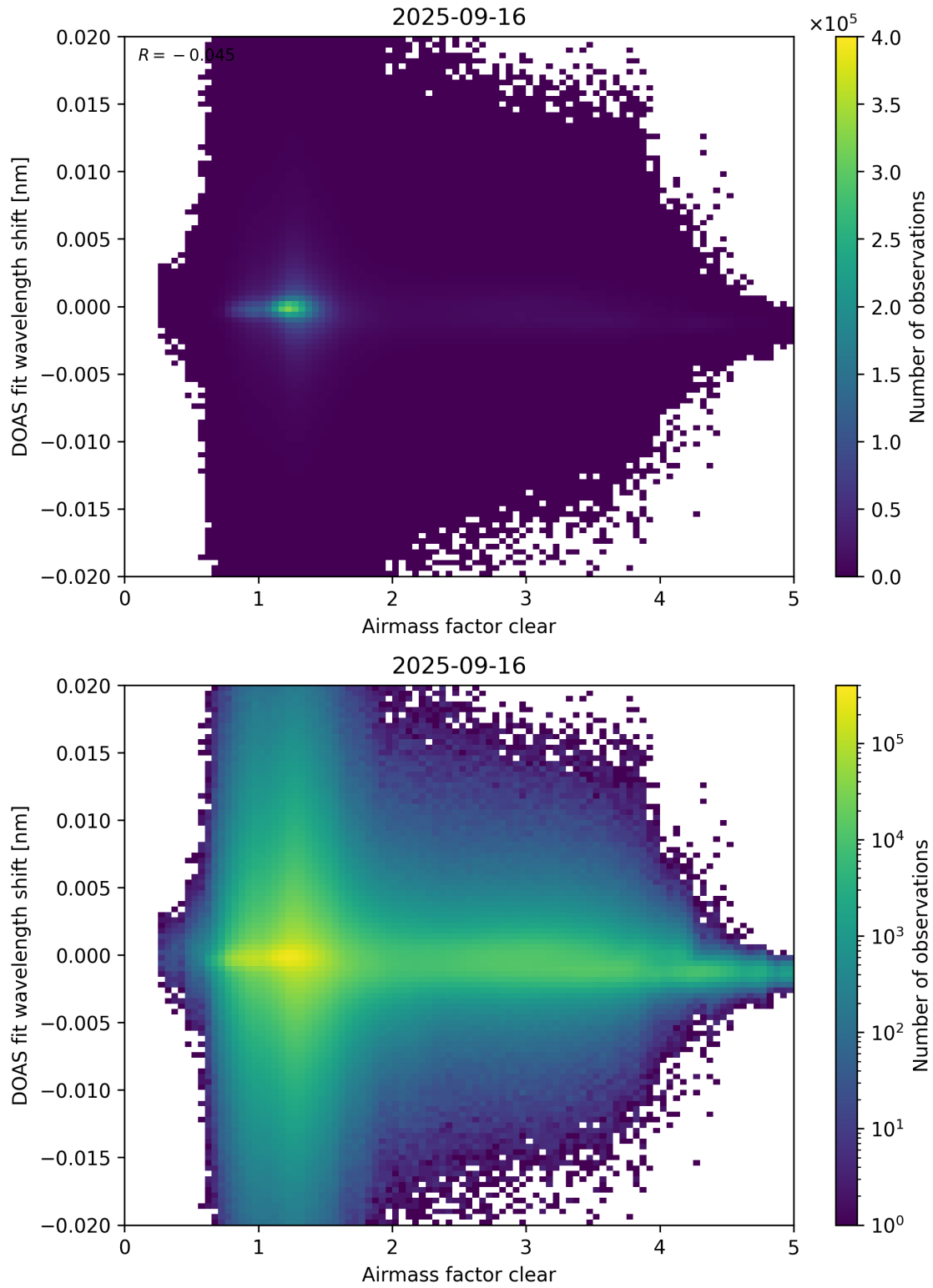
Figure 72: Scatter density plot of “Airmass factor clear” against “DOAS fit wavelength shift” for 2025-09-15 to 2025-09-17.
