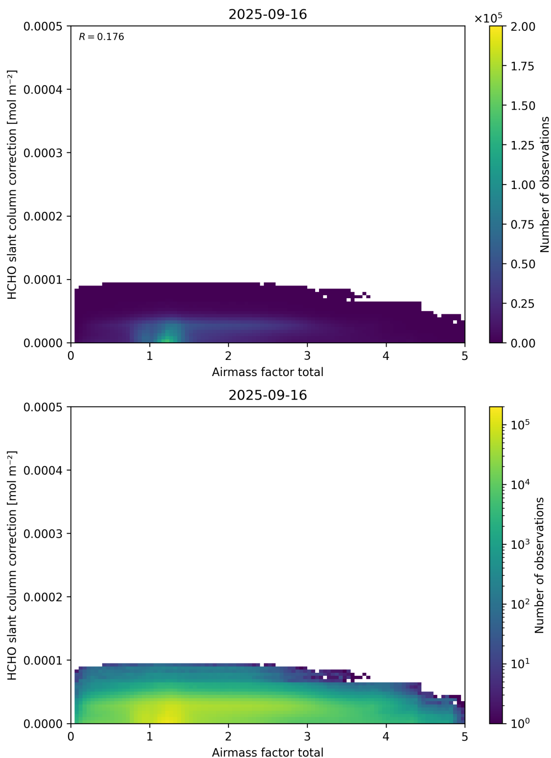
Figure 102: Scatter density plot of “Airmass factor total” against “HCHO slant column correction” for 2025-09-15 to 2025-09-17.
