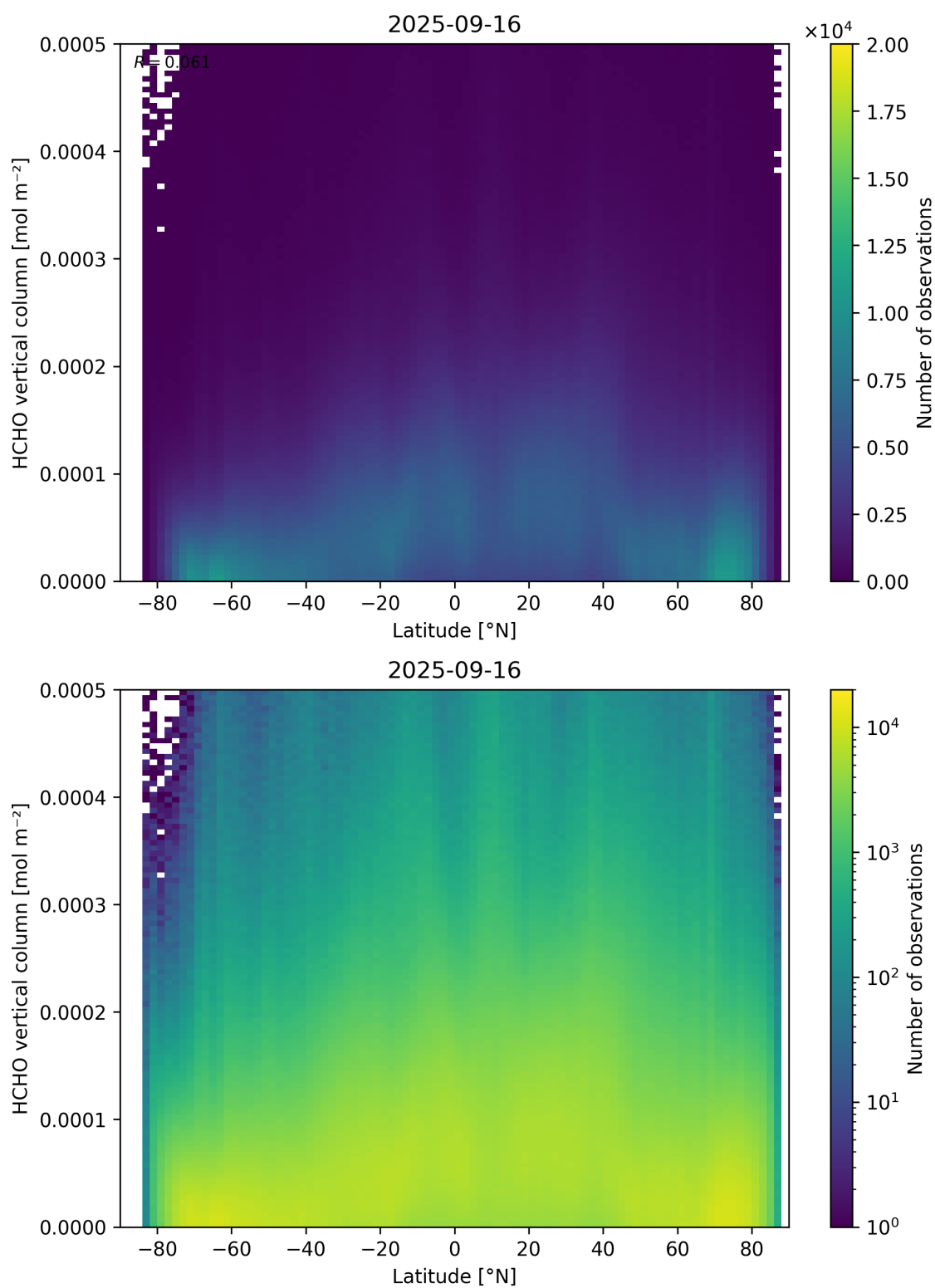
Figure 163: Scatter density plot of “Latitude” against “HCHO vertical column” for 2025-09-15 to 2025-09-17.
