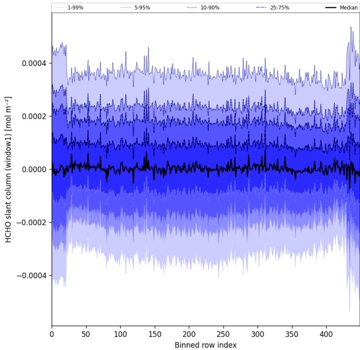
Figure 52: Along track statistics of “HCHO slant column (window1)” for 2025-09-15 to 2025-09-17
