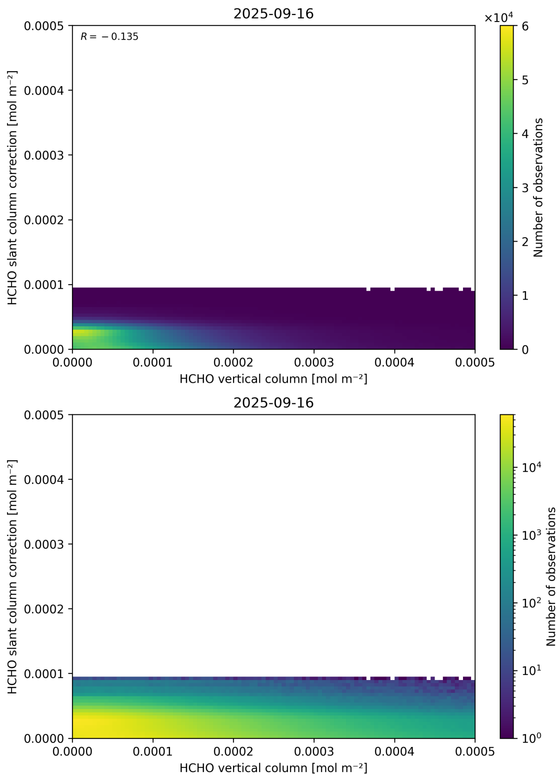
Figure 128: Scatter density plot of “HCHO vertical column” against “HCHO slant column correction” for 2025-09-15 to 2025-09-17.
