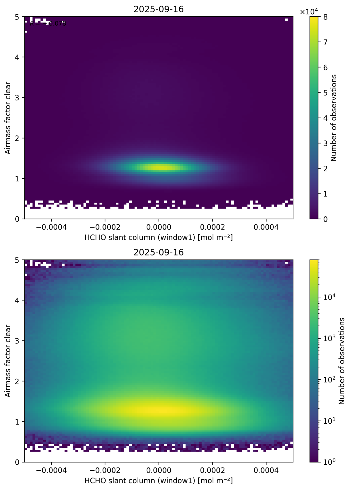
Figure 81: Scatter density plot of “HCHO slant column (window1)” against “Airmass factor clear” for 2025-09-15 to 2025-09-17.
