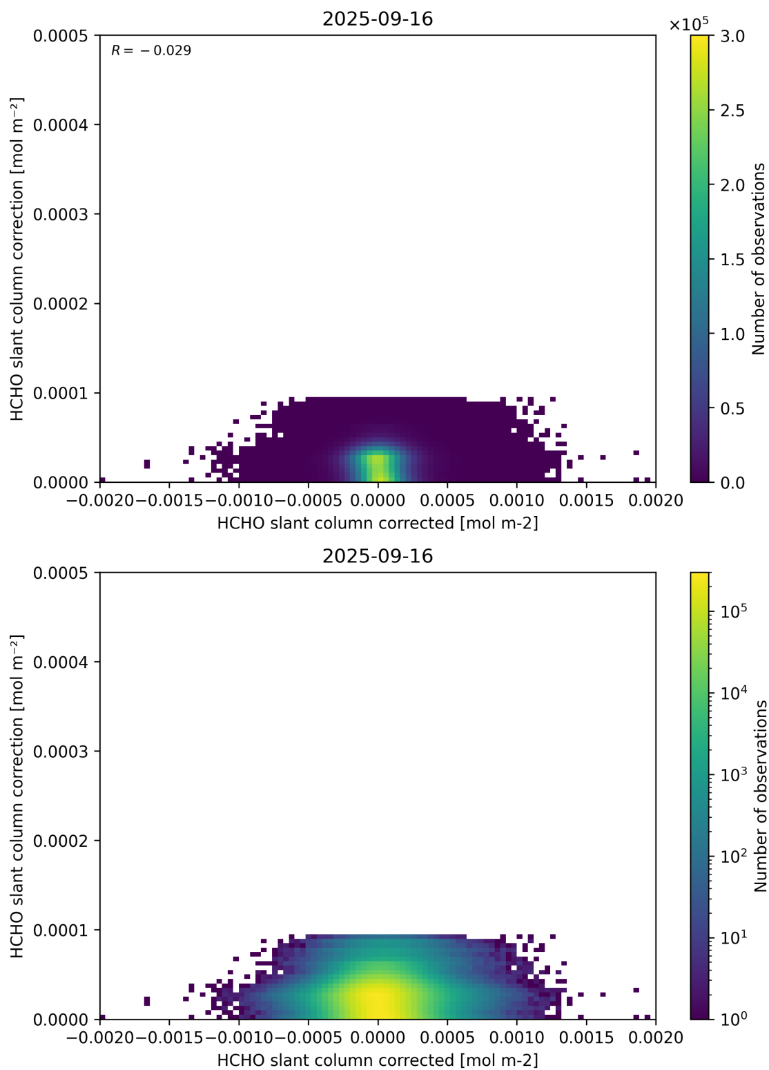
Figure 77: Scatter density plot of “HCHO slant column corrected” against “HCHO slant column correction” for 2025-09-15 to 2025-09-17.
