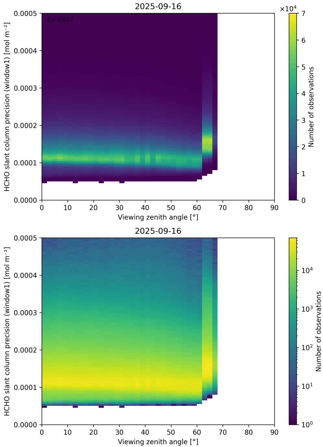
Figure 189: Scatter density plot of “Viewing zenith angle” against “HCHO slant column precision (window1)” for 2025-09-15 to 2025-09-17.
