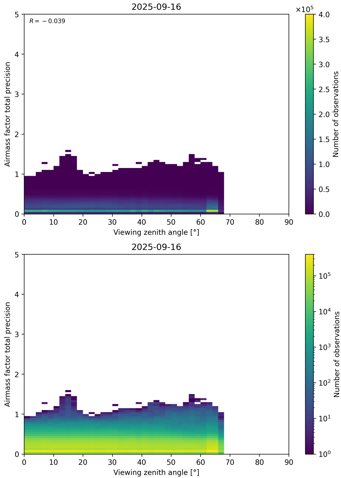
Figure 191: Scatter density plot of “Viewing zenith angle” against “Airmass factor total precision” for 2025-09-15 to 2025-09-17.
