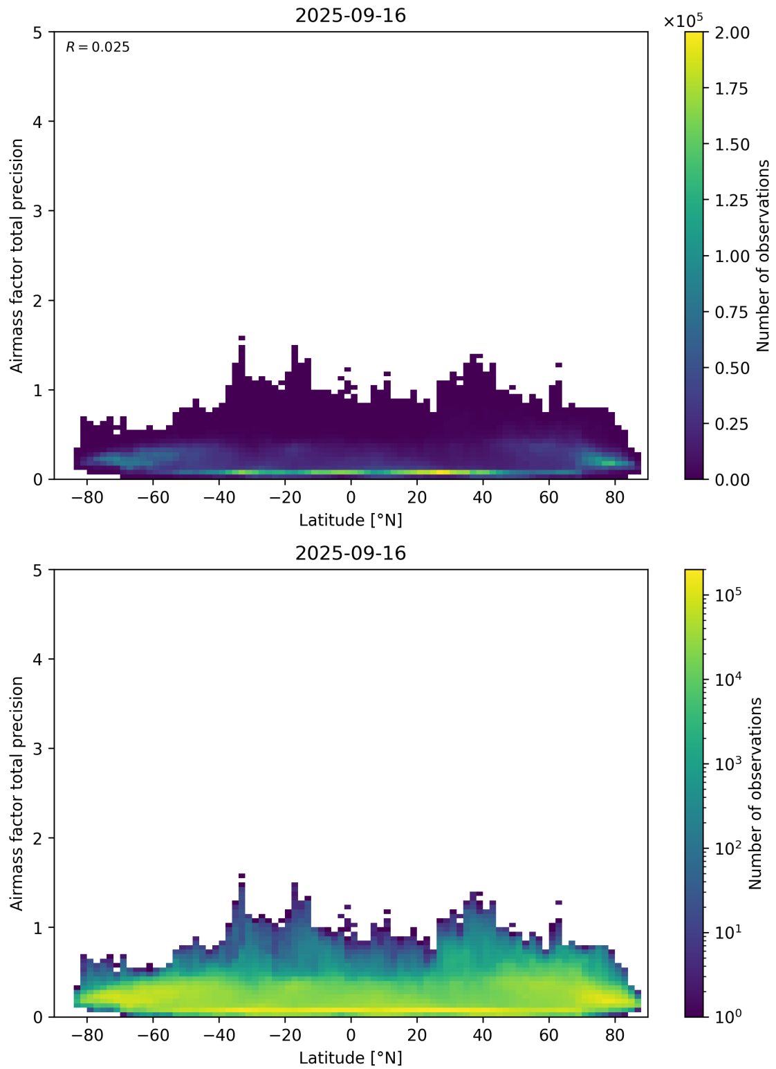
Figure 162: Scatter density plot of “Latitude” against “Airmass factor total precision” for 2025-09-15 to 2025-09-17.
