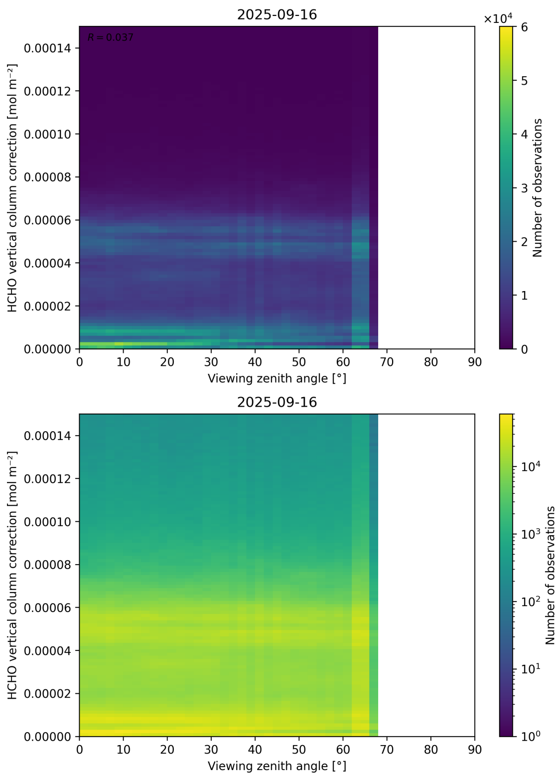
Figure 193: Scatter density plot of “Viewing zenith angle” against “HCHO vertical column correction” for 2025-09-15 to 2025-09-17.
