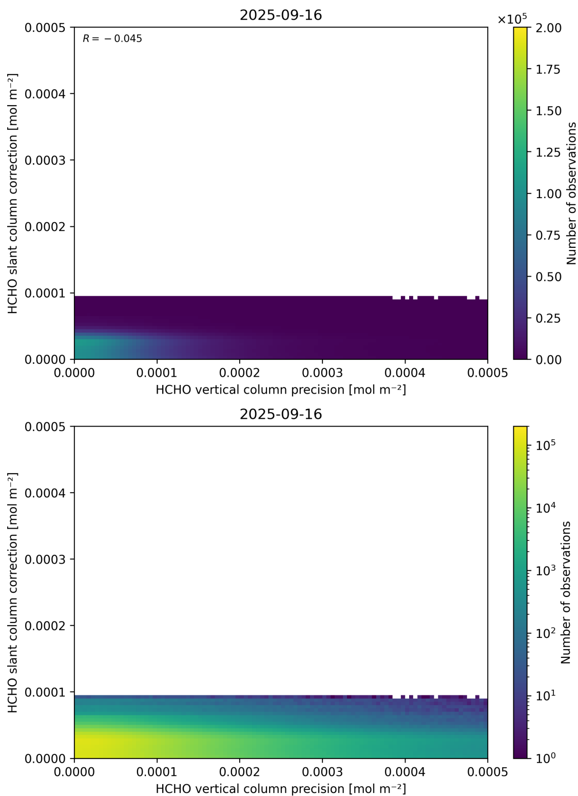
Figure 141: Scatter density plot of “HCHO vertical column precision” against “HCHO slant column correction” for 2025-09-15 to 2025-09-17.
