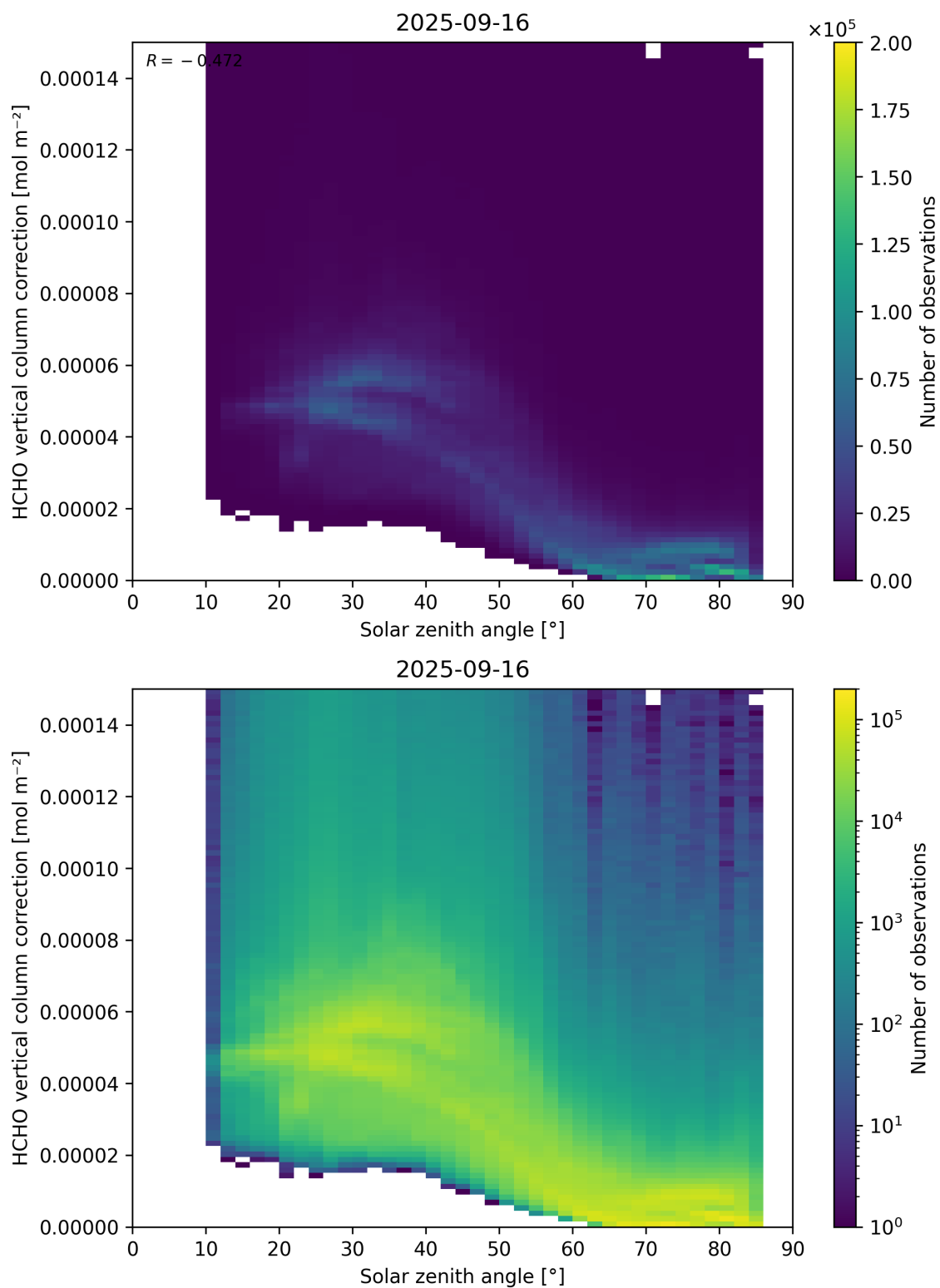
Figure 178: Scatter density plot of “Solar zenith angle” against “HCHO vertical column correction” for 2025-09-15 to 2025-09-17.
