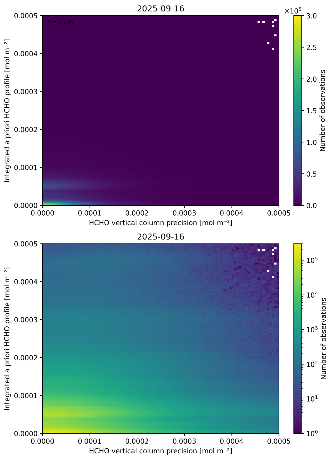
Figure 147: Scatter density plot of “HCHO vertical column precision” against “Integrated a priori HCHO profile” for 2025-09-15 to 2025-09-17.
