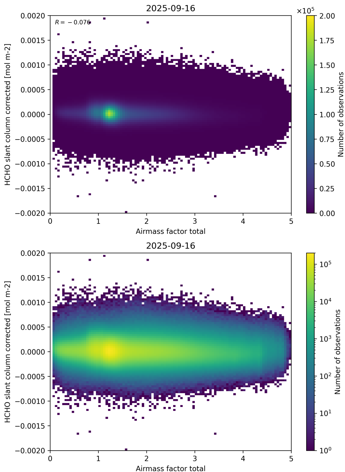
Figure 101: Scatter density plot of “Airmass factor total” against “HCHO slant column corrected” for 2025-09-15 to 2025-09-17.
