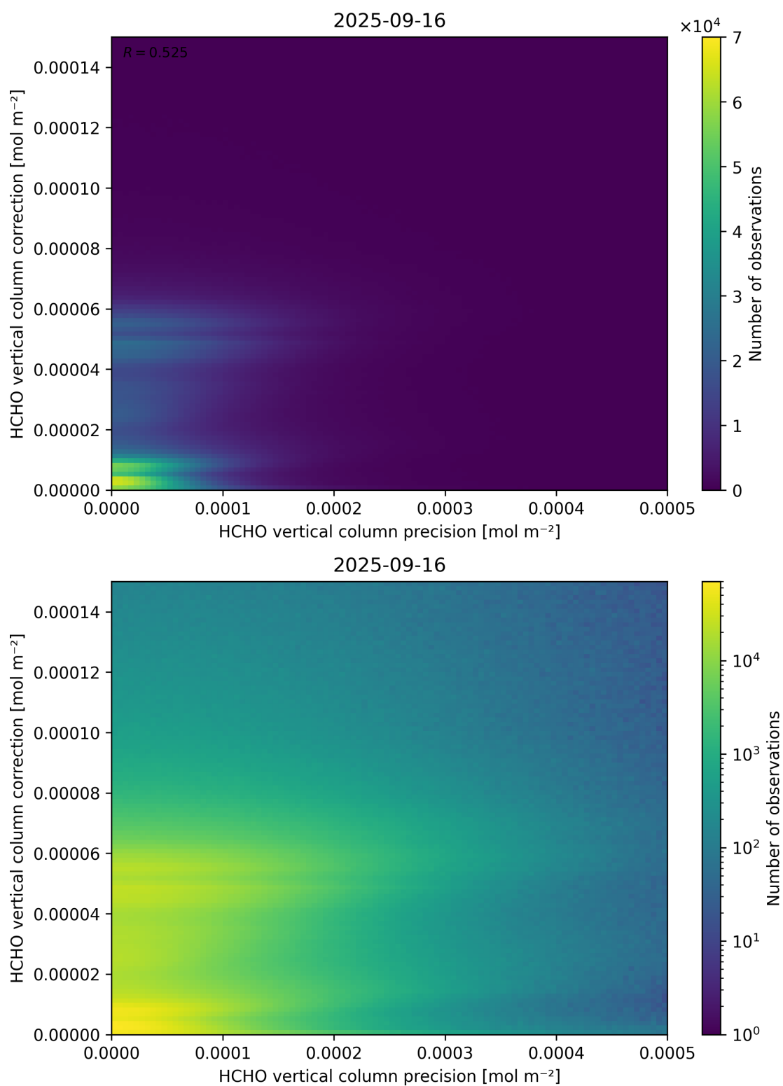
Figure 146: Scatter density plot of “HCHO vertical column precision” against “HCHO vertical column correction” for 2025-09-15 to 2025-09-17.
