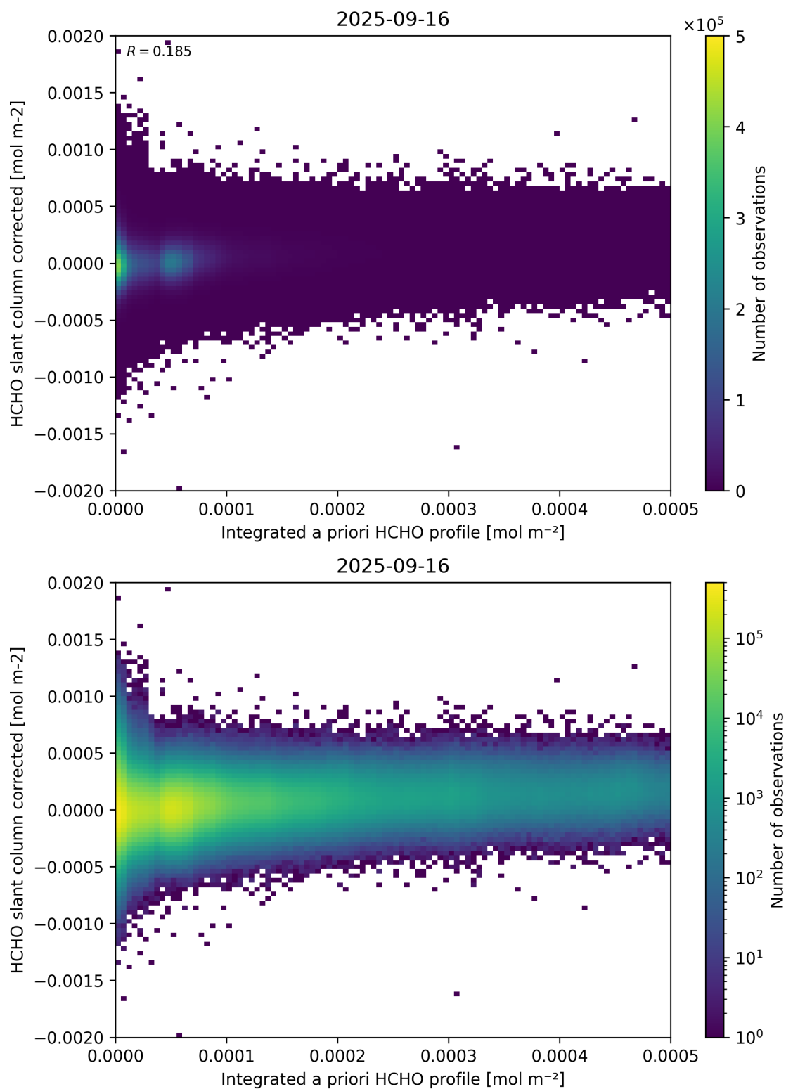
Figure 151: Scatter density plot of “Integrated a priori HCHO profile” against “HCHO slant column corrected” for 2025-09-15 to 2025-09-17.
