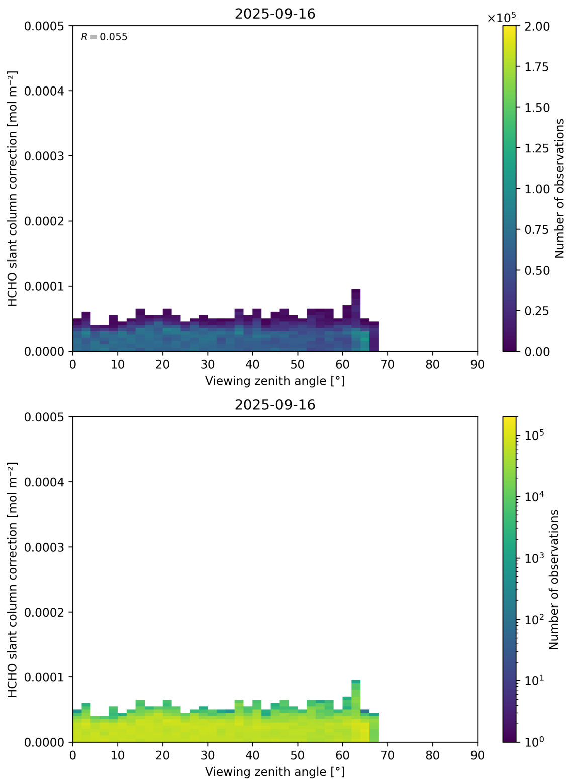
Figure 187: Scatter density plot of “Viewing zenith angle” against “HCHO slant column correction” for 2025-09-15 to 2025-09-17.
