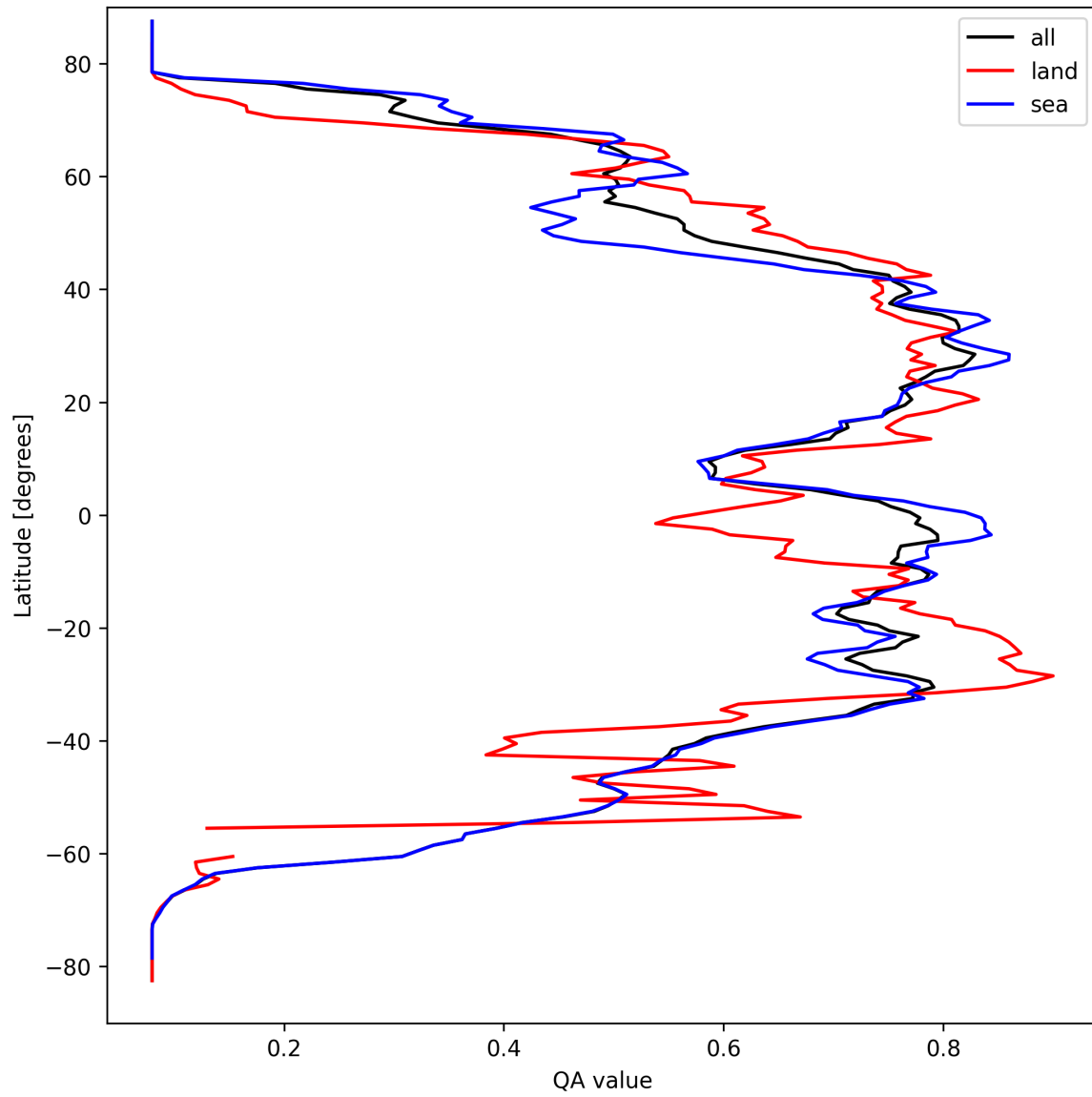
Figure 20: Zonal average of “QA value” for 2025-09-15 to 2025-09-17.
