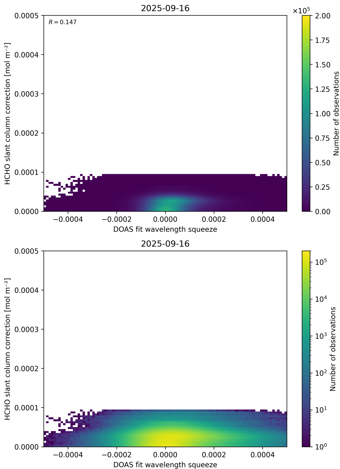
Figure 70: Scatter density plot of “DOAS fit wavelength squeeze” against “HCHO slant column correction” for 2025-09-15 to 2025-09-17.
