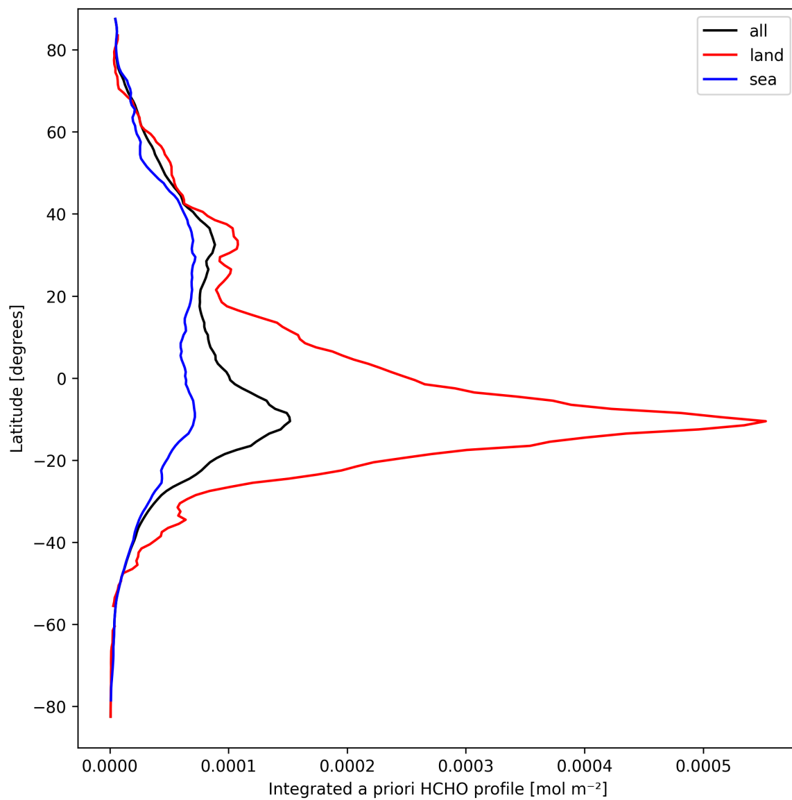
Figure 29: Zonal average of “Integrated a priori HCHO profile” for 2025-09-15 to 2025-09-17.
