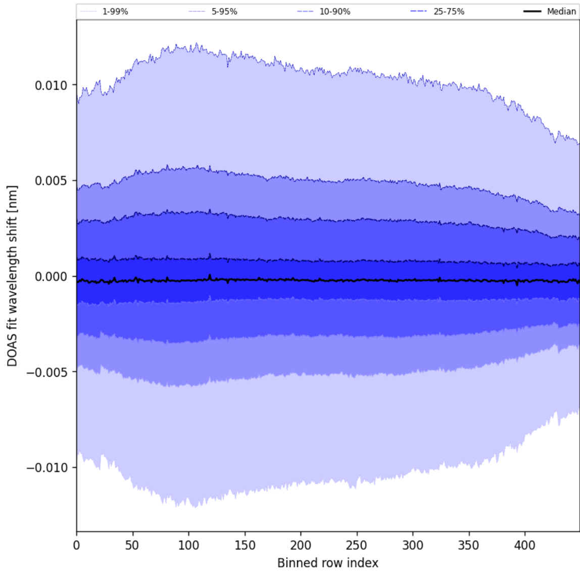
Figure 58: Along track statistics of “DOAS fit wavelength shift” for 2025-09-15 to 2025-09-17
