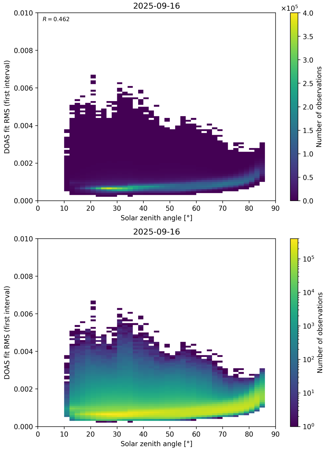
Figure 167: Scatter density plot of “Solar zenith angle” against “DOAS fit RMS (first interval)” for 2025-09-15 to 2025-09-17.
