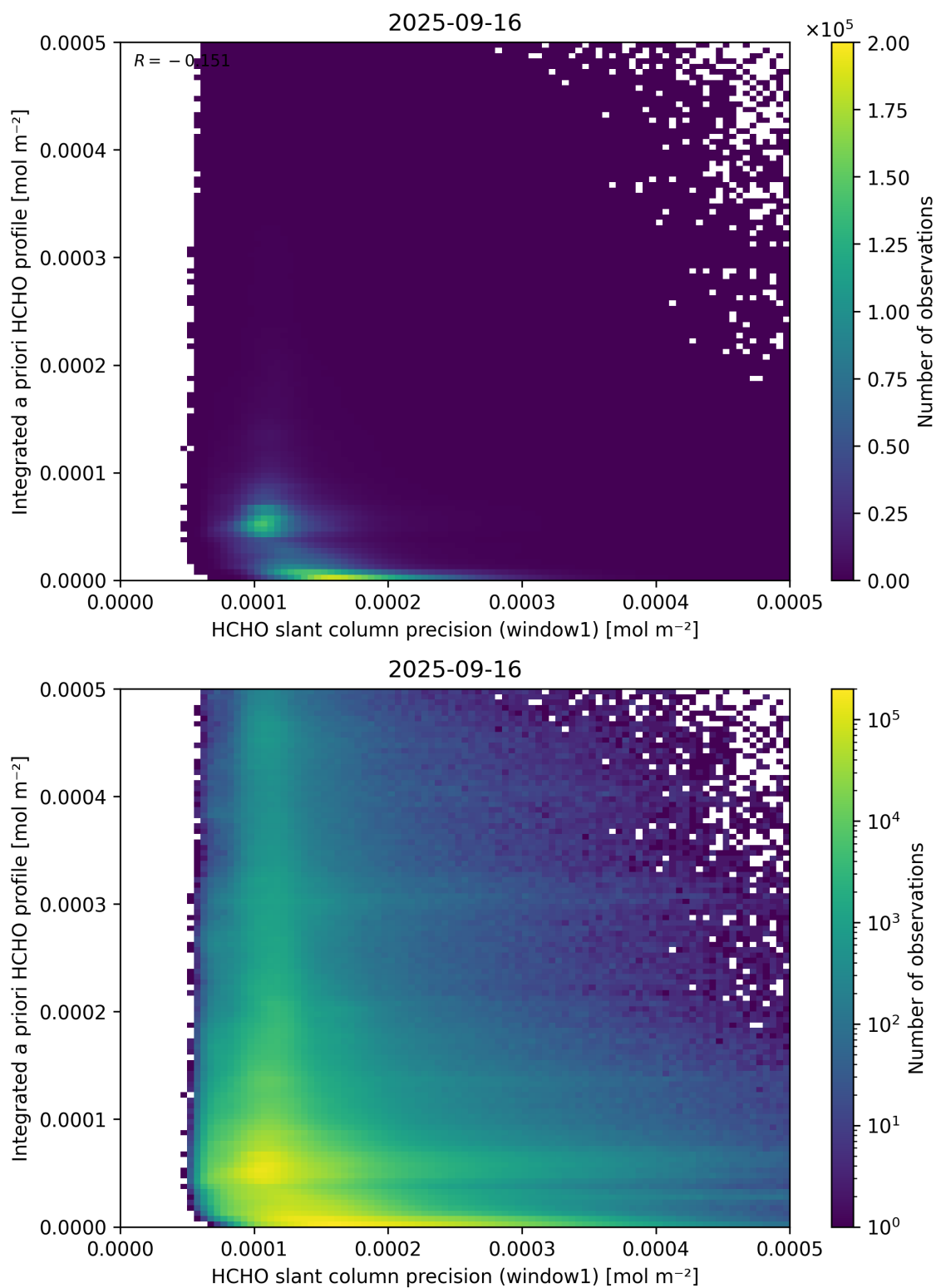
Figure 96: Scatter density plot of “HCHO slant column precision (window1)” against “Integrated a priori HCHO profile” for 2025-09-15 to 2025-09-17.
