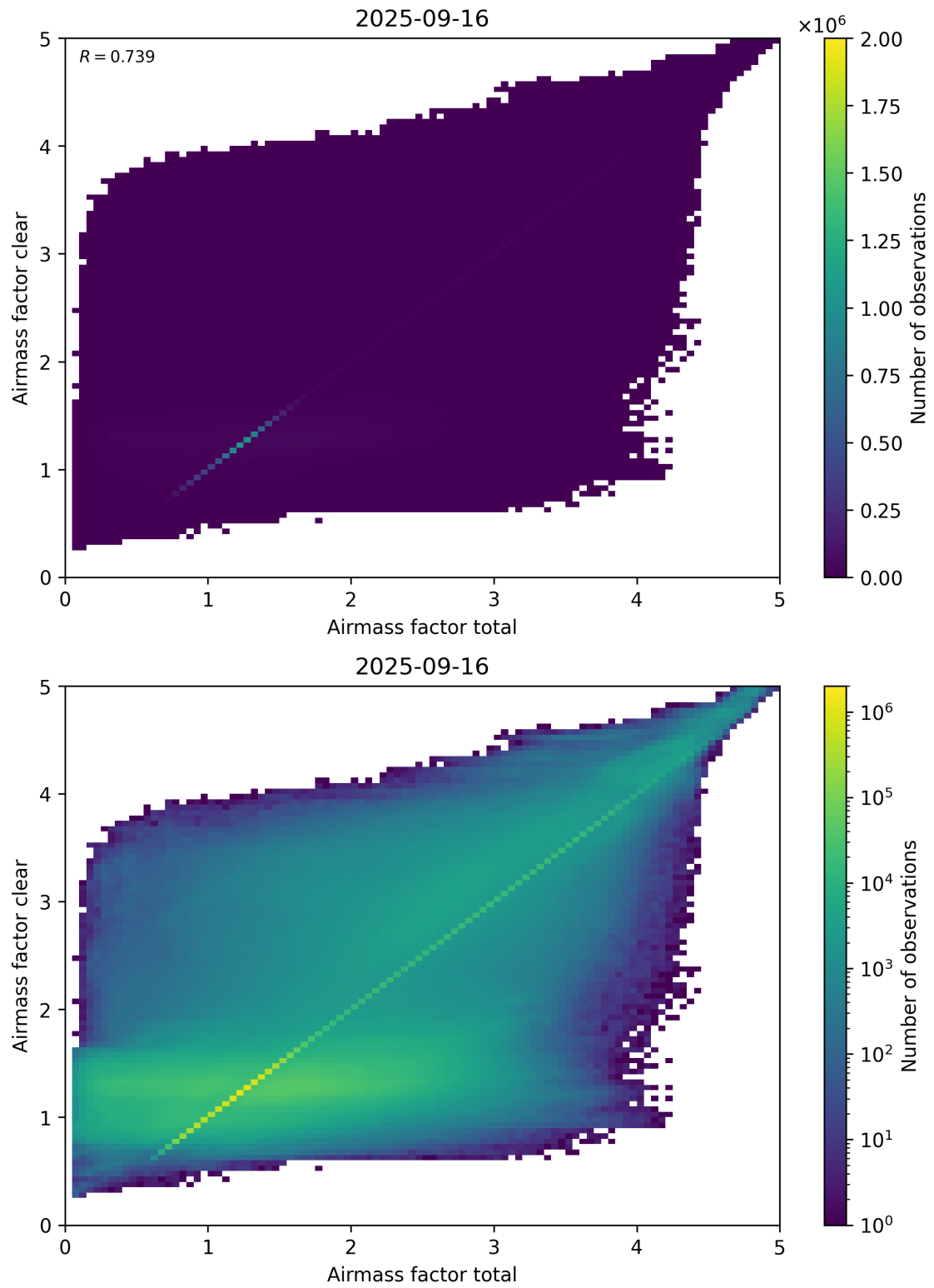
Figure 100: Scatter density plot of “Airmass factor total” against “Airmass factor clear” for 2025-09-15 to 2025-09-17.
