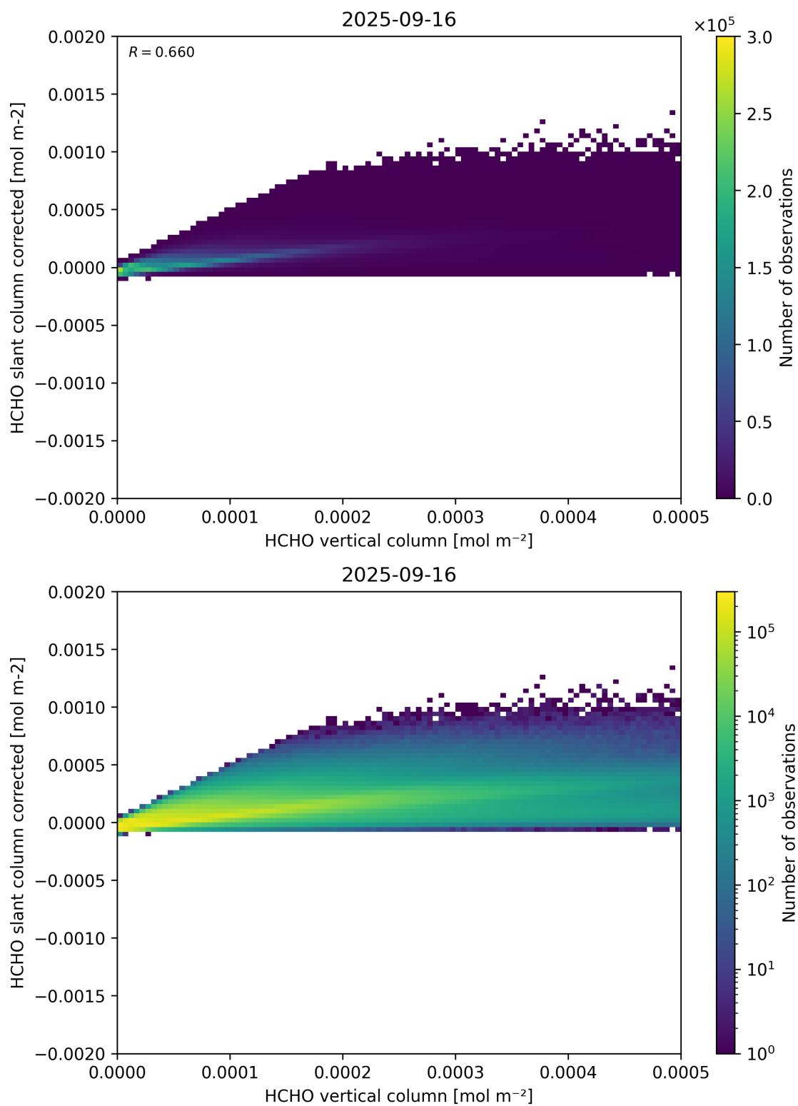
Figure 127: Scatter density plot of “HCHO vertical column” against “HCHO slant column corrected” for 2025-09-15 to 2025-09-17.
