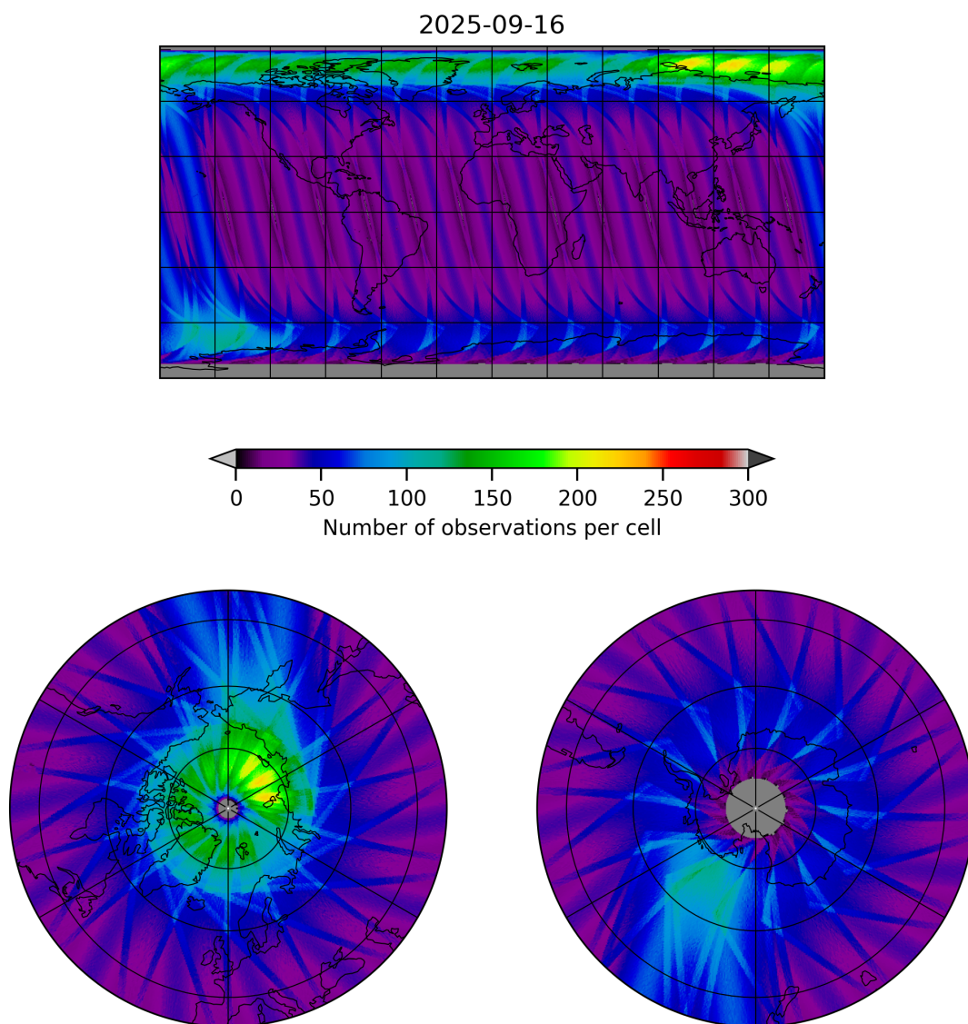
Figure 19: Map of the number of observations for 2025-09-15 to 2025-09-17
