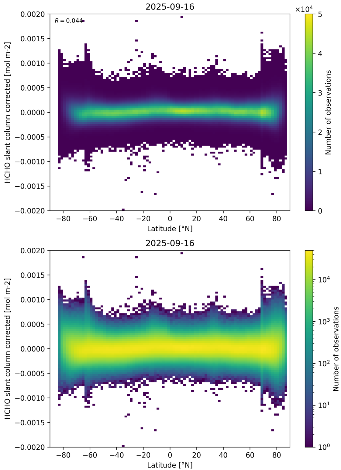
Figure 157: Scatter density plot of “Latitude” against “HCHO slant column corrected” for 2025-09-15 to 2025-09-17.
