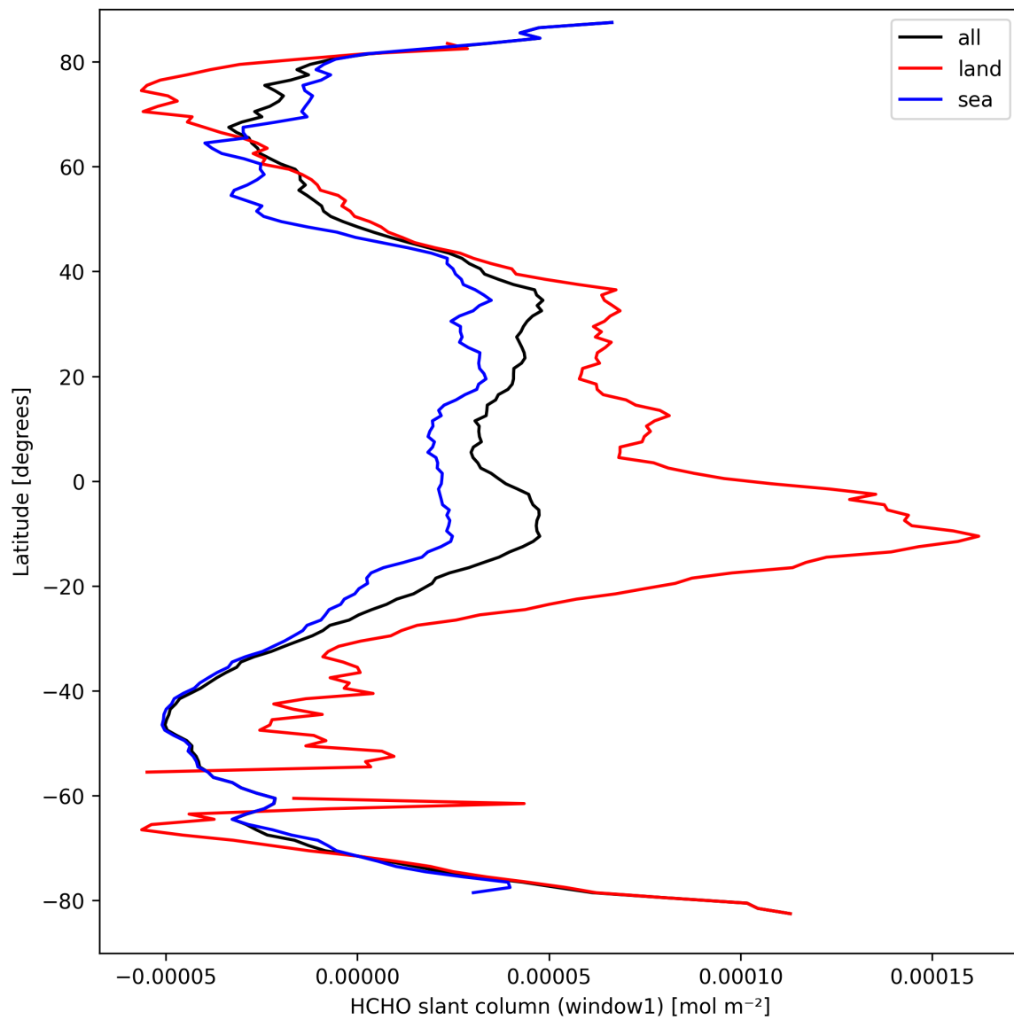
Figure 24: Zonal average of “HCHO slant column (window1)” for 2025-09-15 to 2025-09-17.
