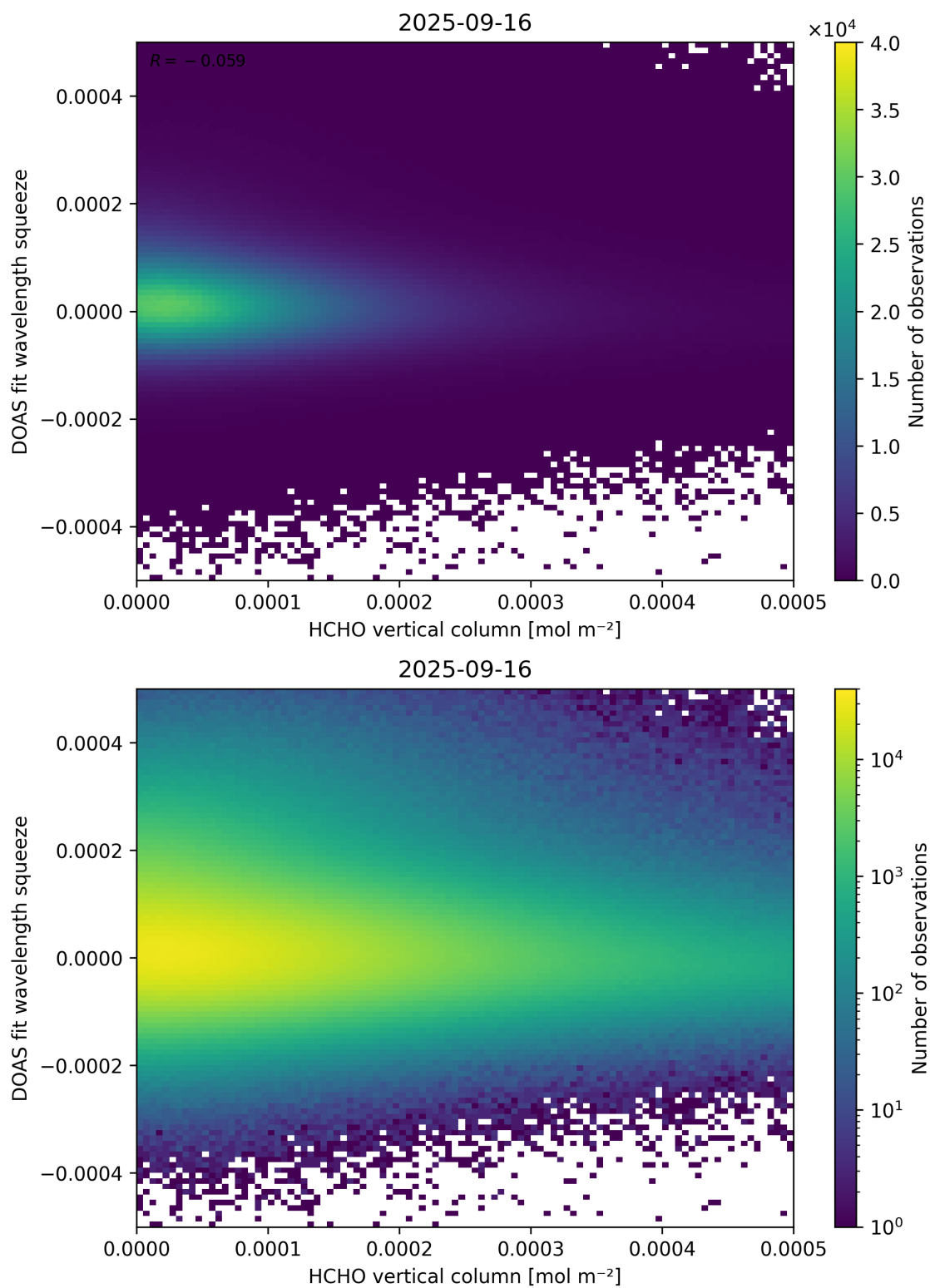
Figure 125: Scatter density plot of “HCHO vertical column” against “DOAS fit wavelength squeeze” for 2025-09-15 to 2025-09-17.
