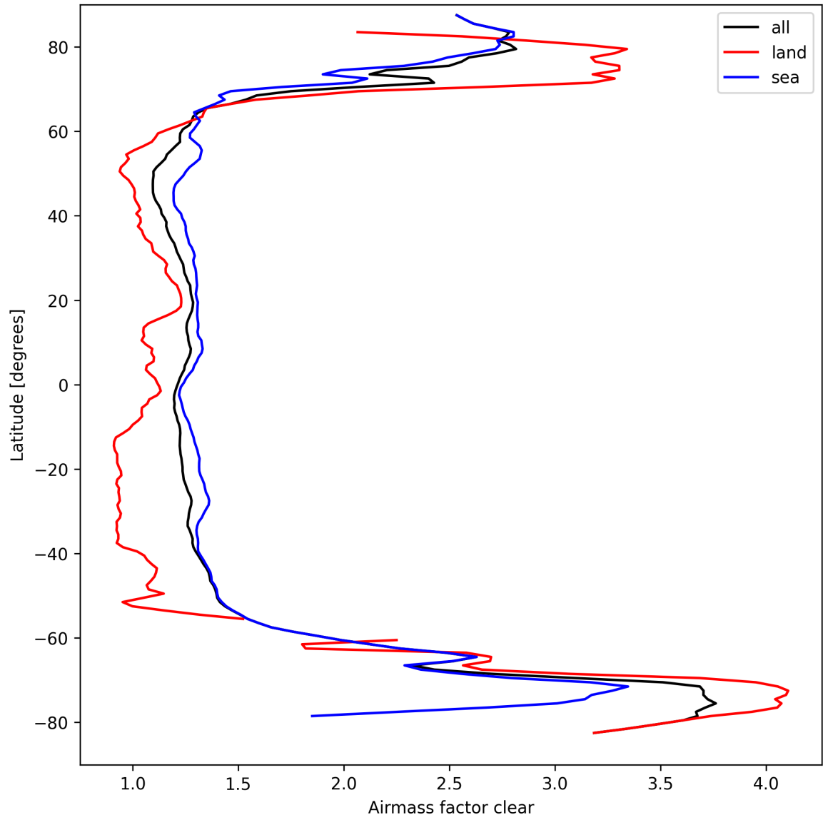
Figure 28: Zonal average of “Airmass factor clear” for 2025-09-15 to 2025-09-17.
