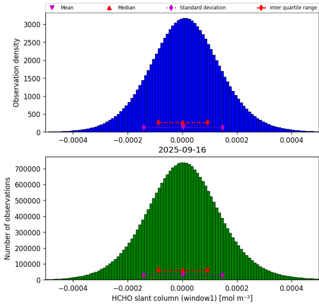
Figure 38: Histogram of “HCHO slant column (window1)” for 2025-09-15 to 2025-09-17
