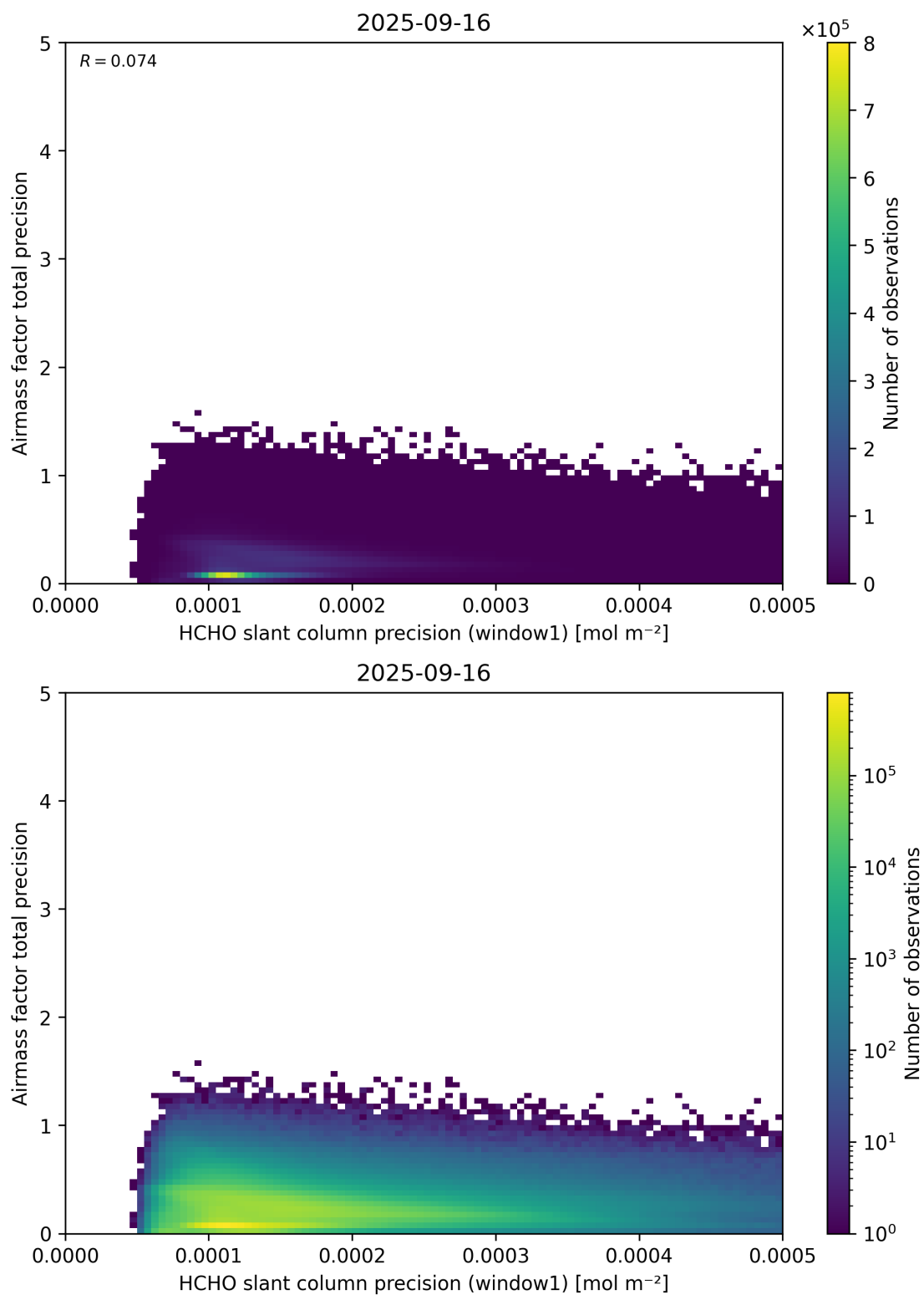
Figure 95: Scatter density plot of “HCHO slant column precision (window1)” against “Airmass factor total precision” for 2025-09-15 to 2025-09-17.
