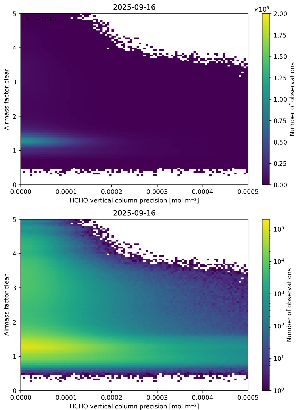
Figure 139: Scatter density plot of “HCHO vertical column precision” against “Airmass factor clear” for 2025-09-15 to 2025-09-17.
