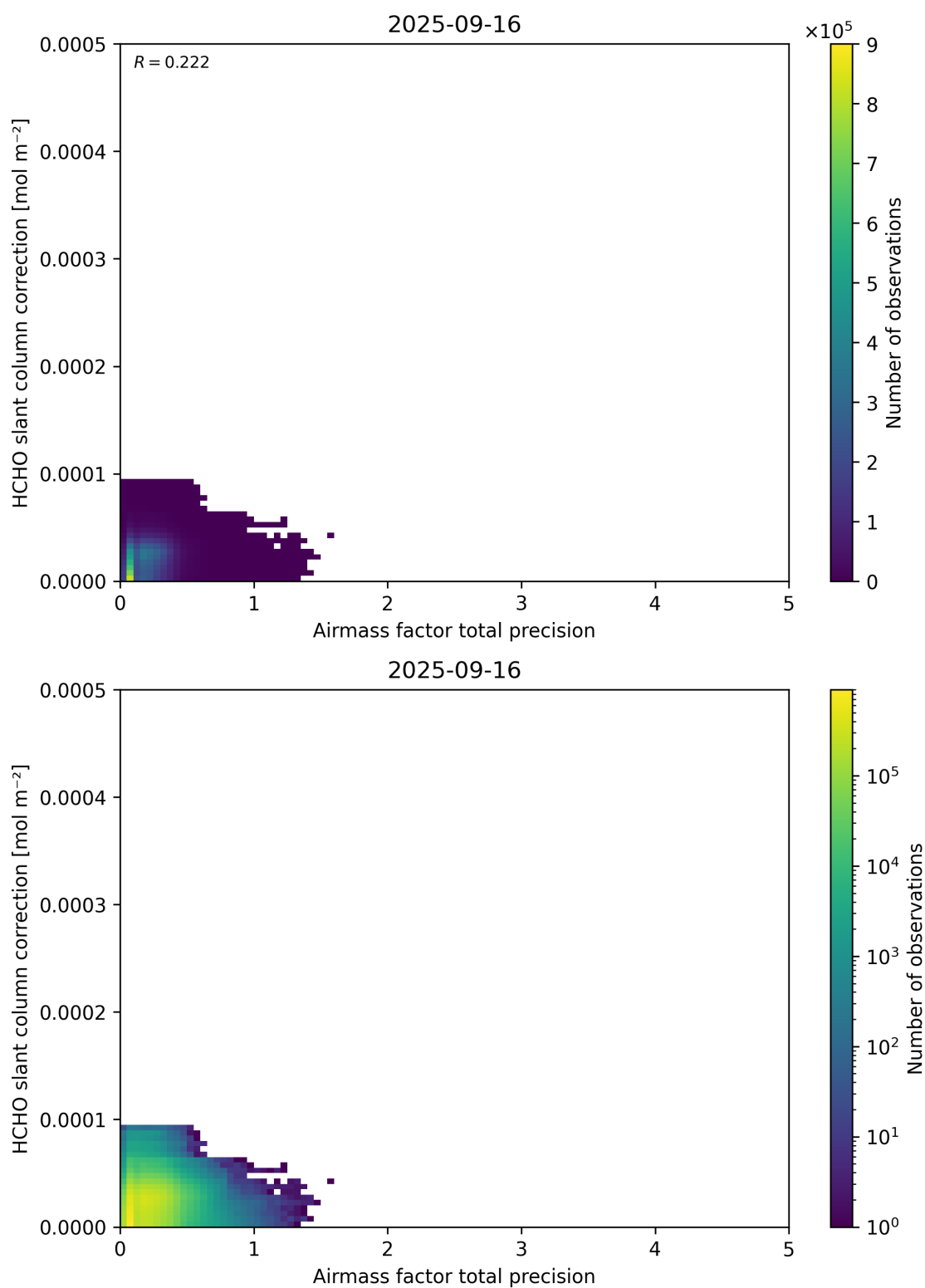
Figure 110: Scatter density plot of “Airmass factor total precision” against “HCHO slant column correction” for 2025-09-15 to 2025-09-17.
