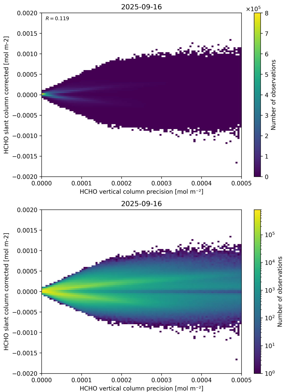
Figure 140: Scatter density plot of “HCHO vertical column precision” against “HCHO slant column corrected” for 2025-09-15 to 2025-09-17.
