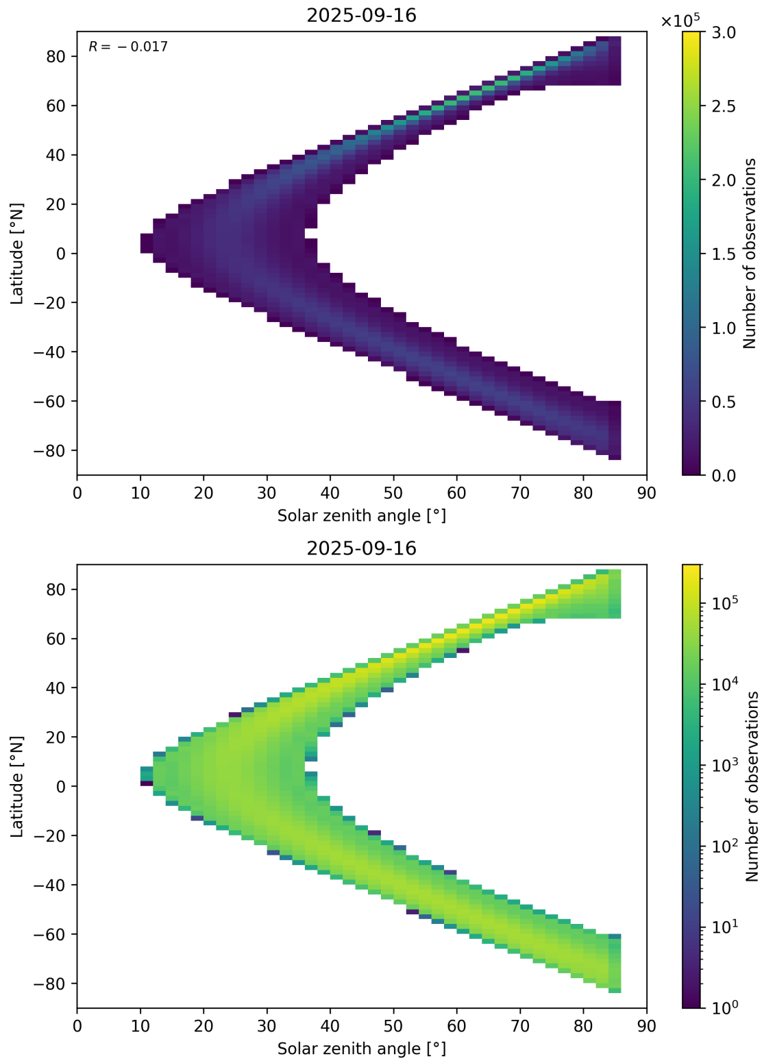
Figure 181: Scatter density plot of “Solar zenith angle” against “Latitude” for 2025-09-15 to 2025-09-17.
