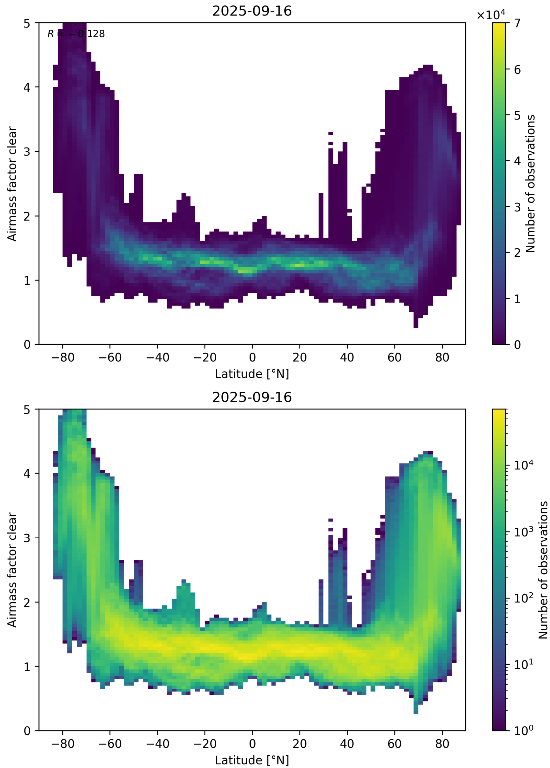
Figure 156: Scatter density plot of “Latitude” against “Airmass factor clear” for 2025-09-15 to 2025-09-17.
