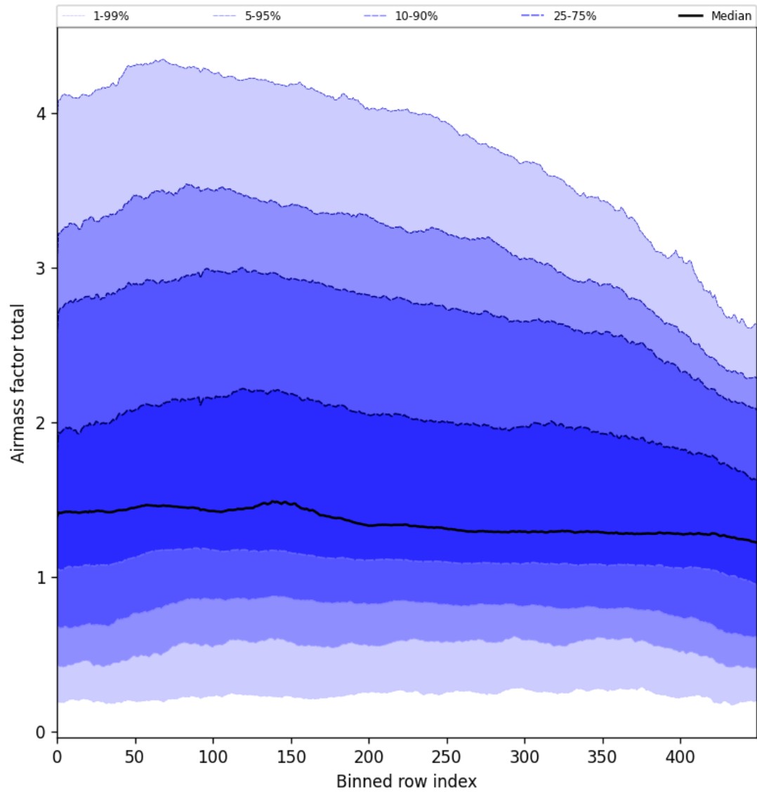
Figure 54: Along track statistics of “Airmass factor total” for 2025-09-15 to 2025-09-17
