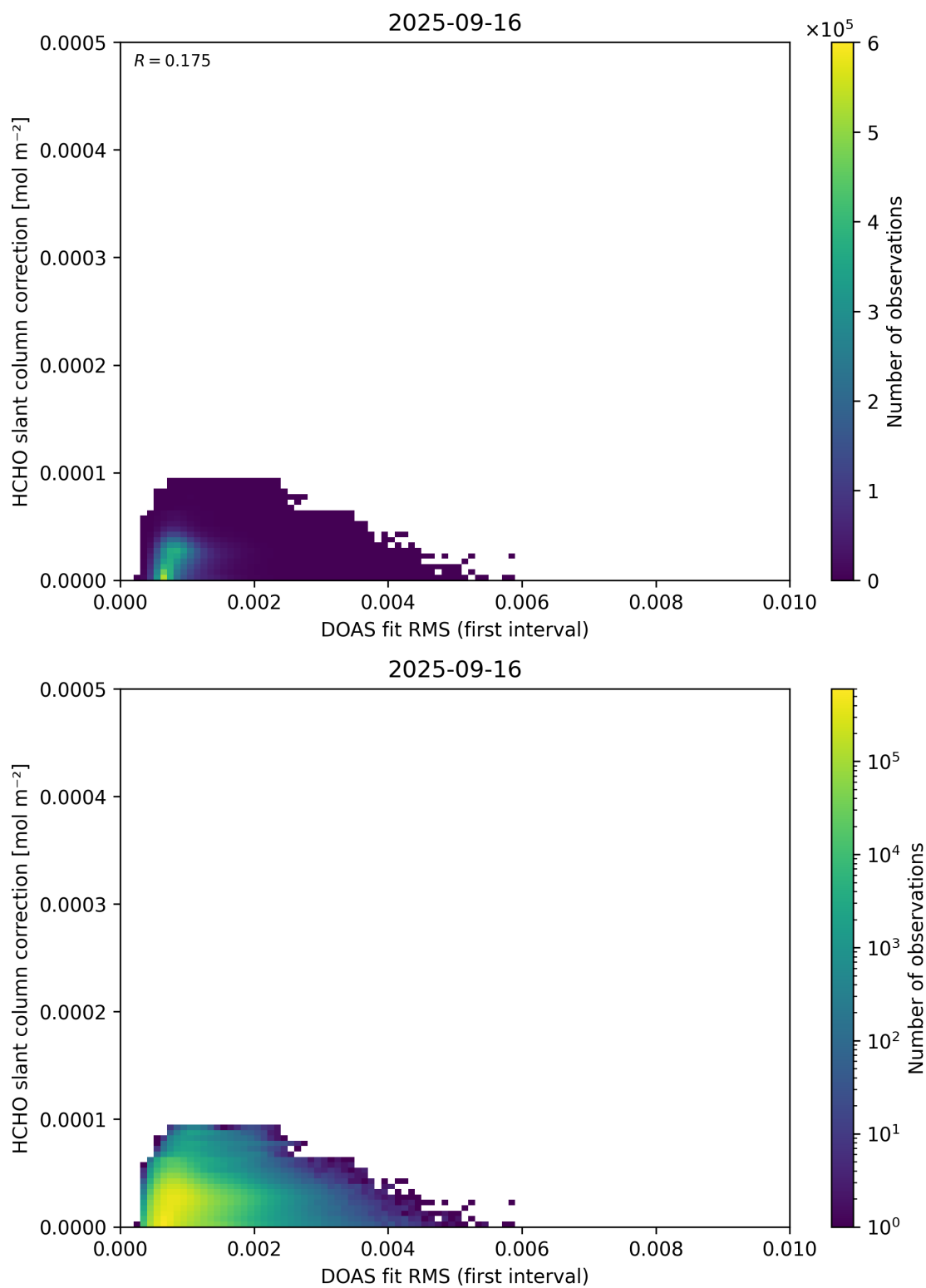
Figure 63: Scatter density plot of “DOAS fit RMS (first interval)” against “HCHO slant column correction” for 2025-09-15 to 2025-09-17.
