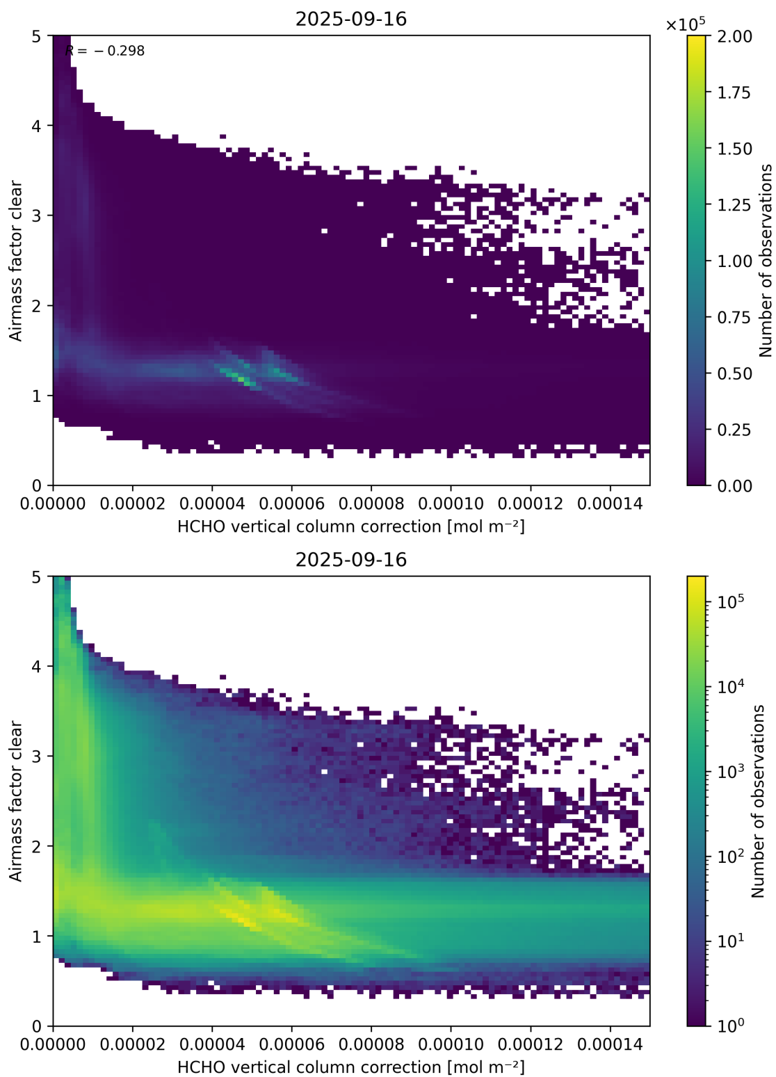
Figure 115: Scatter density plot of “HCHO vertical column correction” against “Airmass factor clear” for 2025-09-15 to 2025-09-17.
