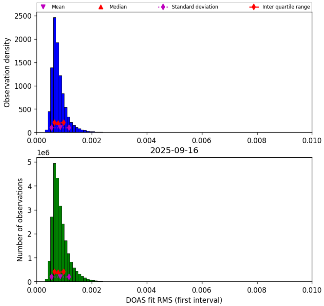
Figure 46: Histogram of “DOAS fit RMS (first interval)” for 2025-09-15 to 2025-09-17
