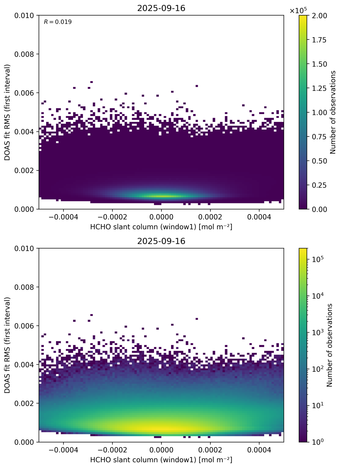
Figure 78: Scatter density plot of “HCHO slant column (window1)” against “DOAS fit RMS (first interval)” for 2025-09-15 to 2025-09-17.
