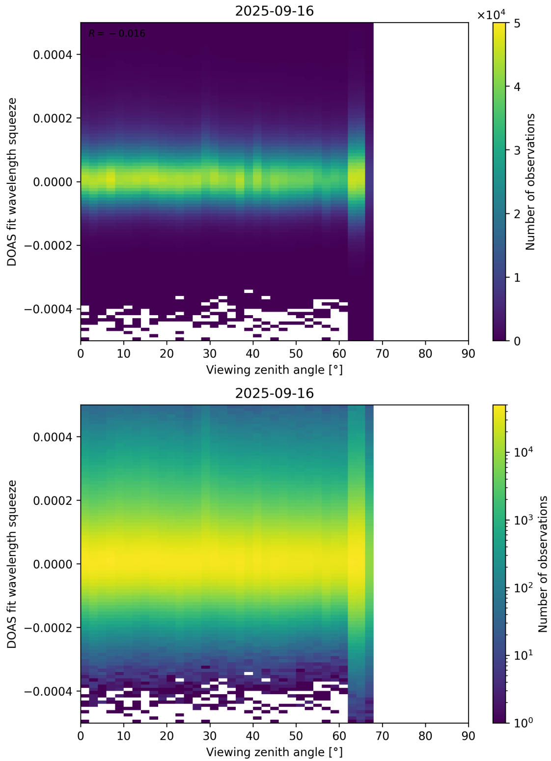
Figure 184: Scatter density plot of “Viewing zenith angle” against “DOAS fit wavelength squeeze” for 2025-09-15 to 2025-09-17.
