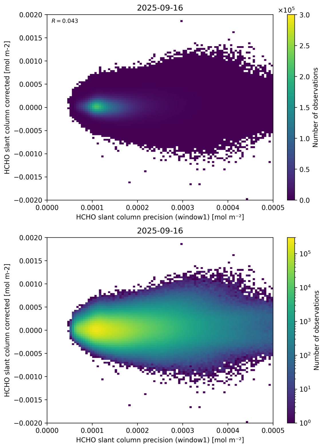
Figure 92: Scatter density plot of “HCHO slant column precision (window1)” against “HCHO slant column corrected” for 2025-09-15 to 2025-09-17.
