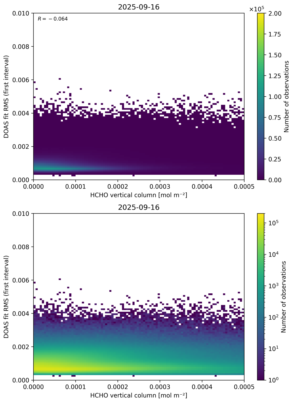
Figure 123: Scatter density plot of “HCHO vertical column” against “DOAS fit RMS (first interval)” for 2025-09-15 to 2025-09-17.
