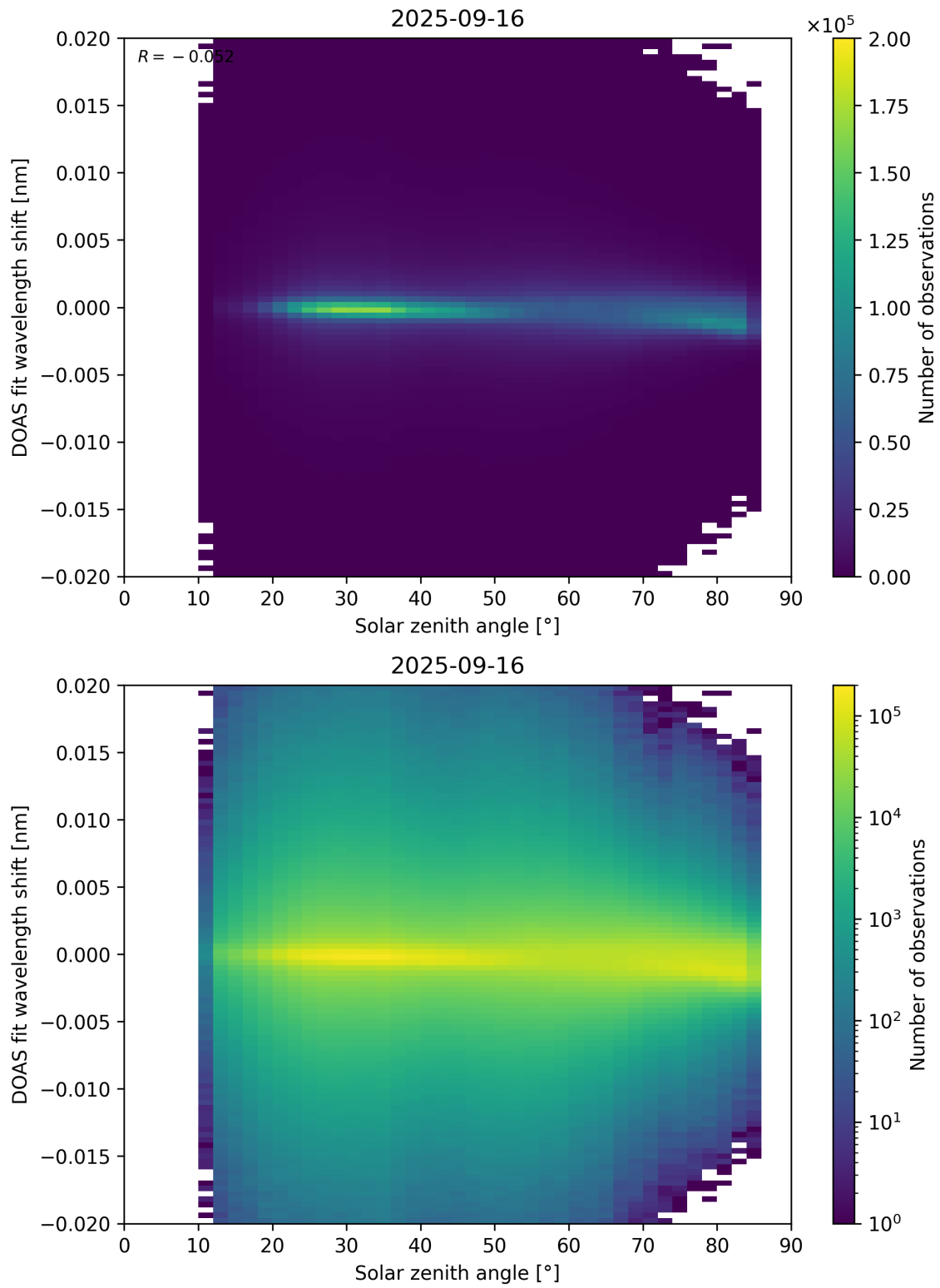
Figure 168: Scatter density plot of “Solar zenith angle” against “DOAS fit wavelength shift” for 2025-09-15 to 2025-09-17.
