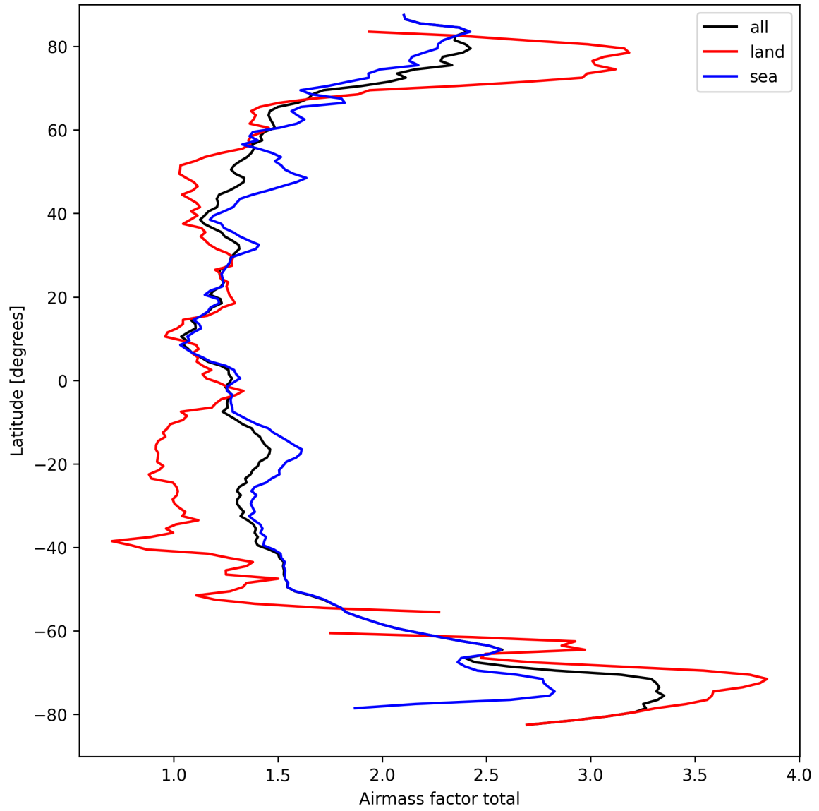
Figure 26: Zonal average of “Airmass factor total” for 2025-09-15 to 2025-09-17.
