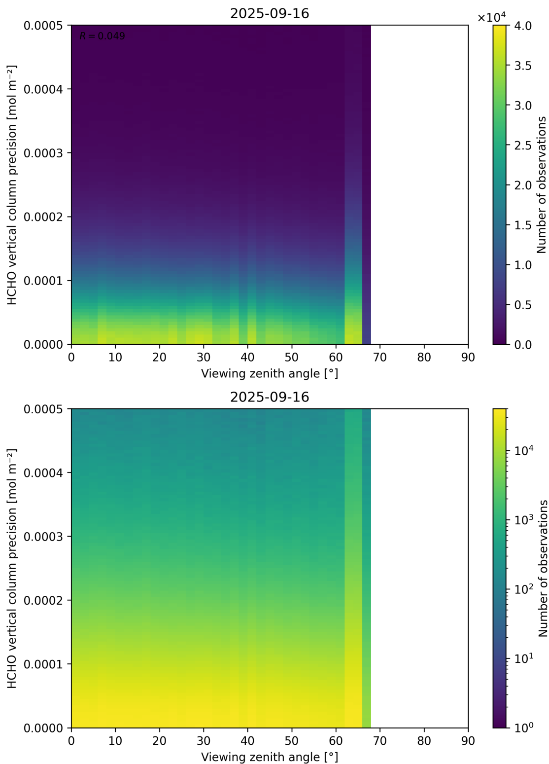
Figure 194: Scatter density plot of “Viewing zenith angle” against “HCHO vertical column precision” for 2025-09-15 to 2025-09-17.
