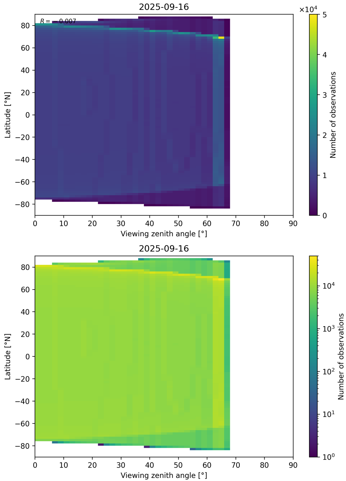
Figure 196: Scatter density plot of “Viewing zenith angle” against “Latitude” for 2025-09-15 to 2025-09-17.
