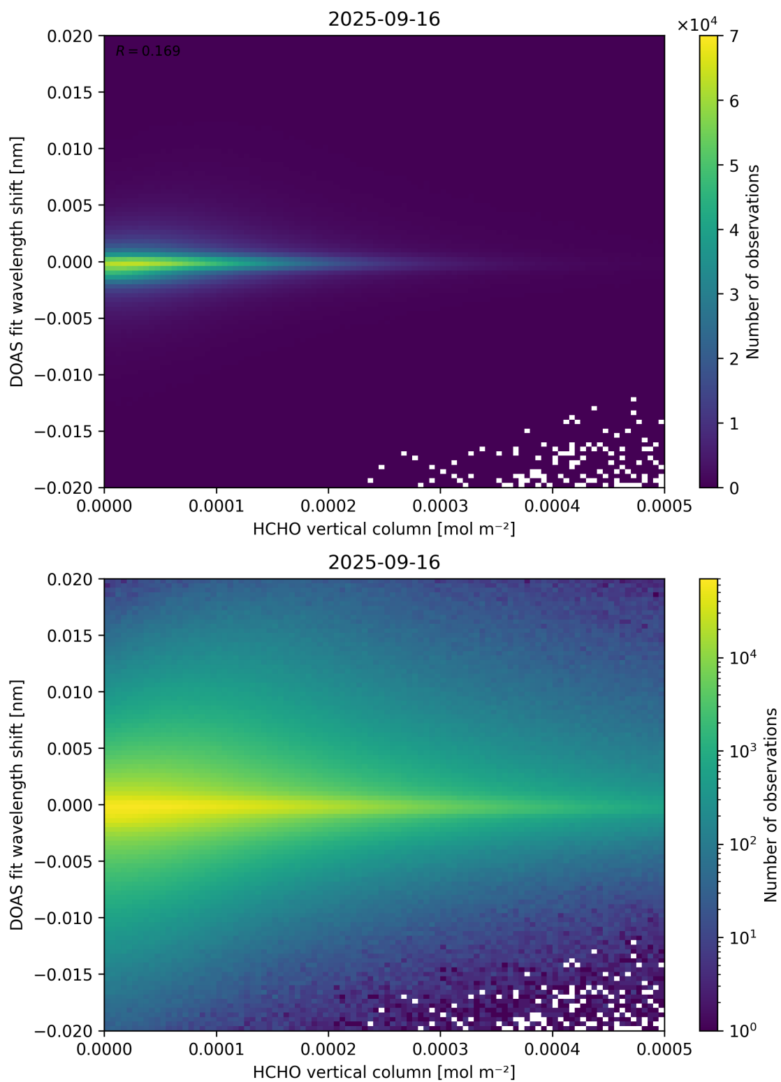
Figure 124: Scatter density plot of “HCHO vertical column” against “DOAS fit wavelength shift” for 2025-09-15 to 2025-09-17.
