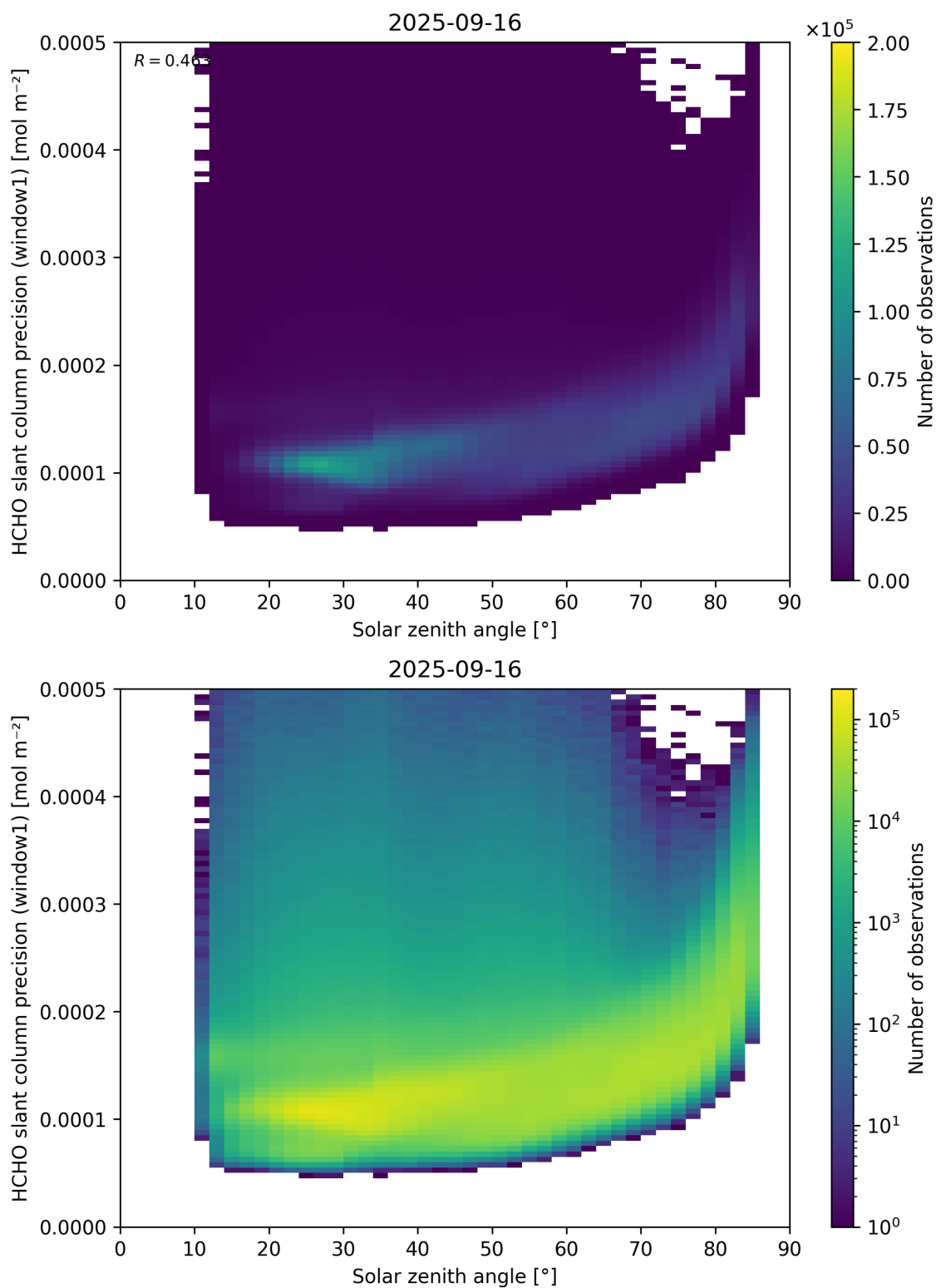
Figure 174: Scatter density plot of “Solar zenith angle” against “HCHO slant column precision (window1)” for 2025-09-15 to 2025-09-17.
