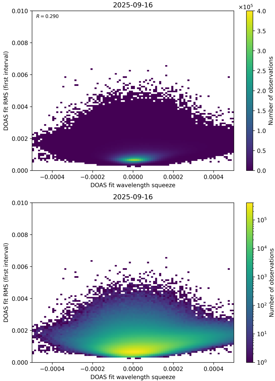
Figure 68: Scatter density plot of “DOAS fit wavelength squeeze” against “DOAS fit RMS (first interval)” for 2025-09-15 to 2025-09-17.
