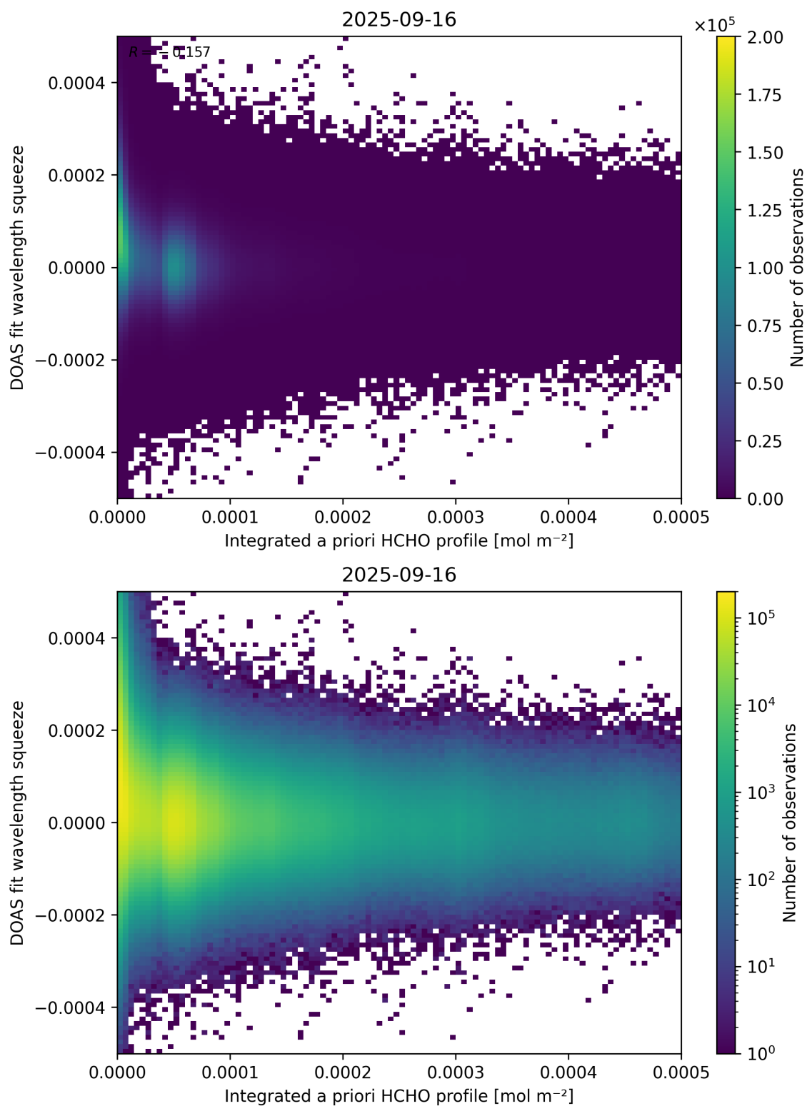
Figure 150: Scatter density plot of “Integrated a priori HCHO profile” against “DOAS fit wavelength squeeze” for 2025-09-15 to 2025-09-17.
