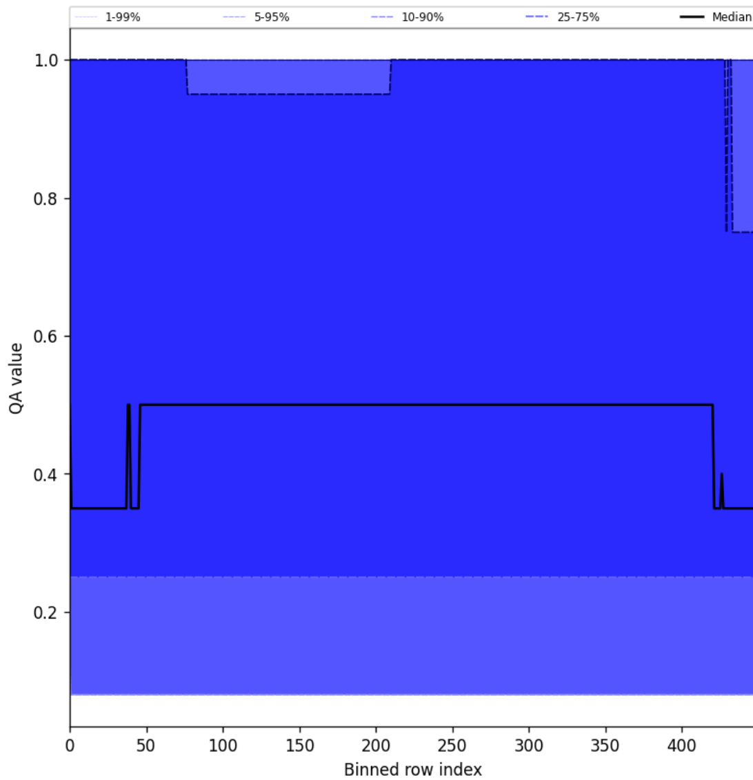
Figure 48: Along track statistics of “QA value” for 2025-09-15 to 2025-09-17
