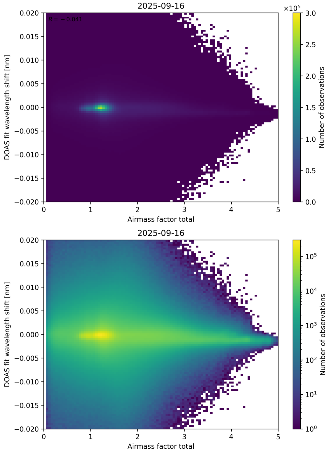
Figure 98: Scatter density plot of “Airmass factor total” against “DOAS fit wavelength shift” for 2025-09-15 to 2025-09-17.
