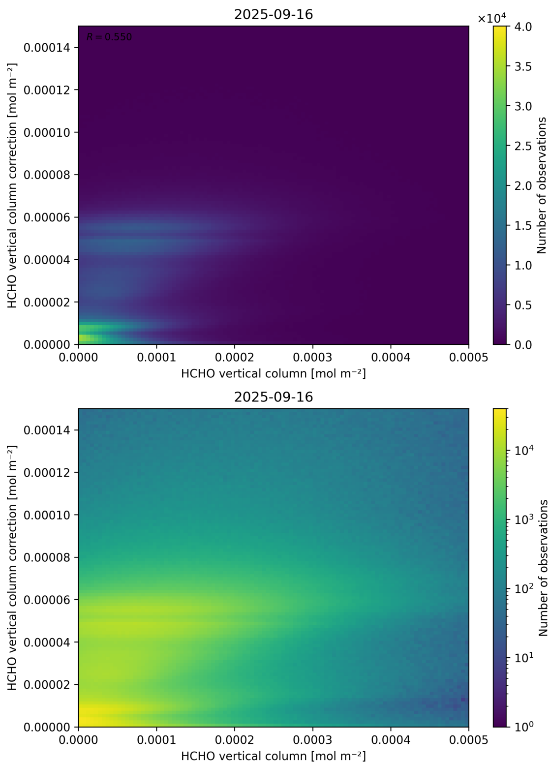
Figure 133: Scatter density plot of “HCHO vertical column” against “HCHO vertical column correction” for 2025-09-15 to 2025-09-17.
