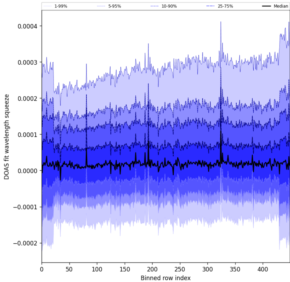
Figure 59: Along track statistics of “DOAS fit wavelength squeeze” for 2025-09-15 to 2025-09-17
