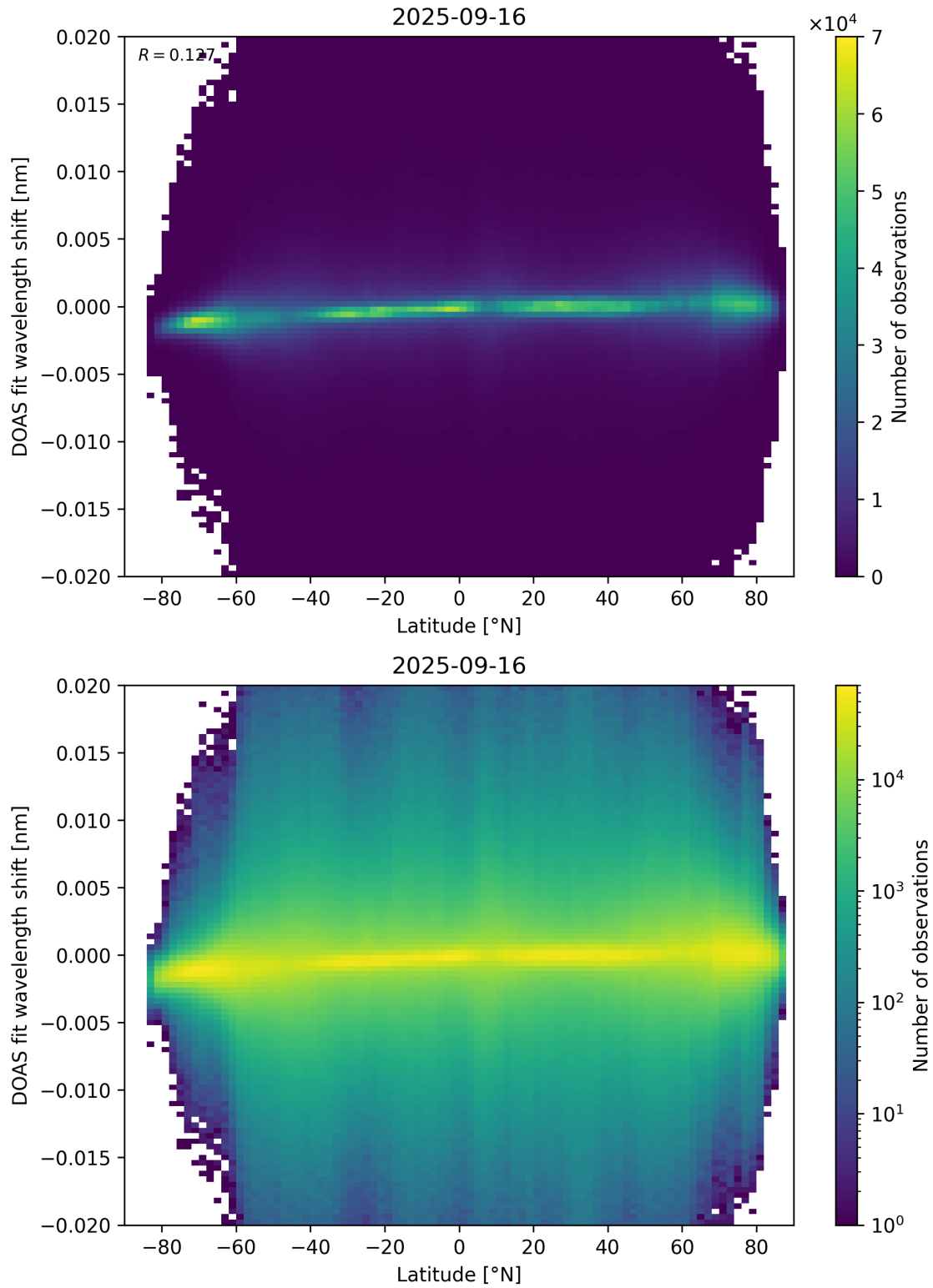
Figure 154: Scatter density plot of “Latitude” against “DOAS fit wavelength shift” for 2025-09-15 to 2025-09-17.
