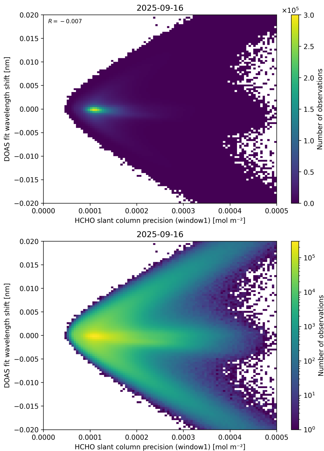
Figure 89: Scatter density plot of “HCHO slant column precision (window1)” against “DOAS fit wavelength shift” for 2025-09-15 to 2025-09-17.
