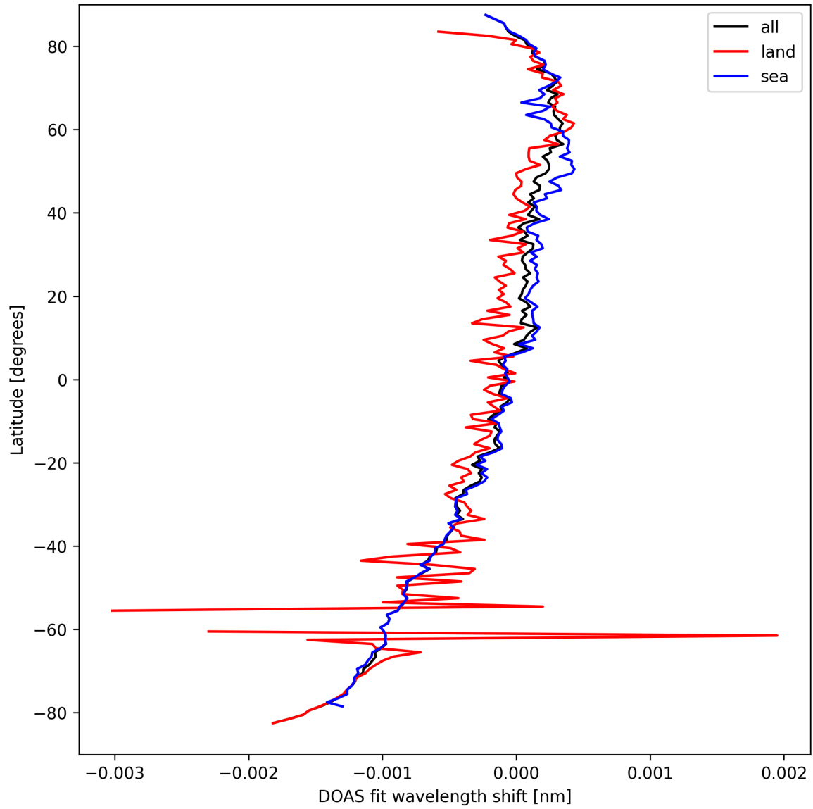
Figure 30: Zonal average of "DOAS fit wavelength shift" for 2025-09-15 to 2025-09-17.
