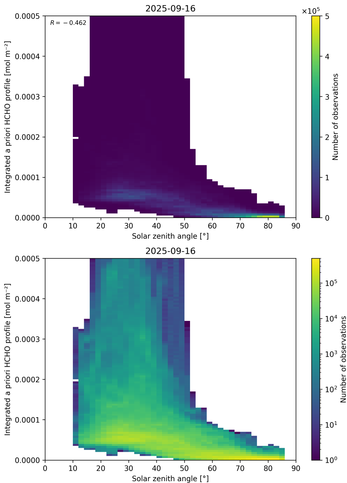
Figure 180: Scatter density plot of “Solar zenith angle” against “Integrated a priori HCHO profile” for 2025-09-15 to 2025-09-17.
