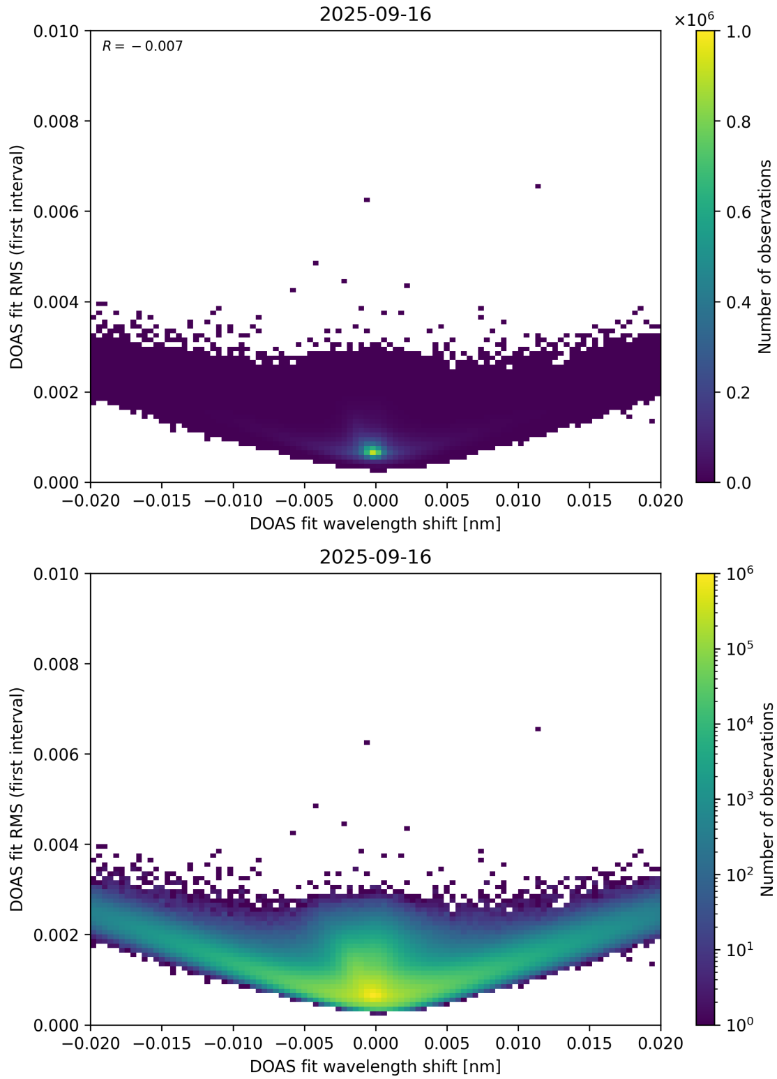
Figure 64: Scatter density plot of “DOAS fit wavelength shift” against “DOAS fit RMS (first interval)” for 2025-09-15 to 2025-09-17.
