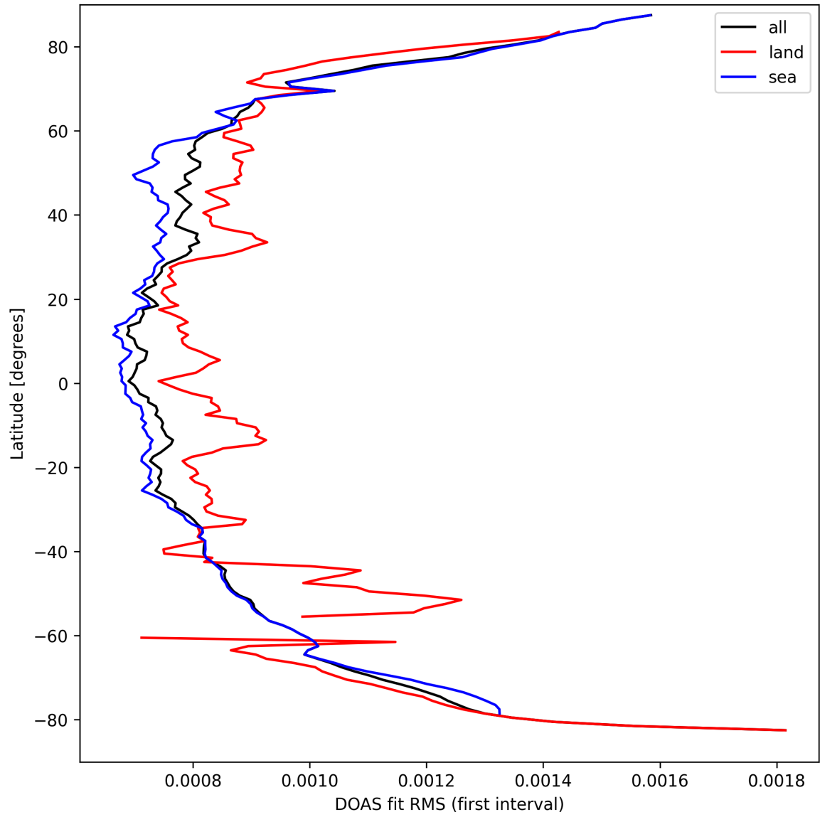
Figure 32: Zonal average of “DOAS fit RMS (first interval)” for 2025-09-15 to 2025-09-17.
