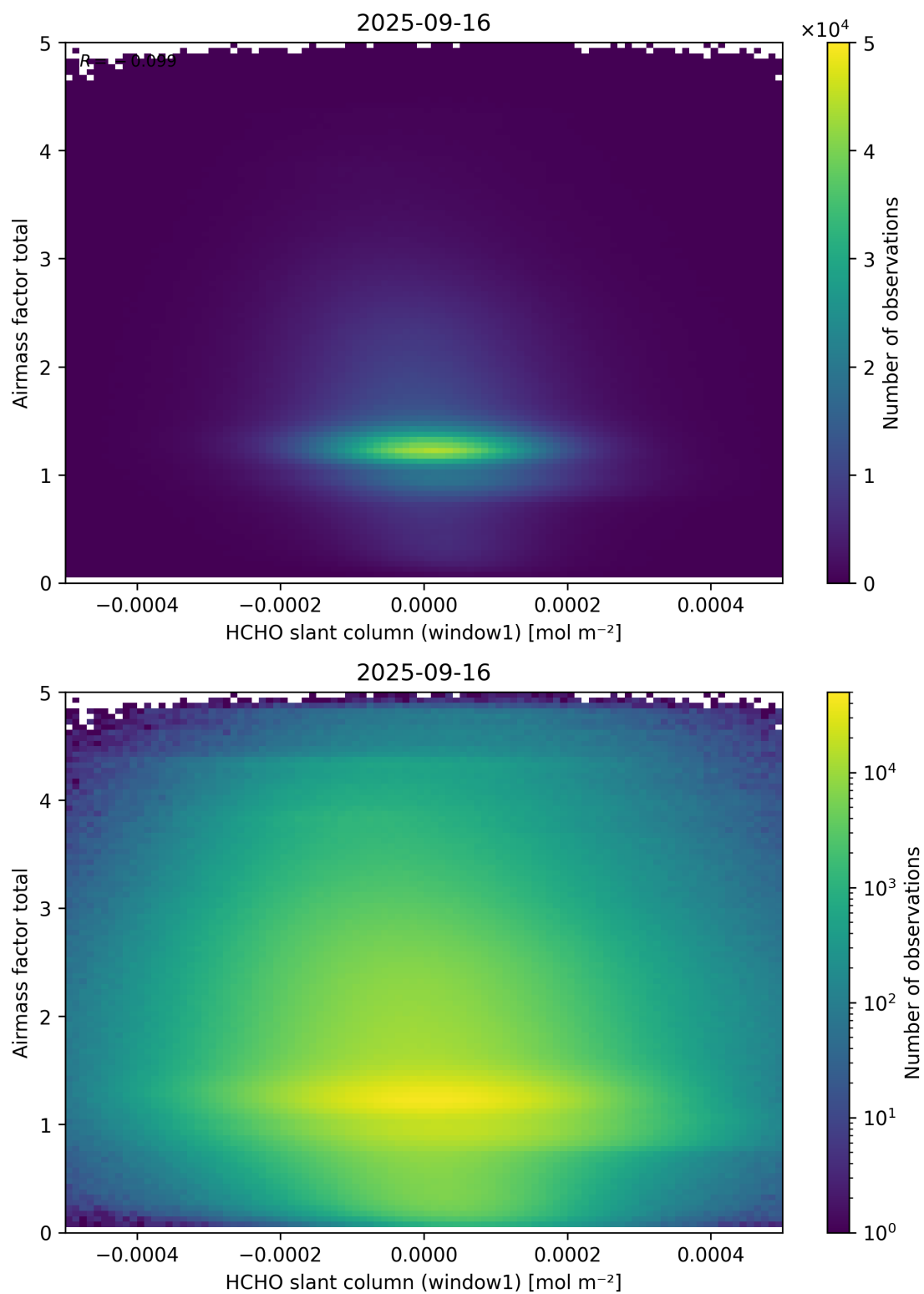
Figure 85: Scatter density plot of “HCHO slant column (window1)” against “Airmass factor total” for 2025-09-15 to 2025-09-17.
