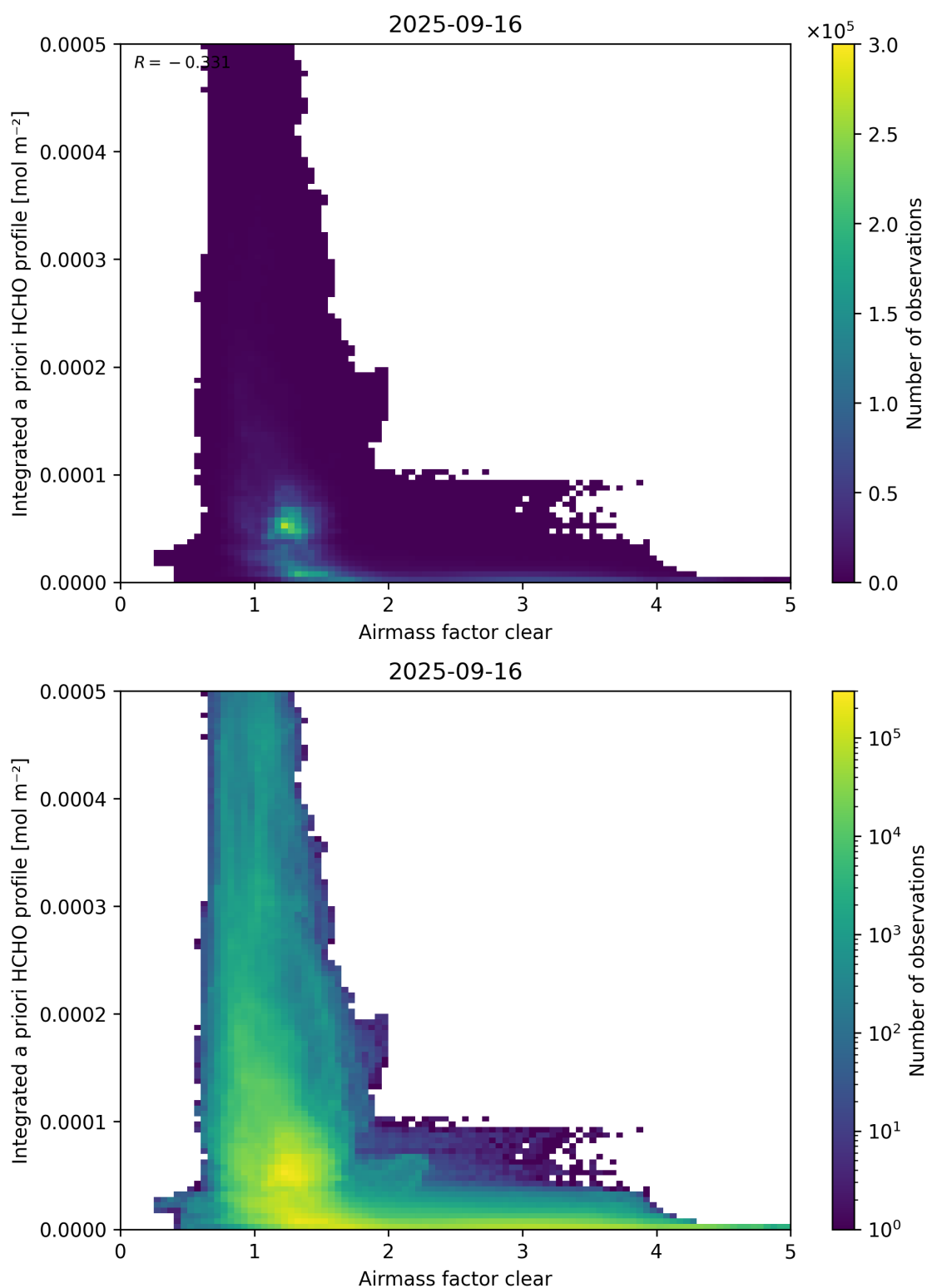
Figure 76: Scatter density plot of “Airmass factor clear” against “Integrated a priori HCHO profile” for 2025-09-15 to 2025-09-17.
