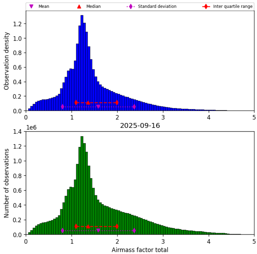
Figure 40: Histogram of “Airmass factor total” for 2025-09-15 to 2025-09-17
