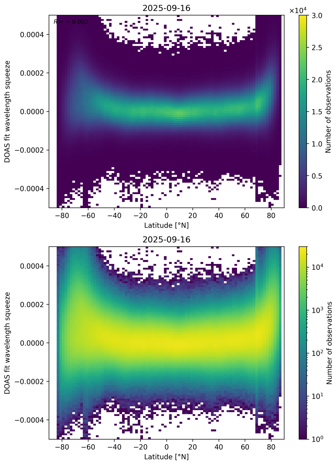
Figure 155: Scatter density plot of “Latitude” against “DOAS fit wavelength squeeze” for 2025-09-15 to 2025-09-17.
