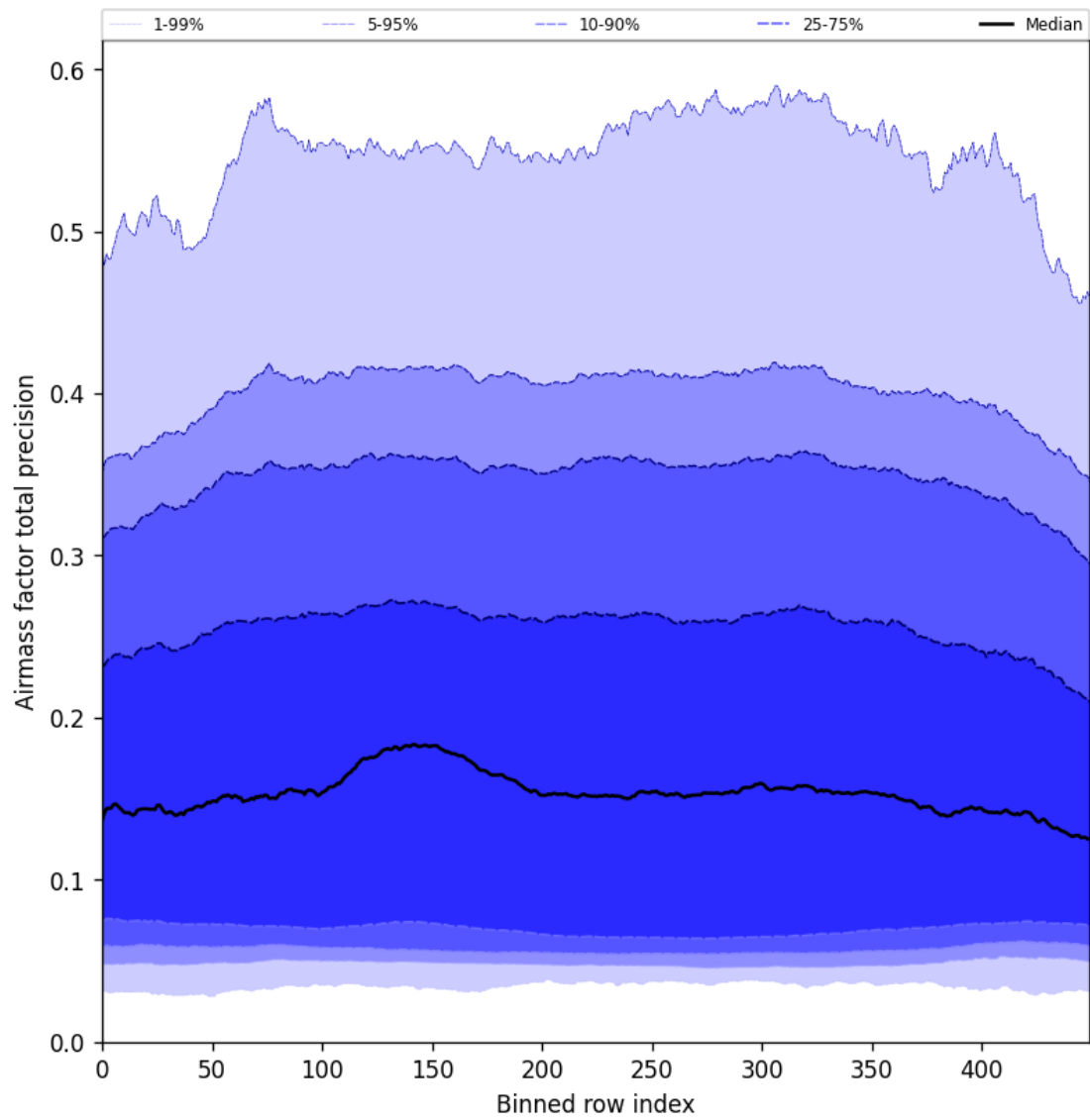
Figure 55: Along track statistics of “Airmass factor total precision” for 2025-09-15 to 2025-09-17
