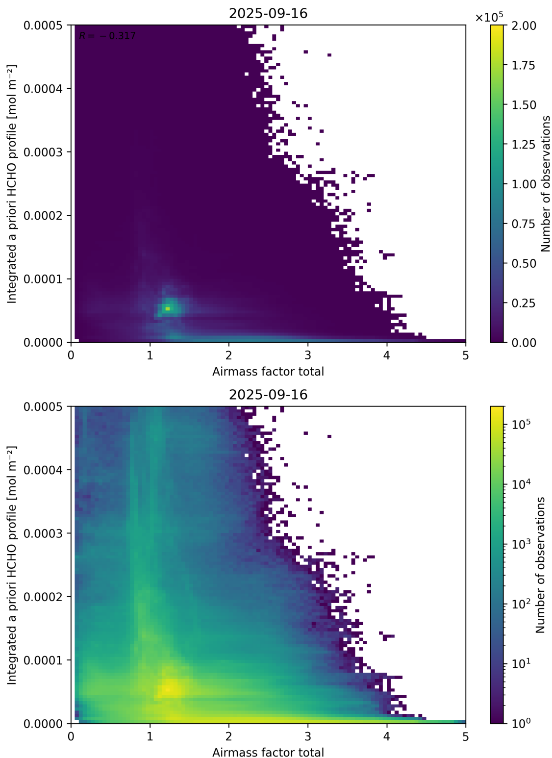
Figure 104: Scatter density plot of “Airmass factor total” against “Integrated a priori HCHO profile” for 2025-09-15 to 2025-09-17.
