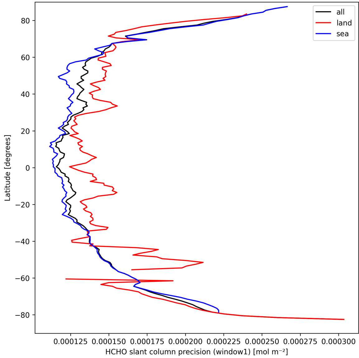
Figure 25: Zonal average of “HCHO slant column precision (window1)” for 2025-09-15 to 2025-09-17.
