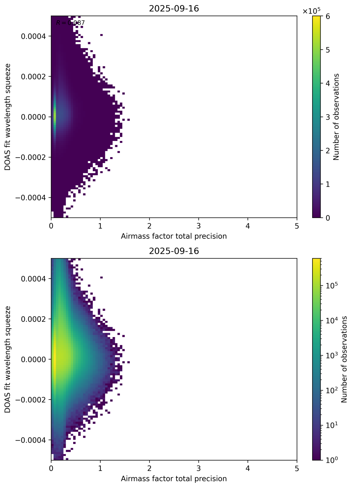
Figure 107: Scatter density plot of “Airmass factor total precision” against “DOAS fit wavelength squeeze” for 2025-09-15 to 2025-09-17.
