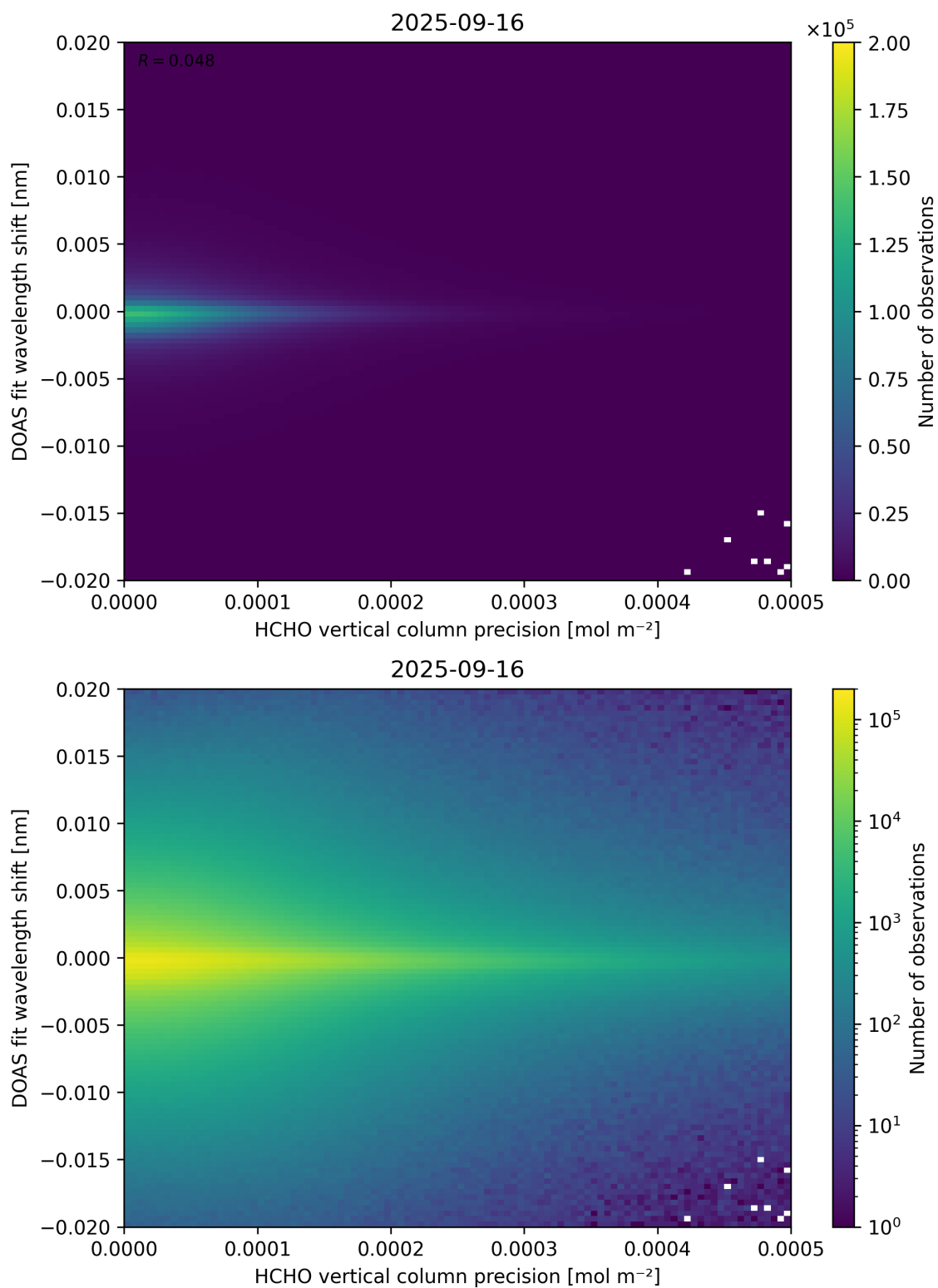
Figure 137: Scatter density plot of “HCHO vertical column precision” against “DOAS fit wavelength shift” for 2025-09-15 to 2025-09-17.
