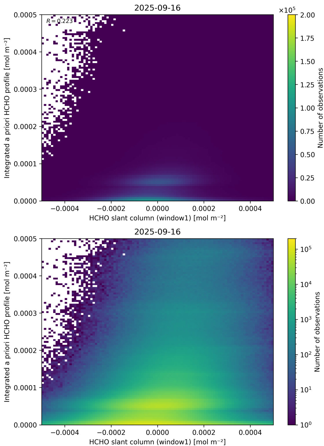
Figure 87: Scatter density plot of “HCHO slant column (window1)” against “Integrated a priori HCHO profile” for 2025-09-15 to 2025-09-17.
