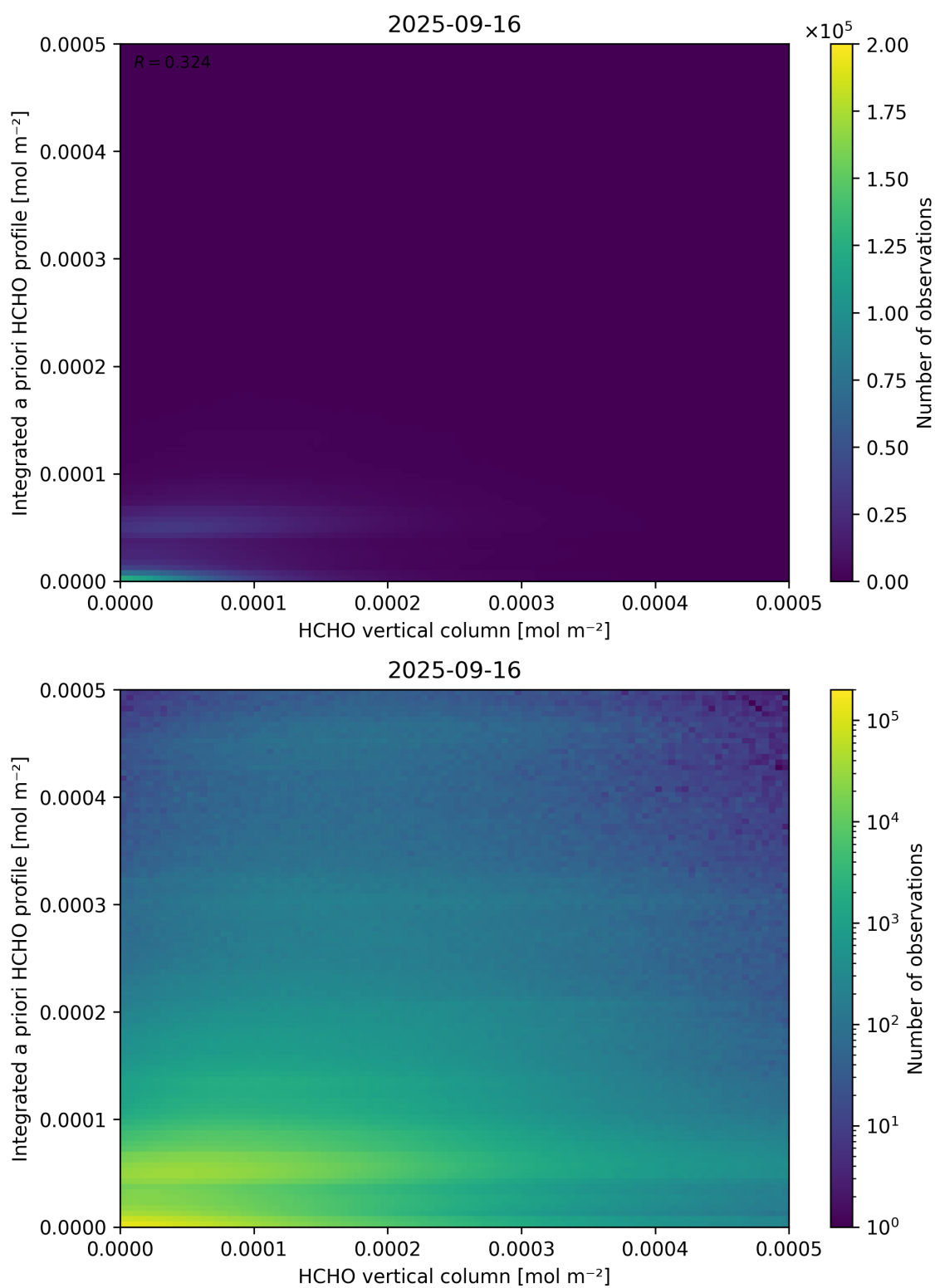
Figure 135: Scatter density plot of “HCHO vertical column” against “Integrated a priori HCHO profile” for 2025-09-15 to 2025-09-17.
