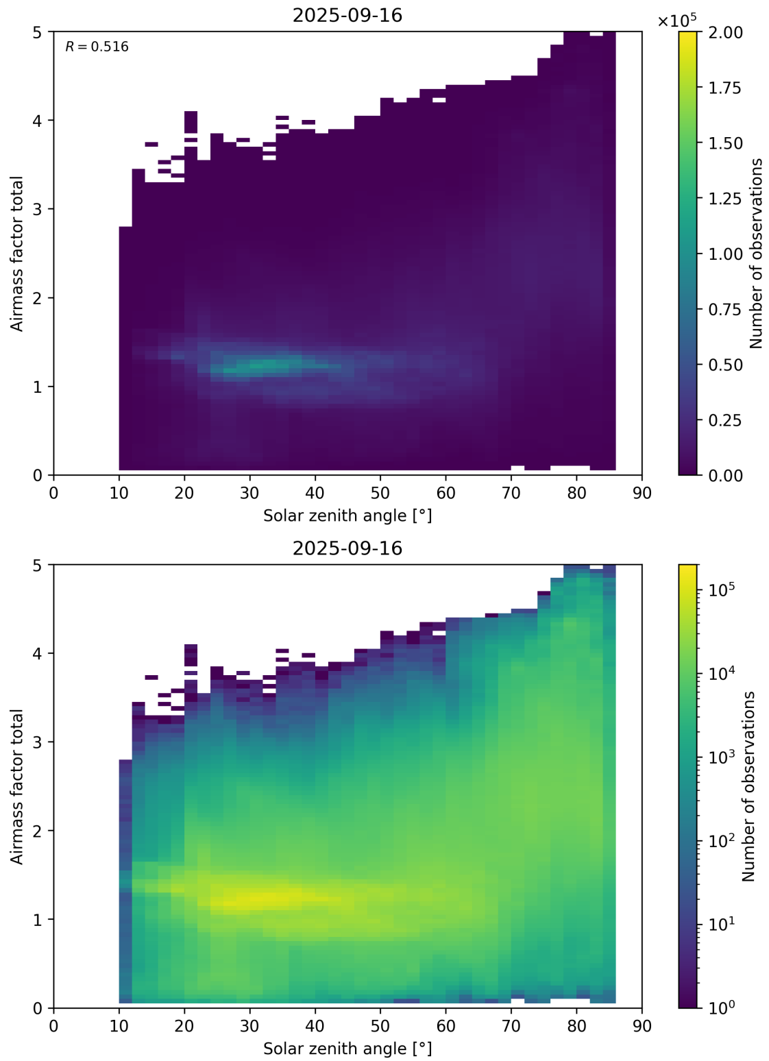
Figure 175: Scatter density plot of “Solar zenith angle” against “Airmass factor total” for 2025-09-15 to 2025-09-17.
