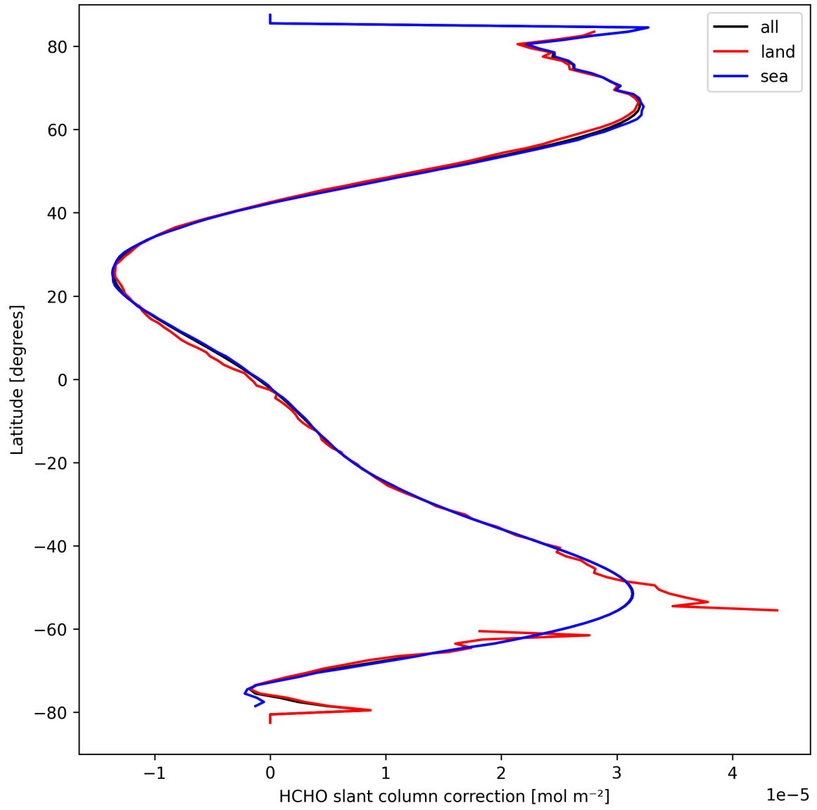
Figure 33: Zonal average of “HCHO slant column correction” for 2025-09-15 to 2025-09-17.
