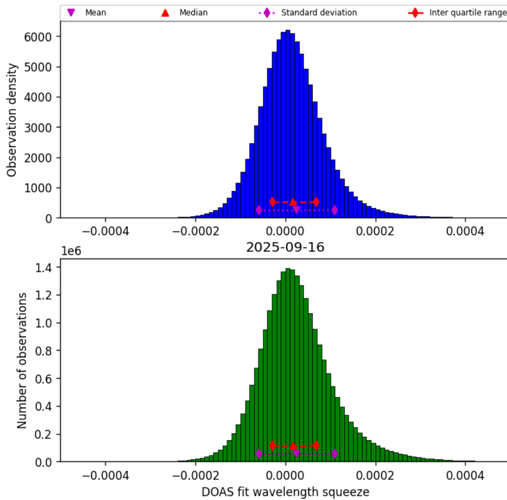
Figure 45: Histogram of “DOAS fit wavelength squeeze” for 2025-09-15 to 2025-09-17
