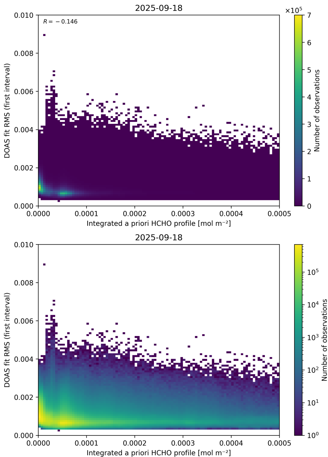
Figure 148: Scatter density plot of “Integrated a priori HCHO profile” against “DOAS fit RMS (first interval)” for 2025-09-17 to 2025-09-19.
