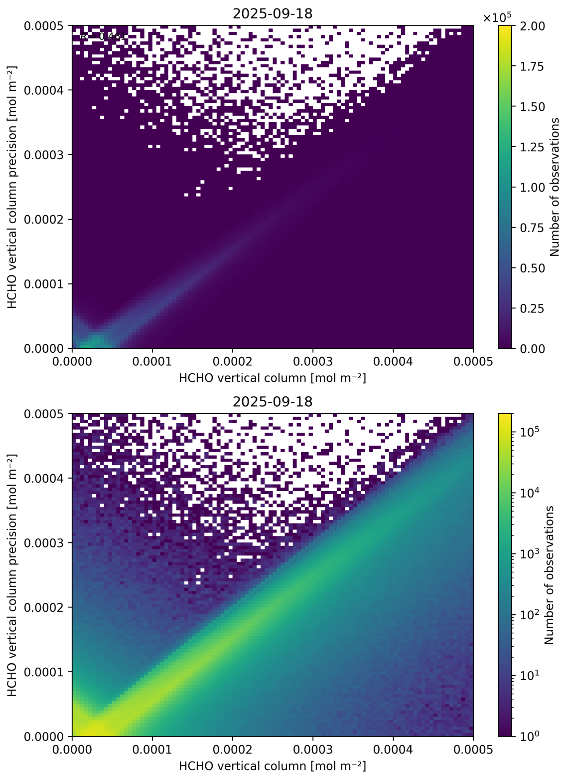
Figure 134: Scatter density plot of “HCHO vertical column” against “HCHO vertical column precision” for 2025-09-17 to 2025-09-19.
