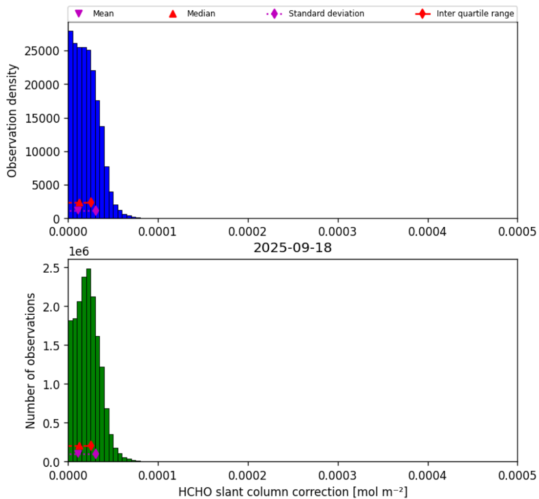
Figure 47: Histogram of “HCHO slant column correction” for 2025-09-17 to 2025-09-19
