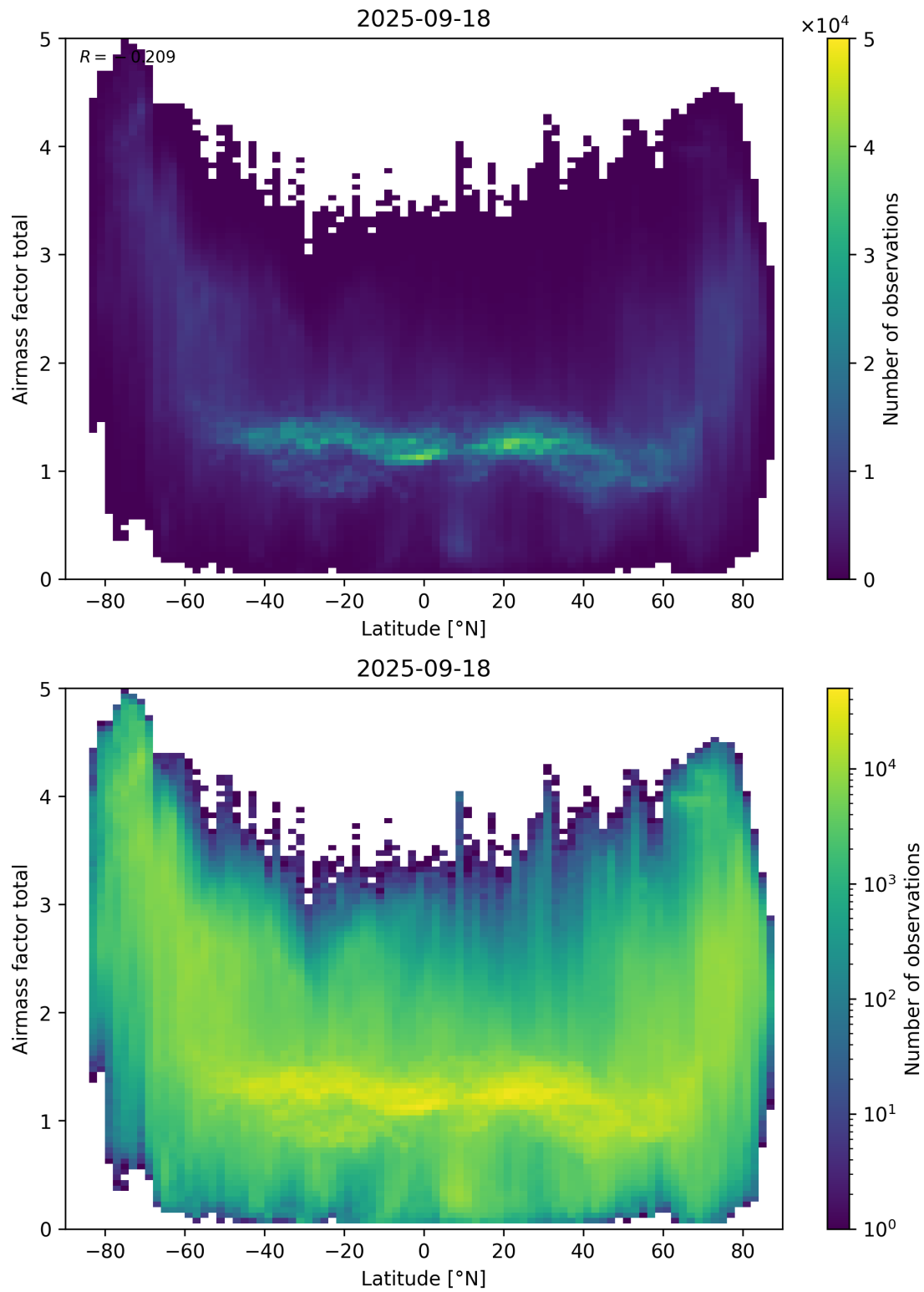
Figure 161: Scatter density plot of “Latitude” against “Airmass factor total” for 2025-09-17 to 2025-09-19.
