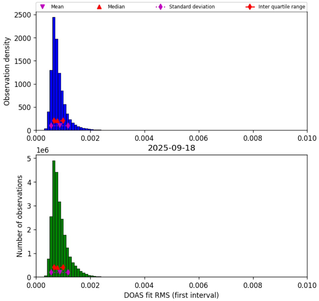
Figure 46: Histogram of “DOAS fit RMS (first interval)” for 2025-09-17 to 2025-09-19
