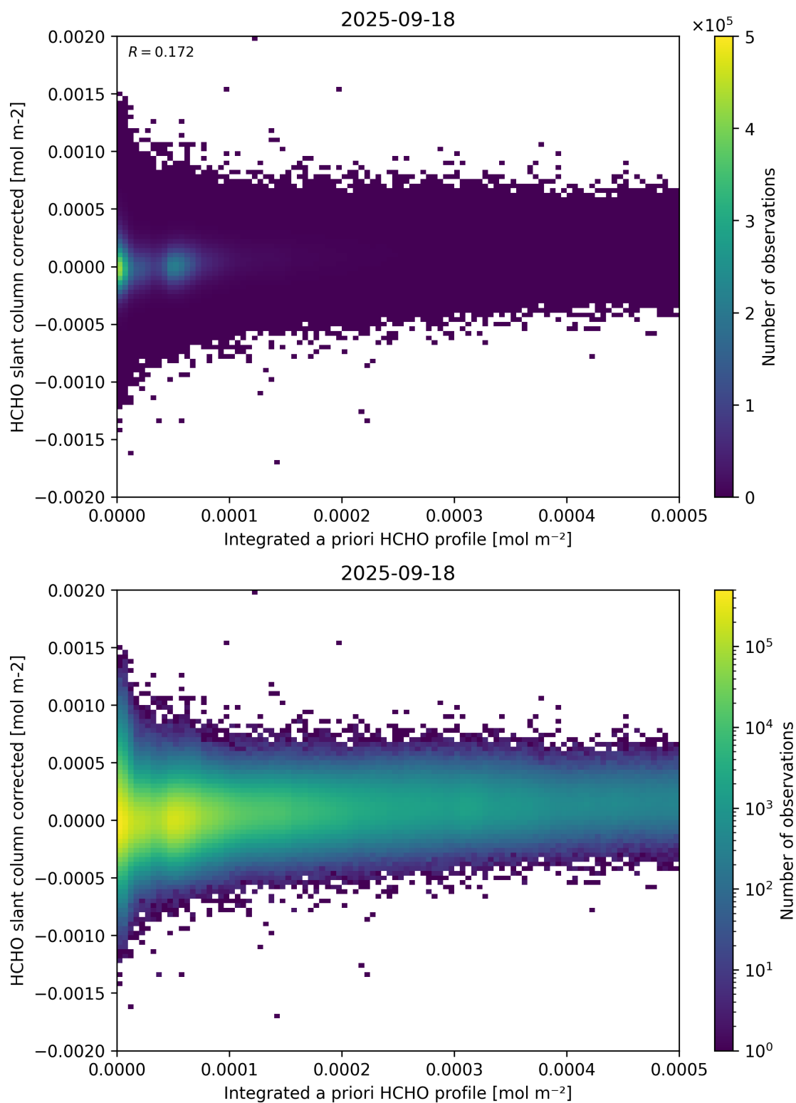
Figure 151: Scatter density plot of “Integrated a priori HCHO profile” against “HCHO slant column corrected” for 2025-09-17 to 2025-09-19.
