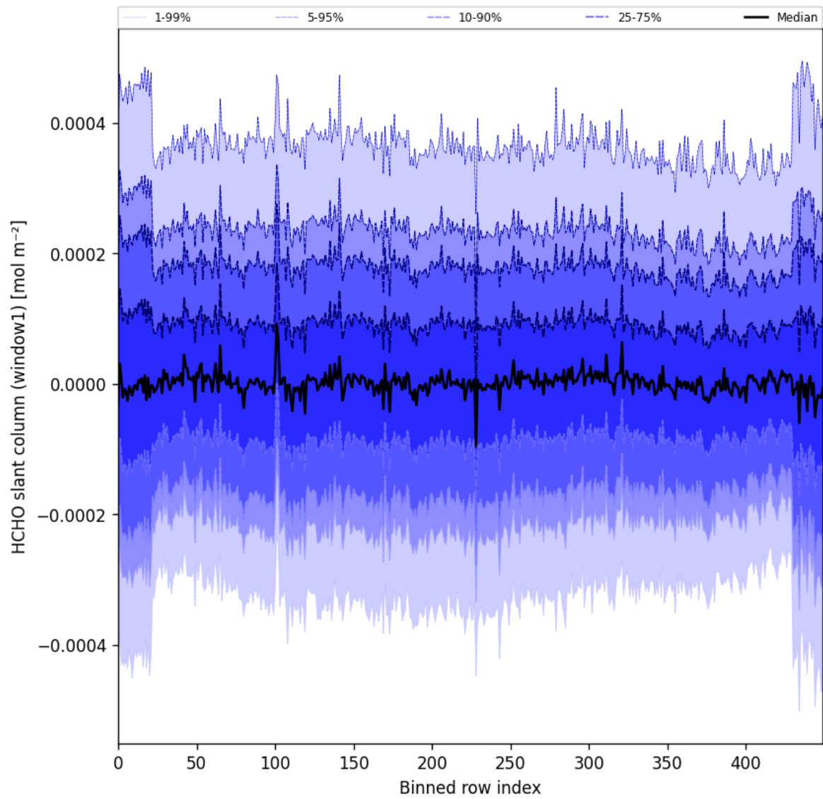
Figure 52: Along track statistics of “HCHO slant column (window1)” for 2025-09-17 to 2025-09-19
