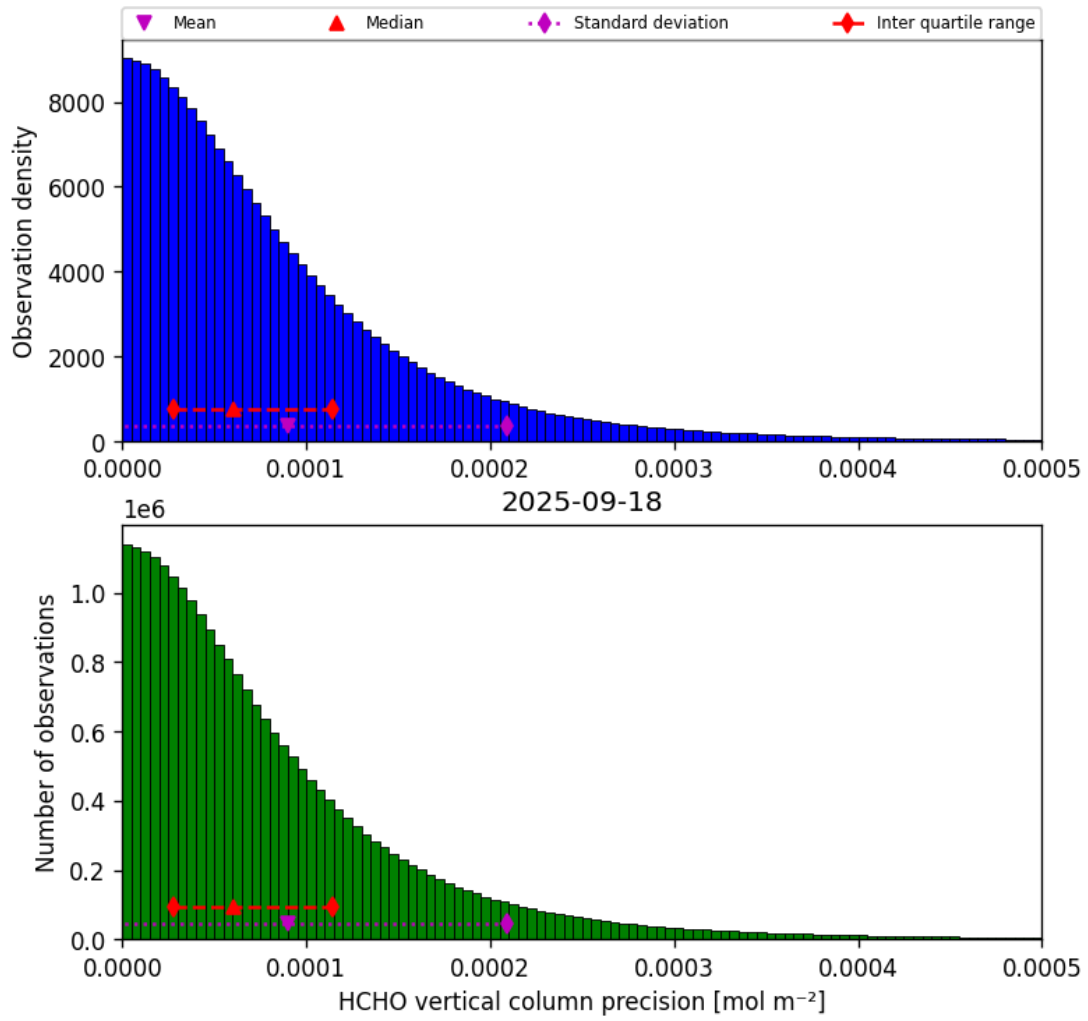
Figure 36: Histogram of “HCHO vertical column precision” for 2025-09-17 to 2025-09-19
