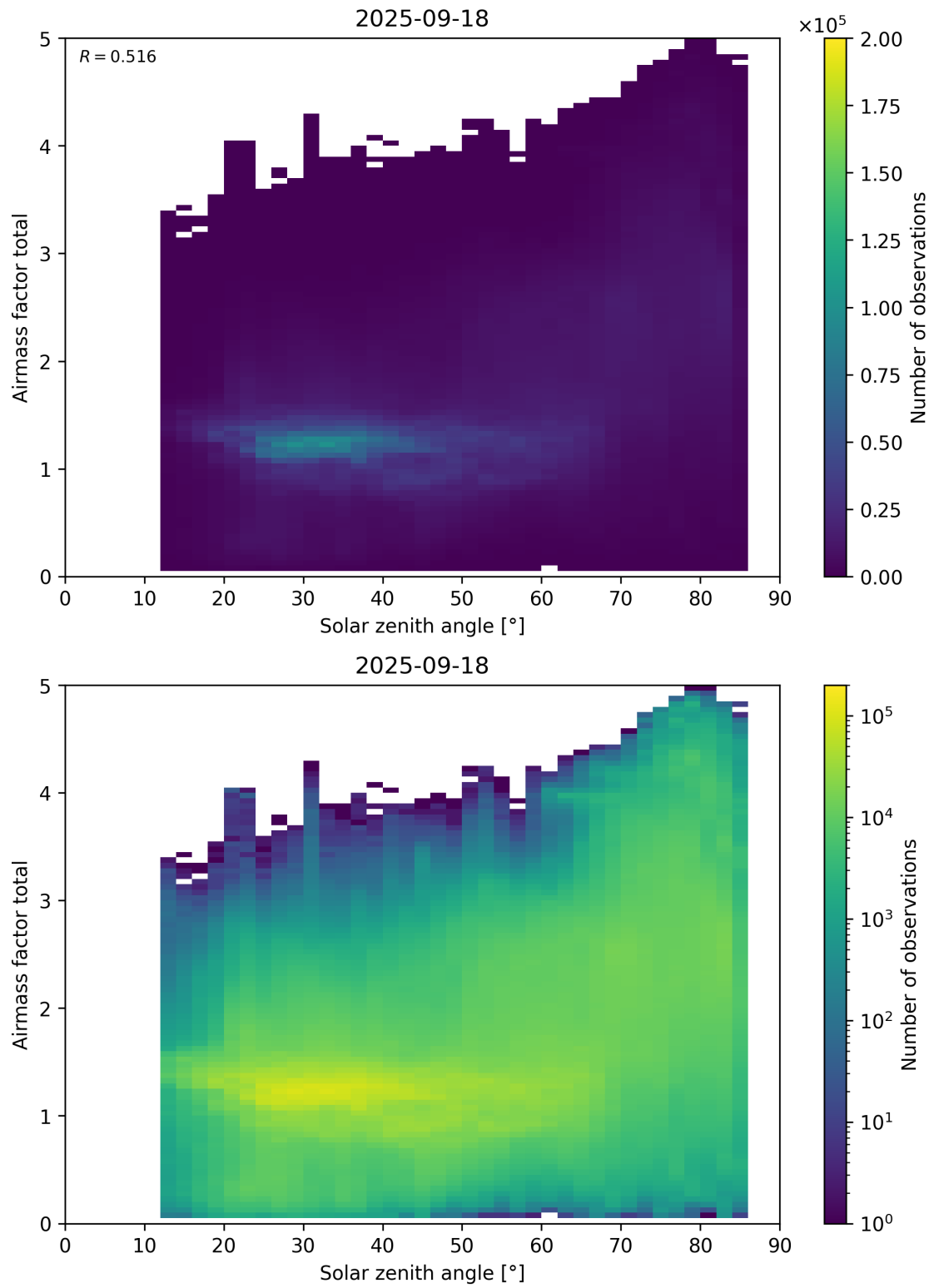
Figure 175: Scatter density plot of “Solar zenith angle” against “Airmass factor total” for 2025-09-17 to 2025-09-19.
