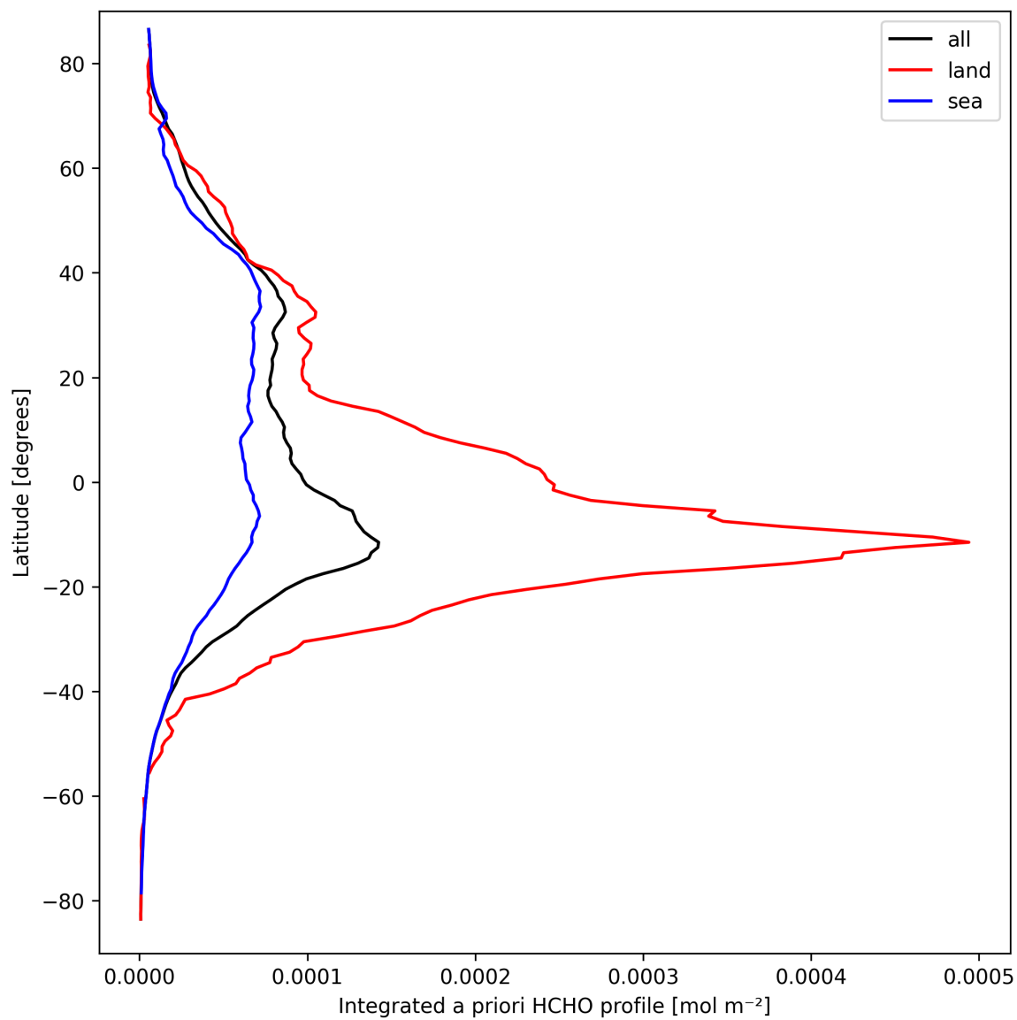
Figure 29: Zonal average of “Integrated a priori HCHO profile” for 2025-09-17 to 2025-09-19.
