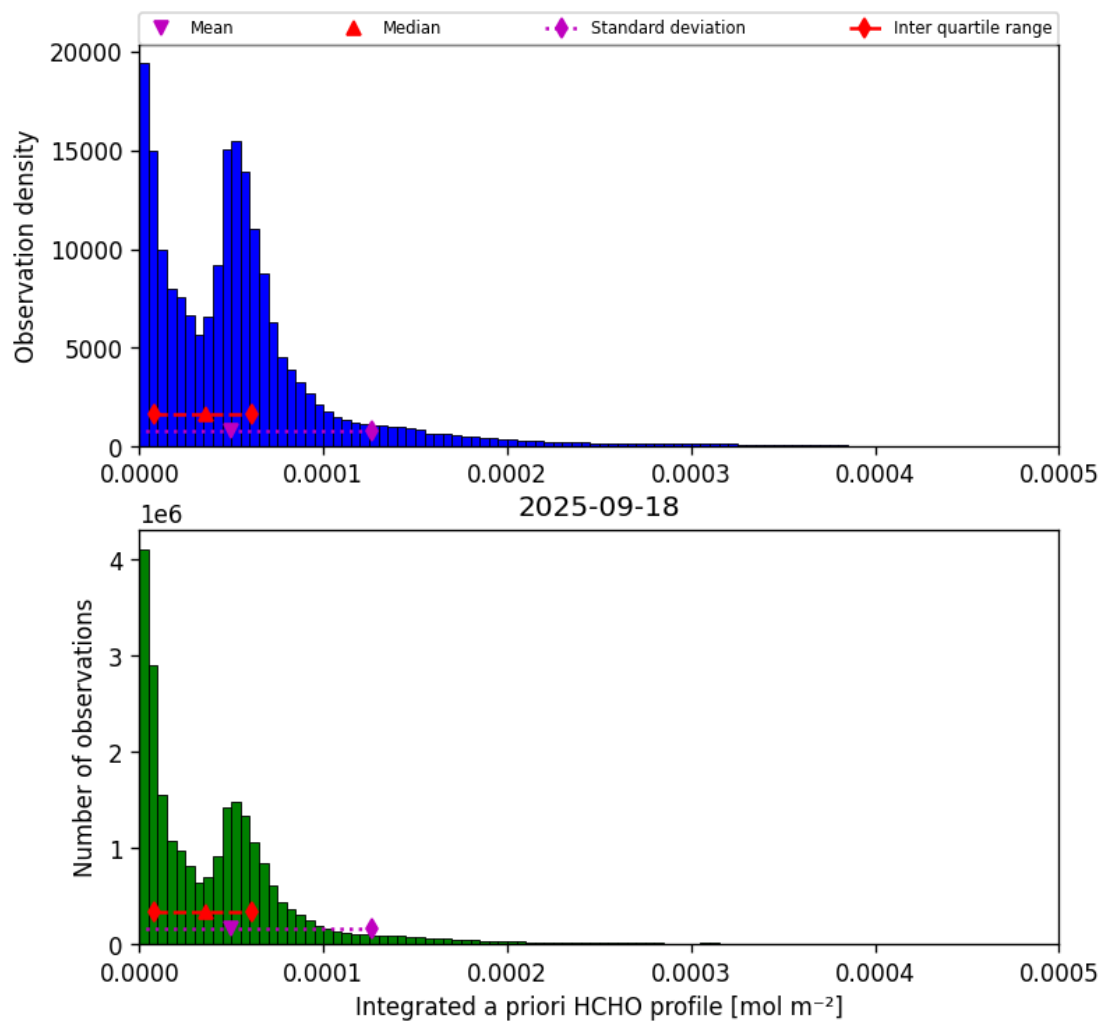
Figure 43: Histogram of “Integrated a priori HCHO profile” for 2025-09-17 to 2025-09-19
