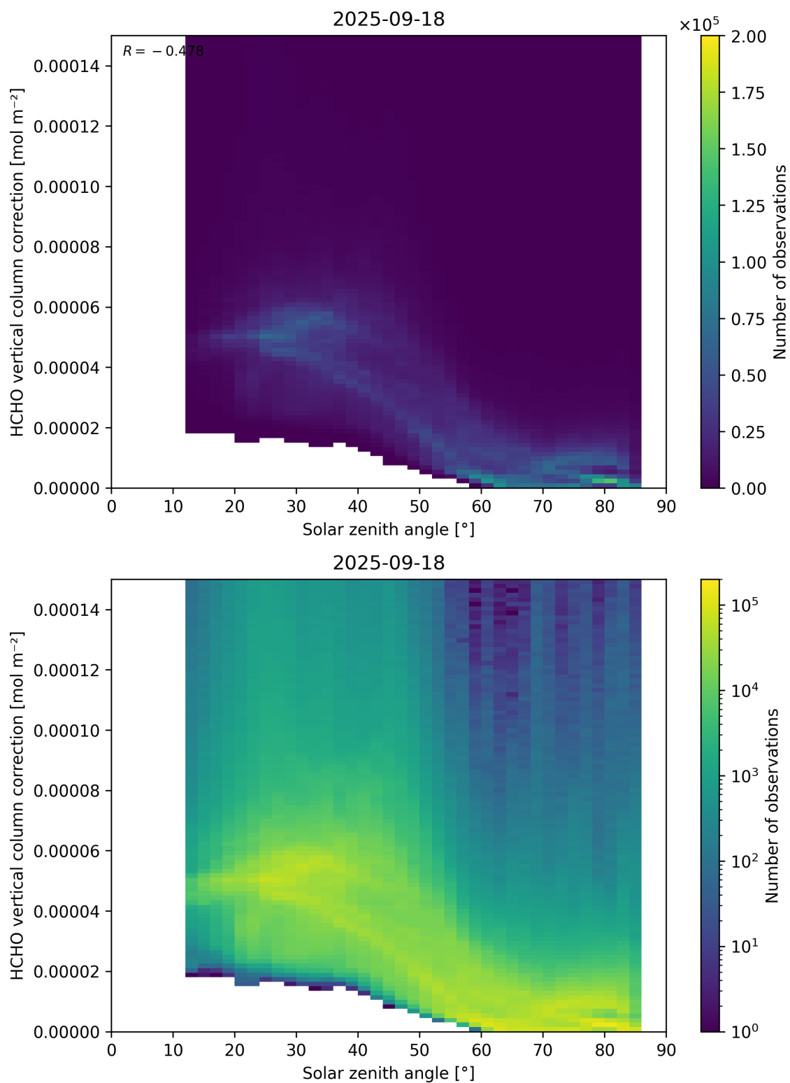
Figure 178: Scatter density plot of “Solar zenith angle” against “HCHO vertical column correction” for 2025-09-17 to 2025-09-19.
