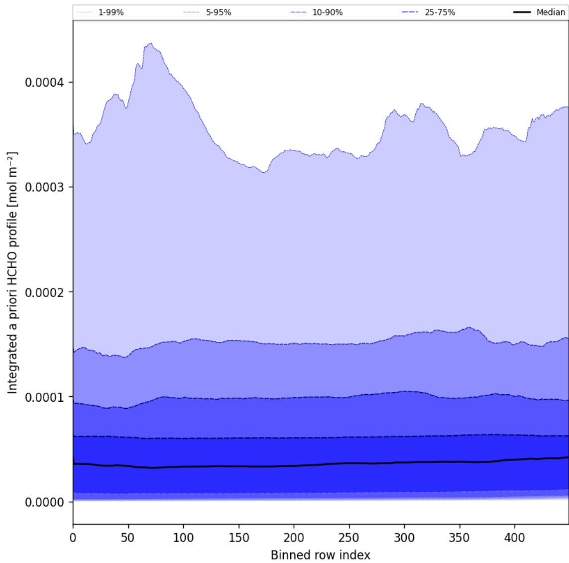
Figure 57: Along track statistics of “Integrated a priori HCHO profile” for 2025-09-17 to 2025-09-19
