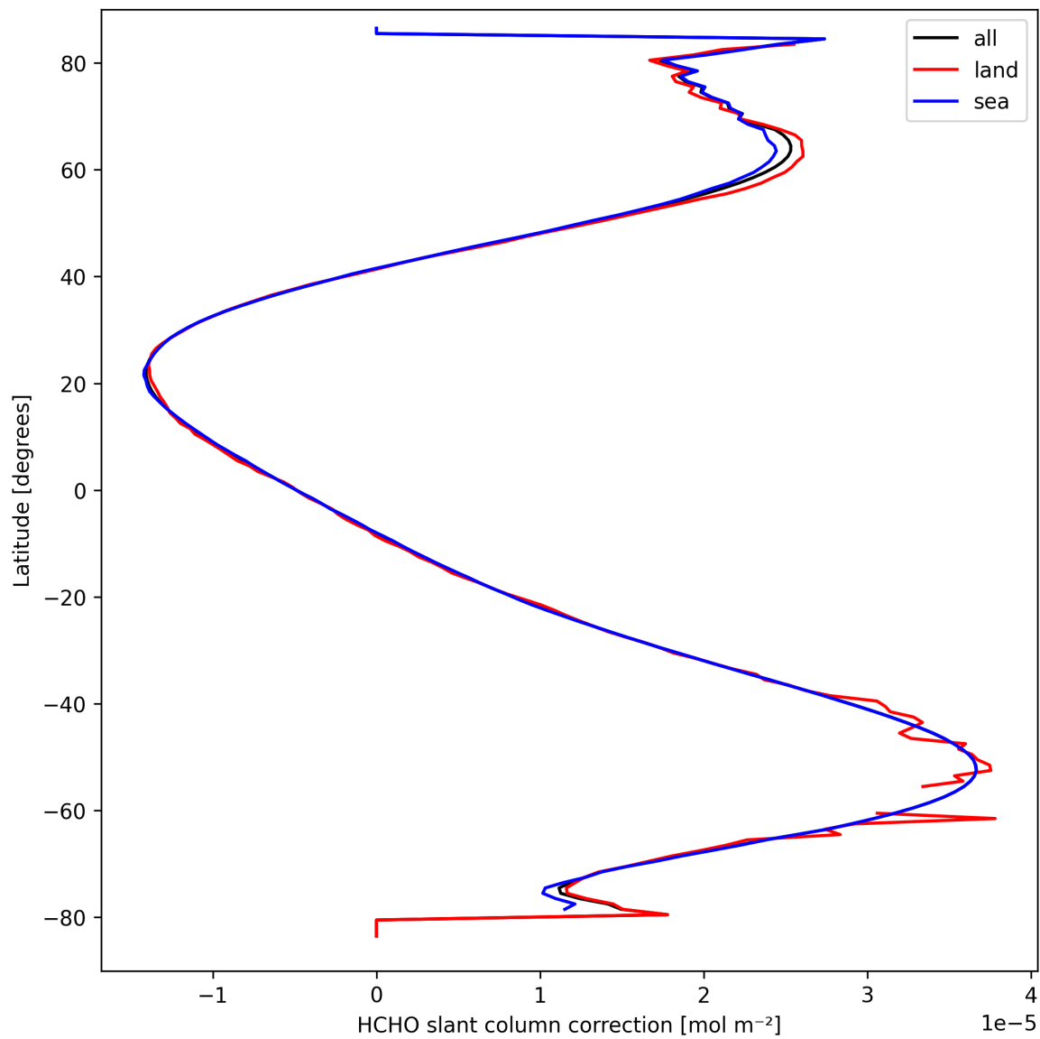
Figure 33: Zonal average of “HCHO slant column correction” for 2025-09-17 to 2025-09-19.
