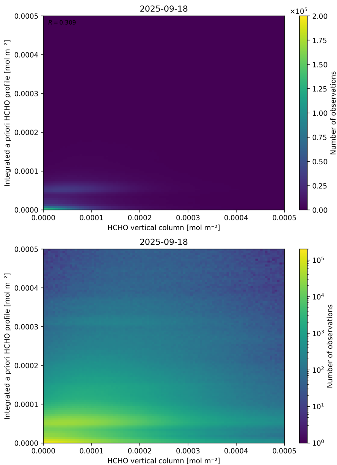
Figure 135: Scatter density plot of “HCHO vertical column” against “Integrated a priori HCHO profile” for 2025-09-17 to 2025-09-19.
