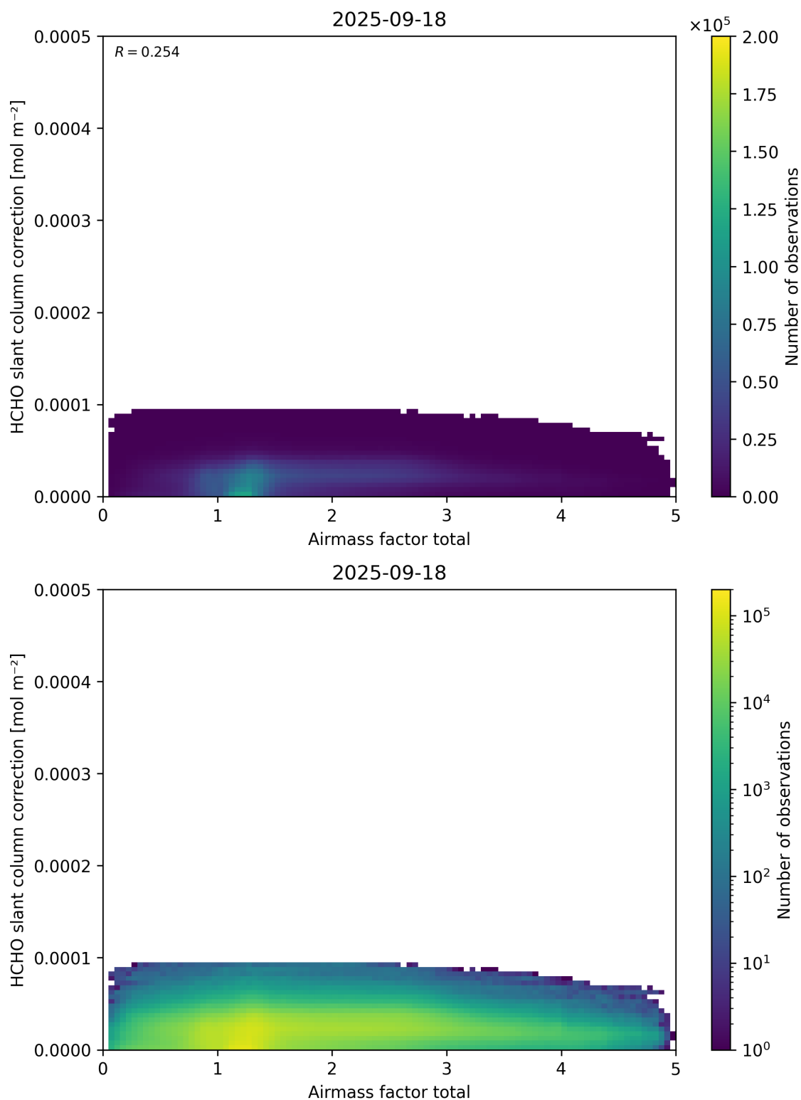
Figure 102: Scatter density plot of “Airmass factor total” against “HCHO slant column correction” for 2025-09-17 to 2025-09-19.
