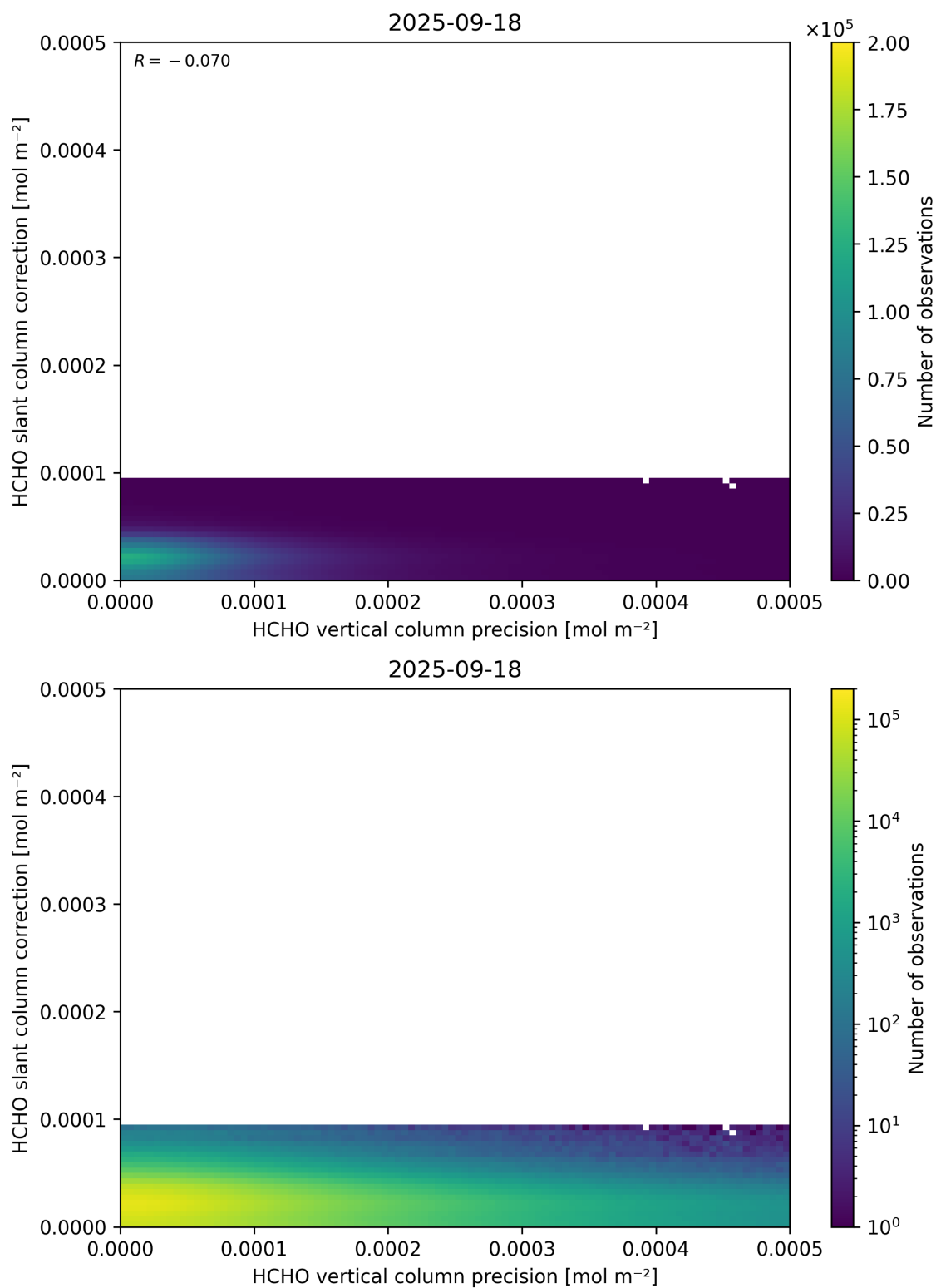
Figure 141: Scatter density plot of “HCHO vertical column precision” against “HCHO slant column correction” for 2025-09-17 to 2025-09-19.
