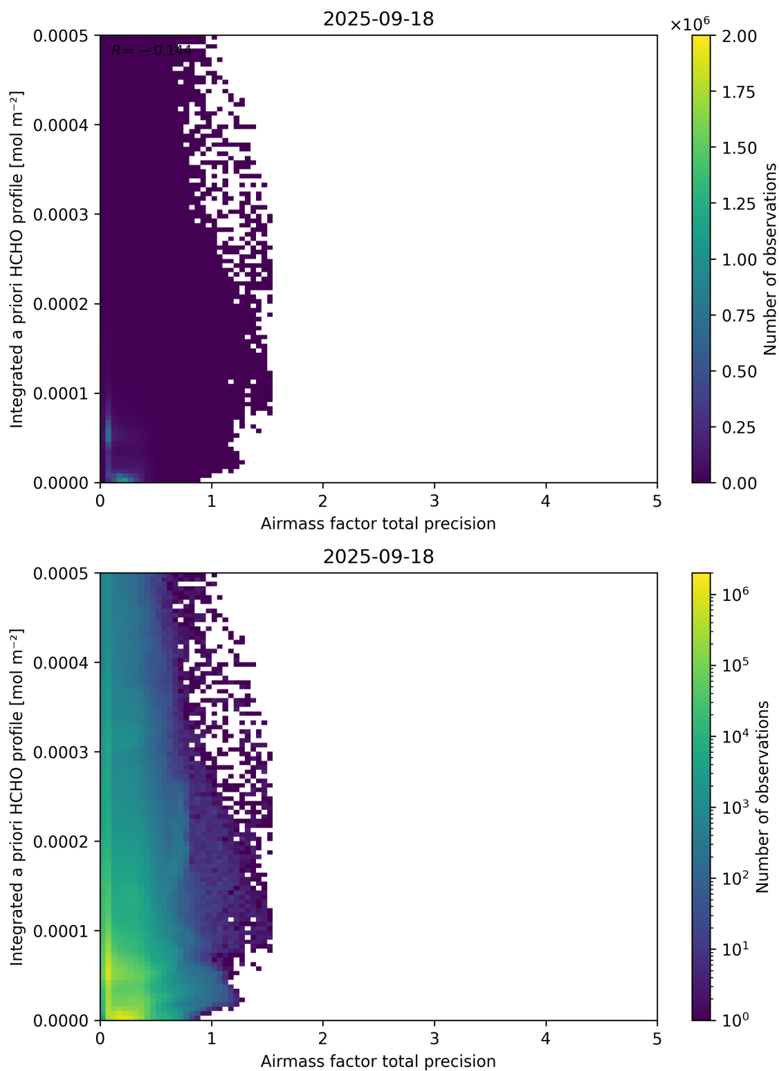
Figure 111: Scatter density plot of “Airmass factor total precision” against “Integrated a priori HCHO profile” for 2025-09-17 to 2025-09-19.
