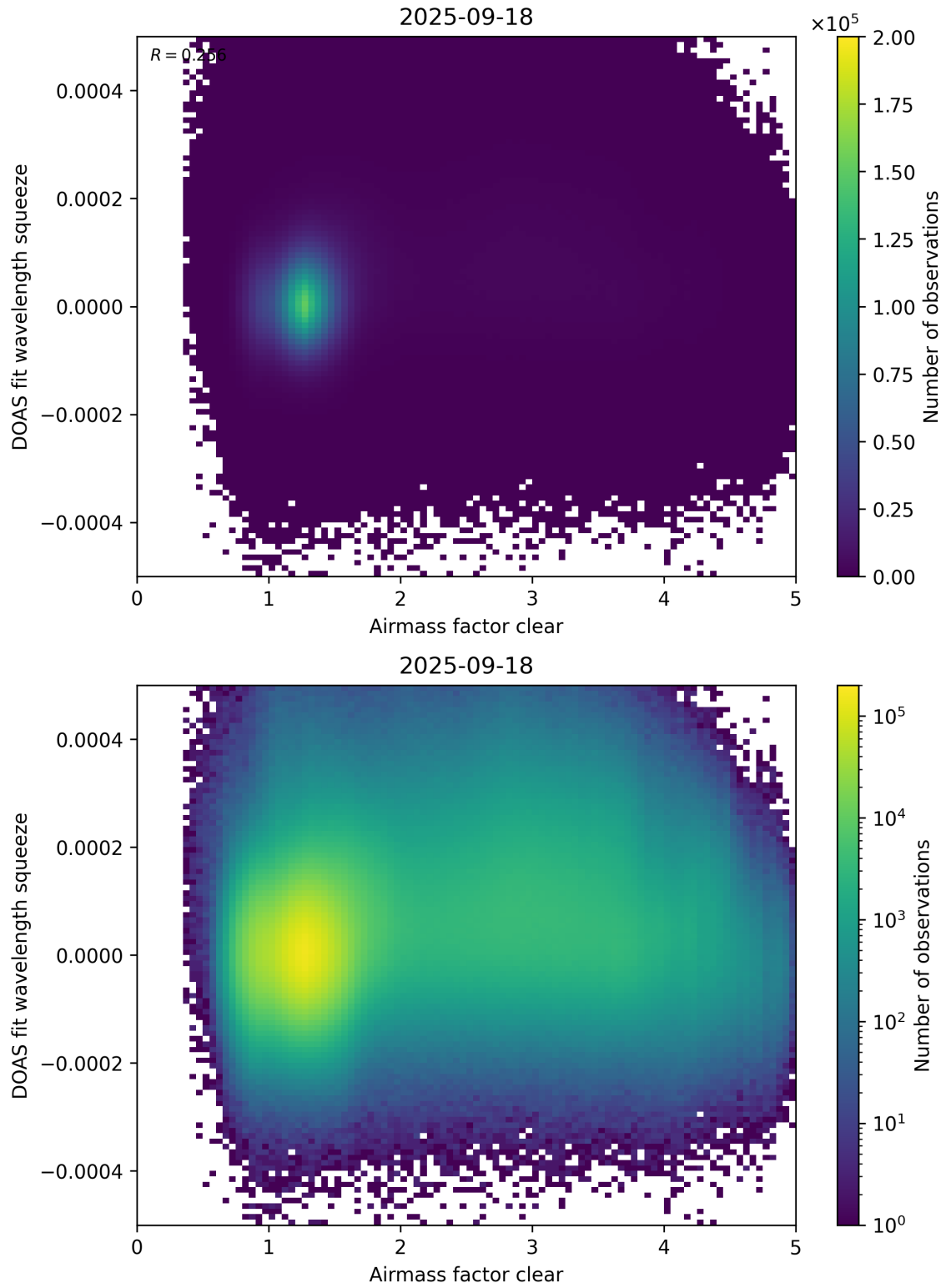
Figure 73: Scatter density plot of “Airmass factor clear” against “DOAS fit wavelength squeeze” for 2025-09-17 to 2025-09-19.
