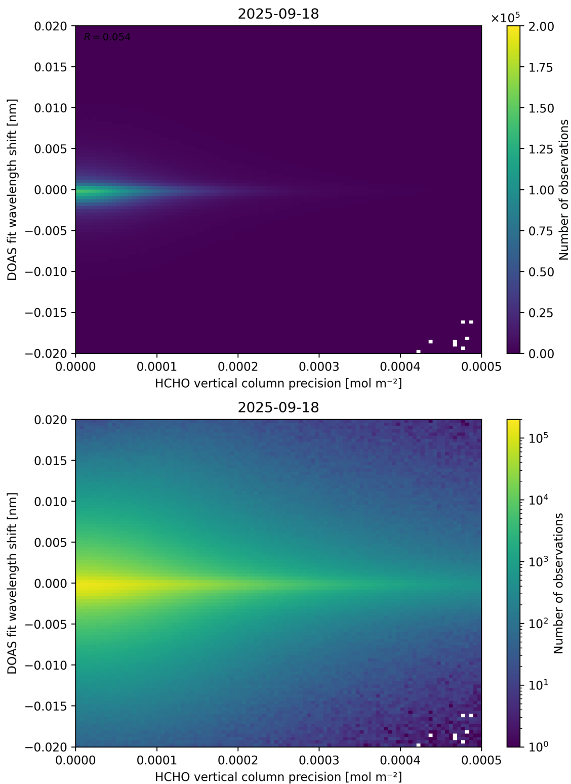
Figure 137: Scatter density plot of “HCHO vertical column precision” against “DOAS fit wavelength shift” for 2025-09-17 to 2025-09-19.
