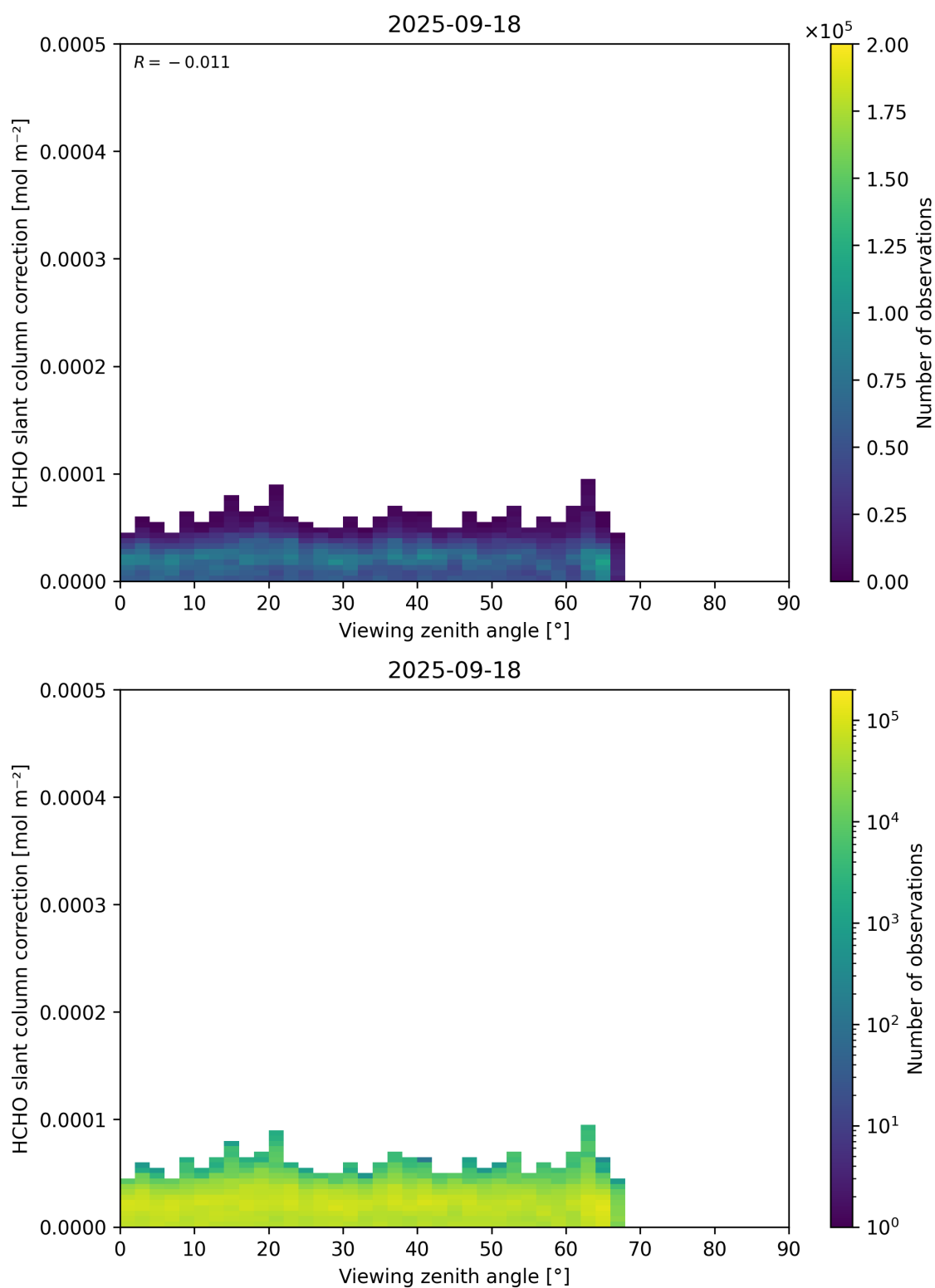
Figure 187: Scatter density plot of “Viewing zenith angle” against “HCHO slant column correction” for 2025-09-17 to 2025-09-19.
