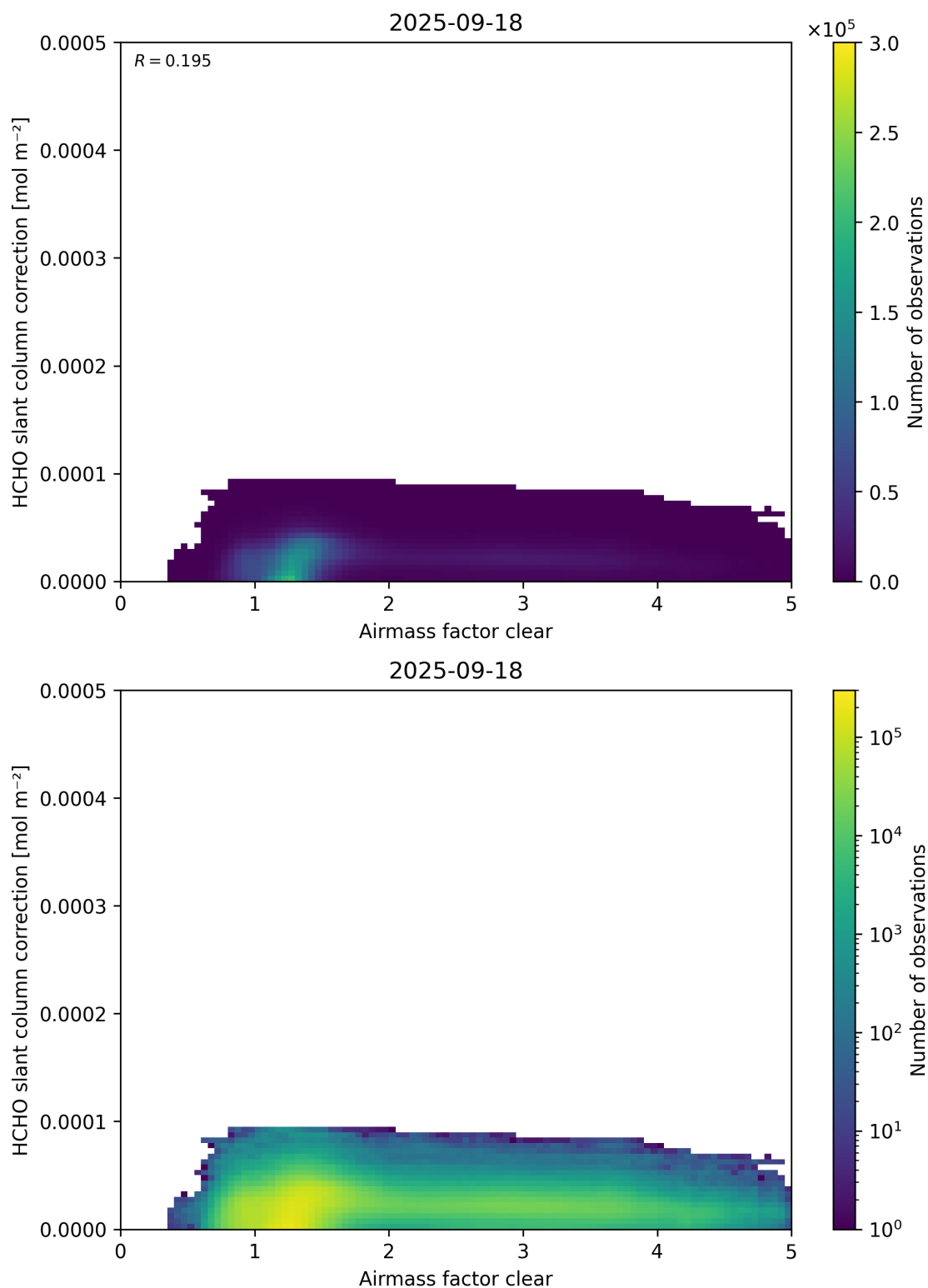
Figure 75: Scatter density plot of “Airmass factor clear” against “HCHO slant column correction” for 2025-09-17 to 2025-09-19.
