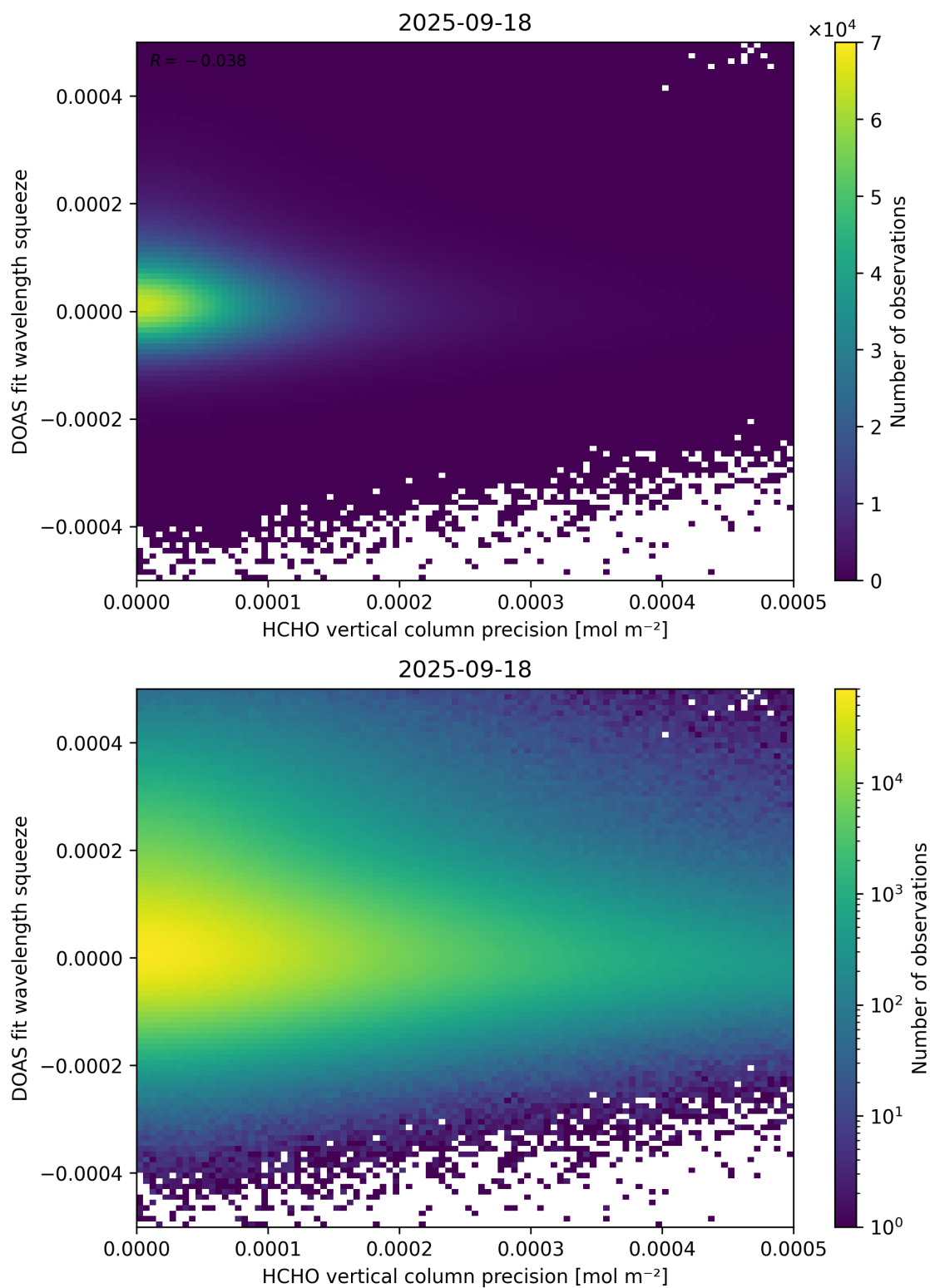
Figure 138: Scatter density plot of “HCHO vertical column precision” against “DOAS fit wavelength squeeze” for 2025-09-17 to 2025-09-19.
