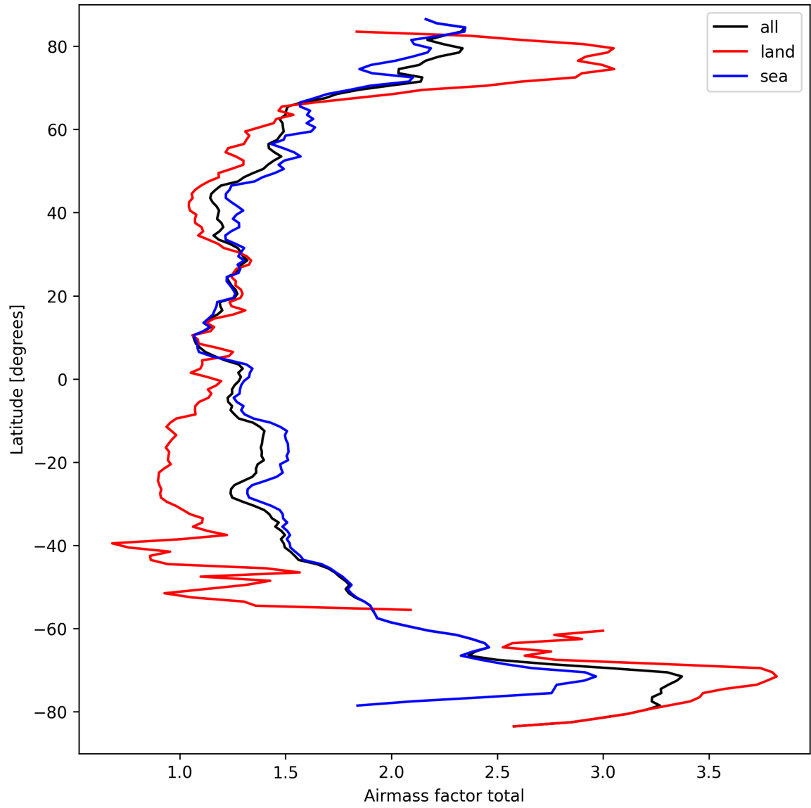
Figure 26: Zonal average of “Airmass factor total” for 2025-09-17 to 2025-09-19.
