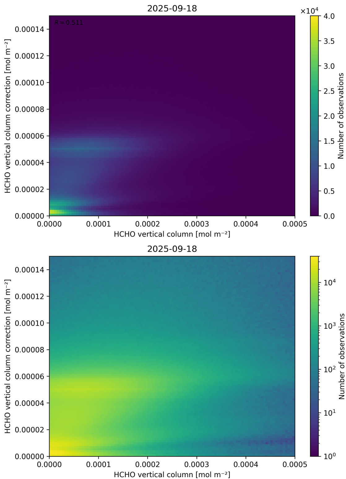
Figure 133: Scatter density plot of “HCHO vertical column” against “HCHO vertical column correction” for 2025-09-17 to 2025-09-19.
