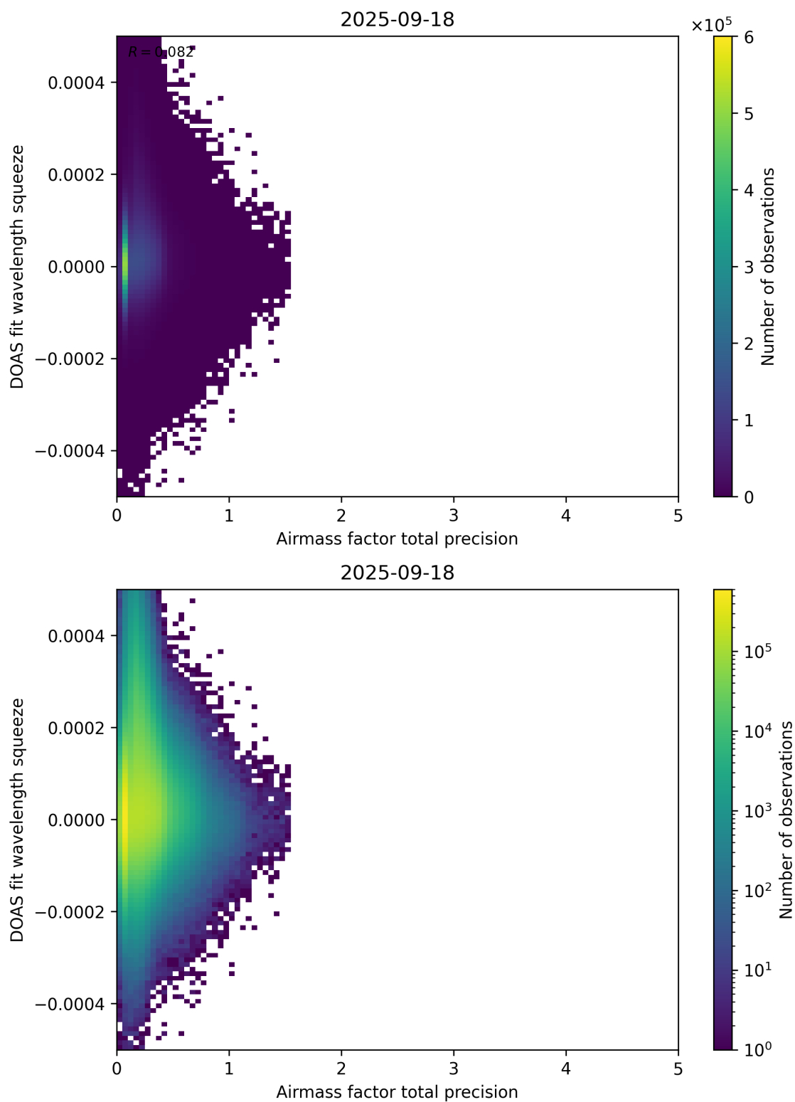
Figure 107: Scatter density plot of “Airmass factor total precision” against “DOAS fit wavelength squeeze” for 2025-09-17 to 2025-09-19.
