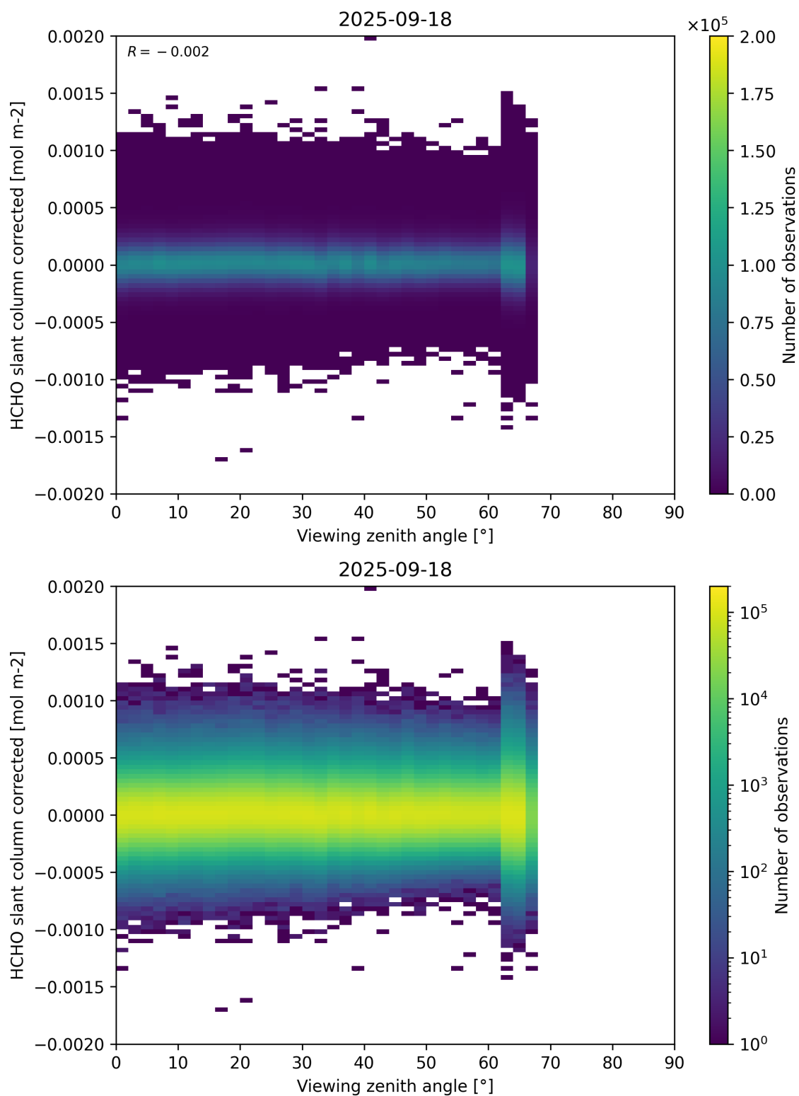
Figure 186: Scatter density plot of “Viewing zenith angle” against “HCHO slant column corrected” for 2025-09-17 to 2025-09-19.
