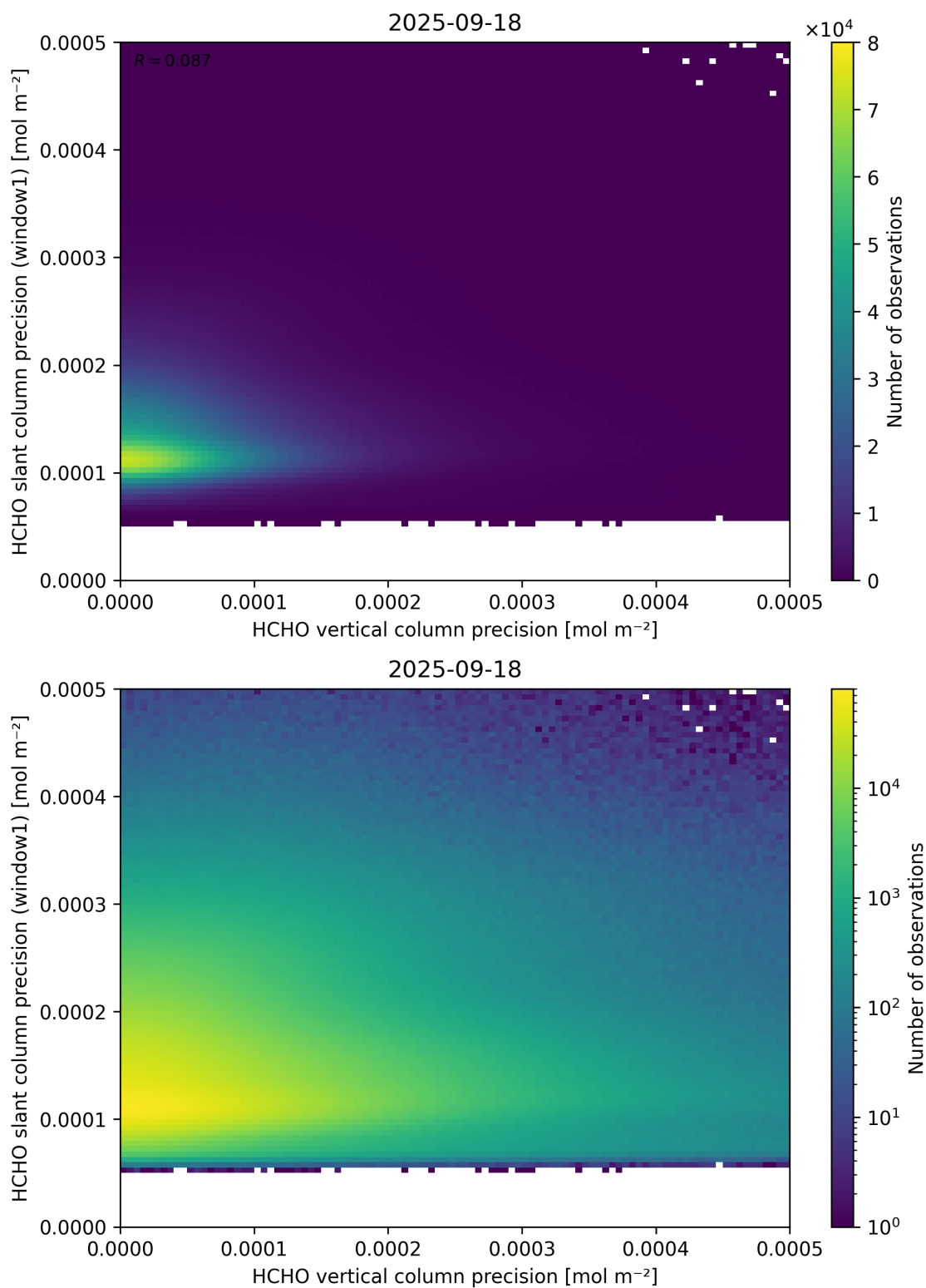
Figure 143: Scatter density plot of “HCHO vertical column precision” against “HCHO slant column precision (window1)” for 2025-09-17 to 2025-09-19.
