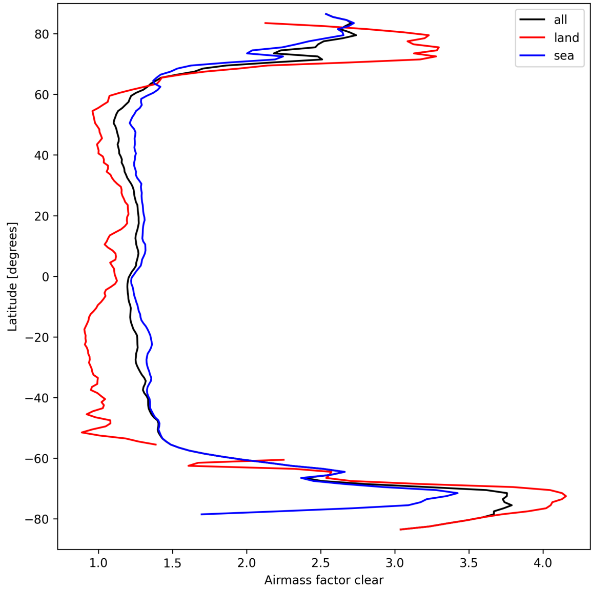
Figure 28: Zonal average of “Airmass factor clear” for 2025-09-17 to 2025-09-19.
