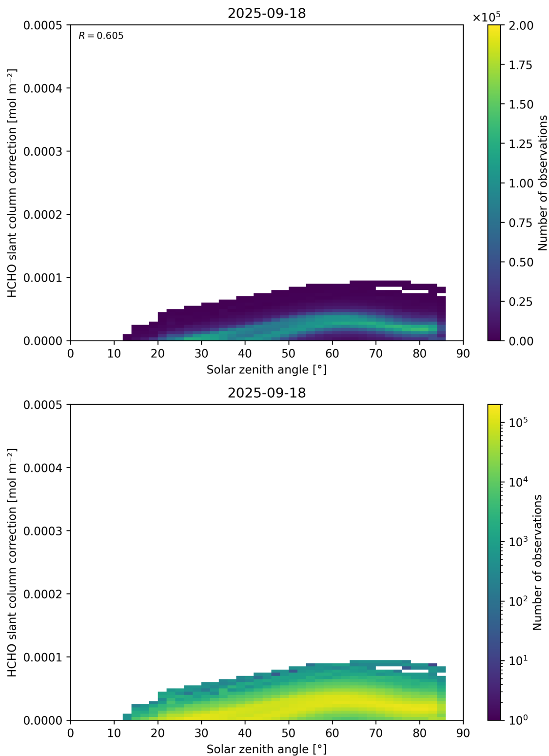
Figure 172: Scatter density plot of “Solar zenith angle” against “HCHO slant column correction” for 2025-09-17 to 2025-09-19.
