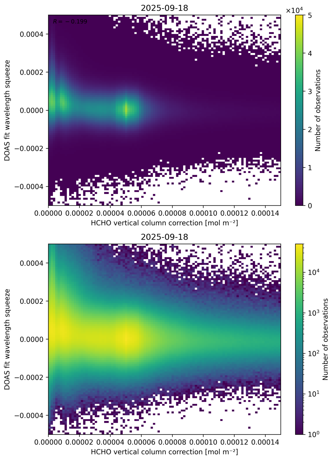
Figure 114: Scatter density plot of “HCHO vertical column correction” against “DOAS fit wavelength squeeze” for 2025-09-17 to 2025-09-19.
