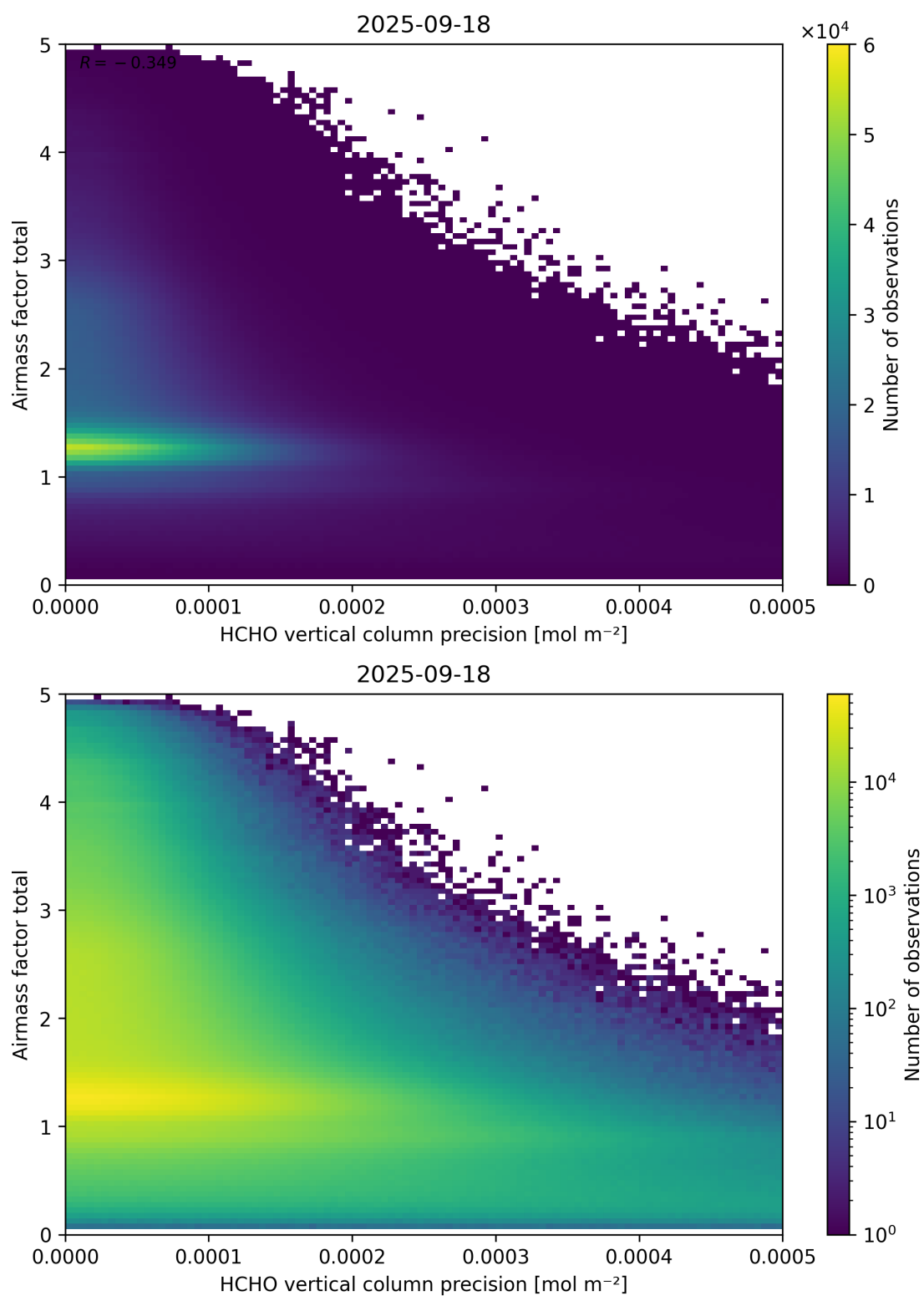
Figure 144: Scatter density plot of “HCHO vertical column precision” against “Airmass factor total” for 2025-09-17 to 2025-09-19.
