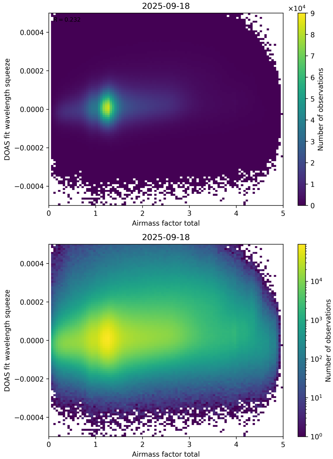
Figure 99: Scatter density plot of “Airmass factor total” against “DOAS fit wavelength squeeze” for 2025-09-17 to 2025-09-19.
