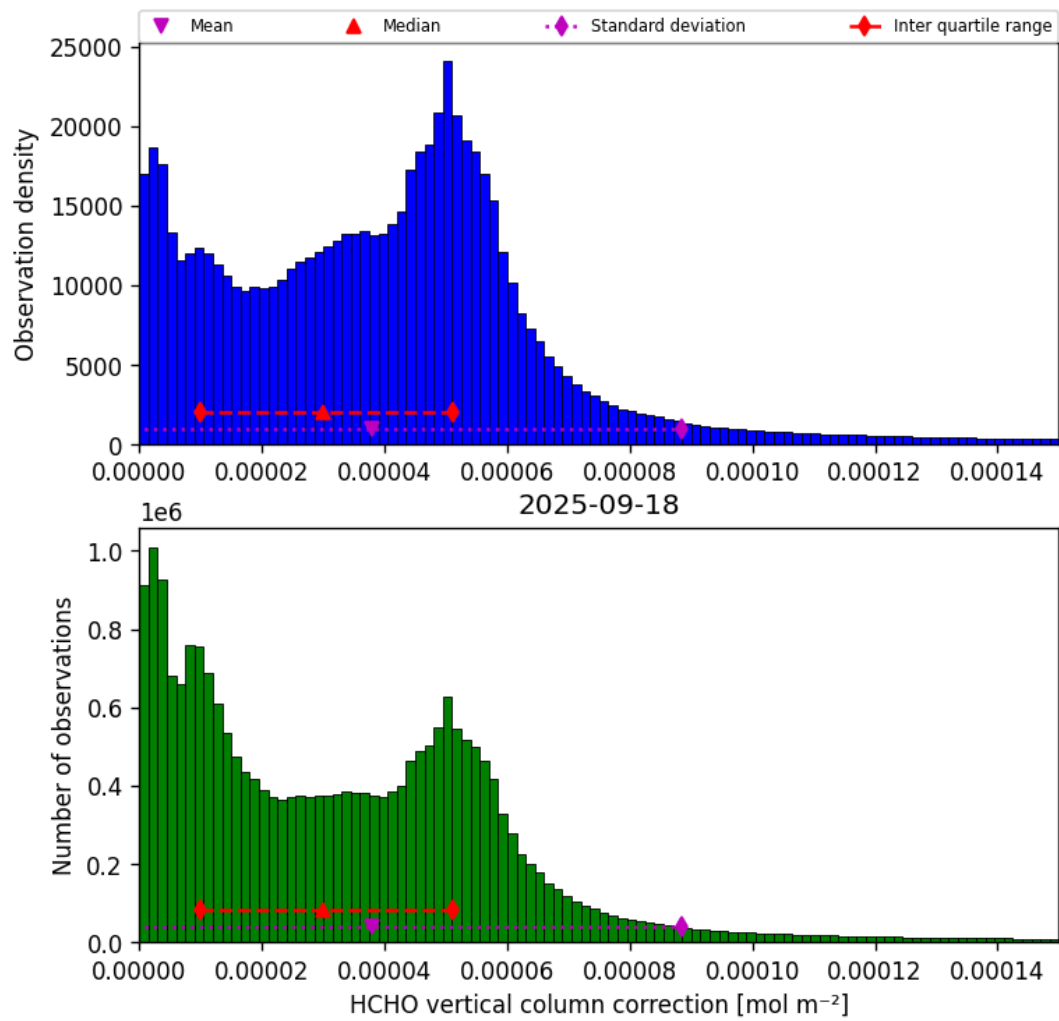
Figure 37: Histogram of “HCHO vertical column correction” for 2025-09-17 to 2025-09-19
