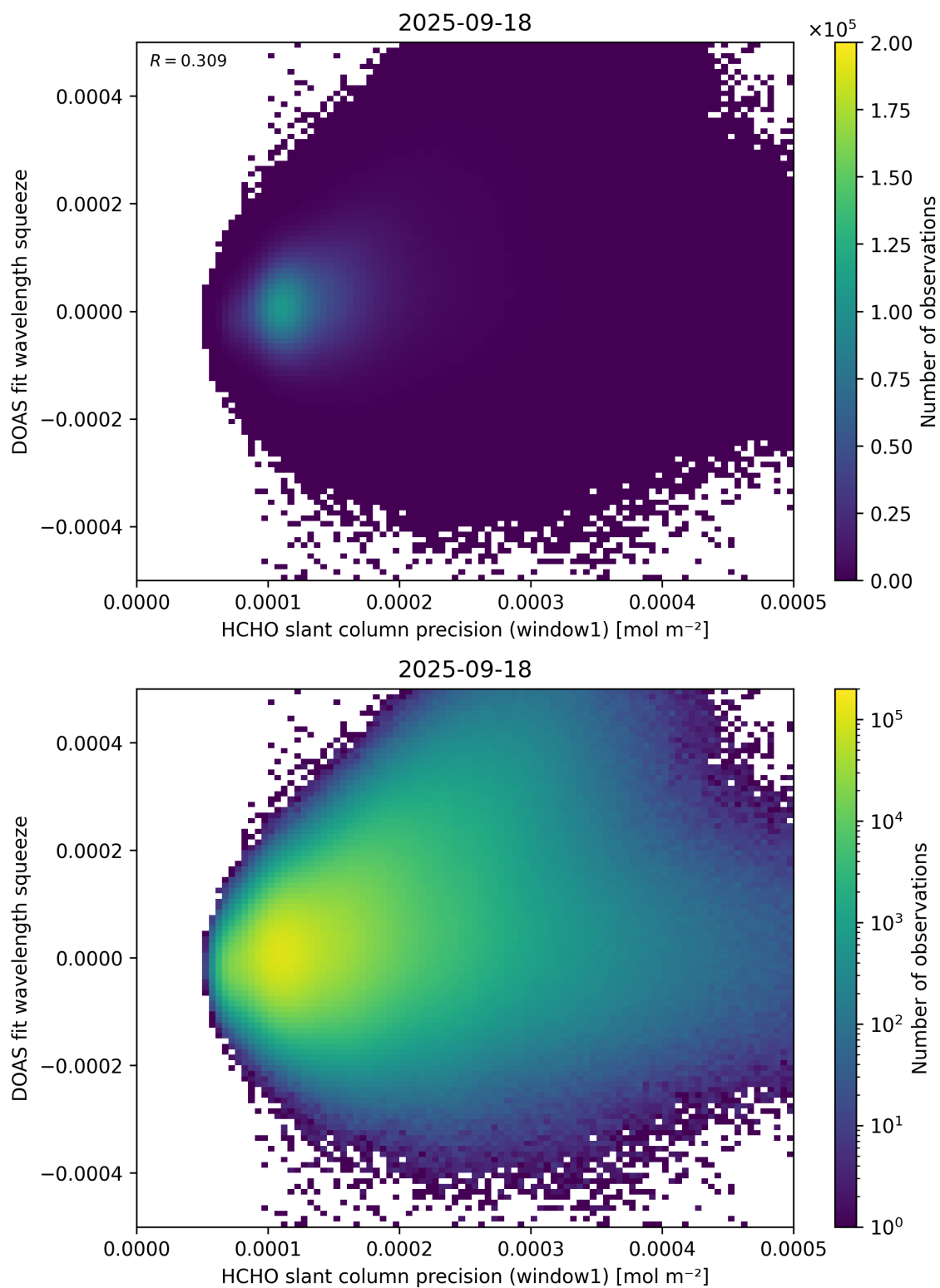
Figure 90: Scatter density plot of “HCHO slant column precision (window1)” against “DOAS fit wavelength squeeze” for 2025-09-17 to 2025-09-19.
