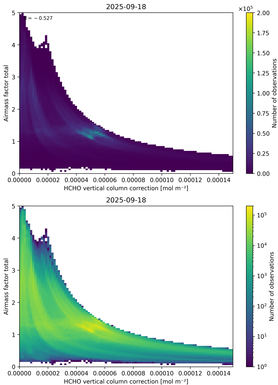
Figure 120: Scatter density plot of “HCHO vertical column correction” against “Airmass factor total” for 2025-09-17 to 2025-09-19.
