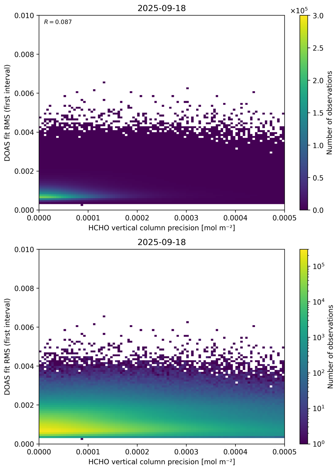
Figure 136: Scatter density plot of “HCHO vertical column precision” against “DOAS fit RMS (first interval)” for 2025-09-17 to 2025-09-19.
