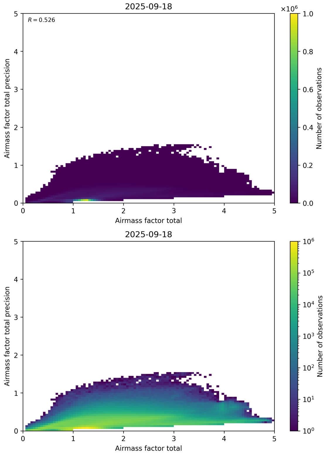
Figure 103: Scatter density plot of “Airmass factor total” against “Airmass factor total precision” for 2025-09-17 to 2025-09-19.
