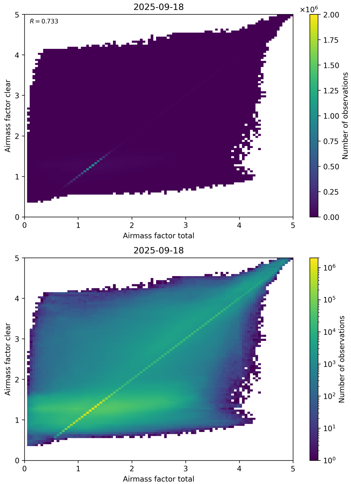
Figure 100: Scatter density plot of “Airmass factor total” against “Airmass factor clear” for 2025-09-17 to 2025-09-19.
