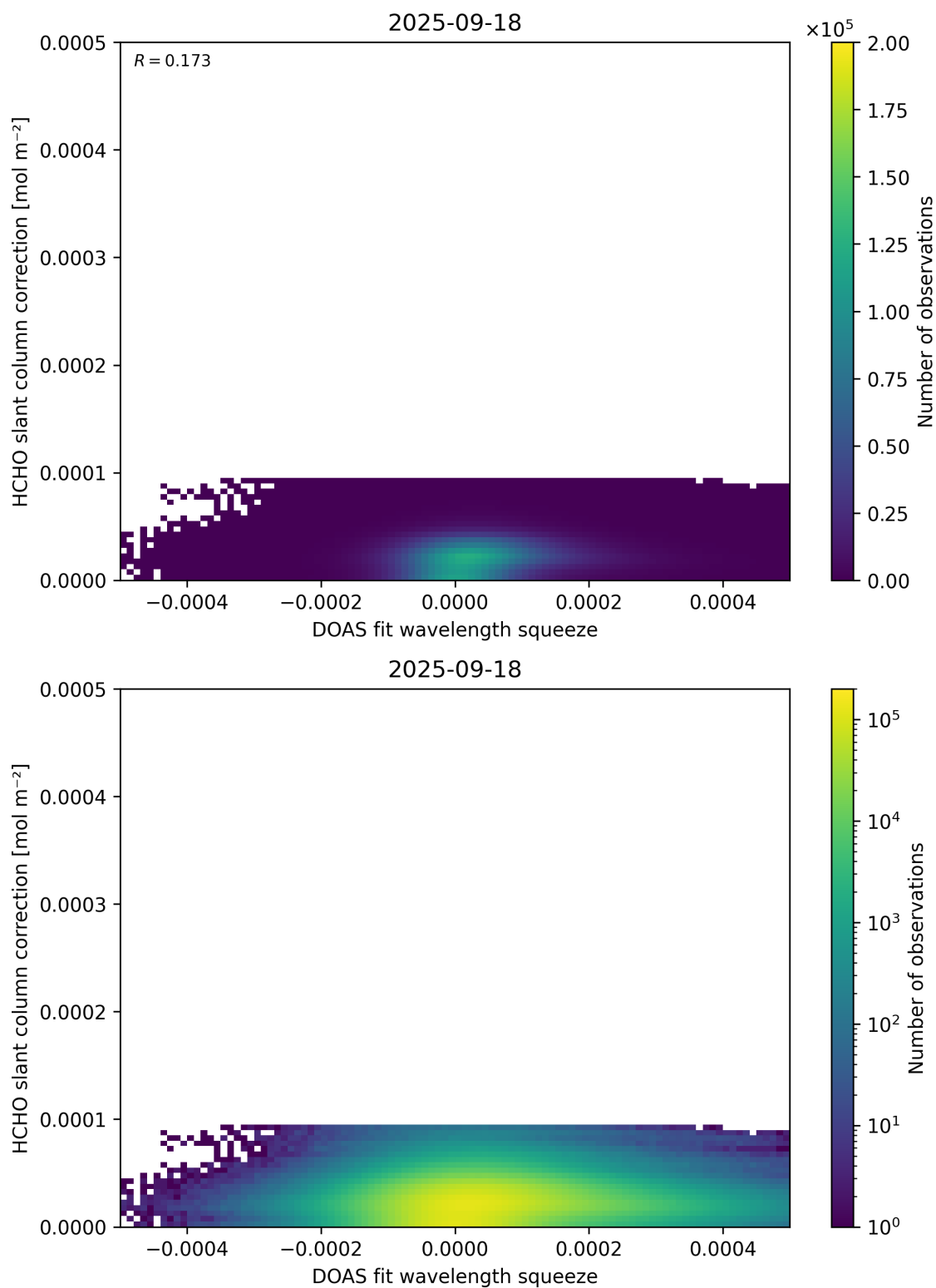
Figure 70: Scatter density plot of “DOAS fit wavelength squeeze” against “HCHO slant column correction” for 2025-09-17 to 2025-09-19.
