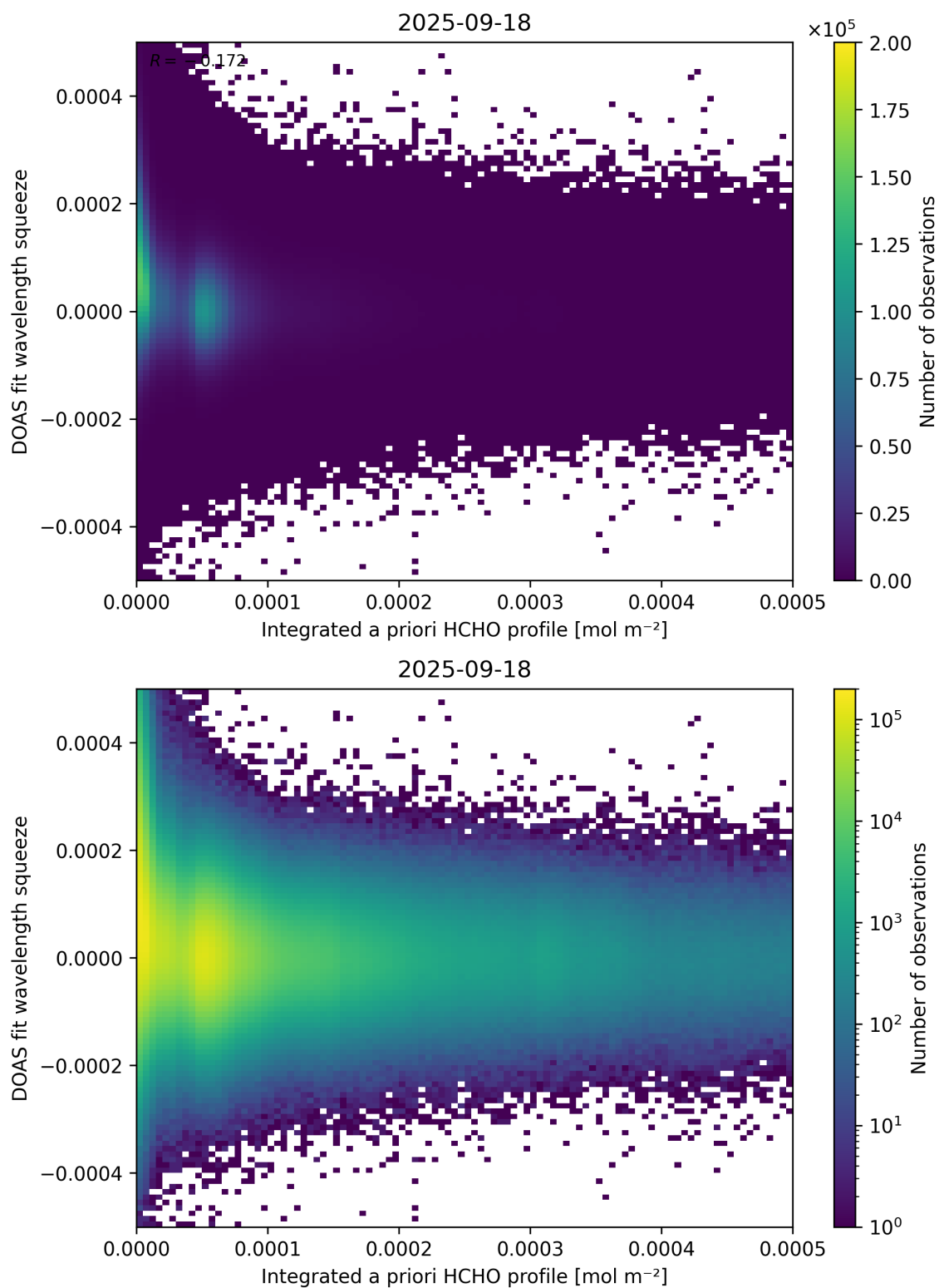
Figure 150: Scatter density plot of “Integrated a priori HCHO profile” against “DOAS fit wavelength squeeze” for 2025-09-17 to 2025-09-19.
