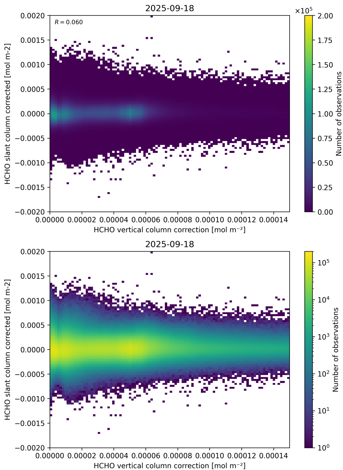
Figure 116: Scatter density plot of “HCHO vertical column correction” against “HCHO slant column corrected” for 2025-09-17 to 2025-09-19.
