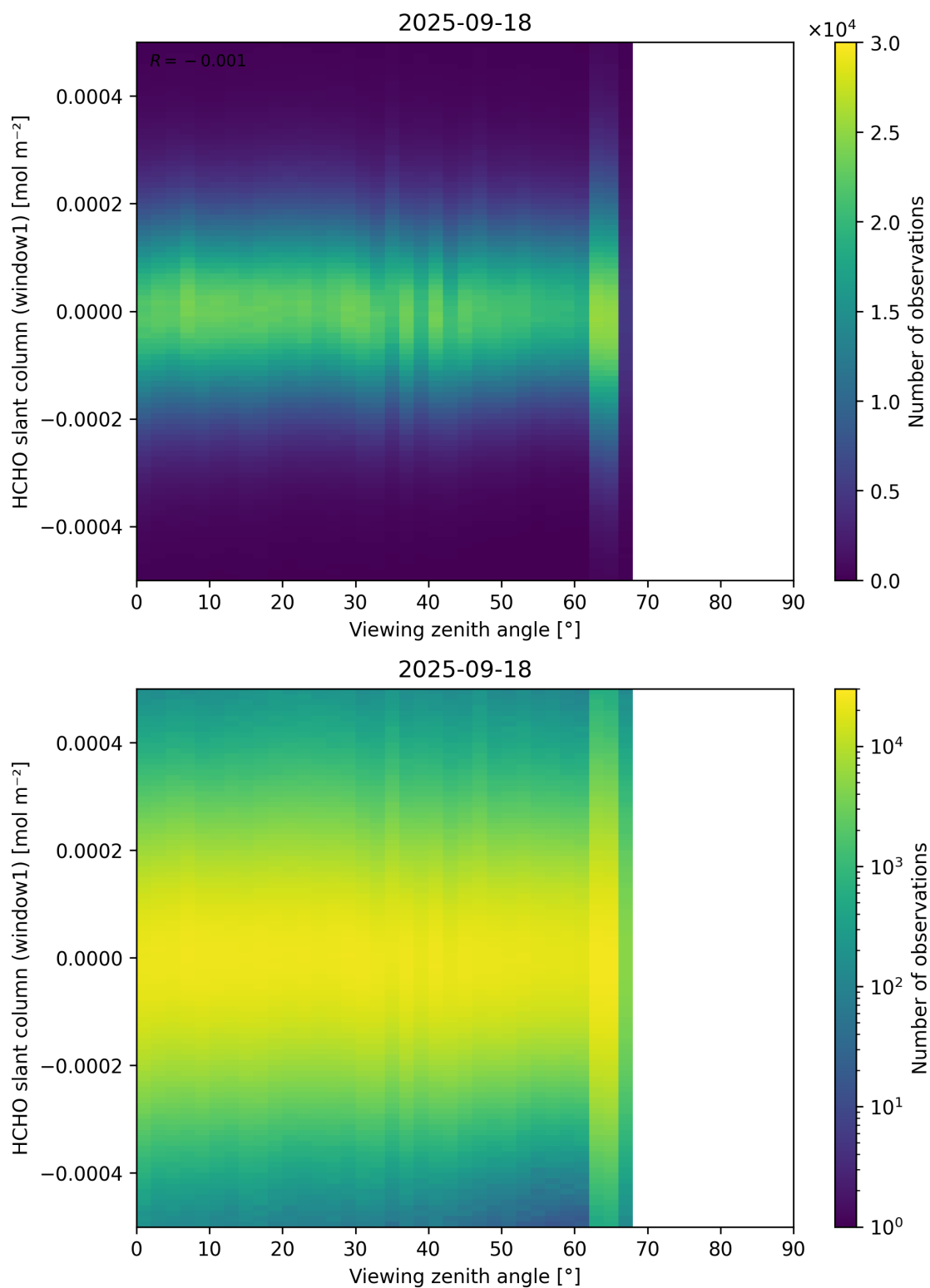
Figure 188: Scatter density plot of “Viewing zenith angle” against “HCHO slant column (window1)” for 2025-09-17 to 2025-09-19.
