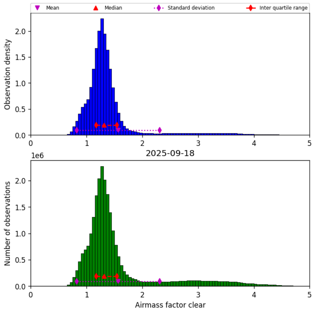
Figure 42: Histogram of “Airmass factor clear” for 2025-09-17 to 2025-09-19
