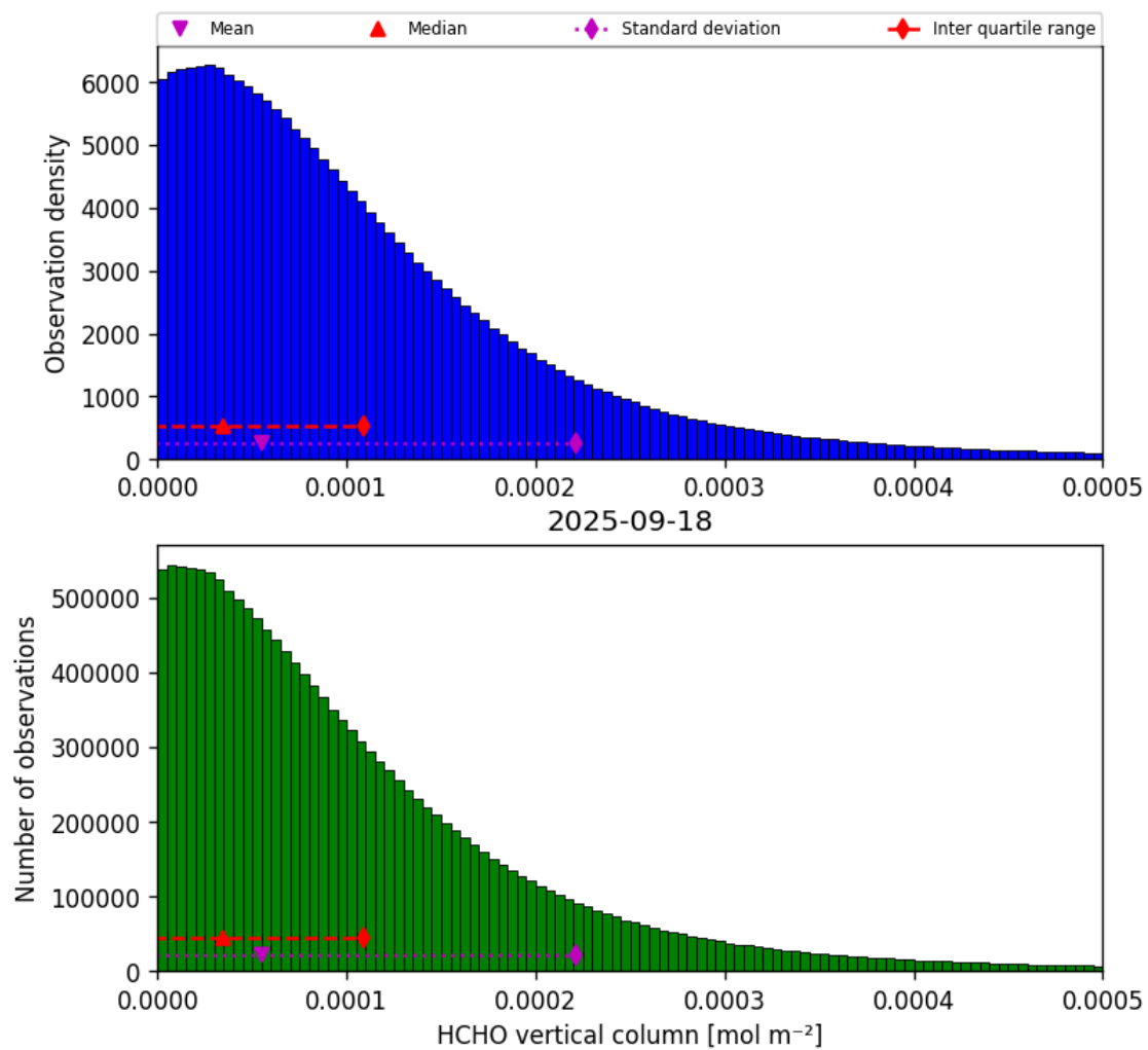
Figure 35: Histogram of “HCHO vertical column” for 2025-09-17 to 2025-09-19
