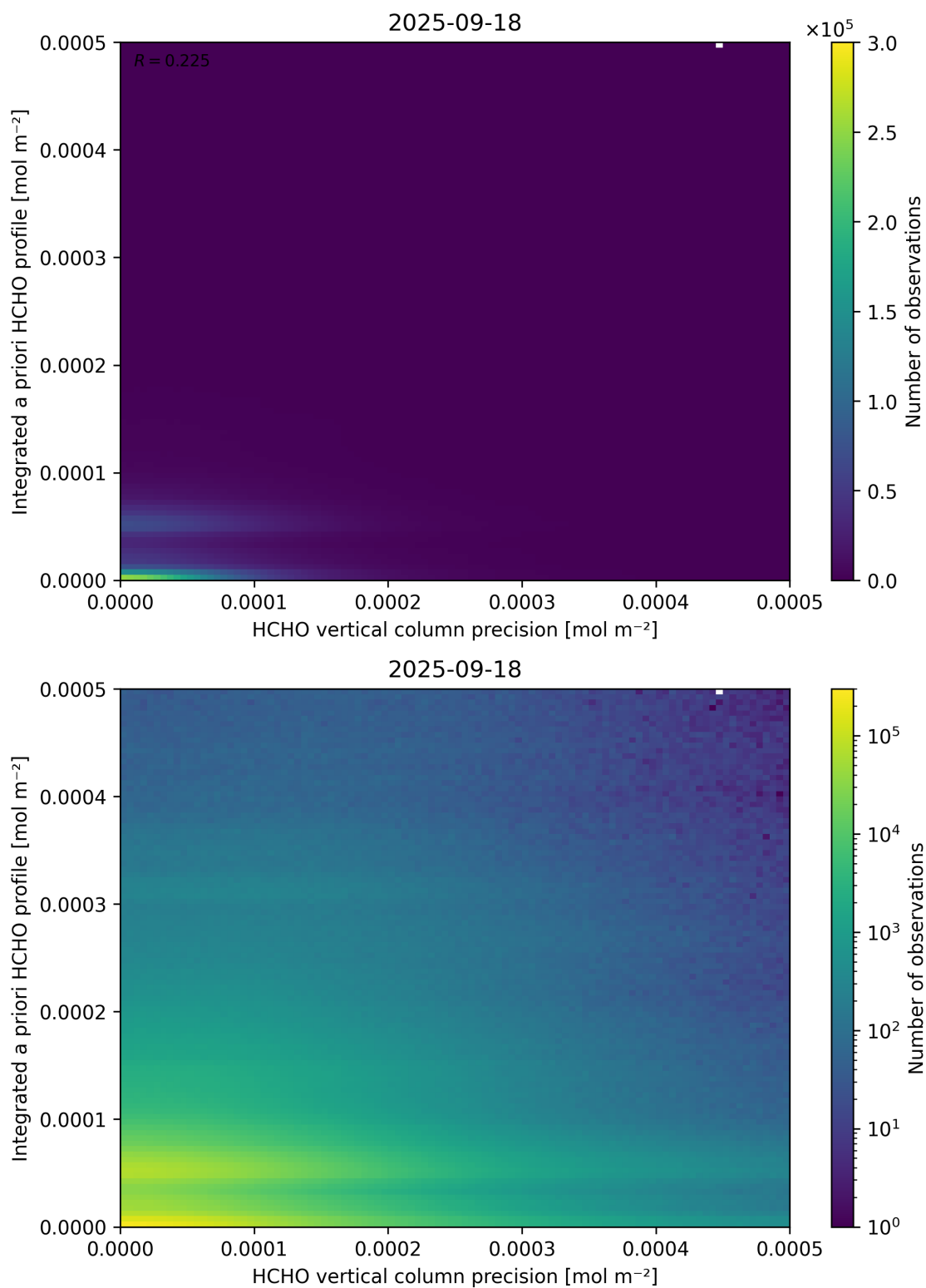
Figure 147: Scatter density plot of “HCHO vertical column precision” against “Integrated a priori HCHO profile” for 2025-09-17 to 2025-09-19.
