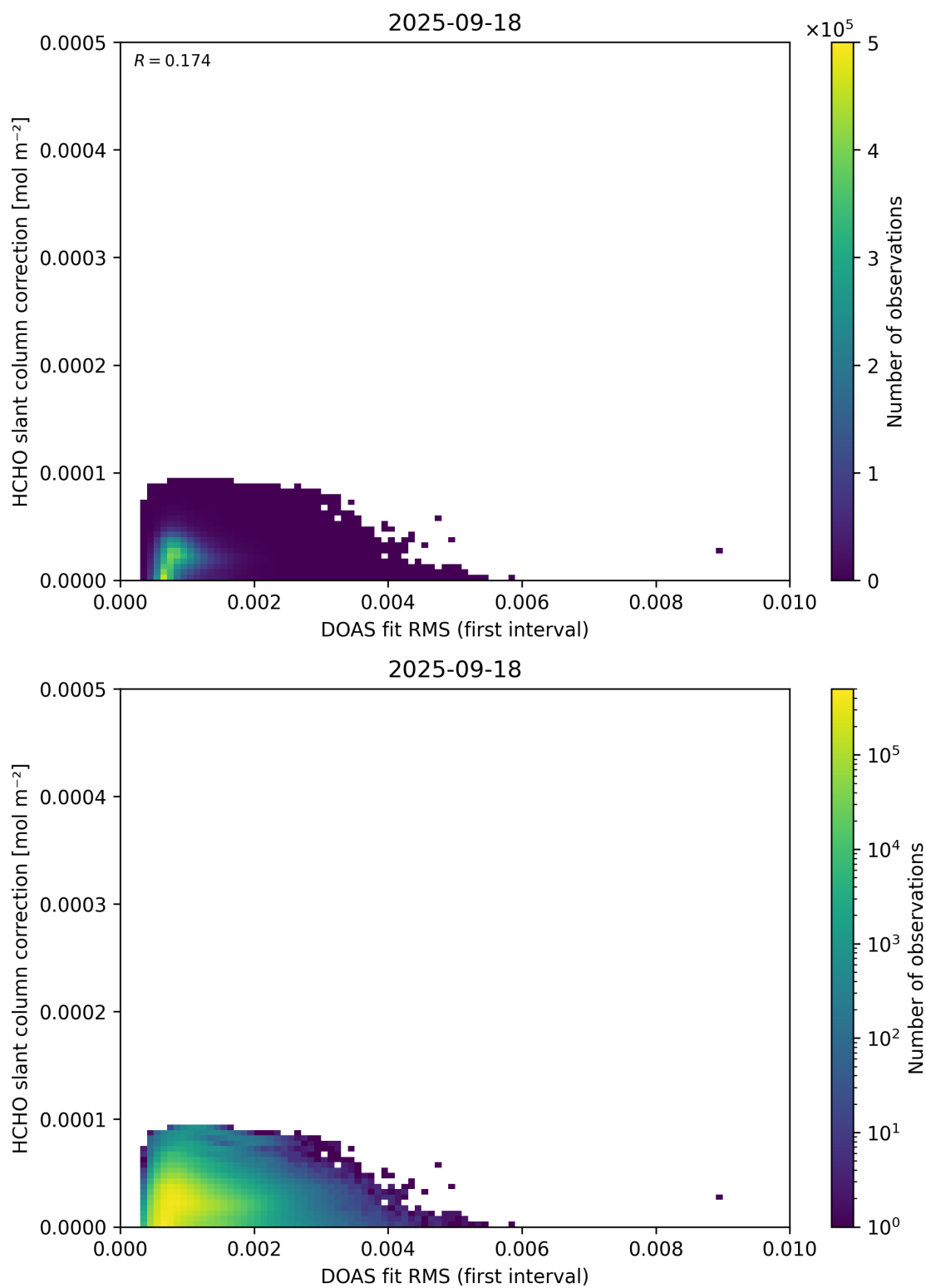
Figure 63: Scatter density plot of “DOAS fit RMS (first interval)” against “HCHO slant column correction” for 2025-09-17 to 2025-09-19.
