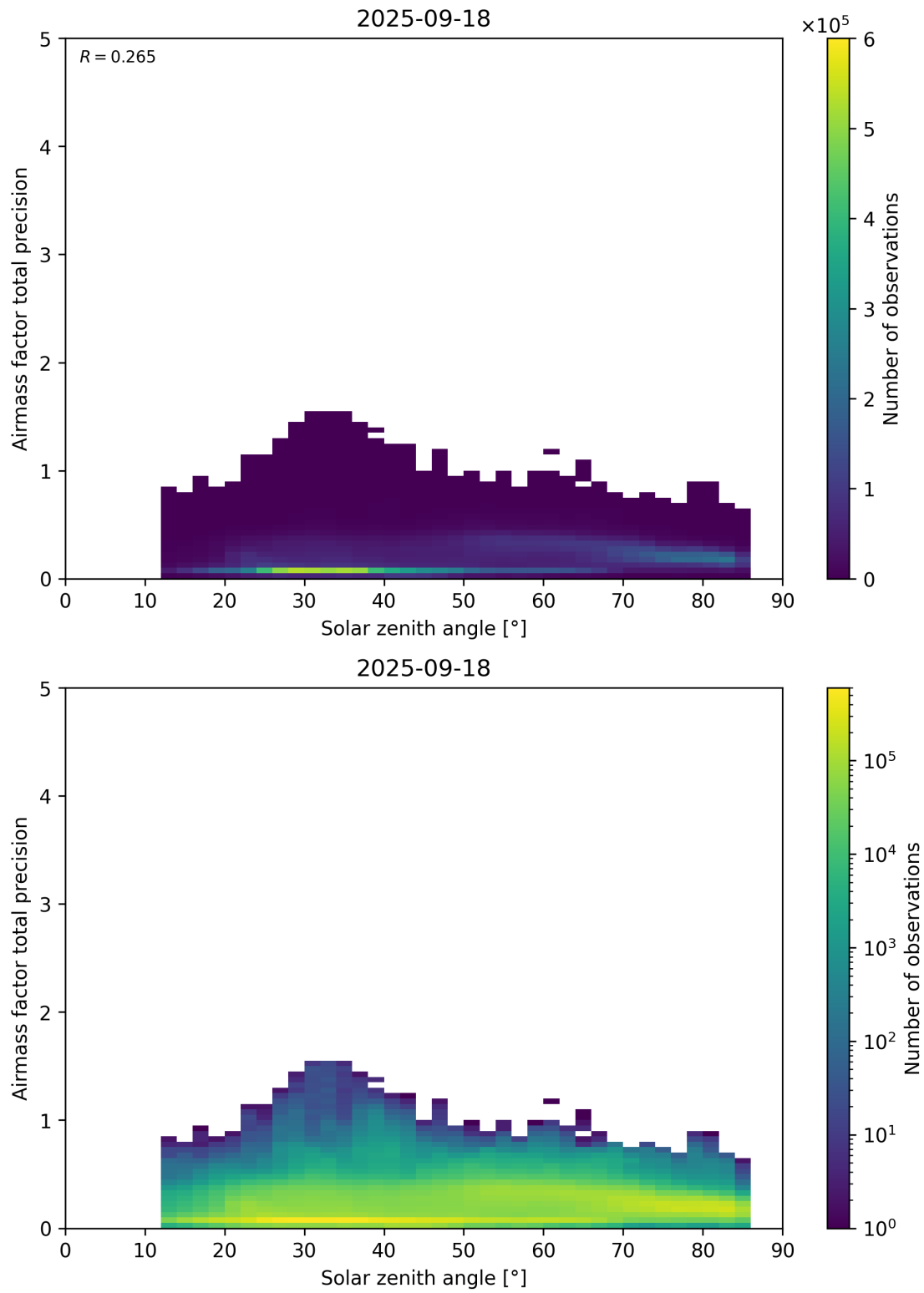
Figure 176: Scatter density plot of “Solar zenith angle” against “Airmass factor total precision” for 2025-09-17 to 2025-09-19.
