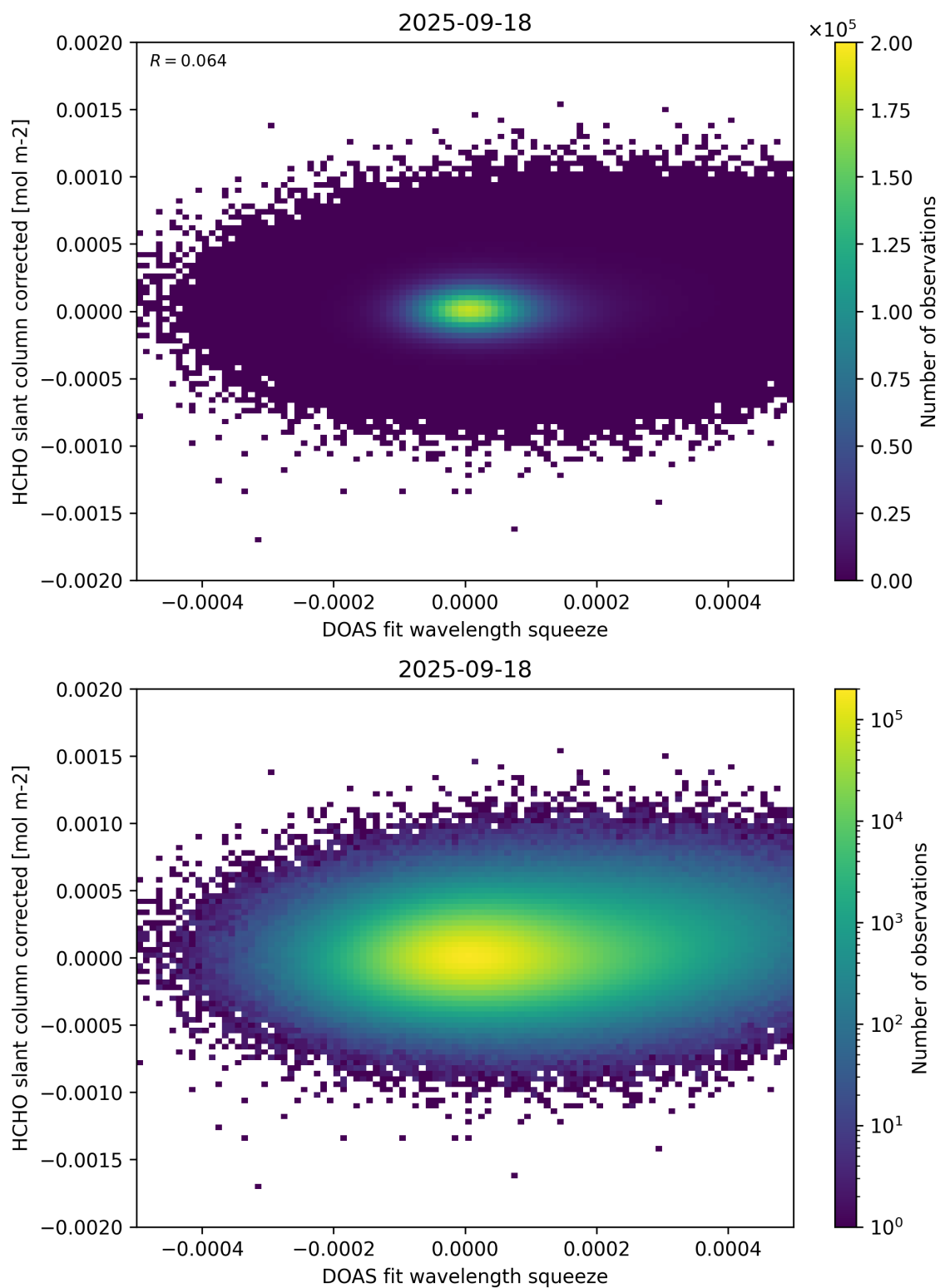
Figure 69: Scatter density plot of “DOAS fit wavelength squeeze” against “HCHO slant column corrected” for 2025-09-17 to 2025-09-19.
