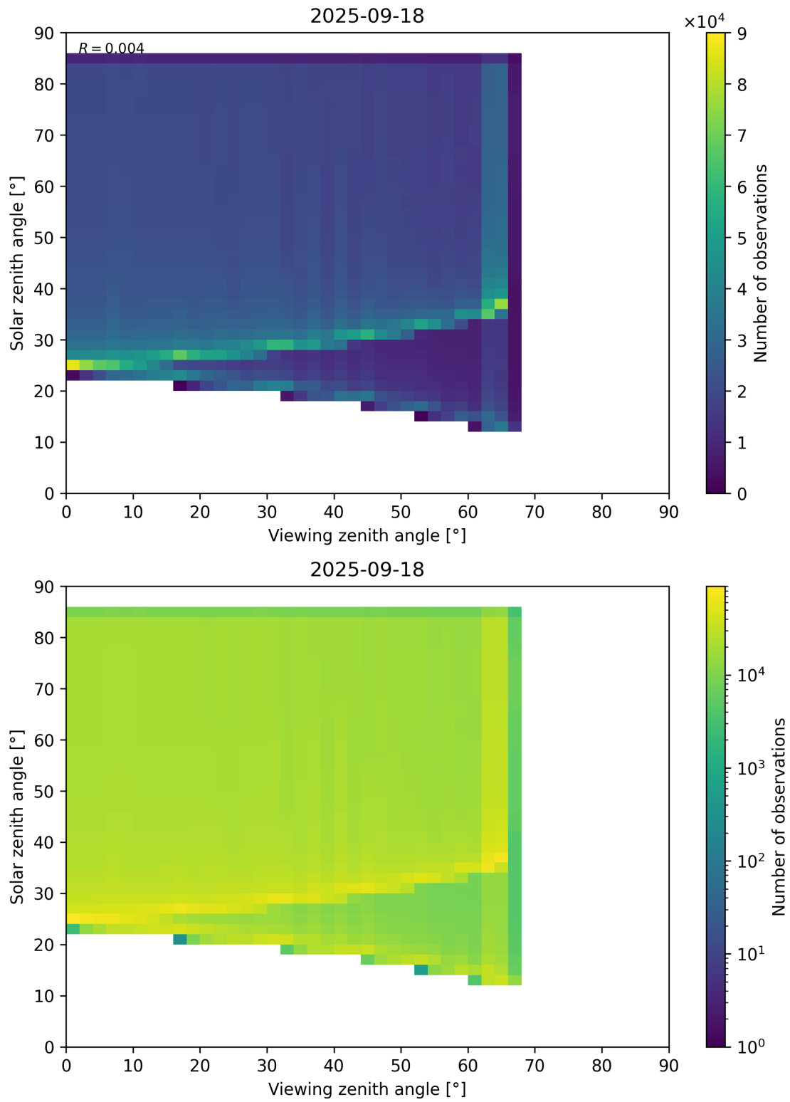
Figure 197: Scatter density plot of “Viewing zenith angle” against “Solar zenith angle” for 2025-09-17 to 2025-09-19.
