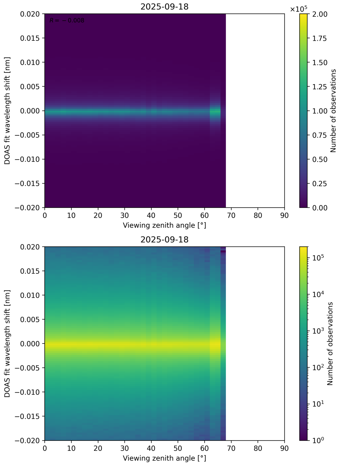
Figure 183: Scatter density plot of “Viewing zenith angle” against “DOAS fit wavelength shift” for 2025-09-17 to 2025-09-19.
