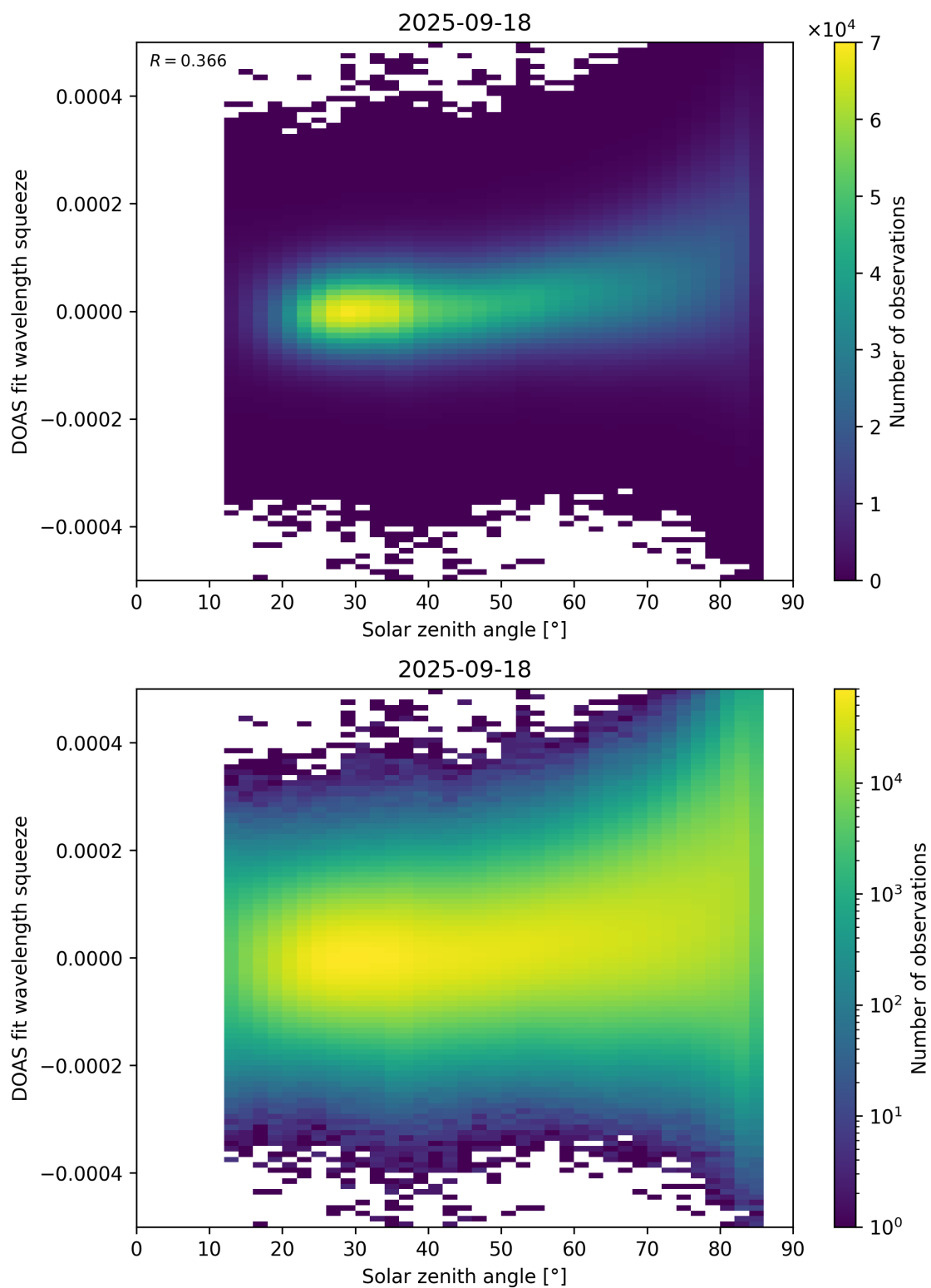
Figure 169: Scatter density plot of “Solar zenith angle” against “DOAS fit wavelength squeeze” for 2025-09-17 to 2025-09-19.
