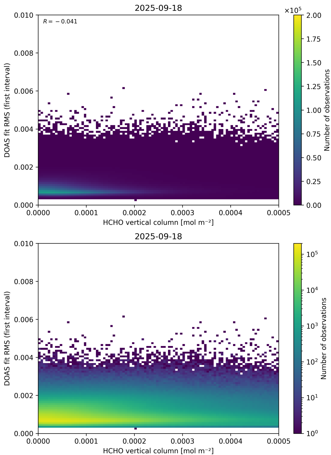
Figure 123: Scatter density plot of “HCHO vertical column” against “DOAS fit RMS (first interval)” for 2025-09-17 to 2025-09-19.
