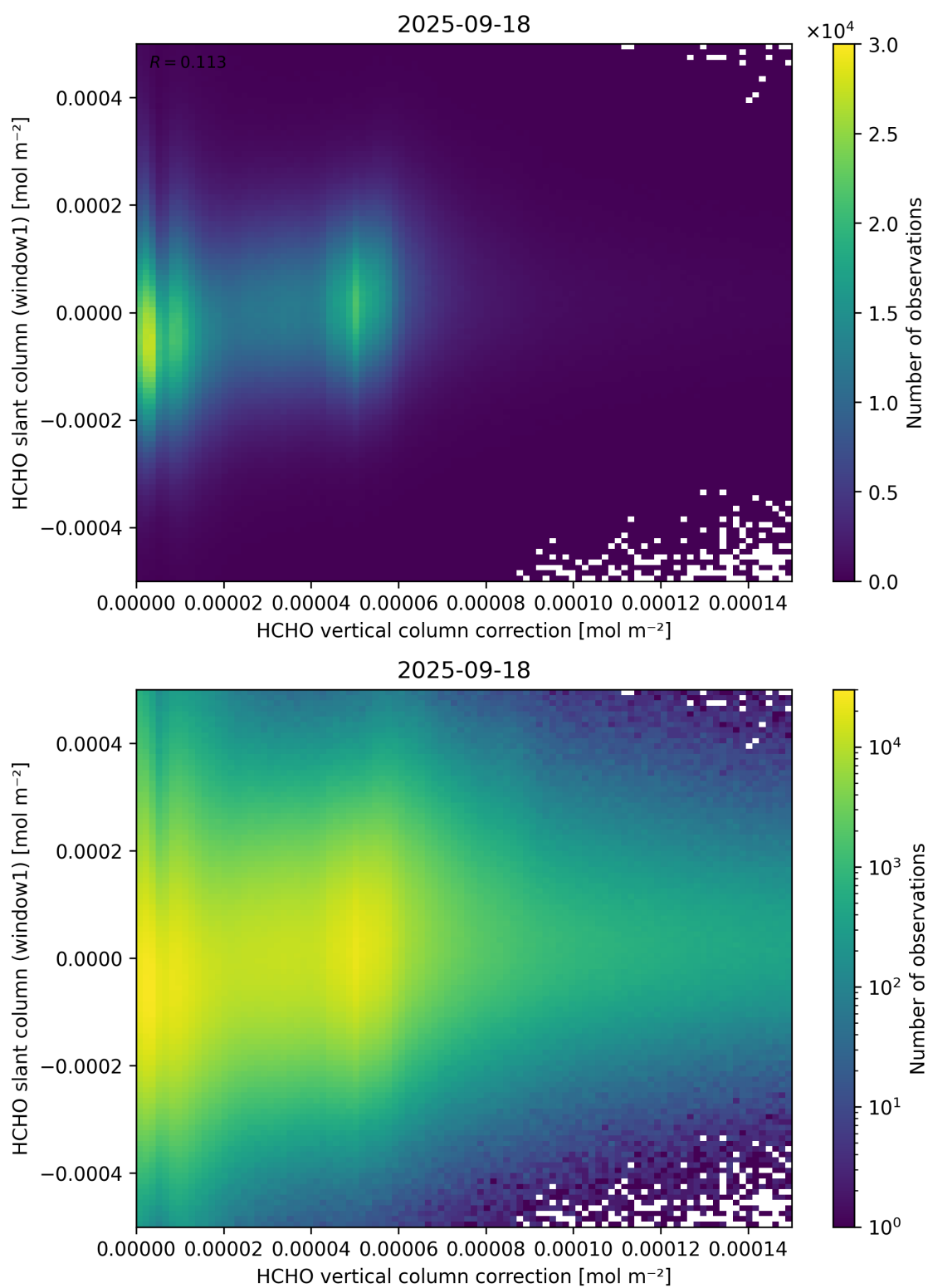
Figure 118: Scatter density plot of “HCHO vertical column correction” against “HCHO slant column (window1)” for 2025-09-17 to 2025-09-19.
