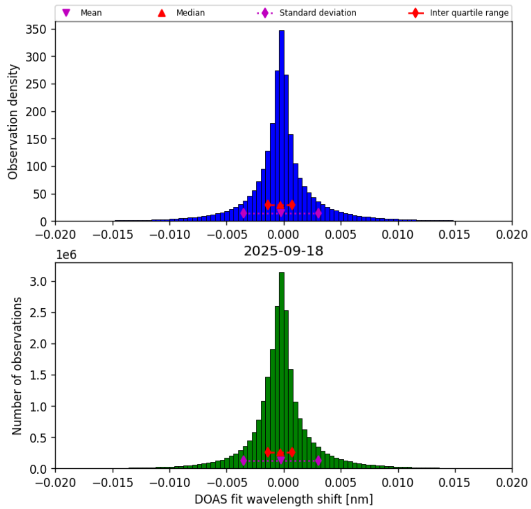
Figure 44: Histogram of “DOAS fit wavelength shift” for 2025-09-17 to 2025-09-19
