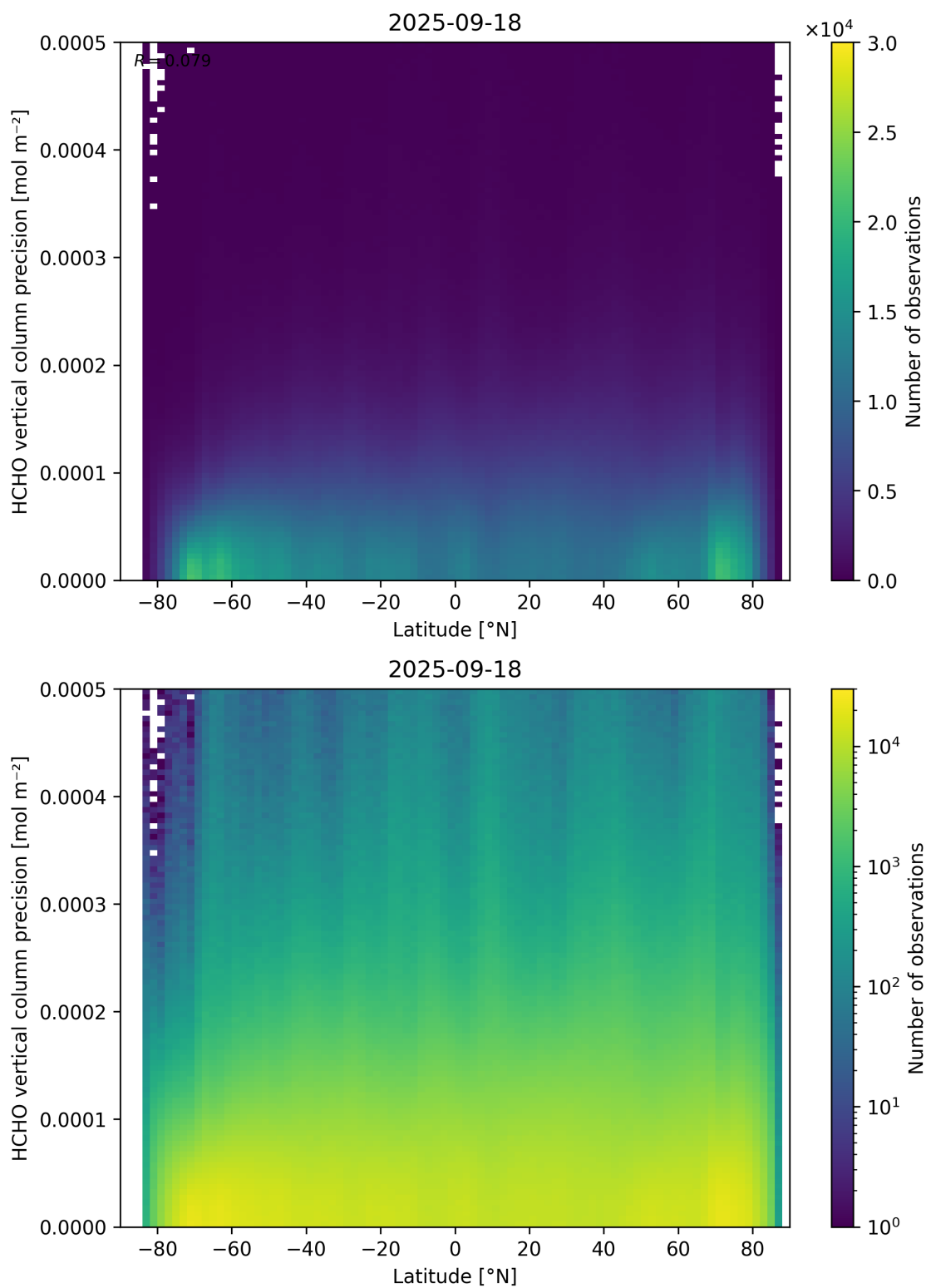
Figure 165: Scatter density plot of “Latitude” against “HCHO vertical column precision” for 2025-09-17 to 2025-09-19.
