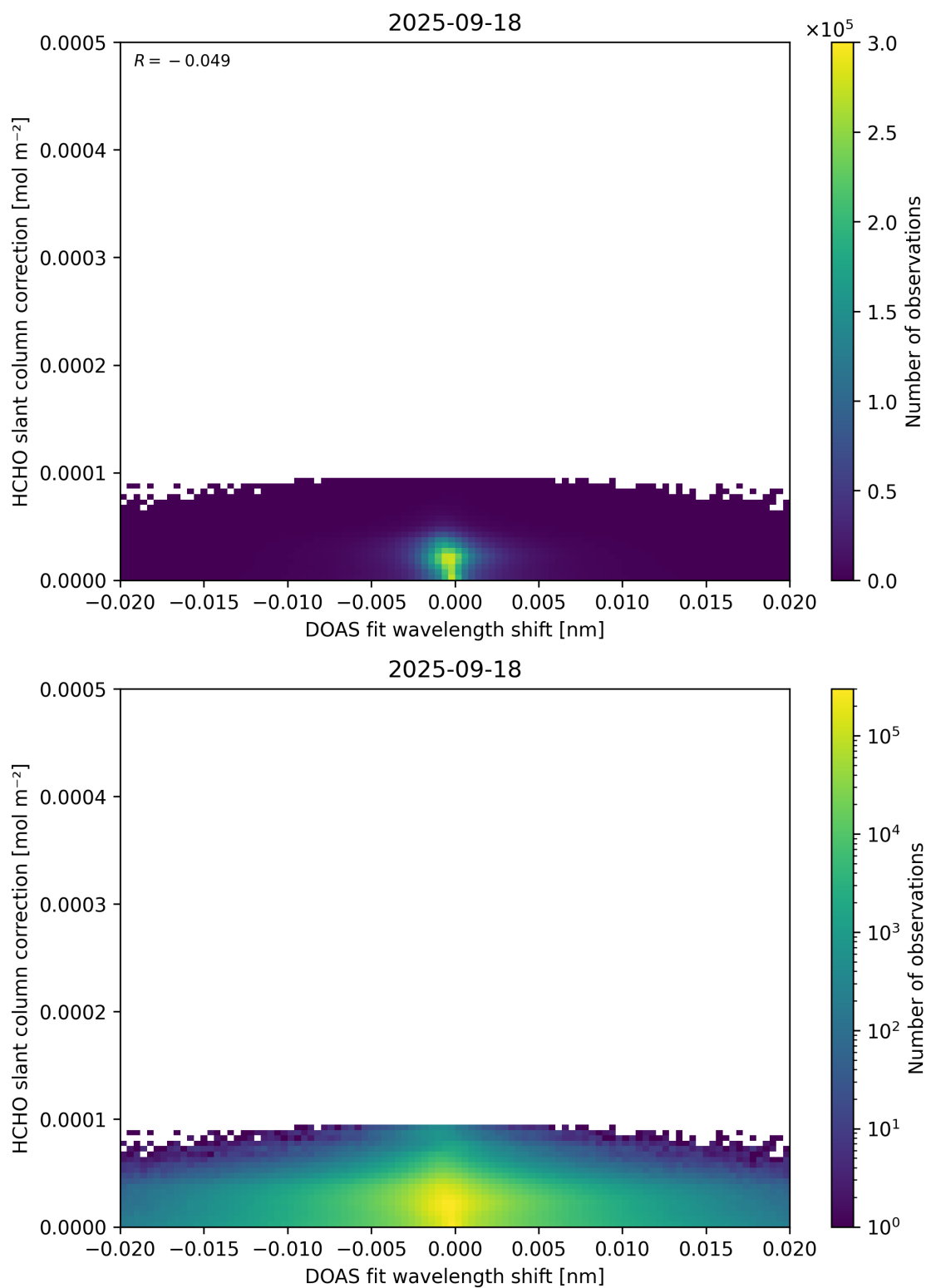
Figure 67: Scatter density plot of “DOAS fit wavelength shift” against “HCHO slant column correction” for 2025-09-17 to 2025-09-19.
