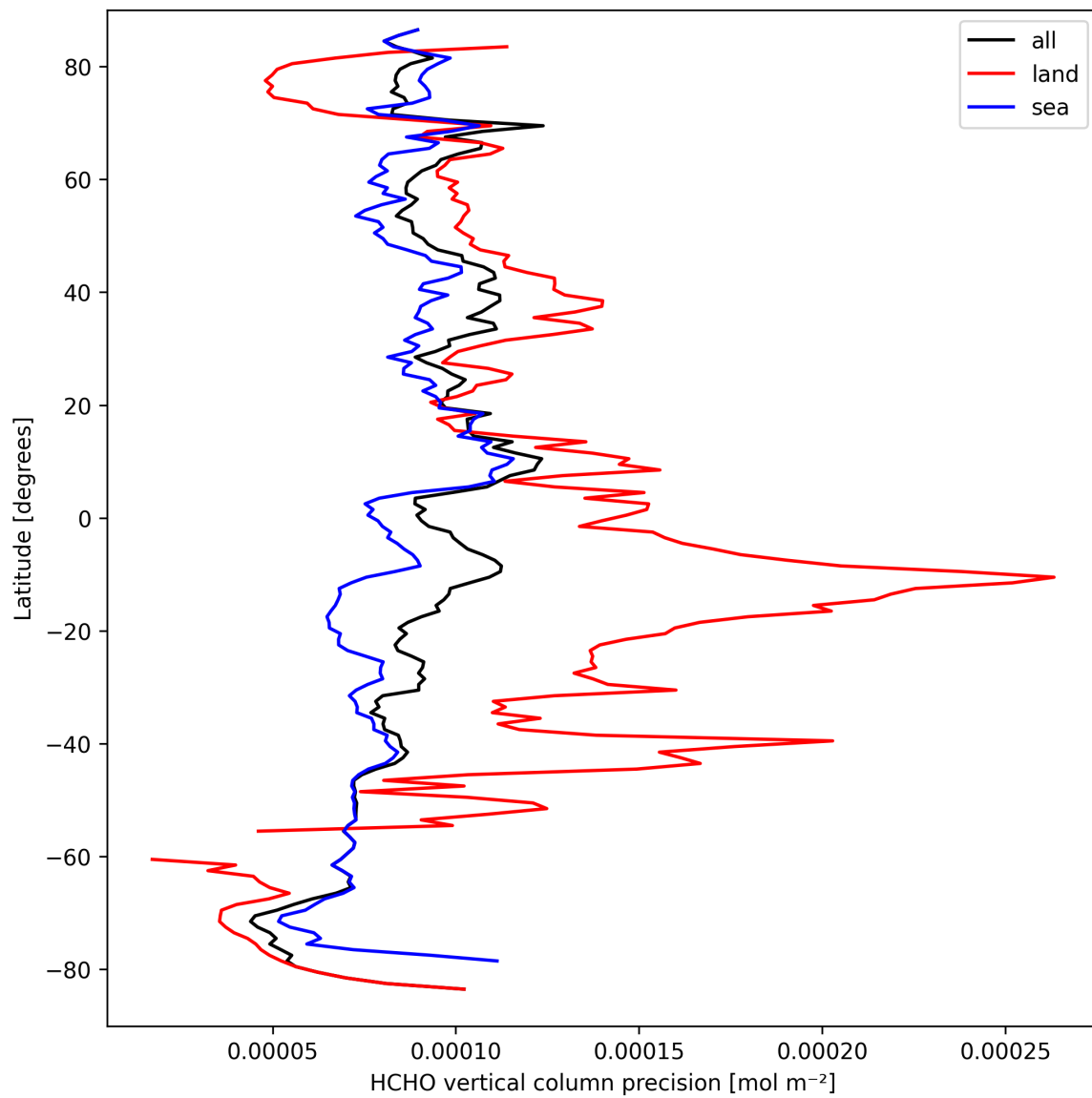
Figure 22: Zonal average of “HCHO vertical column precision” for 2025-09-17 to 2025-09-19.
