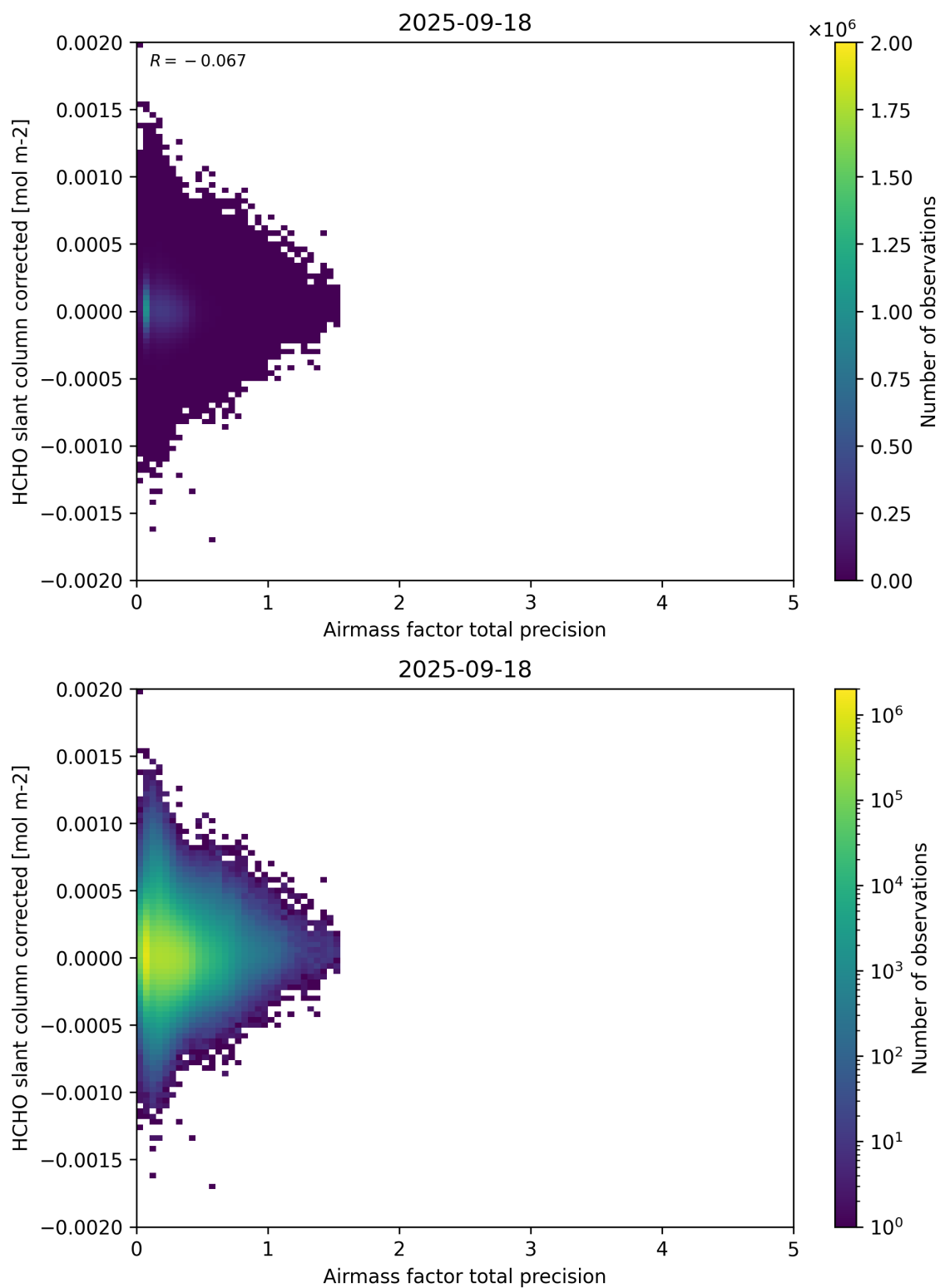
Figure 109: Scatter density plot of “Airmass factor total precision” against “HCHO slant column corrected” for 2025-09-17 to 2025-09-19.
