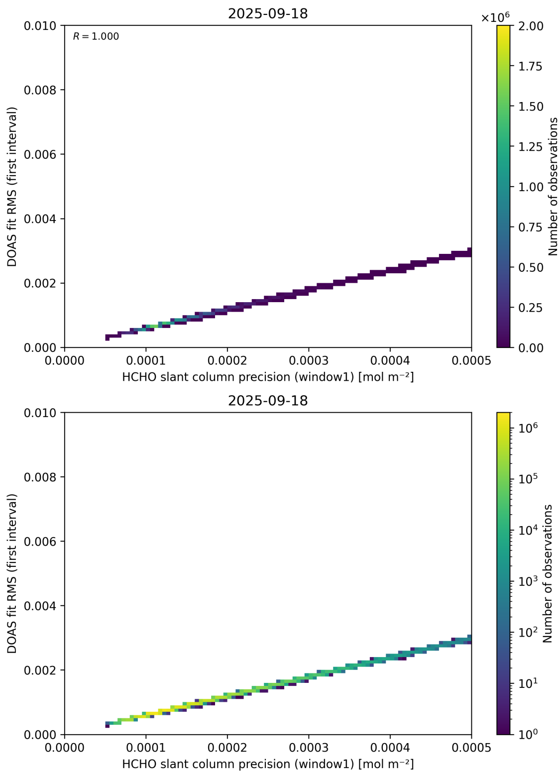
Figure 88: Scatter density plot of “HCHO slant column precision (window1)” against “DOAS fit RMS (first interval)” for 2025-09-17 to 2025-09-19.
