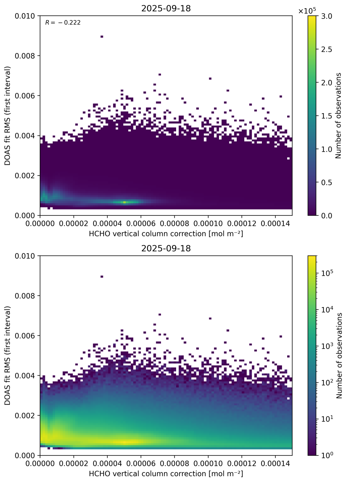
Figure 112: Scatter density plot of “HCHO vertical column correction” against “DOAS fit RMS (first interval)” for 2025-09-17 to 2025-09-19.
