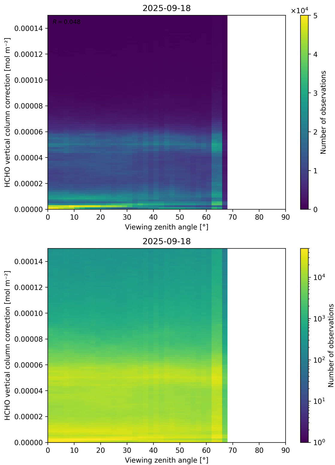
Figure 193: Scatter density plot of “Viewing zenith angle” against “HCHO vertical column correction” for 2025-09-17 to 2025-09-19.
