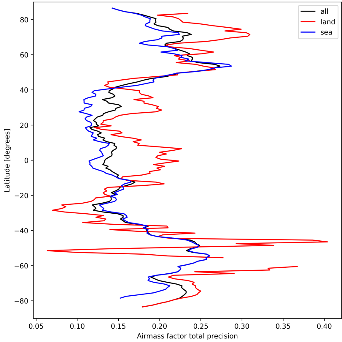
Figure 27: Zonal average of “Airmass factor total precision” for 2025-09-17 to 2025-09-19.
