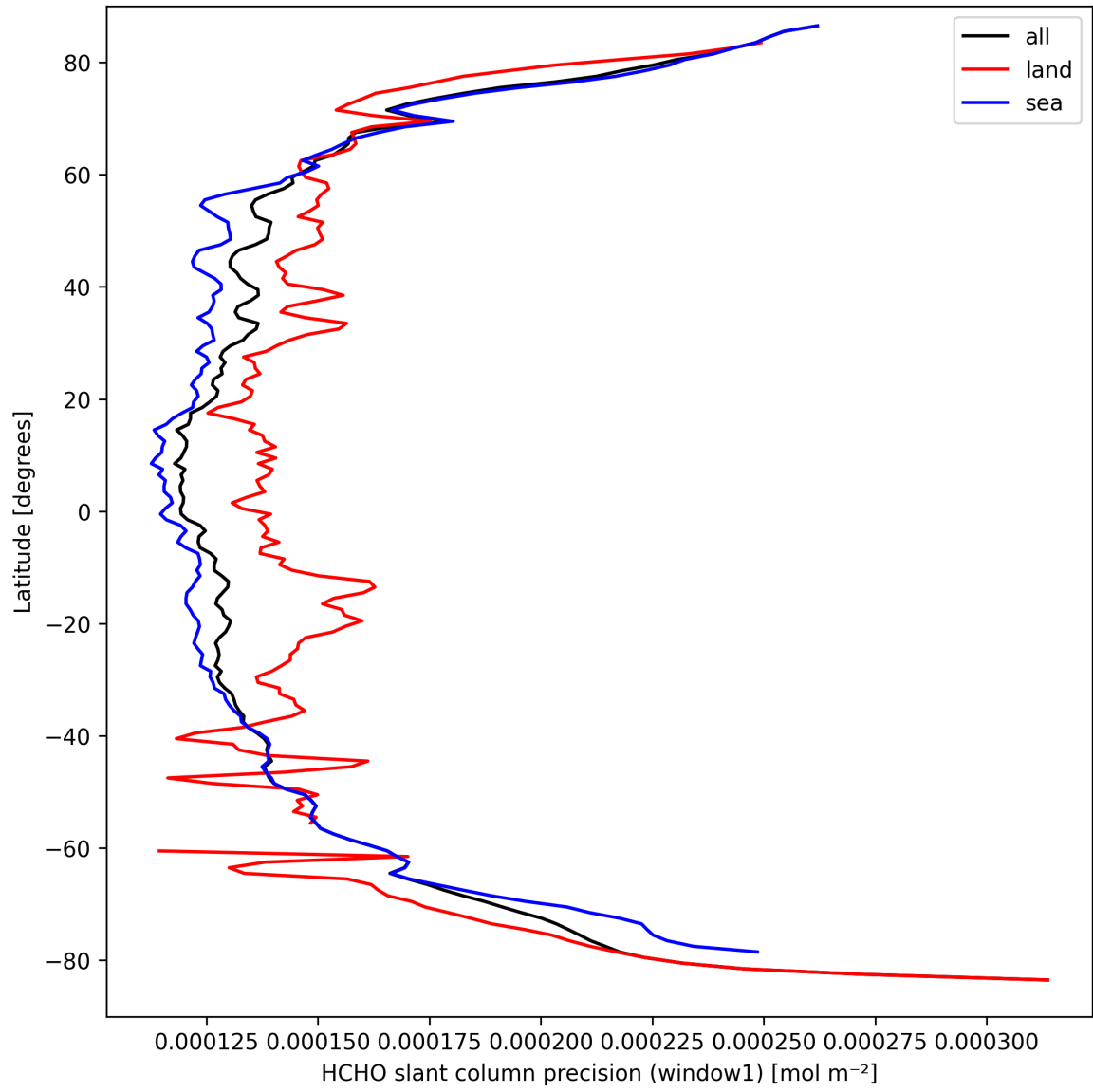
Figure 25: Zonal average of “HCHO slant column precision (window1)” for 2025-09-17 to 2025-09-19.
