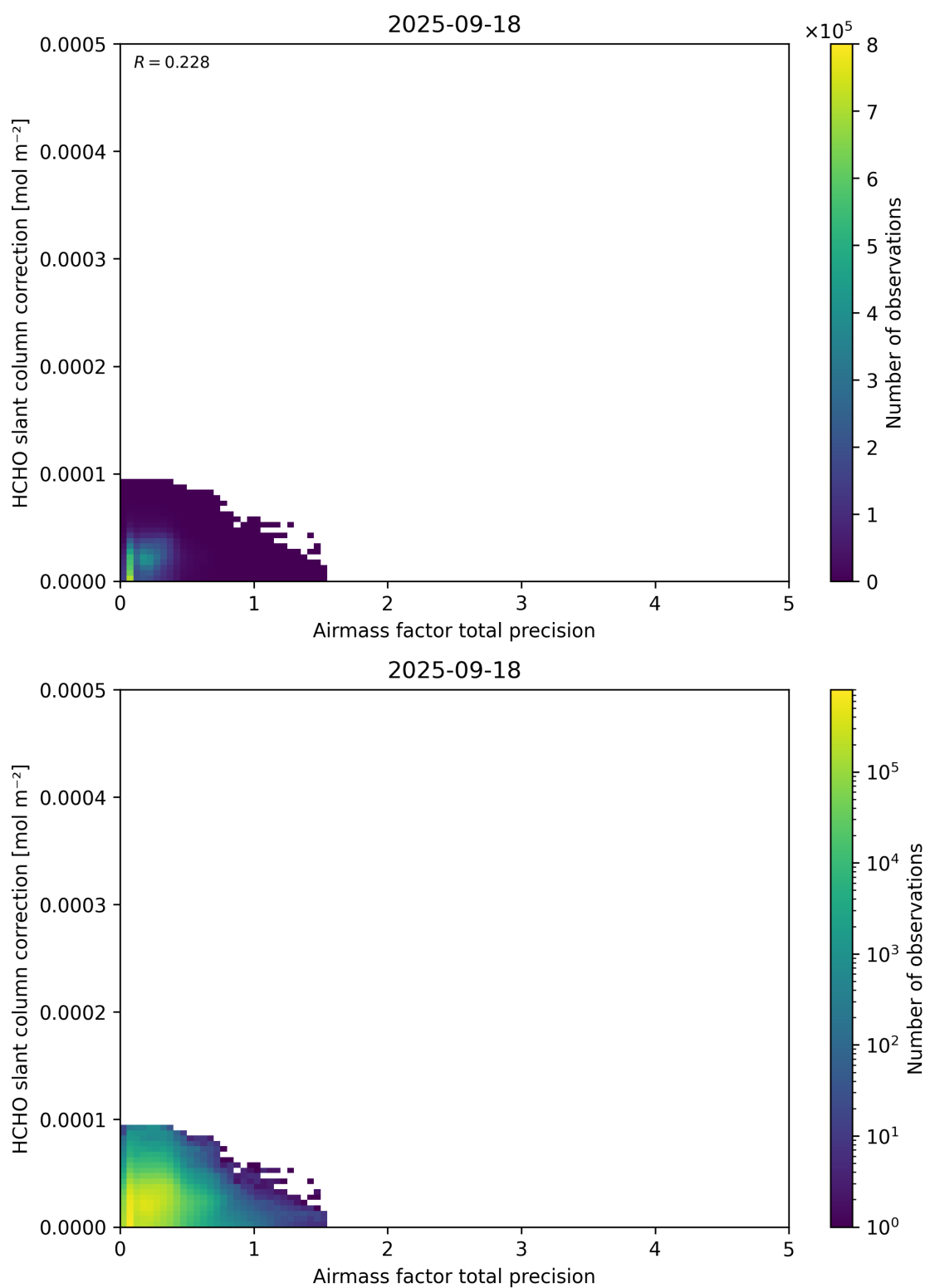
Figure 110: Scatter density plot of “Airmass factor total precision” against “HCHO slant column correction” for 2025-09-17 to 2025-09-19.
