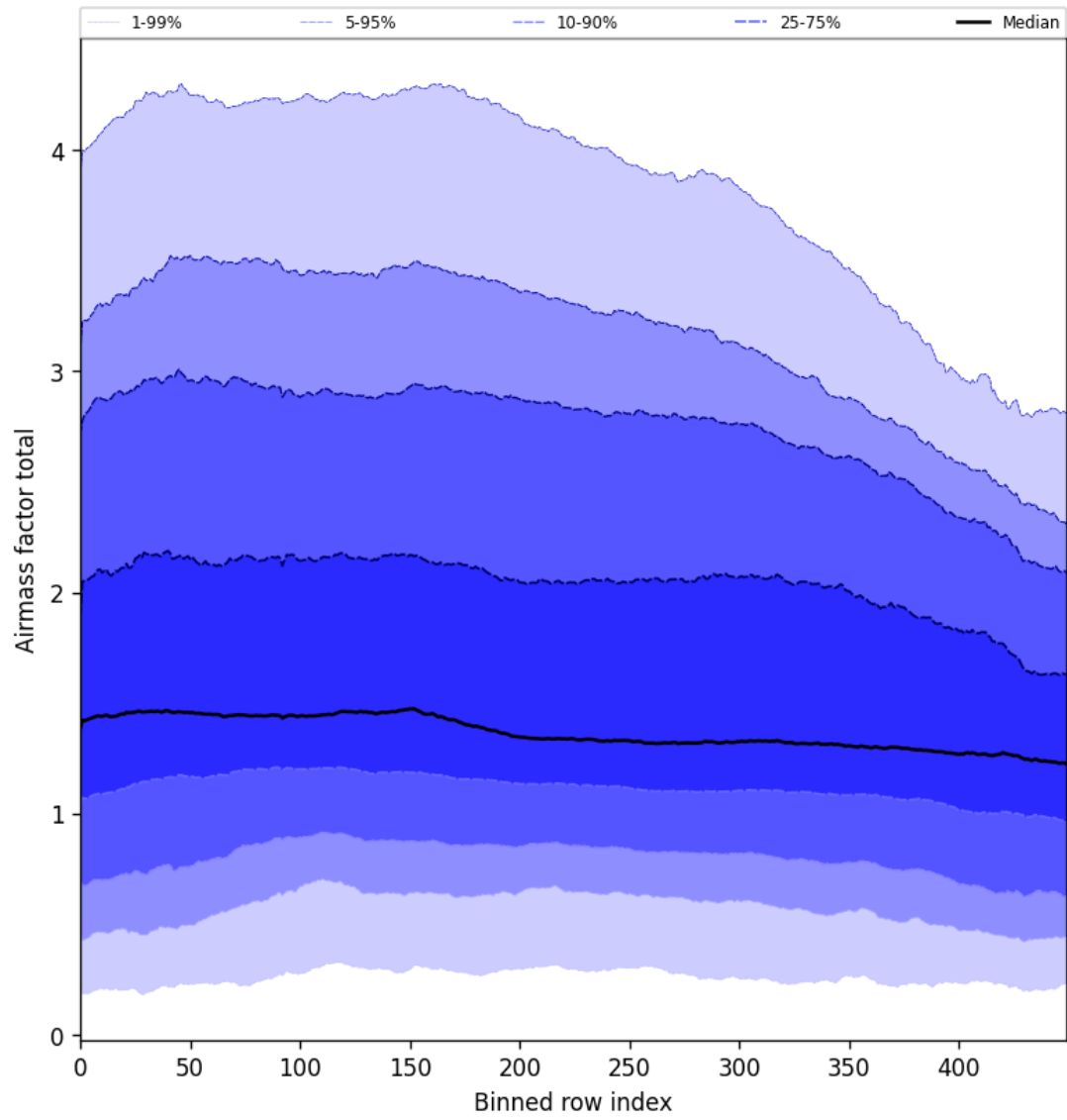
Figure 54: Along track statistics of “Airmass factor total” for 2025-09-17 to 2025-09-19
