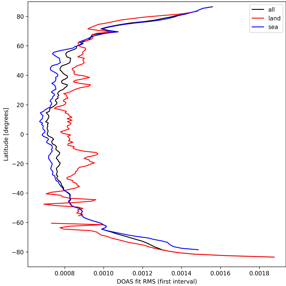
Figure 32: Zonal average of “DOAS fit RMS (first interval)” for 2025-09-17 to 2025-09-19.
