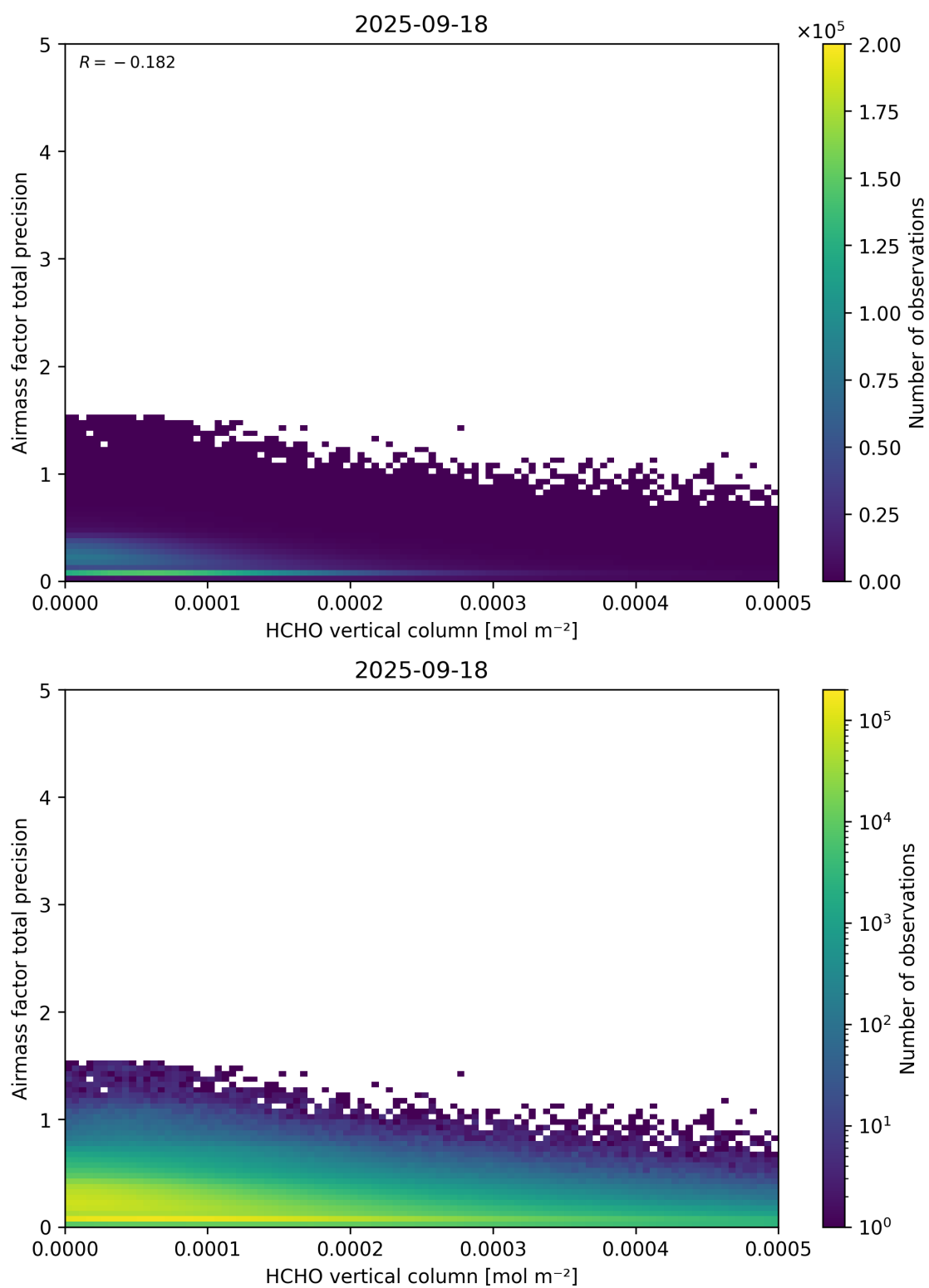
Figure 132: Scatter density plot of “HCHO vertical column” against “Airmass factor total precision” for 2025-09-17 to 2025-09-19.
