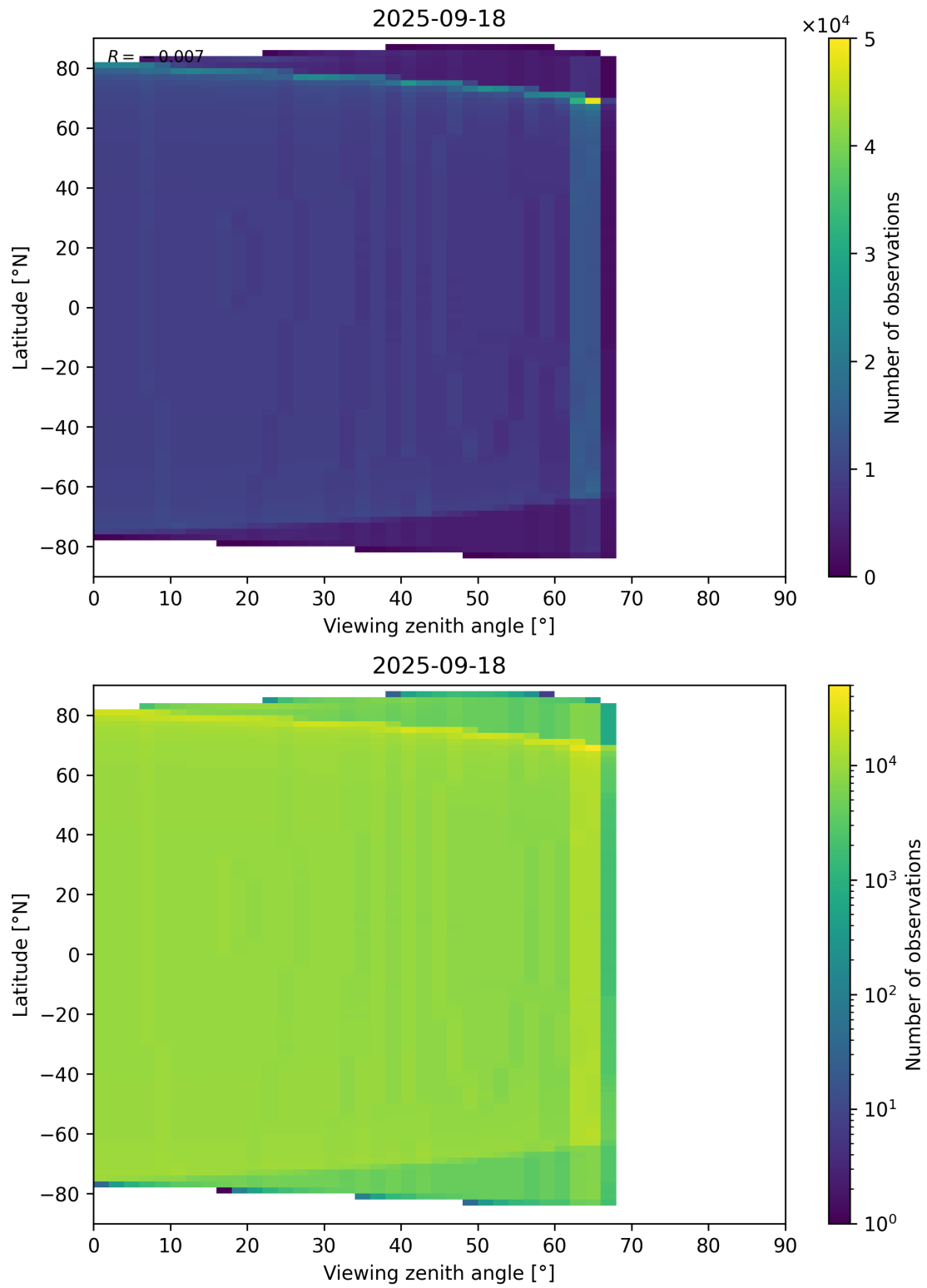
Figure 196: Scatter density plot of “Viewing zenith angle” against “Latitude” for 2025-09-17 to 2025-09-19.
