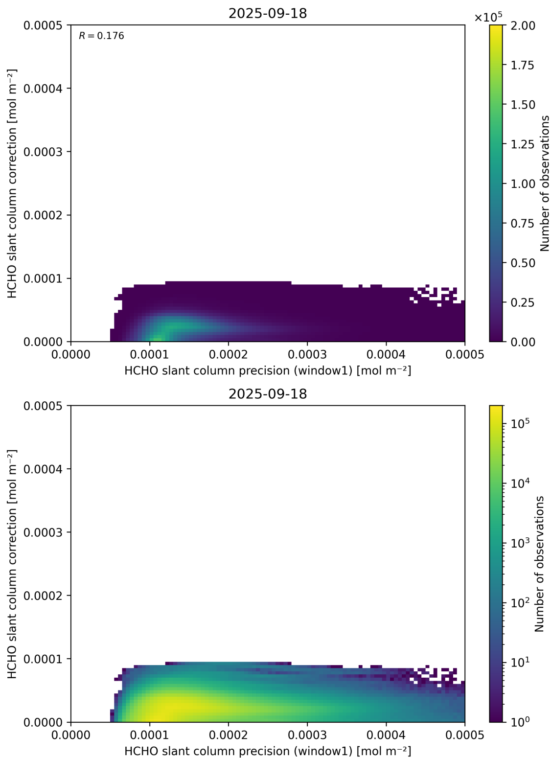
Figure 93: Scatter density plot of “HCHO slant column precision (window1)” against “HCHO slant column correction” for 2025-09-17 to 2025-09-19.
