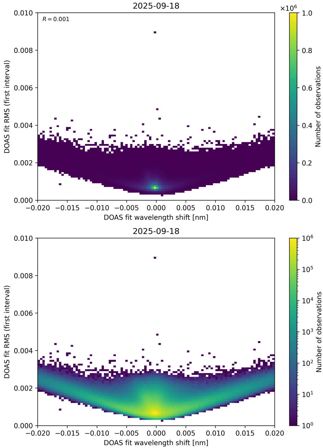
Figure 64: Scatter density plot of “DOAS fit wavelength shift” against “DOAS fit RMS (first interval)” for 2025-09-17 to 2025-09-19.
