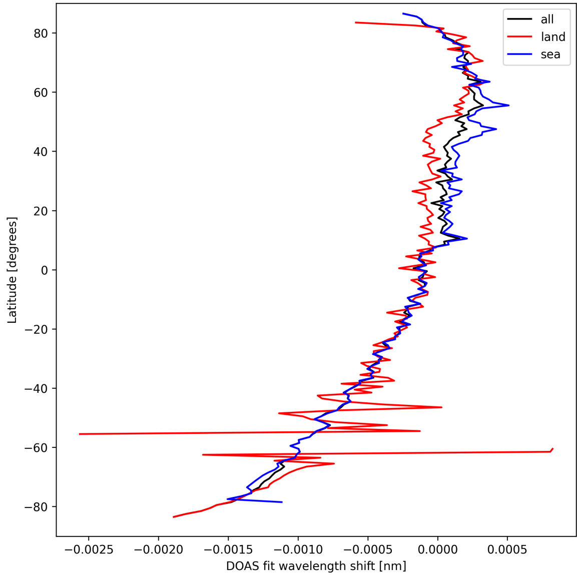
Figure 30: Zonal average of “DOAS fit wavelength shift” for 2025-09-17 to 2025-09-19.
