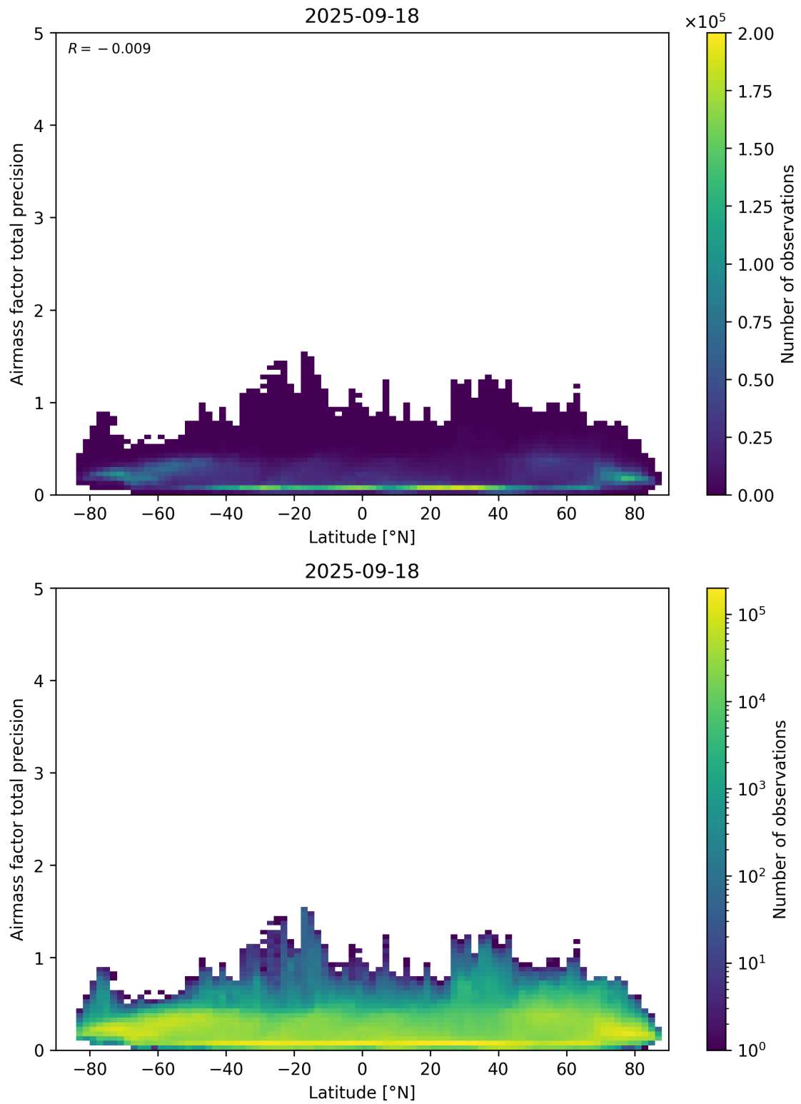
Figure 162: Scatter density plot of “Latitude” against “Airmass factor total precision” for 2025-09-17 to 2025-09-19.
