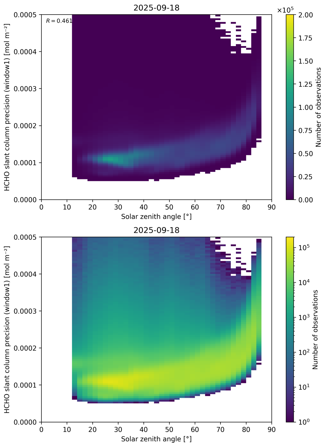
Figure 174: Scatter density plot of “Solar zenith angle” against “HCHO slant column precision (window1)” for 2025-09-17 to 2025-09-19.
