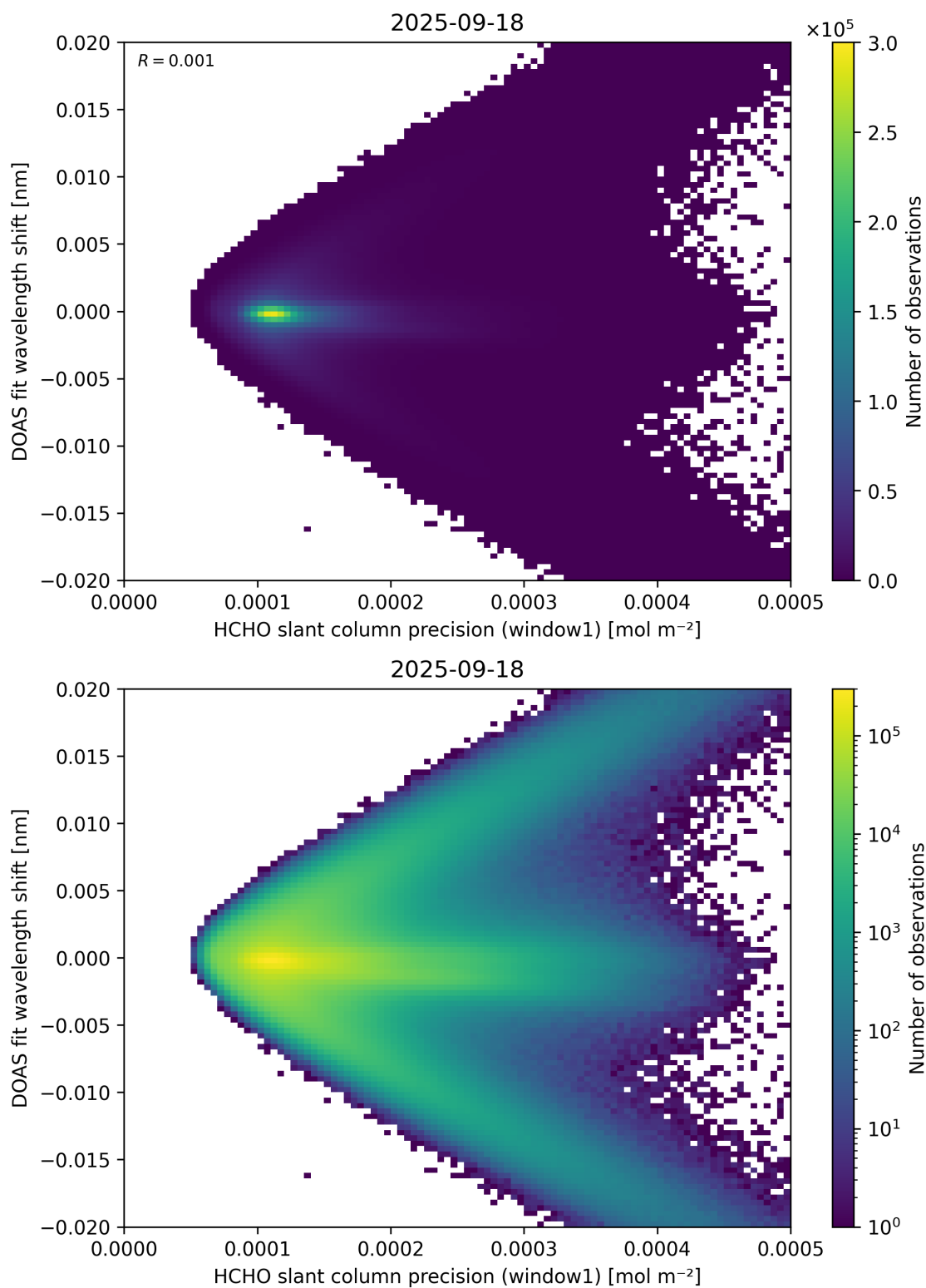
Figure 89: Scatter density plot of “HCHO slant column precision (window1)” against “DOAS fit wavelength shift” for 2025-09-17 to 2025-09-19.
