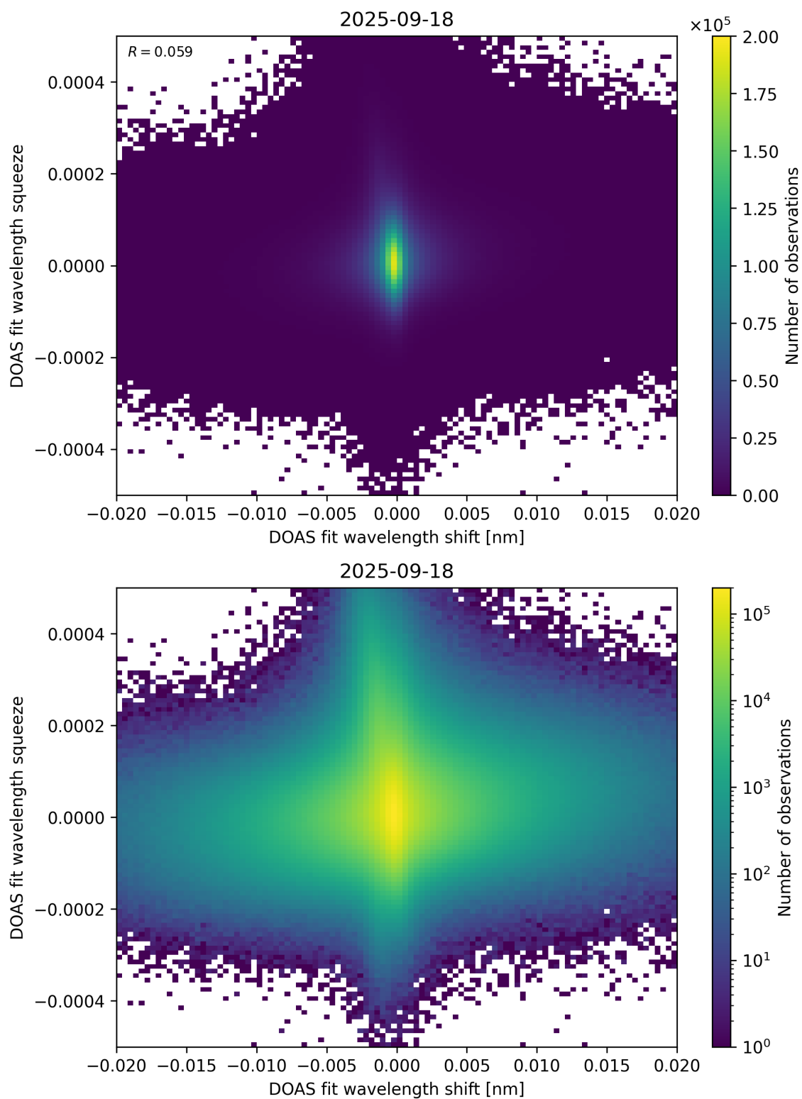
Figure 65: Scatter density plot of “DOAS fit wavelength shift” against “DOAS fit wavelength squeeze” for 2025-09-17 to 2025-09-19.
