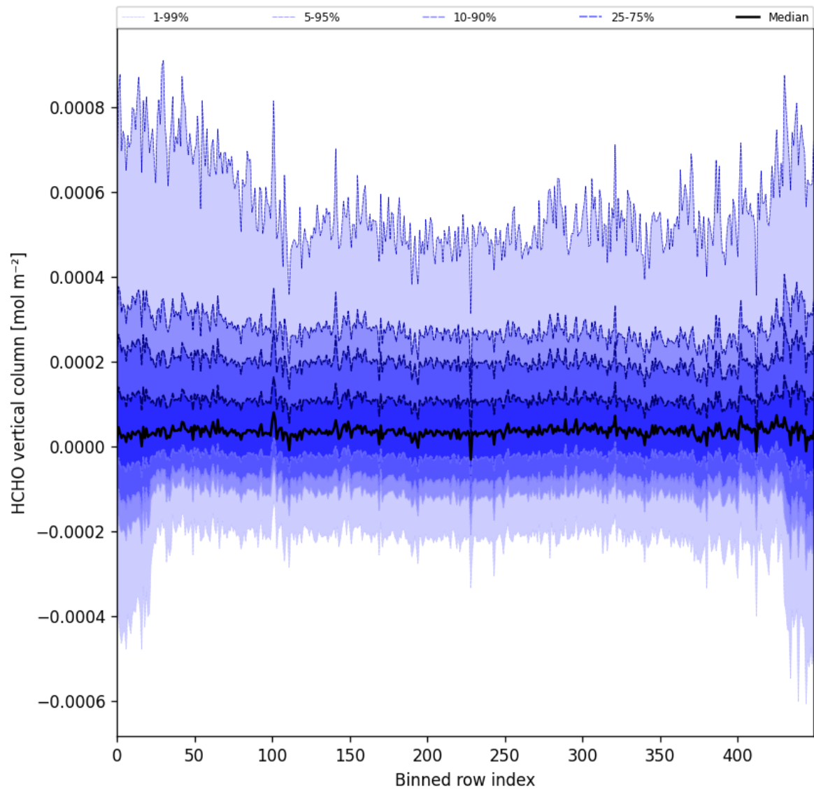
Figure 49: Along track statistics of “HCHO vertical column” for 2025-09-17 to 2025-09-19
