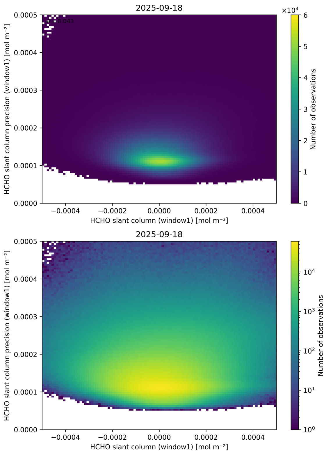
Figure 84: Scatter density plot of “HCHO slant column (window1)” against “HCHO slant column precision (window1)” for 2025-09-17 to 2025-09-19.
