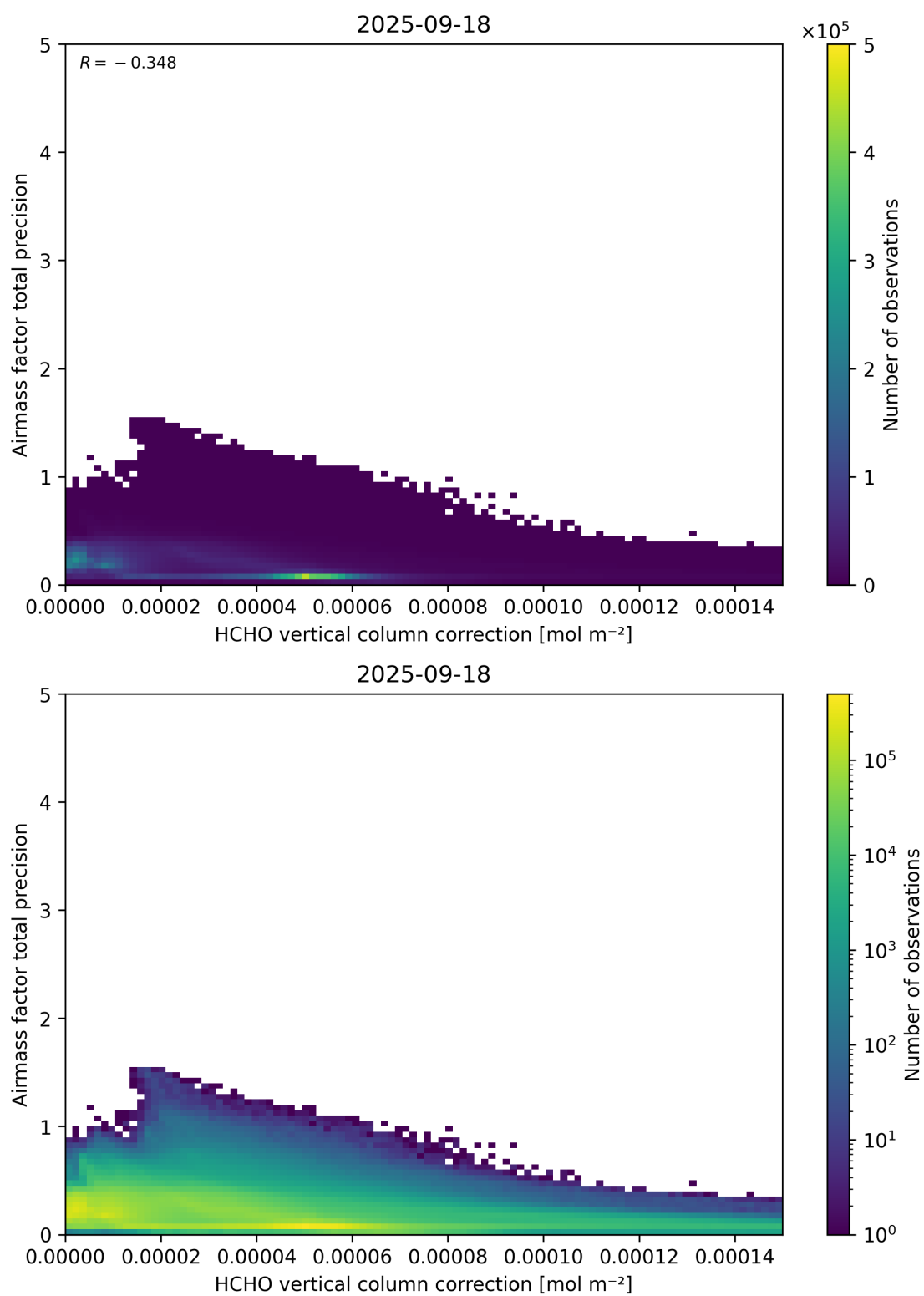
Figure 121: Scatter density plot of “HCHO vertical column correction” against “Airmass factor total precision” for 2025-09-17 to 2025-09-19.
