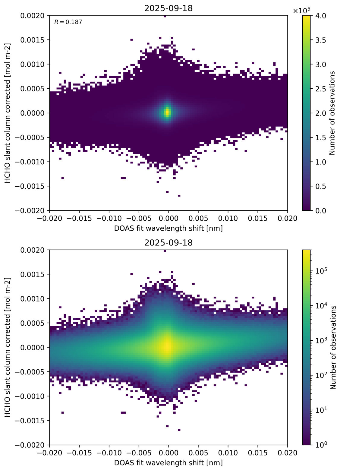
Figure 66: Scatter density plot of “DOAS fit wavelength shift” against “HCHO slant column corrected” for 2025-09-17 to 2025-09-19.
