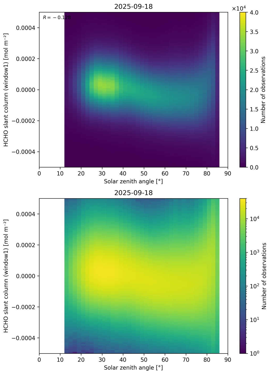
Figure 173: Scatter density plot of “Solar zenith angle” against “HCHO slant column (window1)” for 2025-09-17 to 2025-09-19.
