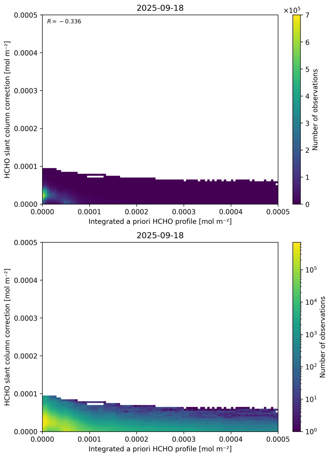
Figure 152: Scatter density plot of “Integrated a priori HCHO profile” against “HCHO slant column correction” for 2025-09-17 to 2025-09-19.
