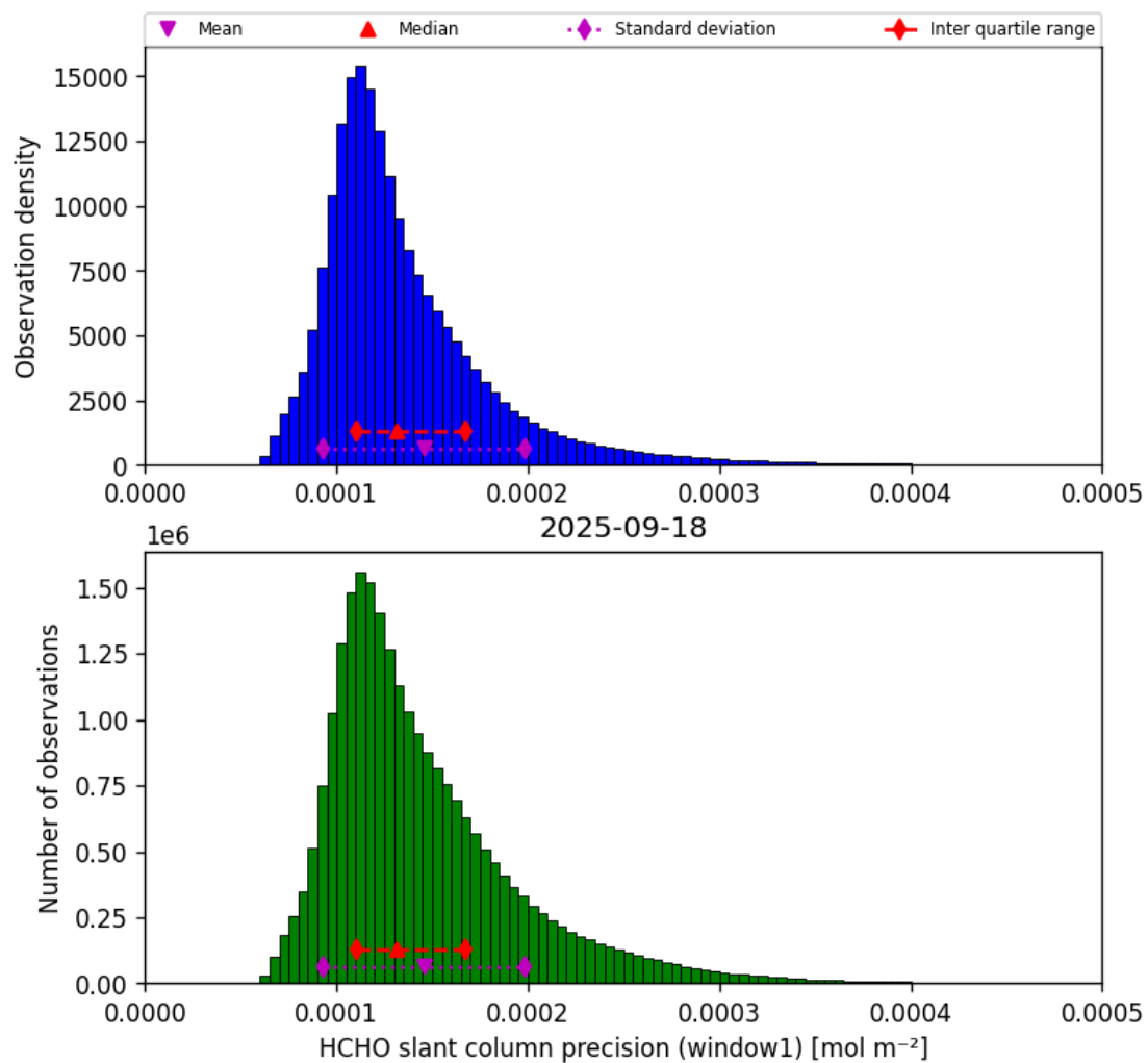
Figure 39: Histogram of “HCHO slant column precision (window1)” for 2025-09-17 to 2025-09-19
