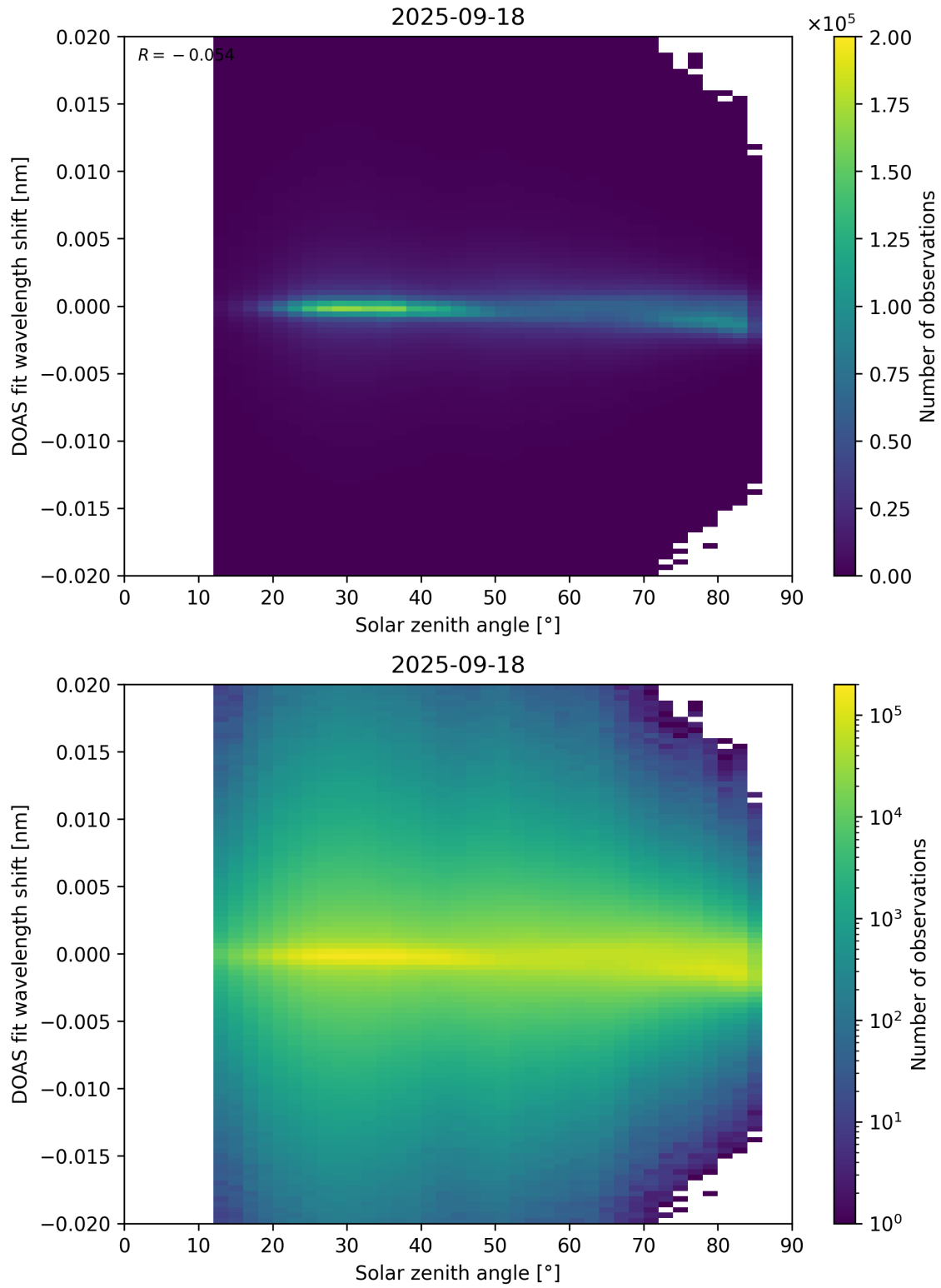
Figure 168: Scatter density plot of “Solar zenith angle” against “DOAS fit wavelength shift” for 2025-09-17 to 2025-09-19.
