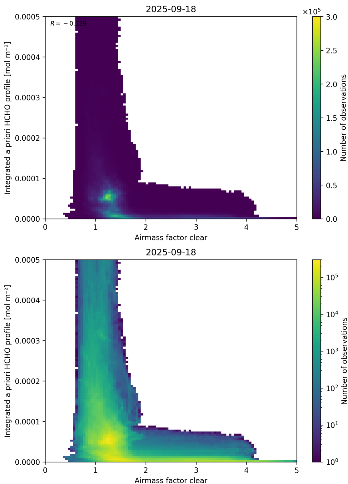
Figure 76: Scatter density plot of “Airmass factor clear” against “Integrated a priori HCHO profile” for 2025-09-17 to 2025-09-19.
