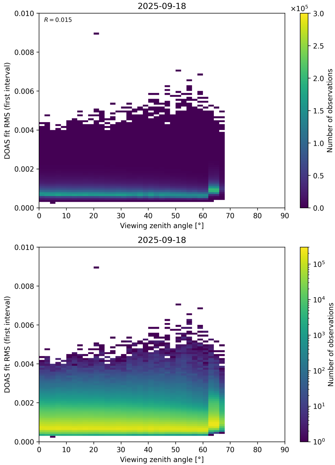
Figure 182: Scatter density plot of “Viewing zenith angle” against “DOAS fit RMS (first interval)” for 2025-09-17 to 2025-09-19.
