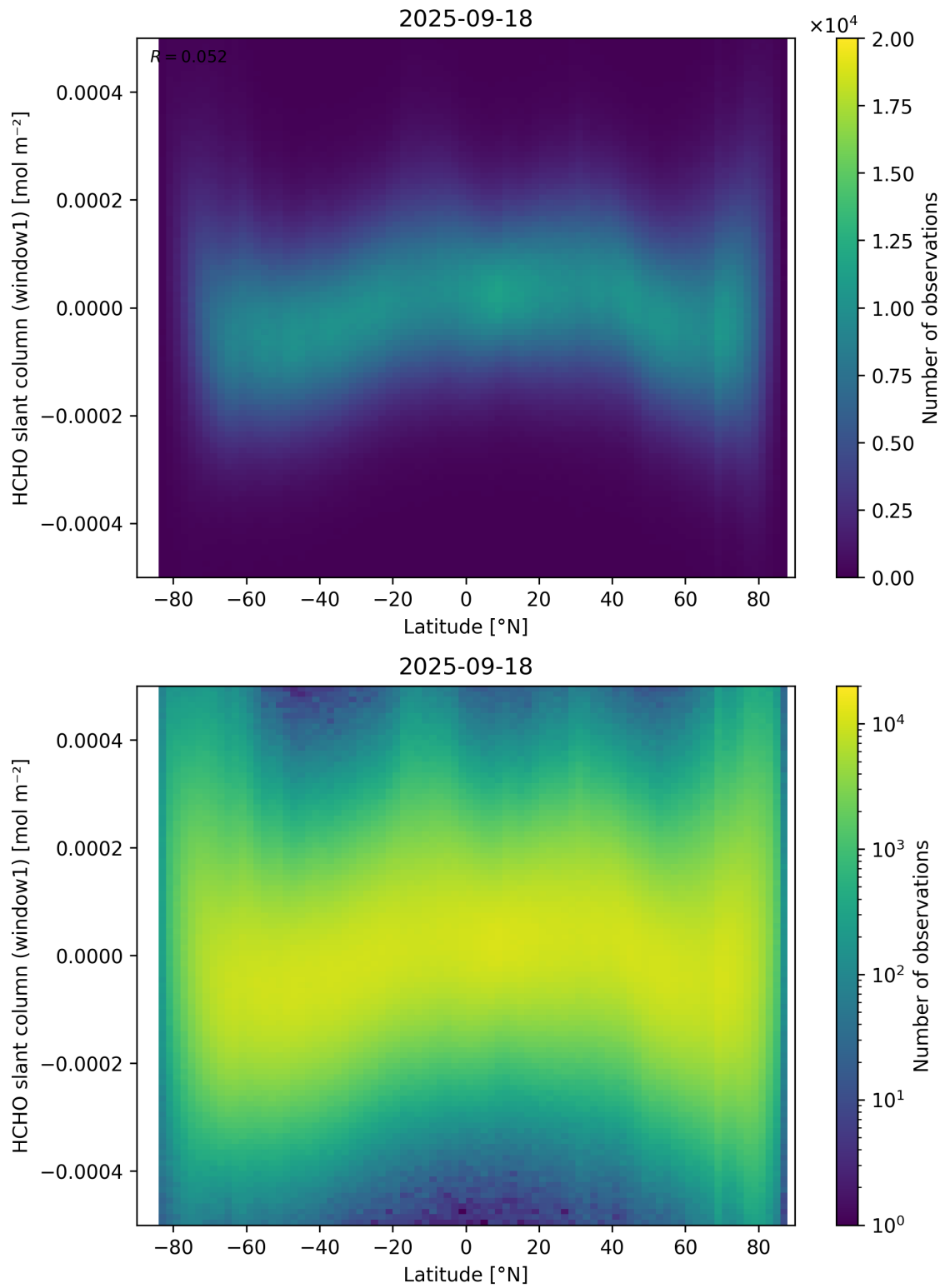
Figure 159: Scatter density plot of “Latitude” against “HCHO slant column (window1)” for 2025-09-17 to 2025-09-19.
