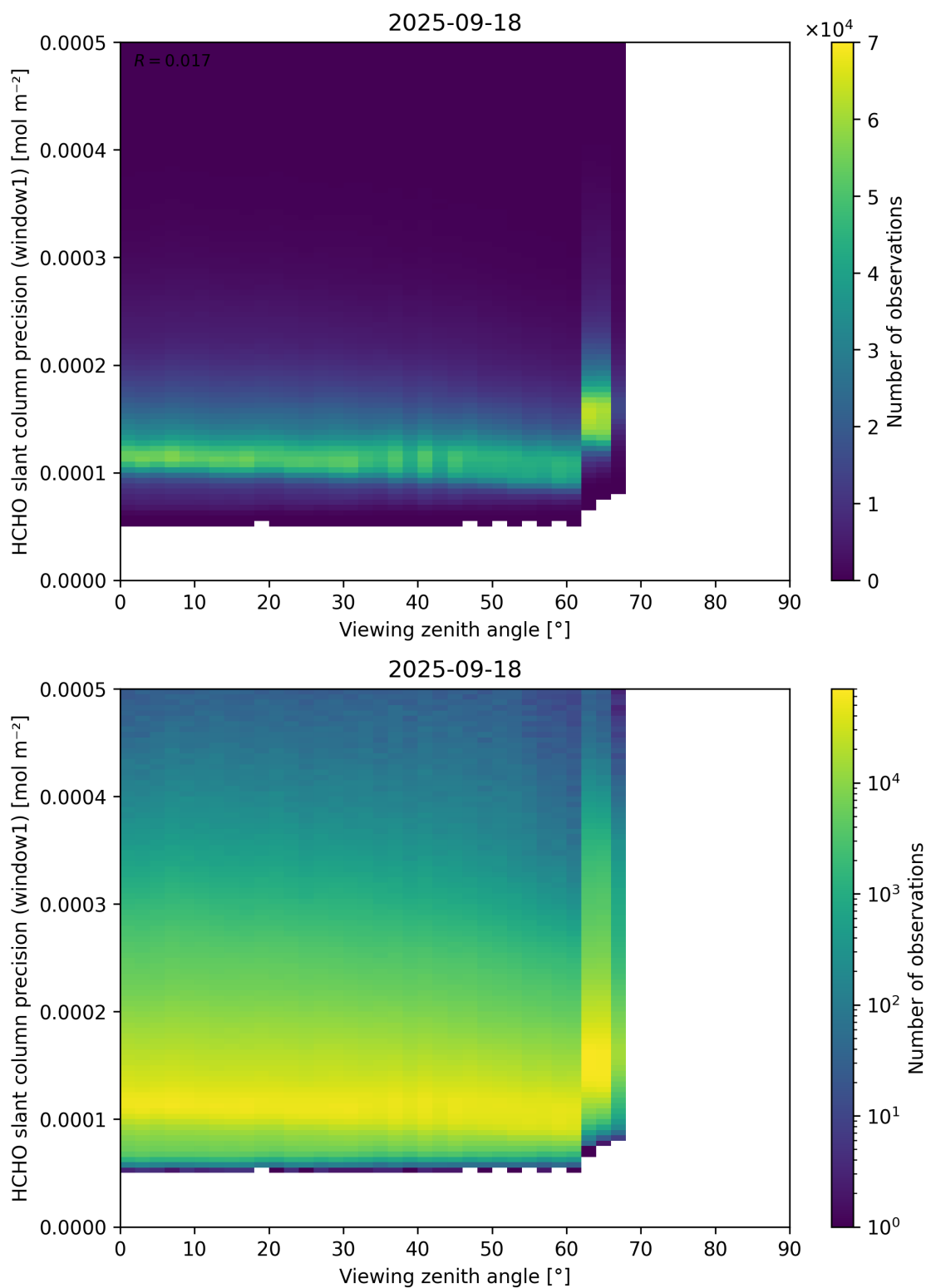
Figure 189: Scatter density plot of “Viewing zenith angle” against “HCHO slant column precision (window1)” for 2025-09-17 to 2025-09-19.
