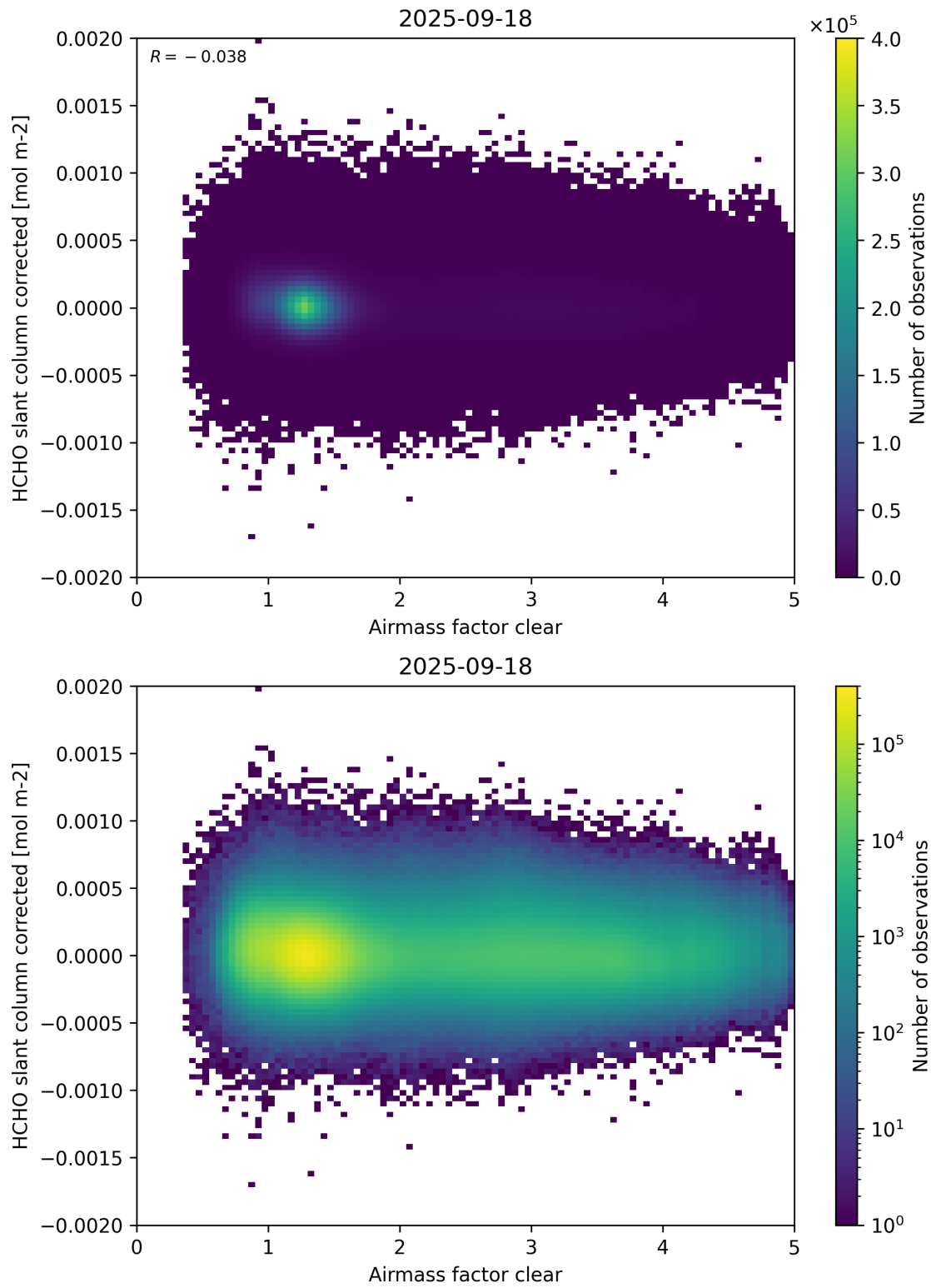
Figure 74: Scatter density plot of “Airmass factor clear” against “HCHO slant column corrected” for 2025-09-17 to 2025-09-19.
