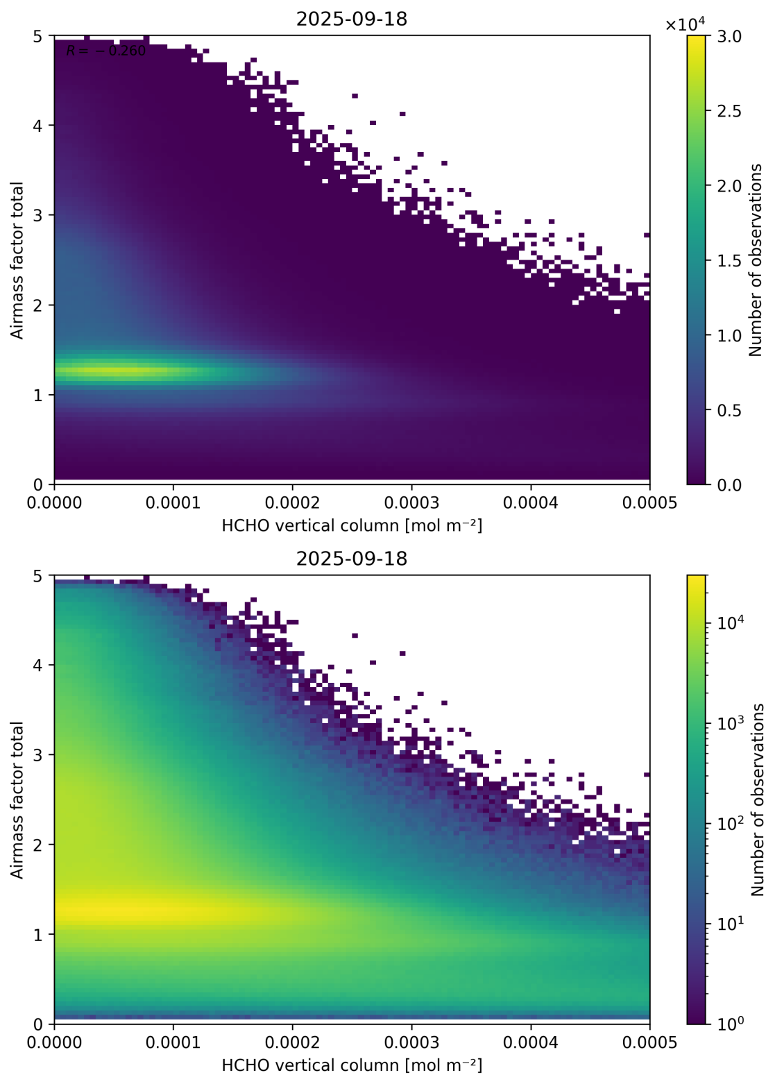
Figure 131: Scatter density plot of “HCHO vertical column” against “Airmass factor total” for 2025-09-17 to 2025-09-19.
