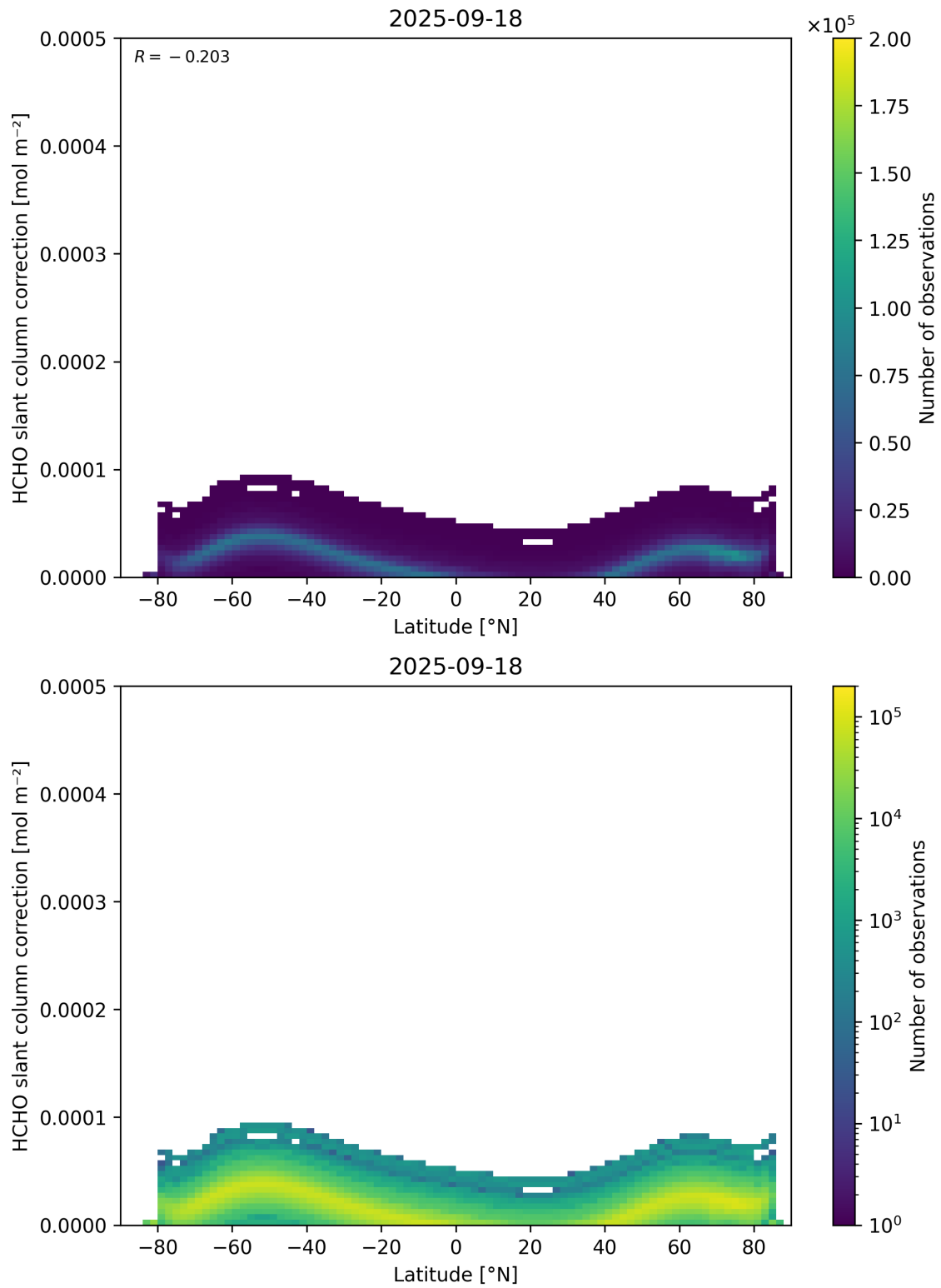
Figure 158: Scatter density plot of “Latitude” against “HCHO slant column correction” for 2025-09-17 to 2025-09-19.
