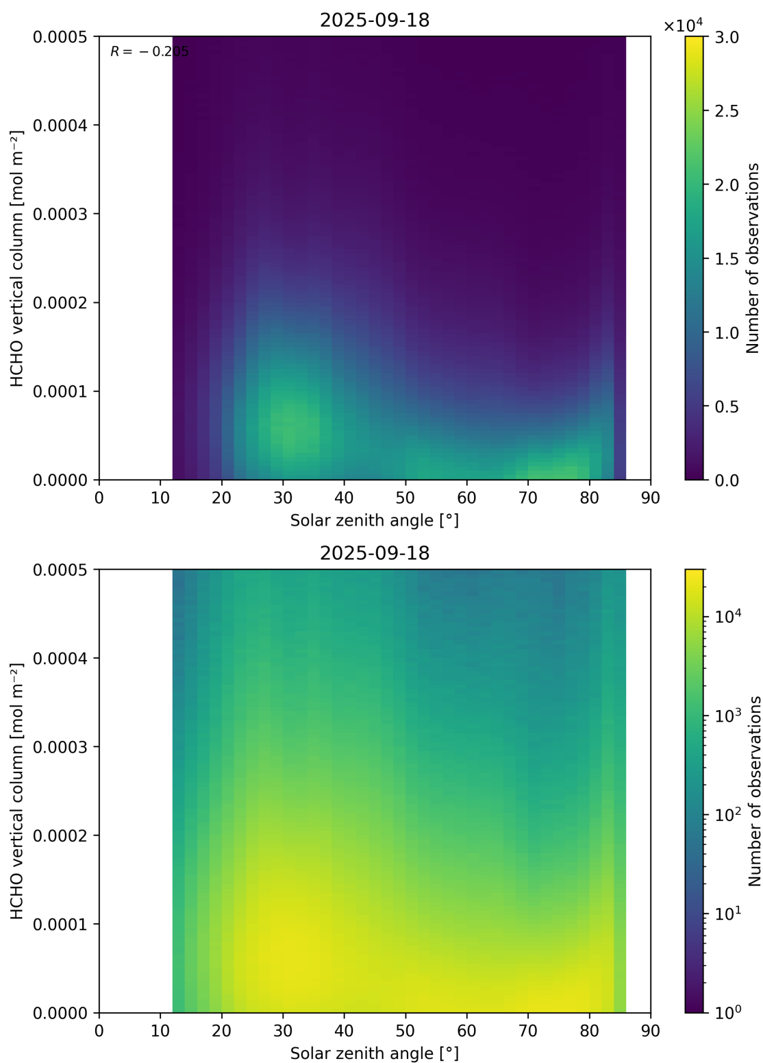
Figure 177: Scatter density plot of “Solar zenith angle” against “HCHO vertical column” for 2025-09-17 to 2025-09-19.
