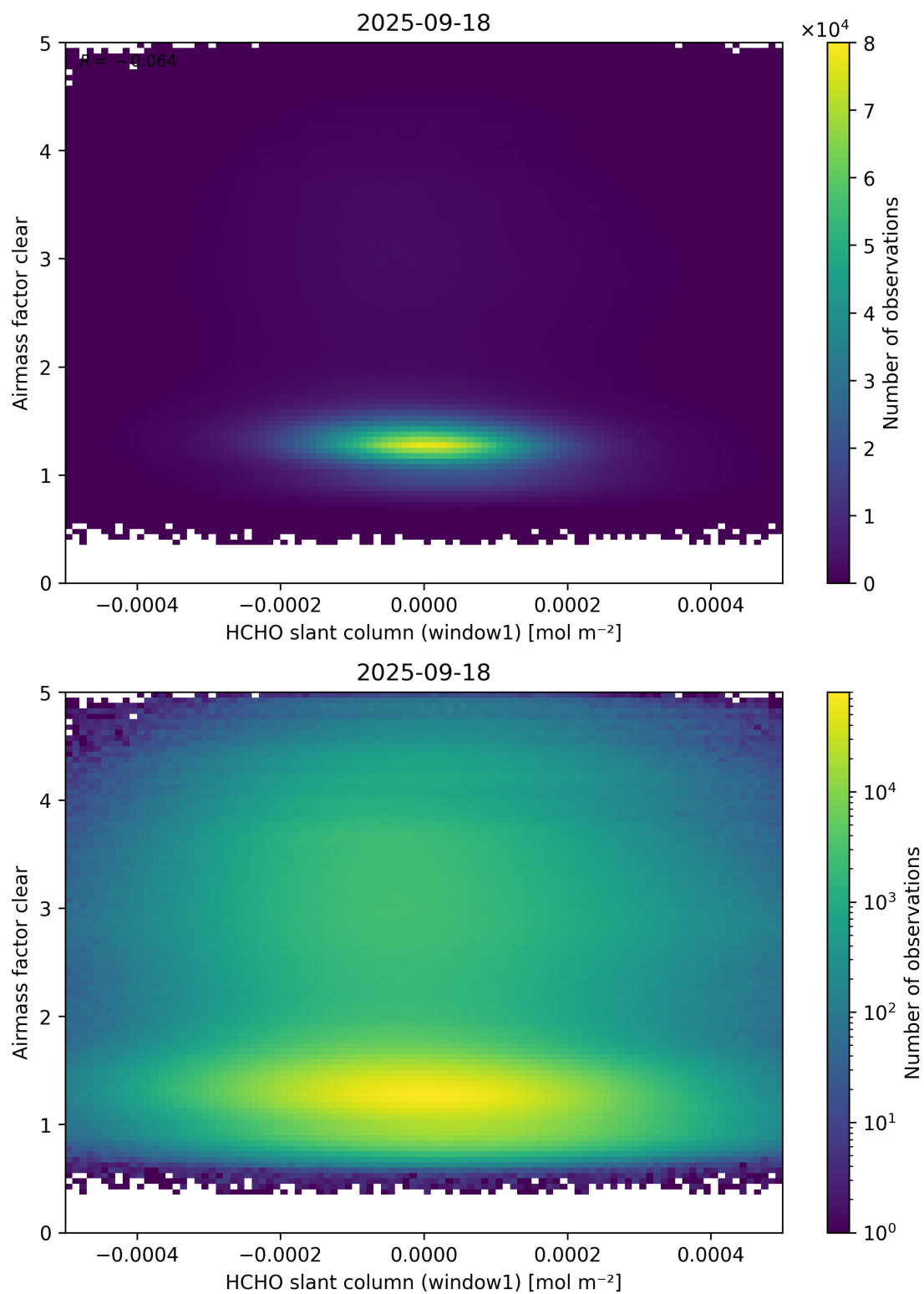
Figure 81: Scatter density plot of “HCHO slant column (window1)” against “Airmass factor clear” for 2025-09-17 to 2025-09-19.
