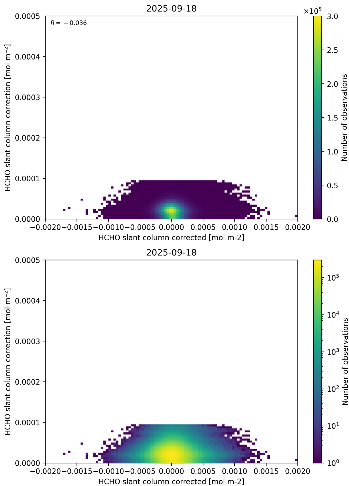
Figure 77: Scatter density plot of “HCHO slant column corrected” against “HCHO slant column correction” for 2025-09-17 to 2025-09-19.
