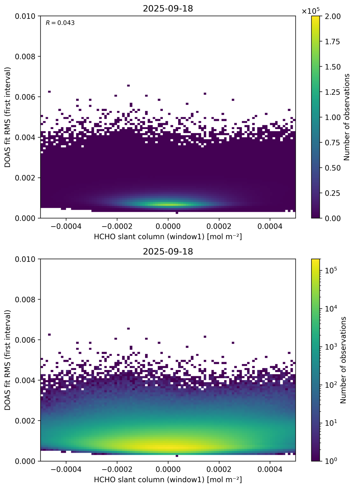
Figure 78: Scatter density plot of “HCHO slant column (window1)” against “DOAS fit RMS (first interval)” for 2025-09-17 to 2025-09-19.
