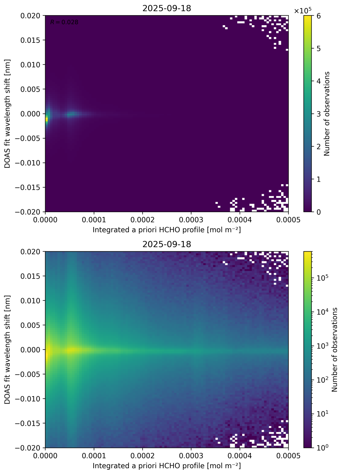
Figure 149: Scatter density plot of “Integrated a priori HCHO profile” against “DOAS fit wavelength shift” for 2025-09-17 to 2025-09-19.
