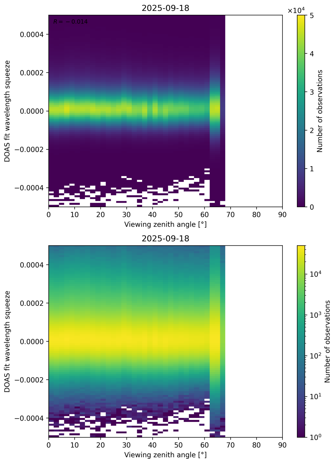
Figure 184: Scatter density plot of “Viewing zenith angle” against “DOAS fit wavelength squeeze” for 2025-09-17 to 2025-09-19.
