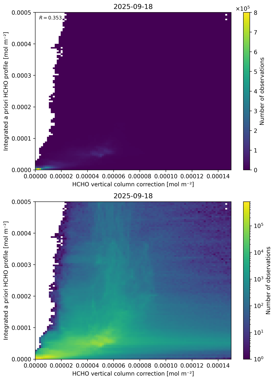
Figure 122: Scatter density plot of “HCHO vertical column correction” against “Integrated a priori HCHO profile” for 2025-09-17 to 2025-09-19.
