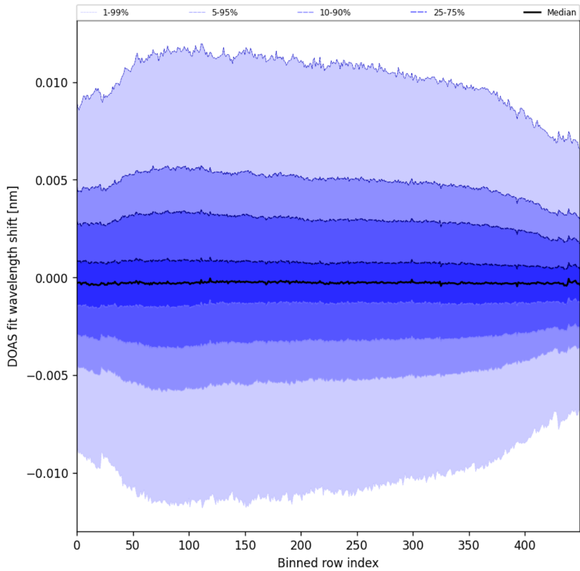
Figure 58: Along track statistics of “DOAS fit wavelength shift” for 2025-09-17 to 2025-09-19
