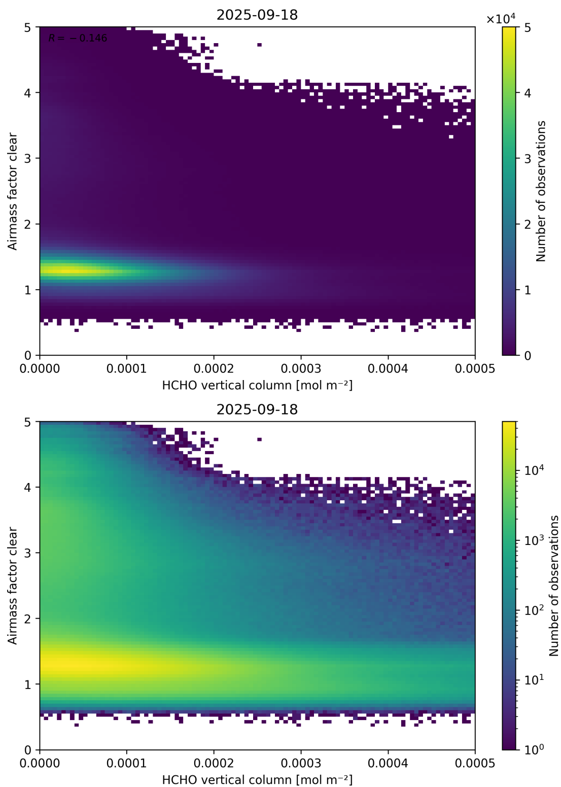
Figure 126: Scatter density plot of “HCHO vertical column” against “Airmass factor clear” for 2025-09-17 to 2025-09-19.
