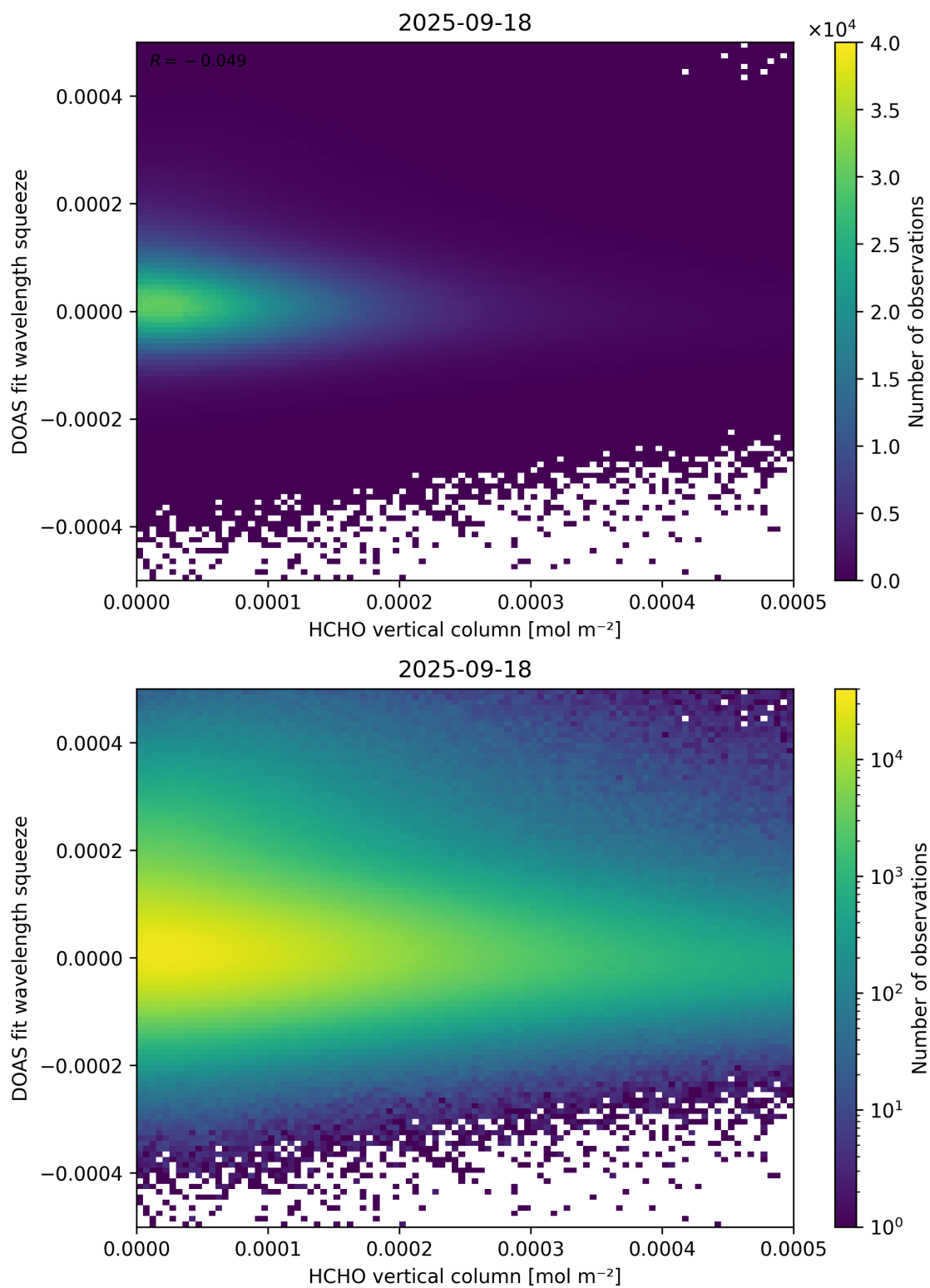
Figure 125: Scatter density plot of “HCHO vertical column” against “DOAS fit wavelength squeeze” for 2025-09-17 to 2025-09-19.
