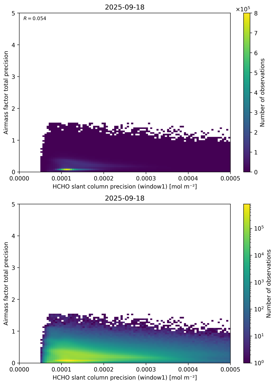
Figure 95: Scatter density plot of “HCHO slant column precision (window1)” against “Airmass factor total precision” for 2025-09-17 to 2025-09-19.
