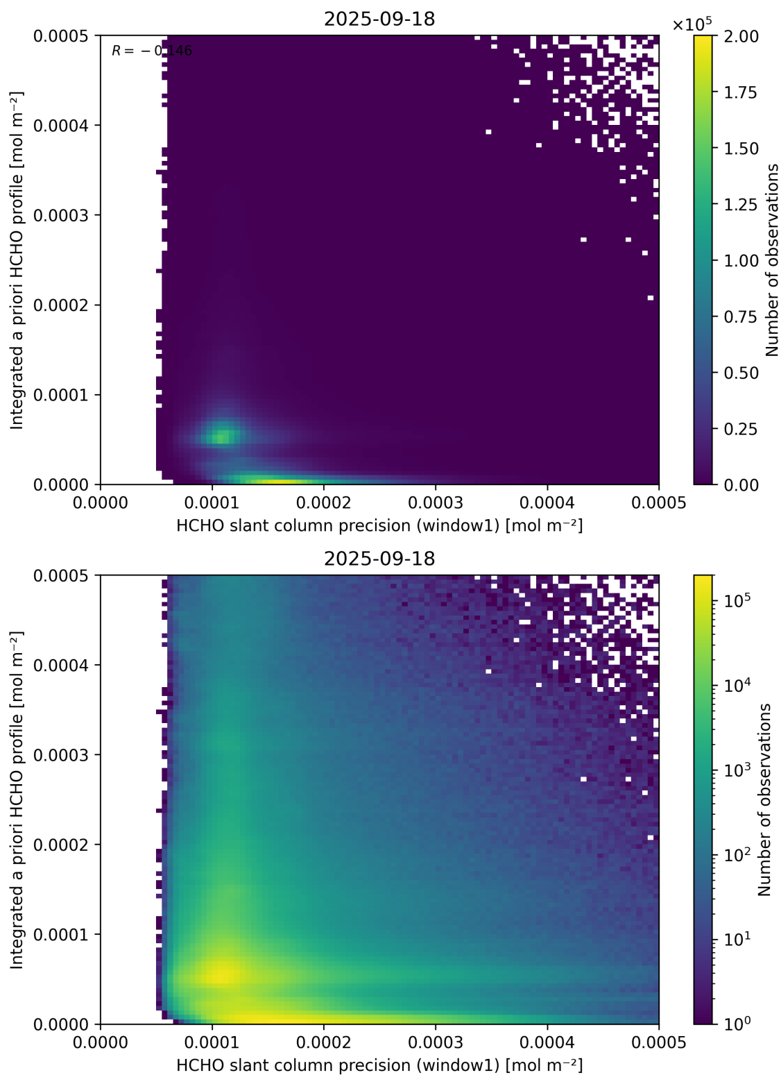
Figure 96: Scatter density plot of “HCHO slant column precision (window1)” against “Integrated a priori HCHO profile” for 2025-09-17 to 2025-09-19.
