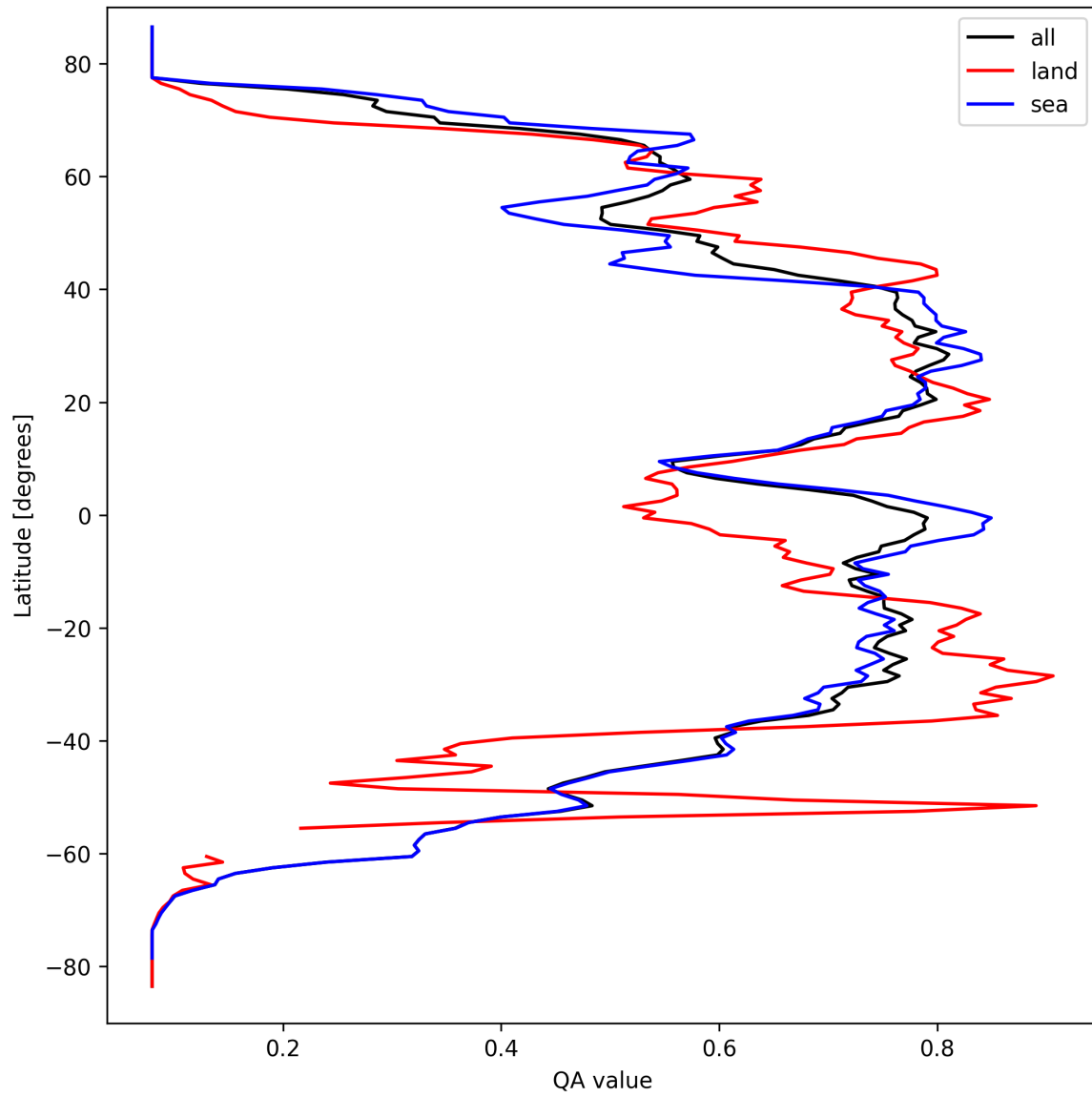
Figure 20: Zonal average of “QA value” for 2025-09-17 to 2025-09-19.
