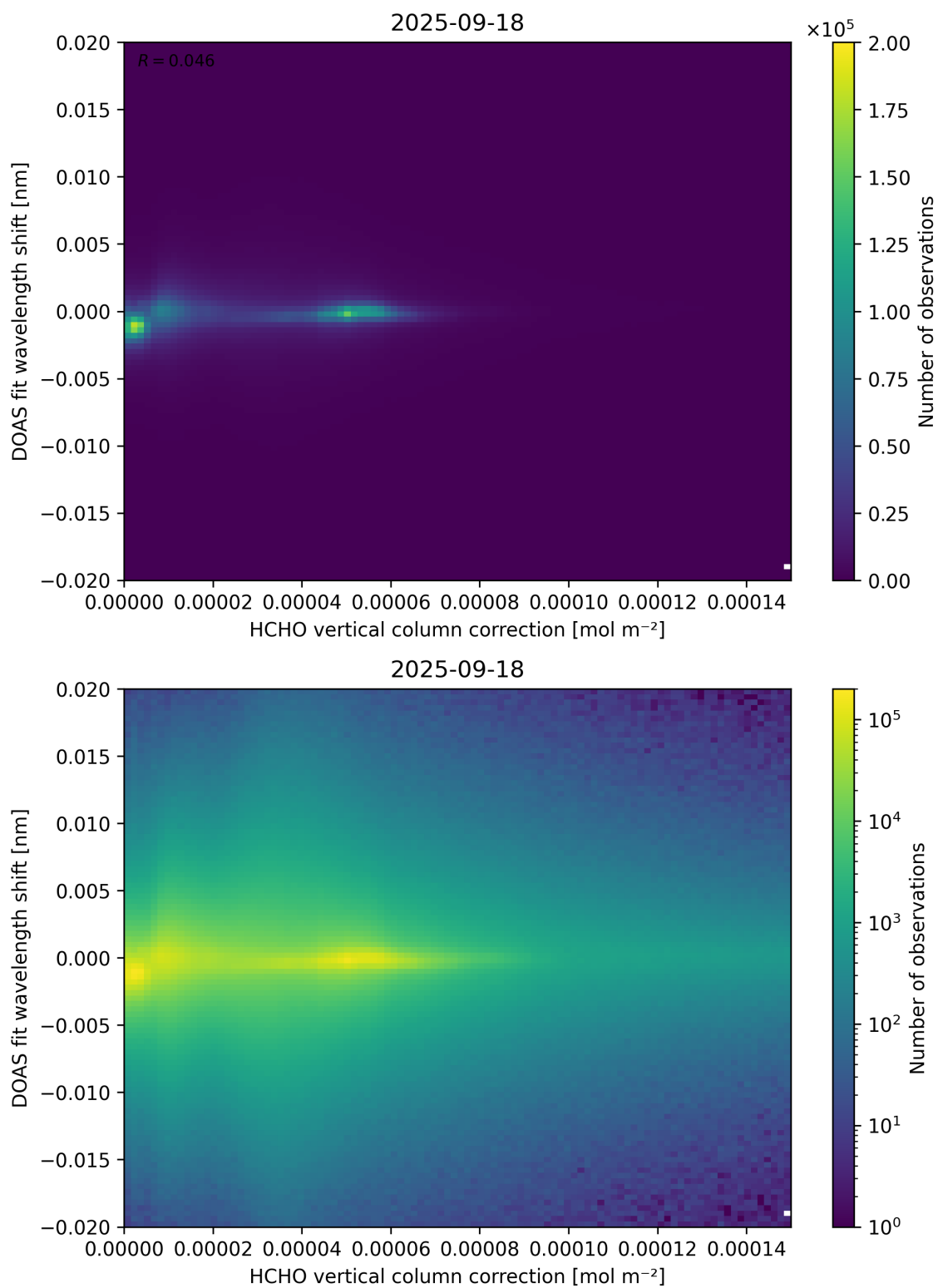
Figure 113: Scatter density plot of “HCHO vertical column correction” against “DOAS fit wavelength shift” for 2025-09-17 to 2025-09-19.
