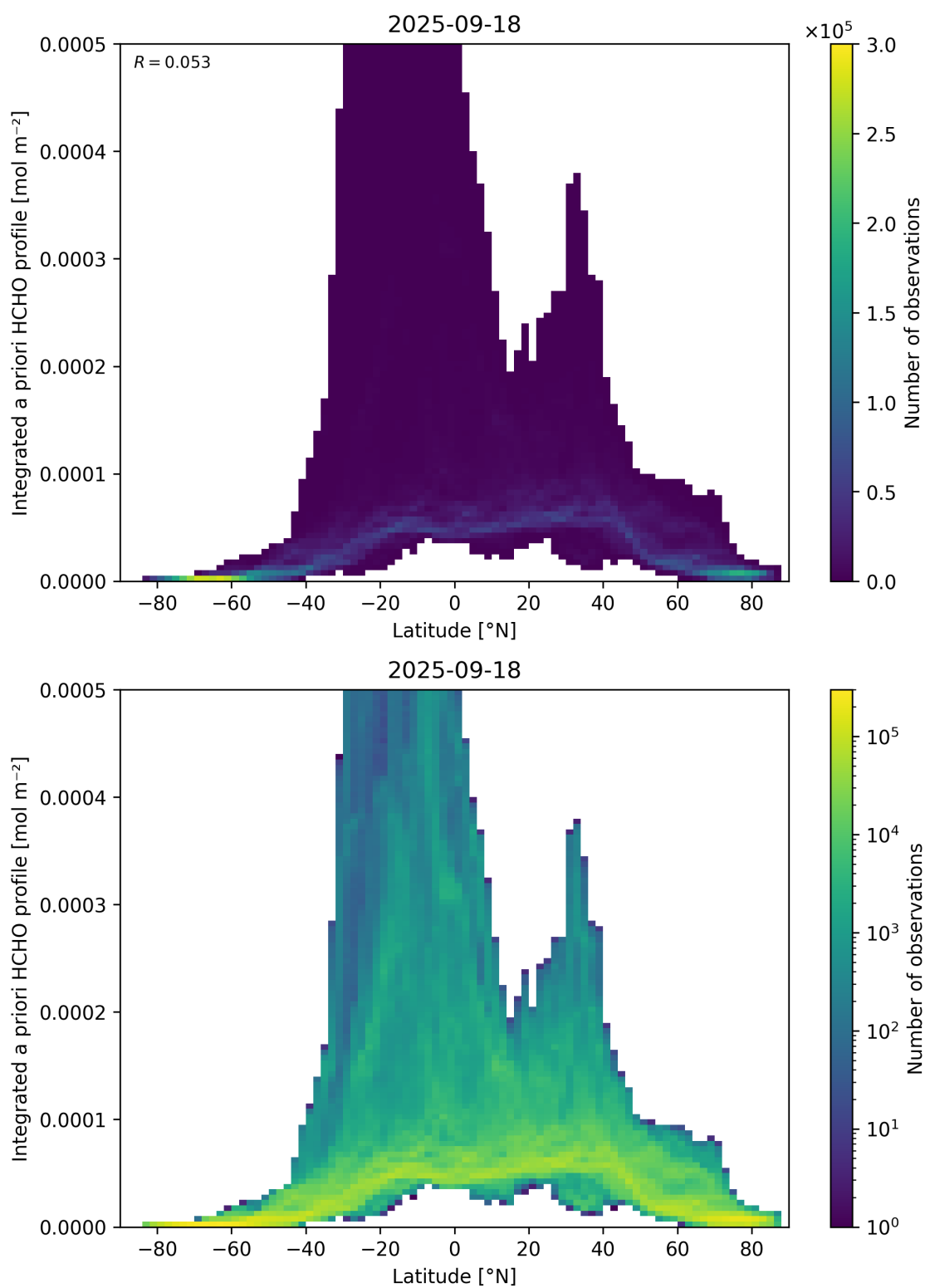
Figure 166: Scatter density plot of “Latitude” against “Integrated a priori HCHO profile” for 2025-09-17 to 2025-09-19.
