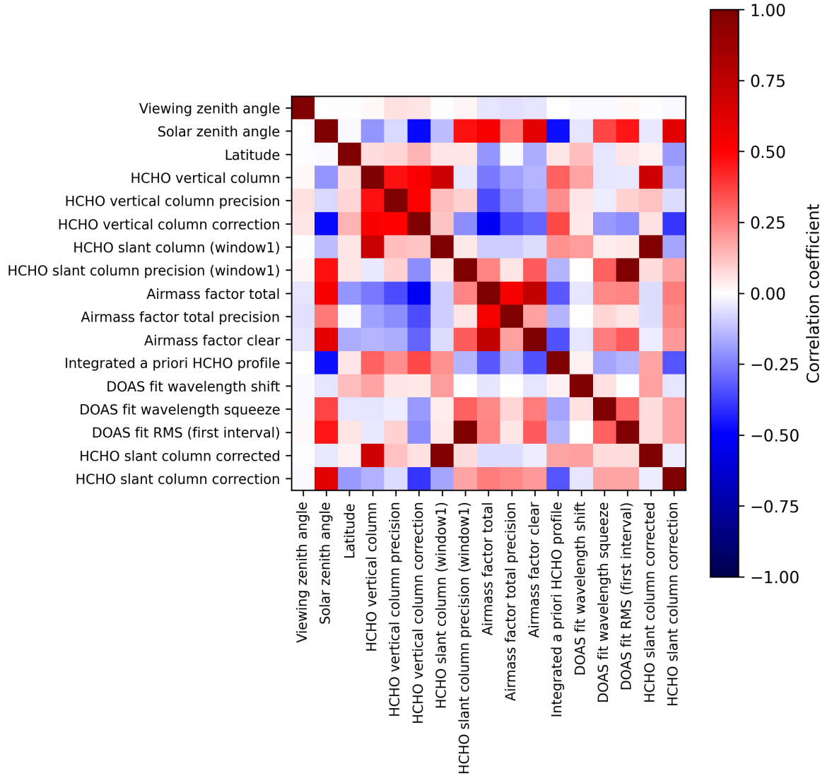
Figure 2: Map of correlation matrix for 2025-09-17 to 2025-09-19.
