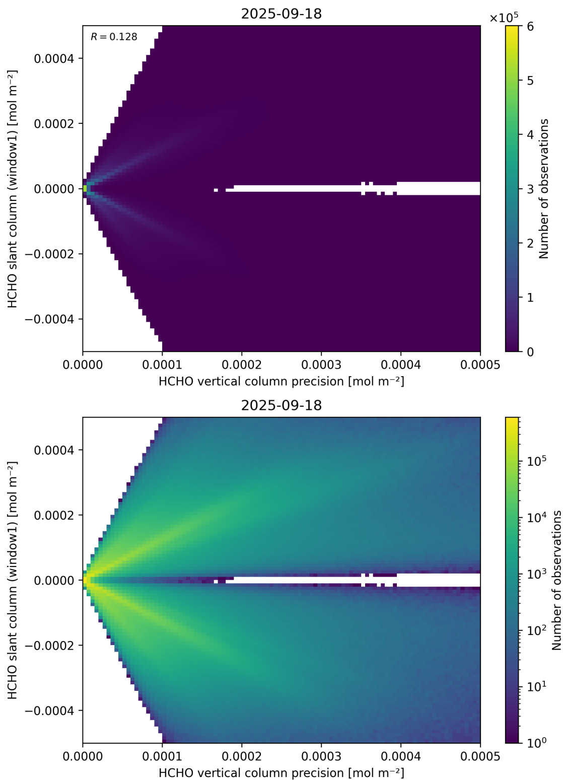
Figure 142: Scatter density plot of “HCHO vertical column precision” against “HCHO slant column (window1)” for 2025-09-17 to 2025-09-19.
