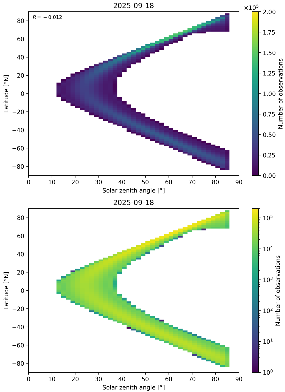
Figure 181: Scatter density plot of “Solar zenith angle” against “Latitude” for 2025-09-17 to 2025-09-19.
