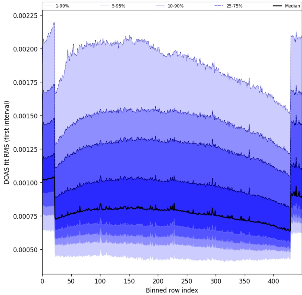
Figure 60: Along track statistics of “DOAS fit RMS (first interval)” for 2025-09-17 to 2025-09-19
