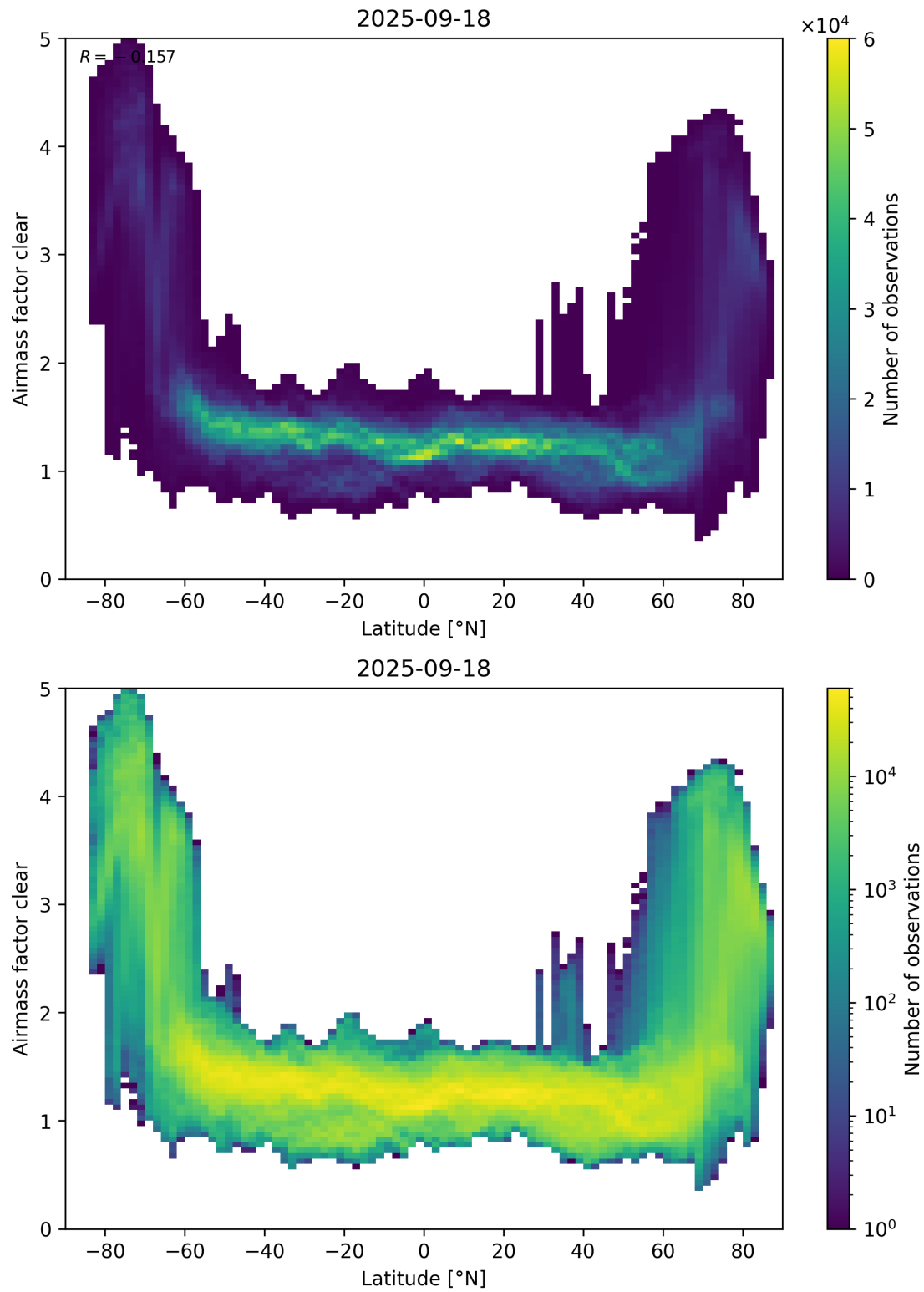
Figure 156: Scatter density plot of “Latitude” against “Airmass factor clear” for 2025-09-17 to 2025-09-19.
