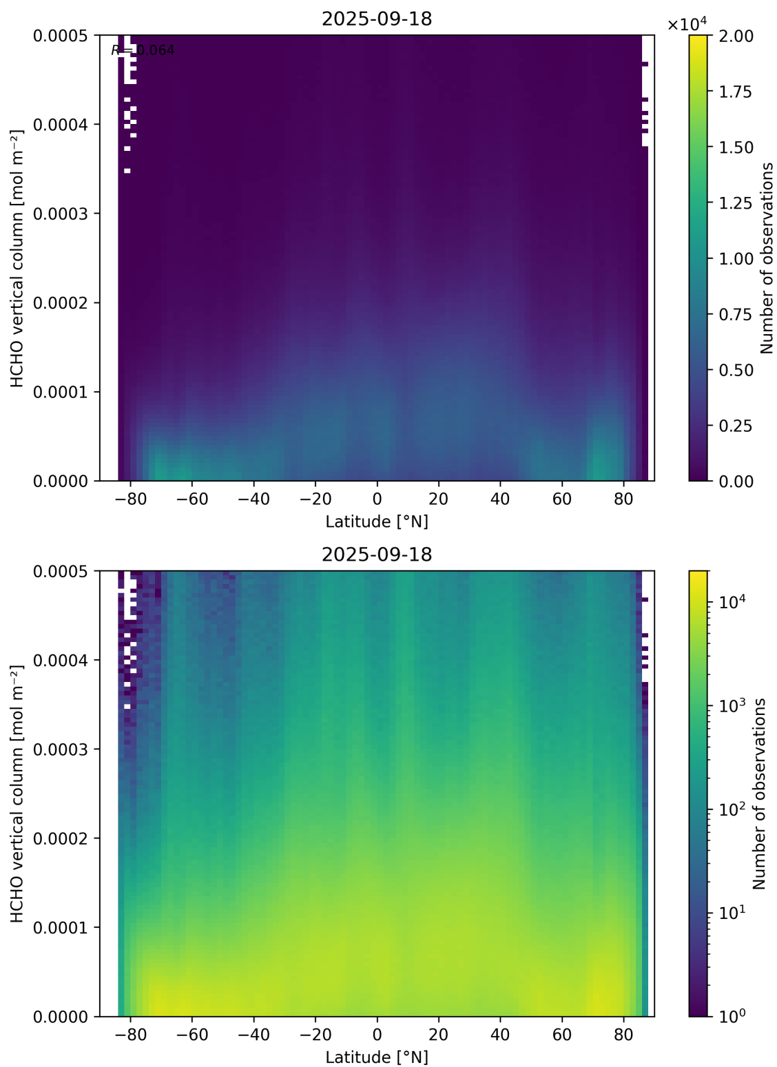
Figure 163: Scatter density plot of “Latitude” against “HCHO vertical column” for 2025-09-17 to 2025-09-19.
