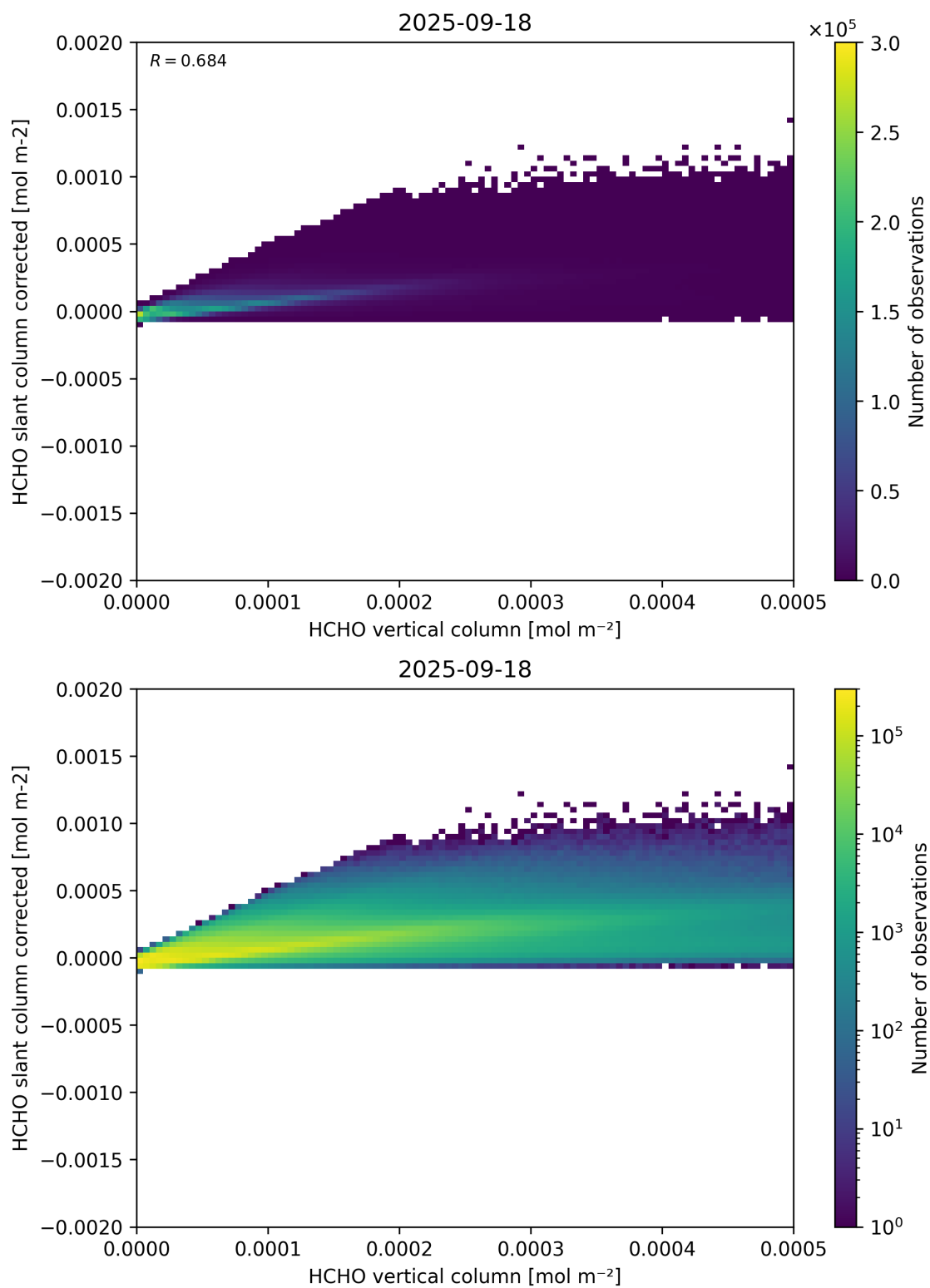
Figure 127: Scatter density plot of “HCHO vertical column” against “HCHO slant column corrected” for 2025-09-17 to 2025-09-19.
