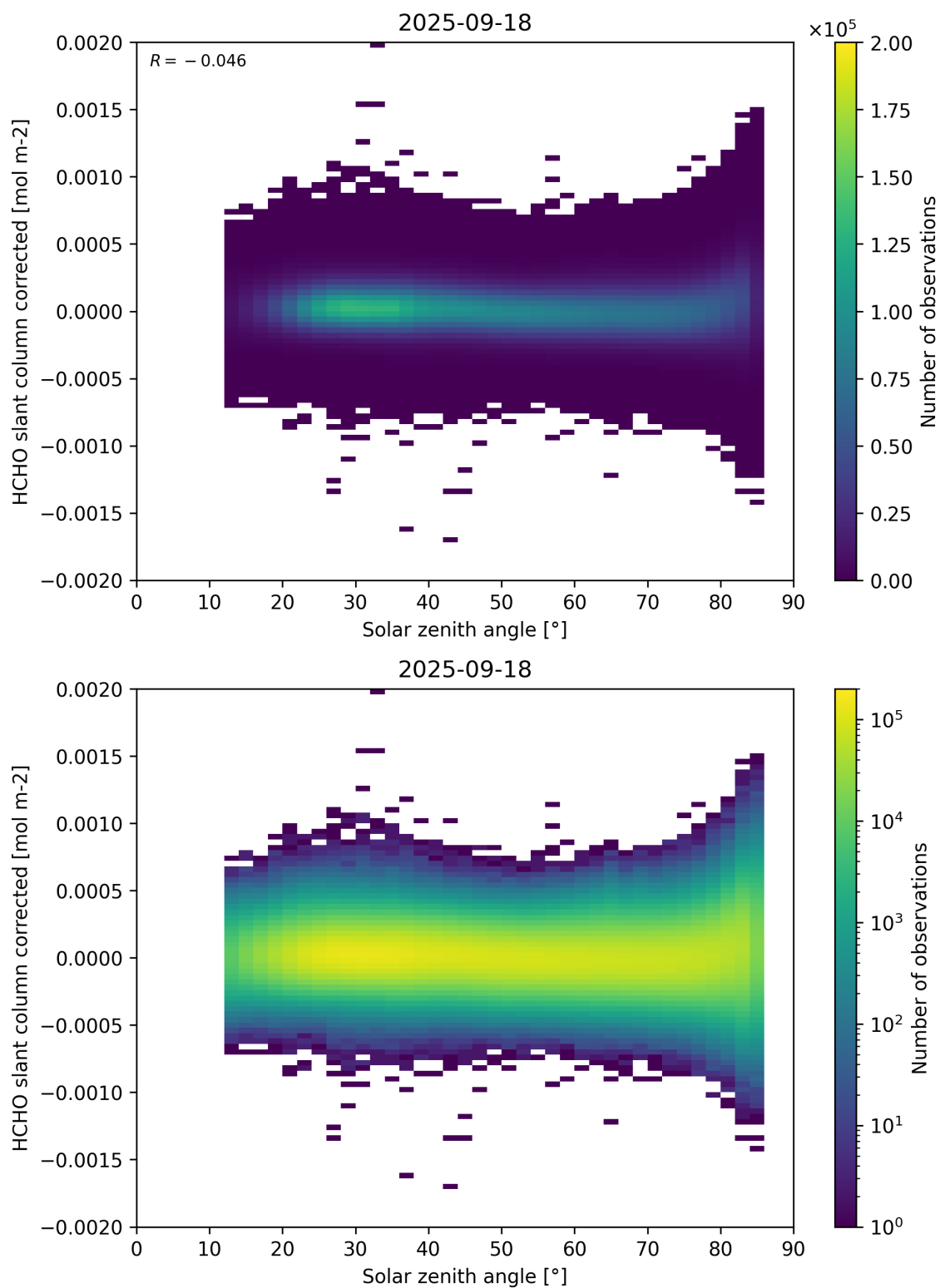
Figure 171: Scatter density plot of “Solar zenith angle” against “HCHO slant column corrected” for 2025-09-17 to 2025-09-19.
