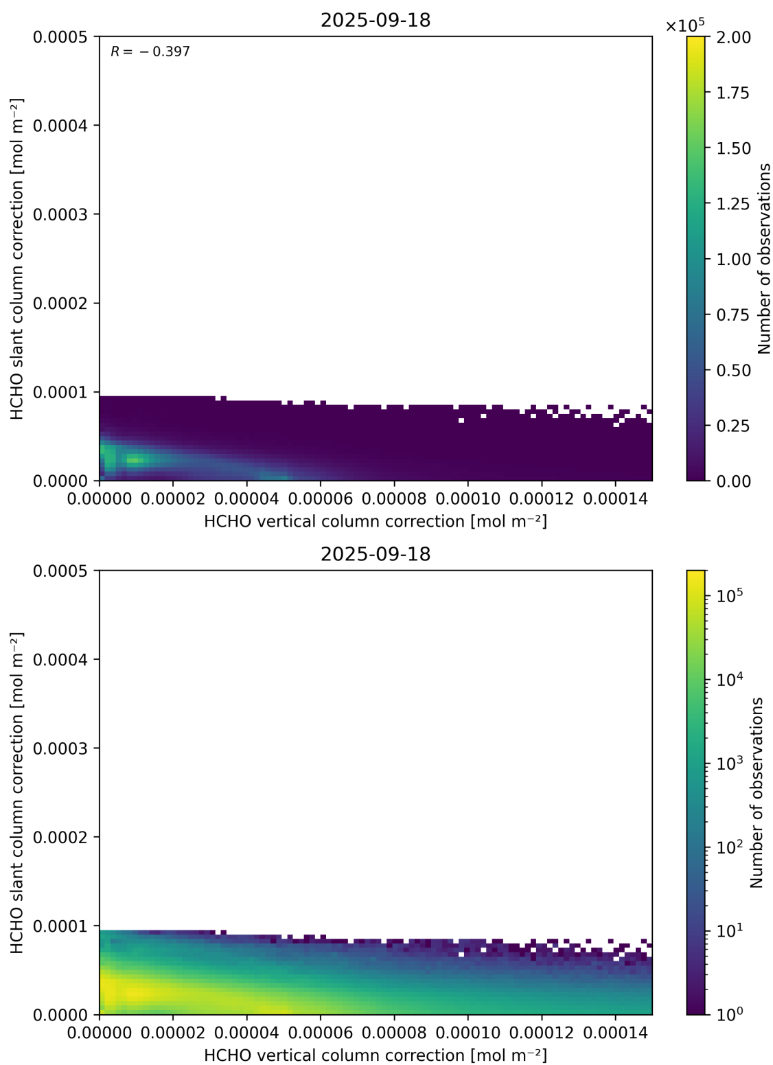
Figure 117: Scatter density plot of “HCHO vertical column correction” against “HCHO slant column correction” for 2025-09-17 to 2025-09-19.
