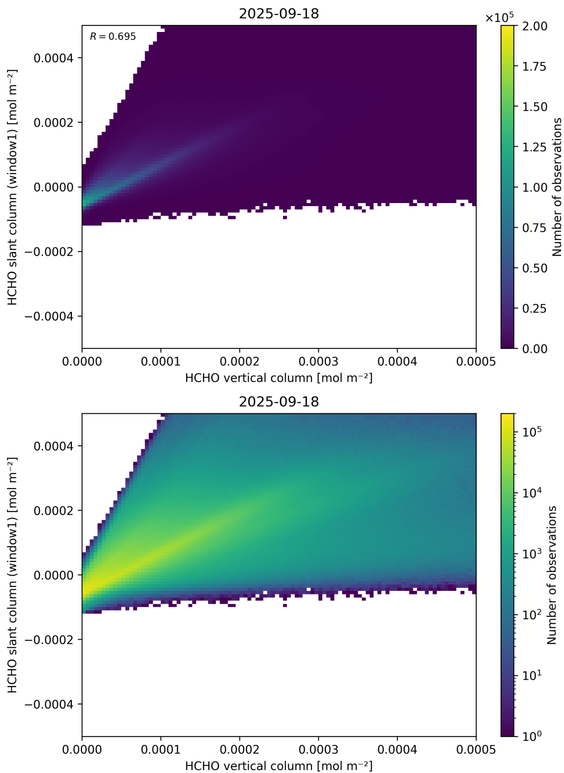
Figure 129: Scatter density plot of “HCHO vertical column” against “HCHO slant column (window1)” for 2025-09-17 to 2025-09-19.
