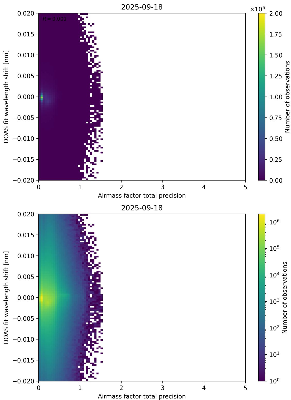
Figure 106: Scatter density plot of “Airmass factor total precision” against “DOAS fit wavelength shift” for 2025-09-17 to 2025-09-19.
