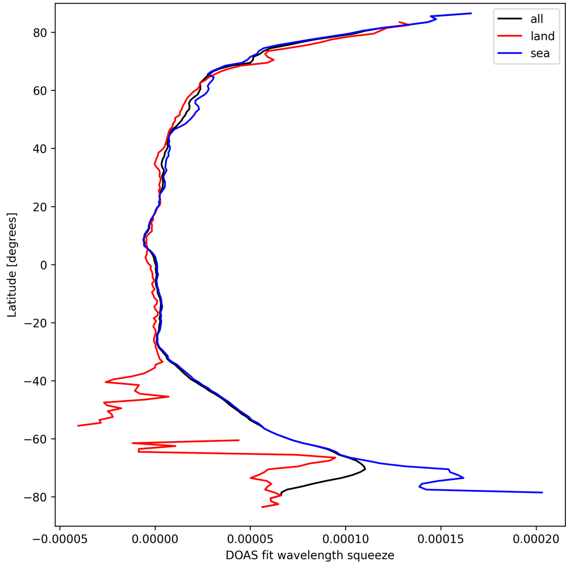
Figure 31: Zonal average of “DOAS fit wavelength squeeze” for 2025-09-17 to 2025-09-19.
