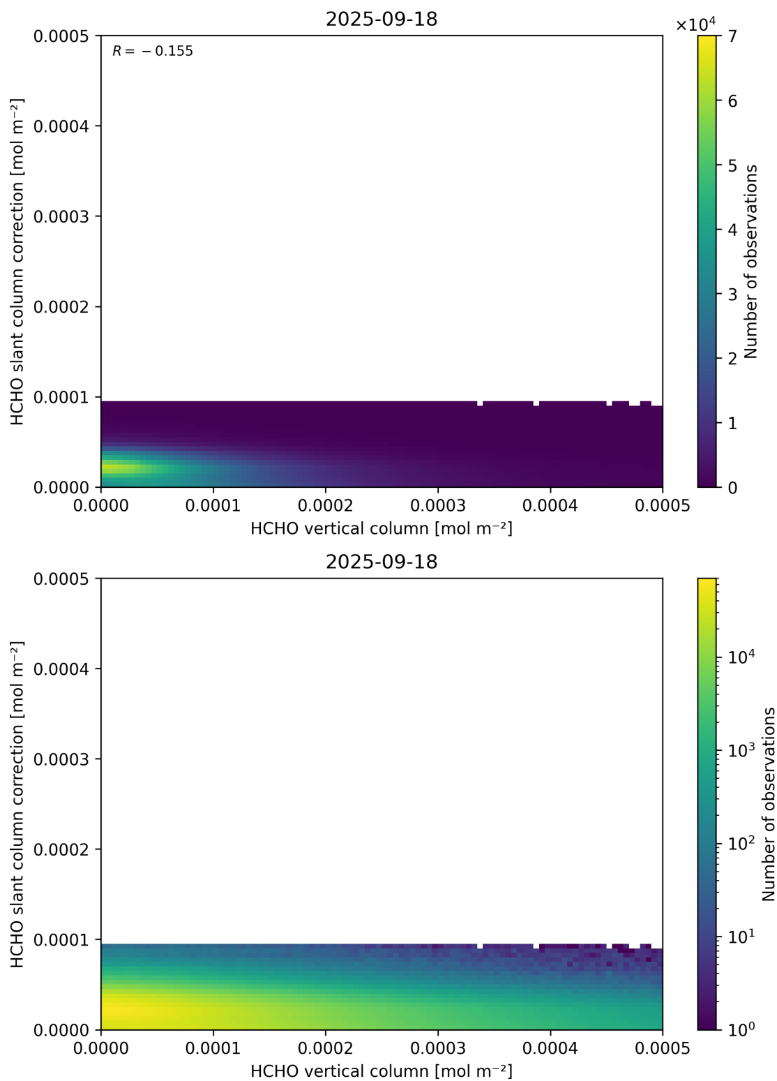
Figure 128: Scatter density plot of “HCHO vertical column” against “HCHO slant column correction” for 2025-09-17 to 2025-09-19.
