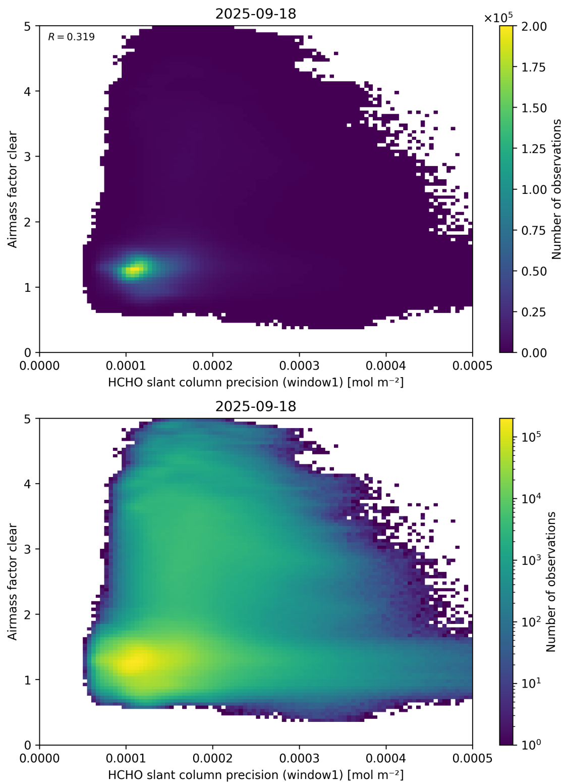
Figure 91: Scatter density plot of “HCHO slant column precision (window1)” against “Airmass factor clear” for 2025-09-17 to 2025-09-19.
