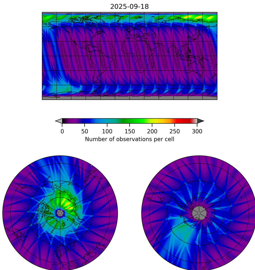
Figure 19: Map of the number of observations for 2025-09-17 to 2025-09-19
