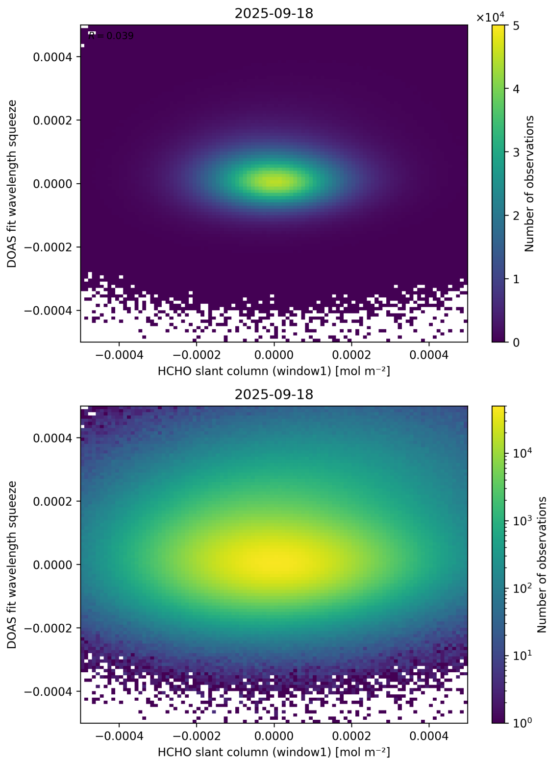
Figure 80: Scatter density plot of “HCHO slant column (window1)” against “DOAS fit wavelength squeeze” for 2025-09-17 to 2025-09-19.
