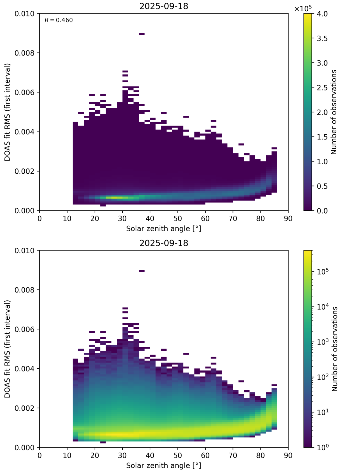
Figure 167: Scatter density plot of “Solar zenith angle” against “DOAS fit RMS (first interval)” for 2025-09-17 to 2025-09-19.
