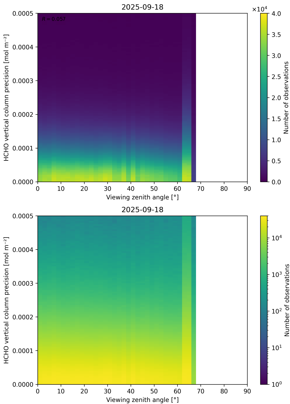
Figure 194: Scatter density plot of “Viewing zenith angle” against “HCHO vertical column precision” for 2025-09-17 to 2025-09-19.
