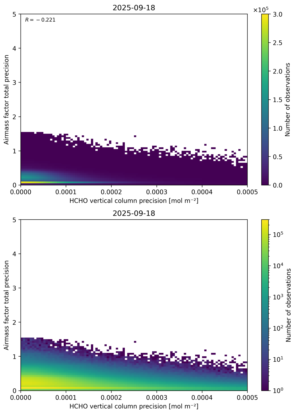
Figure 145: Scatter density plot of “HCHO vertical column precision” against “Airmass factor total precision” for 2025-09-17 to 2025-09-19.
