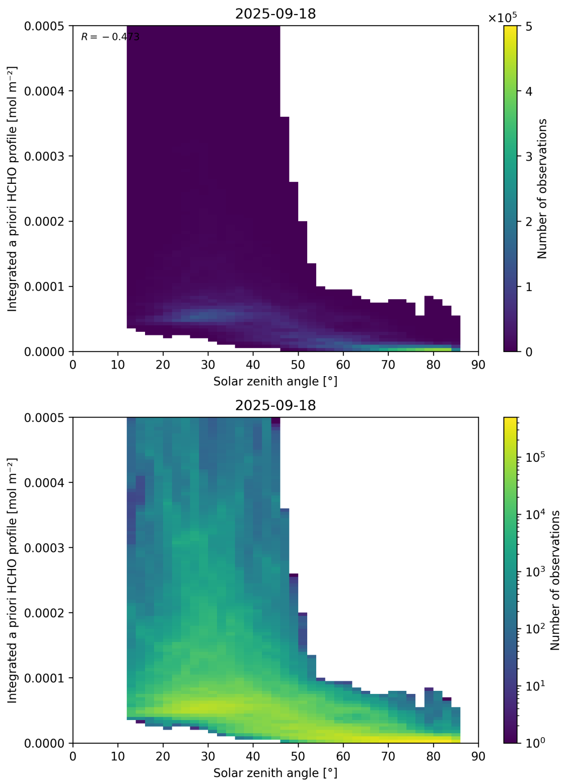
Figure 180: Scatter density plot of “Solar zenith angle” against “Integrated a priori HCHO profile” for 2025-09-17 to 2025-09-19.
