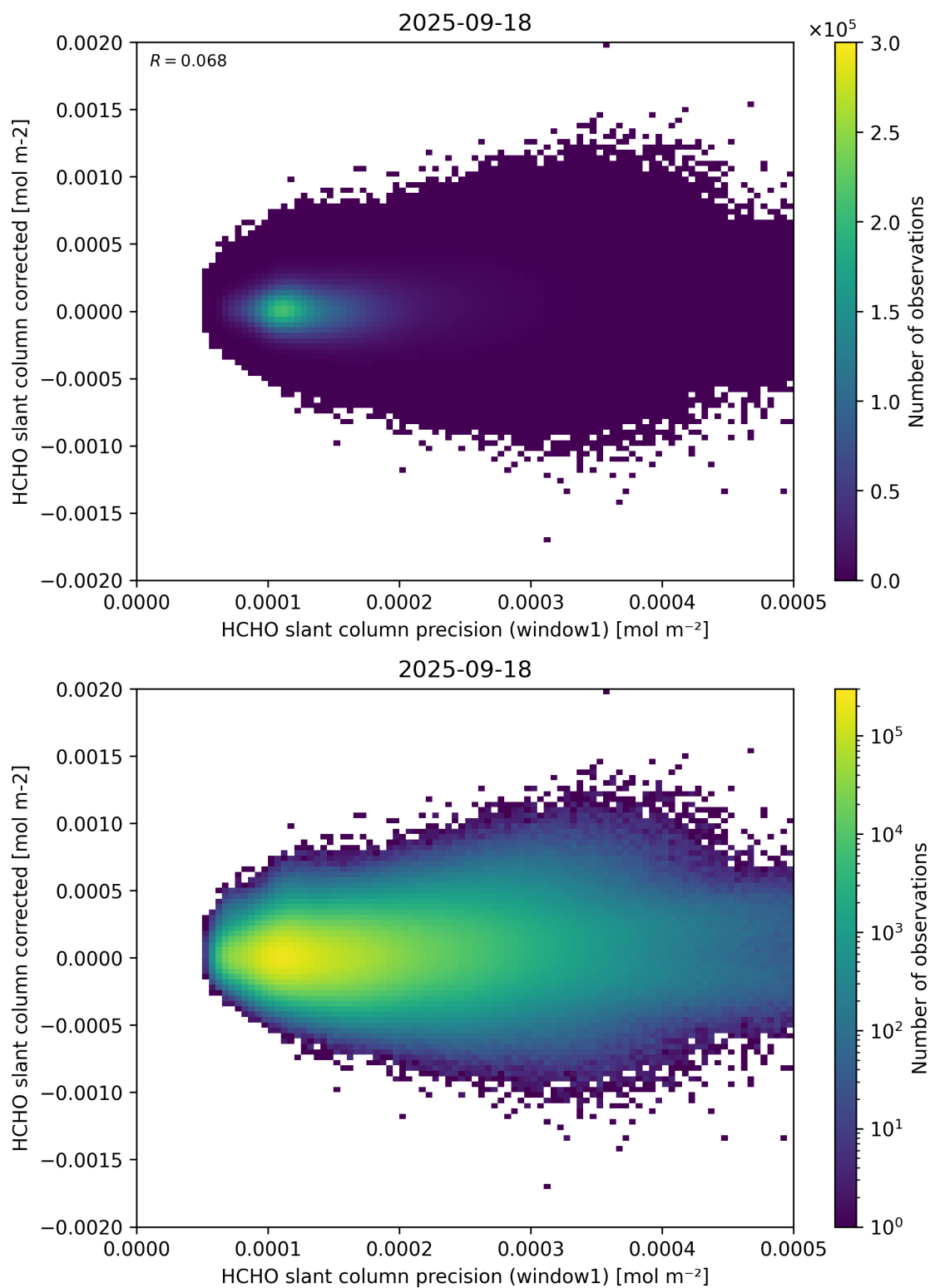
Figure 92: Scatter density plot of “HCHO slant column precision (window1)” against “HCHO slant column corrected” for 2025-09-17 to 2025-09-19.
