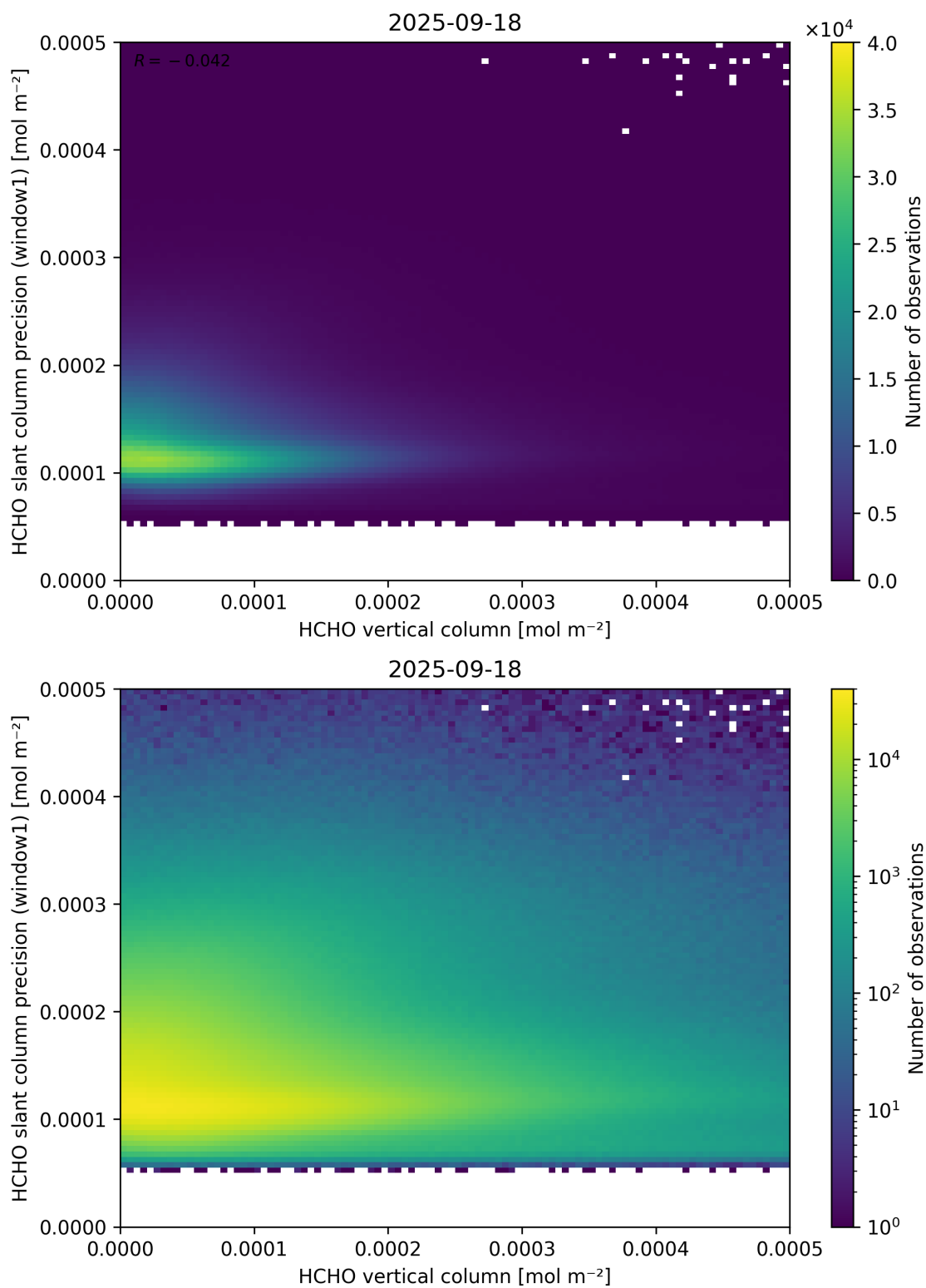
Figure 130: Scatter density plot of “HCHO vertical column” against “HCHO slant column precision (window1)” for 2025-09-17 to 2025-09-19.
