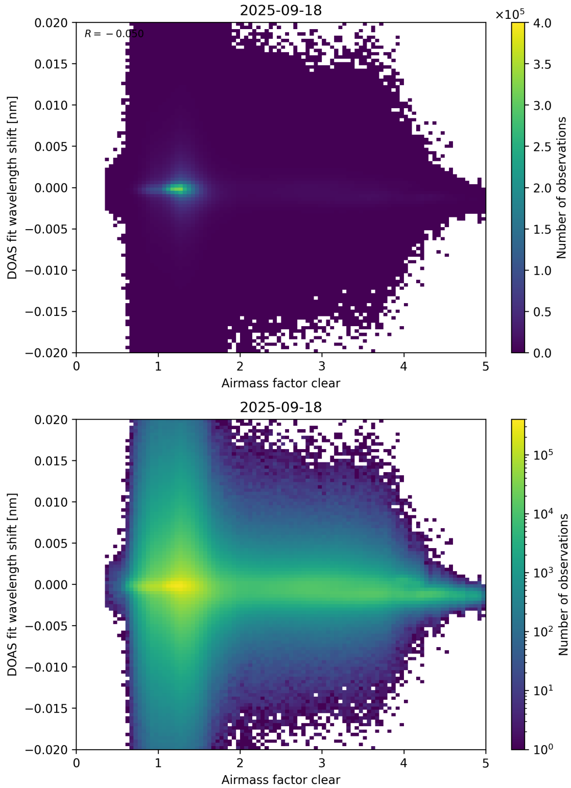
Figure 72: Scatter density plot of “Airmass factor clear” against “DOAS fit wavelength shift” for 2025-09-17 to 2025-09-19.
