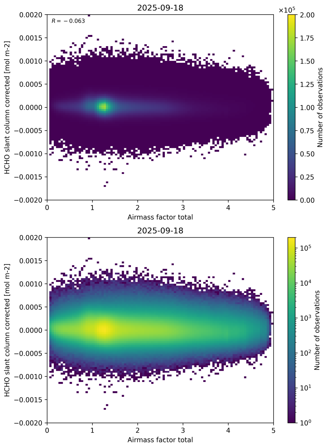
Figure 101: Scatter density plot of “Airmass factor total” against “HCHO slant column corrected” for 2025-09-17 to 2025-09-19.
