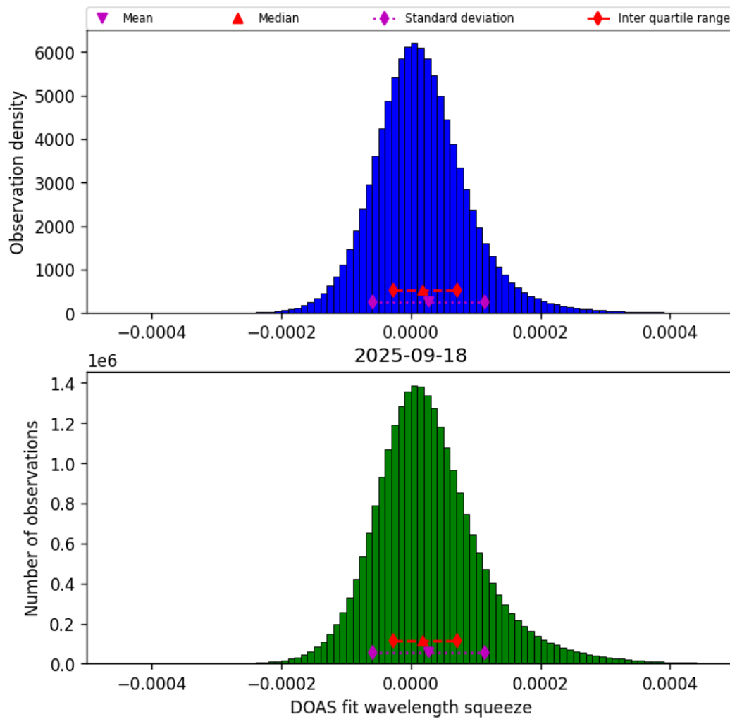
Figure 45: Histogram of “DOAS fit wavelength squeeze” for 2025-09-17 to 2025-09-19
