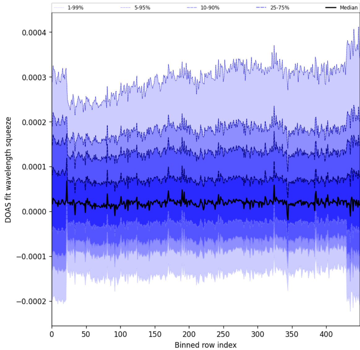
Figure 59: Along track statistics of “DOAS fit wavelength squeeze” for 2025-09-17 to 2025-09-19
