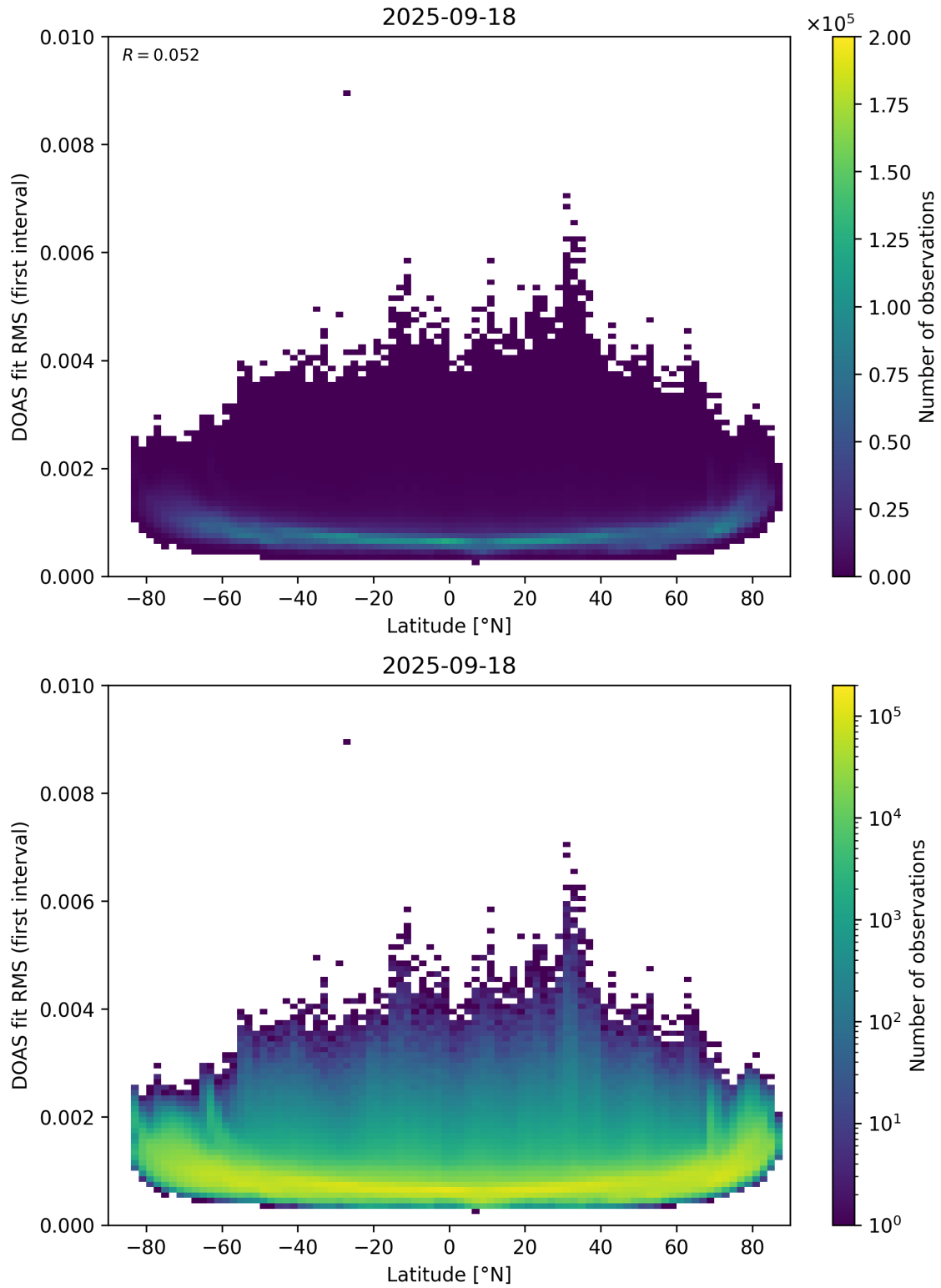
Figure 153: Scatter density plot of “Latitude” against “DOAS fit RMS (first interval)” for 2025-09-17 to 2025-09-19.
