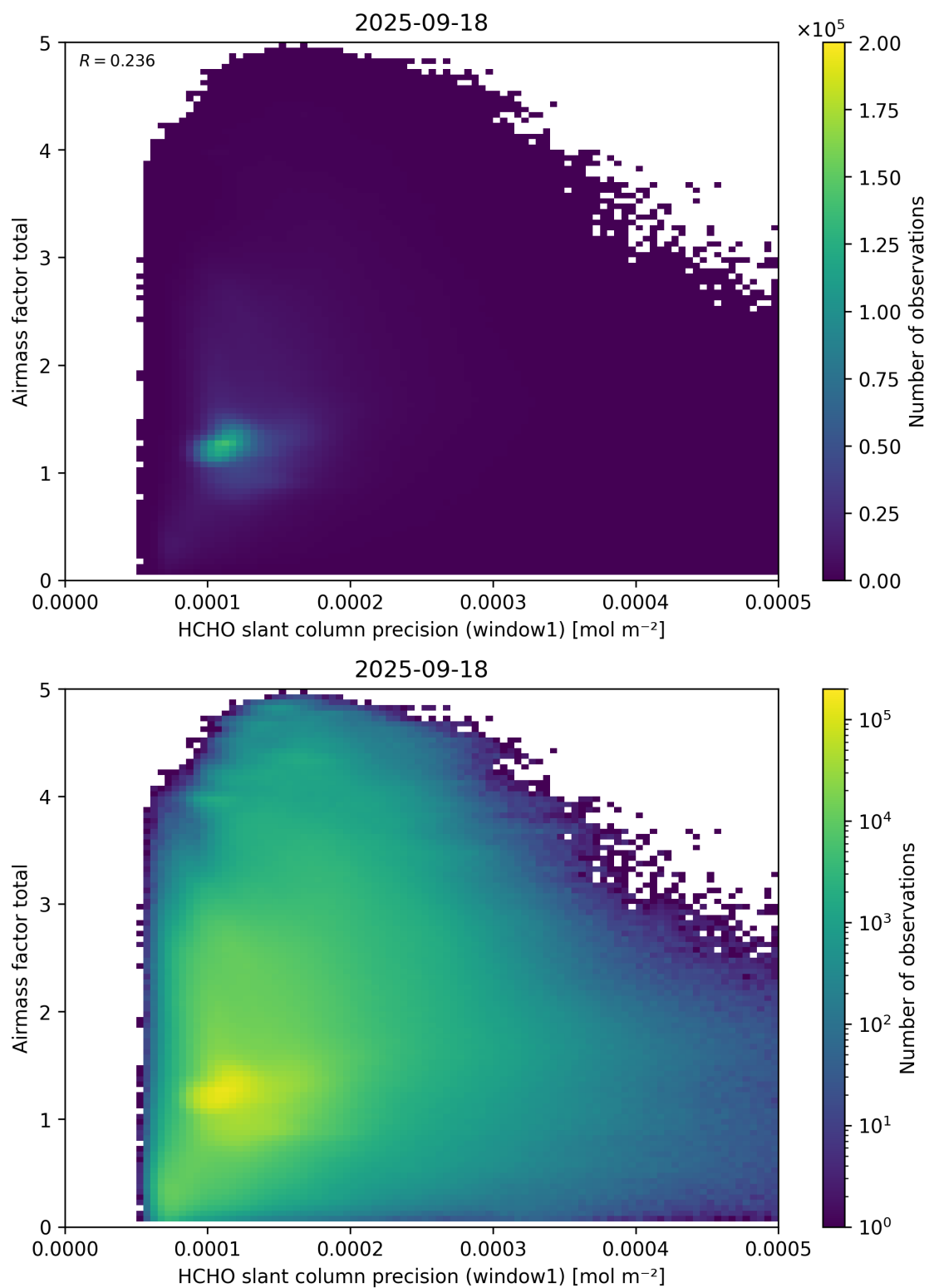
Figure 94: Scatter density plot of “HCHO slant column precision (window1)” against “Airmass factor total” for 2025-09-17 to 2025-09-19.
