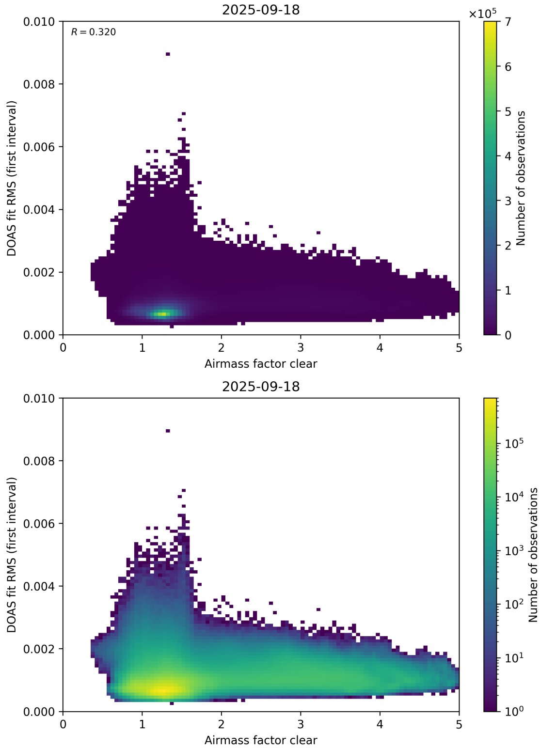
Figure 71: Scatter density plot of “Airmass factor clear” against “DOAS fit RMS (first interval)” for 2025-09-17 to 2025-09-19.
