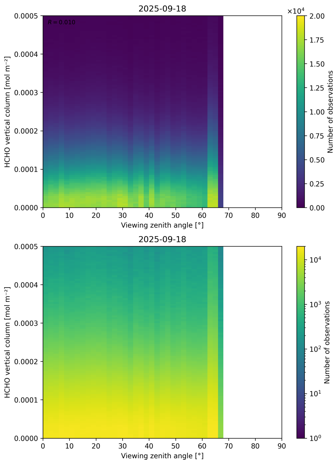
Figure 192: Scatter density plot of “Viewing zenith angle” against “HCHO vertical column” for 2025-09-17 to 2025-09-19.
