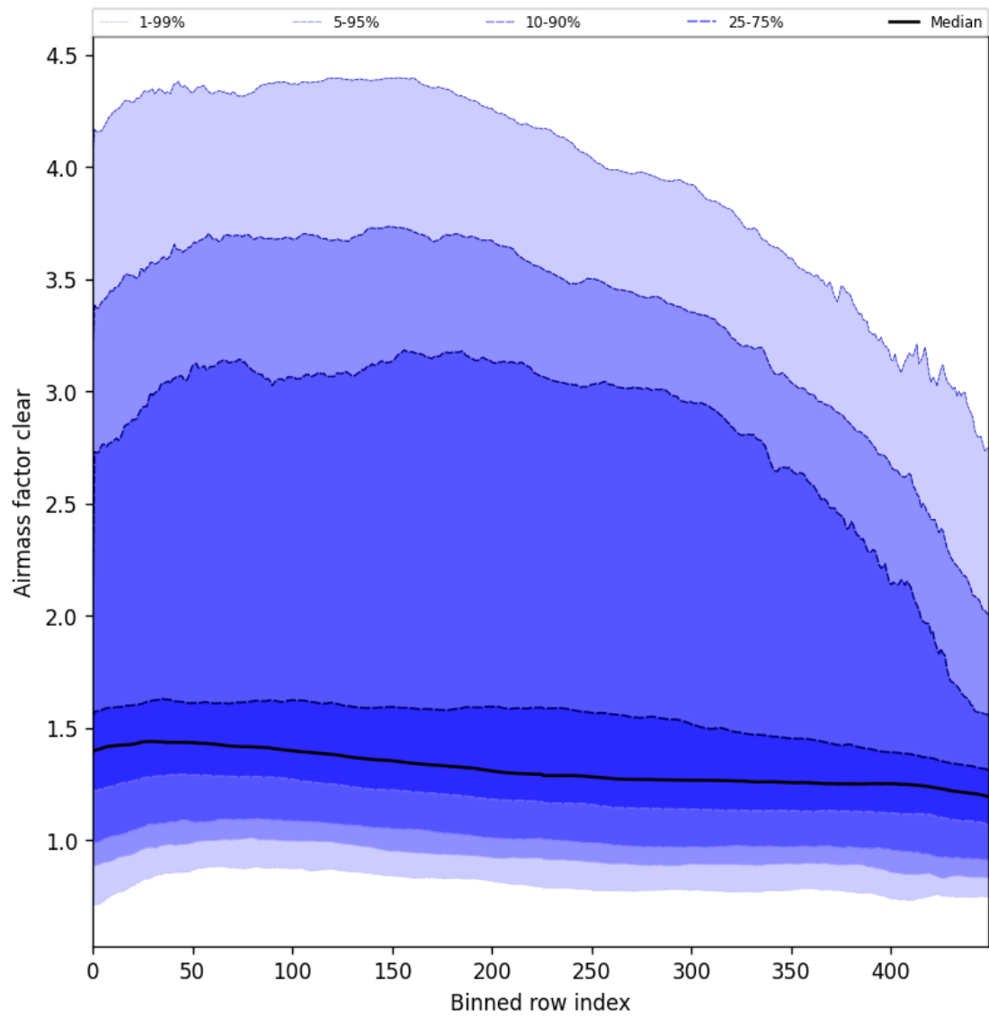
Figure 56: Along track statistics of “Air mass factor clear” for 2025-09-17 to 2025-09-19
