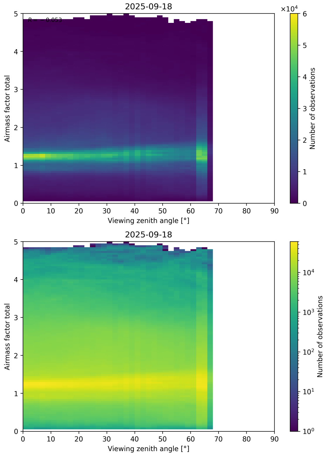
Figure 190: Scatter density plot of “Viewing zenith angle” against “Airmass factor total” for 2025-09-17 to 2025-09-19.
