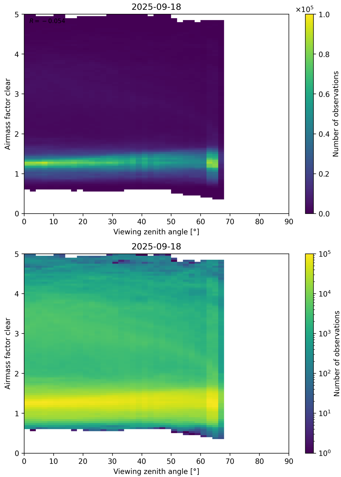
Figure 185: Scatter density plot of “Viewing zenith angle” against “Airmass factor clear” for 2025-09-17 to 2025-09-19.
