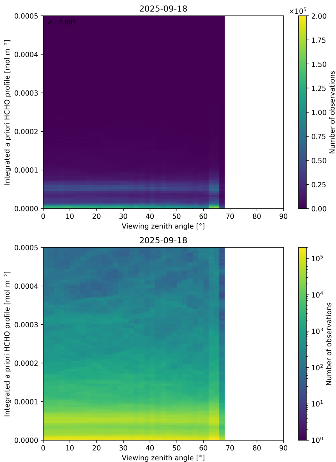
Figure 195: Scatter density plot of “Viewing zenith angle” against “Integrated a priori HCHO profile” for 2025-09-17 to 2025-09-19.
