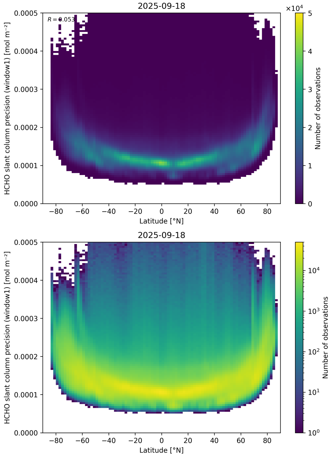
Figure 160: Scatter density plot of “Latitude” against “HCHO slant column precision (window1)” for 2025-09-17 to 2025-09-19.
