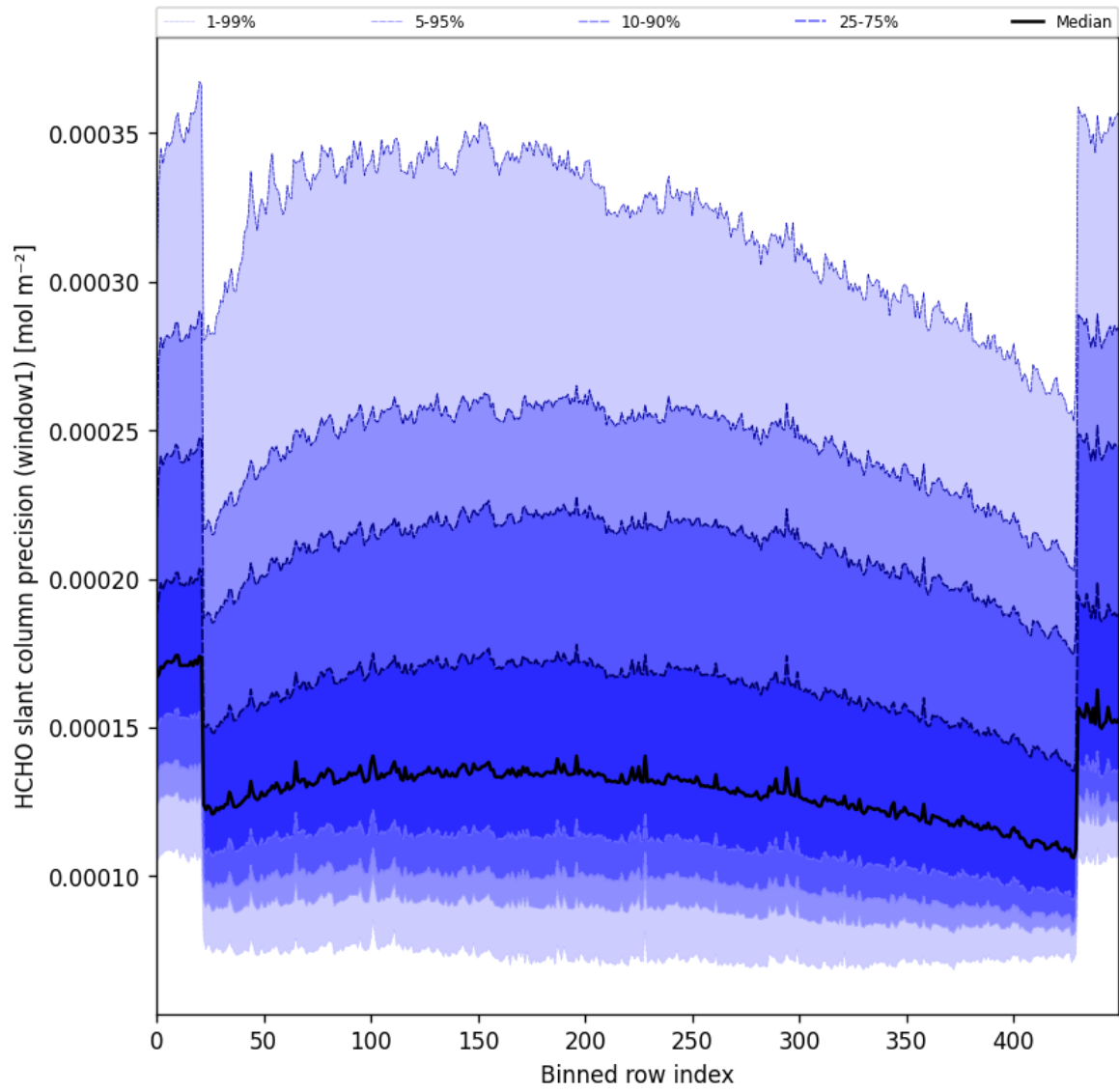
Figure 53: Along track statistics of “HCHO slant column precision (window1)” for 2025-09-17 to 2025-09-19
