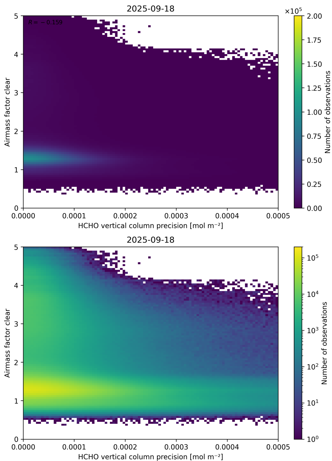
Figure 139: Scatter density plot of “HCHO vertical column precision” against “Airmass factor clear” for 2025-09-17 to 2025-09-19.
