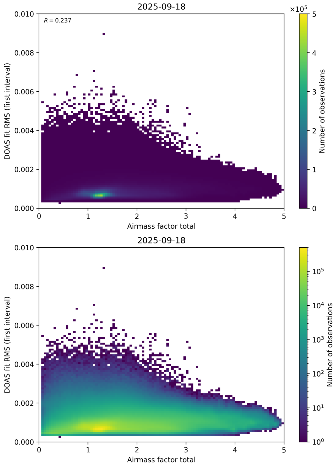
Figure 97: Scatter density plot of “Airmass factor total” against “DOAS fit RMS (first interval)” for 2025-09-17 to 2025-09-19.
