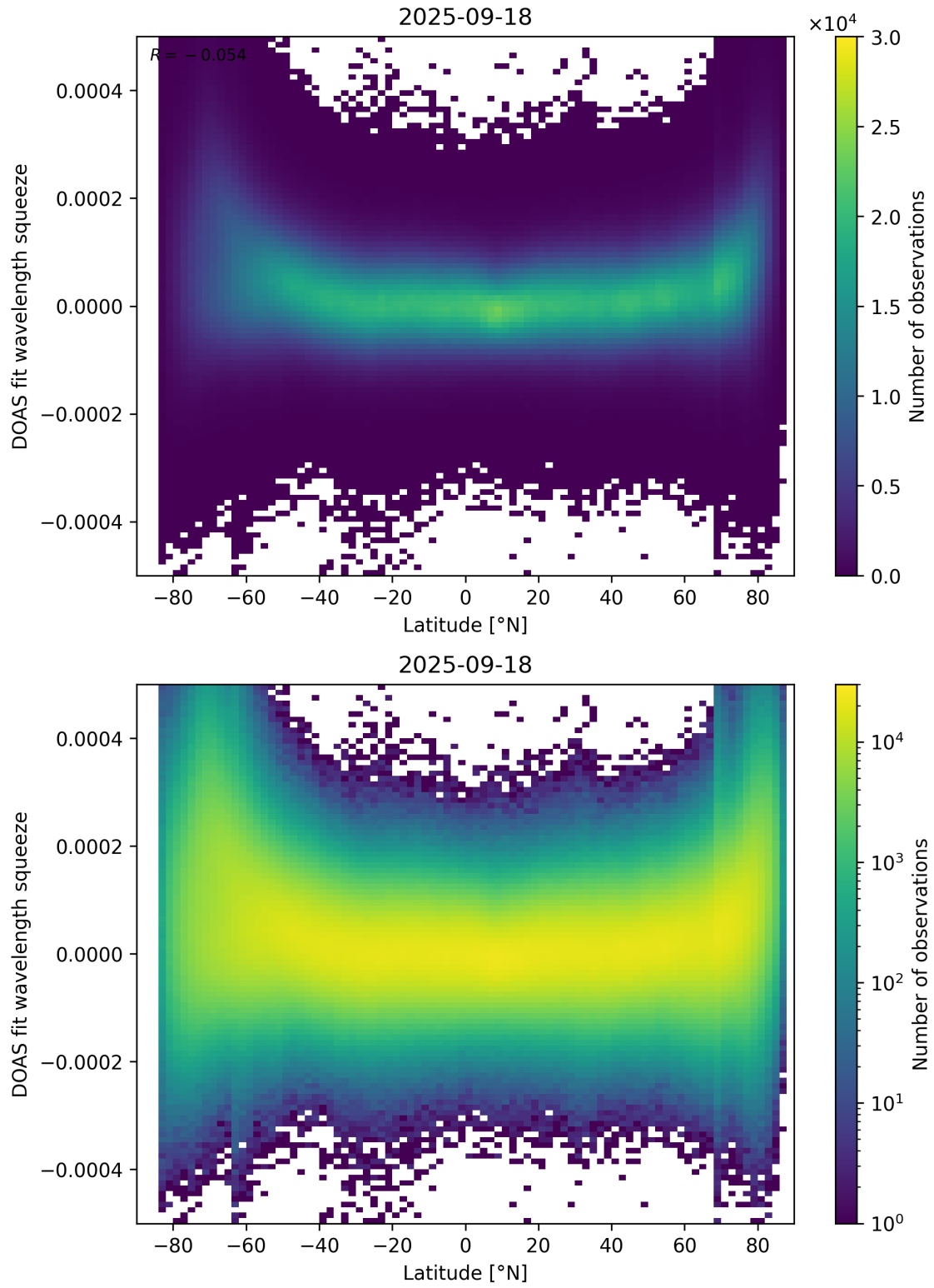
Figure 155: Scatter density plot of “Latitude” against “DOAS fit wavelength squeeze” for 2025-09-17 to 2025-09-19.
