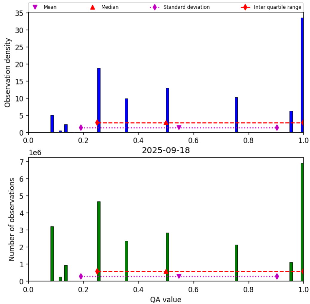
Figure 34: Histogram of “QA value” for 2025-09-17 to 2025-09-19
