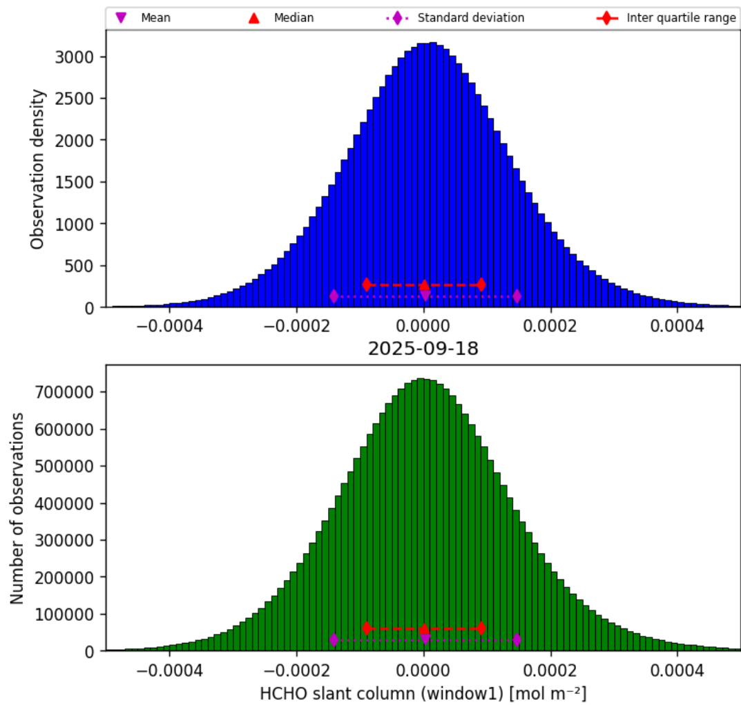
Figure 38: Histogram of “HCHO slant column (window1)” for 2025-09-17 to 2025-09-19
