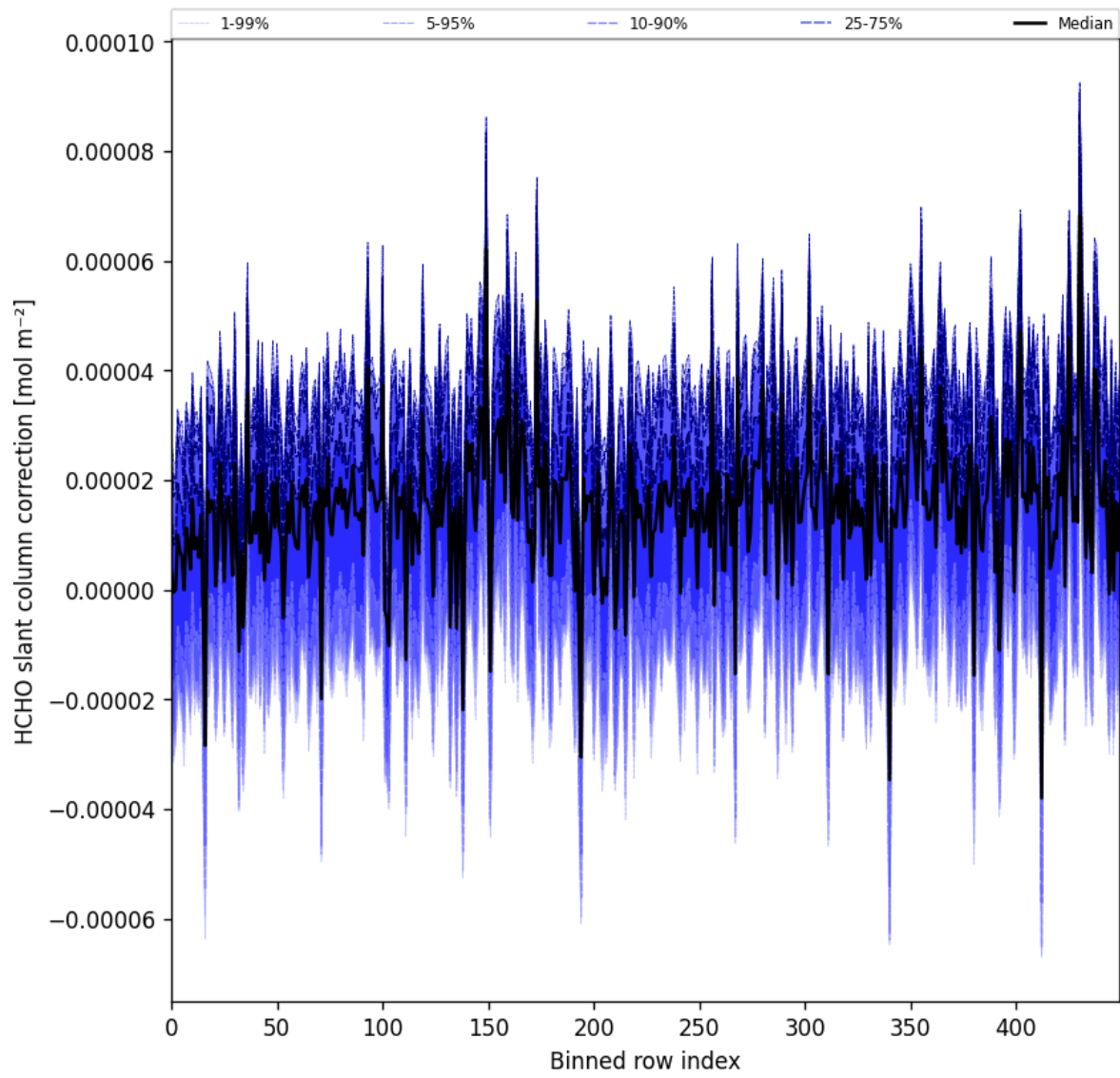
Figure 61: Along track statistics of “HCHO slant column correction” for 2025-09-17 to 2025-09-19
