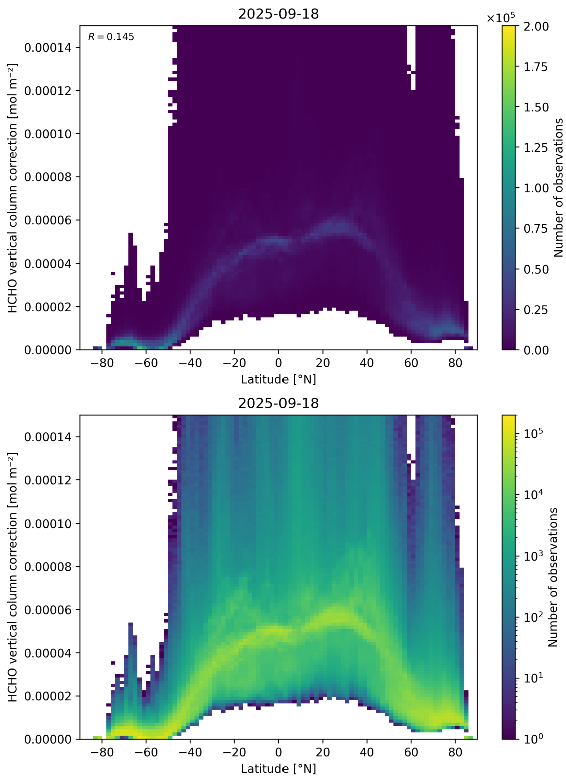
Figure 164: Scatter density plot of “Latitude” against “HCHO vertical column correction” for 2025-09-17 to 2025-09-19.
