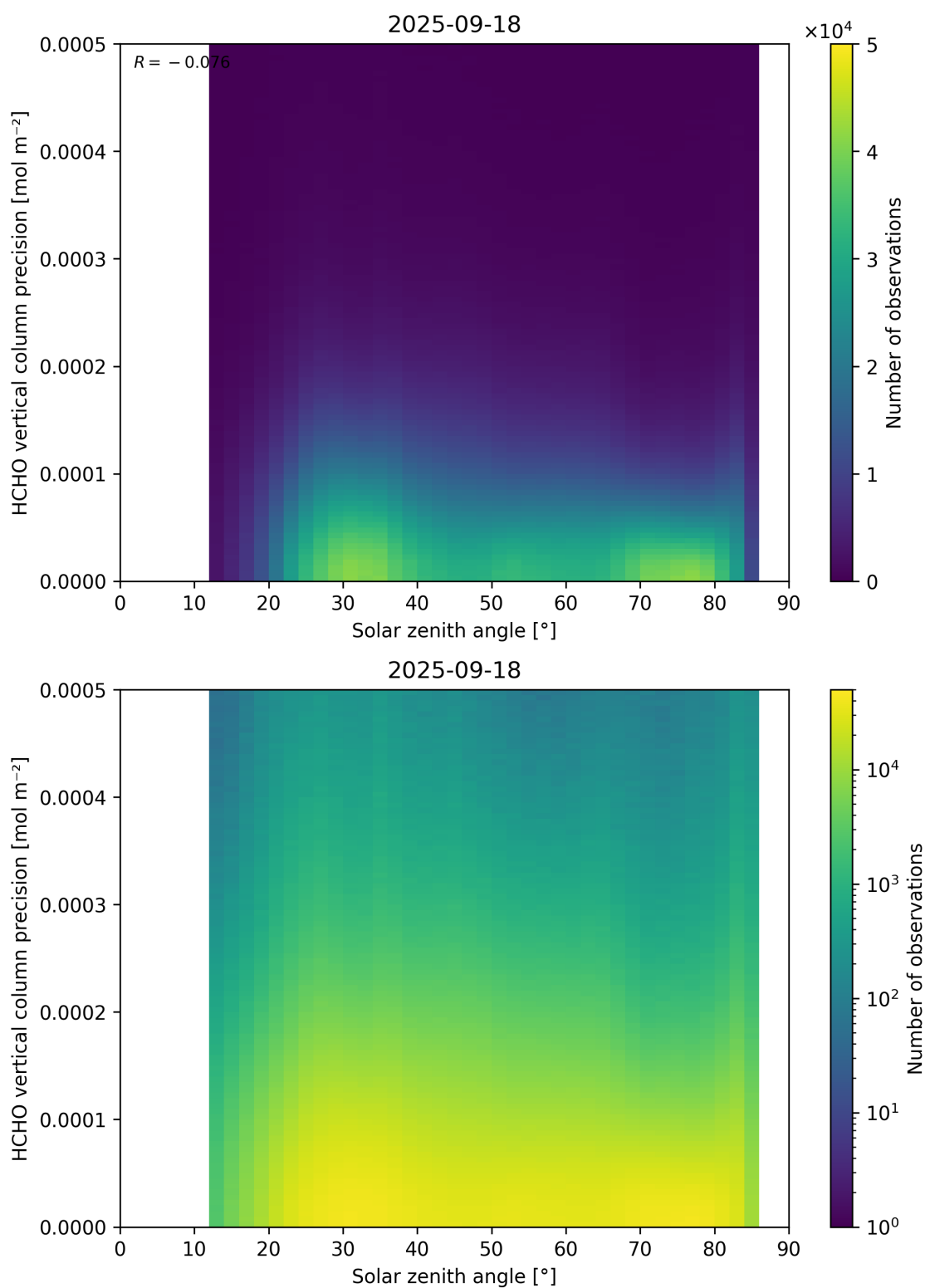
Figure 179: Scatter density plot of “Solar zenith angle” against “HCHO vertical column precision” for 2025-09-17 to 2025-09-19.
