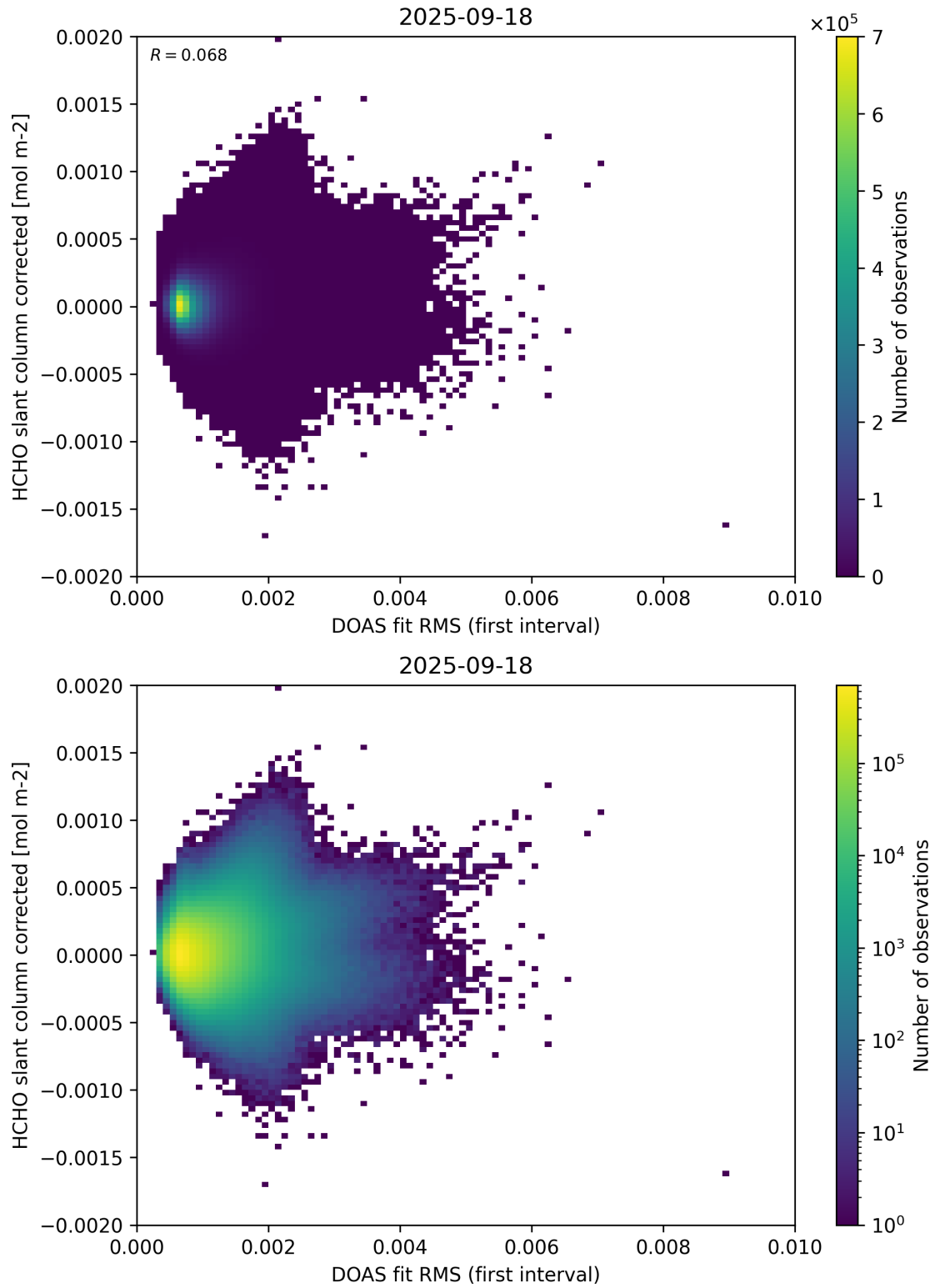
Figure 62: Scatter density plot of “DOAS fit RMS (first interval)” against “HCHO slant column corrected” for 2025-09-17 to 2025-09-19.
