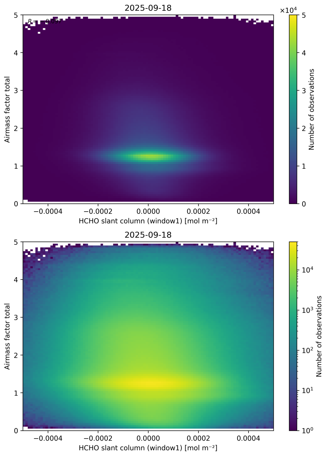
Figure 85: Scatter density plot of “HCHO slant column (window1)” against “Airmass factor total” for 2025-09-17 to 2025-09-19.
