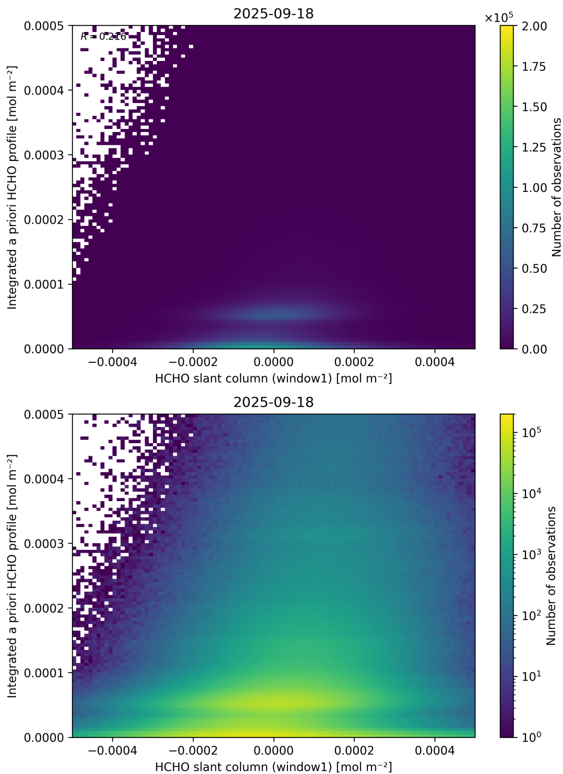
Figure 87: Scatter density plot of “HCHO slant column (window1)” against “Integrated a priori HCHO profile” for 2025-09-17 to 2025-09-19.
