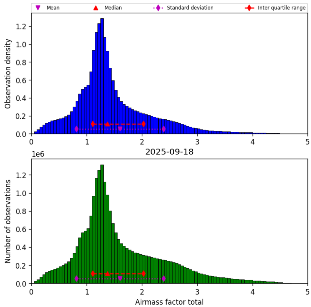
Figure 40: Histogram of “Airmass factor total” for 2025-09-17 to 2025-09-19
