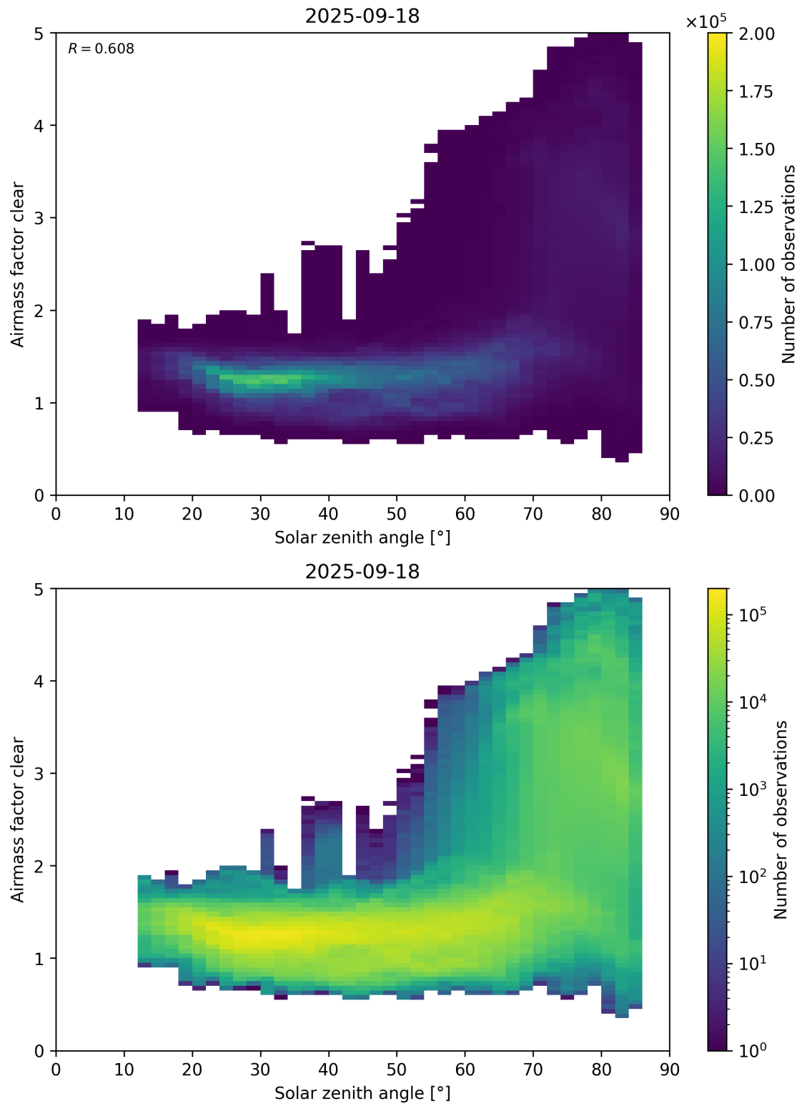
Figure 170: Scatter density plot of “Solar zenith angle” against “Airmass factor clear” for 2025-09-17 to 2025-09-19.
