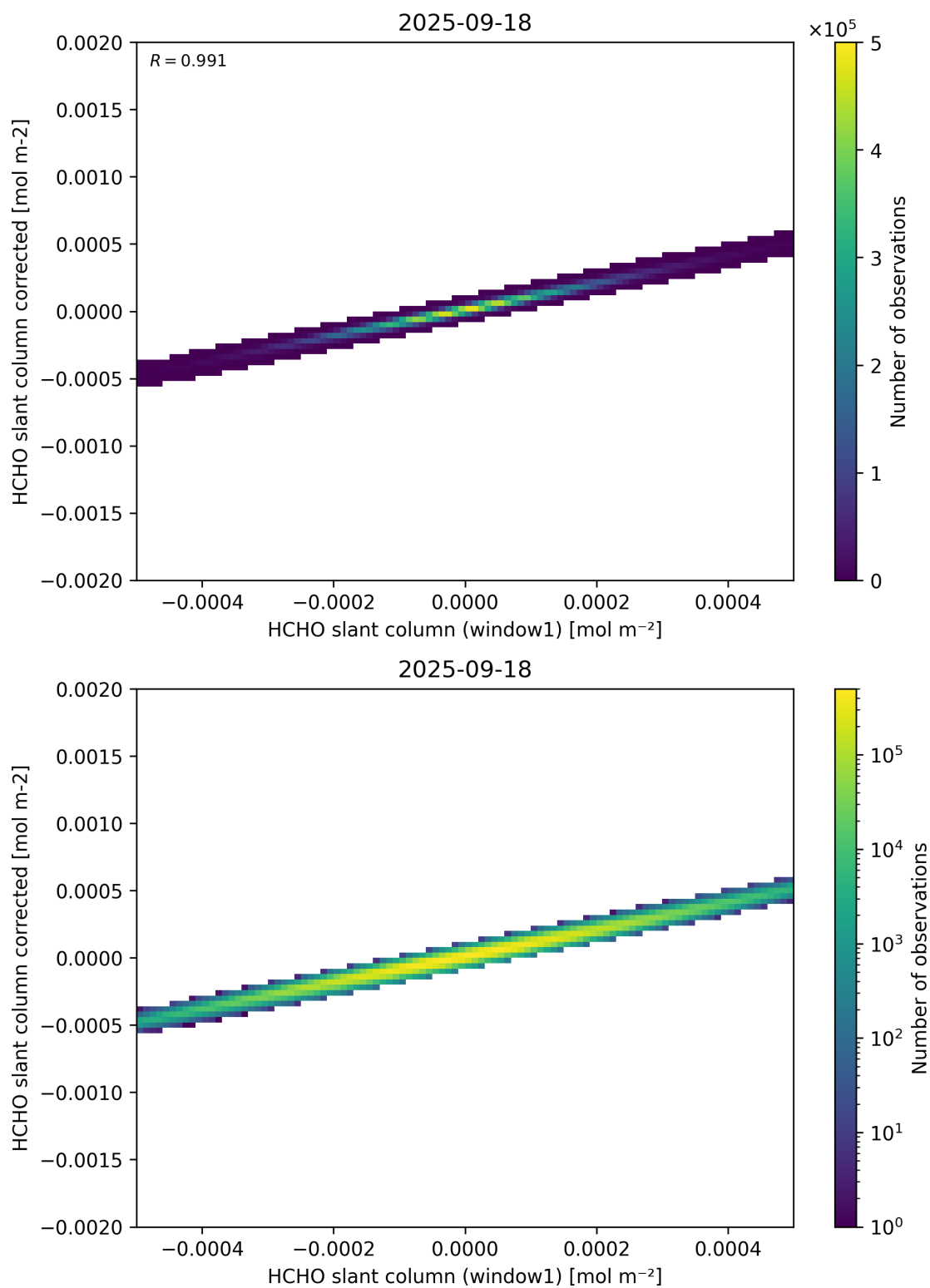
Figure 82: Scatter density plot of “HCHO slant column (window1)” against “HCHO slant column corrected” for 2025-09-17 to 2025-09-19.
