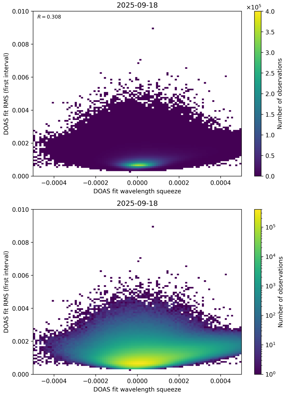
Figure 68: Scatter density plot of “DOAS fit wavelength squeeze” against “DOAS fit RMS (first interval)” for 2025-09-17 to 2025-09-19.
