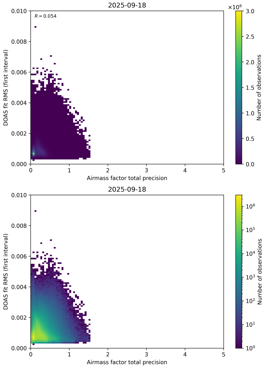
Figure 105: Scatter density plot of “Airmass factor total precision” against “DOAS fit RMS (first interval)” for 2025-09-17 to 2025-09-19.
