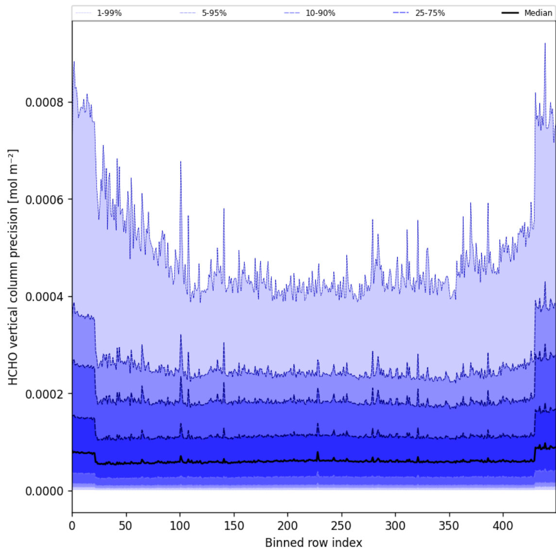
Figure 50: Along track statistics of “HCHO vertical column precision” for 2025-09-17 to 2025-09-19
