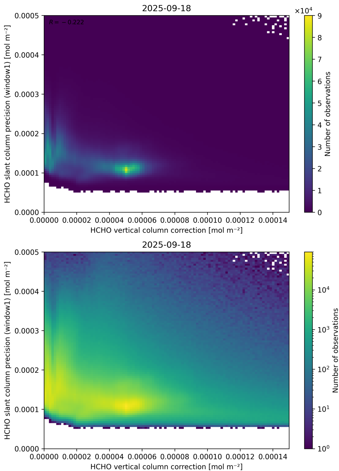
Figure 119: Scatter density plot of “HCHO vertical column correction” against “HCHO slant column precision (window1)” for 2025-09-17 to 2025-09-19.
