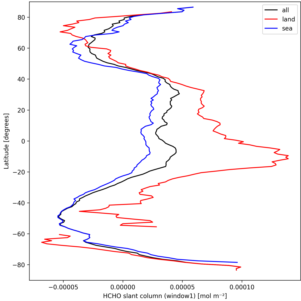
Figure 24: Zonal average of “HCHO slant column (window1)” for 2025-09-17 to 2025-09-19.
