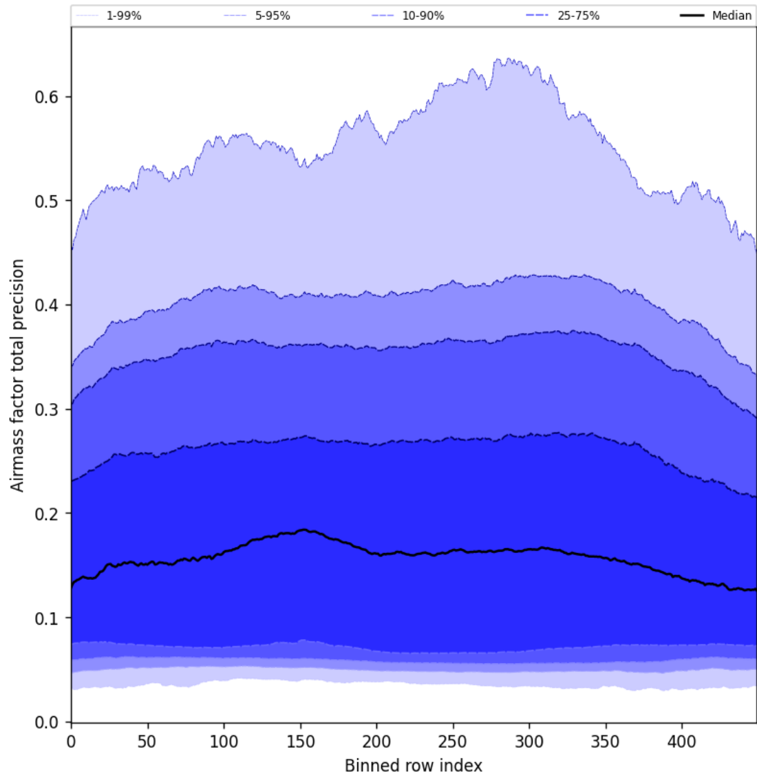
Figure 55: Along track statistics of “Airmass factor total precision” for 2025-09-17 to 2025-09-19
