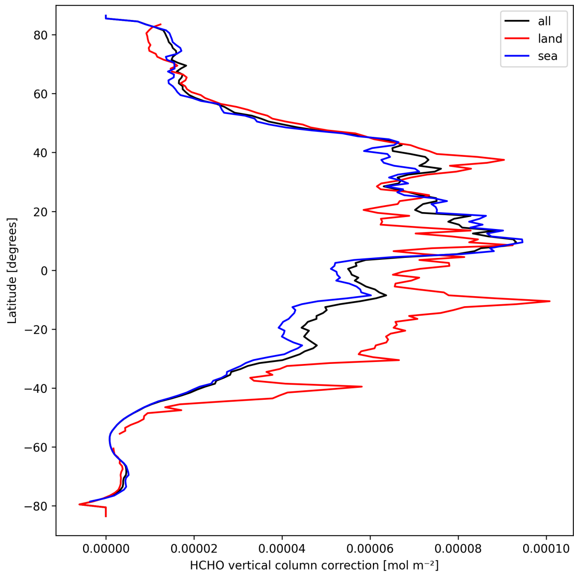
Figure 23: Zonal average of “HCHO vertical column correction” for 2025-09-17 to 2025-09-19.
