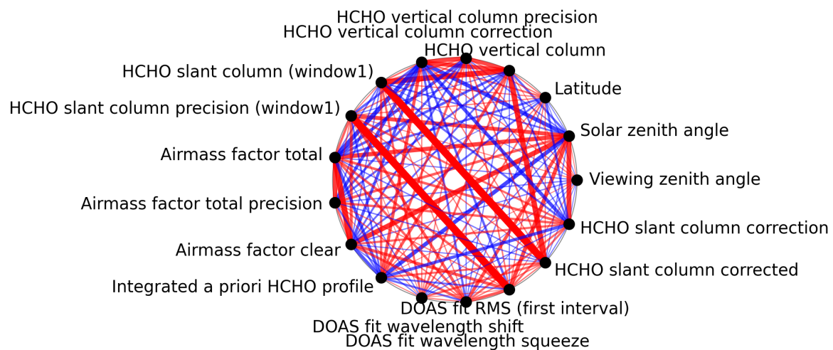
Figure 1: Map of correlation graph for 2025-09-17 to 2025-09-19.
