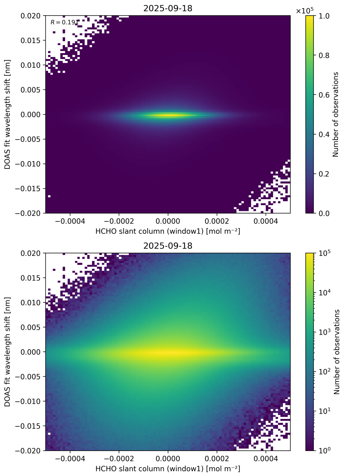
Figure 79: Scatter density plot of “HCHO slant column (window1)” against “DOAS fit wavelength shift” for 2025-09-17 to 2025-09-19.
