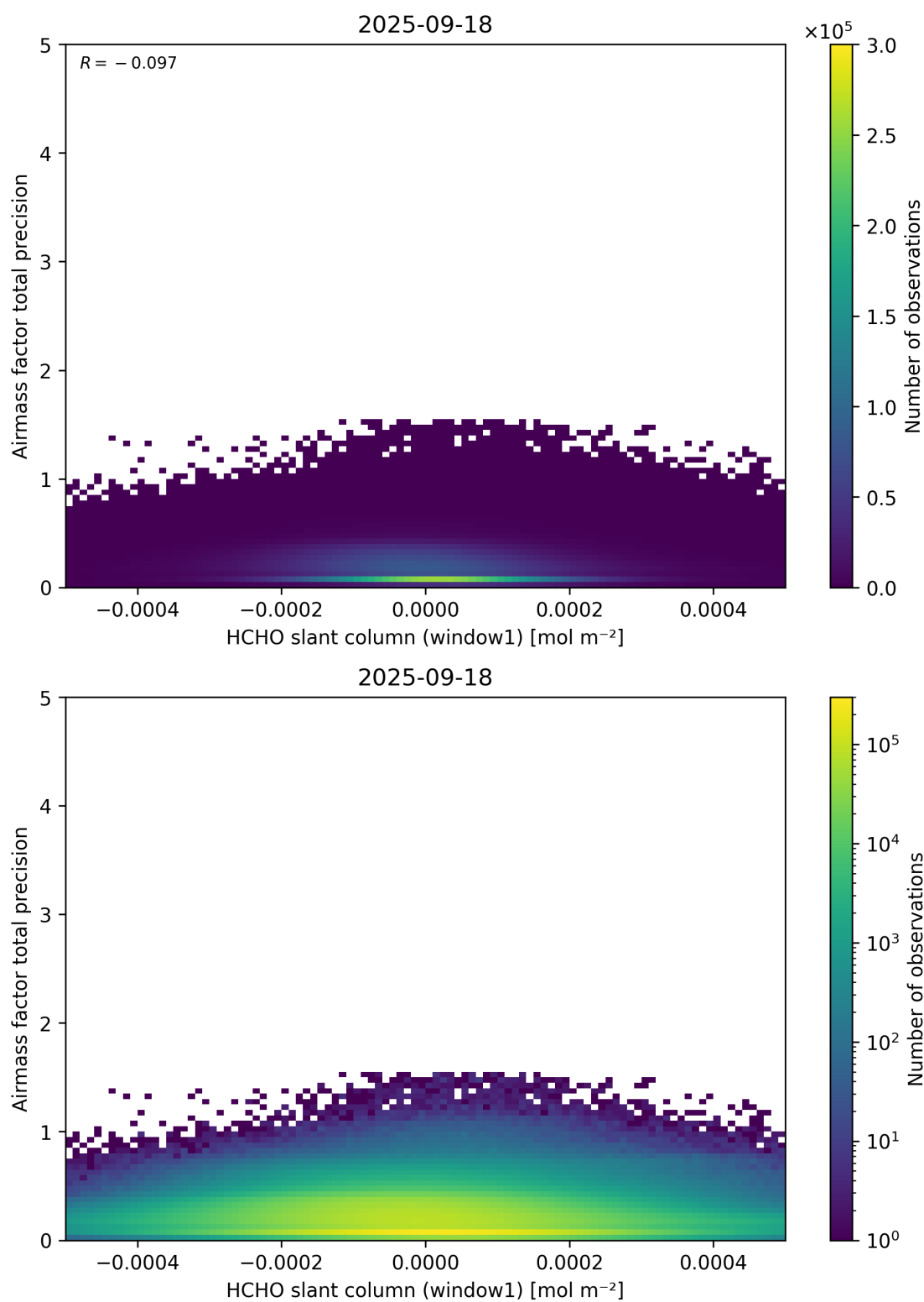
Figure 86: Scatter density plot of “HCHO slant column (window1)” against “Airmass factor total precision” for 2025-09-17 to 2025-09-19.
