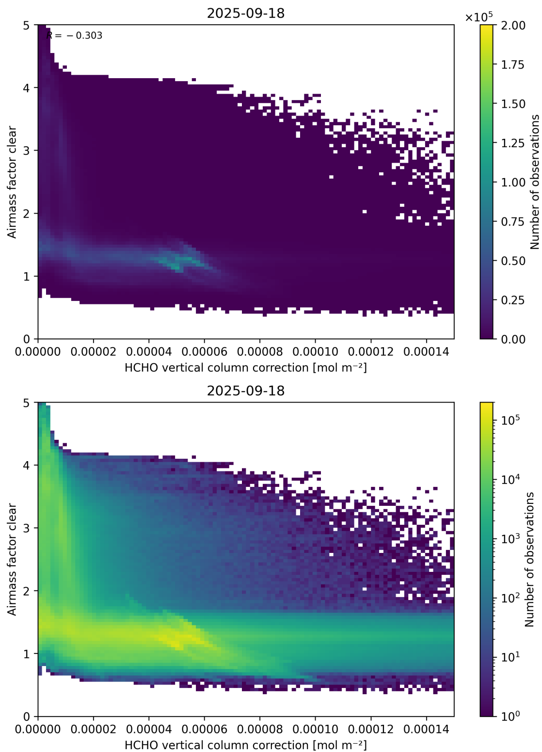
Figure 115: Scatter density plot of “HCHO vertical column correction” against “Airmass factor clear” for 2025-09-17 to 2025-09-19.
