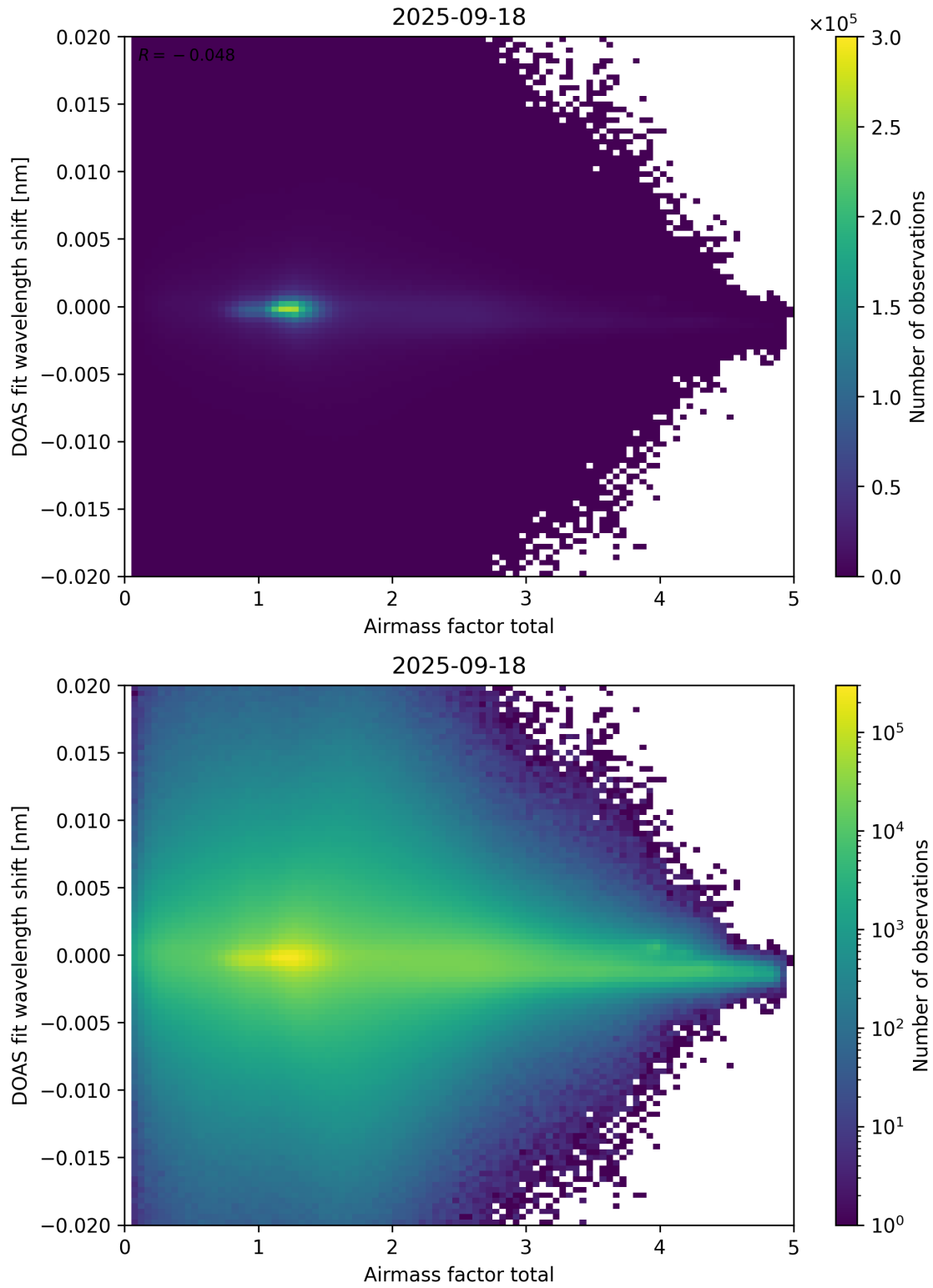
Figure 98: Scatter density plot of “Airmass factor total” against “DOAS fit wavelength shift” for 2025-09-17 to 2025-09-19.
