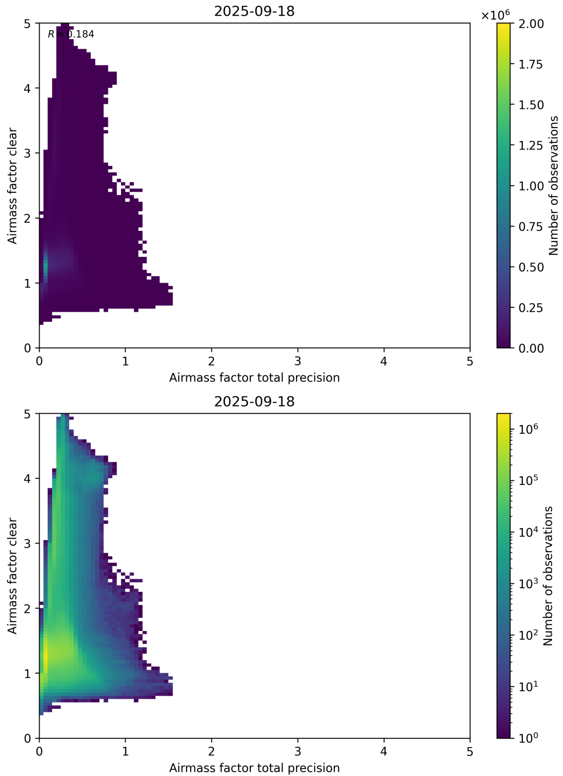
Figure 108: Scatter density plot of “Airmass factor total precision” against “Airmass factor clear” for 2025-09-17 to 2025-09-19.
