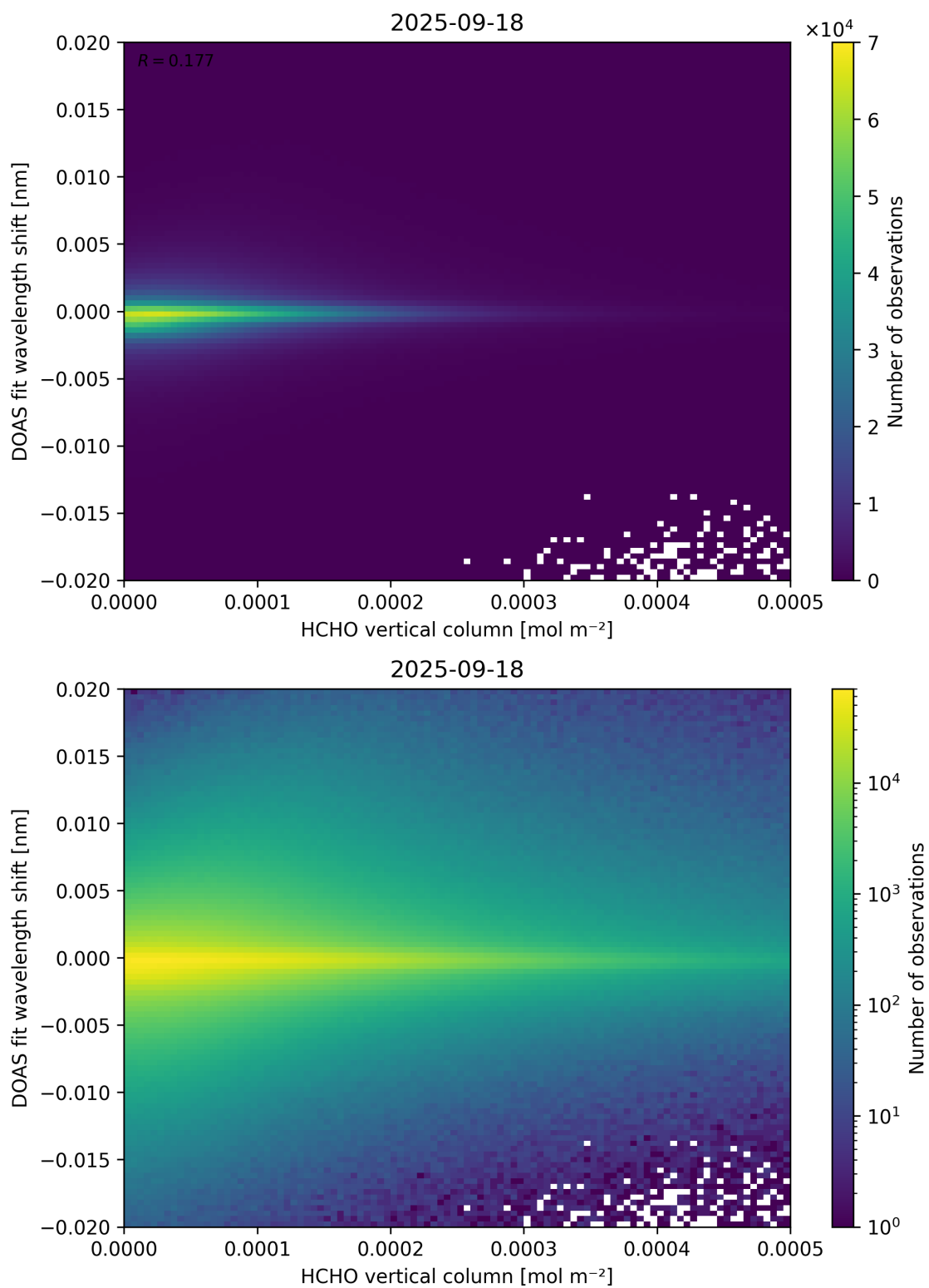
Figure 124: Scatter density plot of “HCHO vertical column” against “DOAS fit wavelength shift” for 2025-09-17 to 2025-09-19.
