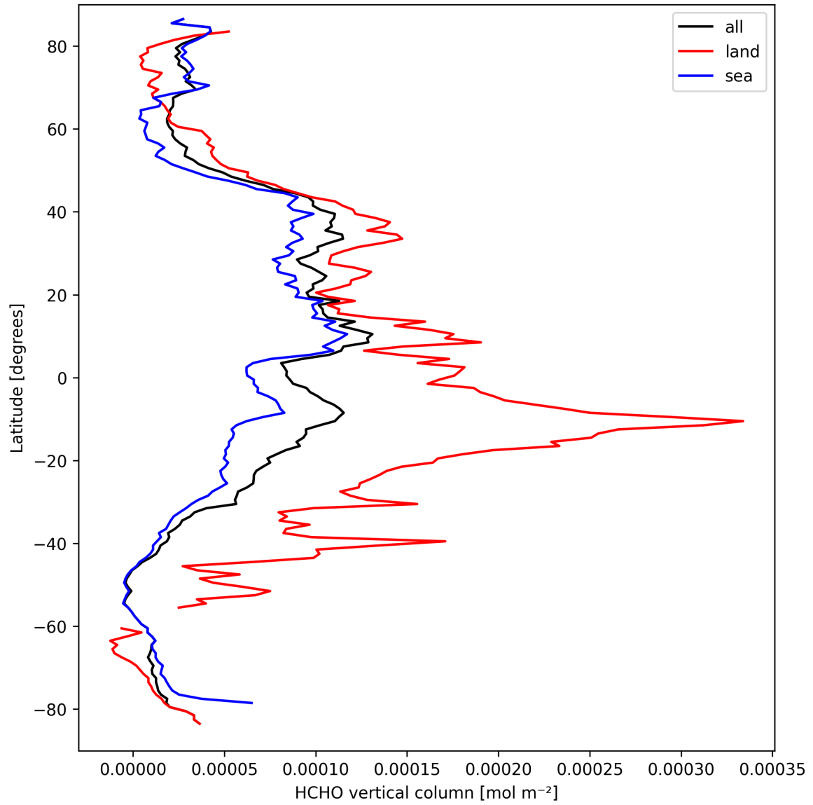
Figure 21: Zonal average of “HCHO vertical column” for 2025-09-17 to 2025-09-19.
