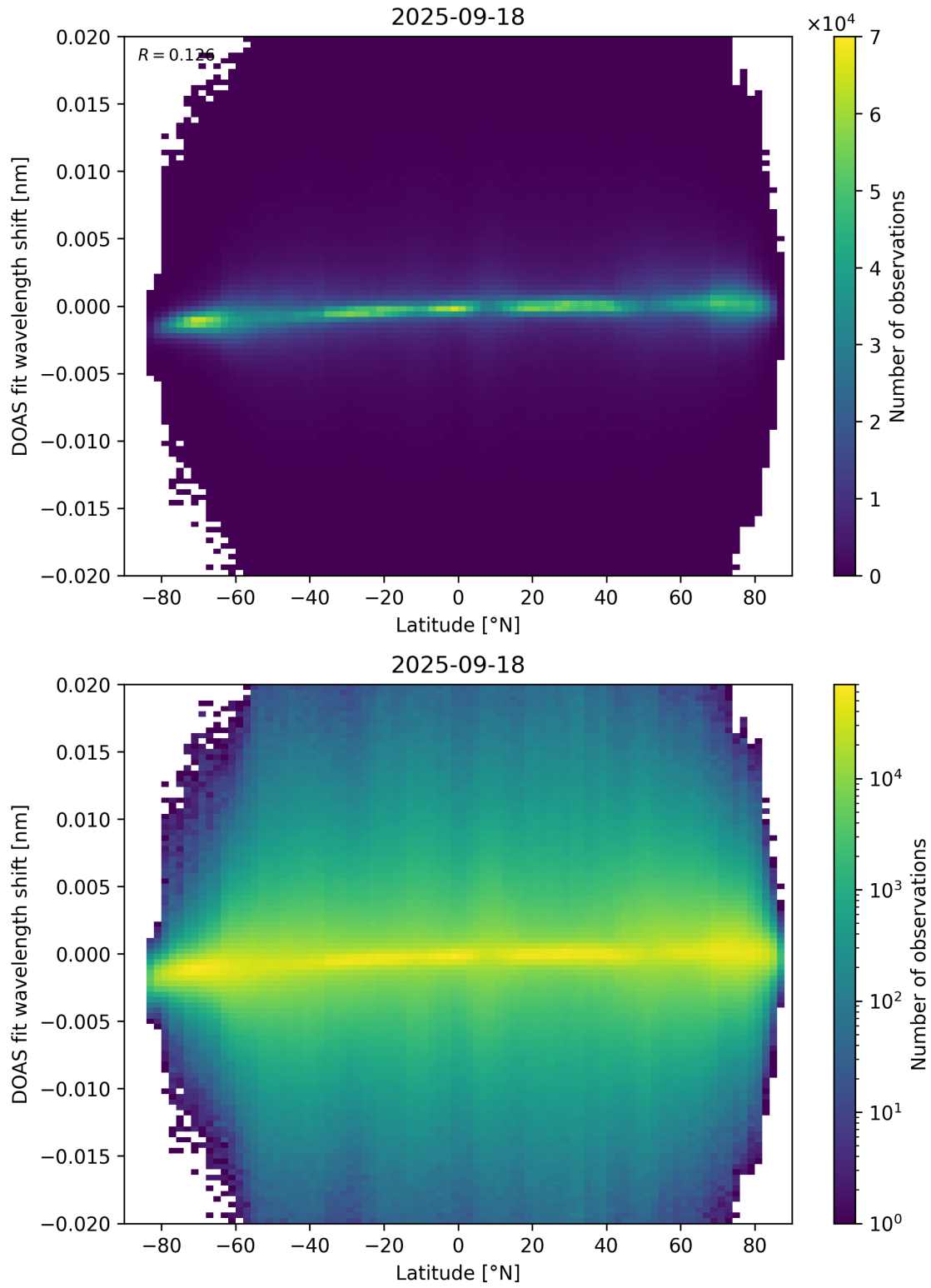
Figure 154: Scatter density plot of “Latitude” against “DOAS fit wavelength shift” for 2025-09-17 to 2025-09-19.
