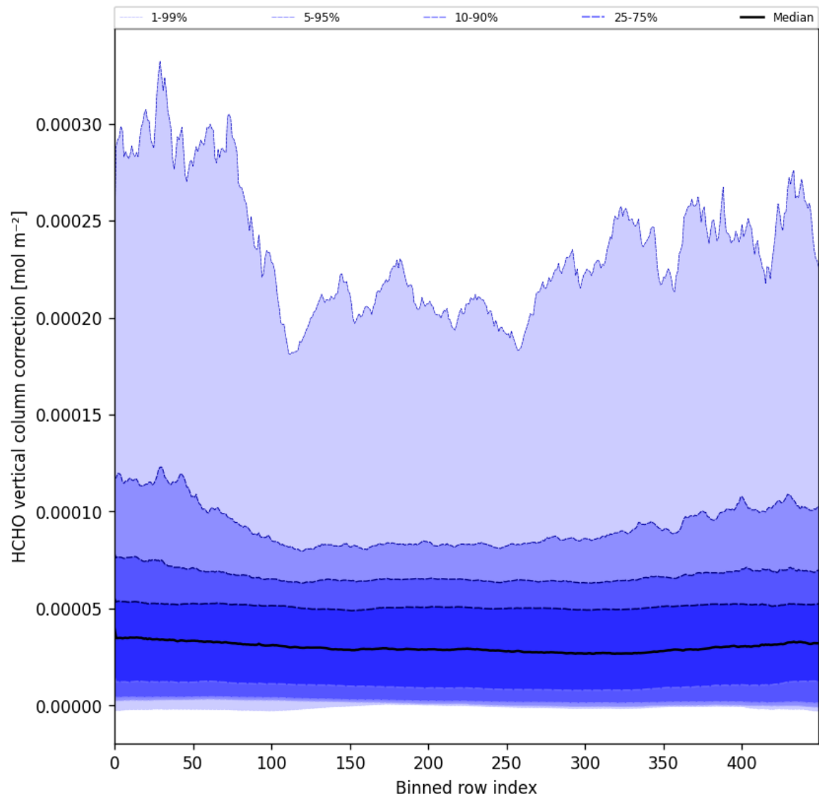
Figure 51: Along track statistics of “HCHO vertical column correction” for 2025-09-17 to 2025-09-19
