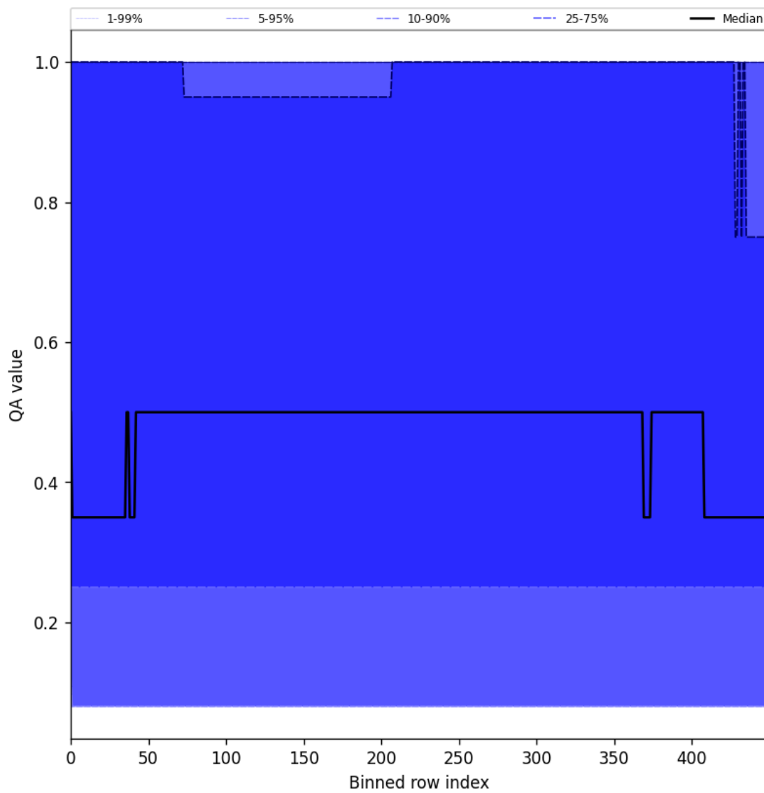
Figure 48: Along track statistics of "QA value" for 2025-09-17 to 2025-09-19
