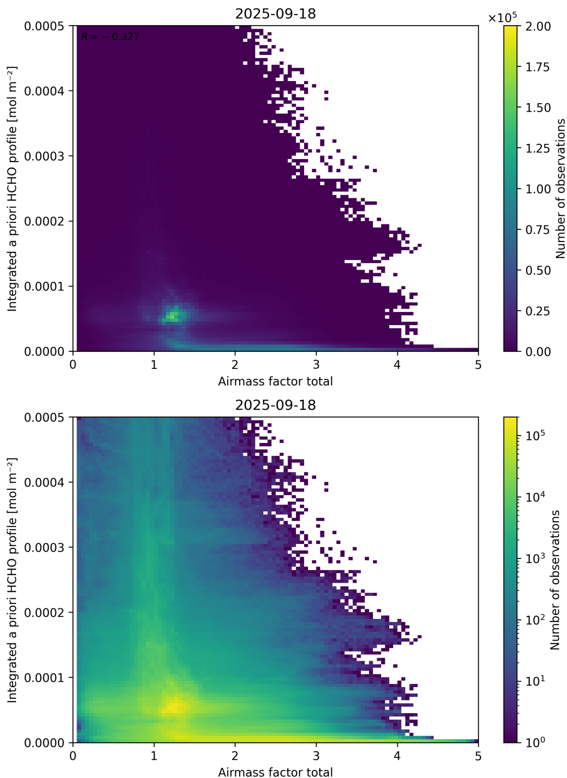
Figure 104: Scatter density plot of “Airmass factor total” against “Integrated a priori HCHO profile” for 2025-09-17 to 2025-09-19.
