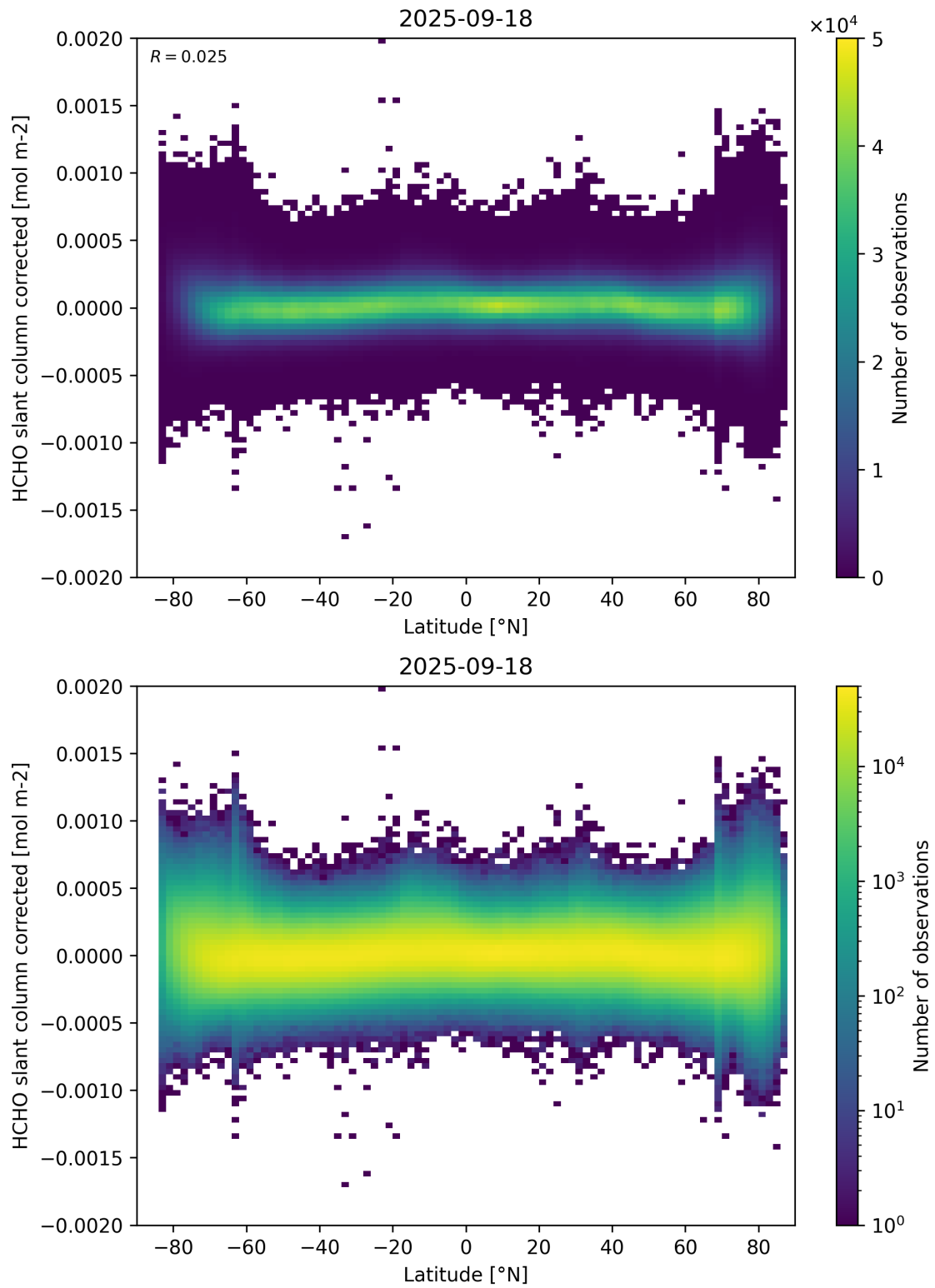
Figure 157: Scatter density plot of “Latitude” against “HCHO slant column corrected” for 2025-09-17 to 2025-09-19.
