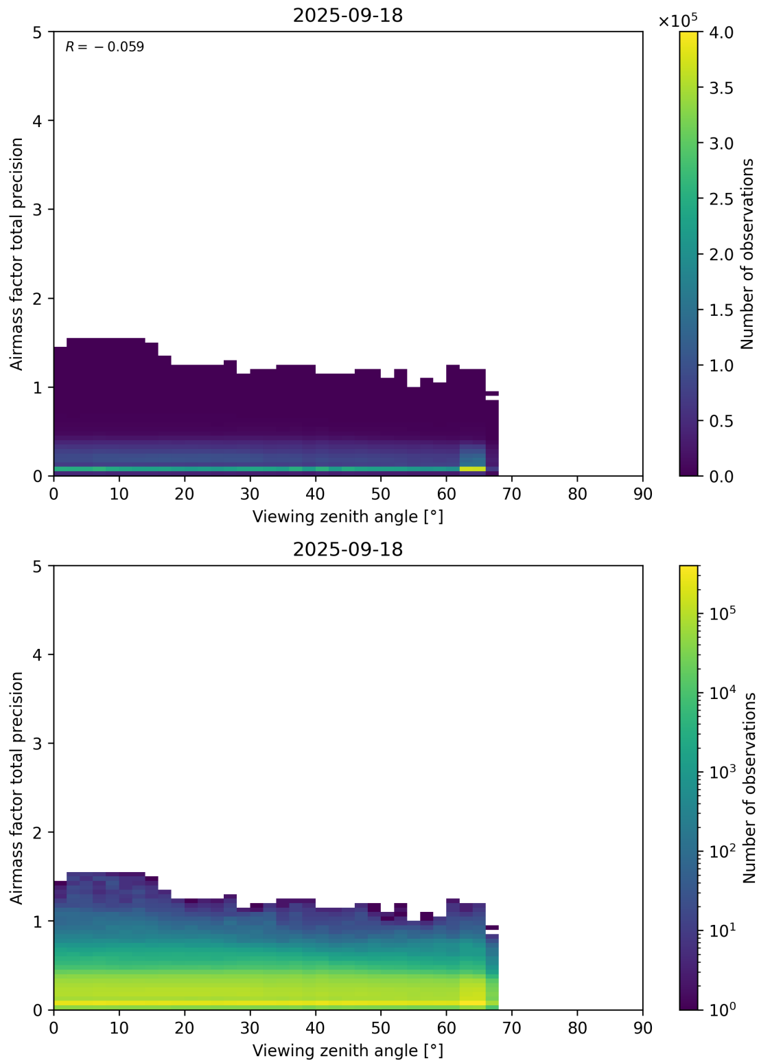
Figure 191: Scatter density plot of “Viewing zenith angle” against “Airmass factor total precision” for 2025-09-17 to 2025-09-19.
