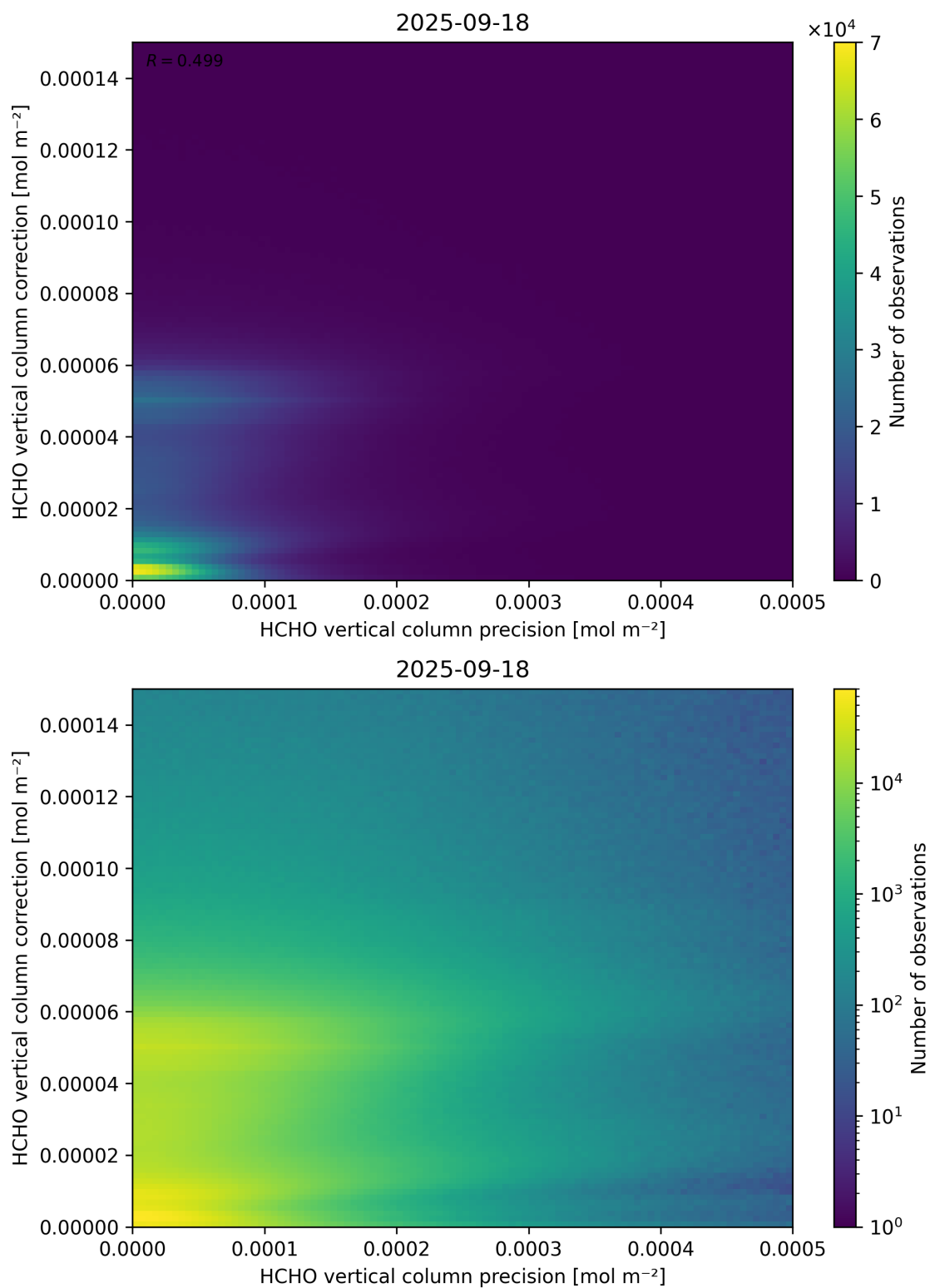
Figure 146: Scatter density plot of “HCHO vertical column precision” against “HCHO vertical column correction” for 2025-09-17 to 2025-09-19.
