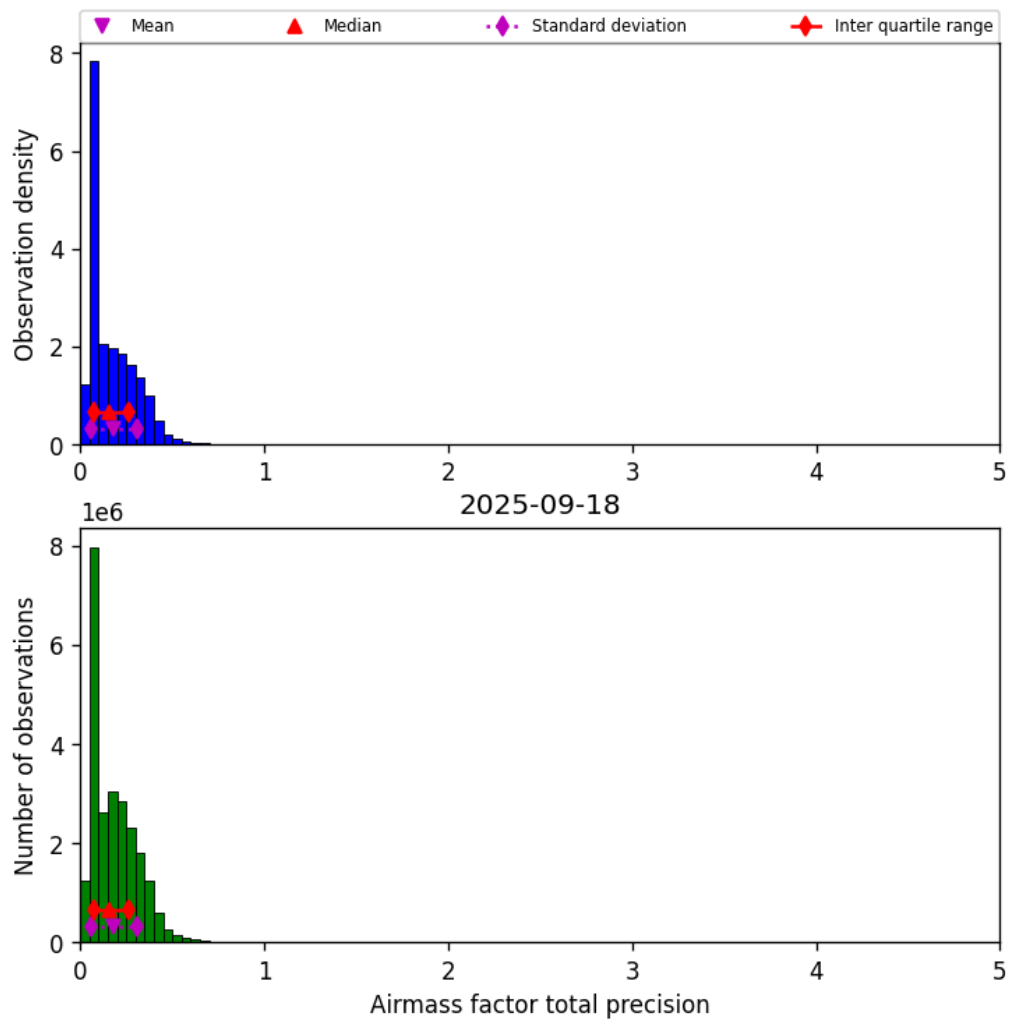
Figure 41: Histogram of “Airmass factor total precision” for 2025-09-17 to 2025-09-19
