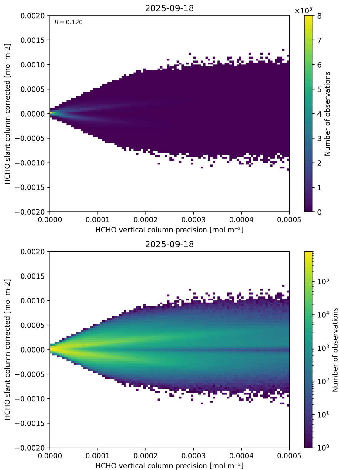
Figure 140: Scatter density plot of “HCHO vertical column precision” against “HCHO slant column corrected” for 2025-09-17 to 2025-09-19.
