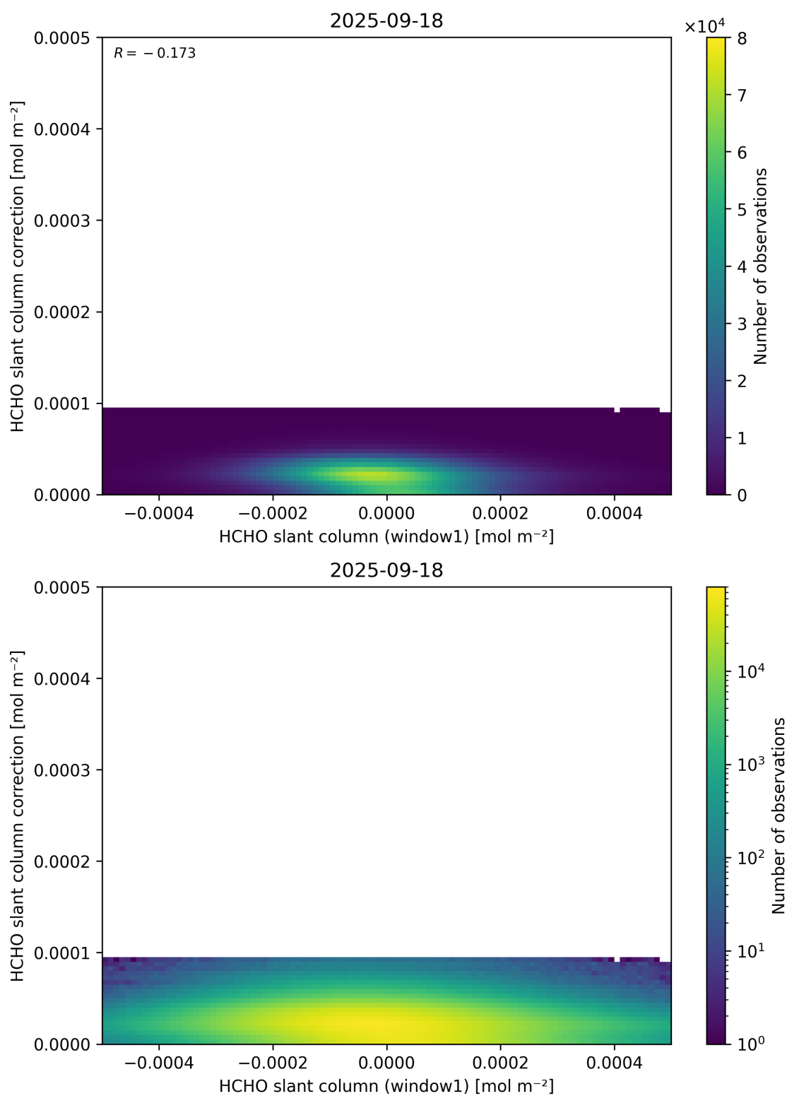
Figure 83: Scatter density plot of “HCHO slant column (window1)” against “HCHO slant column correction” for 2025-09-17 to 2025-09-19.
