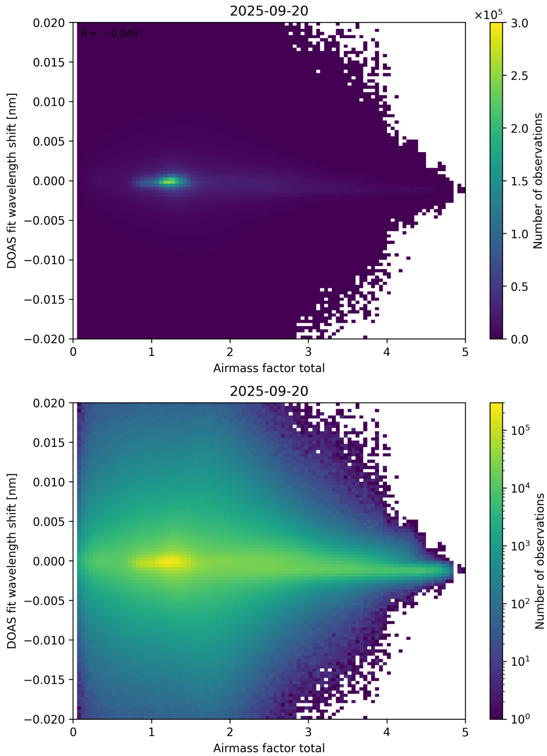
Figure 98: Scatter density plot of “Airmass factor total” against “DOAS fit wavelength shift” for 2025-09-20 to 2025-09-21.
