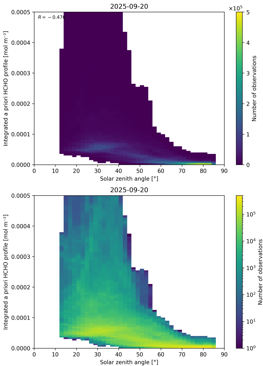
Figure 180: Scatter density plot of “Solar zenith angle” against “Integrated a priori HCHO profile” for 2025-09-20 to 2025-09-21.
