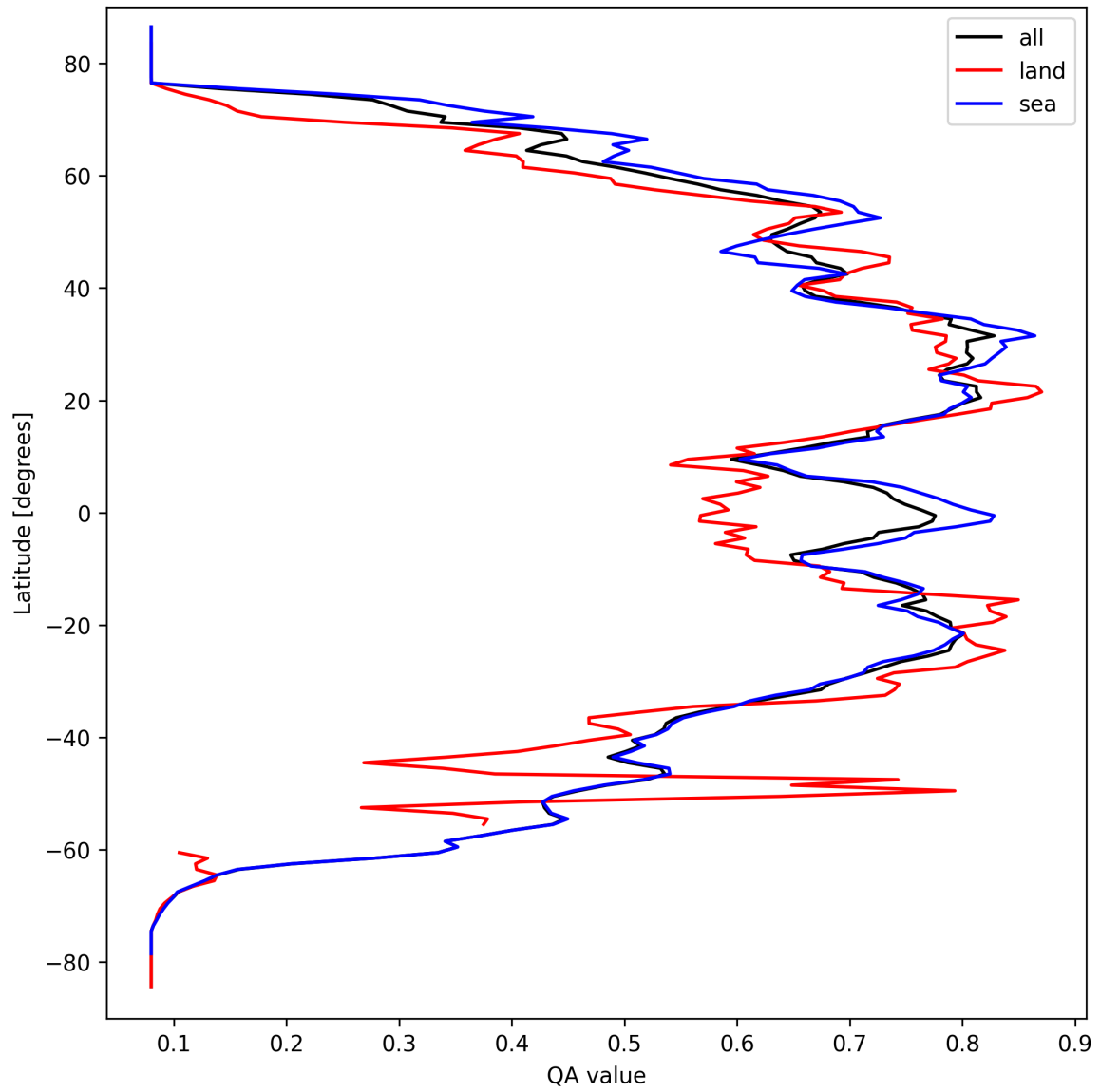
Figure 20: Zonal average of “QA value” for 2025-09-20 to 2025-09-21.
