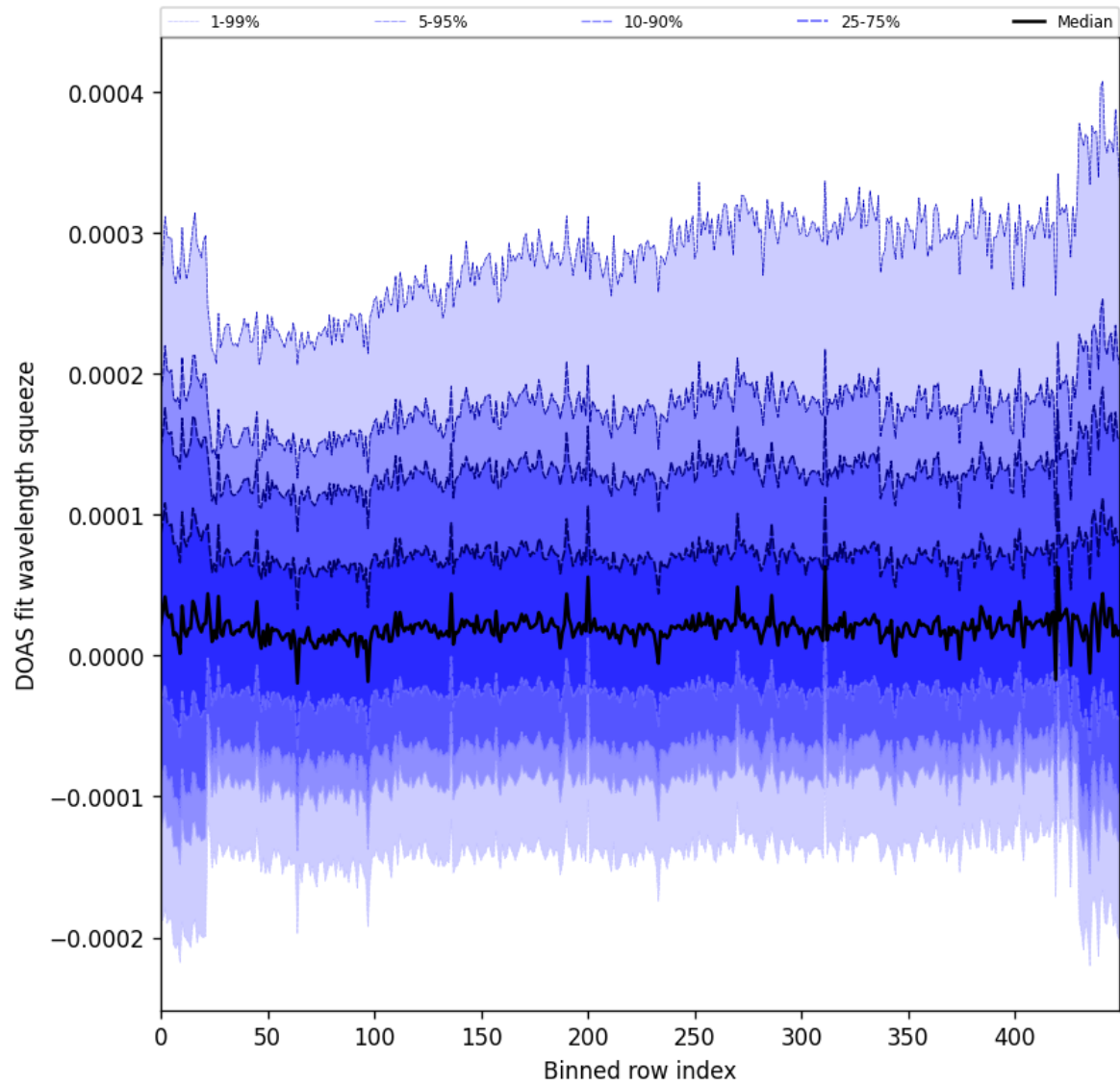
Figure 59: Along track statistics of “DOAS fit wavelength squeeze” for 2025-09-20 to 2025-09-21
