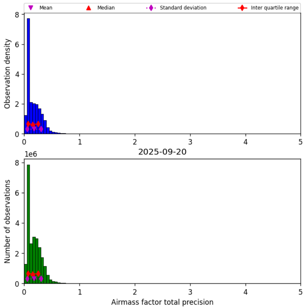
Figure 41: Histogram of “Airmass factor total precision” for 2025-09-20 to 2025-09-21
