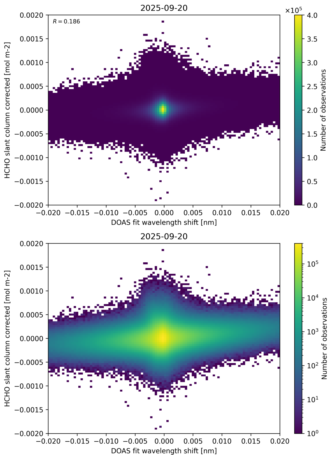
Figure 66: Scatter density plot of “DOAS fit wavelength shift” against “HCHO slant column corrected” for 2025-09-20 to 2025-09-21.
