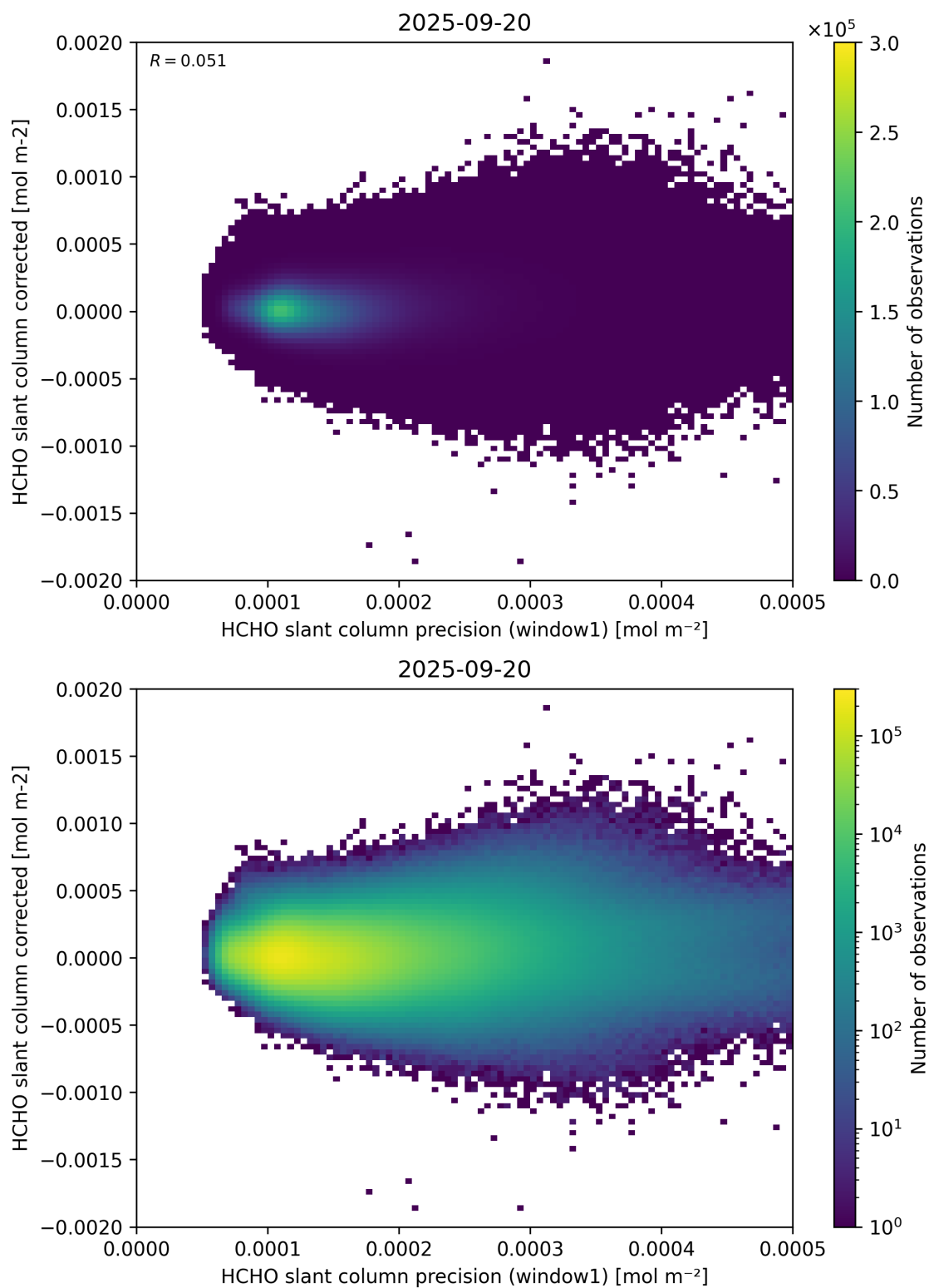
Figure 92: Scatter density plot of “HCHO slant column precision (window1)” against “HCHO slant column corrected” for 2025-09-20 to 2025-09-21.
