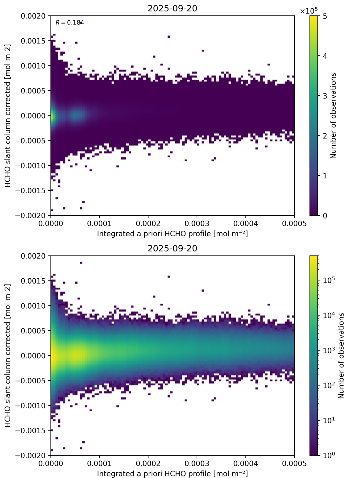
Figure 151: Scatter density plot of “Integrated a priori HCHO profile” against “HCHO slant column corrected” for 2025-09-20 to 2025-09-21.
