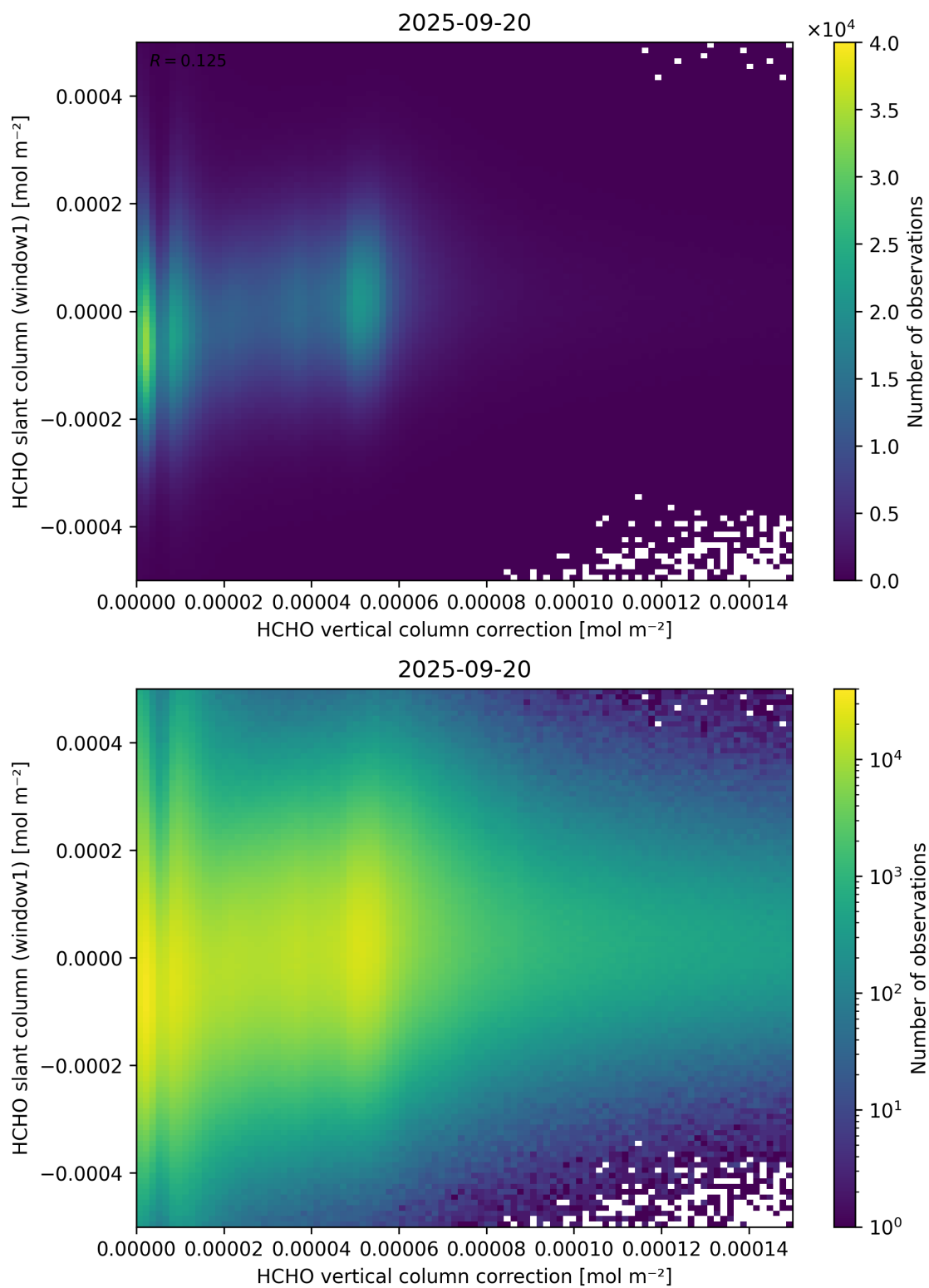
Figure 118: Scatter density plot of “HCHO vertical column correction” against “HCHO slant column (window1)” for 2025-09-20 to 2025-09-21.
