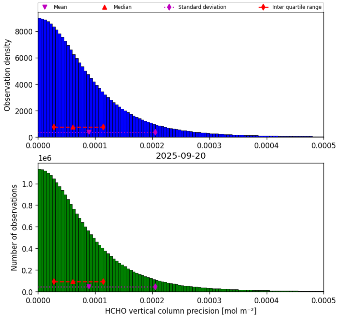
Figure 36: Histogram of “HCHO vertical column precision” for 2025-09-20 to 2025-09-21
