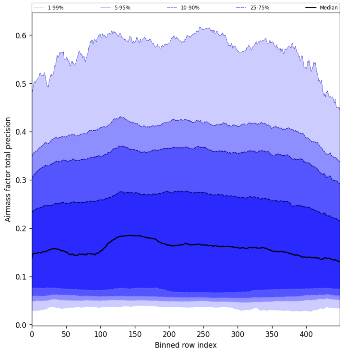
Figure 55: Along track statistics of “Airmass factor total precision” for 2025-09-20 to 2025-09-21
