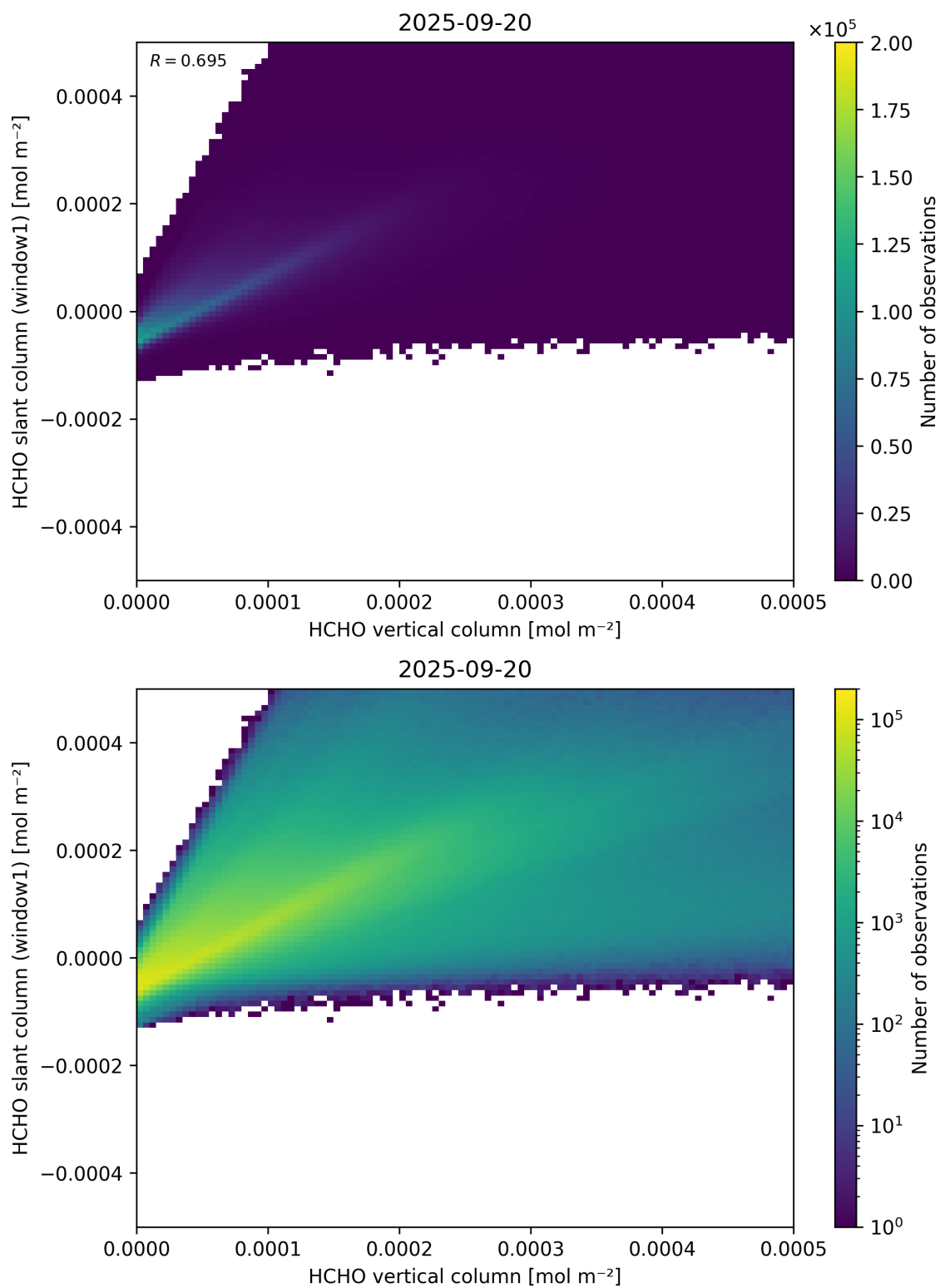
Figure 129: Scatter density plot of “HCHO vertical column” against “HCHO slant column (window1)” for 2025-09-20 to 2025-09-21.
