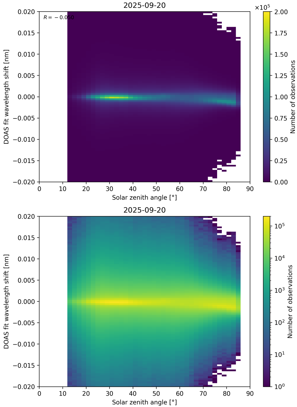
Figure 168: Scatter density plot of “Solar zenith angle” against “DOAS fit wavelength shift” for 2025-09-20 to 2025-09-21.
