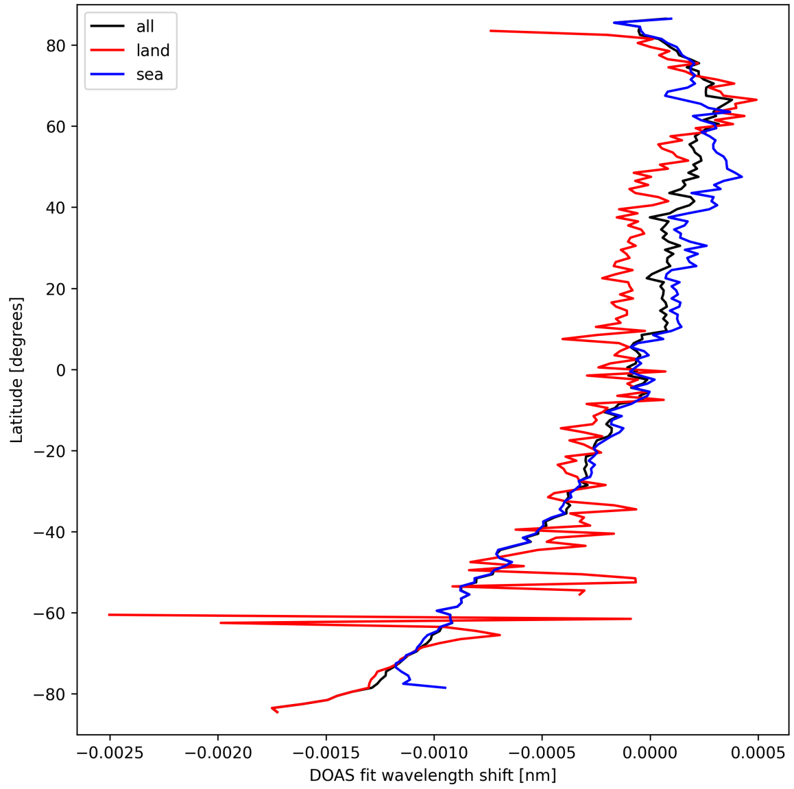
Figure 30: Zonal average of “DOAS fit wavelength shift” for 2025-09-20 to 2025-09-21.
