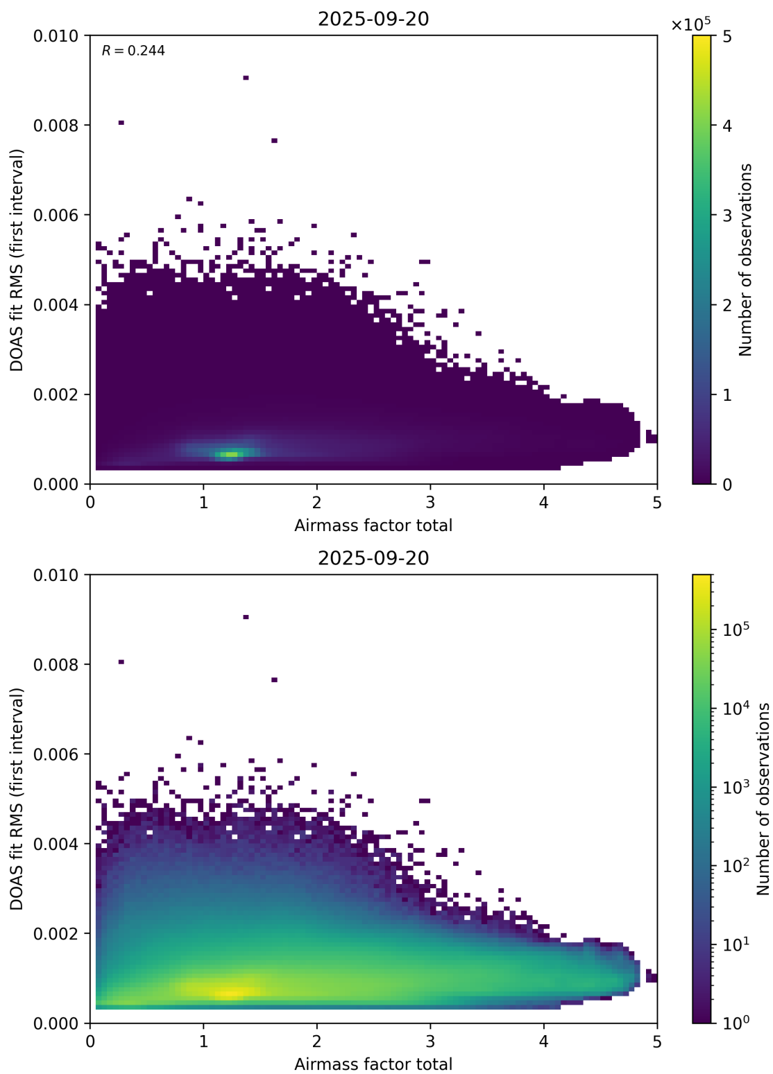
Figure 97: Scatter density plot of “Airmass factor total” against “DOAS fit RMS (first interval)” for 2025-09-20 to 2025-09-21.
