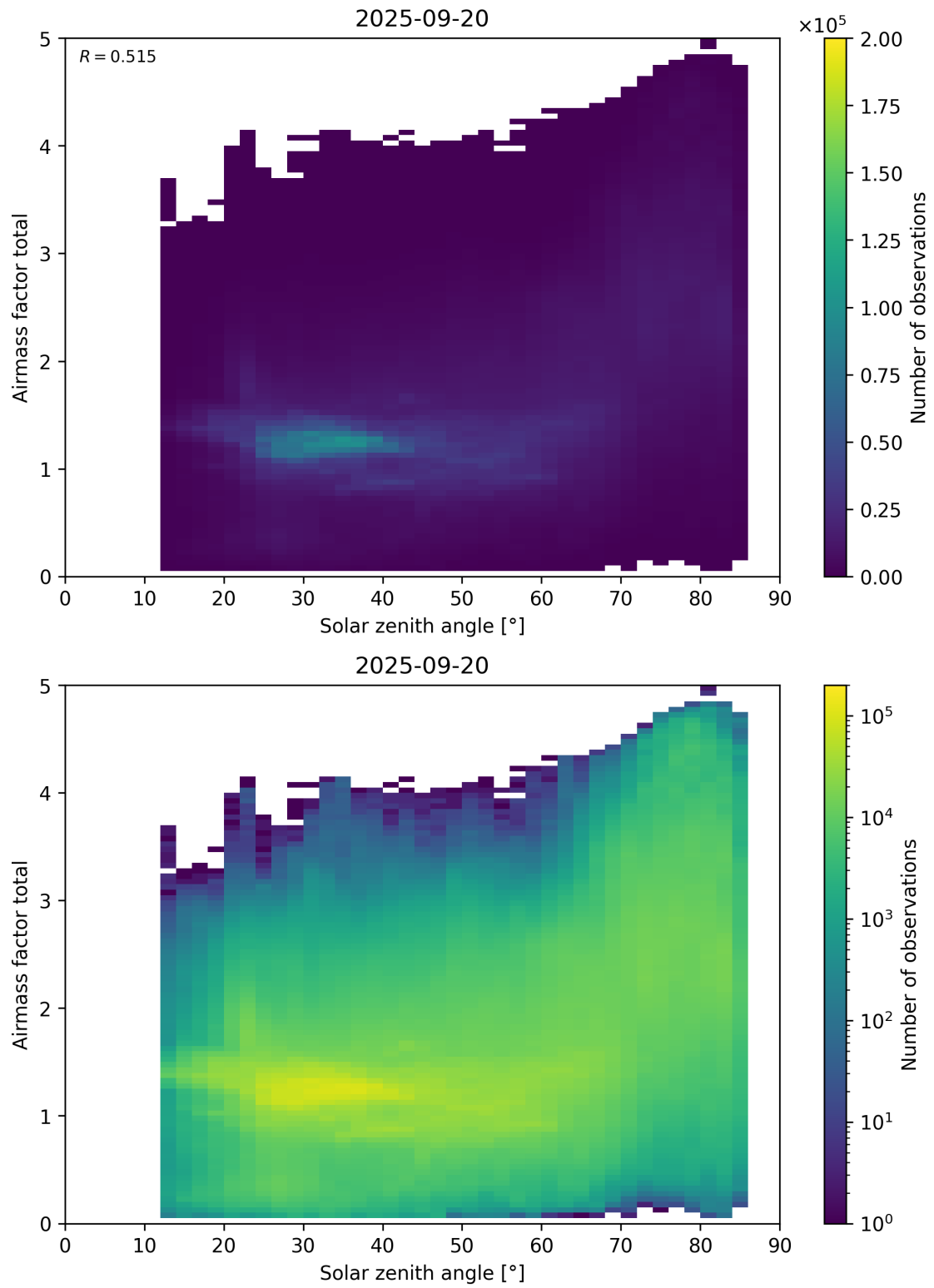
Figure 175: Scatter density plot of “Solar zenith angle” against “Airmass factor total” for 2025-09-20 to 2025-09-21.
