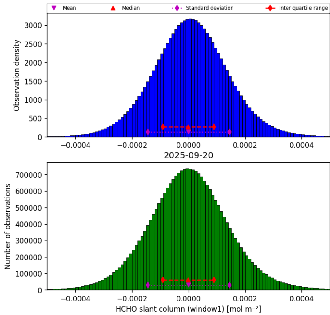
Figure 38: Histogram of “HCHO slant column (window1)” for 2025-09-20 to 2025-09-21
