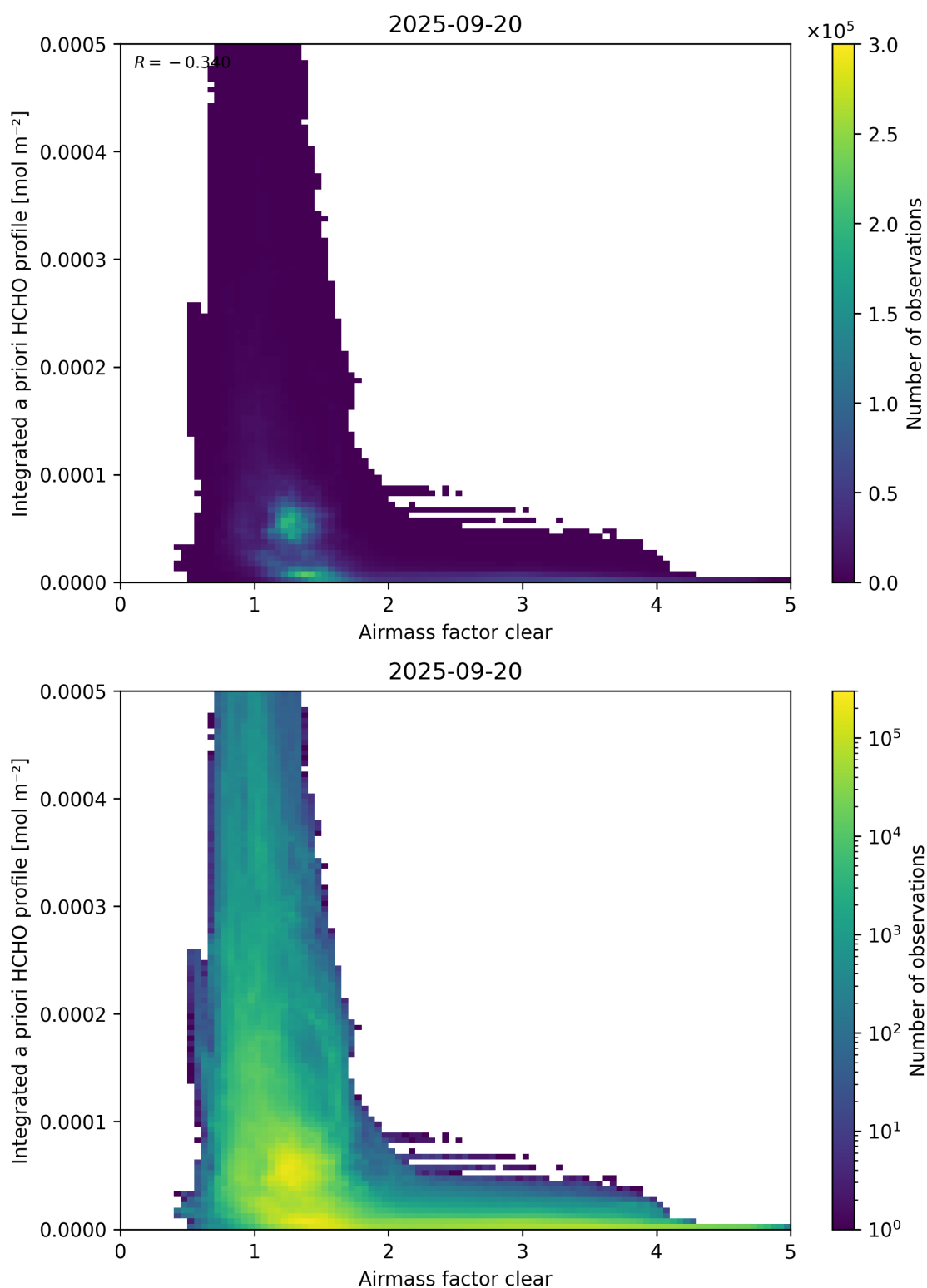
Figure 76: Scatter density plot of “Airmass factor clear” against “Integrated a priori HCHO profile” for 2025-09-20 to 2025-09-21.
