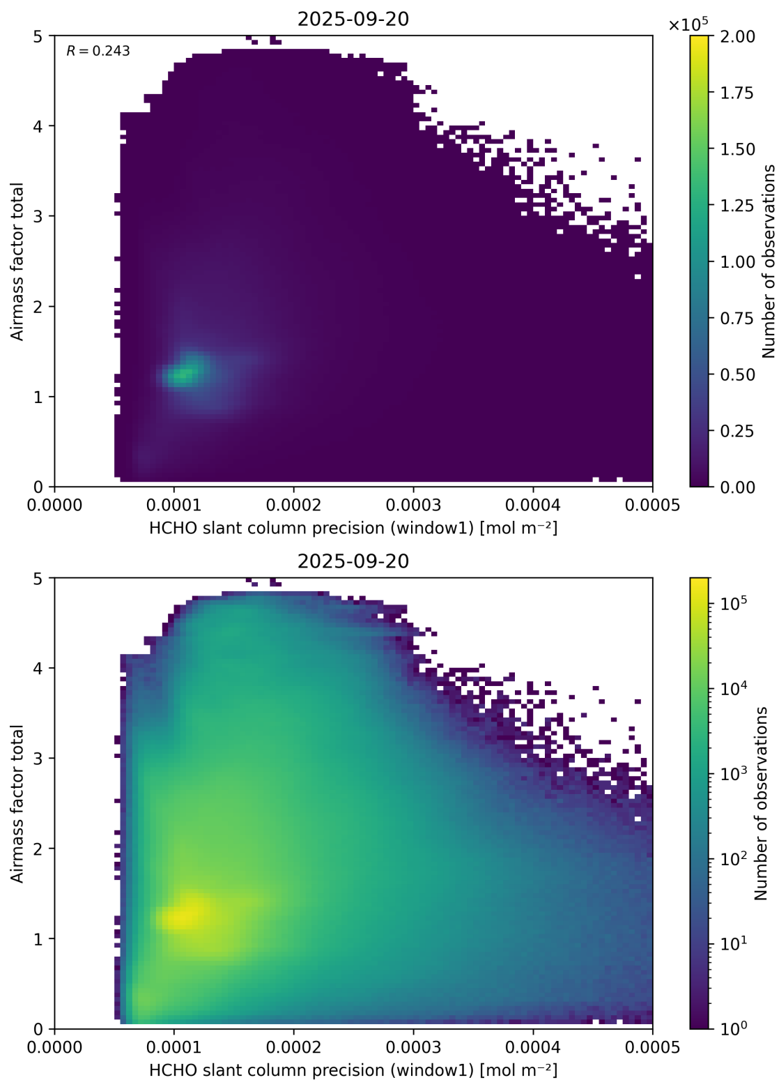
Figure 94: Scatter density plot of “HCHO slant column precision (window1)” against “Airmass factor total” for 2025-09-20 to 2025-09-21.
