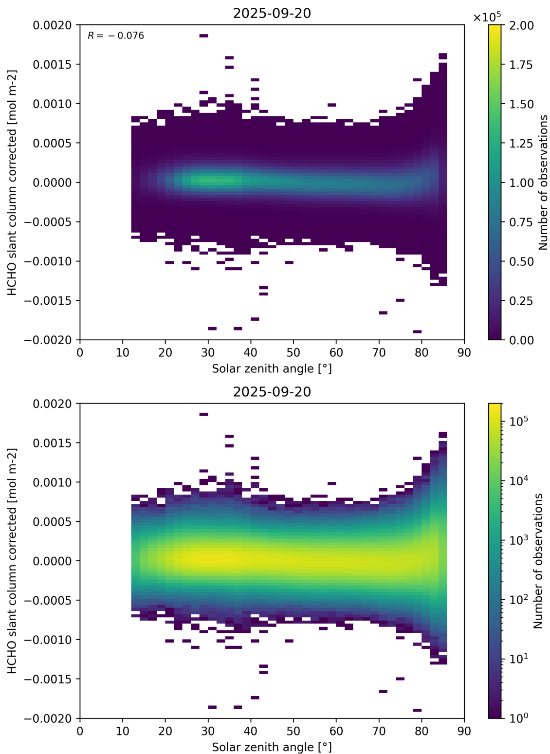
Figure 171: Scatter density plot of “Solar zenith angle” against “HCHO slant column corrected” for 2025-09-20 to 2025-09-21.
