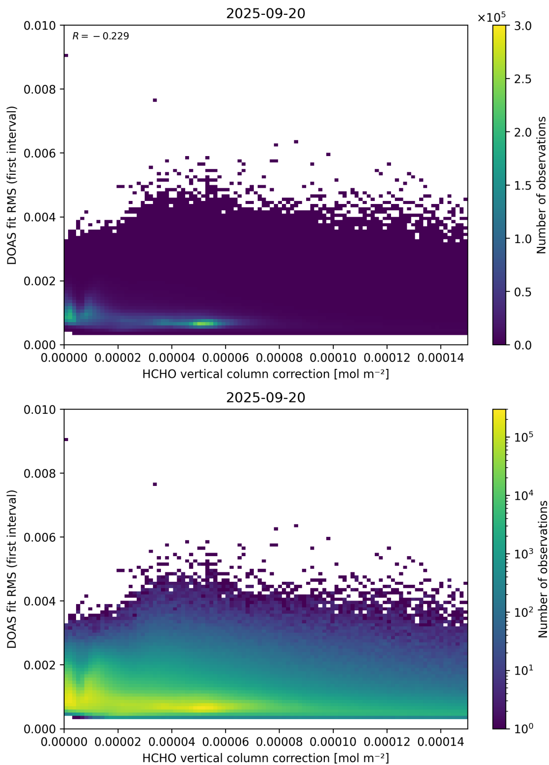
Figure 112: Scatter density plot of “HCHO vertical column correction” against “DOAS fit RMS (first interval)” for 2025-09-20 to 2025-09-21.
