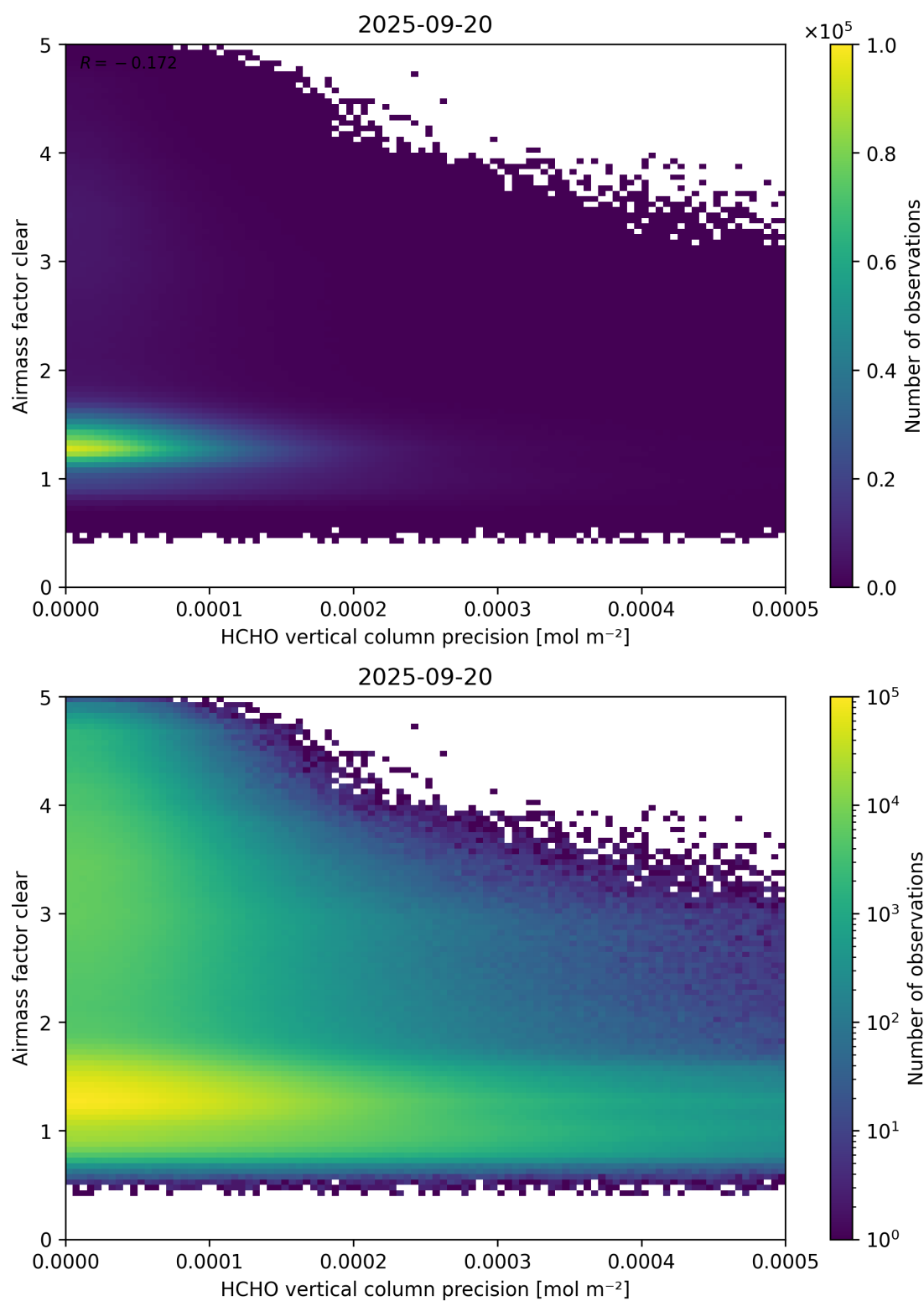
Figure 139: Scatter density plot of “HCHO vertical column precision” against “Airmass factor clear” for 2025-09-20 to 2025-09-21.
