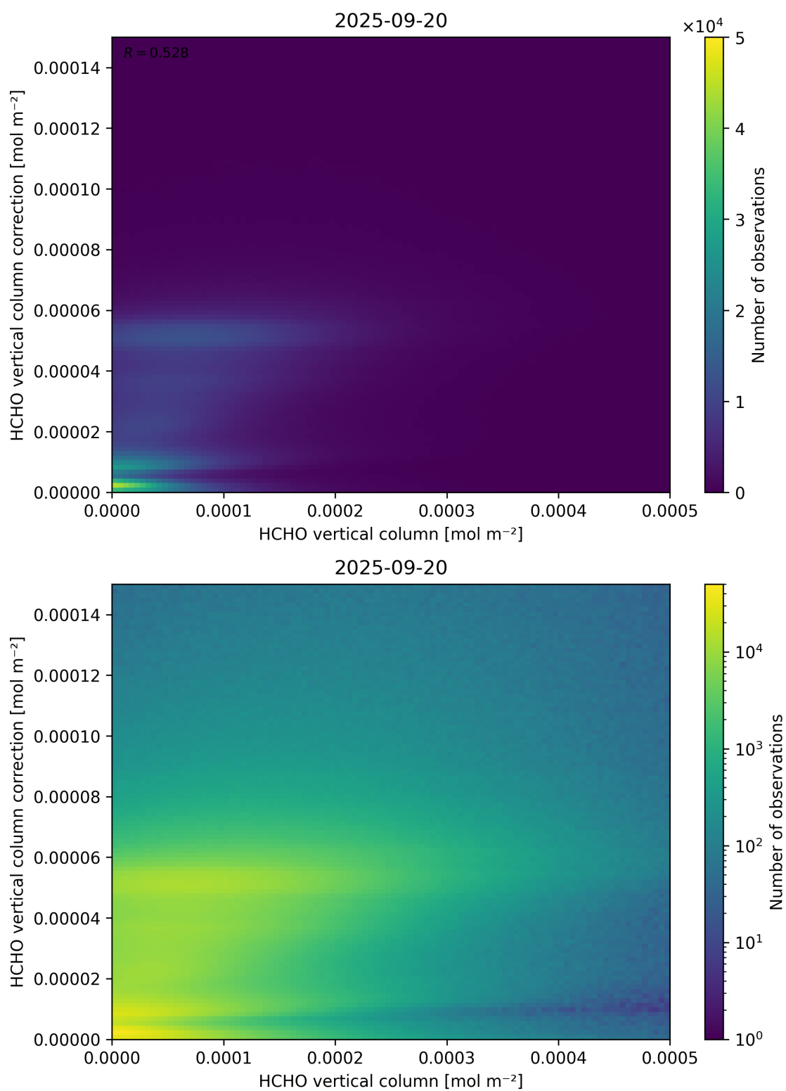
Figure 133: Scatter density plot of “HCHO vertical column” against “HCHO vertical column correction” for 2025-09-20 to 2025-09-21.
