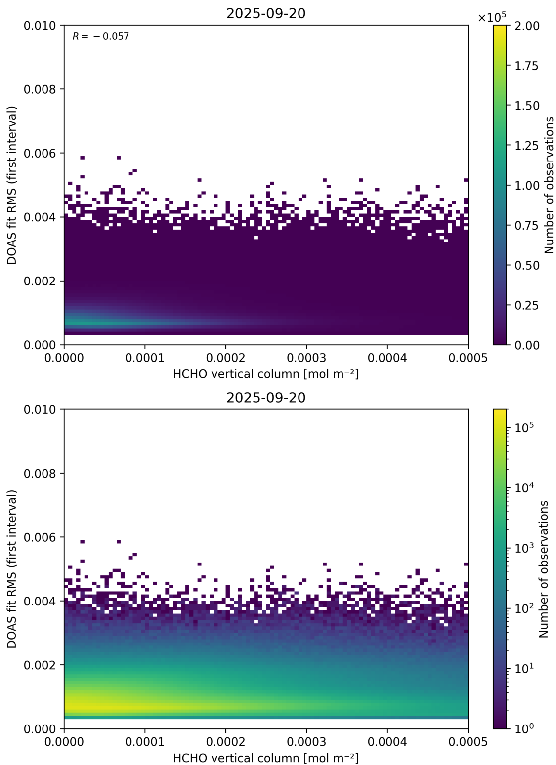
Figure 123: Scatter density plot of “HCHO vertical column” against “DOAS fit RMS (first interval)” for 2025-09-20 to 2025-09-21.
