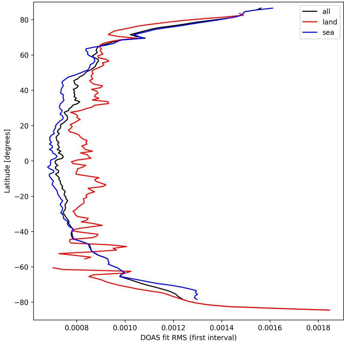
Figure 32: Zonal average of “DOAS fit RMS (first interval)” for 2025-09-20 to 2025-09-21.
