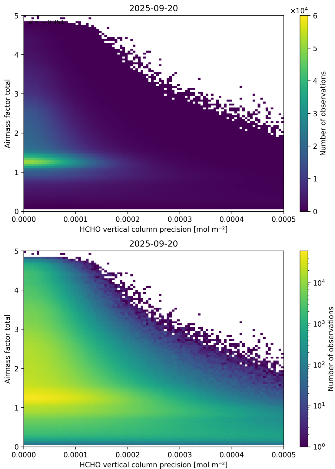
Figure 144: Scatter density plot of “HCHO vertical column precision” against “Airmass factor total” for 2025-09-20 to 2025-09-21.
