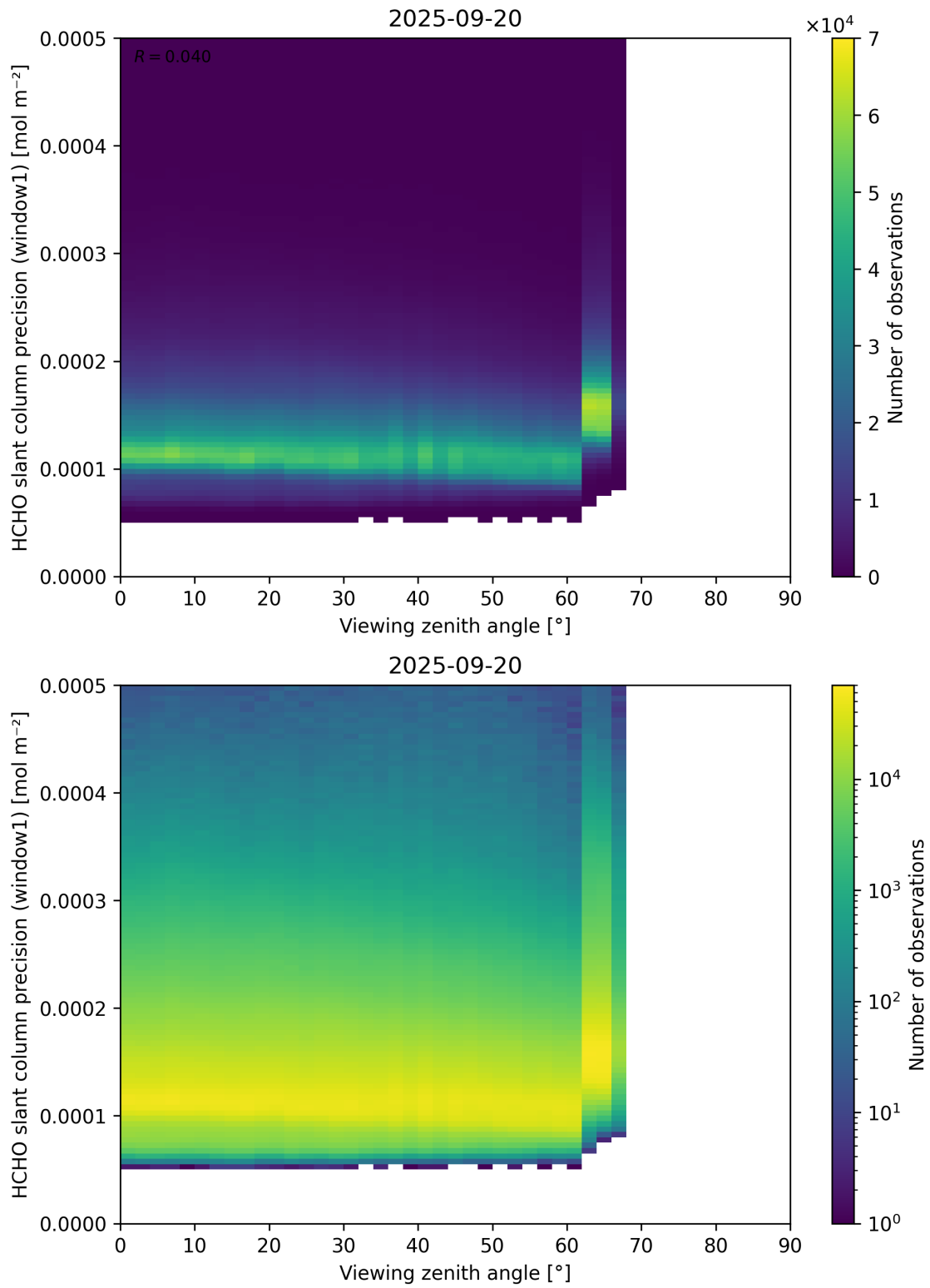
Figure 189: Scatter density plot of “Viewing zenith angle” against “HCHO slant column precision (window1)” for 2025-09-20 to 2025-09-21.
