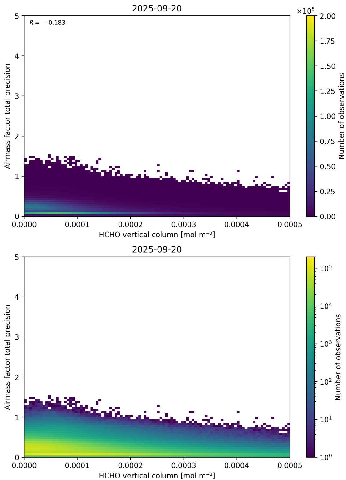
Figure 132: Scatter density plot of “HCHO vertical column” against “Airmass factor total precision” for 2025-09-20 to 2025-09-21.
