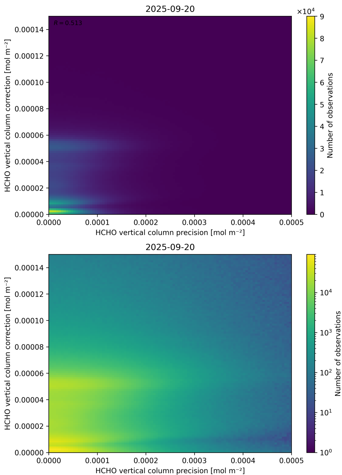
Figure 146: Scatter density plot of “HCHO vertical column precision” against “HCHO vertical column correction” for 2025-09-20 to 2025-09-21.
