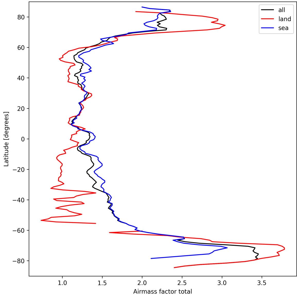
Figure 26: Zonal average of “Airmass factor total” for 2025-09-20 to 2025-09-21.
