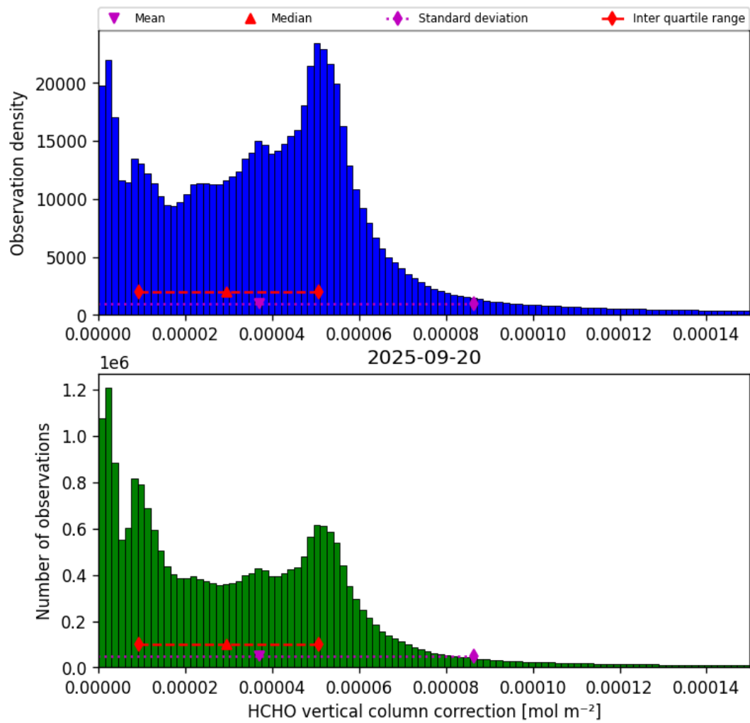
Figure 37: Histogram of “HCHO vertical column correction” for 2025-09-20 to 2025-09-21
