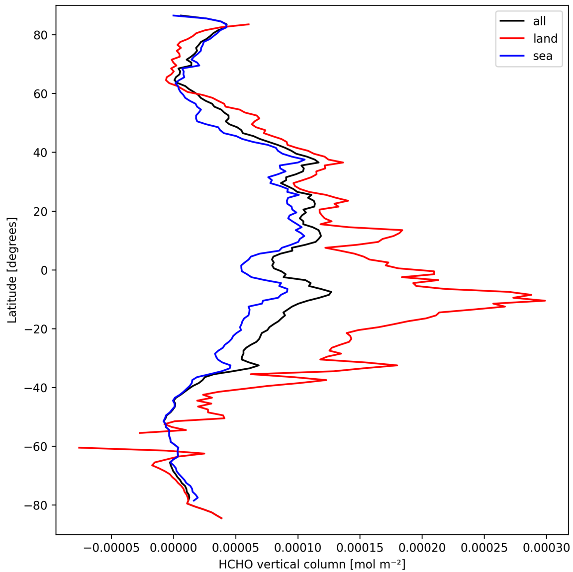
Figure 21: Zonal average of “HCHO vertical column” for 2025-09-20 to 2025-09-21.
