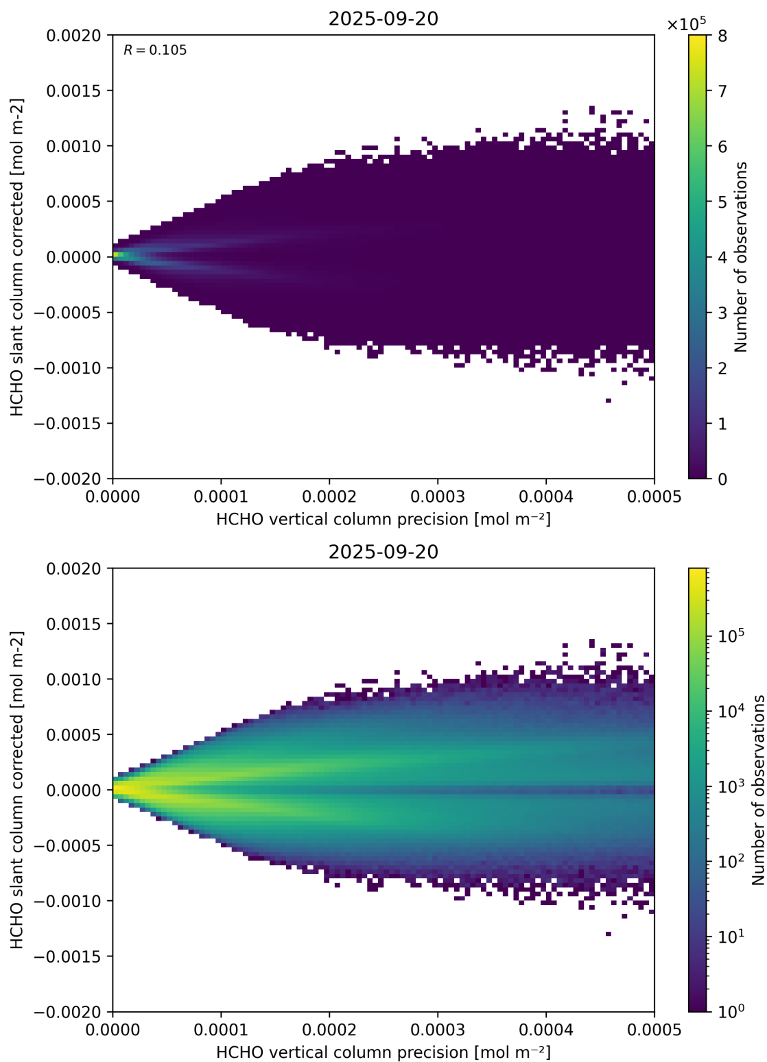
Figure 140: Scatter density plot of “HCHO vertical column precision” against “HCHO slant column corrected” for 2025-09-20 to 2025-09-21.
