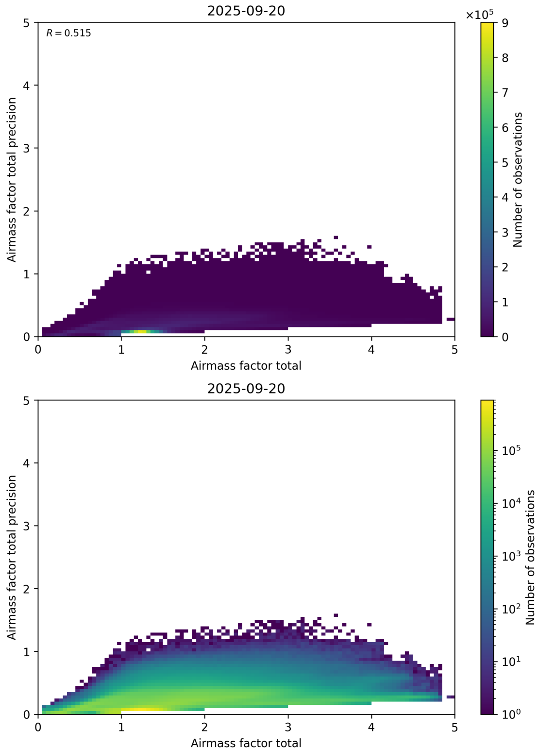
Figure 103: Scatter density plot of “Airmass factor total” against “Airmass factor total precision” for 2025-09-20 to 2025-09-21.
