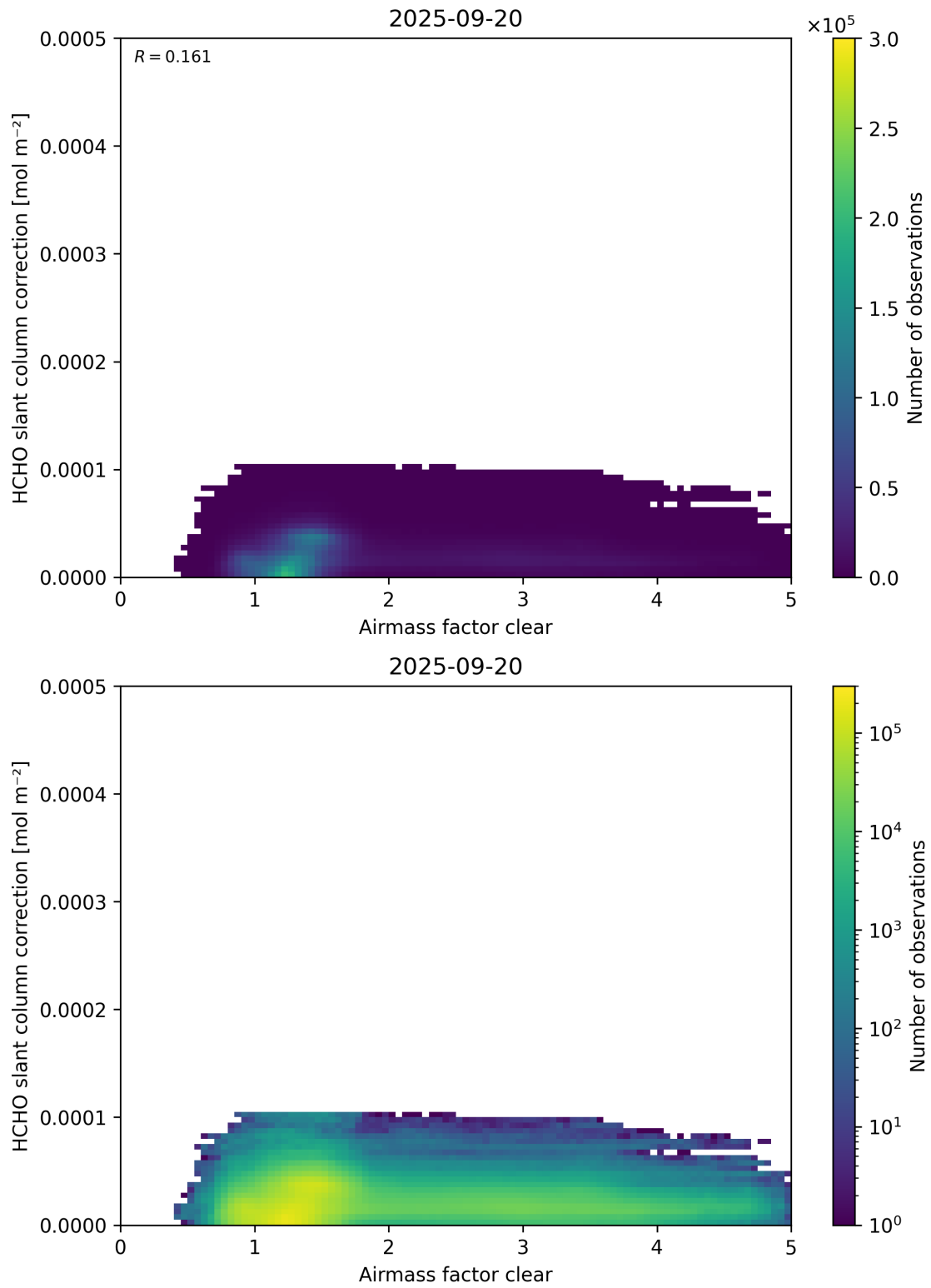
Figure 75: Scatter density plot of “Airmass factor clear” against “HCHO slant column correction” for 2025-09-20 to 2025-09-21.
