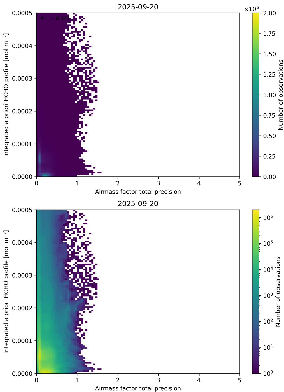
Figure 111: Scatter density plot of “Airmass factor total precision” against “Integrated a priori HCHO profile” for 2025-09-20 to 2025-09-21.
