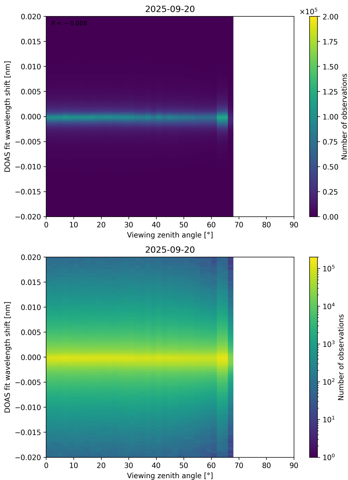
Figure 183: Scatter density plot of “Viewing zenith angle” against “DOAS fit wavelength shift” for 2025-09-20 to 2025-09-21.
