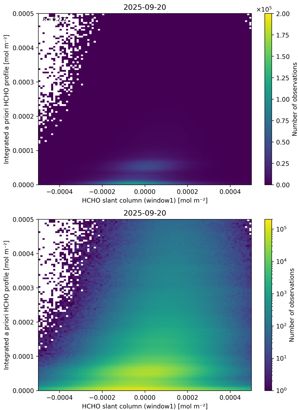
Figure 87: Scatter density plot of “HCHO slant column (window1)” against “Integrated a priori HCHO profile” for 2025-09-20 to 2025-09-21.
