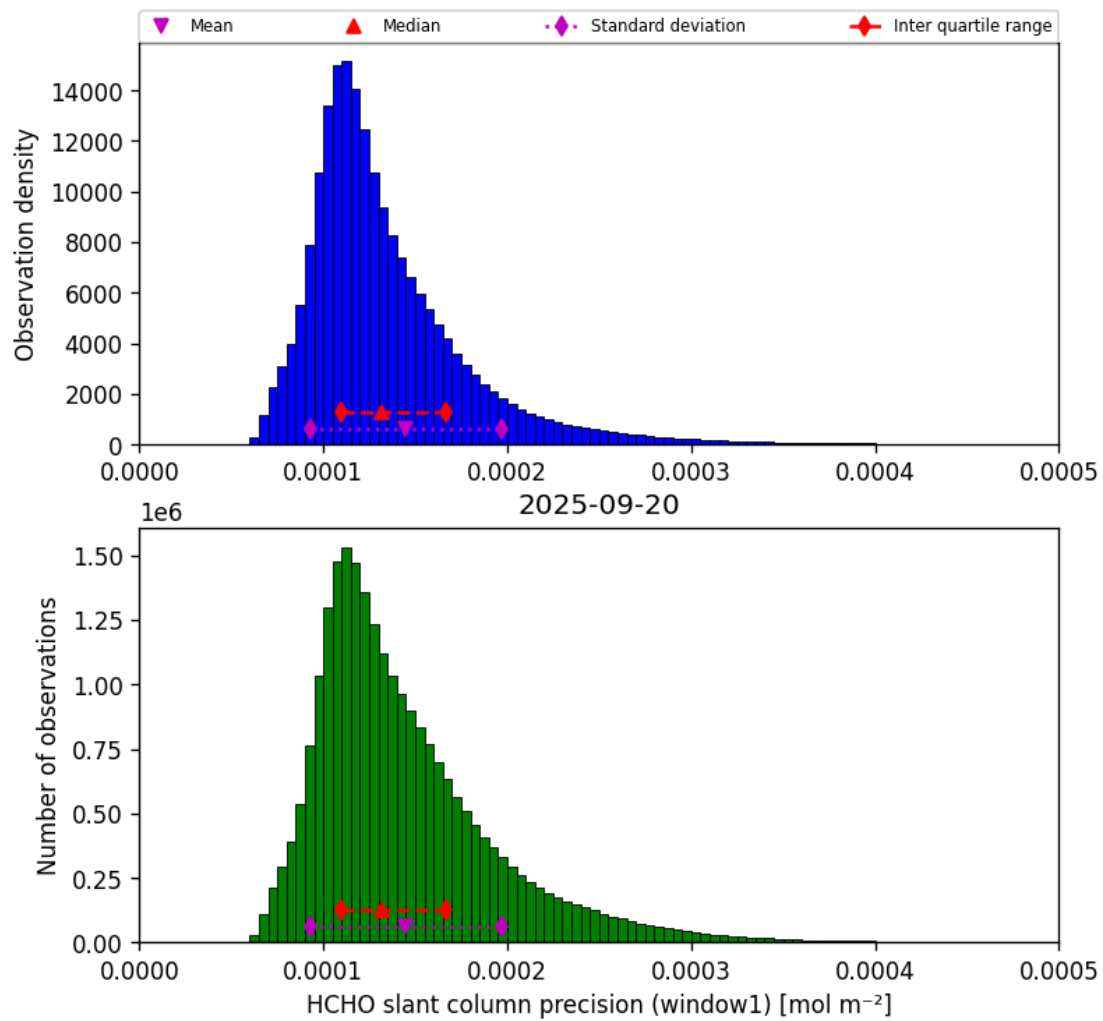
Figure 39: Histogram of “HCHO slant column precision (window1)” for 2025-09-20 to 2025-09-21
