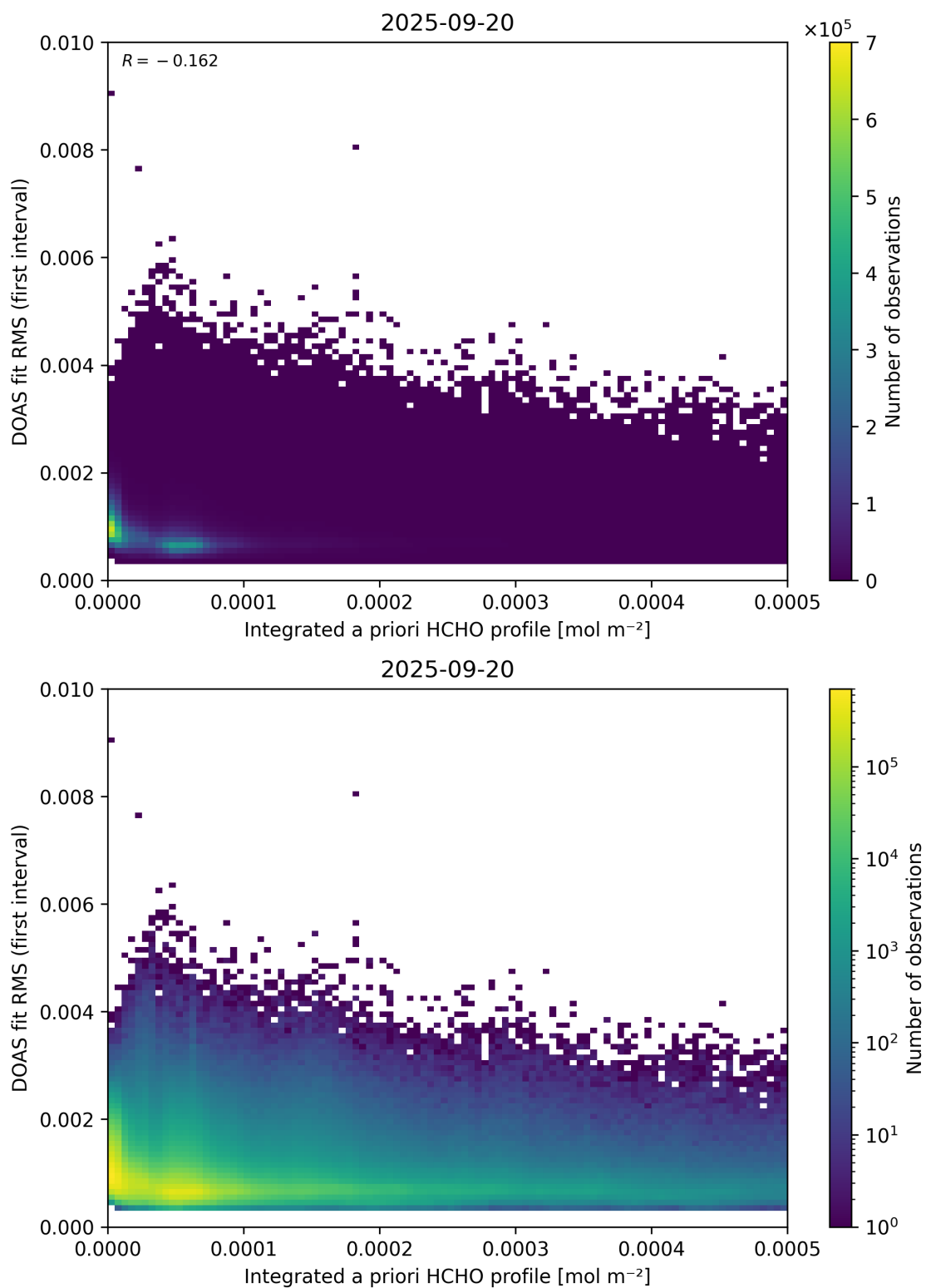
Figure 148: Scatter density plot of “Integrated a priori HCHO profile” against “DOAS fit RMS (first interval)” for 2025-09-20 to 2025-09-21.
