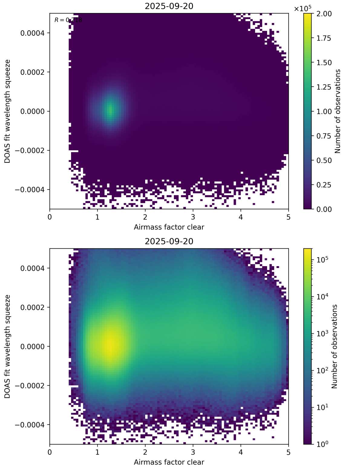
Figure 73: Scatter density plot of “Airmass factor clear” against “DOAS fit wavelength squeeze” for 2025-09-20 to 2025-09-21.
