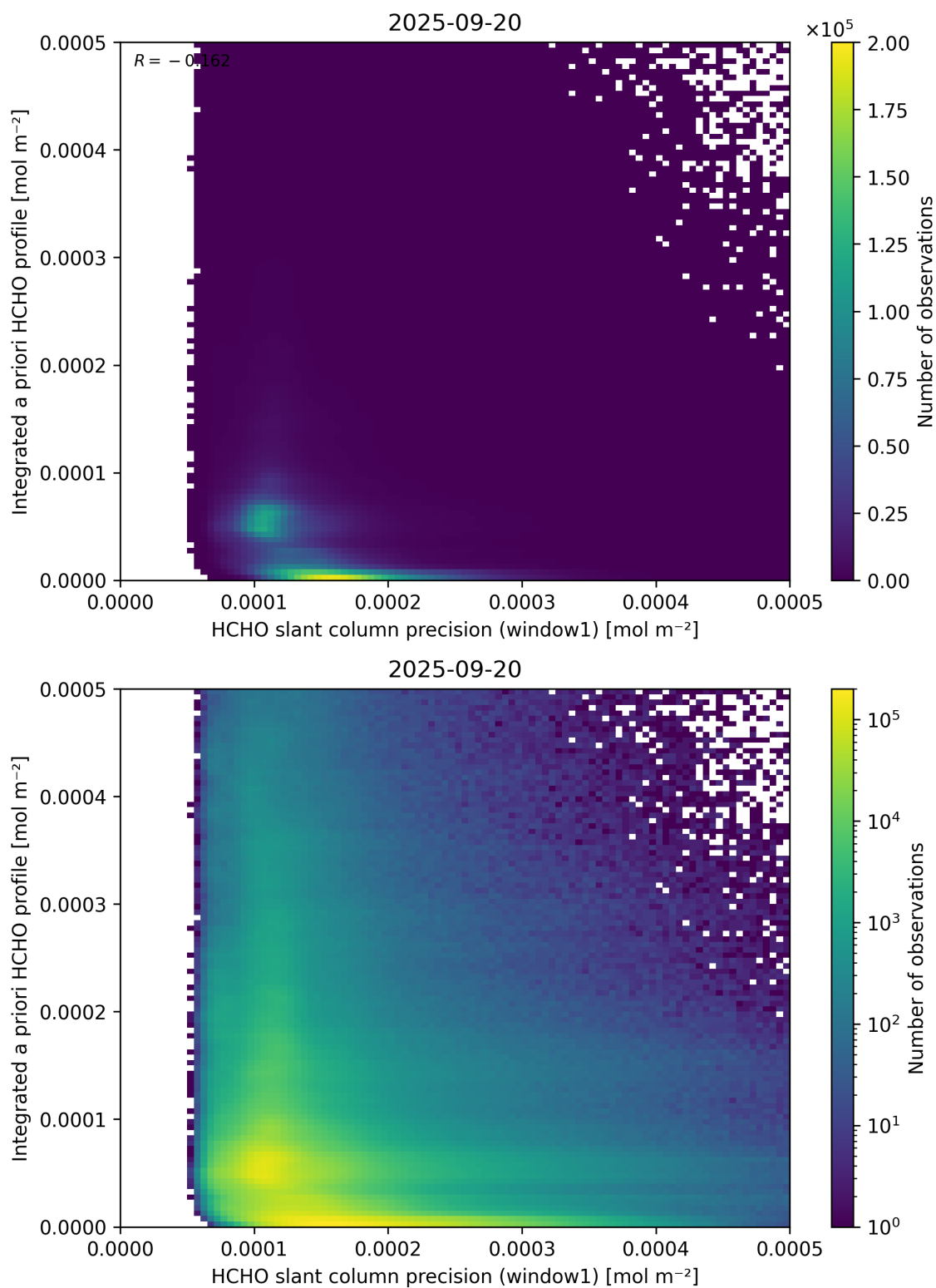
Figure 96: Scatter density plot of “HCHO slant column precision (window1)” against “Integrated a priori HCHO profile” for 2025-09-20 to 2025-09-21.
