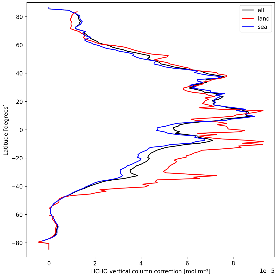
Figure 23: Zonal average of “HCHO vertical column correction” for 2025-09-20 to 2025-09-21.
