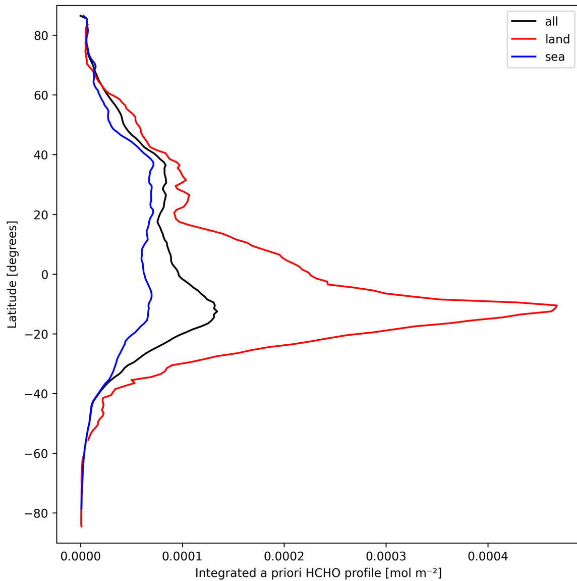
Figure 29: Zonal average of “Integrated a priori HCHO profile” for 2025-09-20 to 2025-09-21.
