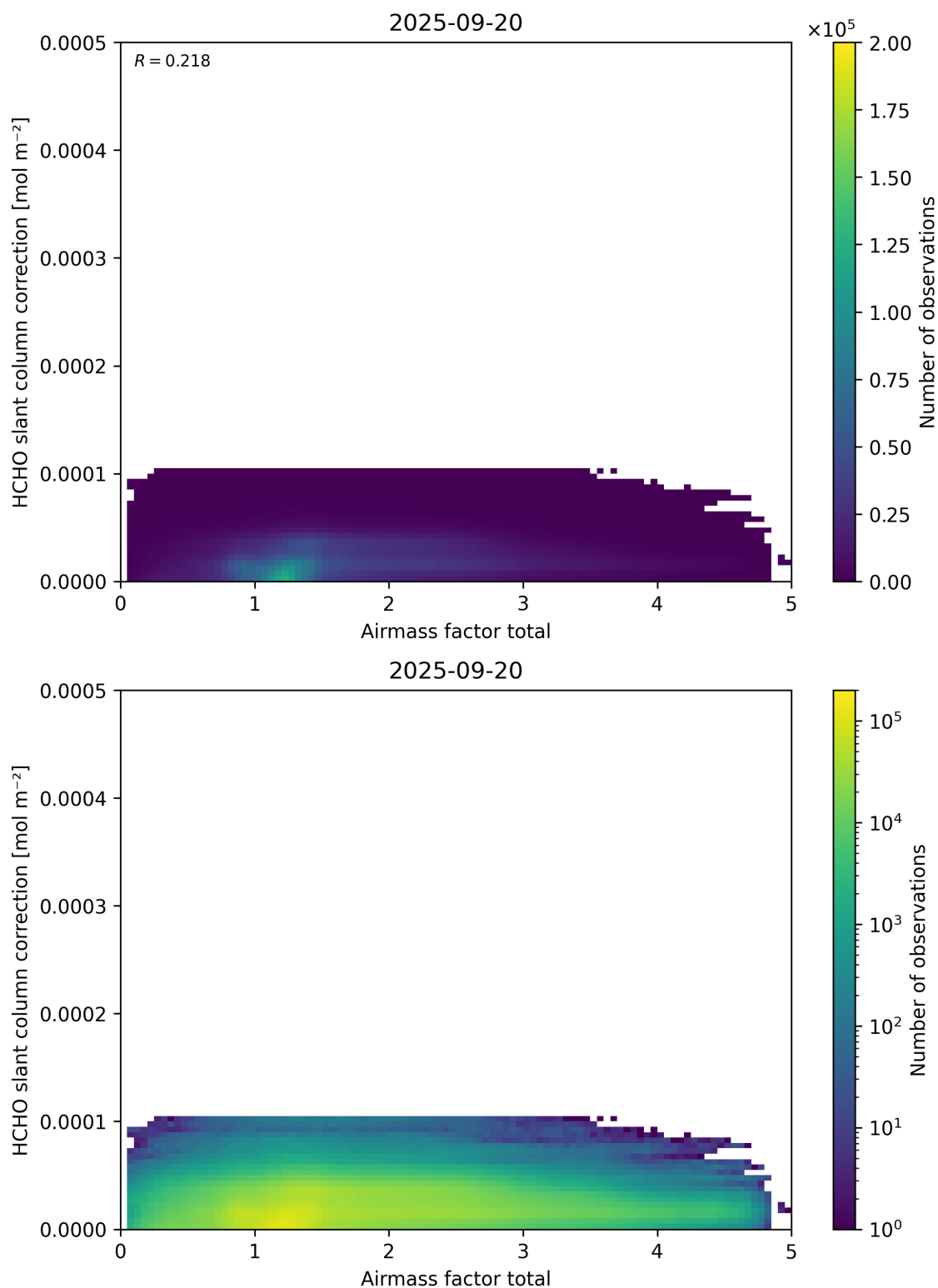
Figure 102: Scatter density plot of “Airmass factor total” against “HCHO slant column correction” for 2025-09-20 to 2025-09-21.
