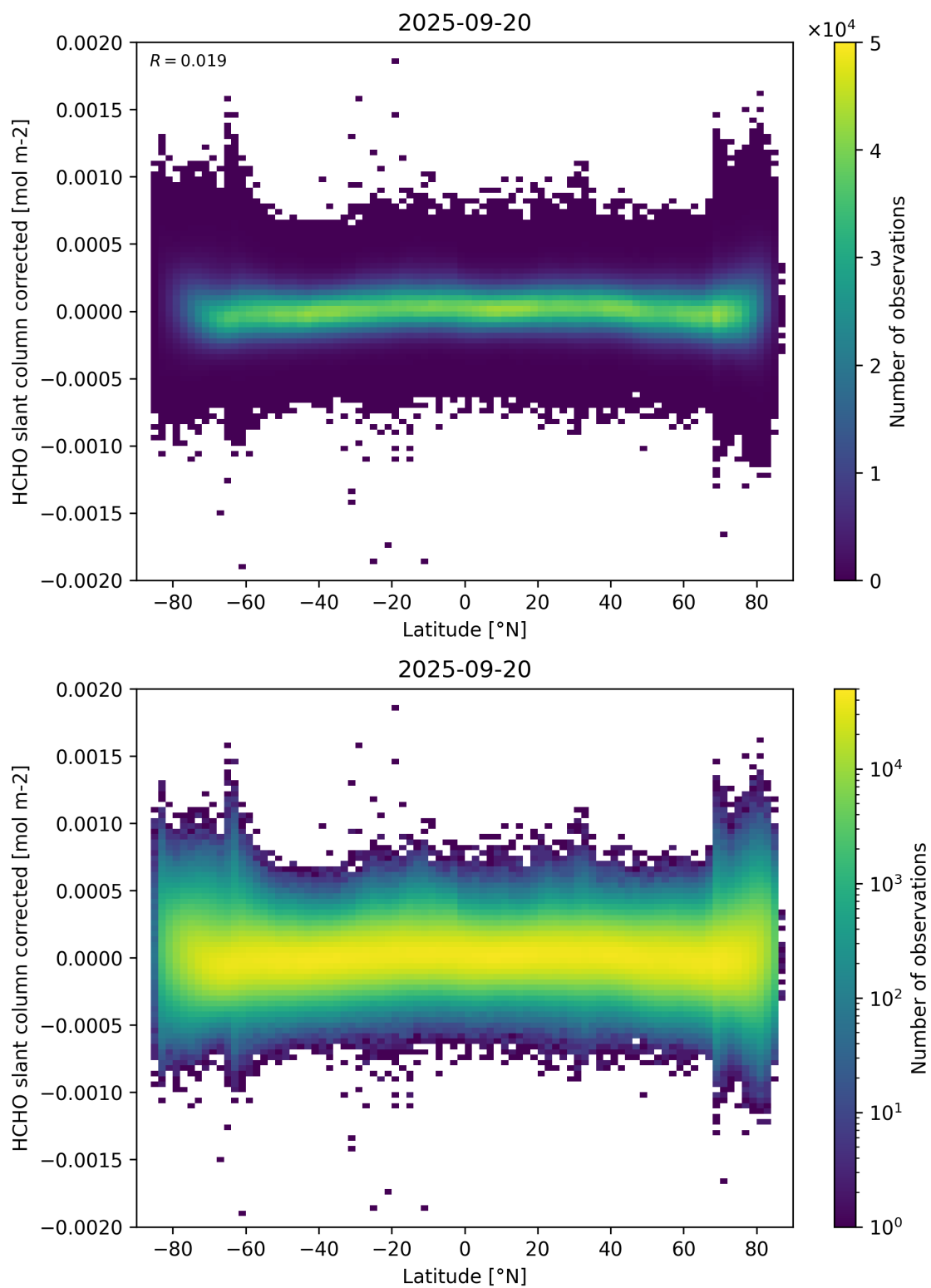
Figure 157: Scatter density plot of “Latitude” against “HCHO slant column corrected” for 2025-09-20 to 2025-09-21.
