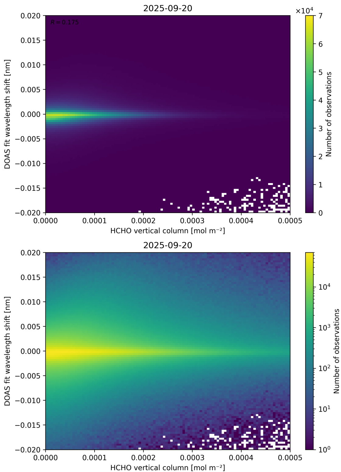
Figure 124: Scatter density plot of “HCHO vertical column” against “DOAS fit wavelength shift” for 2025-09-20 to 2025-09-21.
