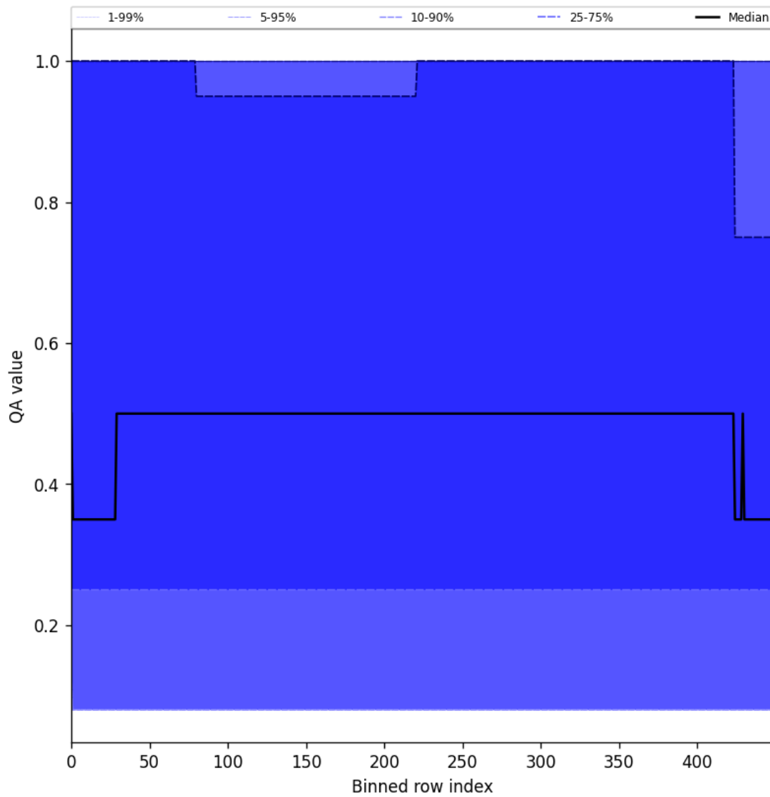
Figure 48: Along track statistics of “QA value” for 2025-09-20 to 2025-09-21
