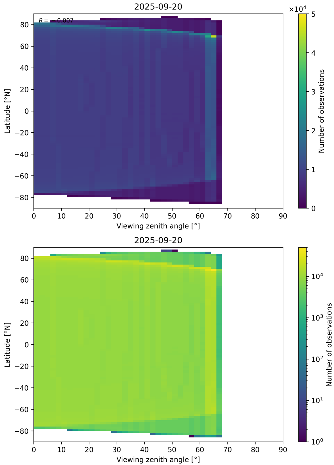
Figure 196: Scatter density plot of “Viewing zenith angle” against “Latitude” for 2025-09-20 to 2025-09-21.
