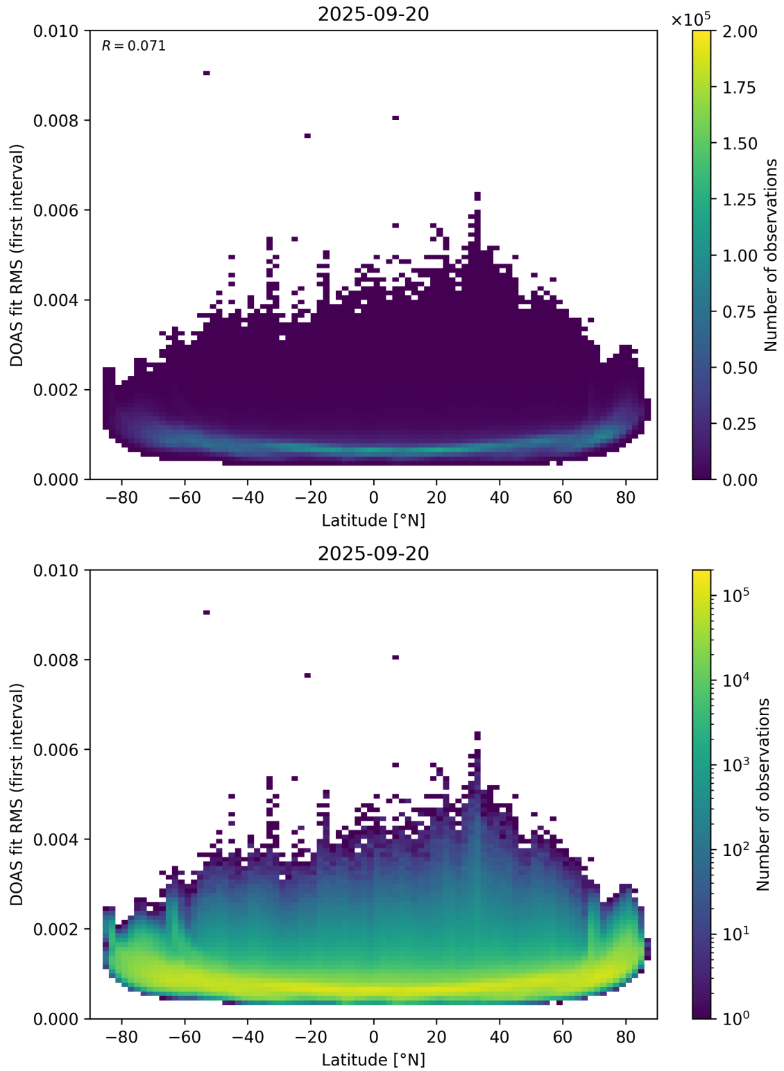
Figure 153: Scatter density plot of “Latitude” against “DOAS fit RMS (first interval)” for 2025-09-20 to 2025-09-21.
