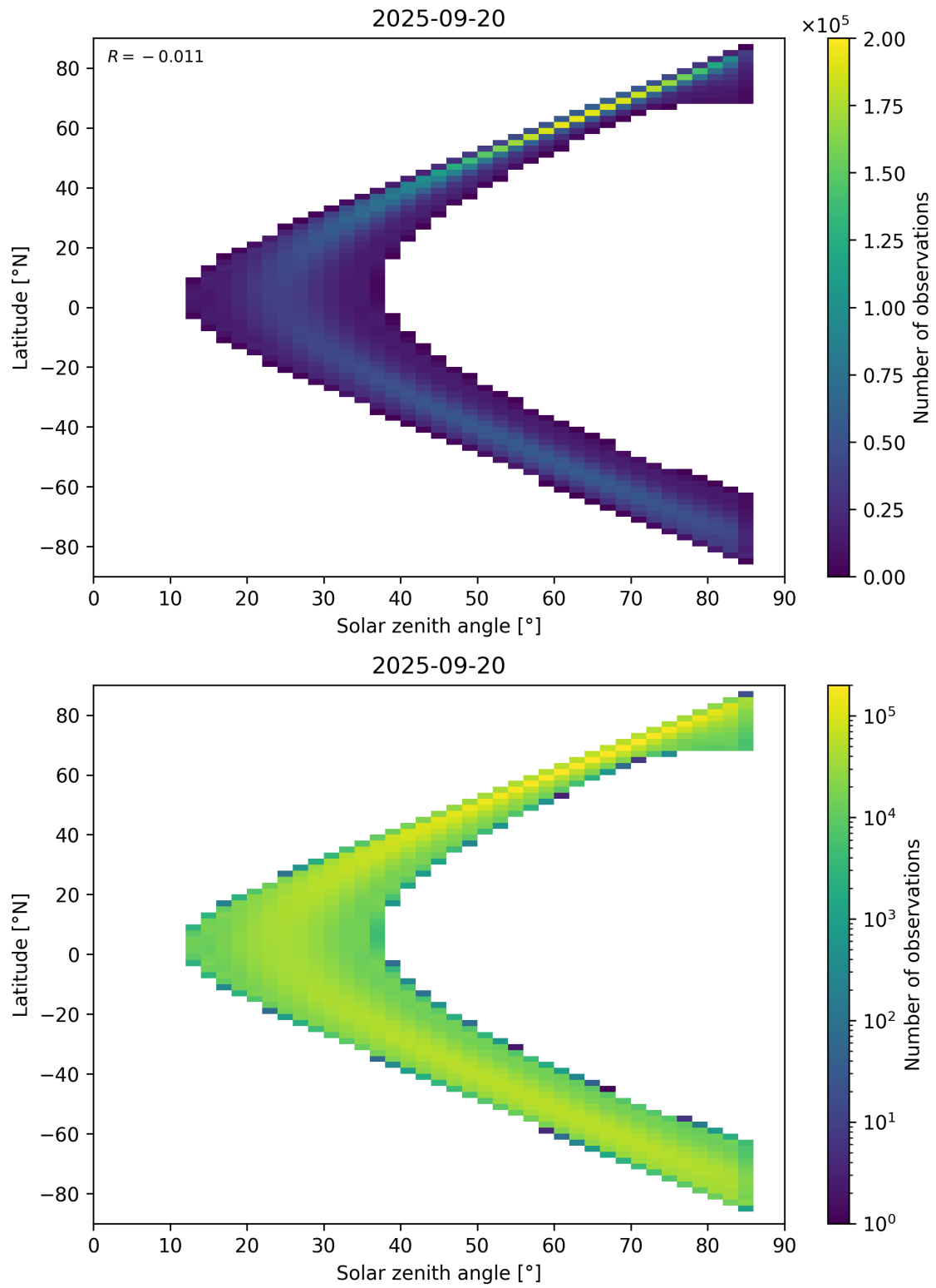
Figure 181: Scatter density plot of “Solar zenith angle” against “Latitude” for 2025-09-20 to 2025-09-21.
