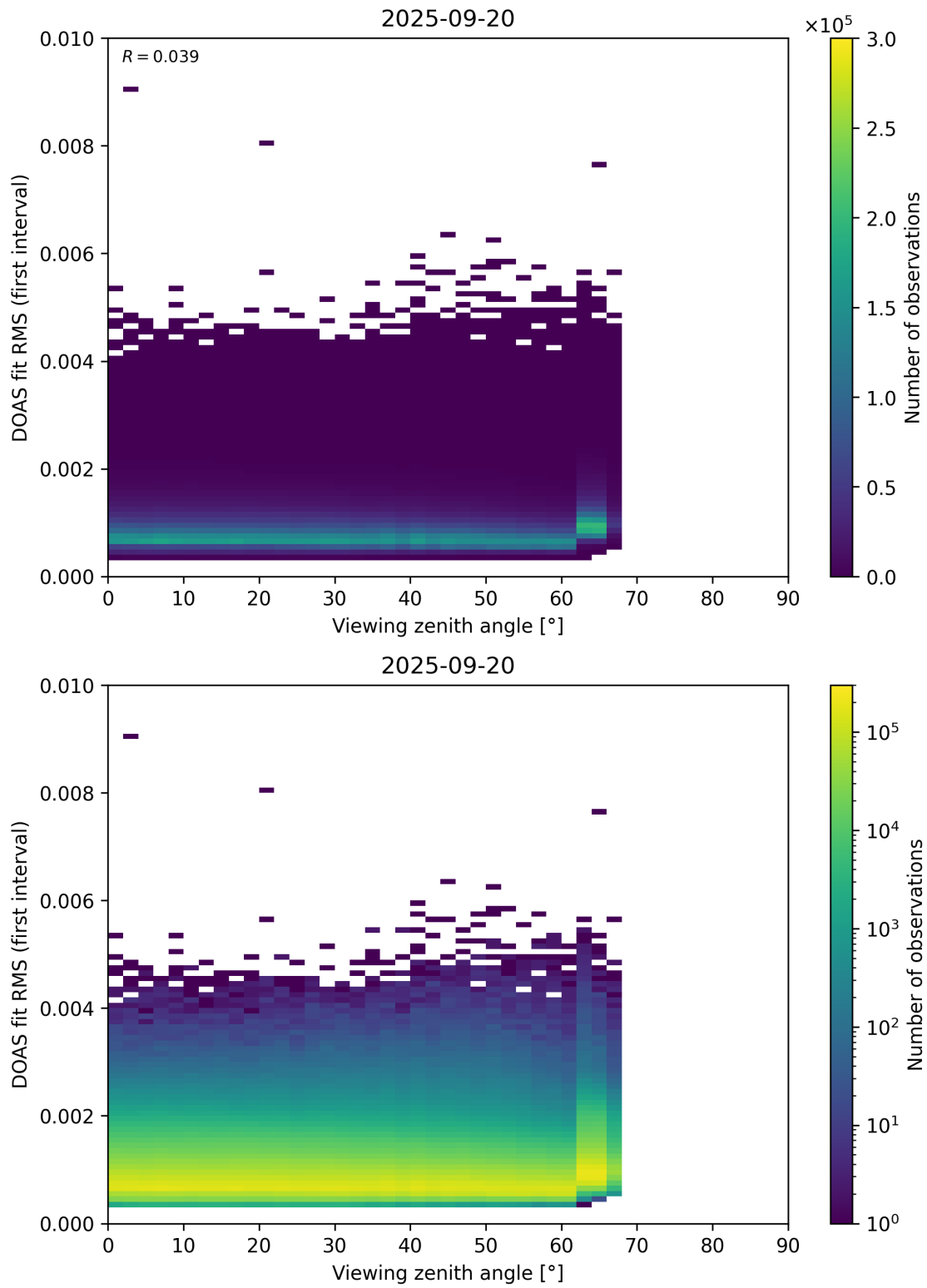
Figure 182: Scatter density plot of “Viewing zenith angle” against “DOAS fit RMS (first interval)” for 2025-09-20 to 2025-09-21.
