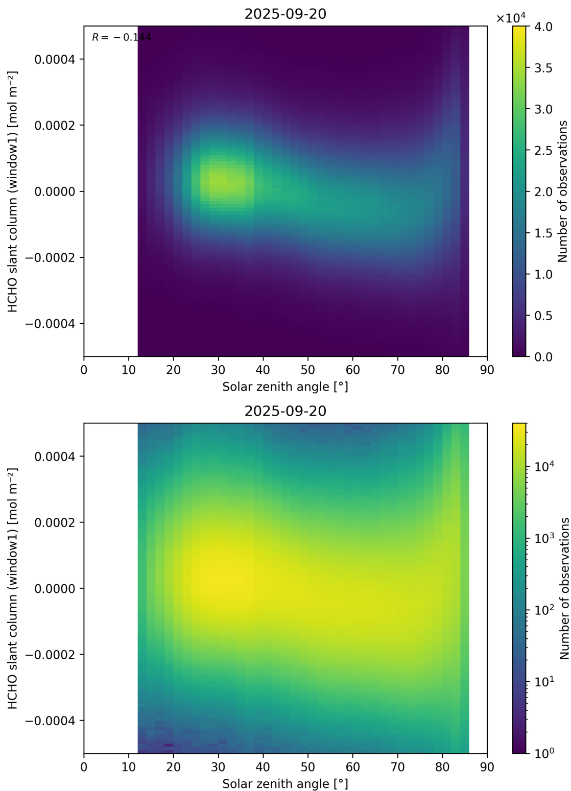
Figure 173: Scatter density plot of “Solar zenith angle” against “HCHO slant column (window1)” for 2025-09-20 to 2025-09-21.
