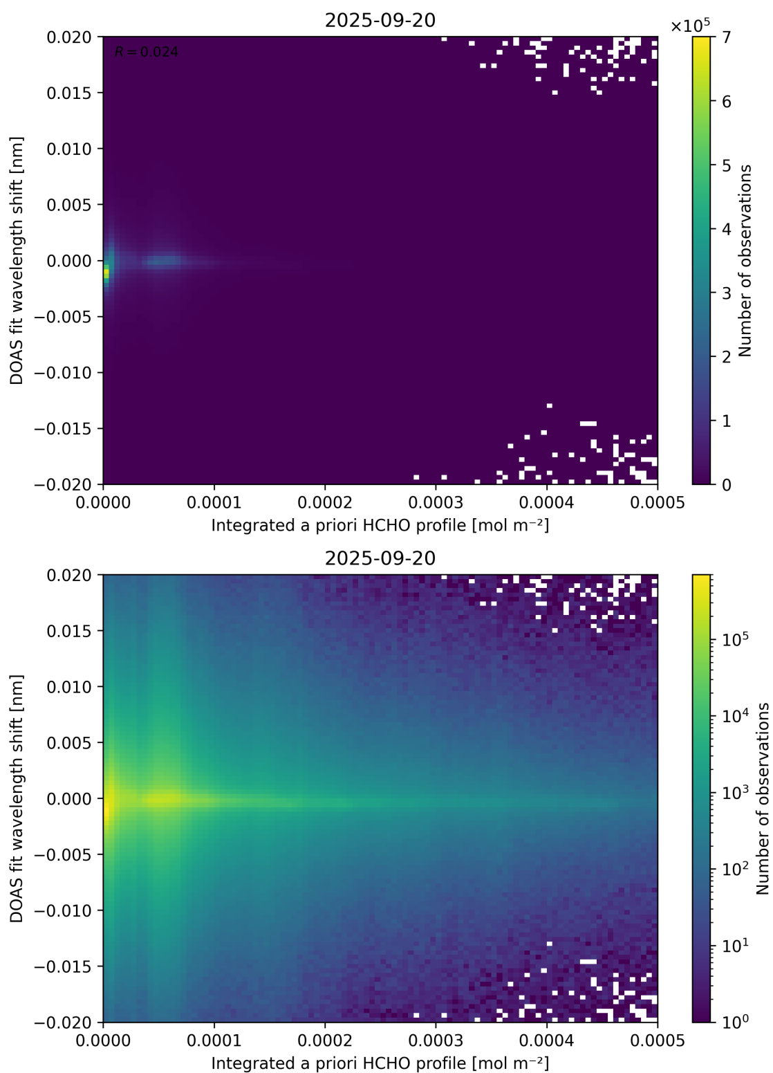
Figure 149: Scatter density plot of “Integrated a priori HCHO profile” against “DOAS fit wavelength shift” for 2025-09-20 to 2025-09-21.
