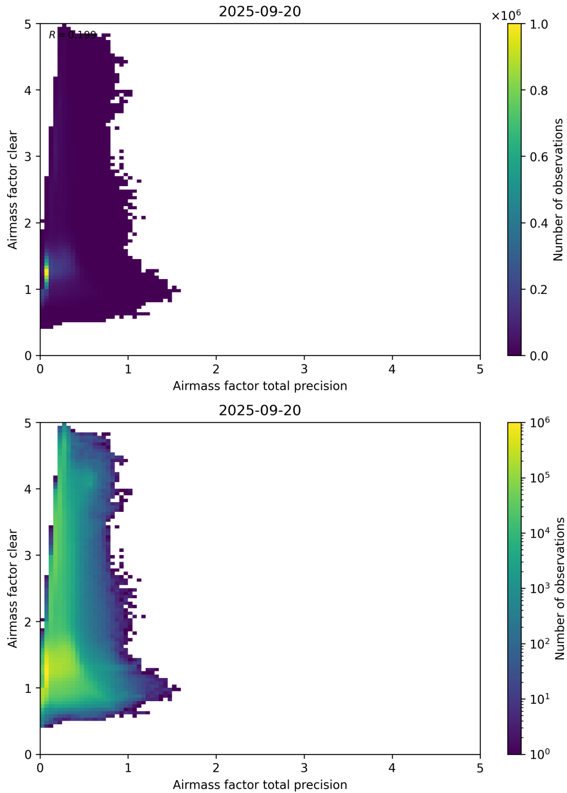
Figure 108: Scatter density plot of “Airmass factor total precision” against “Airmass factor clear” for 2025-09-20 to 2025-09-21.
