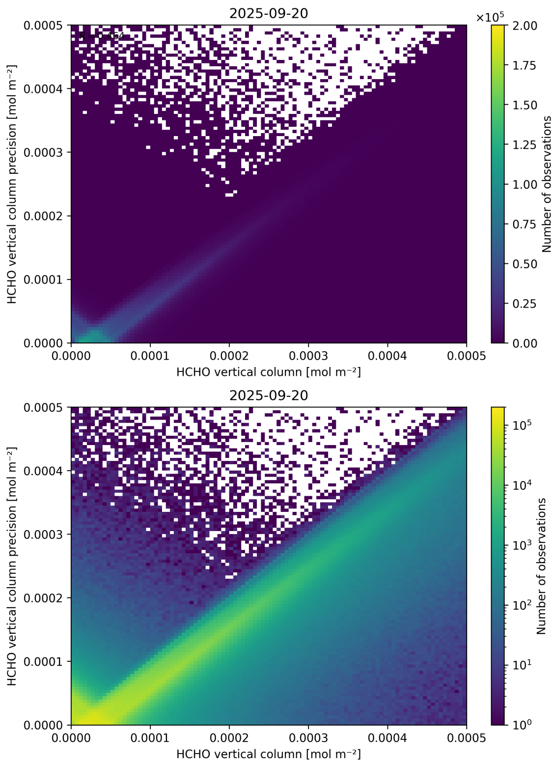
Figure 134: Scatter density plot of “HCHO vertical column” against “HCHO vertical column precision” for 2025-09-20 to 2025-09-21.
