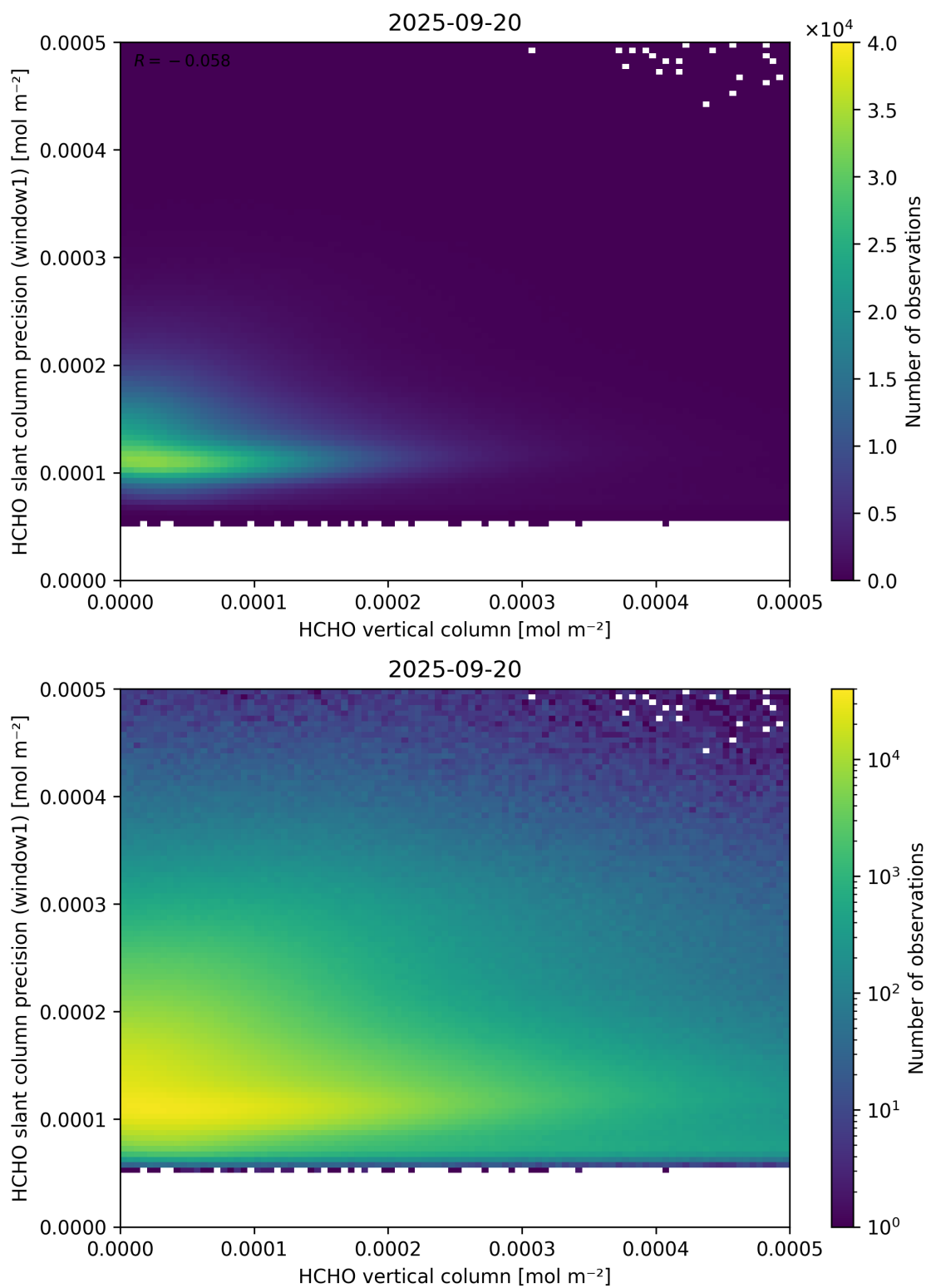
Figure 130: Scatter density plot of “HCHO vertical column” against “HCHO slant column precision (window1)” for 2025-09-20 to 2025-09-21.
