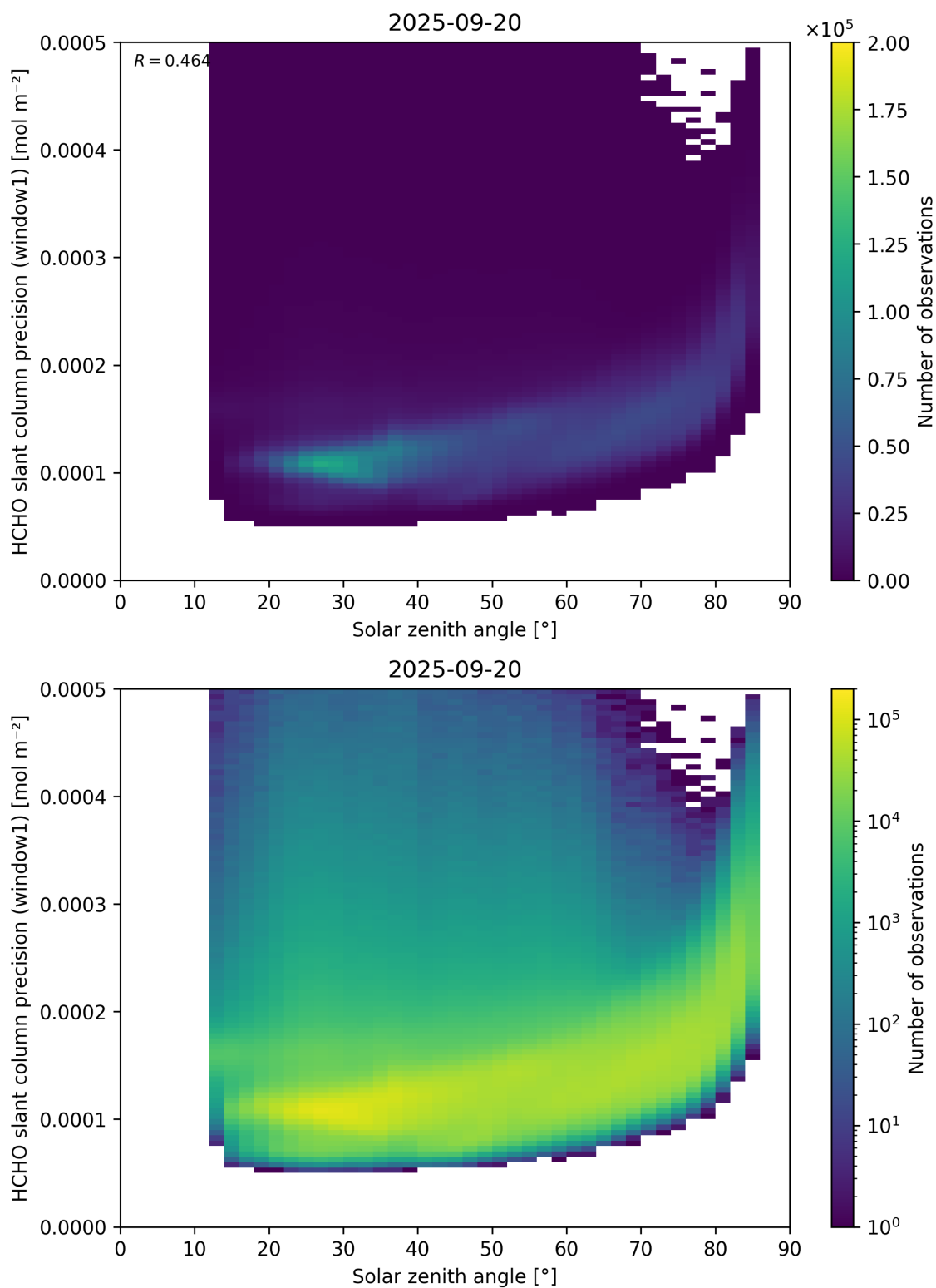
Figure 174: Scatter density plot of “Solar zenith angle” against “HCHO slant column precision (window1)” for 2025-09-20 to 2025-09-21.
