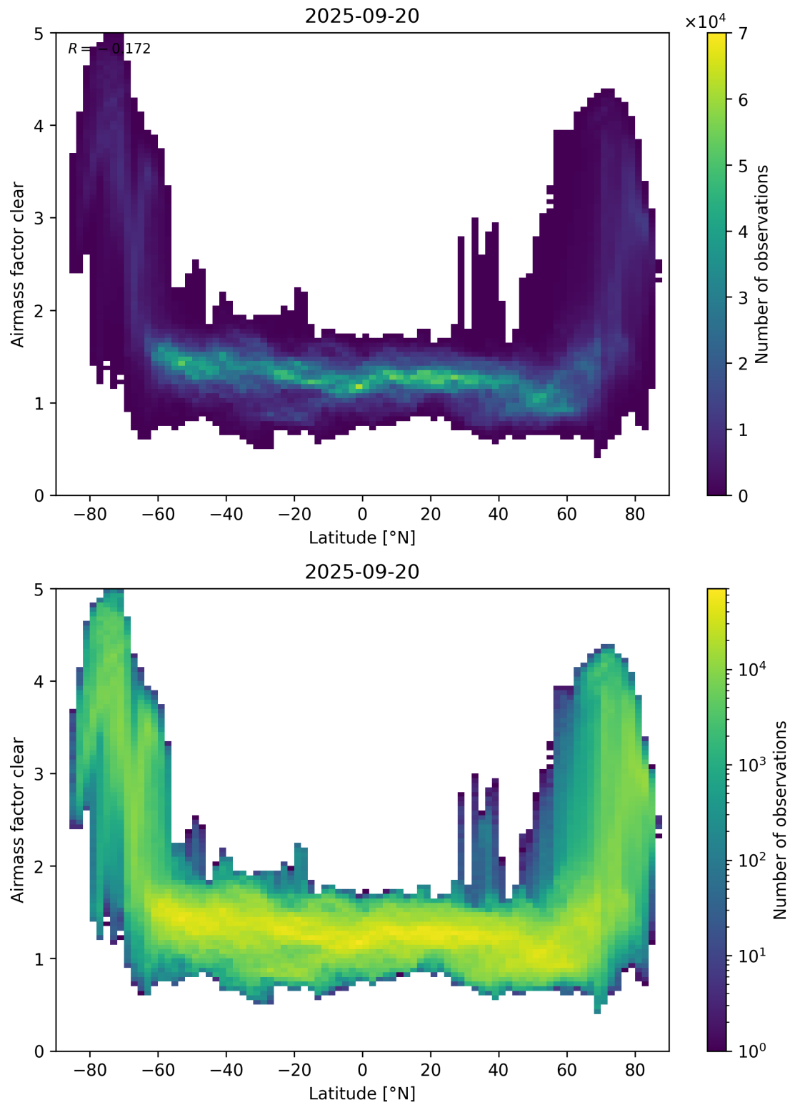
Figure 156: Scatter density plot of “Latitude” against “Airmass factor clear” for 2025-09-20 to 2025-09-21.
