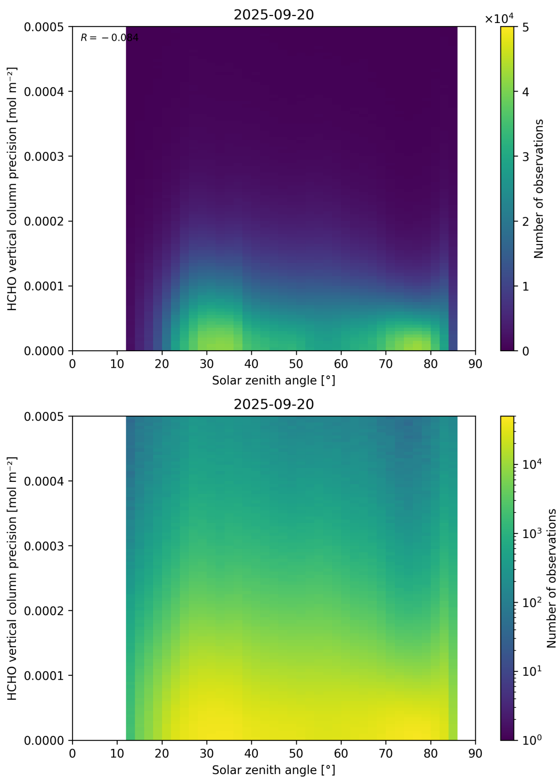
Figure 179: Scatter density plot of “Solar zenith angle” against “HCHO vertical column precision” for 2025-09-20 to 2025-09-21.
