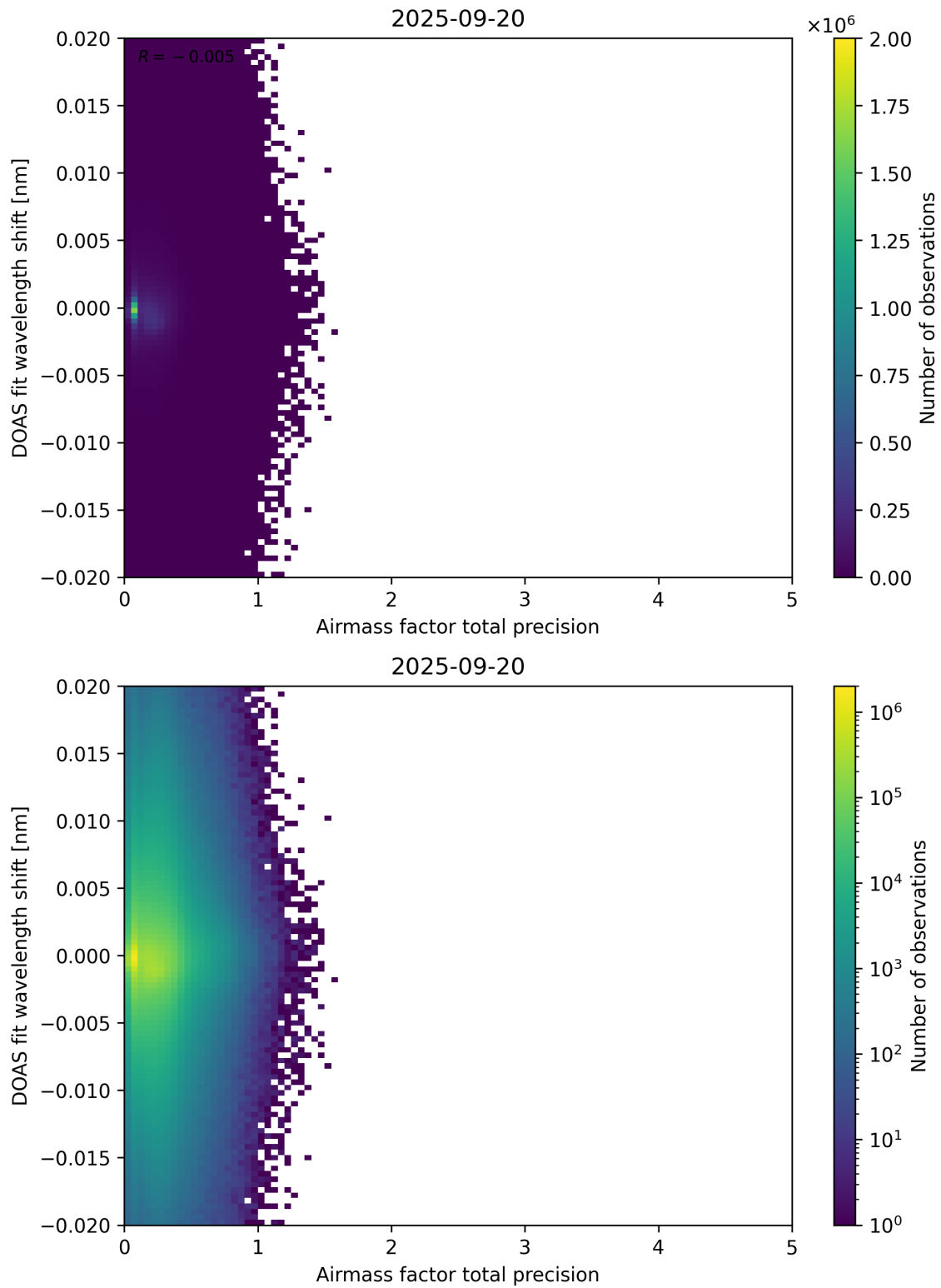
Figure 106: Scatter density plot of “Airmass factor total precision” against “DOAS fit wavelength shift” for 2025-09-20 to 2025-09-21.
