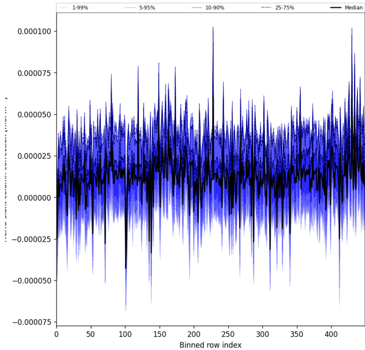
Figure 61: Along track statistics of “HCHO slant column correction” for 2025-09-20 to 2025-09-21
