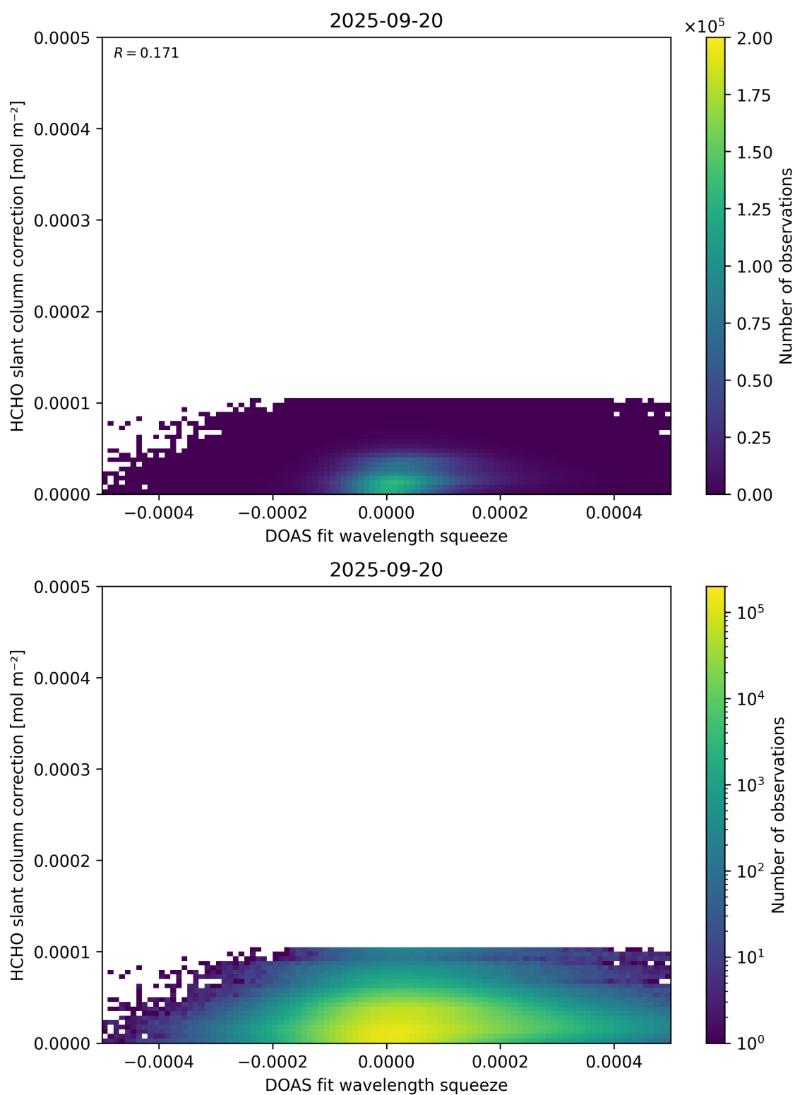
Figure 70: Scatter density plot of “DOAS fit wavelength squeeze” against “HCHO slant column correction” for 2025-09-20 to 2025-09-21.
