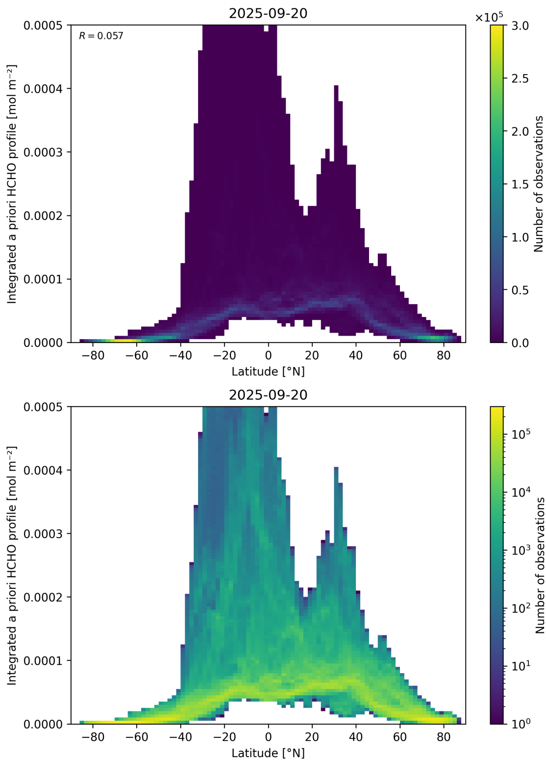
Figure 166: Scatter density plot of “Latitude” against “Integrated a priori HCHO profile” for 2025-09-20 to 2025-09-21.
