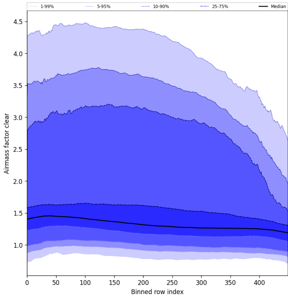
Figure 56: Along track statistics of “Air mass factor clear” for 2025-09-20 to 2025-09-21
