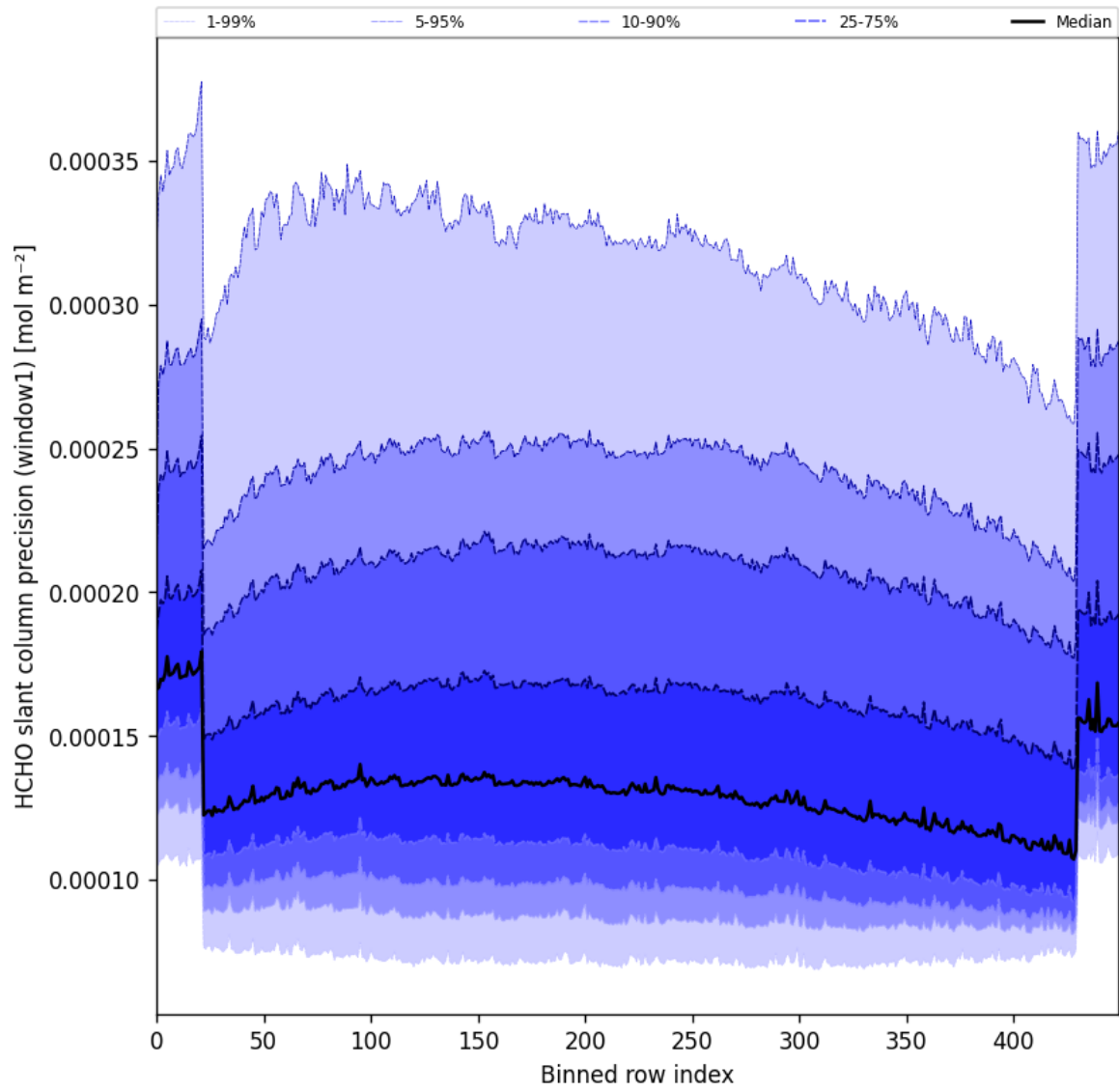
Figure 53: Along track statistics of “HCHO slant column precision (window1)” for 2025-09-20 to 2025-09-21
