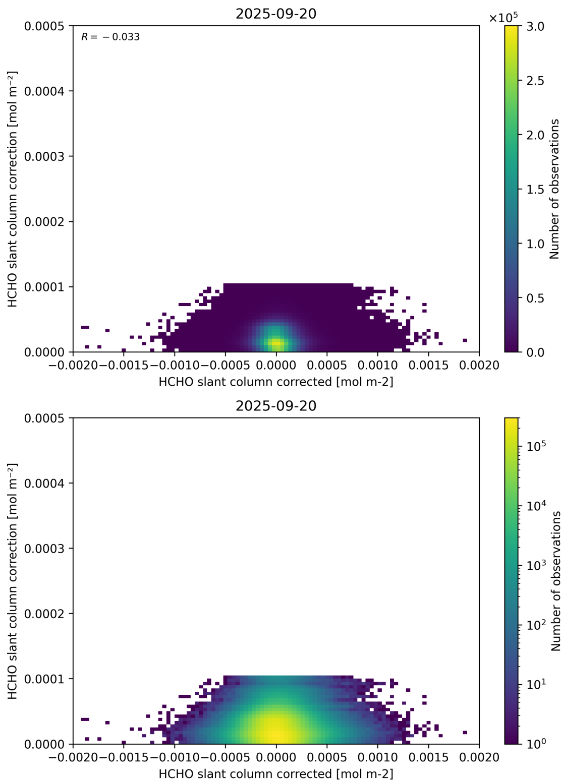
Figure 77: Scatter density plot of “HCHO slant column corrected” against “HCHO slant column correction” for 2025-09-20 to 2025-09-21.
