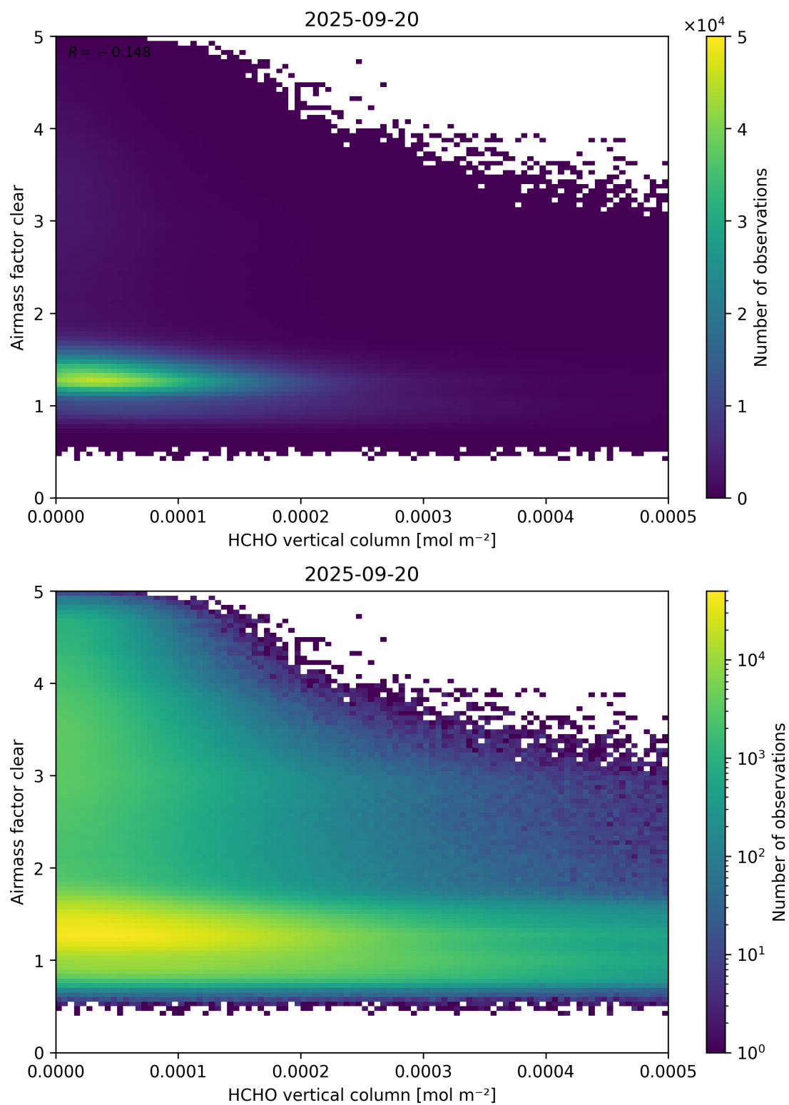
Figure 126: Scatter density plot of “HCHO vertical column” against “Airmass factor clear” for 2025-09-20 to 2025-09-21.
