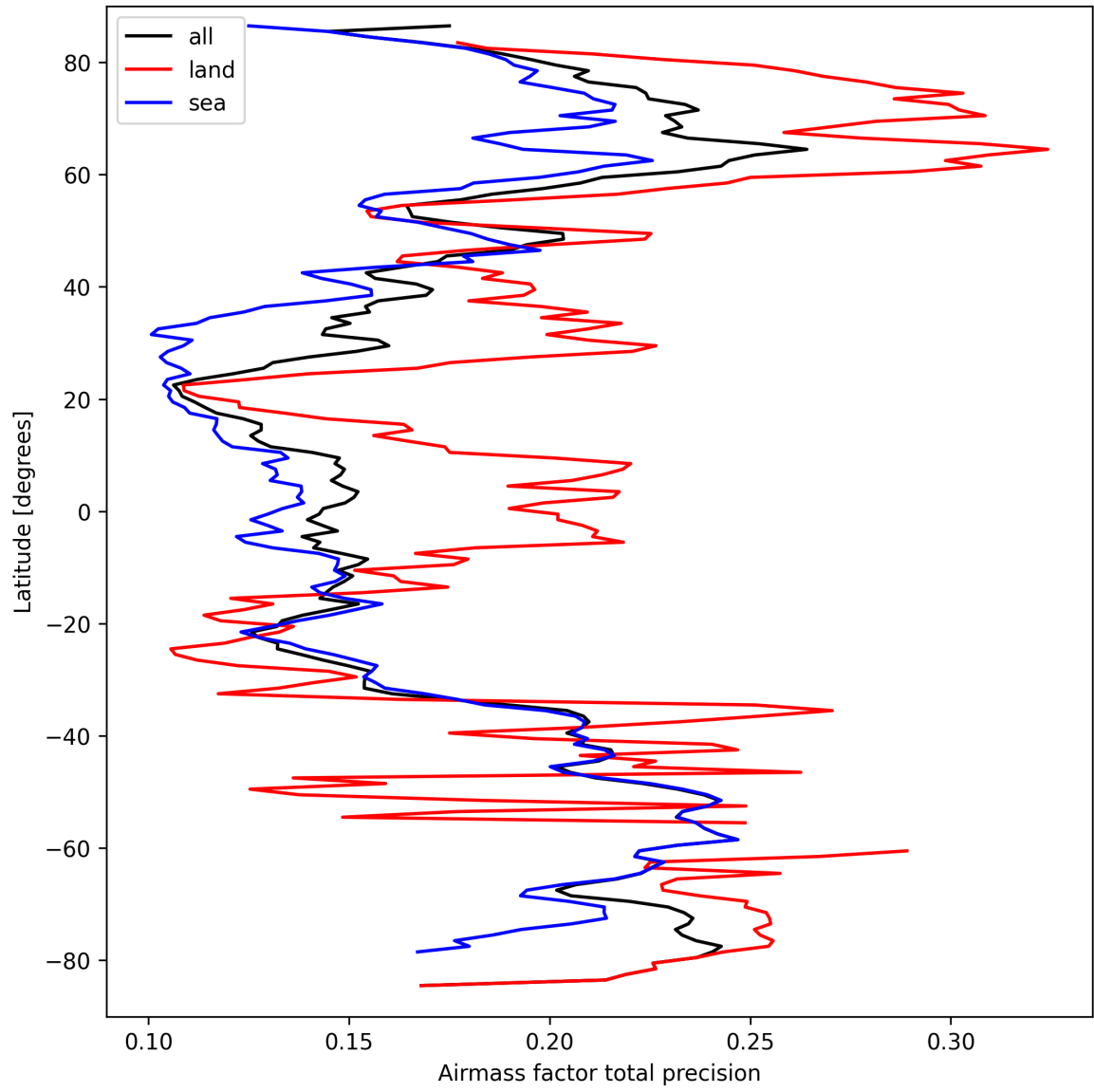
Figure 27: Zonal average of “Airmass factor total precision” for 2025-09-20 to 2025-09-21.
