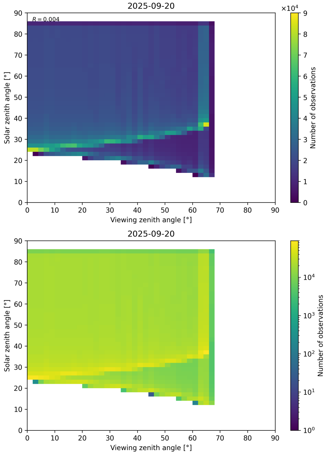
Figure 197: Scatter density plot of “Viewing zenith angle” against “Solar zenith angle” for 2025-09-20 to 2025-09-21.
