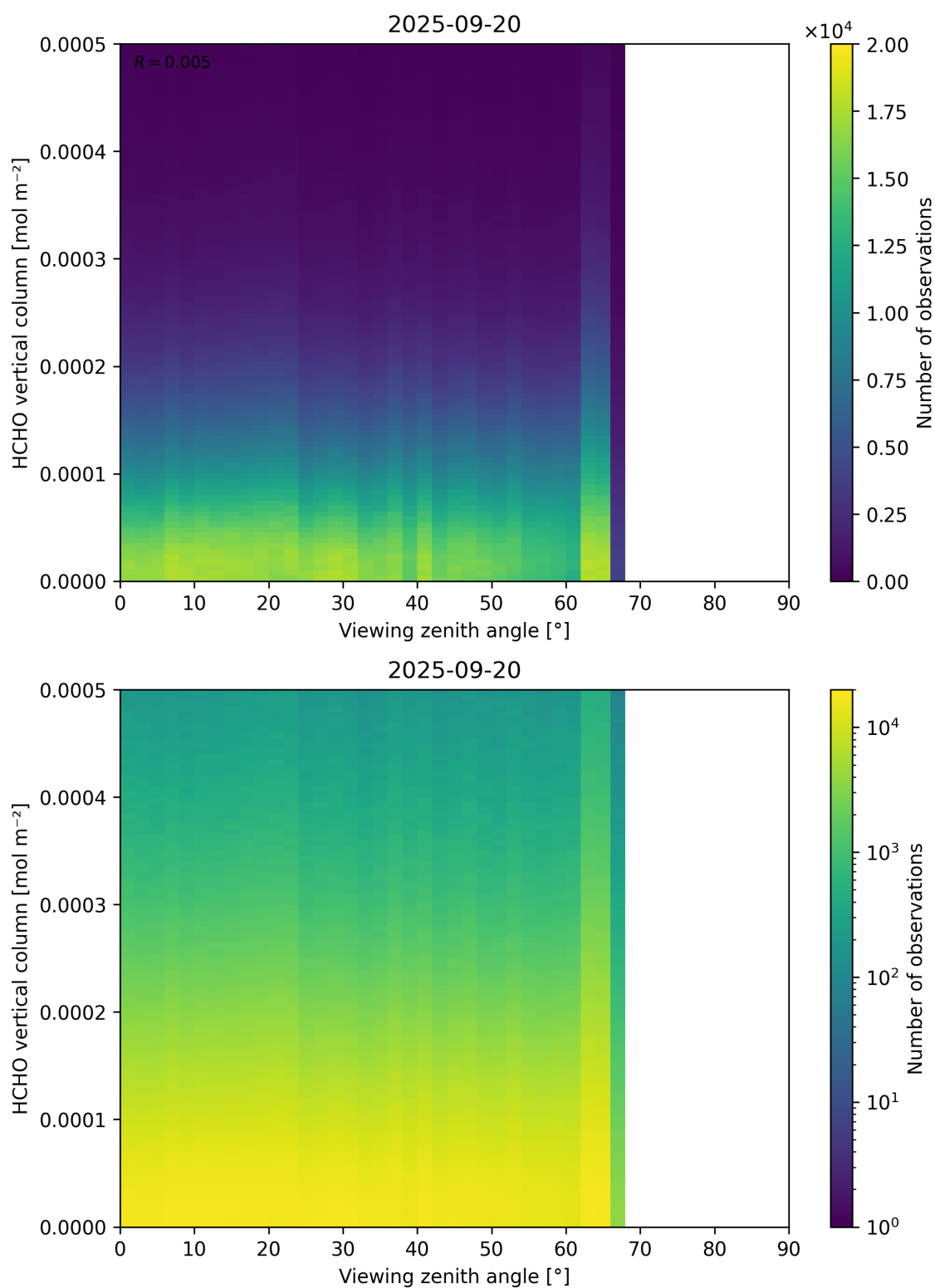
Figure 192: Scatter density plot of “Viewing zenith angle” against “HCHO vertical column” for 2025-09-20 to 2025-09-21.
