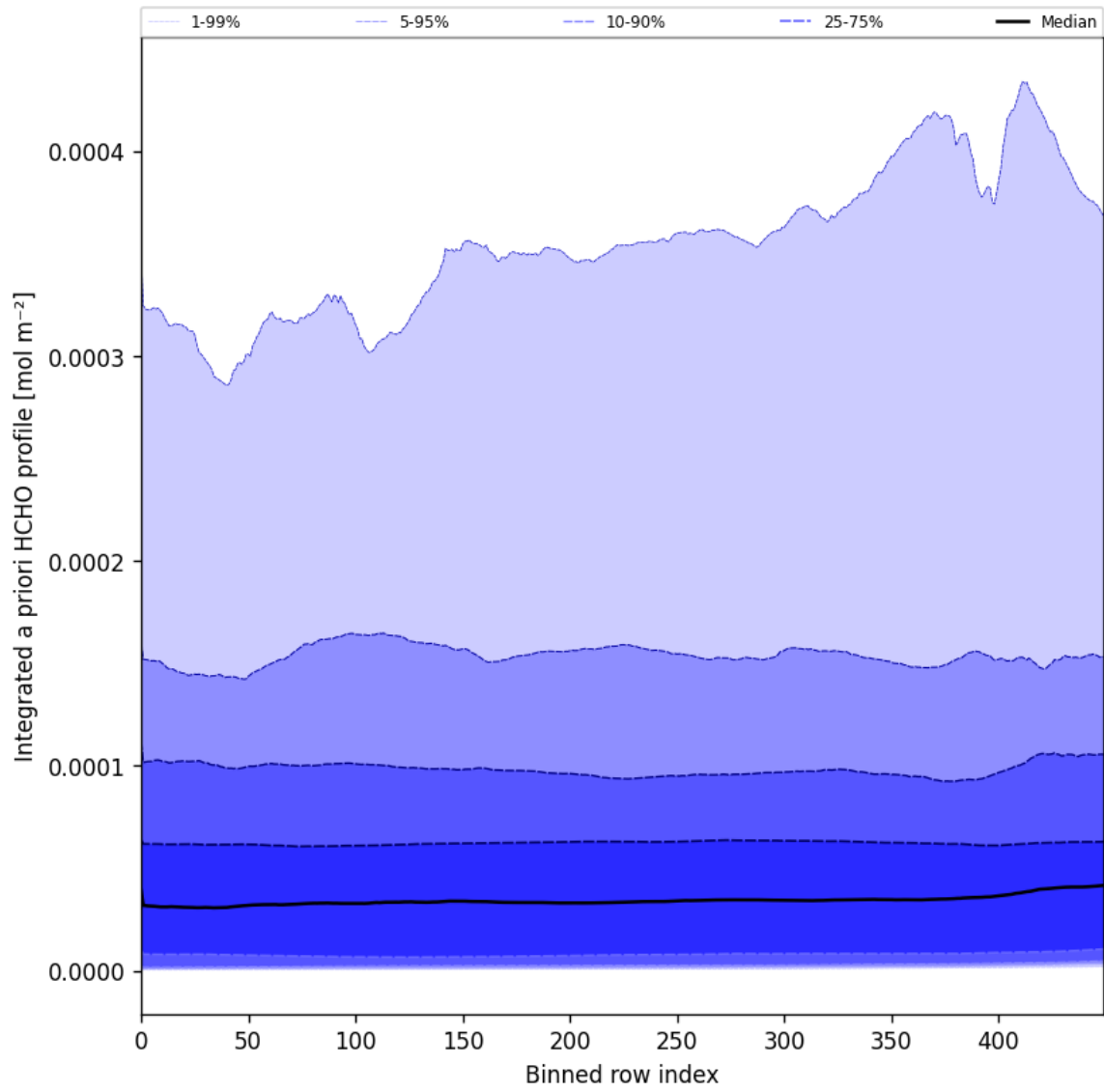
Figure 57: Along track statistics of “Integrated a priori HCHO profile” for 2025-09-20 to 2025-09-21
