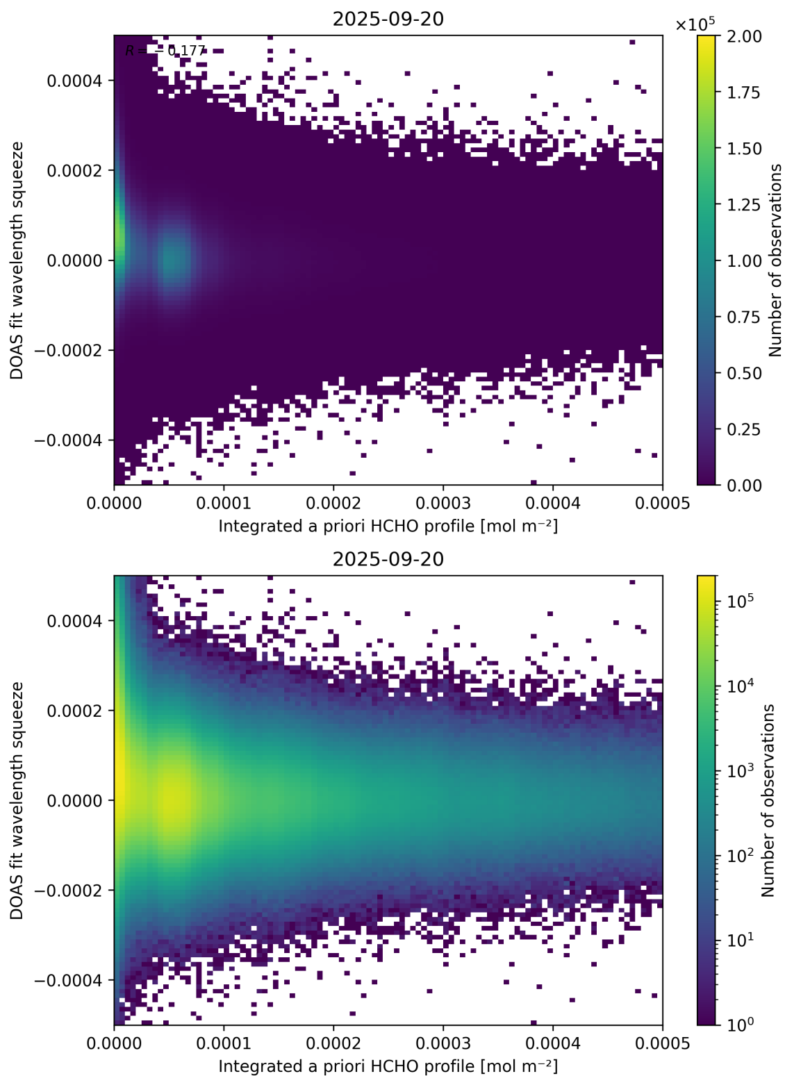
Figure 150: Scatter density plot of “Integrated a priori HCHO profile” against “DOAS fit wavelength squeeze” for 2025-09-20 to 2025-09-21.
