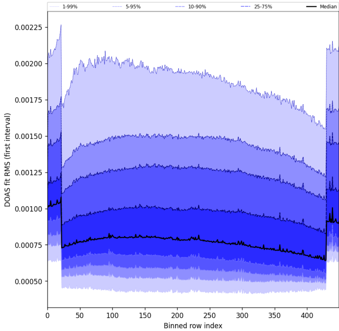
Figure 60: Along track statistics of “DOAS fit RMS (first interval)” for 2025-09-20 to 2025-09-21
