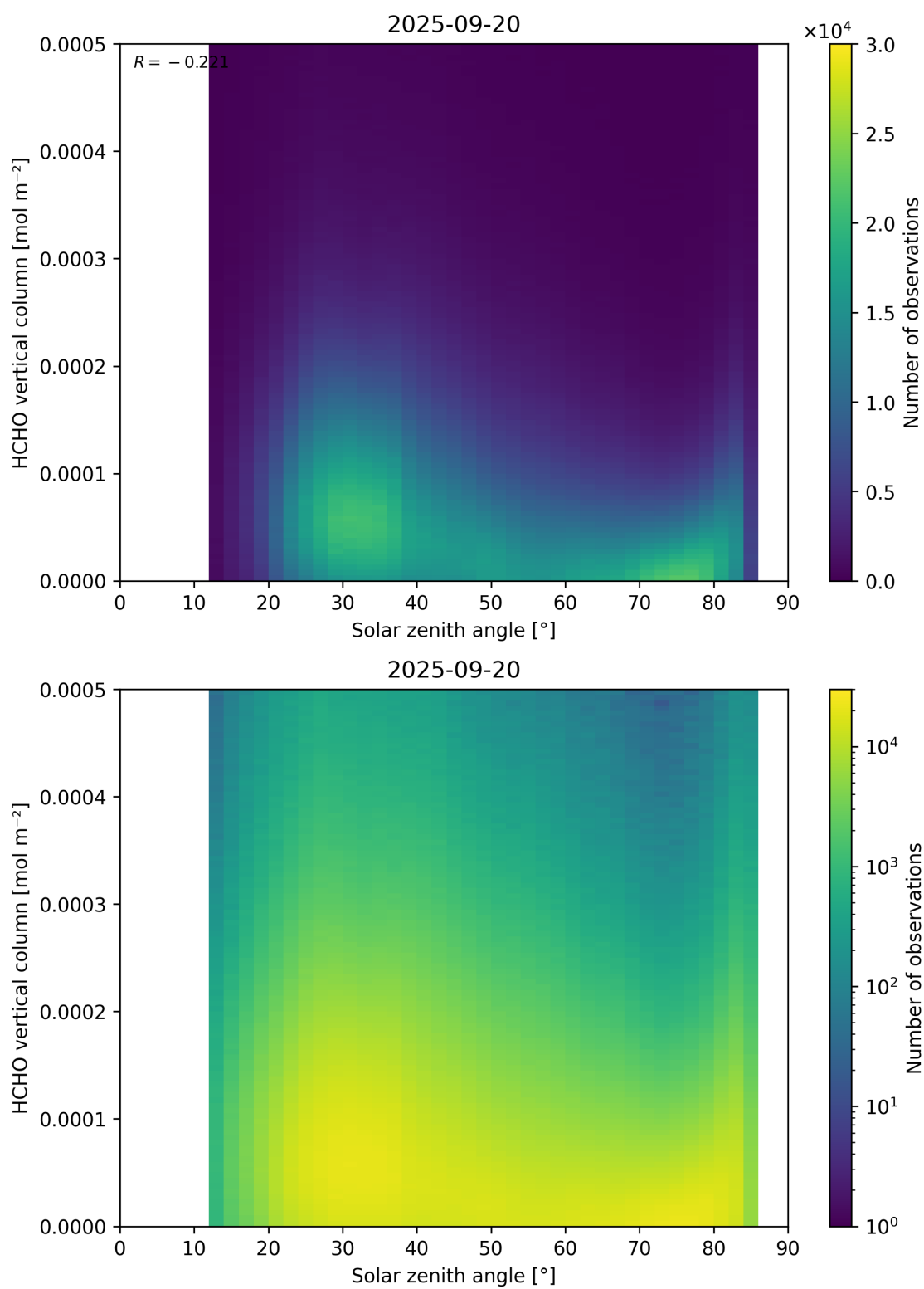
Figure 177: Scatter density plot of “Solar zenith angle” against “HCHO vertical column” for 2025-09-20 to 2025-09-21.
