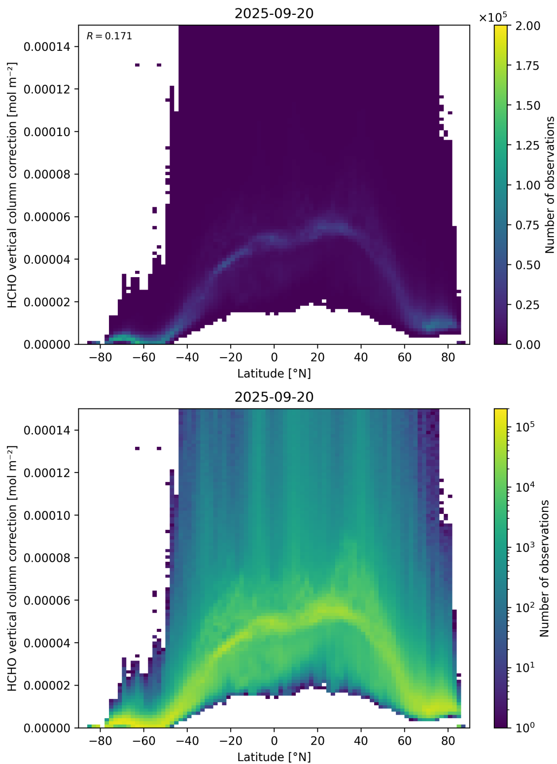
Figure 164: Scatter density plot of “Latitude” against “HCHO vertical column correction” for 2025-09-20 to 2025-09-21.
