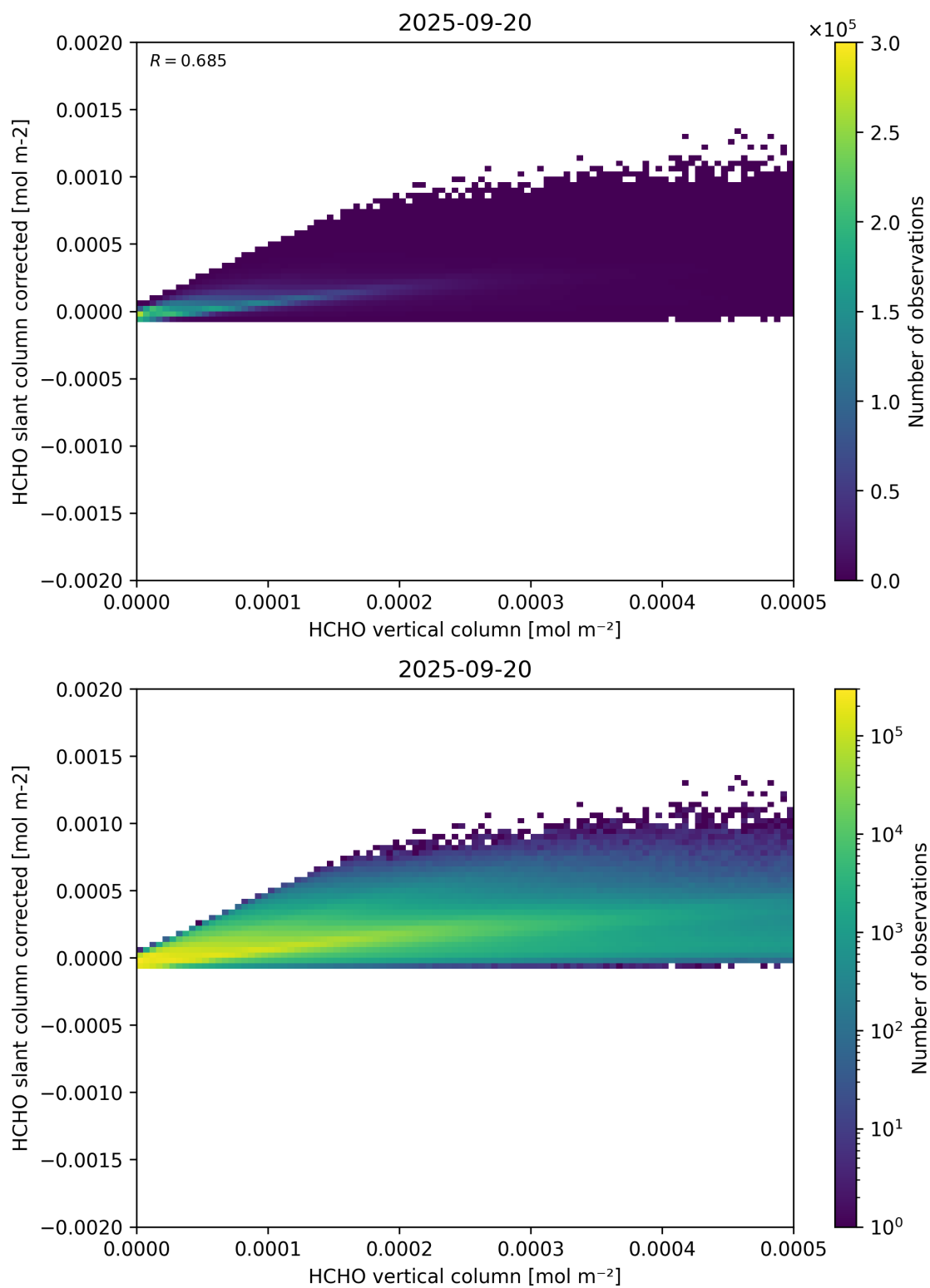
Figure 127: Scatter density plot of “HCHO vertical column” against “HCHO slant column corrected” for 2025-09-20 to 2025-09-21.
