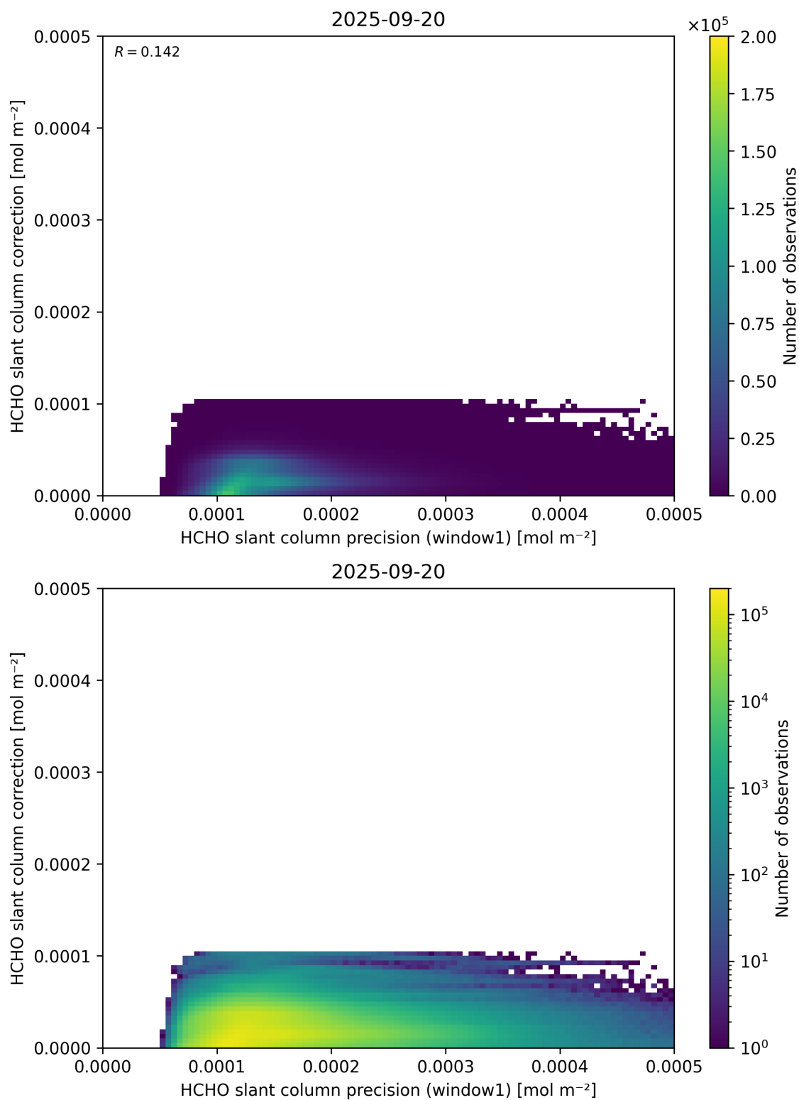
Figure 93: Scatter density plot of “HCHO slant column precision (window1)” against “HCHO slant column correction” for 2025-09-20 to 2025-09-21.
