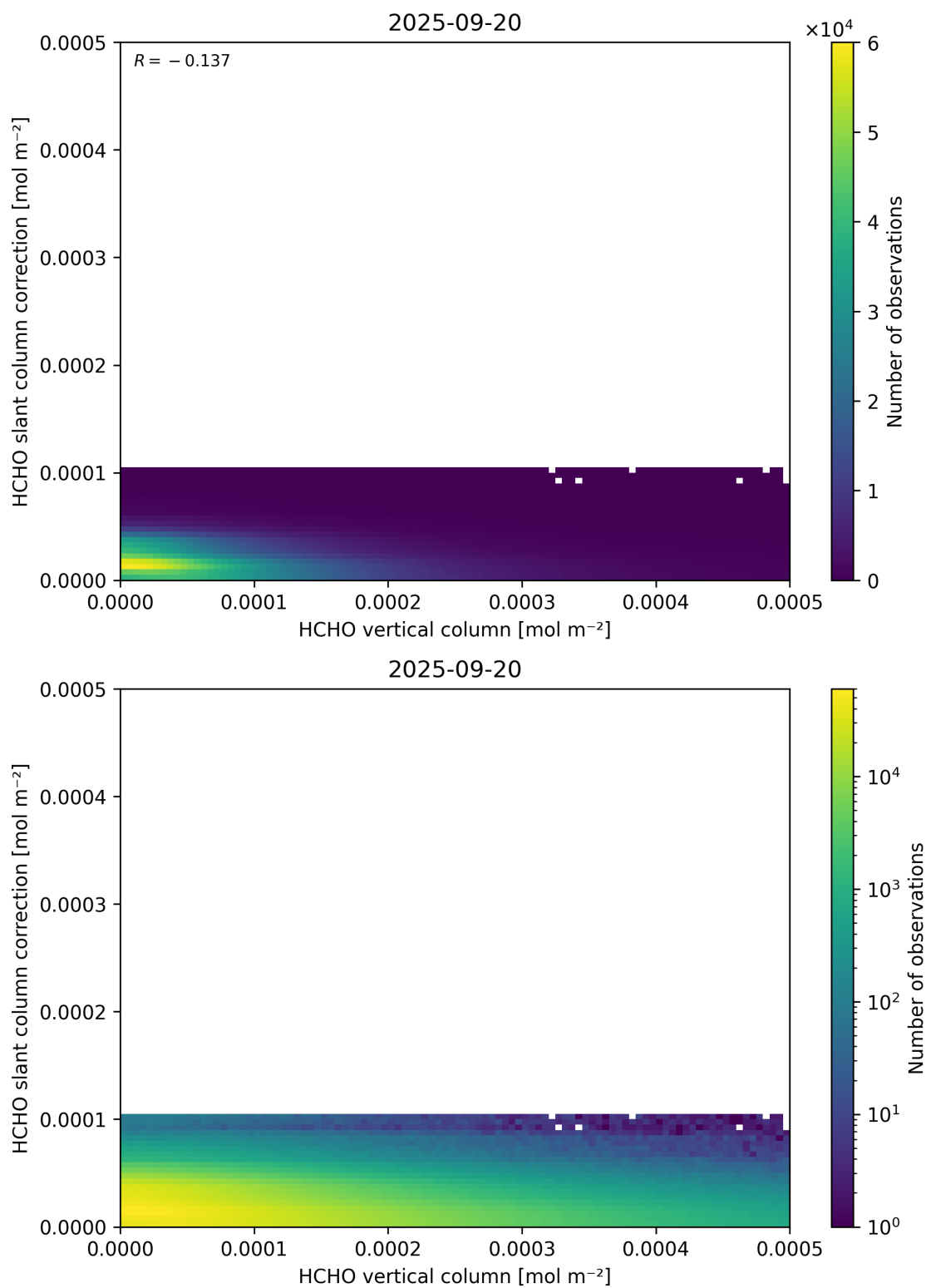
Figure 128: Scatter density plot of “HCHO vertical column” against “HCHO slant column correction” for 2025-09-20 to 2025-09-21.
