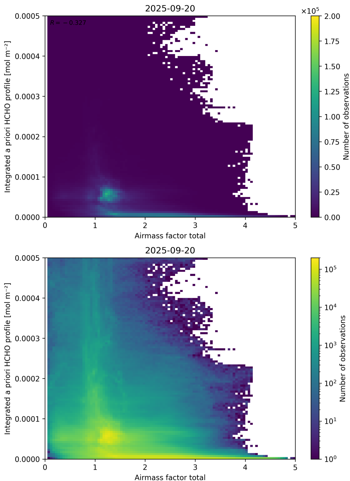
Figure 104: Scatter density plot of “Airmass factor total” against “Integrated a priori HCHO profile” for 2025-09-20 to 2025-09-21.
