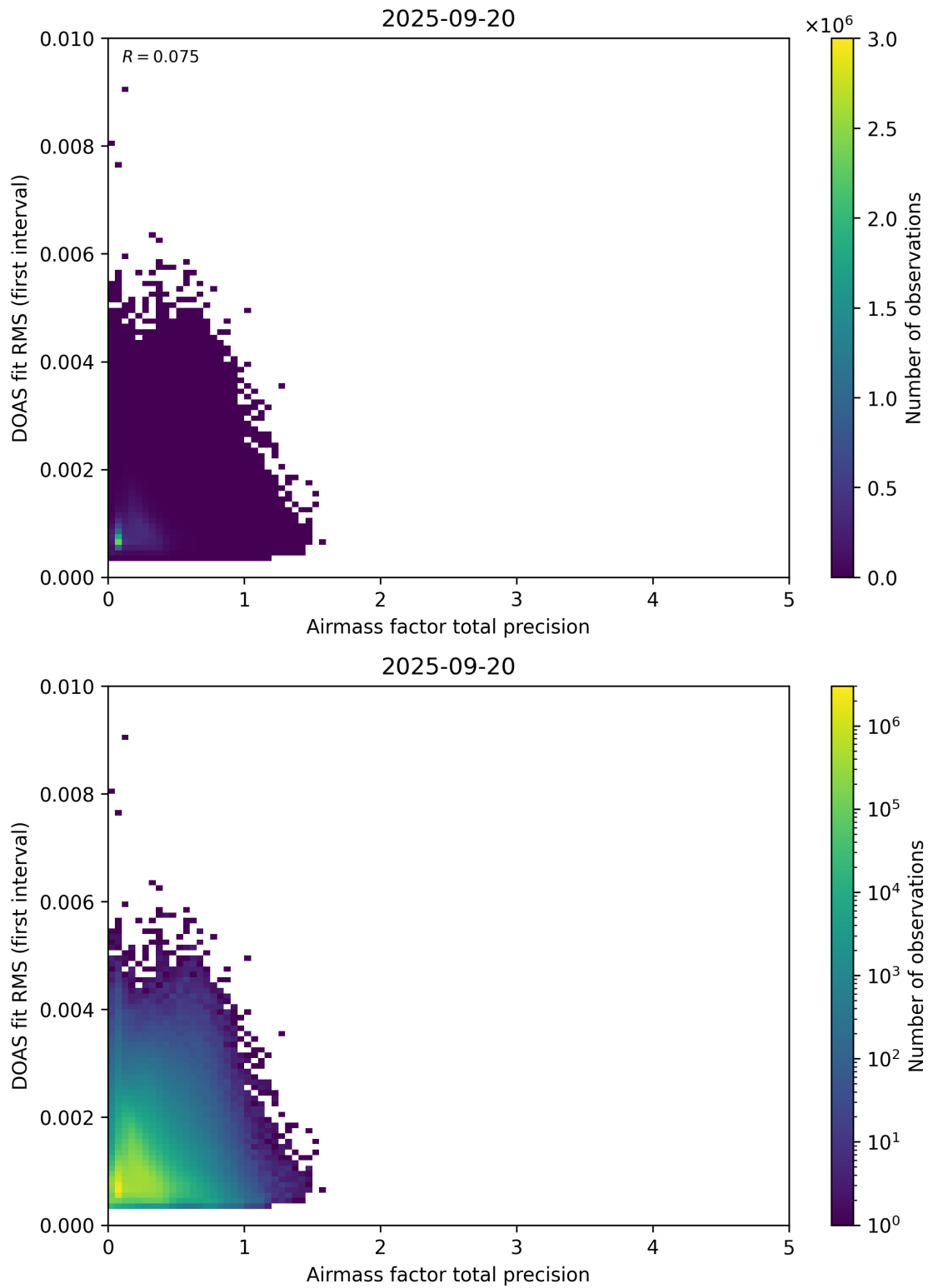
Figure 105: Scatter density plot of “Airmass factor total precision” against “DOAS fit RMS (first interval)” for 2025-09-20 to 2025-09-21.
