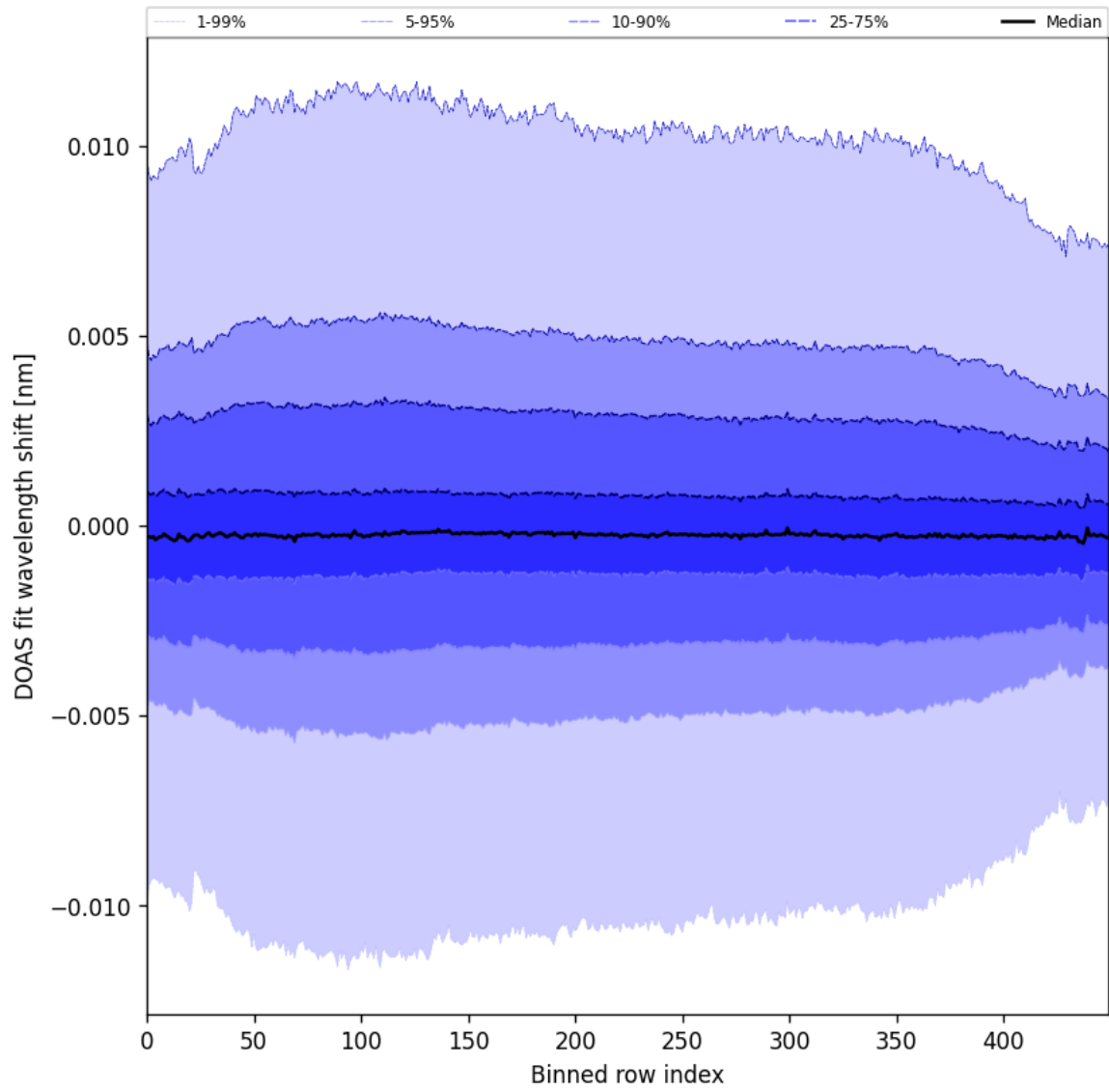
Figure 58: Along track statistics of “DOAS fit wavelength shift” for 2025-09-20 to 2025-09-21
