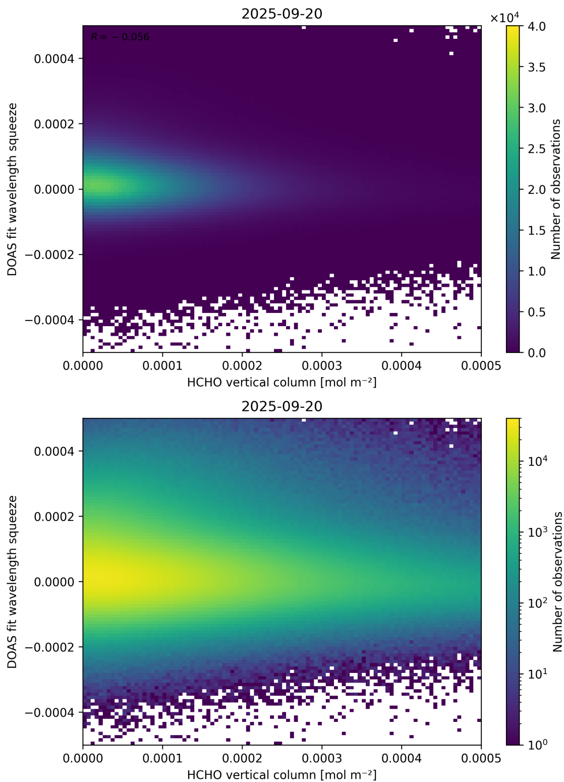
Figure 125: Scatter density plot of “HCHO vertical column” against “DOAS fit wavelength squeeze” for 2025-09-20 to 2025-09-21.
