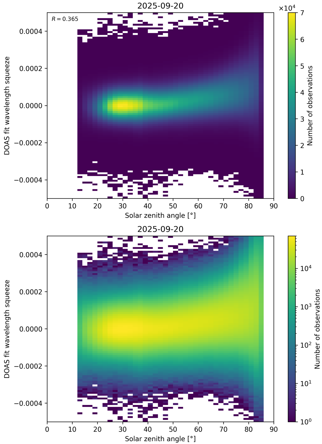
Figure 169: Scatter density plot of “Solar zenith angle” against “DOAS fit wavelength squeeze” for 2025-09-20 to 2025-09-21.
