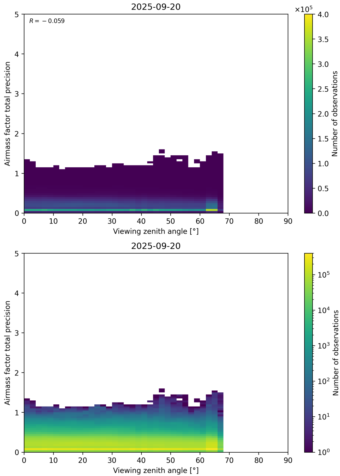
Figure 191: Scatter density plot of “Viewing zenith angle” against “Airmass factor total precision” for 2025-09-20 to 2025-09-21.
