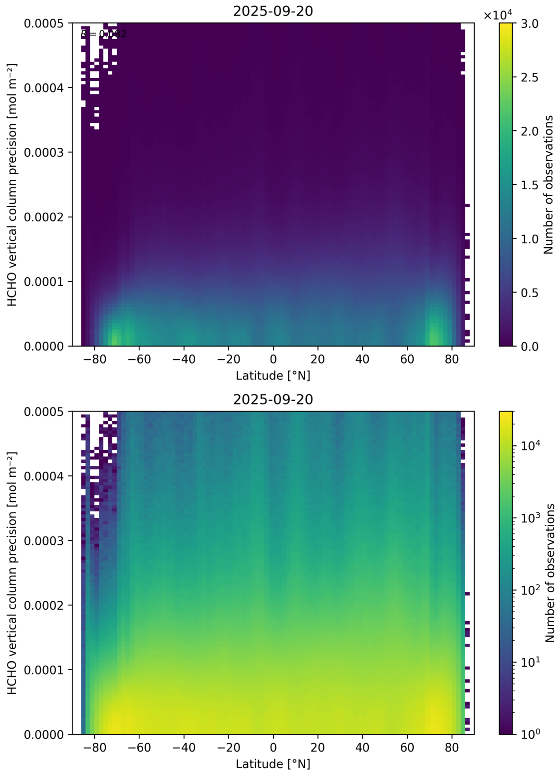
Figure 165: Scatter density plot of “Latitude” against “HCHO vertical column precision” for 2025-09-20 to 2025-09-21.
