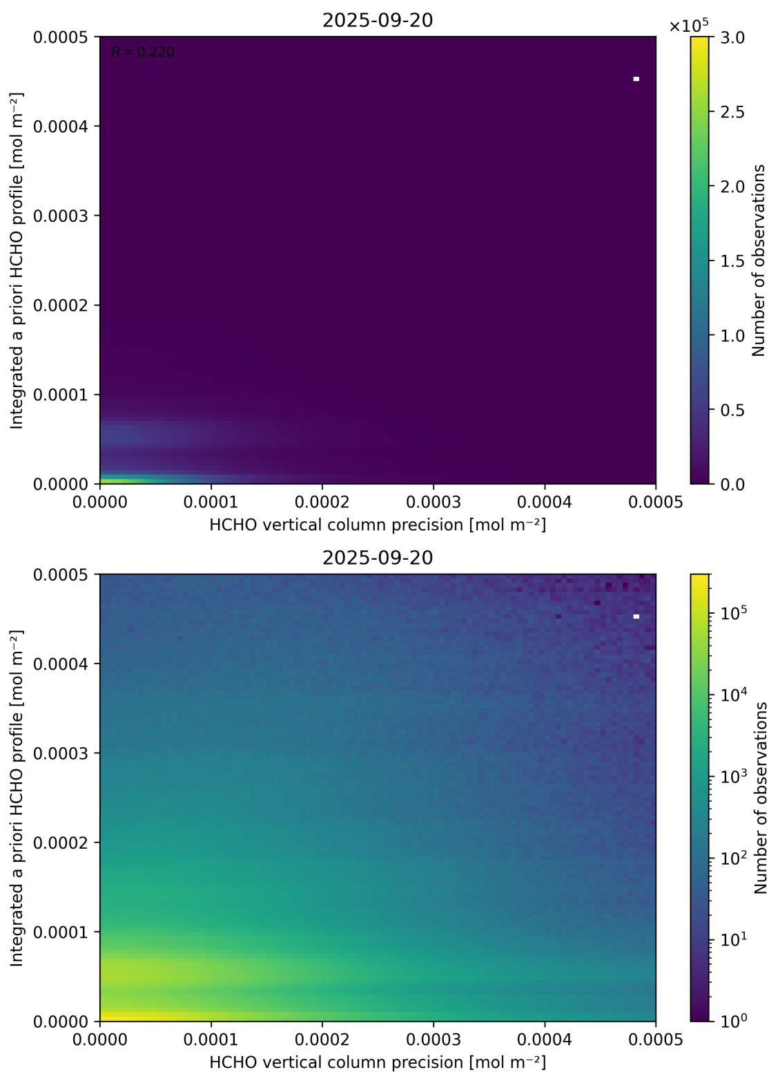
Figure 147: Scatter density plot of “HCHO vertical column precision” against “Integrated a priori HCHO profile” for 2025-09-20 to 2025-09-21.
