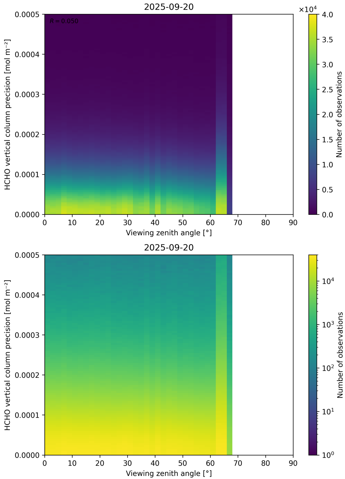
Figure 194: Scatter density plot of “Viewing zenith angle” against “HCHO vertical column precision” for 2025-09-20 to 2025-09-21.
