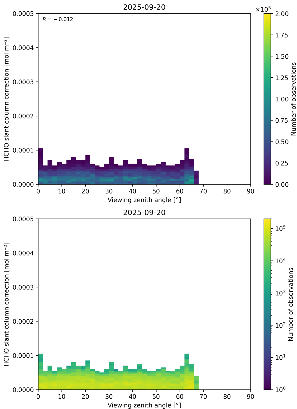
Figure 187: Scatter density plot of “Viewing zenith angle” against “HCHO slant column correction” for 2025-09-20 to 2025-09-21.
