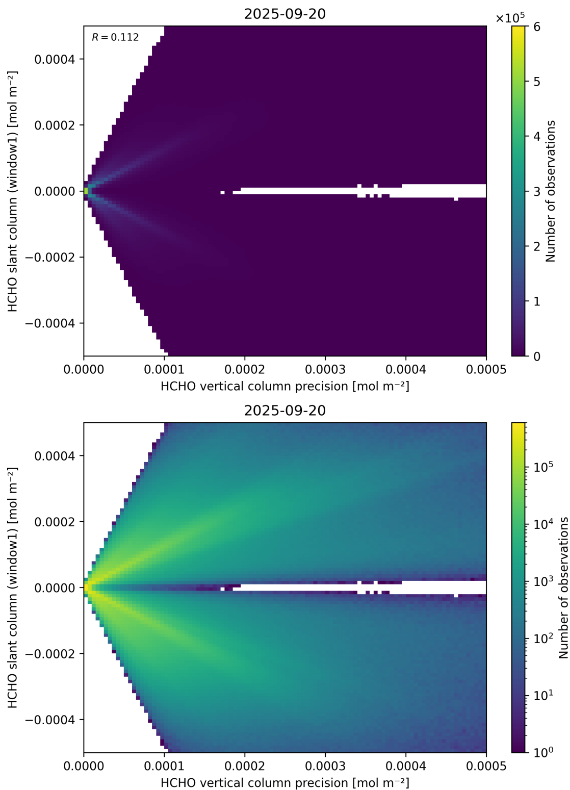
Figure 142: Scatter density plot of “HCHO vertical column precision” against “HCHO slant column (window1)” for 2025-09-20 to 2025-09-21.
