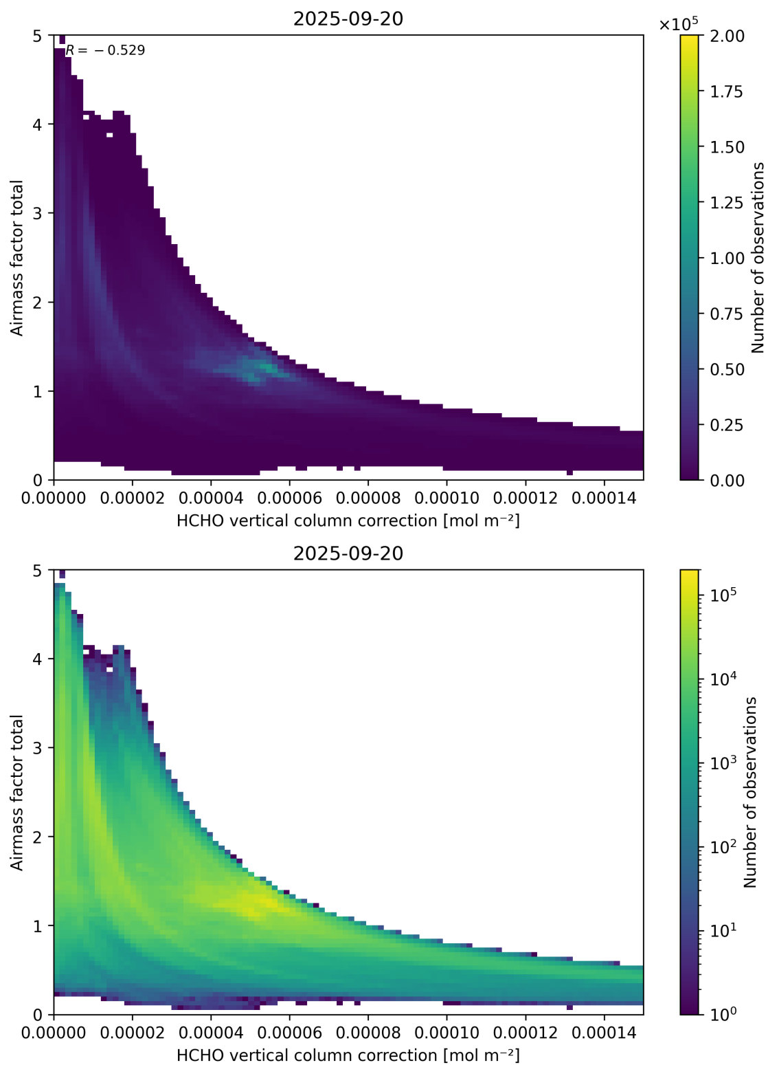
Figure 120: Scatter density plot of “HCHO vertical column correction” against “Airmass factor total” for 2025-09-20 to 2025-09-21.
