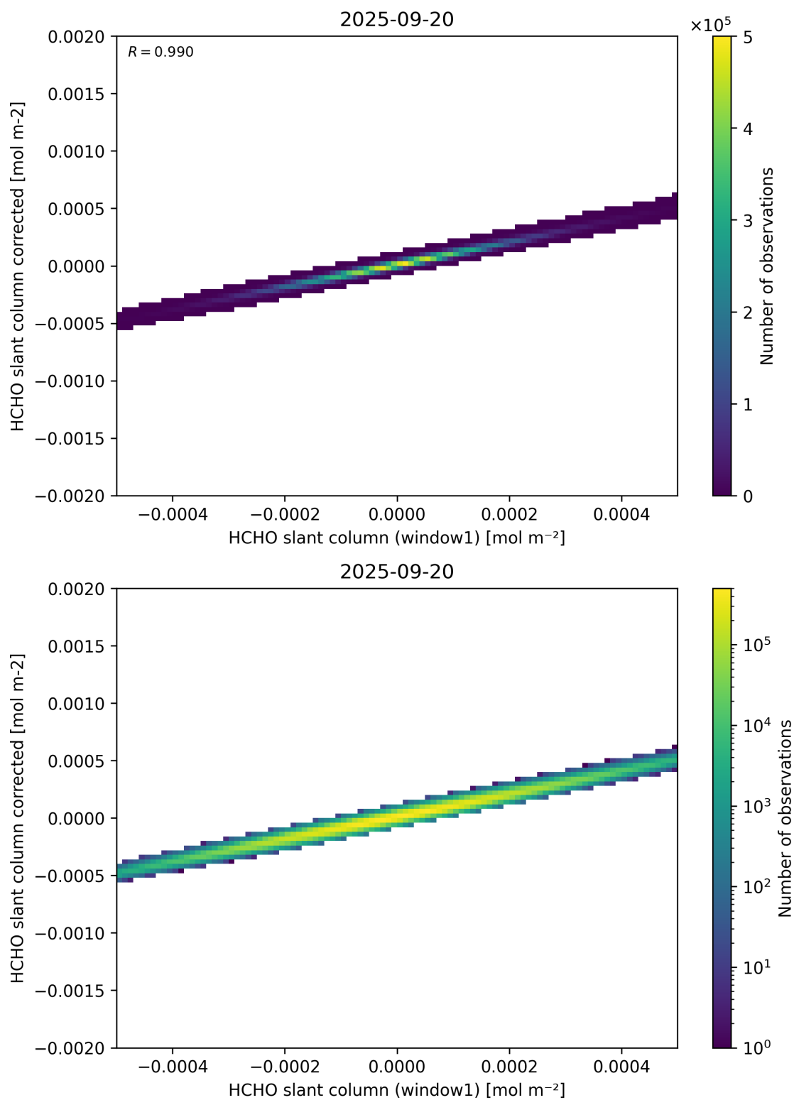
Figure 82: Scatter density plot of “HCHO slant column (window1)” against “HCHO slant column corrected” for 2025-09-20 to 2025-09-21.
