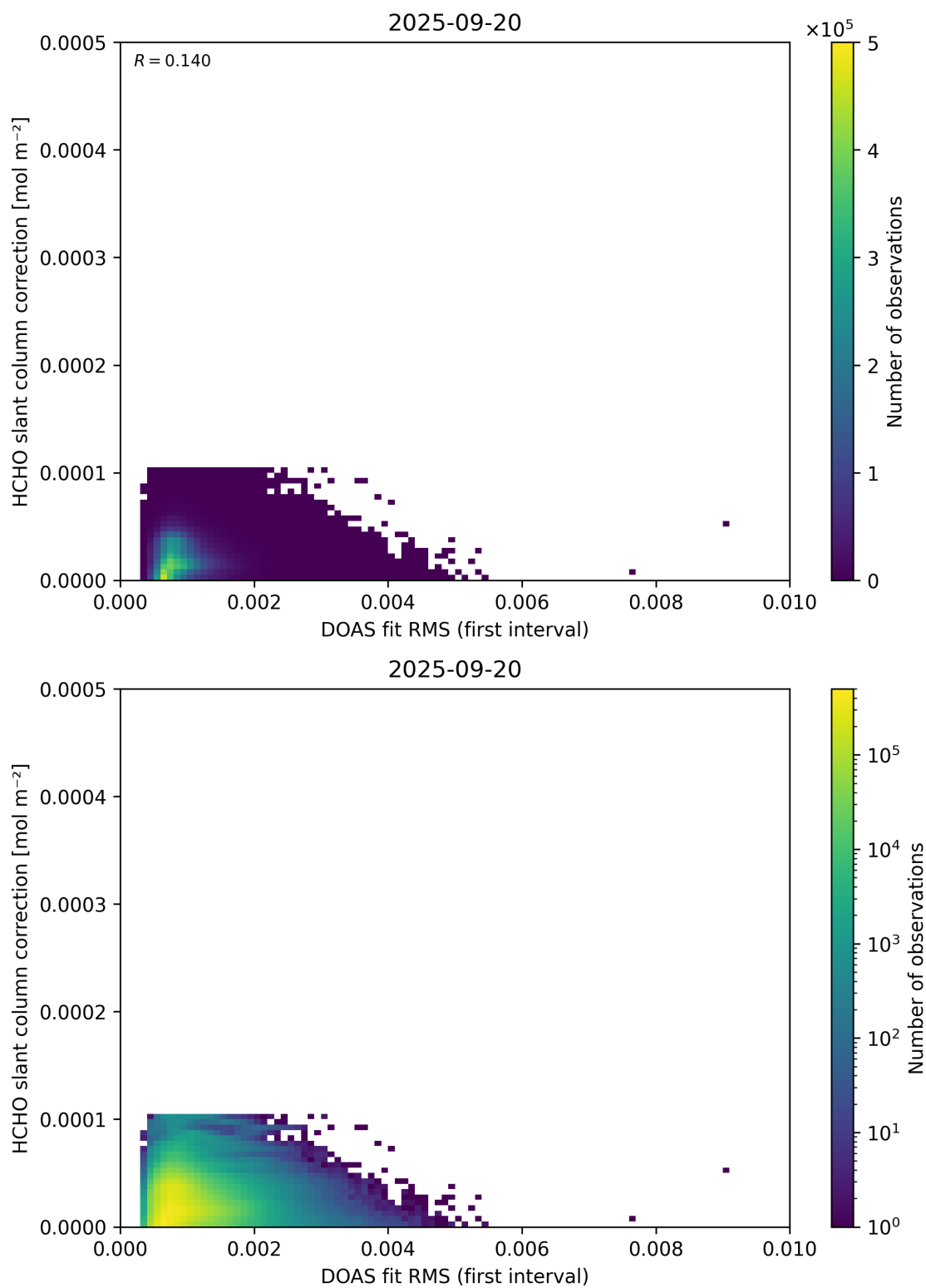
Figure 63: Scatter density plot of “DOAS fit RMS (first interval)” against “HCHO slant column correction” for 2025-09-20 to 2025-09-21.
