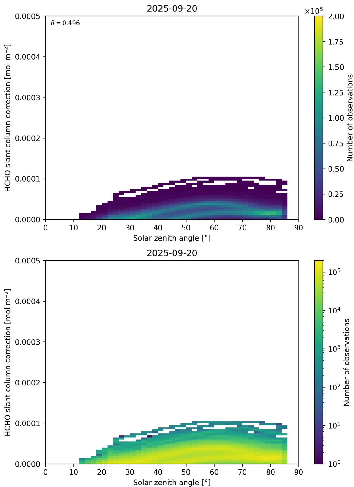
Figure 172: Scatter density plot of “Solar zenith angle” against “HCHO slant column correction” for 2025-09-20 to 2025-09-21.
