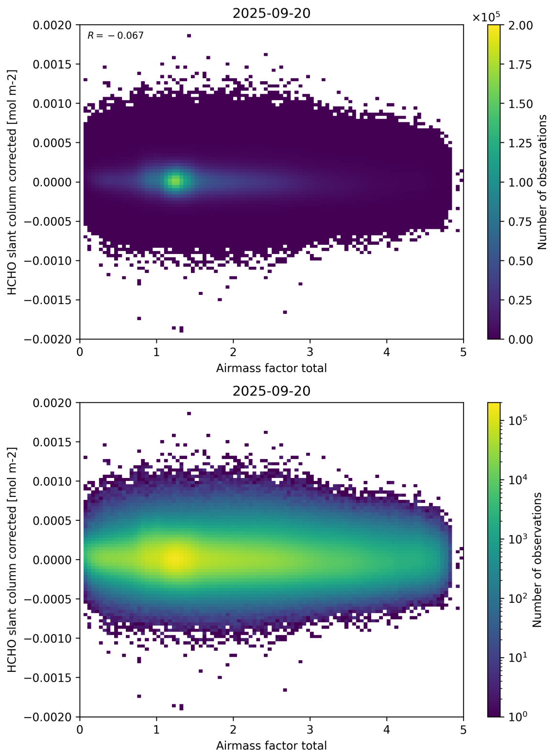
Figure 101: Scatter density plot of “Airmass factor total” against “HCHO slant column corrected” for 2025-09-20 to 2025-09-21.
