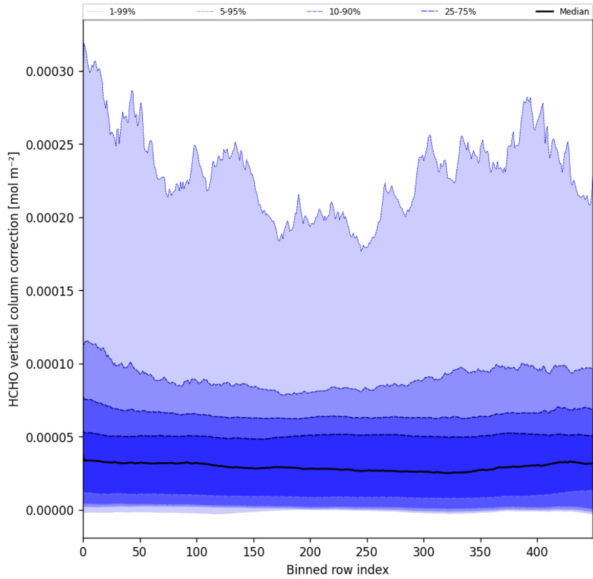
Figure 51: Along track statistics of “HCHO vertical column correction” for 2025-09-20 to 2025-09-21
