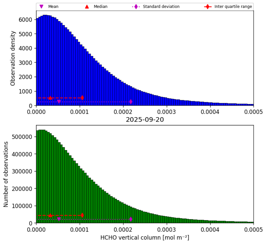
Figure 35: Histogram of “HCHO vertical column” for 2025-09-20 to 2025-09-21
