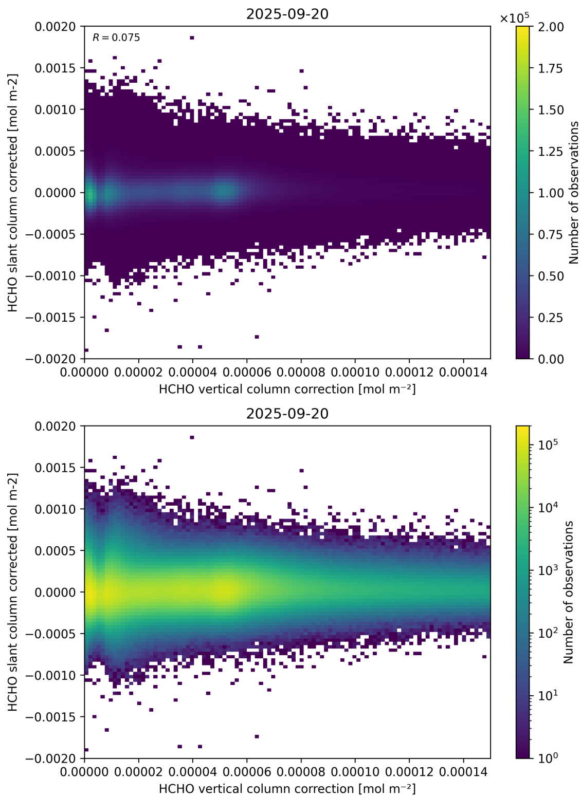
Figure 116: Scatter density plot of “HCHO vertical column correction” against “HCHO slant column corrected” for 2025-09-20 to 2025-09-21.
