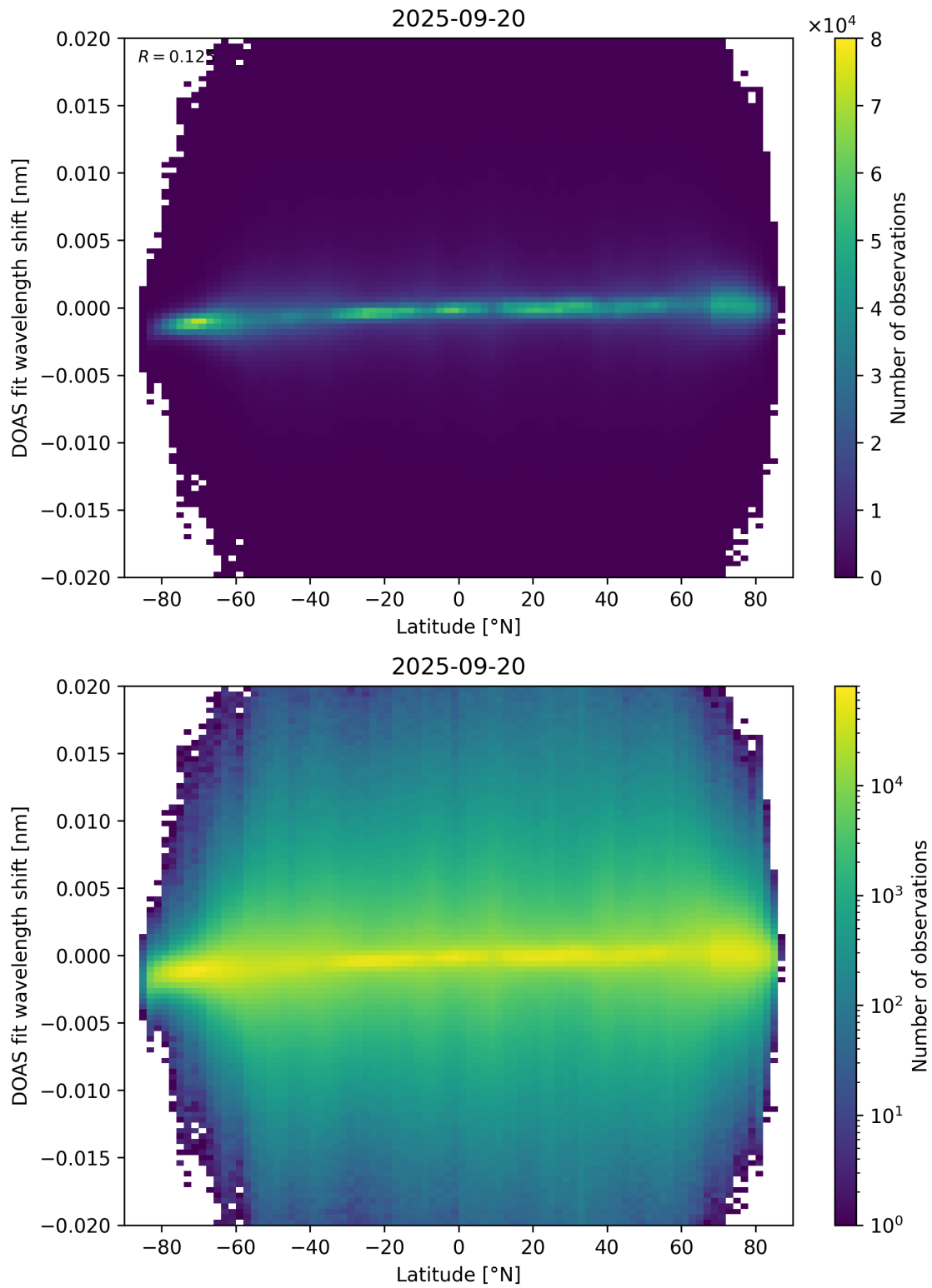
Figure 154: Scatter density plot of “Latitude” against “DOAS fit wavelength shift” for 2025-09-20 to 2025-09-21.
