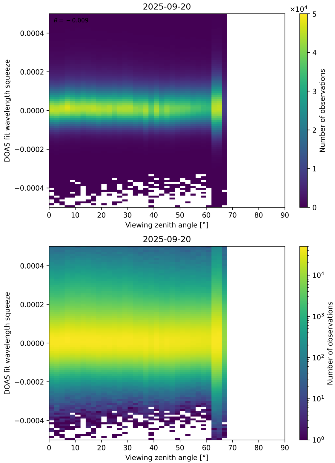
Figure 184: Scatter density plot of “Viewing zenith angle” against “DOAS fit wavelength squeeze” for 2025-09-20 to 2025-09-21.
