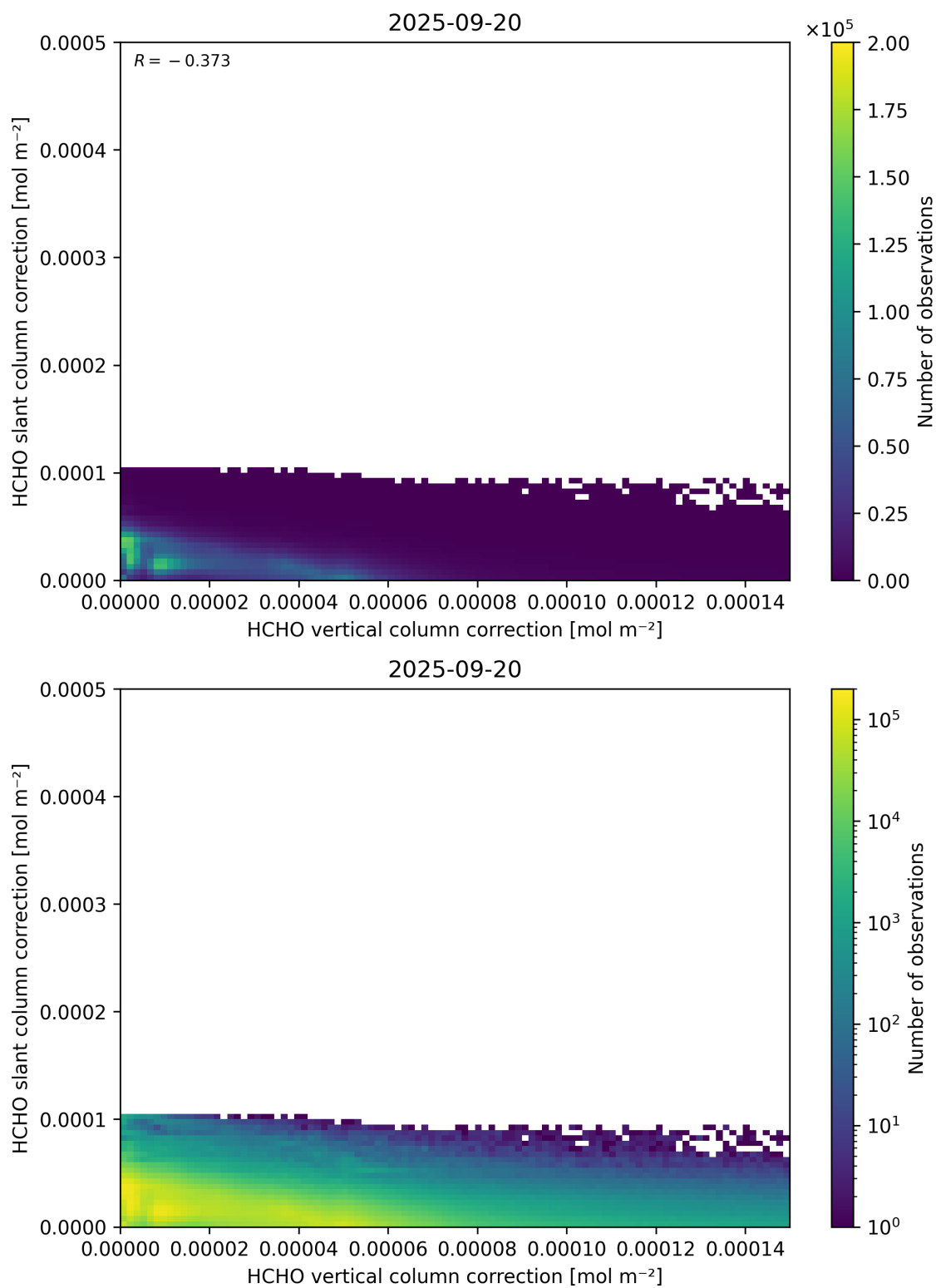
Figure 117: Scatter density plot of “HCHO vertical column correction” against “HCHO slant column correction” for 2025-09-20 to 2025-09-21.
