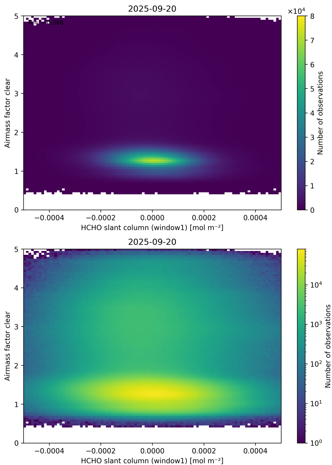
Figure 81: Scatter density plot of “HCHO slant column (window1)” against “Airmass factor clear” for 2025-09-20 to 2025-09-21.
