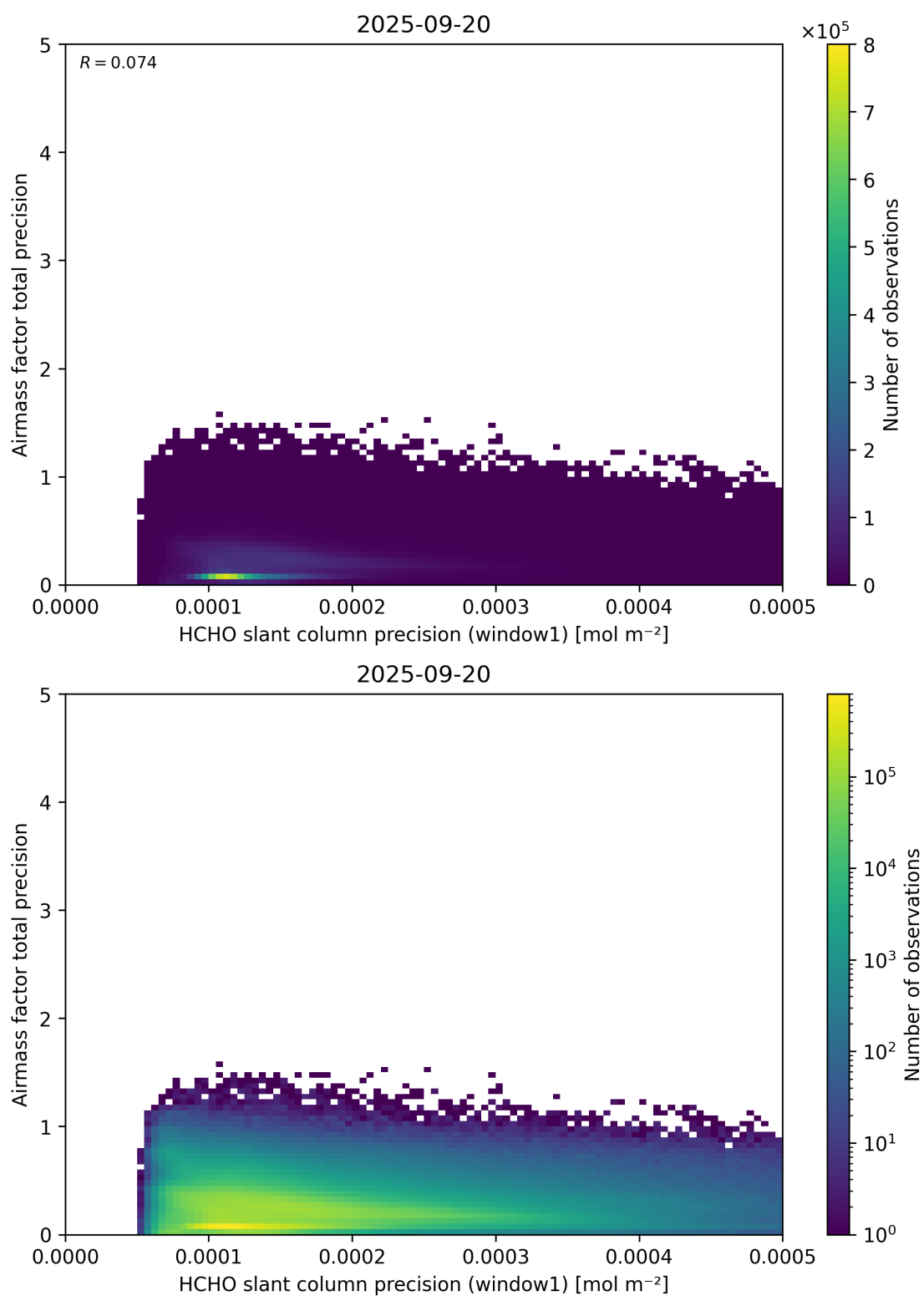
Figure 95: Scatter density plot of “HCHO slant column precision (window1)” against “Airmass factor total precision” for 2025-09-20 to 2025-09-21.
