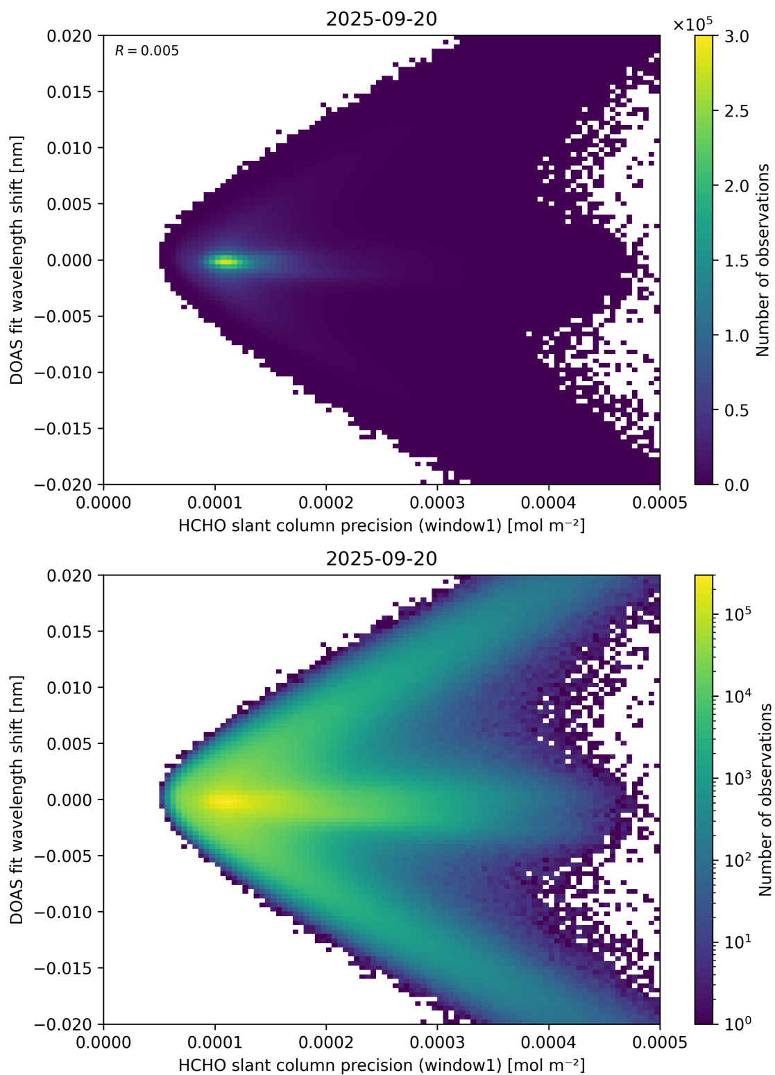
Figure 89: Scatter density plot of “HCHO slant column precision (window1)” against “DOAS fit wavelength shift” for 2025-09-20 to 2025-09-21.
