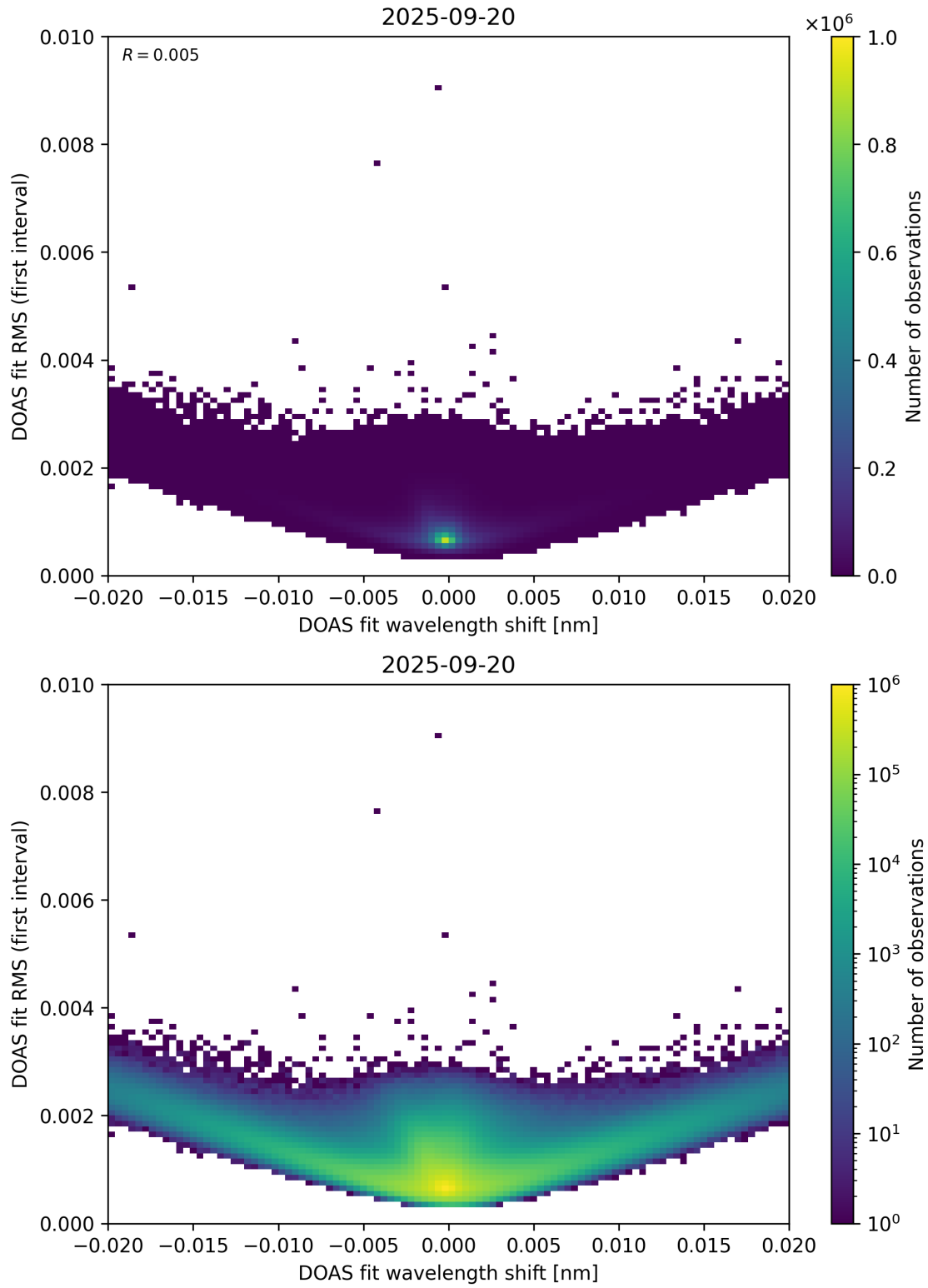
Figure 64: Scatter density plot of “DOAS fit wavelength shift” against “DOAS fit RMS (first interval)” for 2025-09-20 to 2025-09-21.
