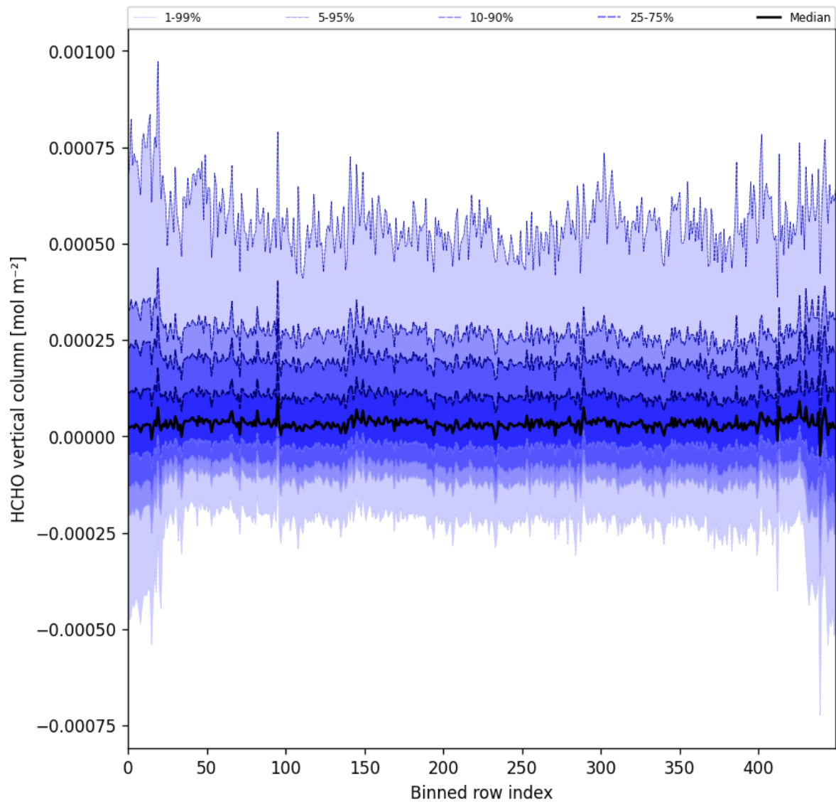
Figure 49: Along track statistics of “HCHO vertical column” for 2025-09-20 to 2025-09-21
