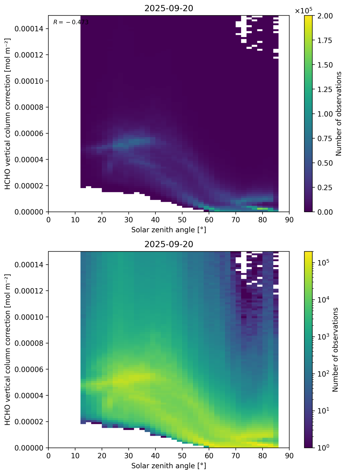
Figure 178: Scatter density plot of “Solar zenith angle” against “HCHO vertical column correction” for 2025-09-20 to 2025-09-21.
