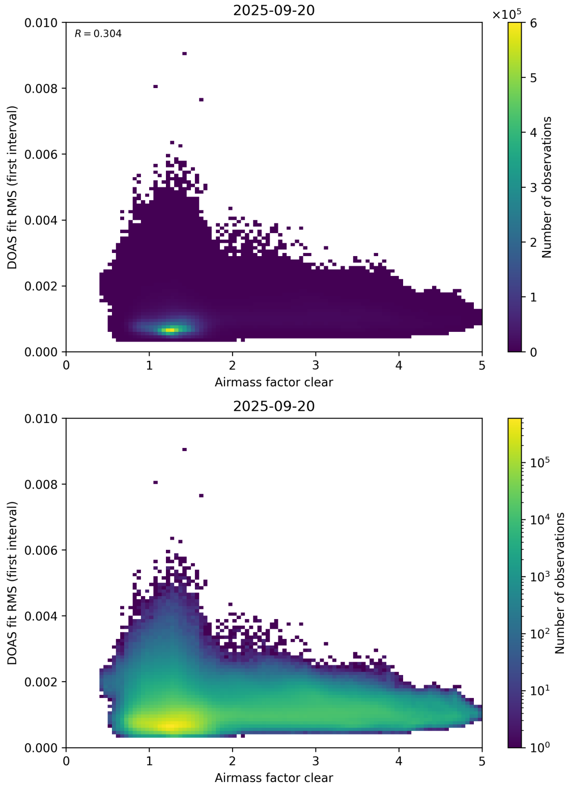
Figure 71: Scatter density plot of “Airmass factor clear” against “DOAS fit RMS (first interval)” for 2025-09-20 to 2025-09-21.
