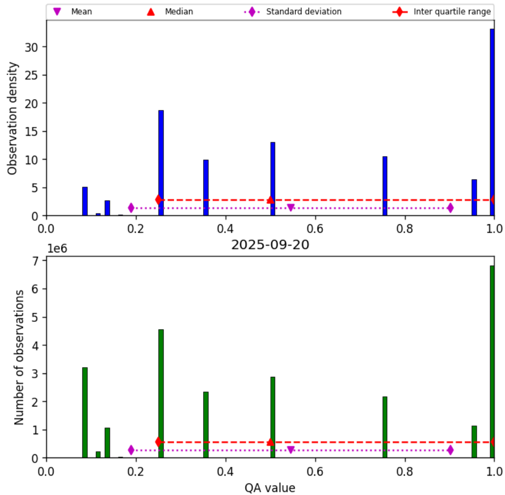
Figure 34: Histogram of “QA value” for 2025-09-20 to 2025-09-21
