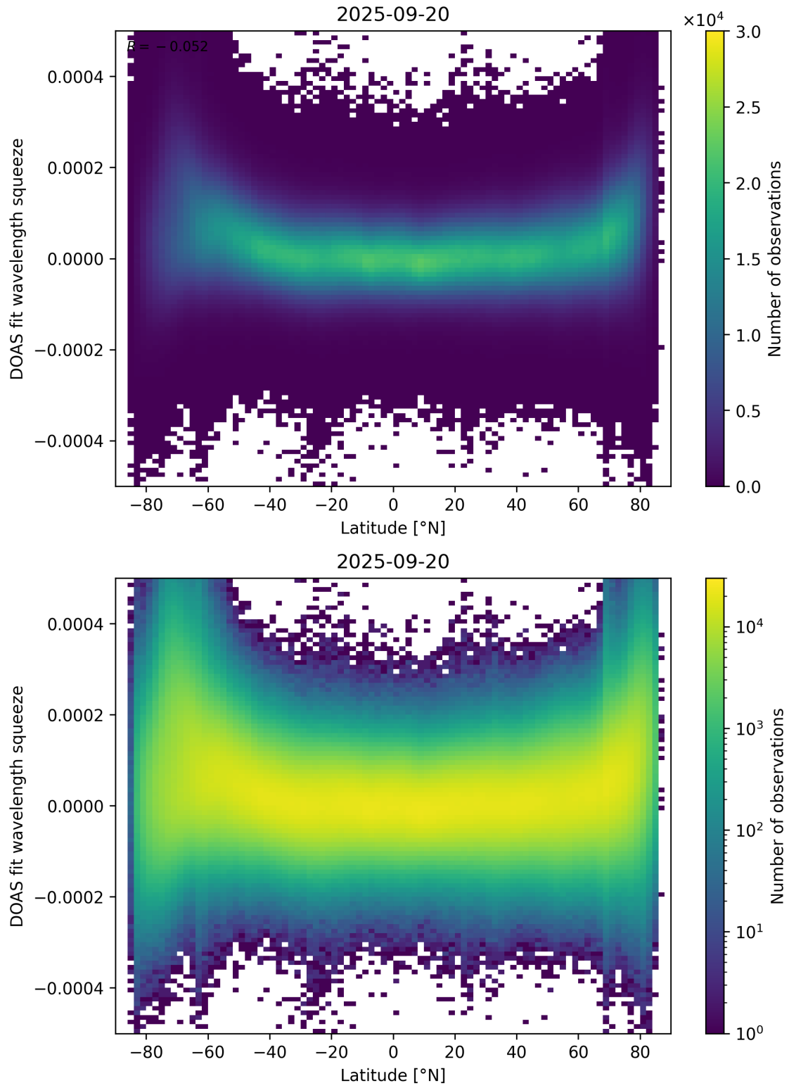
Figure 155: Scatter density plot of “Latitude” against “DOAS fit wavelength squeeze” for 2025-09-20 to 2025-09-21.
