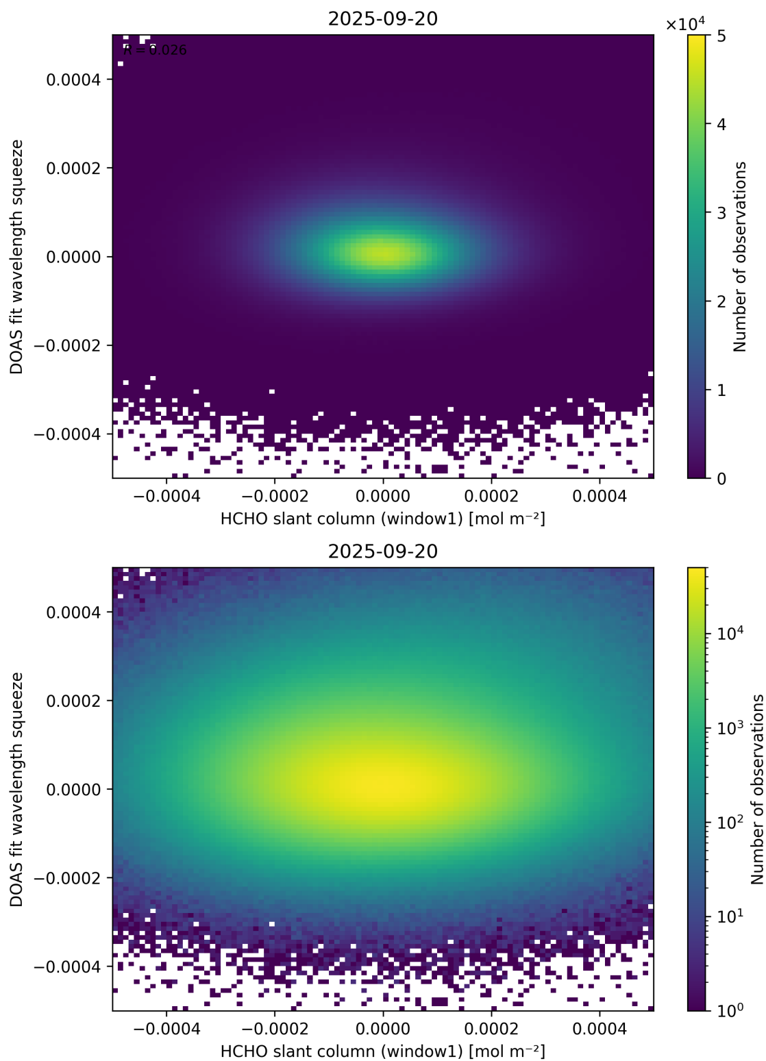
Figure 80: Scatter density plot of “HCHO slant column (window1)” against “DOAS fit wavelength squeeze” for 2025-09-20 to 2025-09-21.
