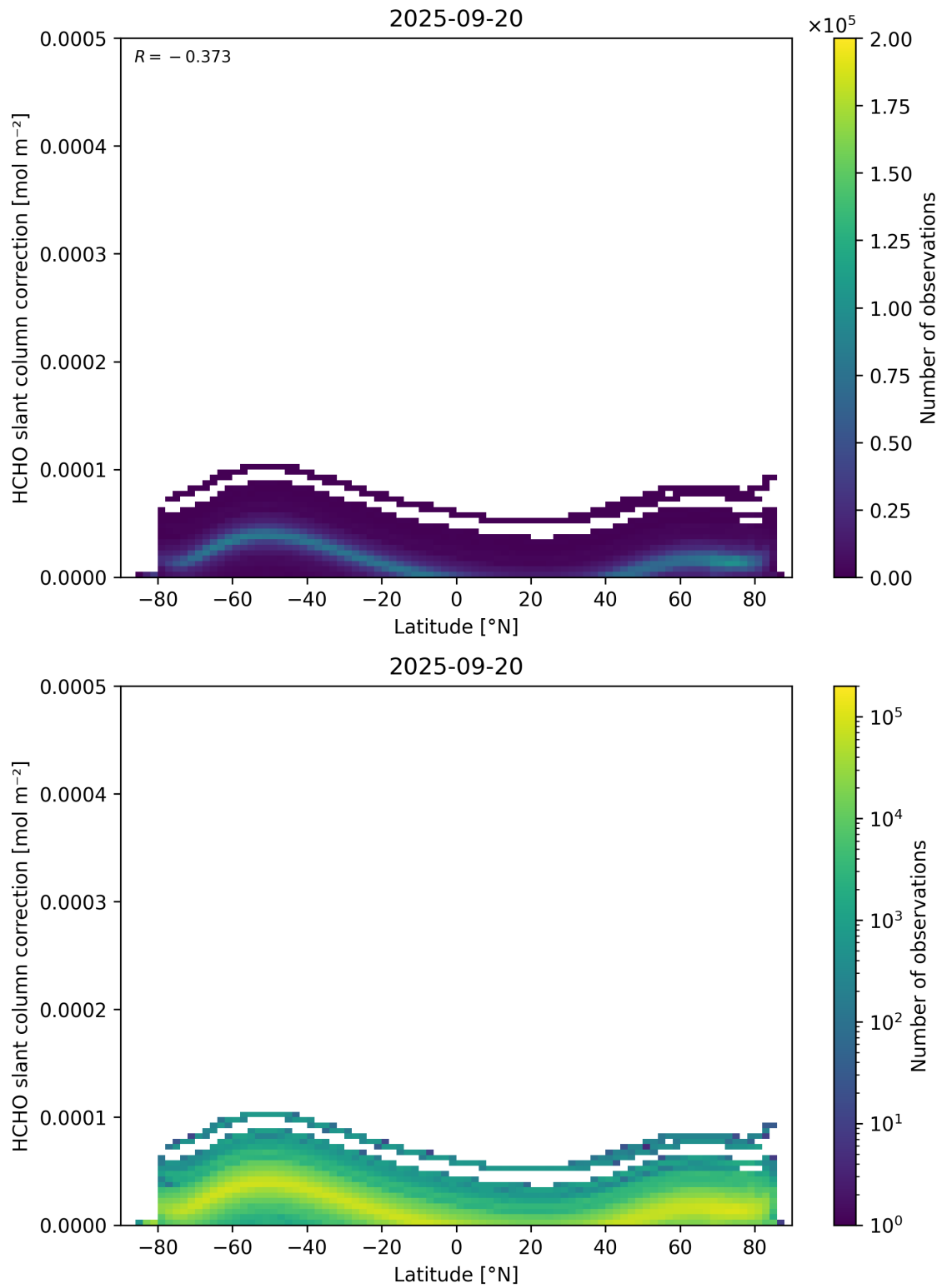
Figure 158: Scatter density plot of “Latitude” against “HCHO slant column correction” for 2025-09-20 to 2025-09-21.
