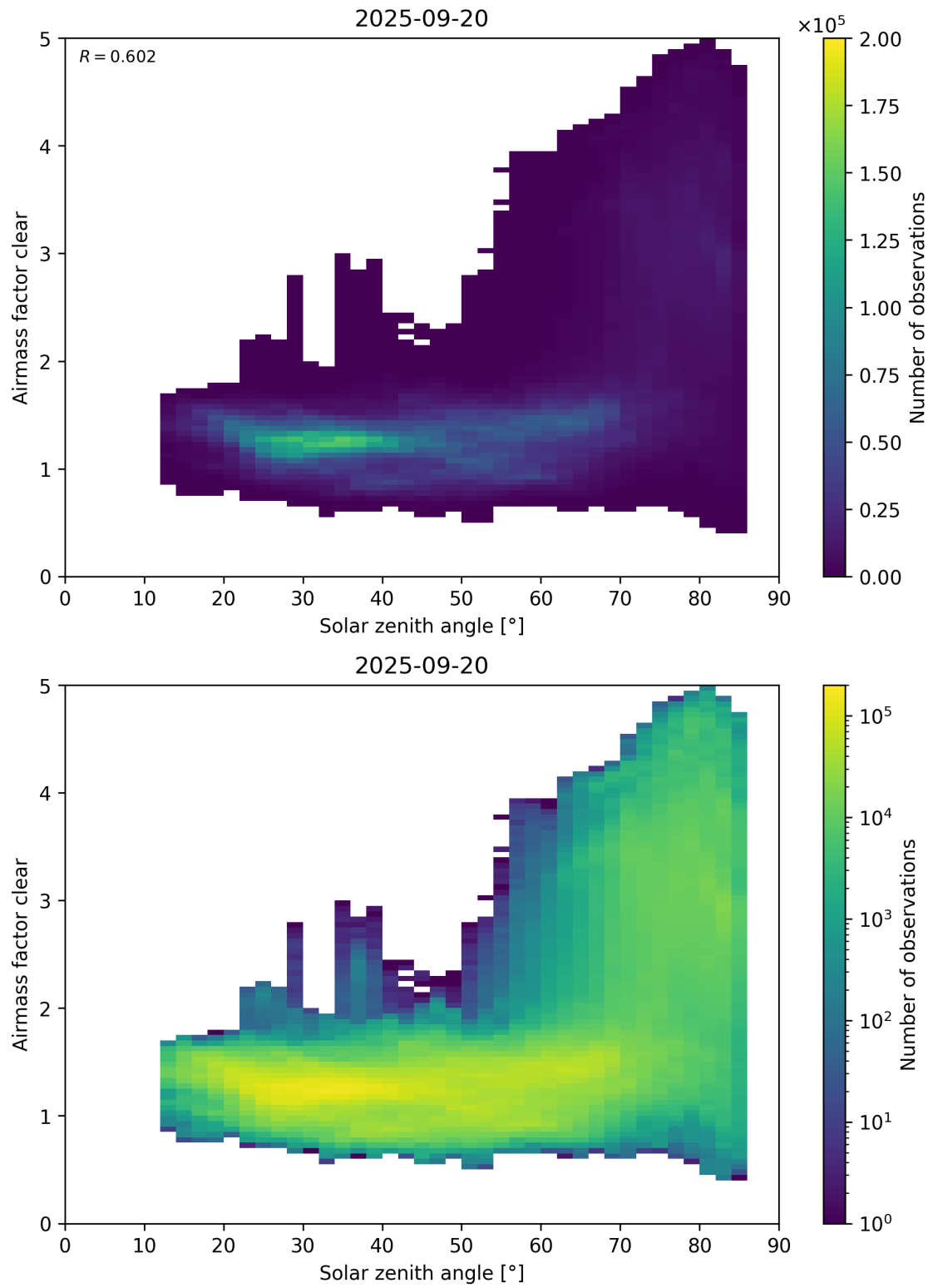
Figure 170: Scatter density plot of “Solar zenith angle” against “Airmass factor clear” for 2025-09-20 to 2025-09-21.
