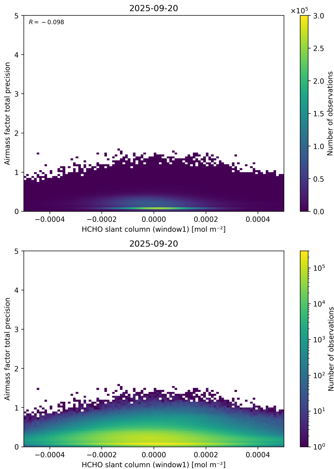
Figure 86: Scatter density plot of “HCHO slant column (window1)” against “Airmass factor total precision” for 2025-09-20 to 2025-09-21.
