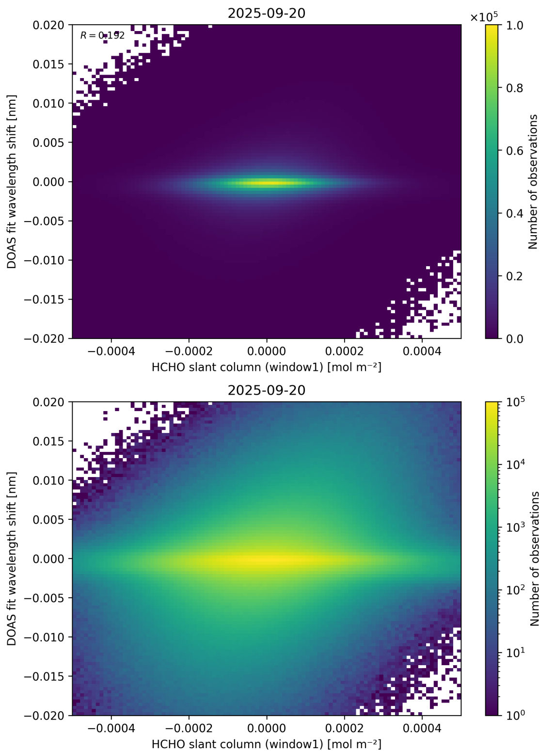
Figure 79: Scatter density plot of “HCHO slant column (window1)” against “DOAS fit wavelength shift” for 2025-09-20 to 2025-09-21.
