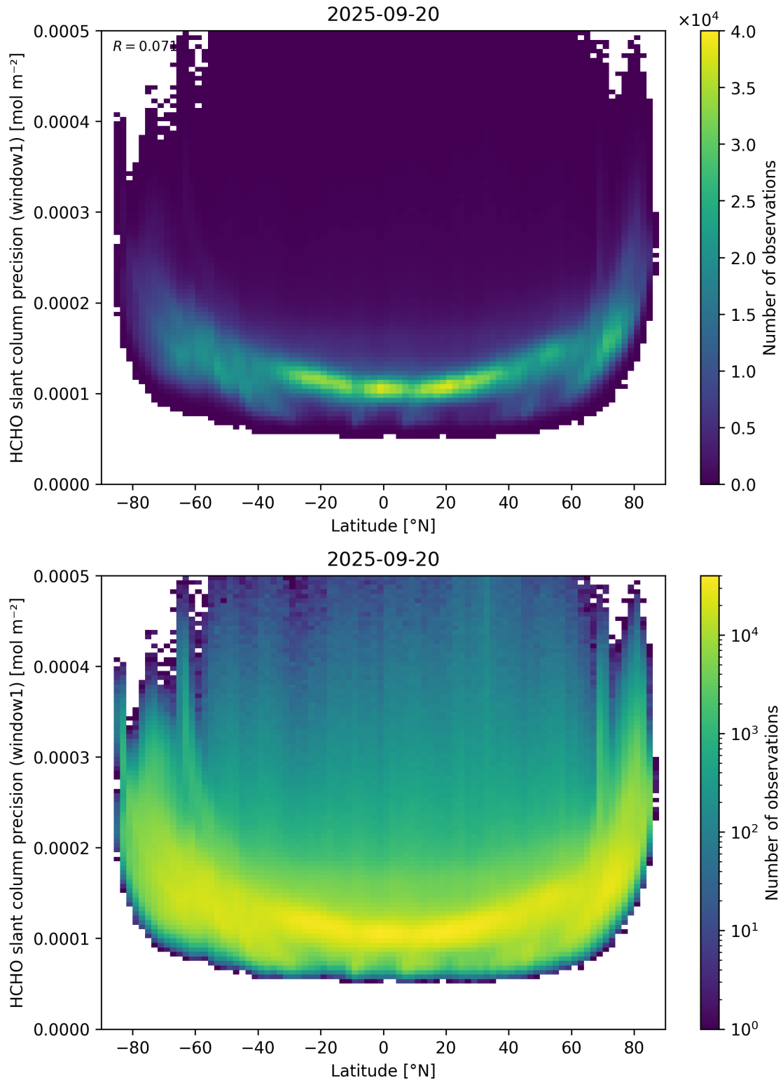
Figure 160: Scatter density plot of “Latitude” against “HCHO slant column precision (window1)” for 2025-09-20 to 2025-09-21.
