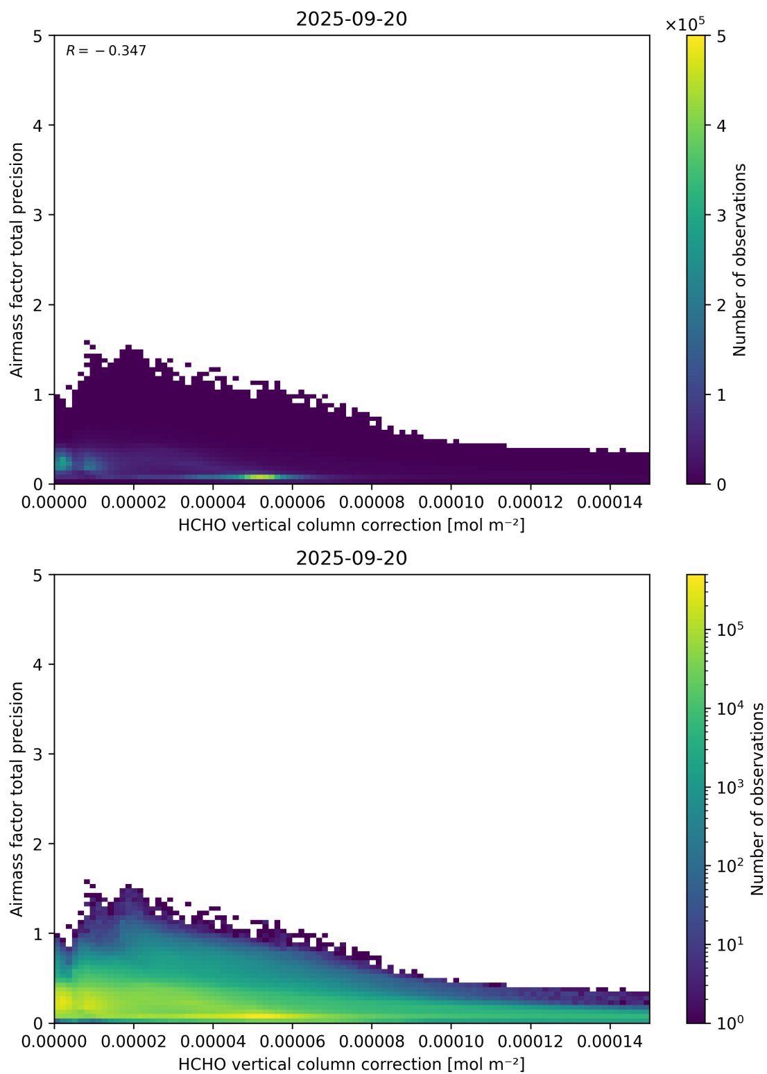
Figure 121: Scatter density plot of “HCHO vertical column correction” against “Airmass factor total precision” for 2025-09-20 to 2025-09-21.
