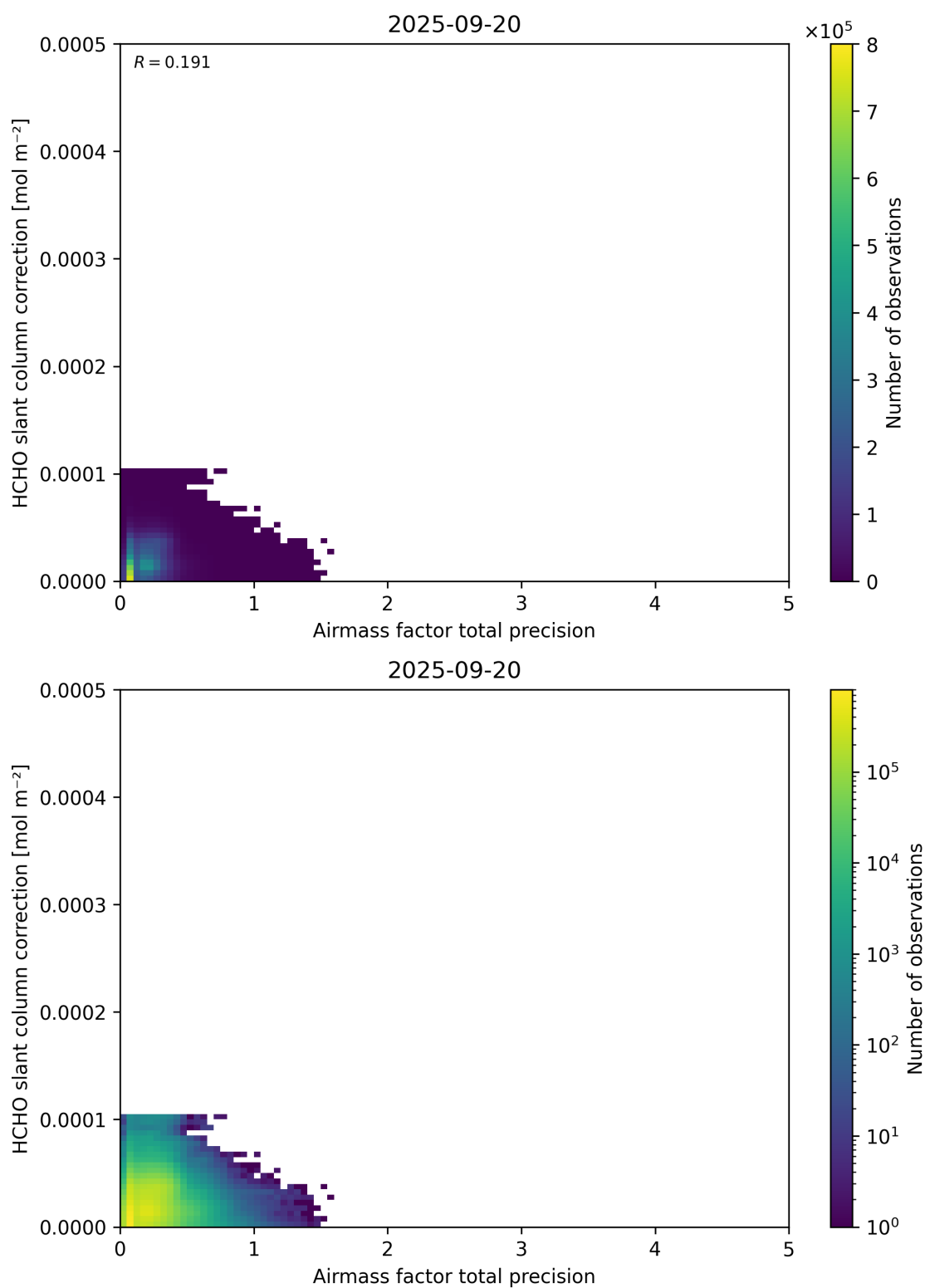
Figure 110: Scatter density plot of “Airmass factor total precision” against “HCHO slant column correction” for 2025-09-20 to 2025-09-21.
