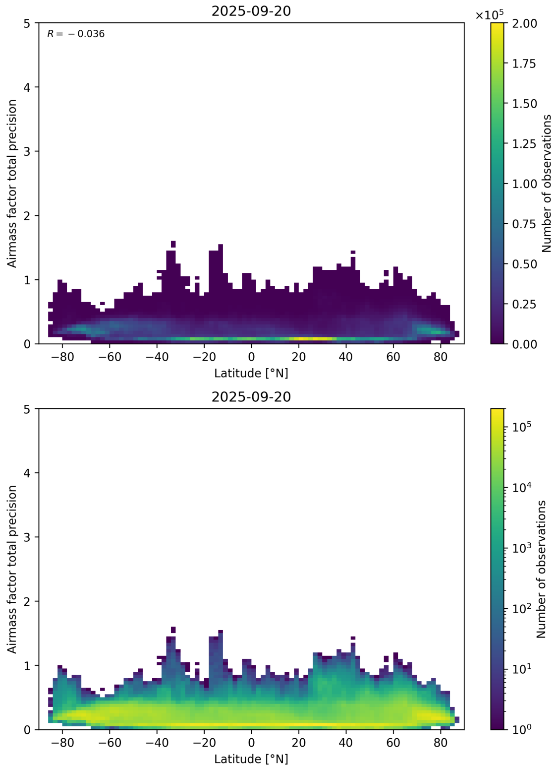
Figure 162: Scatter density plot of “Latitude” against “Airmass factor total precision” for 2025-09-20 to 2025-09-21.
