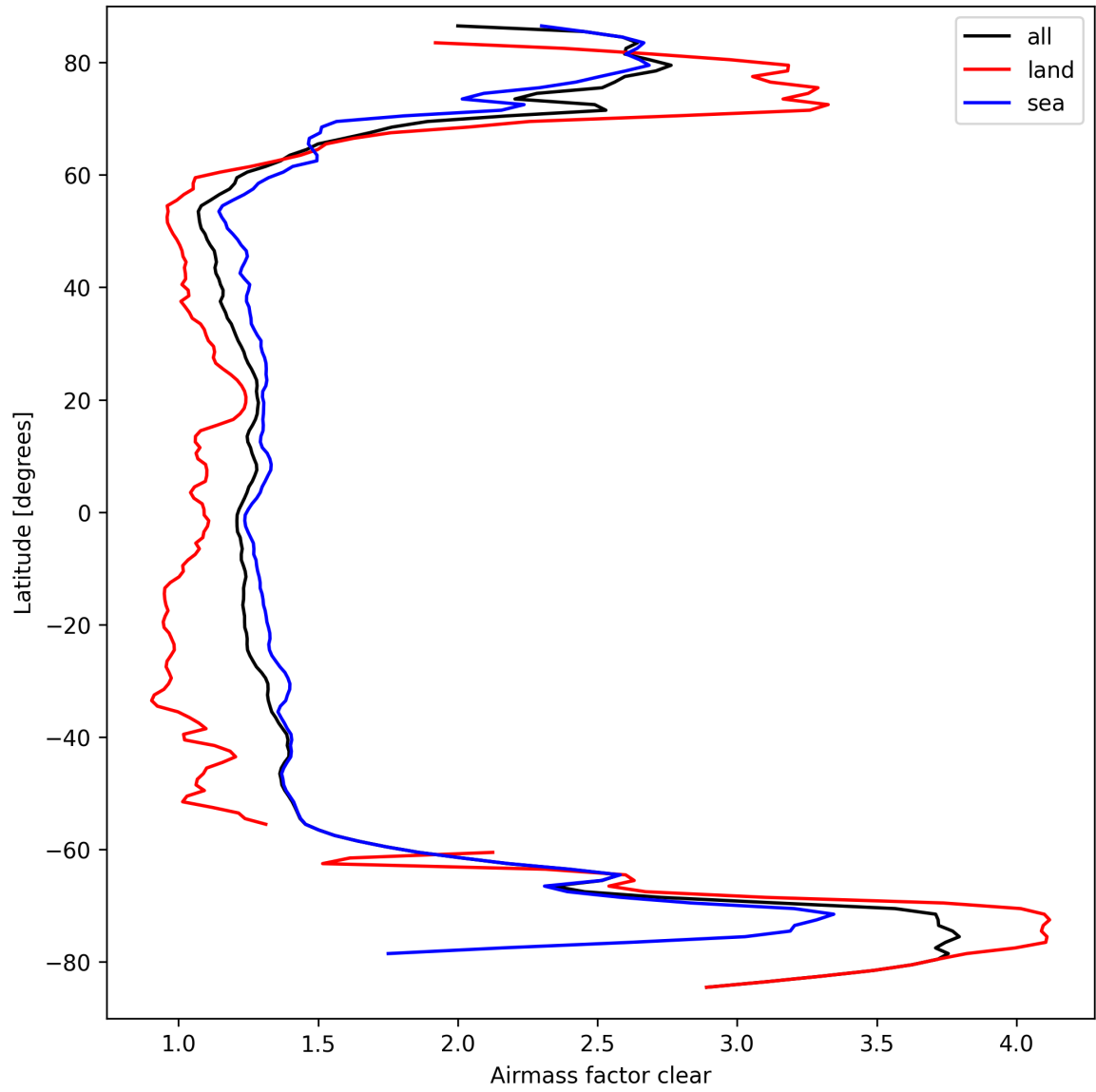
Figure 28: Zonal average of “Airmass factor clear” for 2025-09-20 to 2025-09-21.
