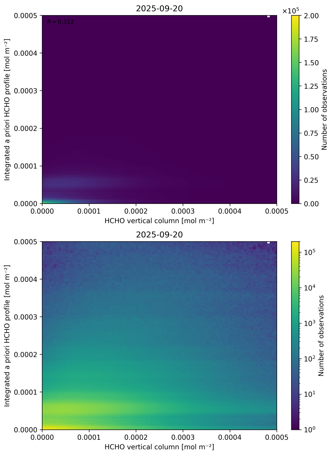
Figure 135: Scatter density plot of “HCHO vertical column” against “Integrated a priori HCHO profile” for 2025-09-20 to 2025-09-21.
