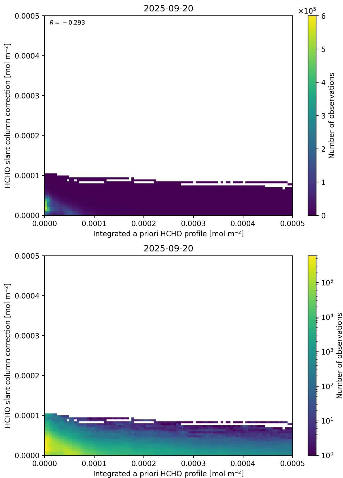
Figure 152: Scatter density plot of “Integrated a priori HCHO profile” against “HCHO slant column correction” for 2025-09-20 to 2025-09-21.
