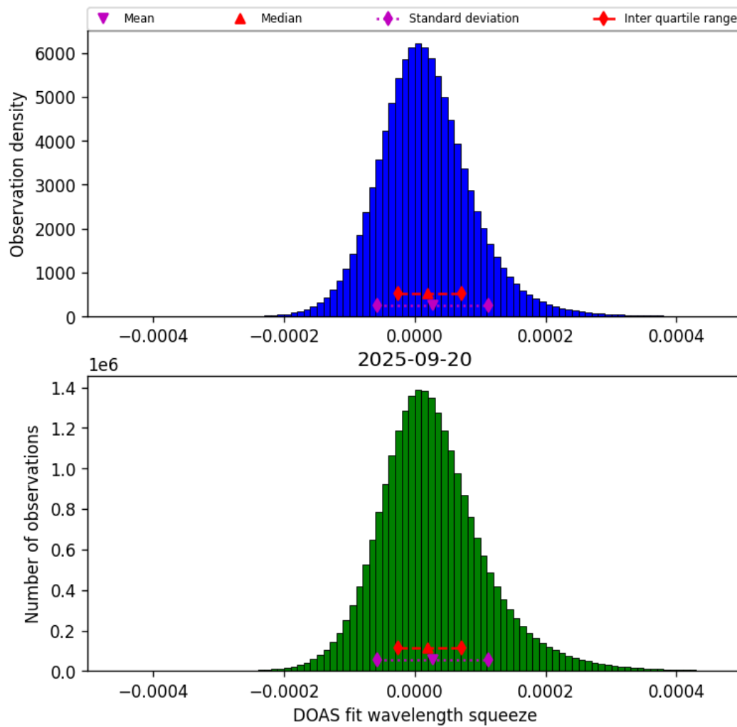
Figure 45: Histogram of “DOAS fit wavelength squeeze” for 2025-09-20 to 2025-09-21
