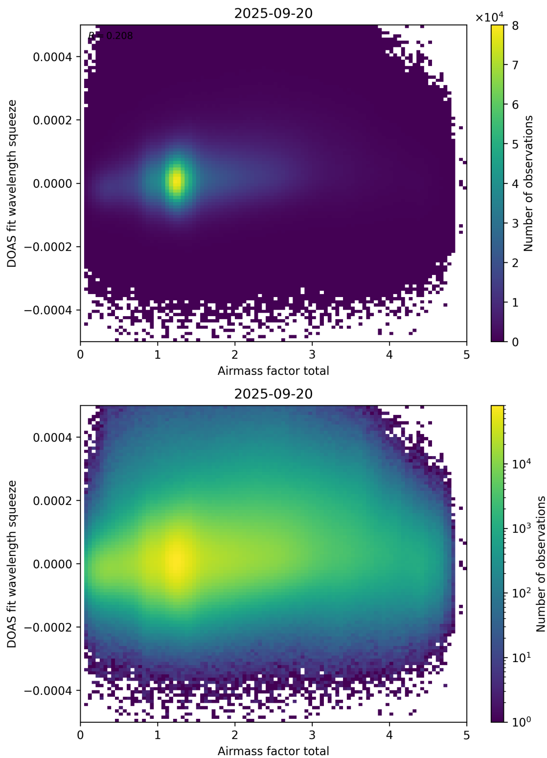
Figure 99: Scatter density plot of “Airmass factor total” against “DOAS fit wavelength squeeze” for 2025-09-20 to 2025-09-21.
