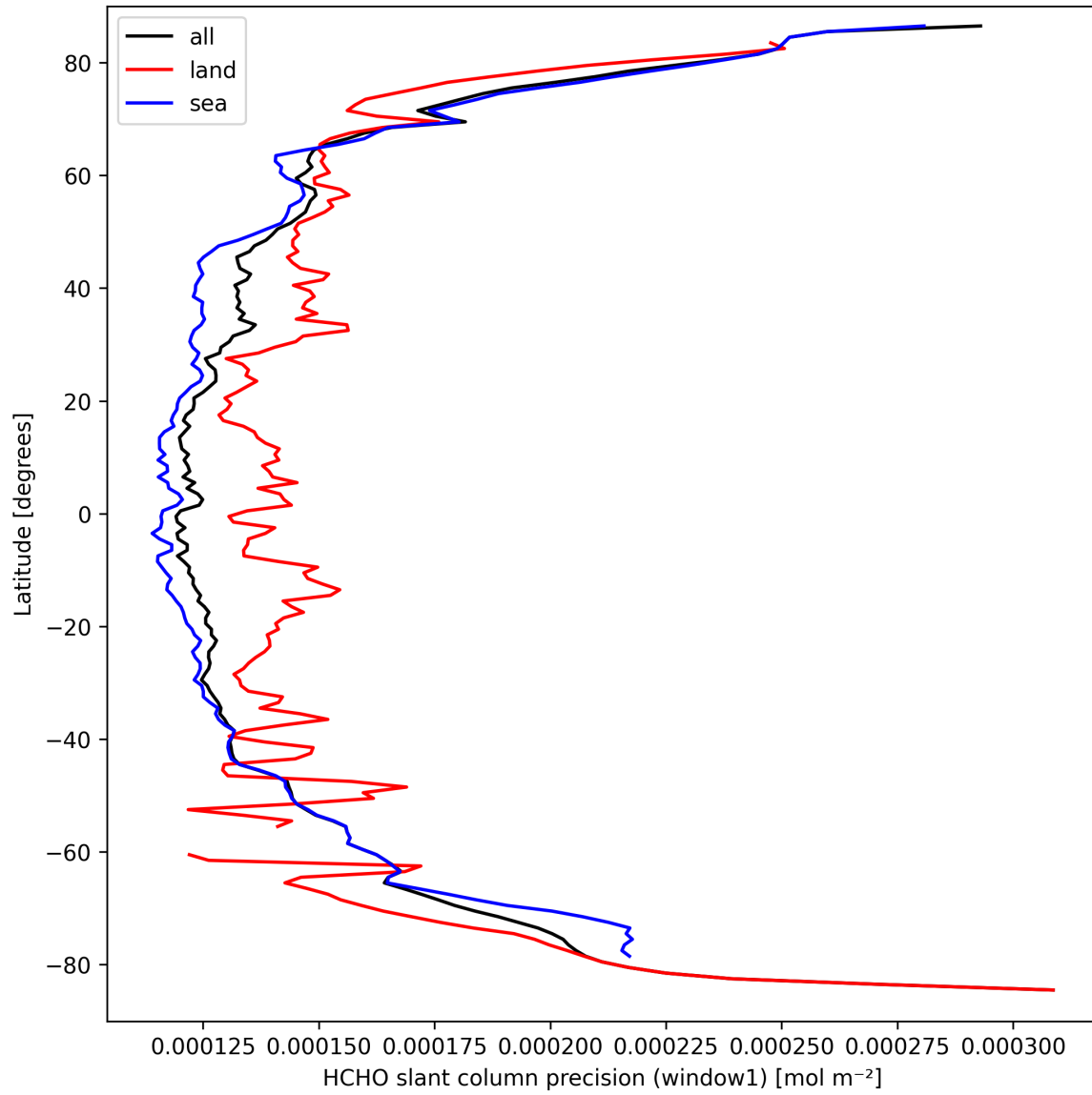
Figure 25: Zonal average of “HCHO slant column precision (window1)” for 2025-09-20 to 2025-09-21.
