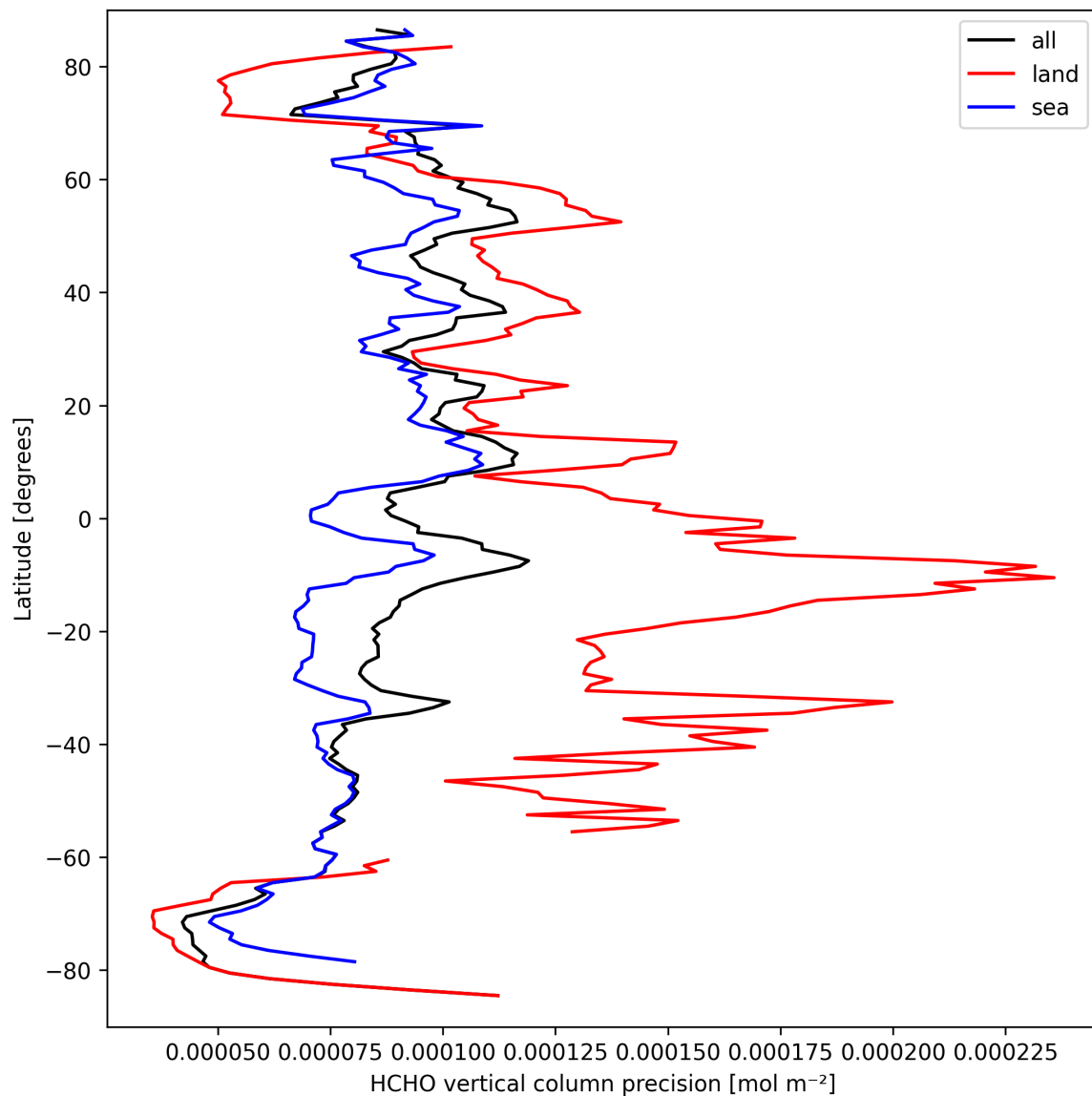
Figure 22: Zonal average of “HCHO vertical column precision” for 2025-09-20 to 2025-09-21.
