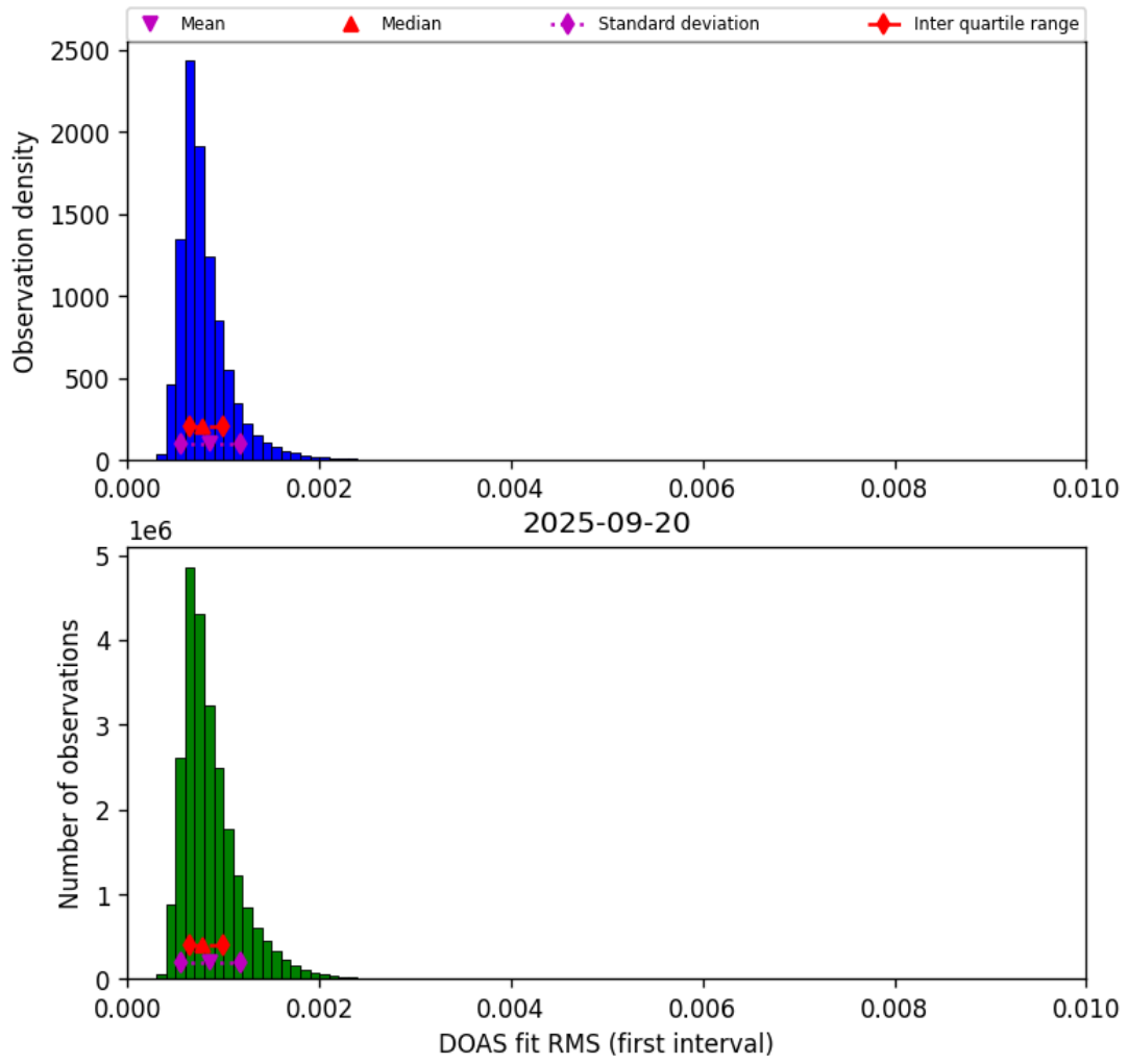
Figure 46: Histogram of “DOAS fit RMS (first interval)” for 2025-09-20 to 2025-09-21
