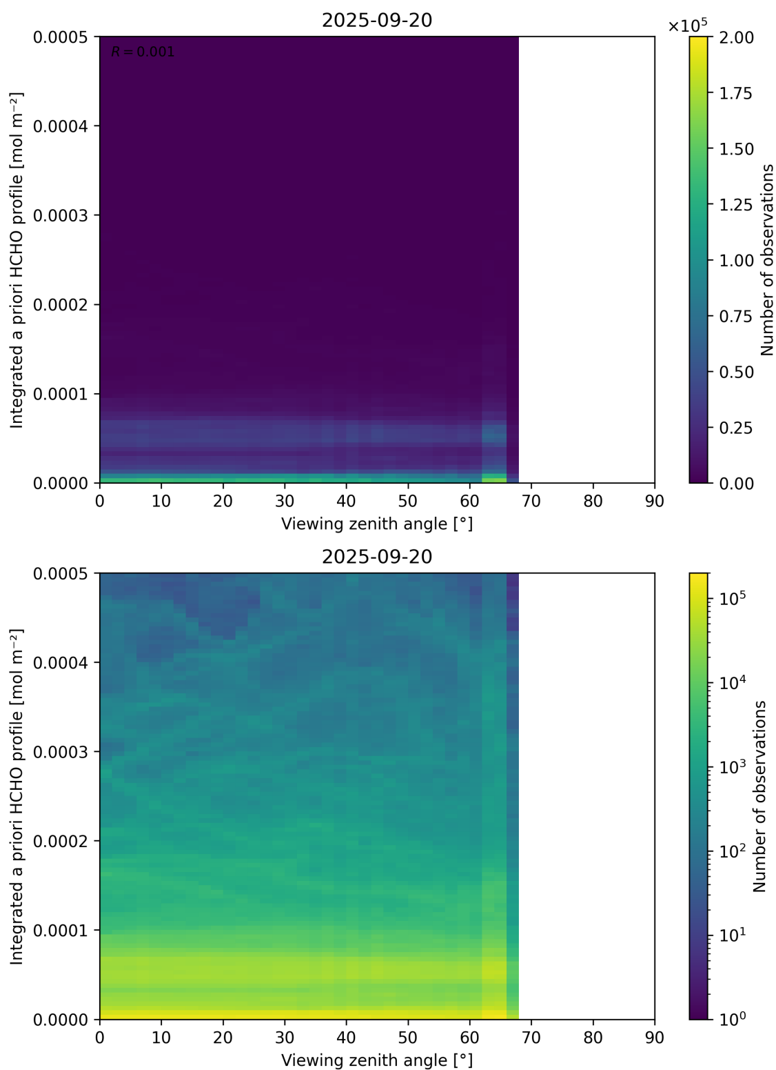
Figure 195: Scatter density plot of “Viewing zenith angle” against “Integrated a priori HCHO profile” for 2025-09-20 to 2025-09-21.
