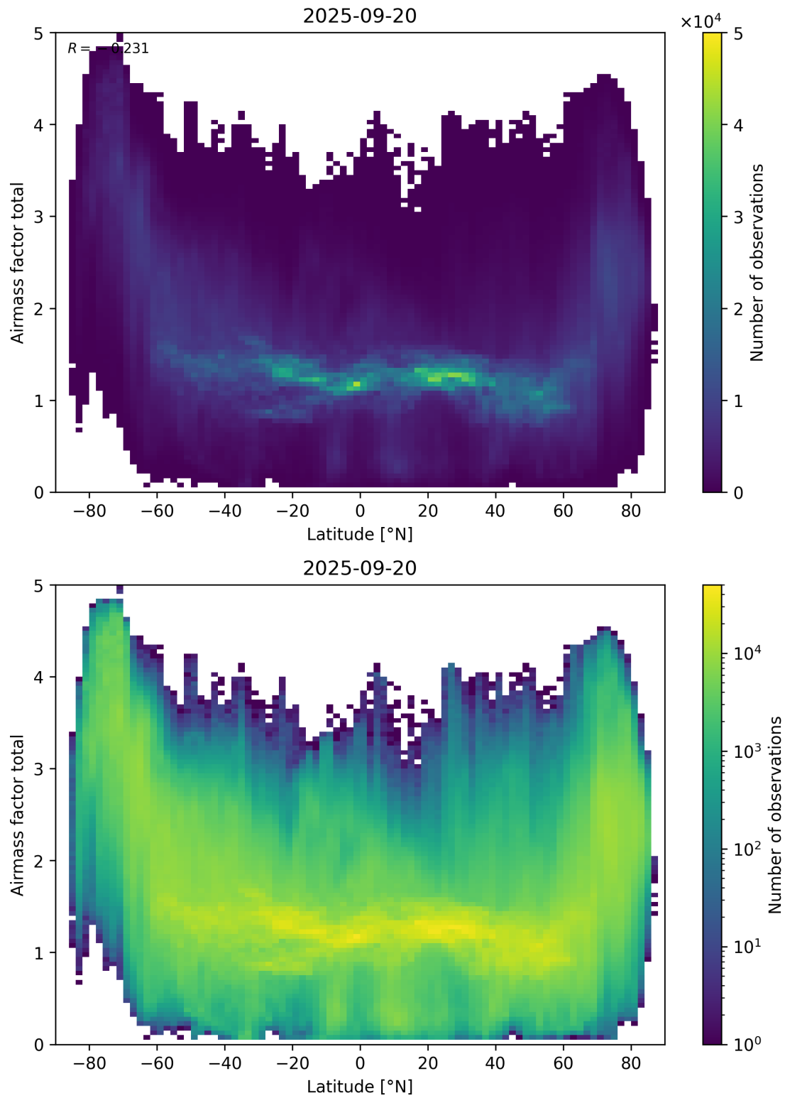
Figure 161: Scatter density plot of “Latitude” against “Airmass factor total” for 2025-09-20 to 2025-09-21.
