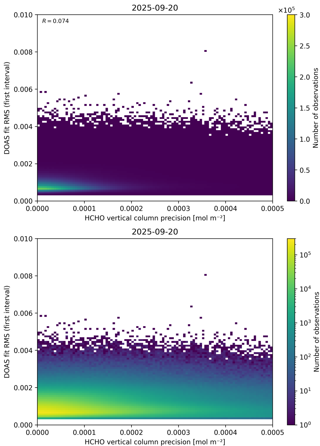
Figure 136: Scatter density plot of “HCHO vertical column precision” against “DOAS fit RMS (first interval)” for 2025-09-20 to 2025-09-21.
