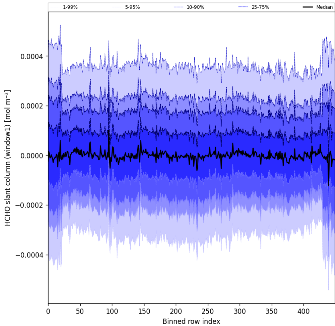
Figure 52: Along track statistics of “HCHO slant column (window1)” for 2025-09-20 to 2025-09-21
