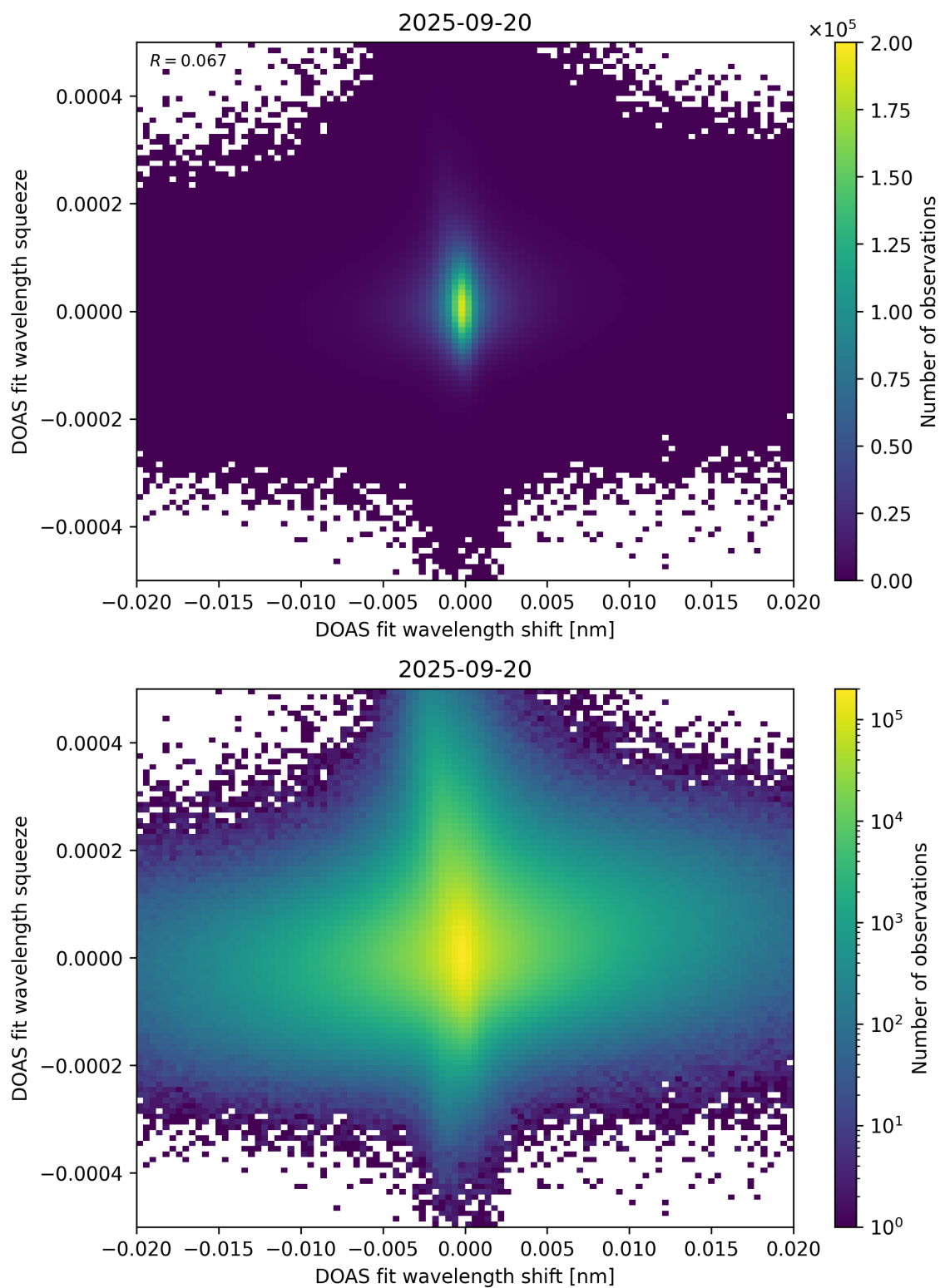
Figure 65: Scatter density plot of “DOAS fit wavelength shift” against “DOAS fit wavelength squeeze” for 2025-09-20 to 2025-09-21.
