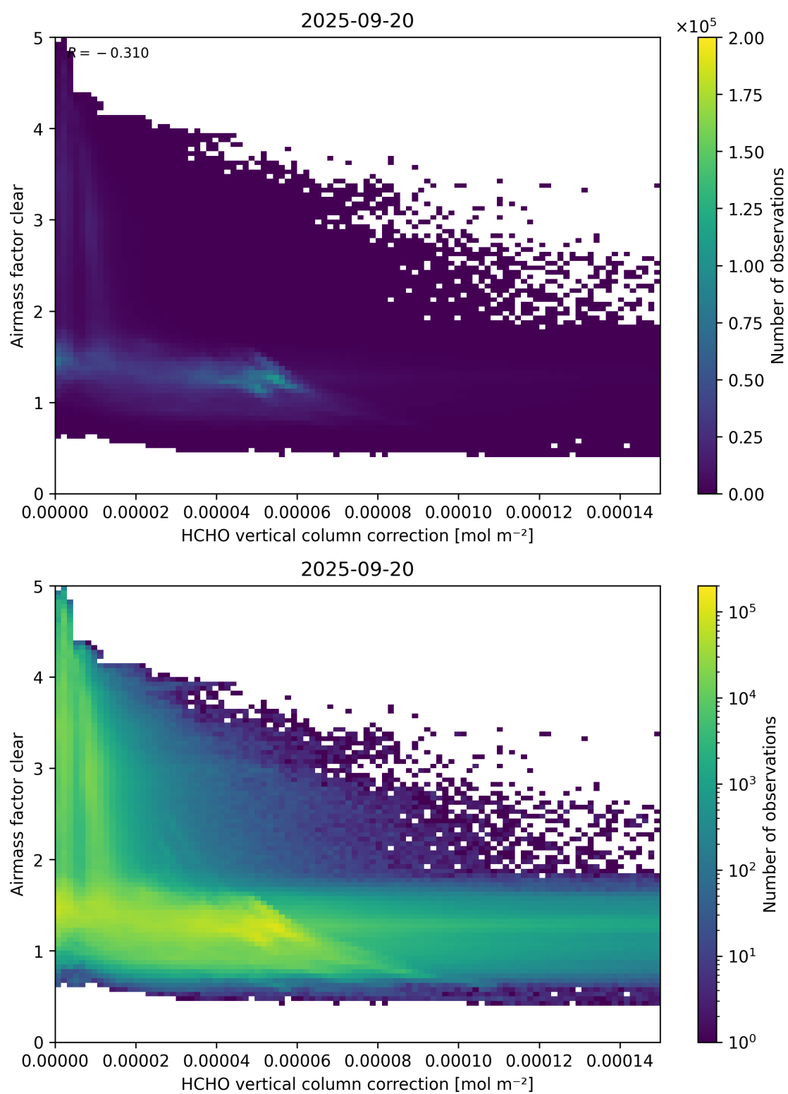
Figure 115: Scatter density plot of “HCHO vertical column correction” against “Airmass factor clear” for 2025-09-20 to 2025-09-21.
