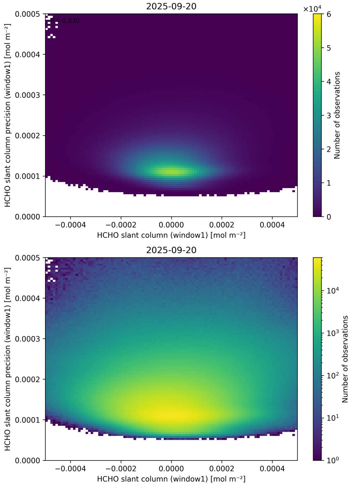
Figure 84: Scatter density plot of “HCHO slant column (window1)” against “HCHO slant column precision (window1)” for 2025-09-20 to 2025-09-21.
