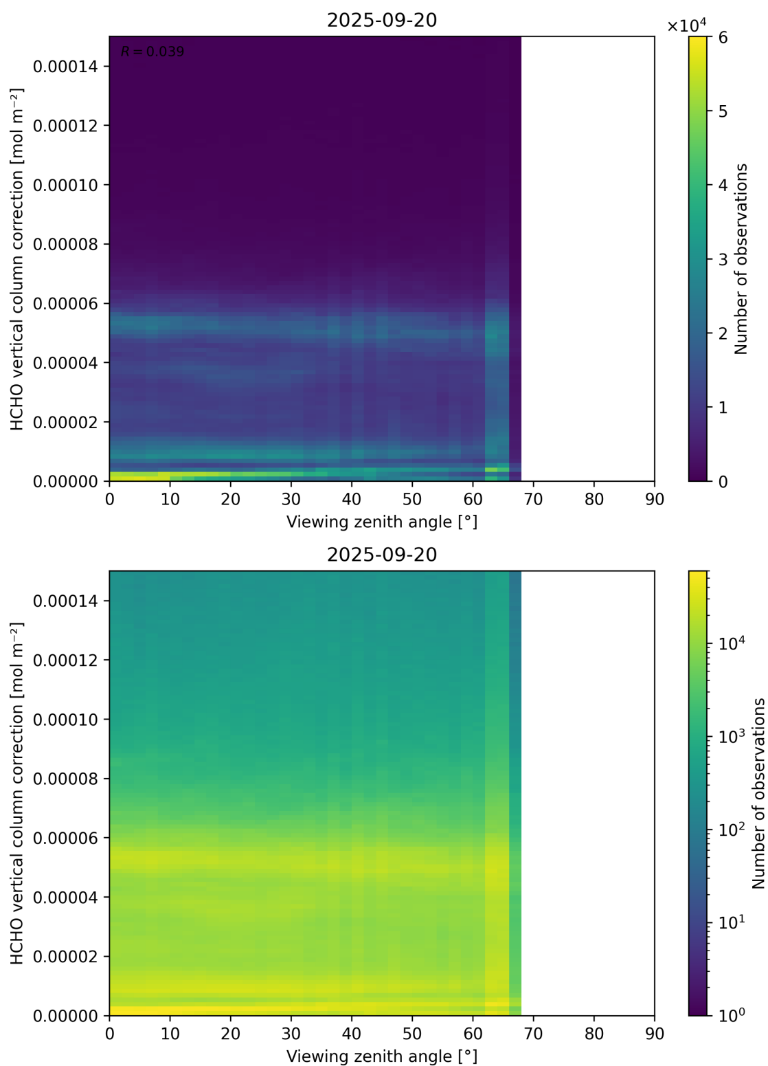
Figure 193: Scatter density plot of “Viewing zenith angle” against “HCHO vertical column correction” for 2025-09-20 to 2025-09-21.
