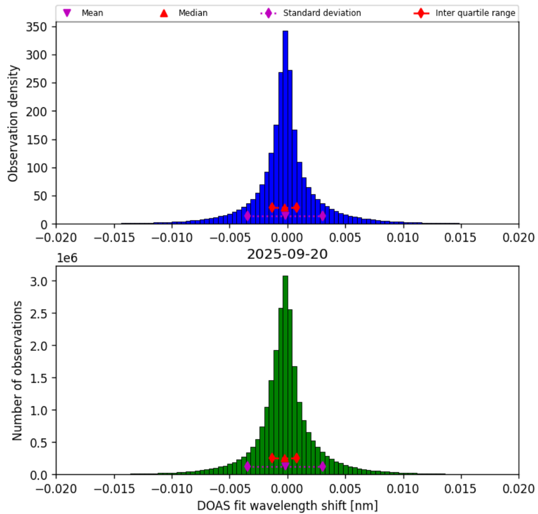
Figure 44: Histogram of “DOAS fit wavelength shift” for 2025-09-20 to 2025-09-21
