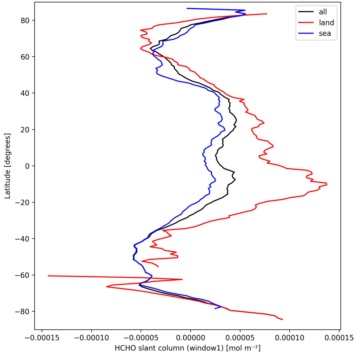
Figure 24: Zonal average of “HCHO slant column (window1)” for 2025-09-20 to 2025-09-21.
