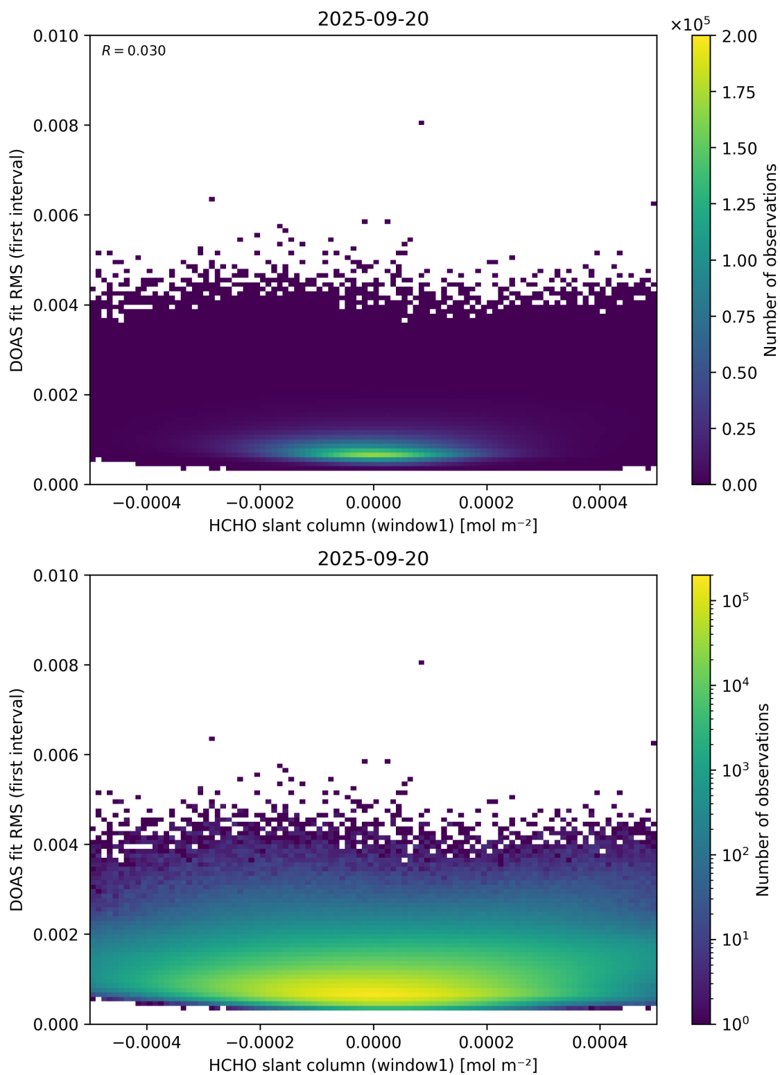
Figure 78: Scatter density plot of “HCHO slant column (window1)” against “DOAS fit RMS (first interval)” for 2025-09-20 to 2025-09-21.
