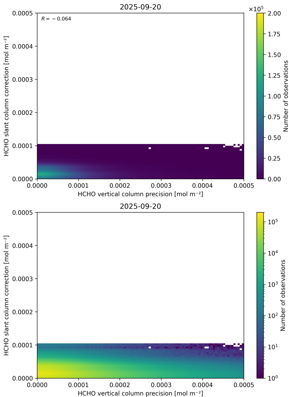
Figure 141: Scatter density plot of “HCHO vertical column precision” against “HCHO slant column correction” for 2025-09-20 to 2025-09-21.
