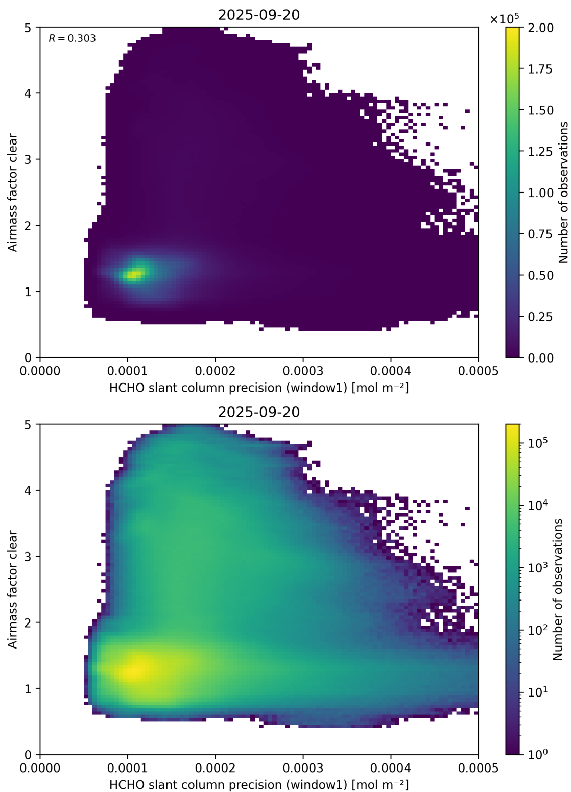
Figure 91: Scatter density plot of “HCHO slant column precision (window1)” against “Airmass factor clear” for 2025-09-20 to 2025-09-21.
