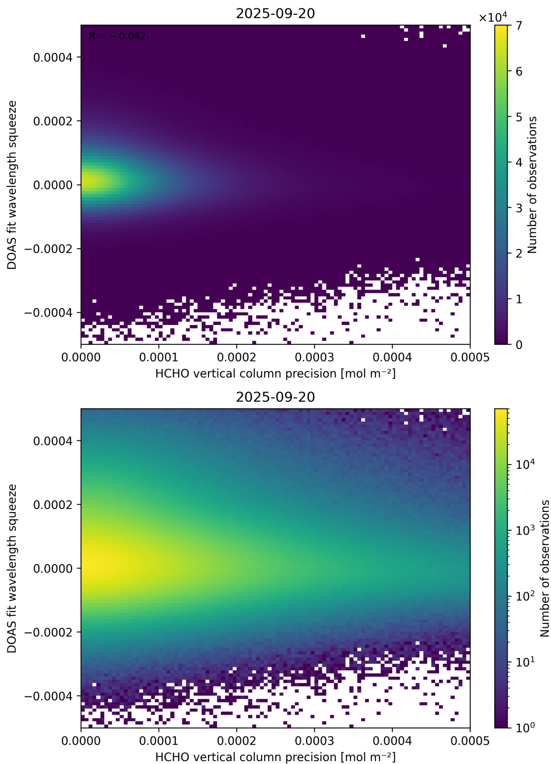
Figure 138: Scatter density plot of “HCHO vertical column precision” against “DOAS fit wavelength squeeze” for 2025-09-20 to 2025-09-21.
