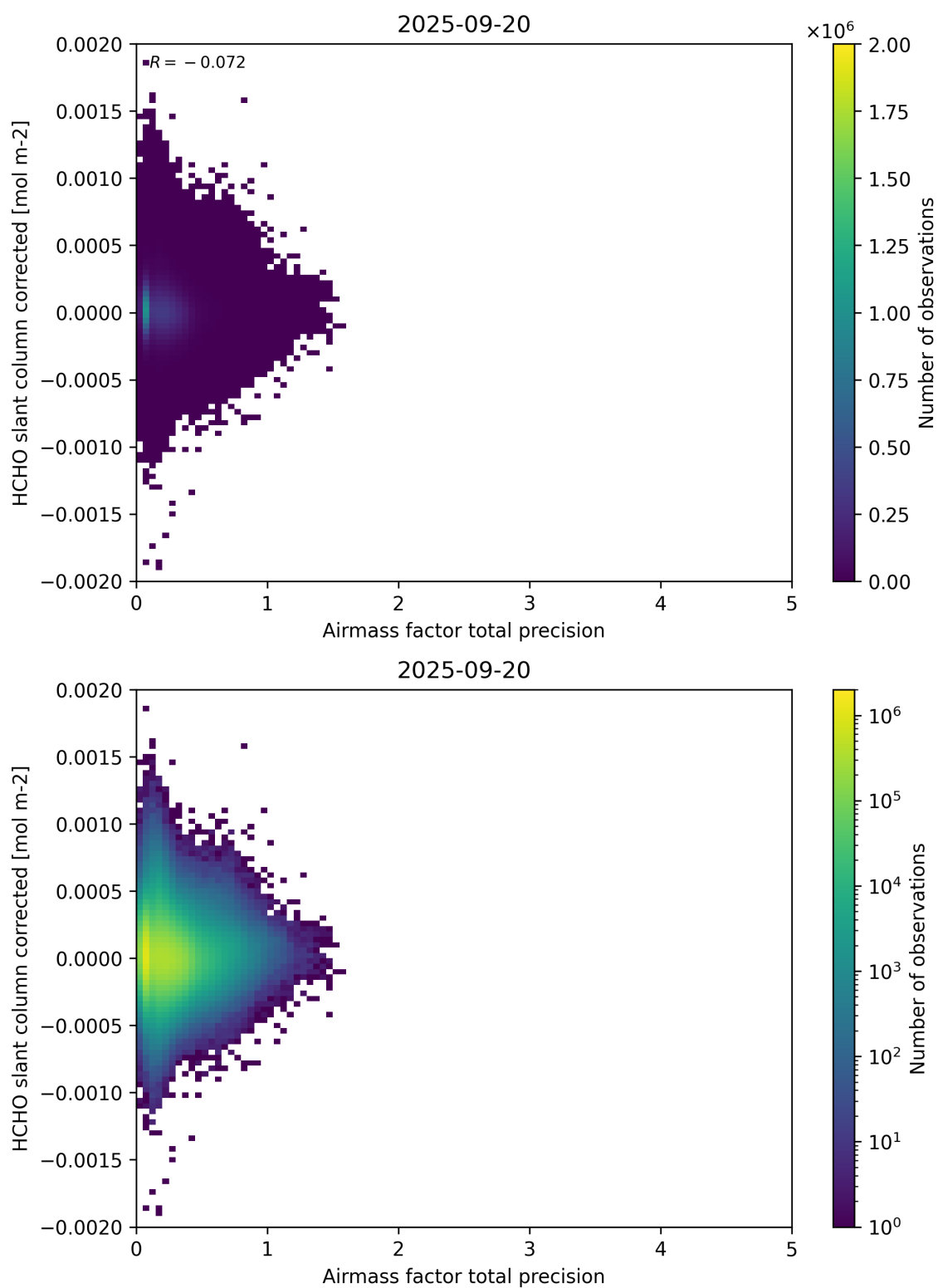
Figure 109: Scatter density plot of “Airmass factor total precision” against “HCHO slant column corrected” for 2025-09-20 to 2025-09-21.
