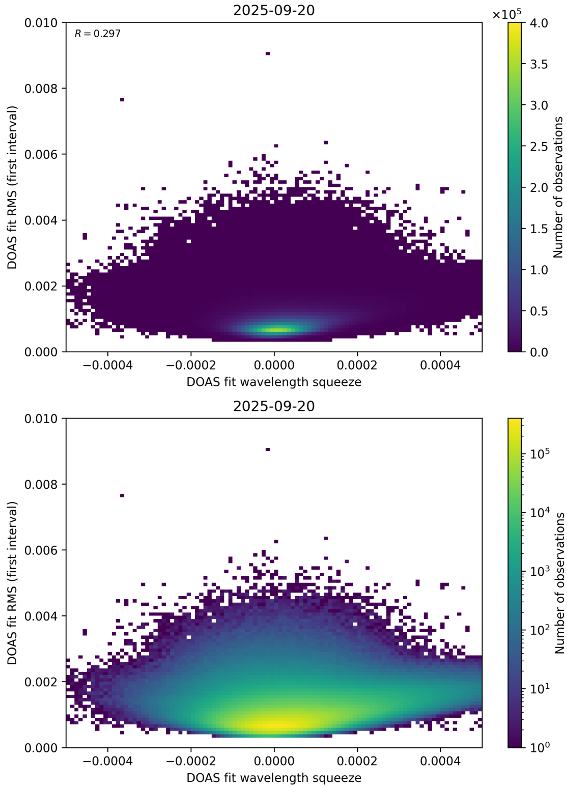
Figure 68: Scatter density plot of “DOAS fit wavelength squeeze” against “DOAS fit RMS (first interval)” for 2025-09-20 to 2025-09-21.
