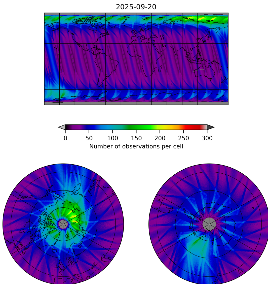
Figure 19: Map of the number of observations for 2025-09-20 to 2025-09-21
