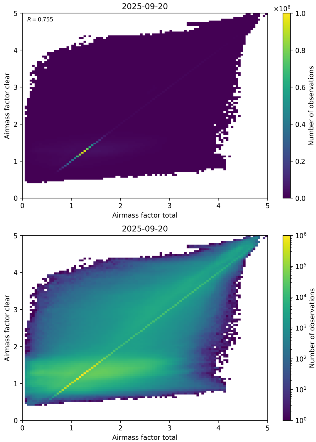
Figure 100: Scatter density plot of “Airmass factor total” against “Airmass factor clear” for 2025-09-20 to 2025-09-21.
