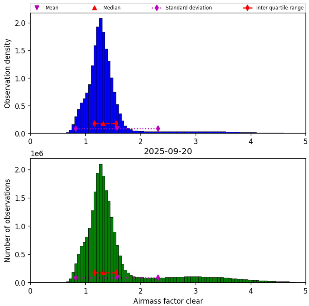
Figure 42: Histogram of “Airmass factor clear” for 2025-09-20 to 2025-09-21
