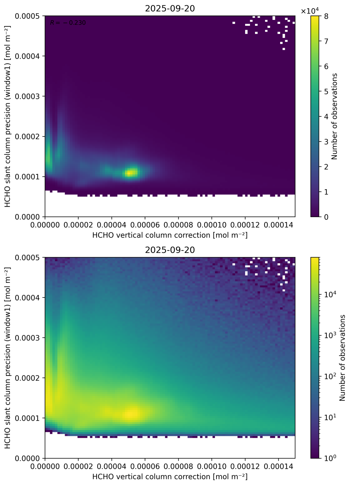
Figure 119: Scatter density plot of “HCHO vertical column correction” against “HCHO slant column precision (window1)” for 2025-09-20 to 2025-09-21.
