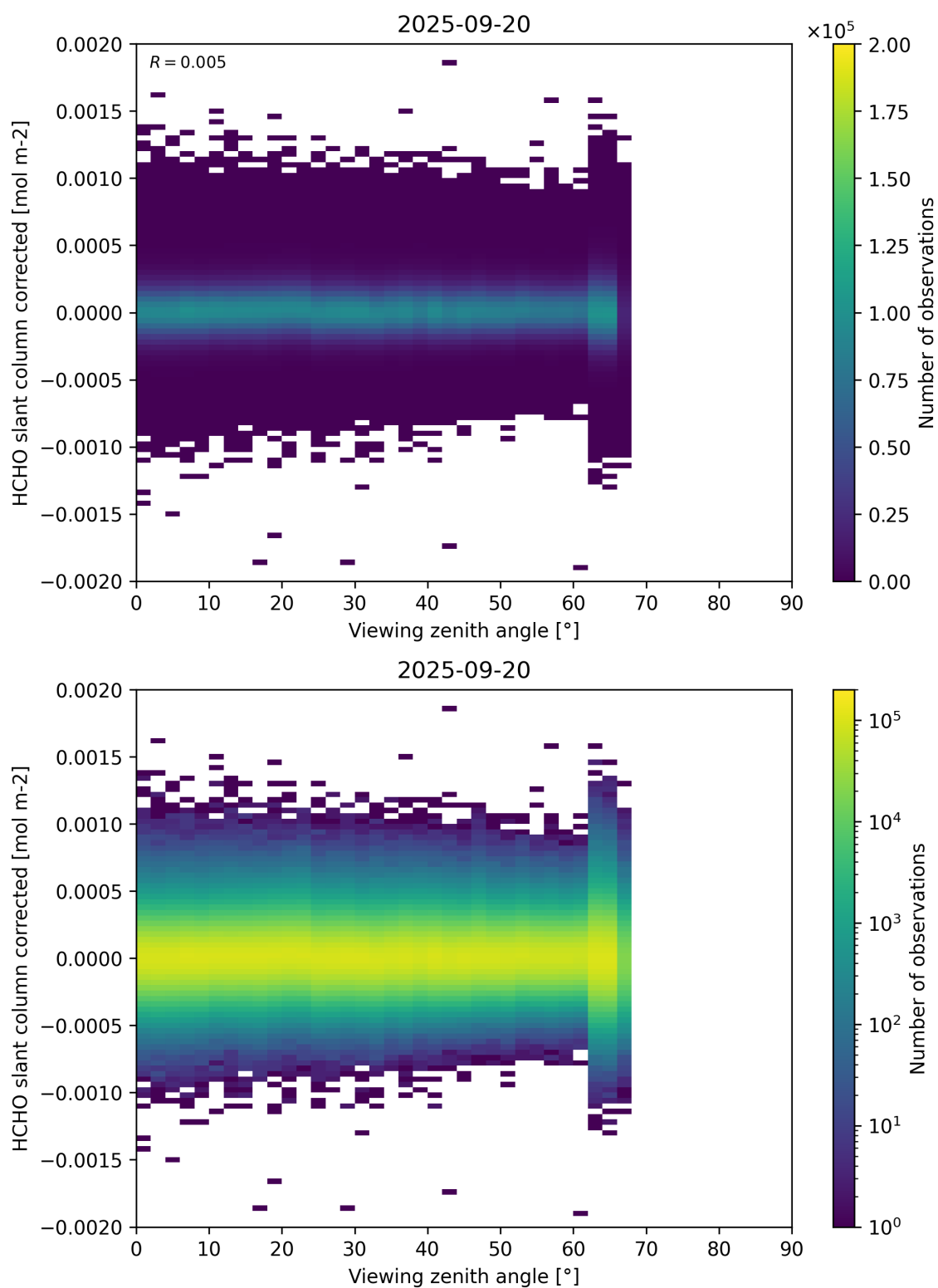
Figure 186: Scatter density plot of “Viewing zenith angle” against “HCHO slant column corrected” for 2025-09-20 to 2025-09-21.
