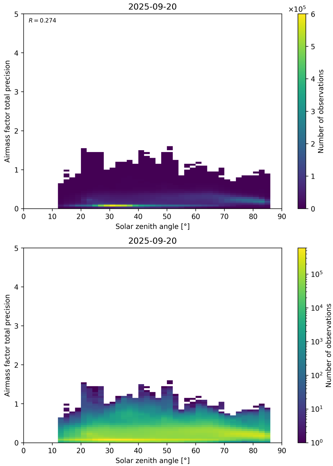
Figure 176: Scatter density plot of “Solar zenith angle” against “Airmass factor total precision” for 2025-09-20 to 2025-09-21.
