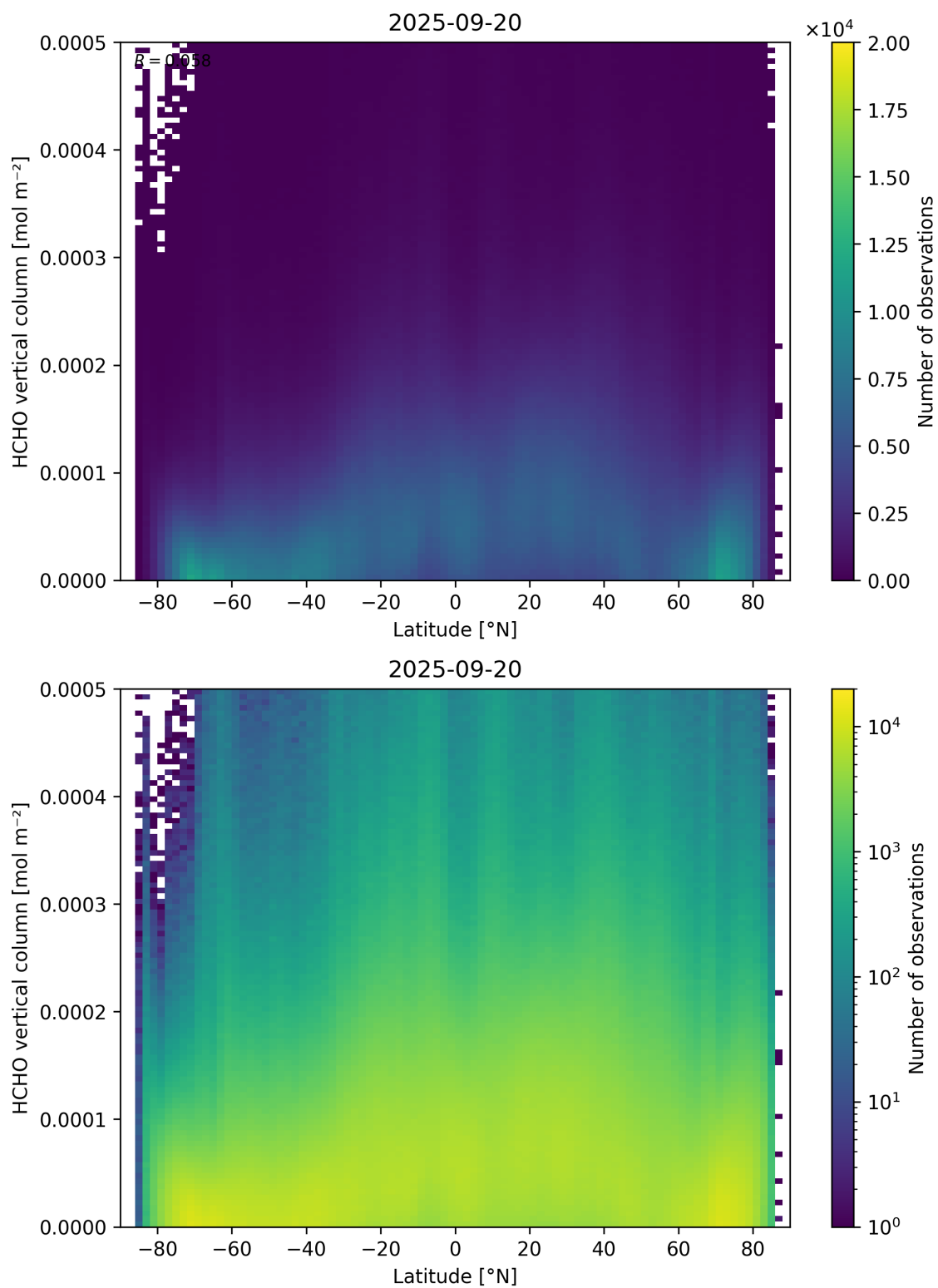
Figure 163: Scatter density plot of “Latitude” against “HCHO vertical column” for 2025-09-20 to 2025-09-21.
