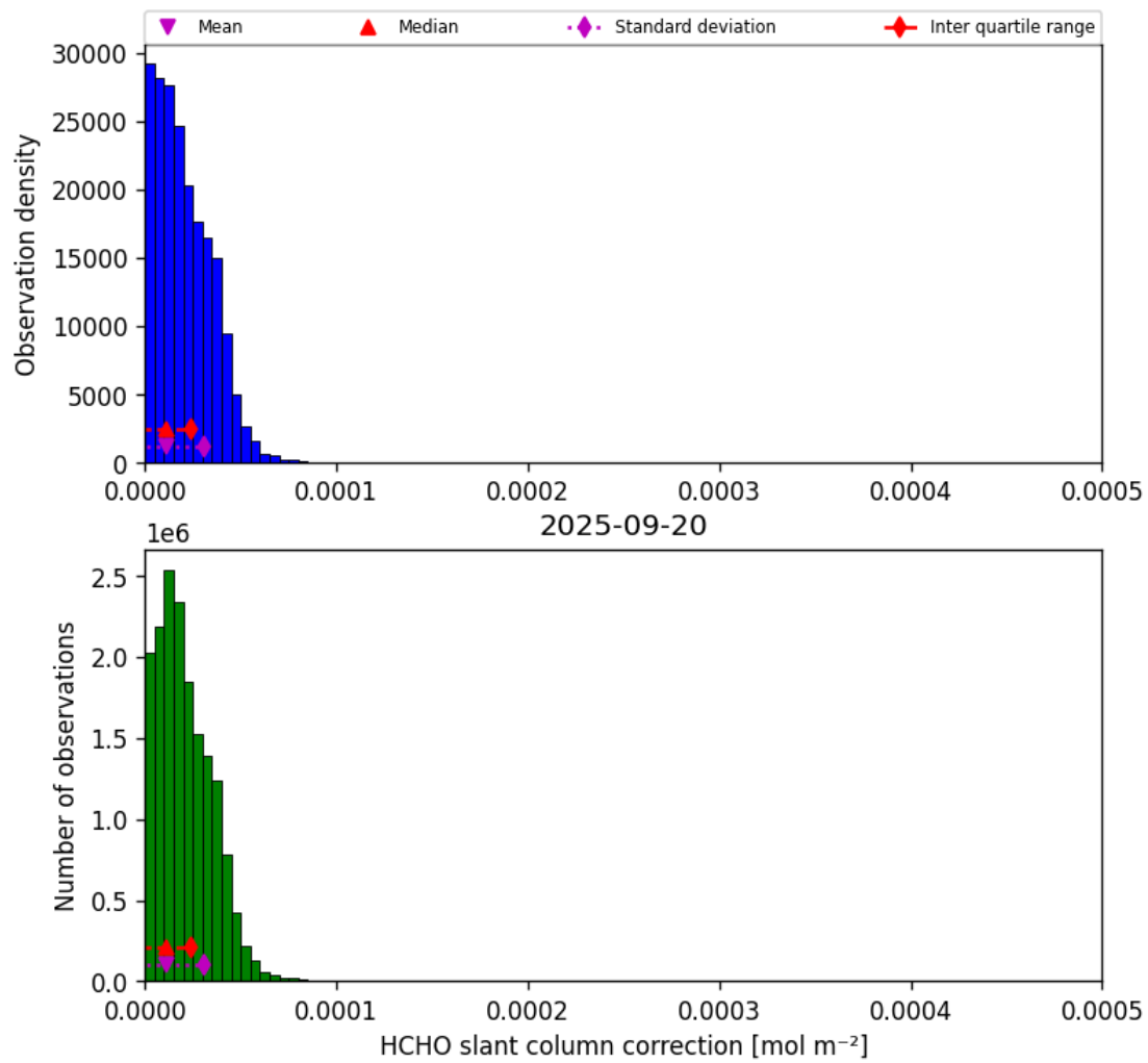
Figure 47: Histogram of “HCHO slant column correction” for 2025-09-20 to 2025-09-21
