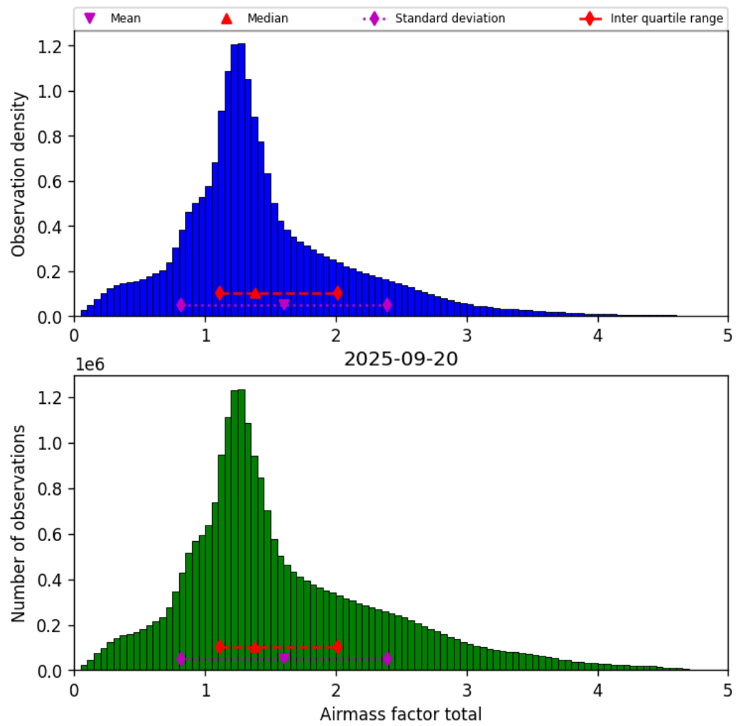
Figure 40: Histogram of “Airmass factor total” for 2025-09-20 to 2025-09-21
