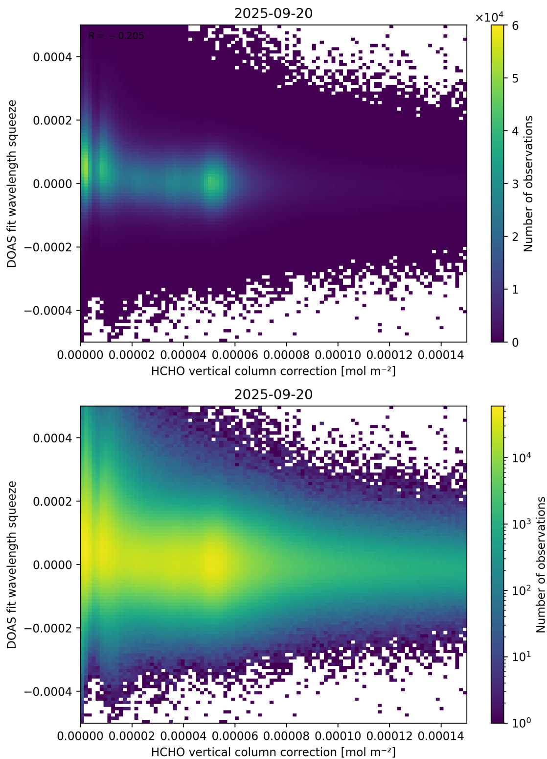
Figure 114: Scatter density plot of “HCHO vertical column correction” against “DOAS fit wavelength squeeze” for 2025-09-20 to 2025-09-21.
