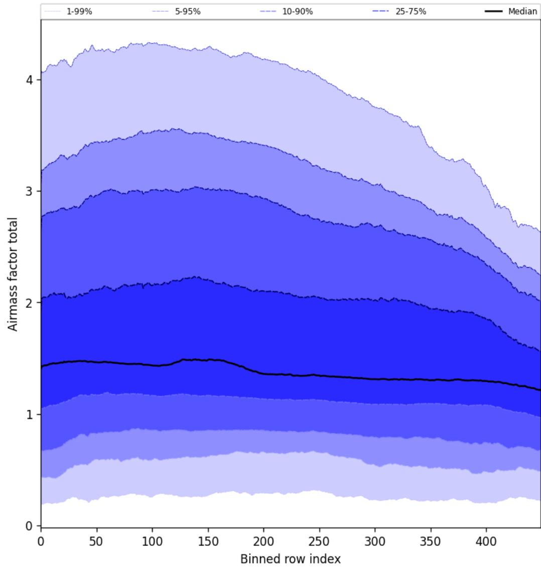
Figure 54: Along track statistics of “Airmass factor total” for 2025-09-20 to 2025-09-21
