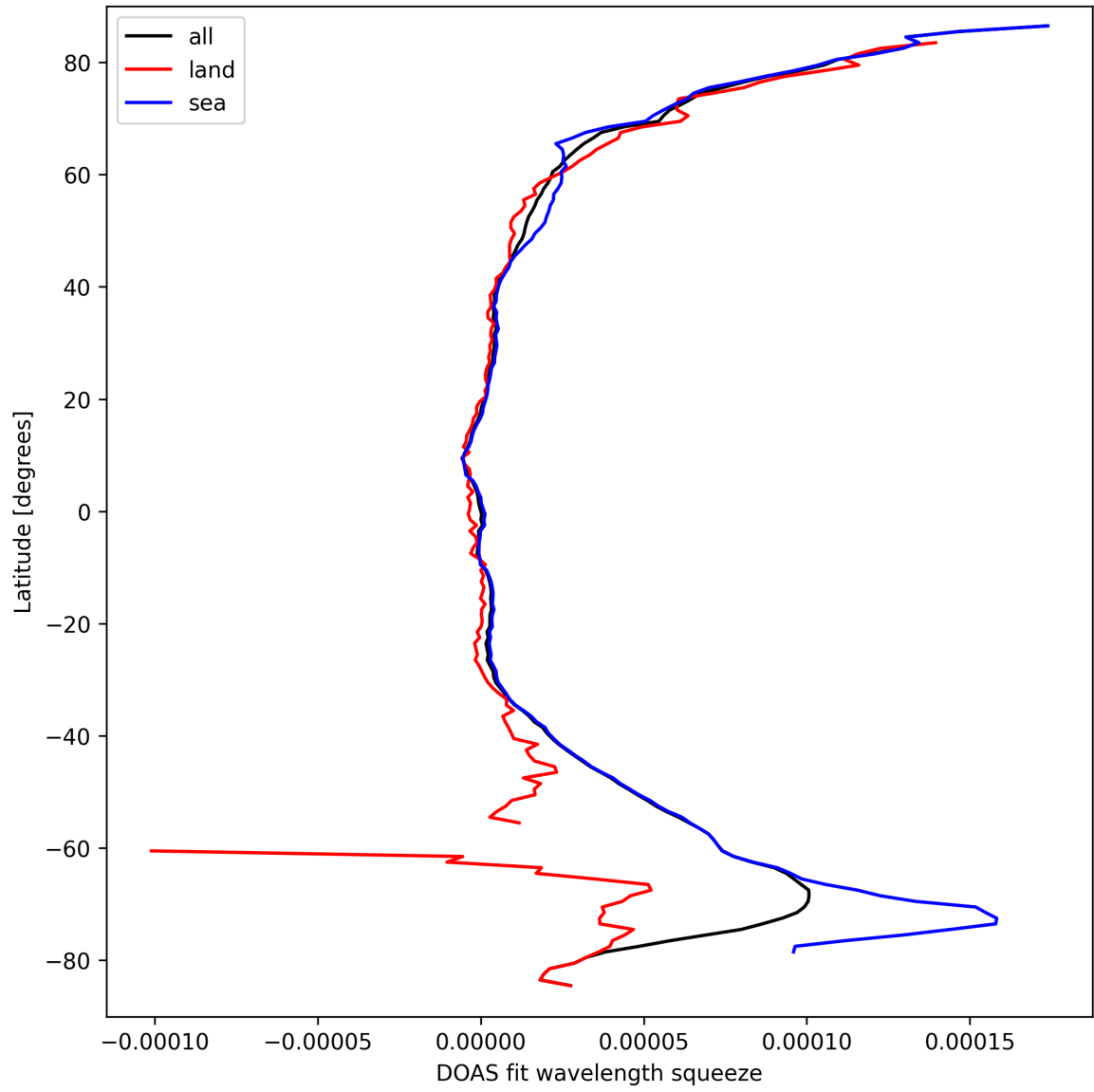
Figure 31: Zonal average of “DOAS fit wavelength squeeze” for 2025-09-20 to 2025-09-21.
