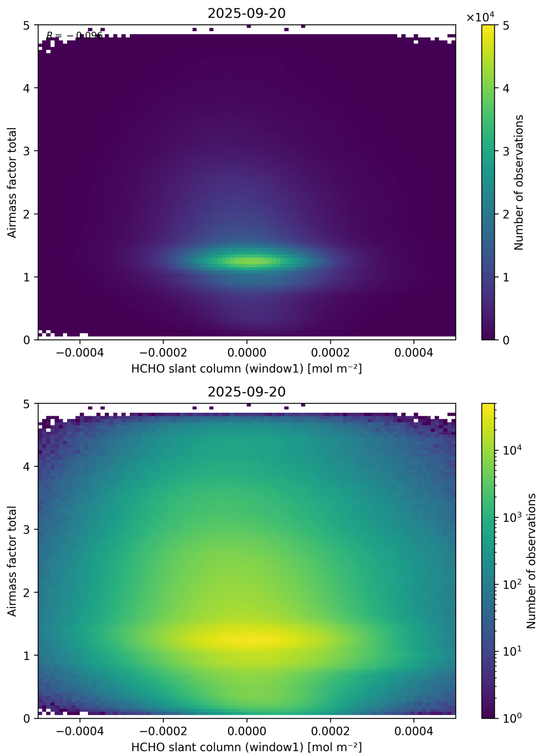
Figure 85: Scatter density plot of “HCHO slant column (window1)” against “Airmass factor total” for 2025-09-20 to 2025-09-21.
