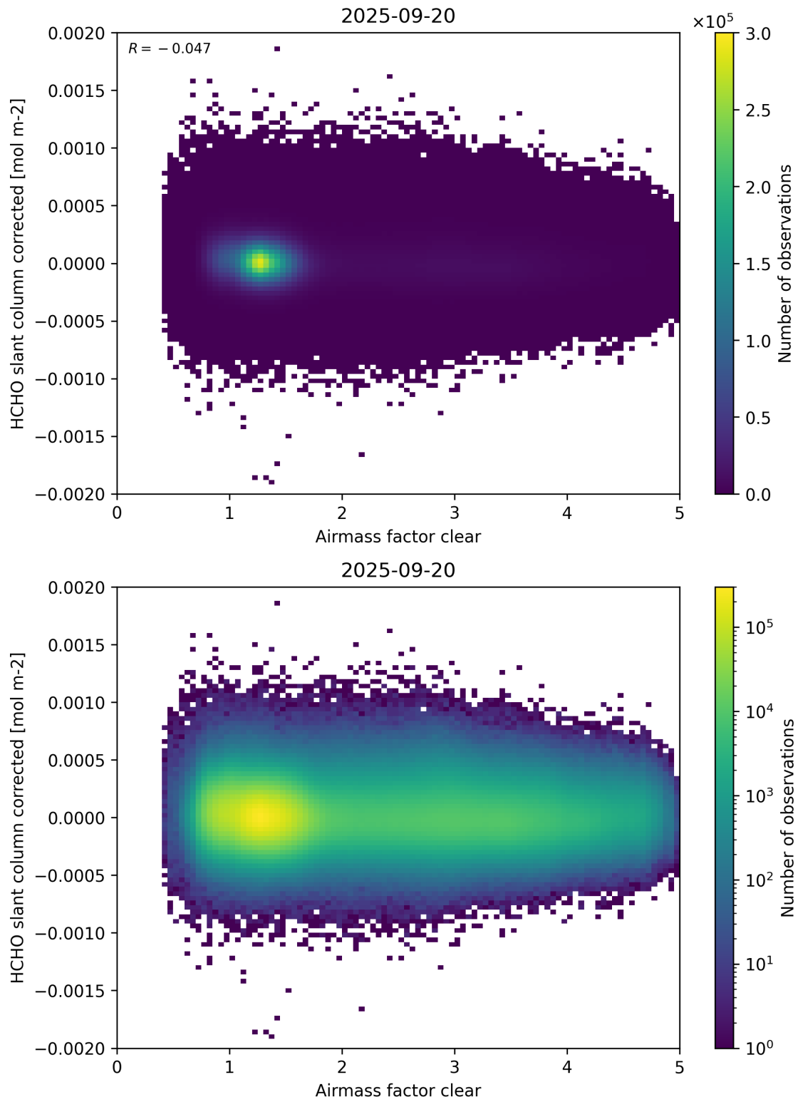
Figure 74: Scatter density plot of “Airmass factor clear” against “HCHO slant column corrected” for 2025-09-20 to 2025-09-21.
