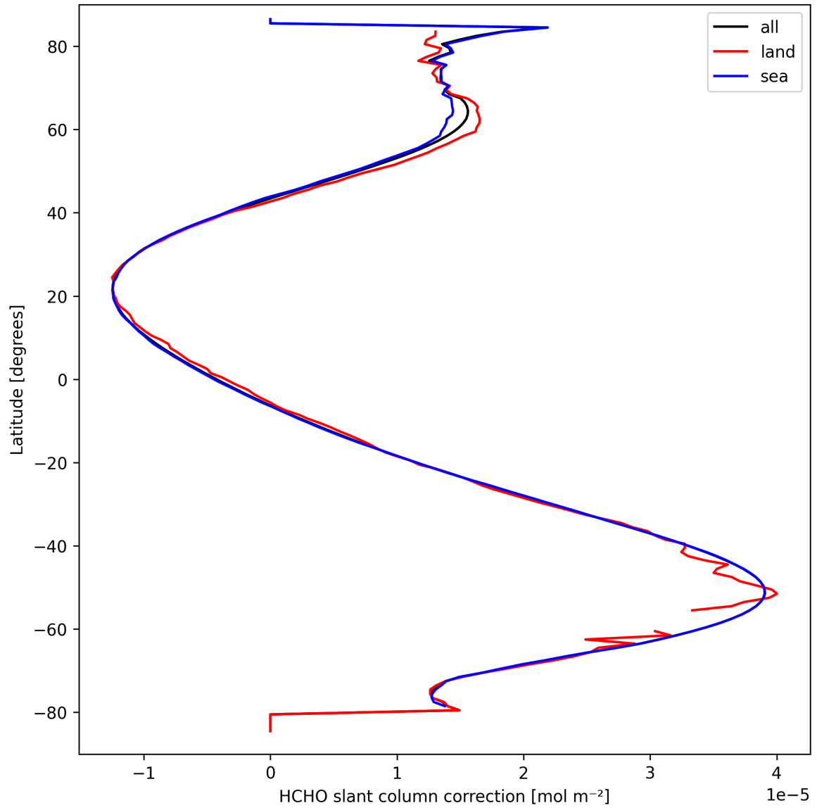
Figure 33: Zonal average of "HCHO slant column correction" for 2025-09-20 to 2025-09-21.
