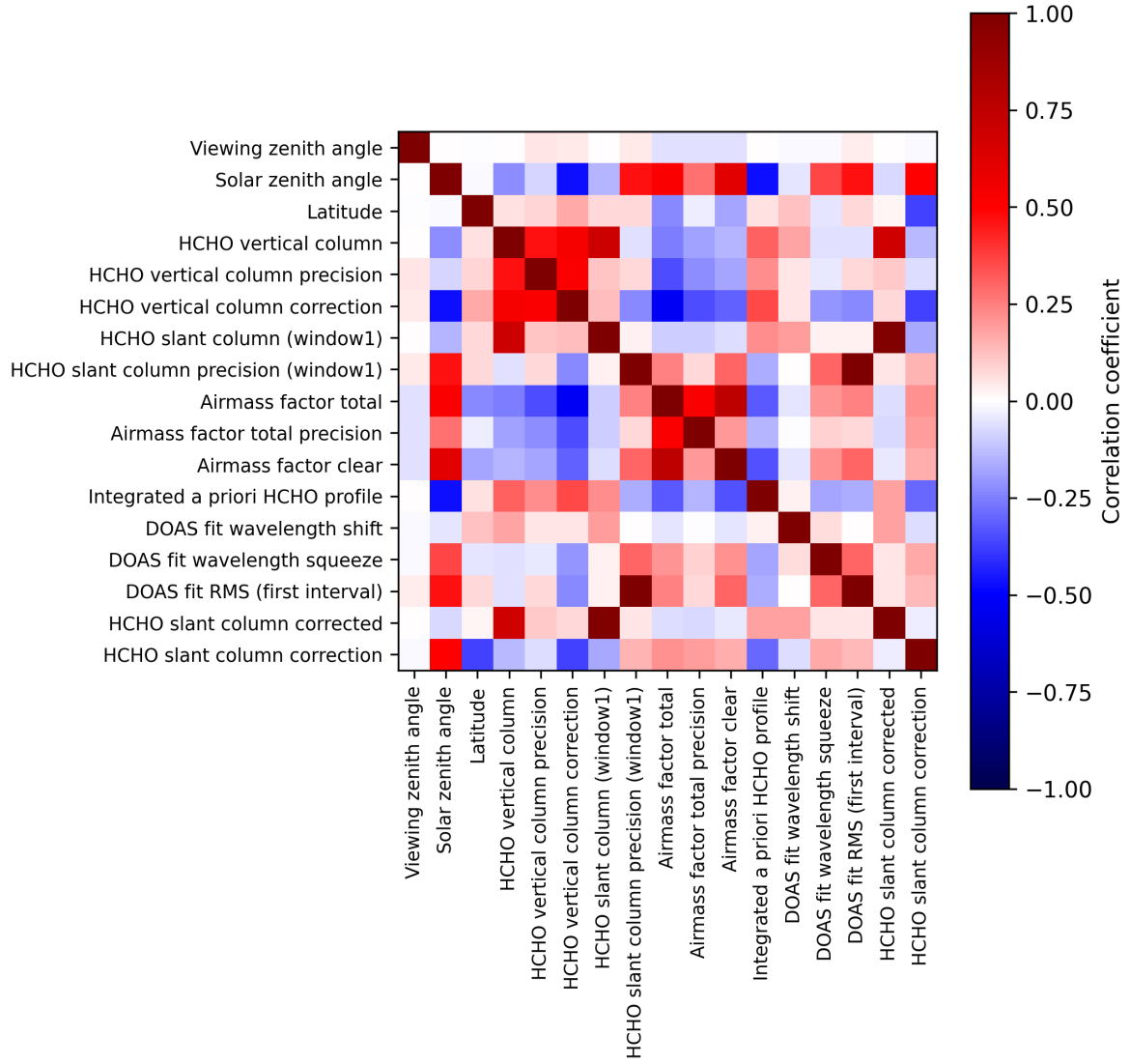
Figure 2: Map of correlation matrix for 2025-09-20 to 2025-09-21.
