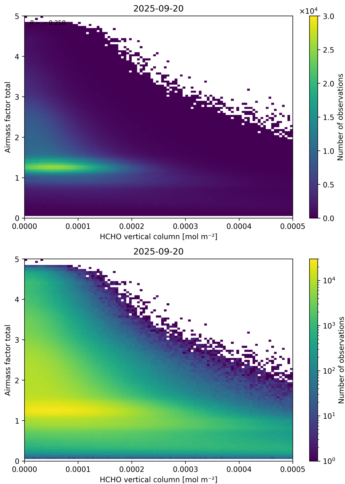
Figure 131: Scatter density plot of “HCHO vertical column” against “Airmass factor total” for 2025-09-20 to 2025-09-21.
