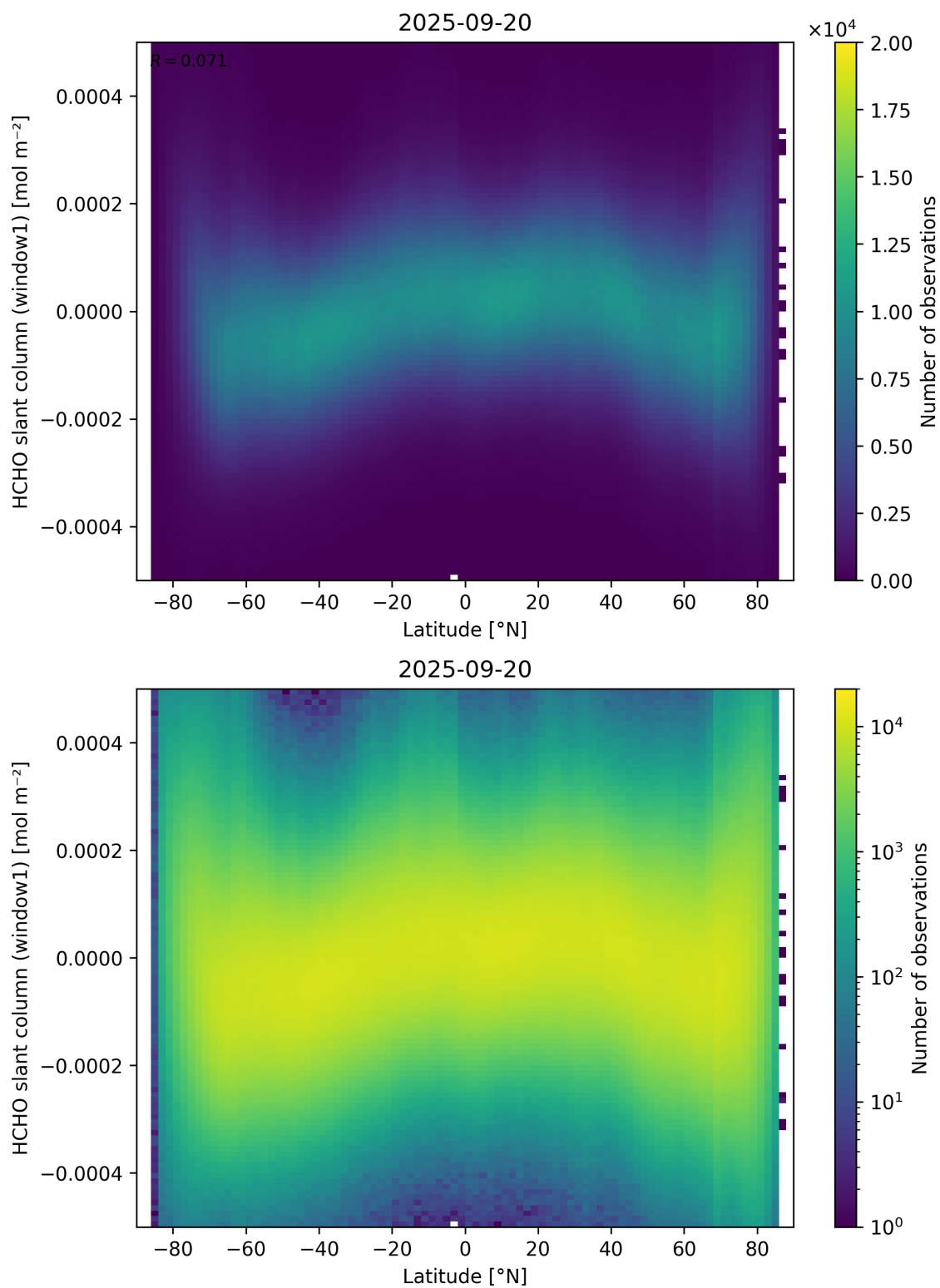
Figure 159: Scatter density plot of “Latitude” against “HCHO slant column (window1)” for 2025-09-20 to 2025-09-21.
