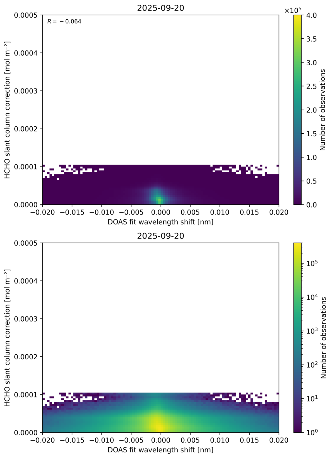
Figure 67: Scatter density plot of “DOAS fit wavelength shift” against “HCHO slant column correction” for 2025-09-20 to 2025-09-21.
