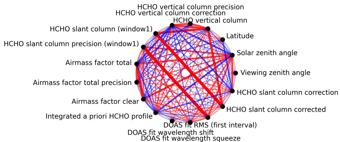
Figure 1: Map of correlation graph for 2025-09-20 to 2025-09-21.
