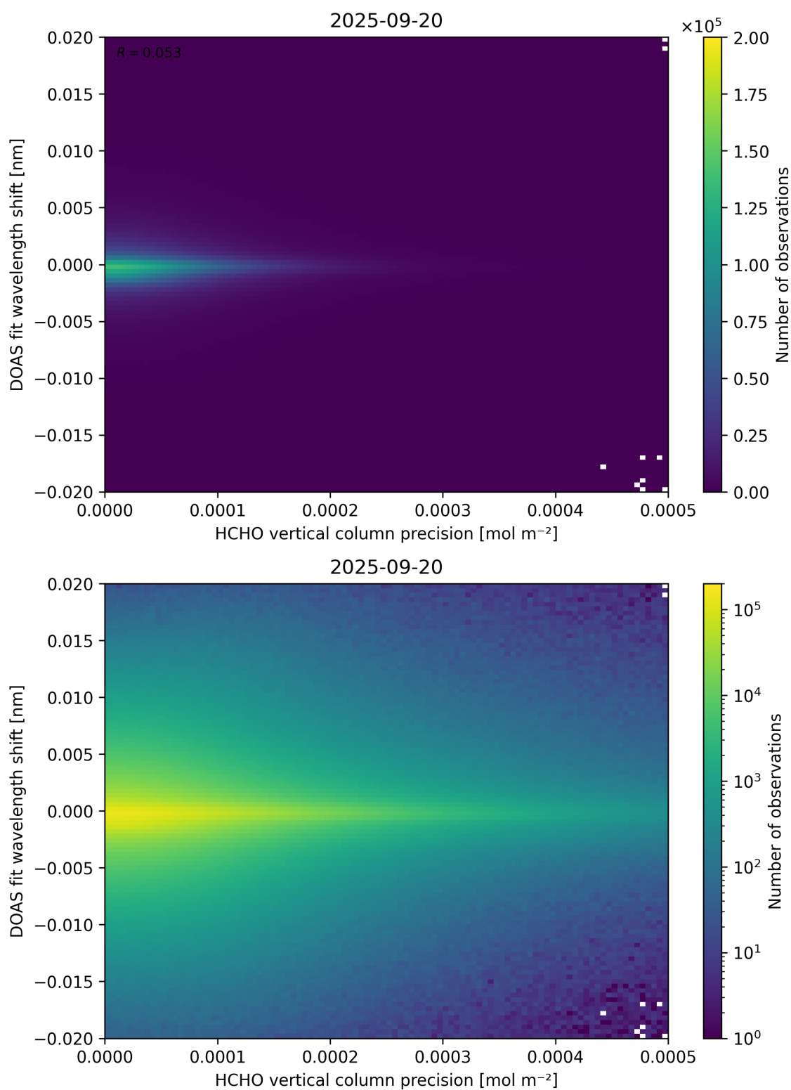
Figure 137: Scatter density plot of “HCHO vertical column precision” against “DOAS fit wavelength shift” for 2025-09-20 to 2025-09-21.
