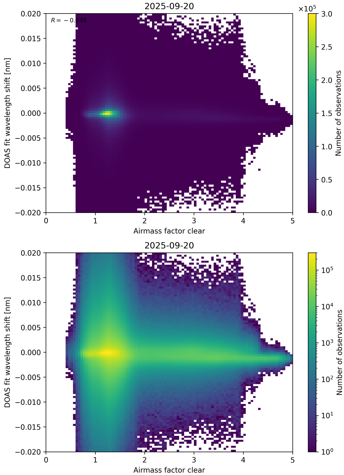
Figure 72: Scatter density plot of “Airmass factor clear” against “DOAS fit wavelength shift” for 2025-09-20 to 2025-09-21.
