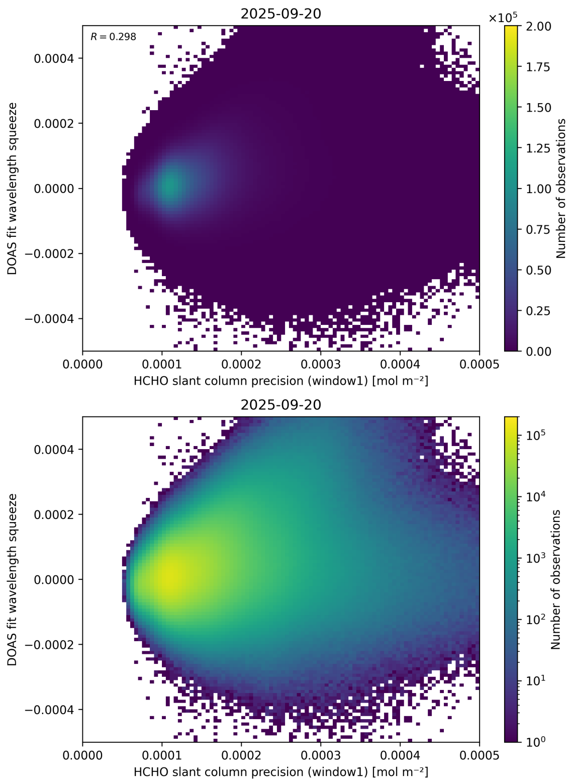
Figure 90: Scatter density plot of “HCHO slant column precision (window1)” against “DOAS fit wavelength squeeze” for 2025-09-20 to 2025-09-21.
