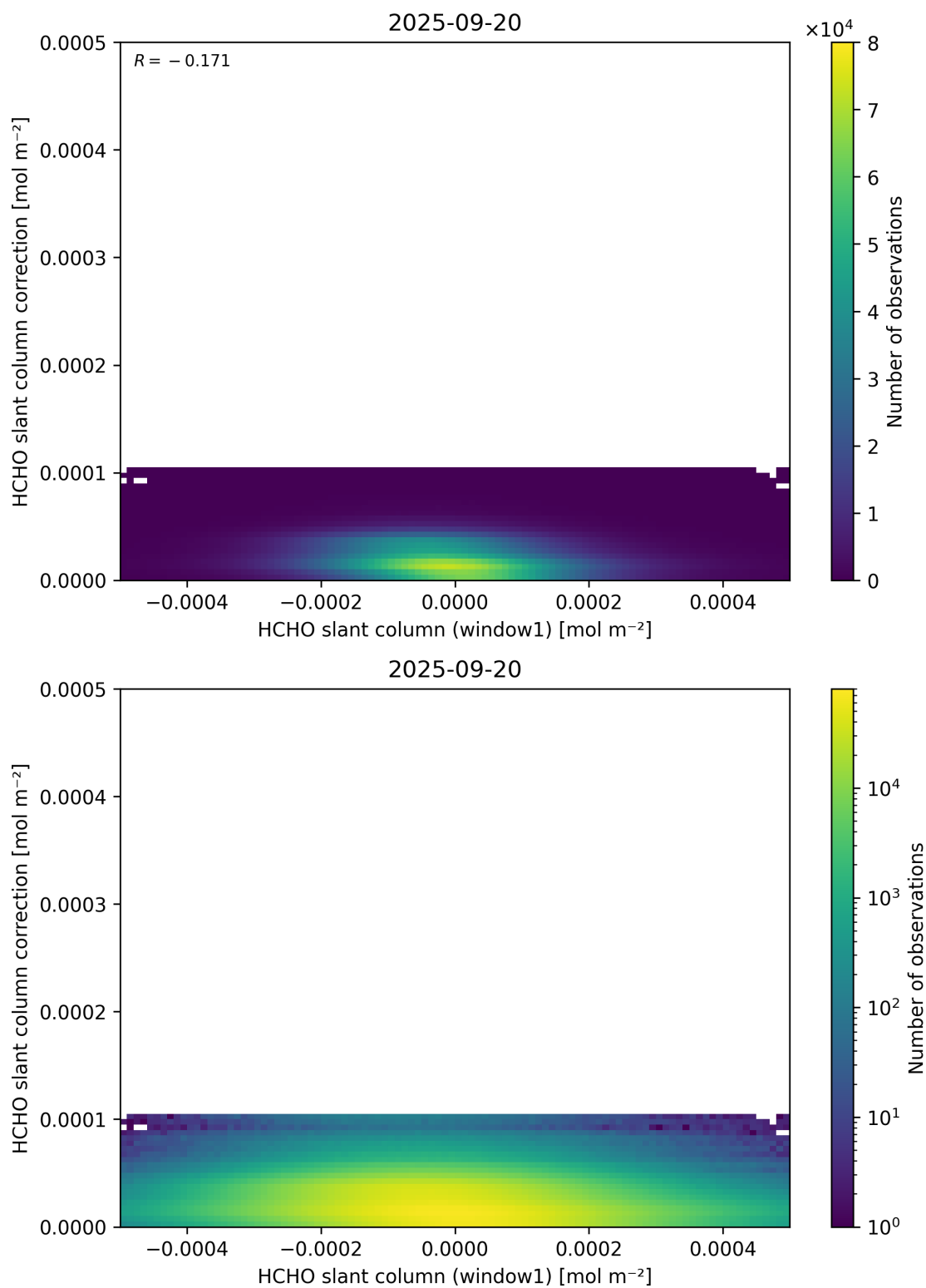
Figure 83: Scatter density plot of “HCHO slant column (window1)” against “HCHO slant column correction” for 2025-09-20 to 2025-09-21.
