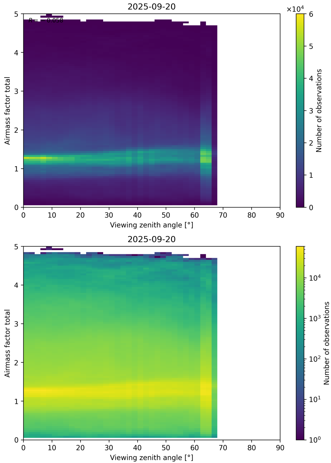
Figure 190: Scatter density plot of “Viewing zenith angle” against “Airmass factor total” for 2025-09-20 to 2025-09-21.
