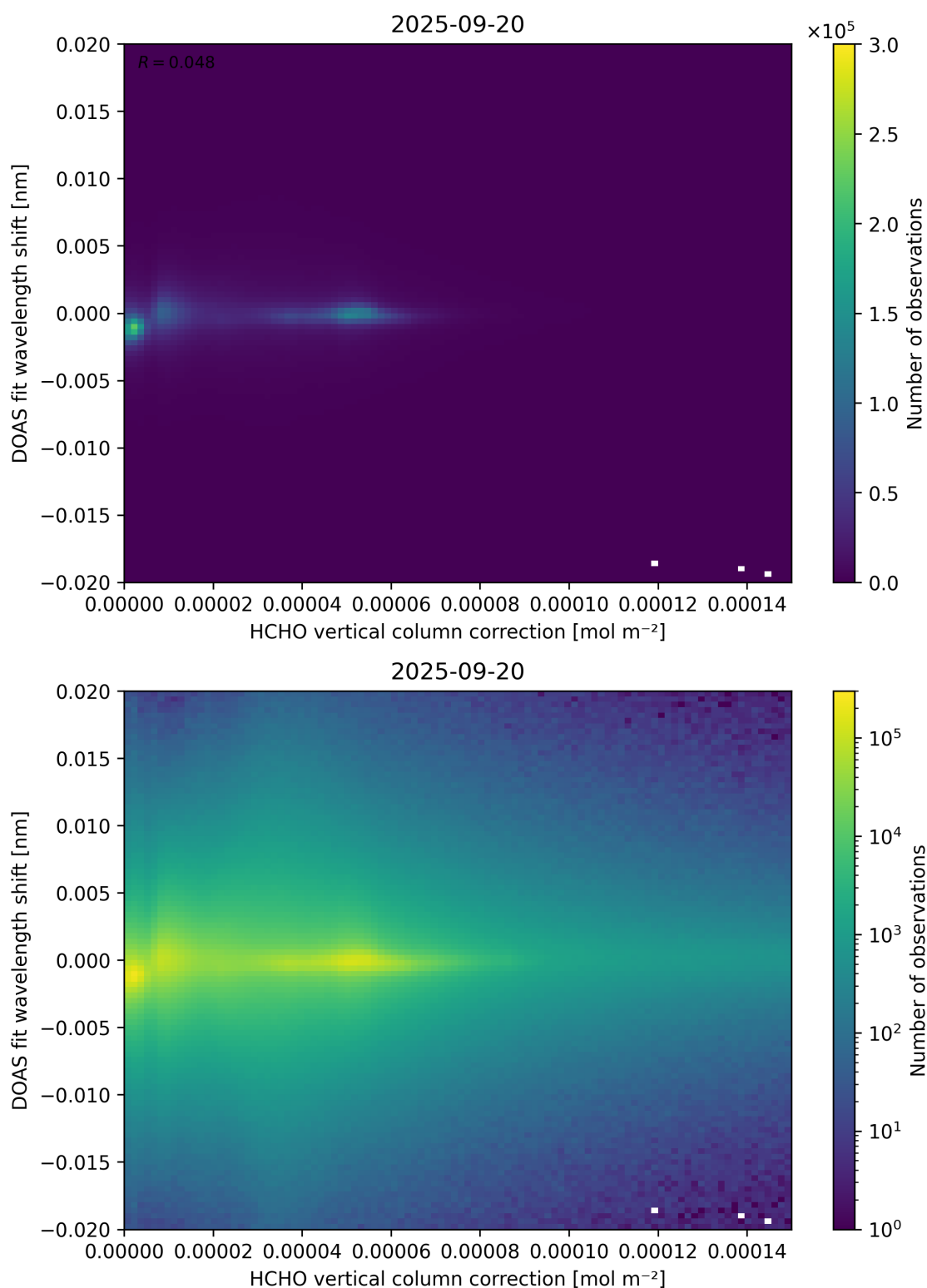
Figure 113: Scatter density plot of “HCHO vertical column correction” against “DOAS fit wavelength shift” for 2025-09-20 to 2025-09-21.
