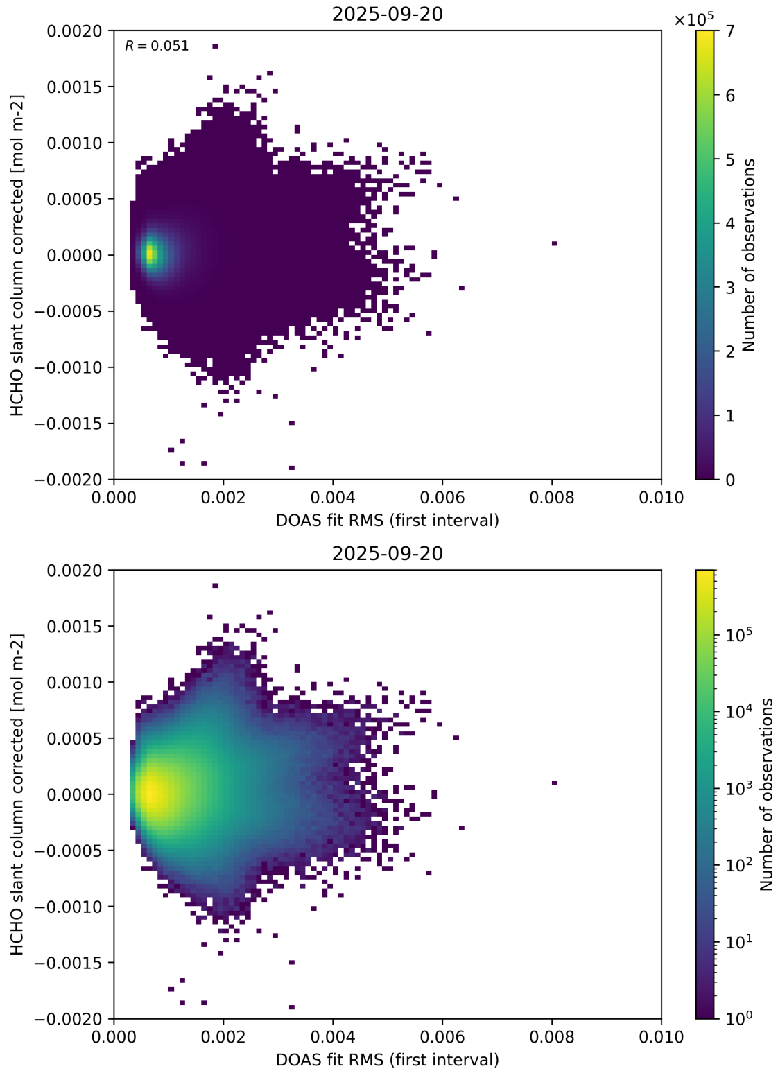
Figure 62: Scatter density plot of “DOAS fit RMS (first interval)” against “HCHO slant column corrected” for 2025-09-20 to 2025-09-21.
