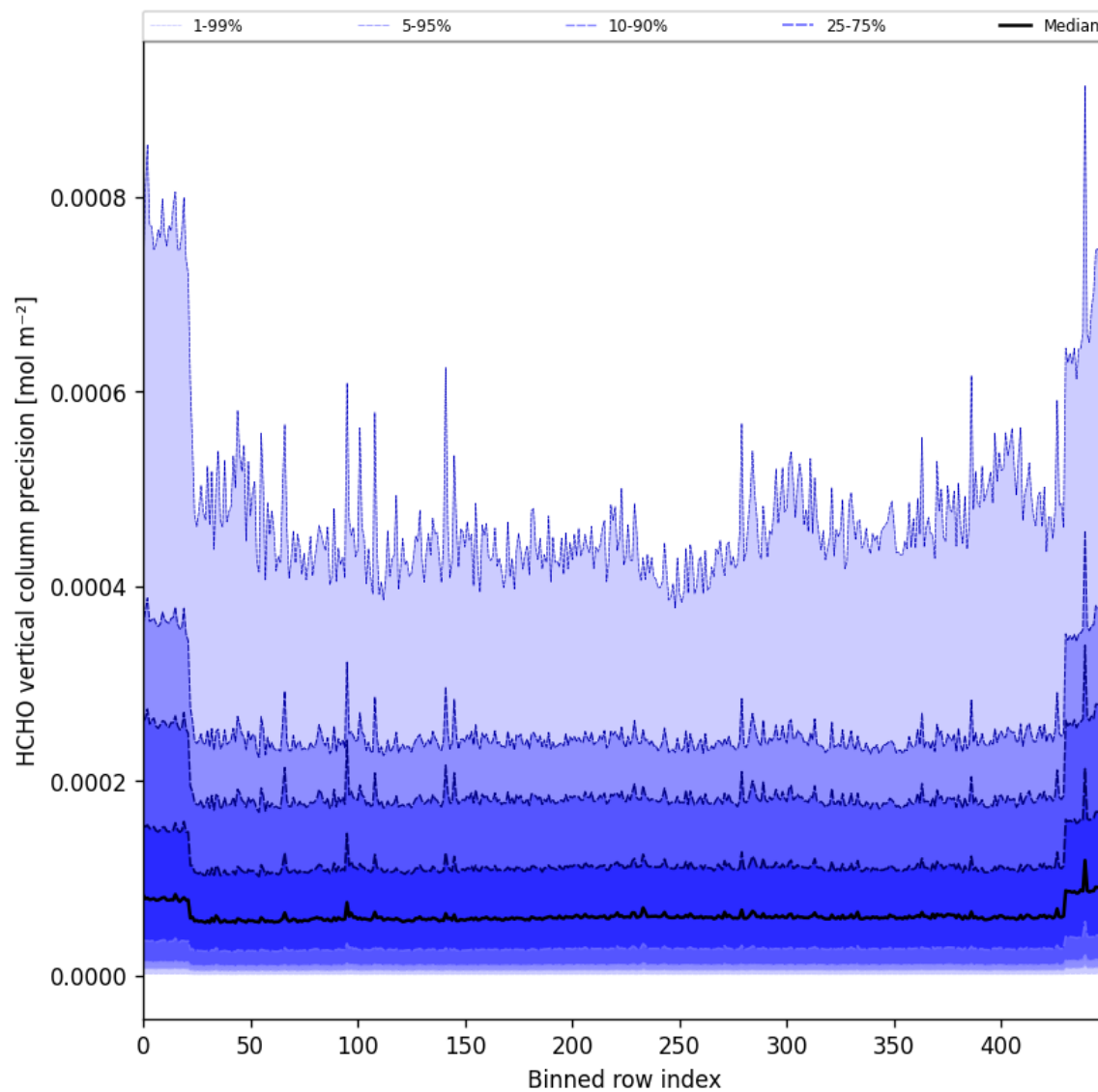
Figure 50: Along track statistics of “HCHO vertical column precision” for 2025-09-20 to 2025-09-21
