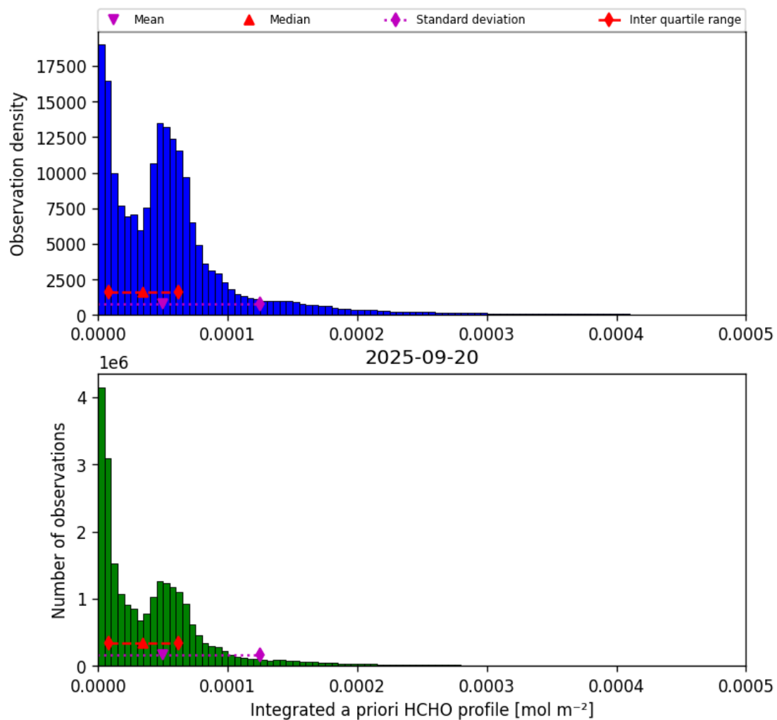
Figure 43: Histogram of “Integrated a priori HCHO profile” for 2025-09-20 to 2025-09-21
