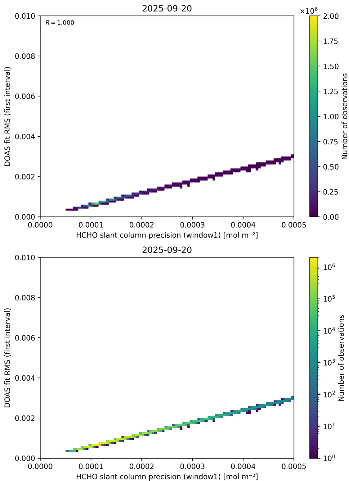
Figure 88: Scatter density plot of “HCHO slant column precision (window1)” against “DOAS fit RMS (first interval)” for 2025-09-20 to 2025-09-21.
