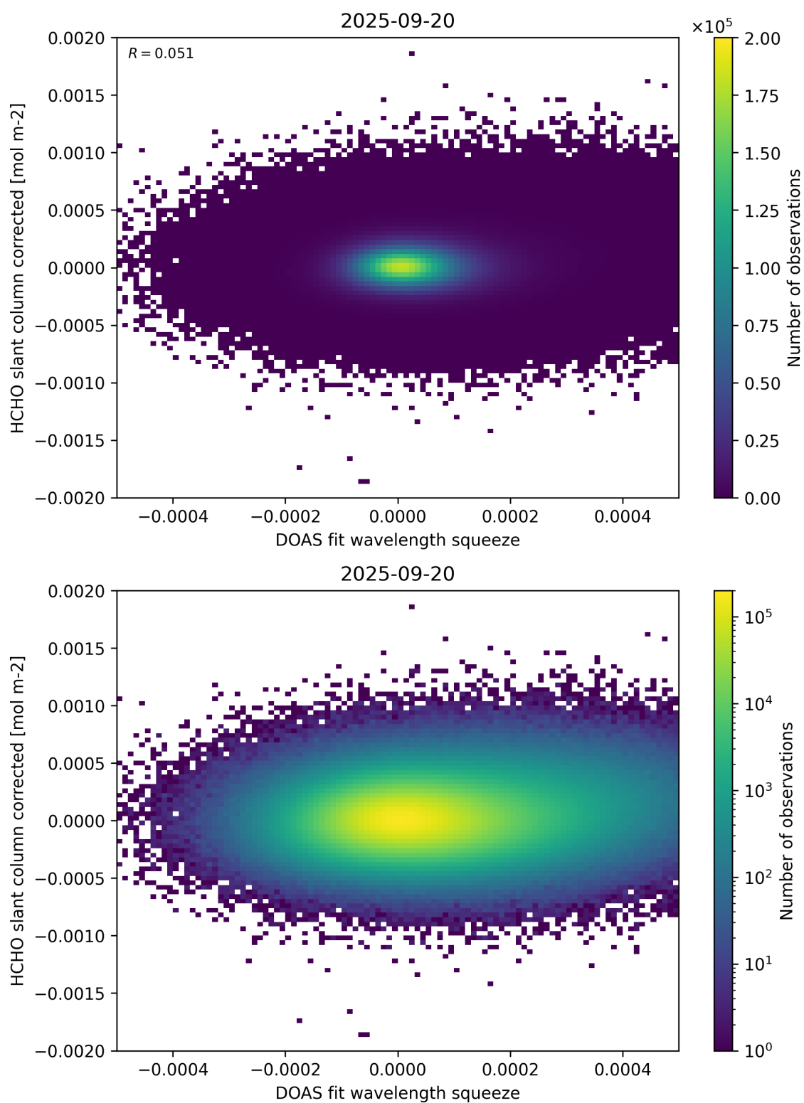
Figure 69: Scatter density plot of “DOAS fit wavelength squeeze” against “HCHO slant column corrected” for 2025-09-20 to 2025-09-21.
