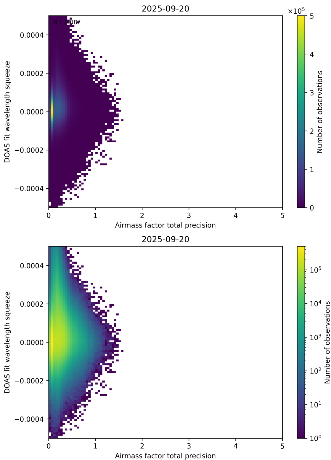
Figure 107: Scatter density plot of “Airmass factor total precision” against “DOAS fit wavelength squeeze” for 2025-09-20 to 2025-09-21.
