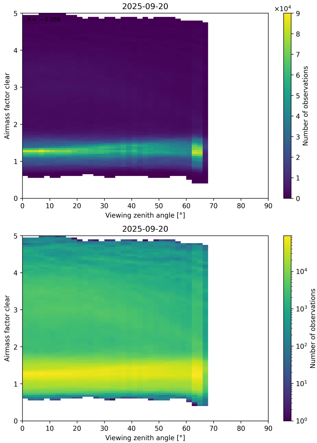
Figure 185: Scatter density plot of “Viewing zenith angle” against “Airmass factor clear” for 2025-09-20 to 2025-09-21.
