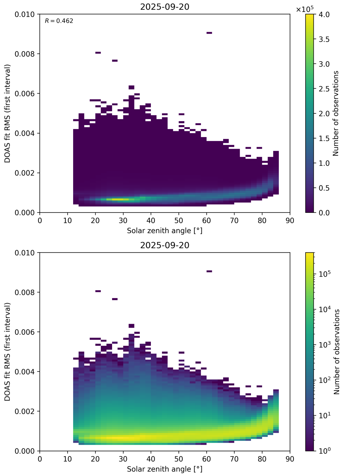
Figure 167: Scatter density plot of “Solar zenith angle” against “DOAS fit RMS (first interval)” for 2025-09-20 to 2025-09-21.
