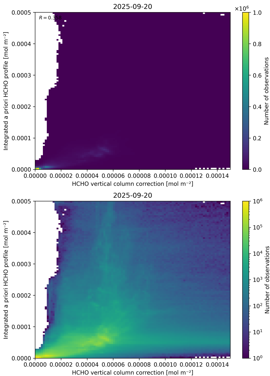
Figure 122: Scatter density plot of “HCHO vertical column correction” against “Integrated a priori HCHO profile” for 2025-09-20 to 2025-09-21.
