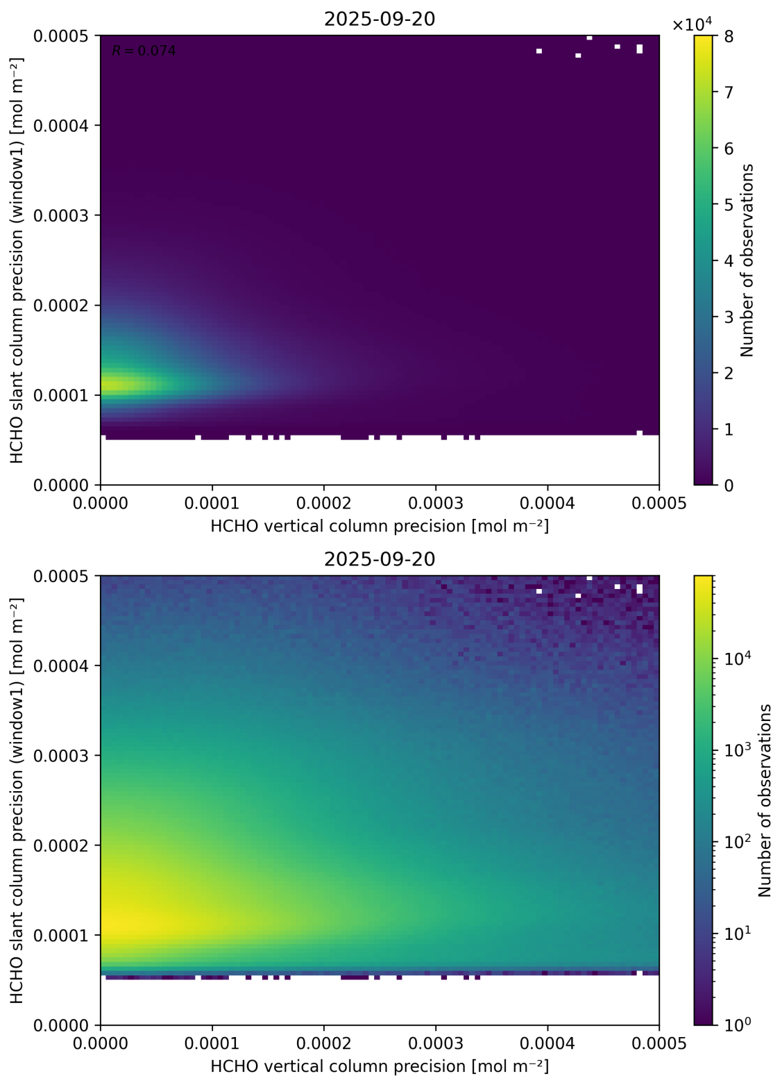
Figure 143: Scatter density plot of “HCHO vertical column precision” against “HCHO slant column precision (window1)” for 2025-09-20 to 2025-09-21.
