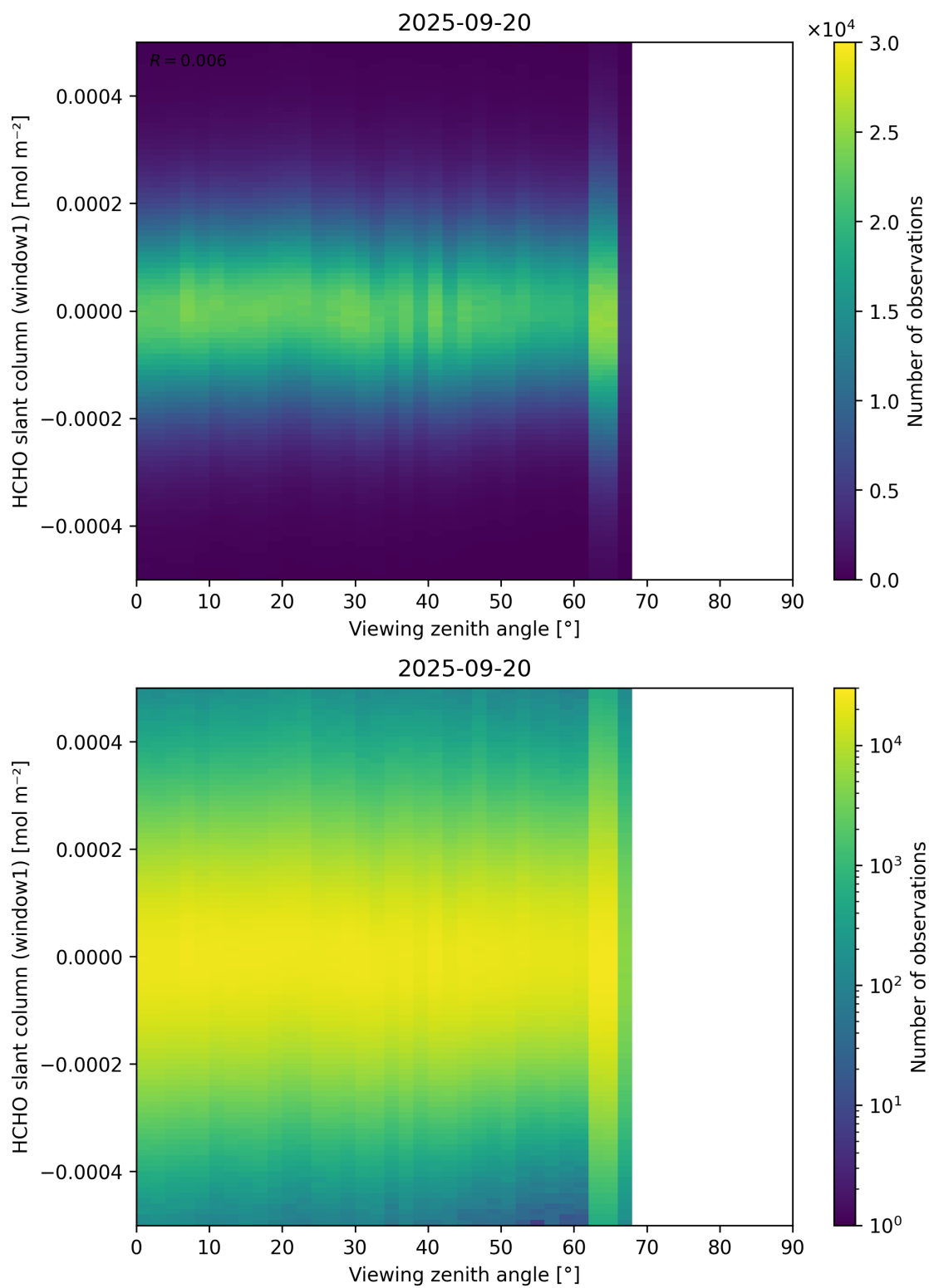
Figure 188: Scatter density plot of “Viewing zenith angle” against “HCHO slant column (window1)” for 2025-09-20 to 2025-09-21.
