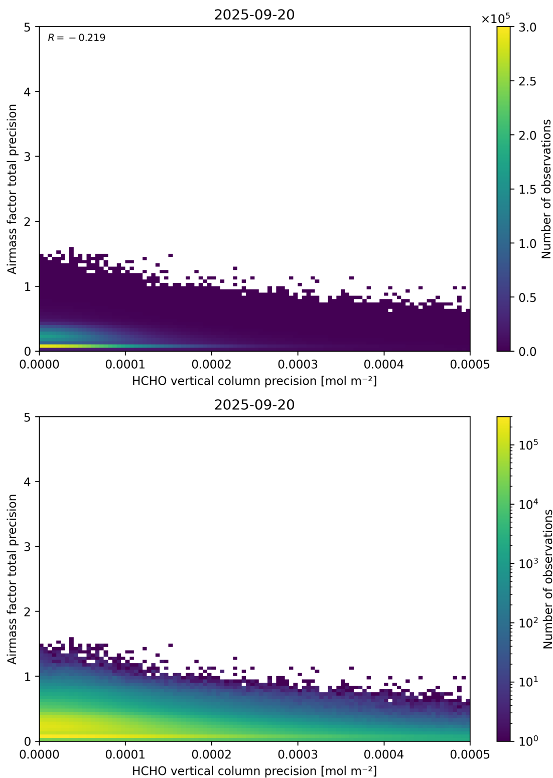
Figure 145: Scatter density plot of “HCHO vertical column precision” against “Airmass factor total precision” for 2025-09-20 to 2025-09-21.
