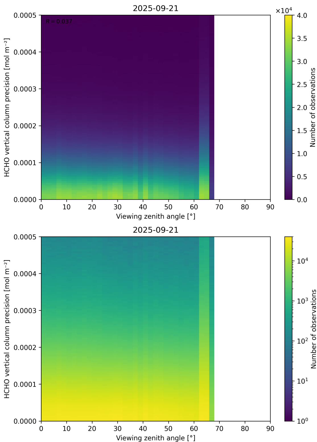
Figure 194: Scatter density plot of “Viewing zenith angle” against “HCHO vertical column precision” for 2025-09-20 to 2025-09-22.
