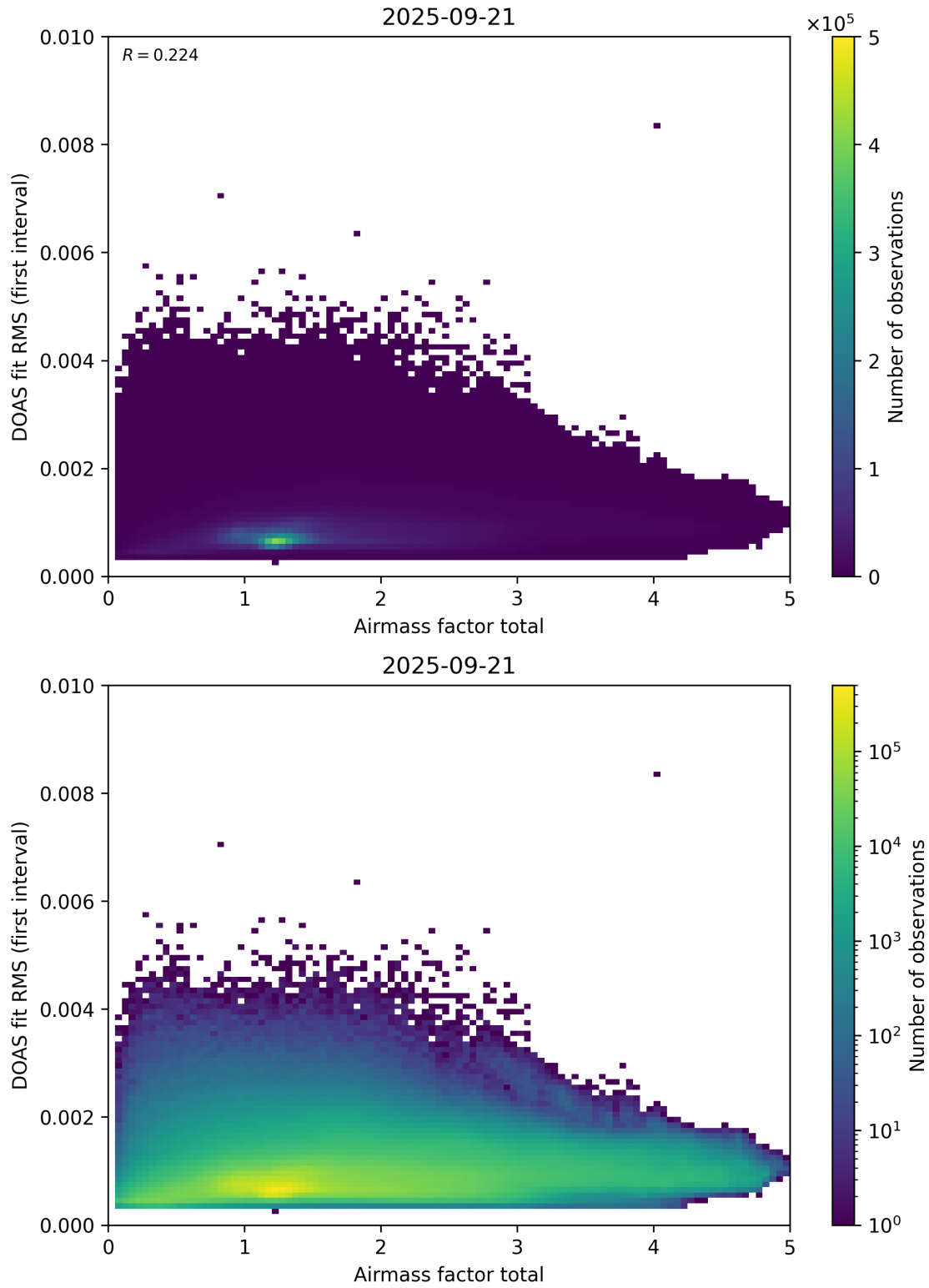
Figure 97: Scatter density plot of “Airmass factor total” against “DOAS fit RMS (first interval)” for 2025-09-20 to 2025-09-22.
