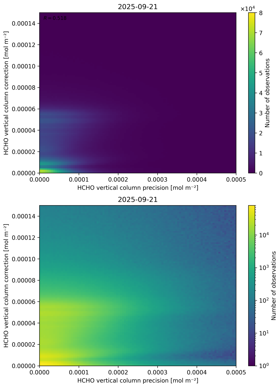
Figure 146: Scatter density plot of “HCHO vertical column precision” against “HCHO vertical column correction” for 2025-09-20 to 2025-09-22.
