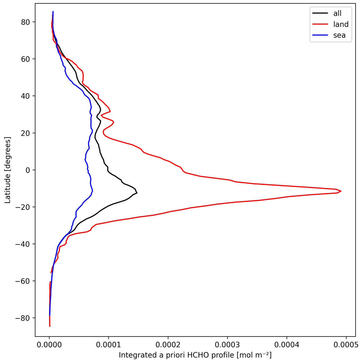
Figure 29: Zonal average of “Integrated a priori HCHO profile” for 2025-09-20 to 2025-09-22.
