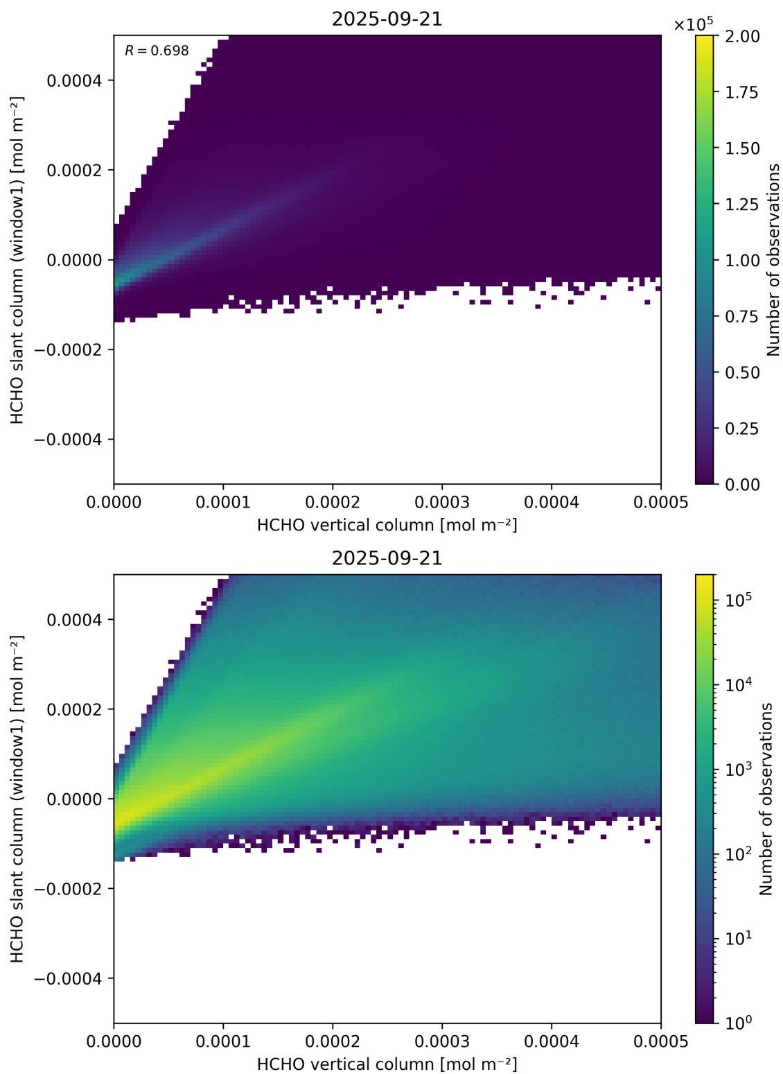
Figure 129: Scatter density plot of “HCHO vertical column” against “HCHO slant column (window1)” for 2025-09-20 to 2025-09-22.
