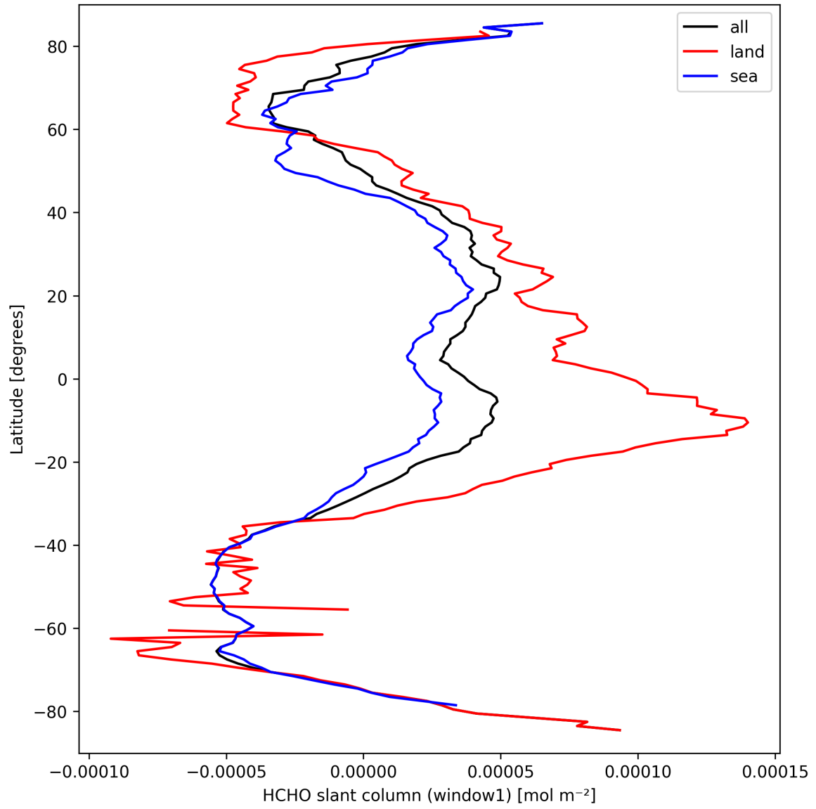
Figure 24: Zonal average of “HCHO slant column (window1)” for 2025-09-20 to 2025-09-22.
