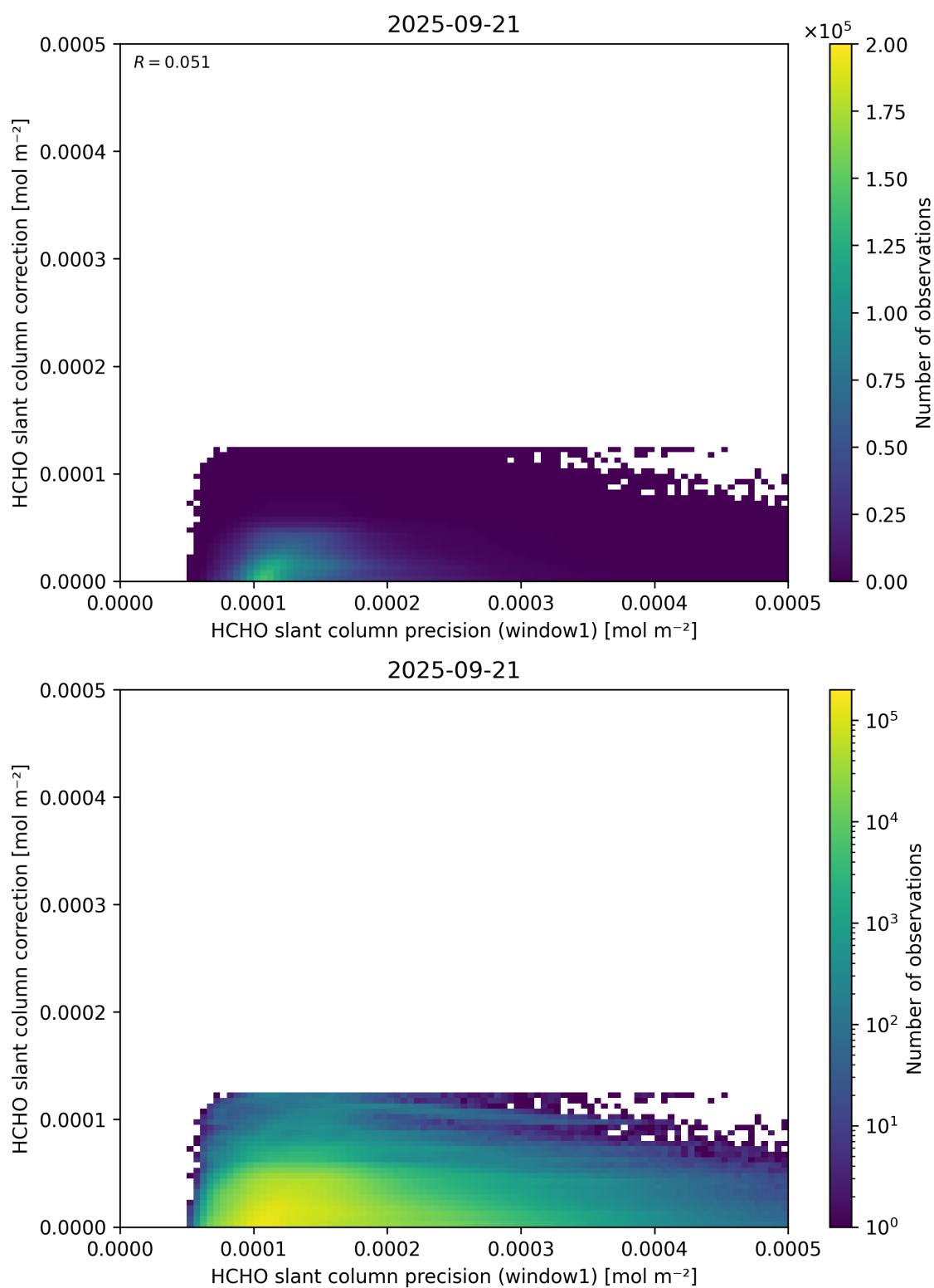
Figure 93: Scatter density plot of “HCHO slant column precision (window1)” against “HCHO slant column correction” for 2025-09-20 to 2025-09-22.
