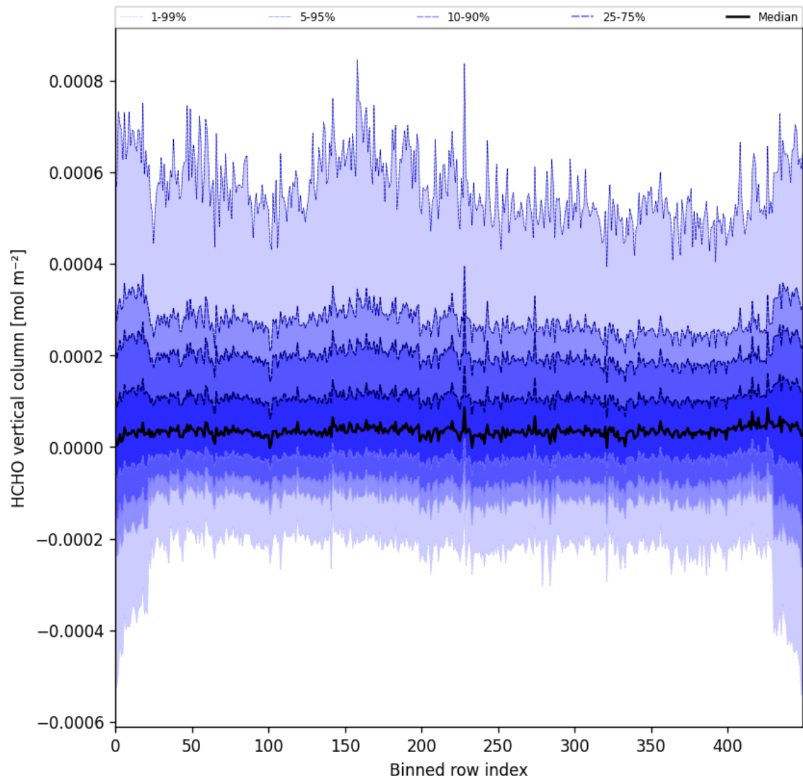
Figure 49: Along track statistics of “HCHO vertical column” for 2025-09-20 to 2025-09-22
