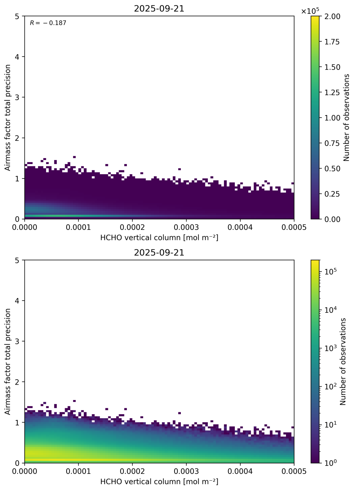
Figure 132: Scatter density plot of “HCHO vertical column” against “Airmass factor total precision” for 2025-09-20 to 2025-09-22.
