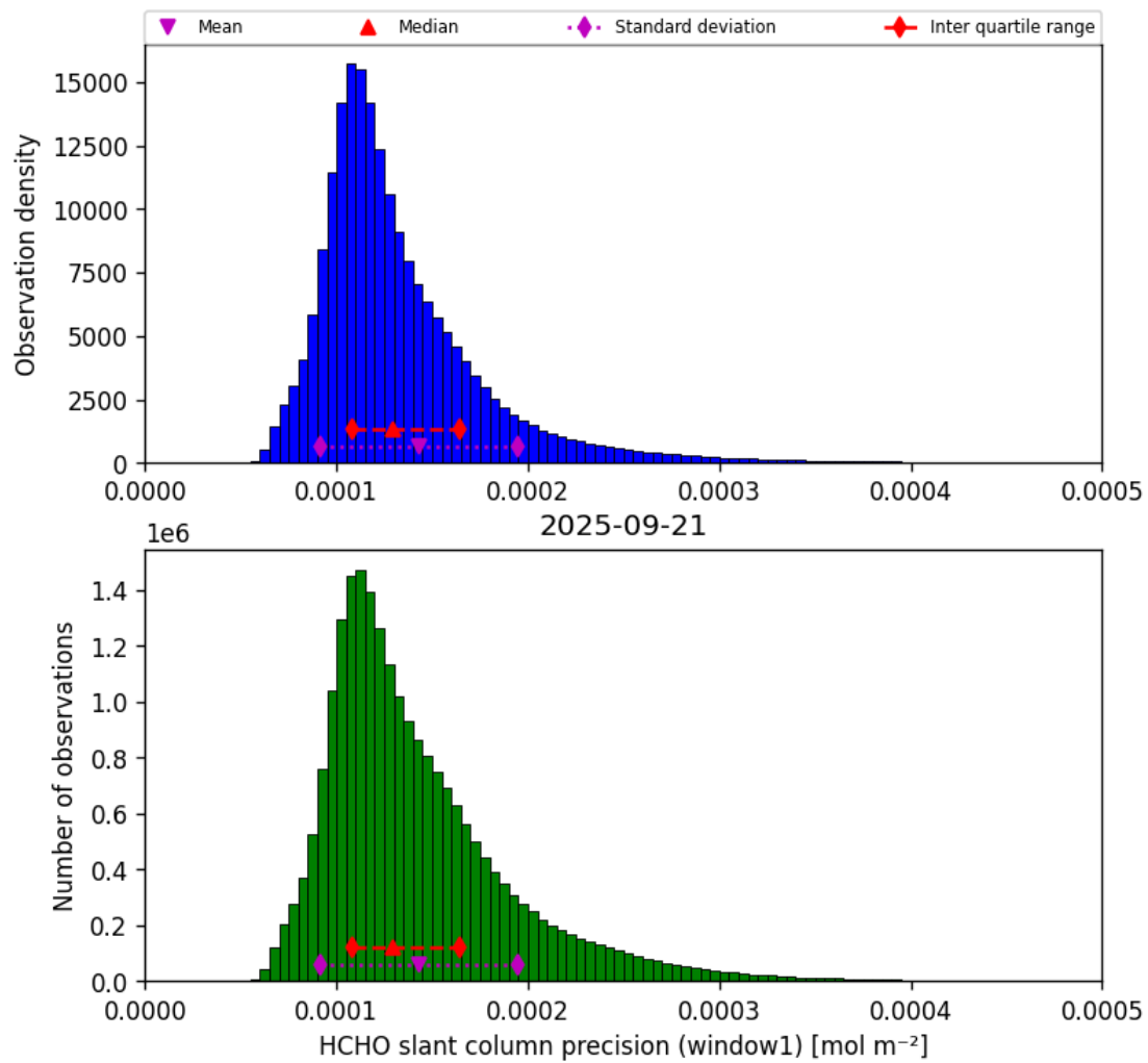
Figure 39: Histogram of “HCHO slant column precision (window1)” for 2025-09-20 to 2025-09-22
