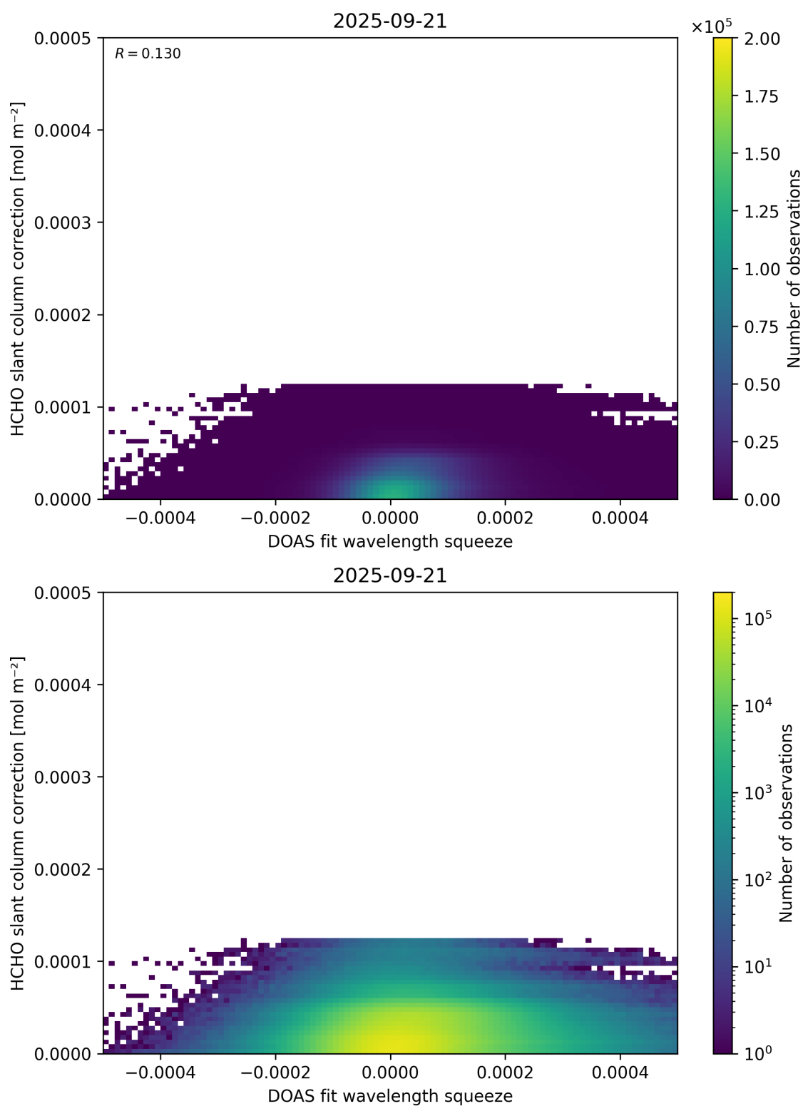
Figure 70: Scatter density plot of “DOAS fit wavelength squeeze” against “HCHO slant column correction” for 2025-09-20 to 2025-09-22.
