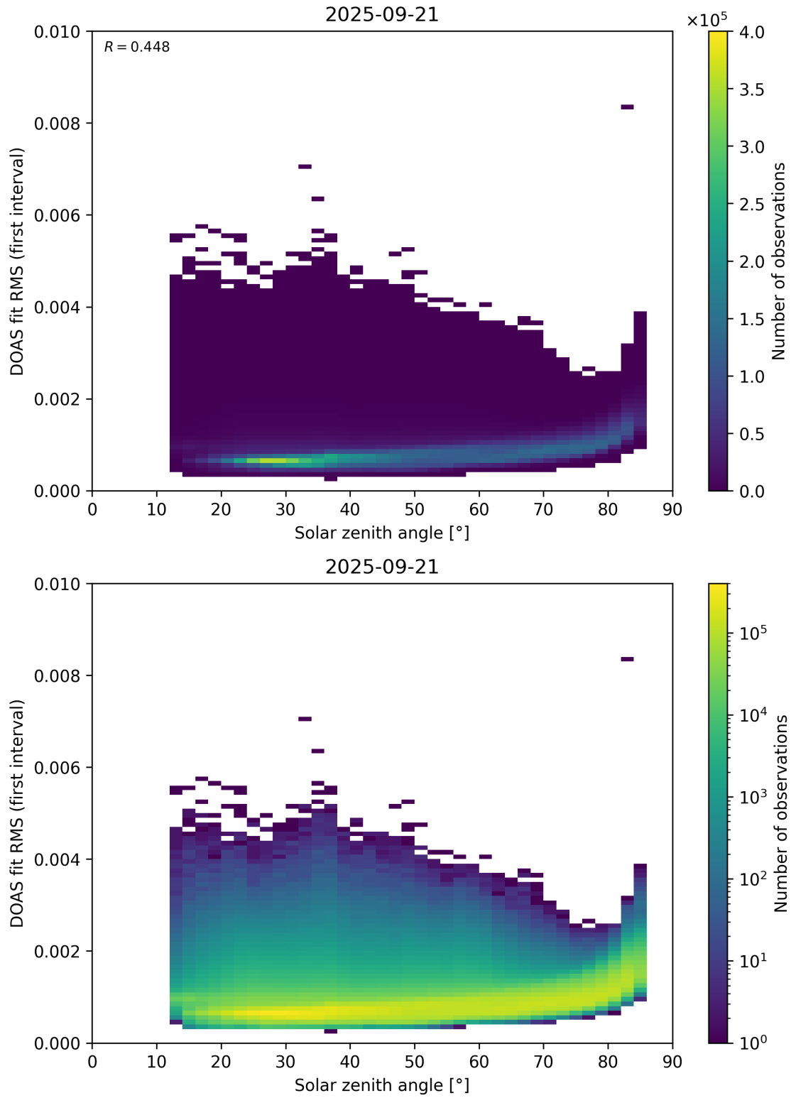
Figure 167: Scatter density plot of “Solar zenith angle” against “DOAS fit RMS (first interval)” for 2025-09-20 to 2025-09-22.
