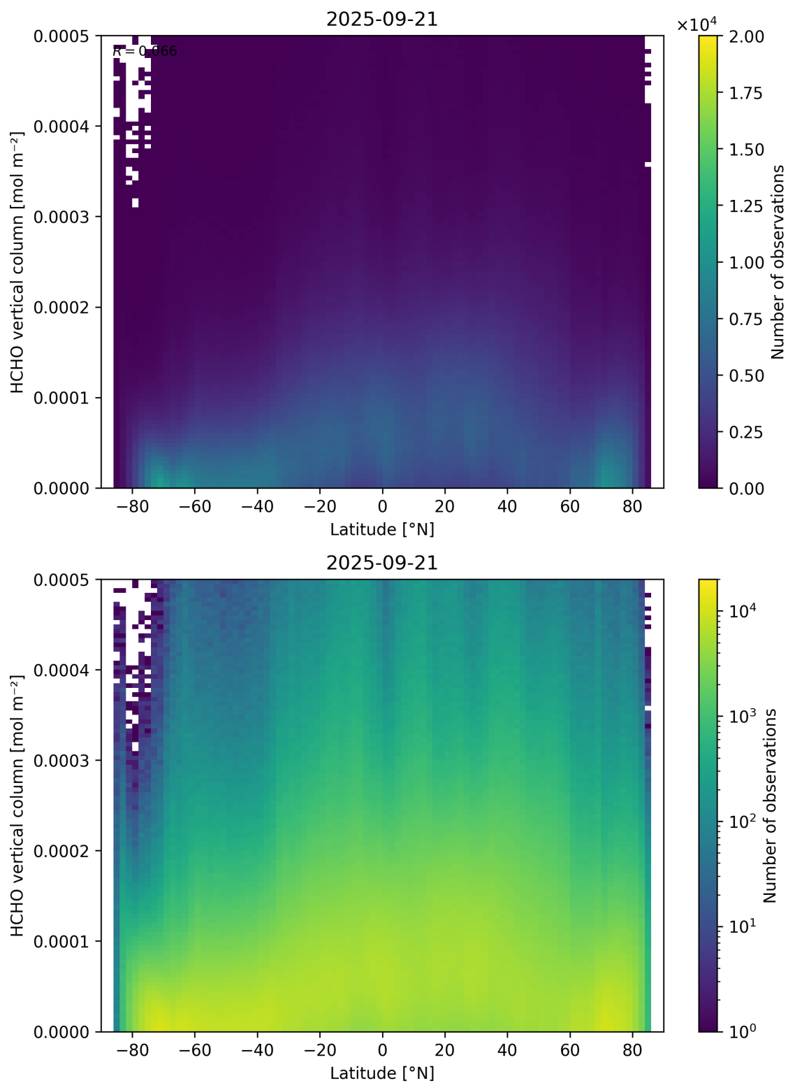
Figure 163: Scatter density plot of “Latitude” against “HCHO vertical column” for 2025-09-20 to 2025-09-22.
