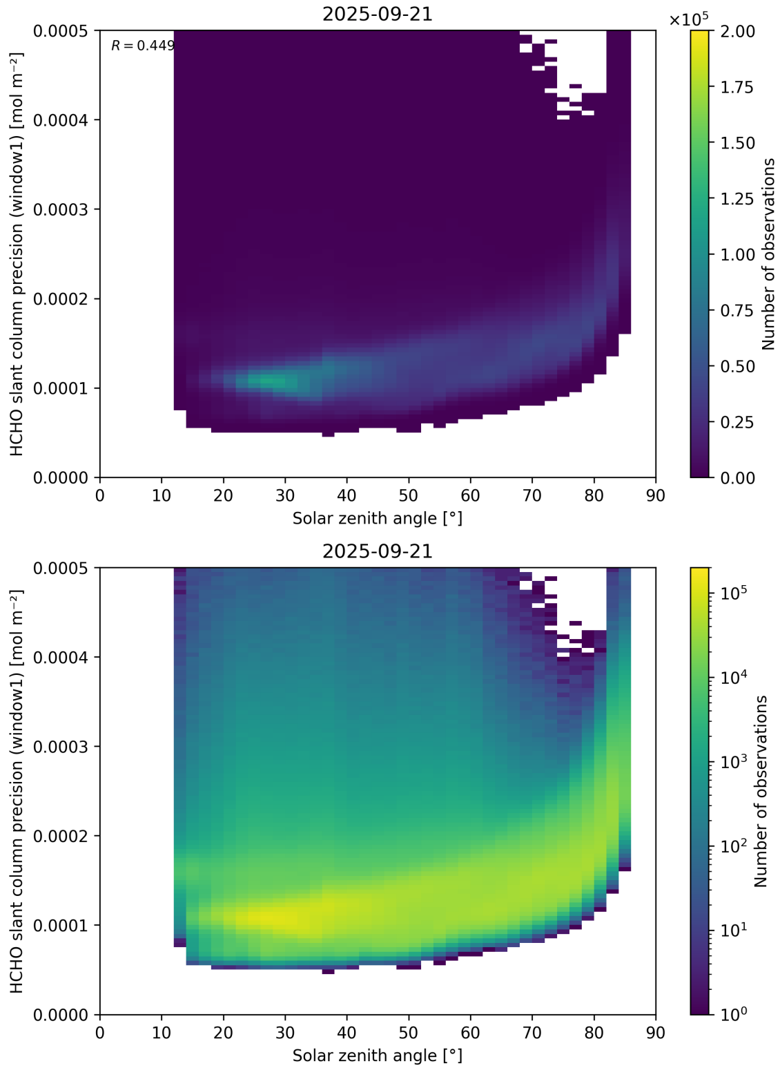
Figure 174: Scatter density plot of “Solar zenith angle” against “HCHO slant column precision (window1)” for 2025-09-20 to 2025-09-22.
