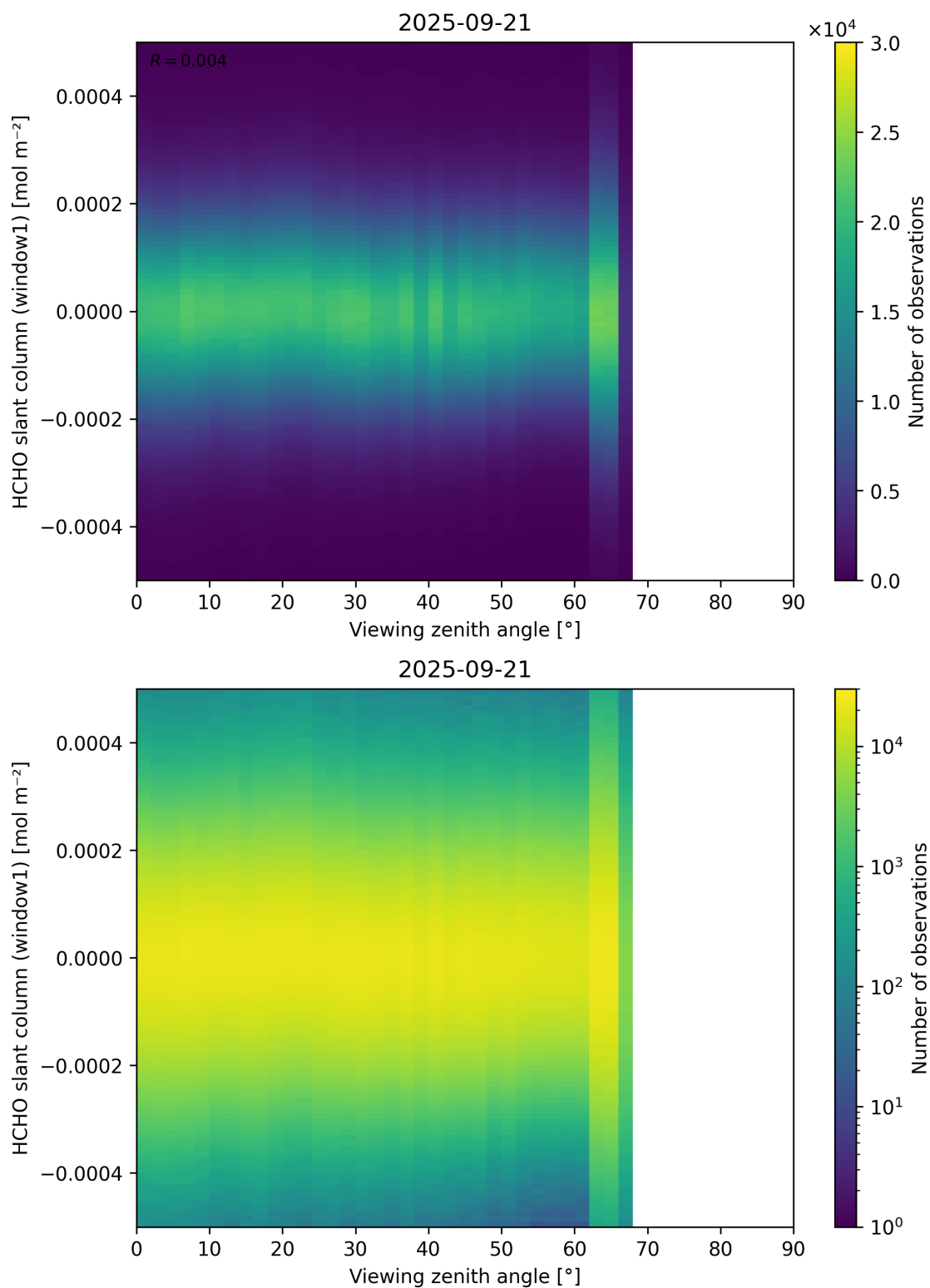
Figure 188: Scatter density plot of “Viewing zenith angle” against “HCHO slant column (window1)” for 2025-09-20 to 2025-09-22.
