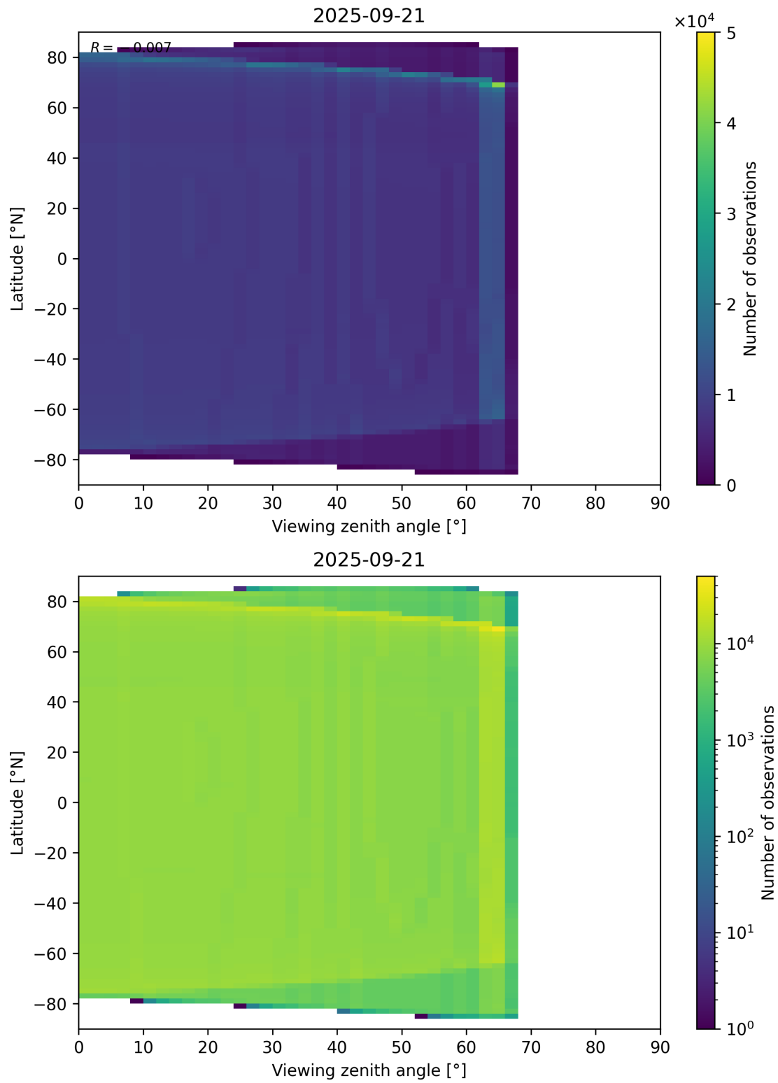
Figure 196: Scatter density plot of “Viewing zenith angle” against “Latitude” for 2025-09-20 to 2025-09-22.
