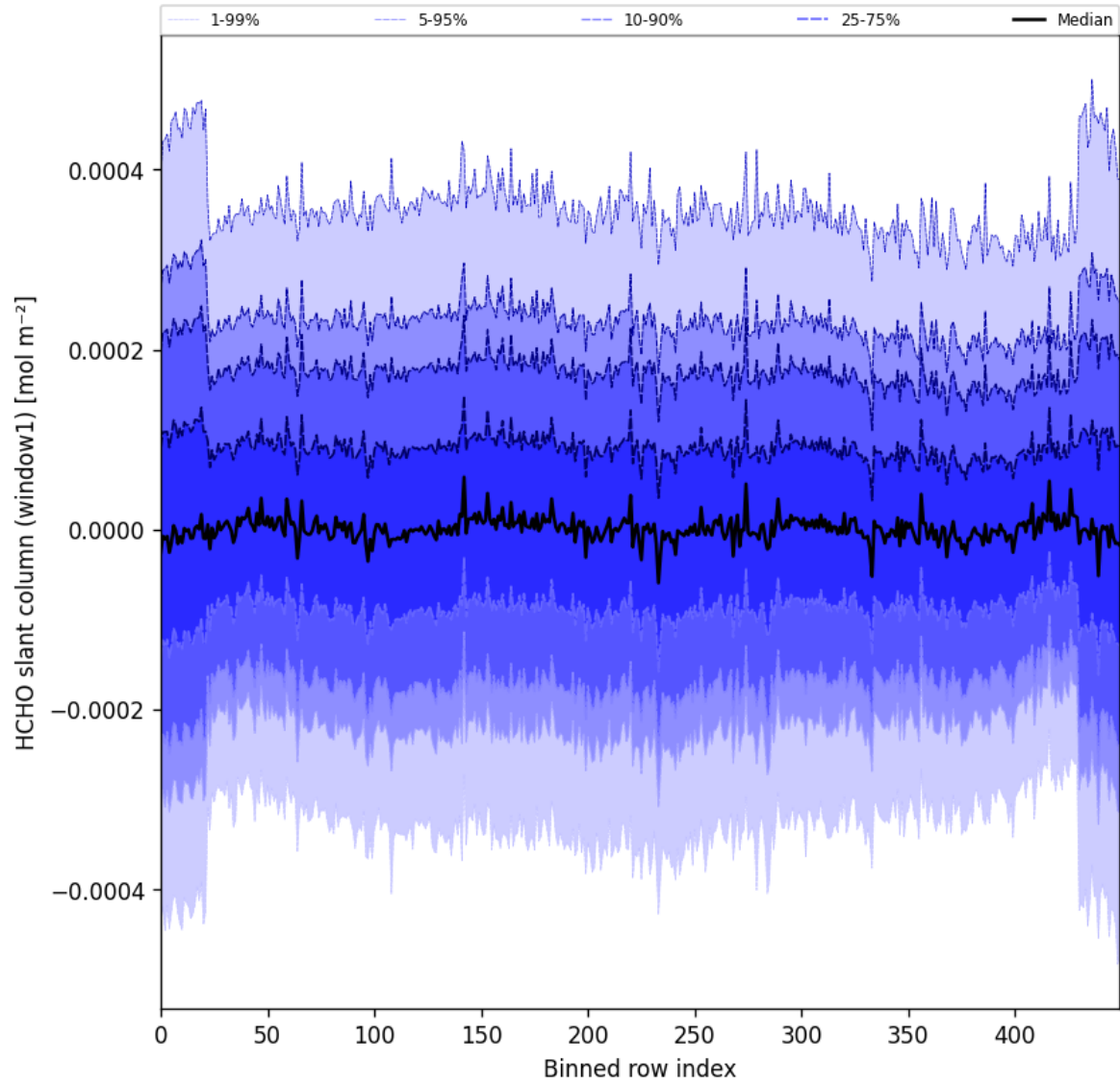
Figure 52: Along track statistics of “HCHO slant column (window1)” for 2025-09-20 to 2025-09-22
