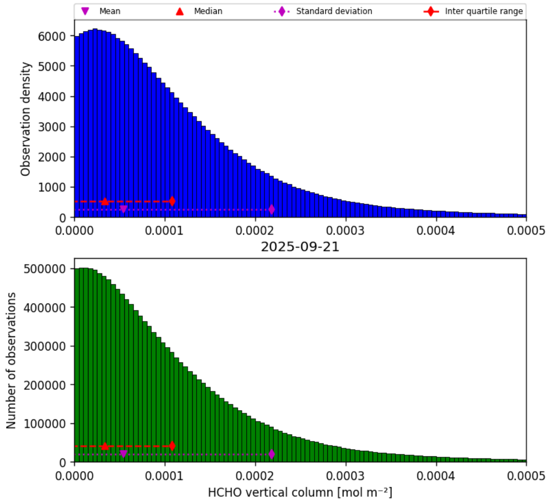
Figure 35: Histogram of “HCHO vertical column” for 2025-09-20 to 2025-09-22
