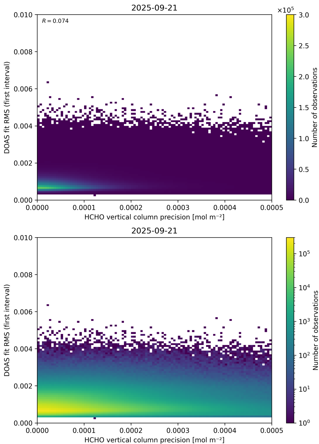
Figure 136: Scatter density plot of “HCHO vertical column precision” against “DOAS fit RMS (first interval)” for 2025-09-20 to 2025-09-22.
