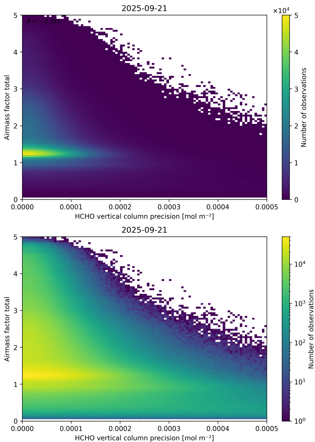
Figure 144: Scatter density plot of “HCHO vertical column precision” against “Airmass factor total” for 2025-09-20 to 2025-09-22.
