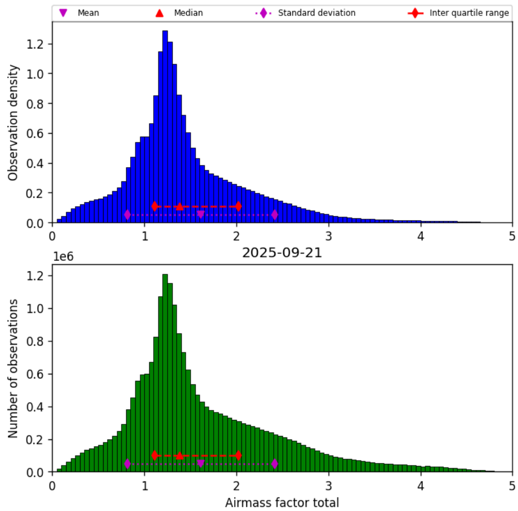
Figure 40: Histogram of “Airmass factor total” for 2025-09-20 to 2025-09-22
