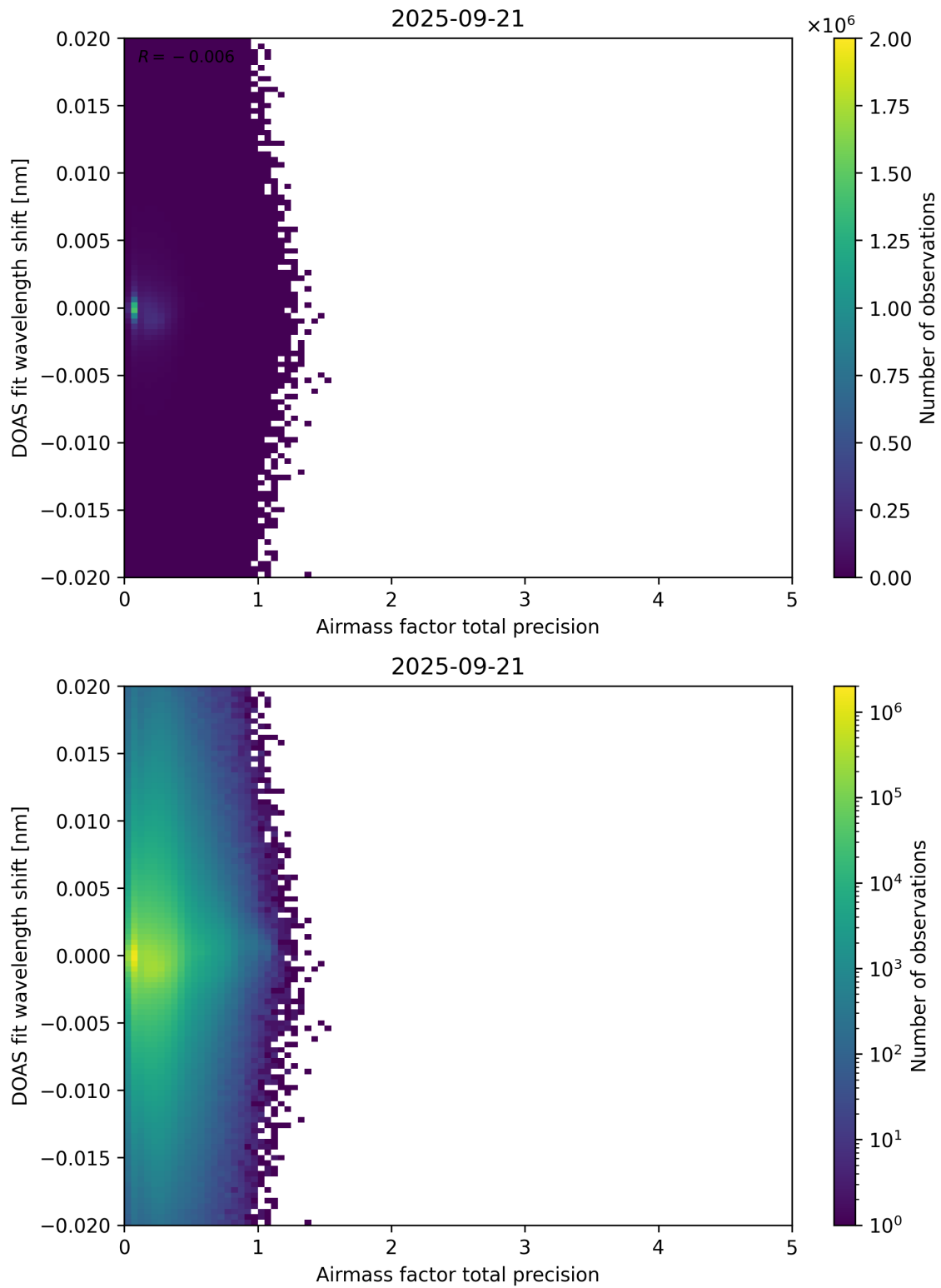
Figure 106: Scatter density plot of “Airmass factor total precision” against “DOAS fit wavelength shift” for 2025-09-20 to 2025-09-22.
