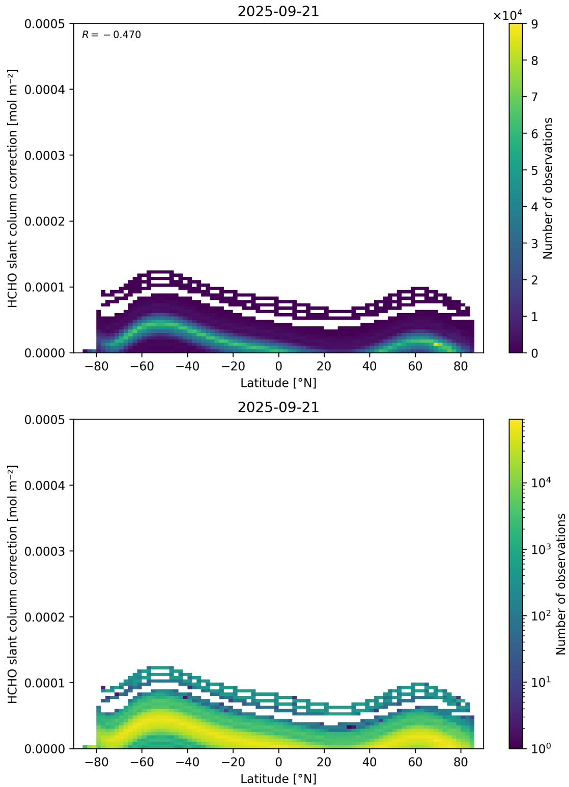
Figure 158: Scatter density plot of “Latitude” against “HCHO slant column correction” for 2025-09-20 to 2025-09-22.
