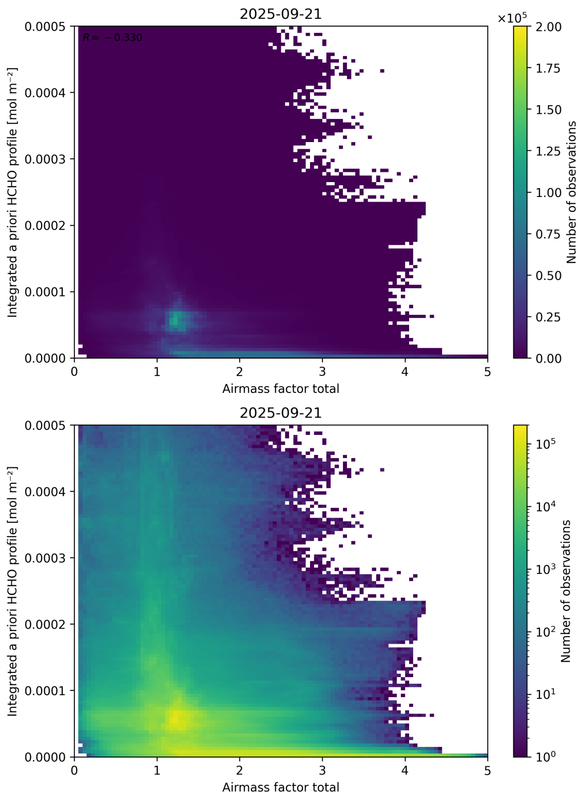
Figure 104: Scatter density plot of “Airmass factor total” against “Integrated a priori HCHO profile” for 2025-09-20 to 2025-09-22.
