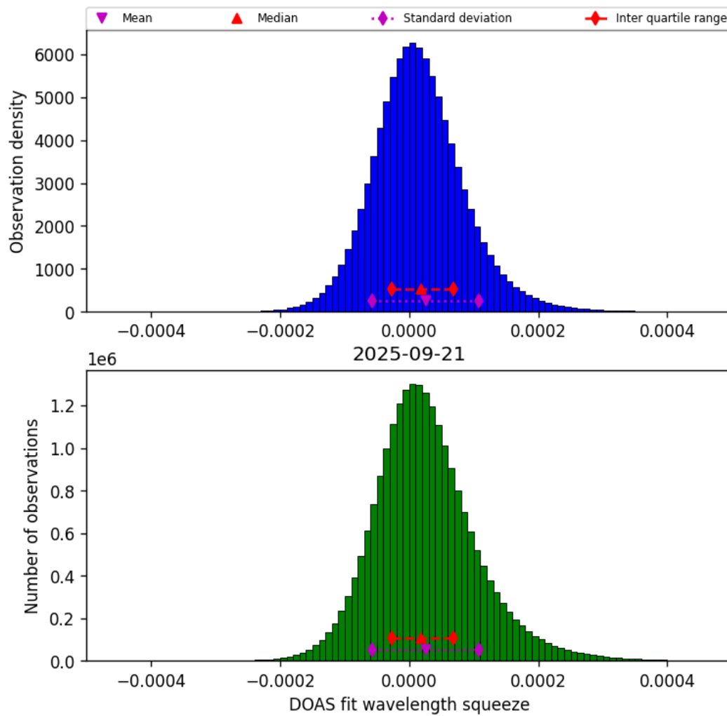
Figure 45: Histogram of “DOAS fit wavelength squeeze” for 2025-09-20 to 2025-09-22
