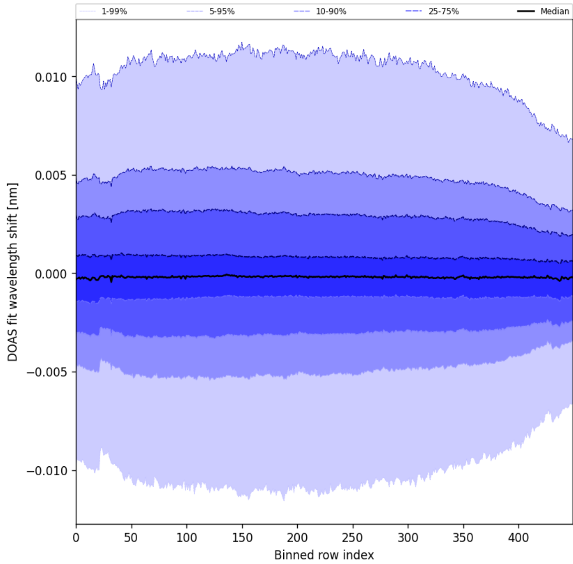
Figure 58: Along track statistics of “DOAS fit wavelength shift” for 2025-09-20 to 2025-09-22
