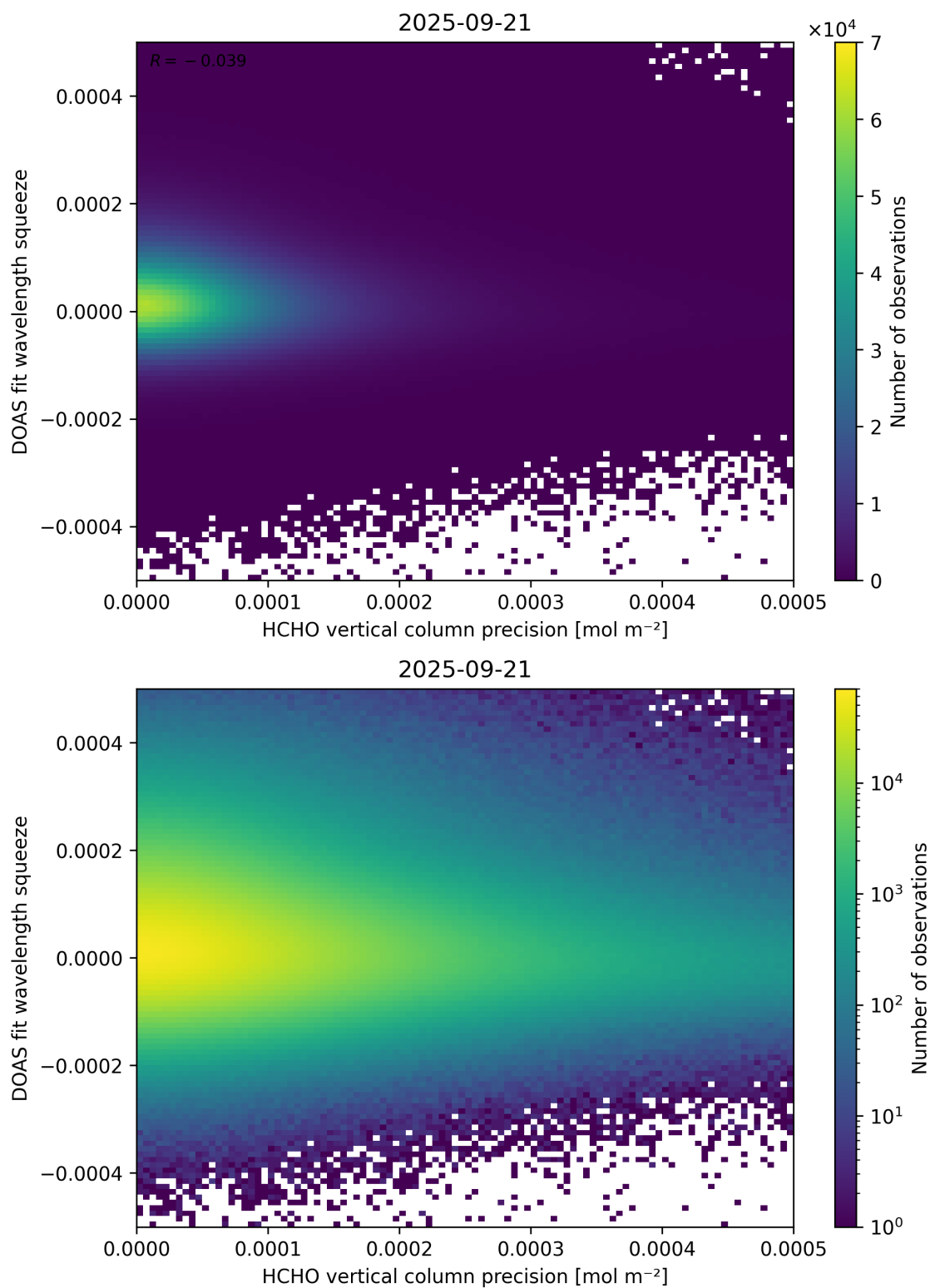
Figure 138: Scatter density plot of “HCHO vertical column precision” against “DOAS fit wavelength squeeze” for 2025-09-20 to 2025-09-22.
