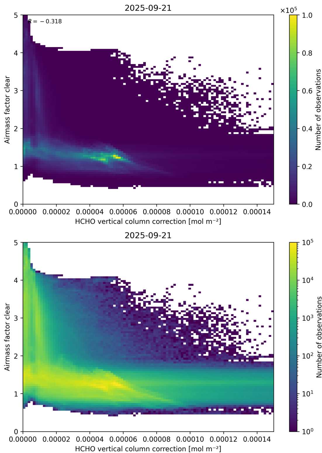
Figure 115: Scatter density plot of “HCHO vertical column correction” against “Airmass factor clear” for 2025-09-20 to 2025-09-22.
