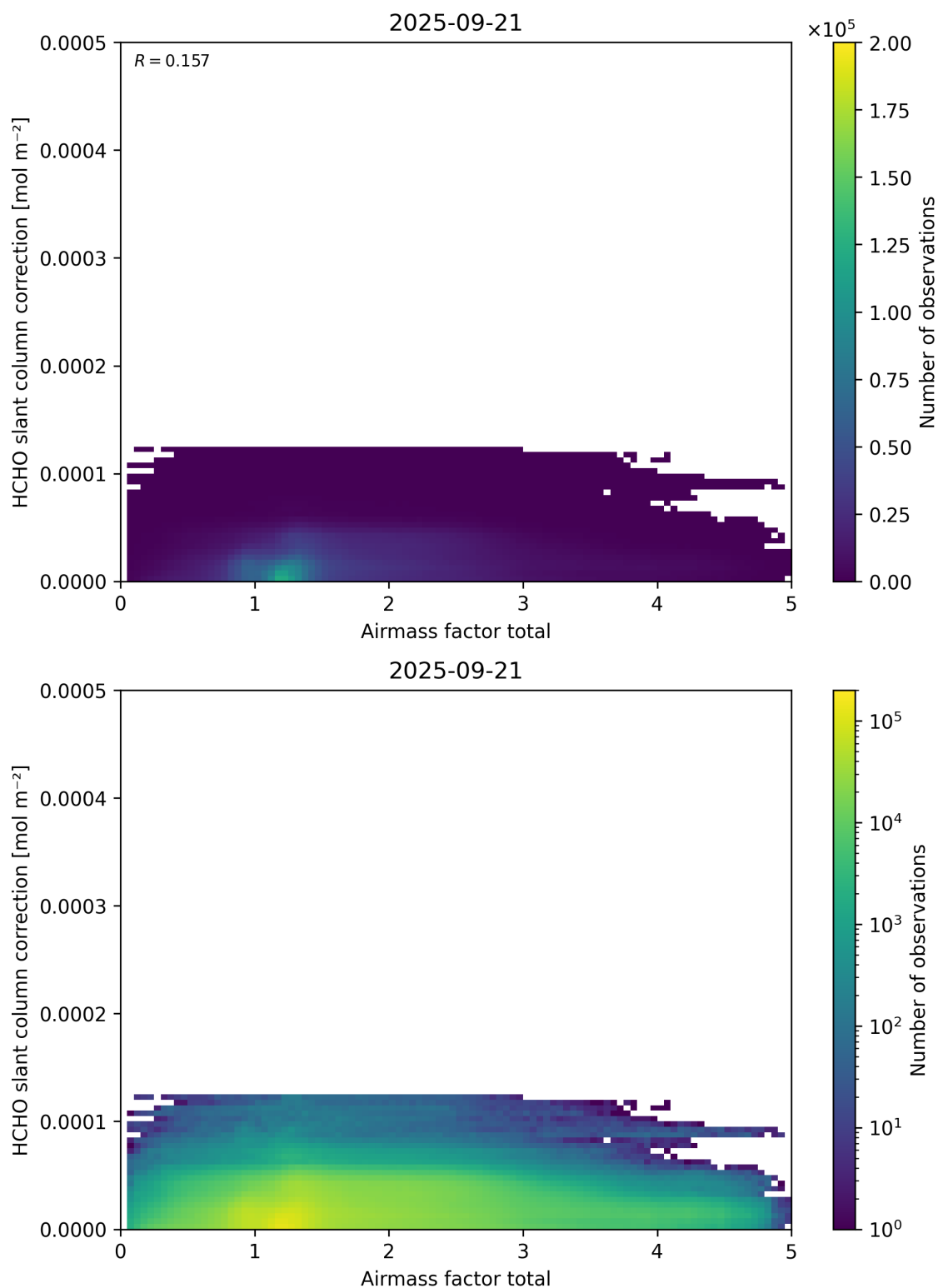
Figure 102: Scatter density plot of “Airmass factor total” against “HCHO slant column correction” for 2025-09-20 to 2025-09-22.
