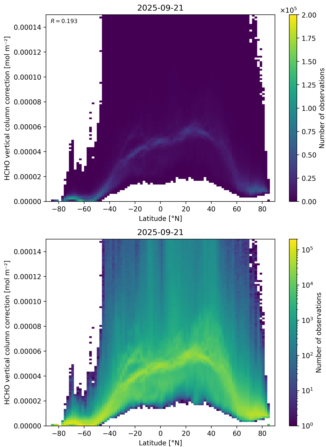
Figure 164: Scatter density plot of “Latitude” against “HCHO vertical column correction” for 2025-09-20 to 2025-09-22.
