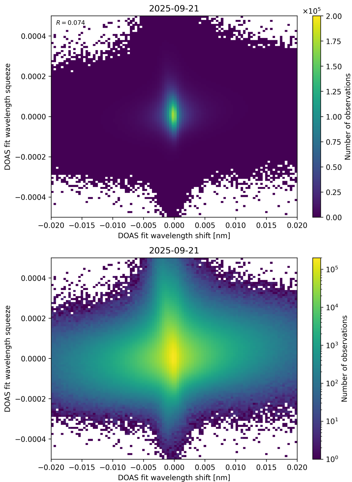
Figure 65: Scatter density plot of “DOAS fit wavelength shift” against “DOAS fit wavelength squeeze” for 2025-09-20 to 2025-09-22.
