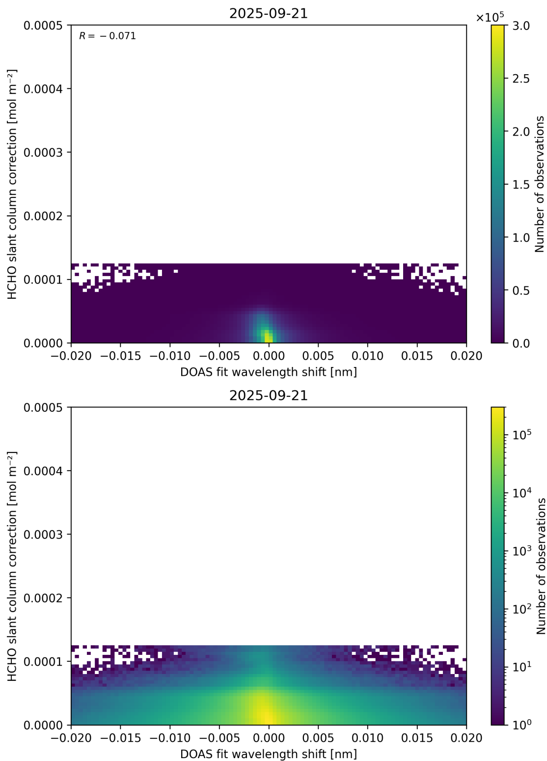
Figure 67: Scatter density plot of “DOAS fit wavelength shift” against “HCHO slant column correction” for 2025-09-20 to 2025-09-22.
