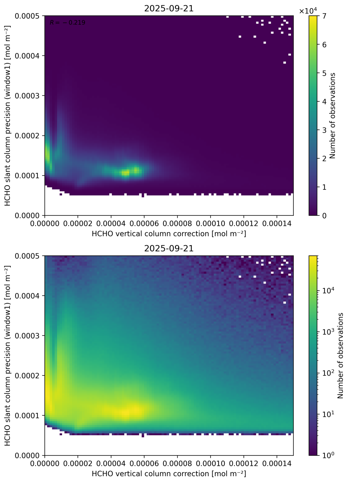
Figure 119: Scatter density plot of “HCHO vertical column correction” against “HCHO slant column precision (window1)” for 2025-09-20 to 2025-09-22.
