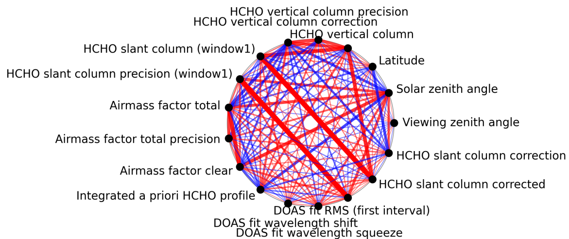
Figure 1: Map of correlation graph for 2025-09-20 to 2025-09-22.
