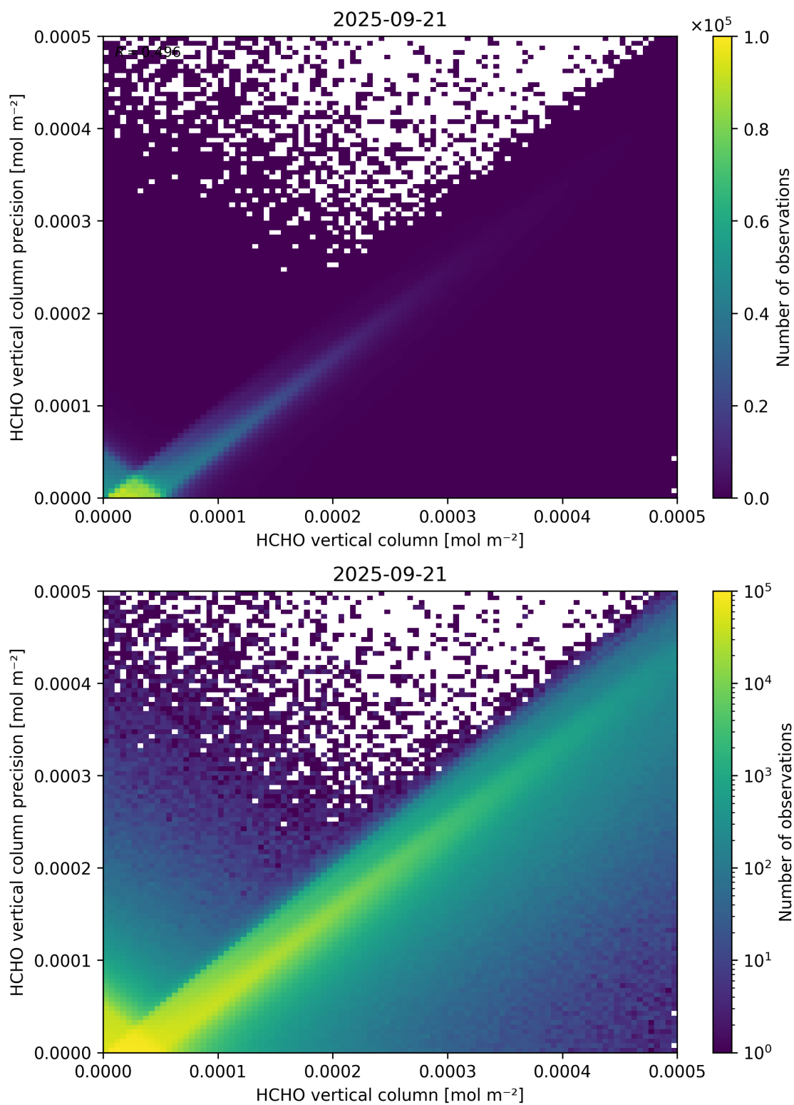
Figure 134: Scatter density plot of “HCHO vertical column” against “HCHO vertical column precision” for 2025-09-20 to 2025-09-22.
