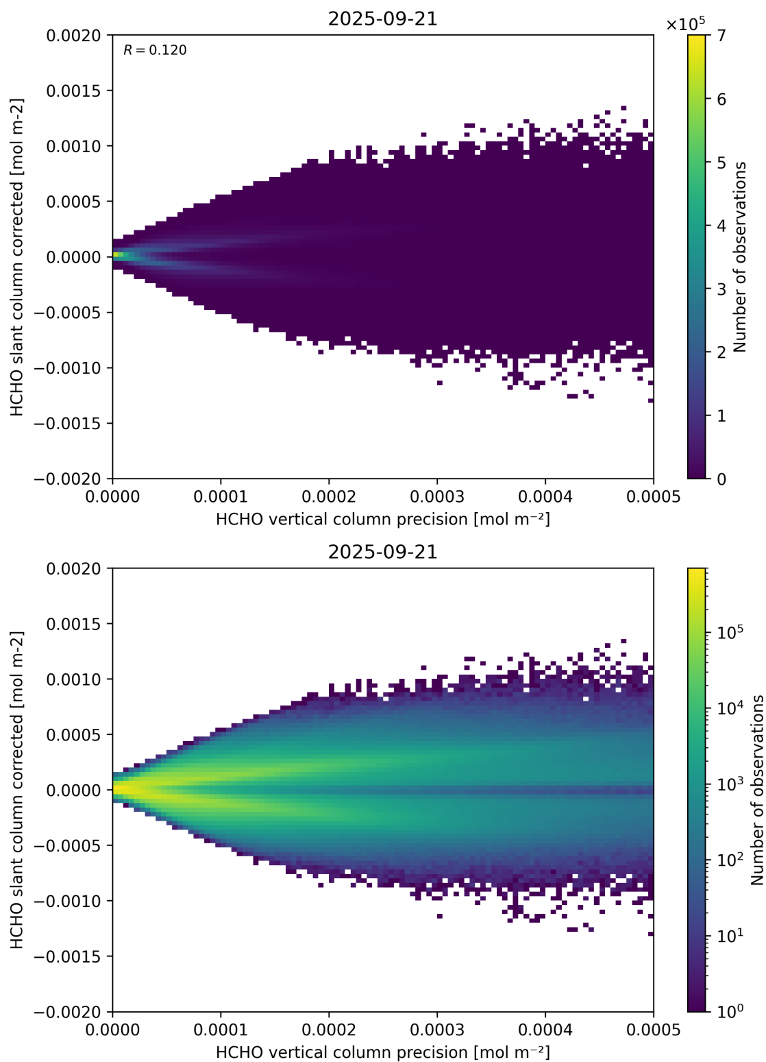
Figure 140: Scatter density plot of “HCHO vertical column precision” against “HCHO slant column corrected” for 2025-09-20 to 2025-09-22.
