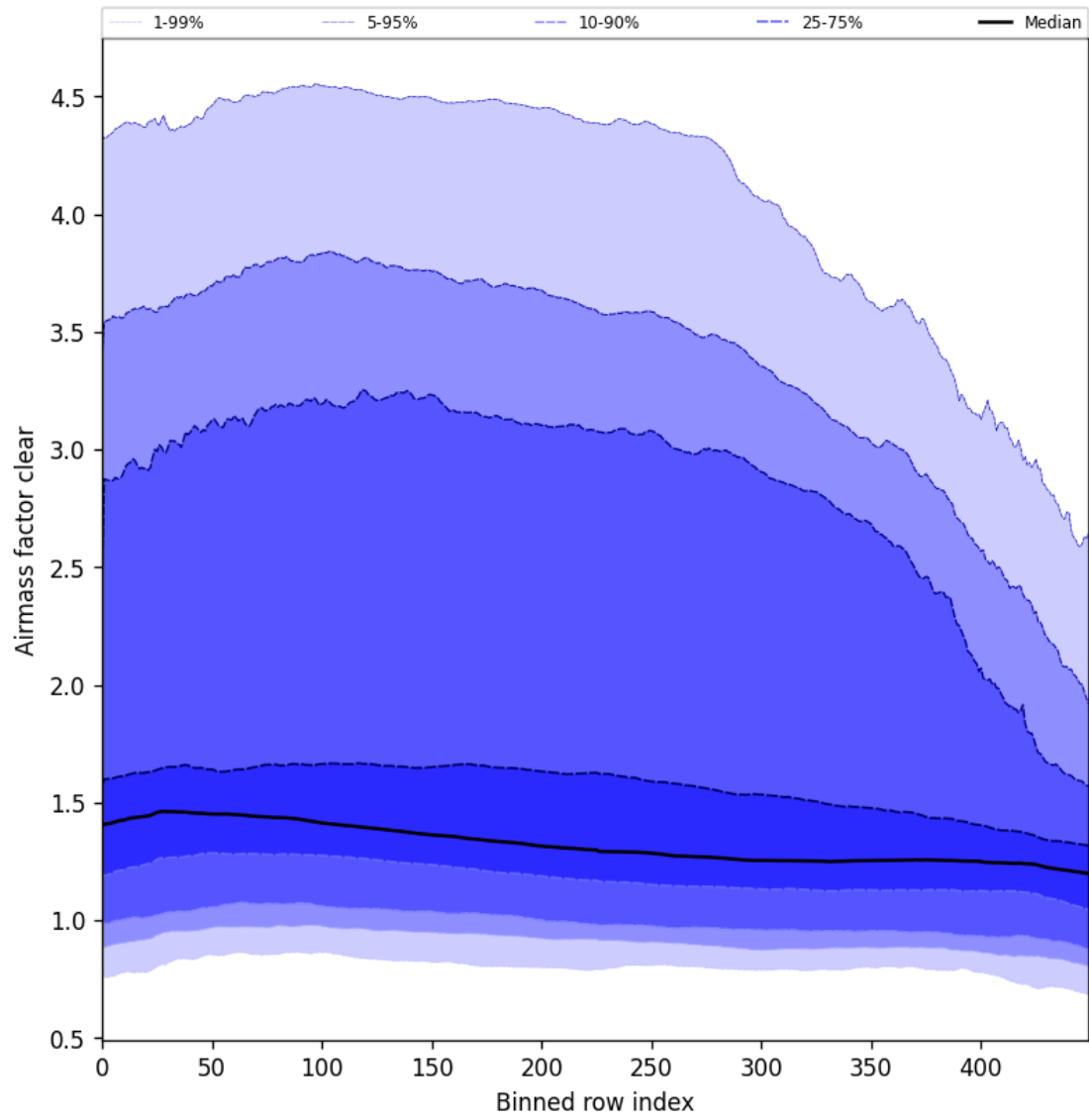
Figure 56: Along track statistics of “Air mass factor clear” for 2025-09-20 to 2025-09-22
