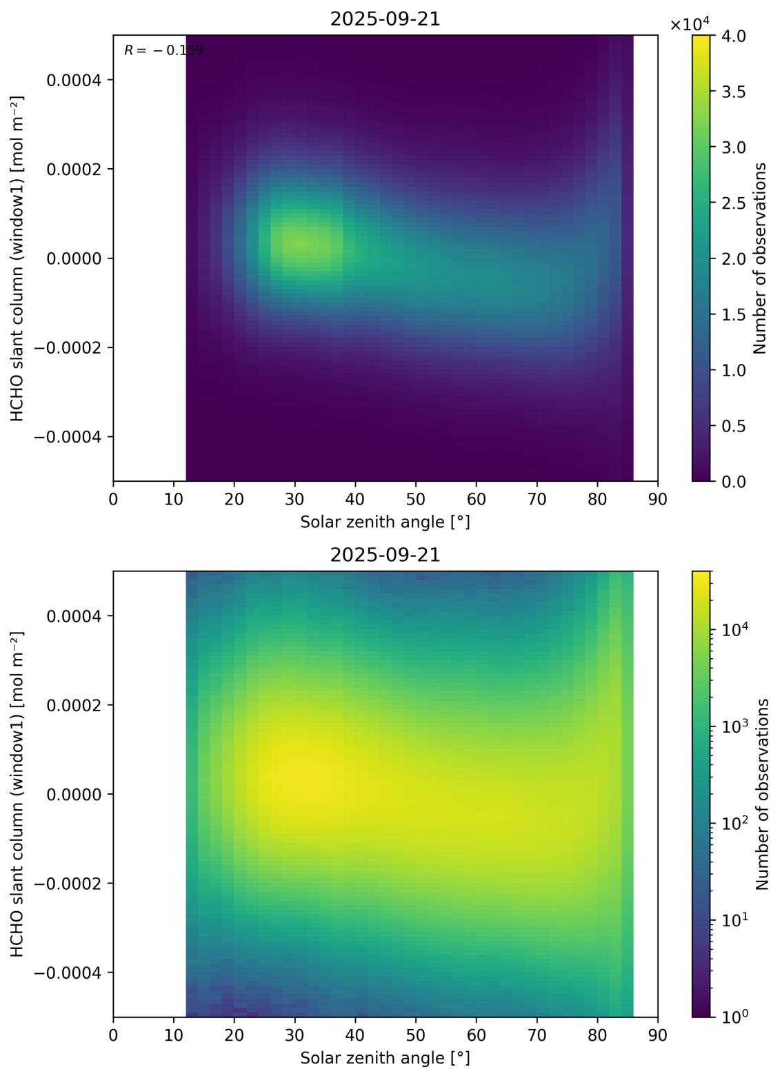
Figure 173: Scatter density plot of “Solar zenith angle” against “HCHO slant column (window1)” for 2025-09-20 to 2025-09-22.
