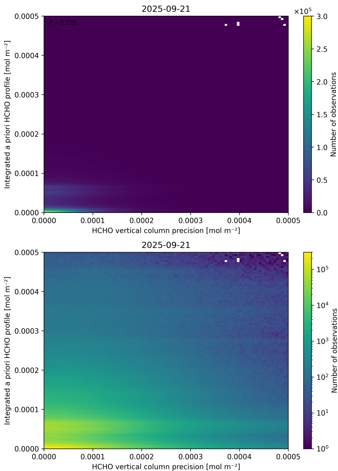
Figure 147: Scatter density plot of “HCHO vertical column precision” against “Integrated a priori HCHO profile” for 2025-09-20 to 2025-09-22.
