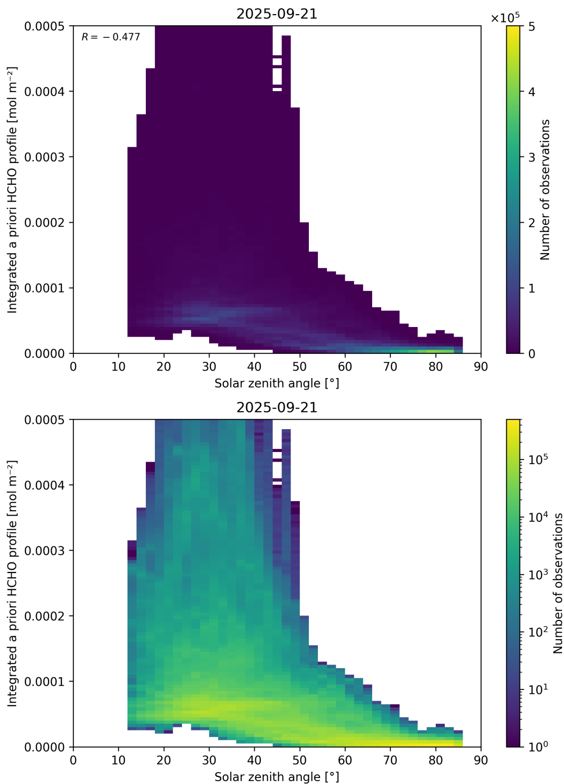
Figure 180: Scatter density plot of “Solar zenith angle” against “Integrated a priori HCHO profile” for 2025-09-20 to 2025-09-22.
