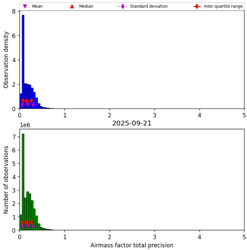
Figure 41: Histogram of “Airmass factor total precision” for 2025-09-20 to 2025-09-22
