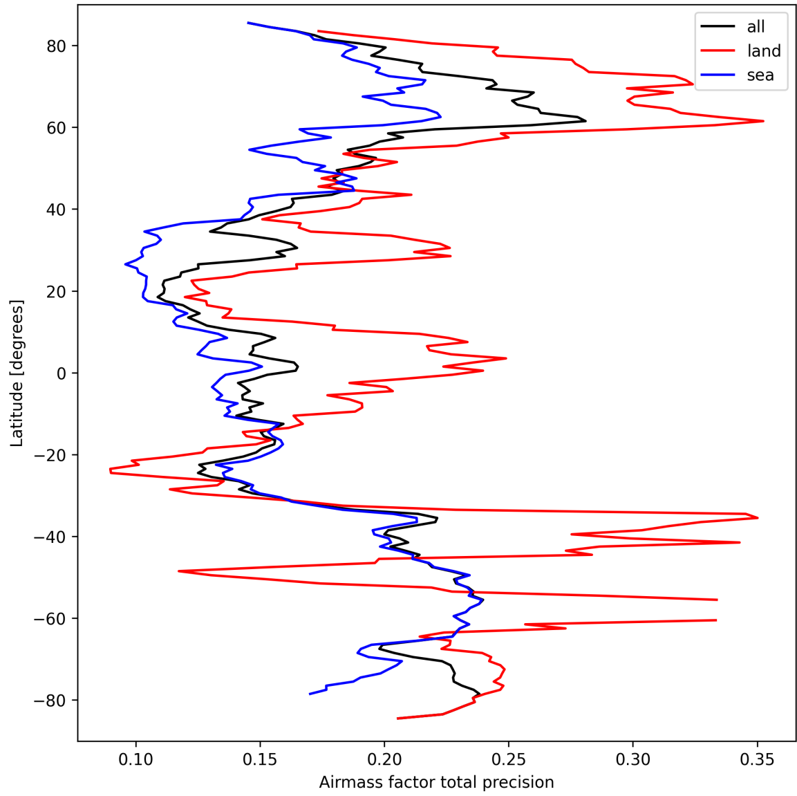
Figure 27: Zonal average of “Airmass factor total precision” for 2025-09-20 to 2025-09-22.
