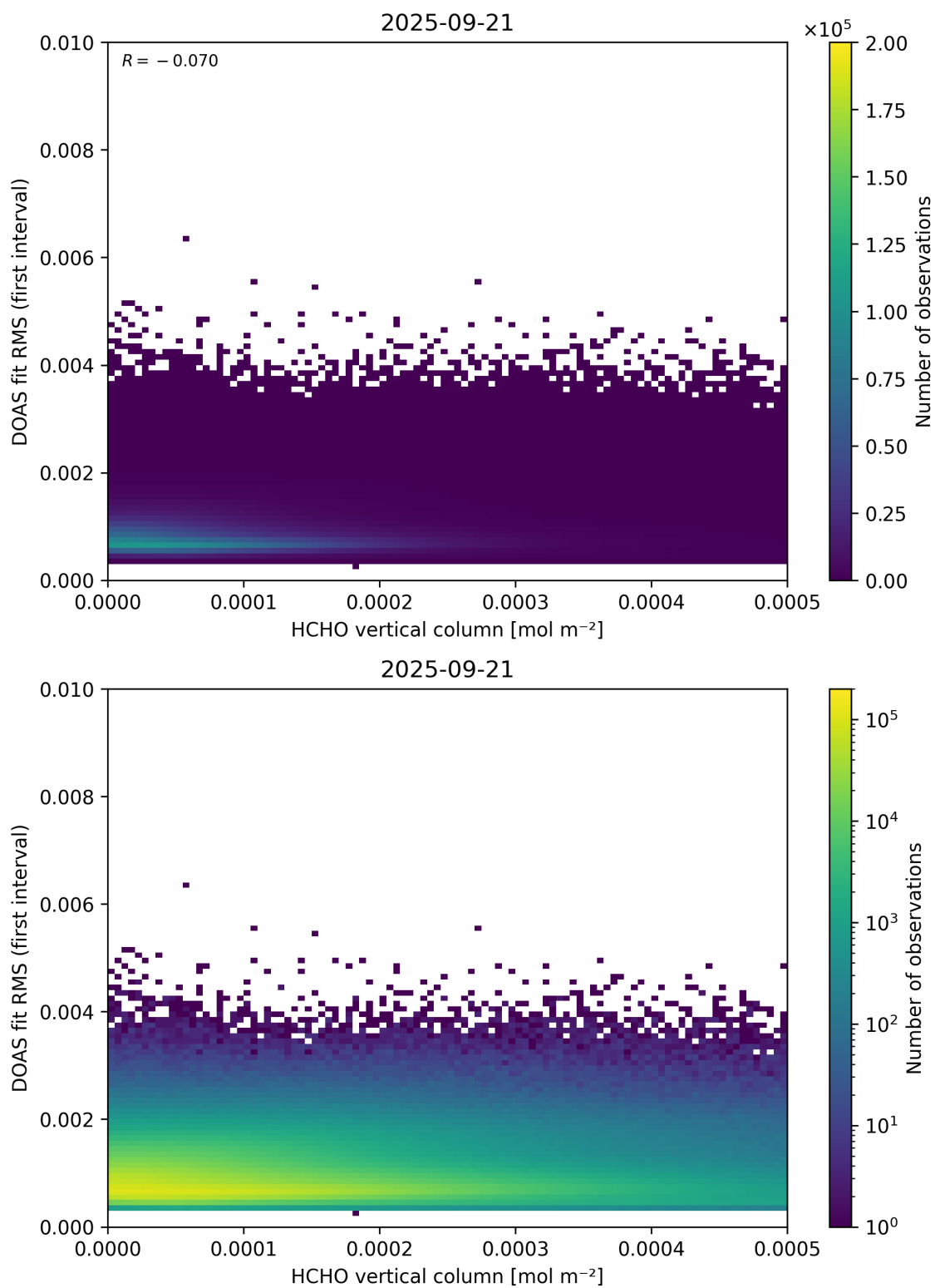
Figure 123: Scatter density plot of “HCHO vertical column” against “DOAS fit RMS (first interval)” for 2025-09-20 to 2025-09-22.
