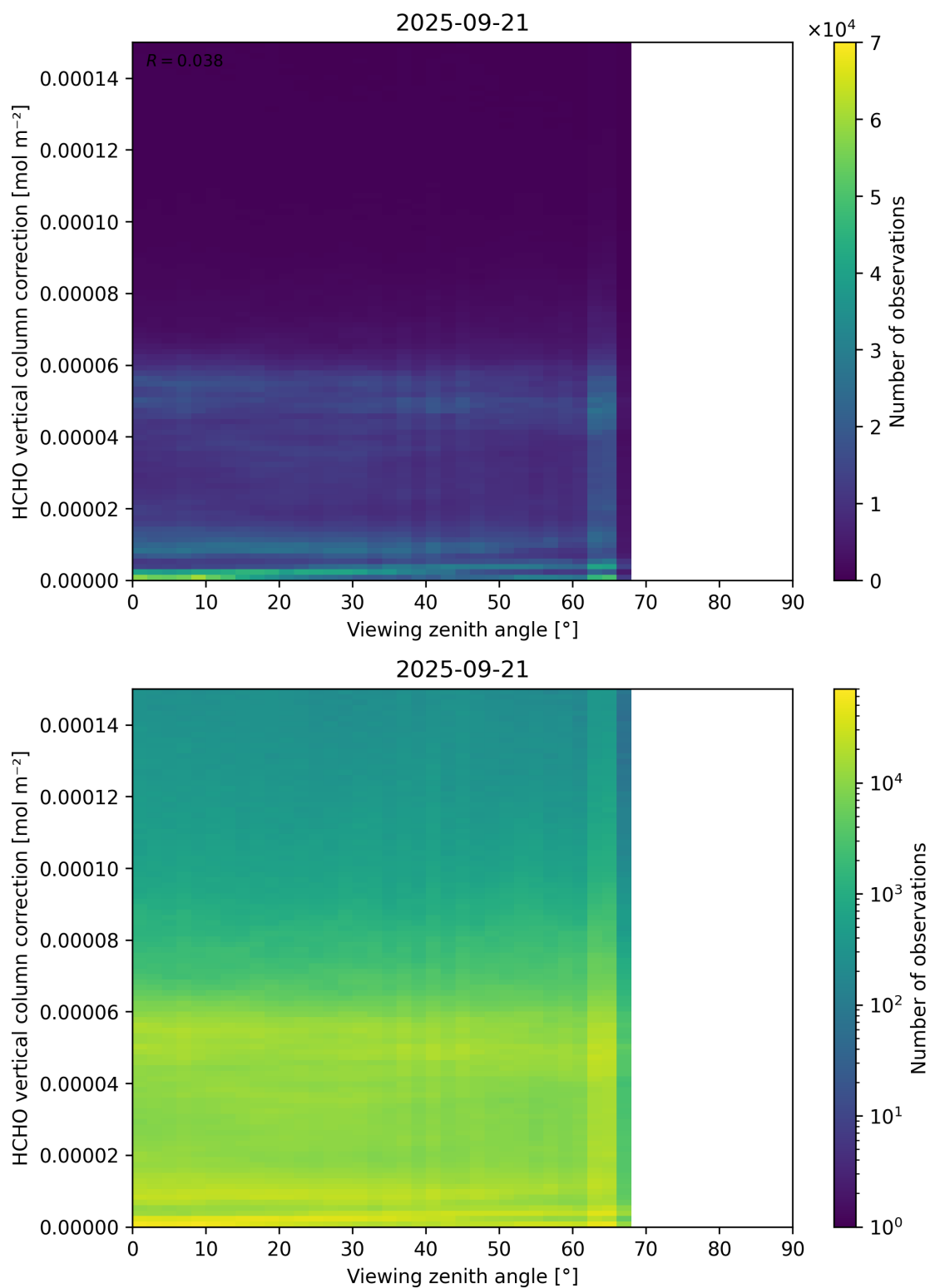
Figure 193: Scatter density plot of “Viewing zenith angle” against “HCHO vertical column correction” for 2025-09-20 to 2025-09-22.
