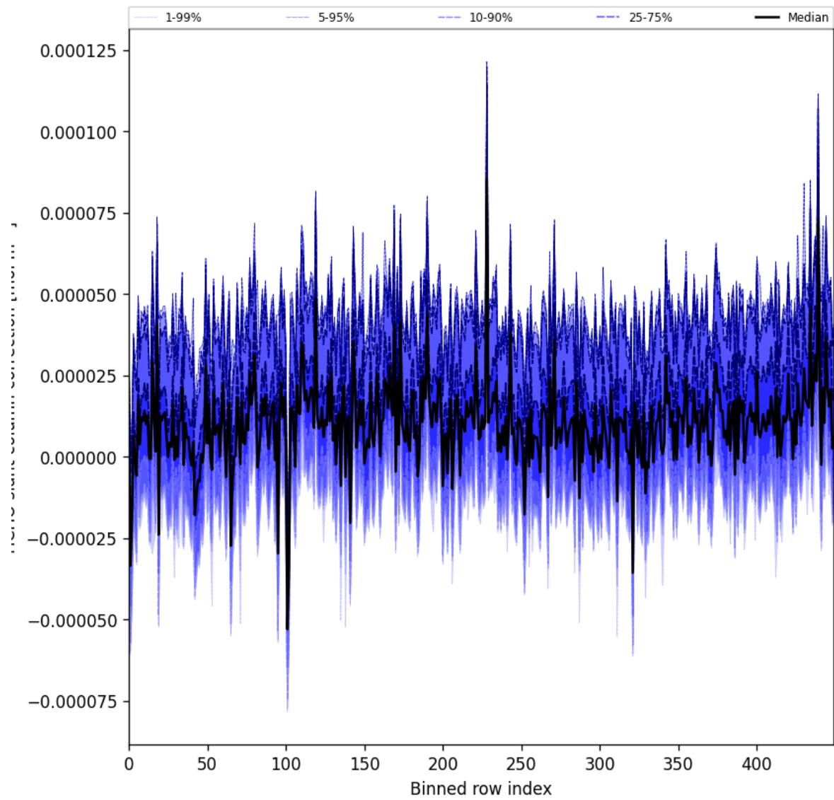
Figure 61: Along track statistics of “HCHO slant column correction” for 2025-09-20 to 2025-09-22
