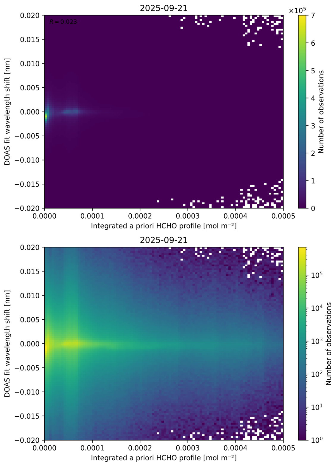
Figure 149: Scatter density plot of “Integrated a priori HCHO profile” against “DOAS fit wavelength shift” for 2025-09-20 to 2025-09-22.
