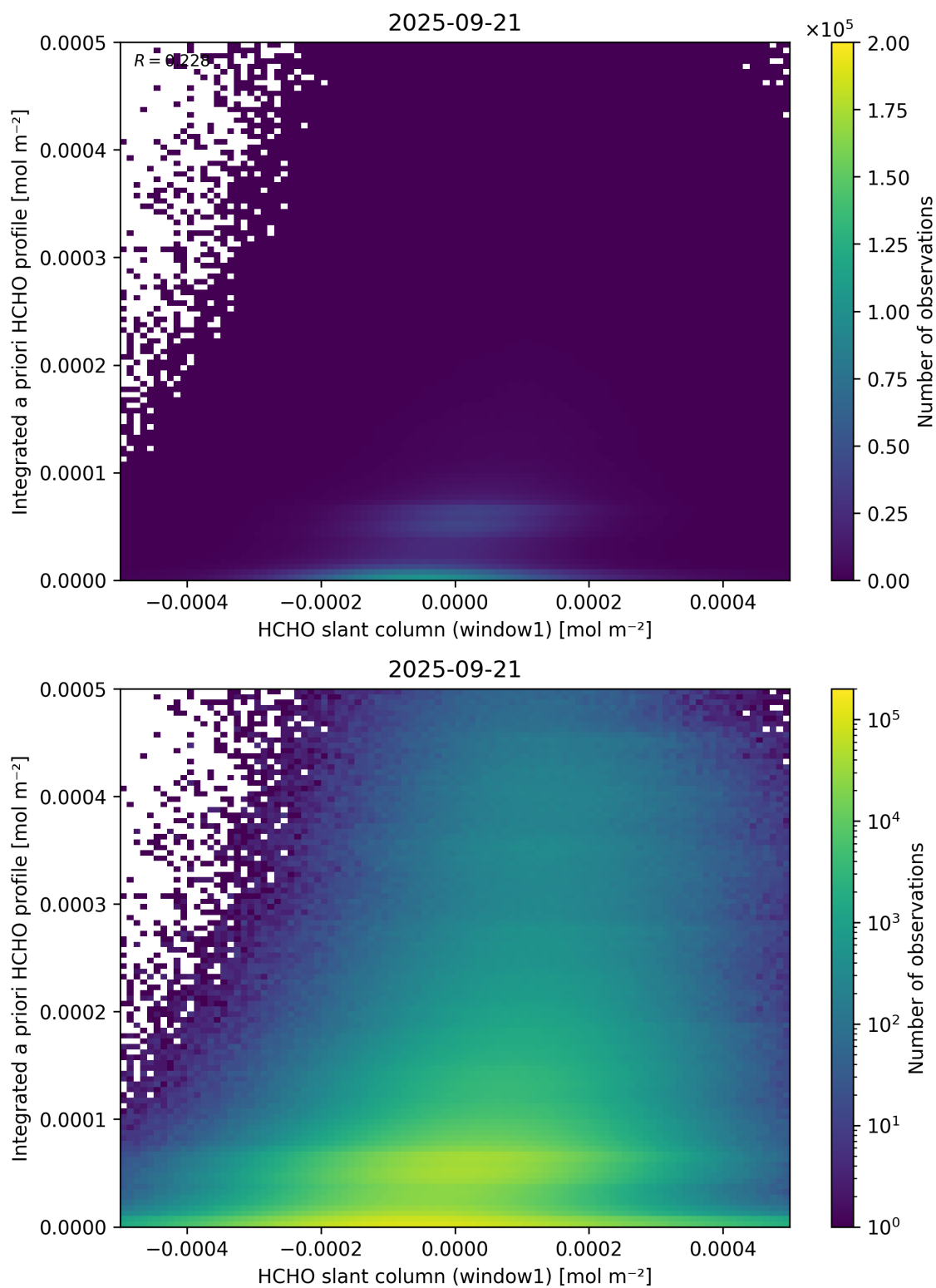
Figure 87: Scatter density plot of “HCHO slant column (window1)” against “Integrated a priori HCHO profile” for 2025-09-20 to 2025-09-22.
