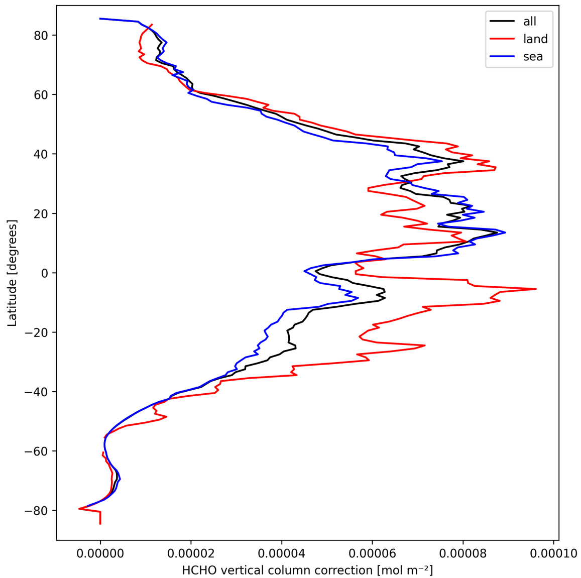
Figure 23: Zonal average of “HCHO vertical column correction” for 2025-09-20 to 2025-09-22.
