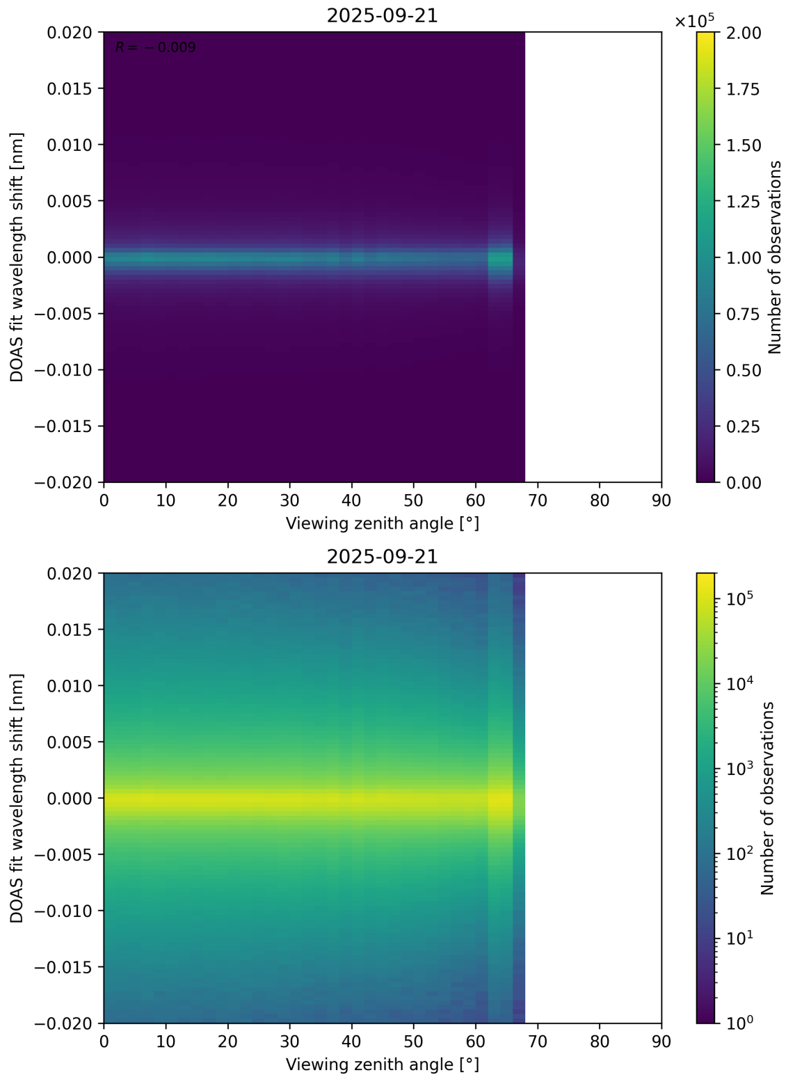
Figure 183: Scatter density plot of “Viewing zenith angle” against “DOAS fit wavelength shift” for 2025-09-20 to 2025-09-22.
