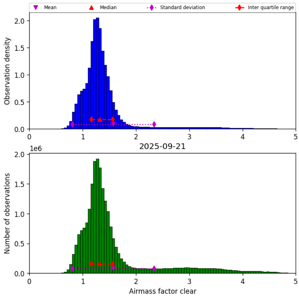
Figure 42: Histogram of “Airmass factor clear” for 2025-09-20 to 2025-09-22
