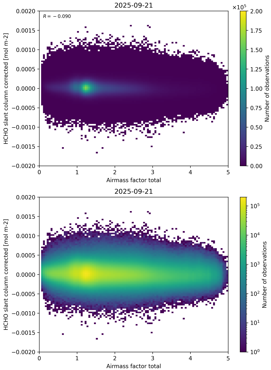
Figure 101: Scatter density plot of “Airmass factor total” against “HCHO slant column corrected” for 2025-09-20 to 2025-09-22.
