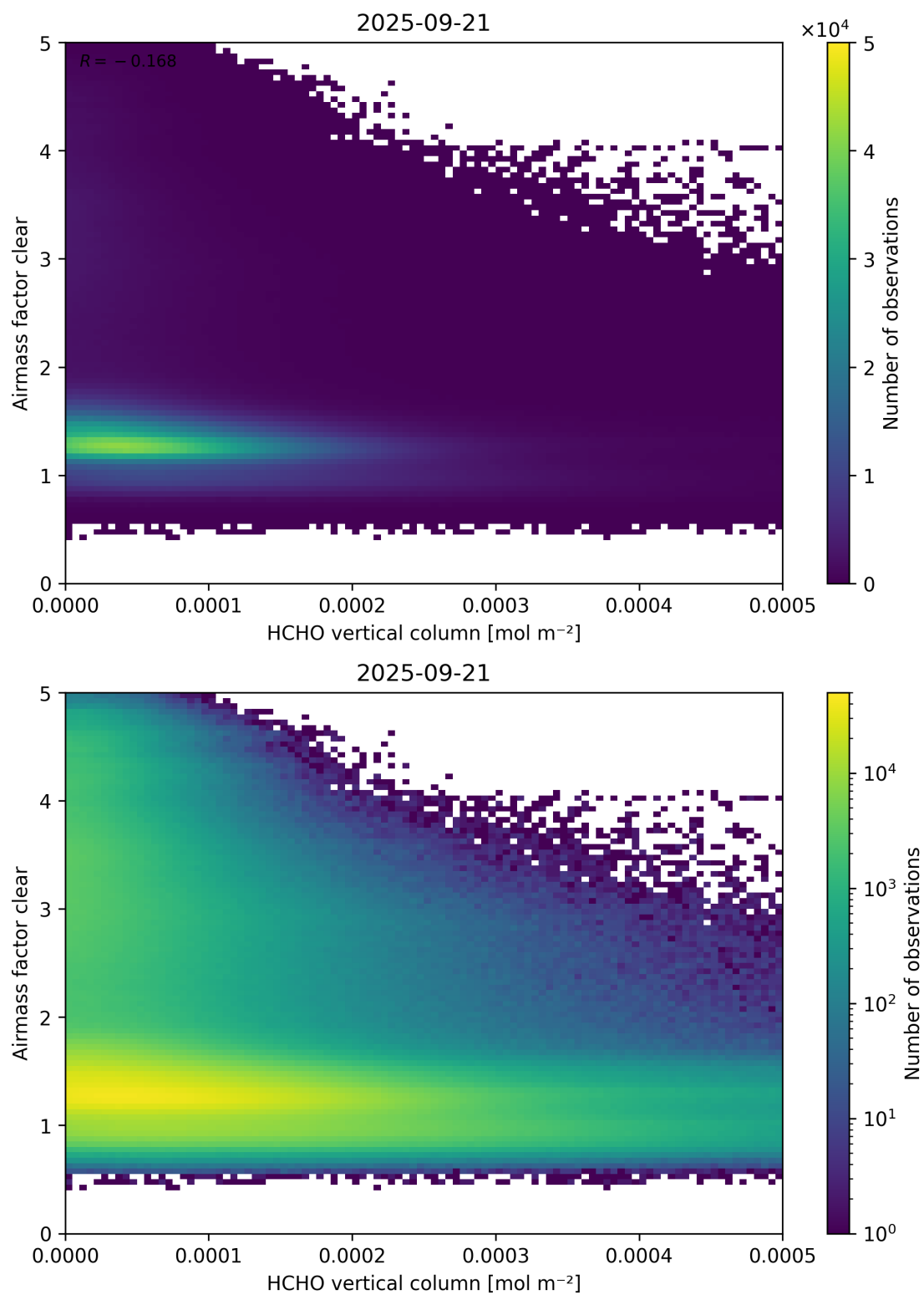
Figure 126: Scatter density plot of “HCHO vertical column” against “Airmass factor clear” for 2025-09-20 to 2025-09-22.
