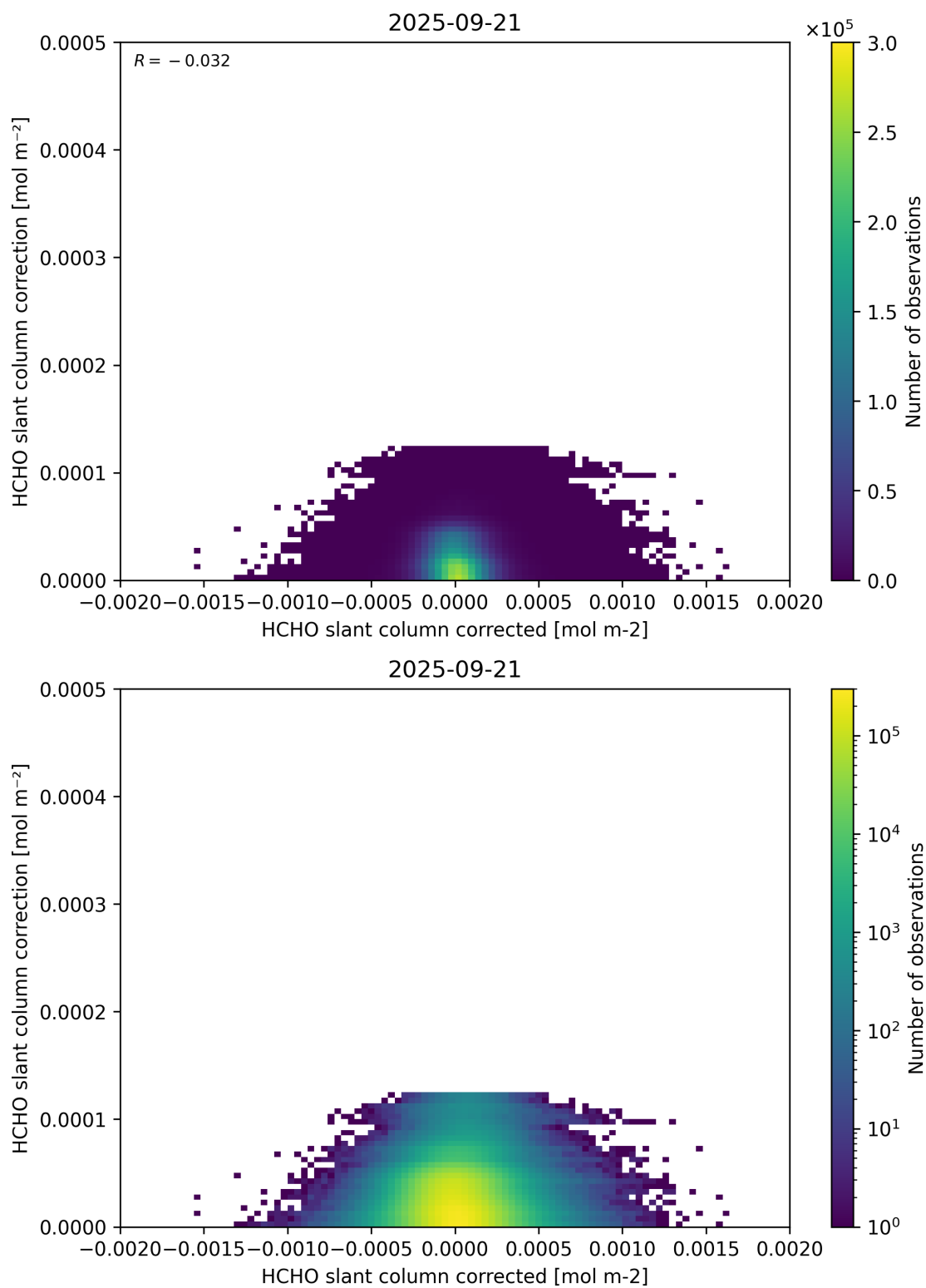
Figure 77: Scatter density plot of “HCHO slant column corrected” against “HCHO slant column correction” for 2025-09-20 to 2025-09-22.
