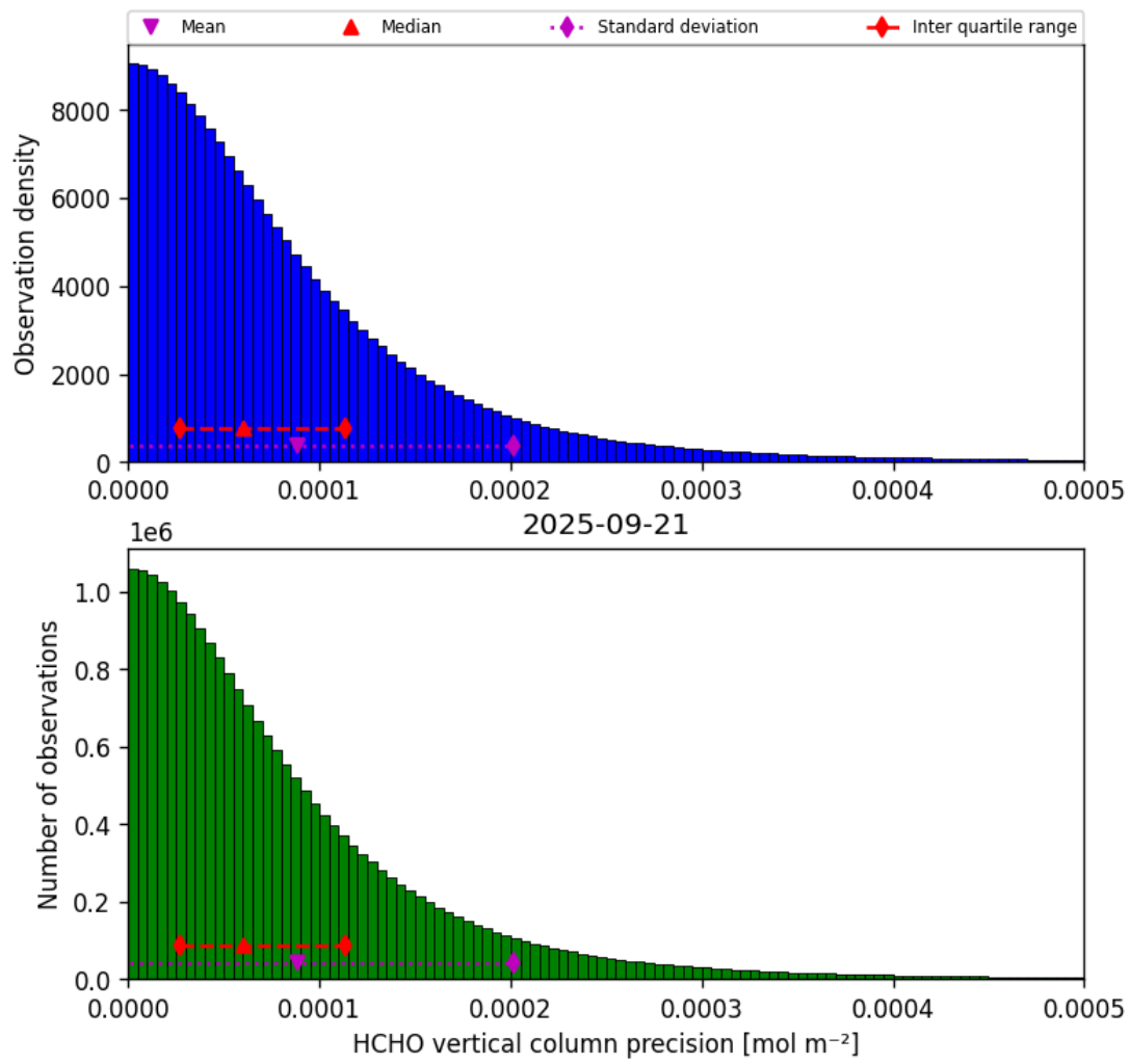
Figure 36: Histogram of “HCHO vertical column precision” for 2025-09-20 to 2025-09-22
