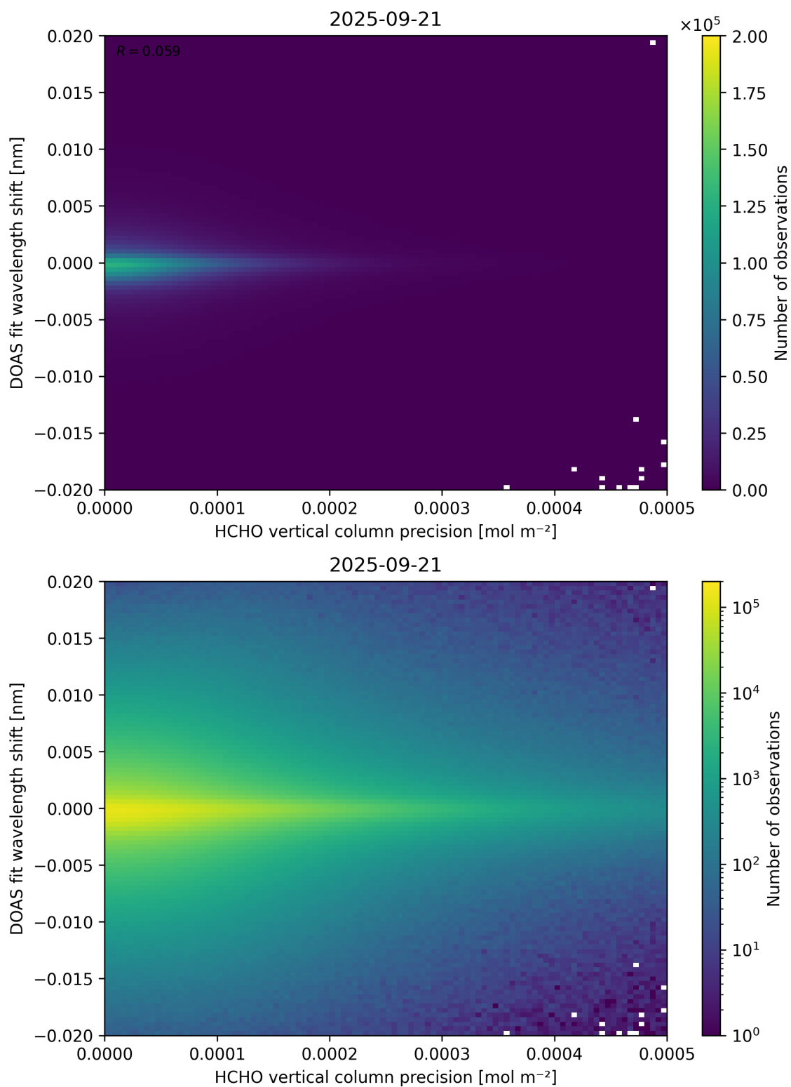
Figure 137: Scatter density plot of “HCHO vertical column precision” against “DOAS fit wavelength shift” for 2025-09-20 to 2025-09-22.
