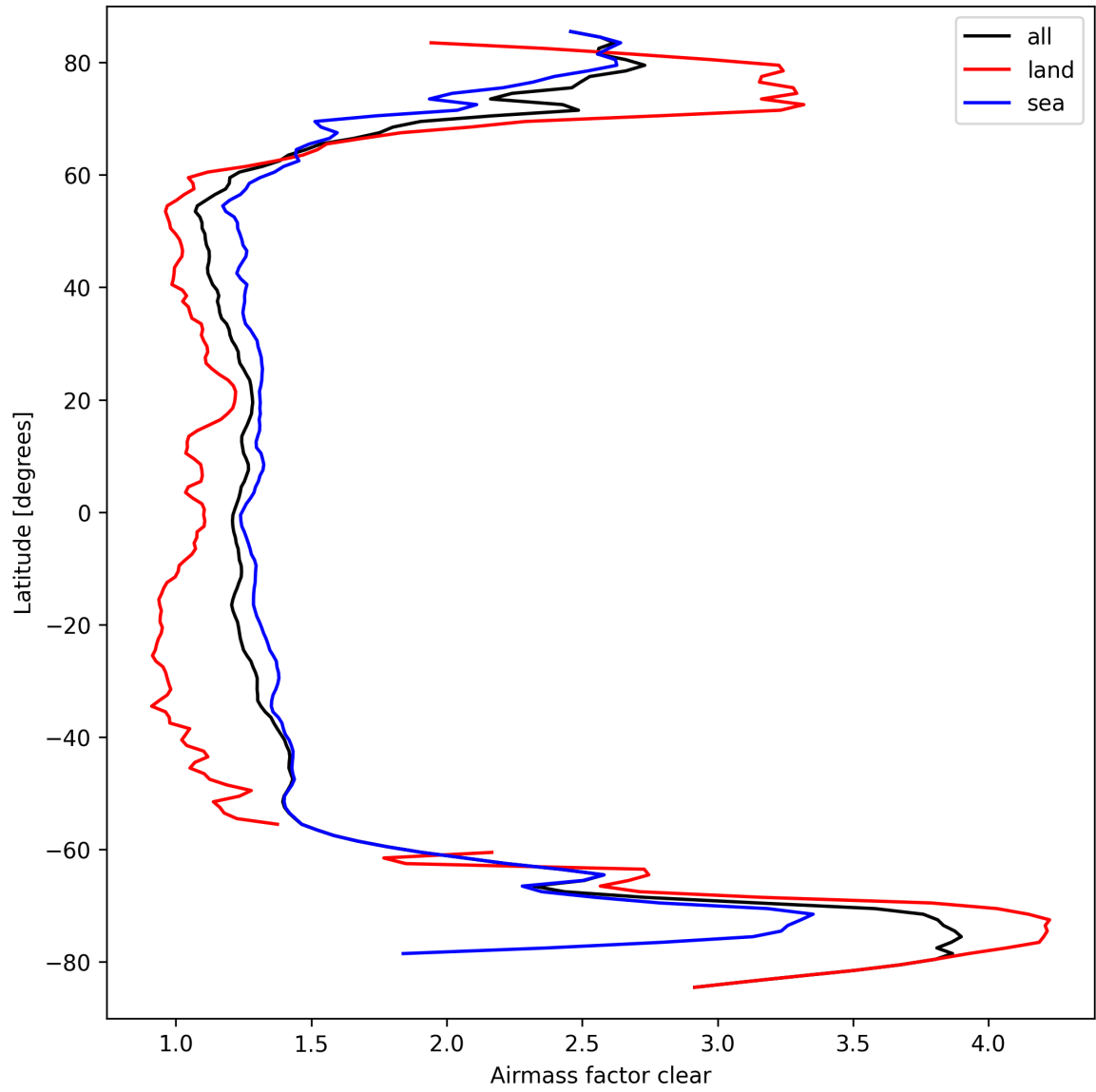
Figure 28: Zonal average of “Airmass factor clear” for 2025-09-20 to 2025-09-22.
