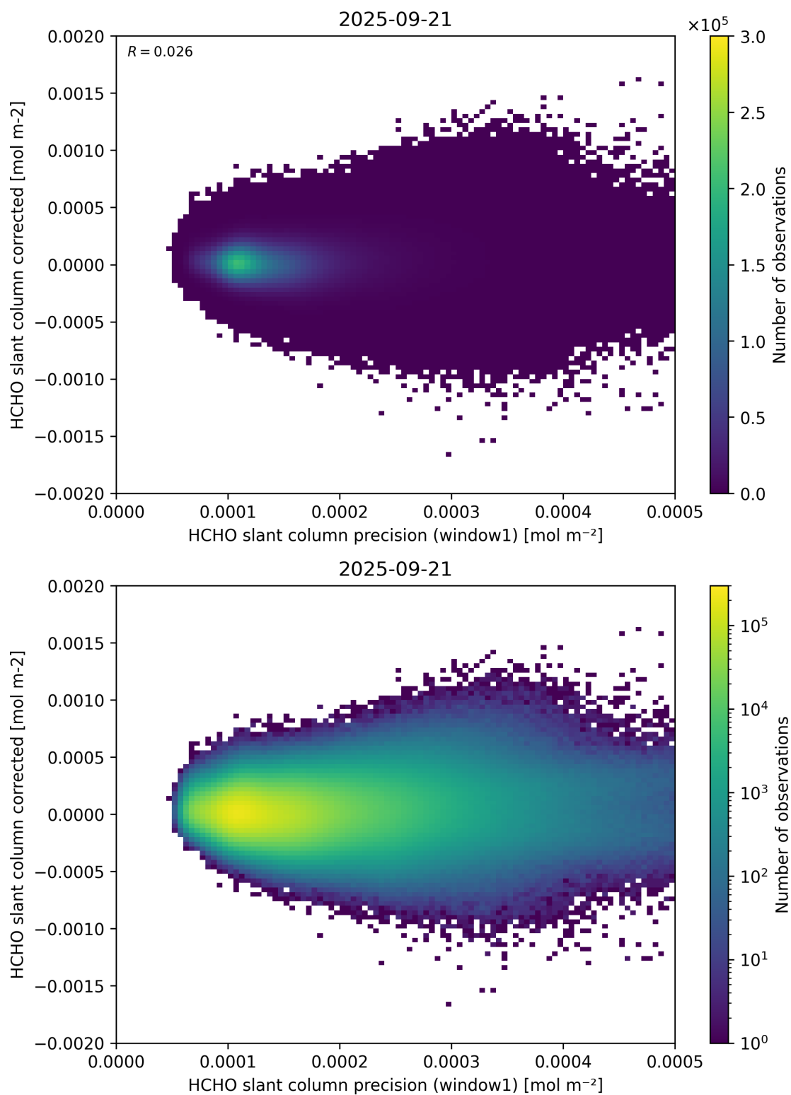
Figure 92: Scatter density plot of “HCHO slant column precision (window1)” against “HCHO slant column corrected” for 2025-09-20 to 2025-09-22.
