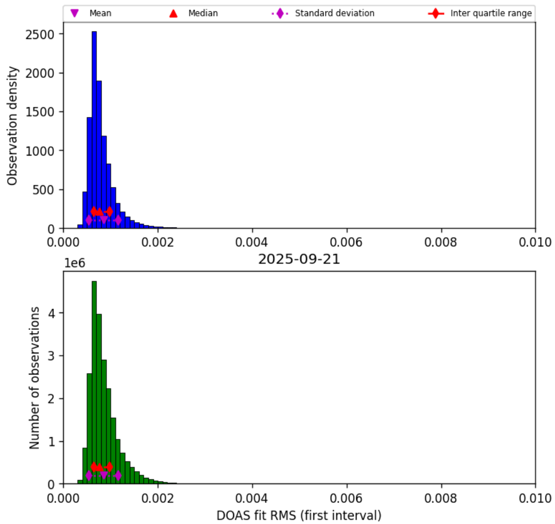
Figure 46: Histogram of “DOAS fit RMS (first interval)” for 2025-09-20 to 2025-09-22
