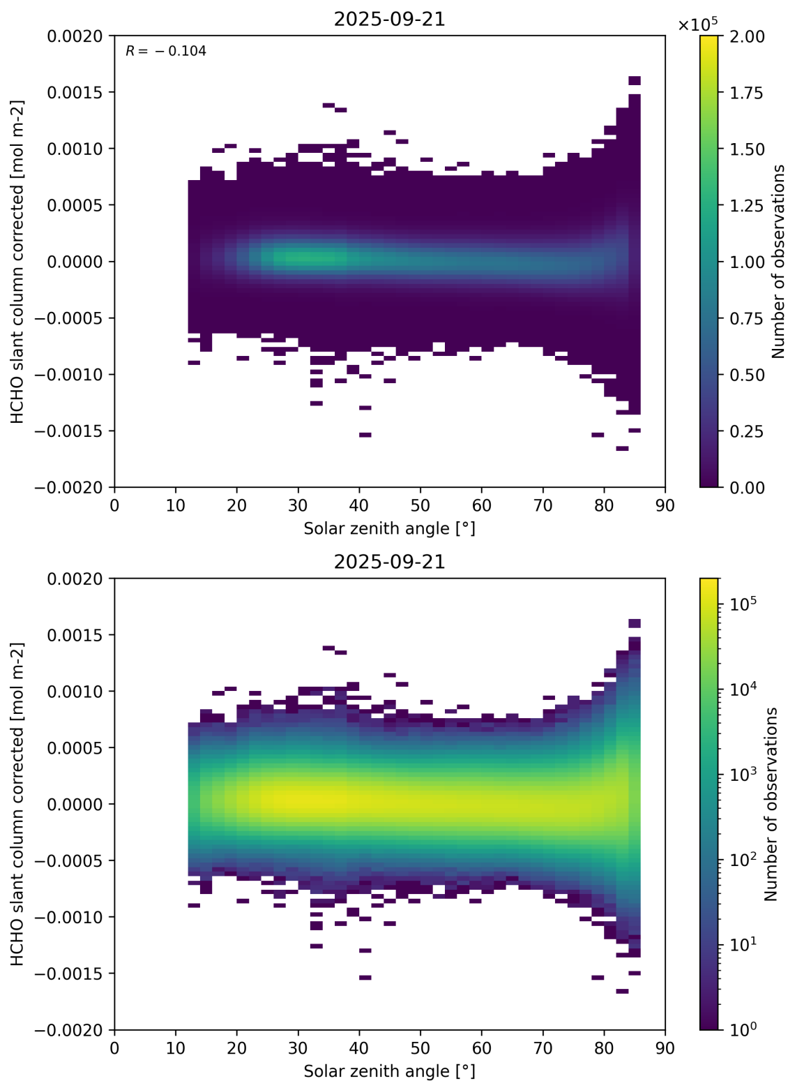
Figure 171: Scatter density plot of “Solar zenith angle” against “HCHO slant column corrected” for 2025-09-20 to 2025-09-22.
