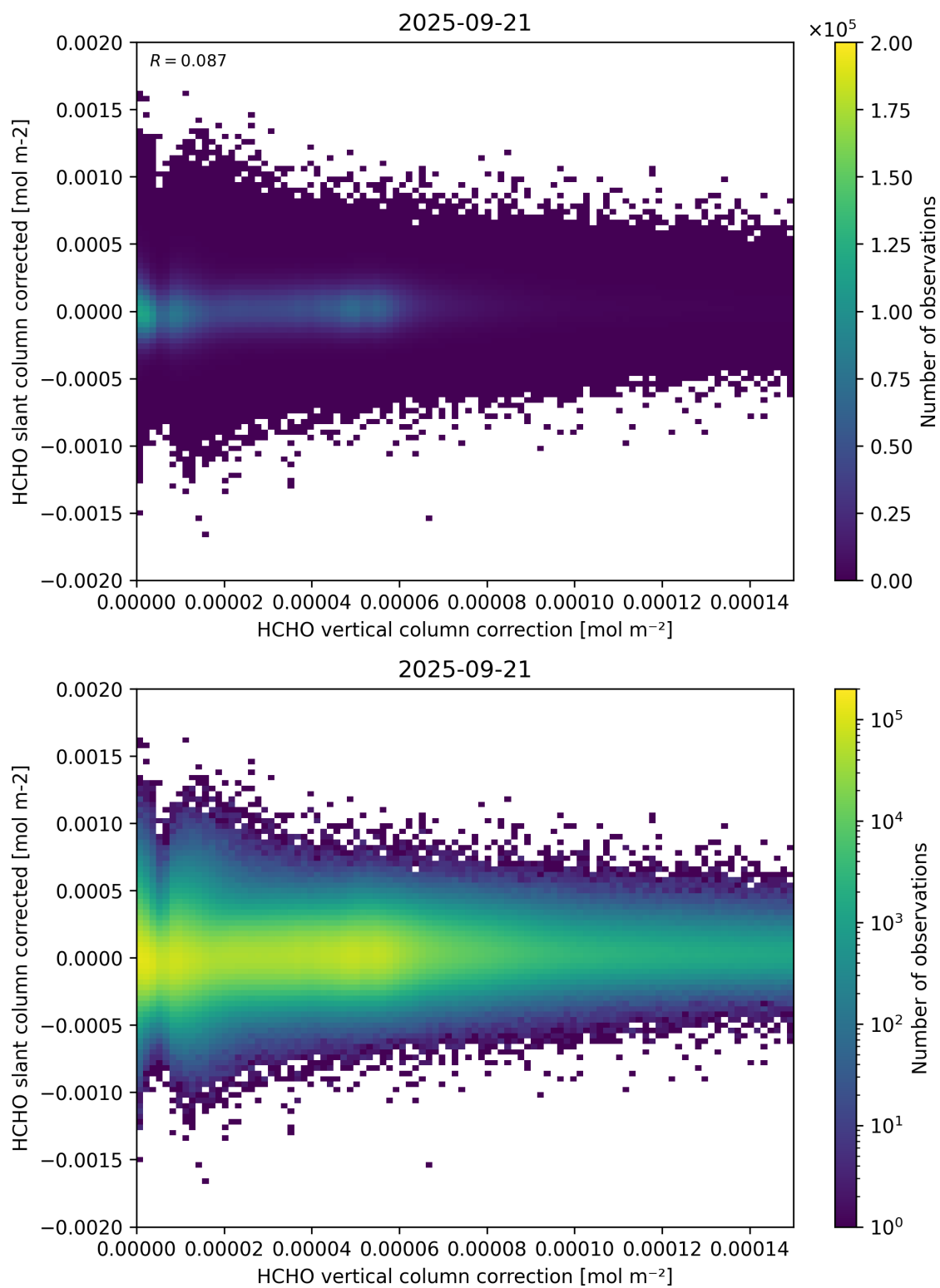
Figure 116: Scatter density plot of “HCHO vertical column correction” against “HCHO slant column corrected” for 2025-09-20 to 2025-09-22.
