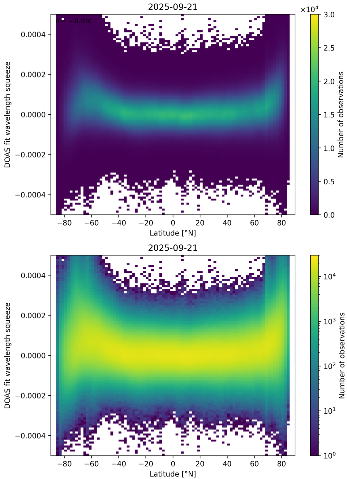
Figure 155: Scatter density plot of “Latitude” against “DOAS fit wavelength squeeze” for 2025-09-20 to 2025-09-22.
