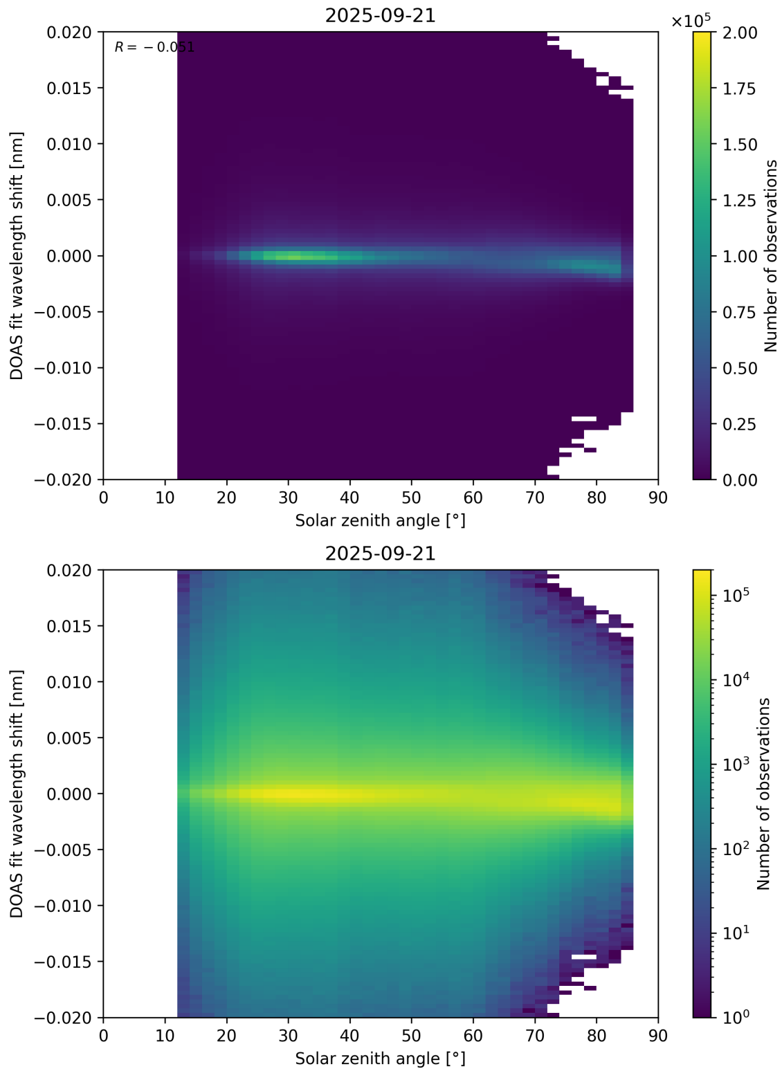
Figure 168: Scatter density plot of “Solar zenith angle” against “DOAS fit wavelength shift” for 2025-09-20 to 2025-09-22.
