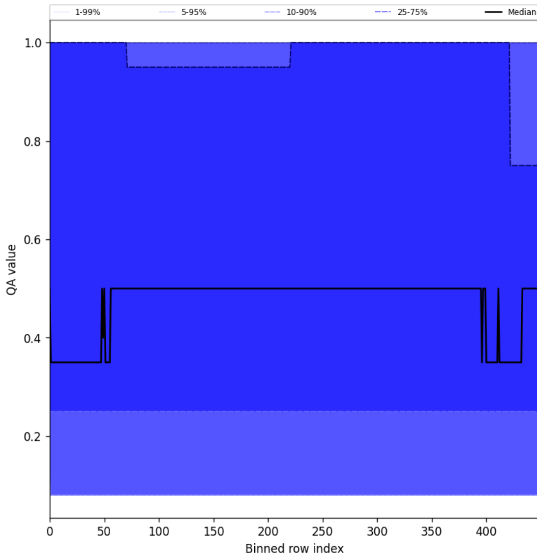
Figure 48: Along track statistics of “QA value” for 2025-09-20 to 2025-09-22
