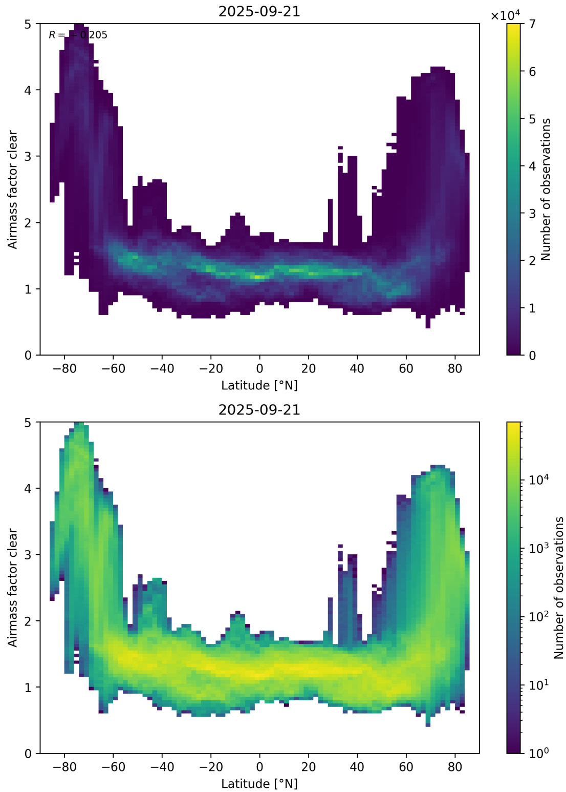
Figure 156: Scatter density plot of “Latitude” against “Airmass factor clear” for 2025-09-20 to 2025-09-22.
