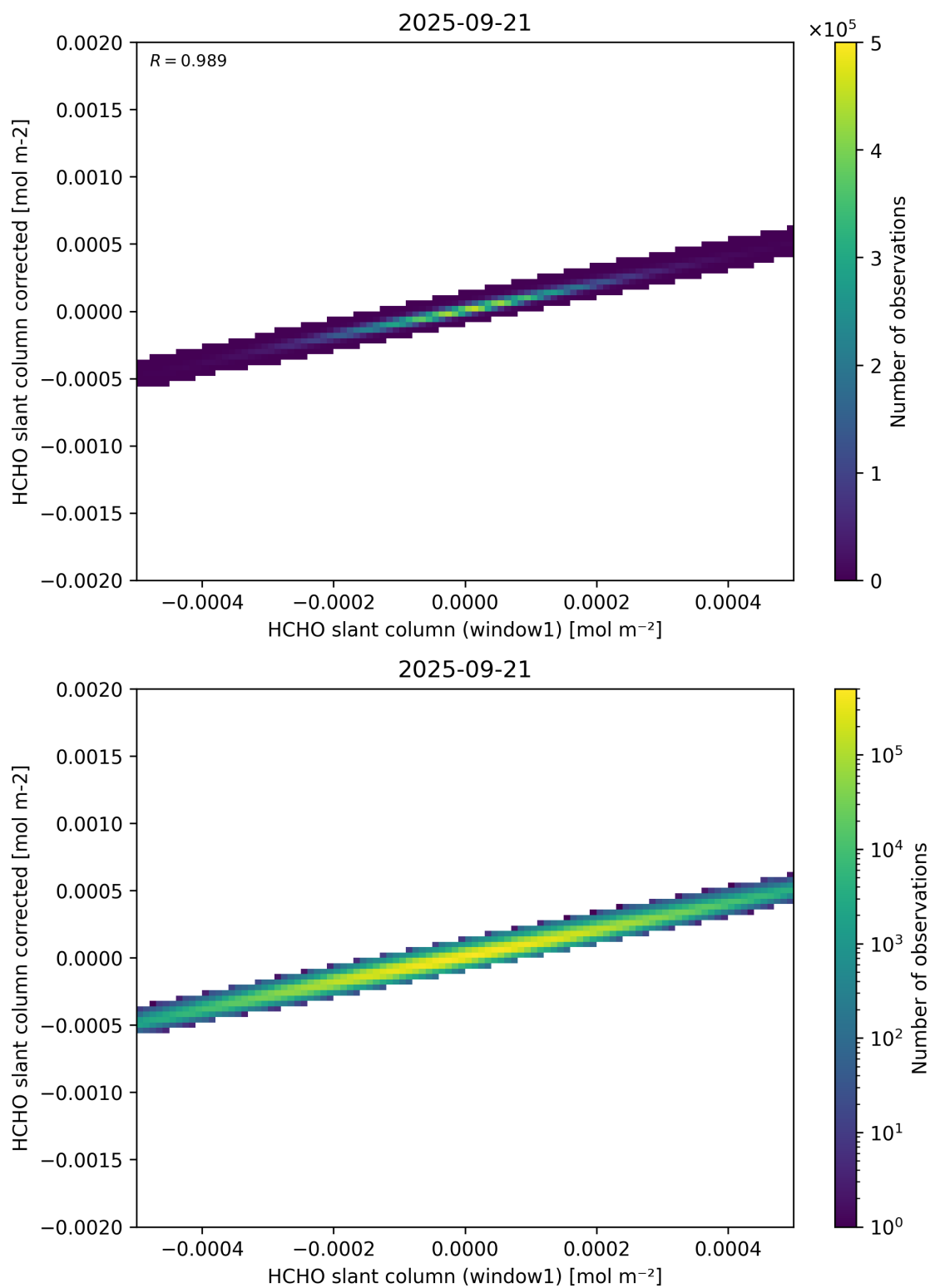
Figure 82: Scatter density plot of “HCHO slant column (window1)” against “HCHO slant column corrected” for 2025-09-20 to 2025-09-22.
