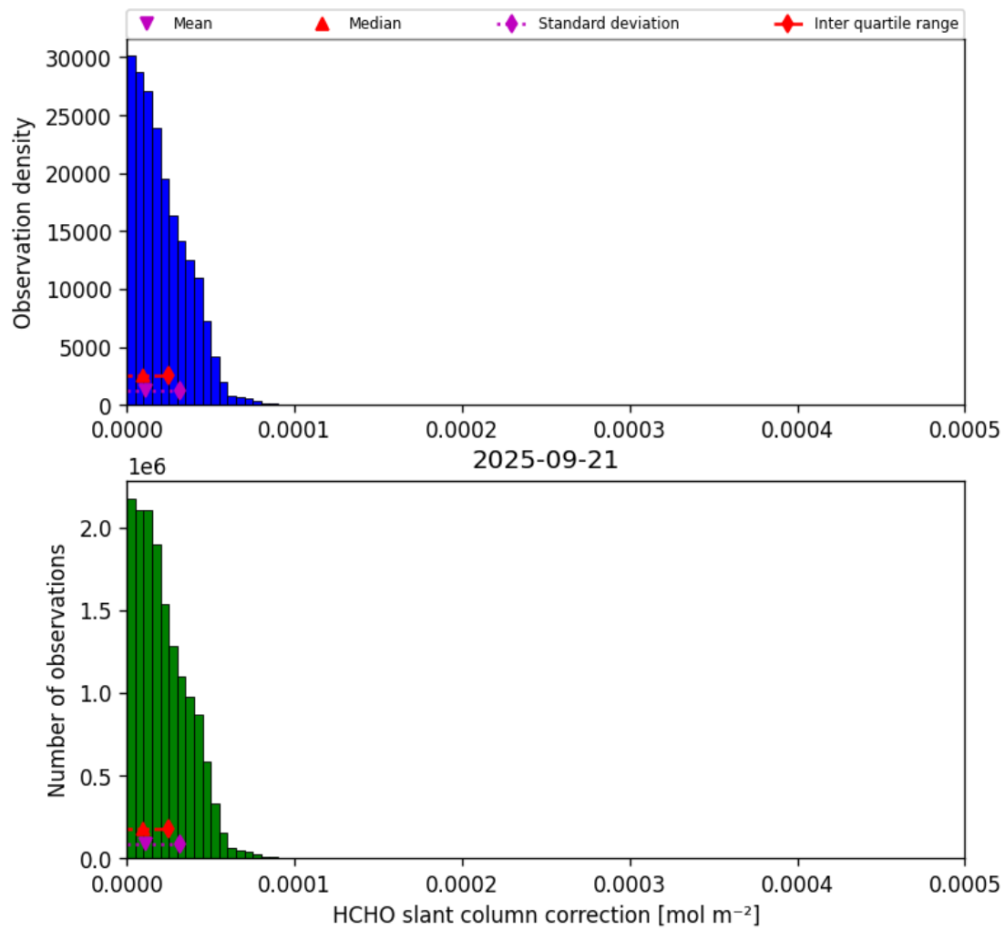
Figure 47: Histogram of “HCHO slant column correction” for 2025-09-20 to 2025-09-22
