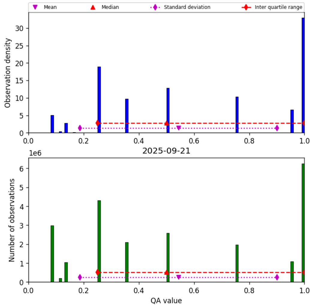
Figure 34: Histogram of “QA value” for 2025-09-20 to 2025-09-22
