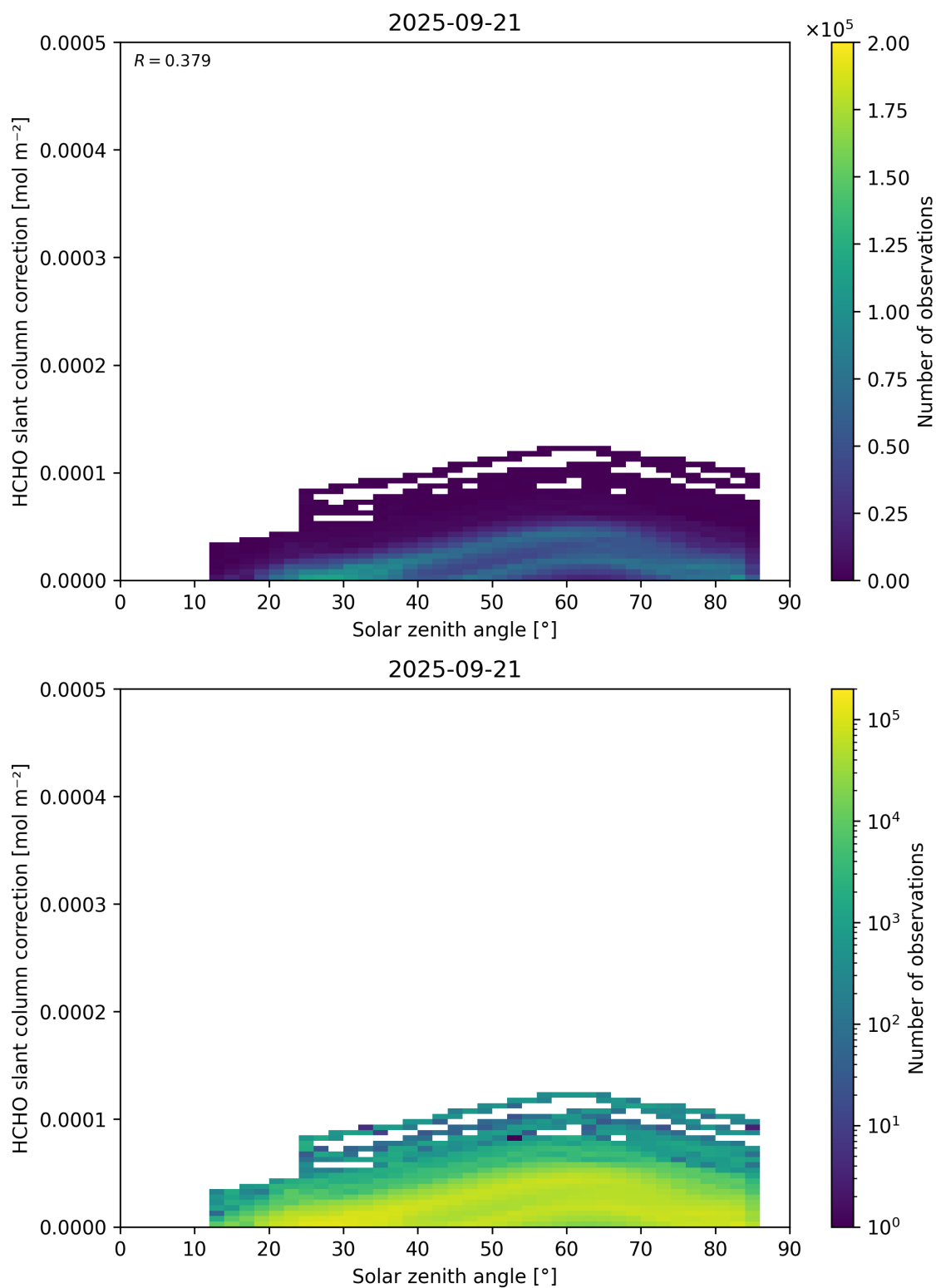
Figure 172: Scatter density plot of “Solar zenith angle” against “HCHO slant column correction” for 2025-09-20 to 2025-09-22.
