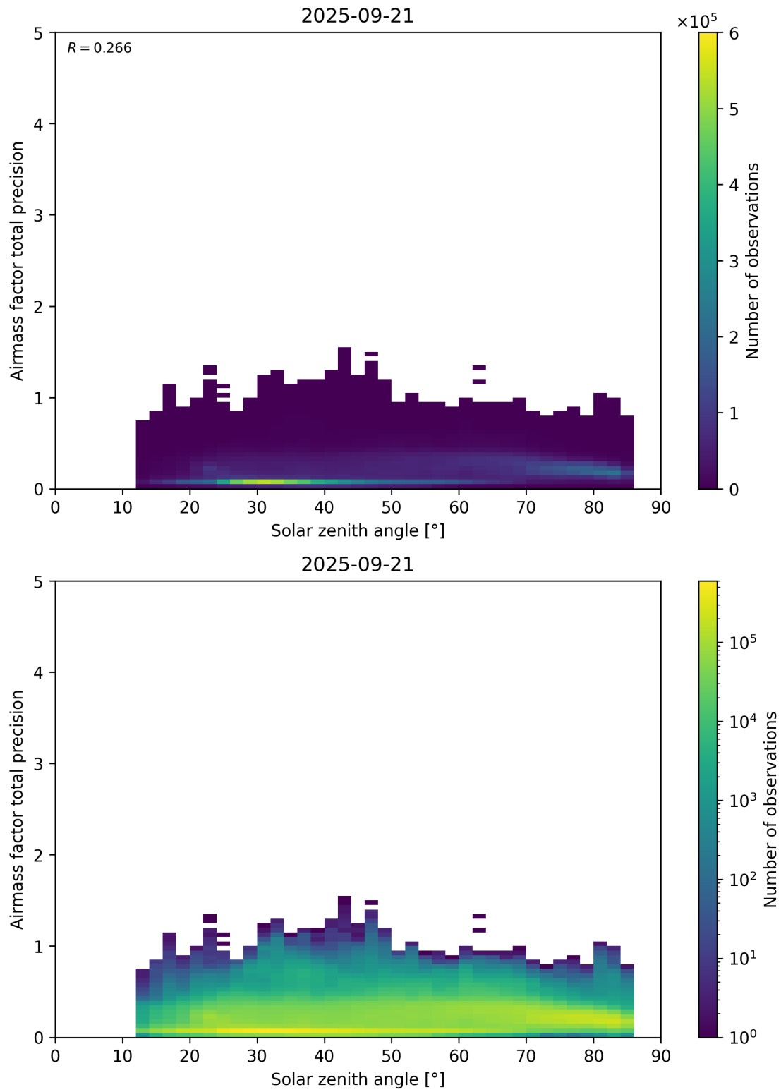
Figure 176: Scatter density plot of “Solar zenith angle” against “Airmass factor total precision” for 2025-09-20 to 2025-09-22.
