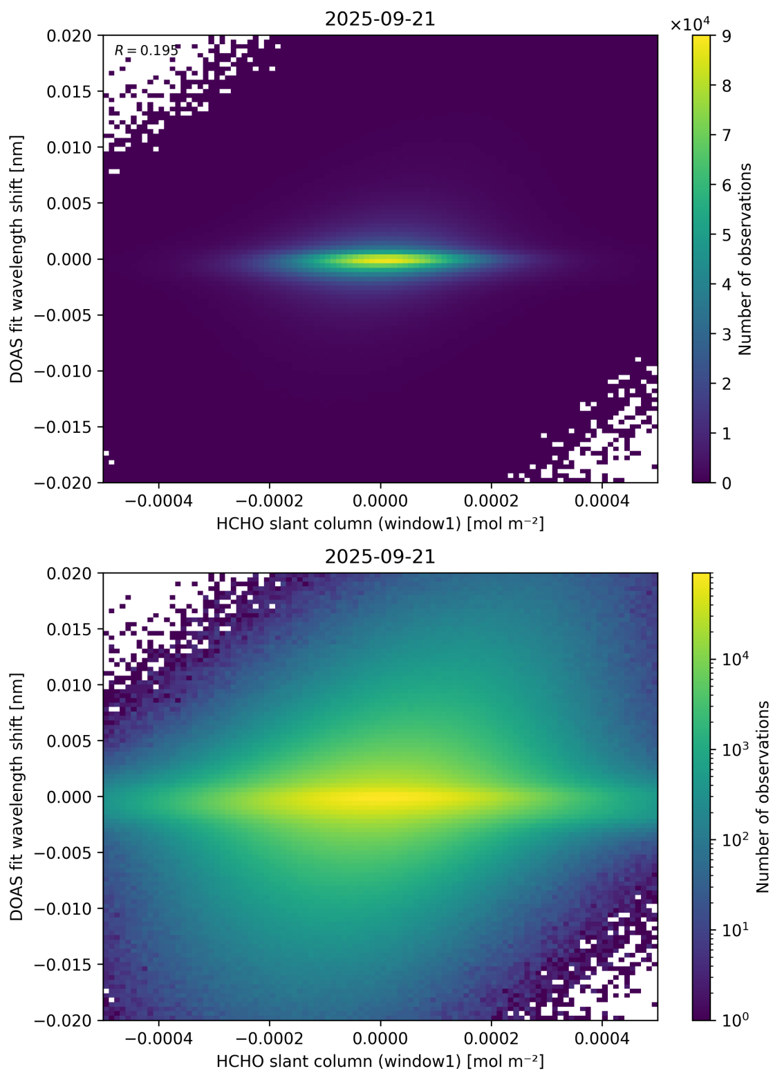
Figure 79: Scatter density plot of “HCHO slant column (window1)” against “DOAS fit wavelength shift” for 2025-09-20 to 2025-09-22.
