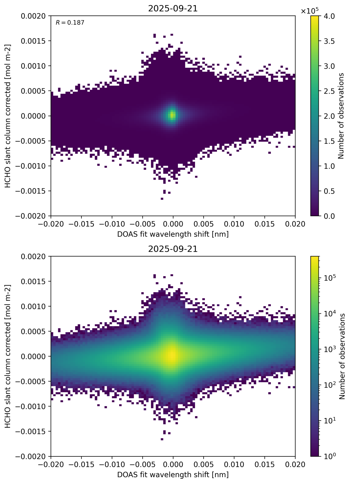
Figure 66: Scatter density plot of “DOAS fit wavelength shift” against “HCHO slant column corrected” for 2025-09-20 to 2025-09-22.
