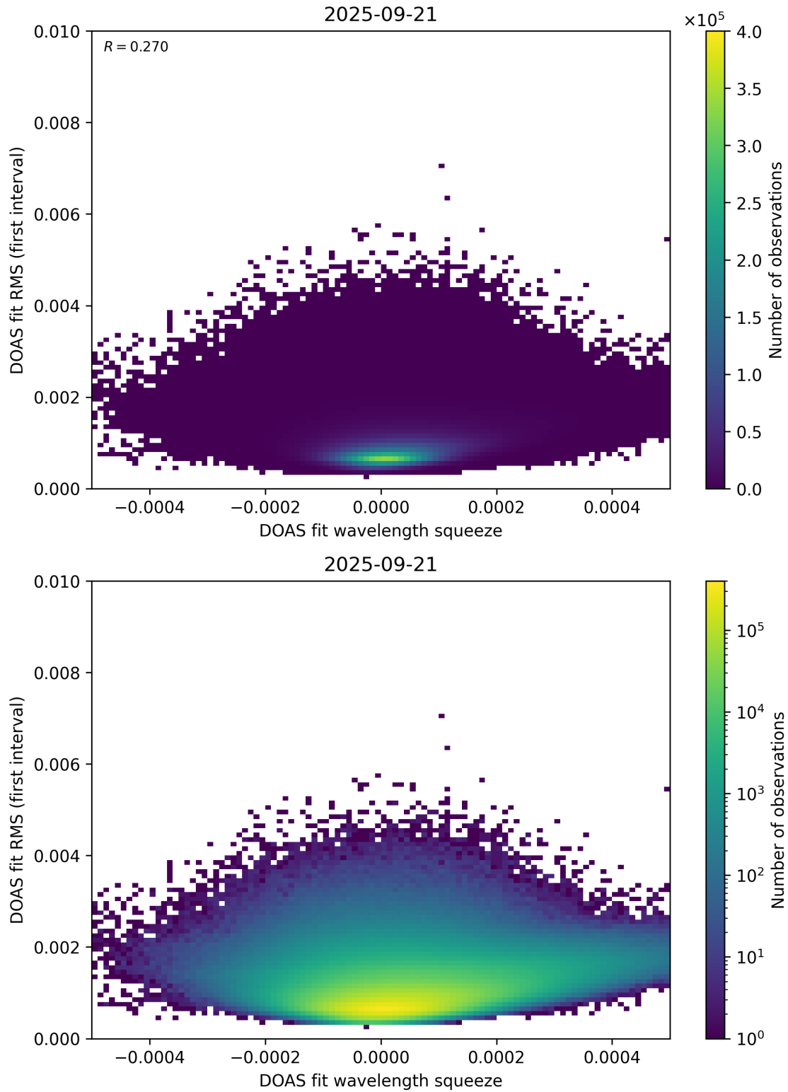
Figure 68: Scatter density plot of “DOAS fit wavelength squeeze” against “DOAS fit RMS (first interval)” for 2025-09-20 to 2025-09-22.
