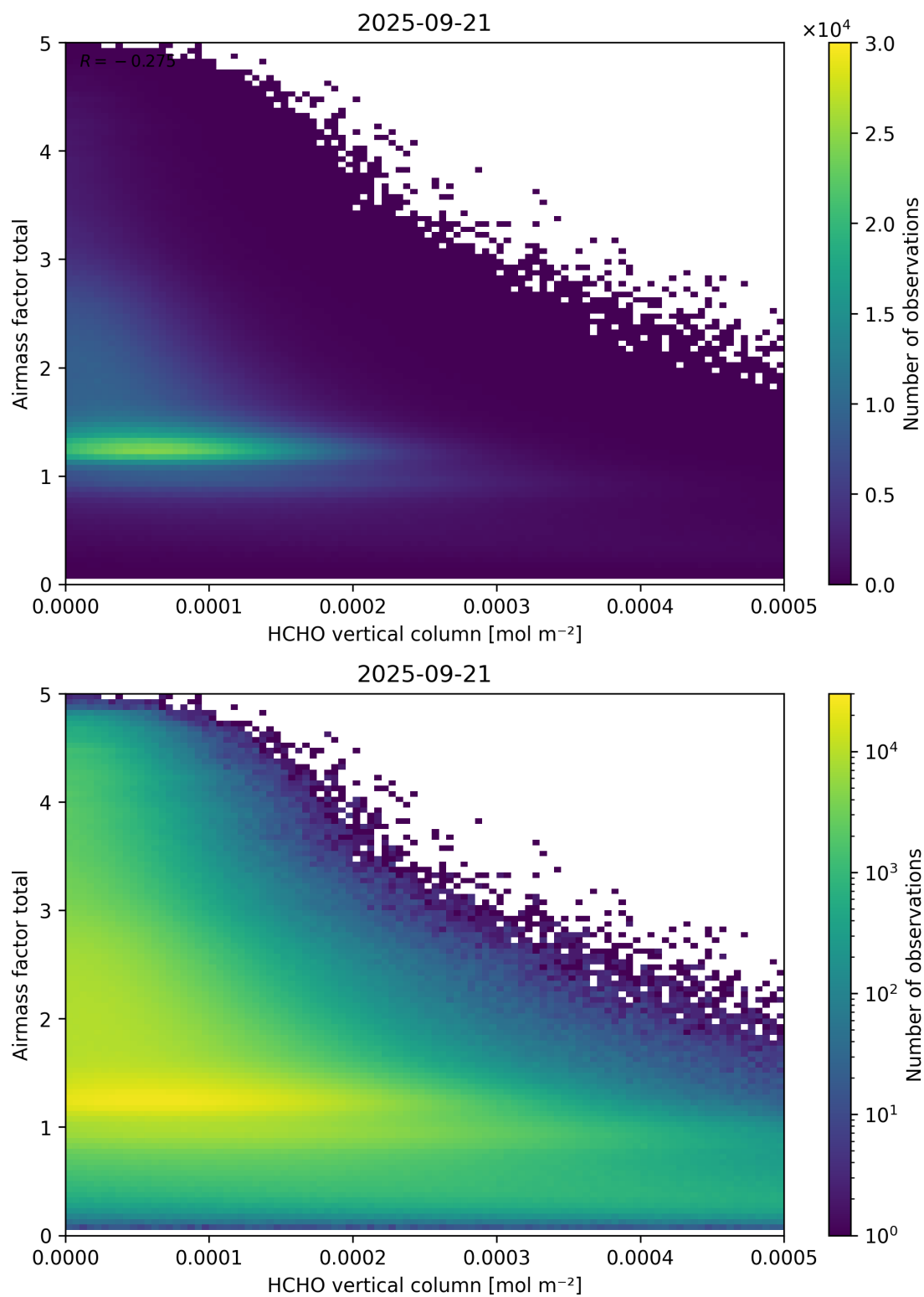
Figure 131: Scatter density plot of “HCHO vertical column” against “Airmass factor total” for 2025-09-20 to 2025-09-22.
