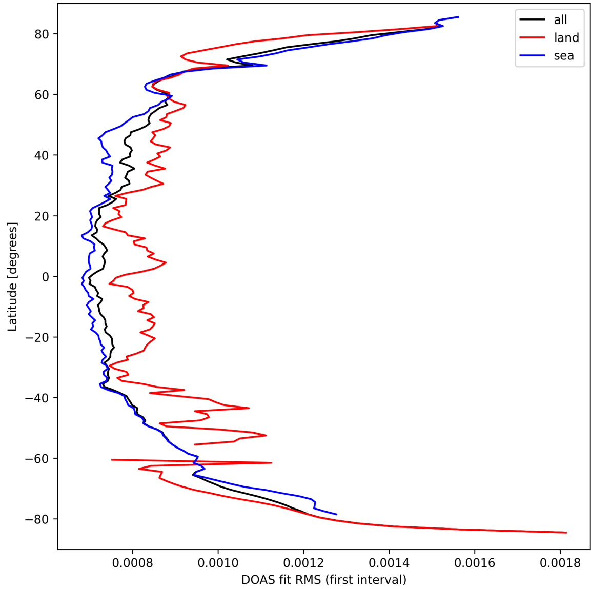
Figure 32: Zonal average of “DOAS fit RMS (first interval)” for 2025-09-20 to 2025-09-22.
