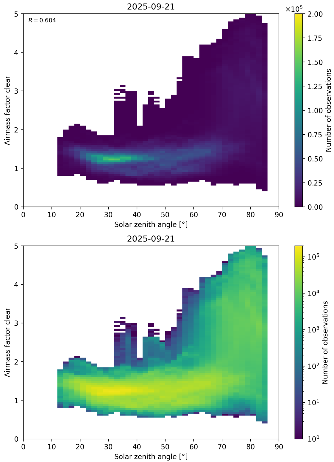
Figure 170: Scatter density plot of “Solar zenith angle” against “Airmass factor clear” for 2025-09-20 to 2025-09-22.
