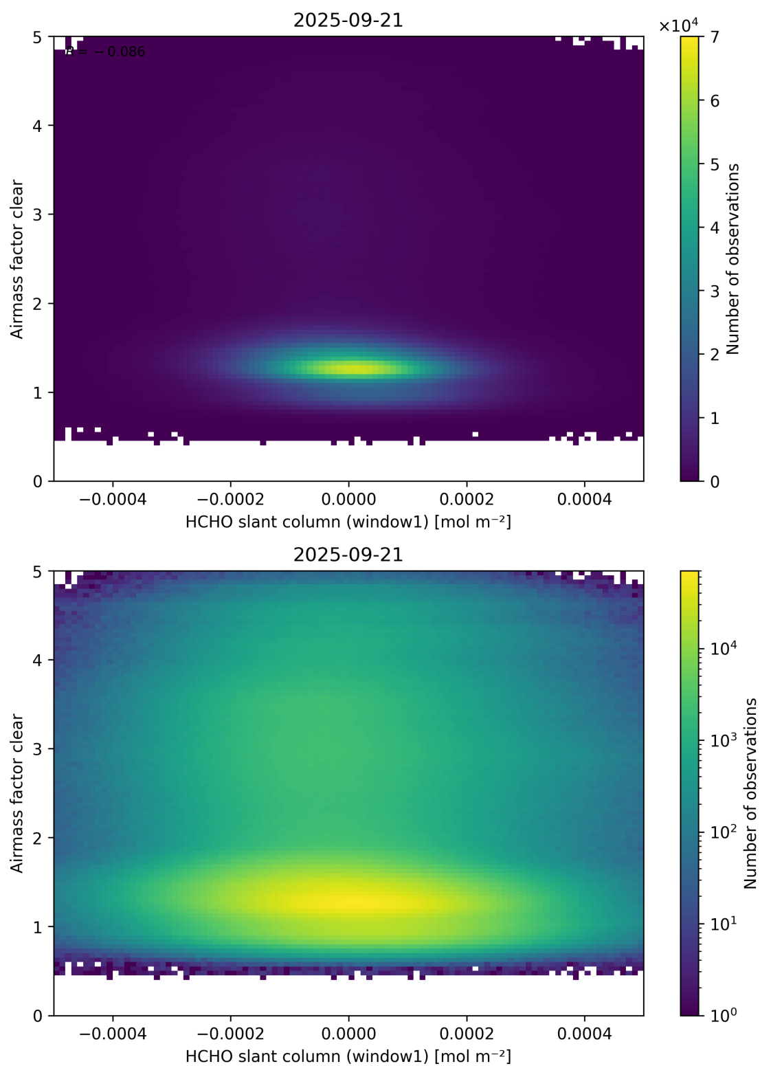
Figure 81: Scatter density plot of “HCHO slant column (window1)” against “Airmass factor clear” for 2025-09-20 to 2025-09-22.
