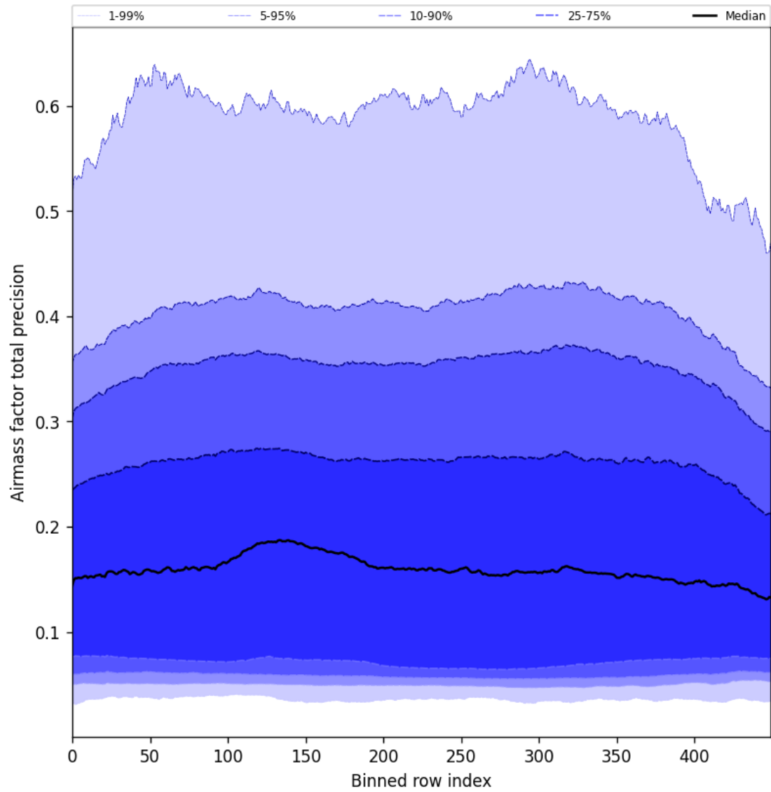
Figure 55: Along track statistics of “Airmass factor total precision” for 2025-09-20 to 2025-09-22
