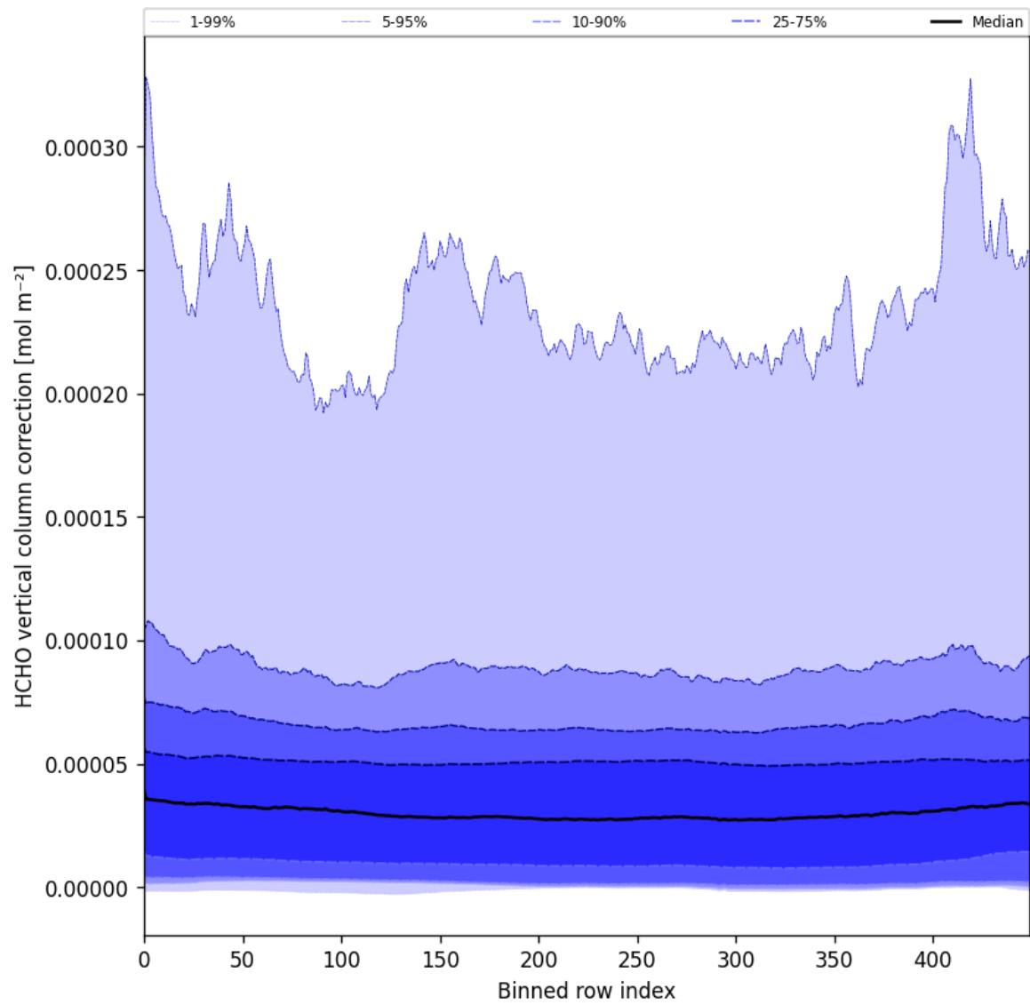
Figure 51: Along track statistics of “HCHO vertical column correction” for 2025-09-20 to 2025-09-22
