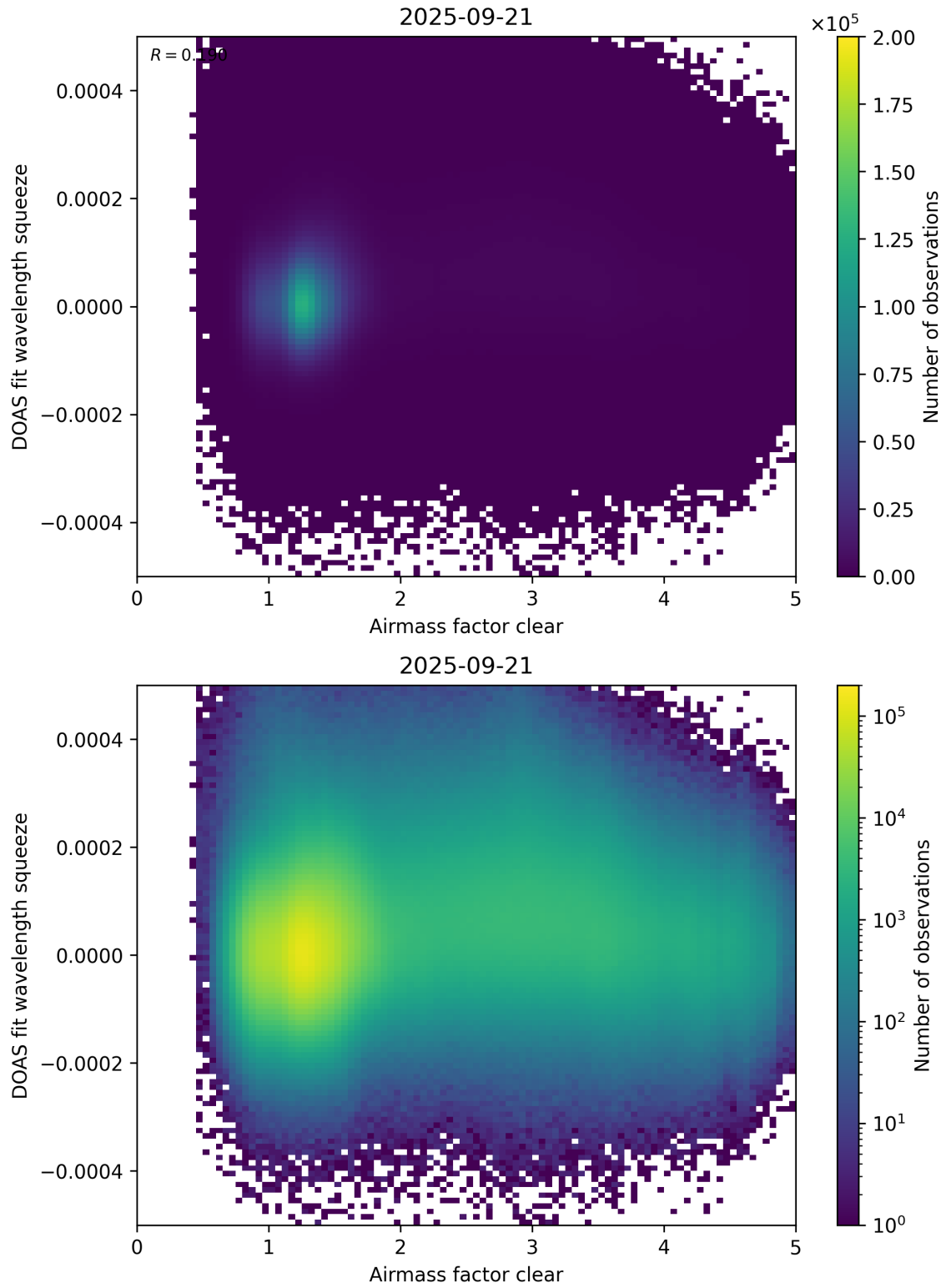
Figure 73: Scatter density plot of “Airmass factor clear” against “DOAS fit wavelength squeeze” for 2025-09-20 to 2025-09-22.
