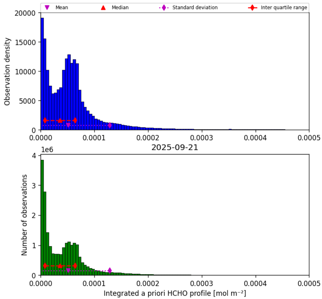
Figure 43: Histogram of “Integrated a priori HCHO profile” for 2025-09-20 to 2025-09-22
