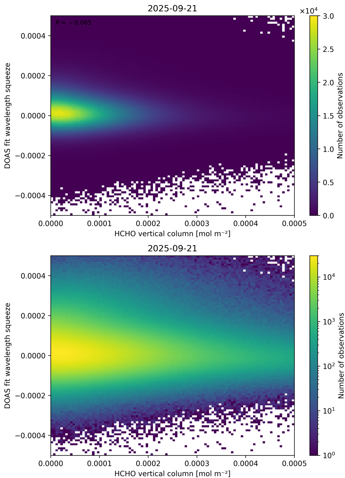
Figure 125: Scatter density plot of “HCHO vertical column” against “DOAS fit wavelength squeeze” for 2025-09-20 to 2025-09-22.
