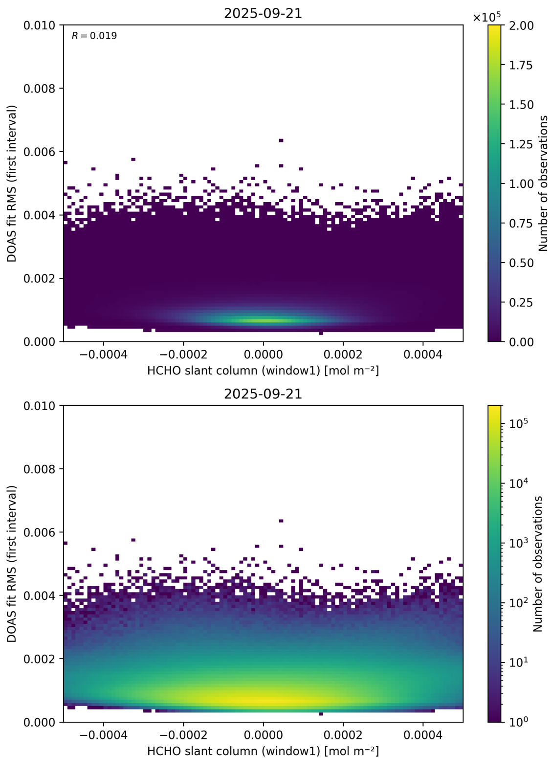
Figure 78: Scatter density plot of “HCHO slant column (window1)” against “DOAS fit RMS (first interval)” for 2025-09-20 to 2025-09-22.
