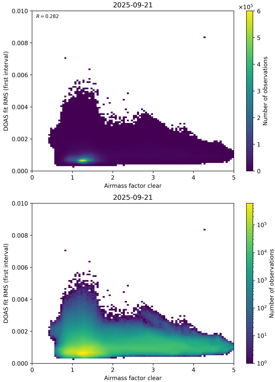
Figure 71: Scatter density plot of “Airmass factor clear” against “DOAS fit RMS (first interval)” for 2025-09-20 to 2025-09-22.
