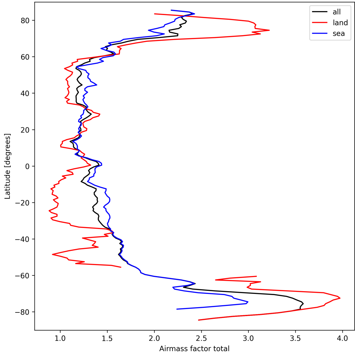
Figure 26: Zonal average of "Airmass factor total" for 2025-09-20 to 2025-09-22.
