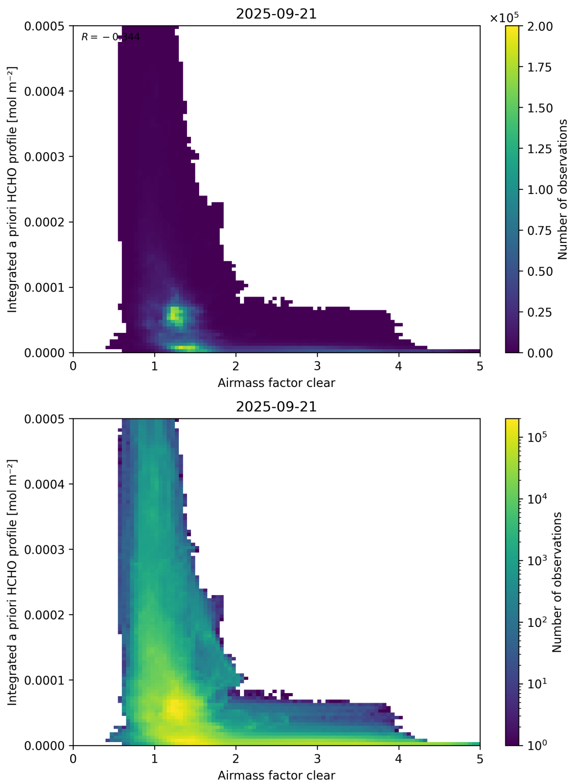
Figure 76: Scatter density plot of “Airmass factor clear” against “Integrated a priori HCHO profile” for 2025-09-20 to 2025-09-22.
