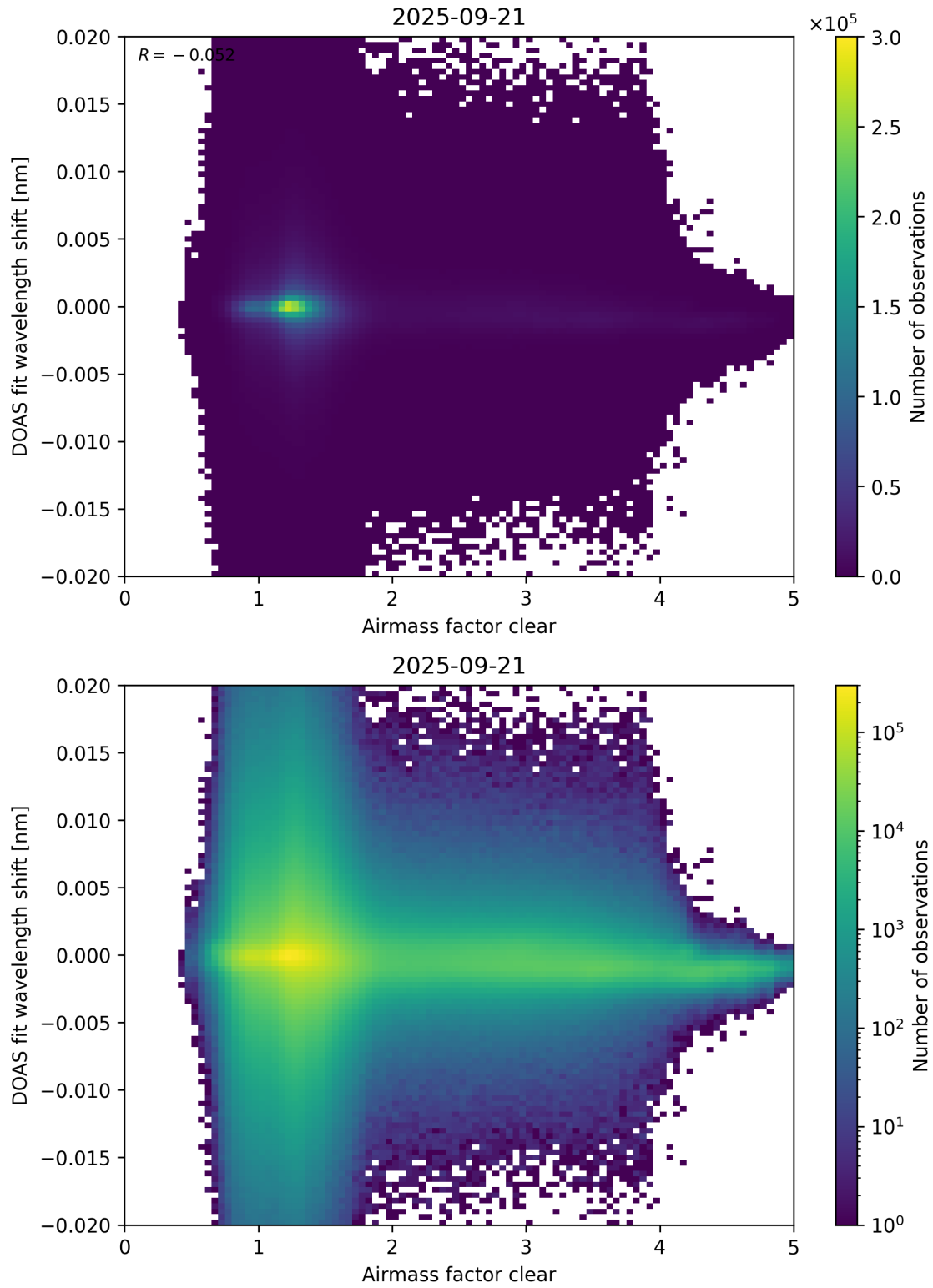
Figure 72: Scatter density plot of “Airmass factor clear” against “DOAS fit wavelength shift” for 2025-09-20 to 2025-09-22.
