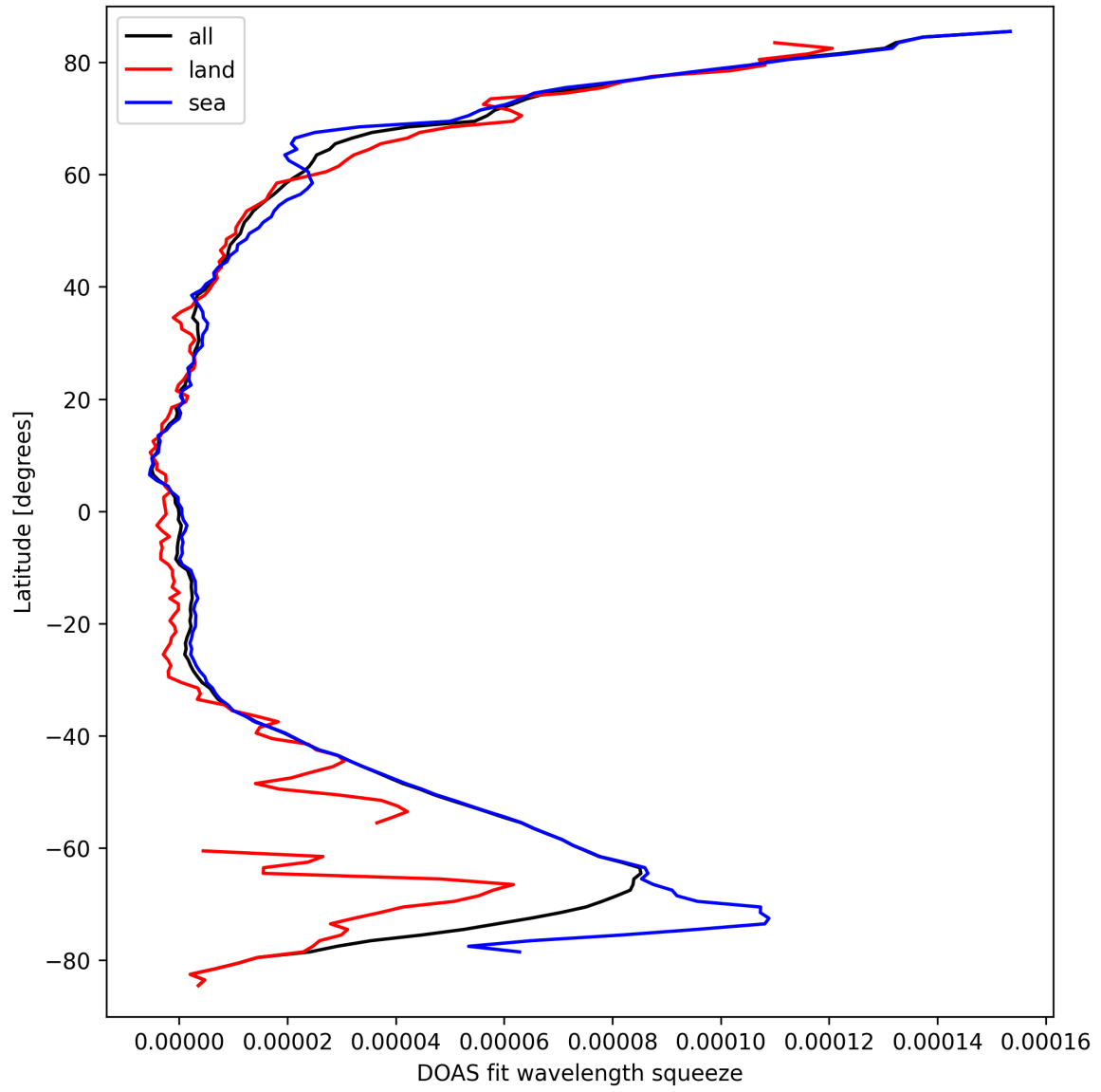
Figure 31: Zonal average of “DOAS fit wavelength squeeze” for 2025-09-20 to 2025-09-22.
