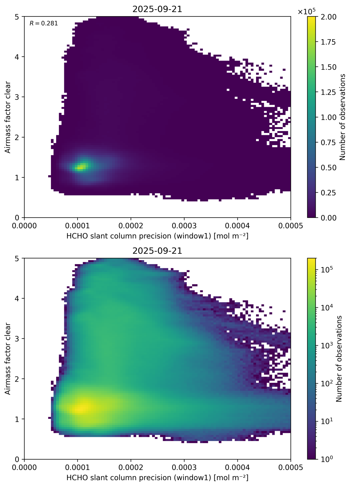
Figure 91: Scatter density plot of “HCHO slant column precision (window1)” against “Airmass factor clear” for 2025-09-20 to 2025-09-22.
