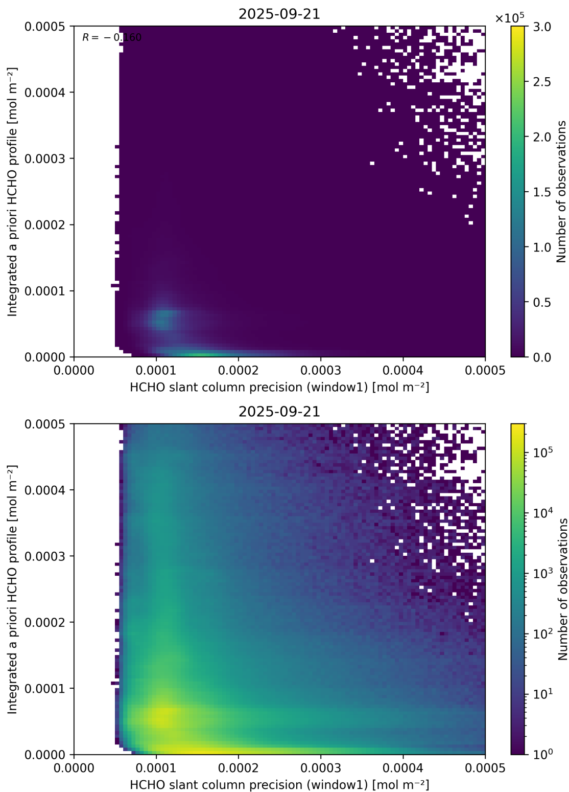
Figure 96: Scatter density plot of “HCHO slant column precision (window1)” against “Integrated a priori HCHO profile” for 2025-09-20 to 2025-09-22.
