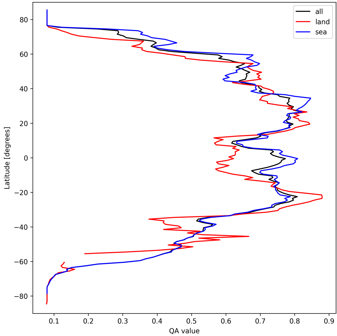
Figure 20: Zonal average of “QA value” for 2025-09-20 to 2025-09-22.
