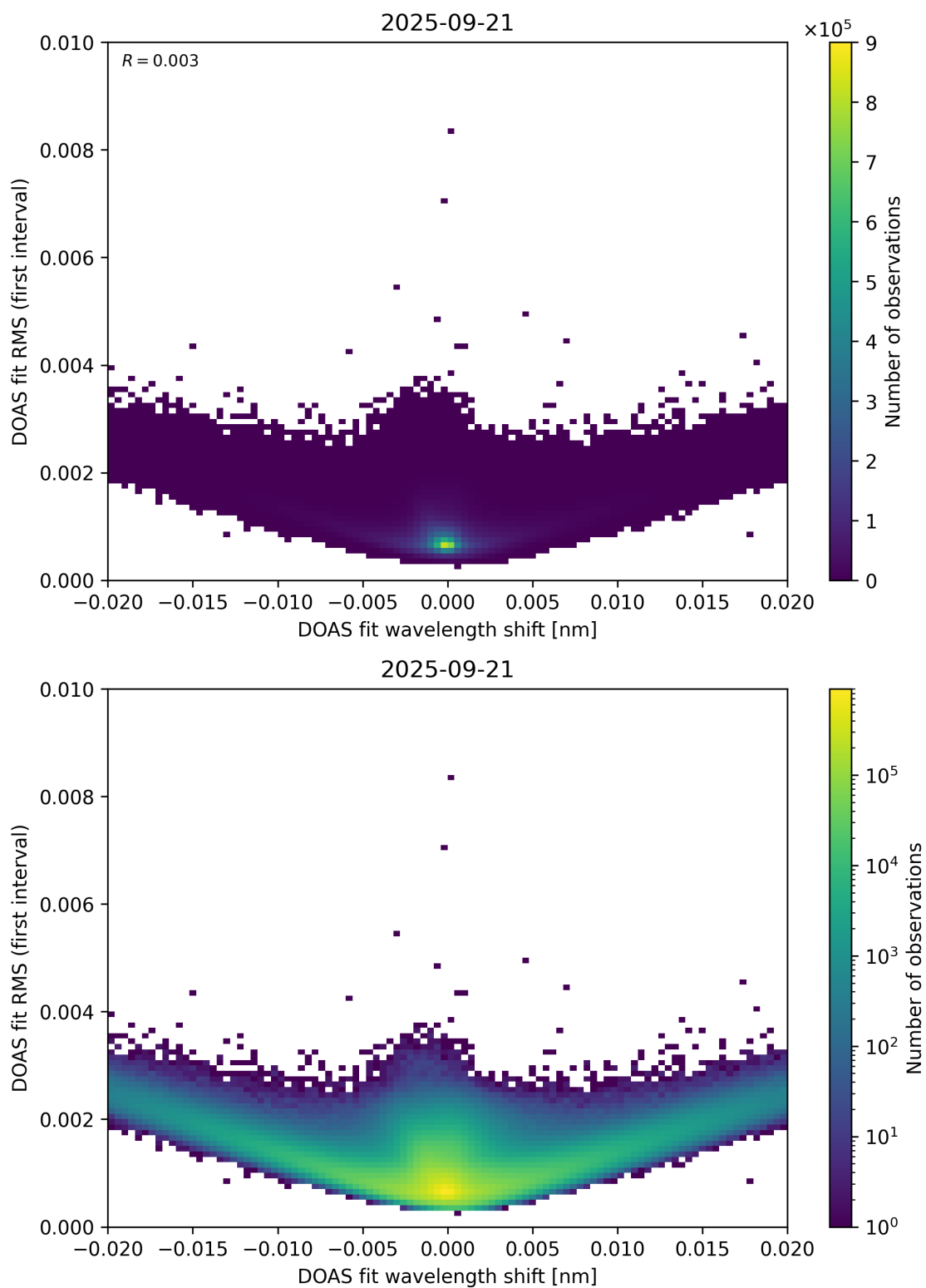
Figure 64: Scatter density plot of “DOAS fit wavelength shift” against “DOAS fit RMS (first interval)” for 2025-09-20 to 2025-09-22.
