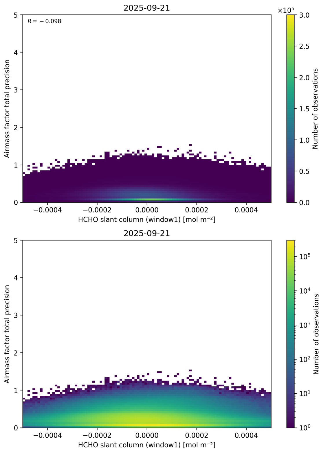
Figure 86: Scatter density plot of “HCHO slant column (window1)” against “Airmass factor total precision” for 2025-09-20 to 2025-09-22.
