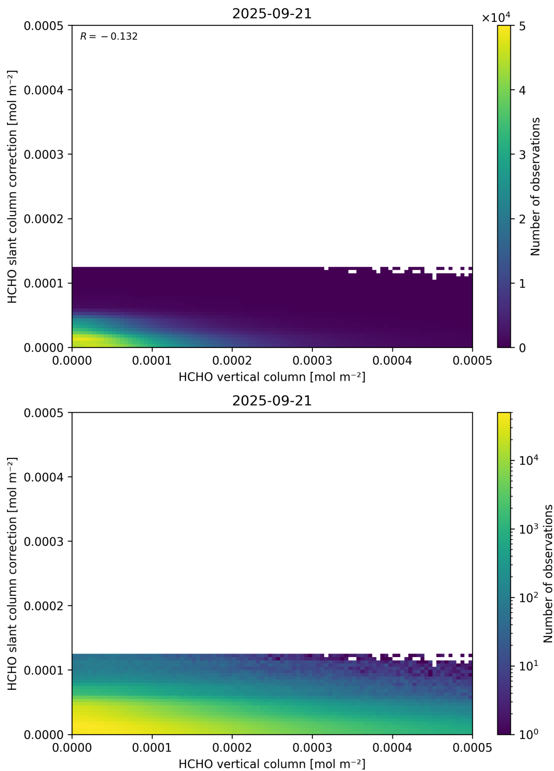
Figure 128: Scatter density plot of “HCHO vertical column” against “HCHO slant column correction” for 2025-09-20 to 2025-09-22.
