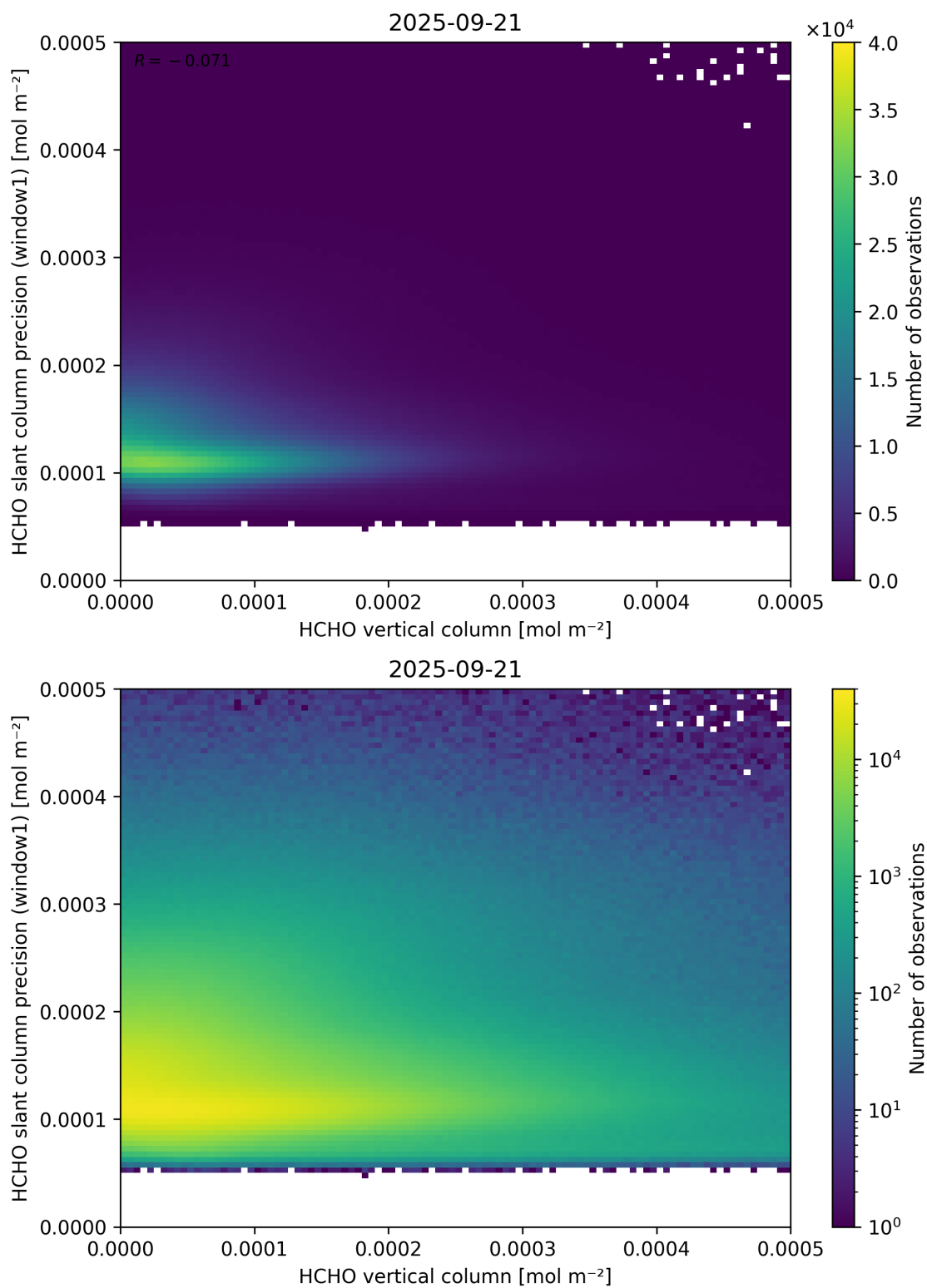
Figure 130: Scatter density plot of “HCHO vertical column” against “HCHO slant column precision (window1)” for 2025-09-20 to 2025-09-22.
