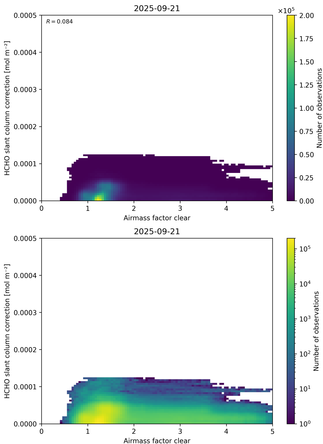
Figure 75: Scatter density plot of “Airmass factor clear” against “HCHO slant column correction” for 2025-09-20 to 2025-09-22.
