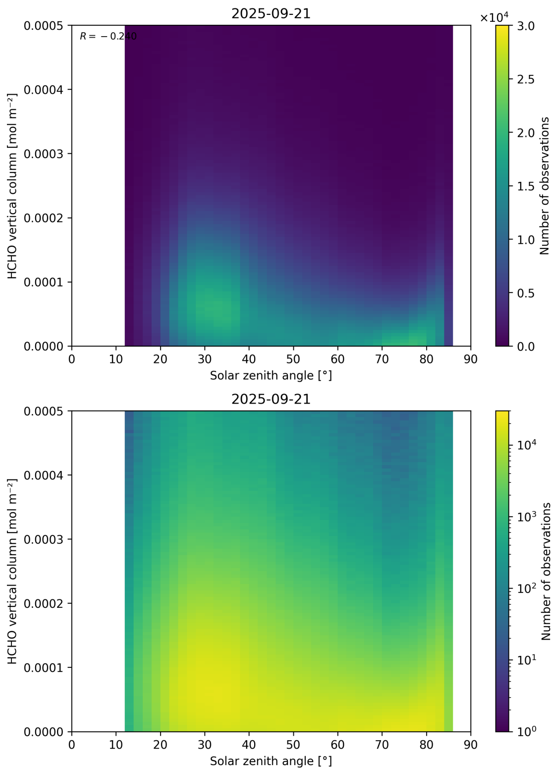
Figure 177: Scatter density plot of “Solar zenith angle” against “HCHO vertical column” for 2025-09-20 to 2025-09-22.
