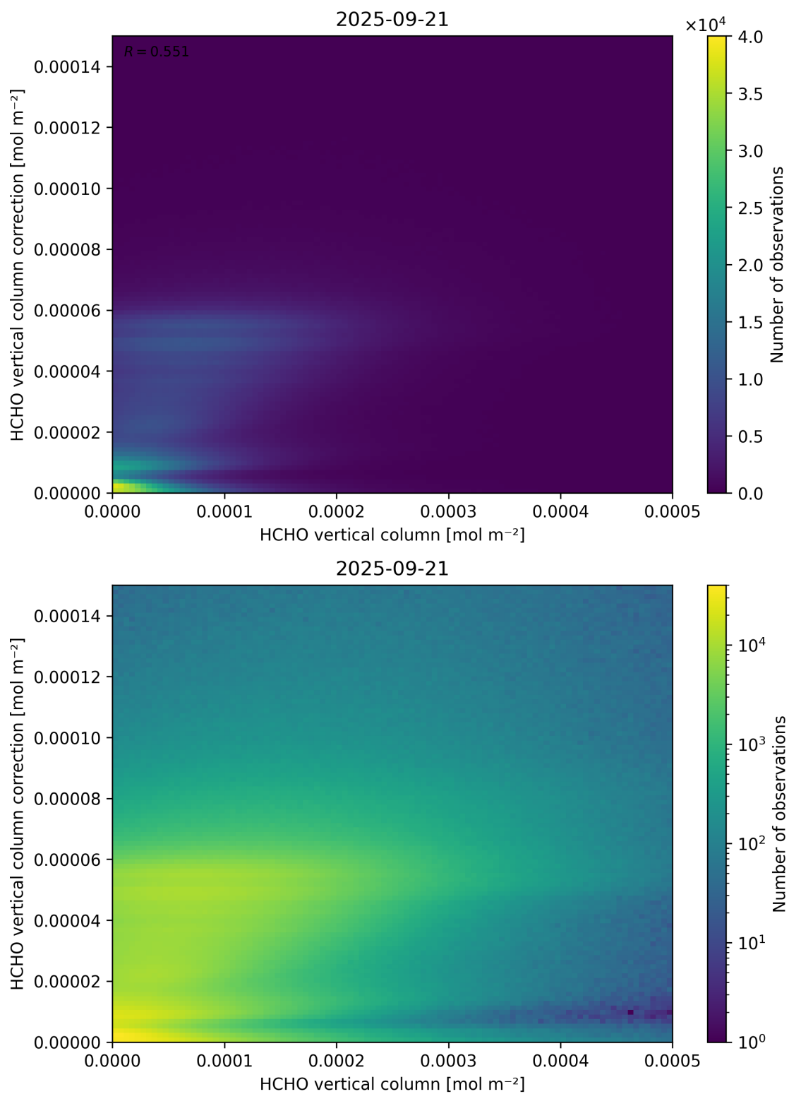
Figure 133: Scatter density plot of “HCHO vertical column” against “HCHO vertical column correction” for 2025-09-20 to 2025-09-22.
