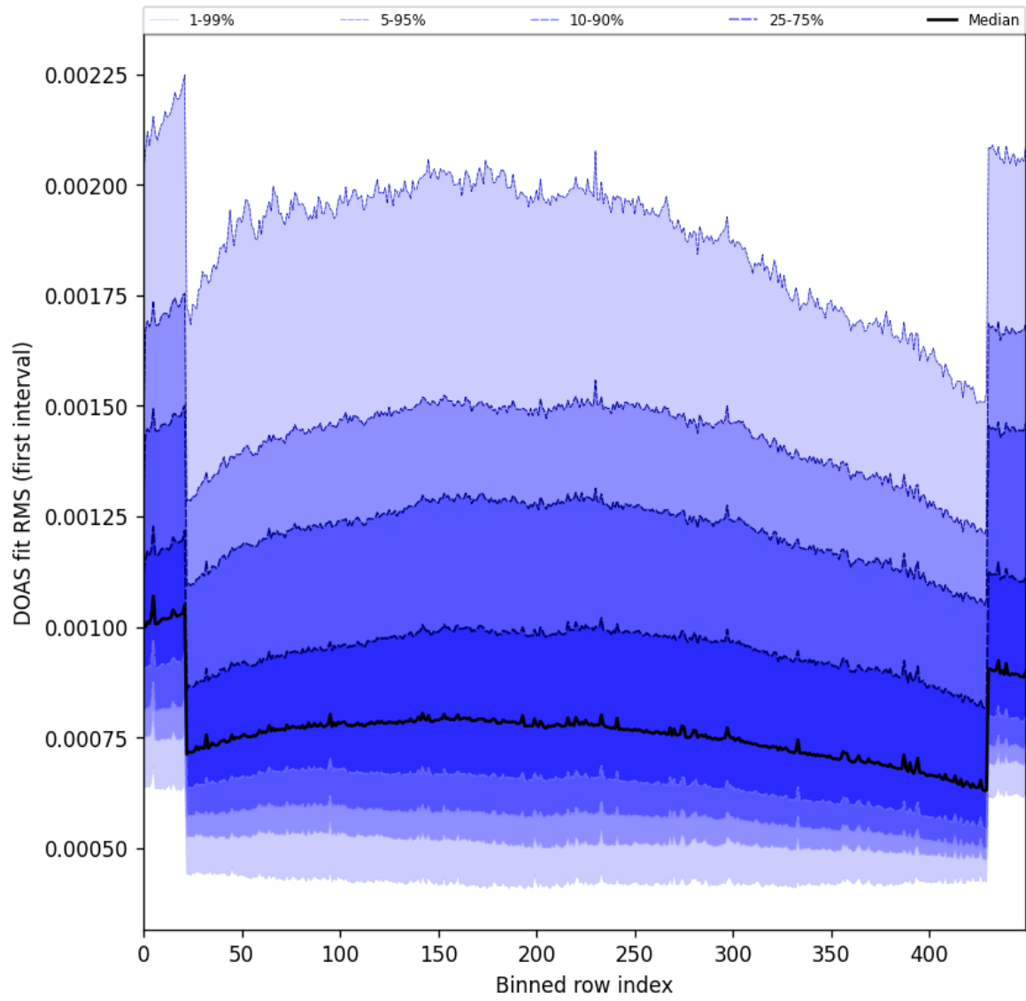
Figure 60: Along track statistics of “DOAS fit RMS (first interval)” for 2025-09-20 to 2025-09-22
