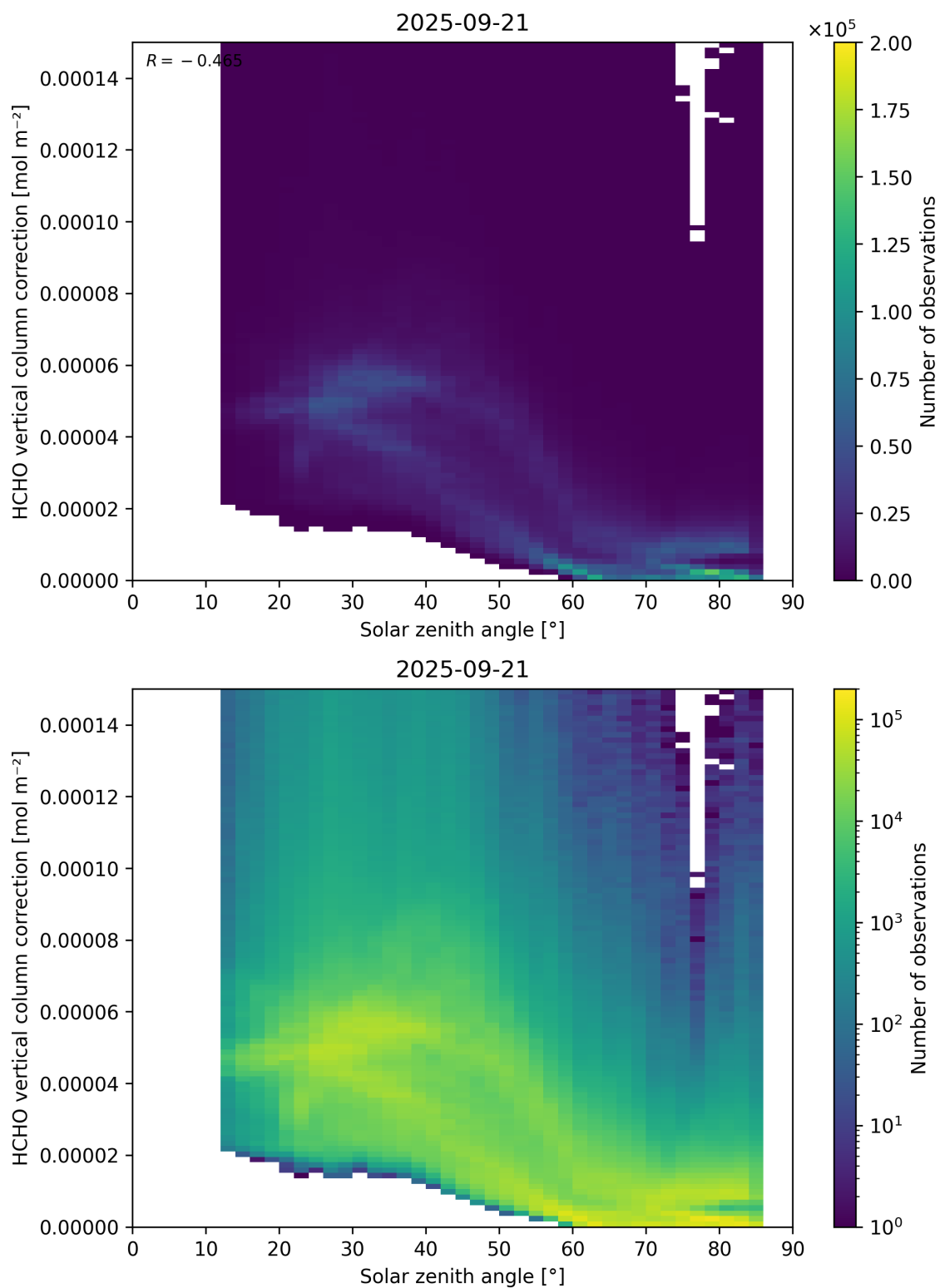
Figure 178: Scatter density plot of “Solar zenith angle” against “HCHO vertical column correction” for 2025-09-20 to 2025-09-22.
