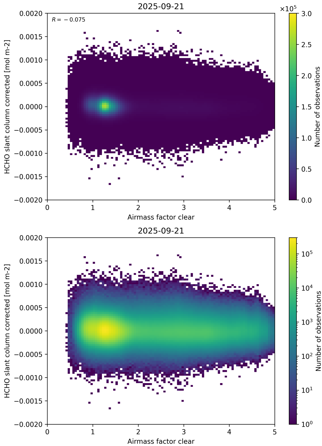
Figure 74: Scatter density plot of “Airmass factor clear” against “HCHO slant column corrected” for 2025-09-20 to 2025-09-22.
