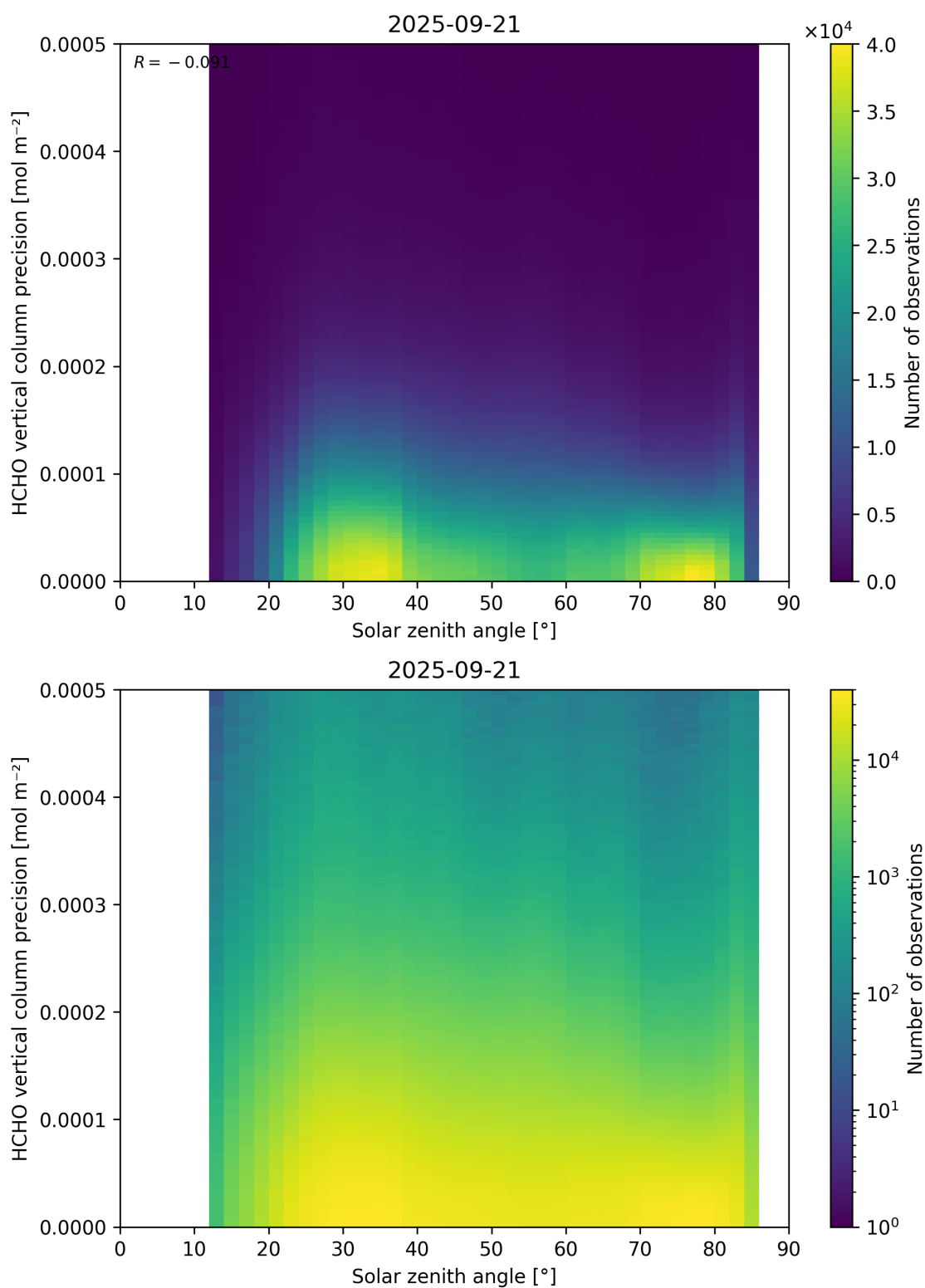
Figure 179: Scatter density plot of “Solar zenith angle” against “HCHO vertical column precision” for 2025-09-20 to 2025-09-22.
