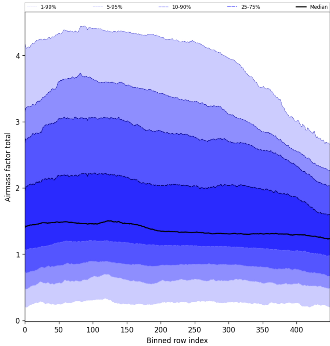
Figure 54: Along track statistics of “Airmass factor total” for 2025-09-20 to 2025-09-22
