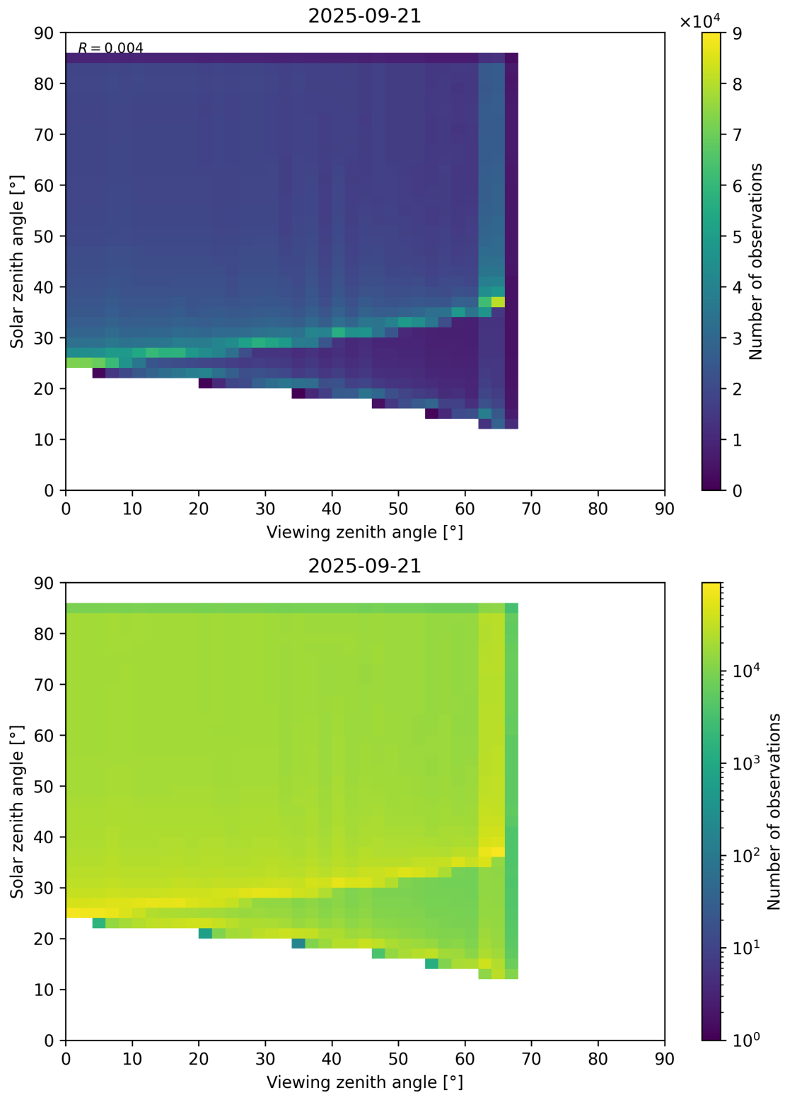
Figure 197: Scatter density plot of “Viewing zenith angle” against “Solar zenith angle” for 2025-09-20 to 2025-09-22.
