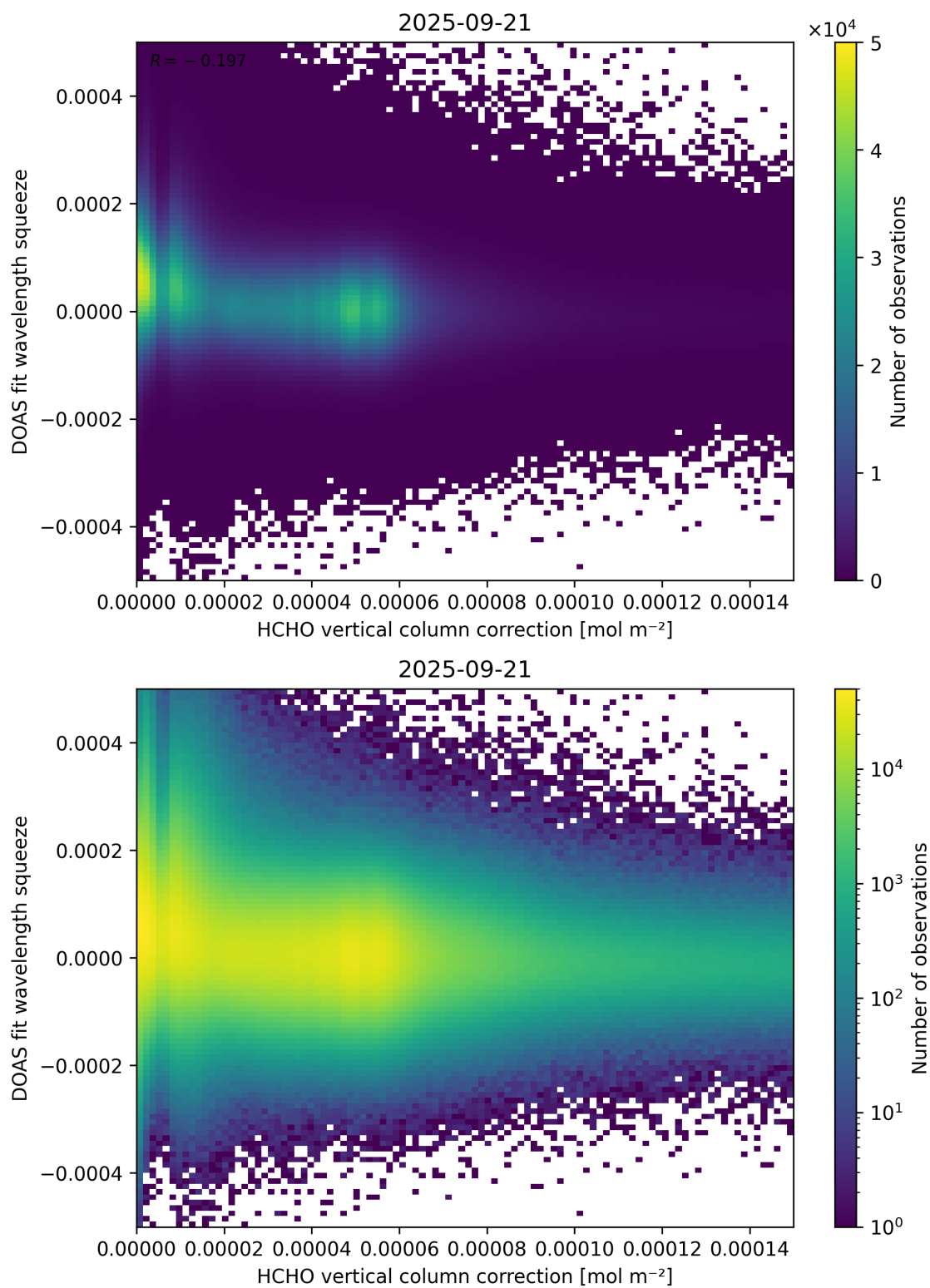
Figure 114: Scatter density plot of “HCHO vertical column correction” against “DOAS fit wavelength squeeze” for 2025-09-20 to 2025-09-22.
