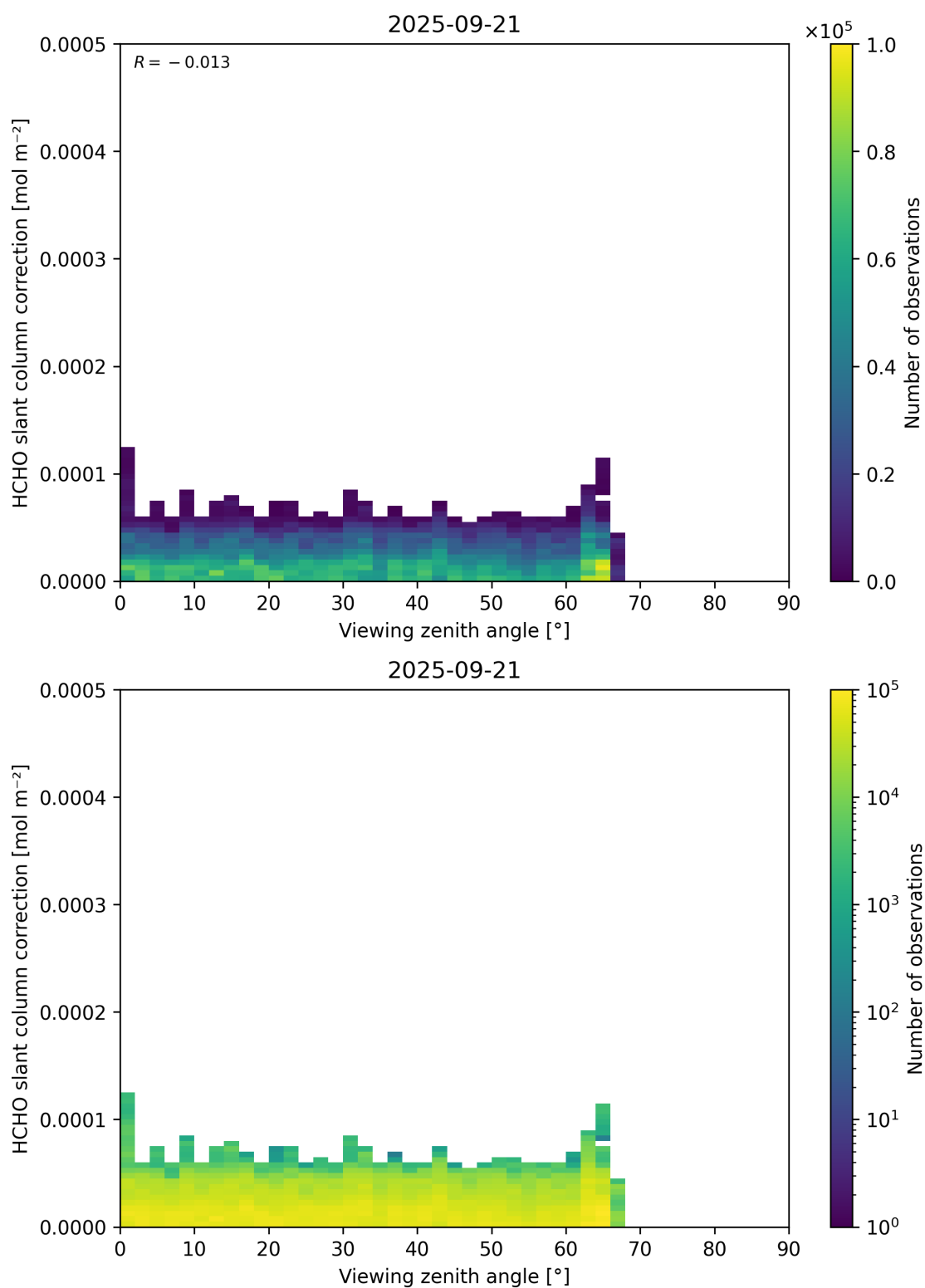
Figure 187: Scatter density plot of “Viewing zenith angle” against “HCHO slant column correction” for 2025-09-20 to 2025-09-22.
