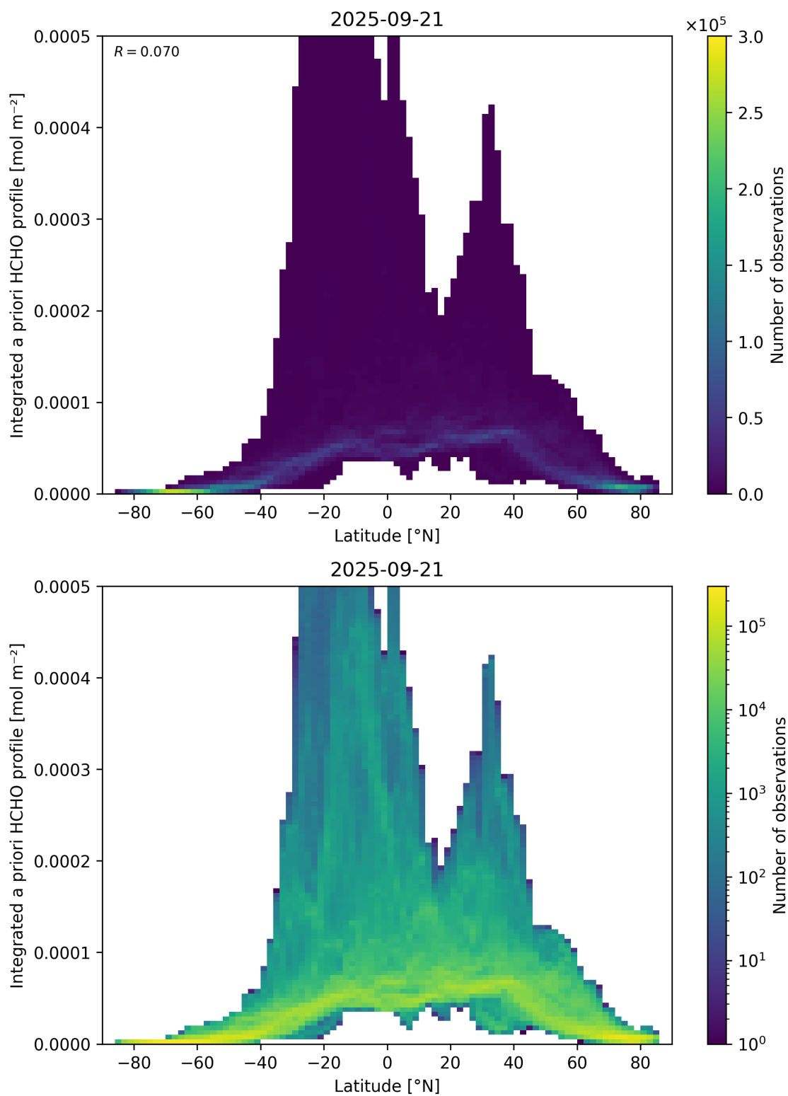
Figure 166: Scatter density plot of “Latitude” against “Integrated a priori HCHO profile” for 2025-09-20 to 2025-09-22.
