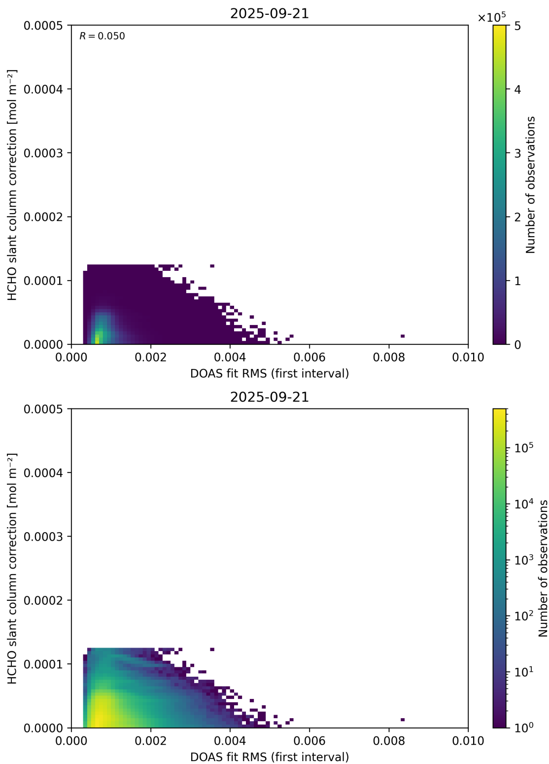
Figure 63: Scatter density plot of “DOAS fit RMS (first interval)” against “HCHO slant column correction” for 2025-09-20 to 2025-09-22.
