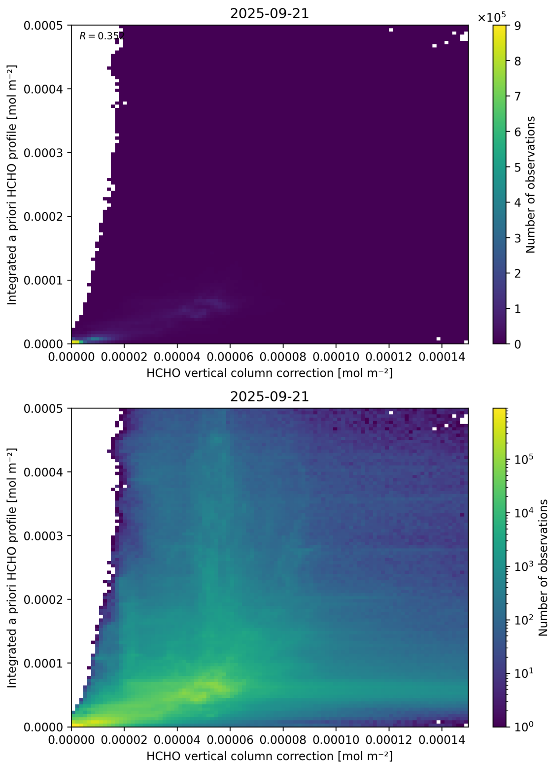
Figure 122: Scatter density plot of “HCHO vertical column correction” against “Integrated a priori HCHO profile” for 2025-09-20 to 2025-09-22.
