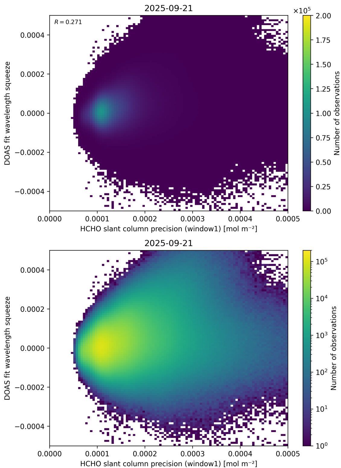
Figure 90: Scatter density plot of “HCHO slant column precision (window1)” against “DOAS fit wavelength squeeze” for 2025-09-20 to 2025-09-22.
