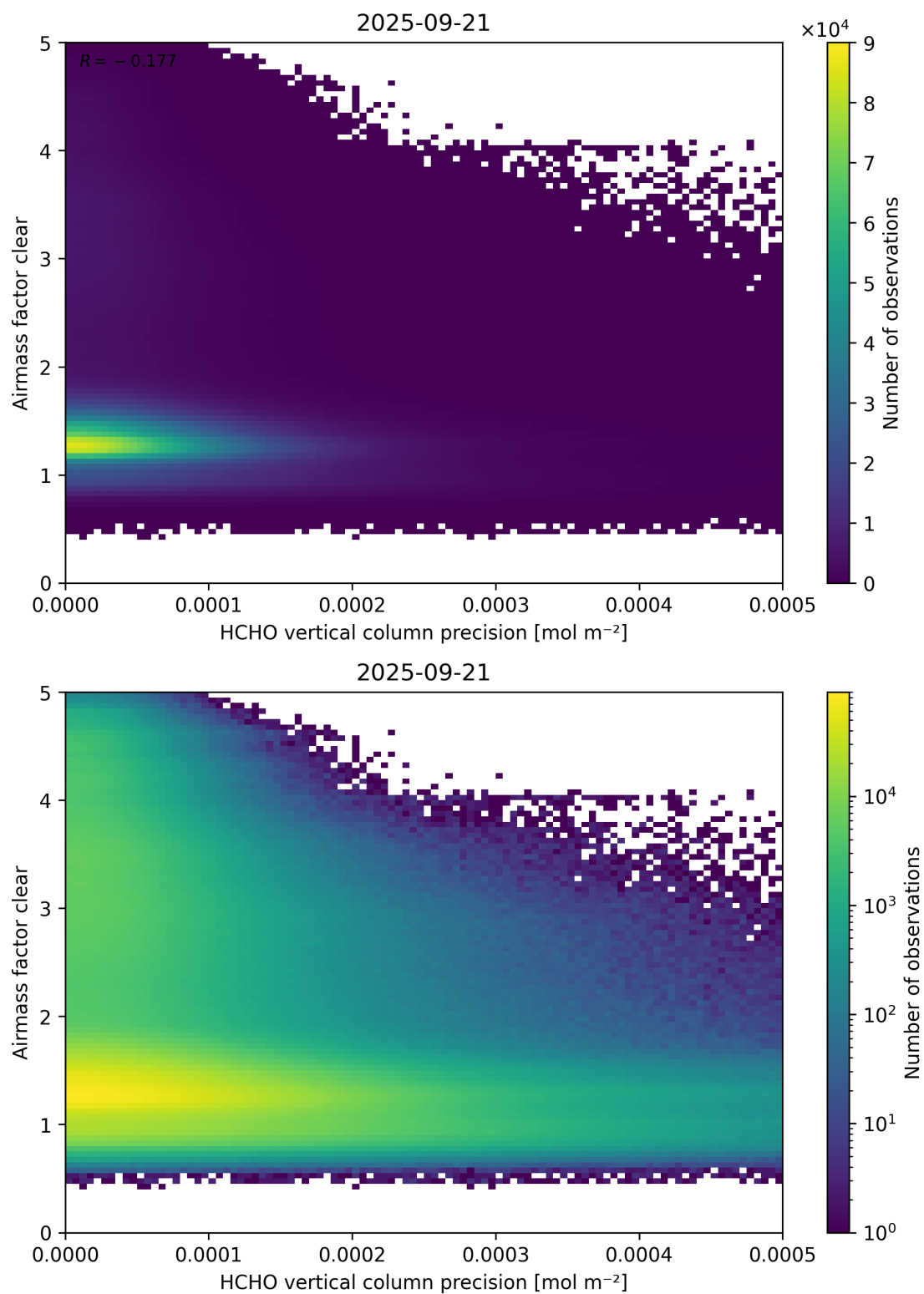
Figure 139: Scatter density plot of “HCHO vertical column precision” against “Airmass factor clear” for 2025-09-20 to 2025-09-22.
