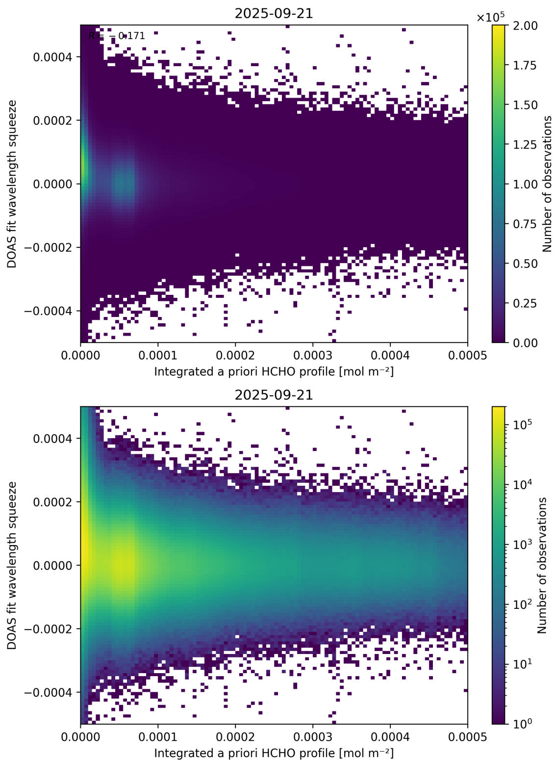
Figure 150: Scatter density plot of “Integrated a priori HCHO profile” against “DOAS fit wavelength squeeze” for 2025-09-20 to 2025-09-22.
