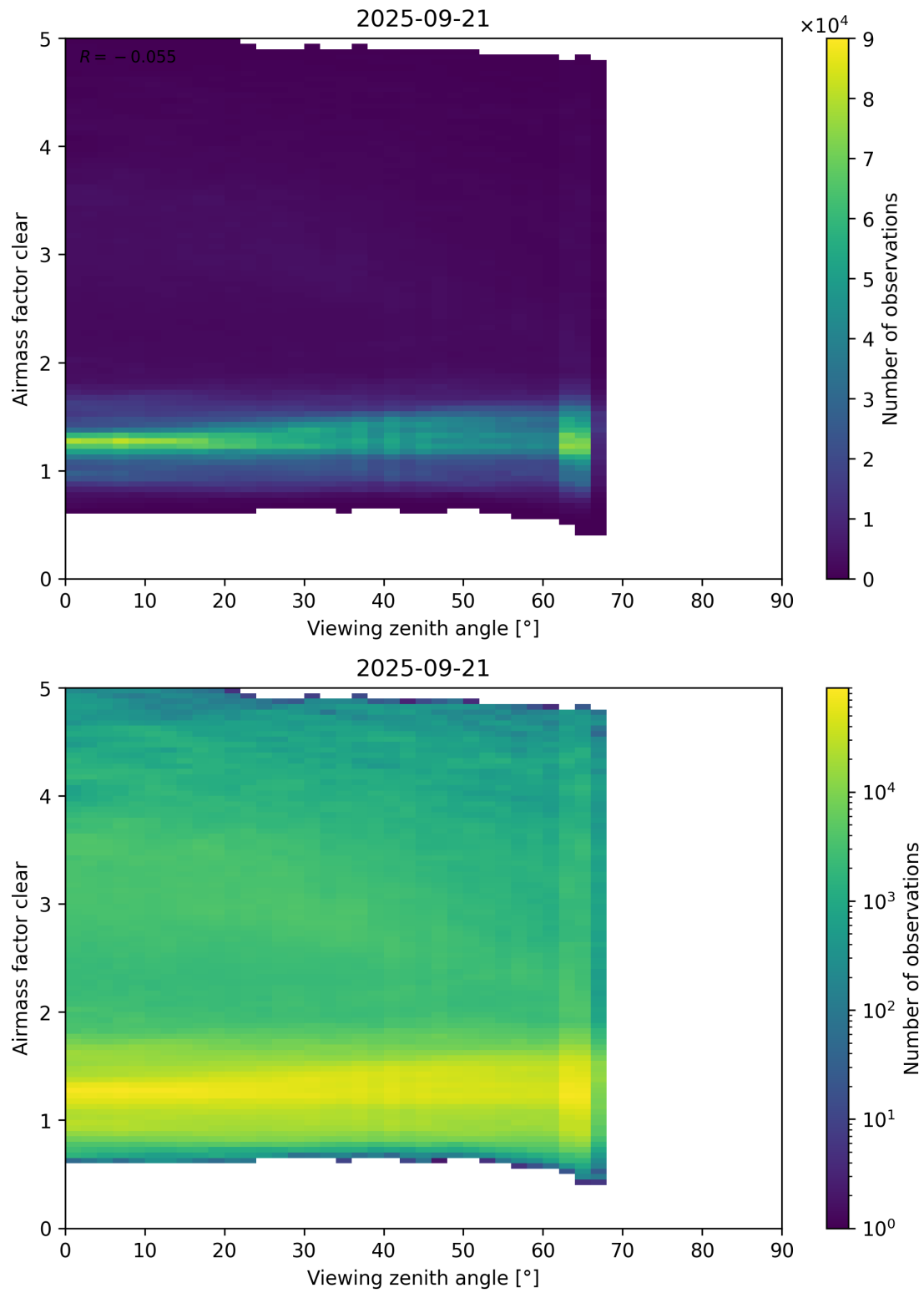
Figure 185: Scatter density plot of “Viewing zenith angle” against “Airmass factor clear” for 2025-09-20 to 2025-09-22.
