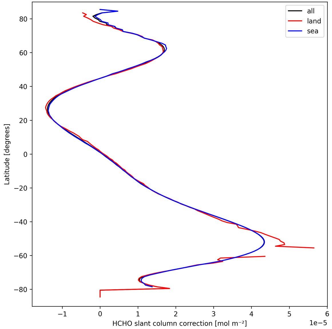
Figure 33: Zonal average of "HCHO slant column correction" for 2025-09-20 to 2025-09-22.
