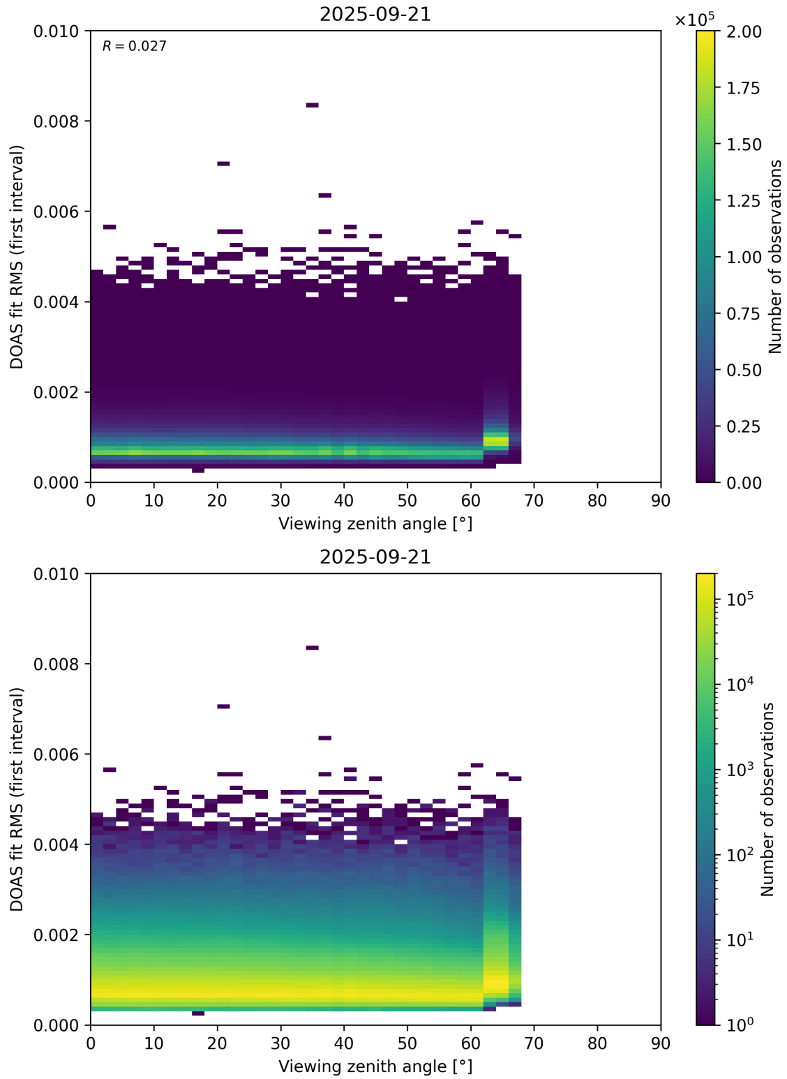
Figure 182: Scatter density plot of “Viewing zenith angle” against “DOAS fit RMS (first interval)” for 2025-09-20 to 2025-09-22.
