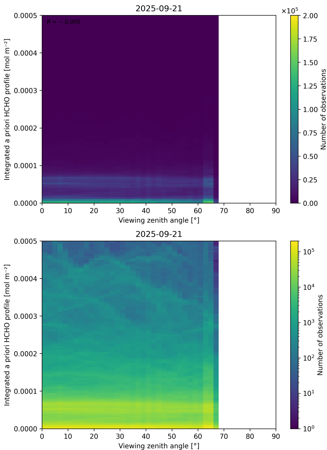
Figure 195: Scatter density plot of “Viewing zenith angle” against “Integrated a priori HCHO profile” for 2025-09-20 to 2025-09-22.
