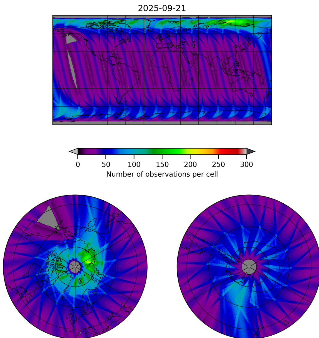
Figure 19: Map of the number of observations for 2025-09-20 to 2025-09-22
