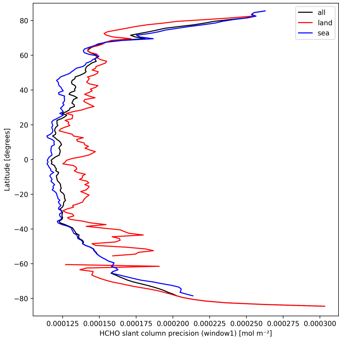
Figure 25: Zonal average of “HCHO slant column precision (window1)” for 2025-09-20 to 2025-09-22.
