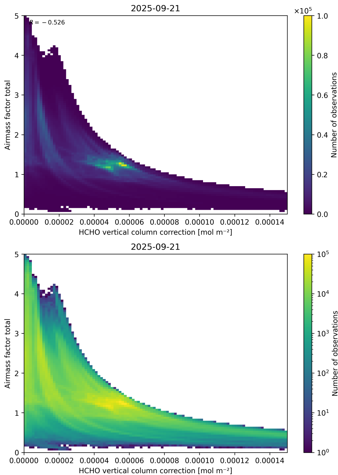
Figure 120: Scatter density plot of “HCHO vertical column correction” against “Airmass factor total” for 2025-09-20 to 2025-09-22.
