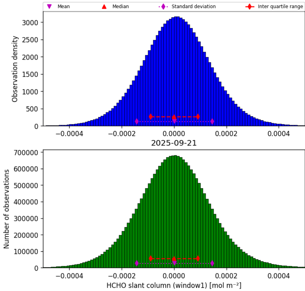
Figure 38: Histogram of “HCHO slant column (window1)” for 2025-09-20 to 2025-09-22
