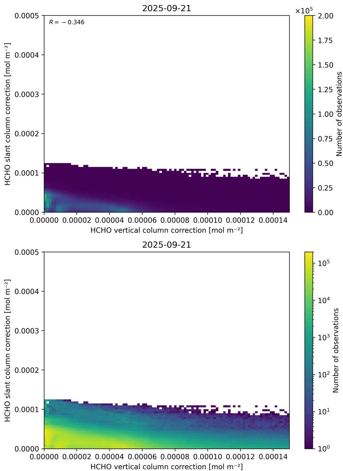
Figure 117: Scatter density plot of “HCHO vertical column correction” against “HCHO slant column correction” for 2025-09-20 to 2025-09-22.
