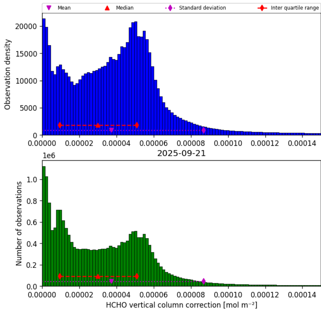
Figure 37: Histogram of “HCHO vertical column correction” for 2025-09-20 to 2025-09-22
