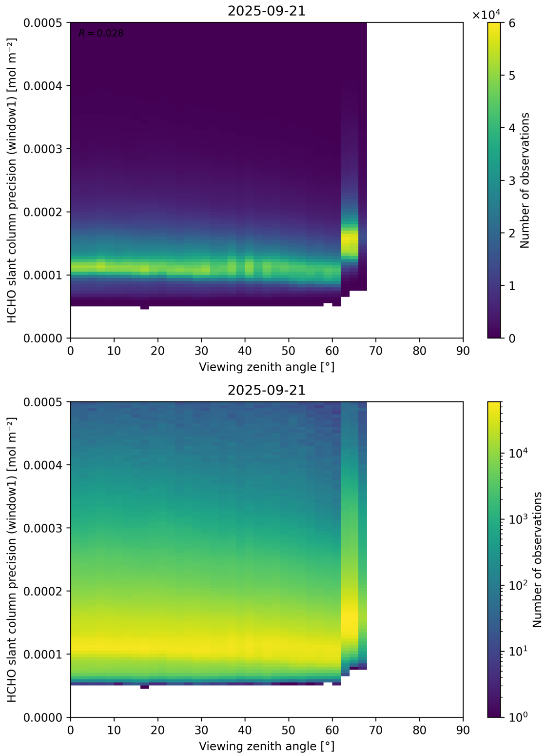
Figure 189: Scatter density plot of “Viewing zenith angle” against “HCHO slant column precision (window1)” for 2025-09-20 to 2025-09-22.
