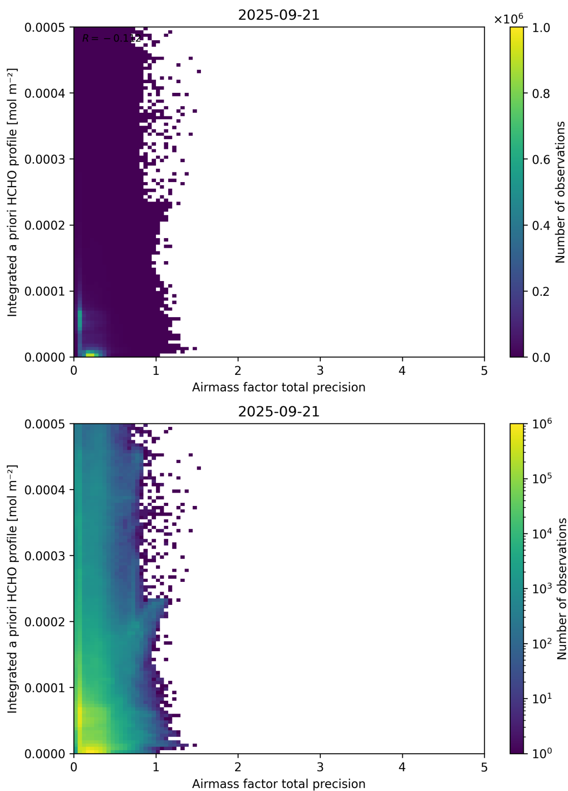
Figure 111: Scatter density plot of “Airmass factor total precision” against “Integrated a priori HCHO profile” for 2025-09-20 to 2025-09-22.
