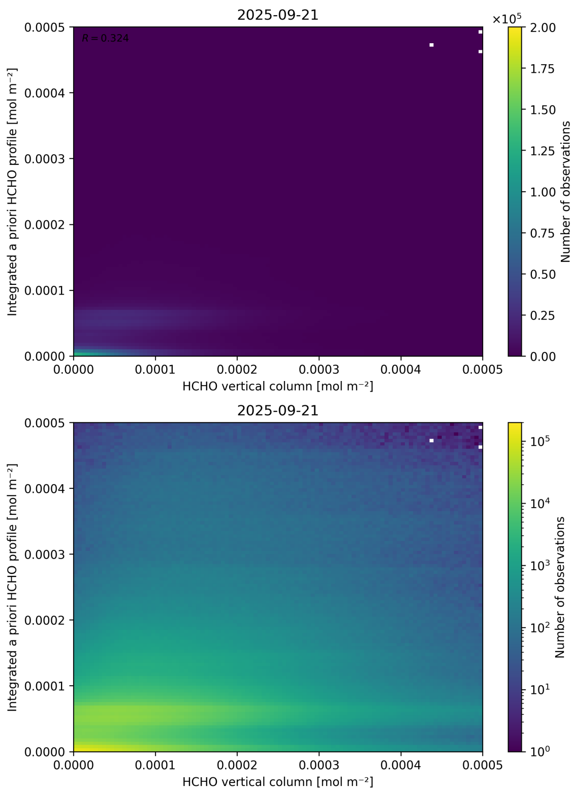
Figure 135: Scatter density plot of “HCHO vertical column” against “Integrated a priori HCHO profile” for 2025-09-20 to 2025-09-22.
