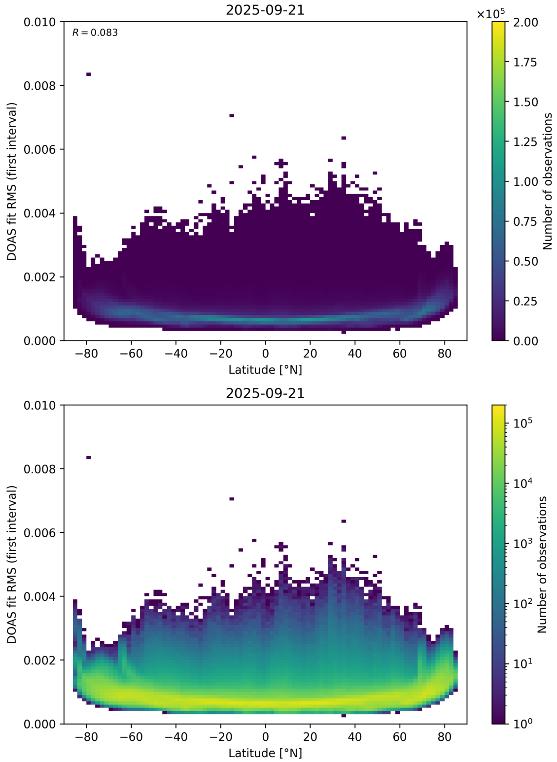
Figure 153: Scatter density plot of “Latitude” against “DOAS fit RMS (first interval)” for 2025-09-20 to 2025-09-22.
