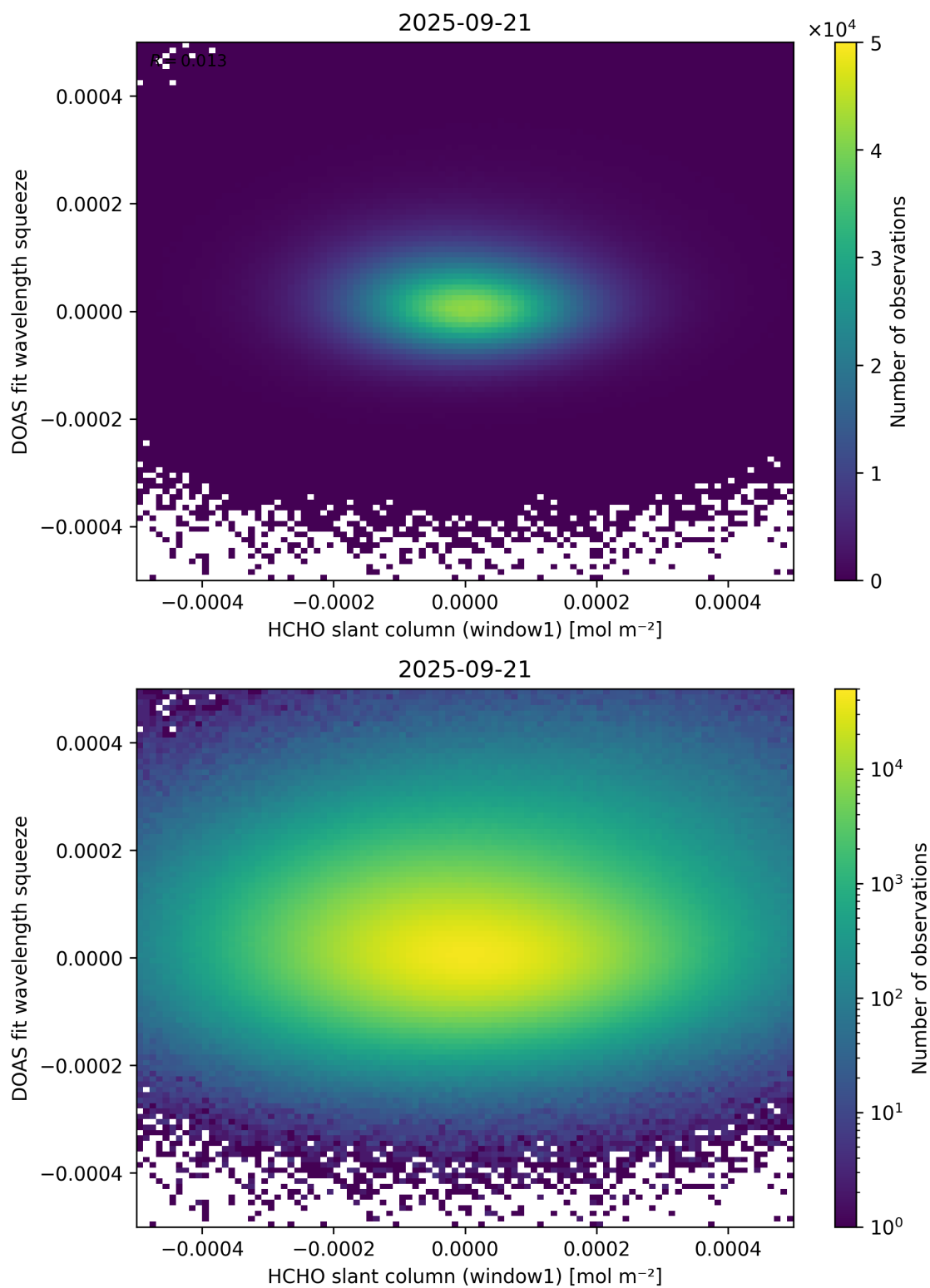
Figure 80: Scatter density plot of “HCHO slant column (window1)” against “DOAS fit wavelength squeeze” for 2025-09-20 to 2025-09-22.
