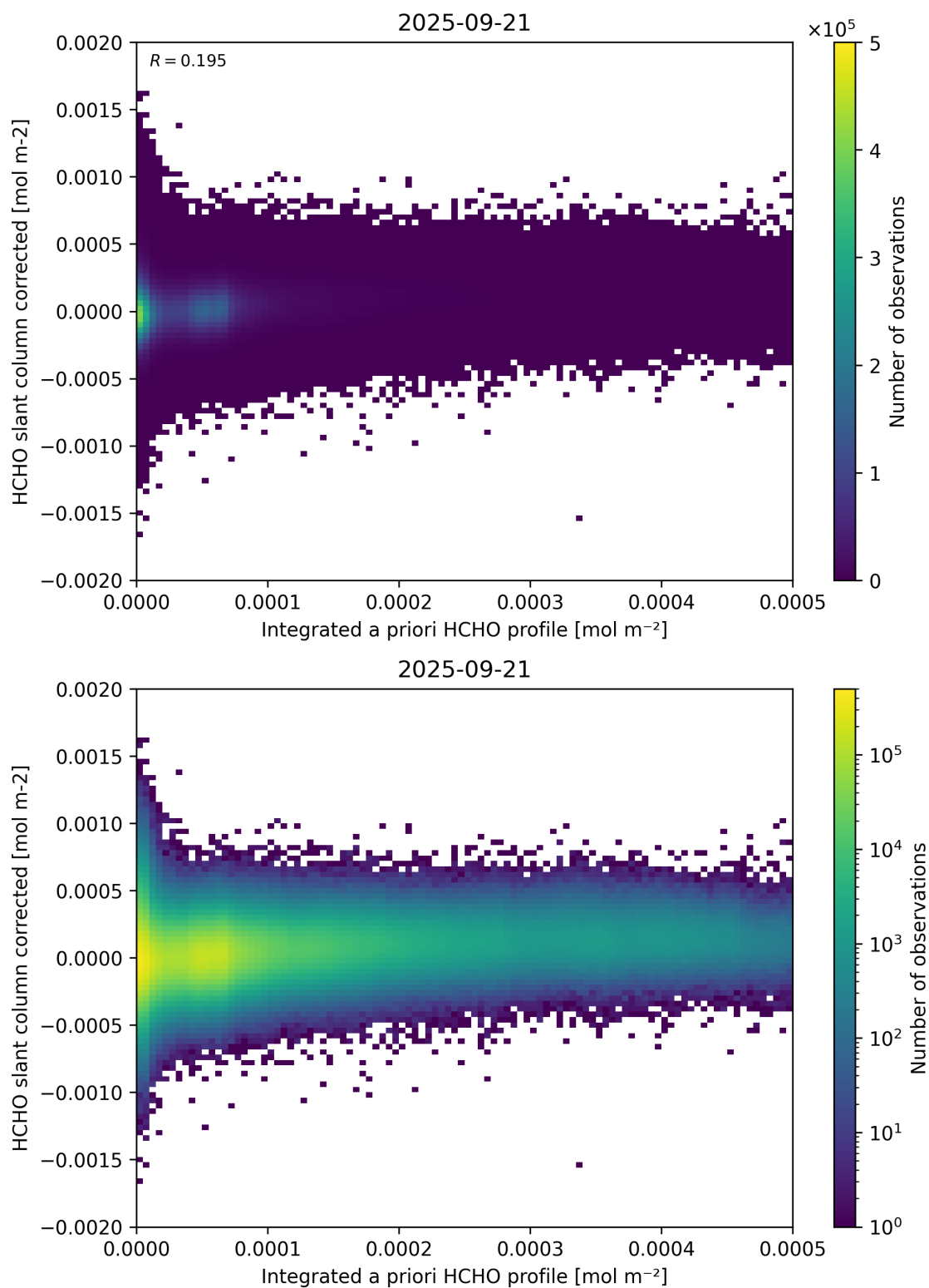
Figure 151: Scatter density plot of “Integrated a priori HCHO profile” against “HCHO slant column corrected” for 2025-09-20 to 2025-09-22.
