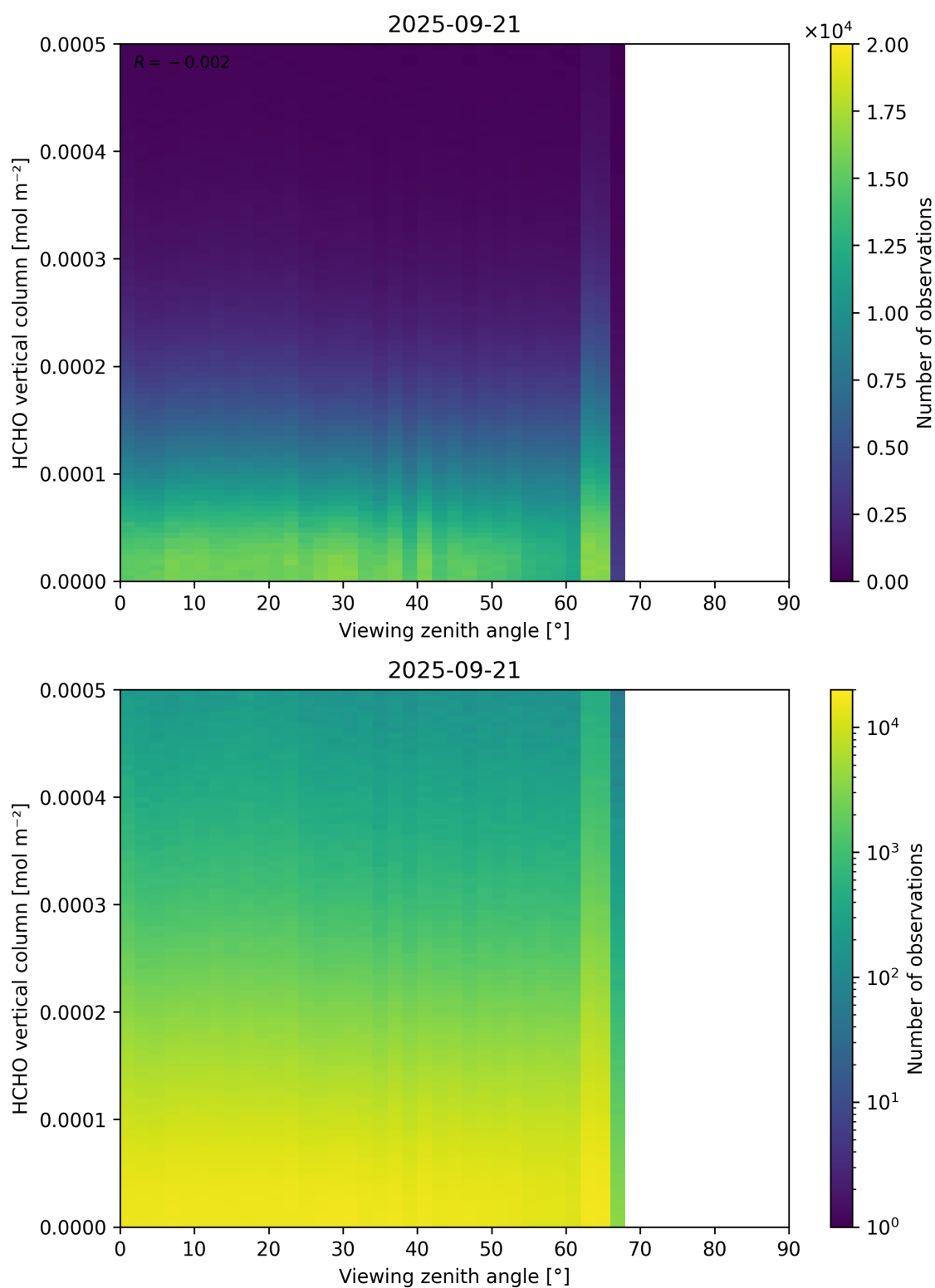
Figure 192: Scatter density plot of “Viewing zenith angle” against “HCHO vertical column” for 2025-09-20 to 2025-09-22.
