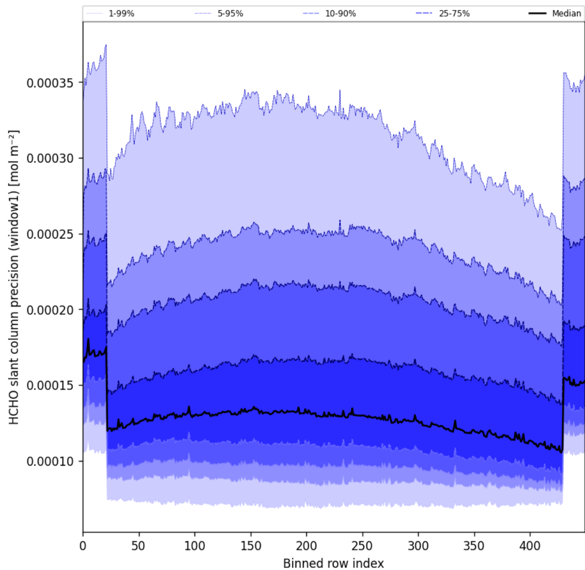
Figure 53: Along track statistics of “HCHO slant column precision (window1)” for 2025-09-20 to 2025-09-22
