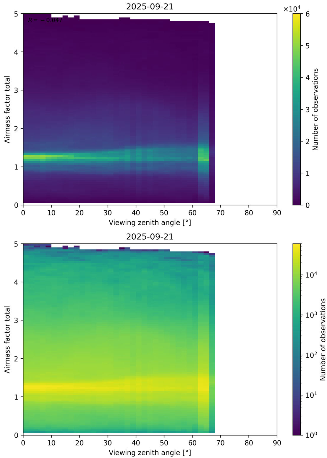
Figure 190: Scatter density plot of “Viewing zenith angle” against “Airmass factor total” for 2025-09-20 to 2025-09-22.
