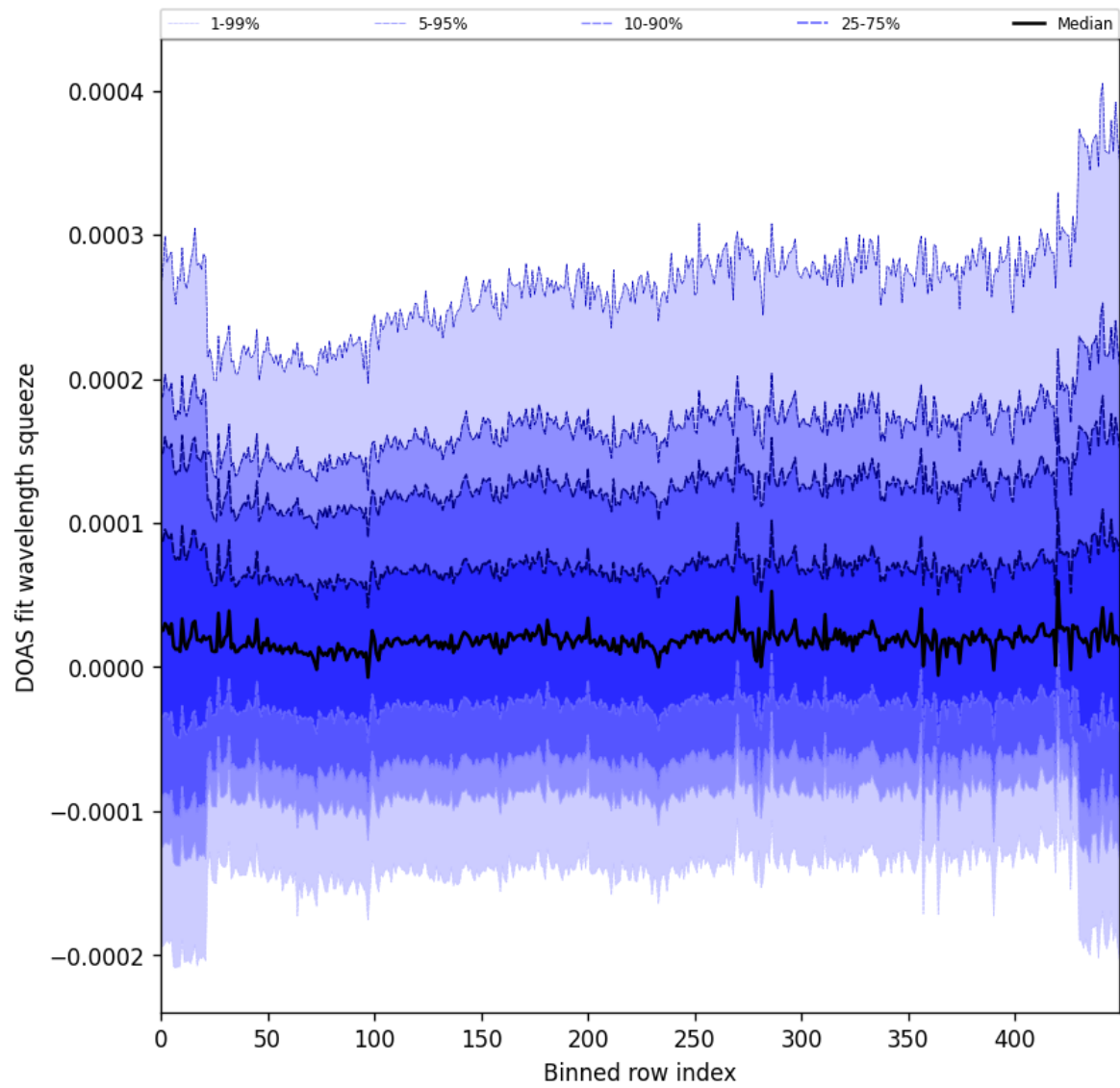
Figure 59: Along track statistics of “DOAS fit wavelength squeeze” for 2025-09-20 to 2025-09-22
