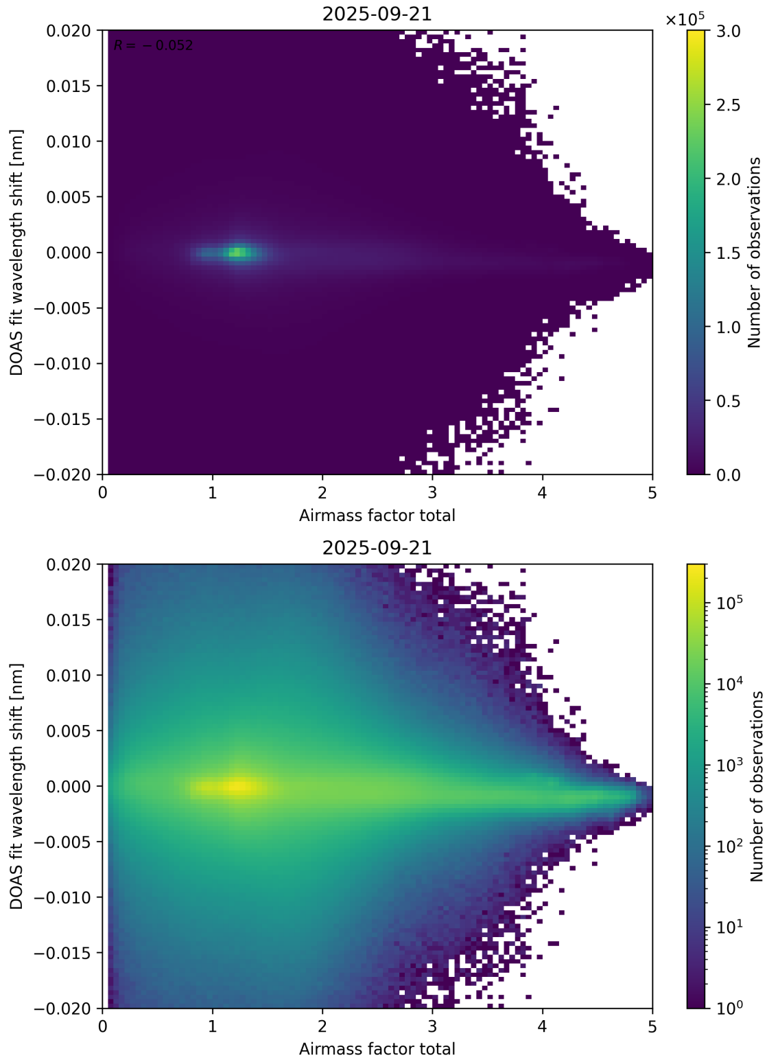
Figure 98: Scatter density plot of “Airmass factor total” against “DOAS fit wavelength shift” for 2025-09-20 to 2025-09-22.
