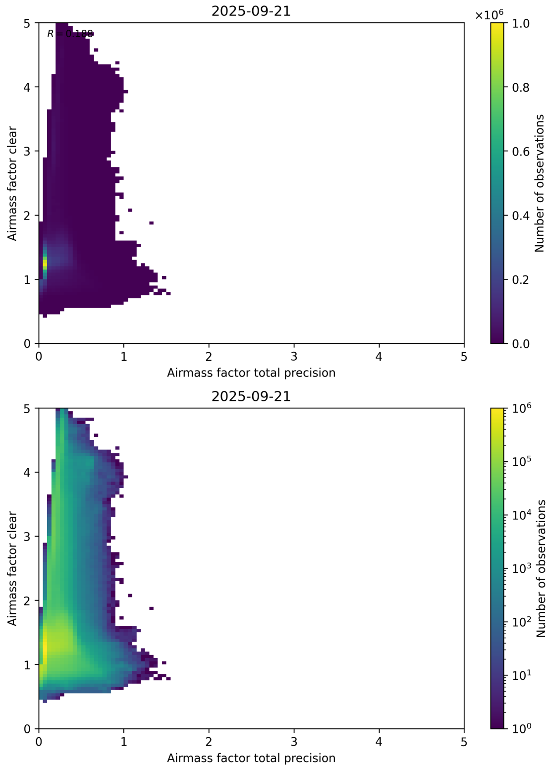
Figure 108: Scatter density plot of “Airmass factor total precision” against “Airmass factor clear” for 2025-09-20 to 2025-09-22.
