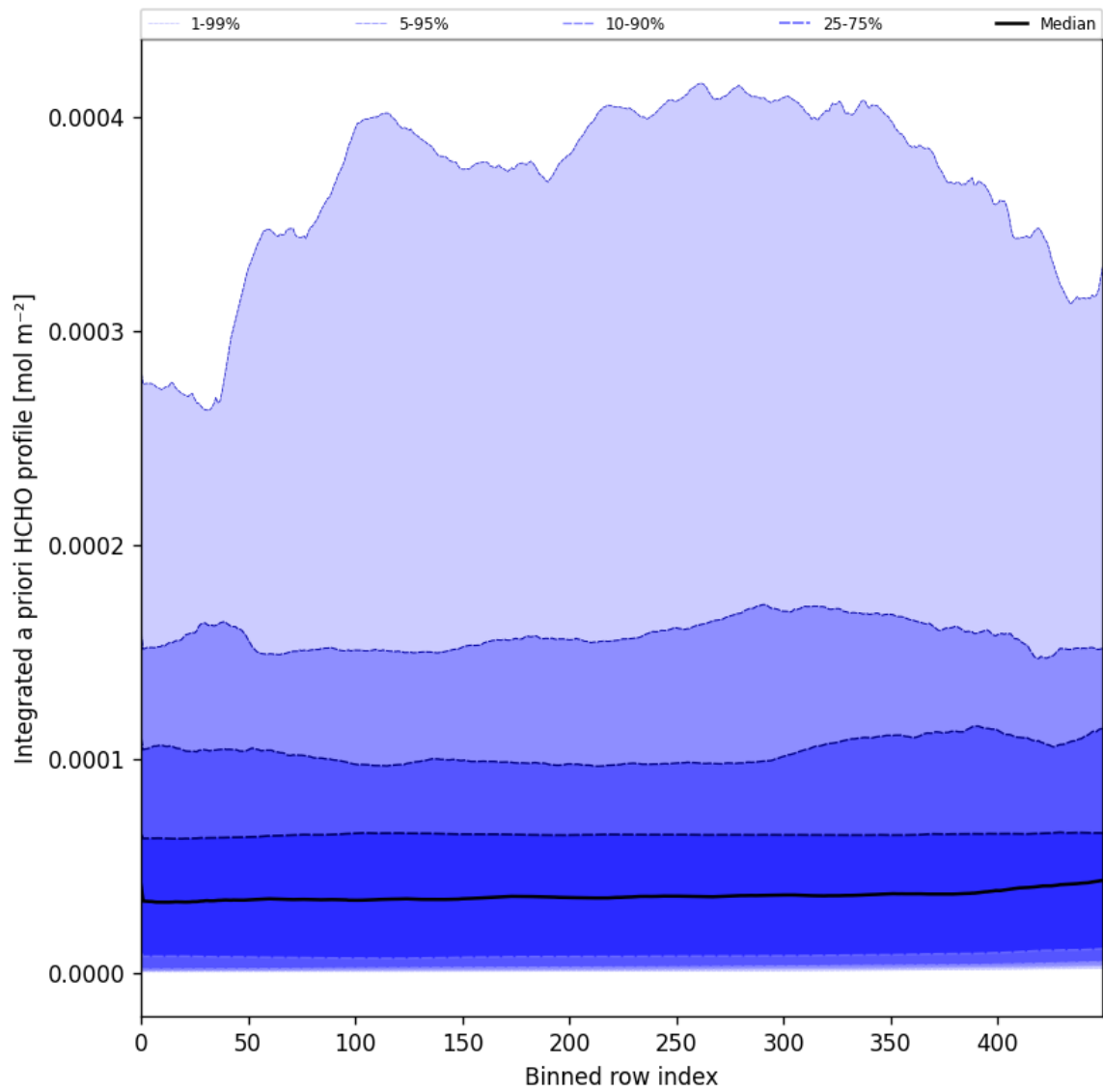
Figure 57: Along track statistics of “Integrated a priori HCHO profile” for 2025-09-20 to 2025-09-22
