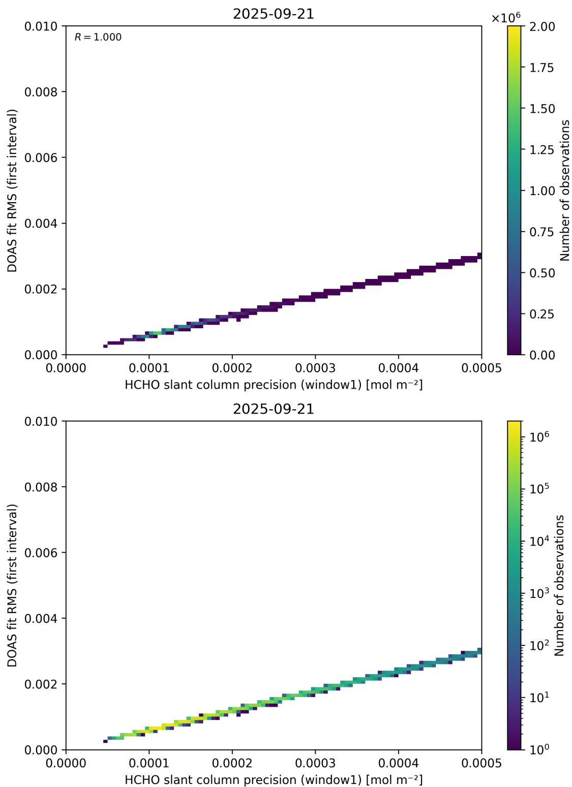
Figure 88: Scatter density plot of “HCHO slant column precision (window1)” against “DOAS fit RMS (first interval)” for 2025-09-20 to 2025-09-22.
