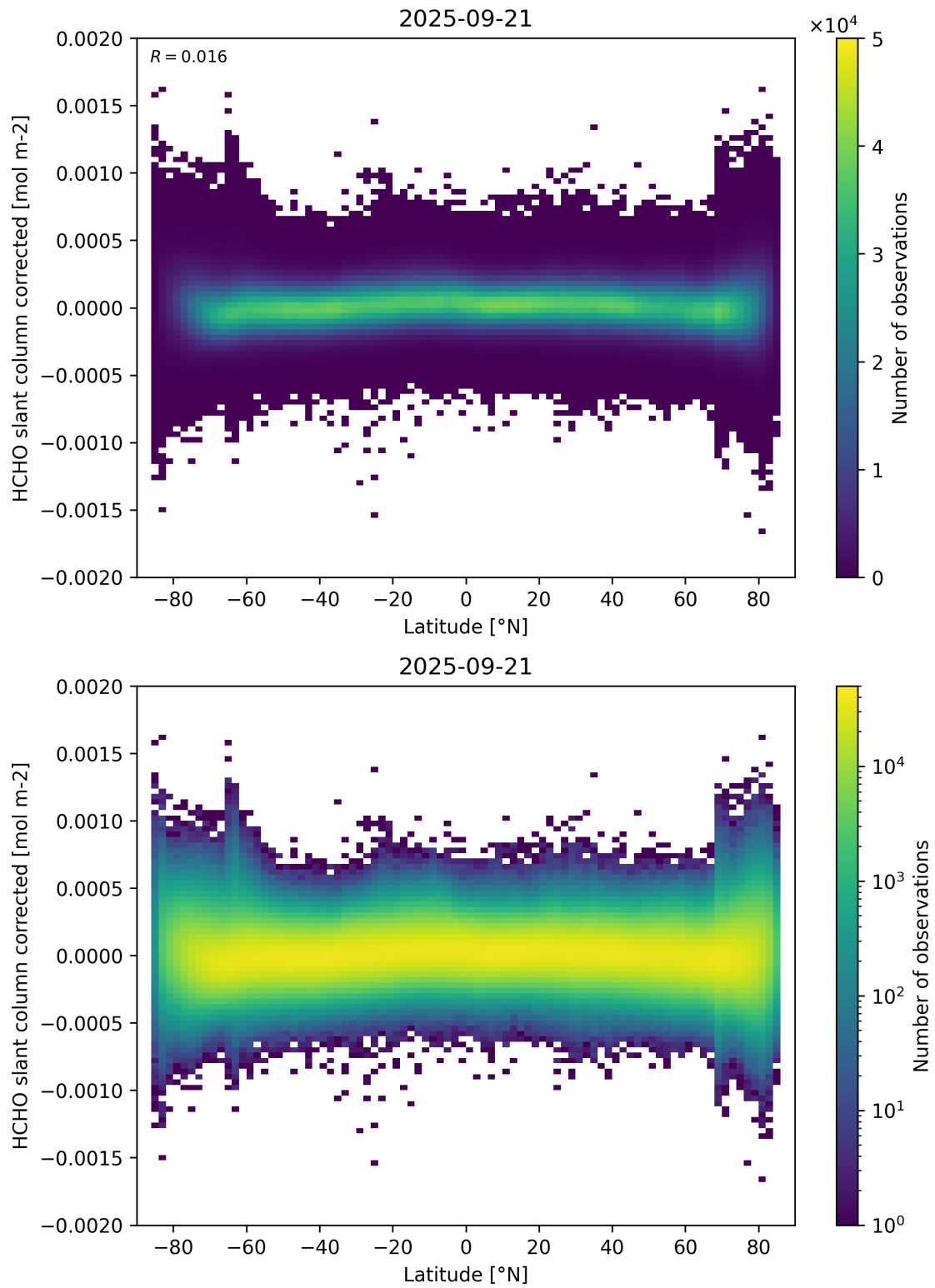
Figure 157: Scatter density plot of “Latitude” against “HCHO slant column corrected” for 2025-09-20 to 2025-09-22.
