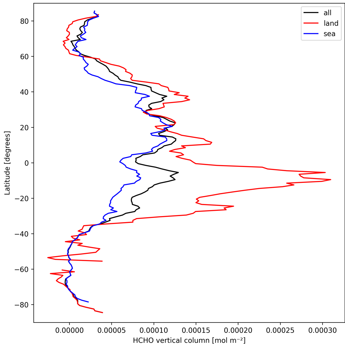
Figure 21: Zonal average of “HCHO vertical column” for 2025-09-20 to 2025-09-22.
