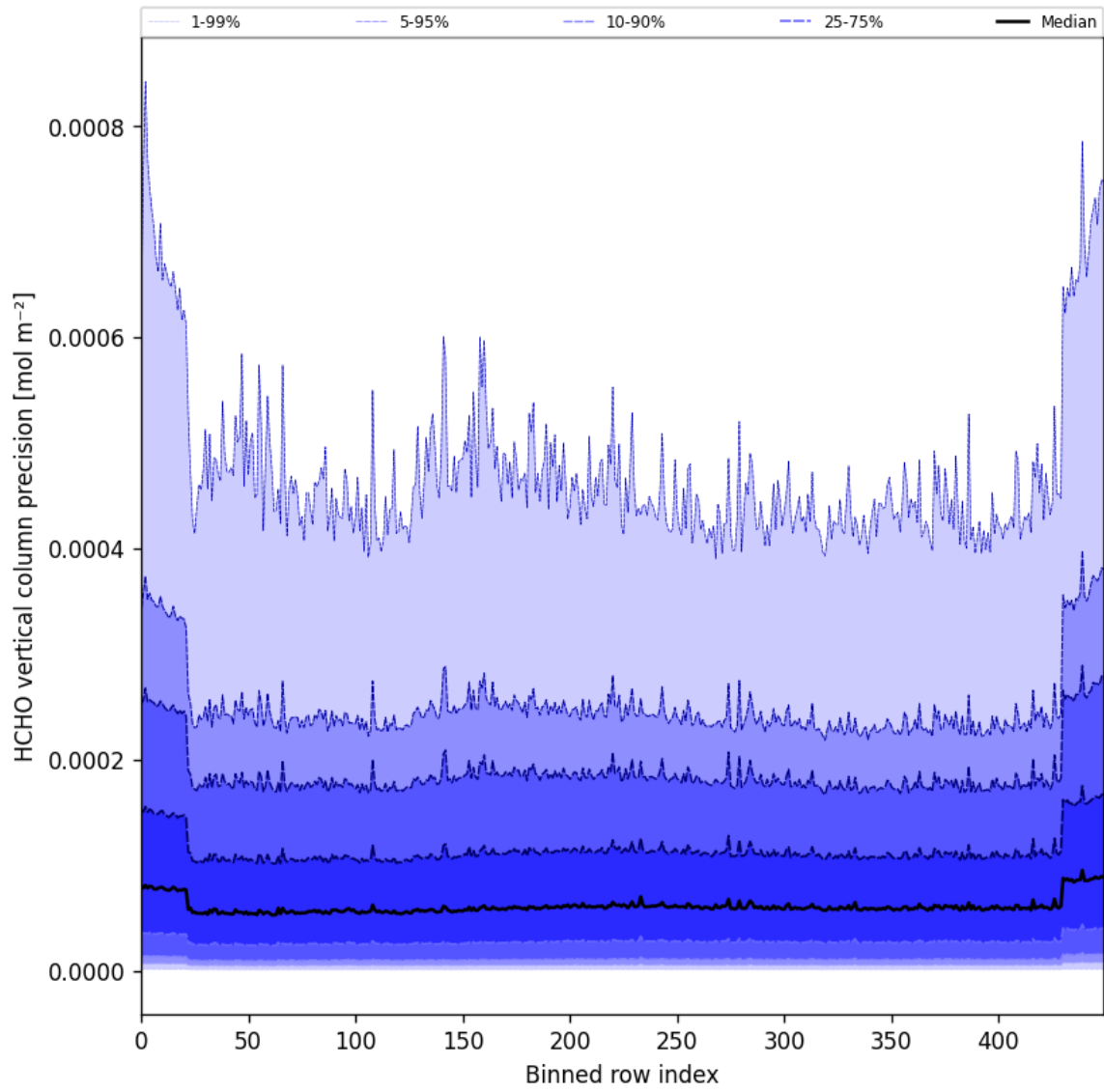
Figure 50: Along track statistics of “HCHO vertical column precision” for 2025-09-20 to 2025-09-22
