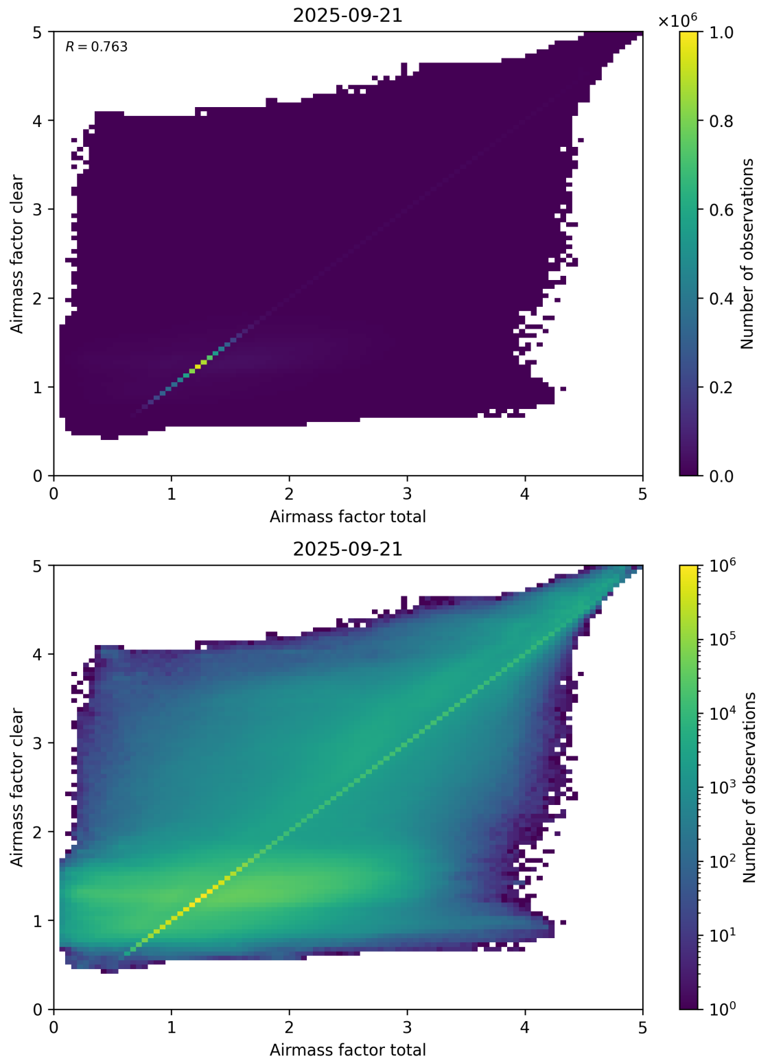
Figure 100: Scatter density plot of “Airmass factor total” against “Airmass factor clear” for 2025-09-20 to 2025-09-22.
