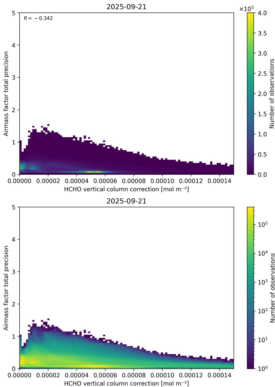
Figure 121: Scatter density plot of “HCHO vertical column correction” against “Airmass factor total precision” for 2025-09-20 to 2025-09-22.
