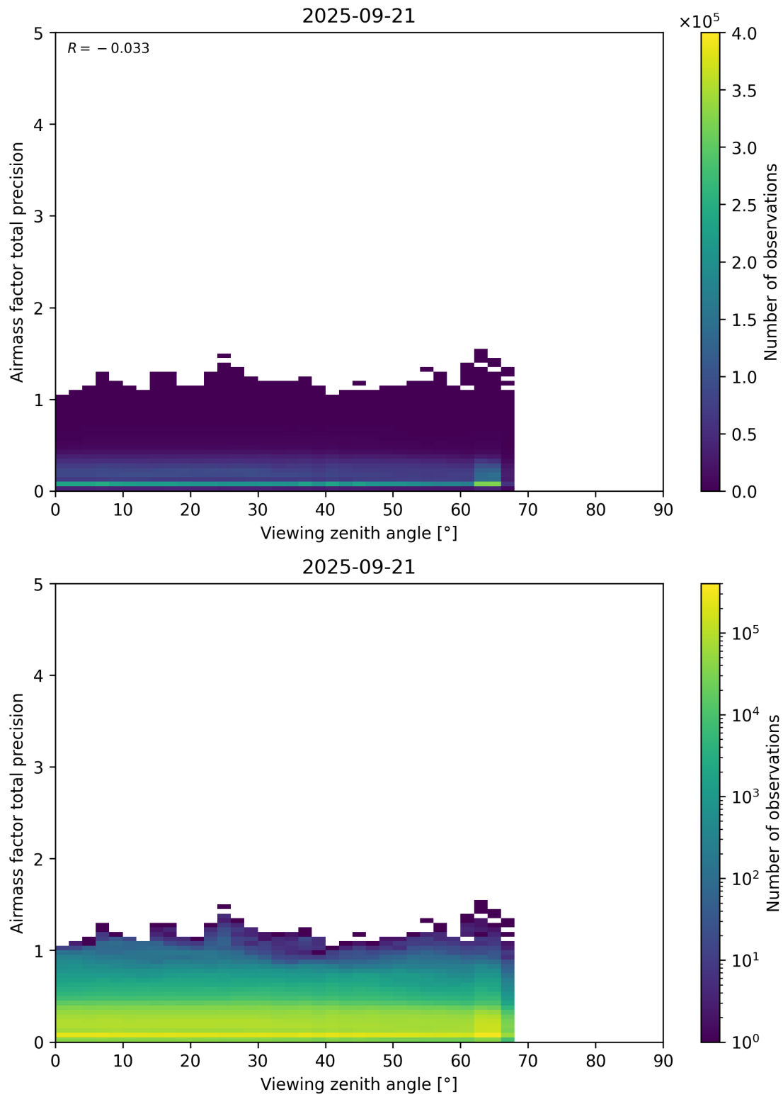
Figure 191: Scatter density plot of “Viewing zenith angle” against “Airmass factor total precision” for 2025-09-20 to 2025-09-22.
