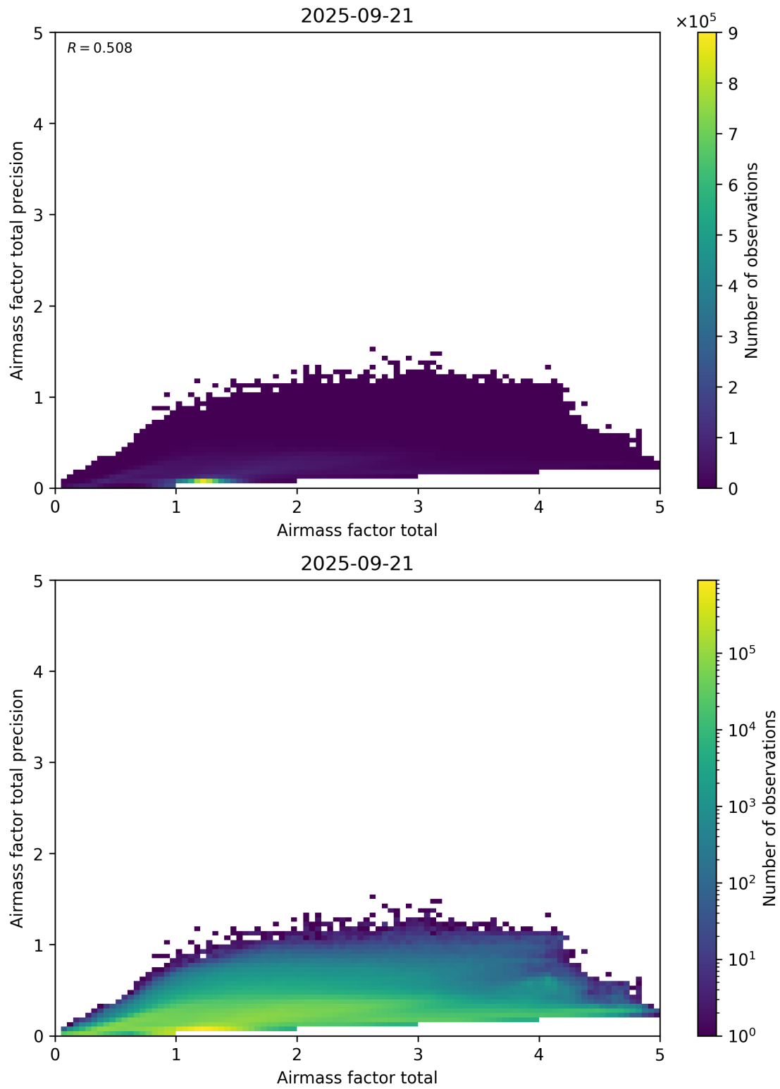
Figure 103: Scatter density plot of “Airmass factor total” against “Airmass factor total precision” for 2025-09-20 to 2025-09-22.
