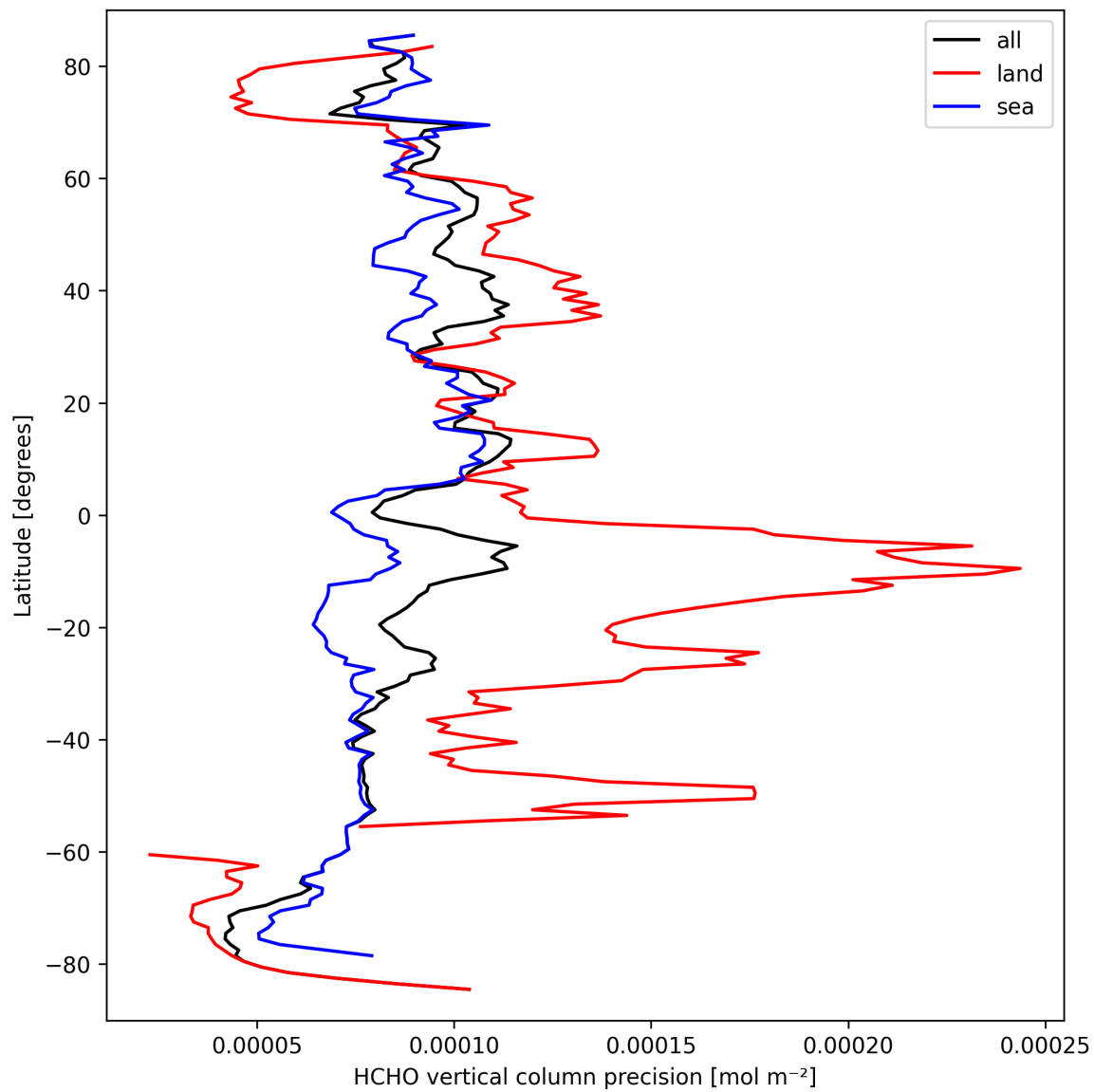
Figure 22: Zonal average of "HCHO vertical column precision" for 2025-09-20 to 2025-09-22.
