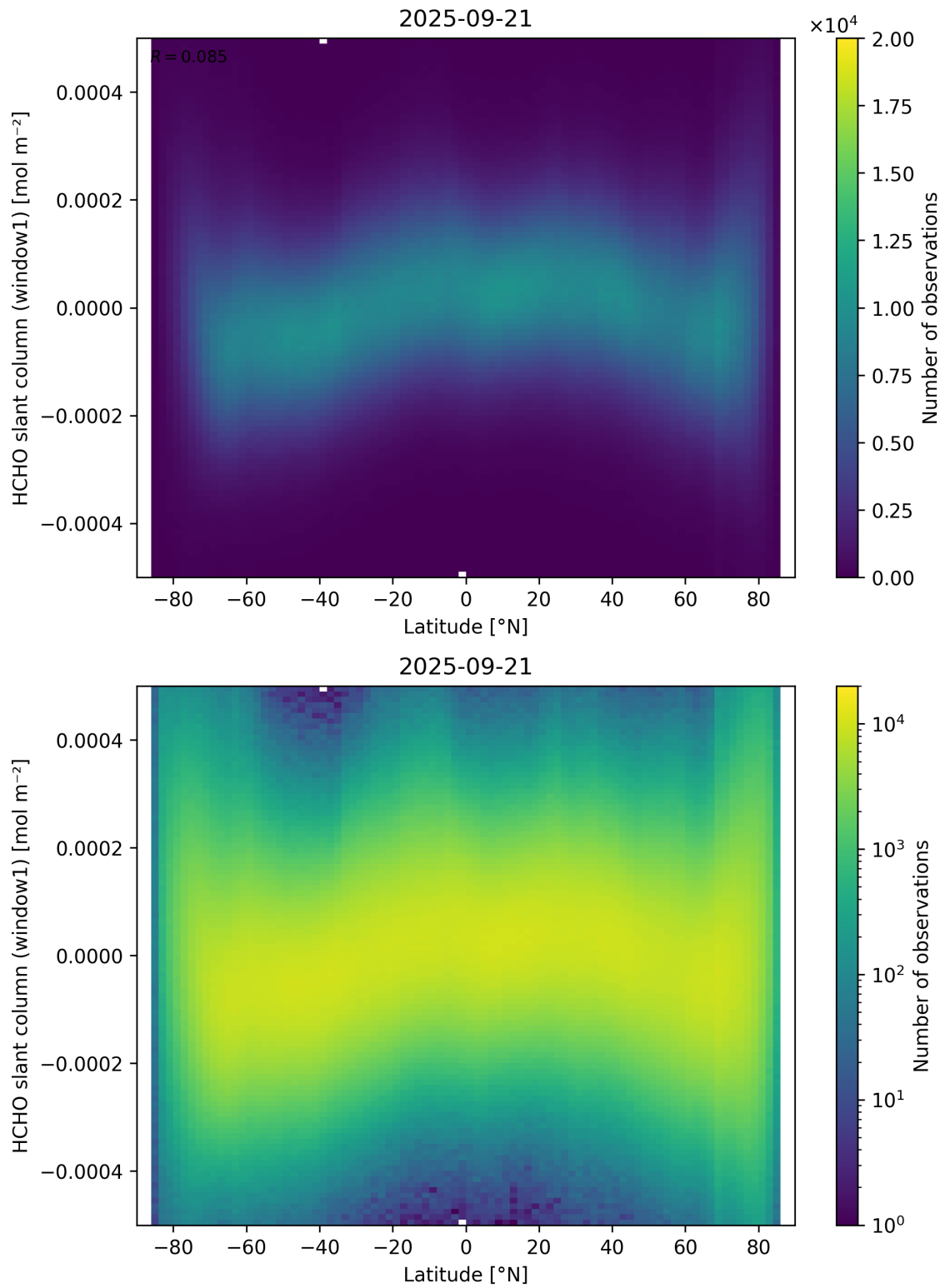
Figure 159: Scatter density plot of “Latitude” against “HCHO slant column (window1)” for 2025-09-20 to 2025-09-22.
