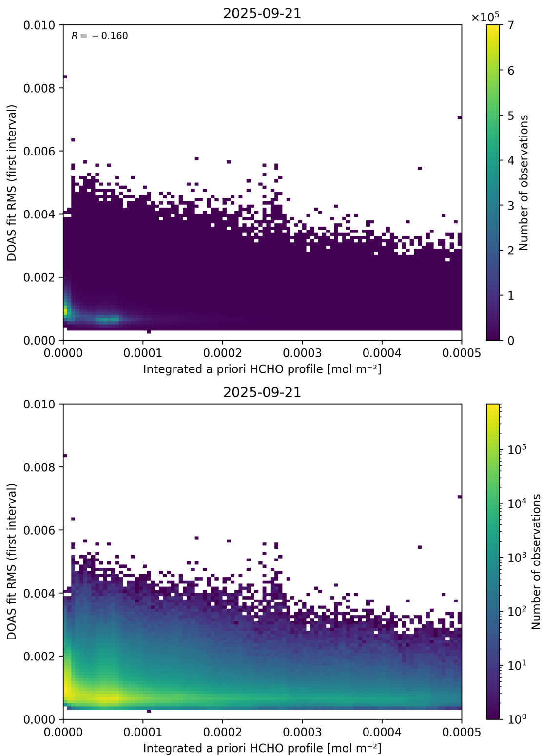
Figure 148: Scatter density plot of “Integrated a priori HCHO profile” against “DOAS fit RMS (first interval)” for 2025-09-20 to 2025-09-22.
