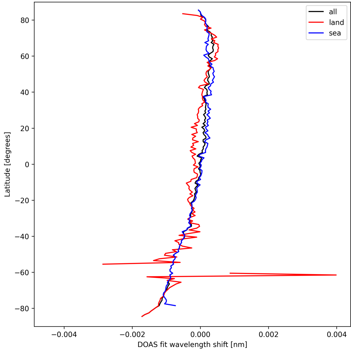
Figure 30: Zonal average of “DOAS fit wavelength shift” for 2025-09-20 to 2025-09-22.
