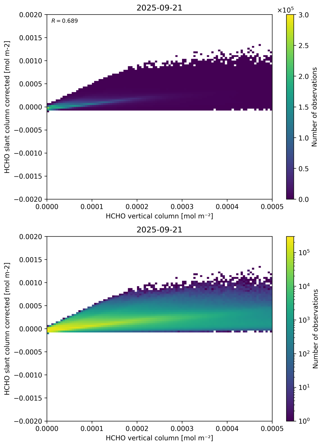
Figure 127: Scatter density plot of “HCHO vertical column” against “HCHO slant column corrected” for 2025-09-20 to 2025-09-22.
