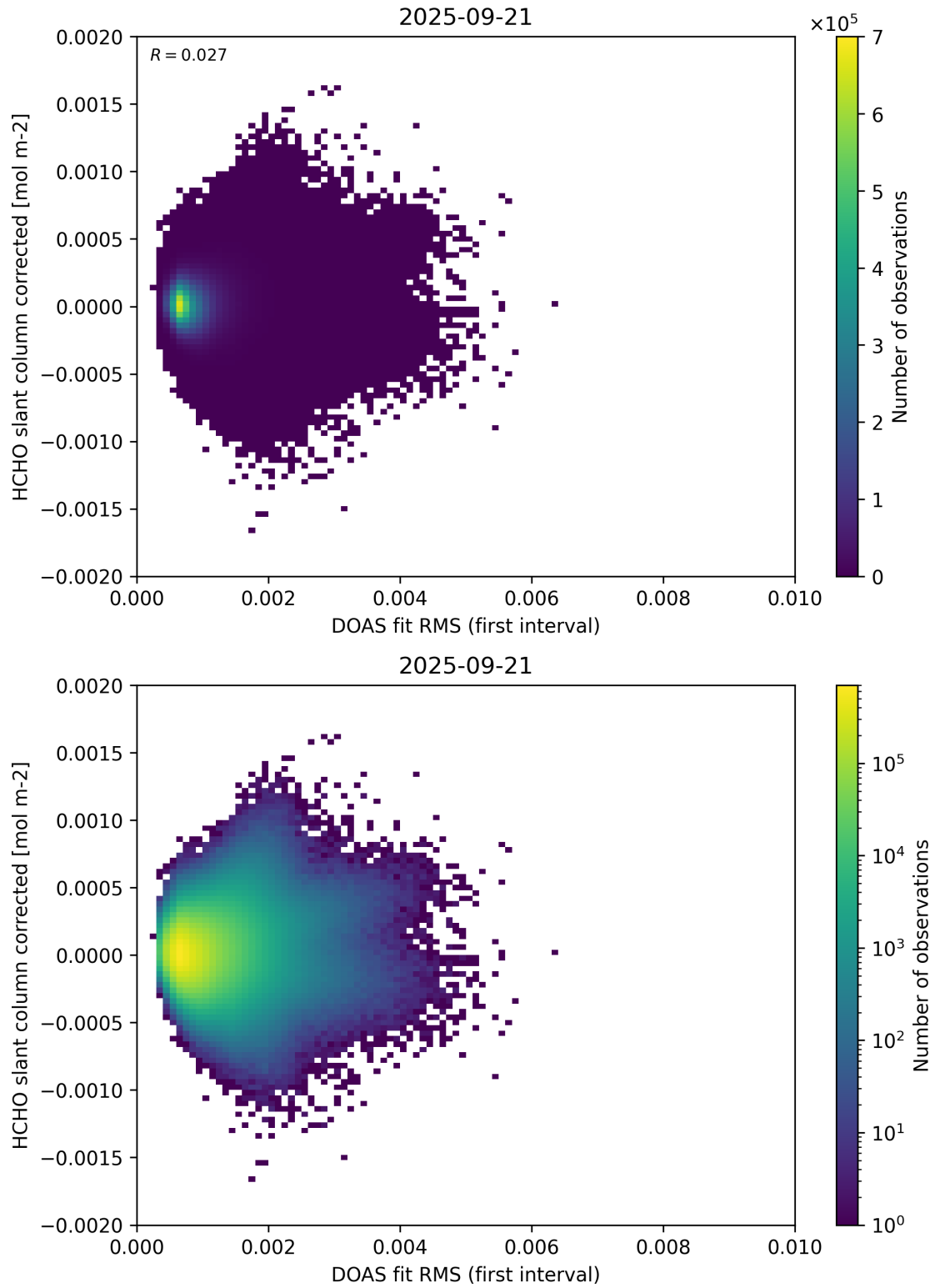
Figure 62: Scatter density plot of “DOAS fit RMS (first interval)” against “HCHO slant column corrected” for 2025-09-20 to 2025-09-22.
