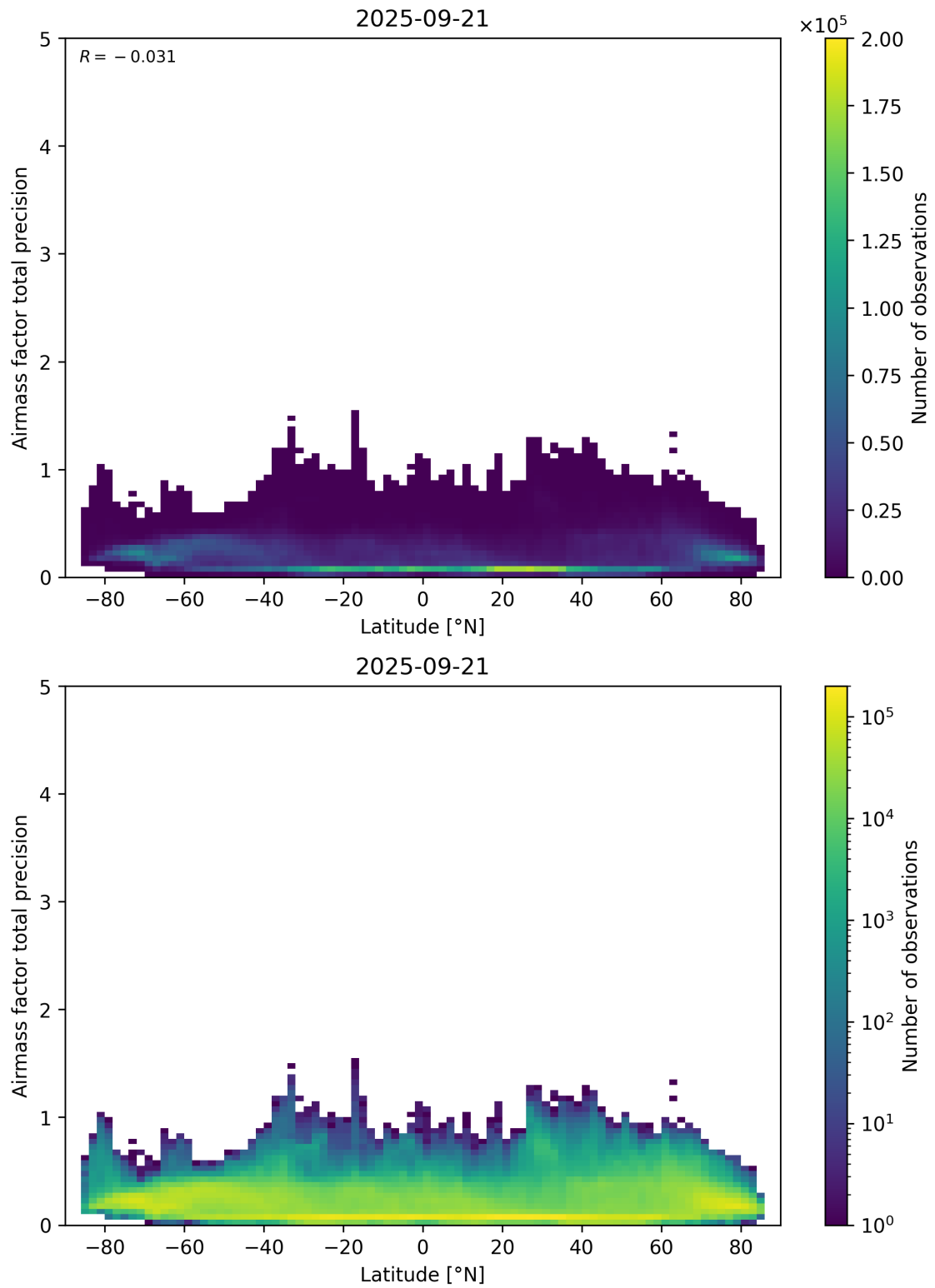
Figure 162: Scatter density plot of “Latitude” against “Airmass factor total precision” for 2025-09-20 to 2025-09-22.
