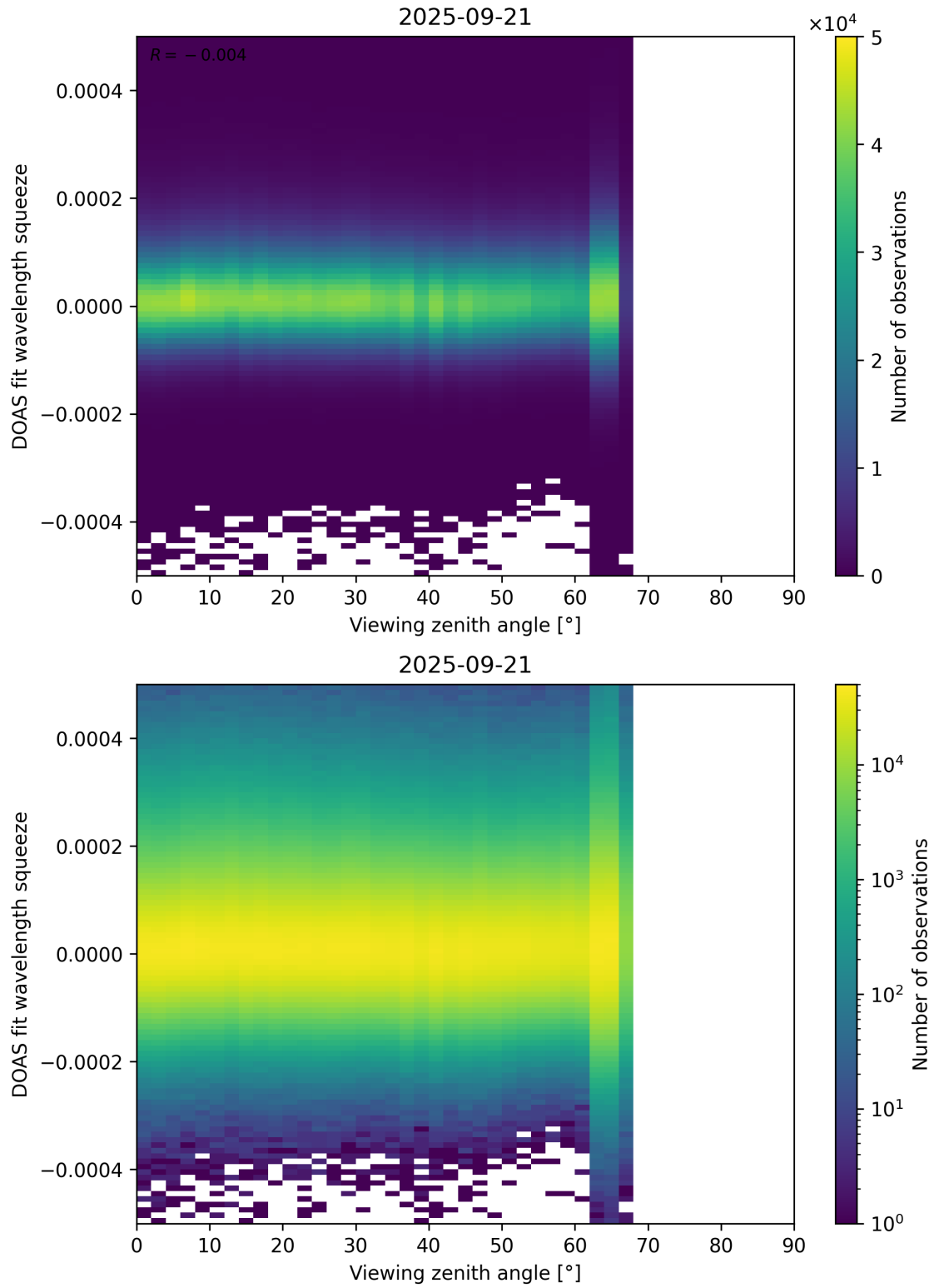
Figure 184: Scatter density plot of “Viewing zenith angle” against “DOAS fit wavelength squeeze” for 2025-09-20 to 2025-09-22.
