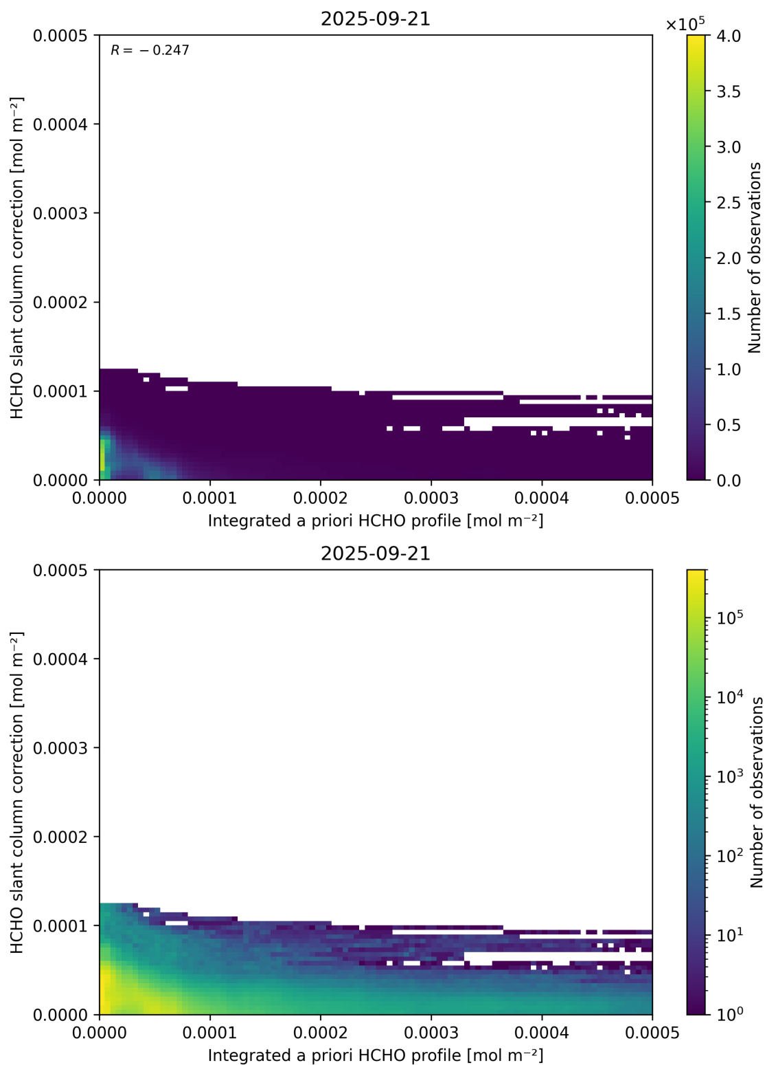
Figure 152: Scatter density plot of “Integrated a priori HCHO profile” against “HCHO slant column correction” for 2025-09-20 to 2025-09-22.
