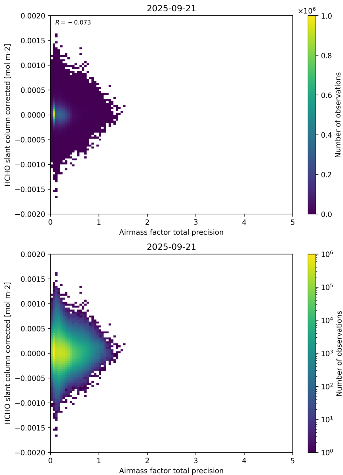
Figure 109: Scatter density plot of “Airmass factor total precision” against “HCHO slant column corrected” for 2025-09-20 to 2025-09-22.
