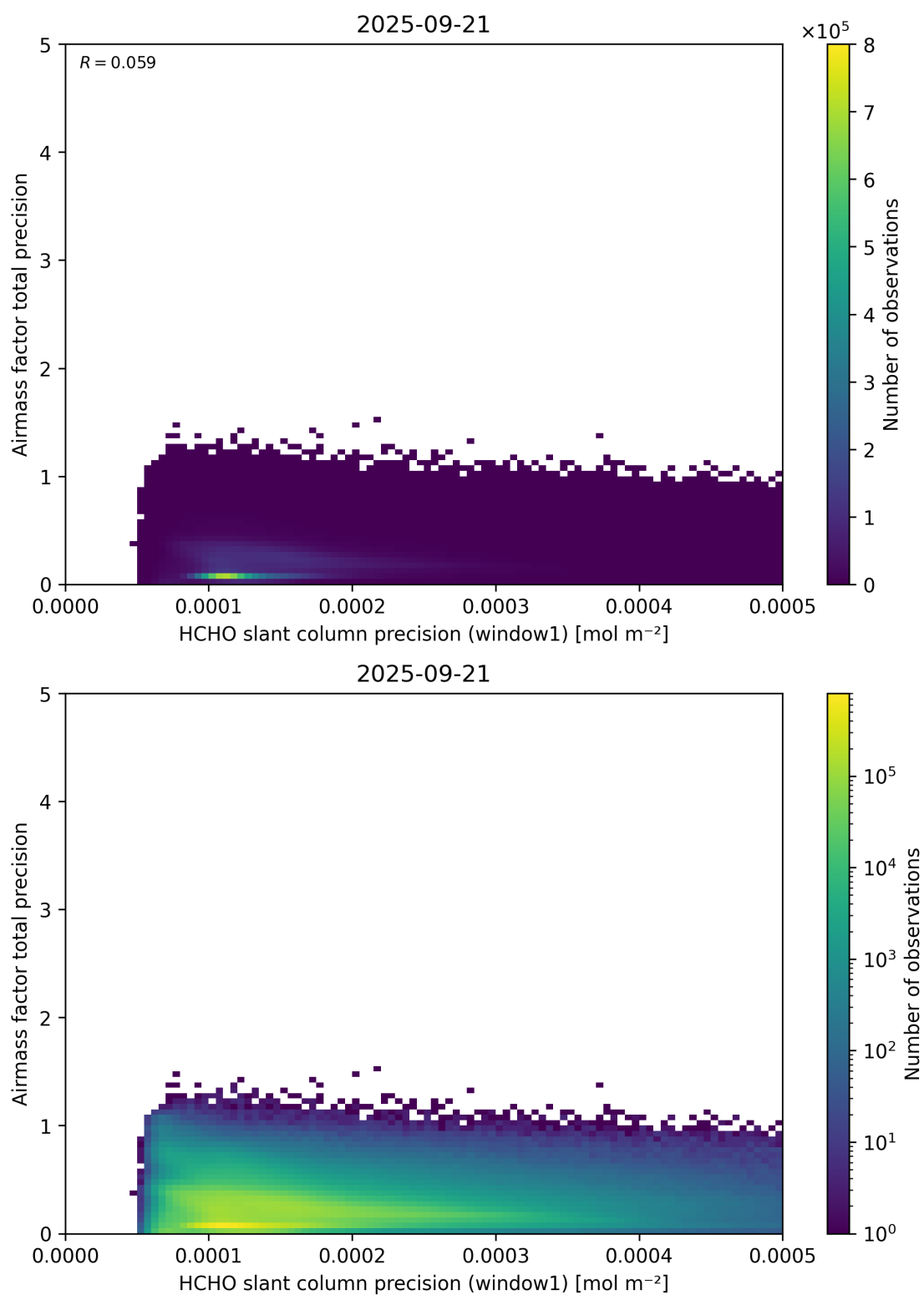
Figure 95: Scatter density plot of “HCHO slant column precision (window1)” against “Airmass factor total precision” for 2025-09-20 to 2025-09-22.
