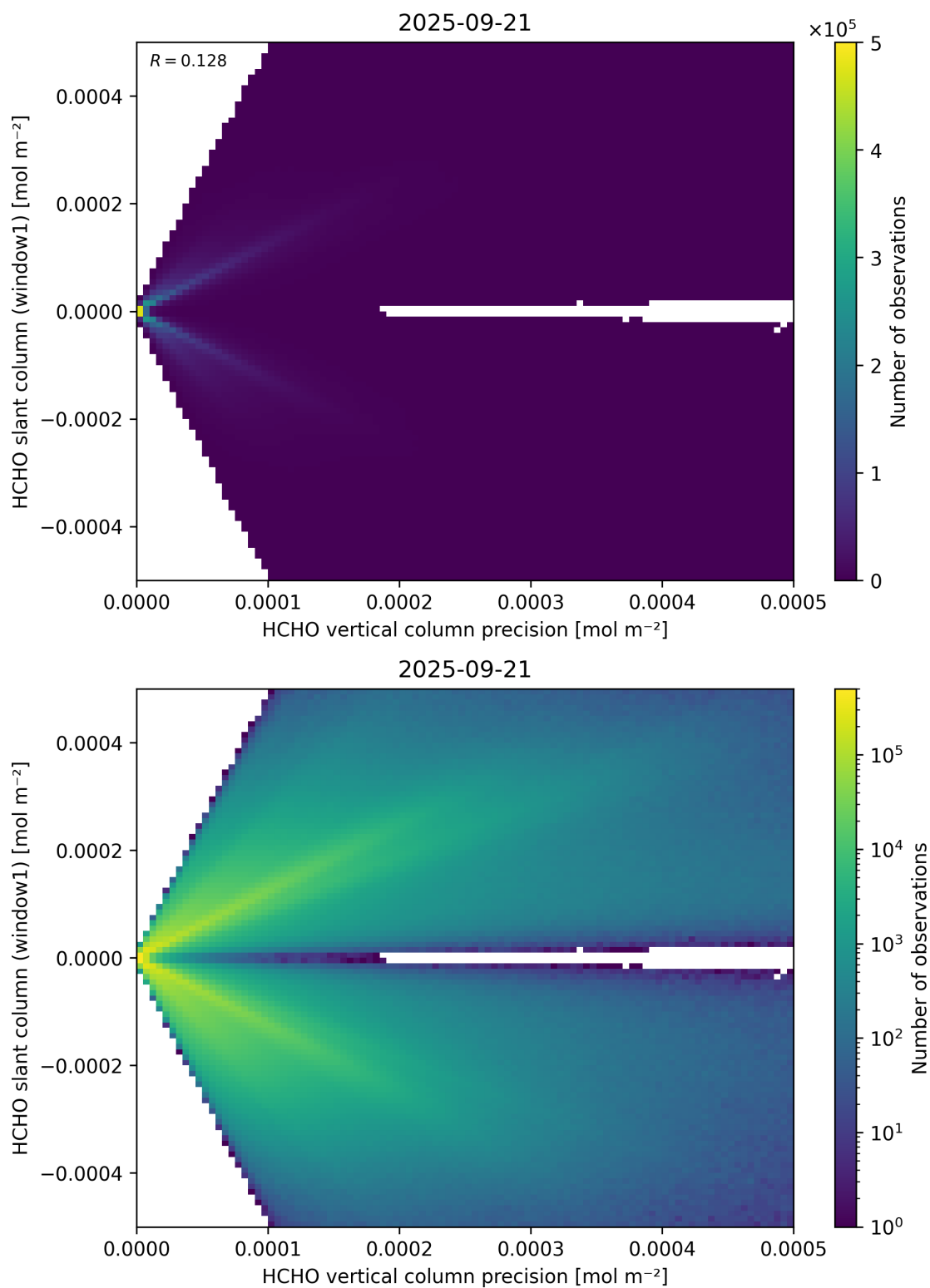
Figure 142: Scatter density plot of “HCHO vertical column precision” against “HCHO slant column (window1)” for 2025-09-20 to 2025-09-22.
