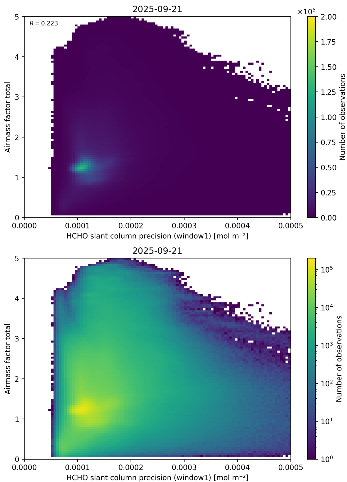
Figure 94: Scatter density plot of “HCHO slant column precision (window1)” against “Airmass factor total” for 2025-09-20 to 2025-09-22.
