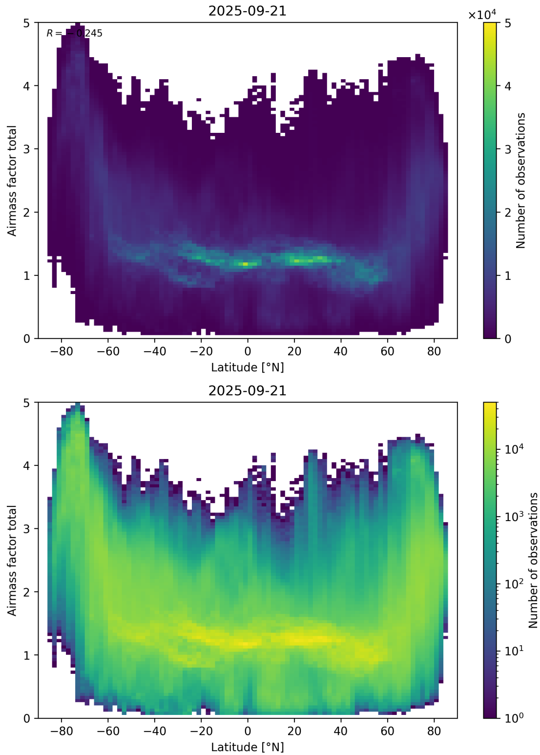
Figure 161: Scatter density plot of “Latitude” against “Airmass factor total” for 2025-09-20 to 2025-09-22.
