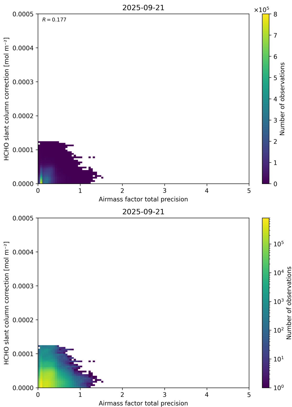
Figure 110: Scatter density plot of “Airmass factor total precision” against “HCHO slant column correction” for 2025-09-20 to 2025-09-22.
