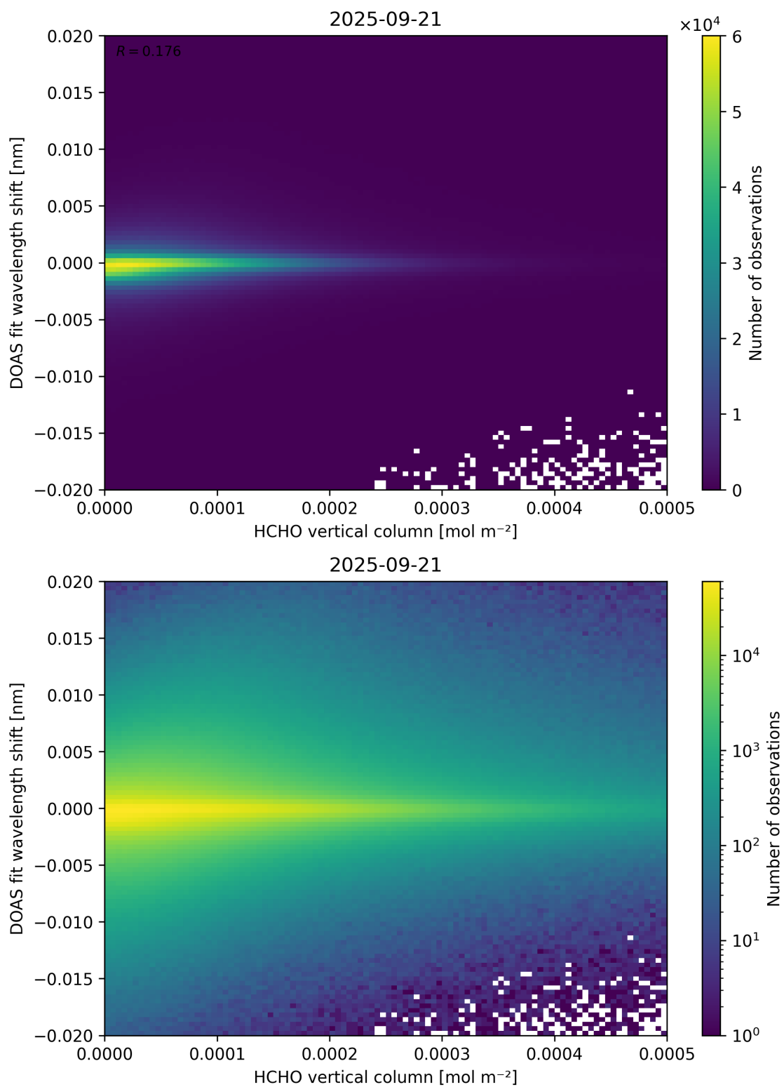
Figure 124: Scatter density plot of “HCHO vertical column” against “DOAS fit wavelength shift” for 2025-09-20 to 2025-09-22.
