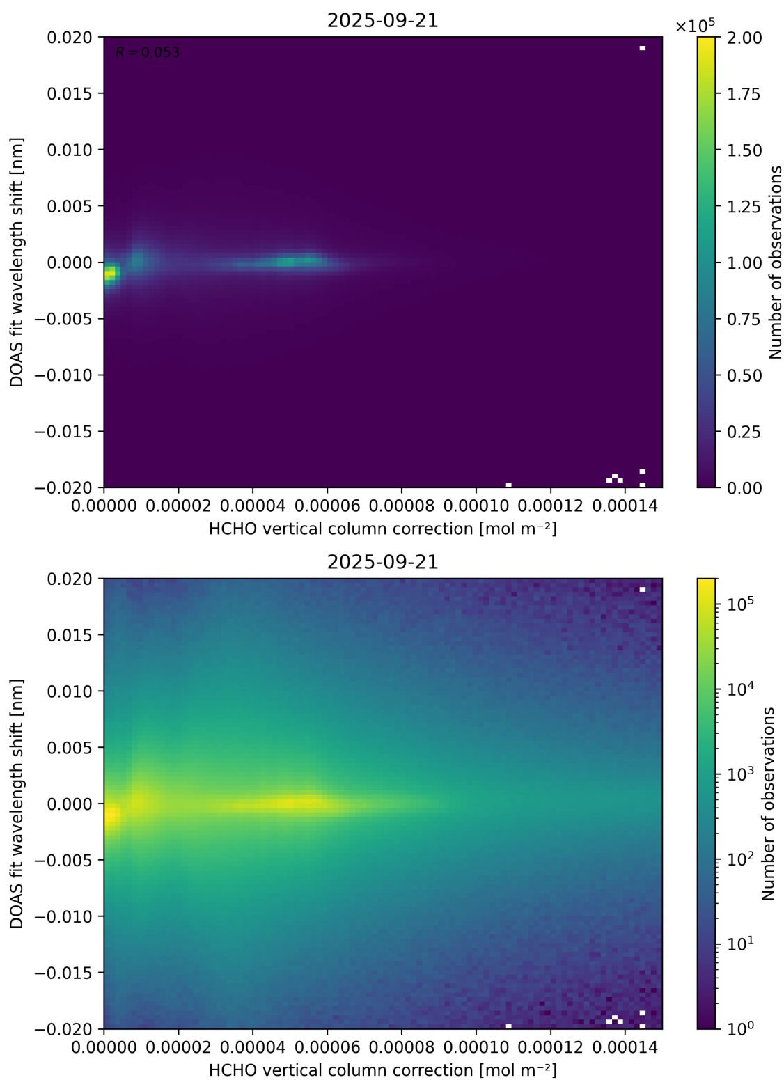
Figure 113: Scatter density plot of “HCHO vertical column correction” against “DOAS fit wavelength shift” for 2025-09-20 to 2025-09-22.
