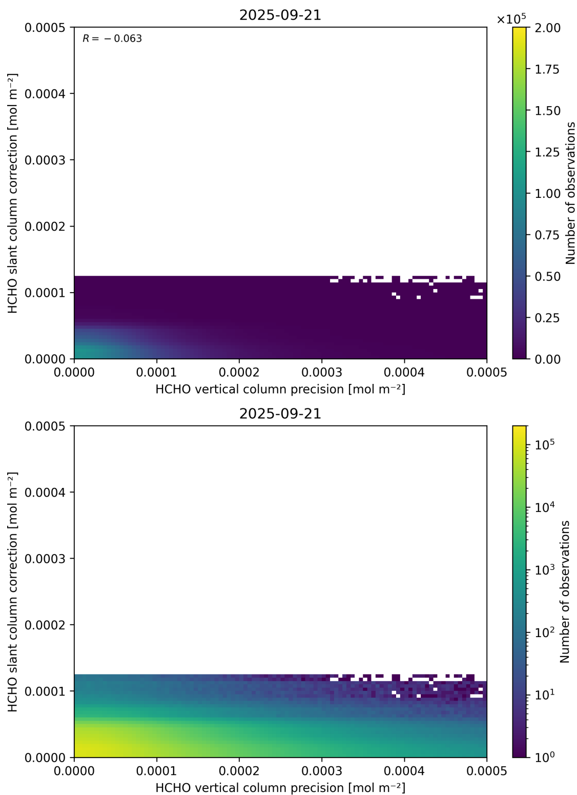
Figure 141: Scatter density plot of “HCHO vertical column precision” against “HCHO slant column correction” for 2025-09-20 to 2025-09-22.
