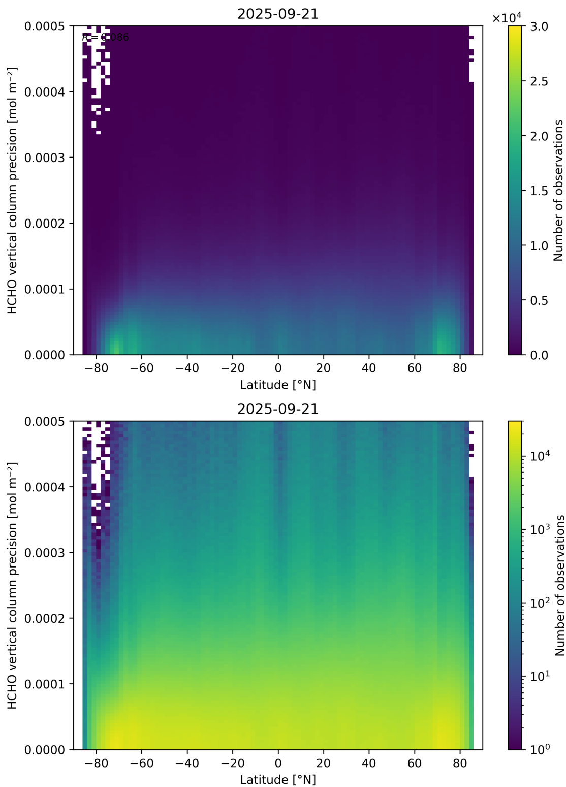
Figure 165: Scatter density plot of “Latitude” against “HCHO vertical column precision” for 2025-09-20 to 2025-09-22.
