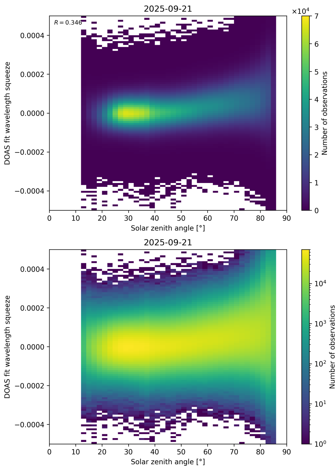
Figure 169: Scatter density plot of “Solar zenith angle” against “DOAS fit wavelength squeeze” for 2025-09-20 to 2025-09-22.
