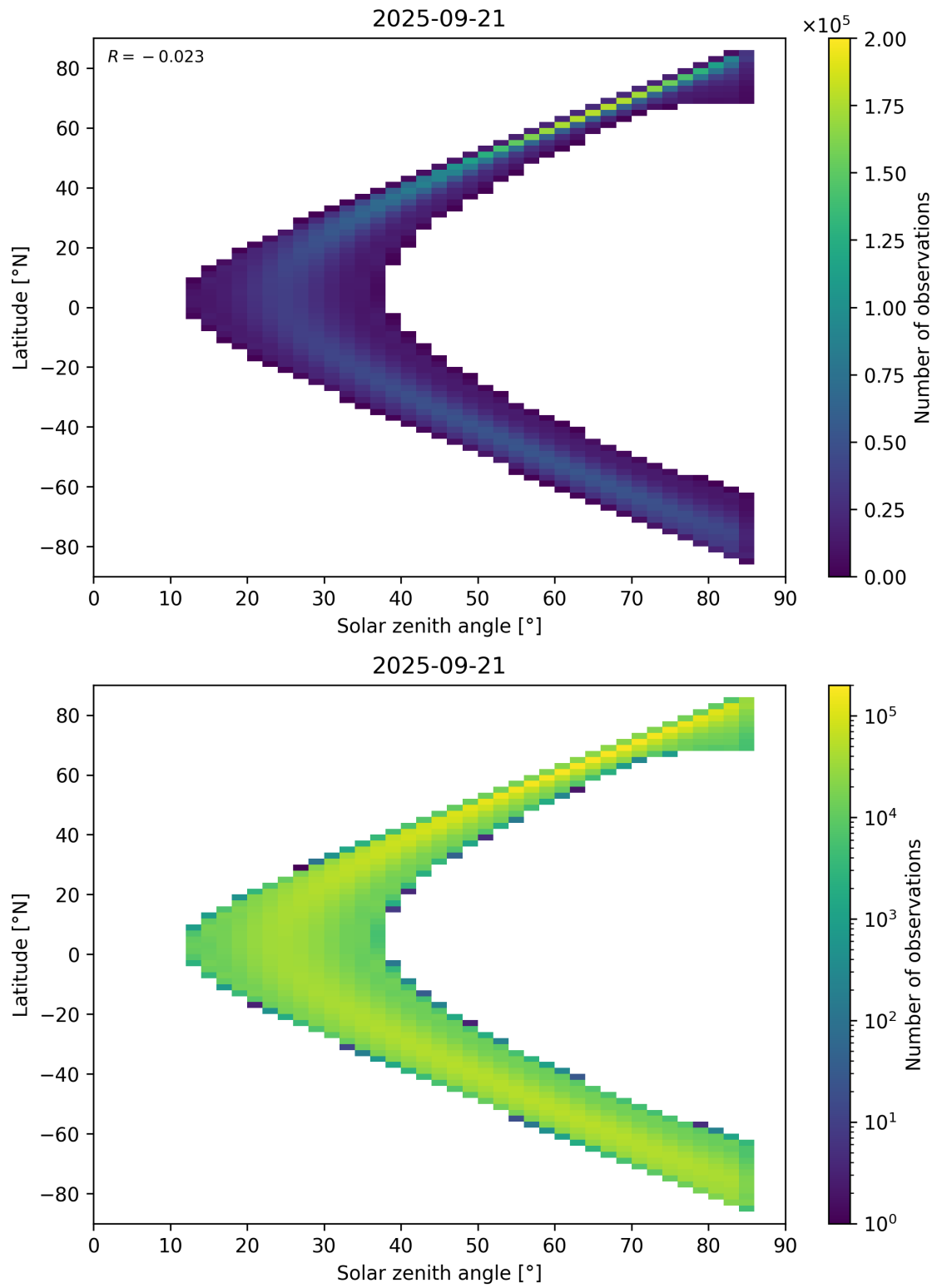
Figure 181: Scatter density plot of “Solar zenith angle” against “Latitude” for 2025-09-20 to 2025-09-22.
