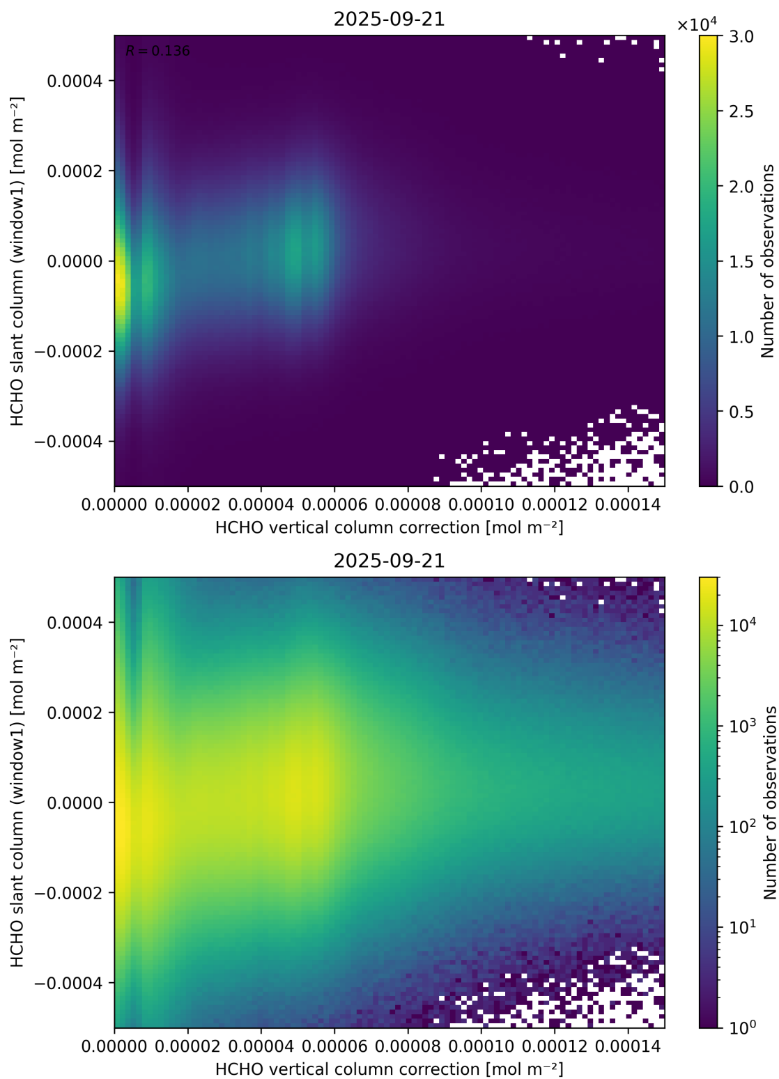
Figure 118: Scatter density plot of “HCHO vertical column correction” against “HCHO slant column (window1)” for 2025-09-20 to 2025-09-22.
