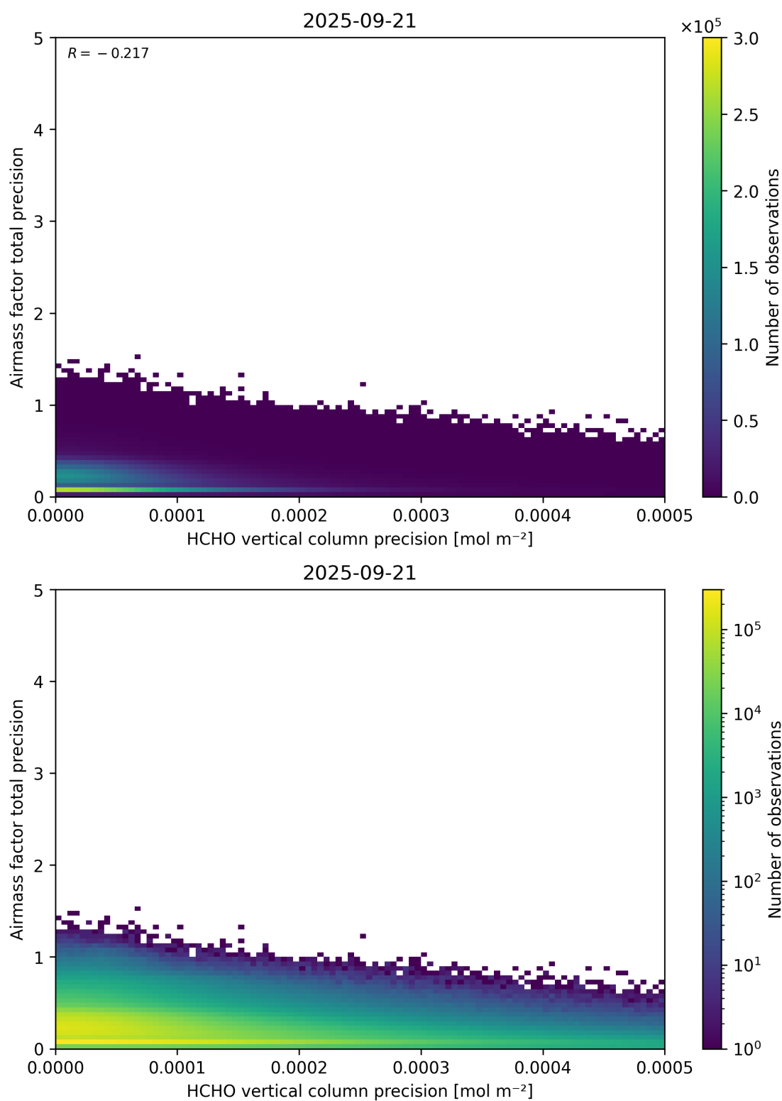
Figure 145: Scatter density plot of “HCHO vertical column precision” against “Airmass factor total precision” for 2025-09-20 to 2025-09-22.
