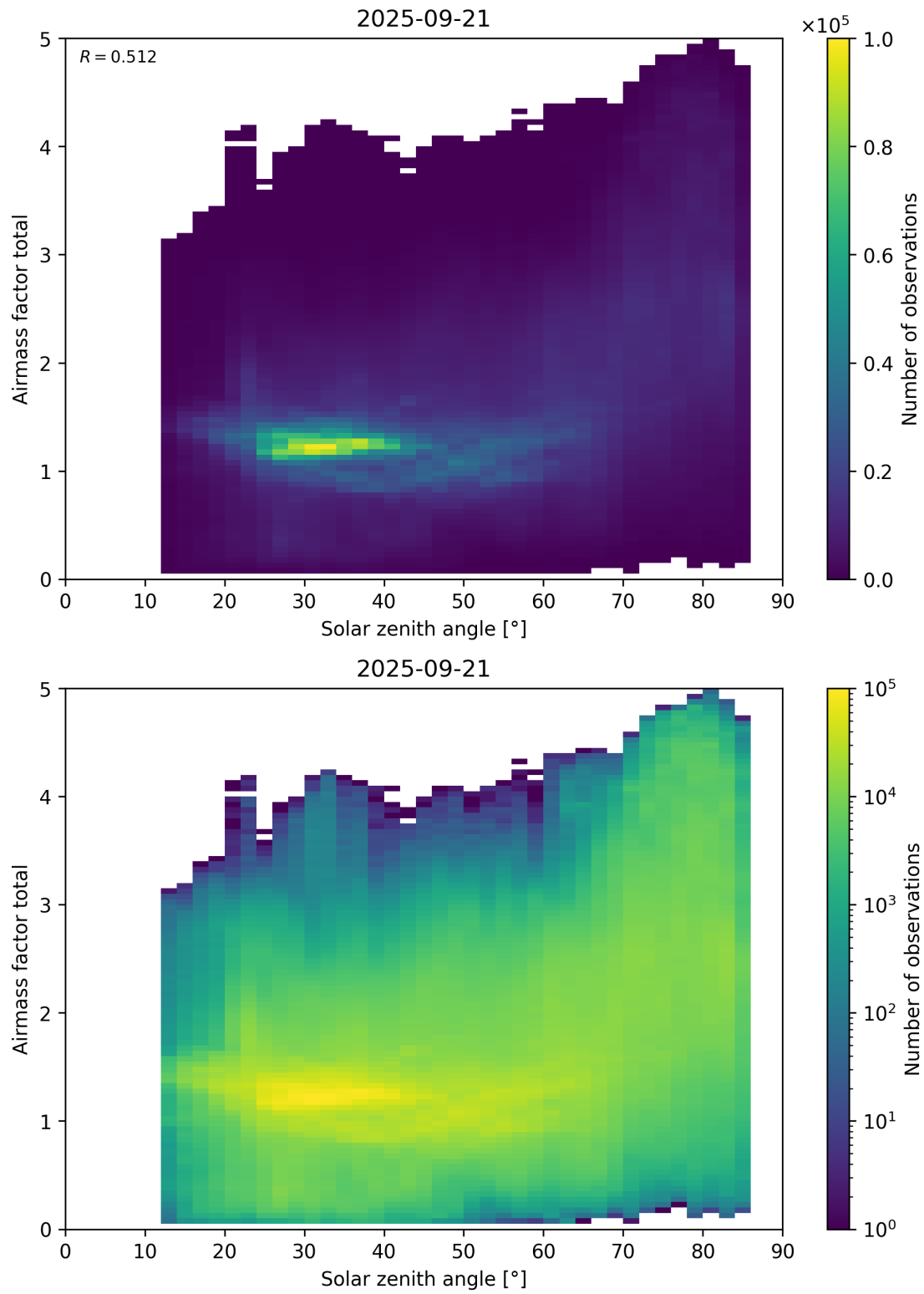
Figure 175: Scatter density plot of “Solar zenith angle” against “Airmass factor total” for 2025-09-20 to 2025-09-22.
