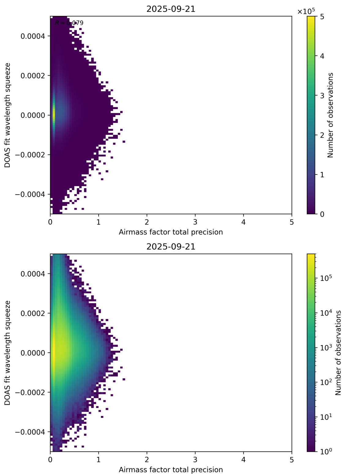
Figure 107: Scatter density plot of “Airmass factor total precision” against “DOAS fit wavelength squeeze” for 2025-09-20 to 2025-09-22.
