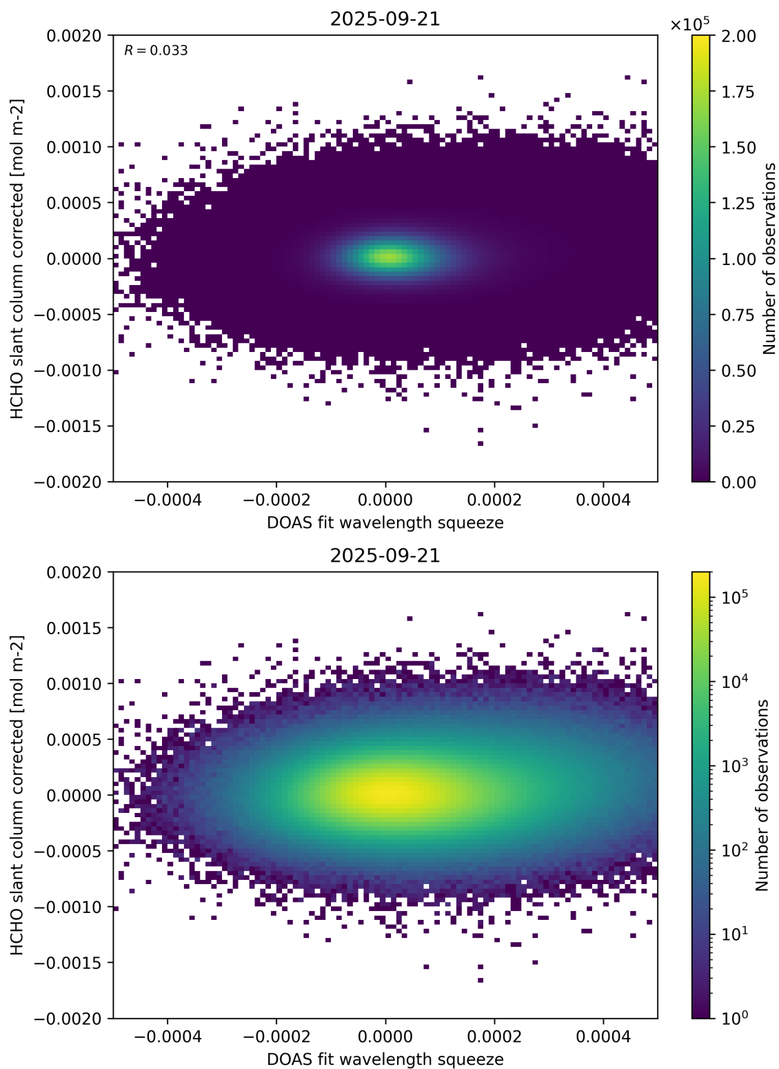
Figure 69: Scatter density plot of “DOAS fit wavelength squeeze” against “HCHO slant column corrected” for 2025-09-20 to 2025-09-22.
