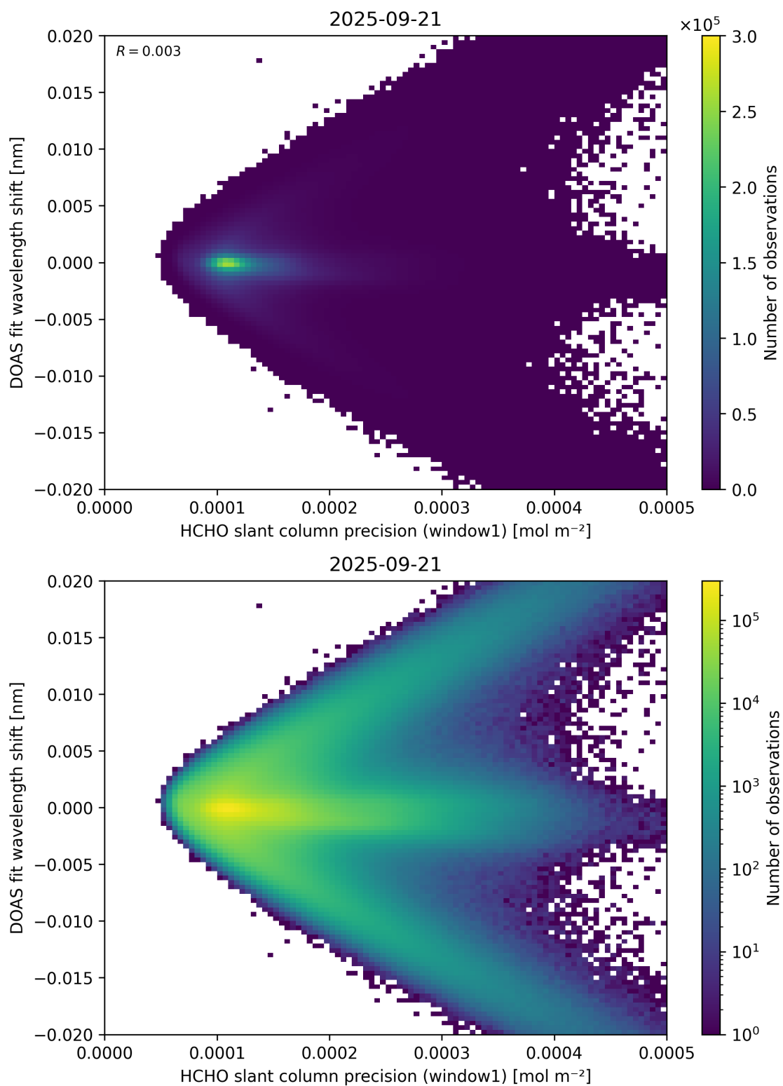
Figure 89: Scatter density plot of “HCHO slant column precision (window1)” against “DOAS fit wavelength shift” for 2025-09-20 to 2025-09-22.
