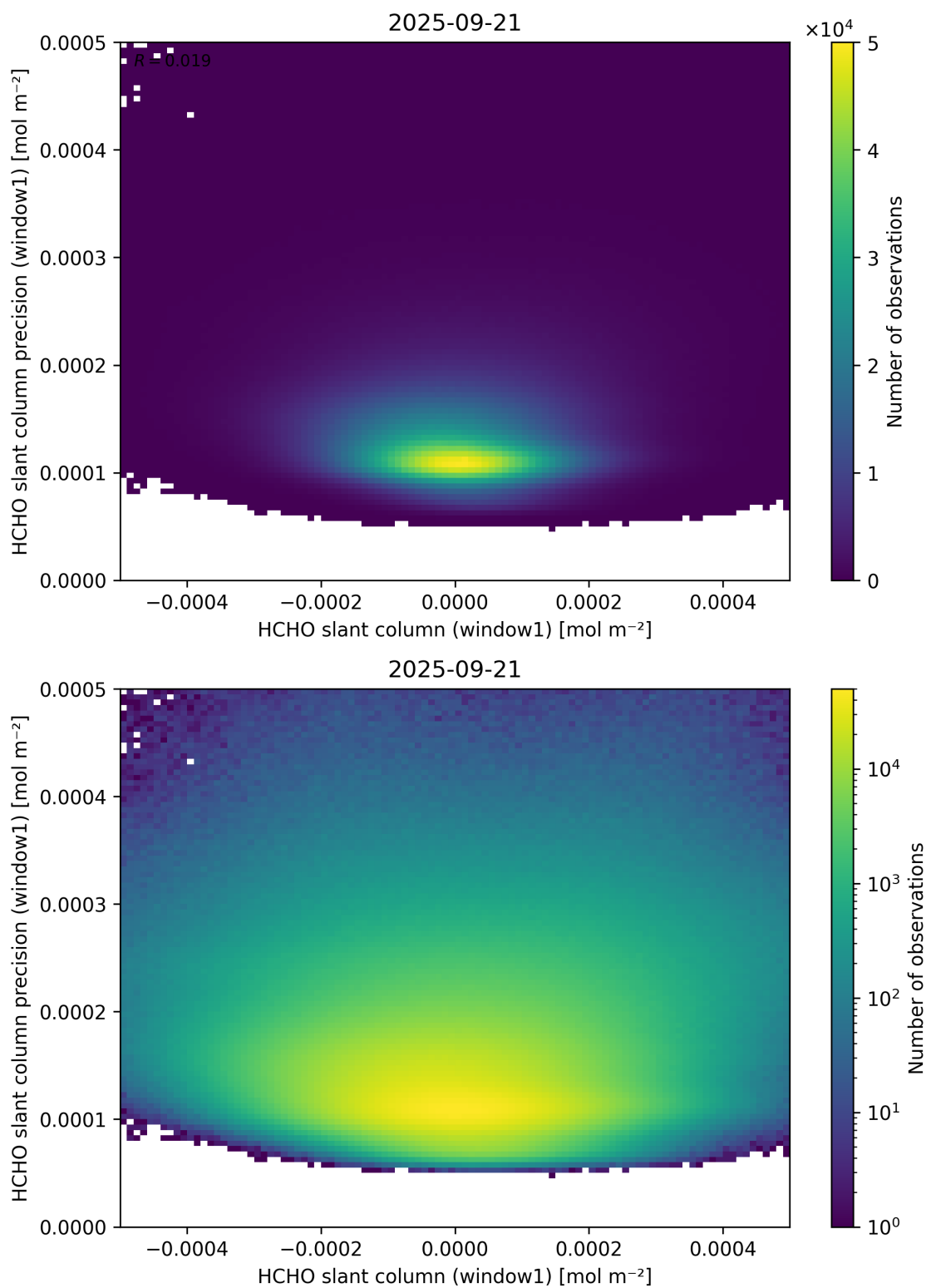
Figure 84: Scatter density plot of “HCHO slant column (window1)” against “HCHO slant column precision (window1)” for 2025-09-20 to 2025-09-22.
