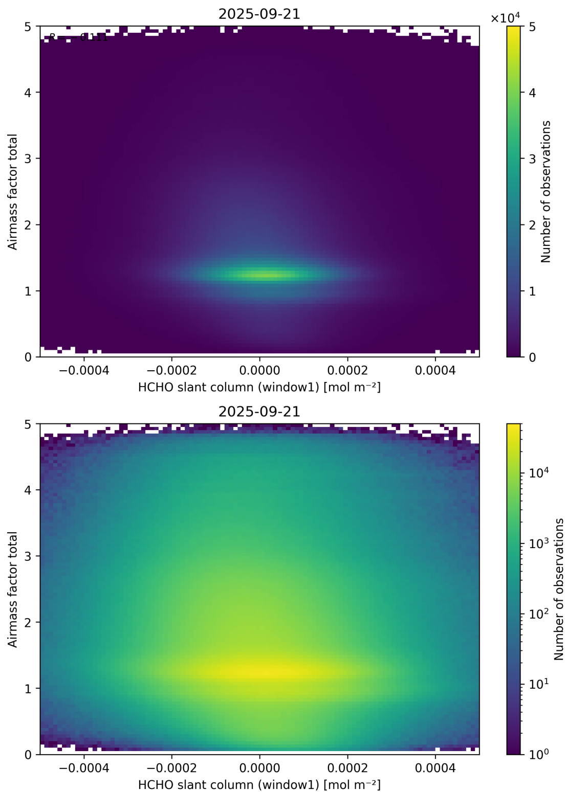
Figure 85: Scatter density plot of “HCHO slant column (window1)” against “Airmass factor total” for 2025-09-20 to 2025-09-22.
