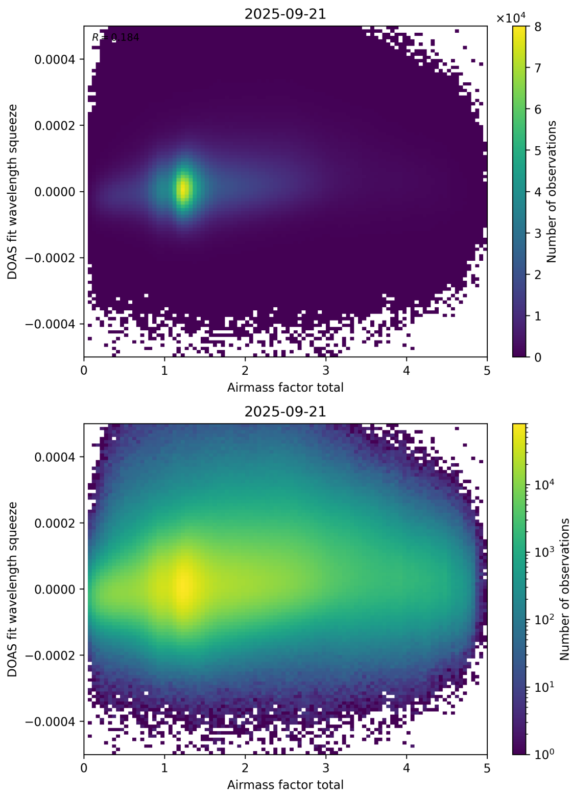
Figure 99: Scatter density plot of “Airmass factor total” against “DOAS fit wavelength squeeze” for 2025-09-20 to 2025-09-22.
