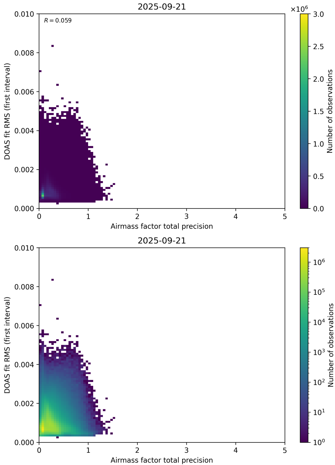
Figure 105: Scatter density plot of “Airmass factor total precision” against “DOAS fit RMS (first interval)” for 2025-09-20 to 2025-09-22.
