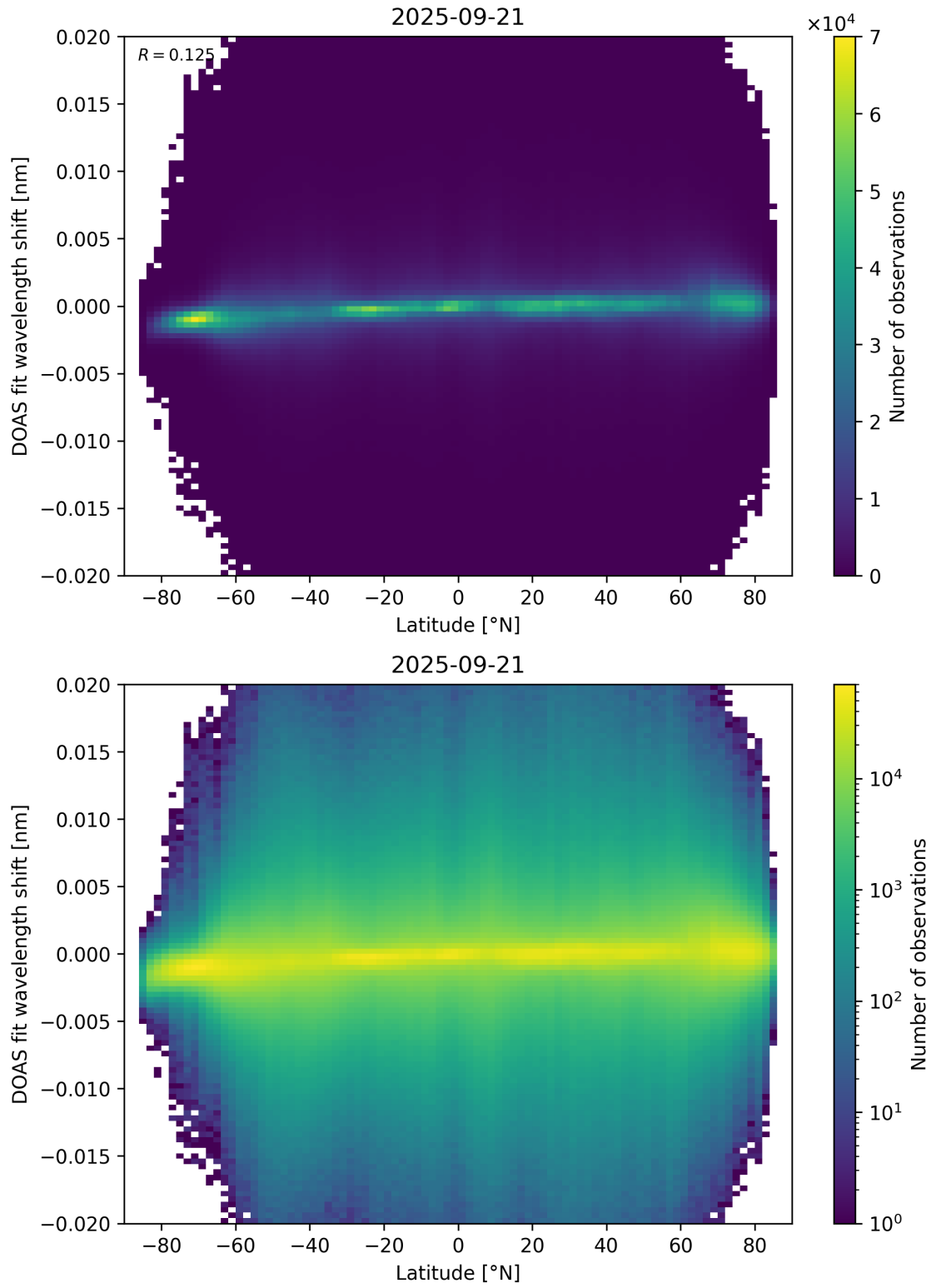
Figure 154: Scatter density plot of “Latitude” against “DOAS fit wavelength shift” for 2025-09-20 to 2025-09-22.
