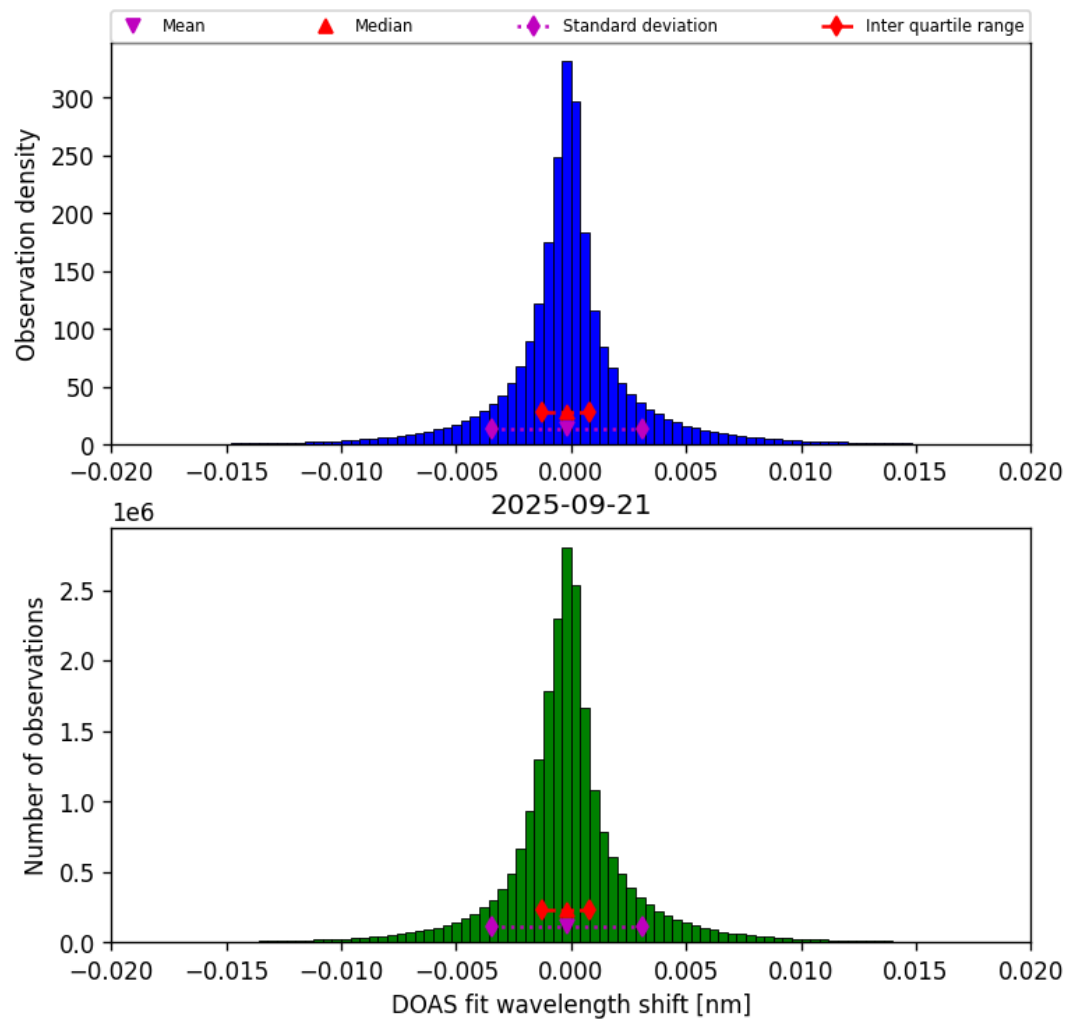
Figure 44: Histogram of “DOAS fit wavelength shift” for 2025-09-20 to 2025-09-22
