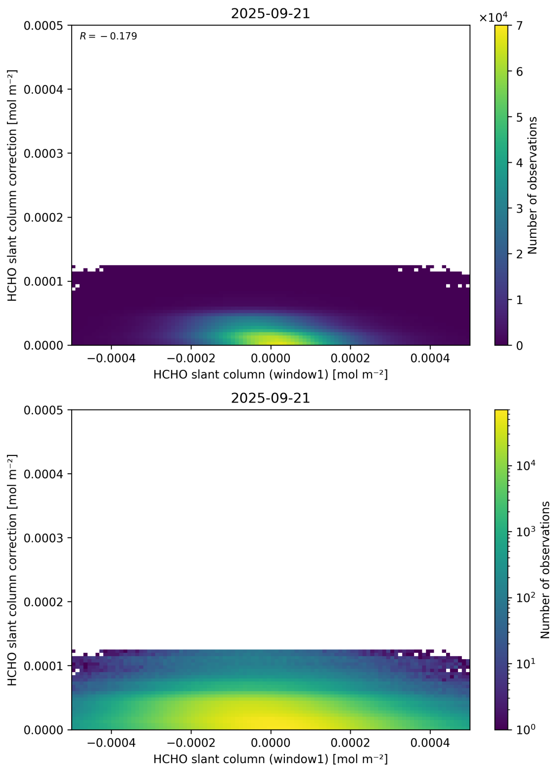
Figure 83: Scatter density plot of “HCHO slant column (window1)” against “HCHO slant column correction” for 2025-09-20 to 2025-09-22.
