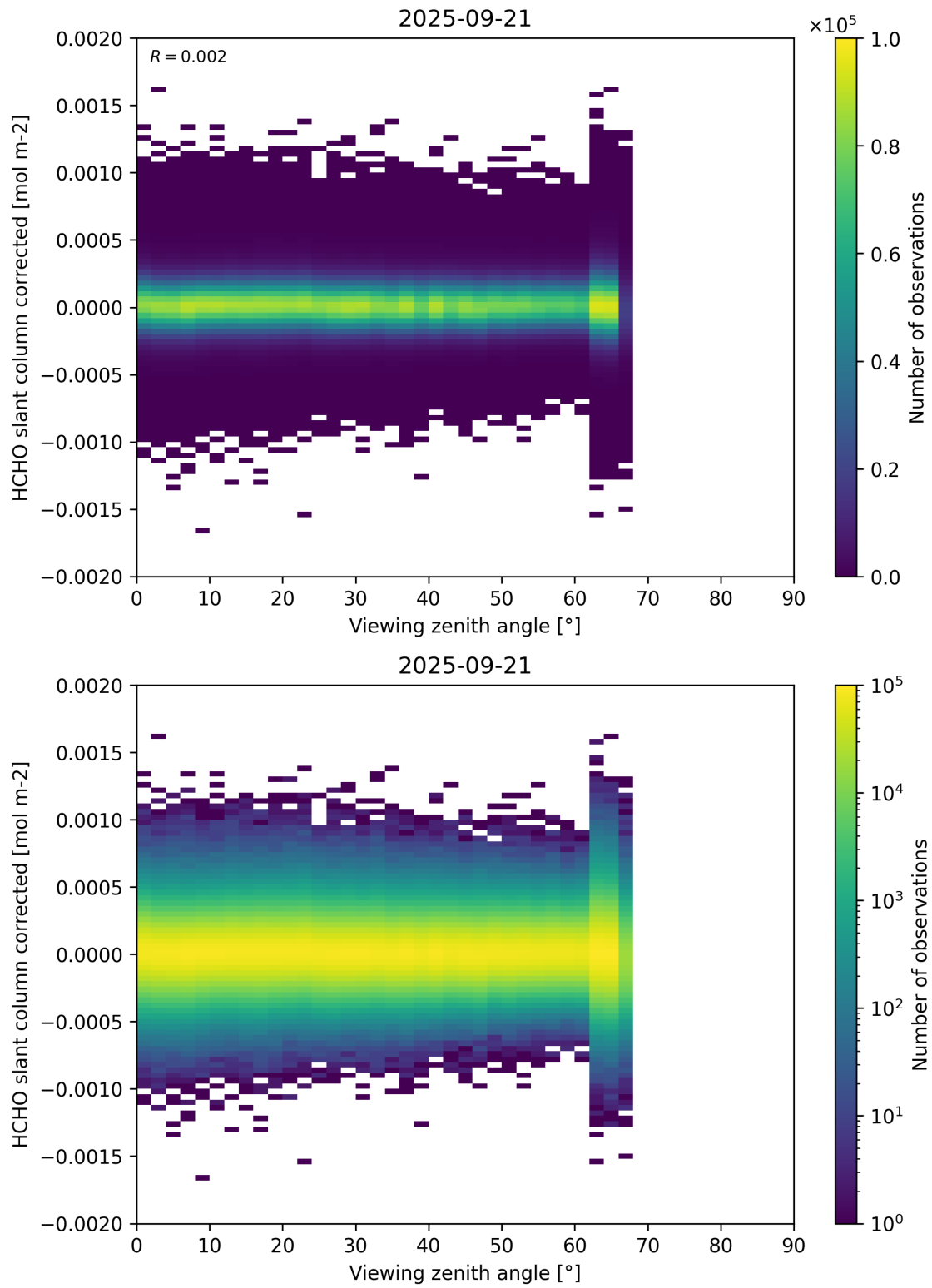
Figure 186: Scatter density plot of “Viewing zenith angle” against “HCHO slant column corrected” for 2025-09-20 to 2025-09-22.
