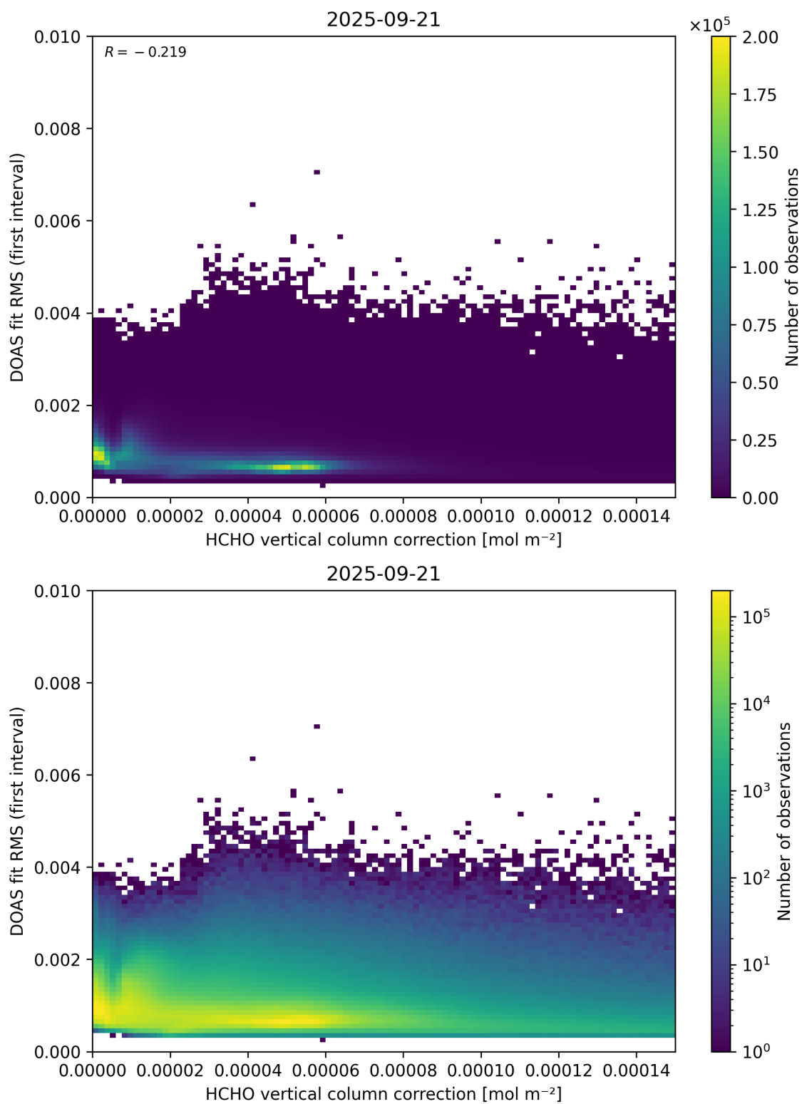
Figure 112: Scatter density plot of “HCHO vertical column correction” against “DOAS fit RMS (first interval)” for 2025-09-20 to 2025-09-22.
