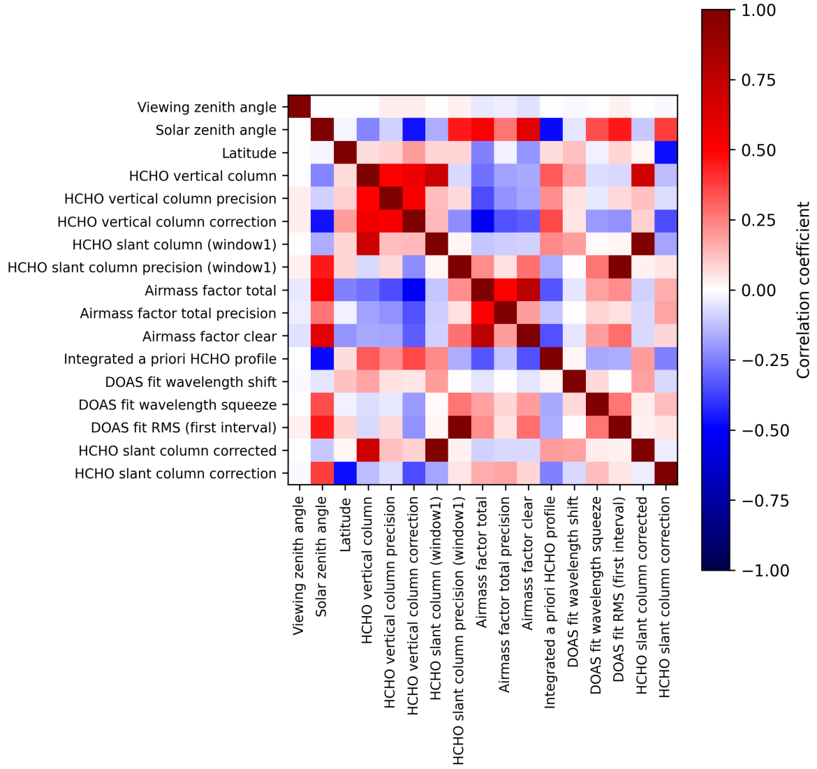
Figure 2: Map of correlation matrix for 2025-09-20 to 2025-09-22.
