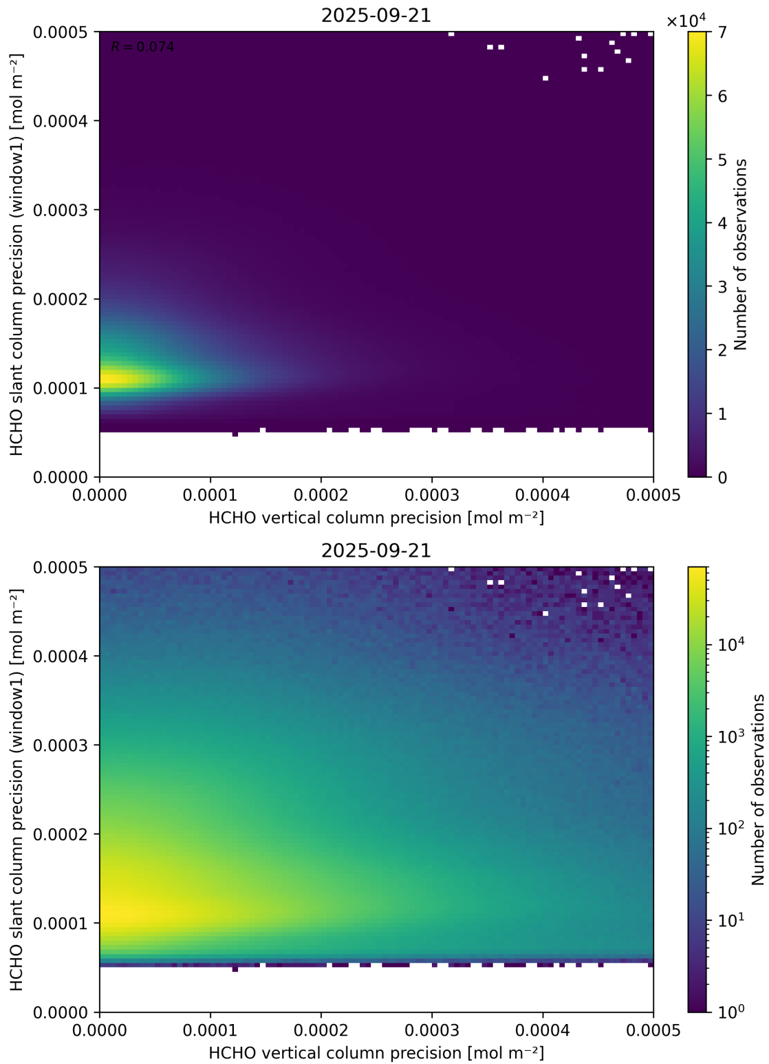
Figure 143: Scatter density plot of “HCHO vertical column precision” against “HCHO slant column precision (window1)” for 2025-09-20 to 2025-09-22.
