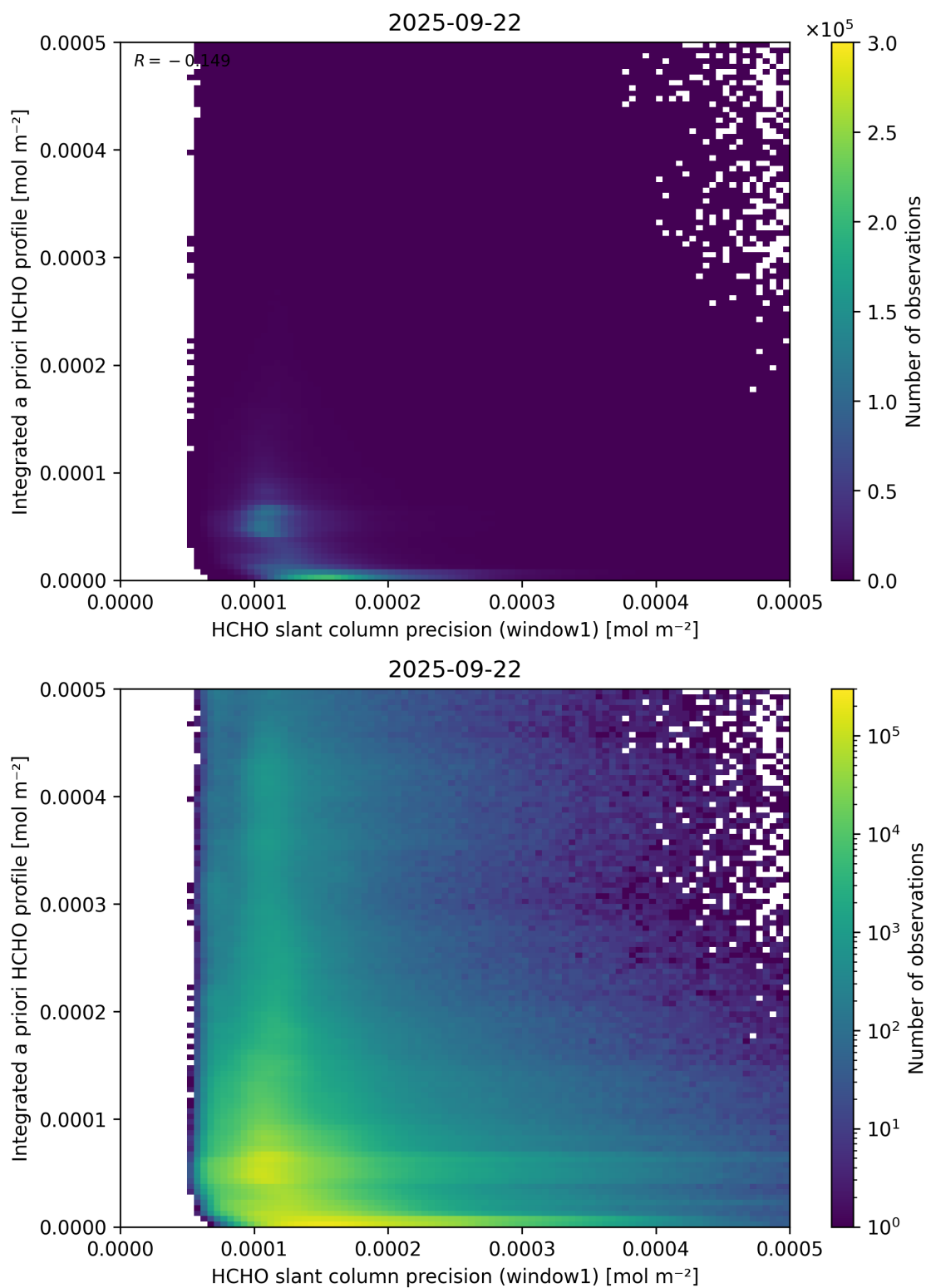
Figure 96: Scatter density plot of “HCHO slant column precision (window1)” against “Integrated a priori HCHO profile” for 2025-09-22 to 2025-09-23.
