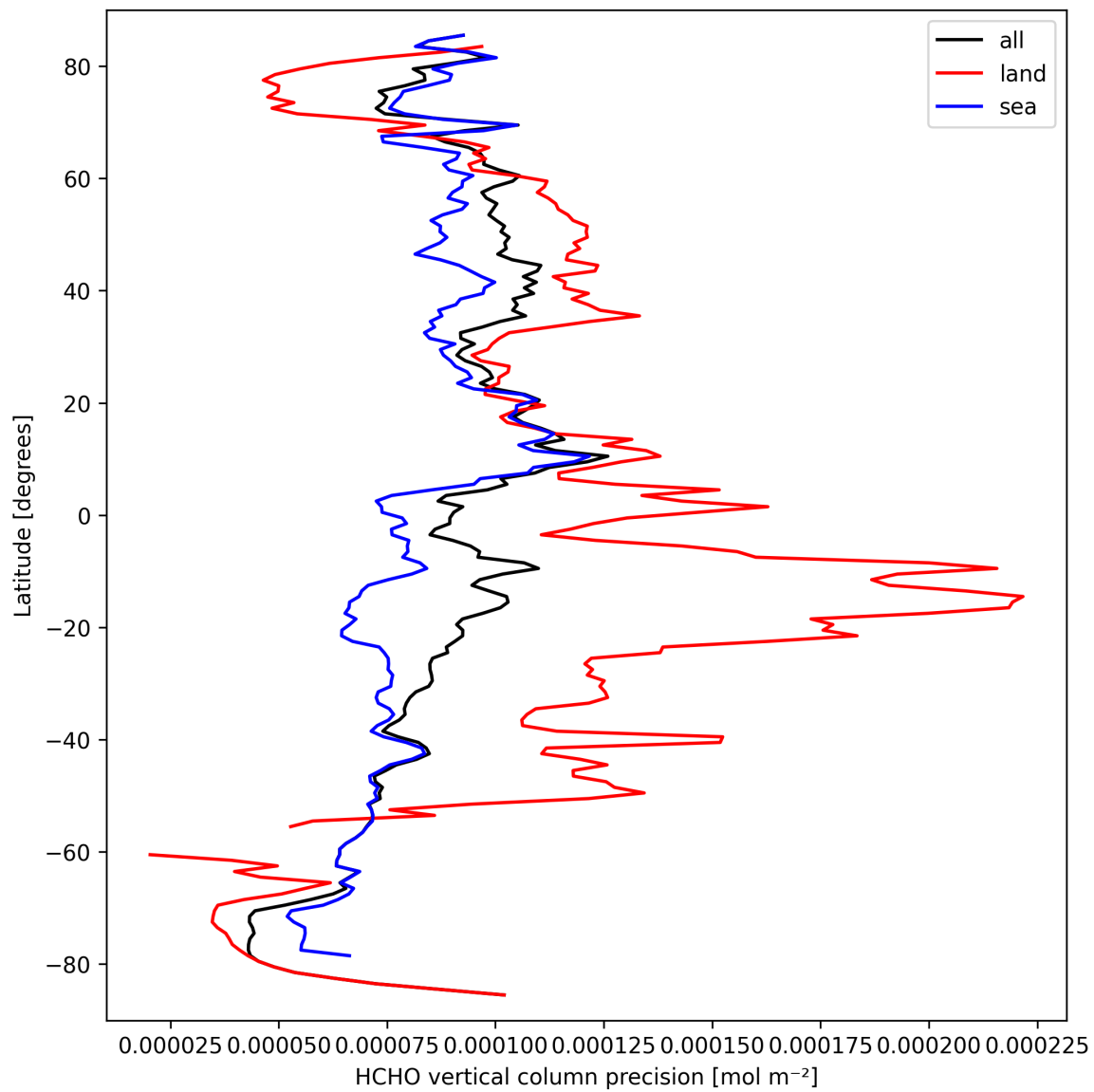
Figure 22: Zonal average of “HCHO vertical column precision” for 2025-09-22 to 2025-09-23.
