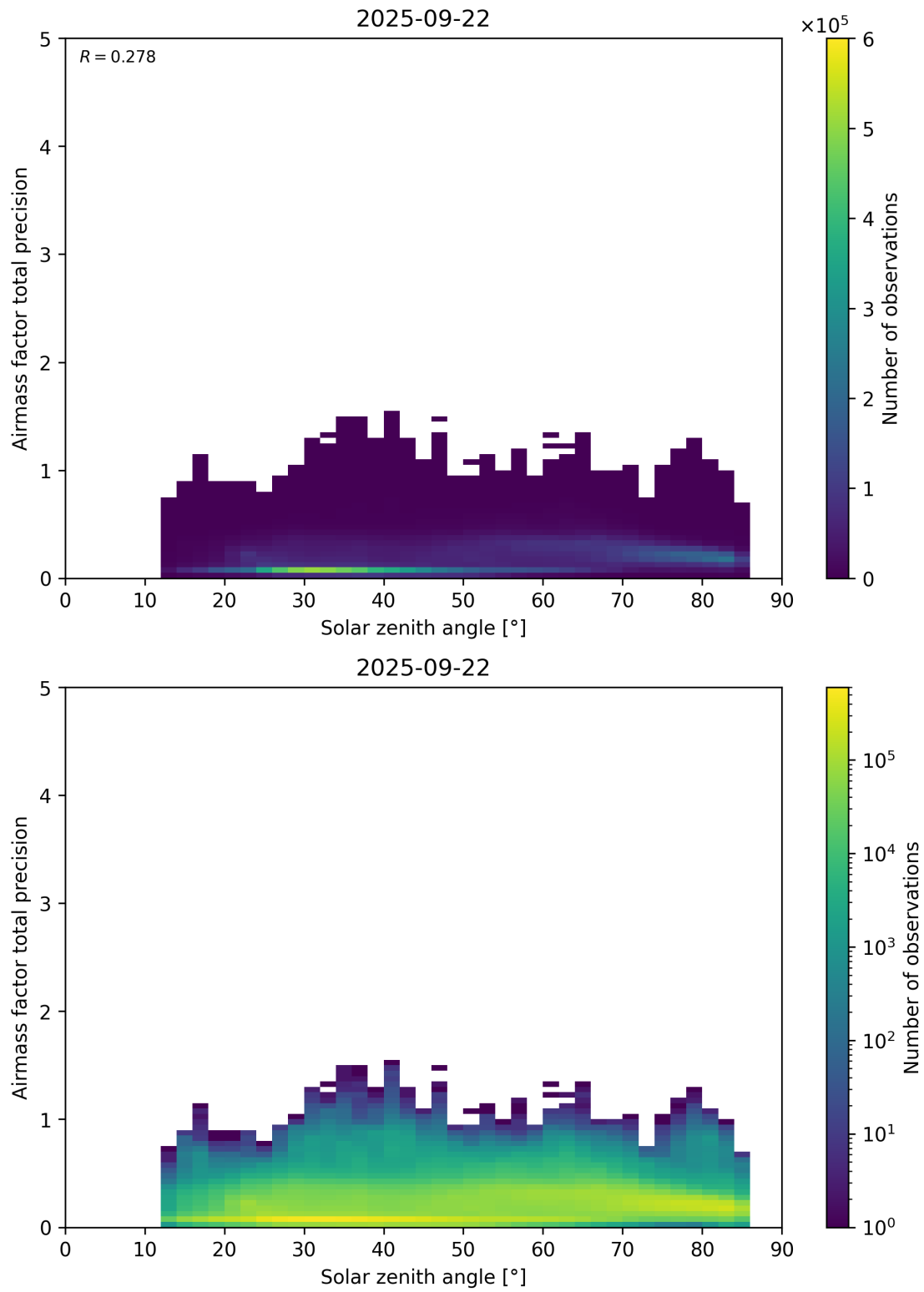
Figure 176: Scatter density plot of “Solar zenith angle” against “Airmass factor total precision” for 2025-09-22 to 2025-09-23.
