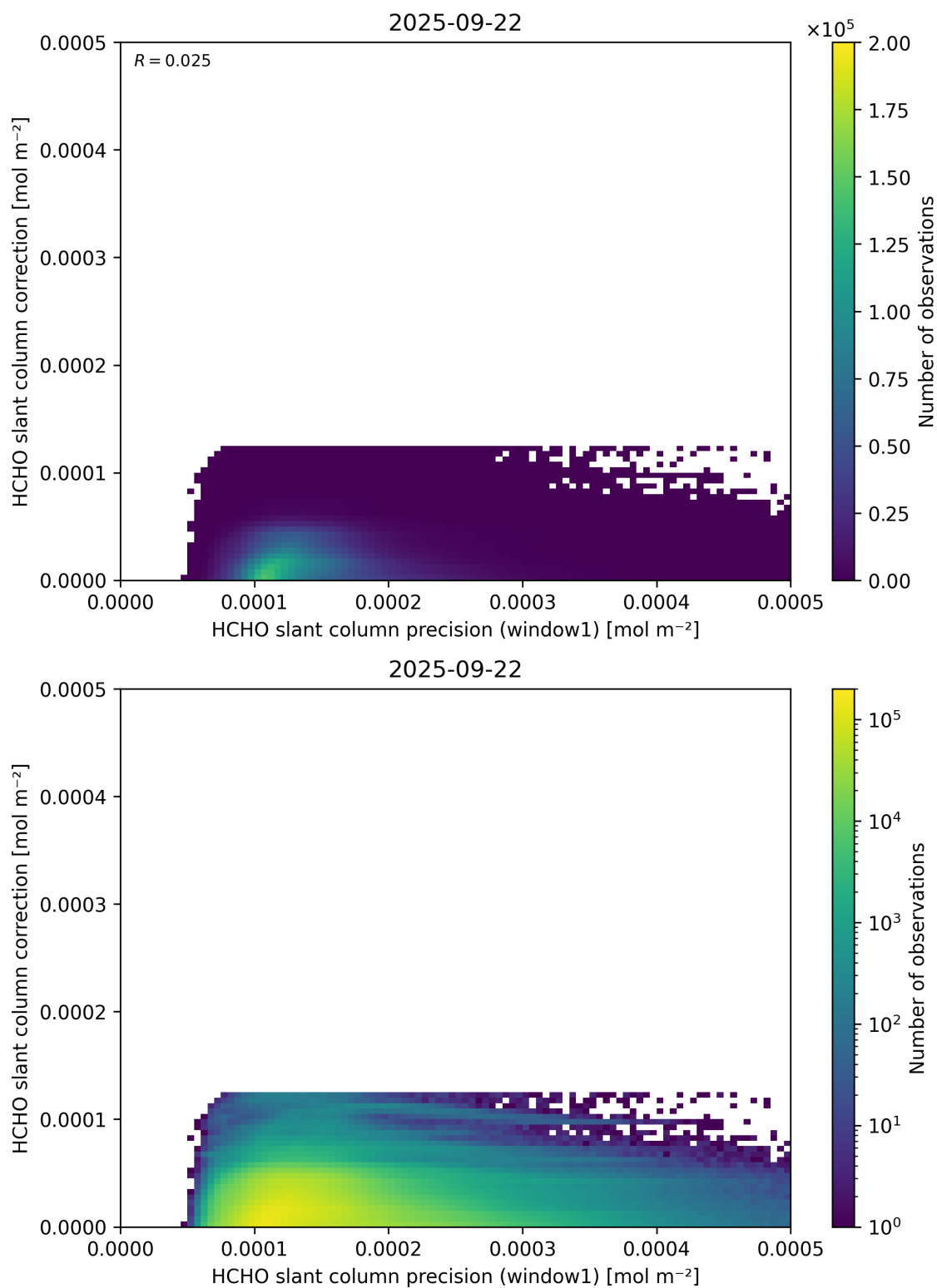
Figure 93: Scatter density plot of “HCHO slant column precision (window1)” against “HCHO slant column correction” for 2025-09-22 to 2025-09-23.
