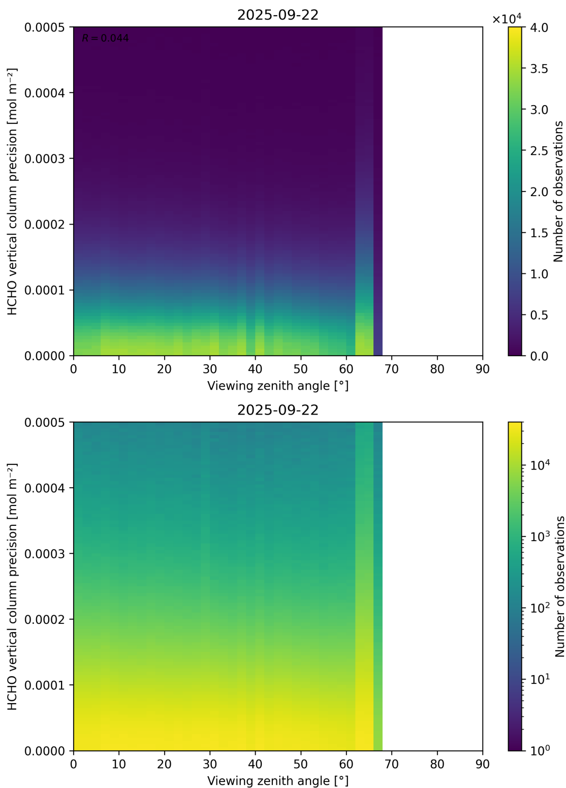
Figure 194: Scatter density plot of “Viewing zenith angle” against “HCHO vertical column precision” for 2025-09-22 to 2025-09-23.
