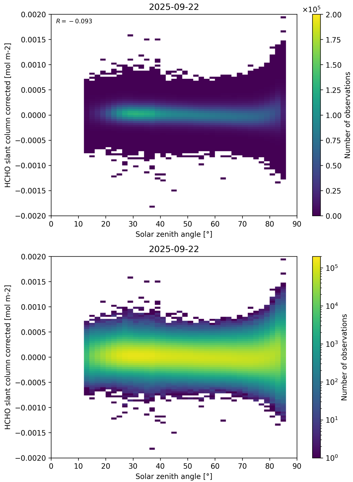
Figure 171: Scatter density plot of “Solar zenith angle” against “HCHO slant column corrected” for 2025-09-22 to 2025-09-23.
