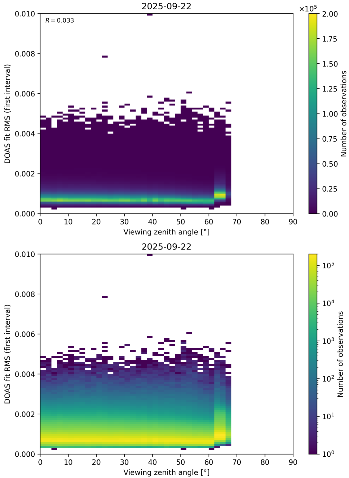
Figure 182: Scatter density plot of “Viewing zenith angle” against “DOAS fit RMS (first interval)” for 2025-09-22 to 2025-09-23.
