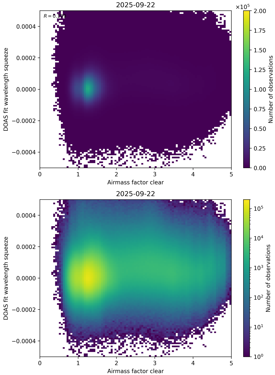
Figure 73: Scatter density plot of “Airmass factor clear” against “DOAS fit wavelength squeeze” for 2025-09-22 to 2025-09-23.
