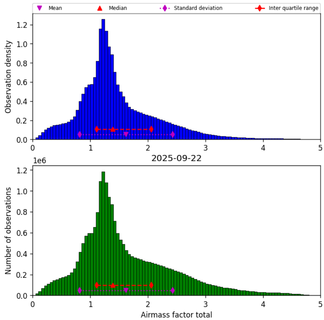
Figure 40: Histogram of “Airmass factor total” for 2025-09-22 to 2025-09-23
