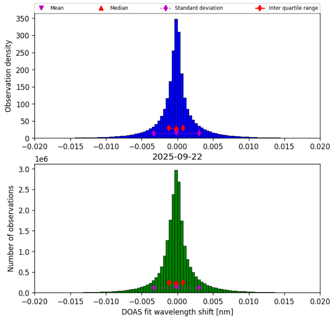
Figure 44: Histogram of “DOAS fit wavelength shift” for 2025-09-22 to 2025-09-23
