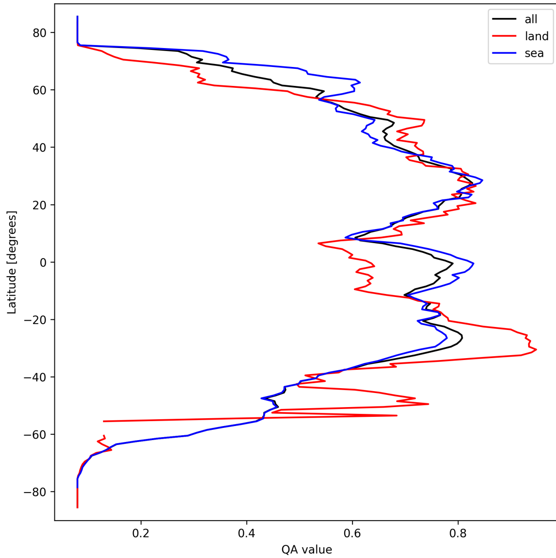
Figure 20: Zonal average of “QA value” for 2025-09-22 to 2025-09-23.
