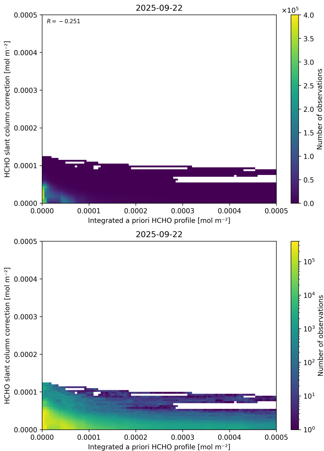
Figure 152: Scatter density plot of “Integrated a priori HCHO profile” against “HCHO slant column correction” for 2025-09-22 to 2025-09-23.
