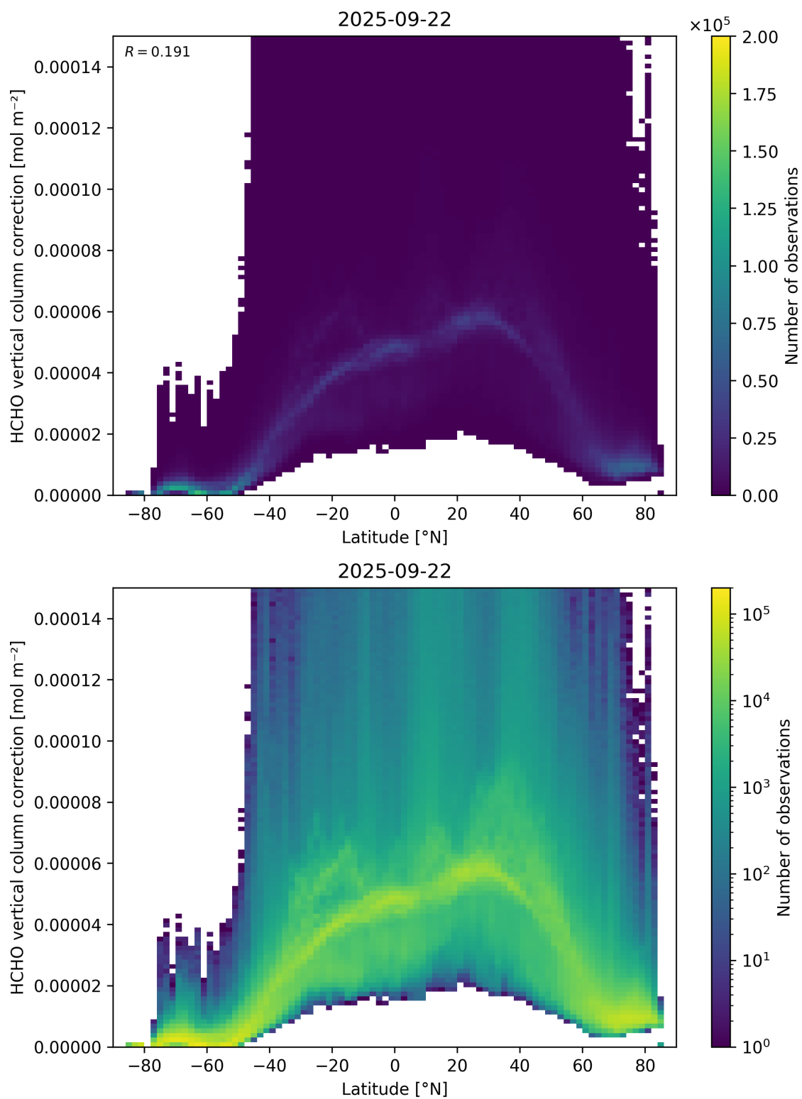
Figure 164: Scatter density plot of “Latitude” against “HCHO vertical column correction” for 2025-09-22 to 2025-09-23.
