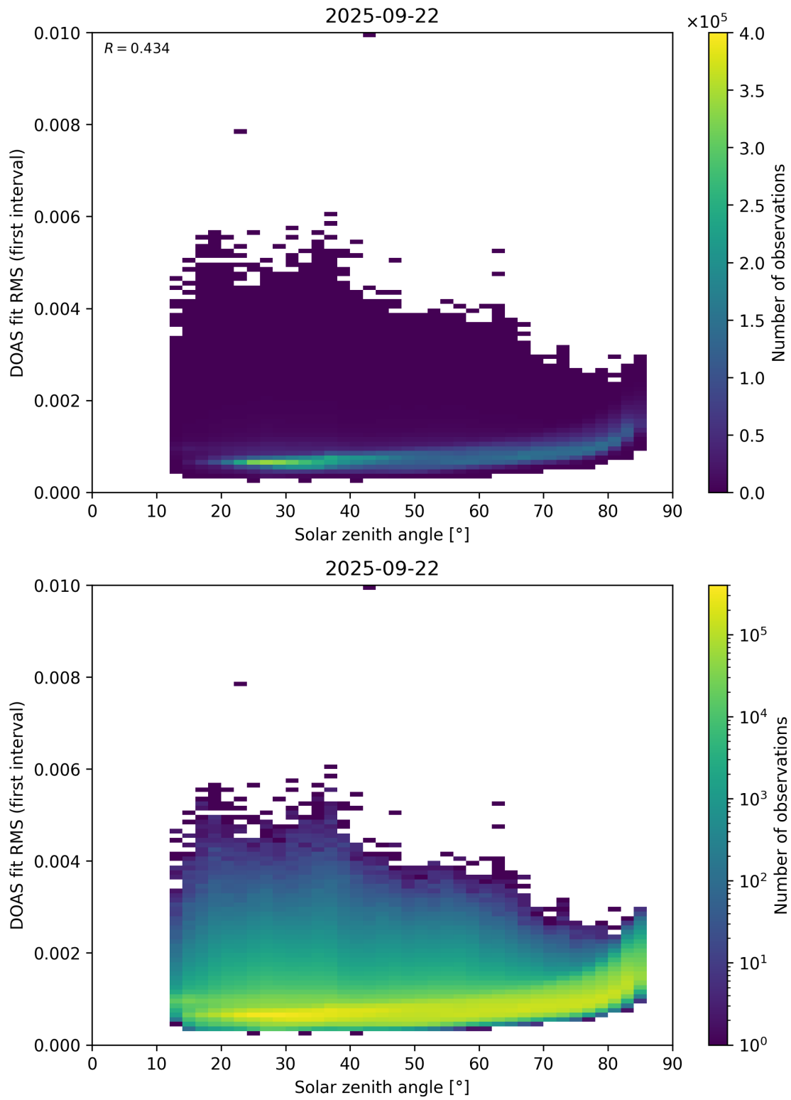
Figure 167: Scatter density plot of “Solar zenith angle” against “DOAS fit RMS (first interval)” for 2025-09-22 to 2025-09-23.
