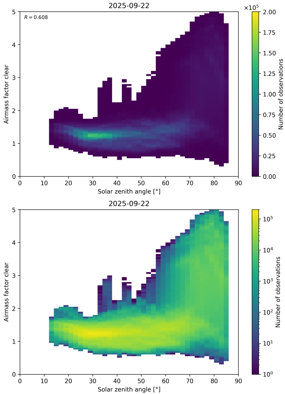
Figure 170: Scatter density plot of “Solar zenith angle” against “Airmass factor clear” for 2025-09-22 to 2025-09-23.
