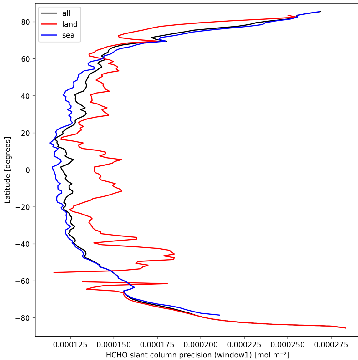
Figure 25: Zonal average of “HCHO slant column precision (window1)” for 2025-09-22 to 2025-09-23.
