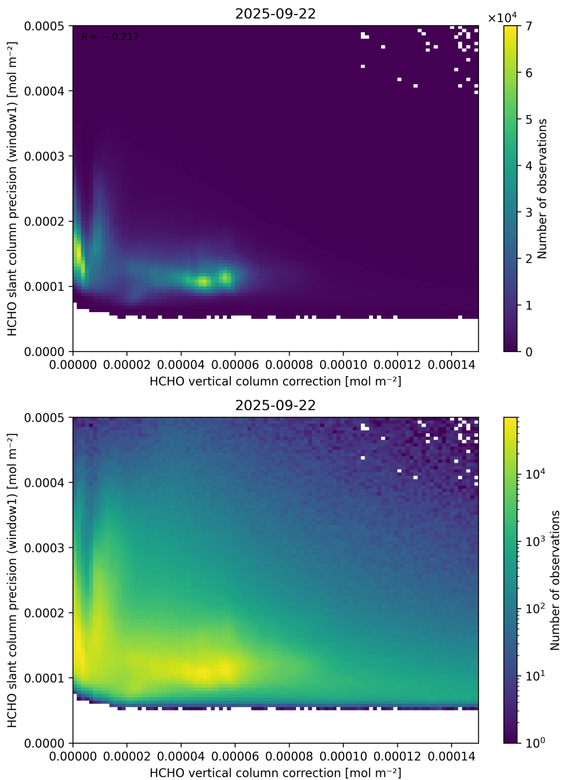
Figure 119: Scatter density plot of “HCHO vertical column correction” against “HCHO slant column precision (window1)” for 2025-09-22 to 2025-09-23.
