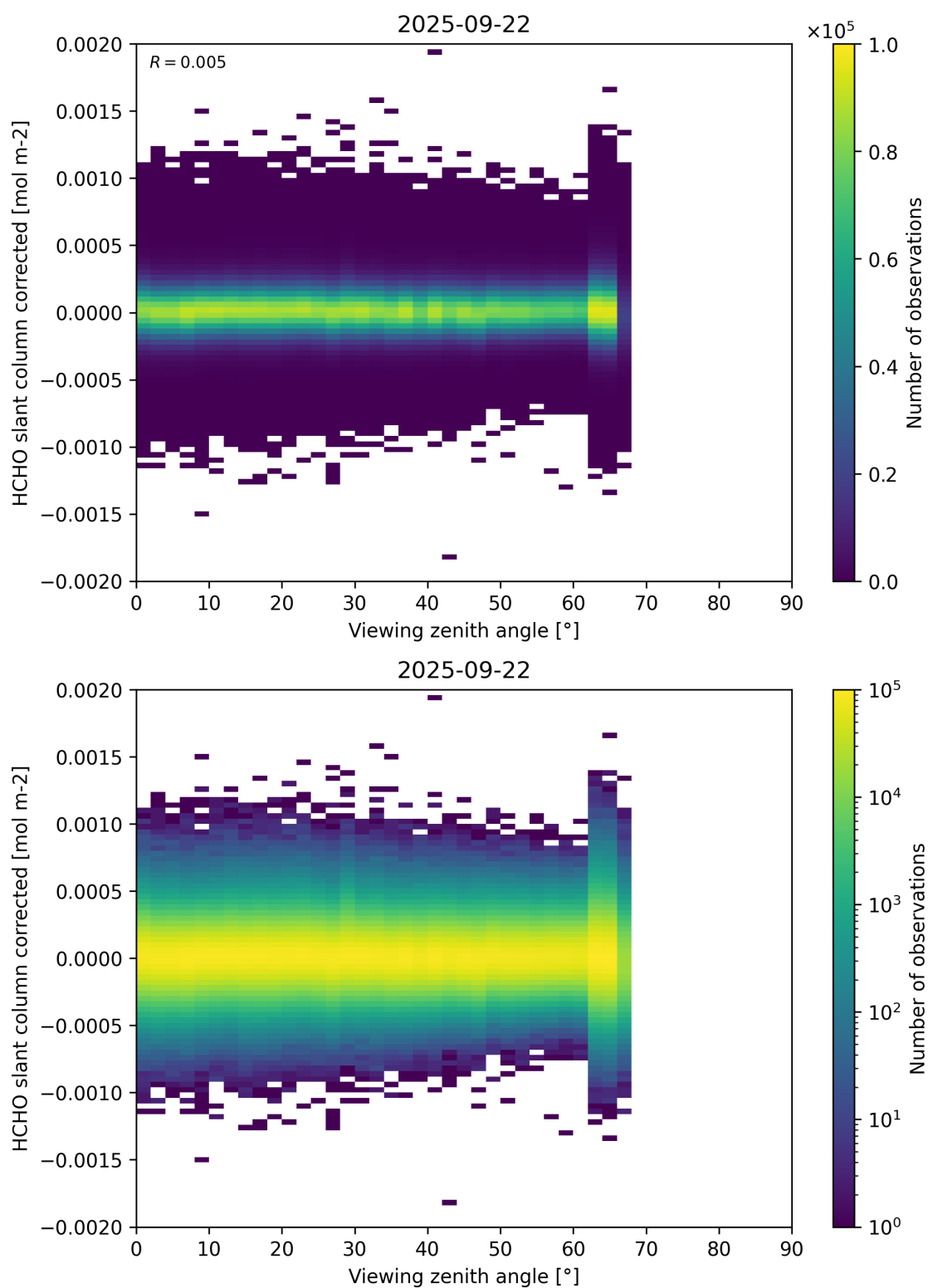
Figure 186: Scatter density plot of “Viewing zenith angle” against “HCHO slant column corrected” for 2025-09-22 to 2025-09-23.
