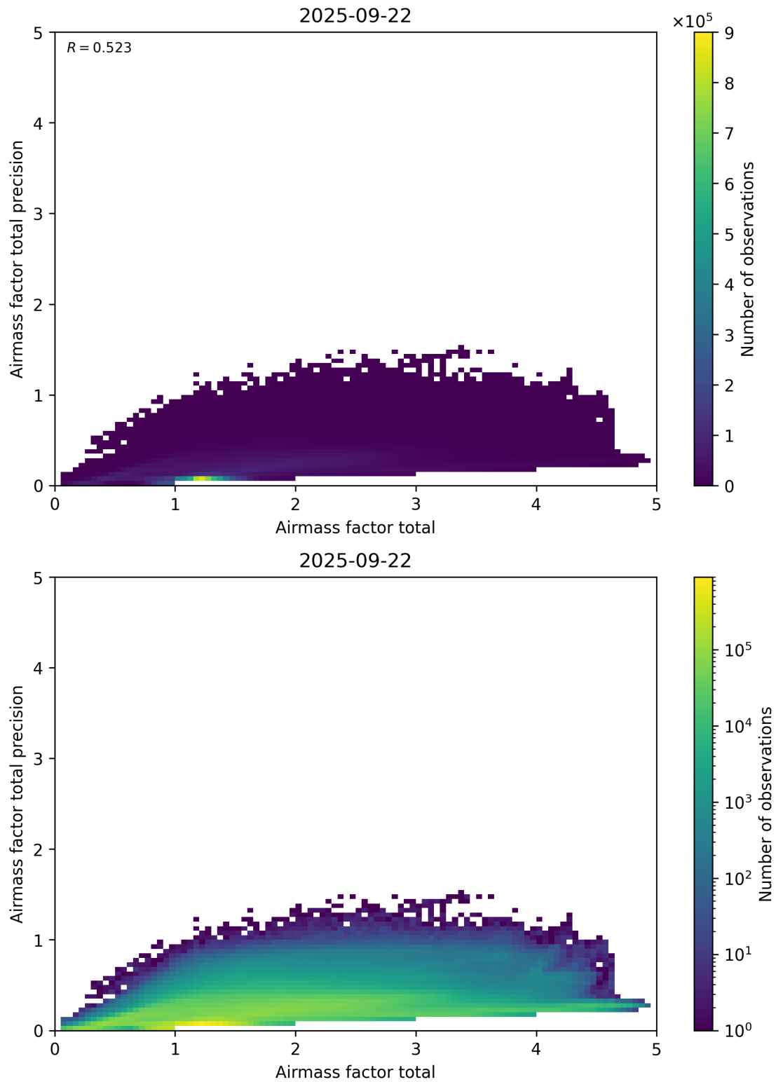
Figure 103: Scatter density plot of “Airmass factor total” against “Airmass factor total precision” for 2025-09-22 to 2025-09-23.
