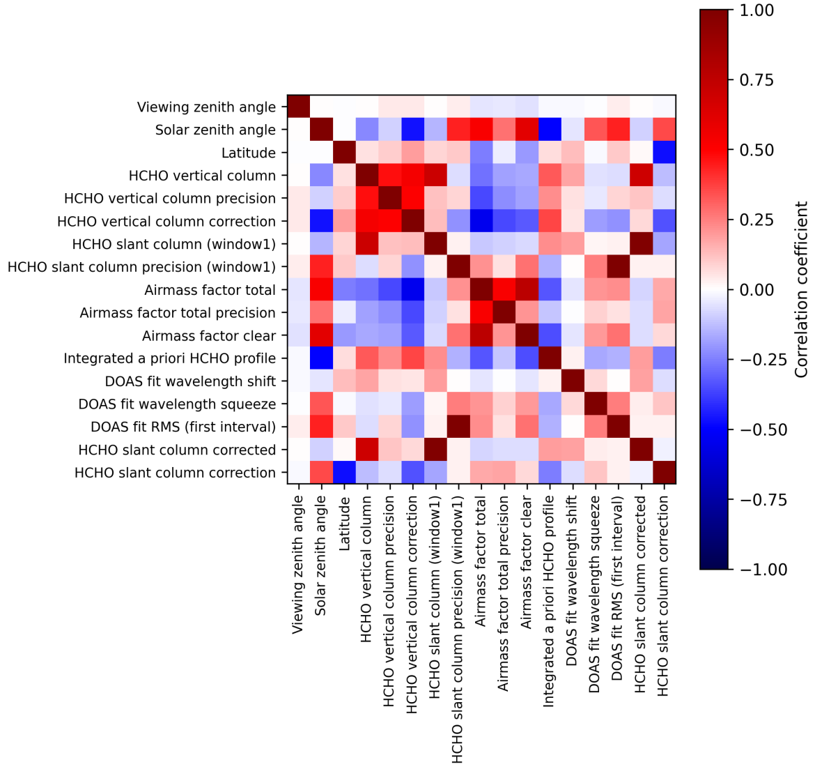
Figure 2: Map of correlation matrix for 2025-09-22 to 2025-09-23.
