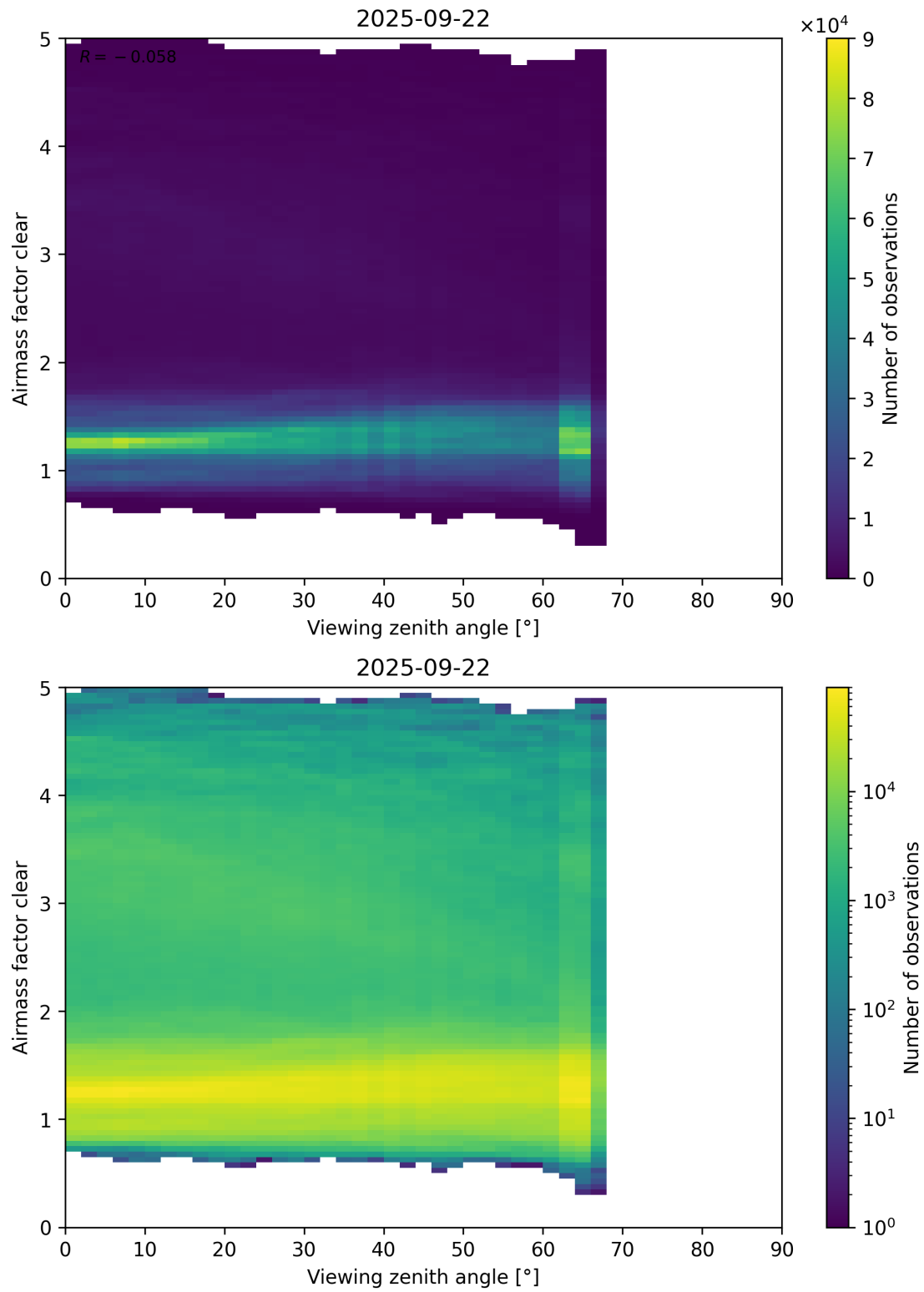
Figure 185: Scatter density plot of “Viewing zenith angle” against “Airmass factor clear” for 2025-09-22 to 2025-09-23.
