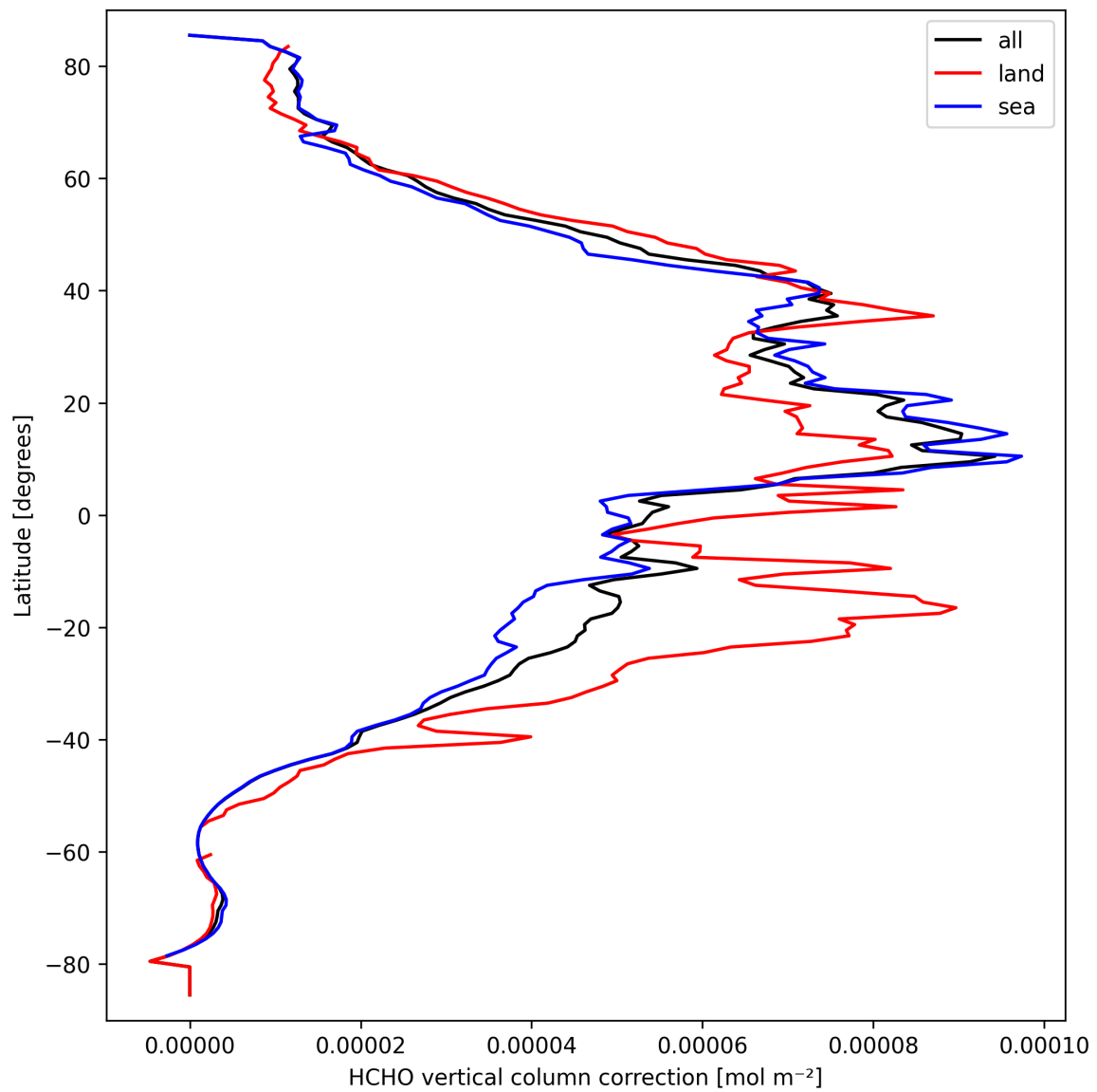
Figure 23: Zonal average of “HCHO vertical column correction” for 2025-09-22 to 2025-09-23.
