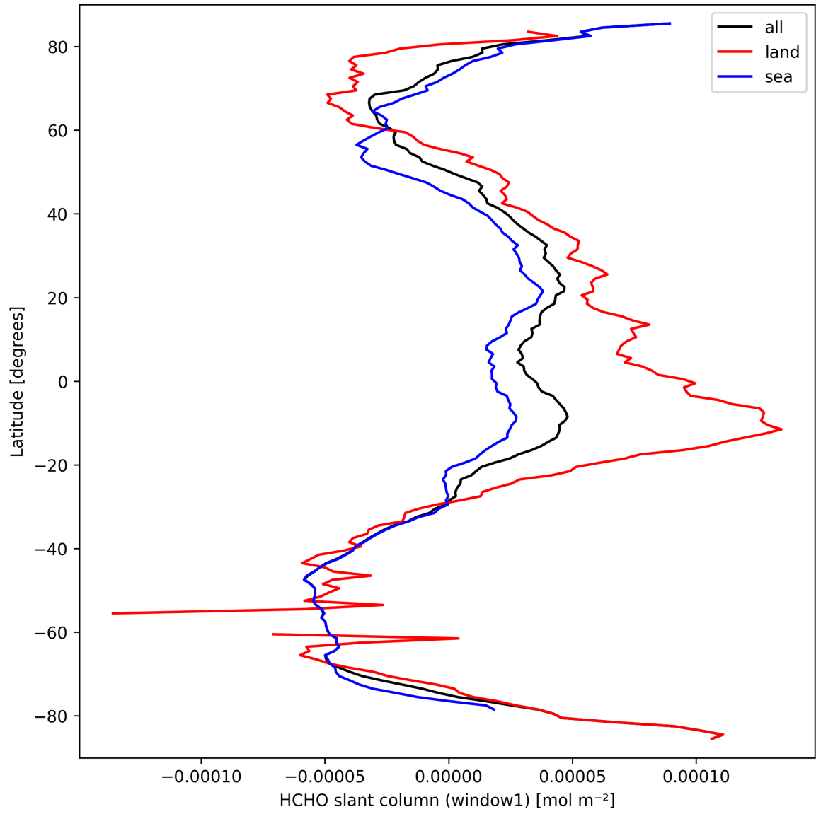
Figure 24: Zonal average of “HCHO slant column (window1)” for 2025-09-22 to 2025-09-23.
