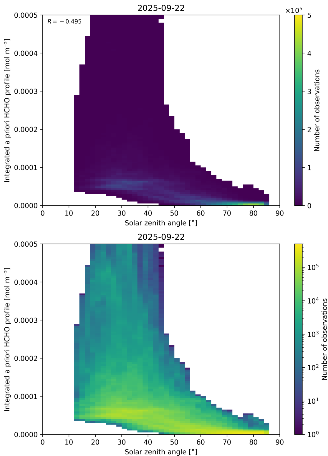
Figure 180: Scatter density plot of “Solar zenith angle” against “Integrated a priori HCHO profile” for 2025-09-22 to 2025-09-23.
