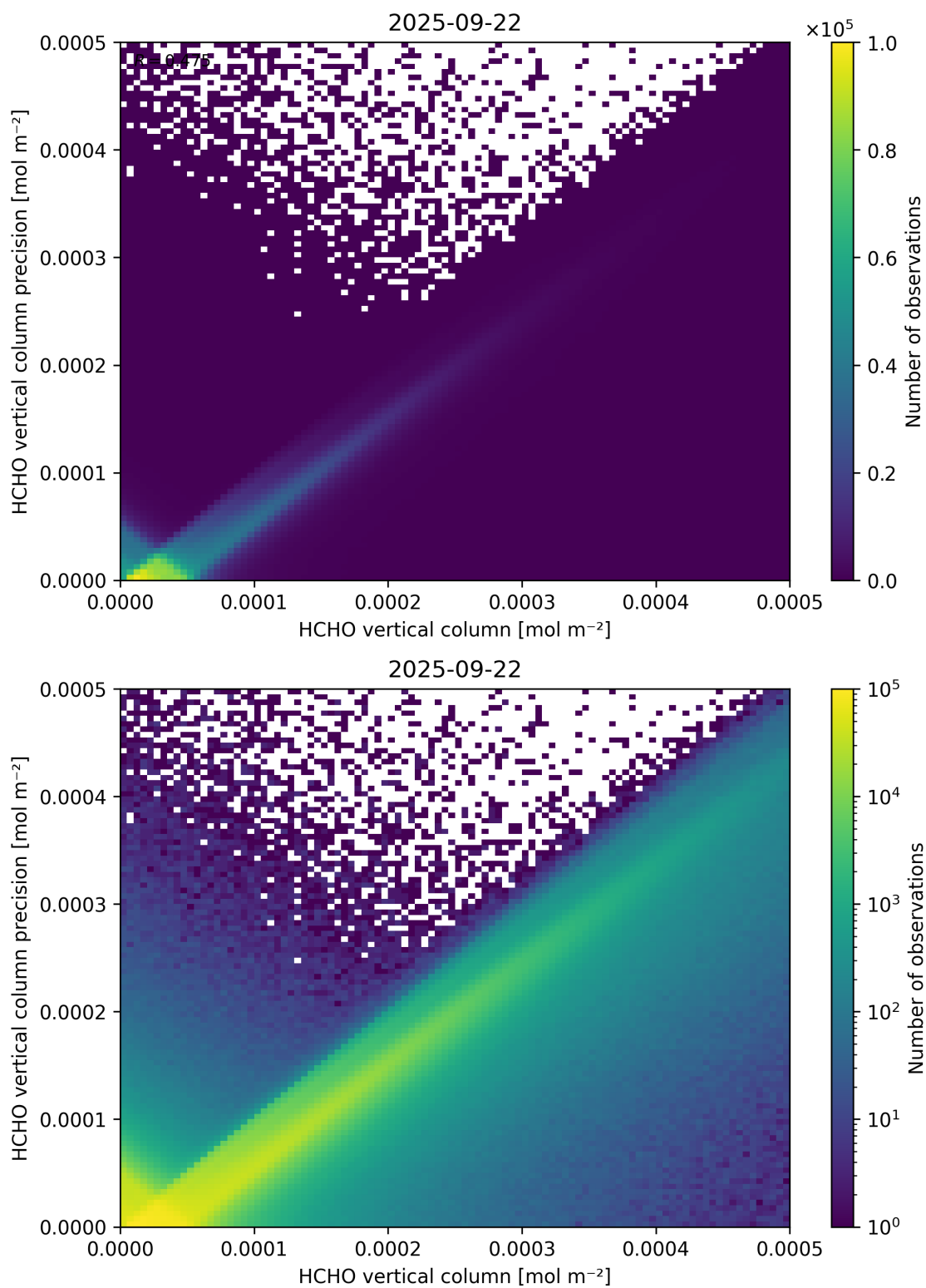
Figure 134: Scatter density plot of “HCHO vertical column” against “HCHO vertical column precision” for 2025-09-22 to 2025-09-23.
