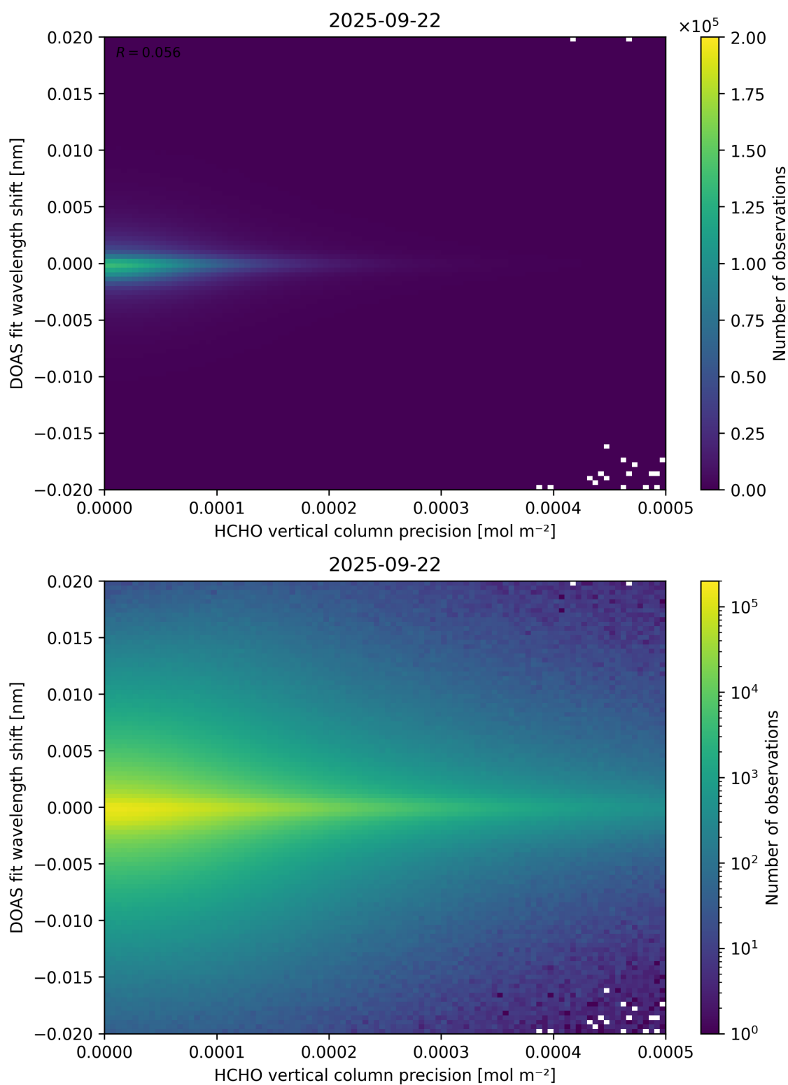
Figure 137: Scatter density plot of “HCHO vertical column precision” against “DOAS fit wavelength shift” for 2025-09-22 to 2025-09-23.
