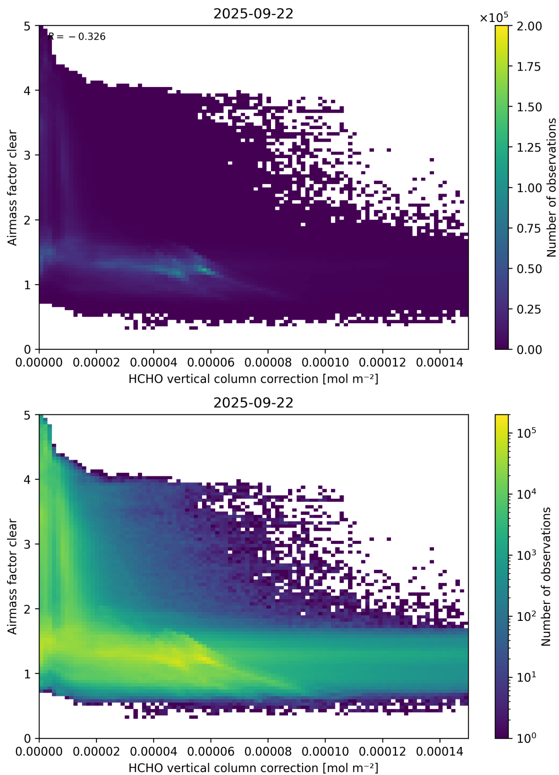
Figure 115: Scatter density plot of “HCHO vertical column correction” against “Airmass factor clear” for 2025-09-22 to 2025-09-23.
