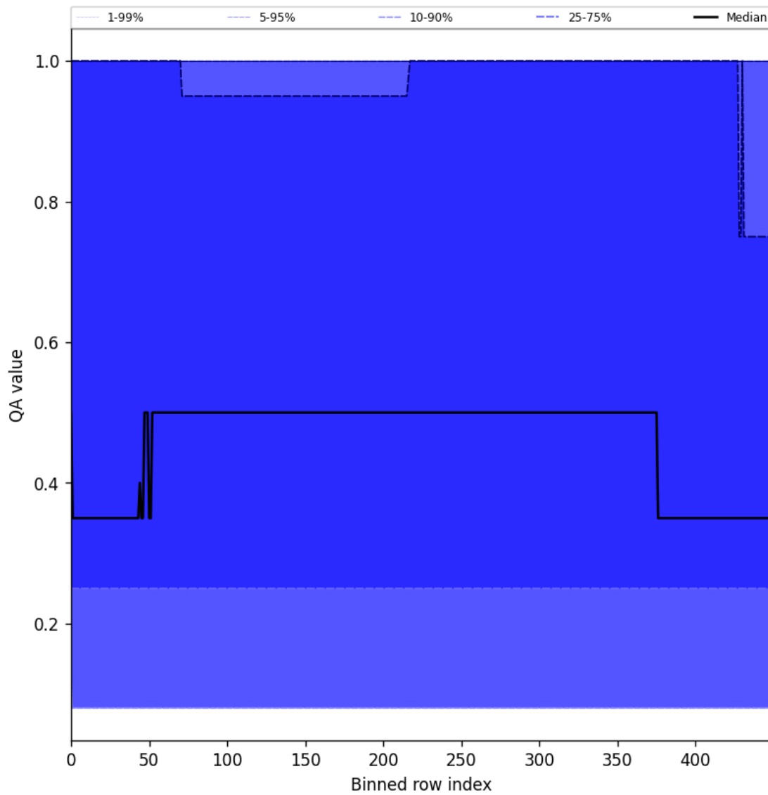
Figure 48: Along track statistics of “QA value” for 2025-09-22 to 2025-09-23
