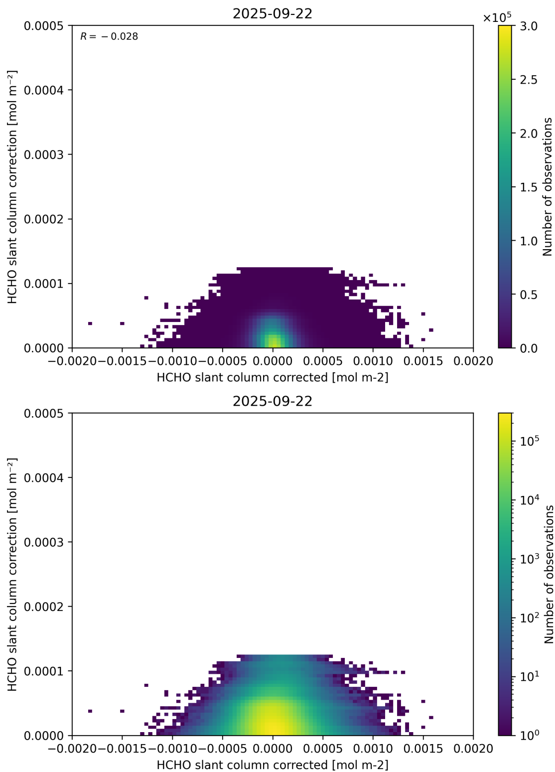
Figure 77: Scatter density plot of “HCHO slant column corrected” against “HCHO slant column correction” for 2025-09-22 to 2025-09-23.
