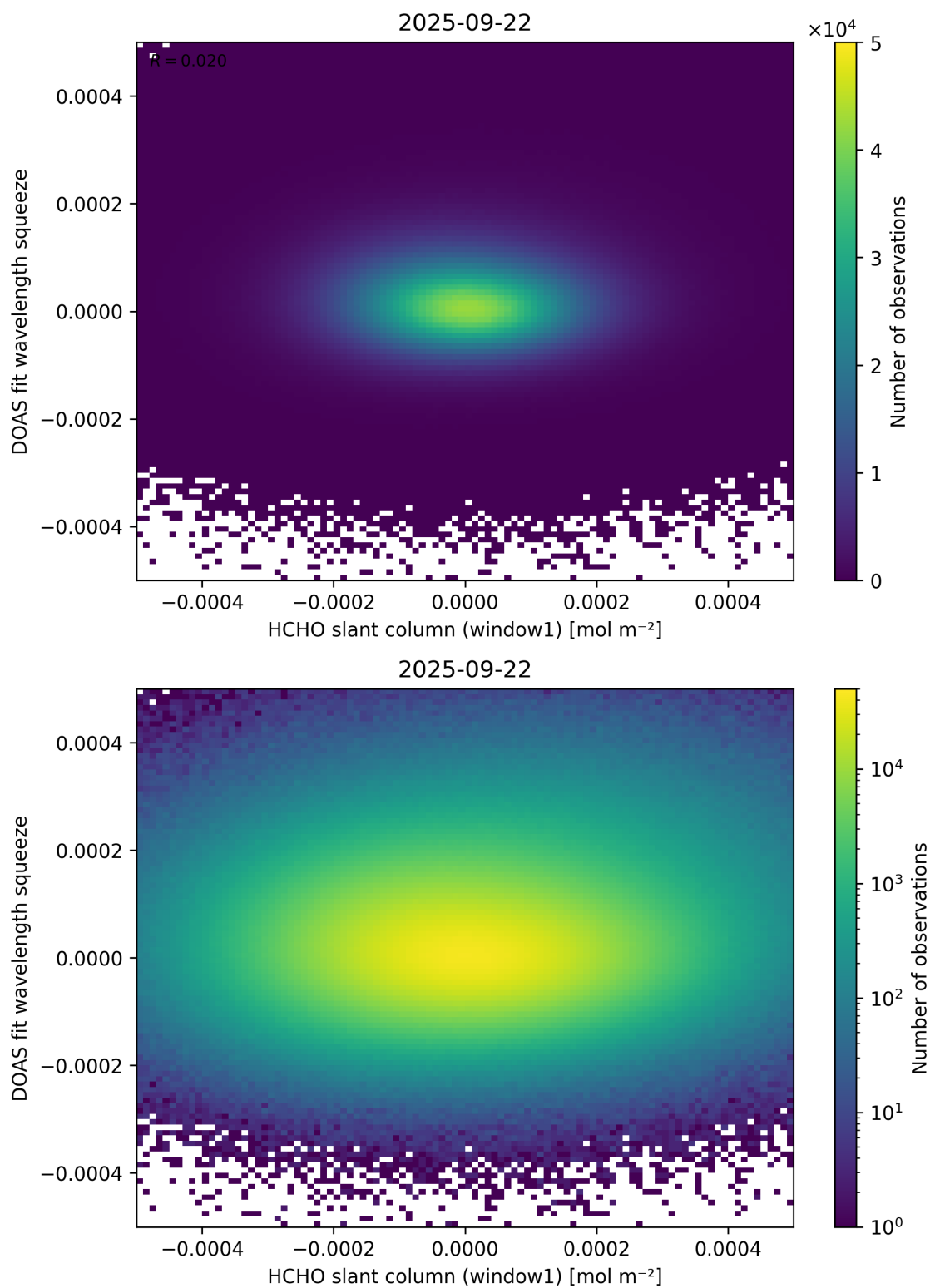
Figure 80: Scatter density plot of “HCHO slant column (window1)” against “DOAS fit wavelength squeeze” for 2025-09-22 to 2025-09-23.
