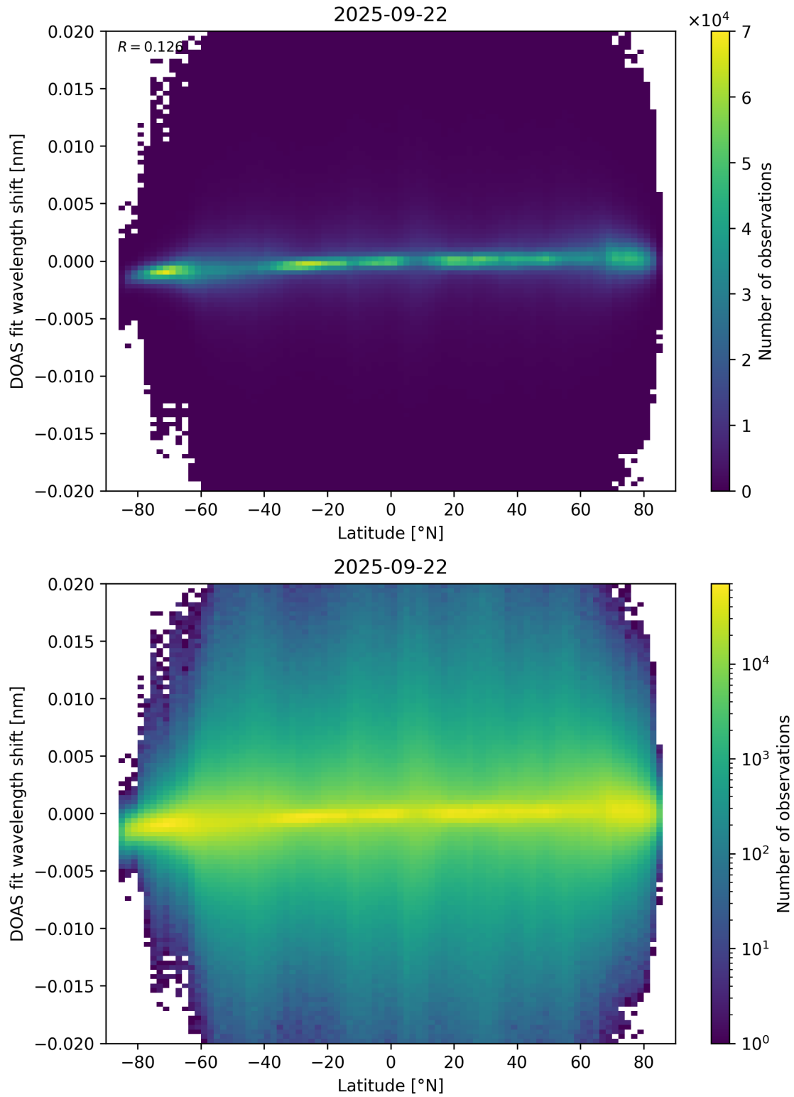
Figure 154: Scatter density plot of “Latitude” against “DOAS fit wavelength shift” for 2025-09-22 to 2025-09-23.
