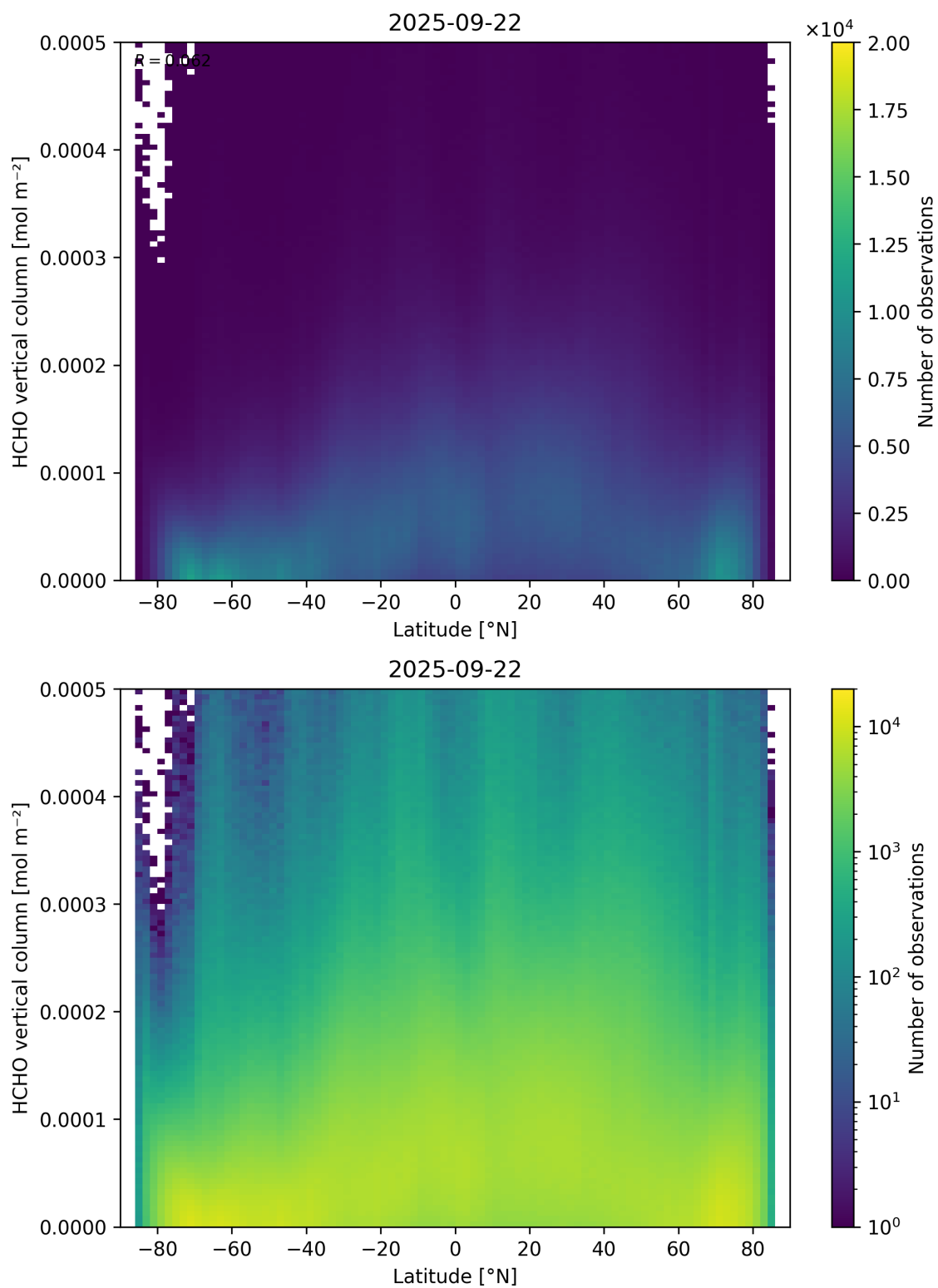
Figure 163: Scatter density plot of “Latitude” against “HCHO vertical column” for 2025-09-22 to 2025-09-23.
