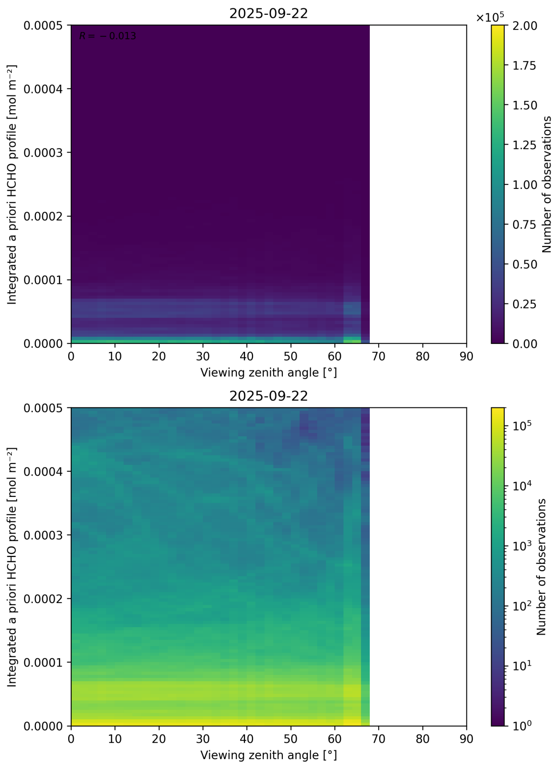
Figure 195: Scatter density plot of “Viewing zenith angle” against “Integrated a priori HCHO profile” for 2025-09-22 to 2025-09-23.
