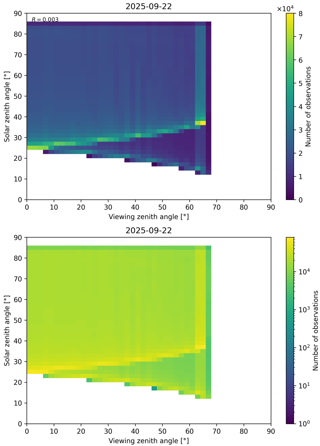
Figure 197: Scatter density plot of “Viewing zenith angle” against “Solar zenith angle” for 2025-09-22 to 2025-09-23.
