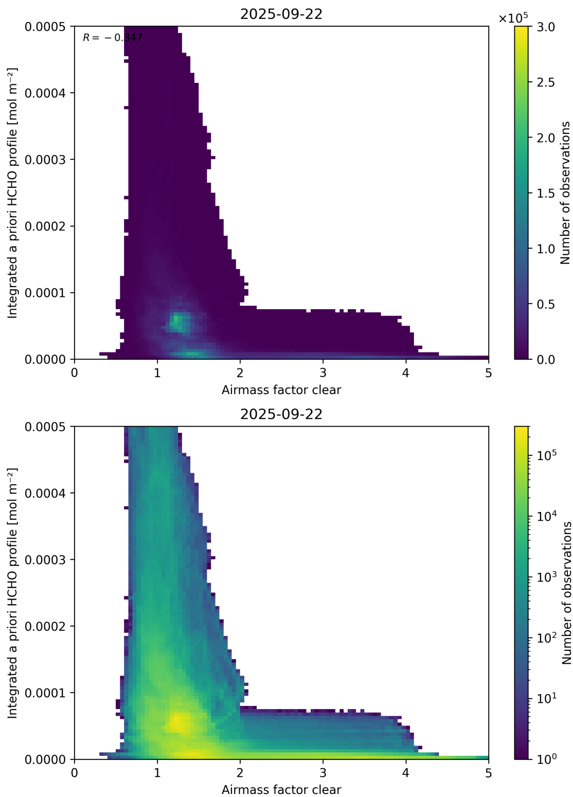
Figure 76: Scatter density plot of “Airmass factor clear” against “Integrated a priori HCHO profile” for 2025-09-22 to 2025-09-23.
