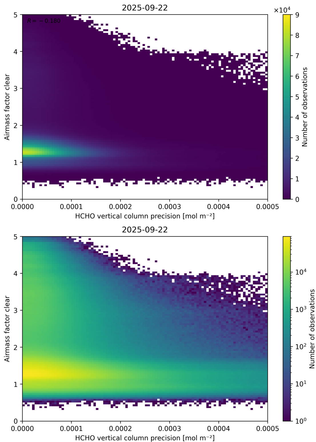
Figure 139: Scatter density plot of “HCHO vertical column precision” against “Airmass factor clear” for 2025-09-22 to 2025-09-23.
