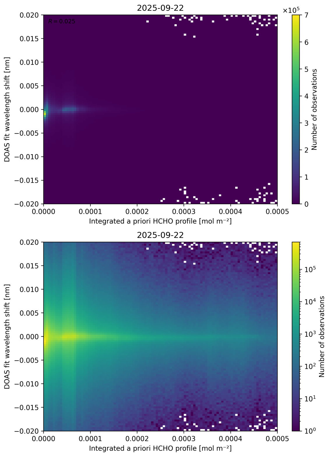
Figure 149: Scatter density plot of “Integrated a priori HCHO profile” against “DOAS fit wavelength shift” for 2025-09-22 to 2025-09-23.
