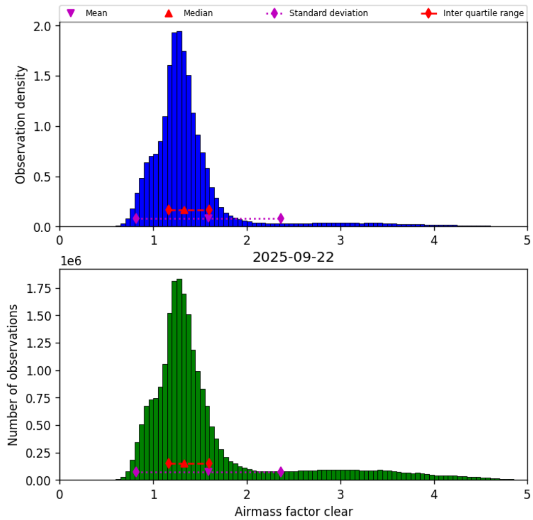
Figure 42: Histogram of “Airmass factor clear” for 2025-09-22 to 2025-09-23
