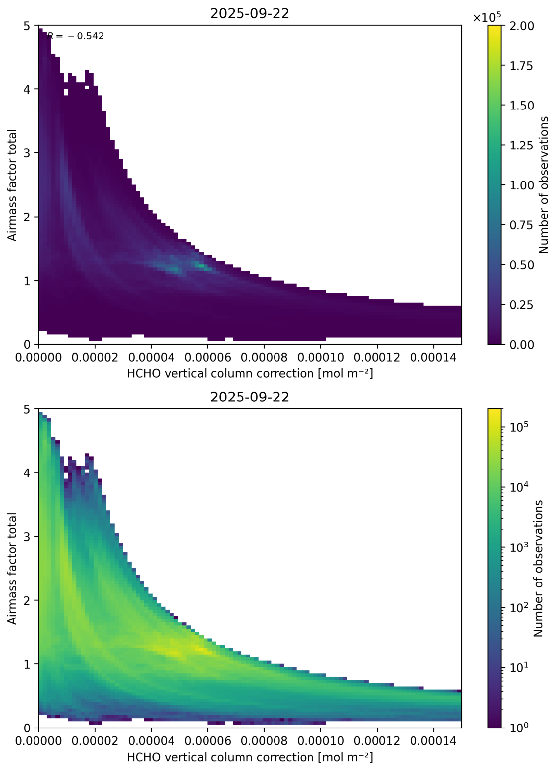
Figure 120: Scatter density plot of “HCHO vertical column correction” against “Airmass factor total” for 2025-09-22 to 2025-09-23.
