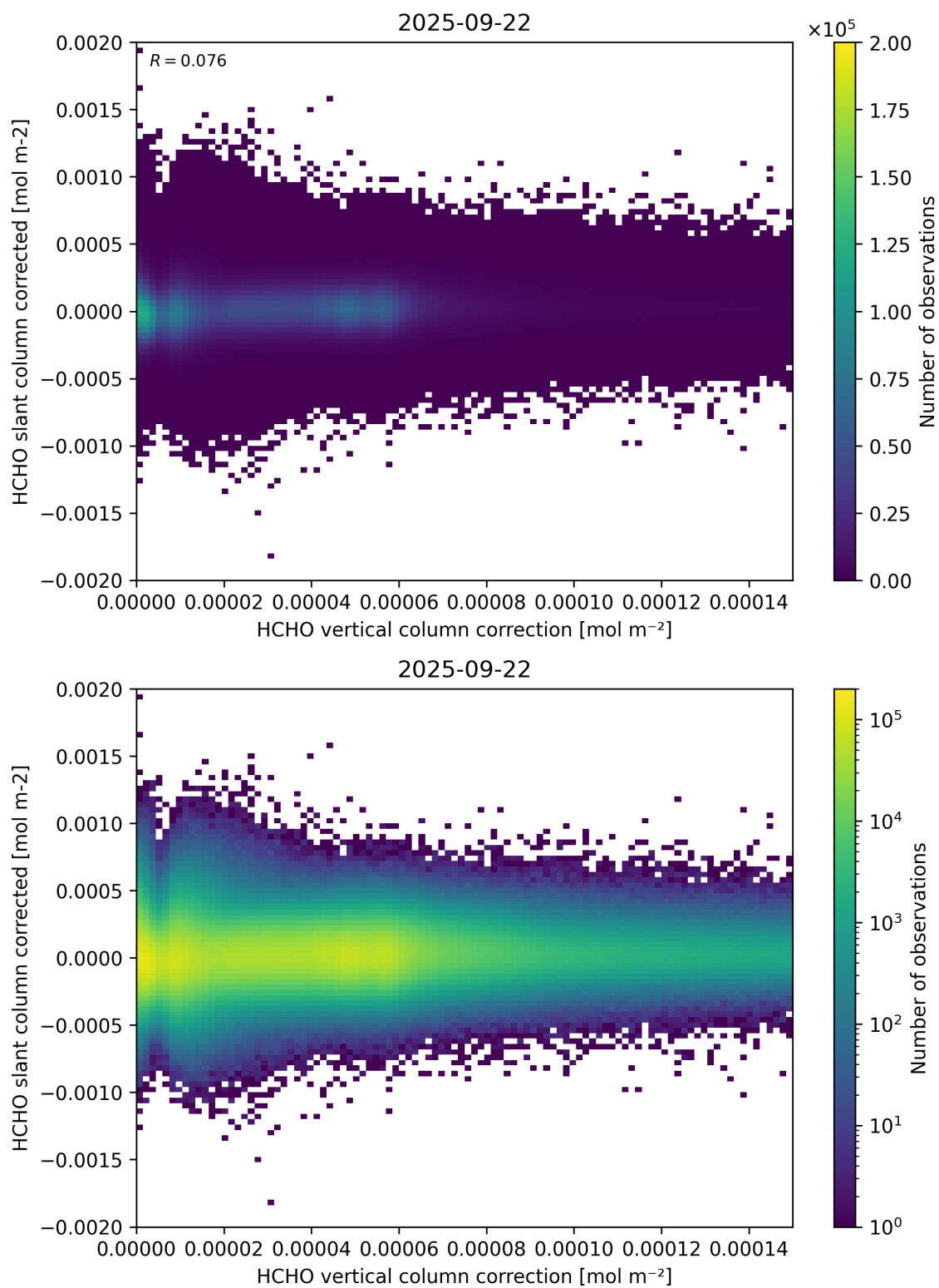
Figure 116: Scatter density plot of “HCHO vertical column correction” against “HCHO slant column corrected” for 2025-09-22 to 2025-09-23.
