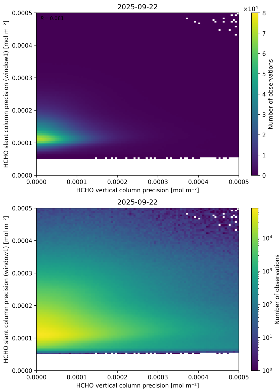
Figure 143: Scatter density plot of “HCHO vertical column precision” against “HCHO slant column precision (window1)” for 2025-09-22 to 2025-09-23.
