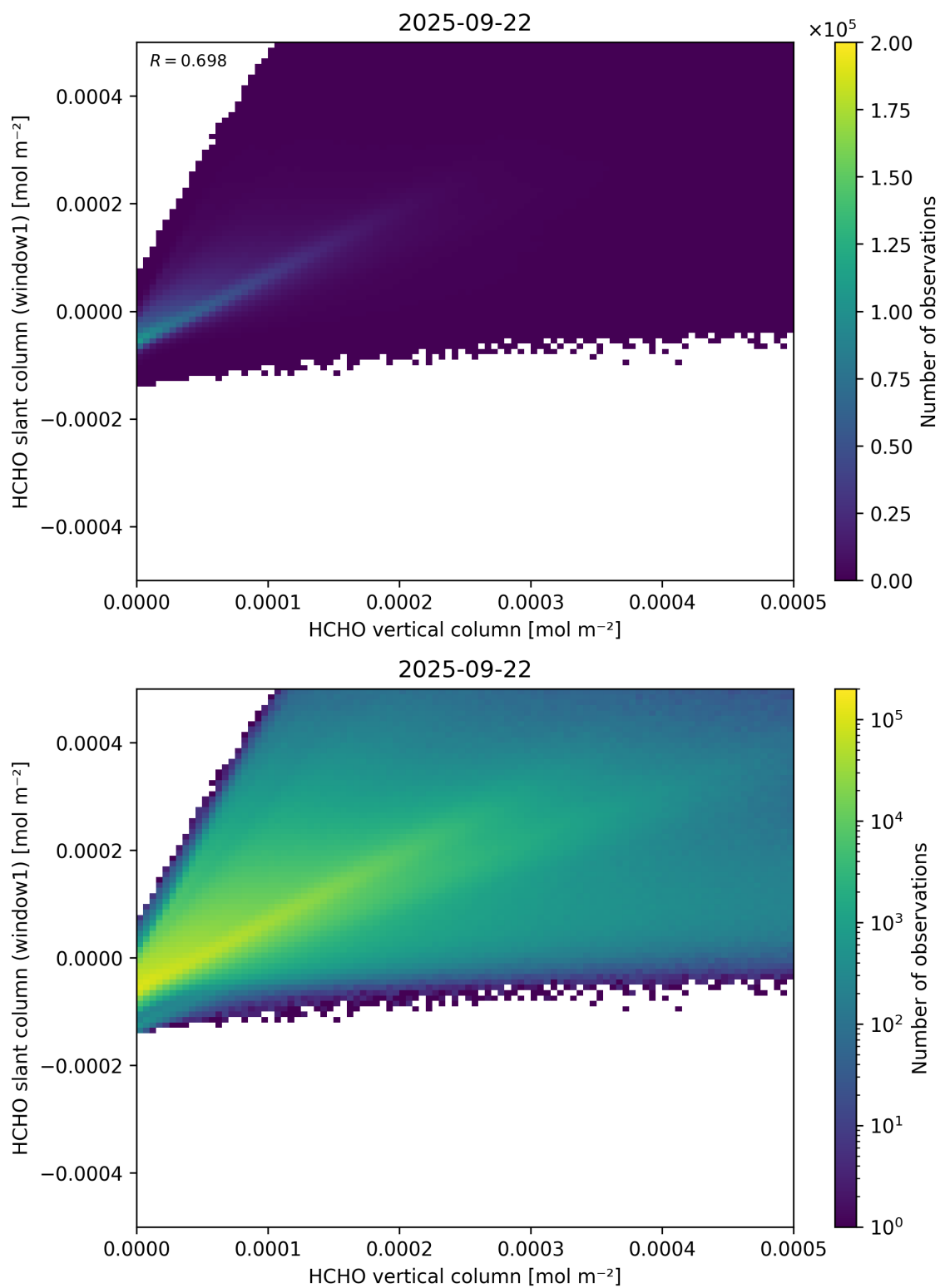
Figure 129: Scatter density plot of “HCHO vertical column” against “HCHO slant column (window1)” for 2025-09-22 to 2025-09-23.
