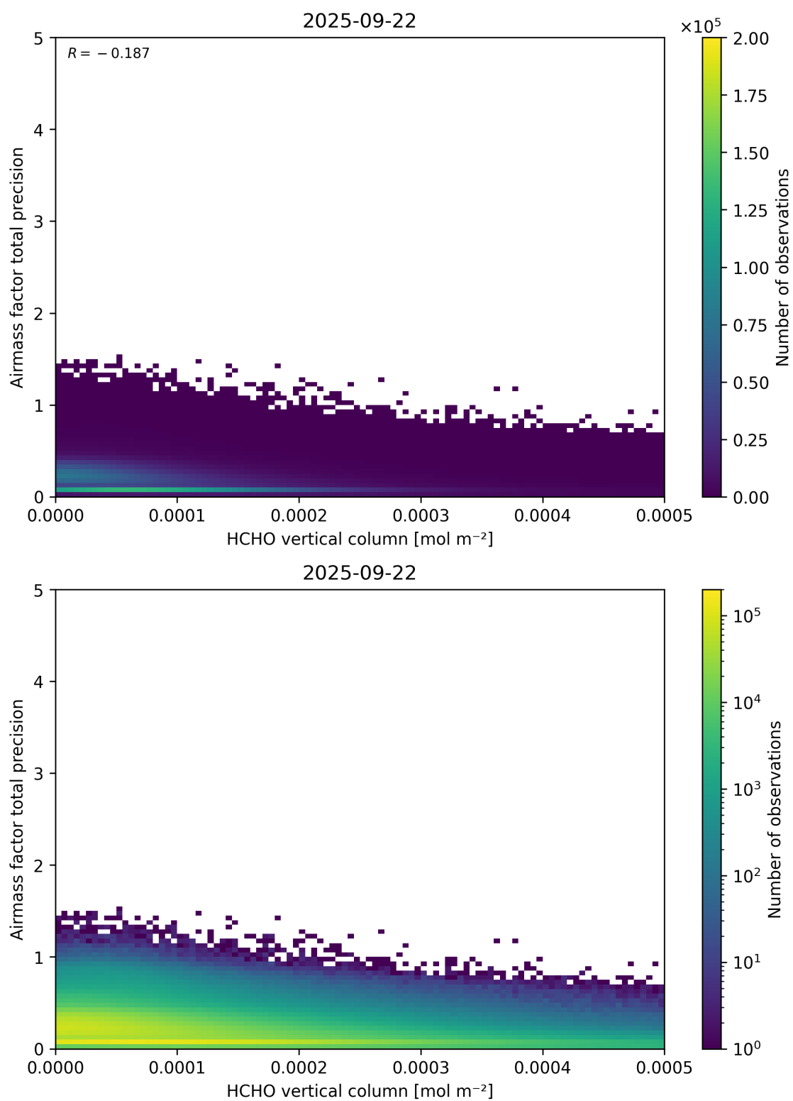
Figure 132: Scatter density plot of “HCHO vertical column” against “Airmass factor total precision” for 2025-09-22 to 2025-09-23.
