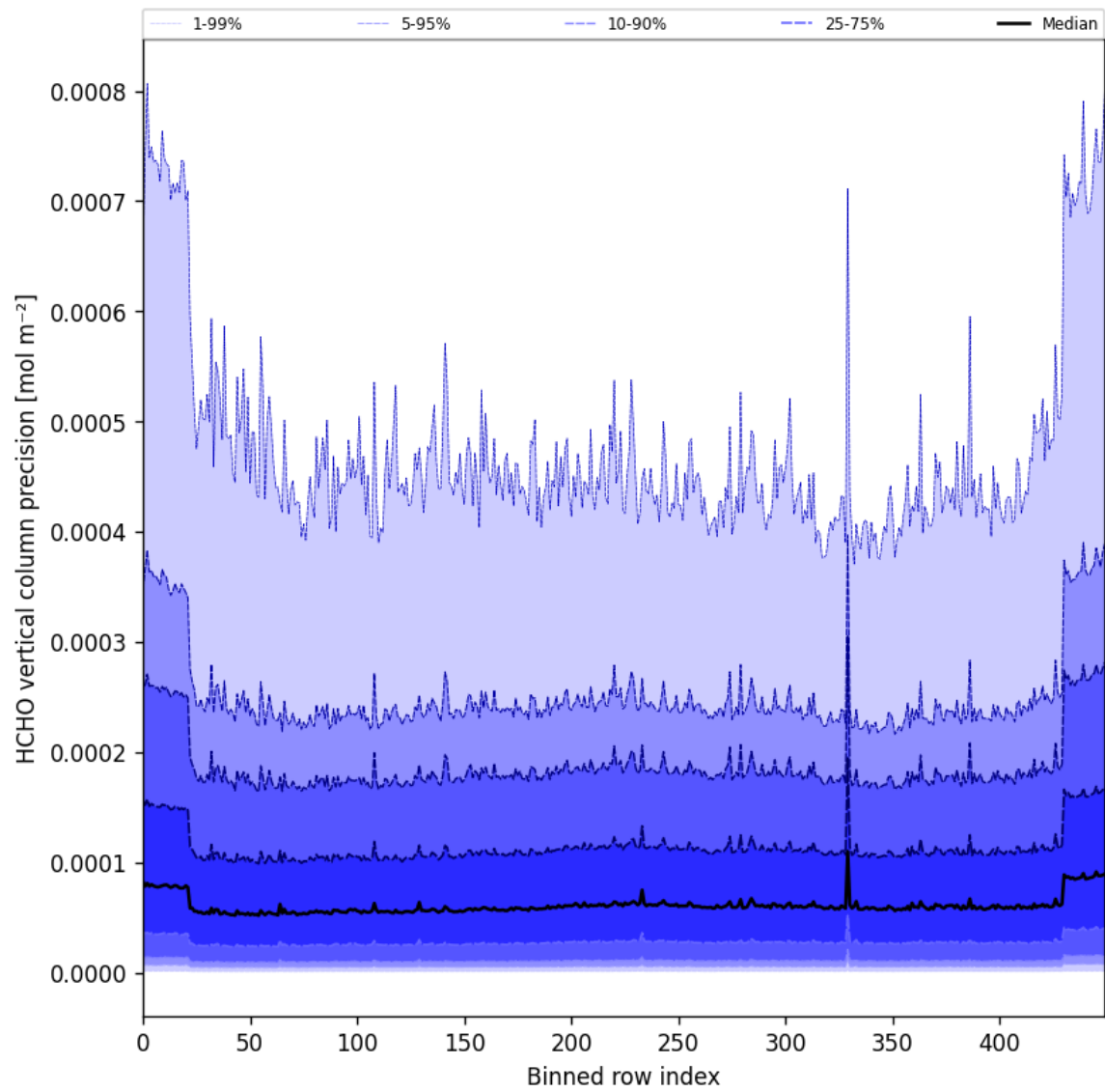
Figure 50: Along track statistics of "HCHO vertical column precision" for 2025-09-22 to 2025-09-23
