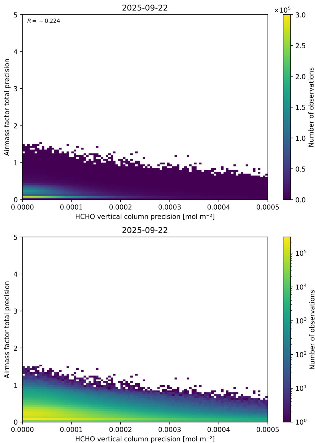
Figure 145: Scatter density plot of “HCHO vertical column precision” against “Airmass factor total precision” for 2025-09-22 to 2025-09-23.
