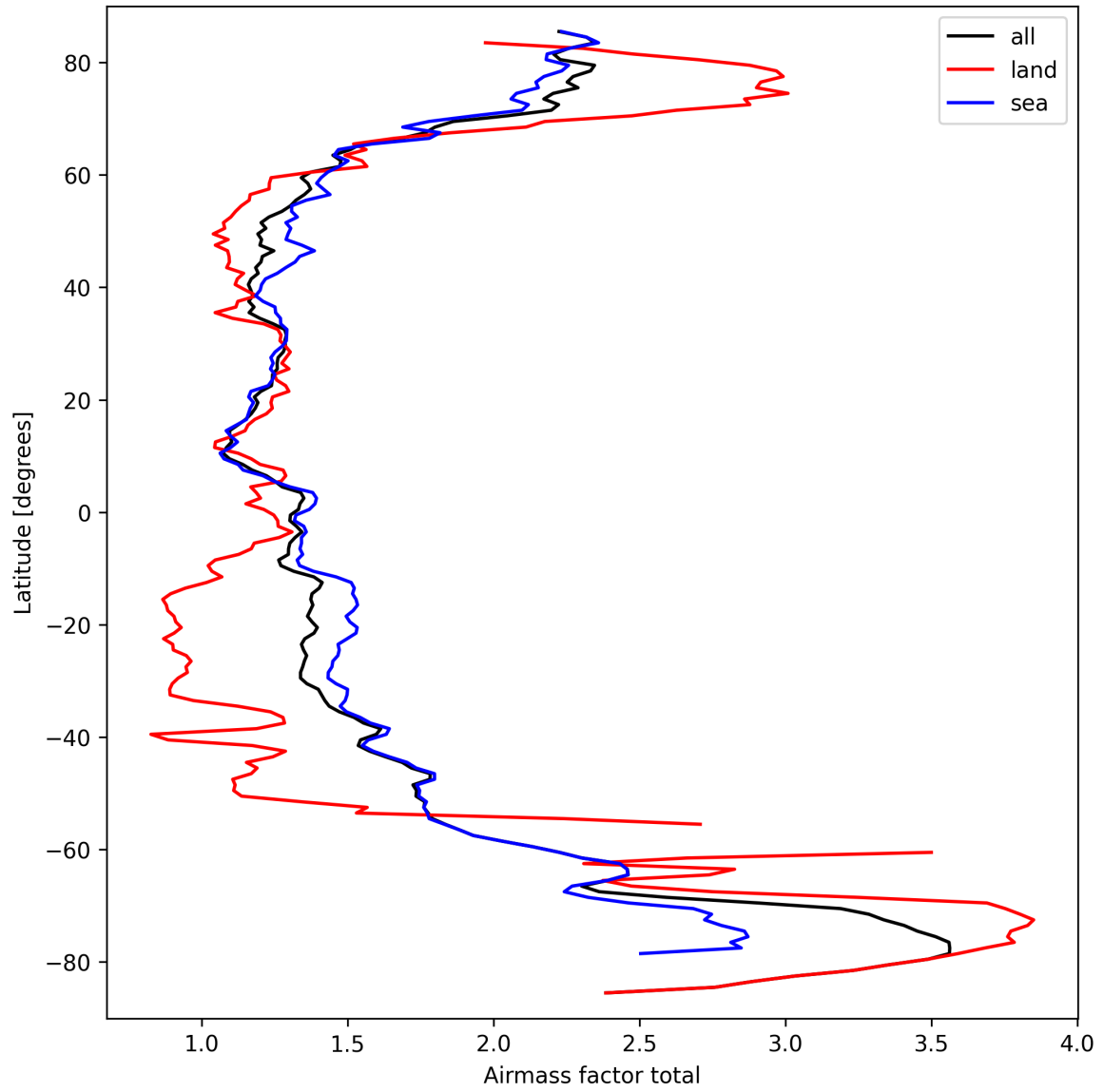
Figure 26: Zonal average of “Airmass factor total” for 2025-09-22 to 2025-09-23.
