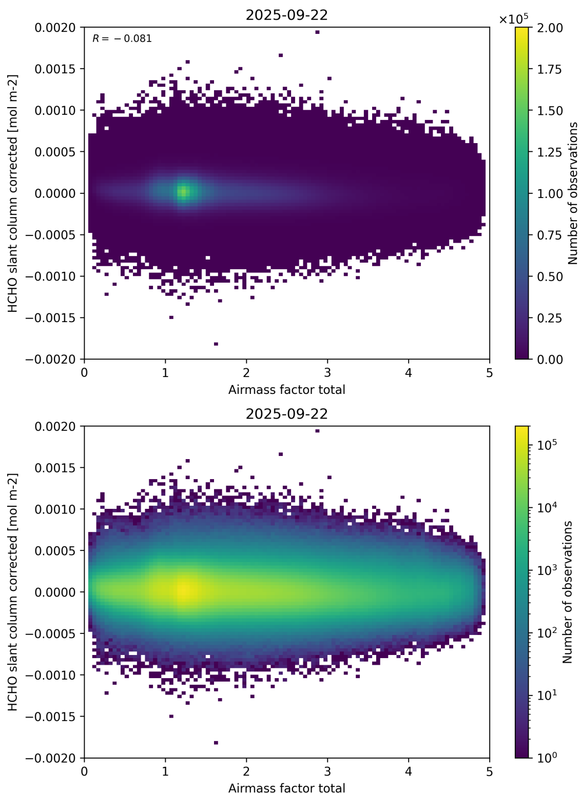
Figure 101: Scatter density plot of “Airmass factor total” against “HCHO slant column corrected” for 2025-09-22 to 2025-09-23.
