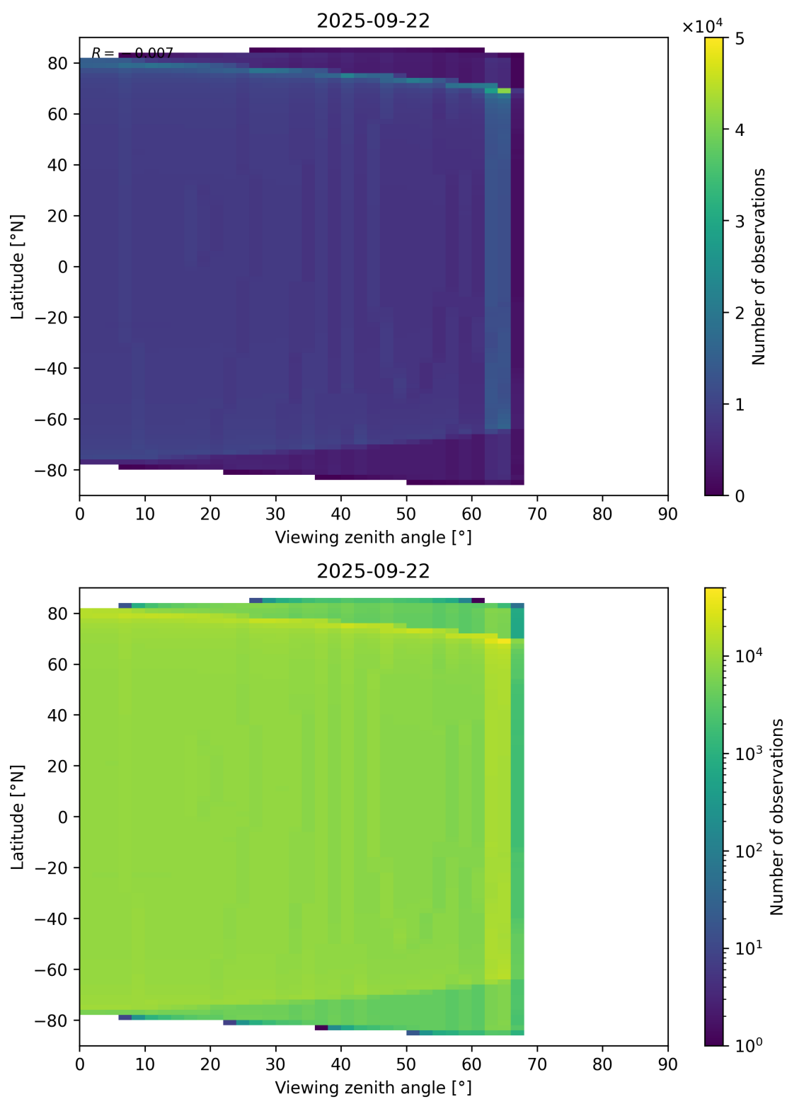
Figure 196: Scatter density plot of “Viewing zenith angle” against “Latitude” for 2025-09-22 to 2025-09-23.
