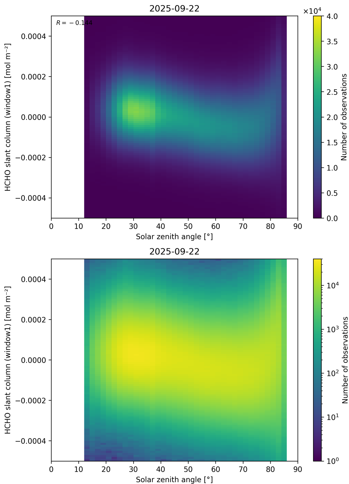
Figure 173: Scatter density plot of “Solar zenith angle” against “HCHO slant column (window1)” for 2025-09-22 to 2025-09-23.
