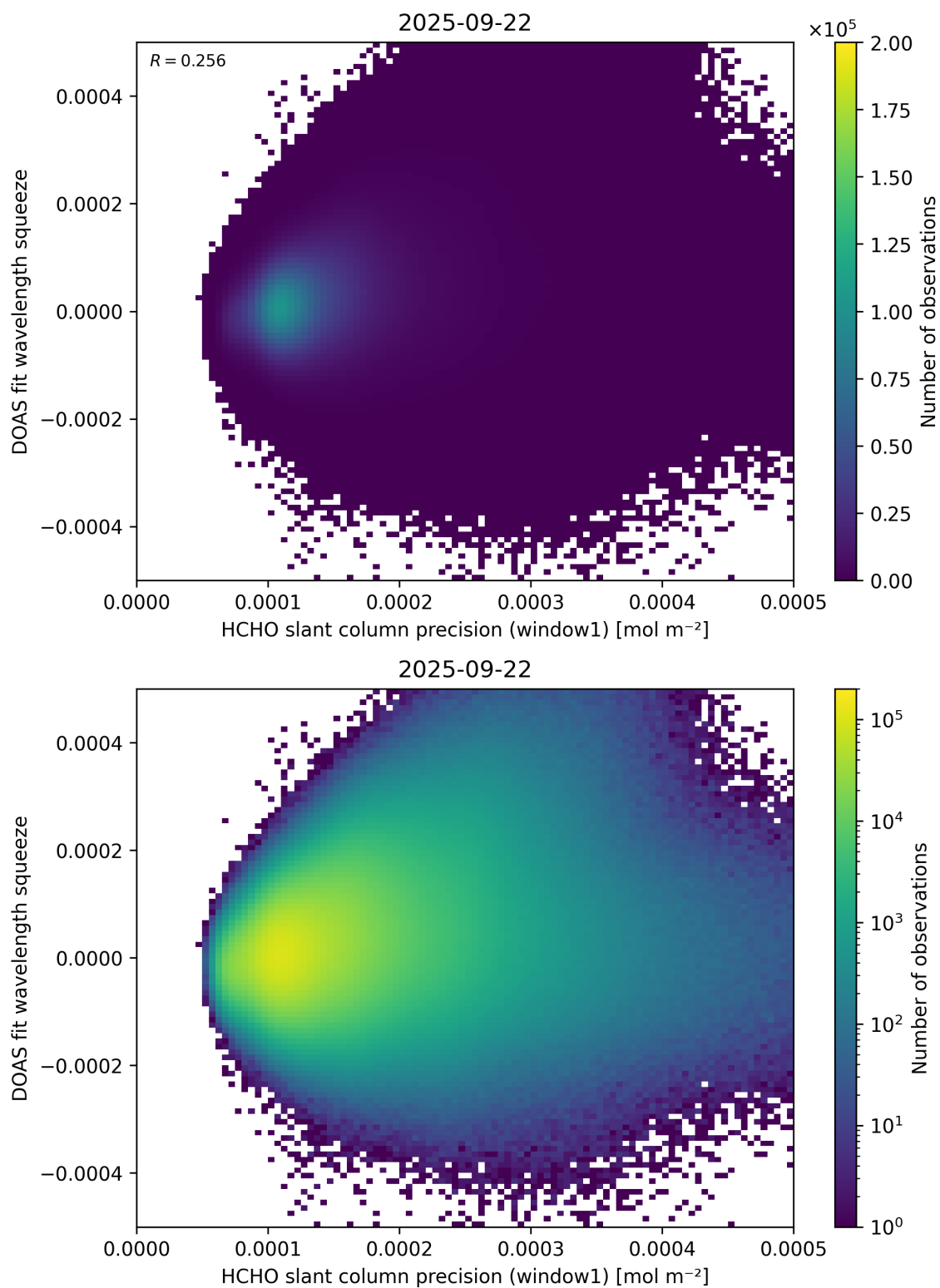
Figure 90: Scatter density plot of “HCHO slant column precision (window1)” against “DOAS fit wavelength squeeze” for 2025-09-22 to 2025-09-23.
