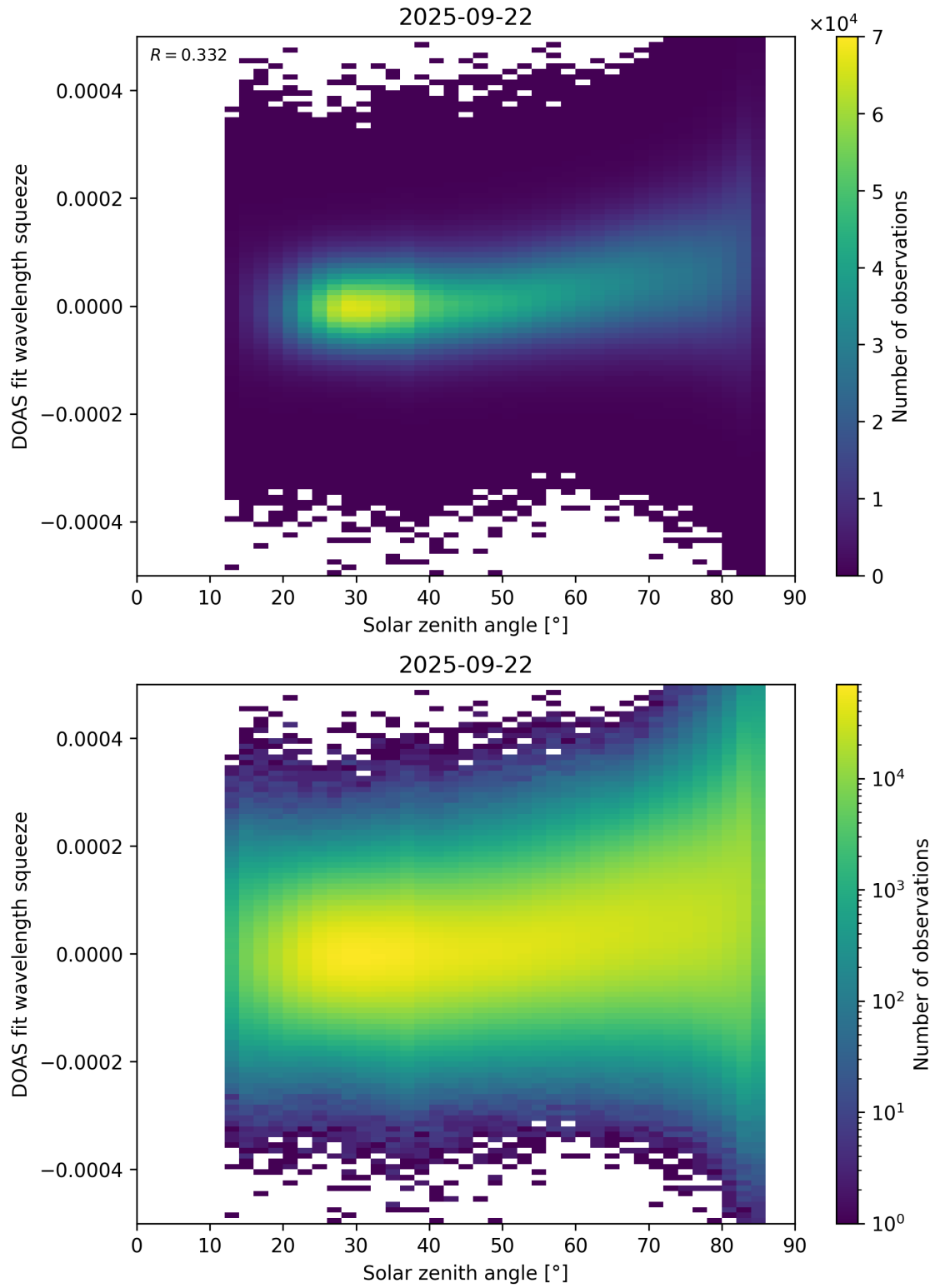
Figure 169: Scatter density plot of “Solar zenith angle” against “DOAS fit wavelength squeeze” for 2025-09-22 to 2025-09-23.
