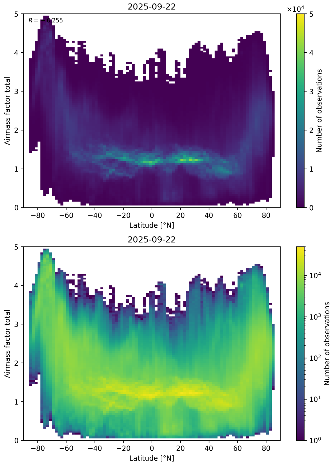
Figure 161: Scatter density plot of “Latitude” against “Airmass factor total” for 2025-09-22 to 2025-09-23.
