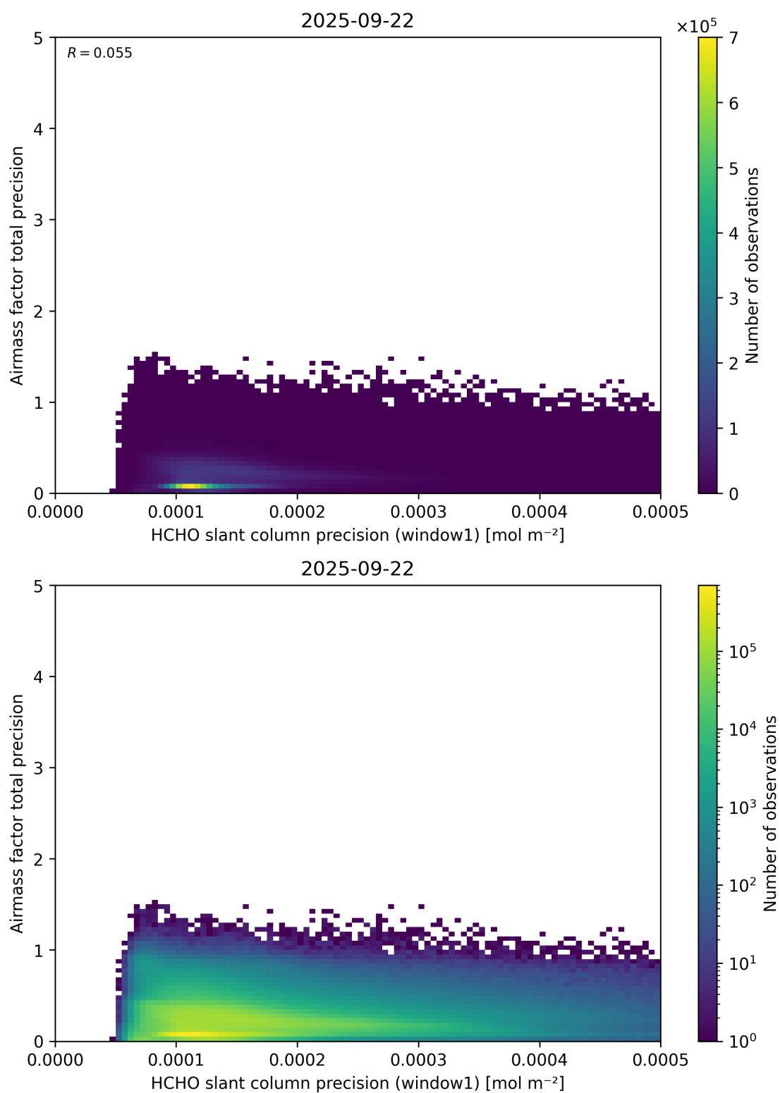
Figure 95: Scatter density plot of “HCHO slant column precision (window1)” against “Airmass factor total precision” for 2025-09-22 to 2025-09-23.
