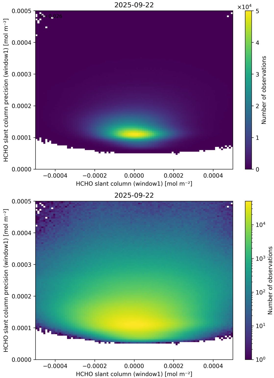
Figure 84: Scatter density plot of “HCHO slant column (window1)” against “HCHO slant column precision (window1)” for 2025-09-22 to 2025-09-23.
