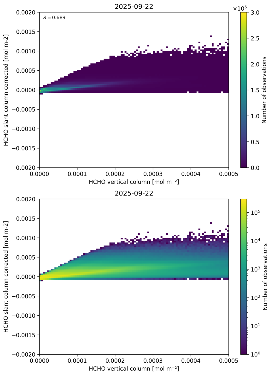
Figure 127: Scatter density plot of “HCHO vertical column” against “HCHO slant column corrected” for 2025-09-22 to 2025-09-23.
