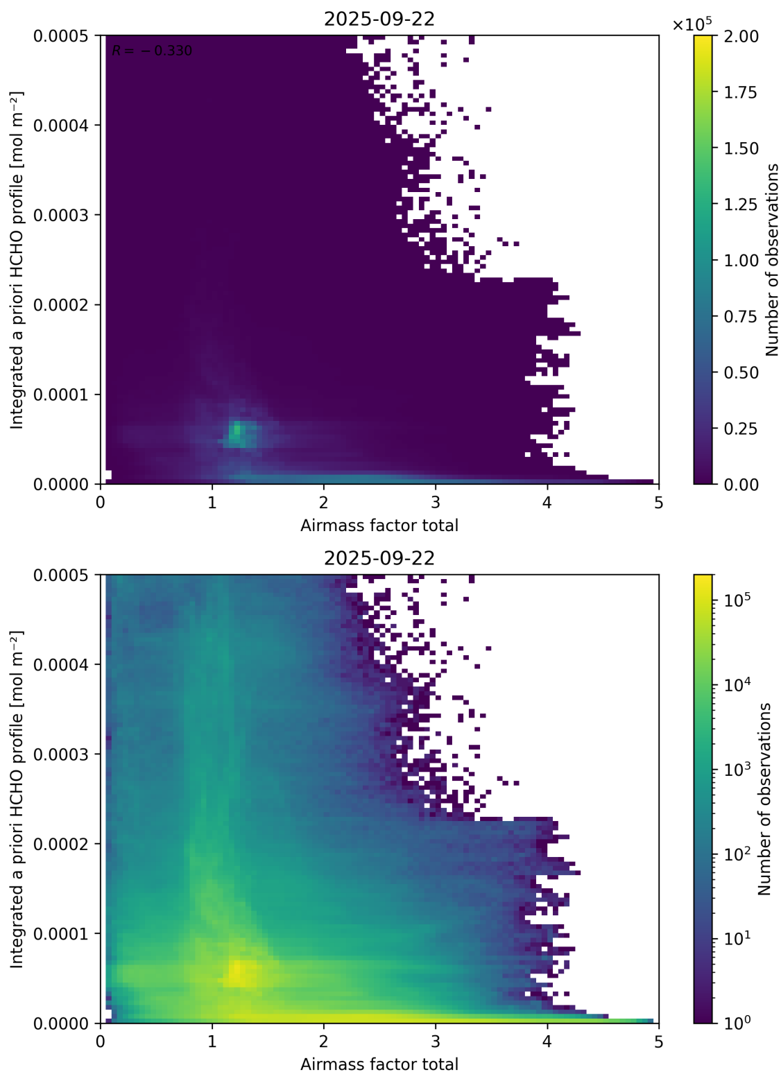
Figure 104: Scatter density plot of “Airmass factor total” against “Integrated a priori HCHO profile” for 2025-09-22 to 2025-09-23.
