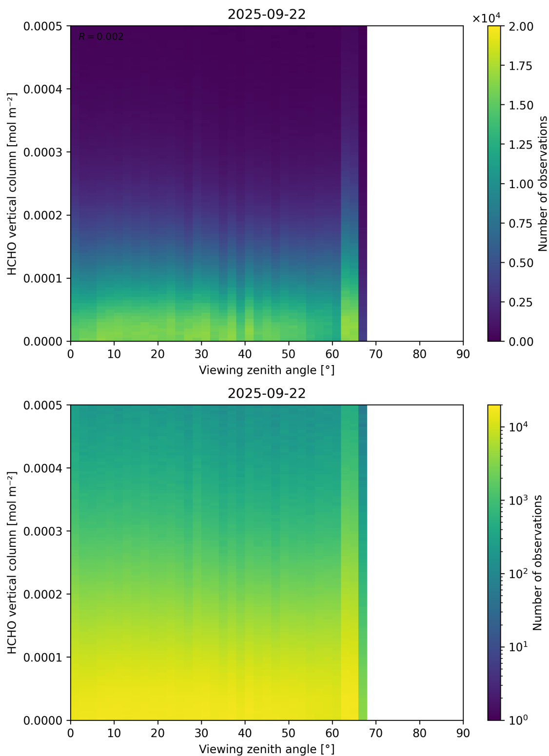
Figure 192: Scatter density plot of “Viewing zenith angle” against “HCHO vertical column” for 2025-09-22 to 2025-09-23.
