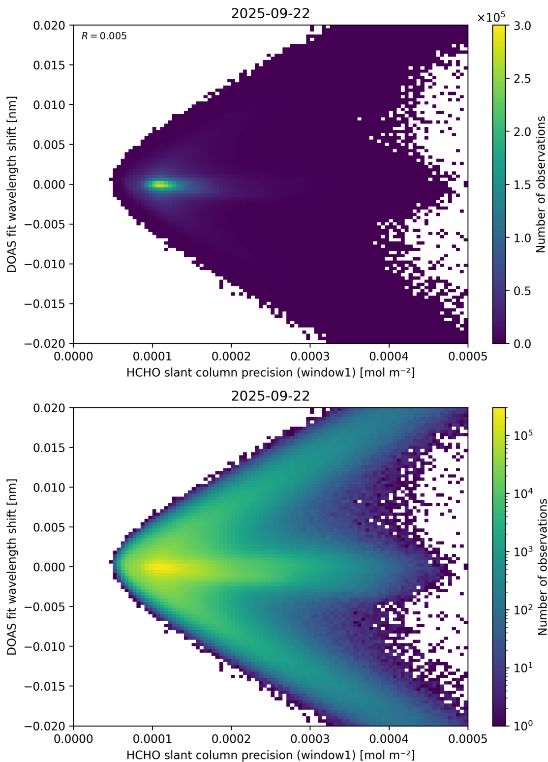
Figure 89: Scatter density plot of “HCHO slant column precision (window1)” against “DOAS fit wavelength shift” for 2025-09-22 to 2025-09-23.
