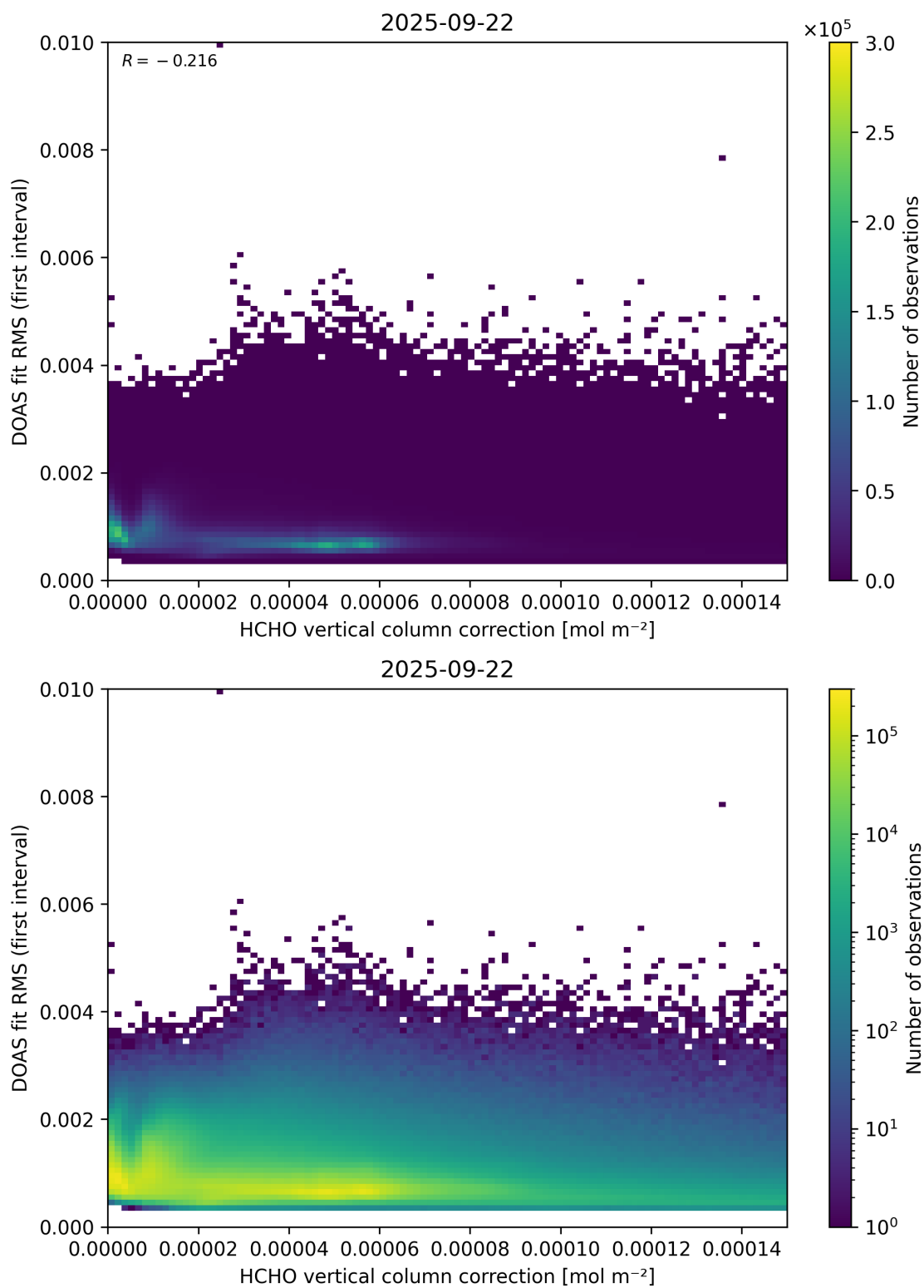
Figure 112: Scatter density plot of “HCHO vertical column correction” against “DOAS fit RMS (first interval)” for 2025-09-22 to 2025-09-23.
