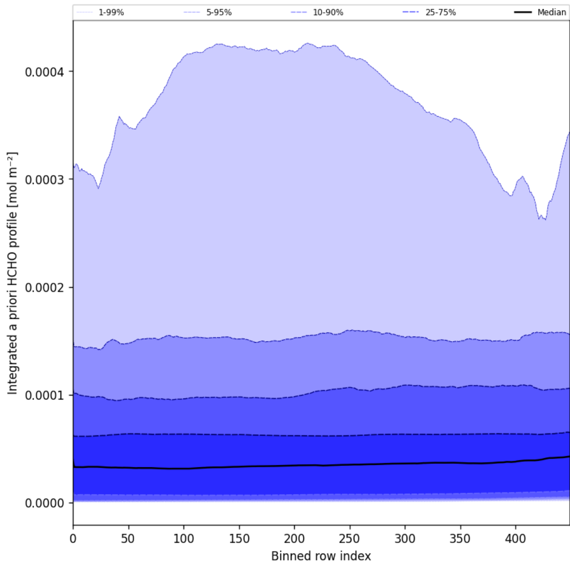
Figure 57: Along track statistics of “Integrated a priori HCHO profile” for 2025-09-22 to 2025-09-23
