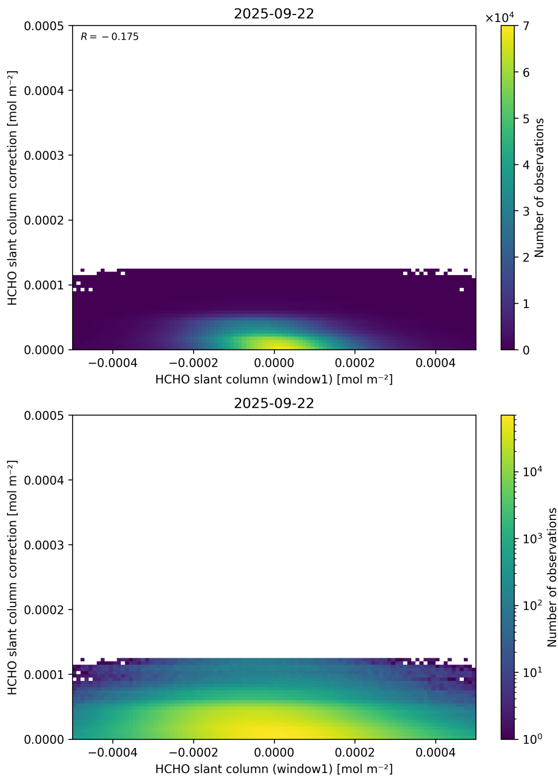
Figure 83: Scatter density plot of “HCHO slant column (window1)” against “HCHO slant column correction” for 2025-09-22 to 2025-09-23.
