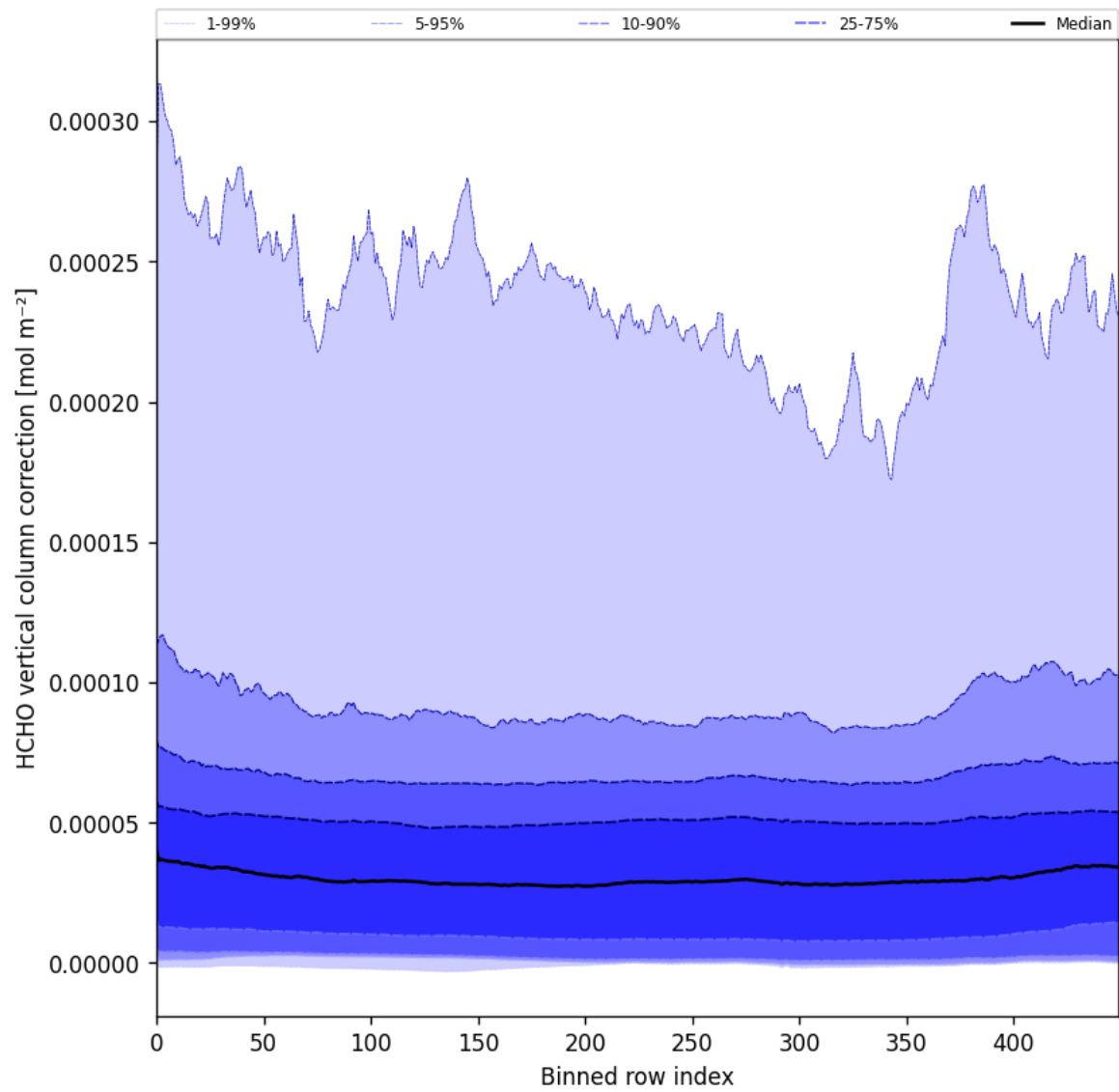
Figure 51: Along track statistics of “HCHO vertical column correction” for 2025-09-22 to 2025-09-23
