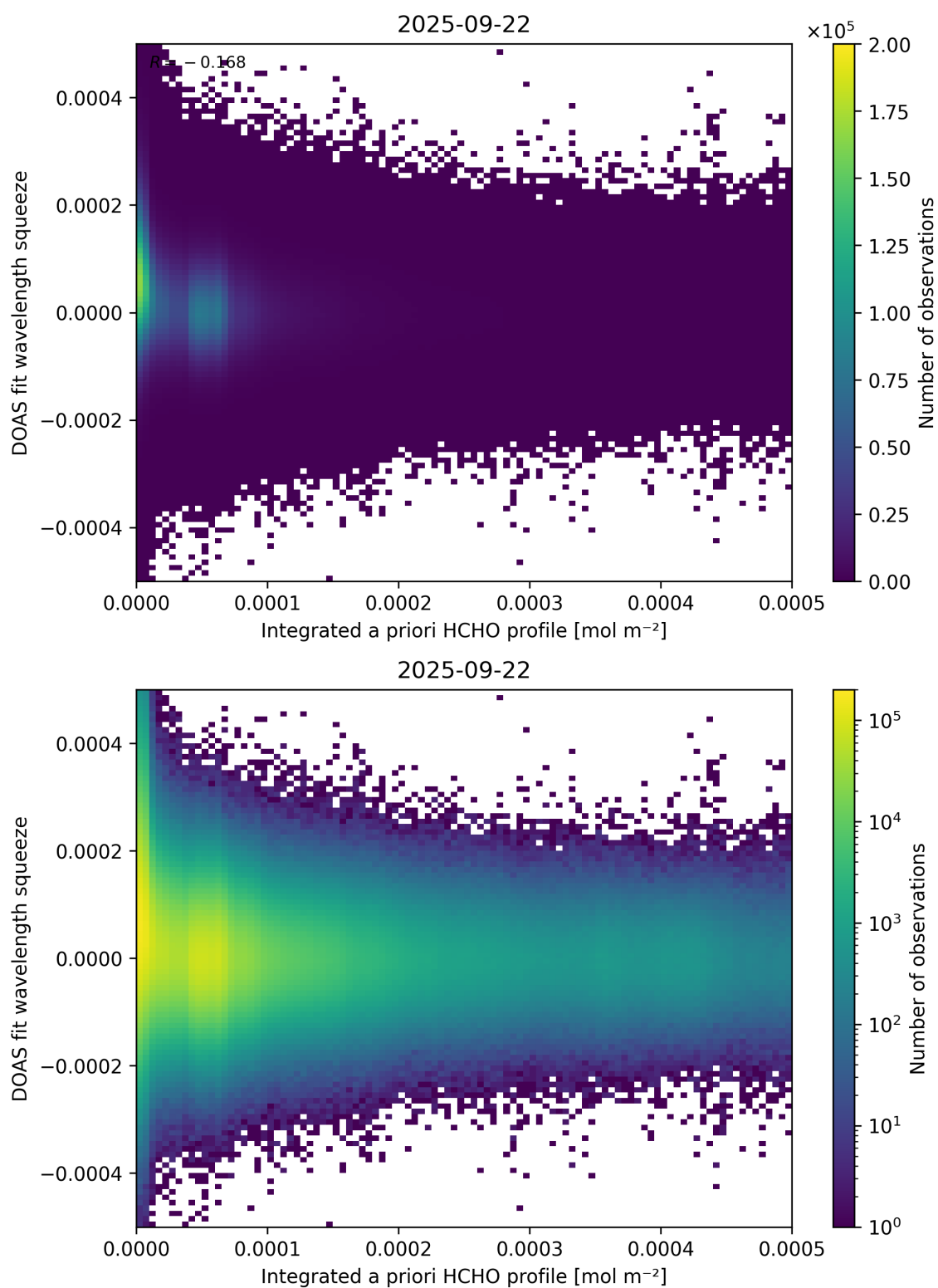
Figure 150: Scatter density plot of “Integrated a priori HCHO profile” against “DOAS fit wavelength squeeze” for 2025-09-22 to 2025-09-23.
