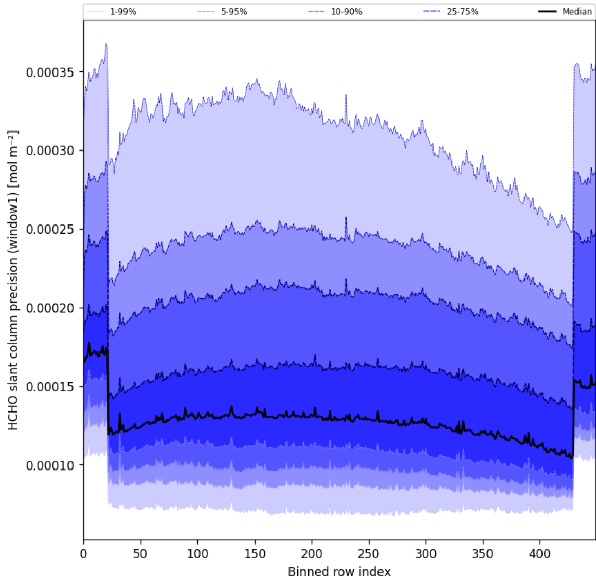
Figure 53: Along track statistics of “HCHO slant column precision (window1)” for 2025-09-22 to 2025-09-23
