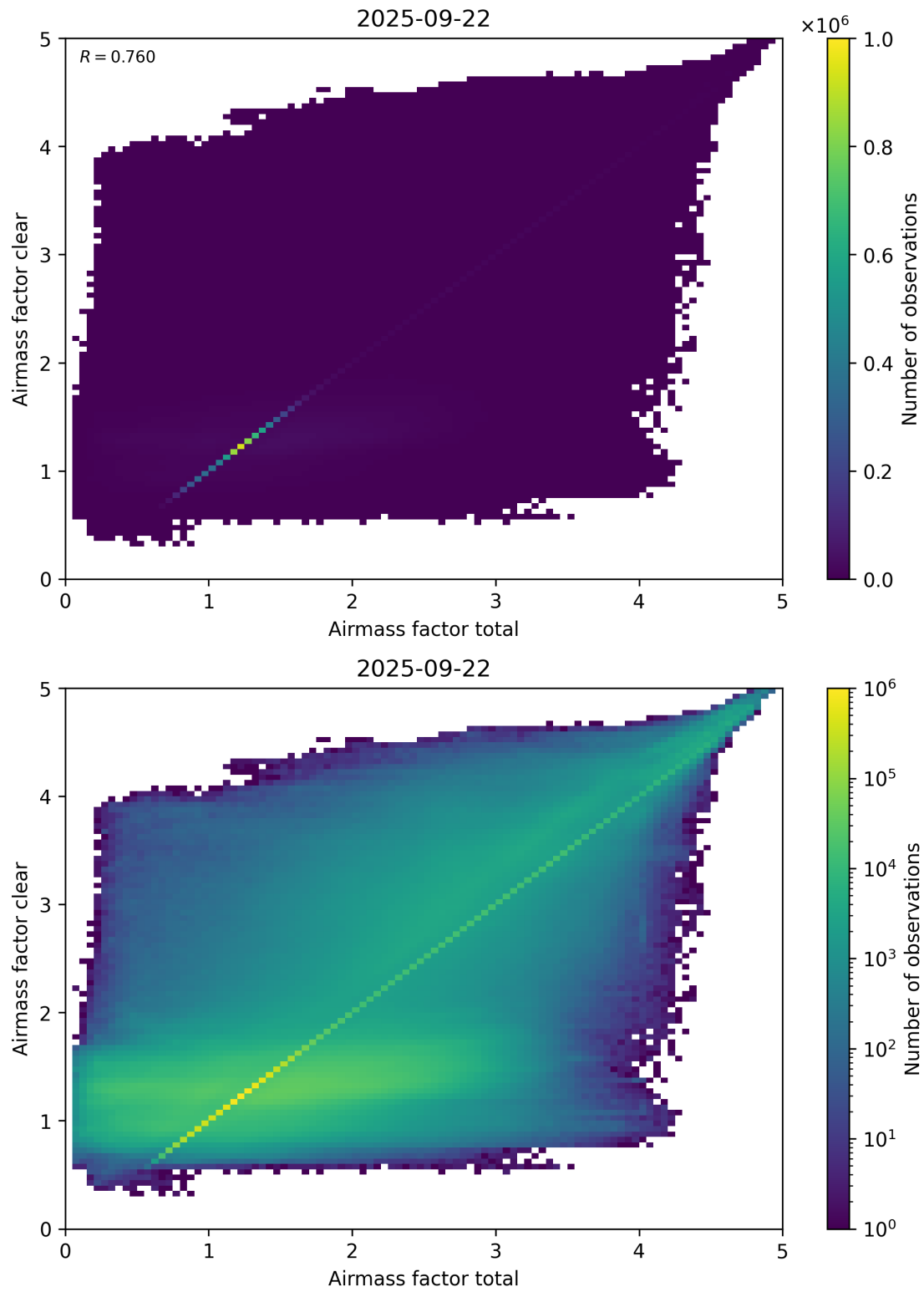
Figure 100: Scatter density plot of “Airmass factor total” against “Airmass factor clear” for 2025-09-22 to 2025-09-23.
