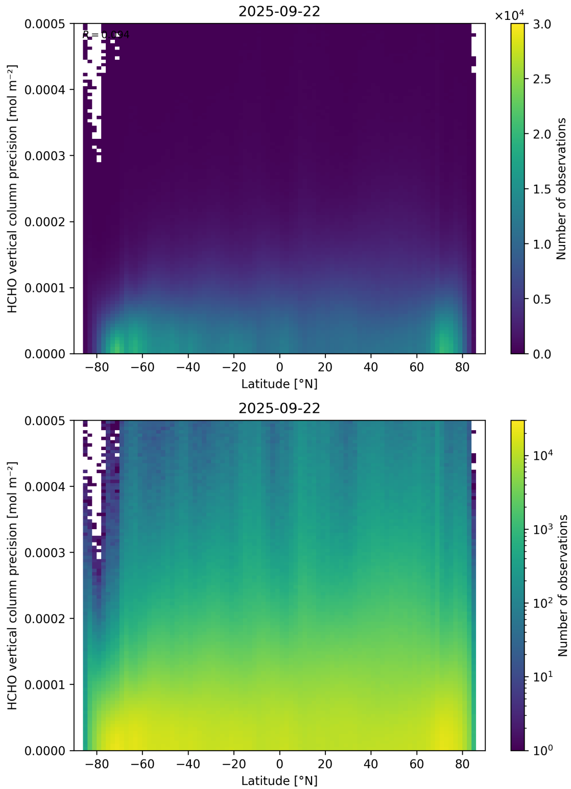
Figure 165: Scatter density plot of “Latitude” against “HCHO vertical column precision” for 2025-09-22 to 2025-09-23.
