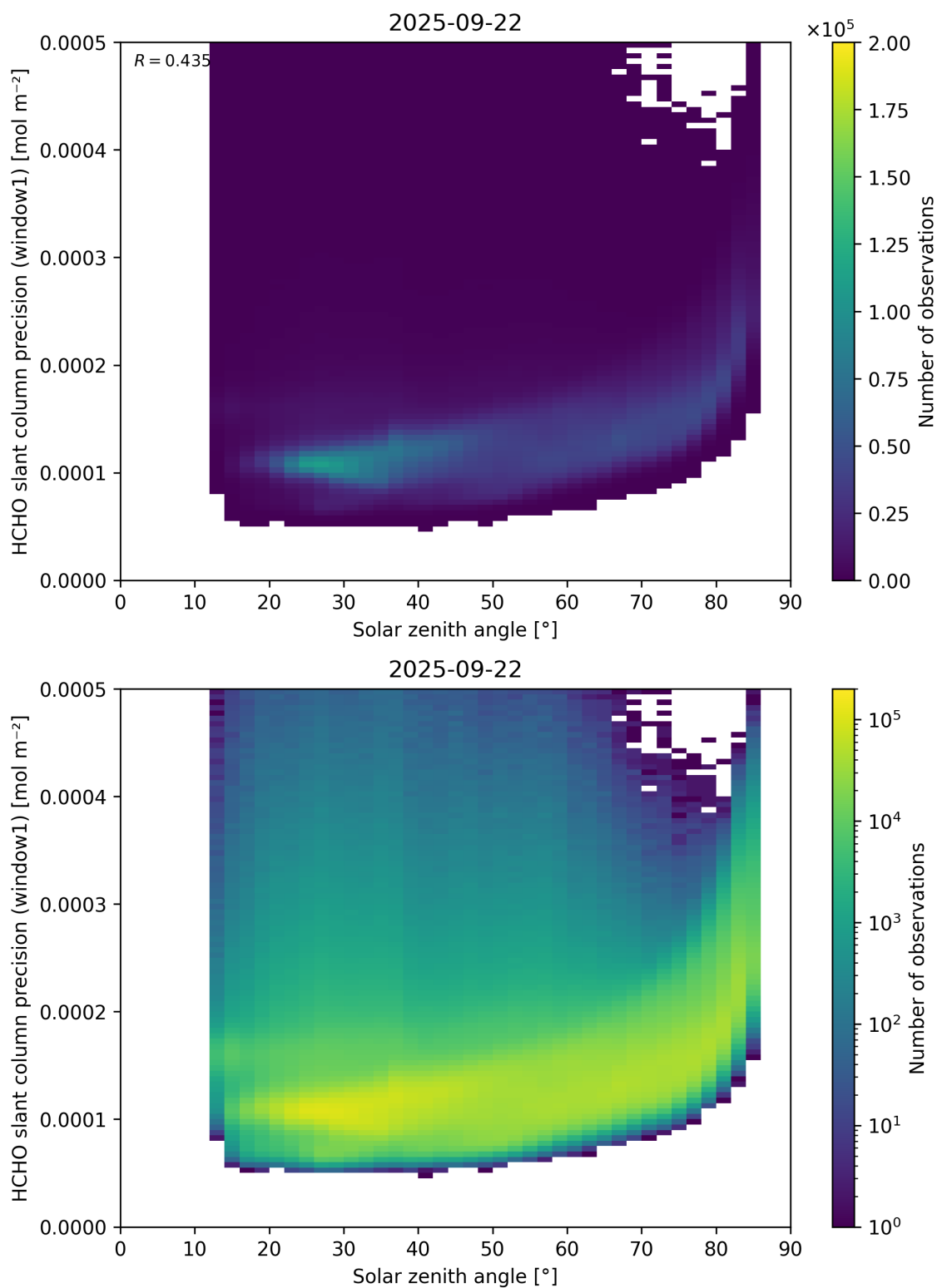
Figure 174: Scatter density plot of “Solar zenith angle” against “HCHO slant column precision (window1)” for 2025-09-22 to 2025-09-23.
