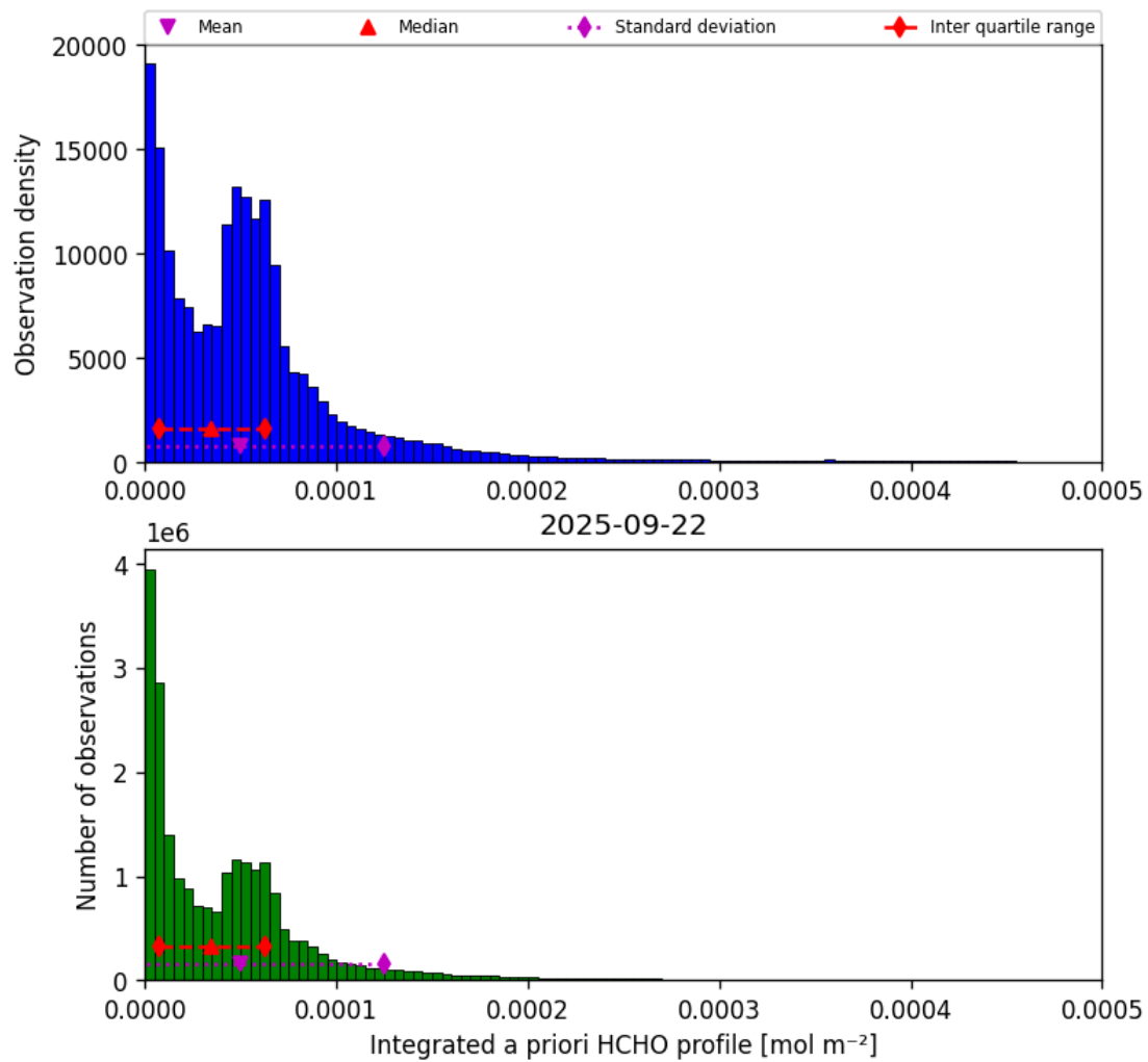
Figure 43: Histogram of “Integrated a priori HCHO profile” for 2025-09-22 to 2025-09-23
