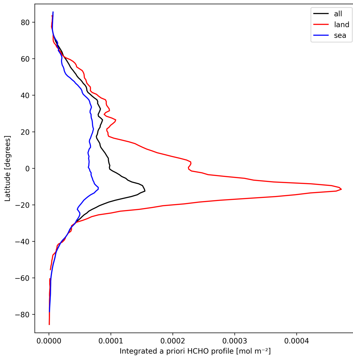
Figure 29: Zonal average of “Integrated a priori HCHO profile” for 2025-09-22 to 2025-09-23.
