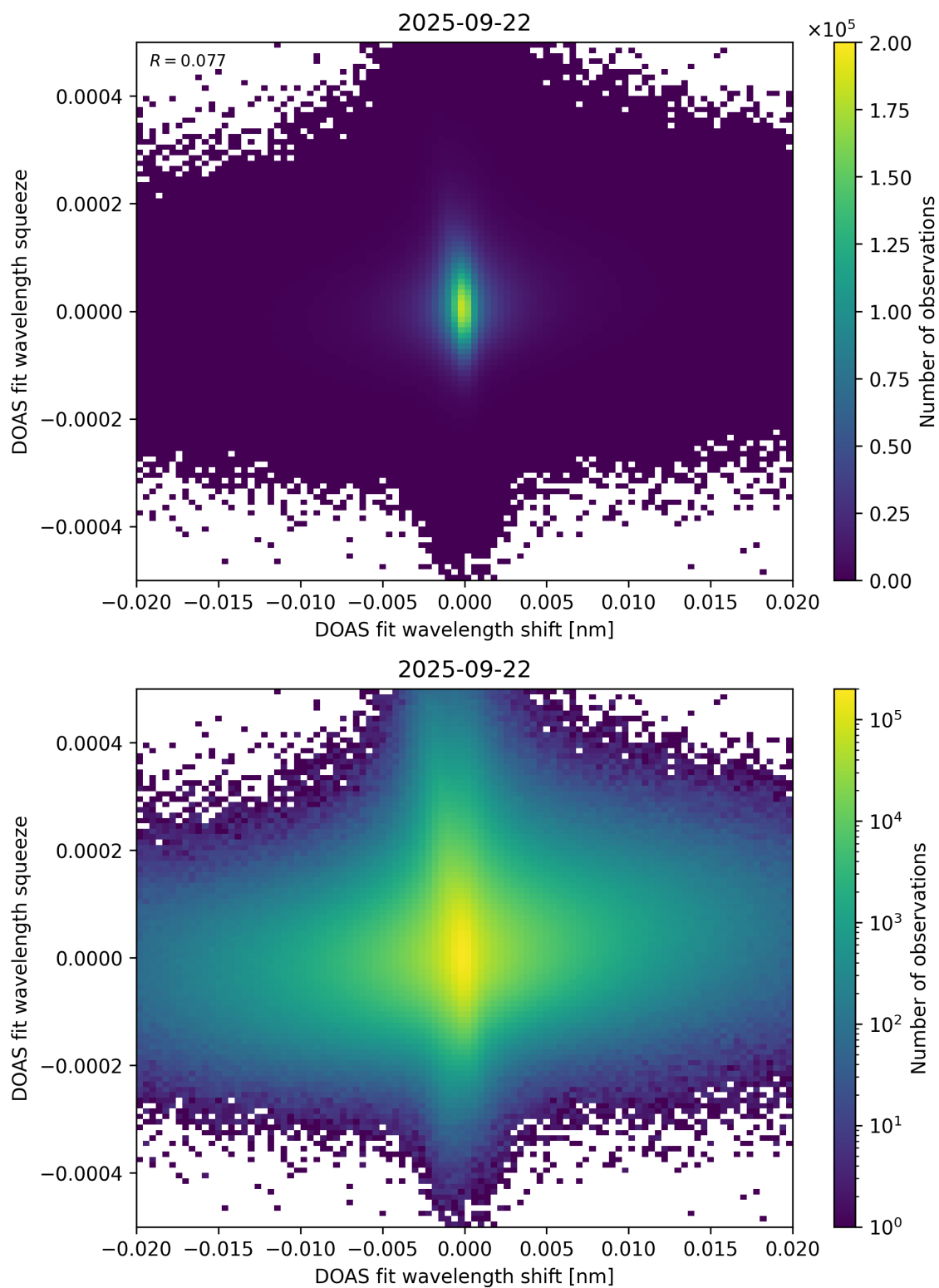
Figure 65: Scatter density plot of “DOAS fit wavelength shift” against “DOAS fit wavelength squeeze” for 2025-09-22 to 2025-09-23.
