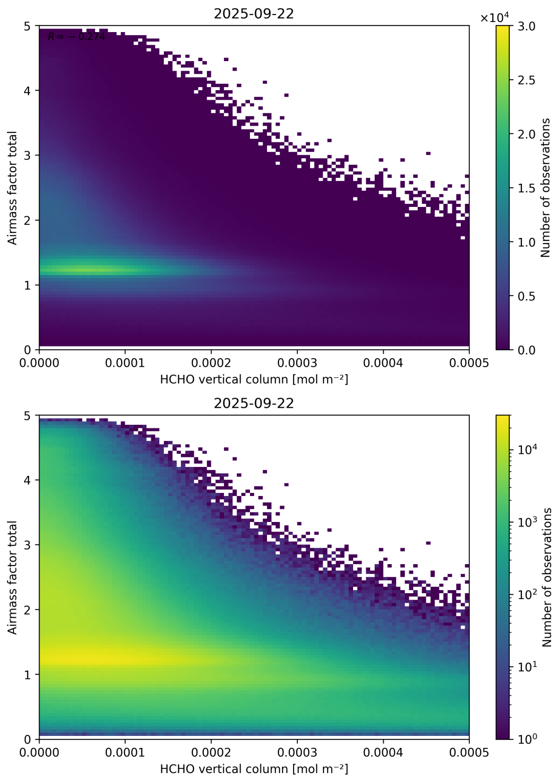
Figure 131: Scatter density plot of “HCHO vertical column” against “Airmass factor total” for 2025-09-22 to 2025-09-23.
