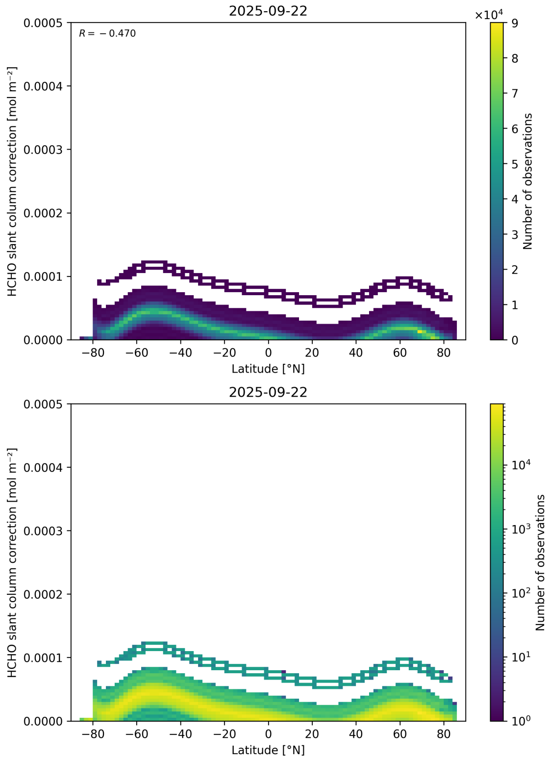
Figure 158: Scatter density plot of “Latitude” against “HCHO slant column correction” for 2025-09-22 to 2025-09-23.
