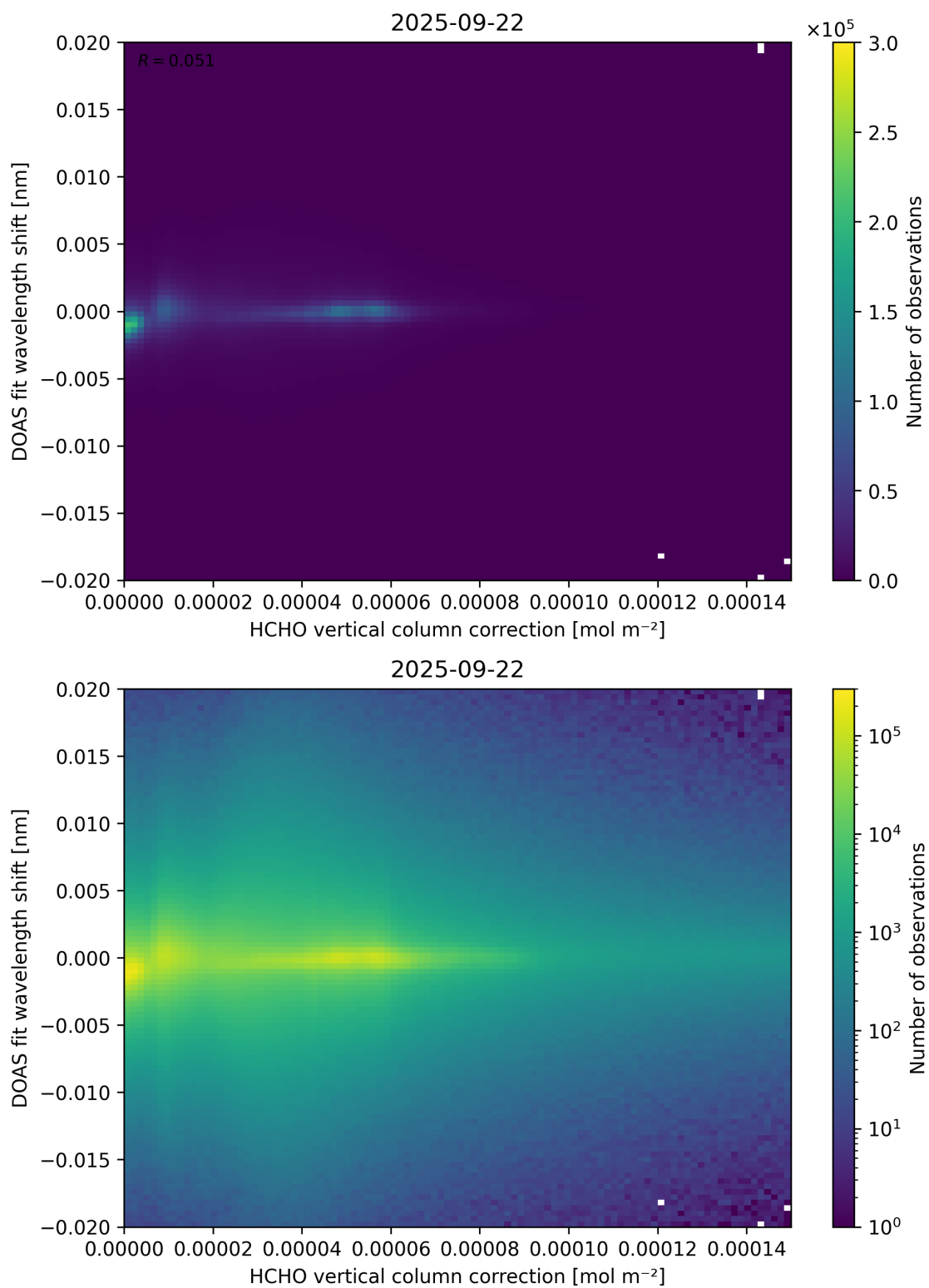
Figure 113: Scatter density plot of “HCHO vertical column correction” against “DOAS fit wavelength shift” for 2025-09-22 to 2025-09-23.
