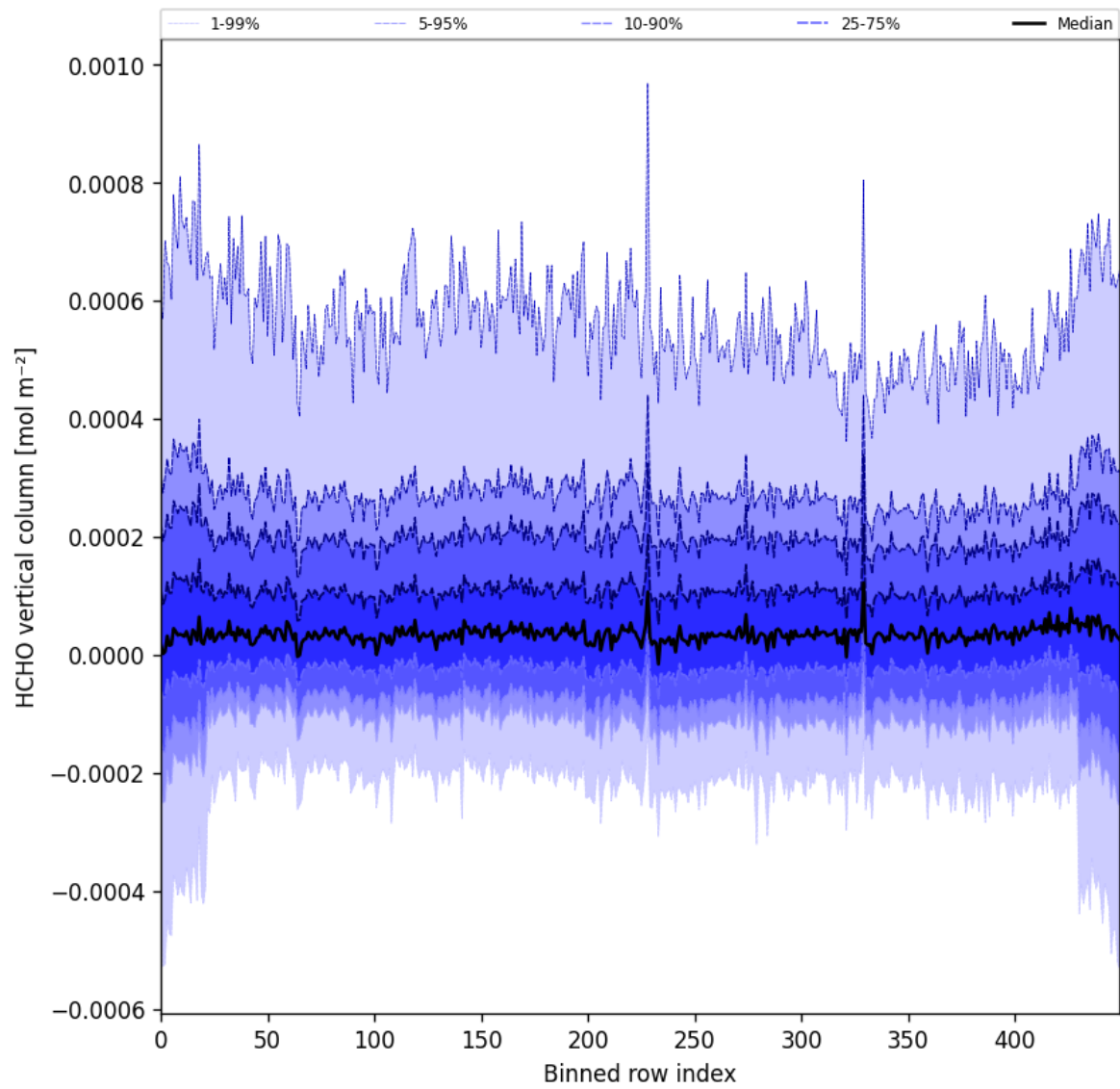
Figure 49: Along track statistics of “HCHO vertical column” for 2025-09-22 to 2025-09-23
