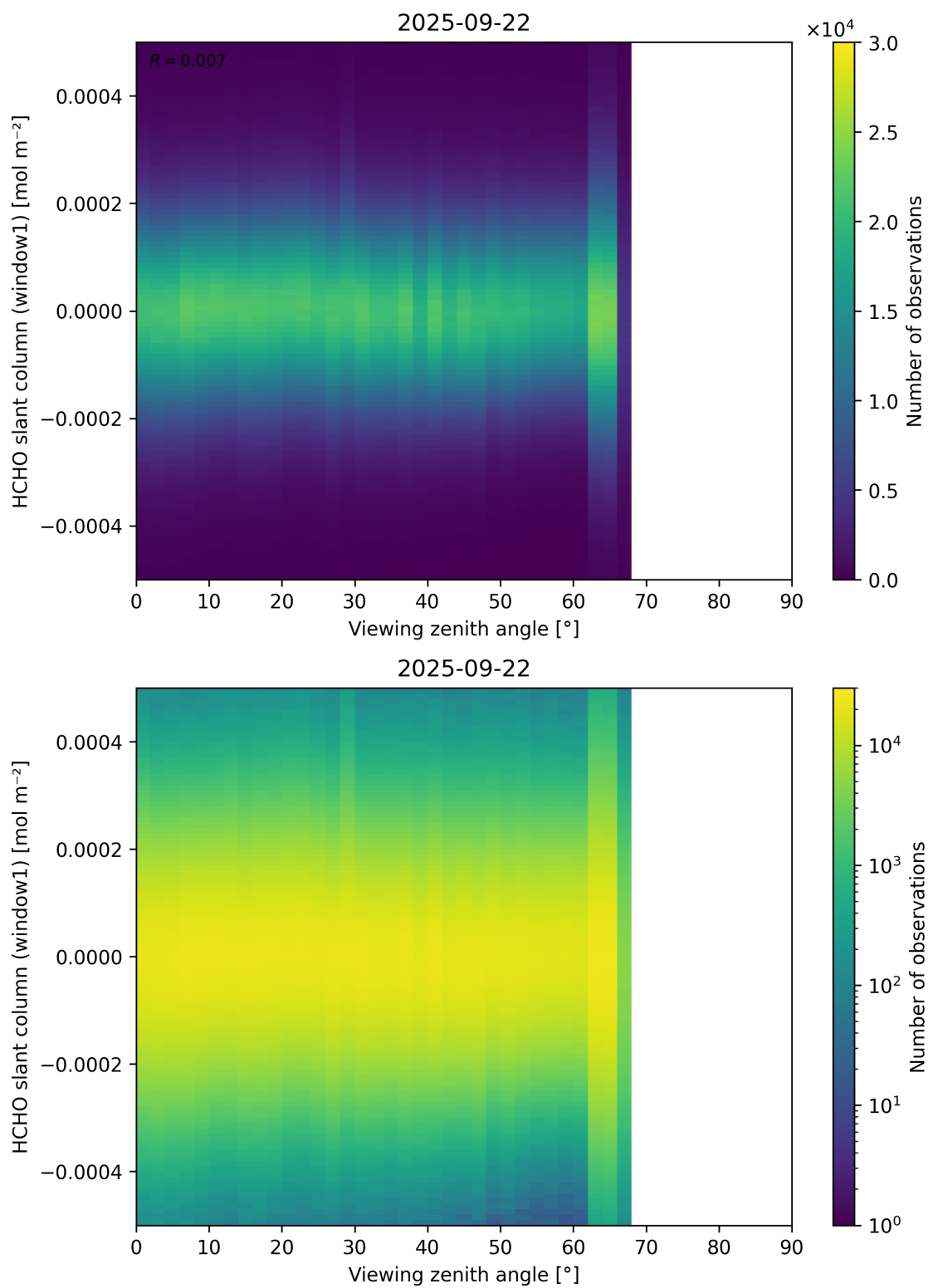
Figure 188: Scatter density plot of “Viewing zenith angle” against “HCHO slant column (window1)” for 2025-09-22 to 2025-09-23.
