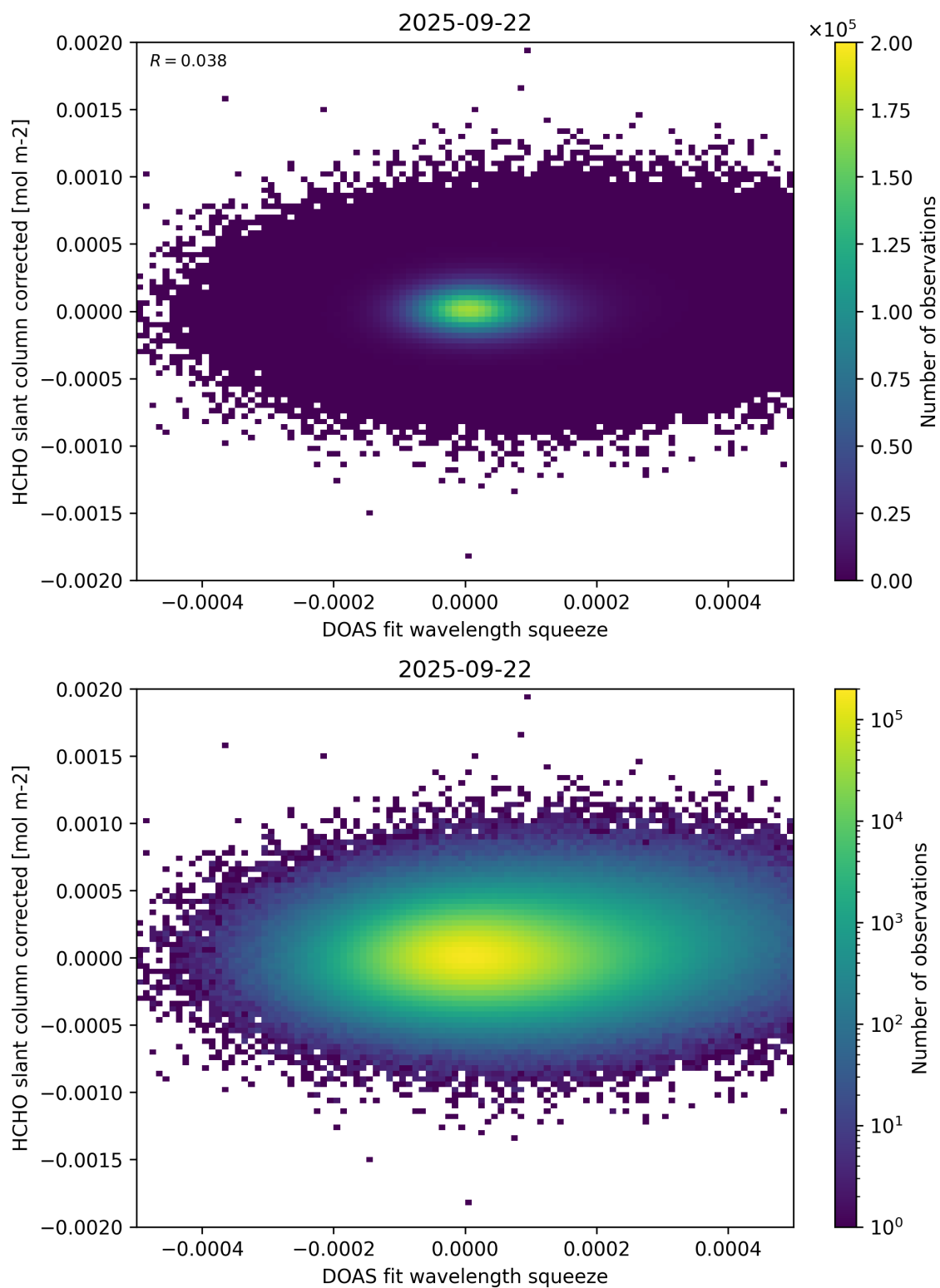
Figure 69: Scatter density plot of “DOAS fit wavelength squeeze” against “HCHO slant column corrected” for 2025-09-22 to 2025-09-23.
