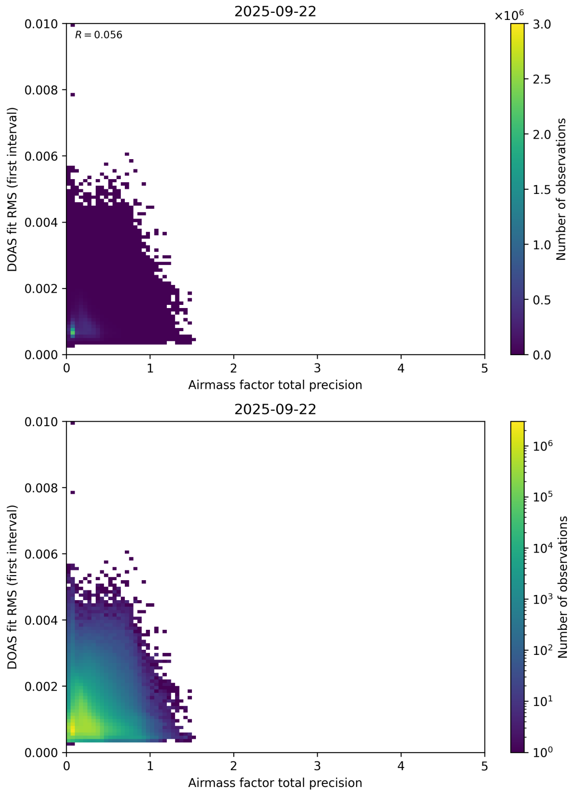
Figure 105: Scatter density plot of “Airmass factor total precision” against “DOAS fit RMS (first interval)” for 2025-09-22 to 2025-09-23.
