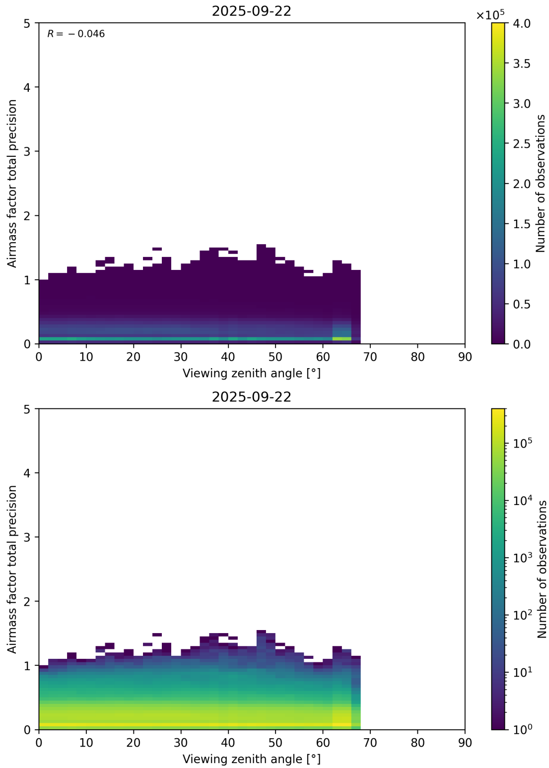
Figure 191: Scatter density plot of “Viewing zenith angle” against “Airmass factor total precision” for 2025-09-22 to 2025-09-23.
