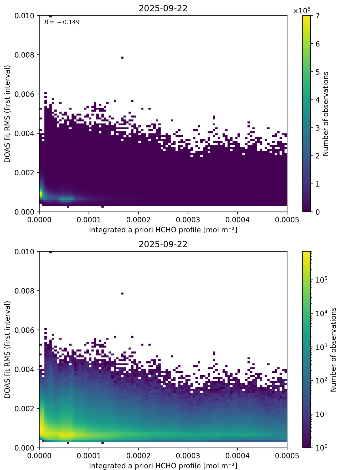
Figure 148: Scatter density plot of “Integrated a priori HCHO profile” against “DOAS fit RMS (first interval)” for 2025-09-22 to 2025-09-23.
