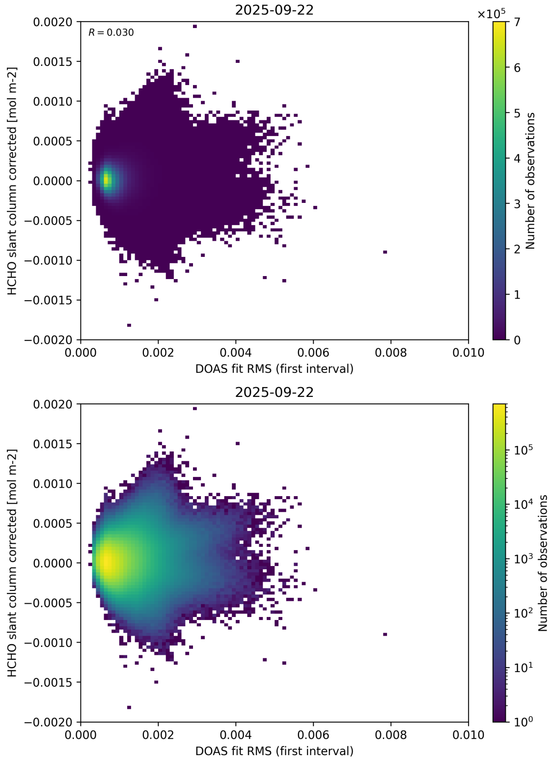
Figure 62: Scatter density plot of “DOAS fit RMS (first interval)” against “HCHO slant column corrected” for 2025-09-22 to 2025-09-23.
