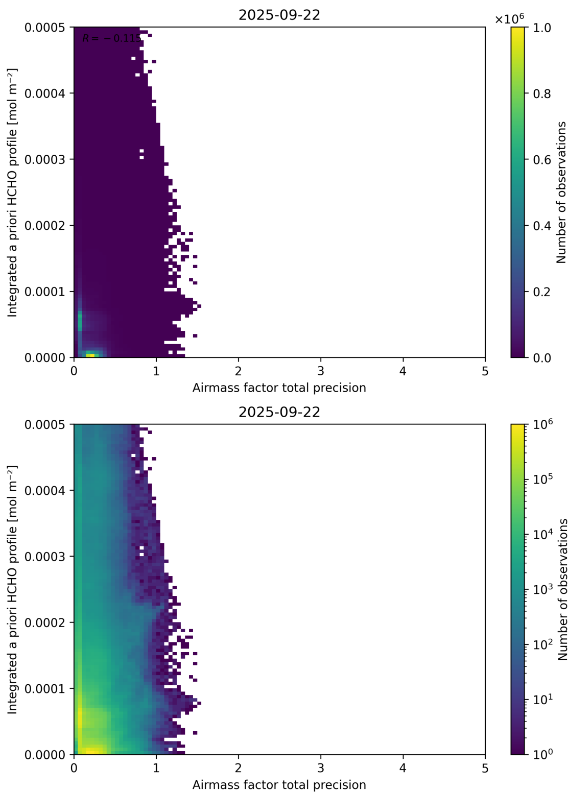
Figure 111: Scatter density plot of “Airmass factor total precision” against “Integrated a priori HCHO profile” for 2025-09-22 to 2025-09-23.
