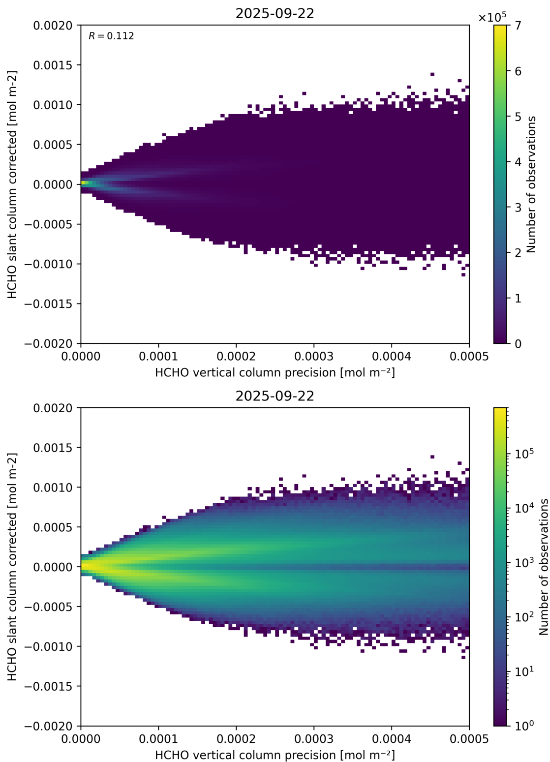
Figure 140: Scatter density plot of “HCHO vertical column precision” against “HCHO slant column corrected” for 2025-09-22 to 2025-09-23.
