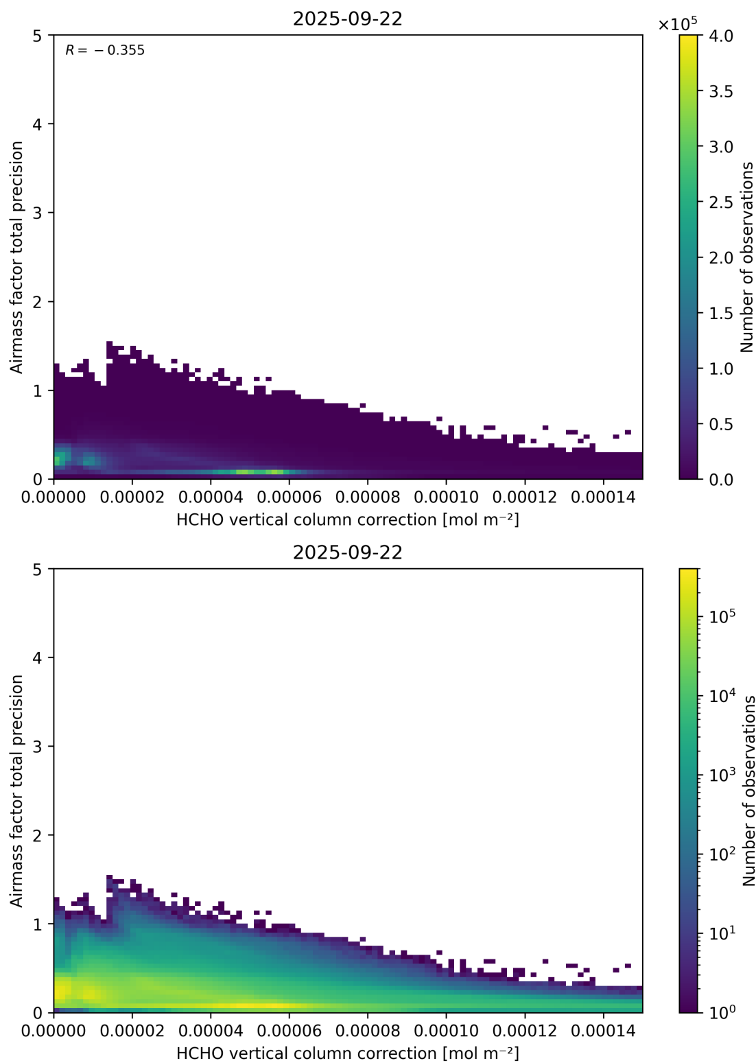
Figure 121: Scatter density plot of “HCHO vertical column correction” against “Airmass factor total precision” for 2025-09-22 to 2025-09-23.
