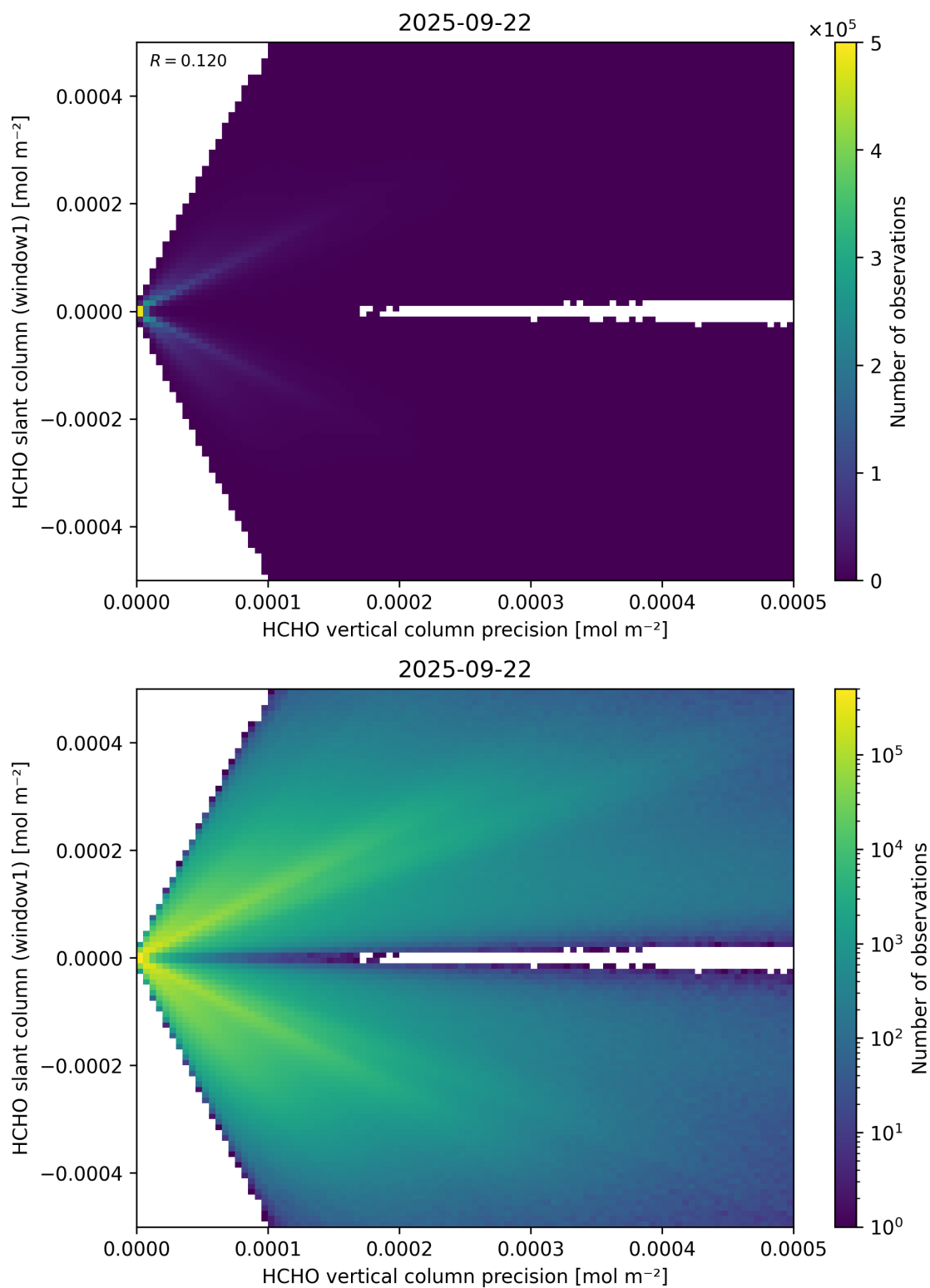
Figure 142: Scatter density plot of “HCHO vertical column precision” against “HCHO slant column (window1)” for 2025-09-22 to 2025-09-23.
