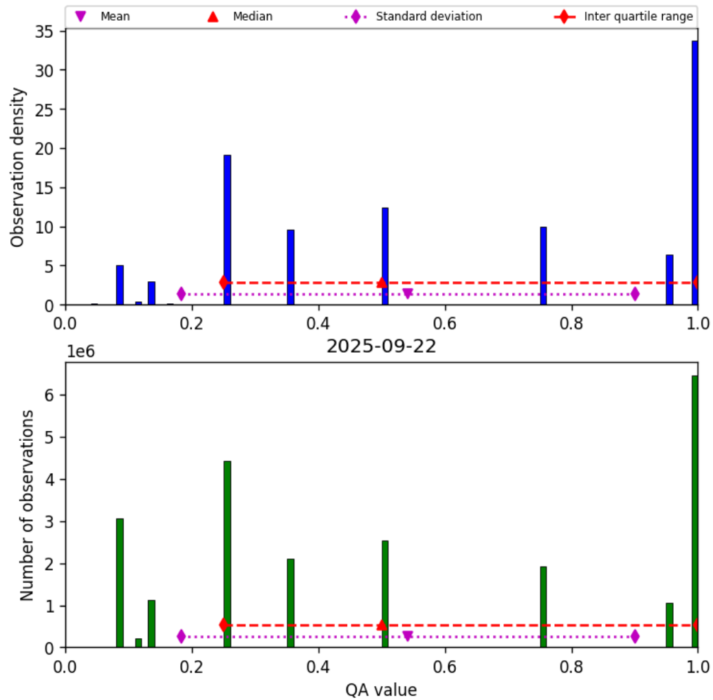
Figure 34: Histogram of “QA value” for 2025-09-22 to 2025-09-23
