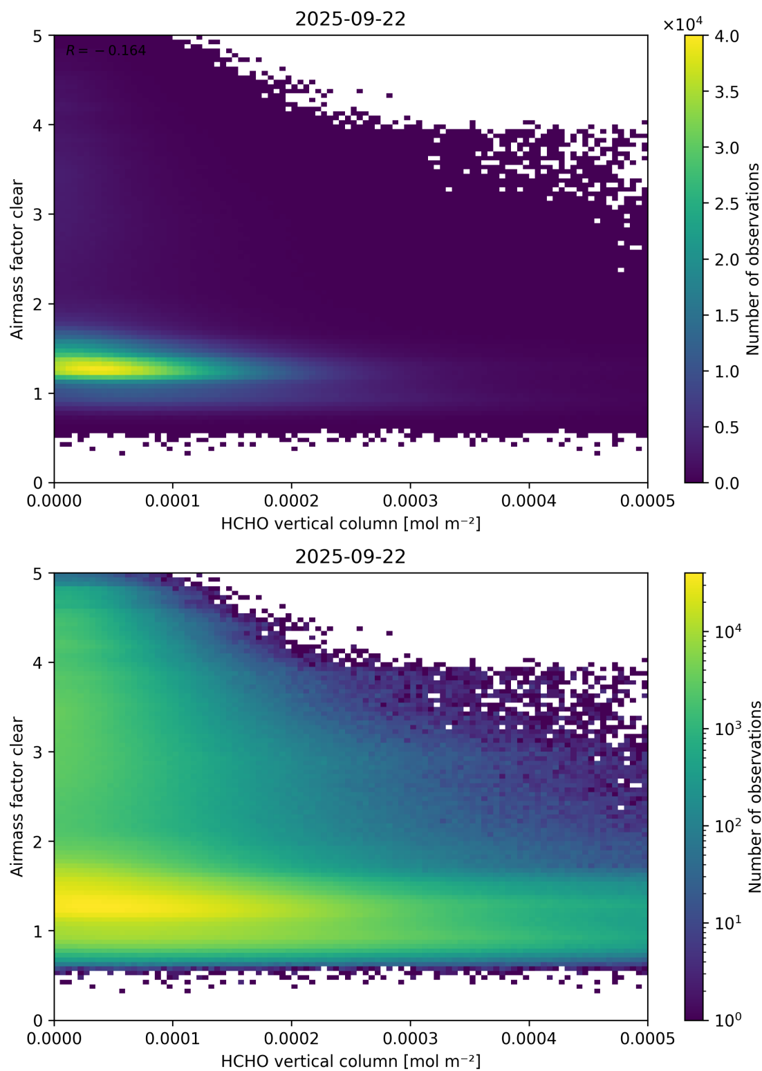
Figure 126: Scatter density plot of “HCHO vertical column” against “Airmass factor clear” for 2025-09-22 to 2025-09-23.
