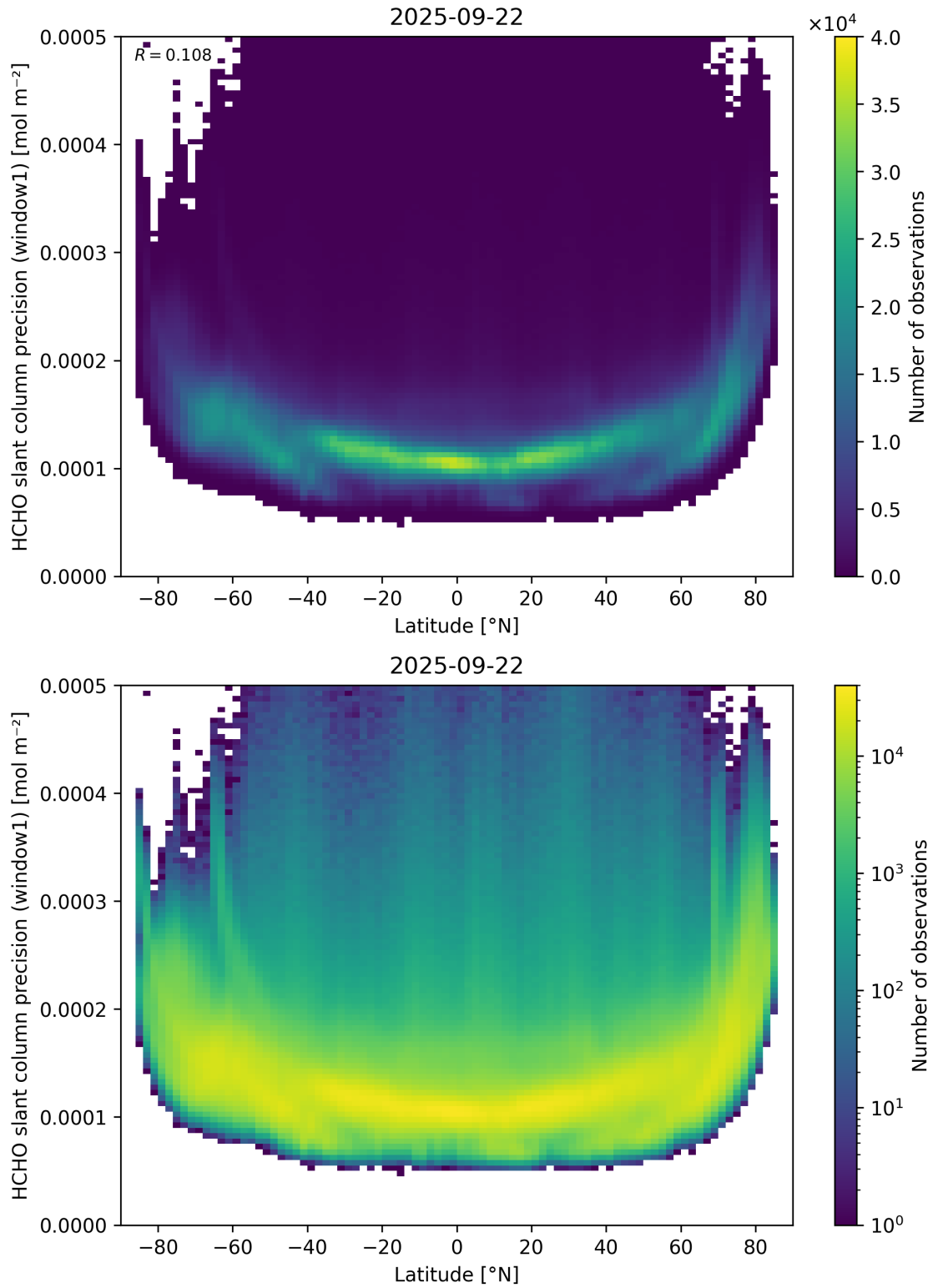
Figure 160: Scatter density plot of “Latitude” against “HCHO slant column precision (window1)” for 2025-09-22 to 2025-09-23.
