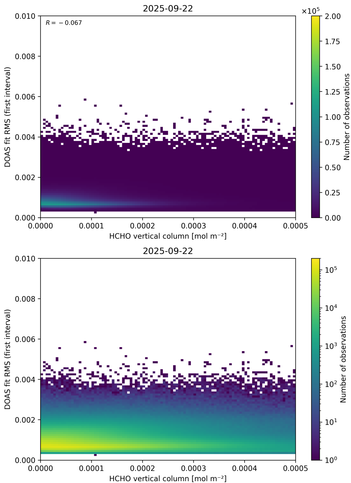
Figure 123: Scatter density plot of “HCHO vertical column” against “DOAS fit RMS (first interval)” for 2025-09-22 to 2025-09-23.
