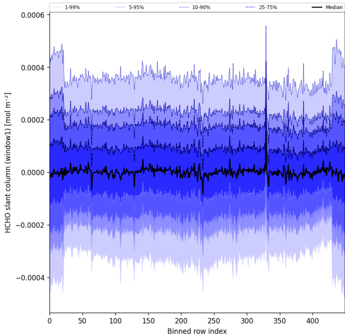
Figure 52: Along track statistics of “HCHO slant column (window1)” for 2025-09-22 to 2025-09-23
