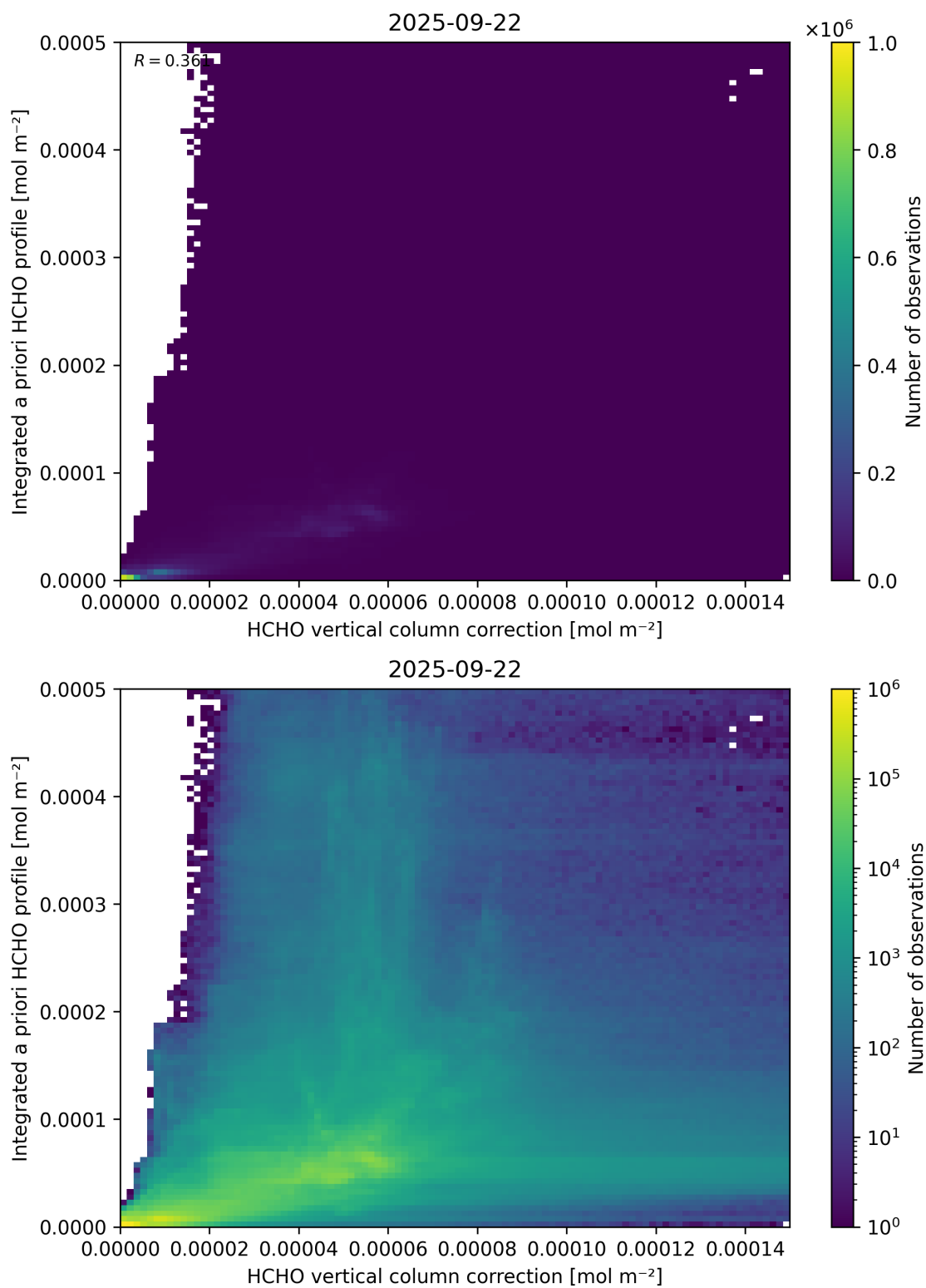
Figure 122: Scatter density plot of “HCHO vertical column correction” against “Integrated a priori HCHO profile” for 2025-09-22 to 2025-09-23.
