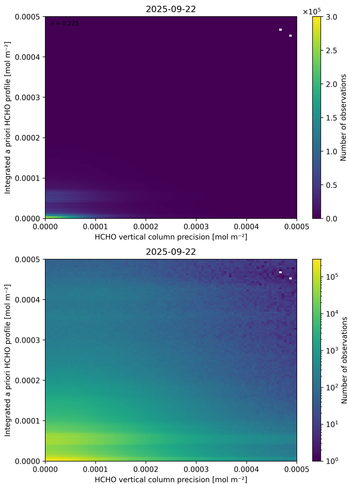
Figure 147: Scatter density plot of “HCHO vertical column precision” against “Integrated a priori HCHO profile” for 2025-09-22 to 2025-09-23.
