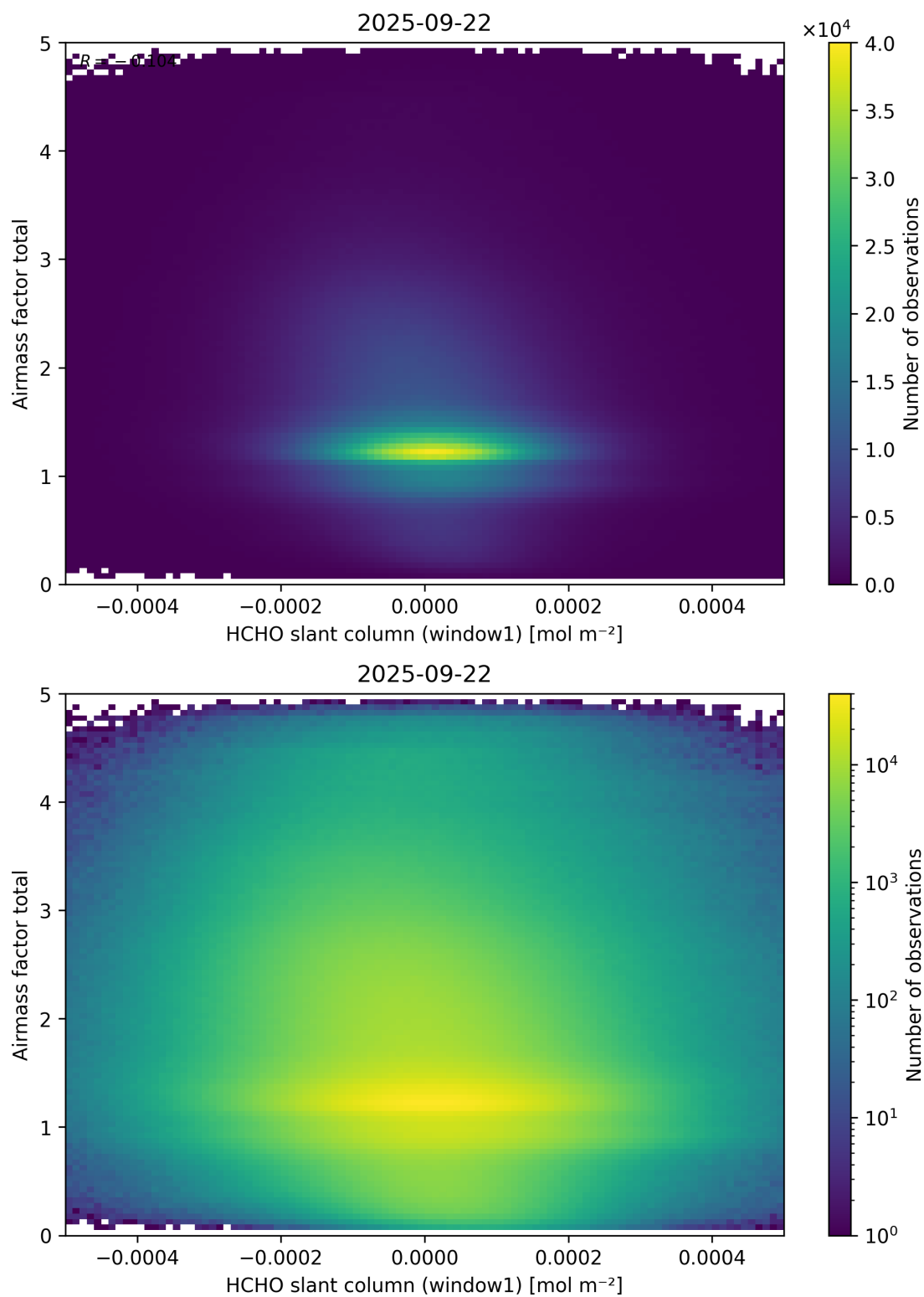
Figure 85: Scatter density plot of “HCHO slant column (window1)” against “Airmass factor total” for 2025-09-22 to 2025-09-23.
