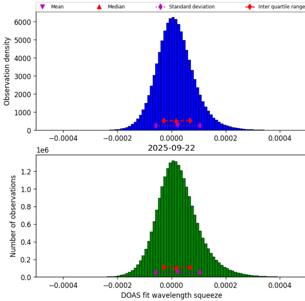
Figure 45: Histogram of “DOAS fit wavelength squeeze” for 2025-09-22 to 2025-09-23
