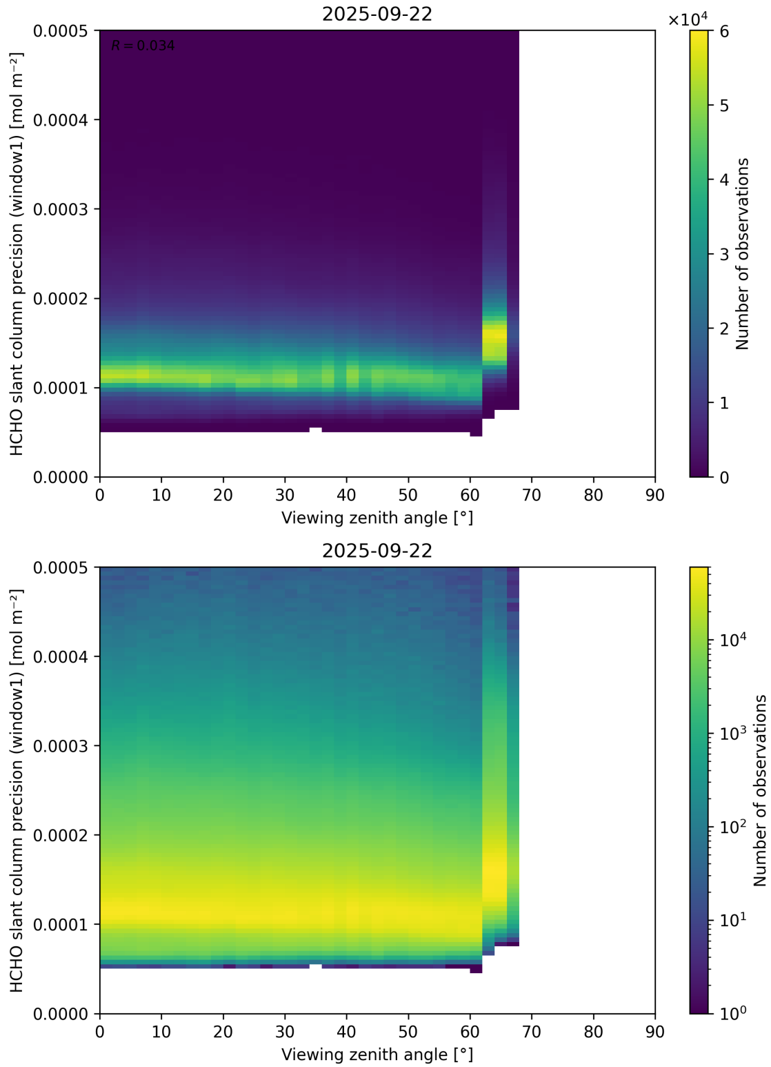
Figure 189: Scatter density plot of “Viewing zenith angle” against “HCHO slant column precision (window1)” for 2025-09-22 to 2025-09-23.
