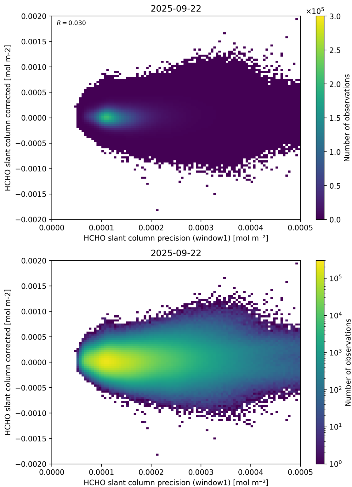
Figure 92: Scatter density plot of “HCHO slant column precision (window1)” against “HCHO slant column corrected” for 2025-09-22 to 2025-09-23.
