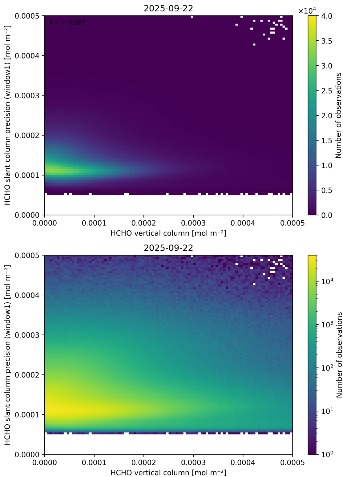
Figure 130: Scatter density plot of “HCHO vertical column” against “HCHO slant column precision (window1)” for 2025-09-22 to 2025-09-23.
