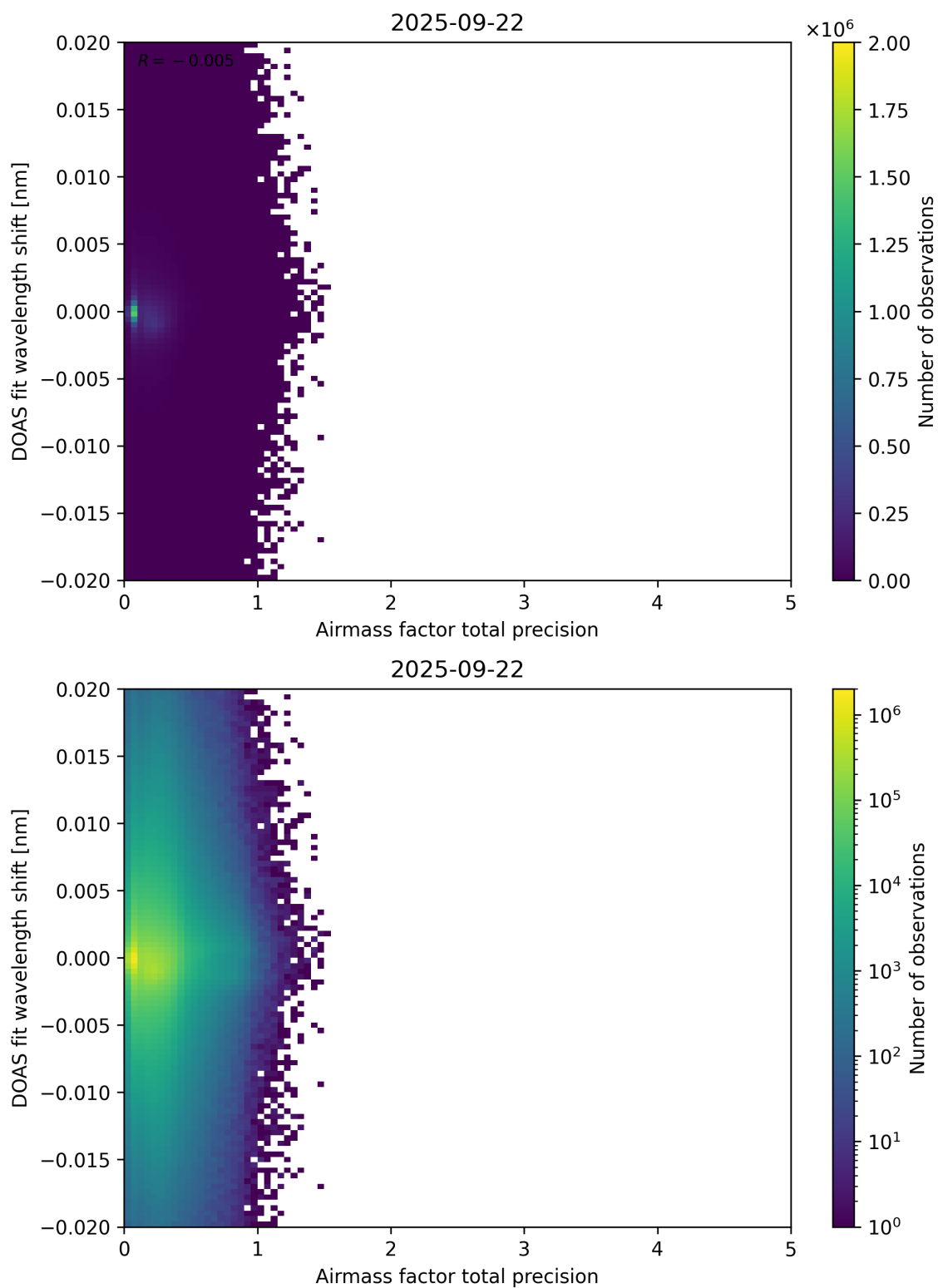
Figure 106: Scatter density plot of “Airmass factor total precision” against “DOAS fit wavelength shift” for 2025-09-22 to 2025-09-23.
