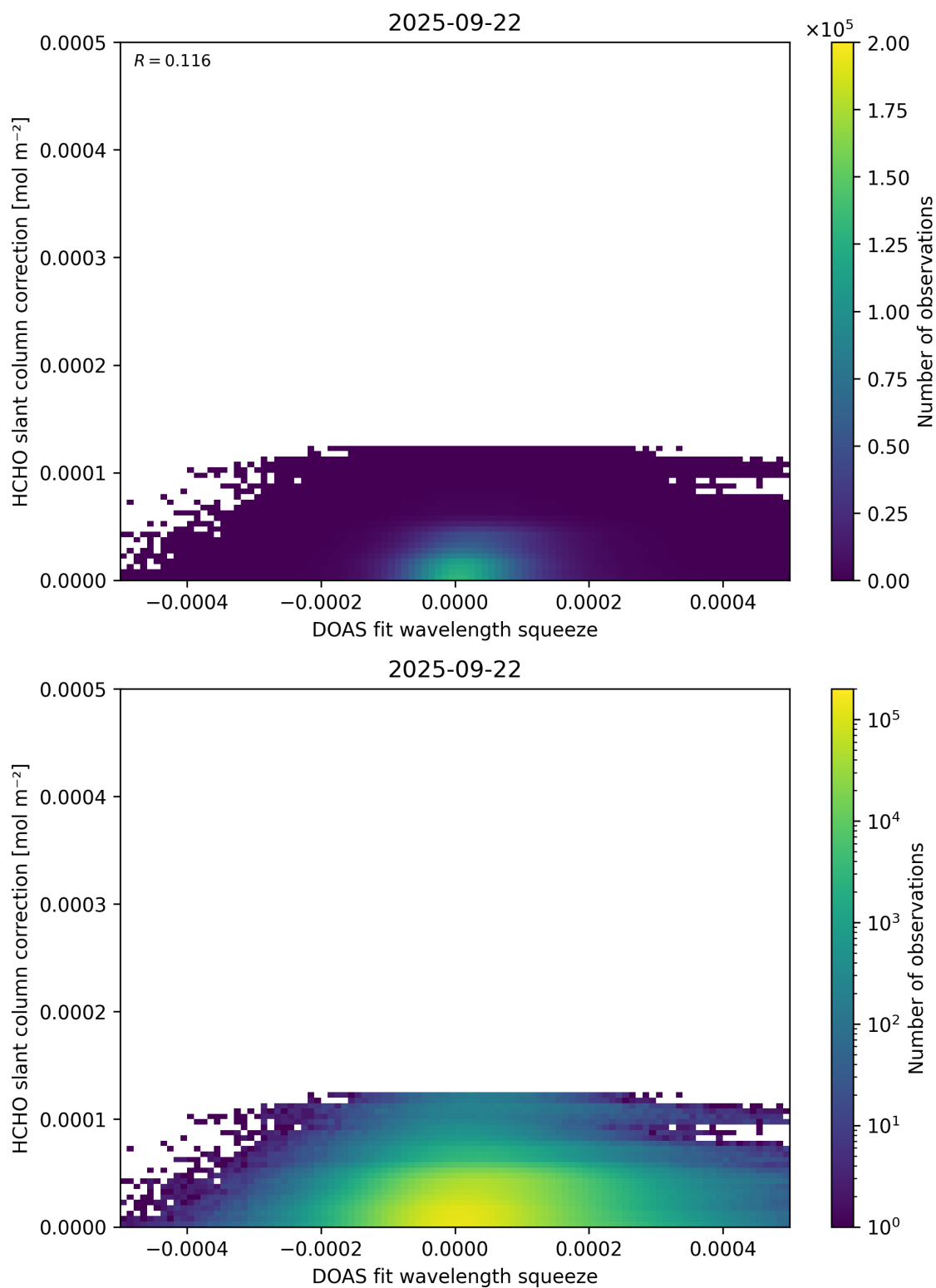
Figure 70: Scatter density plot of “DOAS fit wavelength squeeze” against “HCHO slant column correction” for 2025-09-22 to 2025-09-23.
