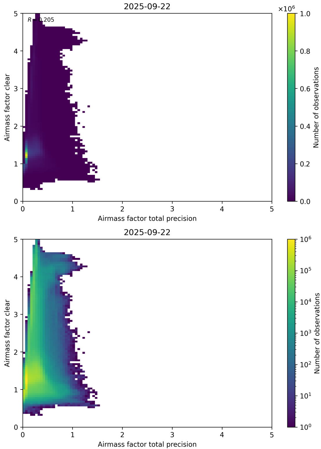
Figure 108: Scatter density plot of “Airmass factor total precision” against “Airmass factor clear” for 2025-09-22 to 2025-09-23.
