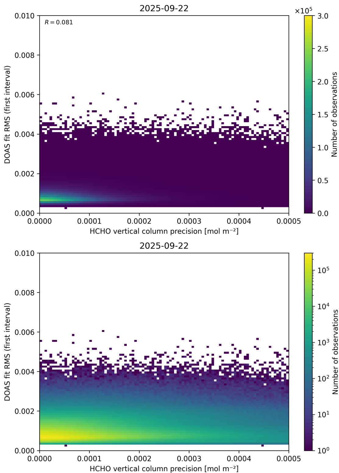
Figure 136: Scatter density plot of “HCHO vertical column precision” against “DOAS fit RMS (first interval)” for 2025-09-22 to 2025-09-23.
