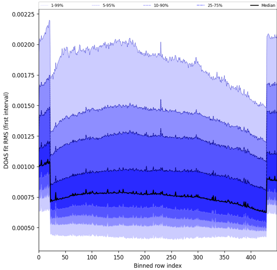
Figure 60: Along track statistics of “DOAS fit RMS (first interval)” for 2025-09-22 to 2025-09-23
