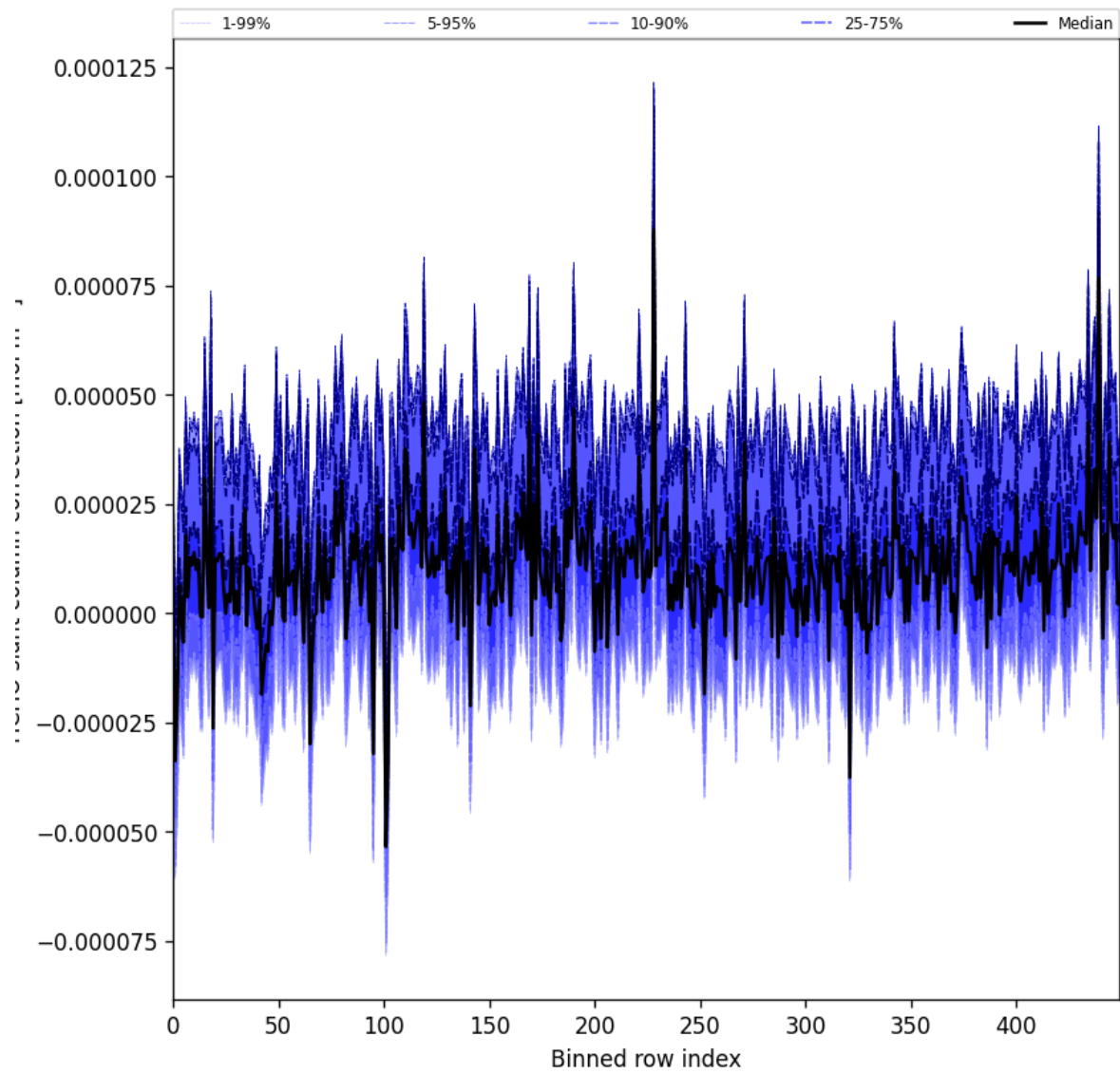
Figure 61: Along track statistics of “HCHO slant column correction” for 2025-09-22 to 2025-09-23
