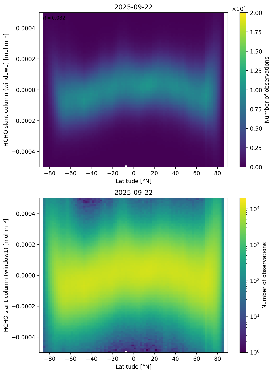
Figure 159: Scatter density plot of “Latitude” against “HCHO slant column (window1)” for 2025-09-22 to 2025-09-23.
