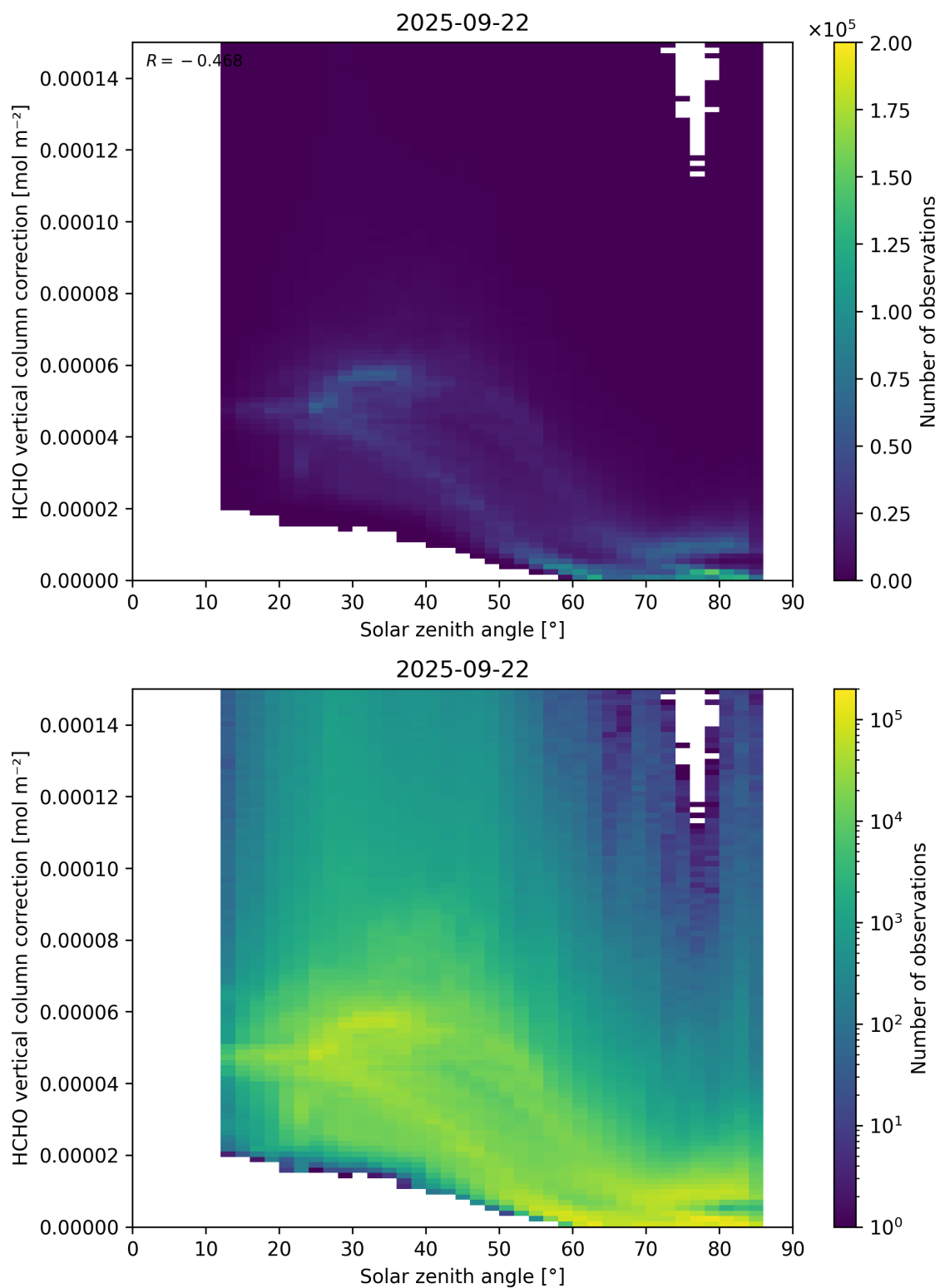
Figure 178: Scatter density plot of “Solar zenith angle” against “HCHO vertical column correction” for 2025-09-22 to 2025-09-23.
