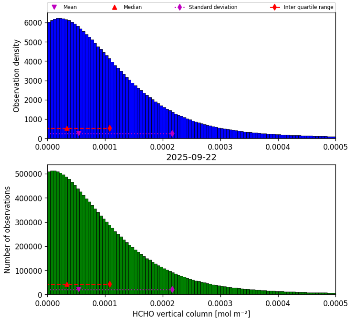
Figure 35: Histogram of “HCHO vertical column” for 2025-09-22 to 2025-09-23
