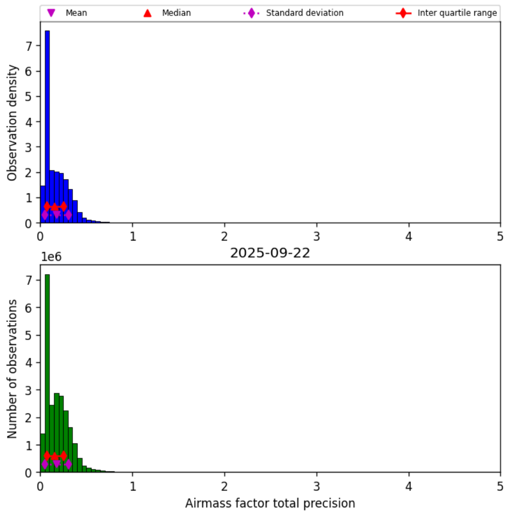
Figure 41: Histogram of “Airmass factor total precision” for 2025-09-22 to 2025-09-23
