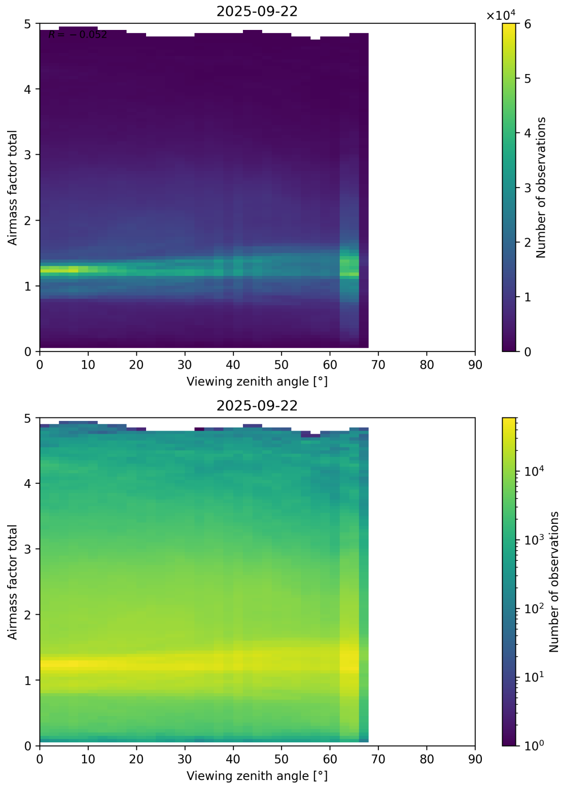
Figure 190: Scatter density plot of “Viewing zenith angle” against “Airmass factor total” for 2025-09-22 to 2025-09-23.
