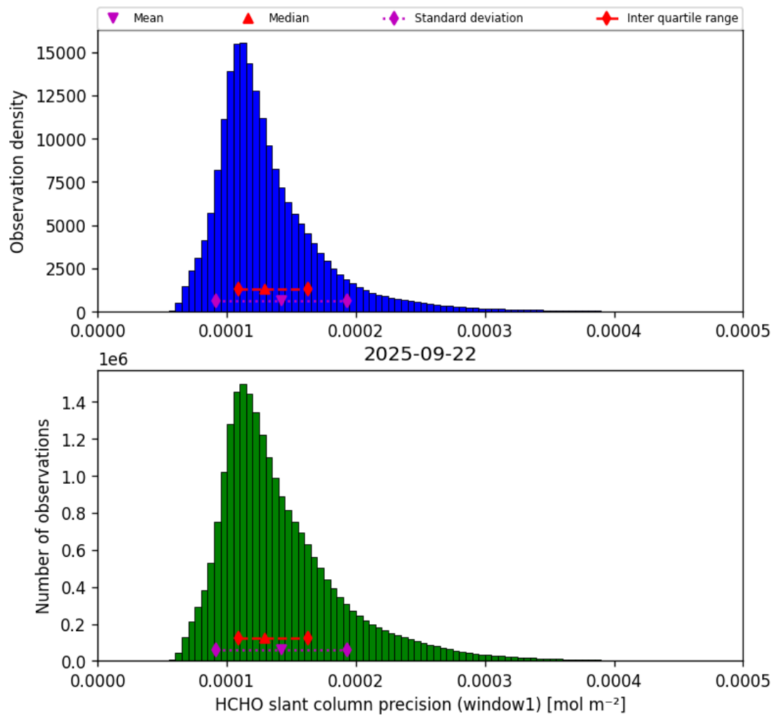
Figure 39: Histogram of “HCHO slant column precision (window1)” for 2025-09-22 to 2025-09-23
