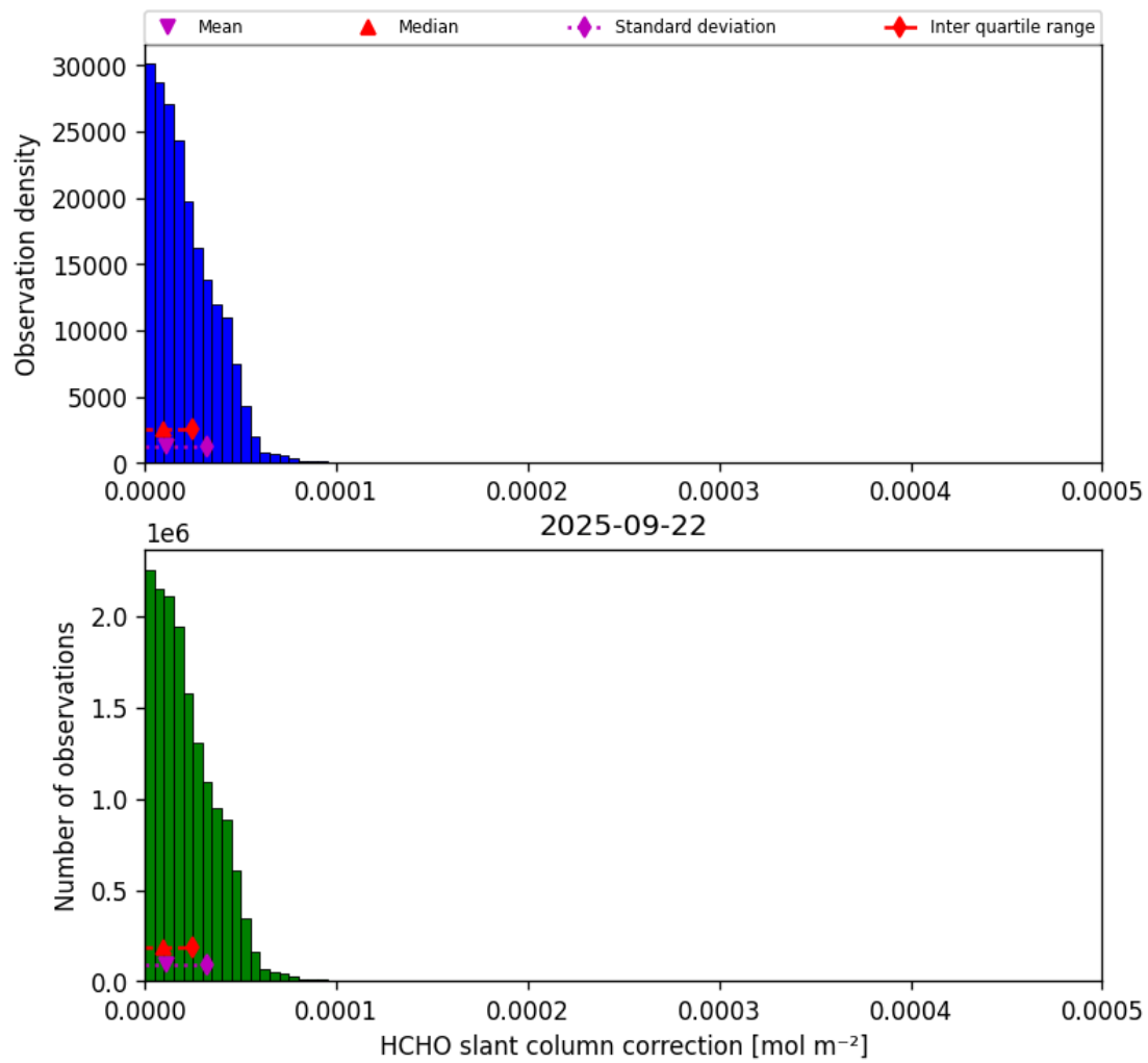
Figure 47: Histogram of “HCHO slant column correction” for 2025-09-22 to 2025-09-23
