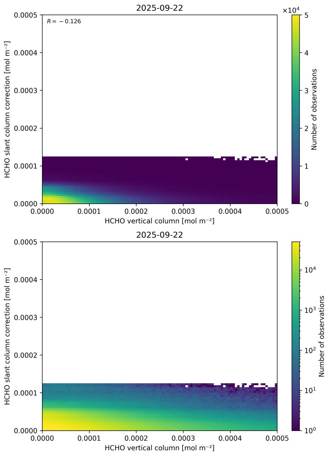
Figure 128: Scatter density plot of “HCHO vertical column” against “HCHO slant column correction” for 2025-09-22 to 2025-09-23.
