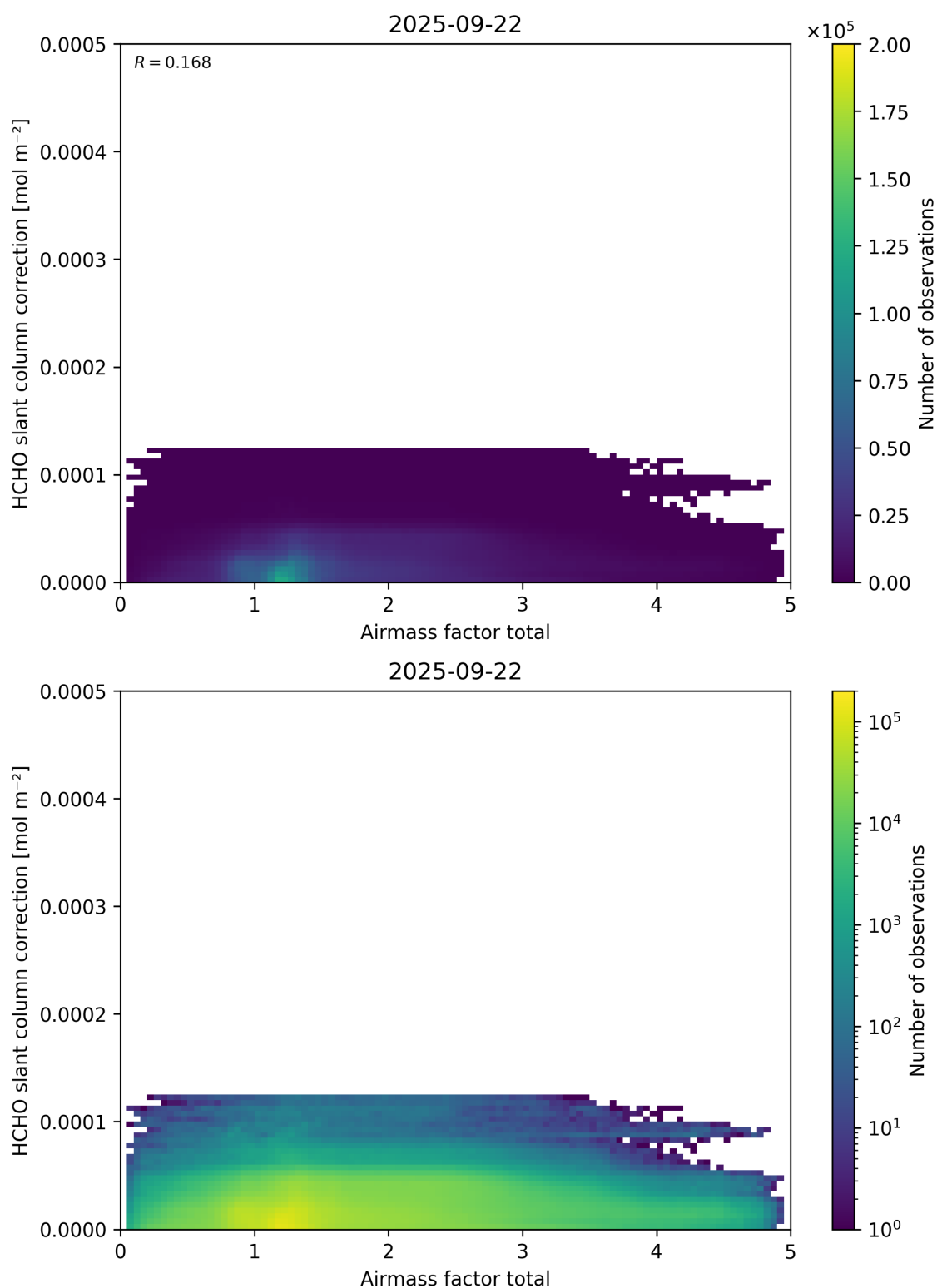
Figure 102: Scatter density plot of “Airmass factor total” against “HCHO slant column correction” for 2025-09-22 to 2025-09-23.
