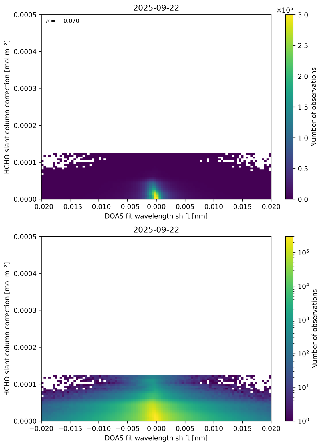
Figure 67: Scatter density plot of “DOAS fit wavelength shift” against “HCHO slant column correction” for 2025-09-22 to 2025-09-23.
