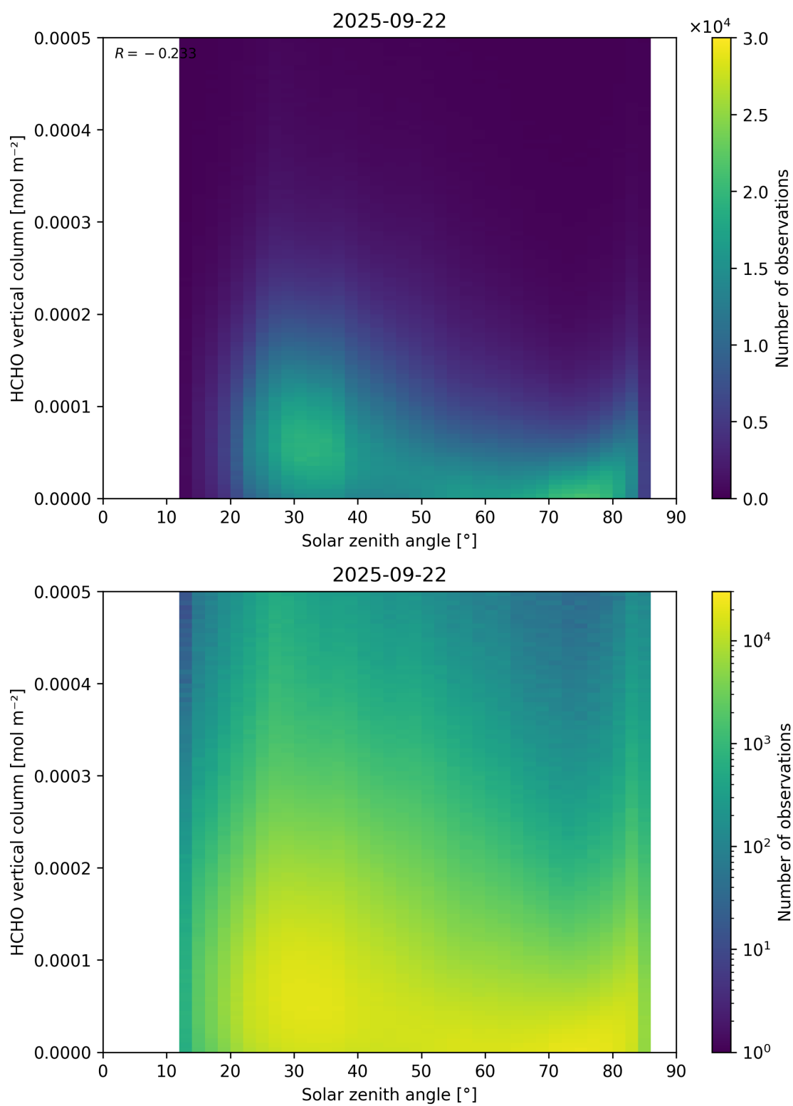
Figure 177: Scatter density plot of “Solar zenith angle” against “HCHO vertical column” for 2025-09-22 to 2025-09-23.
