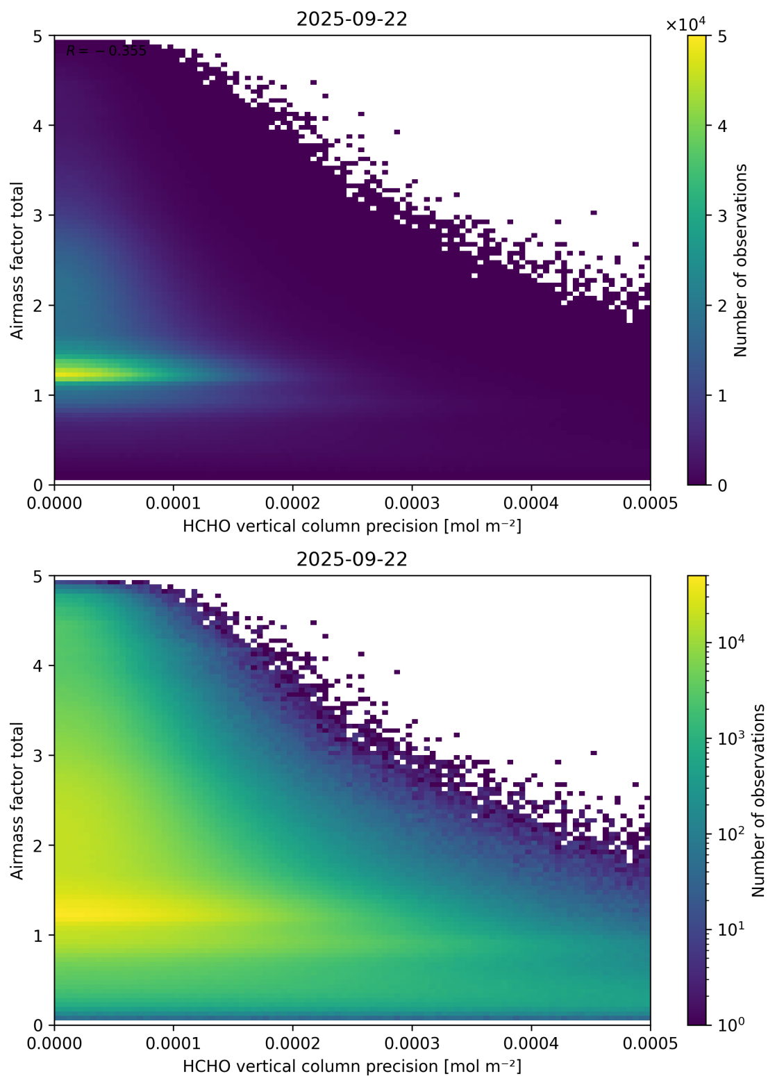
Figure 144: Scatter density plot of “HCHO vertical column precision” against “Airmass factor total” for 2025-09-22 to 2025-09-23.
