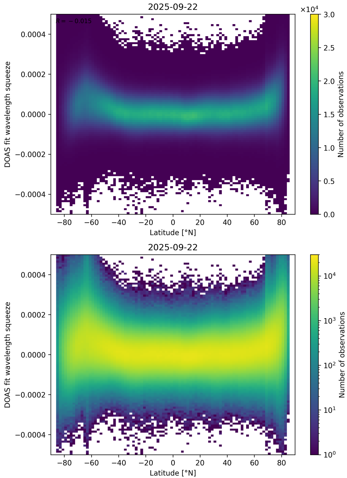
Figure 155: Scatter density plot of “Latitude” against “DOAS fit wavelength squeeze” for 2025-09-22 to 2025-09-23.
