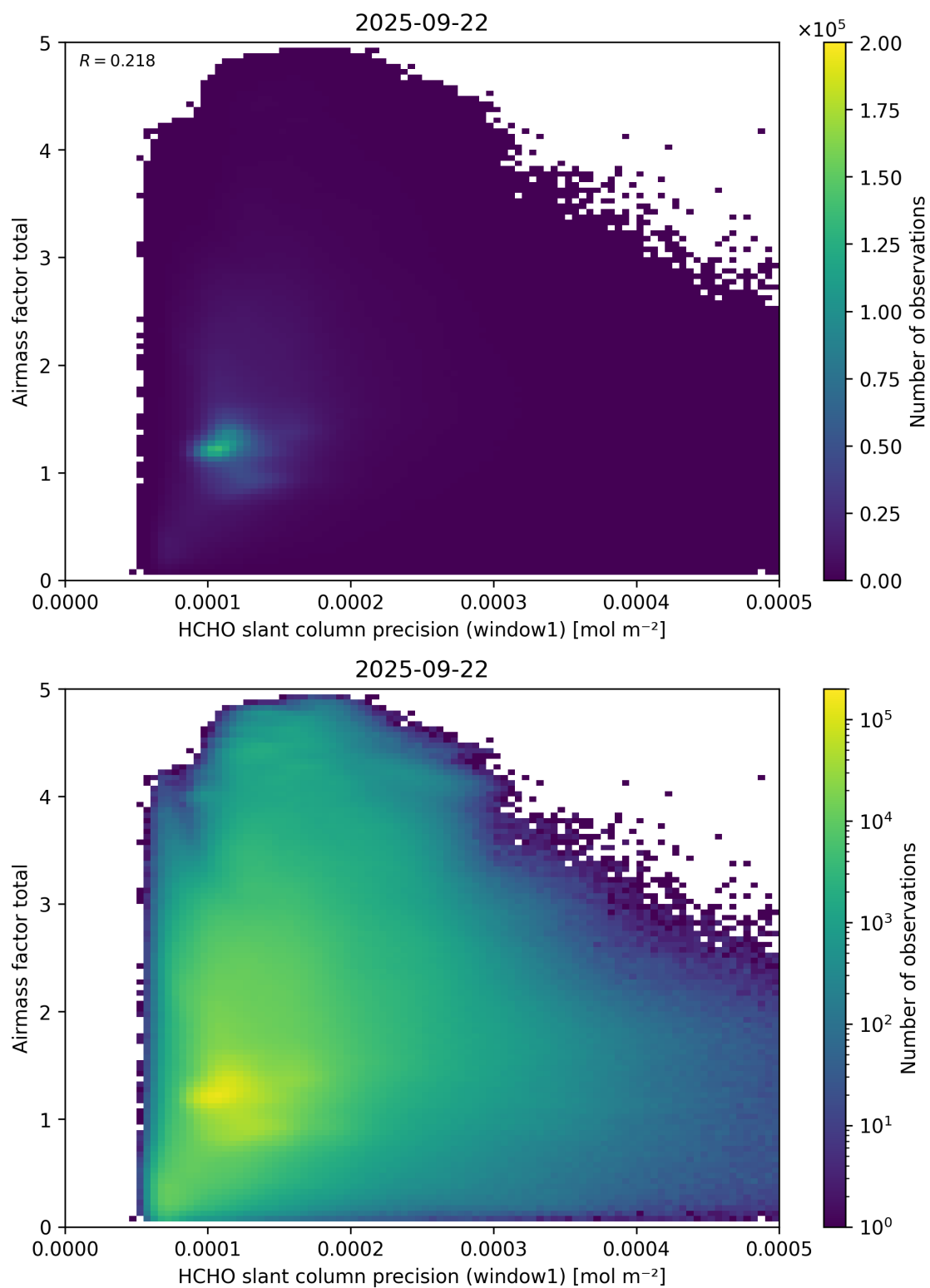
Figure 94: Scatter density plot of “HCHO slant column precision (window1)” against “Airmass factor total” for 2025-09-22 to 2025-09-23.
