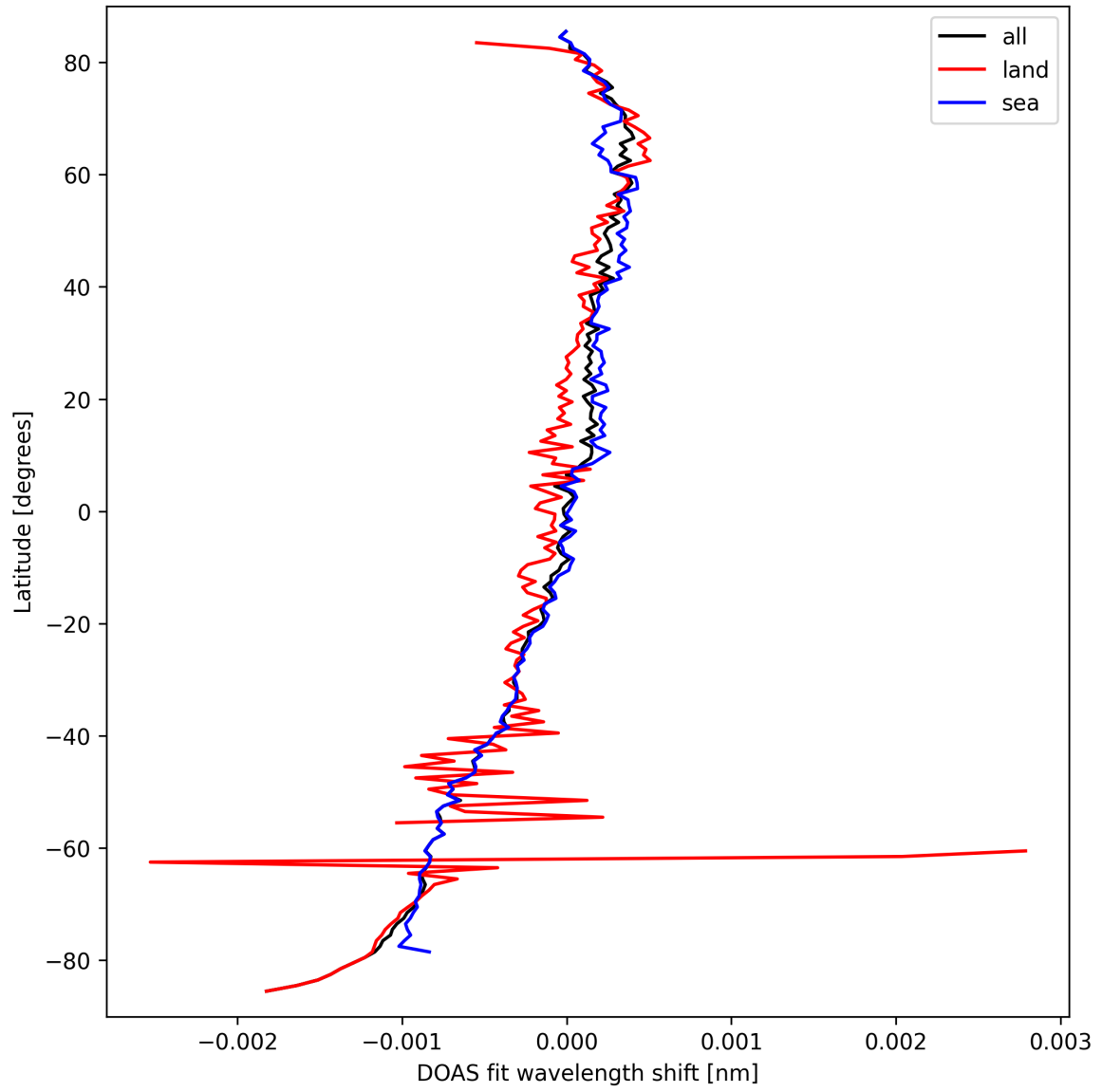
Figure 30: Zonal average of “DOAS fit wavelength shift” for 2025-09-22 to 2025-09-23.
