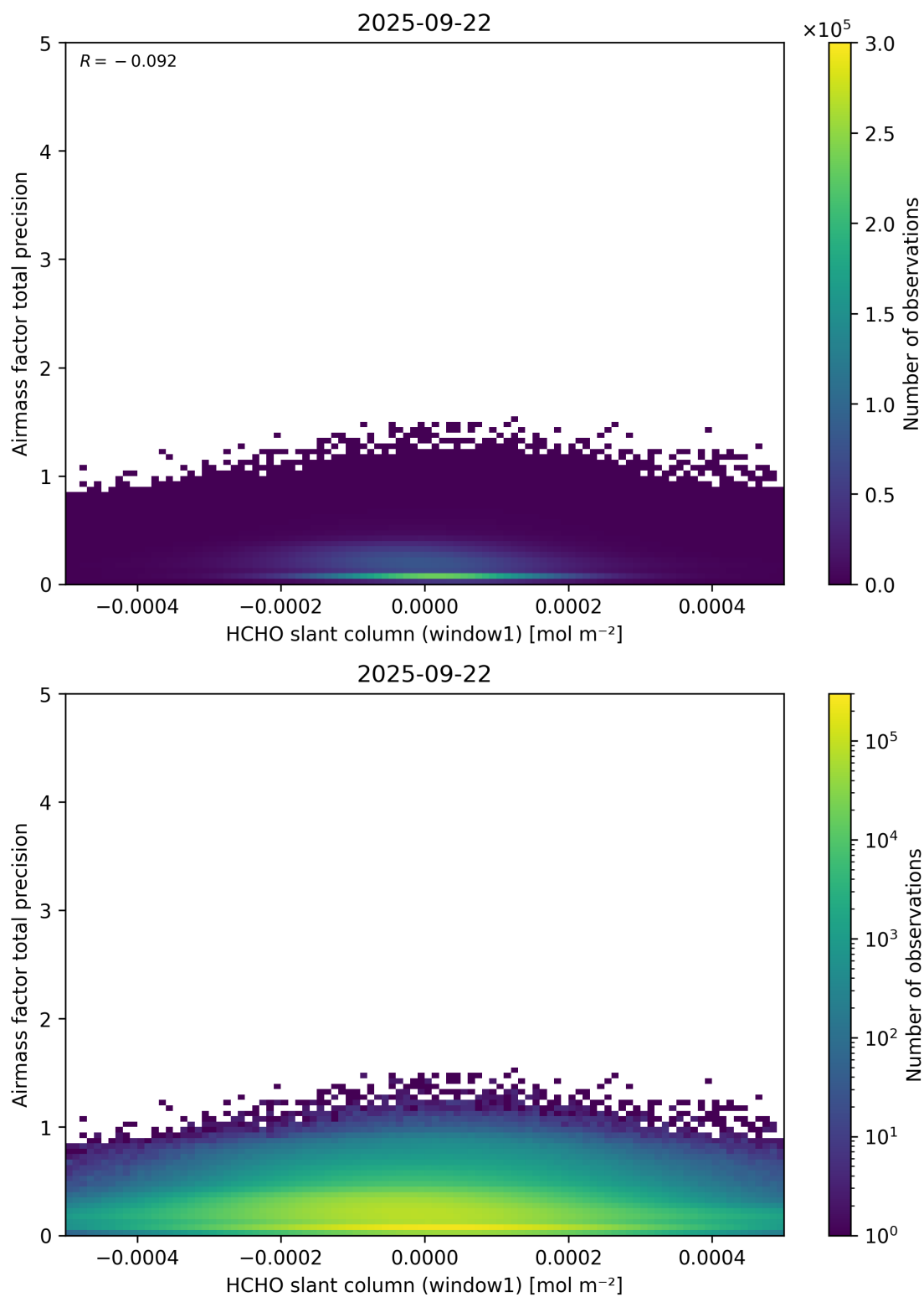
Figure 86: Scatter density plot of “HCHO slant column (window1)” against “Airmass factor total precision” for 2025-09-22 to 2025-09-23.
