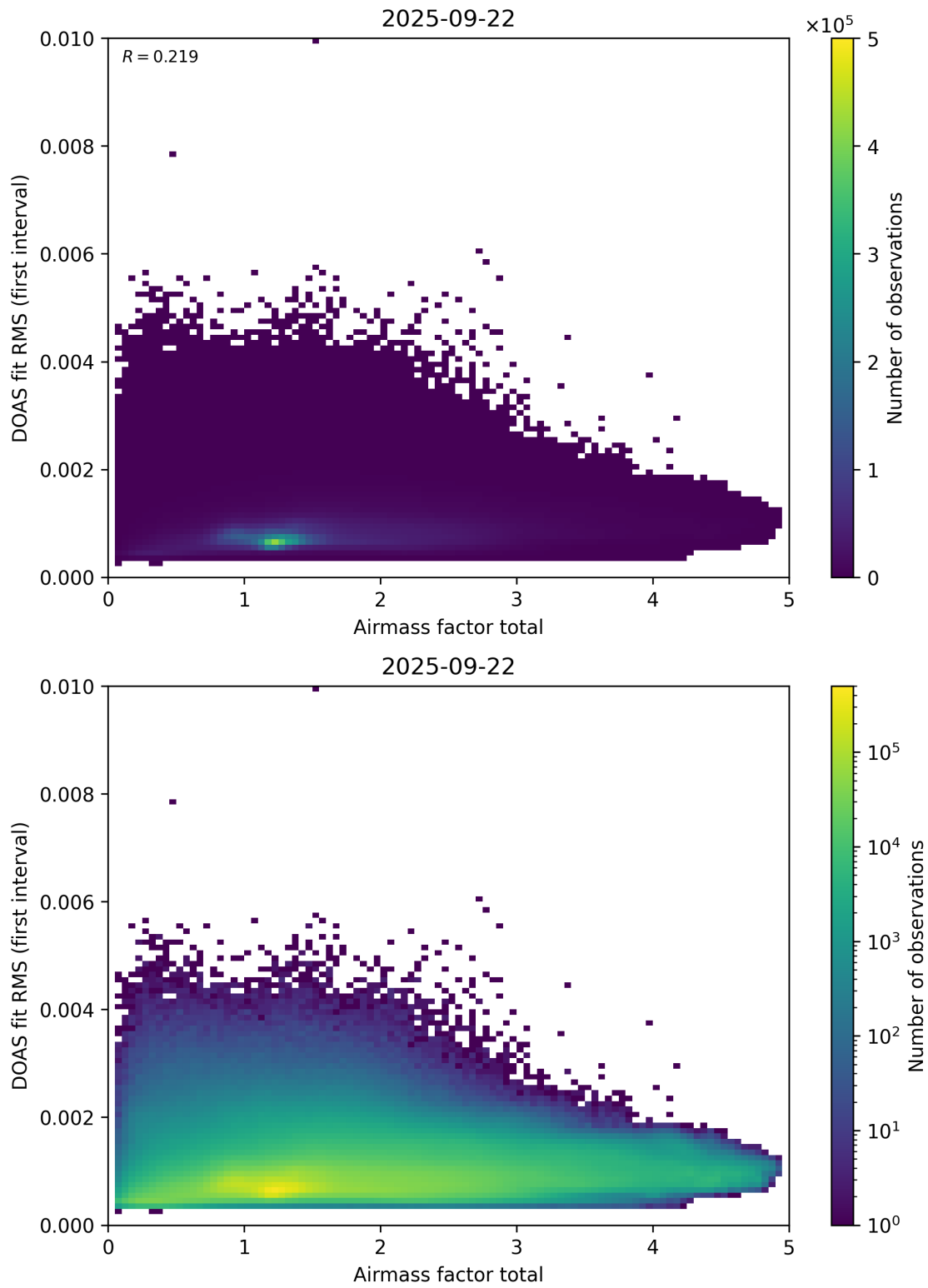
Figure 97: Scatter density plot of “Airmass factor total” against “DOAS fit RMS (first interval)” for 2025-09-22 to 2025-09-23.
