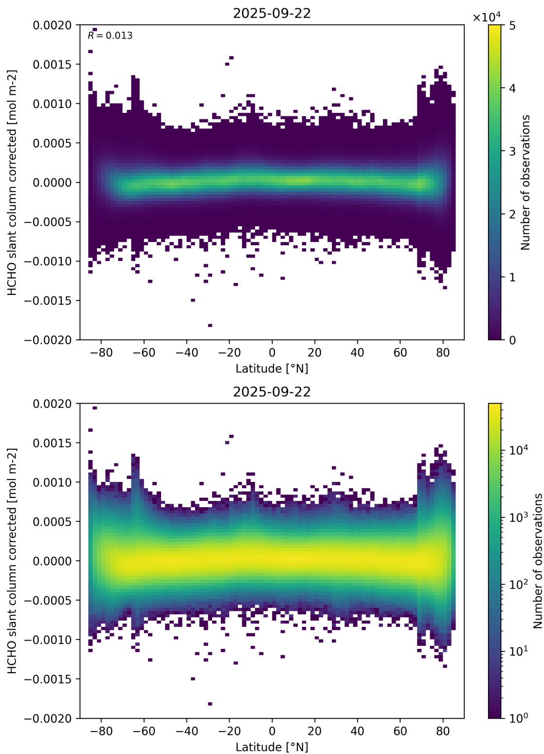
Figure 157: Scatter density plot of “Latitude” against “HCHO slant column corrected” for 2025-09-22 to 2025-09-23.
