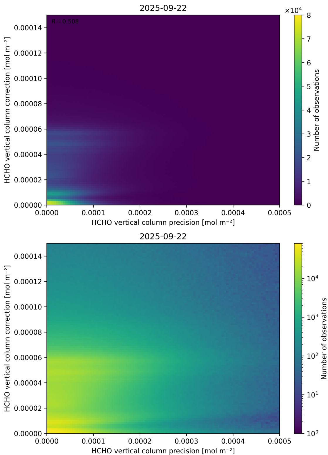
Figure 146: Scatter density plot of “HCHO vertical column precision” against “HCHO vertical column correction” for 2025-09-22 to 2025-09-23.
