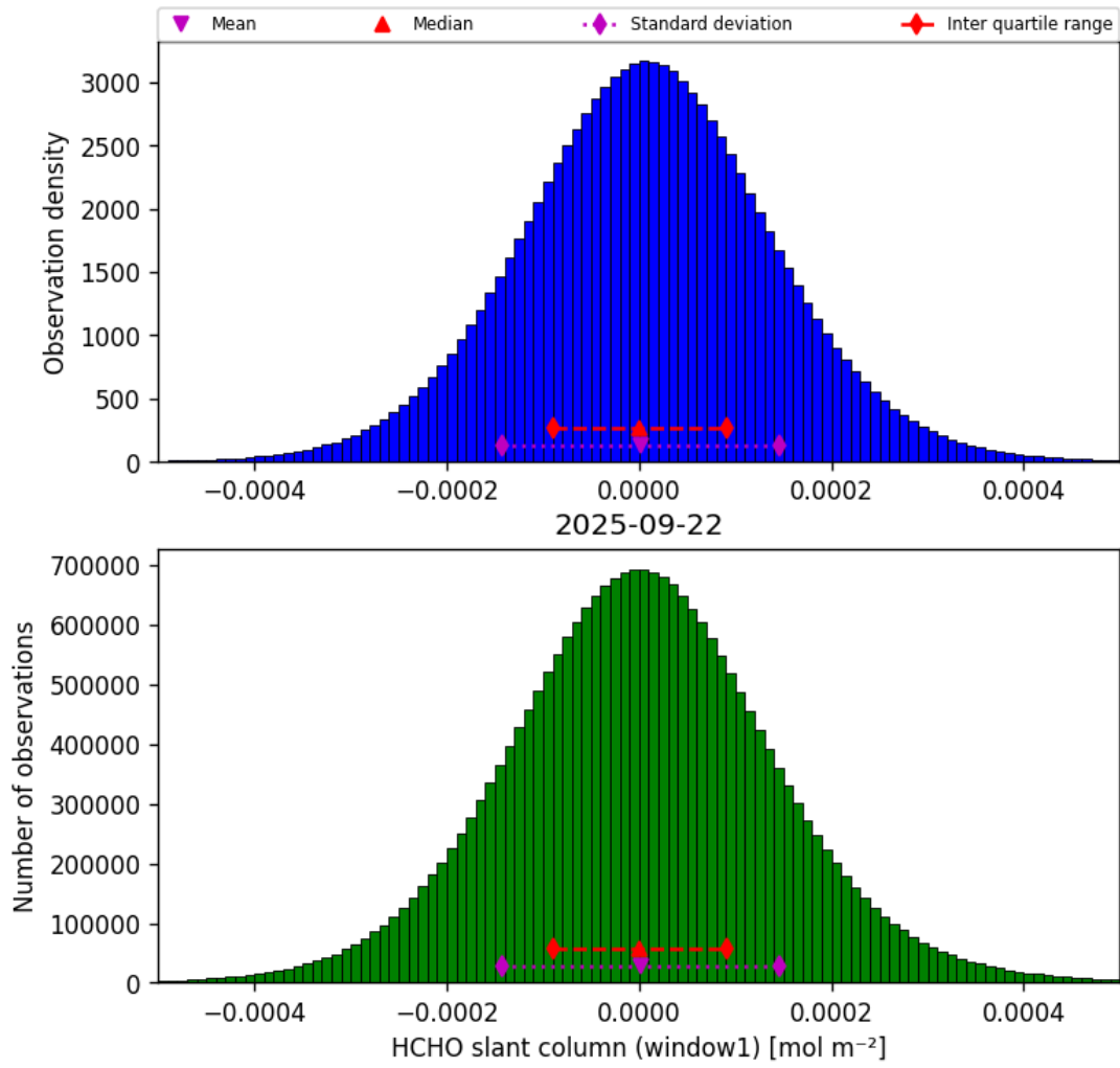
Figure 38: Histogram of “HCHO slant column (window1)” for 2025-09-22 to 2025-09-23
