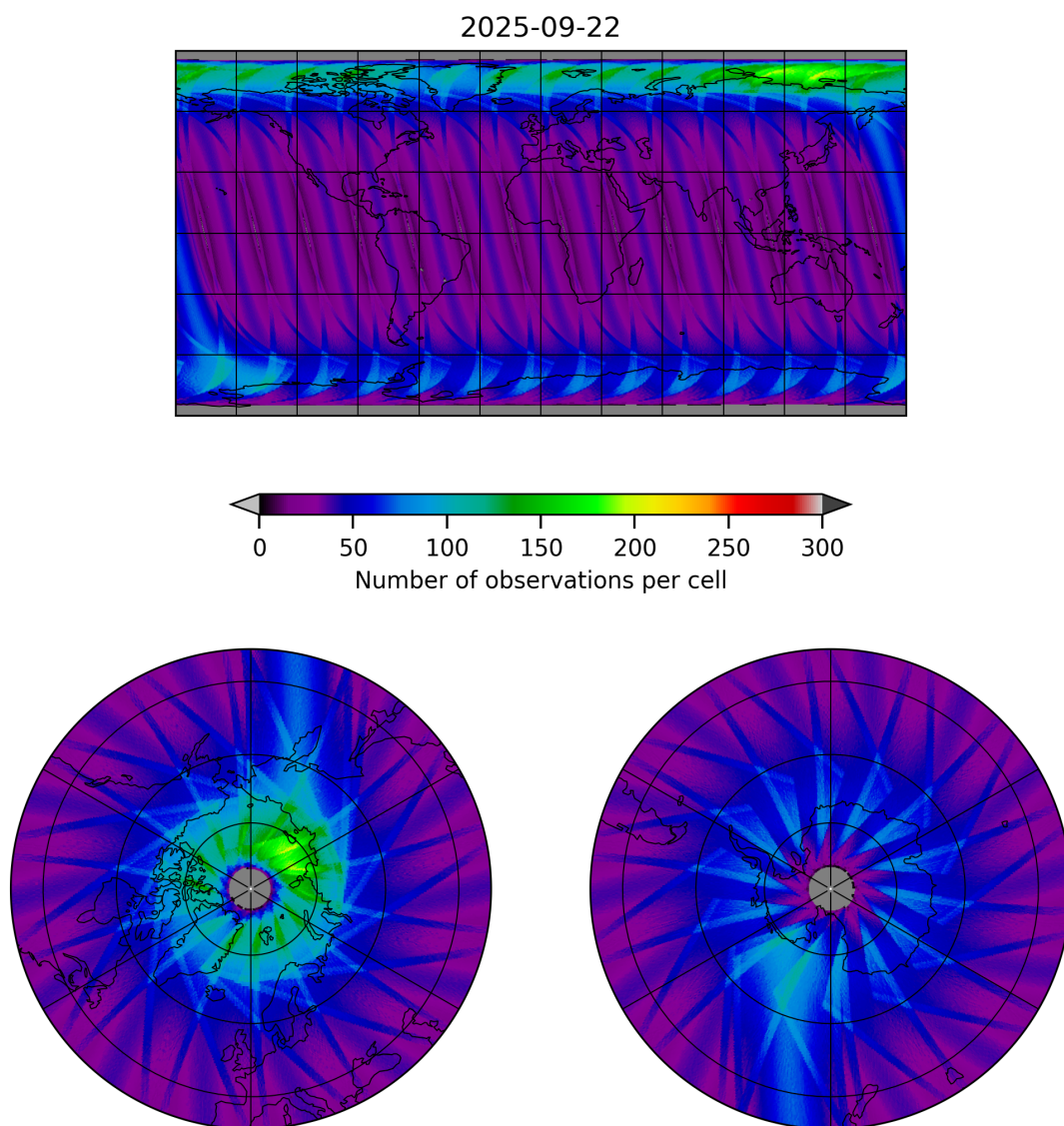
Figure 19: Map of the number of observations for 2025-09-22 to 2025-09-23
