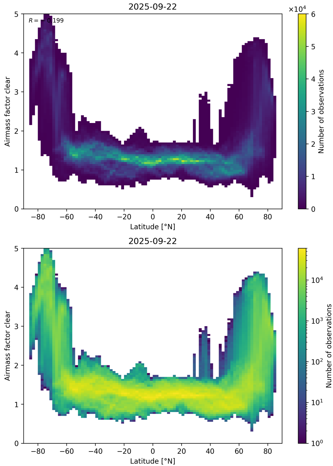
Figure 156: Scatter density plot of “Latitude” against “Airmass factor clear” for 2025-09-22 to 2025-09-23.
