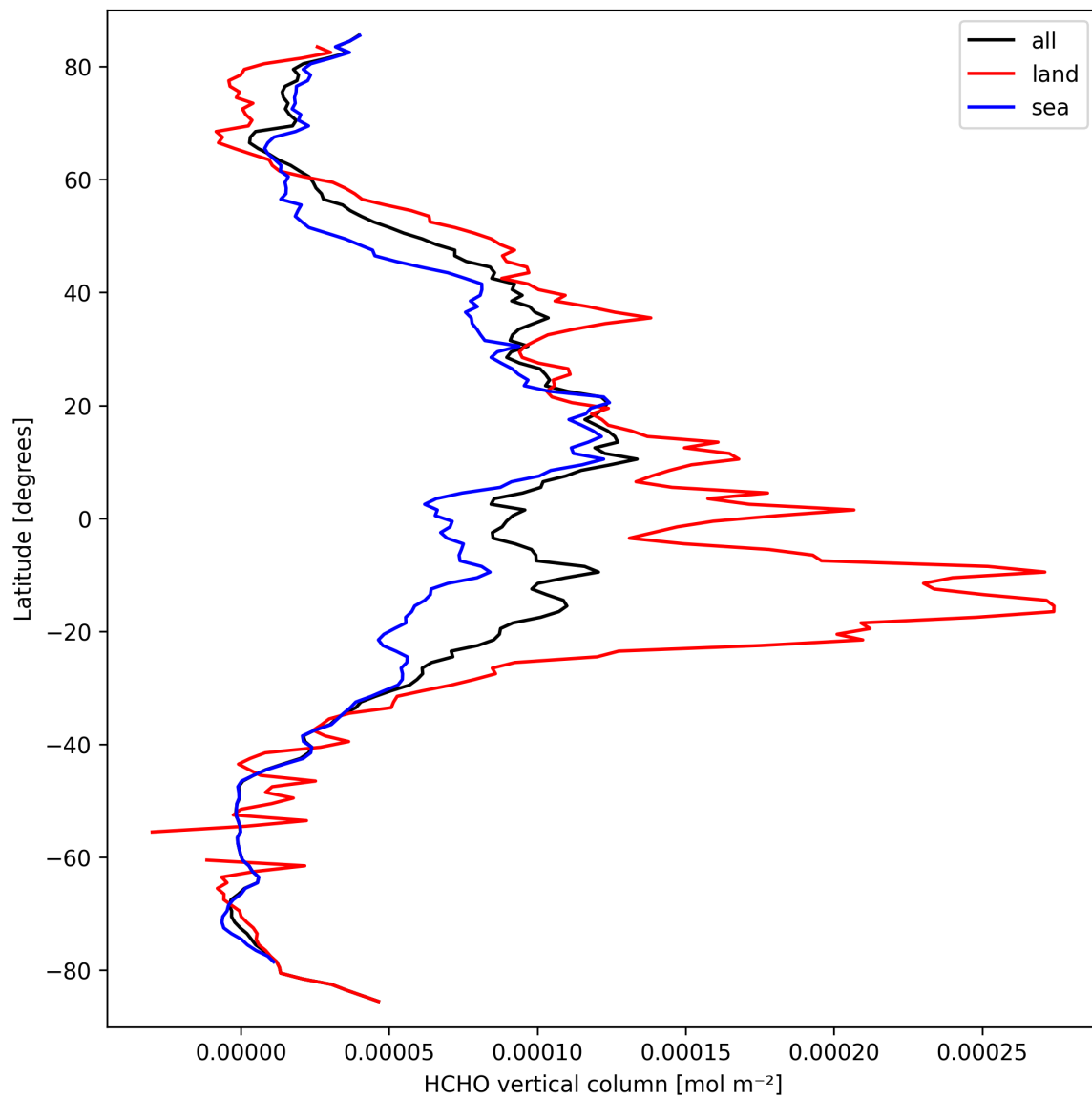
Figure 21: Zonal average of “HCHO vertical column” for 2025-09-22 to 2025-09-23.
