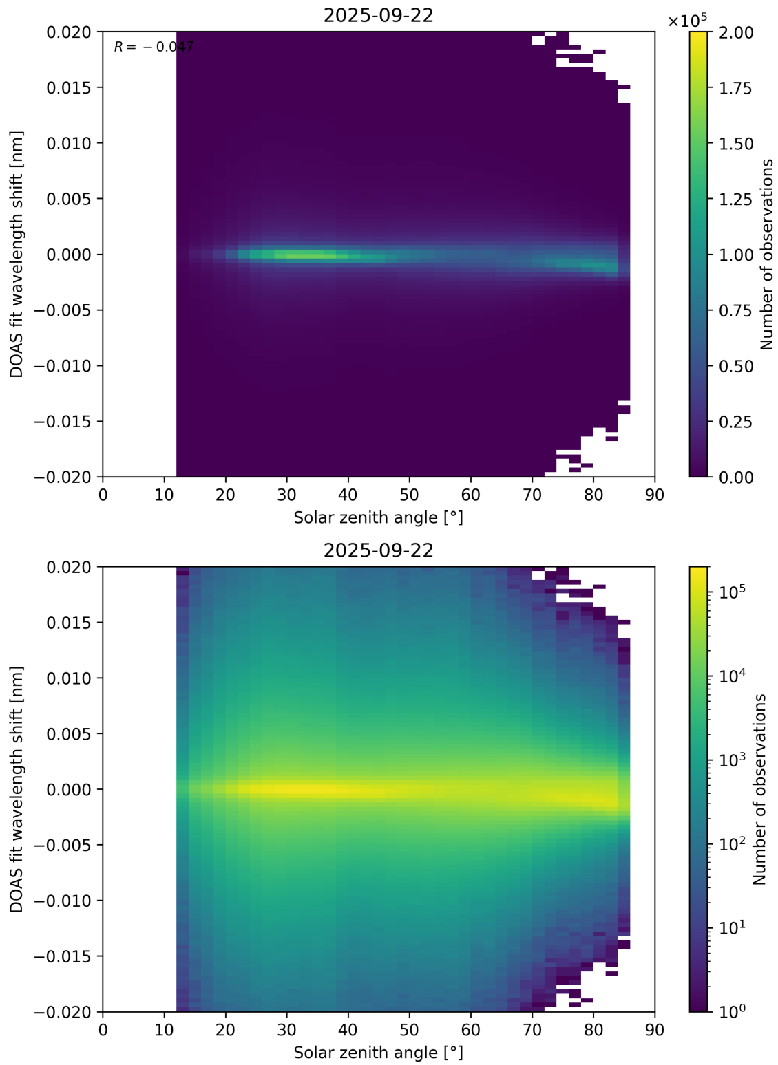
Figure 168: Scatter density plot of “Solar zenith angle” against “DOAS fit wavelength shift” for 2025-09-22 to 2025-09-23.
