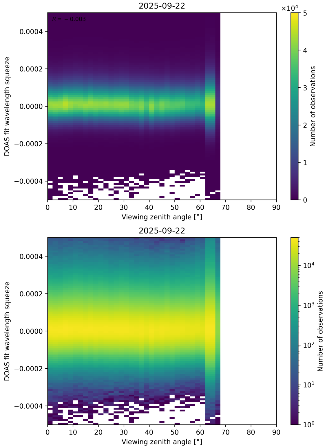
Figure 184: Scatter density plot of “Viewing zenith angle” against “DOAS fit wavelength squeeze” for 2025-09-22 to 2025-09-23.
