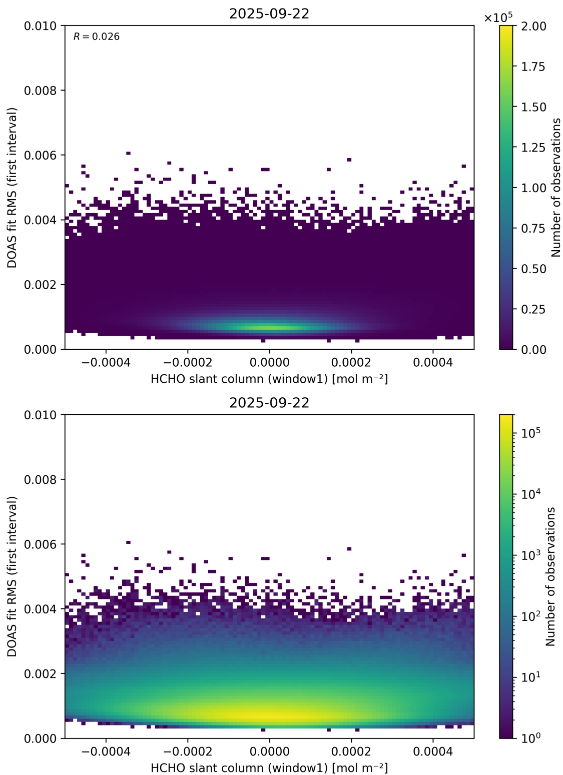
Figure 78: Scatter density plot of “HCHO slant column (window1)” against “DOAS fit RMS (first interval)” for 2025-09-22 to 2025-09-23.
