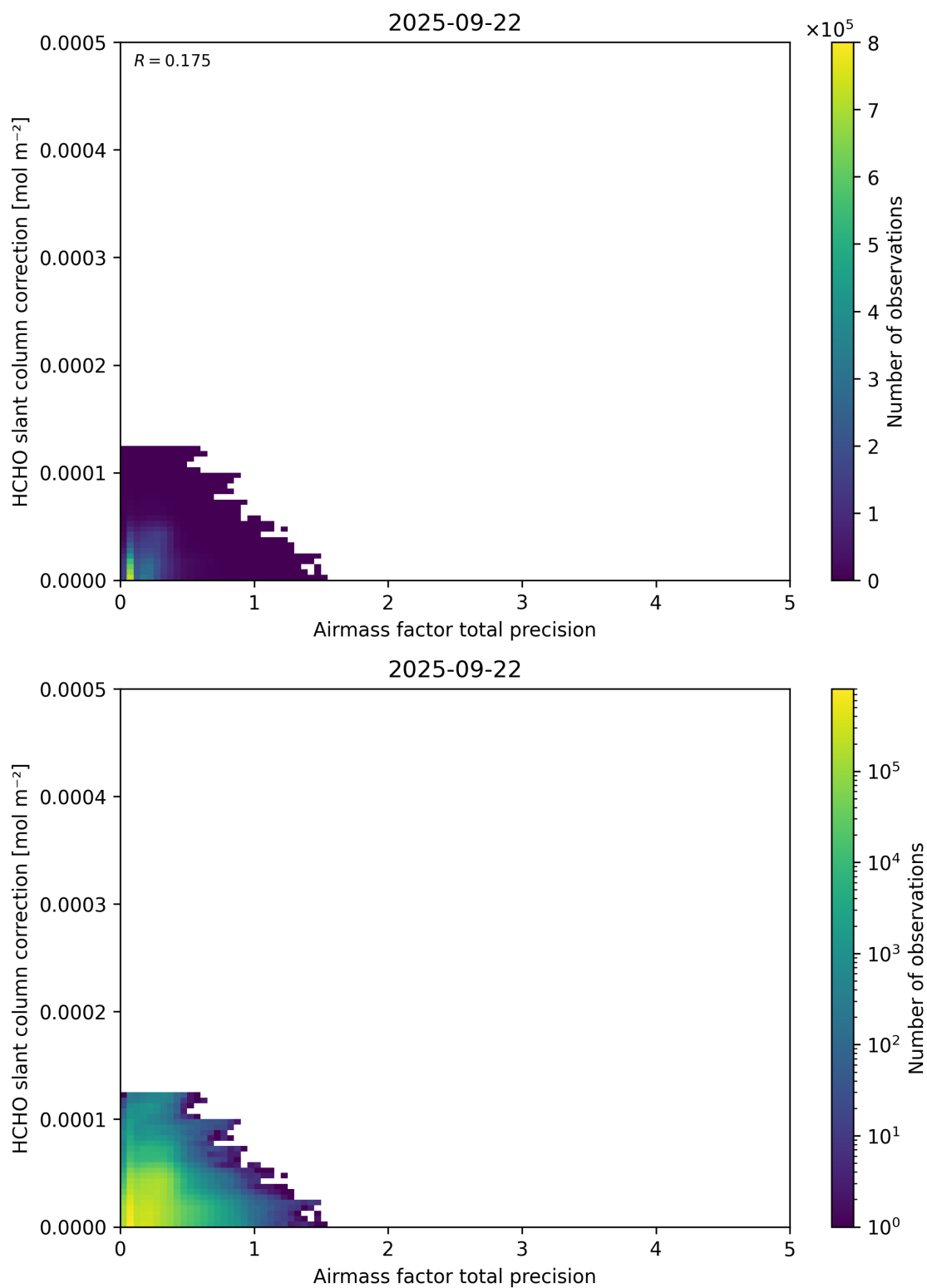
Figure 110: Scatter density plot of “Airmass factor total precision” against “HCHO slant column correction” for 2025-09-22 to 2025-09-23.
