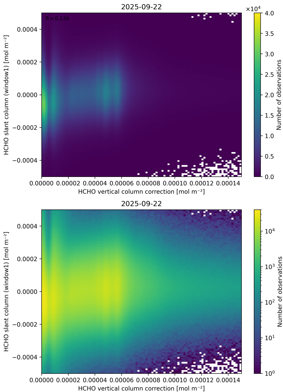
Figure 118: Scatter density plot of “HCHO vertical column correction” against “HCHO slant column (window1)” for 2025-09-22 to 2025-09-23.
