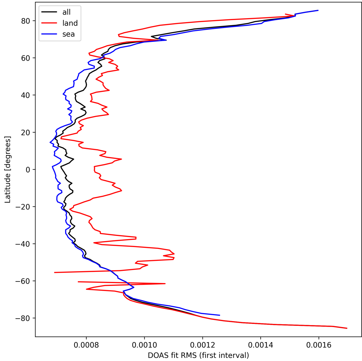
Figure 32: Zonal average of "DOAS fit RMS (first interval)" for 2025-09-22 to 2025-09-23.
