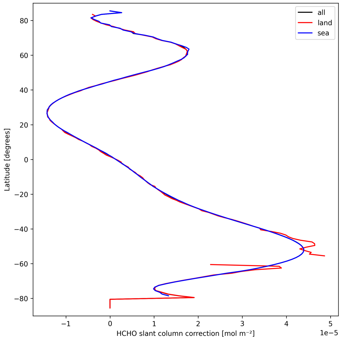
Figure 33: Zonal average of “HCHO slant column correction” for 2025-09-22 to 2025-09-23.
