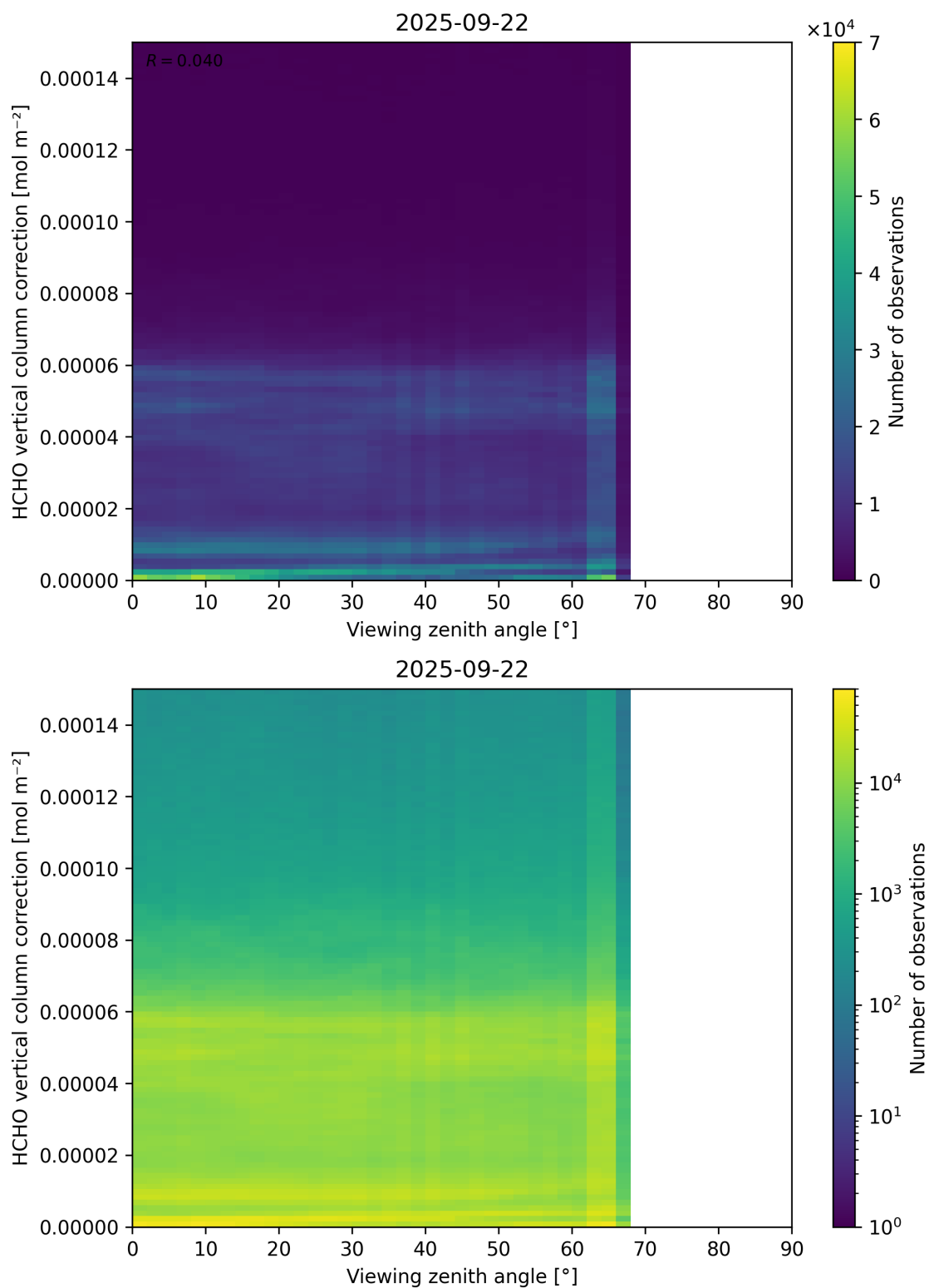
Figure 193: Scatter density plot of “Viewing zenith angle” against “HCHO vertical column correction” for 2025-09-22 to 2025-09-23.
