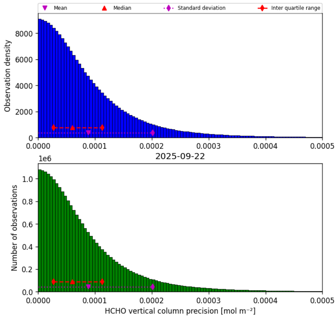
Figure 36: Histogram of “HCHO vertical column precision” for 2025-09-22 to 2025-09-23
