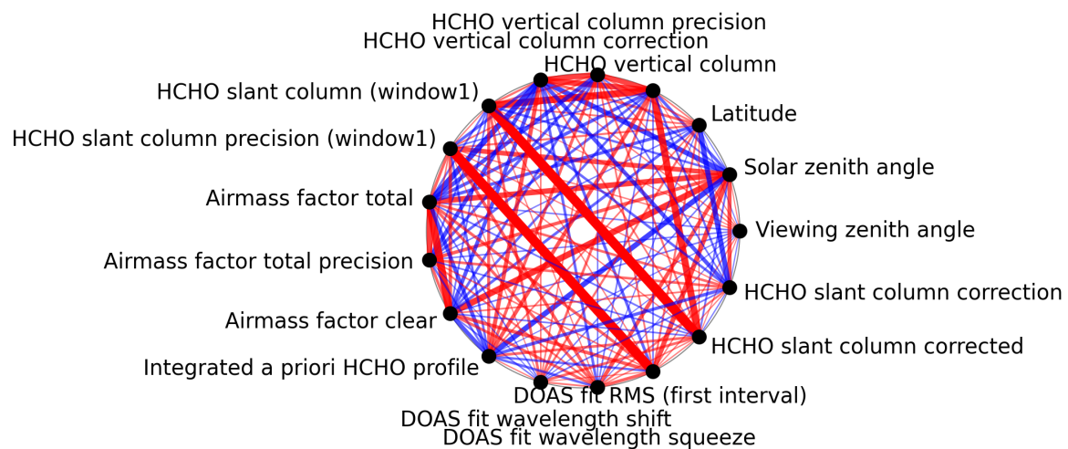
Figure 1: Map of correlation graph for 2025-09-22 to 2025-09-23.
