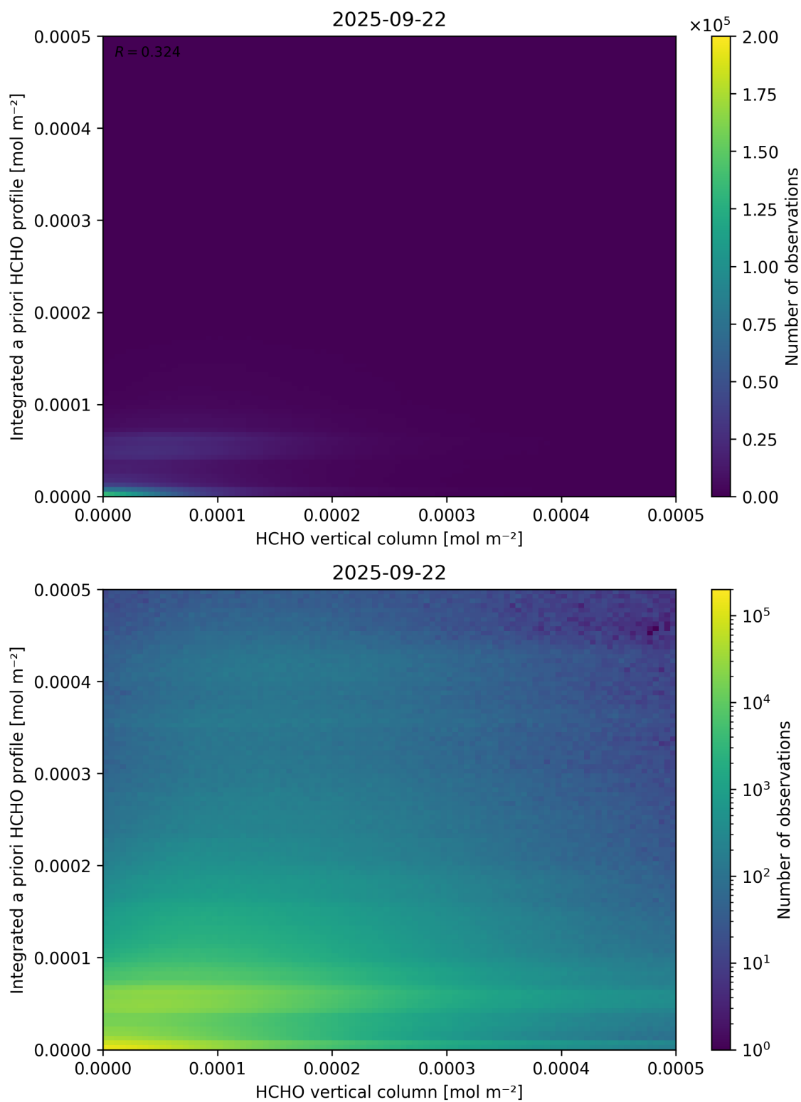
Figure 135: Scatter density plot of “HCHO vertical column” against “Integrated a priori HCHO profile” for 2025-09-22 to 2025-09-23.
