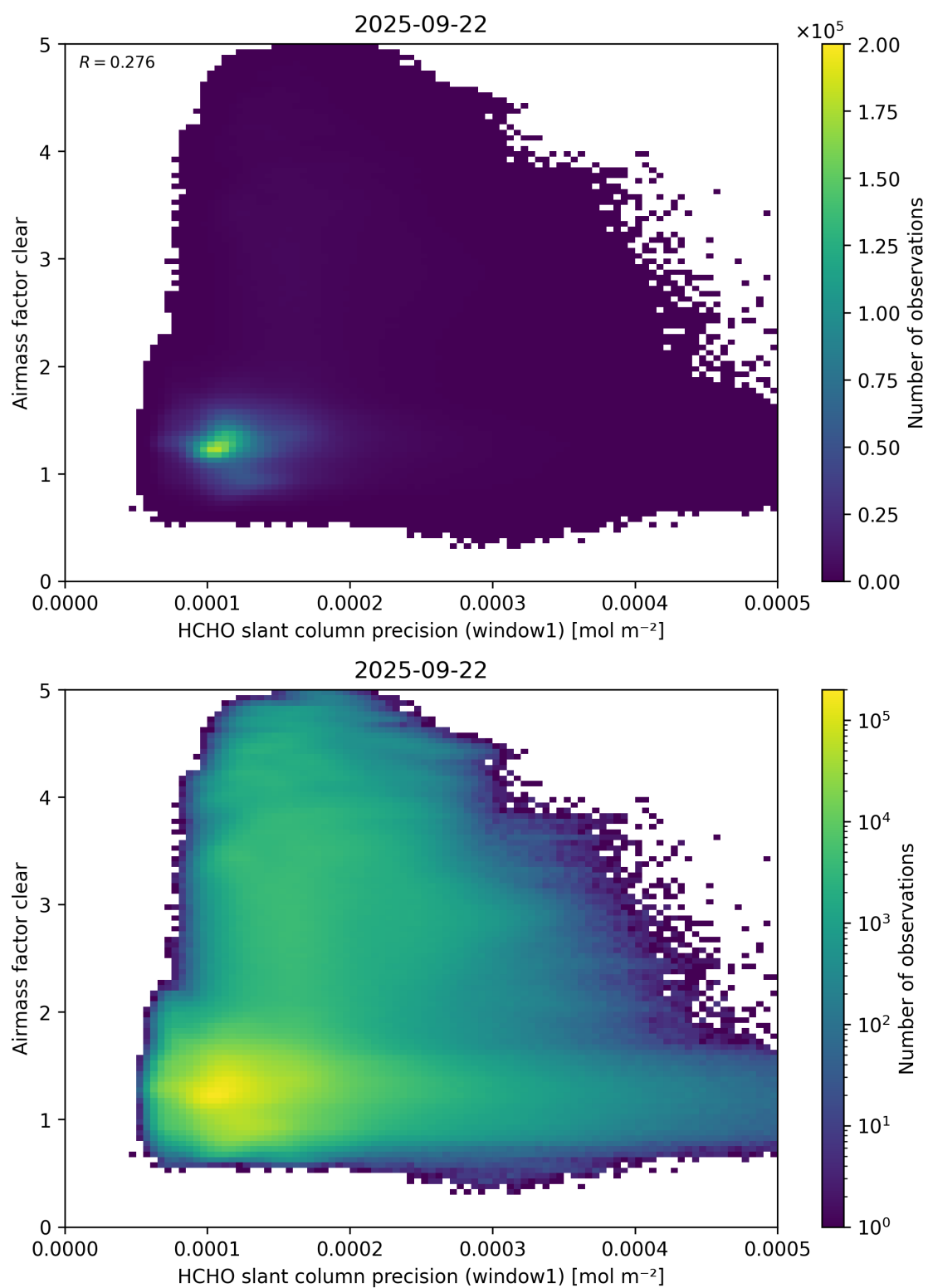
Figure 91: Scatter density plot of “HCHO slant column precision (window1)” against “Airmass factor clear” for 2025-09-22 to 2025-09-23.
