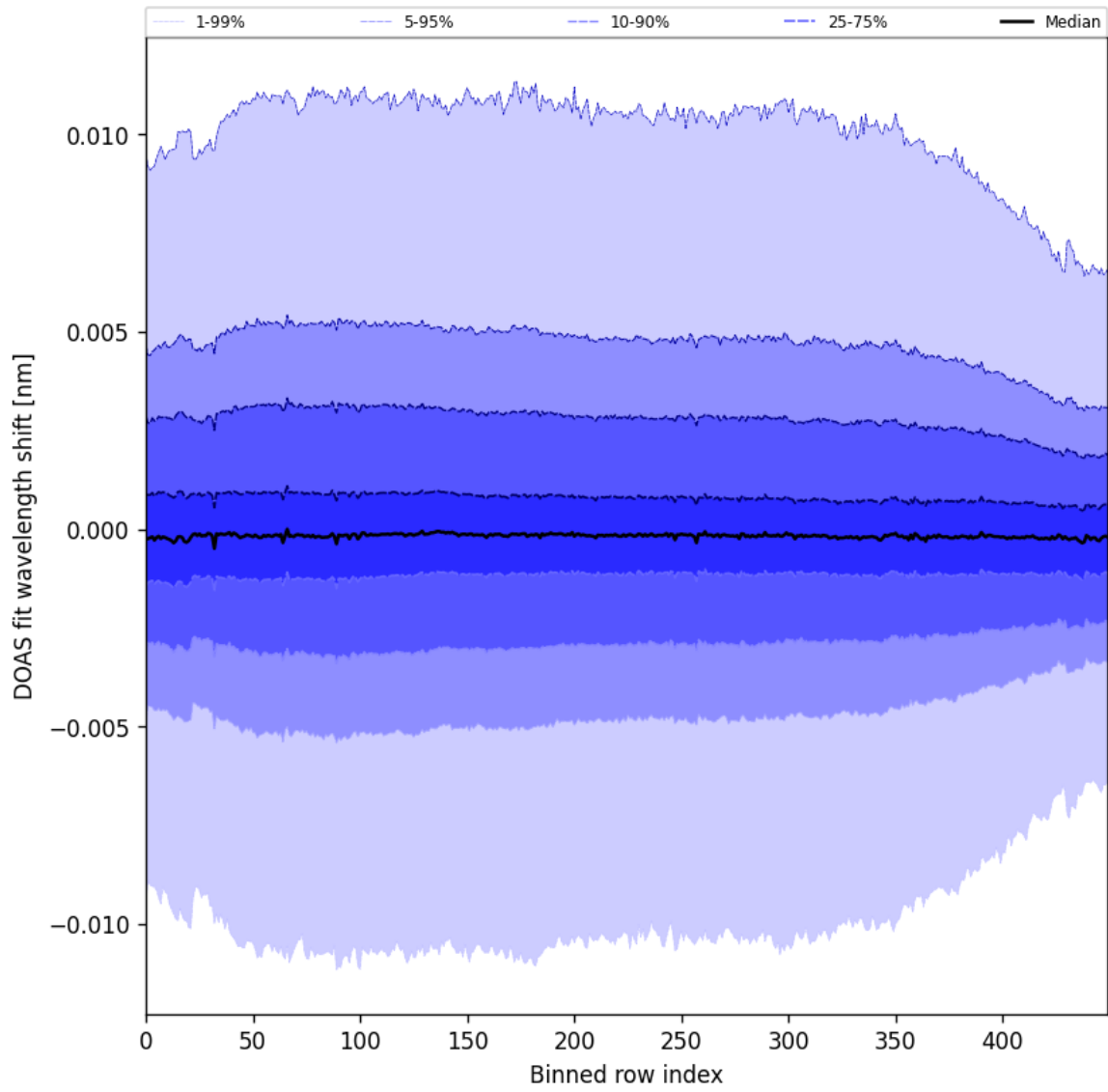
Figure 58: Along track statistics of “DOAS fit wavelength shift” for 2025-09-22 to 2025-09-23
