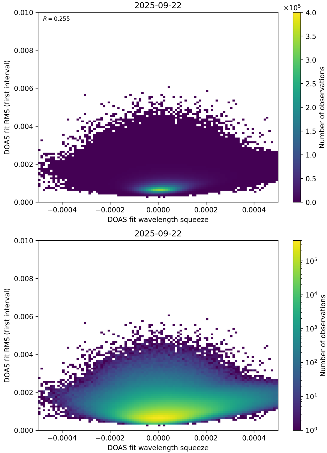
Figure 68: Scatter density plot of “DOAS fit wavelength squeeze” against “DOAS fit RMS (first interval)” for 2025-09-22 to 2025-09-23.
