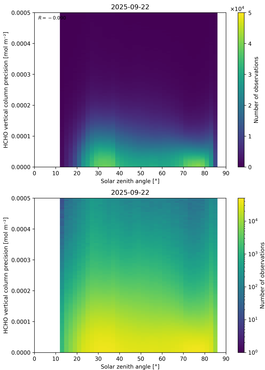
Figure 179: Scatter density plot of “Solar zenith angle” against “HCHO vertical column precision” for 2025-09-22 to 2025-09-23.
