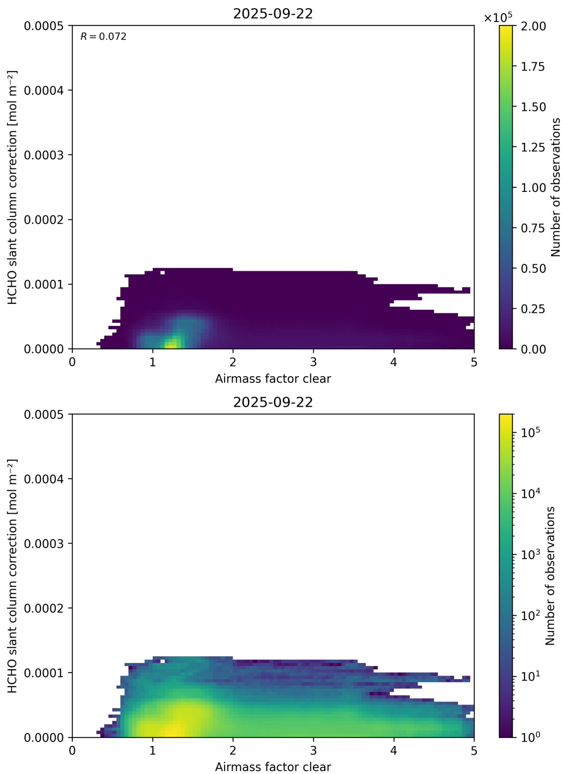
Figure 75: Scatter density plot of “Airmass factor clear” against “HCHO slant column correction” for 2025-09-22 to 2025-09-23.
