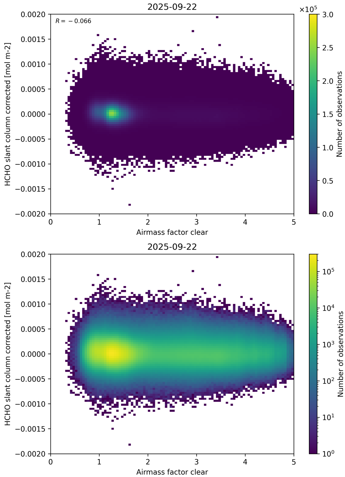
Figure 74: Scatter density plot of “Airmass factor clear” against “HCHO slant column corrected” for 2025-09-22 to 2025-09-23.
