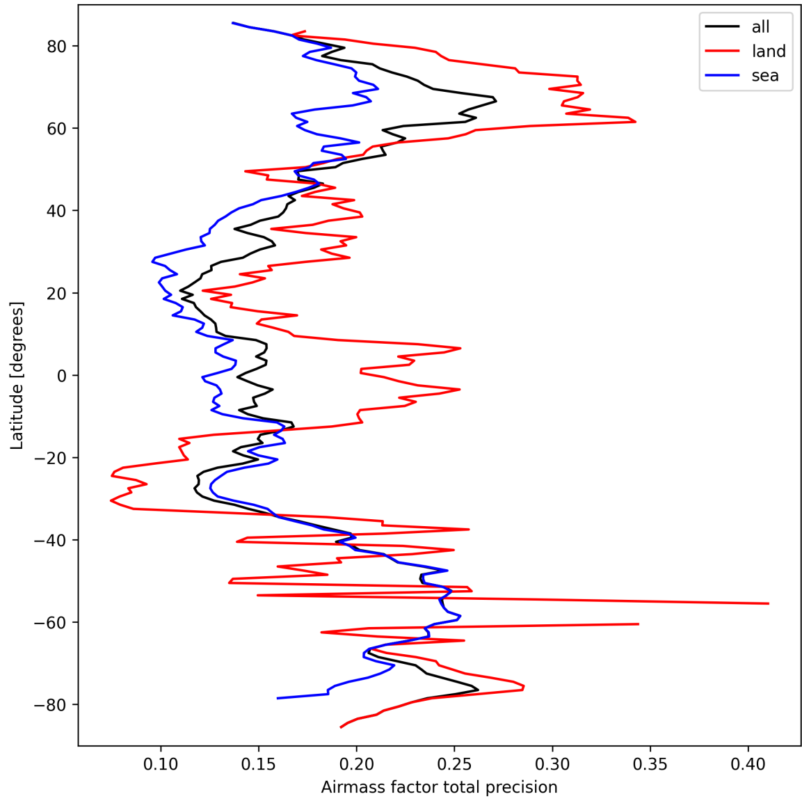
Figure 27: Zonal average of “Airmass factor total precision” for 2025-09-22 to 2025-09-23.
