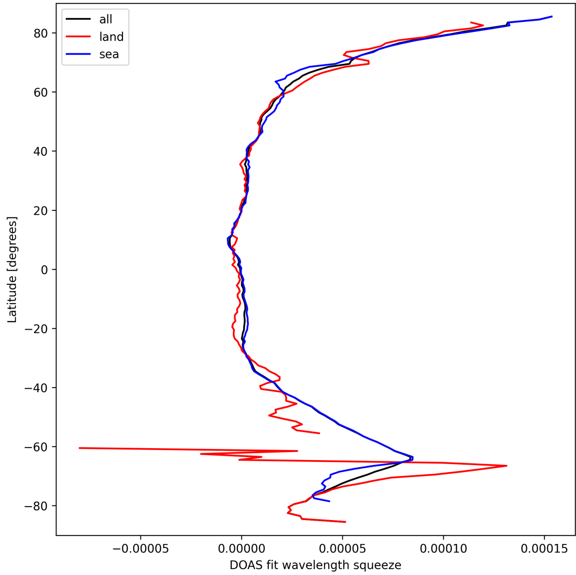
Figure 31: Zonal average of “DOAS fit wavelength squeeze” for 2025-09-22 to 2025-09-23.
