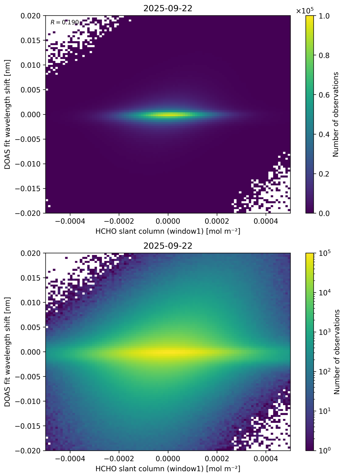
Figure 79: Scatter density plot of “HCHO slant column (window1)” against “DOAS fit wavelength shift” for 2025-09-22 to 2025-09-23.
