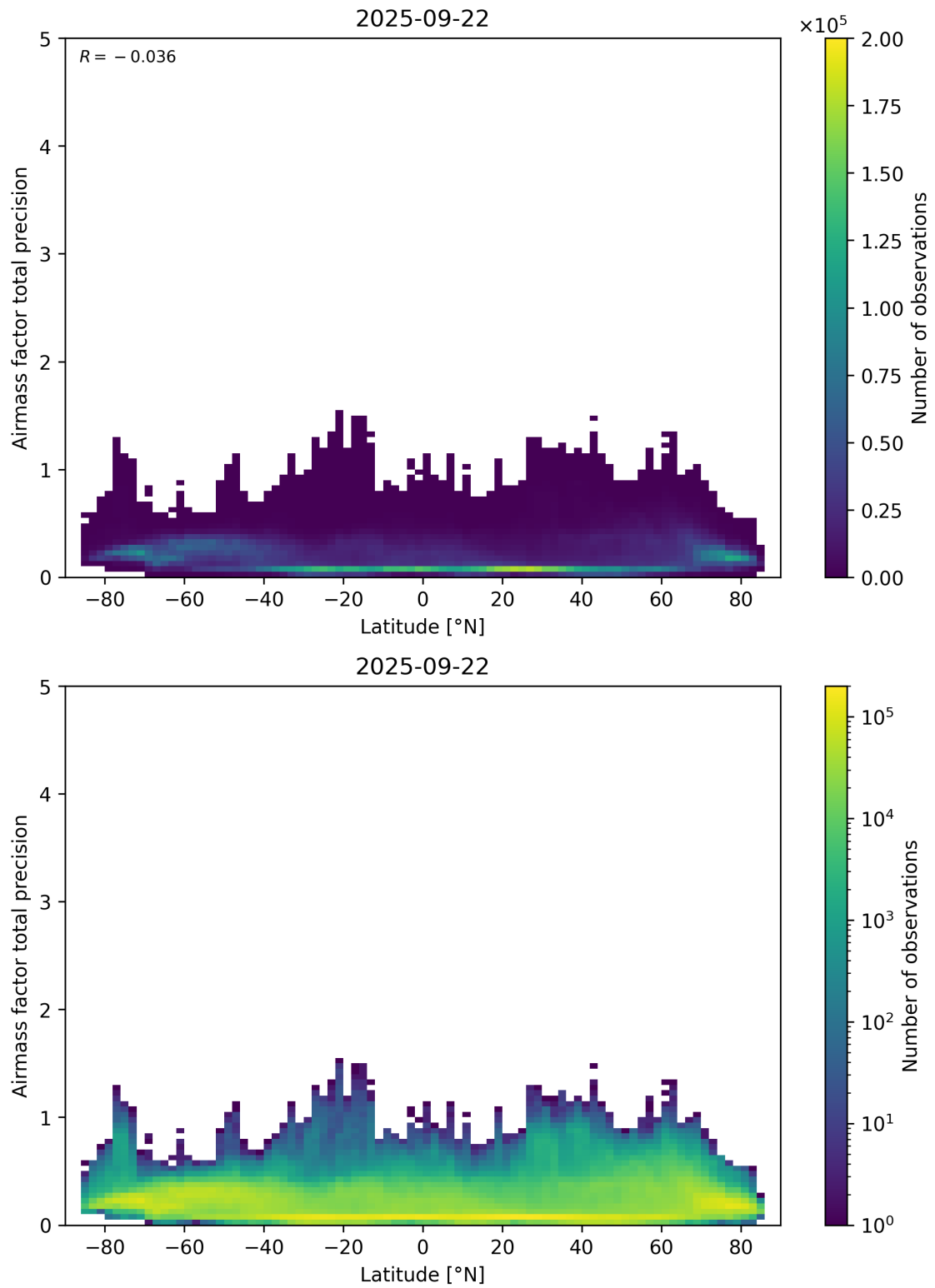
Figure 162: Scatter density plot of “Latitude” against “Airmass factor total precision” for 2025-09-22 to 2025-09-23.
