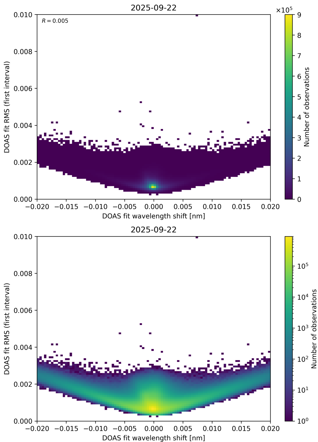
Figure 64: Scatter density plot of “DOAS fit wavelength shift” against “DOAS fit RMS (first interval)” for 2025-09-22 to 2025-09-23.
