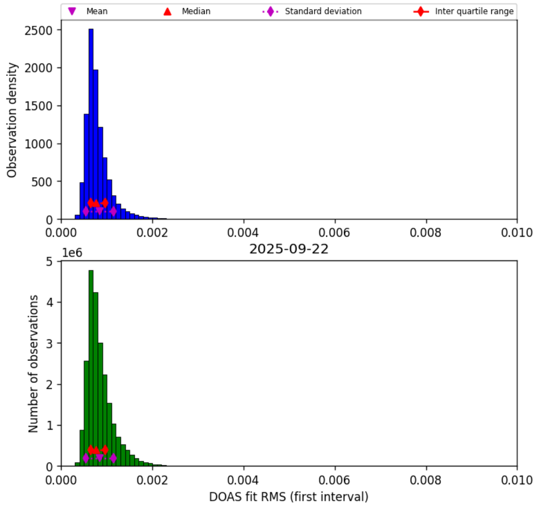
Figure 46: Histogram of "DOAS fit RMS (first interval)" for 2025-09-22 to 2025-09-23
