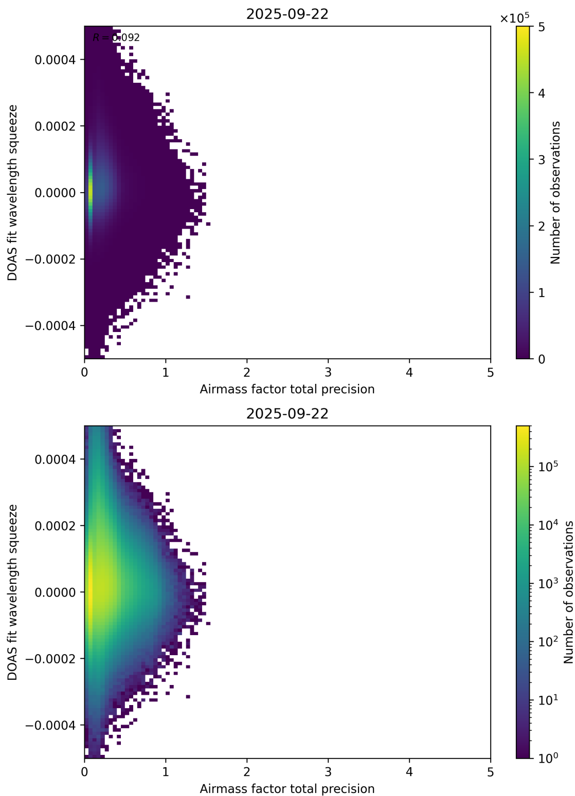
Figure 107: Scatter density plot of “Airmass factor total precision” against “DOAS fit wavelength squeeze” for 2025-09-22 to 2025-09-23.
