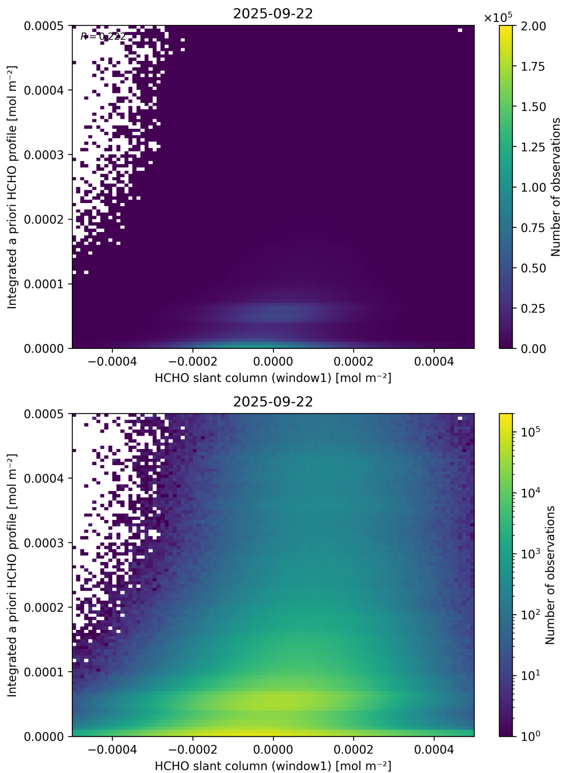
Figure 87: Scatter density plot of “HCHO slant column (window1)” against “Integrated a priori HCHO profile” for 2025-09-22 to 2025-09-23.
