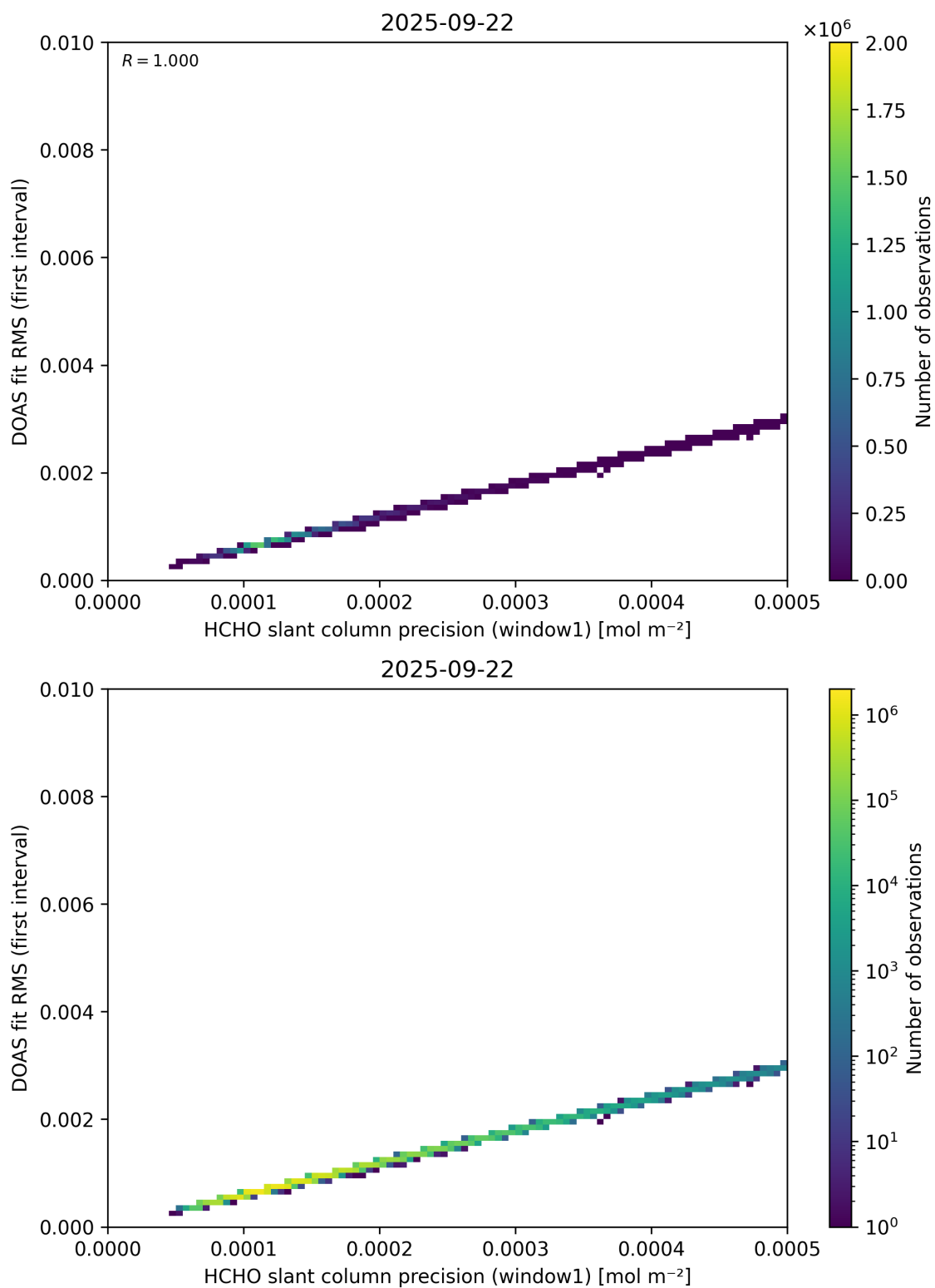
Figure 88: Scatter density plot of “HCHO slant column precision (window1)” against “DOAS fit RMS (first interval)” for 2025-09-22 to 2025-09-23.
