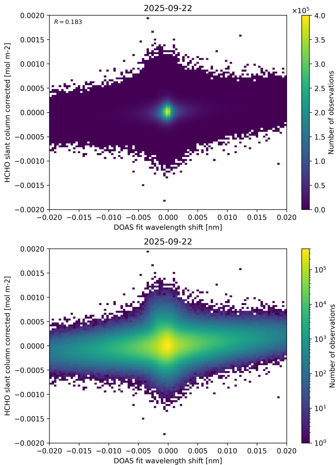
Figure 66: Scatter density plot of “DOAS fit wavelength shift” against “HCHO slant column corrected” for 2025-09-22 to 2025-09-23.
