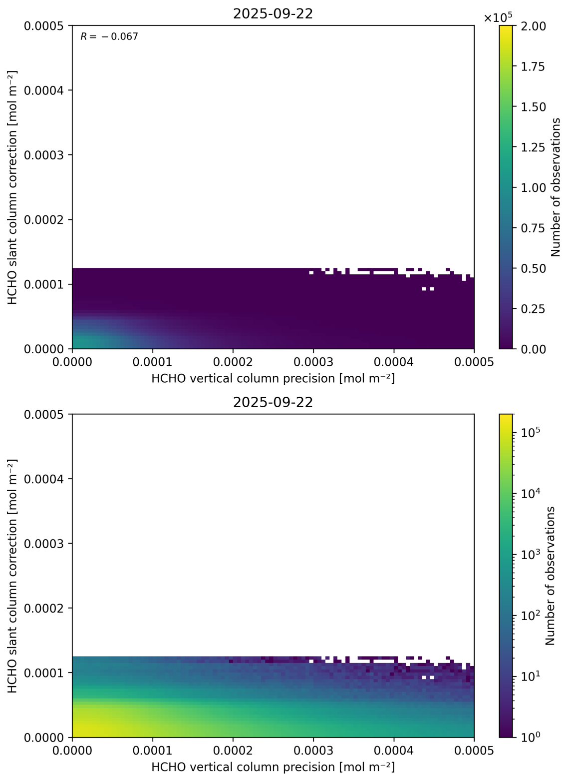
Figure 141: Scatter density plot of “HCHO vertical column precision” against “HCHO slant column correction” for 2025-09-22 to 2025-09-23.
