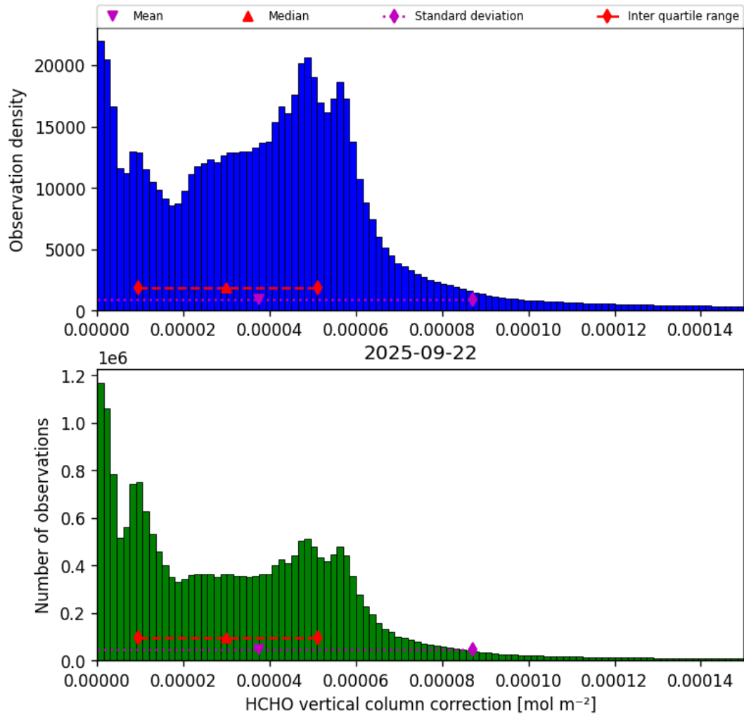
Figure 37: Histogram of “HCHO vertical column correction” for 2025-09-22 to 2025-09-23
