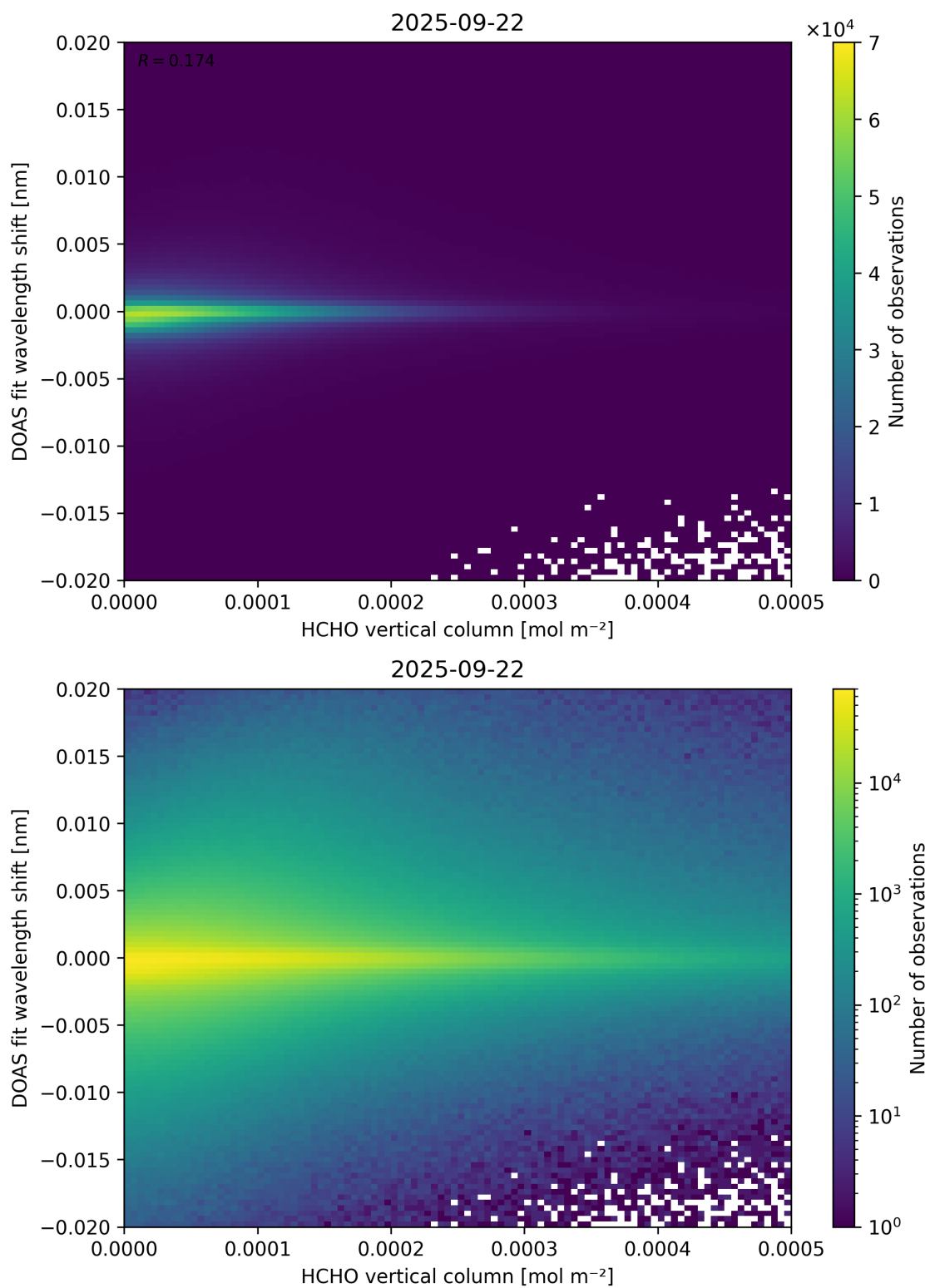
Figure 124: Scatter density plot of “HCHO vertical column” against “DOAS fit wavelength shift” for 2025-09-22 to 2025-09-23.
