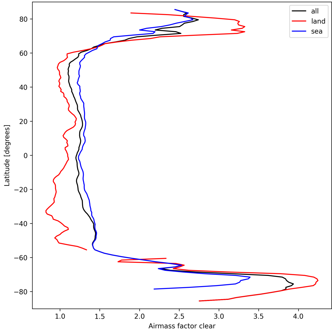
Figure 28: Zonal average of “Airmass factor clear” for 2025-09-22 to 2025-09-23.
