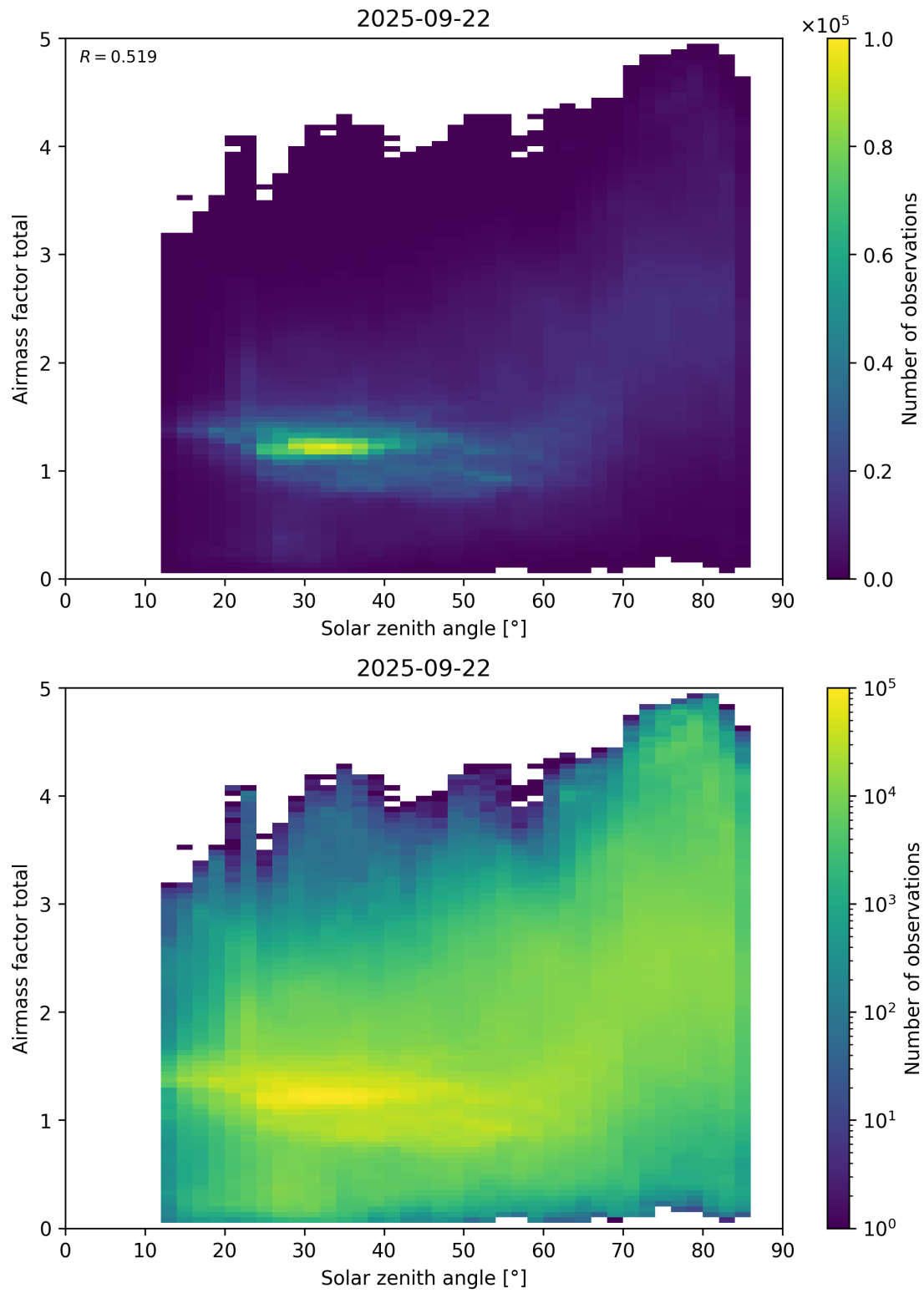
Figure 175: Scatter density plot of “Solar zenith angle” against “Airmass factor total” for 2025-09-22 to 2025-09-23.
