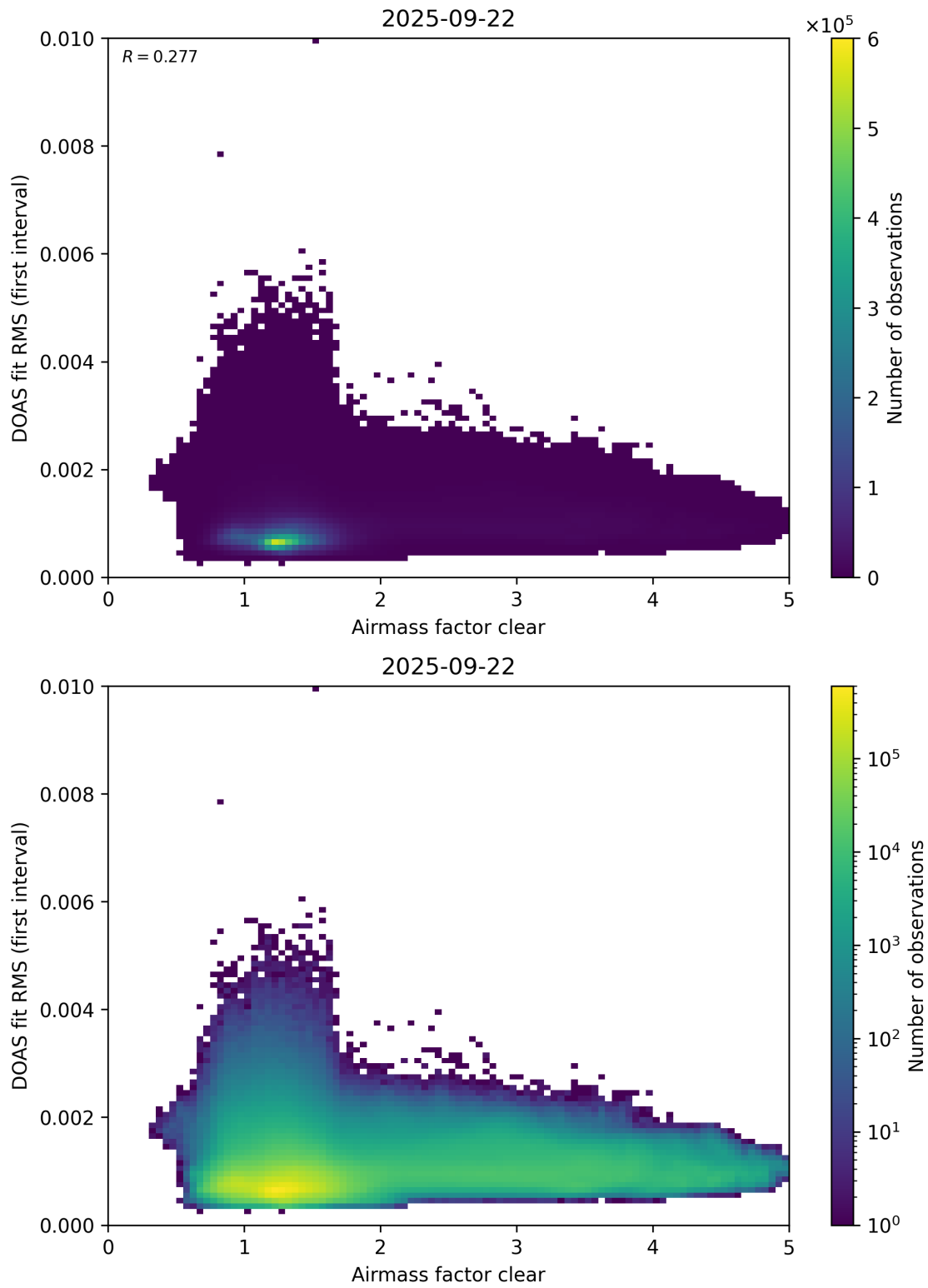
Figure 71: Scatter density plot of “Airmass factor clear” against “DOAS fit RMS (first interval)” for 2025-09-22 to 2025-09-23.
