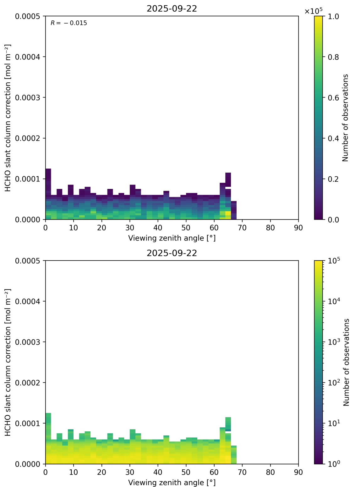
Figure 187: Scatter density plot of “Viewing zenith angle” against “HCHO slant column correction” for 2025-09-22 to 2025-09-23.
