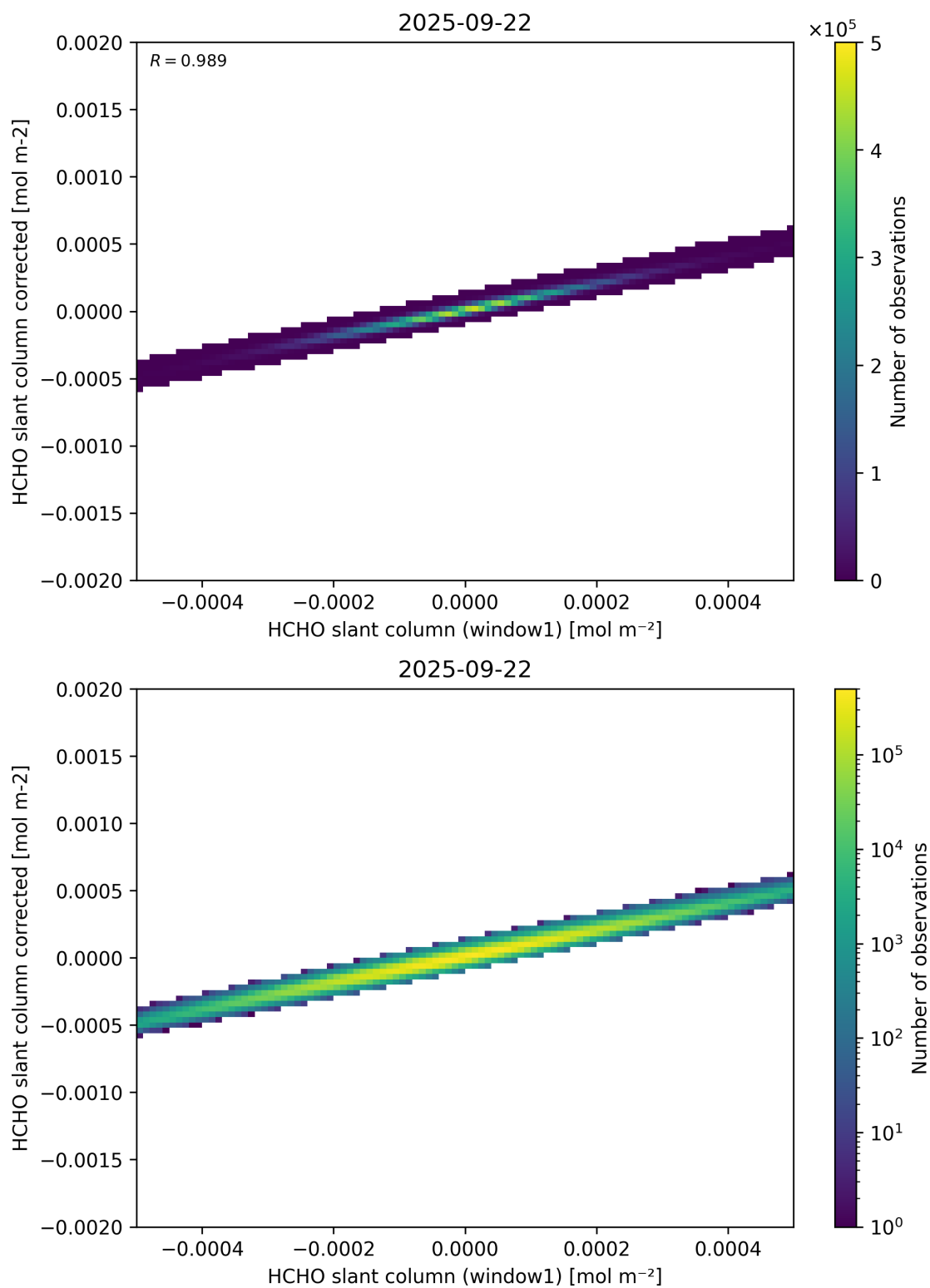
Figure 82: Scatter density plot of “HCHO slant column (window1)” against “HCHO slant column corrected” for 2025-09-22 to 2025-09-23.
