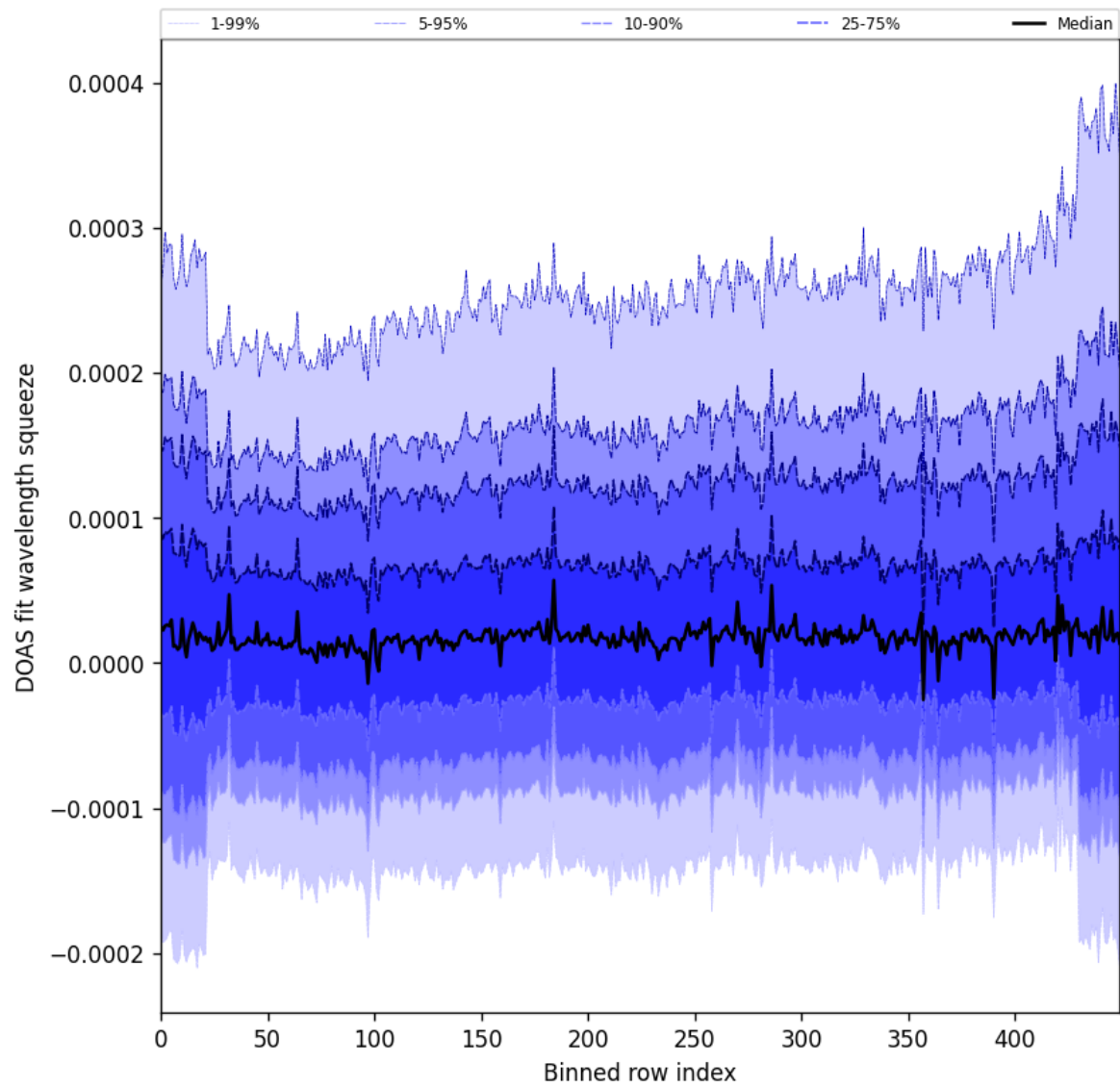
Figure 59: Along track statistics of “DOAS fit wavelength squeeze” for 2025-09-22 to 2025-09-23
