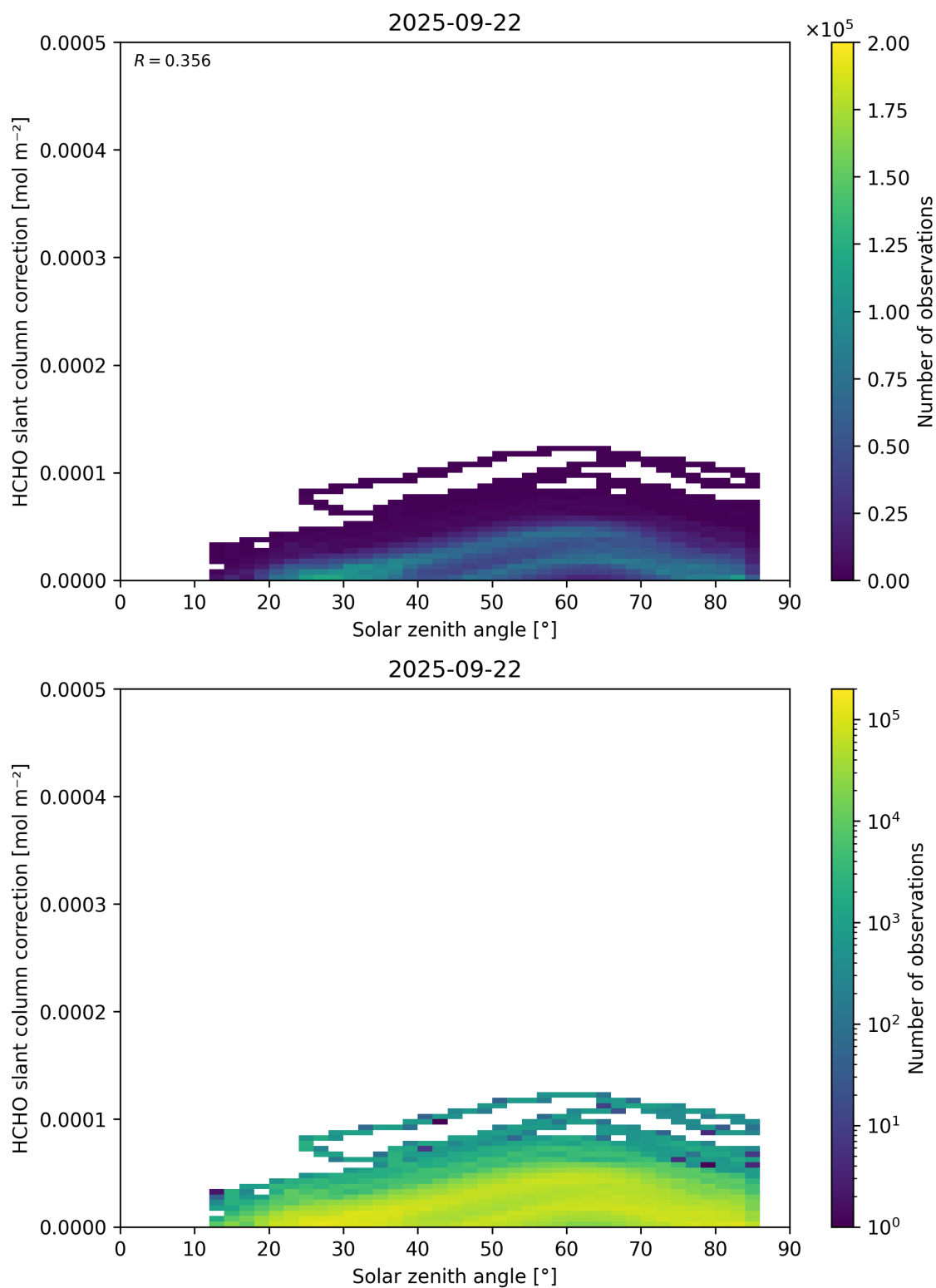
Figure 172: Scatter density plot of “Solar zenith angle” against “HCHO slant column correction” for 2025-09-22 to 2025-09-23.
