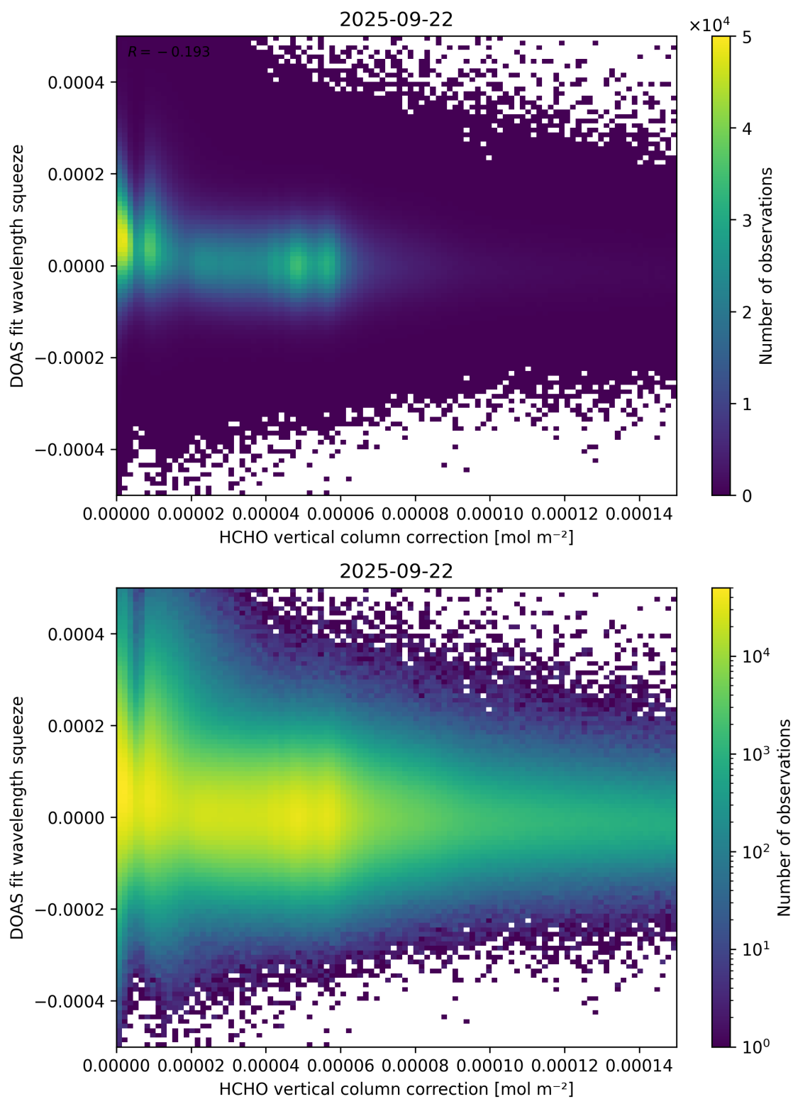
Figure 114: Scatter density plot of “HCHO vertical column correction” against “DOAS fit wavelength squeeze” for 2025-09-22 to 2025-09-23.
