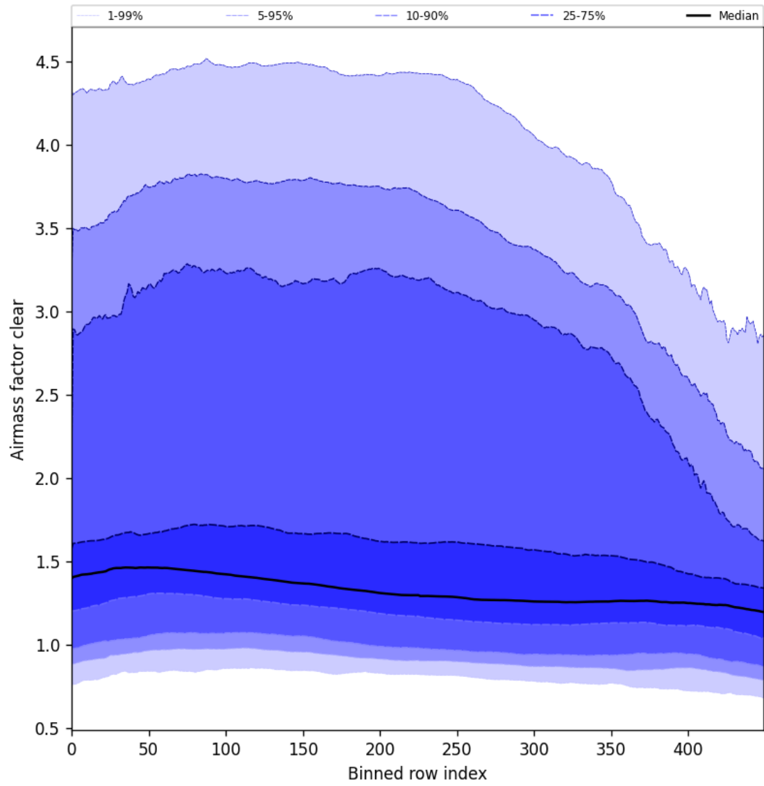
Figure 56: Along track statistics of “Air mass factor clear” for 2025-09-22 to 2025-09-23
