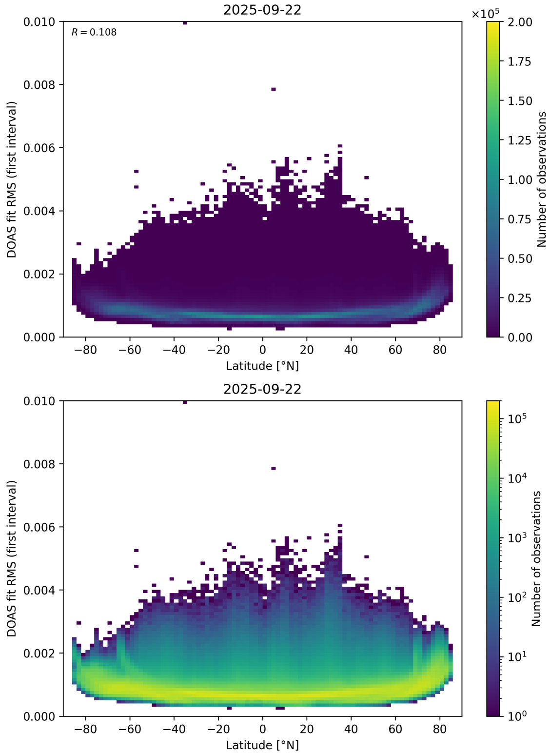
Figure 153: Scatter density plot of “Latitude” against “DOAS fit RMS (first interval)” for 2025-09-22 to 2025-09-23.
