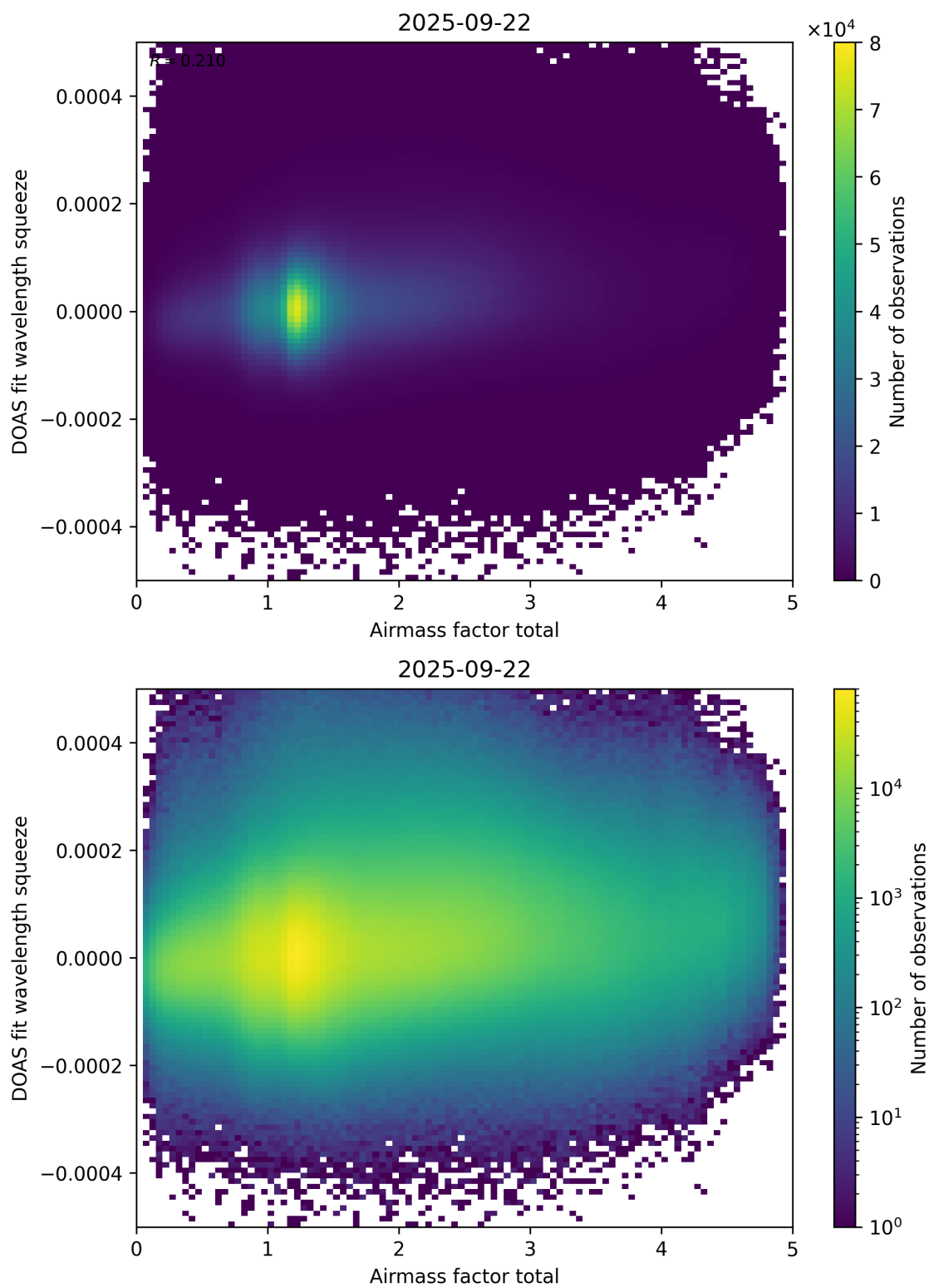
Figure 99: Scatter density plot of “Airmass factor total” against “DOAS fit wavelength squeeze” for 2025-09-22 to 2025-09-23.
