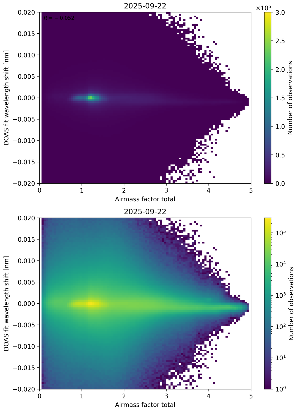
Figure 98: Scatter density plot of “Airmass factor total” against “DOAS fit wavelength shift” for 2025-09-22 to 2025-09-23.
