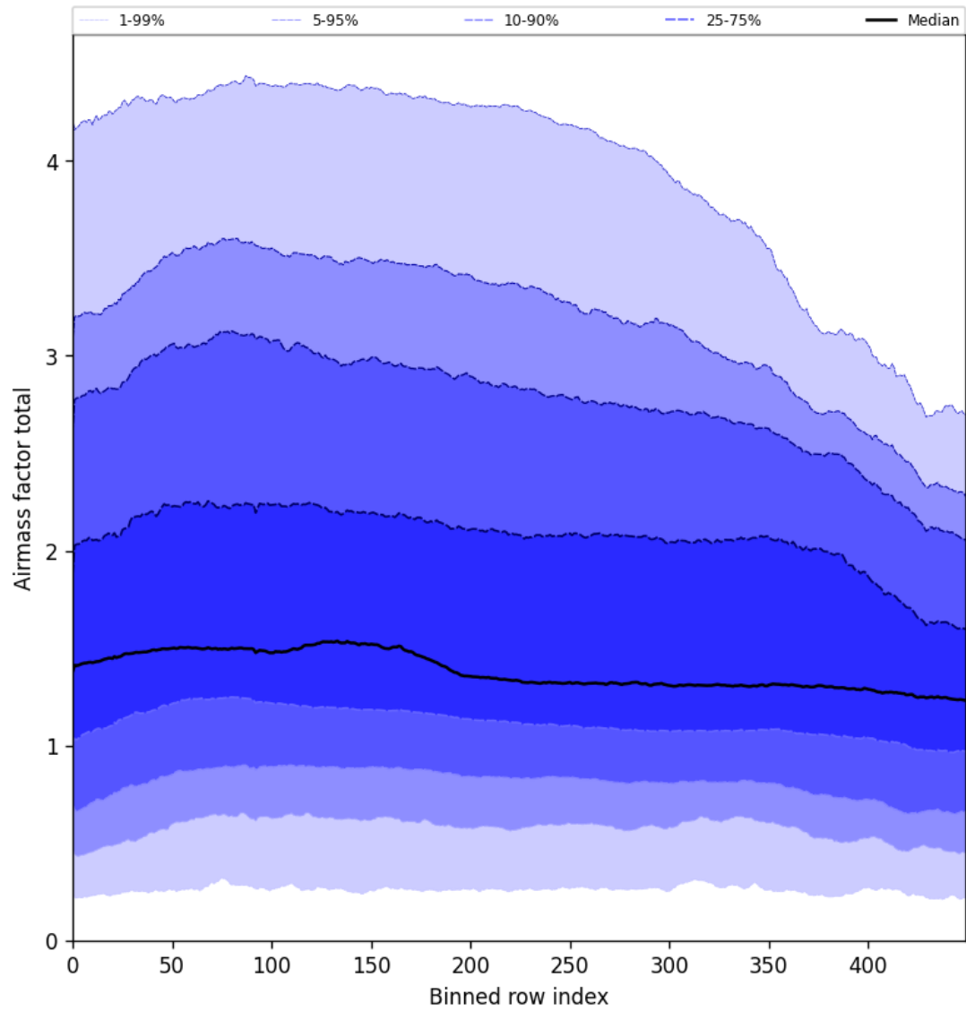
Figure 54: Along track statistics of “Airmass factor total” for 2025-09-22 to 2025-09-23
