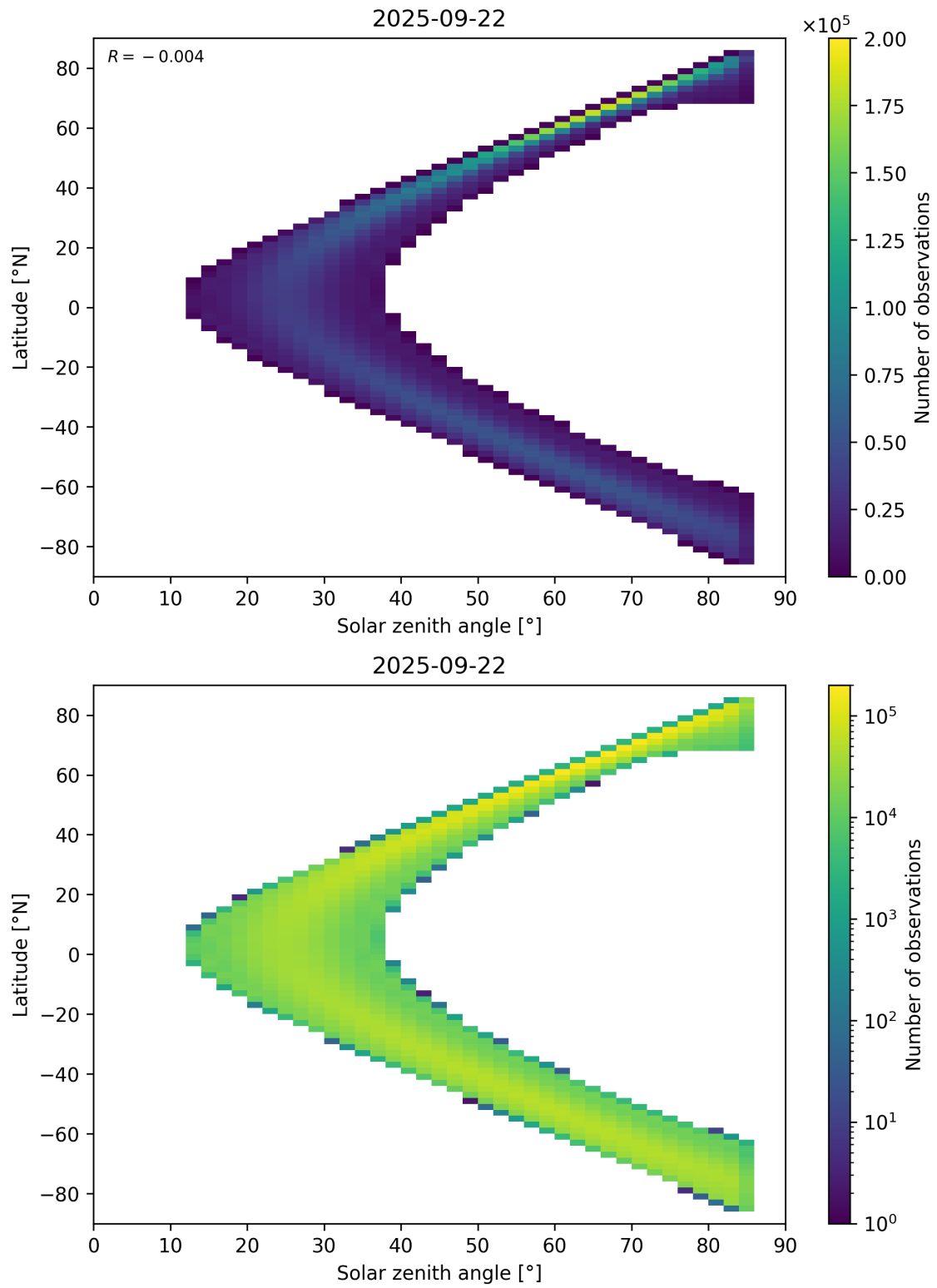
Figure 181: Scatter density plot of “Solar zenith angle” against “Latitude” for 2025-09-22 to 2025-09-23.
