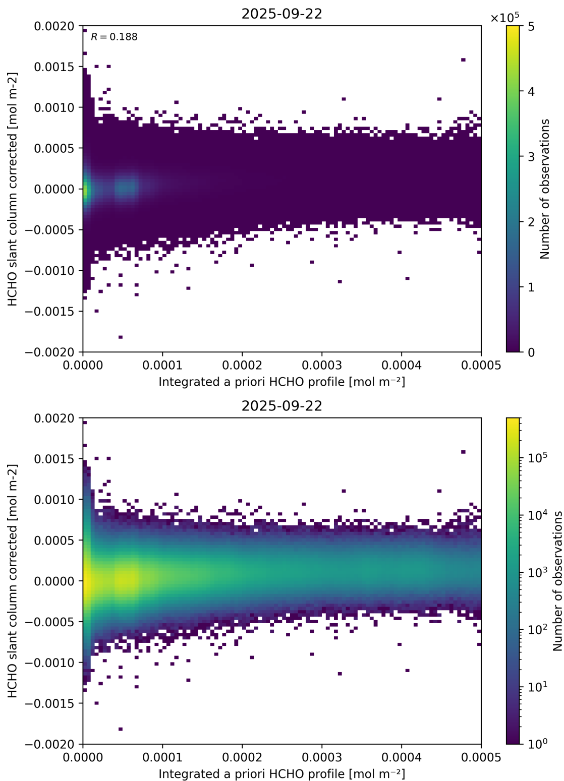
Figure 151: Scatter density plot of “Integrated a priori HCHO profile” against “HCHO slant column corrected” for 2025-09-22 to 2025-09-23.
