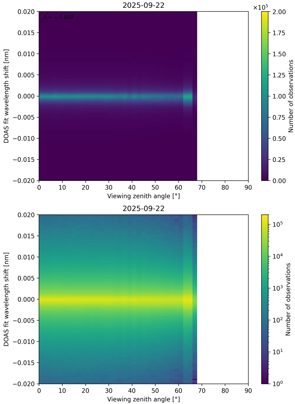
Figure 183: Scatter density plot of “Viewing zenith angle” against “DOAS fit wavelength shift” for 2025-09-22 to 2025-09-23.
