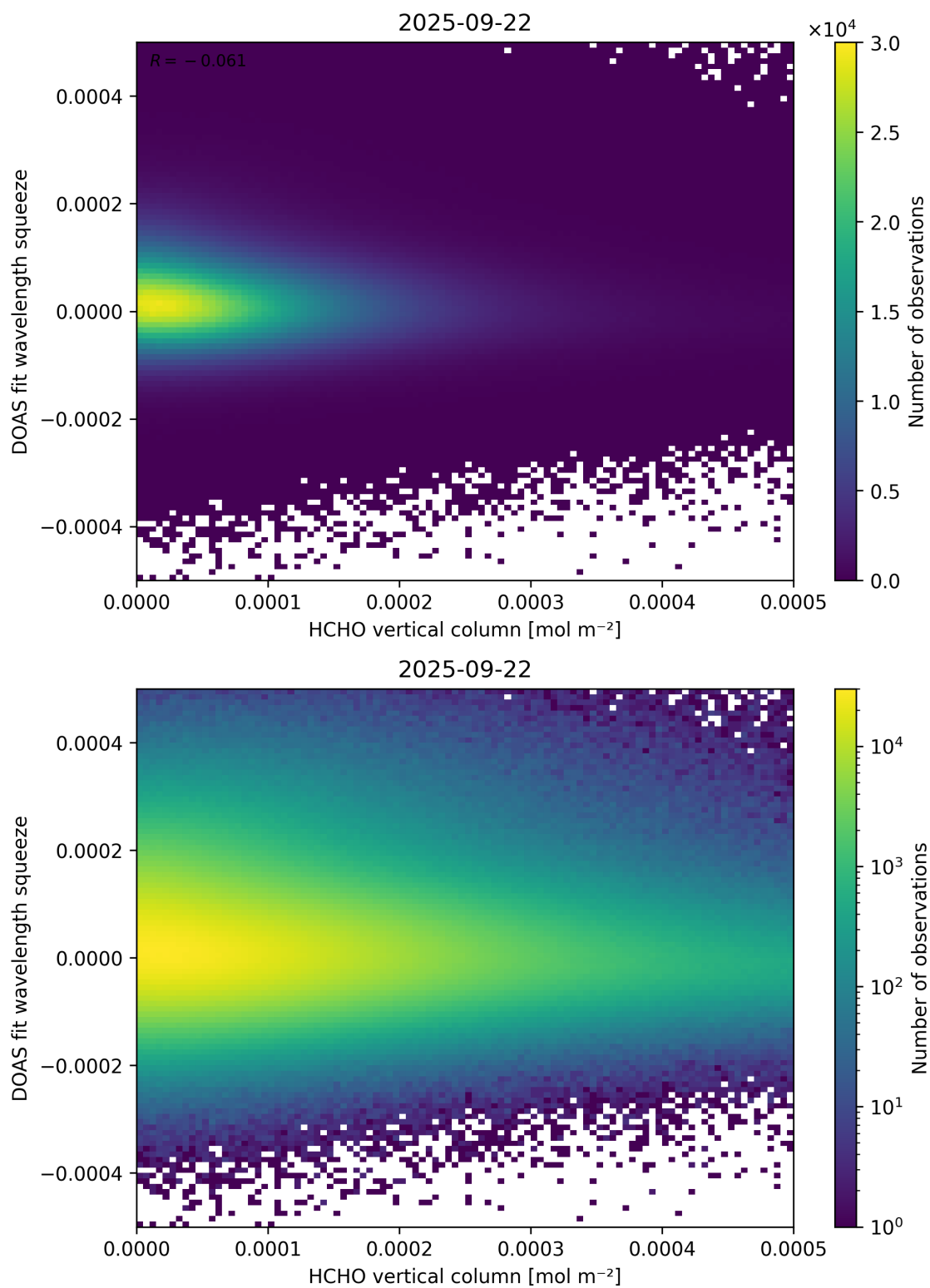
Figure 125: Scatter density plot of “HCHO vertical column” against “DOAS fit wavelength squeeze” for 2025-09-22 to 2025-09-23.
