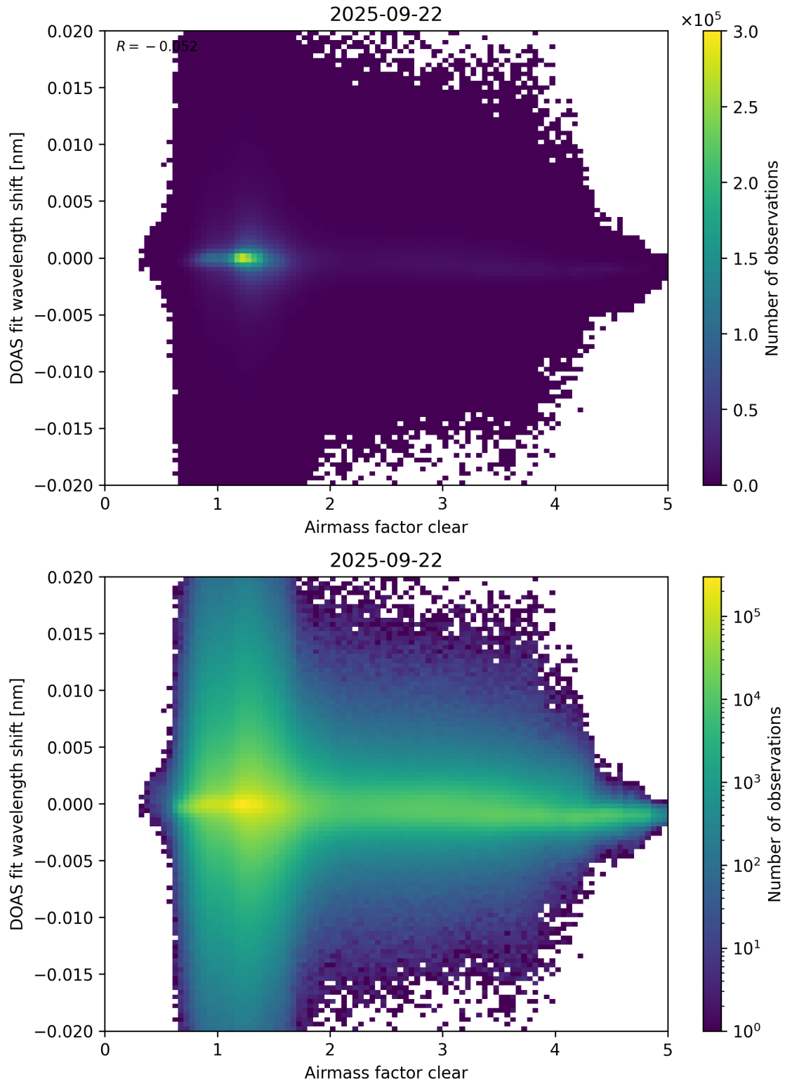
Figure 72: Scatter density plot of “Airmass factor clear” against “DOAS fit wavelength shift” for 2025-09-22 to 2025-09-23.
