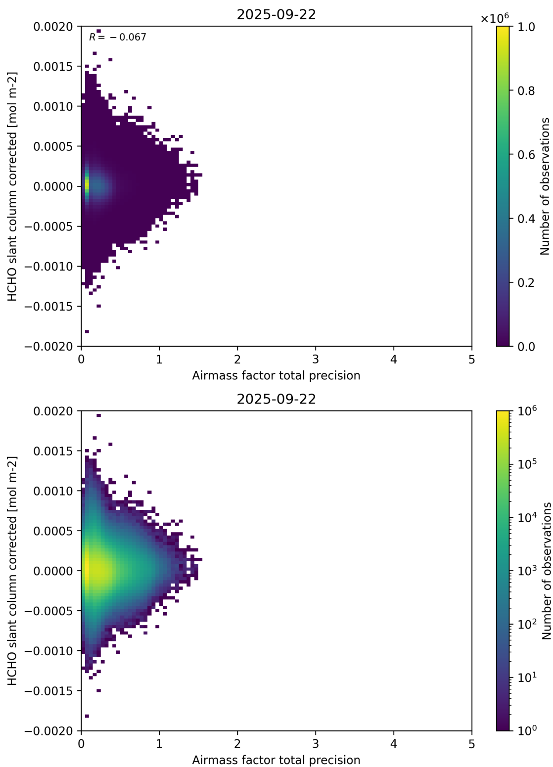
Figure 109: Scatter density plot of “Airmass factor total precision” against “HCHO slant column corrected” for 2025-09-22 to 2025-09-23.
