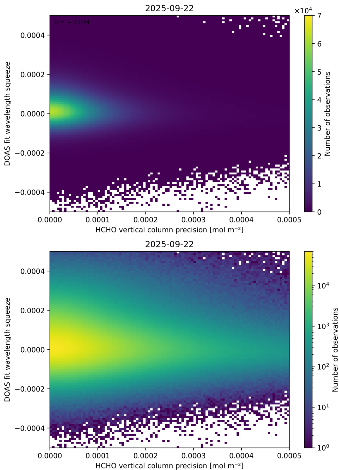
Figure 138: Scatter density plot of “HCHO vertical column precision” against “DOAS fit wavelength squeeze” for 2025-09-22 to 2025-09-23.
