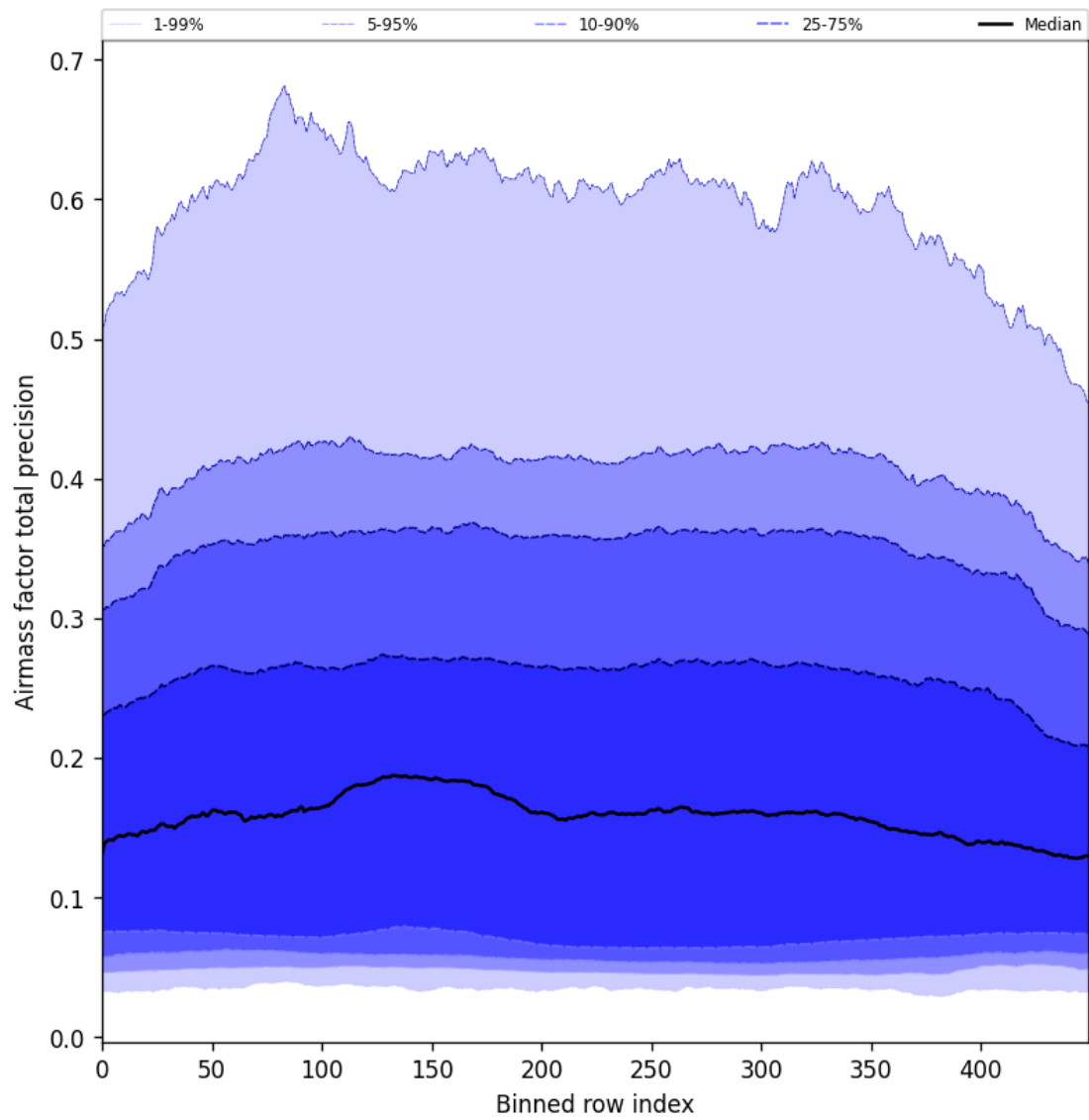
Figure 55: Along track statistics of “Airmass factor total precision” for 2025-09-22 to 2025-09-23
