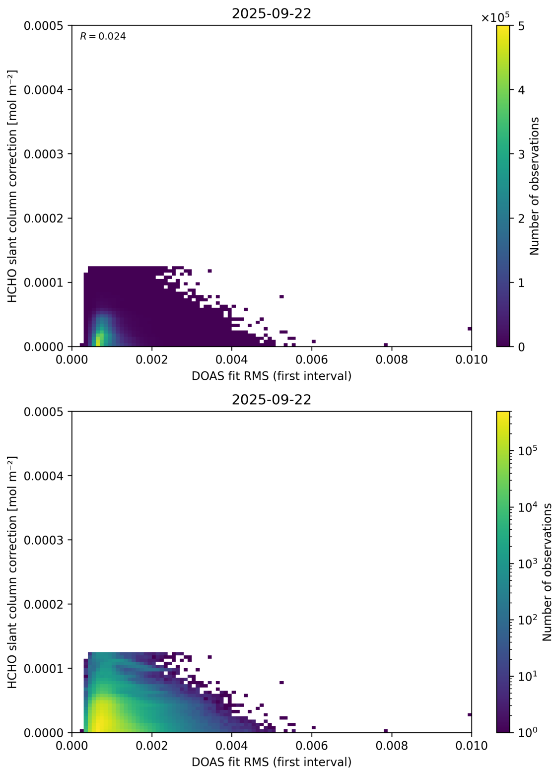
Figure 63: Scatter density plot of “DOAS fit RMS (first interval)” against “HCHO slant column correction” for 2025-09-22 to 2025-09-23.
