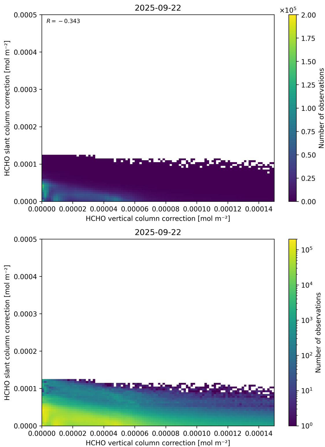
Figure 117: Scatter density plot of “HCHO vertical column correction” against “HCHO slant column correction” for 2025-09-22 to 2025-09-23.
