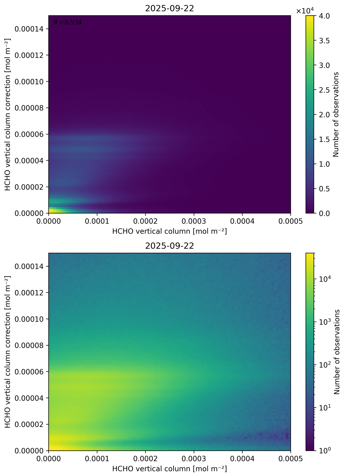
Figure 133: Scatter density plot of “HCHO vertical column” against “HCHO vertical column correction” for 2025-09-22 to 2025-09-23.
