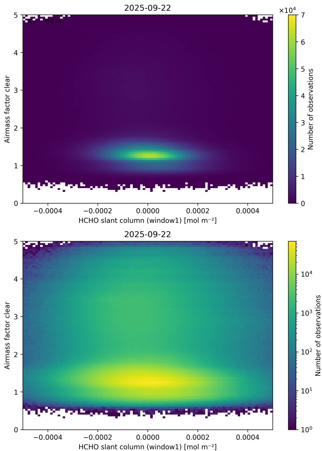
Figure 81: Scatter density plot of “HCHO slant column (window1)” against “Airmass factor clear” for 2025-09-22 to 2025-09-23.
