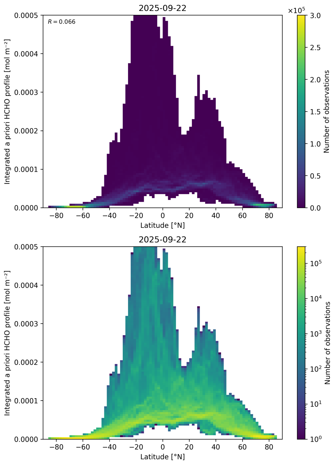
Figure 166: Scatter density plot of “Latitude” against “Integrated a priori HCHO profile” for 2025-09-22 to 2025-09-23.
