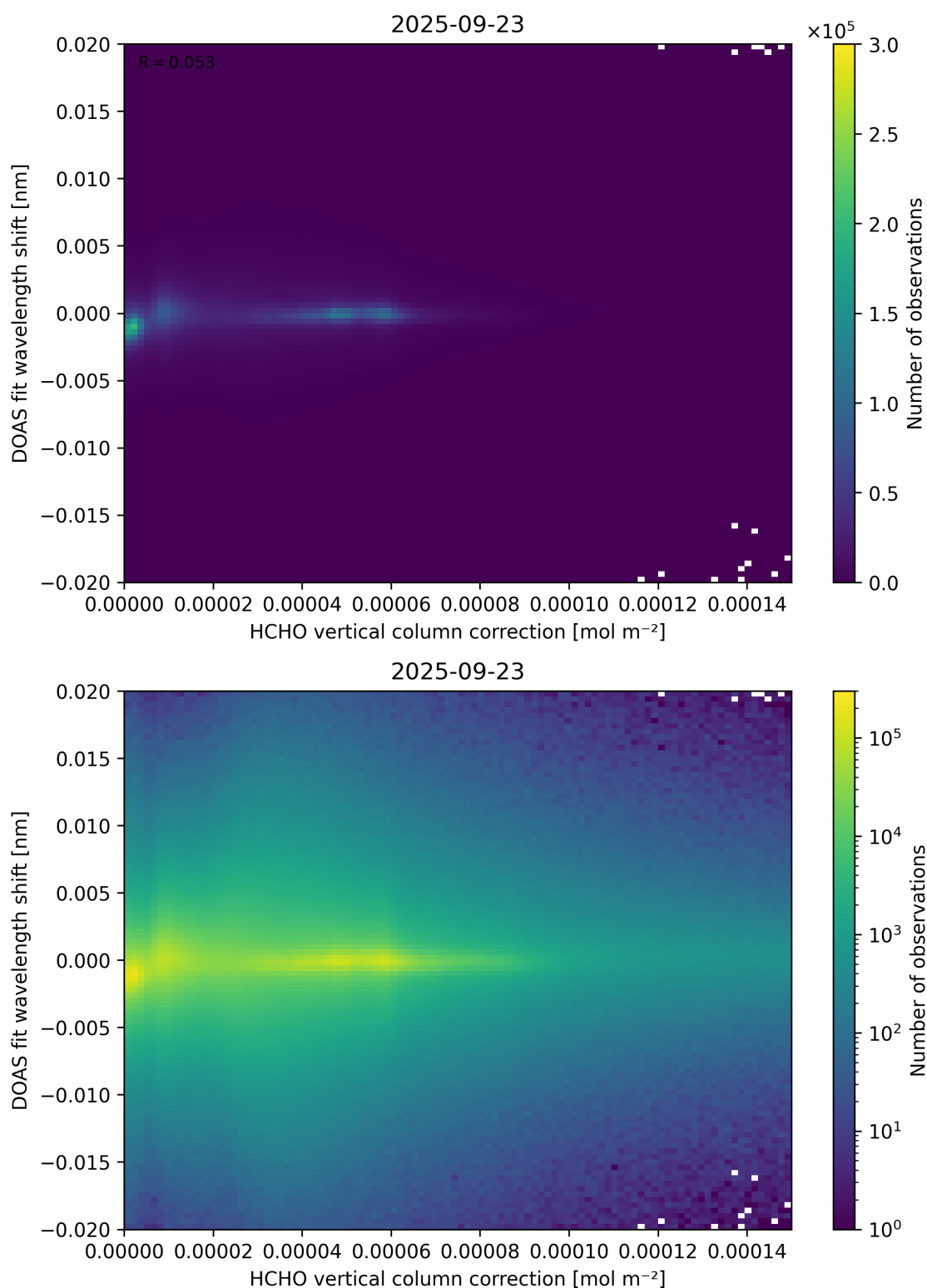
Figure 113: Scatter density plot of “HCHO vertical column correction” against “DOAS fit wavelength shift” for 2025-09-22 to 2025-09-24.
