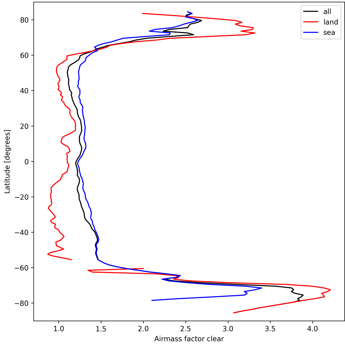
Figure 28: Zonal average of “Airmass factor clear” for 2025-09-22 to 2025-09-24.
