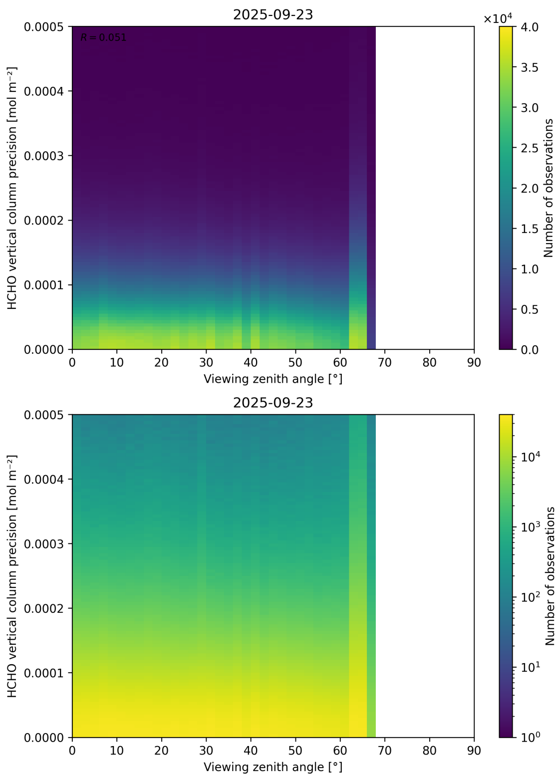
Figure 194: Scatter density plot of “Viewing zenith angle” against “HCHO vertical column precision” for 2025-09-22 to 2025-09-24.
