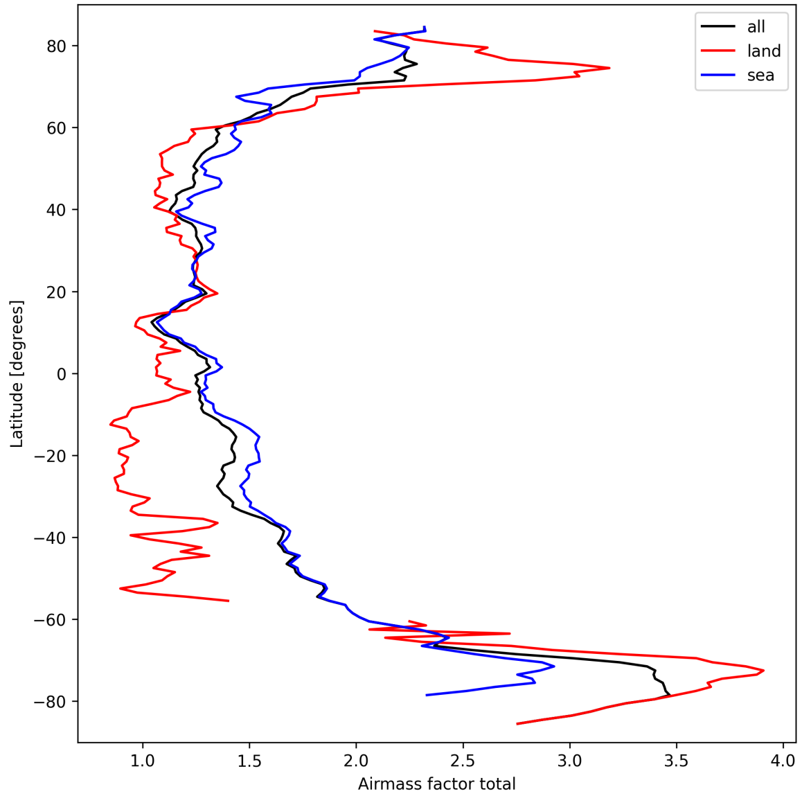
Figure 26: Zonal average of “Airmass factor total” for 2025-09-22 to 2025-09-24.
