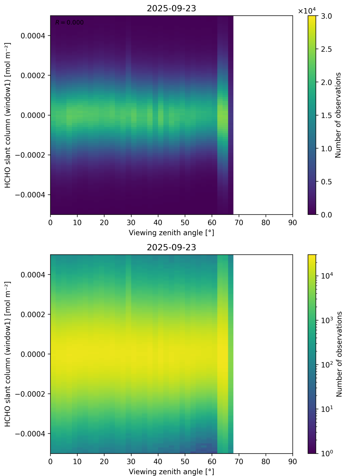
Figure 188: Scatter density plot of “Viewing zenith angle” against “HCHO slant column (window1)” for 2025-09-22 to 2025-09-24.
