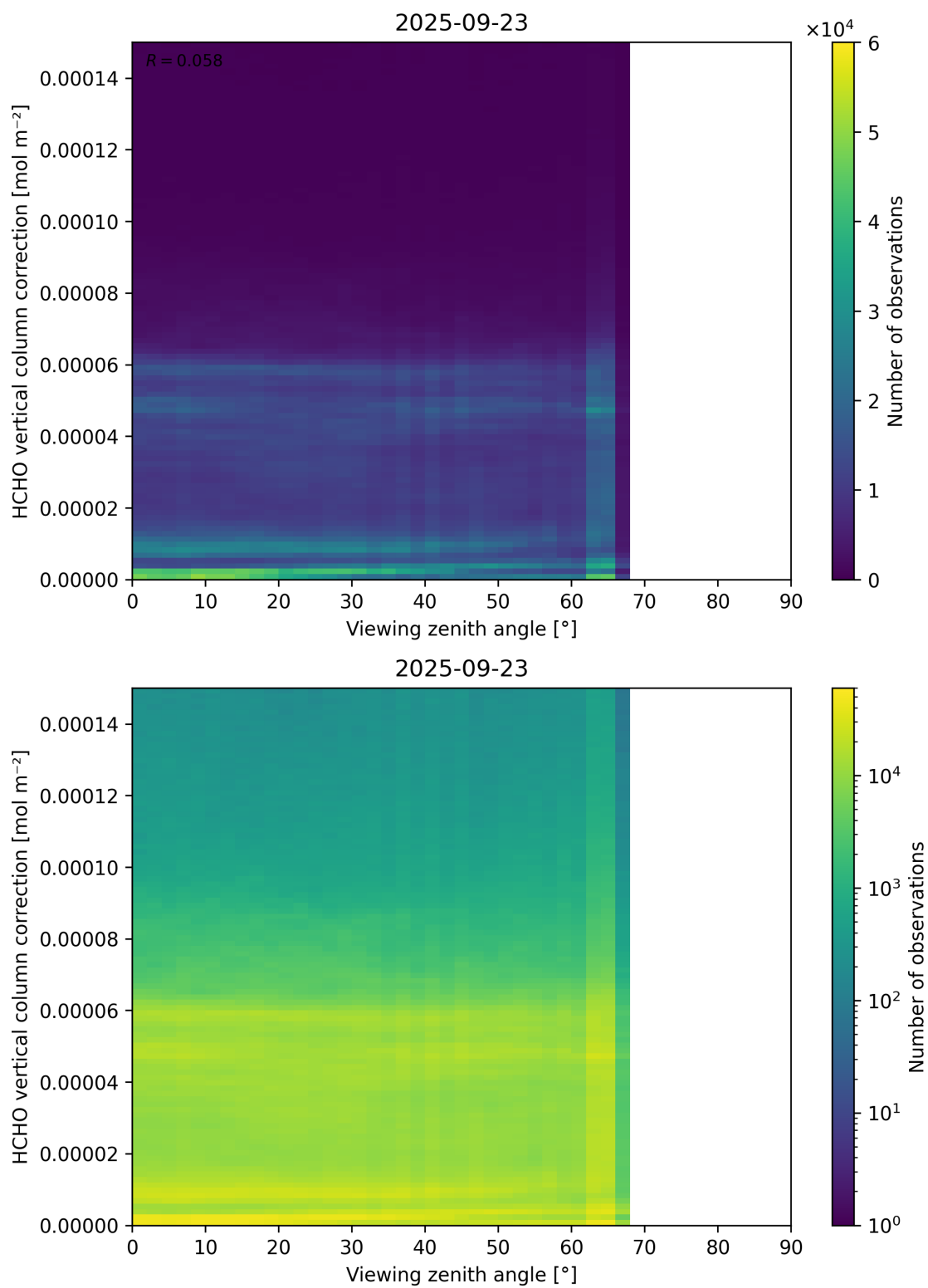
Figure 193: Scatter density plot of “Viewing zenith angle” against “HCHO vertical column correction” for 2025-09-22 to 2025-09-24.
