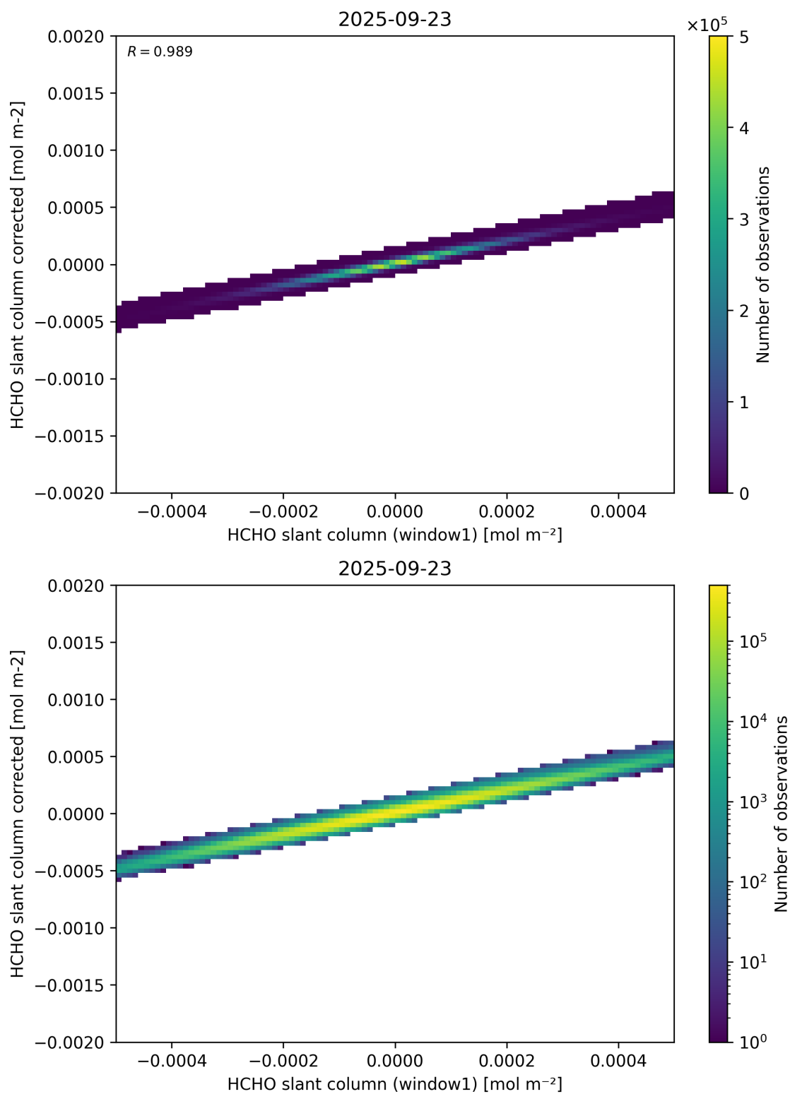
Figure 82: Scatter density plot of “HCHO slant column (window1)” against “HCHO slant column corrected” for 2025-09-22 to 2025-09-24.
