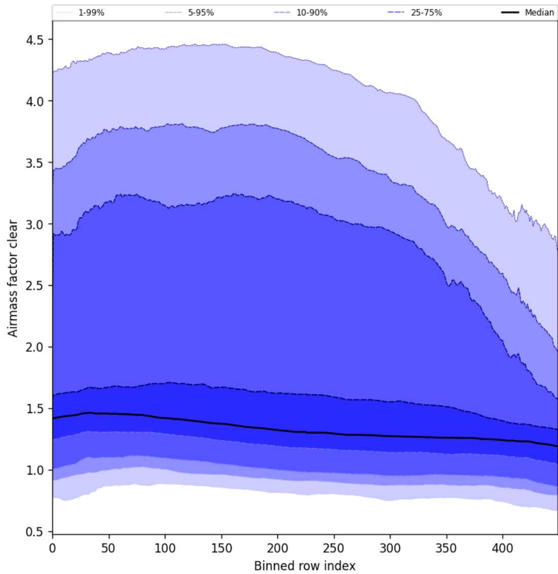
Figure 56: Along track statistics of “Airmass factor clear” for 2025-09-22 to 2025-09-24
