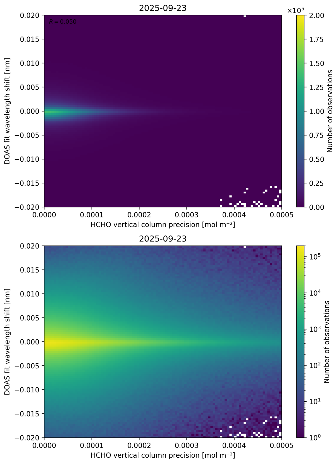
Figure 137: Scatter density plot of “HCHO vertical column precision” against “DOAS fit wavelength shift” for 2025-09-22 to 2025-09-24.
