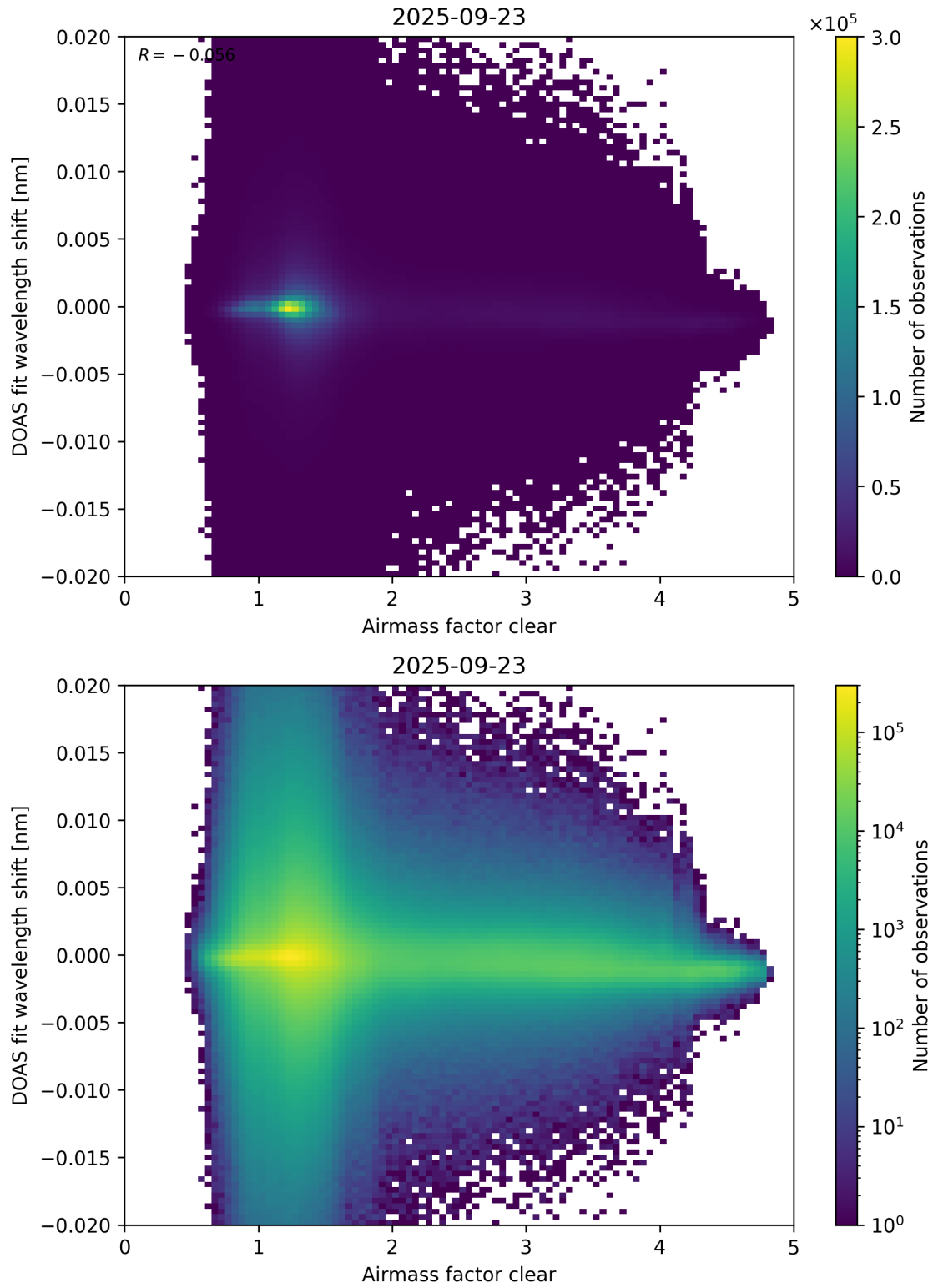
Figure 72: Scatter density plot of “Airmass factor clear” against “DOAS fit wavelength shift” for 2025-09-22 to 2025-09-24.
