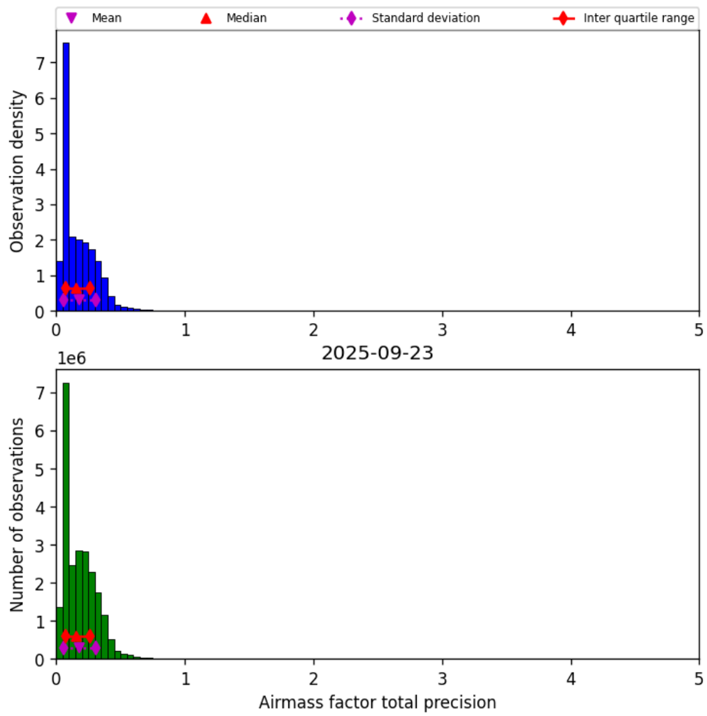
Figure 41: Histogram of “Airmass factor total precision” for 2025-09-22 to 2025-09-24
