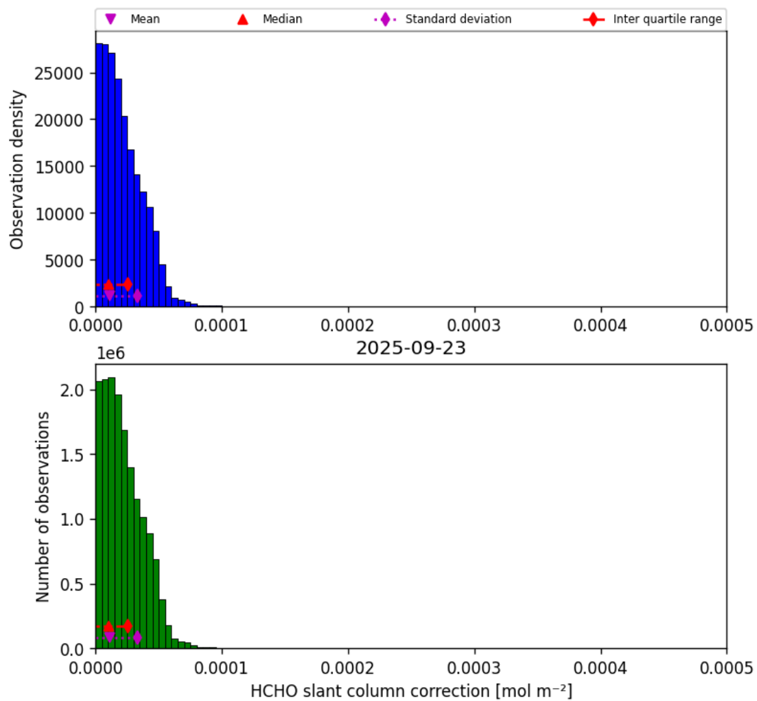
Figure 47: Histogram of “HCHO slant column correction” for 2025-09-22 to 2025-09-24
