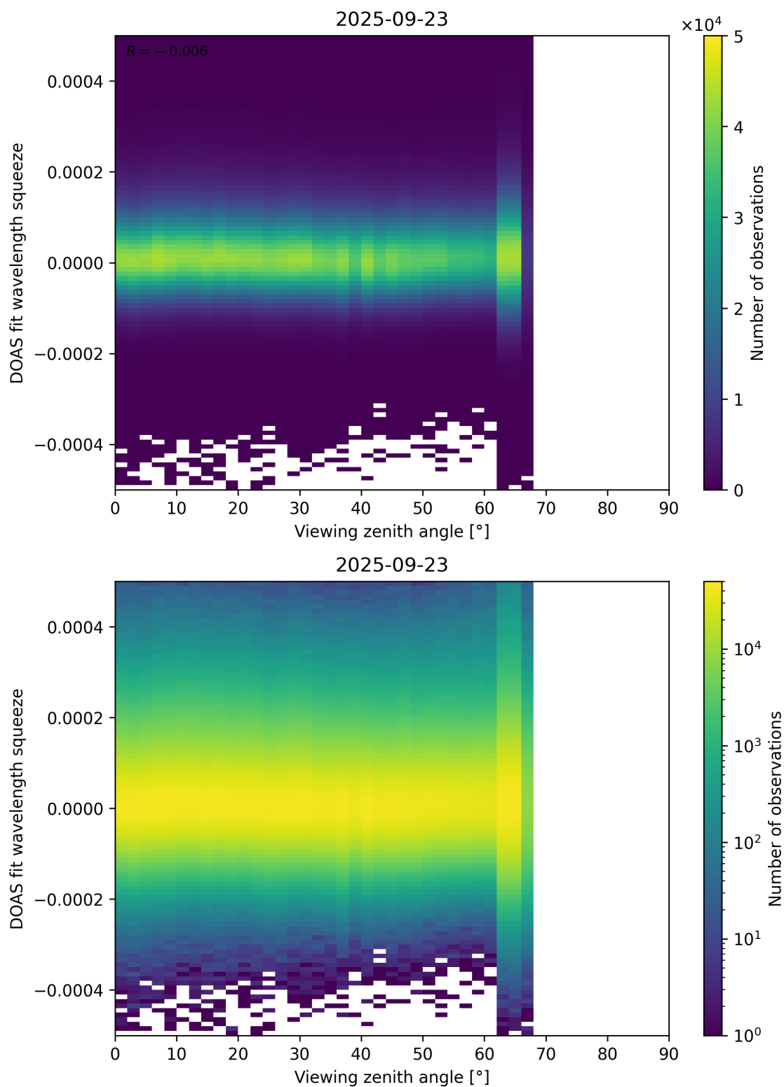
Figure 184: Scatter density plot of “Viewing zenith angle” against “DOAS fit wavelength squeeze” for 2025-09-22 to 2025-09-24.
