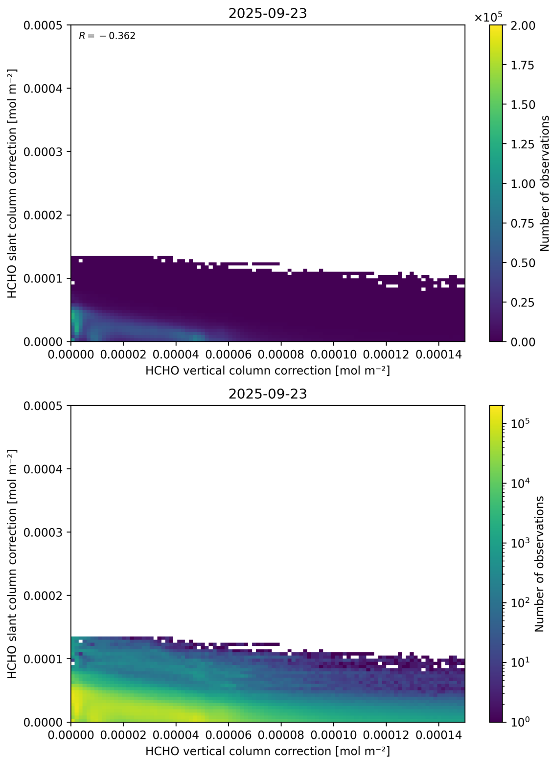
Figure 117: Scatter density plot of “HCHO vertical column correction” against “HCHO slant column correction” for 2025-09-22 to 2025-09-24.
