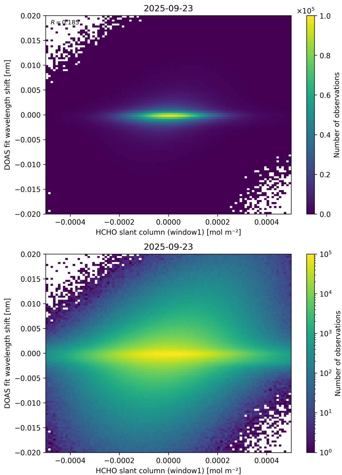
Figure 79: Scatter density plot of “HCHO slant column (window1)” against “DOAS fit wavelength shift” for 2025-09-22 to 2025-09-24.
