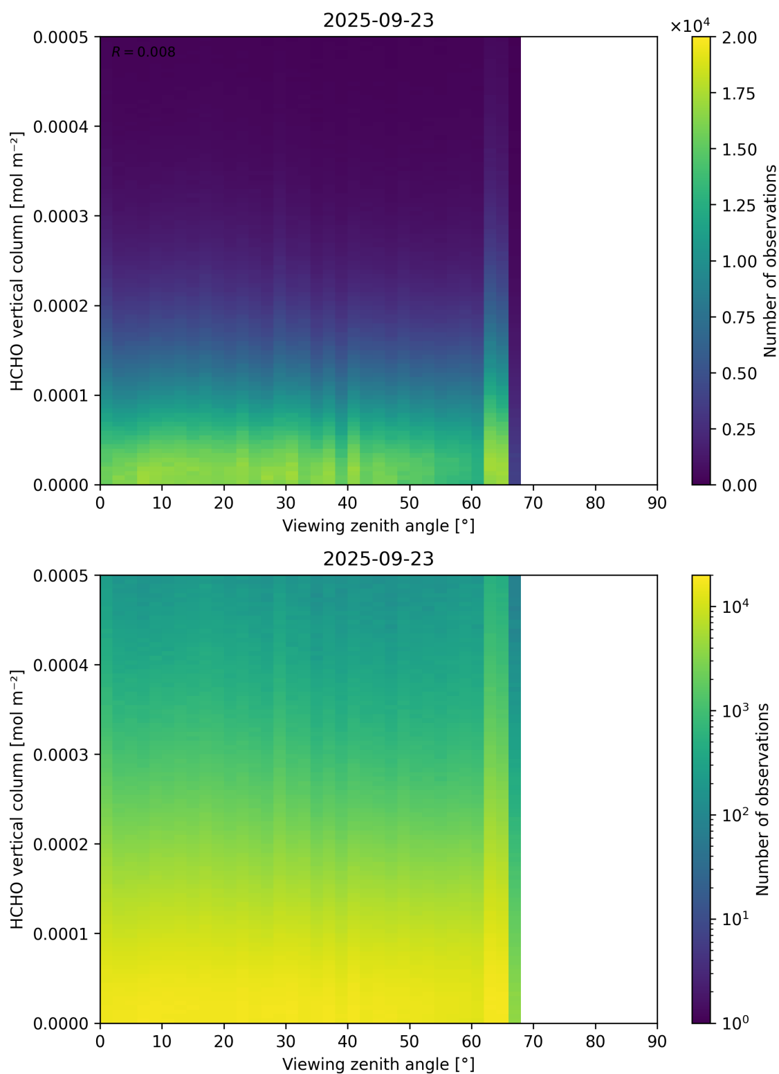
Figure 192: Scatter density plot of “Viewing zenith angle” against “HCHO vertical column” for 2025-09-22 to 2025-09-24.
