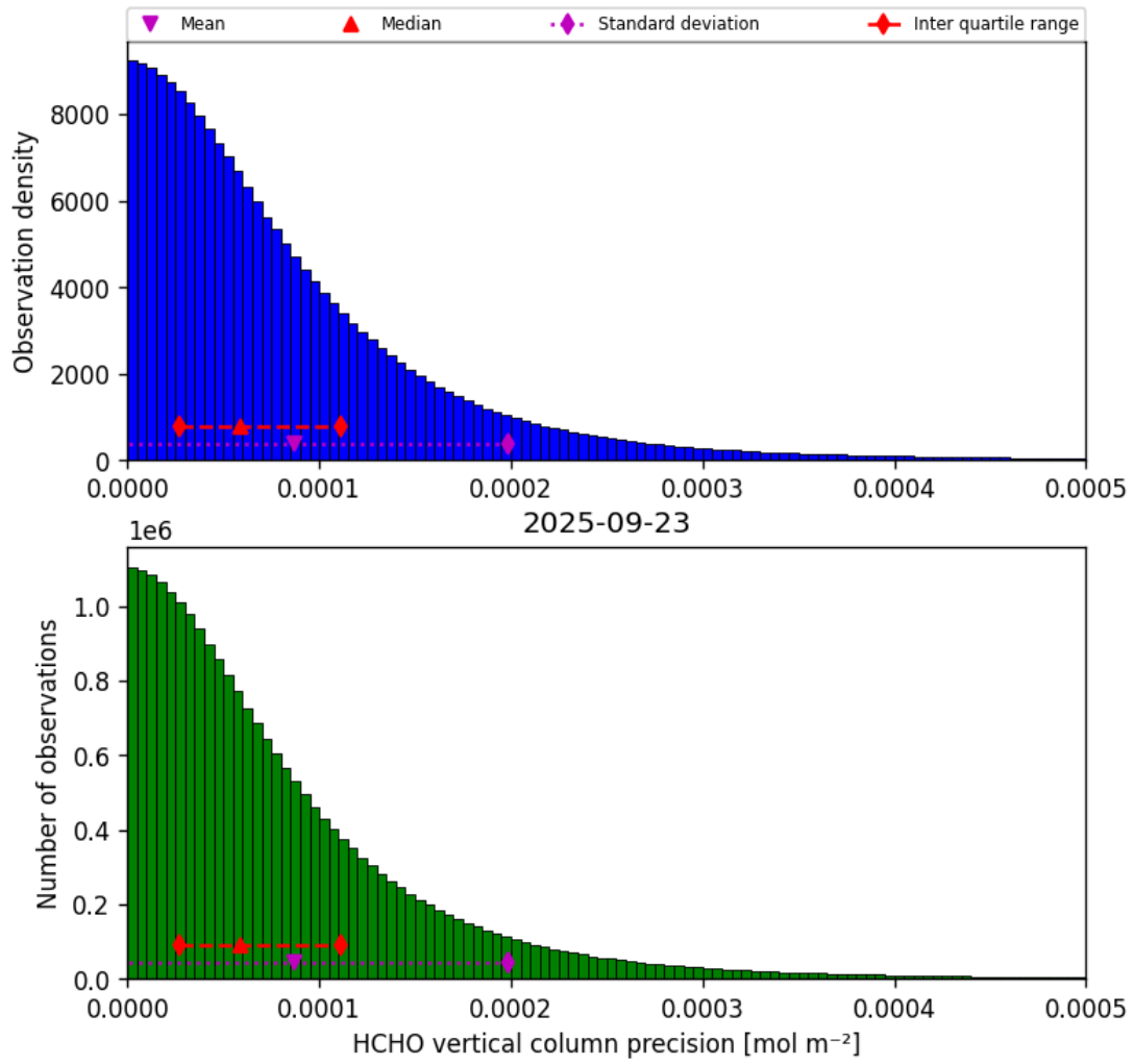
Figure 36: Histogram of “HCHO vertical column precision” for 2025-09-22 to 2025-09-24
