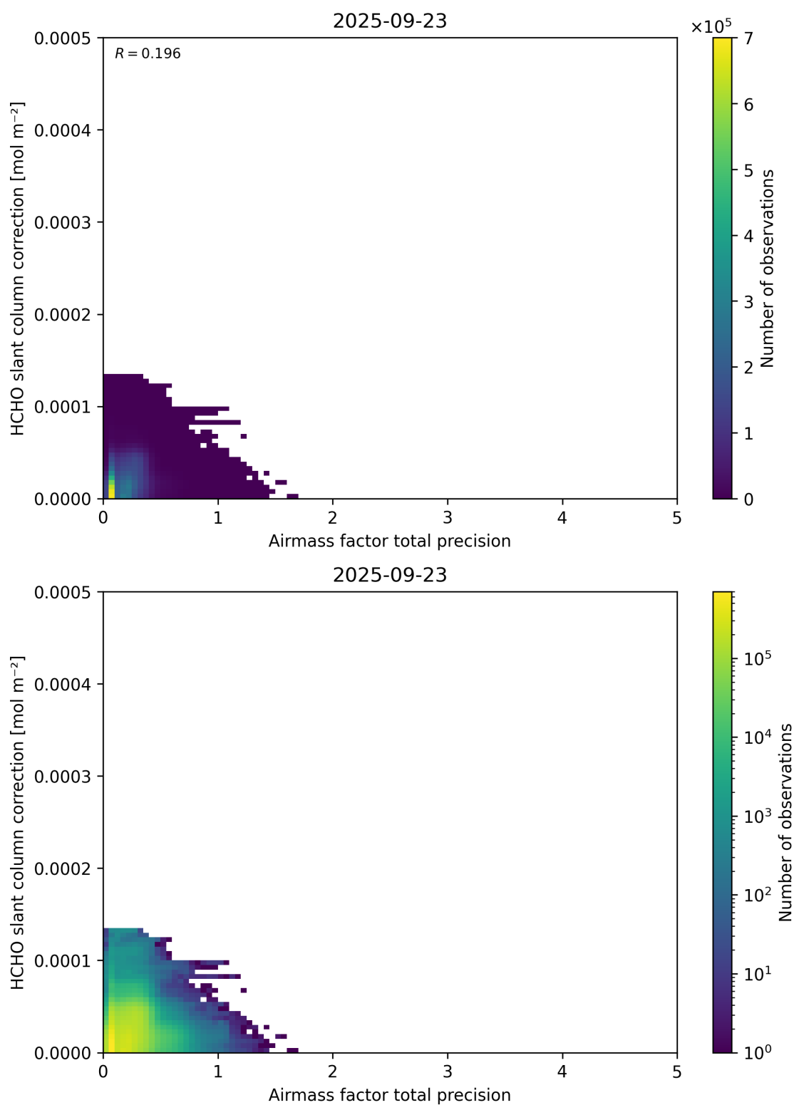
Figure 110: Scatter density plot of “Airmass factor total precision” against “HCHO slant column correction” for 2025-09-22 to 2025-09-24.
