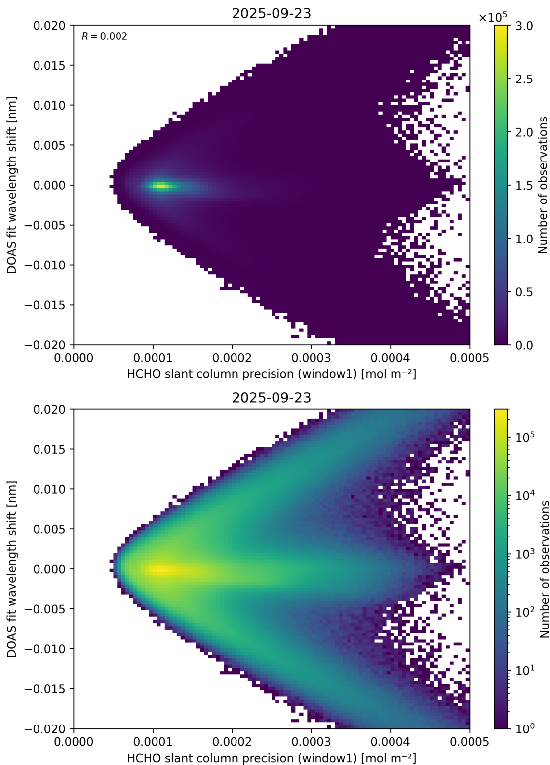
Figure 89: Scatter density plot of “HCHO slant column precision (window1)” against “DOAS fit wavelength shift” for 2025-09-22 to 2025-09-24.
