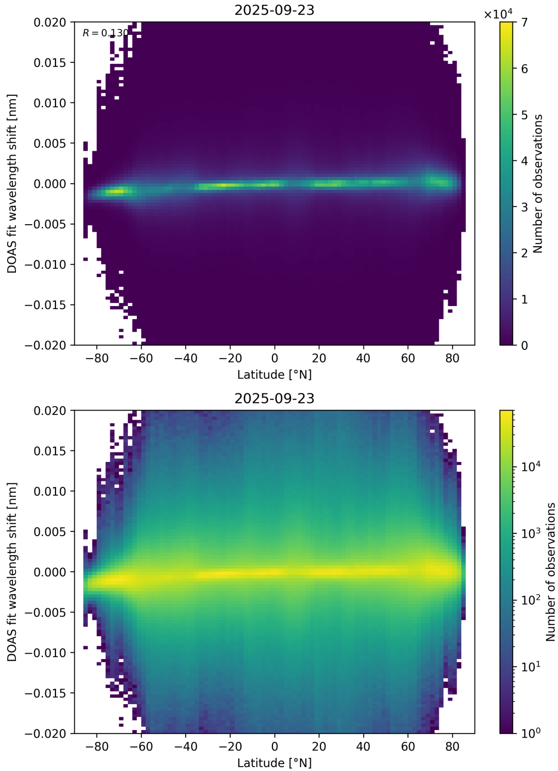
Figure 154: Scatter density plot of “Latitude” against “DOAS fit wavelength shift” for 2025-09-22 to 2025-09-24.
