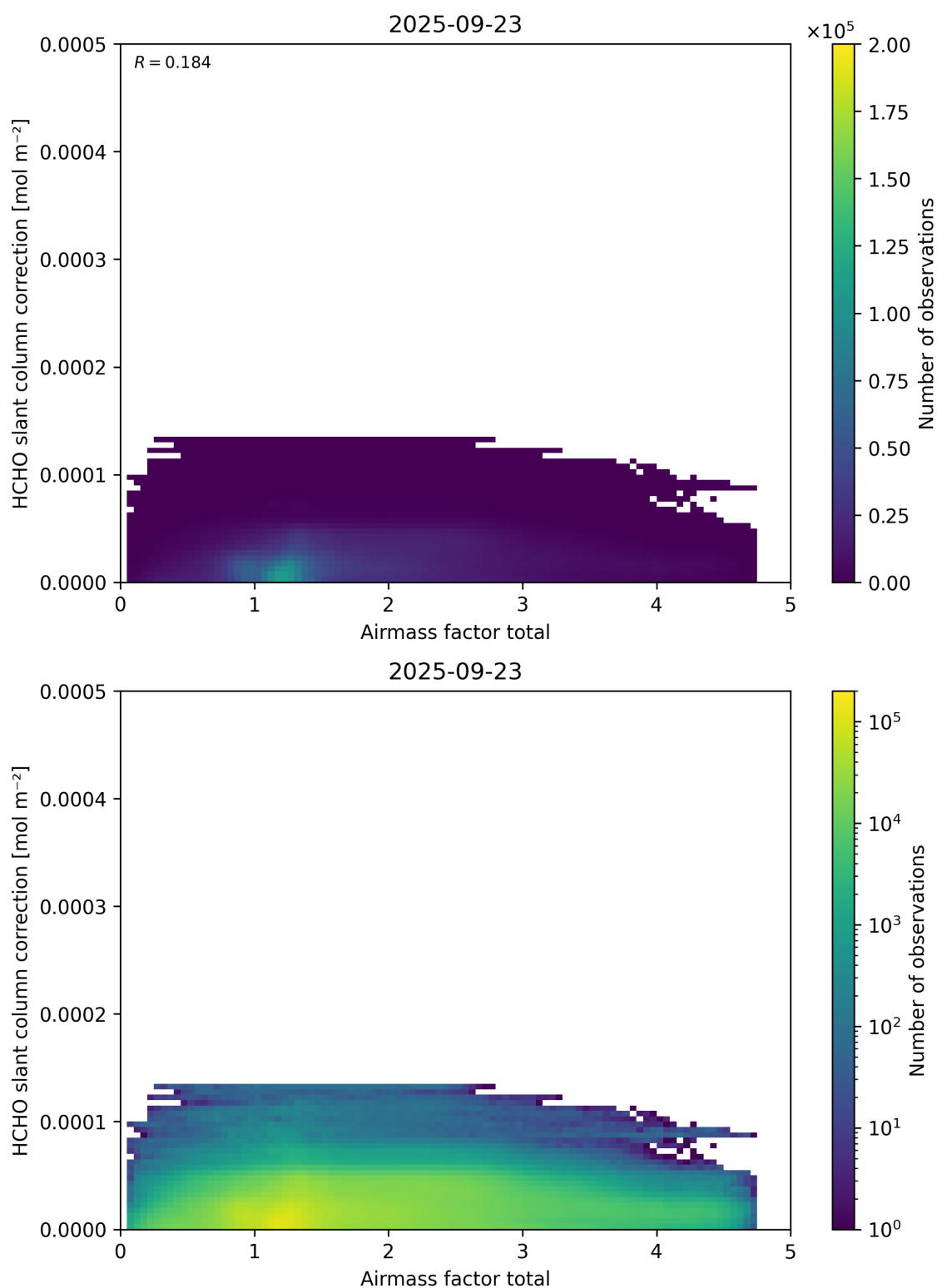
Figure 102: Scatter density plot of “Airmass factor total” against “HCHO slant column correction” for 2025-09-22 to 2025-09-24.
