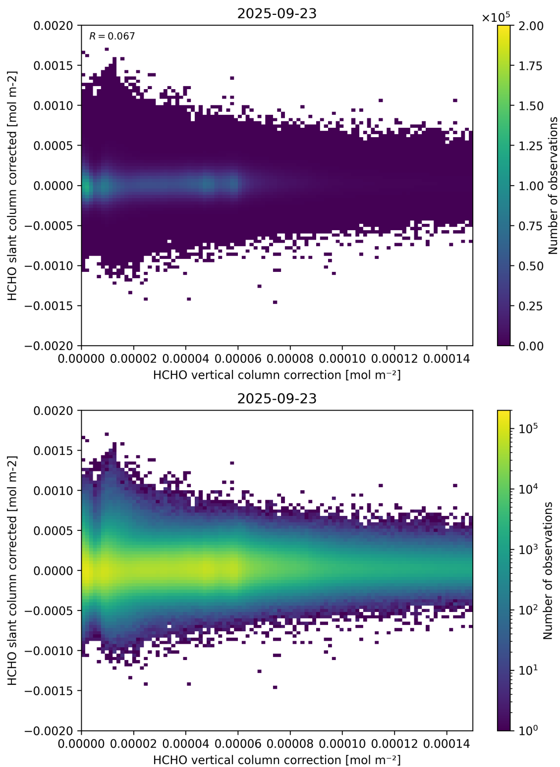
Figure 116: Scatter density plot of “HCHO vertical column correction” against “HCHO slant column corrected” for 2025-09-22 to 2025-09-24.
