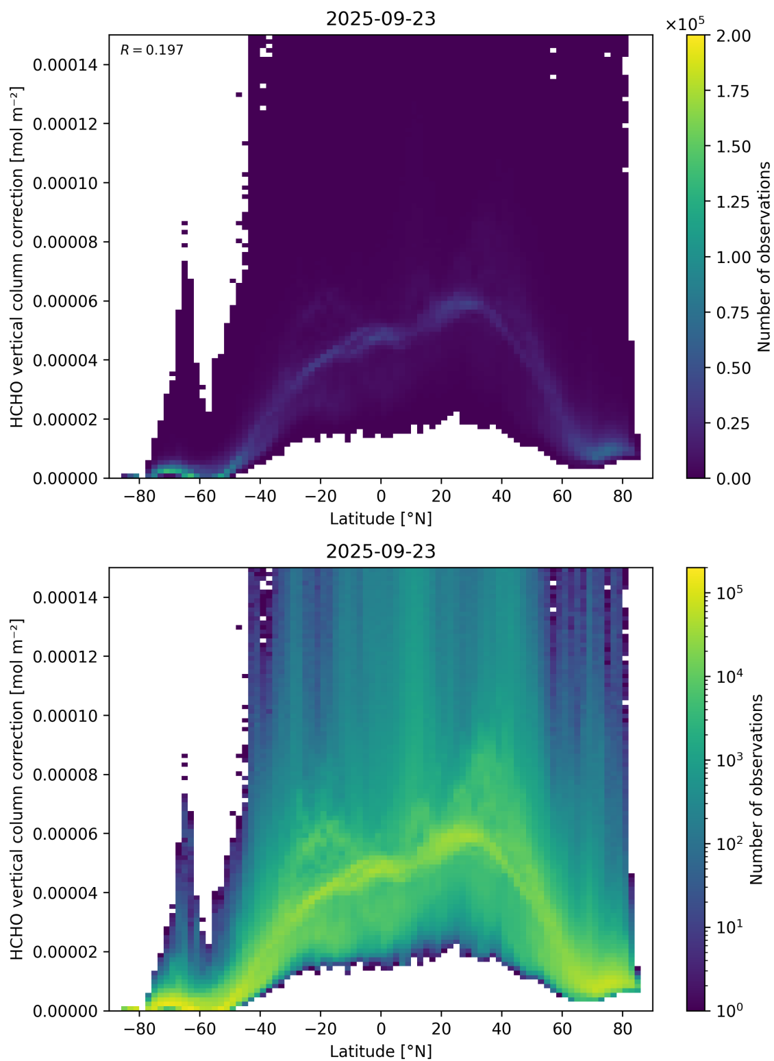
Figure 164: Scatter density plot of “Latitude” against “HCHO vertical column correction” for 2025-09-22 to 2025-09-24.
