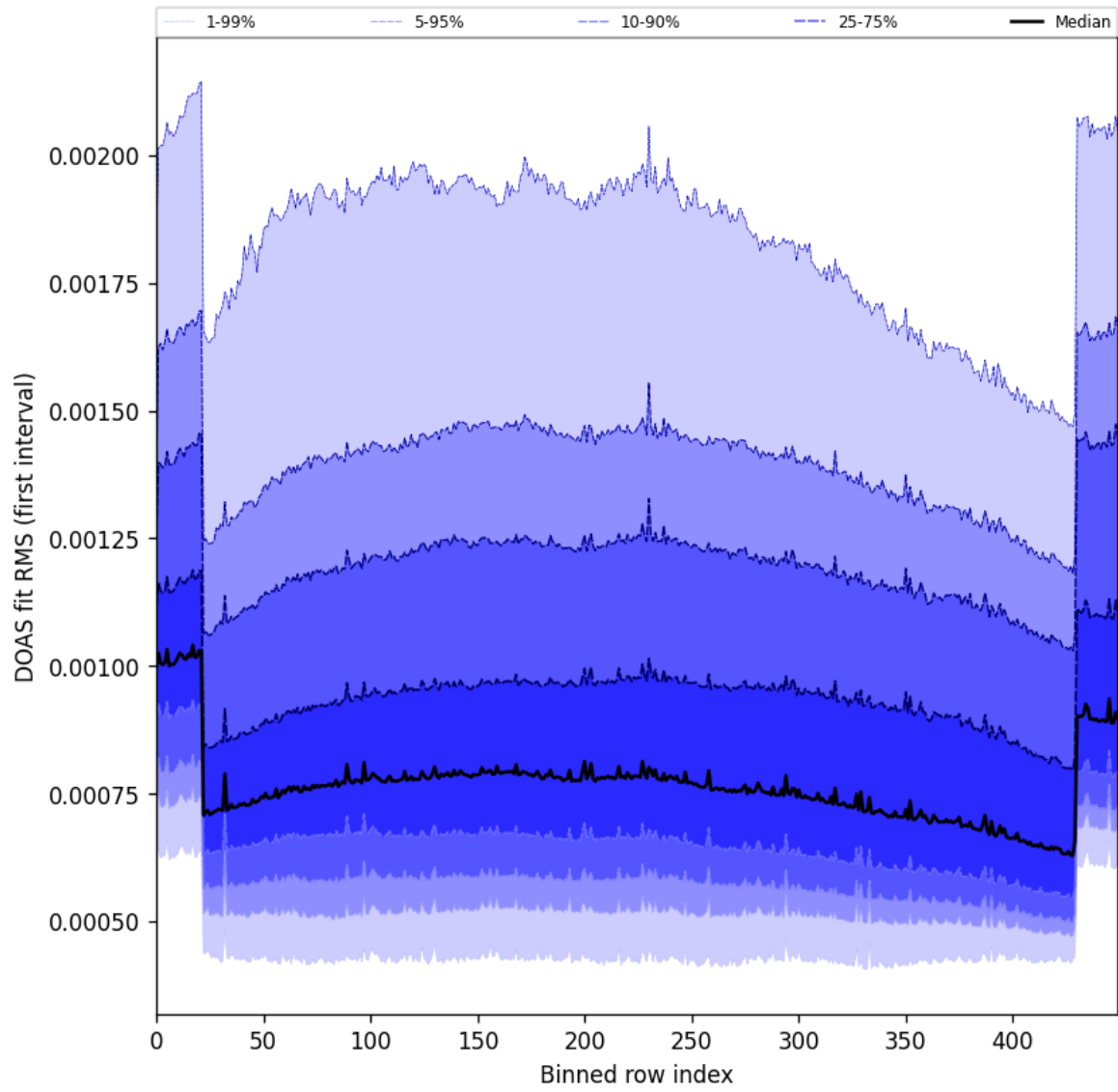
Figure 60: Along track statistics of “DOAS fit RMS (first interval)” for 2025-09-22 to 2025-09-24
