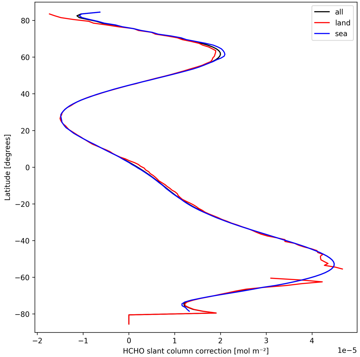
Figure 33: Zonal average of “HCHO slant column correction” for 2025-09-22 to 2025-09-24.
