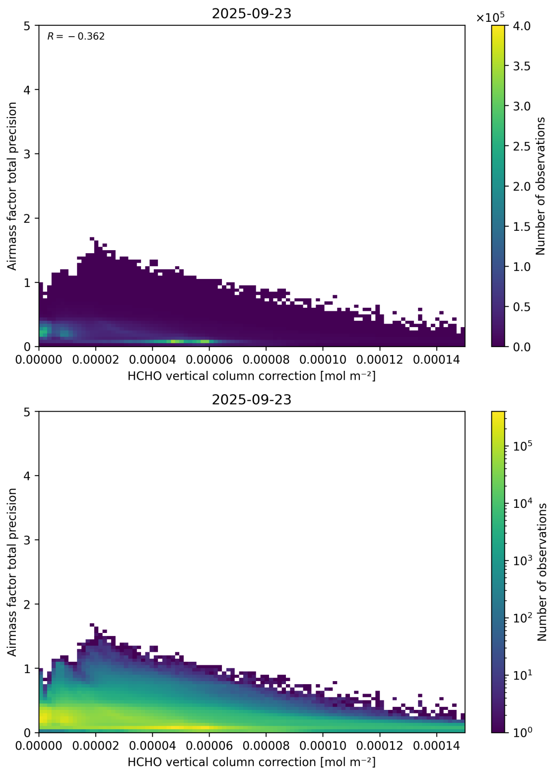
Figure 121: Scatter density plot of “HCHO vertical column correction” against “Airmass factor total precision” for 2025-09-22 to 2025-09-24.
