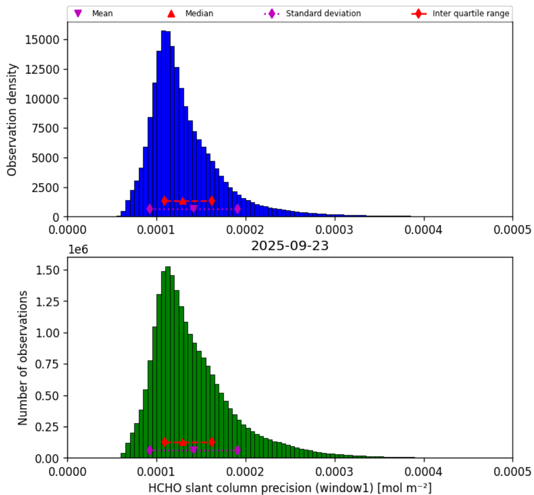
Figure 39: Histogram of “HCHO slant column precision (window1)” for 2025-09-22 to 2025-09-24
