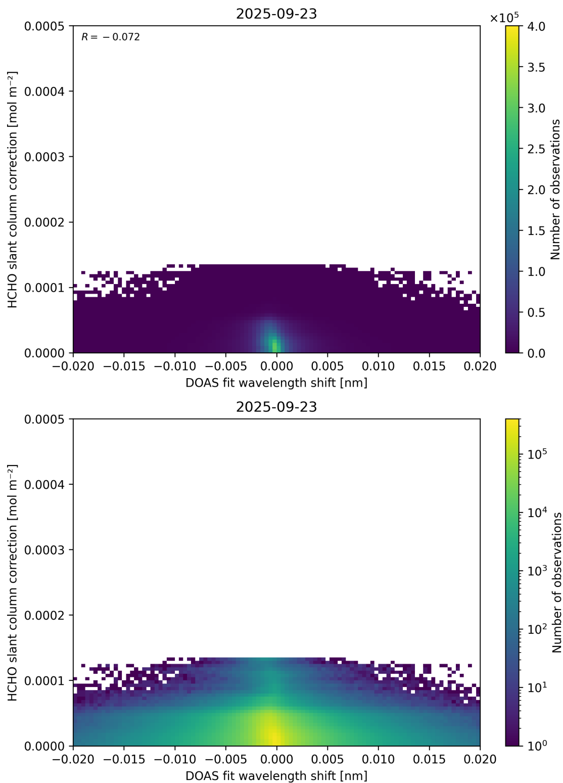
Figure 67: Scatter density plot of “DOAS fit wavelength shift” against “HCHO slant column correction” for 2025-09-22 to 2025-09-24.
