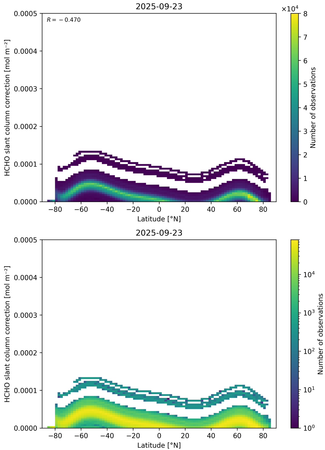
Figure 158: Scatter density plot of “Latitude” against “HCHO slant column correction” for 2025-09-22 to 2025-09-24.
