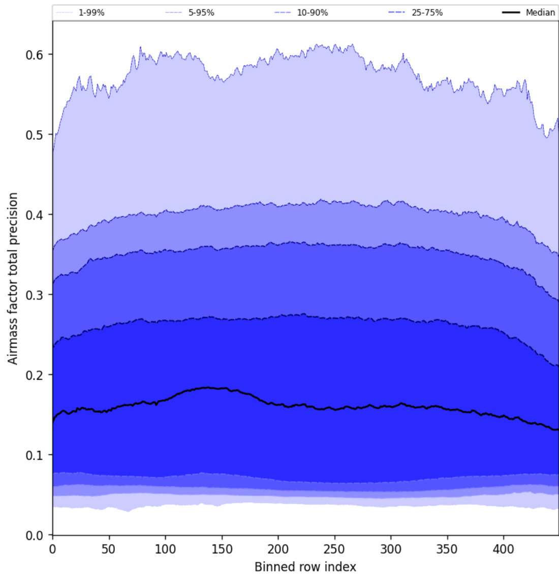
Figure 55: Along track statistics of “Airmass factor total precision” for 2025-09-22 to 2025-09-24
