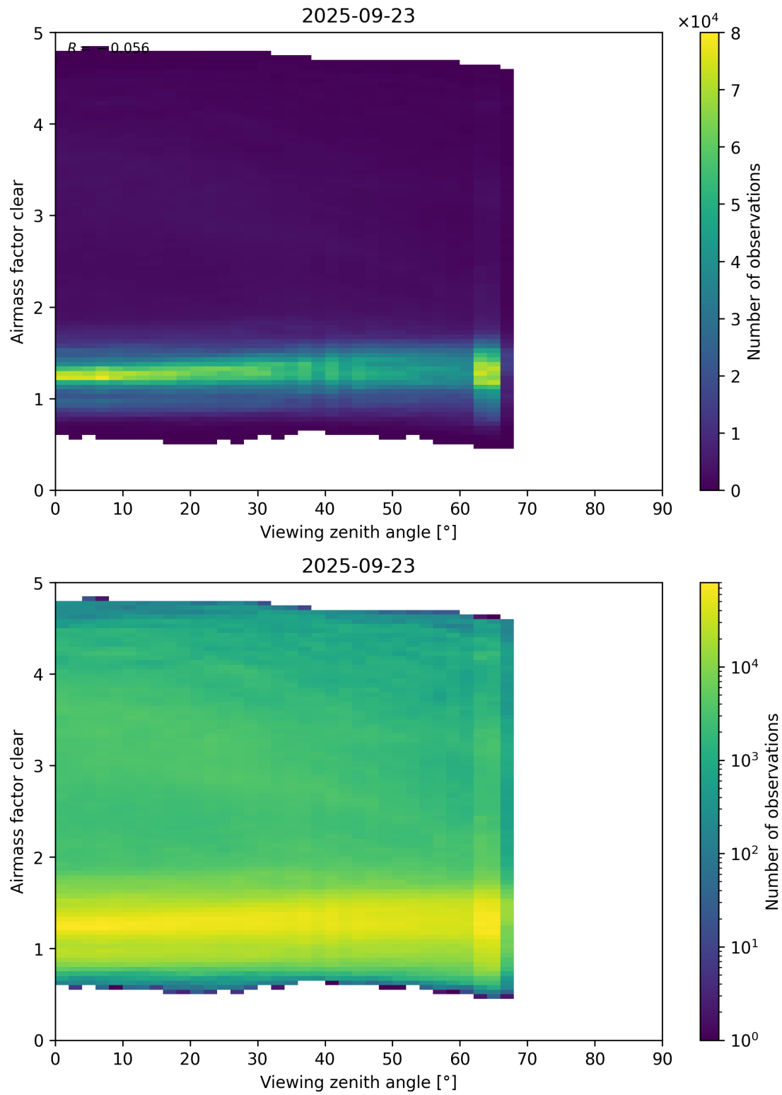
Figure 185: Scatter density plot of “Viewing zenith angle” against “Airmass factor clear” for 2025-09-22 to 2025-09-24.
