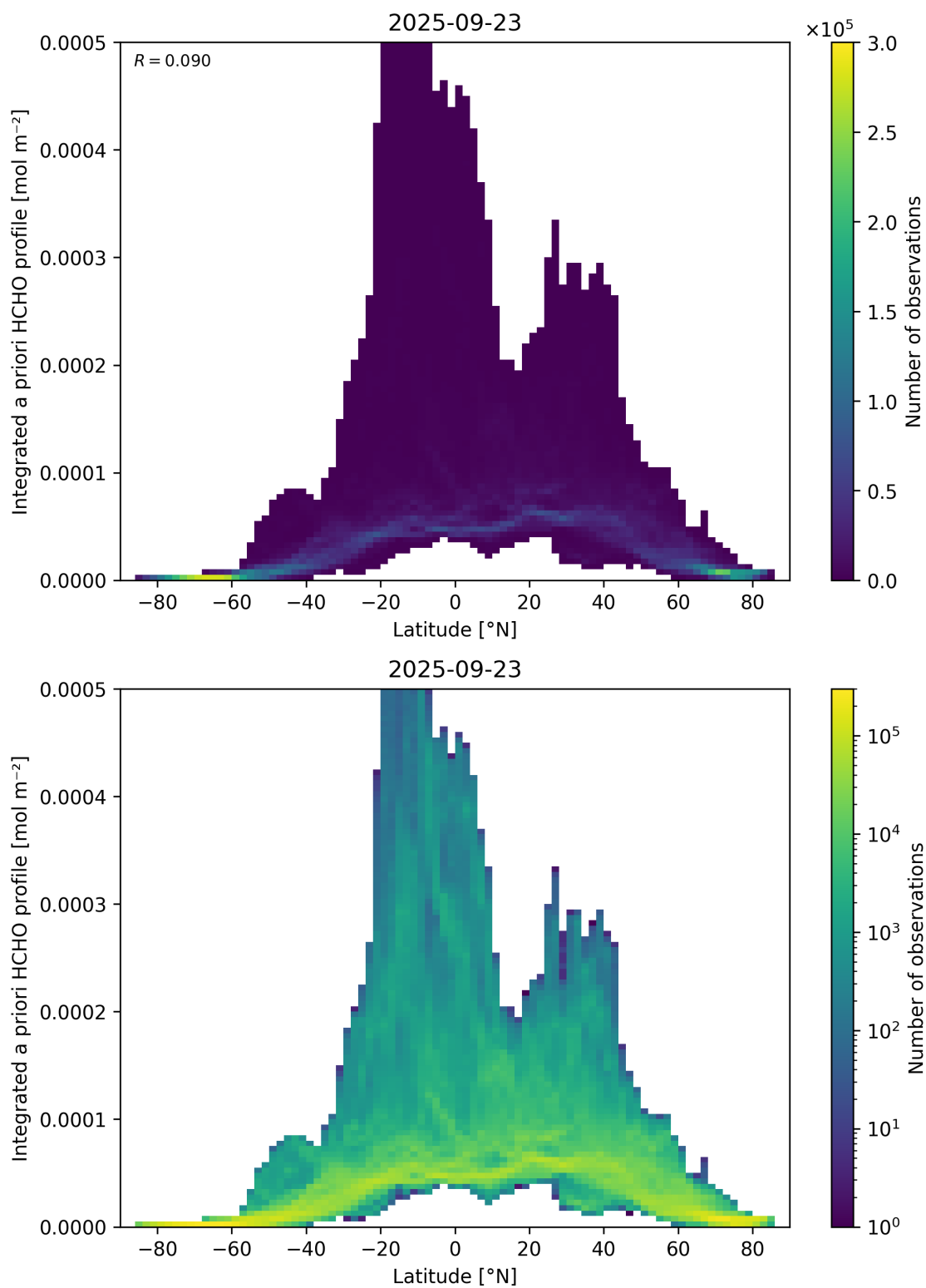
Figure 166: Scatter density plot of “Latitude” against “Integrated a priori HCHO profile” for 2025-09-22 to 2025-09-24.
