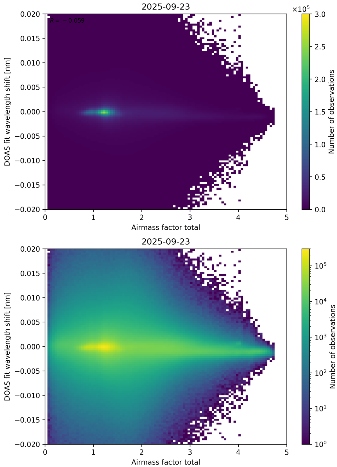
Figure 98: Scatter density plot of “Airmass factor total” against “DOAS fit wavelength shift” for 2025-09-22 to 2025-09-24.
