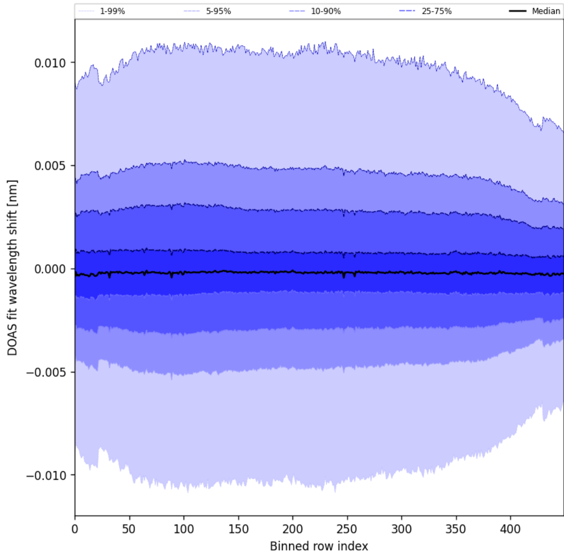
Figure 58: Along track statistics of “DOAS fit wavelength shift” for 2025-09-22 to 2025-09-24
