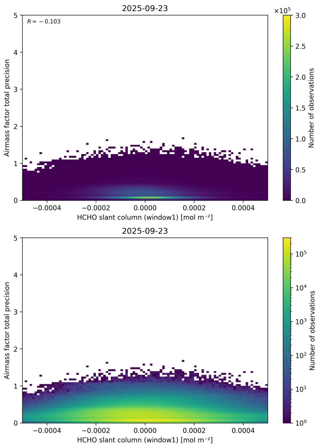
Figure 86: Scatter density plot of “HCHO slant column (window1)” against “Airmass factor total precision” for 2025-09-22 to 2025-09-24.
