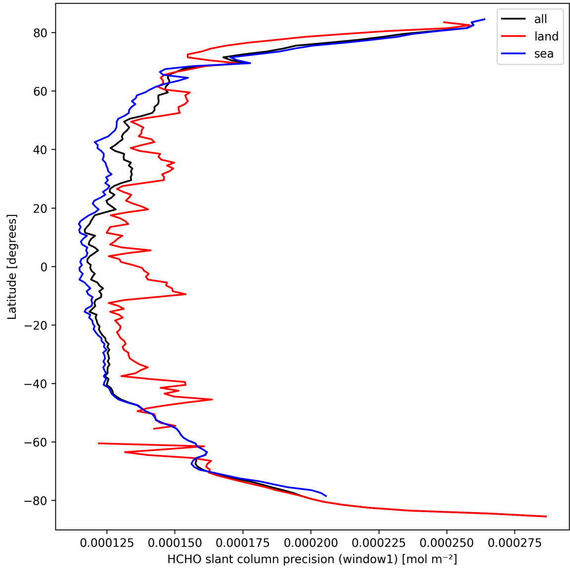
Figure 25: Zonal average of “HCHO slant column precision (window1)” for 2025-09-22 to 2025-09-24.
