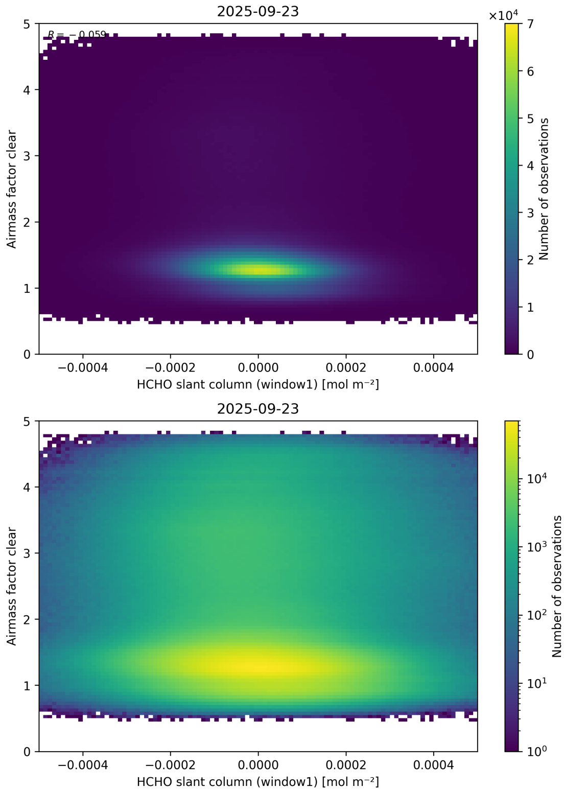
Figure 81: Scatter density plot of “HCHO slant column (window1)” against “Airmass factor clear” for 2025-09-22 to 2025-09-24.
