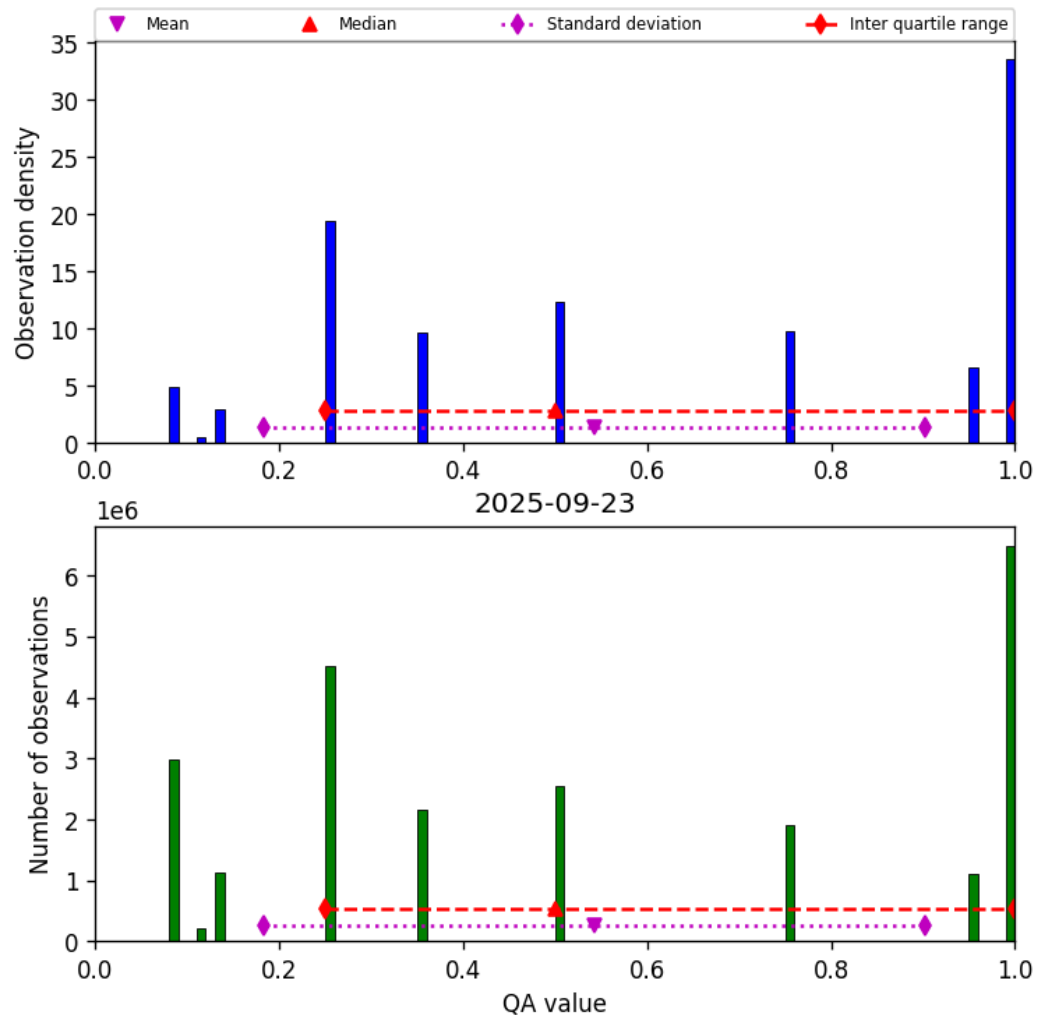
Figure 34: Histogram of “QA value” for 2025-09-22 to 2025-09-24
