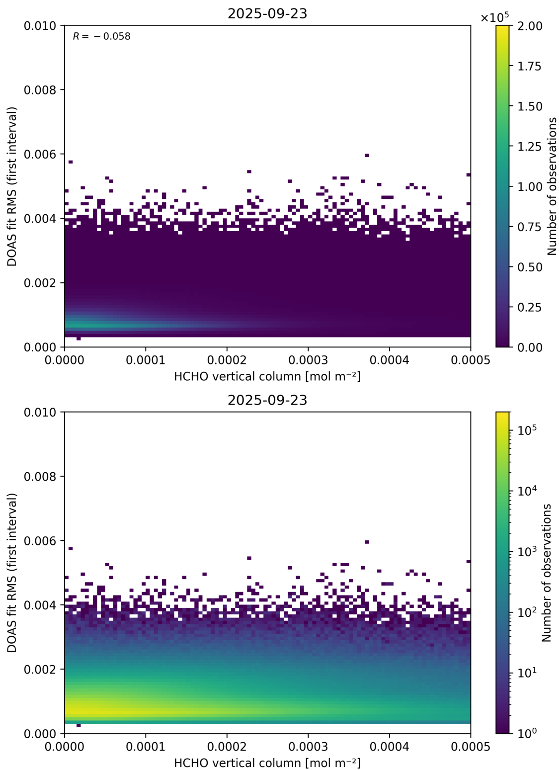
Figure 123: Scatter density plot of “HCHO vertical column” against “DOAS fit RMS (first interval)” for 2025-09-22 to 2025-09-24.
