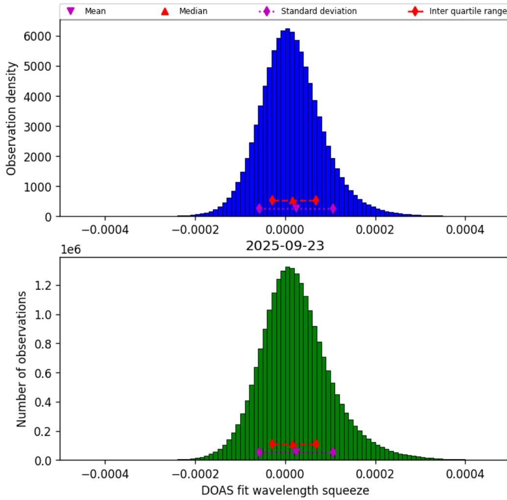
Figure 45: Histogram of “DOAS fit wavelength squeeze” for 2025-09-22 to 2025-09-24
