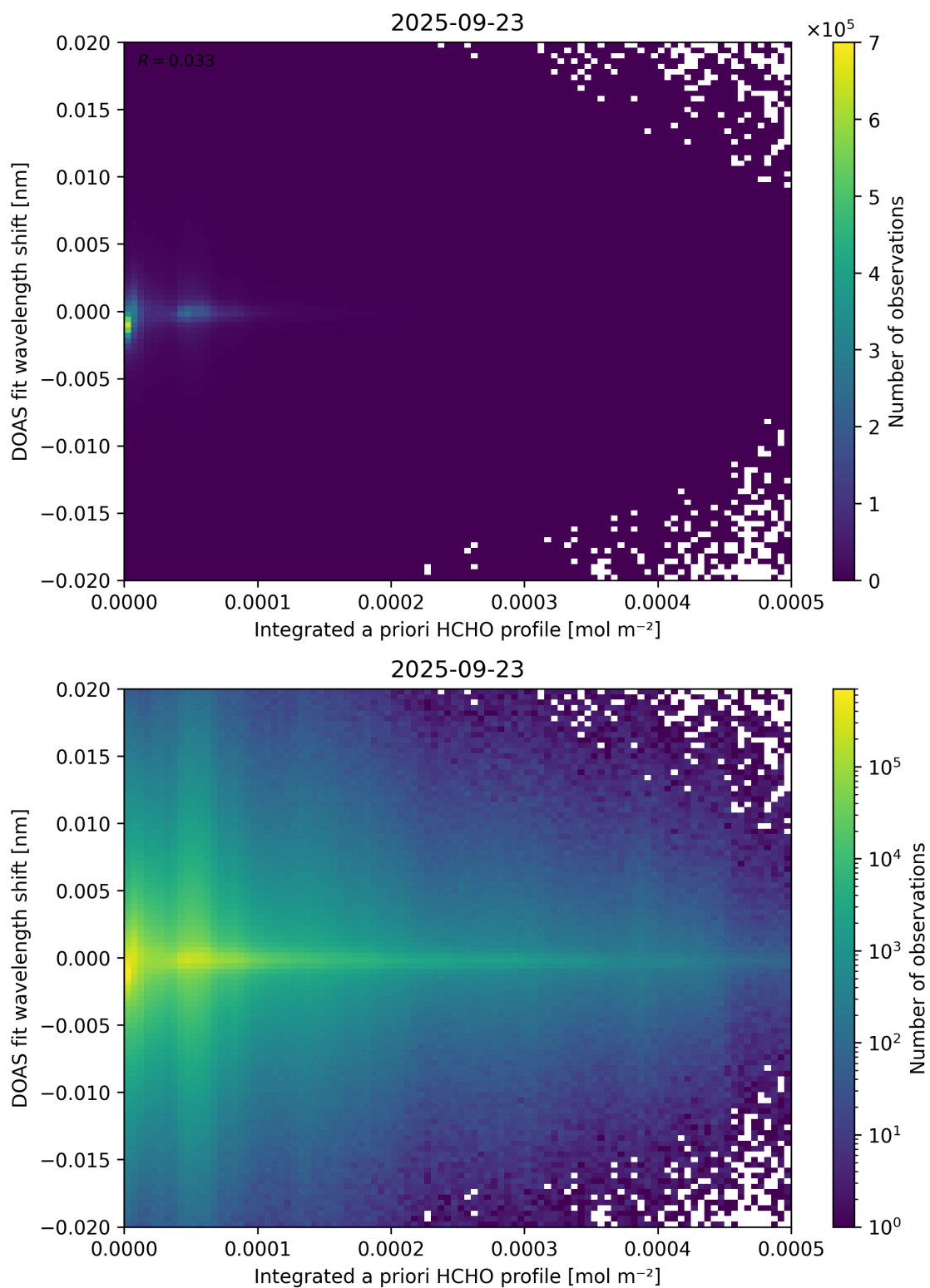
Figure 149: Scatter density plot of “Integrated a priori HCHO profile” against “DOAS fit wavelength shift” for 2025-09-22 to 2025-09-24.
