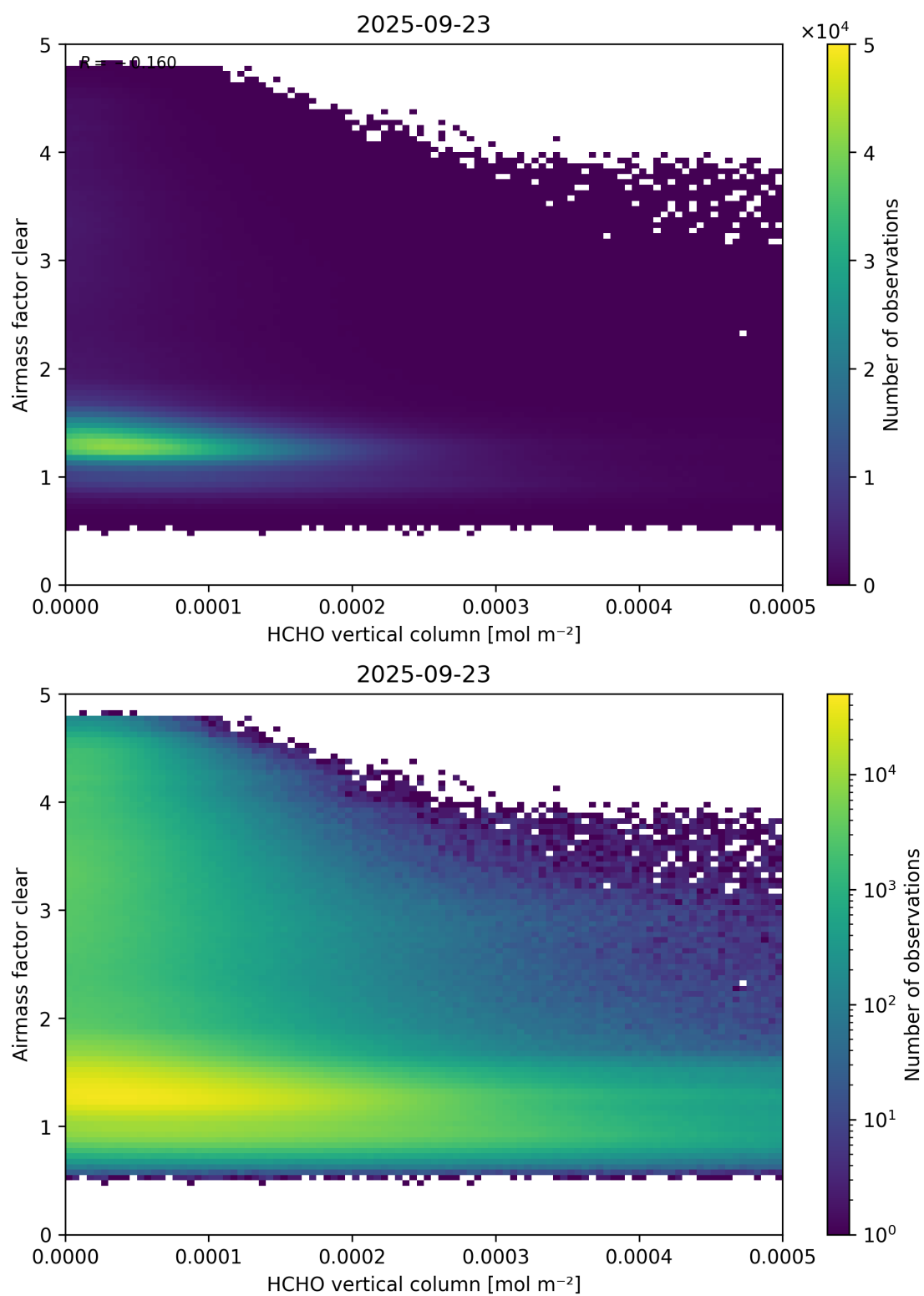
Figure 126: Scatter density plot of “HCHO vertical column” against “Airmass factor clear” for 2025-09-22 to 2025-09-24.
