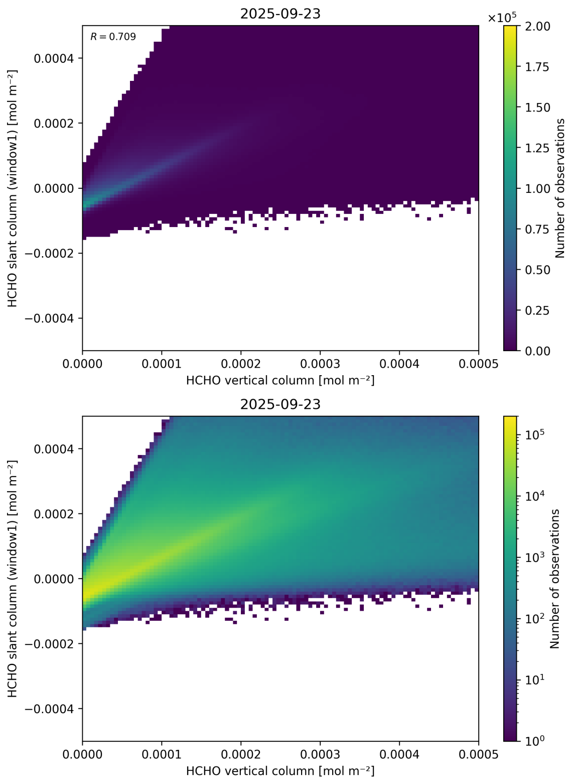
Figure 129: Scatter density plot of “HCHO vertical column” against “HCHO slant column (window1)” for 2025-09-22 to 2025-09-24.
