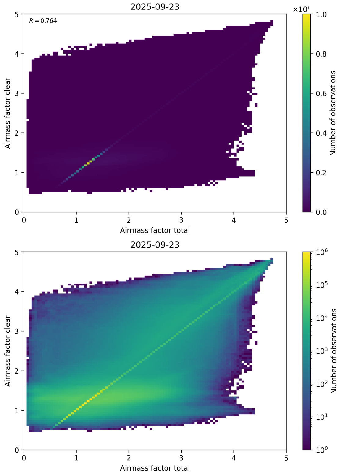
Figure 100: Scatter density plot of “Airmass factor total” against “Airmass factor clear” for 2025-09-22 to 2025-09-24.
