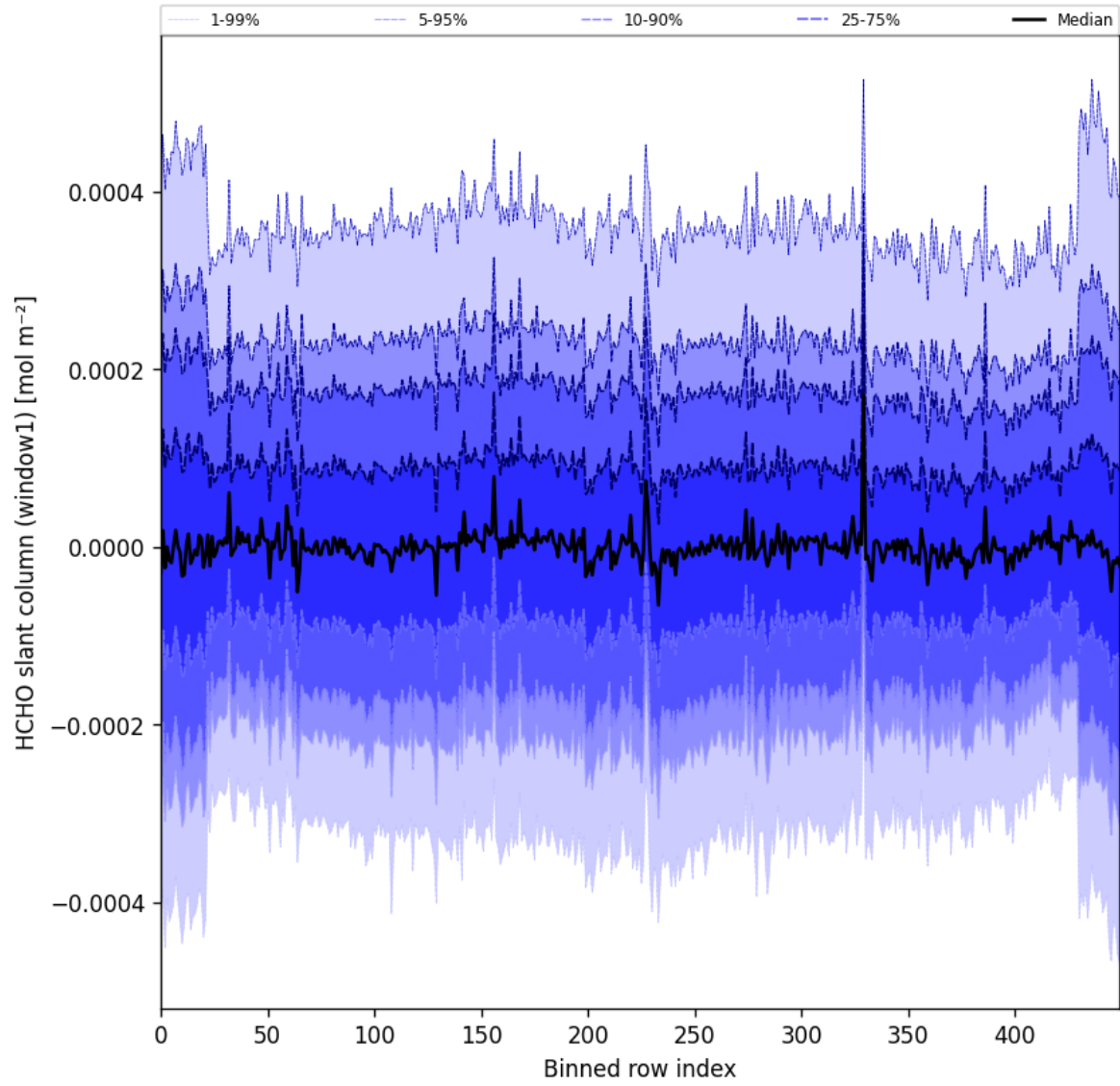
Figure 52: Along track statistics of “HCHO slant column (window1)” for 2025-09-22 to 2025-09-24
