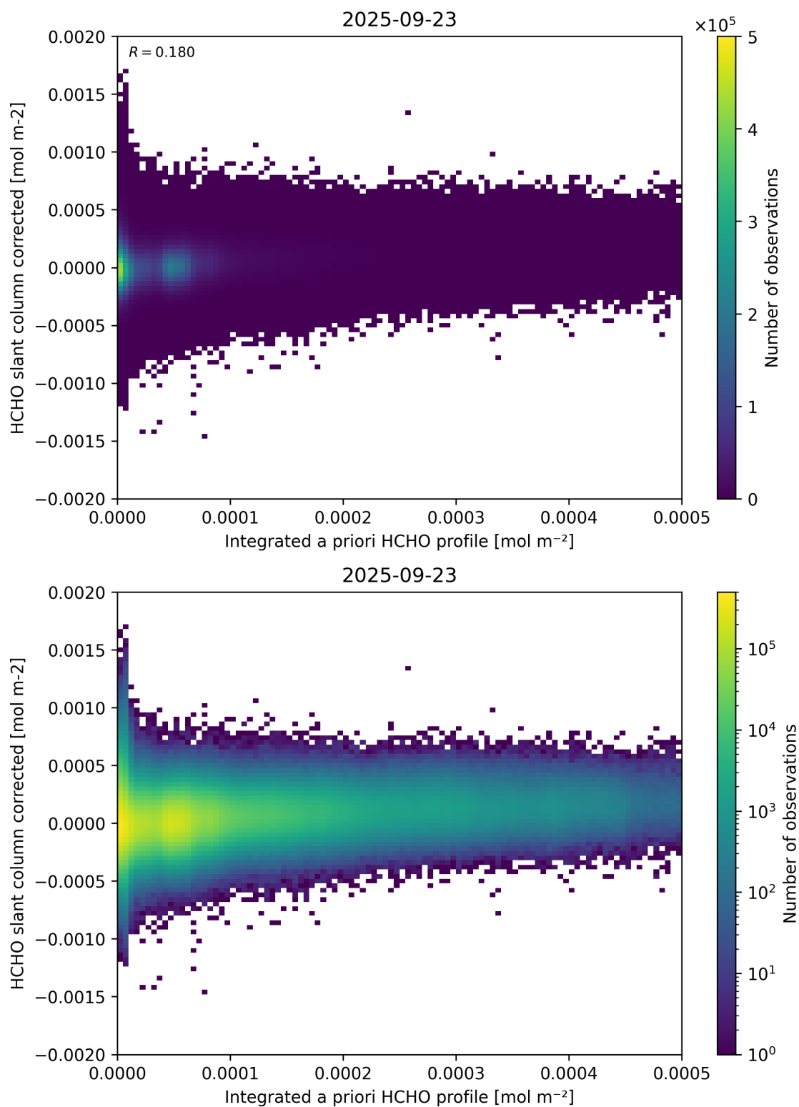
Figure 151: Scatter density plot of “Integrated a priori HCHO profile” against “HCHO slant column corrected” for 2025-09-22 to 2025-09-24.
