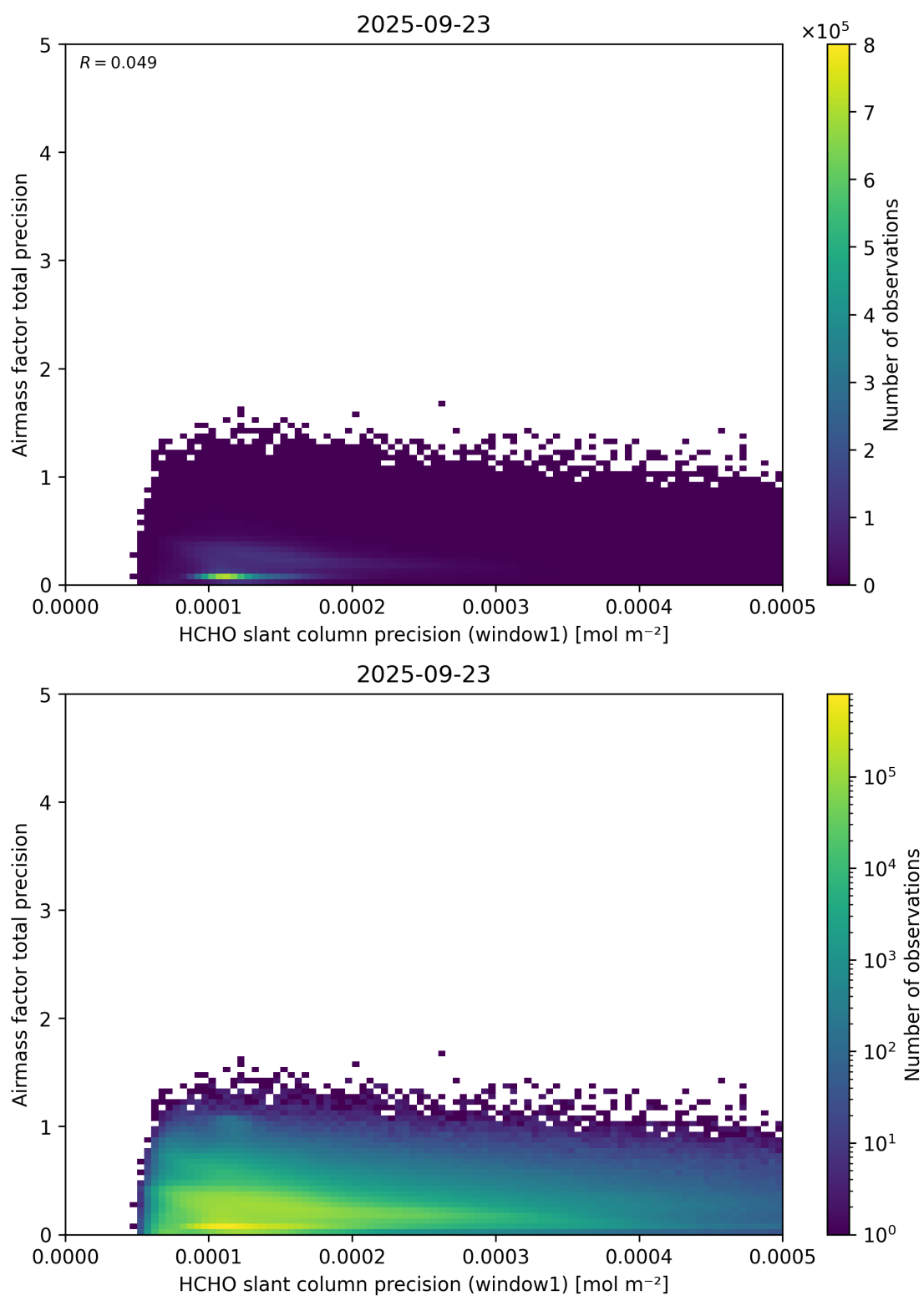
Figure 95: Scatter density plot of “HCHO slant column precision (window1)” against “Airmass factor total precision” for 2025-09-22 to 2025-09-24.
