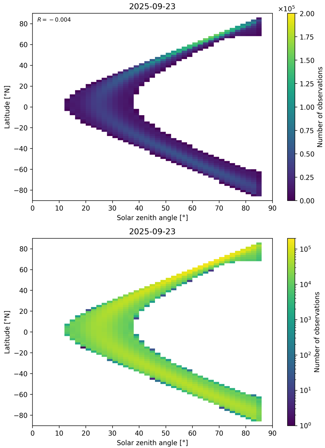
Figure 181: Scatter density plot of “Solar zenith angle” against “Latitude” for 2025-09-22 to 2025-09-24.
