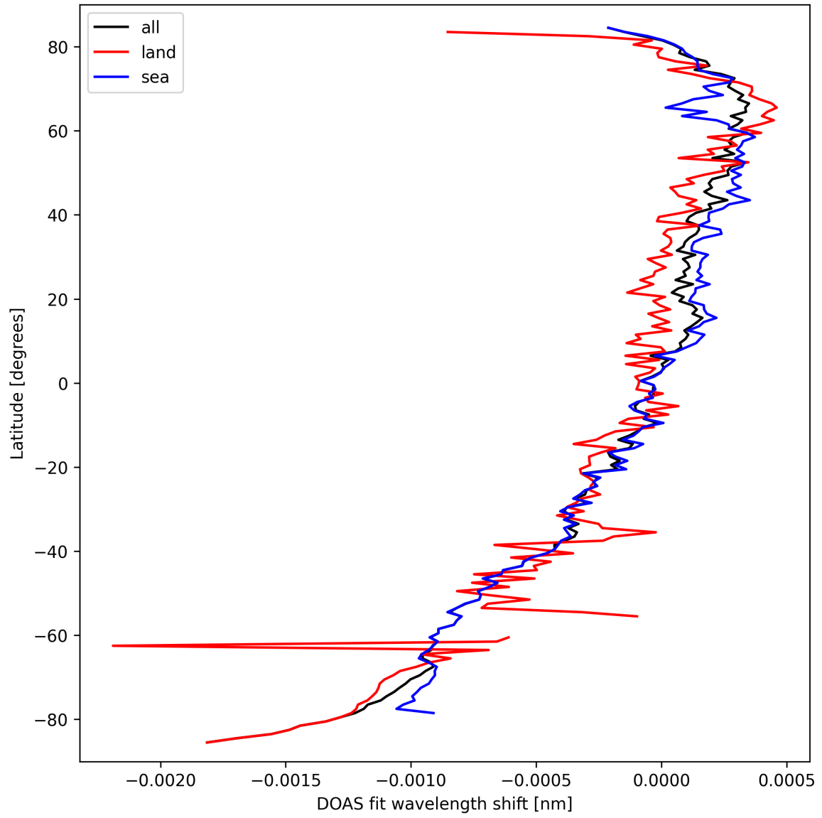
Figure 30: Zonal average of “DOAS fit wavelength shift” for 2025-09-22 to 2025-09-24.
