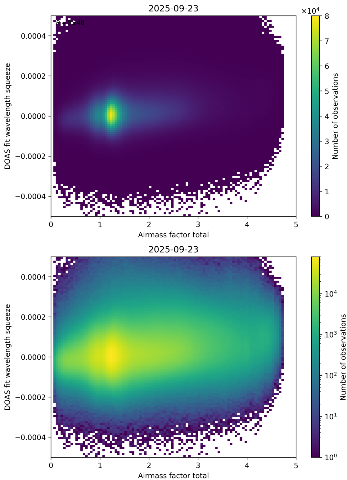
Figure 99: Scatter density plot of “Airmass factor total” against “DOAS fit wavelength squeeze” for 2025-09-22 to 2025-09-24.
