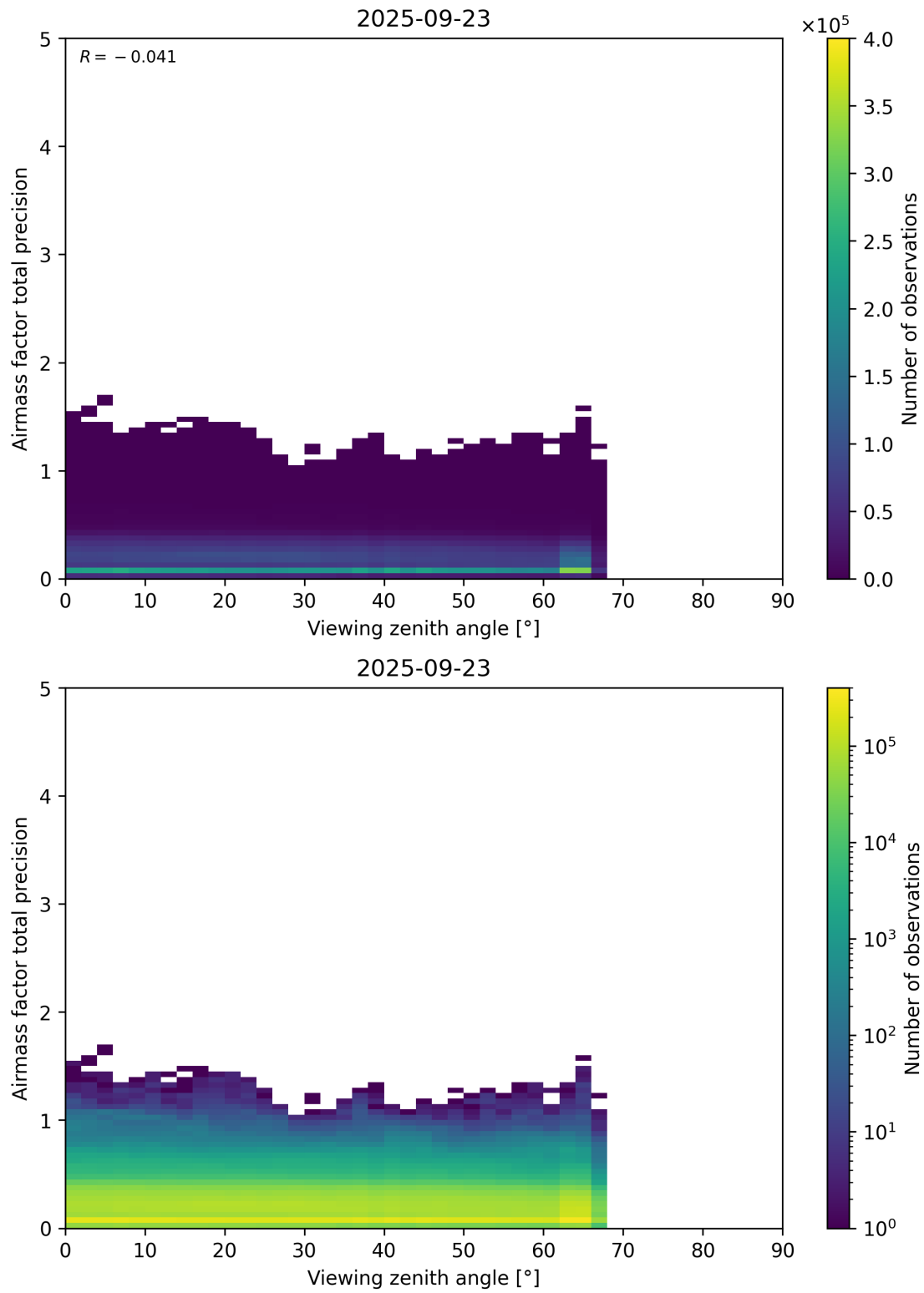
Figure 191: Scatter density plot of “Viewing zenith angle” against “Airmass factor total precision” for 2025-09-22 to 2025-09-24.
