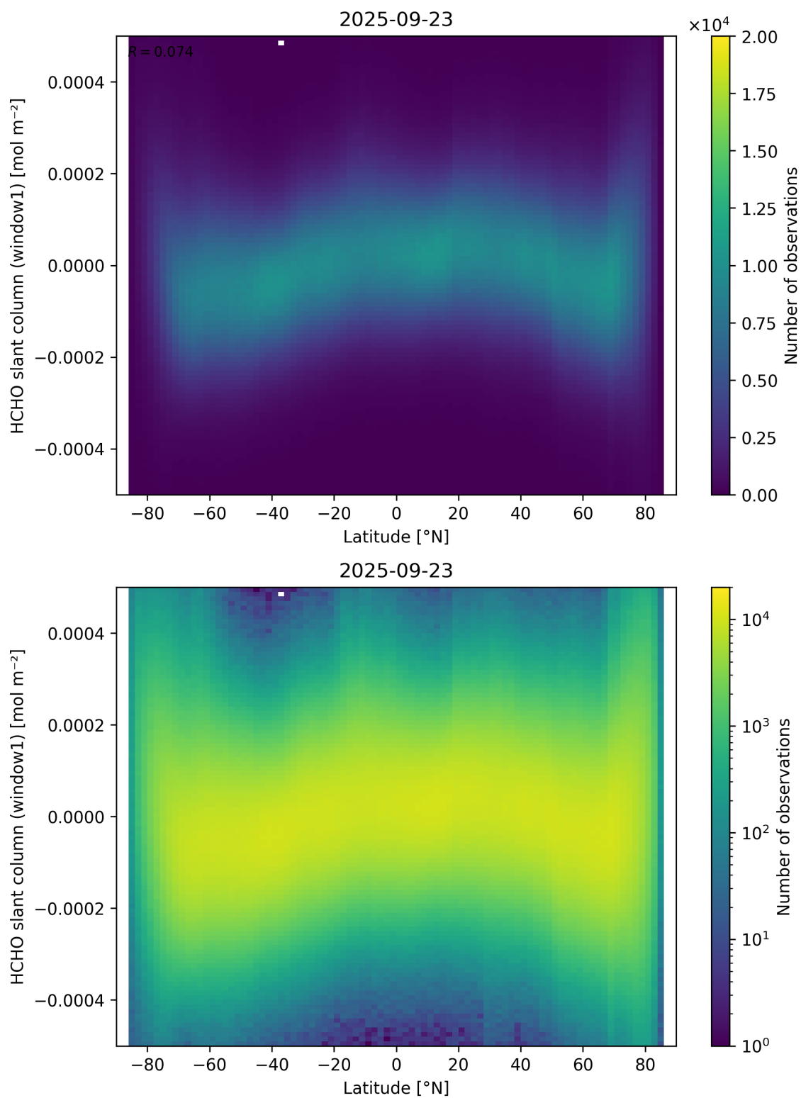
Figure 159: Scatter density plot of “Latitude” against “HCHO slant column (window1)” for 2025-09-22 to 2025-09-24.
