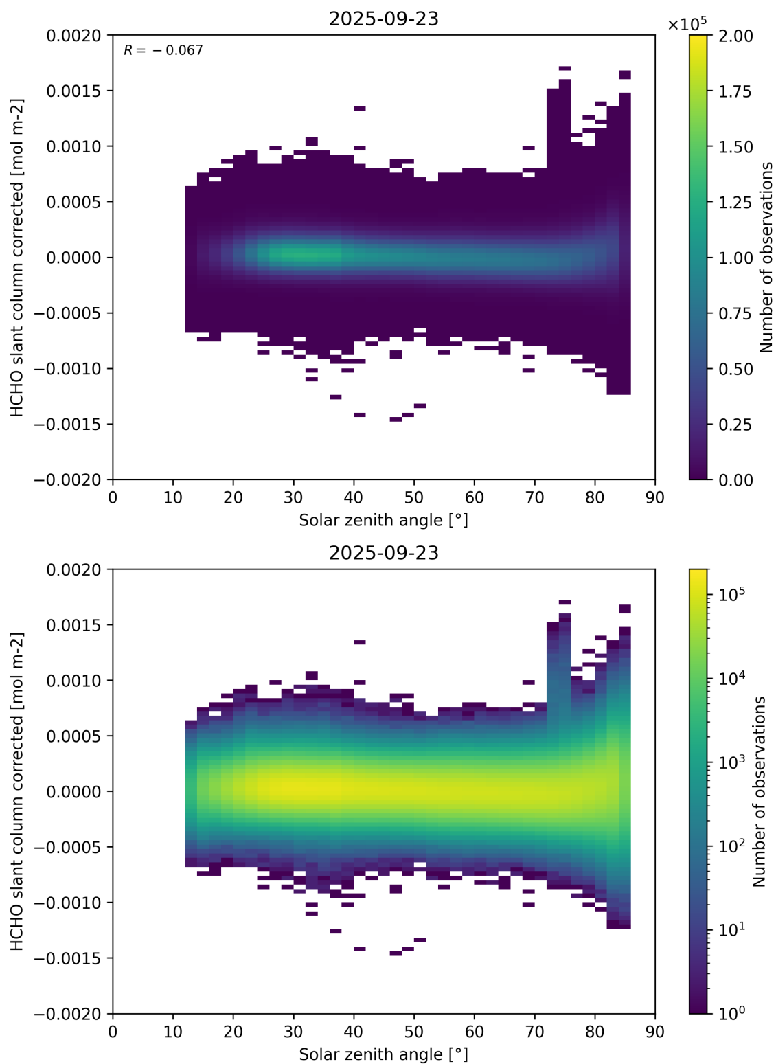
Figure 171: Scatter density plot of “Solar zenith angle” against “HCHO slant column corrected” for 2025-09-22 to 2025-09-24.
