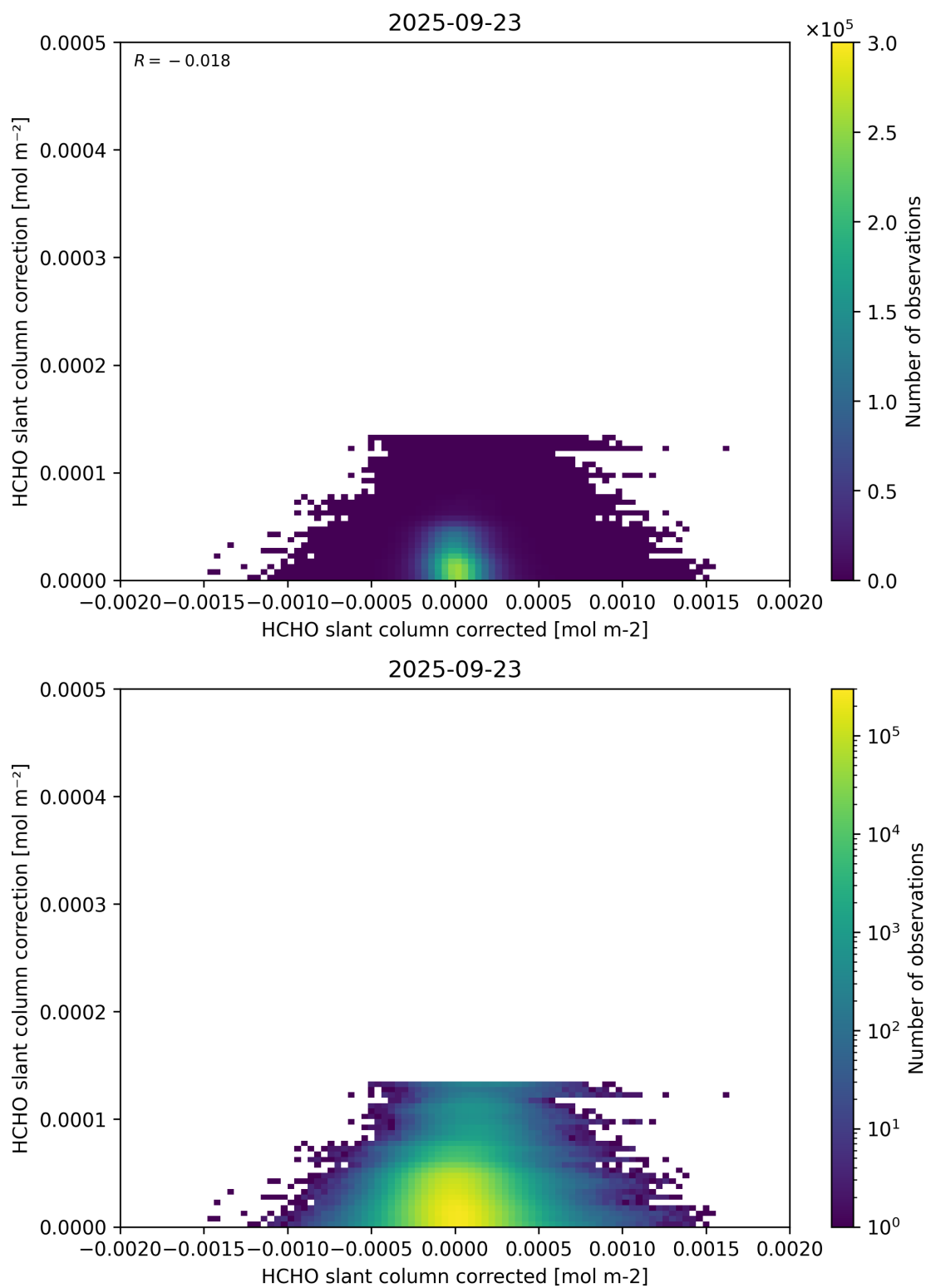
Figure 77: Scatter density plot of “HCHO slant column corrected” against “HCHO slant column correction” for 2025-09-22 to 2025-09-24.
