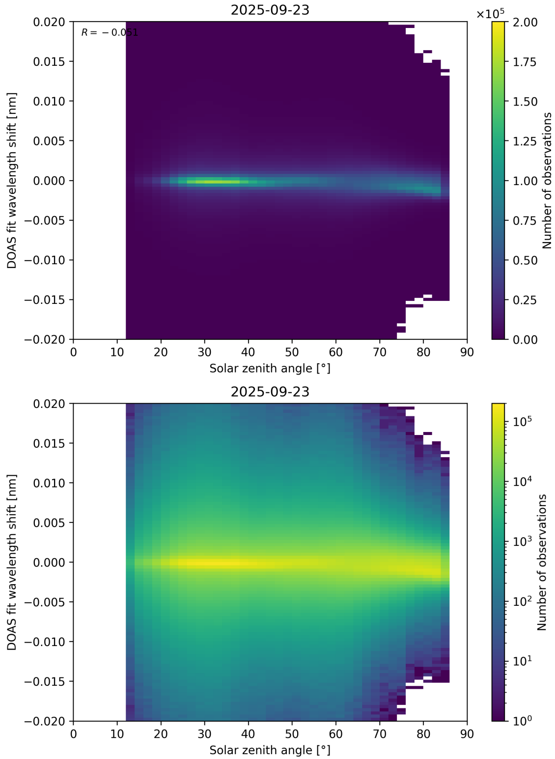
Figure 168: Scatter density plot of “Solar zenith angle” against “DOAS fit wavelength shift” for 2025-09-22 to 2025-09-24.
