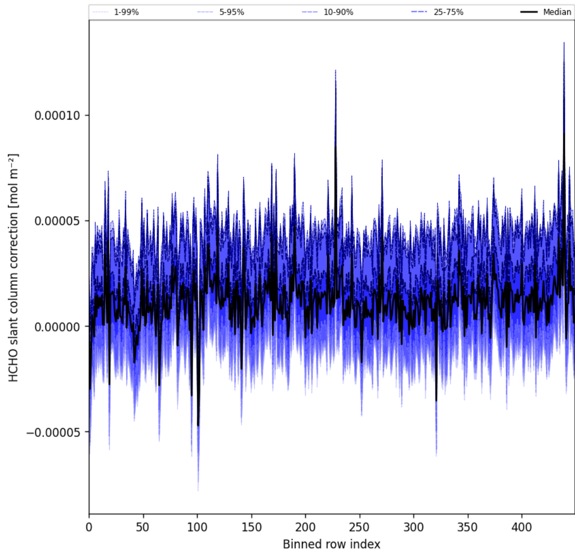
Figure 61: Along track statistics of “HCHO slant column correction” for 2025-09-22 to 2025-09-24
