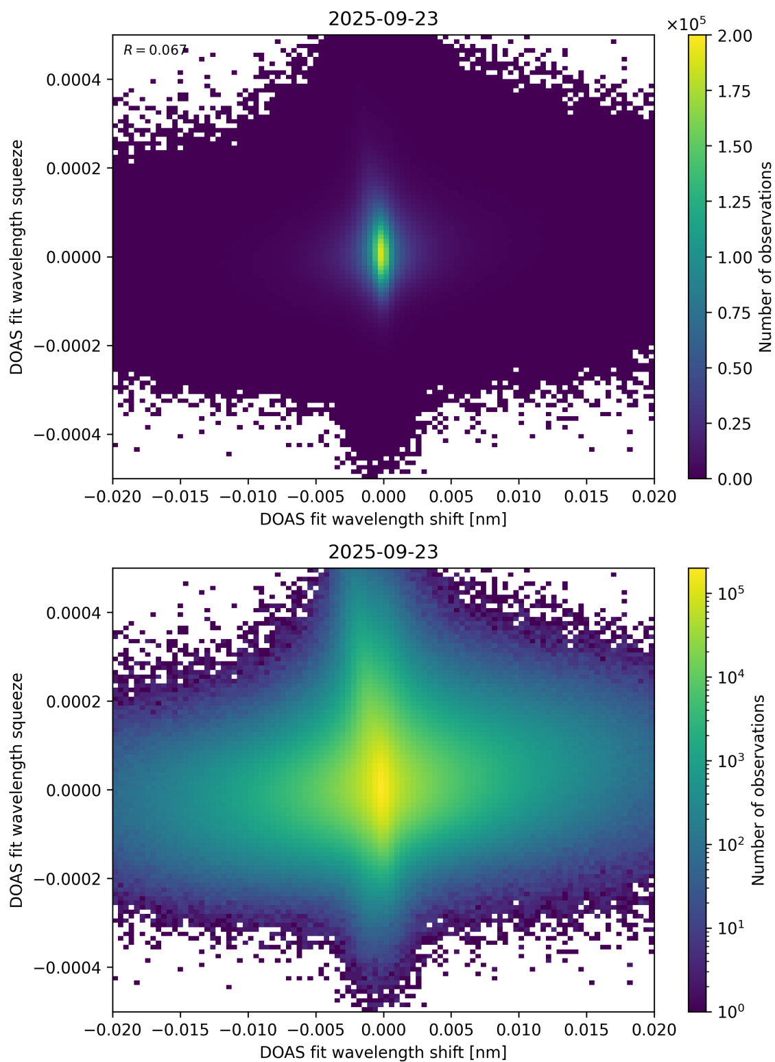
Figure 65: Scatter density plot of “DOAS fit wavelength shift” against “DOAS fit wavelength squeeze” for 2025-09-22 to 2025-09-24.
