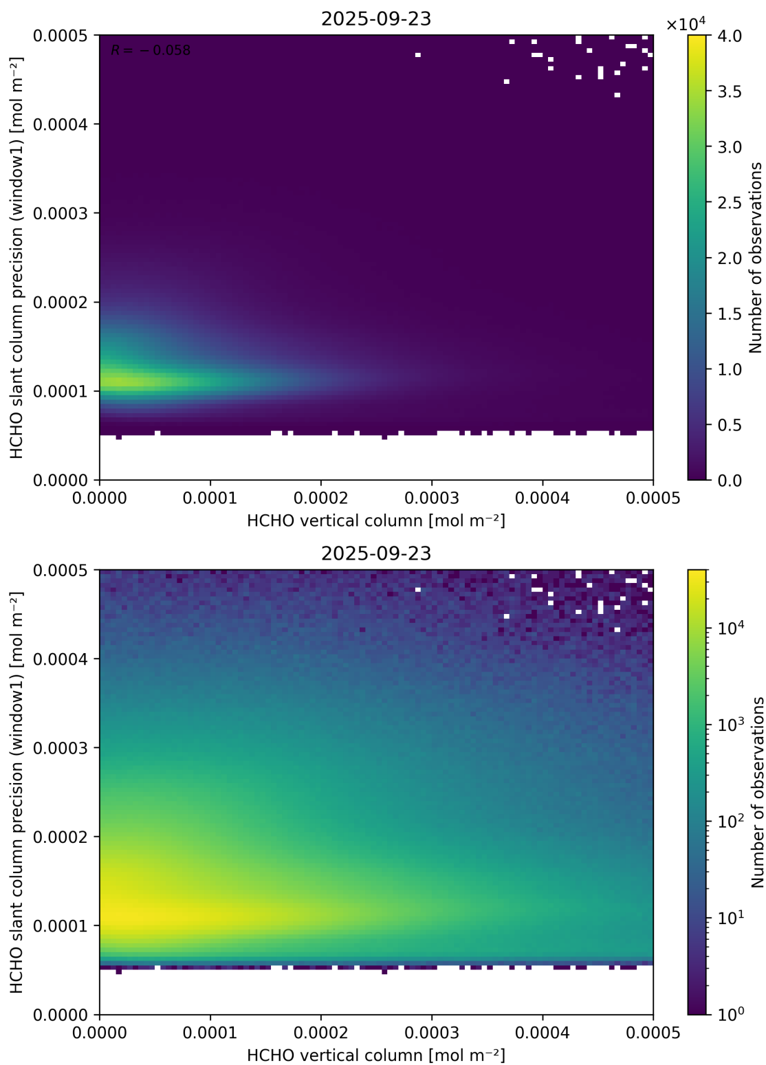
Figure 130: Scatter density plot of “HCHO vertical column” against “HCHO slant column precision (window1)” for 2025-09-22 to 2025-09-24.
