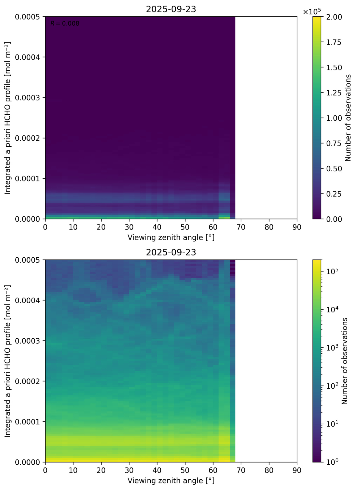
Figure 195: Scatter density plot of “Viewing zenith angle” against “Integrated a priori HCHO profile” for 2025-09-22 to 2025-09-24.
