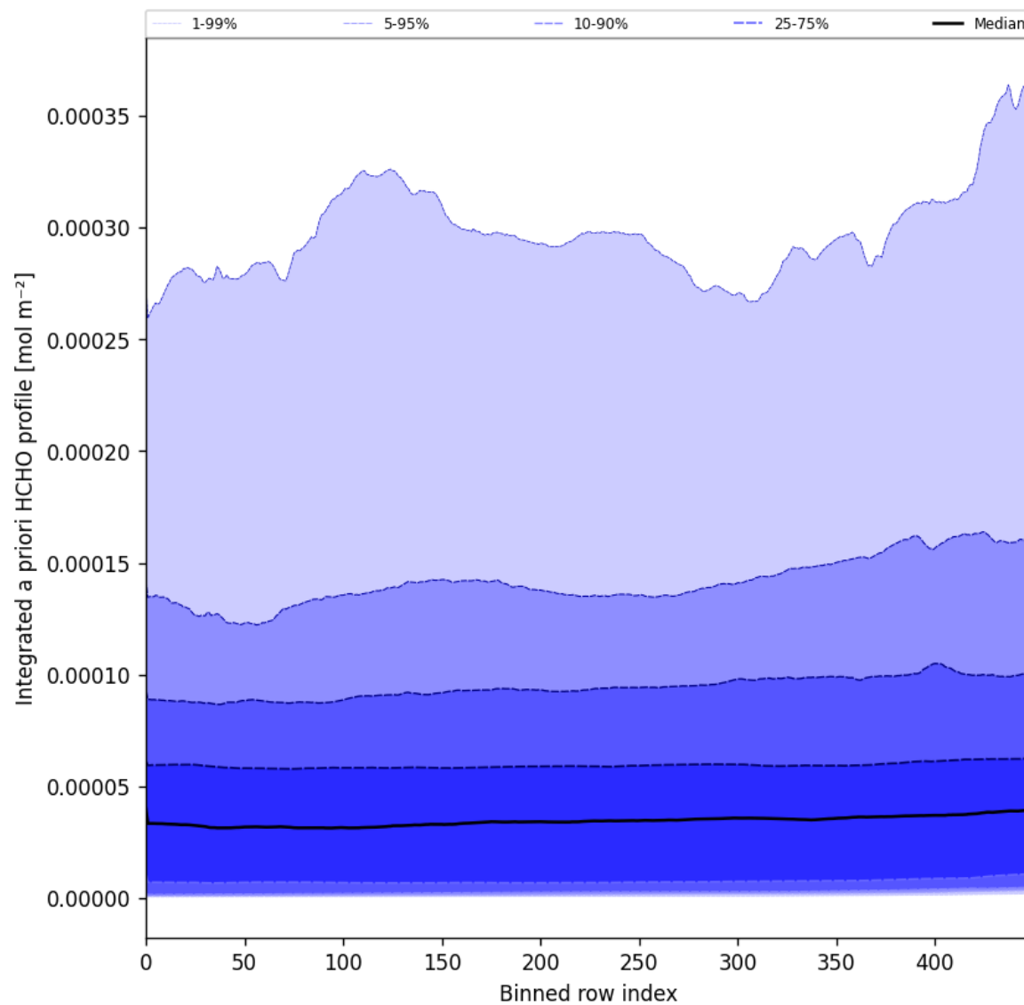
Figure 57: Along track statistics of “Integrated a priori HCHO profile” for 2025-09-22 to 2025-09-24
