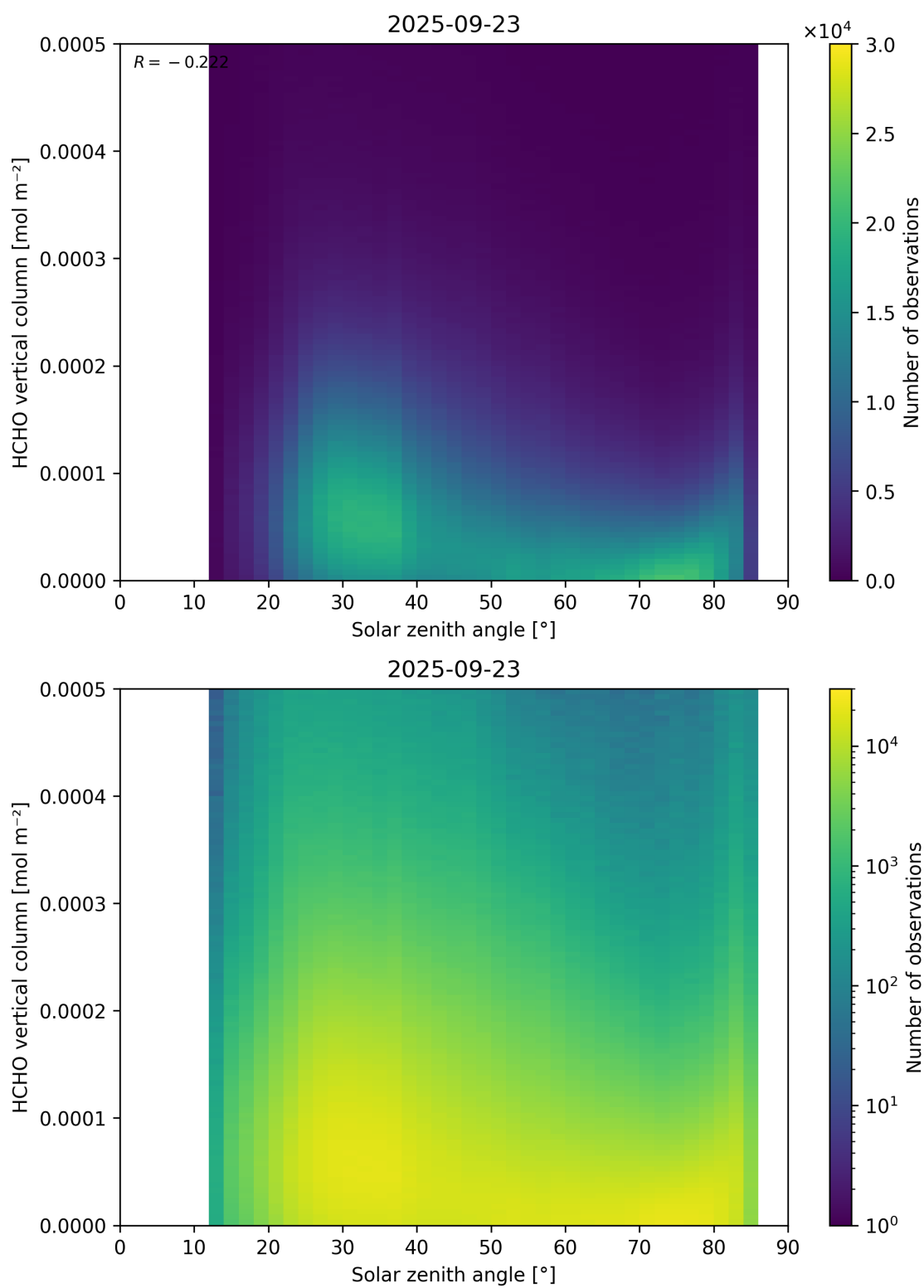
Figure 177: Scatter density plot of “Solar zenith angle” against “HCHO vertical column” for 2025-09-22 to 2025-09-24.
