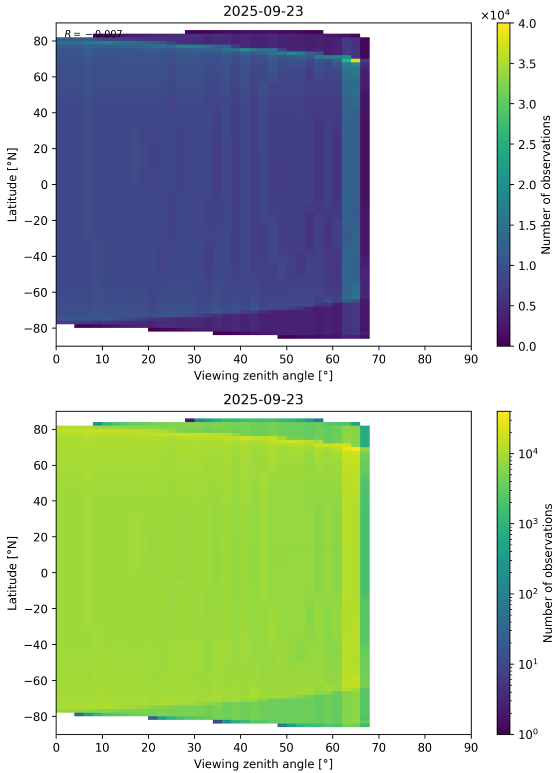
Figure 196: Scatter density plot of “Viewing zenith angle” against “Latitude” for 2025-09-22 to 2025-09-24.
