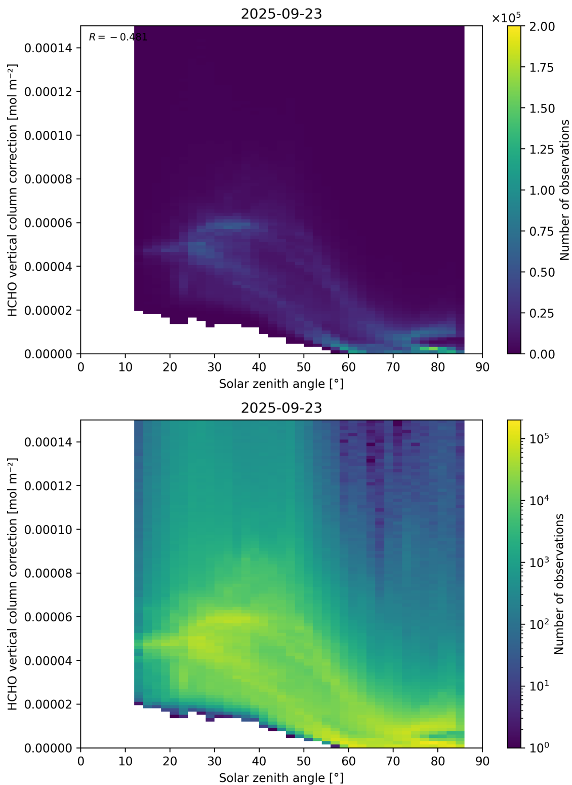
Figure 178: Scatter density plot of “Solar zenith angle” against “HCHO vertical column correction” for 2025-09-22 to 2025-09-24.
