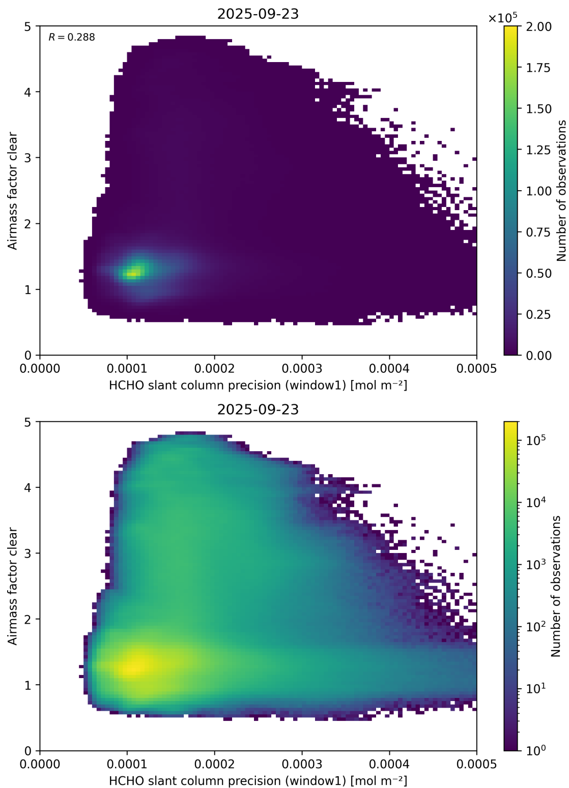
Figure 91: Scatter density plot of “HCHO slant column precision (window1)” against “Airmass factor clear” for 2025-09-22 to 2025-09-24.
