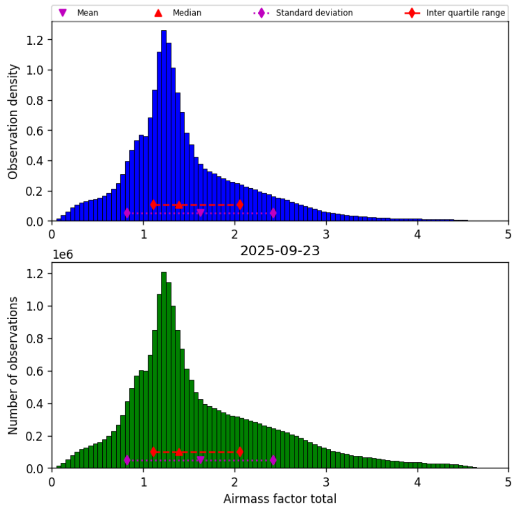
Figure 40: Histogram of "Airmass factor total" for 2025-09-22 to 2025-09-24
