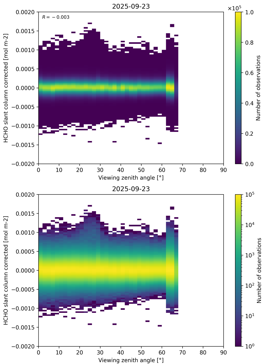
Figure 186: Scatter density plot of “Viewing zenith angle” against “HCHO slant column corrected” for 2025-09-22 to 2025-09-24.
