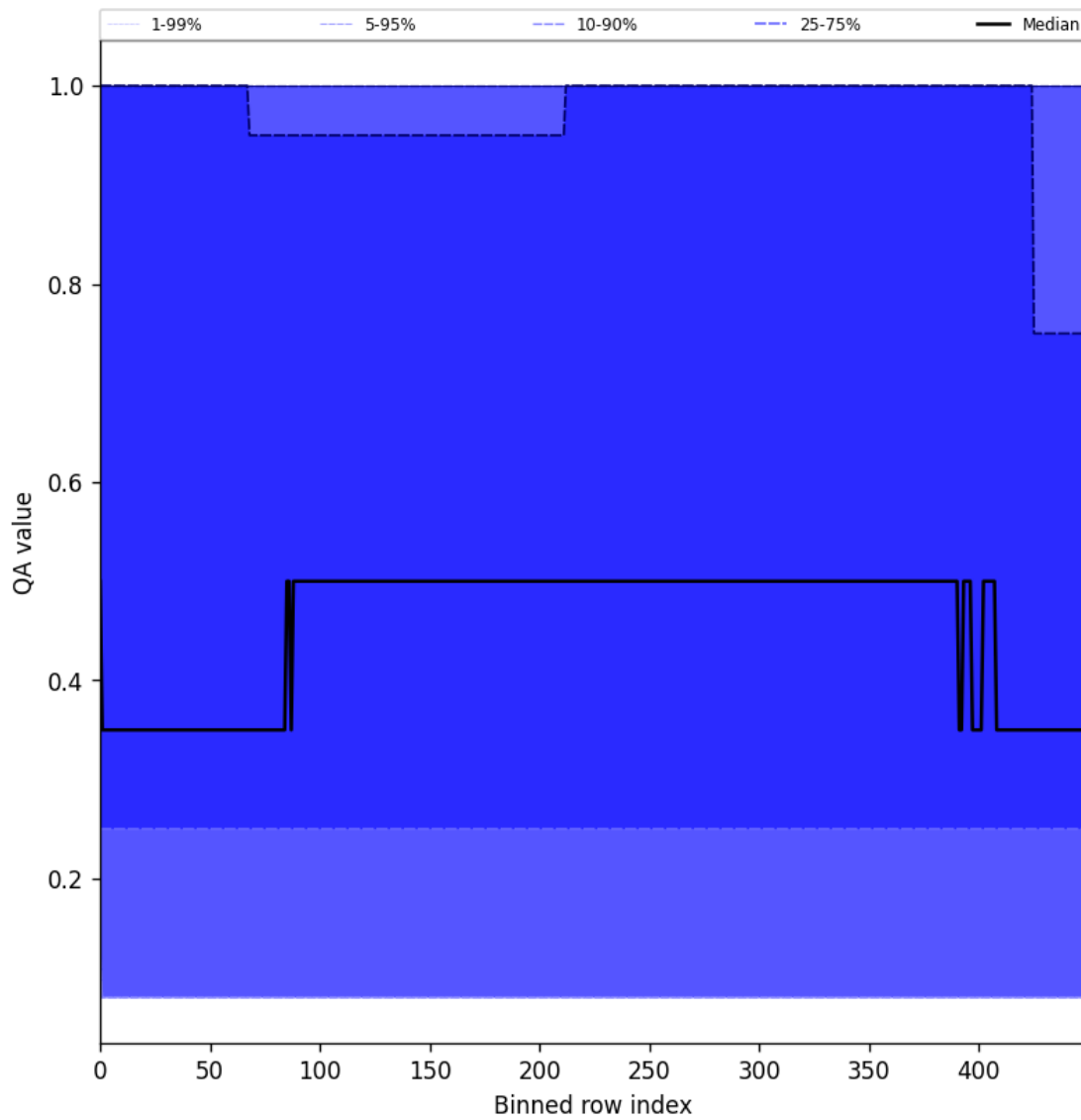
Figure 48: Along track statistics of “QA value” for 2025-09-22 to 2025-09-24
