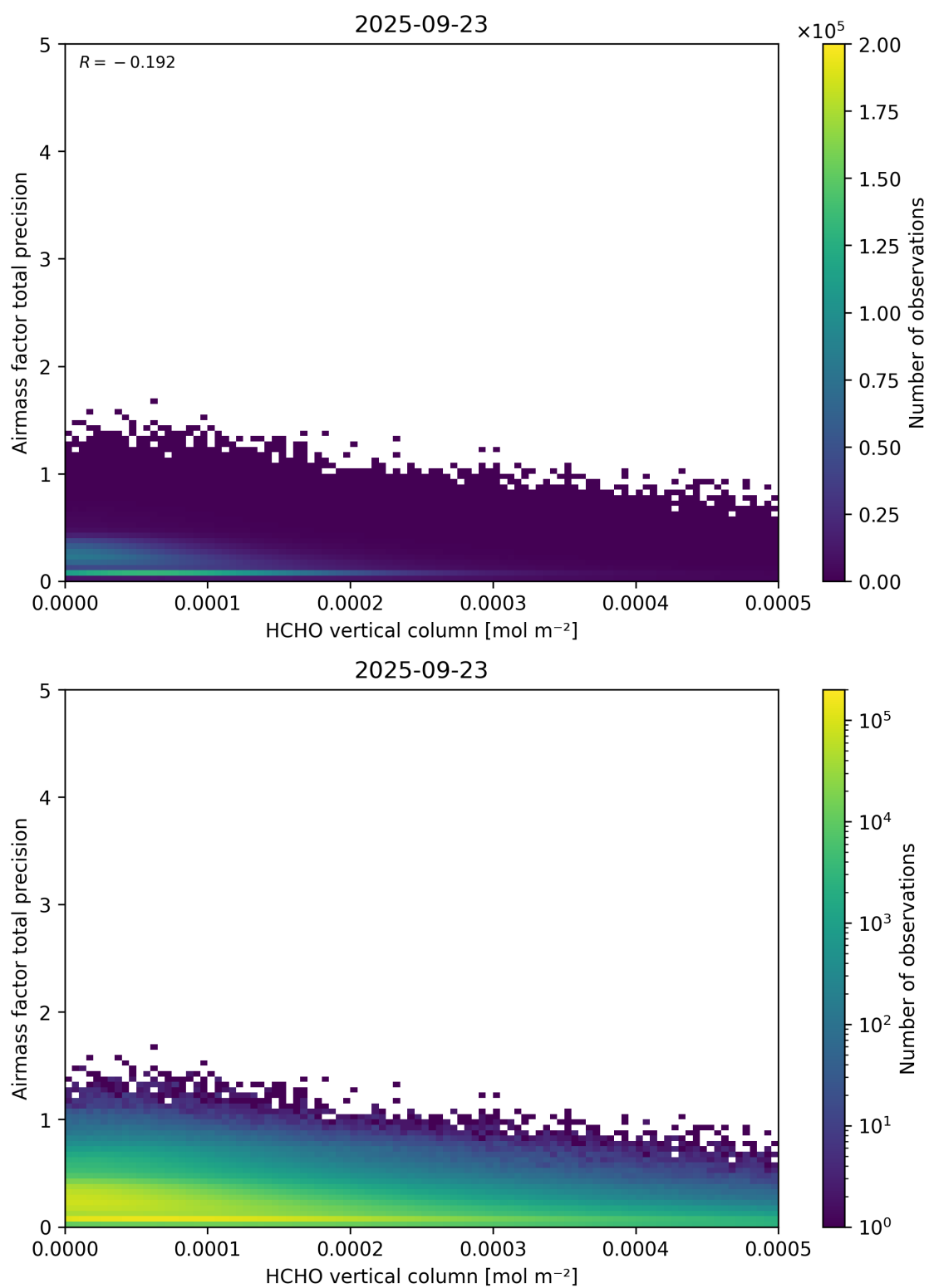
Figure 132: Scatter density plot of “HCHO vertical column” against “Airmass factor total precision” for 2025-09-22 to 2025-09-24.
