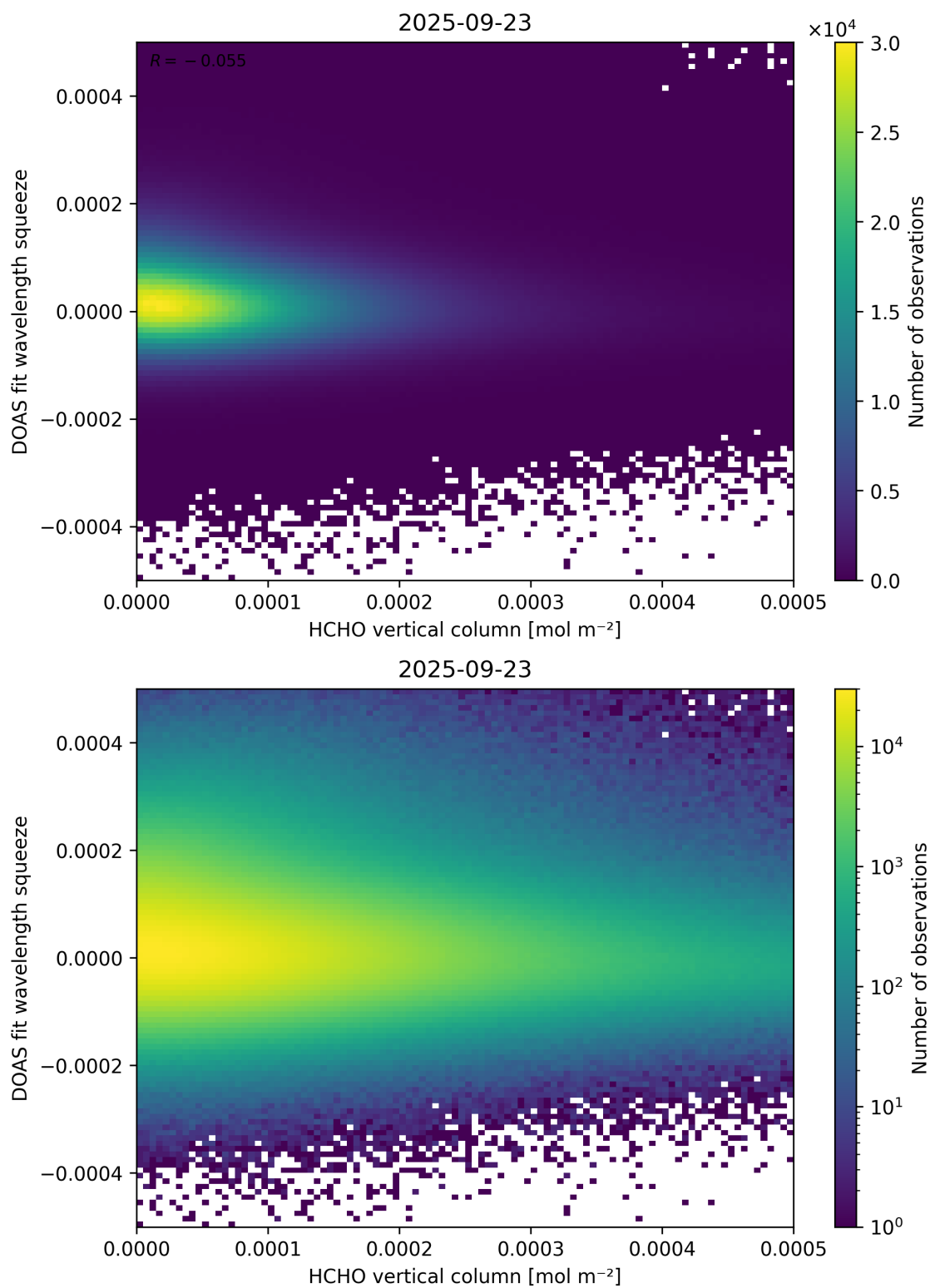
Figure 125: Scatter density plot of “HCHO vertical column” against “DOAS fit wavelength squeeze” for 2025-09-22 to 2025-09-24.
