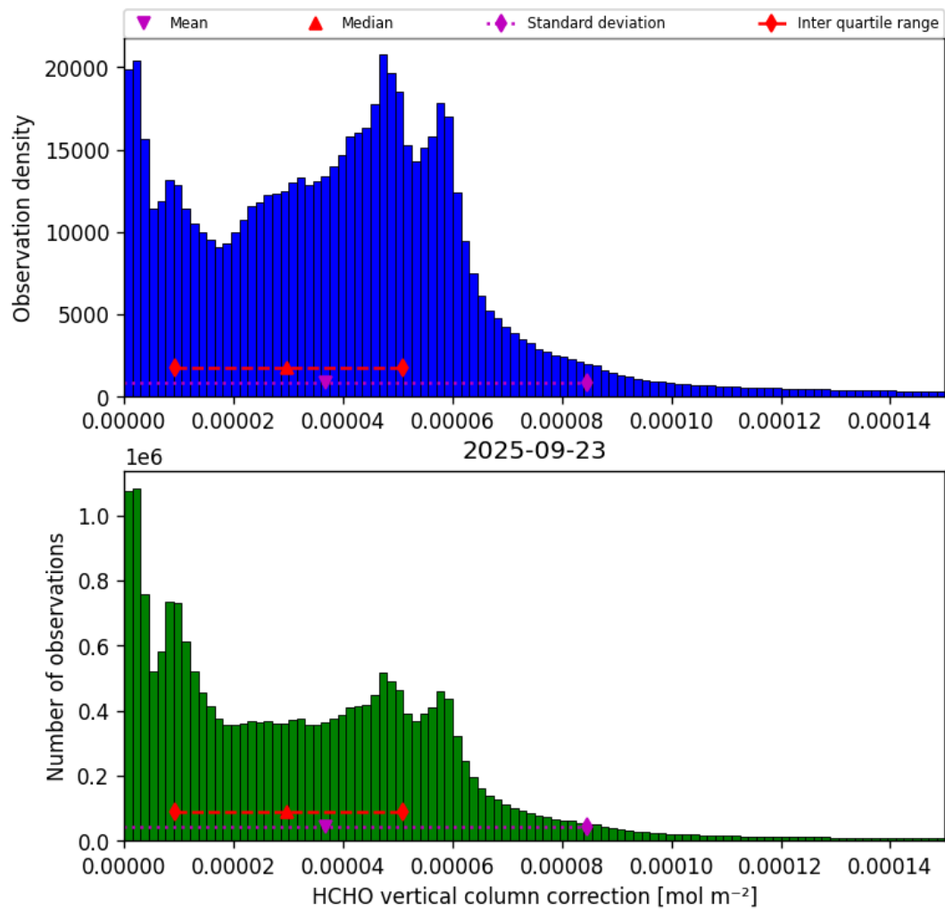
Figure 37: Histogram of “HCHO vertical column correction” for 2025-09-22 to 2025-09-24
