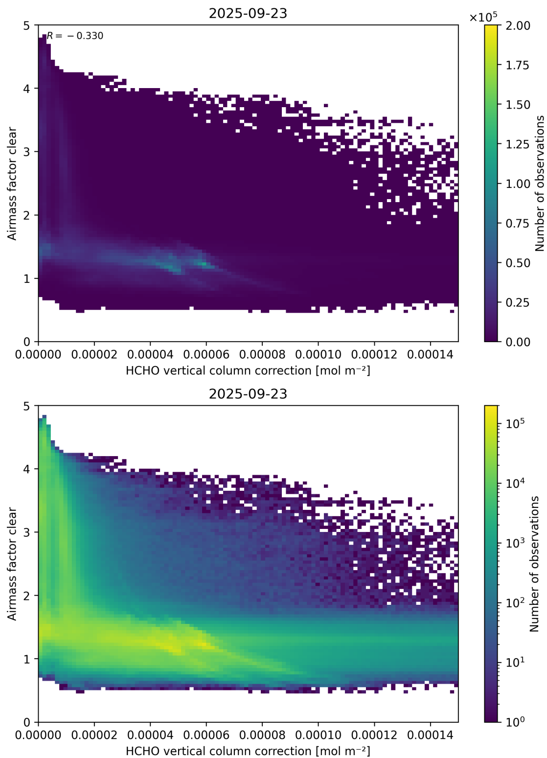
Figure 115: Scatter density plot of “HCHO vertical column correction” against “Airmass factor clear” for 2025-09-22 to 2025-09-24.
