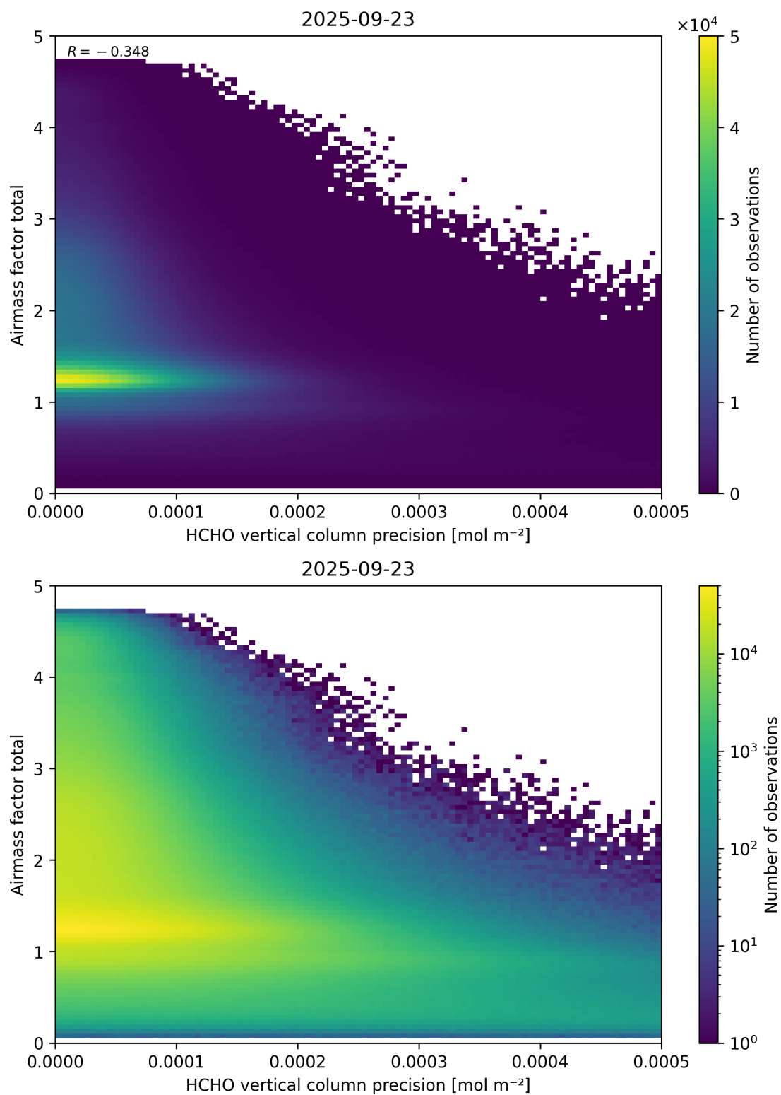
Figure 144: Scatter density plot of “HCHO vertical column precision” against “Airmass factor total” for 2025-09-22 to 2025-09-24.
