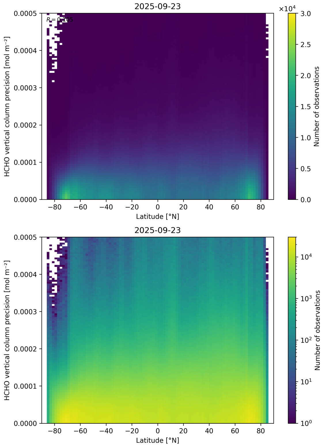
Figure 165: Scatter density plot of “Latitude” against “HCHO vertical column precision” for 2025-09-22 to 2025-09-24.
