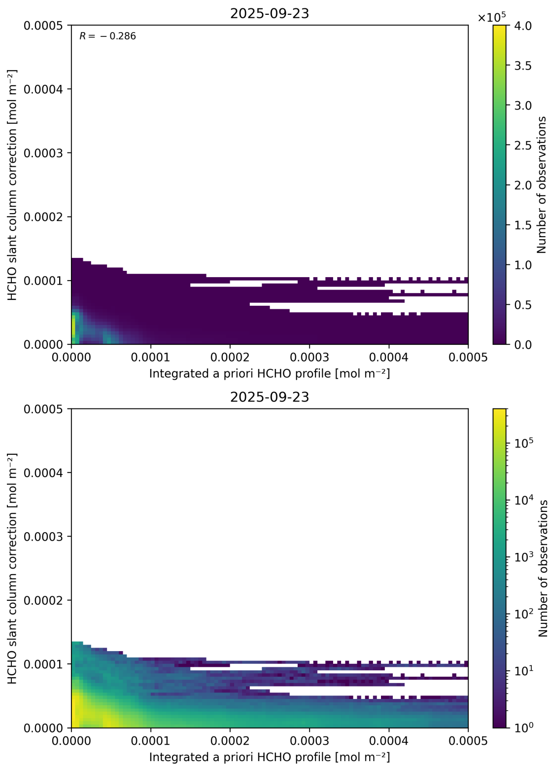
Figure 152: Scatter density plot of “Integrated a priori HCHO profile” against “HCHO slant column correction” for 2025-09-22 to 2025-09-24.
