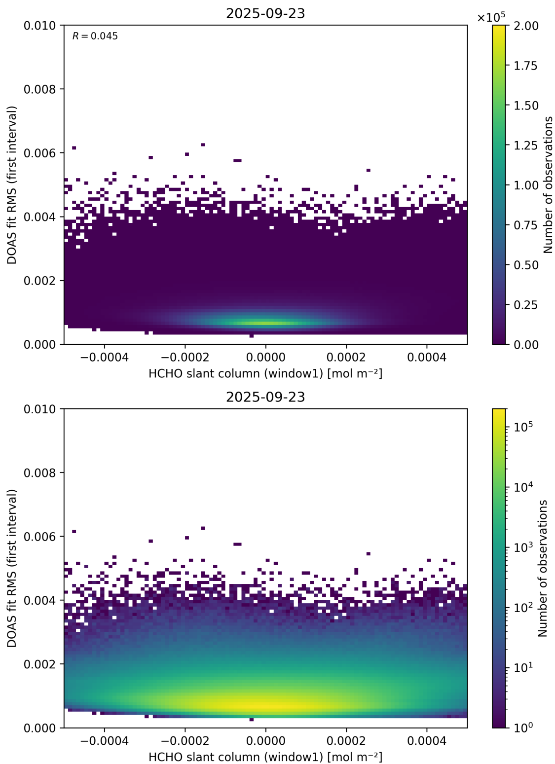
Figure 78: Scatter density plot of “HCHO slant column (window1)” against “DOAS fit RMS (first interval)” for 2025-09-22 to 2025-09-24.
