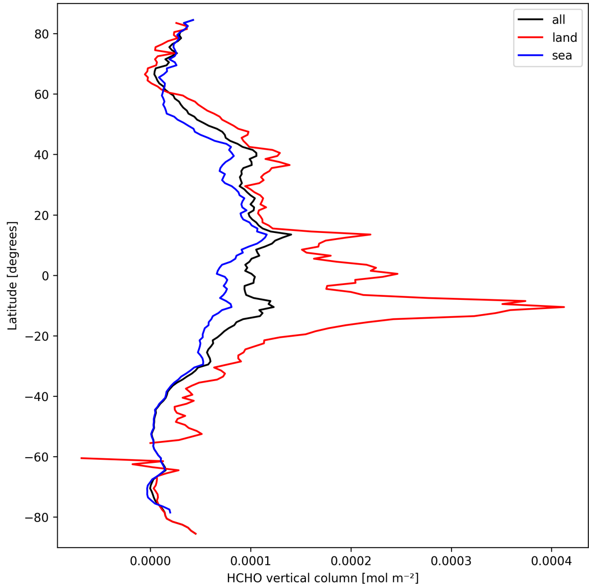
Figure 21: Zonal average of “HCHO vertical column” for 2025-09-22 to 2025-09-24.
