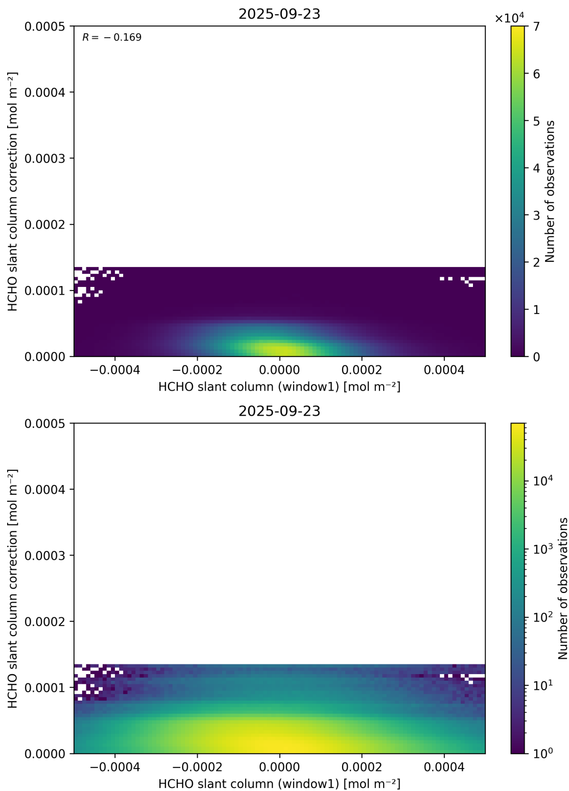
Figure 83: Scatter density plot of “HCHO slant column (window1)” against “HCHO slant column correction” for 2025-09-22 to 2025-09-24.
