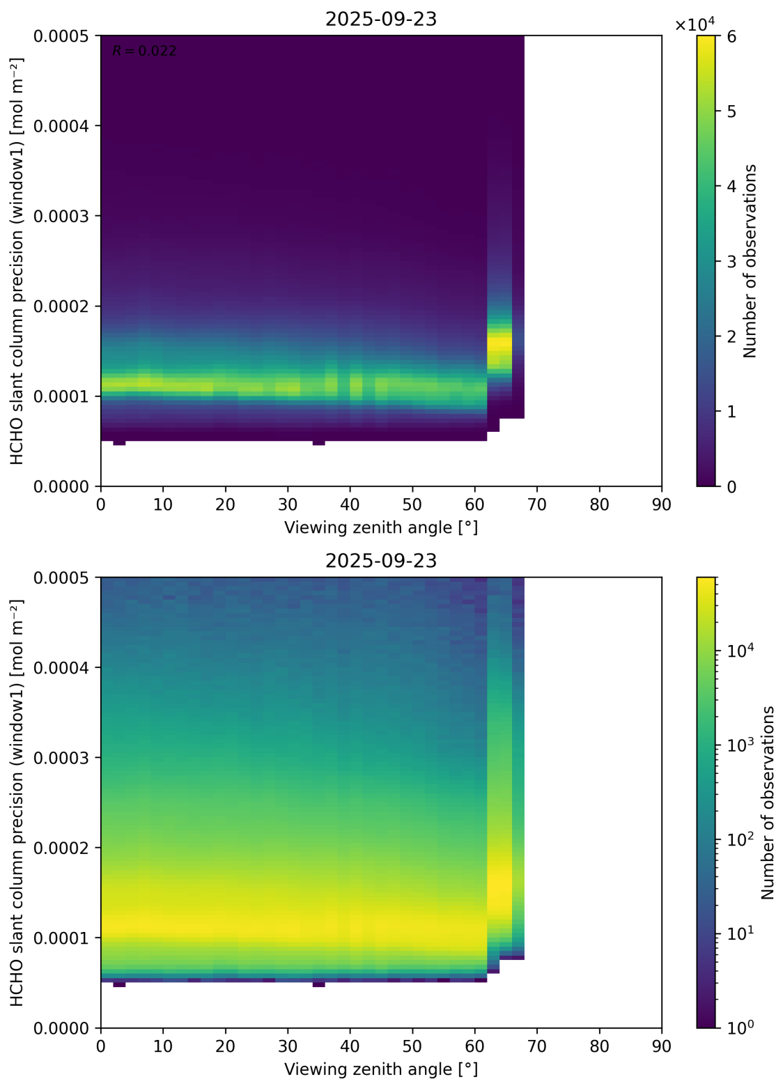
Figure 189: Scatter density plot of “Viewing zenith angle” against “HCHO slant column precision (window1)” for 2025-09-22 to 2025-09-24.
