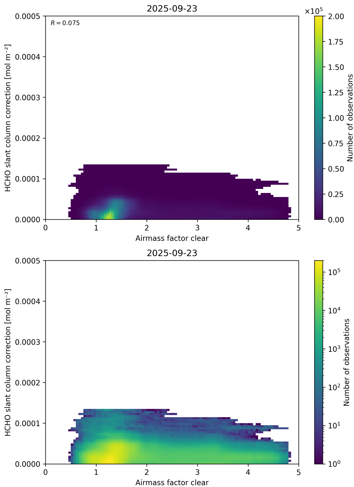
Figure 75: Scatter density plot of “Airmass factor clear” against “HCHO slant column correction” for 2025-09-22 to 2025-09-24.
