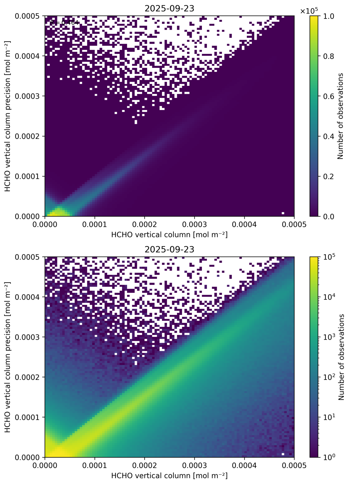
Figure 134: Scatter density plot of “HCHO vertical column” against “HCHO vertical column precision” for 2025-09-22 to 2025-09-24.
