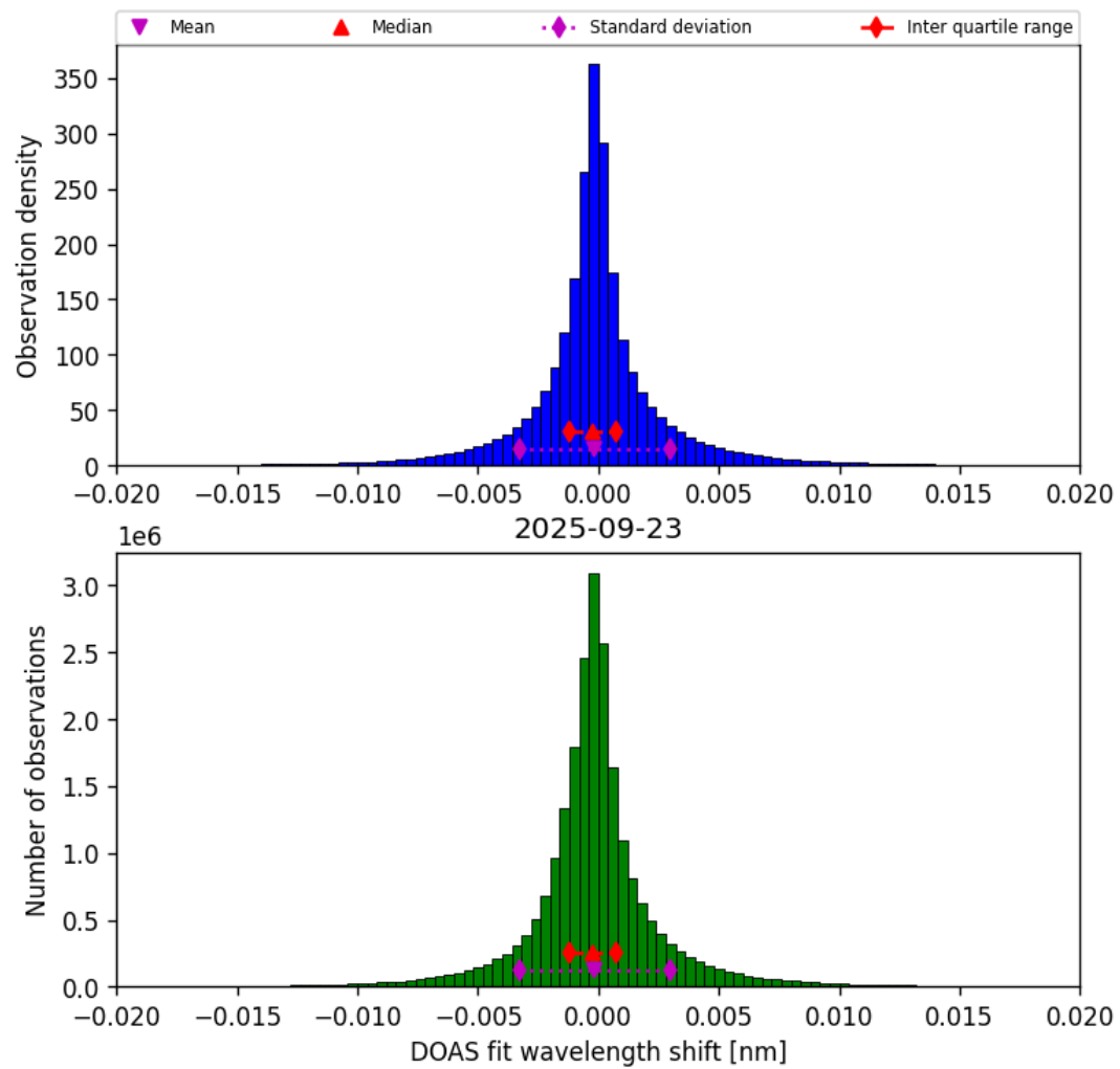
Figure 44: Histogram of “DOAS fit wavelength shift” for 2025-09-22 to 2025-09-24
