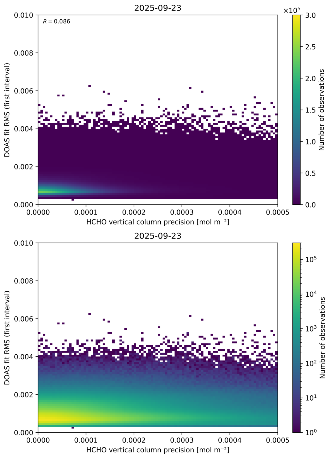
Figure 136: Scatter density plot of “HCHO vertical column precision” against “DOAS fit RMS (first interval)” for 2025-09-22 to 2025-09-24.
