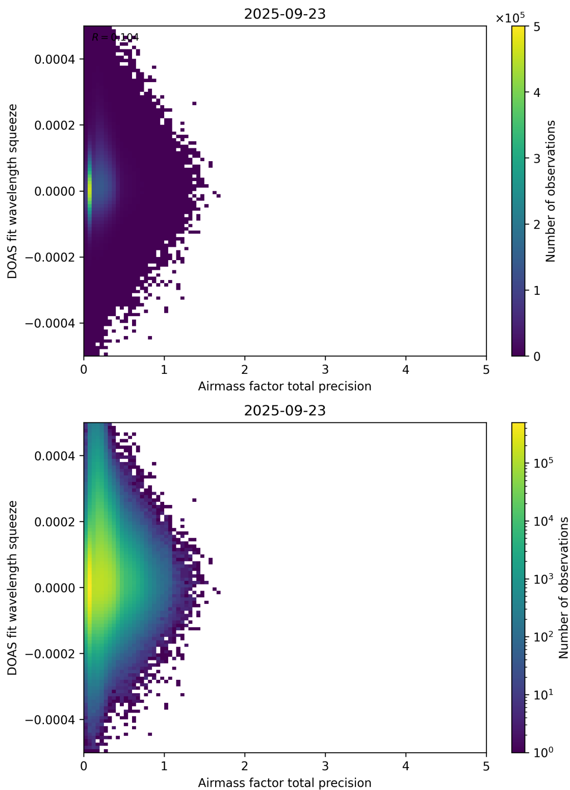
Figure 107: Scatter density plot of “Airmass factor total precision” against “DOAS fit wavelength squeeze” for 2025-09-22 to 2025-09-24.
