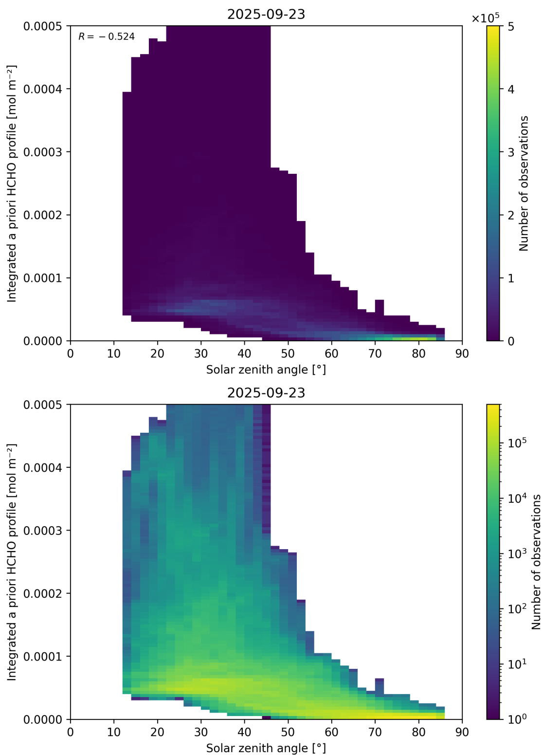
Figure 180: Scatter density plot of “Solar zenith angle” against “Integrated a priori HCHO profile” for 2025-09-22 to 2025-09-24.
