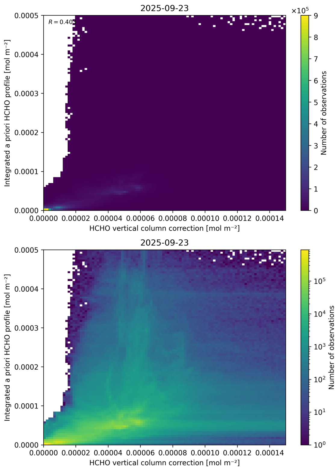
Figure 122: Scatter density plot of “HCHO vertical column correction” against “Integrated a priori HCHO profile” for 2025-09-22 to 2025-09-24.
