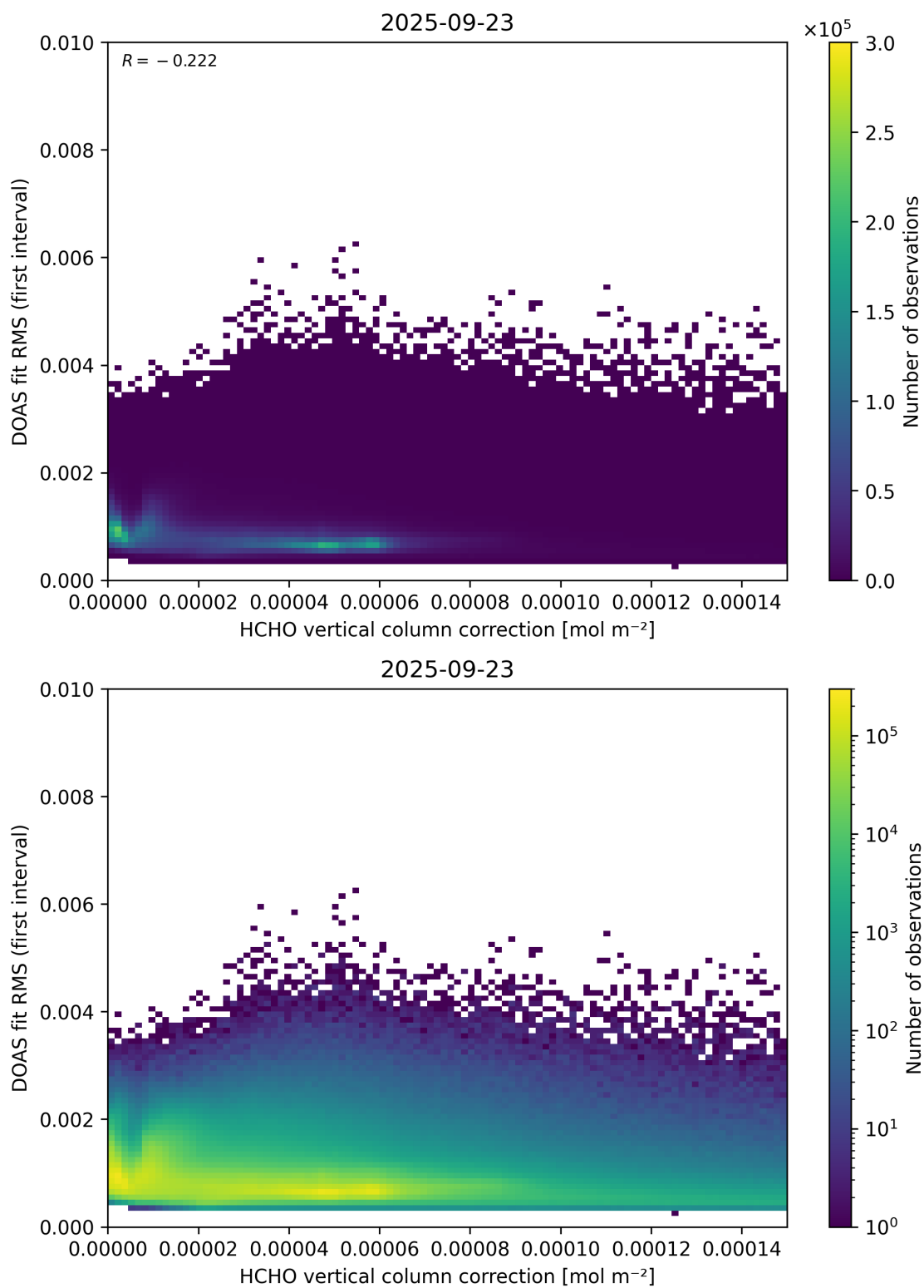
Figure 112: Scatter density plot of “HCHO vertical column correction” against “DOAS fit RMS (first interval)” for 2025-09-22 to 2025-09-24.
