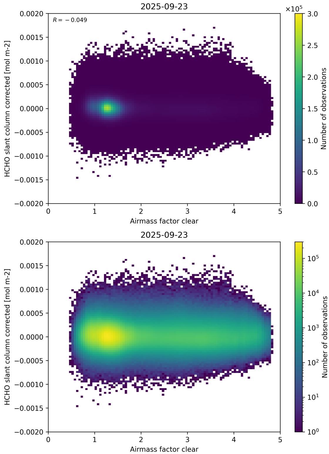
Figure 74: Scatter density plot of “Airmass factor clear” against “HCHO slant column corrected” for 2025-09-22 to 2025-09-24.
