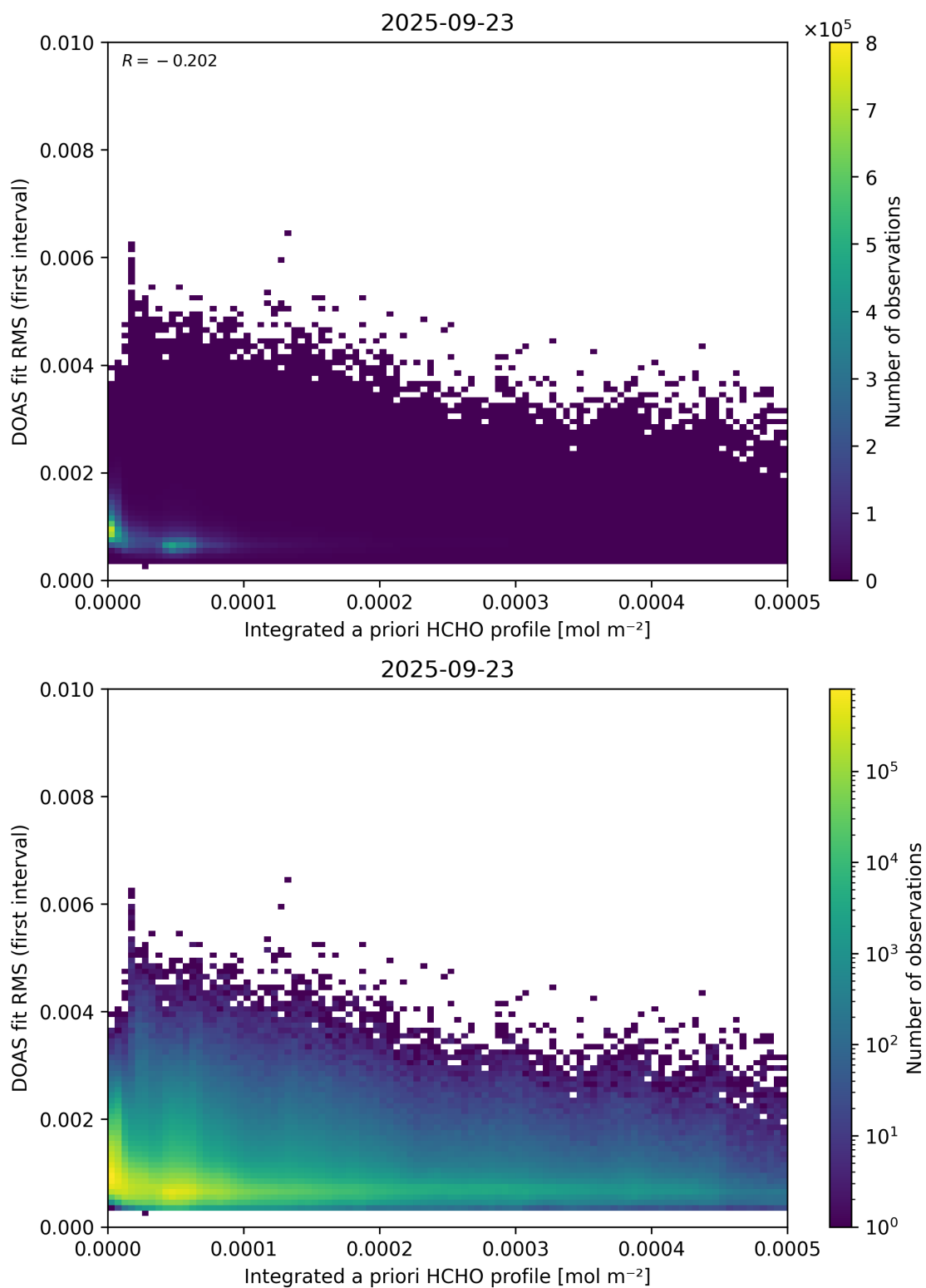
Figure 148: Scatter density plot of “Integrated a priori HCHO profile” against “DOAS fit RMS (first interval)” for 2025-09-22 to 2025-09-24.
