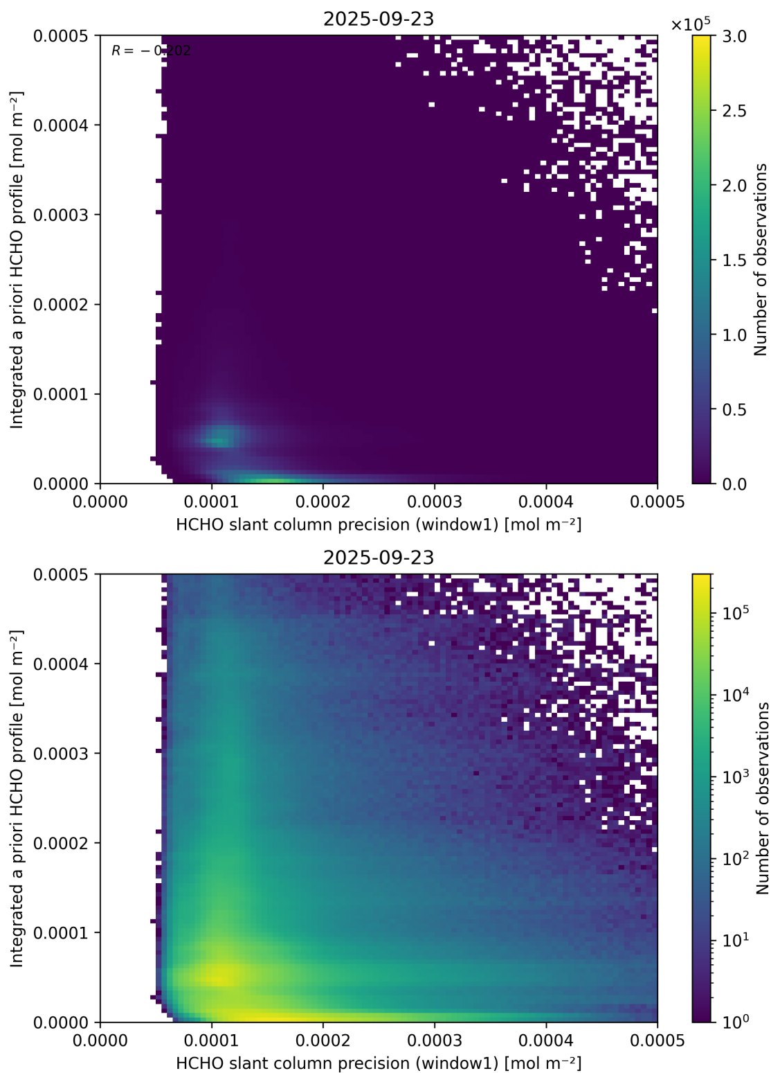
Figure 96: Scatter density plot of “HCHO slant column precision (window1)” against “Integrated a priori HCHO profile” for 2025-09-22 to 2025-09-24.
