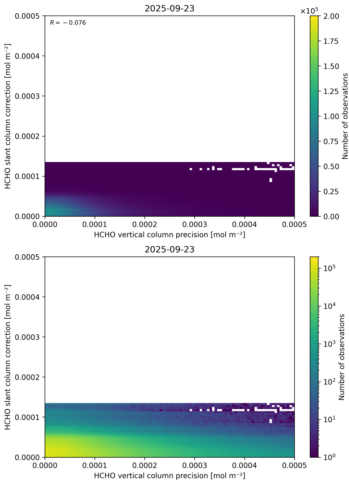
Figure 141: Scatter density plot of “HCHO vertical column precision” against “HCHO slant column correction” for 2025-09-22 to 2025-09-24.
