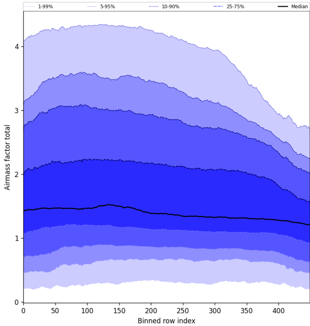
Figure 54: Along track statistics of “Airmass factor total” for 2025-09-22 to 2025-09-24
