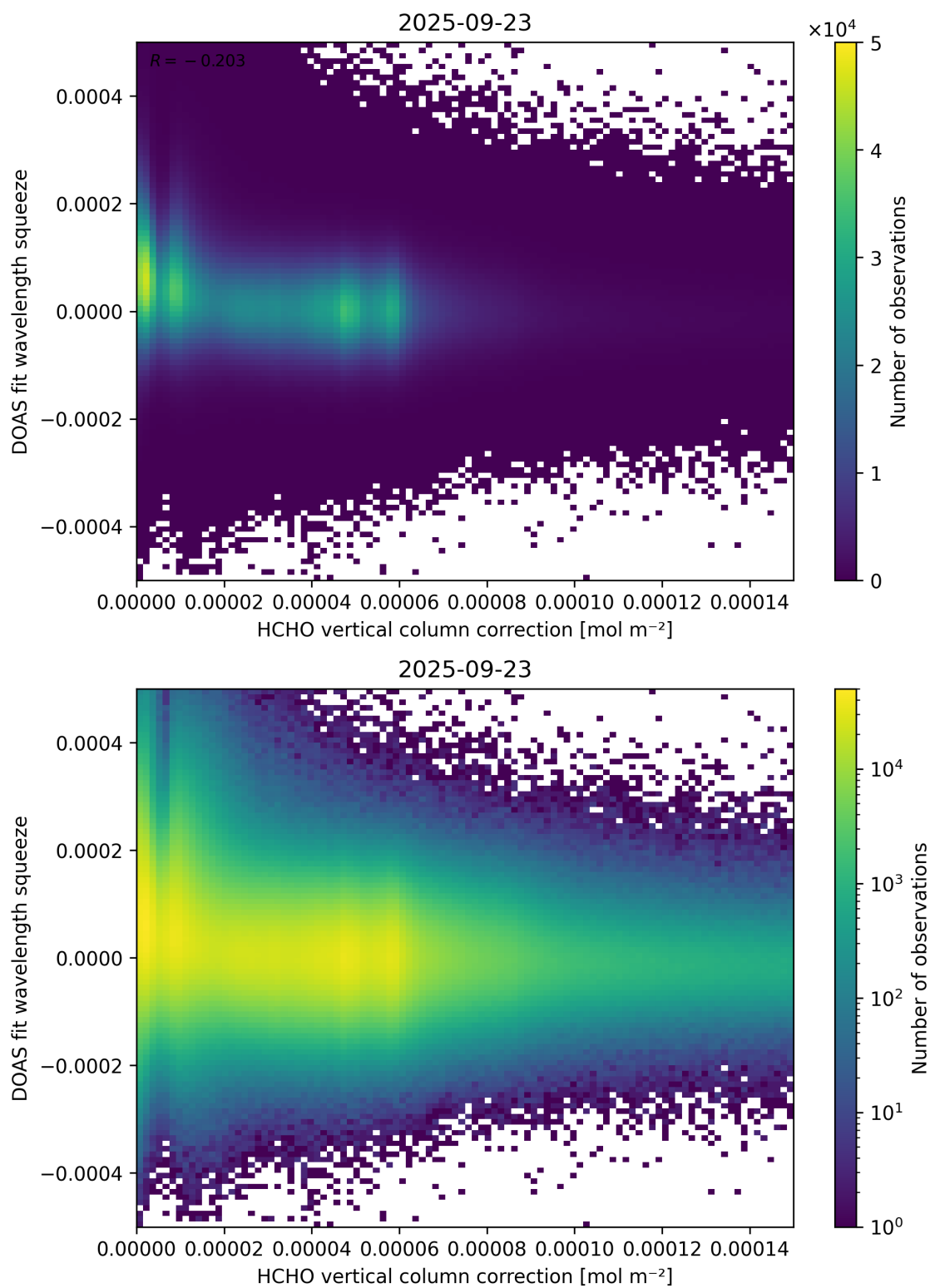
Figure 114: Scatter density plot of “HCHO vertical column correction” against “DOAS fit wavelength squeeze” for 2025-09-22 to 2025-09-24.
