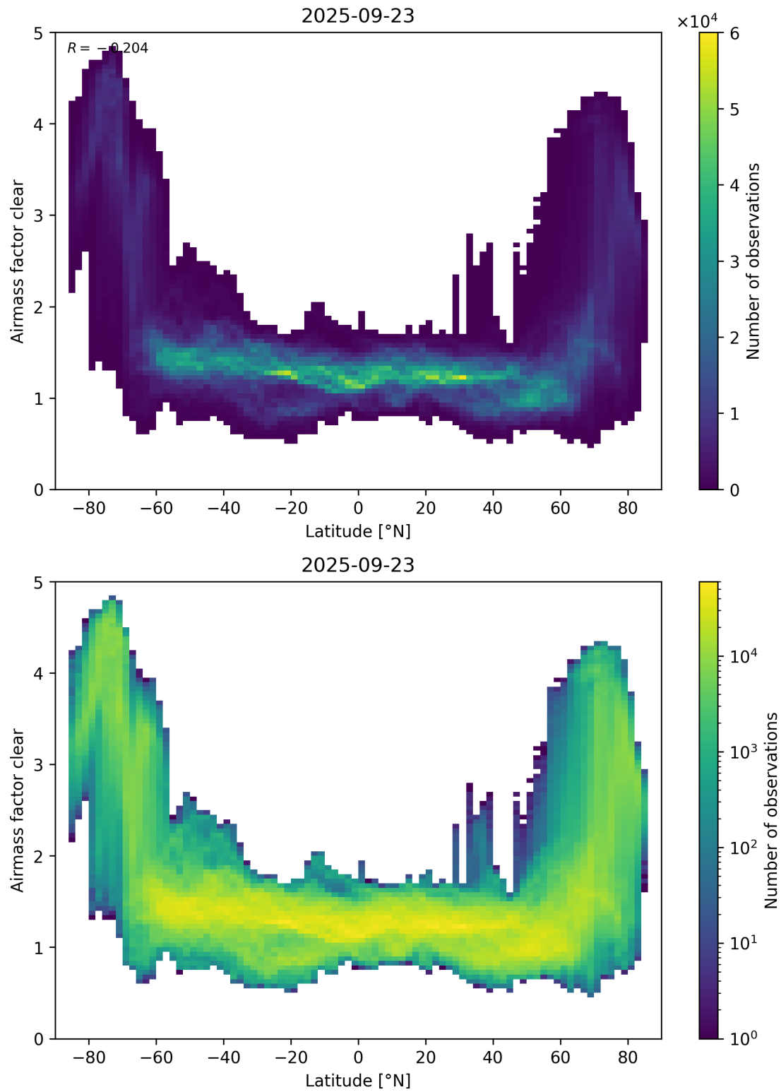
Figure 156: Scatter density plot of “Latitude” against “Airmass factor clear” for 2025-09-22 to 2025-09-24.
