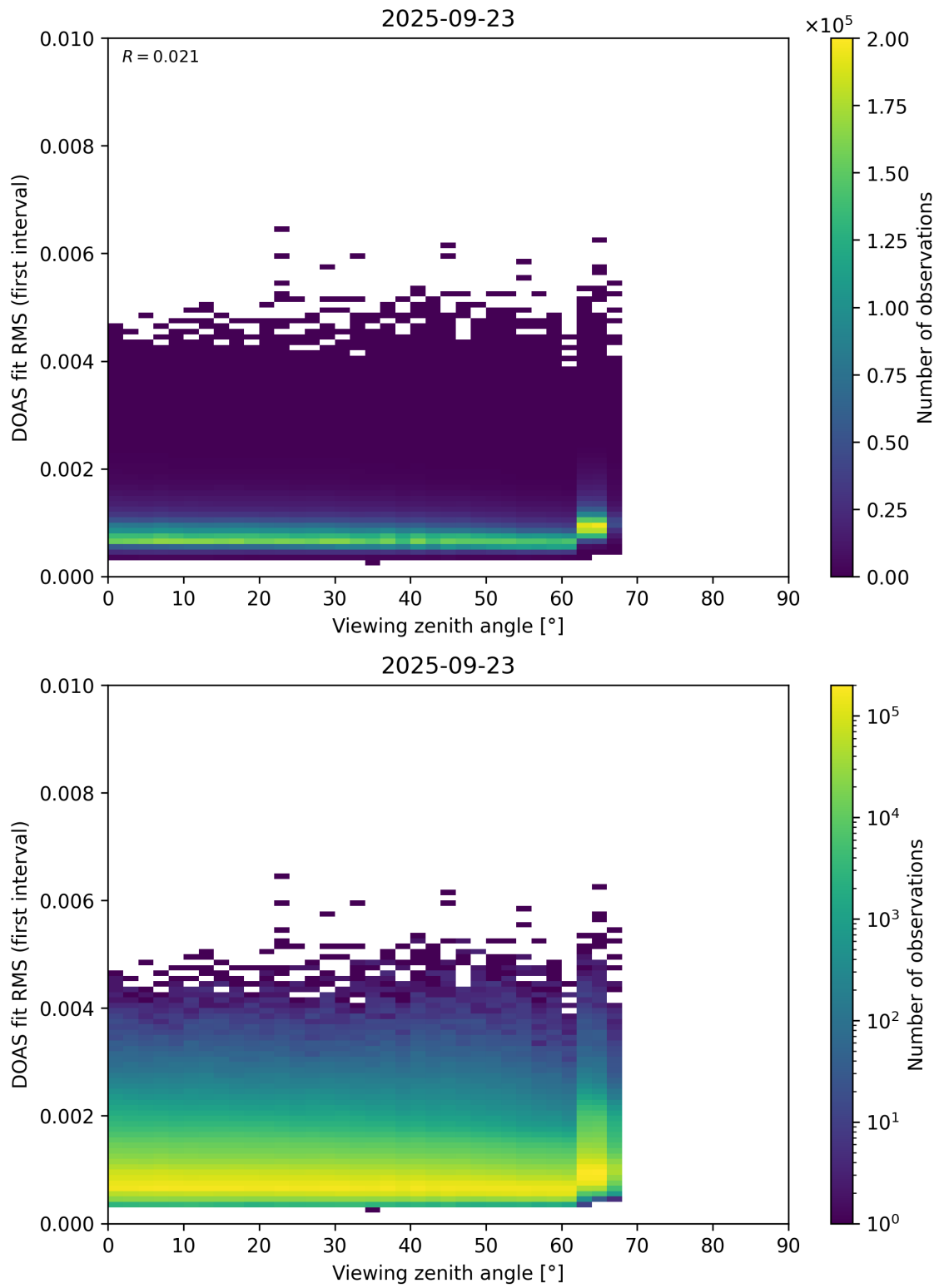
Figure 182: Scatter density plot of “Viewing zenith angle” against “DOAS fit RMS (first interval)” for 2025-09-22 to 2025-09-24.
