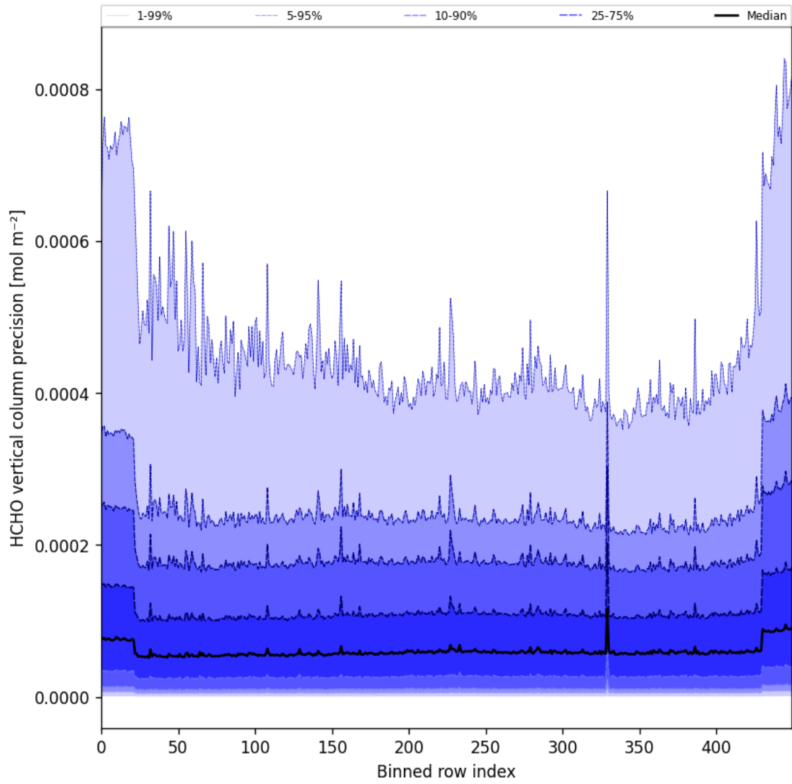
Figure 50: Along track statistics of “HCHO vertical column precision” for 2025-09-22 to 2025-09-24
