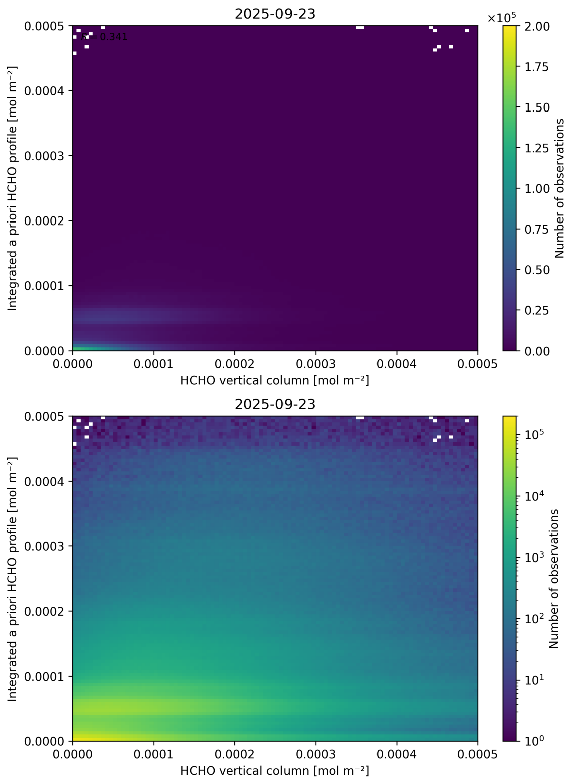
Figure 135: Scatter density plot of “HCHO vertical column” against “Integrated a priori HCHO profile” for 2025-09-22 to 2025-09-24.
