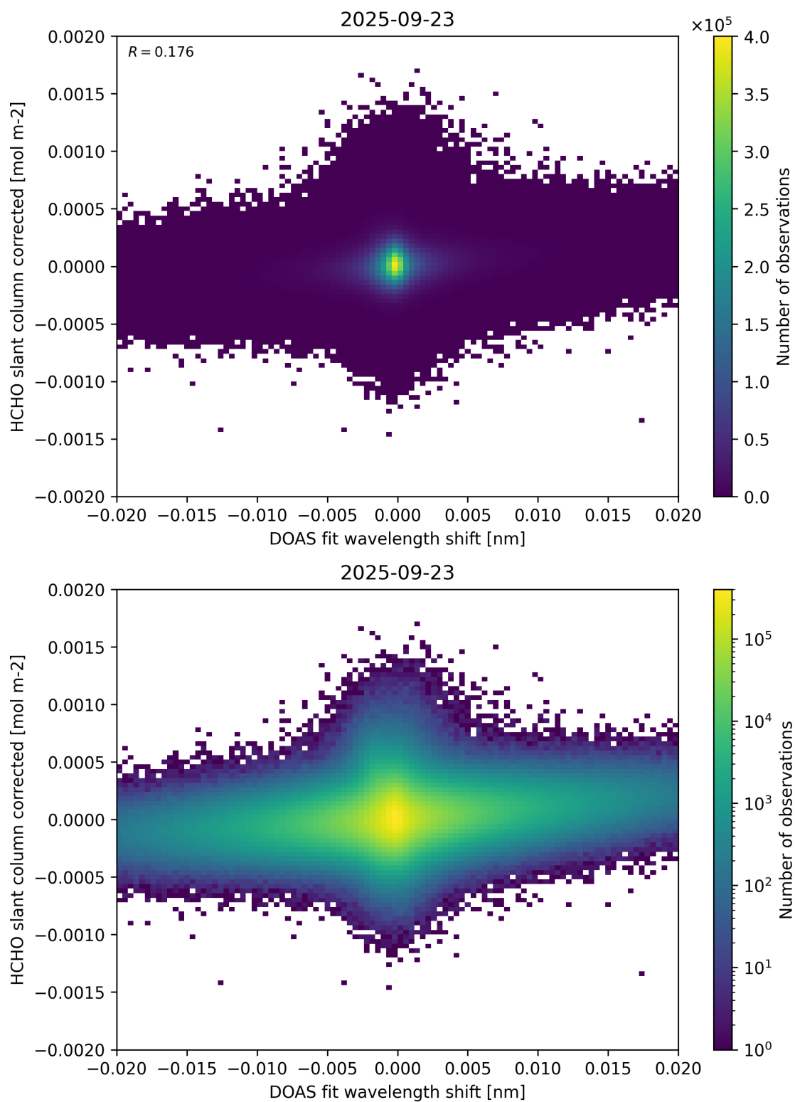
Figure 66: Scatter density plot of “DOAS fit wavelength shift” against “HCHO slant column corrected” for 2025-09-22 to 2025-09-24.
