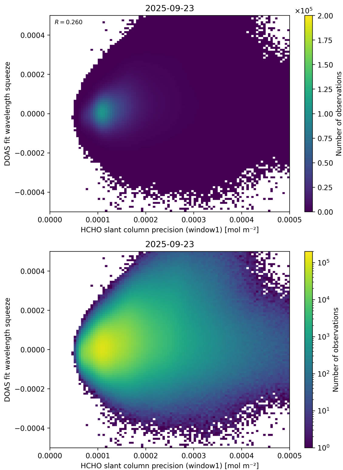
Figure 90: Scatter density plot of “HCHO slant column precision (window1)” against “DOAS fit wavelength squeeze” for 2025-09-22 to 2025-09-24.
