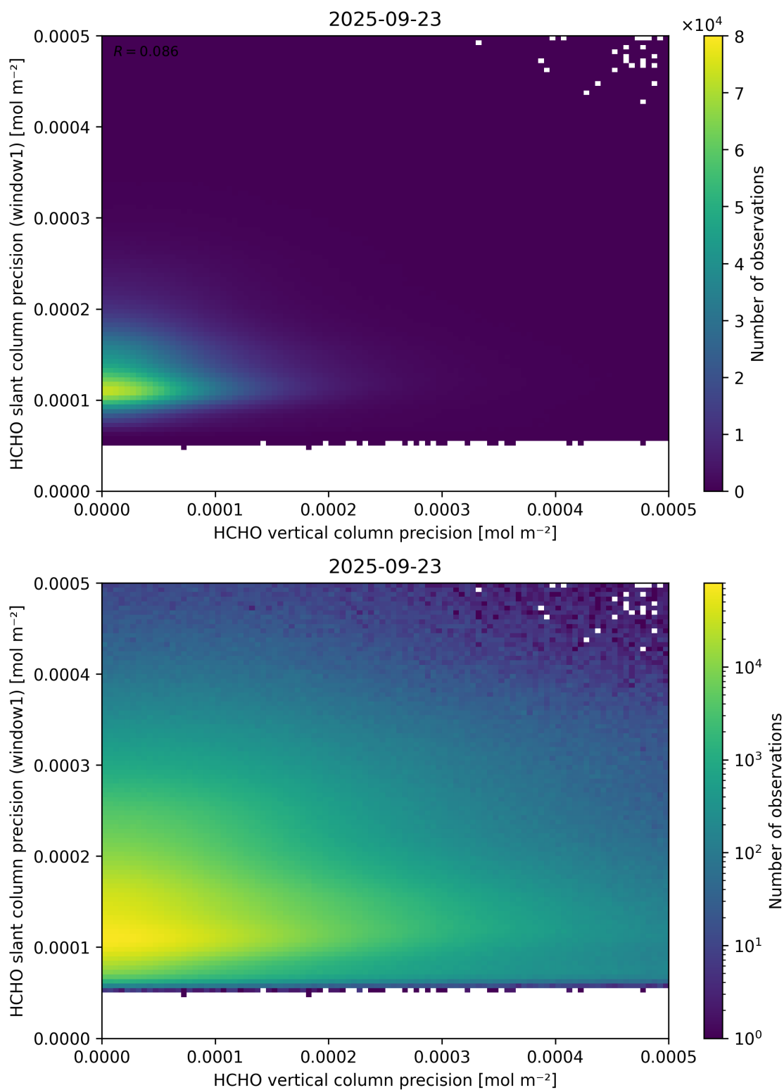
Figure 143: Scatter density plot of “HCHO vertical column precision” against “HCHO slant column precision (window1)” for 2025-09-22 to 2025-09-24.
