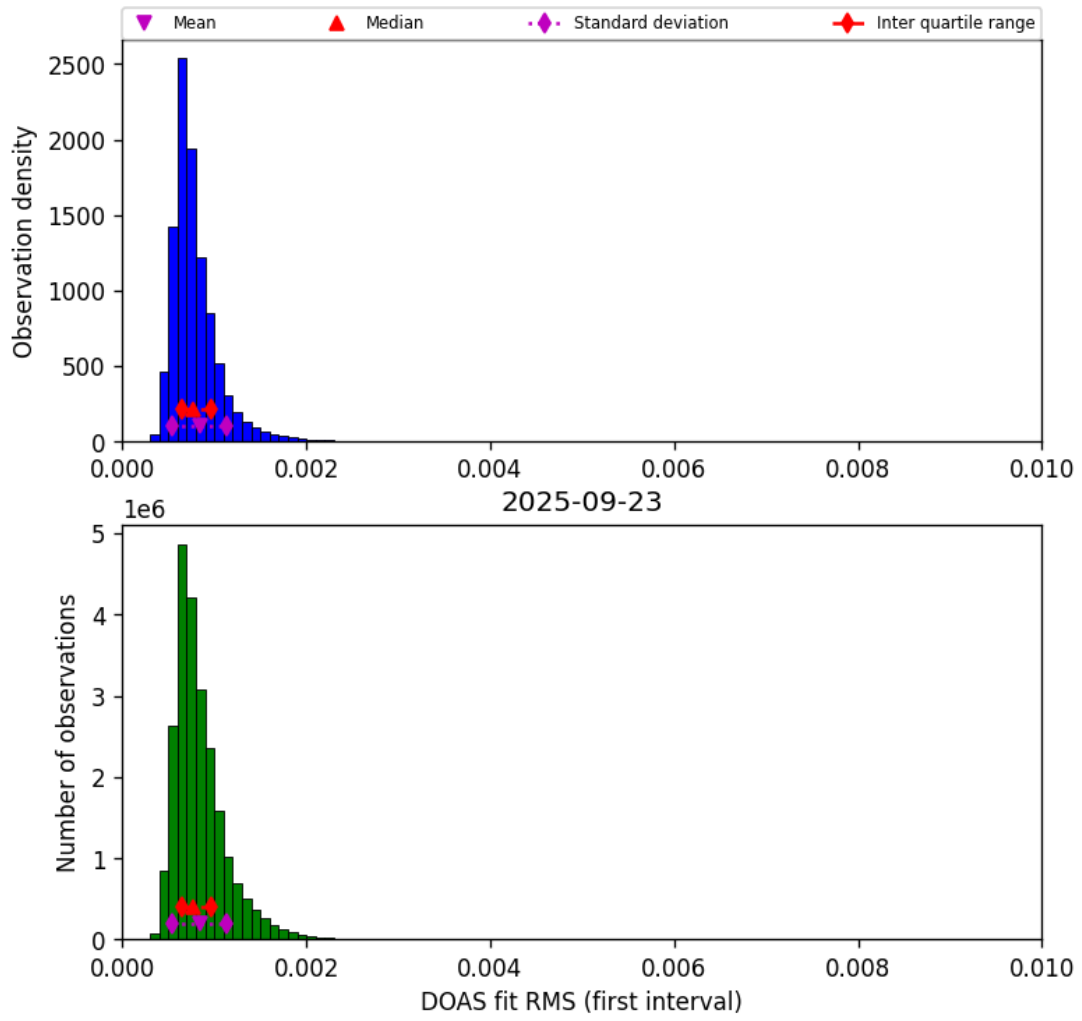
Figure 46: Histogram of “DOAS fit RMS (first interval)” for 2025-09-22 to 2025-09-24
