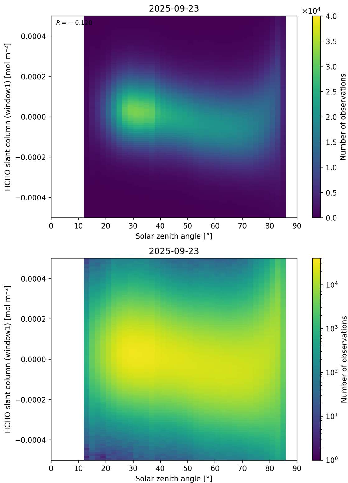
Figure 173: Scatter density plot of “Solar zenith angle” against “HCHO slant column (window1)” for 2025-09-22 to 2025-09-24.
