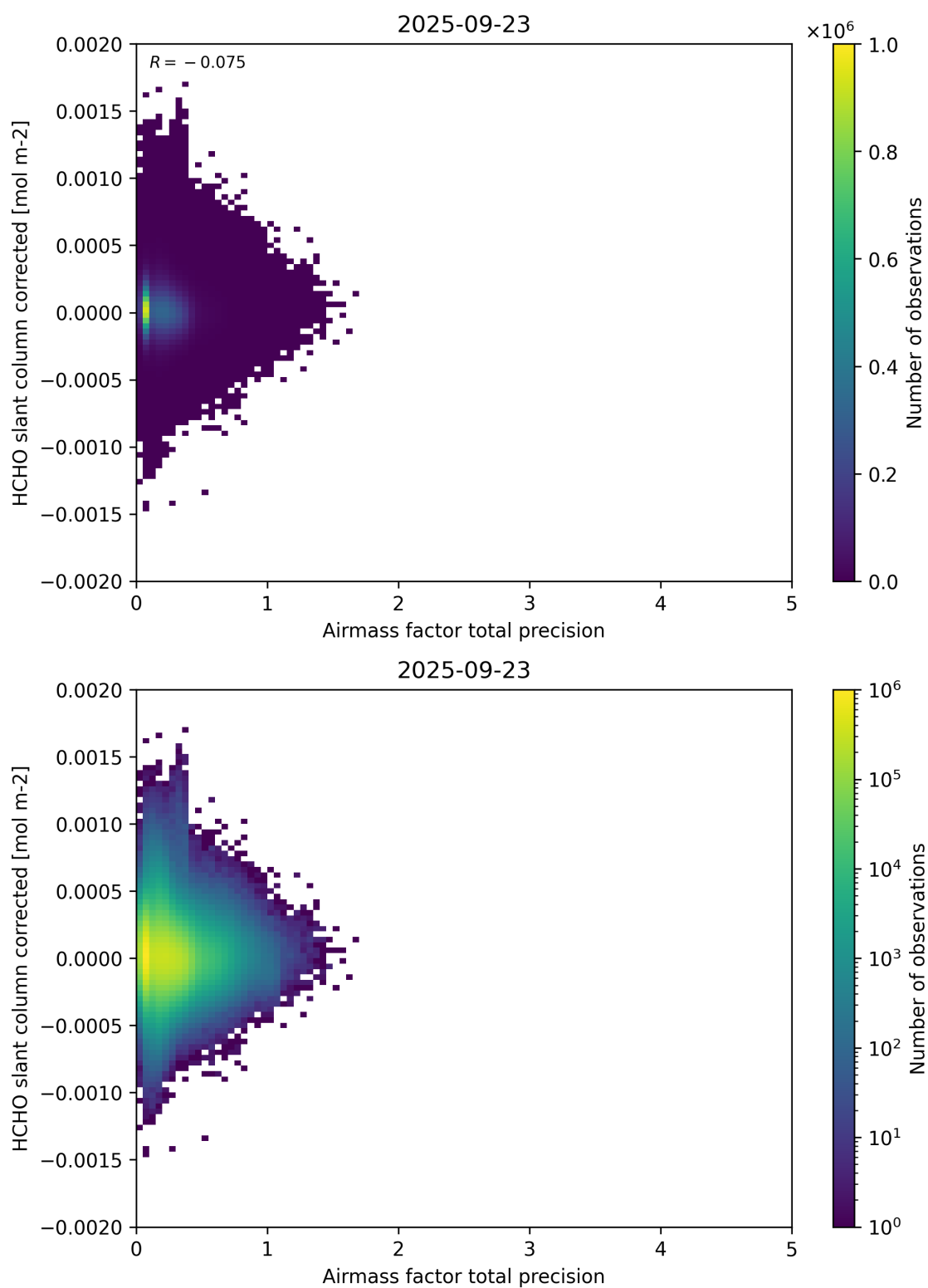
Figure 109: Scatter density plot of “Airmass factor total precision” against “HCHO slant column corrected” for 2025-09-22 to 2025-09-24.
