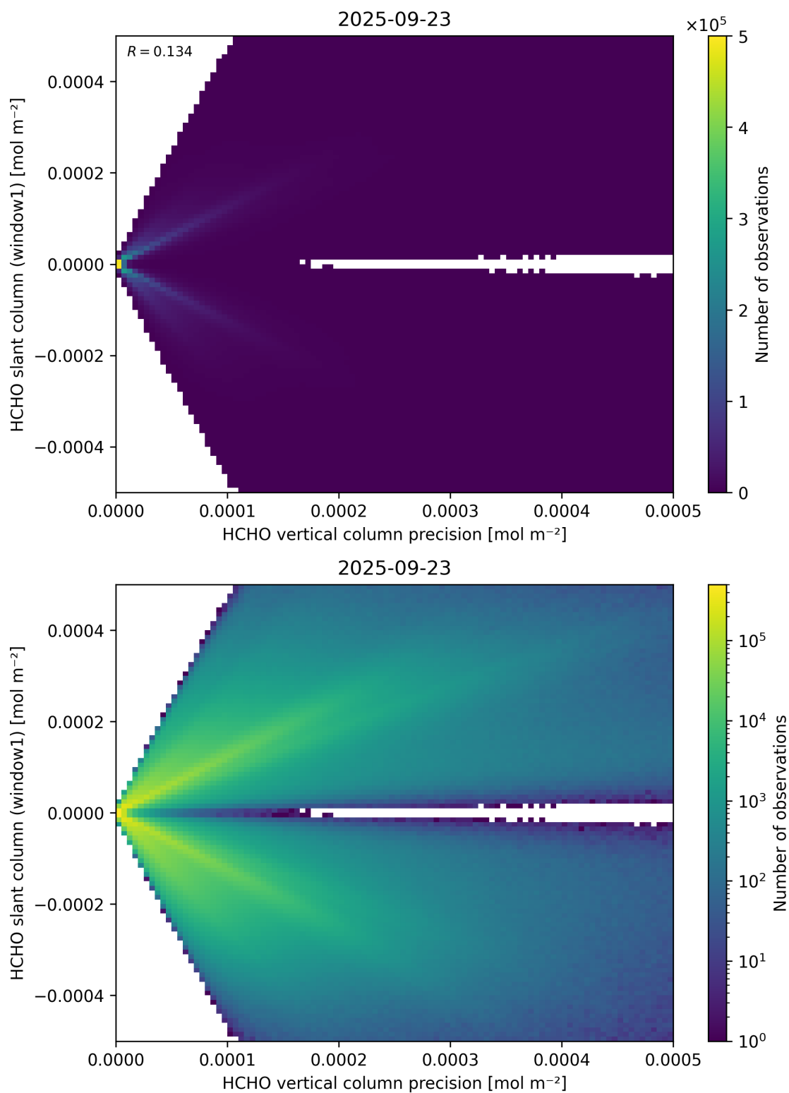
Figure 142: Scatter density plot of “HCHO vertical column precision” against “HCHO slant column (window1)” for 2025-09-22 to 2025-09-24.
