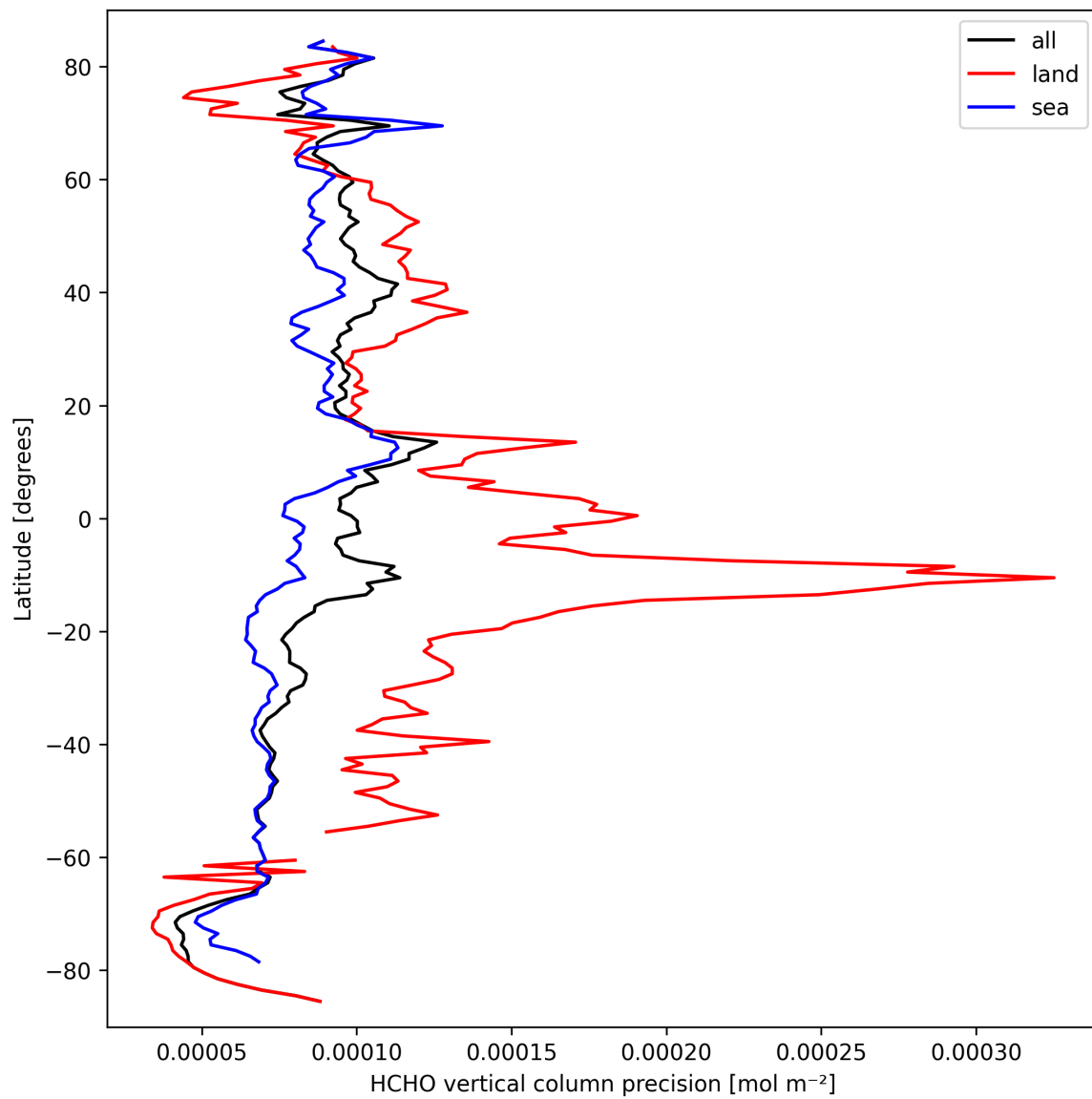
Figure 22: Zonal average of “HCHO vertical column precision” for 2025-09-22 to 2025-09-24.
