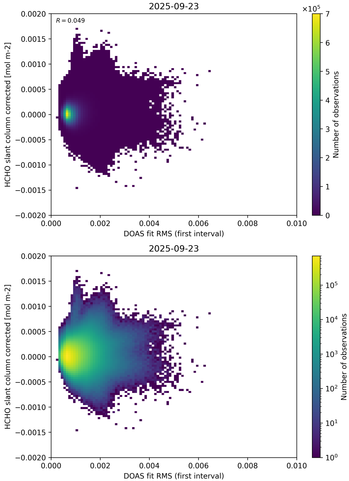
Figure 62: Scatter density plot of “DOAS fit RMS (first interval)” against “HCHO slant column corrected” for 2025-09-22 to 2025-09-24.
