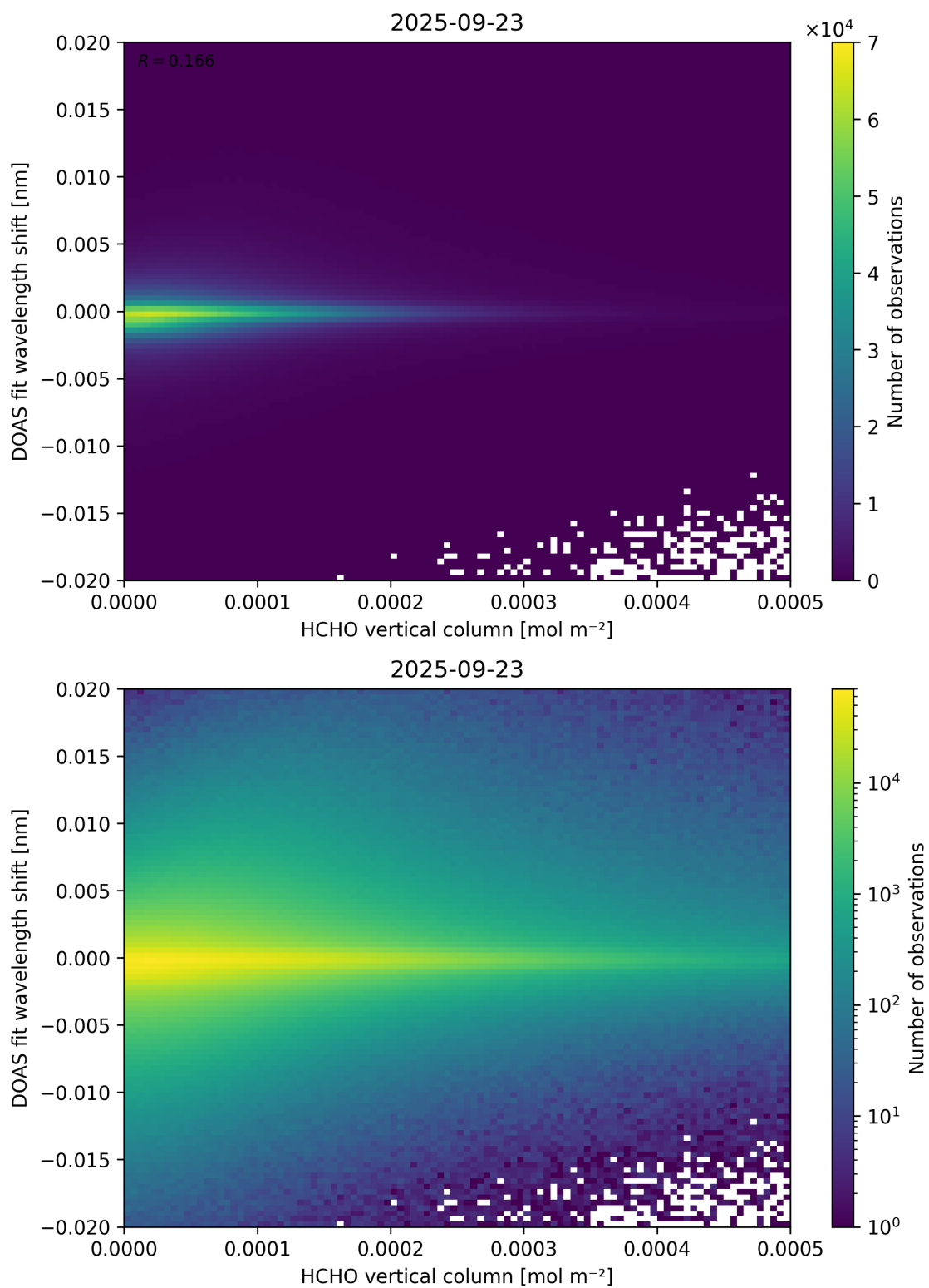
Figure 124: Scatter density plot of “HCHO vertical column” against “DOAS fit wavelength shift” for 2025-09-22 to 2025-09-24.
