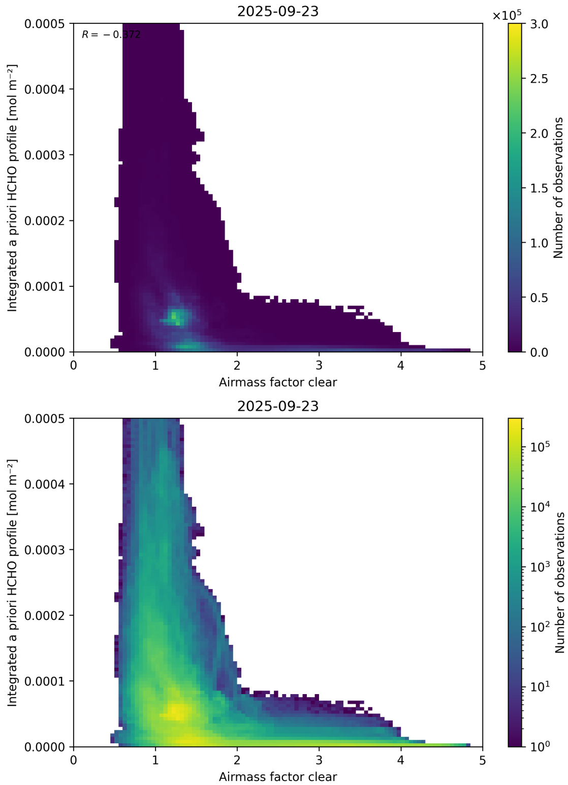
Figure 76: Scatter density plot of “Airmass factor clear” against “Integrated a priori HCHO profile” for 2025-09-22 to 2025-09-24.
