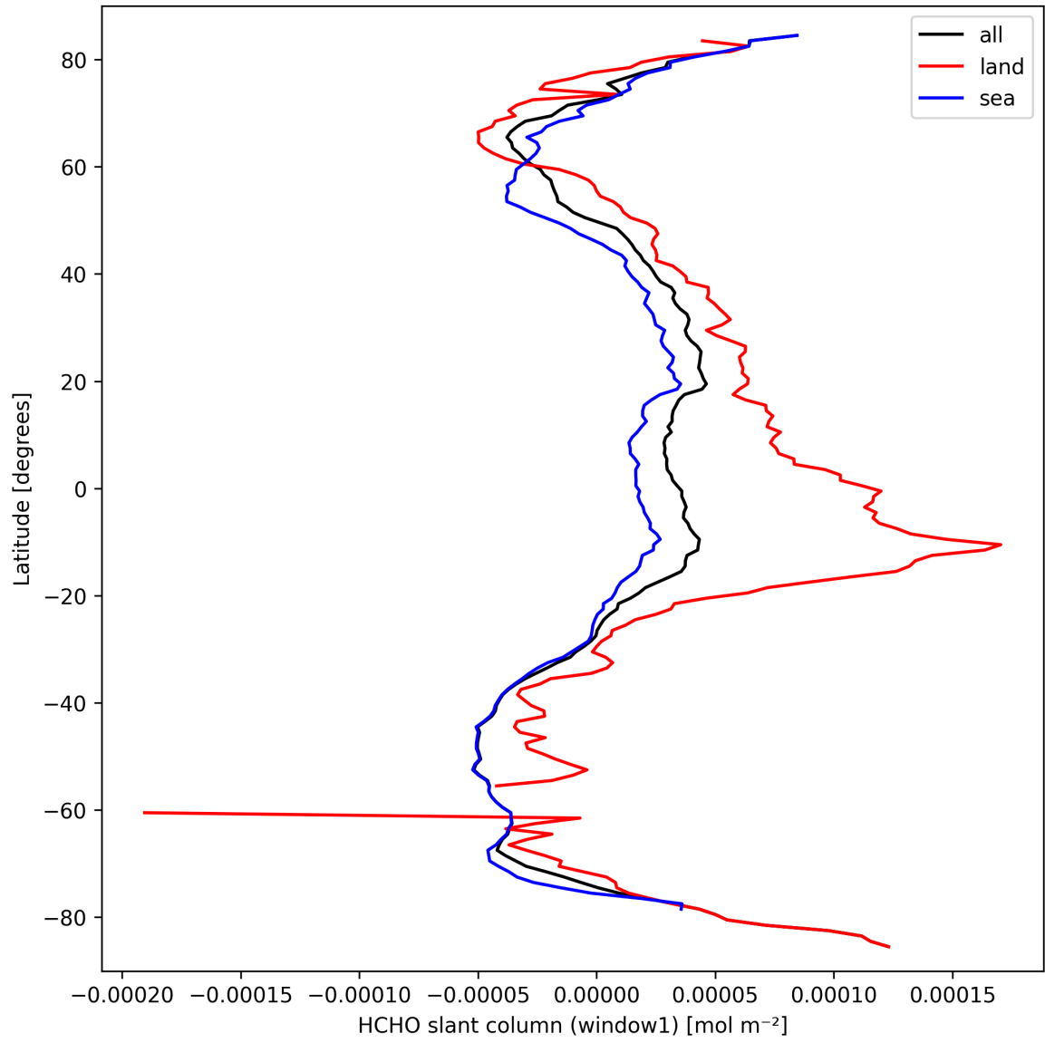
Figure 24: Zonal average of “HCHO slant column (window1)” for 2025-09-22 to 2025-09-24.
