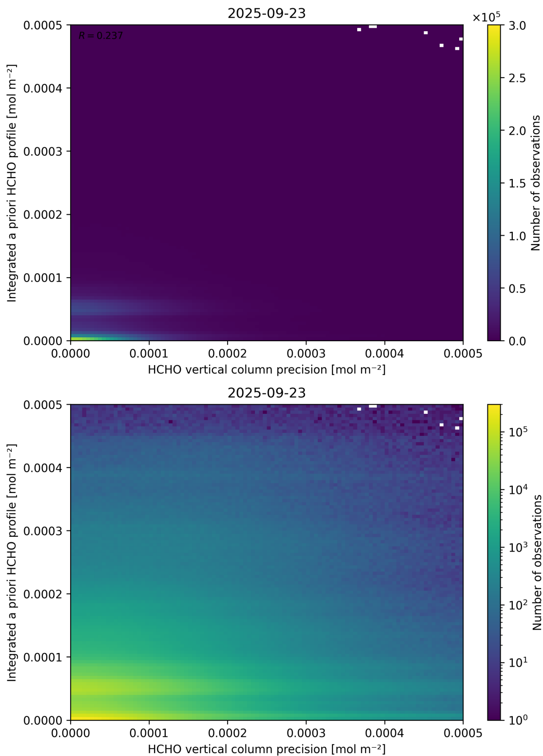
Figure 147: Scatter density plot of “HCHO vertical column precision” against “Integrated a priori HCHO profile” for 2025-09-22 to 2025-09-24.
