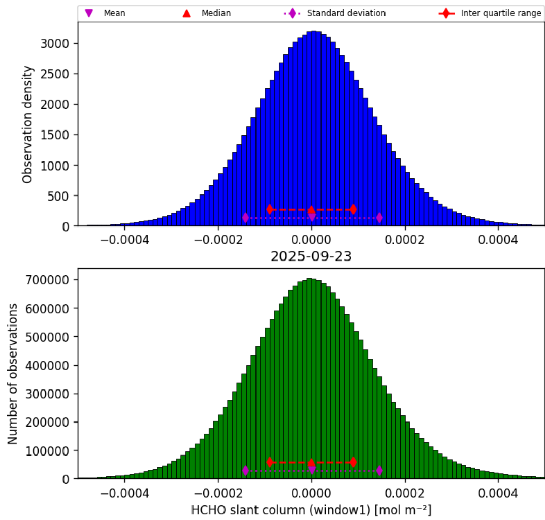
Figure 38: Histogram of “HCHO slant column (window1)” for 2025-09-22 to 2025-09-24
