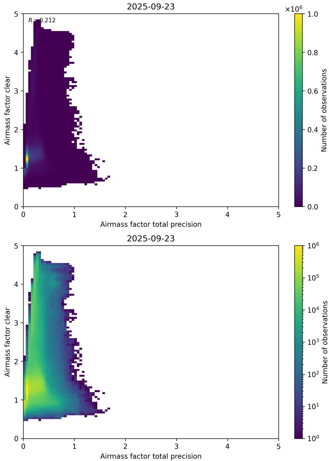
Figure 108: Scatter density plot of “Airmass factor total precision” against “Airmass factor clear” for 2025-09-22 to 2025-09-24.
