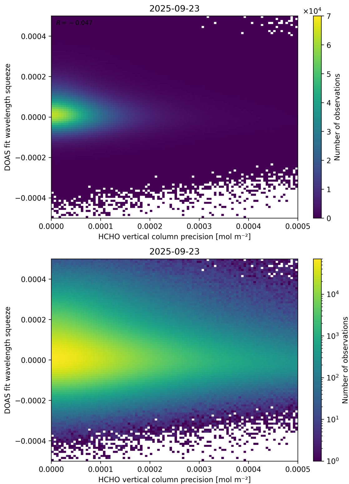
Figure 138: Scatter density plot of “HCHO vertical column precision” against “DOAS fit wavelength squeeze” for 2025-09-22 to 2025-09-24.
