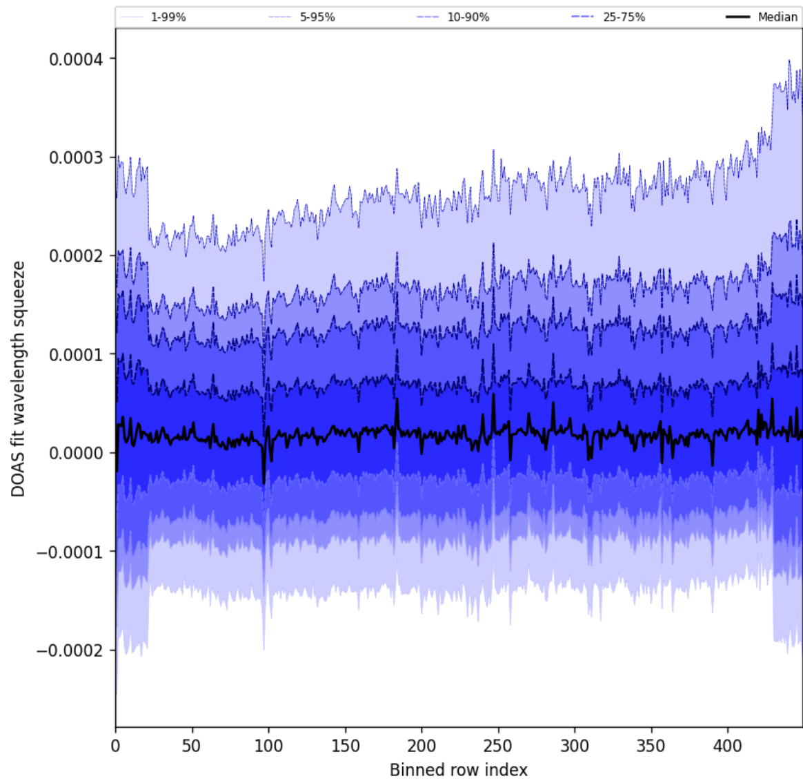
Figure 59: Along track statistics of “DOAS fit wavelength squeeze” for 2025-09-22 to 2025-09-24
