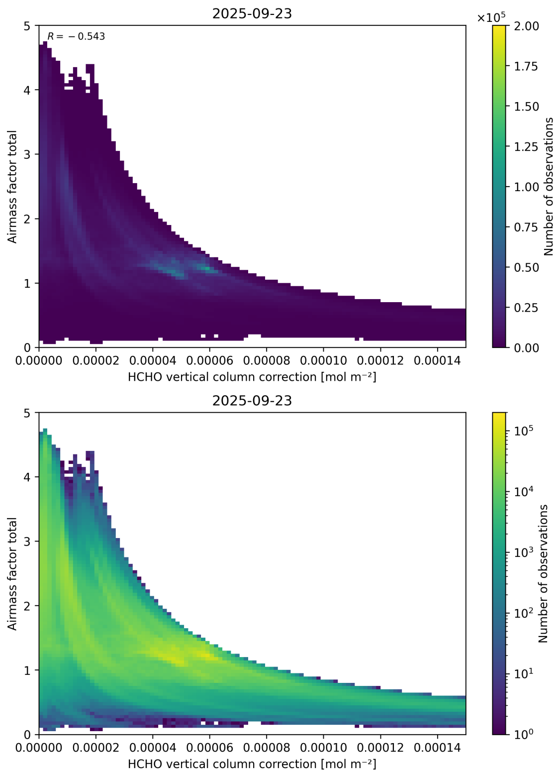
Figure 120: Scatter density plot of “HCHO vertical column correction” against “Airmass factor total” for 2025-09-22 to 2025-09-24.
