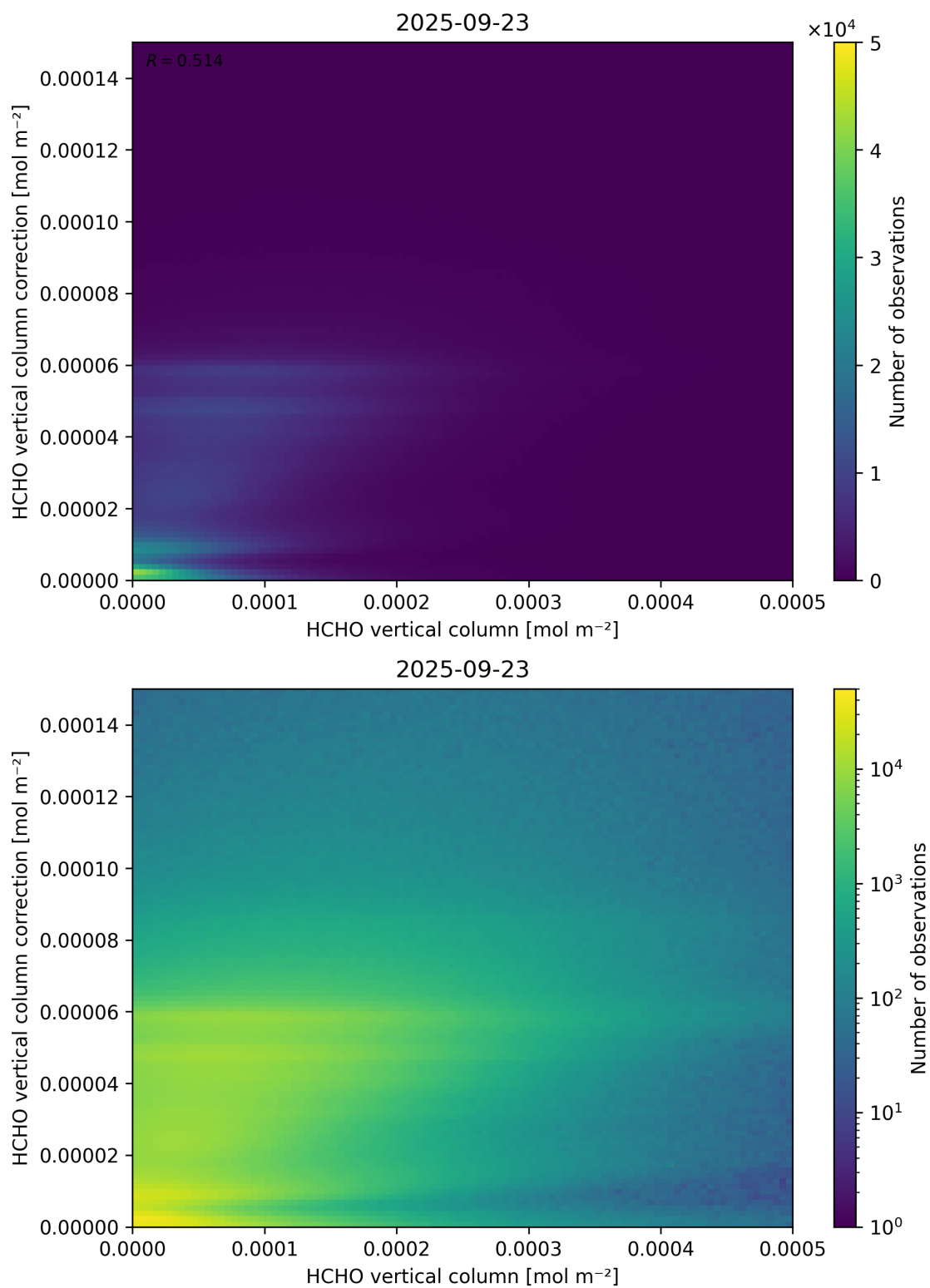
Figure 133: Scatter density plot of “HCHO vertical column” against “HCHO vertical column correction” for 2025-09-22 to 2025-09-24.
