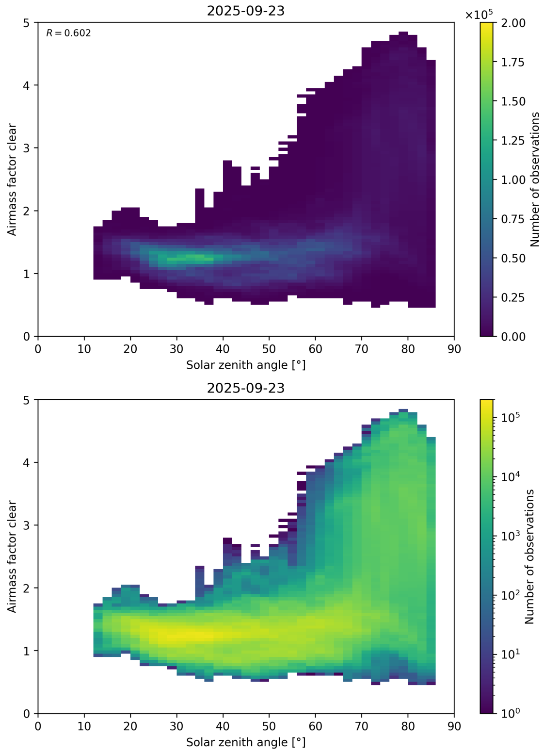
Figure 170: Scatter density plot of “Solar zenith angle” against “Airmass factor clear” for 2025-09-22 to 2025-09-24.
