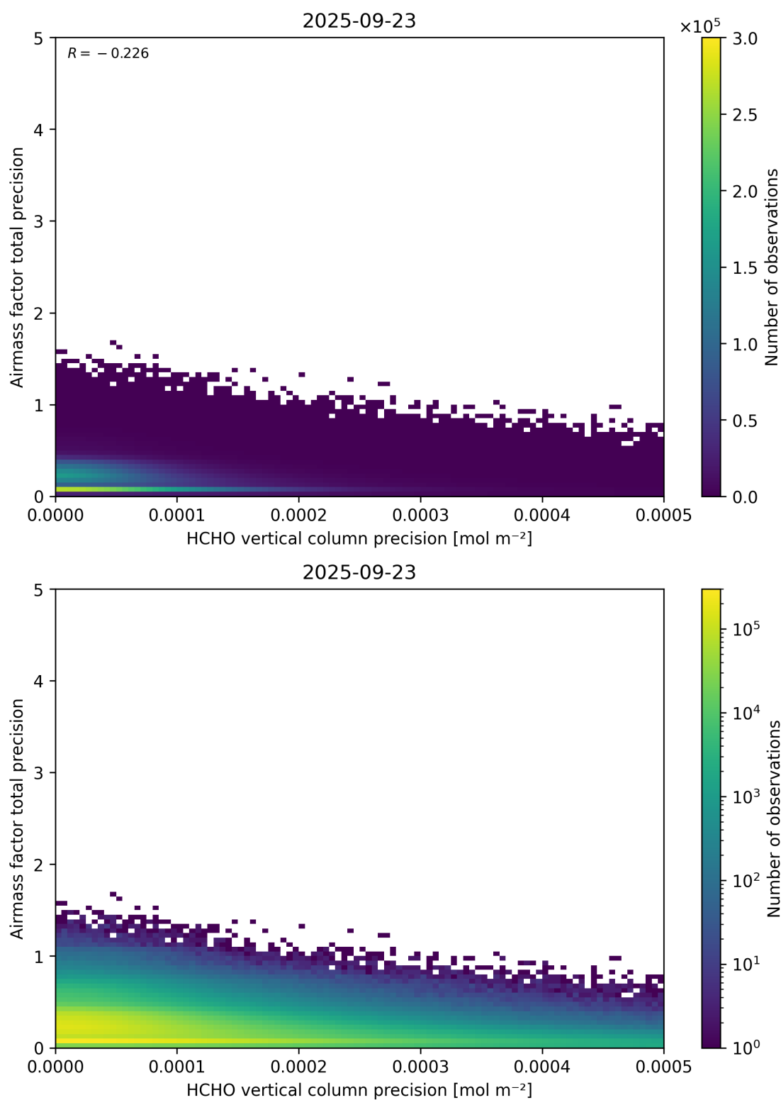
Figure 145: Scatter density plot of “HCHO vertical column precision” against “Airmass factor total precision” for 2025-09-22 to 2025-09-24.
