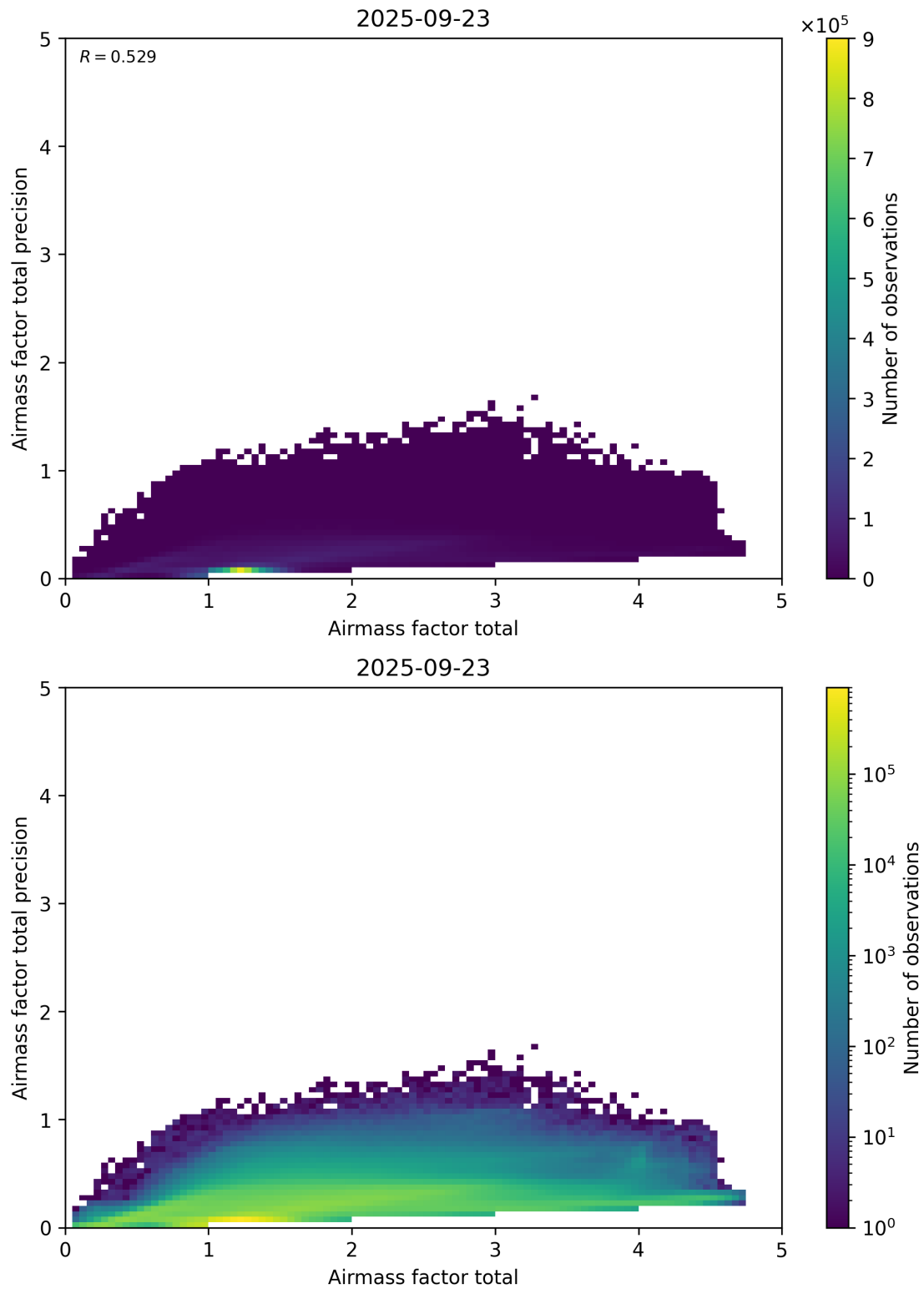
Figure 103: Scatter density plot of “Airmass factor total” against “Airmass factor total precision” for 2025-09-22 to 2025-09-24.
