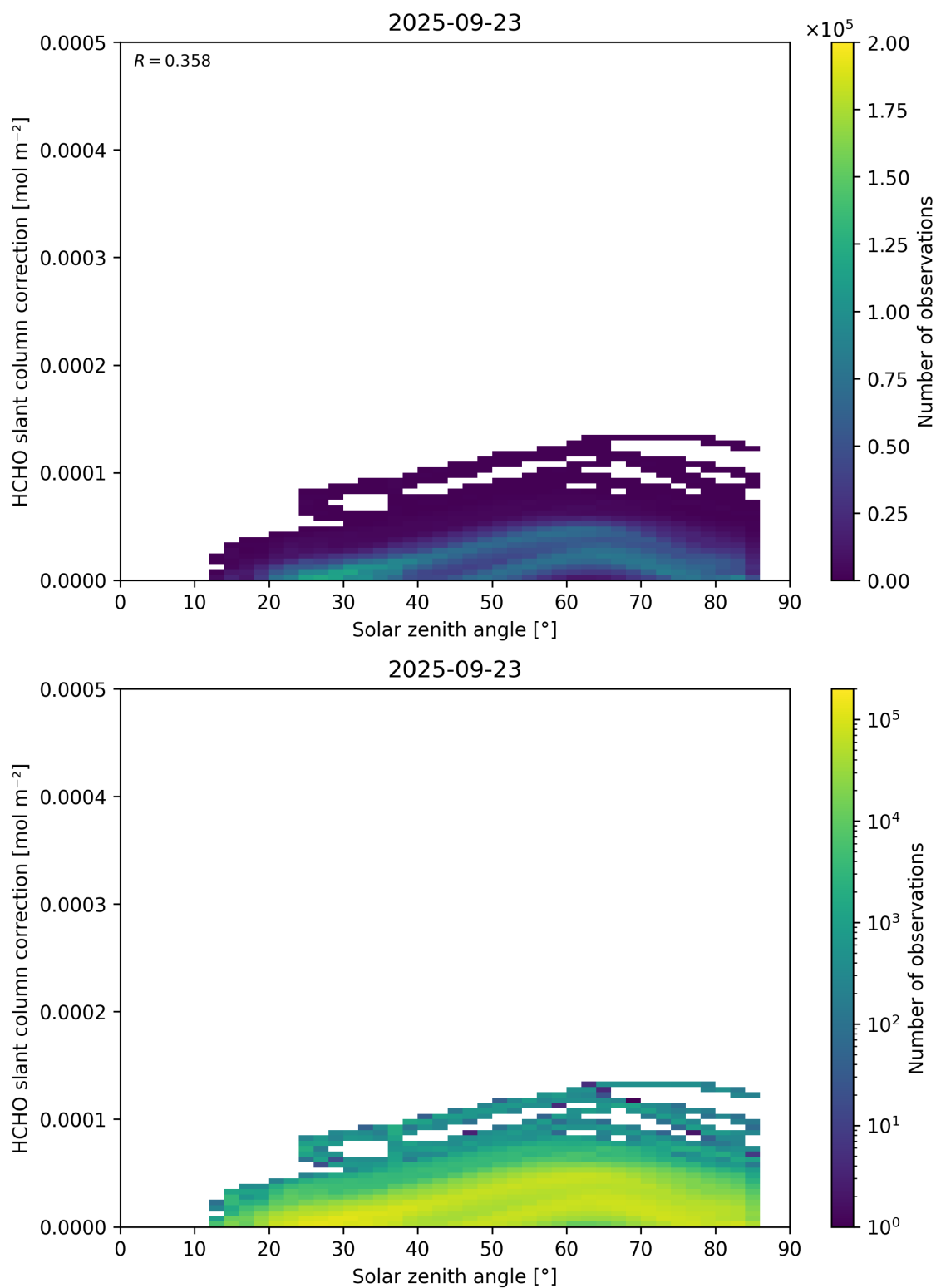
Figure 172: Scatter density plot of “Solar zenith angle” against “HCHO slant column correction” for 2025-09-22 to 2025-09-24.
