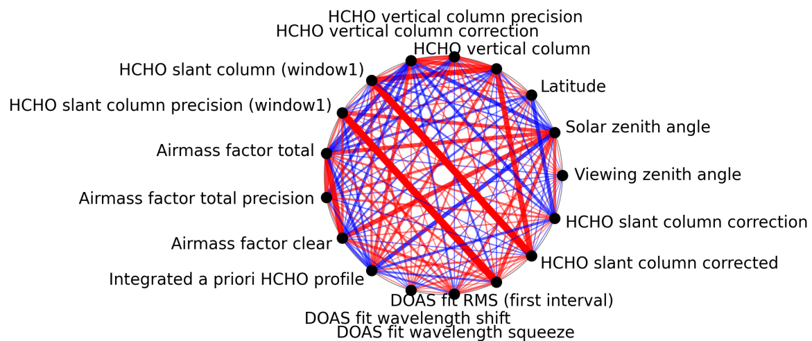
Figure 1: Map of correlation graph for 2025-09-22 to 2025-09-24.
