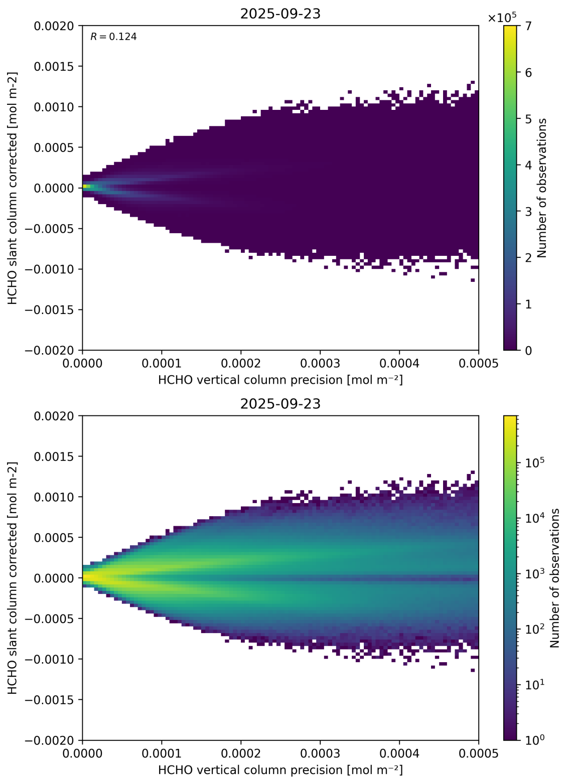
Figure 140: Scatter density plot of “HCHO vertical column precision” against “HCHO slant column corrected” for 2025-09-22 to 2025-09-24.
