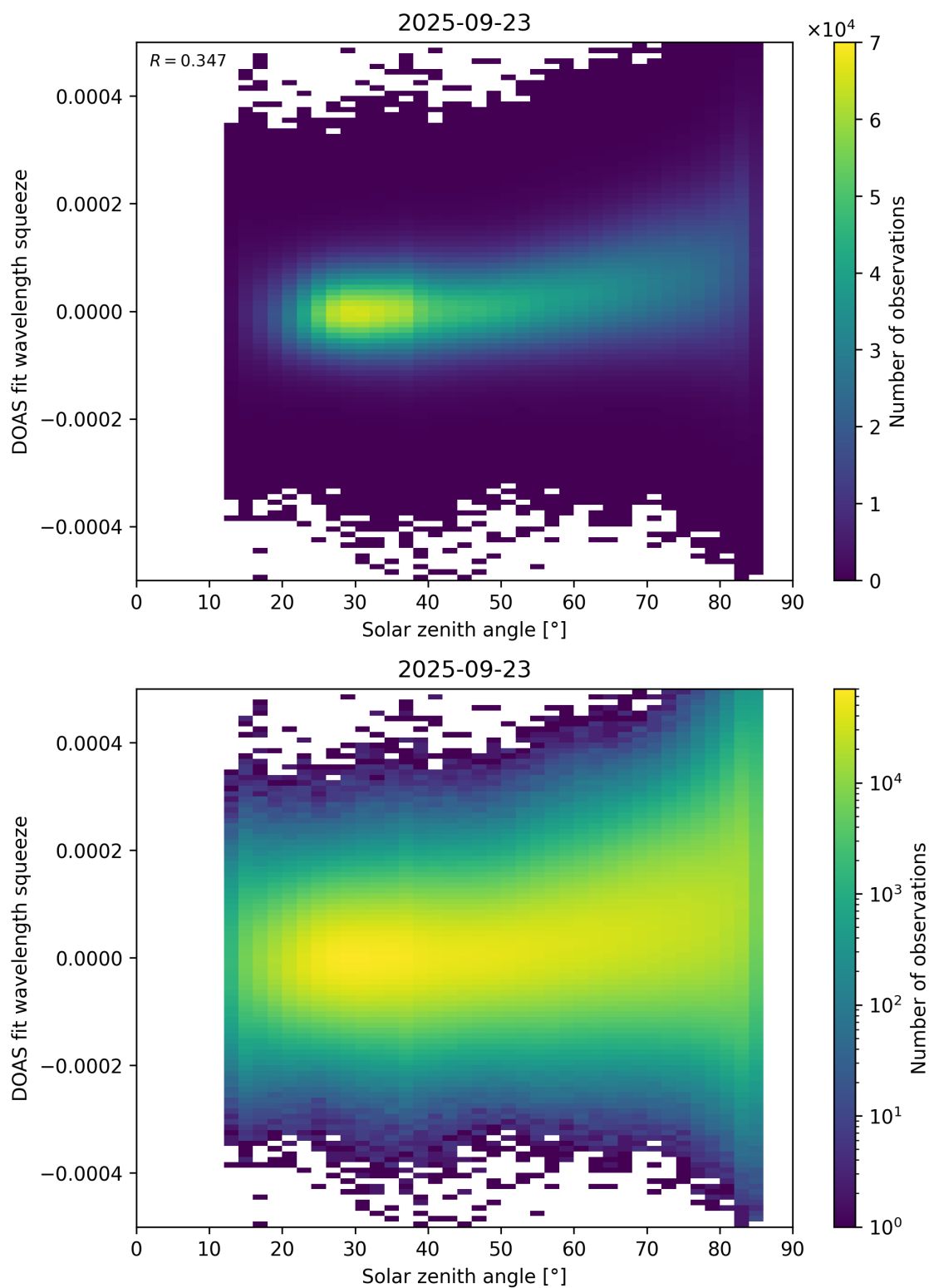
Figure 169: Scatter density plot of “Solar zenith angle” against “DOAS fit wavelength squeeze” for 2025-09-22 to 2025-09-24.
