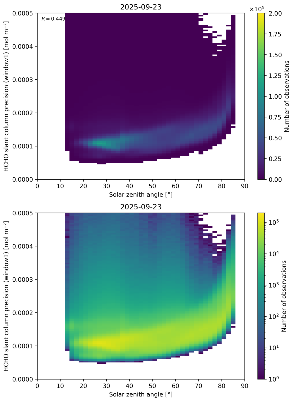
Figure 174: Scatter density plot of “Solar zenith angle” against “HCHO slant column precision (window1)” for 2025-09-22 to 2025-09-24.
