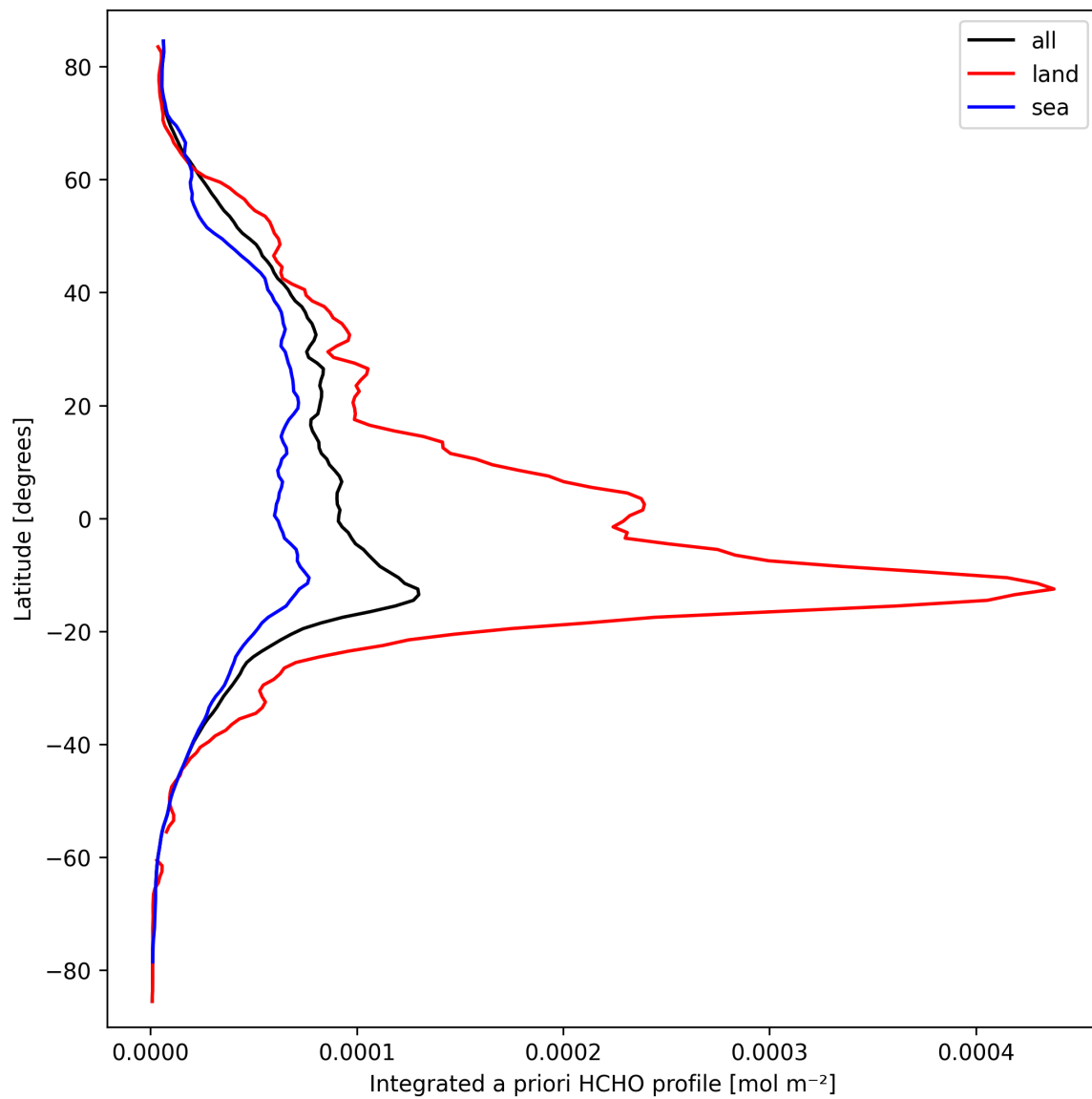
Figure 29: Zonal average of “Integrated a priori HCHO profile” for 2025-09-22 to 2025-09-24.
