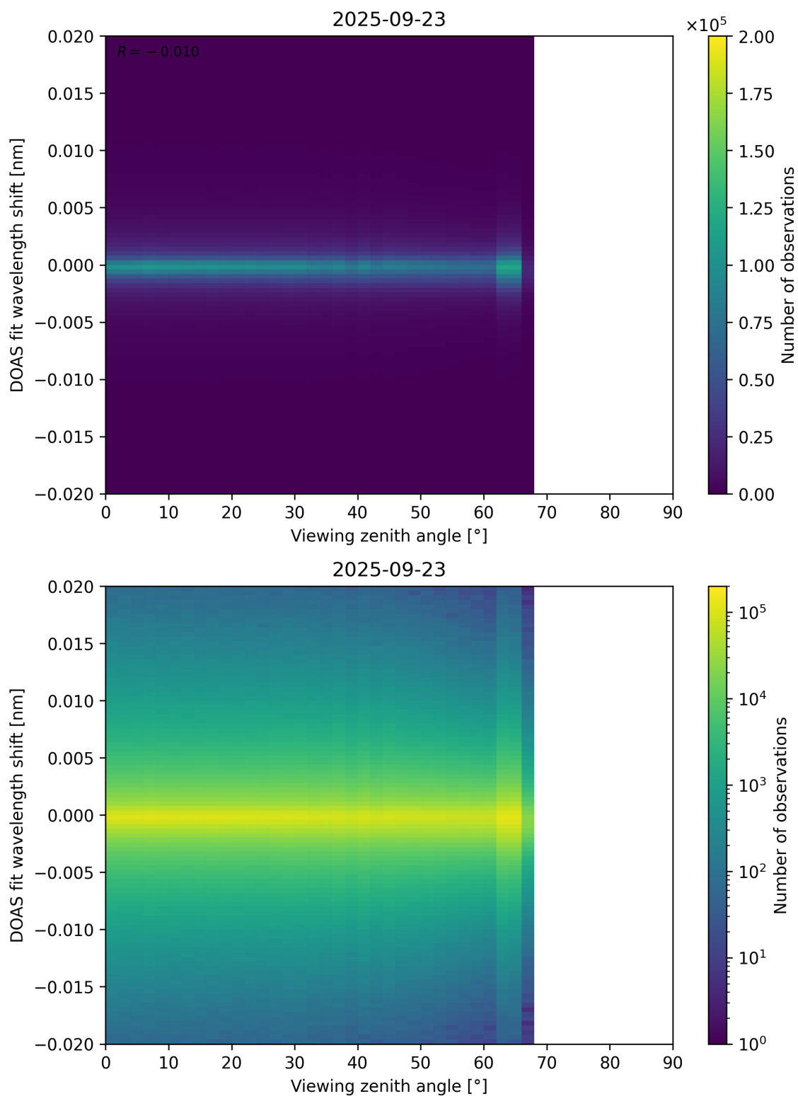
Figure 183: Scatter density plot of “Viewing zenith angle” against “DOAS fit wavelength shift” for 2025-09-22 to 2025-09-24.
