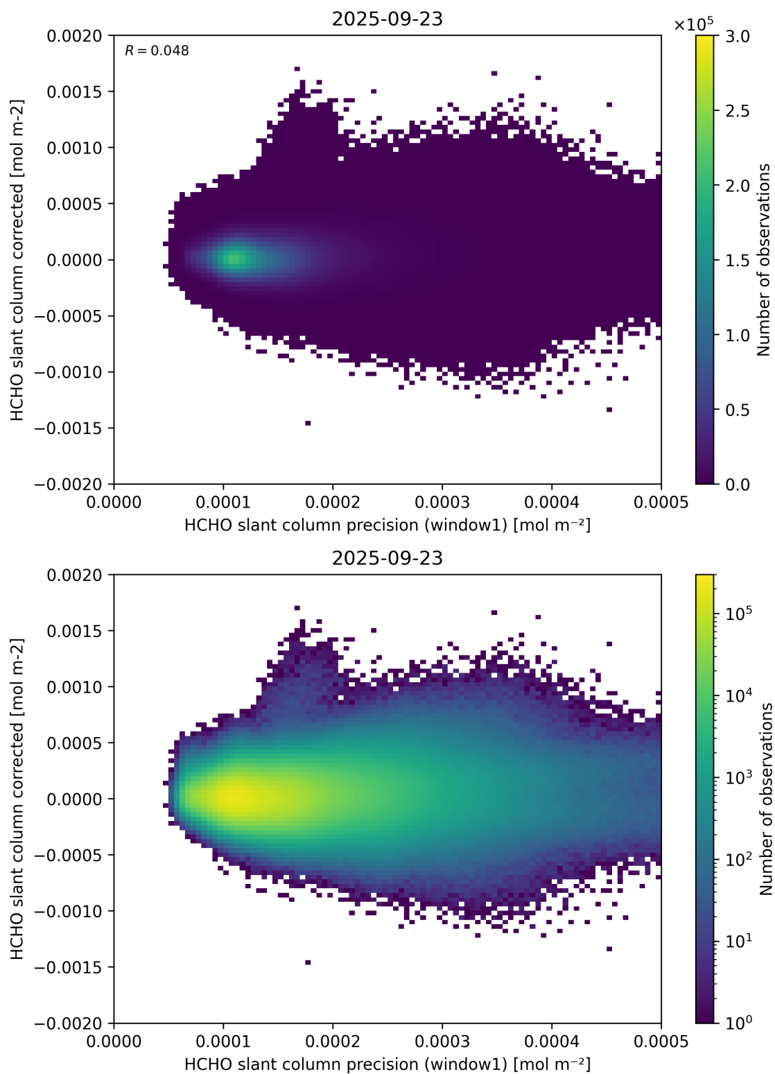
Figure 92: Scatter density plot of “HCHO slant column precision (window1)” against “HCHO slant column corrected” for 2025-09-22 to 2025-09-24.
