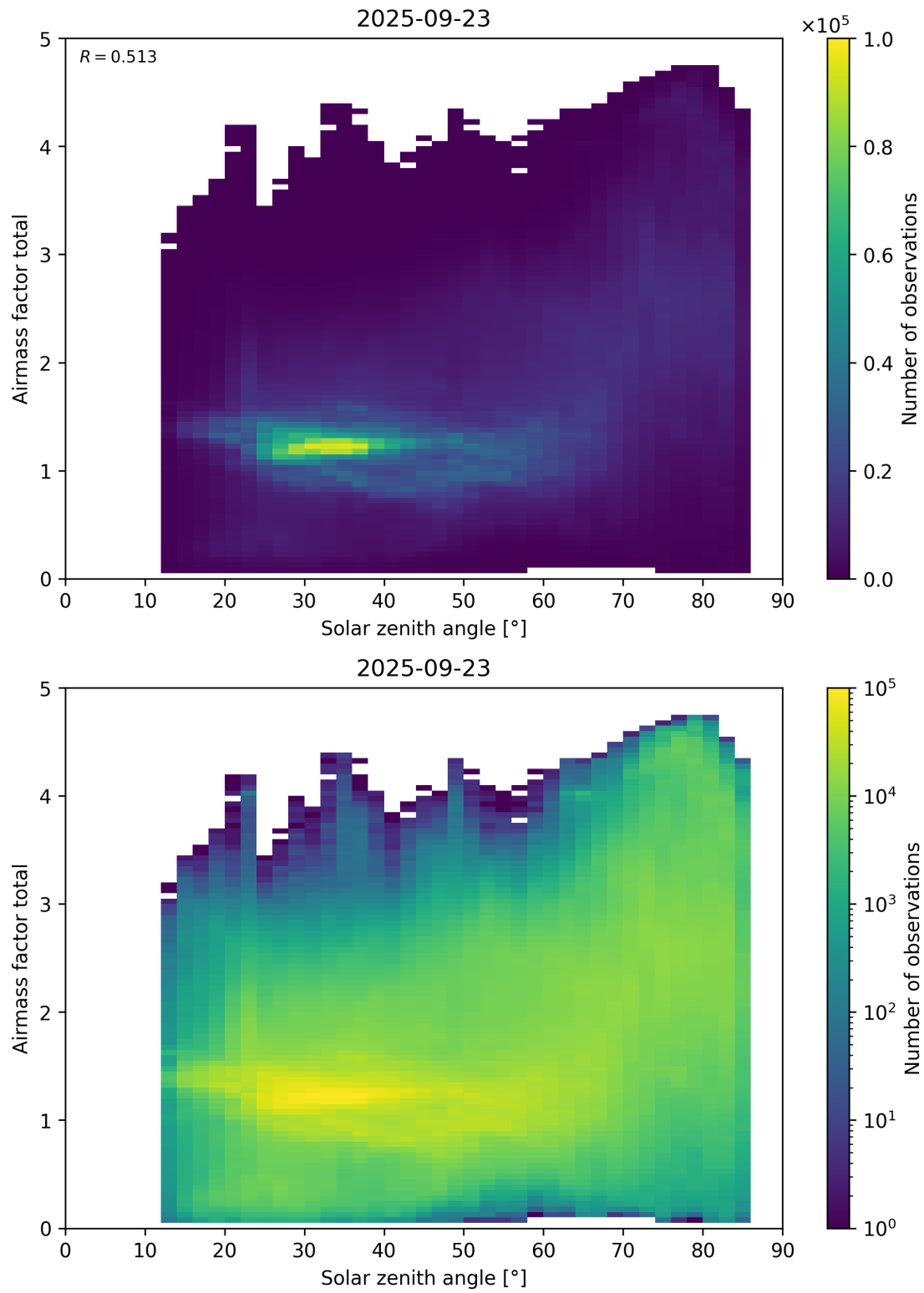
Figure 175: Scatter density plot of “Solar zenith angle” against “Airmass factor total” for 2025-09-22 to 2025-09-24.
