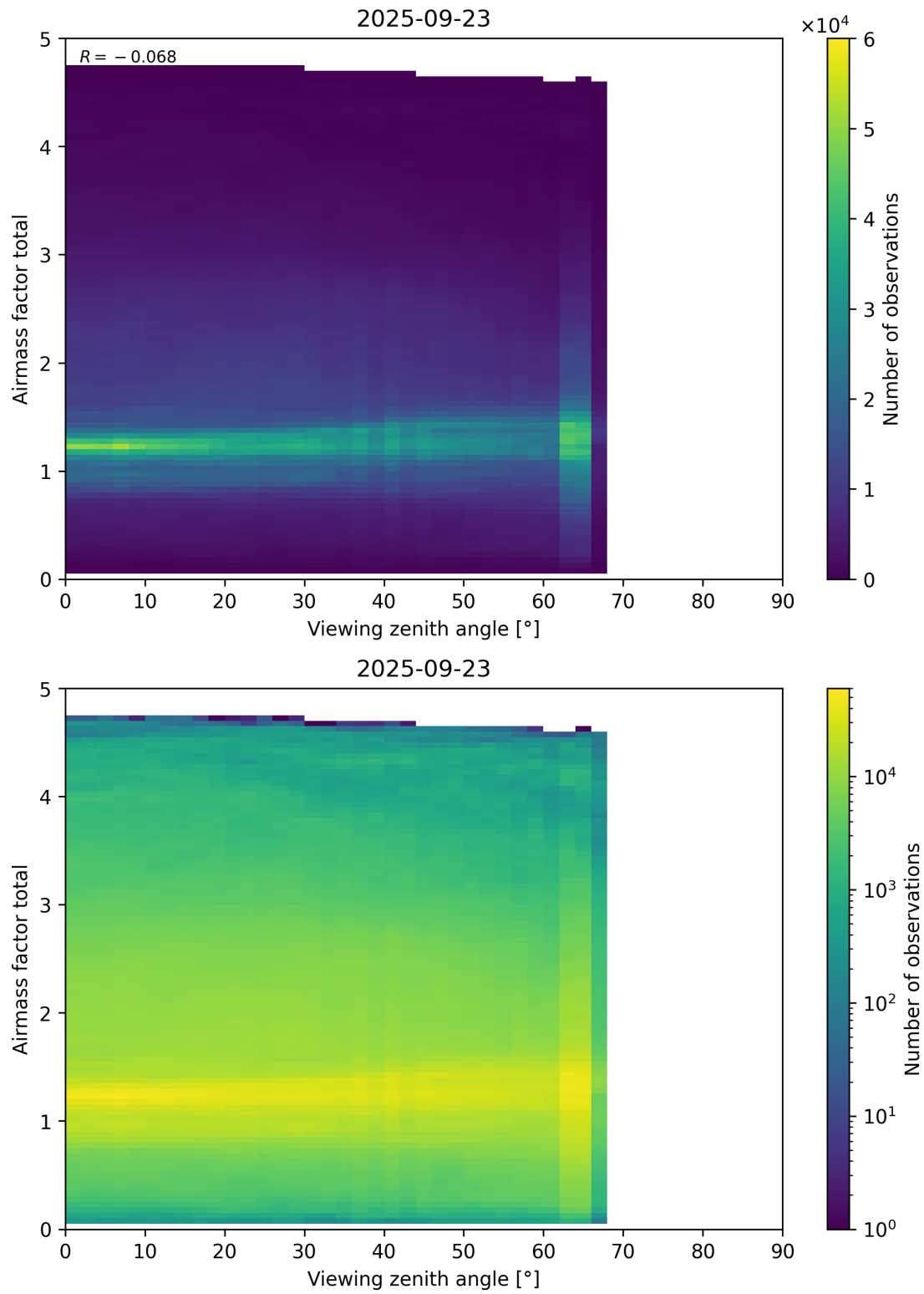
Figure 190: Scatter density plot of “Viewing zenith angle” against “Airmass factor total” for 2025-09-22 to 2025-09-24.
