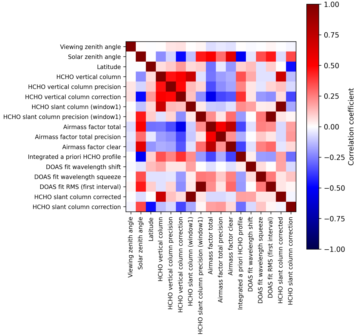
Figure 2: Map of correlation matrix for 2025-09-22 to 2025-09-24.
