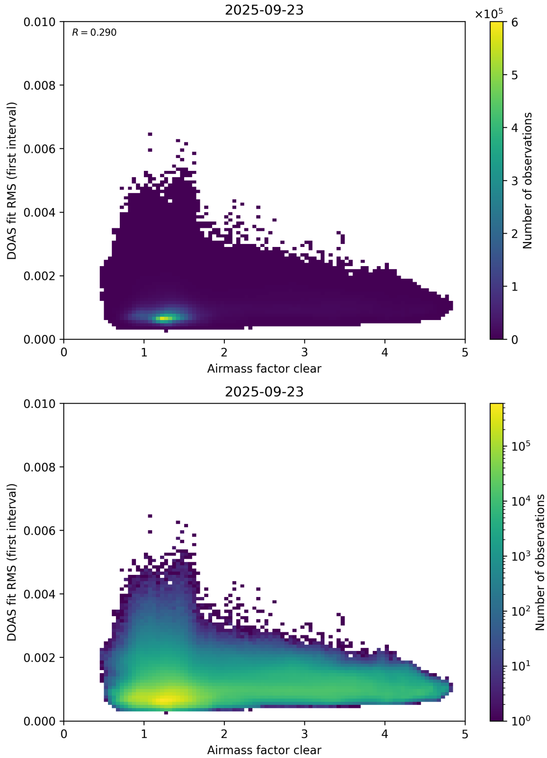
Figure 71: Scatter density plot of “Airmass factor clear” against “DOAS fit RMS (first interval)” for 2025-09-22 to 2025-09-24.
