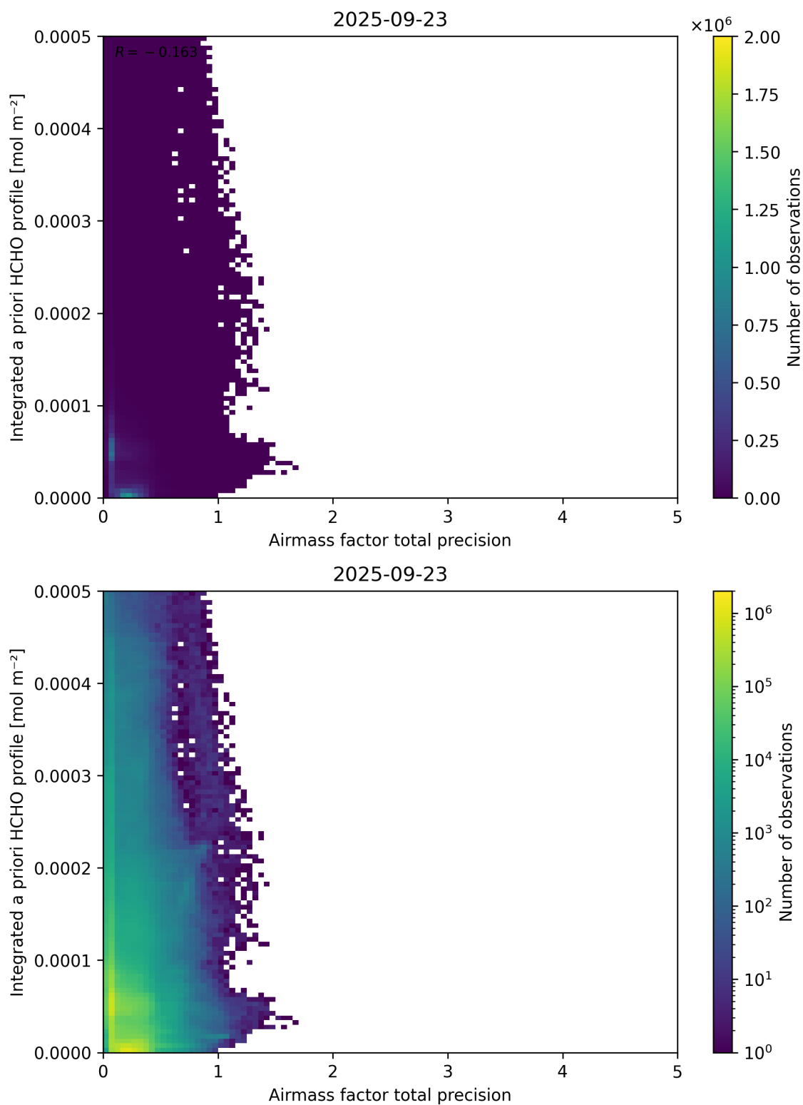
Figure 111: Scatter density plot of “Airmass factor total precision” against “Integrated a priori HCHO profile” for 2025-09-22 to 2025-09-24.
