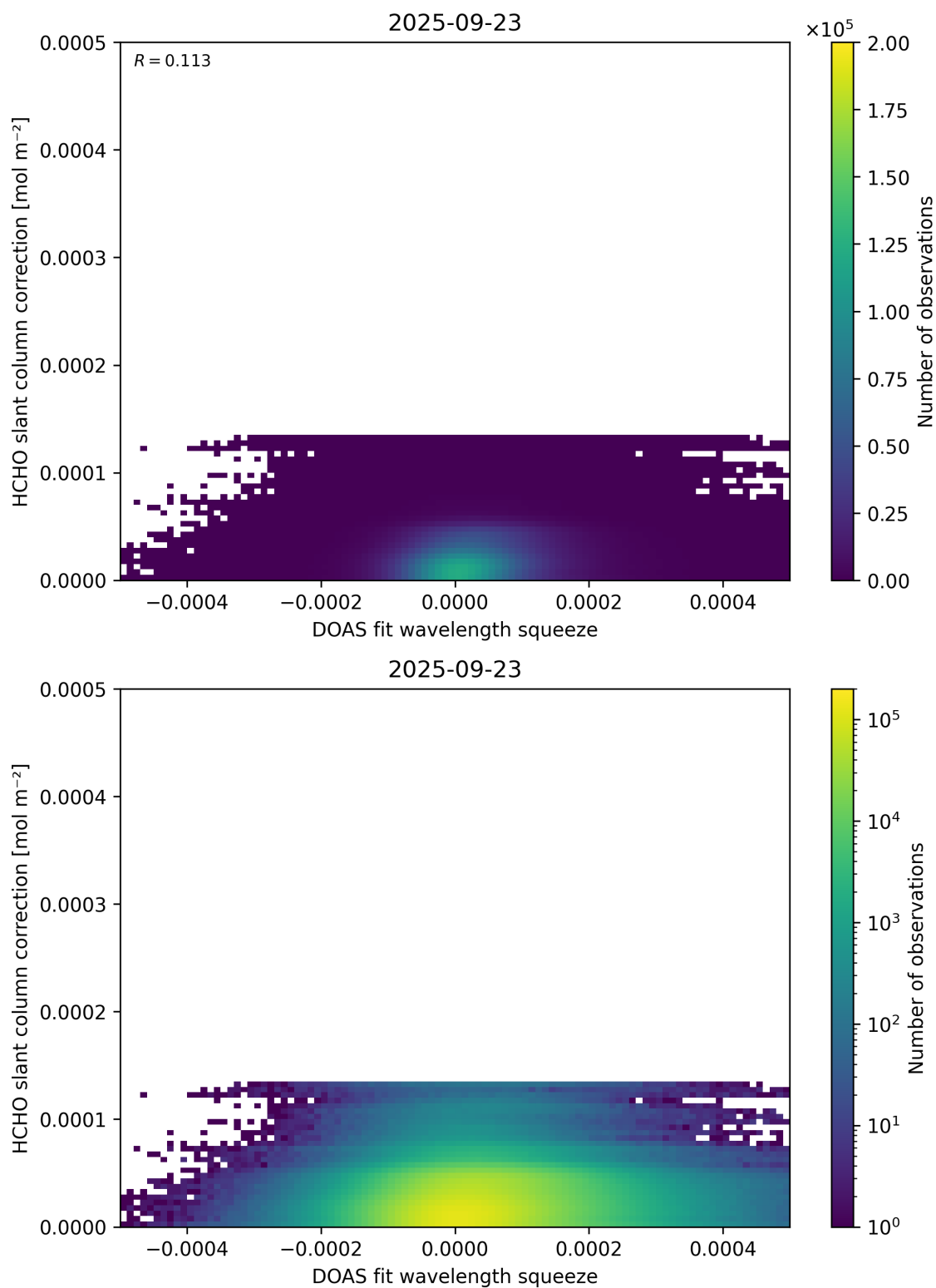
Figure 70: Scatter density plot of “DOAS fit wavelength squeeze” against “HCHO slant column correction” for 2025-09-22 to 2025-09-24.
