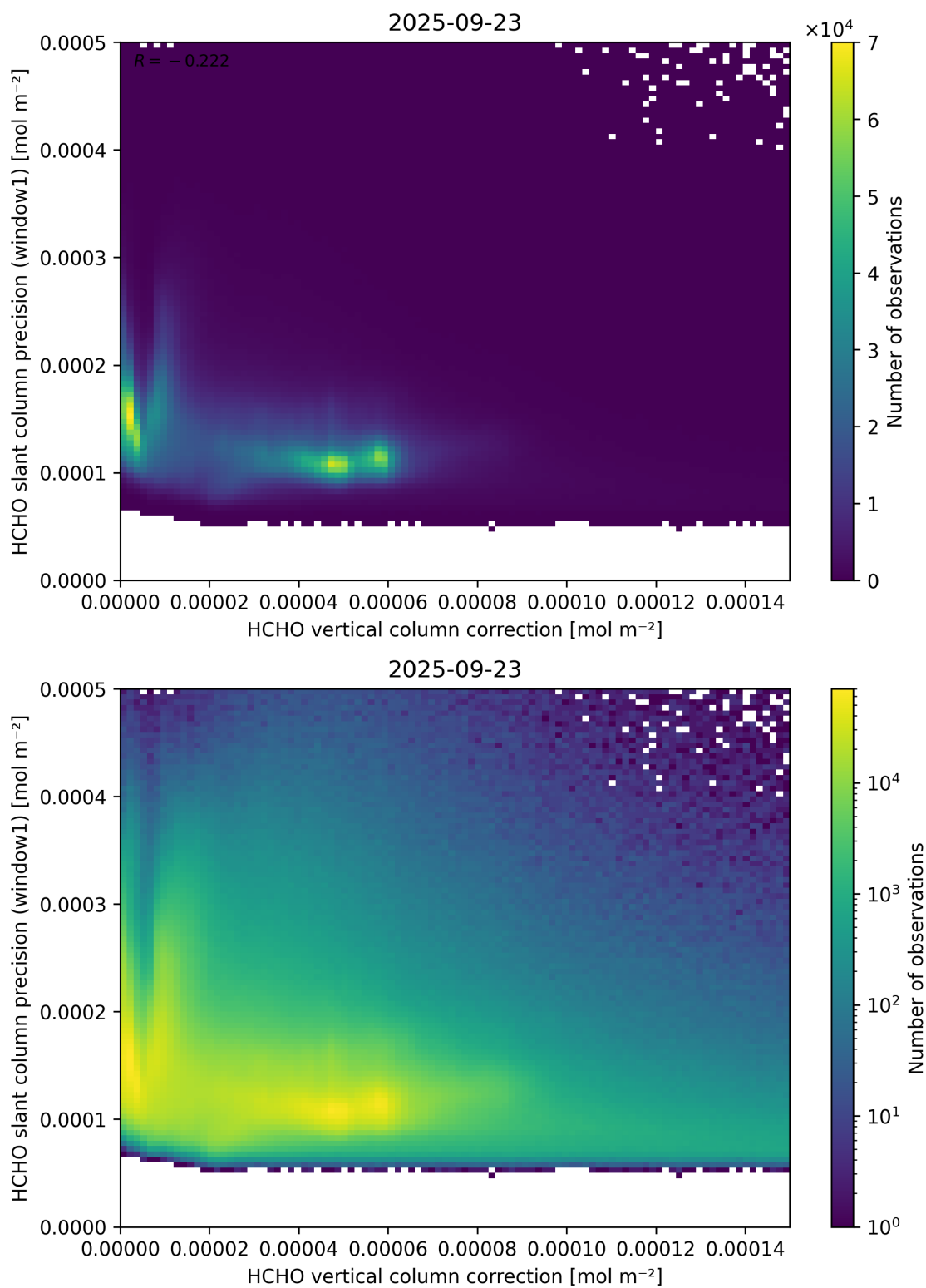
Figure 119: Scatter density plot of “HCHO vertical column correction” against “HCHO slant column precision (window1)” for 2025-09-22 to 2025-09-24.
