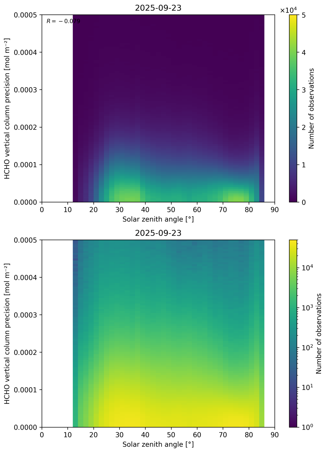
Figure 179: Scatter density plot of “Solar zenith angle” against “HCHO vertical column precision” for 2025-09-22 to 2025-09-24.
