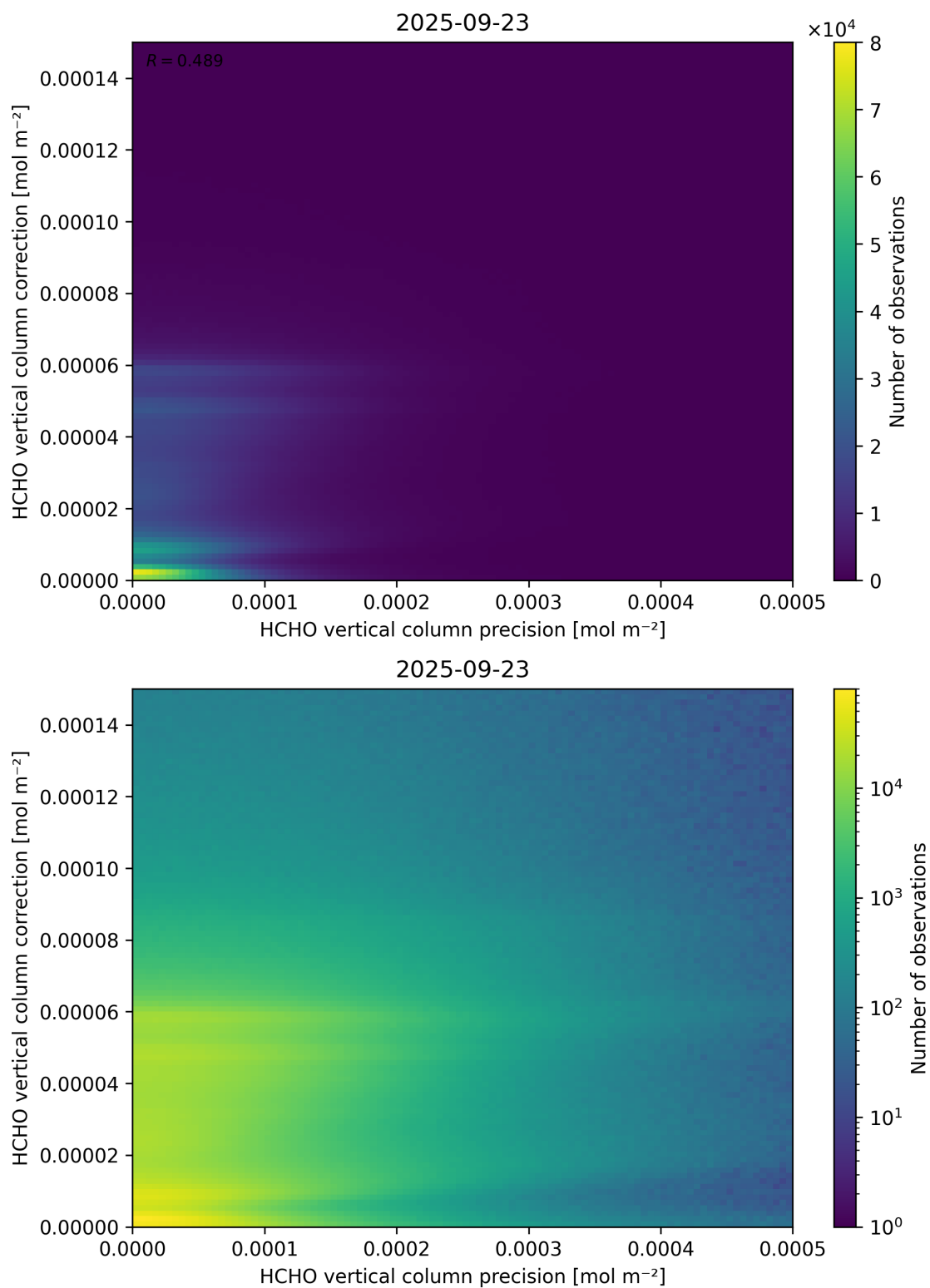
Figure 146: Scatter density plot of “HCHO vertical column precision” against “HCHO vertical column correction” for 2025-09-22 to 2025-09-24.
