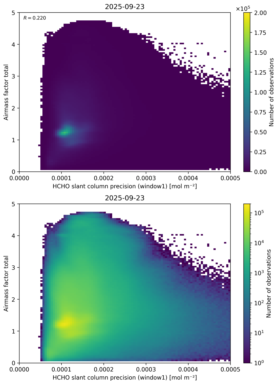
Figure 94: Scatter density plot of “HCHO slant column precision (window1)” against “Airmass factor total” for 2025-09-22 to 2025-09-24.
