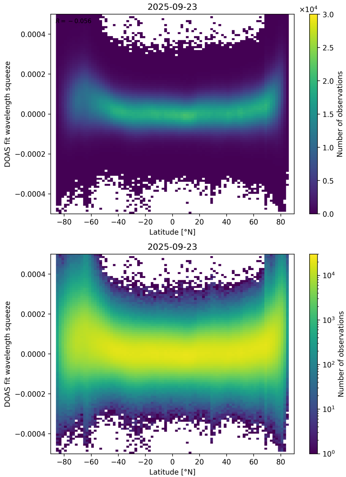
Figure 155: Scatter density plot of “Latitude” against “DOAS fit wavelength squeeze” for 2025-09-22 to 2025-09-24.
