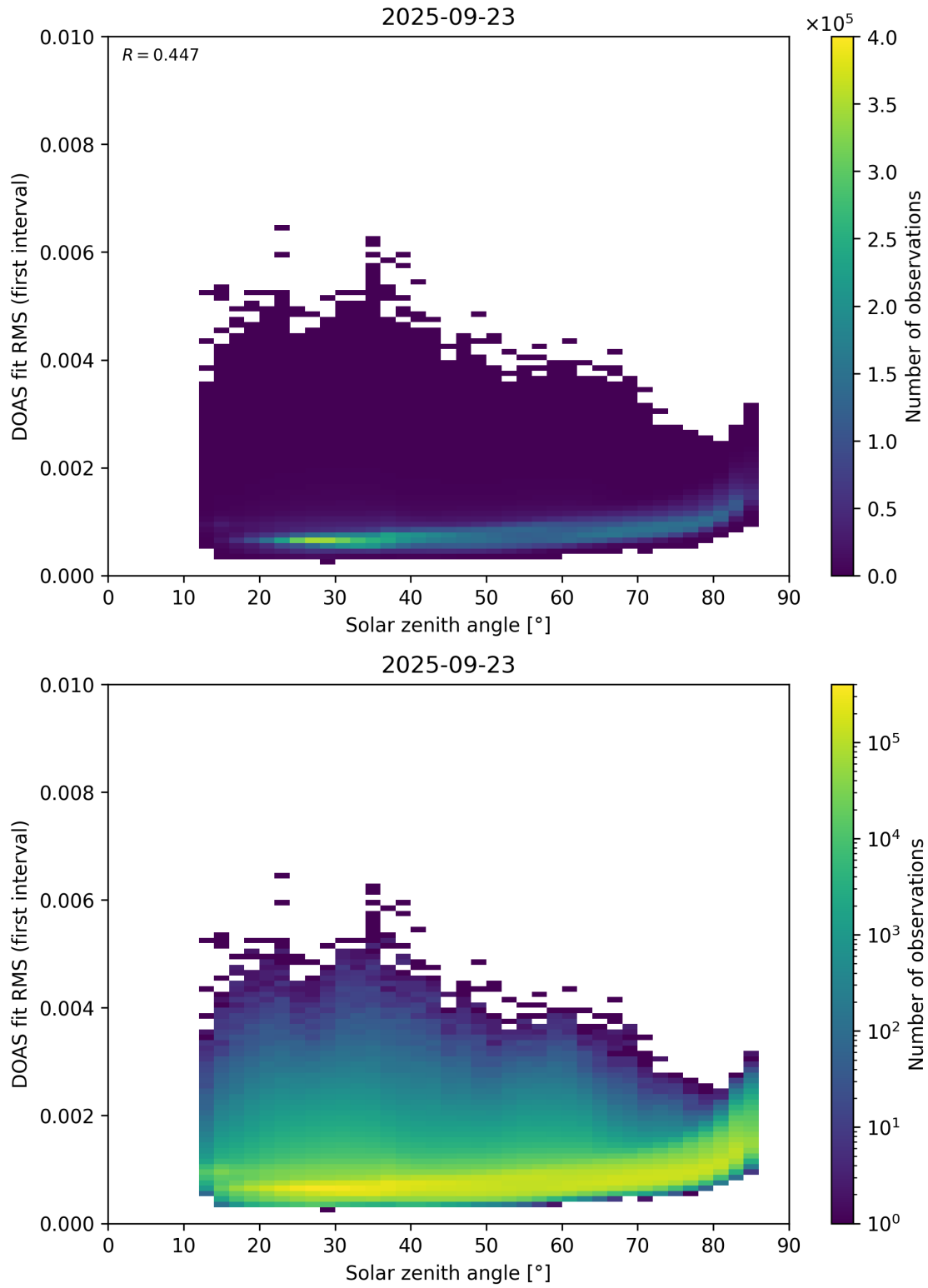
Figure 167: Scatter density plot of “Solar zenith angle” against “DOAS fit RMS (first interval)” for 2025-09-22 to 2025-09-24.
