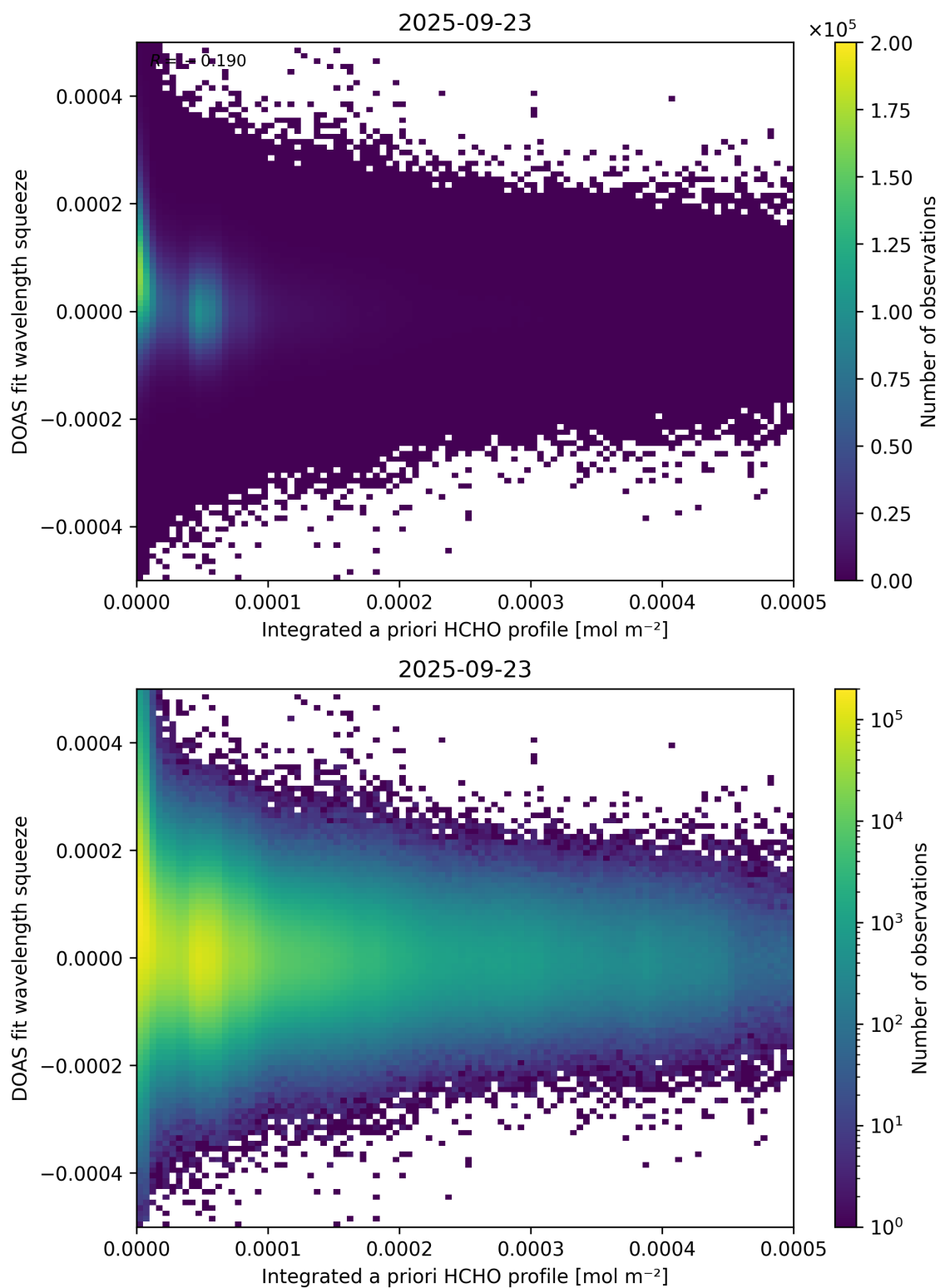
Figure 150: Scatter density plot of “Integrated a priori HCHO profile” against “DOAS fit wavelength squeeze” for 2025-09-22 to 2025-09-24.
