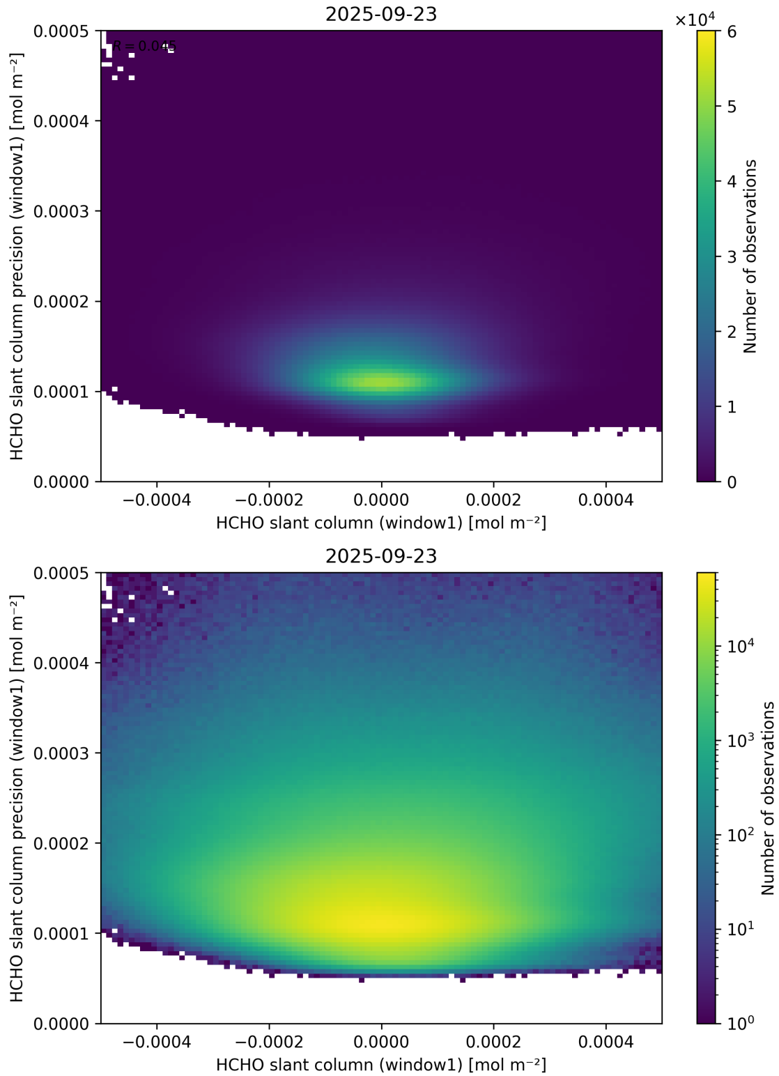
Figure 84: Scatter density plot of “HCHO slant column (window1)” against “HCHO slant column precision (window1)” for 2025-09-22 to 2025-09-24.
