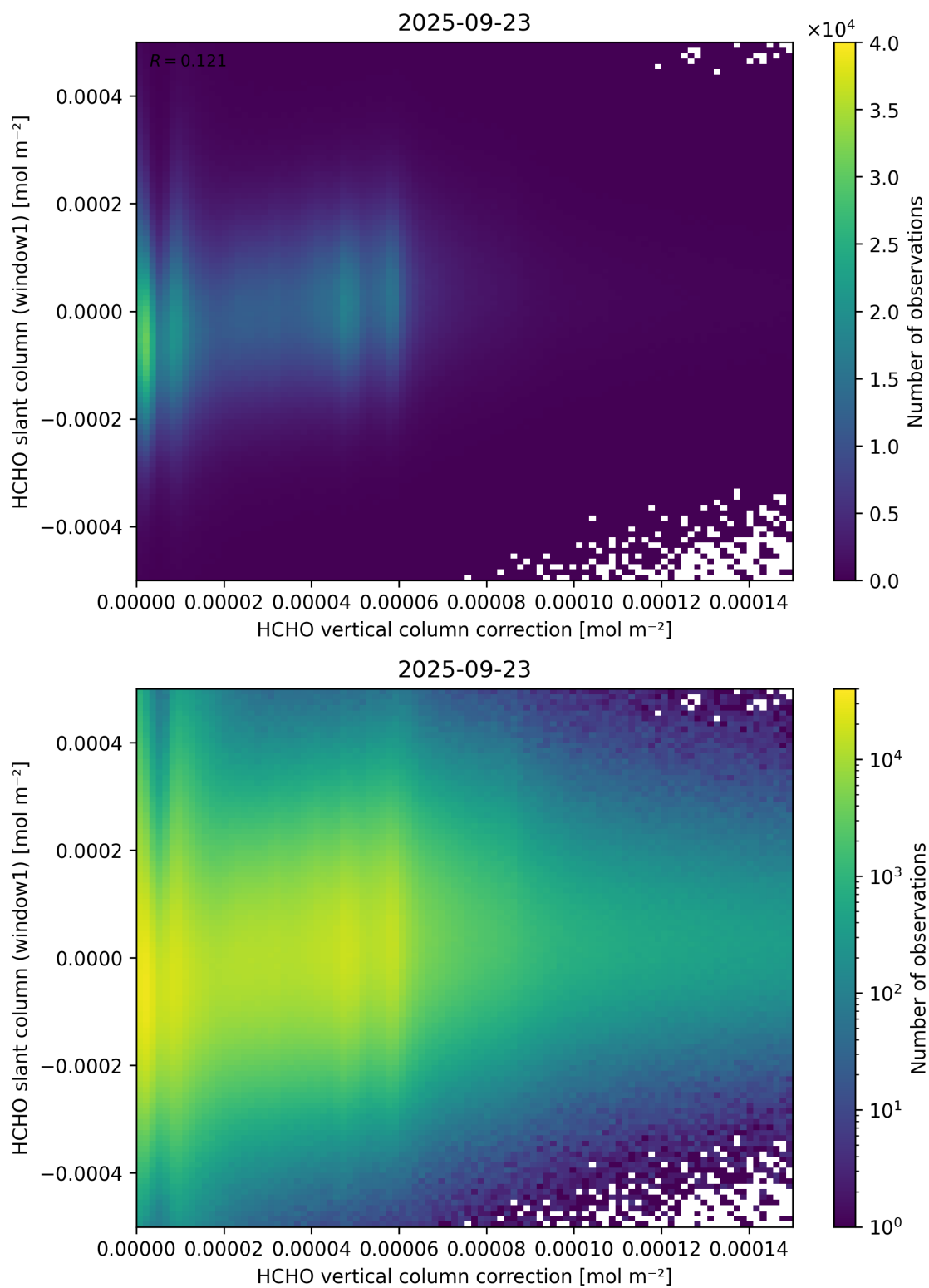
Figure 118: Scatter density plot of “HCHO vertical column correction” against “HCHO slant column (window1)” for 2025-09-22 to 2025-09-24.
