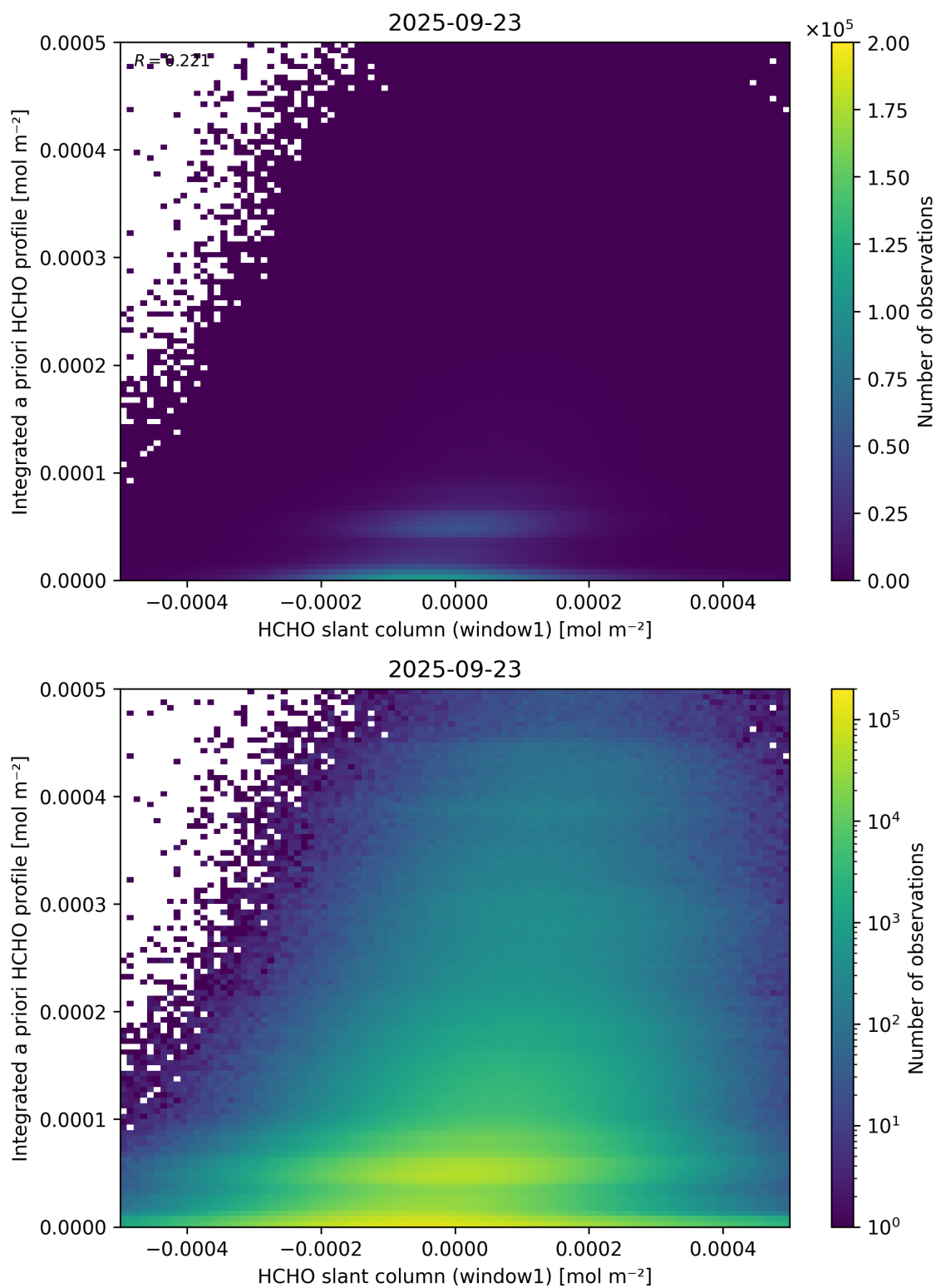
Figure 87: Scatter density plot of “HCHO slant column (window1)” against “Integrated a priori HCHO profile” for 2025-09-22 to 2025-09-24.
