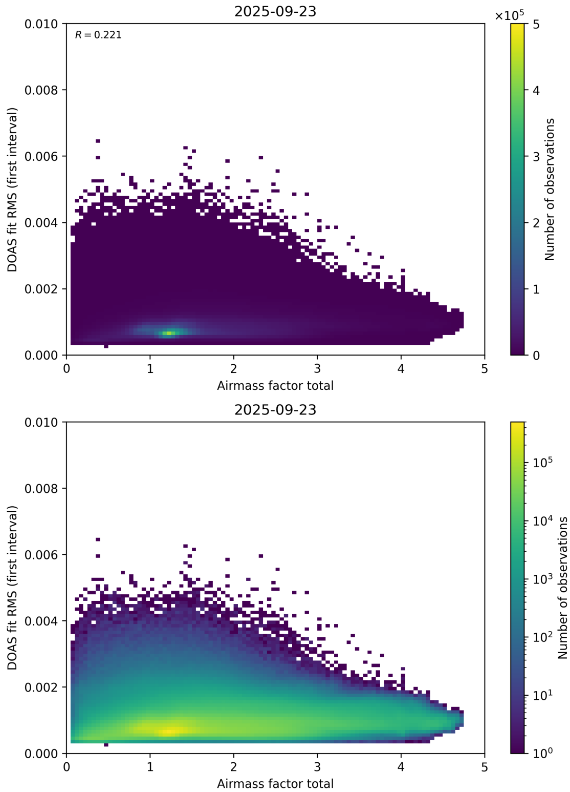
Figure 97: Scatter density plot of “Airmass factor total” against “DOAS fit RMS (first interval)” for 2025-09-22 to 2025-09-24.
