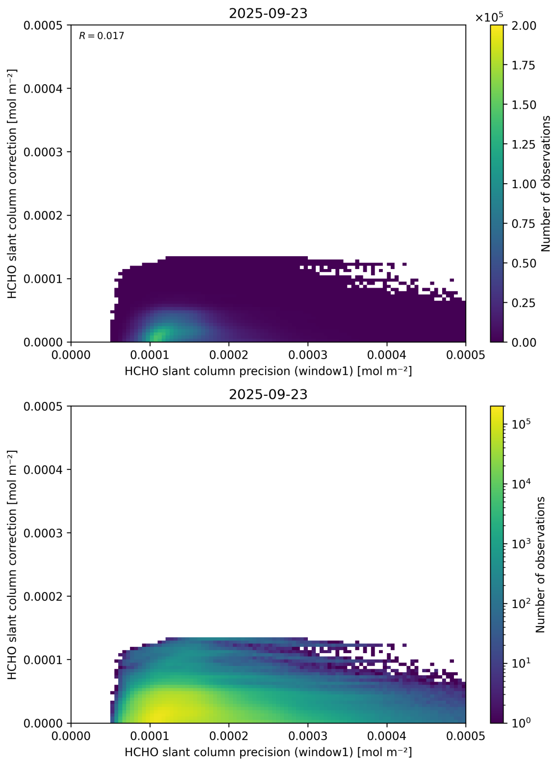
Figure 93: Scatter density plot of “HCHO slant column precision (window1)” against “HCHO slant column correction” for 2025-09-22 to 2025-09-24.
