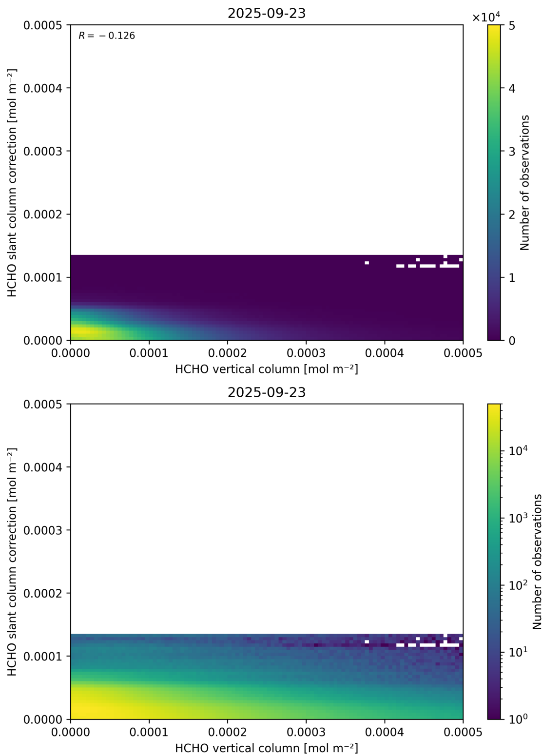
Figure 128: Scatter density plot of “HCHO vertical column” against “HCHO slant column correction” for 2025-09-22 to 2025-09-24.
