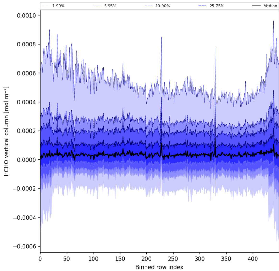
Figure 49: Along track statistics of “HCHO vertical column” for 2025-09-22 to 2025-09-24
