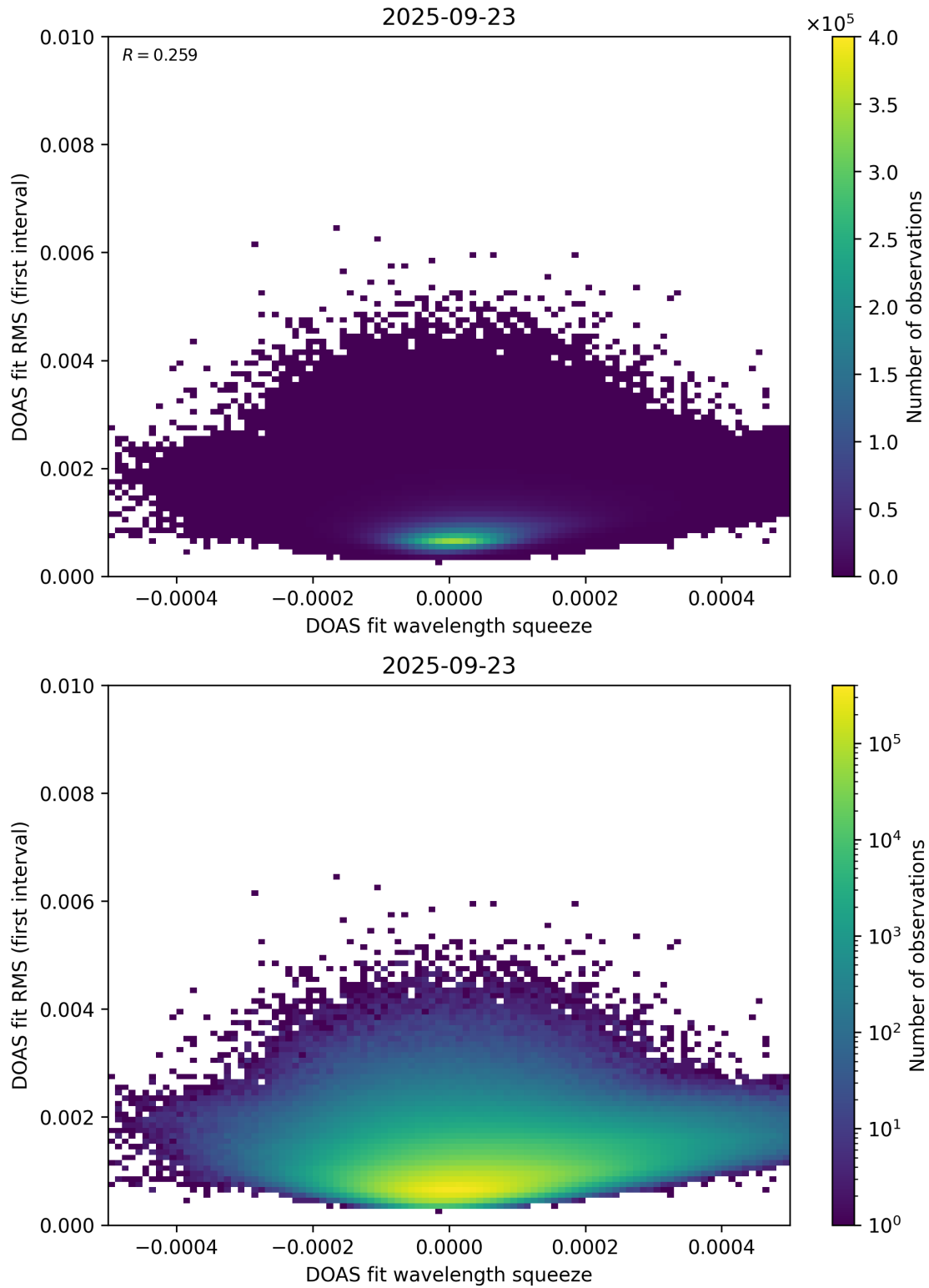
Figure 68: Scatter density plot of “DOAS fit wavelength squeeze” against “DOAS fit RMS (first interval)” for 2025-09-22 to 2025-09-24.
