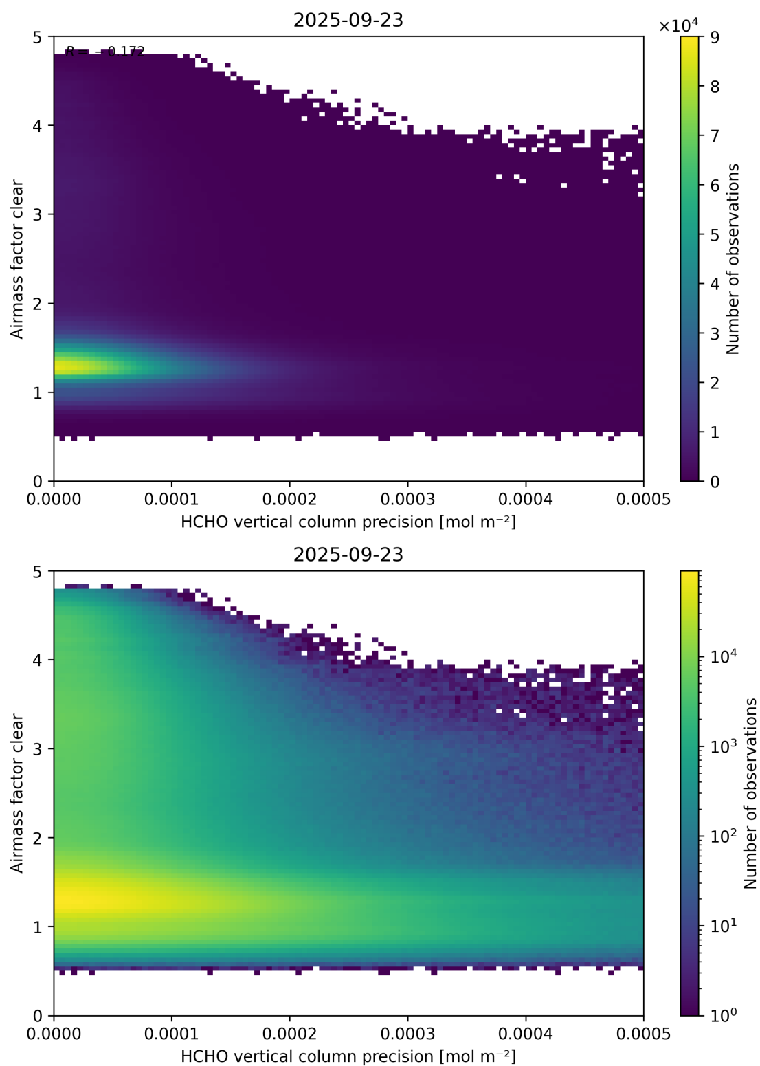
Figure 139: Scatter density plot of “HCHO vertical column precision” against “Airmass factor clear” for 2025-09-22 to 2025-09-24.
