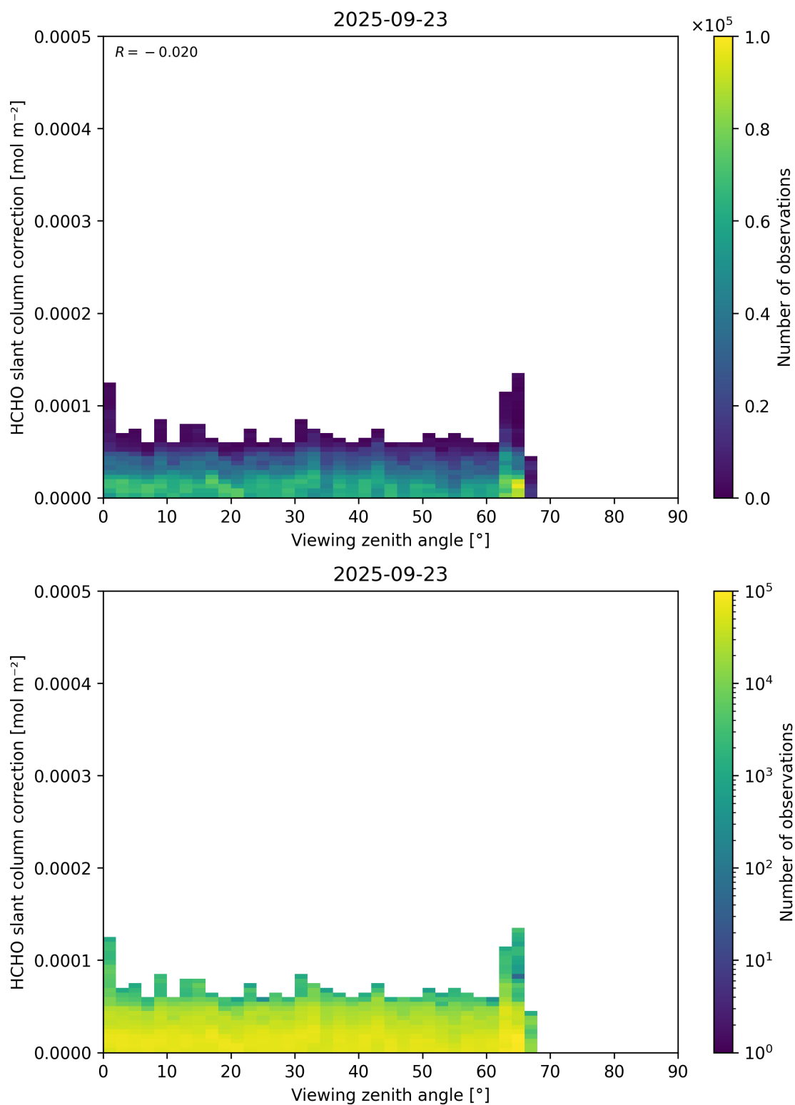
Figure 187: Scatter density plot of “Viewing zenith angle” against “HCHO slant column correction” for 2025-09-22 to 2025-09-24.
