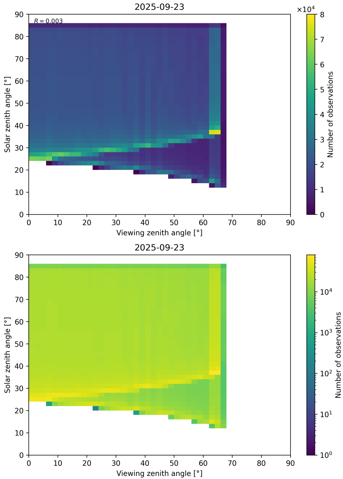
Figure 197: Scatter density plot of “Viewing zenith angle” against “Solar zenith angle” for 2025-09-22 to 2025-09-24.
