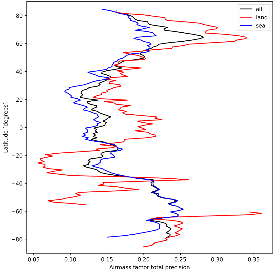
Figure 27: Zonal average of “Airmass factor total precision” for 2025-09-22 to 2025-09-24.
