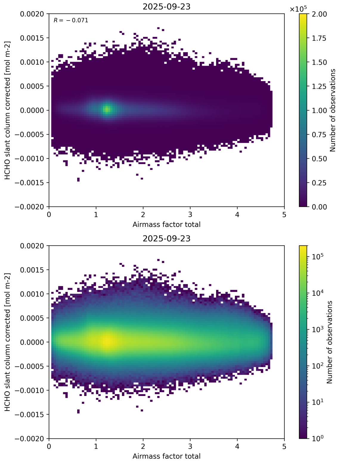
Figure 101: Scatter density plot of “Airmass factor total” against “HCHO slant column corrected” for 2025-09-22 to 2025-09-24.
