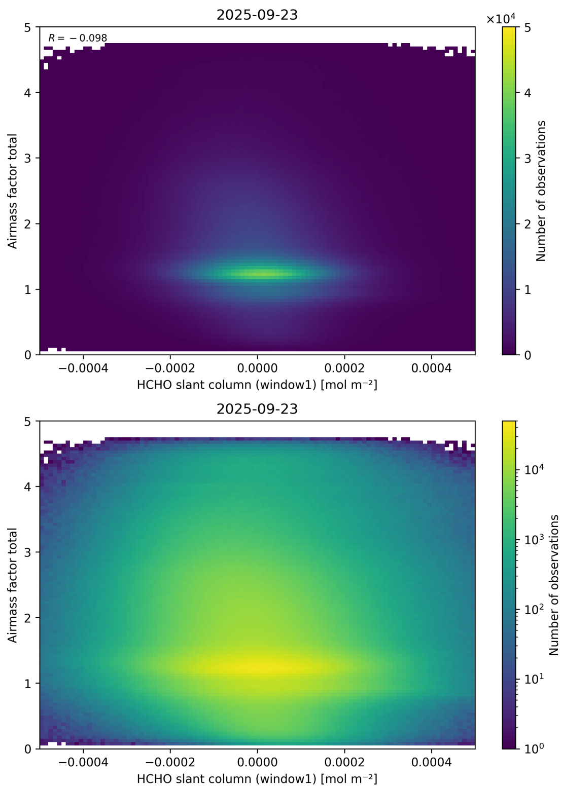
Figure 85: Scatter density plot of “HCHO slant column (window1)” against “Airmass factor total” for 2025-09-22 to 2025-09-24.
