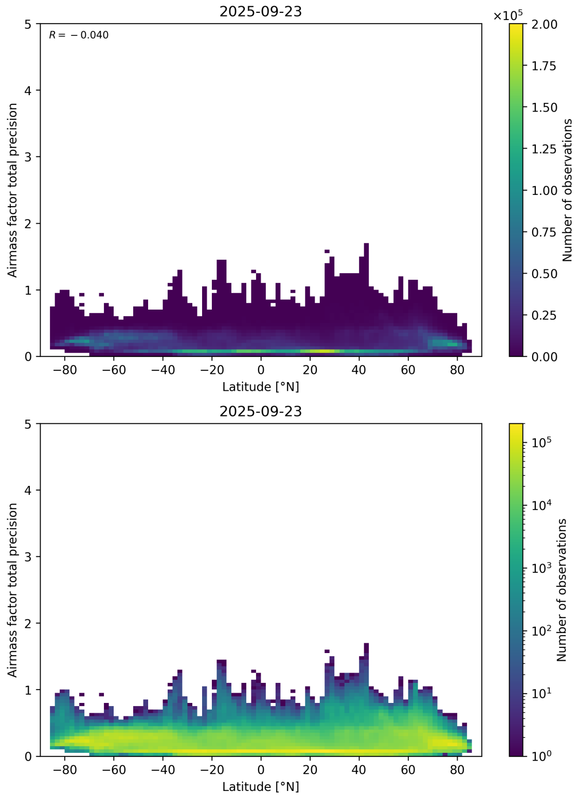
Figure 162: Scatter density plot of “Latitude” against “Airmass factor total precision” for 2025-09-22 to 2025-09-24.
