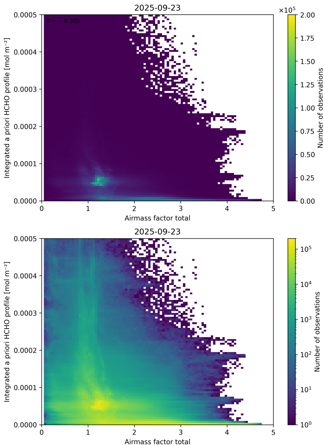
Figure 104: Scatter density plot of “Airmass factor total” against “Integrated a priori HCHO profile” for 2025-09-22 to 2025-09-24.
