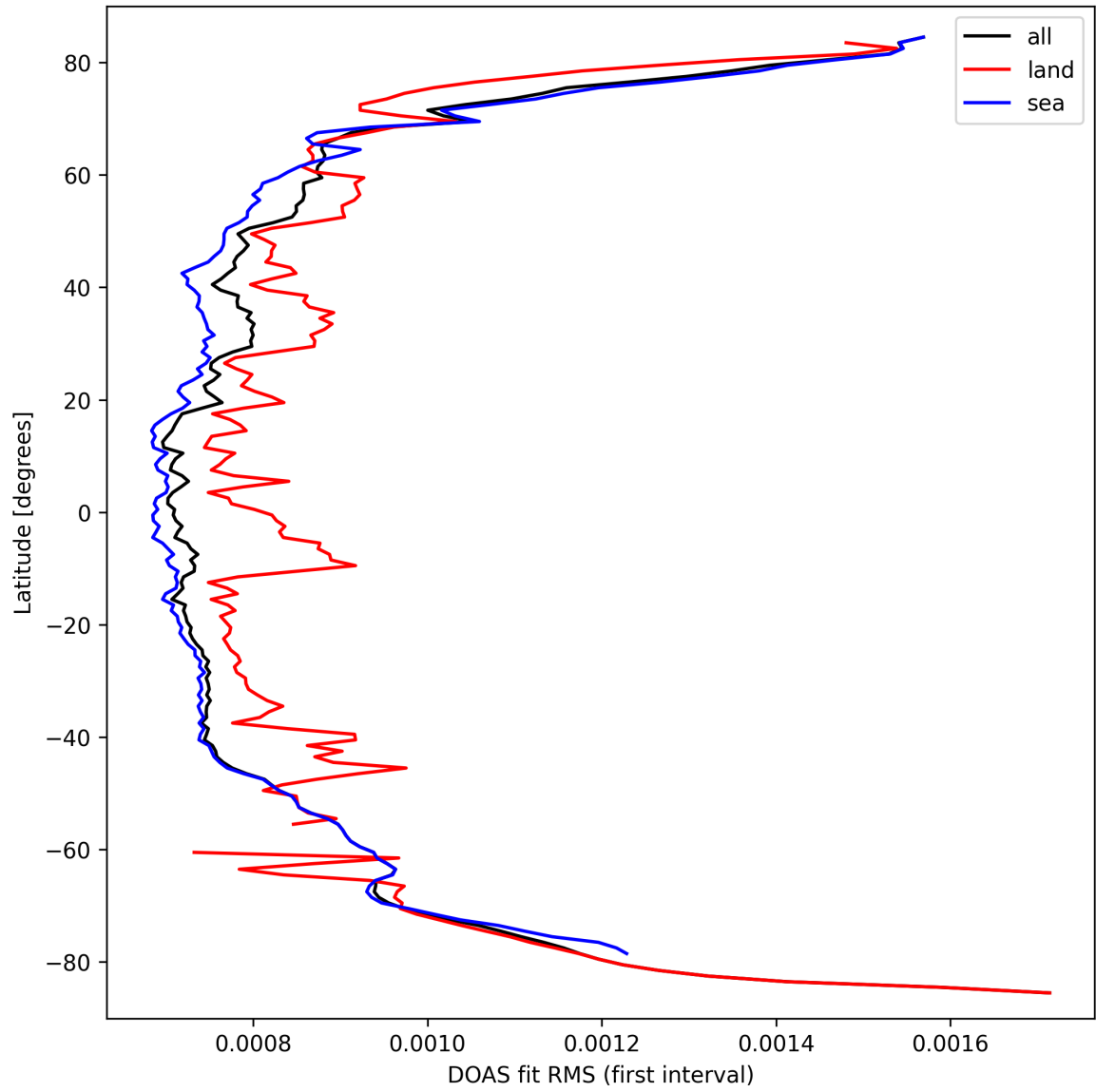
Figure 32: Zonal average of “DOAS fit RMS (first interval)” for 2025-09-22 to 2025-09-24.
