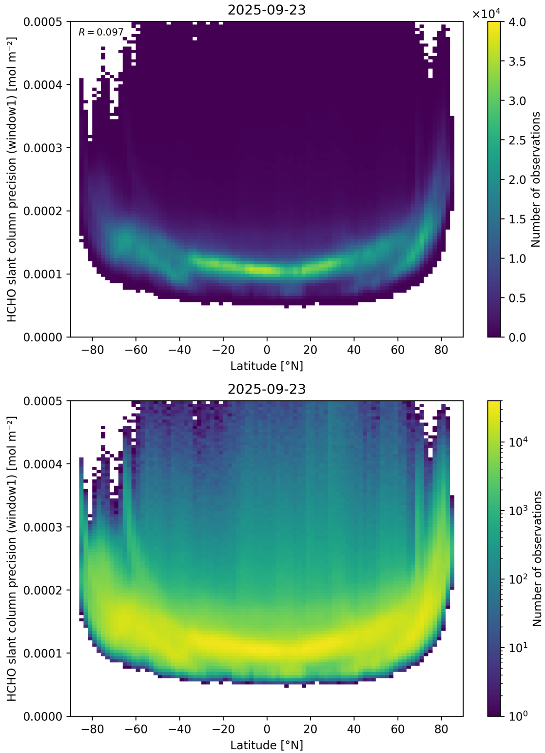
Figure 160: Scatter density plot of “Latitude” against “HCHO slant column precision (window1)” for 2025-09-22 to 2025-09-24.
