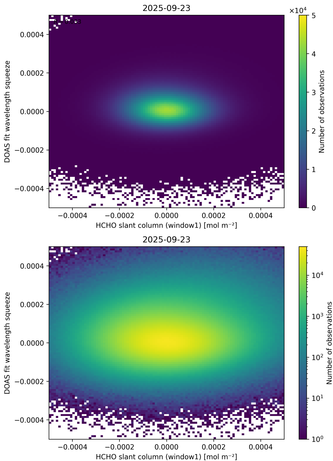
Figure 80: Scatter density plot of “HCHO slant column (window1)” against “DOAS fit wavelength squeeze” for 2025-09-22 to 2025-09-24.
