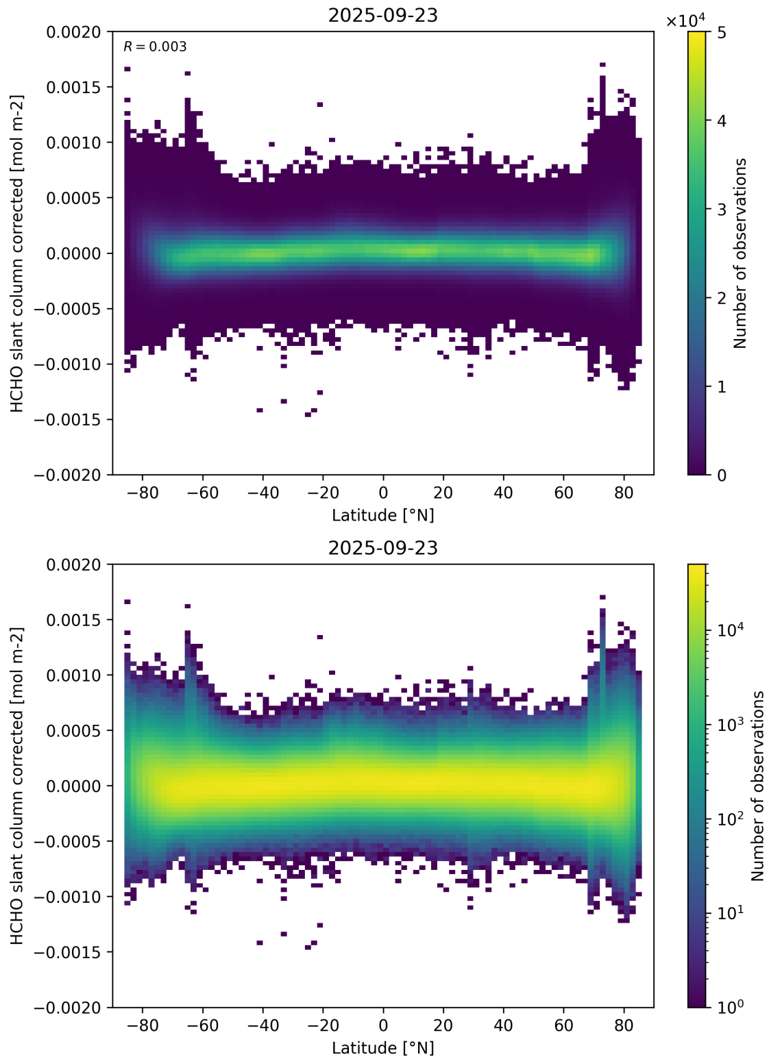
Figure 157: Scatter density plot of “Latitude” against “HCHO slant column corrected” for 2025-09-22 to 2025-09-24.
