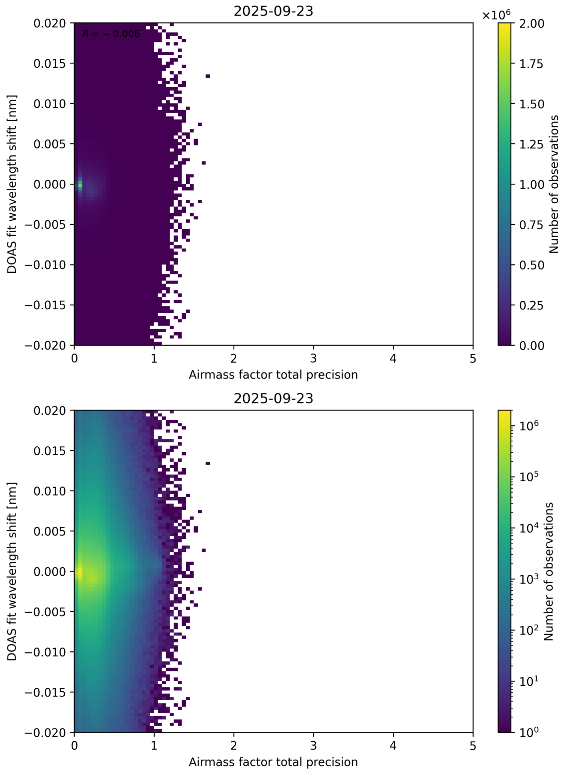
Figure 106: Scatter density plot of “Airmass factor total precision” against “DOAS fit wavelength shift” for 2025-09-22 to 2025-09-24.
