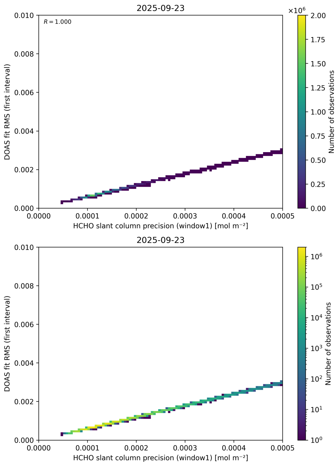
Figure 88: Scatter density plot of “HCHO slant column precision (window1)” against “DOAS fit RMS (first interval)” for 2025-09-22 to 2025-09-24.
