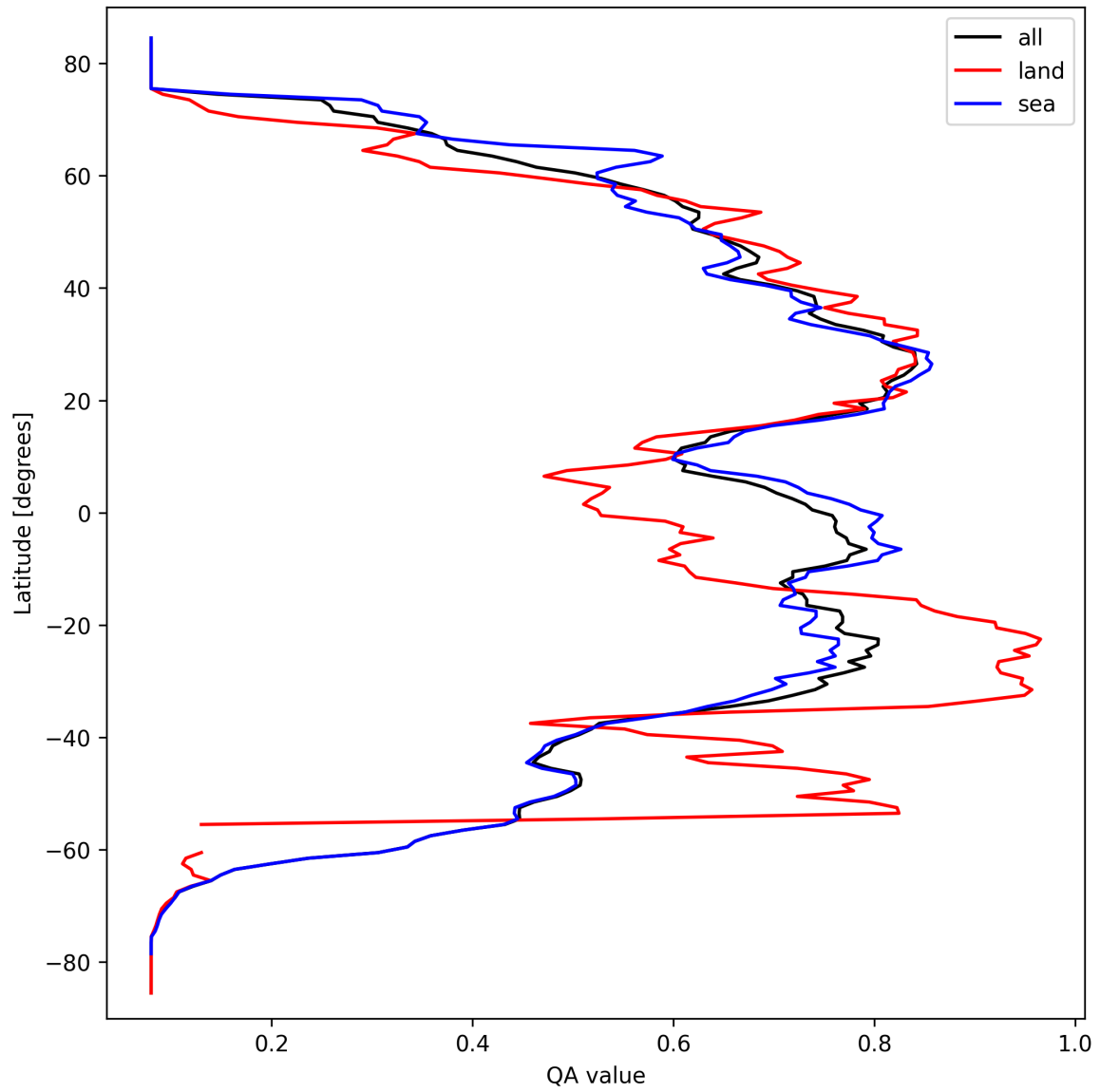
Figure 20: Zonal average of “QA value” for 2025-09-22 to 2025-09-24.
