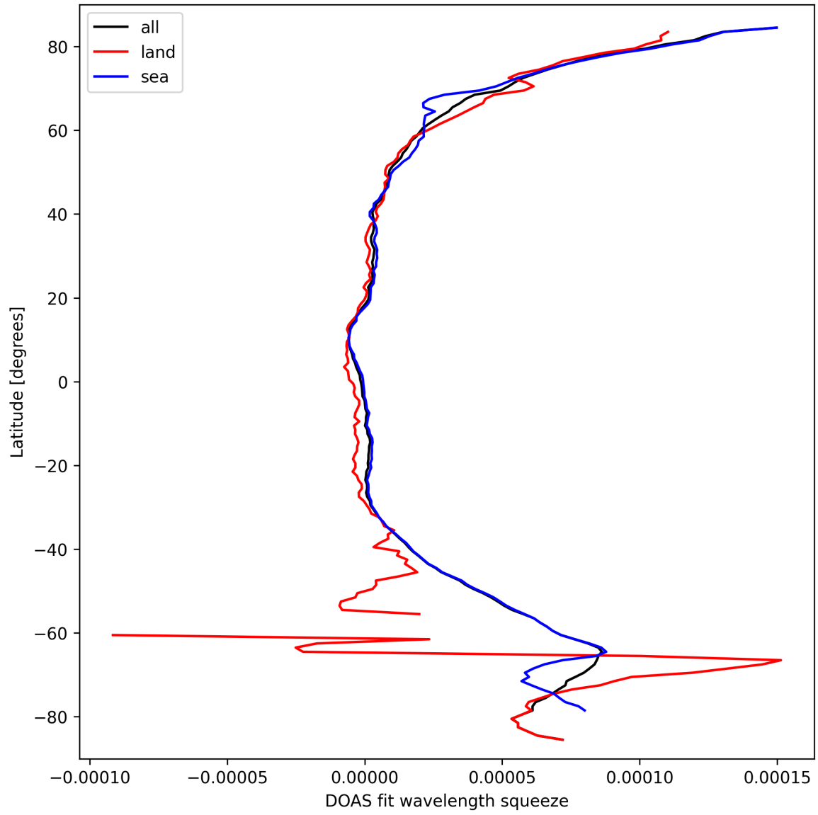
Figure 31: Zonal average of “DOAS fit wavelength squeeze” for 2025-09-22 to 2025-09-24.
