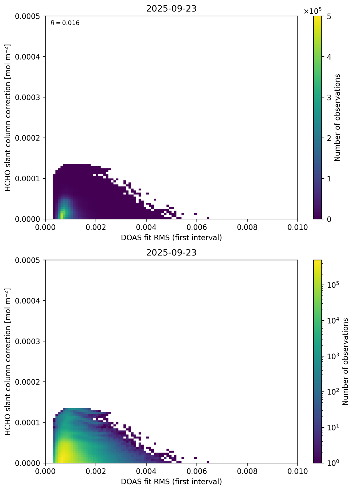
Figure 63: Scatter density plot of “DOAS fit RMS (first interval)” against “HCHO slant column correction” for 2025-09-22 to 2025-09-24.
