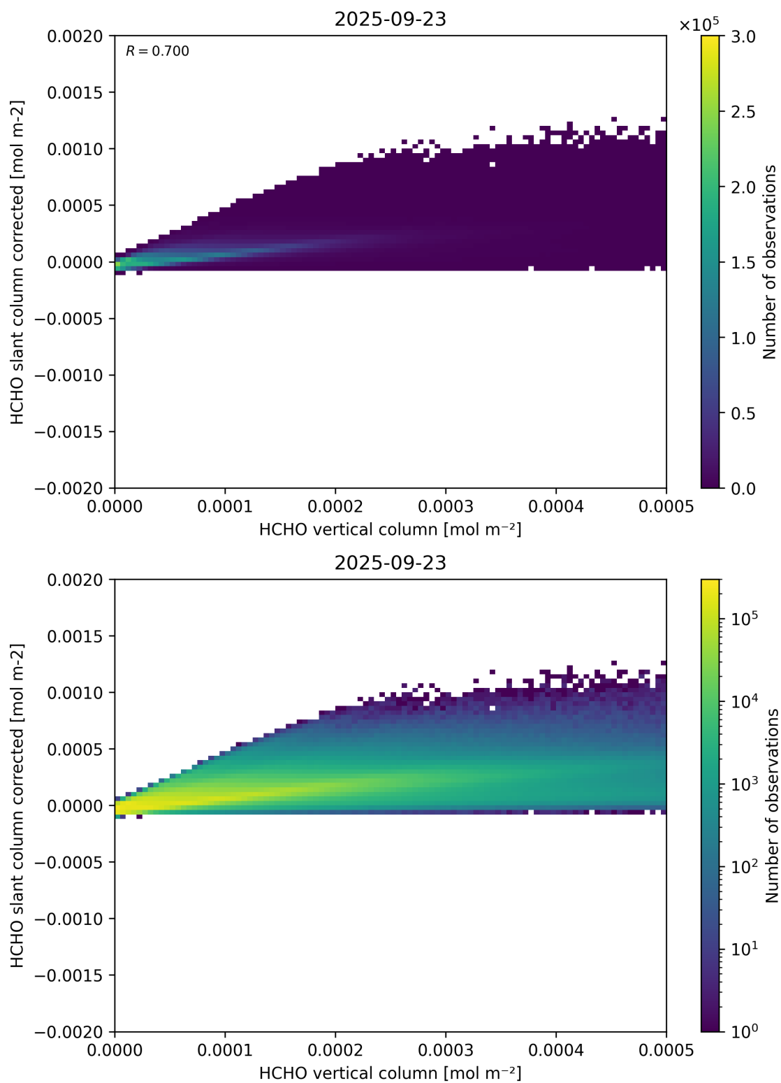
Figure 127: Scatter density plot of “HCHO vertical column” against “HCHO slant column corrected” for 2025-09-22 to 2025-09-24.
