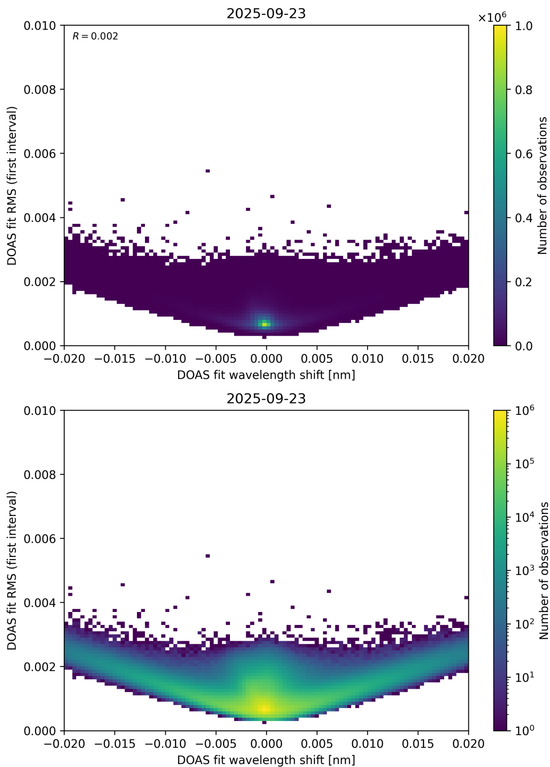
Figure 64: Scatter density plot of “DOAS fit wavelength shift” against “DOAS fit RMS (first interval)” for 2025-09-22 to 2025-09-24.
