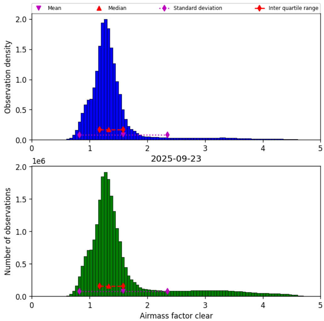
Figure 42: Histogram of “Airmass factor clear” for 2025-09-22 to 2025-09-24
