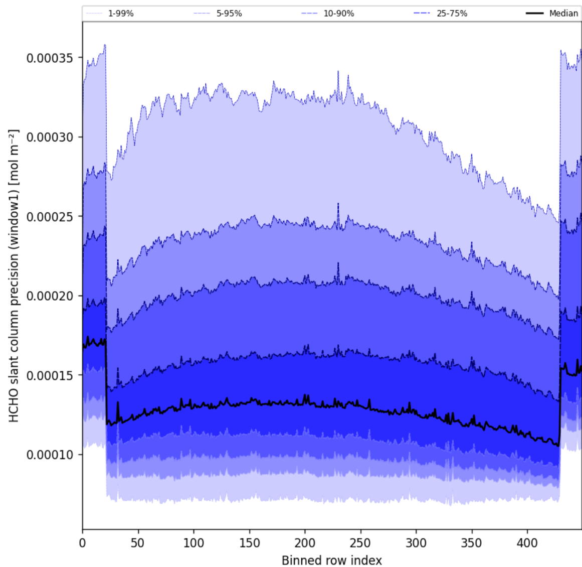
Figure 53: Along track statistics of “HCHO slant column precision (window1)” for 2025-09-22 to 2025-09-24
