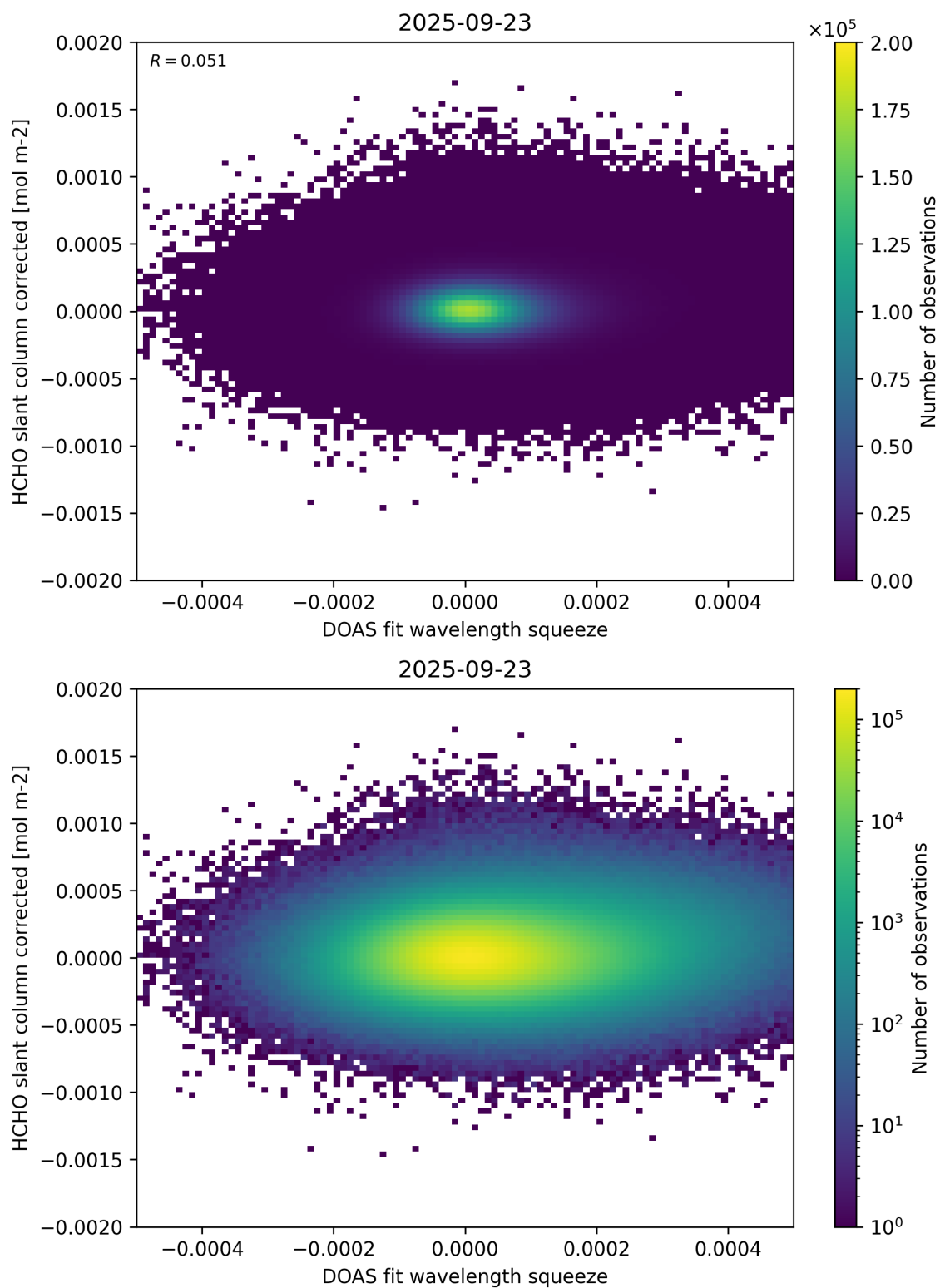
Figure 69: Scatter density plot of “DOAS fit wavelength squeeze” against “HCHO slant column corrected” for 2025-09-22 to 2025-09-24.
