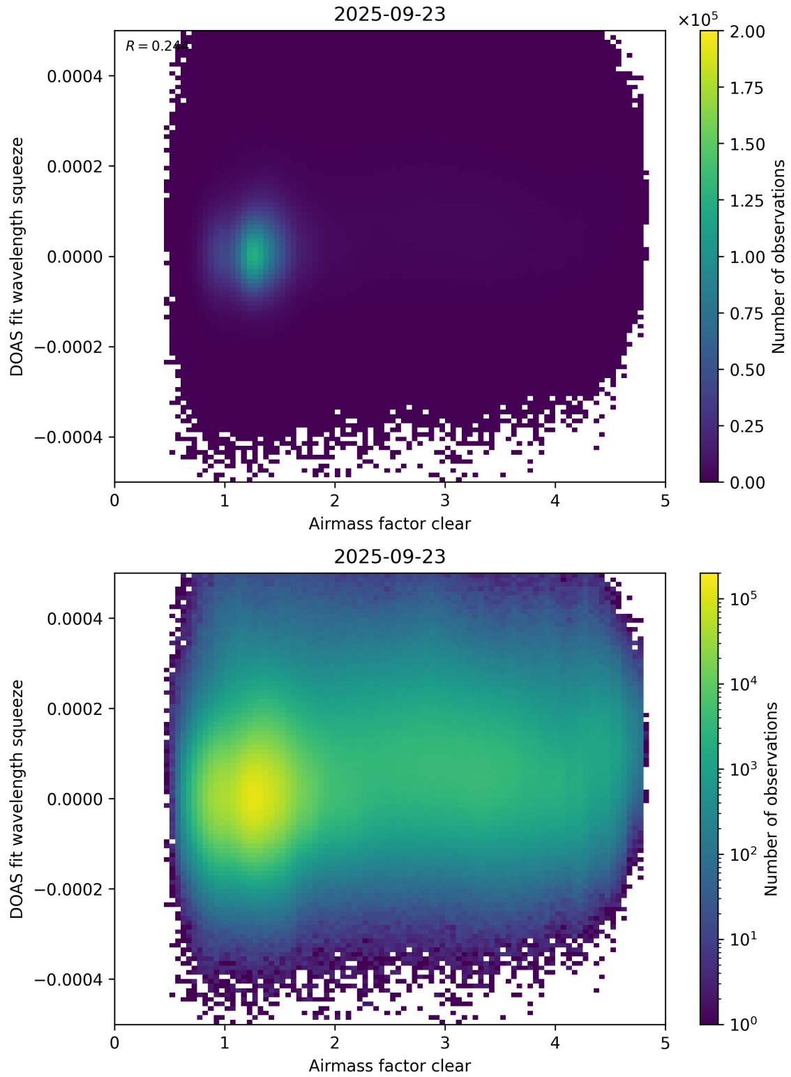
Figure 73: Scatter density plot of “Airmass factor clear” against “DOAS fit wavelength squeeze” for 2025-09-22 to 2025-09-24.
