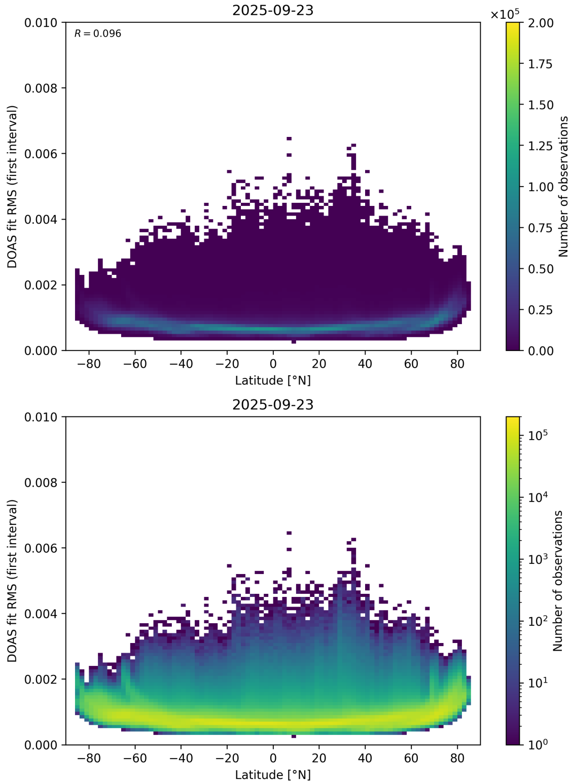
Figure 153: Scatter density plot of “Latitude” against “DOAS fit RMS (first interval)” for 2025-09-22 to 2025-09-24.
