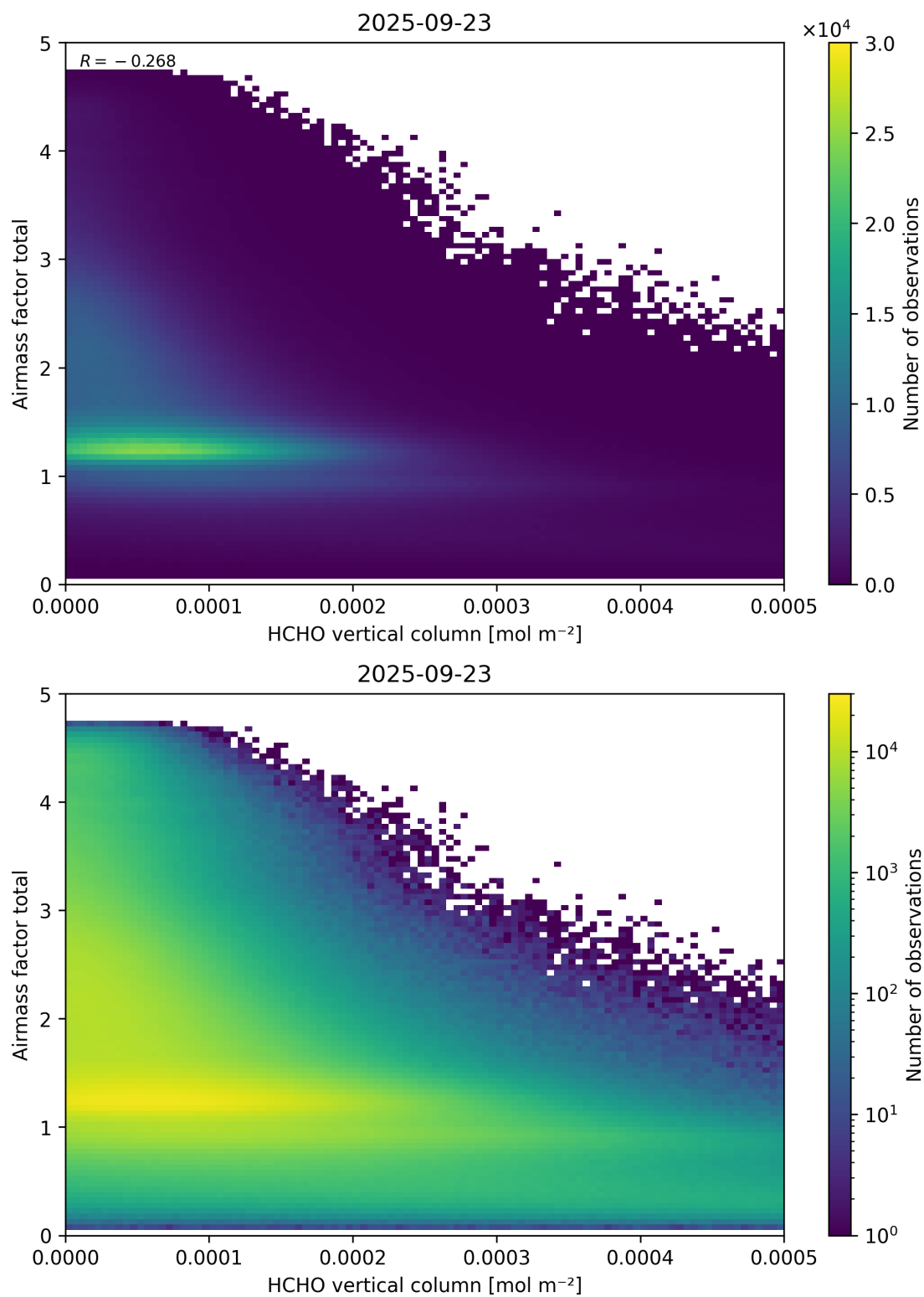
Figure 131: Scatter density plot of “HCHO vertical column” against “Airmass factor total” for 2025-09-22 to 2025-09-24.
