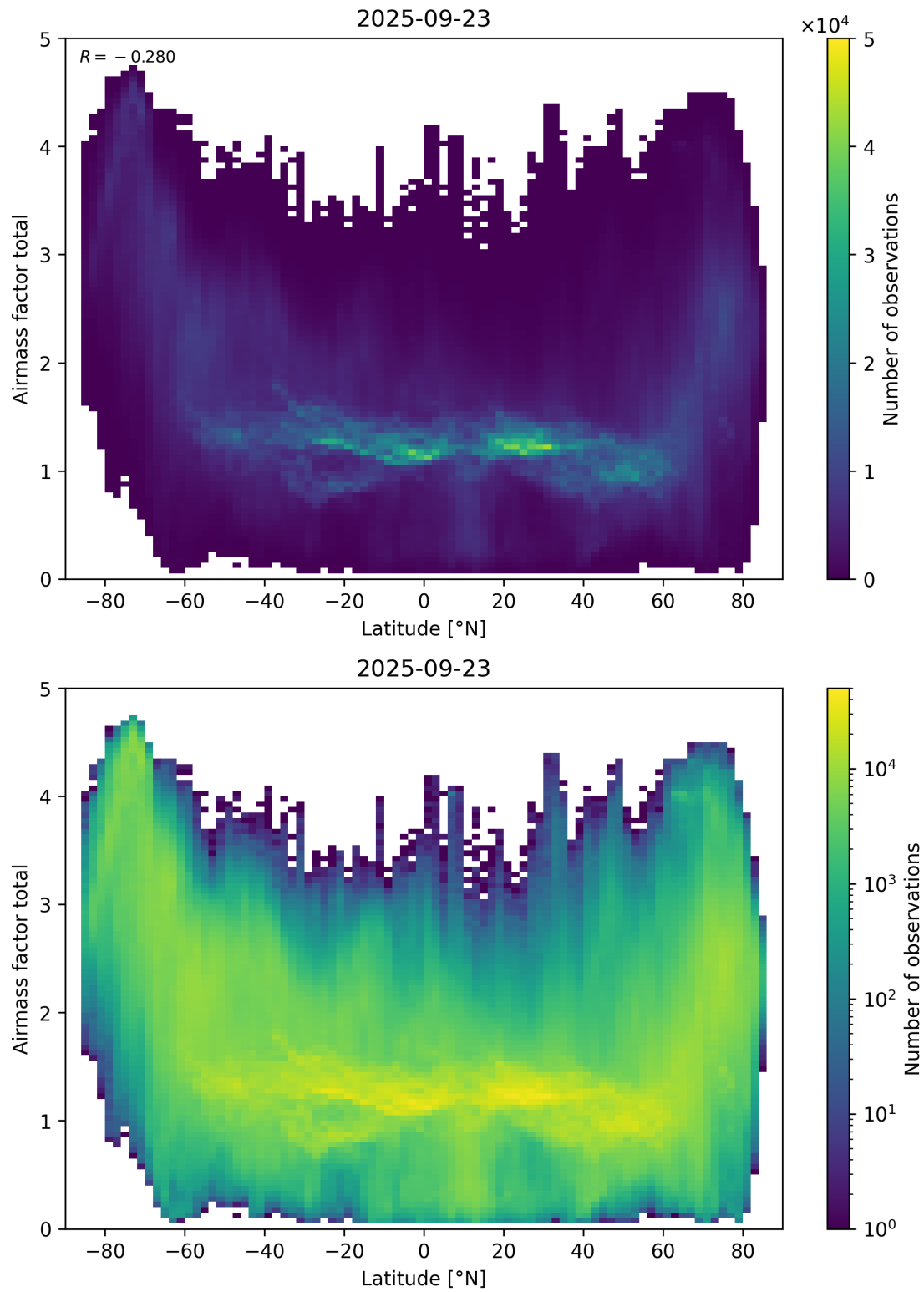
Figure 161: Scatter density plot of “Latitude” against “Airmass factor total” for 2025-09-22 to 2025-09-24.
