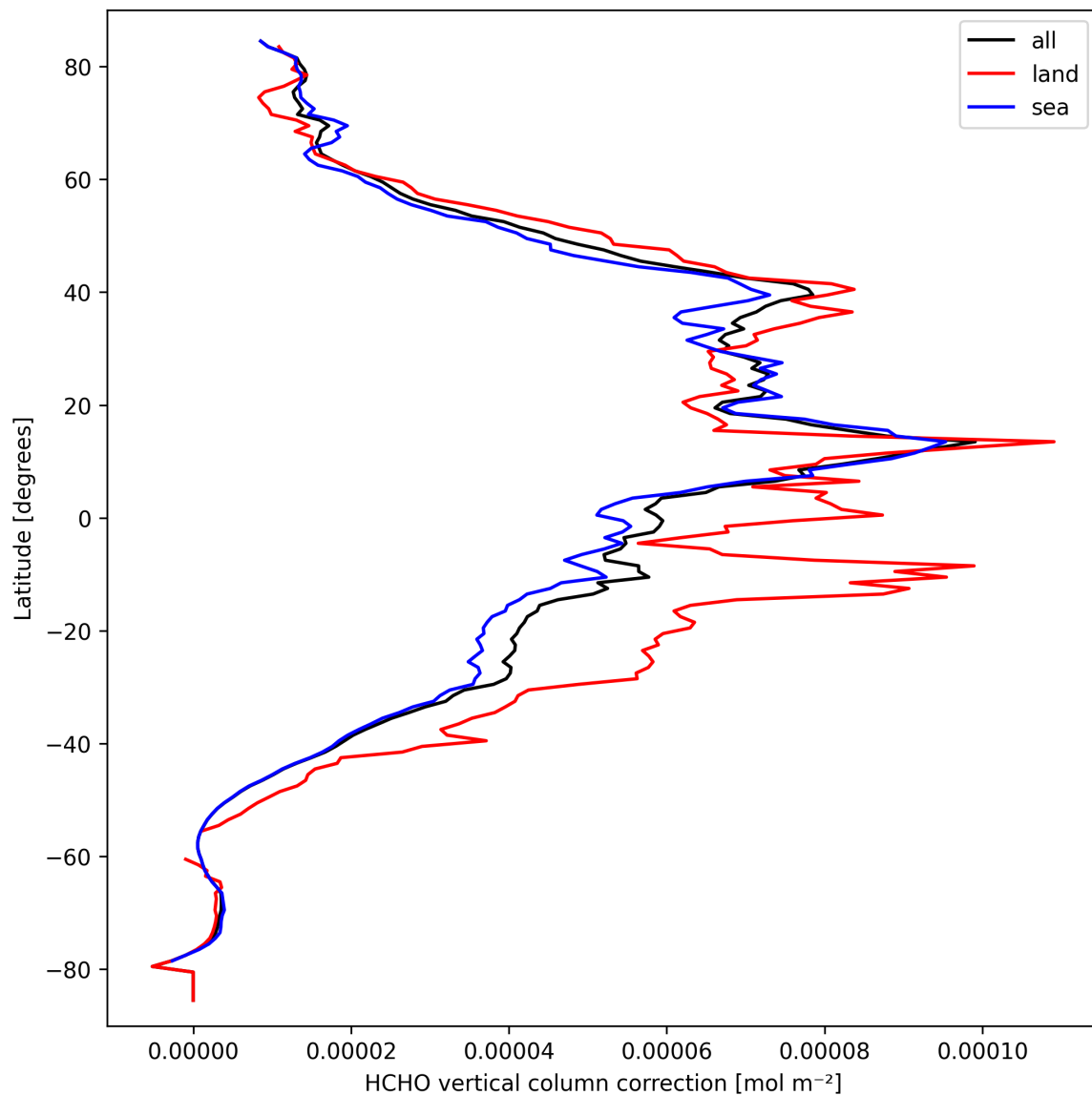
Figure 23: Zonal average of “HCHO vertical column correction” for 2025-09-22 to 2025-09-24.
