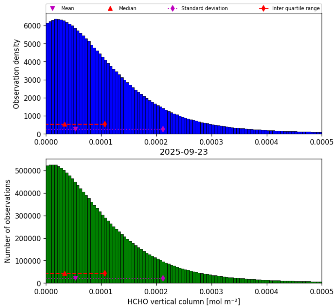
Figure 35: Histogram of “HCHO vertical column” for 2025-09-22 to 2025-09-24
