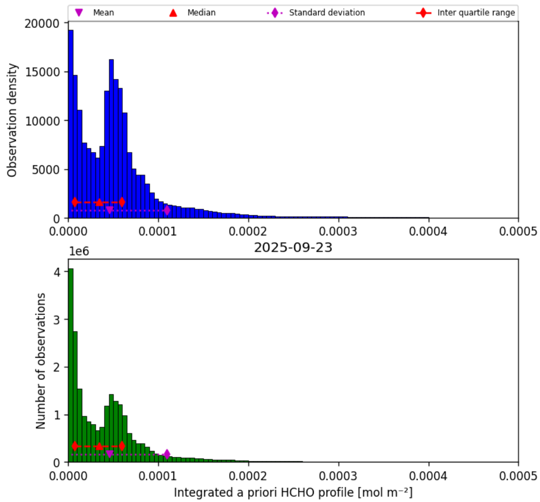
Figure 43: Histogram of “Integrated a priori HCHO profile” for 2025-09-22 to 2025-09-24
