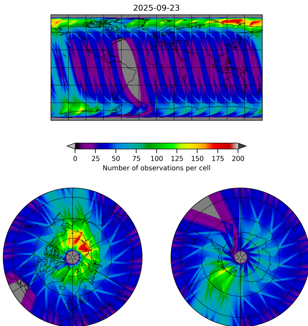
Figure 19: Map of the number of observations for 2025-09-22 to 2025-09-24
