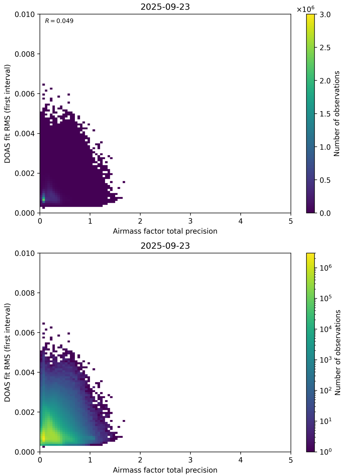
Figure 105: Scatter density plot of “Airmass factor total precision” against “DOAS fit RMS (first interval)” for 2025-09-22 to 2025-09-24.
