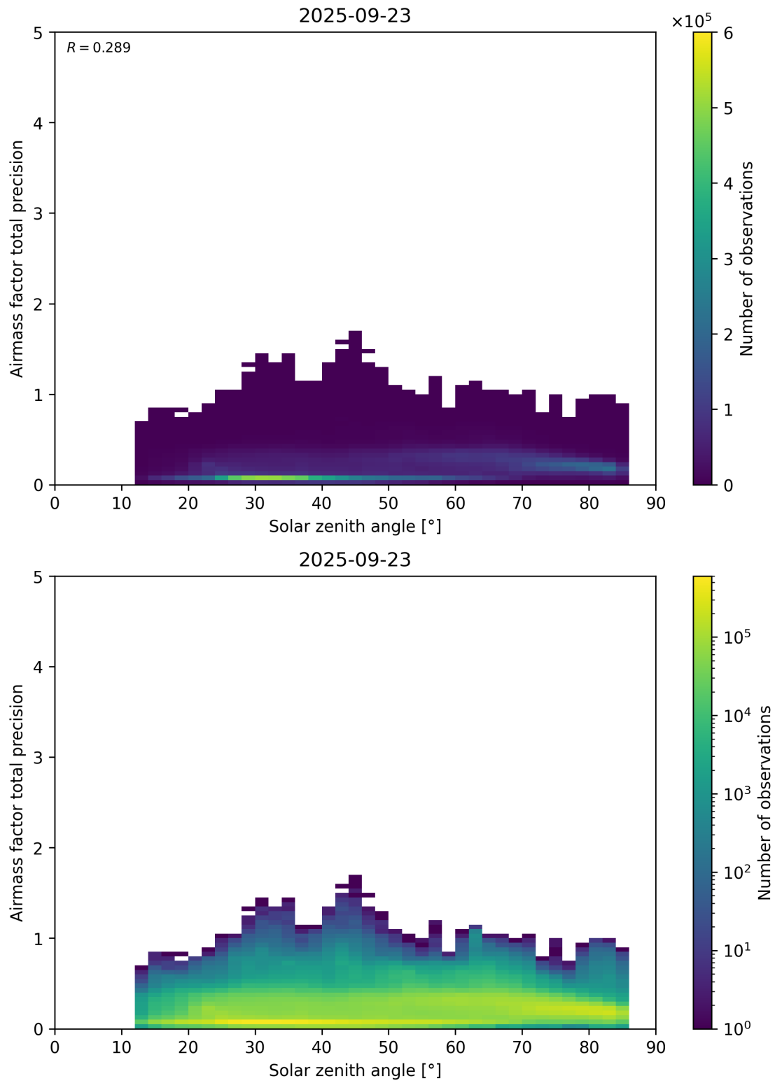
Figure 176: Scatter density plot of “Solar zenith angle” against “Airmass factor total precision” for 2025-09-22 to 2025-09-24.
