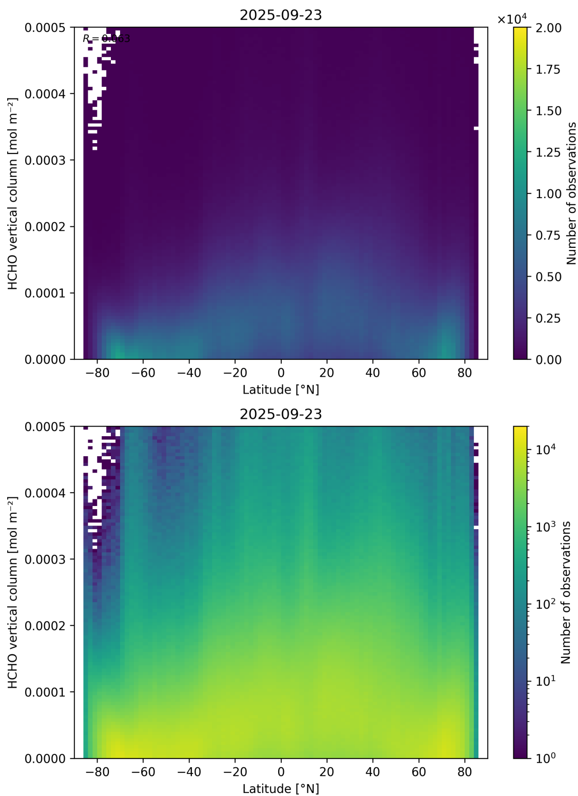
Figure 163: Scatter density plot of “Latitude” against “HCHO vertical column” for 2025-09-22 to 2025-09-24.
