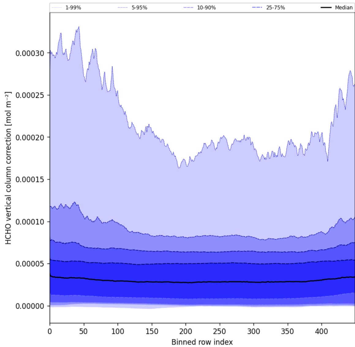
Figure 51: Along track statistics of “HCHO vertical column correction” for 2025-09-22 to 2025-09-24
