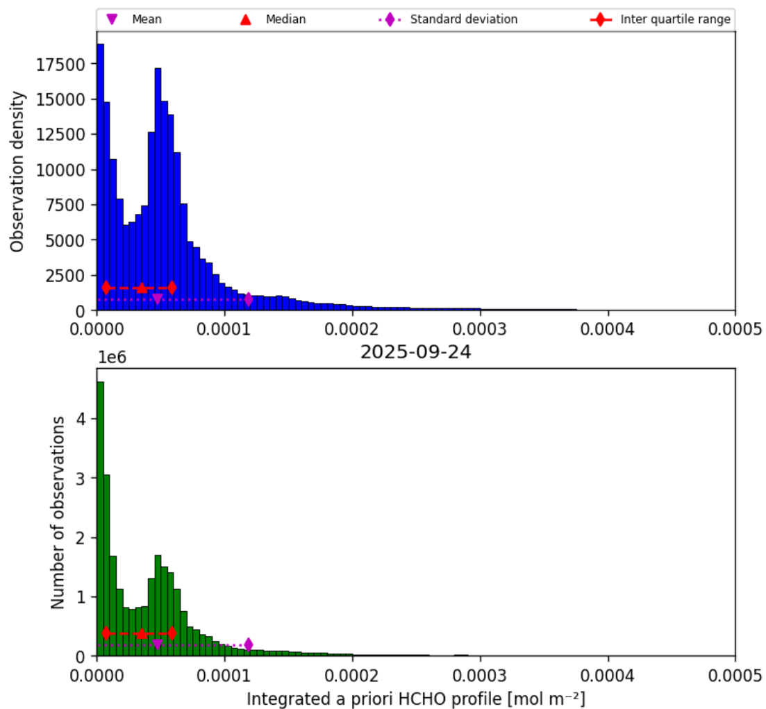
Figure 43: Histogram of “Integrated a priori HCHO profile” for 2025-09-23 to 2025-09-25
