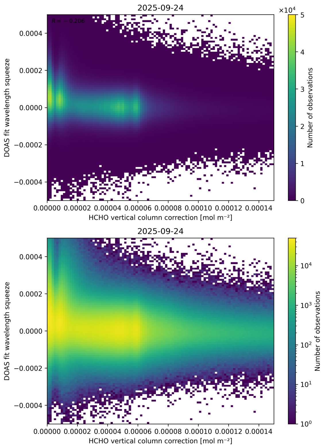
Figure 114: Scatter density plot of “HCHO vertical column correction” against “DOAS fit wavelength squeeze” for 2025-09-23 to 2025-09-25.
