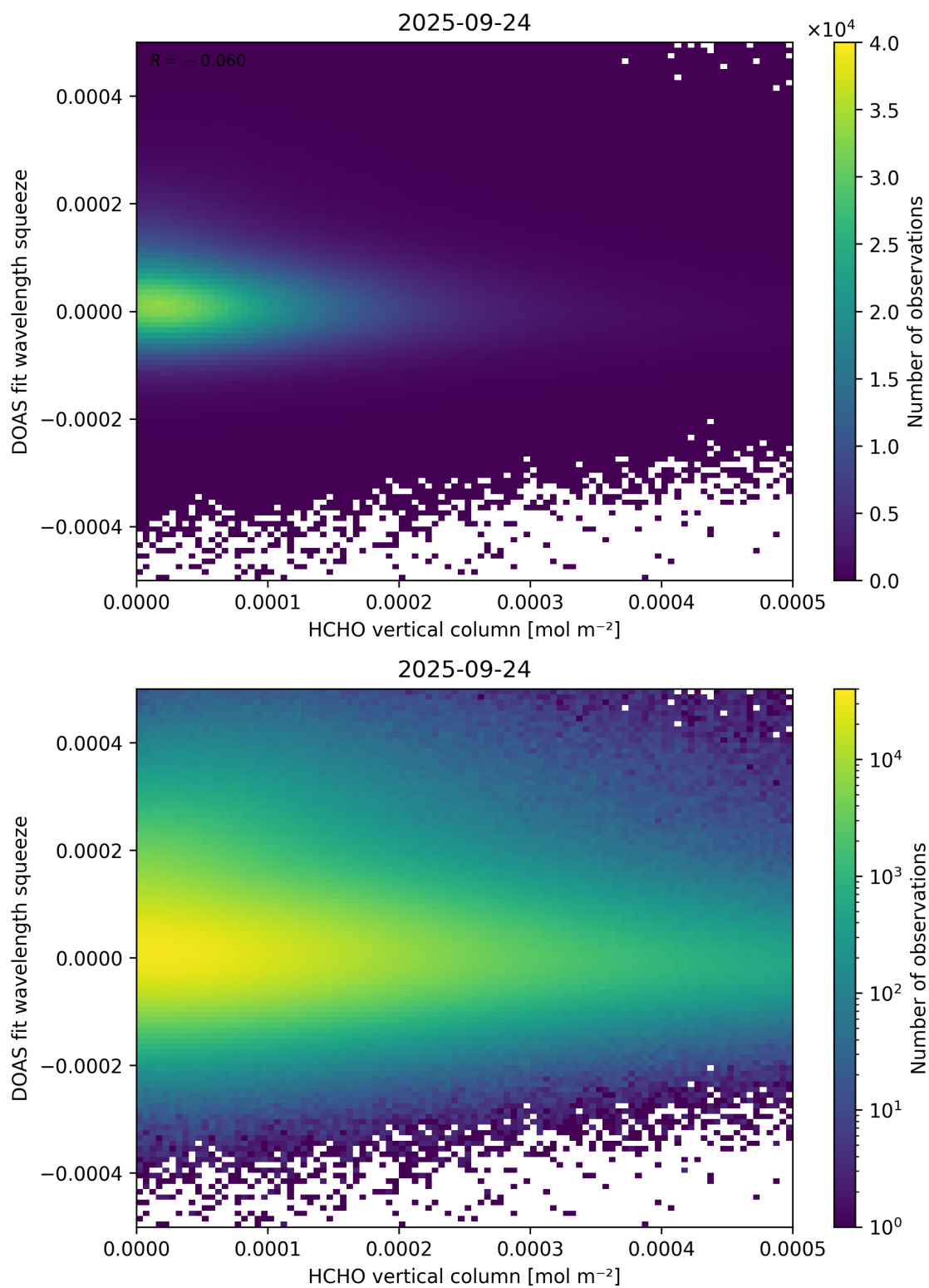
Figure 125: Scatter density plot of “HCHO vertical column” against “DOAS fit wavelength squeeze” for 2025-09-23 to 2025-09-25.
