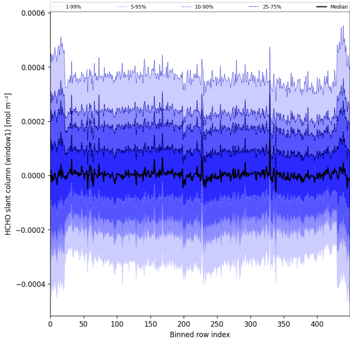
Figure 52: Along track statistics of “HCHO slant column (window1)” for 2025-09-23 to 2025-09-25
