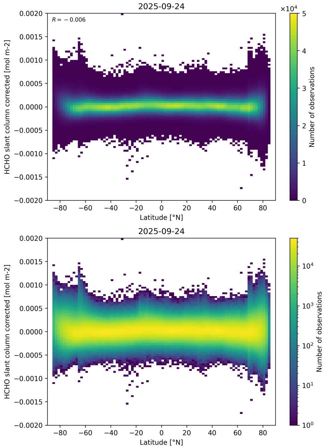
Figure 157: Scatter density plot of “Latitude” against “HCHO slant column corrected” for 2025-09-23 to 2025-09-25.
