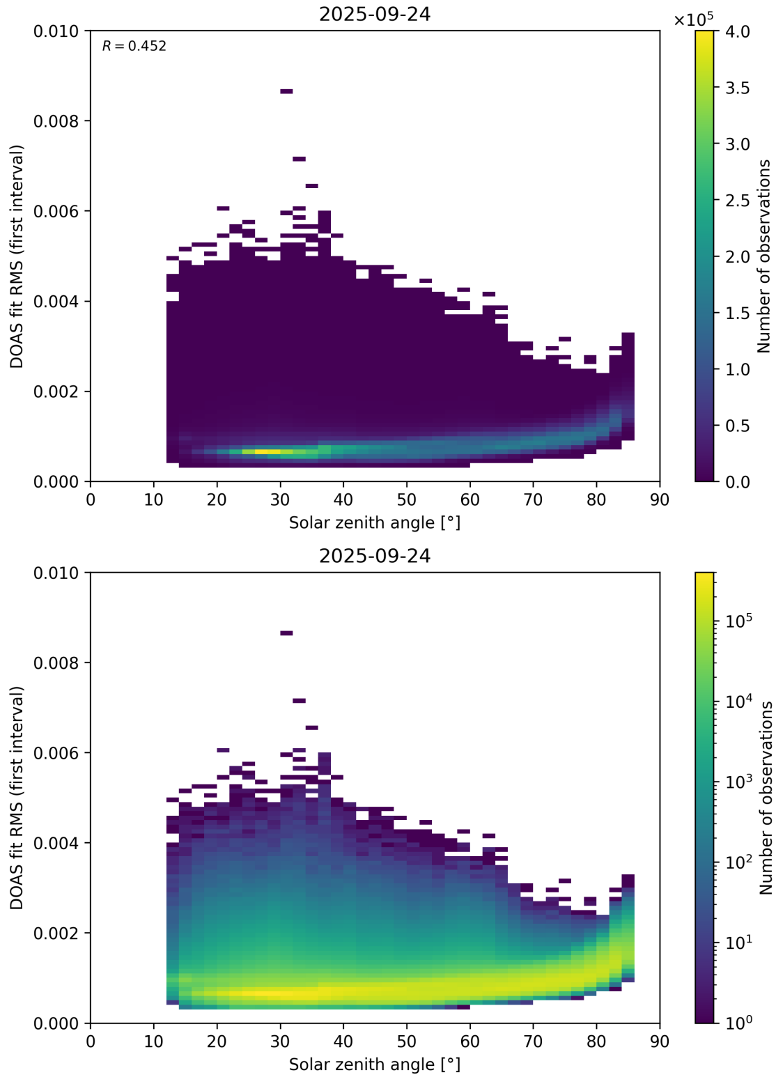
Figure 167: Scatter density plot of “Solar zenith angle” against “DOAS fit RMS (first interval)” for 2025-09-23 to 2025-09-25.
