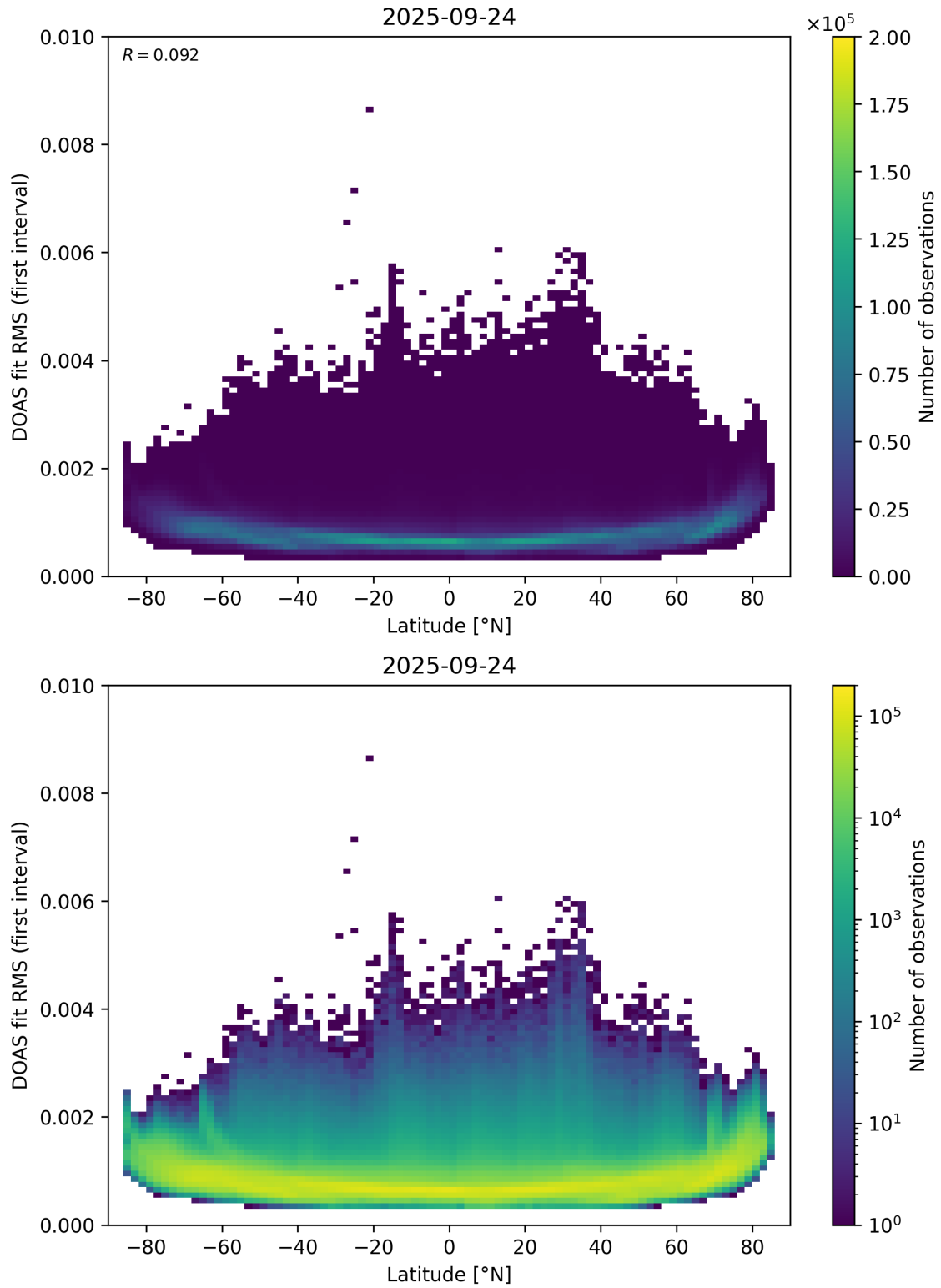
Figure 153: Scatter density plot of “Latitude” against “DOAS fit RMS (first interval)” for 2025-09-23 to 2025-09-25.
