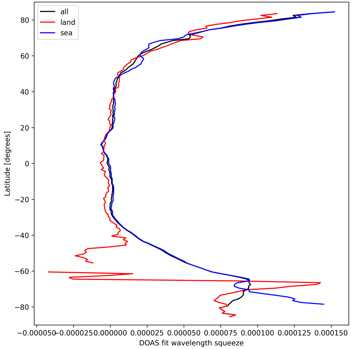
Figure 31: Zonal average of “DOAS fit wavelength squeeze” for 2025-09-23 to 2025-09-25.
