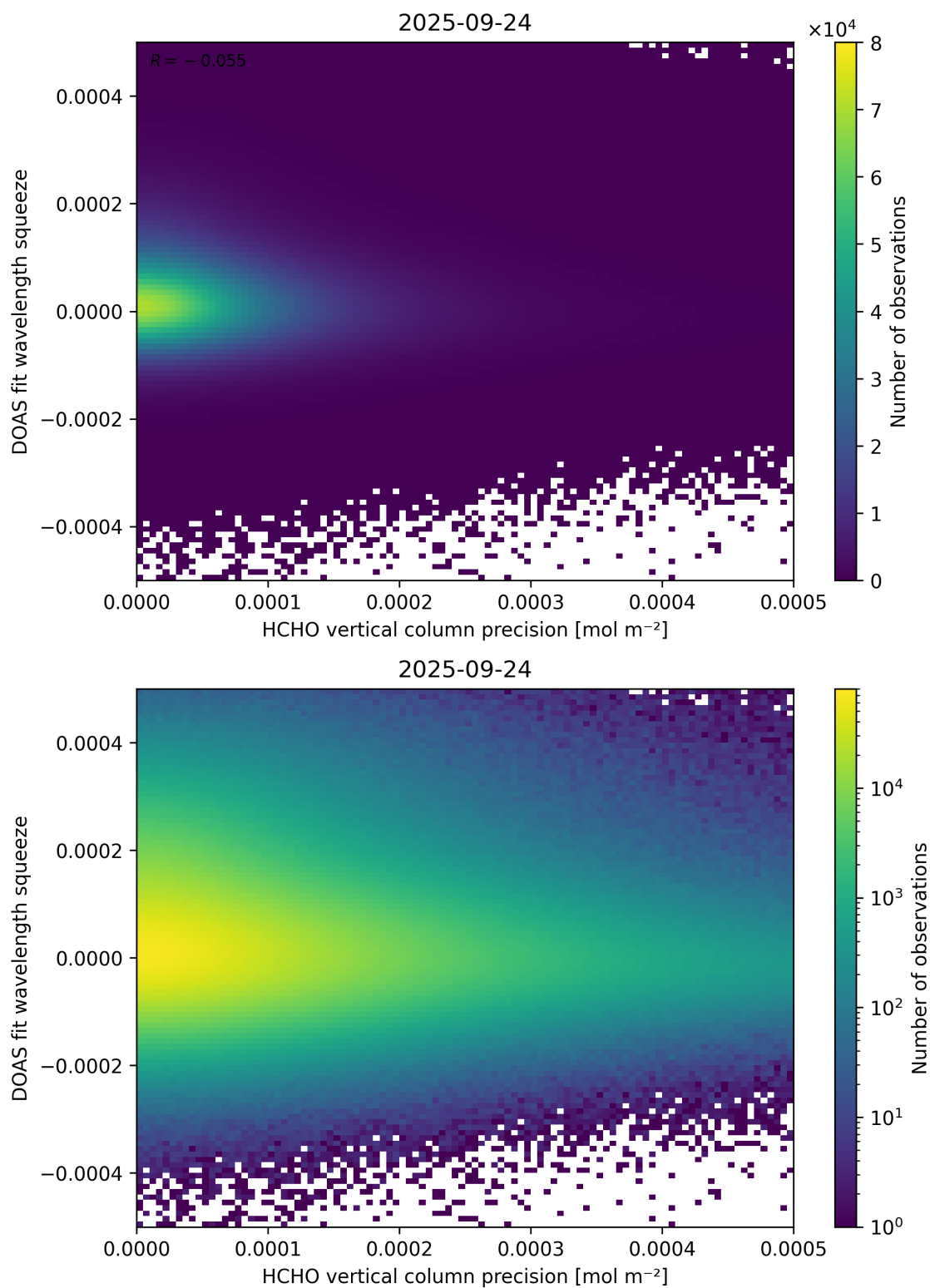
Figure 138: Scatter density plot of “HCHO vertical column precision” against “DOAS fit wavelength squeeze” for 2025-09-23 to 2025-09-25.
