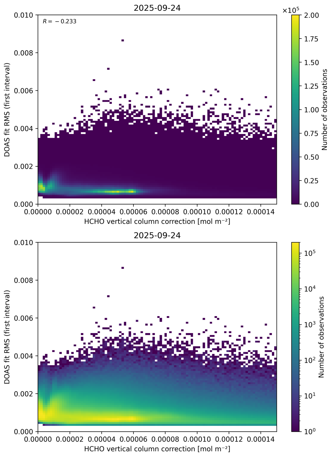
Figure 112: Scatter density plot of “HCHO vertical column correction” against “DOAS fit RMS (first interval)” for 2025-09-23 to 2025-09-25.
