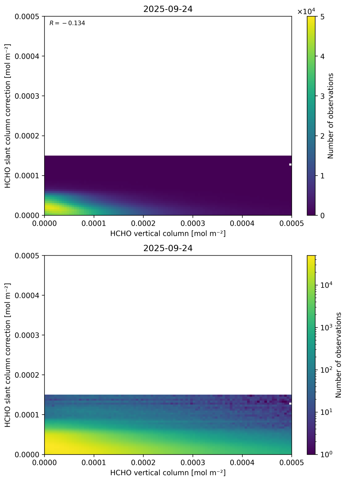
Figure 128: Scatter density plot of “HCHO vertical column” against “HCHO slant column correction” for 2025-09-23 to 2025-09-25.
