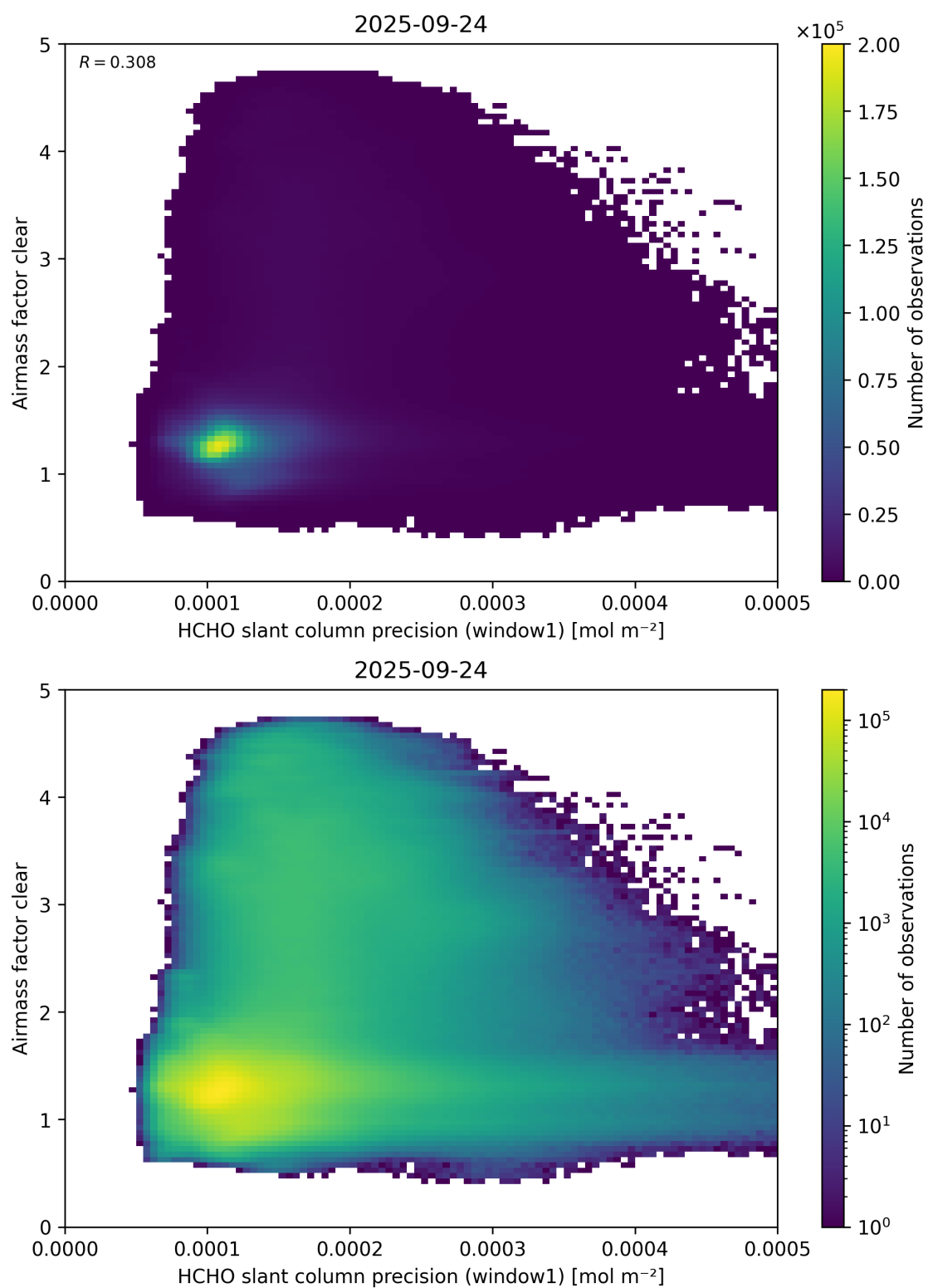
Figure 91: Scatter density plot of “HCHO slant column precision (window1)” against “Airmass factor clear” for 2025-09-23 to 2025-09-25.
