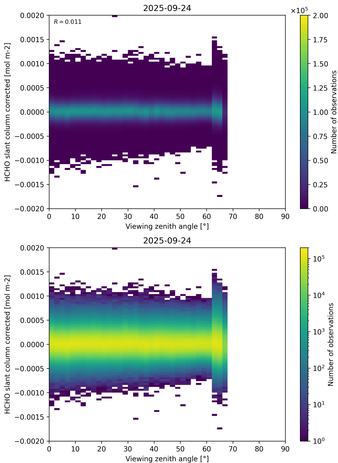
Figure 186: Scatter density plot of “Viewing zenith angle” against “HCHO slant column corrected” for 2025-09-23 to 2025-09-25.
