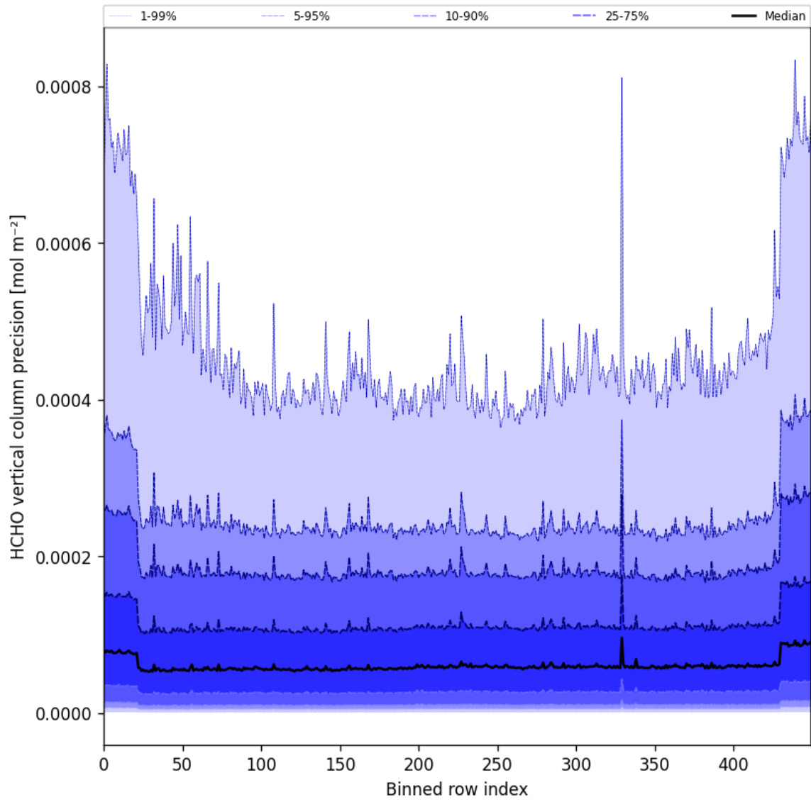
Figure 50: Along track statistics of “HCHO vertical column precision” for 2025-09-23 to 2025-09-25
