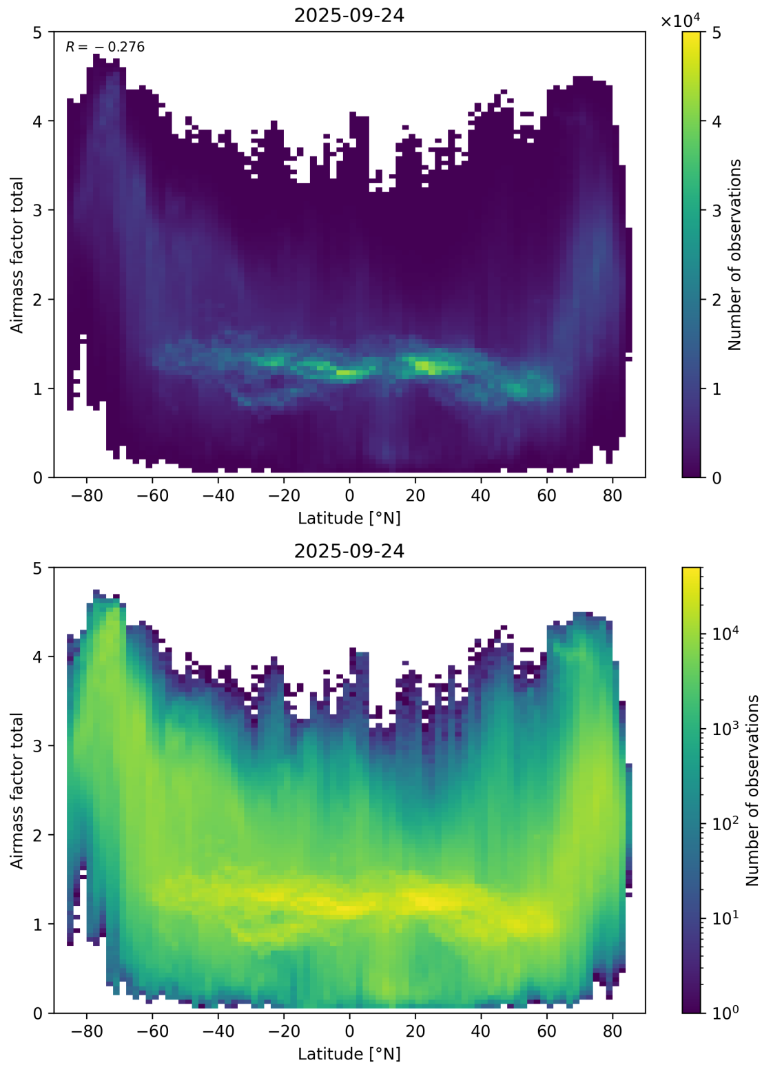
Figure 161: Scatter density plot of “Latitude” against “Airmass factor total” for 2025-09-23 to 2025-09-25.
