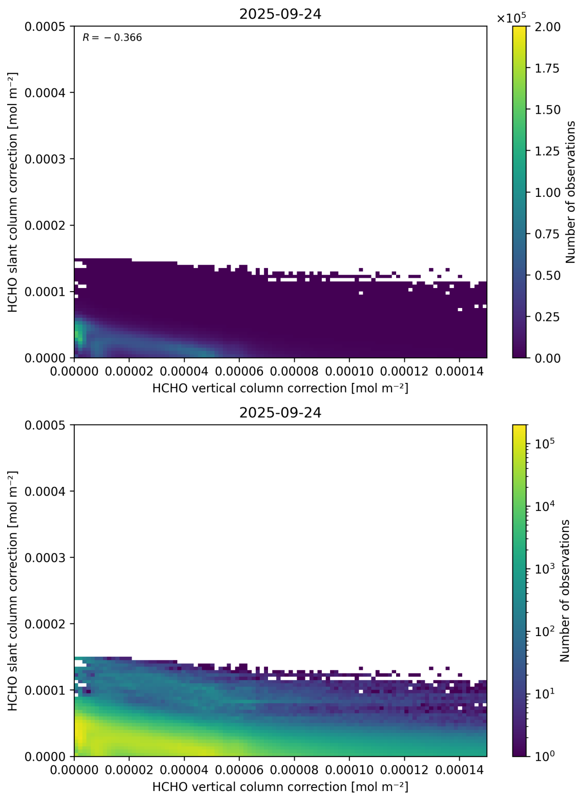
Figure 117: Scatter density plot of “HCHO vertical column correction” against “HCHO slant column correction” for 2025-09-23 to 2025-09-25.
