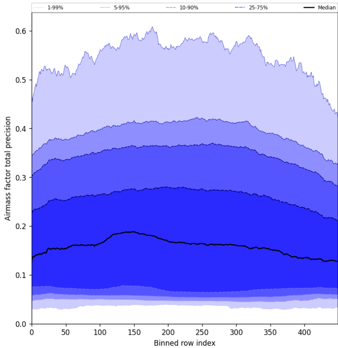
Figure 55: Along track statistics of “Airmass factor total precision” for 2025-09-23 to 2025-09-25
