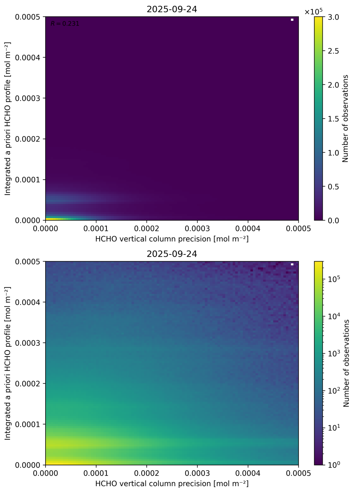
Figure 147: Scatter density plot of “HCHO vertical column precision” against “Integrated a priori HCHO profile” for 2025-09-23 to 2025-09-25.
