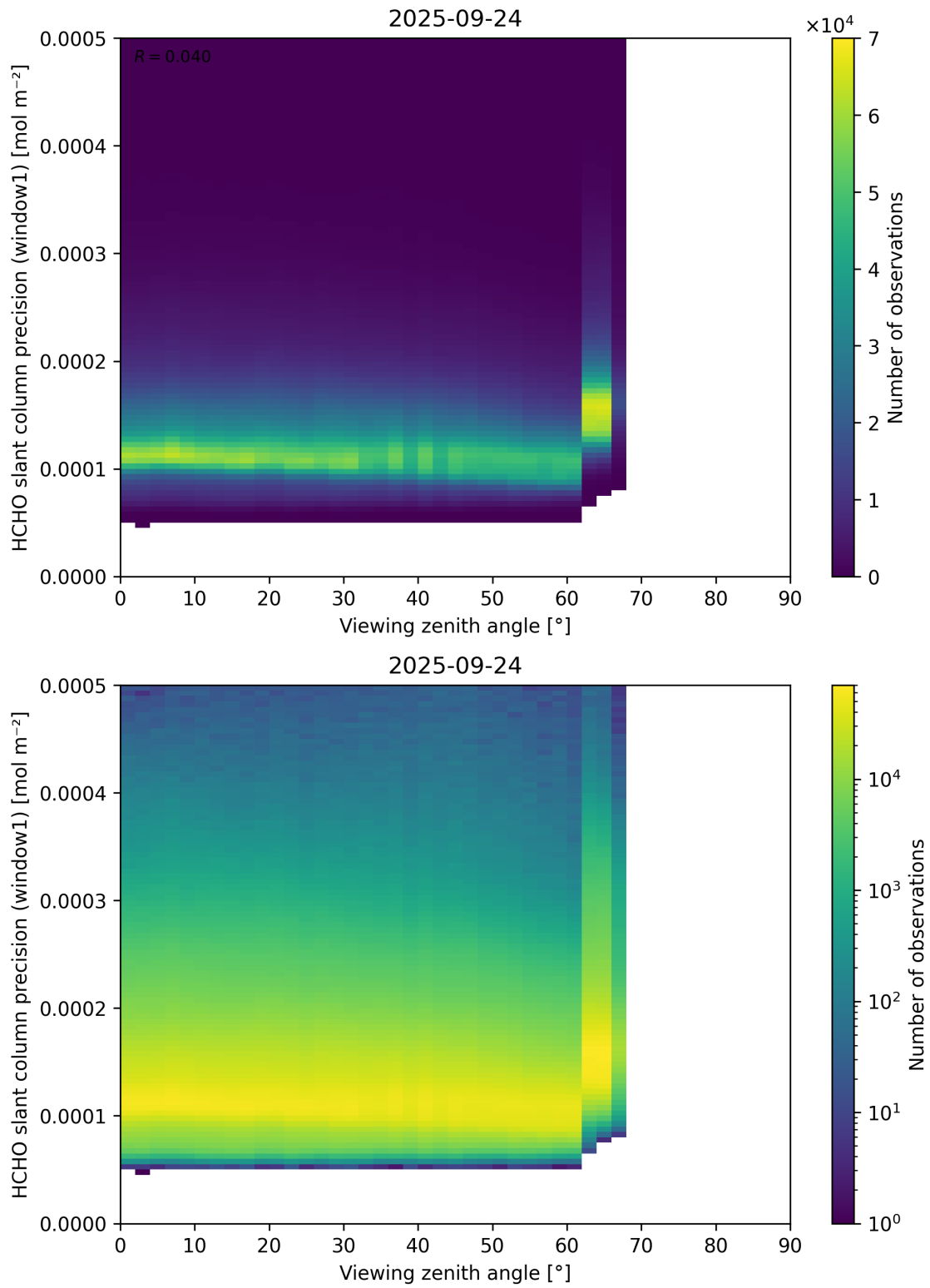
Figure 189: Scatter density plot of “Viewing zenith angle” against “HCHO slant column precision (window1)” for 2025-09-23 to 2025-09-25.
