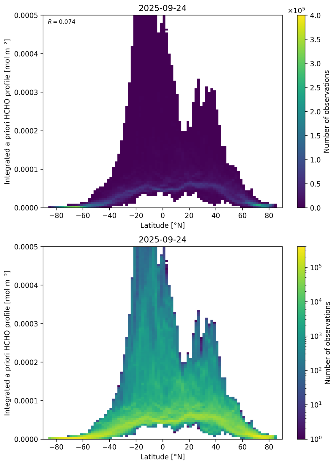
Figure 166: Scatter density plot of “Latitude” against “Integrated a priori HCHO profile” for 2025-09-23 to 2025-09-25.
