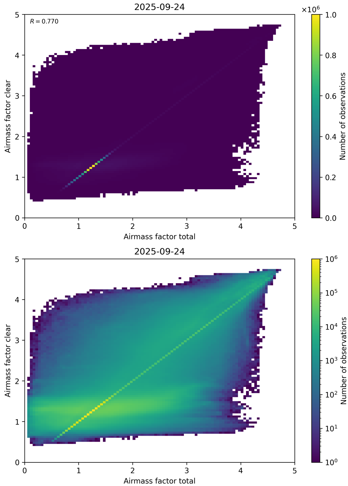
Figure 100: Scatter density plot of “Airmass factor total” against “Airmass factor clear” for 2025-09-23 to 2025-09-25.
