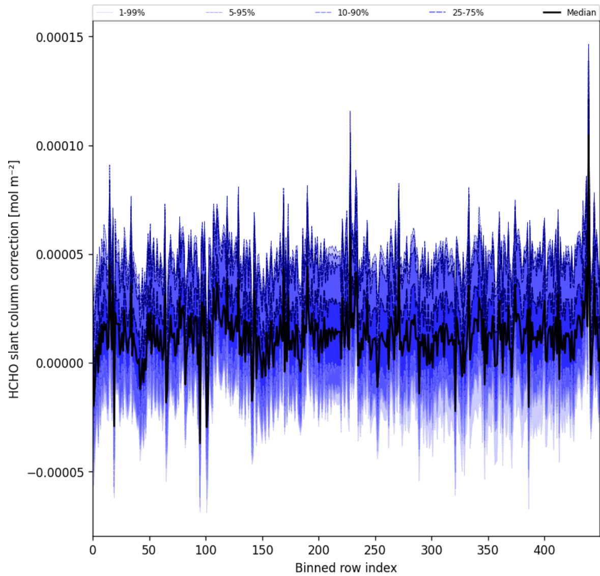
Figure 61: Along track statistics of “HCHO slant column correction” for 2025-09-23 to 2025-09-25
