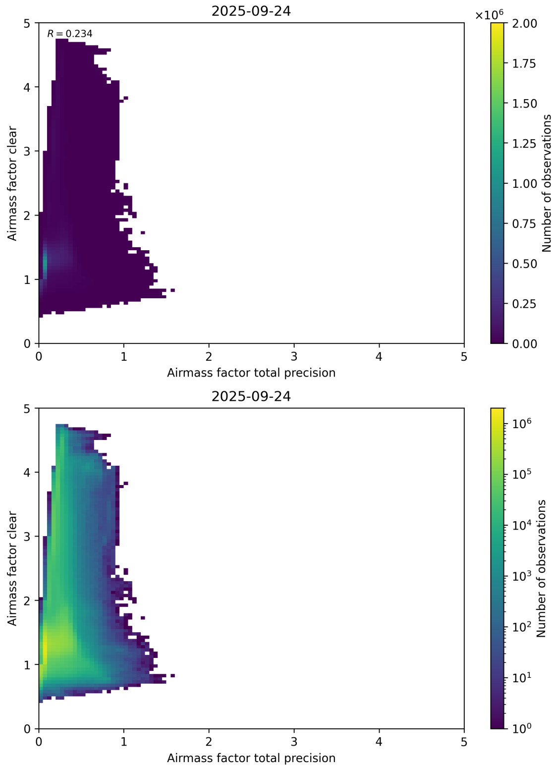
Figure 108: Scatter density plot of “Airmass factor total precision” against “Airmass factor clear” for 2025-09-23 to 2025-09-25.
