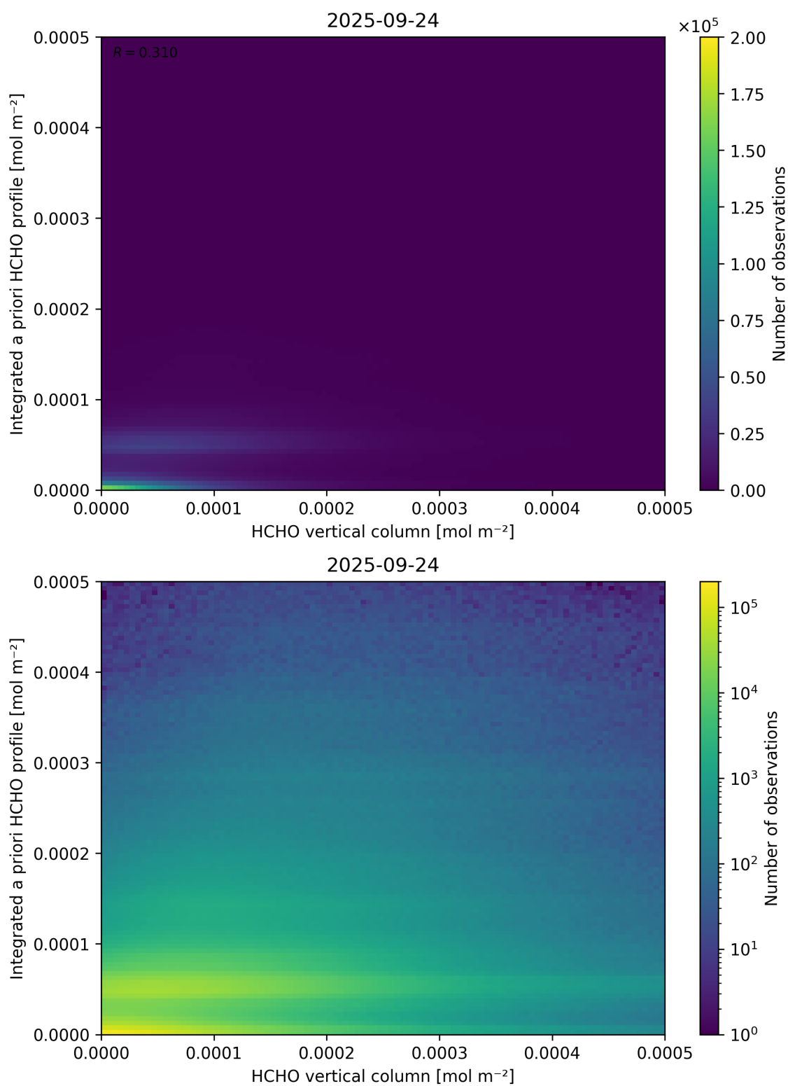
Figure 135: Scatter density plot of “HCHO vertical column” against “Integrated a priori HCHO profile” for 2025-09-23 to 2025-09-25.
