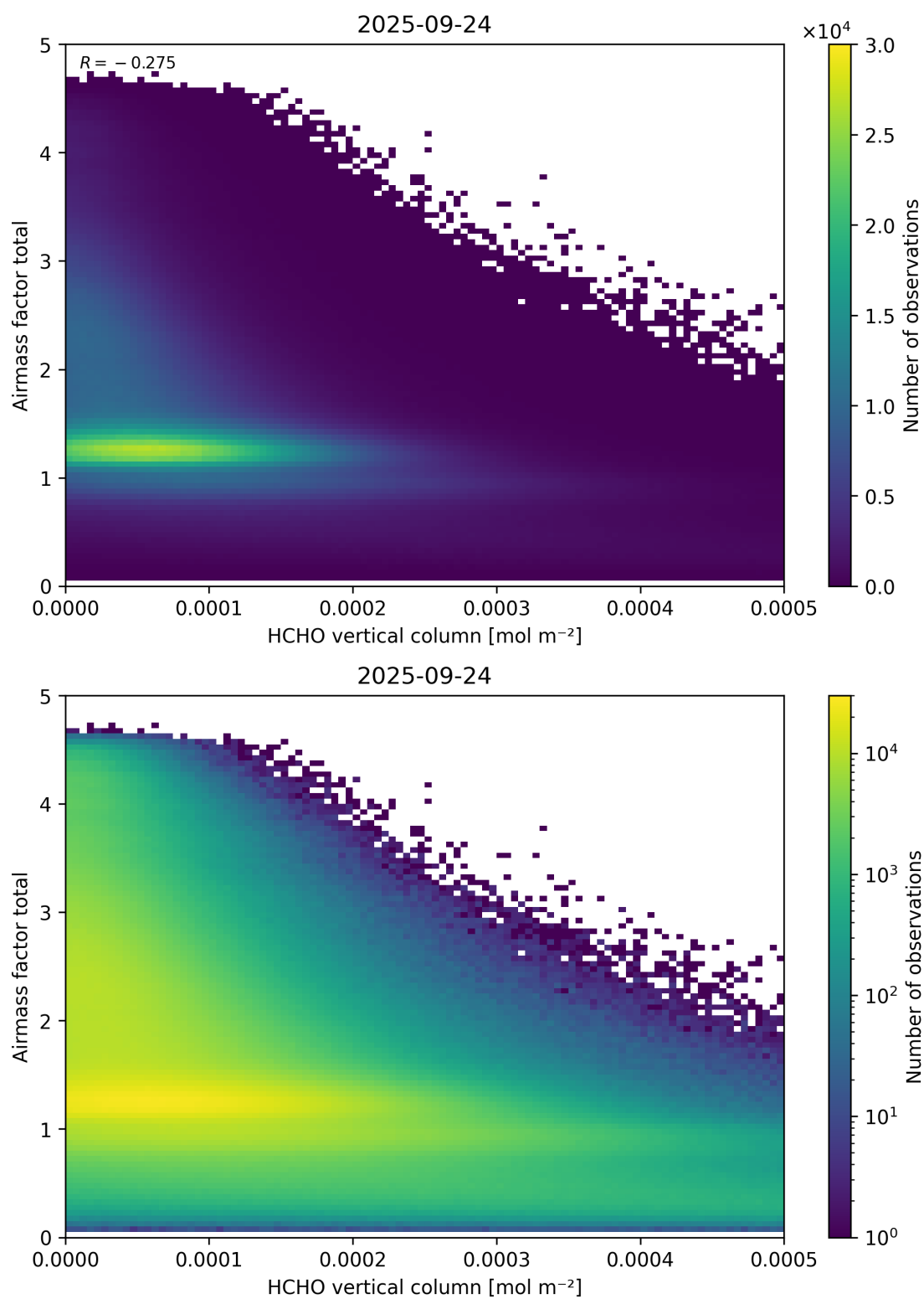
Figure 131: Scatter density plot of “HCHO vertical column” against “Airmass factor total” for 2025-09-23 to 2025-09-25.
