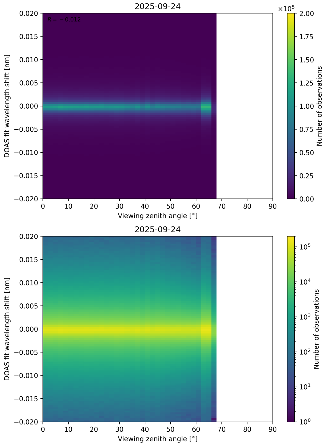
Figure 183: Scatter density plot of “Viewing zenith angle” against “DOAS fit wavelength shift” for 2025-09-23 to 2025-09-25.
