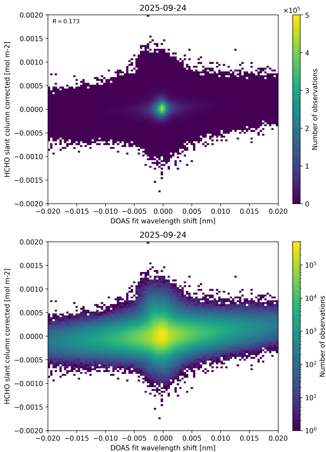
Figure 66: Scatter density plot of “DOAS fit wavelength shift” against “HCHO slant column corrected” for 2025-09-23 to 2025-09-25.
