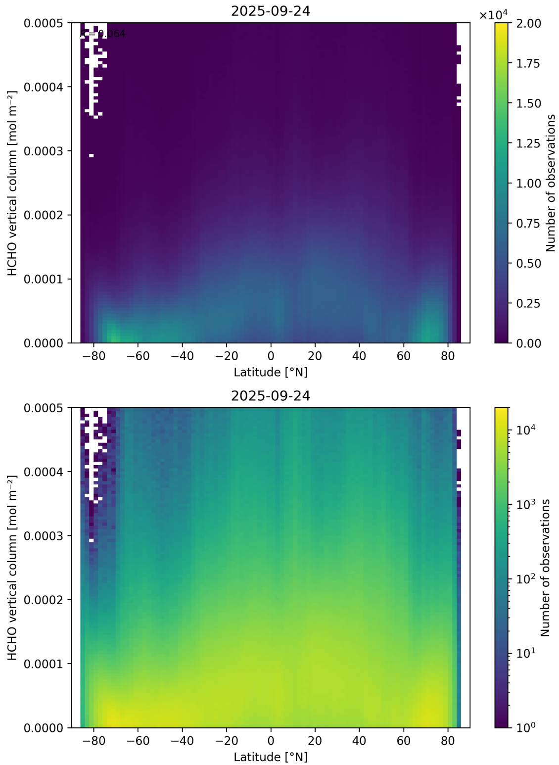
Figure 163: Scatter density plot of “Latitude” against “HCHO vertical column” for 2025-09-23 to 2025-09-25.
