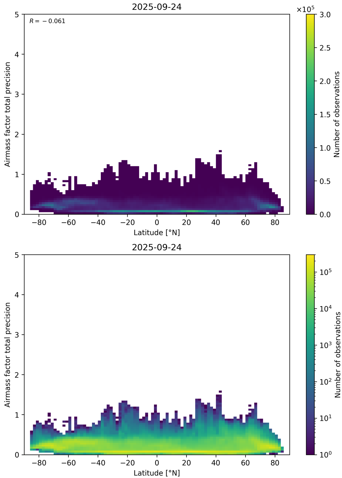
Figure 162: Scatter density plot of “Latitude” against “Airmass factor total precision” for 2025-09-23 to 2025-09-25.
