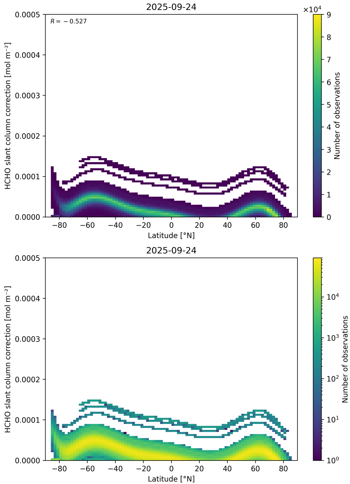
Figure 158: Scatter density plot of “Latitude” against “HCHO slant column correction” for 2025-09-23 to 2025-09-25.
