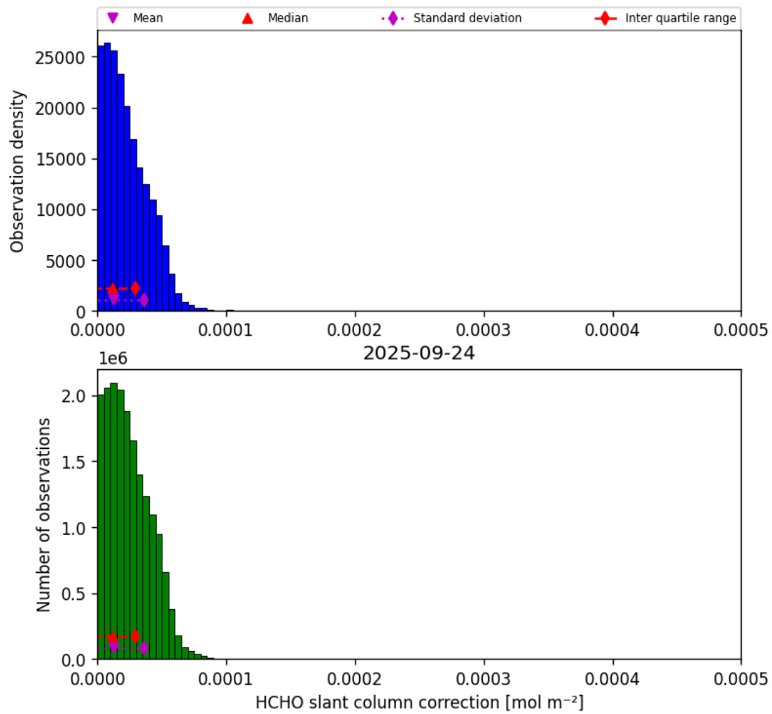
Figure 47: Histogram of “HCHO slant column correction” for 2025-09-23 to 2025-09-25
