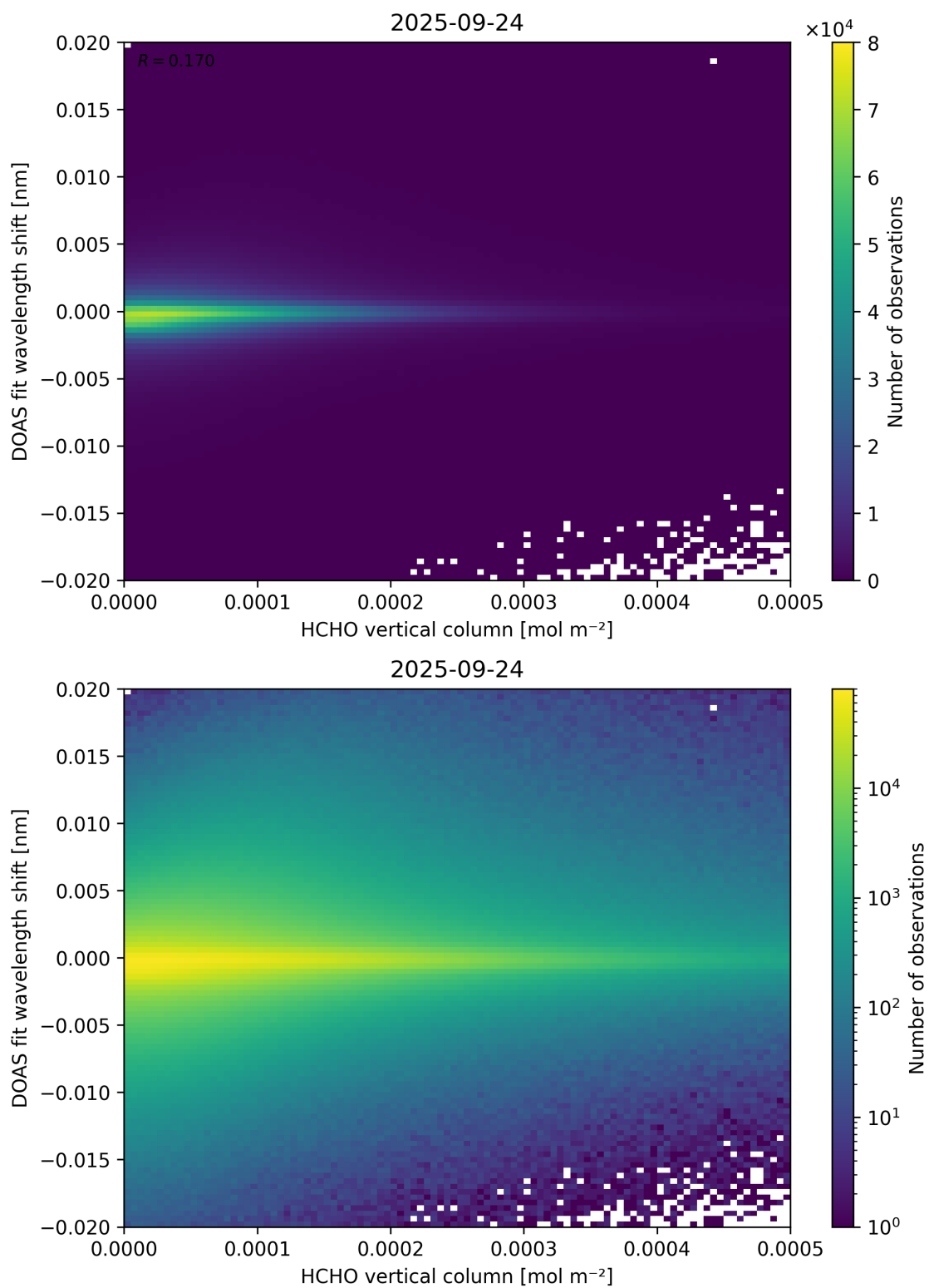
Figure 124: Scatter density plot of “HCHO vertical column” against “DOAS fit wavelength shift” for 2025-09-23 to 2025-09-25.
