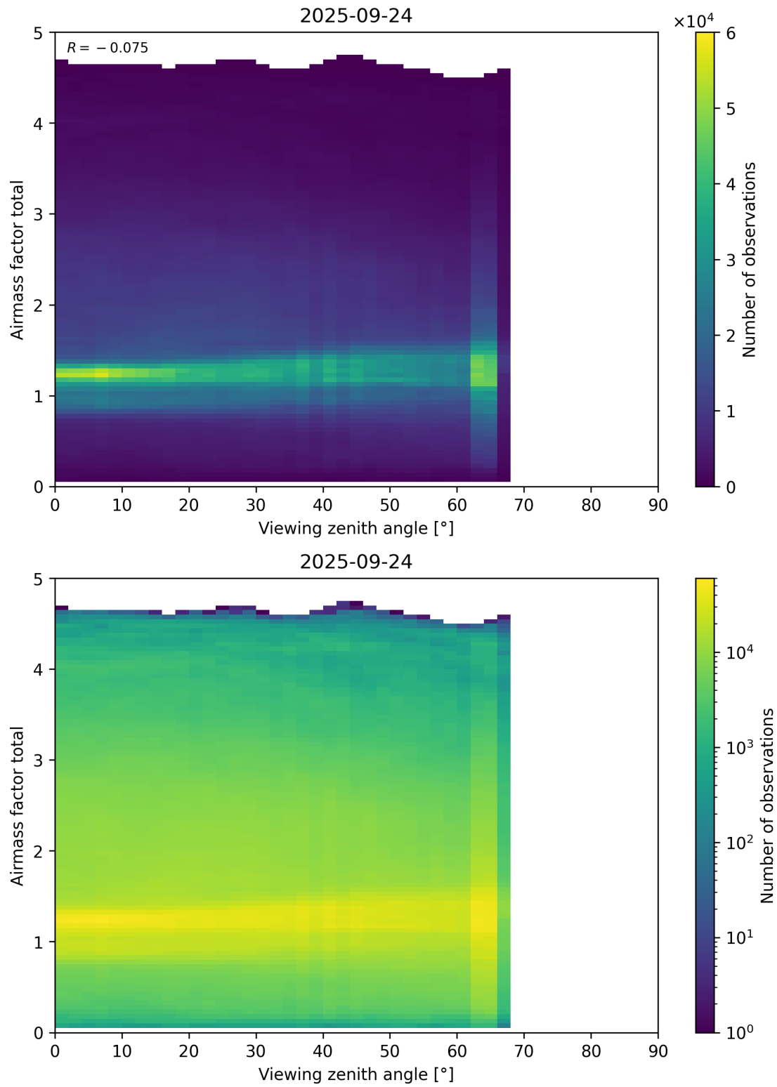
Figure 190: Scatter density plot of “Viewing zenith angle” against “Airmass factor total” for 2025-09-23 to 2025-09-25.
