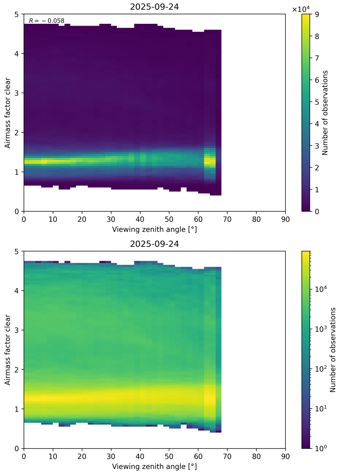
Figure 185: Scatter density plot of “Viewing zenith angle” against “Airmass factor clear” for 2025-09-23 to 2025-09-25.
