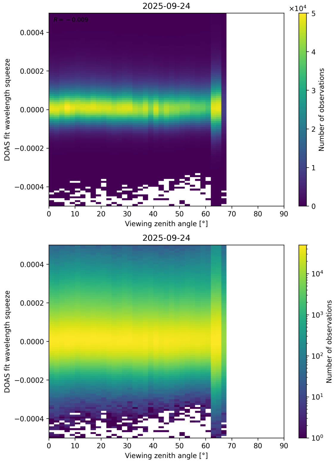
Figure 184: Scatter density plot of “Viewing zenith angle” against “DOAS fit wavelength squeeze” for 2025-09-23 to 2025-09-25.
