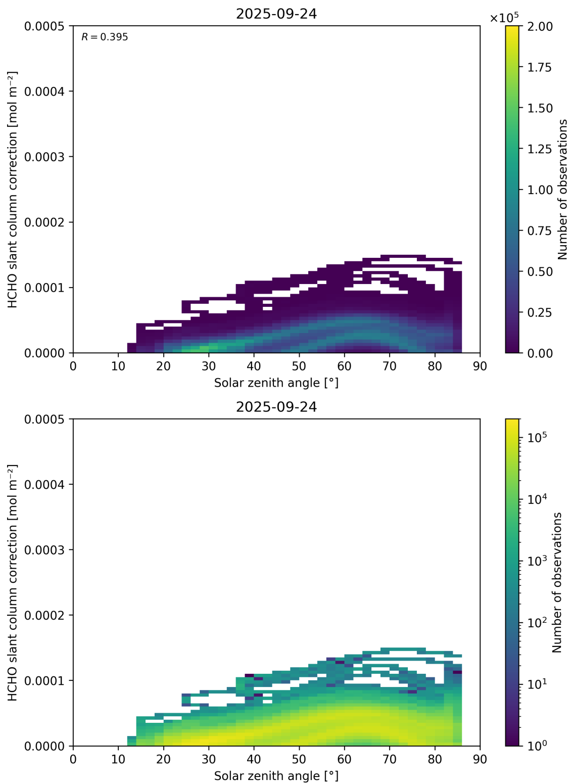
Figure 172: Scatter density plot of “Solar zenith angle” against “HCHO slant column correction” for 2025-09-23 to 2025-09-25.
