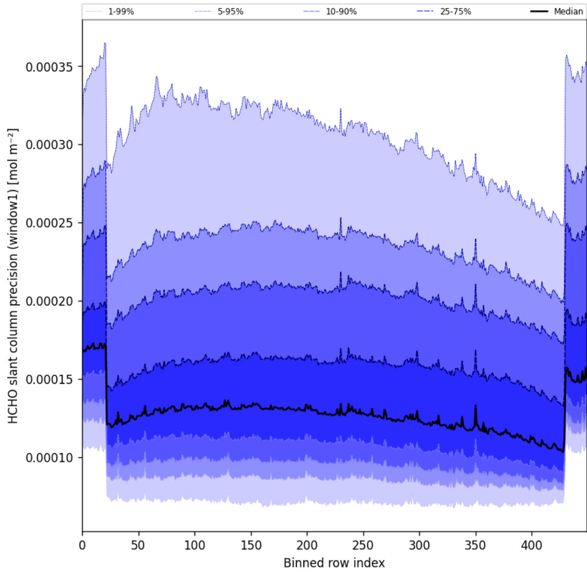
Figure 53: Along track statistics of “HCHO slant column precision (window1)” for 2025-09-23 to 2025-09-25
