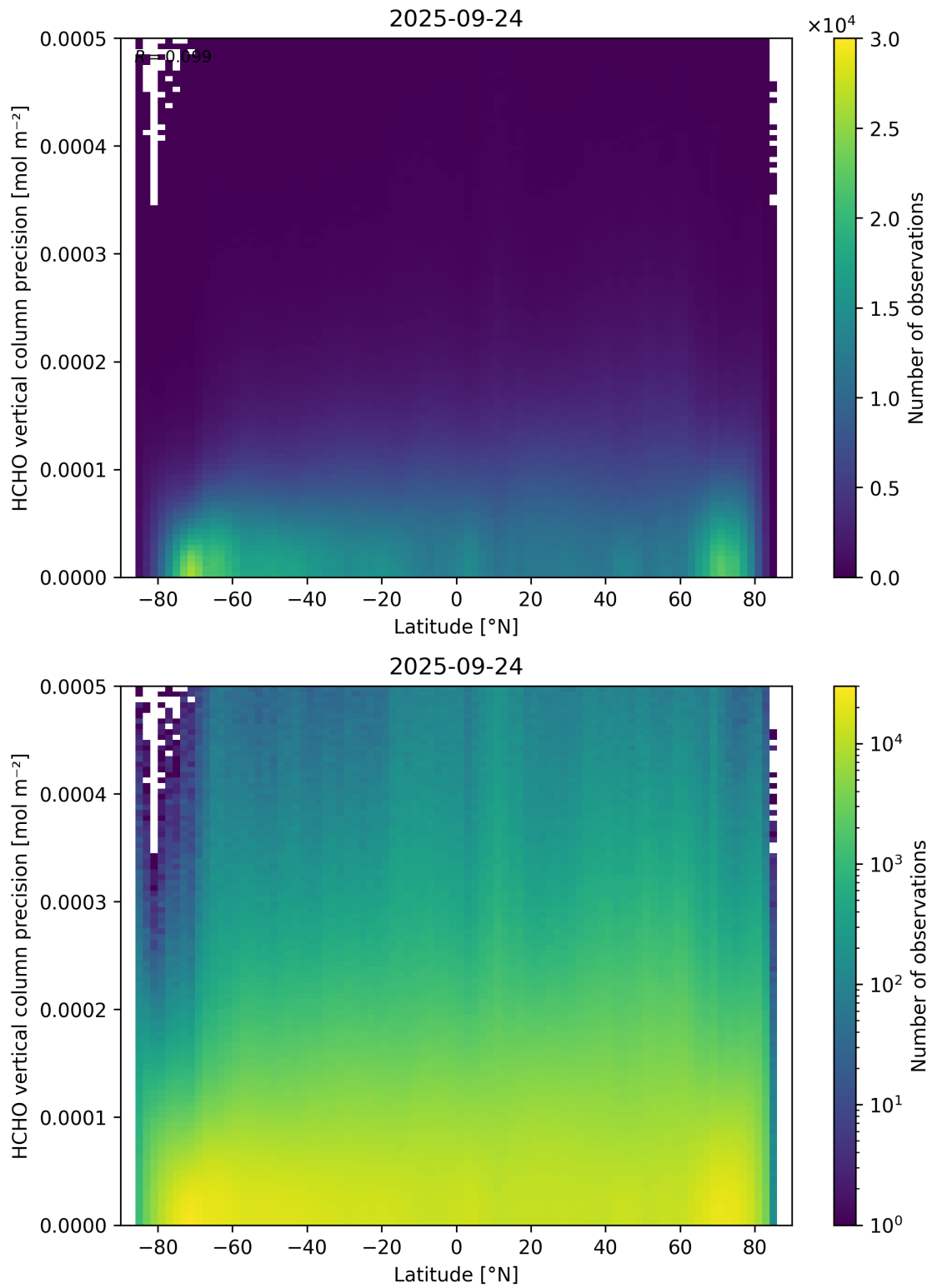
Figure 165: Scatter density plot of “Latitude” against “HCHO vertical column precision” for 2025-09-23 to 2025-09-25.
