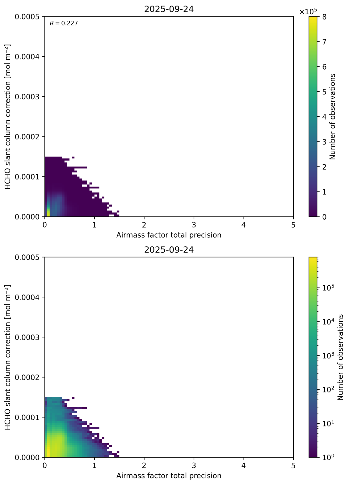
Figure 110: Scatter density plot of “Airmass factor total precision” against “HCHO slant column correction” for 2025-09-23 to 2025-09-25.
