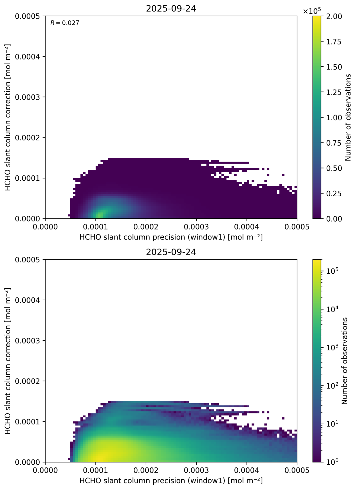
Figure 93: Scatter density plot of “HCHO slant column precision (window1)” against “HCHO slant column correction” for 2025-09-23 to 2025-09-25.
