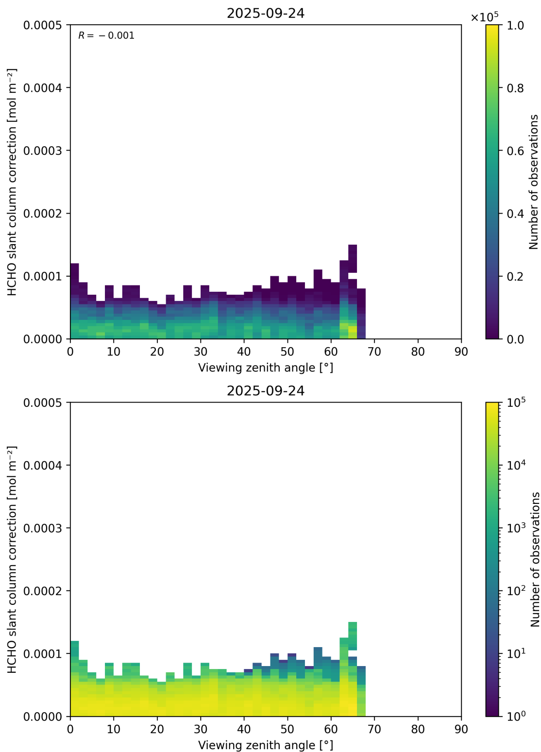
Figure 187: Scatter density plot of “Viewing zenith angle” against “HCHO slant column correction” for 2025-09-23 to 2025-09-25.
