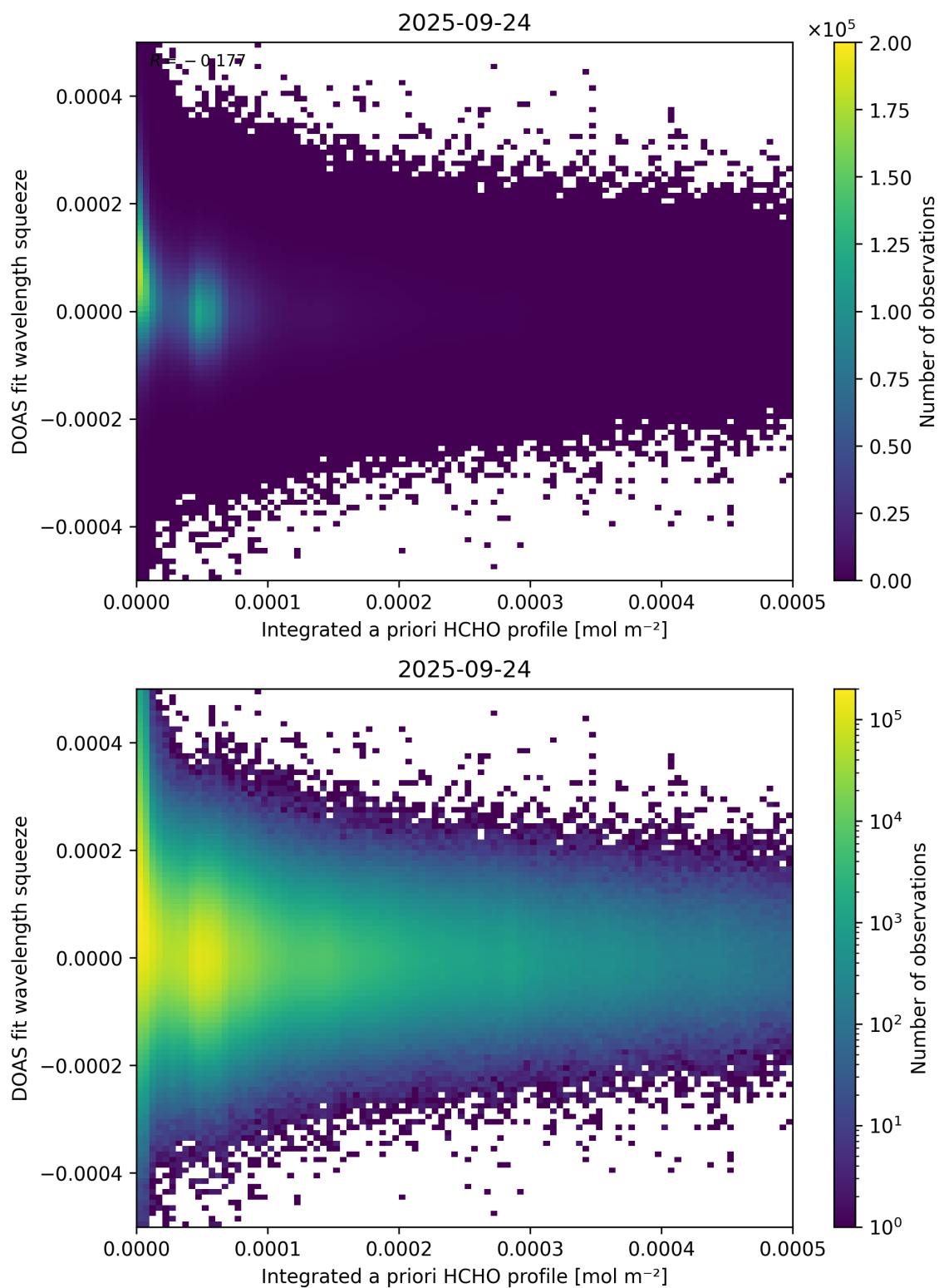
Figure 150: Scatter density plot of “Integrated a priori HCHO profile” against “DOAS fit wavelength squeeze” for 2025-09-23 to 2025-09-25.
