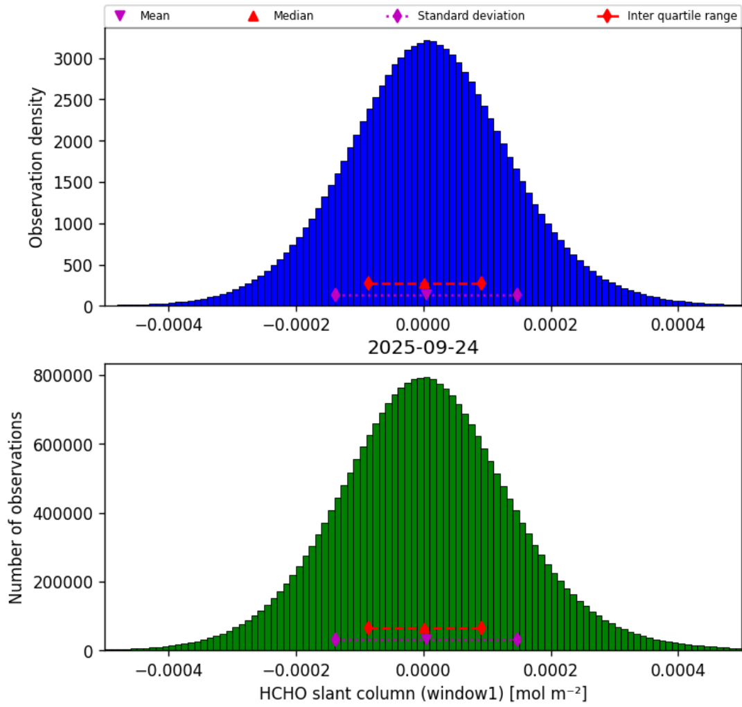
Figure 38: Histogram of “HCHO slant column (window1)” for 2025-09-23 to 2025-09-25
