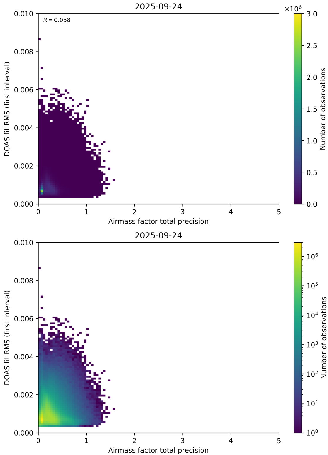
Figure 105: Scatter density plot of “Airmass factor total precision” against “DOAS fit RMS (first interval)” for 2025-09-23 to 2025-09-25.
