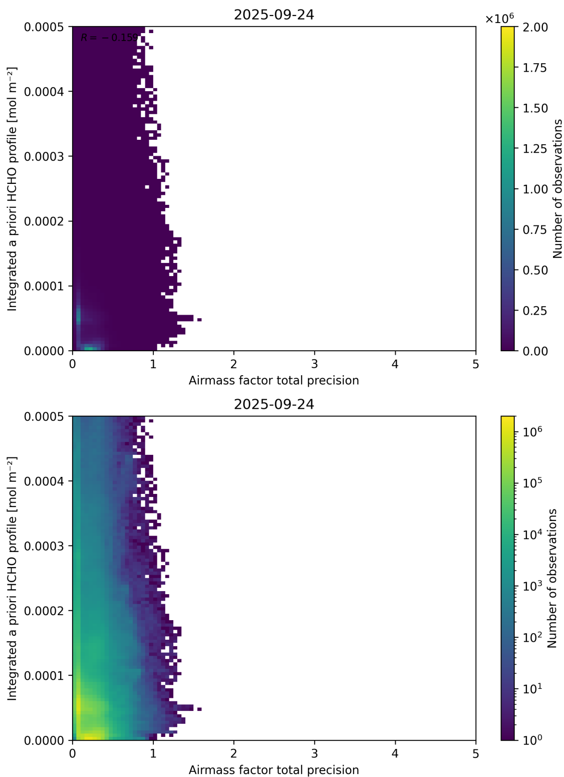
Figure 111: Scatter density plot of “Airmass factor total precision” against “Integrated a priori HCHO profile” for 2025-09-23 to 2025-09-25.
