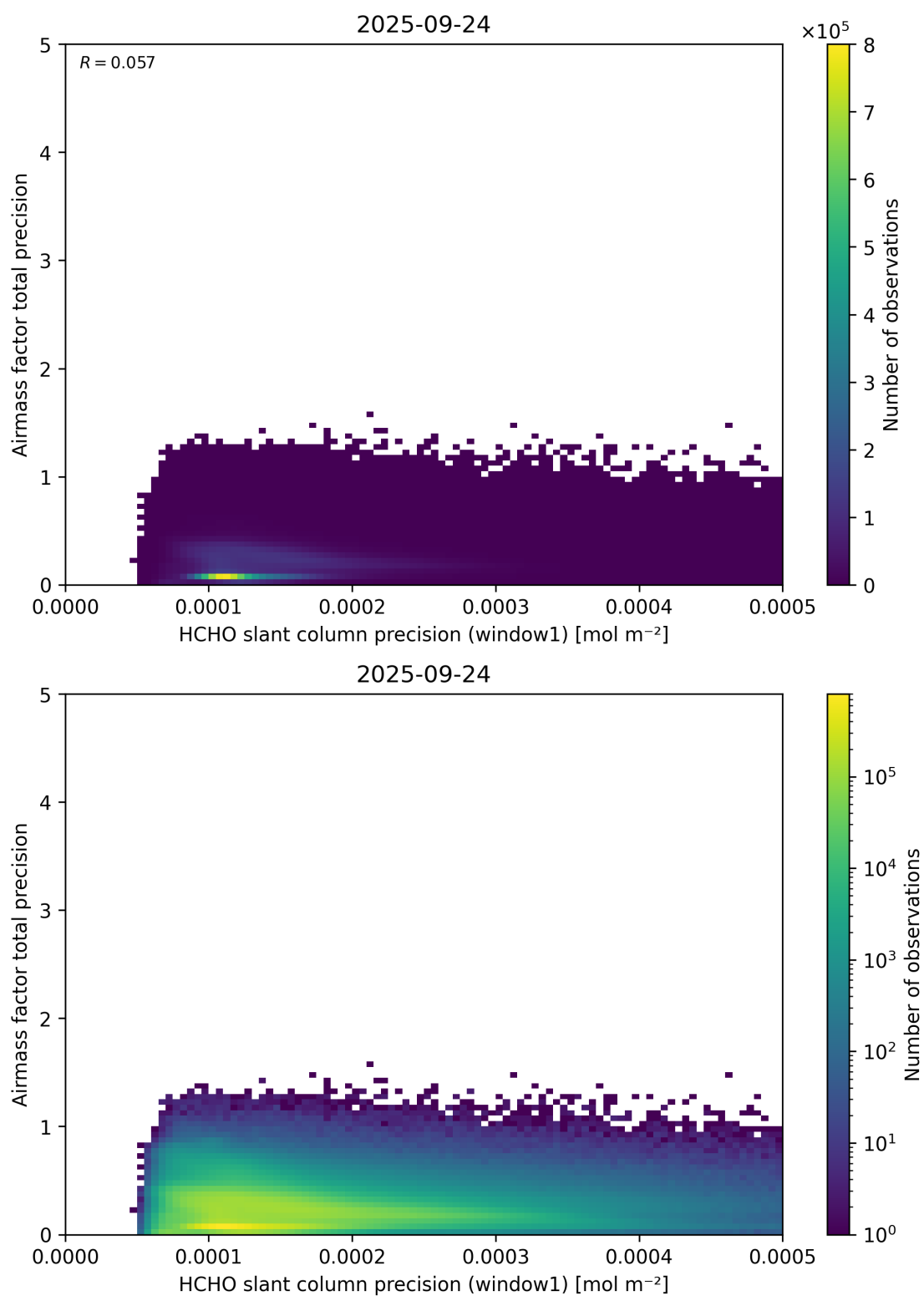
Figure 95: Scatter density plot of “HCHO slant column precision (window1)” against “Airmass factor total precision” for 2025-09-23 to 2025-09-25.
