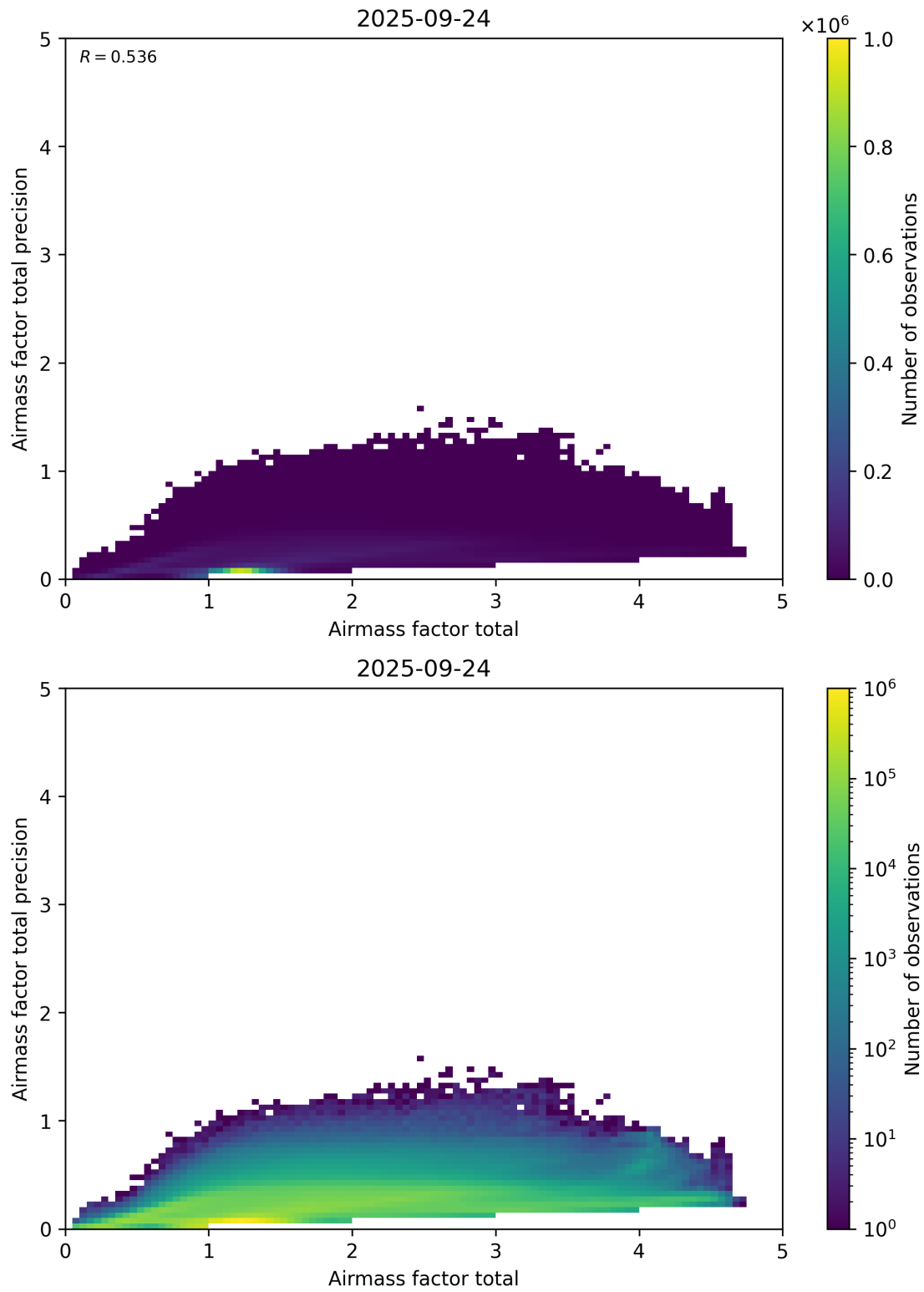
Figure 103: Scatter density plot of “Airmass factor total” against “Airmass factor total precision” for 2025-09-23 to 2025-09-25.
