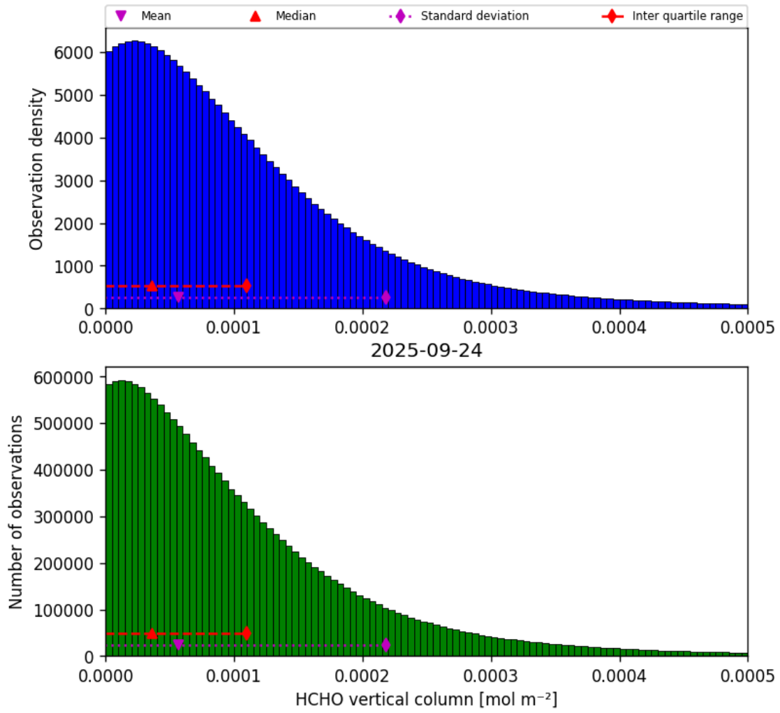
Figure 35: Histogram of “HCHO vertical column” for 2025-09-23 to 2025-09-25
