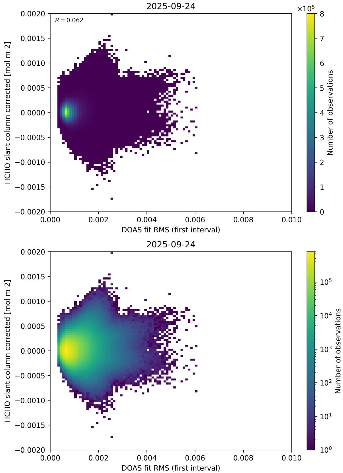
Figure 62: Scatter density plot of “DOAS fit RMS (first interval)” against “HCHO slant column corrected” for 2025-09-23 to 2025-09-25.
