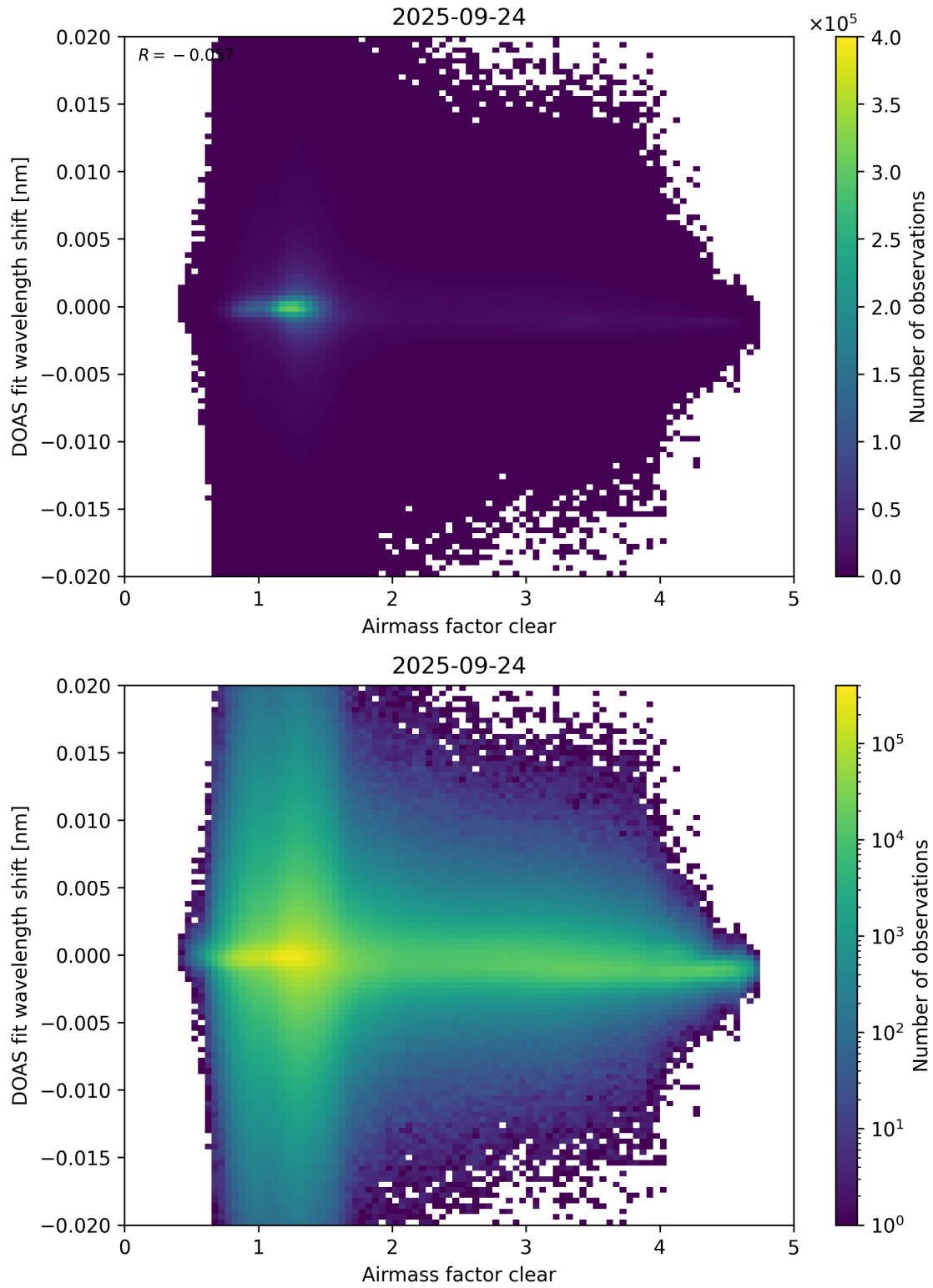
Figure 72: Scatter density plot of “Airmass factor clear” against “DOAS fit wavelength shift” for 2025-09-23 to 2025-09-25.
