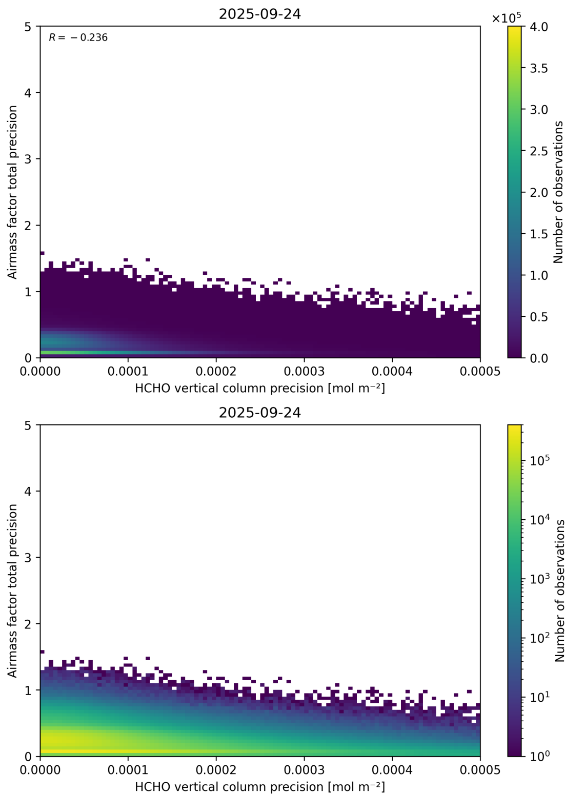
Figure 145: Scatter density plot of “HCHO vertical column precision” against “Airmass factor total precision” for 2025-09-23 to 2025-09-25.
