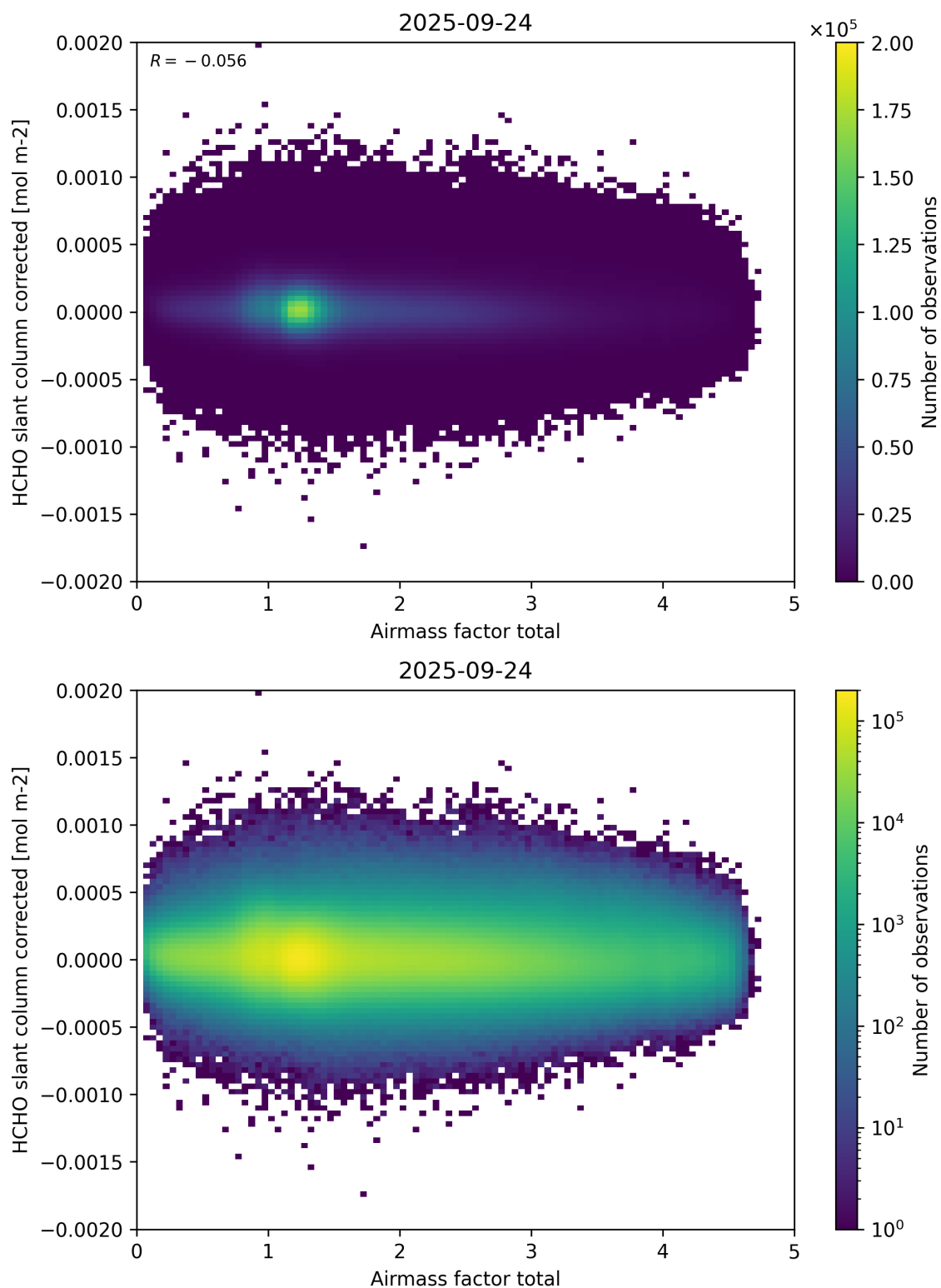
Figure 101: Scatter density plot of “Airmass factor total” against “HCHO slant column corrected” for 2025-09-23 to 2025-09-25.
