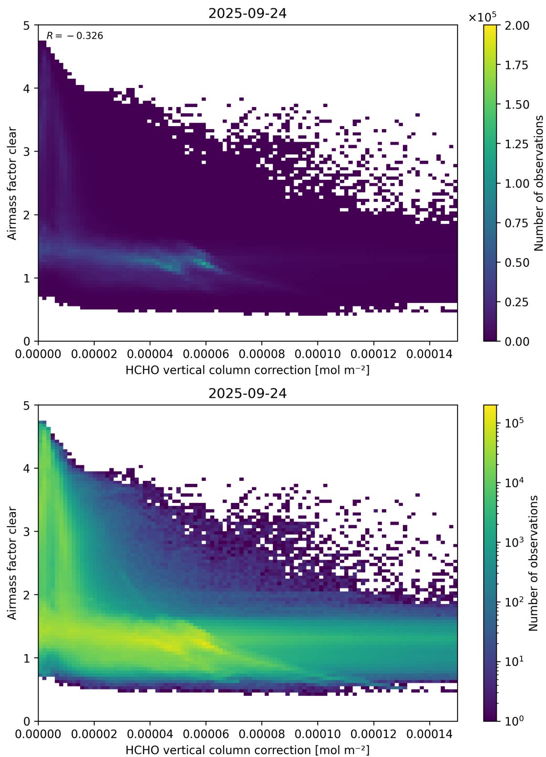
Figure 115: Scatter density plot of “HCHO vertical column correction” against “Airmass factor clear” for 2025-09-23 to 2025-09-25.
