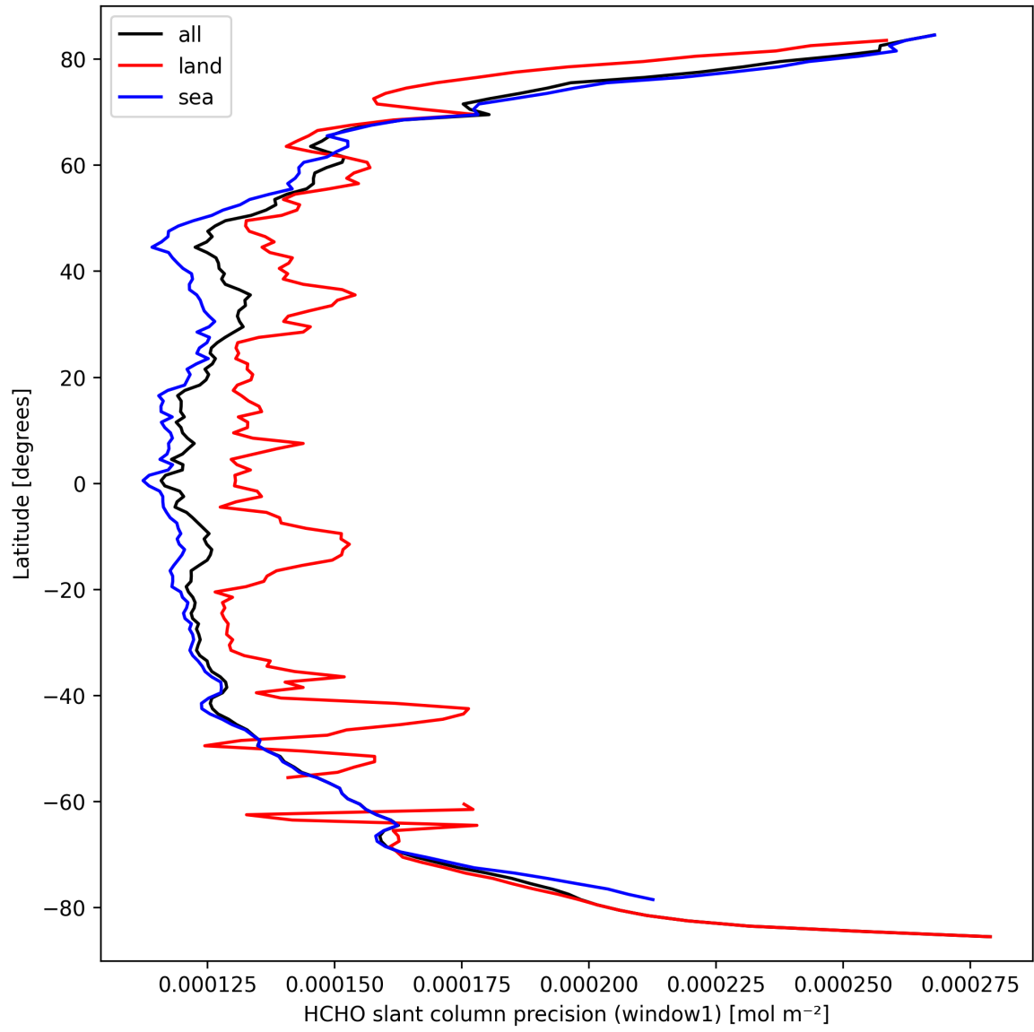
Figure 25: Zonal average of “HCHO slant column precision (window1)” for 2025-09-23 to 2025-09-25.
