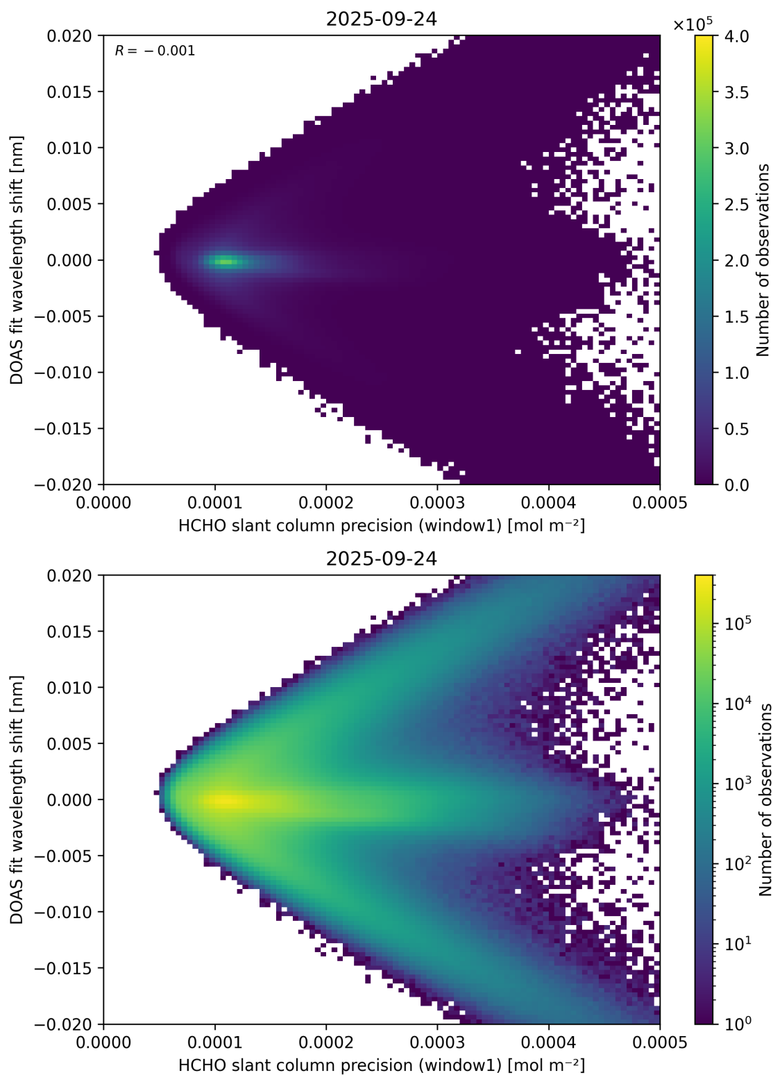
Figure 89: Scatter density plot of “HCHO slant column precision (window1)” against “DOAS fit wavelength shift” for 2025-09-23 to 2025-09-25.
