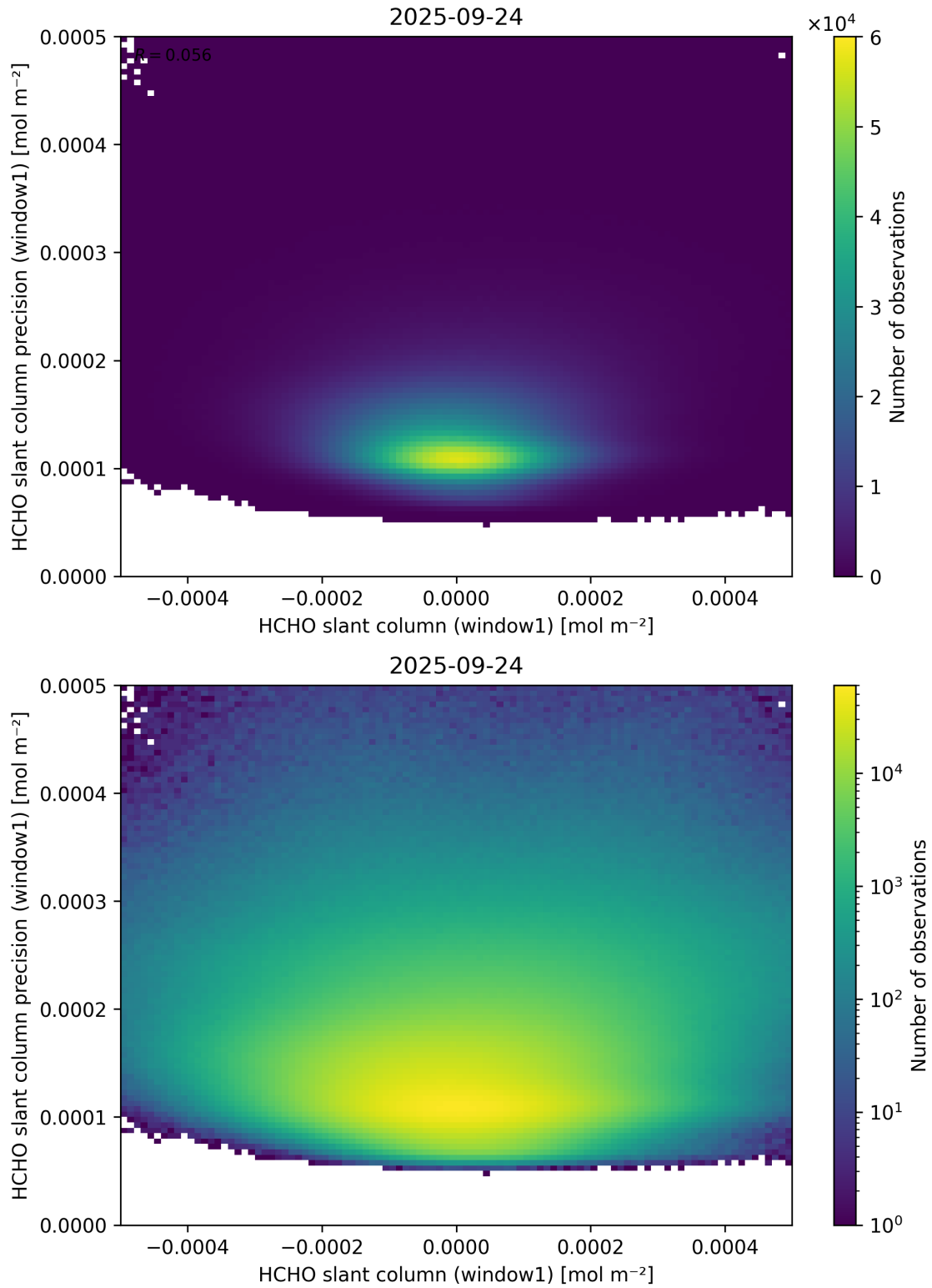
Figure 84: Scatter density plot of “HCHO slant column (window1)” against “HCHO slant column precision (window1)” for 2025-09-23 to 2025-09-25.
