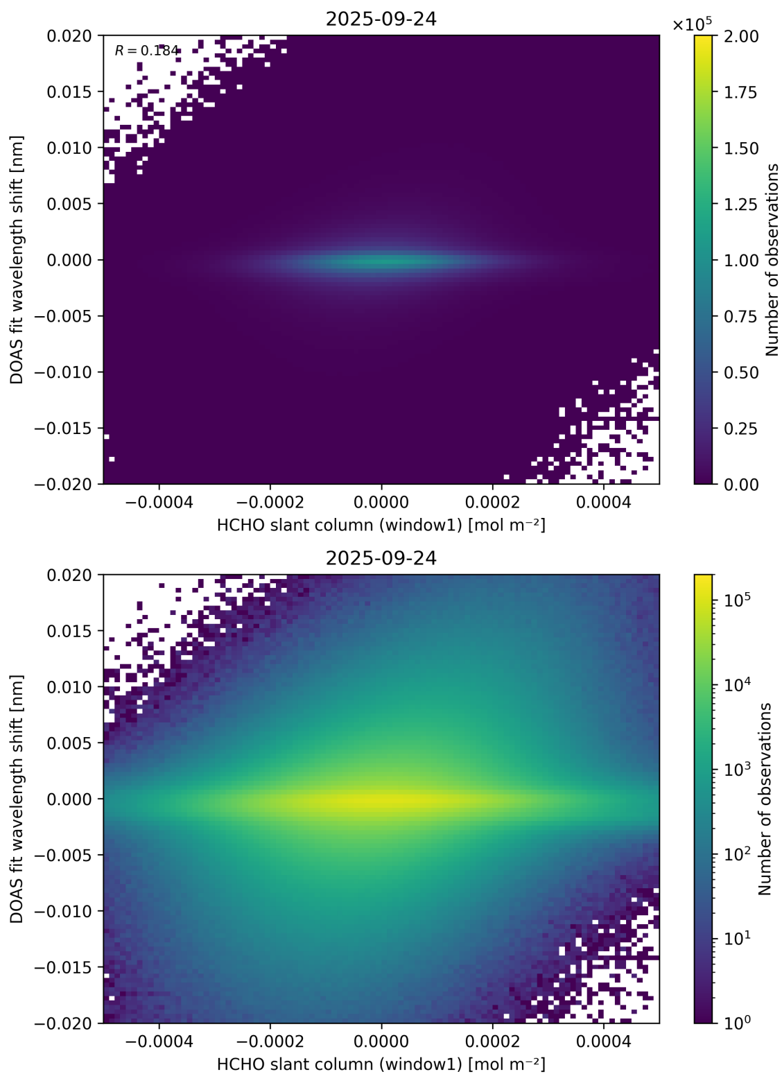
Figure 79: Scatter density plot of “HCHO slant column (window1)” against “DOAS fit wavelength shift” for 2025-09-23 to 2025-09-25.
