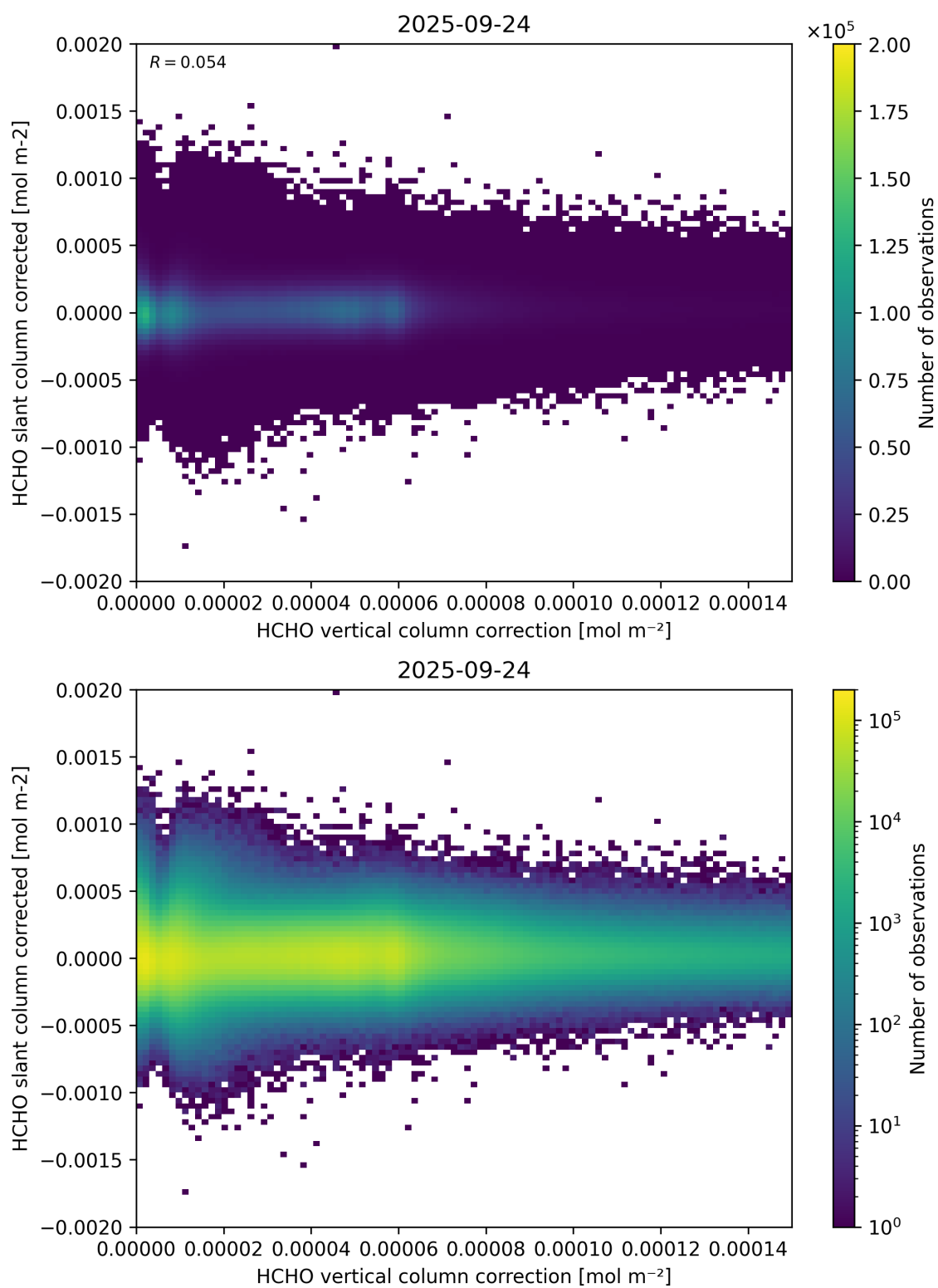
Figure 116: Scatter density plot of “HCHO vertical column correction” against “HCHO slant column corrected” for 2025-09-23 to 2025-09-25.
