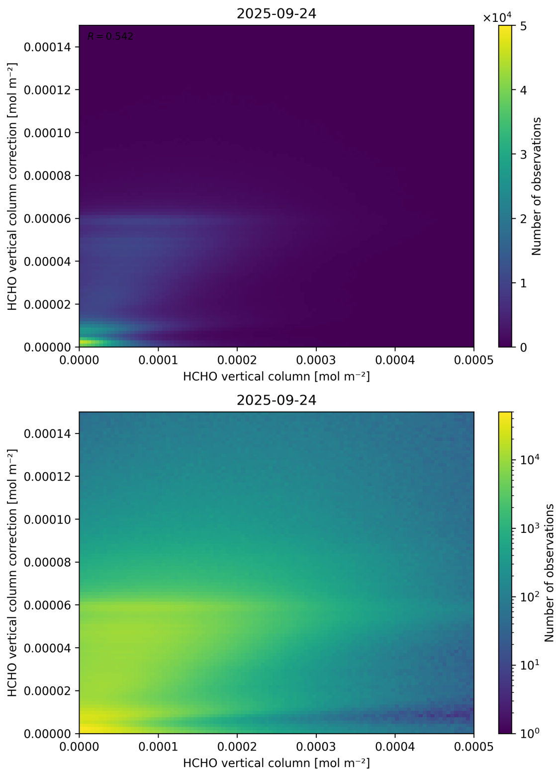
Figure 133: Scatter density plot of “HCHO vertical column” against “HCHO vertical column correction” for 2025-09-23 to 2025-09-25.
