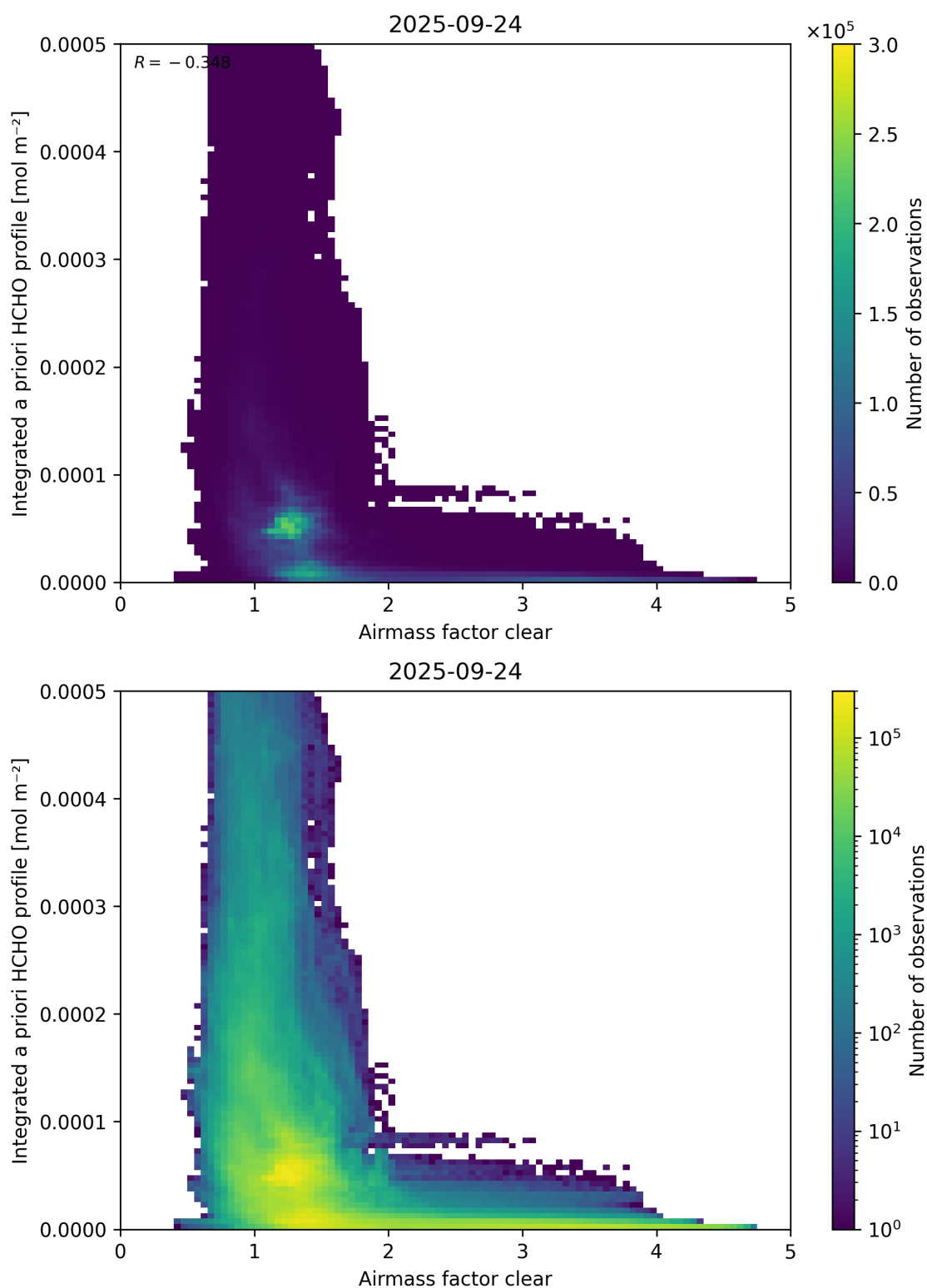
Figure 76: Scatter density plot of “Airmass factor clear” against “Integrated a priori HCHO profile” for 2025-09-23 to 2025-09-25.
