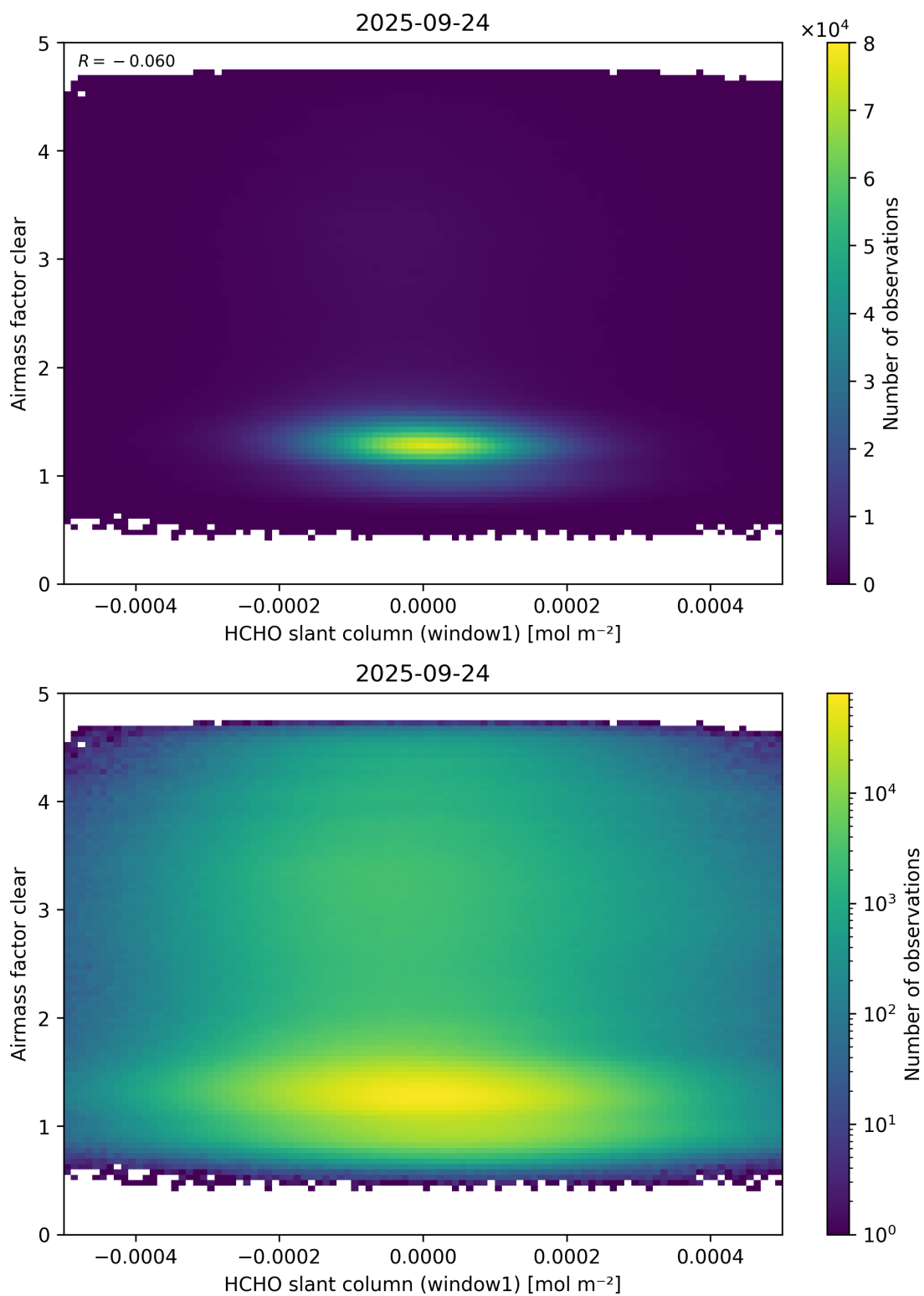
Figure 81: Scatter density plot of “HCHO slant column (window1)” against “Airmass factor clear” for 2025-09-23 to 2025-09-25.
