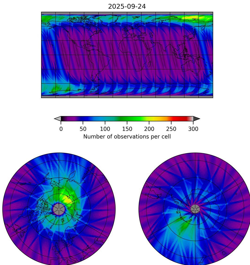
Figure 19: Map of the number of observations for 2025-09-23 to 2025-09-25
