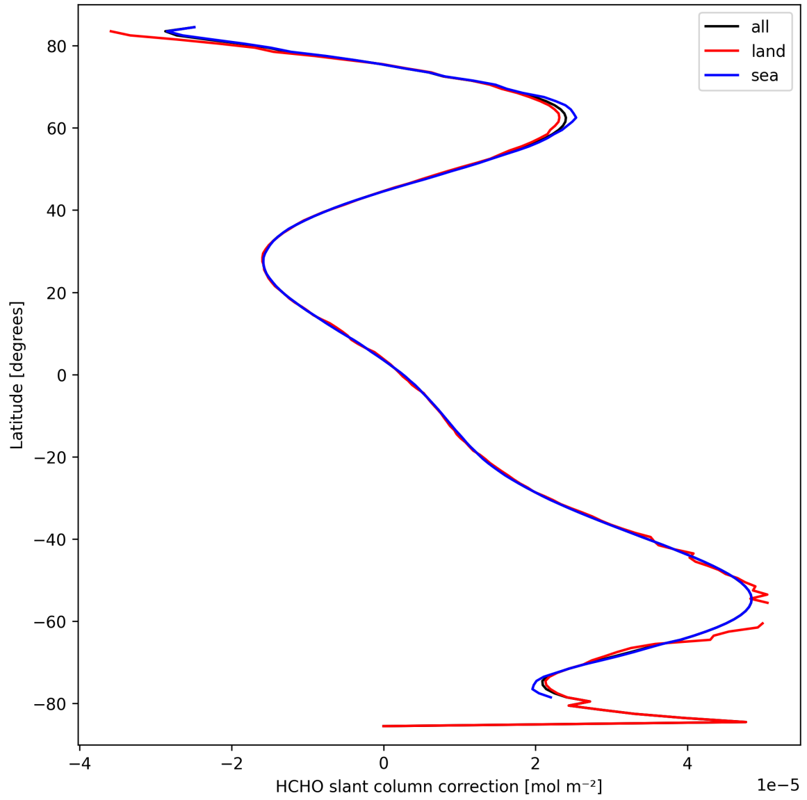
Figure 33: Zonal average of "HCHO slant column correction" for 2025-09-23 to 2025-09-25.
