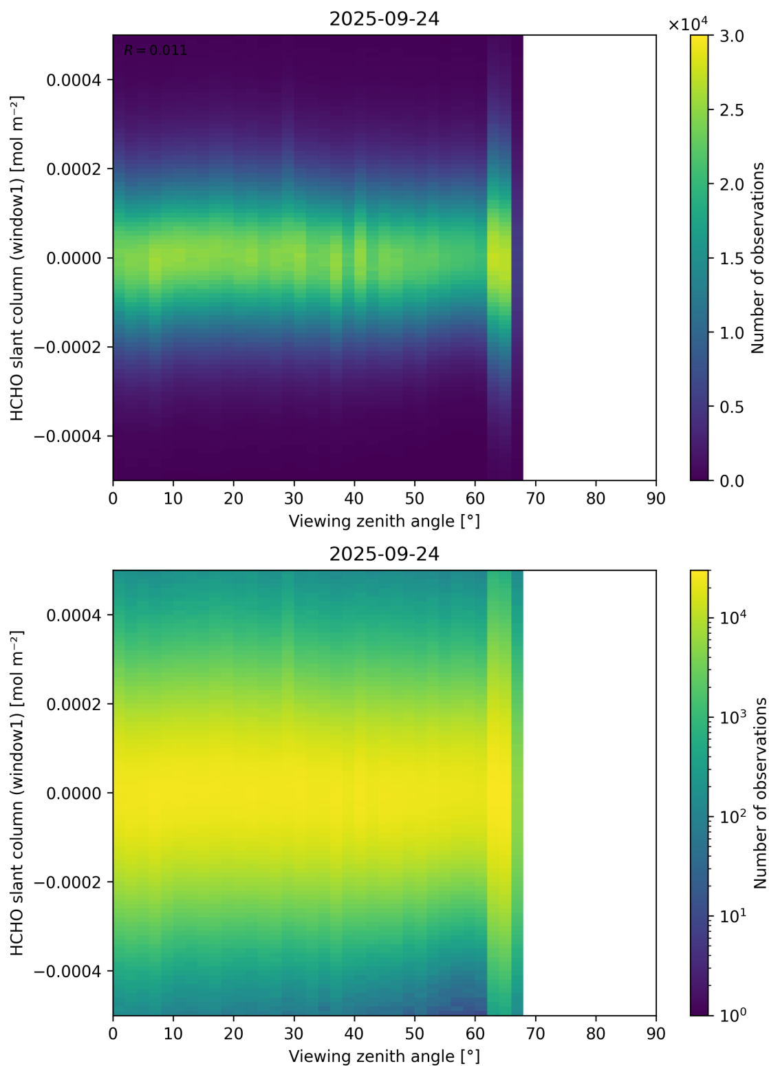
Figure 188: Scatter density plot of “Viewing zenith angle” against “HCHO slant column (window1)” for 2025-09-23 to 2025-09-25.
