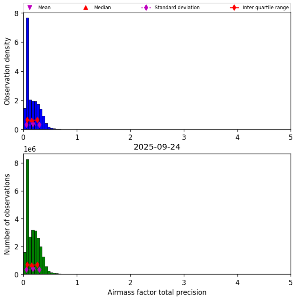
Figure 41: Histogram of “Airmass factor total precision” for 2025-09-23 to 2025-09-25
