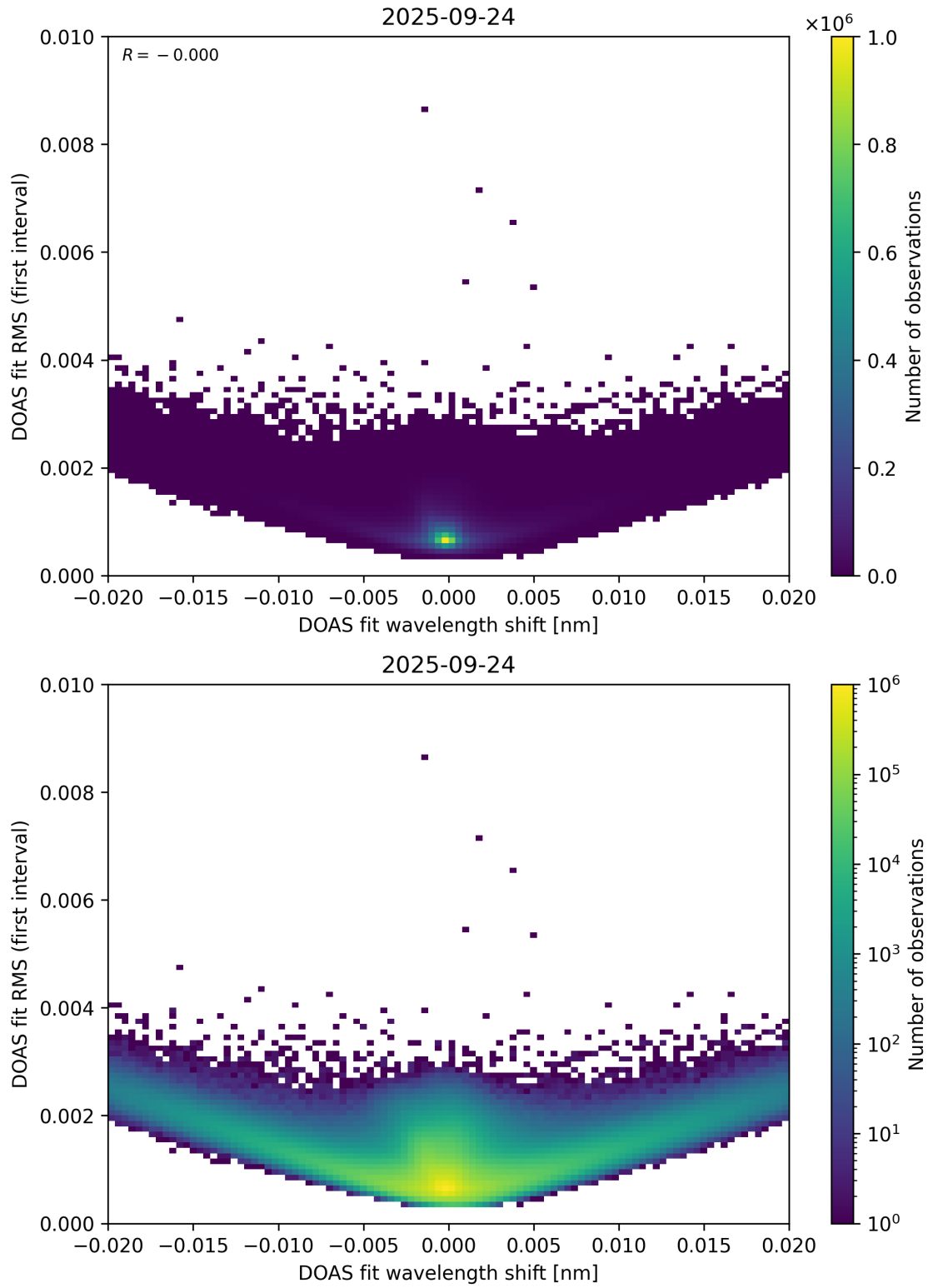
Figure 64: Scatter density plot of “DOAS fit wavelength shift” against “DOAS fit RMS (first interval)” for 2025-09-23 to 2025-09-25.
