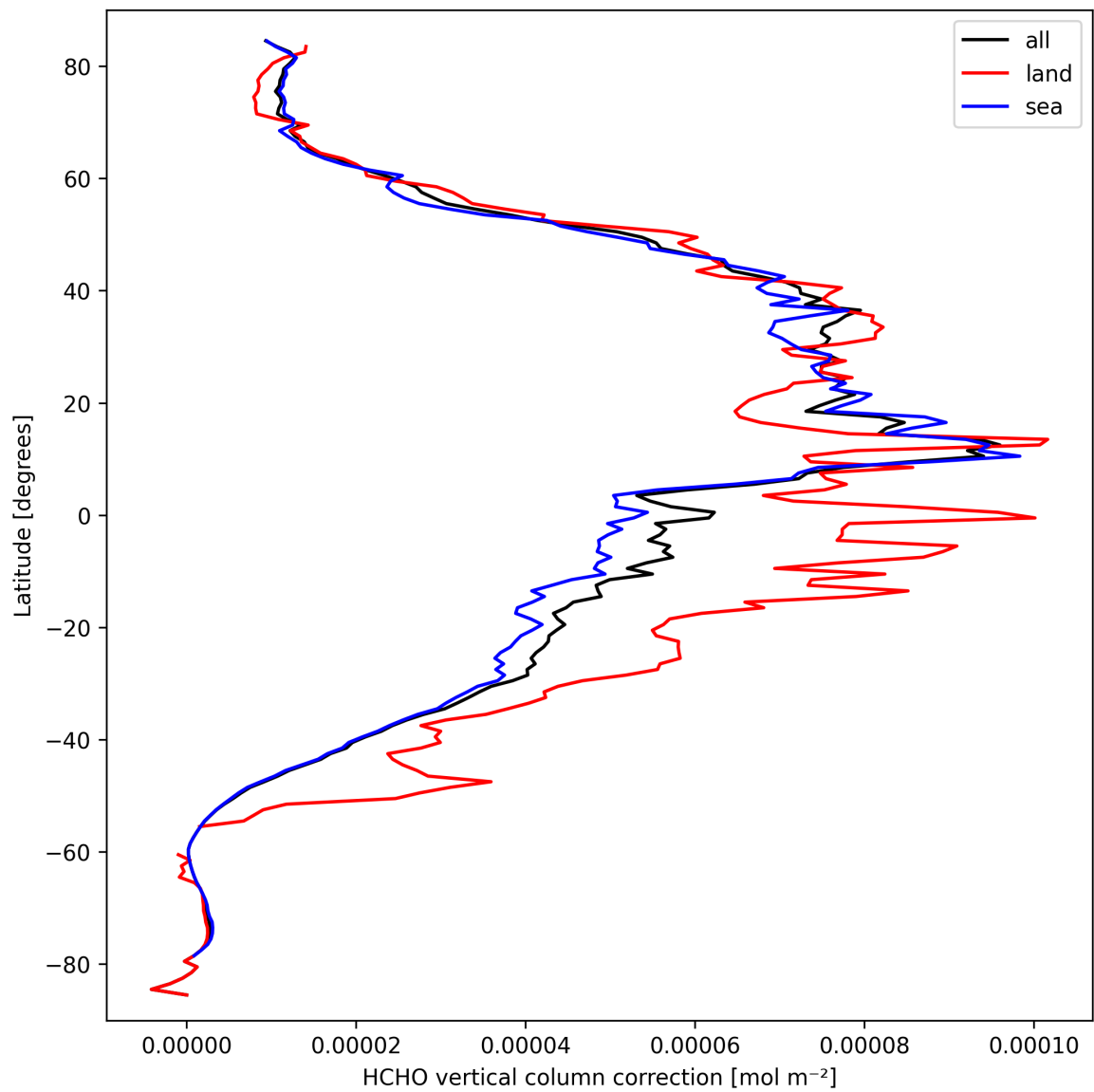
Figure 23: Zonal average of “HCHO vertical column correction” for 2025-09-23 to 2025-09-25.
