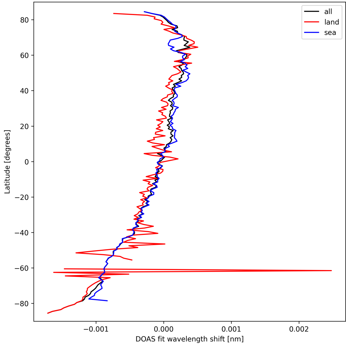
Figure 30: Zonal average of "DOAS fit wavelength shift" for 2025-09-23 to 2025-09-25.
