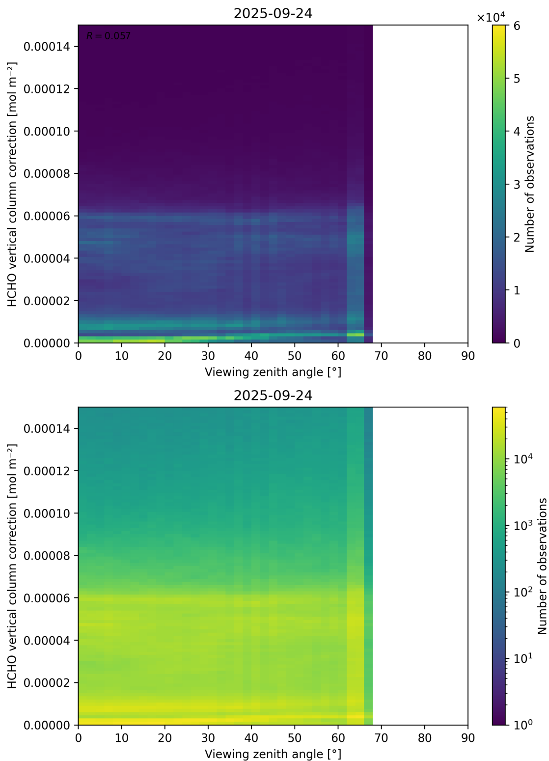
Figure 193: Scatter density plot of “Viewing zenith angle” against “HCHO vertical column correction” for 2025-09-23 to 2025-09-25.
