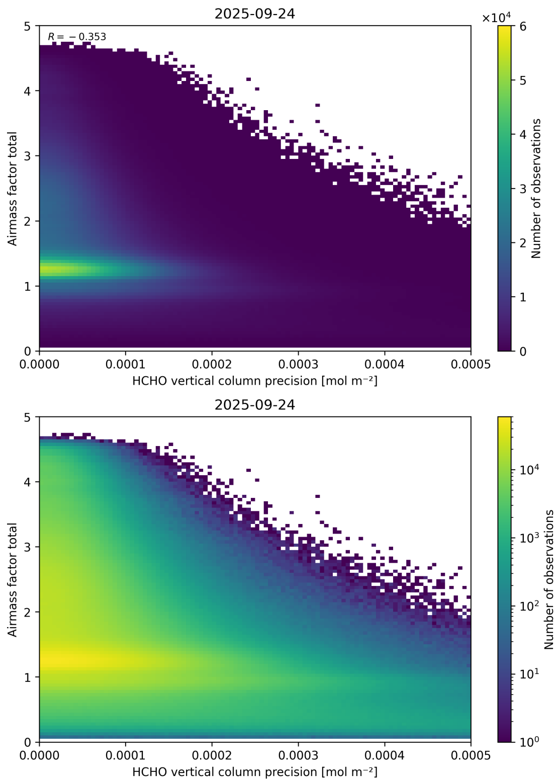
Figure 144: Scatter density plot of “HCHO vertical column precision” against “Airmass factor total” for 2025-09-23 to 2025-09-25.
