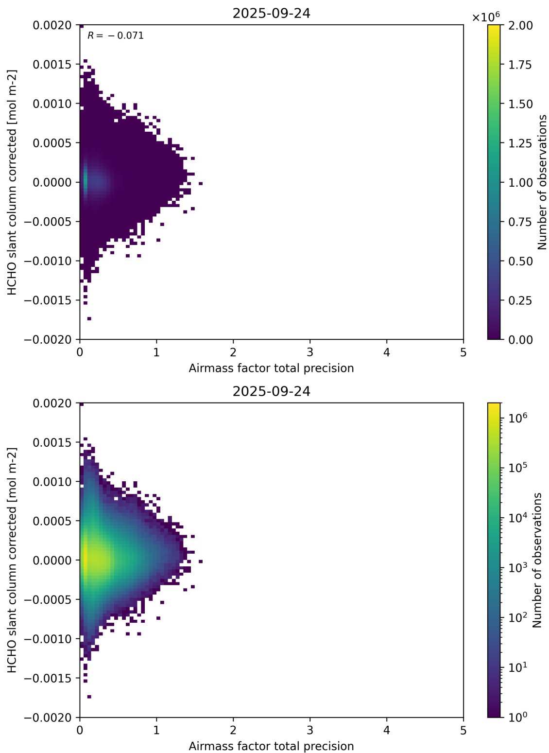
Figure 109: Scatter density plot of “Airmass factor total precision” against “HCHO slant column corrected” for 2025-09-23 to 2025-09-25.
