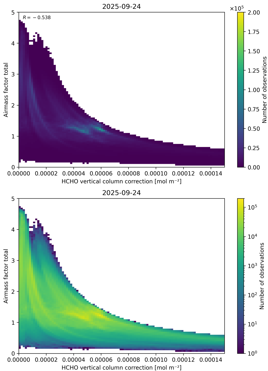
Figure 120: Scatter density plot of “HCHO vertical column correction” against “Airmass factor total” for 2025-09-23 to 2025-09-25.
