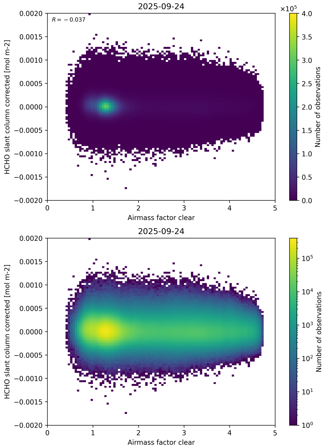
Figure 74: Scatter density plot of “Airmass factor clear” against “HCHO slant column corrected” for 2025-09-23 to 2025-09-25.
