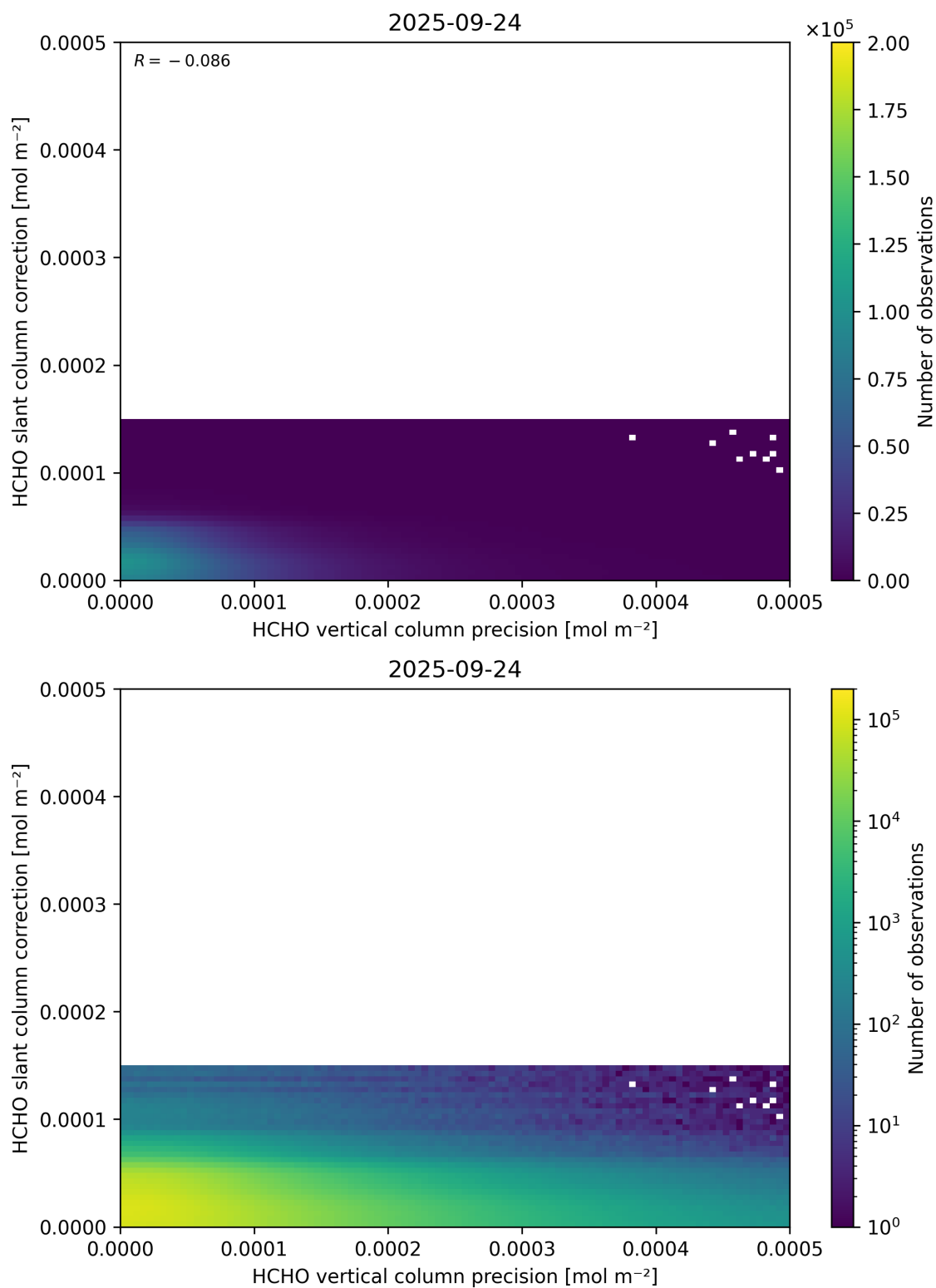
Figure 141: Scatter density plot of “HCHO vertical column precision” against “HCHO slant column correction” for 2025-09-23 to 2025-09-25.
