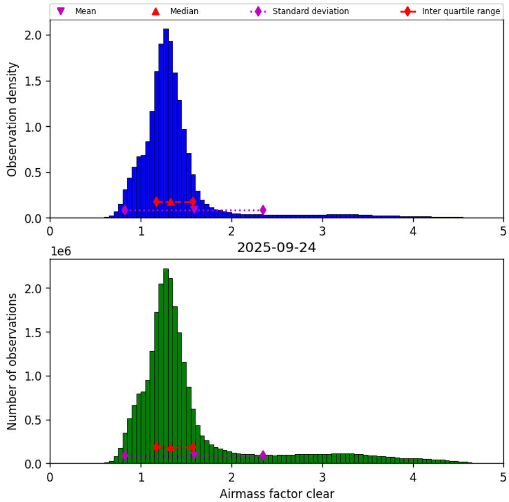
Figure 42: Histogram of “Airmass factor clear” for 2025-09-23 to 2025-09-25
