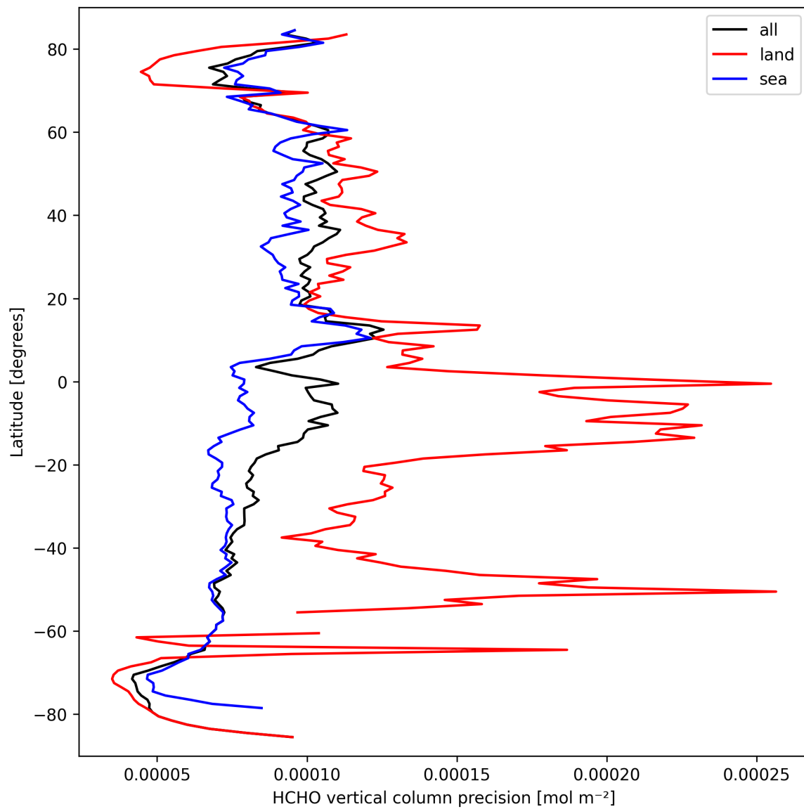
Figure 22: Zonal average of “HCHO vertical column precision” for 2025-09-23 to 2025-09-25.
