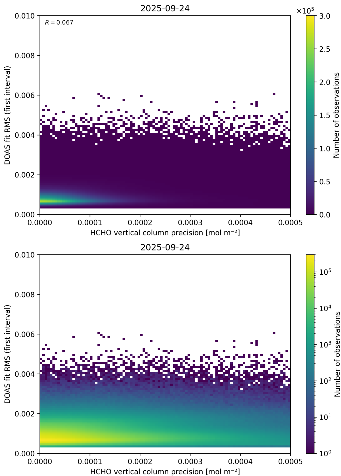
Figure 136: Scatter density plot of “HCHO vertical column precision” against “DOAS fit RMS (first interval)” for 2025-09-23 to 2025-09-25.
