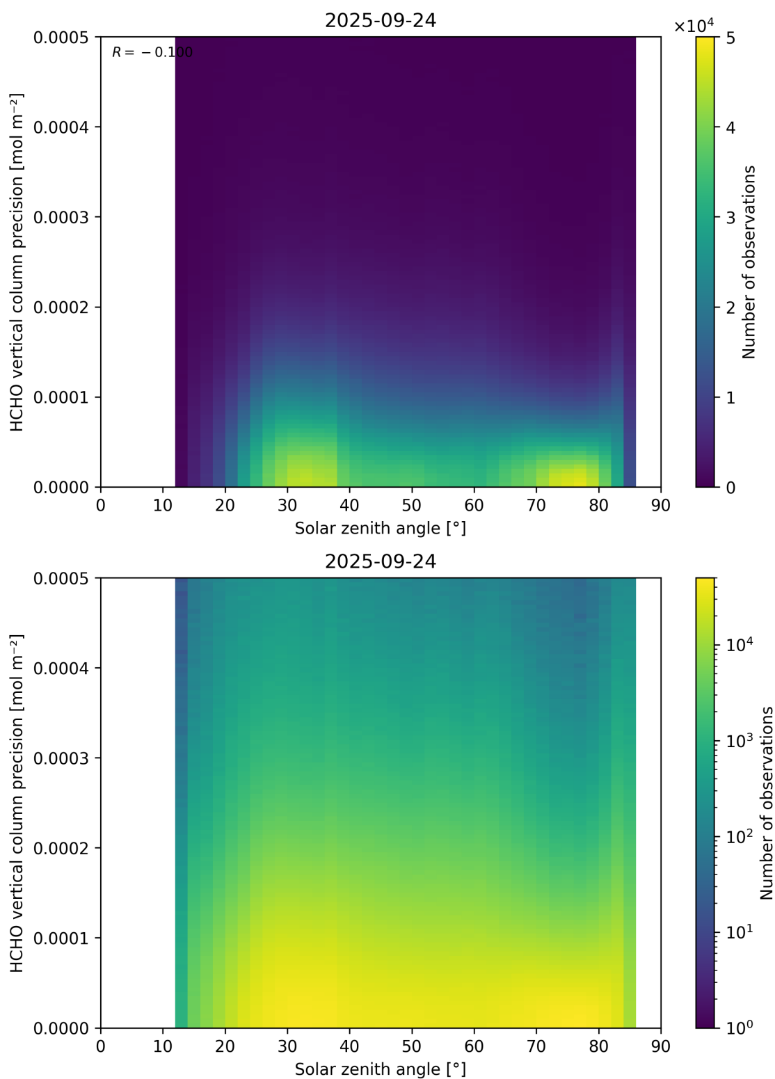
Figure 179: Scatter density plot of “Solar zenith angle” against “HCHO vertical column precision” for 2025-09-23 to 2025-09-25.
