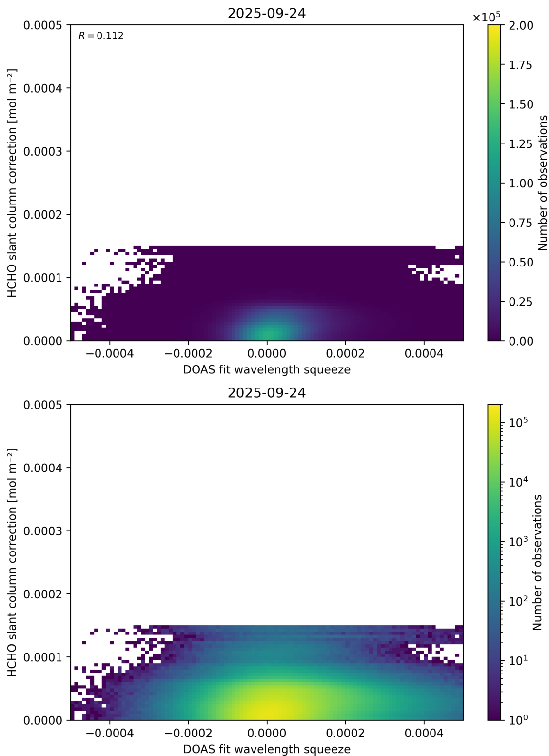
Figure 70: Scatter density plot of “DOAS fit wavelength squeeze” against “HCHO slant column correction” for 2025-09-23 to 2025-09-25.
