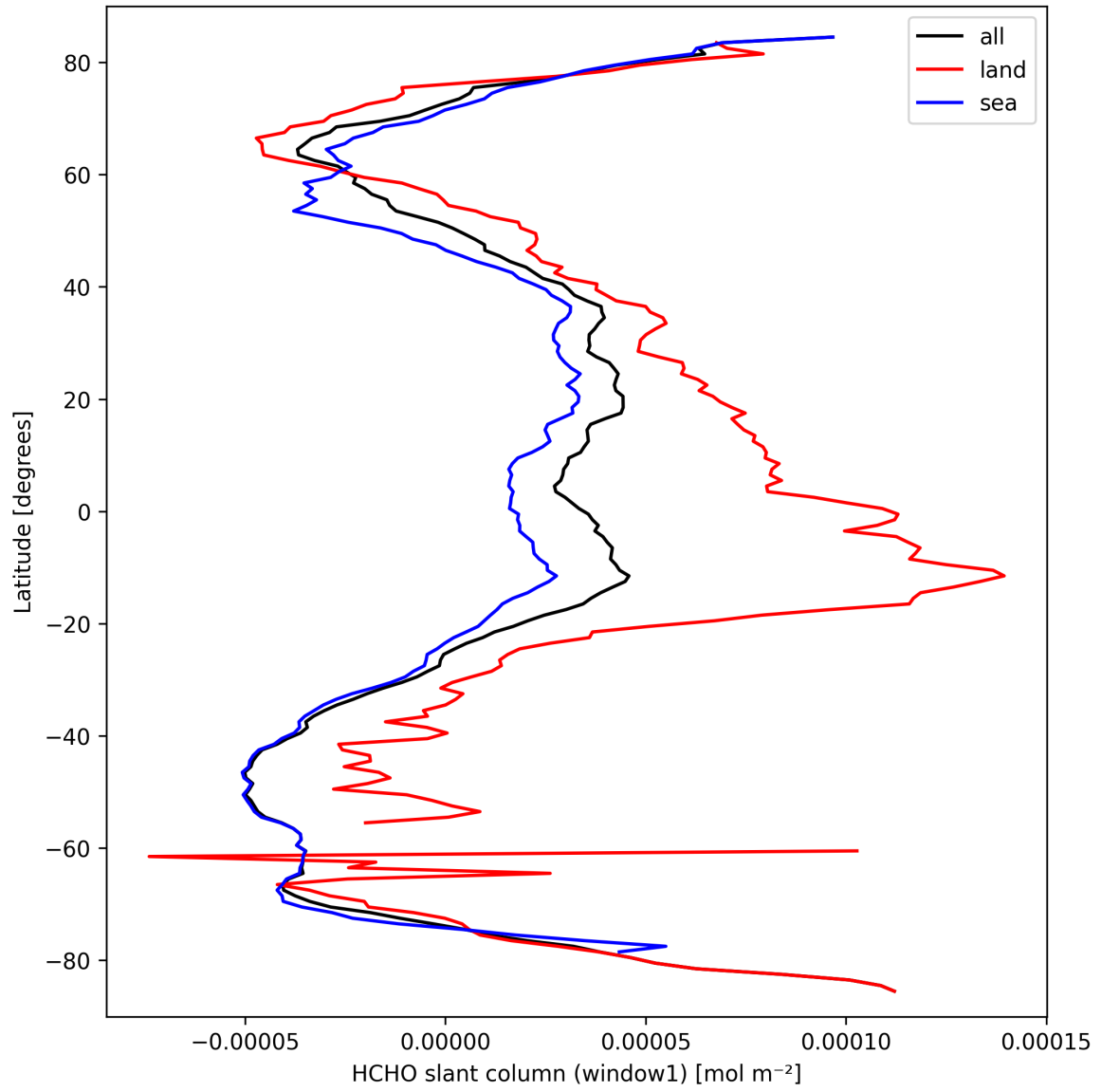
Figure 24: Zonal average of "HCHO slant column (window1)" for 2025-09-23 to 2025-09-25.
