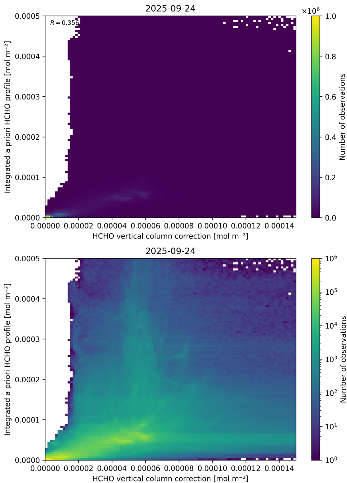
Figure 122: Scatter density plot of “HCHO vertical column correction” against “Integrated a priori HCHO profile” for 2025-09-23 to 2025-09-25.
