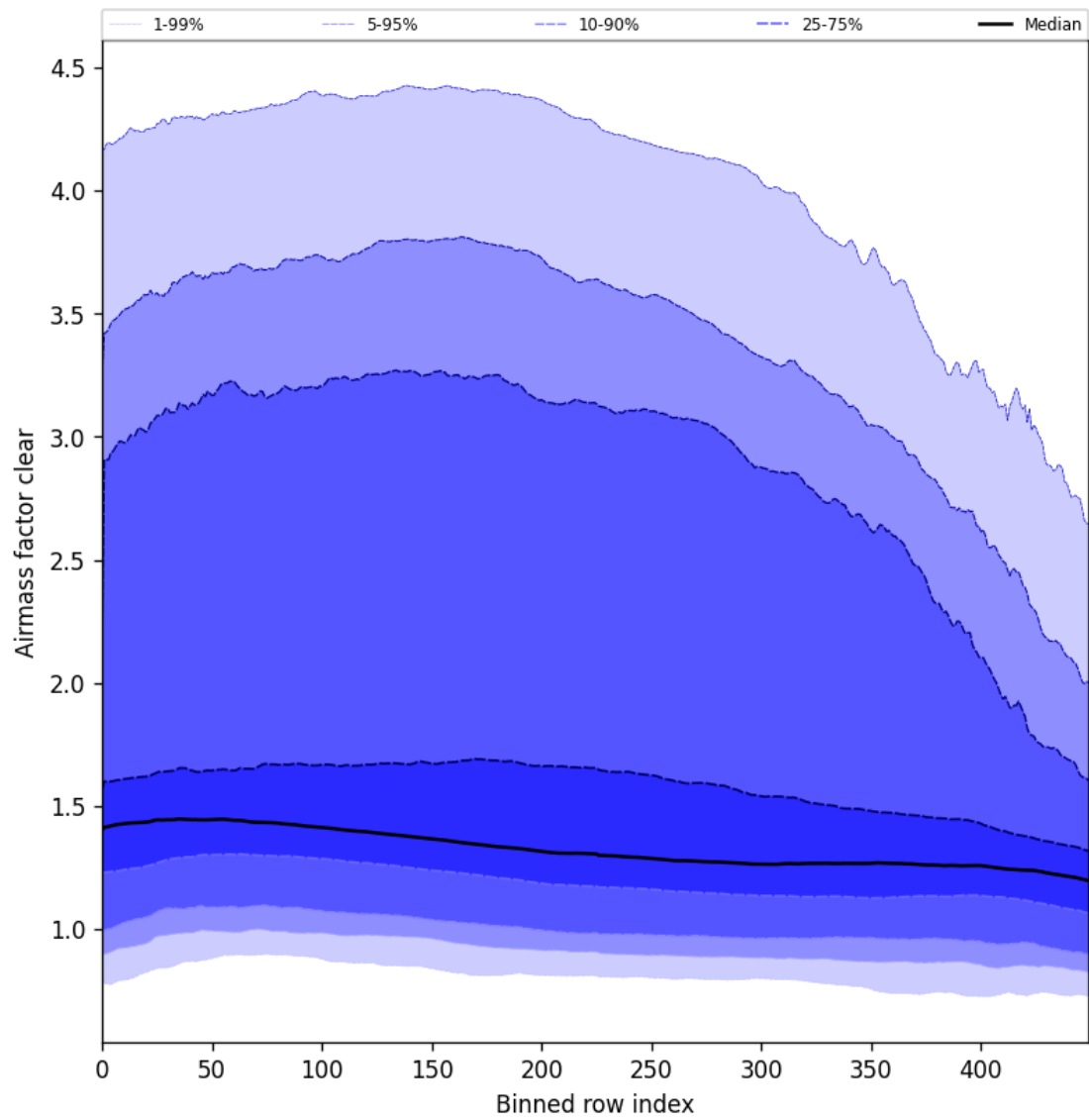
Figure 56: Along track statistics of “Air mass factor clear” for 2025-09-23 to 2025-09-25
