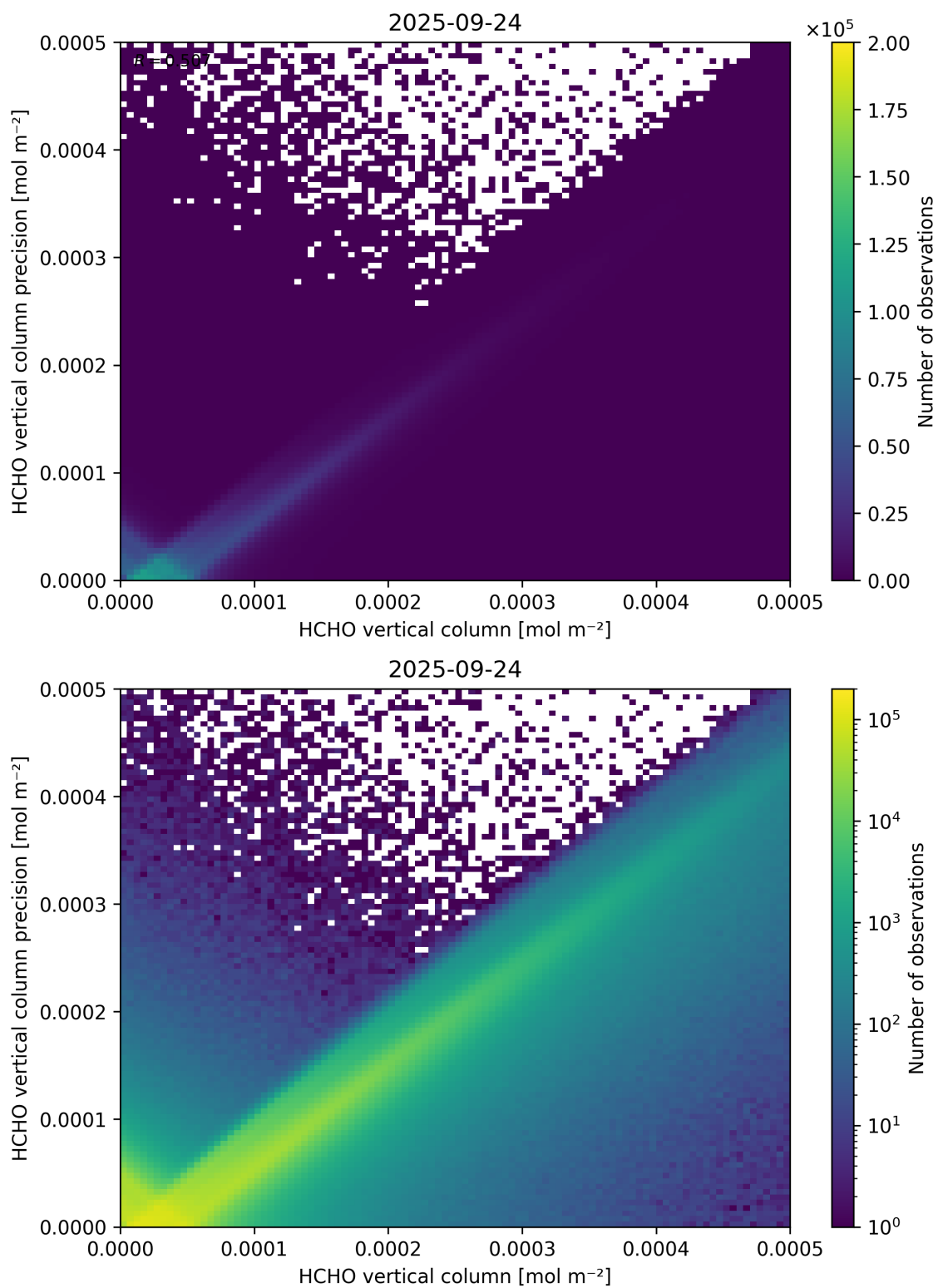
Figure 134: Scatter density plot of “HCHO vertical column” against “HCHO vertical column precision” for 2025-09-23 to 2025-09-25.
