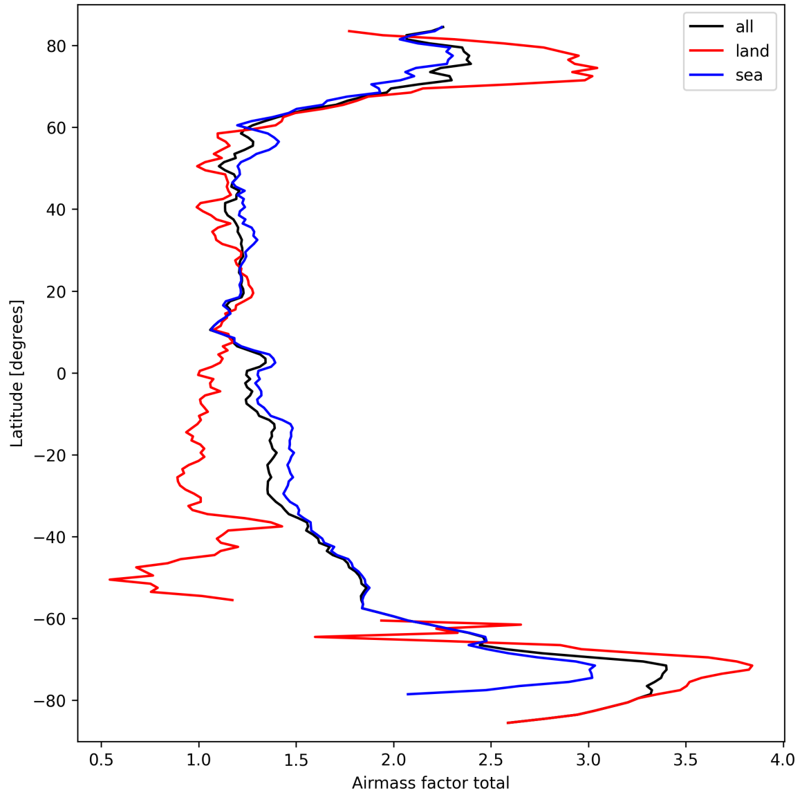
Figure 26: Zonal average of “Airmass factor total” for 2025-09-23 to 2025-09-25.
