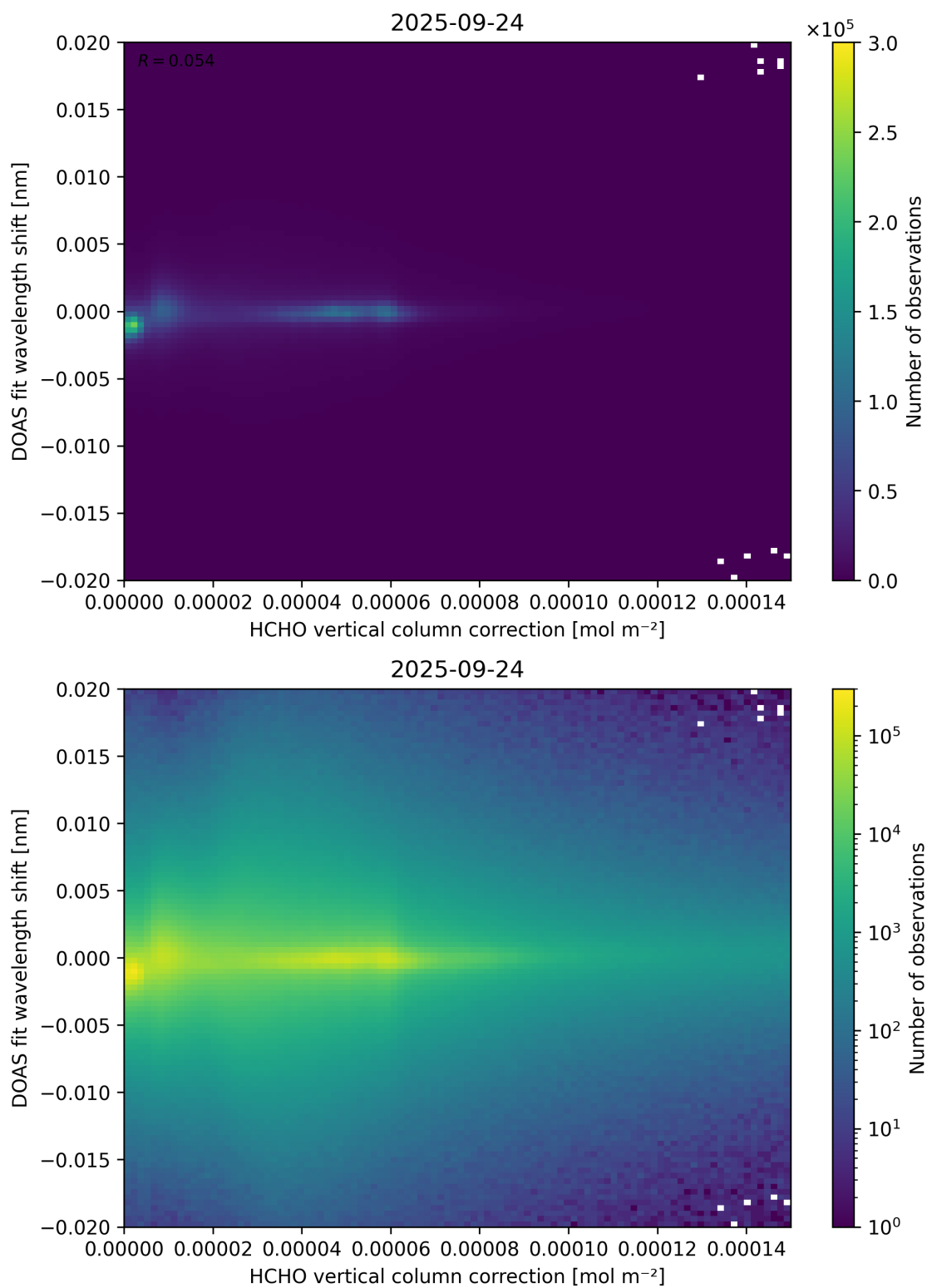
Figure 113: Scatter density plot of “HCHO vertical column correction” against “DOAS fit wavelength shift” for 2025-09-23 to 2025-09-25.
