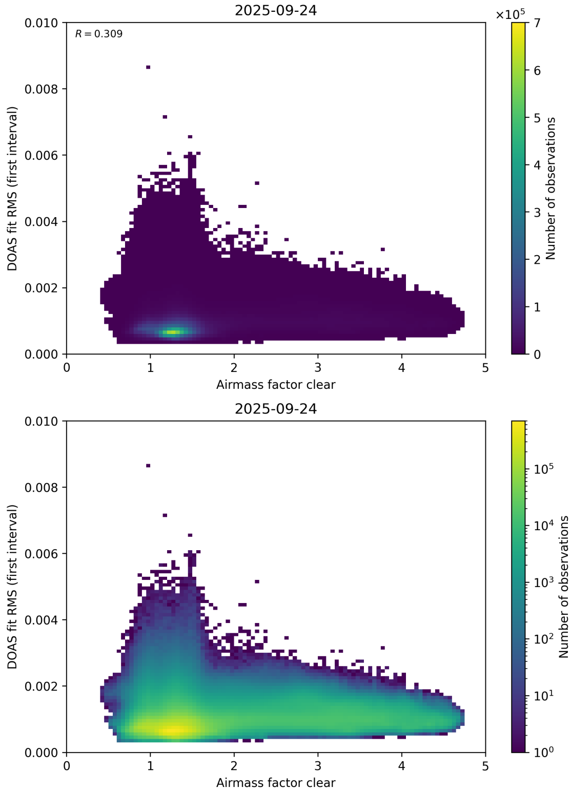
Figure 71: Scatter density plot of “Airmass factor clear” against “DOAS fit RMS (first interval)” for 2025-09-23 to 2025-09-25.
