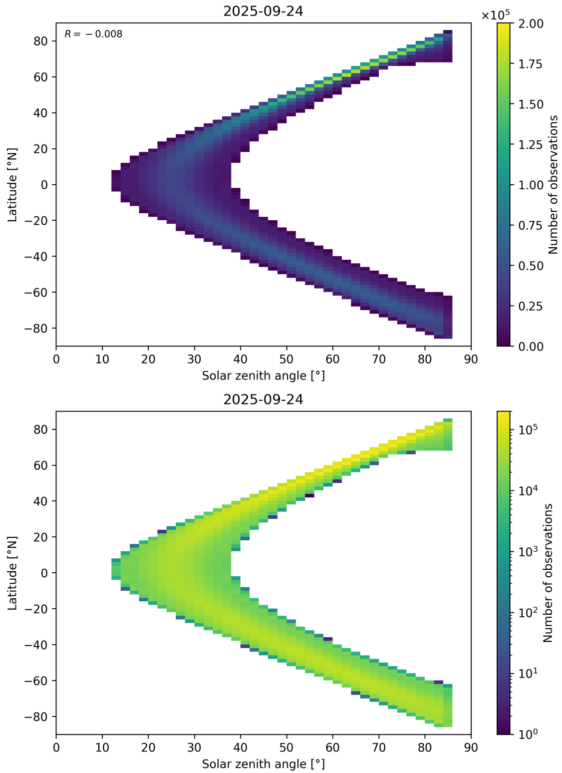
Figure 181: Scatter density plot of “Solar zenith angle” against “Latitude” for 2025-09-23 to 2025-09-25.
