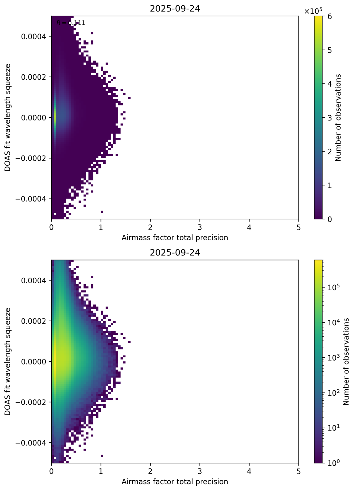
Figure 107: Scatter density plot of “Airmass factor total precision” against “DOAS fit wavelength squeeze” for 2025-09-23 to 2025-09-25.
