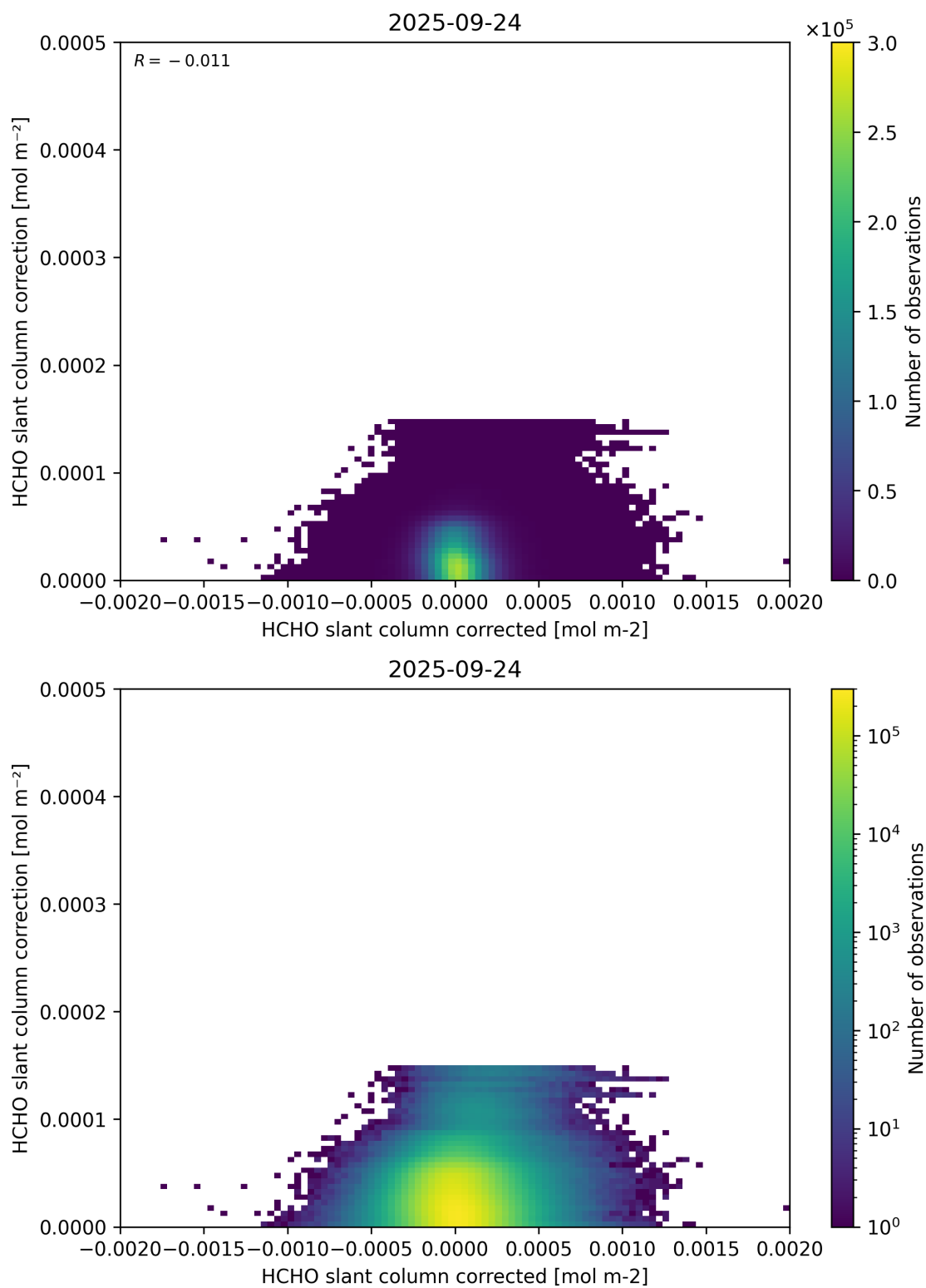
Figure 77: Scatter density plot of “HCHO slant column corrected” against “HCHO slant column correction” for 2025-09-23 to 2025-09-25.
