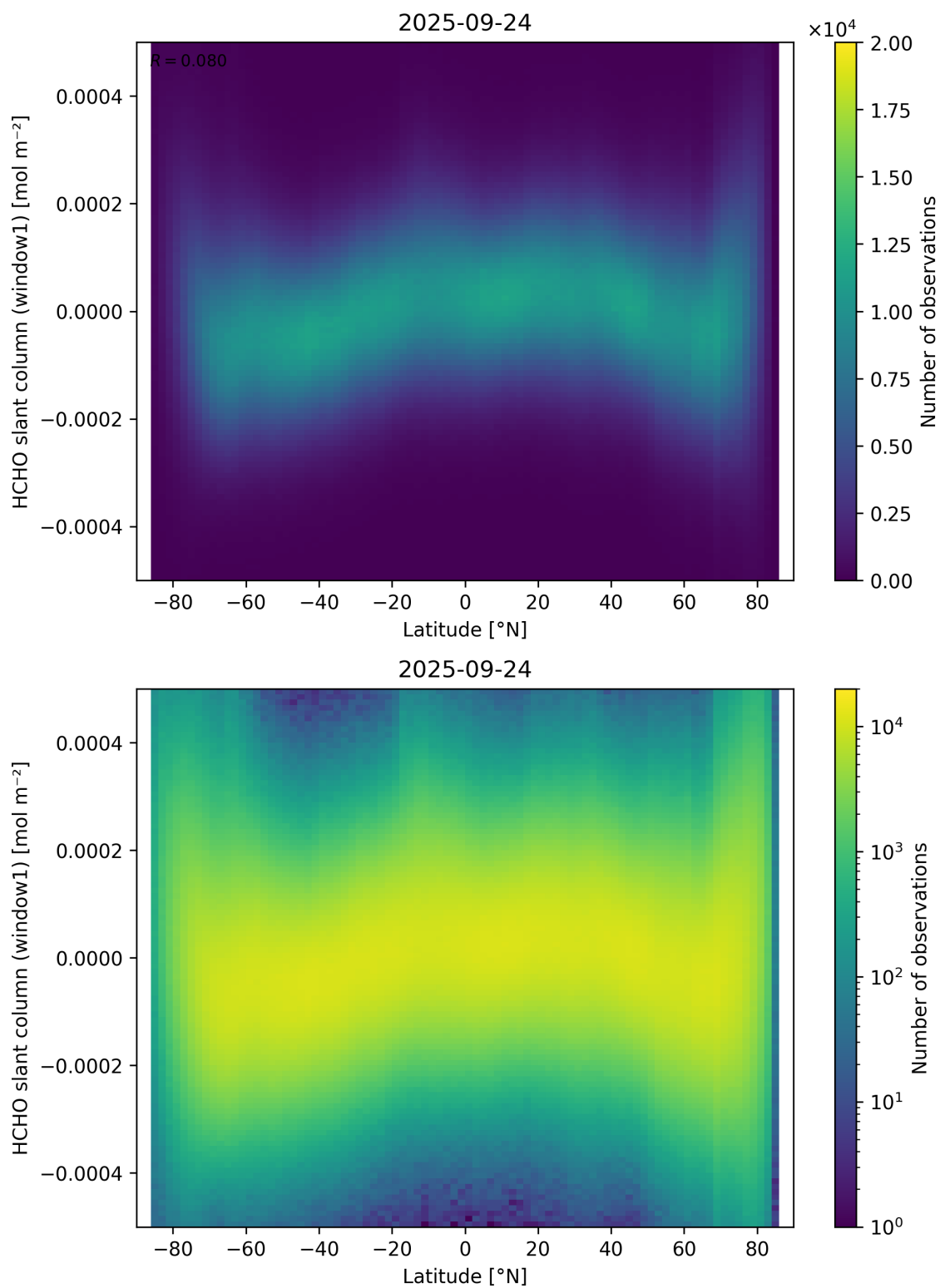
Figure 159: Scatter density plot of “Latitude” against “HCHO slant column (window1)” for 2025-09-23 to 2025-09-25.
