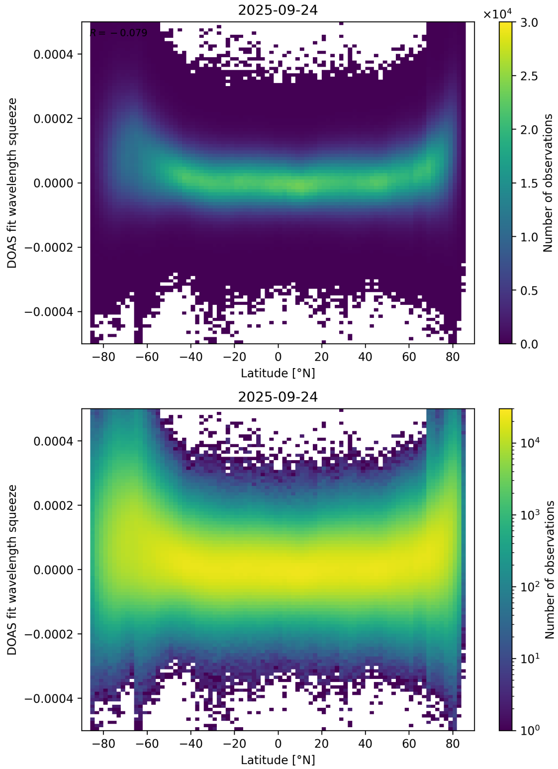
Figure 155: Scatter density plot of “Latitude” against “DOAS fit wavelength squeeze” for 2025-09-23 to 2025-09-25.
