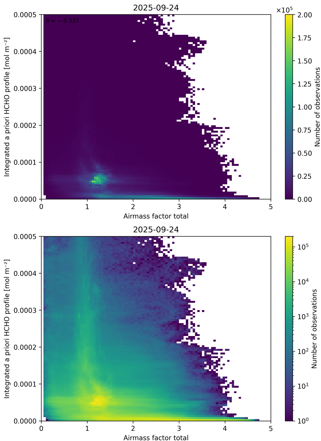
Figure 104: Scatter density plot of “Airmass factor total” against “Integrated a priori HCHO profile” for 2025-09-23 to 2025-09-25.
