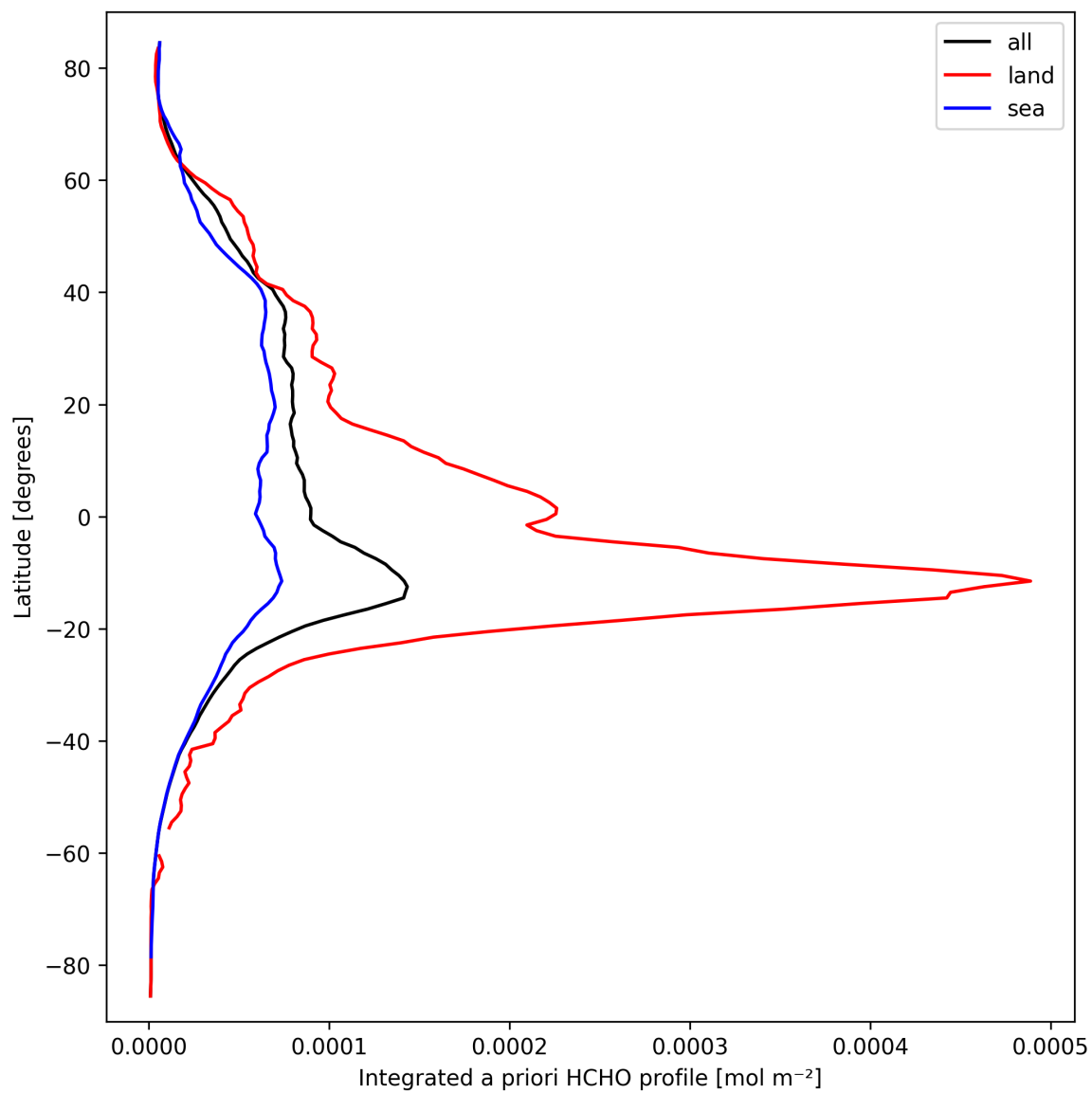
Figure 29: Zonal average of “Integrated a priori HCHO profile” for 2025-09-23 to 2025-09-25.
