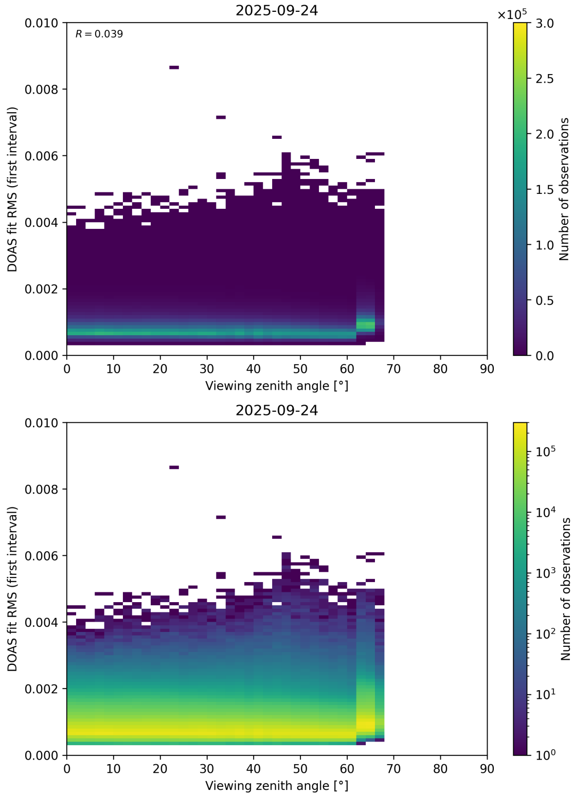
Figure 182: Scatter density plot of “Viewing zenith angle” against “DOAS fit RMS (first interval)” for 2025-09-23 to 2025-09-25.
