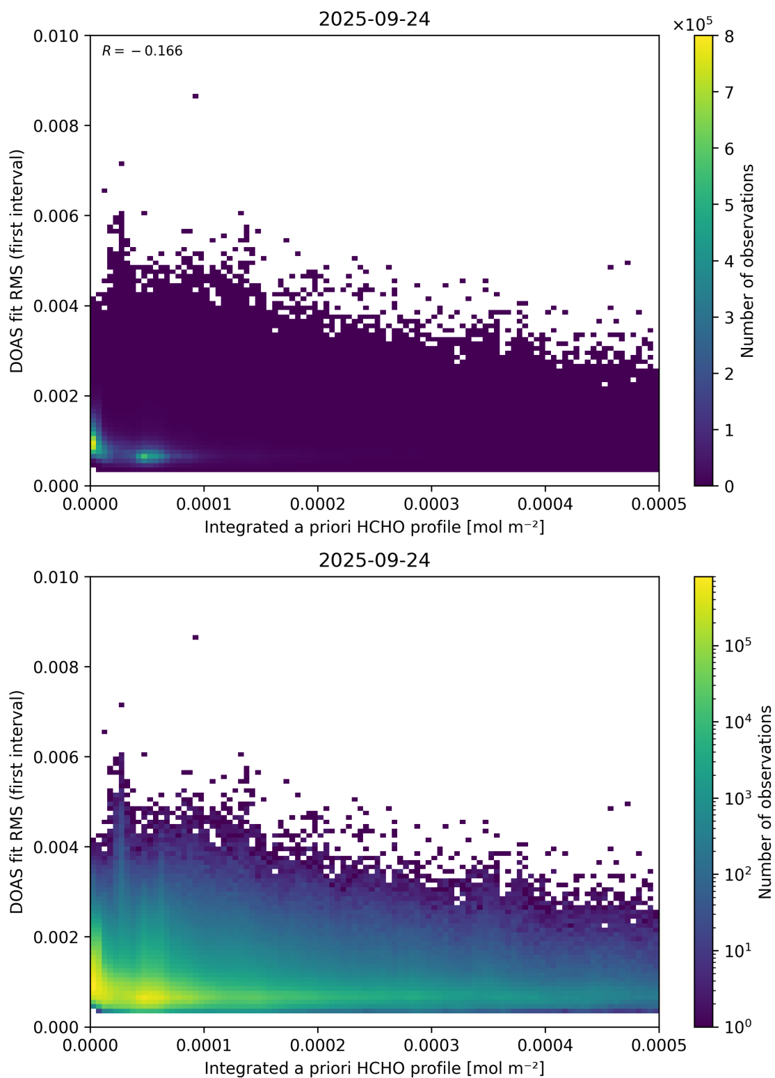
Figure 148: Scatter density plot of “Integrated a priori HCHO profile” against “DOAS fit RMS (first interval)” for 2025-09-23 to 2025-09-25.
