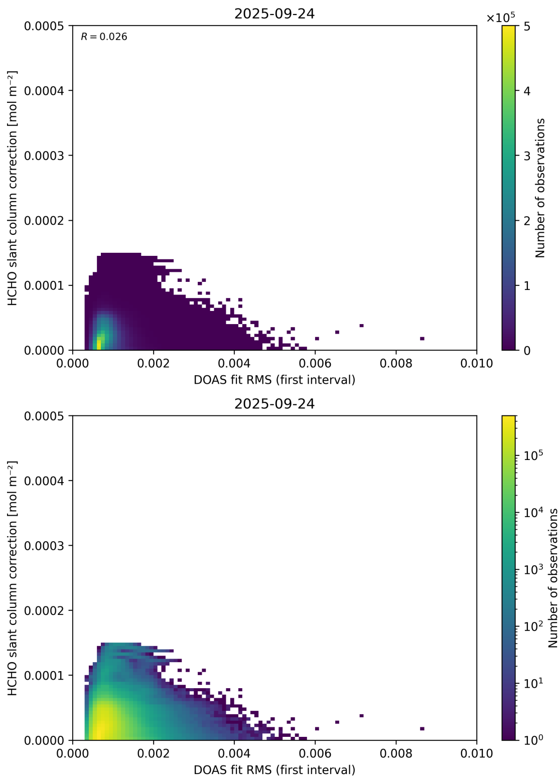
Figure 63: Scatter density plot of “DOAS fit RMS (first interval)” against “HCHO slant column correction” for 2025-09-23 to 2025-09-25.
