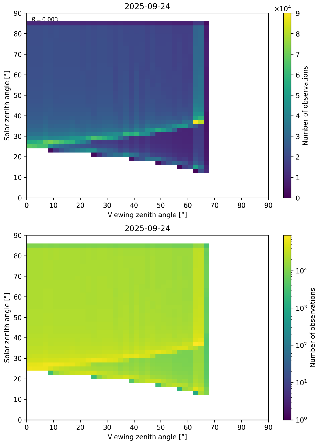
Figure 197: Scatter density plot of “Viewing zenith angle” against “Solar zenith angle” for 2025-09-23 to 2025-09-25.
