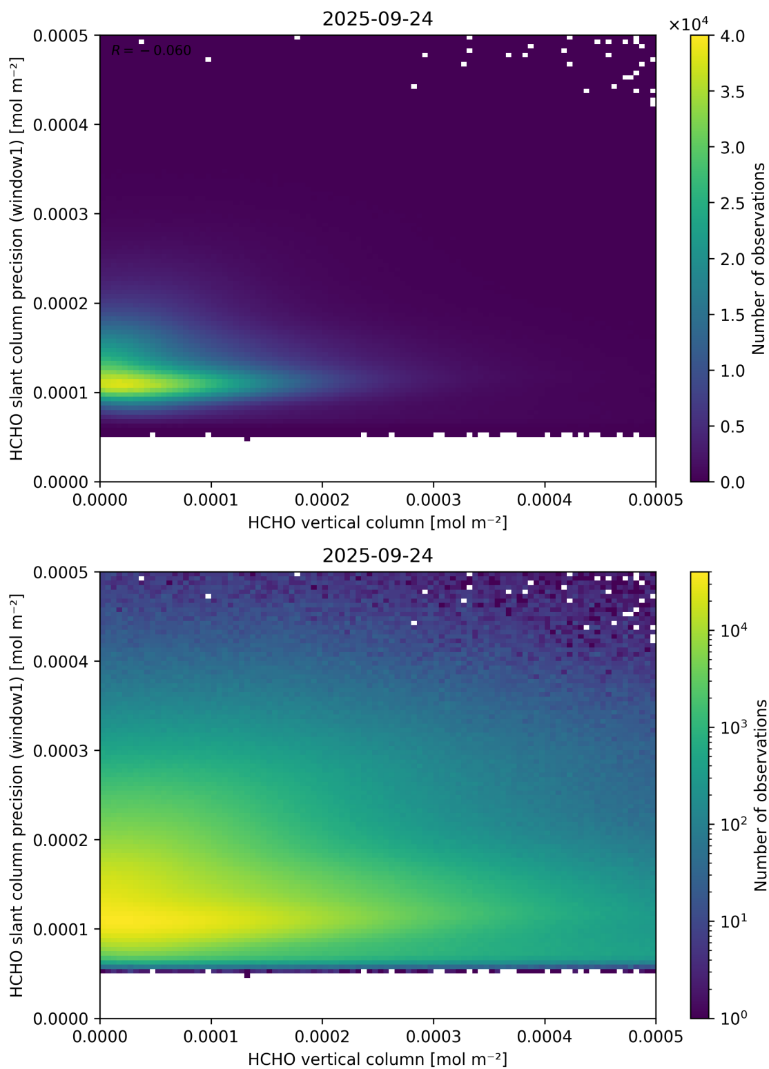
Figure 130: Scatter density plot of “HCHO vertical column” against “HCHO slant column precision (window1)” for 2025-09-23 to 2025-09-25.
