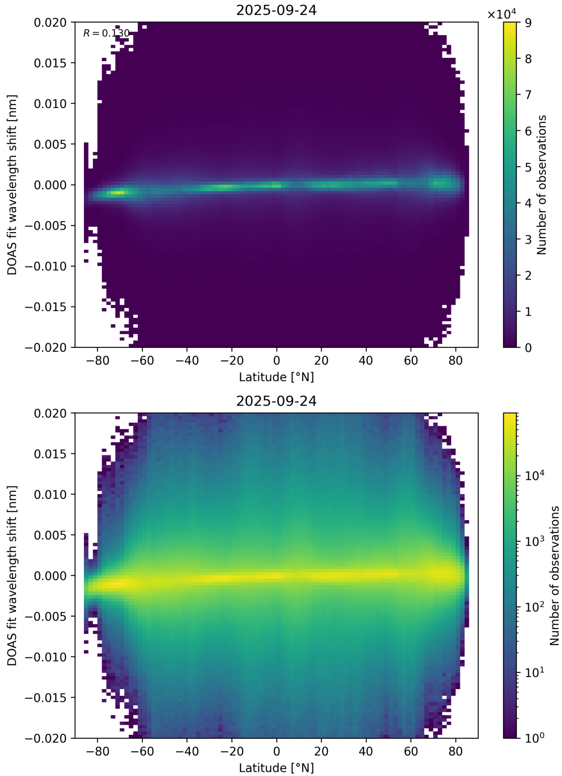
Figure 154: Scatter density plot of “Latitude” against “DOAS fit wavelength shift” for 2025-09-23 to 2025-09-25.
