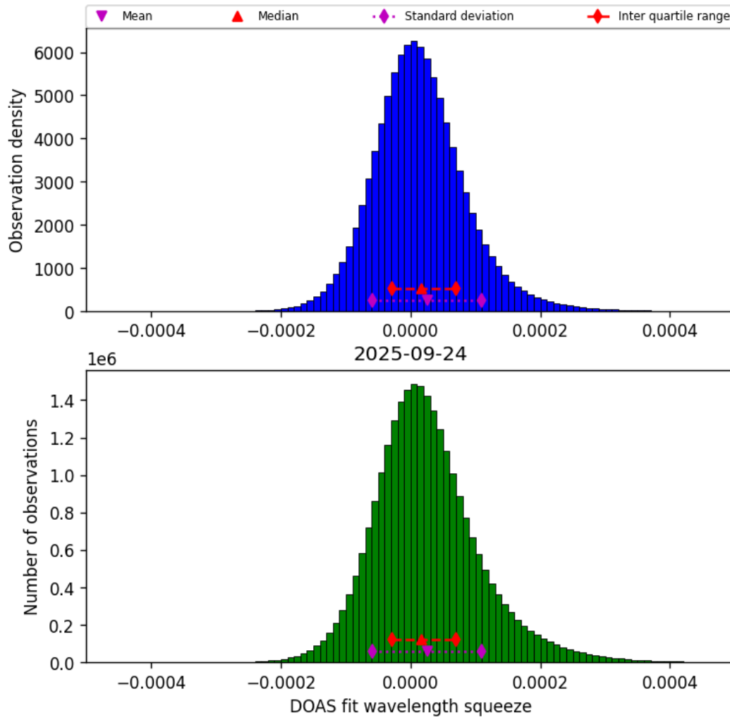
Figure 45: Histogram of “DOAS fit wavelength squeeze” for 2025-09-23 to 2025-09-25
