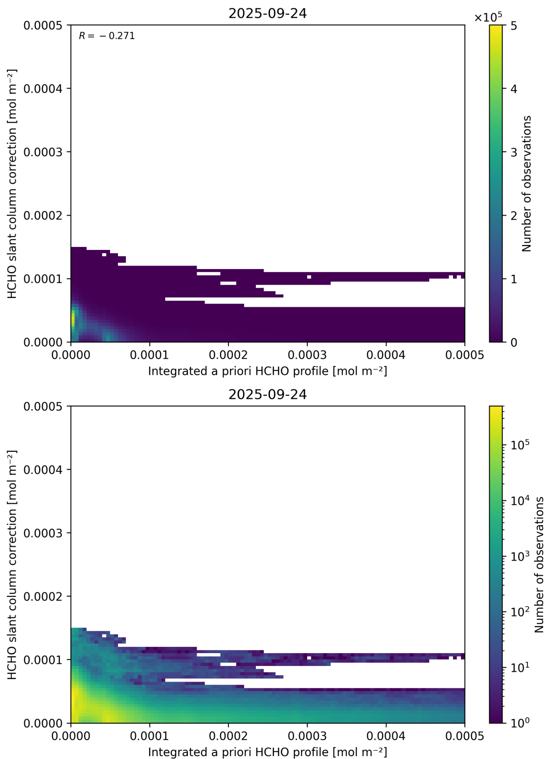
Figure 152: Scatter density plot of “Integrated a priori HCHO profile” against “HCHO slant column correction” for 2025-09-23 to 2025-09-25.
