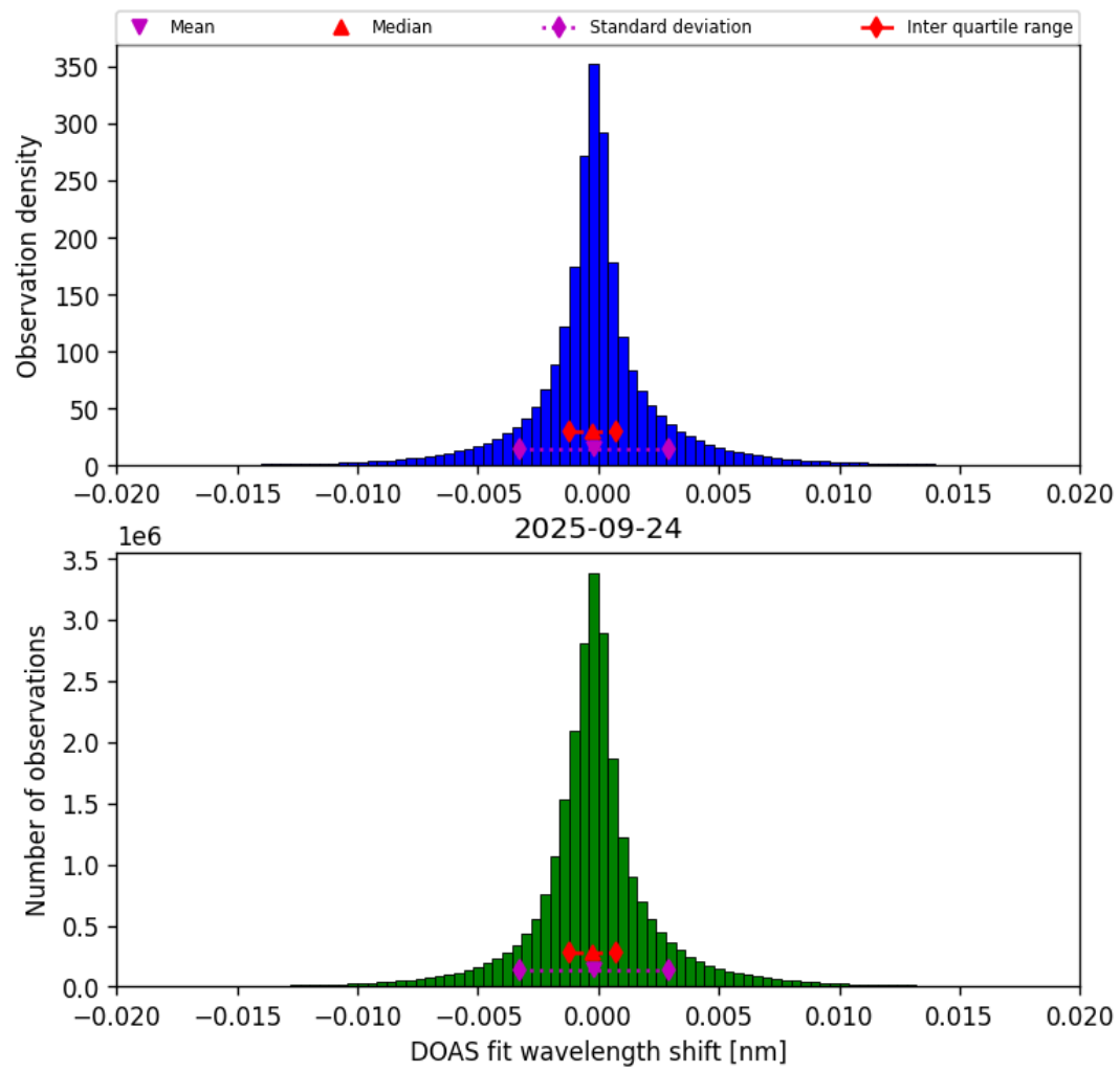
Figure 44: Histogram of “DOAS fit wavelength shift” for 2025-09-23 to 2025-09-25
