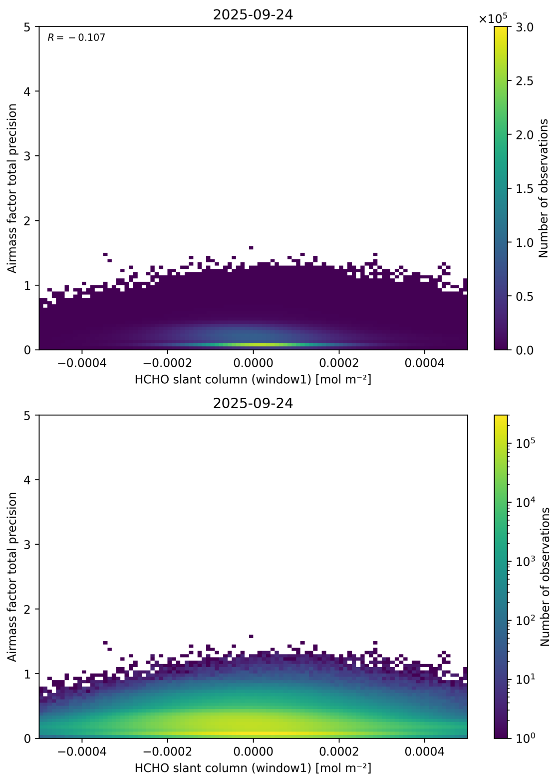
Figure 86: Scatter density plot of “HCHO slant column (window1)” against “Airmass factor total precision” for 2025-09-23 to 2025-09-25.
