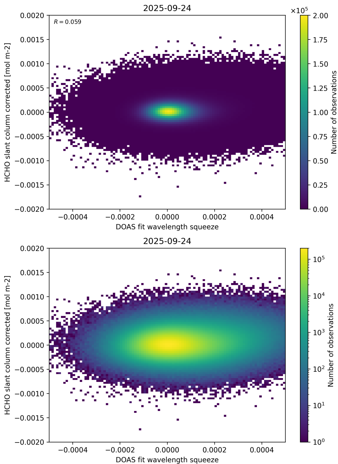
Figure 69: Scatter density plot of “DOAS fit wavelength squeeze” against “HCHO slant column corrected” for 2025-09-23 to 2025-09-25.
