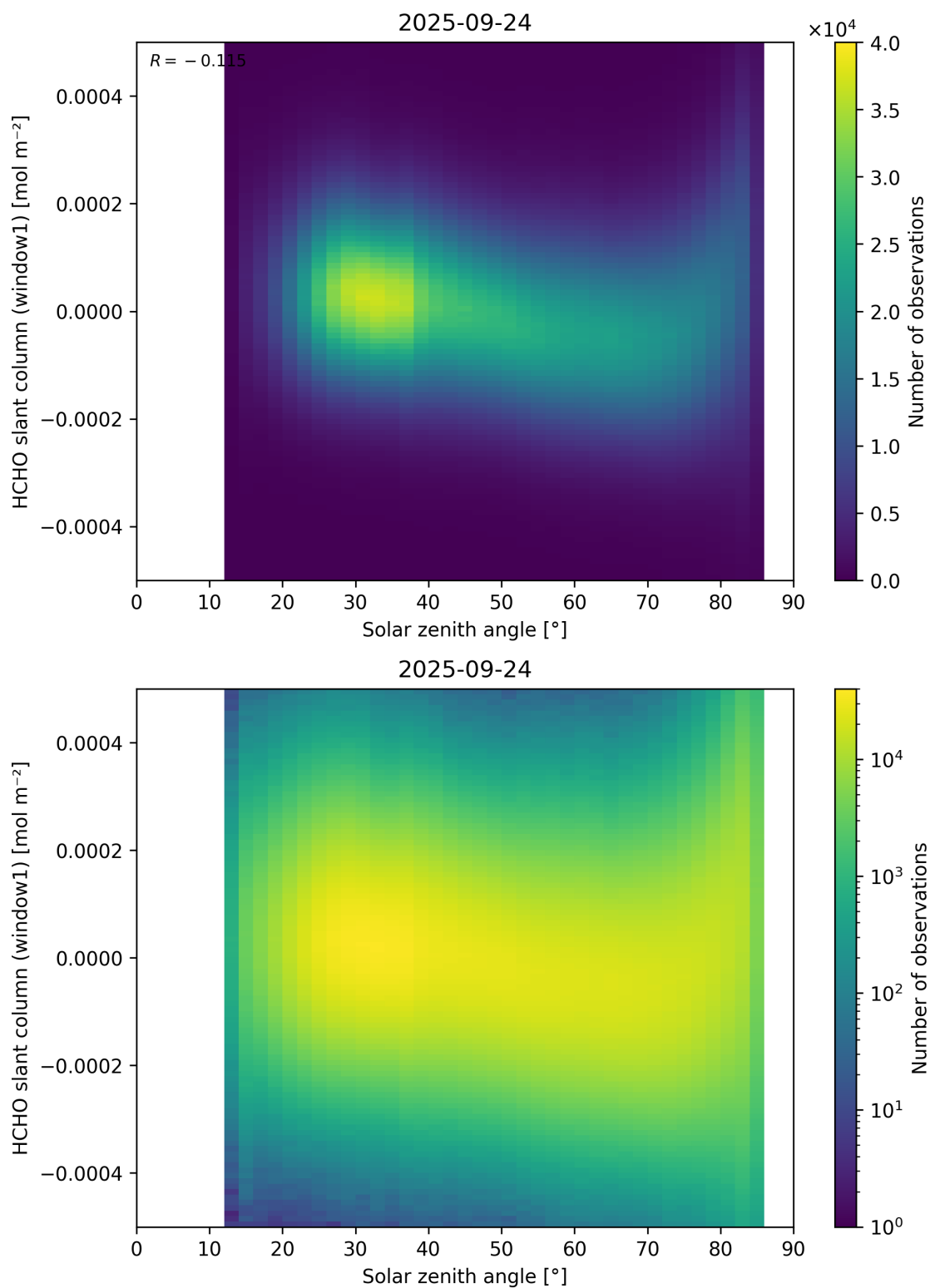
Figure 173: Scatter density plot of “Solar zenith angle” against “HCHO slant column (window1)” for 2025-09-23 to 2025-09-25.
