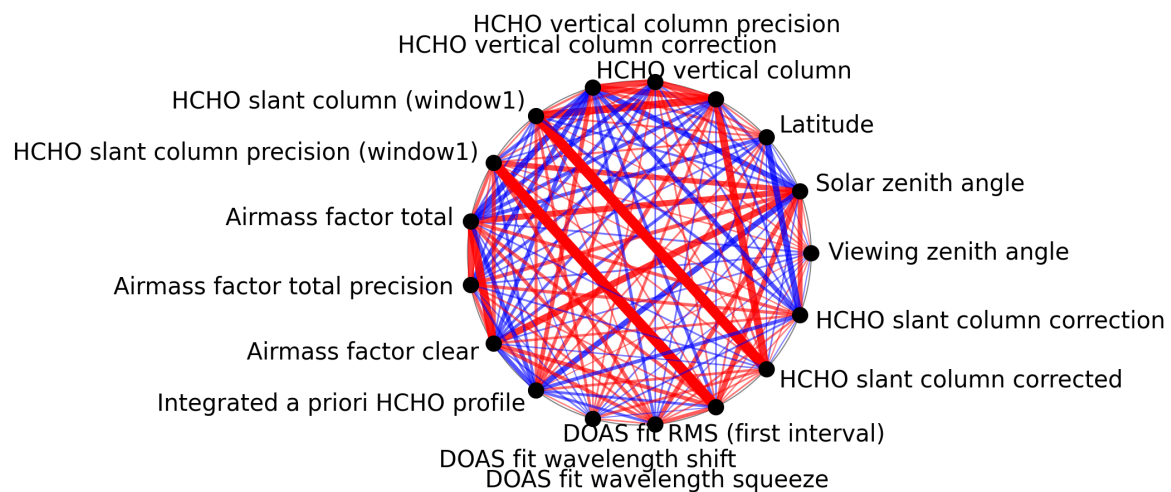
Figure 1: Map of correlation graph for 2025-09-23 to 2025-09-25.
