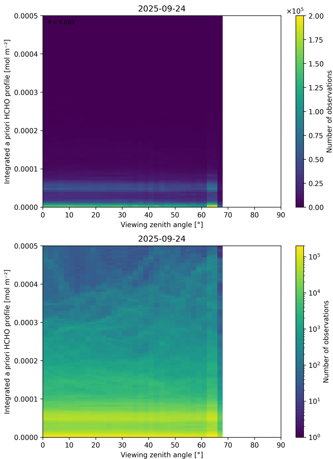
Figure 195: Scatter density plot of “Viewing zenith angle” against “Integrated a priori HCHO profile” for 2025-09-23 to 2025-09-25.
