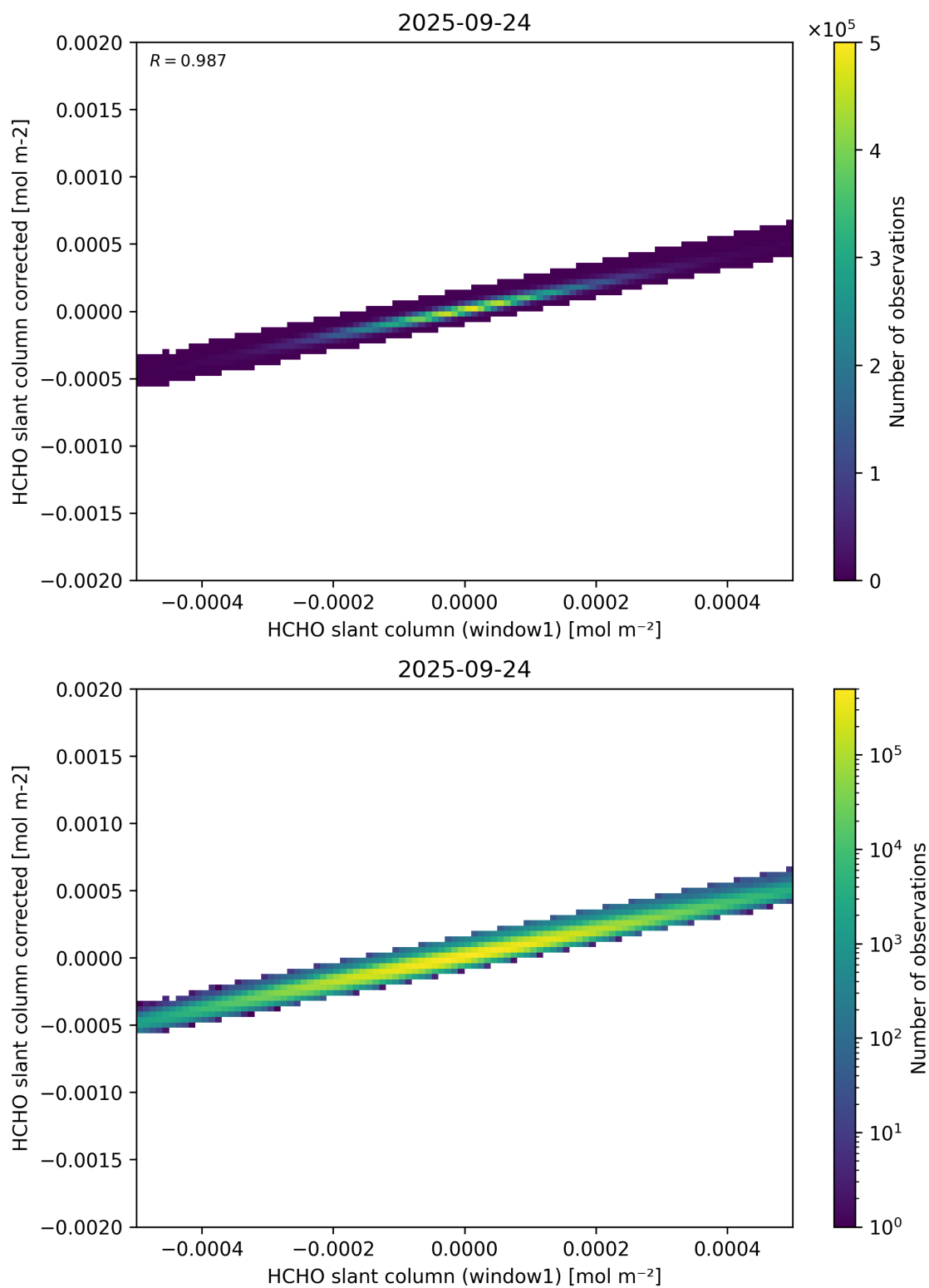
Figure 82: Scatter density plot of “HCHO slant column (window1)” against “HCHO slant column corrected” for 2025-09-23 to 2025-09-25.
