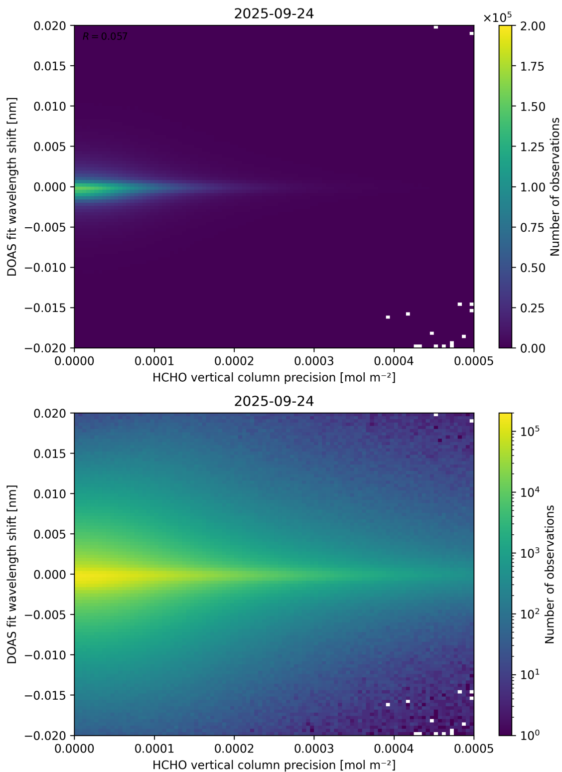
Figure 137: Scatter density plot of “HCHO vertical column precision” against “DOAS fit wavelength shift” for 2025-09-23 to 2025-09-25.
