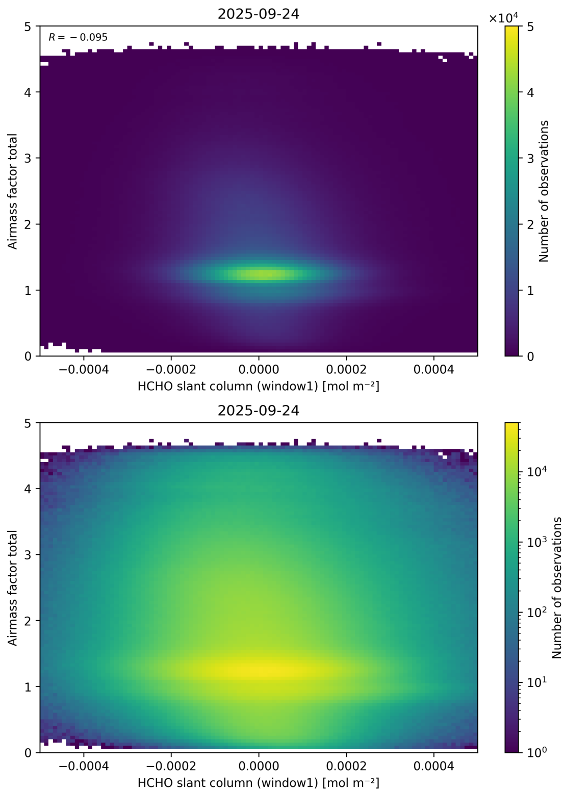
Figure 85: Scatter density plot of “HCHO slant column (window1)” against “Airmass factor total” for 2025-09-23 to 2025-09-25.
