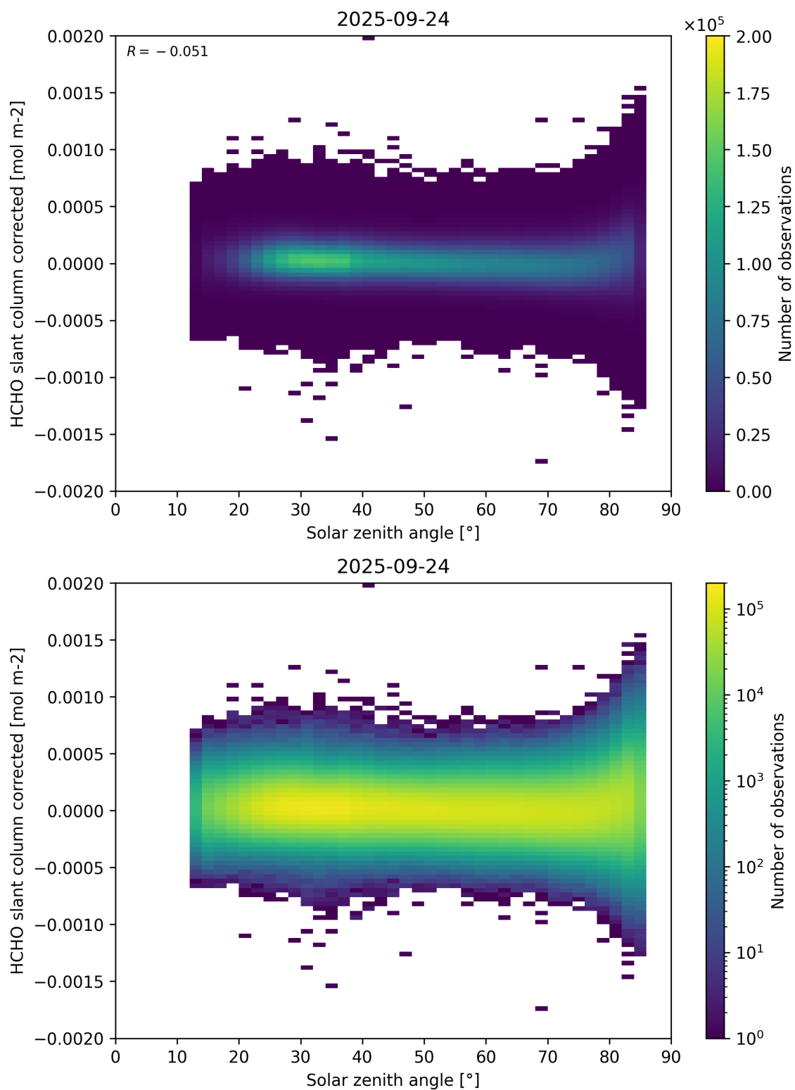
Figure 171: Scatter density plot of “Solar zenith angle” against “HCHO slant column corrected” for 2025-09-23 to 2025-09-25.
