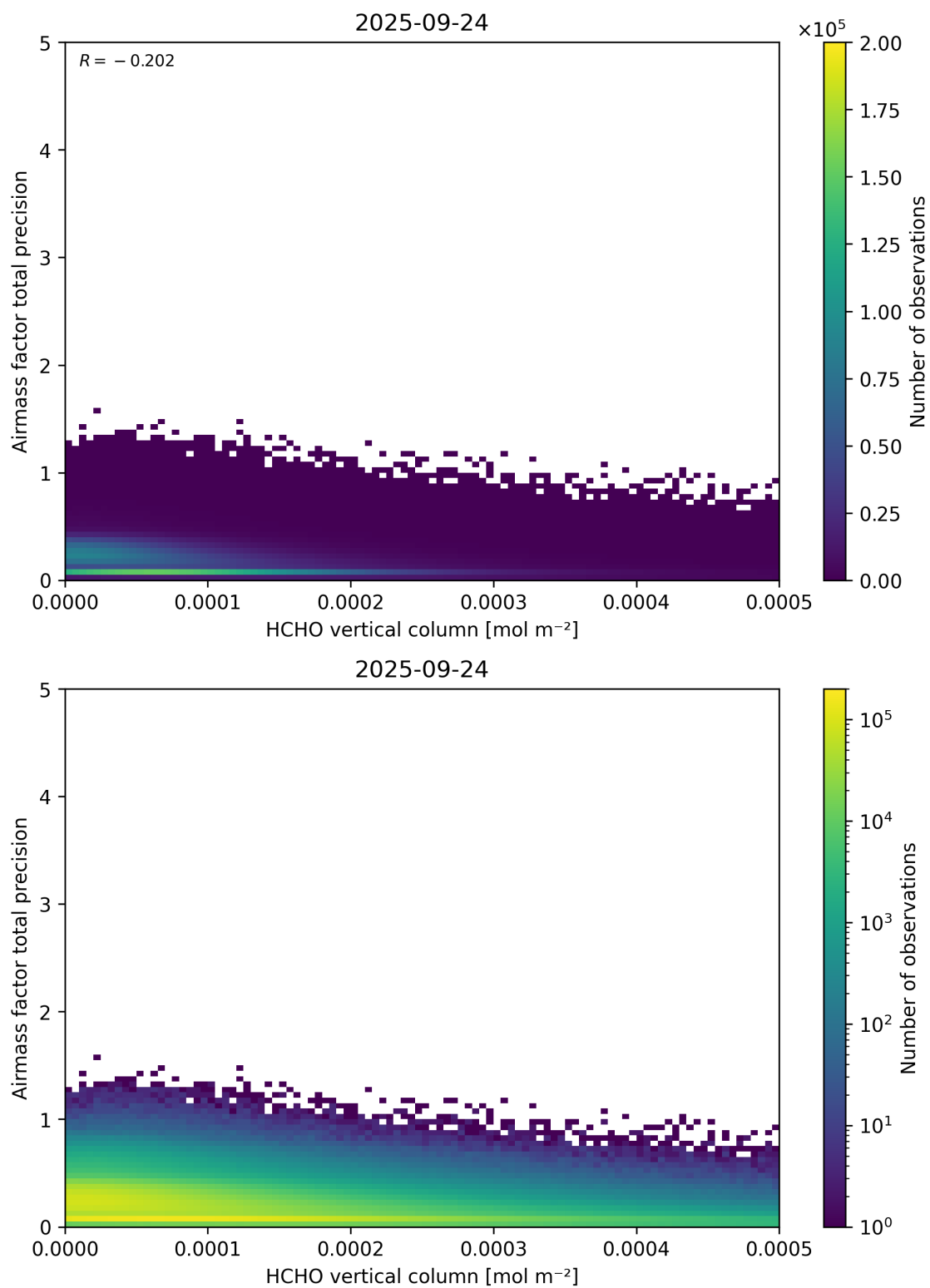
Figure 132: Scatter density plot of “HCHO vertical column” against “Airmass factor total precision” for 2025-09-23 to 2025-09-25.
