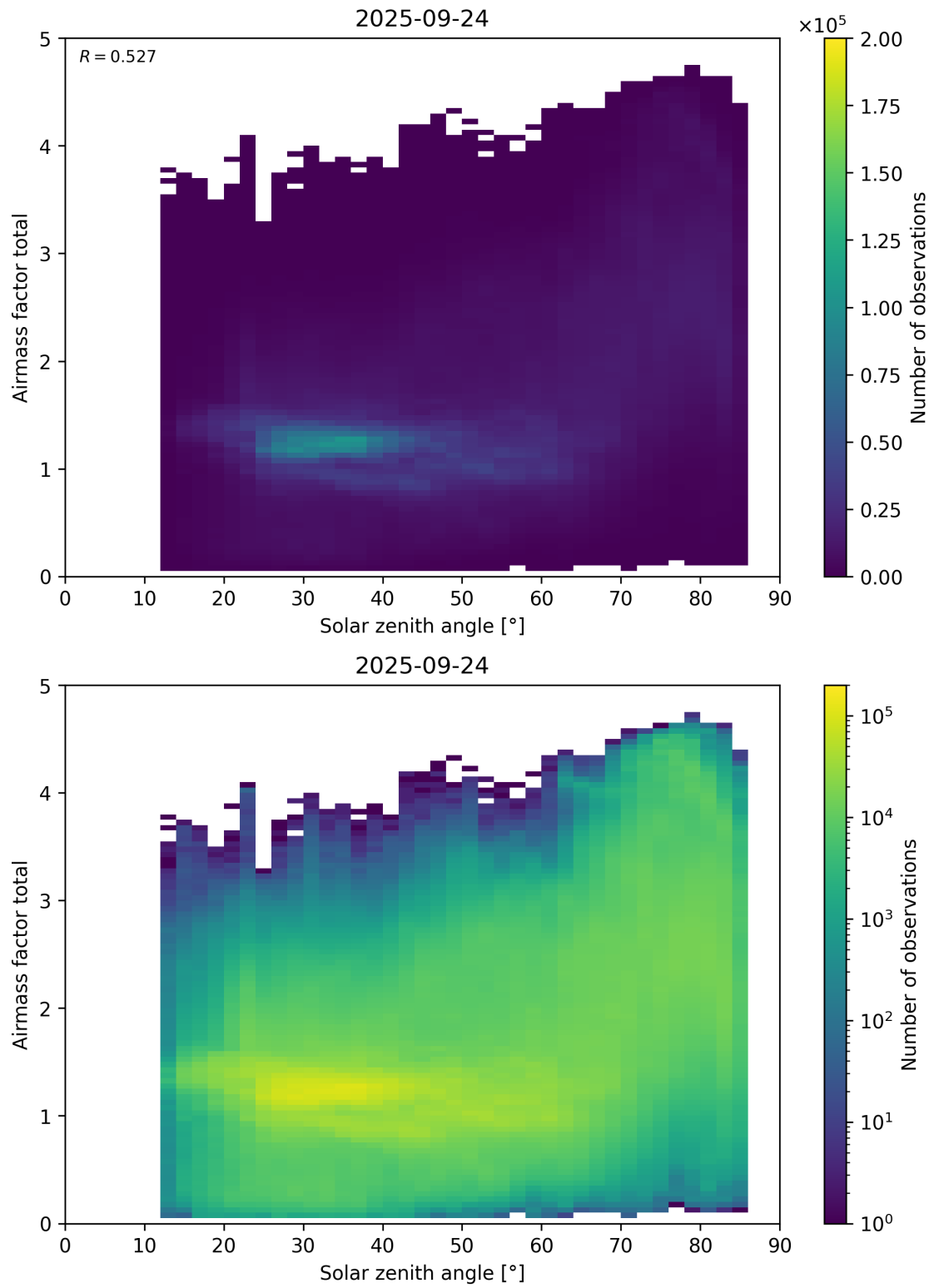
Figure 175: Scatter density plot of “Solar zenith angle” against “Airmass factor total” for 2025-09-23 to 2025-09-25.
