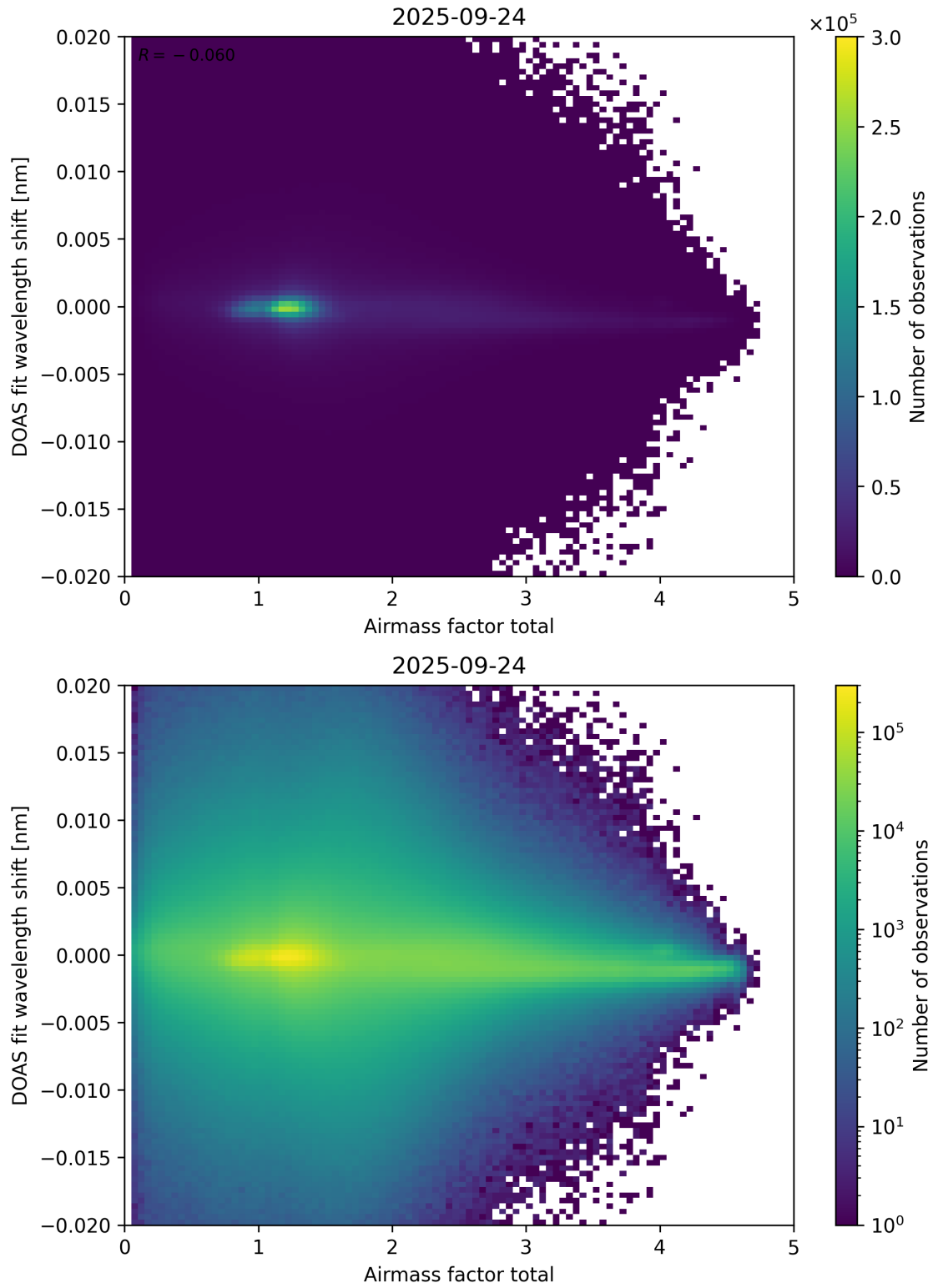
Figure 98: Scatter density plot of “Airmass factor total” against “DOAS fit wavelength shift” for 2025-09-23 to 2025-09-25.
