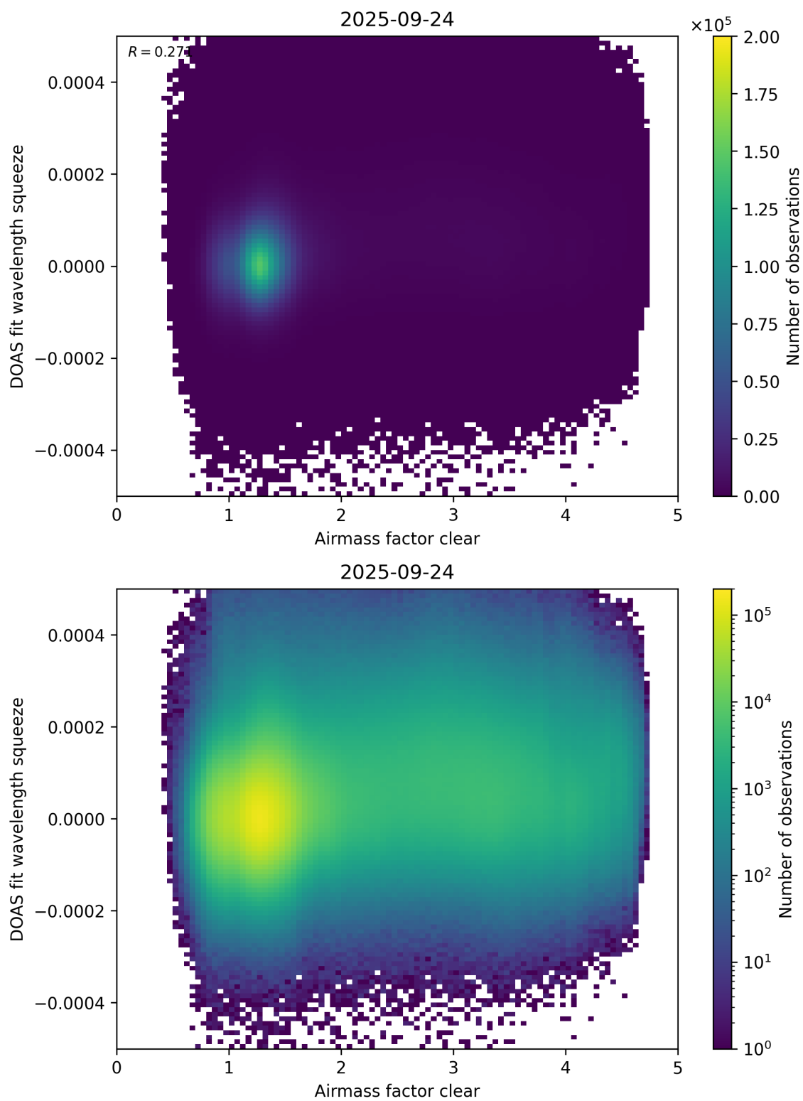
Figure 73: Scatter density plot of “Airmass factor clear” against “DOAS fit wavelength squeeze” for 2025-09-23 to 2025-09-25.
