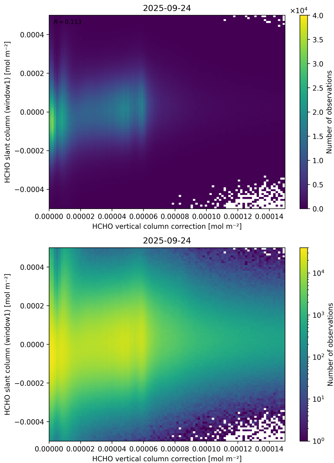
Figure 118: Scatter density plot of “HCHO vertical column correction” against “HCHO slant column (window1)” for 2025-09-23 to 2025-09-25.
