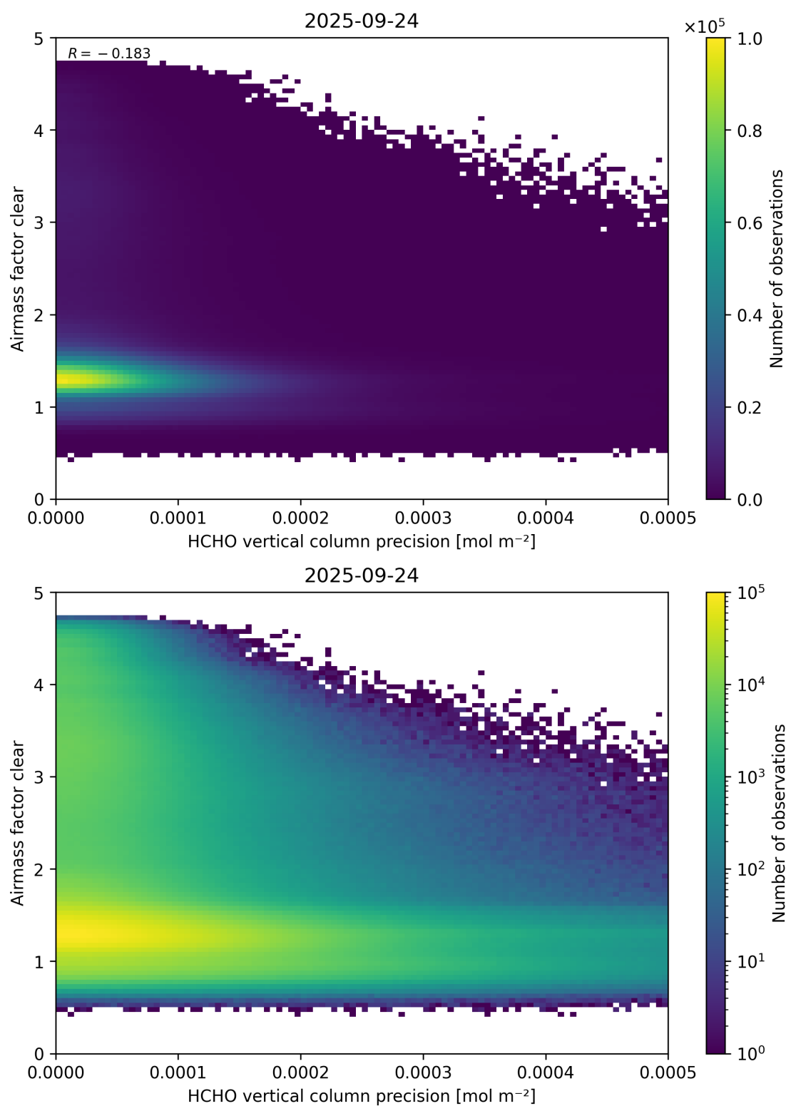
Figure 139: Scatter density plot of “HCHO vertical column precision” against “Airmass factor clear” for 2025-09-23 to 2025-09-25.
