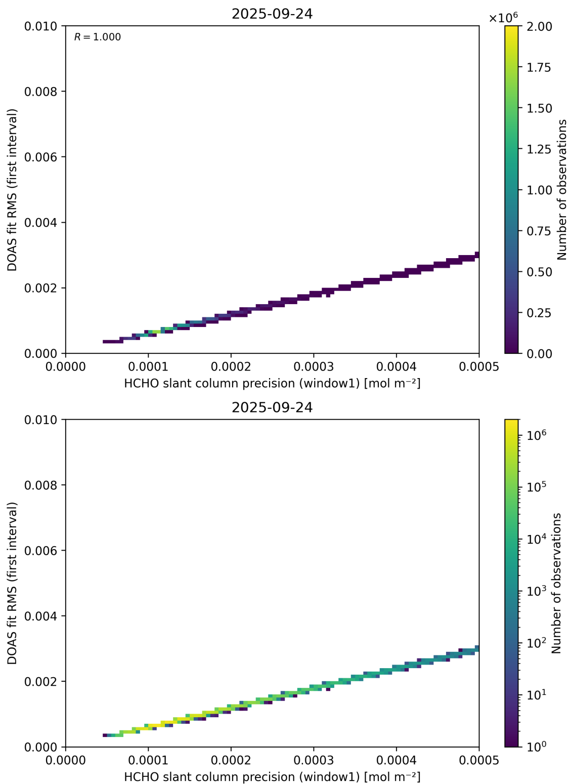
Figure 88: Scatter density plot of “HCHO slant column precision (window1)” against “DOAS fit RMS (first interval)” for 2025-09-23 to 2025-09-25.
