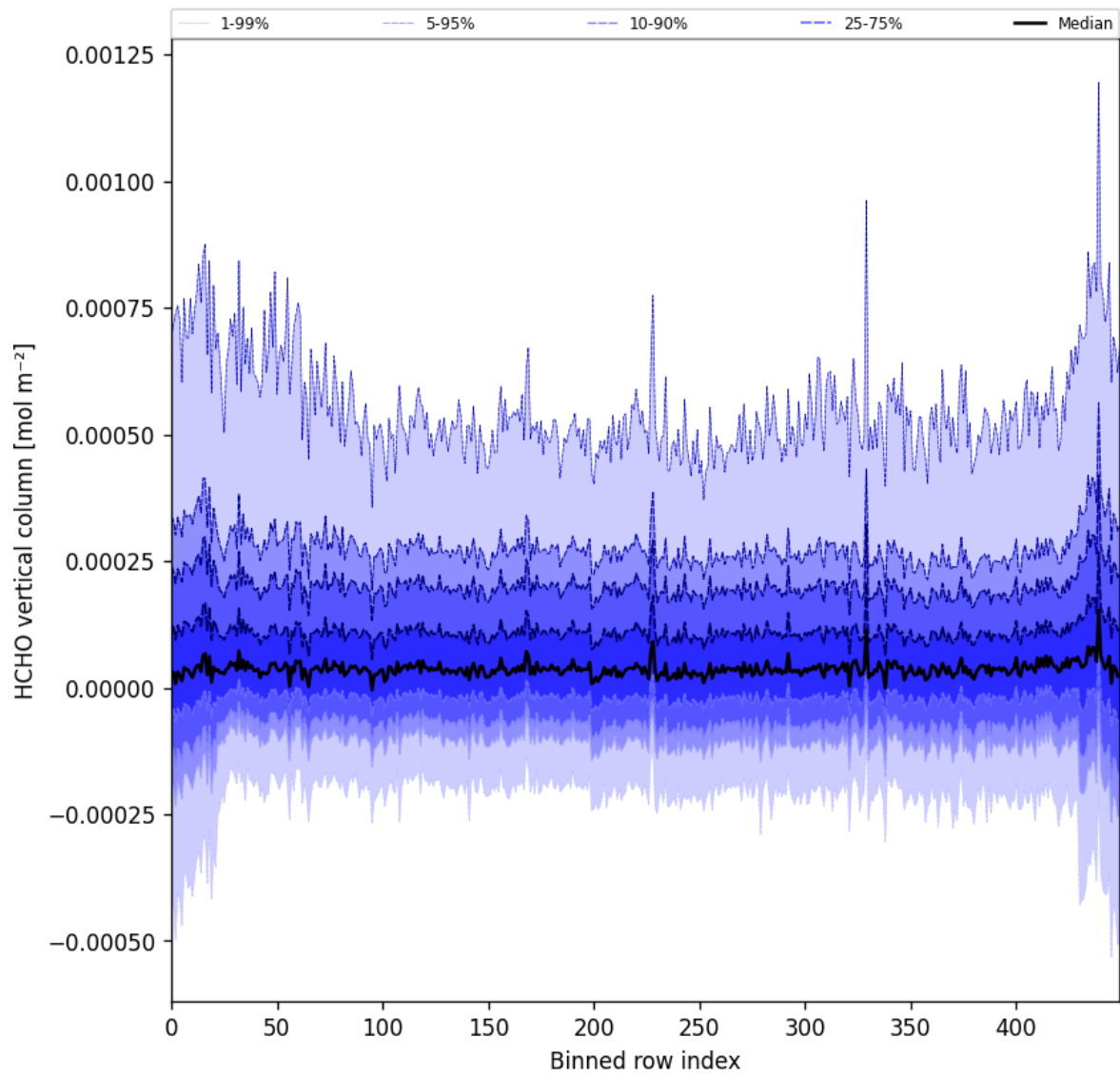
Figure 49: Along track statistics of “HCHO vertical column” for 2025-09-23 to 2025-09-25
