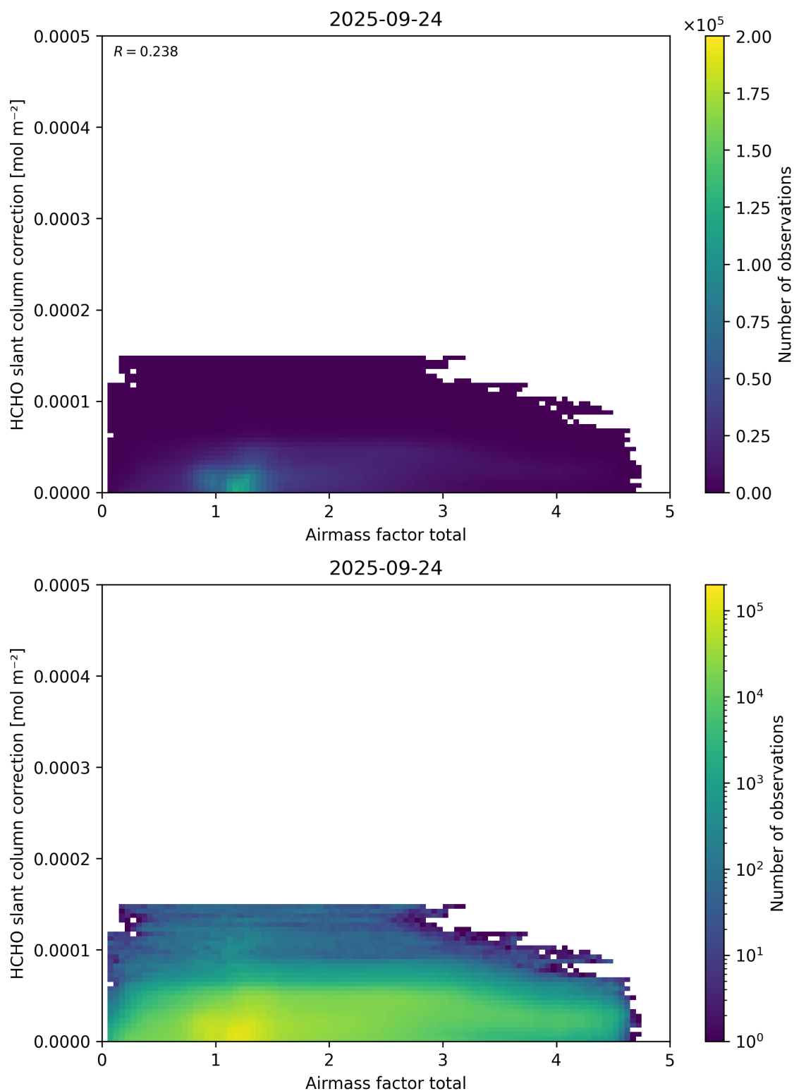
Figure 102: Scatter density plot of “Airmass factor total” against “HCHO slant column correction” for 2025-09-23 to 2025-09-25.
