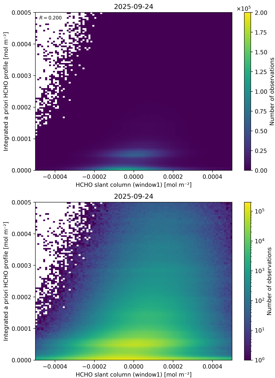
Figure 87: Scatter density plot of “HCHO slant column (window1)” against “Integrated a priori HCHO profile” for 2025-09-23 to 2025-09-25.
