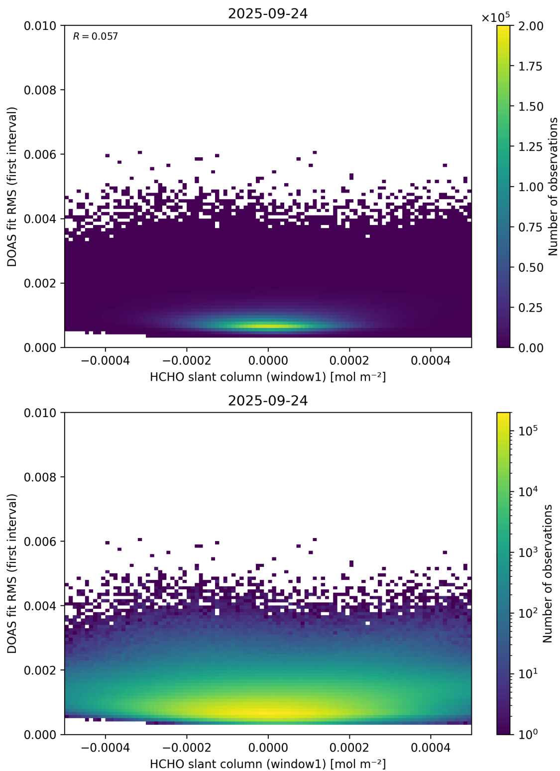
Figure 78: Scatter density plot of “HCHO slant column (window1)” against “DOAS fit RMS (first interval)” for 2025-09-23 to 2025-09-25.
