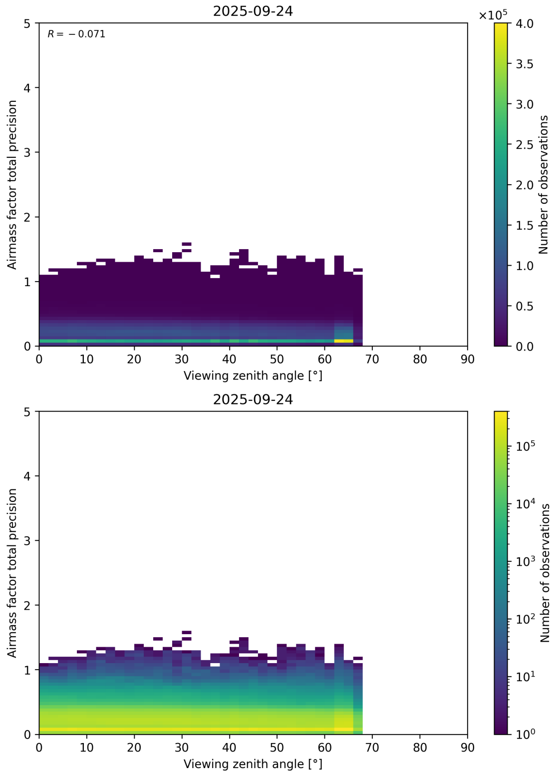
Figure 191: Scatter density plot of “Viewing zenith angle” against “Airmass factor total precision” for 2025-09-23 to 2025-09-25.
