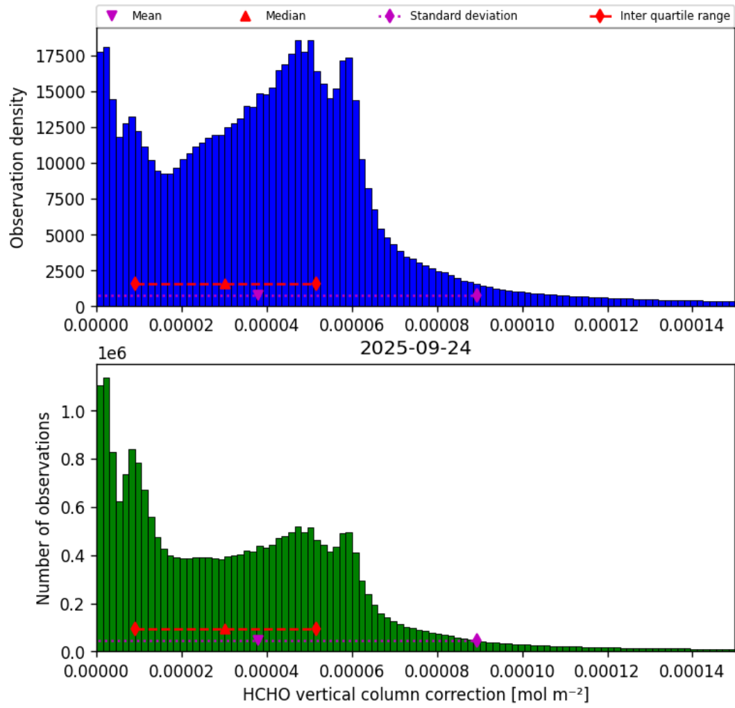
Figure 37: Histogram of “HCHO vertical column correction” for 2025-09-23 to 2025-09-25
