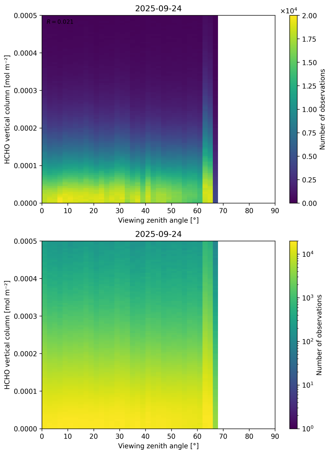
Figure 192: Scatter density plot of “Viewing zenith angle” against “HCHO vertical column” for 2025-09-23 to 2025-09-25.
