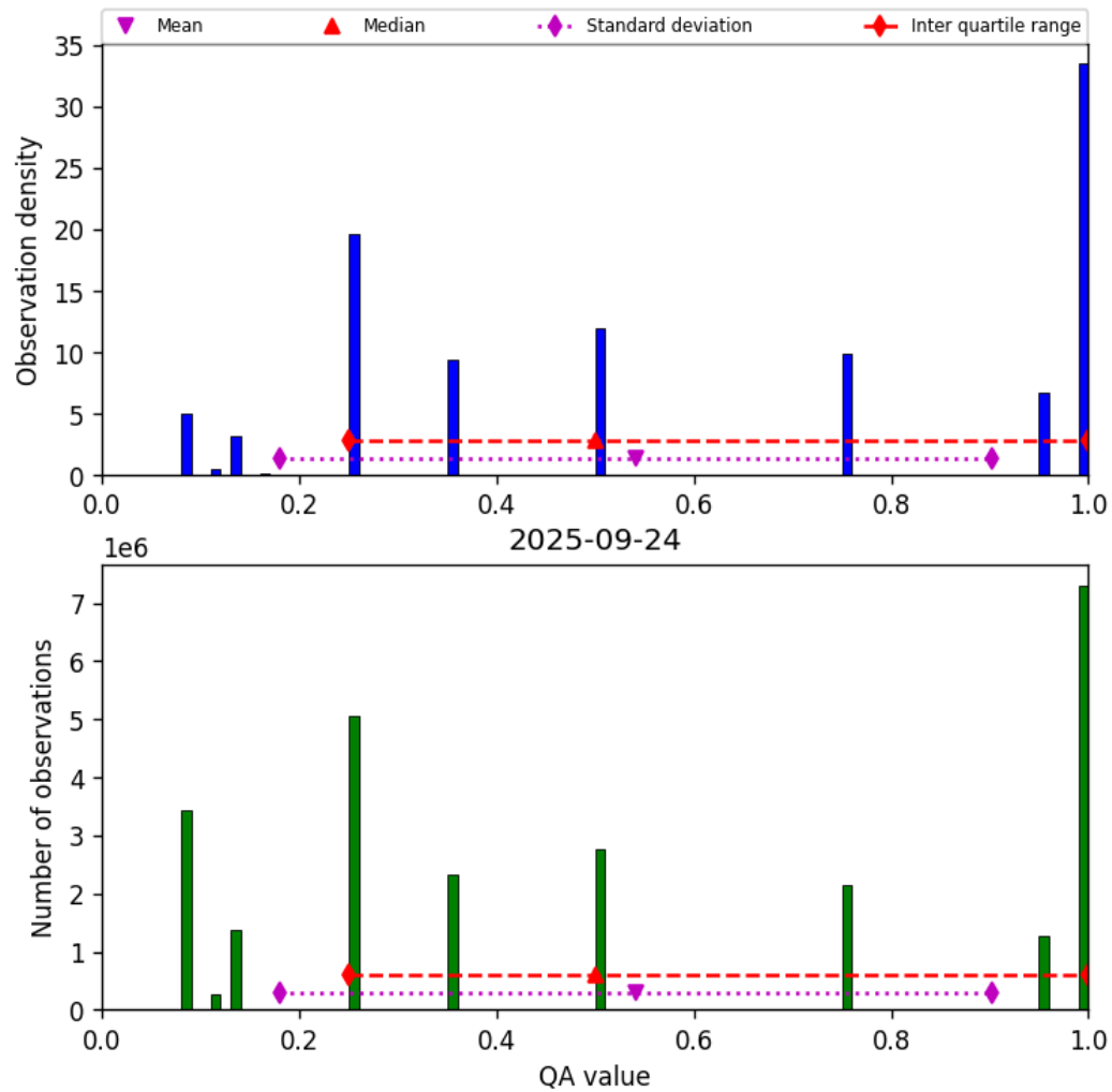
Figure 34: Histogram of “QA value” for 2025-09-23 to 2025-09-25
