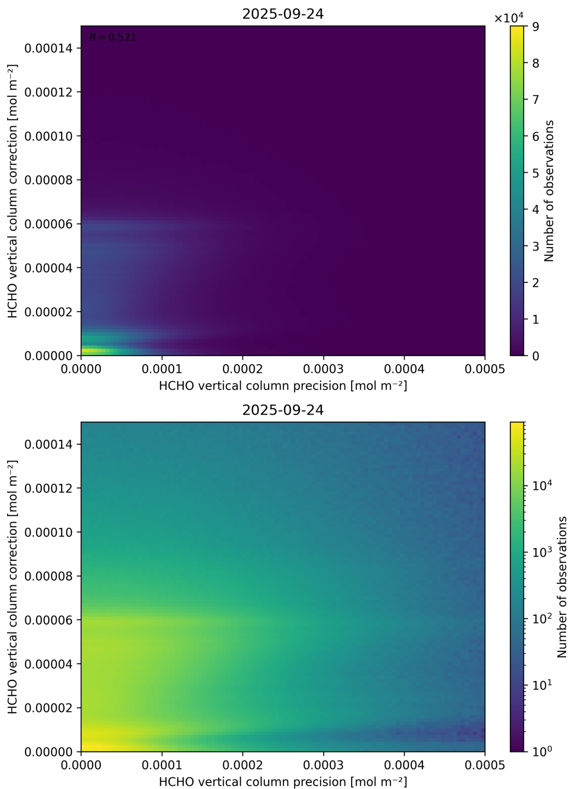
Figure 146: Scatter density plot of “HCHO vertical column precision” against “HCHO vertical column correction” for 2025-09-23 to 2025-09-25.
