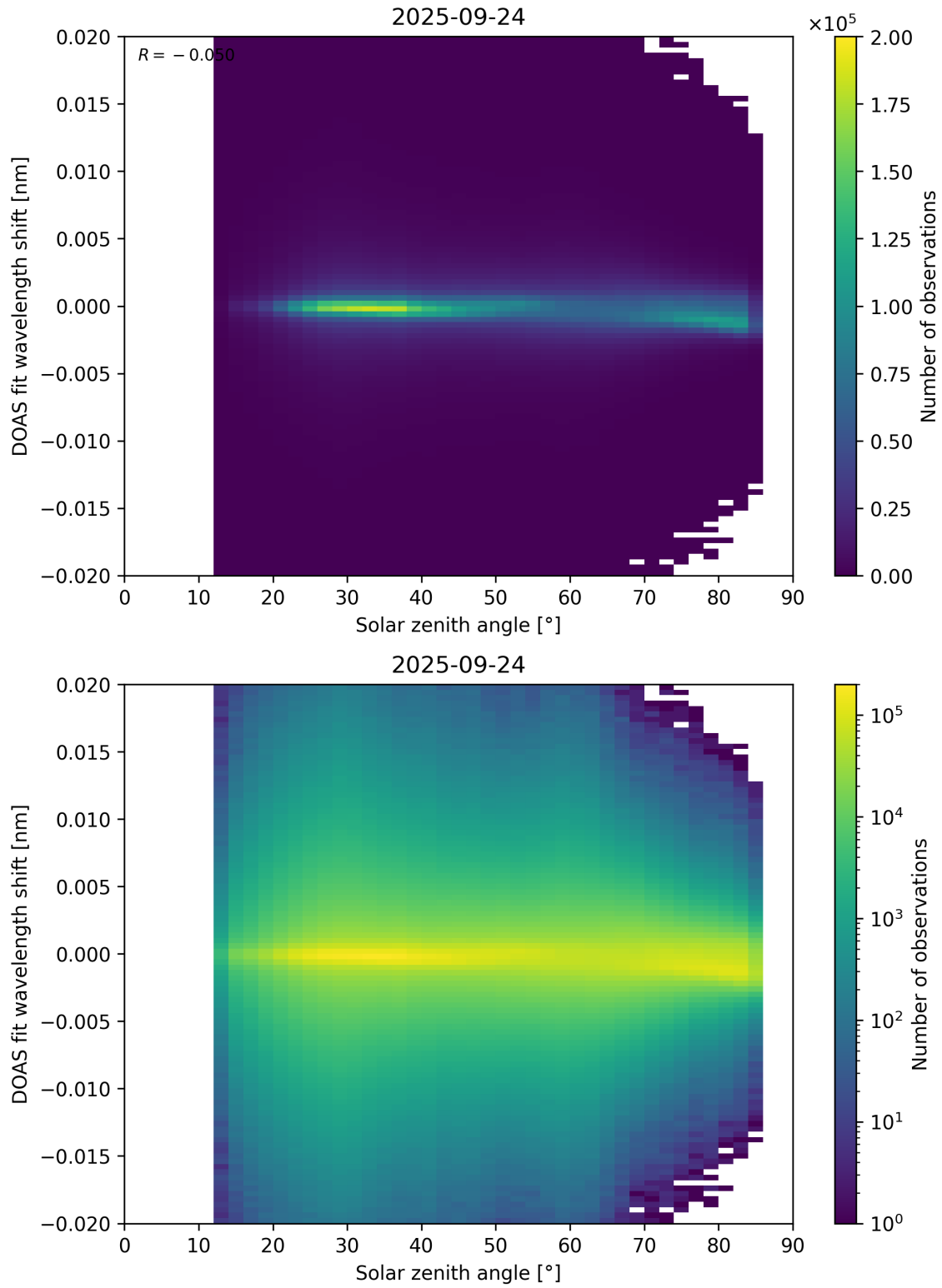
Figure 168: Scatter density plot of “Solar zenith angle” against “DOAS fit wavelength shift” for 2025-09-23 to 2025-09-25.
