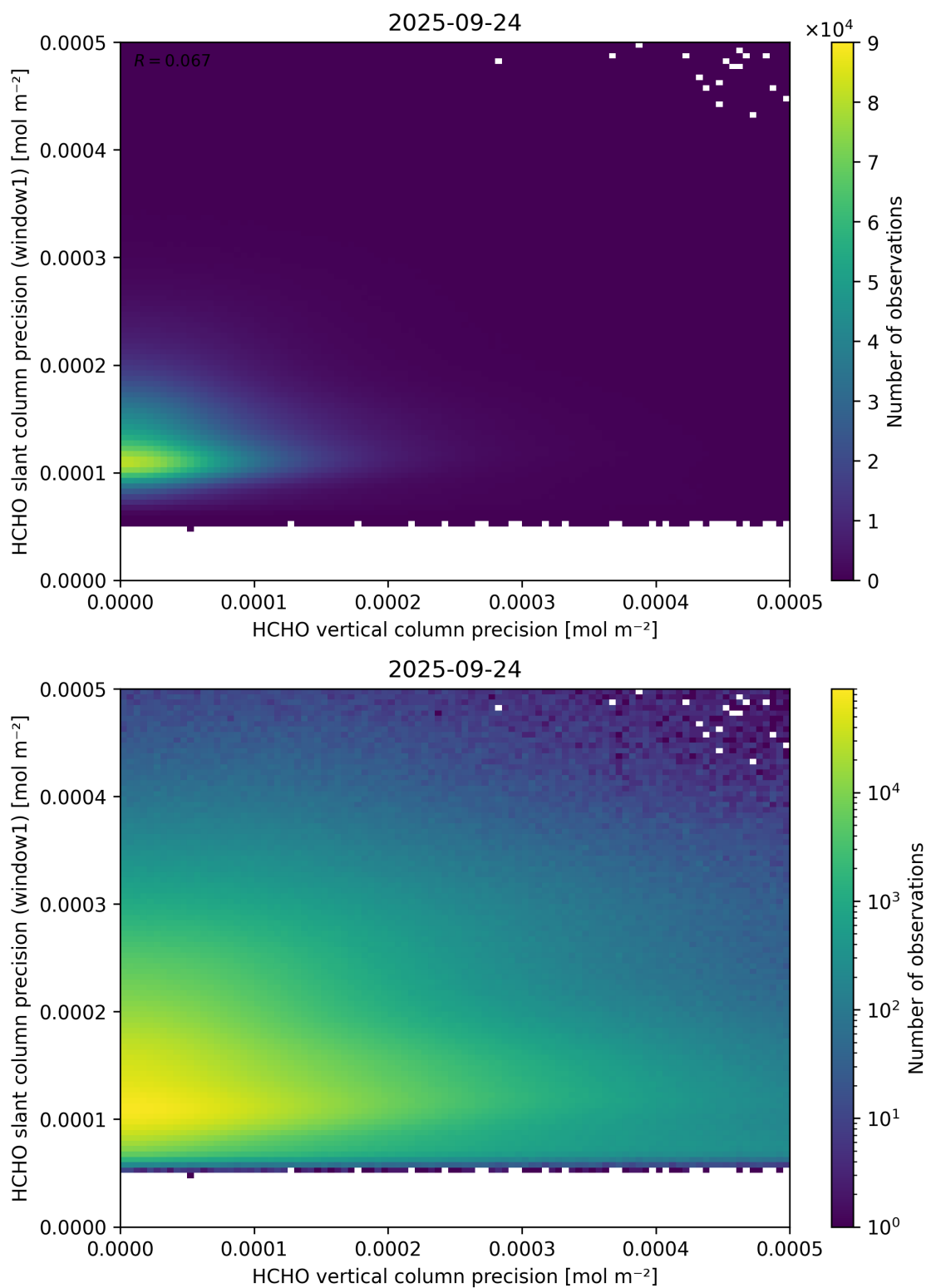
Figure 143: Scatter density plot of “HCHO vertical column precision” against “HCHO slant column precision (window1)” for 2025-09-23 to 2025-09-25.
