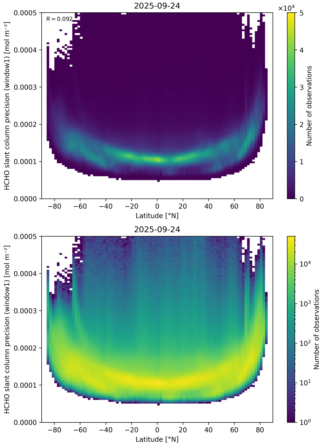
Figure 160: Scatter density plot of “Latitude” against “HCHO slant column precision (window1)” for 2025-09-23 to 2025-09-25.
