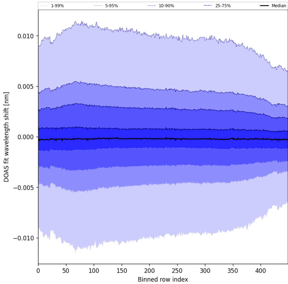
Figure 58: Along track statistics of “DOAS fit wavelength shift” for 2025-09-23 to 2025-09-25
