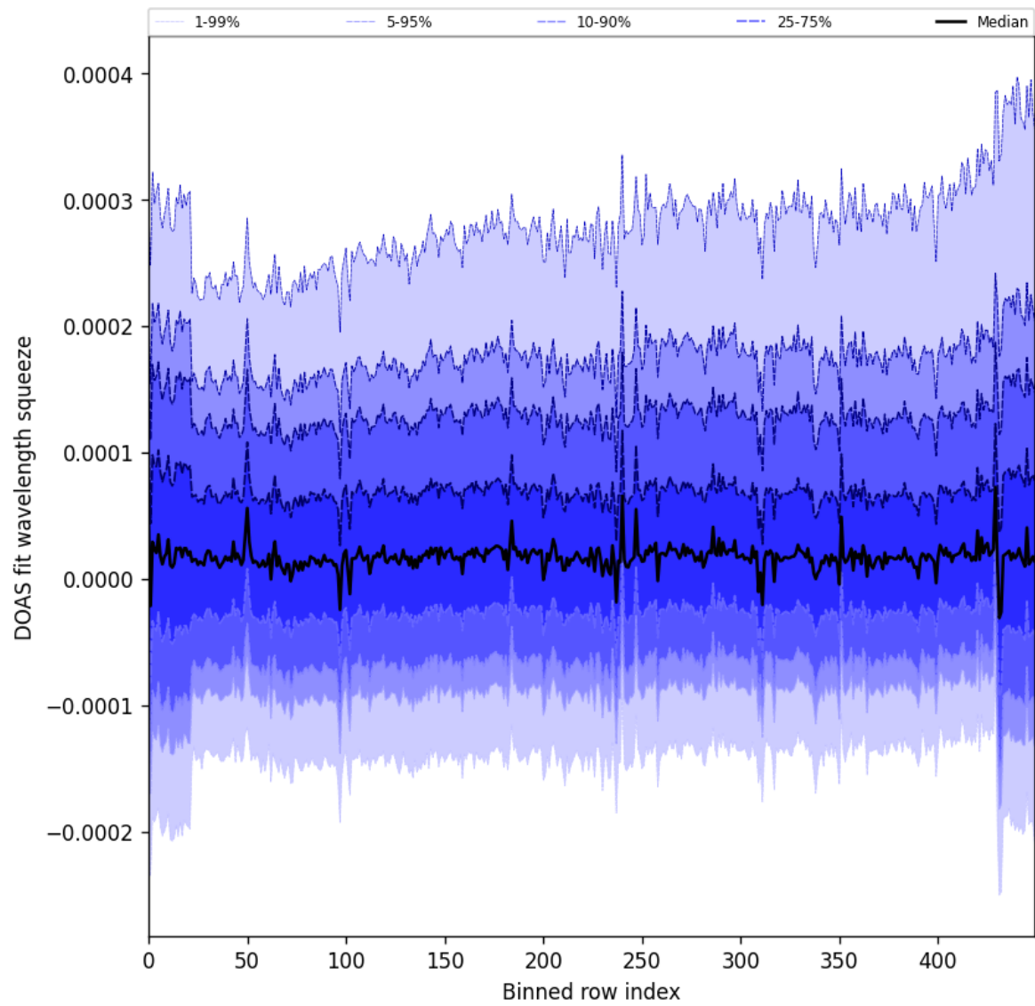
Figure 59: Along track statistics of “DOAS fit wavelength squeeze” for 2025-09-23 to 2025-09-25
