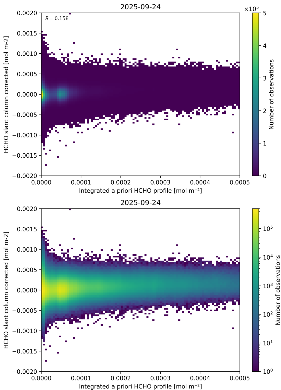
Figure 151: Scatter density plot of “Integrated a priori HCHO profile” against “HCHO slant column corrected” for 2025-09-23 to 2025-09-25.
