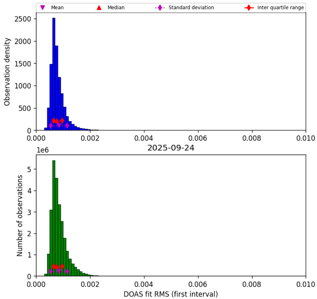
Figure 46: Histogram of “DOAS fit RMS (first interval)” for 2025-09-23 to 2025-09-25
