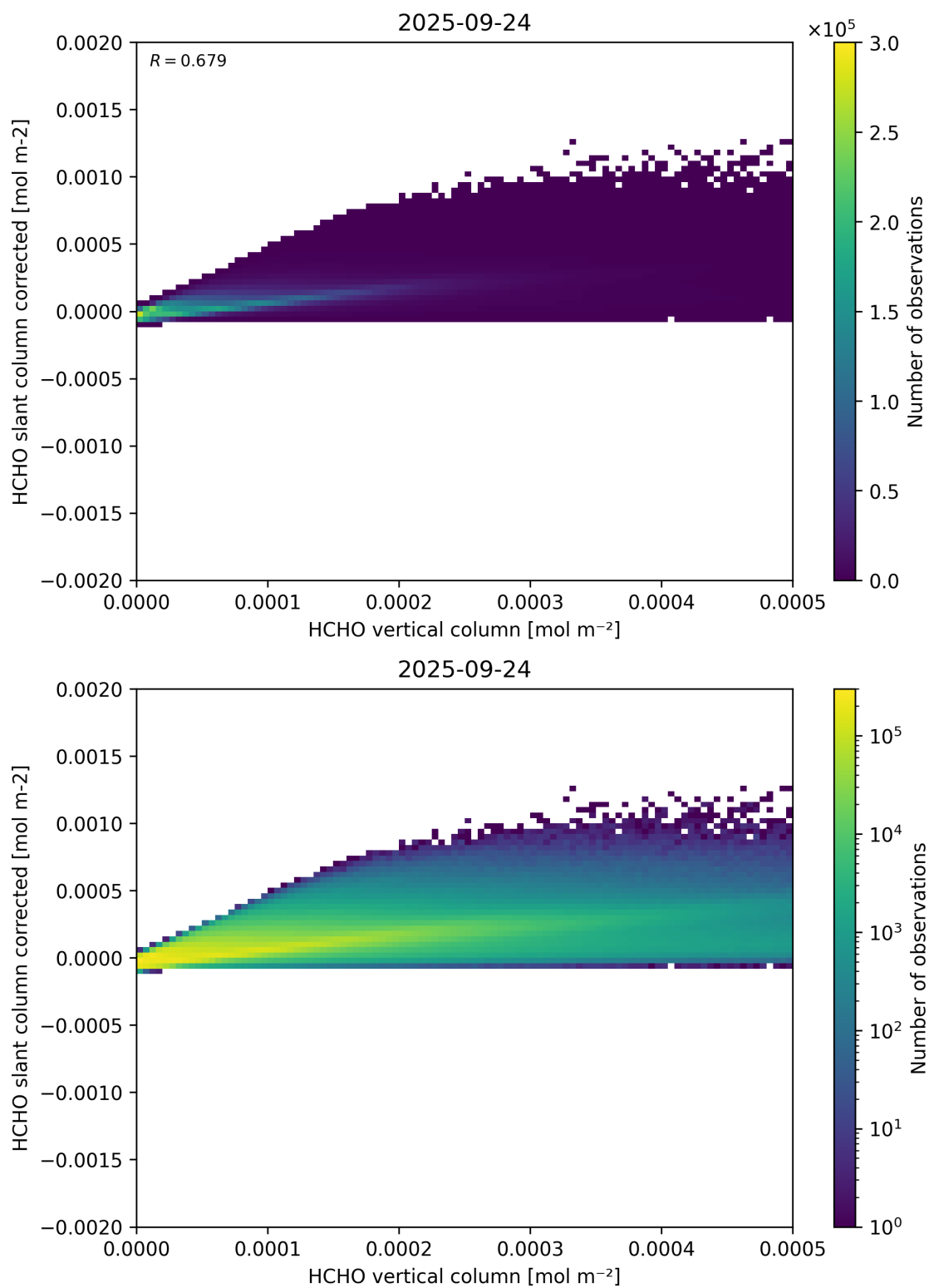
Figure 127: Scatter density plot of “HCHO vertical column” against “HCHO slant column corrected” for 2025-09-23 to 2025-09-25.
