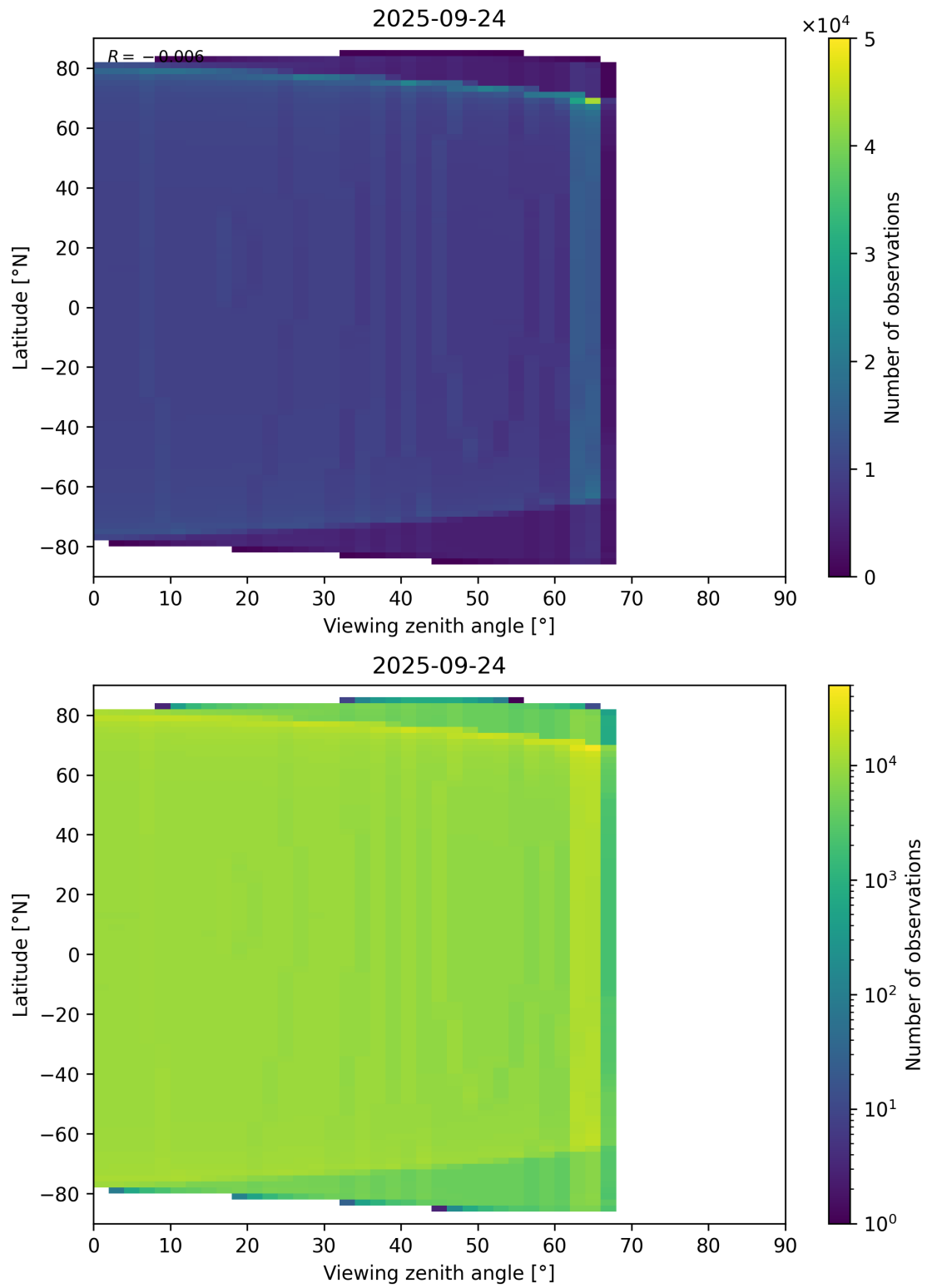
Figure 196: Scatter density plot of “Viewing zenith angle” against “Latitude” for 2025-09-23 to 2025-09-25.
