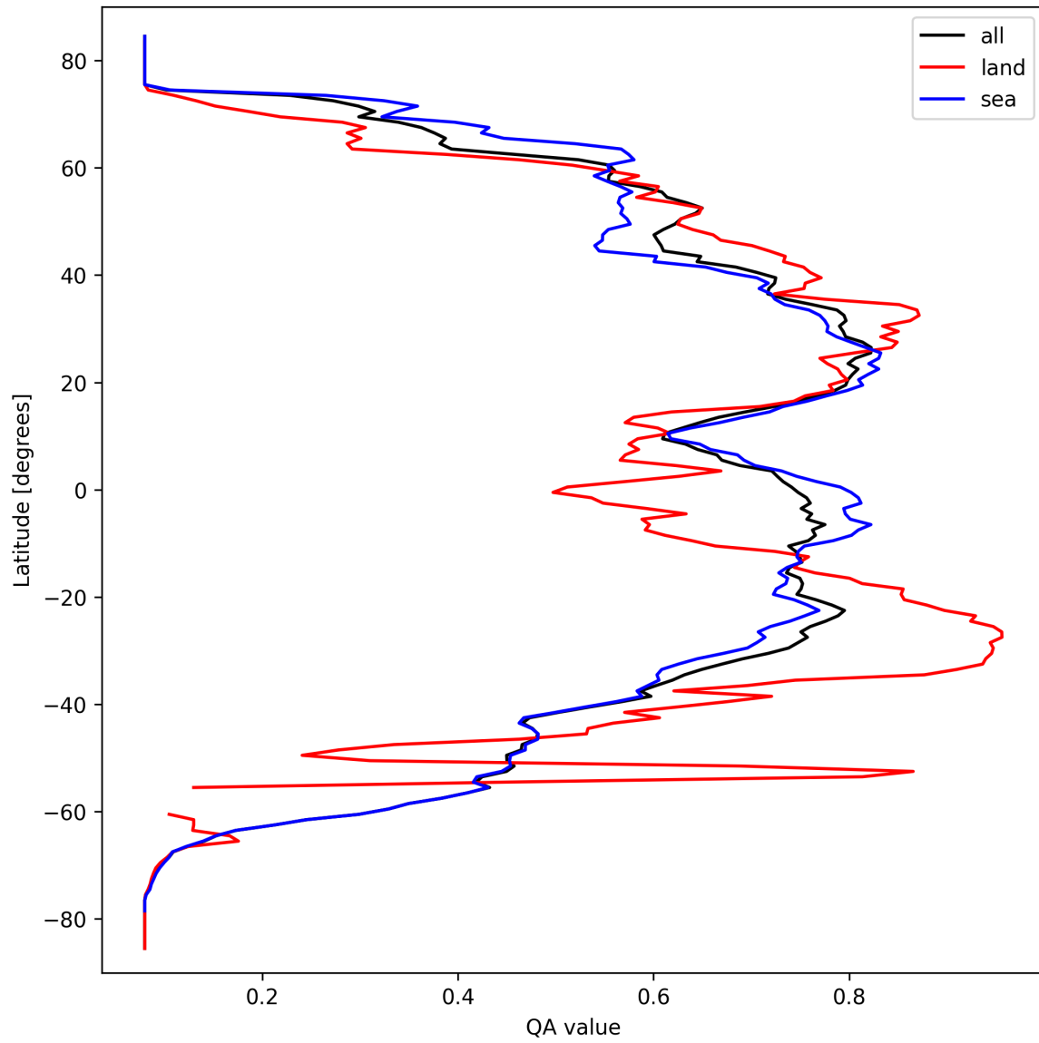
Figure 20: Zonal average of “QA value” for 2025-09-23 to 2025-09-25.
