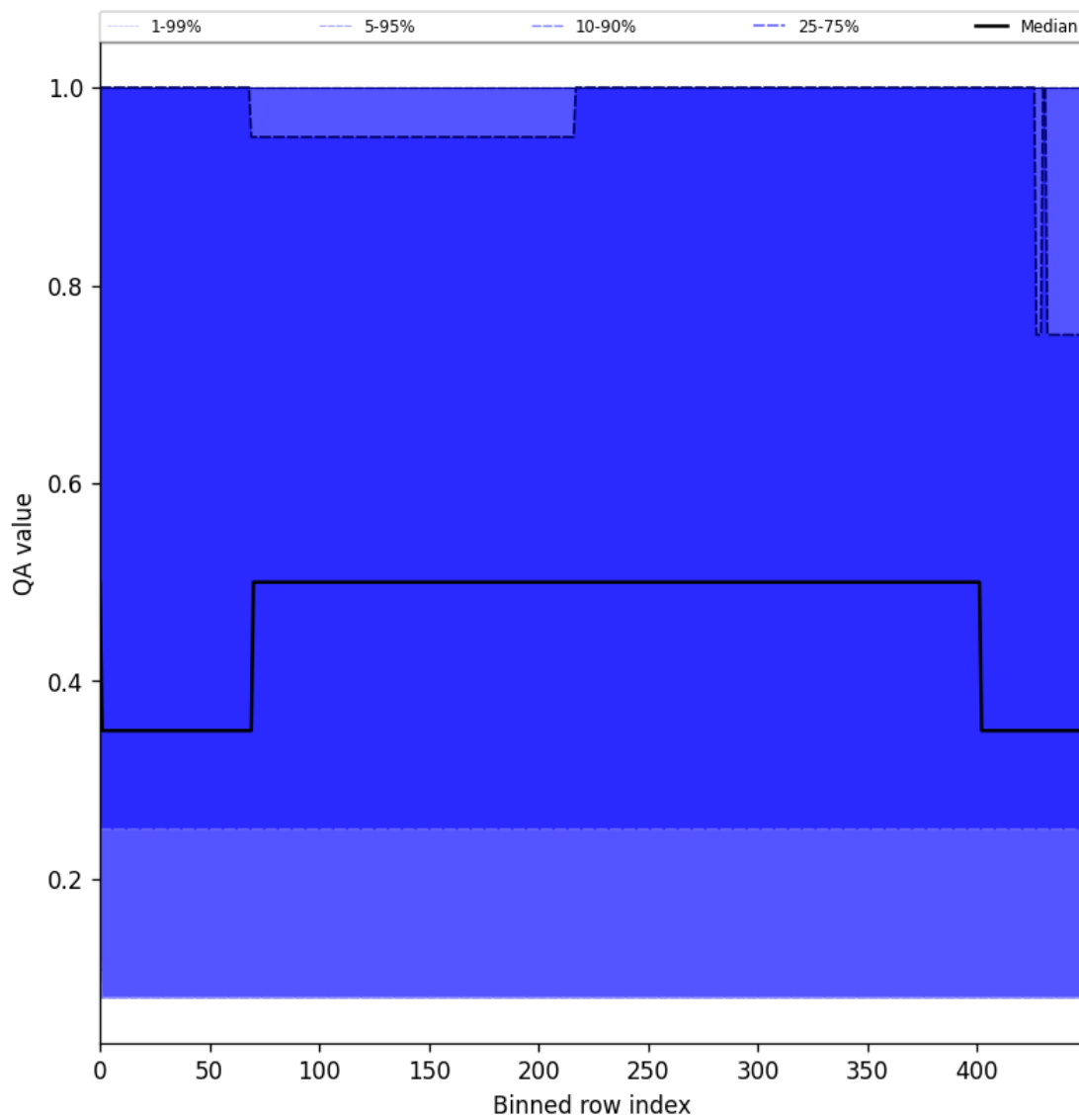
Figure 48: Along track statistics of “QA value” for 2025-09-23 to 2025-09-25
