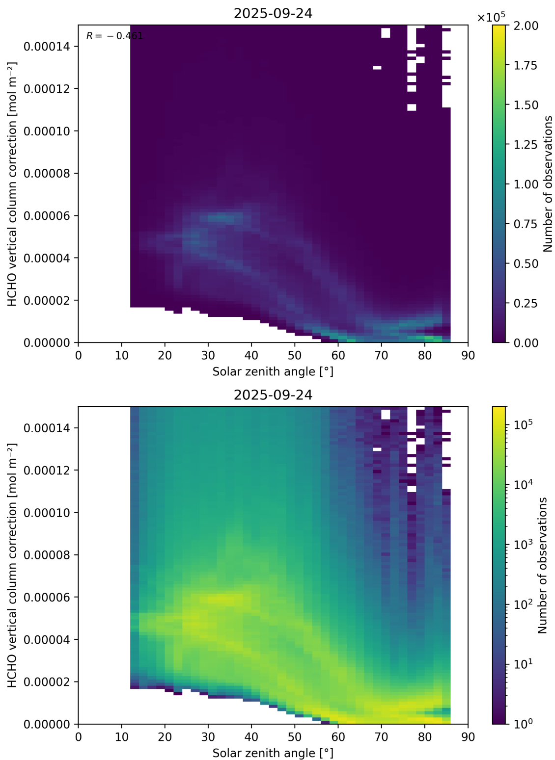
Figure 178: Scatter density plot of “Solar zenith angle” against “HCHO vertical column correction” for 2025-09-23 to 2025-09-25.
