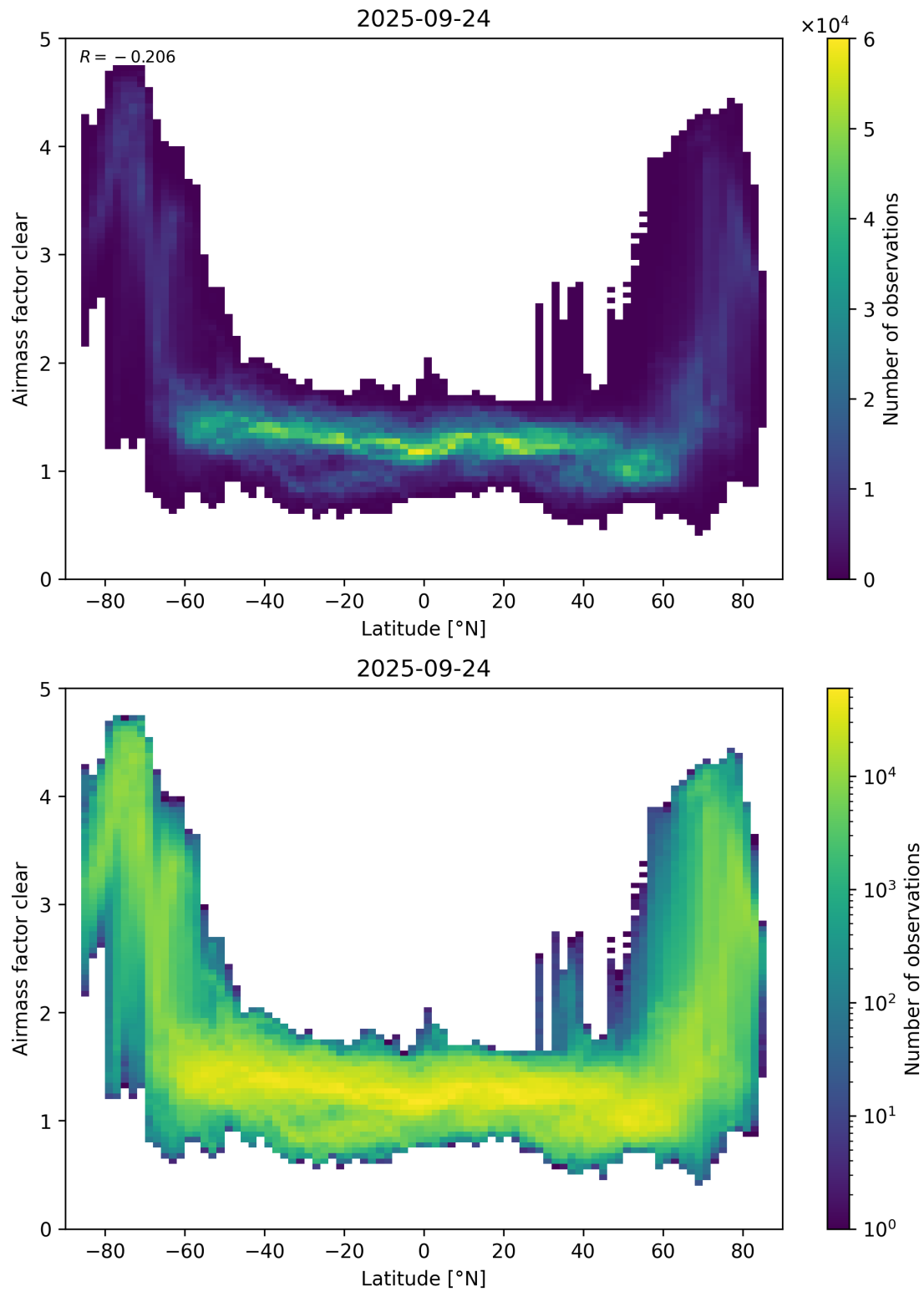
Figure 156: Scatter density plot of “Latitude” against “Airmass factor clear” for 2025-09-23 to 2025-09-25.
