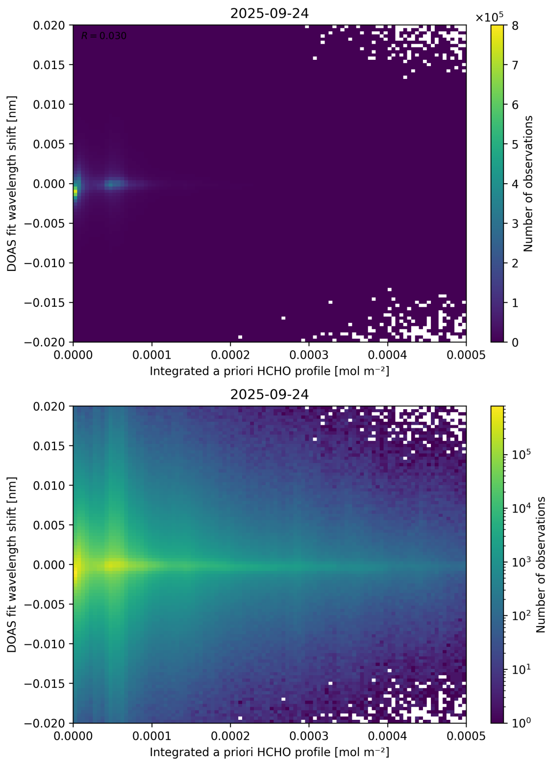
Figure 149: Scatter density plot of “Integrated a priori HCHO profile” against “DOAS fit wavelength shift” for 2025-09-23 to 2025-09-25.
