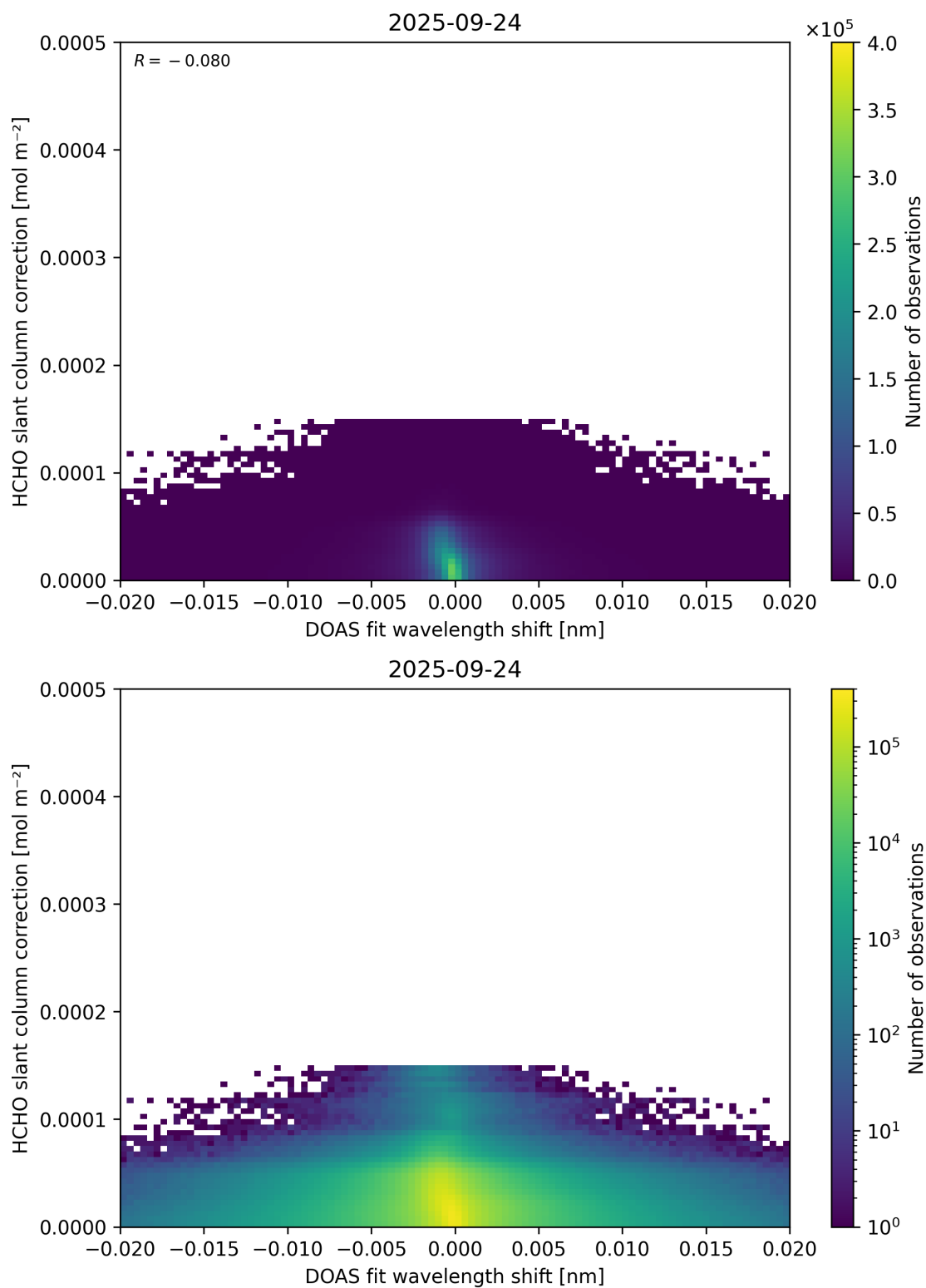
Figure 67: Scatter density plot of “DOAS fit wavelength shift” against “HCHO slant column correction” for 2025-09-23 to 2025-09-25.
