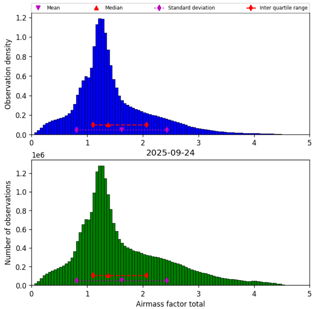
Figure 40: Histogram of “Airmass factor total” for 2025-09-23 to 2025-09-25
