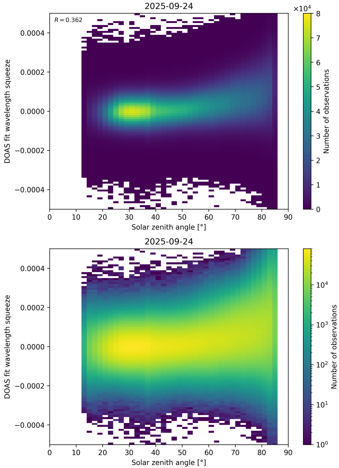
Figure 169: Scatter density plot of “Solar zenith angle” against “DOAS fit wavelength squeeze” for 2025-09-23 to 2025-09-25.
