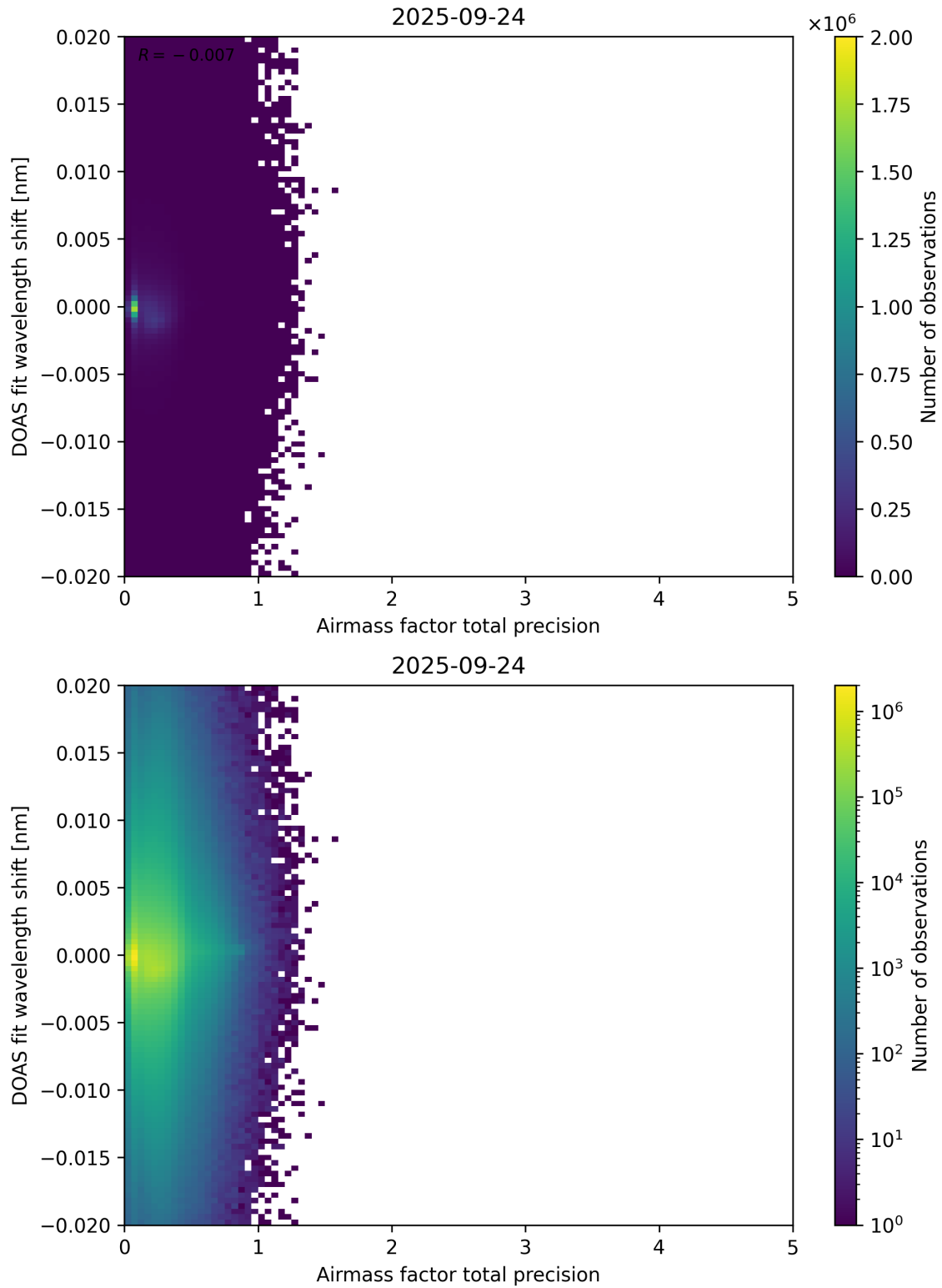
Figure 106: Scatter density plot of “Airmass factor total precision” against “DOAS fit wavelength shift” for 2025-09-23 to 2025-09-25.
