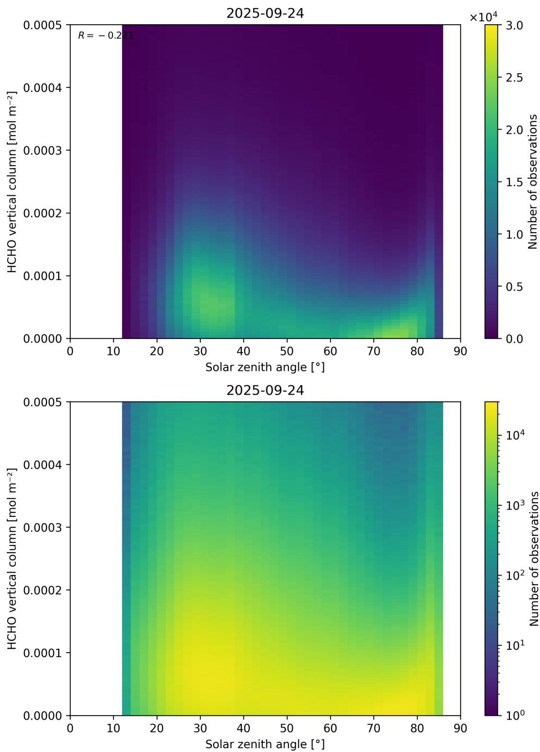
Figure 177: Scatter density plot of “Solar zenith angle” against “HCHO vertical column” for 2025-09-23 to 2025-09-25.
