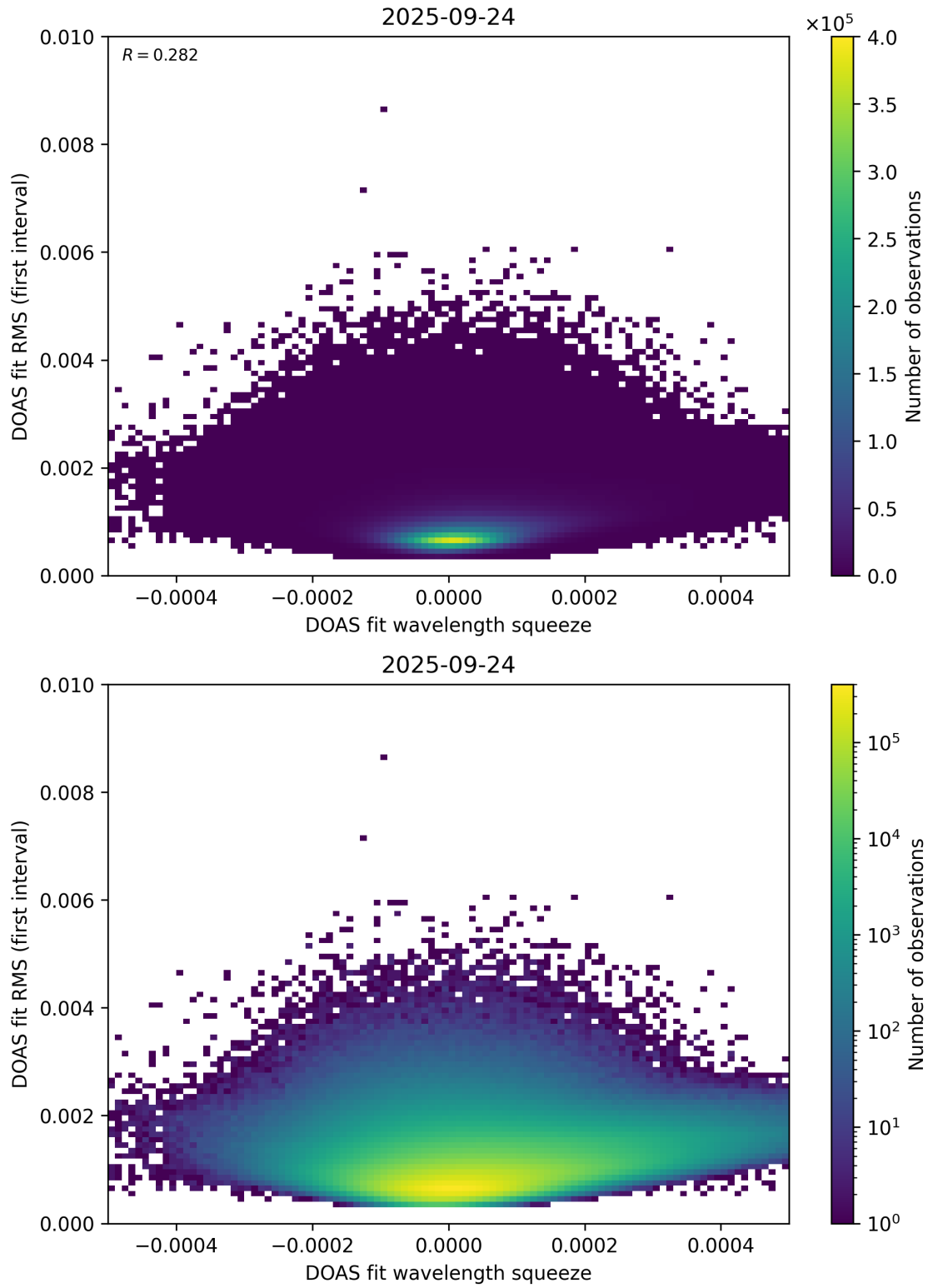
Figure 68: Scatter density plot of “DOAS fit wavelength squeeze” against “DOAS fit RMS (first interval)” for 2025-09-23 to 2025-09-25.
