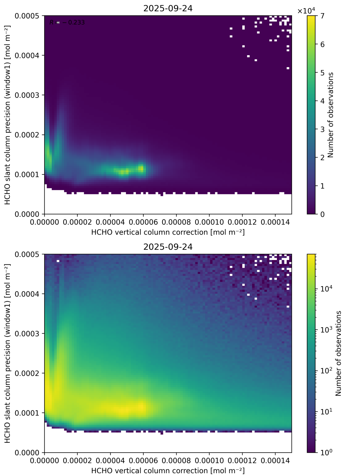
Figure 119: Scatter density plot of “HCHO vertical column correction” against “HCHO slant column precision (window1)” for 2025-09-23 to 2025-09-25.
