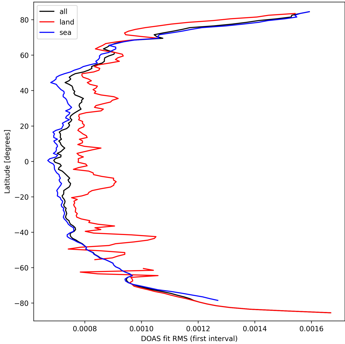
Figure 32: Zonal average of “DOAS fit RMS (first interval)” for 2025-09-23 to 2025-09-25.
