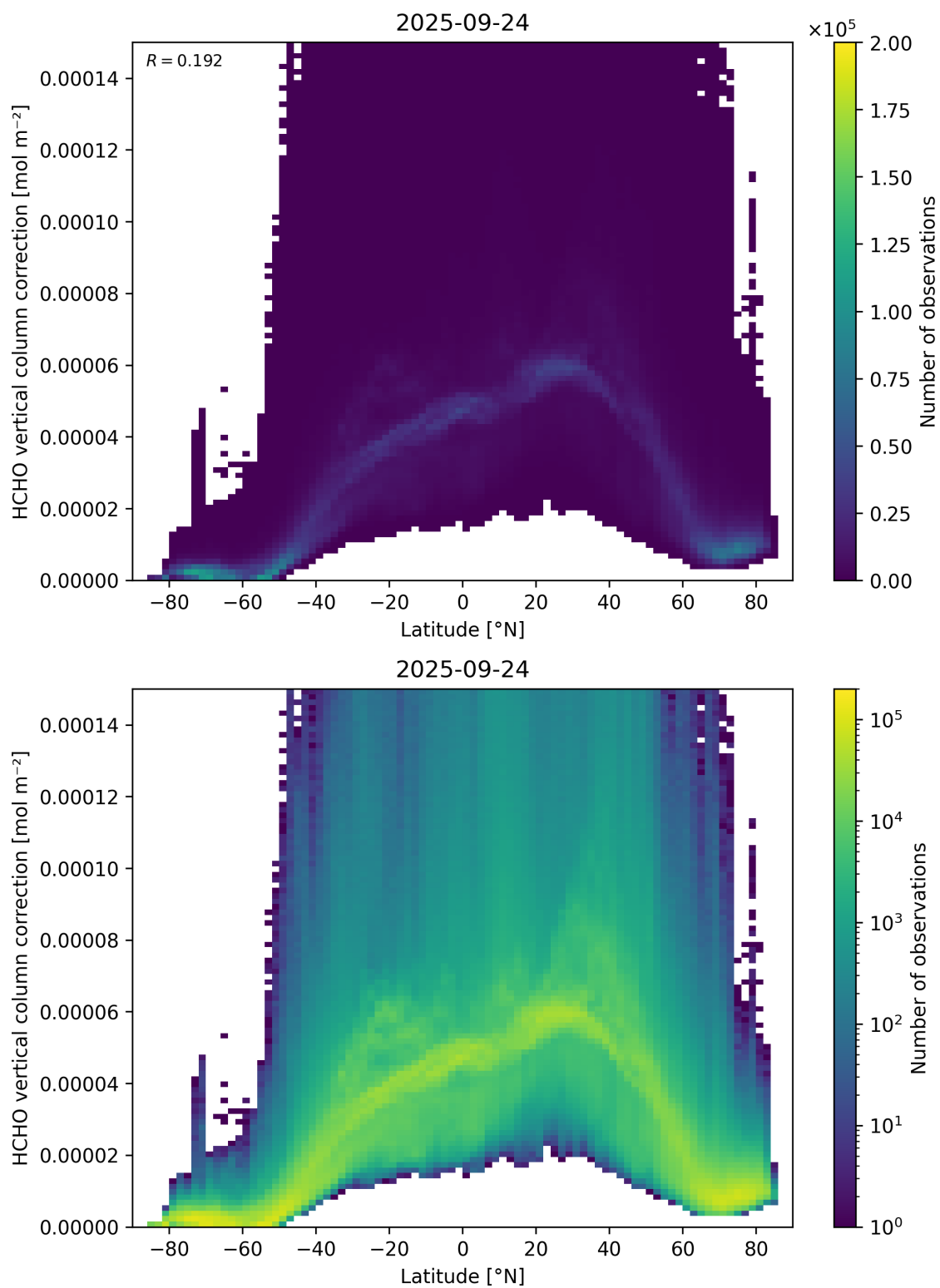
Figure 164: Scatter density plot of “Latitude” against “HCHO vertical column correction” for 2025-09-23 to 2025-09-25.
