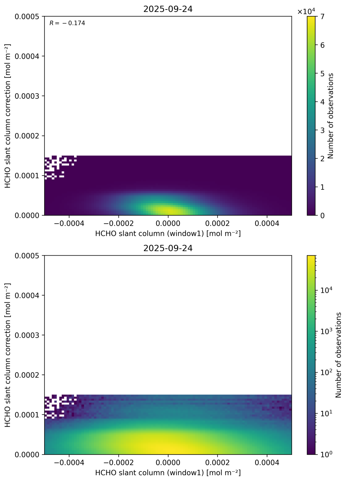
Figure 83: Scatter density plot of “HCHO slant column (window1)” against “HCHO slant column correction” for 2025-09-23 to 2025-09-25.
