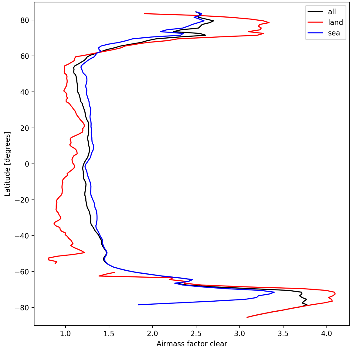
Figure 28: Zonal average of “Airmass factor clear” for 2025-09-23 to 2025-09-25.
