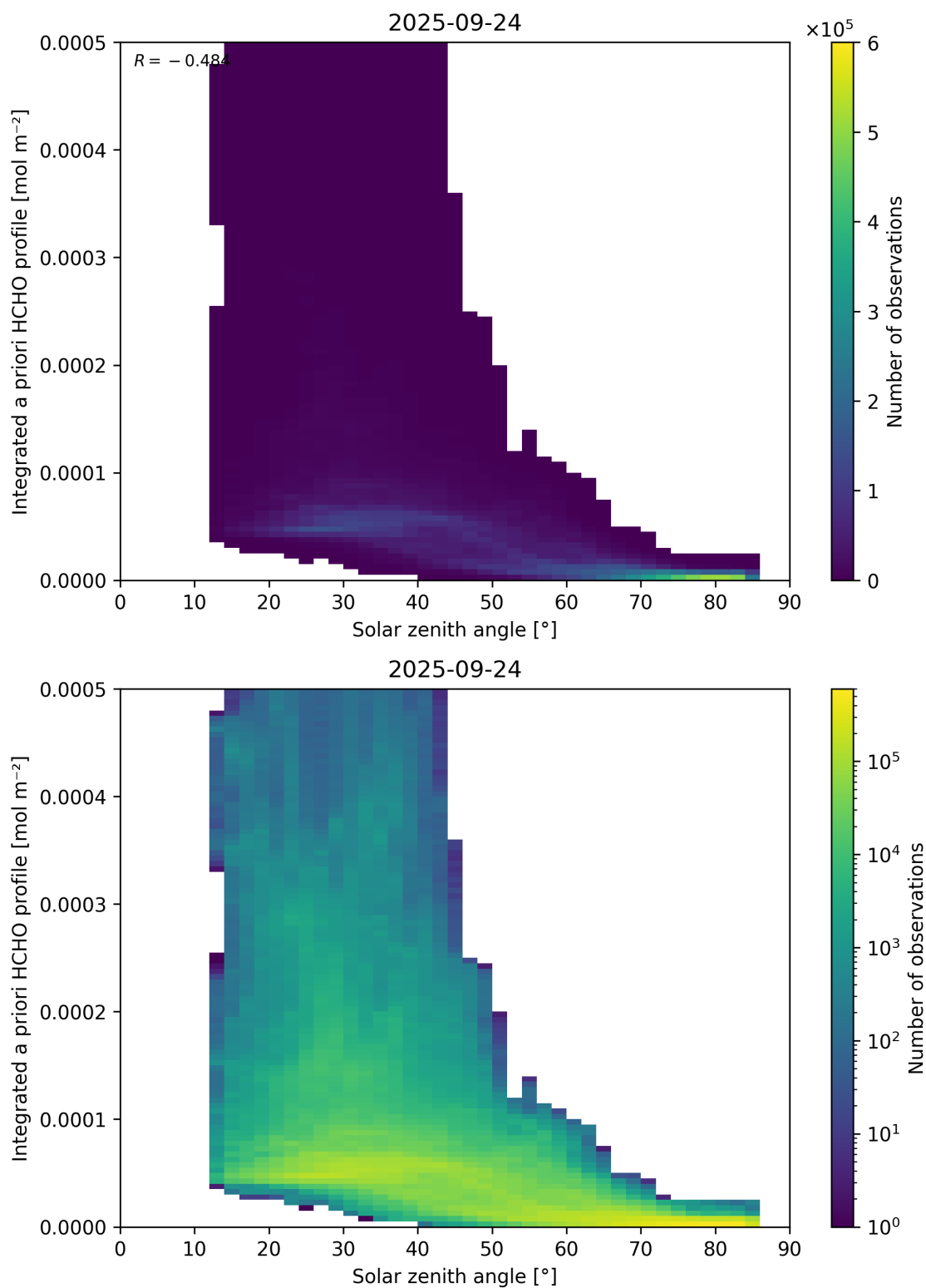
Figure 180: Scatter density plot of “Solar zenith angle” against “Integrated a priori HCHO profile” for 2025-09-23 to 2025-09-25.
