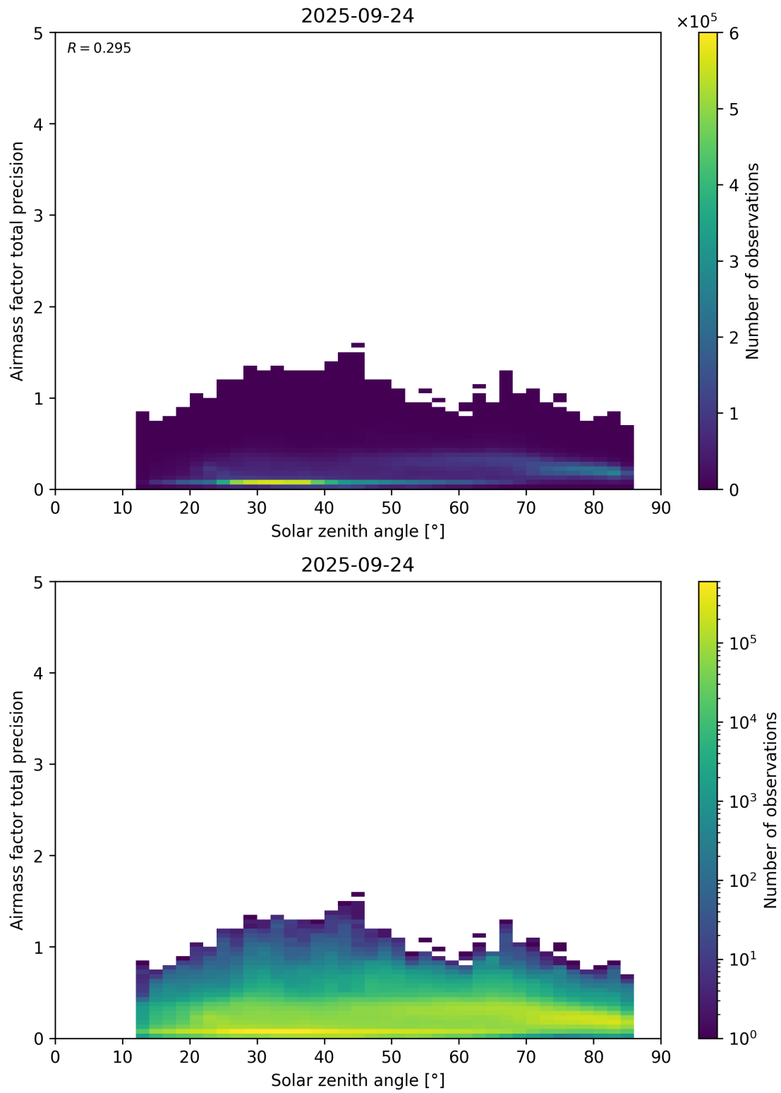
Figure 176: Scatter density plot of “Solar zenith angle” against “Airmass factor total precision” for 2025-09-23 to 2025-09-25.
