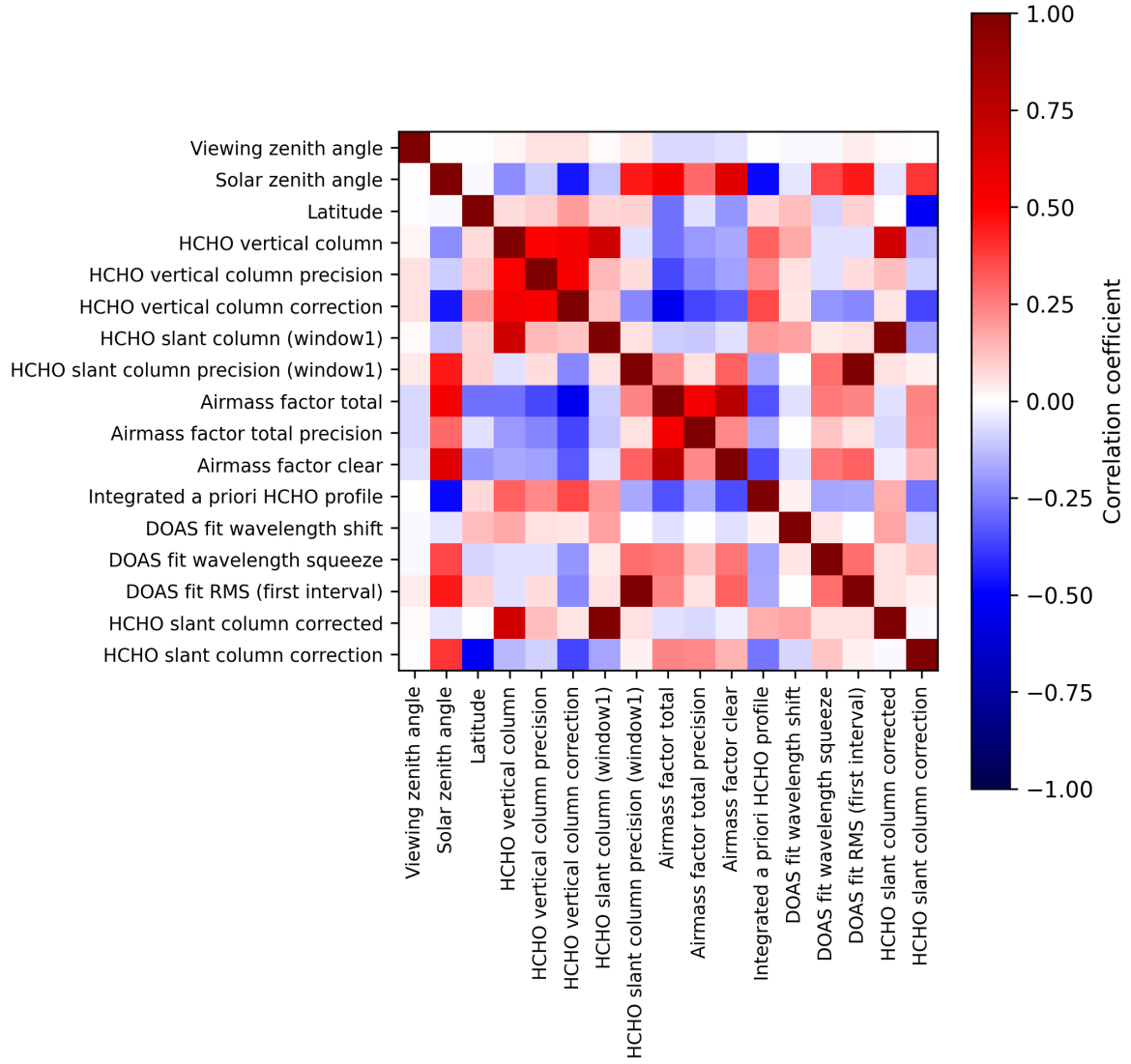
Figure 2: Map of correlation matrix for 2025-09-23 to 2025-09-25.
