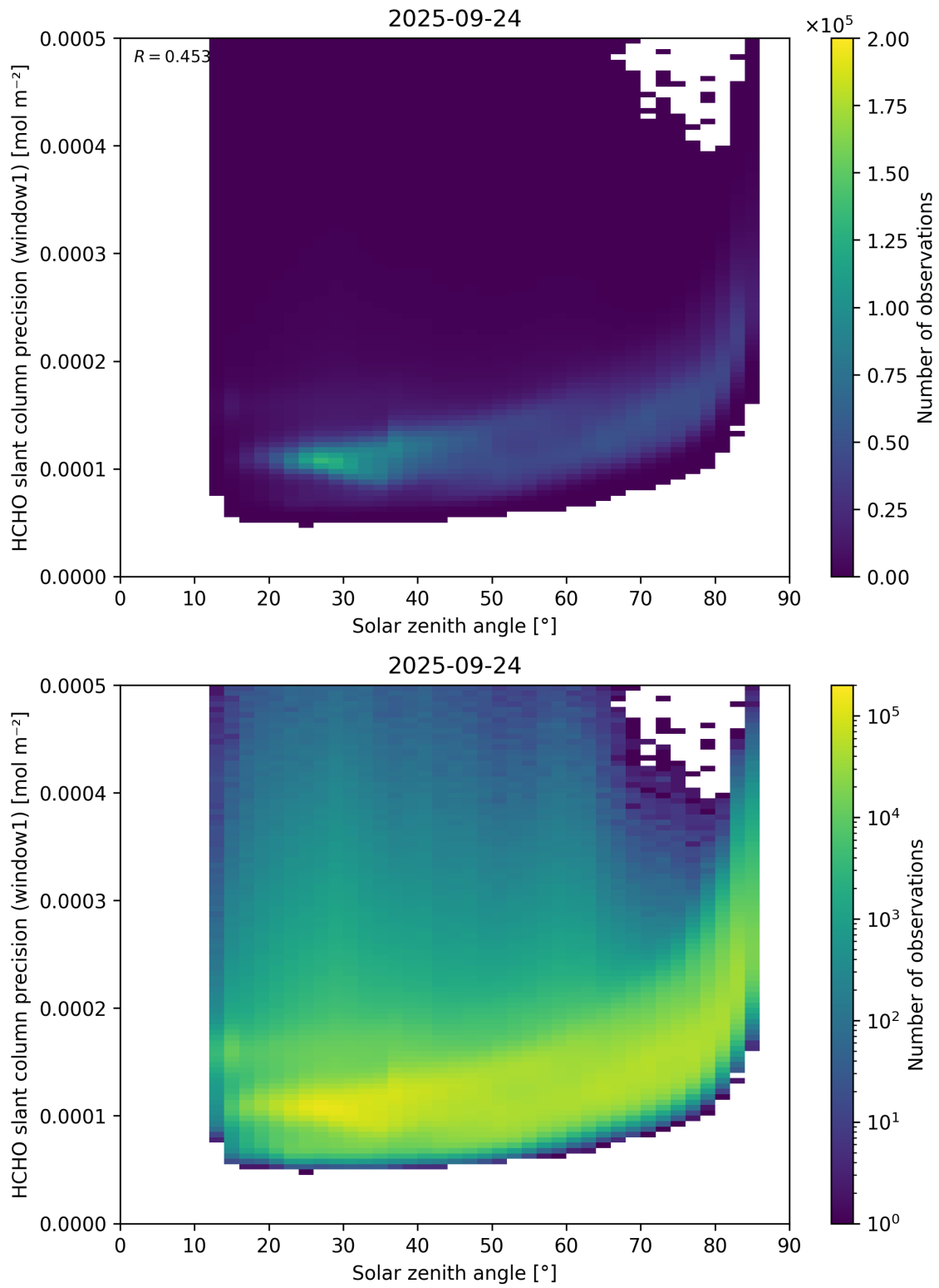
Figure 174: Scatter density plot of “Solar zenith angle” against “HCHO slant column precision (window1)” for 2025-09-23 to 2025-09-25.
