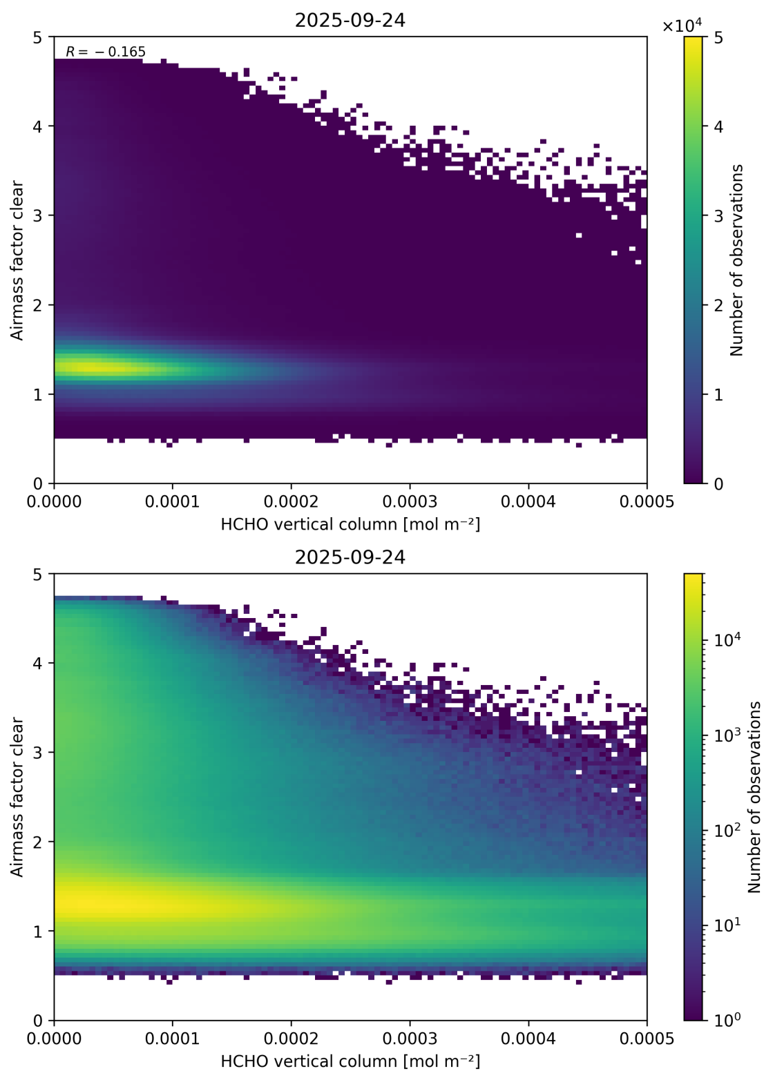
Figure 126: Scatter density plot of “HCHO vertical column” against “Airmass factor clear” for 2025-09-23 to 2025-09-25.
