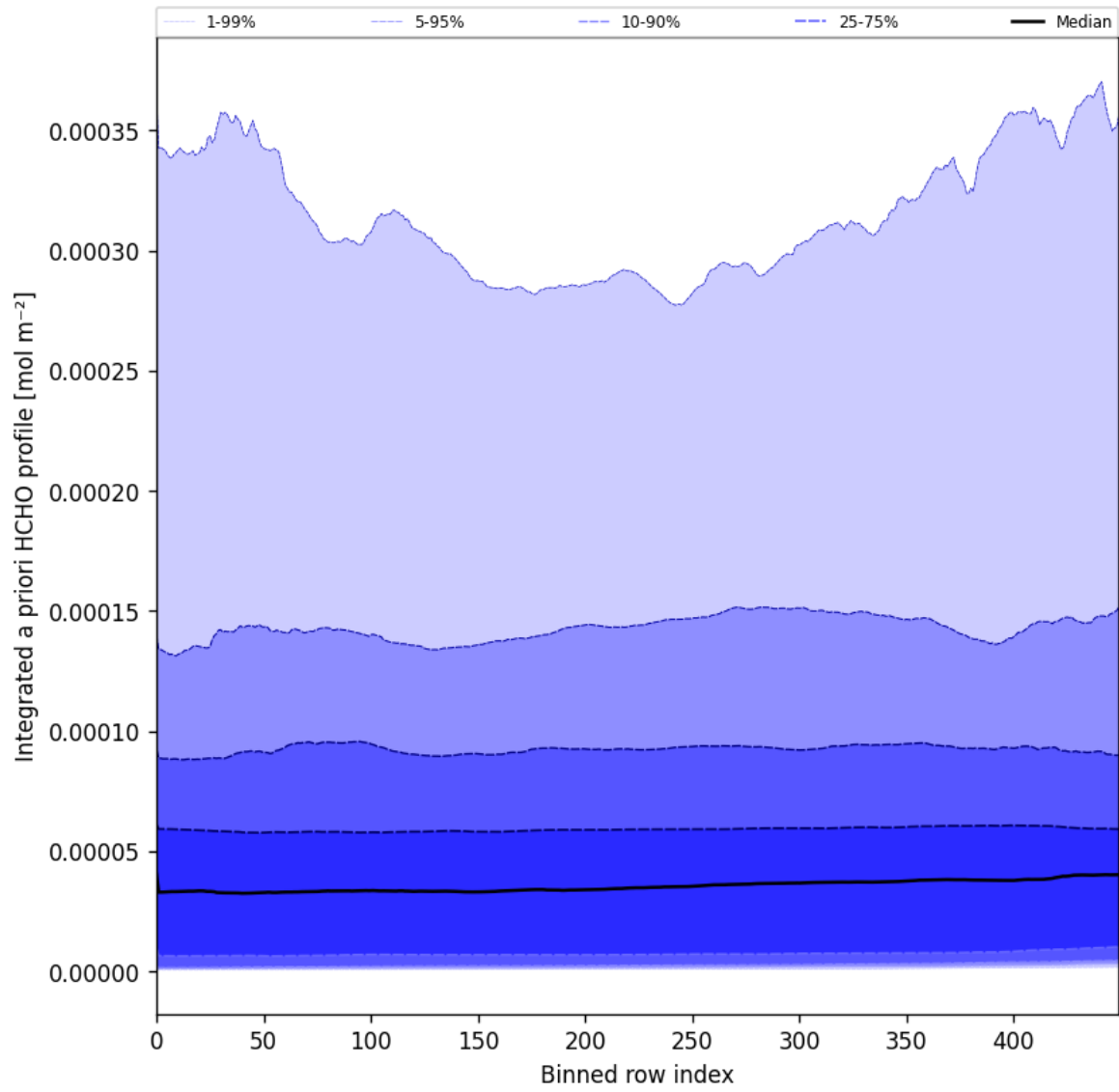
Figure 57: Along track statistics of "Integrated a priori HCHO profile" for 2025-09-23 to 2025-09-25
