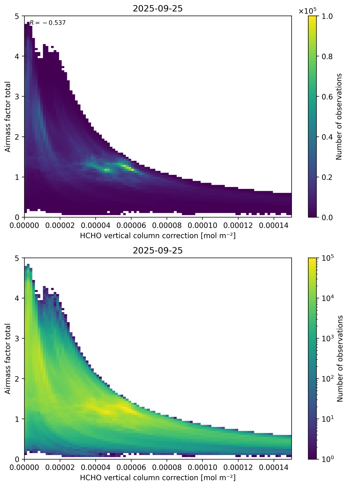
Figure 120: Scatter density plot of “HCHO vertical column correction” against “Airmass factor total” for 2025-09-25 to 2025-09-26.
