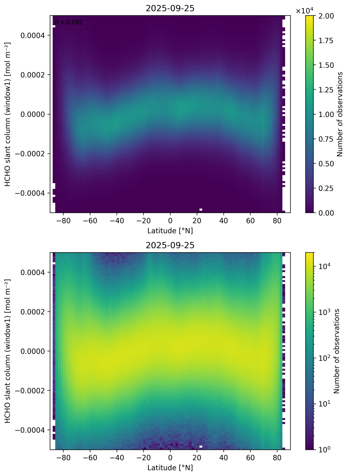
Figure 159: Scatter density plot of “Latitude” against “HCHO slant column (window1)” for 2025-09-25 to 2025-09-26.
