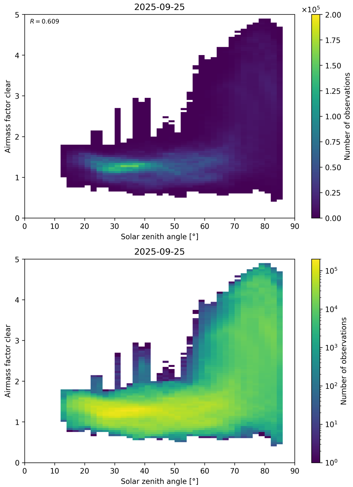
Figure 170: Scatter density plot of “Solar zenith angle” against “Airmass factor clear” for 2025-09-25 to 2025-09-26.
