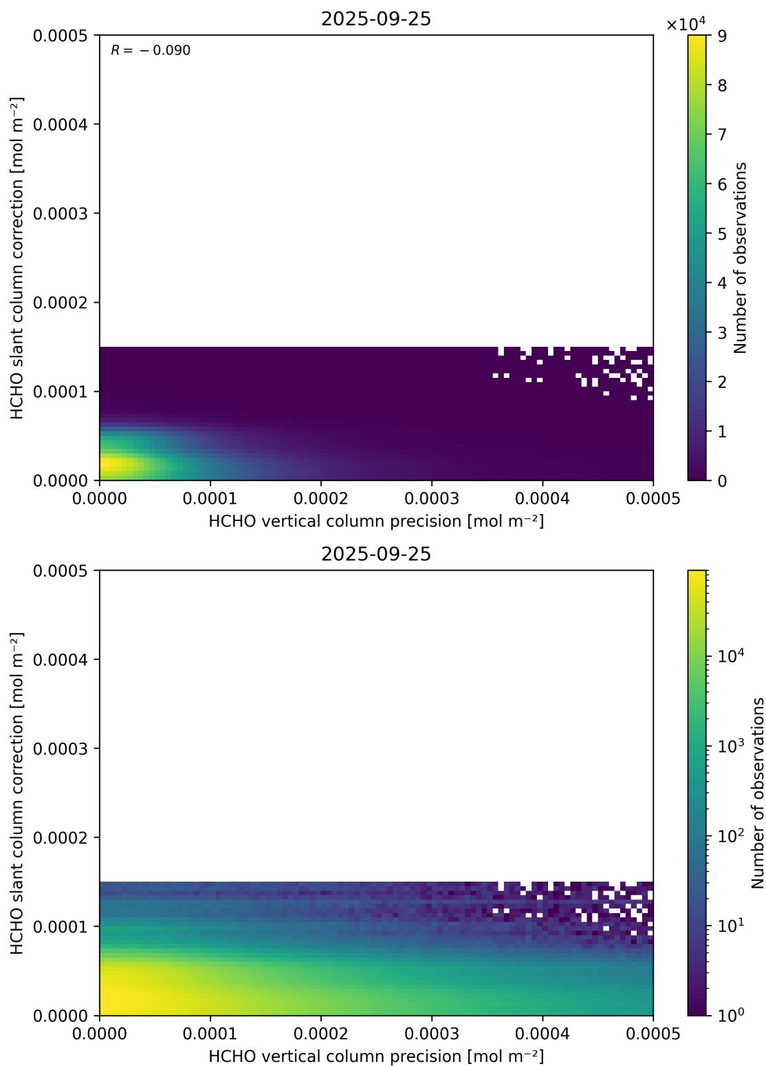
Figure 141: Scatter density plot of “HCHO vertical column precision” against “HCHO slant column correction” for 2025-09-25 to 2025-09-26.
