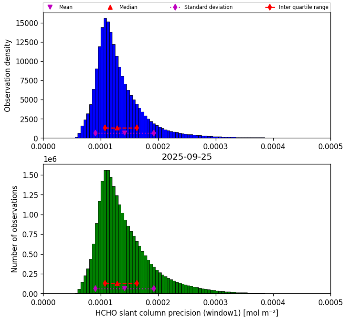
Figure 39: Histogram of “HCHO slant column precision (window1)” for 2025-09-25 to 2025-09-26
