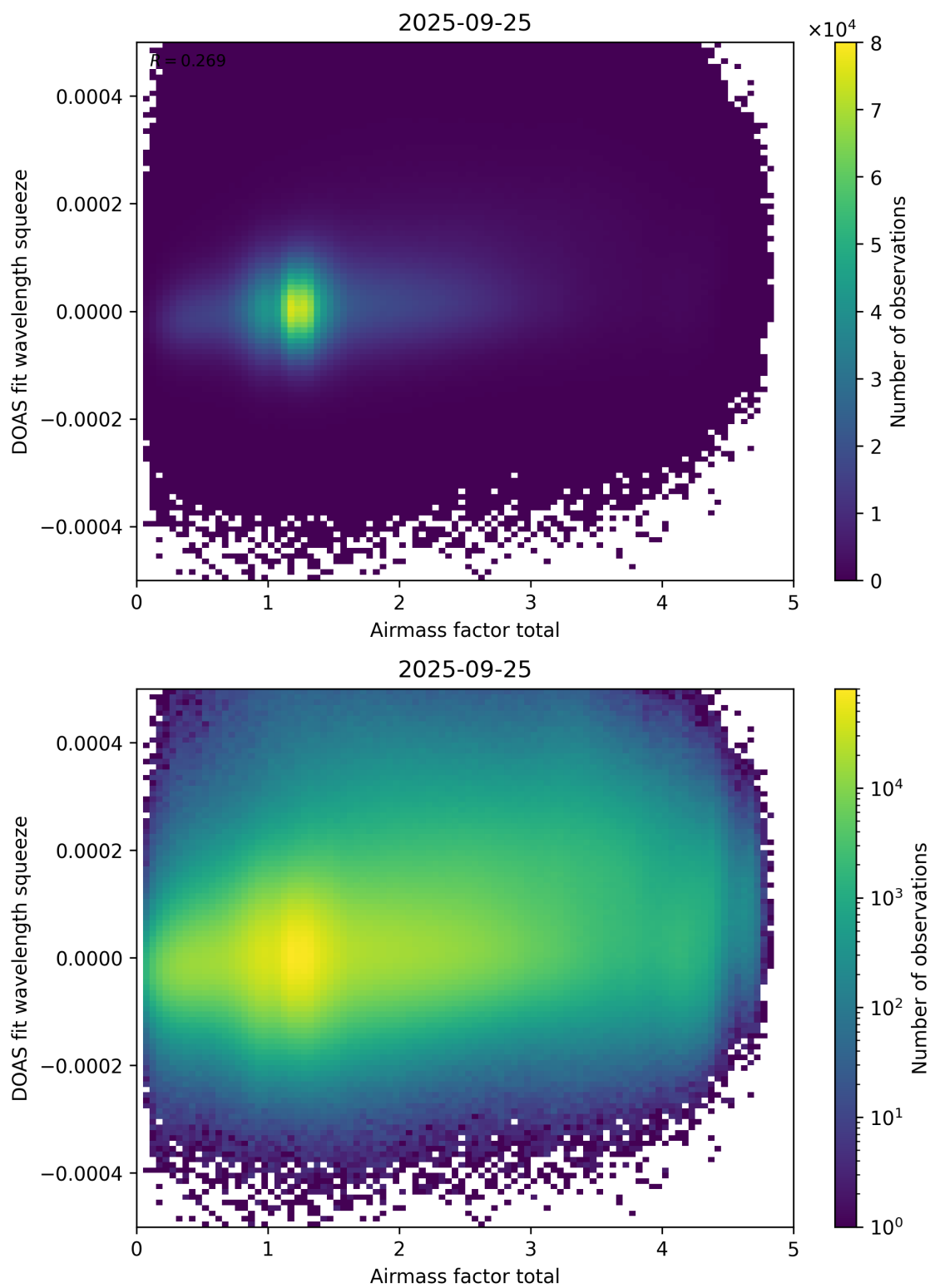
Figure 99: Scatter density plot of “Airmass factor total” against “DOAS fit wavelength squeeze” for 2025-09-25 to 2025-09-26.
