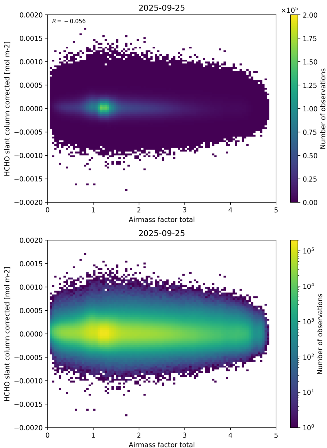
Figure 101: Scatter density plot of “Airmass factor total” against “HCHO slant column corrected” for 2025-09-25 to 2025-09-26.
