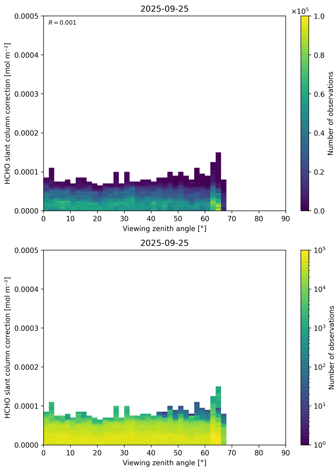
Figure 187: Scatter density plot of “Viewing zenith angle” against “HCHO slant column correction” for 2025-09-25 to 2025-09-26.
