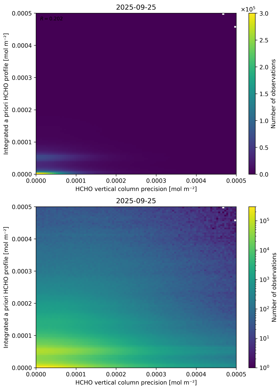
Figure 147: Scatter density plot of “HCHO vertical column precision” against “Integrated a priori HCHO profile” for 2025-09-25 to 2025-09-26.
