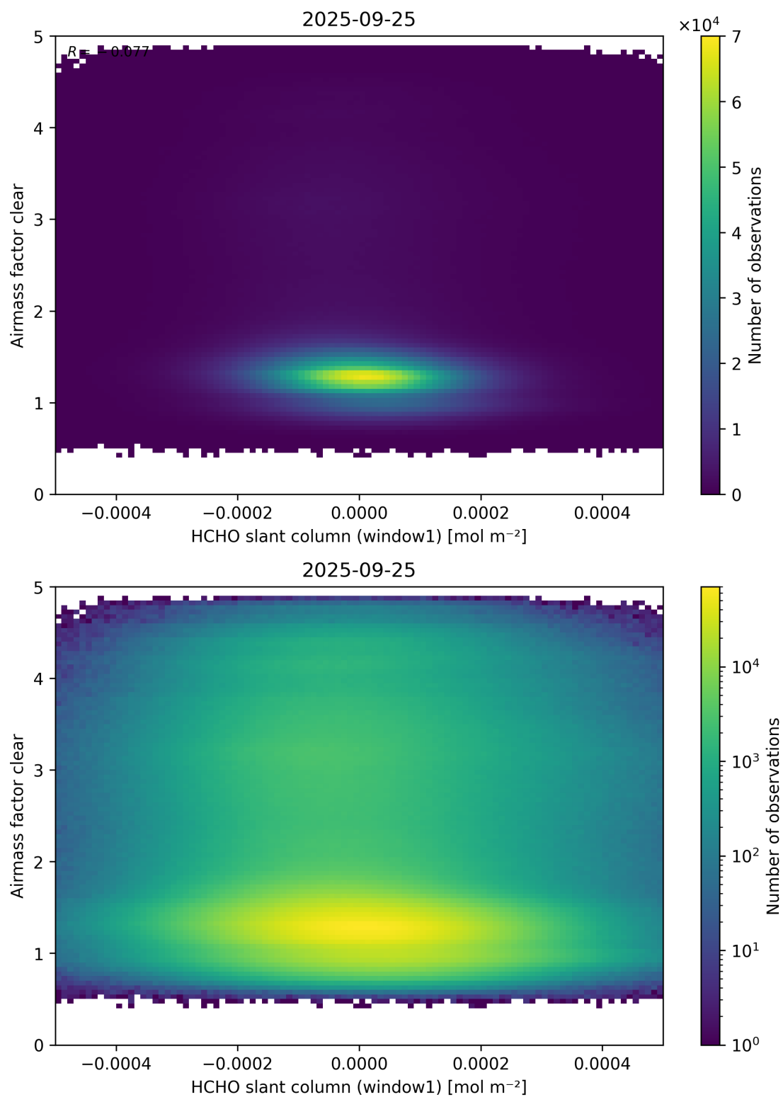
Figure 81: Scatter density plot of “HCHO slant column (window1)” against “Airmass factor clear” for 2025-09-25 to 2025-09-26.
