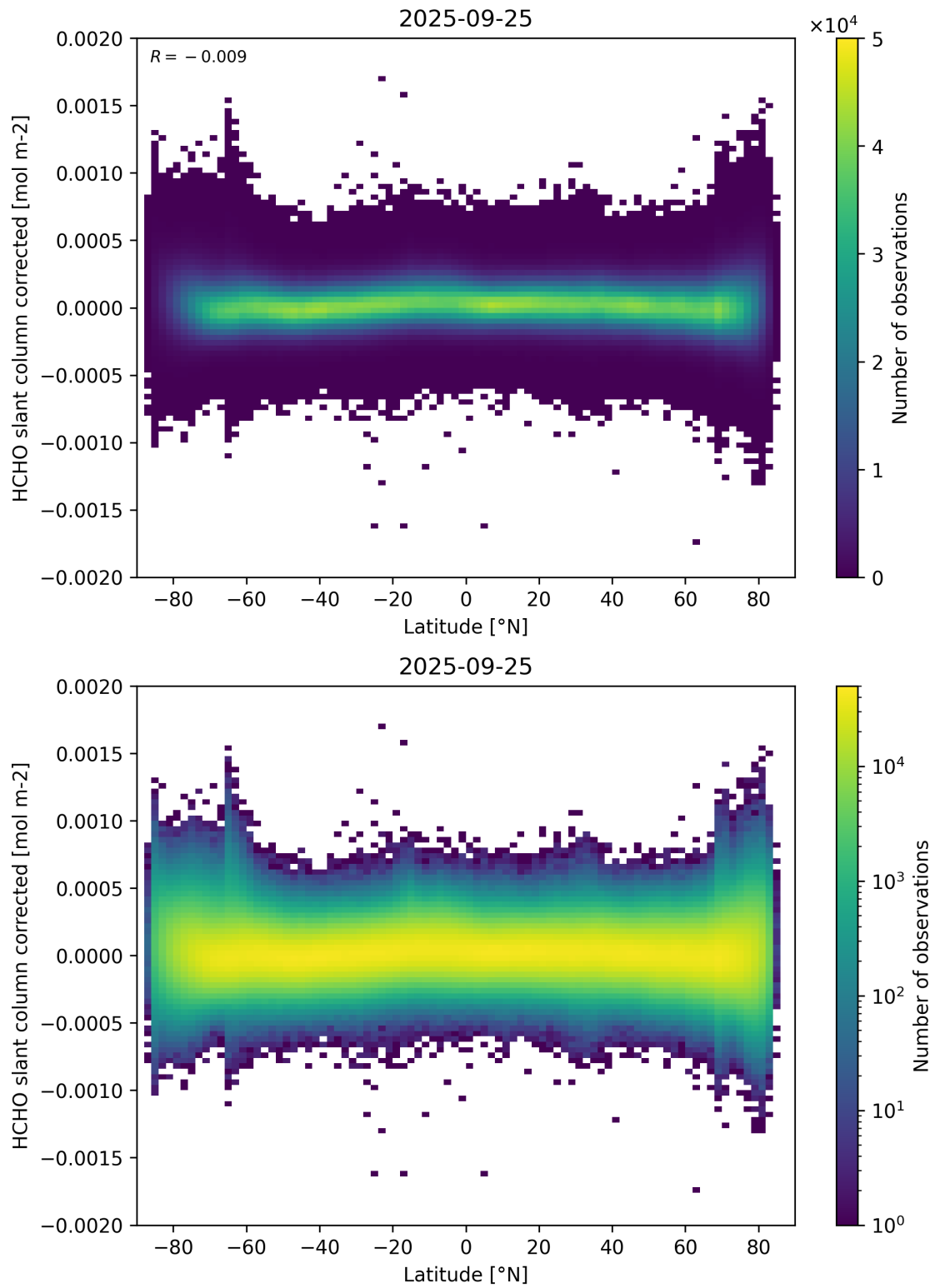
Figure 157: Scatter density plot of “Latitude” against “HCHO slant column corrected” for 2025-09-25 to 2025-09-26.
