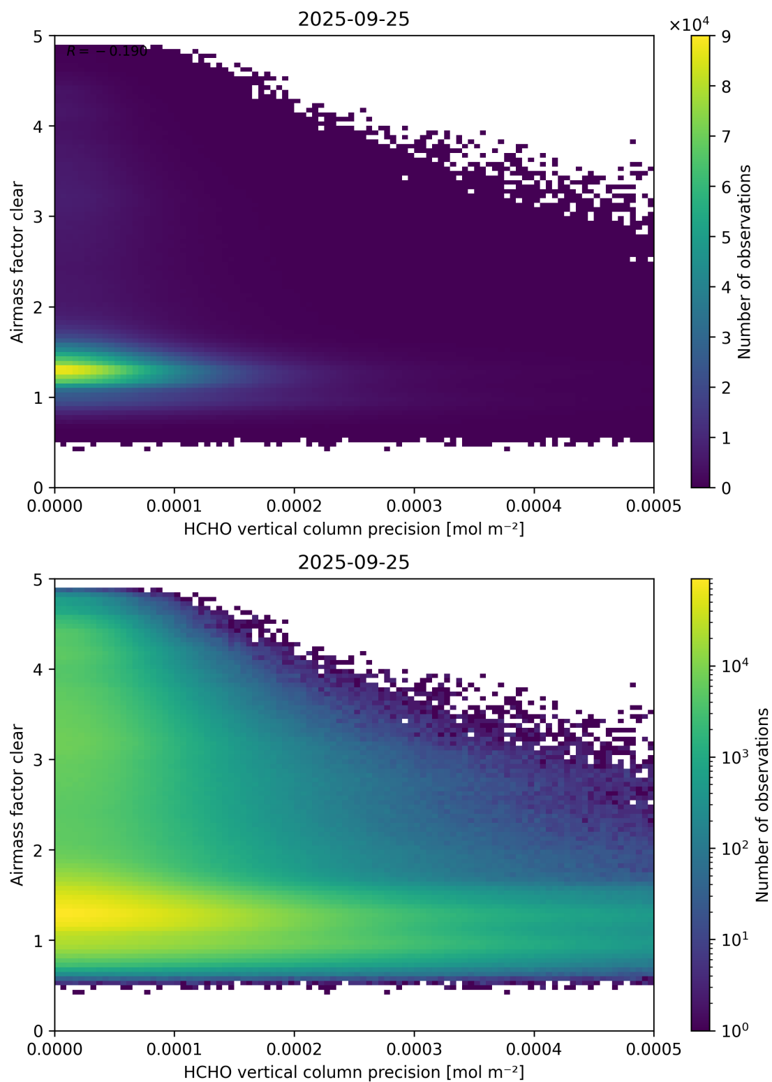
Figure 139: Scatter density plot of “HCHO vertical column precision” against “Airmass factor clear” for 2025-09-25 to 2025-09-26.
