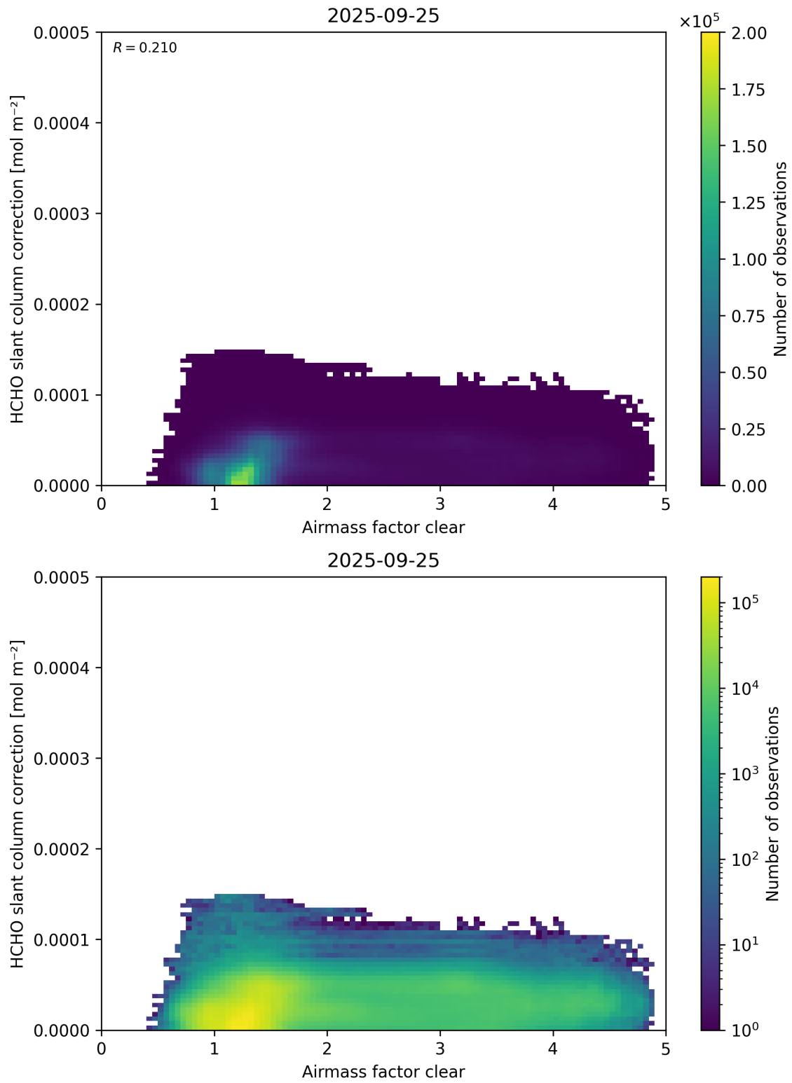
Figure 75: Scatter density plot of “Airmass factor clear” against “HCHO slant column correction” for 2025-09-25 to 2025-09-26.
