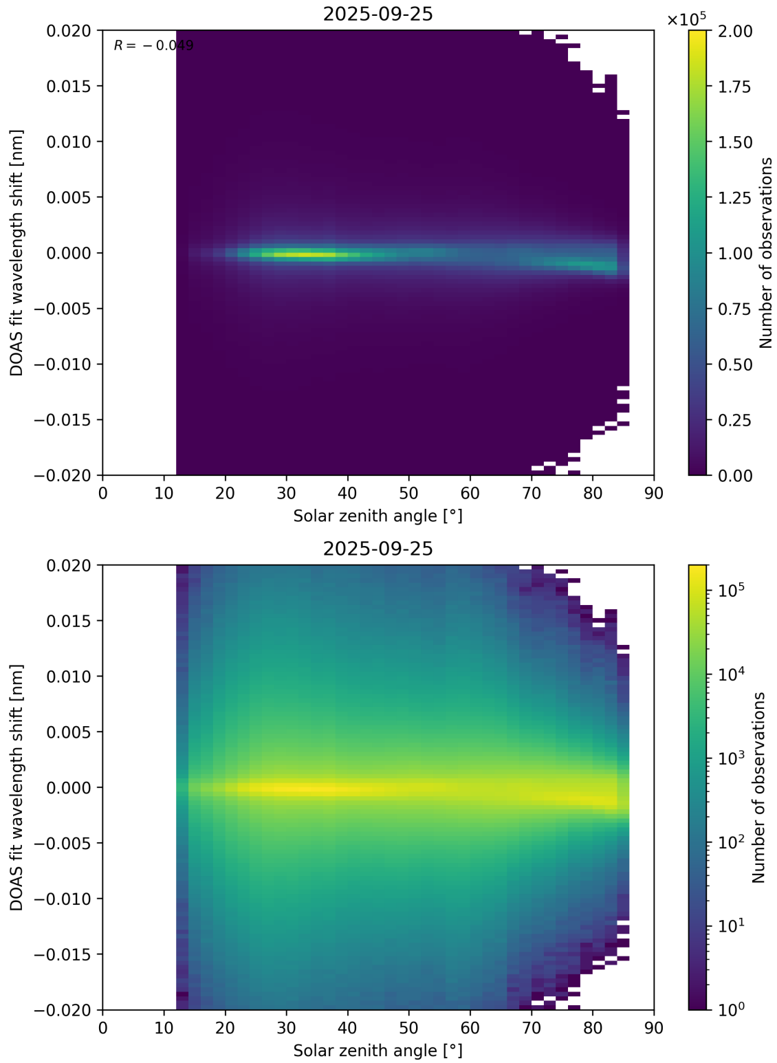
Figure 168: Scatter density plot of “Solar zenith angle” against “DOAS fit wavelength shift” for 2025-09-25 to 2025-09-26.
