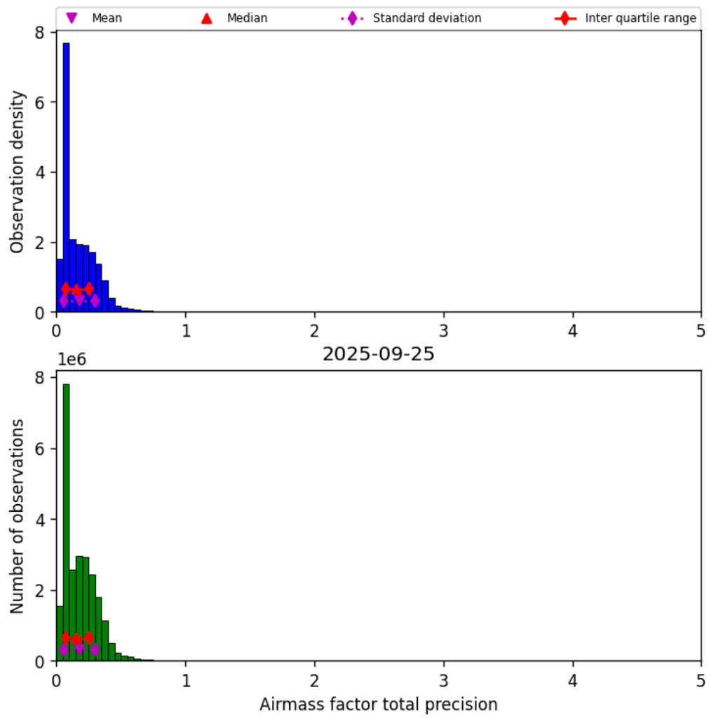
Figure 41: Histogram of “Airmass factor total precision” for 2025-09-25 to 2025-09-26
