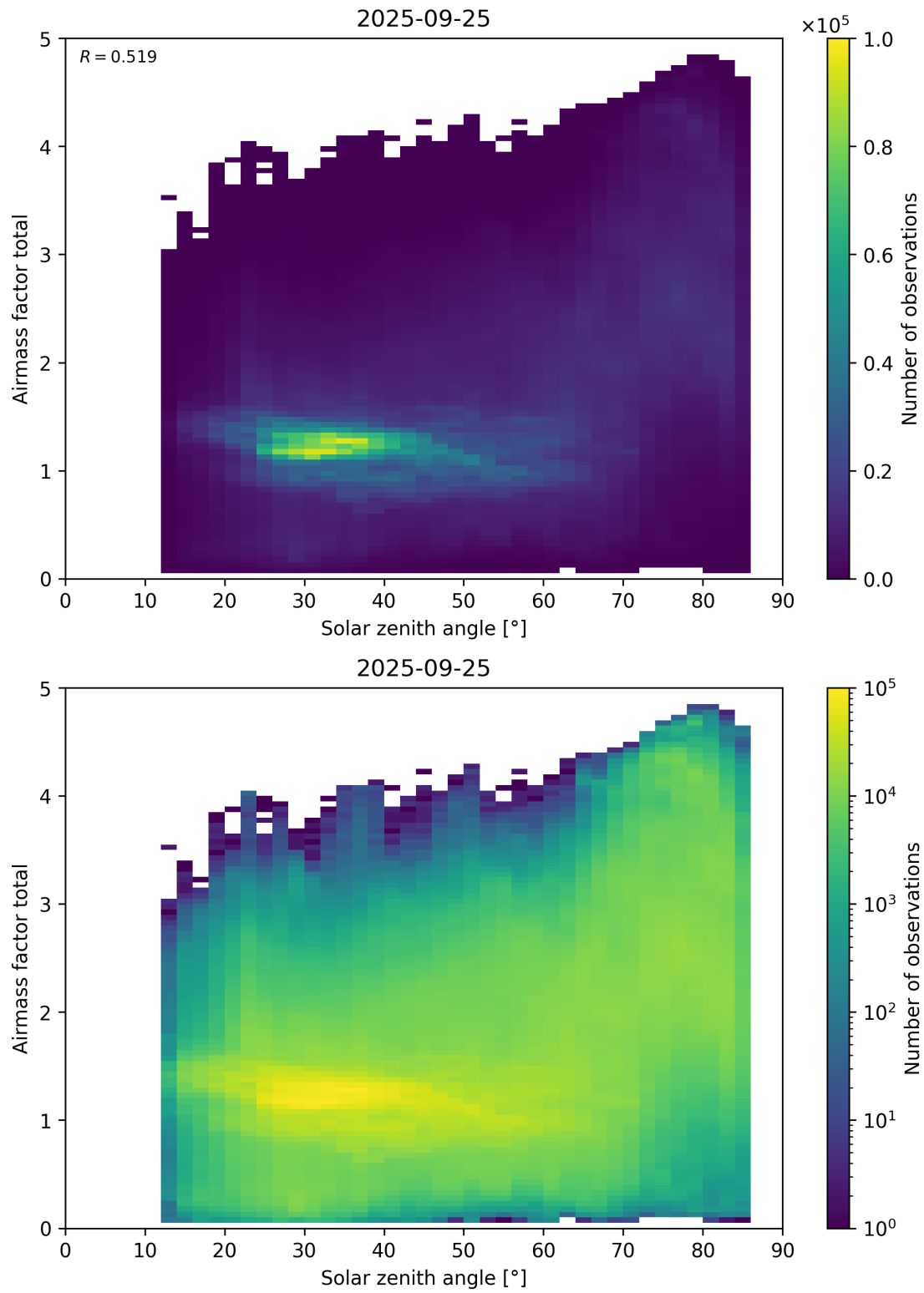
Figure 175: Scatter density plot of “Solar zenith angle” against “Airmass factor total” for 2025-09-25 to 2025-09-26.
