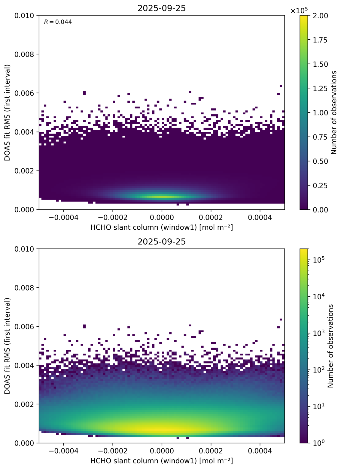
Figure 78: Scatter density plot of “HCHO slant column (window1)” against “DOAS fit RMS (first interval)” for 2025-09-25 to 2025-09-26.
