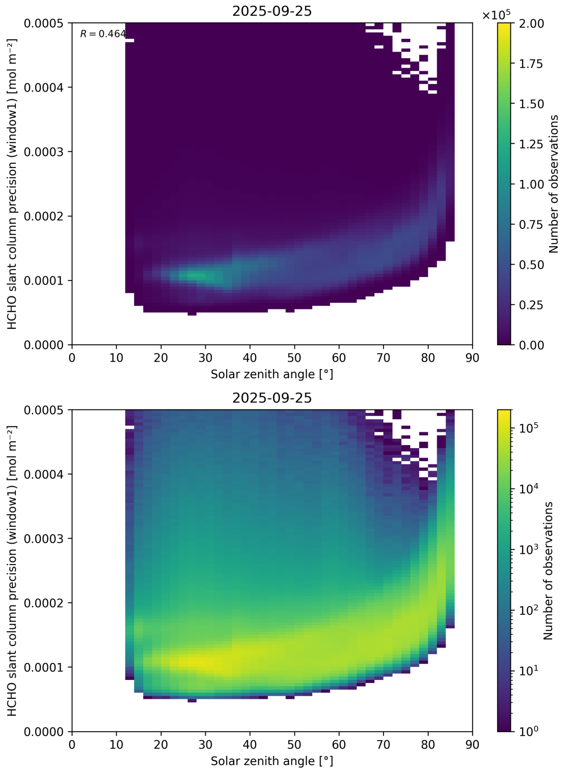
Figure 174: Scatter density plot of “Solar zenith angle” against “HCHO slant column precision (window1)” for 2025-09-25 to 2025-09-26.
