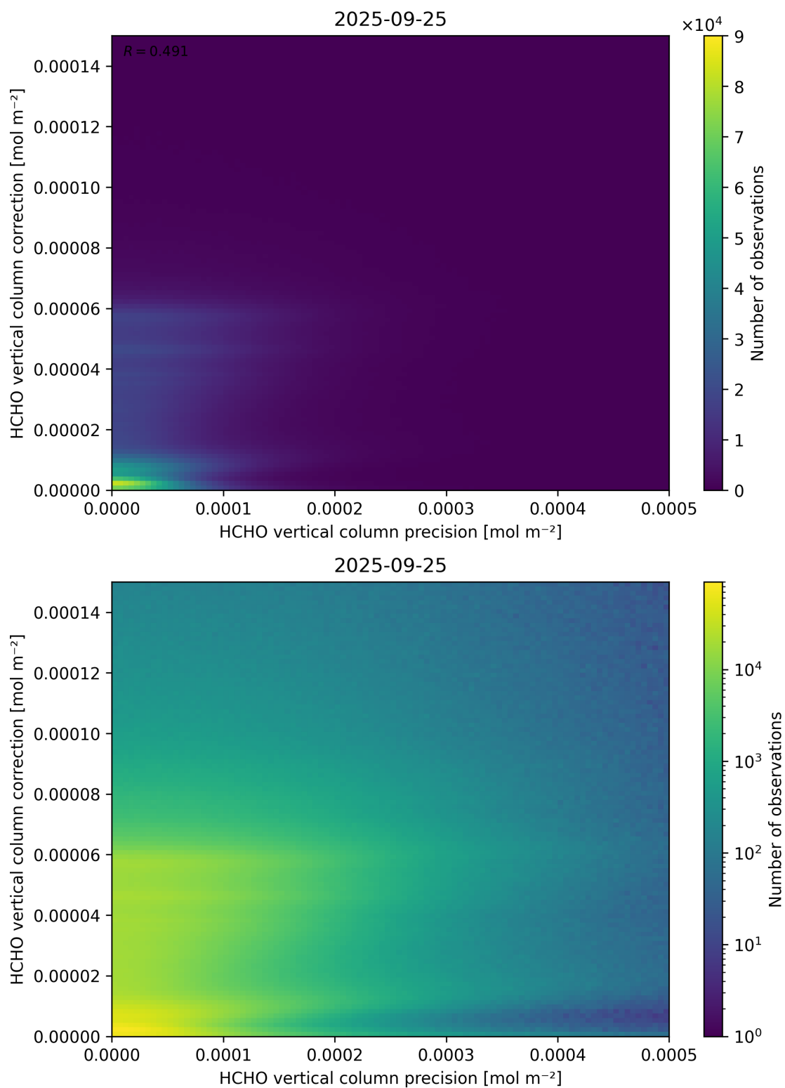
Figure 146: Scatter density plot of “HCHO vertical column precision” against “HCHO vertical column correction” for 2025-09-25 to 2025-09-26.
