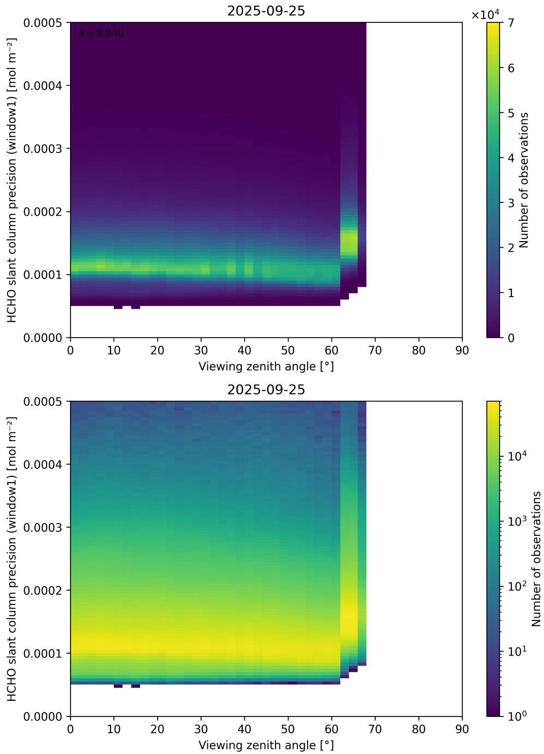
Figure 189: Scatter density plot of “Viewing zenith angle” against “HCHO slant column precision (window1)” for 2025-09-25 to 2025-09-26.
