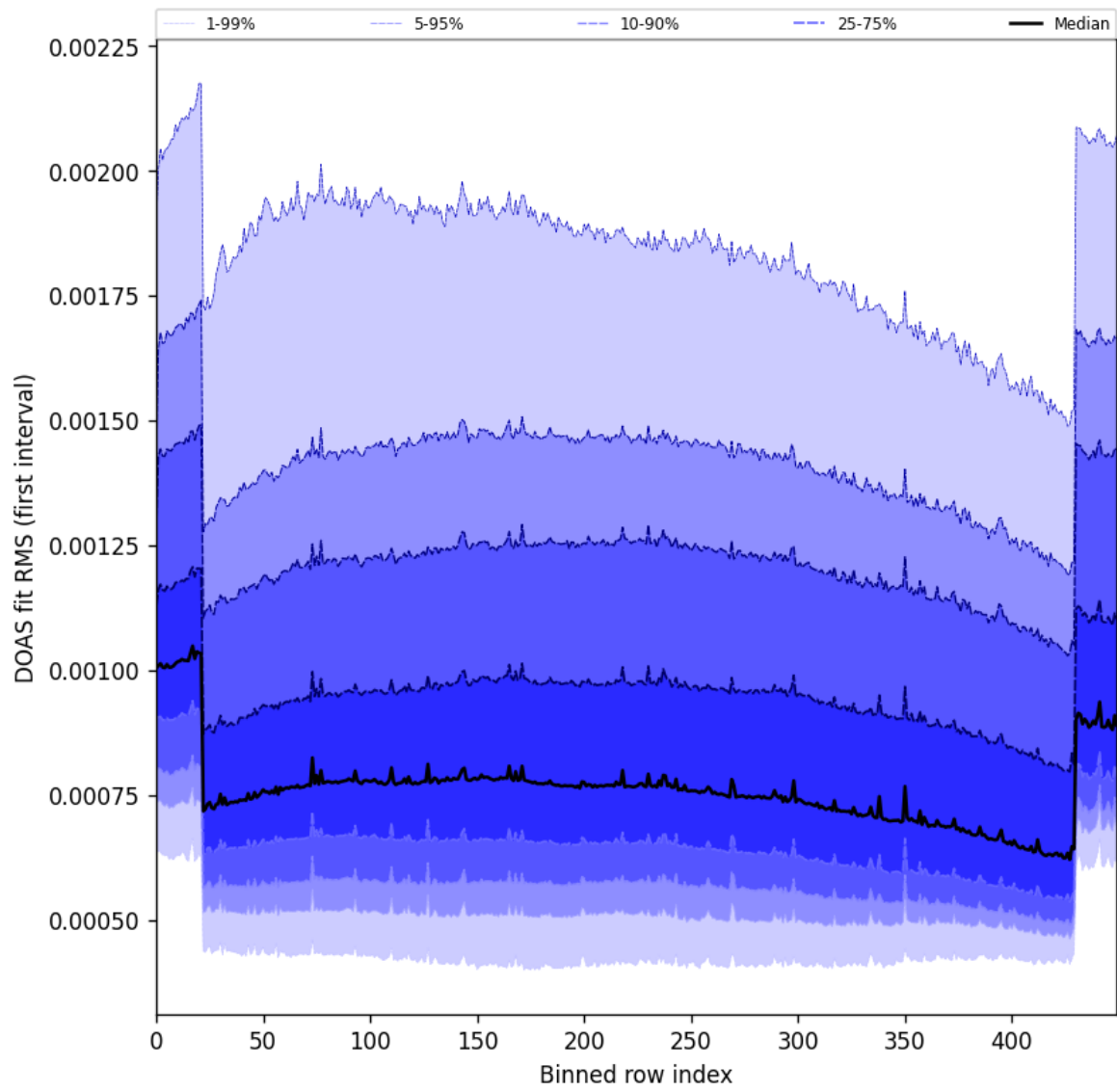
Figure 60: Along track statistics of “DOAS fit RMS (first interval)” for 2025-09-25 to 2025-09-26
