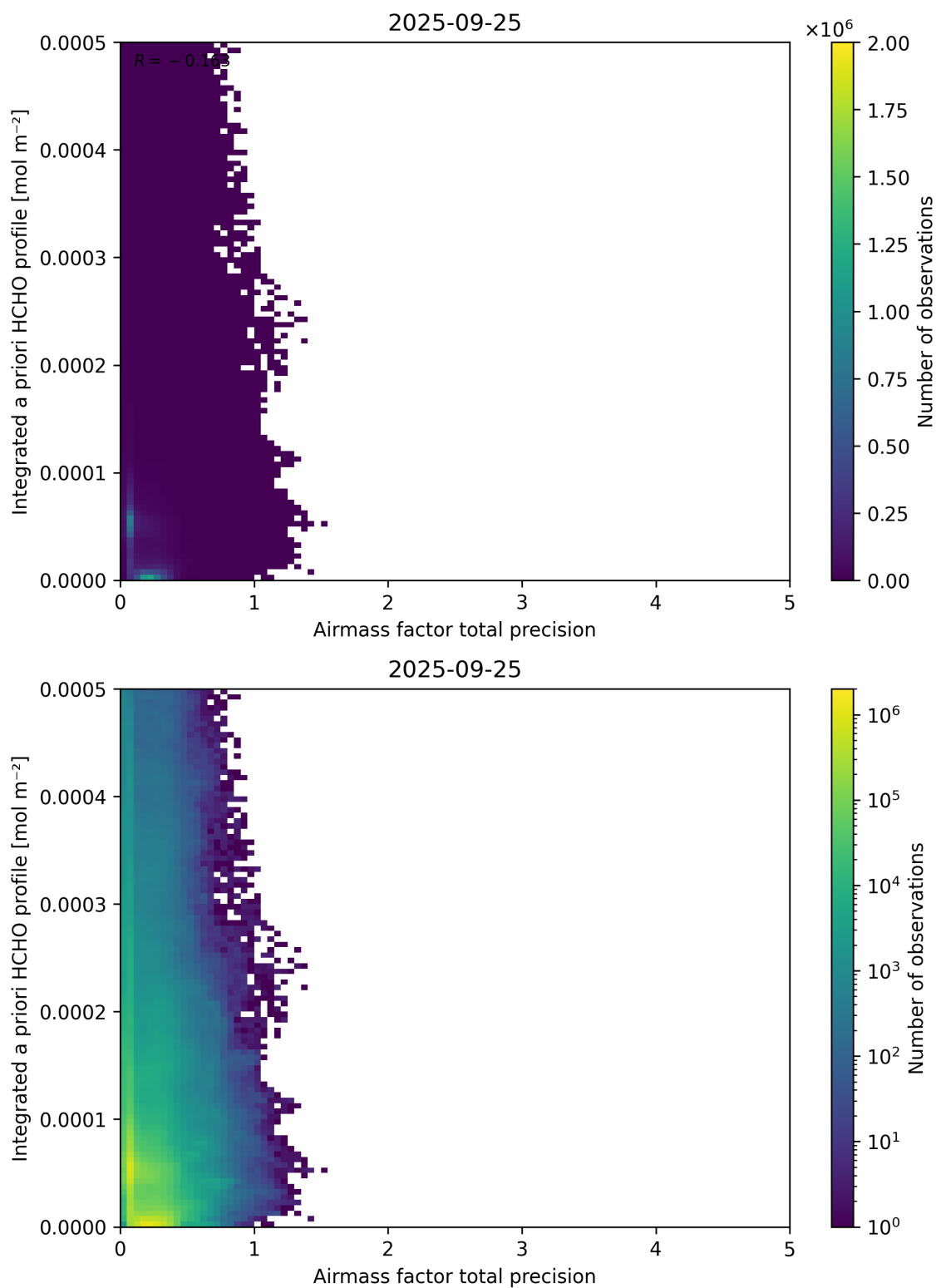
Figure 111: Scatter density plot of “Airmass factor total precision” against “Integrated a priori HCHO profile” for 2025-09-25 to 2025-09-26.
