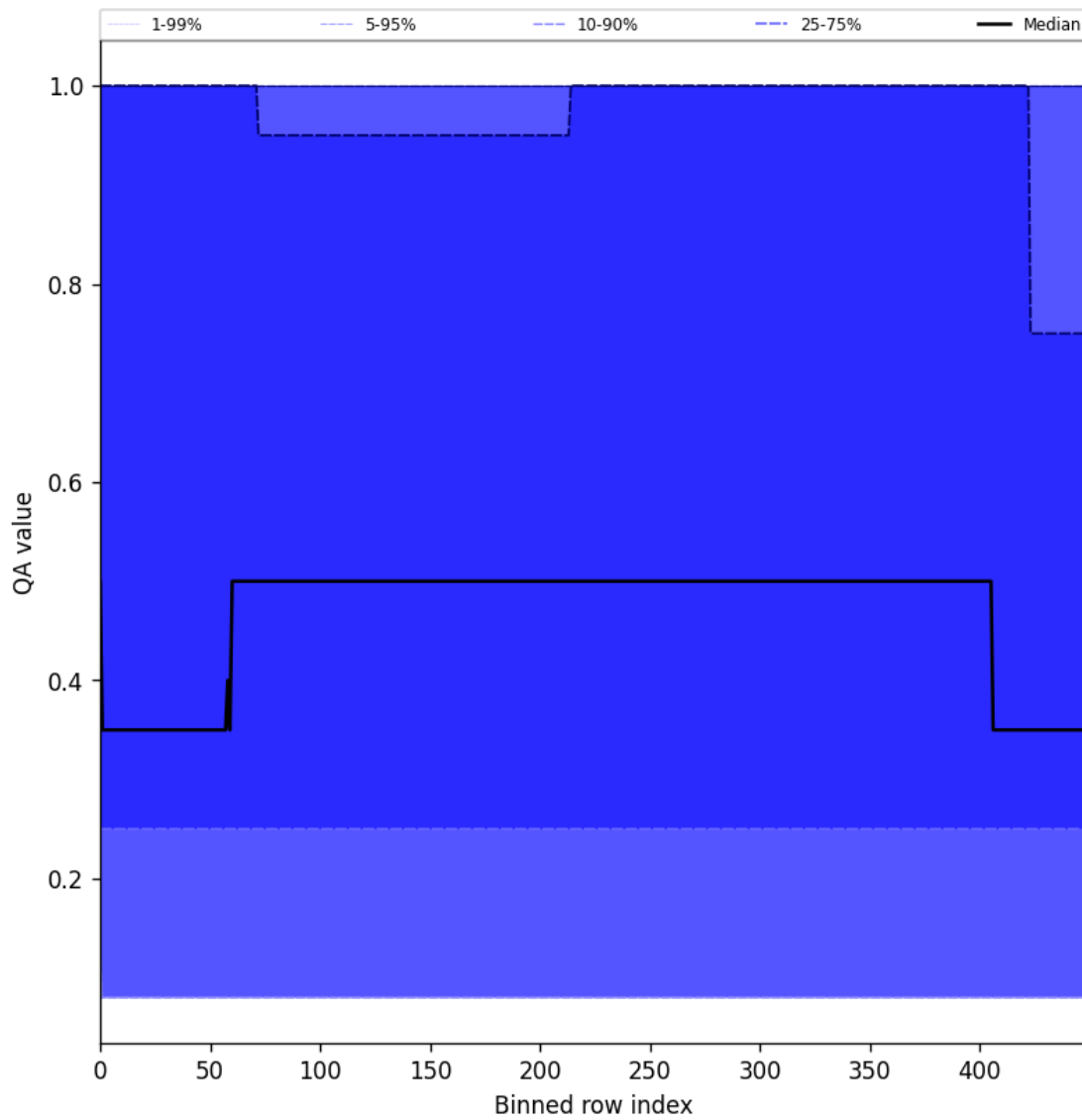
Figure 48: Along track statistics of “QA value” for 2025-09-25 to 2025-09-26
