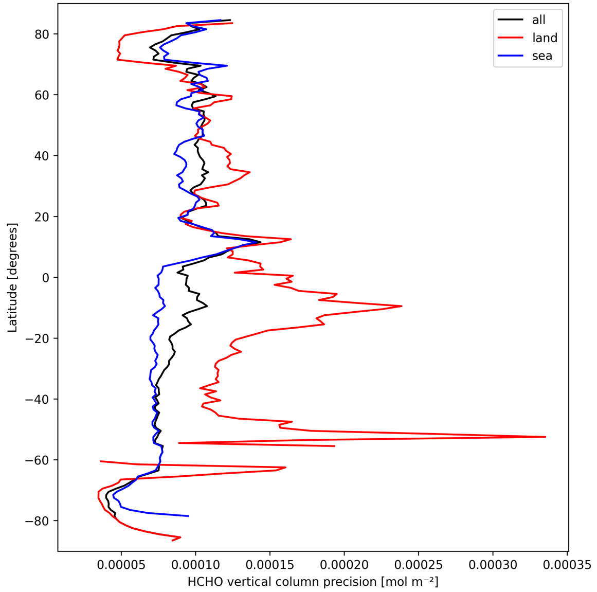
Figure 22: Zonal average of “HCHO vertical column precision” for 2025-09-25 to 2025-09-26.
