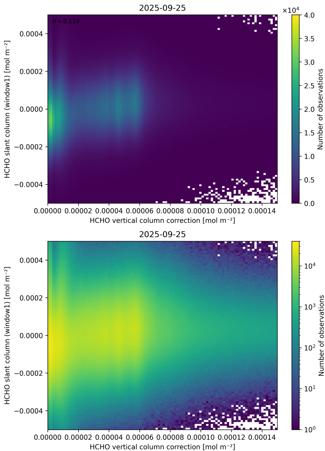
Figure 118: Scatter density plot of “HCHO vertical column correction” against “HCHO slant column (window1)” for 2025-09-25 to 2025-09-26.
