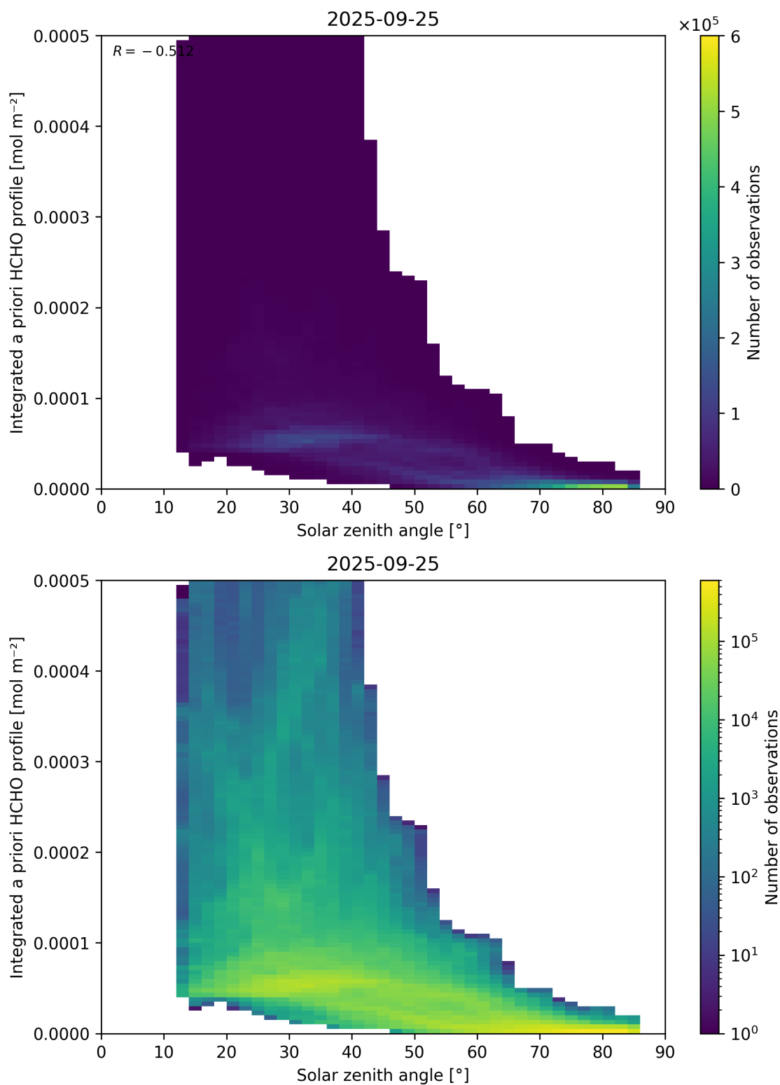
Figure 180: Scatter density plot of “Solar zenith angle” against “Integrated a priori HCHO profile” for 2025-09-25 to 2025-09-26.
