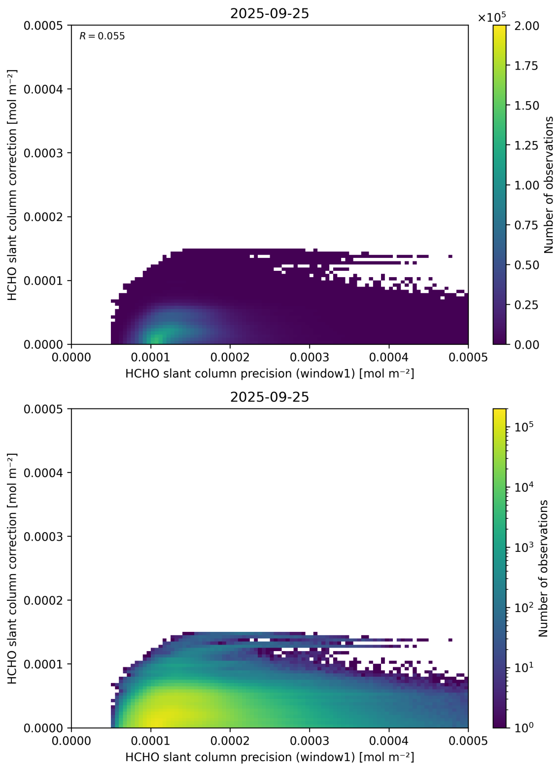
Figure 93: Scatter density plot of “HCHO slant column precision (window1)” against “HCHO slant column correction” for 2025-09-25 to 2025-09-26.
