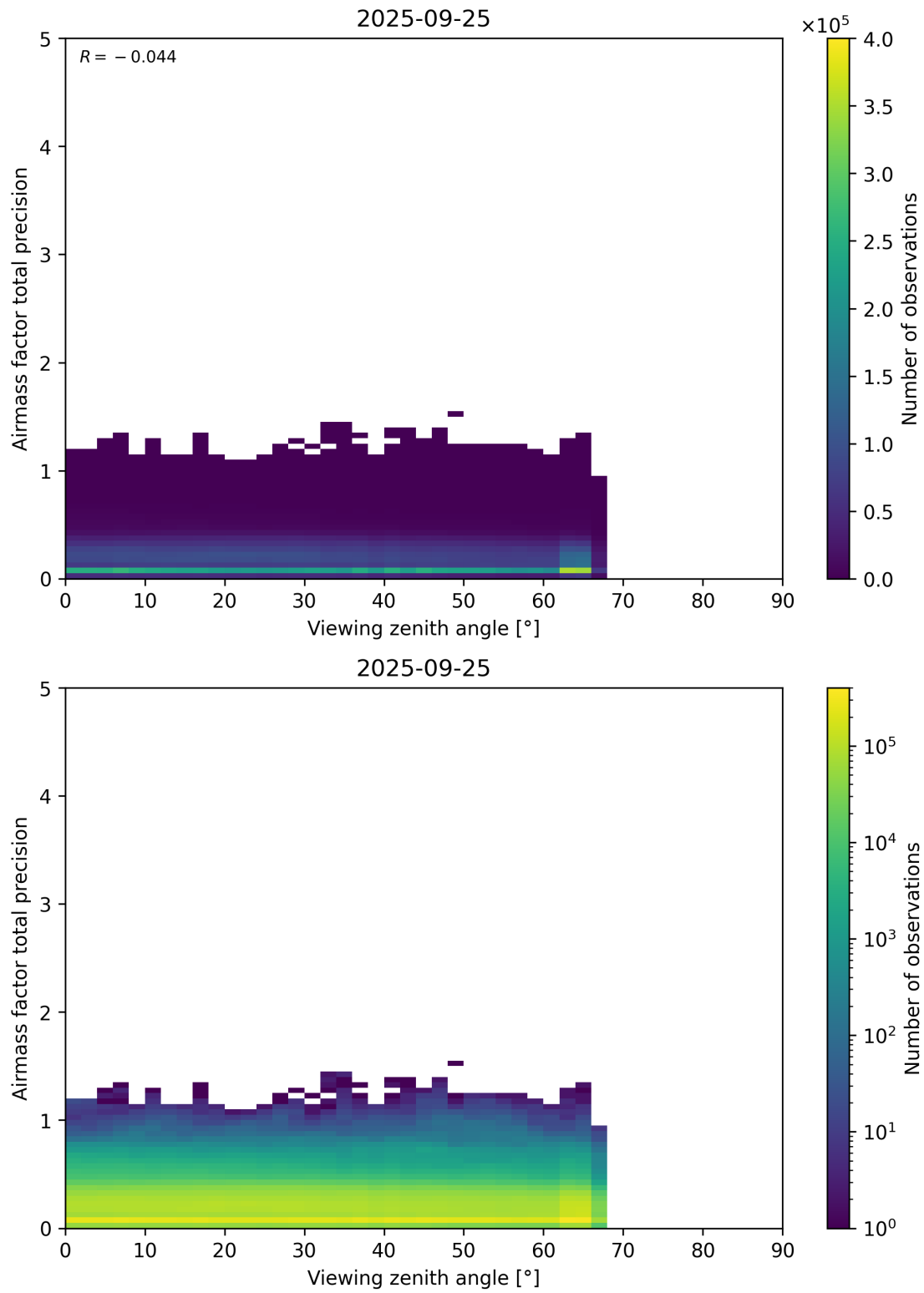
Figure 191: Scatter density plot of “Viewing zenith angle” against “Airmass factor total precision” for 2025-09-25 to 2025-09-26.
