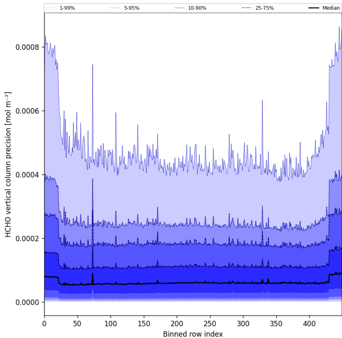
Figure 50: Along track statistics of “HCHO vertical column precision” for 2025-09-25 to 2025-09-26
