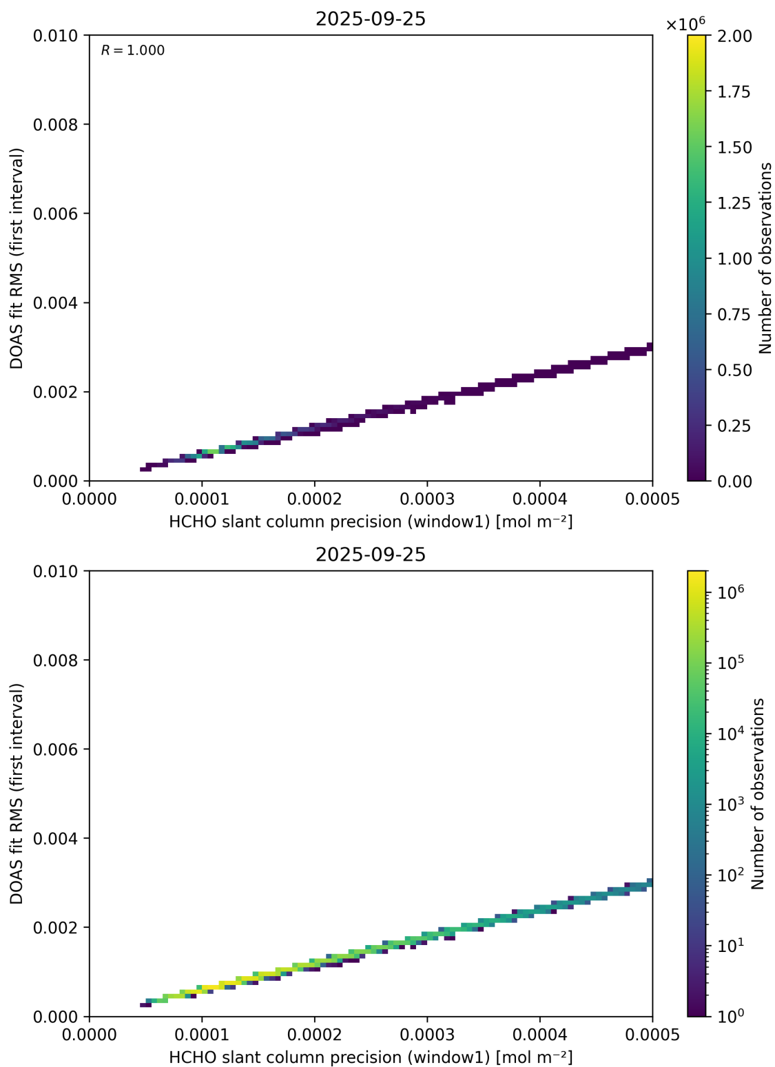
Figure 88: Scatter density plot of “HCHO slant column precision (window1)” against “DOAS fit RMS (first interval)” for 2025-09-25 to 2025-09-26.
