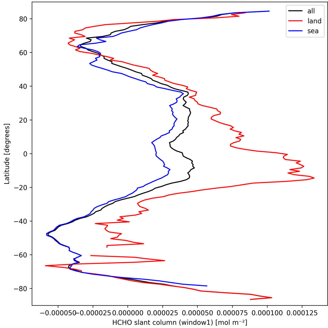
Figure 24: Zonal average of “HCHO slant column (window1)” for 2025-09-25 to 2025-09-26.
