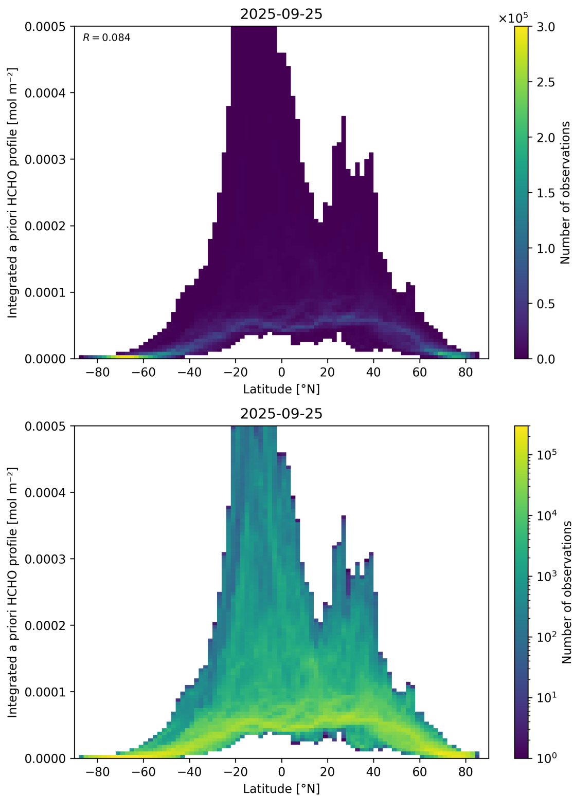
Figure 166: Scatter density plot of “Latitude” against “Integrated a priori HCHO profile” for 2025-09-25 to 2025-09-26.
