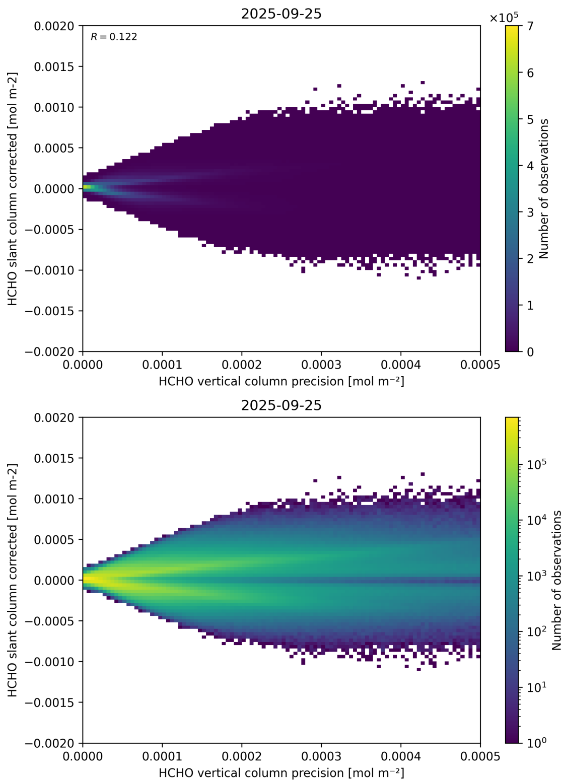
Figure 140: Scatter density plot of “HCHO vertical column precision” against “HCHO slant column corrected” for 2025-09-25 to 2025-09-26.
