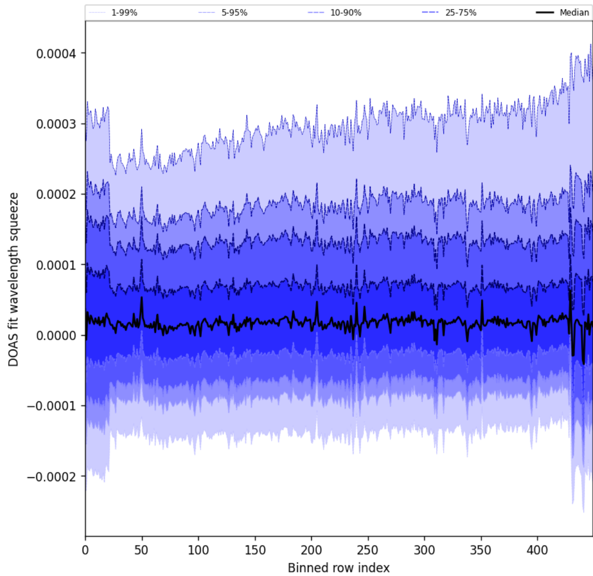
Figure 59: Along track statistics of “DOAS fit wavelength squeeze” for 2025-09-25 to 2025-09-26
