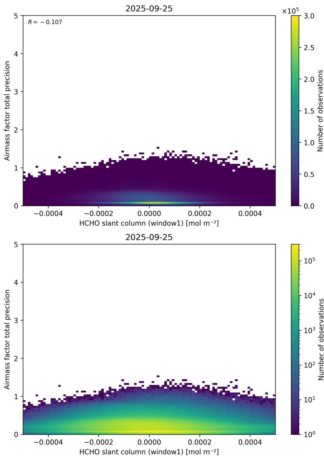
Figure 86: Scatter density plot of “HCHO slant column (window1)” against “Airmass factor total precision” for 2025-09-25 to 2025-09-26.
