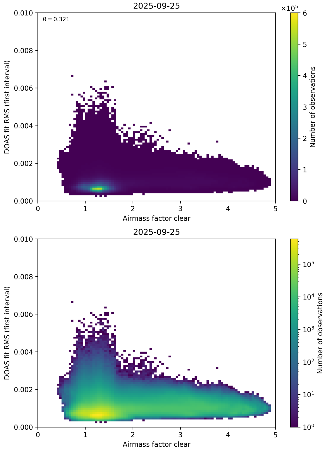
Figure 71: Scatter density plot of “Airmass factor clear” against “DOAS fit RMS (first interval)” for 2025-09-25 to 2025-09-26.
