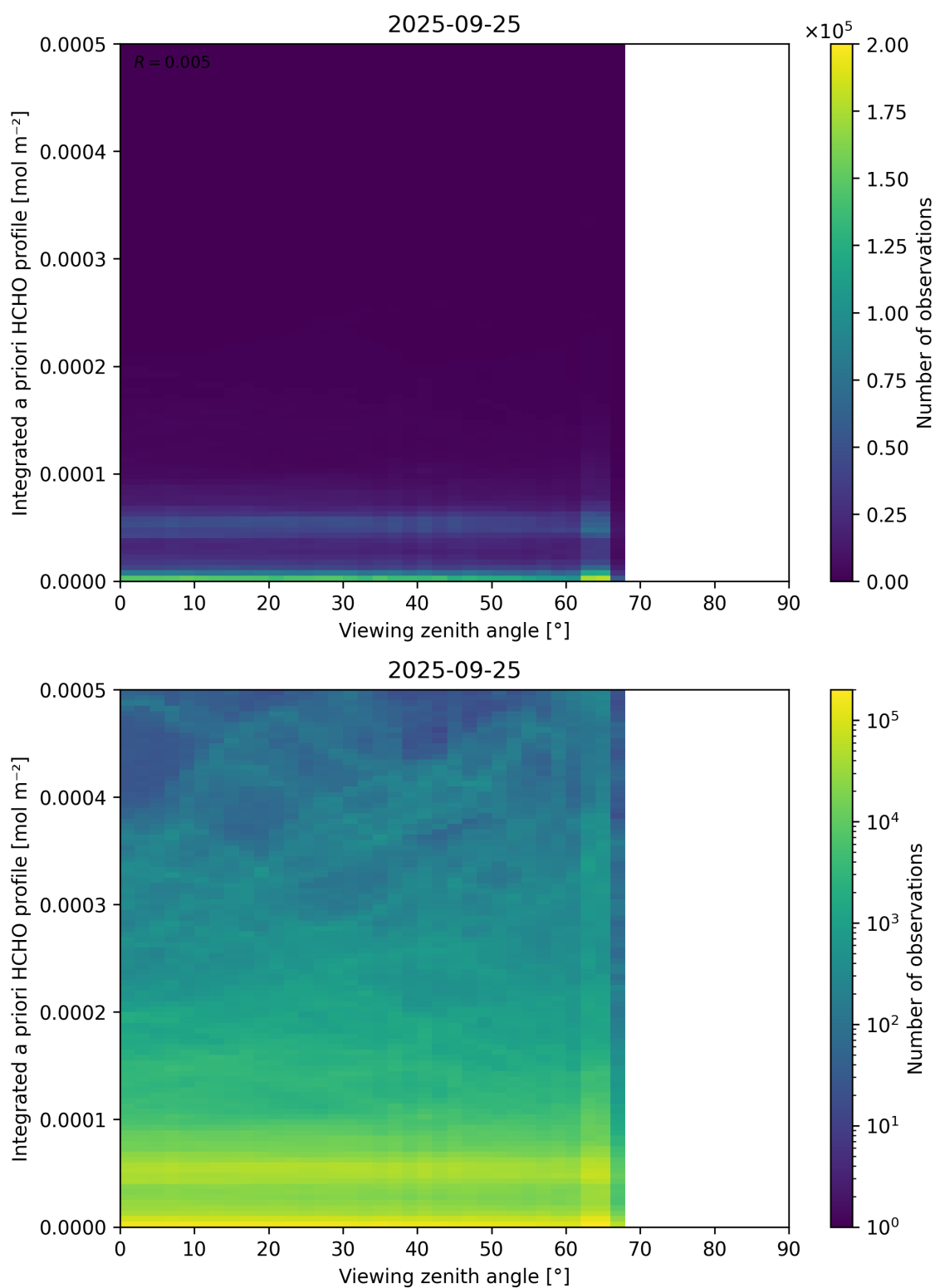
Figure 195: Scatter density plot of “Viewing zenith angle” against “Integrated a priori HCHO profile” for 2025-09-25 to 2025-09-26.
