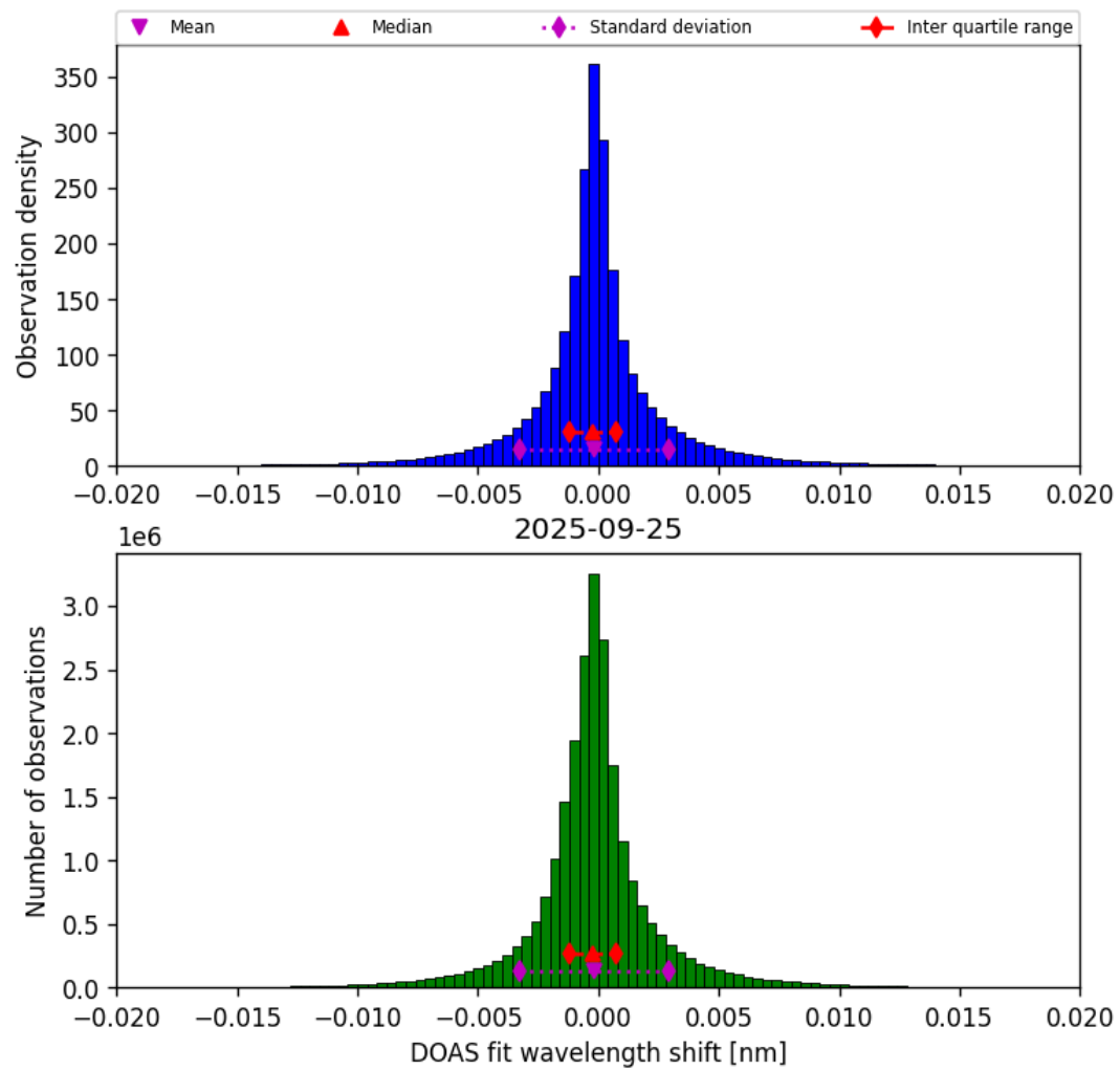
Figure 44: Histogram of “DOAS fit wavelength shift” for 2025-09-25 to 2025-09-26
