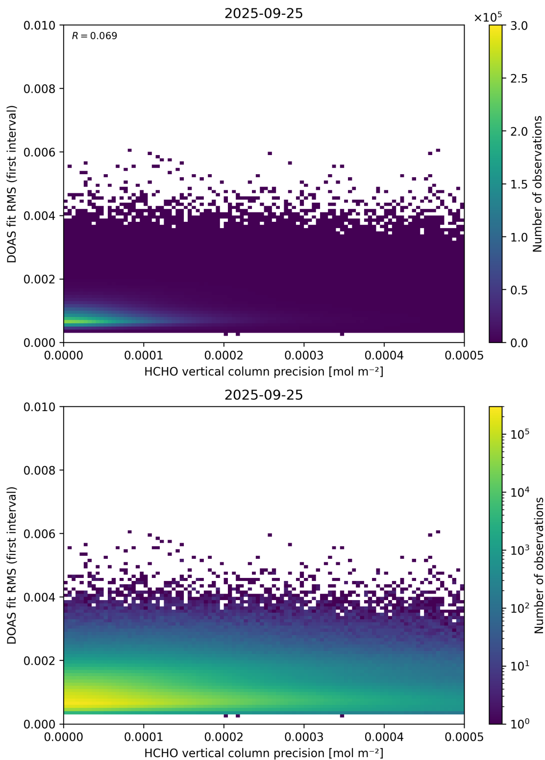
Figure 136: Scatter density plot of “HCHO vertical column precision” against “DOAS fit RMS (first interval)” for 2025-09-25 to 2025-09-26.
