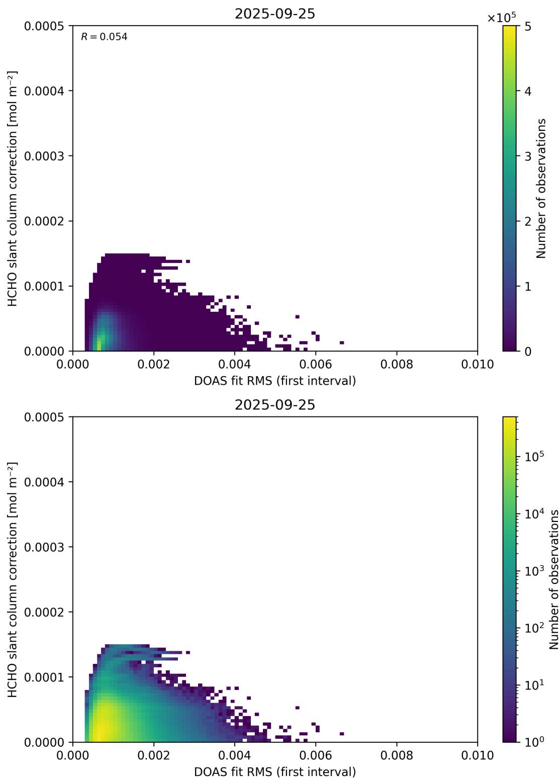
Figure 63: Scatter density plot of “DOAS fit RMS (first interval)” against “HCHO slant column correction” for 2025-09-25 to 2025-09-26.
