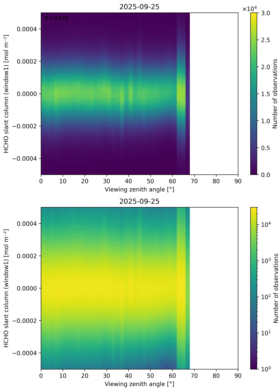
Figure 188: Scatter density plot of “Viewing zenith angle” against “HCHO slant column (window1)” for 2025-09-25 to 2025-09-26.
