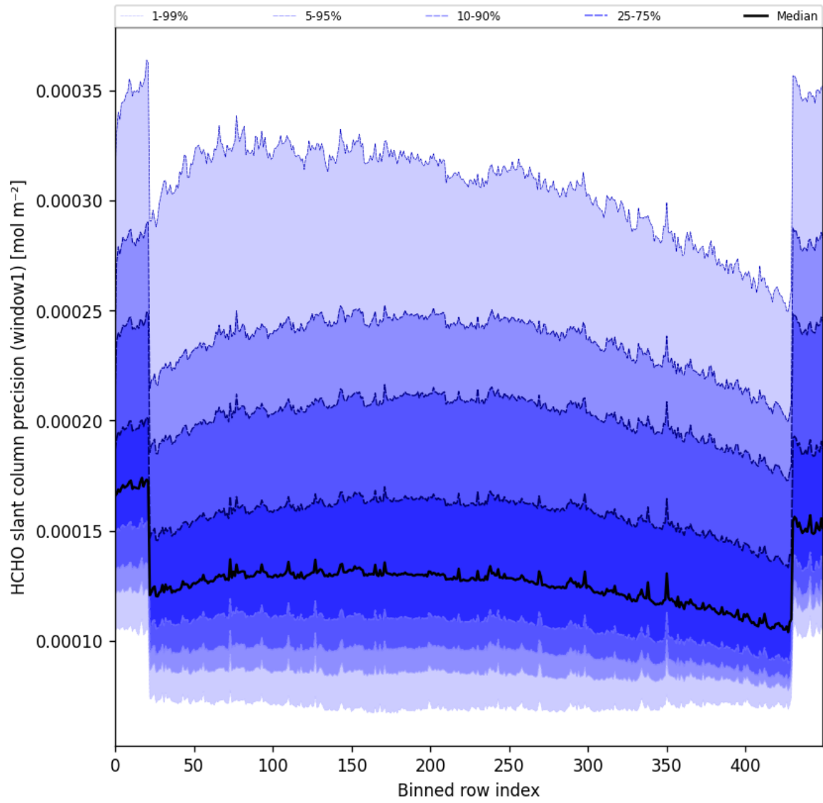
Figure 53: Along track statistics of “HCHO slant column precision (window1)” for 2025-09-25 to 2025-09-26
