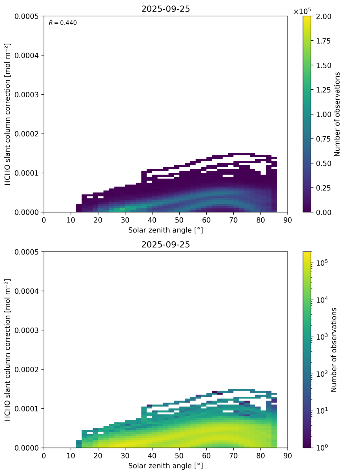
Figure 172: Scatter density plot of “Solar zenith angle” against “HCHO slant column correction” for 2025-09-25 to 2025-09-26.
