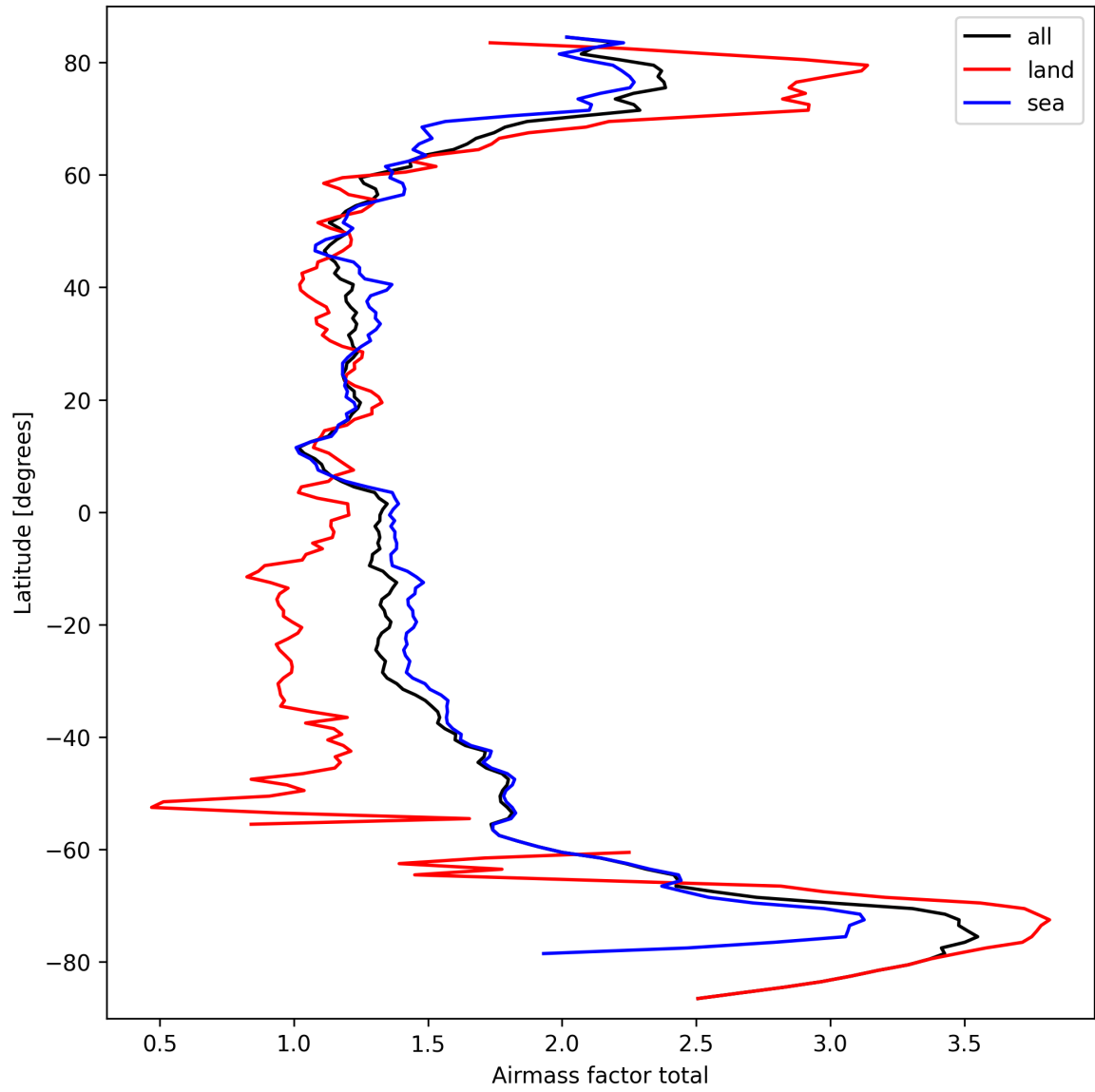
Figure 26: Zonal average of “Airmass factor total” for 2025-09-25 to 2025-09-26.
