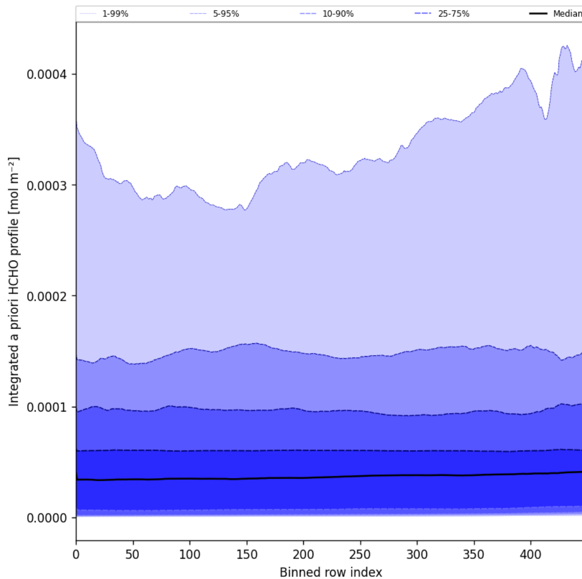
Figure 57: Along track statistics of “Integrated a priori HCHO profile” for 2025-09-25 to 2025-09-26
