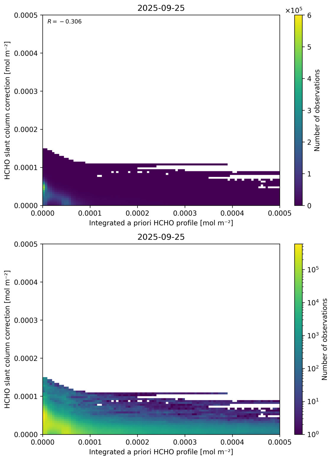
Figure 152: Scatter density plot of “Integrated a priori HCHO profile” against “HCHO slant column correction” for 2025-09-25 to 2025-09-26.
