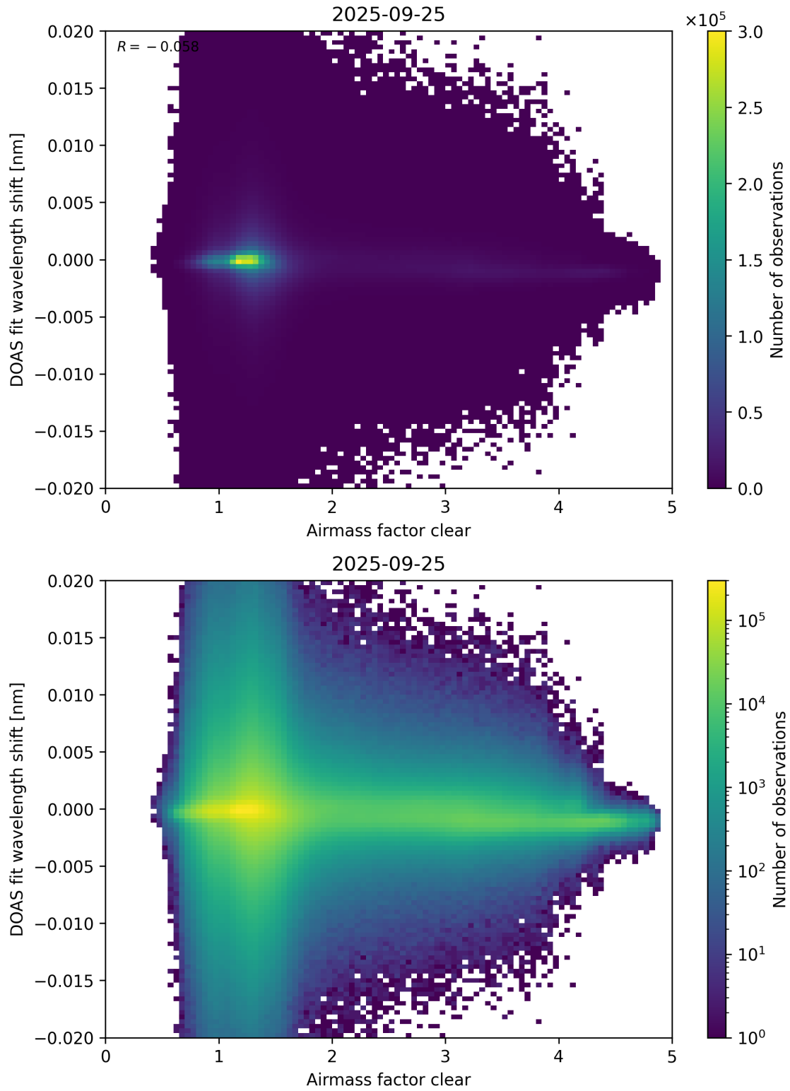
Figure 72: Scatter density plot of “Airmass factor clear” against “DOAS fit wavelength shift” for 2025-09-25 to 2025-09-26.
