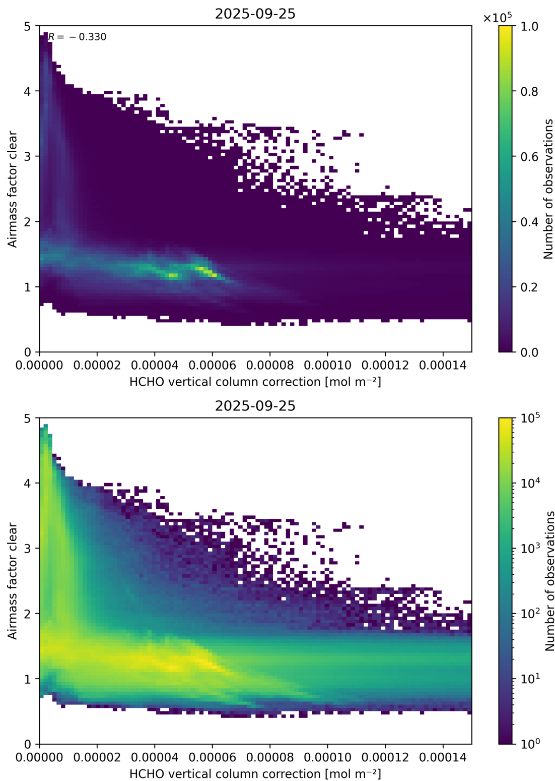
Figure 115: Scatter density plot of “HCHO vertical column correction” against “Airmass factor clear” for 2025-09-25 to 2025-09-26.
