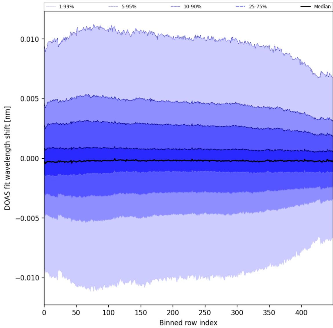
Figure 58: Along track statistics of “DOAS fit wavelength shift” for 2025-09-25 to 2025-09-26
