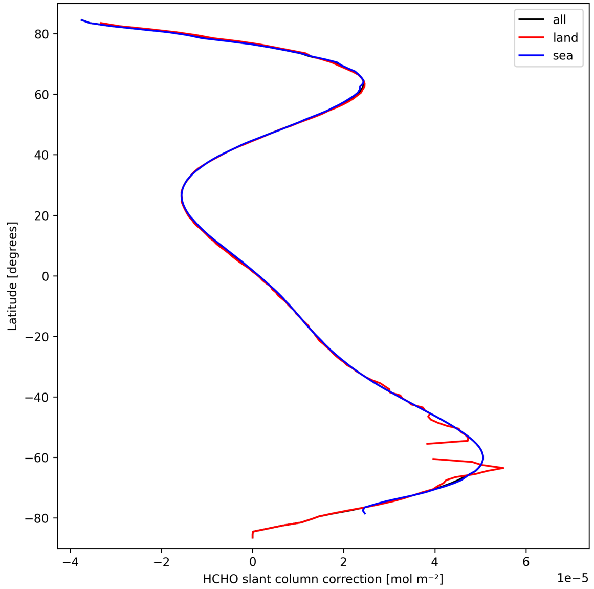
Figure 33: Zonal average of “HCHO slant column correction” for 2025-09-25 to 2025-09-26.
