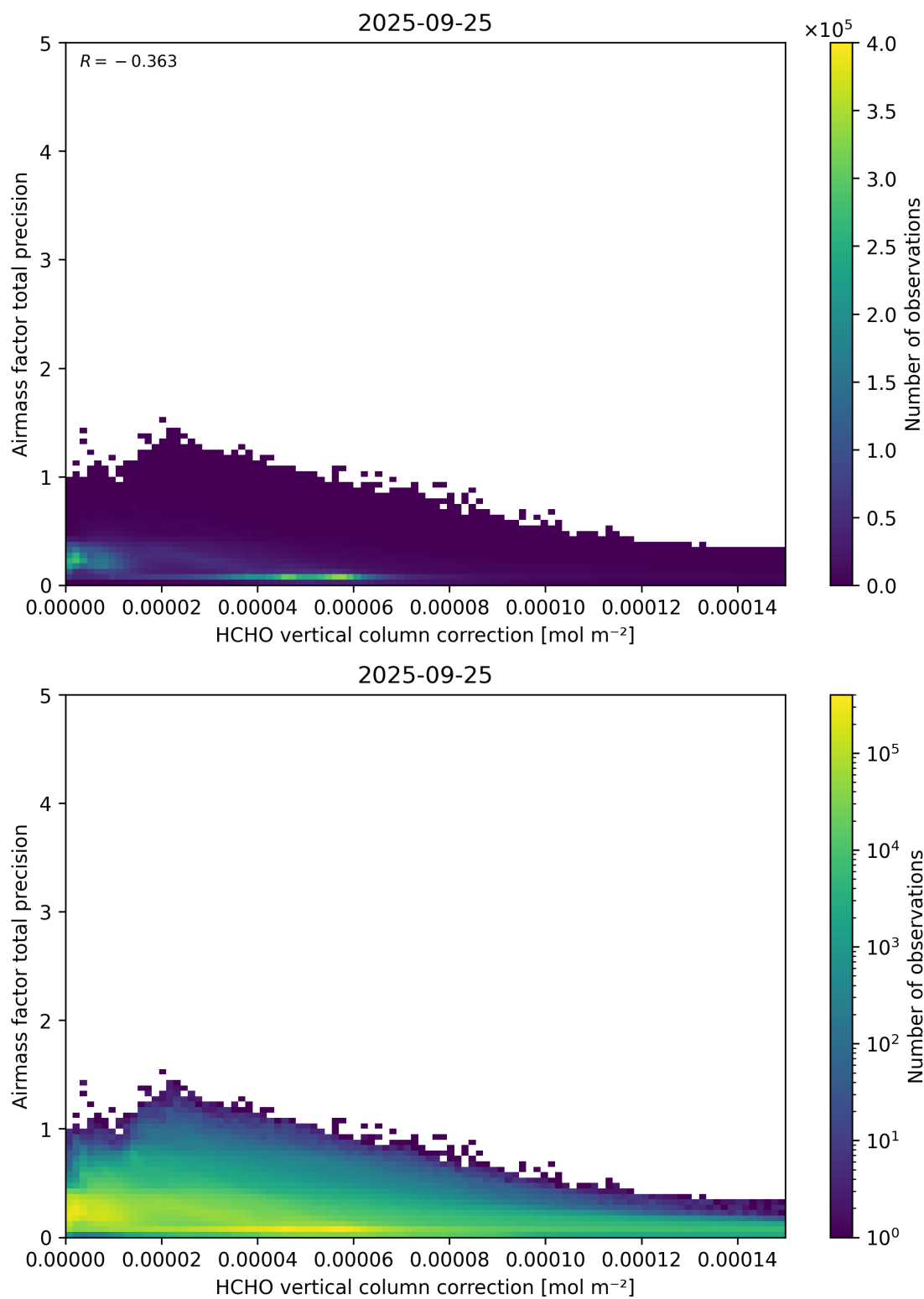
Figure 121: Scatter density plot of “HCHO vertical column correction” against “Airmass factor total precision” for 2025-09-25 to 2025-09-26.
