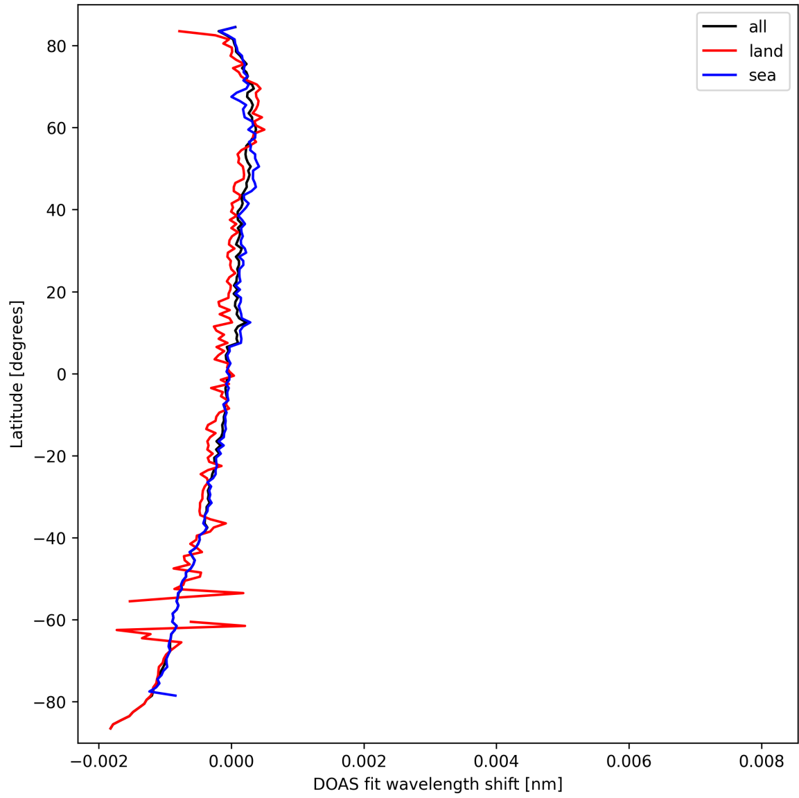
Figure 30: Zonal average of "DOAS fit wavelength shift" for 2025-09-25 to 2025-09-26.
