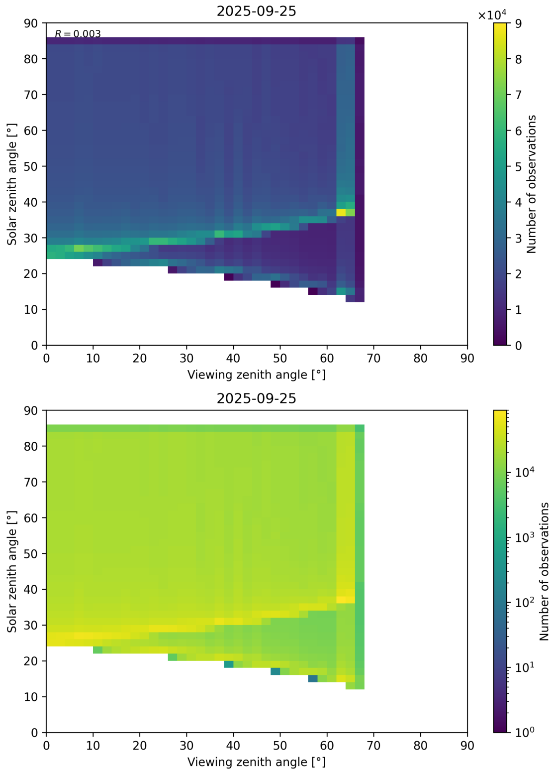
Figure 197: Scatter density plot of “Viewing zenith angle” against “Solar zenith angle” for 2025-09-25 to 2025-09-26.
