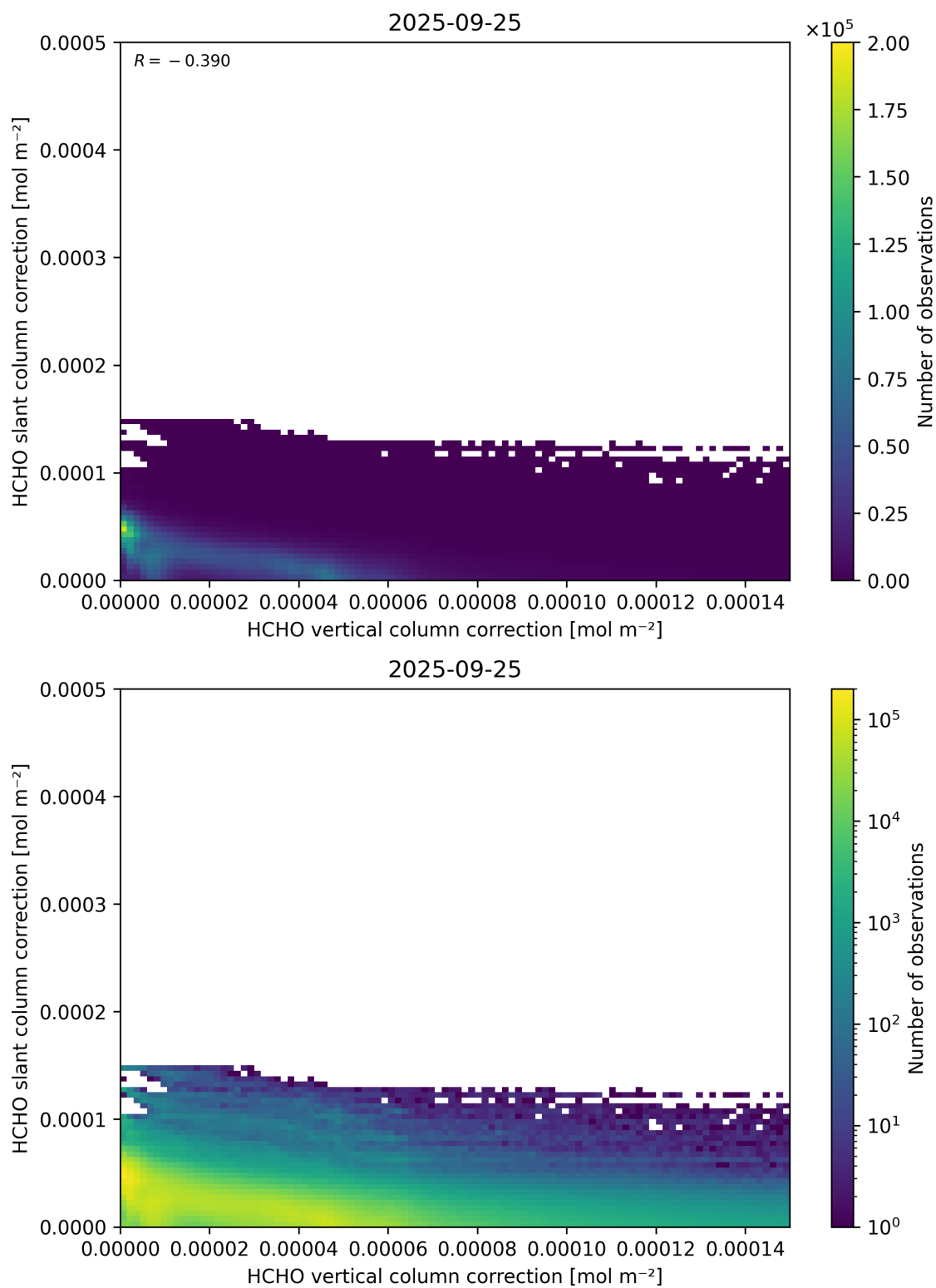
Figure 117: Scatter density plot of “HCHO vertical column correction” against “HCHO slant column correction” for 2025-09-25 to 2025-09-26.
