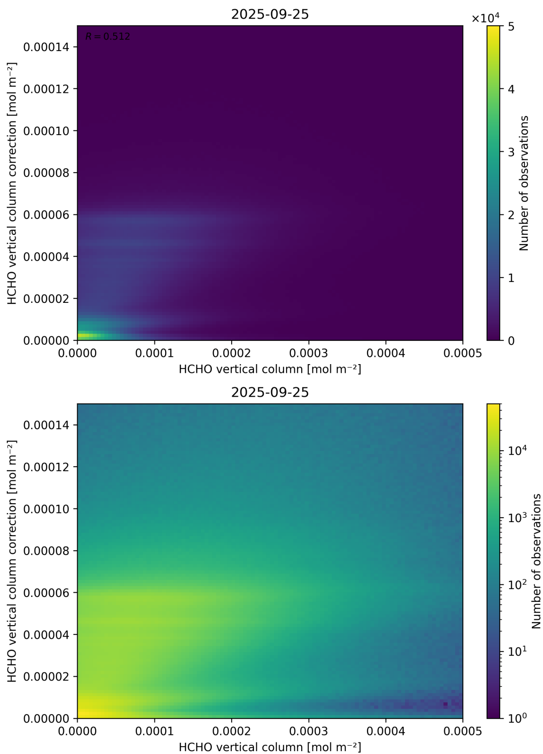
Figure 133: Scatter density plot of “HCHO vertical column” against “HCHO vertical column correction” for 2025-09-25 to 2025-09-26.
