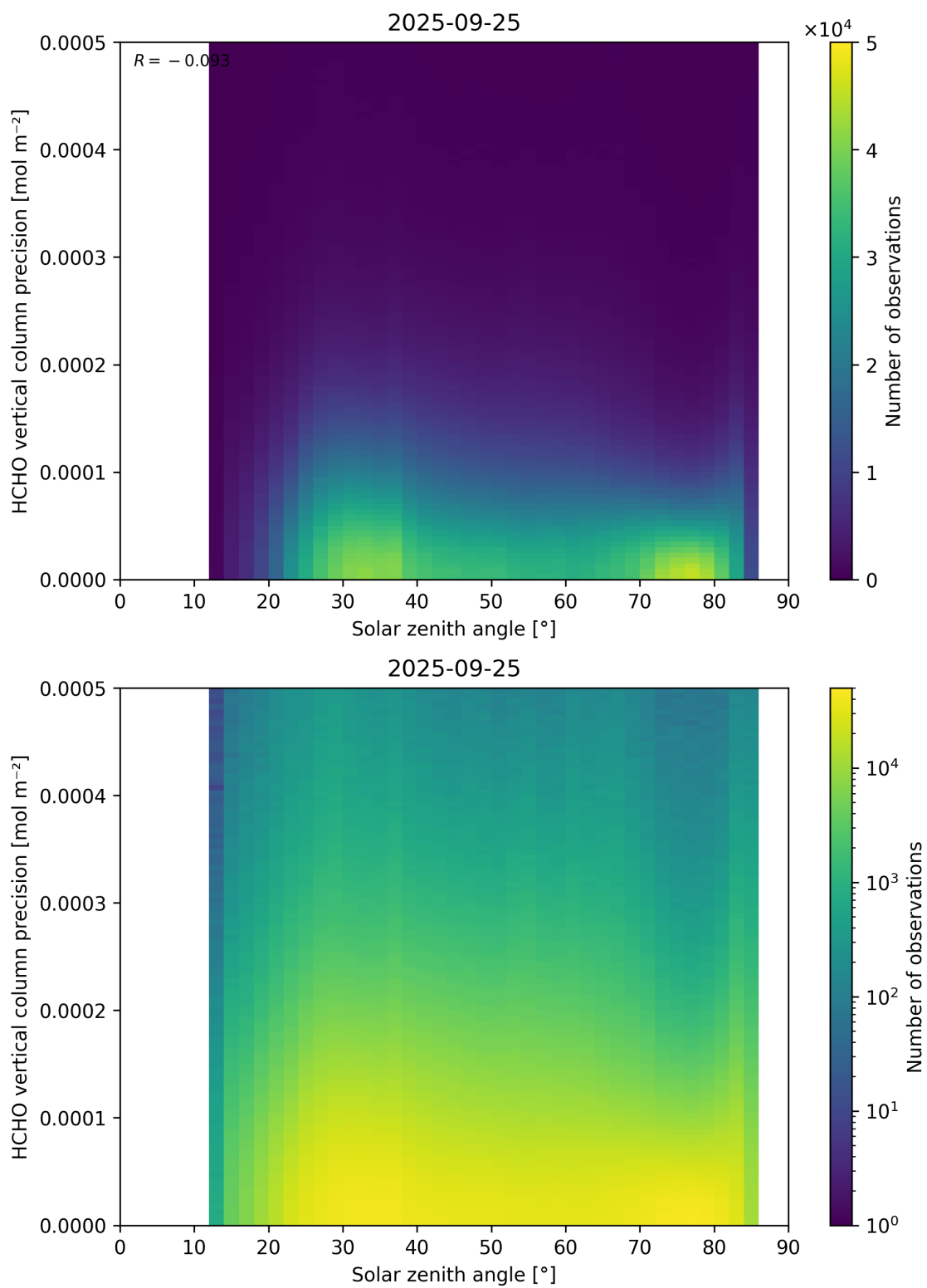
Figure 179: Scatter density plot of “Solar zenith angle” against “HCHO vertical column precision” for 2025-09-25 to 2025-09-26.
