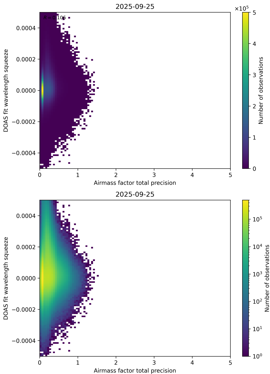
Figure 107: Scatter density plot of “Airmass factor total precision” against “DOAS fit wavelength squeeze” for 2025-09-25 to 2025-09-26.
