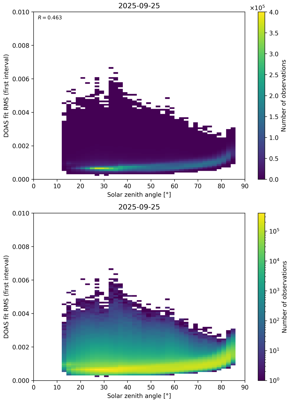
Figure 167: Scatter density plot of “Solar zenith angle” against “DOAS fit RMS (first interval)” for 2025-09-25 to 2025-09-26.
