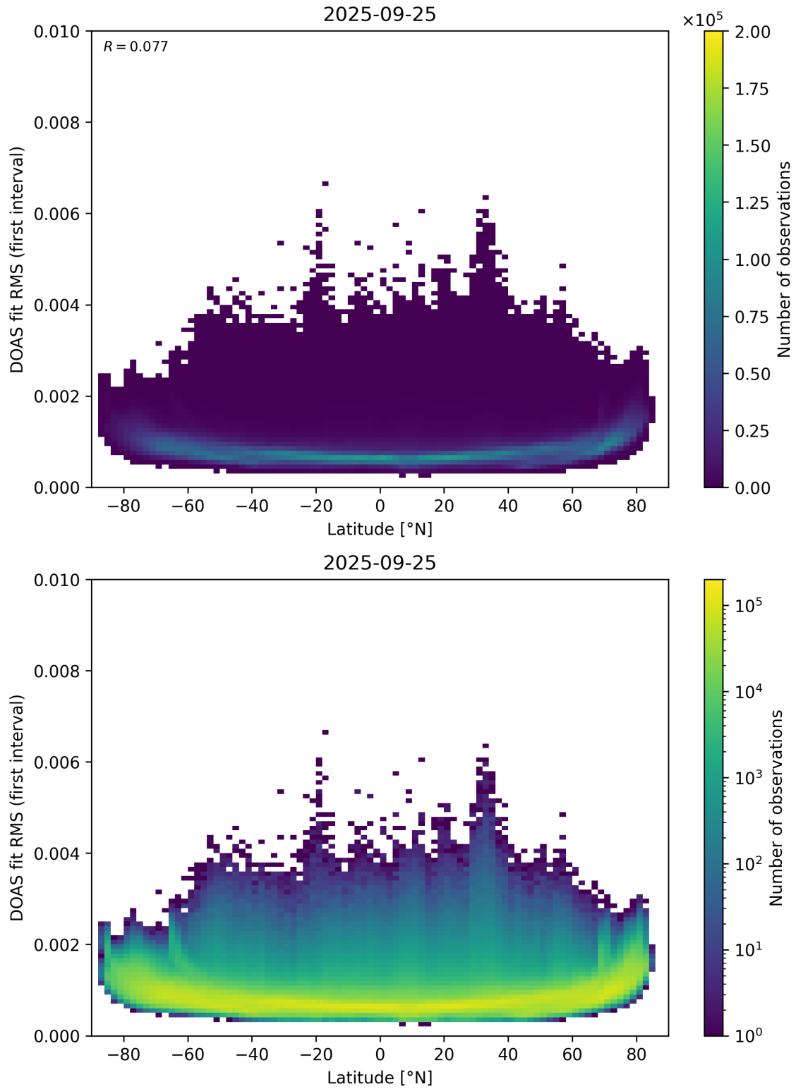
Figure 153: Scatter density plot of “Latitude” against “DOAS fit RMS (first interval)” for 2025-09-25 to 2025-09-26.
