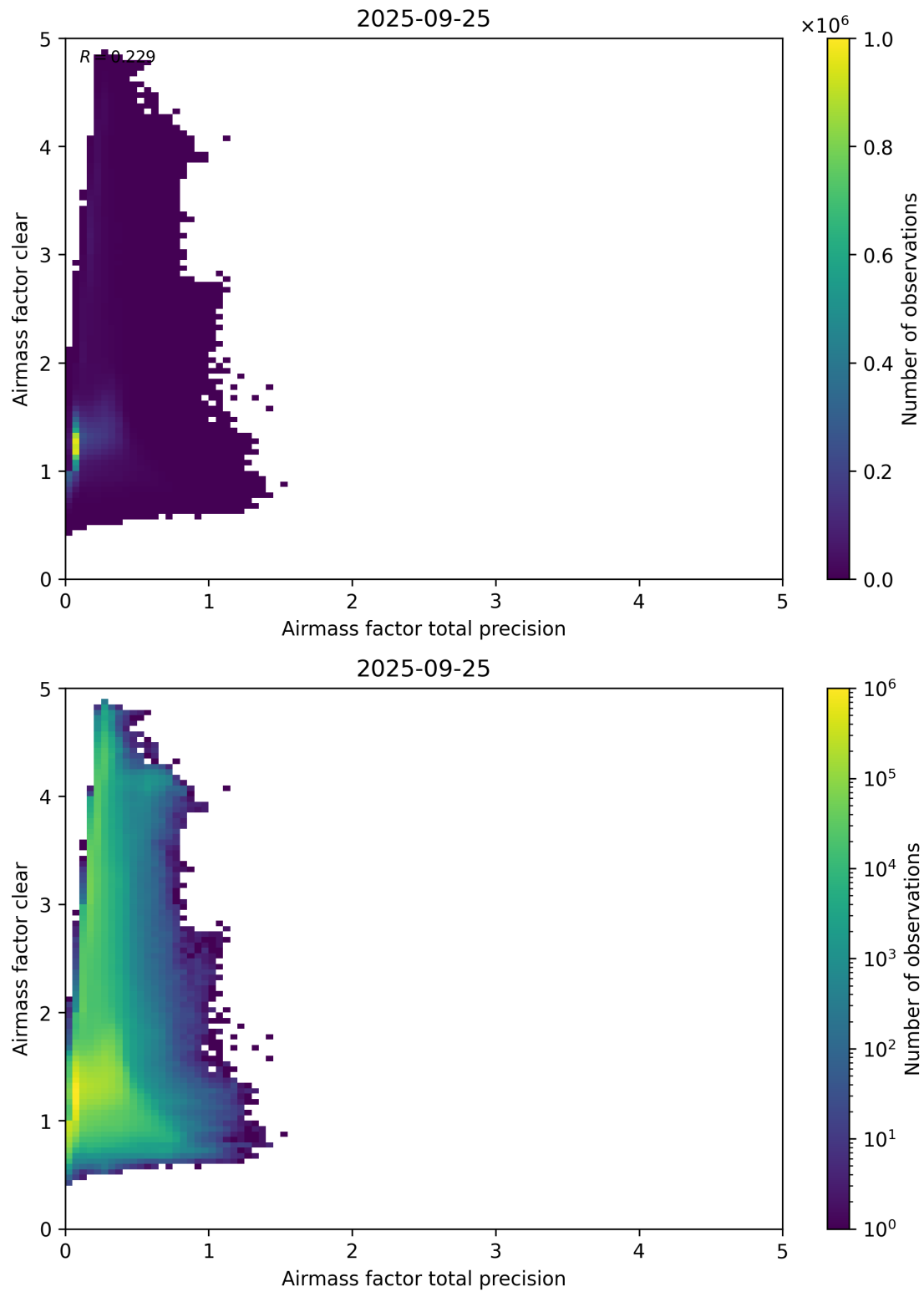
Figure 108: Scatter density plot of “Airmass factor total precision” against “Airmass factor clear” for 2025-09-25 to 2025-09-26.
