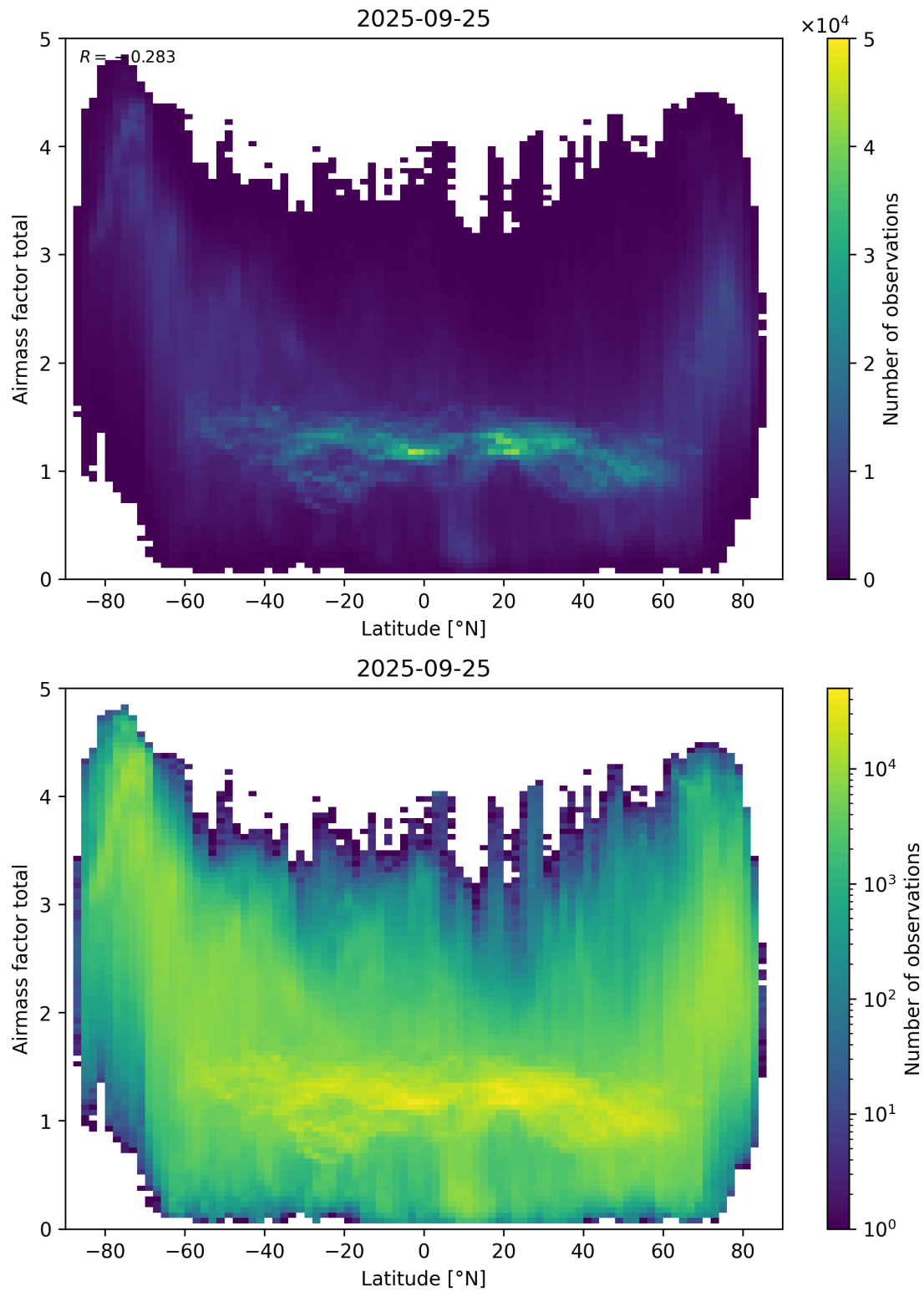
Figure 161: Scatter density plot of “Latitude” against “Airmass factor total” for 2025-09-25 to 2025-09-26.
