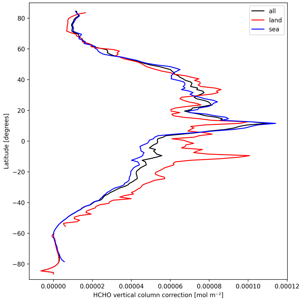
Figure 23: Zonal average of “HCHO vertical column correction” for 2025-09-25 to 2025-09-26.
