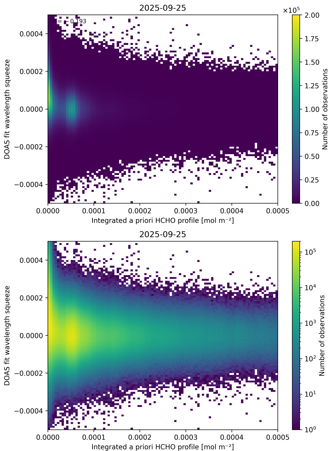
Figure 150: Scatter density plot of “Integrated a priori HCHO profile” against “DOAS fit wavelength squeeze” for 2025-09-25 to 2025-09-26.
