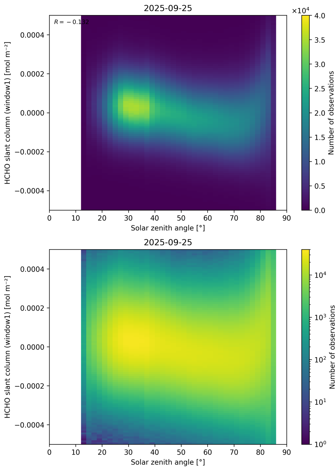
Figure 173: Scatter density plot of “Solar zenith angle” against “HCHO slant column (window1)” for 2025-09-25 to 2025-09-26.
