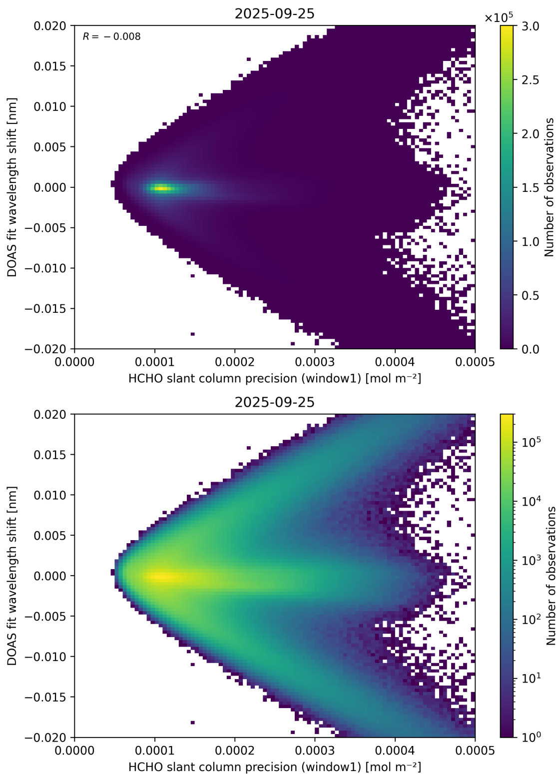
Figure 89: Scatter density plot of “HCHO slant column precision (window1)” against “DOAS fit wavelength shift” for 2025-09-25 to 2025-09-26.
