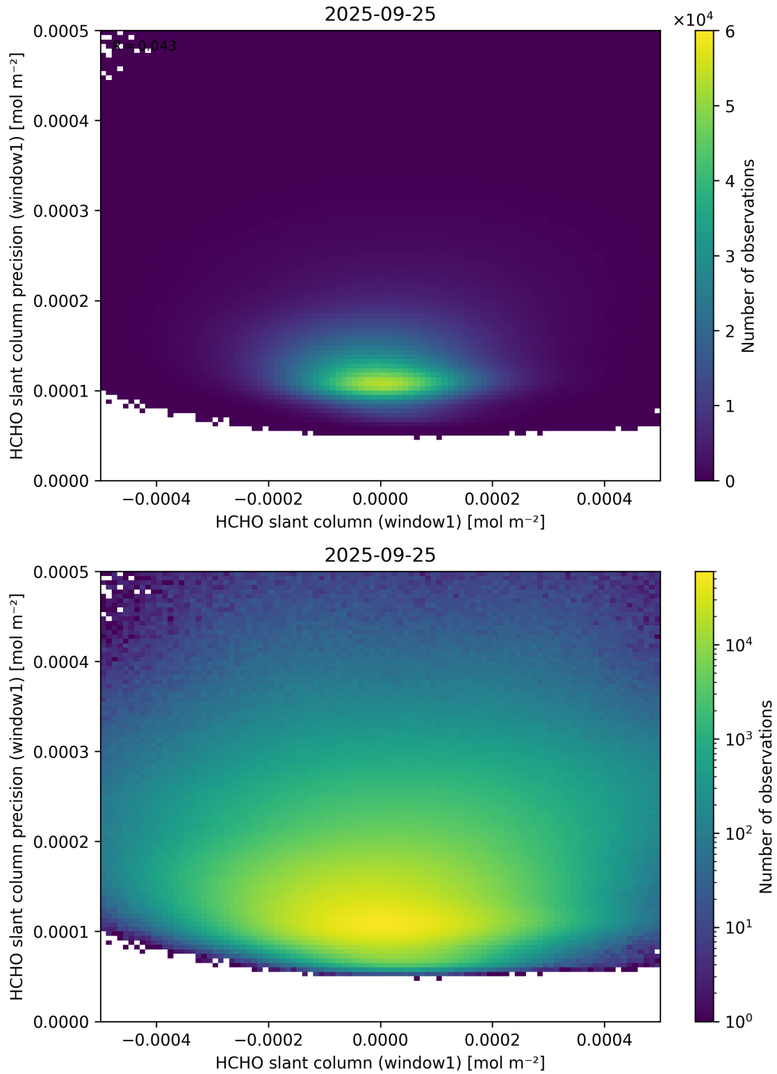
Figure 84: Scatter density plot of “HCHO slant column (window1)” against “HCHO slant column precision (window1)” for 2025-09-25 to 2025-09-26.
