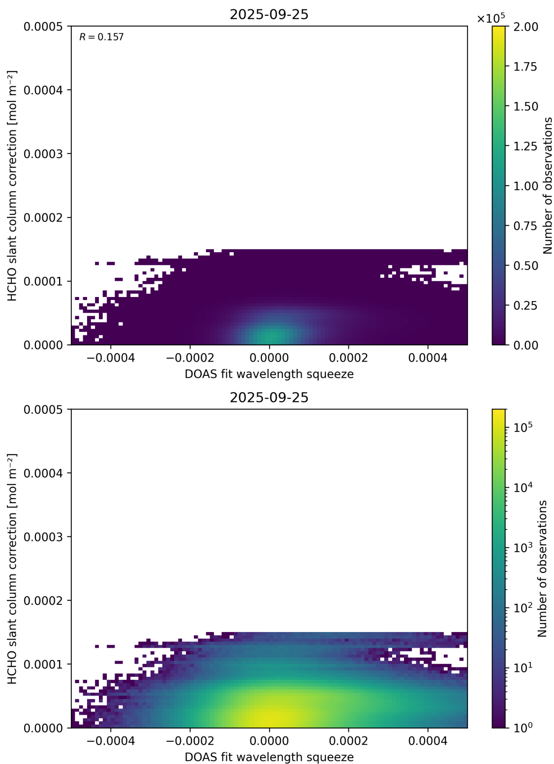
Figure 70: Scatter density plot of “DOAS fit wavelength squeeze” against “HCHO slant column correction” for 2025-09-25 to 2025-09-26.
