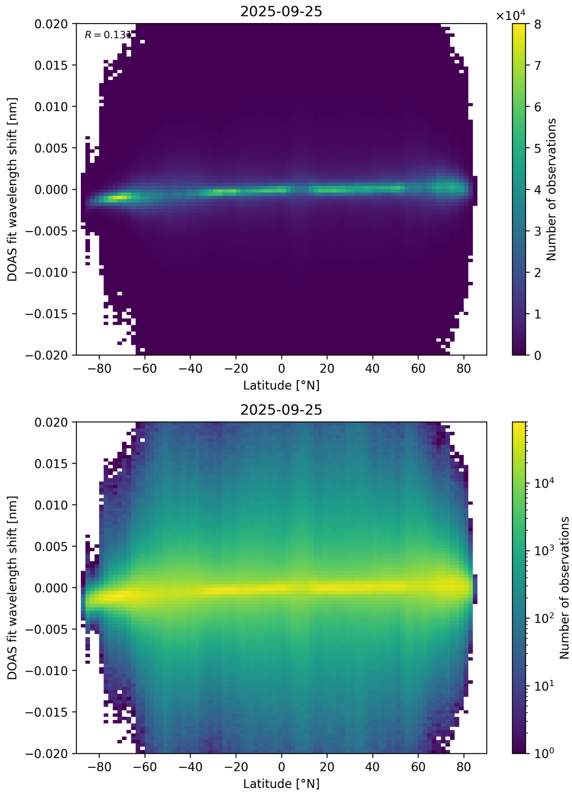
Figure 154: Scatter density plot of “Latitude” against “DOAS fit wavelength shift” for 2025-09-25 to 2025-09-26.
