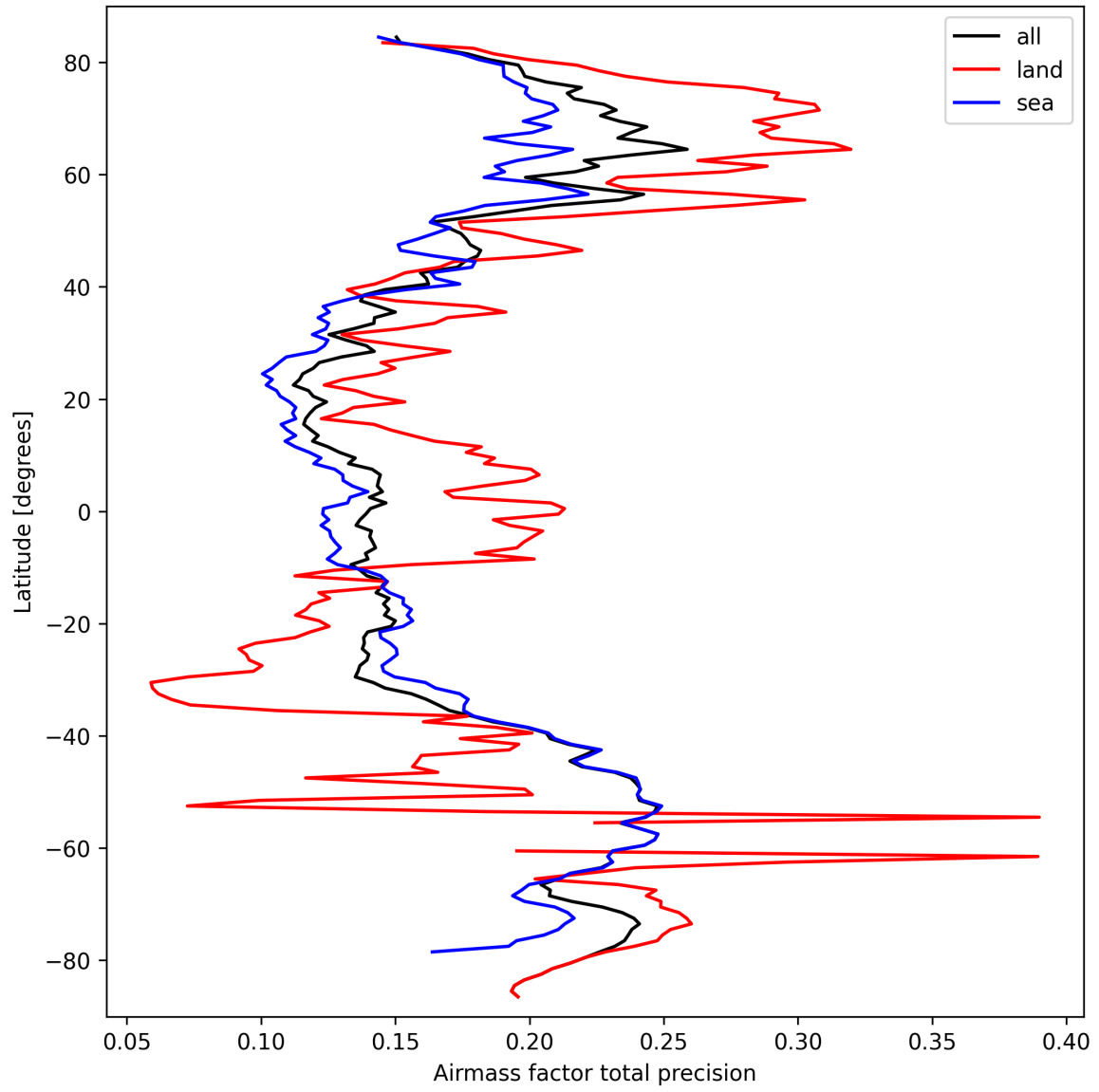
Figure 27: Zonal average of “Airmass factor total precision” for 2025-09-25 to 2025-09-26.
