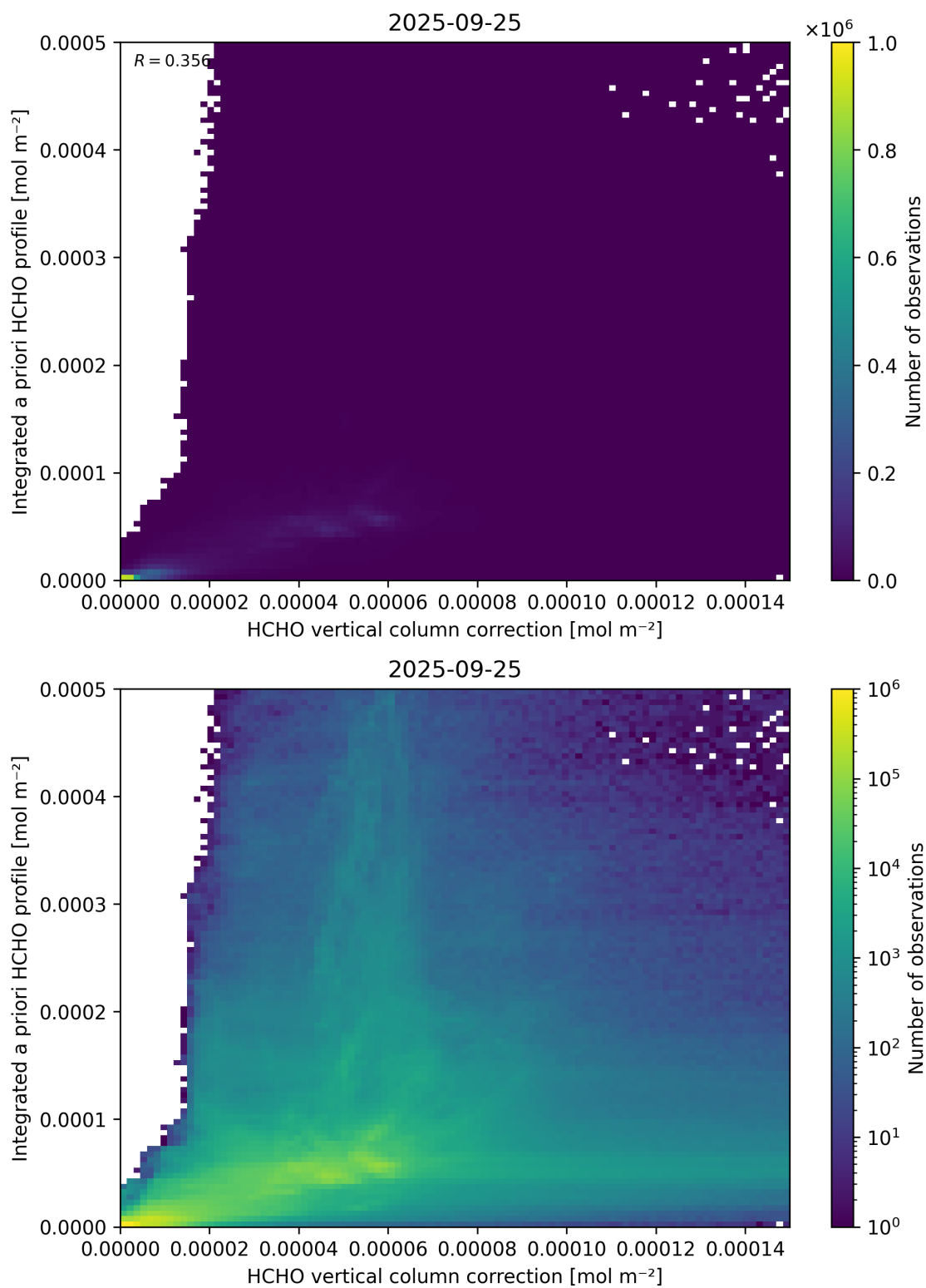
Figure 122: Scatter density plot of “HCHO vertical column correction” against “Integrated a priori HCHO profile” for 2025-09-25 to 2025-09-26.
