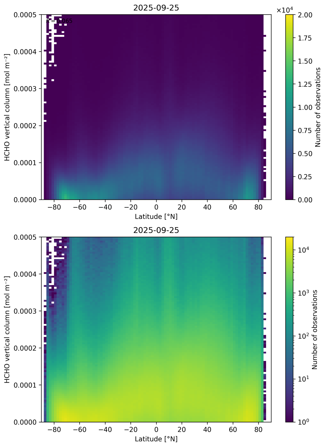
Figure 163: Scatter density plot of “Latitude” against “HCHO vertical column” for 2025-09-25 to 2025-09-26.
