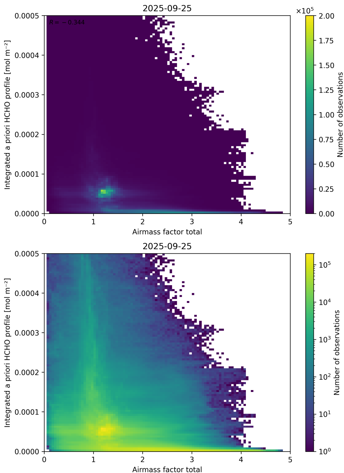
Figure 104: Scatter density plot of “Airmass factor total” against “Integrated a priori HCHO profile” for 2025-09-25 to 2025-09-26.
