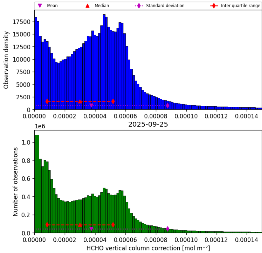
Figure 37: Histogram of “HCHO vertical column correction” for 2025-09-25 to 2025-09-26
