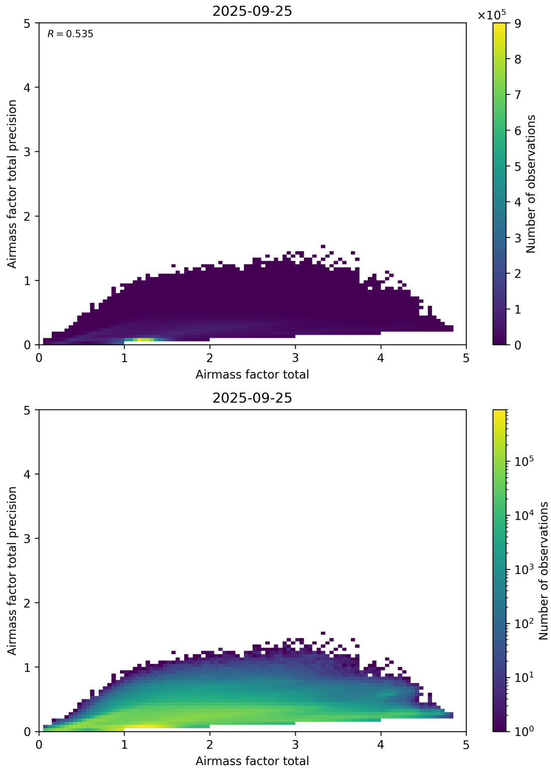
Figure 103: Scatter density plot of “Airmass factor total” against “Airmass factor total precision” for 2025-09-25 to 2025-09-26.
