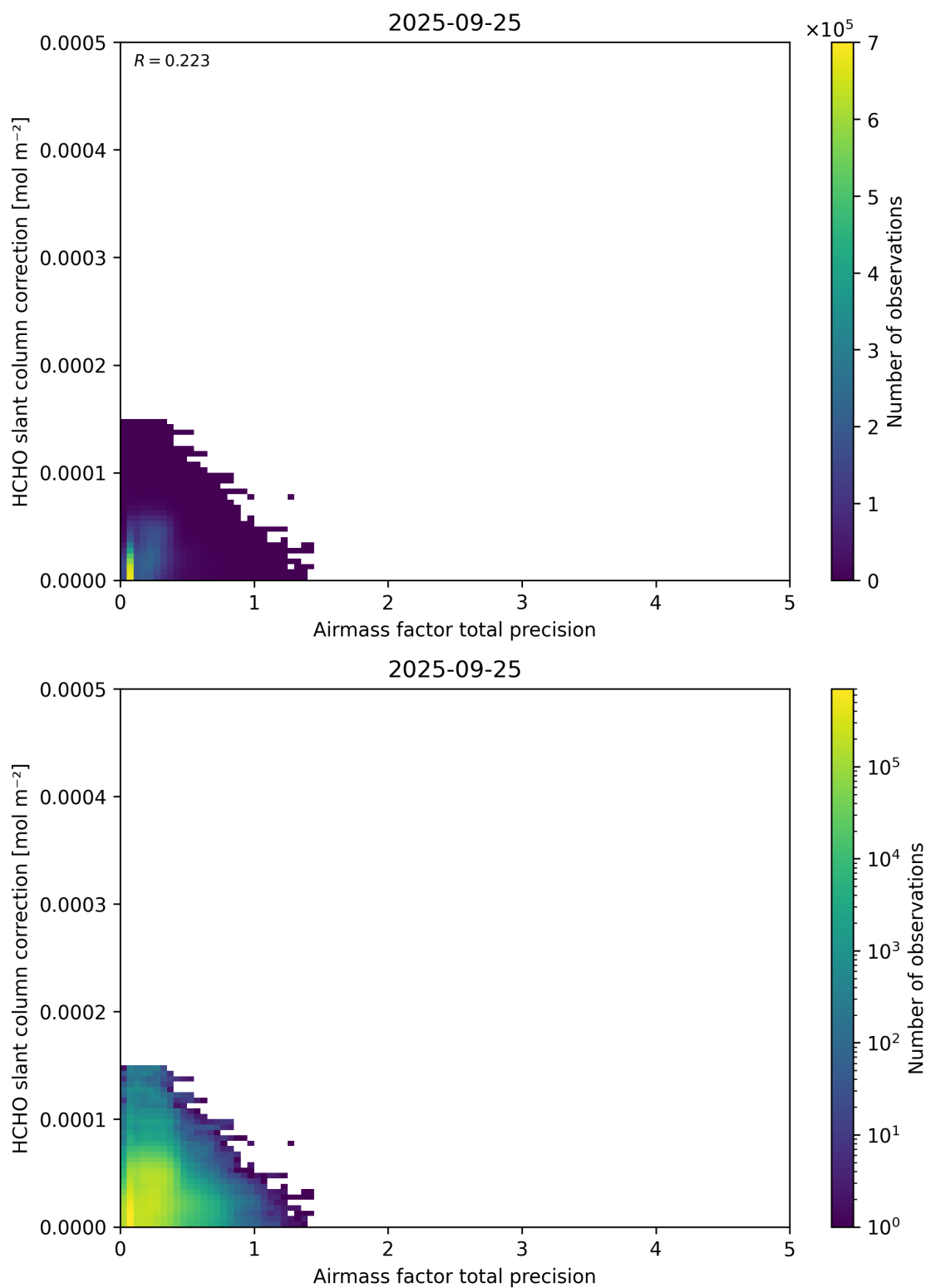
Figure 110: Scatter density plot of “Airmass factor total precision” against “HCHO slant column correction” for 2025-09-25 to 2025-09-26.
