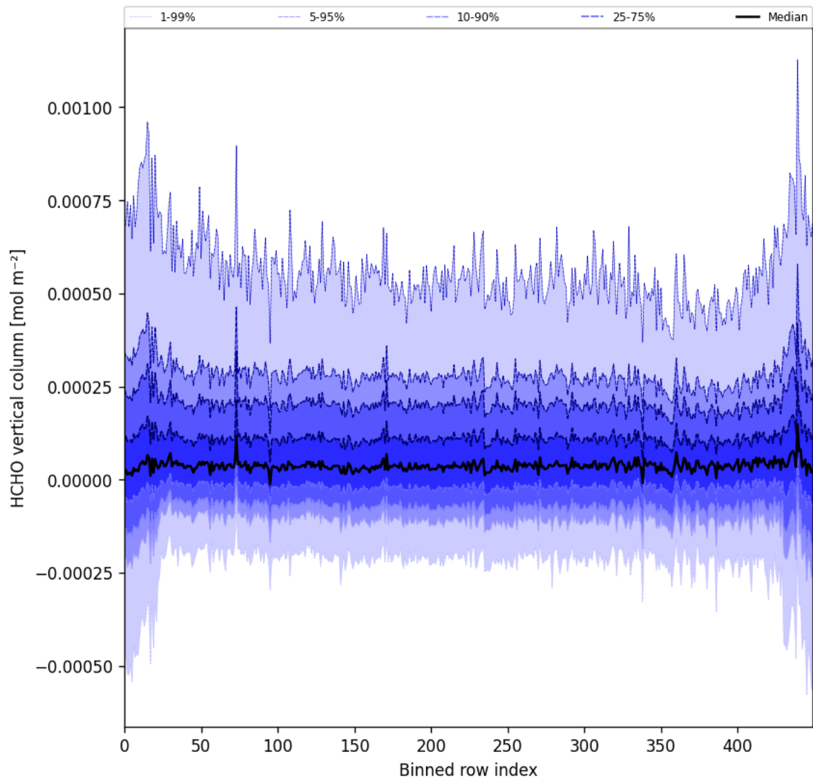
Figure 49: Along track statistics of “HCHO vertical column” for 2025-09-25 to 2025-09-26
