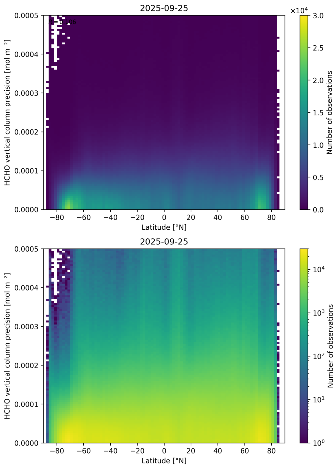
Figure 165: Scatter density plot of “Latitude” against “HCHO vertical column precision” for 2025-09-25 to 2025-09-26.
