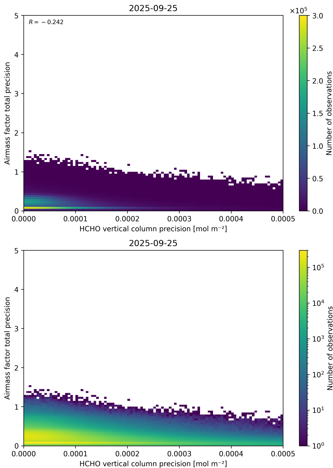
Figure 145: Scatter density plot of “HCHO vertical column precision” against “Airmass factor total precision” for 2025-09-25 to 2025-09-26.
