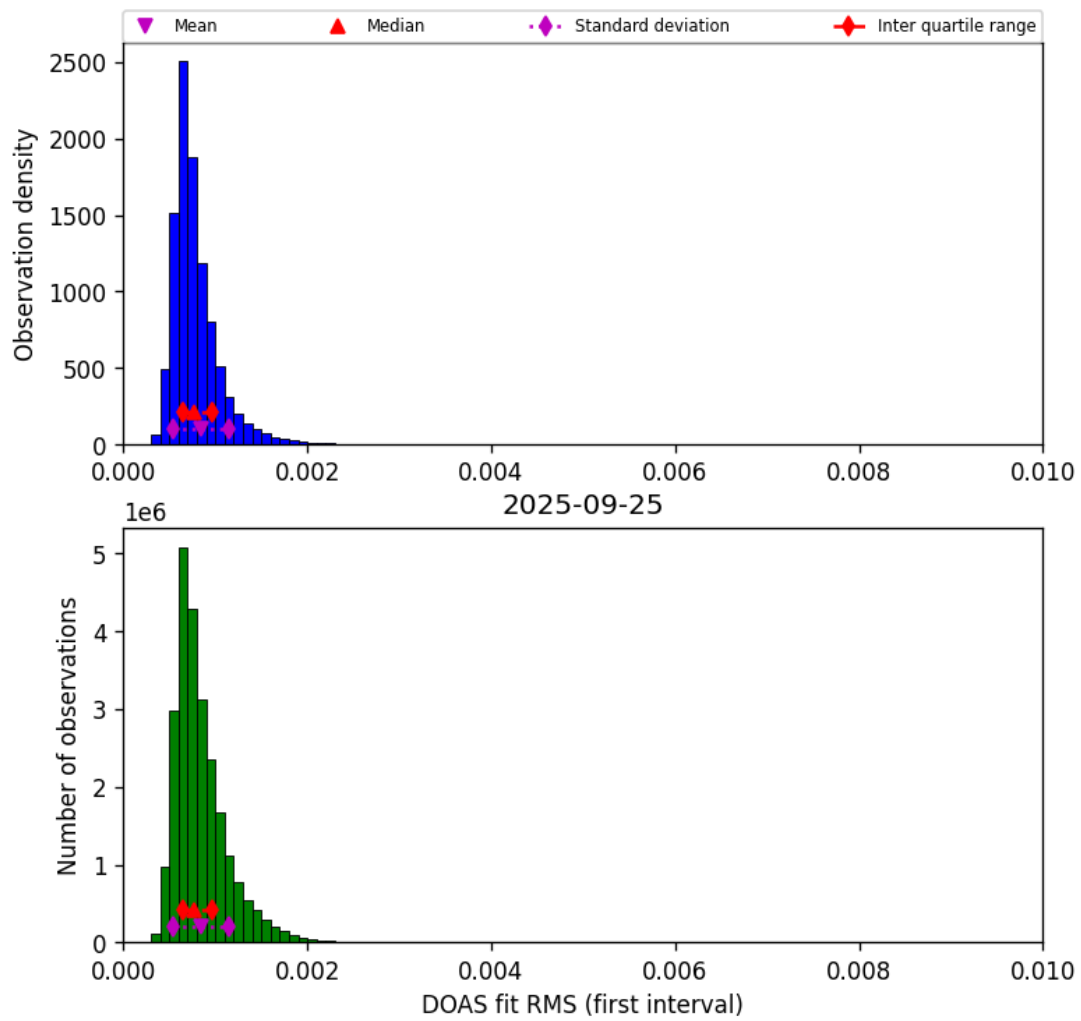
Figure 46: Histogram of “DOAS fit RMS (first interval)” for 2025-09-25 to 2025-09-26
