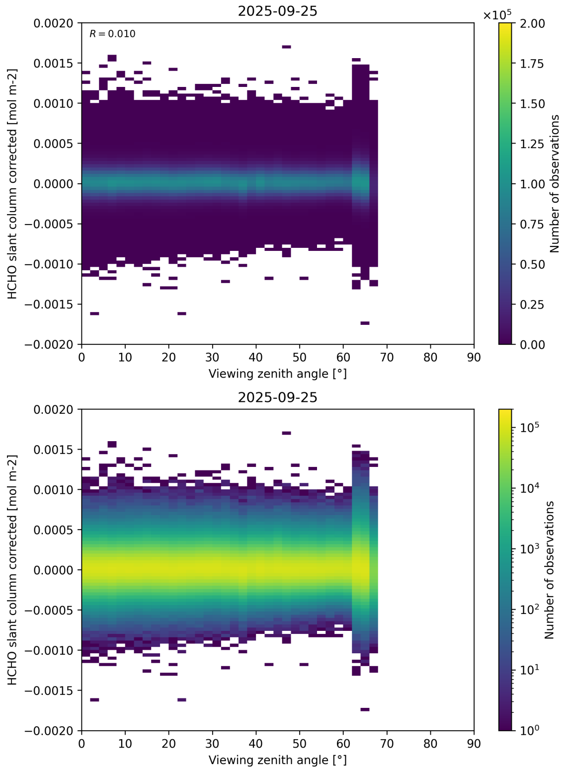
Figure 186: Scatter density plot of “Viewing zenith angle” against “HCHO slant column corrected” for 2025-09-25 to 2025-09-26.
