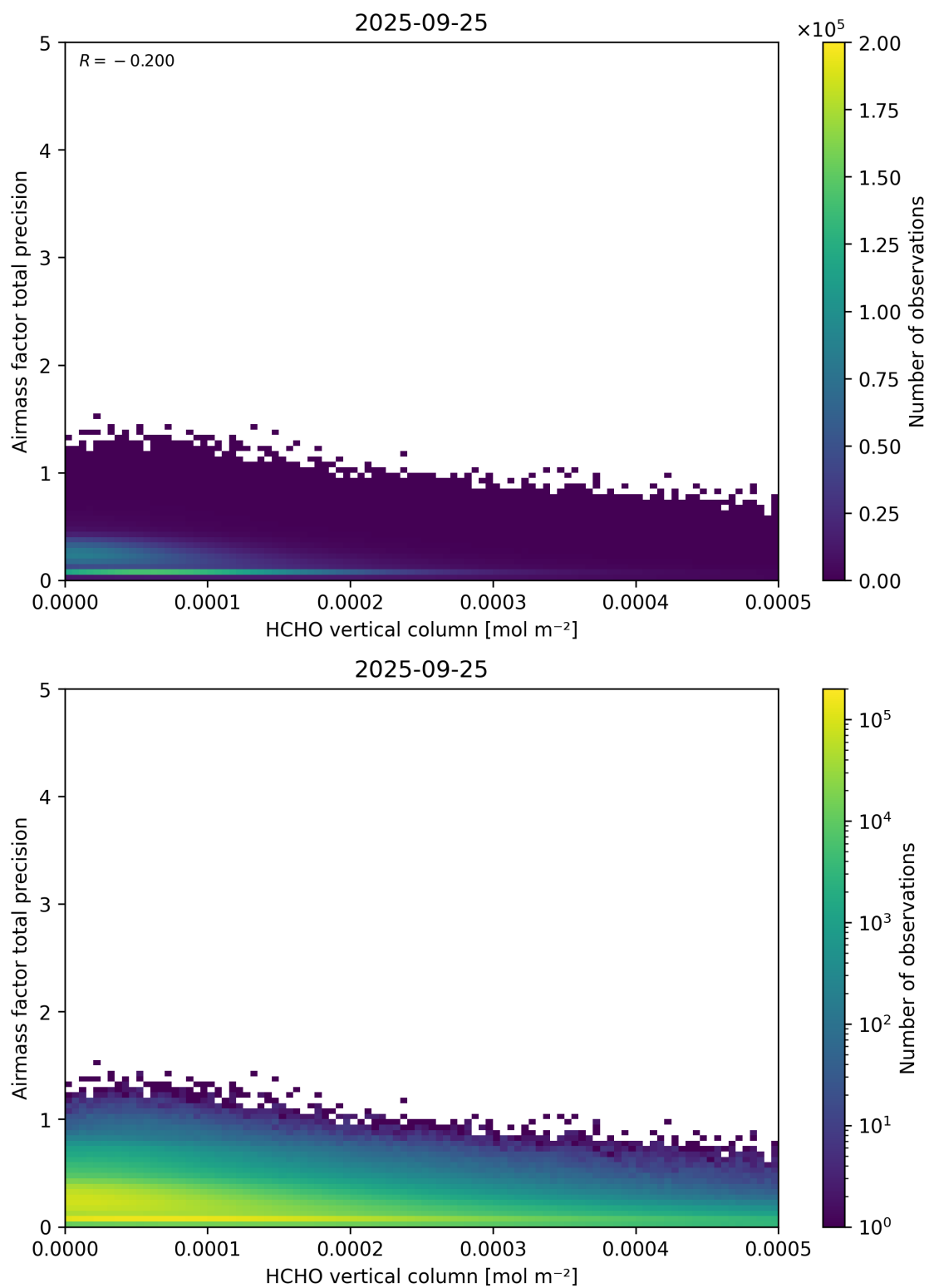
Figure 132: Scatter density plot of “HCHO vertical column” against “Airmass factor total precision” for 2025-09-25 to 2025-09-26.
