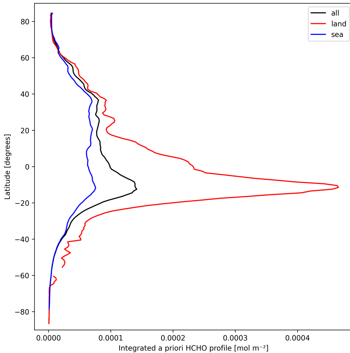
Figure 29: Zonal average of “Integrated a priori HCHO profile” for 2025-09-25 to 2025-09-26.
