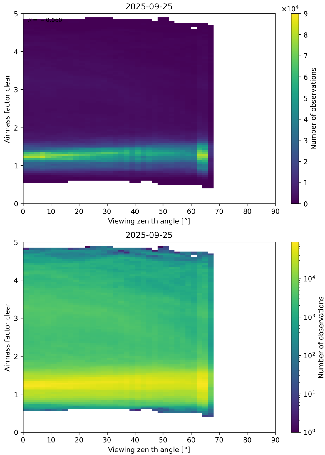
Figure 185: Scatter density plot of “Viewing zenith angle” against “Airmass factor clear” for 2025-09-25 to 2025-09-26.
