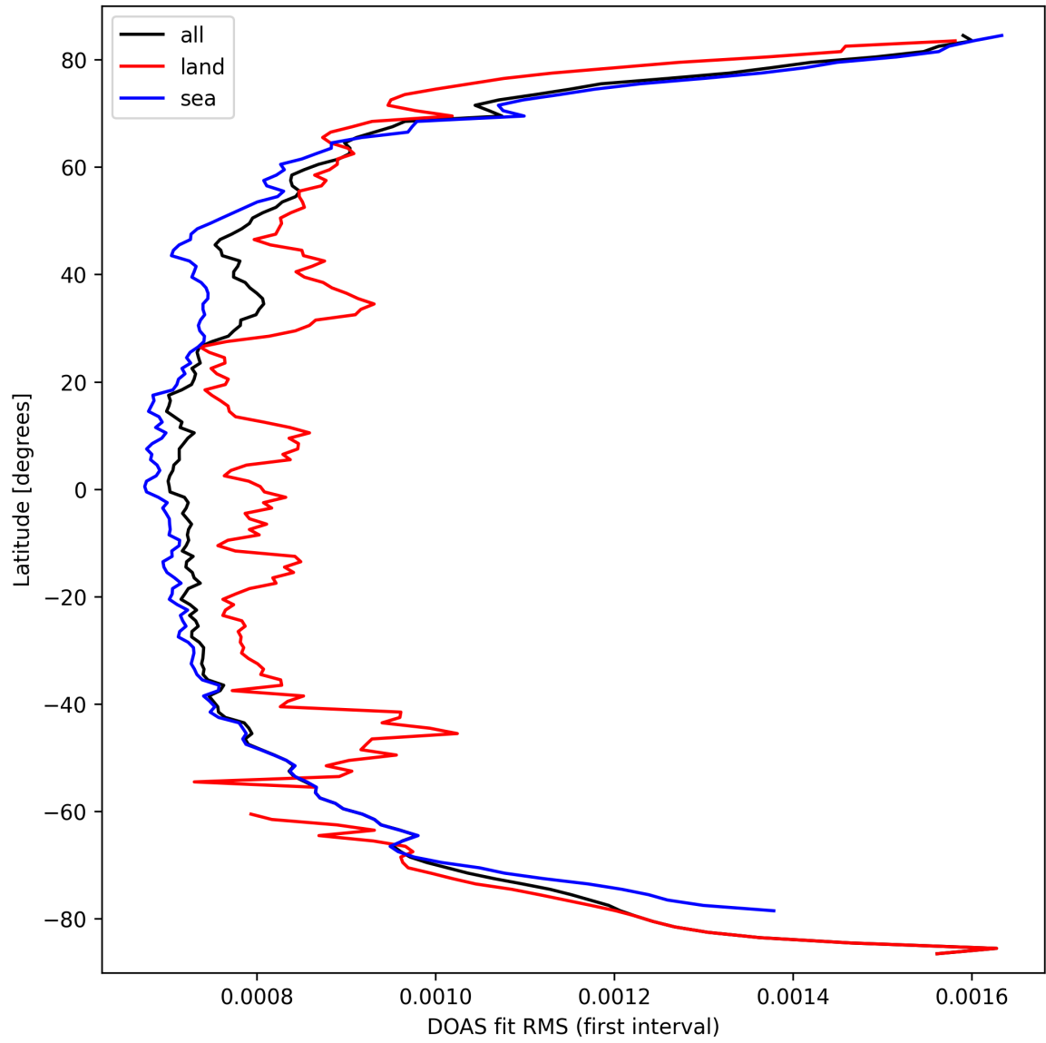
Figure 32: Zonal average of "DOAS fit RMS (first interval)" for 2025-09-25 to 2025-09-26.
