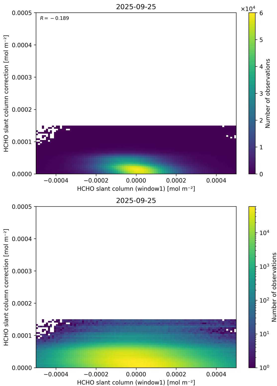
Figure 83: Scatter density plot of “HCHO slant column (window1)” against “HCHO slant column correction” for 2025-09-25 to 2025-09-26.
