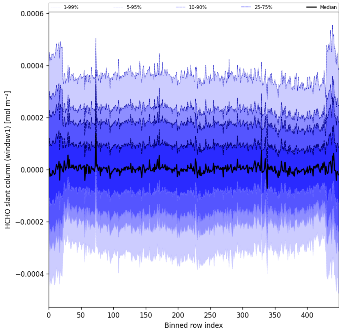
Figure 52: Along track statistics of “HCHO slant column (window1)” for 2025-09-25 to 2025-09-26
