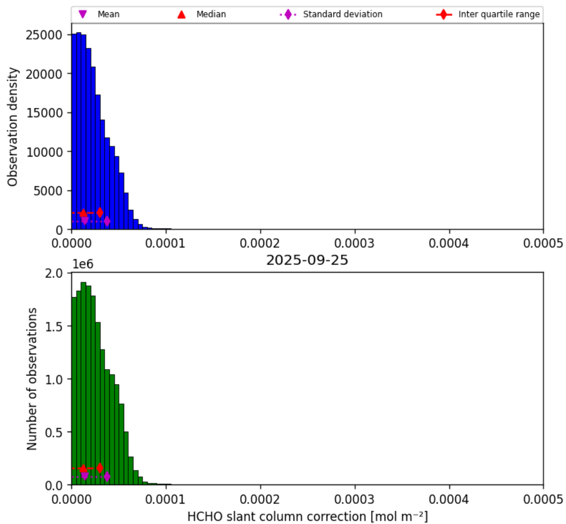
Figure 47: Histogram of “HCHO slant column correction” for 2025-09-25 to 2025-09-26
