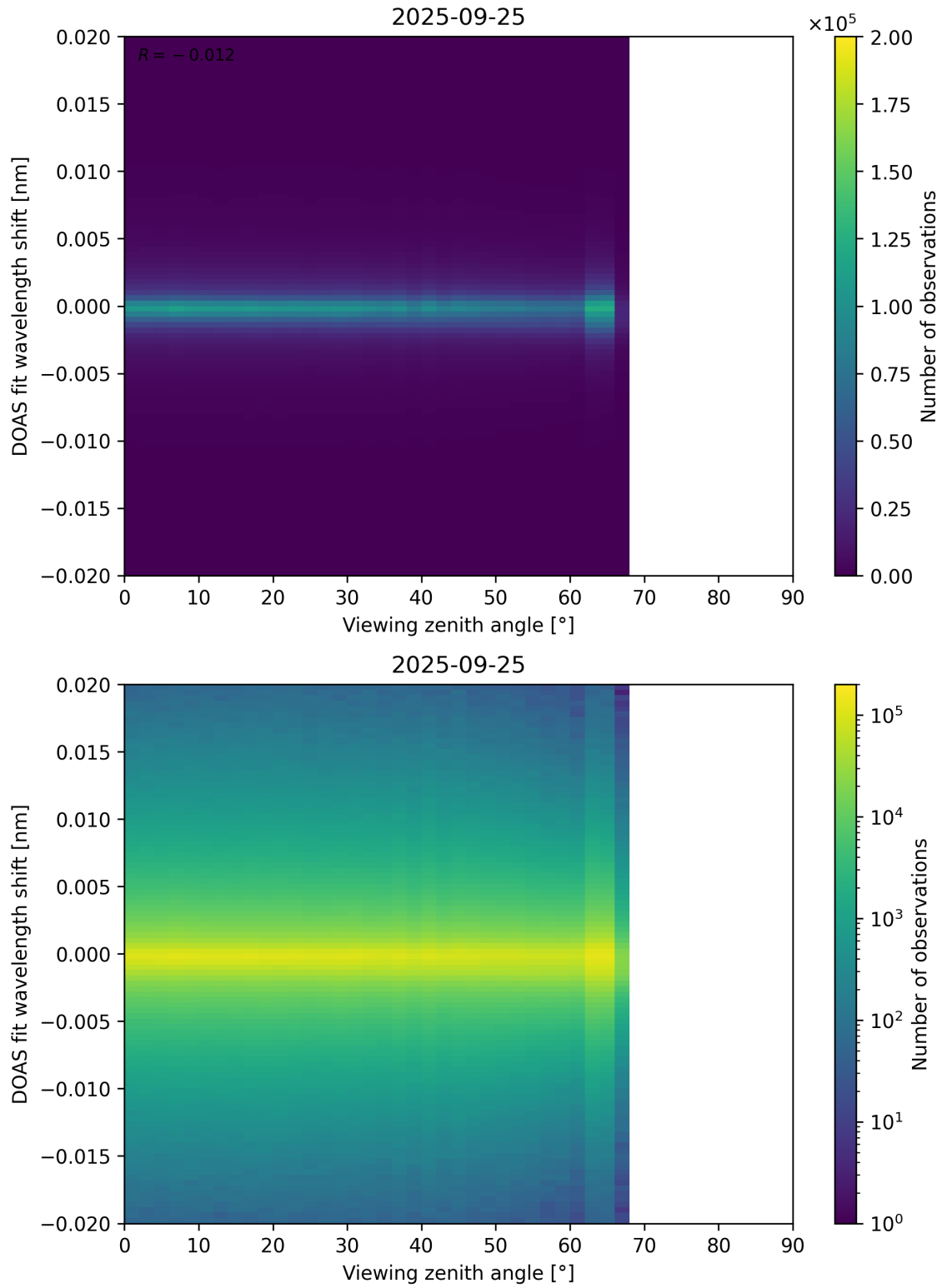
Figure 183: Scatter density plot of “Viewing zenith angle” against “DOAS fit wavelength shift” for 2025-09-25 to 2025-09-26.
