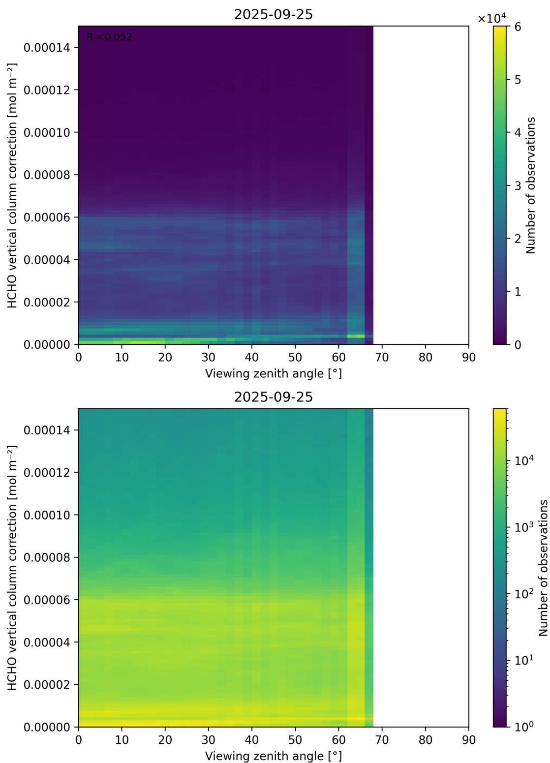
Figure 193: Scatter density plot of “Viewing zenith angle” against “HCHO vertical column correction” for 2025-09-25 to 2025-09-26.
