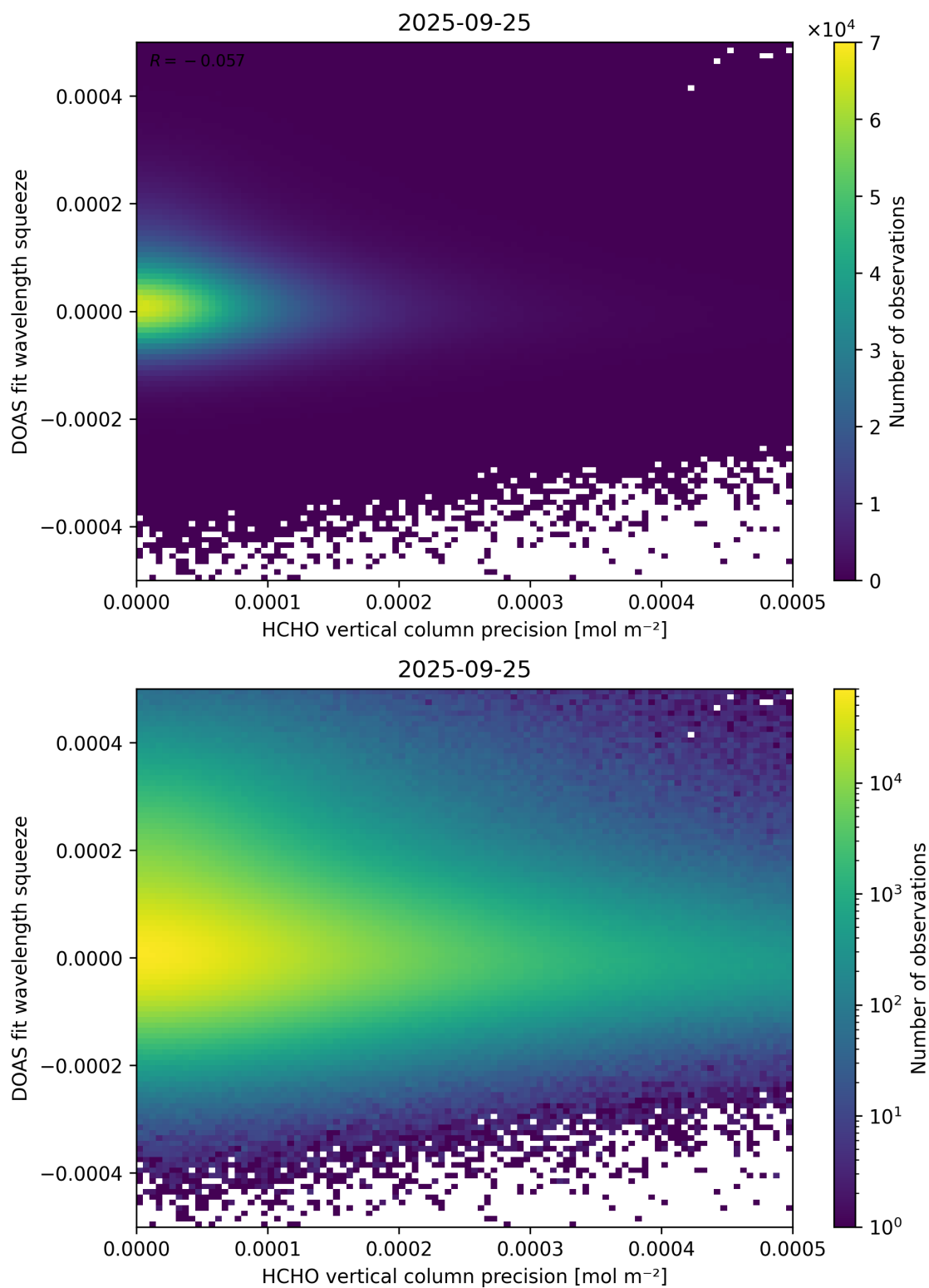
Figure 138: Scatter density plot of “HCHO vertical column precision” against “DOAS fit wavelength squeeze” for 2025-09-25 to 2025-09-26.
