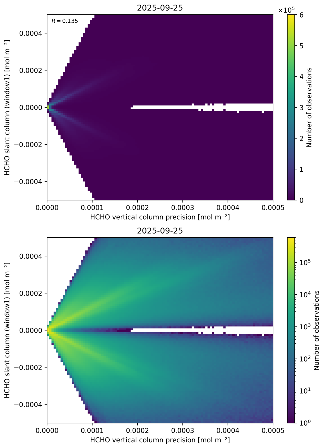
Figure 142: Scatter density plot of “HCHO vertical column precision” against “HCHO slant column (window1)” for 2025-09-25 to 2025-09-26.
