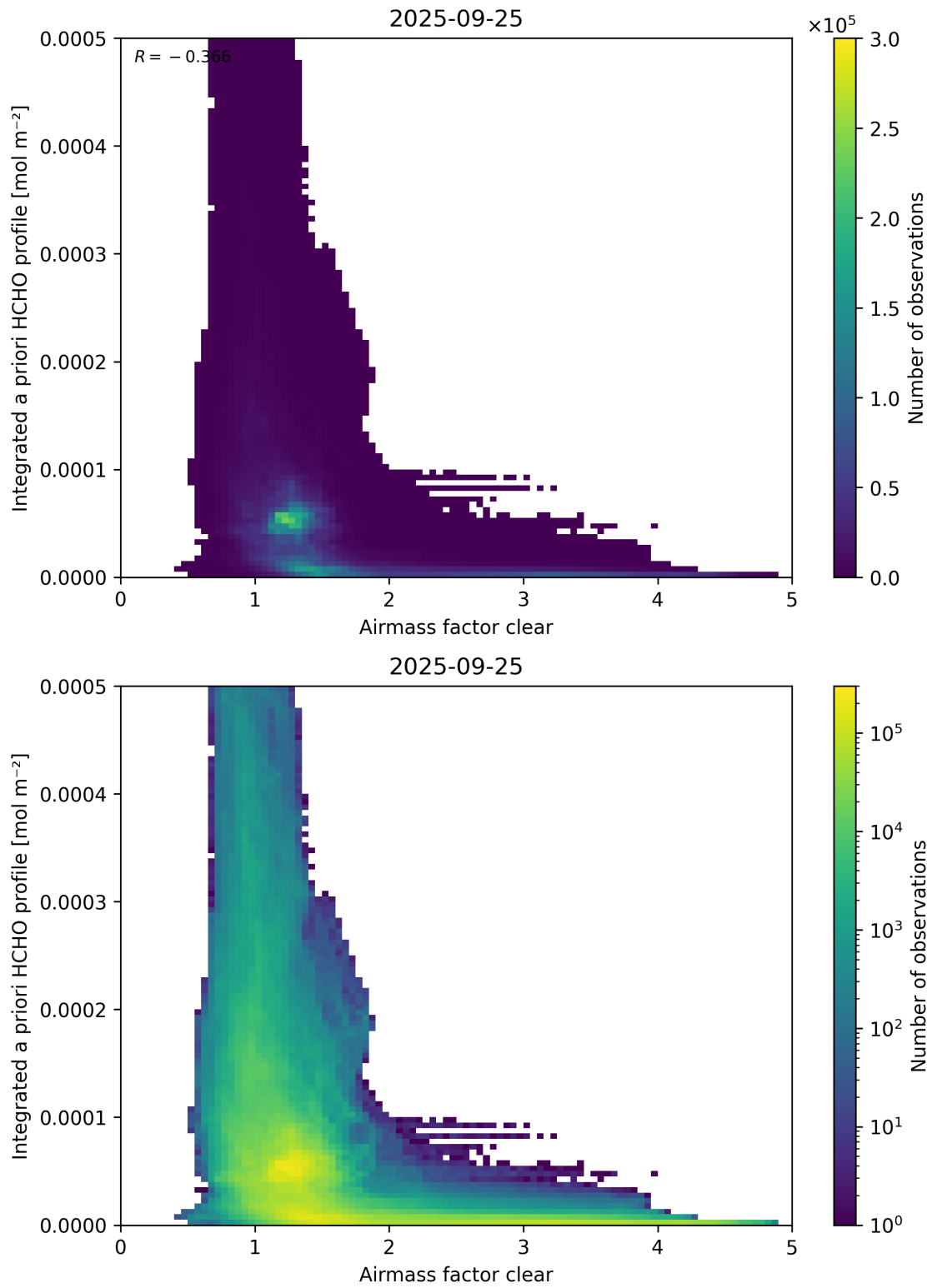
Figure 76: Scatter density plot of “Airmass factor clear” against “Integrated a priori HCHO profile” for 2025-09-25 to 2025-09-26.
