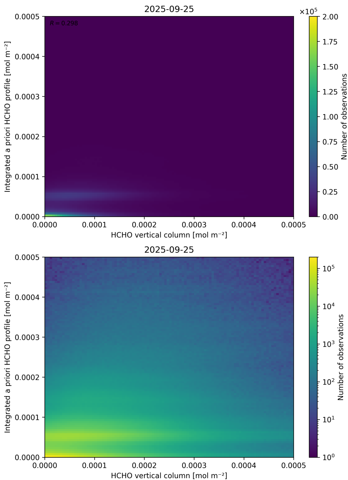
Figure 135: Scatter density plot of “HCHO vertical column” against “Integrated a priori HCHO profile” for 2025-09-25 to 2025-09-26.
