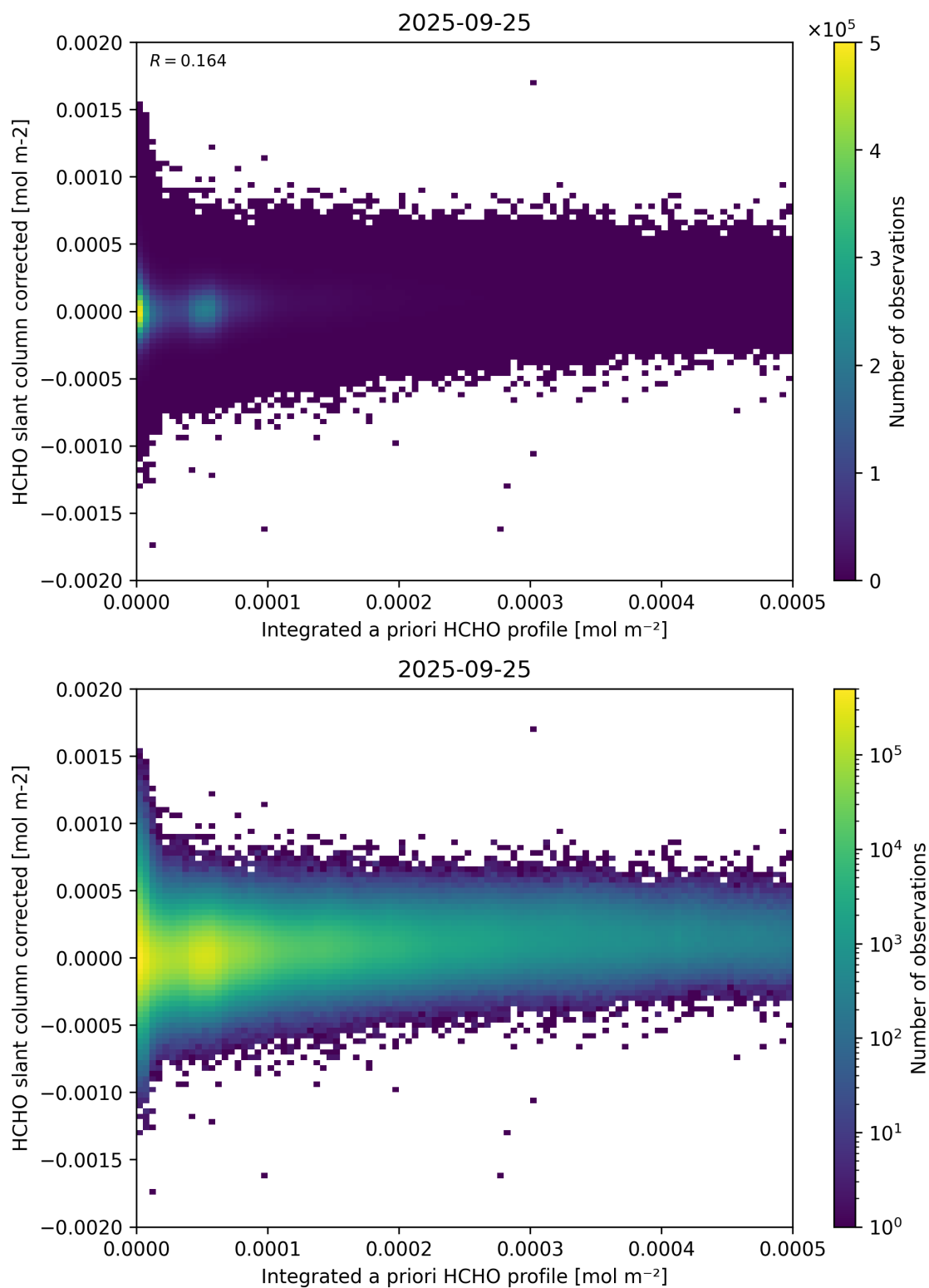
Figure 151: Scatter density plot of “Integrated a priori HCHO profile” against “HCHO slant column corrected” for 2025-09-25 to 2025-09-26.
