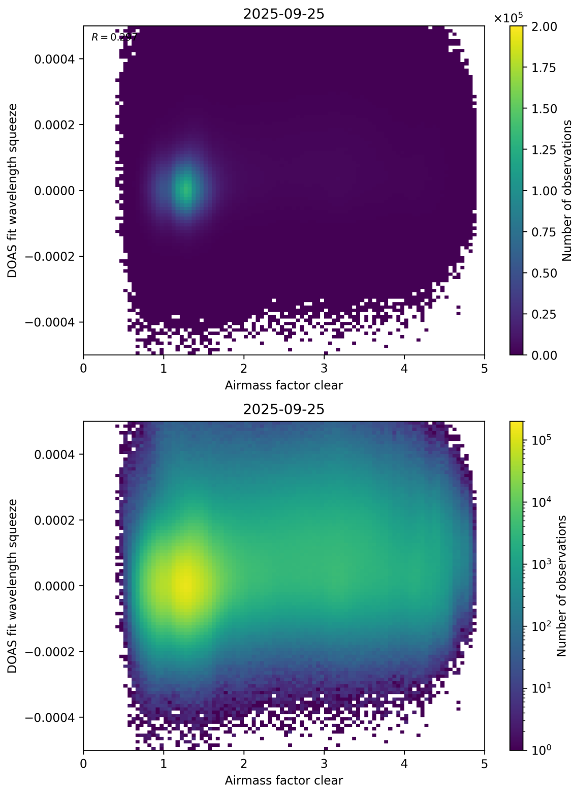
Figure 73: Scatter density plot of “Airmass factor clear” against “DOAS fit wavelength squeeze” for 2025-09-25 to 2025-09-26.
