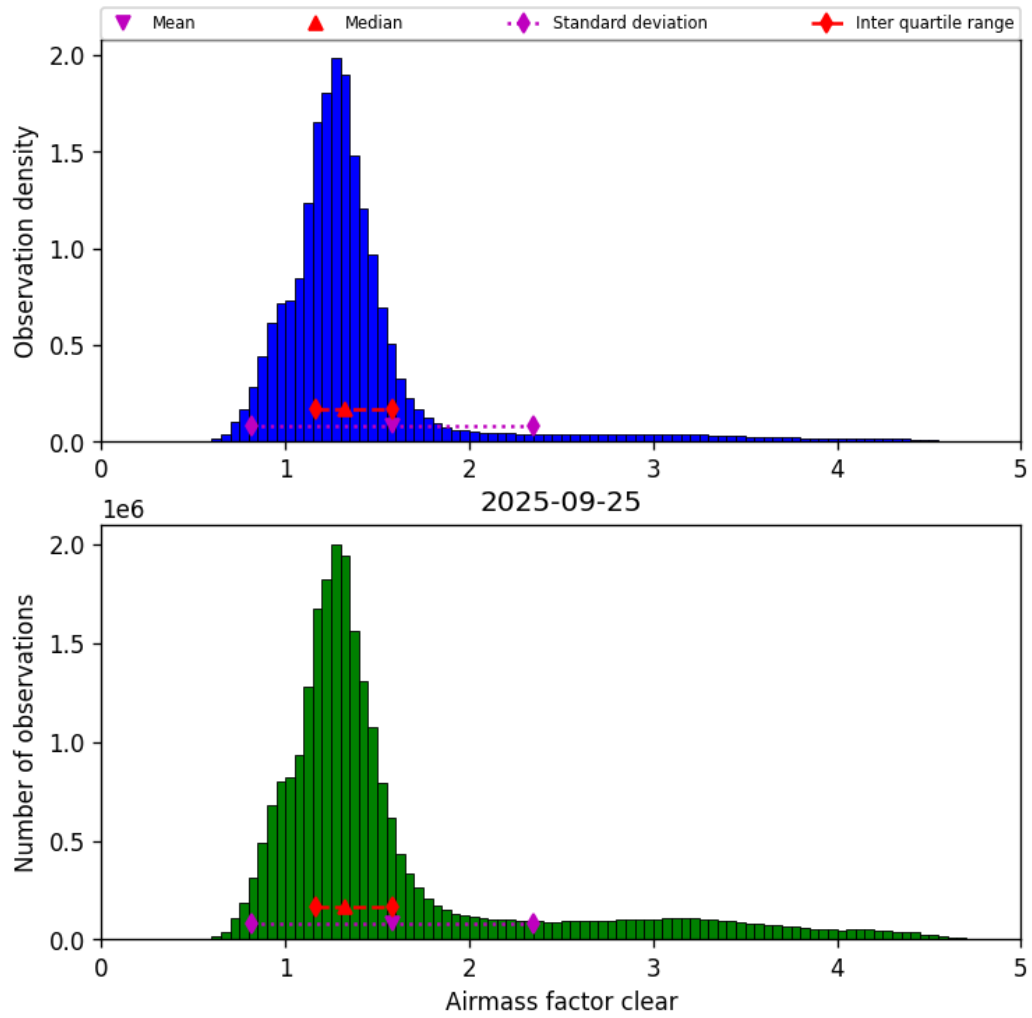
Figure 42: Histogram of “Airmass factor clear” for 2025-09-25 to 2025-09-26
