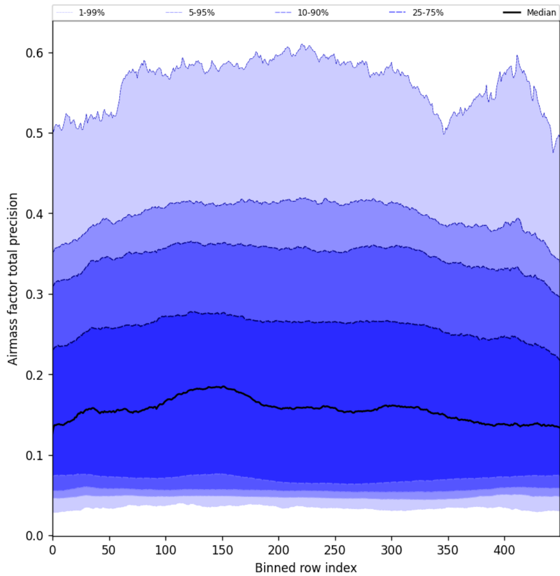
Figure 55: Along track statistics of “Airmass factor total precision” for 2025-09-25 to 2025-09-26
