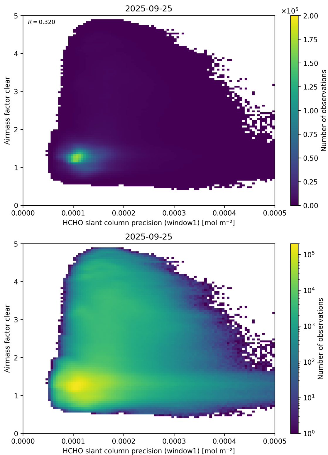
Figure 91: Scatter density plot of “HCHO slant column precision (window1)” against “Airmass factor clear” for 2025-09-25 to 2025-09-26.
