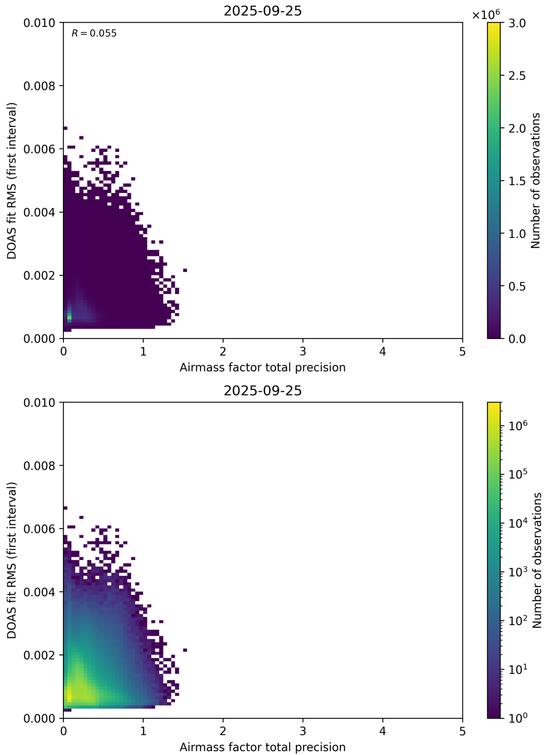
Figure 105: Scatter density plot of “Airmass factor total precision” against “DOAS fit RMS (first interval)” for 2025-09-25 to 2025-09-26.
