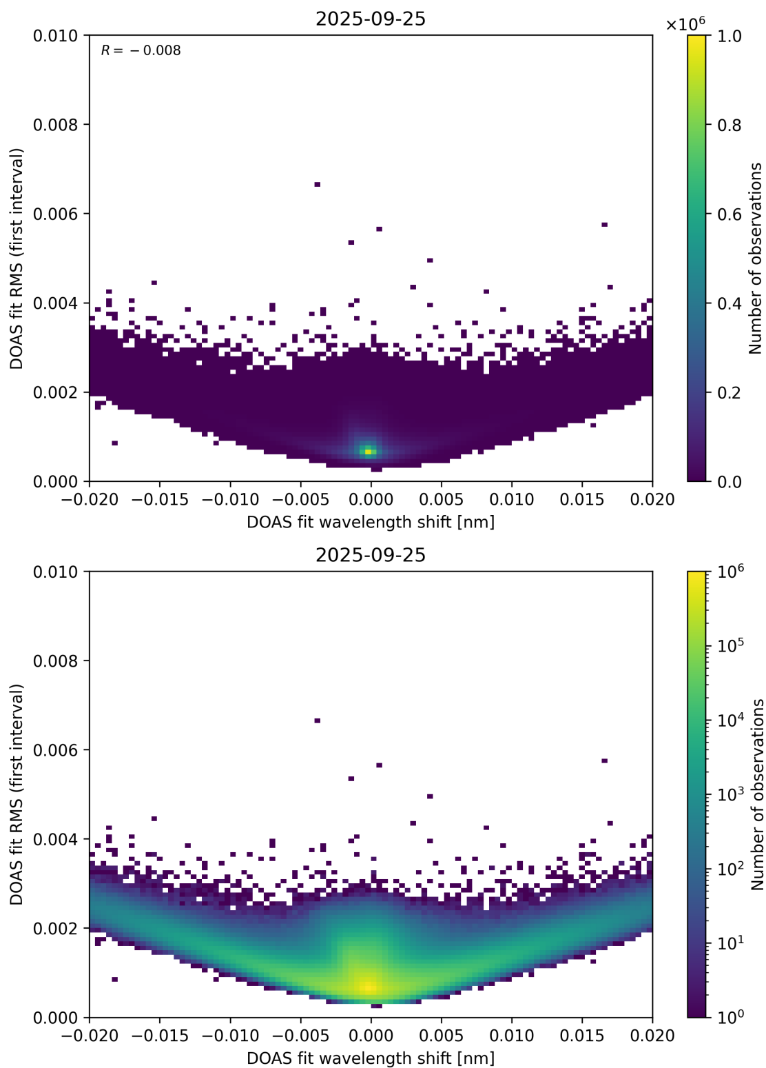
Figure 64: Scatter density plot of “DOAS fit wavelength shift” against “DOAS fit RMS (first interval)” for 2025-09-25 to 2025-09-26.
