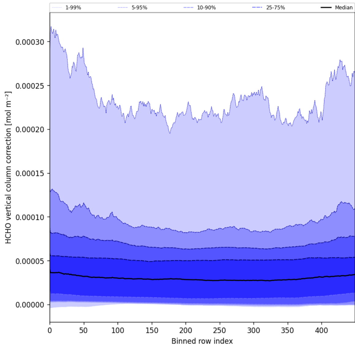
Figure 51: Along track statistics of “HCHO vertical column correction” for 2025-09-25 to 2025-09-26
