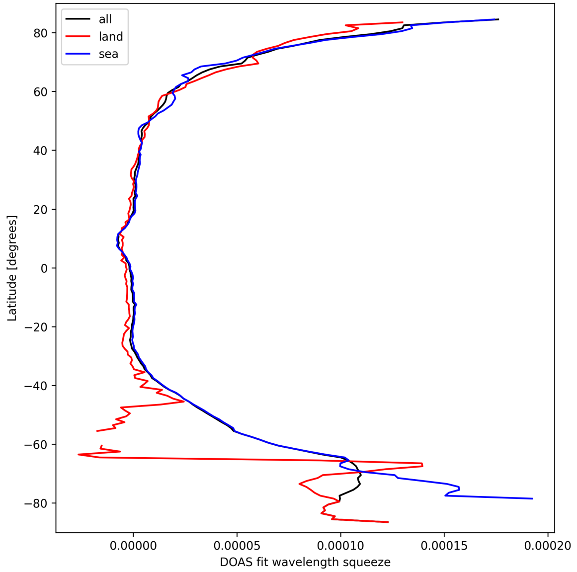
Figure 31: Zonal average of “DOAS fit wavelength squeeze” for 2025-09-25 to 2025-09-26.
