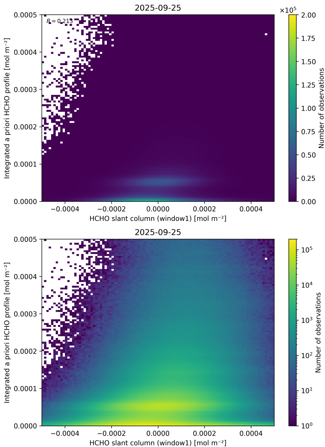
Figure 87: Scatter density plot of “HCHO slant column (window1)” against “Integrated a priori HCHO profile” for 2025-09-25 to 2025-09-26.
