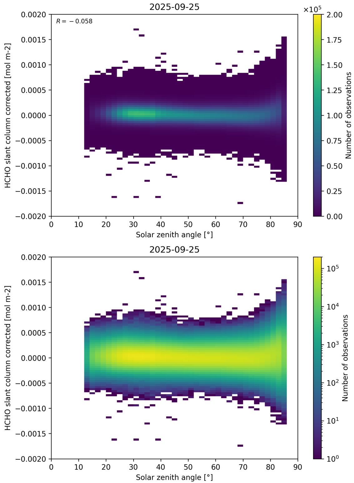
Figure 171: Scatter density plot of “Solar zenith angle” against “HCHO slant column corrected” for 2025-09-25 to 2025-09-26.
