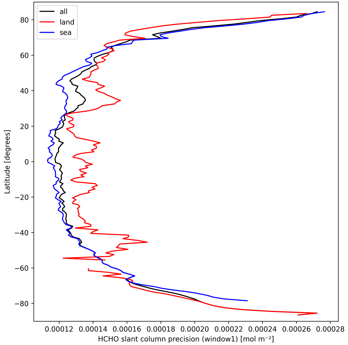
Figure 25: Zonal average of “HCHO slant column precision (window1)” for 2025-09-25 to 2025-09-26.
