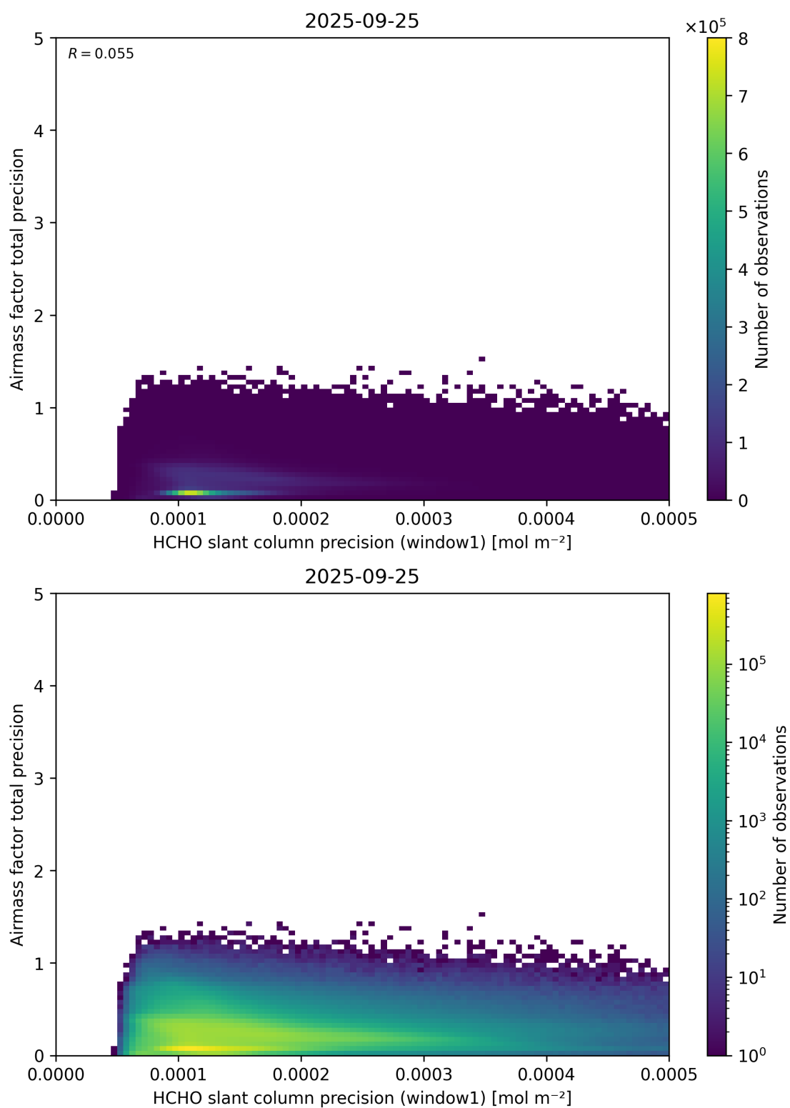
Figure 95: Scatter density plot of “HCHO slant column precision (window1)” against “Airmass factor total precision” for 2025-09-25 to 2025-09-26.
