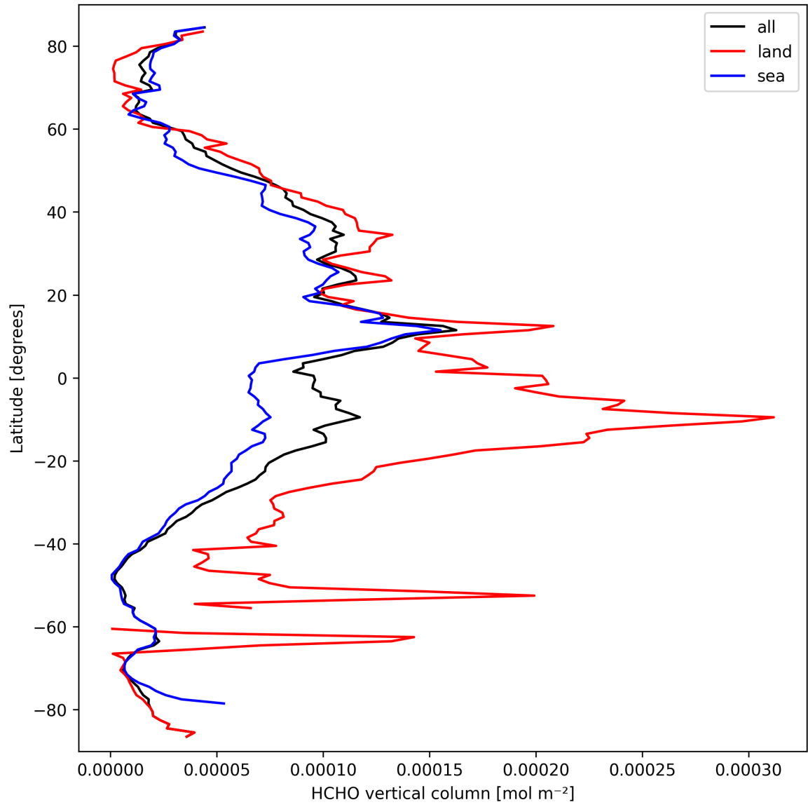
Figure 21: Zonal average of “HCHO vertical column” for 2025-09-25 to 2025-09-26.
