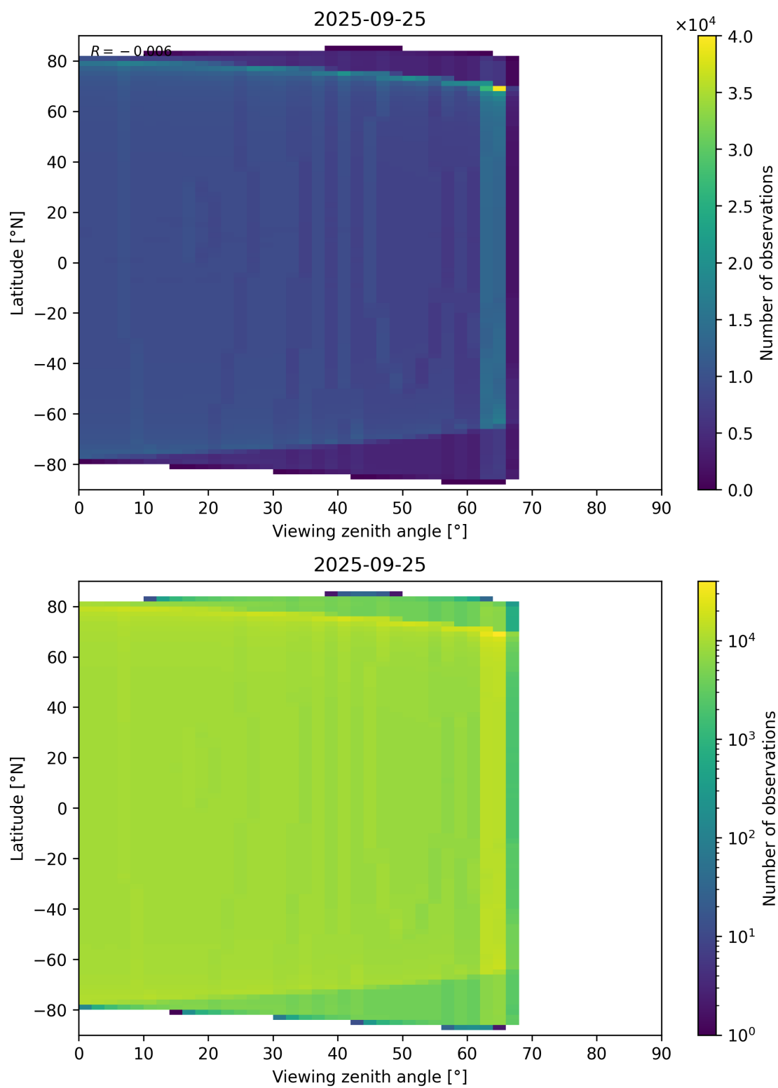
Figure 196: Scatter density plot of “Viewing zenith angle” against “Latitude” for 2025-09-25 to 2025-09-26.
