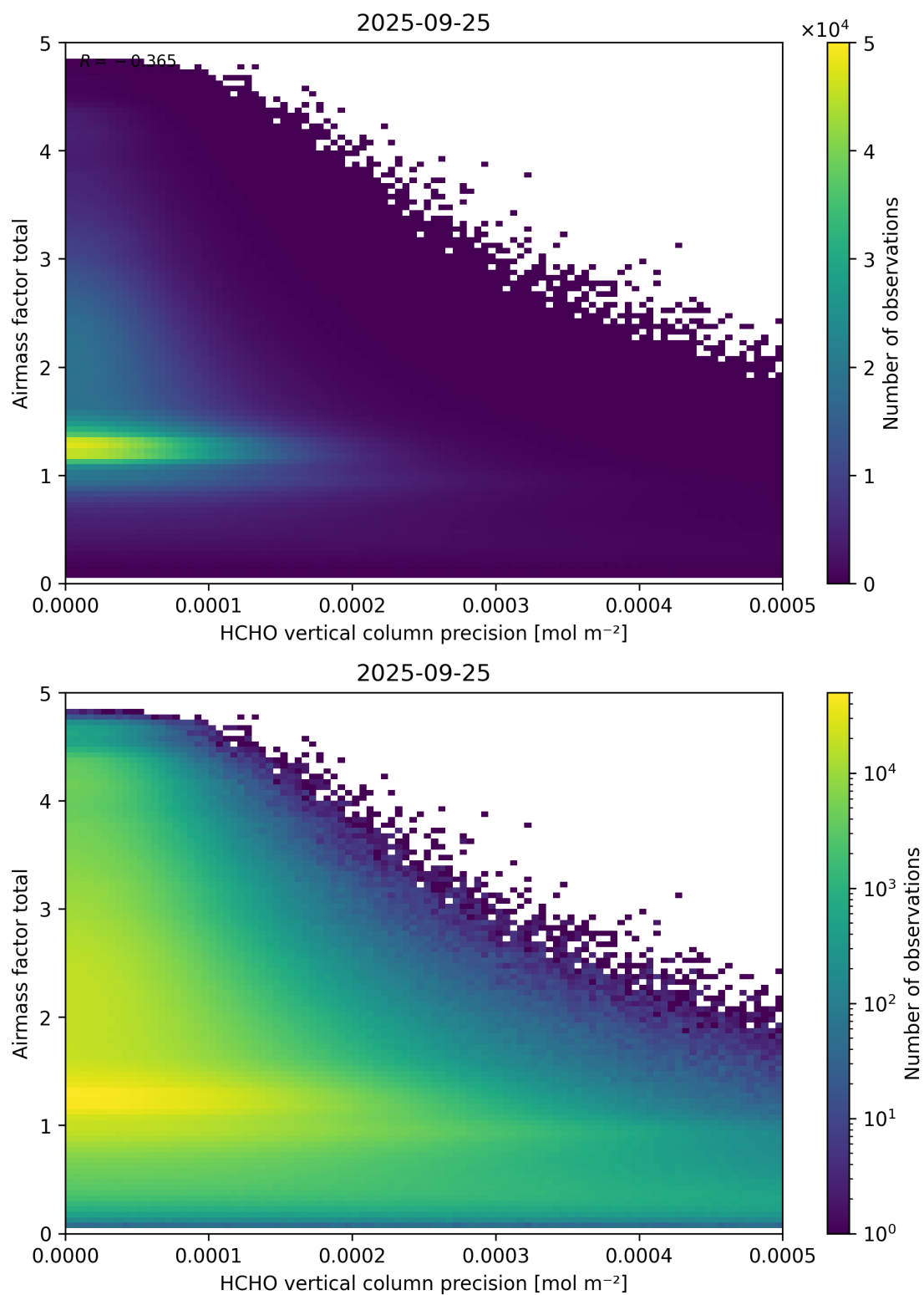
Figure 144: Scatter density plot of “HCHO vertical column precision” against “Airmass factor total” for 2025-09-25 to 2025-09-26.
