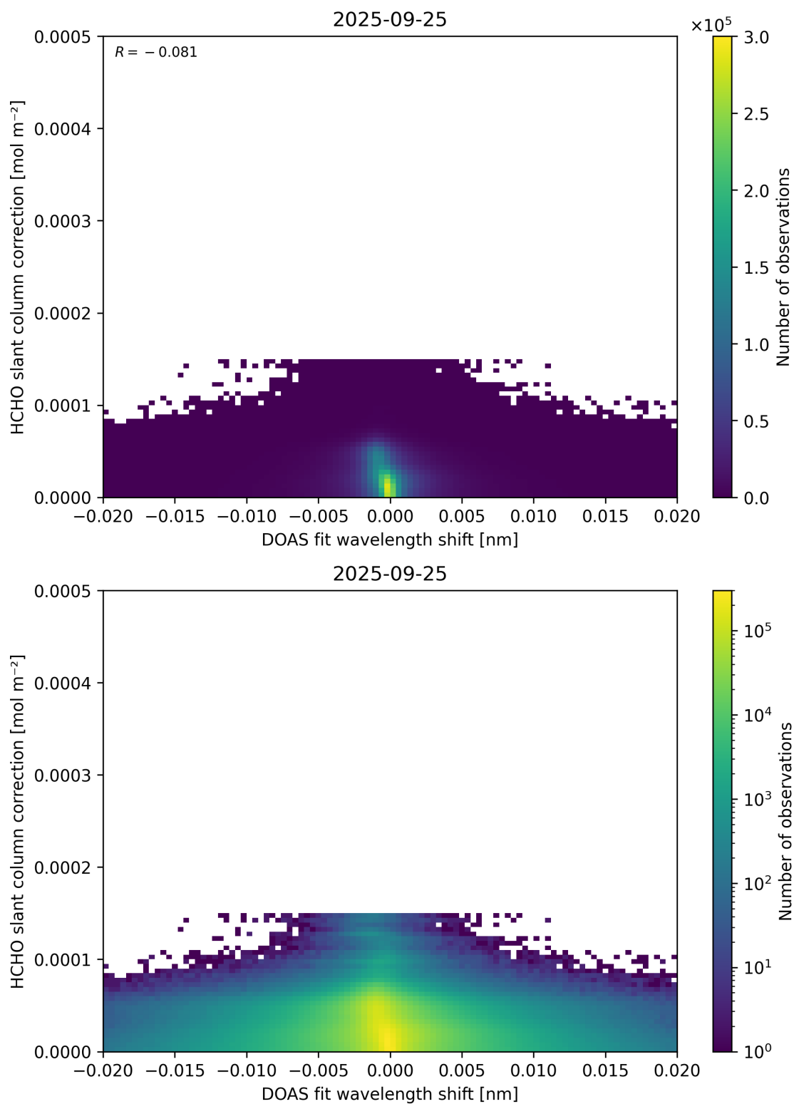
Figure 67: Scatter density plot of “DOAS fit wavelength shift” against “HCHO slant column correction” for 2025-09-25 to 2025-09-26.
