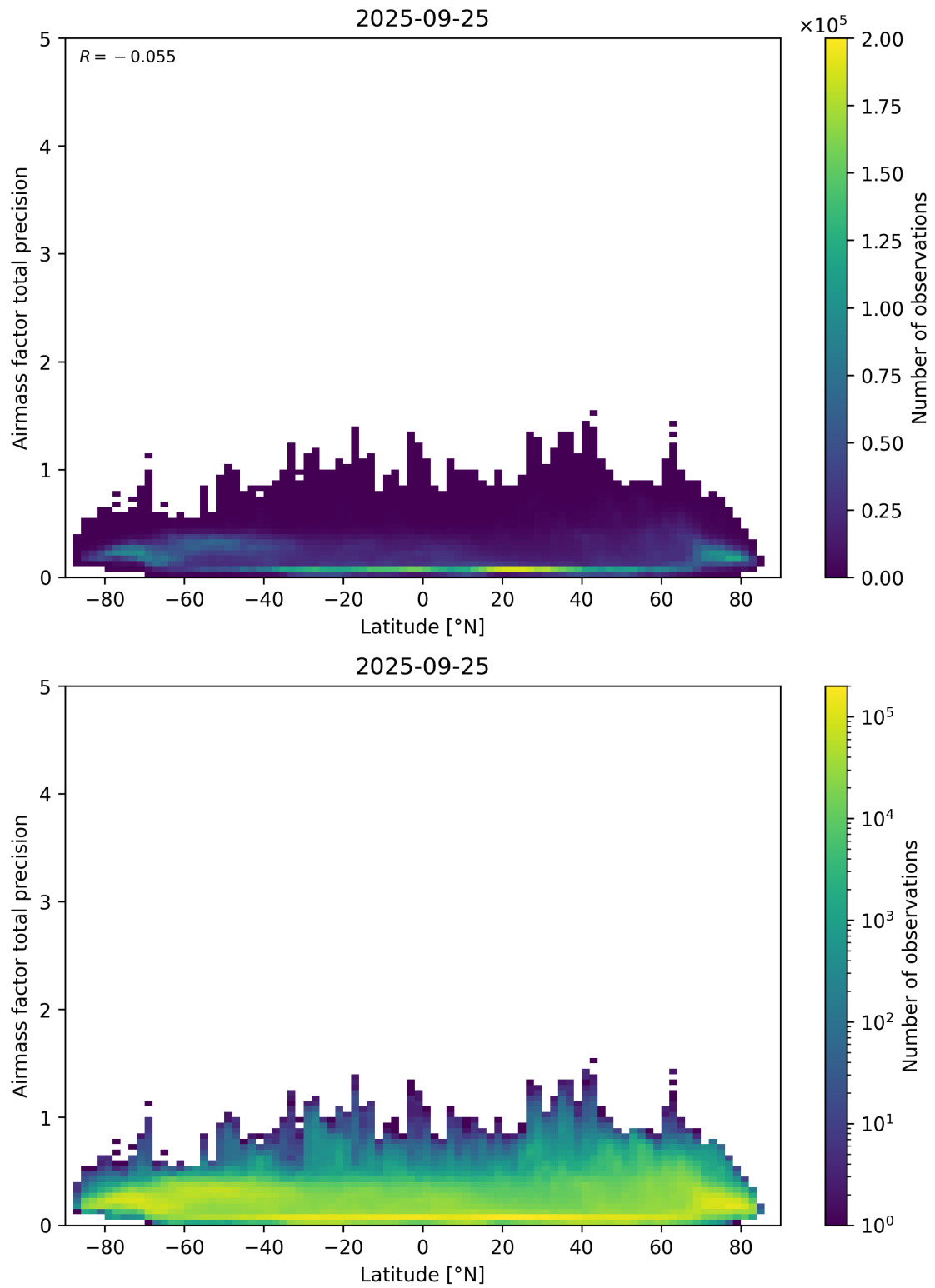
Figure 162: Scatter density plot of “Latitude” against “Airmass factor total precision” for 2025-09-25 to 2025-09-26.
