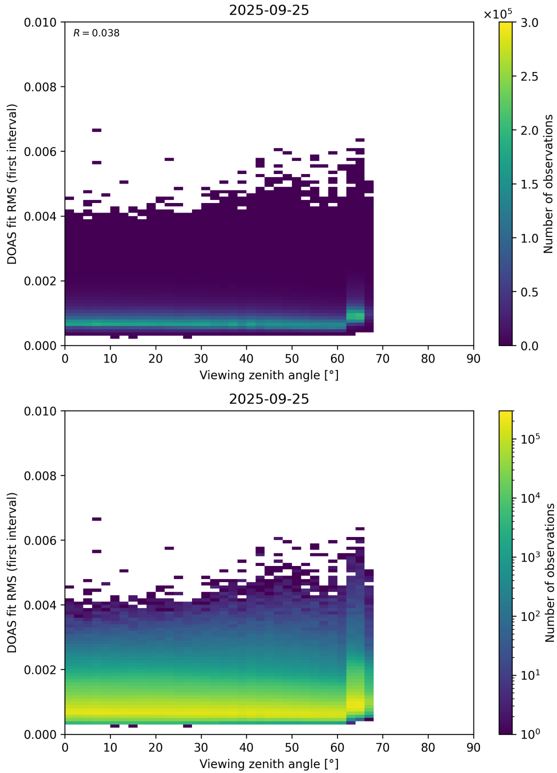
Figure 182: Scatter density plot of “Viewing zenith angle” against “DOAS fit RMS (first interval)” for 2025-09-25 to 2025-09-26.
