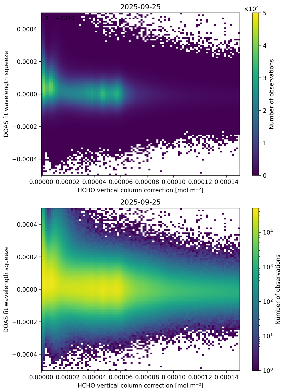
Figure 114: Scatter density plot of “HCHO vertical column correction” against “DOAS fit wavelength squeeze” for 2025-09-25 to 2025-09-26.
