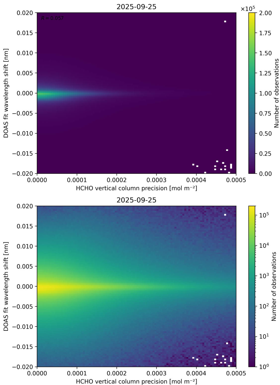
Figure 137: Scatter density plot of “HCHO vertical column precision” against “DOAS fit wavelength shift” for 2025-09-25 to 2025-09-26.
