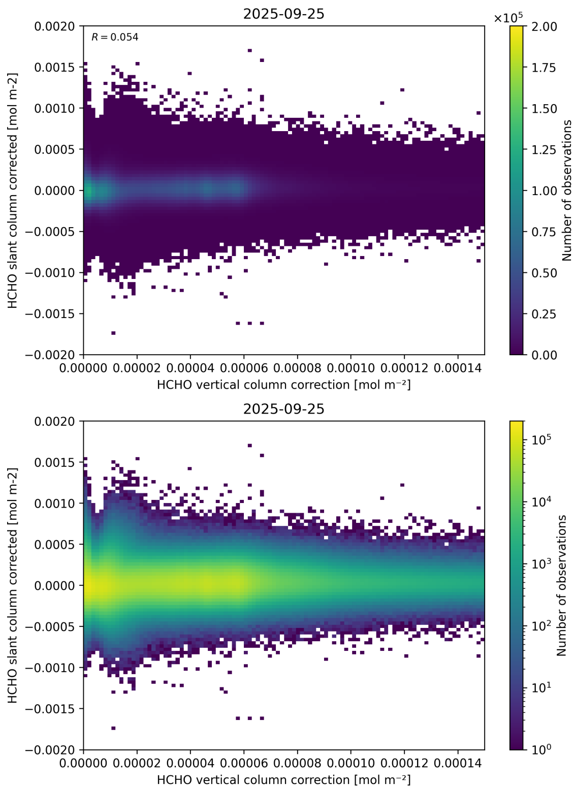
Figure 116: Scatter density plot of “HCHO vertical column correction” against “HCHO slant column corrected” for 2025-09-25 to 2025-09-26.
