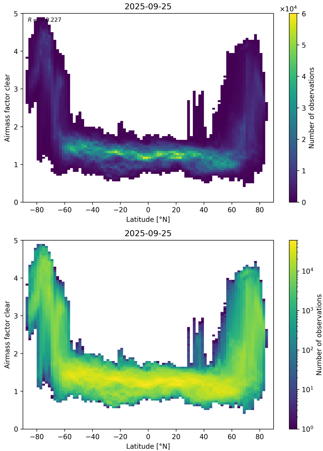
Figure 156: Scatter density plot of “Latitude” against “Airmass factor clear” for 2025-09-25 to 2025-09-26.
