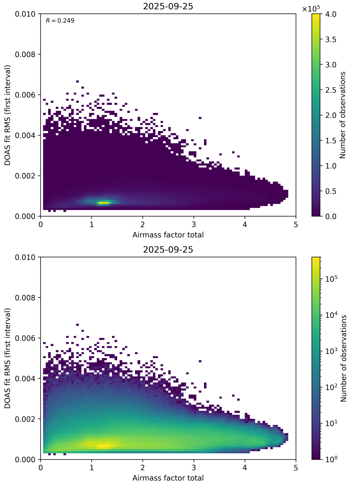
Figure 97: Scatter density plot of “Airmass factor total” against “DOAS fit RMS (first interval)” for 2025-09-25 to 2025-09-26.
