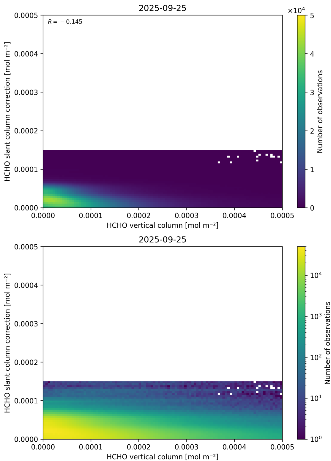
Figure 128: Scatter density plot of “HCHO vertical column” against “HCHO slant column correction” for 2025-09-25 to 2025-09-26.
