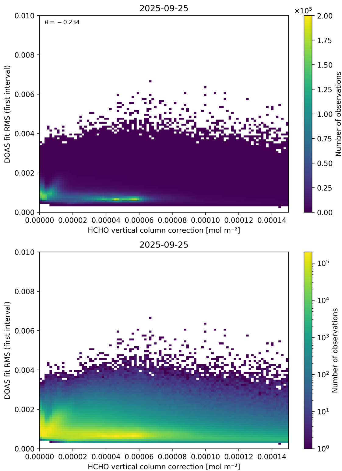
Figure 112: Scatter density plot of “HCHO vertical column correction” against “DOAS fit RMS (first interval)” for 2025-09-25 to 2025-09-26.
