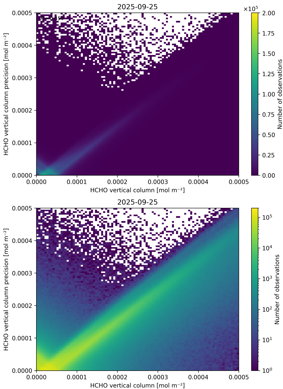
Figure 134: Scatter density plot of “HCHO vertical column” against “HCHO vertical column precision” for 2025-09-25 to 2025-09-26.
