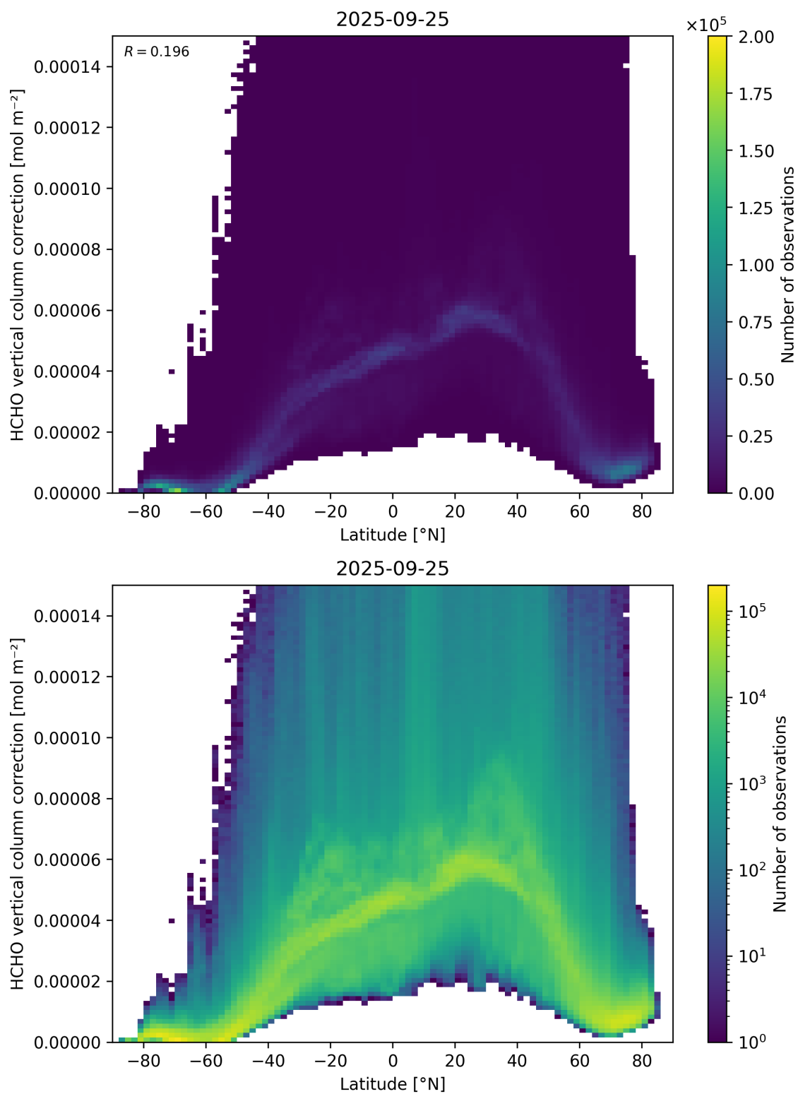
Figure 164: Scatter density plot of “Latitude” against “HCHO vertical column correction” for 2025-09-25 to 2025-09-26.
