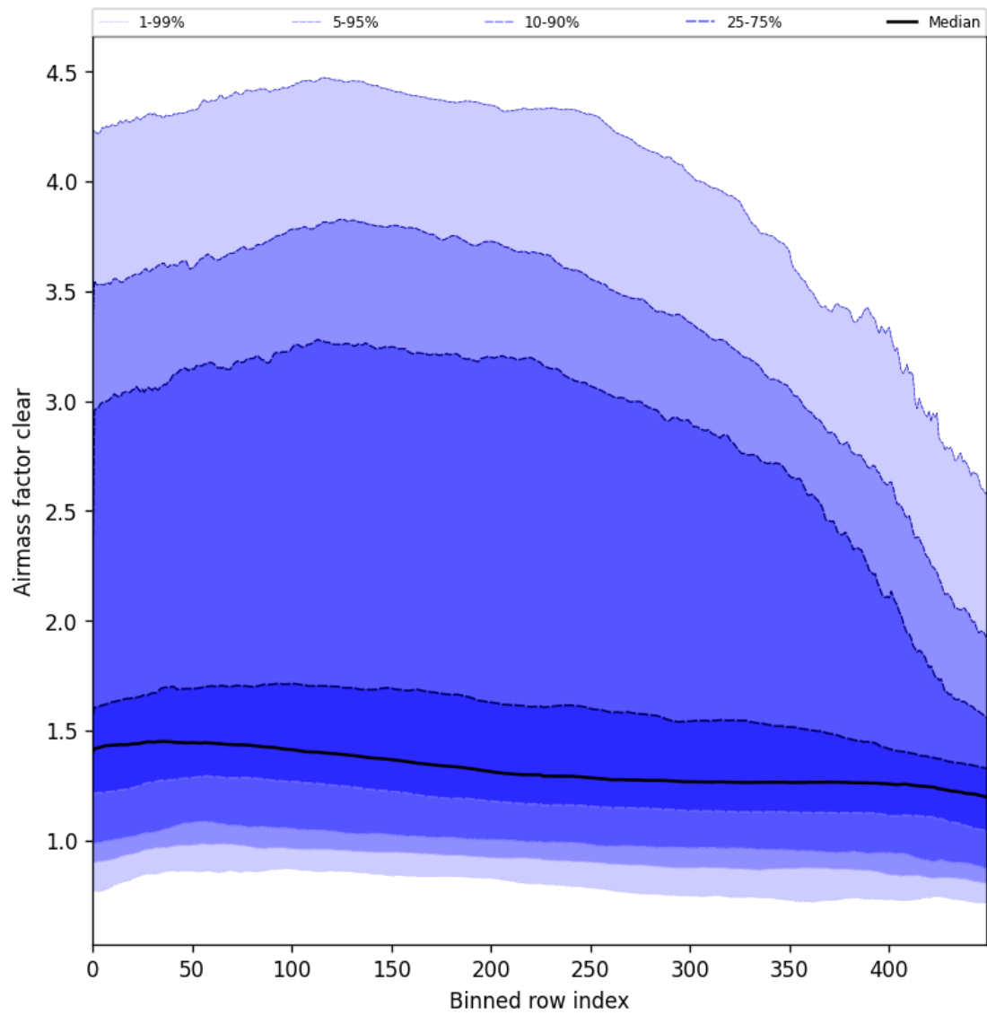
Figure 56: Along track statistics of “Airmass factor clear” for 2025-09-25 to 2025-09-26
