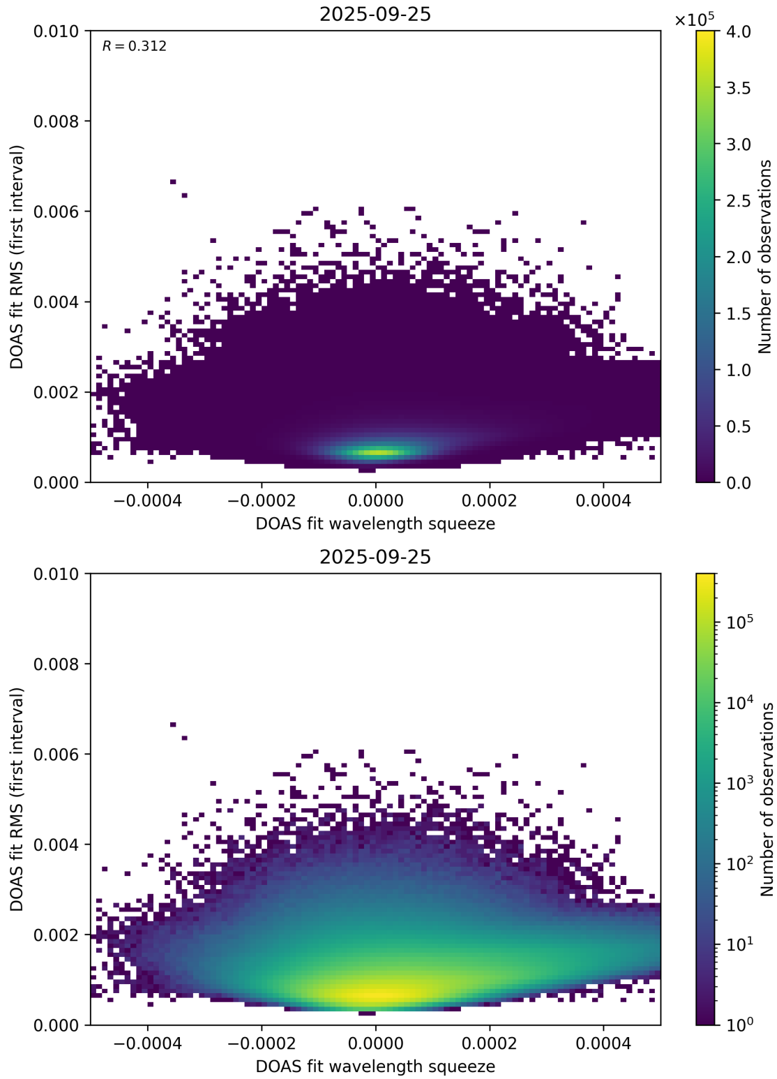
Figure 68: Scatter density plot of “DOAS fit wavelength squeeze” against “DOAS fit RMS (first interval)” for 2025-09-25 to 2025-09-26.
