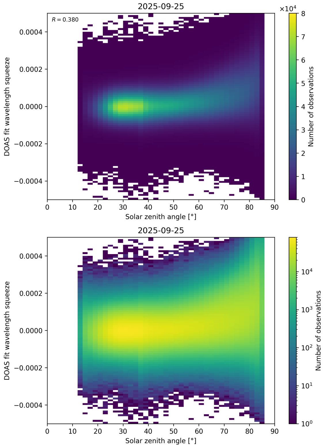
Figure 169: Scatter density plot of “Solar zenith angle” against “DOAS fit wavelength squeeze” for 2025-09-25 to 2025-09-26.
