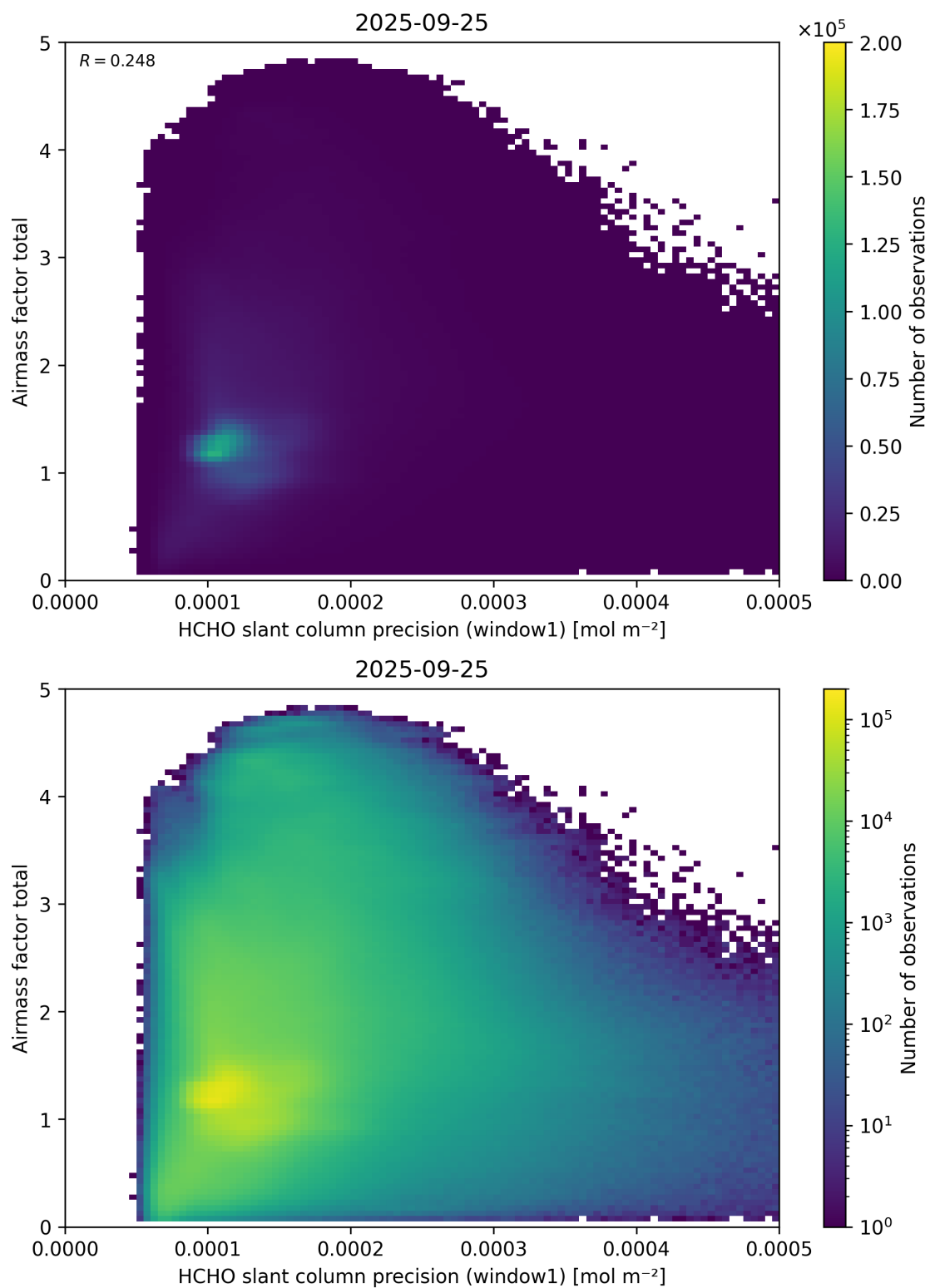
Figure 94: Scatter density plot of “HCHO slant column precision (window1)” against “Airmass factor total” for 2025-09-25 to 2025-09-26.
