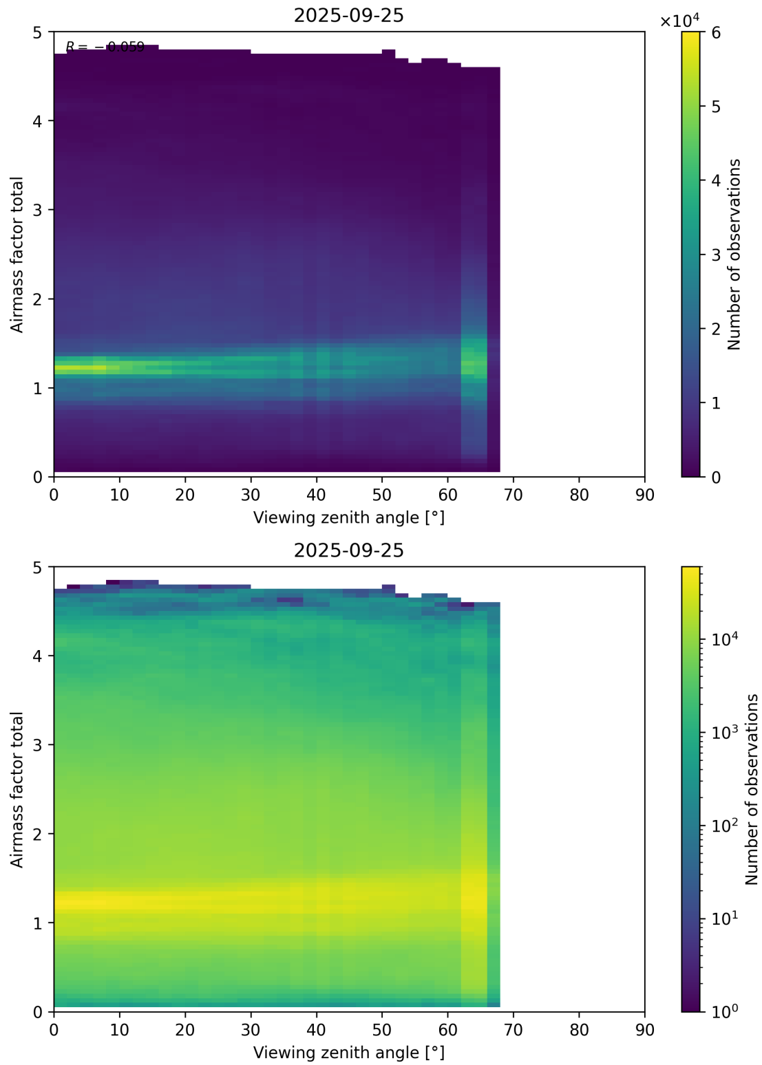
Figure 190: Scatter density plot of “Viewing zenith angle” against “Airmass factor total” for 2025-09-25 to 2025-09-26.
