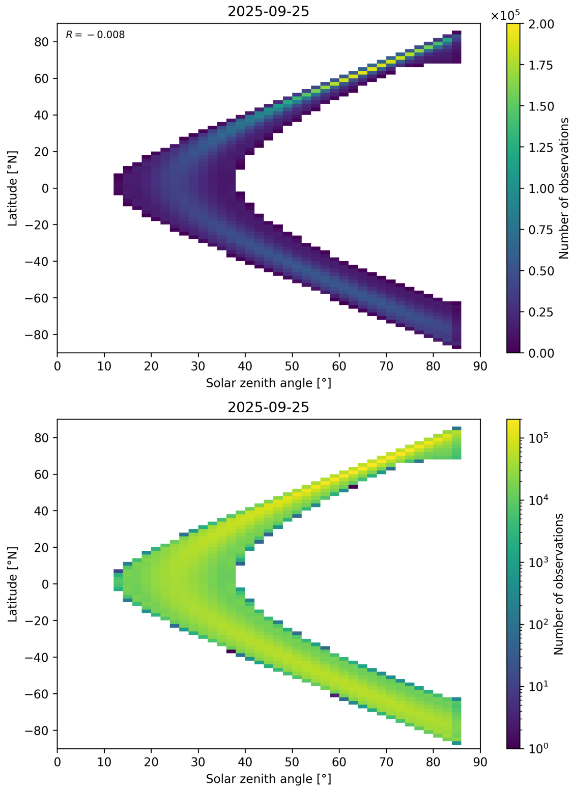
Figure 181: Scatter density plot of “Solar zenith angle” against “Latitude” for 2025-09-25 to 2025-09-26.
