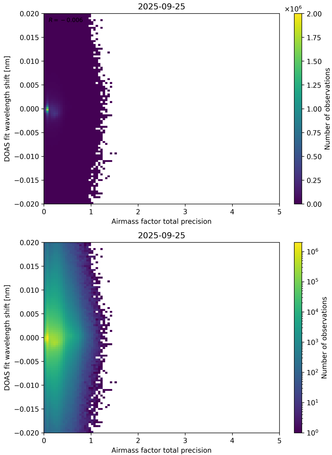
Figure 106: Scatter density plot of “Airmass factor total precision” against “DOAS fit wavelength shift” for 2025-09-25 to 2025-09-26.
