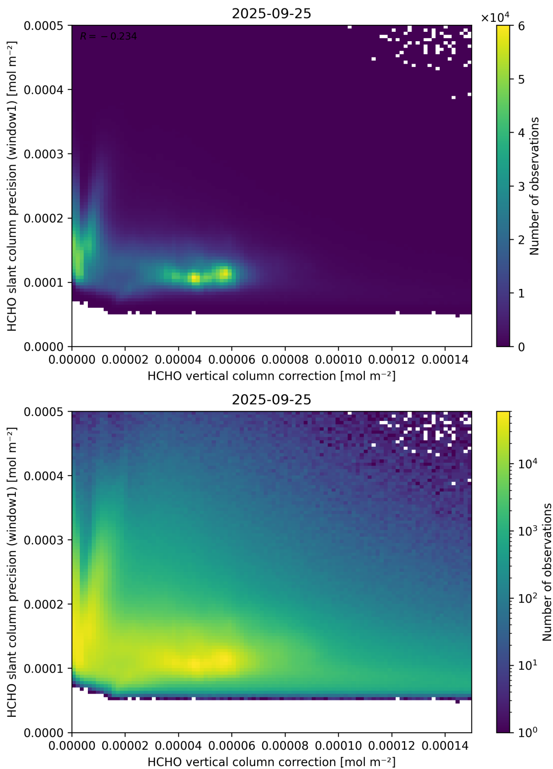
Figure 119: Scatter density plot of “HCHO vertical column correction” against “HCHO slant column precision (window1)” for 2025-09-25 to 2025-09-26.
