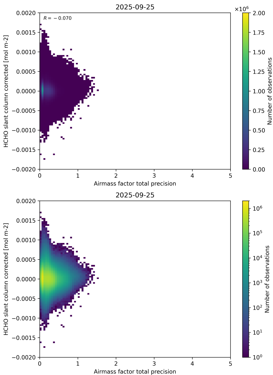
Figure 109: Scatter density plot of “Airmass factor total precision” against “HCHO slant column corrected” for 2025-09-25 to 2025-09-26.
