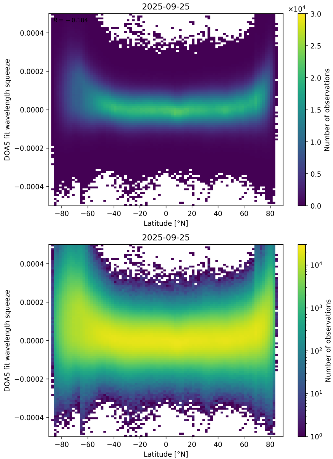
Figure 155: Scatter density plot of “Latitude” against “DOAS fit wavelength squeeze” for 2025-09-25 to 2025-09-26.
