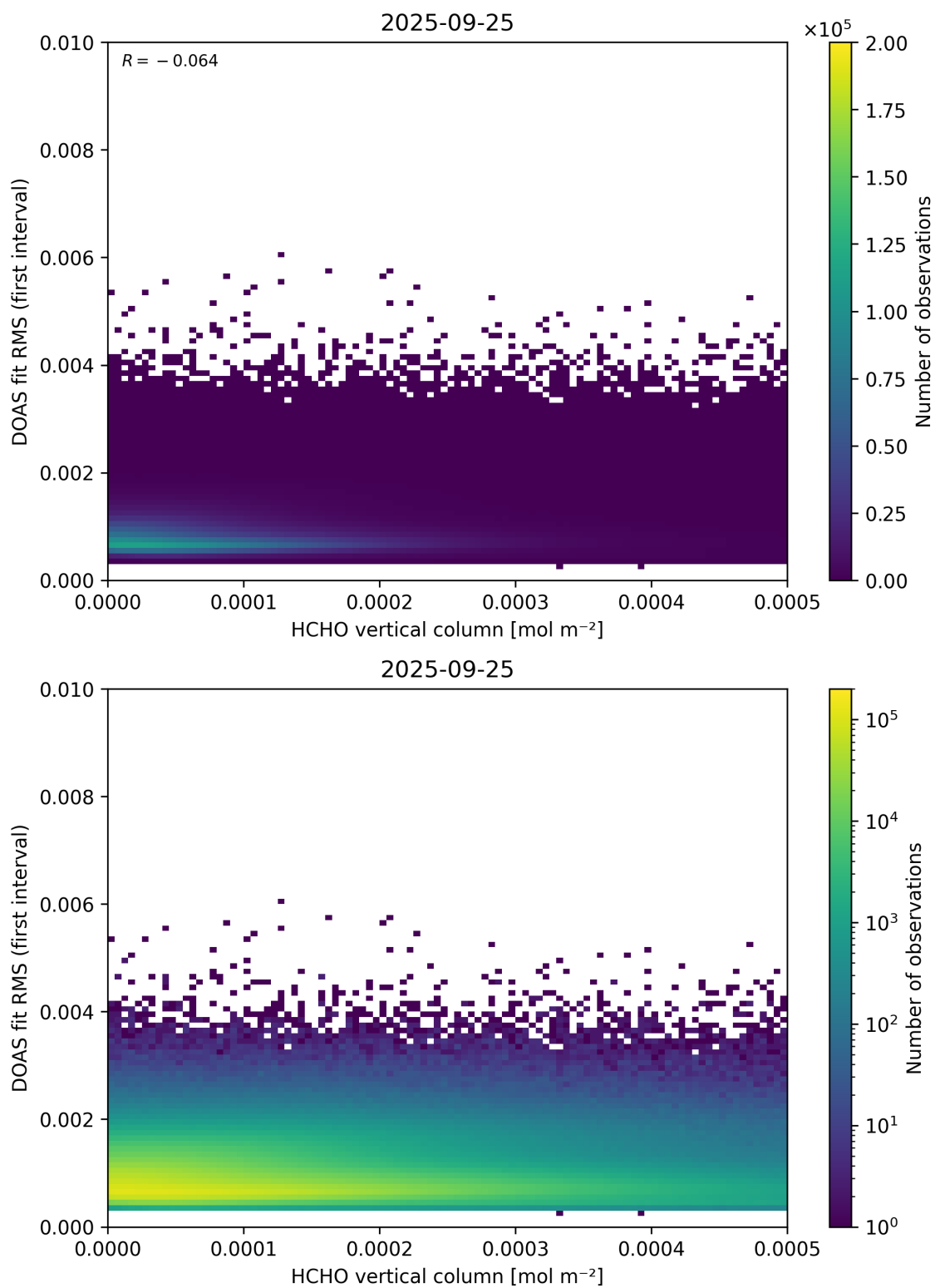
Figure 123: Scatter density plot of “HCHO vertical column” against “DOAS fit RMS (first interval)” for 2025-09-25 to 2025-09-26.
