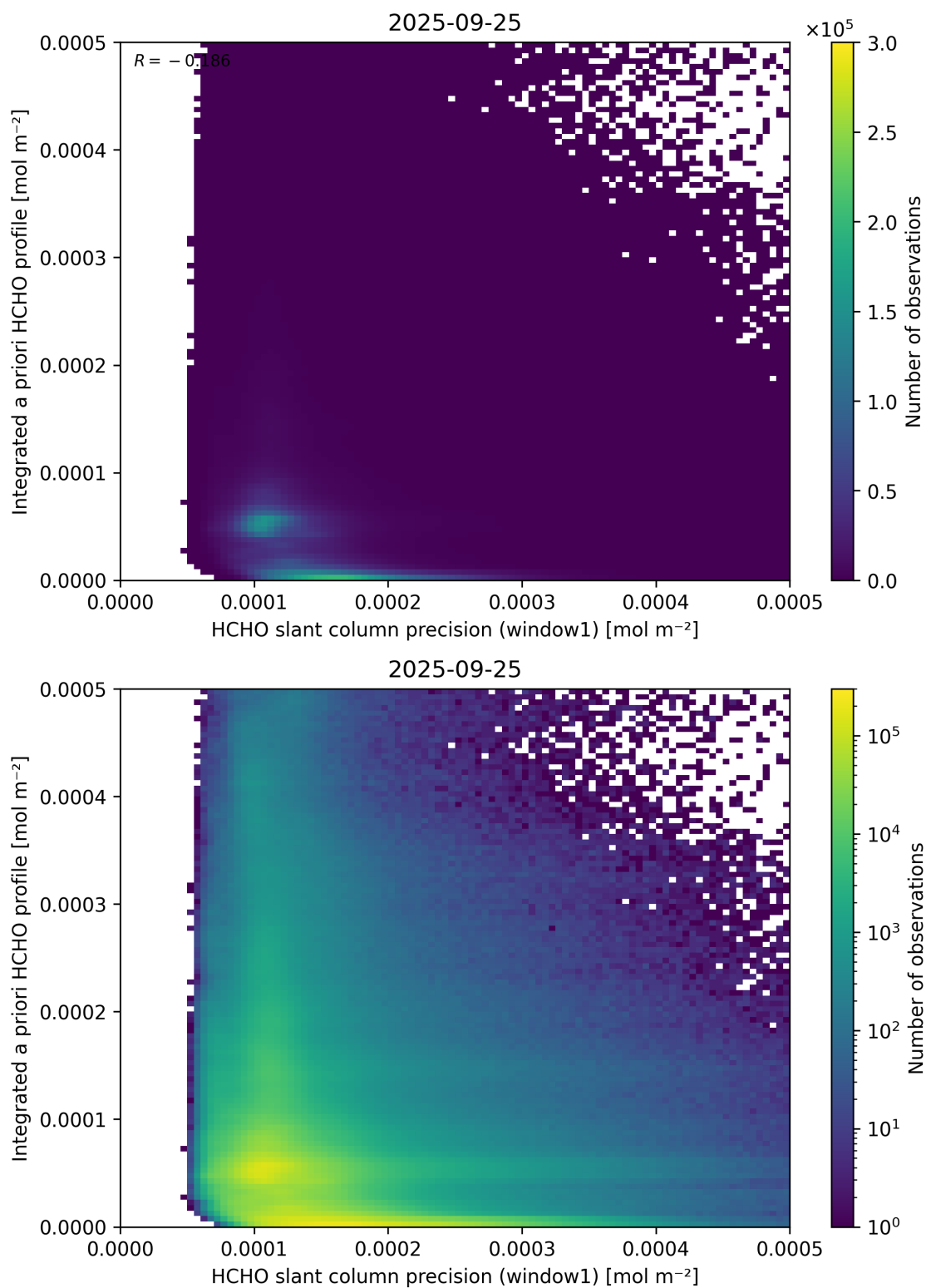
Figure 96: Scatter density plot of “HCHO slant column precision (window1)” against “Integrated a priori HCHO profile” for 2025-09-25 to 2025-09-26.
