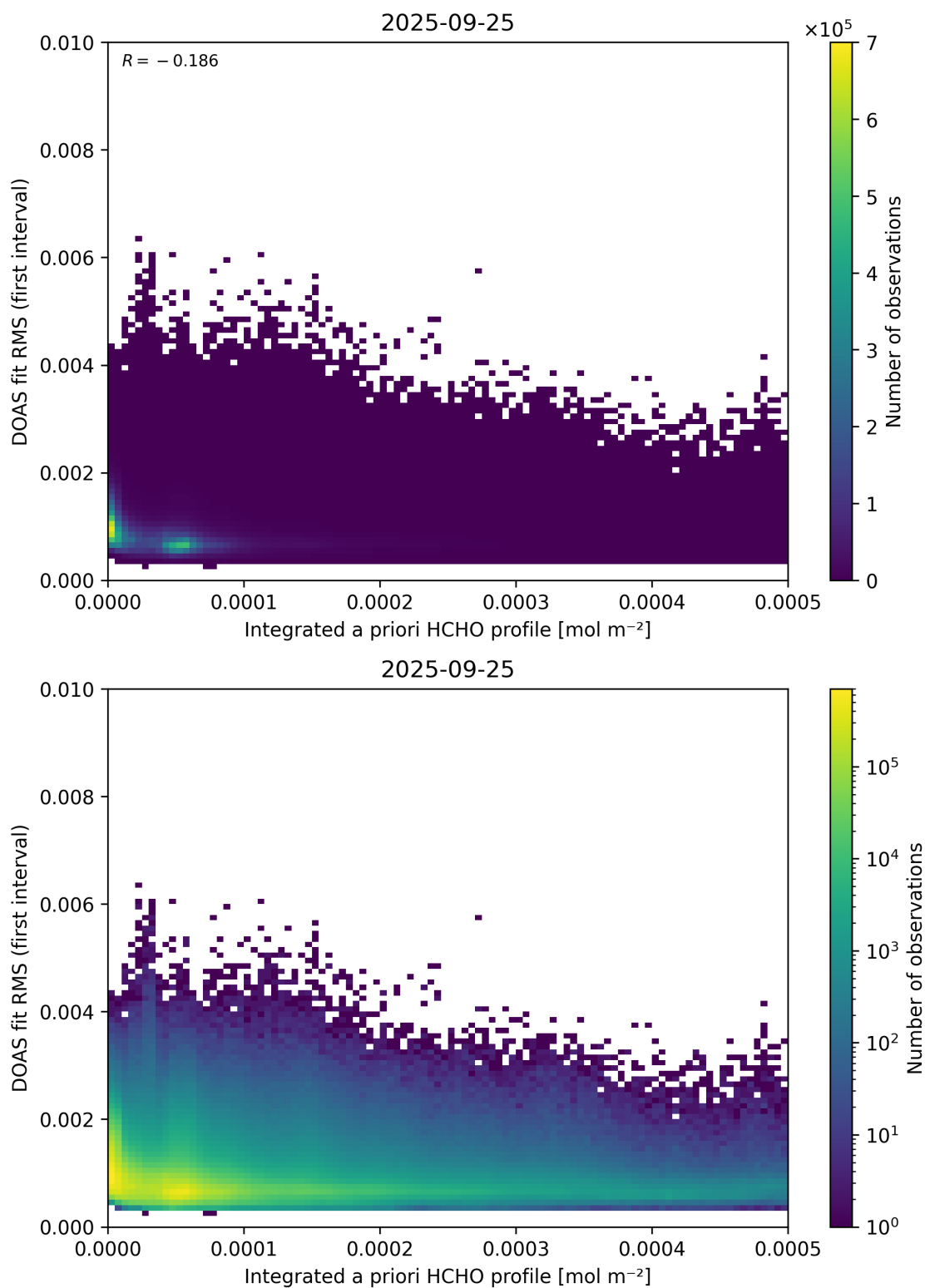
Figure 148: Scatter density plot of “Integrated a priori HCHO profile” against “DOAS fit RMS (first interval)” for 2025-09-25 to 2025-09-26.
