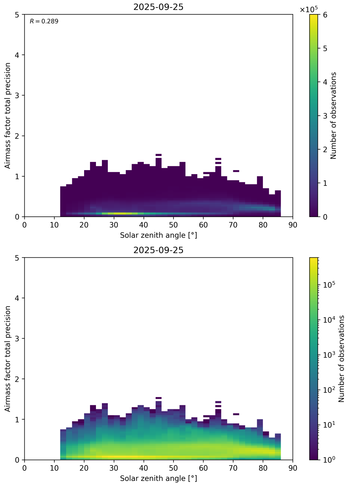
Figure 176: Scatter density plot of “Solar zenith angle” against “Airmass factor total precision” for 2025-09-25 to 2025-09-26.
