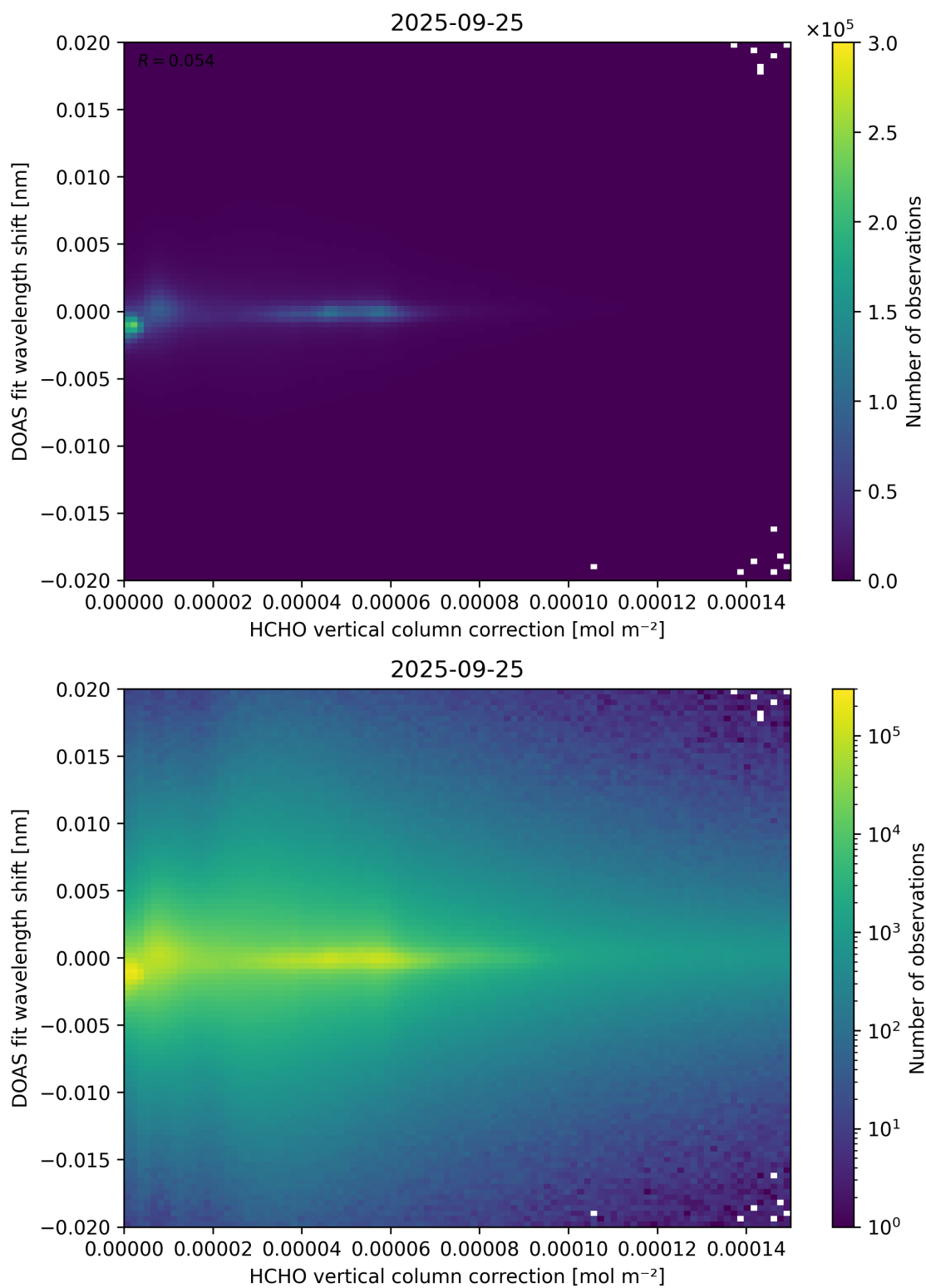
Figure 113: Scatter density plot of “HCHO vertical column correction” against “DOAS fit wavelength shift” for 2025-09-25 to 2025-09-26.
