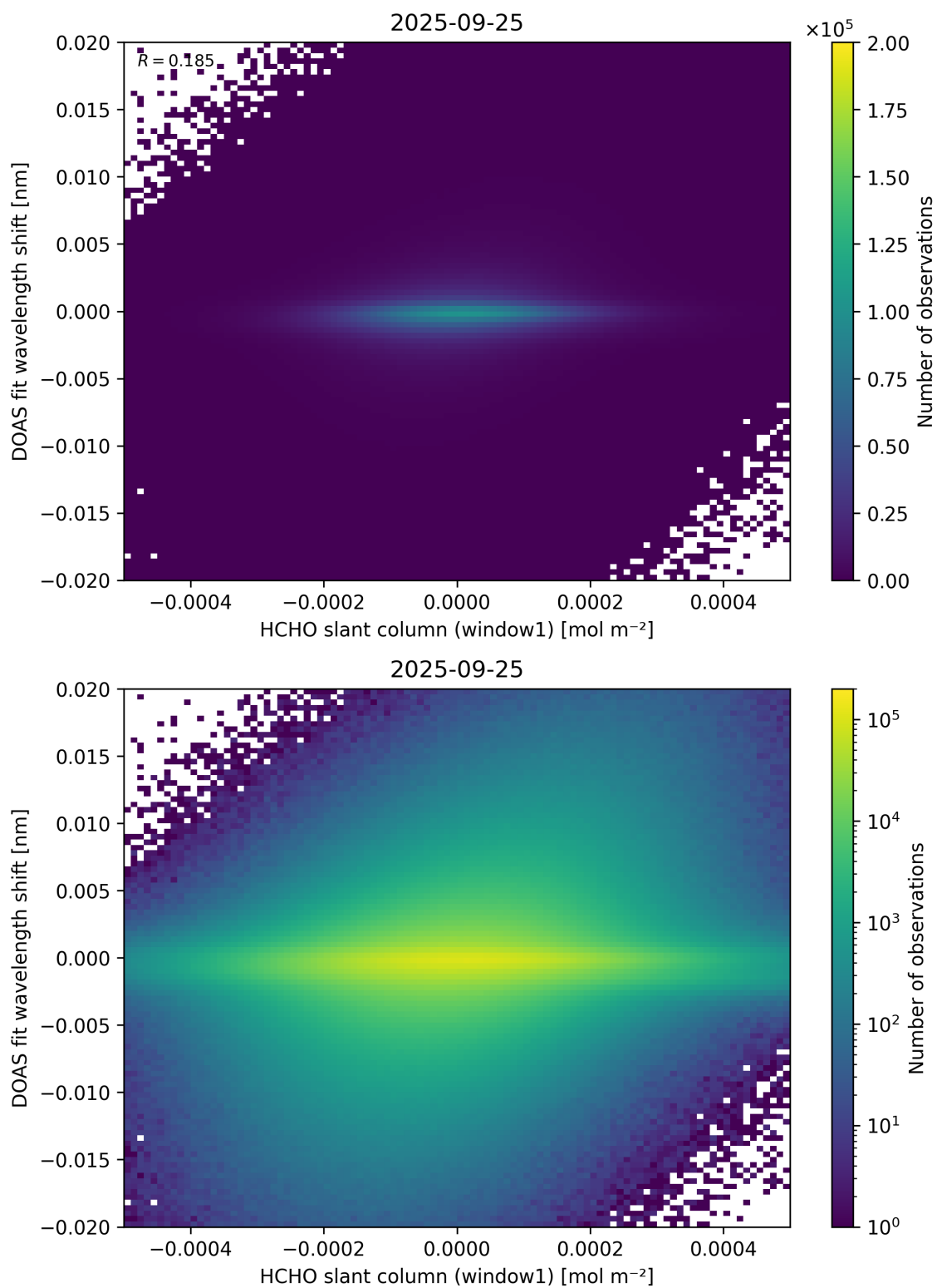
Figure 79: Scatter density plot of “HCHO slant column (window1)” against “DOAS fit wavelength shift” for 2025-09-25 to 2025-09-26.
