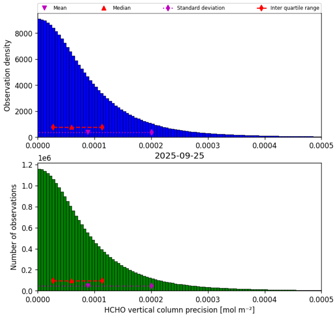
Figure 36: Histogram of “HCHO vertical column precision” for 2025-09-25 to 2025-09-26
