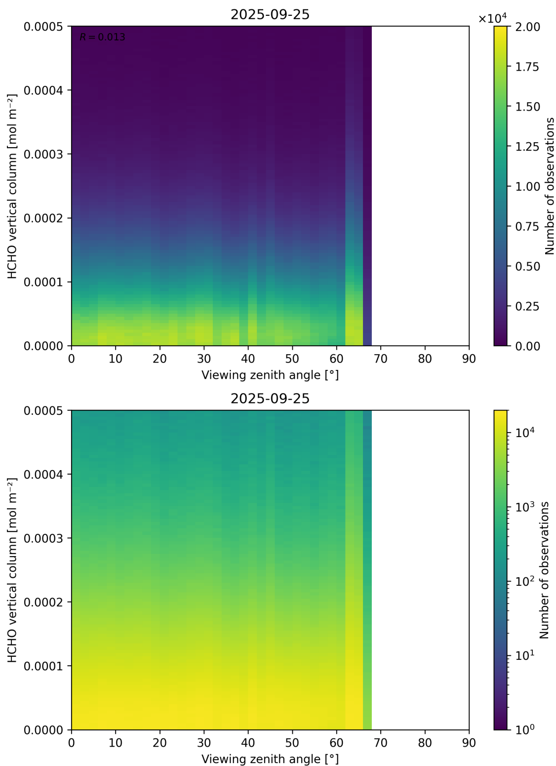
Figure 192: Scatter density plot of “Viewing zenith angle” against “HCHO vertical column” for 2025-09-25 to 2025-09-26.
