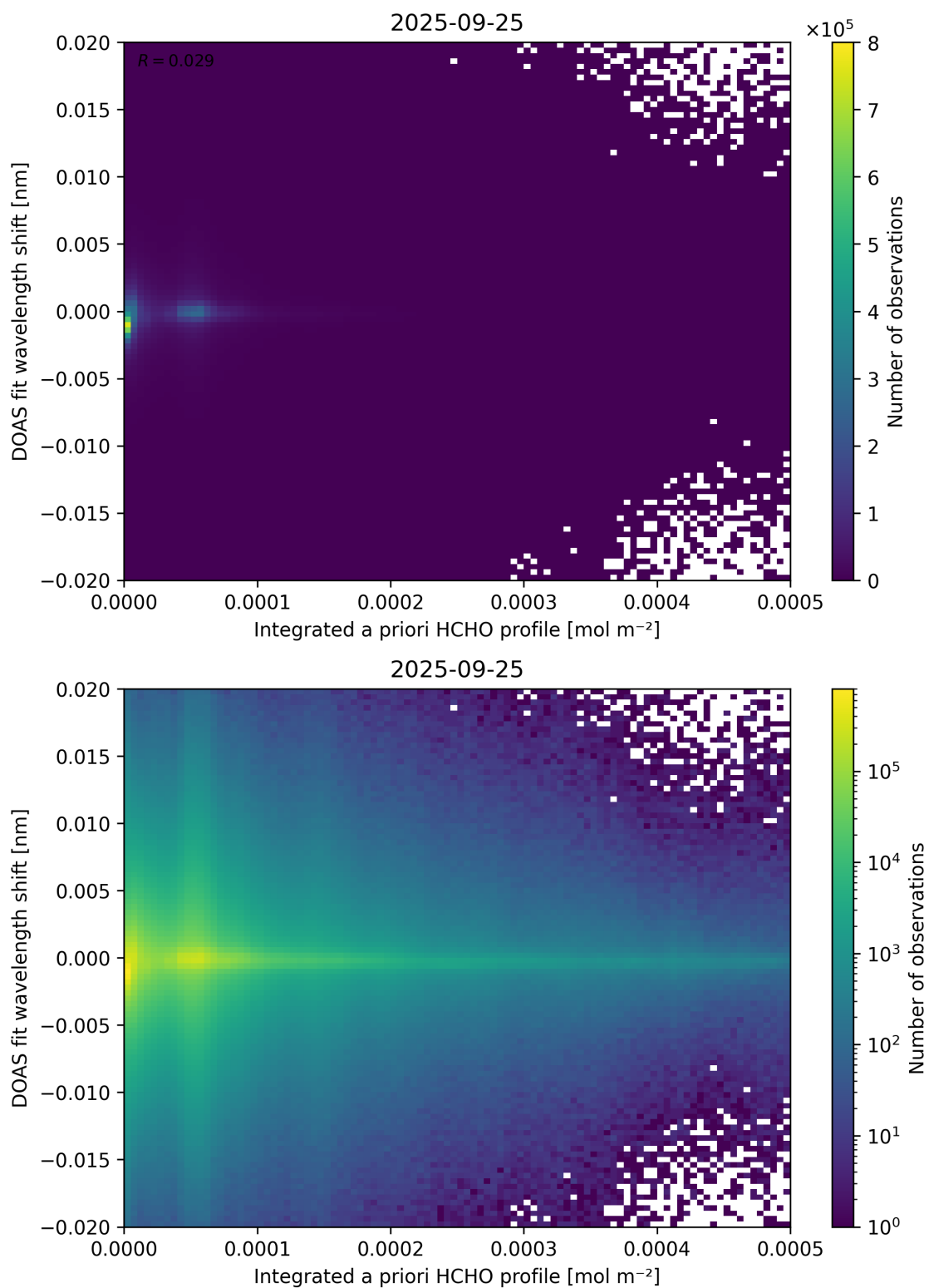
Figure 149: Scatter density plot of “Integrated a priori HCHO profile” against “DOAS fit wavelength shift” for 2025-09-25 to 2025-09-26.
