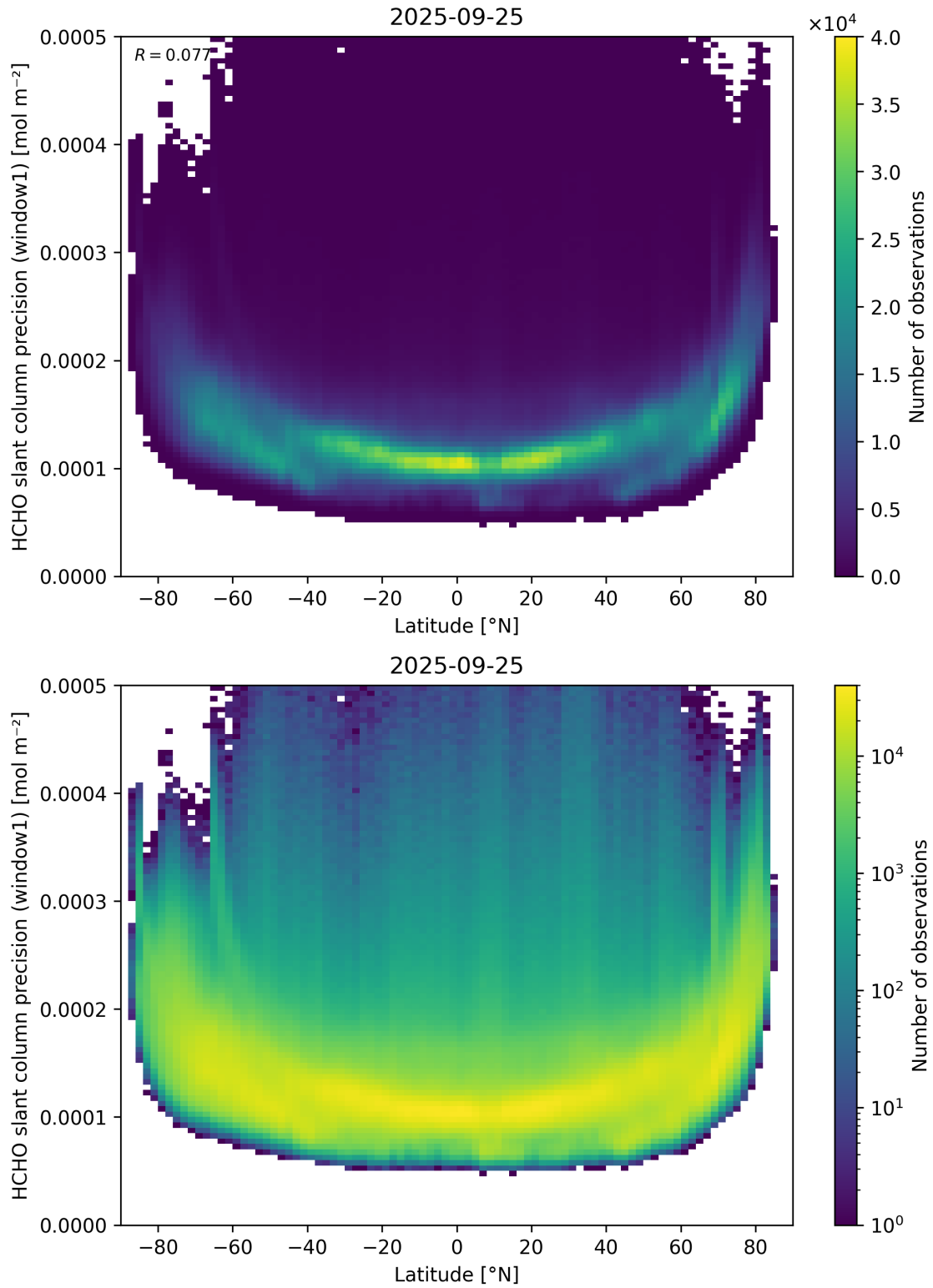
Figure 160: Scatter density plot of “Latitude” against “HCHO slant column precision (window1)” for 2025-09-25 to 2025-09-26.
