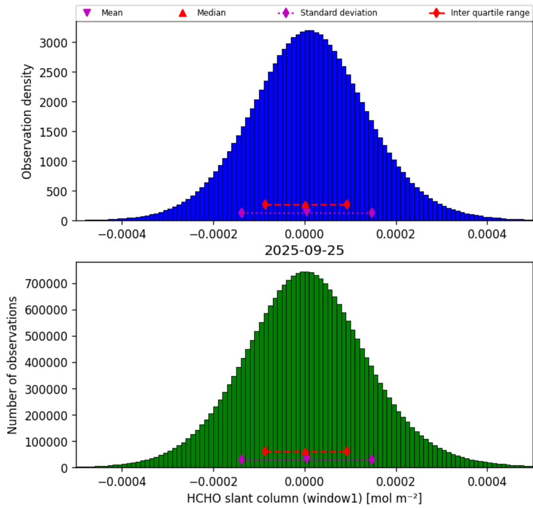
Figure 38: Histogram of “HCHO slant column (window1)” for 2025-09-25 to 2025-09-26
