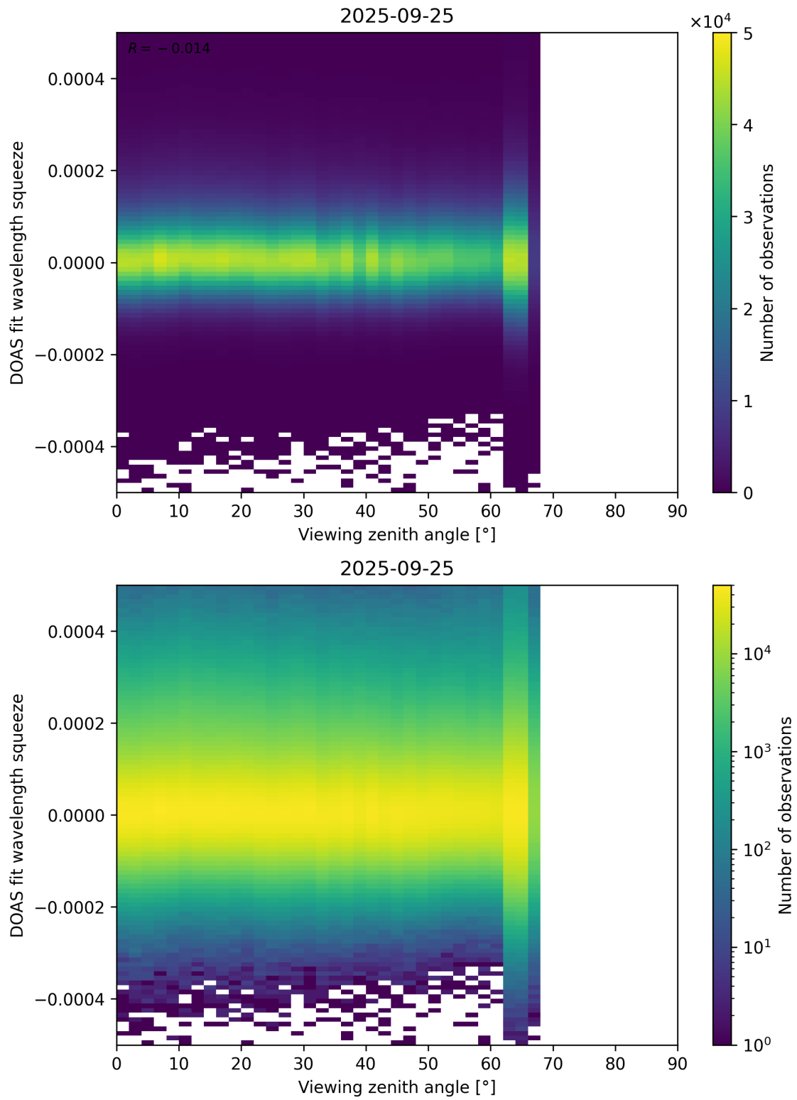
Figure 184: Scatter density plot of “Viewing zenith angle” against “DOAS fit wavelength squeeze” for 2025-09-25 to 2025-09-26.
