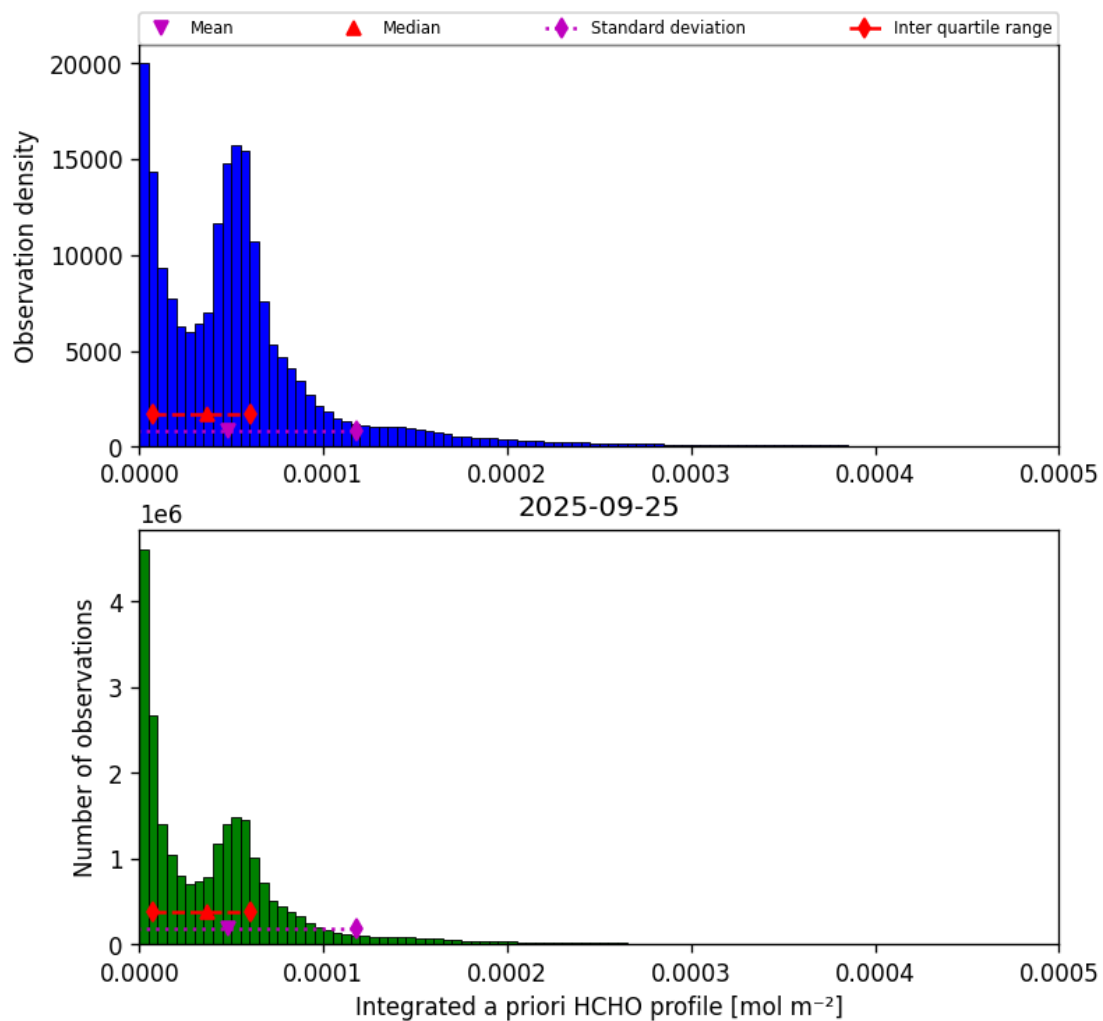
Figure 43: Histogram of “Integrated a priori HCHO profile” for 2025-09-25 to 2025-09-26
