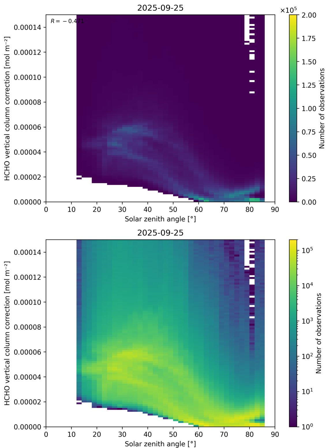
Figure 178: Scatter density plot of “Solar zenith angle” against “HCHO vertical column correction” for 2025-09-25 to 2025-09-26.
