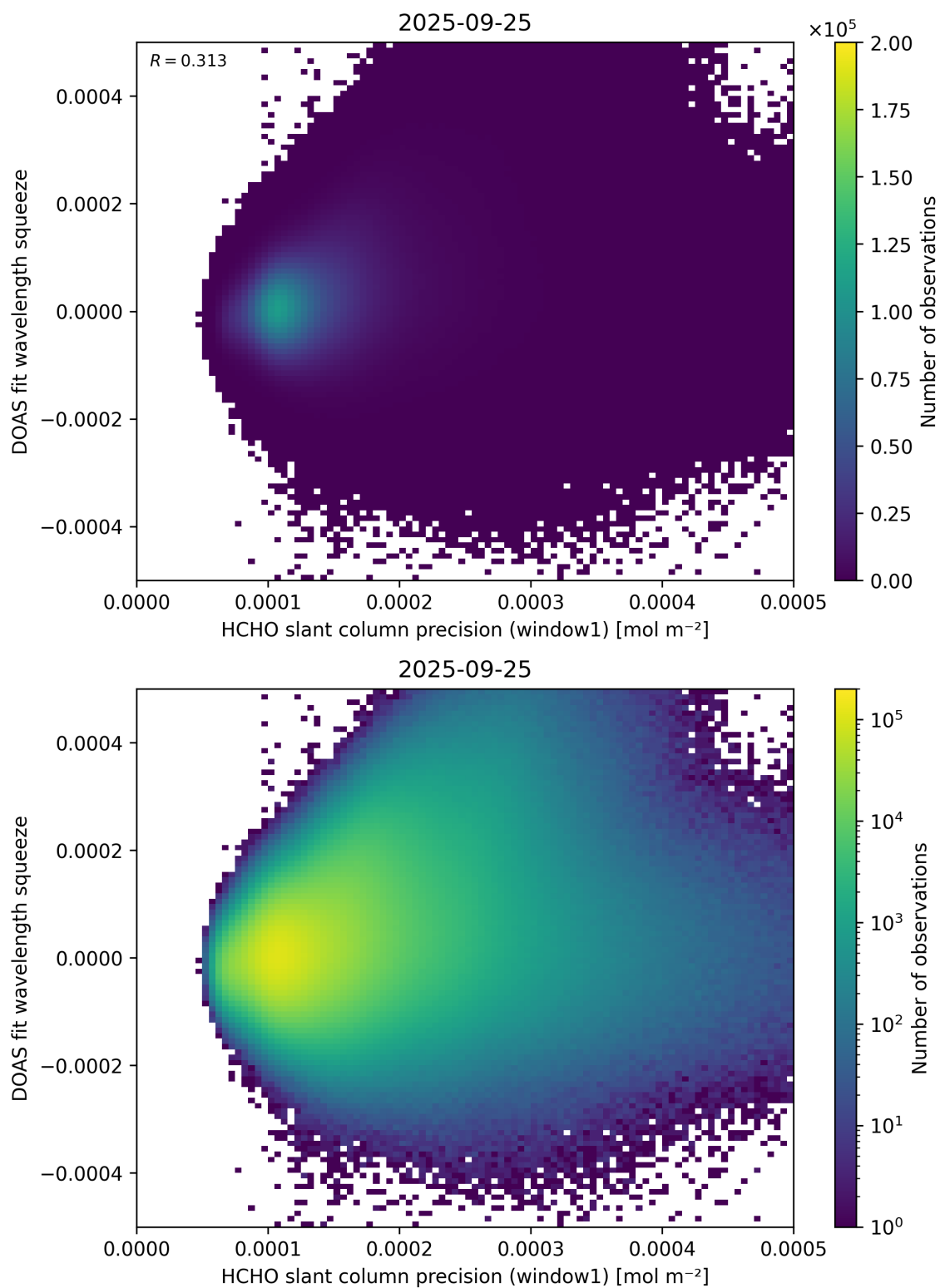
Figure 90: Scatter density plot of “HCHO slant column precision (window1)” against “DOAS fit wavelength squeeze” for 2025-09-25 to 2025-09-26.
