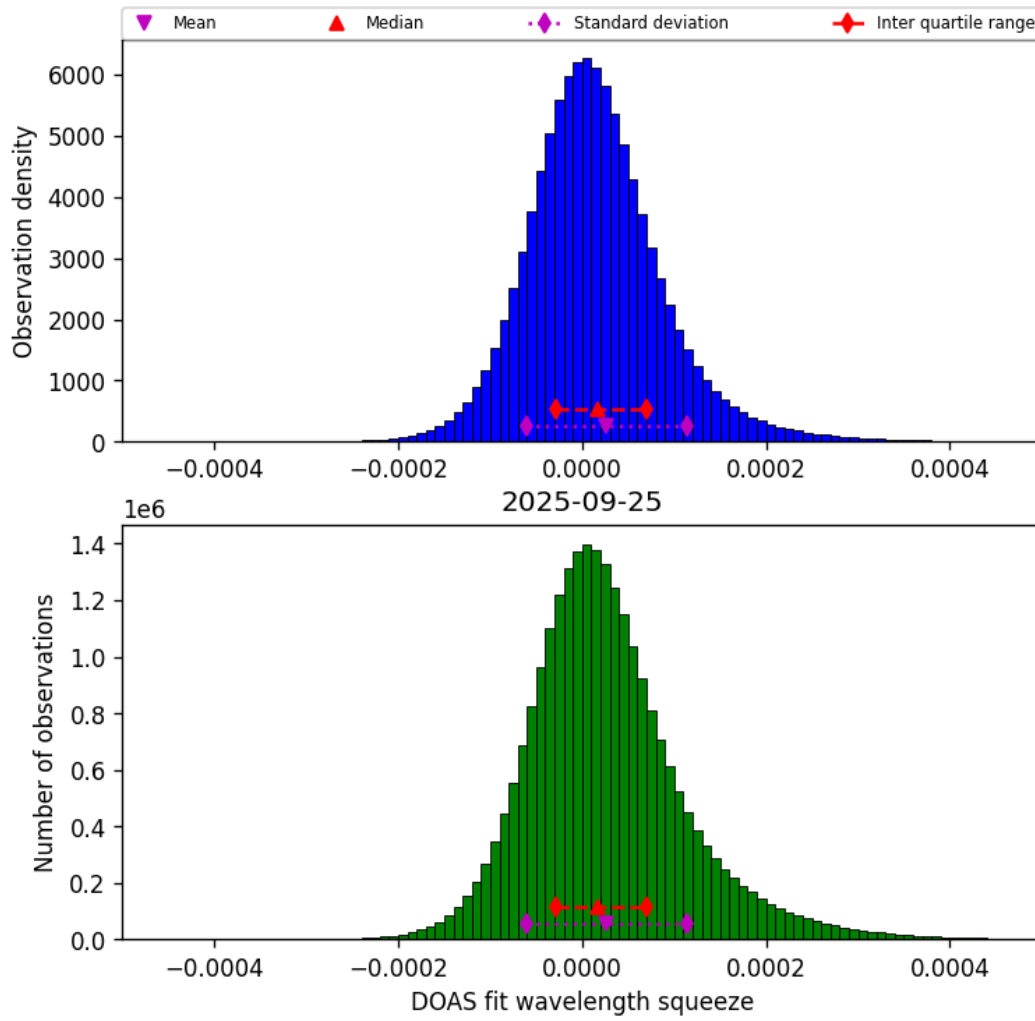
Figure 45: Histogram of “DOAS fit wavelength squeeze” for 2025-09-25 to 2025-09-26
