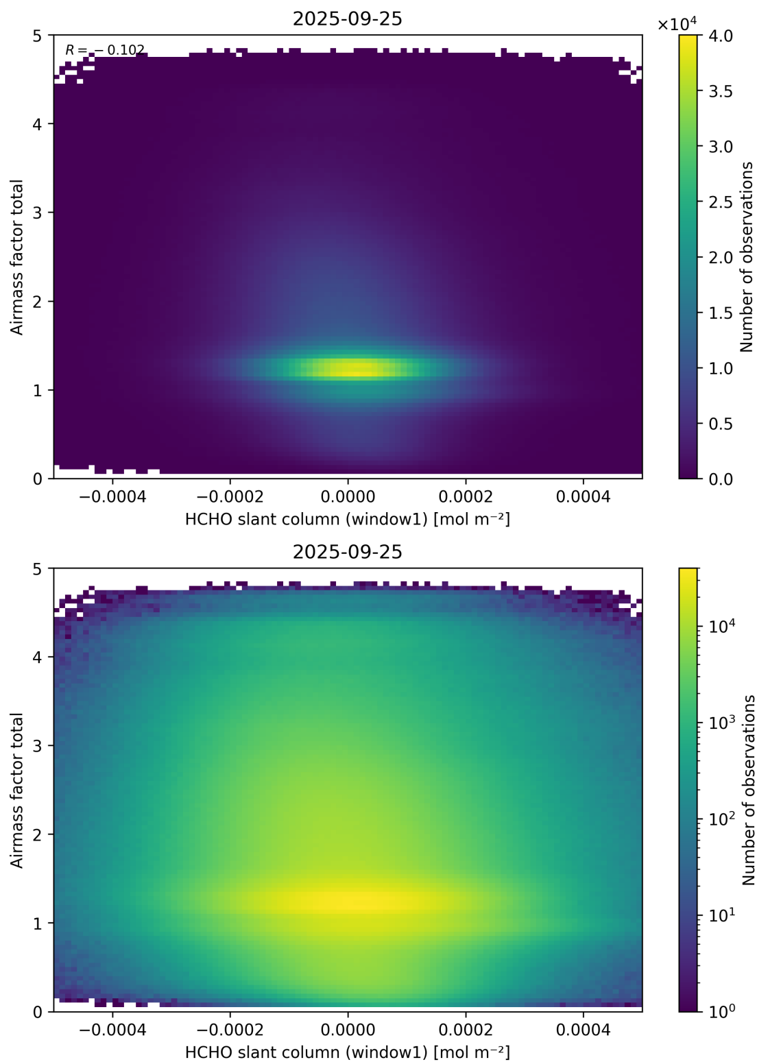
Figure 85: Scatter density plot of “HCHO slant column (window1)” against “Airmass factor total” for 2025-09-25 to 2025-09-26.
