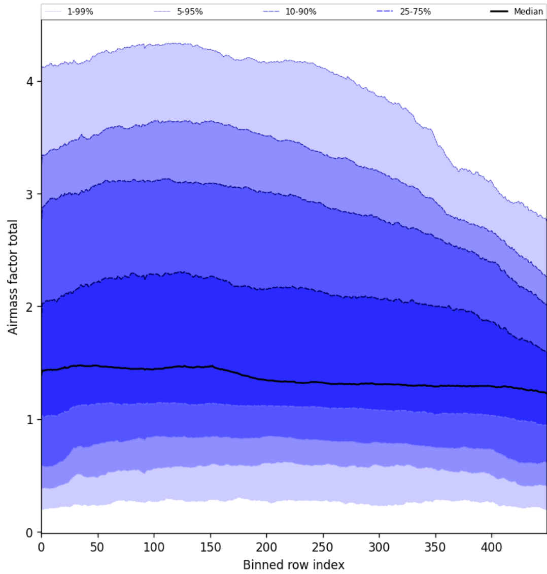
Figure 54: Along track statistics of “Airmass factor total” for 2025-09-25 to 2025-09-26
