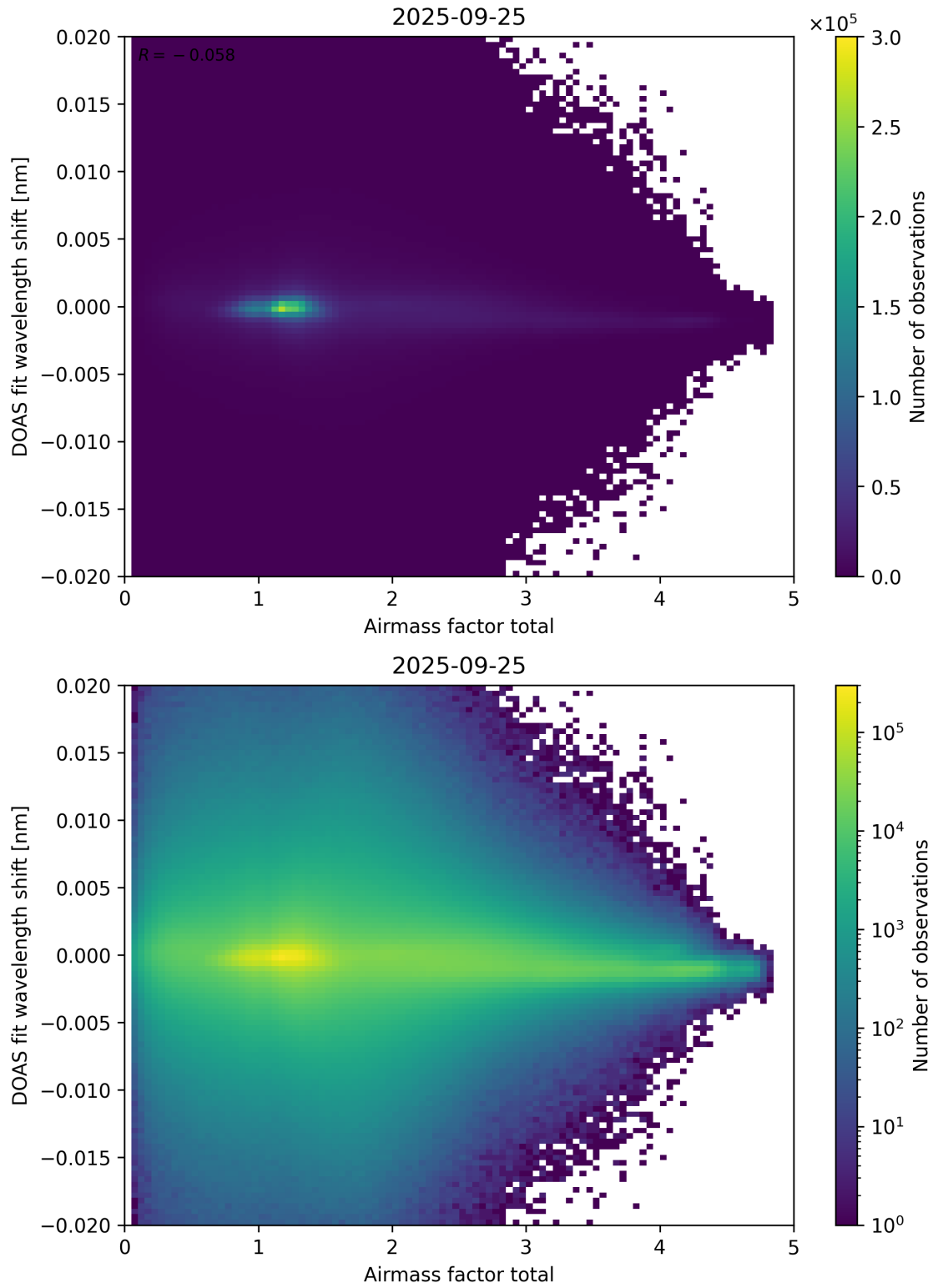
Figure 98: Scatter density plot of “Airmass factor total” against “DOAS fit wavelength shift” for 2025-09-25 to 2025-09-26.
