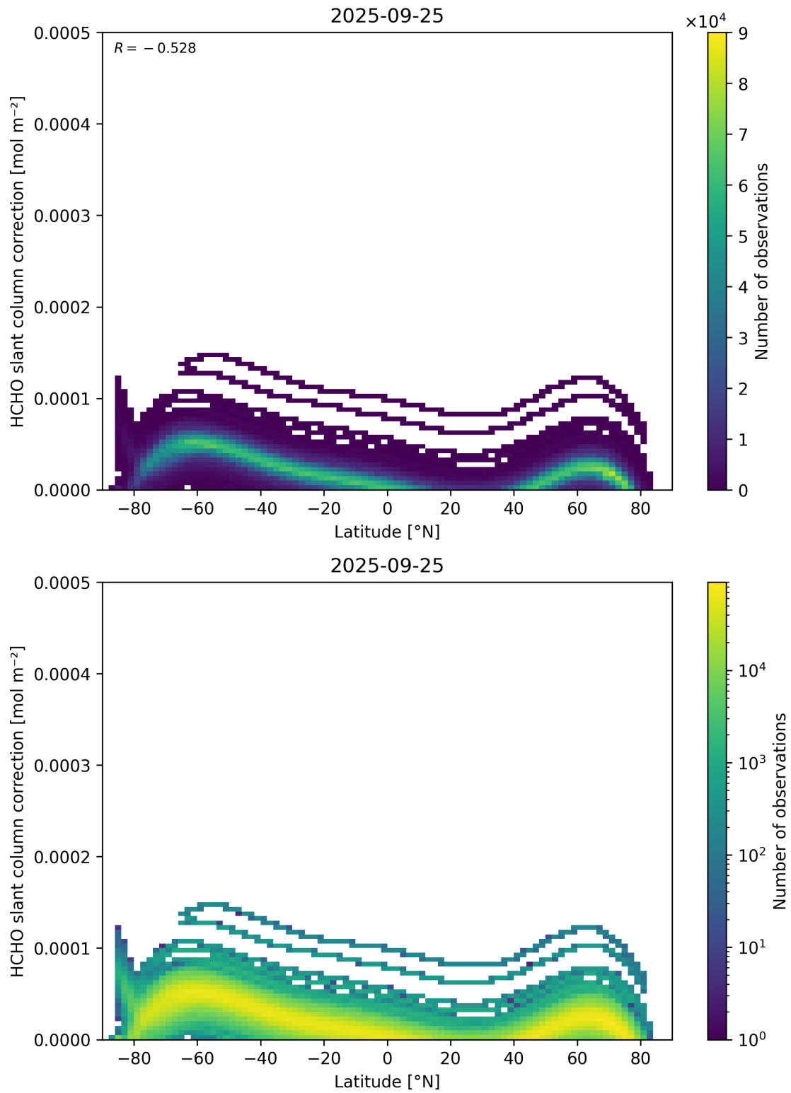
Figure 158: Scatter density plot of “Latitude” against “HCHO slant column correction” for 2025-09-25 to 2025-09-26.
