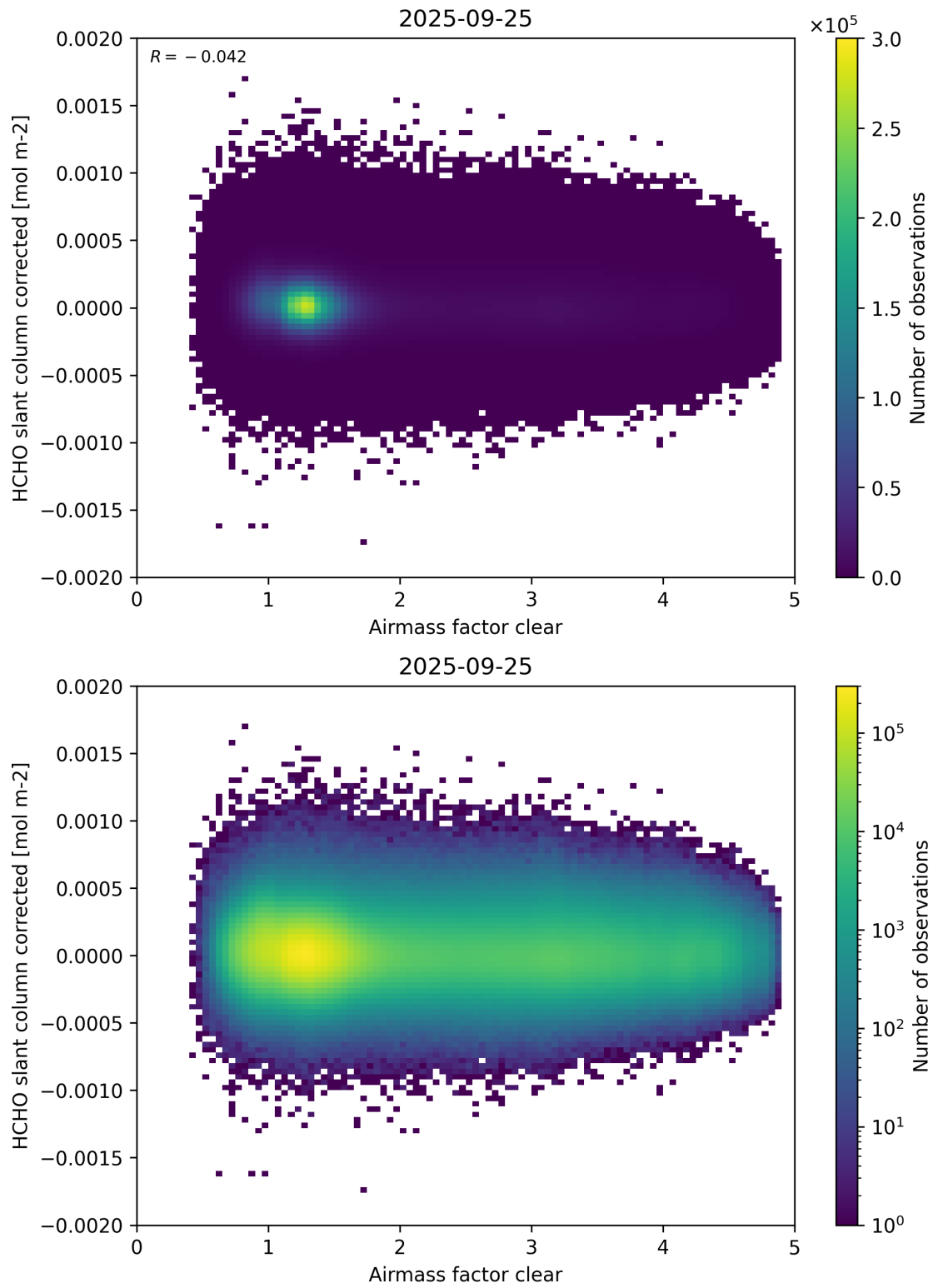
Figure 74: Scatter density plot of “Airmass factor clear” against “HCHO slant column corrected” for 2025-09-25 to 2025-09-26.
