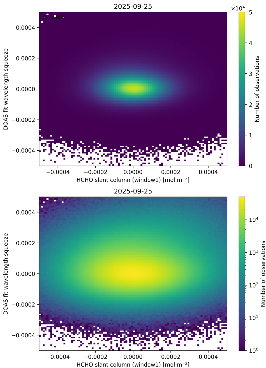
Figure 80: Scatter density plot of “HCHO slant column (window1)” against “DOAS fit wavelength squeeze” for 2025-09-25 to 2025-09-26.
