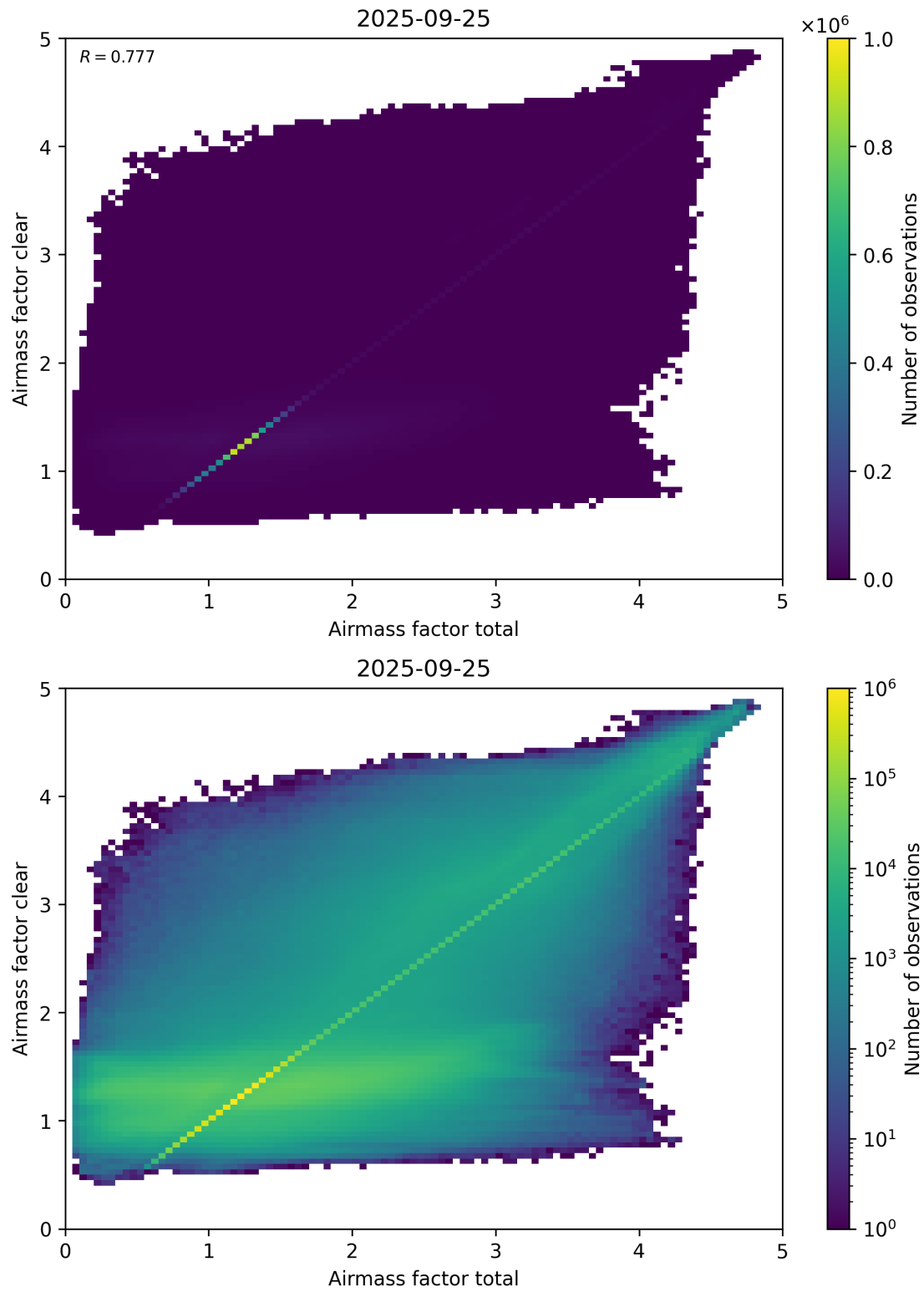
Figure 100: Scatter density plot of “Airmass factor total” against “Airmass factor clear” for 2025-09-25 to 2025-09-26.
