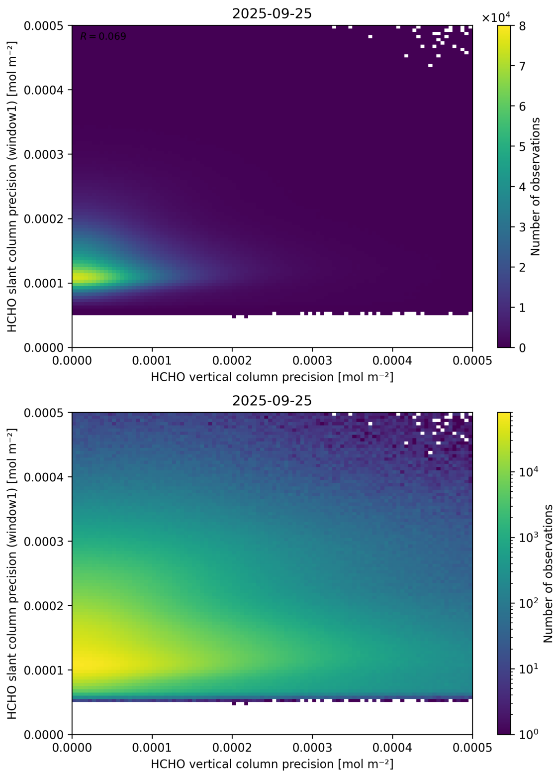
Figure 143: Scatter density plot of “HCHO vertical column precision” against “HCHO slant column precision (window1)” for 2025-09-25 to 2025-09-26.
