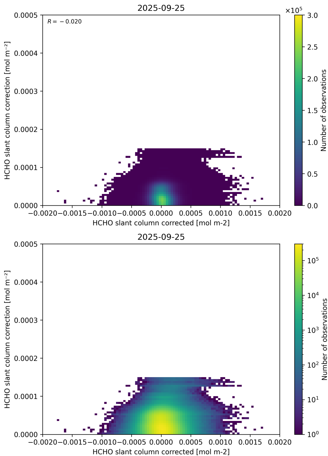
Figure 77: Scatter density plot of “HCHO slant column corrected” against “HCHO slant column correction” for 2025-09-25 to 2025-09-26.
