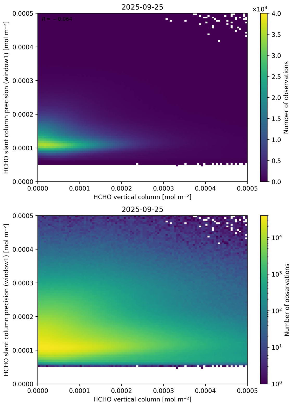
Figure 130: Scatter density plot of “HCHO vertical column” against “HCHO slant column precision (window1)” for 2025-09-25 to 2025-09-26.
