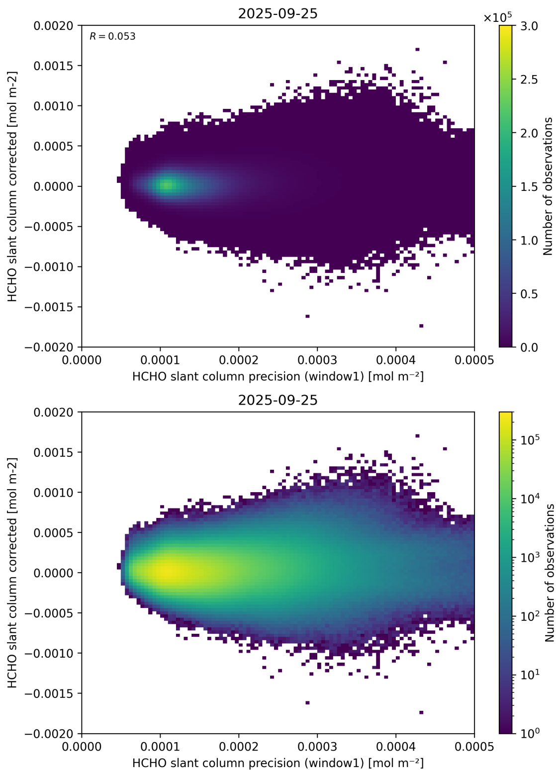
Figure 92: Scatter density plot of “HCHO slant column precision (window1)” against “HCHO slant column corrected” for 2025-09-25 to 2025-09-26.
