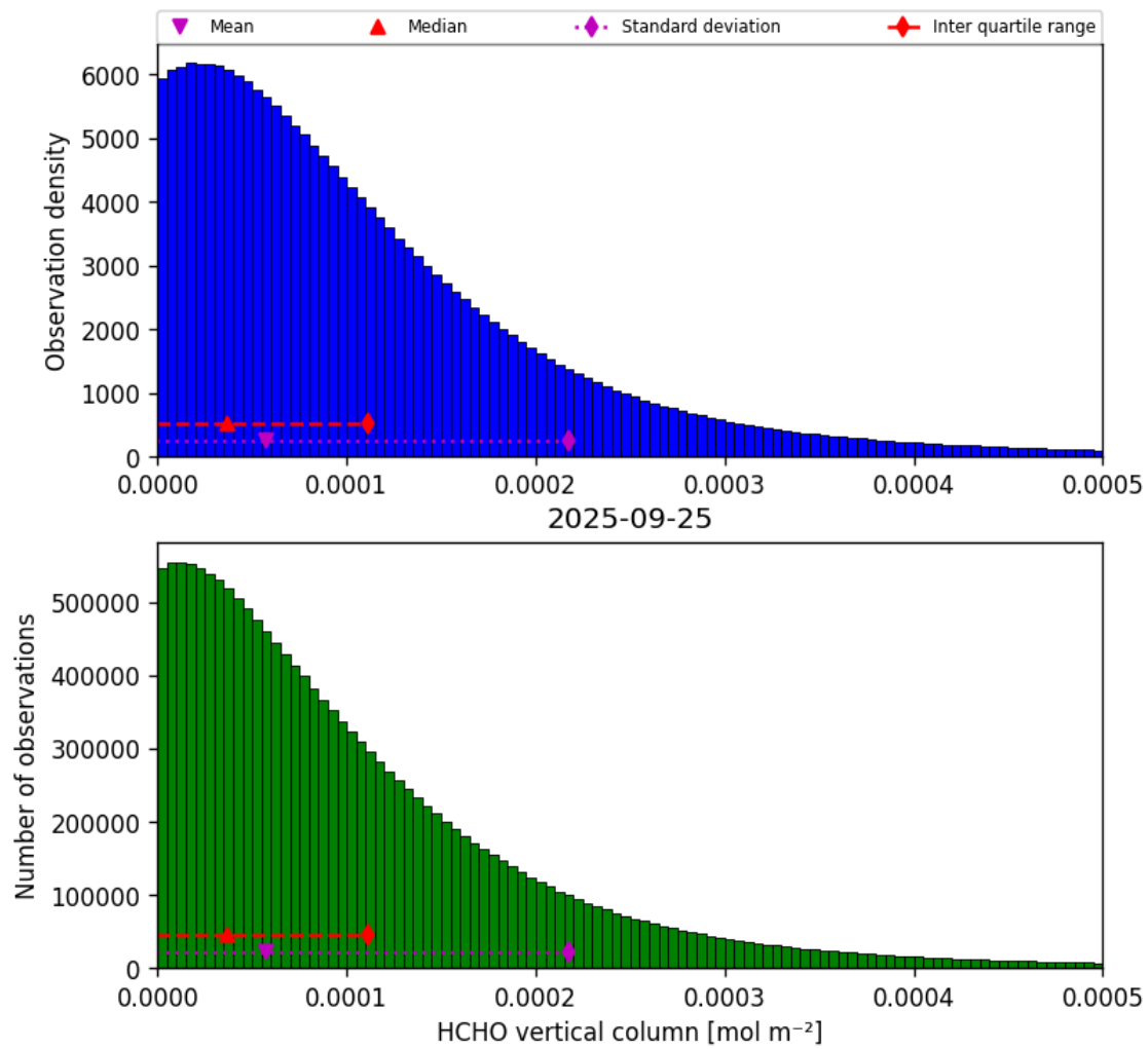
Figure 35: Histogram of “HCHO vertical column” for 2025-09-25 to 2025-09-26
