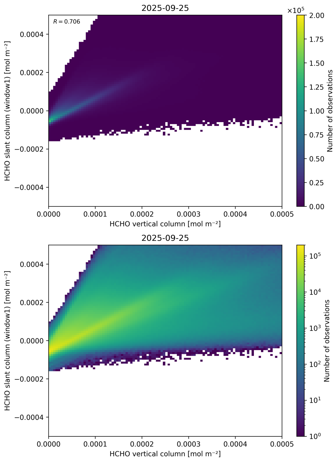
Figure 129: Scatter density plot of “HCHO vertical column” against “HCHO slant column (window1)” for 2025-09-25 to 2025-09-26.
