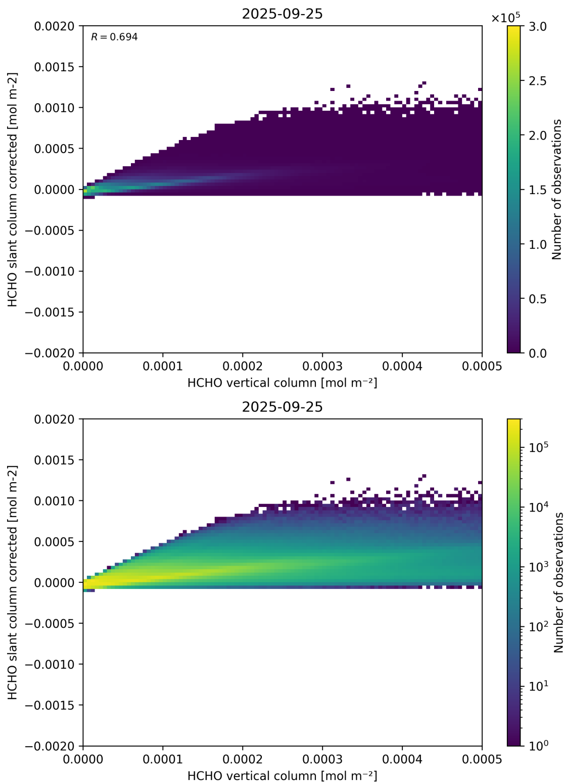
Figure 127: Scatter density plot of “HCHO vertical column” against “HCHO slant column corrected” for 2025-09-25 to 2025-09-26.
