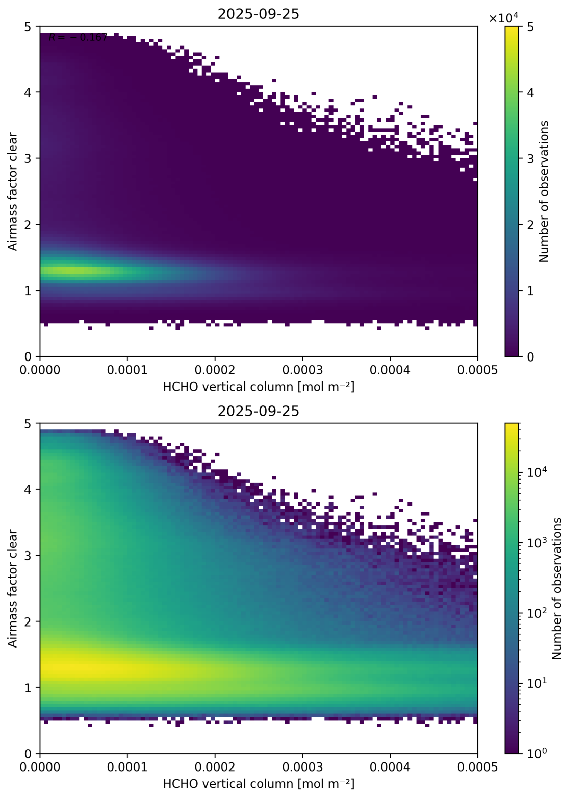
Figure 126: Scatter density plot of “HCHO vertical column” against “Airmass factor clear” for 2025-09-25 to 2025-09-26.
