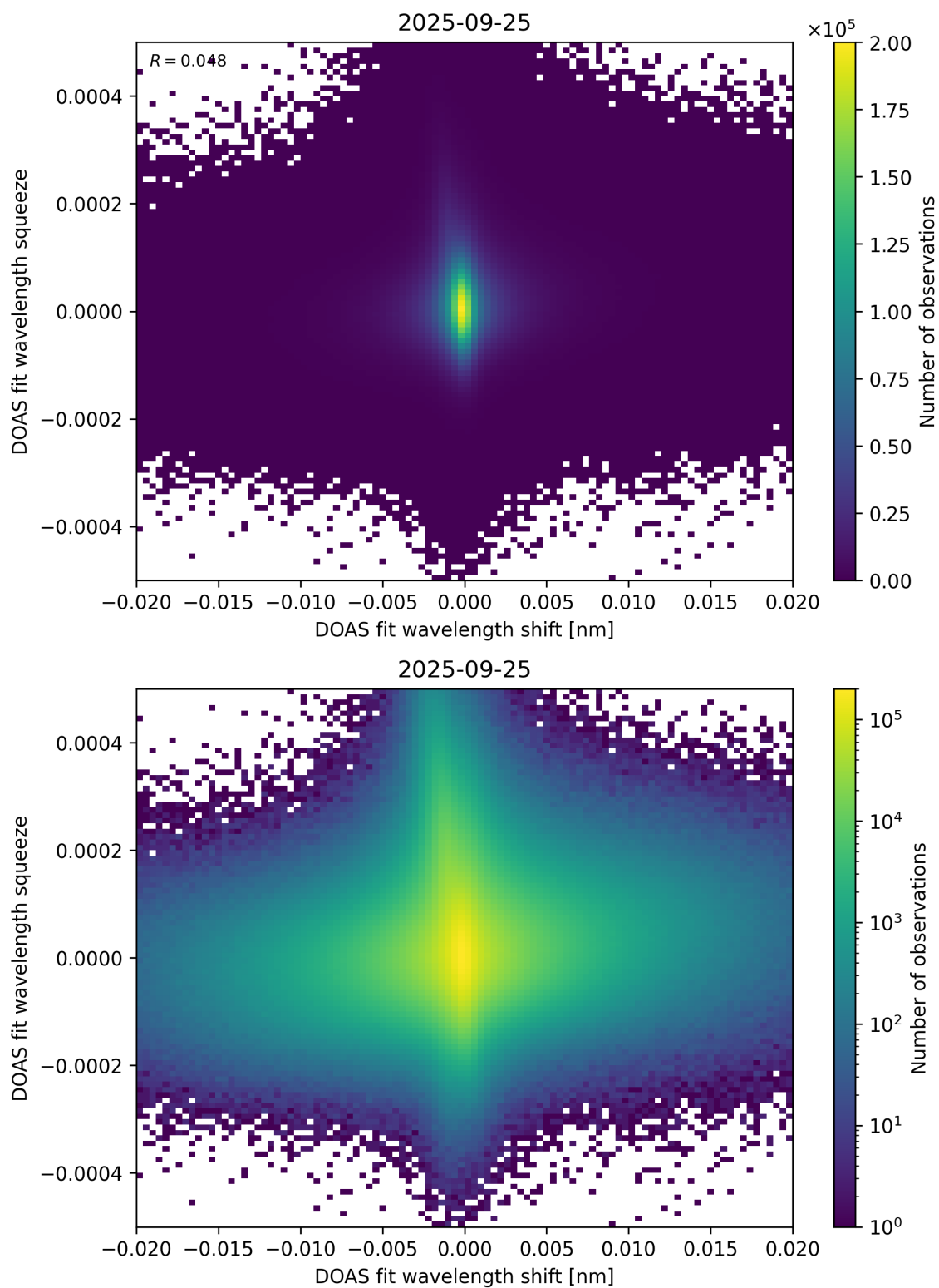
Figure 65: Scatter density plot of “DOAS fit wavelength shift” against “DOAS fit wavelength squeeze” for 2025-09-25 to 2025-09-26.
