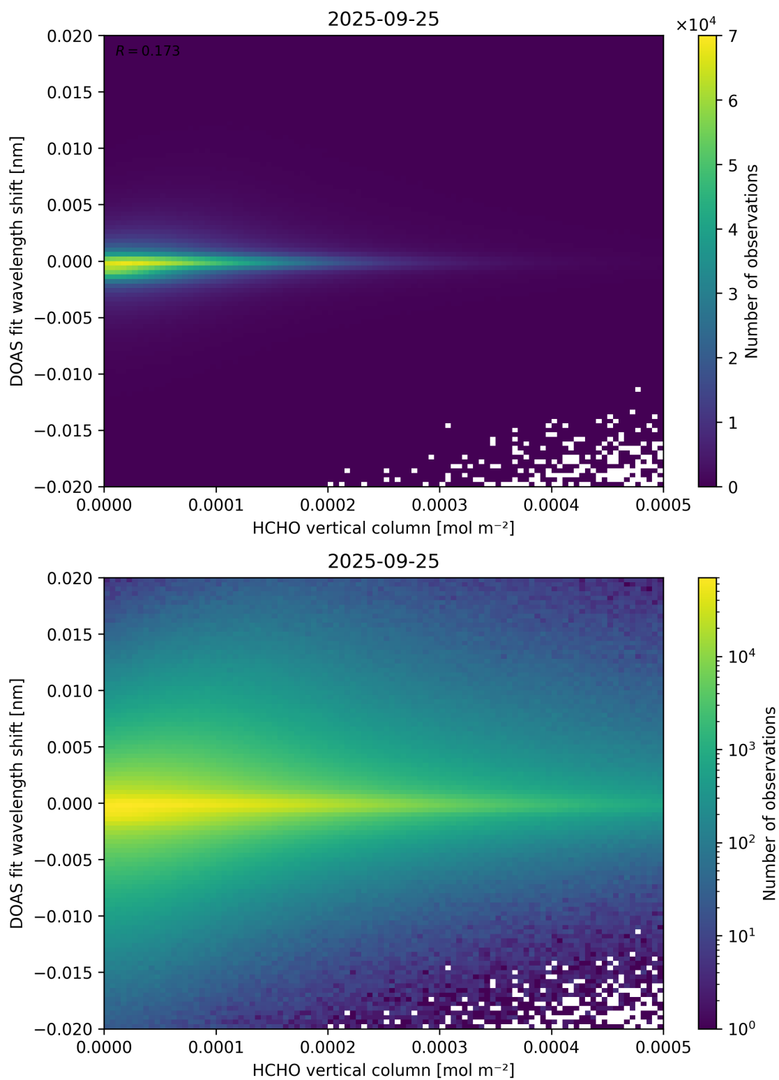
Figure 124: Scatter density plot of “HCHO vertical column” against “DOAS fit wavelength shift” for 2025-09-25 to 2025-09-26.
