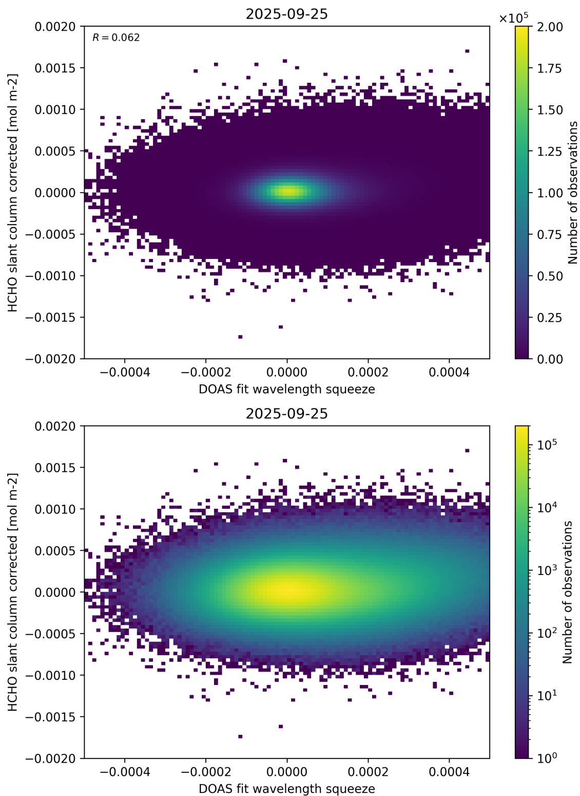
Figure 69: Scatter density plot of “DOAS fit wavelength squeeze” against “HCHO slant column corrected” for 2025-09-25 to 2025-09-26.
