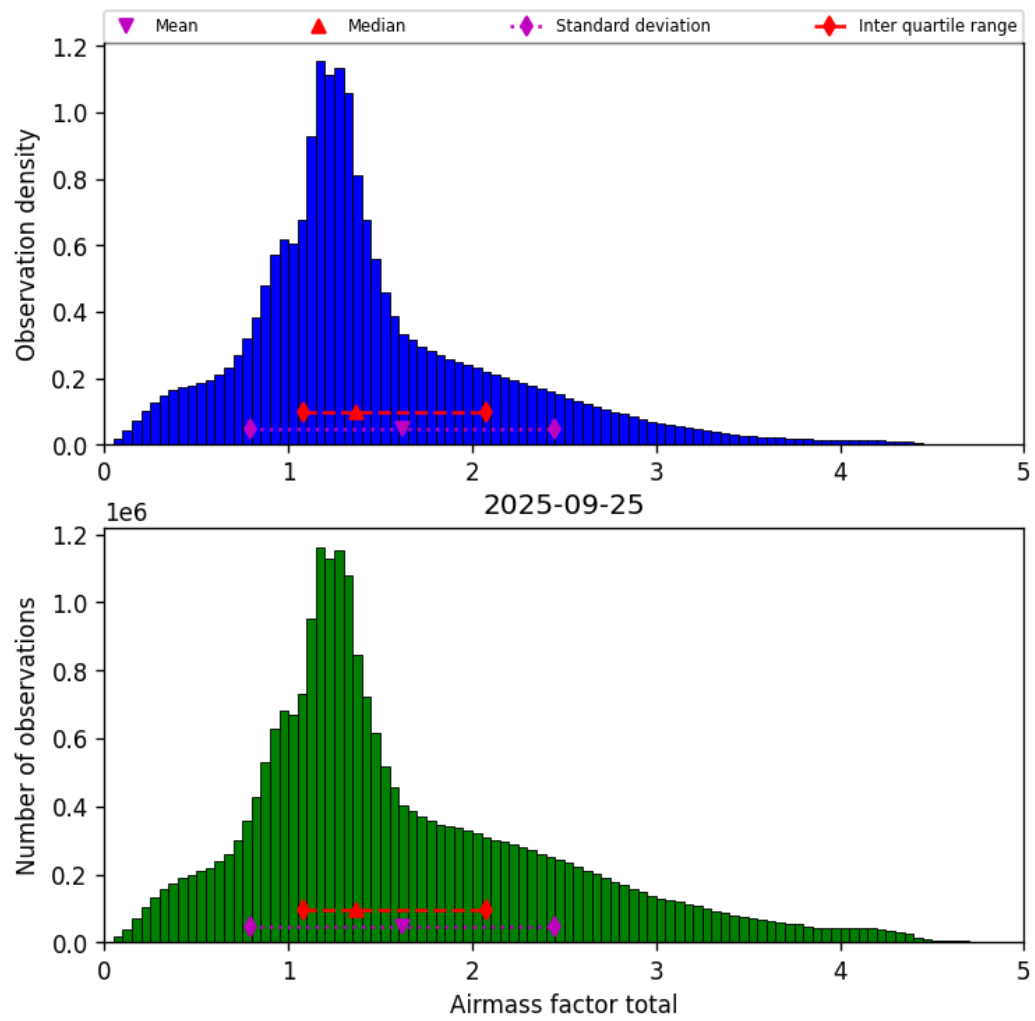
Figure 40: Histogram of “Airmass factor total” for 2025-09-25 to 2025-09-26
