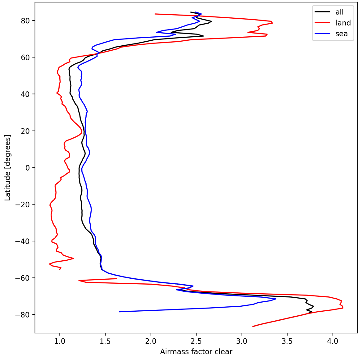
Figure 28: Zonal average of “Airmass factor clear” for 2025-09-25 to 2025-09-26.
