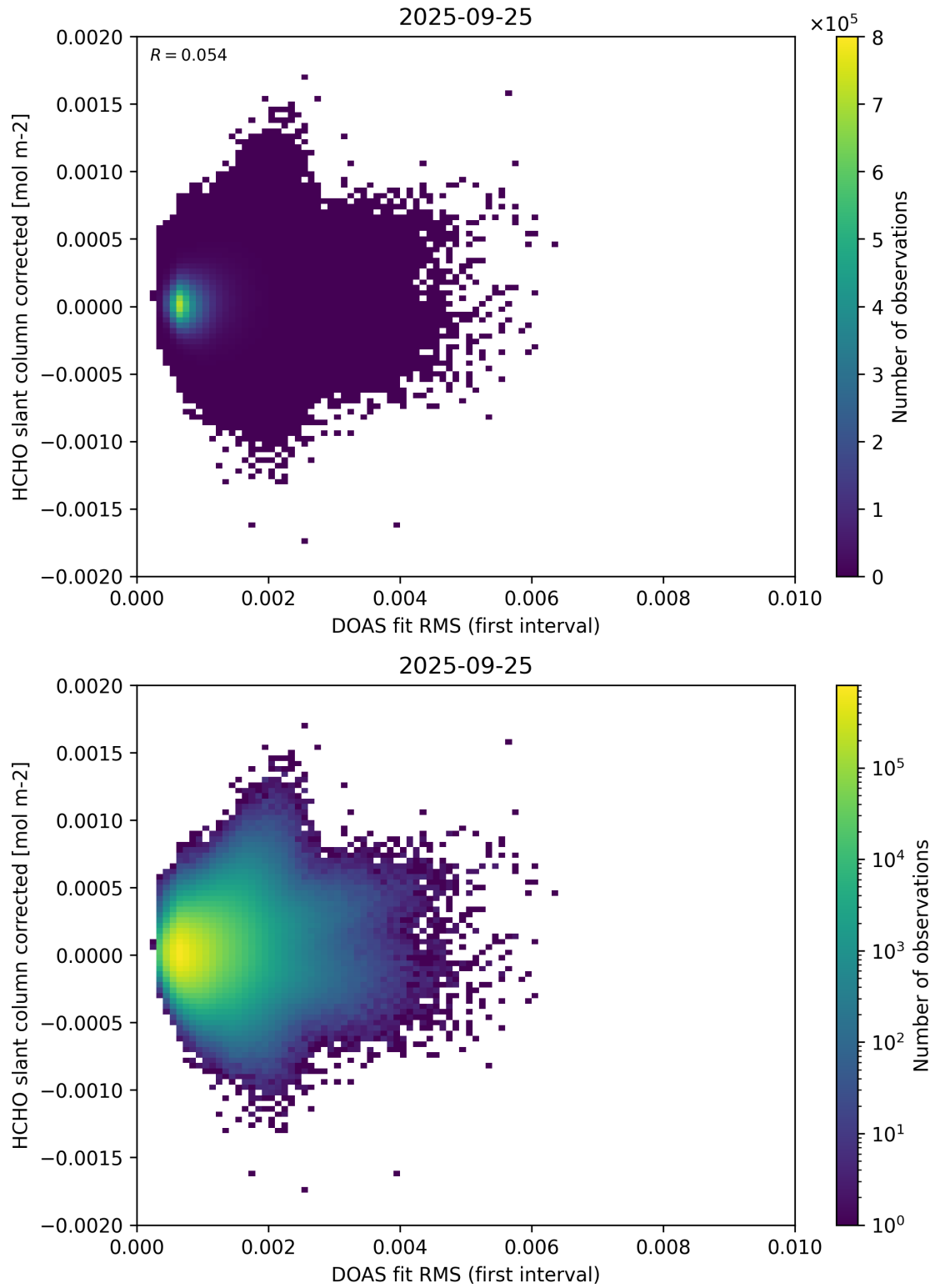
Figure 62: Scatter density plot of “DOAS fit RMS (first interval)” against “HCHO slant column corrected” for 2025-09-25 to 2025-09-26.
