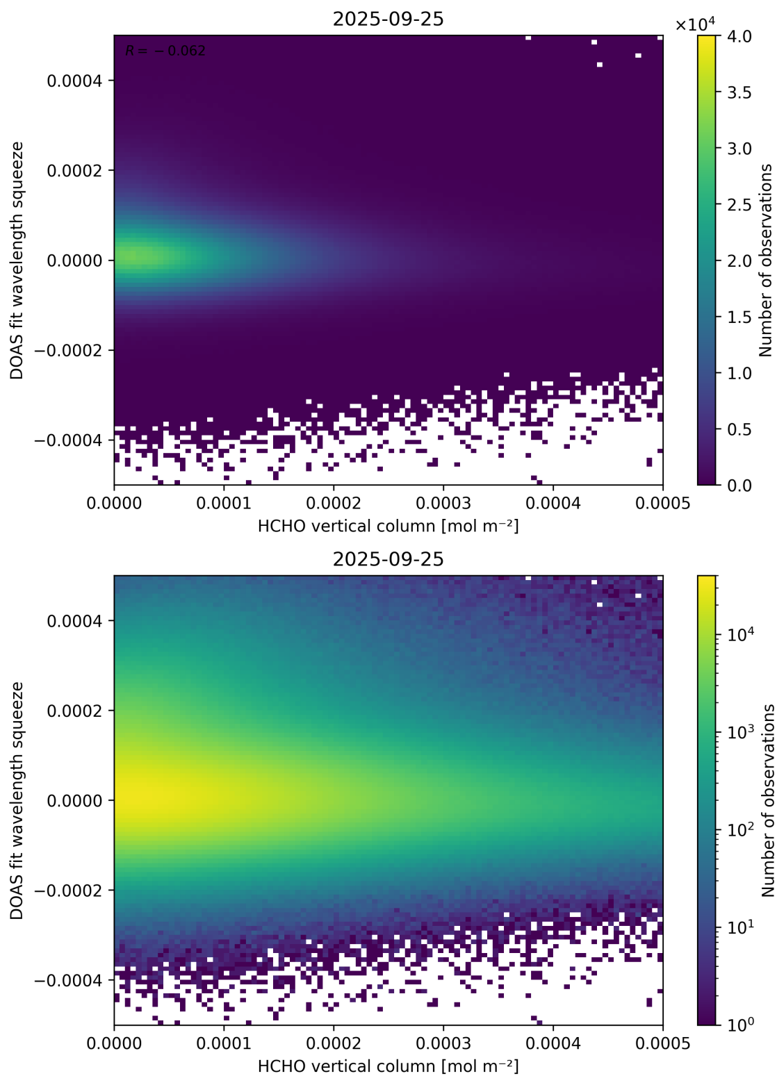
Figure 125: Scatter density plot of “HCHO vertical column” against “DOAS fit wavelength squeeze” for 2025-09-25 to 2025-09-26.
