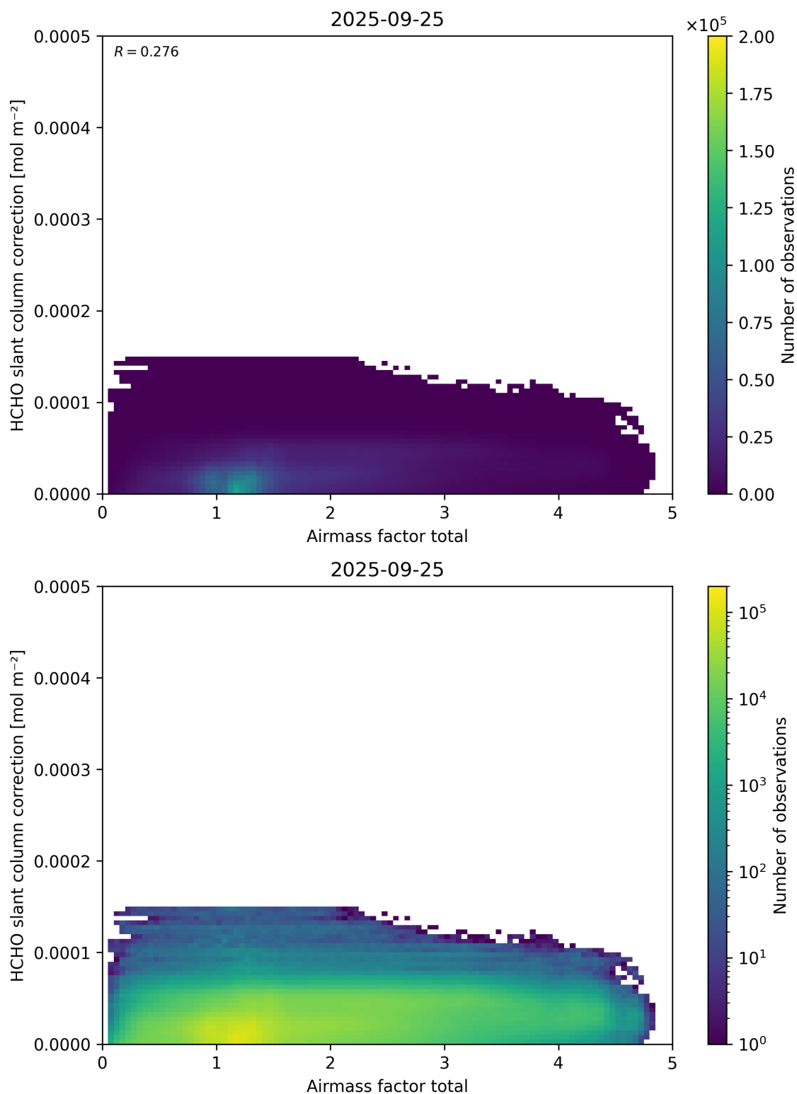
Figure 102: Scatter density plot of “Airmass factor total” against “HCHO slant column correction” for 2025-09-25 to 2025-09-26.
