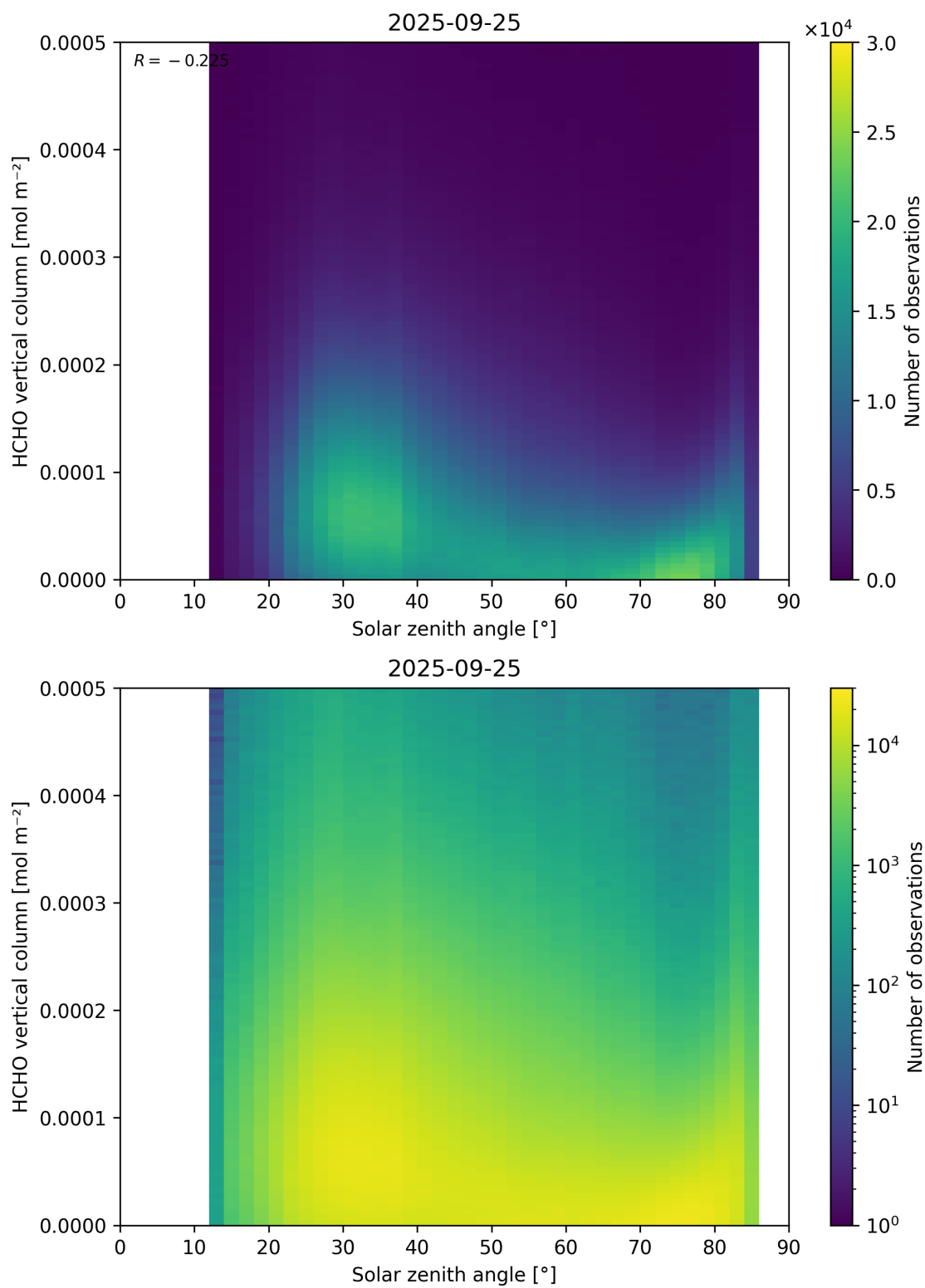
Figure 177: Scatter density plot of “Solar zenith angle” against “HCHO vertical column” for 2025-09-25 to 2025-09-26.
