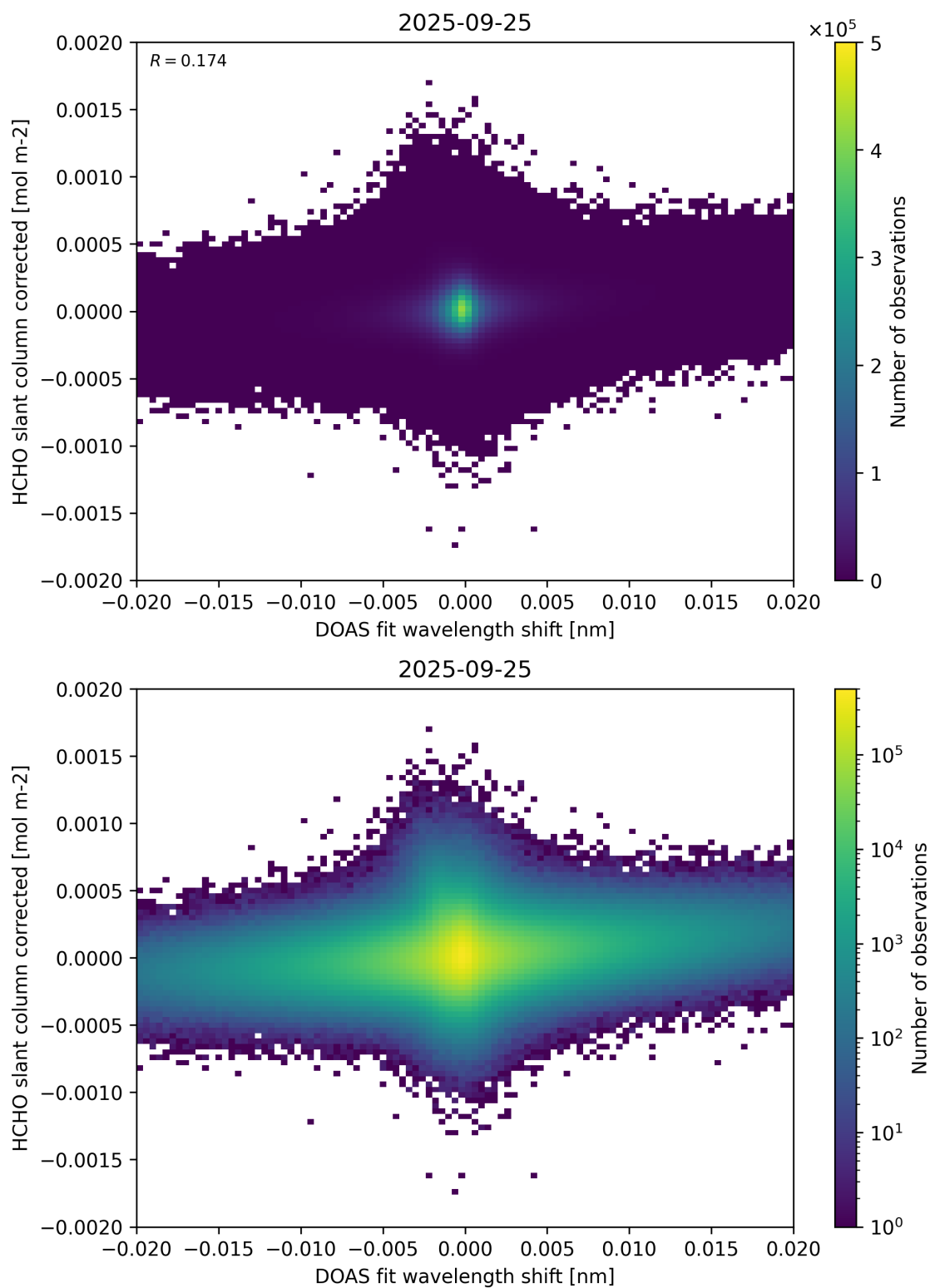
Figure 66: Scatter density plot of “DOAS fit wavelength shift” against “HCHO slant column corrected” for 2025-09-25 to 2025-09-26.
