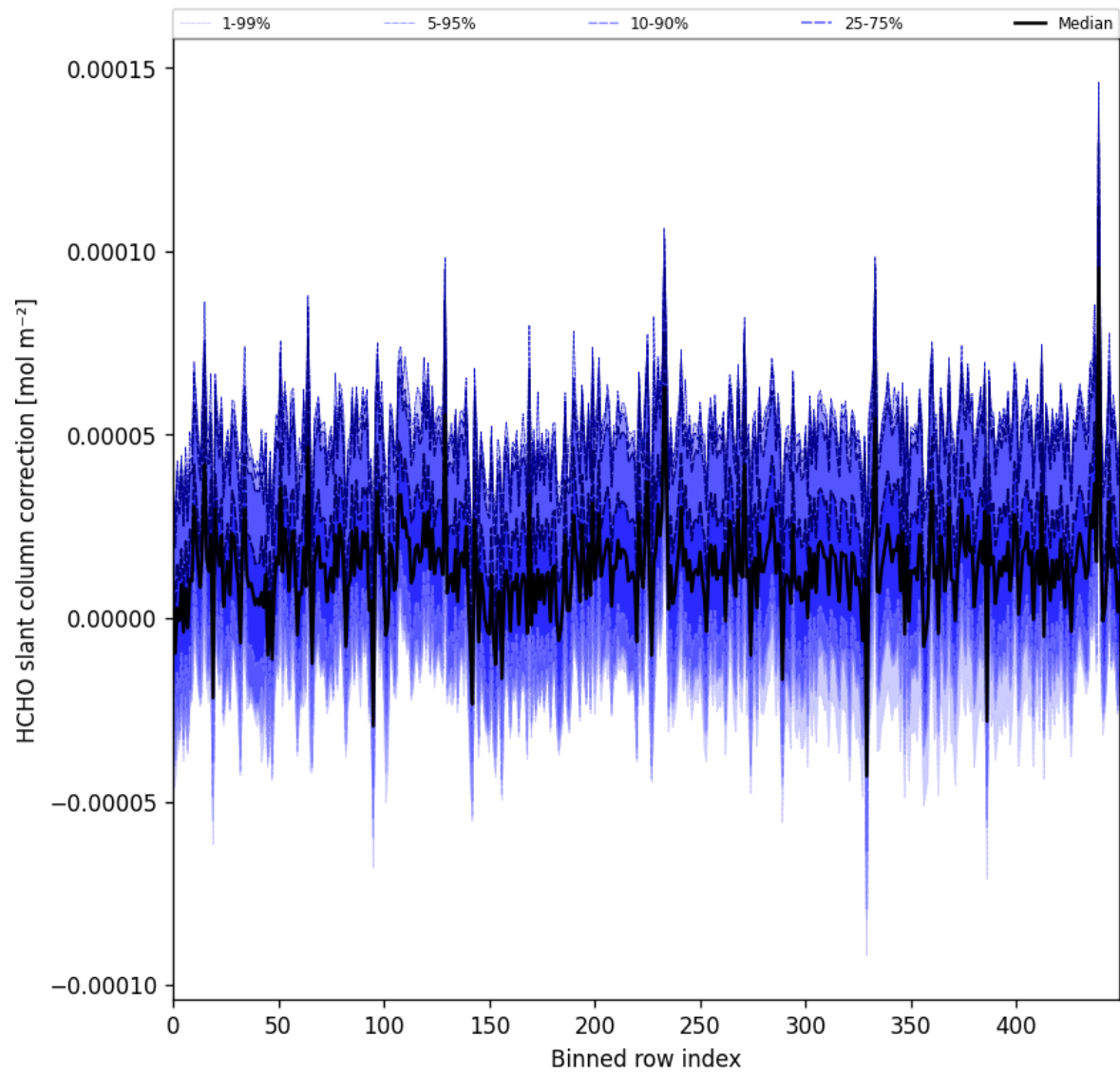
Figure 61: Along track statistics of “HCHO slant column correction” for 2025-09-25 to 2025-09-26
