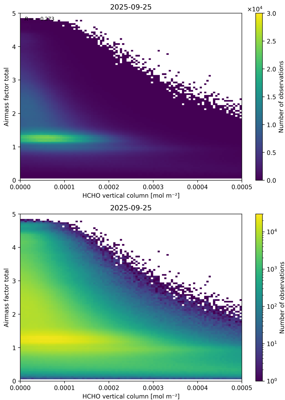
Figure 131: Scatter density plot of “HCHO vertical column” against “Airmass factor total” for 2025-09-25 to 2025-09-26.
