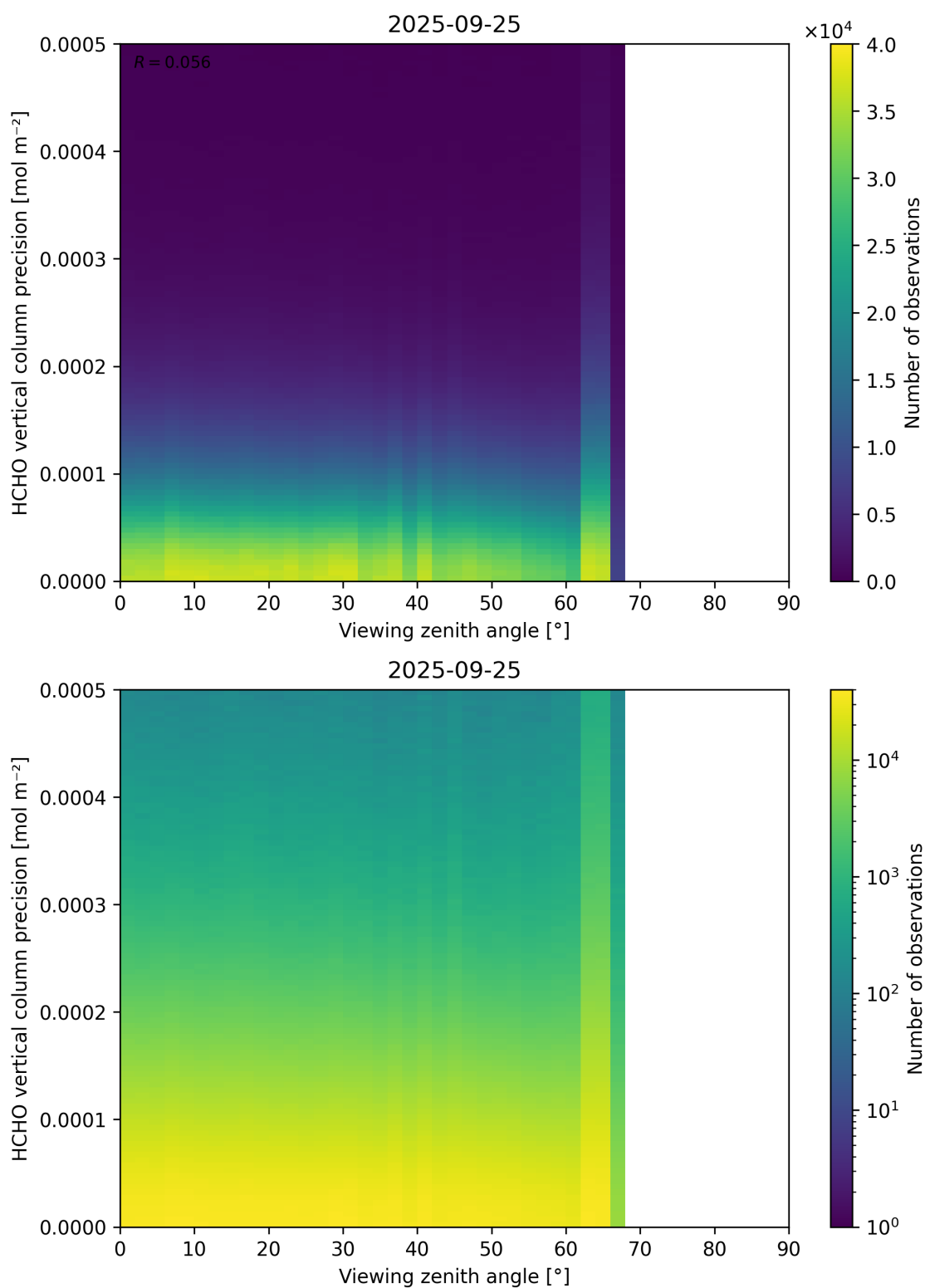
Figure 194: Scatter density plot of “Viewing zenith angle” against “HCHO vertical column precision” for 2025-09-25 to 2025-09-26.
