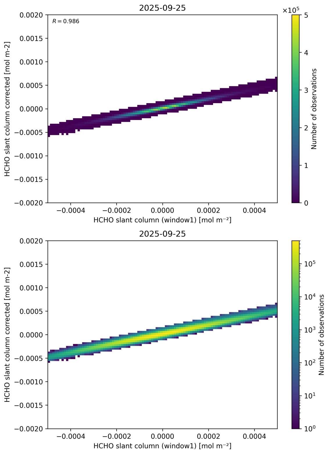
Figure 82: Scatter density plot of “HCHO slant column (window1)” against “HCHO slant column corrected” for 2025-09-25 to 2025-09-26.
