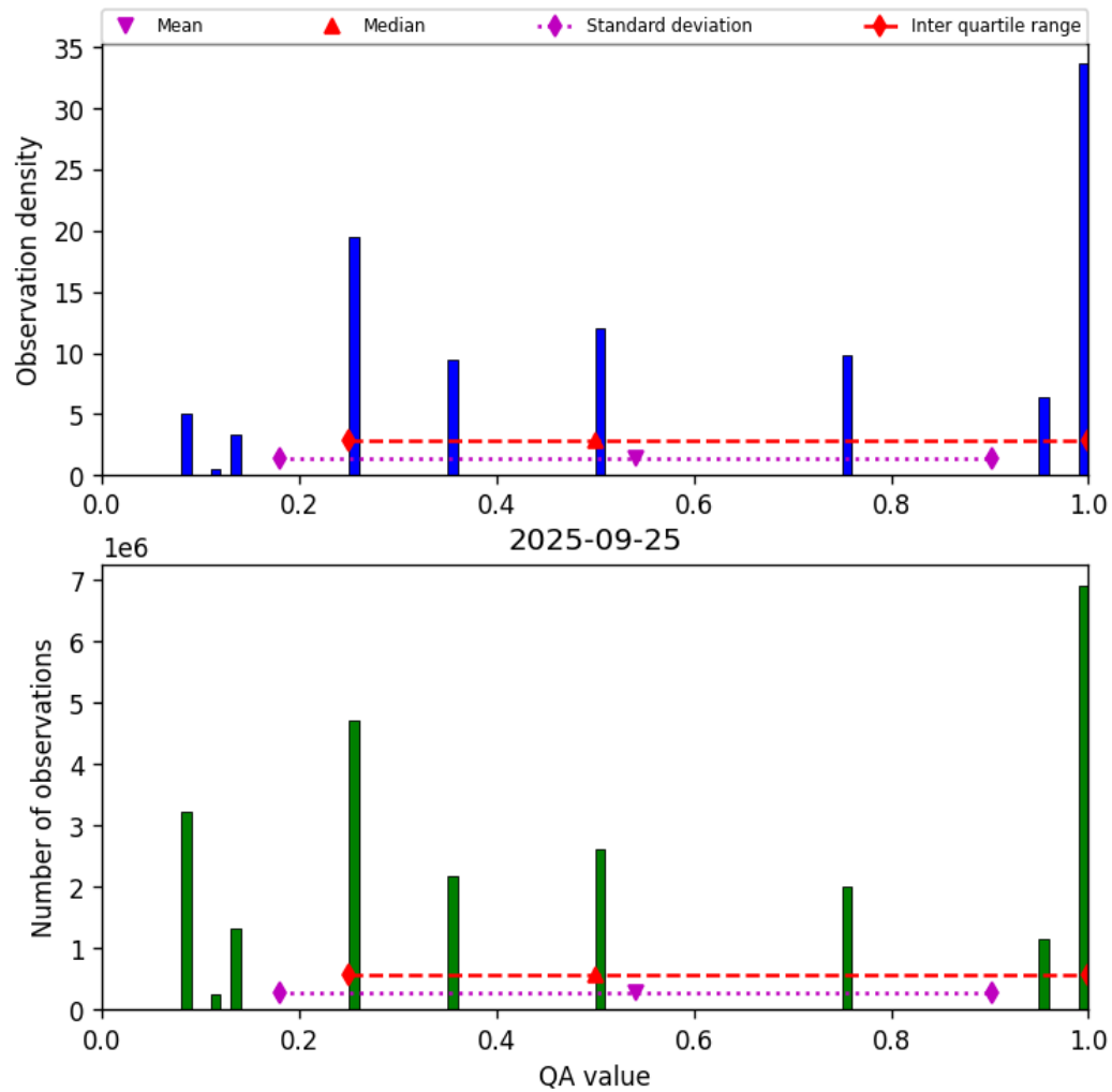
Figure 34: Histogram of “QA value” for 2025-09-25 to 2025-09-26
