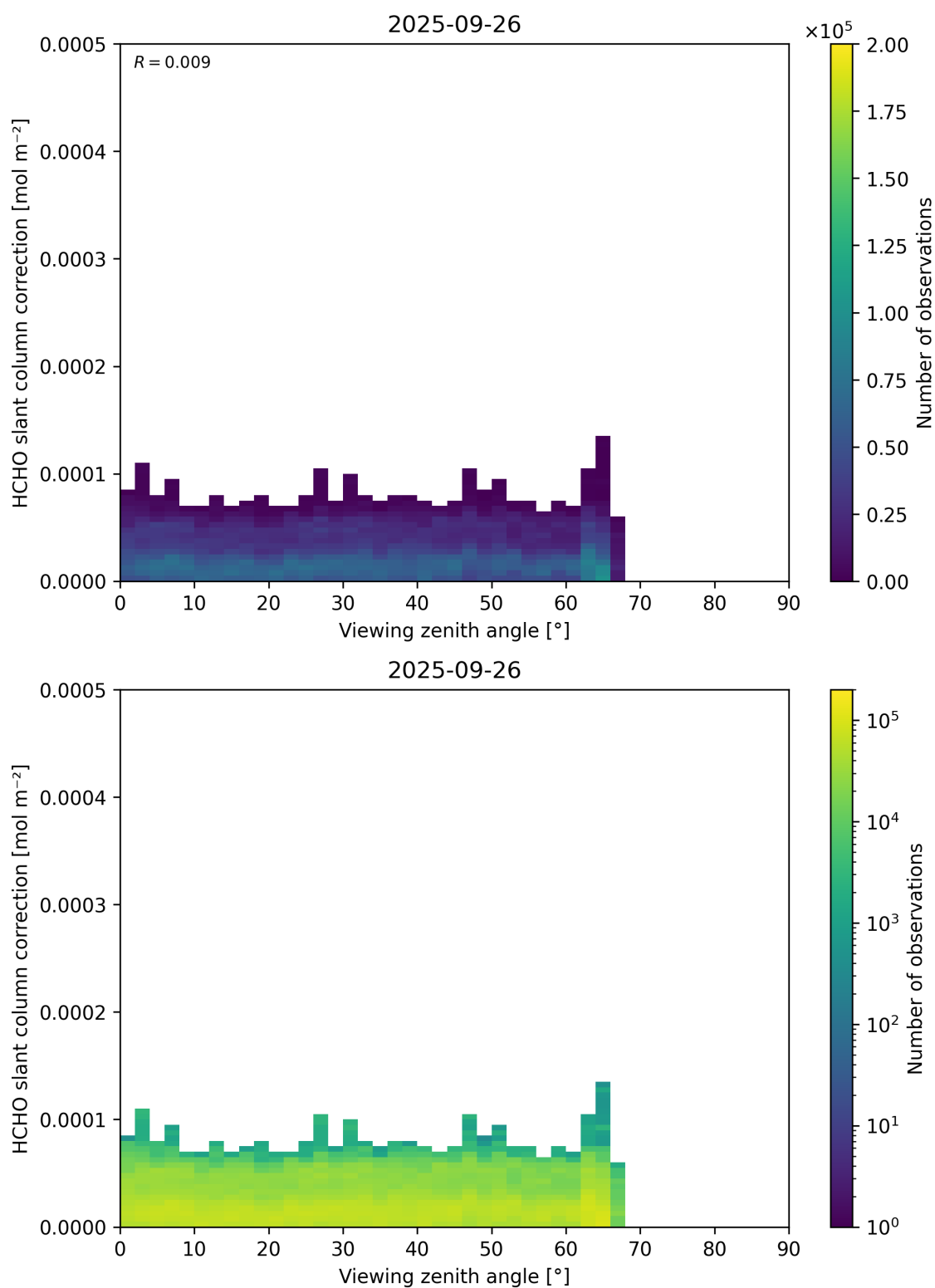
Figure 187: Scatter density plot of “Viewing zenith angle” against “HCHO slant column correction” for 2025-09-26 to 2025-09-27.
