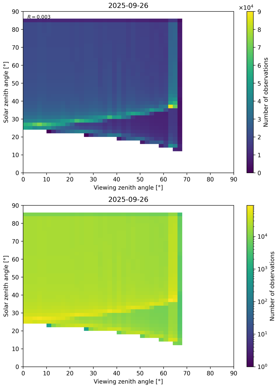
Figure 197: Scatter density plot of “Viewing zenith angle” against “Solar zenith angle” for 2025-09-26 to 2025-09-27.
