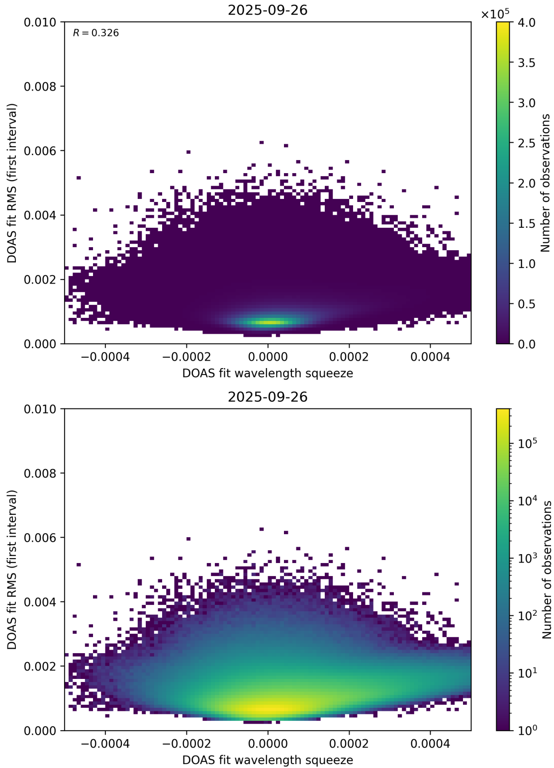
Figure 68: Scatter density plot of “DOAS fit wavelength squeeze” against “DOAS fit RMS (first interval)” for 2025-09-26 to 2025-09-27.
