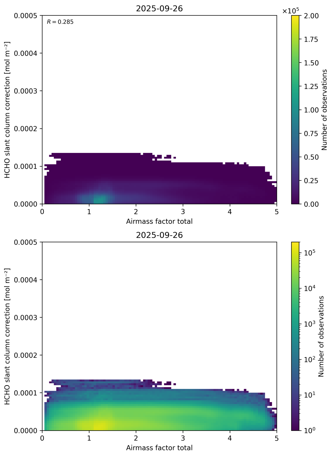
Figure 102: Scatter density plot of “Airmass factor total” against “HCHO slant column correction” for 2025-09-26 to 2025-09-27.
