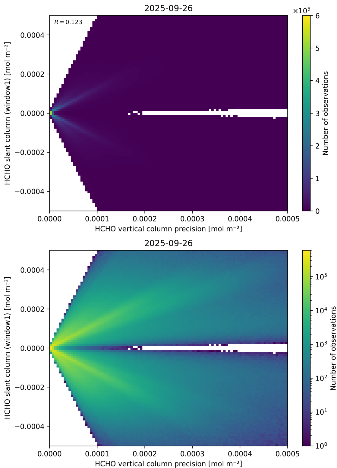
Figure 142: Scatter density plot of “HCHO vertical column precision” against “HCHO slant column (window1)” for 2025-09-26 to 2025-09-27.
