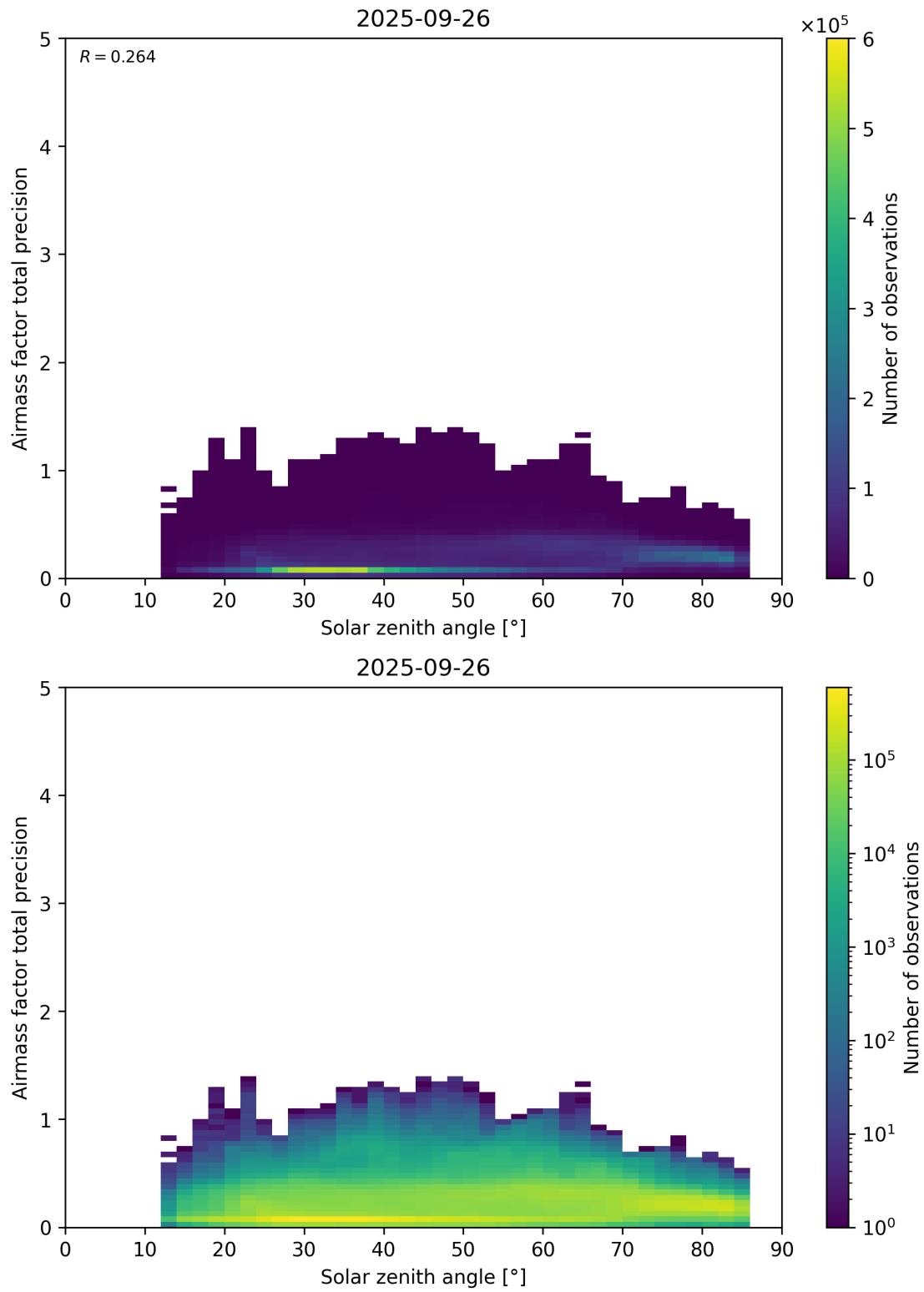
Figure 176: Scatter density plot of “Solar zenith angle” against “Airmass factor total precision” for 2025-09-26 to 2025-09-27.
