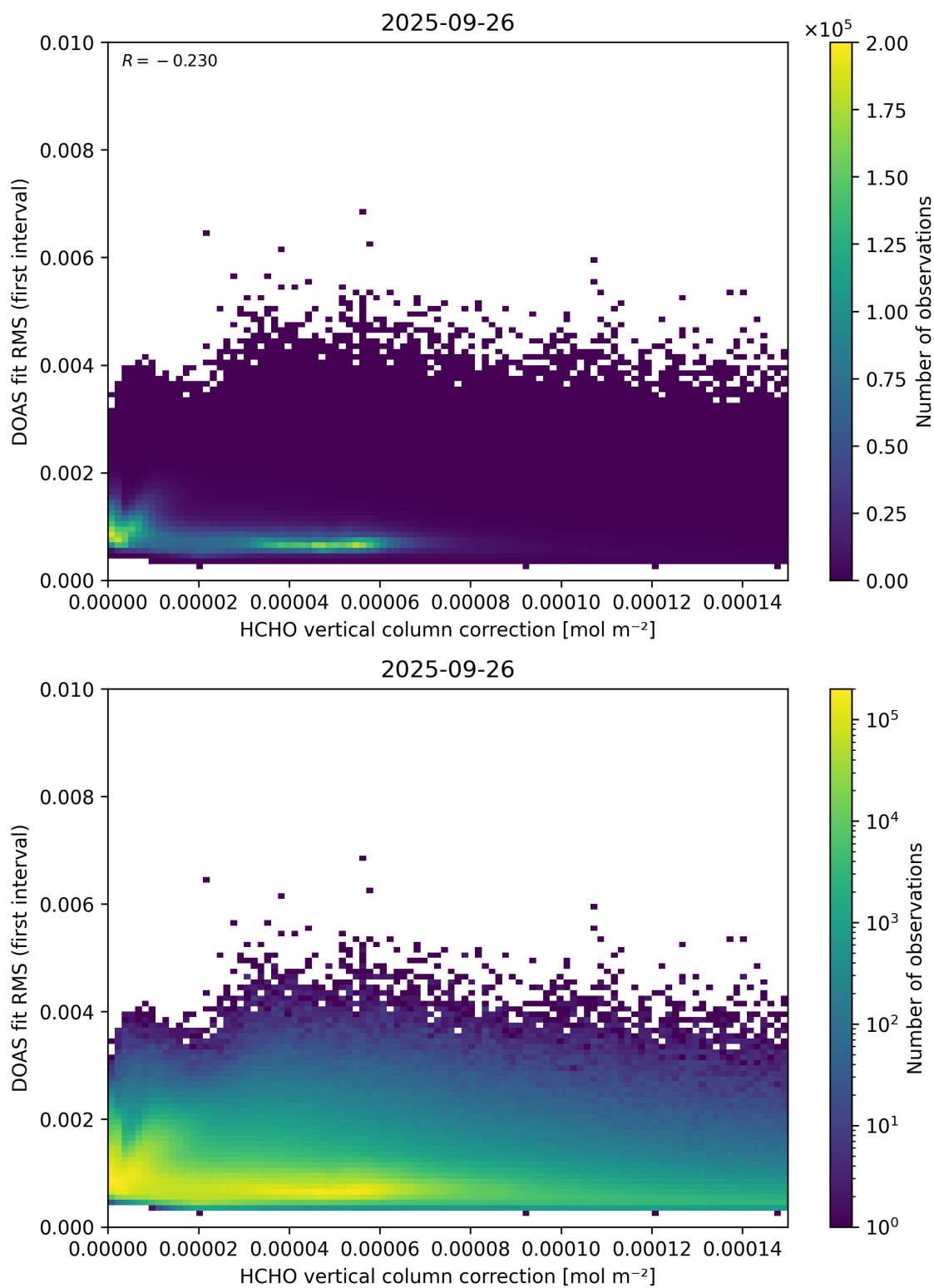
Figure 112: Scatter density plot of “HCHO vertical column correction” against “DOAS fit RMS (first interval)” for 2025-09-26 to 2025-09-27.
