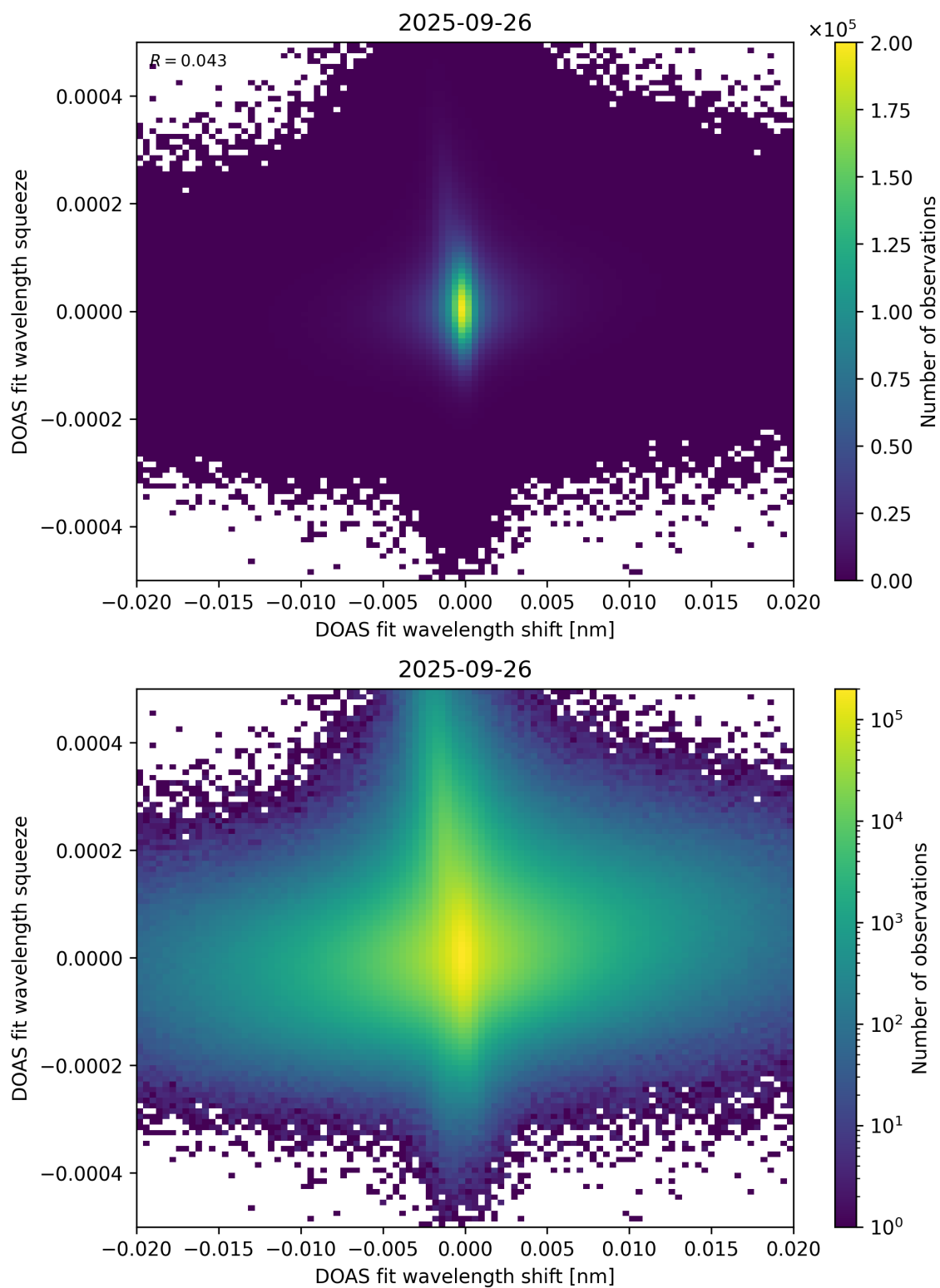
Figure 65: Scatter density plot of “DOAS fit wavelength shift” against “DOAS fit wavelength squeeze” for 2025-09-26 to 2025-09-27.
