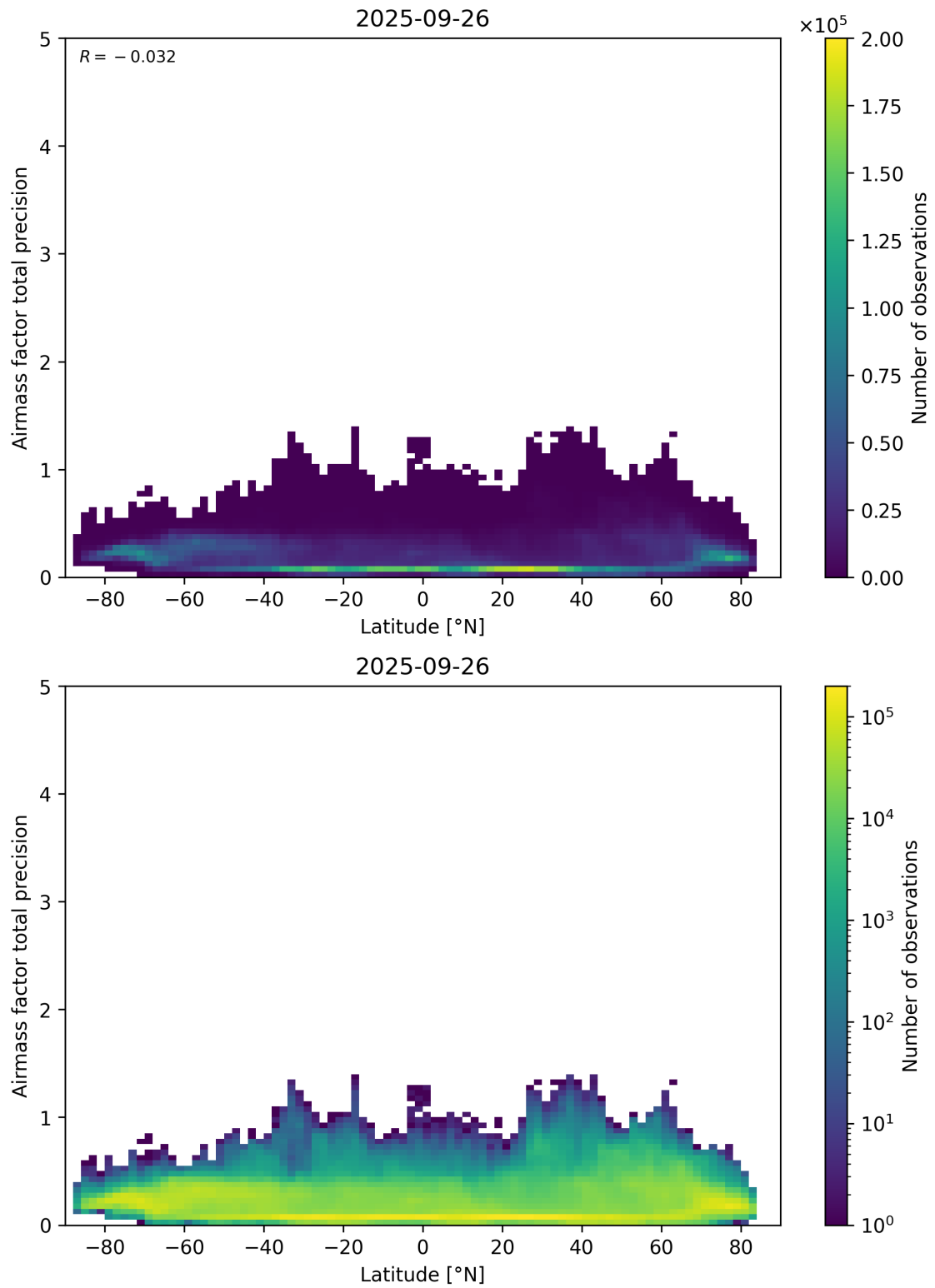
Figure 162: Scatter density plot of “Latitude” against “Airmass factor total precision” for 2025-09-26 to 2025-09-27.
