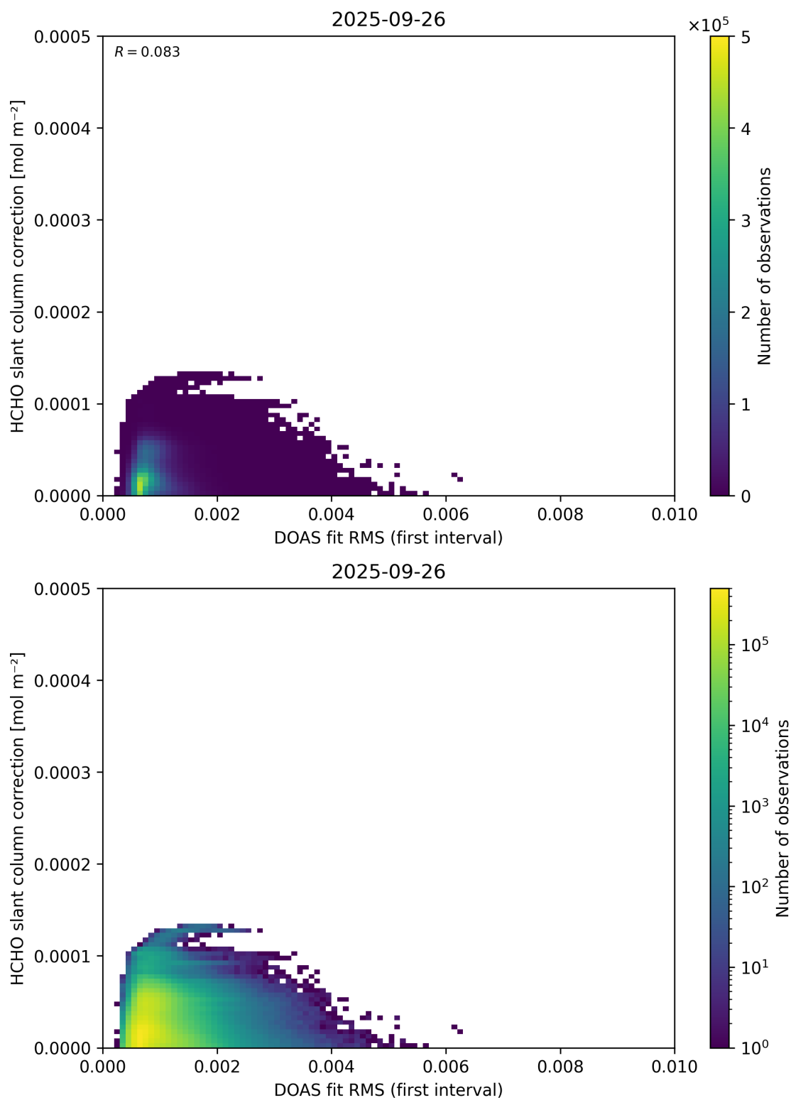
Figure 63: Scatter density plot of “DOAS fit RMS (first interval)” against “HCHO slant column correction” for 2025-09-26 to 2025-09-27.
