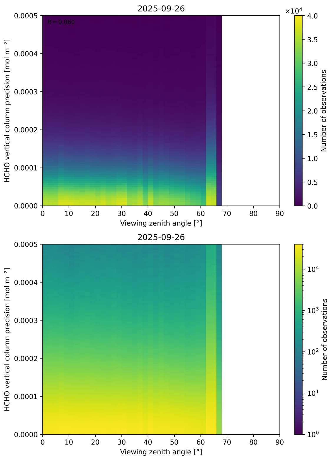
Figure 194: Scatter density plot of “Viewing zenith angle” against “HCHO vertical column precision” for 2025-09-26 to 2025-09-27.
