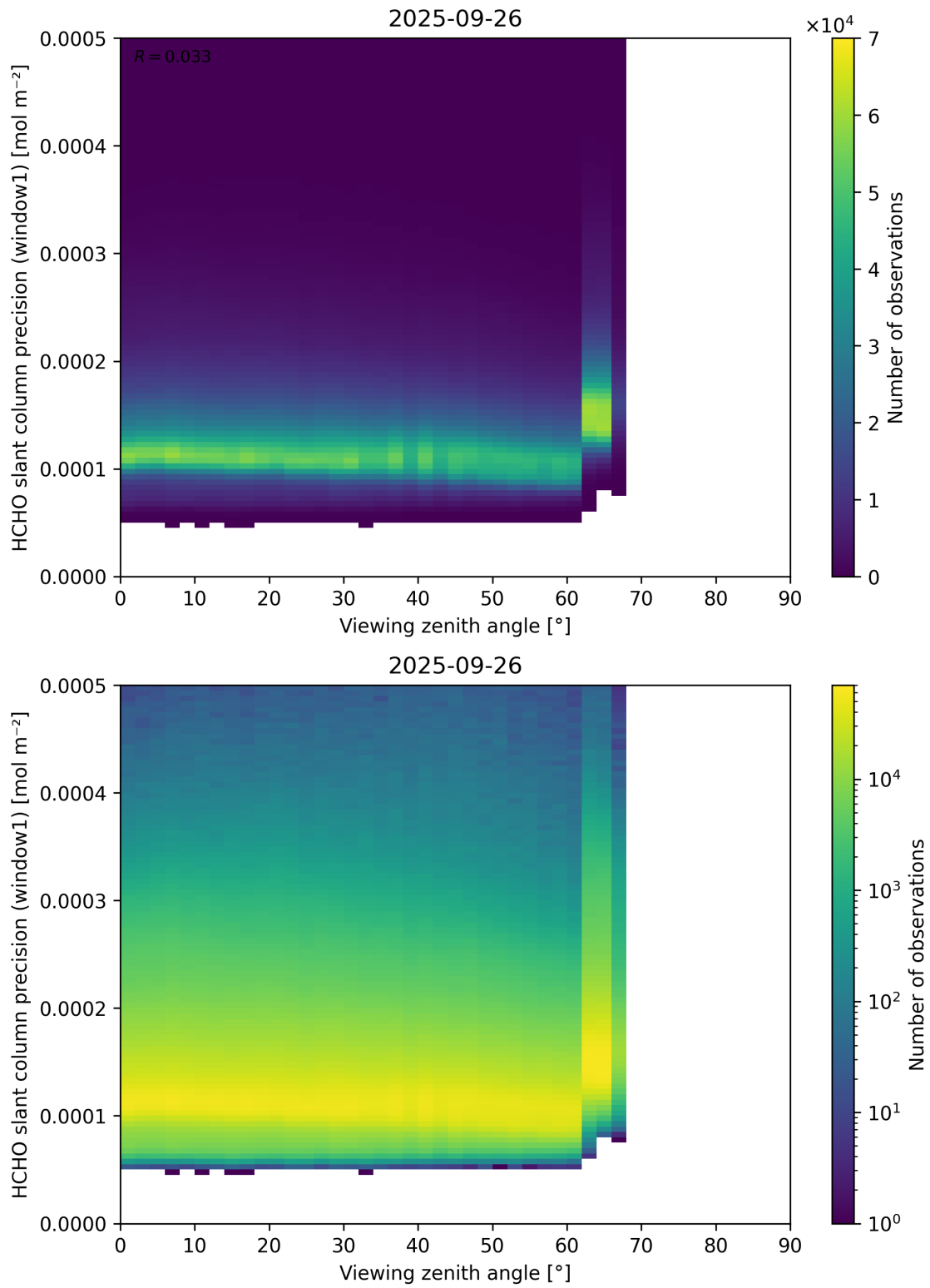
Figure 189: Scatter density plot of “Viewing zenith angle” against “HCHO slant column precision (window1)” for 2025-09-26 to 2025-09-27.
