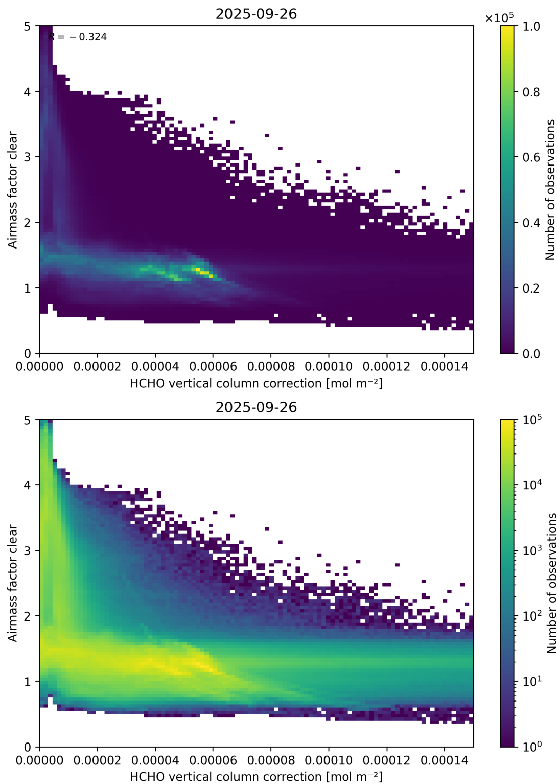
Figure 115: Scatter density plot of “HCHO vertical column correction” against “Airmass factor clear” for 2025-09-26 to 2025-09-27.
