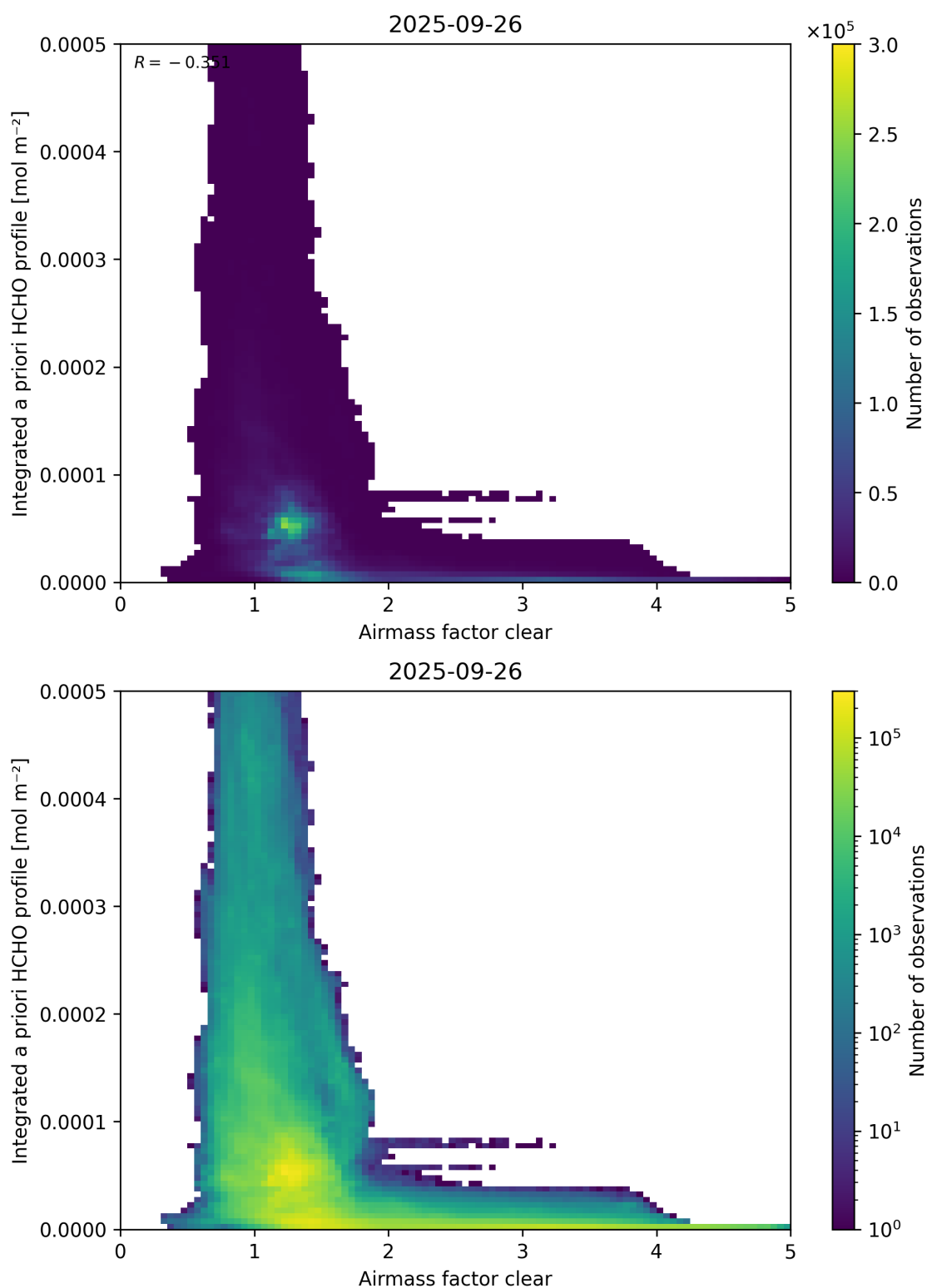
Figure 76: Scatter density plot of “Airmass factor clear” against “Integrated a priori HCHO profile” for 2025-09-26 to 2025-09-27.
