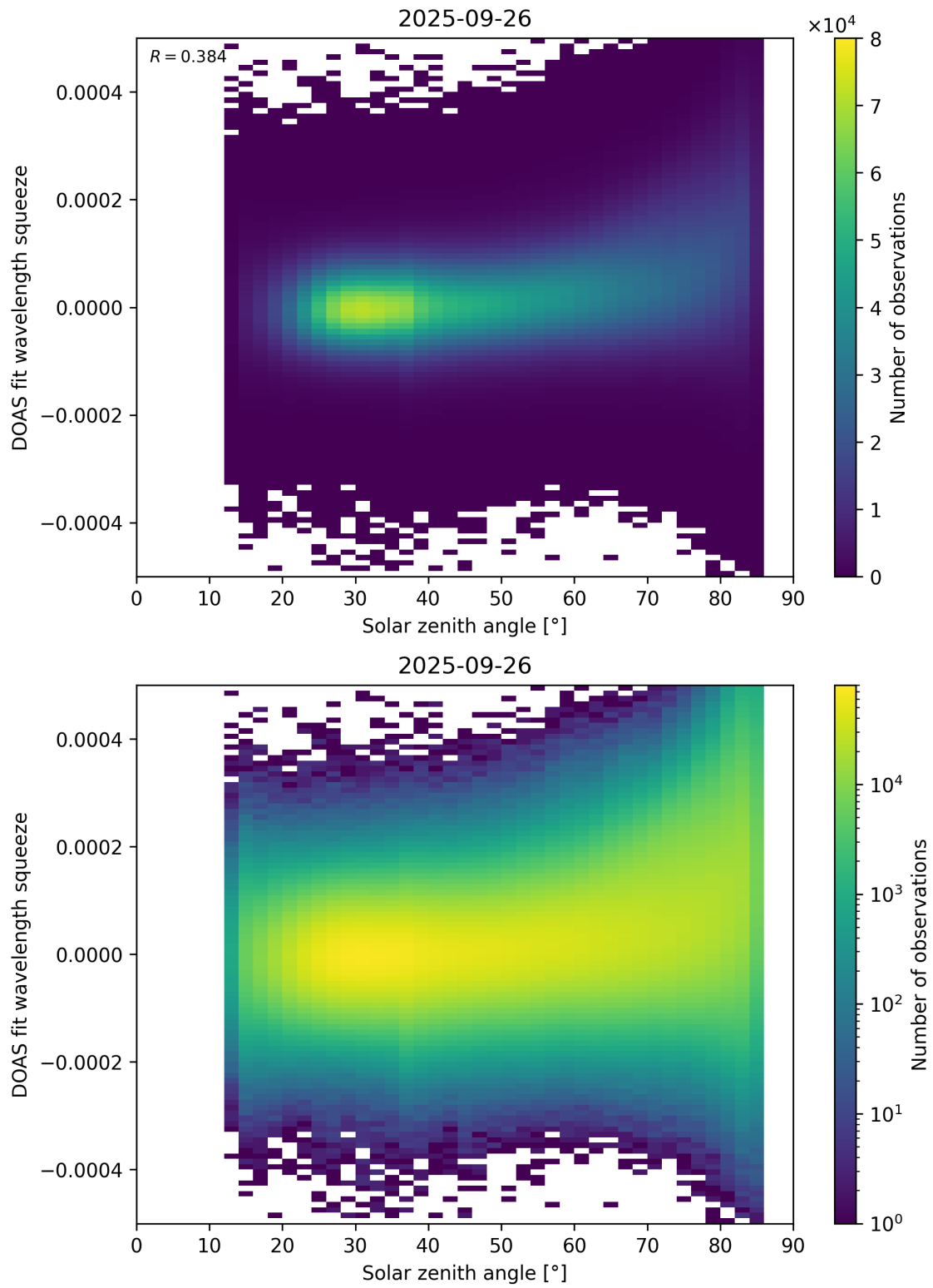
Figure 169: Scatter density plot of “Solar zenith angle” against “DOAS fit wavelength squeeze” for 2025-09-26 to 2025-09-27.
