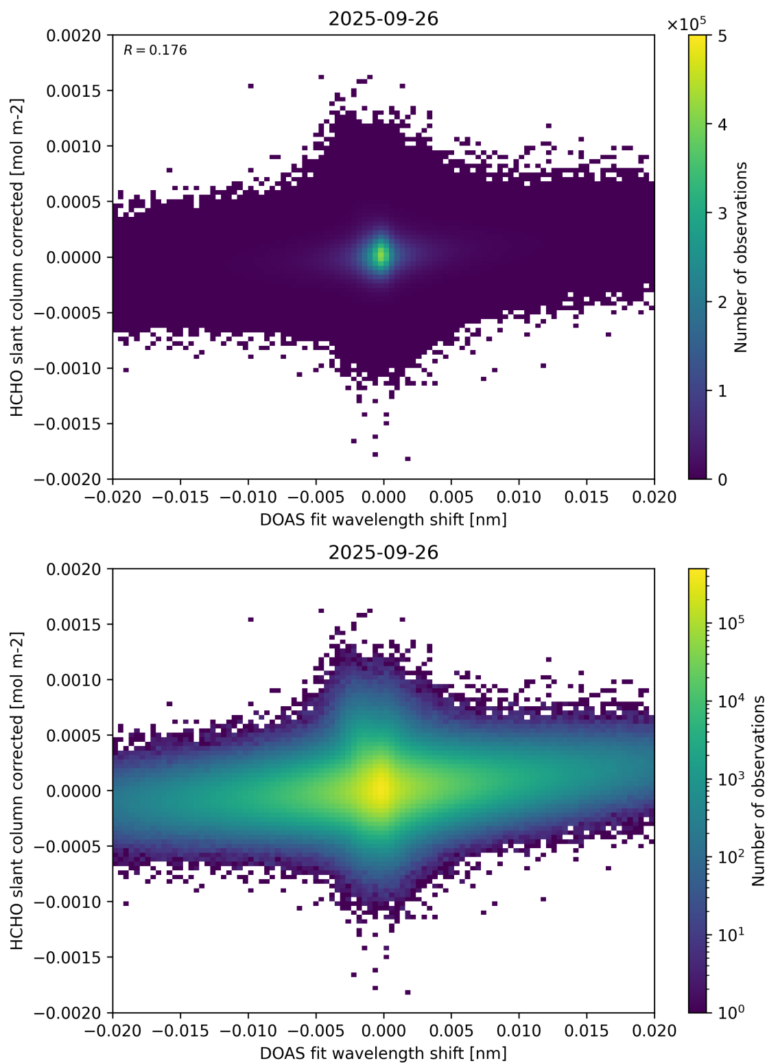
Figure 66: Scatter density plot of “DOAS fit wavelength shift” against “HCHO slant column corrected” for 2025-09-26 to 2025-09-27.
