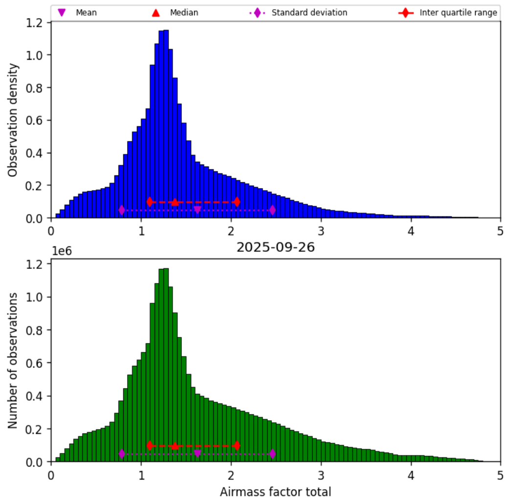
Figure 40: Histogram of “Airmass factor total” for 2025-09-26 to 2025-09-27
