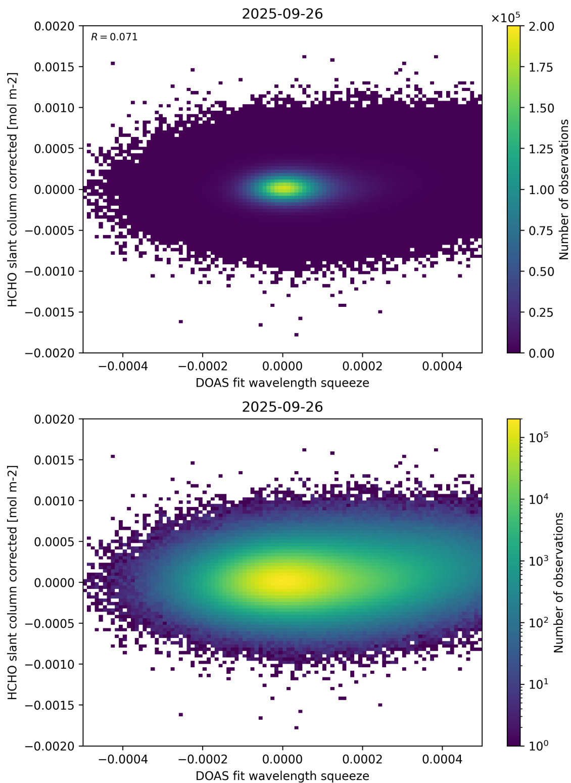
Figure 69: Scatter density plot of “DOAS fit wavelength squeeze” against “HCHO slant column corrected” for 2025-09-26 to 2025-09-27.
