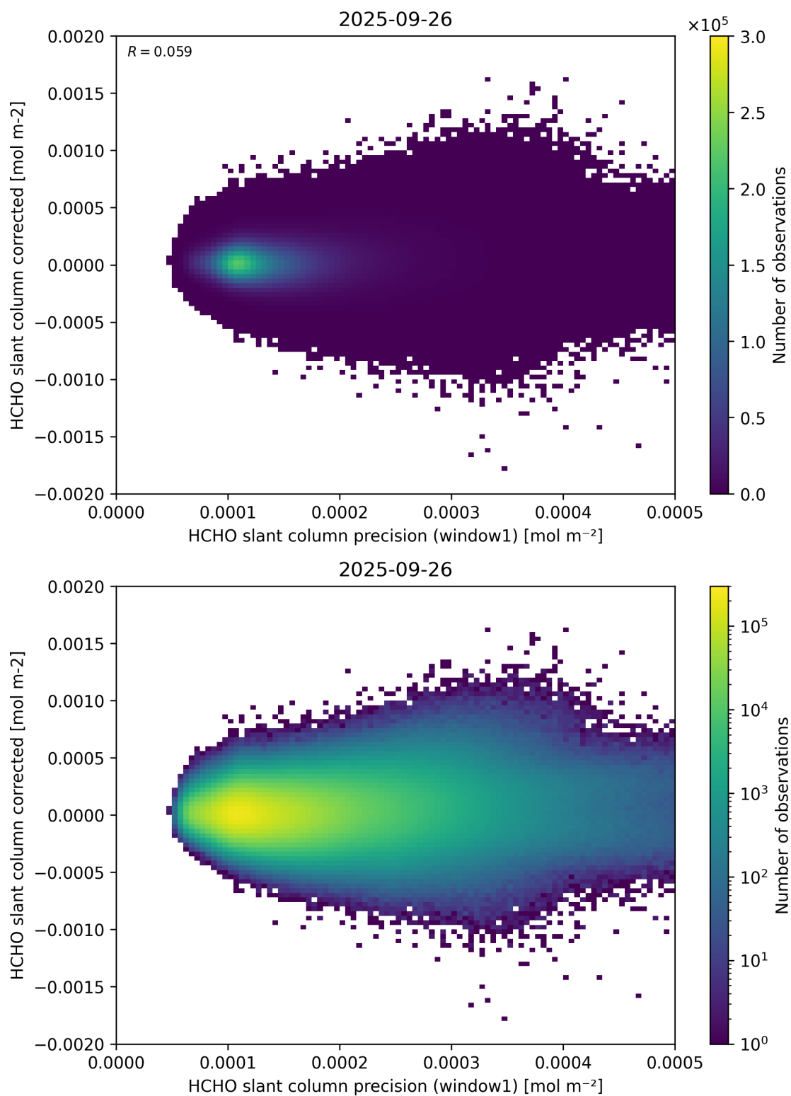
Figure 92: Scatter density plot of “HCHO slant column precision (window1)” against “HCHO slant column corrected” for 2025-09-26 to 2025-09-27.
