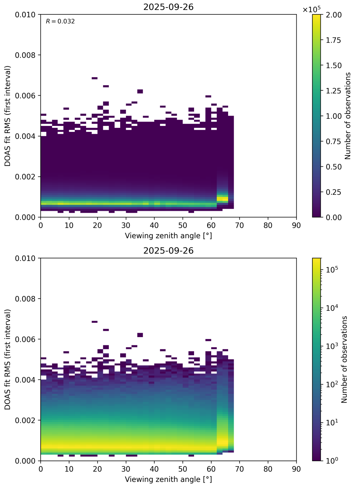
Figure 182: Scatter density plot of “Viewing zenith angle” against “DOAS fit RMS (first interval)” for 2025-09-26 to 2025-09-27.
