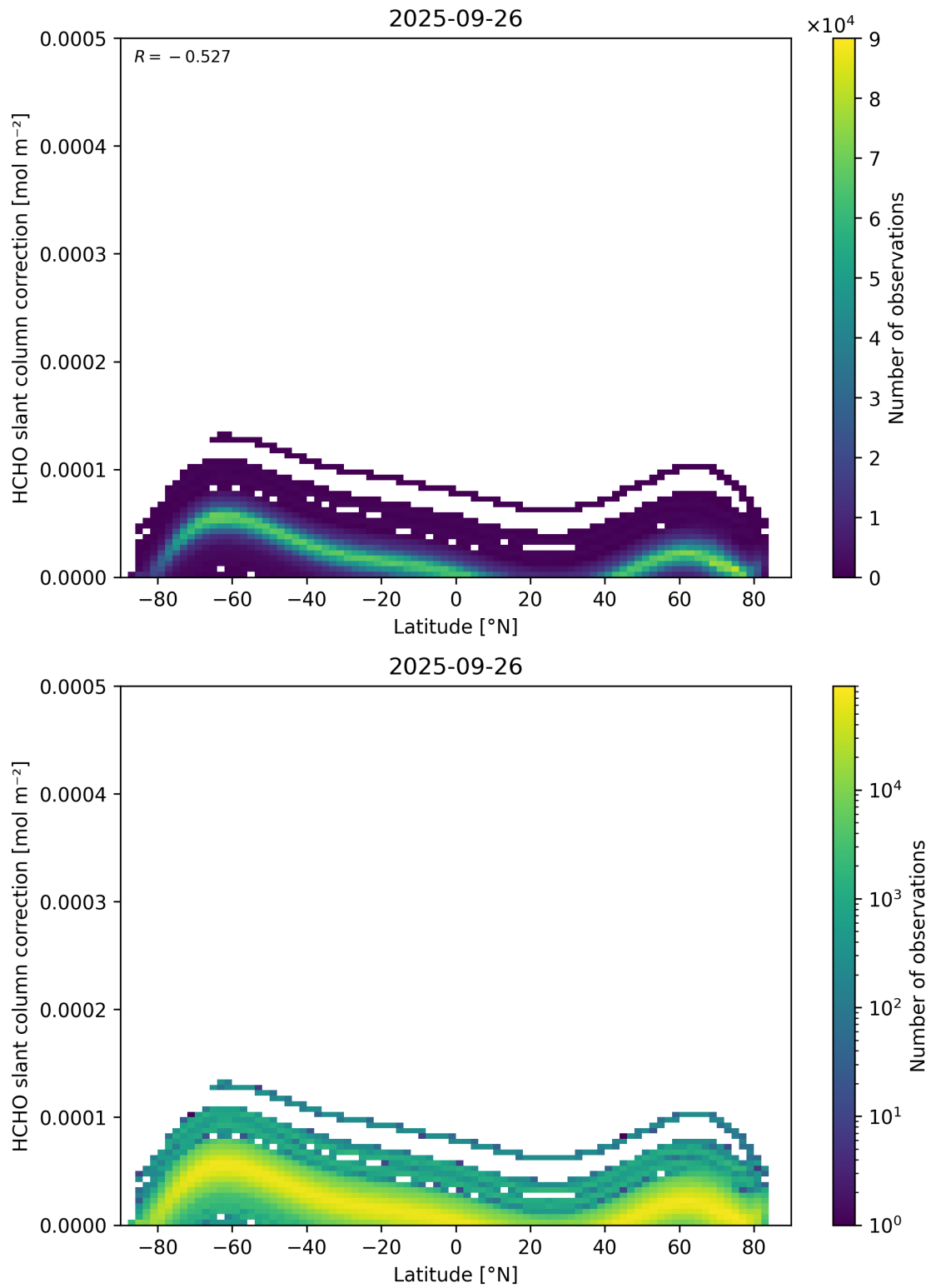
Figure 158: Scatter density plot of “Latitude” against “HCHO slant column correction” for 2025-09-26 to 2025-09-27.
