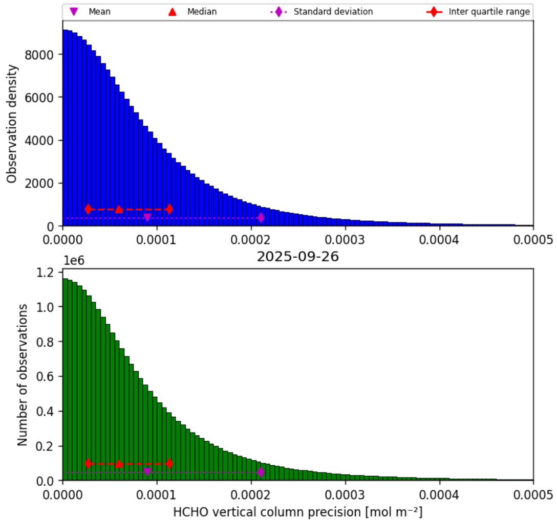
Figure 36: Histogram of “HCHO vertical column precision” for 2025-09-26 to 2025-09-27
