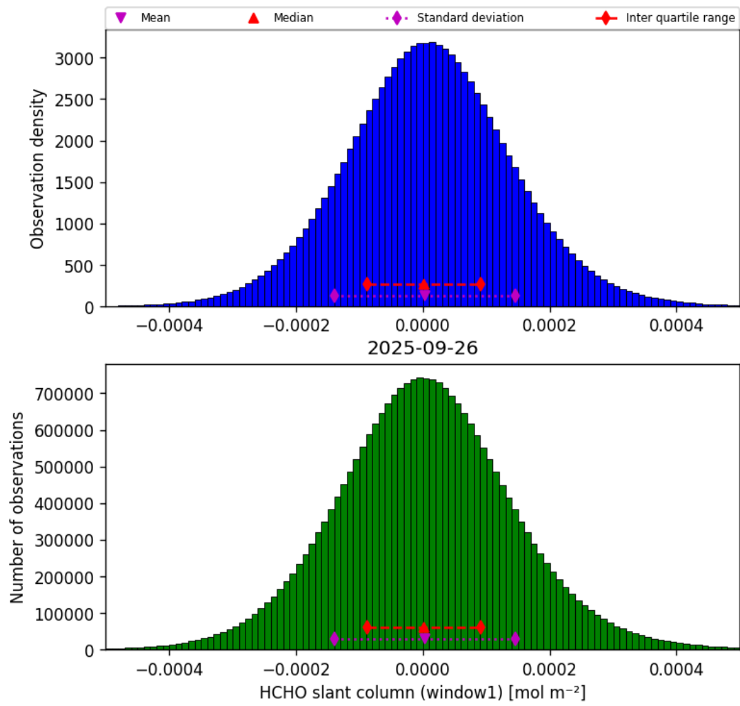
Figure 38: Histogram of “HCHO slant column (window1)” for 2025-09-26 to 2025-09-27
