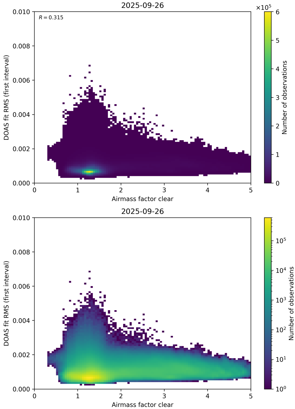
Figure 71: Scatter density plot of “Airmass factor clear” against “DOAS fit RMS (first interval)” for 2025-09-26 to 2025-09-27.
