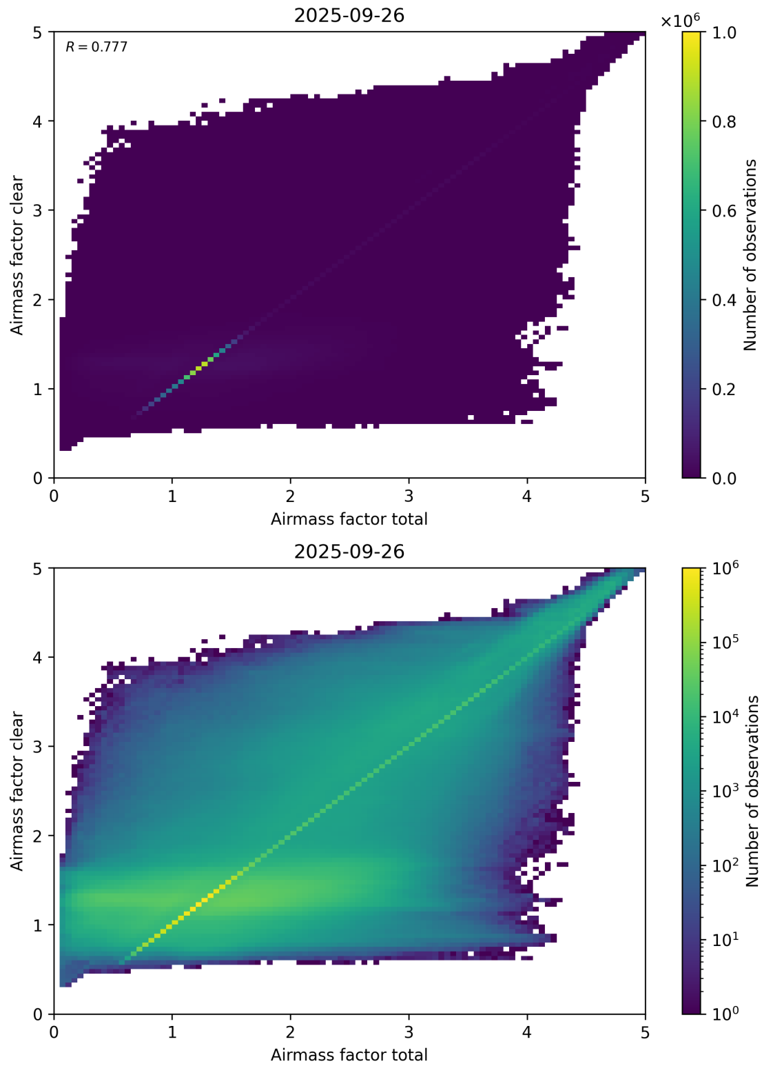
Figure 100: Scatter density plot of “Airmass factor total” against “Airmass factor clear” for 2025-09-26 to 2025-09-27.
