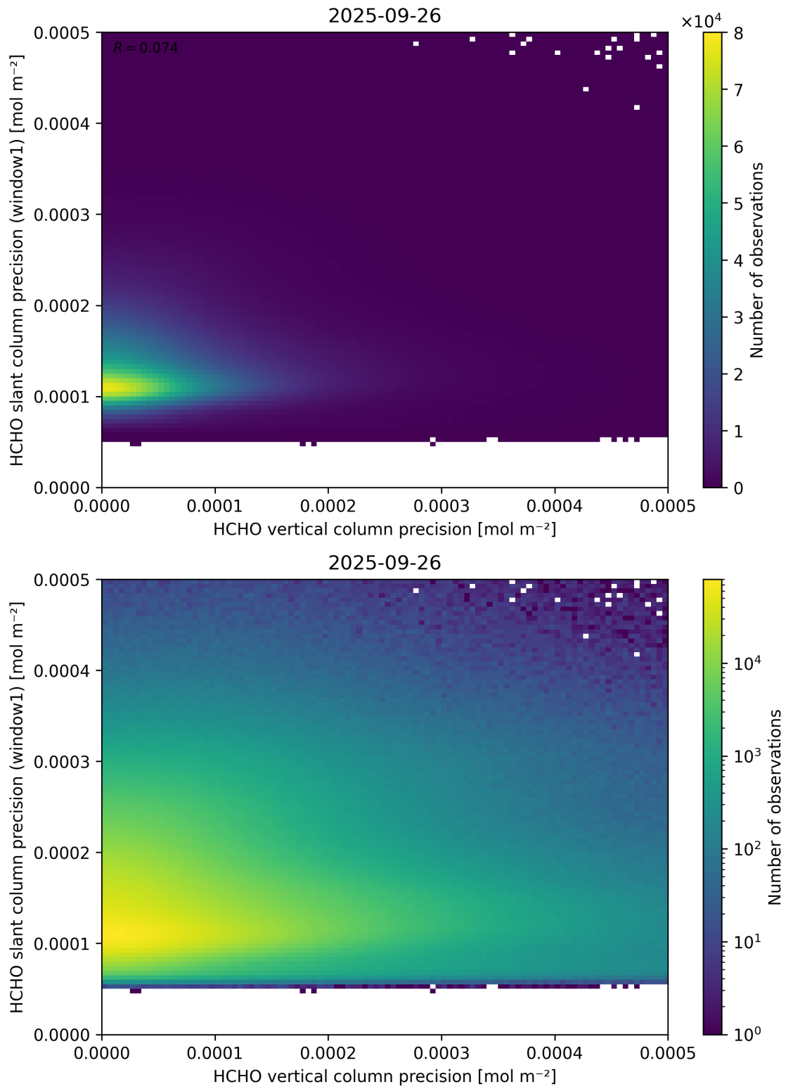
Figure 143: Scatter density plot of “HCHO vertical column precision” against “HCHO slant column precision (window1)” for 2025-09-26 to 2025-09-27.
