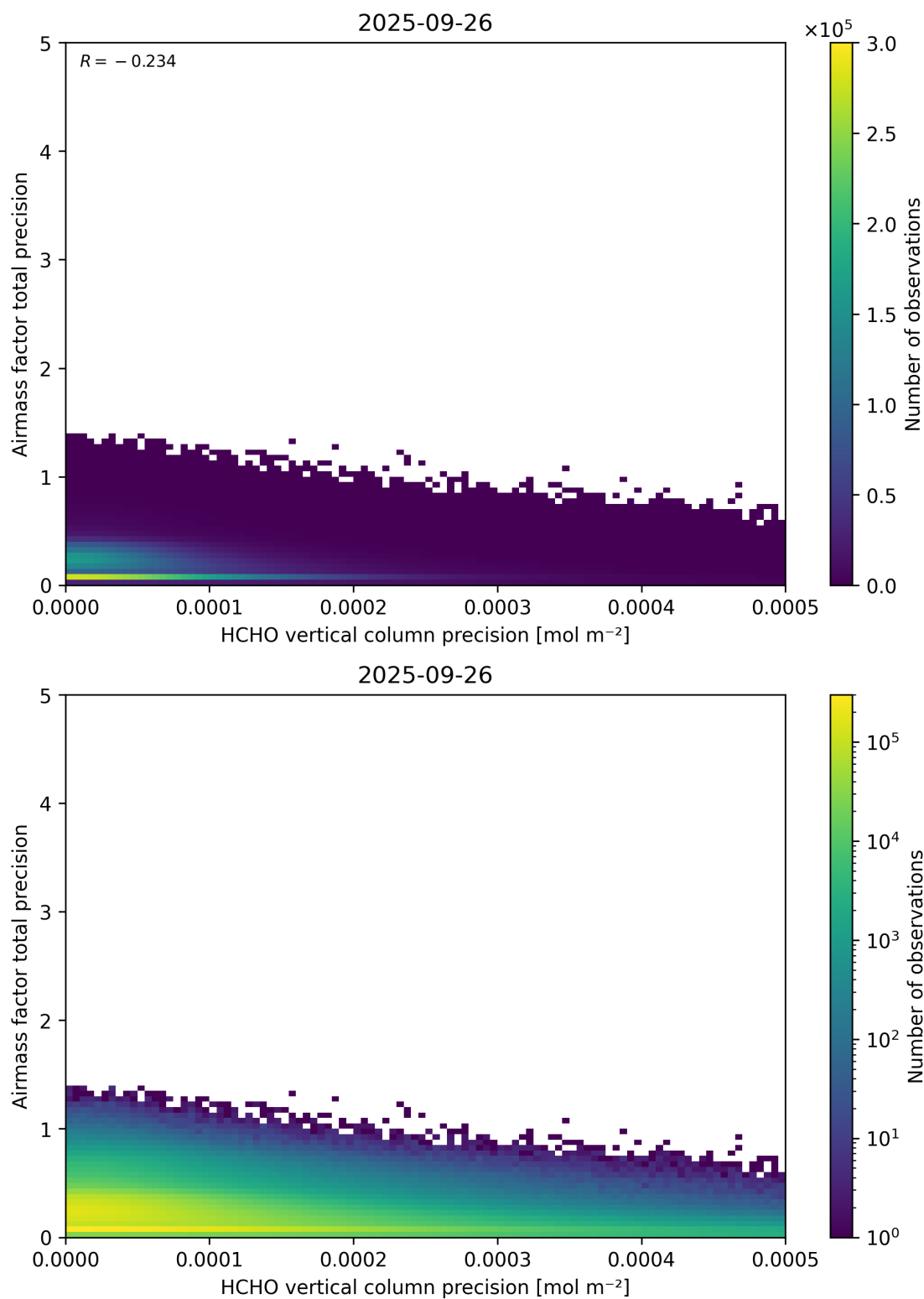
Figure 145: Scatter density plot of “HCHO vertical column precision” against “Airmass factor total precision” for 2025-09-26 to 2025-09-27.
