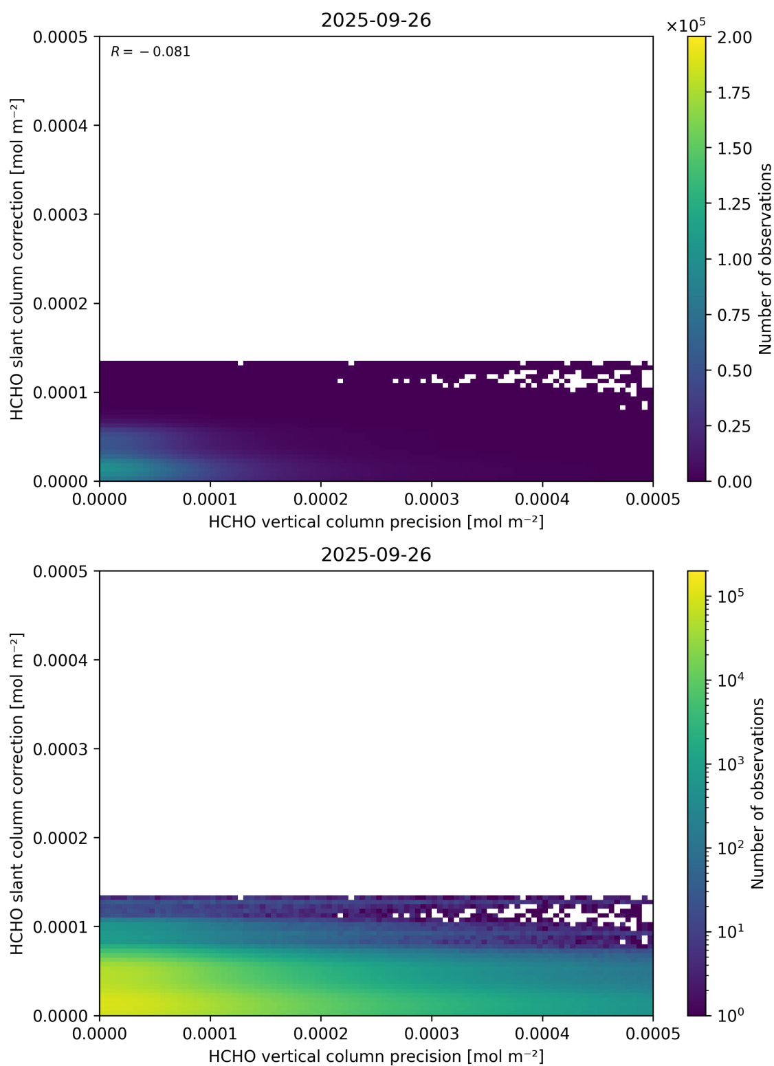
Figure 141: Scatter density plot of “HCHO vertical column precision” against “HCHO slant column correction” for 2025-09-26 to 2025-09-27.
