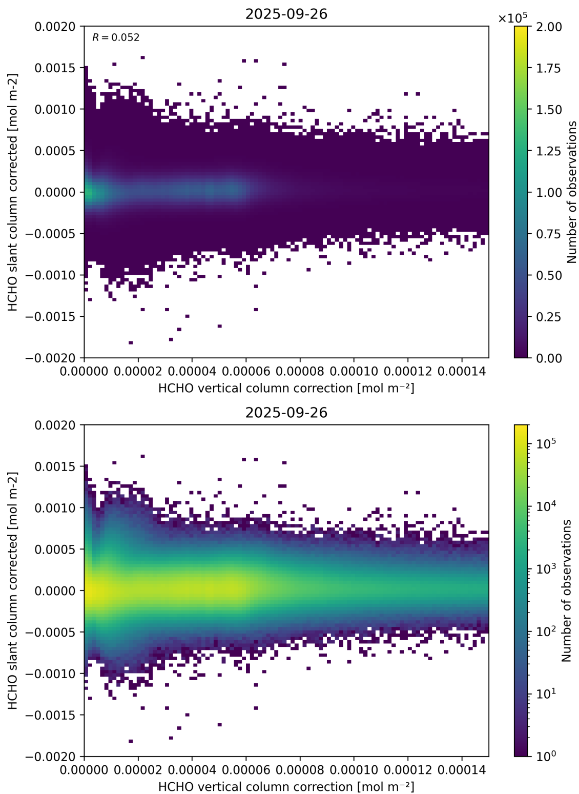
Figure 116: Scatter density plot of “HCHO vertical column correction” against “HCHO slant column corrected” for 2025-09-26 to 2025-09-27.
