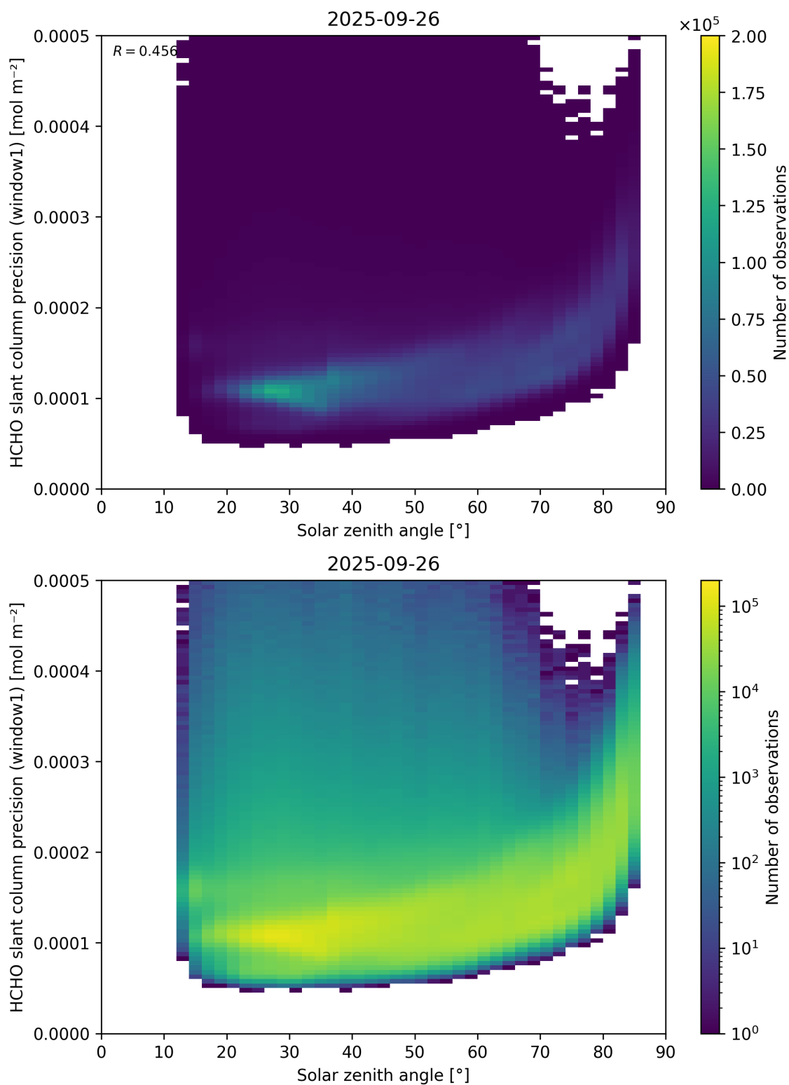
Figure 174: Scatter density plot of “Solar zenith angle” against “HCHO slant column precision (window1)” for 2025-09-26 to 2025-09-27.
