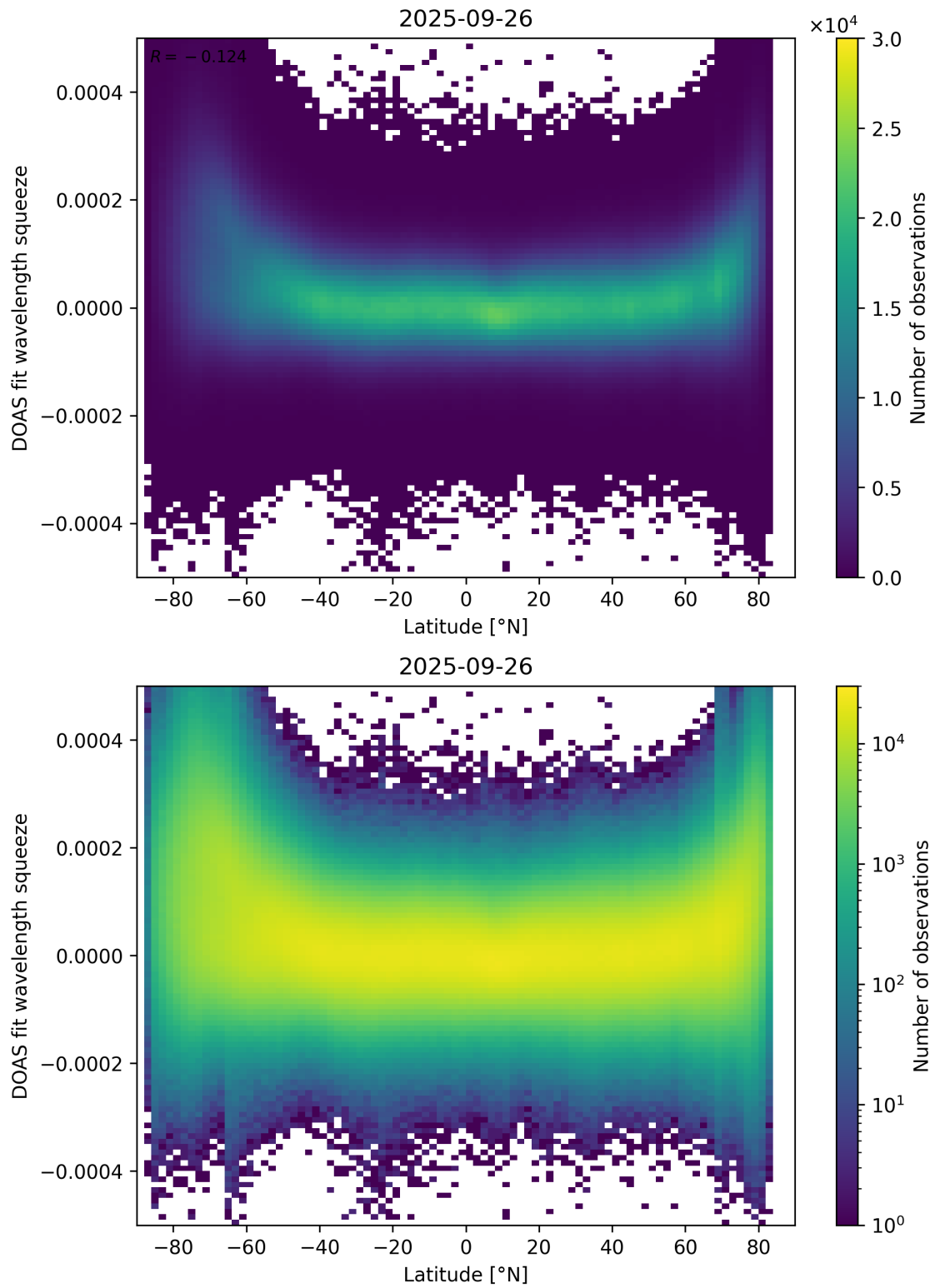
Figure 155: Scatter density plot of “Latitude” against “DOAS fit wavelength squeeze” for 2025-09-26 to 2025-09-27.
