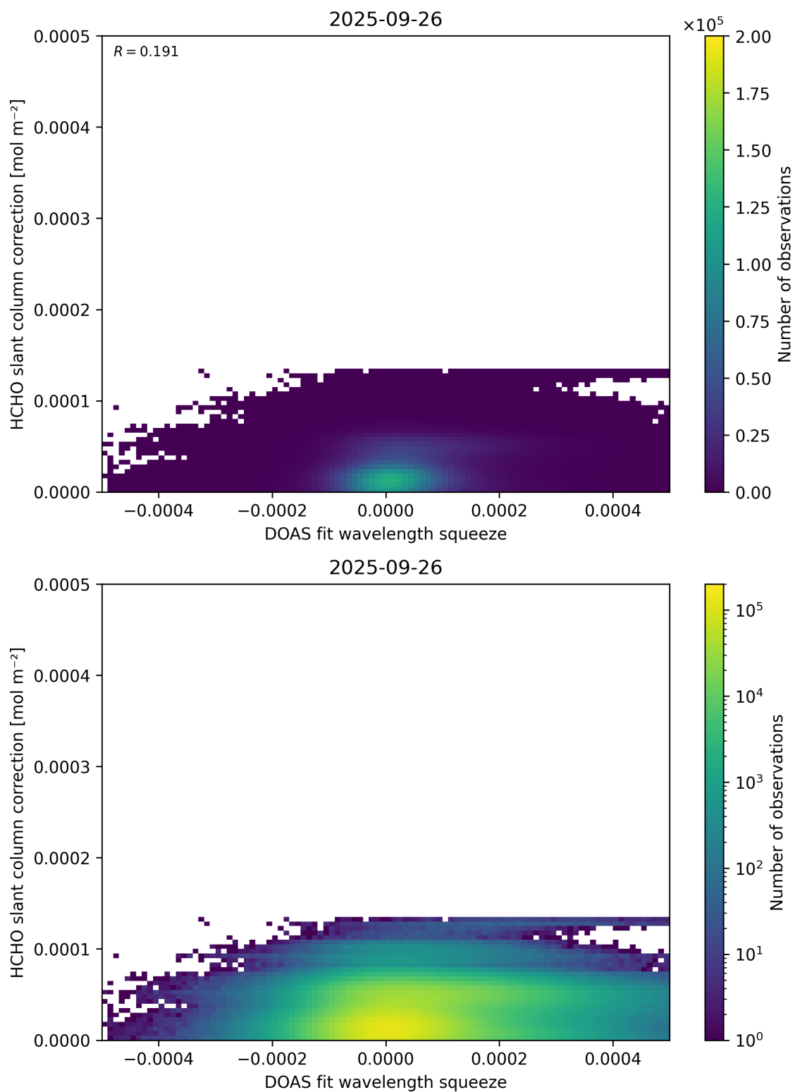
Figure 70: Scatter density plot of “DOAS fit wavelength squeeze” against “HCHO slant column correction” for 2025-09-26 to 2025-09-27.
