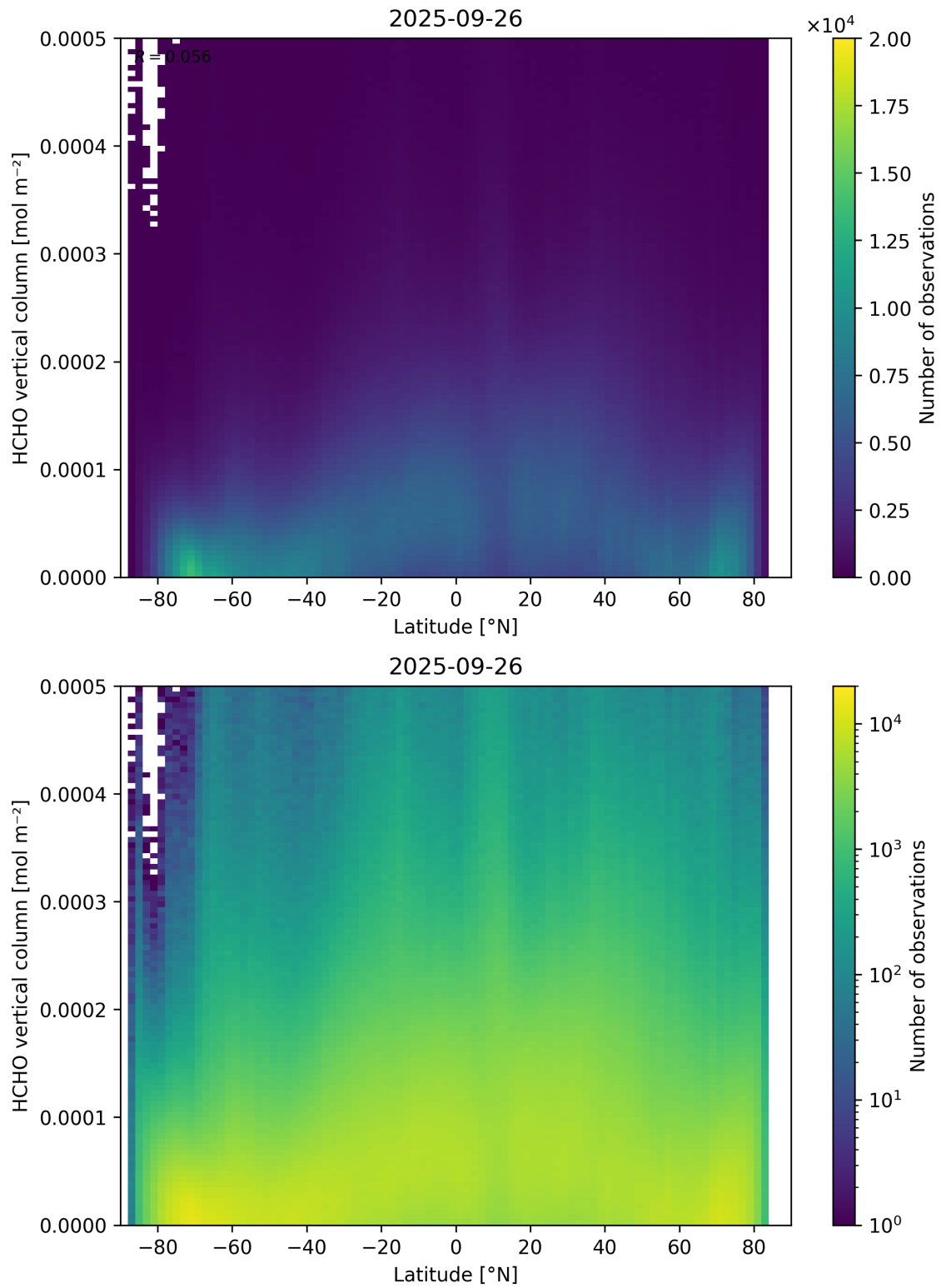
Figure 163: Scatter density plot of “Latitude” against “HCHO vertical column” for 2025-09-26 to 2025-09-27.
