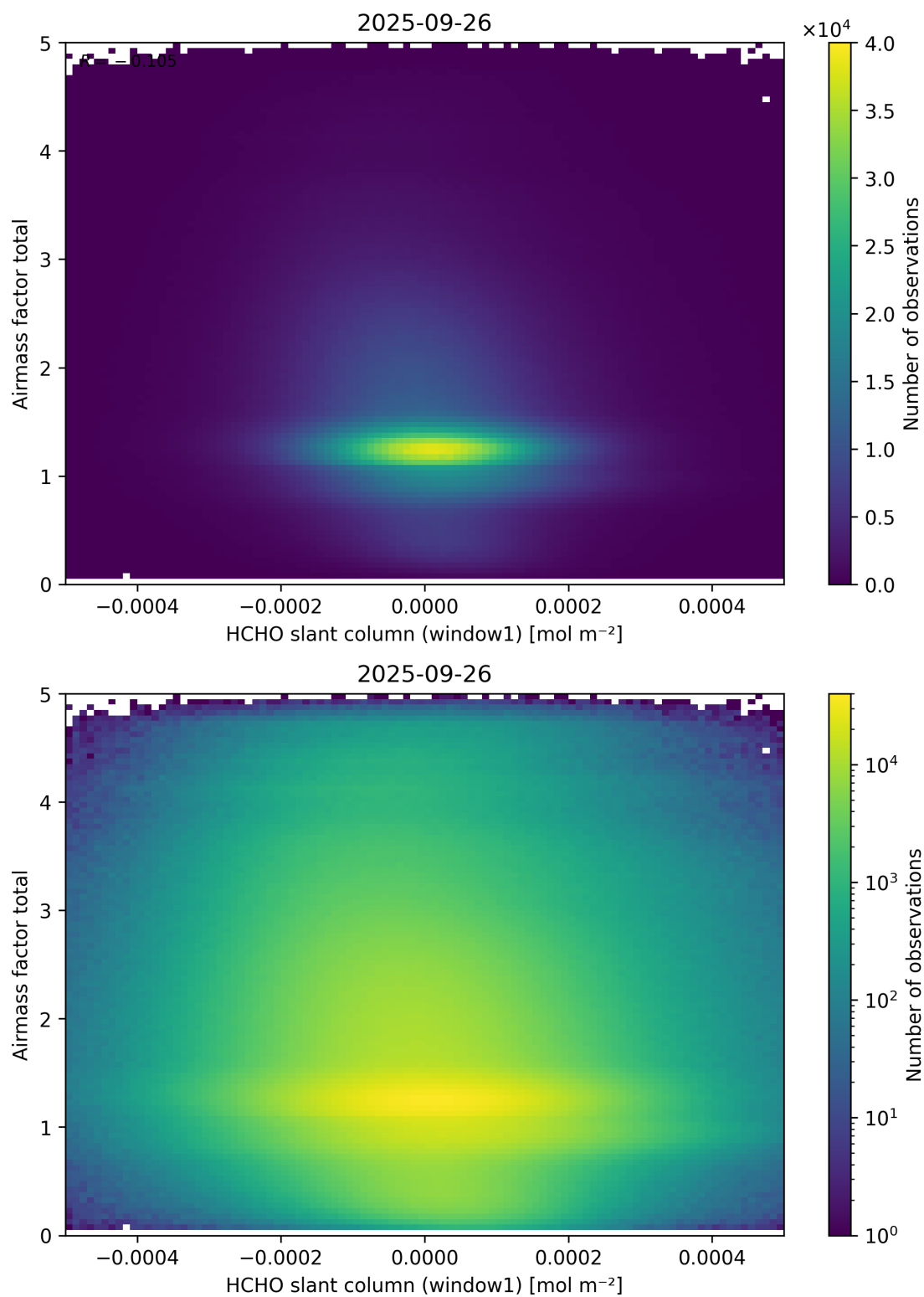
Figure 85: Scatter density plot of “HCHO slant column (window1)” against “Airmass factor total” for 2025-09-26 to 2025-09-27.
