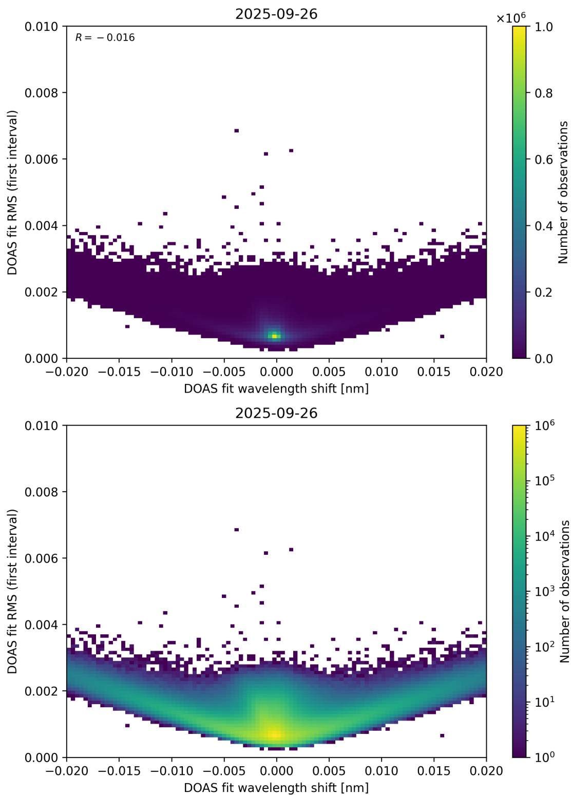
Figure 64: Scatter density plot of “DOAS fit wavelength shift” against “DOAS fit RMS (first interval)” for 2025-09-26 to 2025-09-27.
