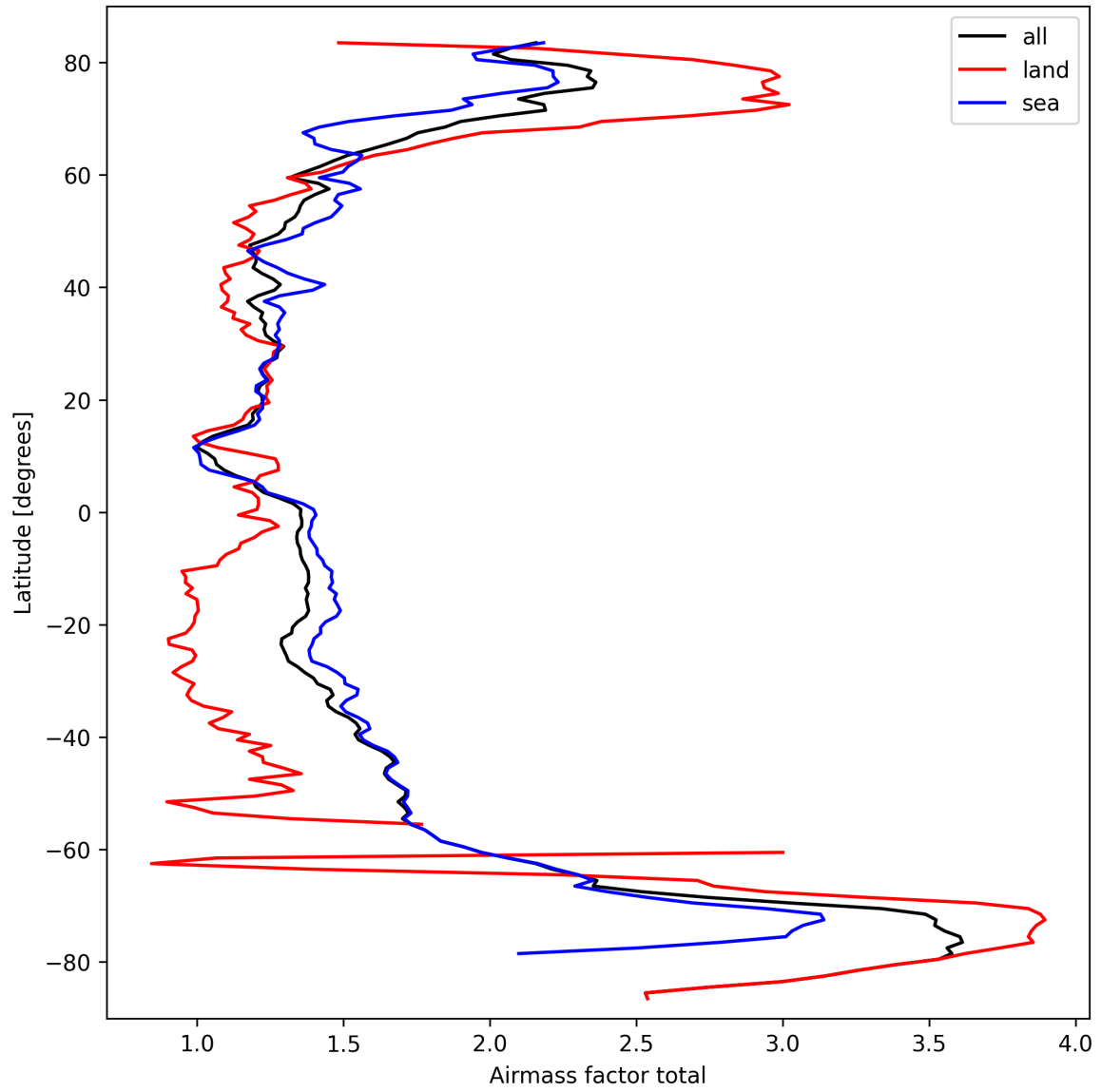
Figure 26: Zonal average of “Airmass factor total” for 2025-09-26 to 2025-09-27.
