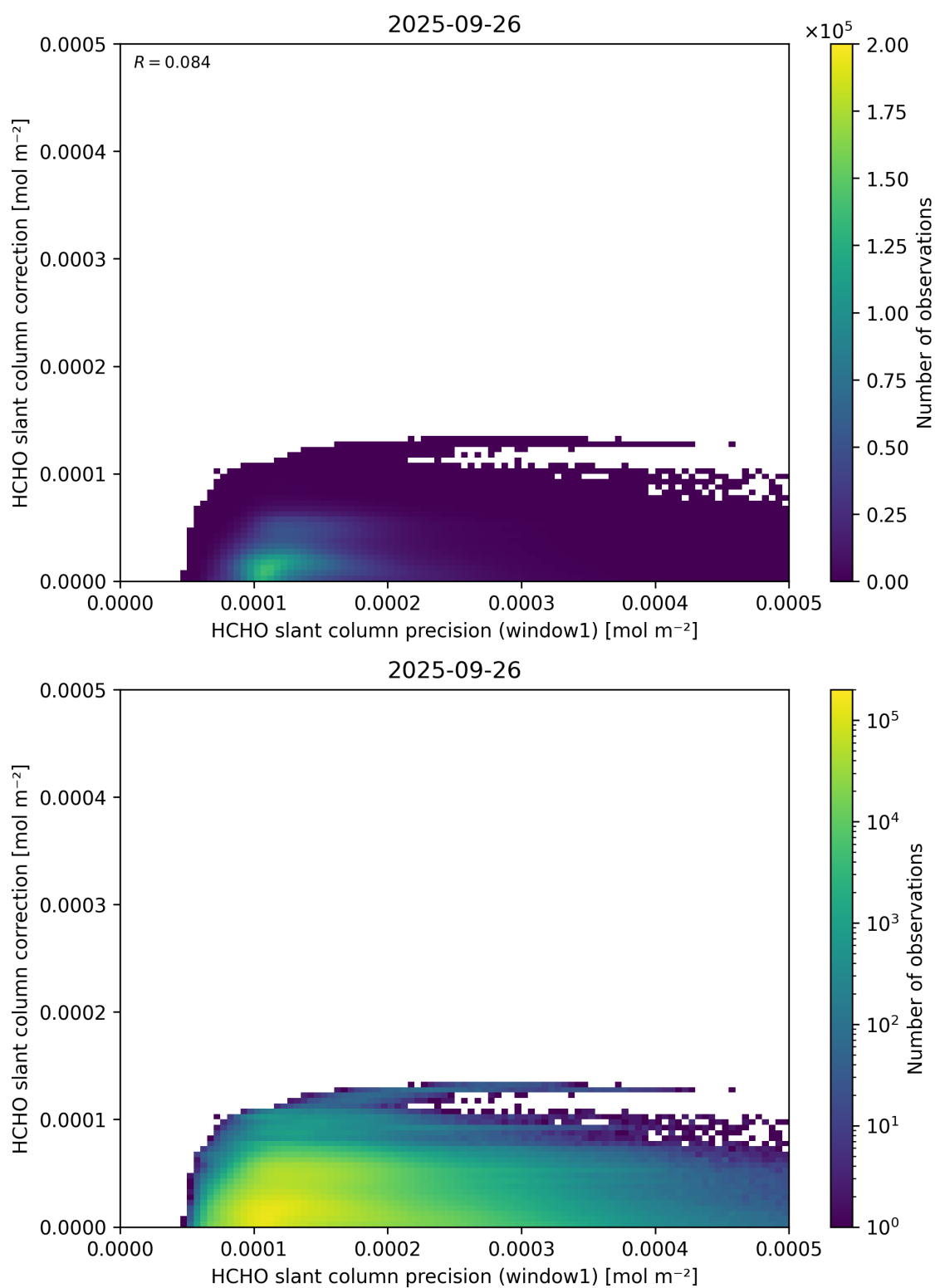
Figure 93: Scatter density plot of “HCHO slant column precision (window1)” against “HCHO slant column correction” for 2025-09-26 to 2025-09-27.
