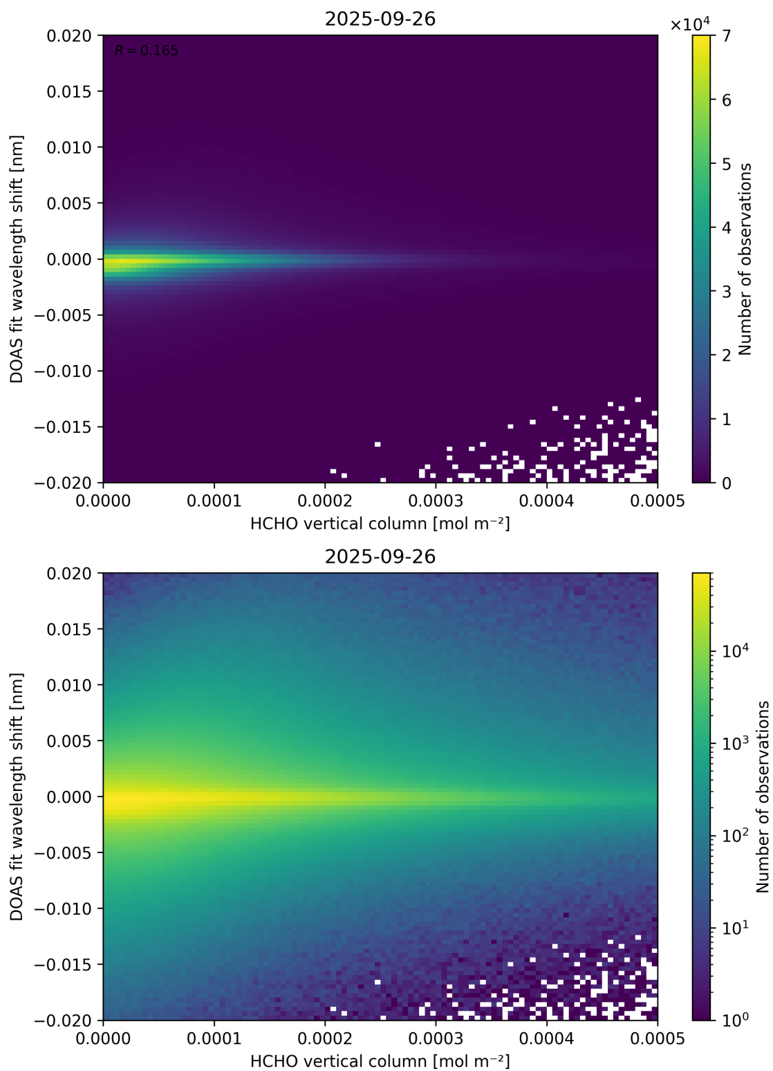
Figure 124: Scatter density plot of “HCHO vertical column” against “DOAS fit wavelength shift” for 2025-09-26 to 2025-09-27.
