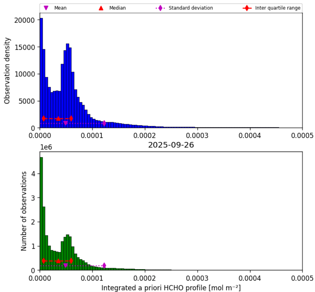
Figure 43: Histogram of “Integrated a priori HCHO profile” for 2025-09-26 to 2025-09-27
