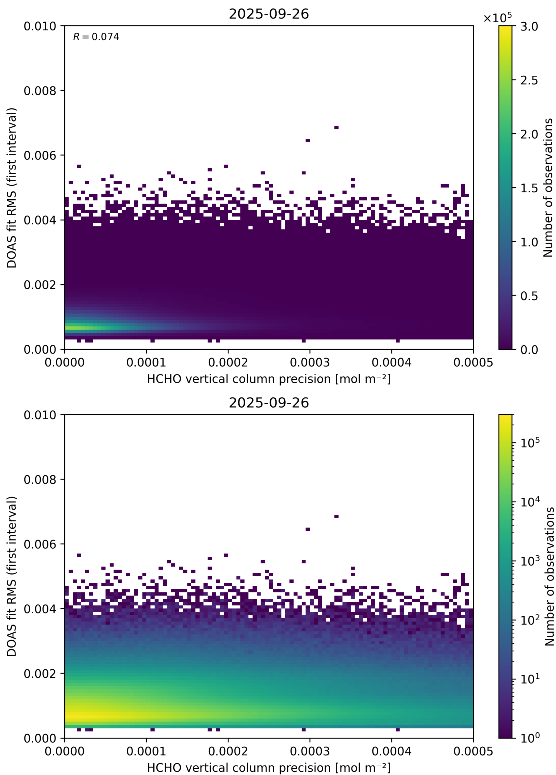
Figure 136: Scatter density plot of “HCHO vertical column precision” against “DOAS fit RMS (first interval)” for 2025-09-26 to 2025-09-27.
