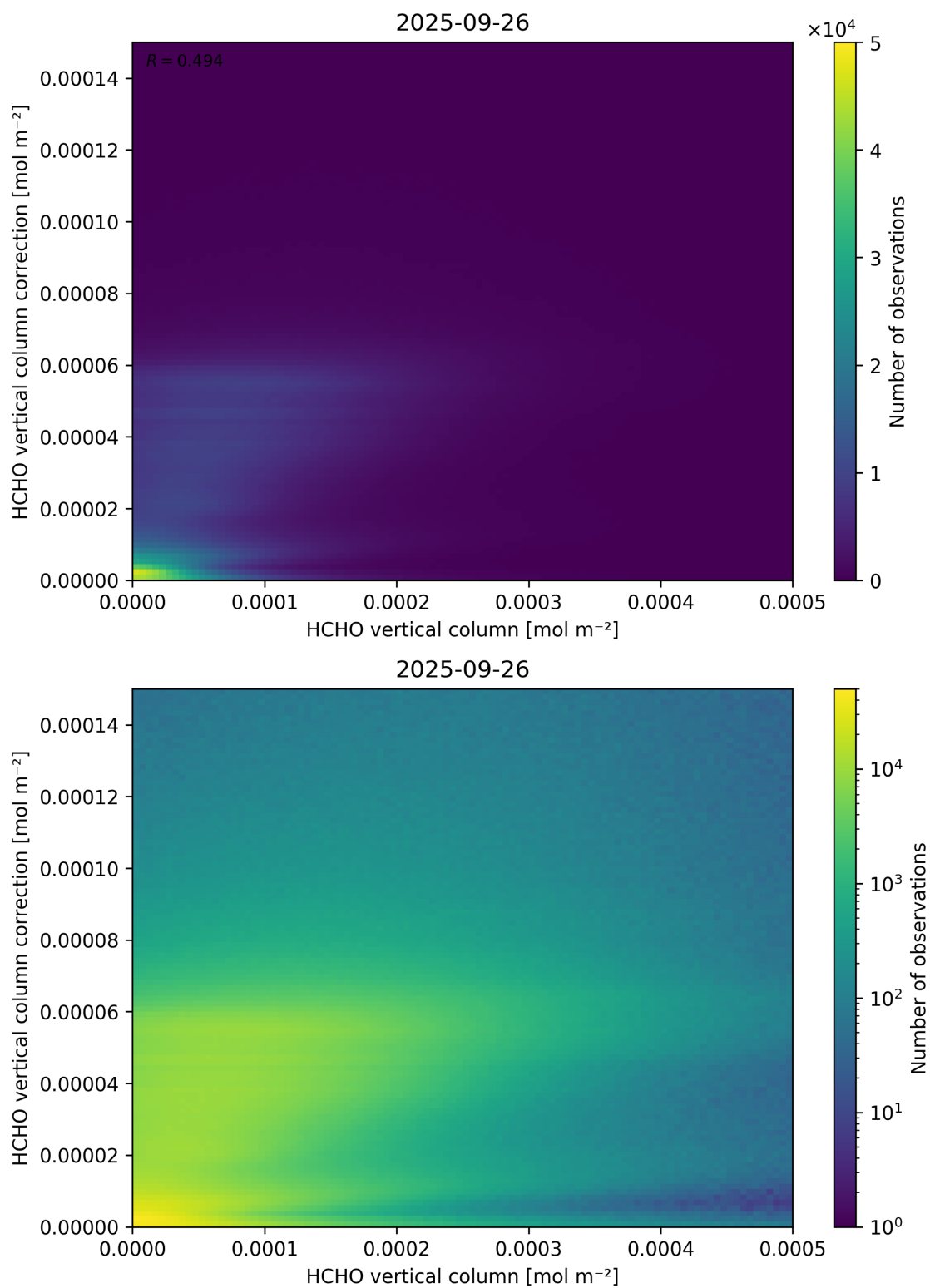
Figure 133: Scatter density plot of “HCHO vertical column” against “HCHO vertical column correction” for 2025-09-26 to 2025-09-27.
