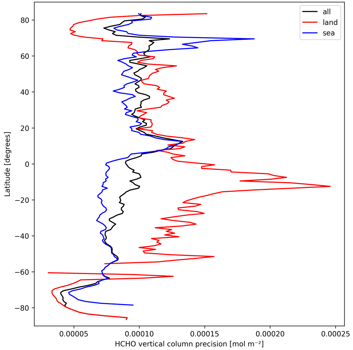
Figure 22: Zonal average of "HCHO vertical column precision" for 2025-09-26 to 2025-09-27.
