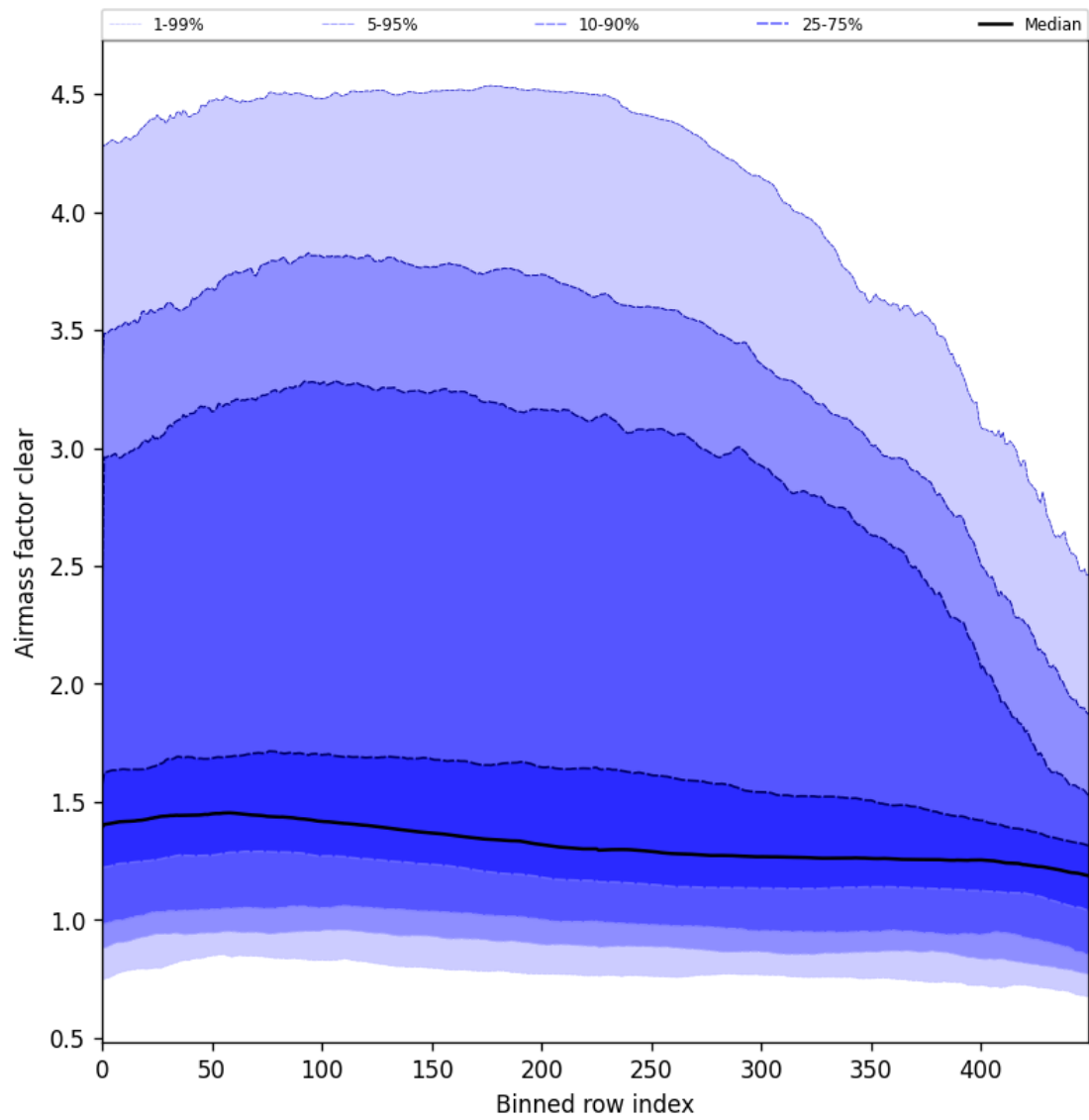
Figure 56: Along track statistics of “Air mass factor clear” for 2025-09-26 to 2025-09-27
