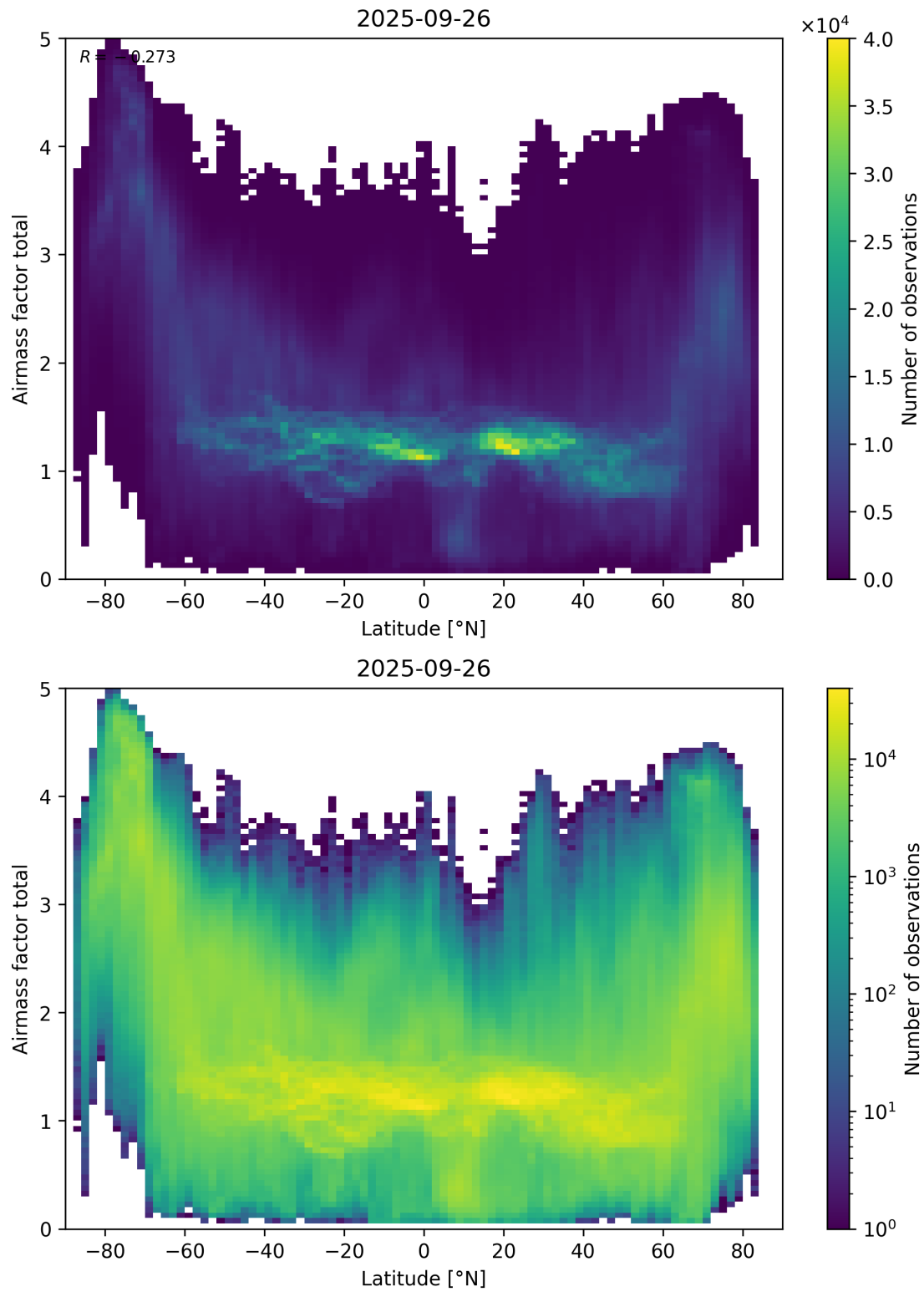
Figure 161: Scatter density plot of “Latitude” against “Airmass factor total” for 2025-09-26 to 2025-09-27.
