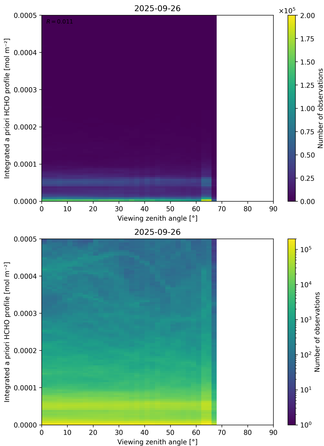
Figure 195: Scatter density plot of “Viewing zenith angle” against “Integrated a priori HCHO profile” for 2025-09-26 to 2025-09-27.
