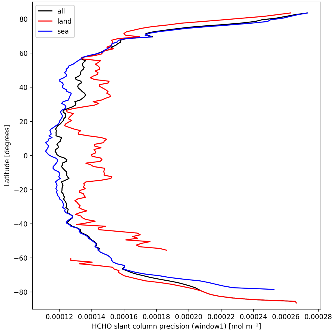
Figure 25: Zonal average of “HCHO slant column precision (window1)” for 2025-09-26 to 2025-09-27.
