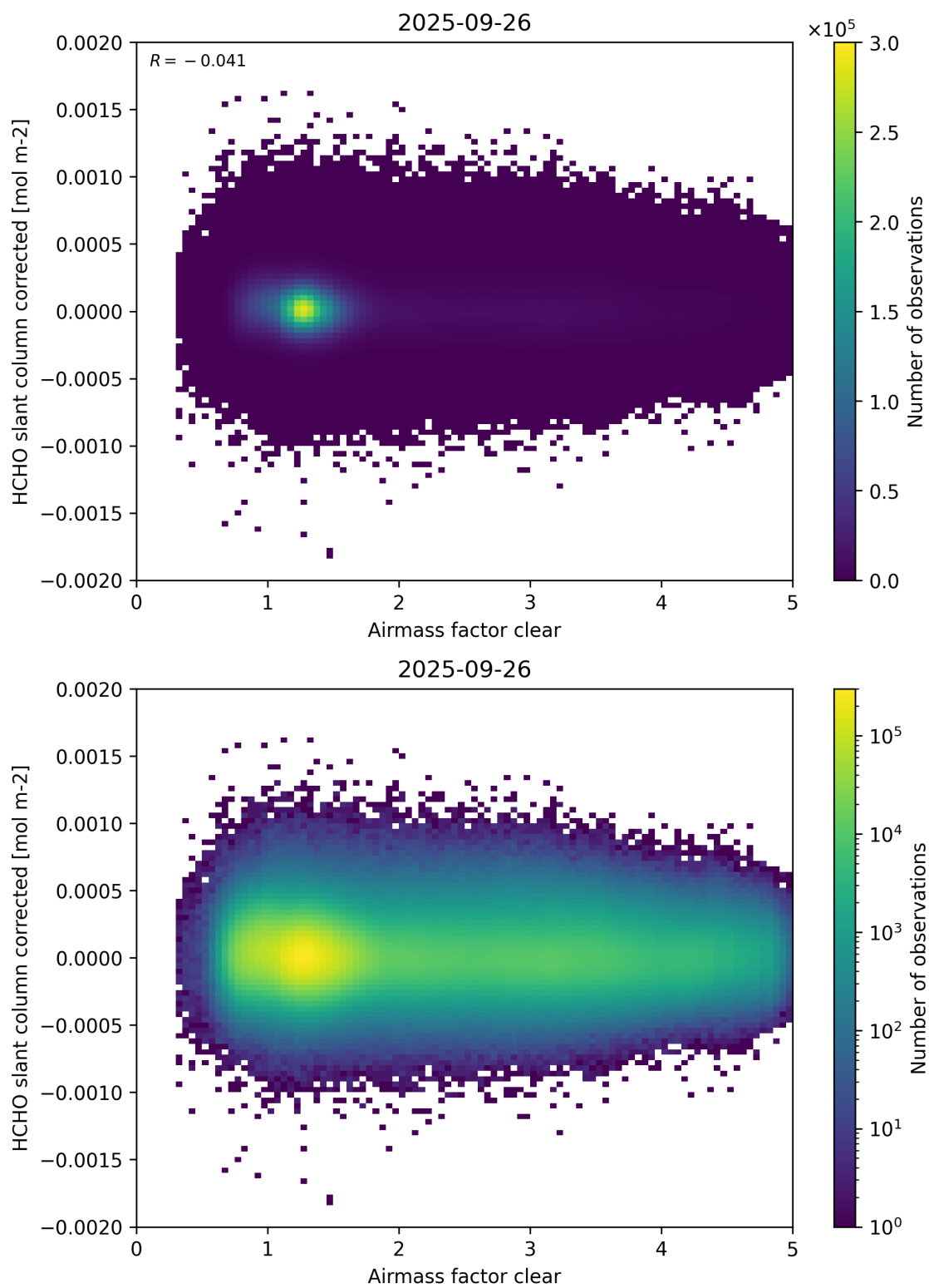
Figure 74: Scatter density plot of “Airmass factor clear” against “HCHO slant column corrected” for 2025-09-26 to 2025-09-27.
