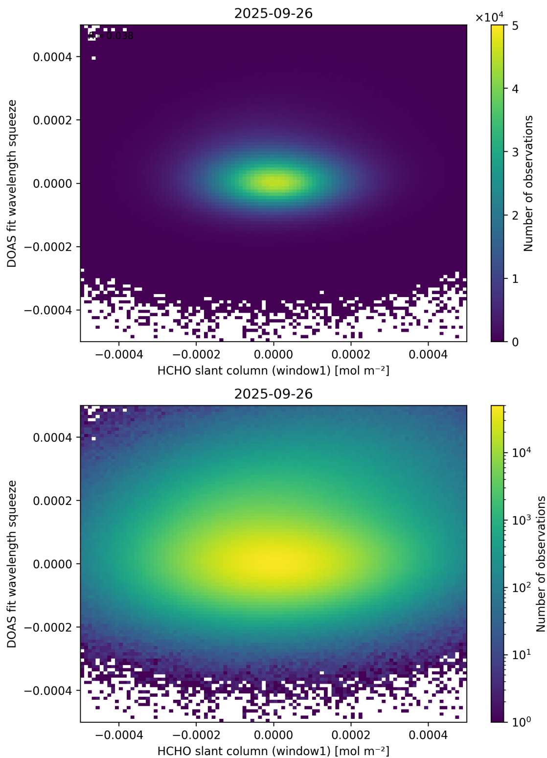
Figure 80: Scatter density plot of “HCHO slant column (window1)” against “DOAS fit wavelength squeeze” for 2025-09-26 to 2025-09-27.
