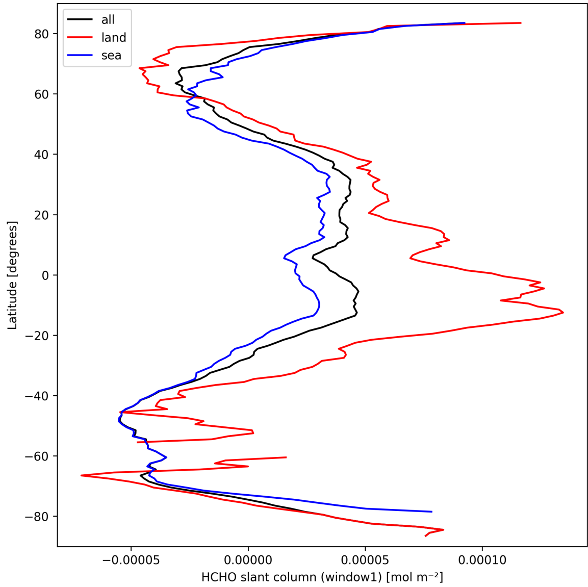
Figure 24: Zonal average of “HCHO slant column (window1)” for 2025-09-26 to 2025-09-27.
