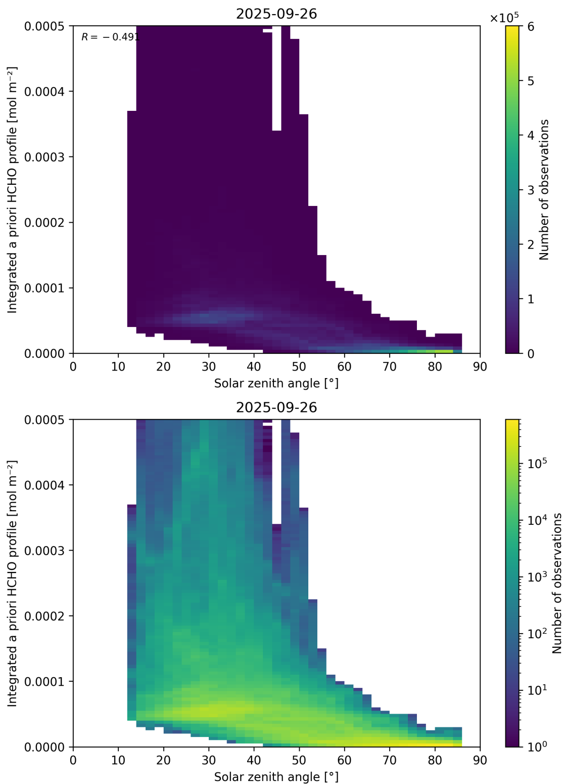
Figure 180: Scatter density plot of “Solar zenith angle” against “Integrated a priori HCHO profile” for 2025-09-26 to 2025-09-27.
