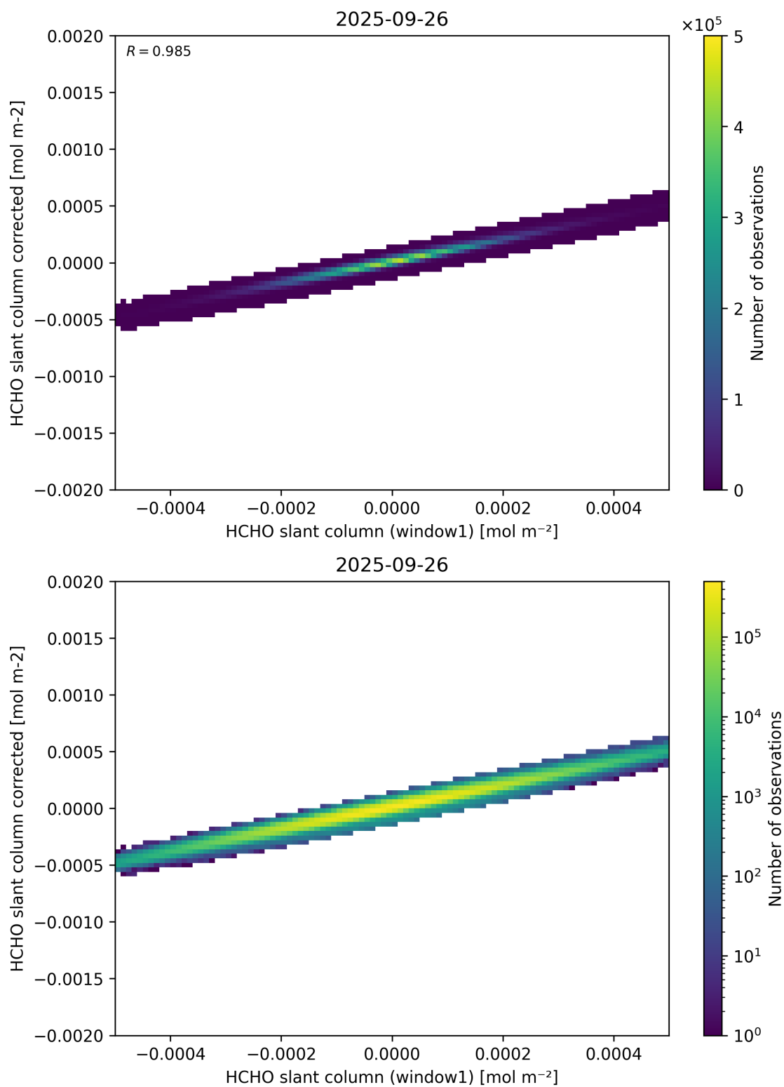
Figure 82: Scatter density plot of “HCHO slant column (window1)” against “HCHO slant column corrected” for 2025-09-26 to 2025-09-27.
