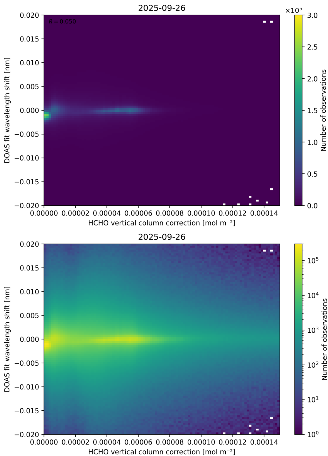
Figure 113: Scatter density plot of “HCHO vertical column correction” against “DOAS fit wavelength shift” for 2025-09-26 to 2025-09-27.
