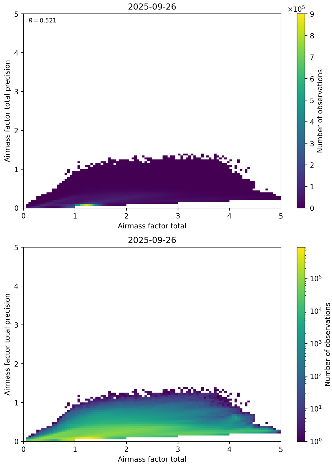
Figure 103: Scatter density plot of “Airmass factor total” against “Airmass factor total precision” for 2025-09-26 to 2025-09-27.
