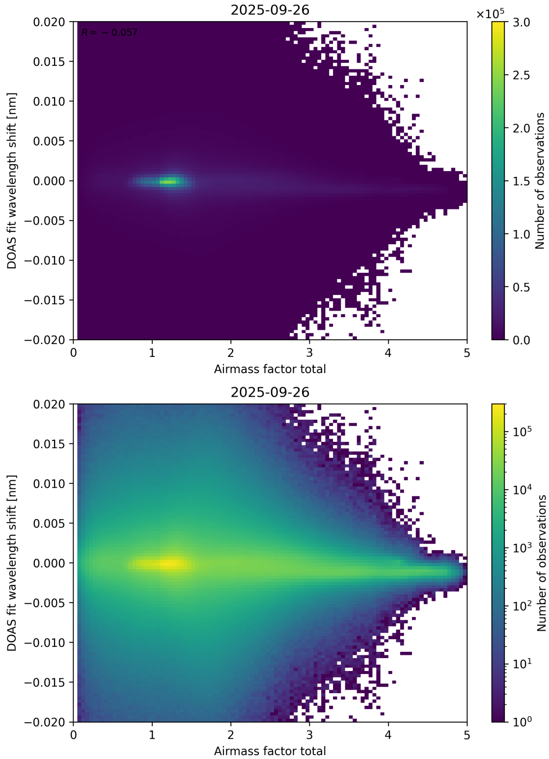
Figure 98: Scatter density plot of “Airmass factor total” against “DOAS fit wavelength shift” for 2025-09-26 to 2025-09-27.
