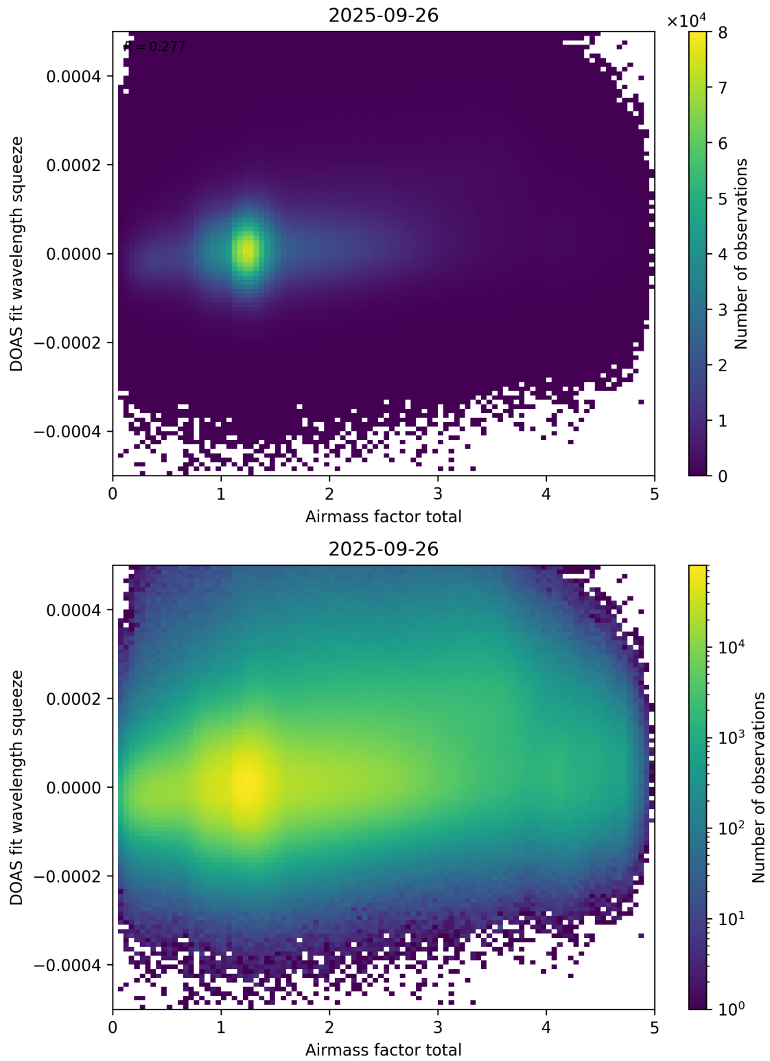
Figure 99: Scatter density plot of “Airmass factor total” against “DOAS fit wavelength squeeze” for 2025-09-26 to 2025-09-27.
