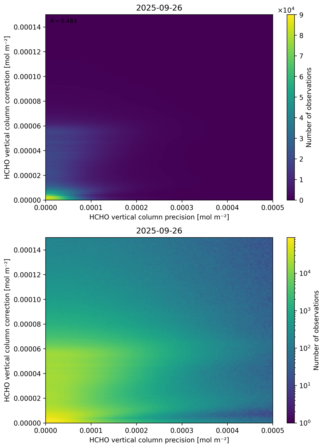
Figure 146: Scatter density plot of “HCHO vertical column precision” against “HCHO vertical column correction” for 2025-09-26 to 2025-09-27.
