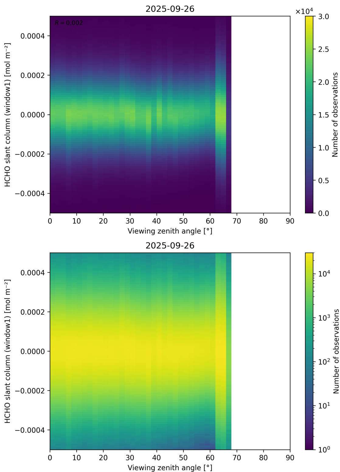
Figure 188: Scatter density plot of “Viewing zenith angle” against “HCHO slant column (window1)” for 2025-09-26 to 2025-09-27.
