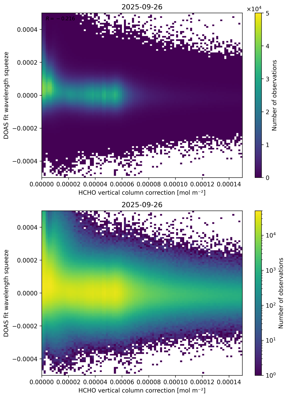
Figure 114: Scatter density plot of “HCHO vertical column correction” against “DOAS fit wavelength squeeze” for 2025-09-26 to 2025-09-27.
