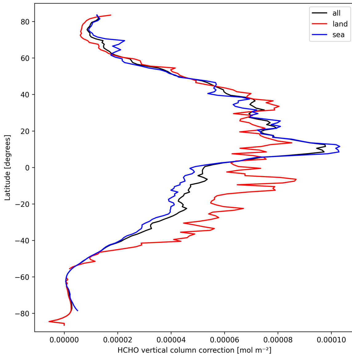
Figure 23: Zonal average of “HCHO vertical column correction” for 2025-09-26 to 2025-09-27.
