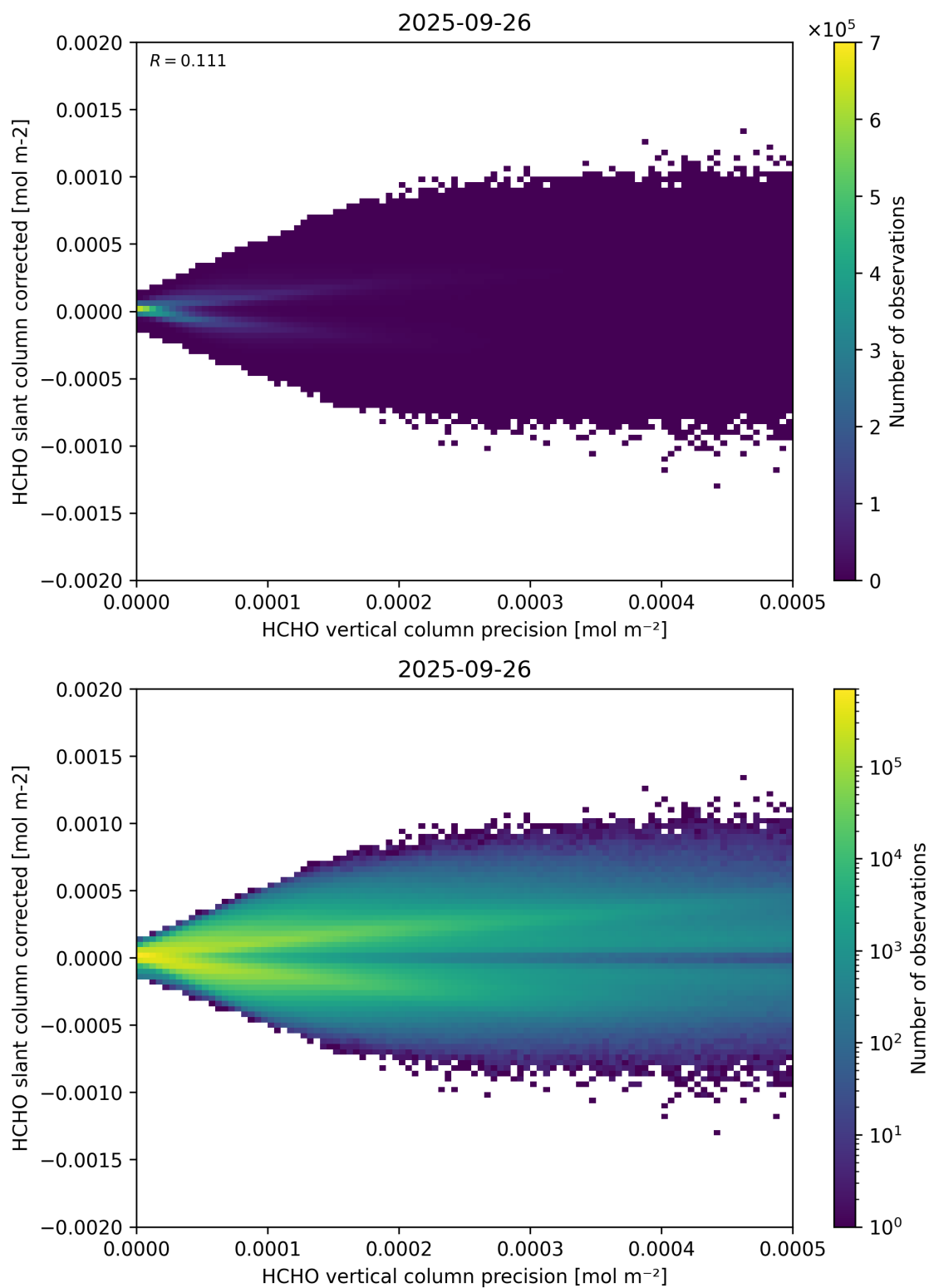
Figure 140: Scatter density plot of “HCHO vertical column precision” against “HCHO slant column corrected” for 2025-09-26 to 2025-09-27.
