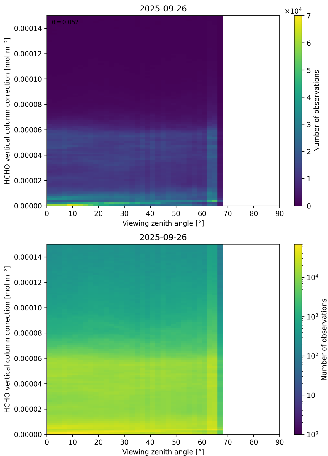
Figure 193: Scatter density plot of “Viewing zenith angle” against “HCHO vertical column correction” for 2025-09-26 to 2025-09-27.
