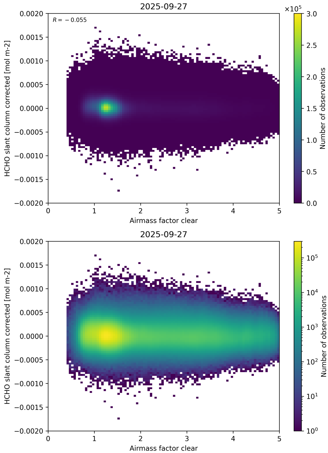
Figure 74: Scatter density plot of “Airmass factor clear” against “HCHO slant column corrected” for 2025-09-26 to 2025-09-28.
