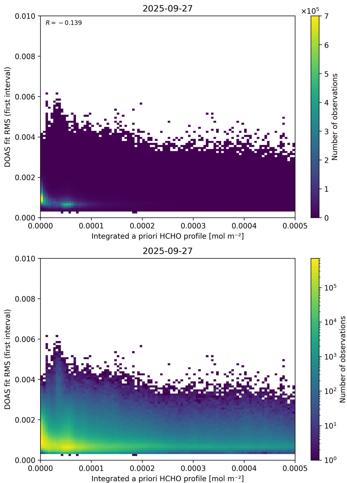
Figure 148: Scatter density plot of “Integrated a priori HCHO profile” against “DOAS fit RMS (first interval)” for 2025-09-26 to 2025-09-28.
