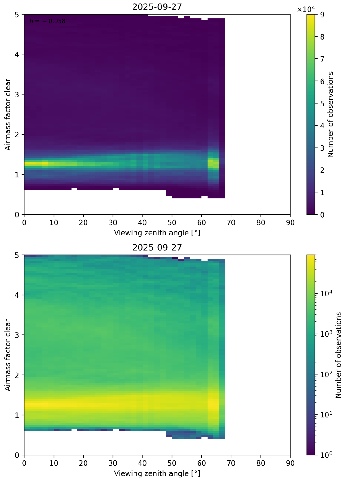
Figure 185: Scatter density plot of “Viewing zenith angle” against “Airmass factor clear” for 2025-09-26 to 2025-09-28.
