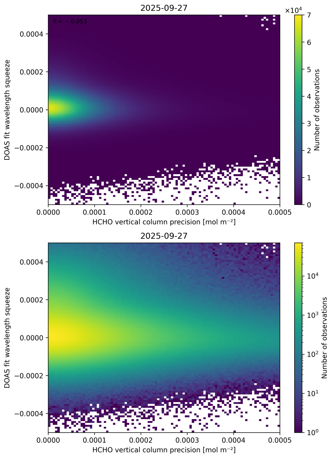
Figure 138: Scatter density plot of “HCHO vertical column precision” against “DOAS fit wavelength squeeze” for 2025-09-26 to 2025-09-28.
