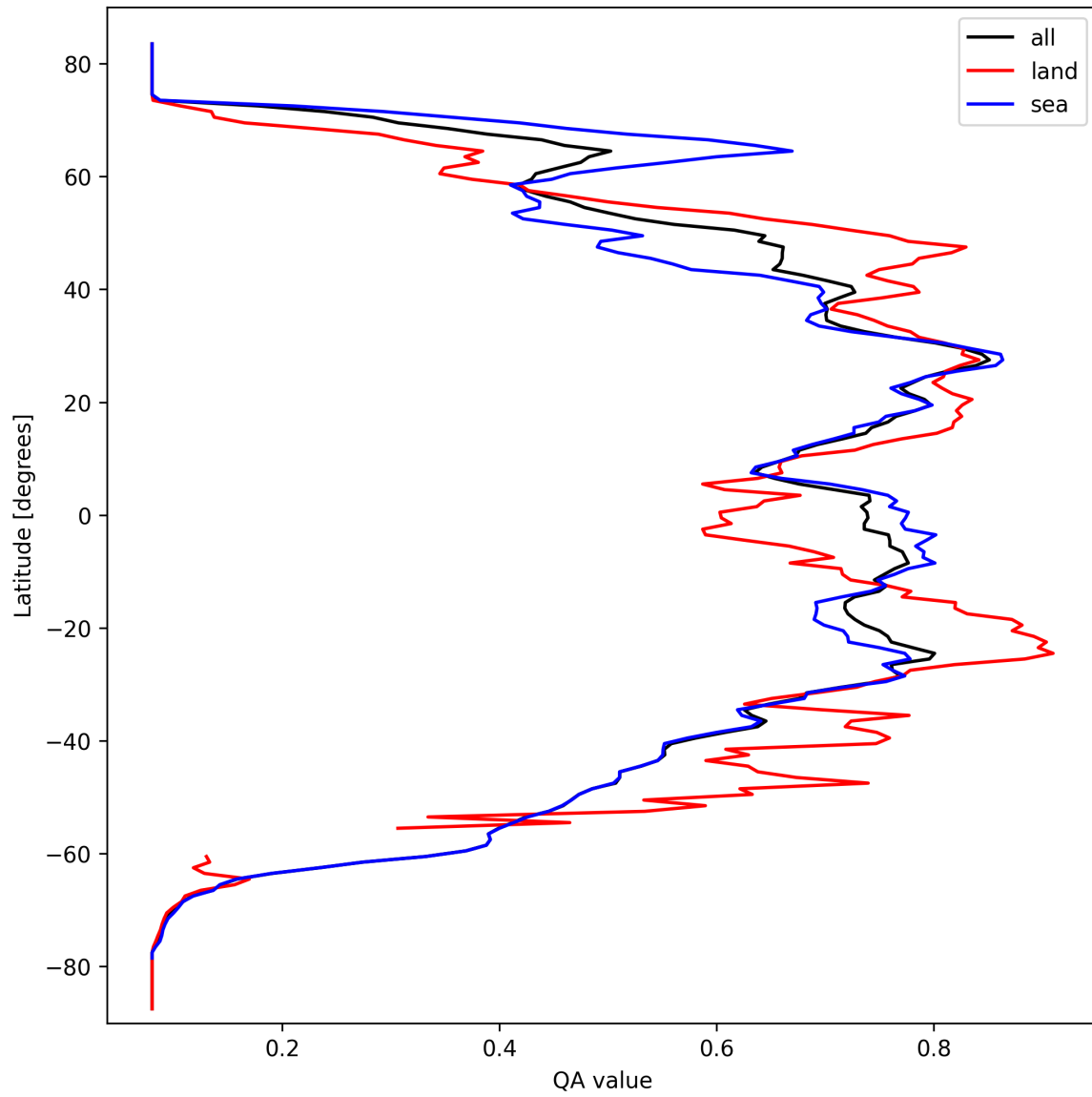
Figure 20: Zonal average of “QA value” for 2025-09-26 to 2025-09-28.
