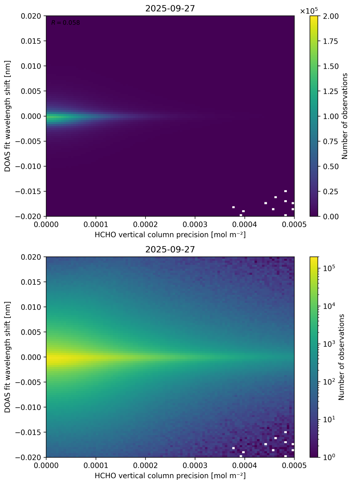
Figure 137: Scatter density plot of “HCHO vertical column precision” against “DOAS fit wavelength shift” for 2025-09-26 to 2025-09-28.
