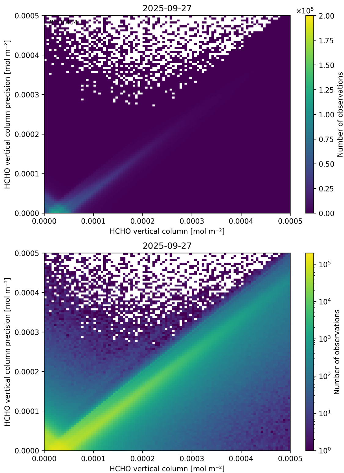
Figure 134: Scatter density plot of “HCHO vertical column” against “HCHO vertical column precision” for 2025-09-26 to 2025-09-28.
