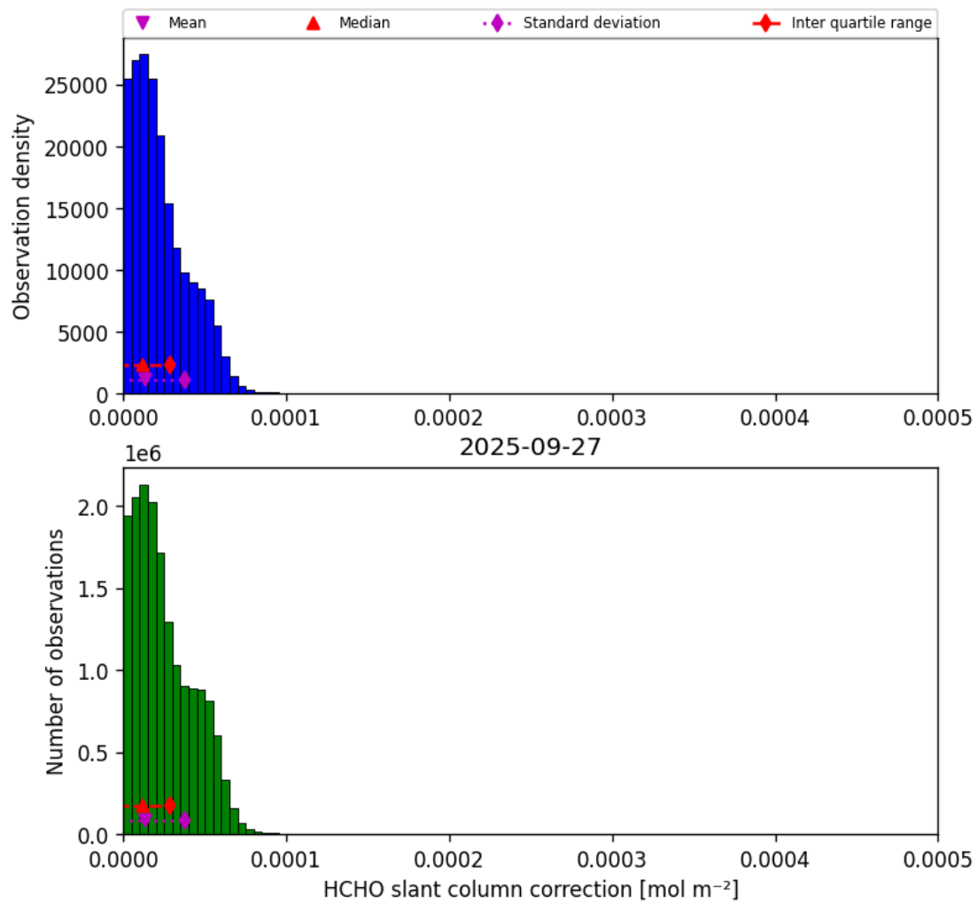
Figure 47: Histogram of “HCHO slant column correction” for 2025-09-26 to 2025-09-28
