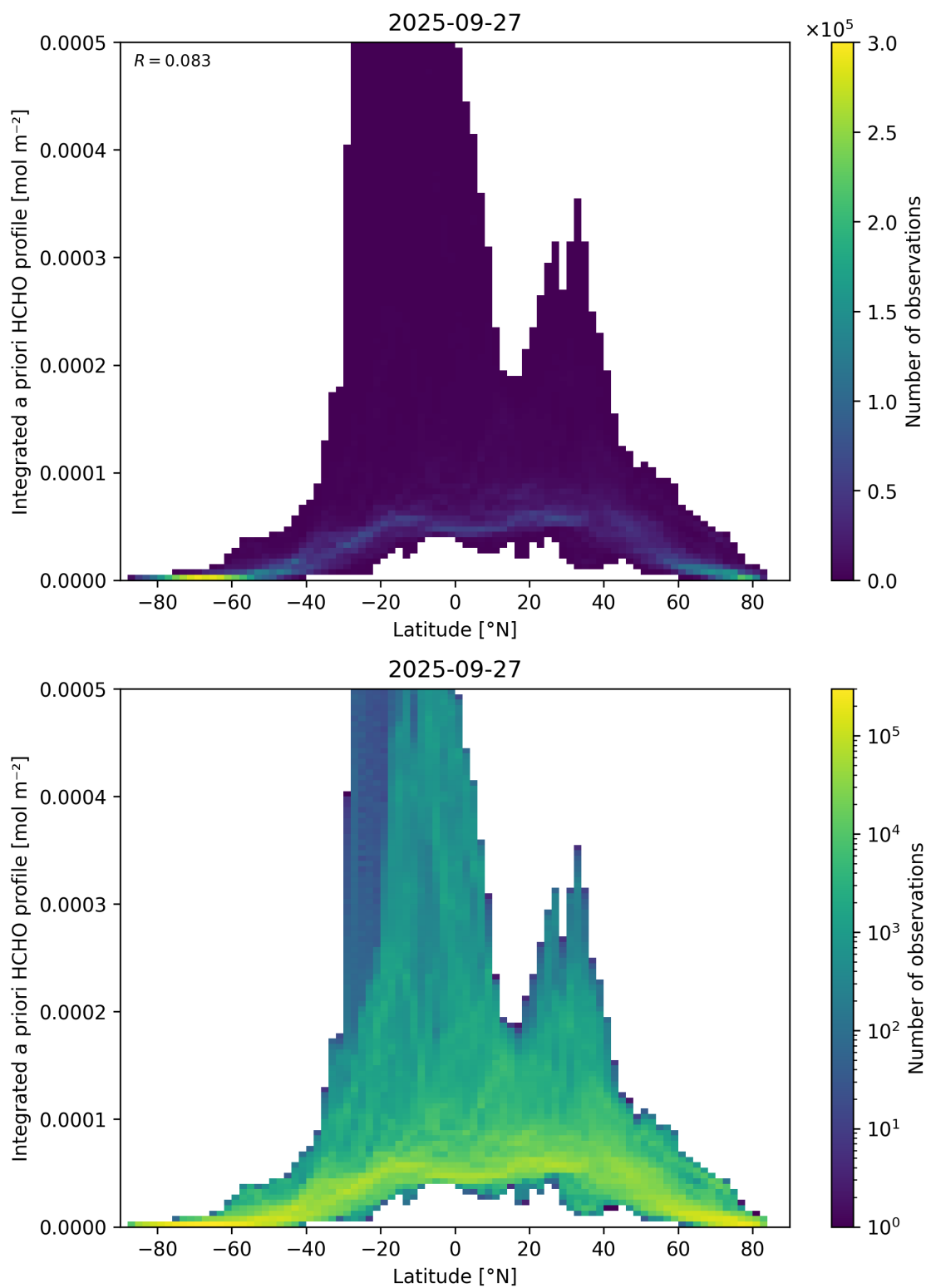
Figure 166: Scatter density plot of “Latitude” against “Integrated a priori HCHO profile” for 2025-09-26 to 2025-09-28.
