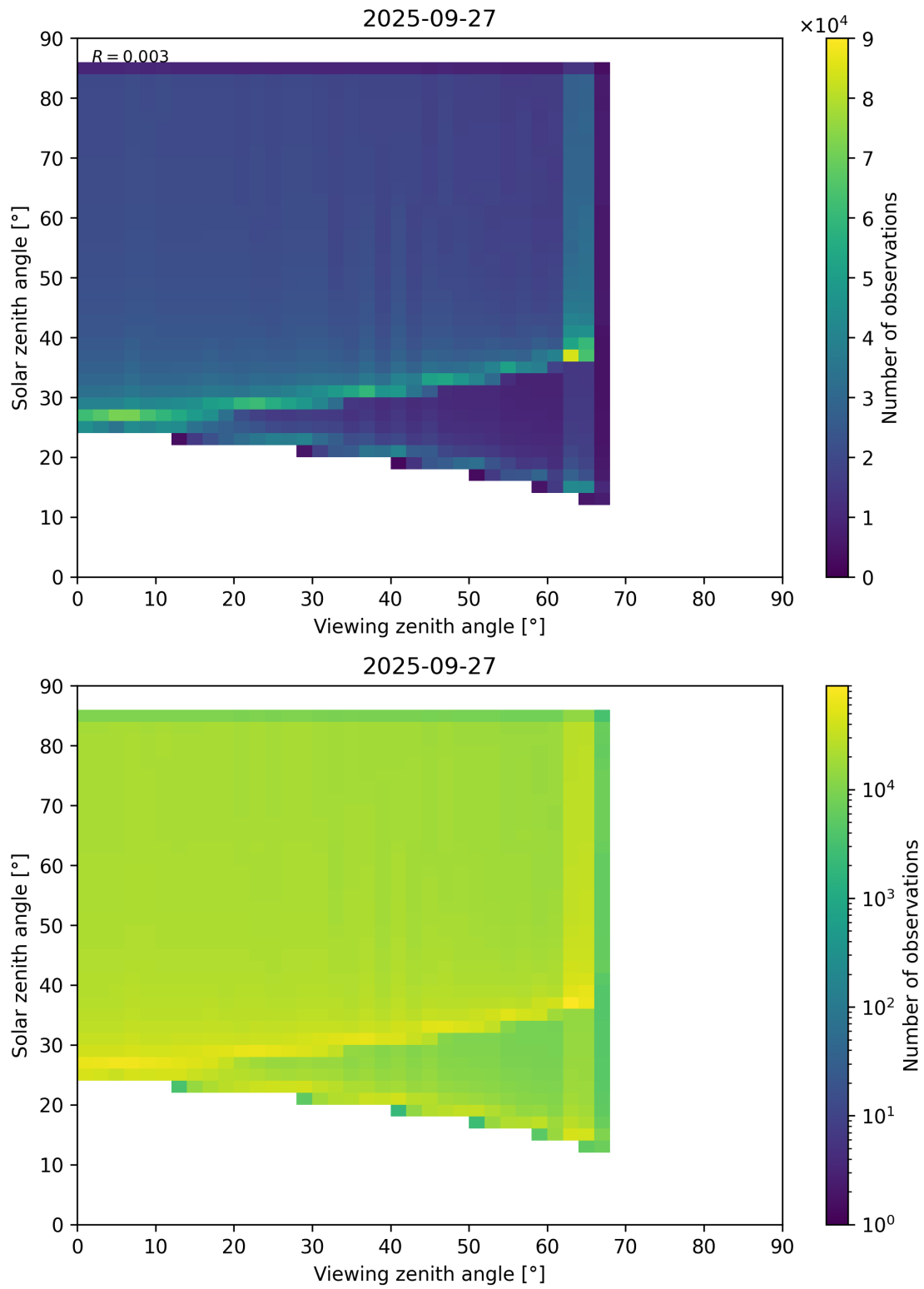
Figure 197: Scatter density plot of “Viewing zenith angle” against “Solar zenith angle” for 2025-09-26 to 2025-09-28.
