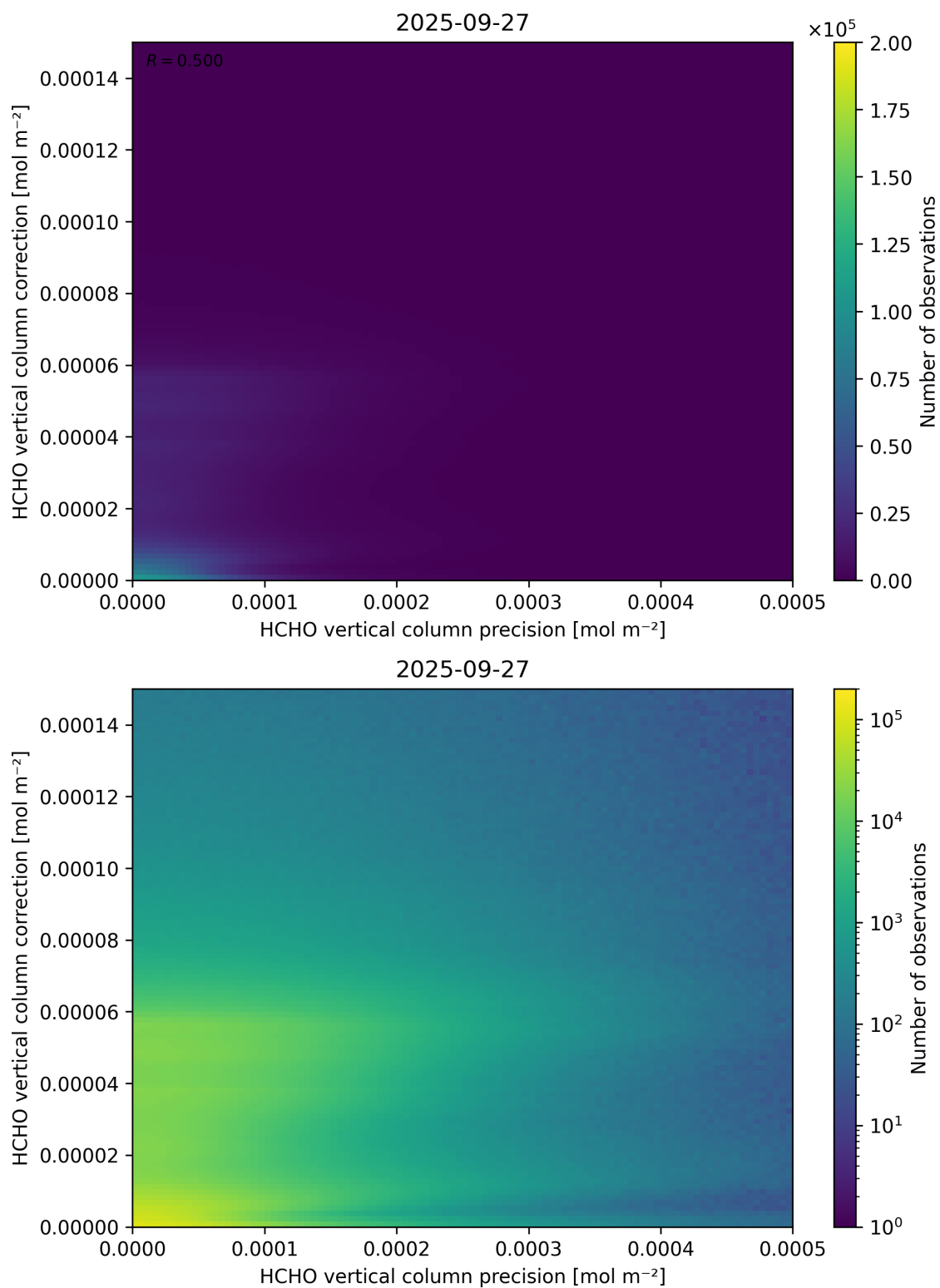
Figure 146: Scatter density plot of “HCHO vertical column precision” against “HCHO vertical column correction” for 2025-09-26 to 2025-09-28.
