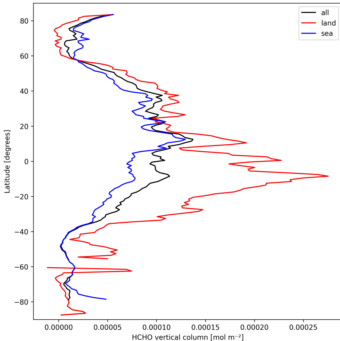
Figure 21: Zonal average of “HCHO vertical column” for 2025-09-26 to 2025-09-28.
