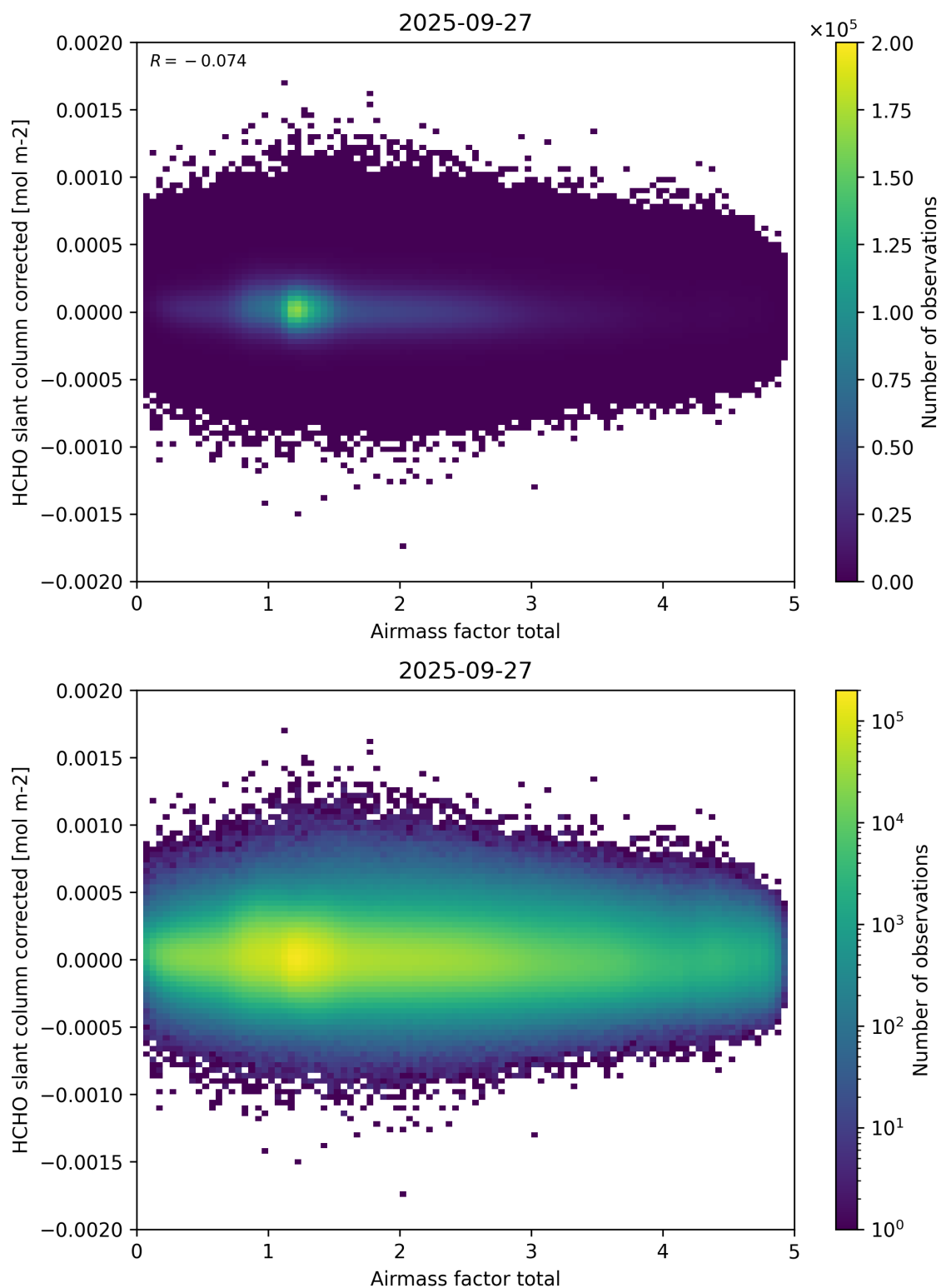
Figure 101: Scatter density plot of “Airmass factor total” against “HCHO slant column corrected” for 2025-09-26 to 2025-09-28.
