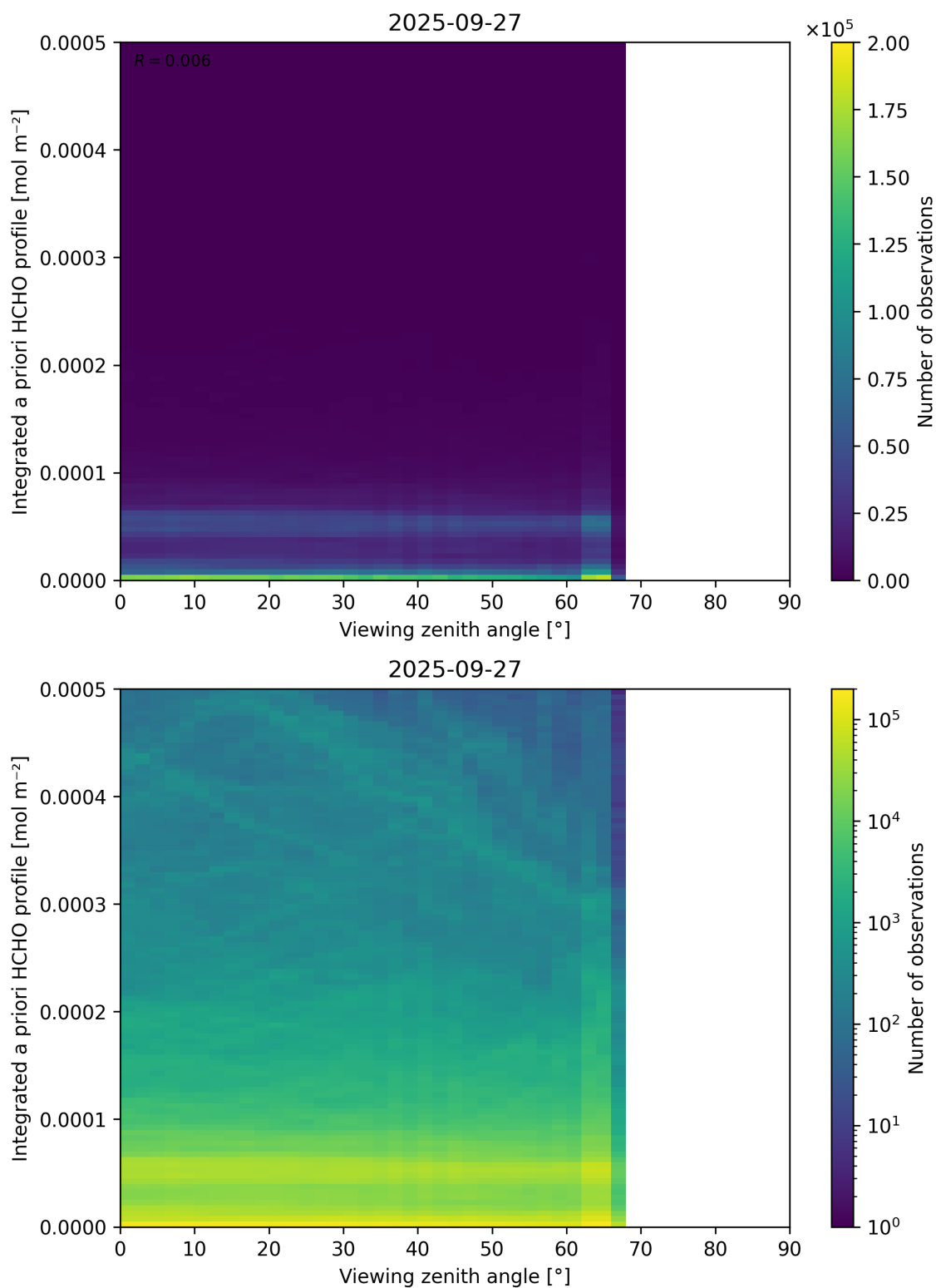
Figure 195: Scatter density plot of “Viewing zenith angle” against “Integrated a priori HCHO profile” for 2025-09-26 to 2025-09-28.
