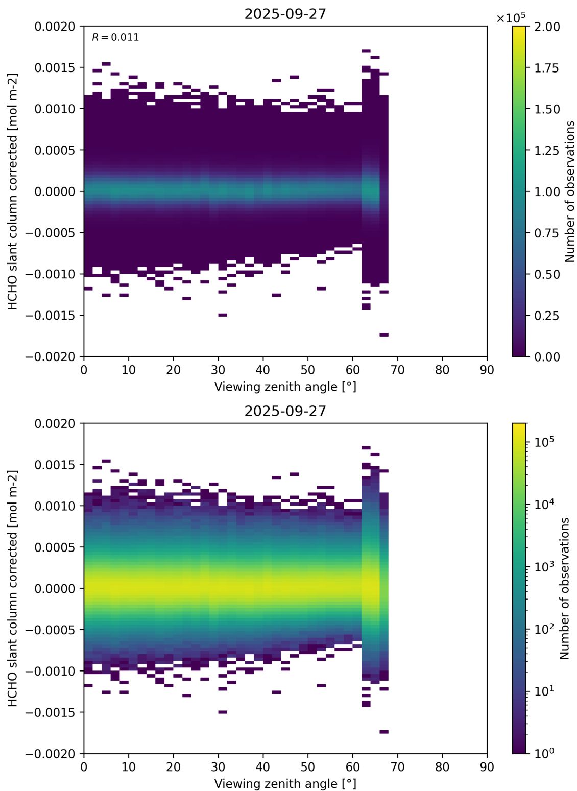
Figure 186: Scatter density plot of “Viewing zenith angle” against “HCHO slant column corrected” for 2025-09-26 to 2025-09-28.
