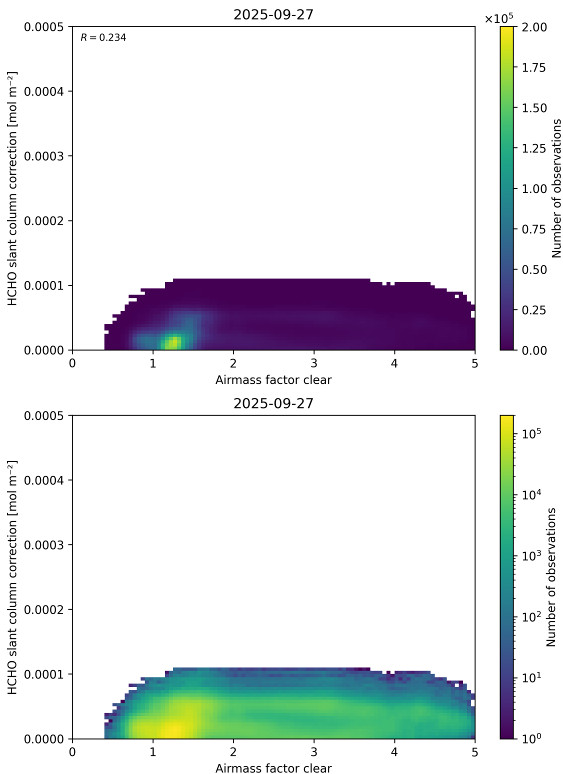
Figure 75: Scatter density plot of “Airmass factor clear” against “HCHO slant column correction” for 2025-09-26 to 2025-09-28.
