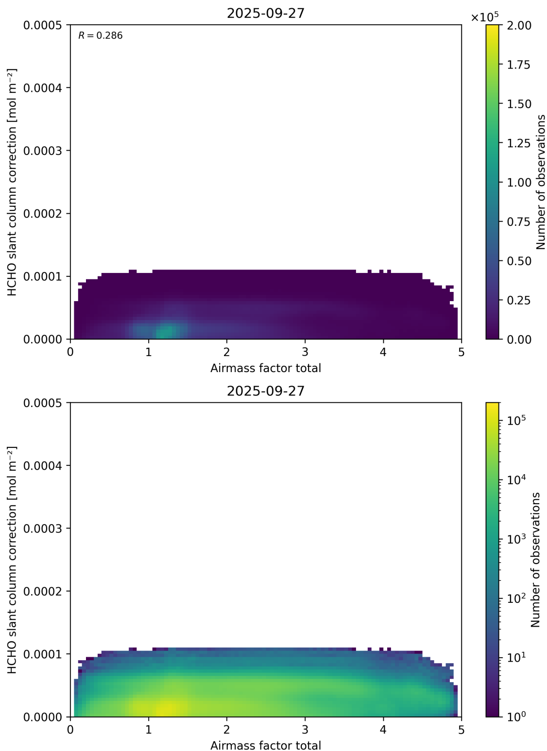
Figure 102: Scatter density plot of “Airmass factor total” against “HCHO slant column correction” for 2025-09-26 to 2025-09-28.
