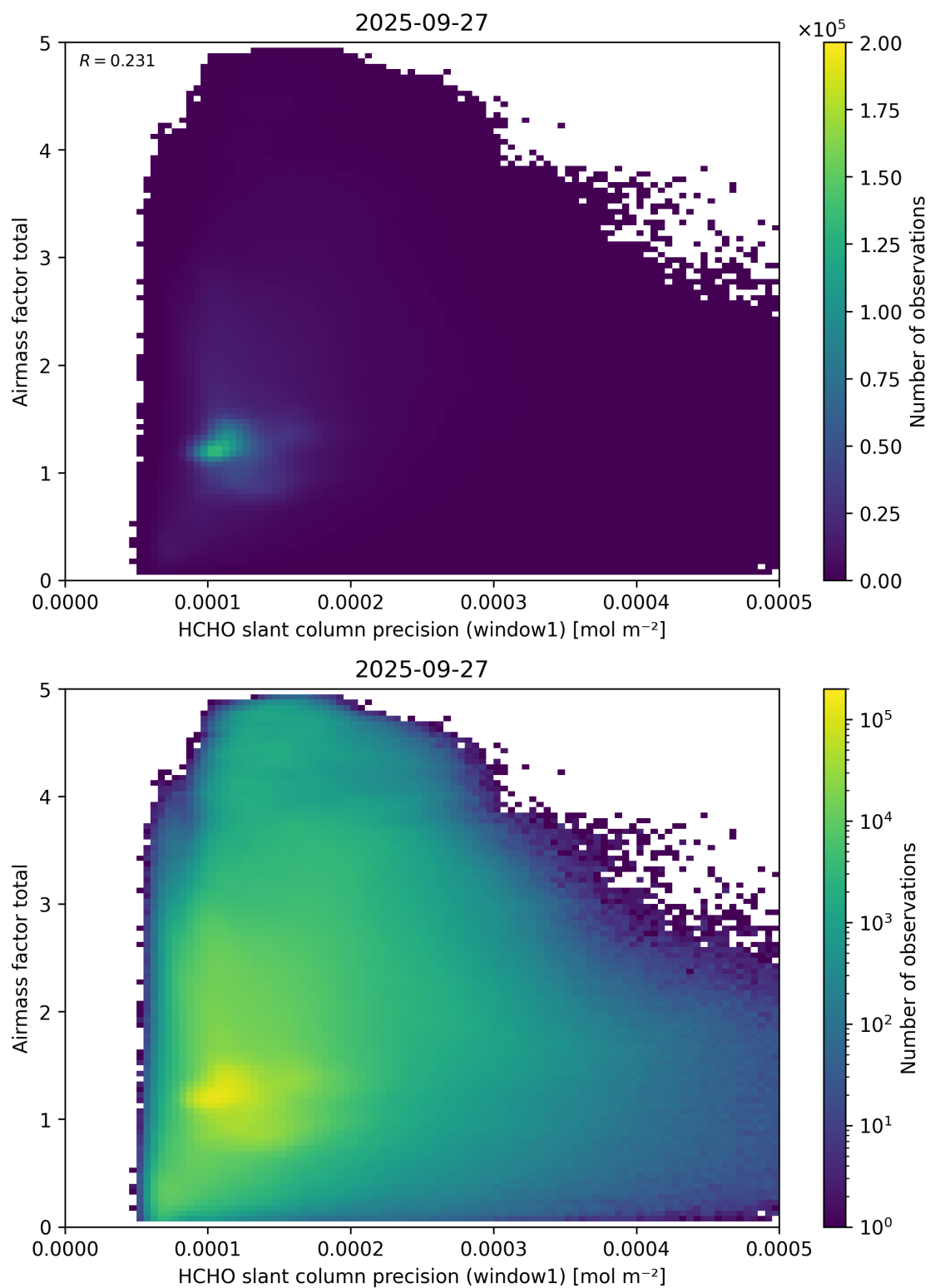
Figure 94: Scatter density plot of “HCHO slant column precision (window1)” against “Airmass factor total” for 2025-09-26 to 2025-09-28.
