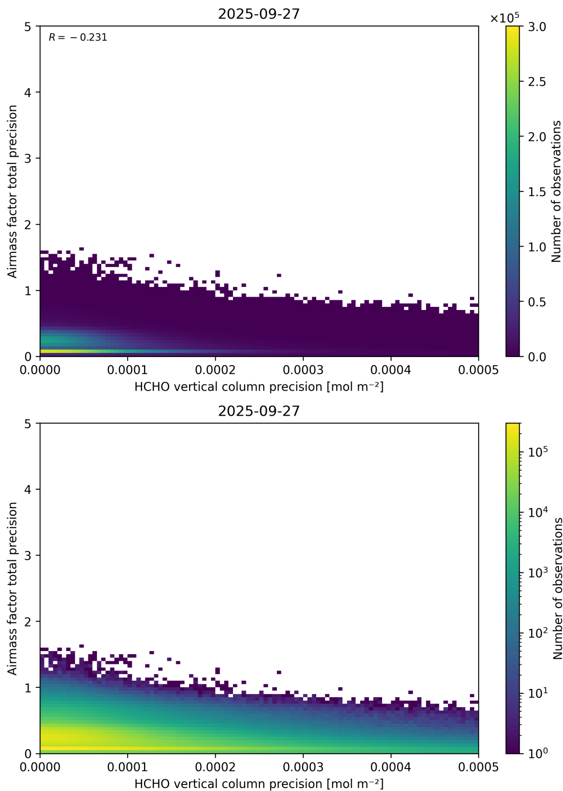
Figure 145: Scatter density plot of “HCHO vertical column precision” against “Airmass factor total precision” for 2025-09-26 to 2025-09-28.
