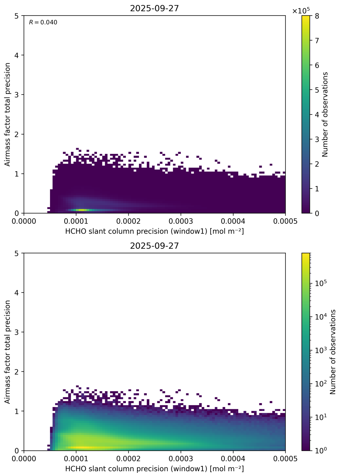
Figure 95: Scatter density plot of “HCHO slant column precision (window1)” against “Airmass factor total precision” for 2025-09-26 to 2025-09-28.
