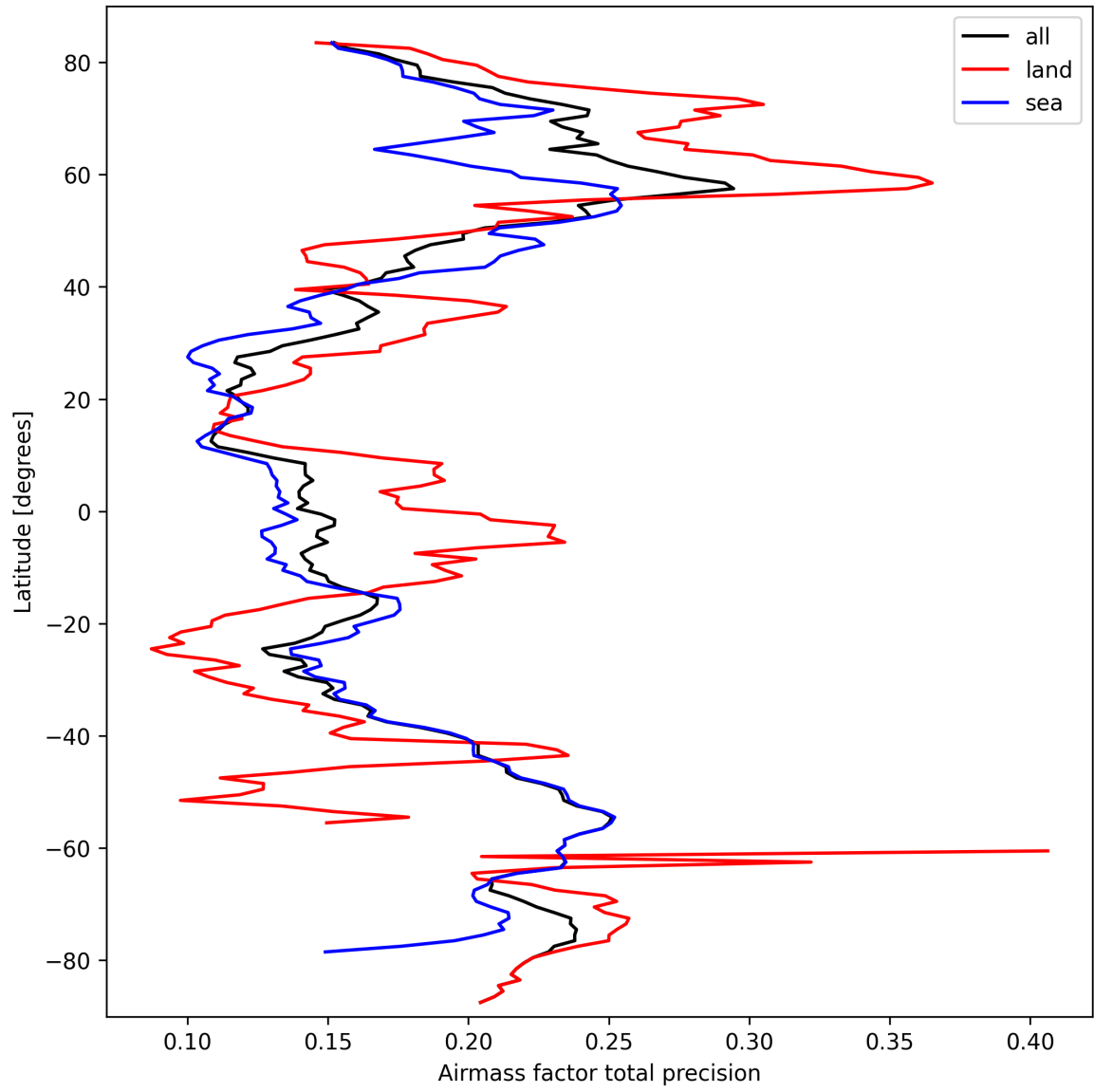
Figure 27: Zonal average of “Airmass factor total precision” for 2025-09-26 to 2025-09-28.
