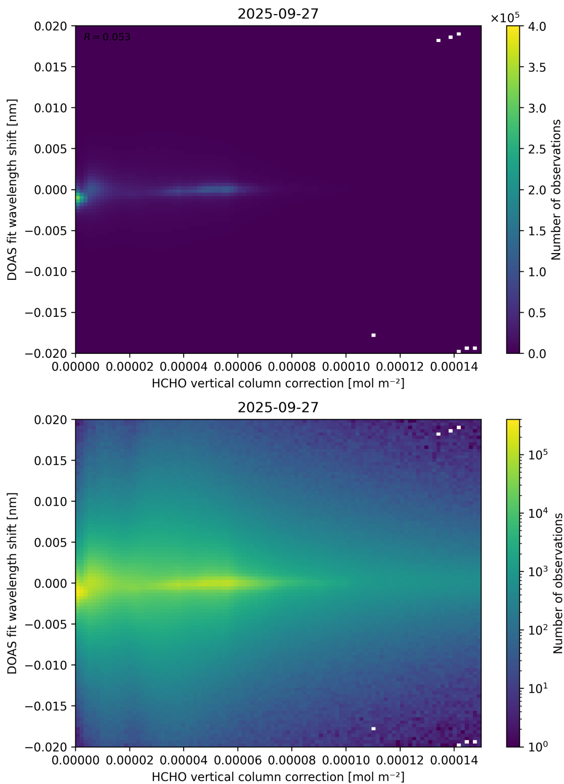
Figure 113: Scatter density plot of “HCHO vertical column correction” against “DOAS fit wavelength shift” for 2025-09-26 to 2025-09-28.
