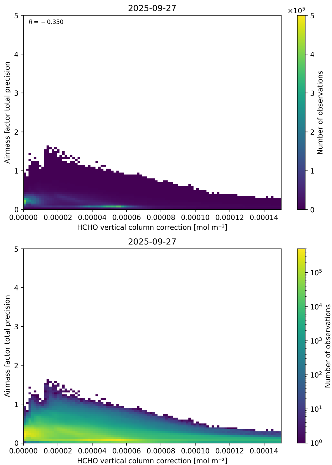
Figure 121: Scatter density plot of “HCHO vertical column correction” against “Airmass factor total precision” for 2025-09-26 to 2025-09-28.
