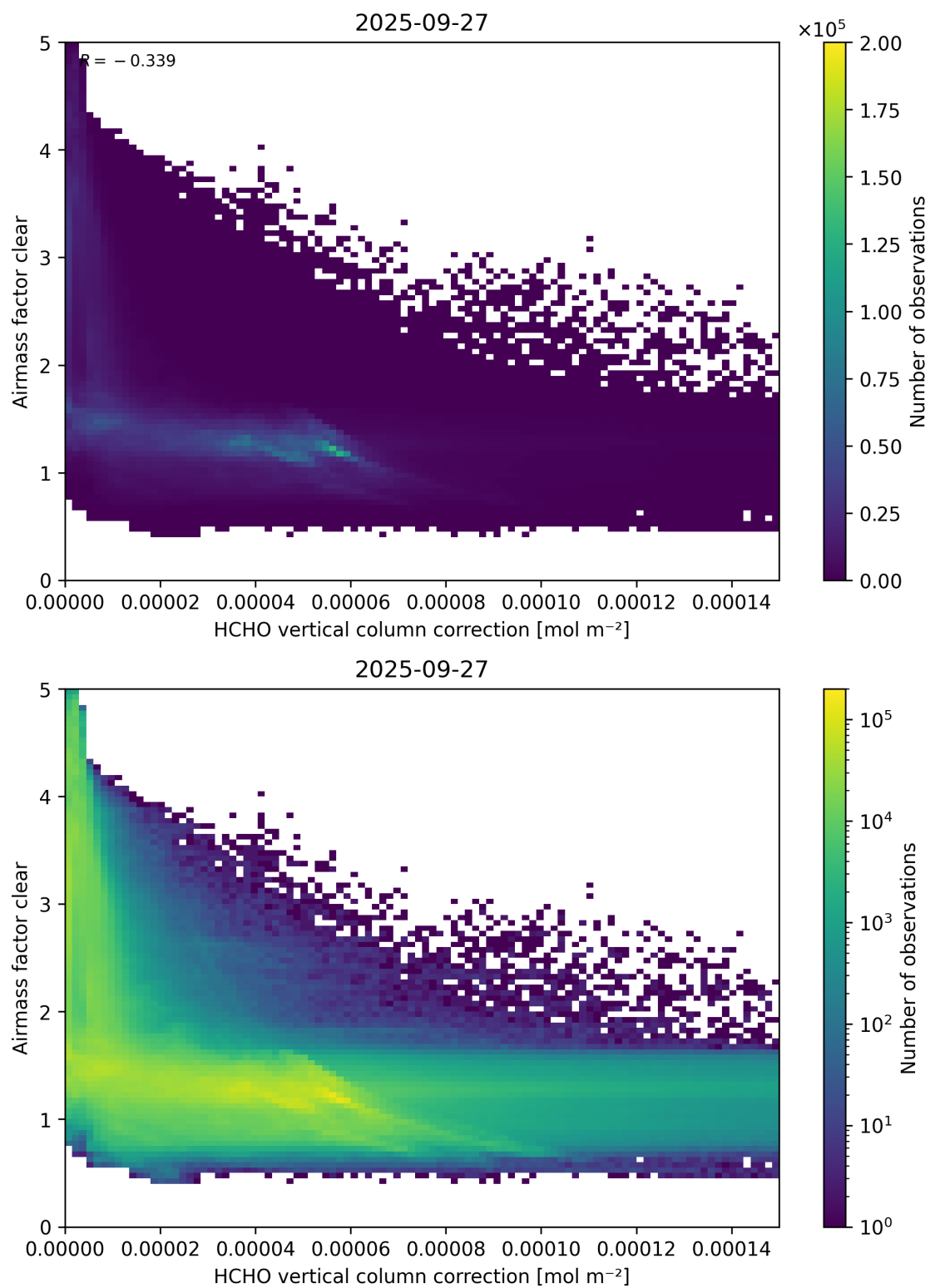
Figure 115: Scatter density plot of “HCHO vertical column correction” against “Airmass factor clear” for 2025-09-26 to 2025-09-28.
