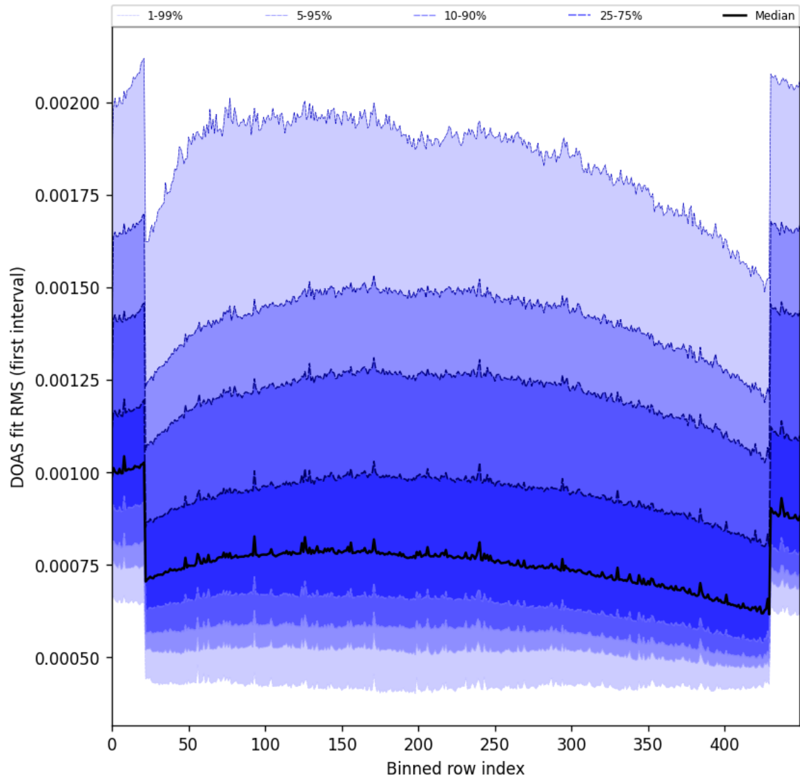
Figure 60: Along track statistics of “DOAS fit RMS (first interval)” for 2025-09-26 to 2025-09-28
