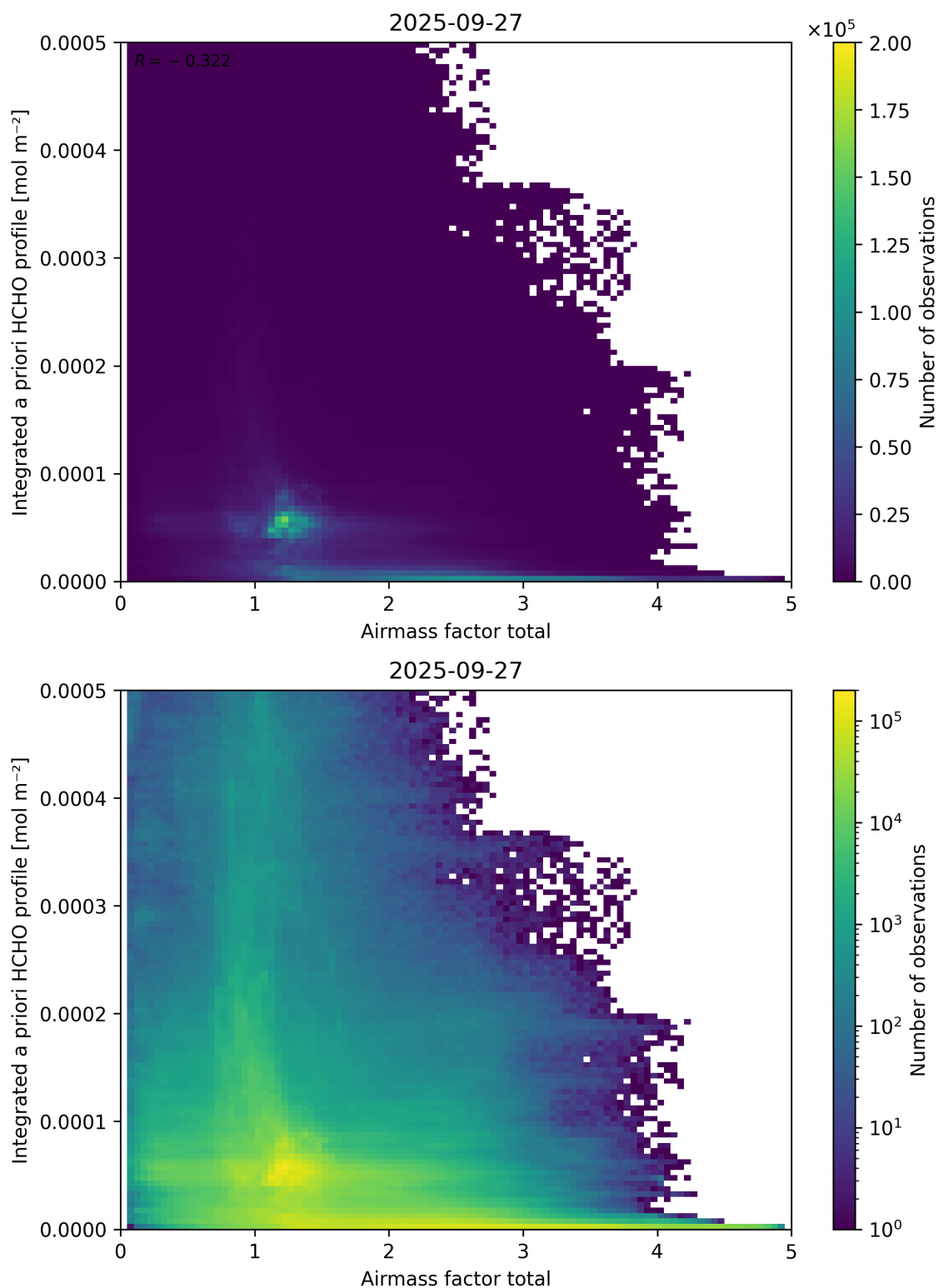
Figure 104: Scatter density plot of “Airmass factor total” against “Integrated a priori HCHO profile” for 2025-09-26 to 2025-09-28.
