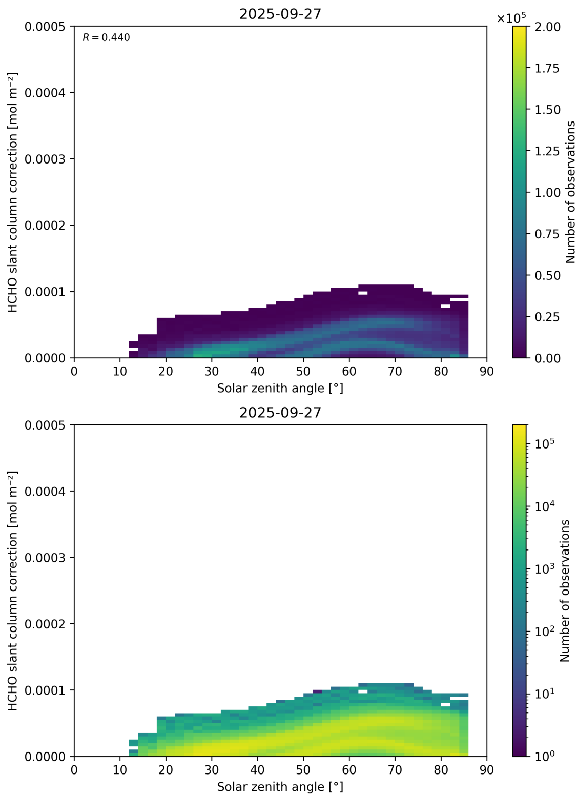
Figure 172: Scatter density plot of “Solar zenith angle” against “HCHO slant column correction” for 2025-09-26 to 2025-09-28.
