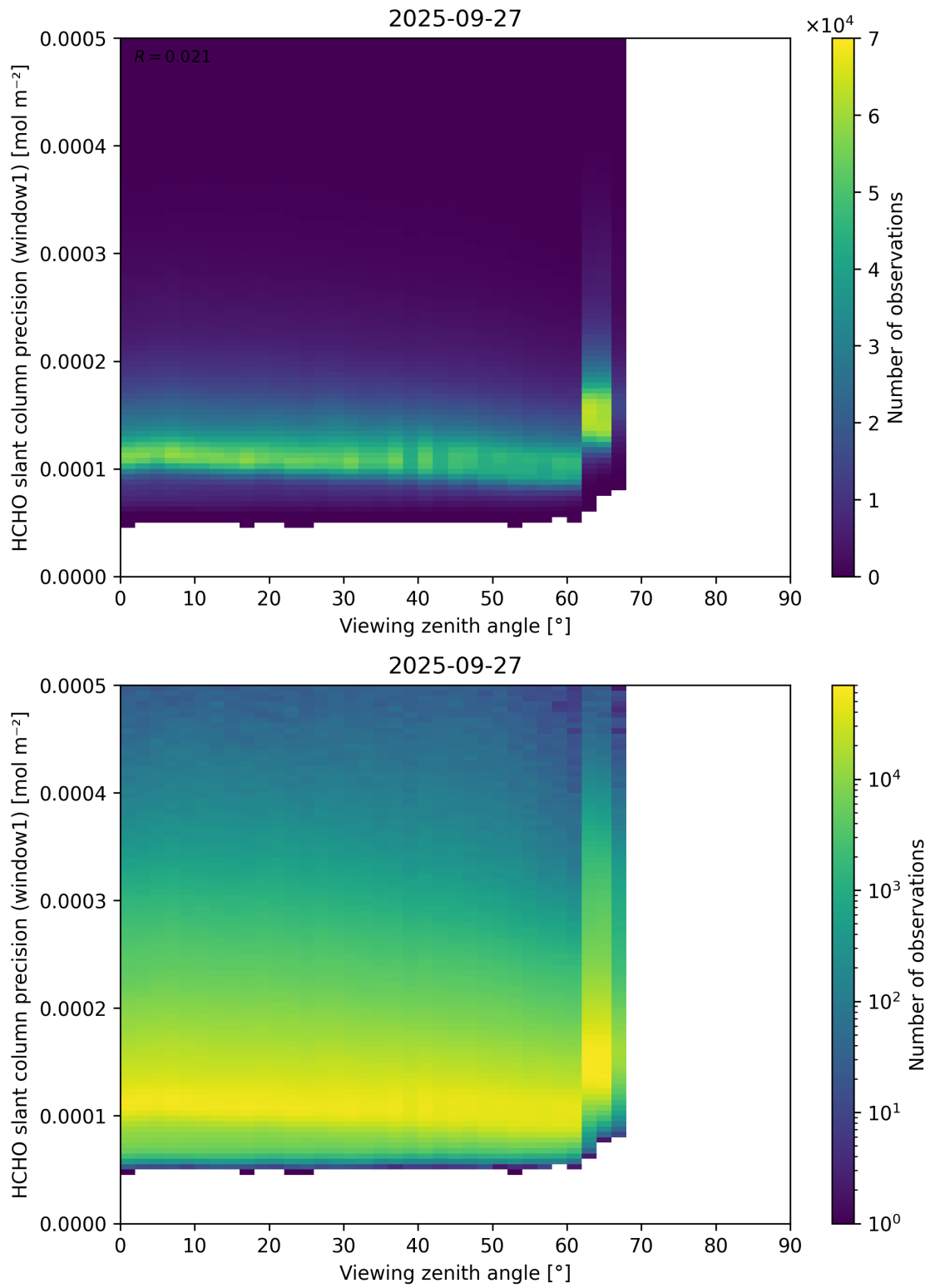
Figure 189: Scatter density plot of “Viewing zenith angle” against “HCHO slant column precision (window1)” for 2025-09-26 to 2025-09-28.
