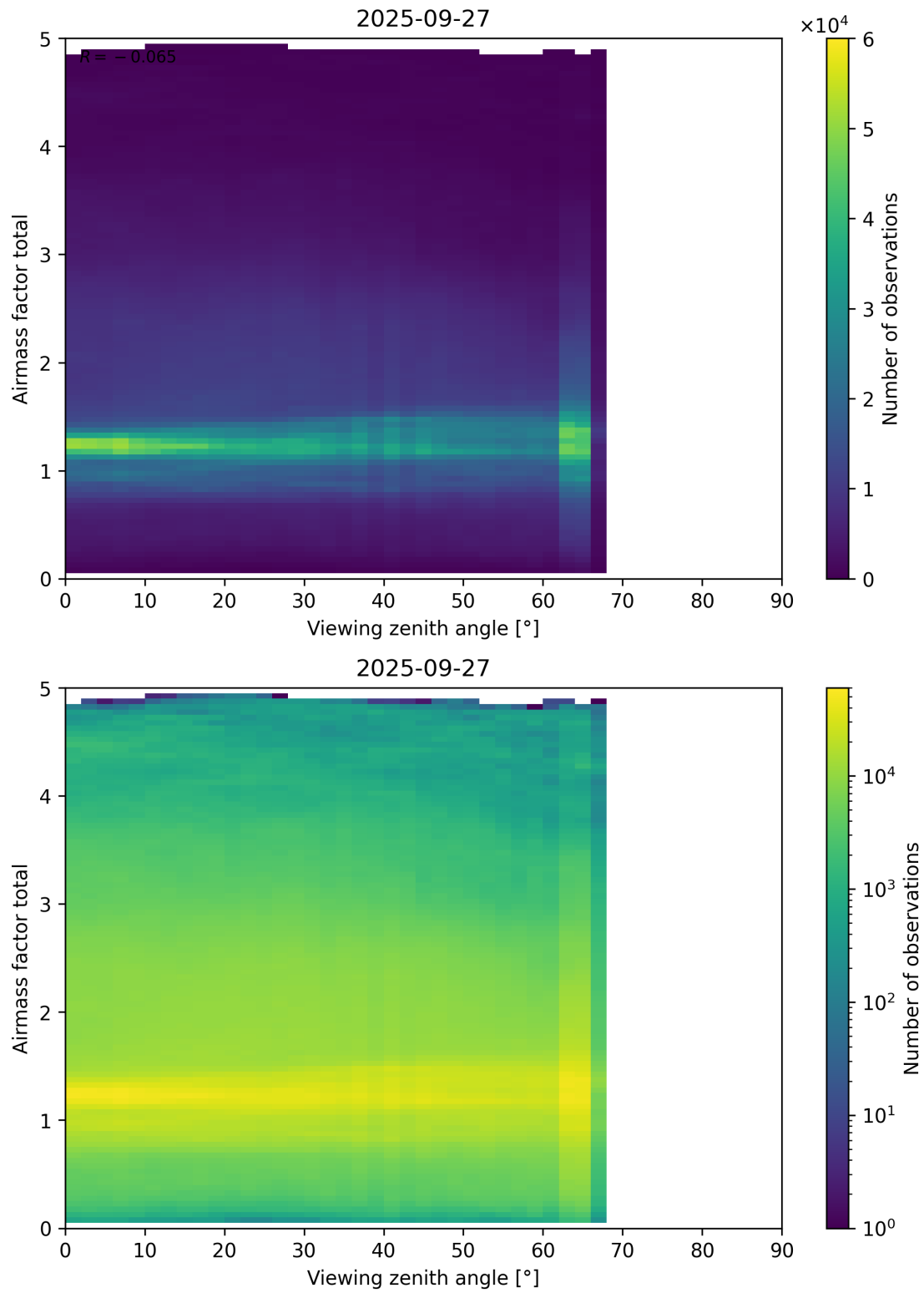
Figure 190: Scatter density plot of “Viewing zenith angle” against “Airmass factor total” for 2025-09-26 to 2025-09-28.
