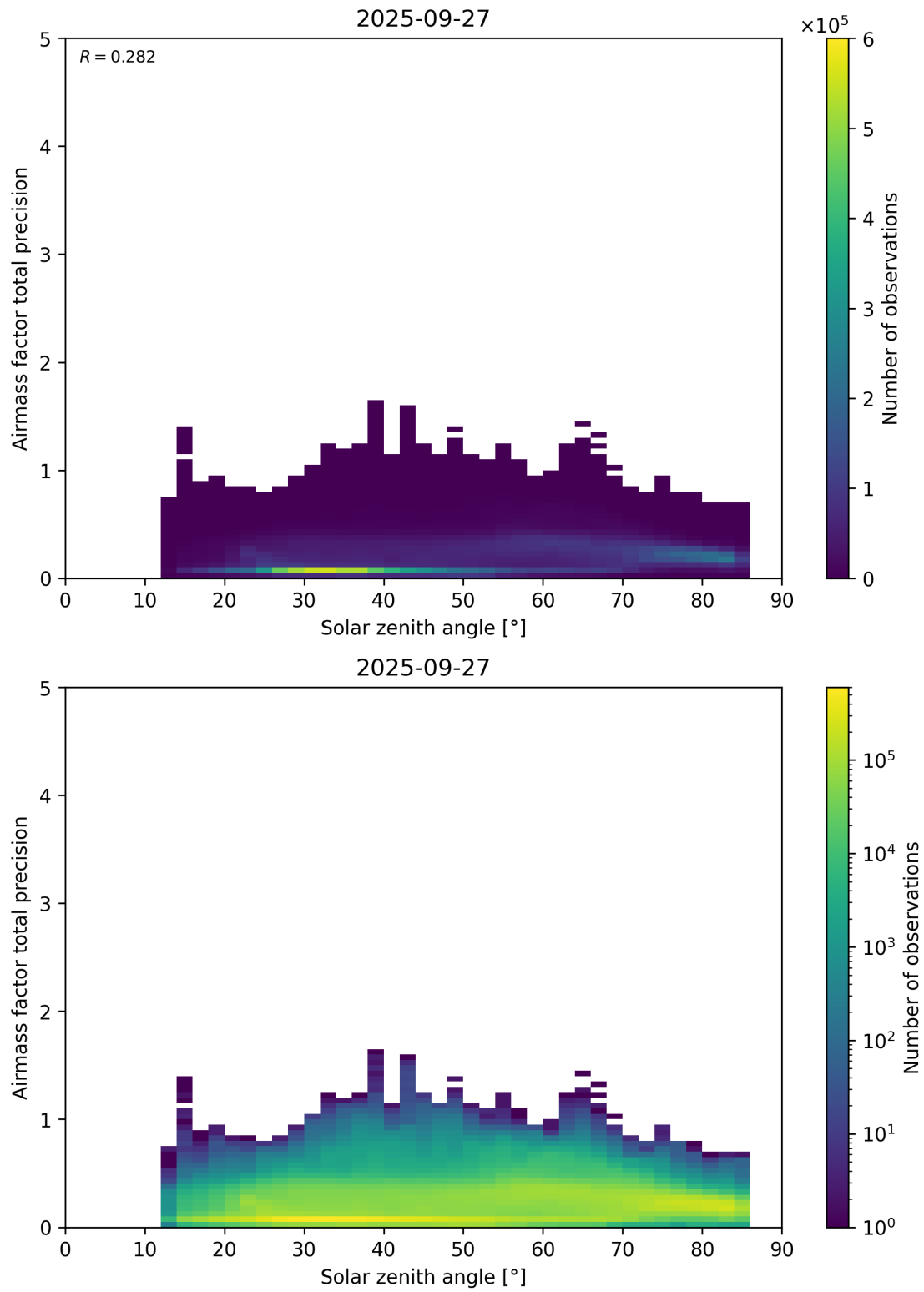
Figure 176: Scatter density plot of “Solar zenith angle” against “Airmass factor total precision” for 2025-09-26 to 2025-09-28.
