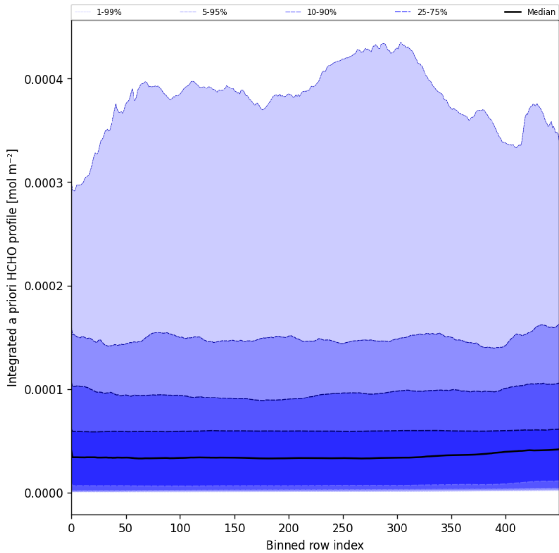
Figure 57: Along track statistics of “Integrated a priori HCHO profile” for 2025-09-26 to 2025-09-28
