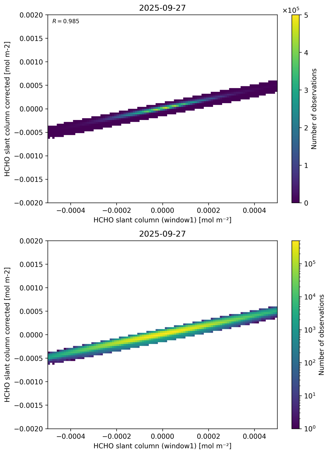
Figure 82: Scatter density plot of “HCHO slant column (window1)” against “HCHO slant column corrected” for 2025-09-26 to 2025-09-28.
