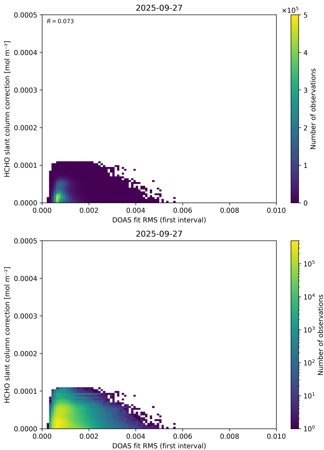
Figure 63: Scatter density plot of “DOAS fit RMS (first interval)” against “HCHO slant column correction” for 2025-09-26 to 2025-09-28.
