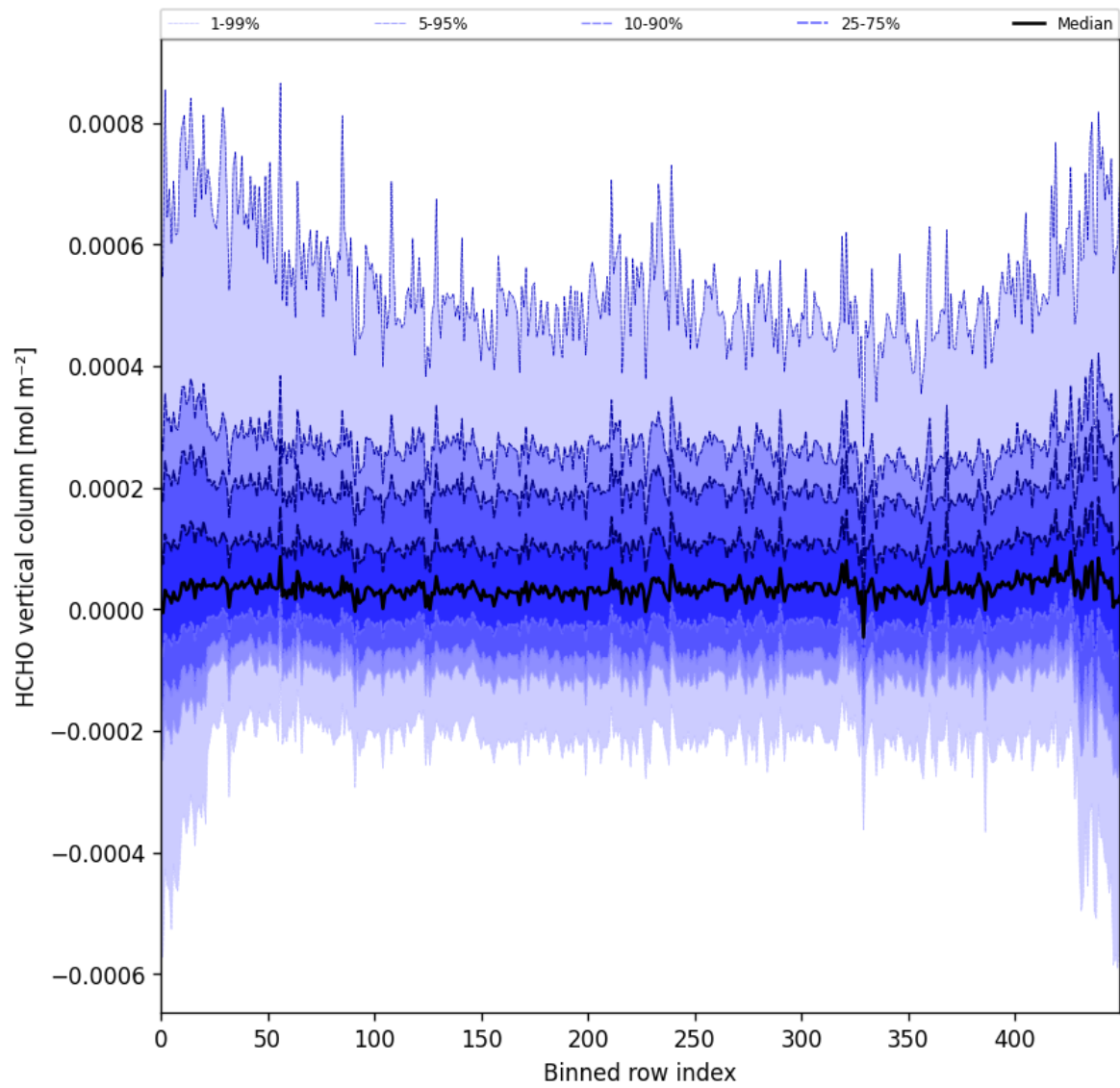
Figure 49: Along track statistics of “HCHO vertical column” for 2025-09-26 to 2025-09-28
