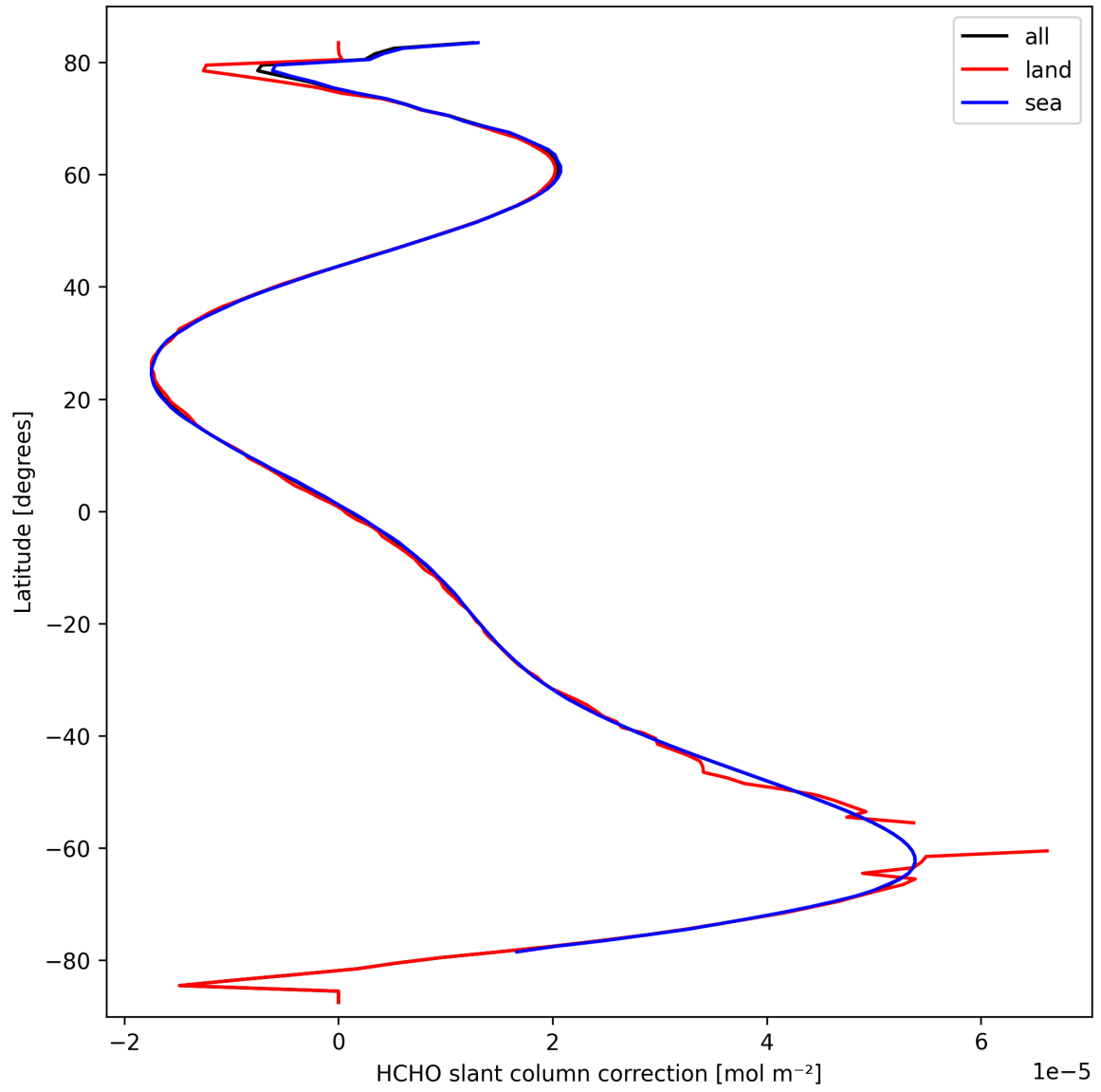
Figure 33: Zonal average of “HCHO slant column correction” for 2025-09-26 to 2025-09-28.
