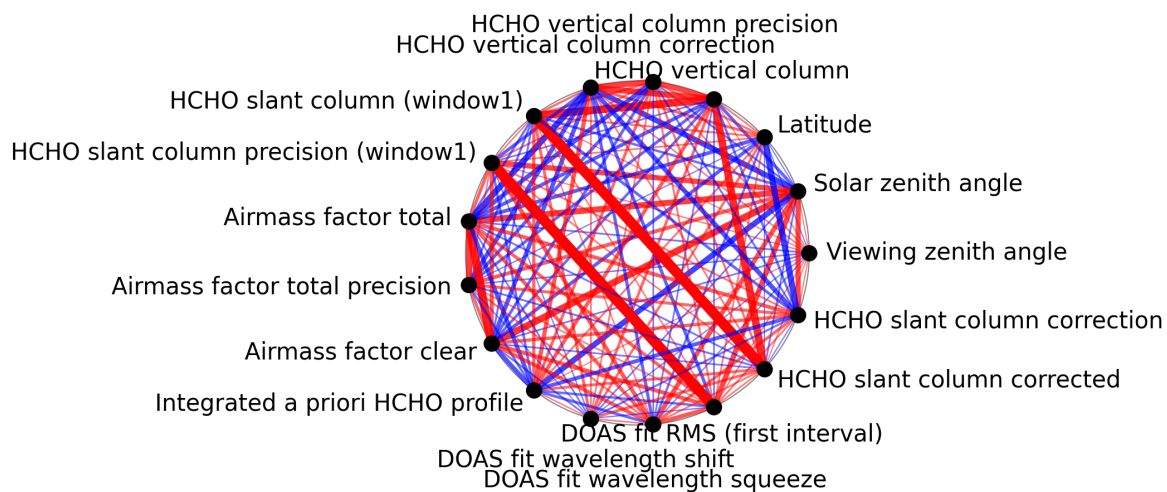
Figure 1: Map of correlation graph for 2025-09-26 to 2025-09-28.
