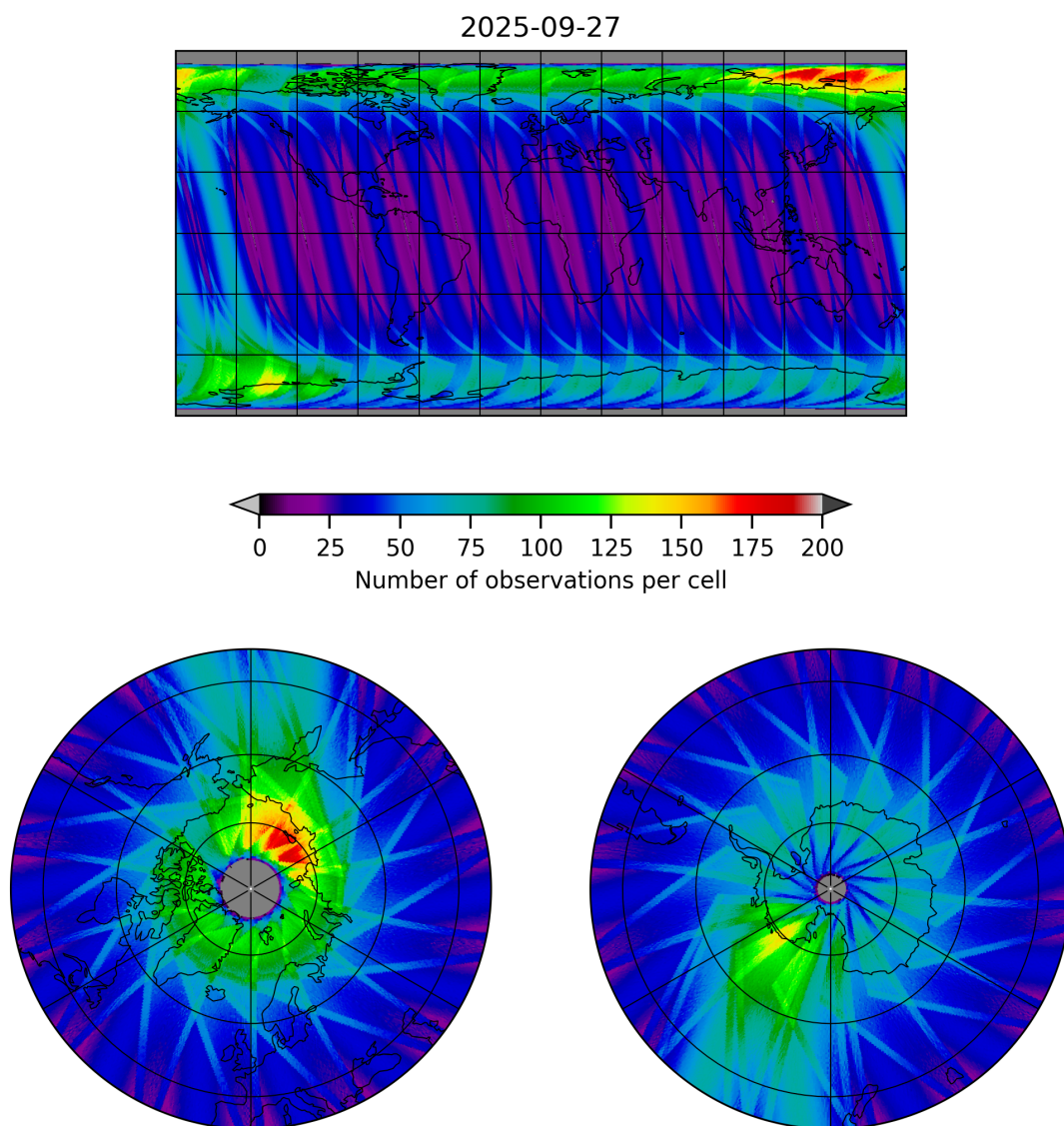
Figure 19: Map of the number of observations for 2025-09-26 to 2025-09-28
