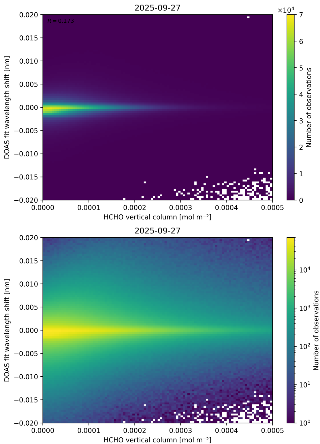
Figure 124: Scatter density plot of “HCHO vertical column” against “DOAS fit wavelength shift” for 2025-09-26 to 2025-09-28.
