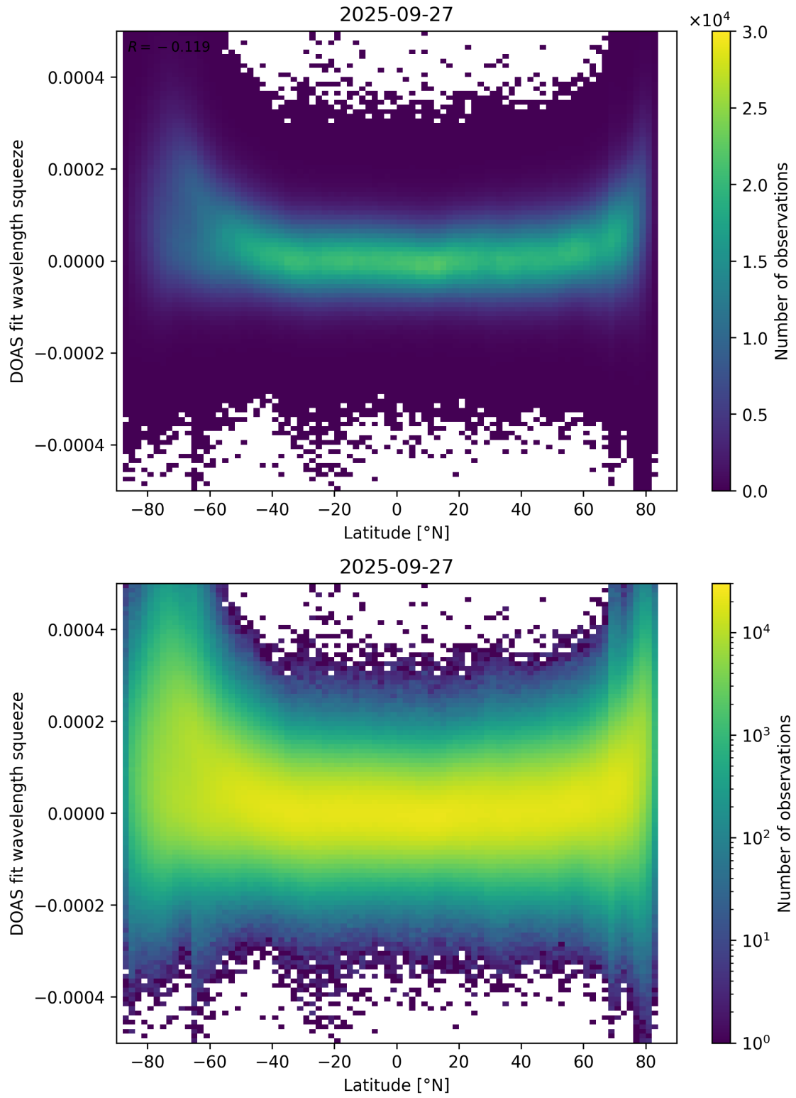
Figure 155: Scatter density plot of “Latitude” against “DOAS fit wavelength squeeze” for 2025-09-26 to 2025-09-28.
