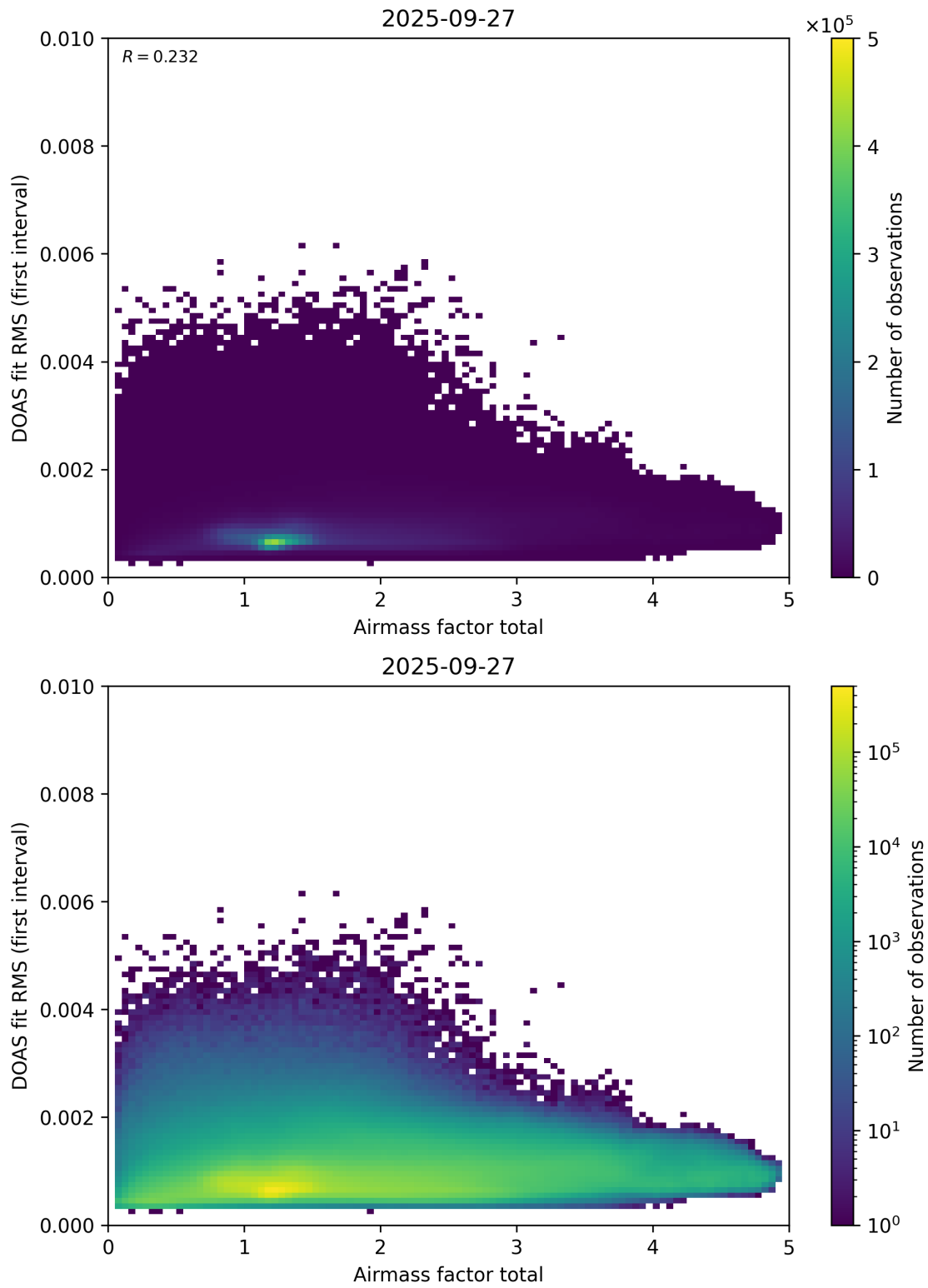
Figure 97: Scatter density plot of “Airmass factor total” against “DOAS fit RMS (first interval)” for 2025-09-26 to 2025-09-28.
