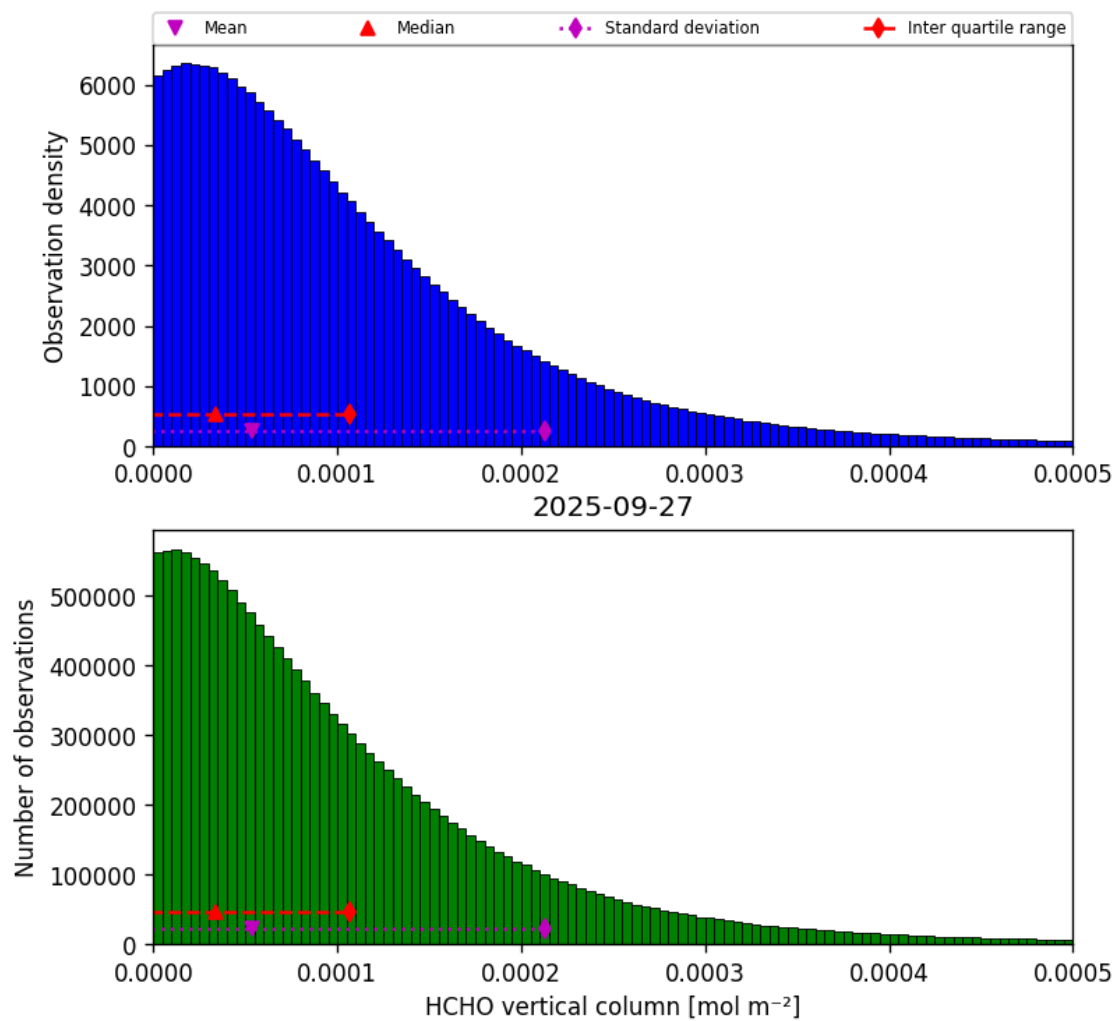
Figure 35: Histogram of “HCHO vertical column” for 2025-09-26 to 2025-09-28
