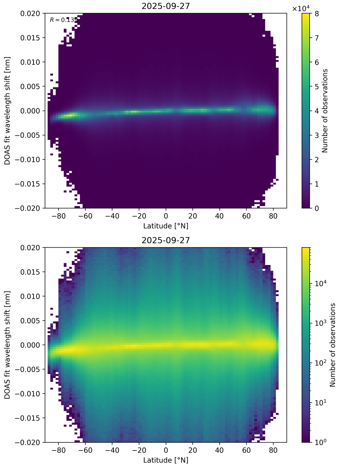
Figure 154: Scatter density plot of “Latitude” against “DOAS fit wavelength shift” for 2025-09-26 to 2025-09-28.
