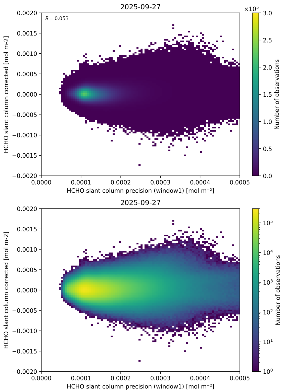
Figure 92: Scatter density plot of “HCHO slant column precision (window1)” against “HCHO slant column corrected” for 2025-09-26 to 2025-09-28.
