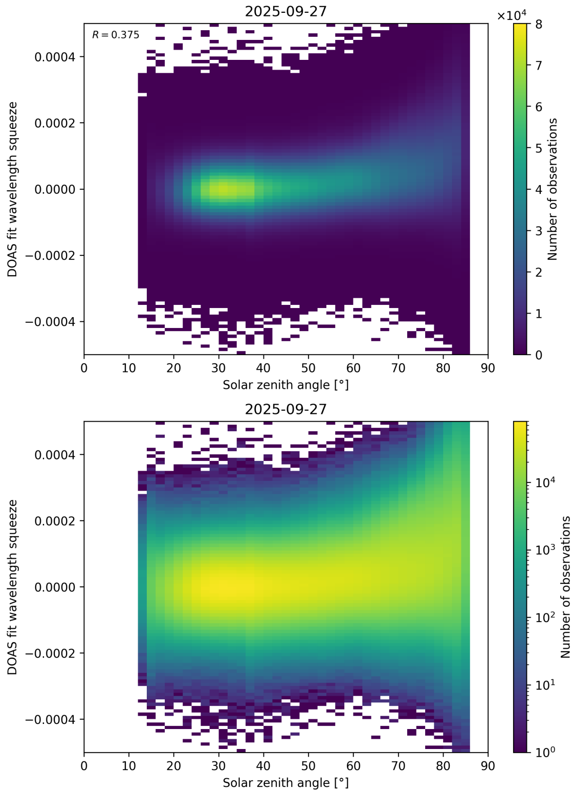
Figure 169: Scatter density plot of “Solar zenith angle” against “DOAS fit wavelength squeeze” for 2025-09-26 to 2025-09-28.
