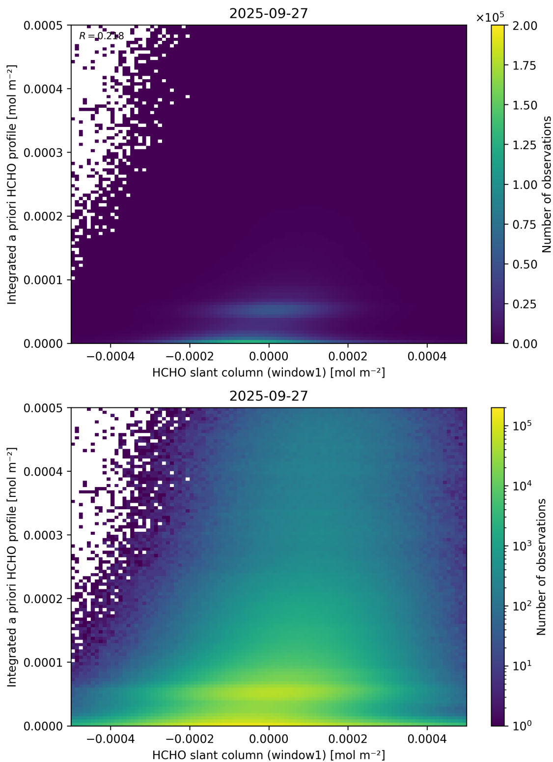
Figure 87: Scatter density plot of “HCHO slant column (window1)” against “Integrated a priori HCHO profile” for 2025-09-26 to 2025-09-28.
