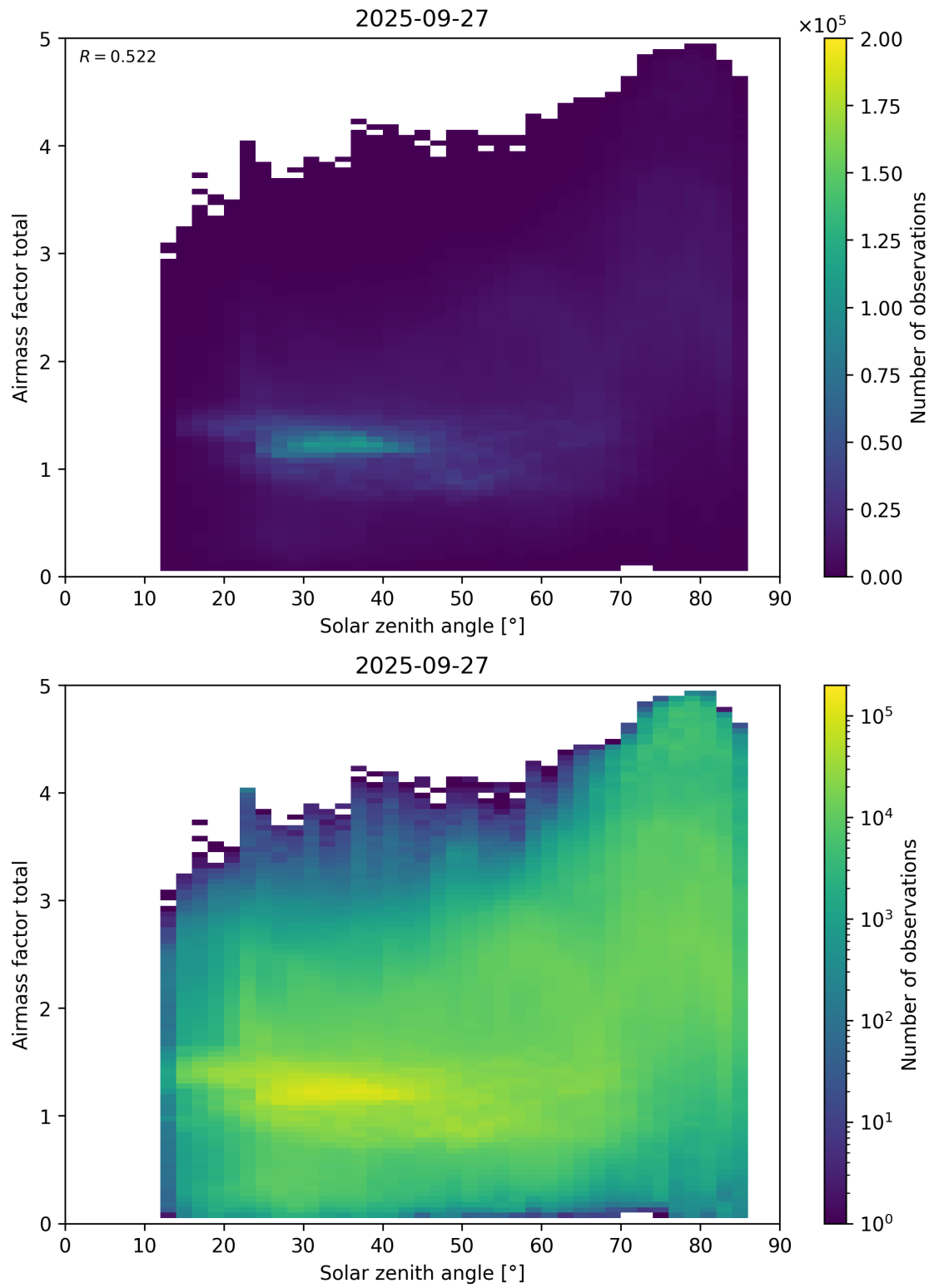
Figure 175: Scatter density plot of “Solar zenith angle” against “Airmass factor total” for 2025-09-26 to 2025-09-28.
