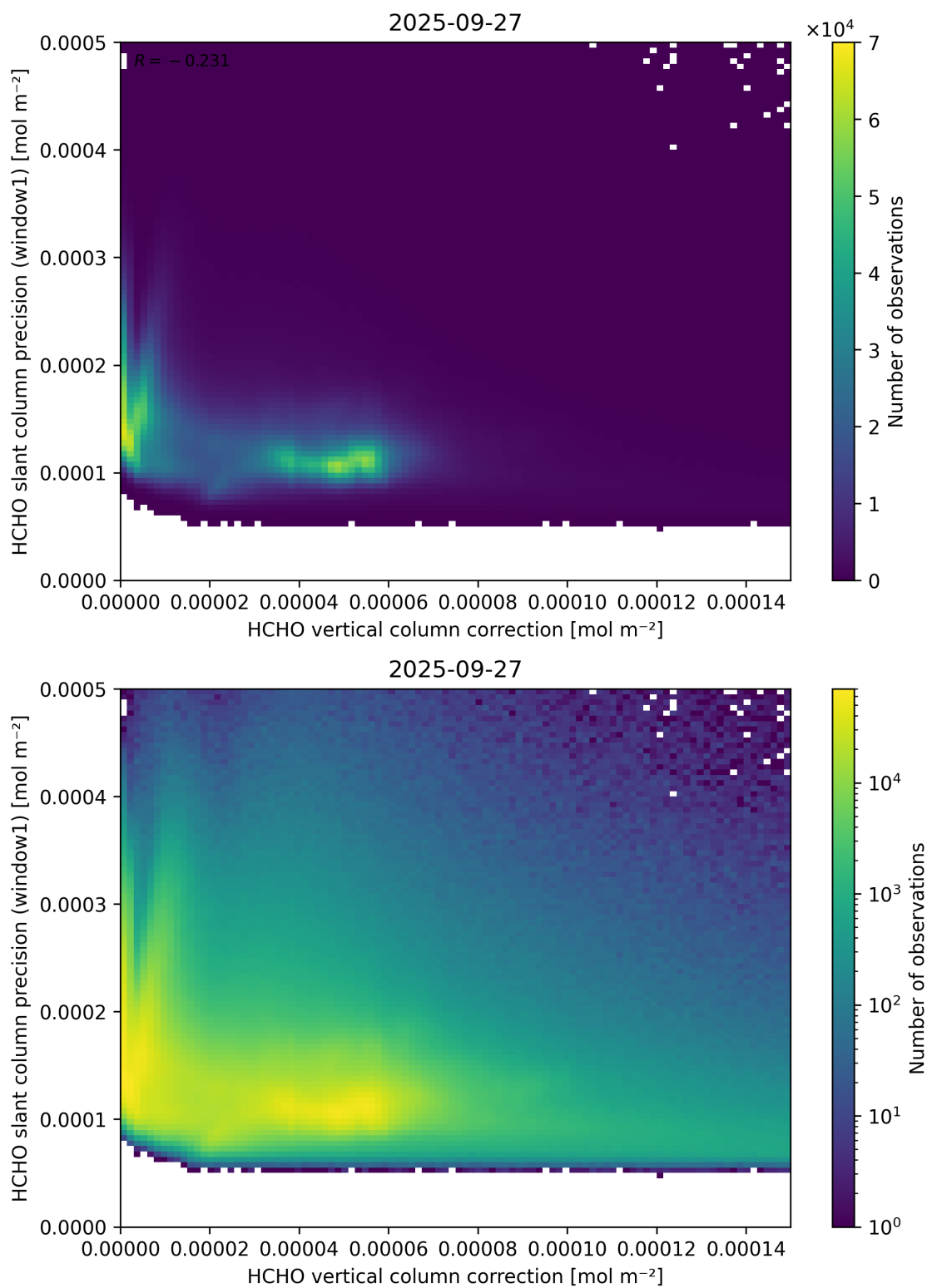
Figure 119: Scatter density plot of “HCHO vertical column correction” against “HCHO slant column precision (window1)” for 2025-09-26 to 2025-09-28.
