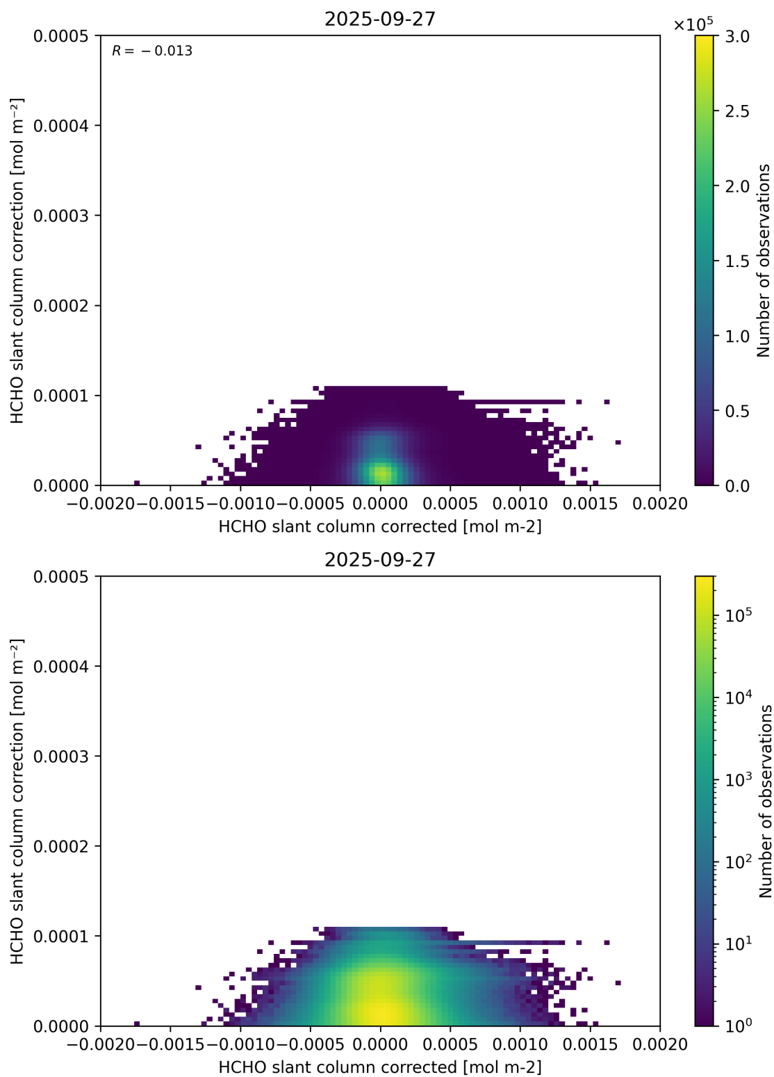
Figure 77: Scatter density plot of “HCHO slant column corrected” against “HCHO slant column correction” for 2025-09-26 to 2025-09-28.
