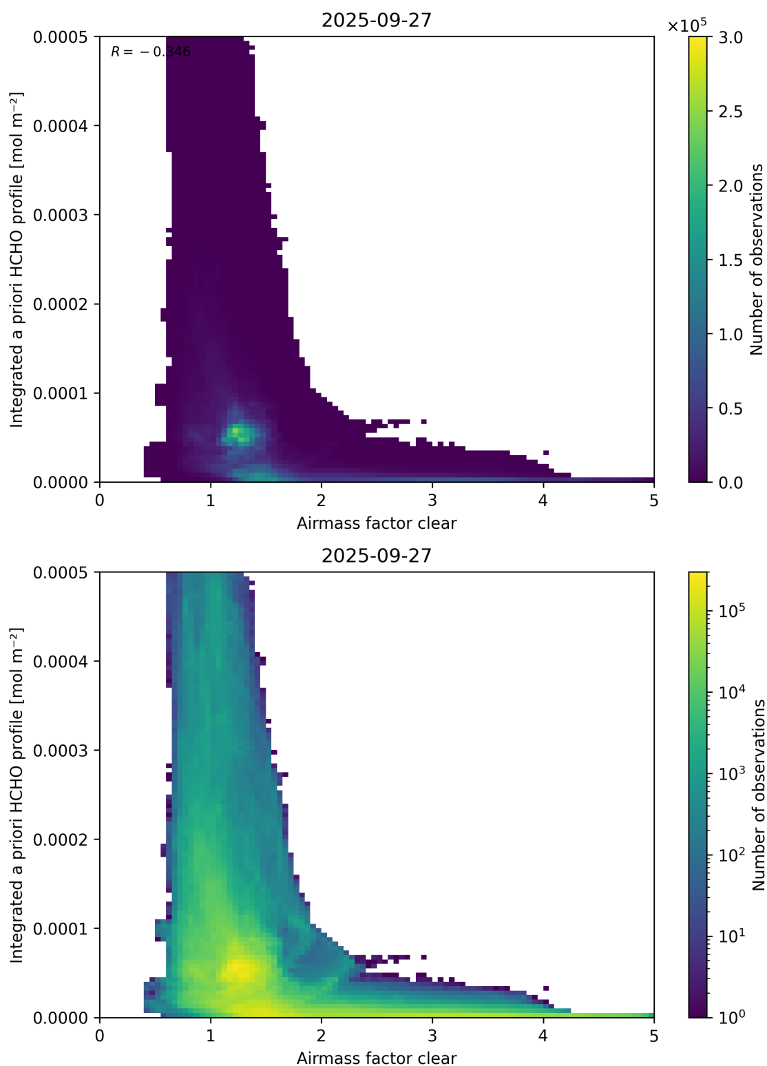
Figure 76: Scatter density plot of “Airmass factor clear” against “Integrated a priori HCHO profile” for 2025-09-26 to 2025-09-28.
