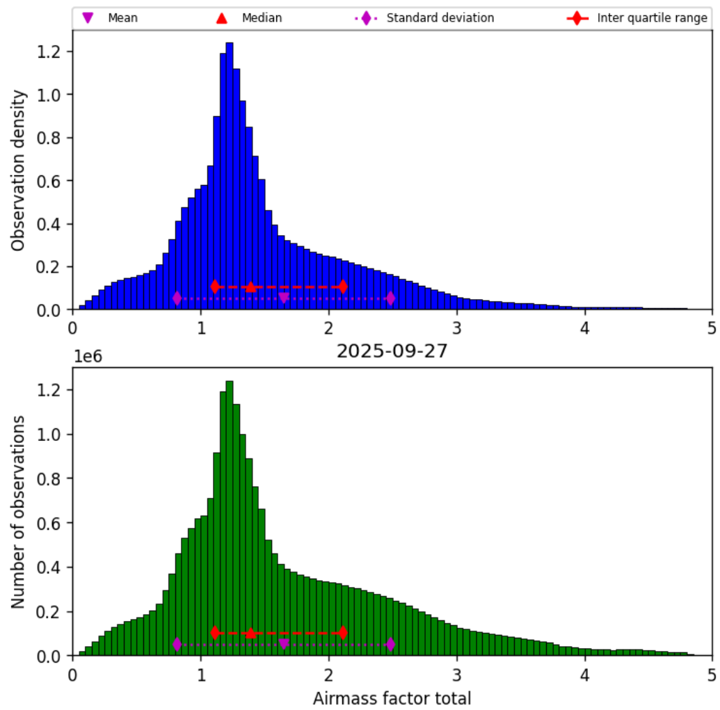
Figure 40: Histogram of “Airmass factor total” for 2025-09-26 to 2025-09-28
