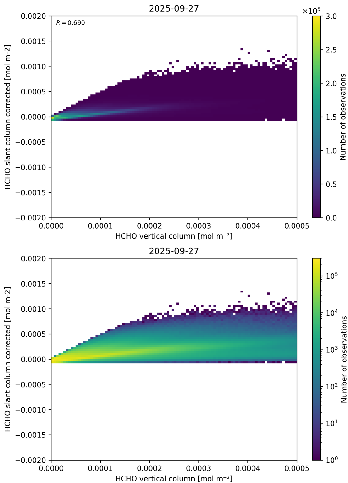
Figure 127: Scatter density plot of “HCHO vertical column” against “HCHO slant column corrected” for 2025-09-26 to 2025-09-28.
