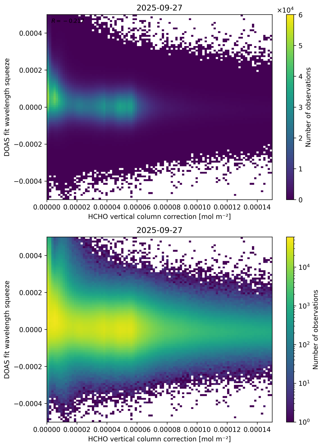
Figure 114: Scatter density plot of “HCHO vertical column correction” against “DOAS fit wavelength squeeze” for 2025-09-26 to 2025-09-28.
