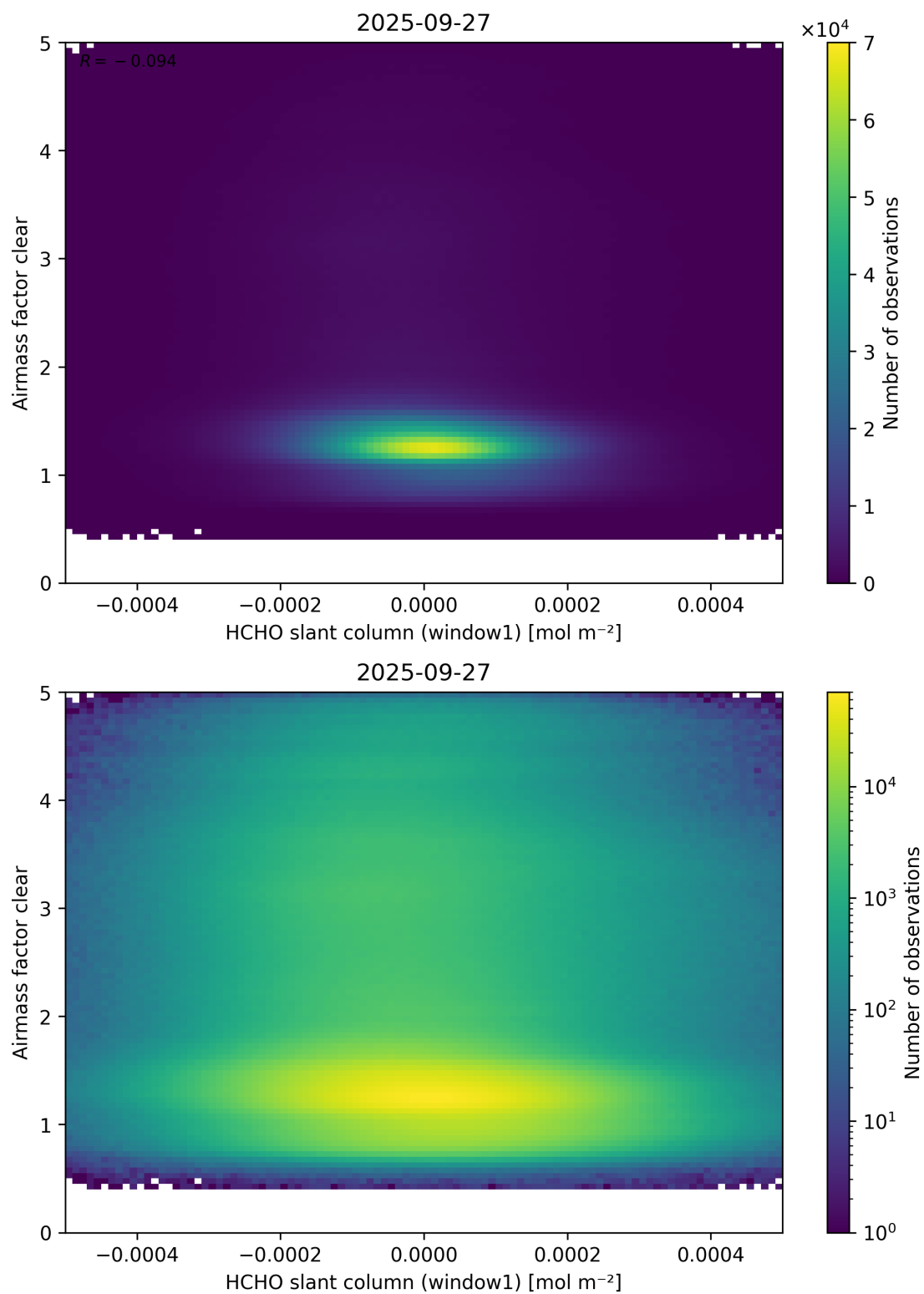
Figure 81: Scatter density plot of “HCHO slant column (window1)” against “Airmass factor clear” for 2025-09-26 to 2025-09-28.
