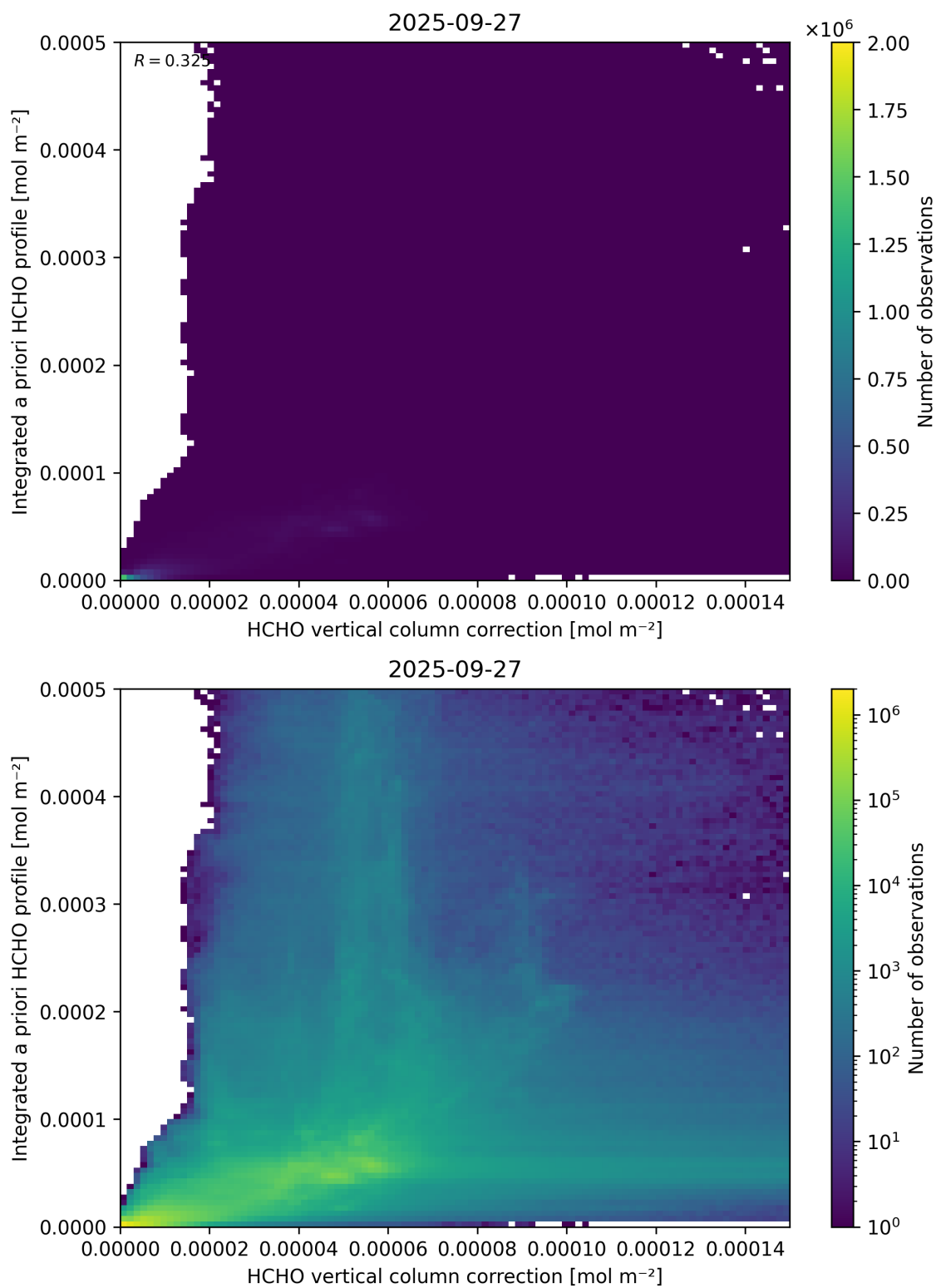
Figure 122: Scatter density plot of “HCHO vertical column correction” against “Integrated a priori HCHO profile” for 2025-09-26 to 2025-09-28.
