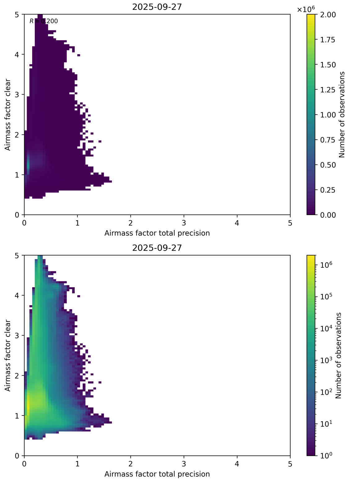
Figure 108: Scatter density plot of “Airmass factor total precision” against “Airmass factor clear” for 2025-09-26 to 2025-09-28.
