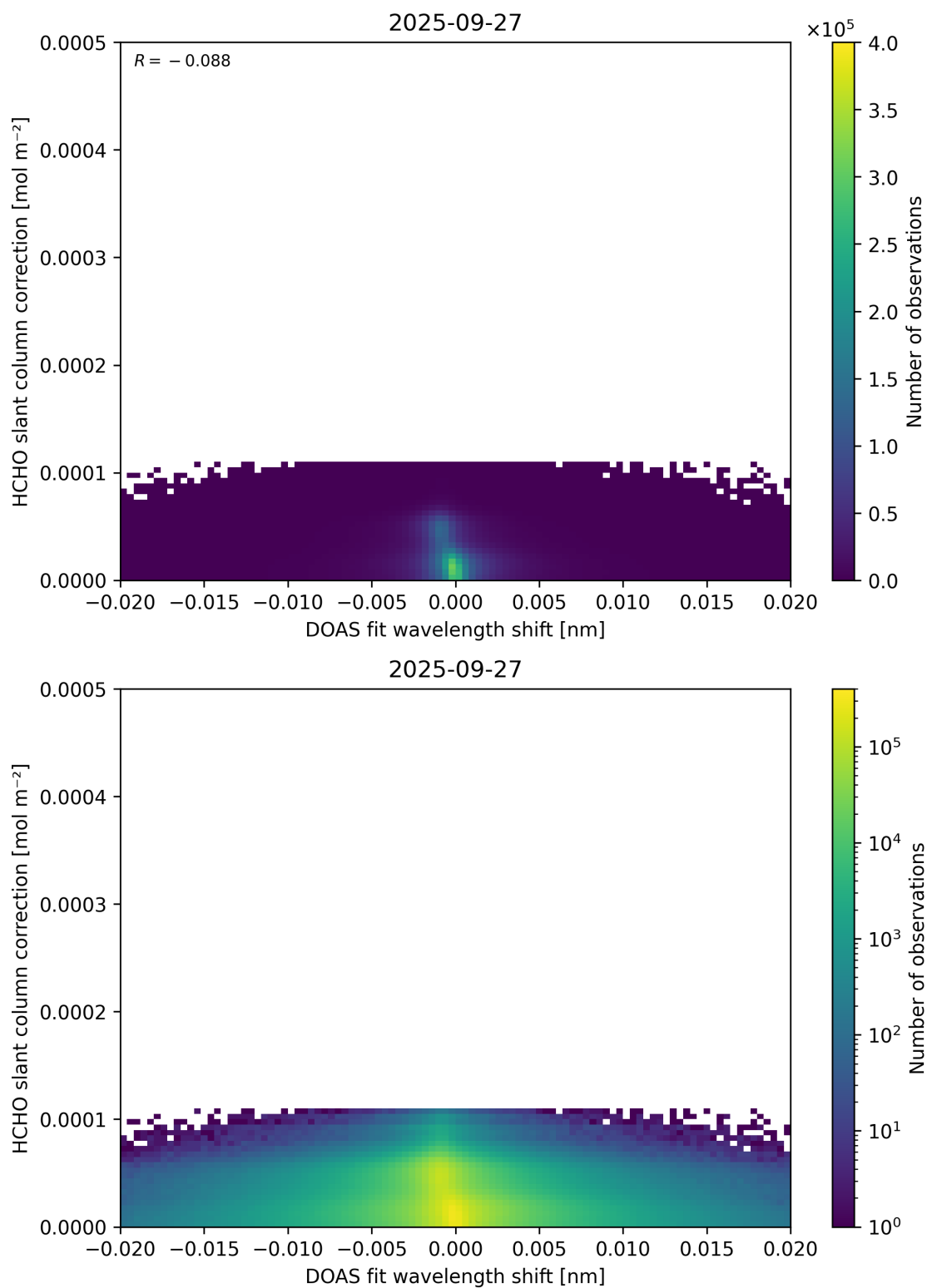
Figure 67: Scatter density plot of “DOAS fit wavelength shift” against “HCHO slant column correction” for 2025-09-26 to 2025-09-28.
