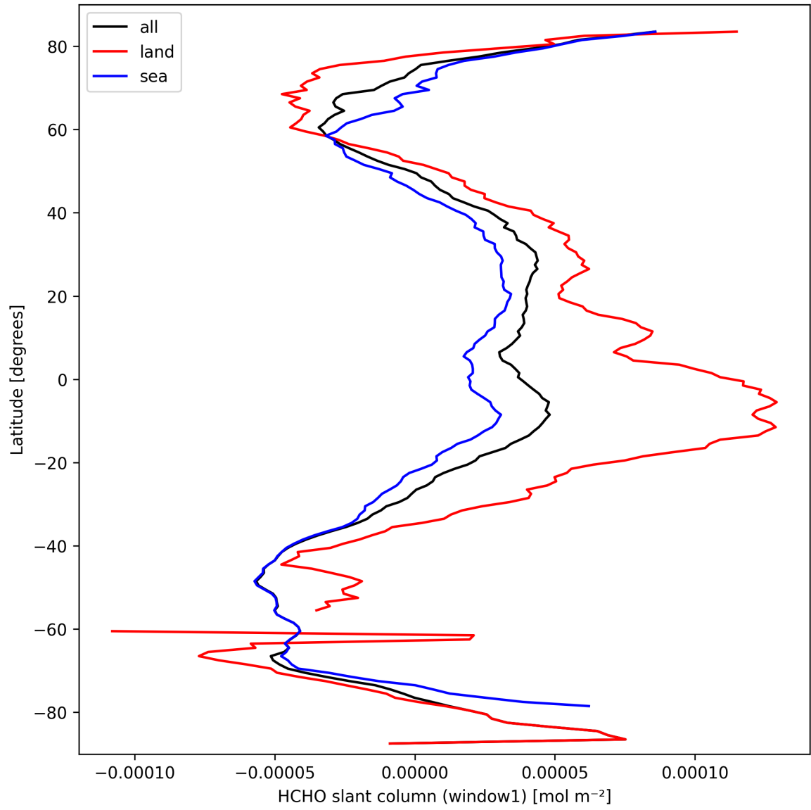
Figure 24: Zonal average of “HCHO slant column (window1)” for 2025-09-26 to 2025-09-28.
