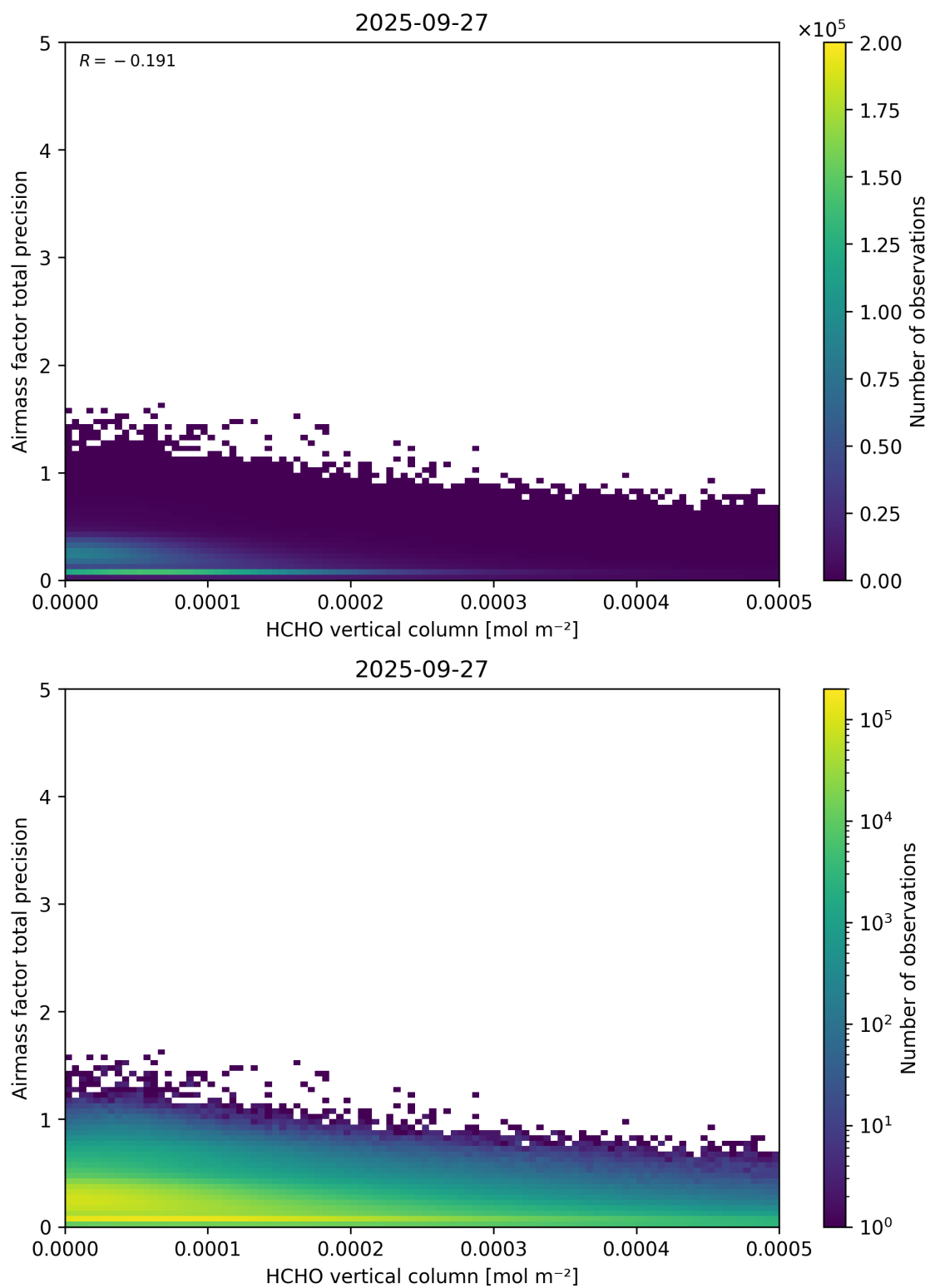
Figure 132: Scatter density plot of “HCHO vertical column” against “Airmass factor total precision” for 2025-09-26 to 2025-09-28.
