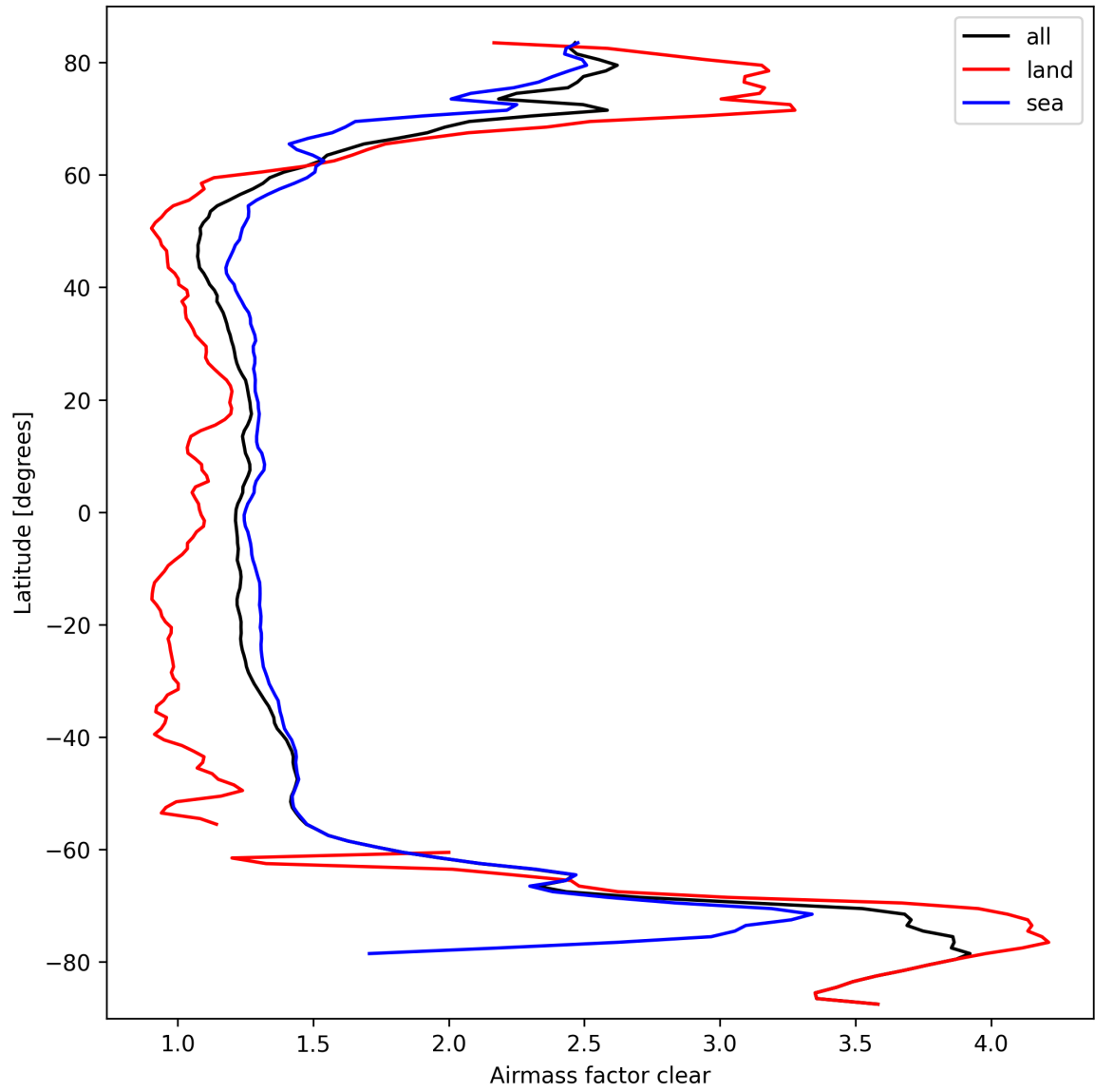
Figure 28: Zonal average of “Airmass factor clear” for 2025-09-26 to 2025-09-28.
