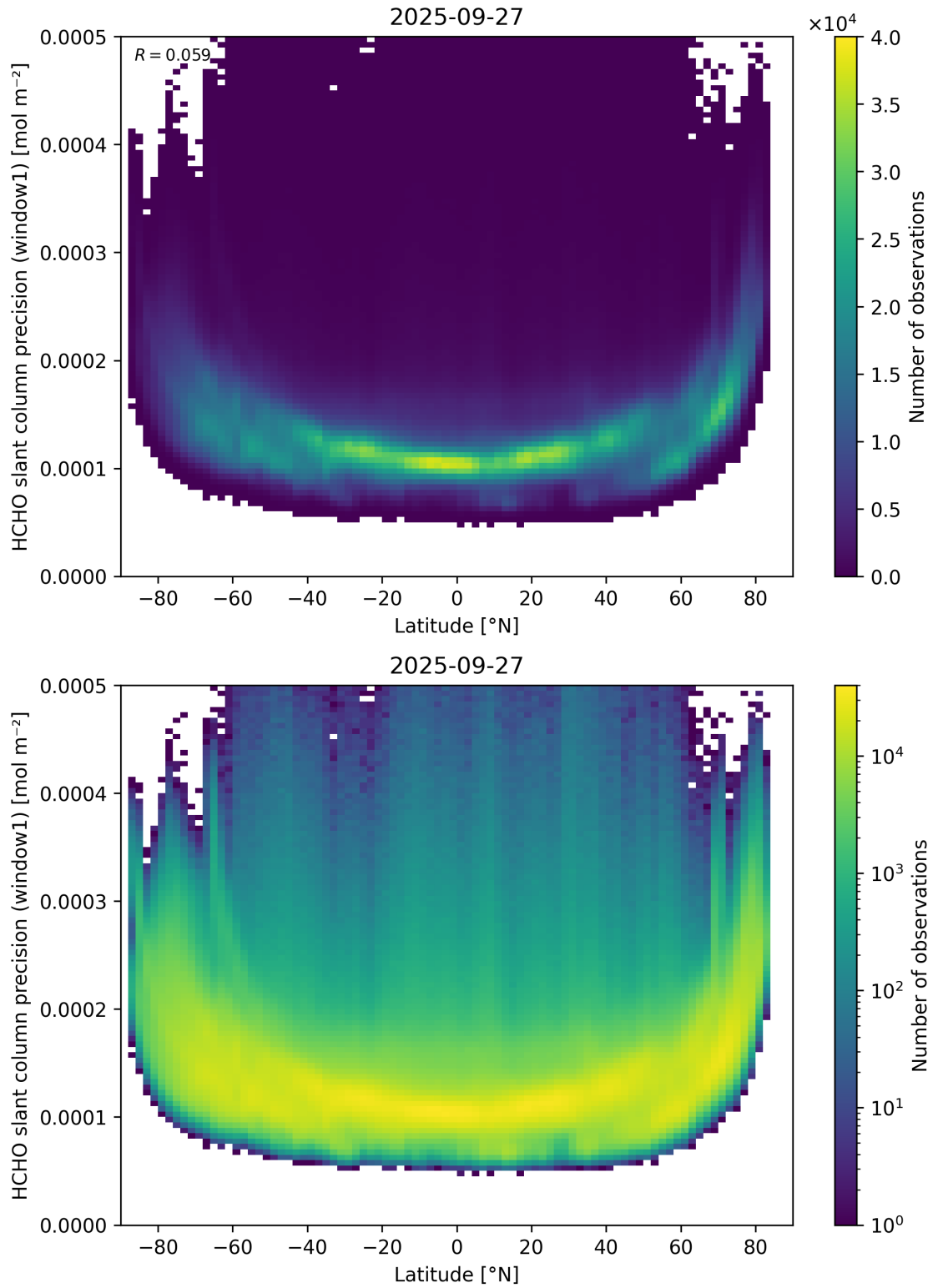
Figure 160: Scatter density plot of “Latitude” against “HCHO slant column precision (window1)” for 2025-09-26 to 2025-09-28.
