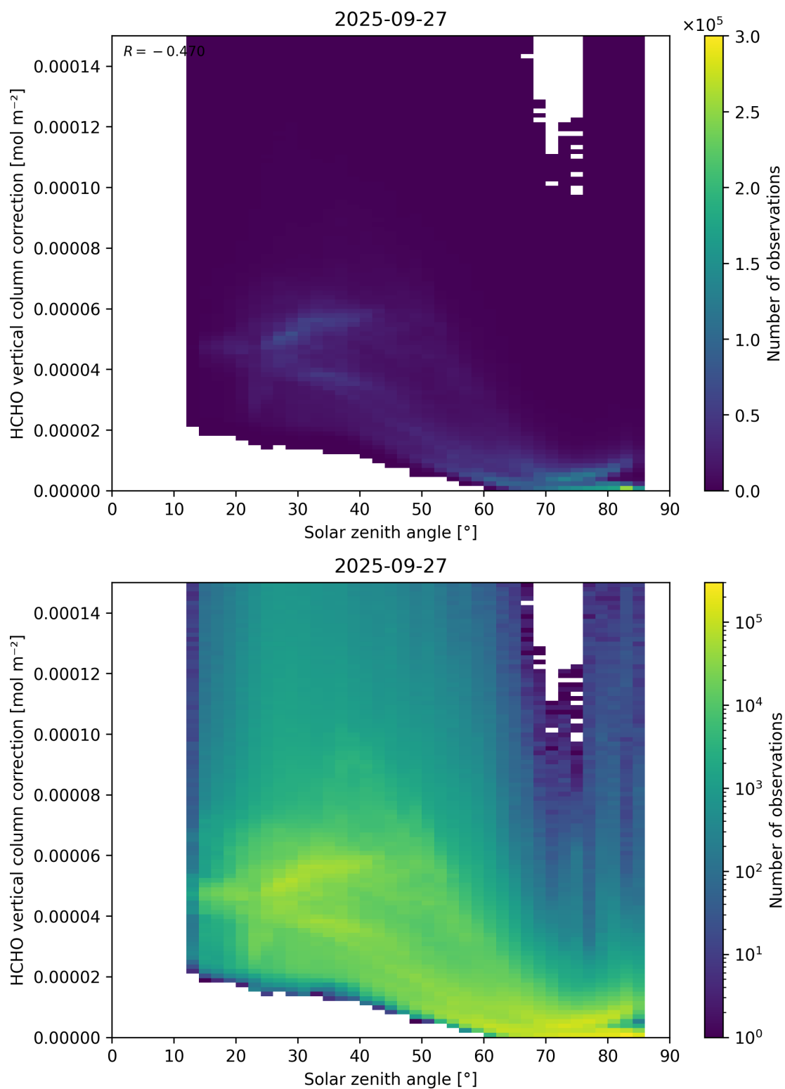
Figure 178: Scatter density plot of “Solar zenith angle” against “HCHO vertical column correction” for 2025-09-26 to 2025-09-28.
