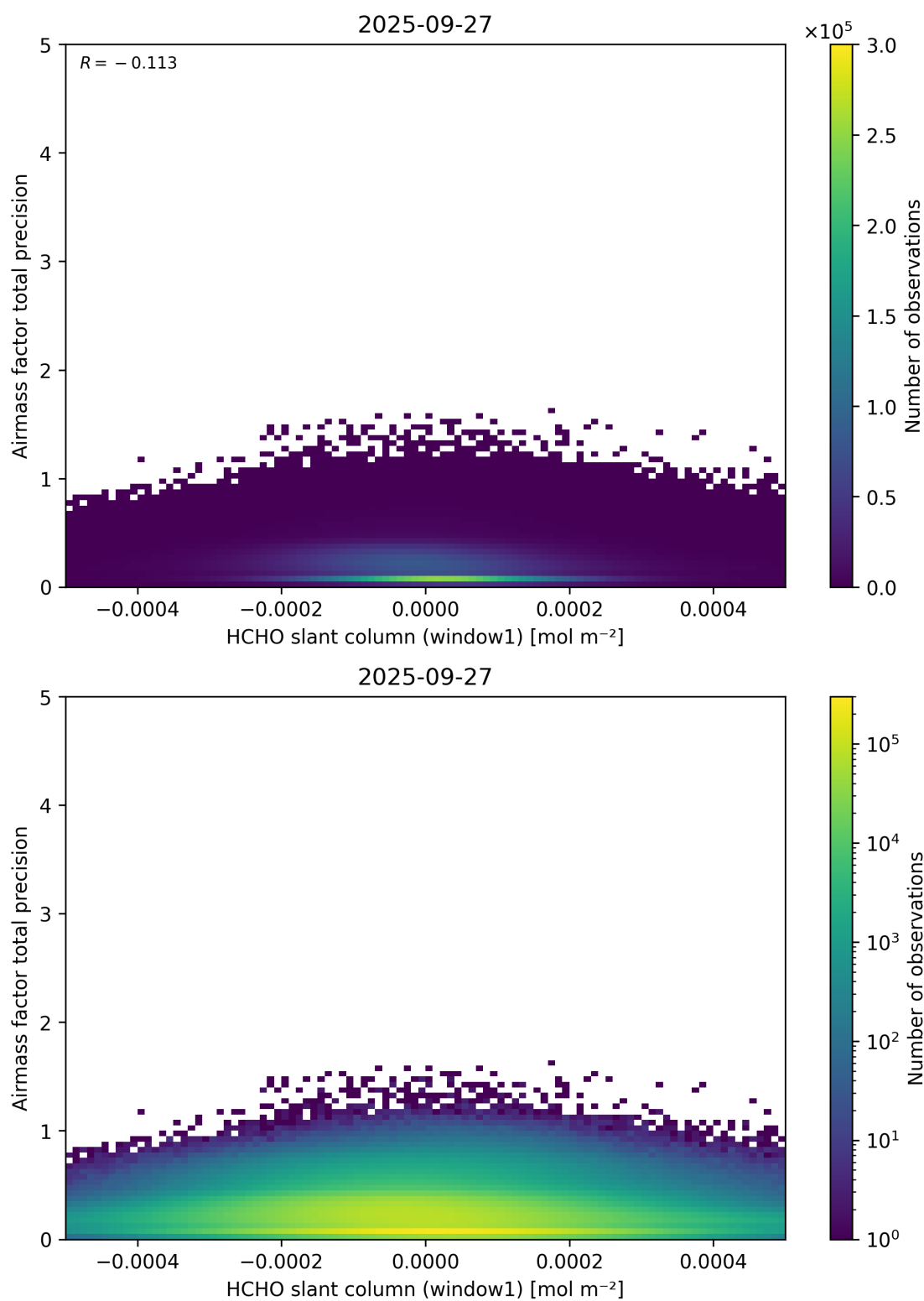
Figure 86: Scatter density plot of “HCHO slant column (window1)” against “Airmass factor total precision” for 2025-09-26 to 2025-09-28.
