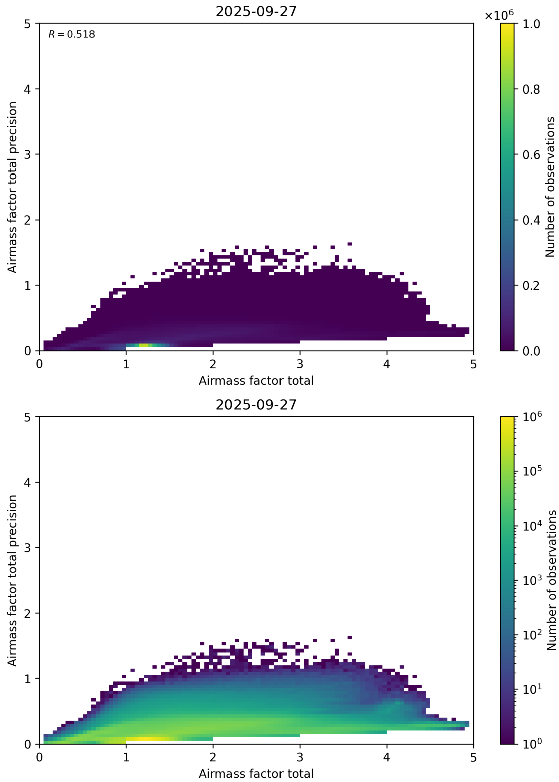
Figure 103: Scatter density plot of “Airmass factor total” against “Airmass factor total precision” for 2025-09-26 to 2025-09-28.
