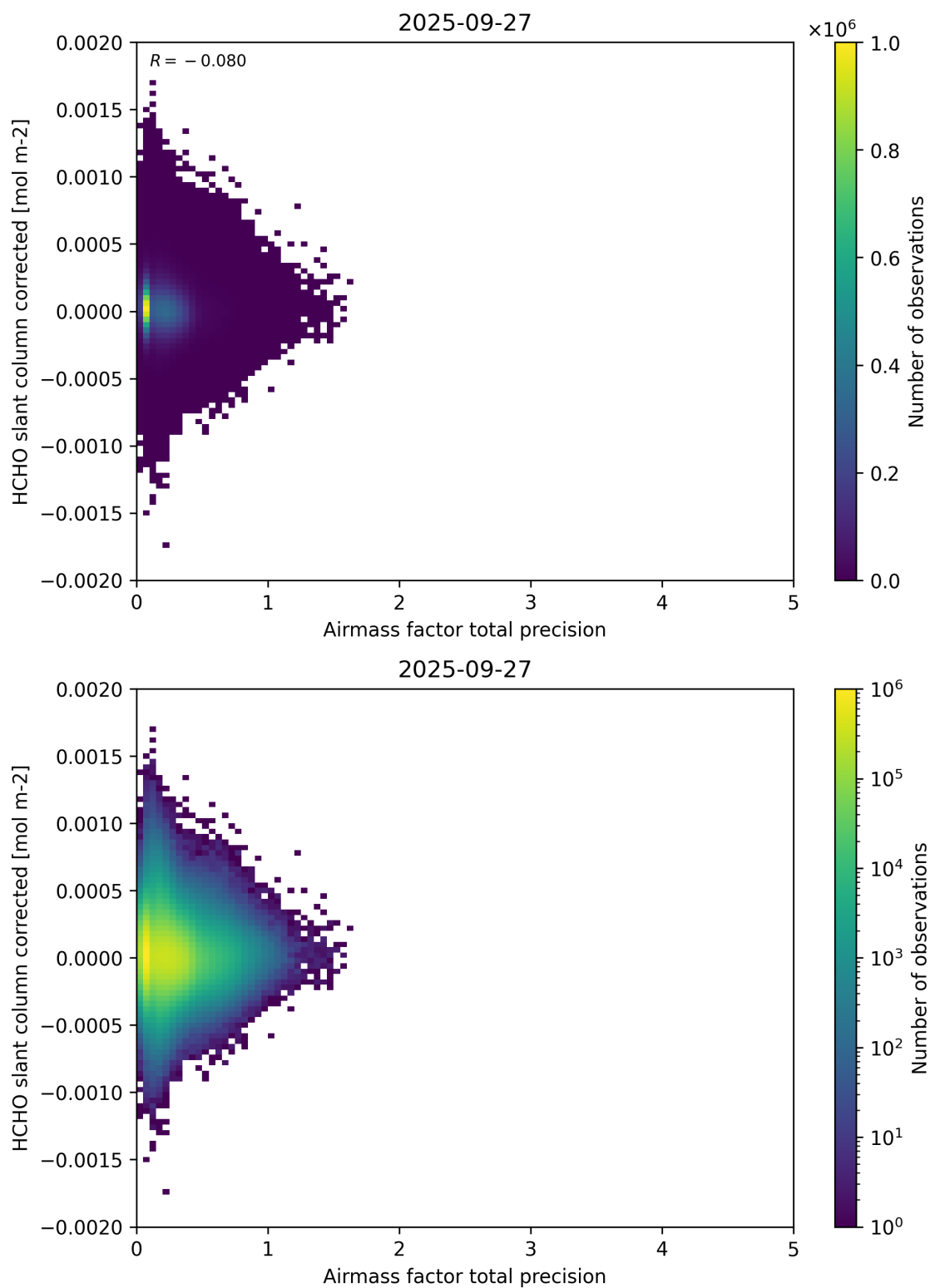
Figure 109: Scatter density plot of “Airmass factor total precision” against “HCHO slant column corrected” for 2025-09-26 to 2025-09-28.
