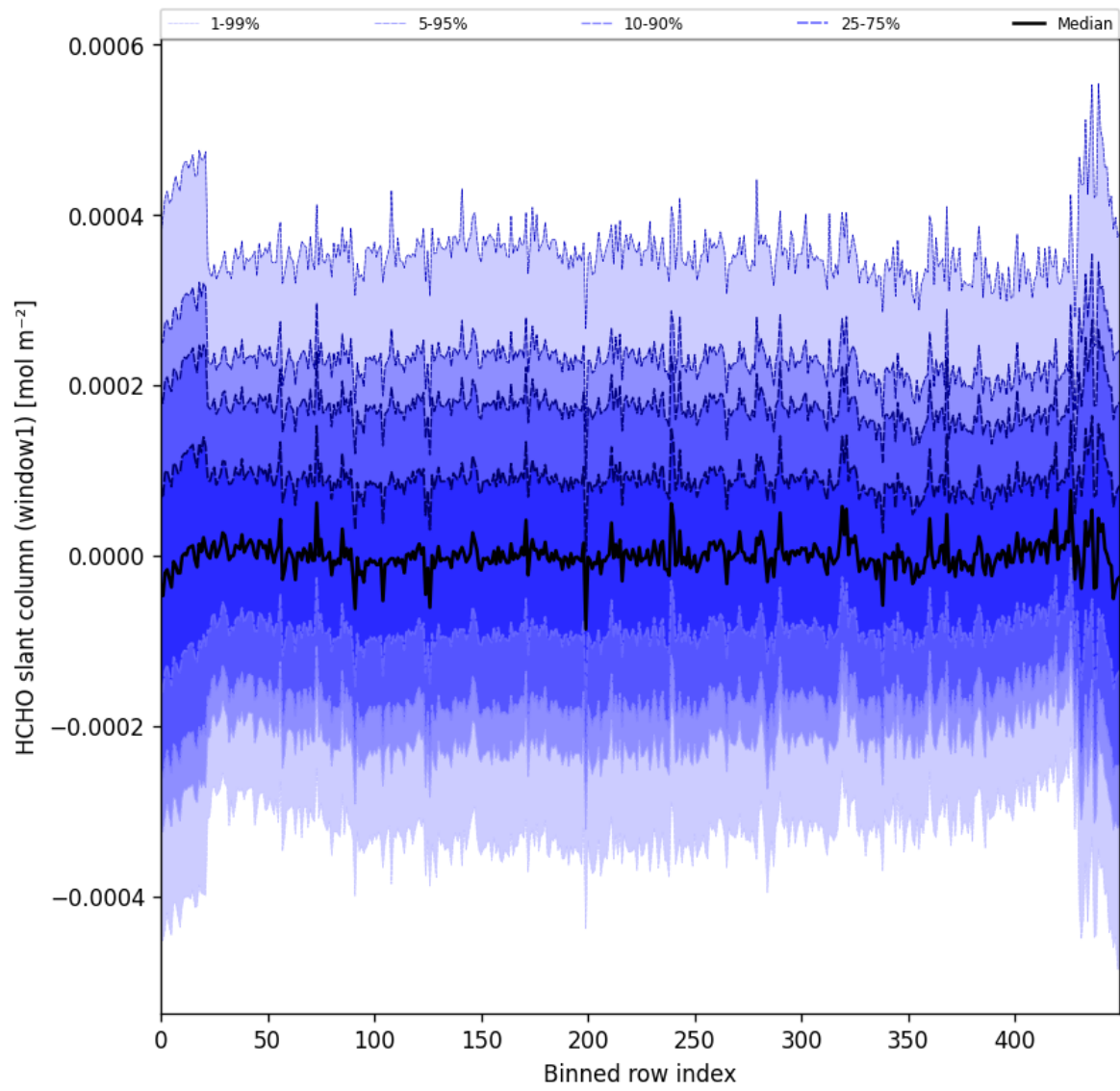
Figure 52: Along track statistics of “HCHO slant column (window1)” for 2025-09-26 to 2025-09-28
