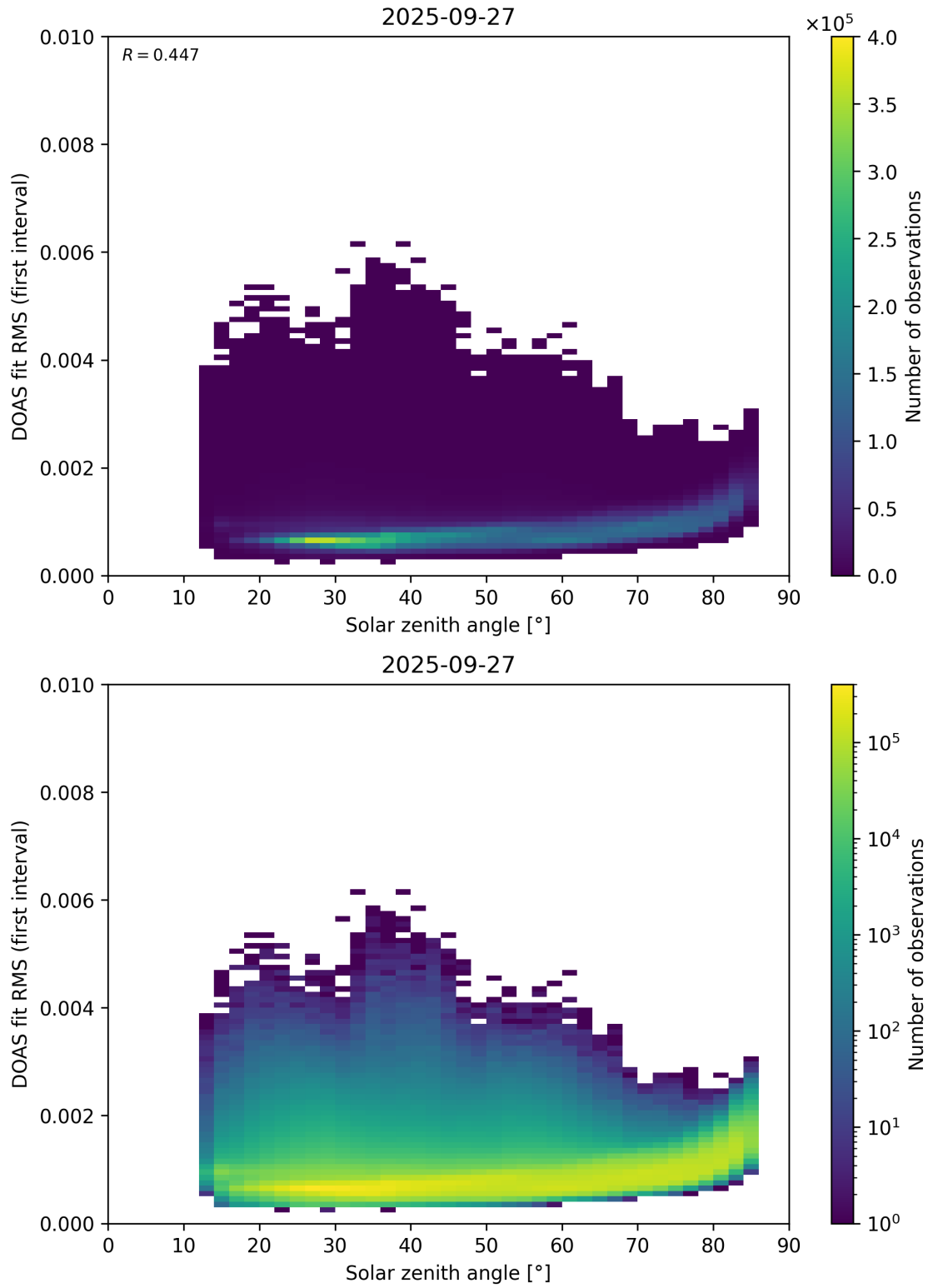
Figure 167: Scatter density plot of “Solar zenith angle” against “DOAS fit RMS (first interval)” for 2025-09-26 to 2025-09-28.
