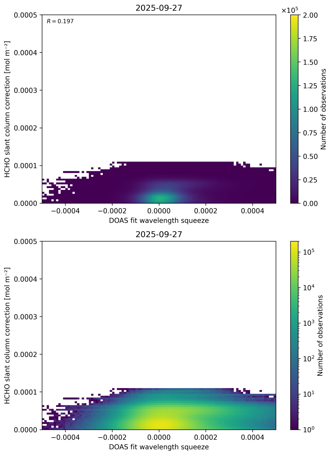
Figure 70: Scatter density plot of “DOAS fit wavelength squeeze” against “HCHO slant column correction” for 2025-09-26 to 2025-09-28.
