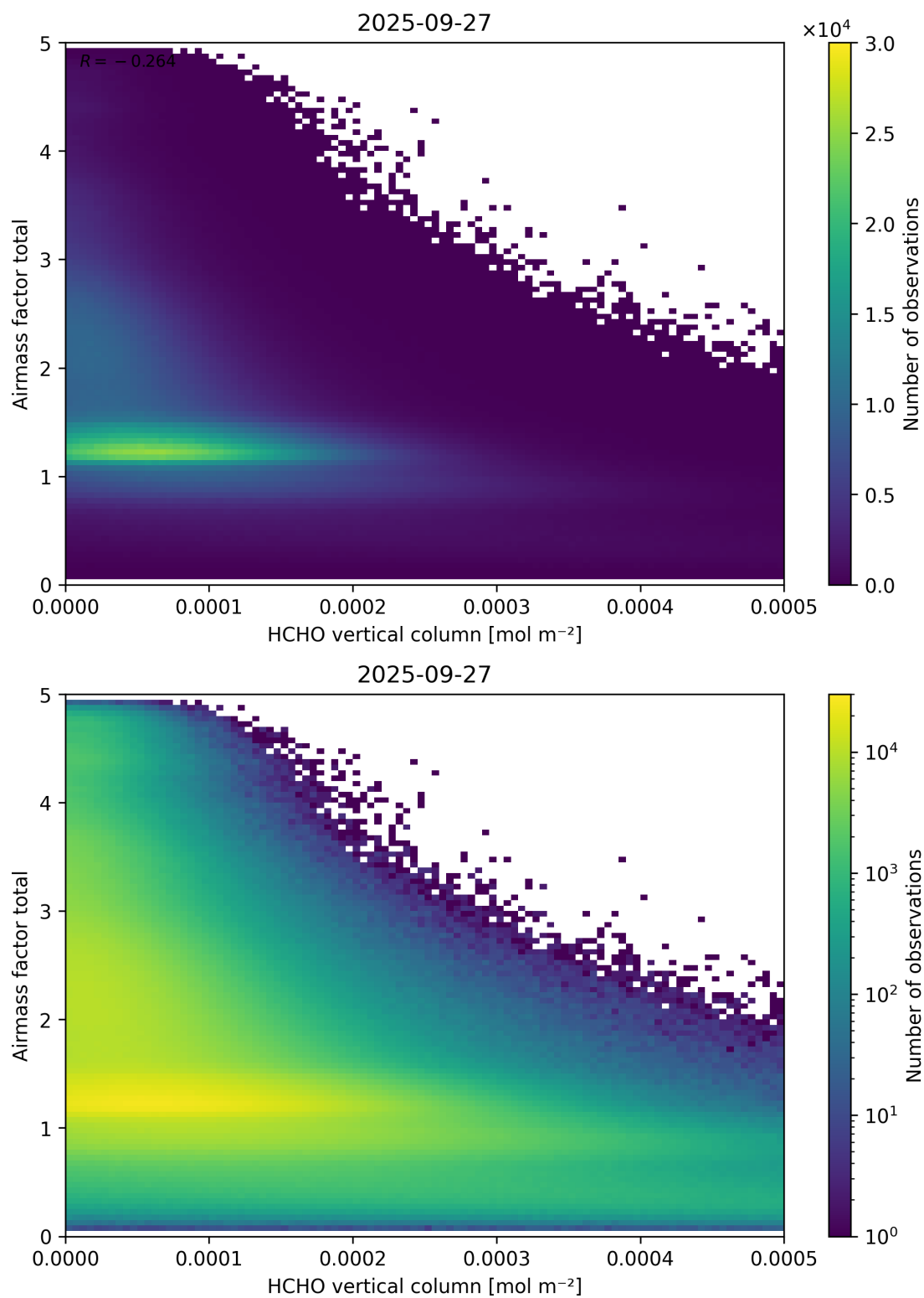
Figure 131: Scatter density plot of “HCHO vertical column” against “Airmass factor total” for 2025-09-26 to 2025-09-28.
