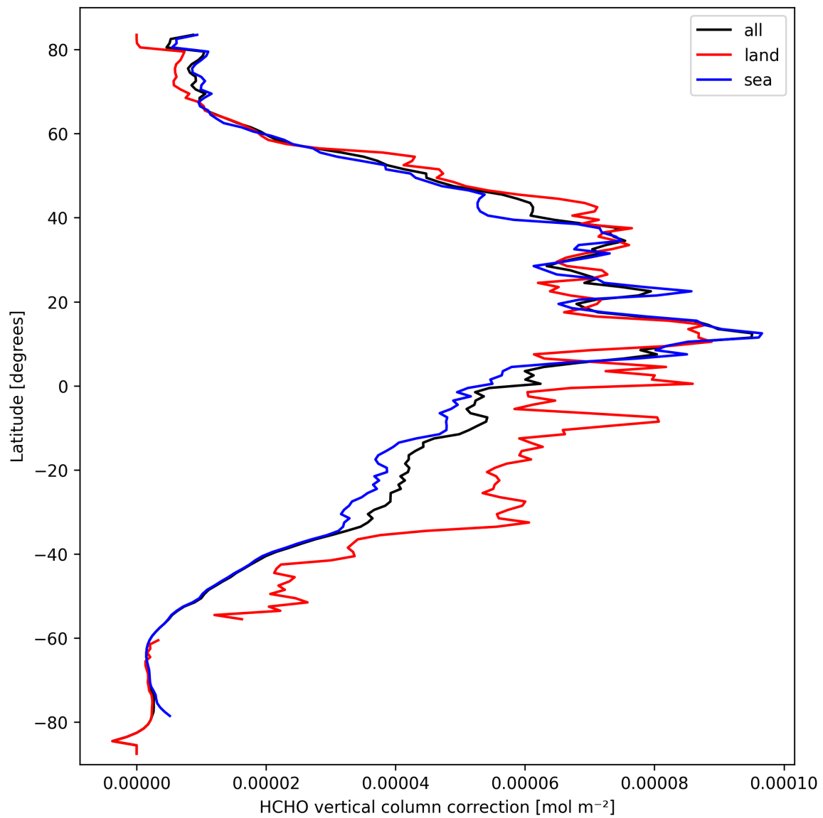
Figure 23: Zonal average of “HCHO vertical column correction” for 2025-09-26 to 2025-09-28.
