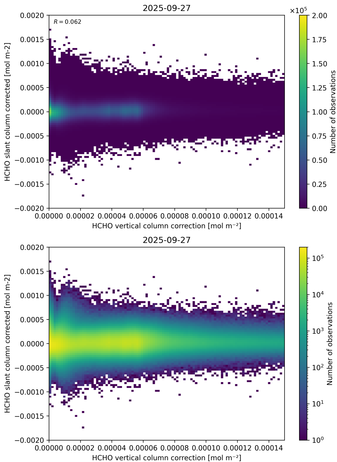
Figure 116: Scatter density plot of “HCHO vertical column correction” against “HCHO slant column corrected” for 2025-09-26 to 2025-09-28.
