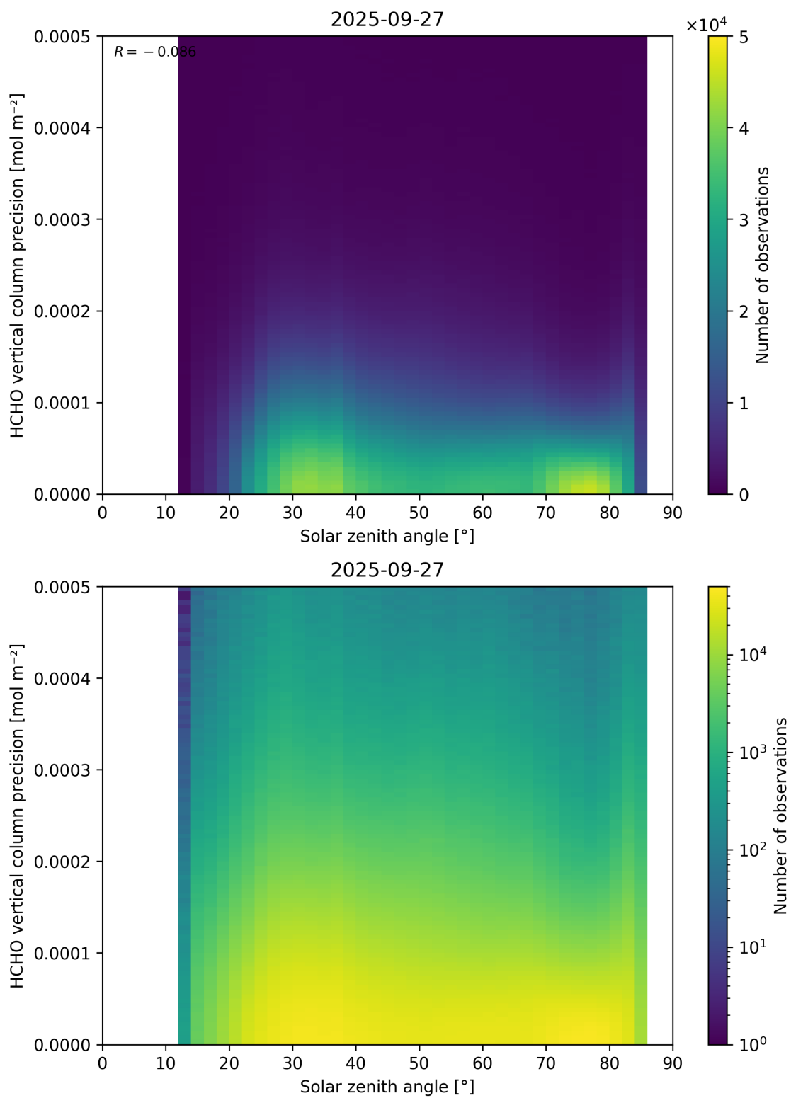
Figure 179: Scatter density plot of “Solar zenith angle” against “HCHO vertical column precision” for 2025-09-26 to 2025-09-28.
