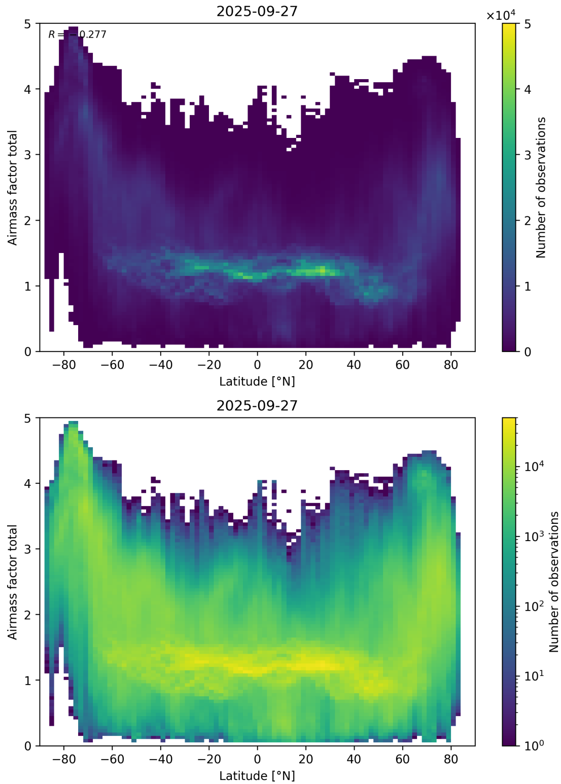
Figure 161: Scatter density plot of “Latitude” against “Airmass factor total” for 2025-09-26 to 2025-09-28.
