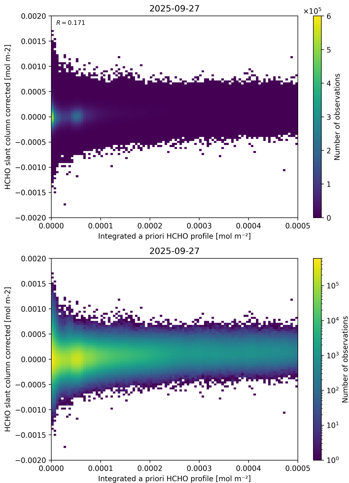
Figure 151: Scatter density plot of “Integrated a priori HCHO profile” against “HCHO slant column corrected” for 2025-09-26 to 2025-09-28.
