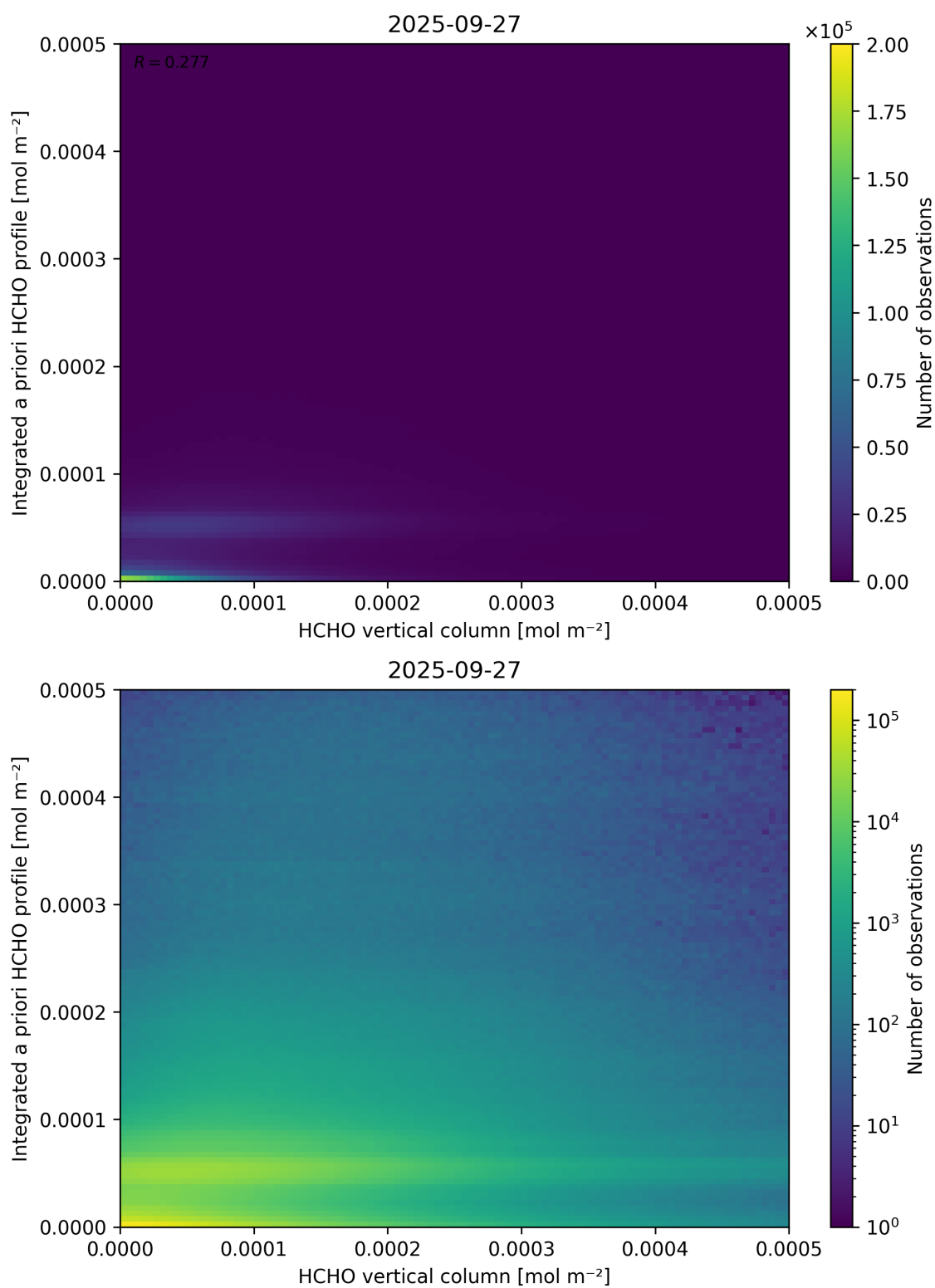
Figure 135: Scatter density plot of “HCHO vertical column” against “Integrated a priori HCHO profile” for 2025-09-26 to 2025-09-28.
