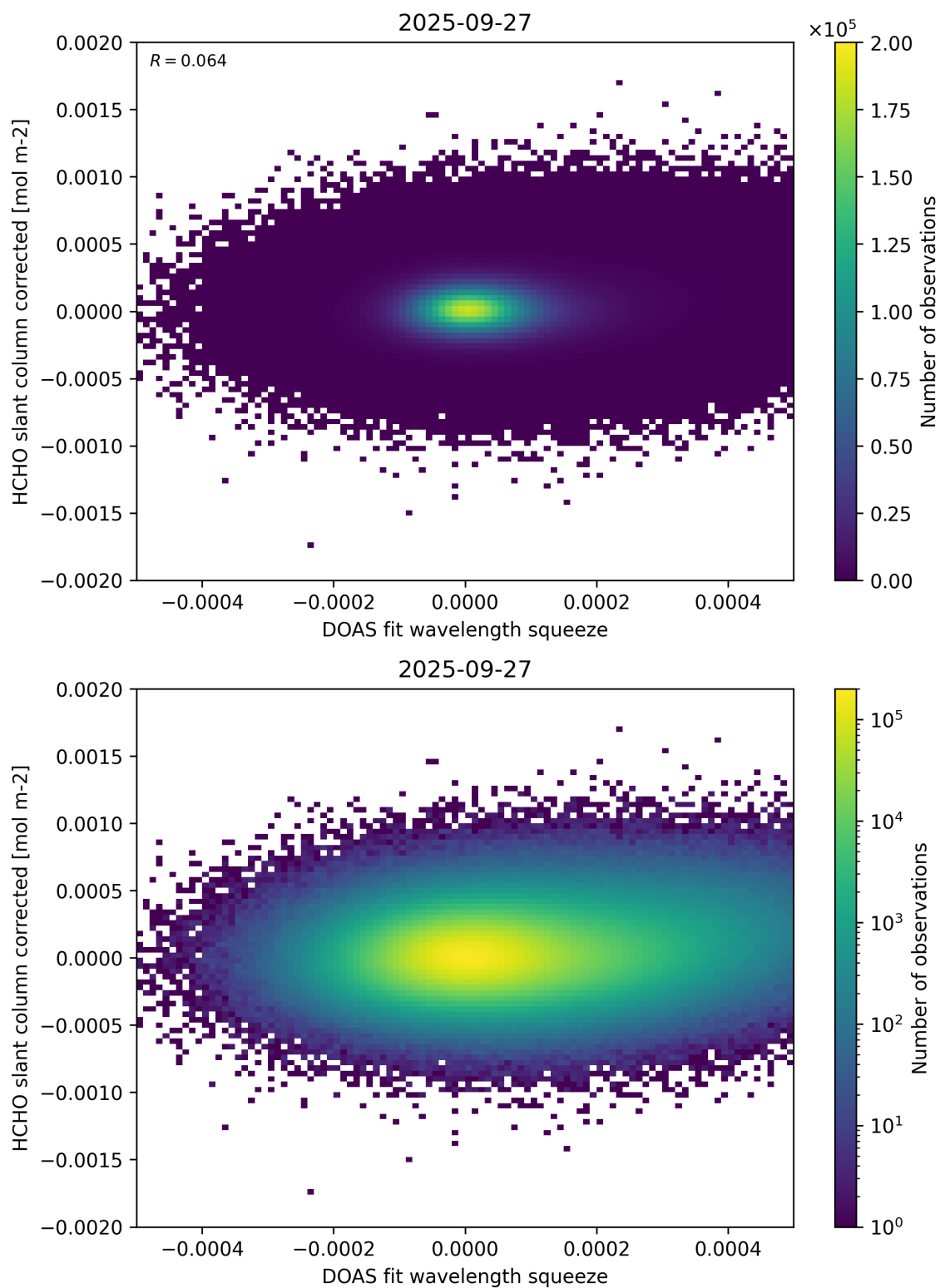
Figure 69: Scatter density plot of “DOAS fit wavelength squeeze” against “HCHO slant column corrected” for 2025-09-26 to 2025-09-28.
