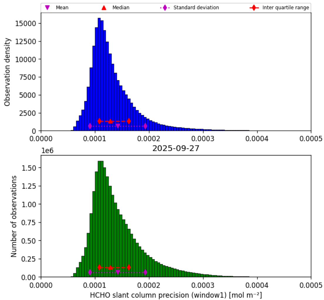
Figure 39: Histogram of “HCHO slant column precision (window1)” for 2025-09-26 to 2025-09-28
