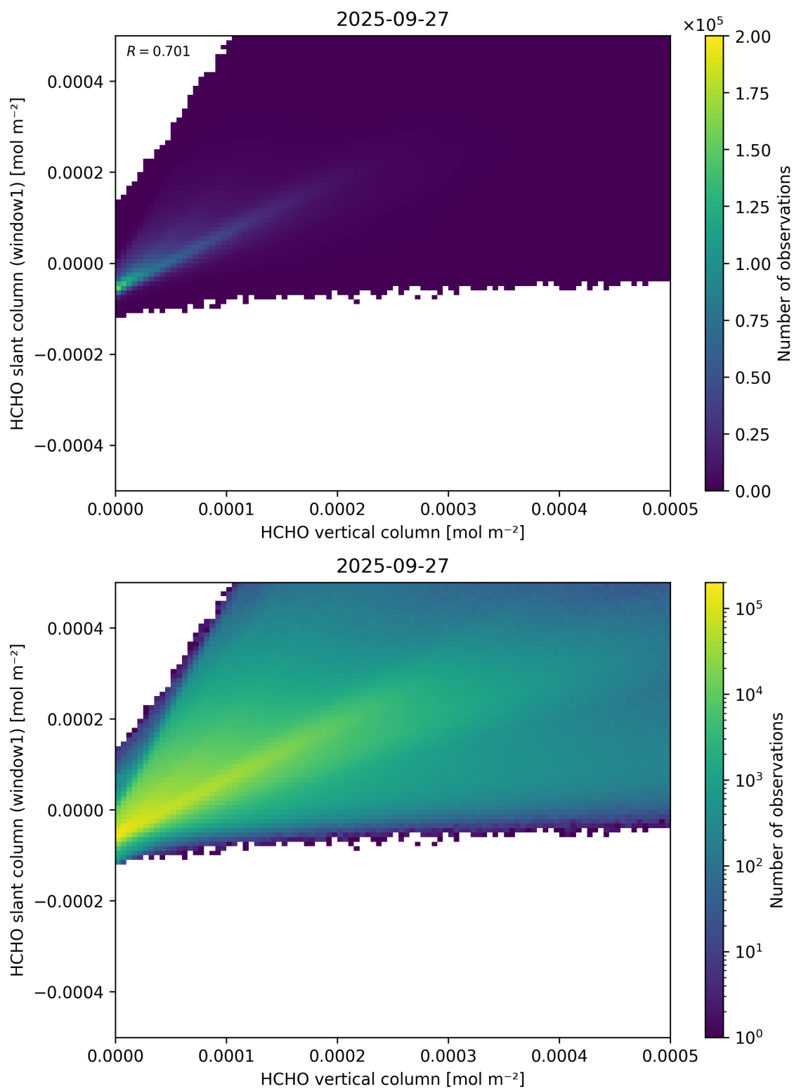
Figure 129: Scatter density plot of “HCHO vertical column” against “HCHO slant column (window1)” for 2025-09-26 to 2025-09-28.
