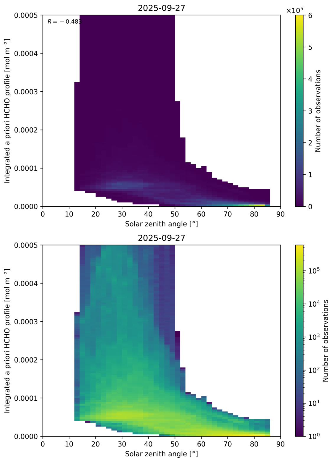
Figure 180: Scatter density plot of “Solar zenith angle” against “Integrated a priori HCHO profile” for 2025-09-26 to 2025-09-28.
