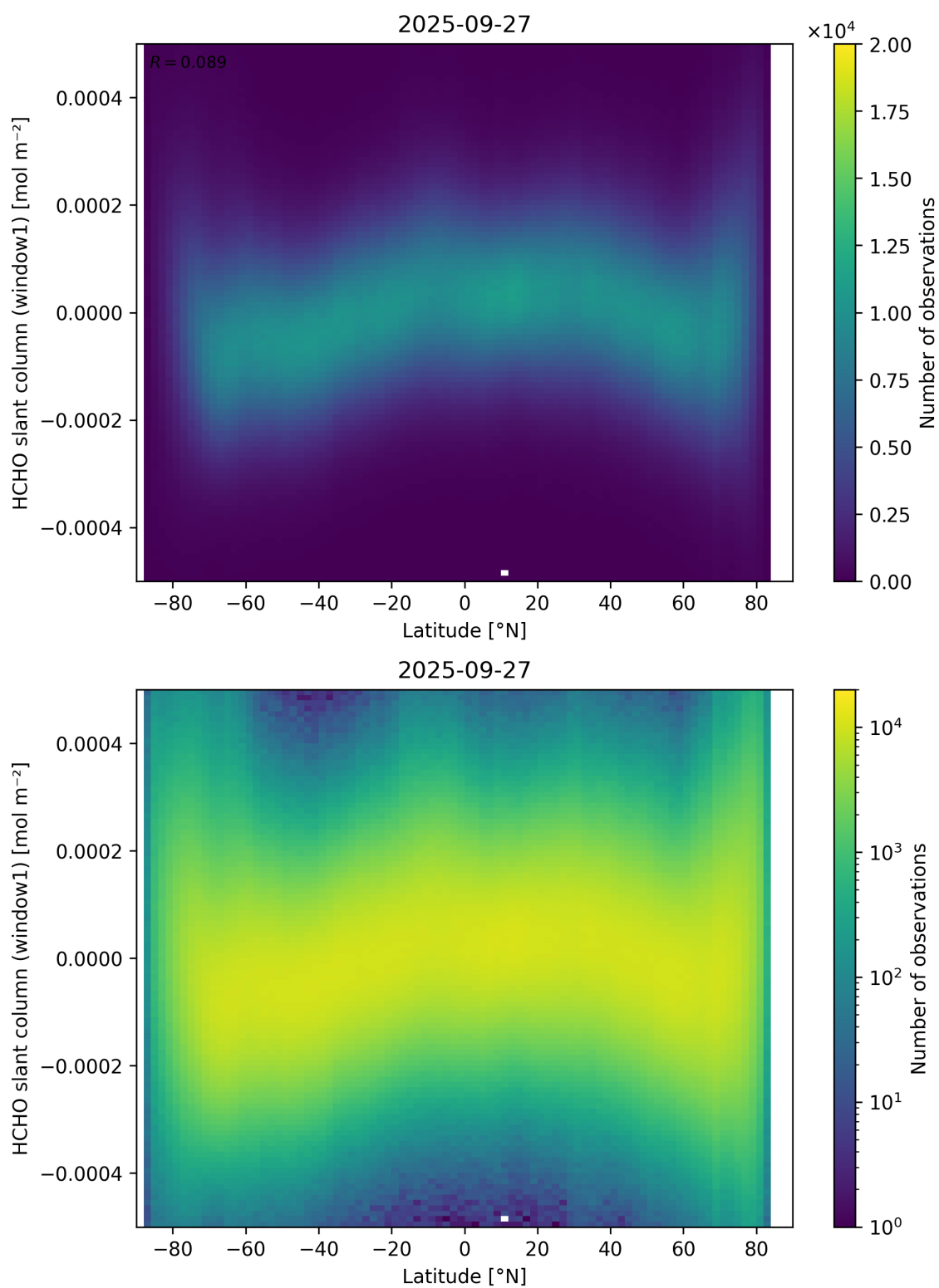
Figure 159: Scatter density plot of “Latitude” against “HCHO slant column (window1)” for 2025-09-26 to 2025-09-28.
