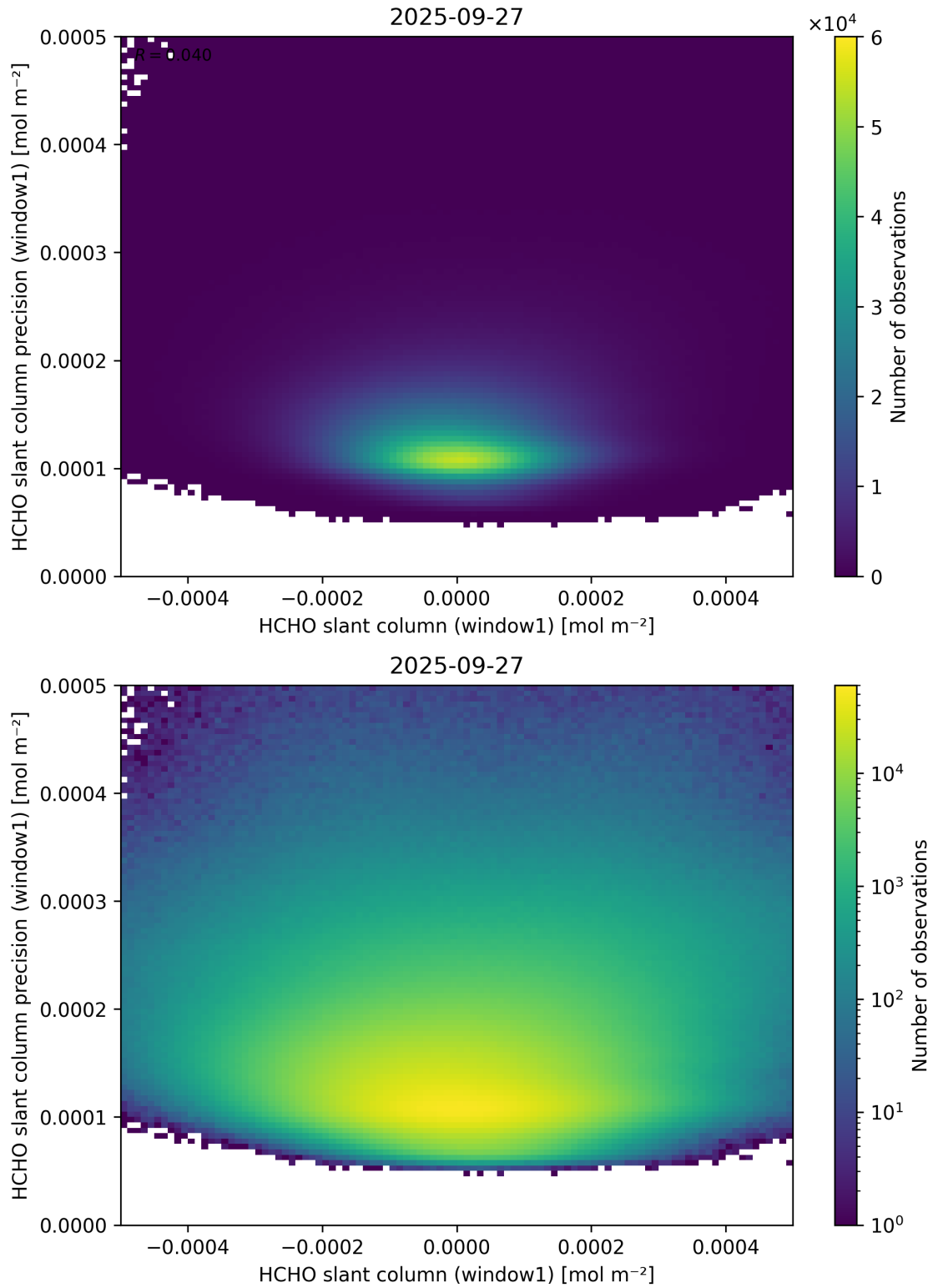
Figure 84: Scatter density plot of “HCHO slant column (window1)” against “HCHO slant column precision (window1)” for 2025-09-26 to 2025-09-28.
