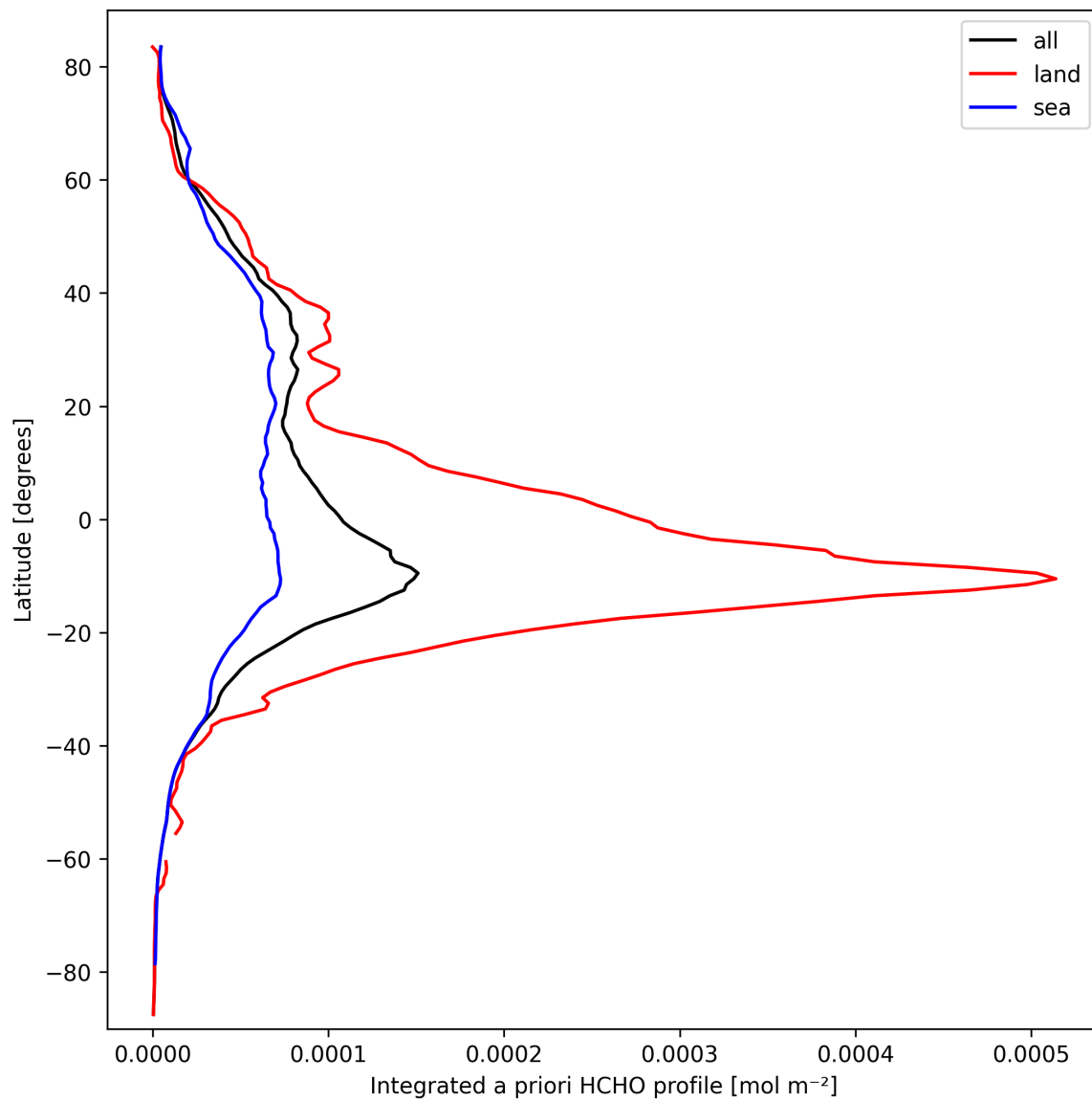
Figure 29: Zonal average of “Integrated a priori HCHO profile” for 2025-09-26 to 2025-09-28.
