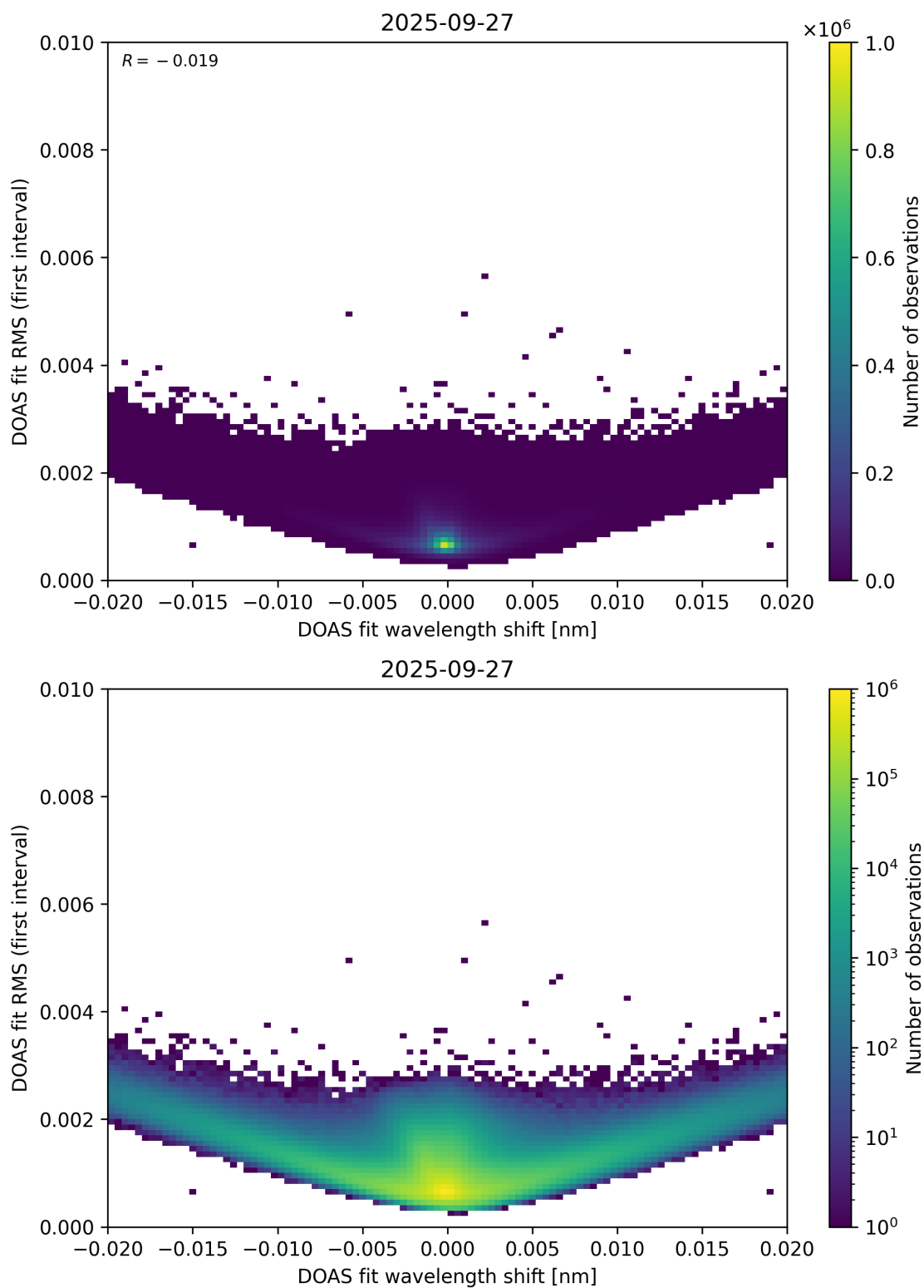
Figure 64: Scatter density plot of “DOAS fit wavelength shift” against “DOAS fit RMS (first interval)” for 2025-09-26 to 2025-09-28.
