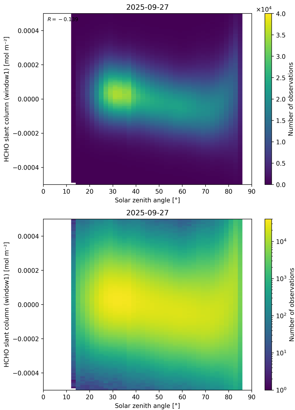
Figure 173: Scatter density plot of “Solar zenith angle” against “HCHO slant column (window1)” for 2025-09-26 to 2025-09-28.
