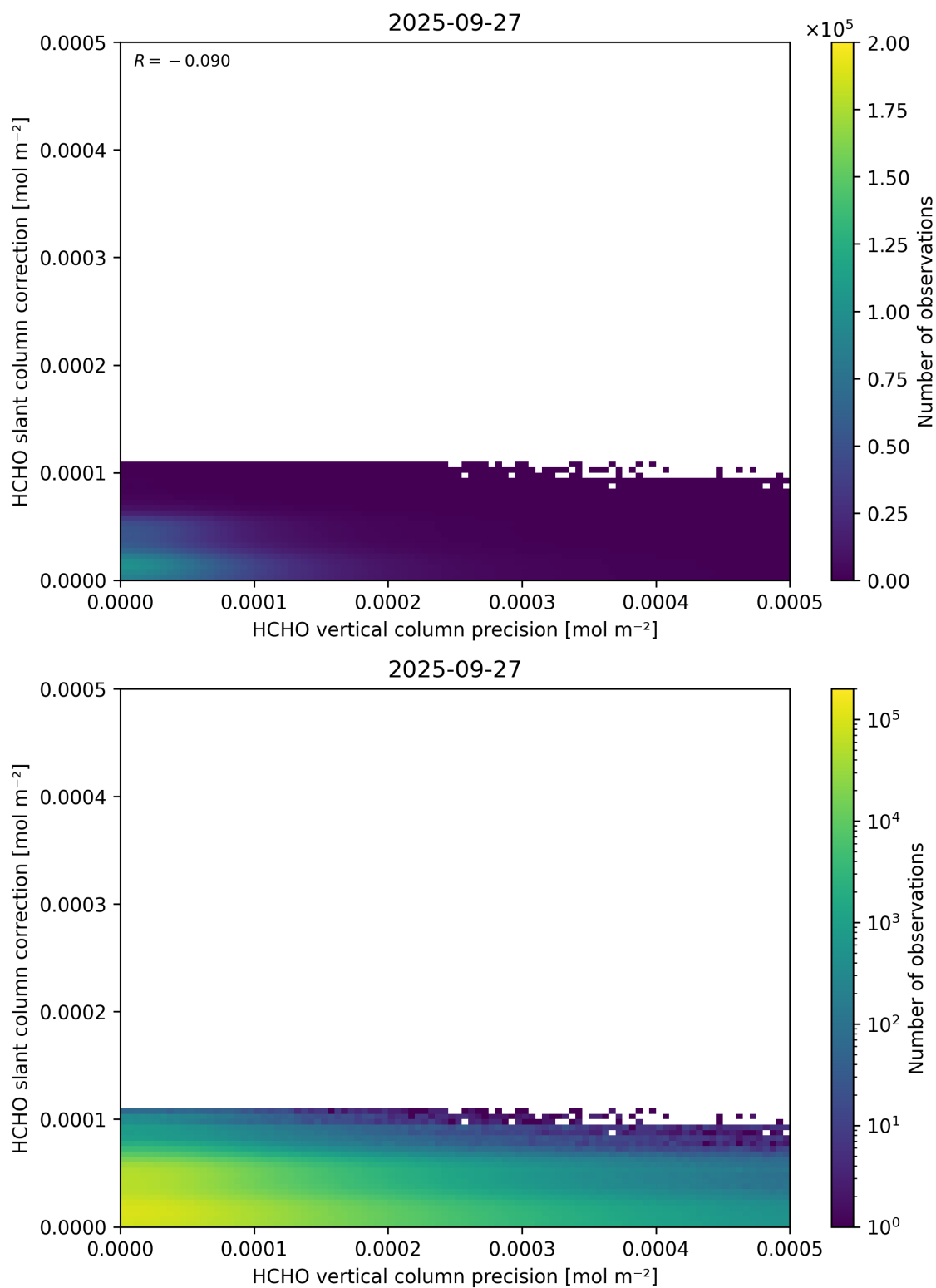
Figure 141: Scatter density plot of “HCHO vertical column precision” against “HCHO slant column correction” for 2025-09-26 to 2025-09-28.
