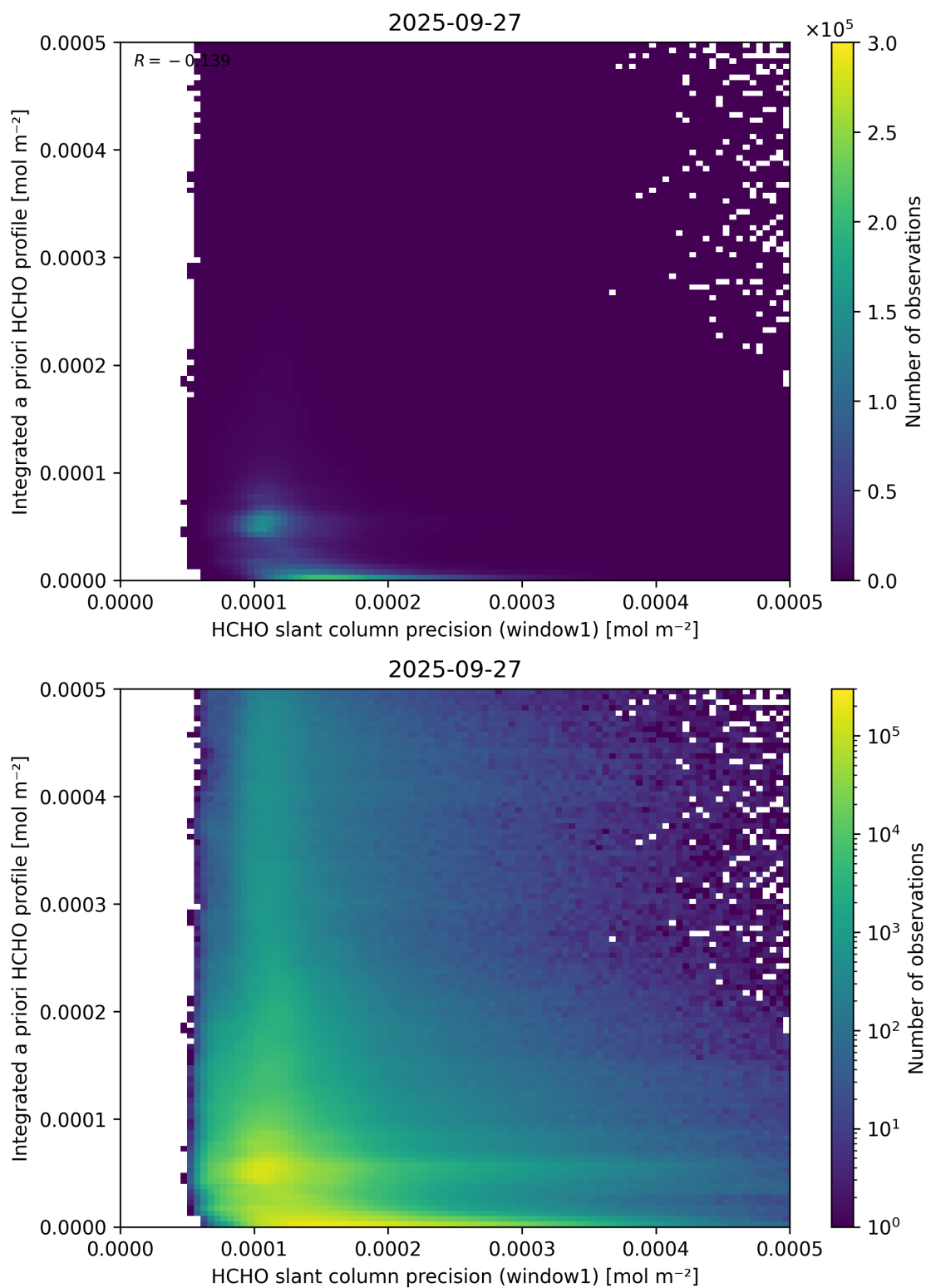
Figure 96: Scatter density plot of “HCHO slant column precision (window1)” against “Integrated a priori HCHO profile” for 2025-09-26 to 2025-09-28.
