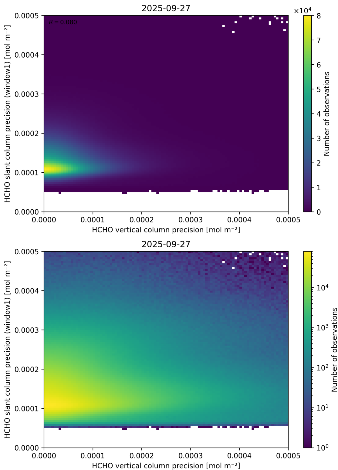
Figure 143: Scatter density plot of “HCHO vertical column precision” against “HCHO slant column precision (window1)” for 2025-09-26 to 2025-09-28.
