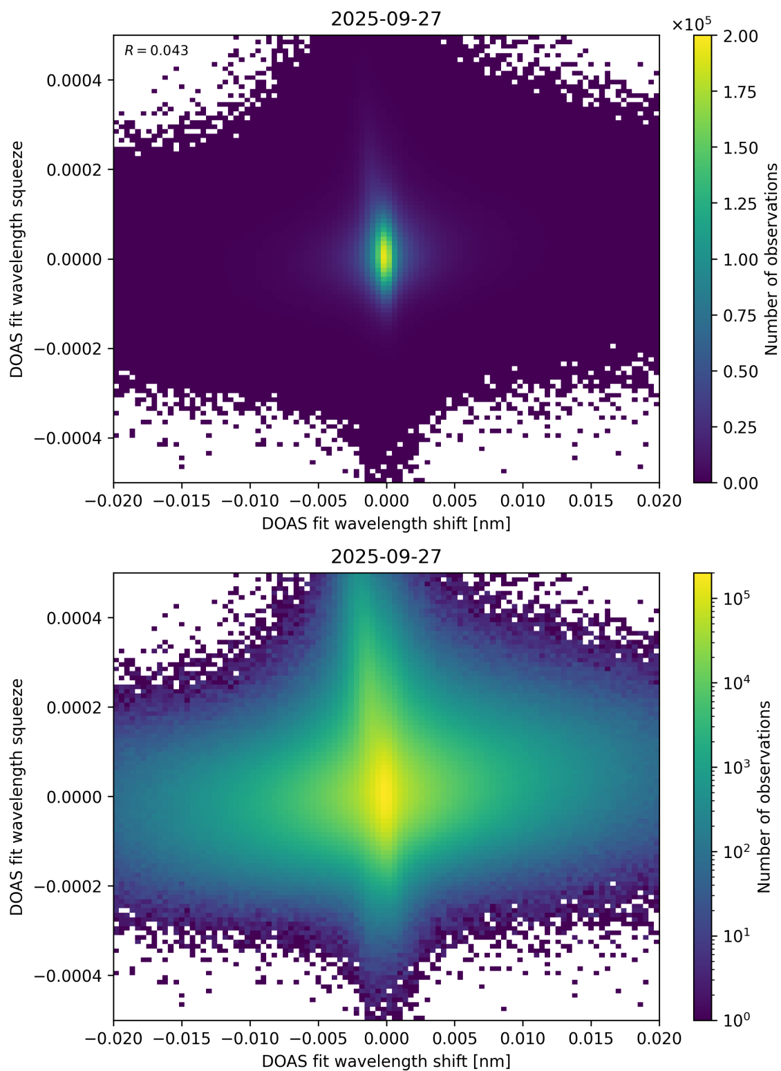
Figure 65: Scatter density plot of “DOAS fit wavelength shift” against “DOAS fit wavelength squeeze” for 2025-09-26 to 2025-09-28.
