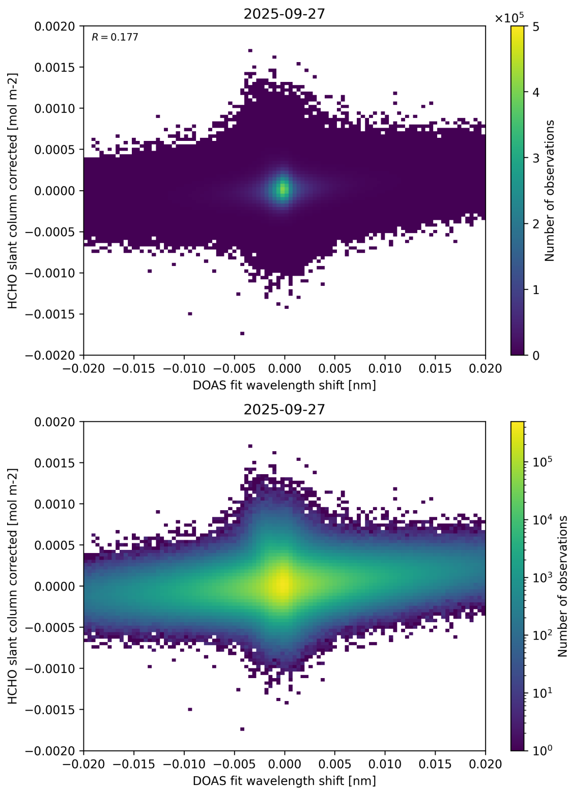
Figure 66: Scatter density plot of “DOAS fit wavelength shift” against “HCHO slant column corrected” for 2025-09-26 to 2025-09-28.
