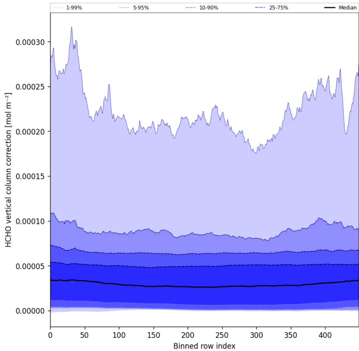
Figure 51: Along track statistics of “HCHO vertical column correction” for 2025-09-26 to 2025-09-28
