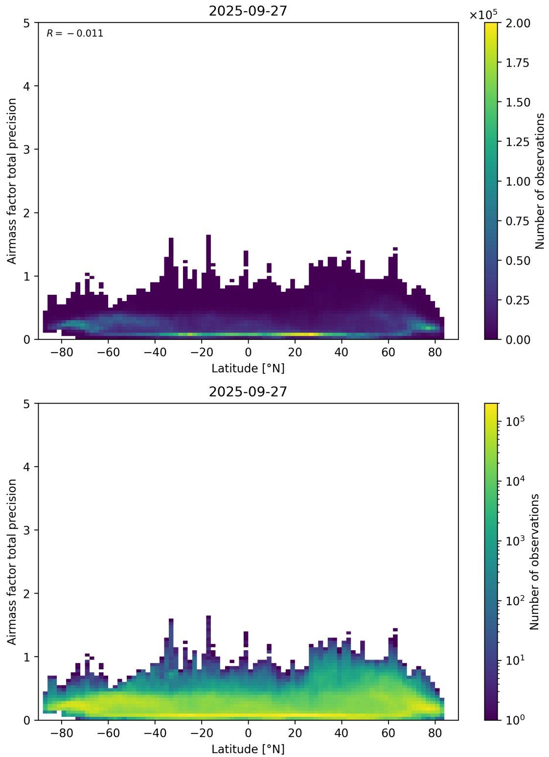
Figure 162: Scatter density plot of “Latitude” against “Airmass factor total precision” for 2025-09-26 to 2025-09-28.
