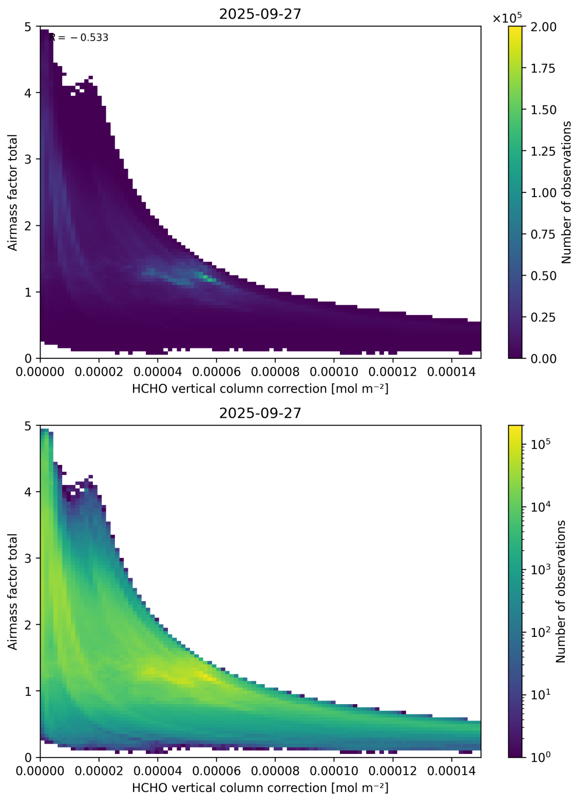
Figure 120: Scatter density plot of “HCHO vertical column correction” against “Airmass factor total” for 2025-09-26 to 2025-09-28.
