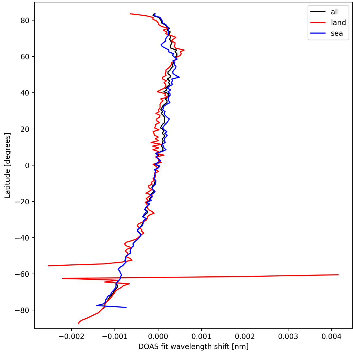
Figure 30: Zonal average of “DOAS fit wavelength shift” for 2025-09-26 to 2025-09-28.
