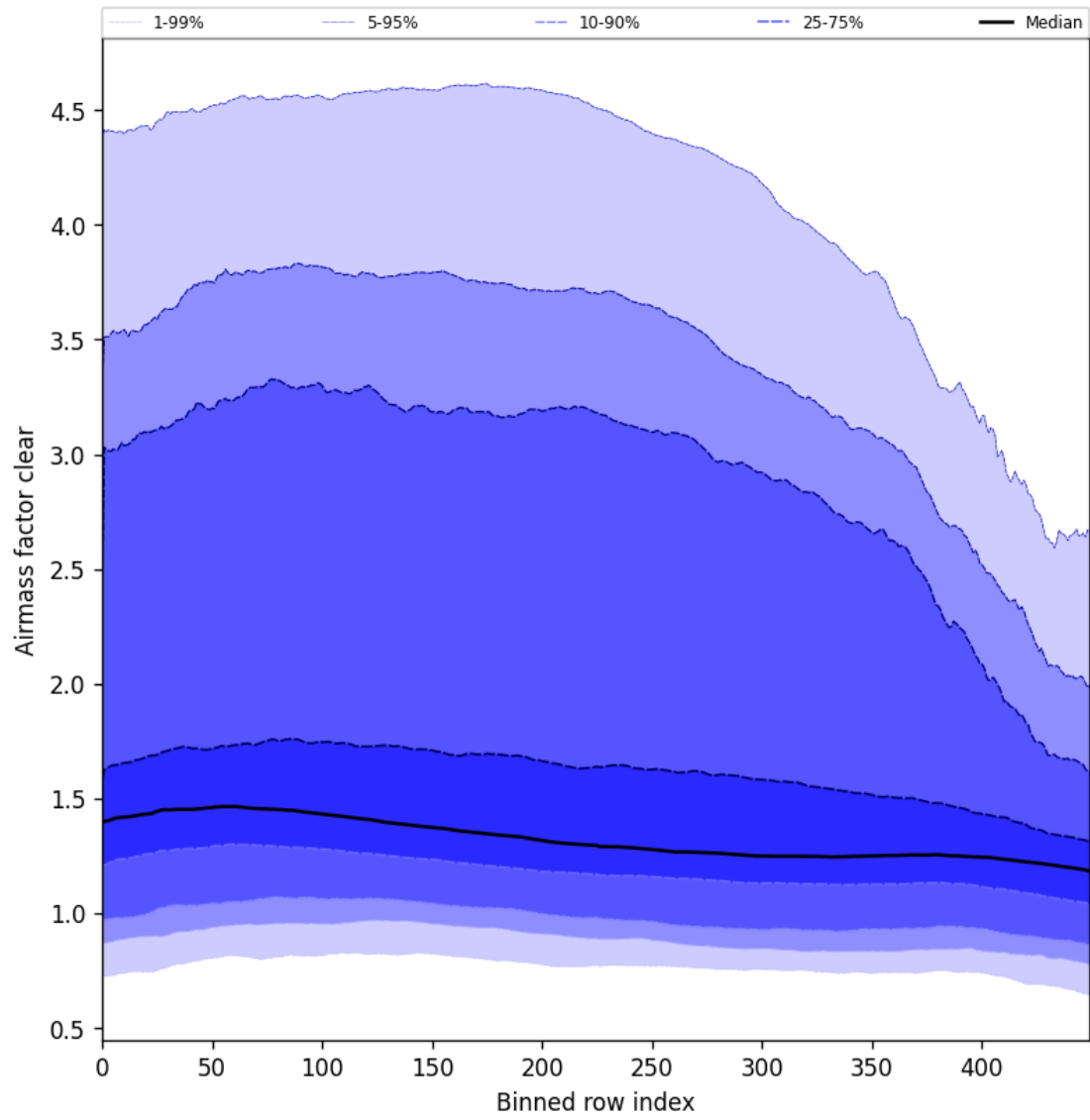
Figure 56: Along track statistics of “Airmass factor clear” for 2025-09-26 to 2025-09-28
