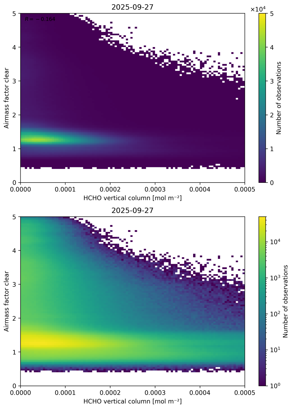
Figure 126: Scatter density plot of “HCHO vertical column” against “Airmass factor clear” for 2025-09-26 to 2025-09-28.
