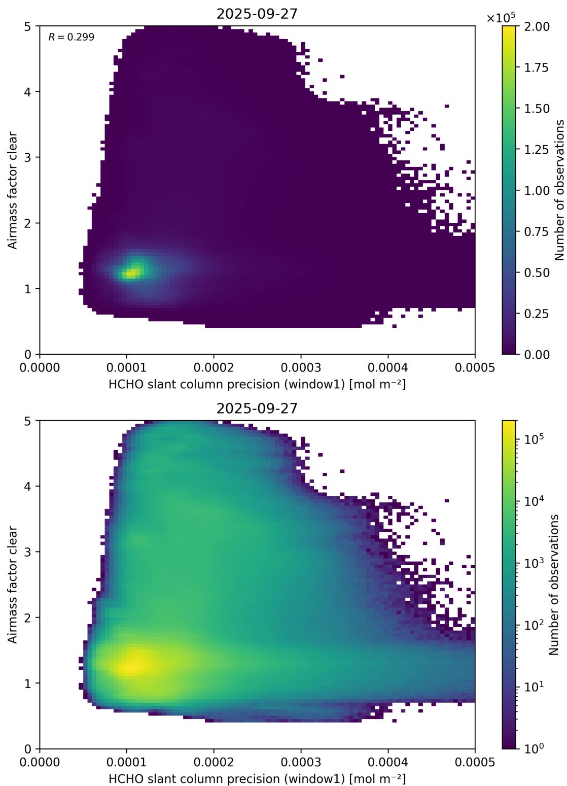
Figure 91: Scatter density plot of “HCHO slant column precision (window1)” against “Airmass factor clear” for 2025-09-26 to 2025-09-28.
