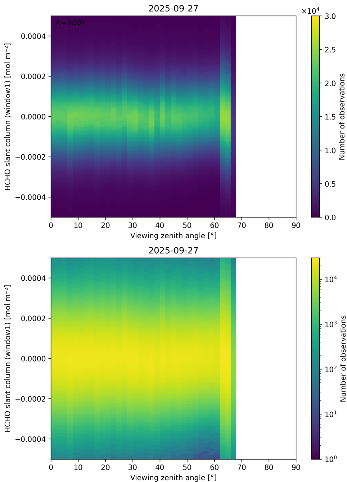
Figure 188: Scatter density plot of “Viewing zenith angle” against “HCHO slant column (window1)” for 2025-09-26 to 2025-09-28.
