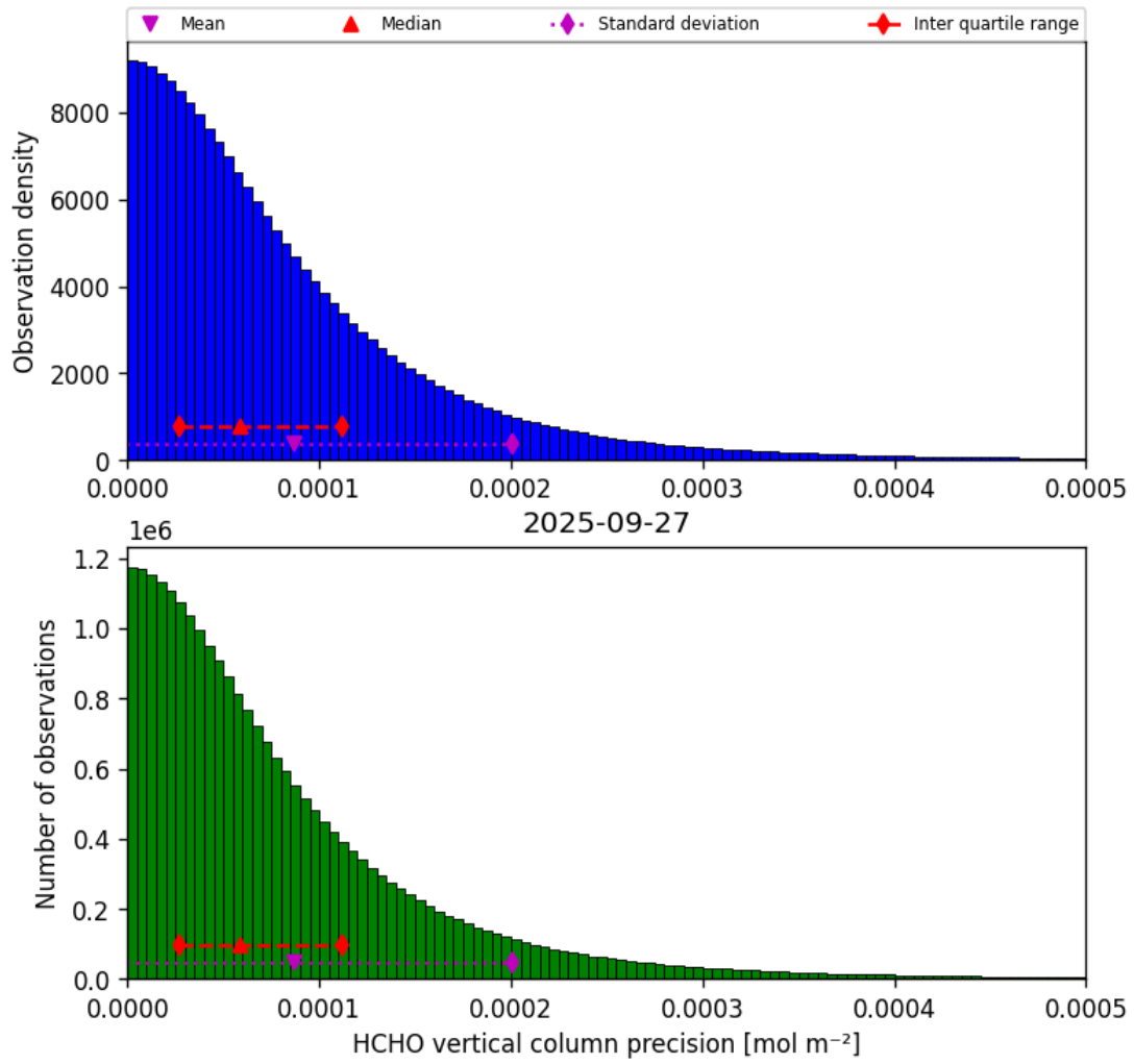
Figure 36: Histogram of “HCHO vertical column precision” for 2025-09-26 to 2025-09-28
