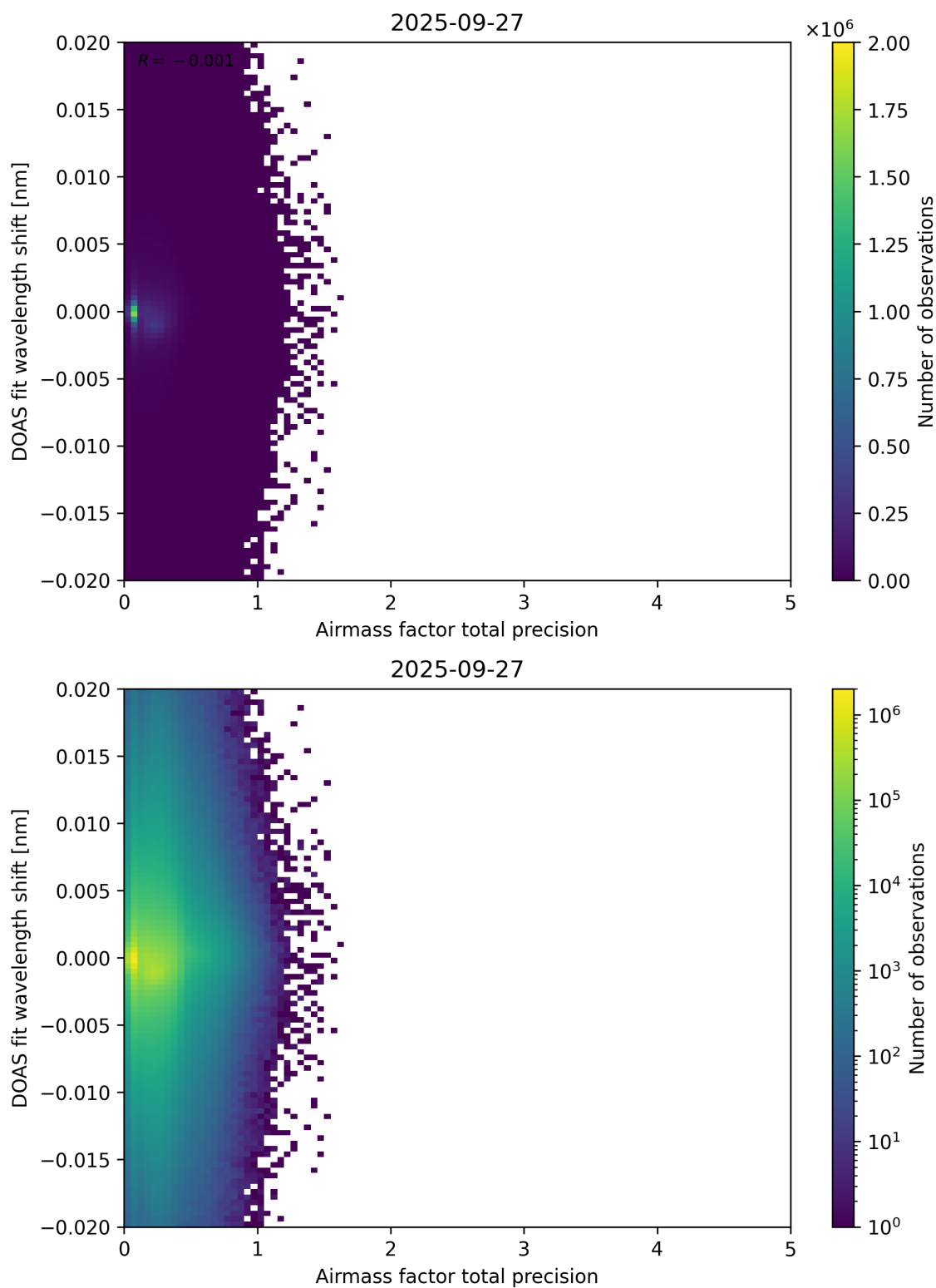
Figure 106: Scatter density plot of “Airmass factor total precision” against “DOAS fit wavelength shift” for 2025-09-26 to 2025-09-28.
