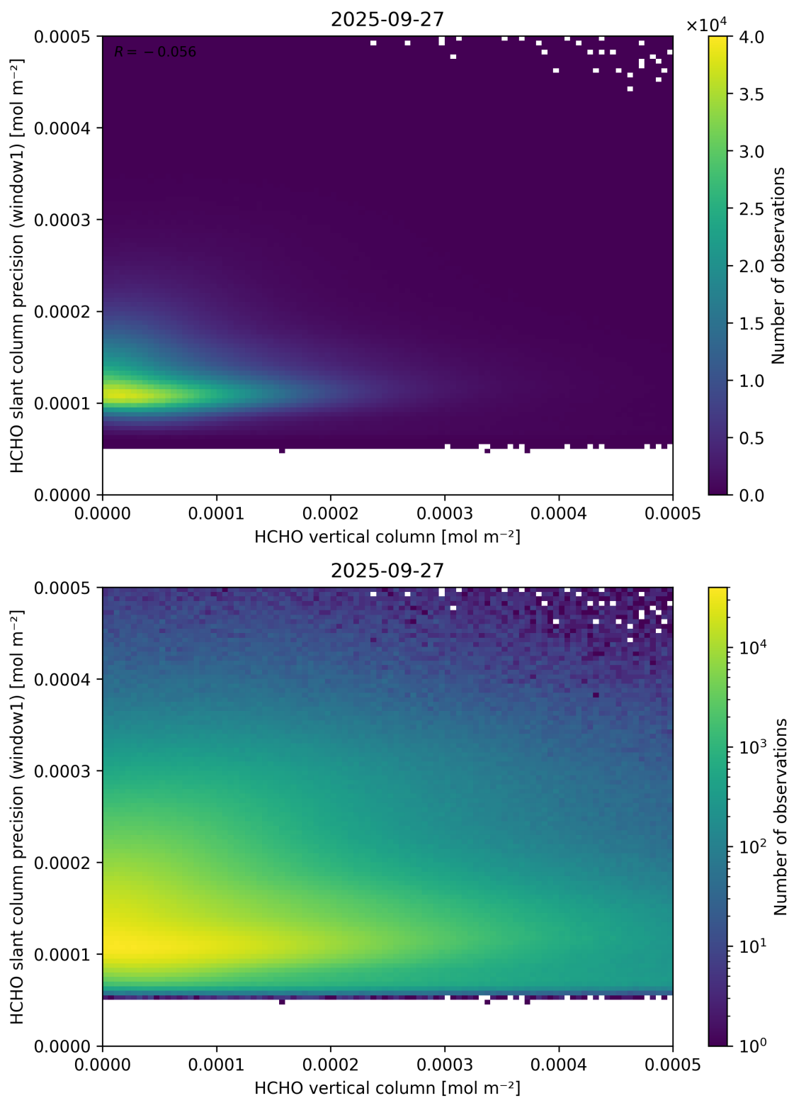
Figure 130: Scatter density plot of “HCHO vertical column” against “HCHO slant column precision (window1)” for 2025-09-26 to 2025-09-28.
