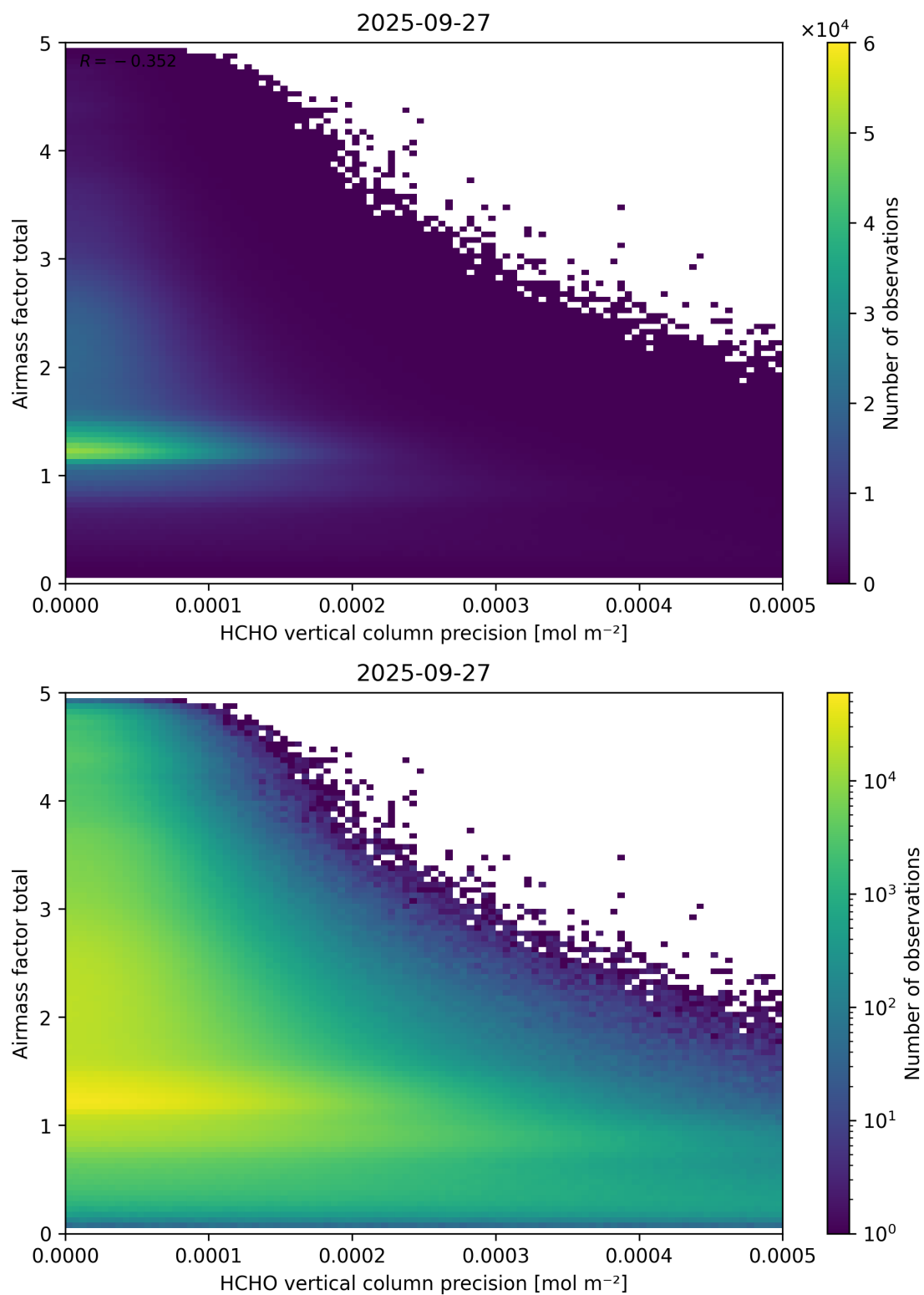
Figure 144: Scatter density plot of “HCHO vertical column precision” against “Airmass factor total” for 2025-09-26 to 2025-09-28.
