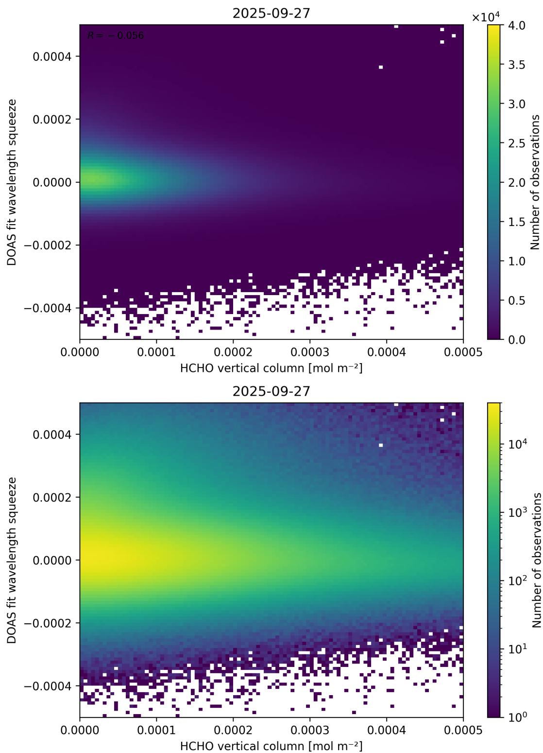
Figure 125: Scatter density plot of “HCHO vertical column” against “DOAS fit wavelength squeeze” for 2025-09-26 to 2025-09-28.
