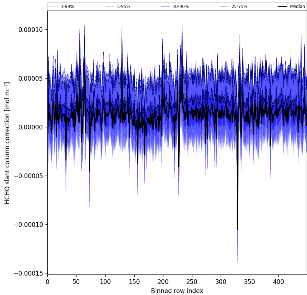
Figure 61: Along track statistics of “HCHO slant column correction” for 2025-09-26 to 2025-09-28
