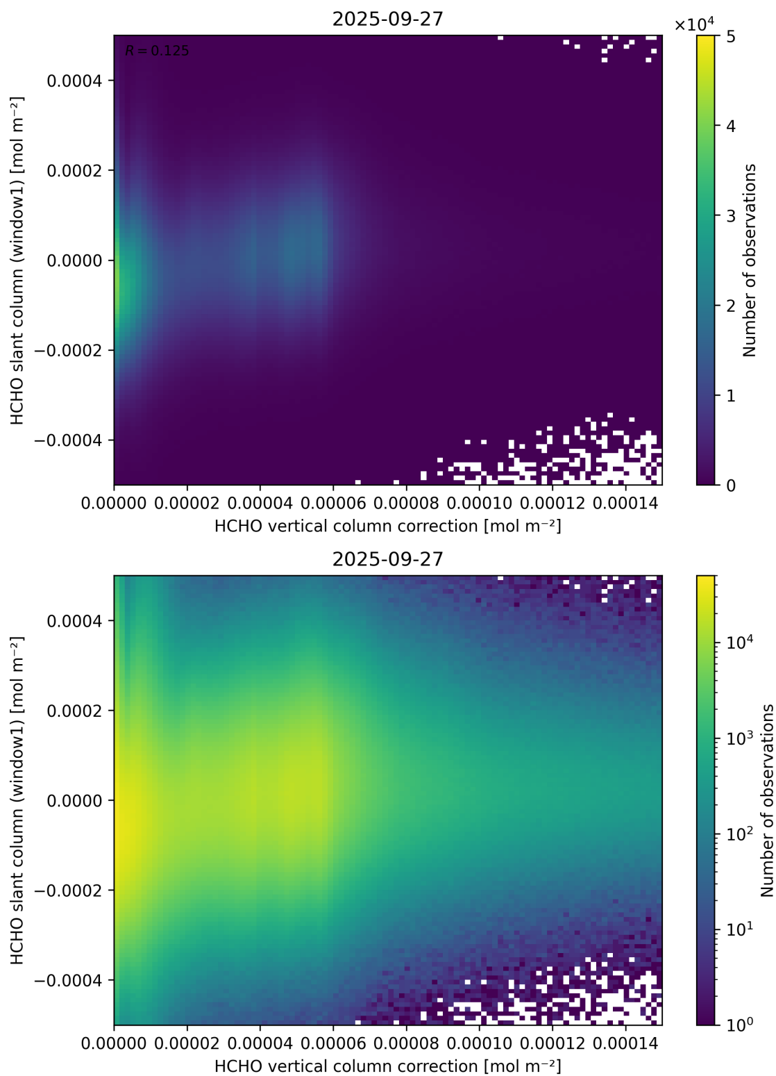
Figure 118: Scatter density plot of “HCHO vertical column correction” against “HCHO slant column (window1)” for 2025-09-26 to 2025-09-28.
