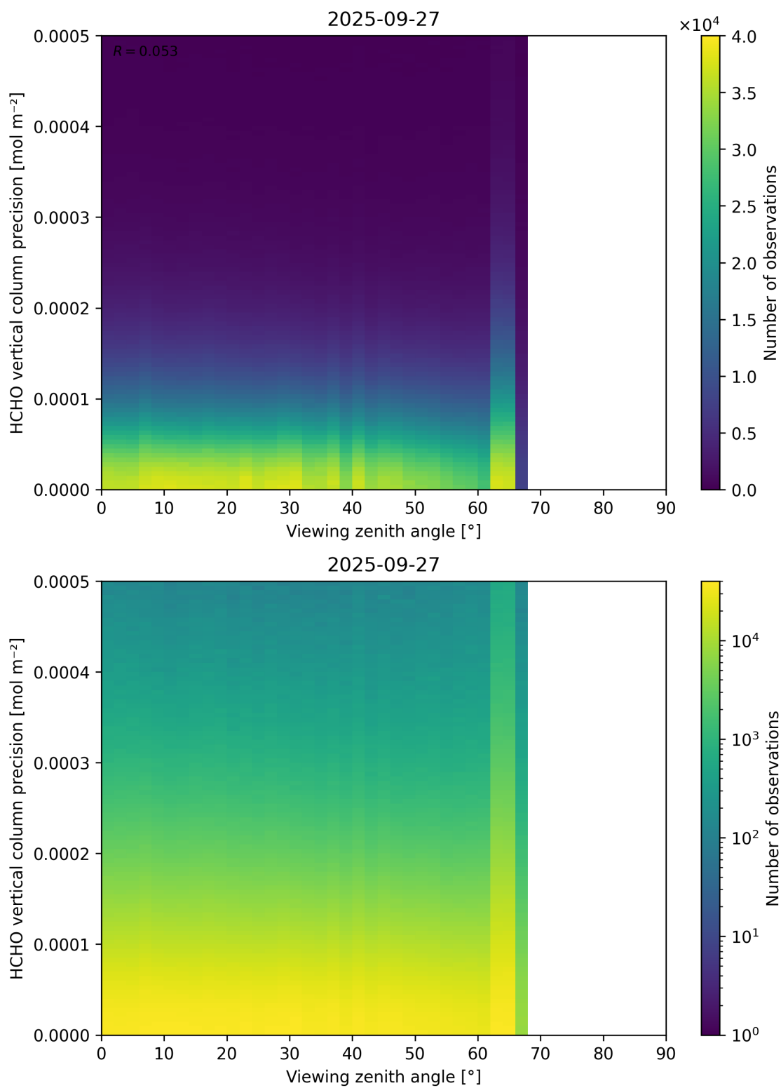
Figure 194: Scatter density plot of “Viewing zenith angle” against “HCHO vertical column precision” for 2025-09-26 to 2025-09-28.
