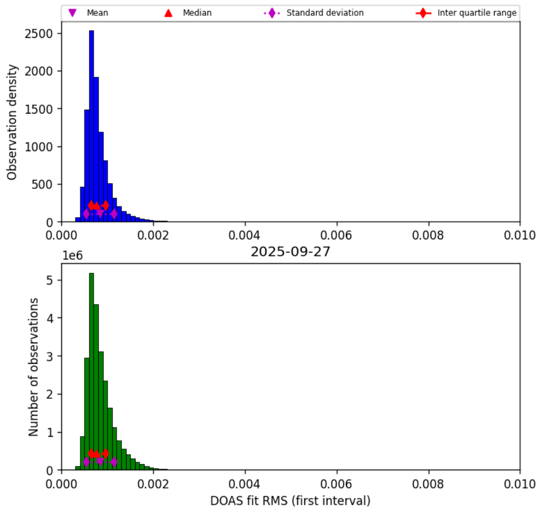
Figure 46: Histogram of “DOAS fit RMS (first interval)” for 2025-09-26 to 2025-09-28
