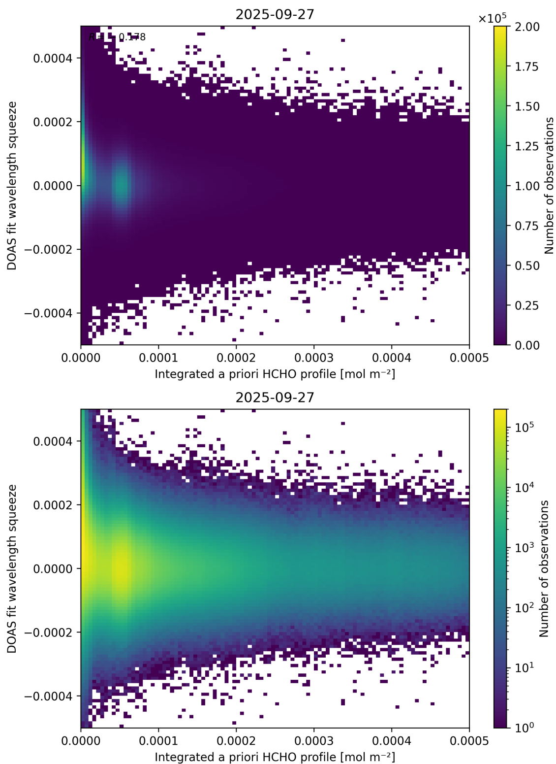
Figure 150: Scatter density plot of “Integrated a priori HCHO profile” against “DOAS fit wavelength squeeze” for 2025-09-26 to 2025-09-28.
