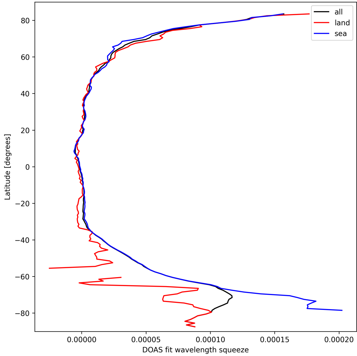
Figure 31: Zonal average of “DOAS fit wavelength squeeze” for 2025-09-26 to 2025-09-28.
