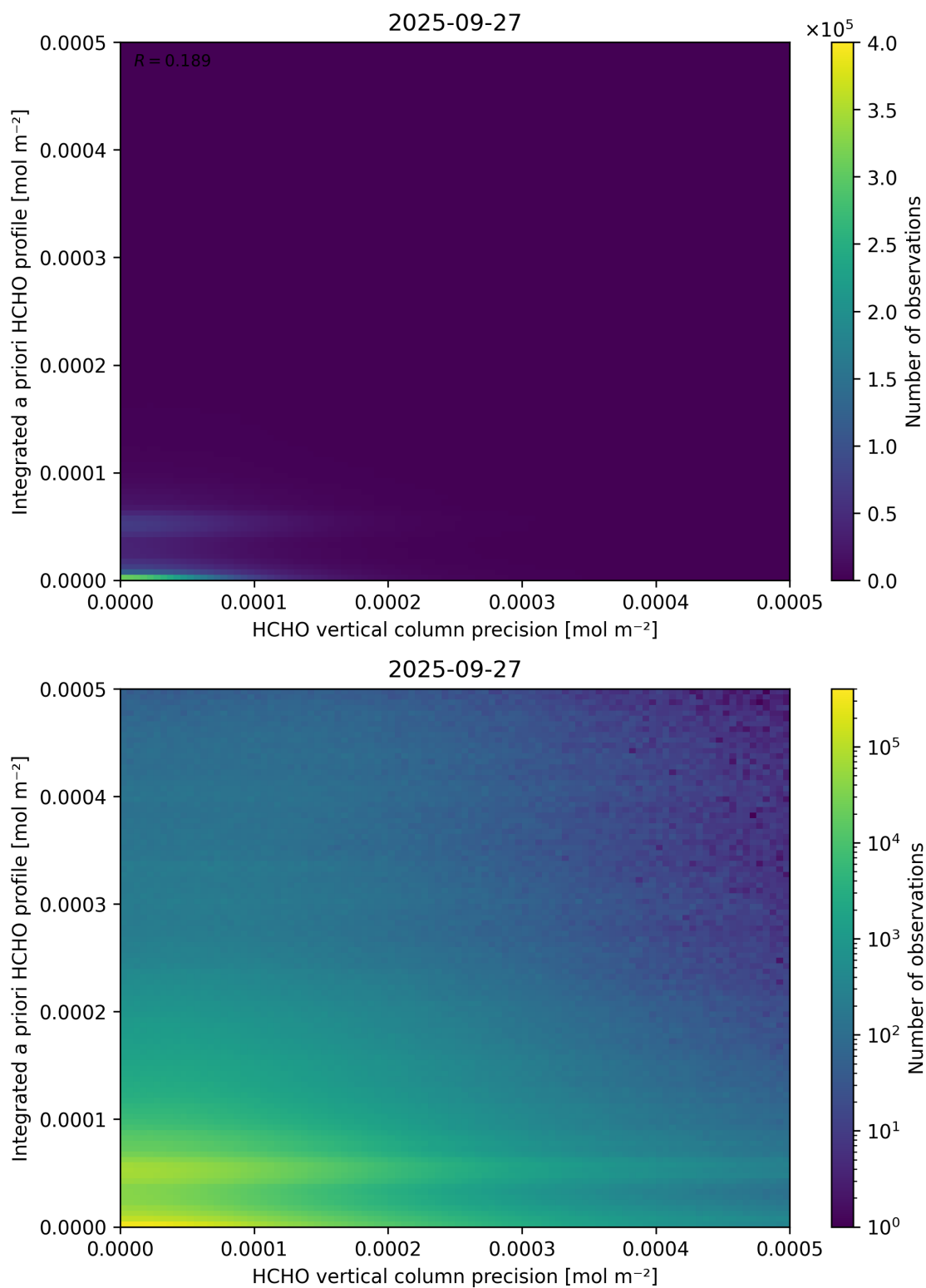
Figure 147: Scatter density plot of “HCHO vertical column precision” against “Integrated a priori HCHO profile” for 2025-09-26 to 2025-09-28.
