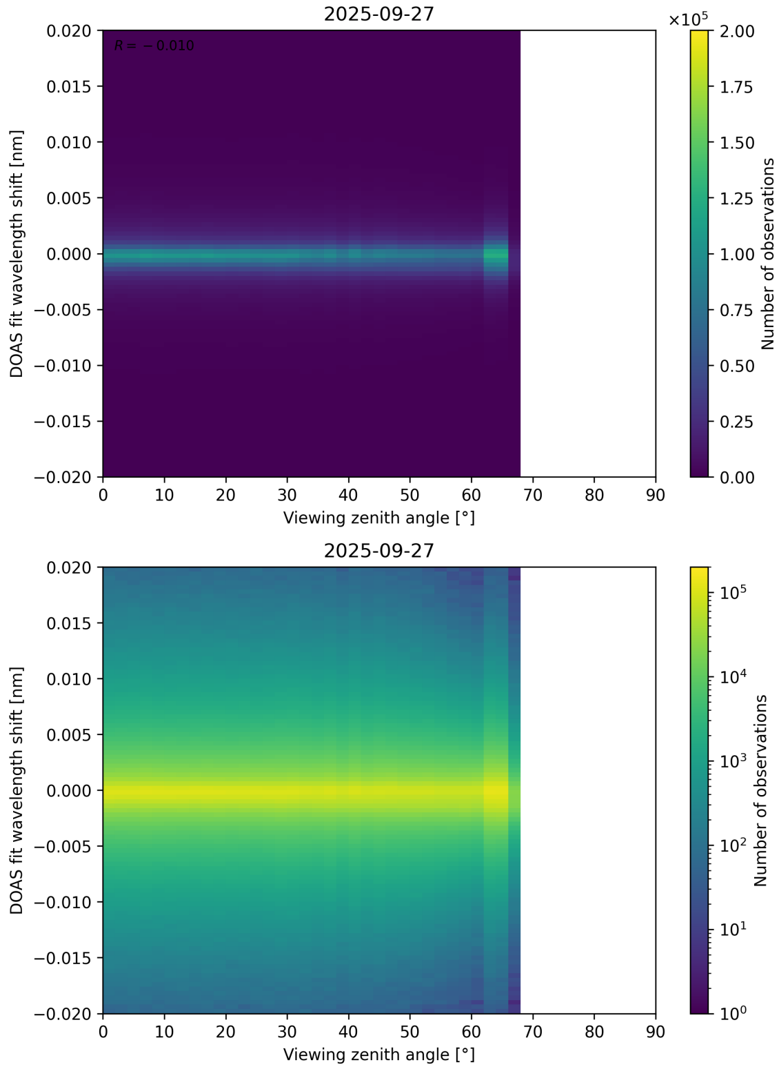
Figure 183: Scatter density plot of “Viewing zenith angle” against “DOAS fit wavelength shift” for 2025-09-26 to 2025-09-28.
