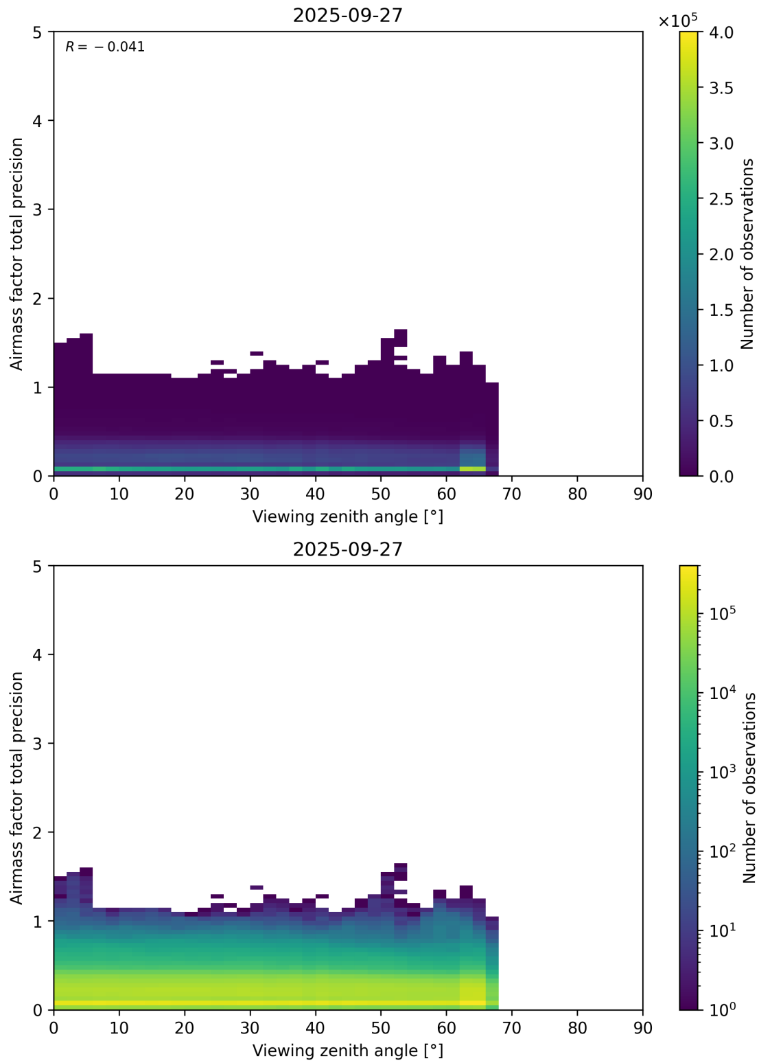
Figure 191: Scatter density plot of “Viewing zenith angle” against “Airmass factor total precision” for 2025-09-26 to 2025-09-28.
