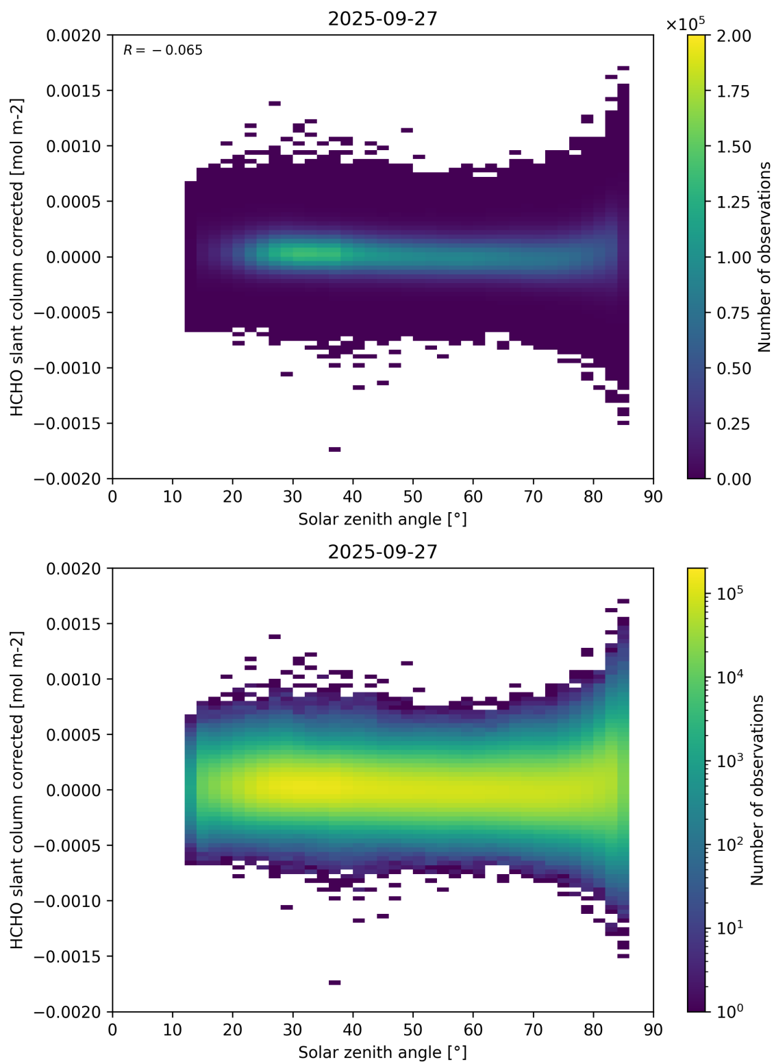
Figure 171: Scatter density plot of “Solar zenith angle” against “HCHO slant column corrected” for 2025-09-26 to 2025-09-28.
