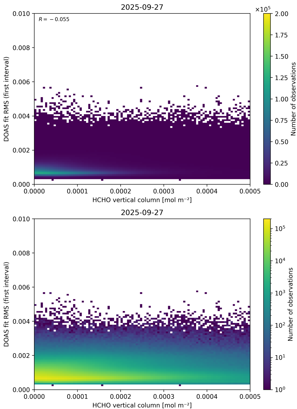
Figure 123: Scatter density plot of “HCHO vertical column” against “DOAS fit RMS (first interval)” for 2025-09-26 to 2025-09-28.
