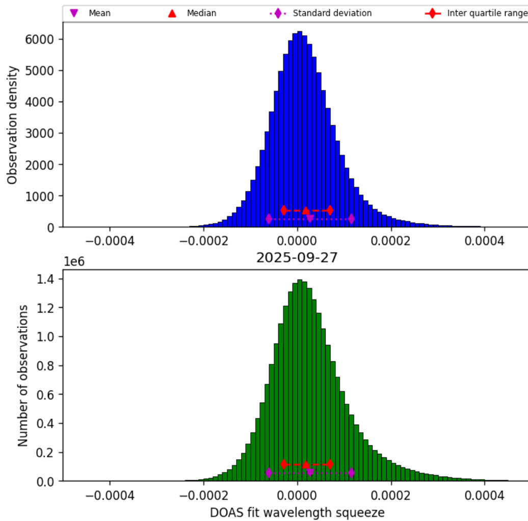
Figure 45: Histogram of “DOAS fit wavelength squeeze” for 2025-09-26 to 2025-09-28
