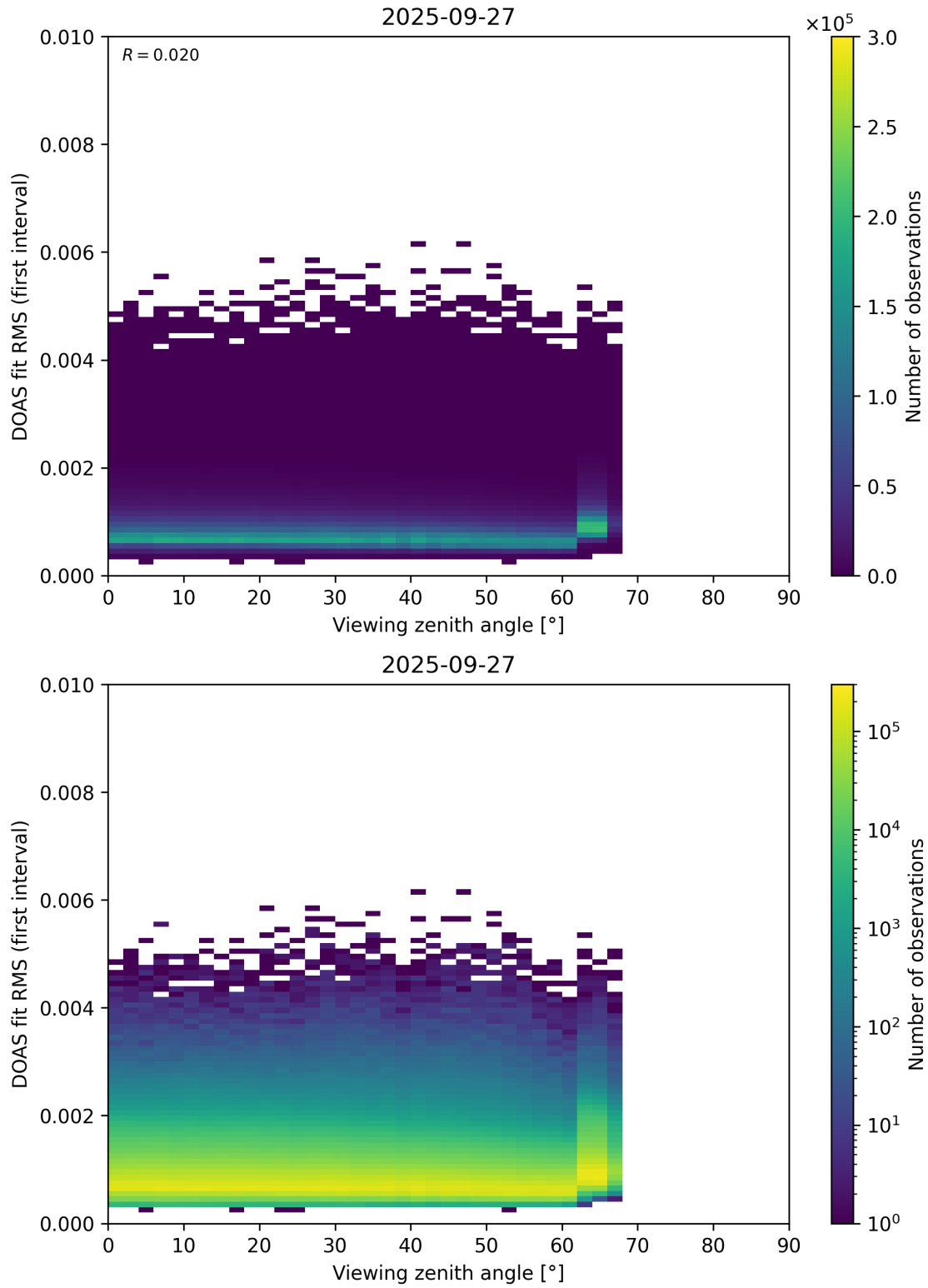
Figure 182: Scatter density plot of “Viewing zenith angle” against “DOAS fit RMS (first interval)” for 2025-09-26 to 2025-09-28.
