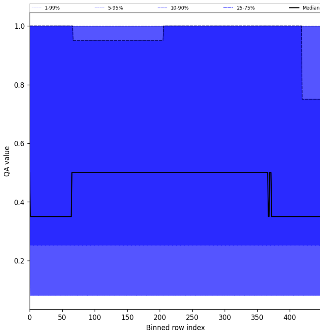
Figure 48: Along track statistics of “QA value” for 2025-09-26 to 2025-09-28
