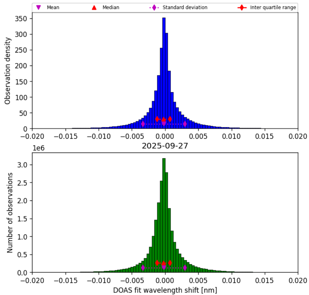
Figure 44: Histogram of “DOAS fit wavelength shift” for 2025-09-26 to 2025-09-28
