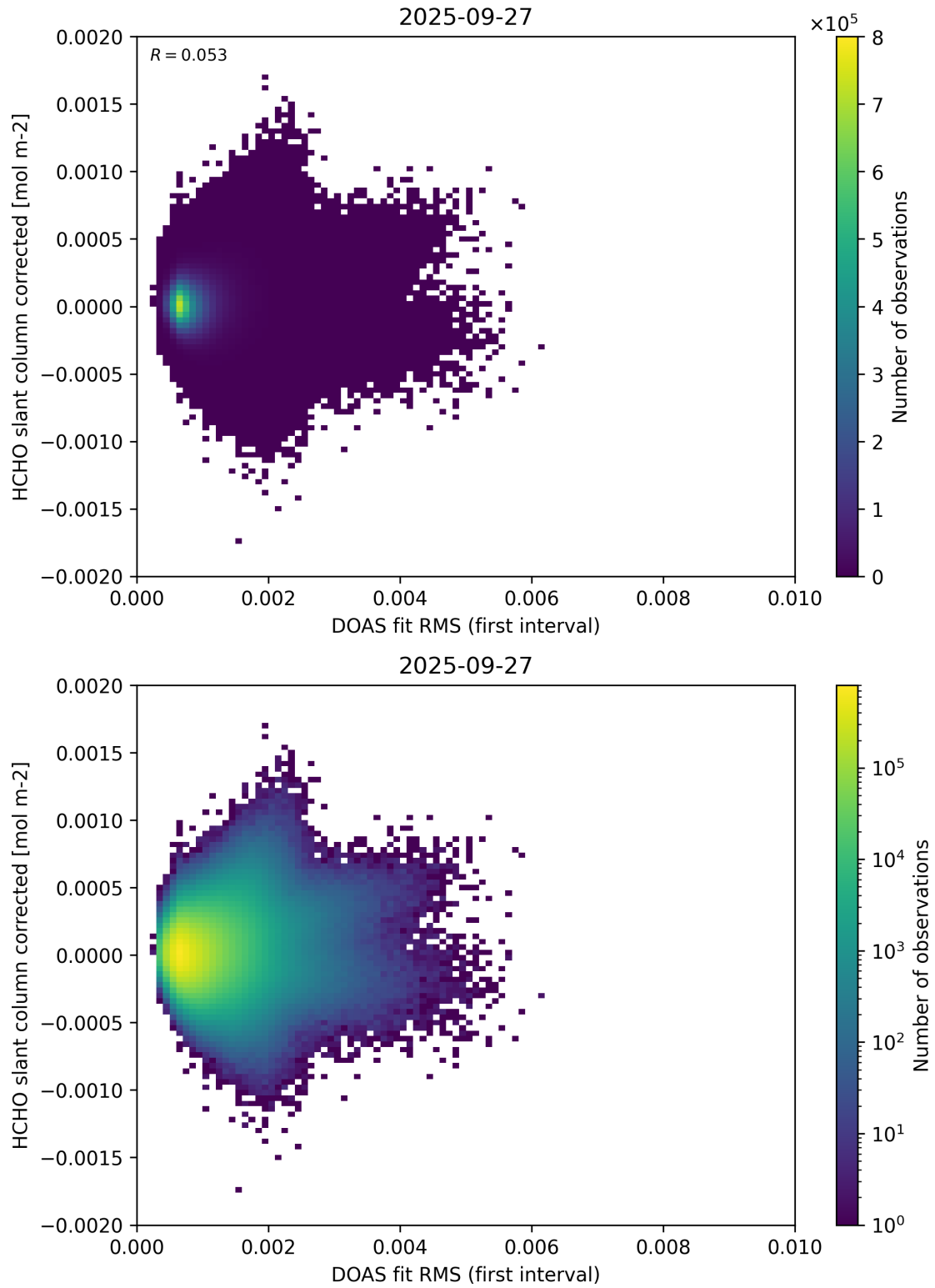
Figure 62: Scatter density plot of “DOAS fit RMS (first interval)” against “HCHO slant column corrected” for 2025-09-26 to 2025-09-28.
