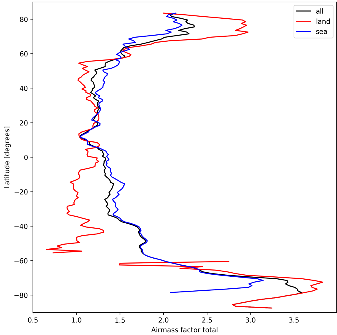
Figure 26: Zonal average of “Airmass factor total” for 2025-09-26 to 2025-09-28.
