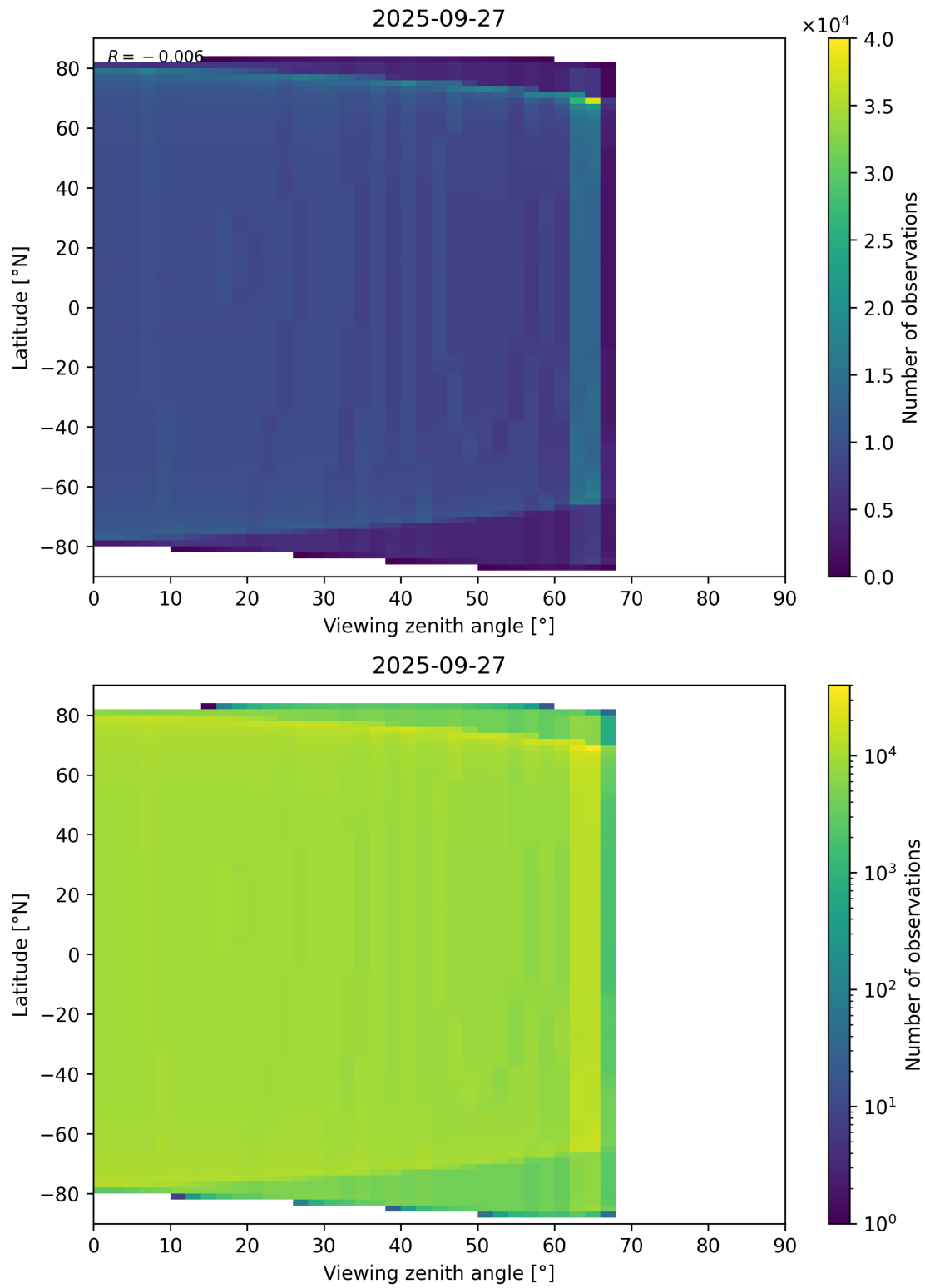
Figure 196: Scatter density plot of “Viewing zenith angle” against “Latitude” for 2025-09-26 to 2025-09-28.
