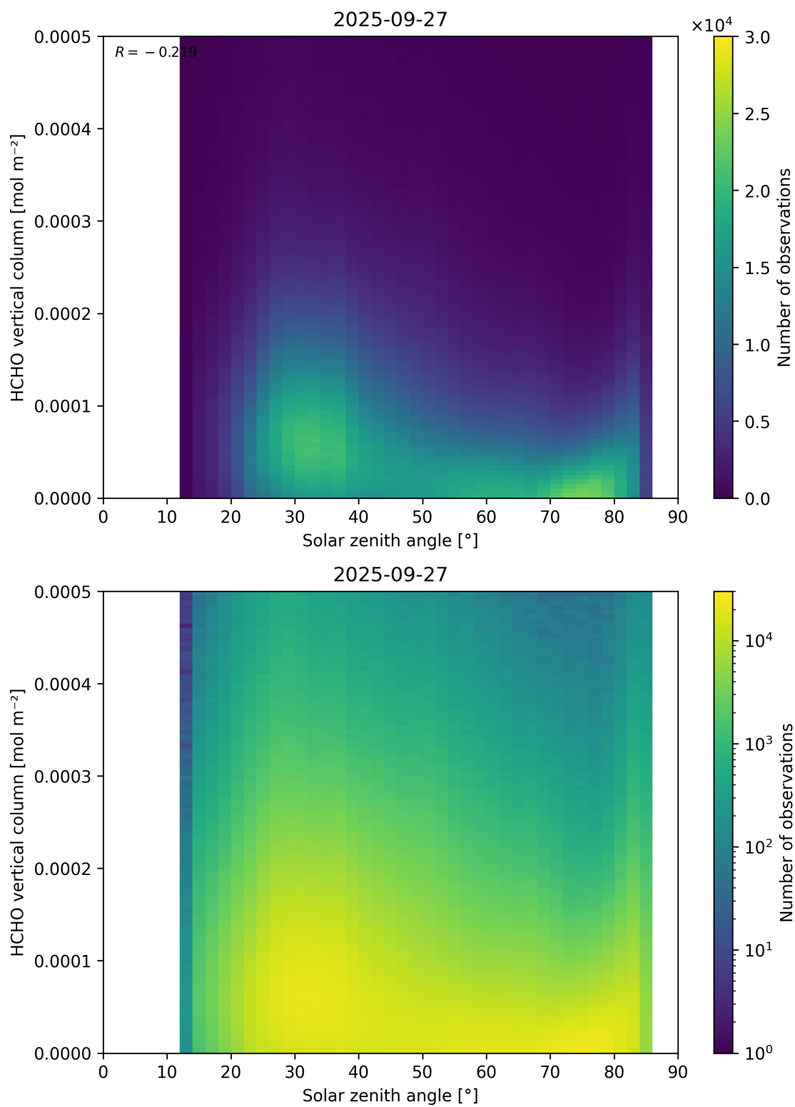
Figure 177: Scatter density plot of “Solar zenith angle” against “HCHO vertical column” for 2025-09-26 to 2025-09-28.
