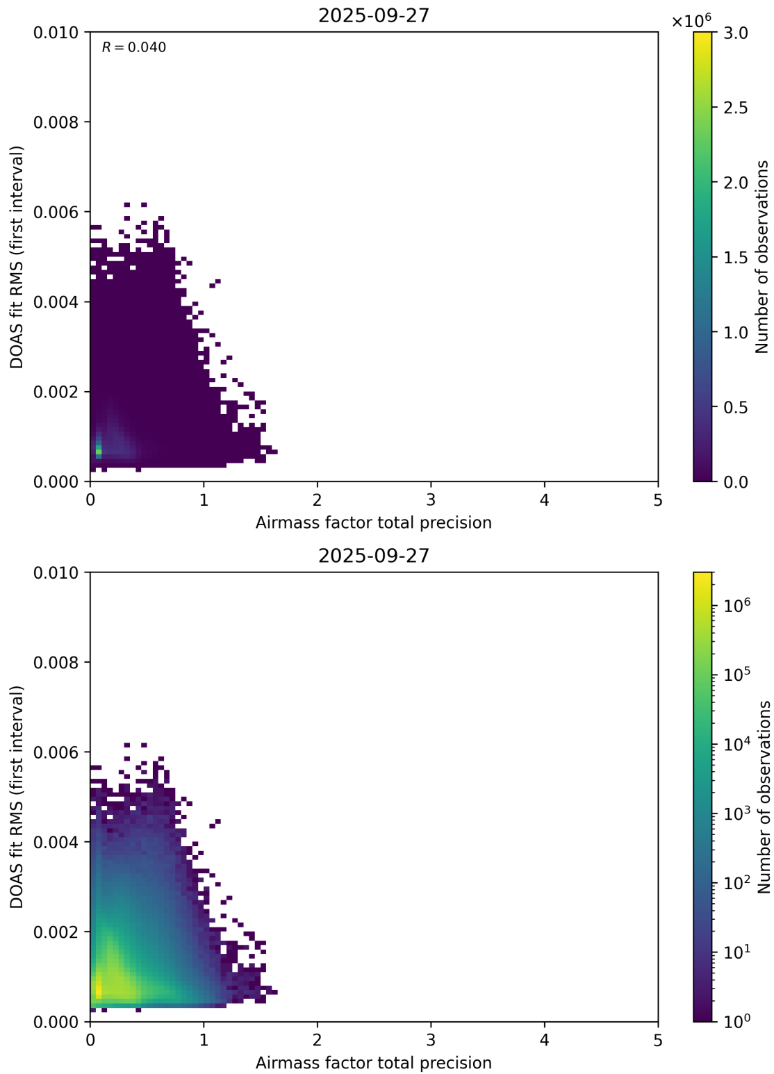
Figure 105: Scatter density plot of “Airmass factor total precision” against “DOAS fit RMS (first interval)” for 2025-09-26 to 2025-09-28.
