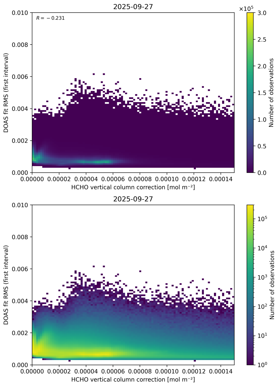
Figure 112: Scatter density plot of “HCHO vertical column correction” against “DOAS fit RMS (first interval)” for 2025-09-26 to 2025-09-28.
