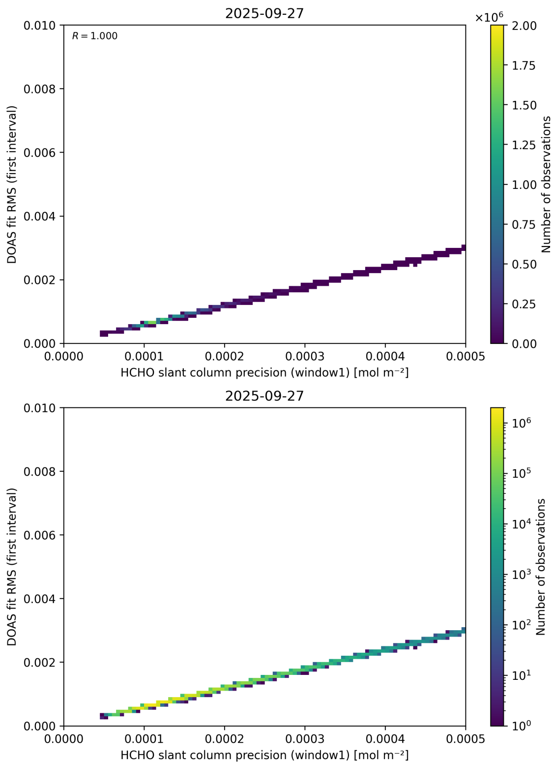
Figure 88: Scatter density plot of “HCHO slant column precision (window1)” against “DOAS fit RMS (first interval)” for 2025-09-26 to 2025-09-28.
