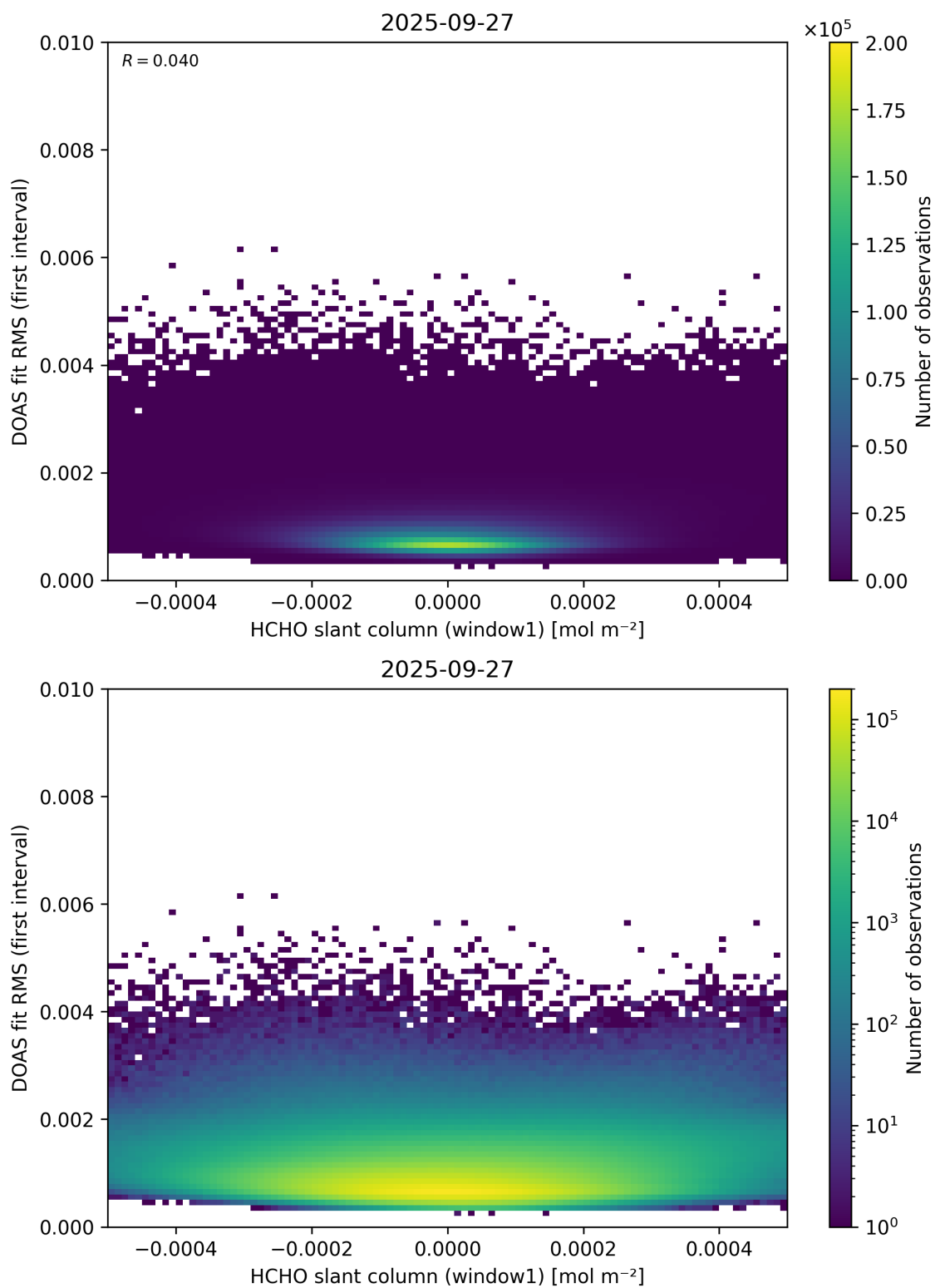
Figure 78: Scatter density plot of “HCHO slant column (window1)” against “DOAS fit RMS (first interval)” for 2025-09-26 to 2025-09-28.
