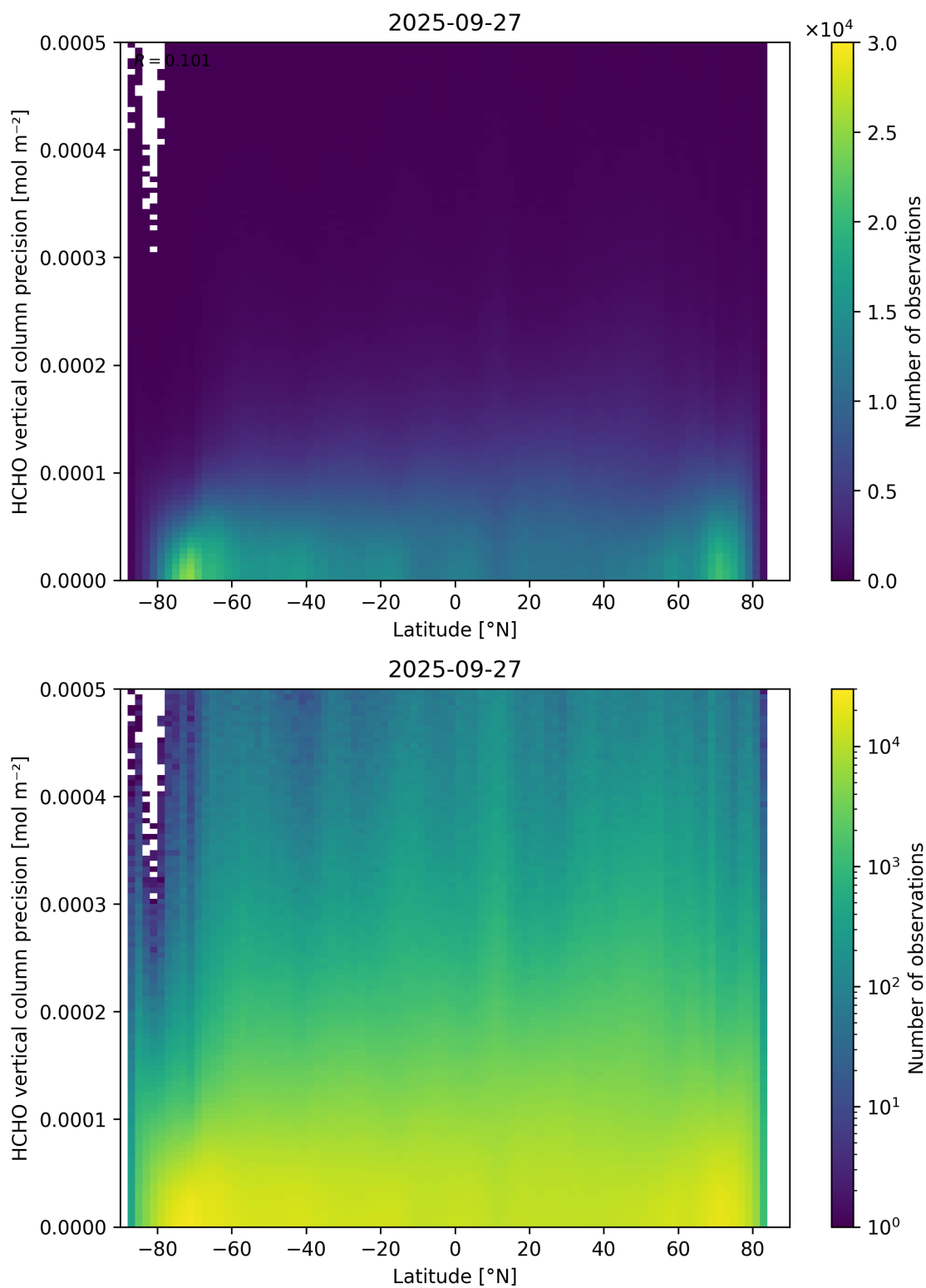
Figure 165: Scatter density plot of “Latitude” against “HCHO vertical column precision” for 2025-09-26 to 2025-09-28.
