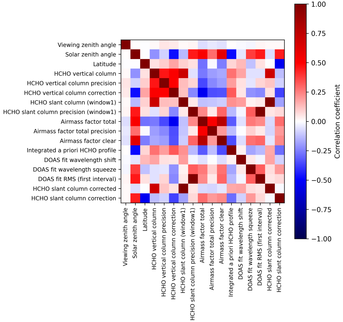
Figure 2: Map of correlation matrix for 2025-09-26 to 2025-09-28.
