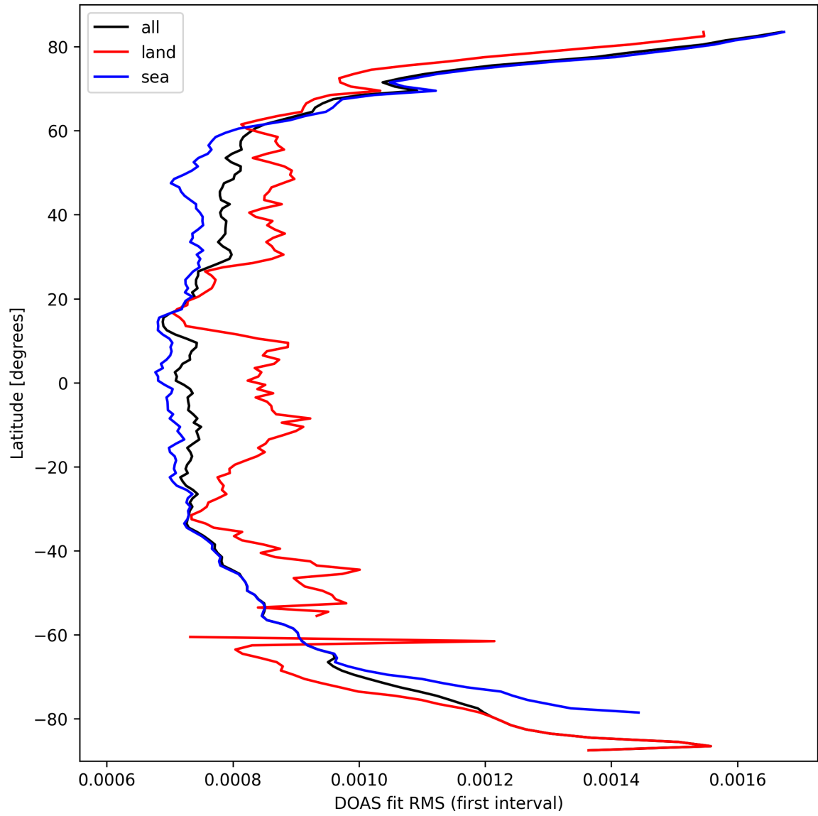
Figure 32: Zonal average of “DOAS fit RMS (first interval)” for 2025-09-26 to 2025-09-28.
