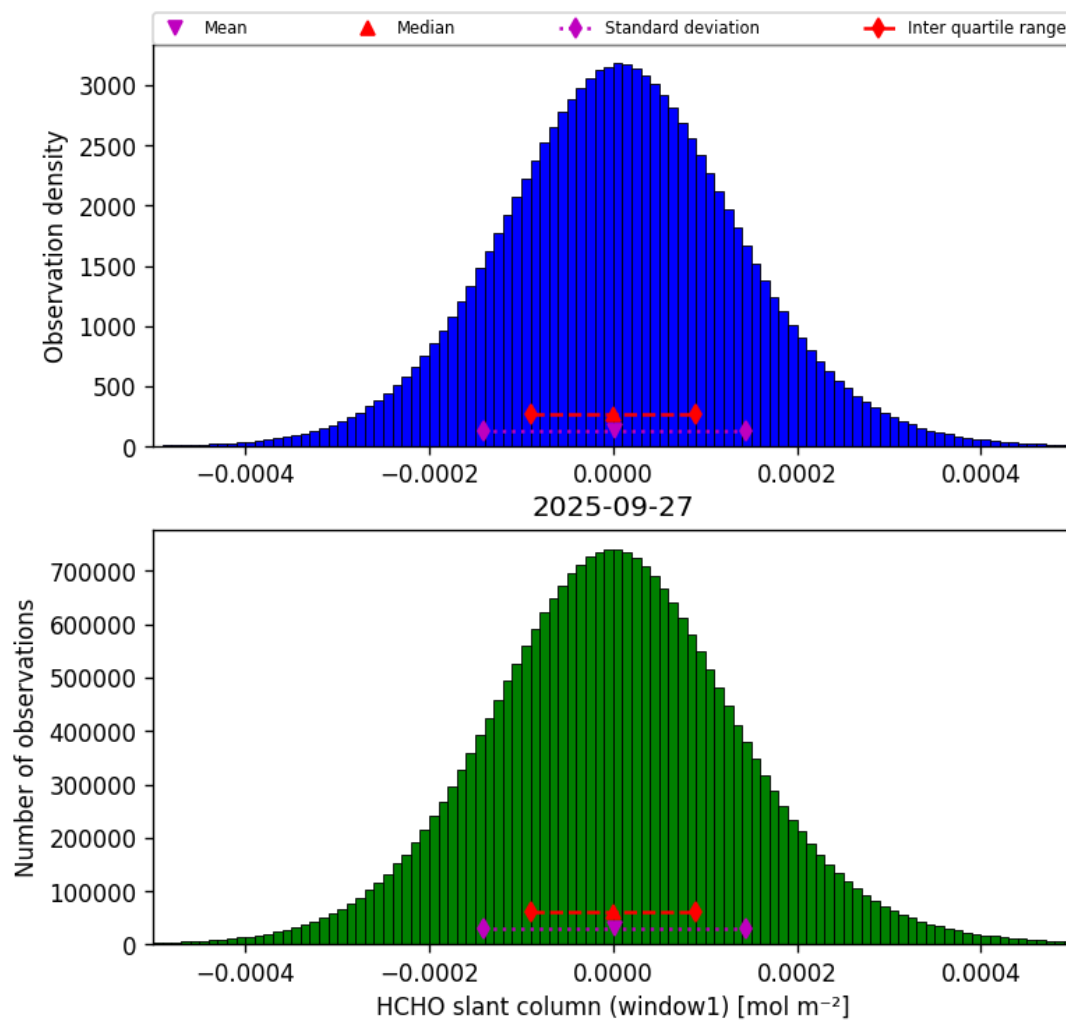
Figure 38: Histogram of “HCHO slant column (window1)” for 2025-09-26 to 2025-09-28
