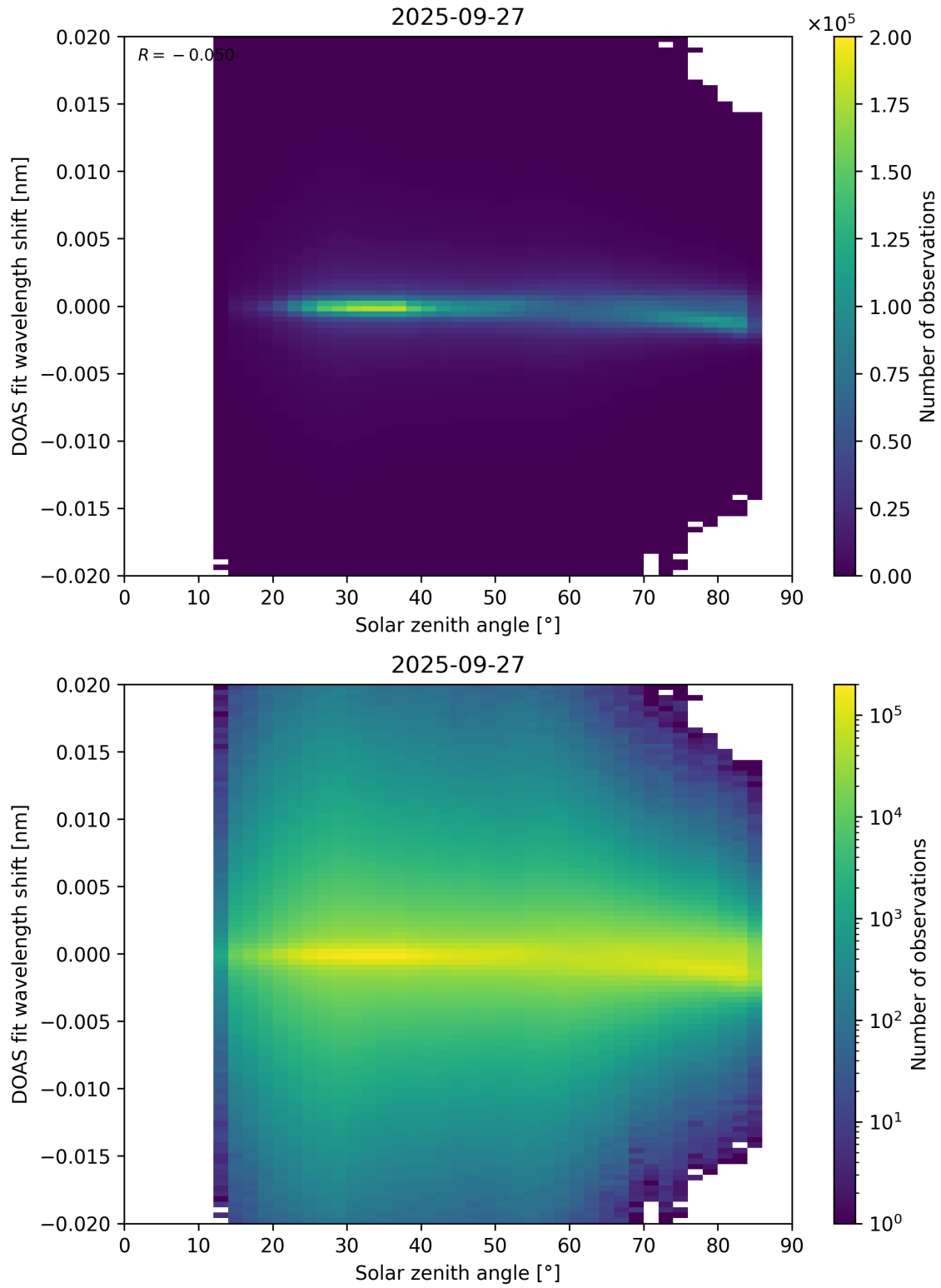
Figure 168: Scatter density plot of “Solar zenith angle” against “DOAS fit wavelength shift” for 2025-09-26 to 2025-09-28.
