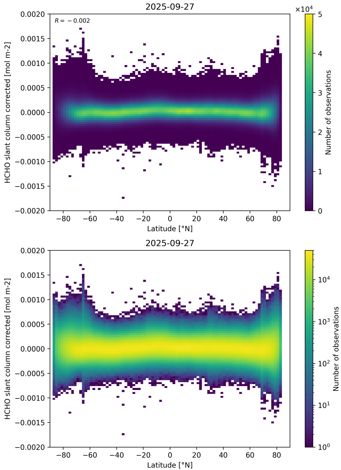
Figure 157: Scatter density plot of “Latitude” against “HCHO slant column corrected” for 2025-09-26 to 2025-09-28.
