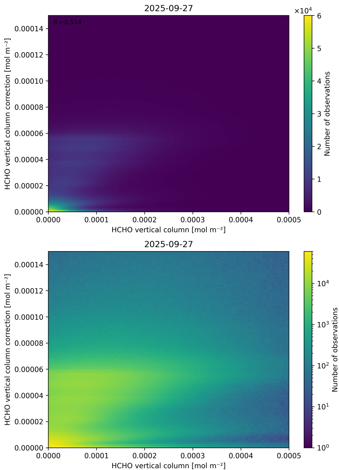
Figure 133: Scatter density plot of “HCHO vertical column” against “HCHO vertical column correction” for 2025-09-26 to 2025-09-28.
