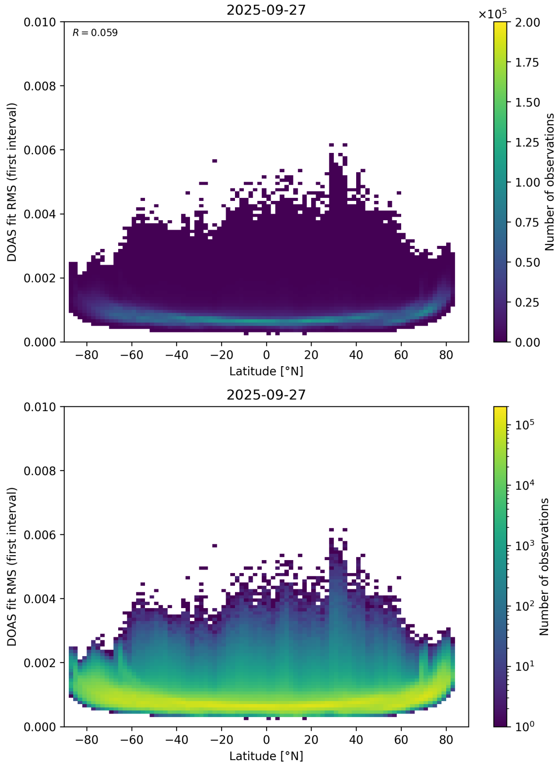
Figure 153: Scatter density plot of “Latitude” against “DOAS fit RMS (first interval)” for 2025-09-26 to 2025-09-28.
