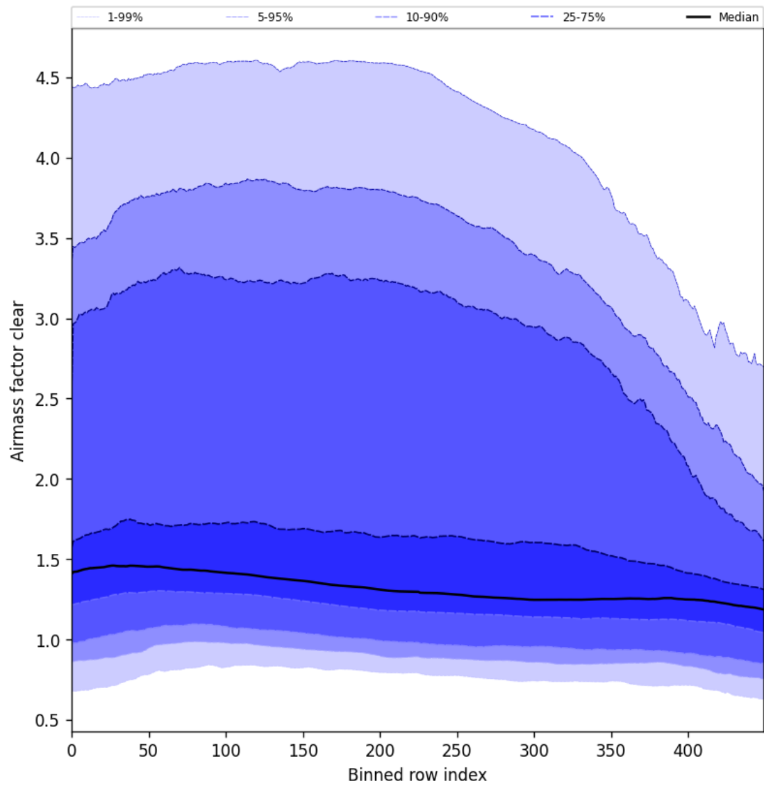
Figure 56: Along track statistics of “Air mass factor clear” for 2025-09-27 to 2025-09-29
