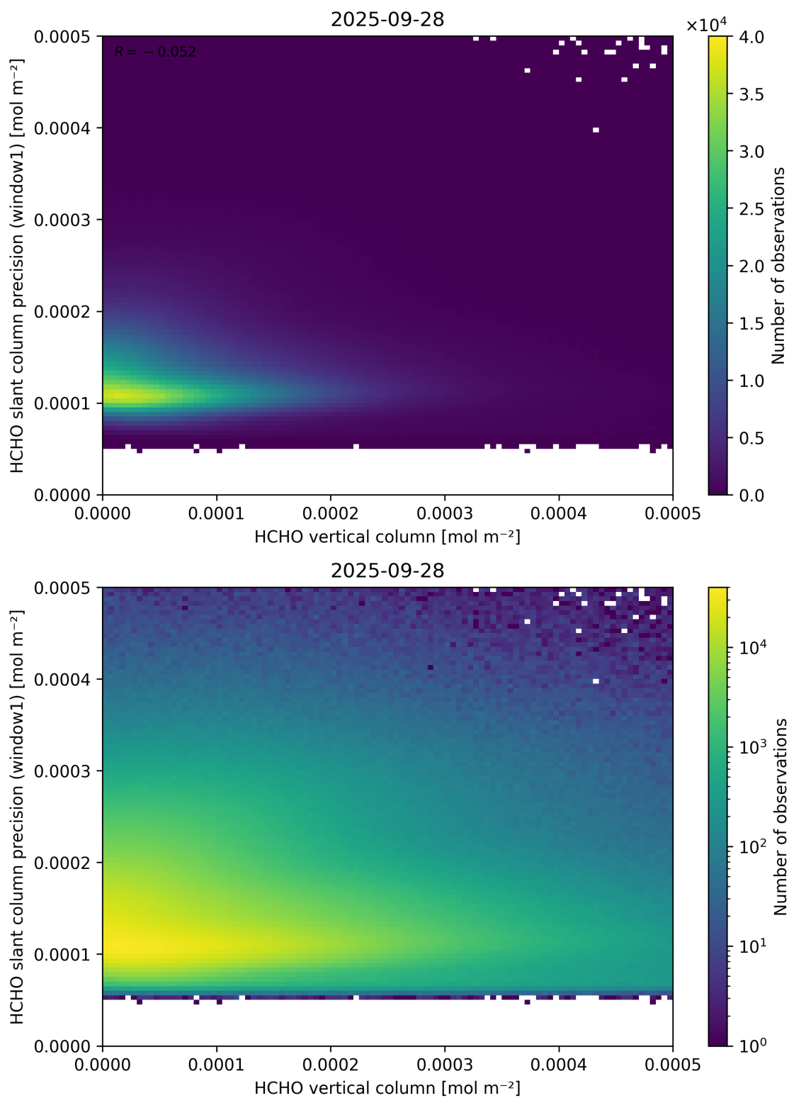
Figure 130: Scatter density plot of “HCHO vertical column” against “HCHO slant column precision (window1)” for 2025-09-27 to 2025-09-29.
