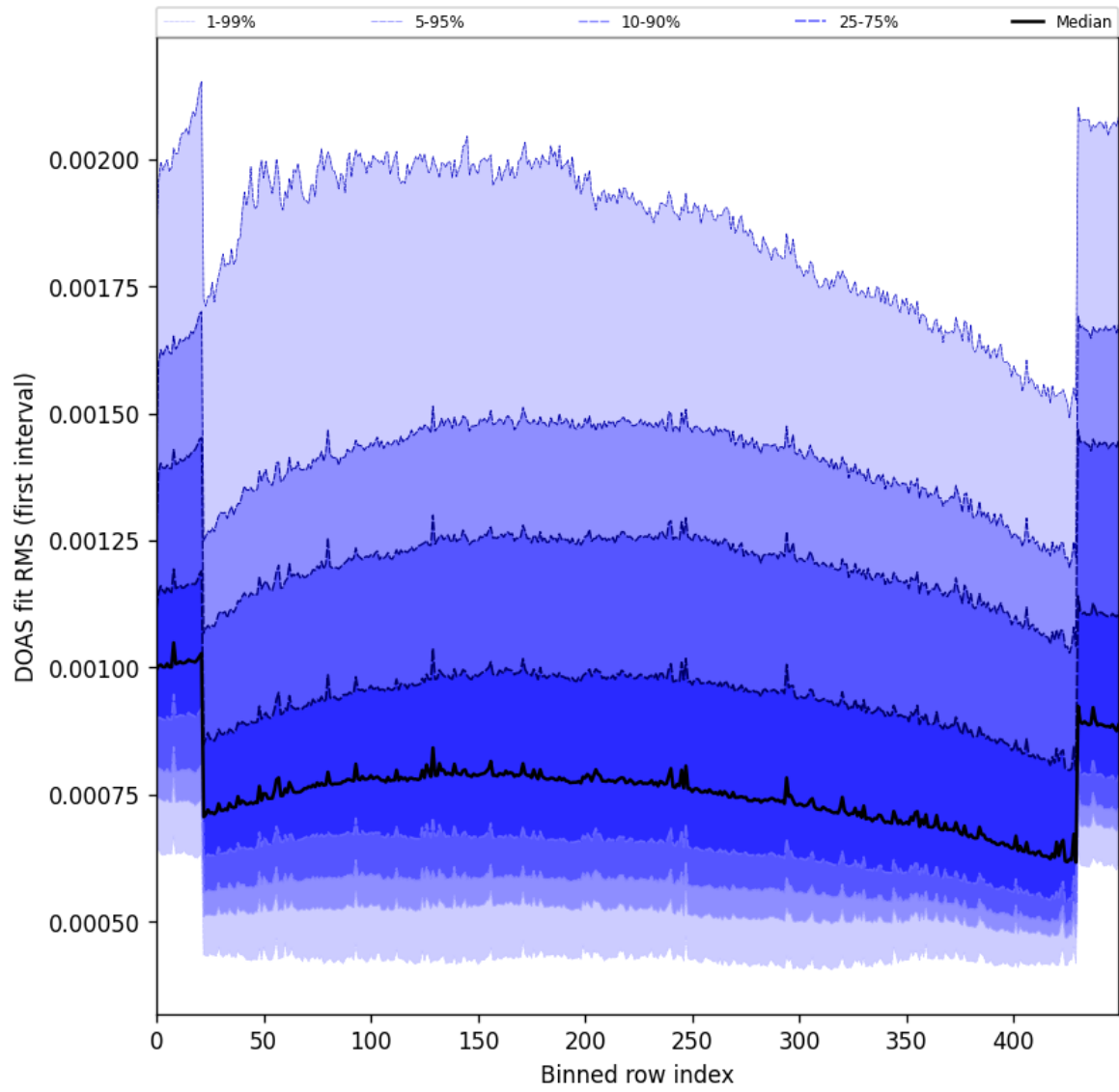
Figure 60: Along track statistics of “DOAS fit RMS (first interval)” for 2025-09-27 to 2025-09-29
