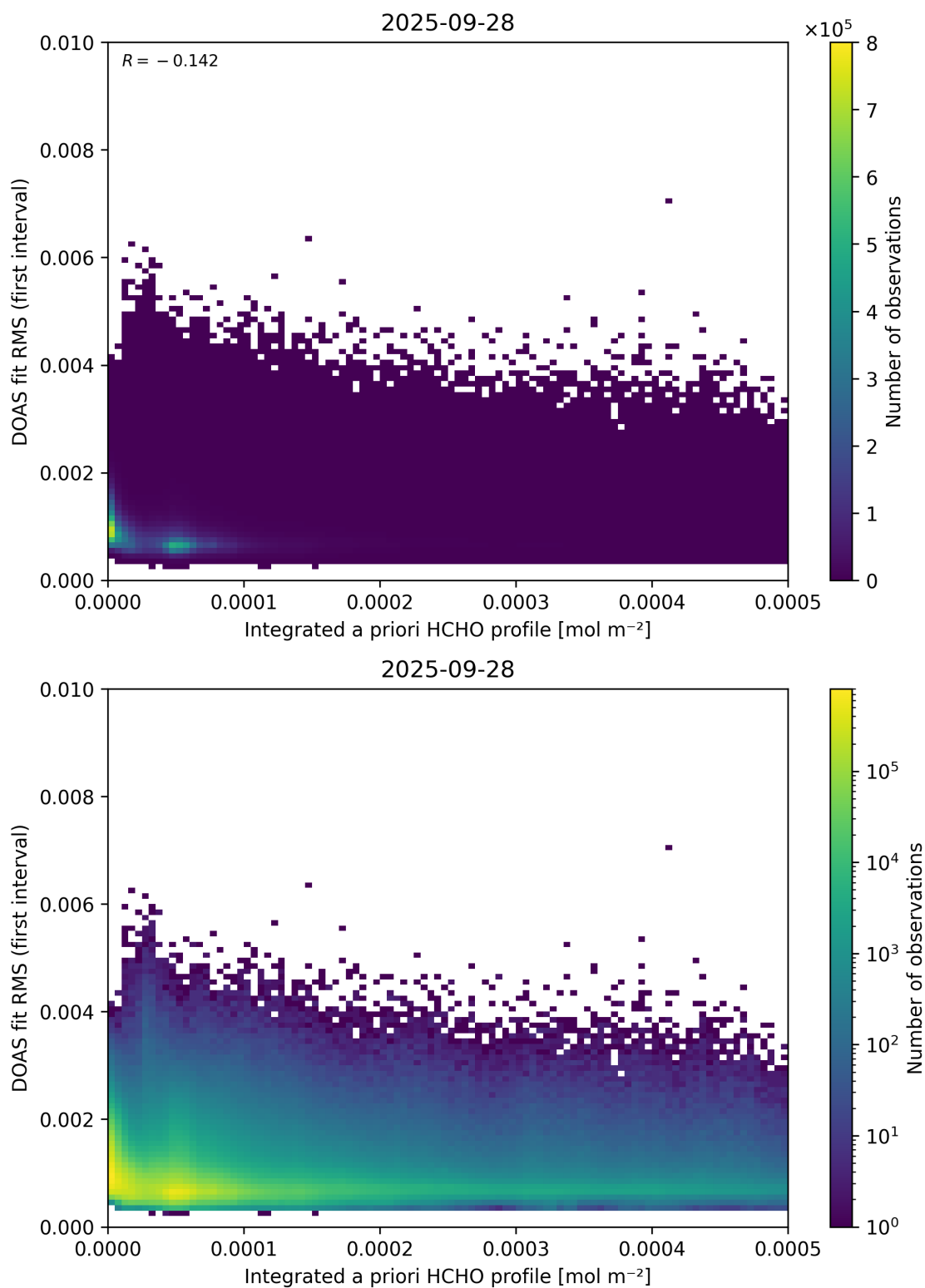
Figure 148: Scatter density plot of “Integrated a priori HCHO profile” against “DOAS fit RMS (first interval)” for 2025-09-27 to 2025-09-29.
