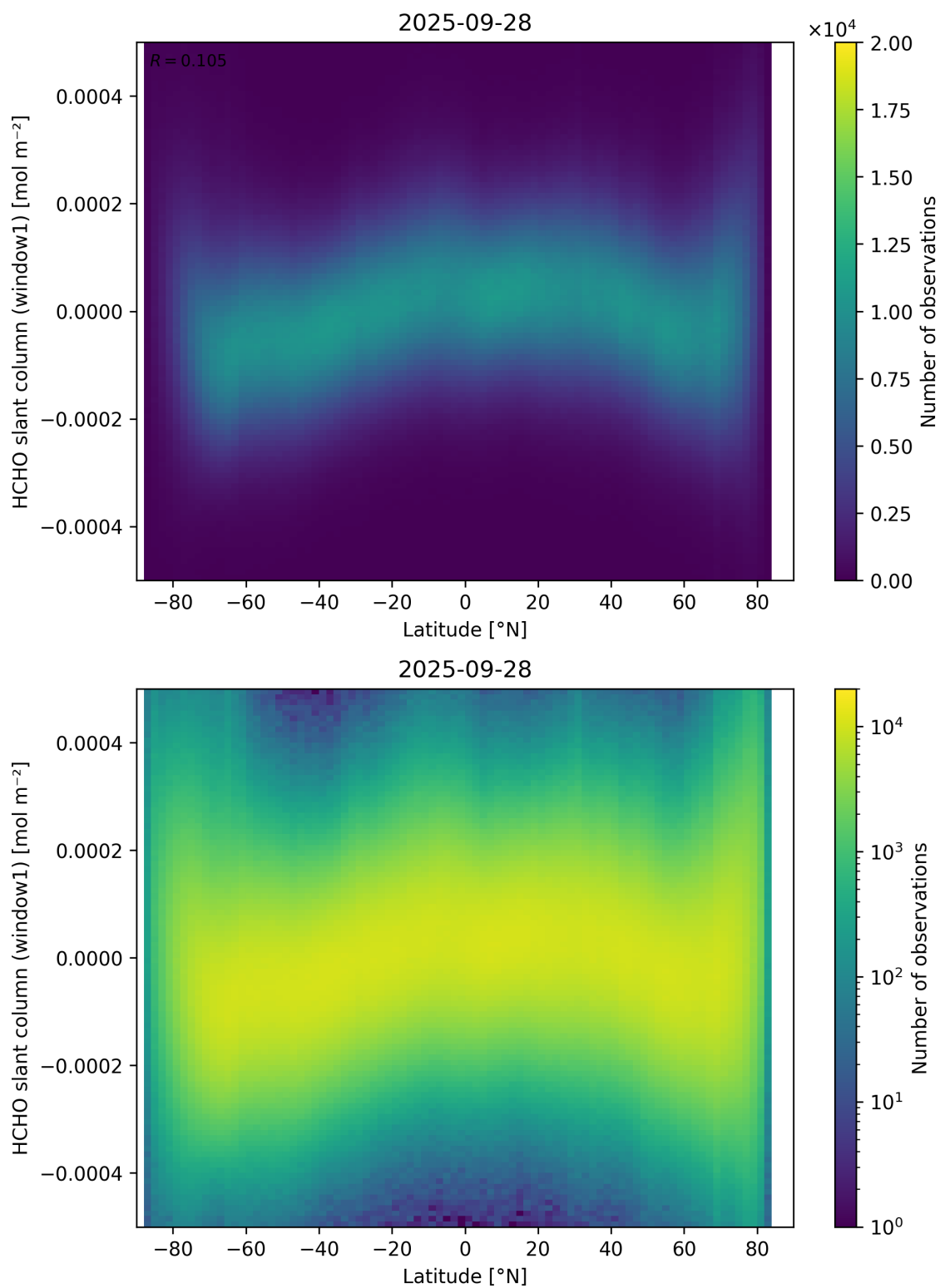
Figure 159: Scatter density plot of “Latitude” against “HCHO slant column (window1)” for 2025-09-27 to 2025-09-29.
