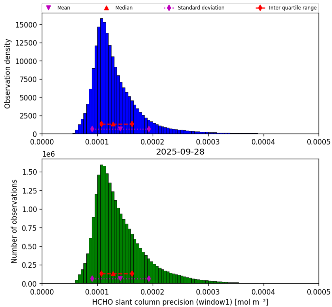
Figure 39: Histogram of “HCHO slant column precision (window1)” for 2025-09-27 to 2025-09-29
