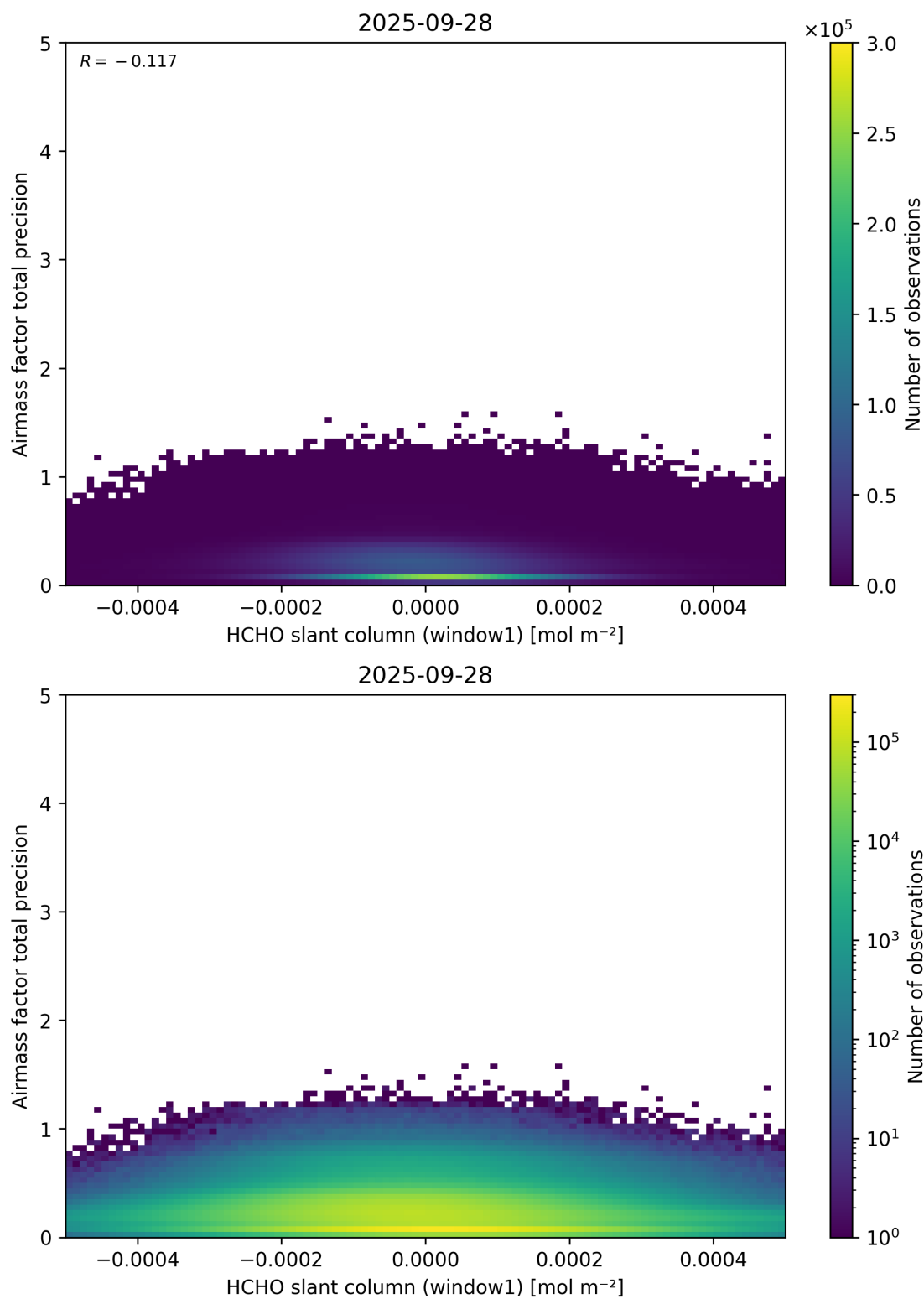
Figure 86: Scatter density plot of “HCHO slant column (window1)” against “Airmass factor total precision” for 2025-09-27 to 2025-09-29.
