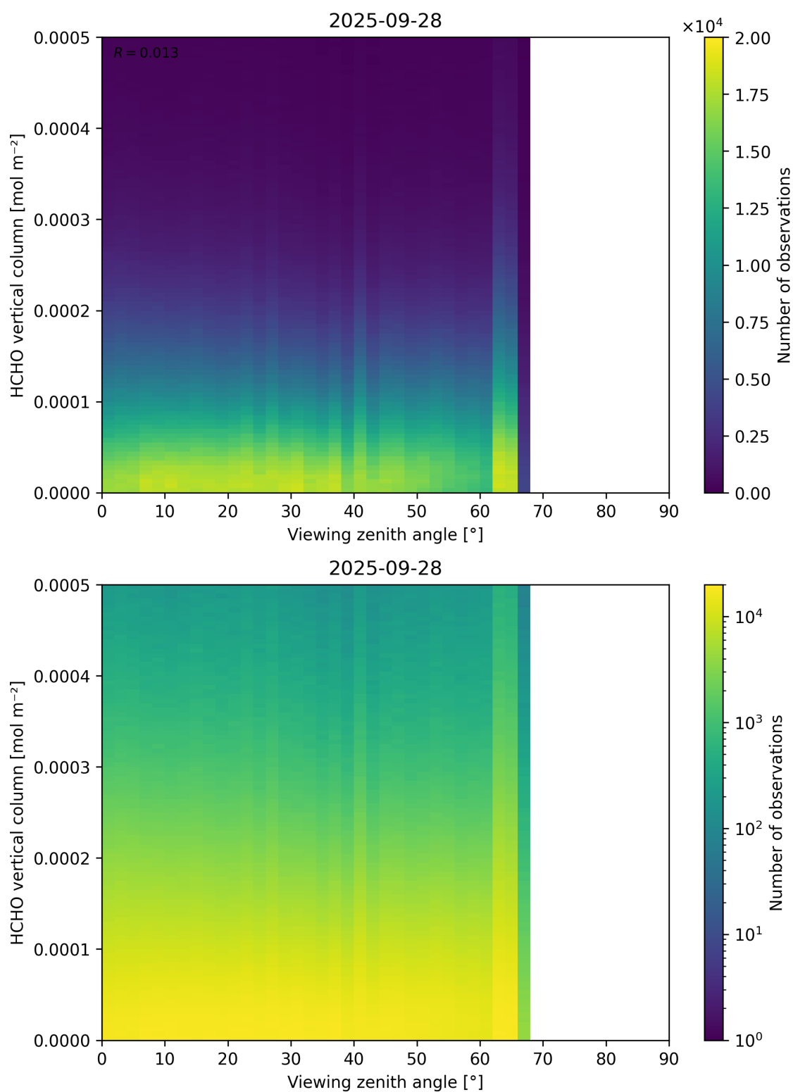
Figure 192: Scatter density plot of “Viewing zenith angle” against “HCHO vertical column” for 2025-09-27 to 2025-09-29.
