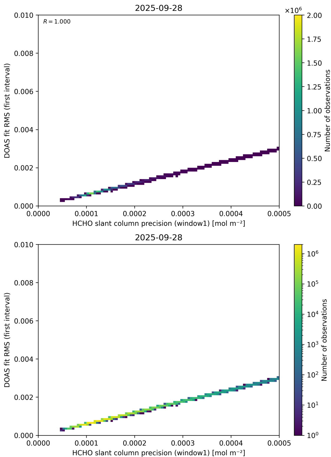
Figure 88: Scatter density plot of “HCHO slant column precision (window1)” against “DOAS fit RMS (first interval)” for 2025-09-27 to 2025-09-29.
