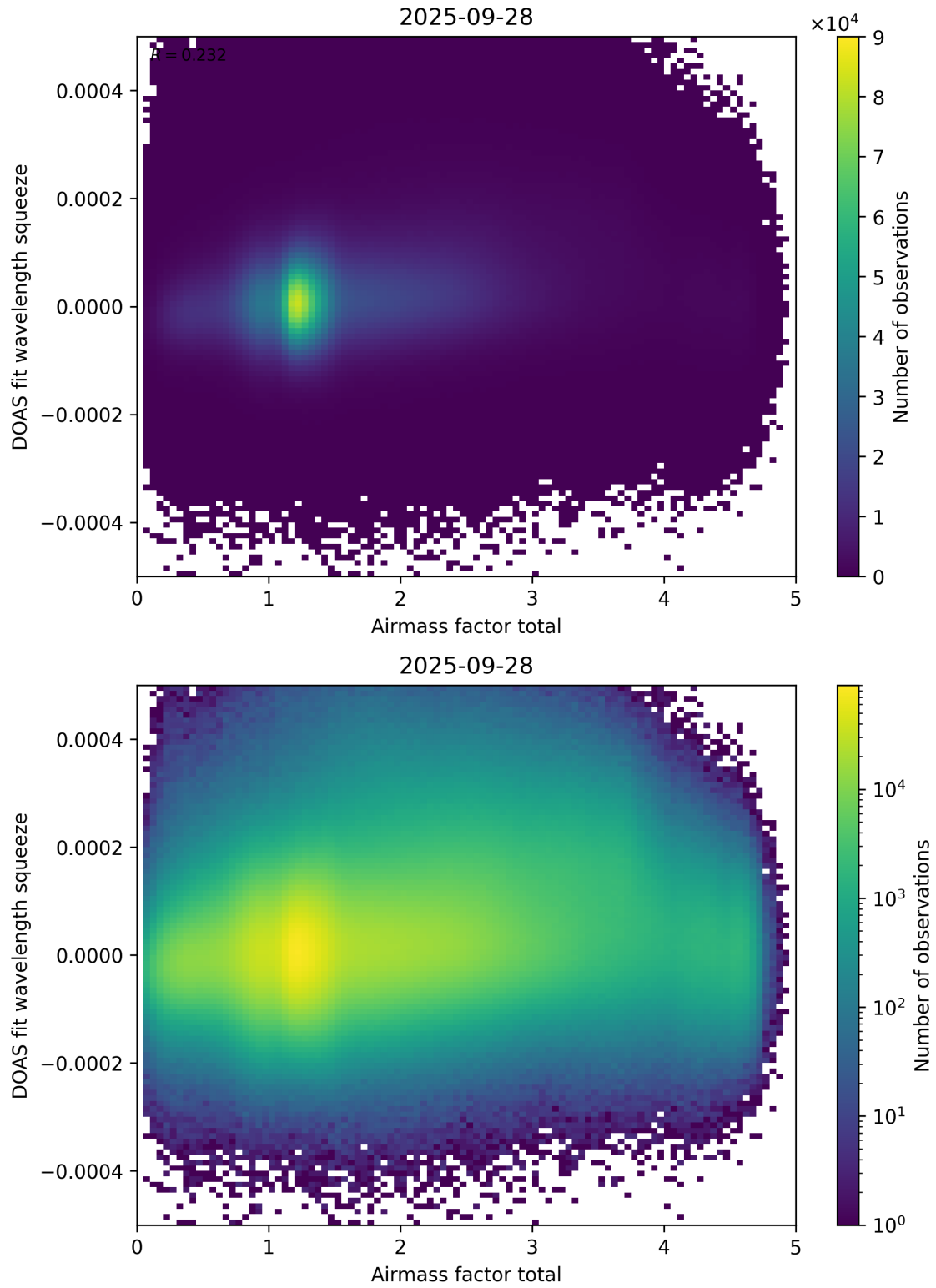
Figure 99: Scatter density plot of “Airmass factor total” against “DOAS fit wavelength squeeze” for 2025-09-27 to 2025-09-29.
