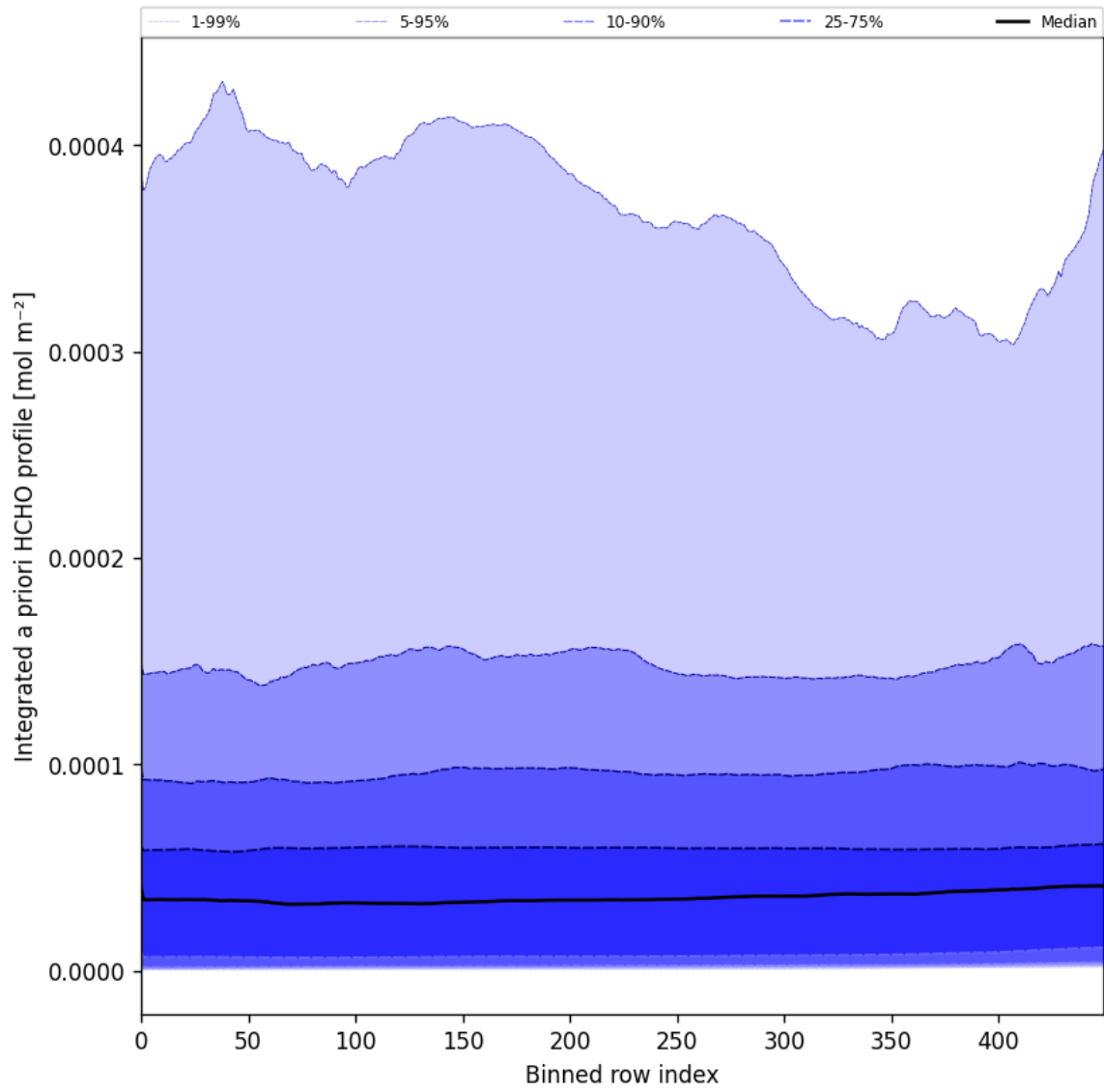
Figure 57: Along track statistics of "Integrated a priori HCHO profile" for 2025-09-27 to 2025-09-29
