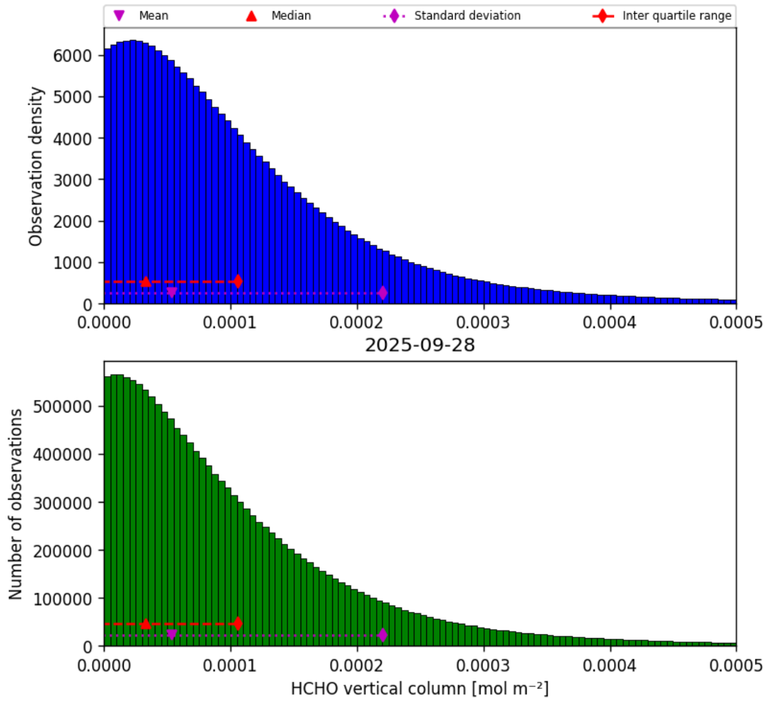
Figure 35: Histogram of “HCHO vertical column” for 2025-09-27 to 2025-09-29
