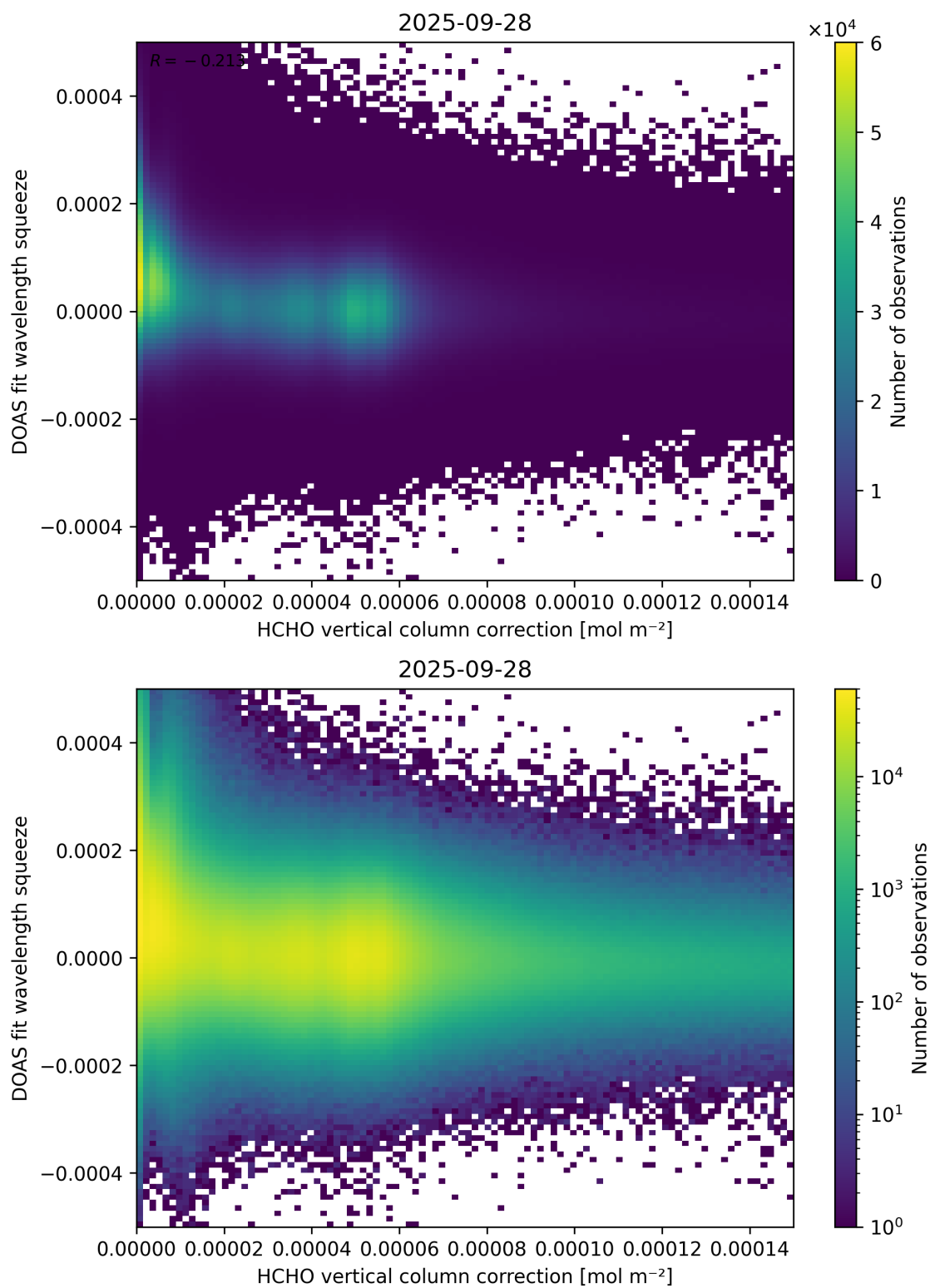
Figure 114: Scatter density plot of “HCHO vertical column correction” against “DOAS fit wavelength squeeze” for 2025-09-27 to 2025-09-29.
