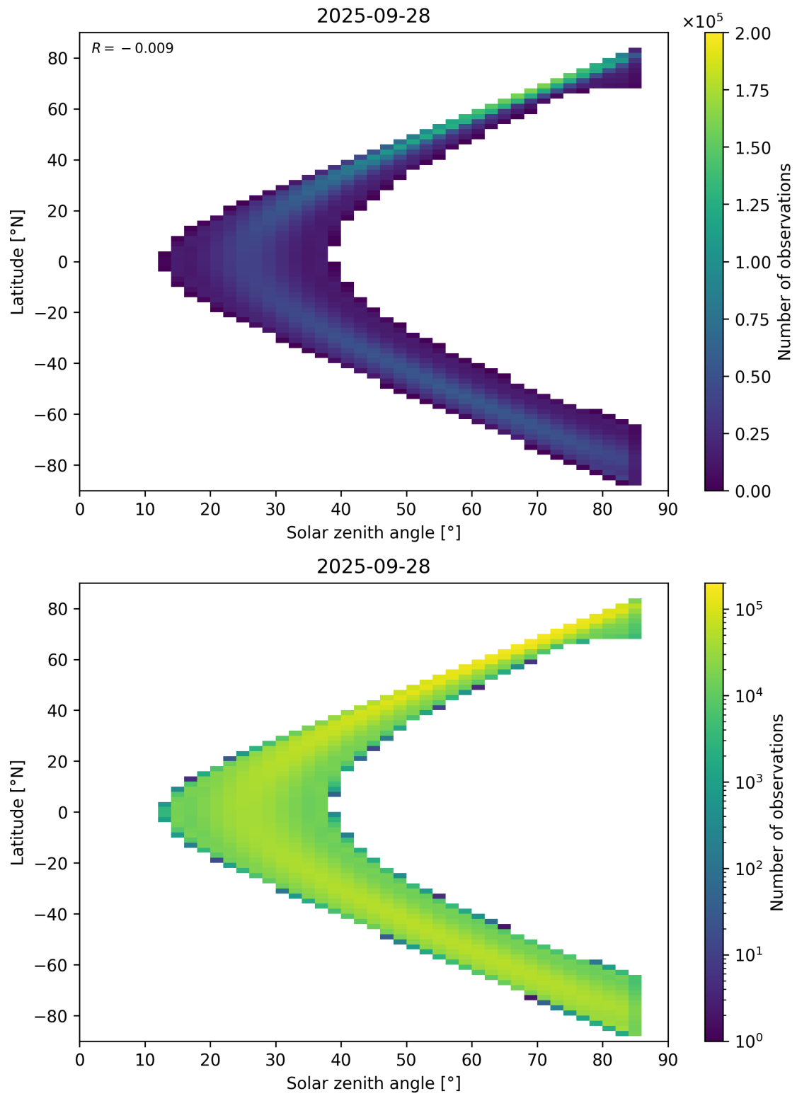
Figure 181: Scatter density plot of “Solar zenith angle” against “Latitude” for 2025-09-27 to 2025-09-29.
