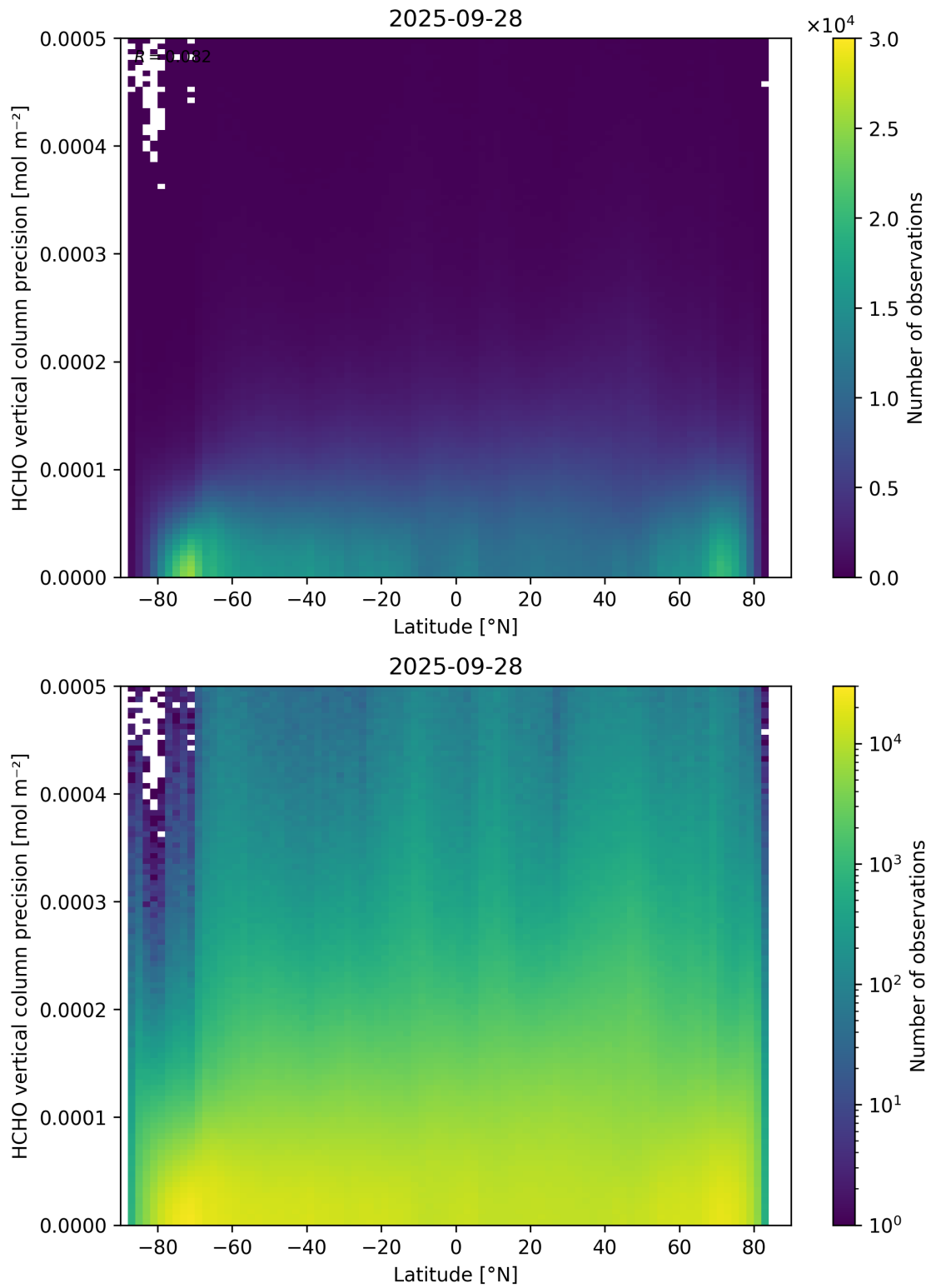
Figure 165: Scatter density plot of “Latitude” against “HCHO vertical column precision” for 2025-09-27 to 2025-09-29.
