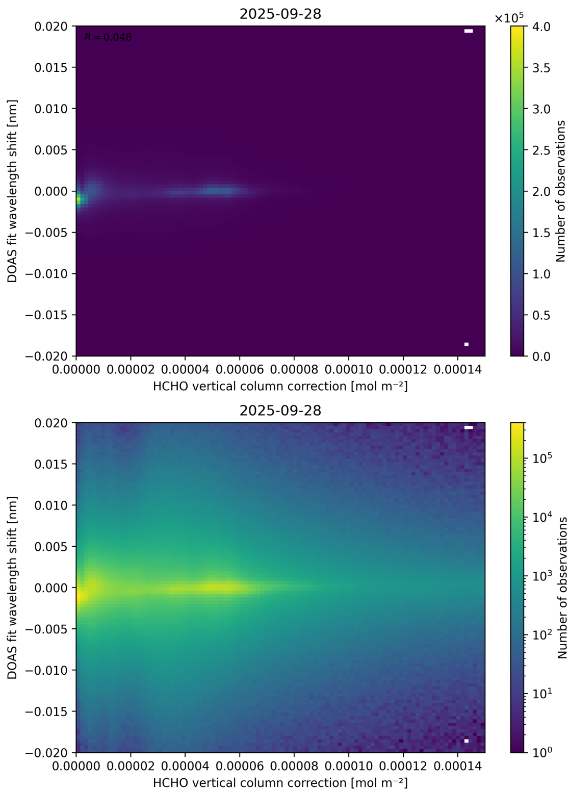
Figure 113: Scatter density plot of “HCHO vertical column correction” against “DOAS fit wavelength shift” for 2025-09-27 to 2025-09-29.
