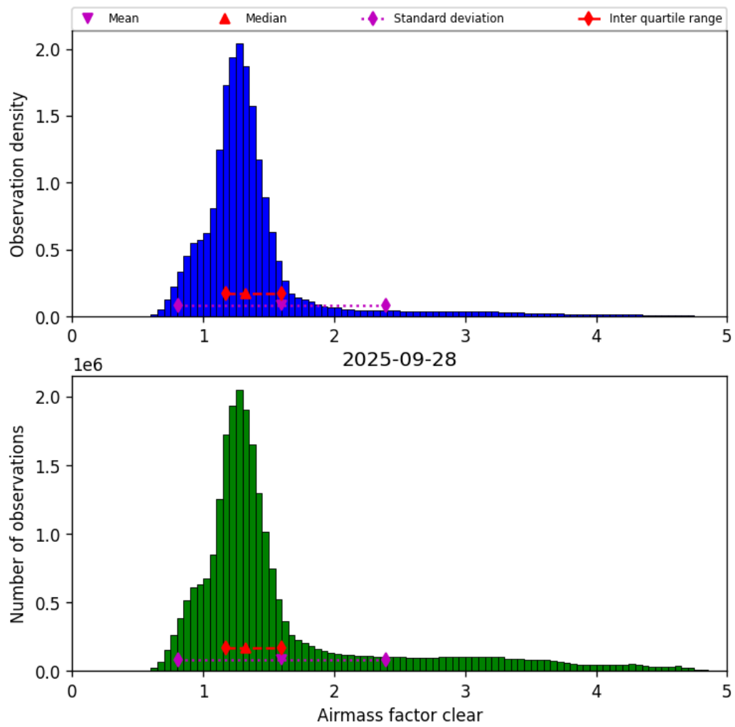
Figure 42: Histogram of “Airmass factor clear” for 2025-09-27 to 2025-09-29
