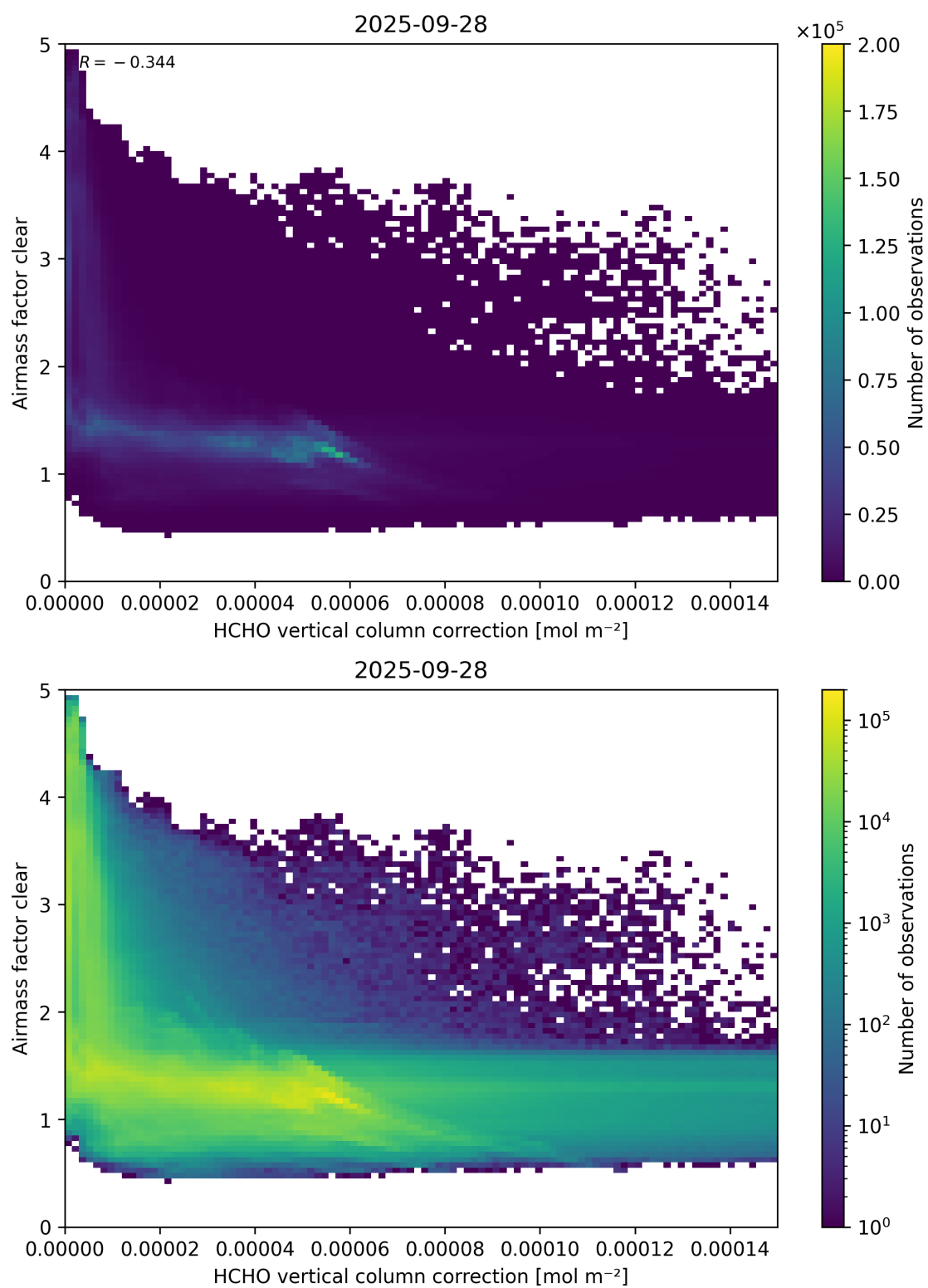
Figure 115: Scatter density plot of “HCHO vertical column correction” against “Airmass factor clear” for 2025-09-27 to 2025-09-29.
