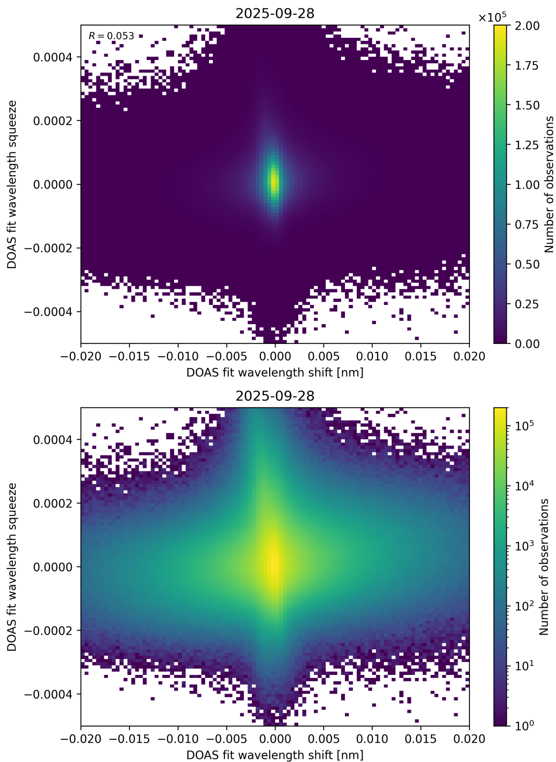
Figure 65: Scatter density plot of “DOAS fit wavelength shift” against “DOAS fit wavelength squeeze” for 2025-09-27 to 2025-09-29.
