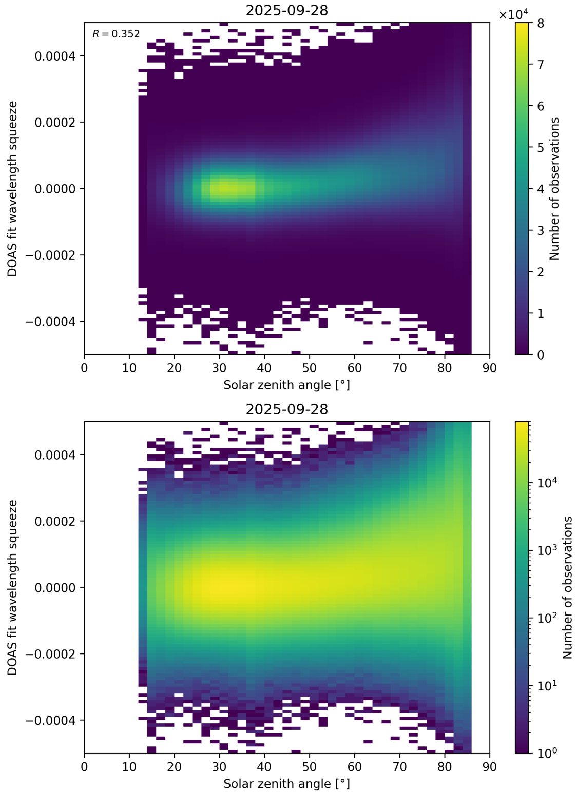
Figure 169: Scatter density plot of “Solar zenith angle” against “DOAS fit wavelength squeeze” for 2025-09-27 to 2025-09-29.
