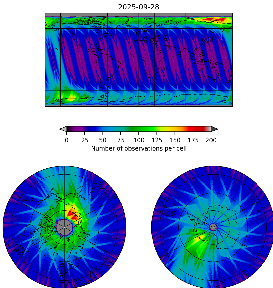
Figure 19: Map of the number of observations for 2025-09-27 to 2025-09-29
