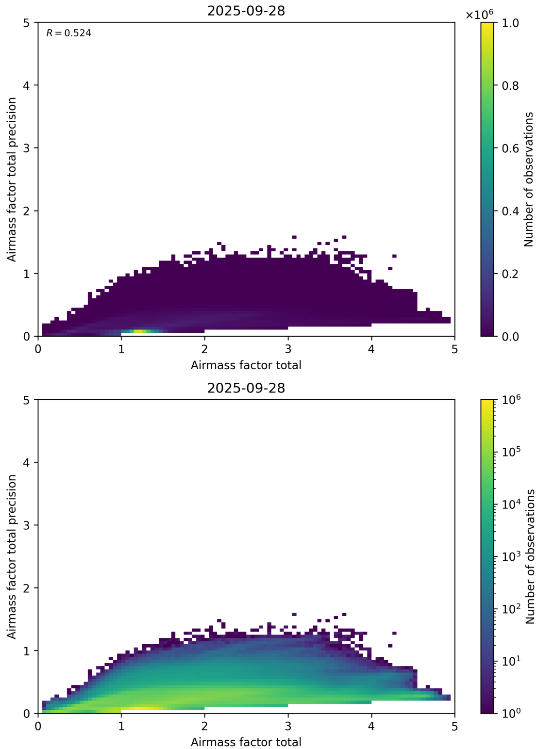
Figure 103: Scatter density plot of “Airmass factor total” against “Airmass factor total precision” for 2025-09-27 to 2025-09-29.
