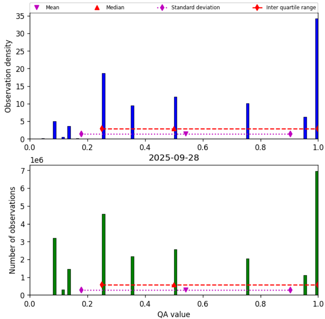
Figure 34: Histogram of “QA value” for 2025-09-27 to 2025-09-29
