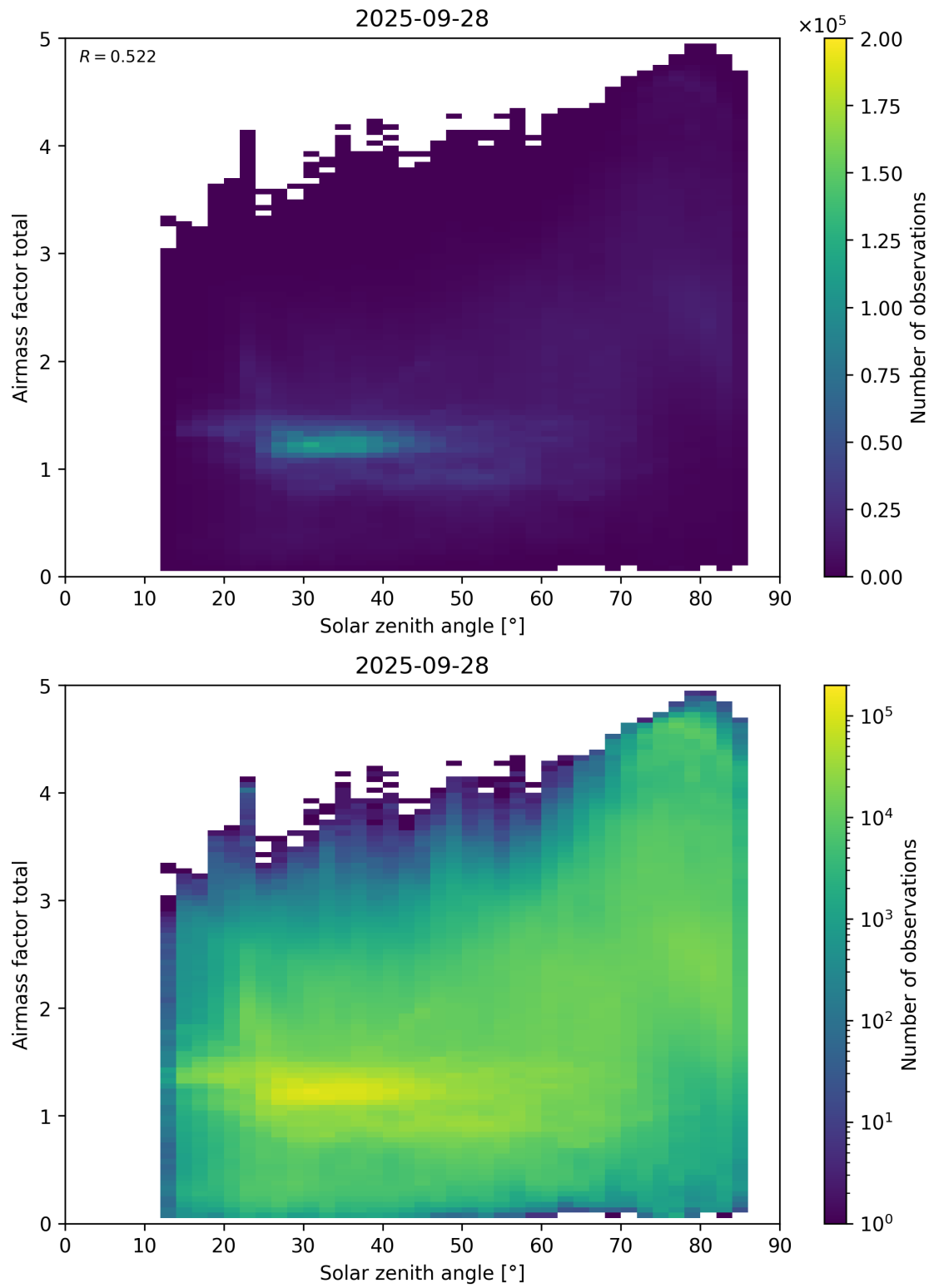
Figure 175: Scatter density plot of “Solar zenith angle” against “Airmass factor total” for 2025-09-27 to 2025-09-29.
