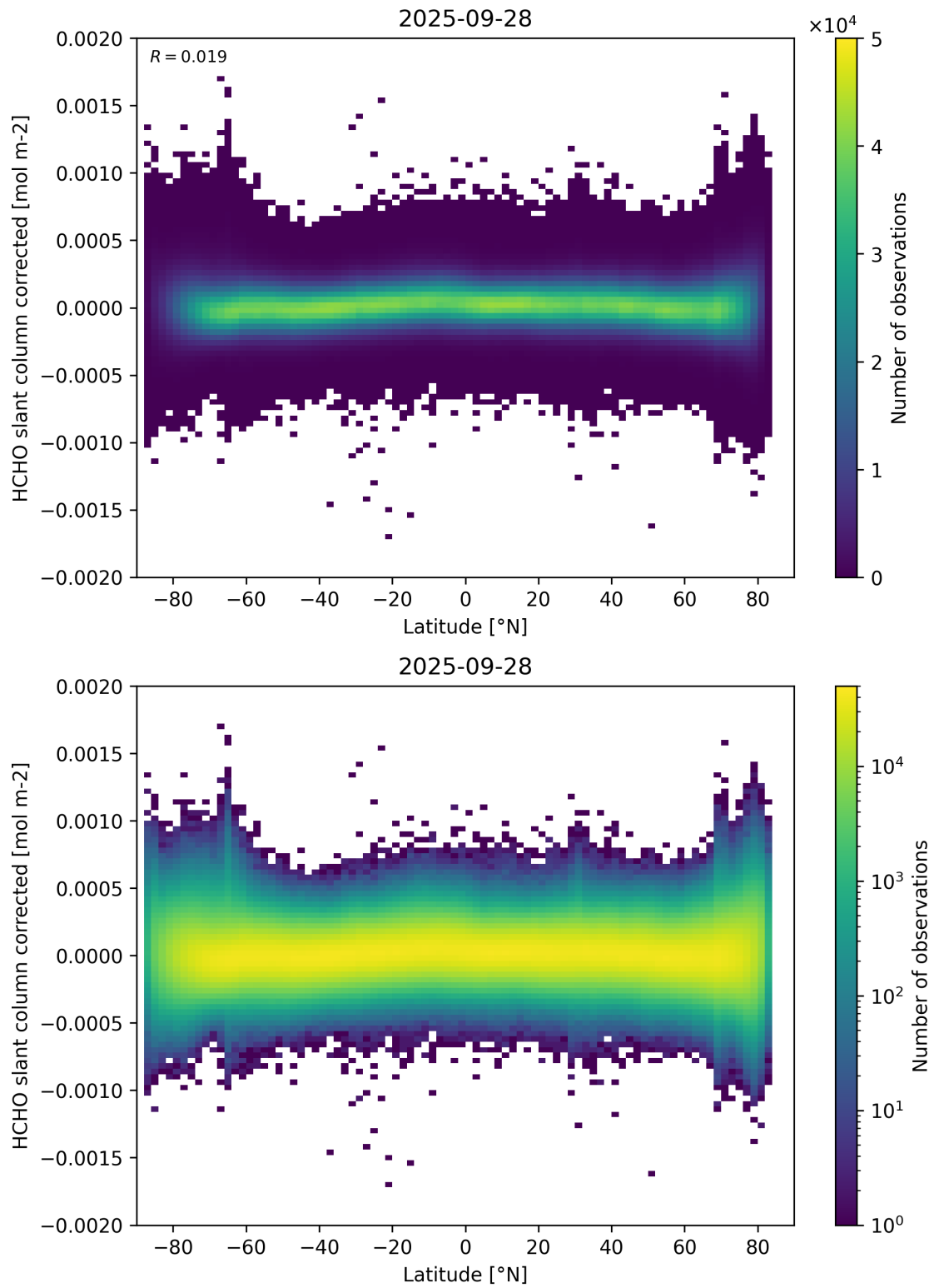
Figure 157: Scatter density plot of “Latitude” against “HCHO slant column corrected” for 2025-09-27 to 2025-09-29.
