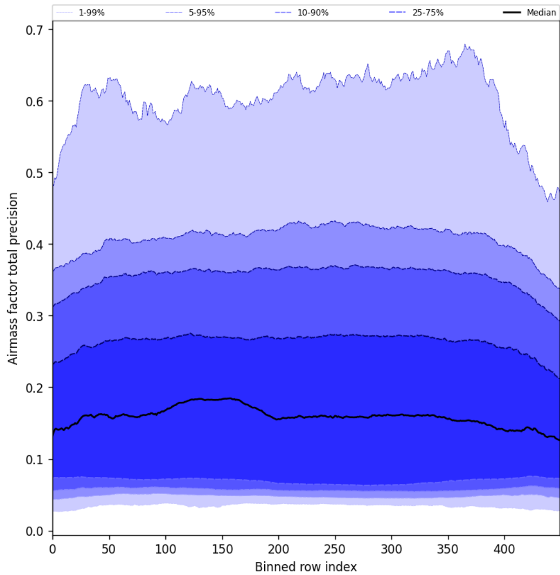
Figure 55: Along track statistics of “Airmass factor total precision” for 2025-09-27 to 2025-09-29
