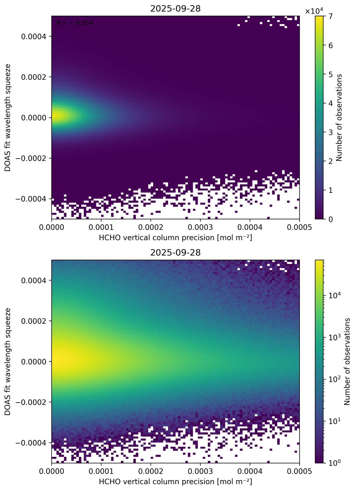
Figure 138: Scatter density plot of “HCHO vertical column precision” against “DOAS fit wavelength squeeze” for 2025-09-27 to 2025-09-29.
