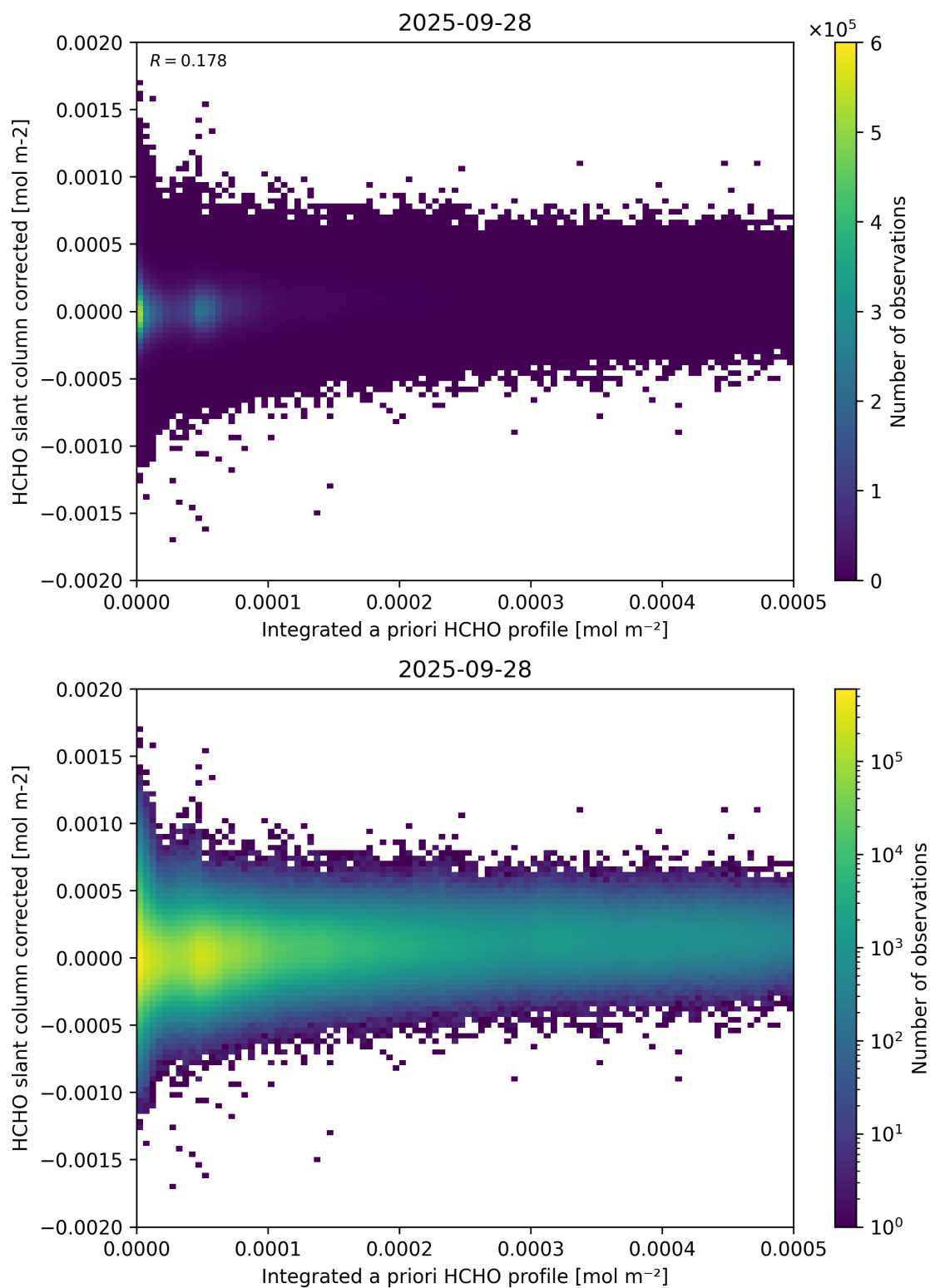
Figure 151: Scatter density plot of “Integrated a priori HCHO profile” against “HCHO slant column corrected” for 2025-09-27 to 2025-09-29.
