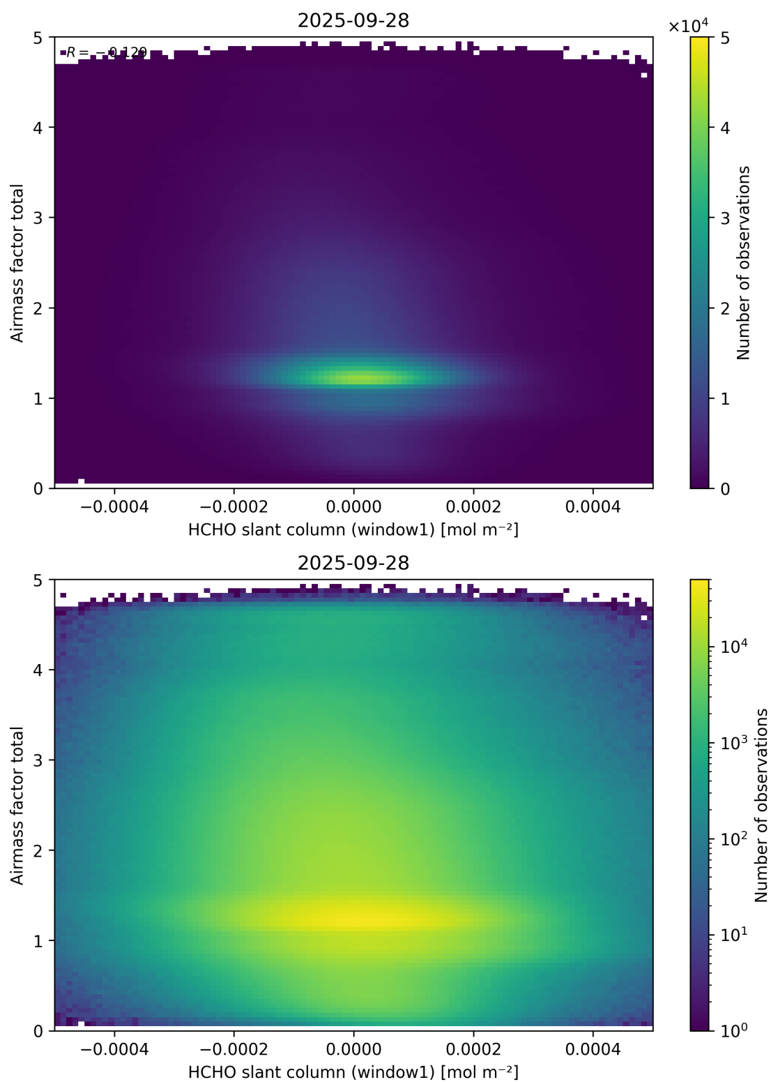
Figure 85: Scatter density plot of “HCHO slant column (window1)” against “Airmass factor total” for 2025-09-27 to 2025-09-29.
