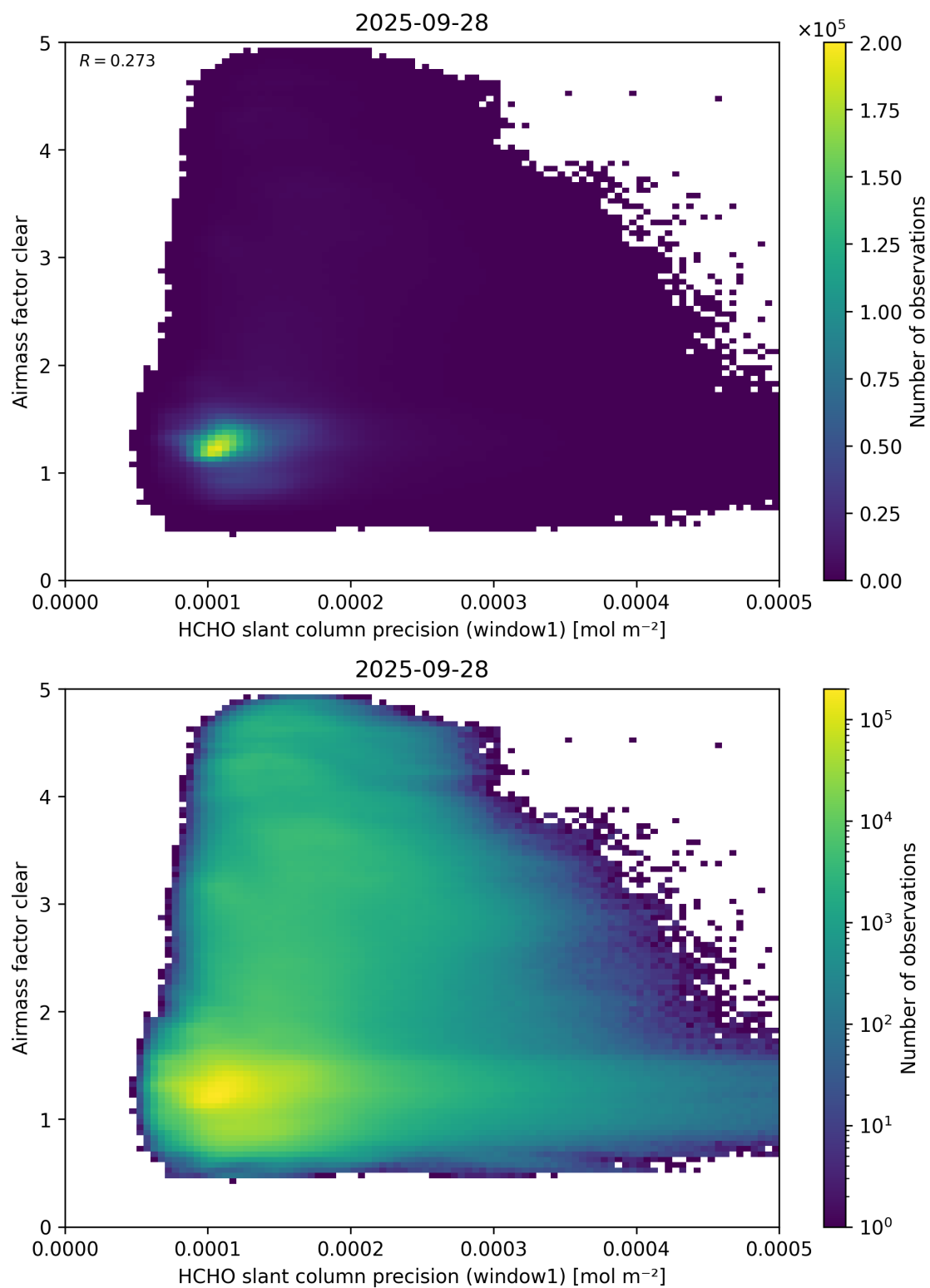
Figure 91: Scatter density plot of “HCHO slant column precision (window1)” against “Airmass factor clear” for 2025-09-27 to 2025-09-29.
