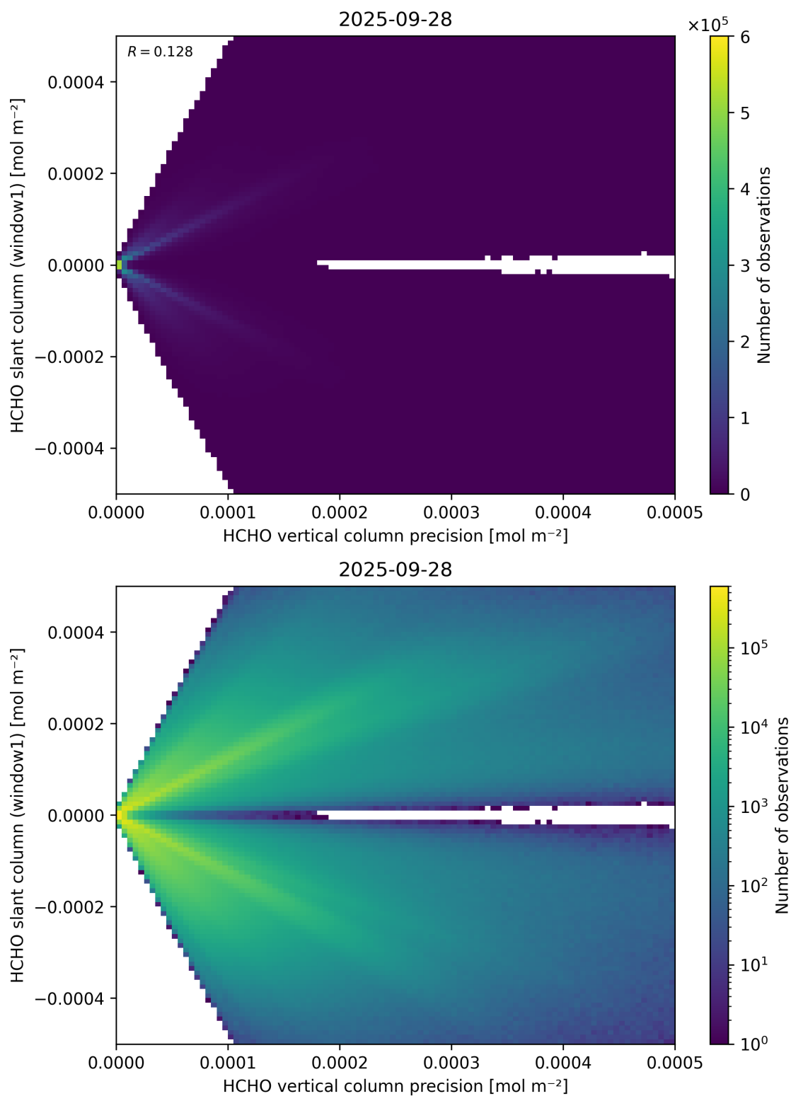
Figure 142: Scatter density plot of “HCHO vertical column precision” against “HCHO slant column (window1)” for 2025-09-27 to 2025-09-29.
