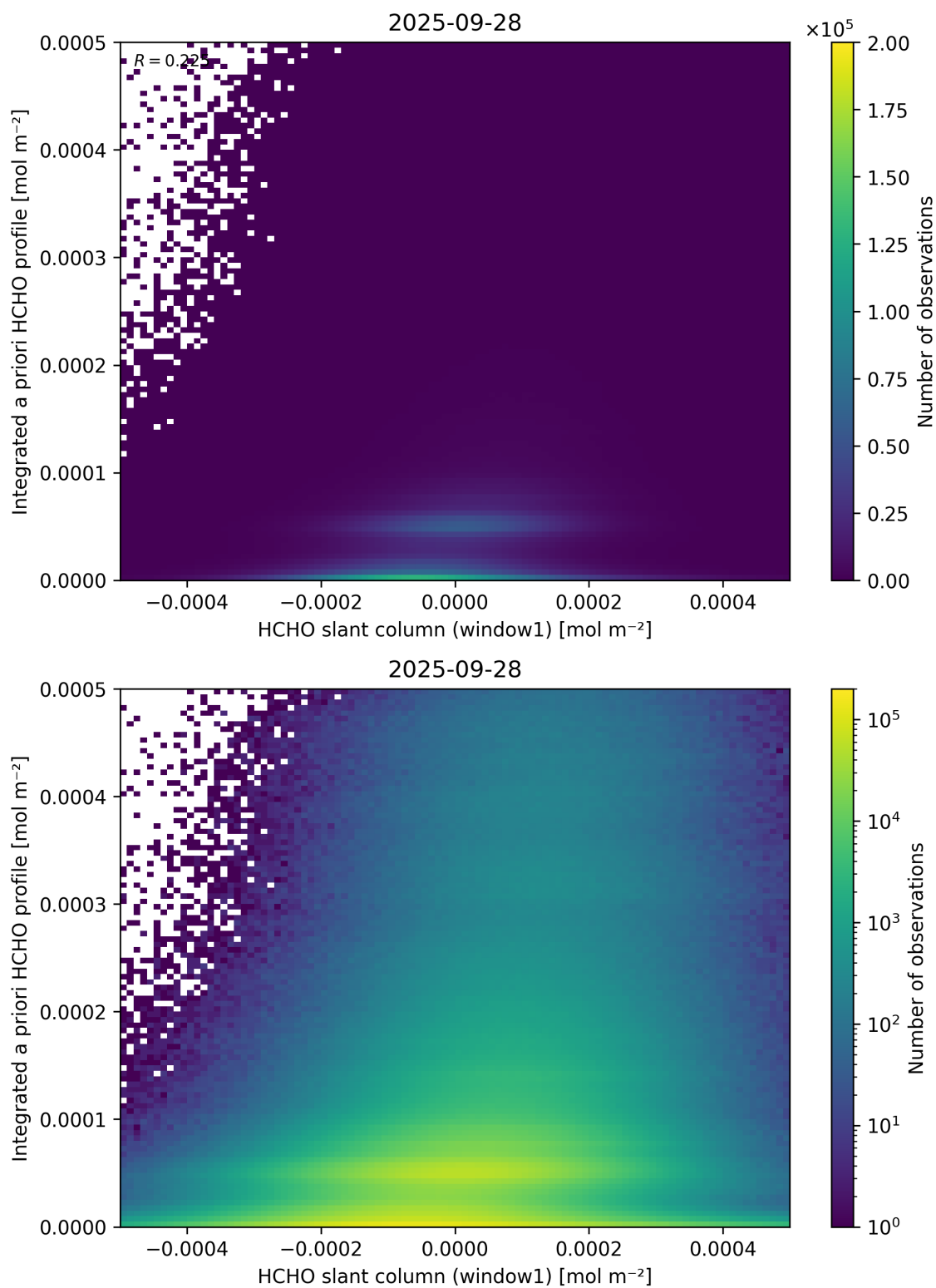
Figure 87: Scatter density plot of “HCHO slant column (window1)” against “Integrated a priori HCHO profile” for 2025-09-27 to 2025-09-29.
