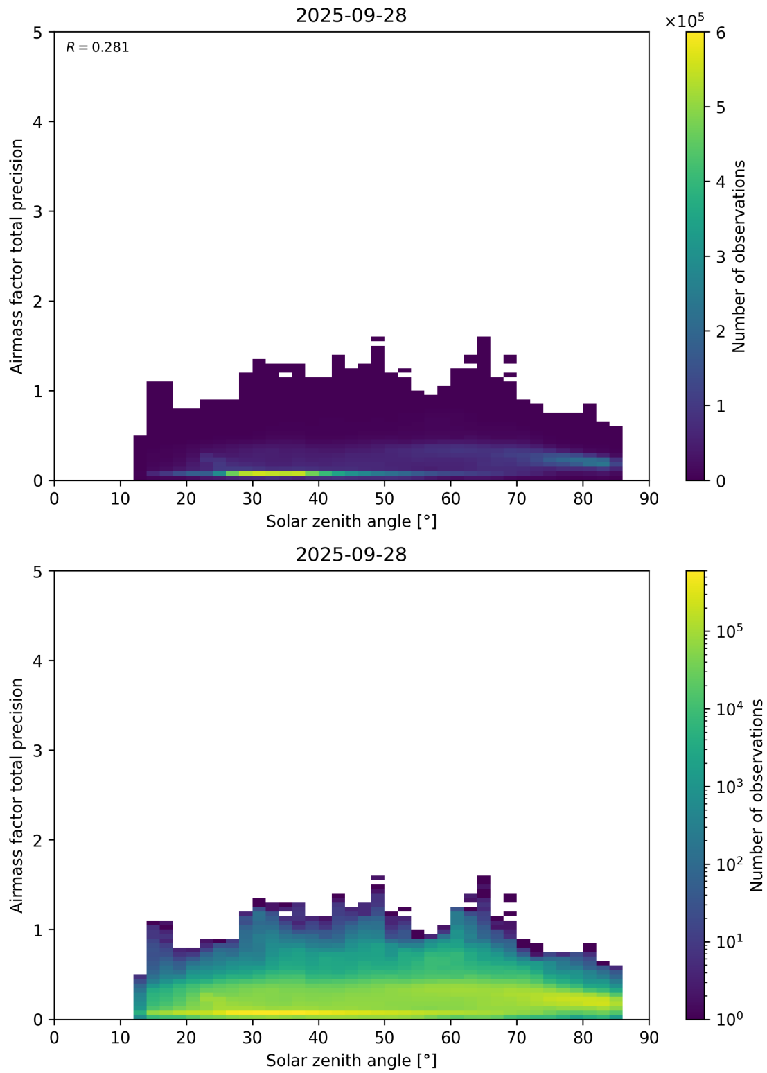
Figure 176: Scatter density plot of “Solar zenith angle” against “Airmass factor total precision” for 2025-09-27 to 2025-09-29.
