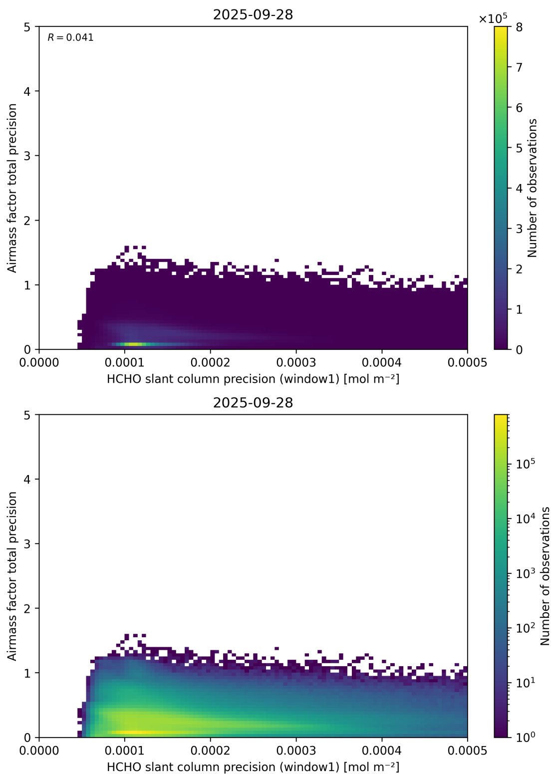
Figure 95: Scatter density plot of “HCHO slant column precision (window1)” against “Airmass factor total precision” for 2025-09-27 to 2025-09-29.
