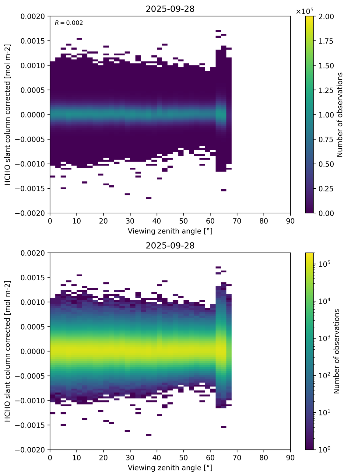
Figure 186: Scatter density plot of “Viewing zenith angle” against “HCHO slant column corrected” for 2025-09-27 to 2025-09-29.
