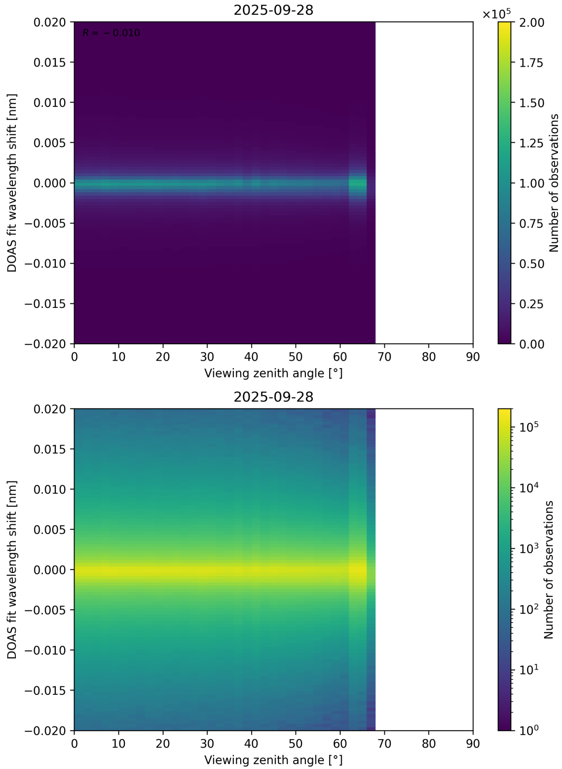
Figure 183: Scatter density plot of “Viewing zenith angle” against “DOAS fit wavelength shift” for 2025-09-27 to 2025-09-29.
