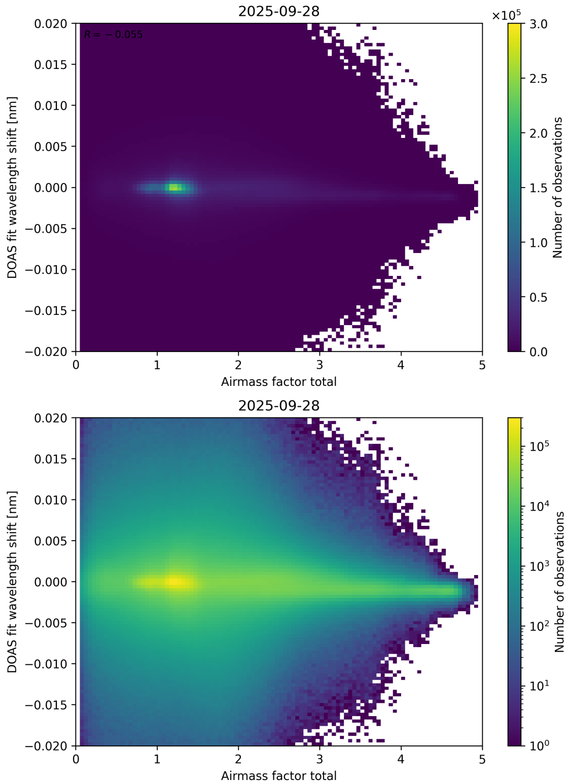
Figure 98: Scatter density plot of “Airmass factor total” against “DOAS fit wavelength shift” for 2025-09-27 to 2025-09-29.
