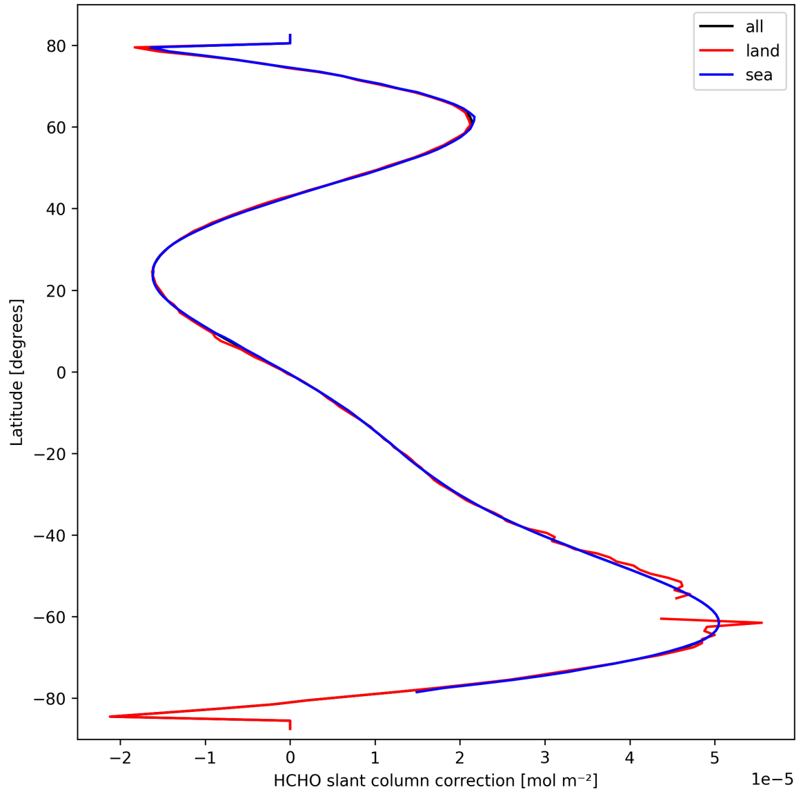
Figure 33: Zonal average of “HCHO slant column correction” for 2025-09-27 to 2025-09-29.
