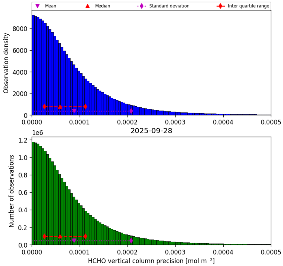
Figure 36: Histogram of “HCHO vertical column precision” for 2025-09-27 to 2025-09-29
