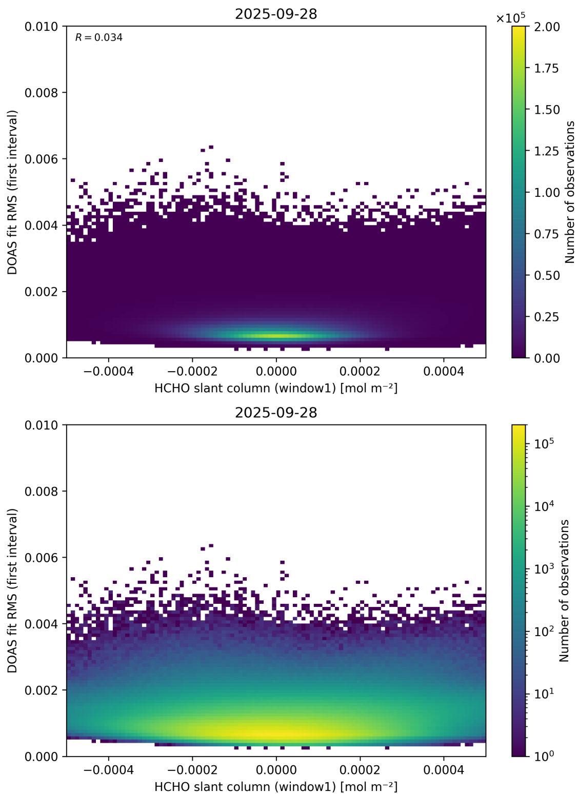
Figure 78: Scatter density plot of “HCHO slant column (window1)” against “DOAS fit RMS (first interval)” for 2025-09-27 to 2025-09-29.
