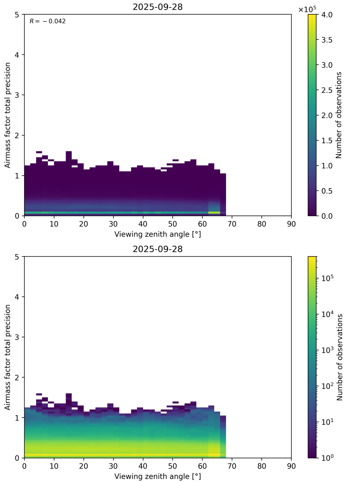
Figure 191: Scatter density plot of “Viewing zenith angle” against “Airmass factor total precision” for 2025-09-27 to 2025-09-29.
