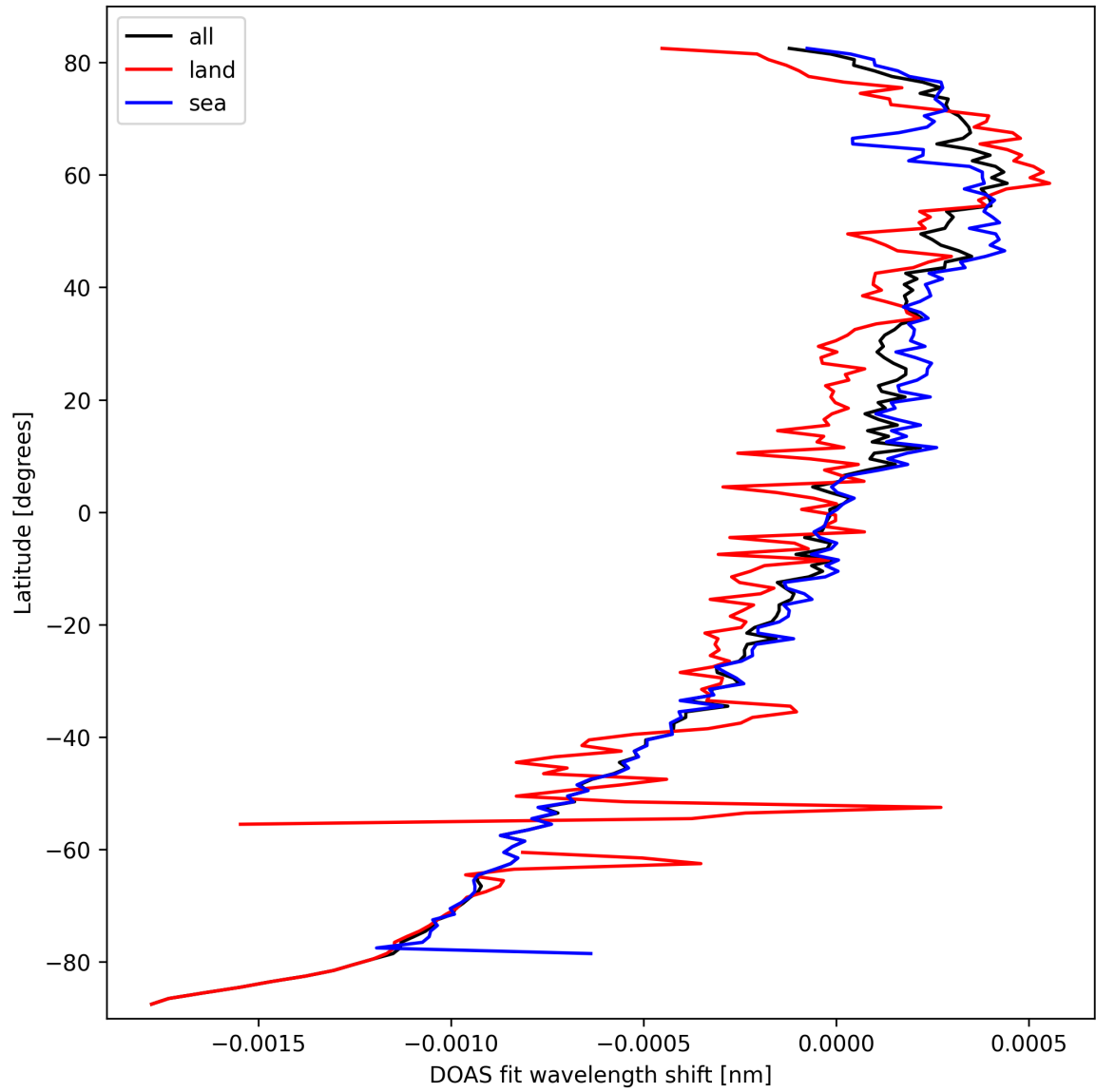
Figure 30: Zonal average of “DOAS fit wavelength shift” for 2025-09-27 to 2025-09-29.
