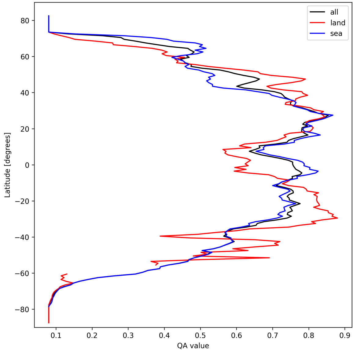
Figure 20: Zonal average of “QA value” for 2025-09-27 to 2025-09-29.
