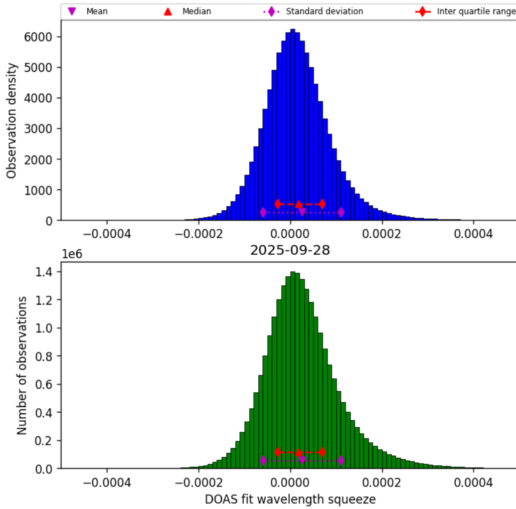
Figure 45: Histogram of “DOAS fit wavelength squeeze” for 2025-09-27 to 2025-09-29
