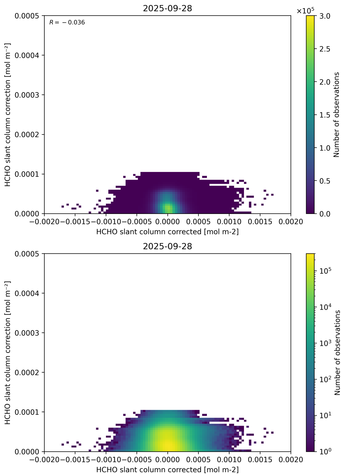
Figure 77: Scatter density plot of “HCHO slant column corrected” against “HCHO slant column correction” for 2025-09-27 to 2025-09-29.
