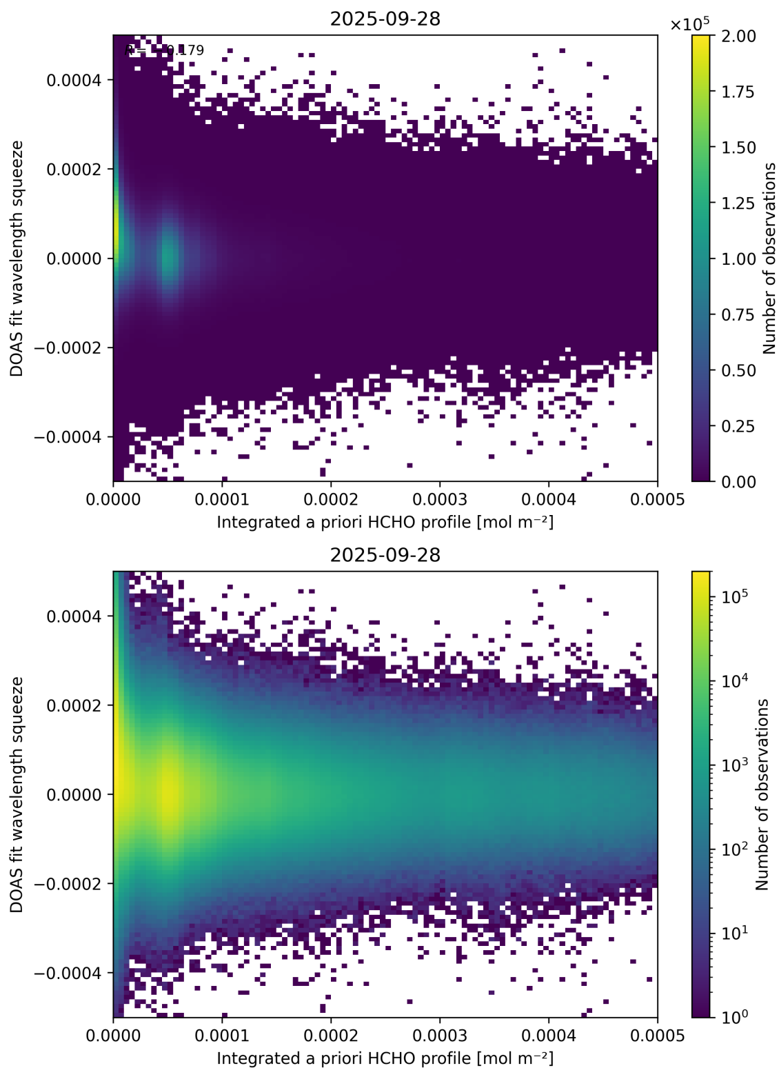
Figure 150: Scatter density plot of “Integrated a priori HCHO profile” against “DOAS fit wavelength squeeze” for 2025-09-27 to 2025-09-29.
