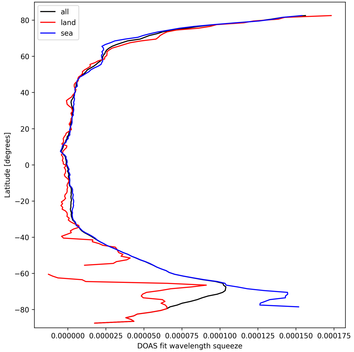
Figure 31: Zonal average of “DOAS fit wavelength squeeze” for 2025-09-27 to 2025-09-29.
