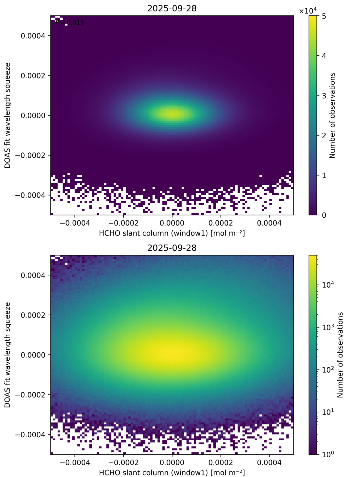
Figure 80: Scatter density plot of “HCHO slant column (window1)” against “DOAS fit wavelength squeeze” for 2025-09-27 to 2025-09-29.
