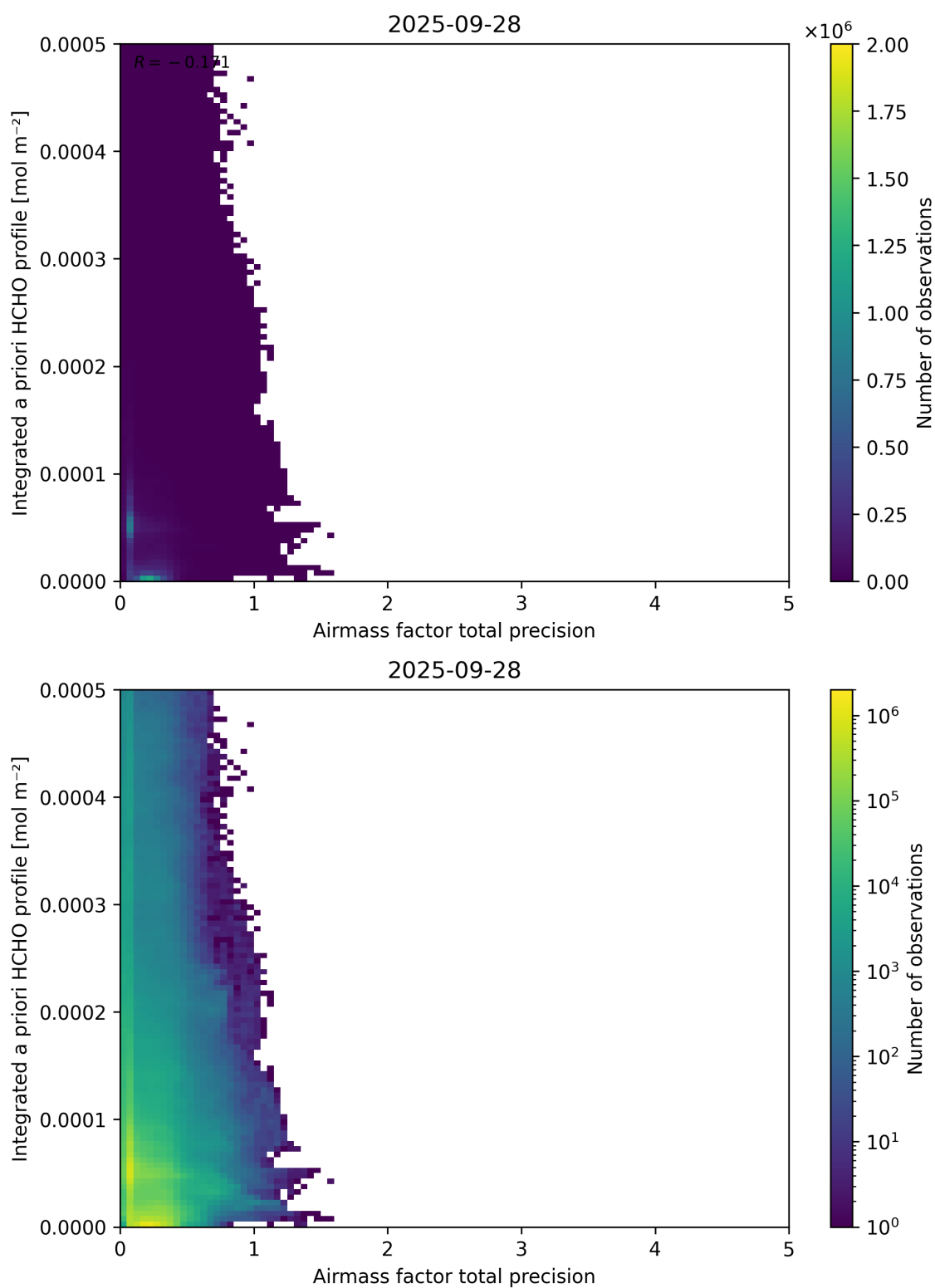
Figure 111: Scatter density plot of “Airmass factor total precision” against “Integrated a priori HCHO profile” for 2025-09-27 to 2025-09-29.
