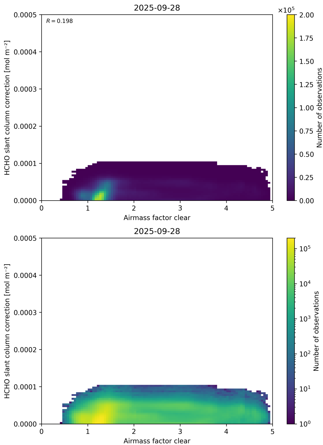
Figure 75: Scatter density plot of “Airmass factor clear” against “HCHO slant column correction” for 2025-09-27 to 2025-09-29.
