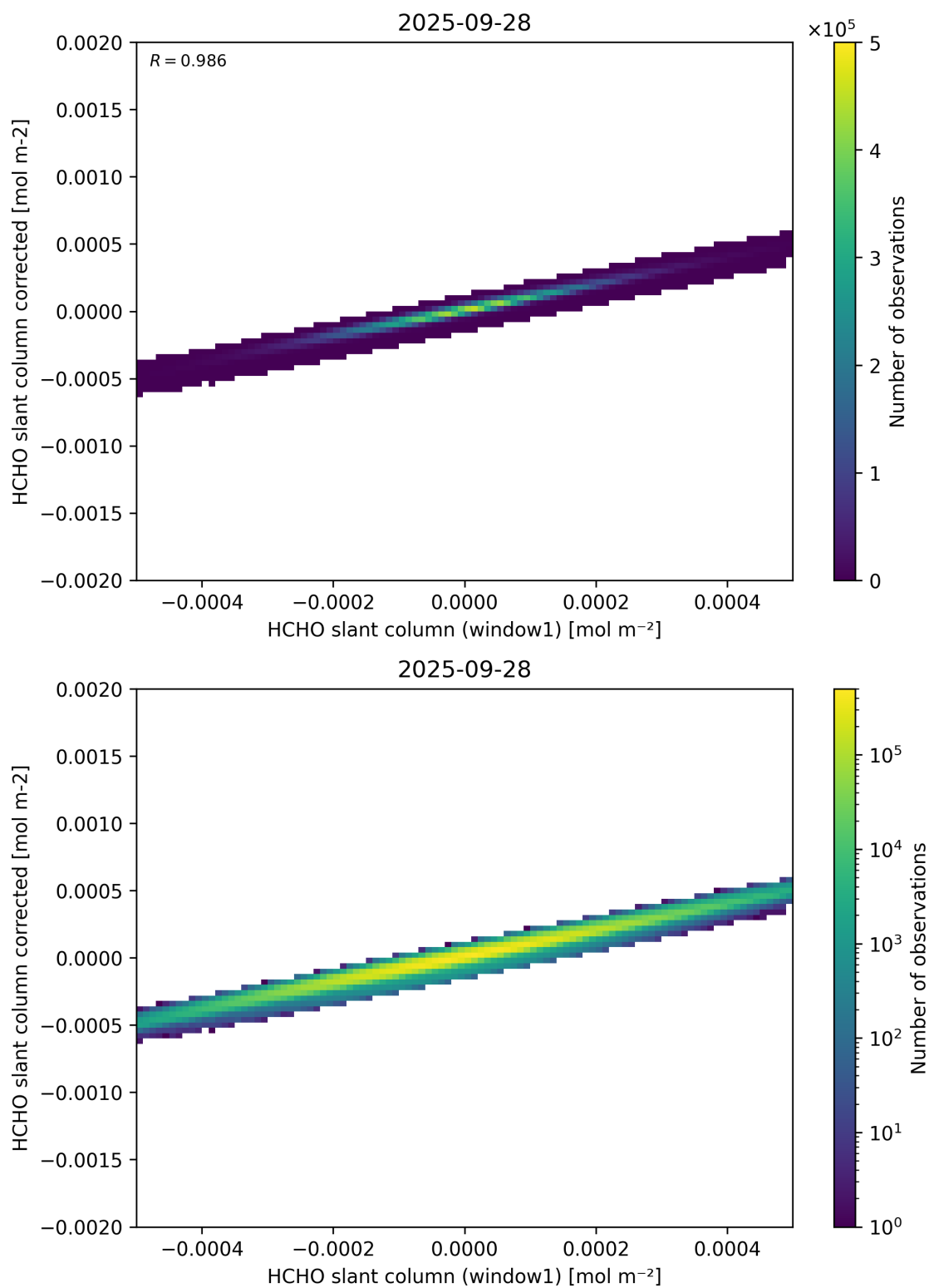
Figure 82: Scatter density plot of “HCHO slant column (window1)” against “HCHO slant column corrected” for 2025-09-27 to 2025-09-29.
