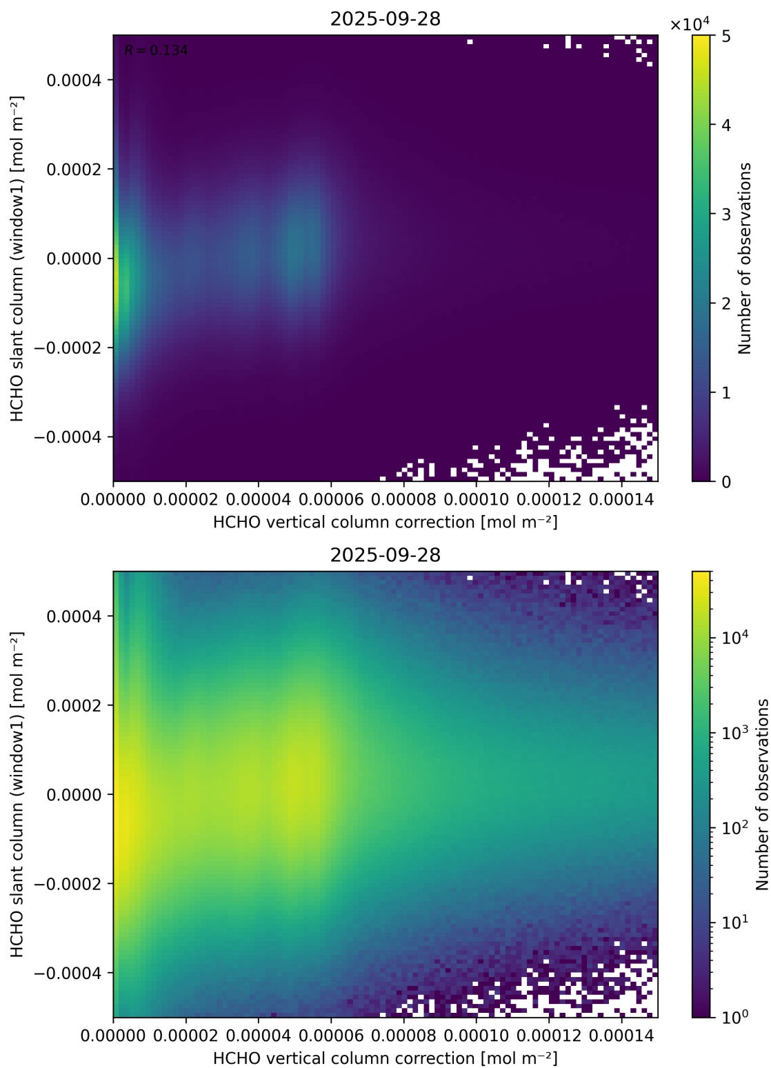
Figure 118: Scatter density plot of “HCHO vertical column correction” against “HCHO slant column (window1)” for 2025-09-27 to 2025-09-29.
