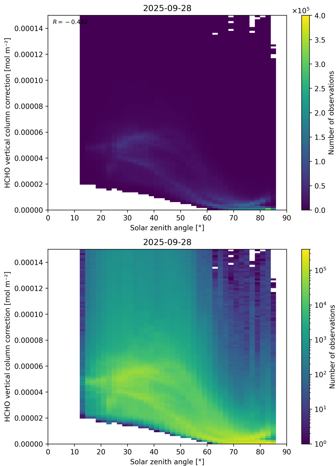
Figure 178: Scatter density plot of “Solar zenith angle” against “HCHO vertical column correction” for 2025-09-27 to 2025-09-29.
