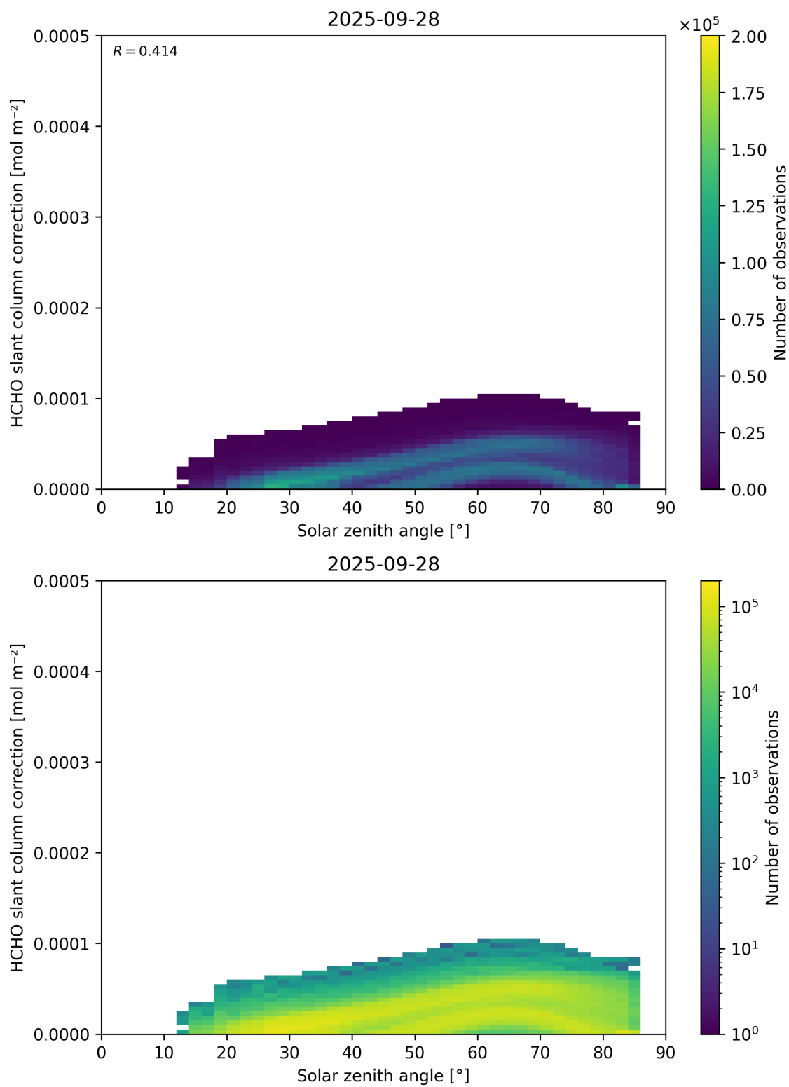
Figure 172: Scatter density plot of “Solar zenith angle” against “HCHO slant column correction” for 2025-09-27 to 2025-09-29.
