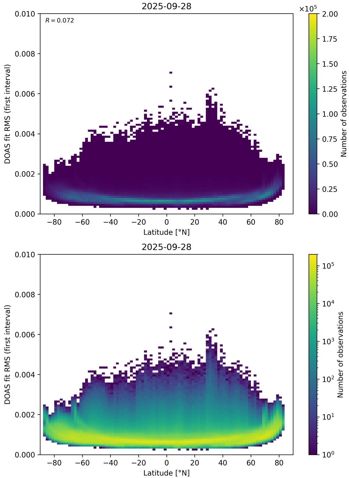
Figure 153: Scatter density plot of “Latitude” against “DOAS fit RMS (first interval)” for 2025-09-27 to 2025-09-29.
