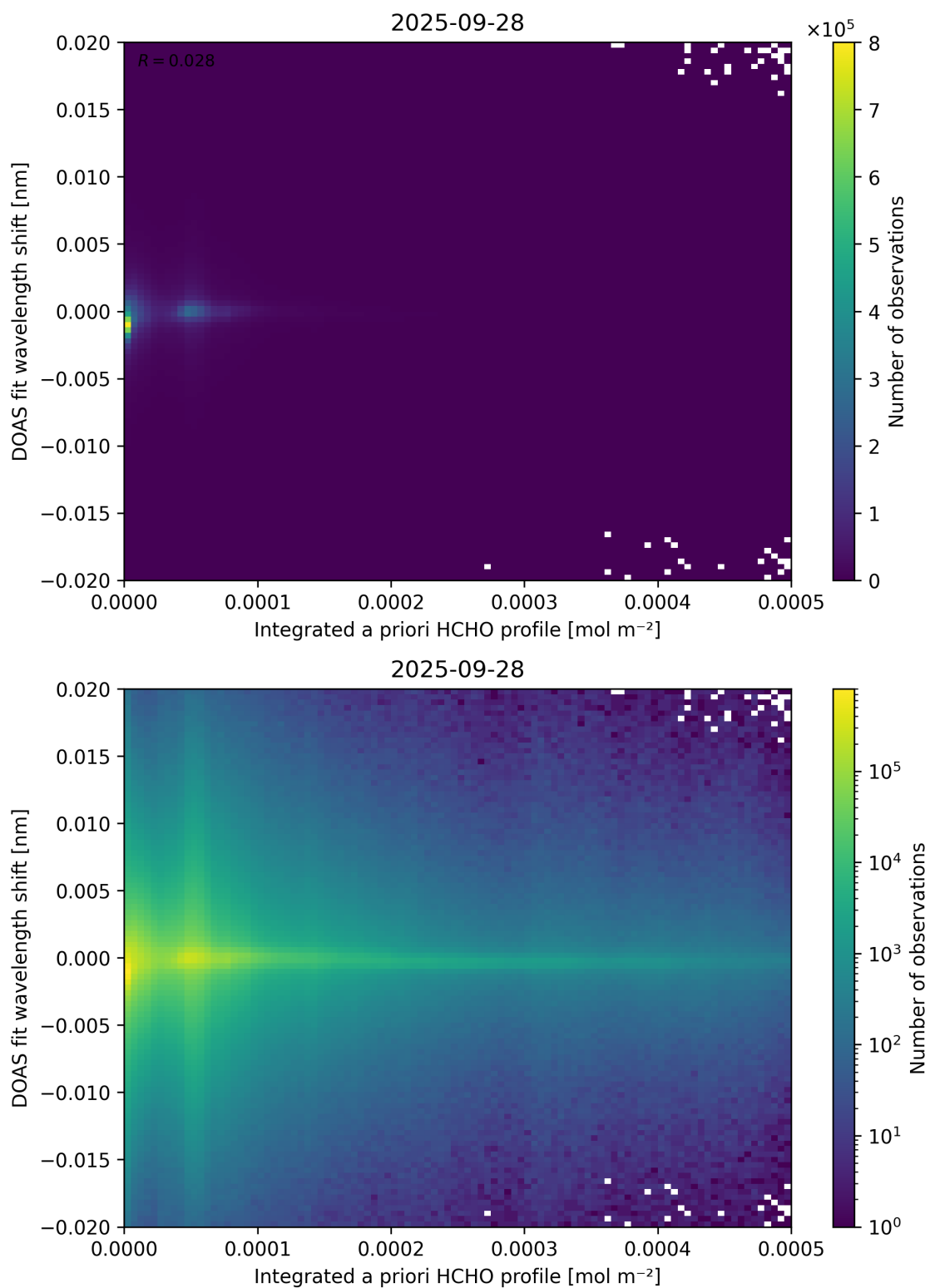
Figure 149: Scatter density plot of “Integrated a priori HCHO profile” against “DOAS fit wavelength shift” for 2025-09-27 to 2025-09-29.
