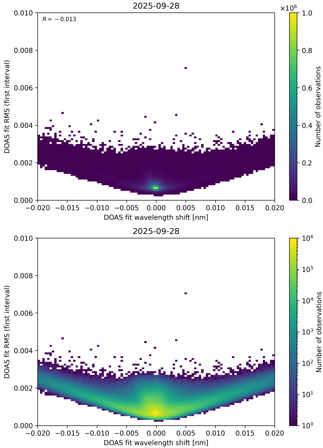
Figure 64: Scatter density plot of “DOAS fit wavelength shift” against “DOAS fit RMS (first interval)” for 2025-09-27 to 2025-09-29.
