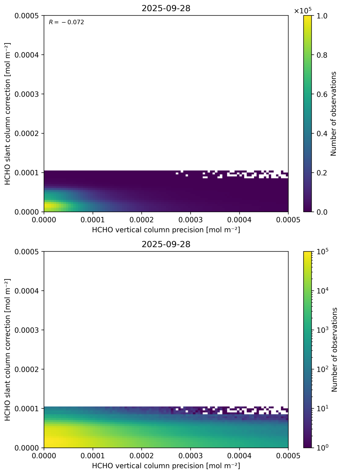
Figure 141: Scatter density plot of “HCHO vertical column precision” against “HCHO slant column correction” for 2025-09-27 to 2025-09-29.
