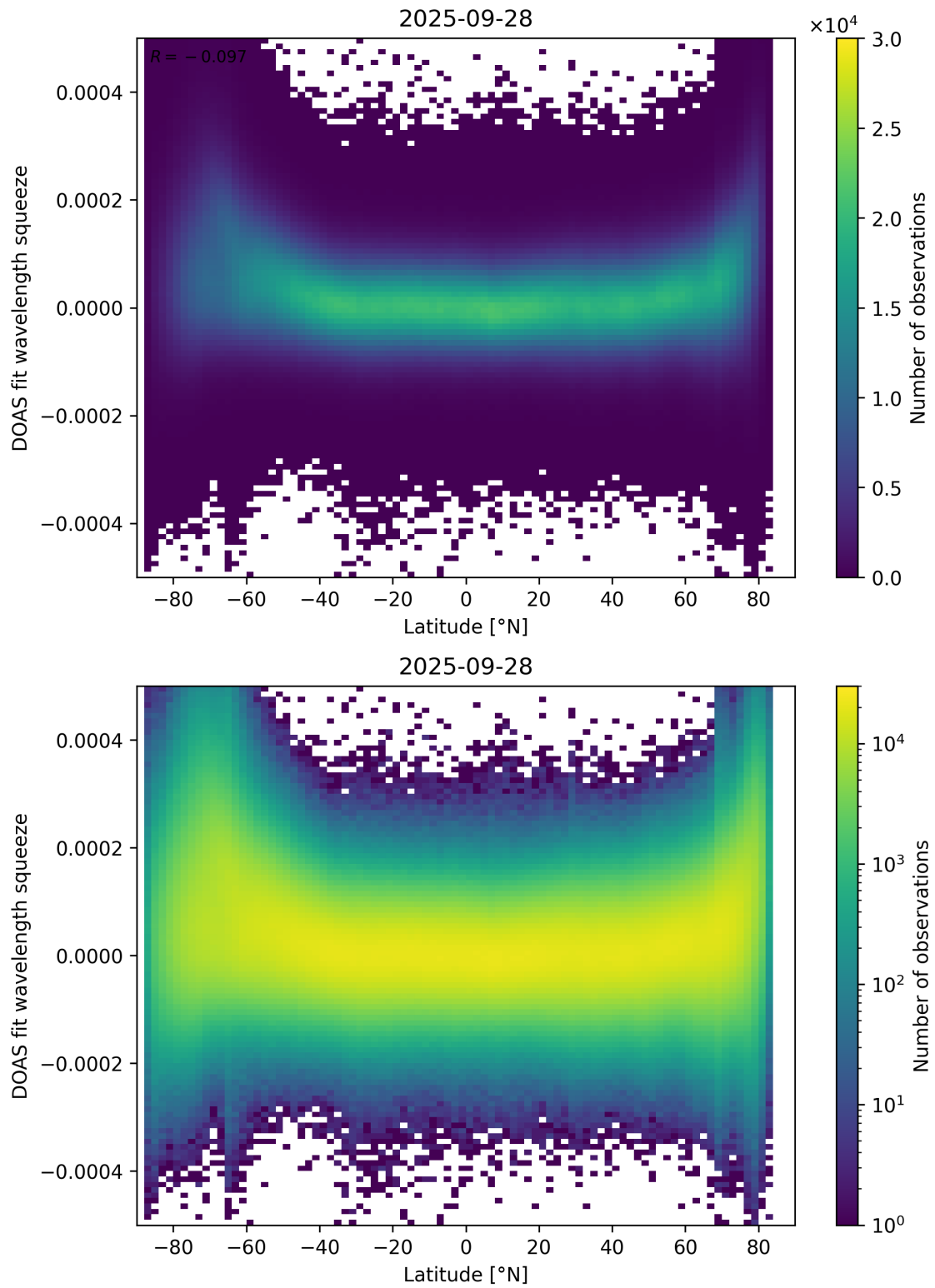
Figure 155: Scatter density plot of “Latitude” against “DOAS fit wavelength squeeze” for 2025-09-27 to 2025-09-29.
