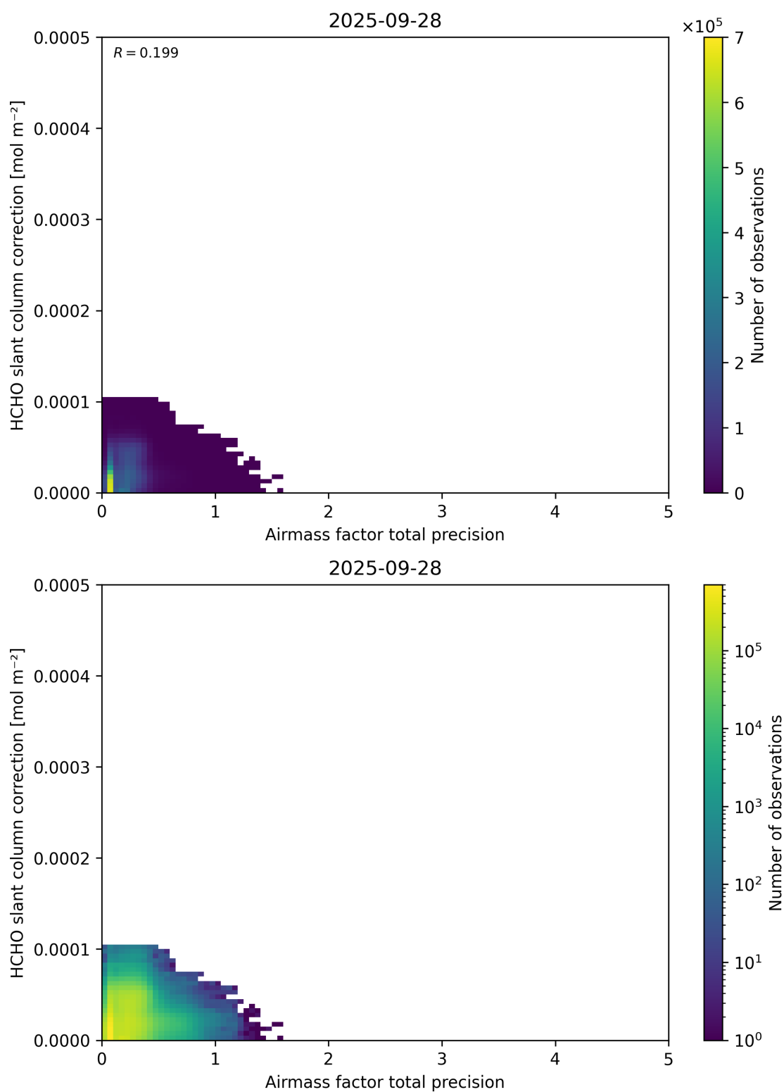
Figure 110: Scatter density plot of “Airmass factor total precision” against “HCHO slant column correction” for 2025-09-27 to 2025-09-29.
