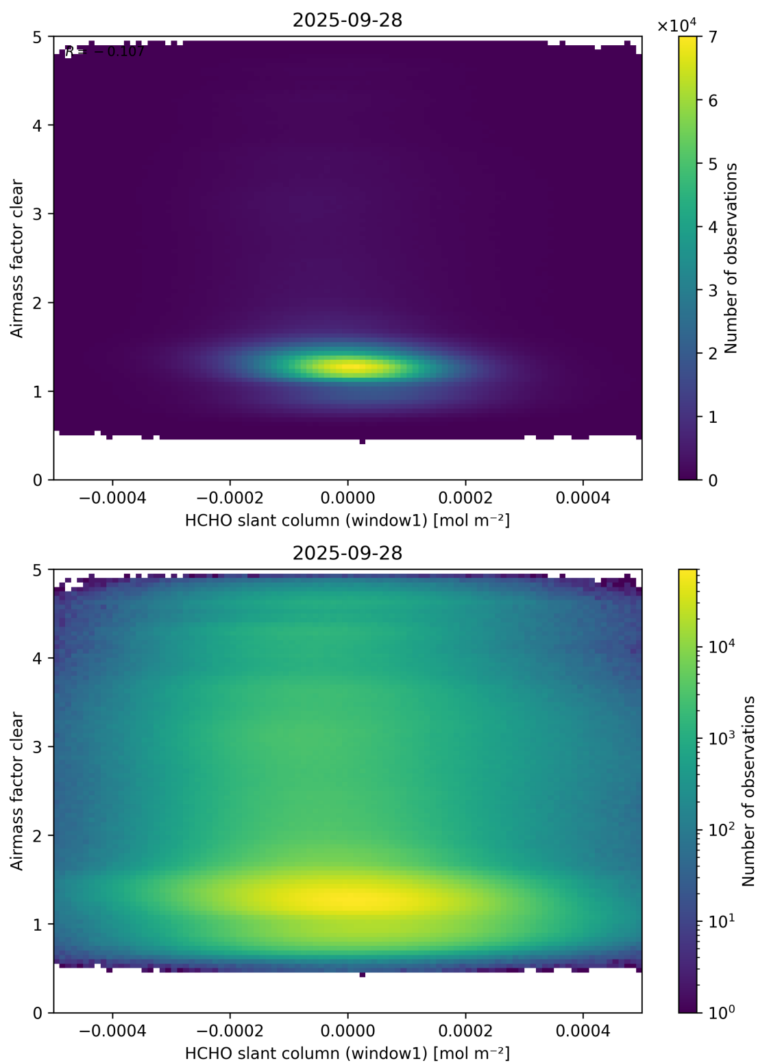
Figure 81: Scatter density plot of “HCHO slant column (window1)” against “Airmass factor clear” for 2025-09-27 to 2025-09-29.
