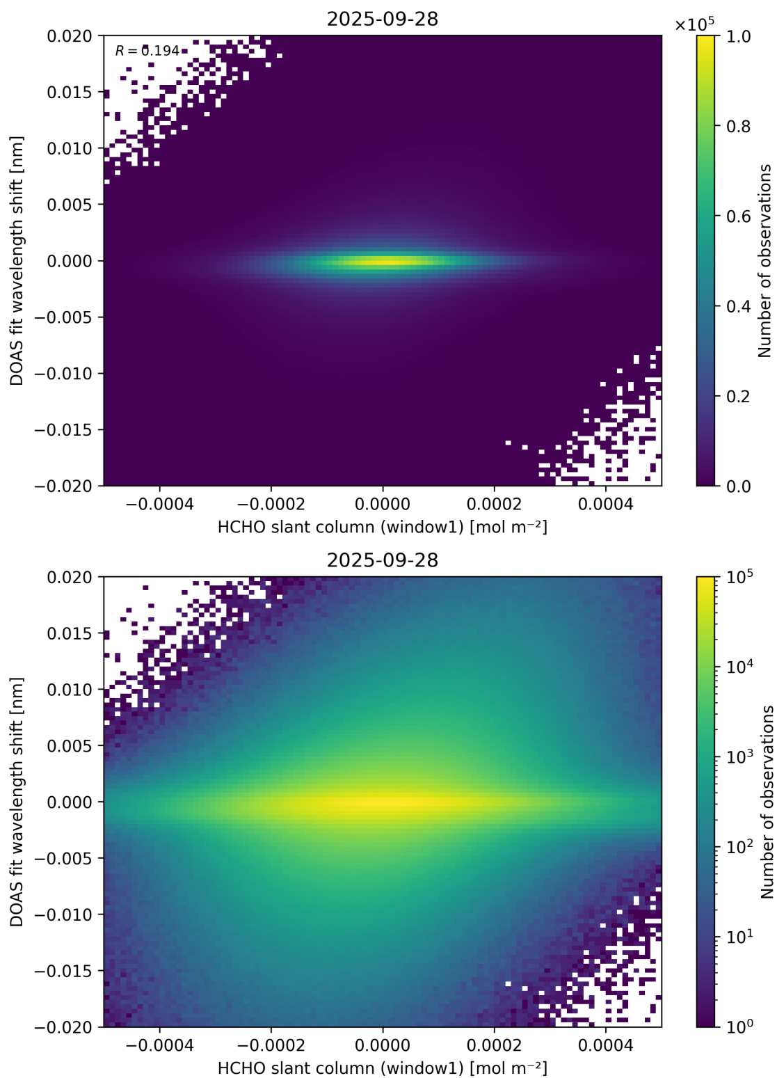
Figure 79: Scatter density plot of “HCHO slant column (window1)” against “DOAS fit wavelength shift” for 2025-09-27 to 2025-09-29.
