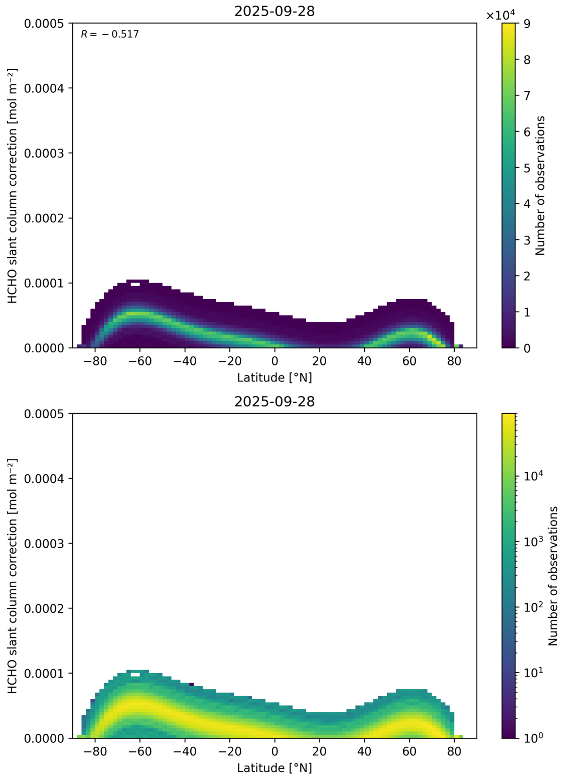
Figure 158: Scatter density plot of “Latitude” against “HCHO slant column correction” for 2025-09-27 to 2025-09-29.
