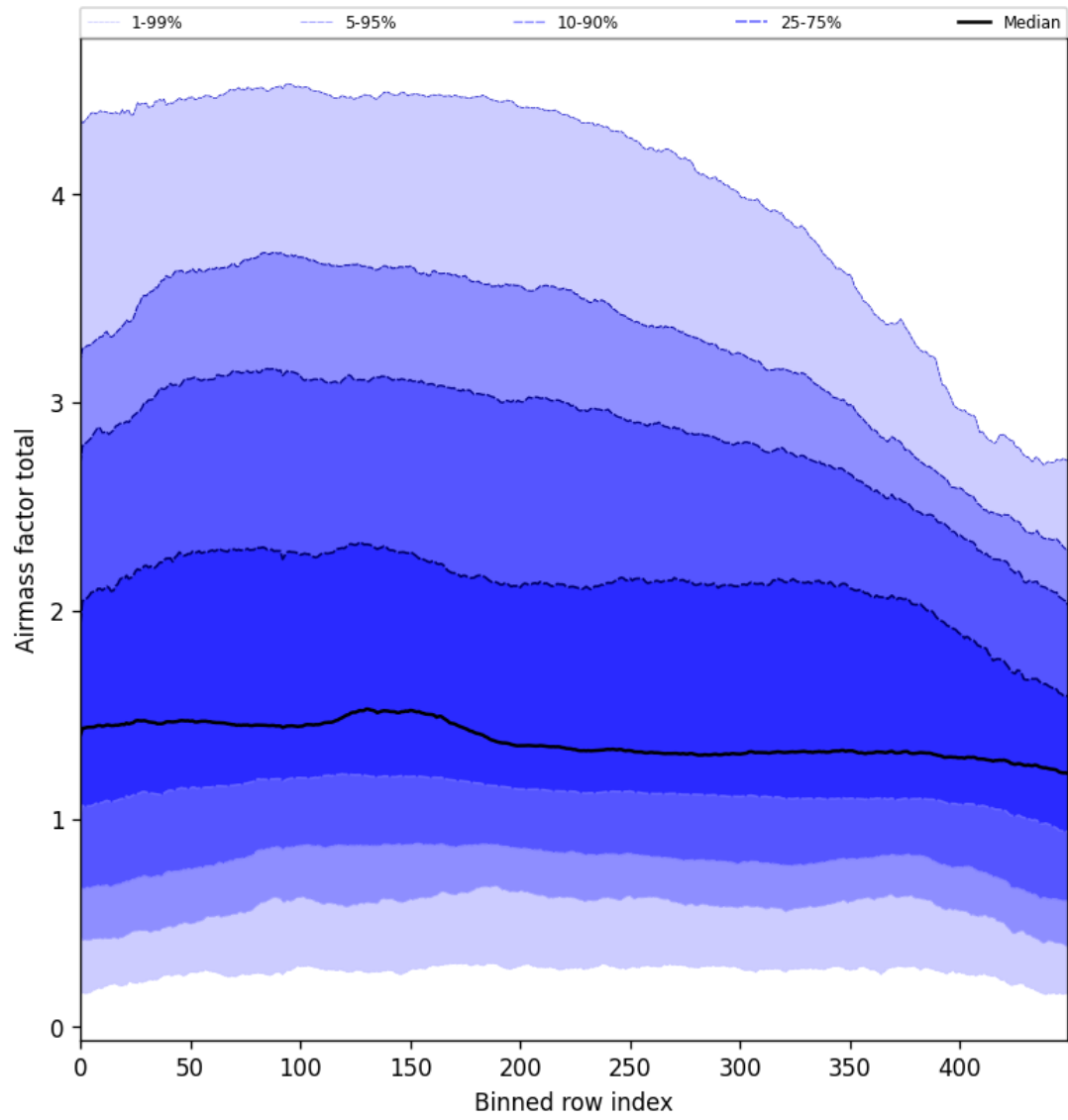
Figure 54: Along track statistics of “Airmass factor total” for 2025-09-27 to 2025-09-29
