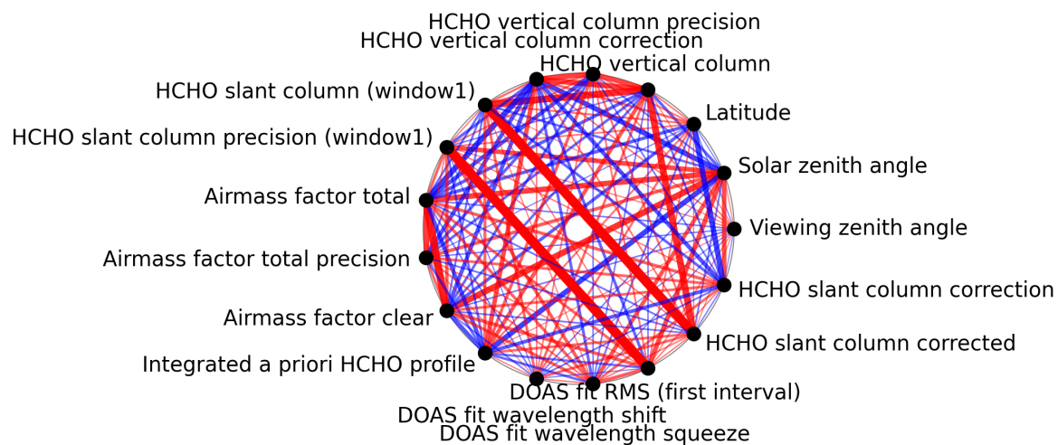
Figure 1: Map of correlation graph for 2025-09-27 to 2025-09-29.
