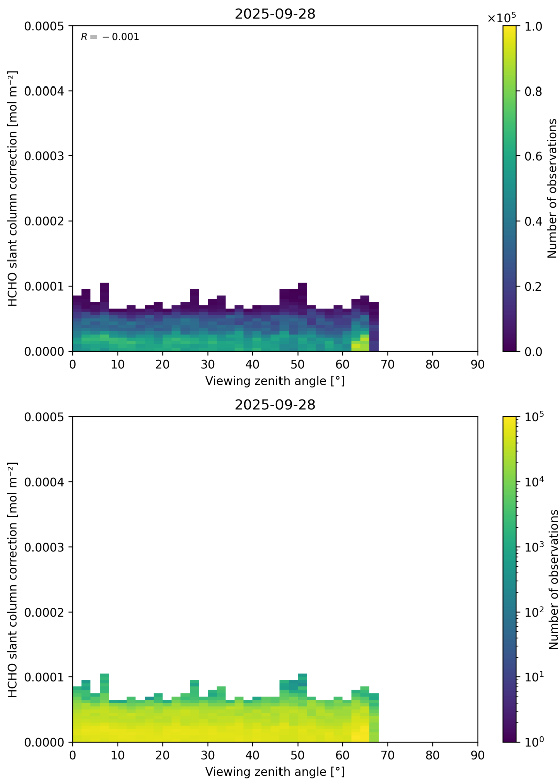
Figure 187: Scatter density plot of “Viewing zenith angle” against “HCHO slant column correction” for 2025-09-27 to 2025-09-29.
