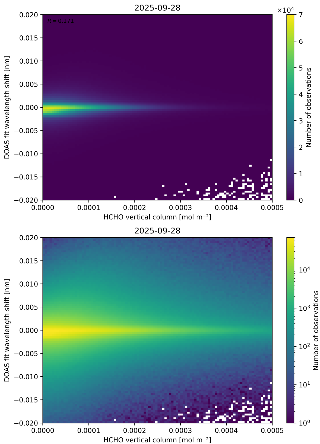
Figure 124: Scatter density plot of “HCHO vertical column” against “DOAS fit wavelength shift” for 2025-09-27 to 2025-09-29.
