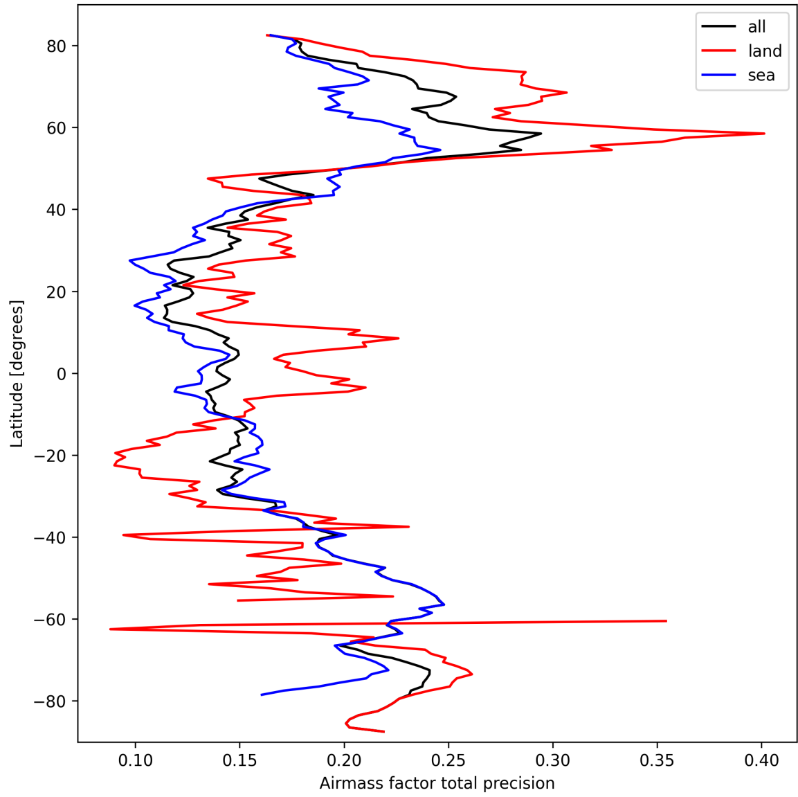
Figure 27: Zonal average of “Airmass factor total precision” for 2025-09-27 to 2025-09-29.
