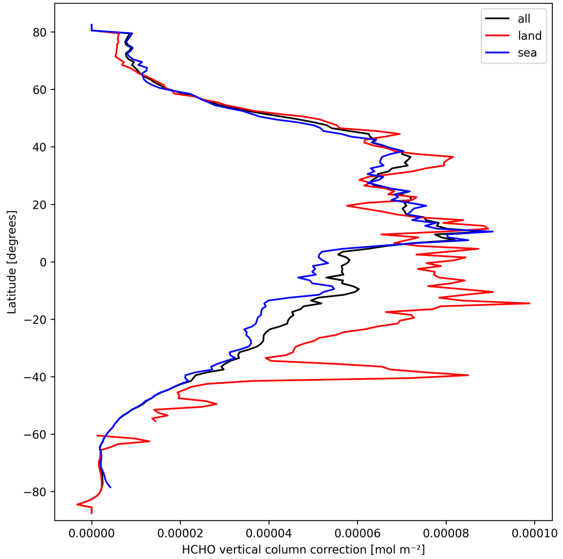
Figure 23: Zonal average of “HCHO vertical column correction” for 2025-09-27 to 2025-09-29.
