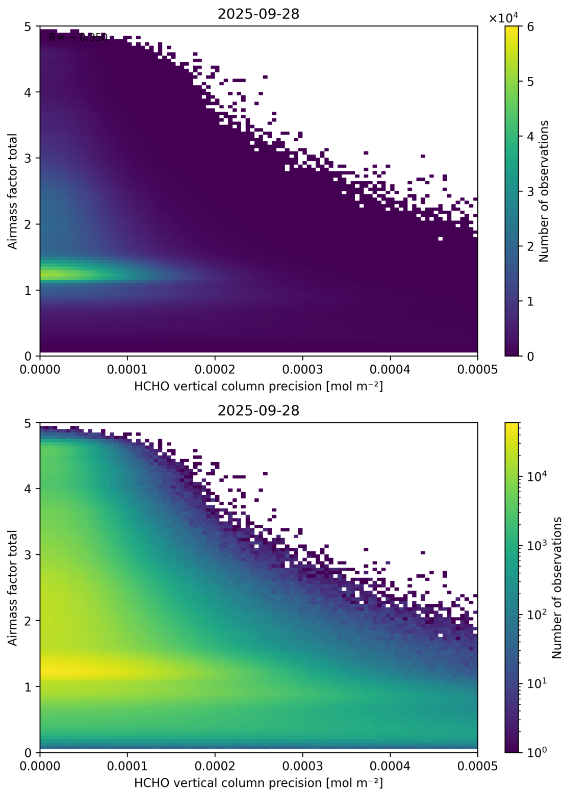
Figure 144: Scatter density plot of “HCHO vertical column precision” against “Airmass factor total” for 2025-09-27 to 2025-09-29.
