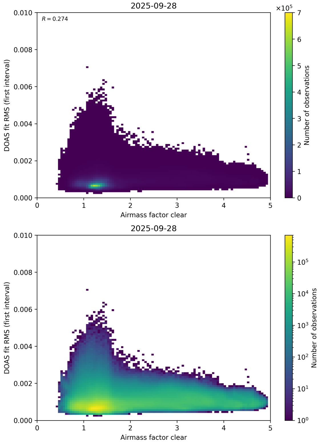
Figure 71: Scatter density plot of “Airmass factor clear” against “DOAS fit RMS (first interval)” for 2025-09-27 to 2025-09-29.
