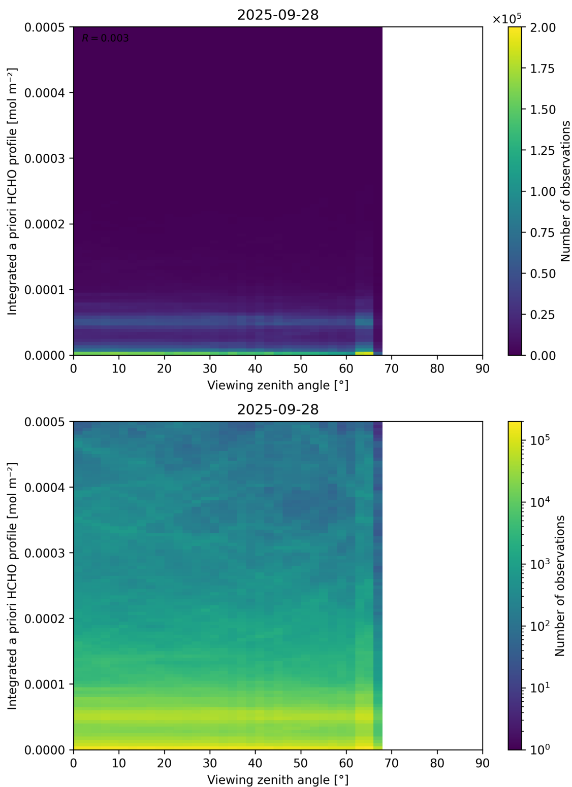
Figure 195: Scatter density plot of “Viewing zenith angle” against “Integrated a priori HCHO profile” for 2025-09-27 to 2025-09-29.
