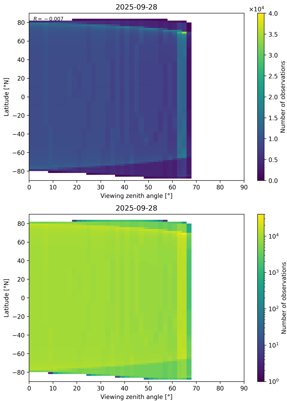
Figure 196: Scatter density plot of “Viewing zenith angle” against “Latitude” for 2025-09-27 to 2025-09-29.
