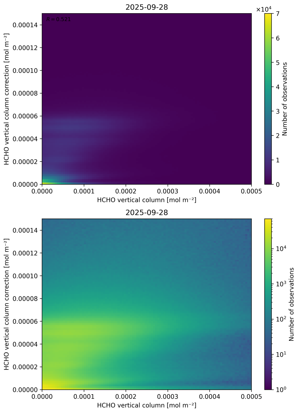
Figure 133: Scatter density plot of “HCHO vertical column” against “HCHO vertical column correction” for 2025-09-27 to 2025-09-29.
