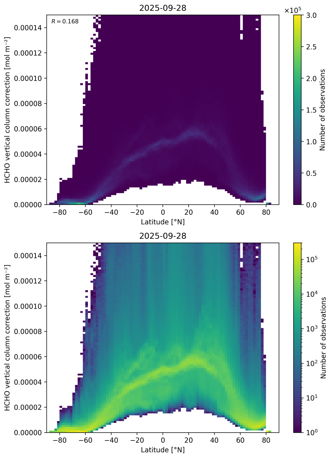
Figure 164: Scatter density plot of “Latitude” against “HCHO vertical column correction” for 2025-09-27 to 2025-09-29.
