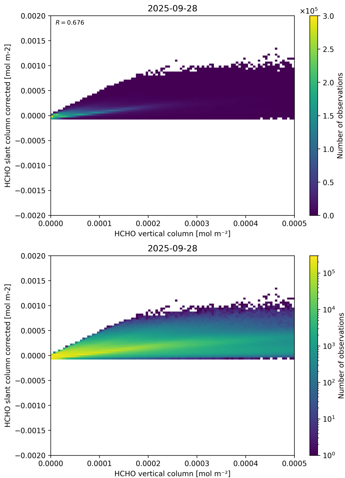
Figure 127: Scatter density plot of “HCHO vertical column” against “HCHO slant column corrected” for 2025-09-27 to 2025-09-29.
