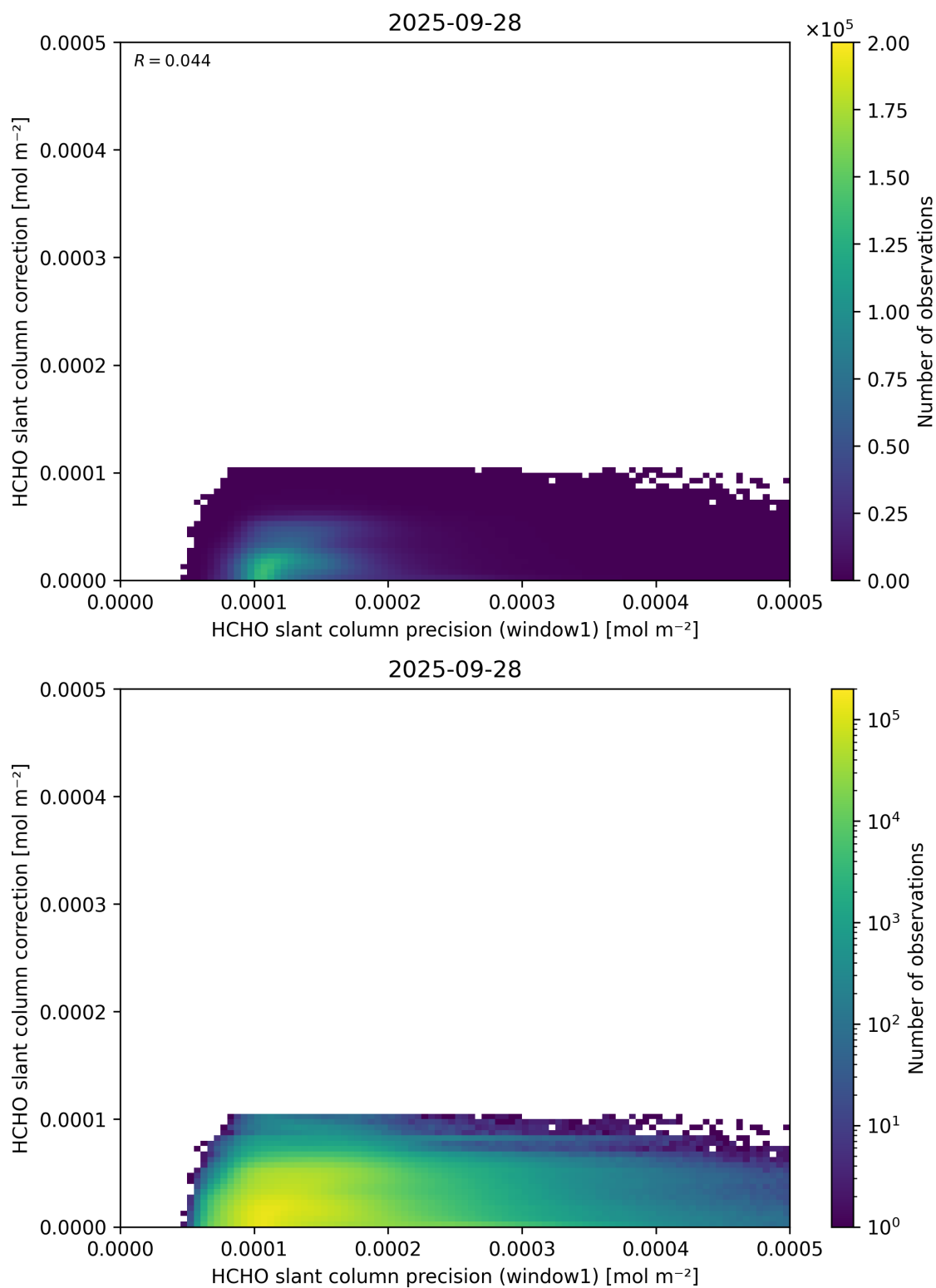
Figure 93: Scatter density plot of “HCHO slant column precision (window1)” against “HCHO slant column correction” for 2025-09-27 to 2025-09-29.
