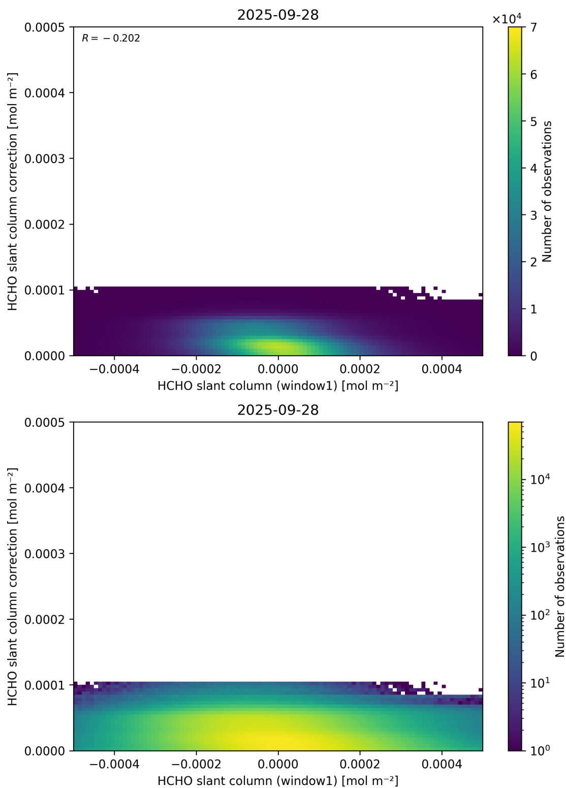
Figure 83: Scatter density plot of “HCHO slant column (window1)” against “HCHO slant column correction” for 2025-09-27 to 2025-09-29.
