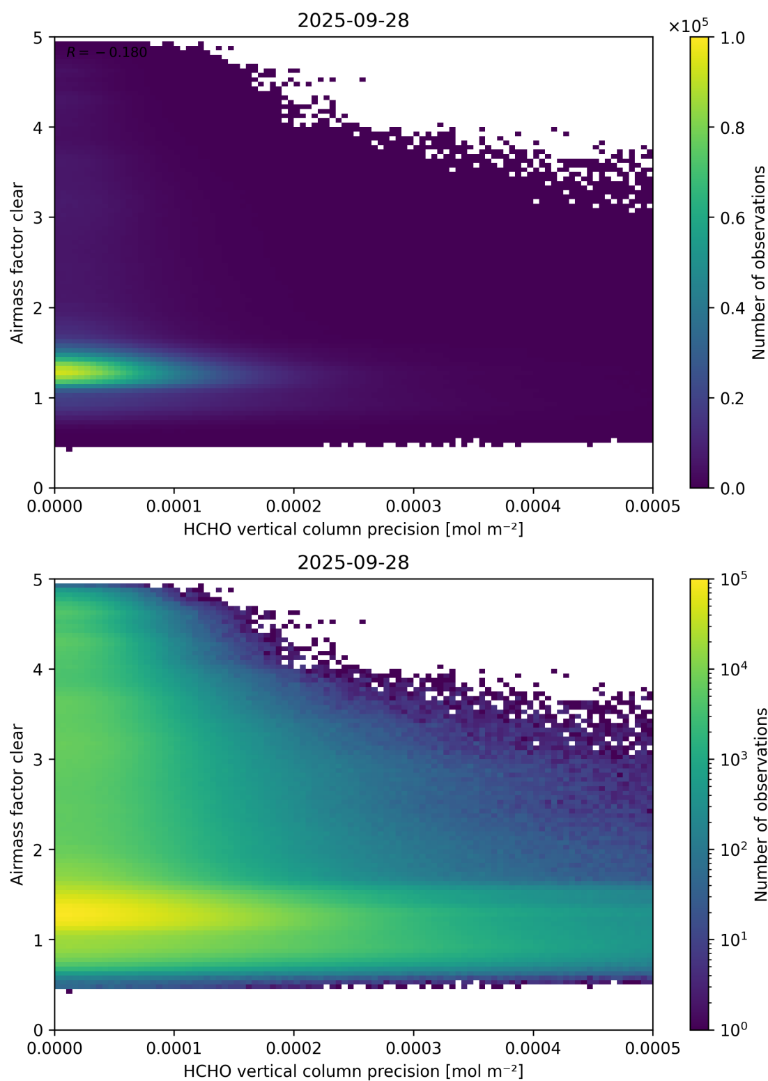
Figure 139: Scatter density plot of “HCHO vertical column precision” against “Airmass factor clear” for 2025-09-27 to 2025-09-29.
