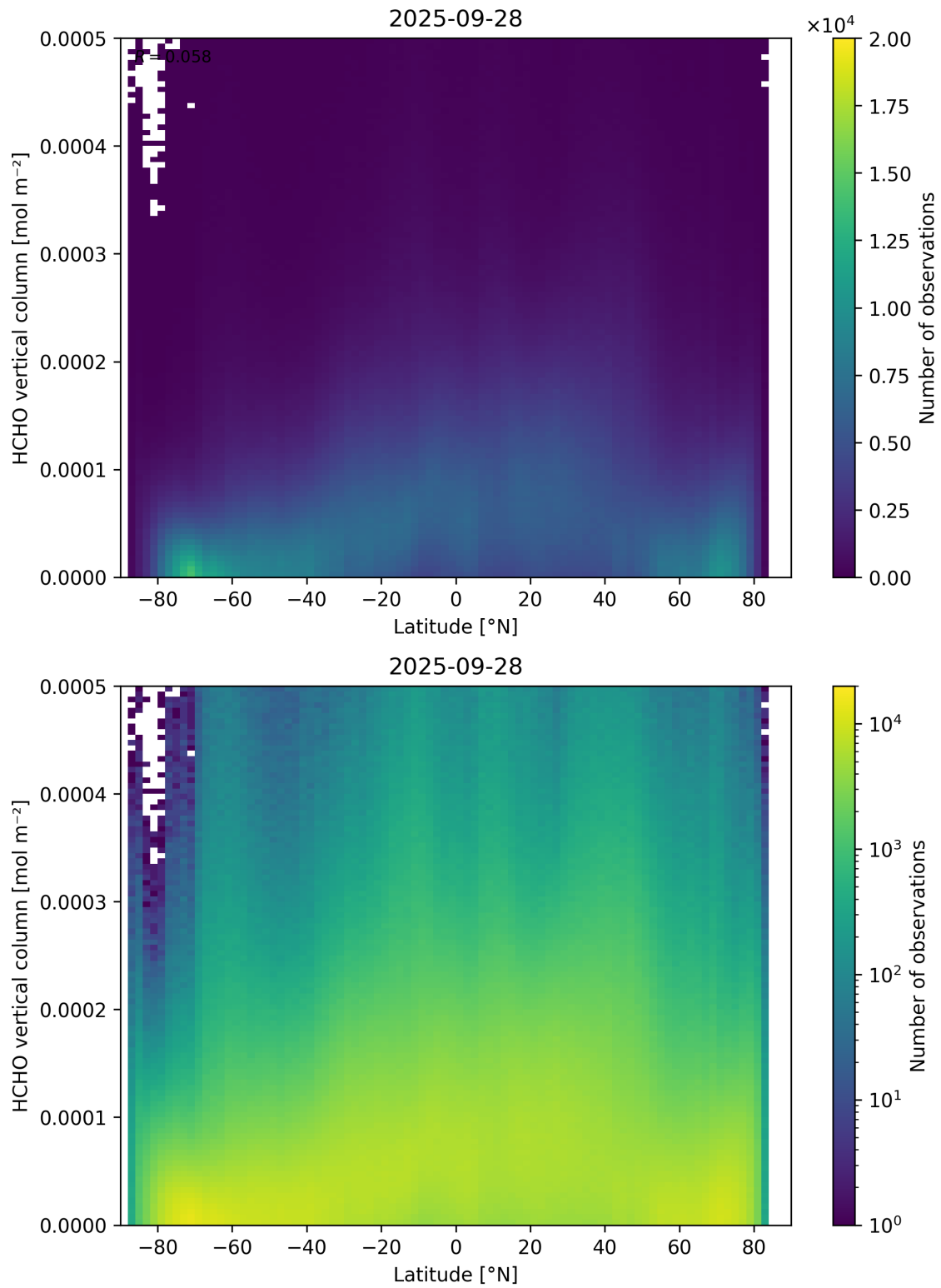
Figure 163: Scatter density plot of “Latitude” against “HCHO vertical column” for 2025-09-27 to 2025-09-29.
