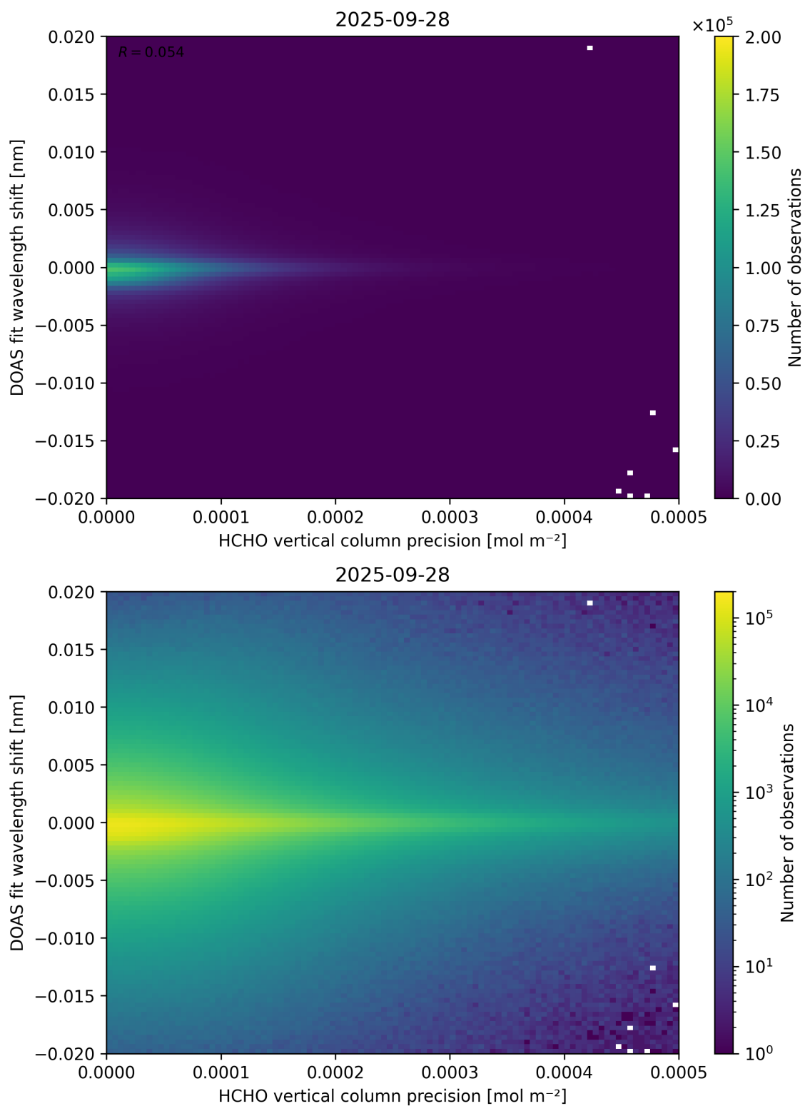
Figure 137: Scatter density plot of “HCHO vertical column precision” against “DOAS fit wavelength shift” for 2025-09-27 to 2025-09-29.
