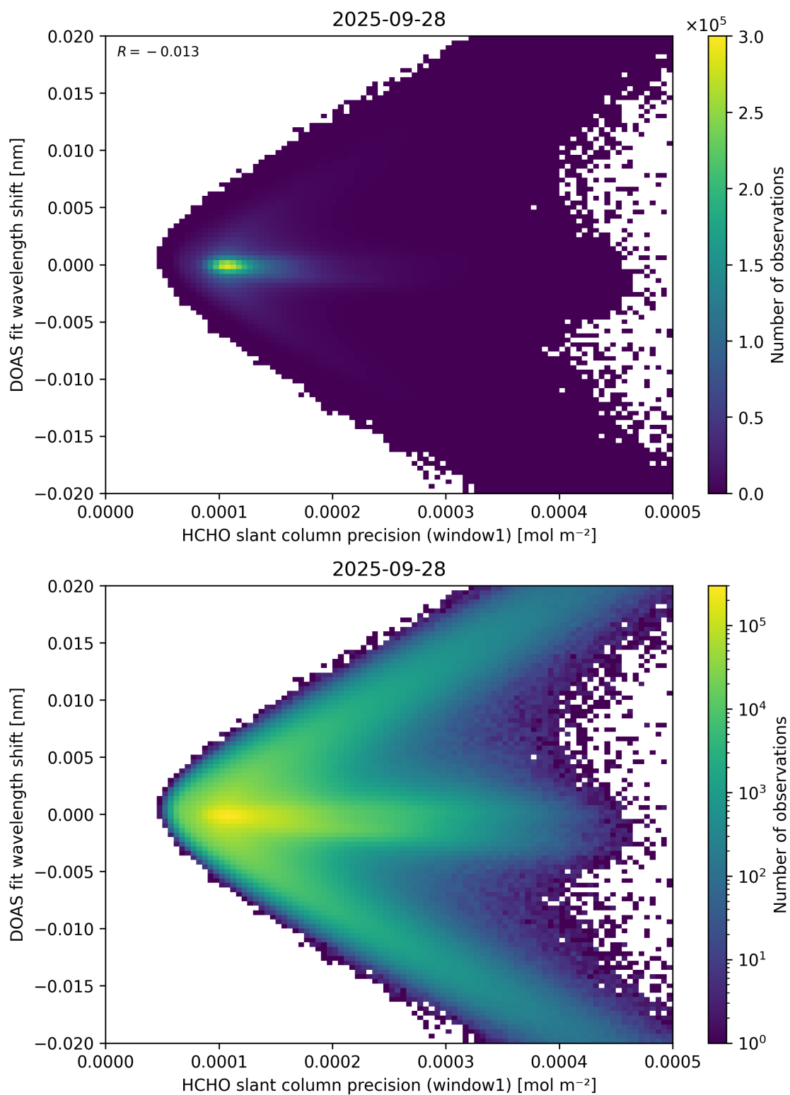
Figure 89: Scatter density plot of “HCHO slant column precision (window1)” against “DOAS fit wavelength shift” for 2025-09-27 to 2025-09-29.
