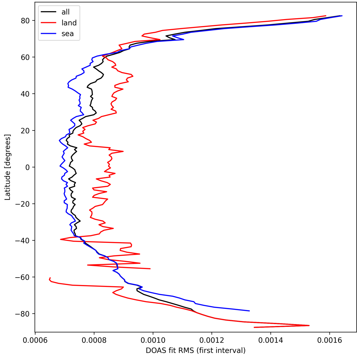
Figure 32: Zonal average of “DOAS fit RMS (first interval)” for 2025-09-27 to 2025-09-29.
