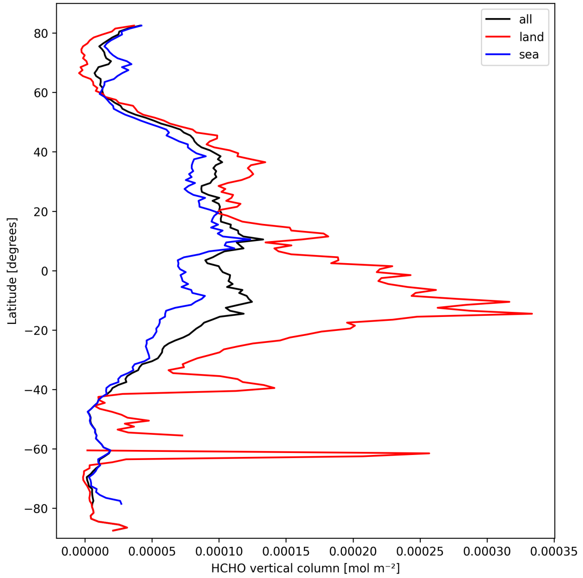
Figure 21: Zonal average of “HCHO vertical column” for 2025-09-27 to 2025-09-29.
