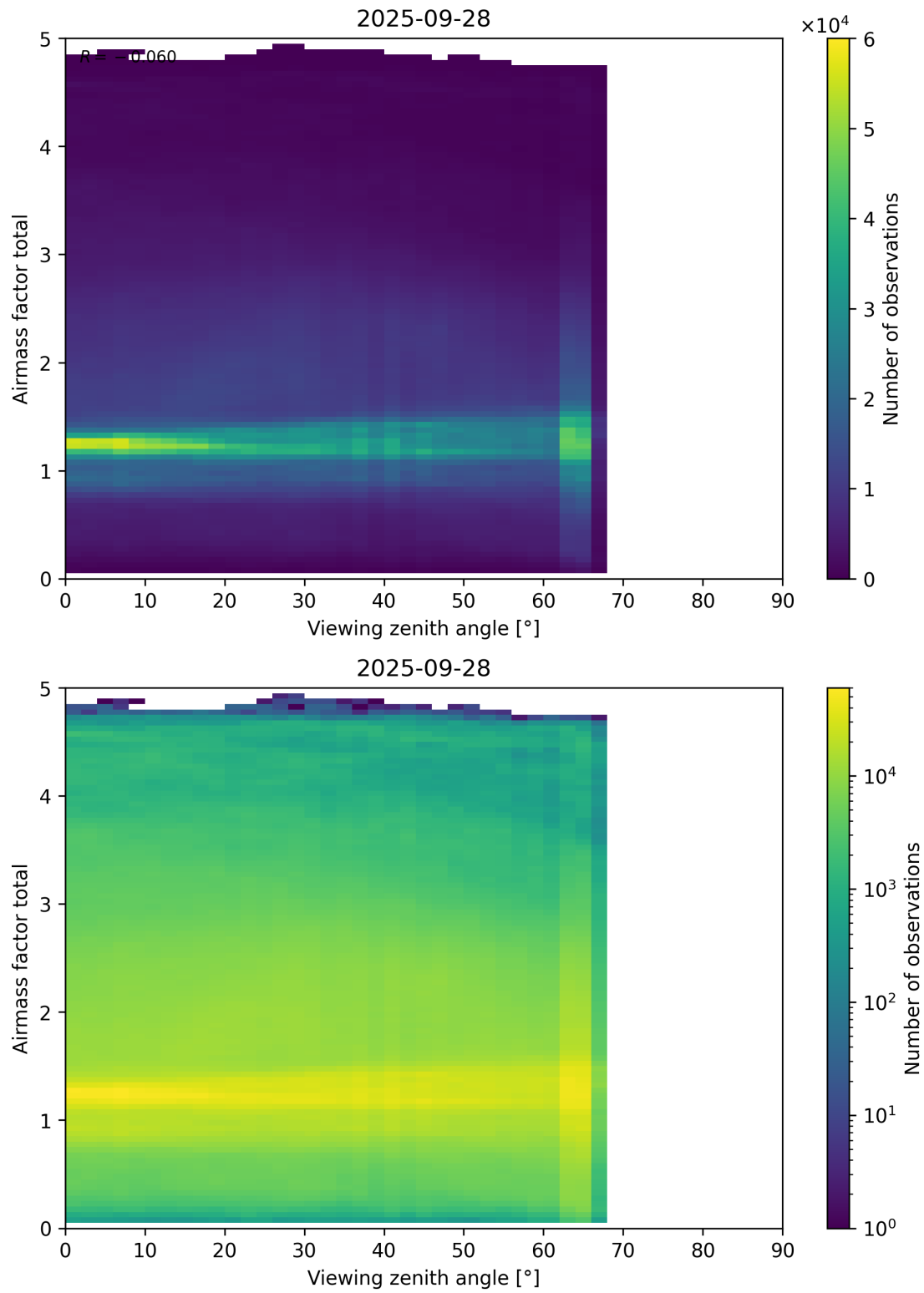
Figure 190: Scatter density plot of “Viewing zenith angle” against “Airmass factor total” for 2025-09-27 to 2025-09-29.
