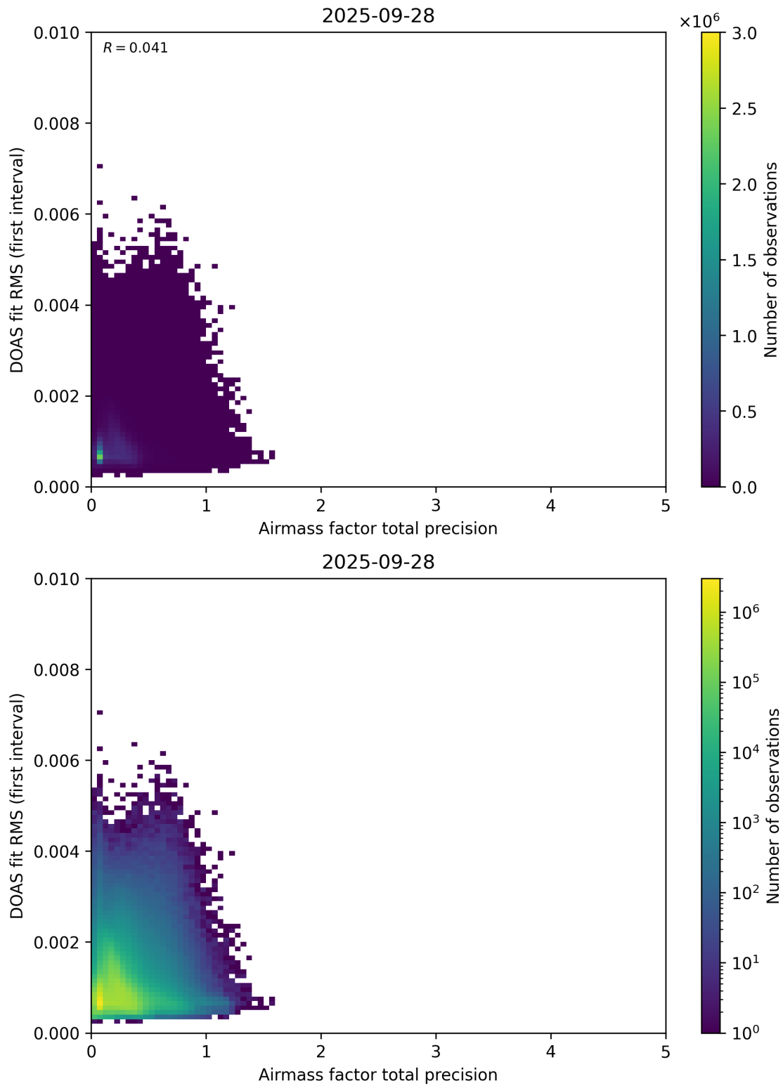
Figure 105: Scatter density plot of “Airmass factor total precision” against “DOAS fit RMS (first interval)” for 2025-09-27 to 2025-09-29.
