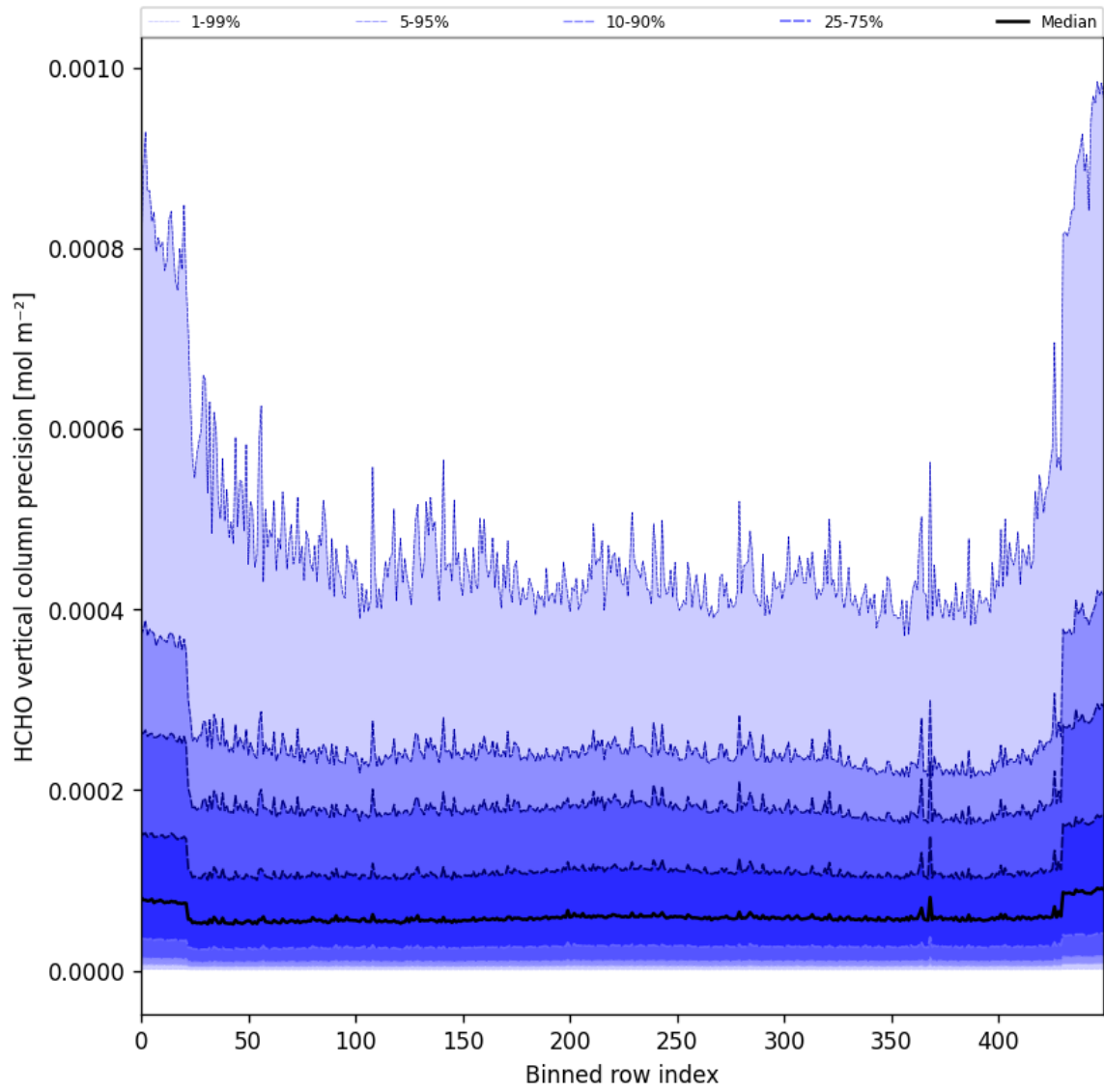
Figure 50: Along track statistics of “HCHO vertical column precision” for 2025-09-27 to 2025-09-29
