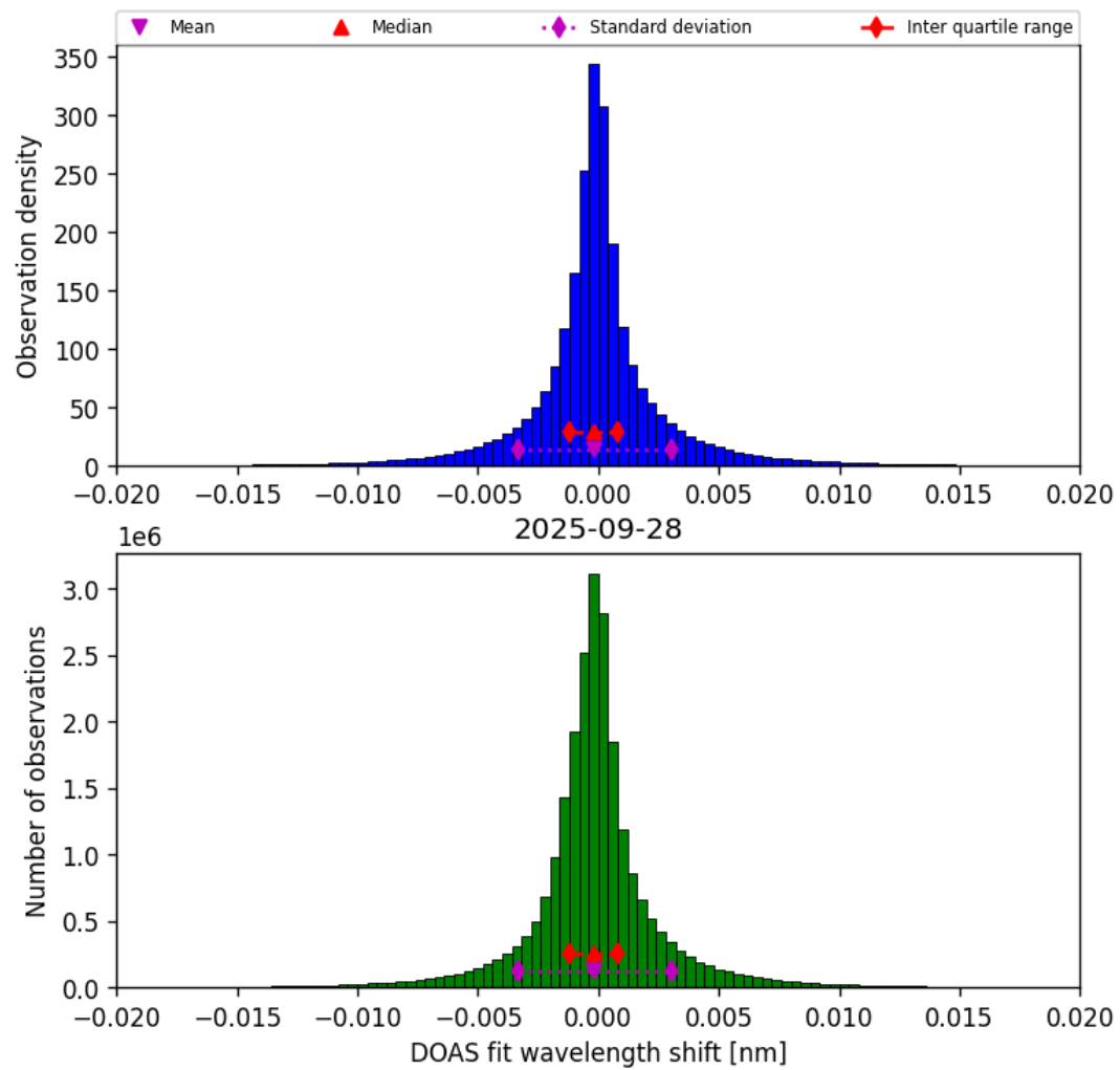
Figure 44: Histogram of “DOAS fit wavelength shift” for 2025-09-27 to 2025-09-29
