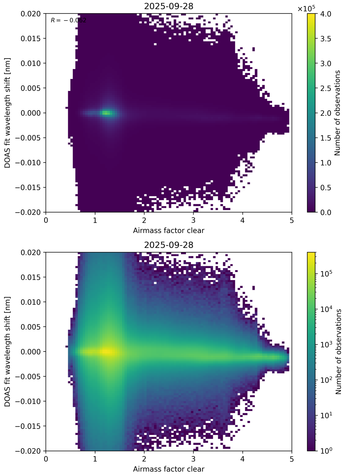
Figure 72: Scatter density plot of “Airmass factor clear” against “DOAS fit wavelength shift” for 2025-09-27 to 2025-09-29.
