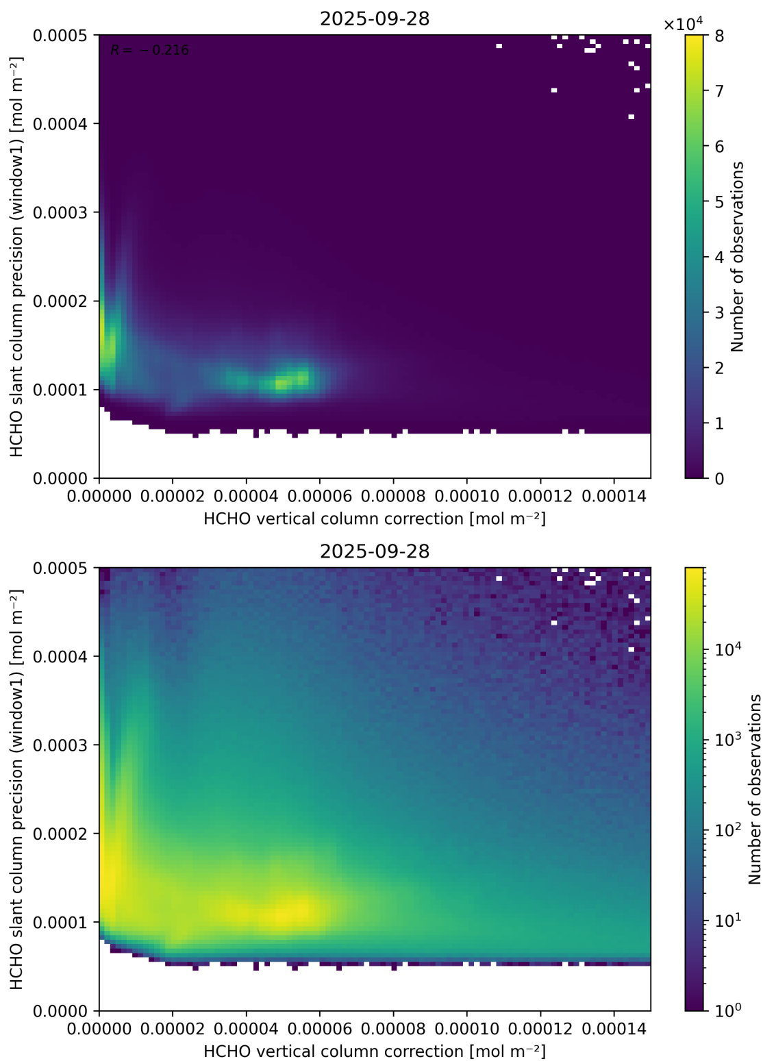
Figure 119: Scatter density plot of “HCHO vertical column correction” against “HCHO slant column precision (window1)” for 2025-09-27 to 2025-09-29.
