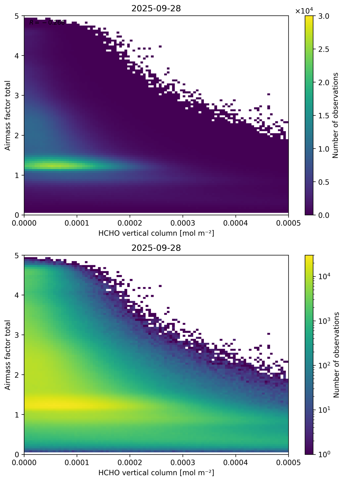
Figure 131: Scatter density plot of “HCHO vertical column” against “Airmass factor total” for 2025-09-27 to 2025-09-29.
