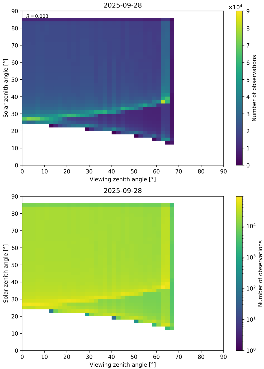
Figure 197: Scatter density plot of “Viewing zenith angle” against “Solar zenith angle” for 2025-09-27 to 2025-09-29.
