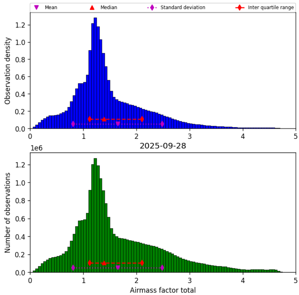
Figure 40: Histogram of “Airmass factor total” for 2025-09-27 to 2025-09-29
