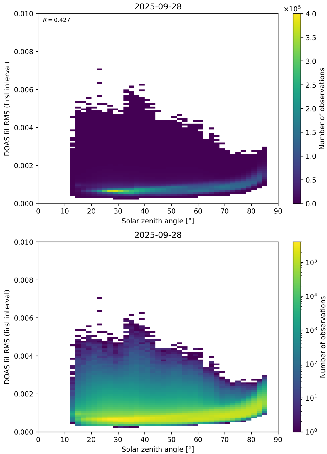
Figure 167: Scatter density plot of “Solar zenith angle” against “DOAS fit RMS (first interval)” for 2025-09-27 to 2025-09-29.
