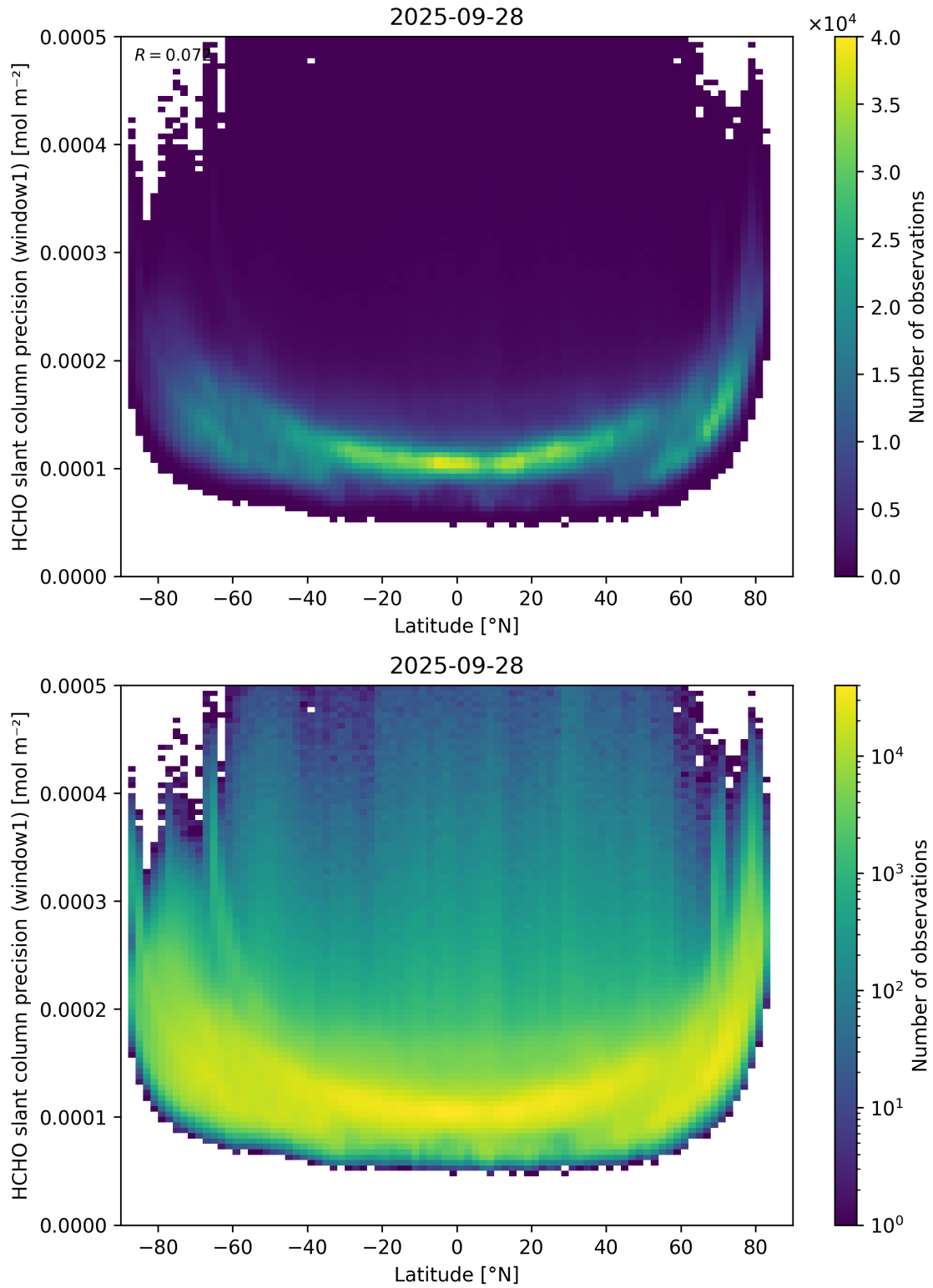
Figure 160: Scatter density plot of “Latitude” against “HCHO slant column precision (window1)” for 2025-09-27 to 2025-09-29.
