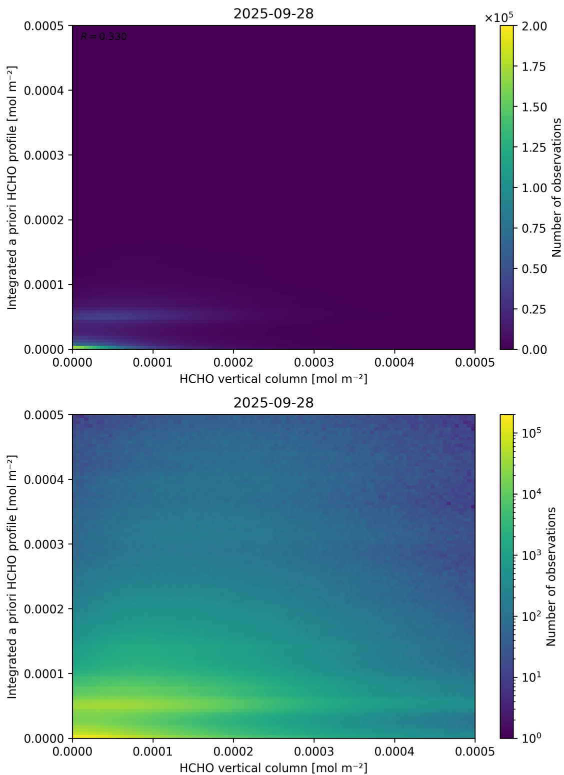
Figure 135: Scatter density plot of “HCHO vertical column” against “Integrated a priori HCHO profile” for 2025-09-27 to 2025-09-29.
