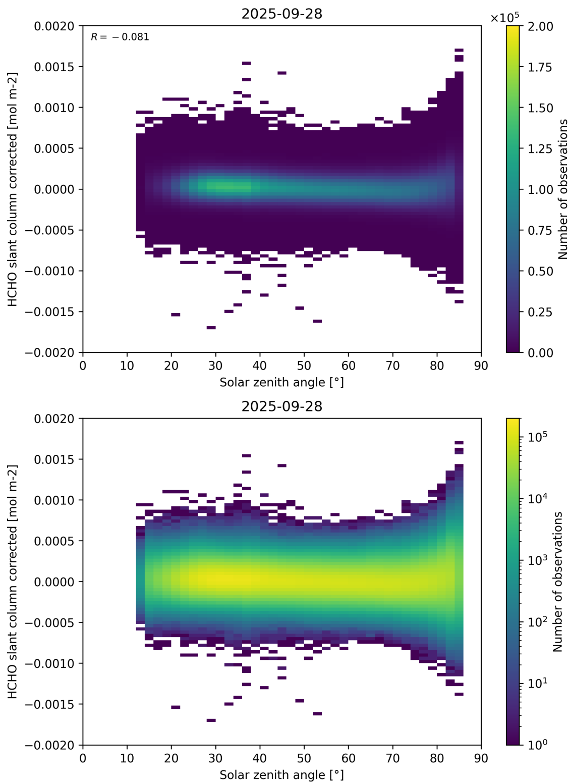
Figure 171: Scatter density plot of “Solar zenith angle” against “HCHO slant column corrected” for 2025-09-27 to 2025-09-29.
