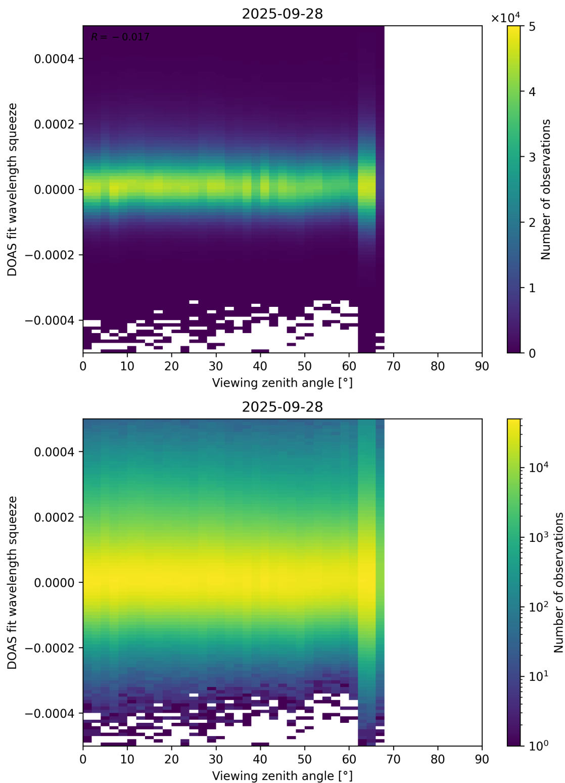
Figure 184: Scatter density plot of “Viewing zenith angle” against “DOAS fit wavelength squeeze” for 2025-09-27 to 2025-09-29.
