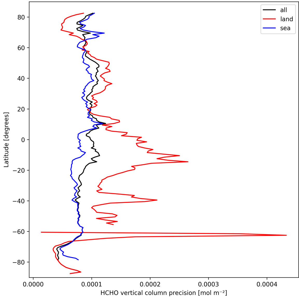
Figure 22: Zonal average of “HCHO vertical column precision” for 2025-09-27 to 2025-09-29.
