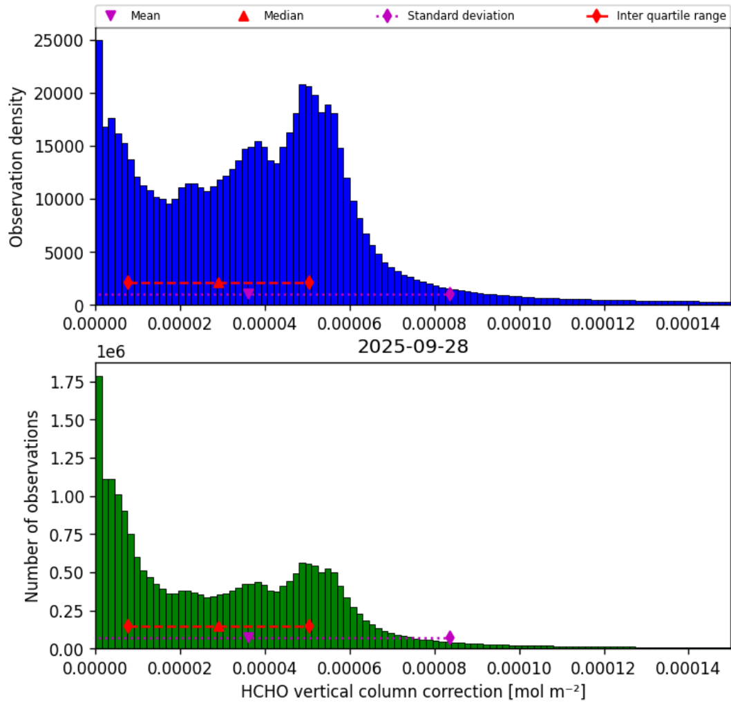
Figure 37: Histogram of “HCHO vertical column correction” for 2025-09-27 to 2025-09-29
