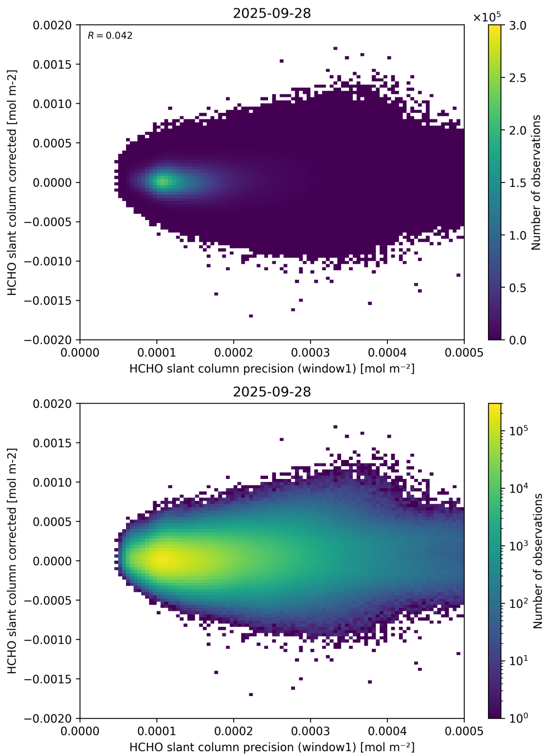
Figure 92: Scatter density plot of “HCHO slant column precision (window1)” against “HCHO slant column corrected” for 2025-09-27 to 2025-09-29.
