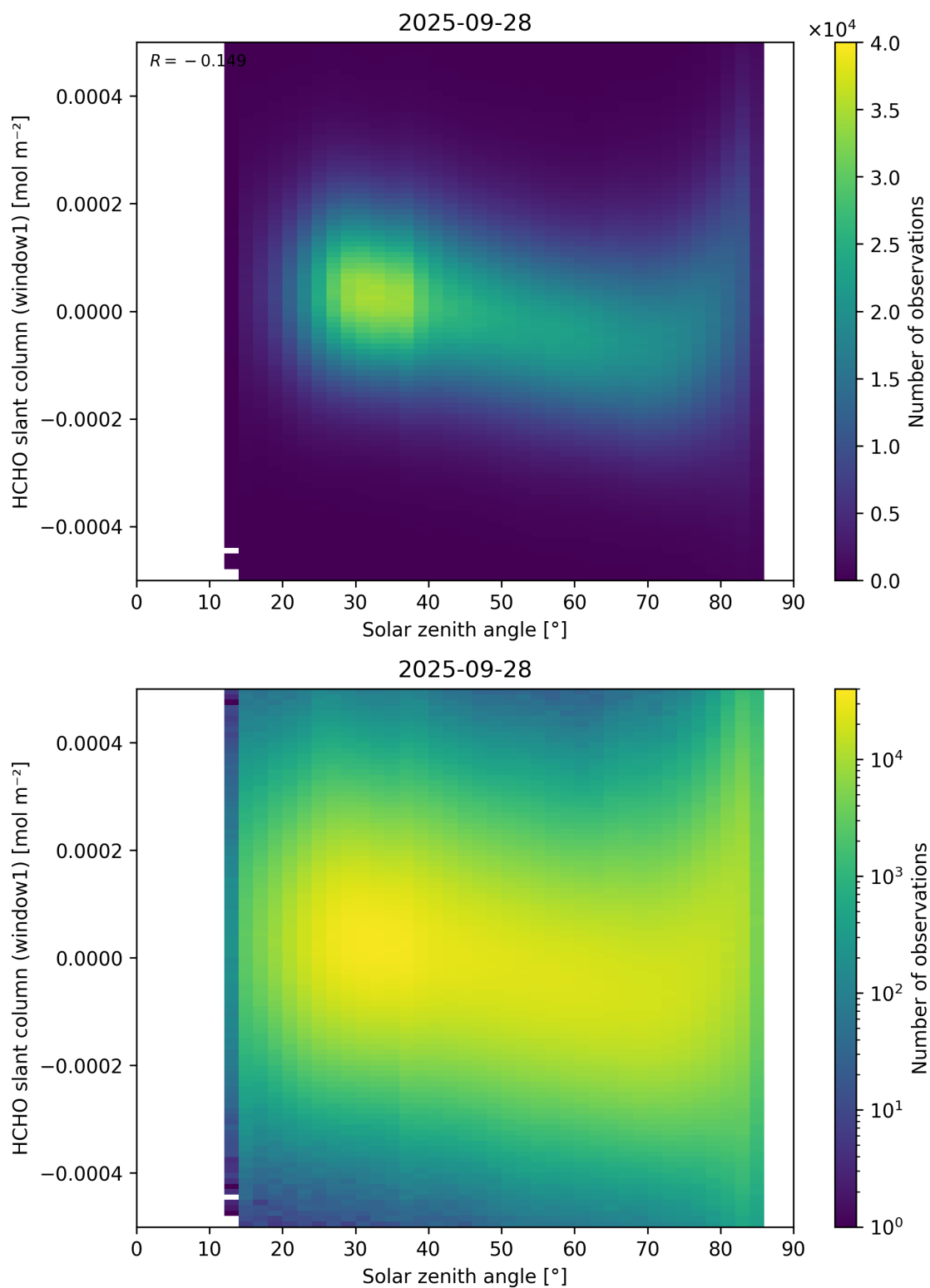
Figure 173: Scatter density plot of “Solar zenith angle” against “HCHO slant column (window1)” for 2025-09-27 to 2025-09-29.
