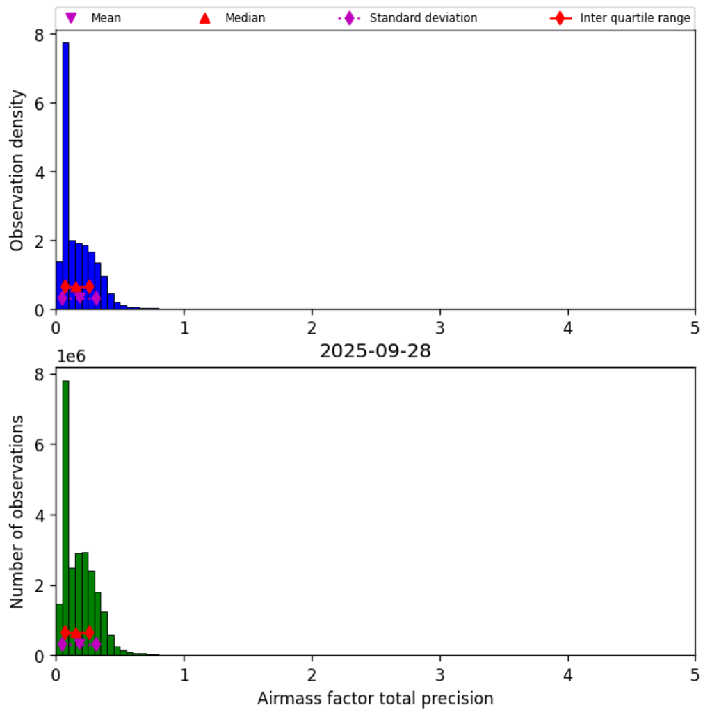
Figure 41: Histogram of “Airmass factor total precision” for 2025-09-27 to 2025-09-29
