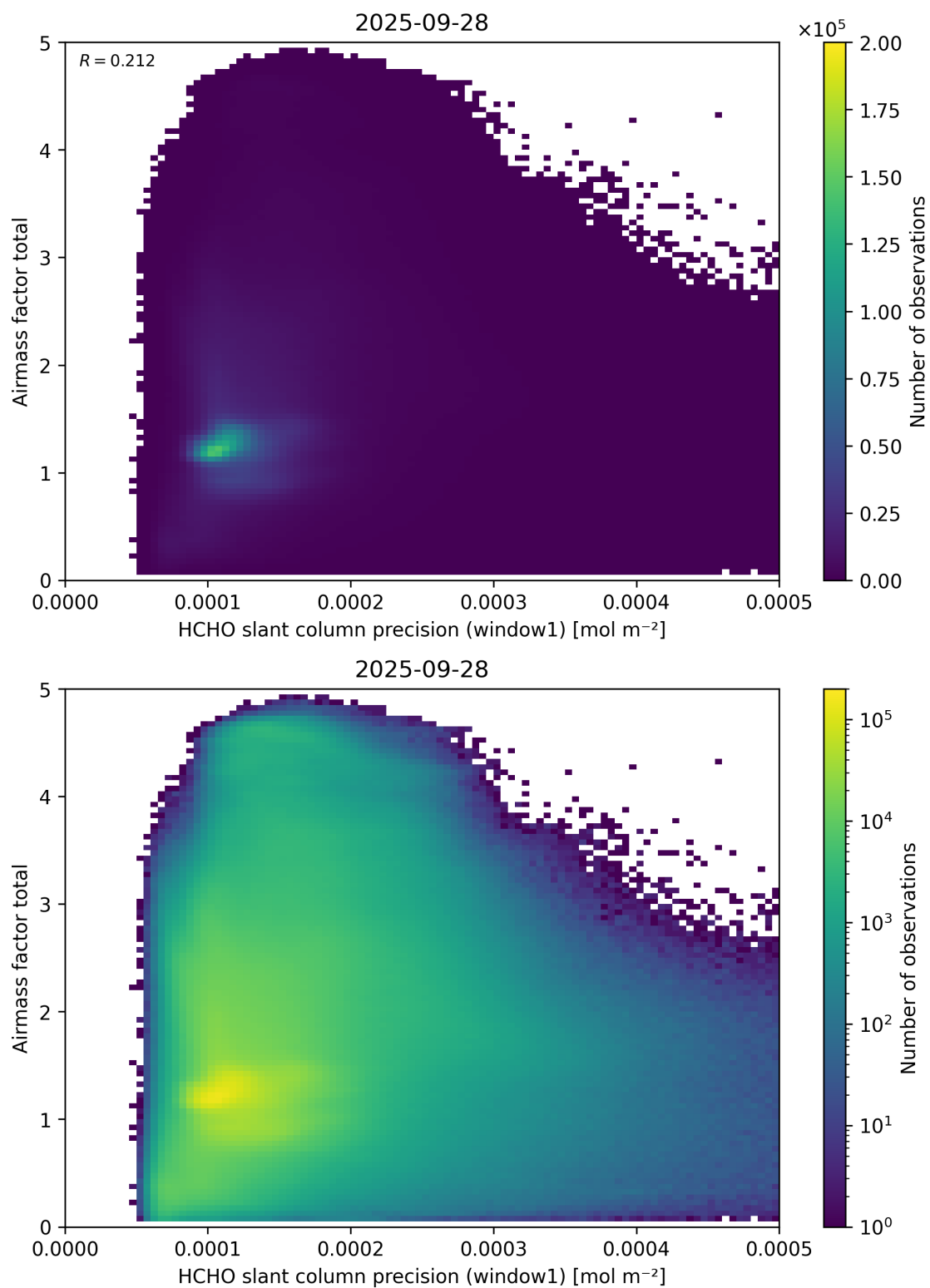
Figure 94: Scatter density plot of “HCHO slant column precision (window1)” against “Airmass factor total” for 2025-09-27 to 2025-09-29.
