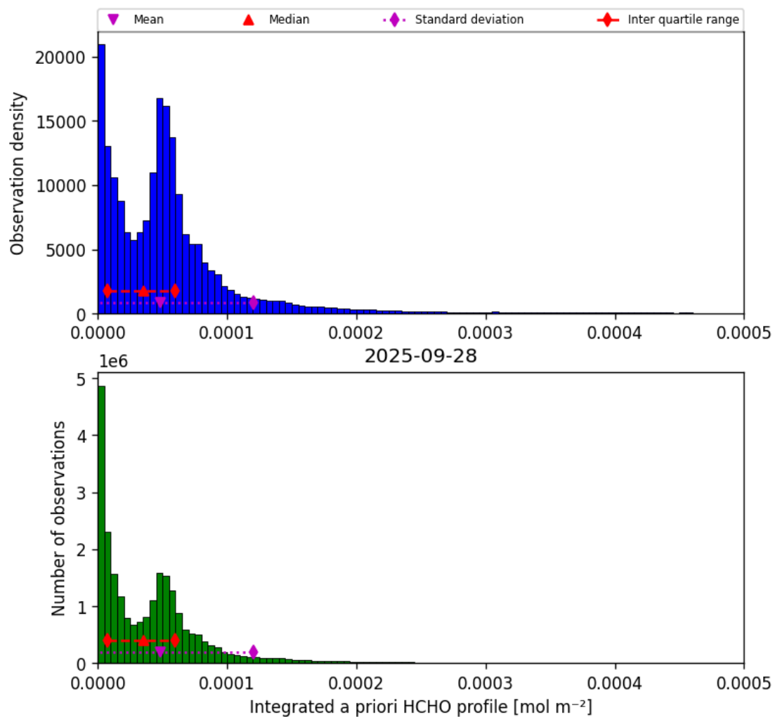
Figure 43: Histogram of “Integrated a priori HCHO profile” for 2025-09-27 to 2025-09-29
