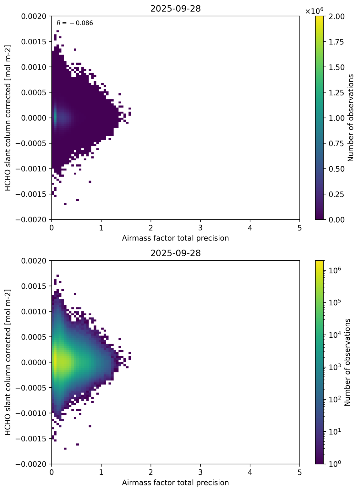
Figure 109: Scatter density plot of “Airmass factor total precision” against “HCHO slant column corrected” for 2025-09-27 to 2025-09-29.
