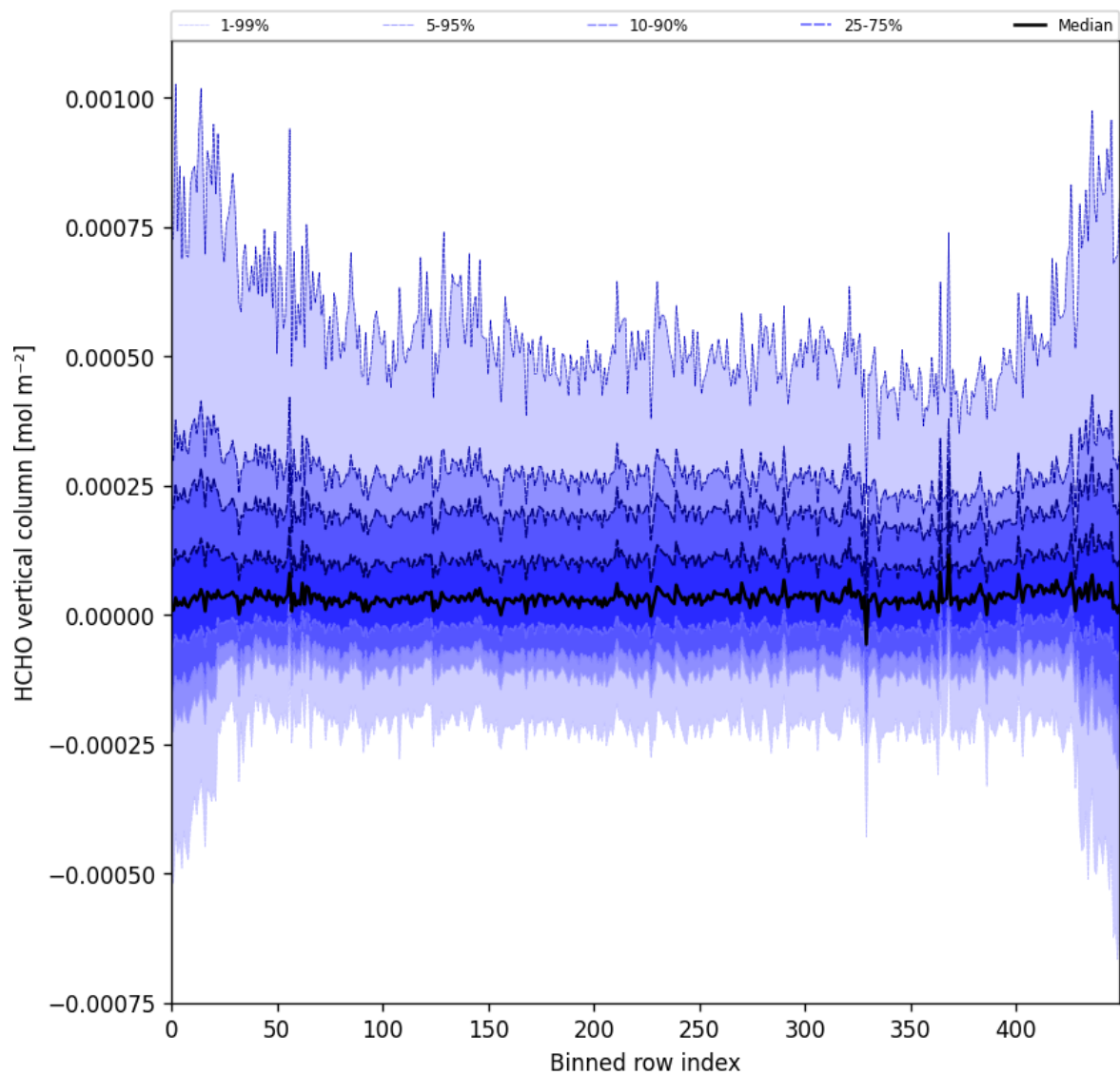
Figure 49: Along track statistics of “HCHO vertical column” for 2025-09-27 to 2025-09-29
