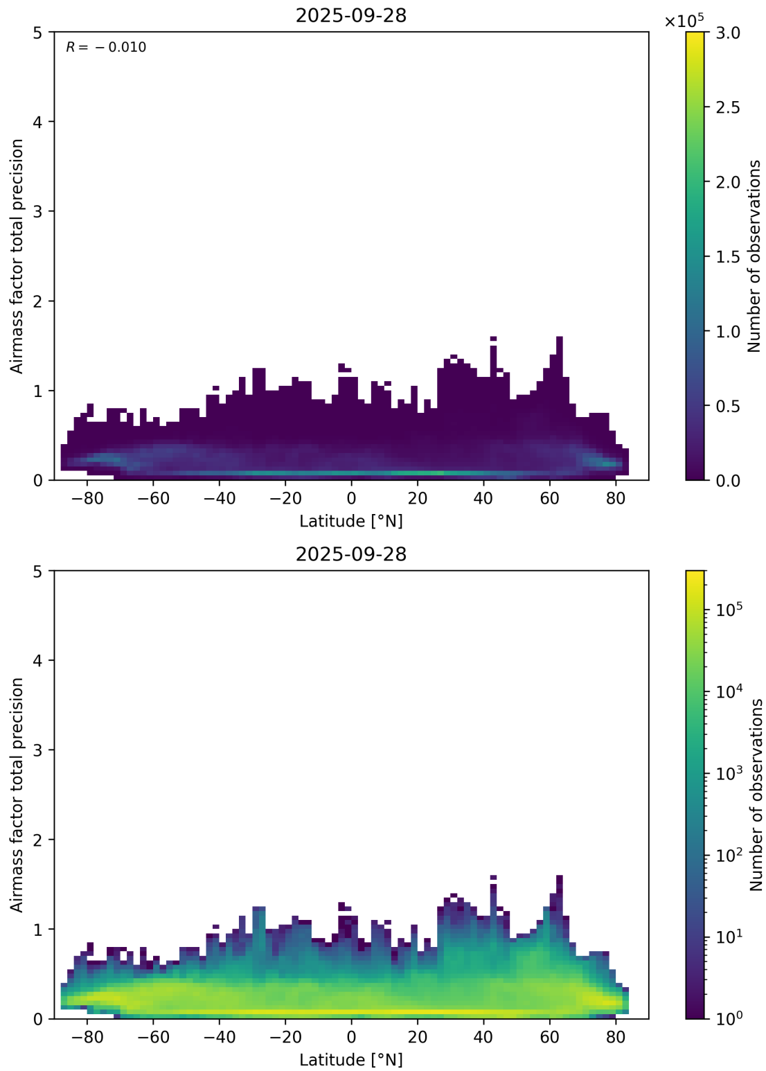
Figure 162: Scatter density plot of “Latitude” against “Airmass factor total precision” for 2025-09-27 to 2025-09-29.
