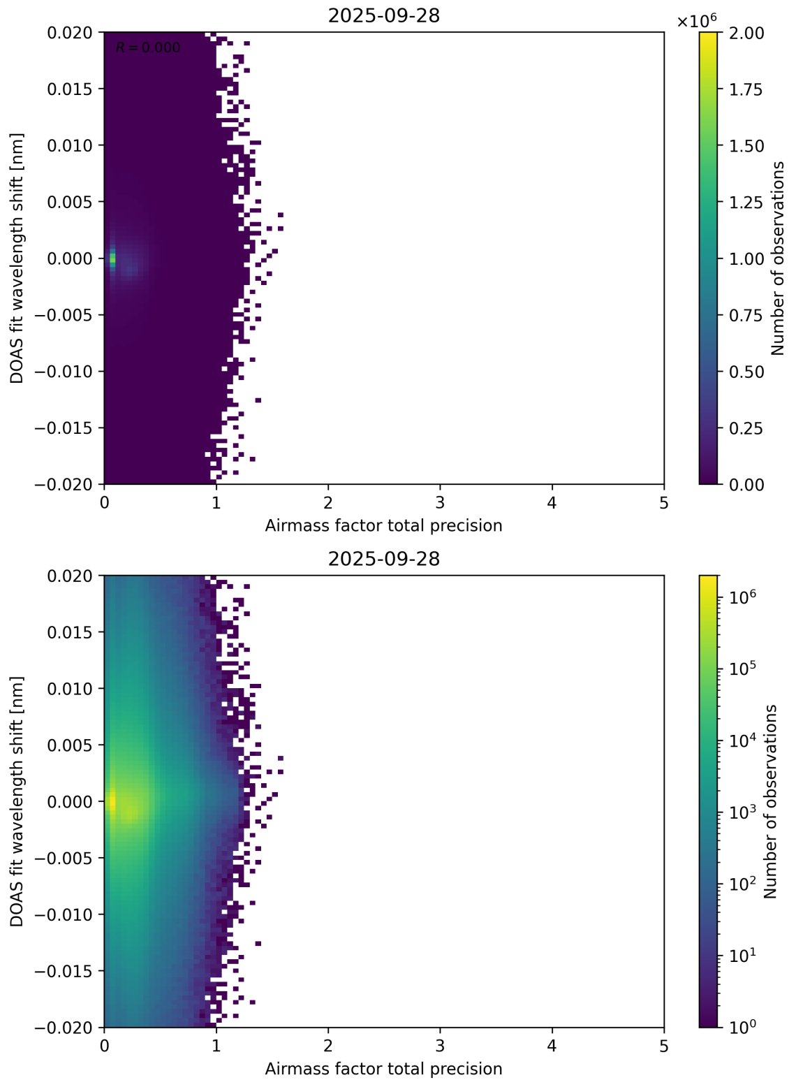
Figure 106: Scatter density plot of “Airmass factor total precision” against “DOAS fit wavelength shift” for 2025-09-27 to 2025-09-29.
