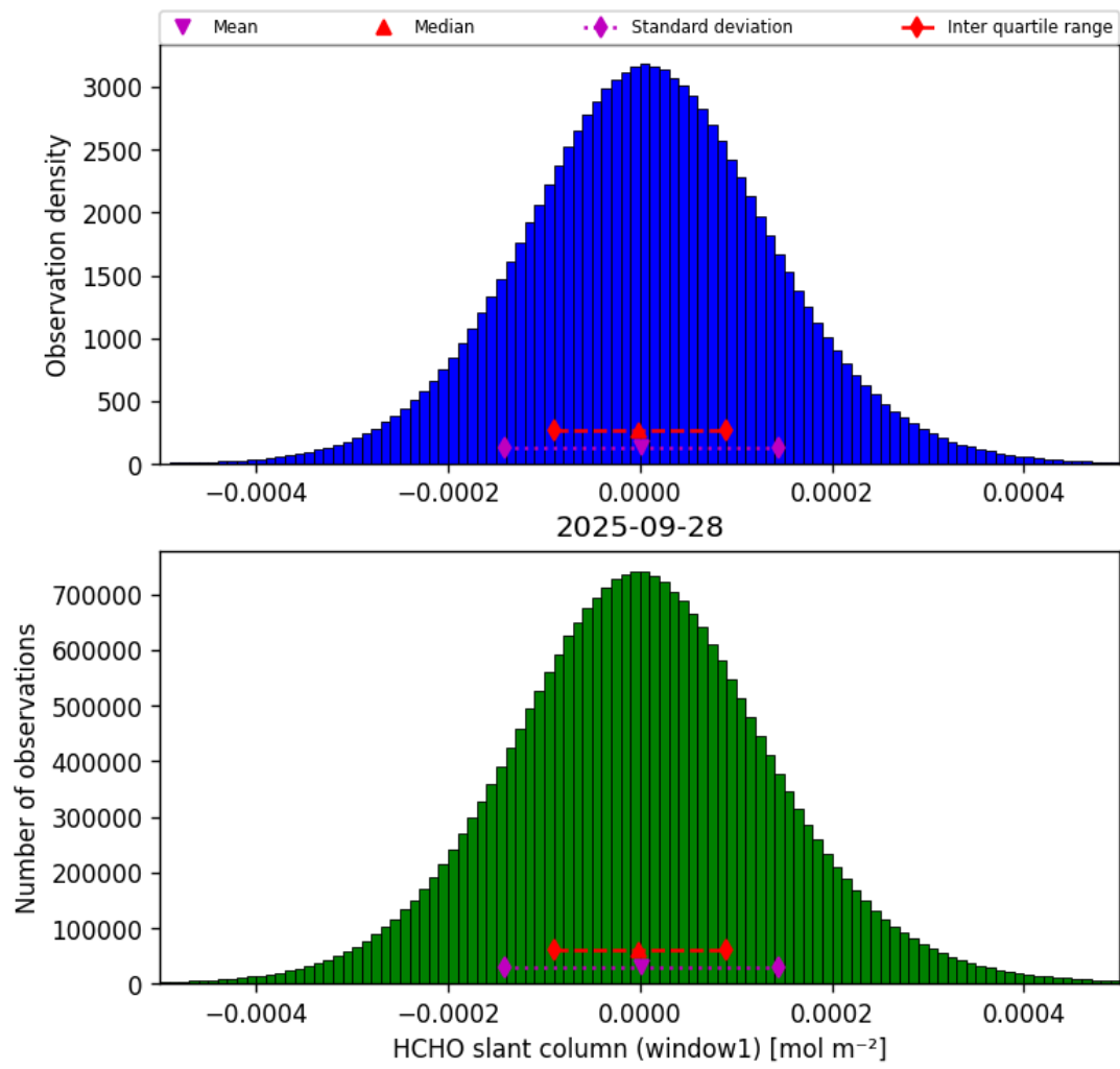
Figure 38: Histogram of “HCHO slant column (window1)” for 2025-09-27 to 2025-09-29
