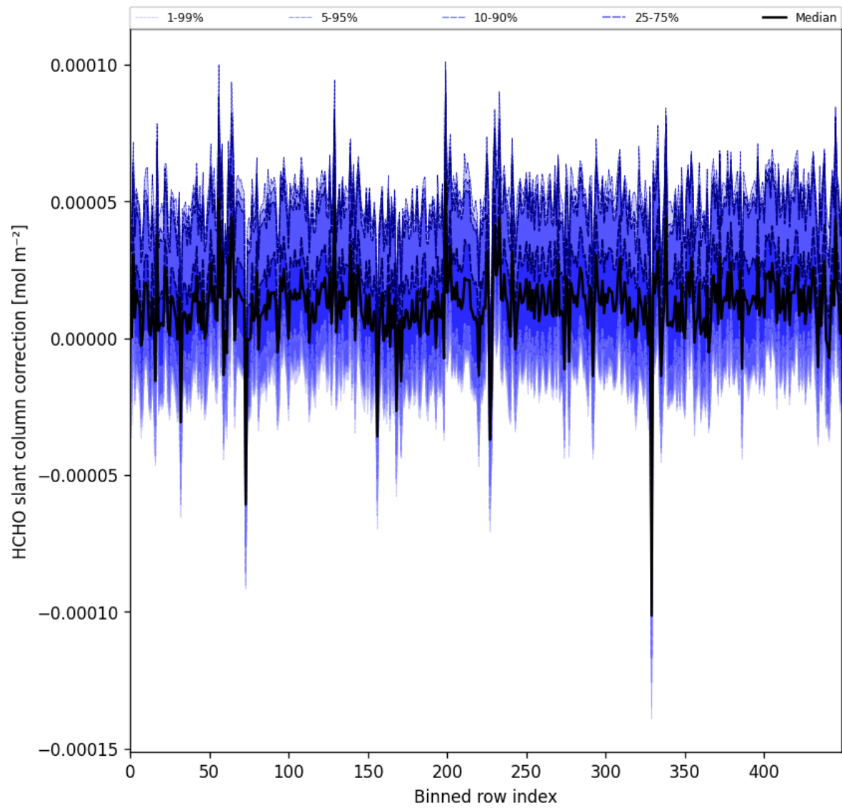
Figure 61: Along track statistics of “HCHO slant column correction” for 2025-09-27 to 2025-09-29
