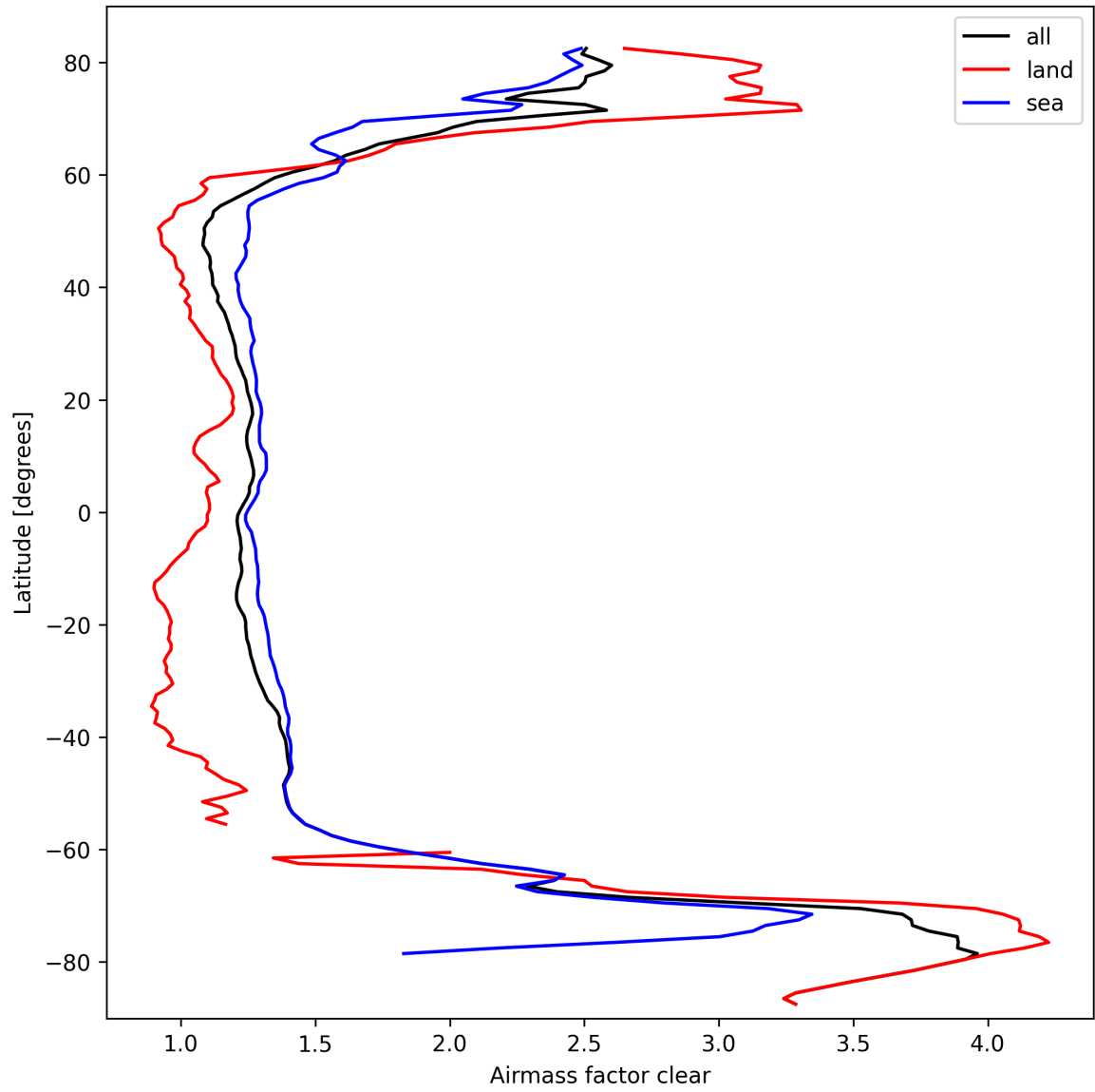
Figure 28: Zonal average of “Airmass factor clear” for 2025-09-27 to 2025-09-29.
