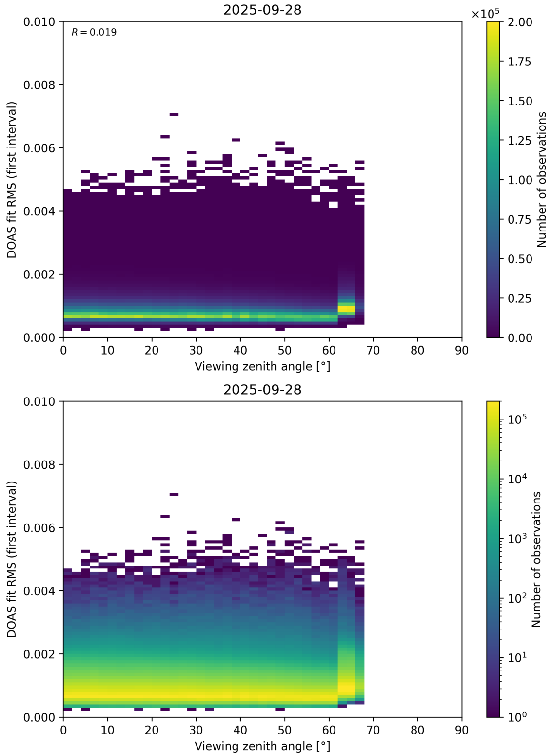
Figure 182: Scatter density plot of “Viewing zenith angle” against “DOAS fit RMS (first interval)” for 2025-09-27 to 2025-09-29.
