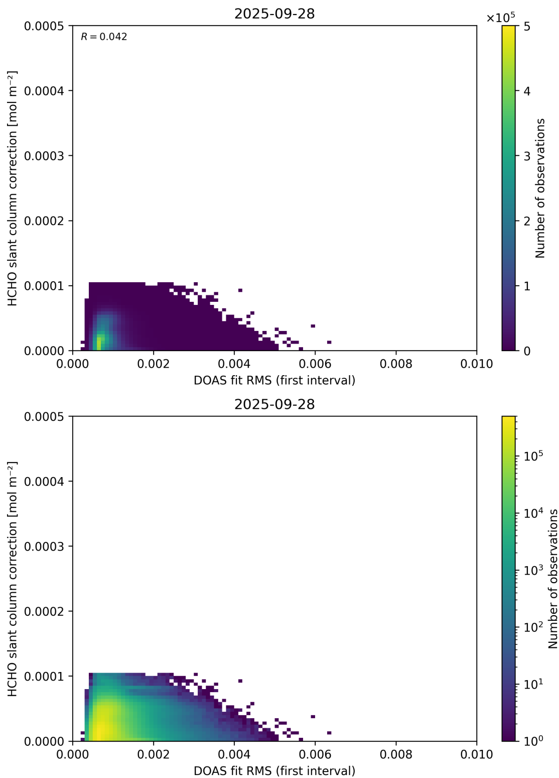
Figure 63: Scatter density plot of “DOAS fit RMS (first interval)” against “HCHO slant column correction” for 2025-09-27 to 2025-09-29.
