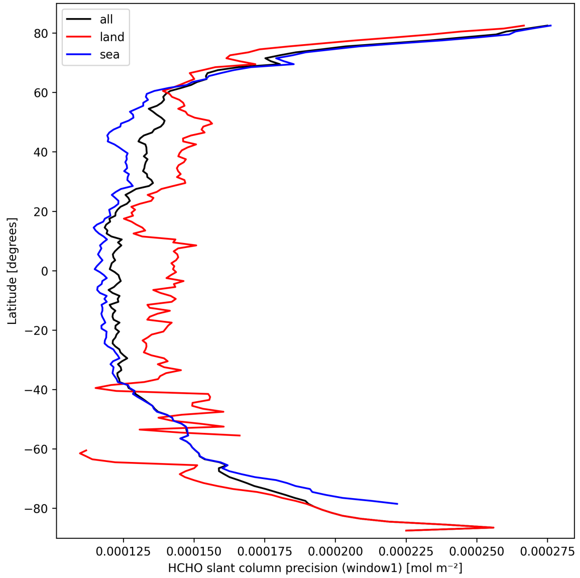
Figure 25: Zonal average of “HCHO slant column precision (window1)” for 2025-09-27 to 2025-09-29.
