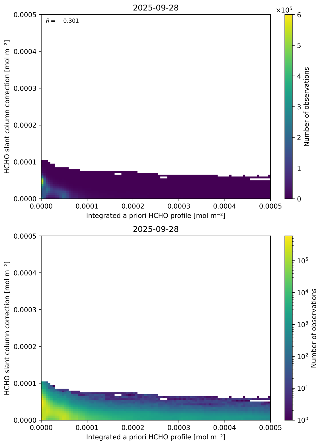
Figure 152: Scatter density plot of “Integrated a priori HCHO profile” against “HCHO slant column correction” for 2025-09-27 to 2025-09-29.
