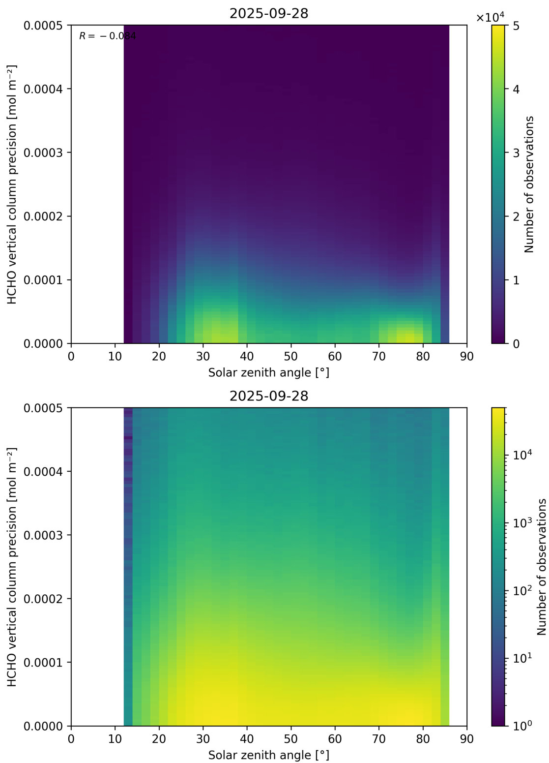
Figure 179: Scatter density plot of “Solar zenith angle” against “HCHO vertical column precision” for 2025-09-27 to 2025-09-29.
