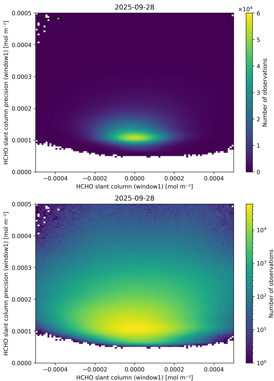
Figure 84: Scatter density plot of “HCHO slant column (window1)” against “HCHO slant column precision (window1)” for 2025-09-27 to 2025-09-29.
