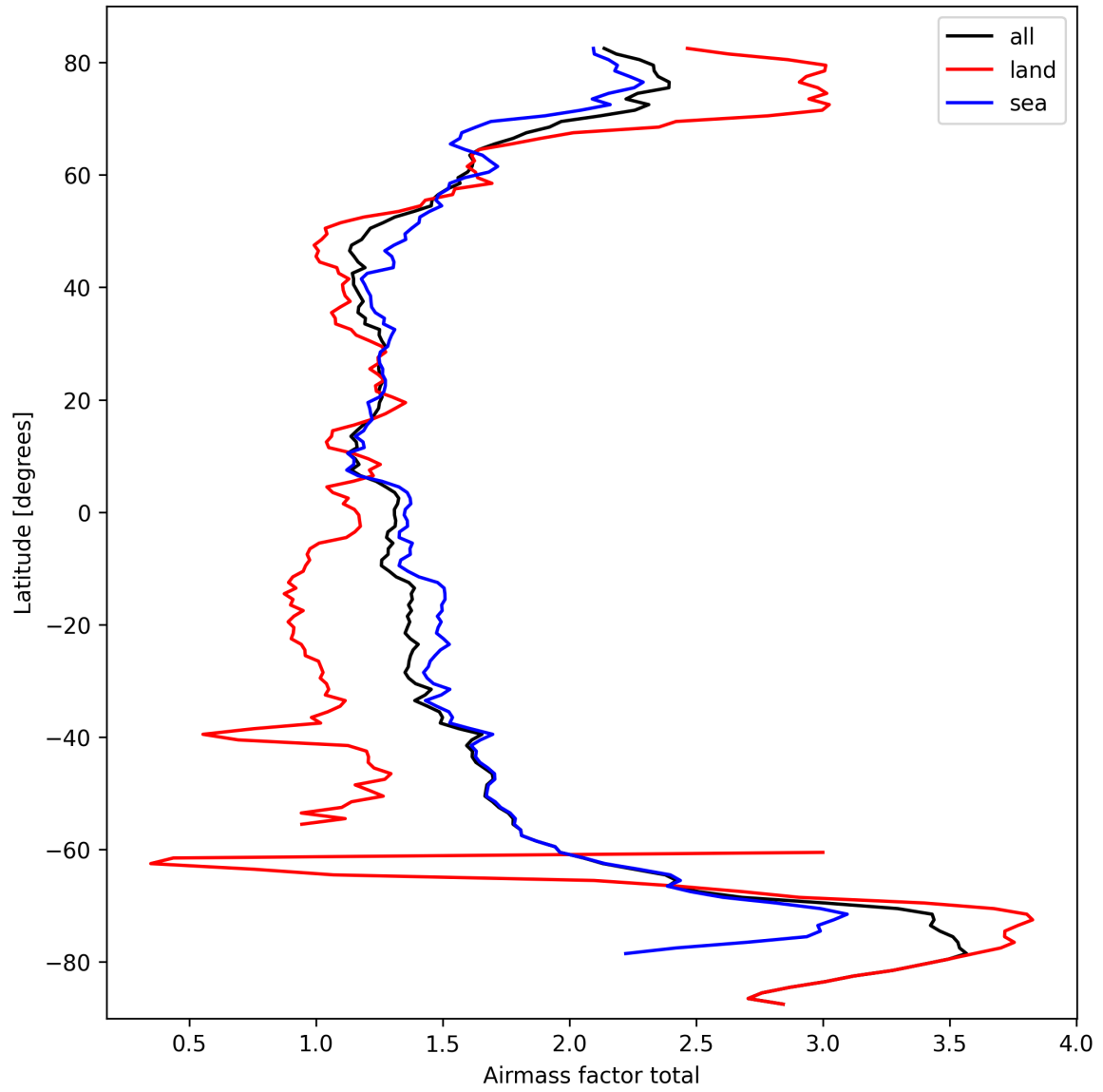
Figure 26: Zonal average of “Airmass factor total” for 2025-09-27 to 2025-09-29.
