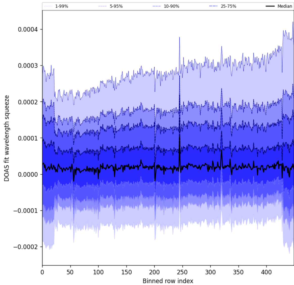
Figure 59: Along track statistics of “DOAS fit wavelength squeeze” for 2025-09-27 to 2025-09-29
