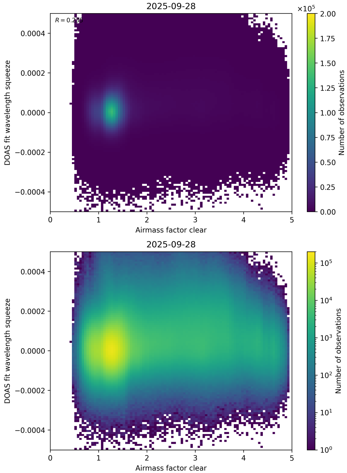
Figure 73: Scatter density plot of “Airmass factor clear” against “DOAS fit wavelength squeeze” for 2025-09-27 to 2025-09-29.
