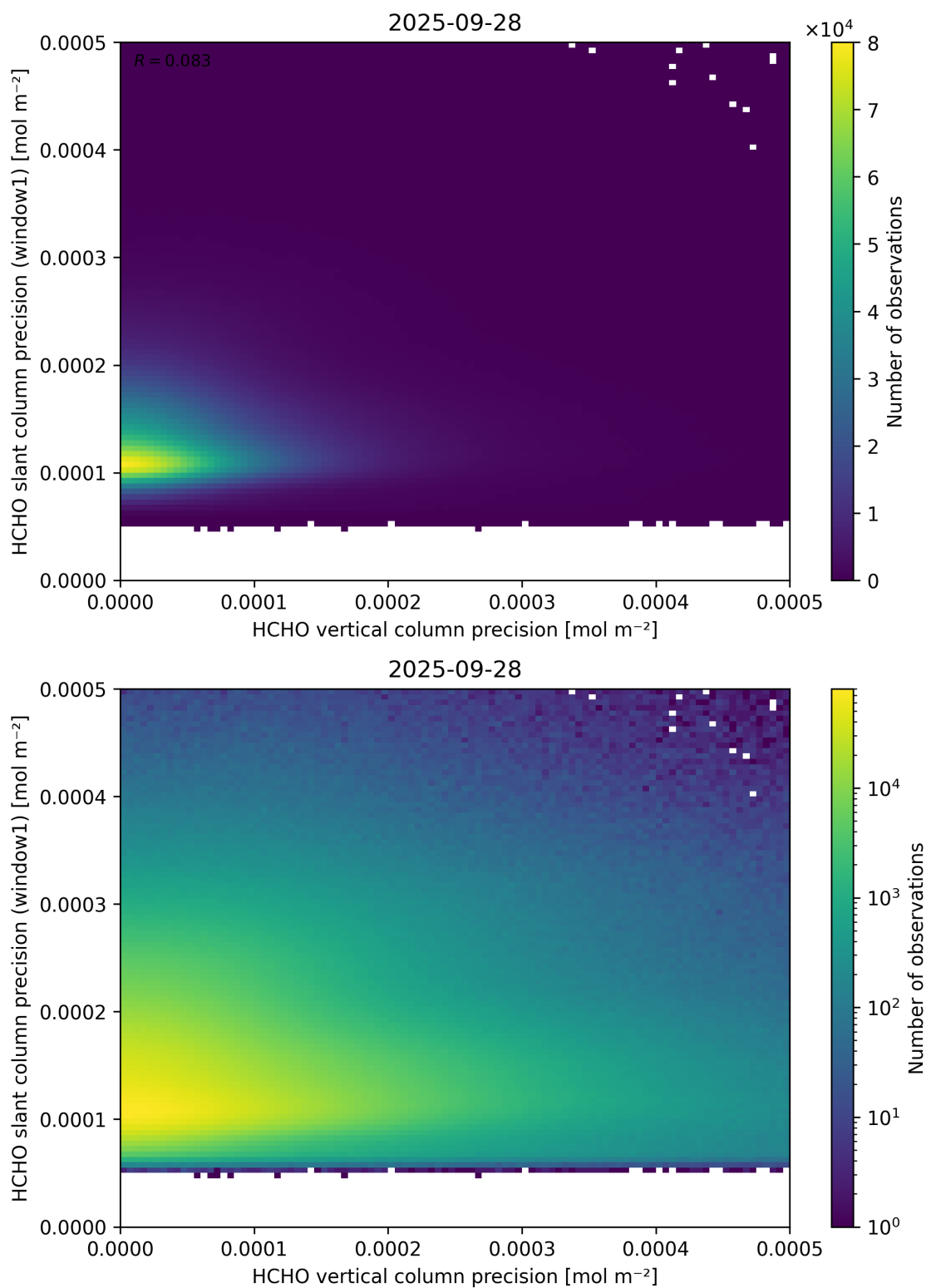
Figure 143: Scatter density plot of “HCHO vertical column precision” against “HCHO slant column precision (window1)” for 2025-09-27 to 2025-09-29.
