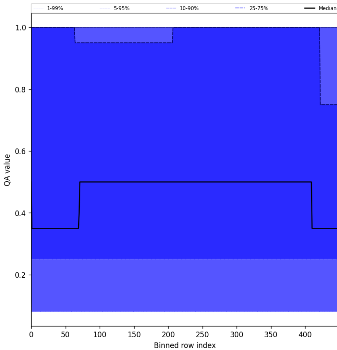
Figure 48: Along track statistics of “QA value” for 2025-09-27 to 2025-09-29
