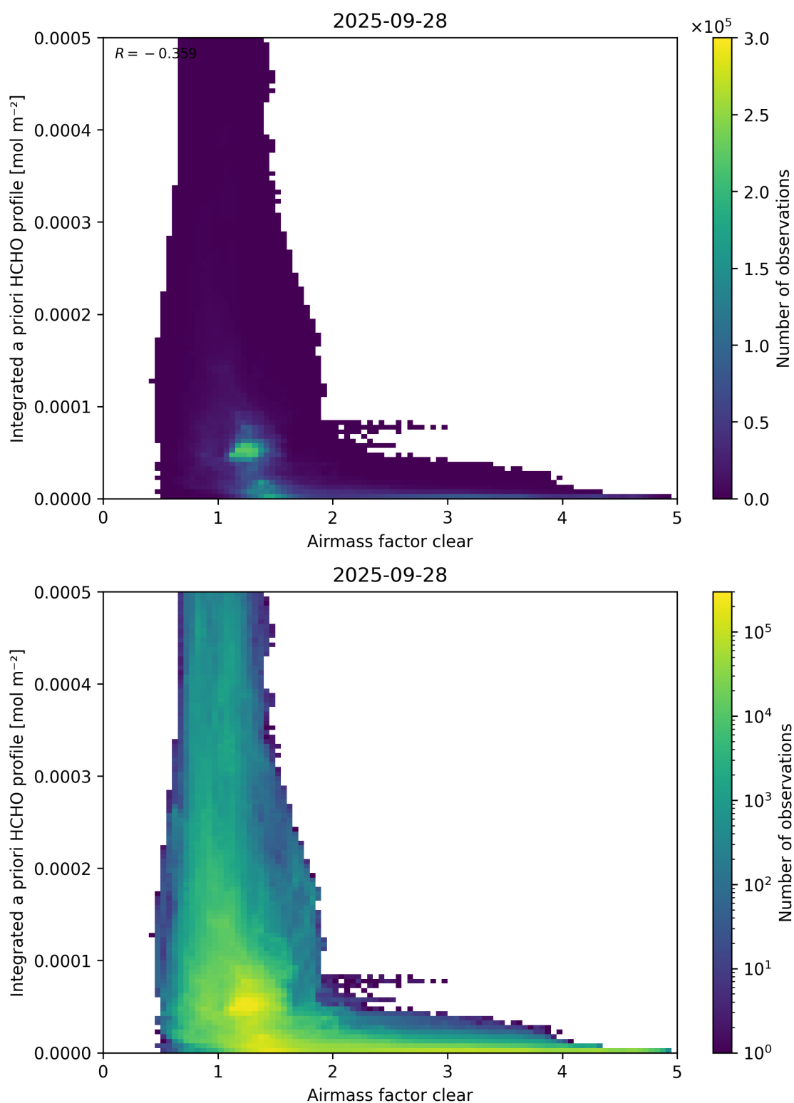
Figure 76: Scatter density plot of “Airmass factor clear” against “Integrated a priori HCHO profile” for 2025-09-27 to 2025-09-29.
