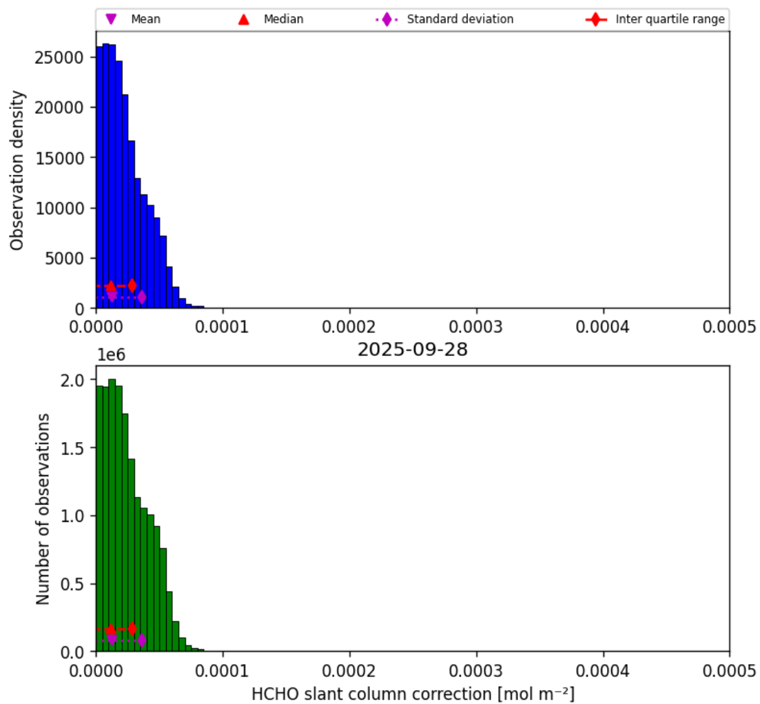
Figure 47: Histogram of “HCHO slant column correction” for 2025-09-27 to 2025-09-29
