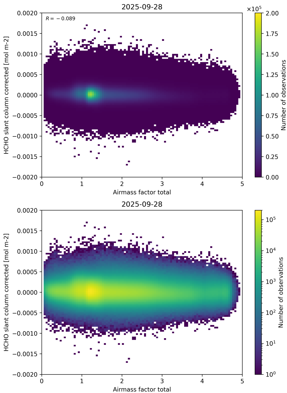
Figure 101: Scatter density plot of “Airmass factor total” against “HCHO slant column corrected” for 2025-09-27 to 2025-09-29.
