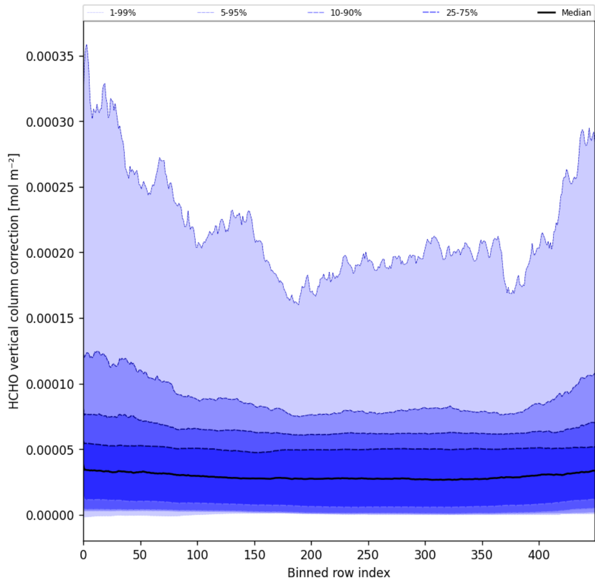
Figure 51: Along track statistics of “HCHO vertical column correction” for 2025-09-27 to 2025-09-29
