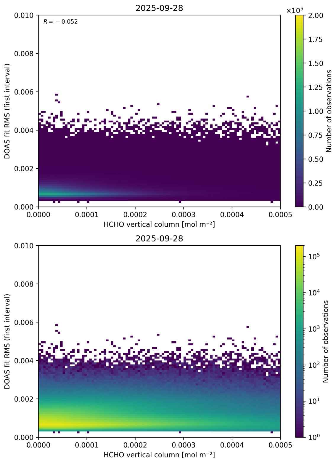
Figure 123: Scatter density plot of “HCHO vertical column” against “DOAS fit RMS (first interval)” for 2025-09-27 to 2025-09-29.
