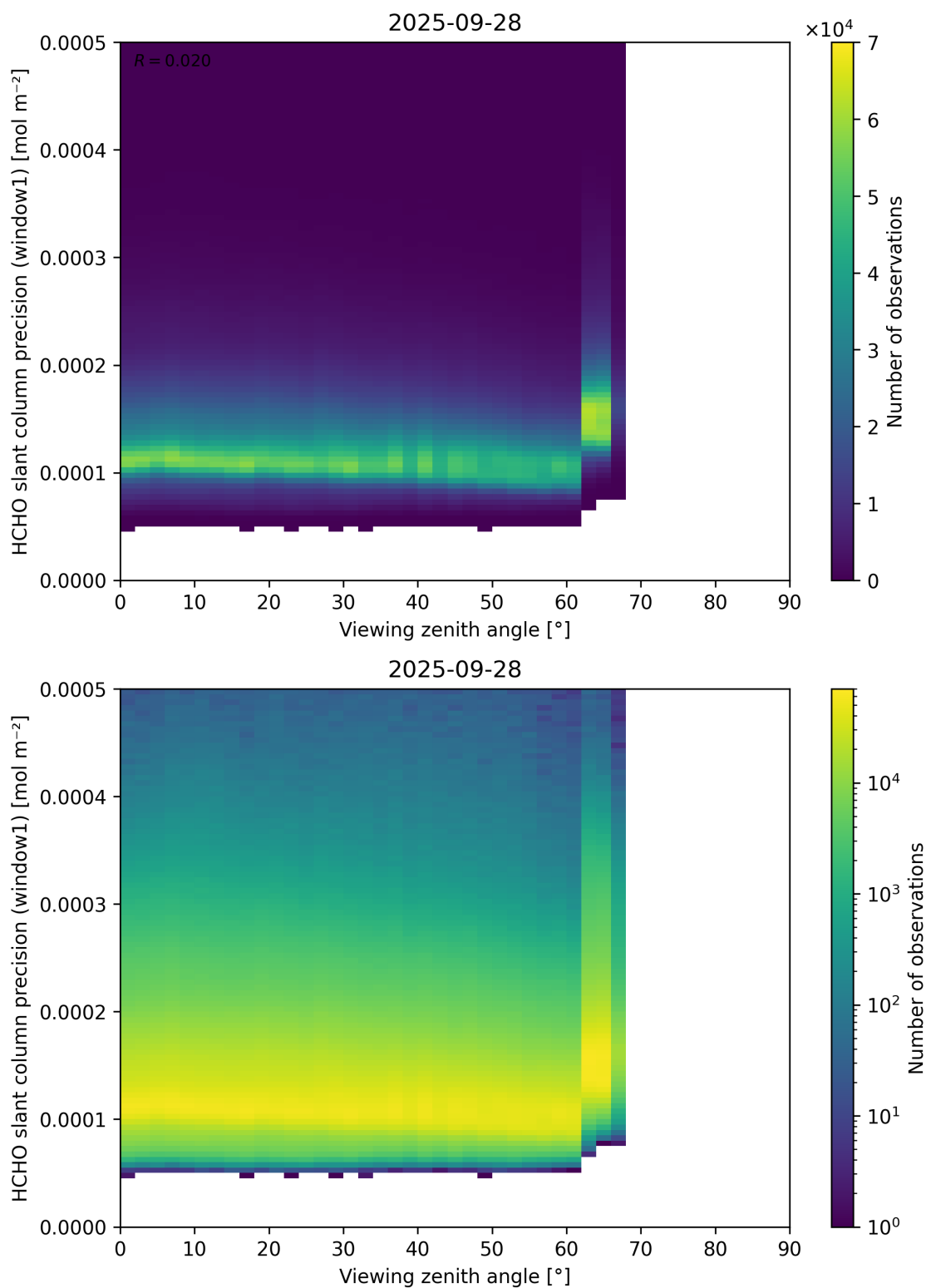
Figure 189: Scatter density plot of “Viewing zenith angle” against “HCHO slant column precision (window1)” for 2025-09-27 to 2025-09-29.
