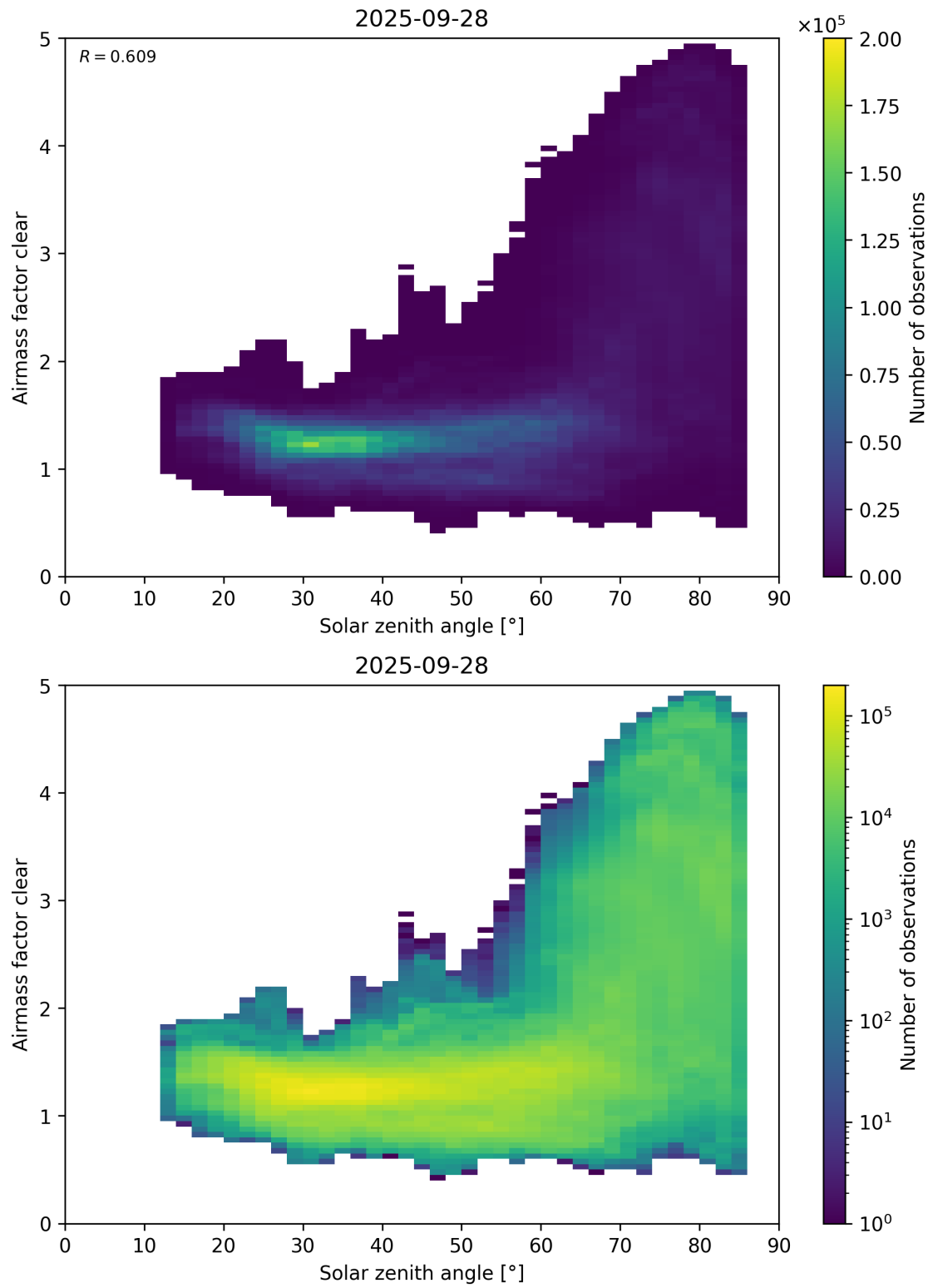
Figure 170: Scatter density plot of “Solar zenith angle” against “Airmass factor clear” for 2025-09-27 to 2025-09-29.
