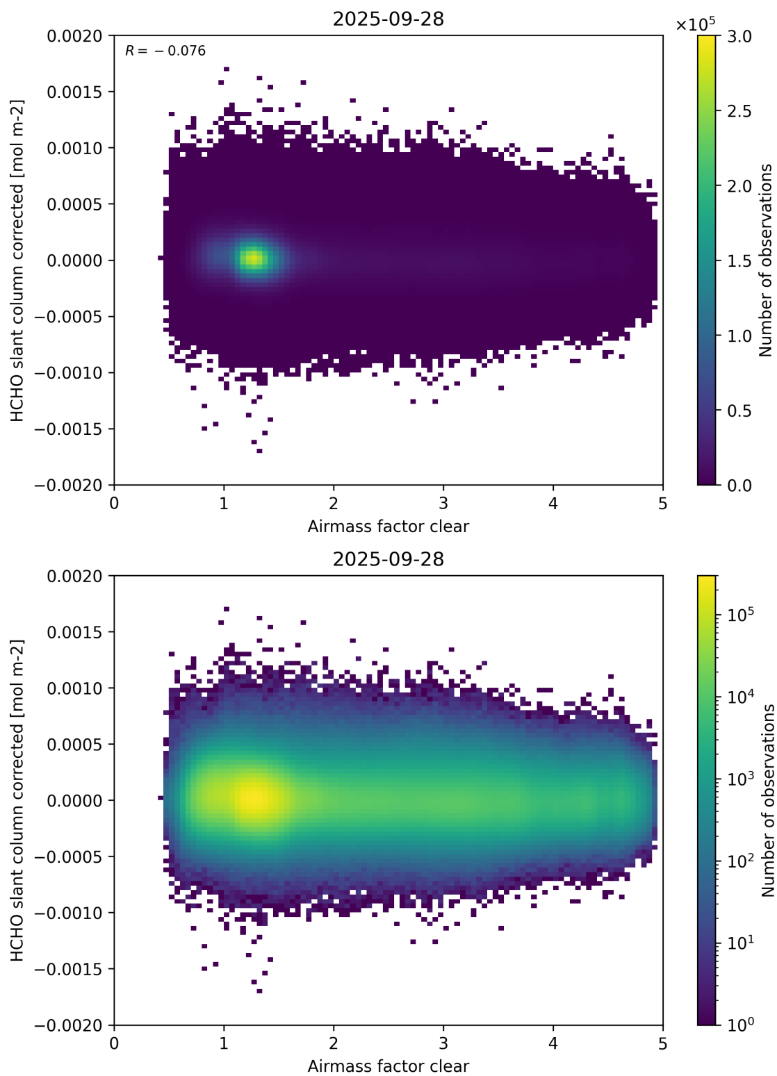
Figure 74: Scatter density plot of “Airmass factor clear” against “HCHO slant column corrected” for 2025-09-27 to 2025-09-29.
