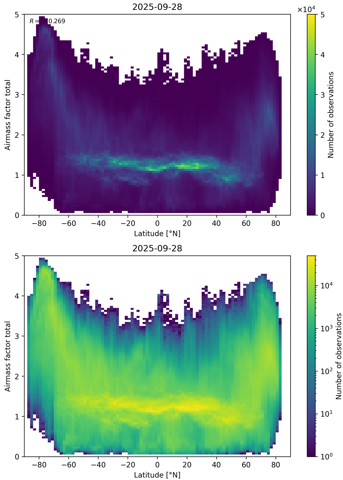
Figure 161: Scatter density plot of “Latitude” against “Airmass factor total” for 2025-09-27 to 2025-09-29.
