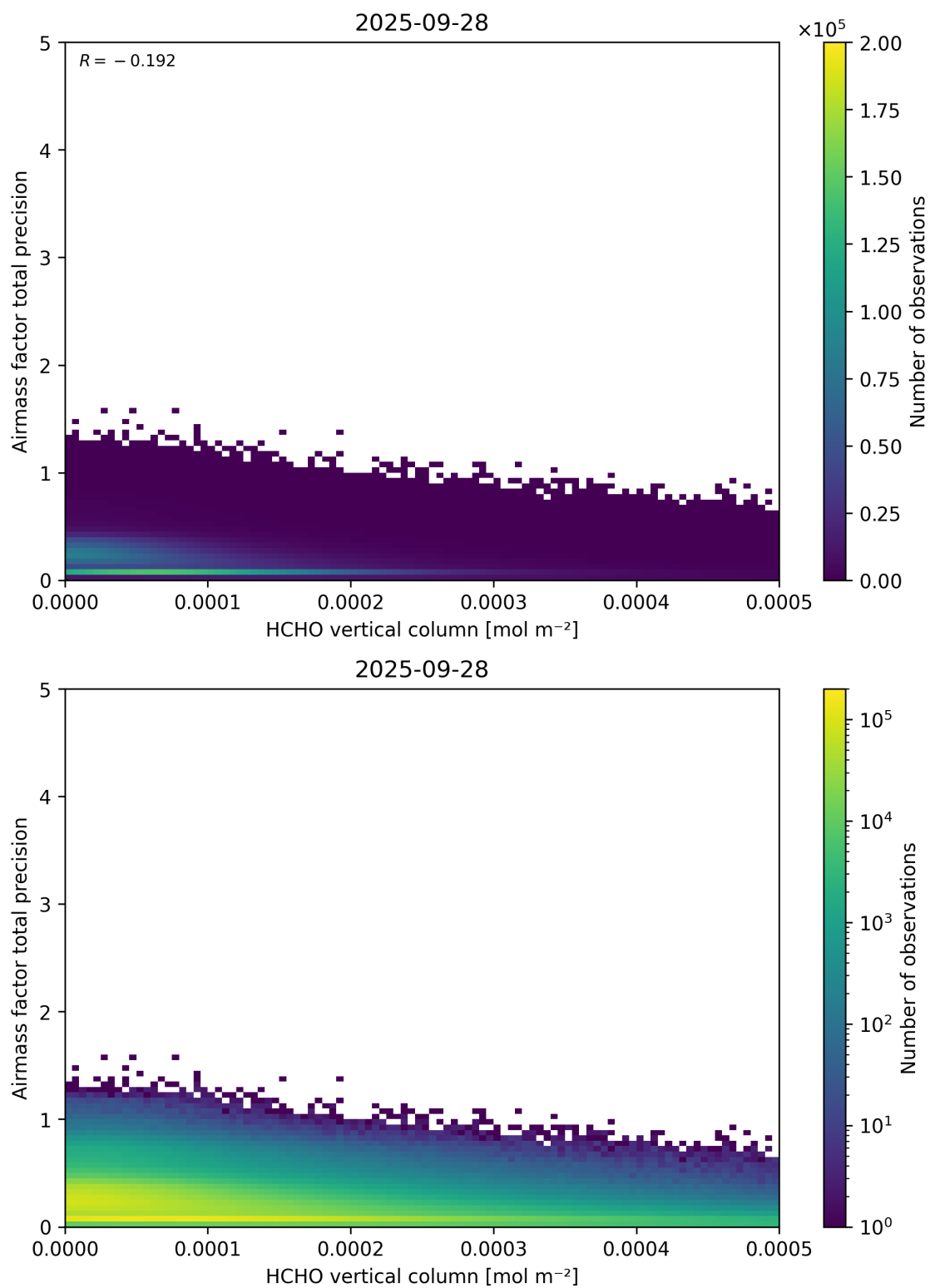
Figure 132: Scatter density plot of “HCHO vertical column” against “Airmass factor total precision” for 2025-09-27 to 2025-09-29.
