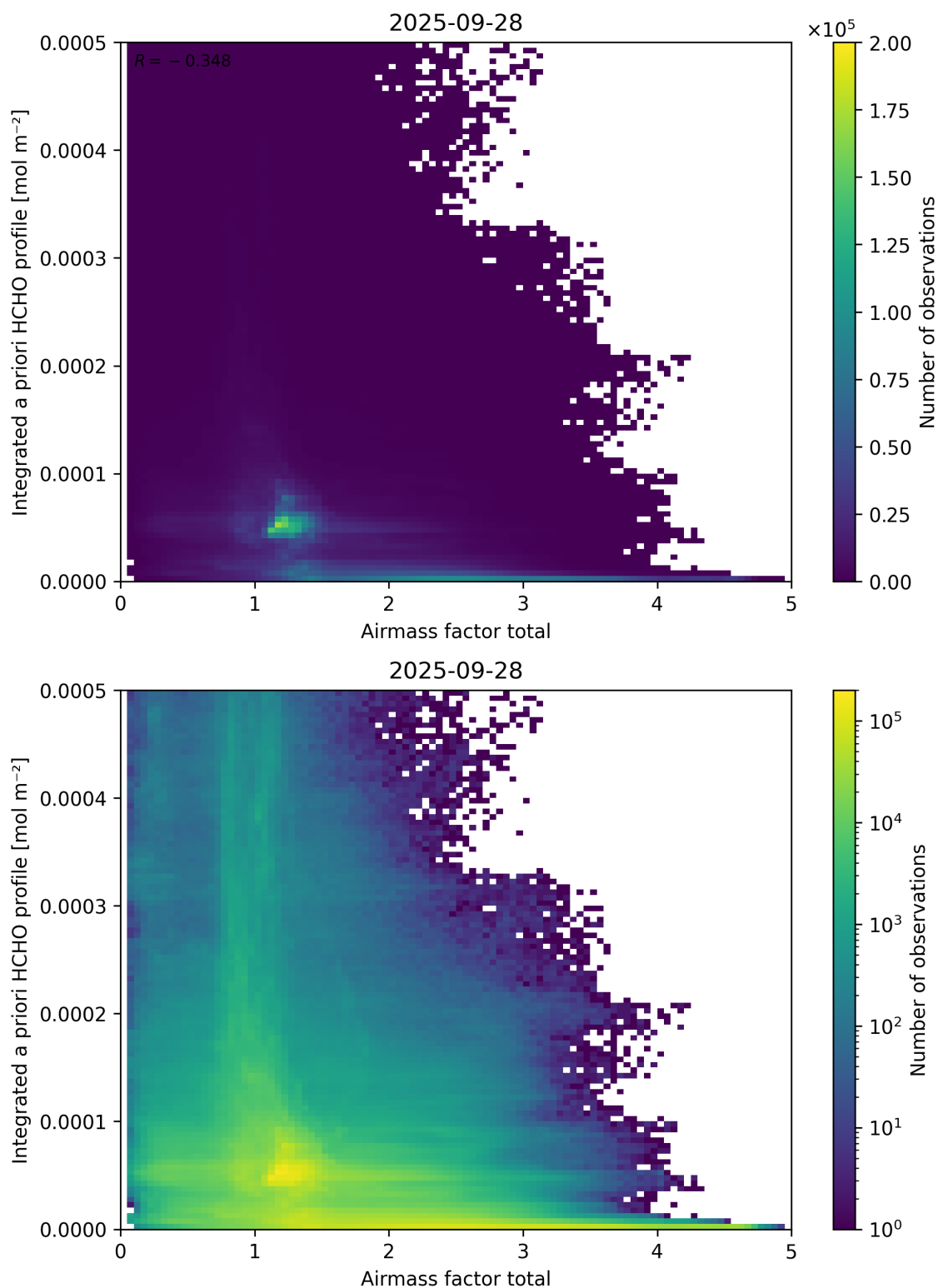
Figure 104: Scatter density plot of “Airmass factor total” against “Integrated a priori HCHO profile” for 2025-09-27 to 2025-09-29.
