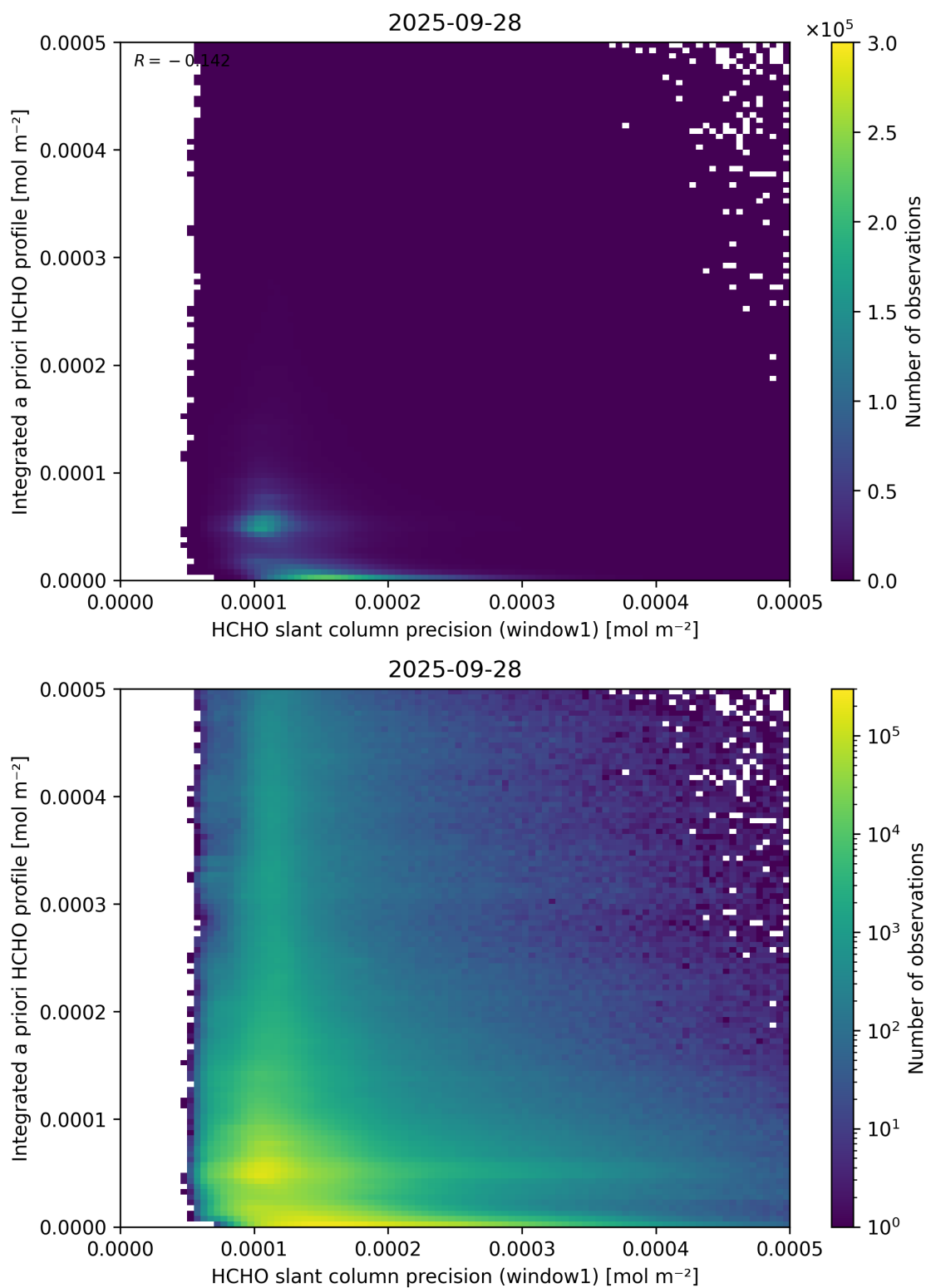
Figure 96: Scatter density plot of “HCHO slant column precision (window1)” against “Integrated a priori HCHO profile” for 2025-09-27 to 2025-09-29.
