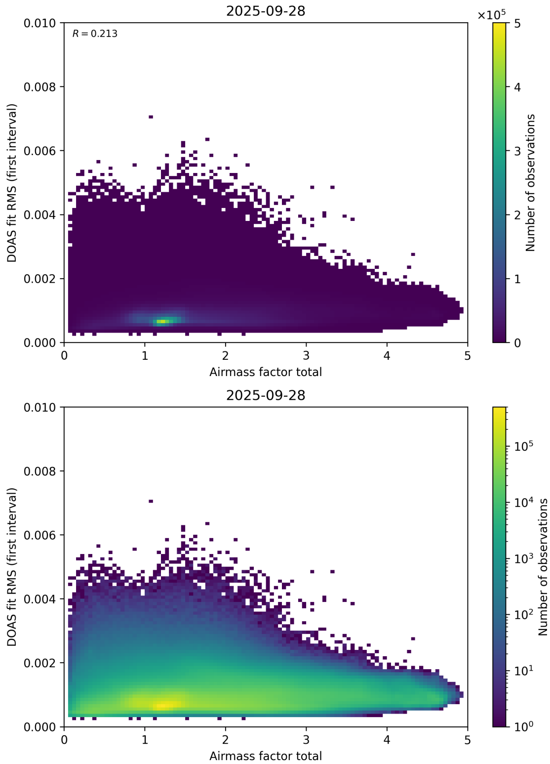
Figure 97: Scatter density plot of “Airmass factor total” against “DOAS fit RMS (first interval)” for 2025-09-27 to 2025-09-29.
