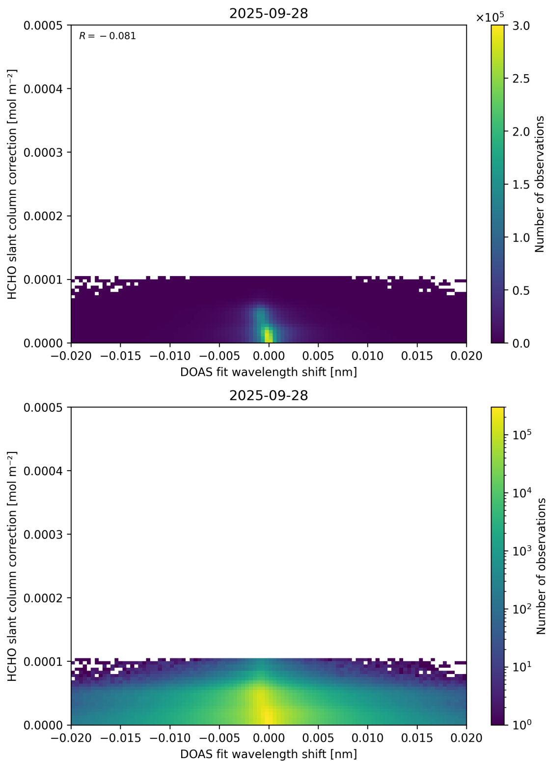
Figure 67: Scatter density plot of “DOAS fit wavelength shift” against “HCHO slant column correction” for 2025-09-27 to 2025-09-29.
