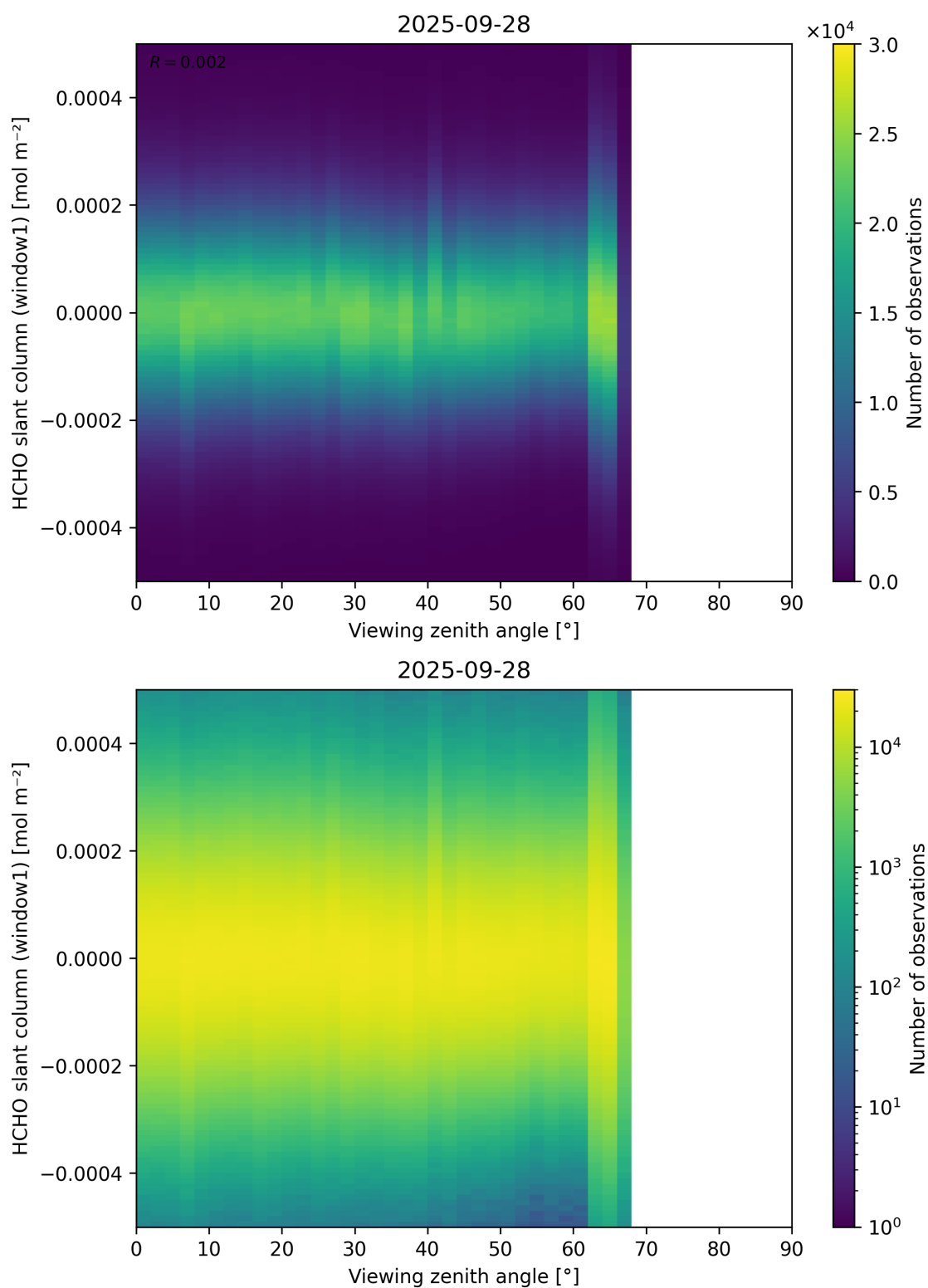
Figure 188: Scatter density plot of “Viewing zenith angle” against “HCHO slant column (window1)” for 2025-09-27 to 2025-09-29.
