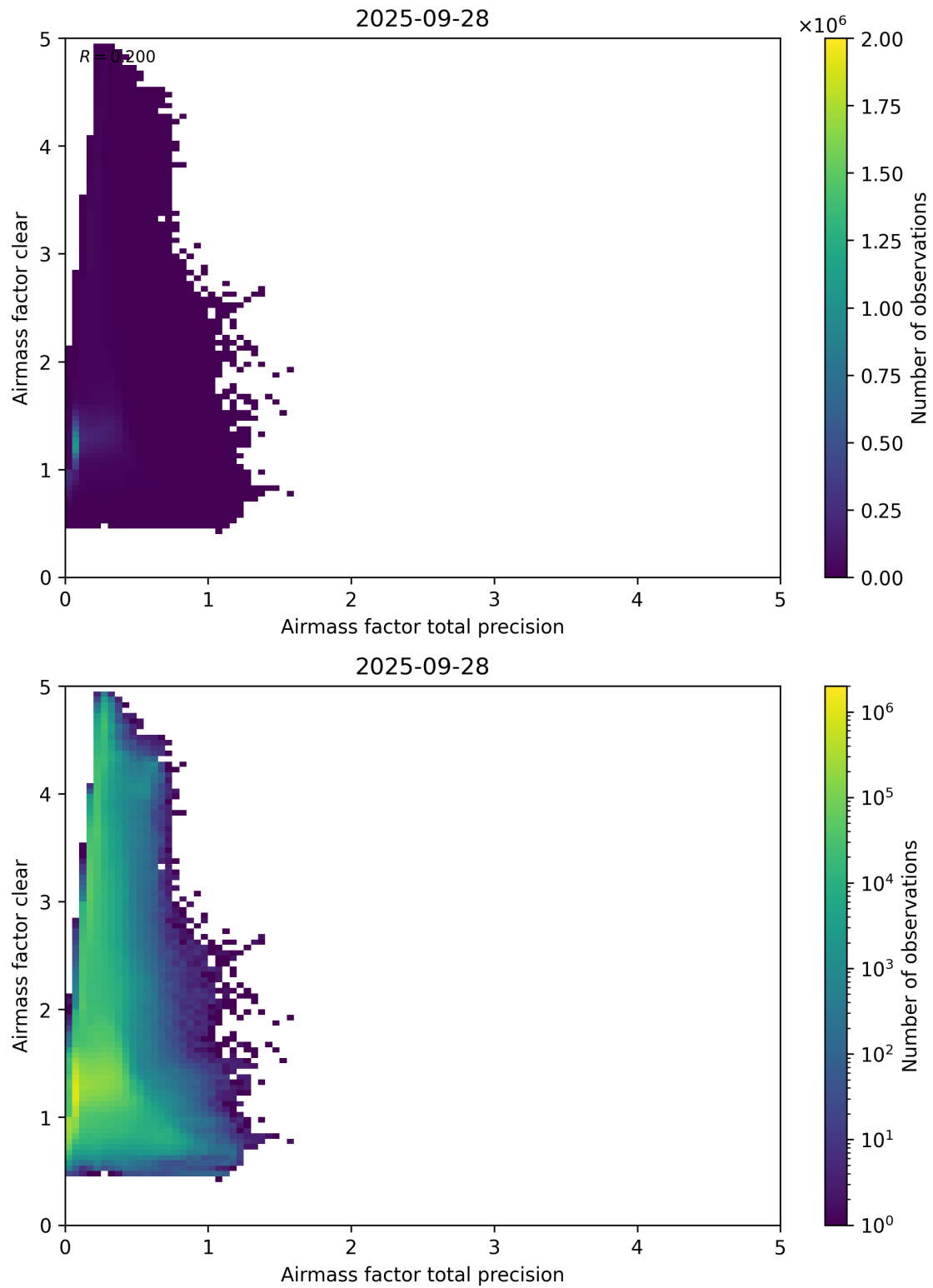
Figure 108: Scatter density plot of “Airmass factor total precision” against “Airmass factor clear” for 2025-09-27 to 2025-09-29.
