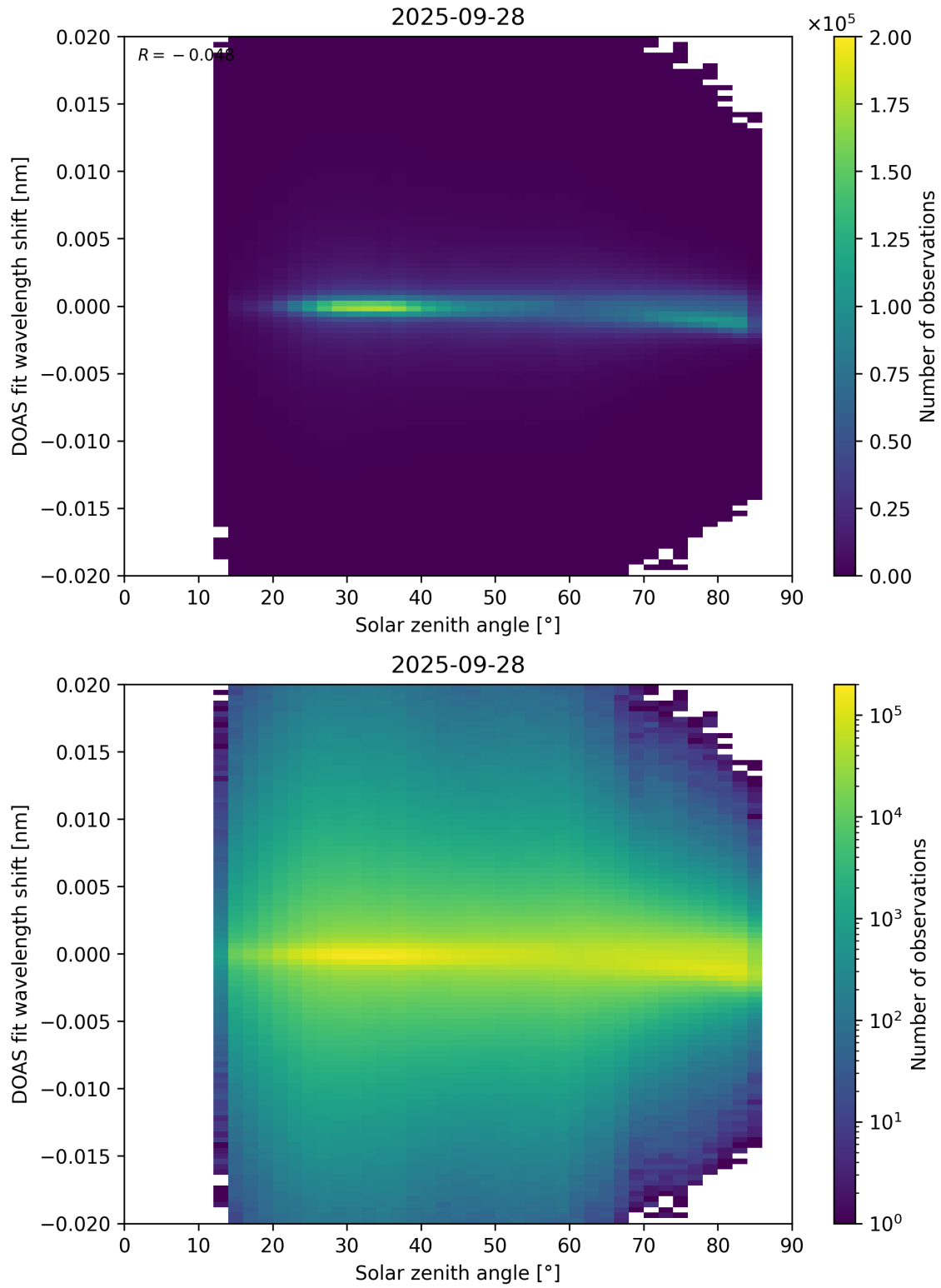
Figure 168: Scatter density plot of “Solar zenith angle” against “DOAS fit wavelength shift” for 2025-09-27 to 2025-09-29.
