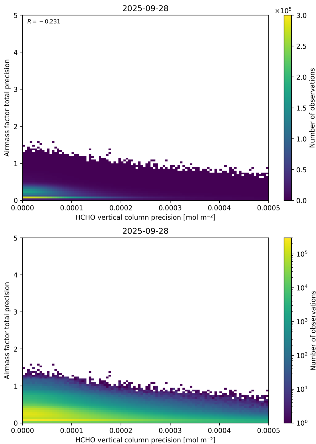
Figure 145: Scatter density plot of “HCHO vertical column precision” against “Airmass factor total precision” for 2025-09-27 to 2025-09-29.
