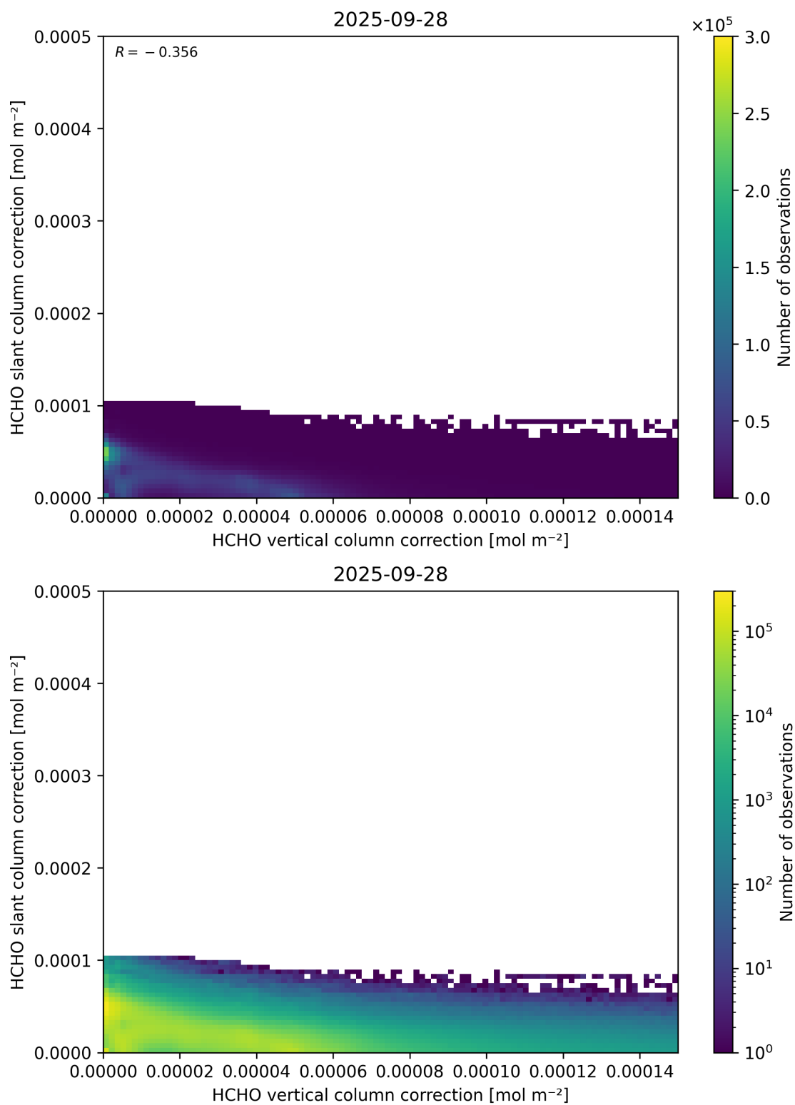
Figure 117: Scatter density plot of “HCHO vertical column correction” against “HCHO slant column correction” for 2025-09-27 to 2025-09-29.
