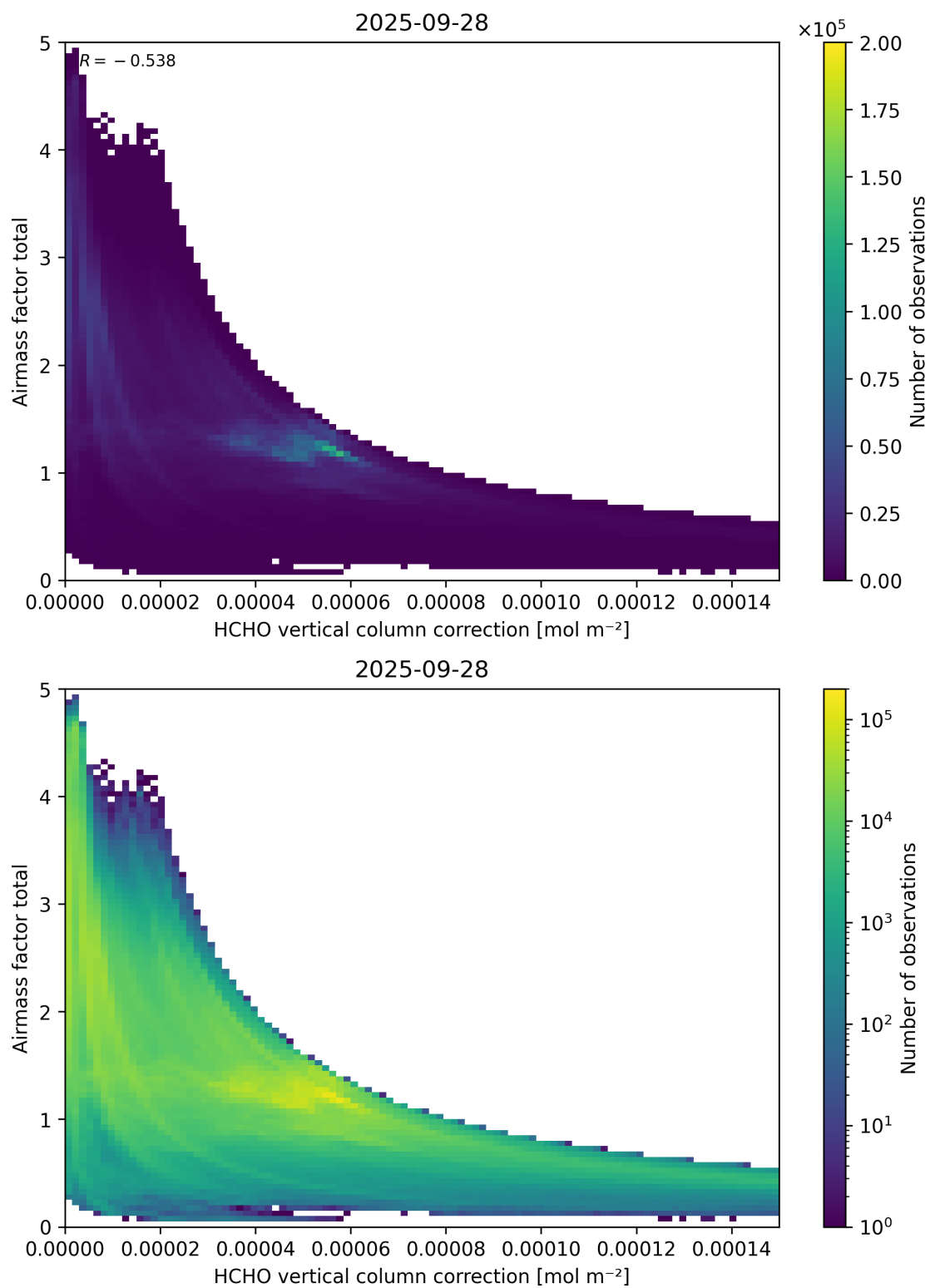
Figure 120: Scatter density plot of “HCHO vertical column correction” against “Airmass factor total” for 2025-09-27 to 2025-09-29.
