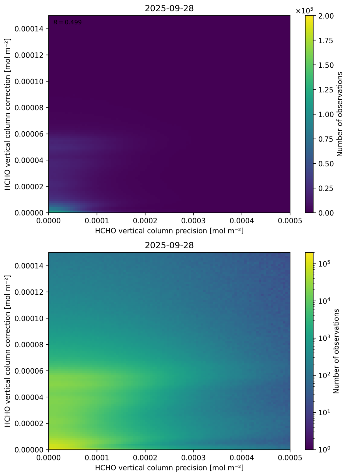
Figure 146: Scatter density plot of “HCHO vertical column precision” against “HCHO vertical column correction” for 2025-09-27 to 2025-09-29.
