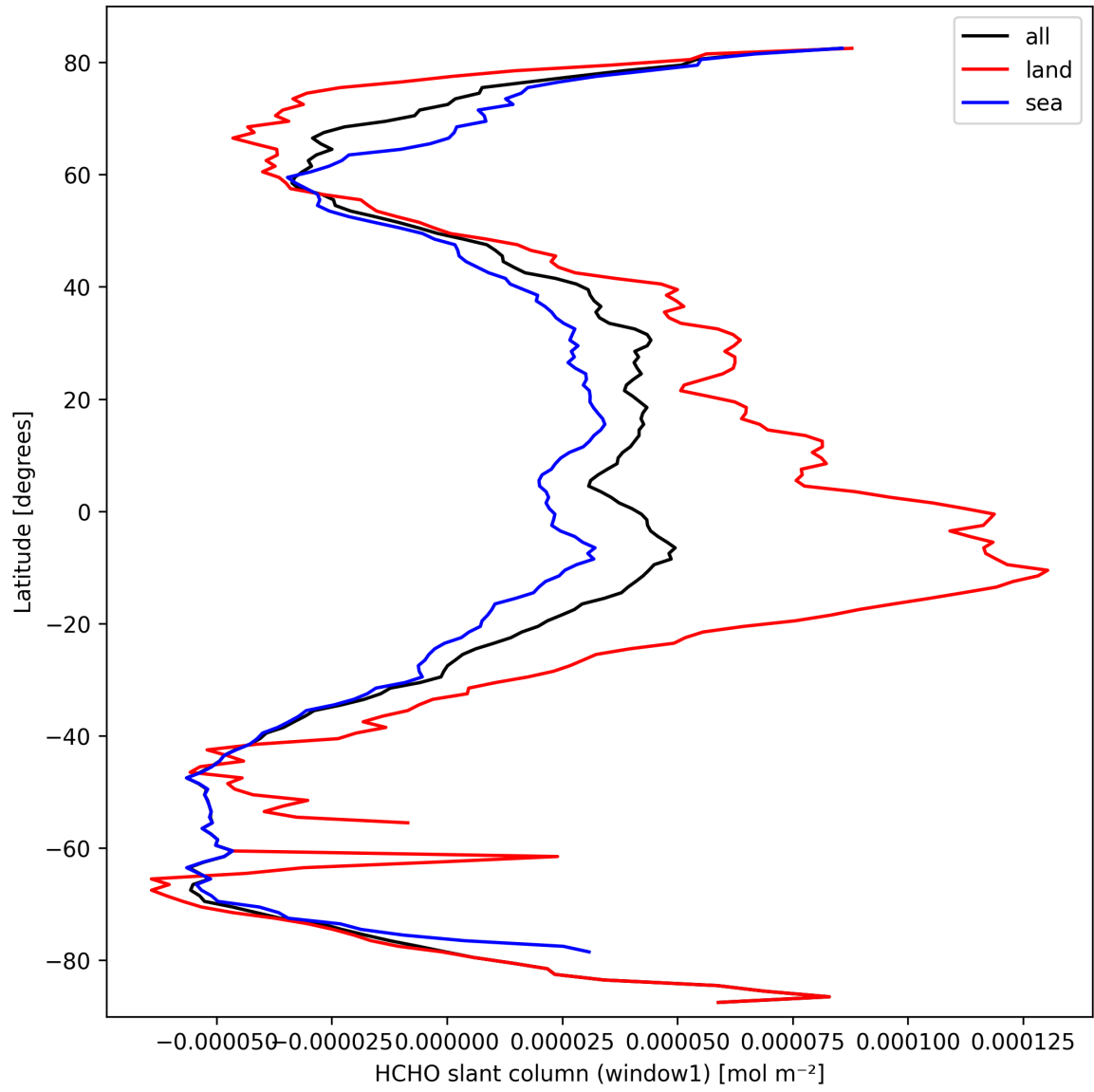
Figure 24: Zonal average of “HCHO slant column (window1)” for 2025-09-27 to 2025-09-29.
