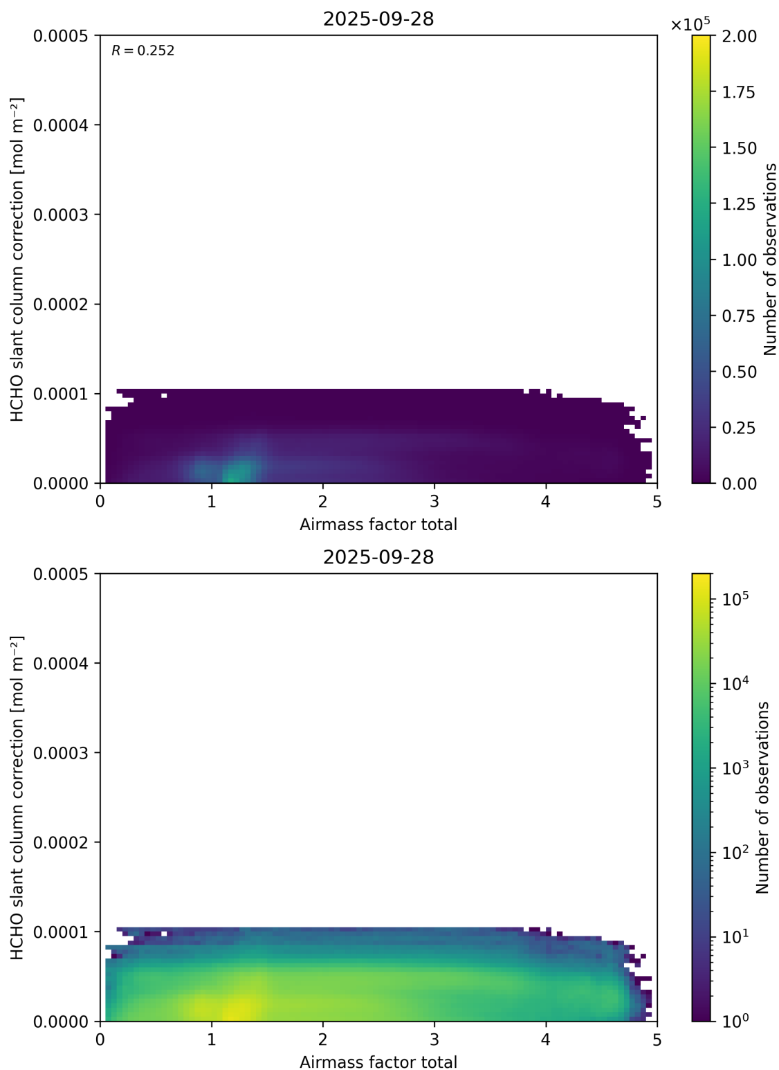
Figure 102: Scatter density plot of “Airmass factor total” against “HCHO slant column correction” for 2025-09-27 to 2025-09-29.
