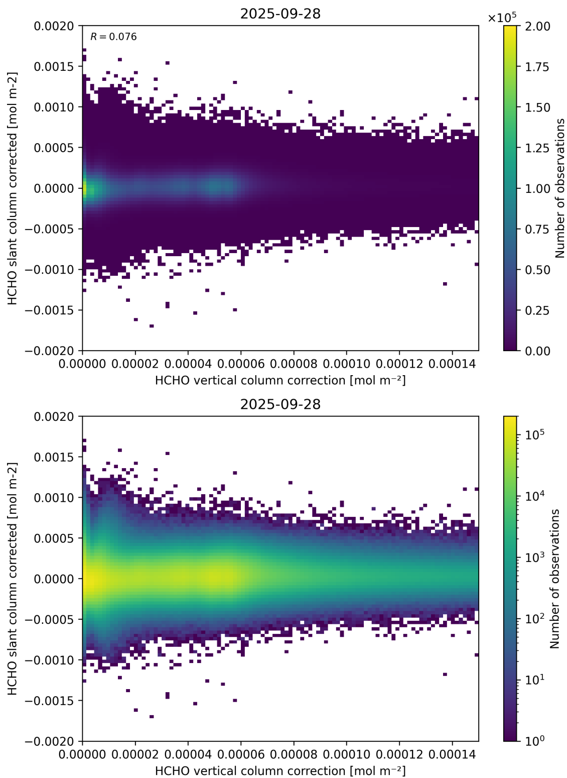
Figure 116: Scatter density plot of “HCHO vertical column correction” against “HCHO slant column corrected” for 2025-09-27 to 2025-09-29.
