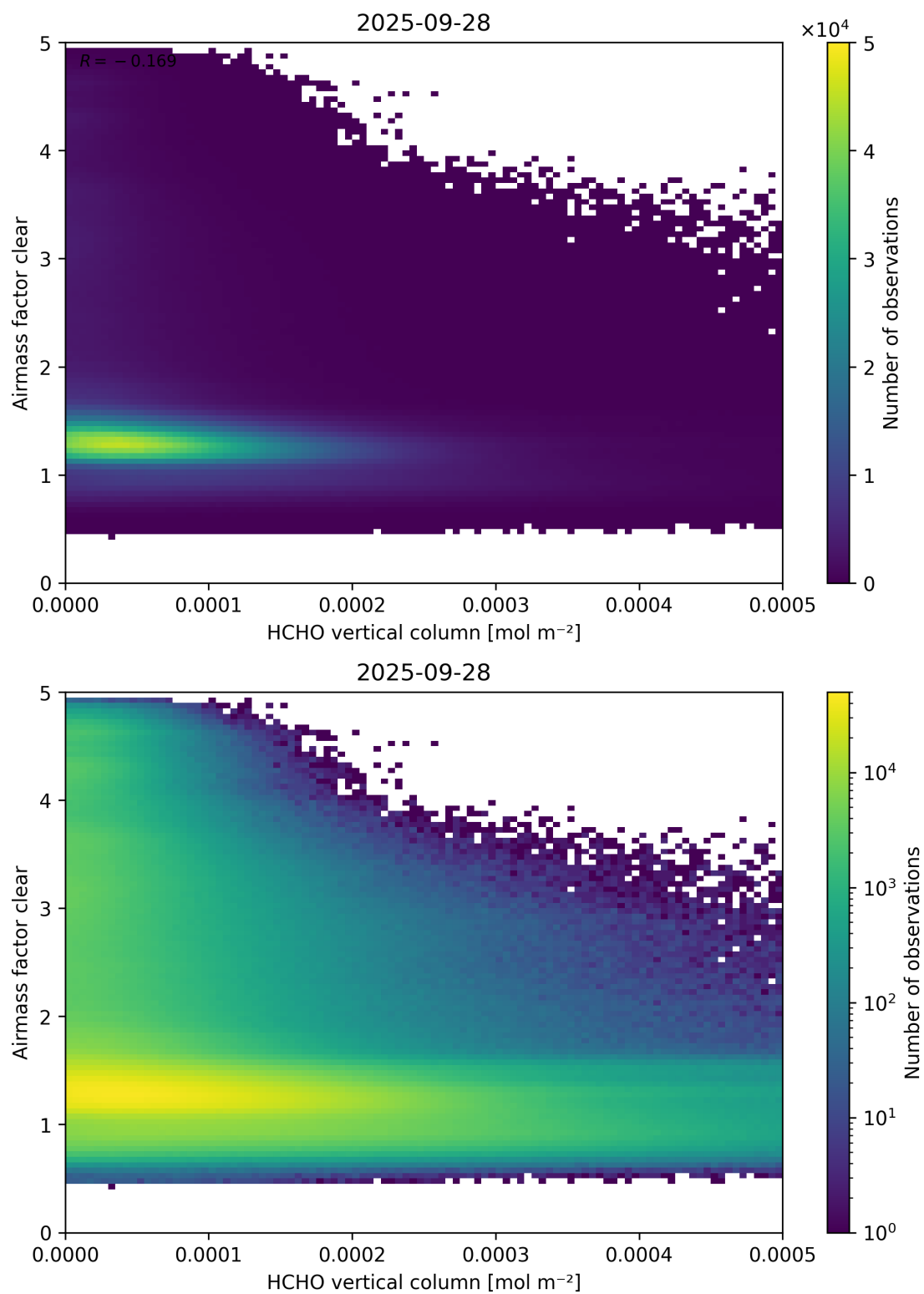
Figure 126: Scatter density plot of “HCHO vertical column” against “Airmass factor clear” for 2025-09-27 to 2025-09-29.
