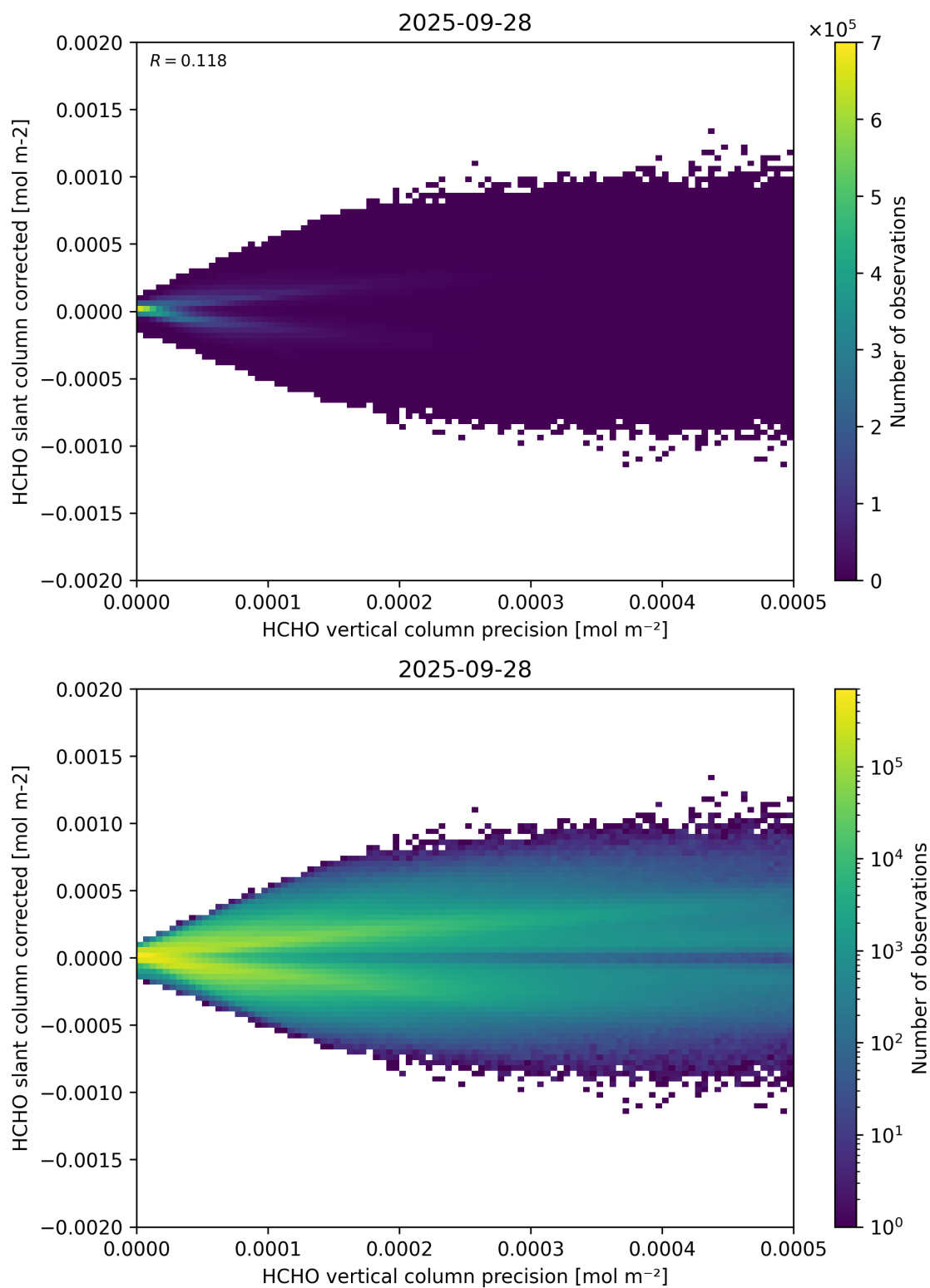
Figure 140: Scatter density plot of “HCHO vertical column precision” against “HCHO slant column corrected” for 2025-09-27 to 2025-09-29.
