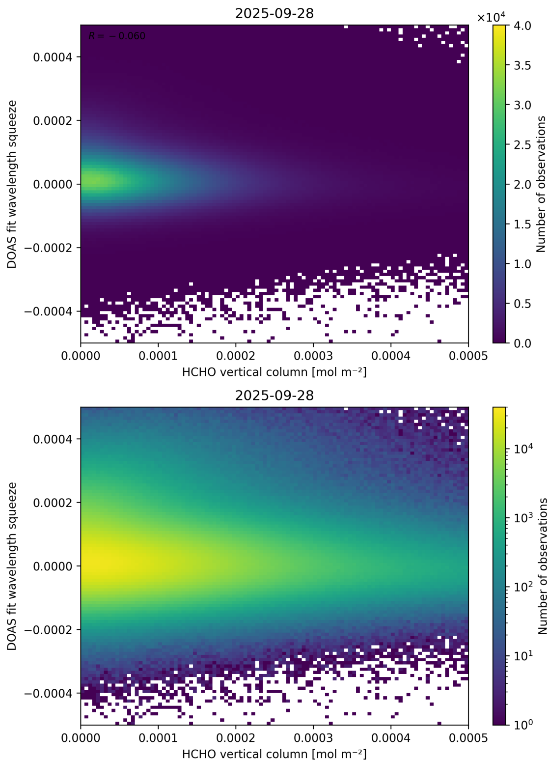
Figure 125: Scatter density plot of “HCHO vertical column” against “DOAS fit wavelength squeeze” for 2025-09-27 to 2025-09-29.
