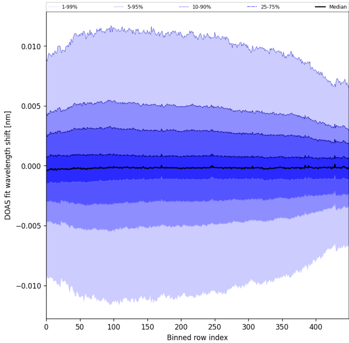
Figure 58: Along track statistics of “DOAS fit wavelength shift” for 2025-09-27 to 2025-09-29
