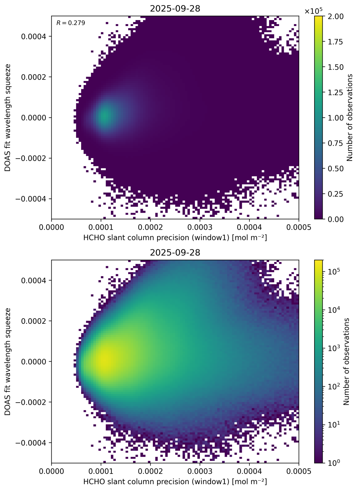
Figure 90: Scatter density plot of “HCHO slant column precision (window1)” against “DOAS fit wavelength squeeze” for 2025-09-27 to 2025-09-29.
