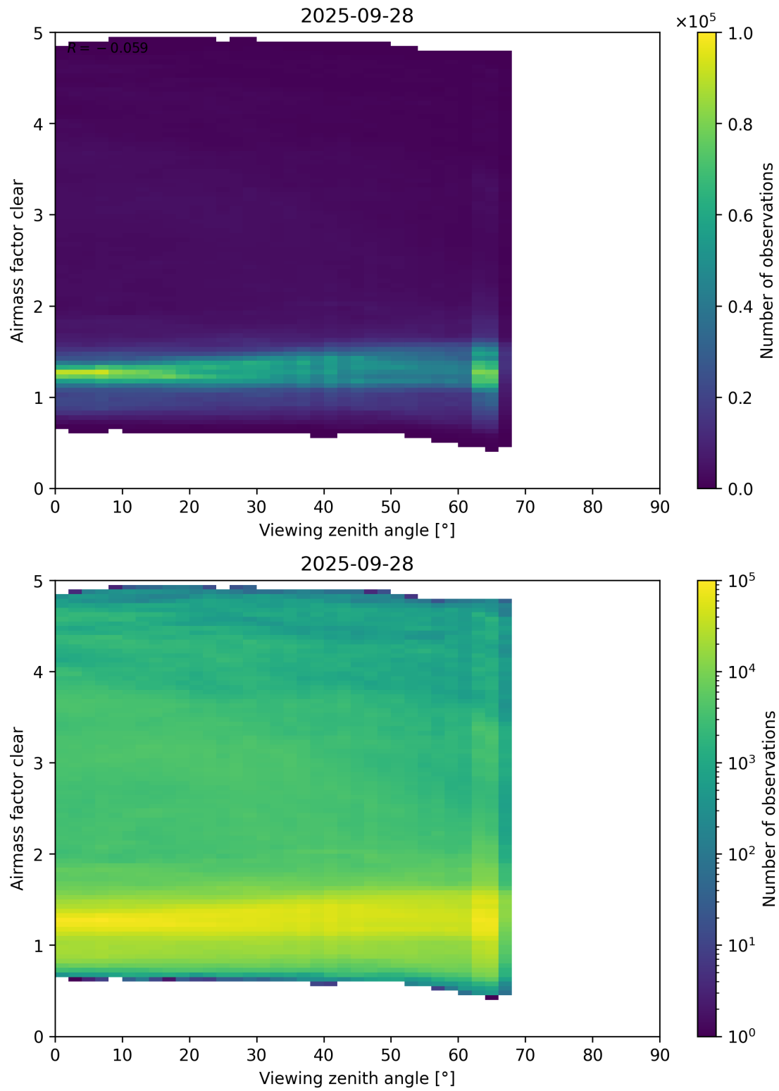
Figure 185: Scatter density plot of “Viewing zenith angle” against “Airmass factor clear” for 2025-09-27 to 2025-09-29.
