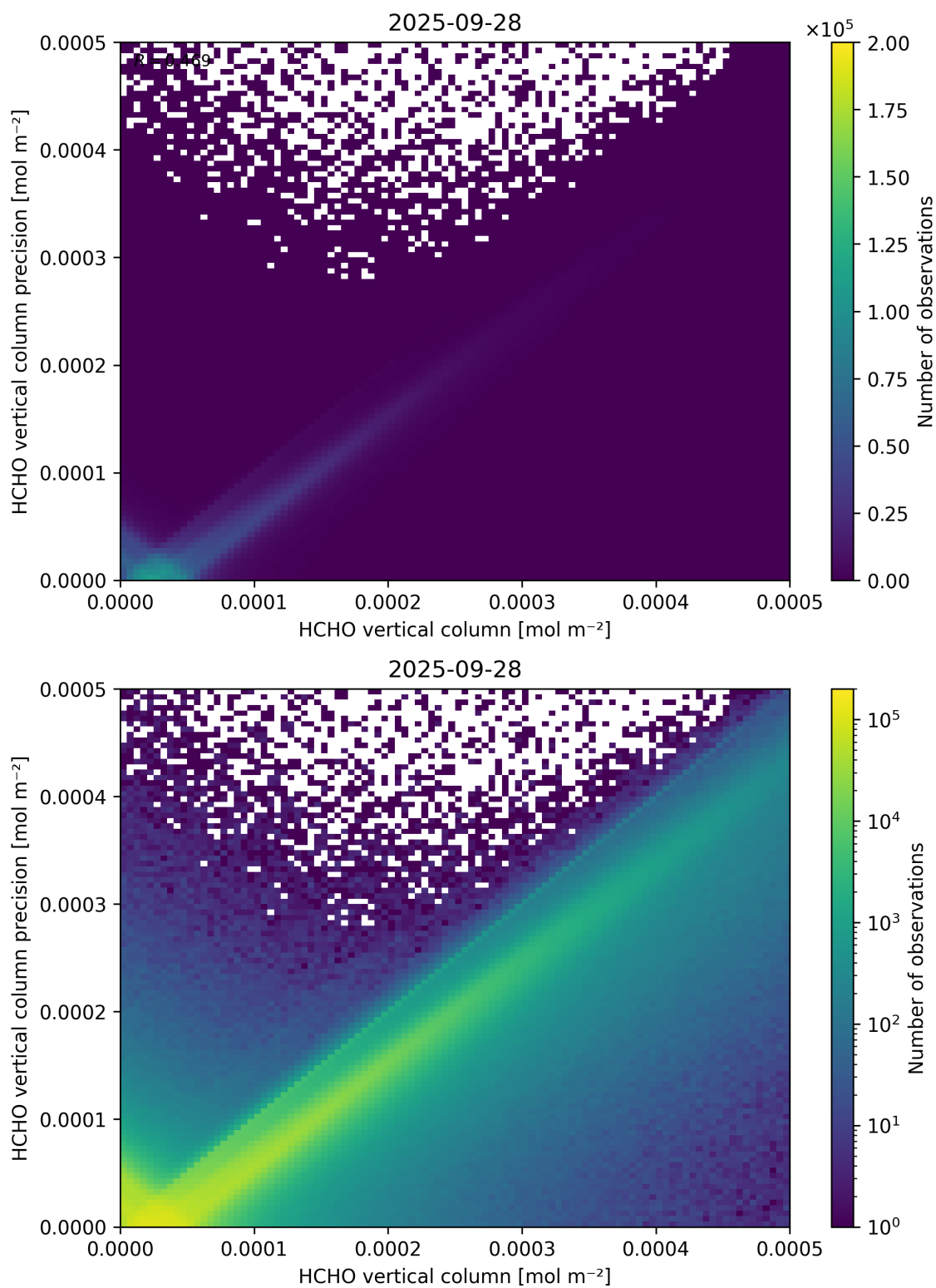
Figure 134: Scatter density plot of “HCHO vertical column” against “HCHO vertical column precision” for 2025-09-27 to 2025-09-29.
