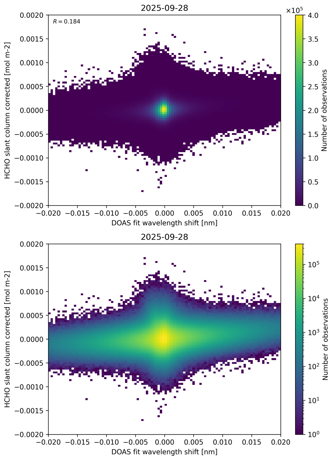
Figure 66: Scatter density plot of “DOAS fit wavelength shift” against “HCHO slant column corrected” for 2025-09-27 to 2025-09-29.
