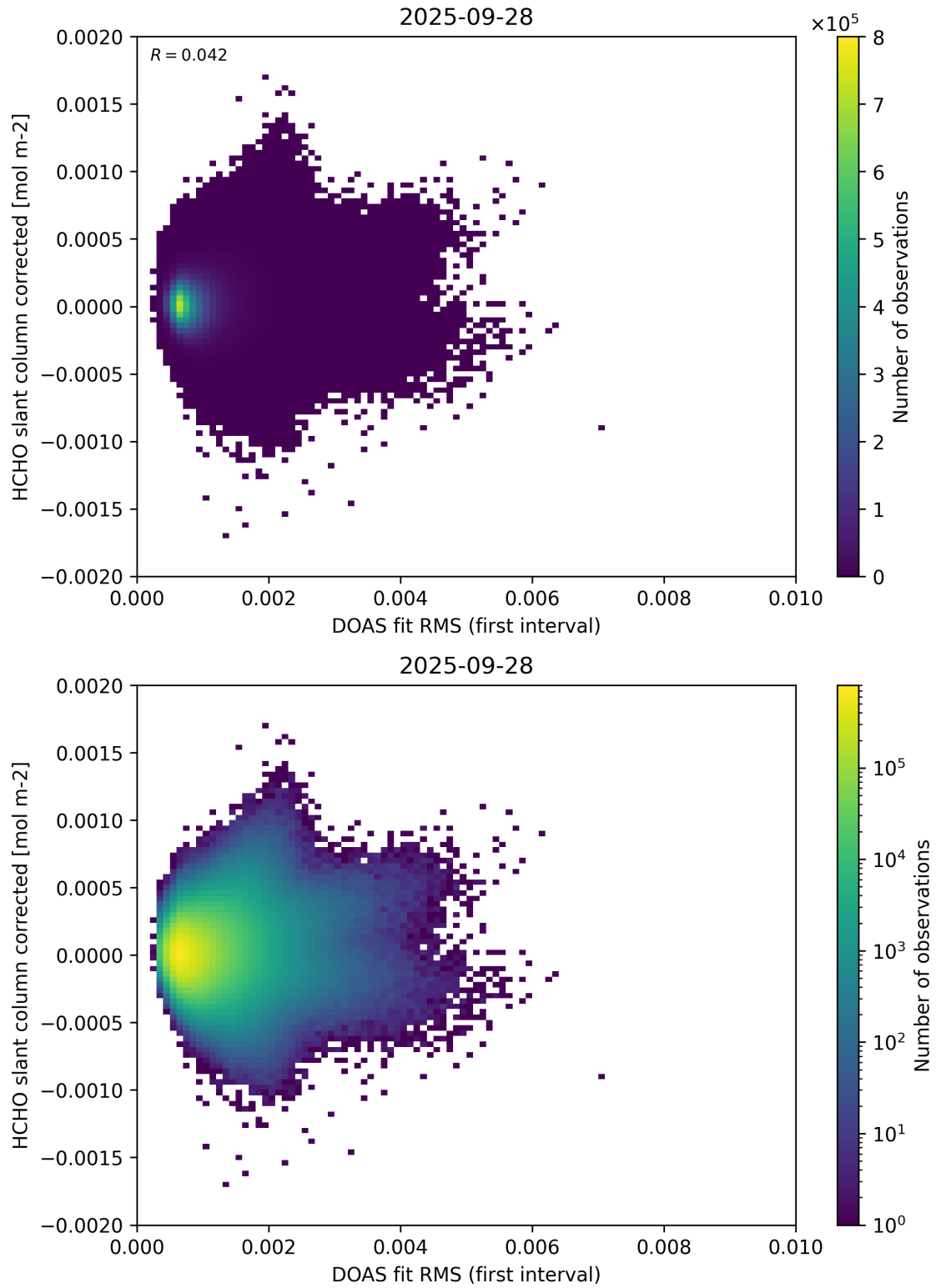
Figure 62: Scatter density plot of “DOAS fit RMS (first interval)” against “HCHO slant column corrected” for 2025-09-27 to 2025-09-29.
