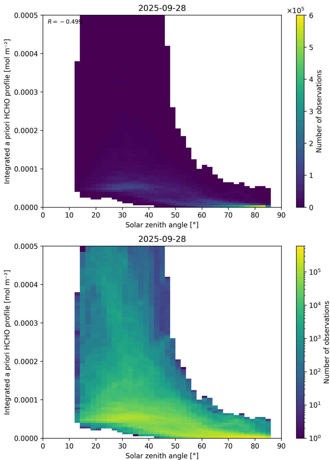
Figure 180: Scatter density plot of “Solar zenith angle” against “Integrated a priori HCHO profile” for 2025-09-27 to 2025-09-29.
