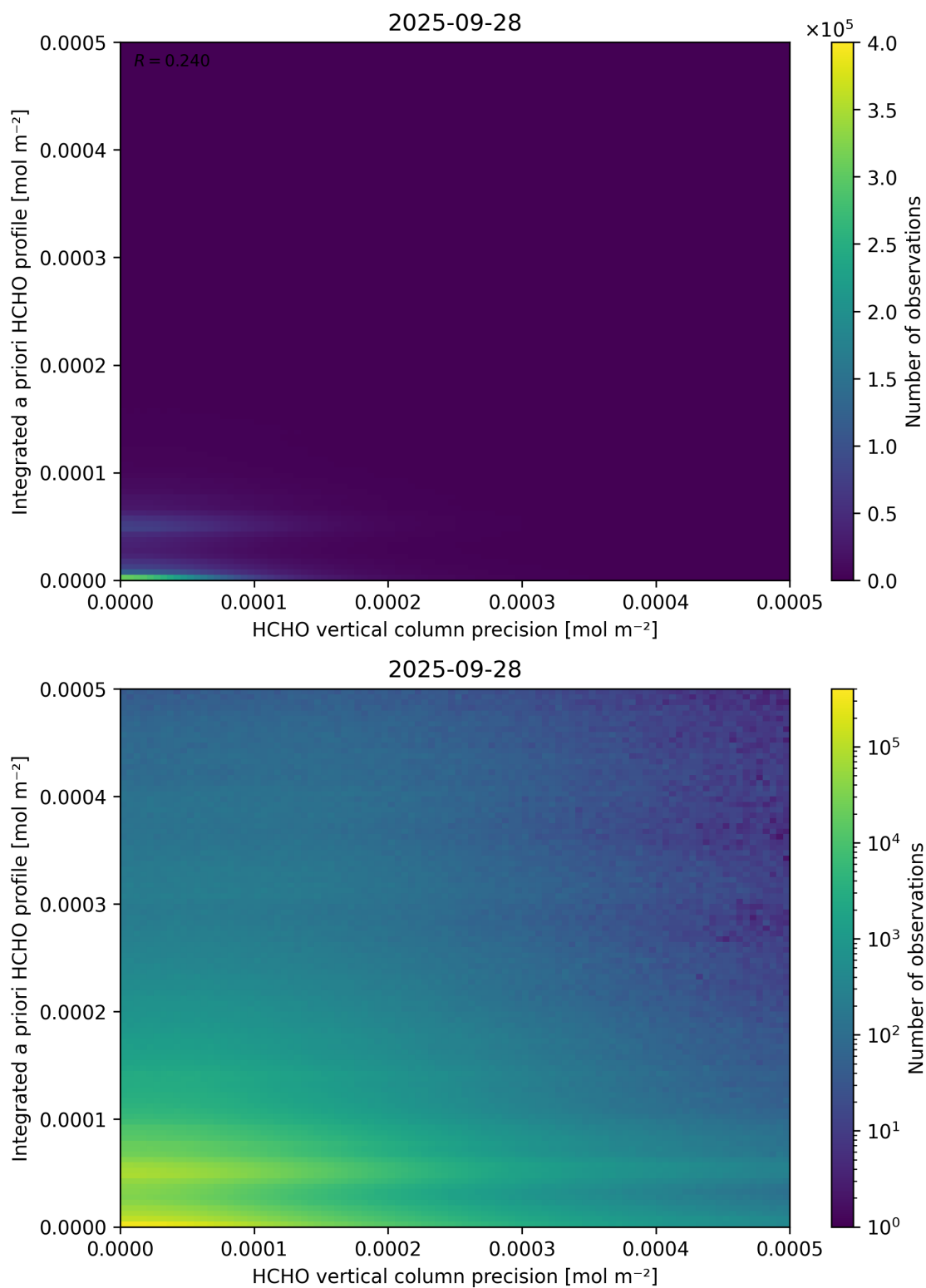
Figure 147: Scatter density plot of “HCHO vertical column precision” against “Integrated a priori HCHO profile” for 2025-09-27 to 2025-09-29.
