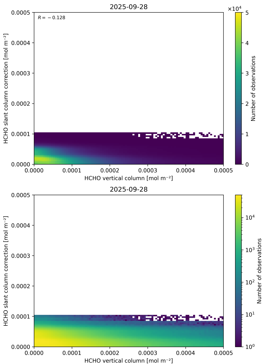
Figure 128: Scatter density plot of “HCHO vertical column” against “HCHO slant column correction” for 2025-09-27 to 2025-09-29.
