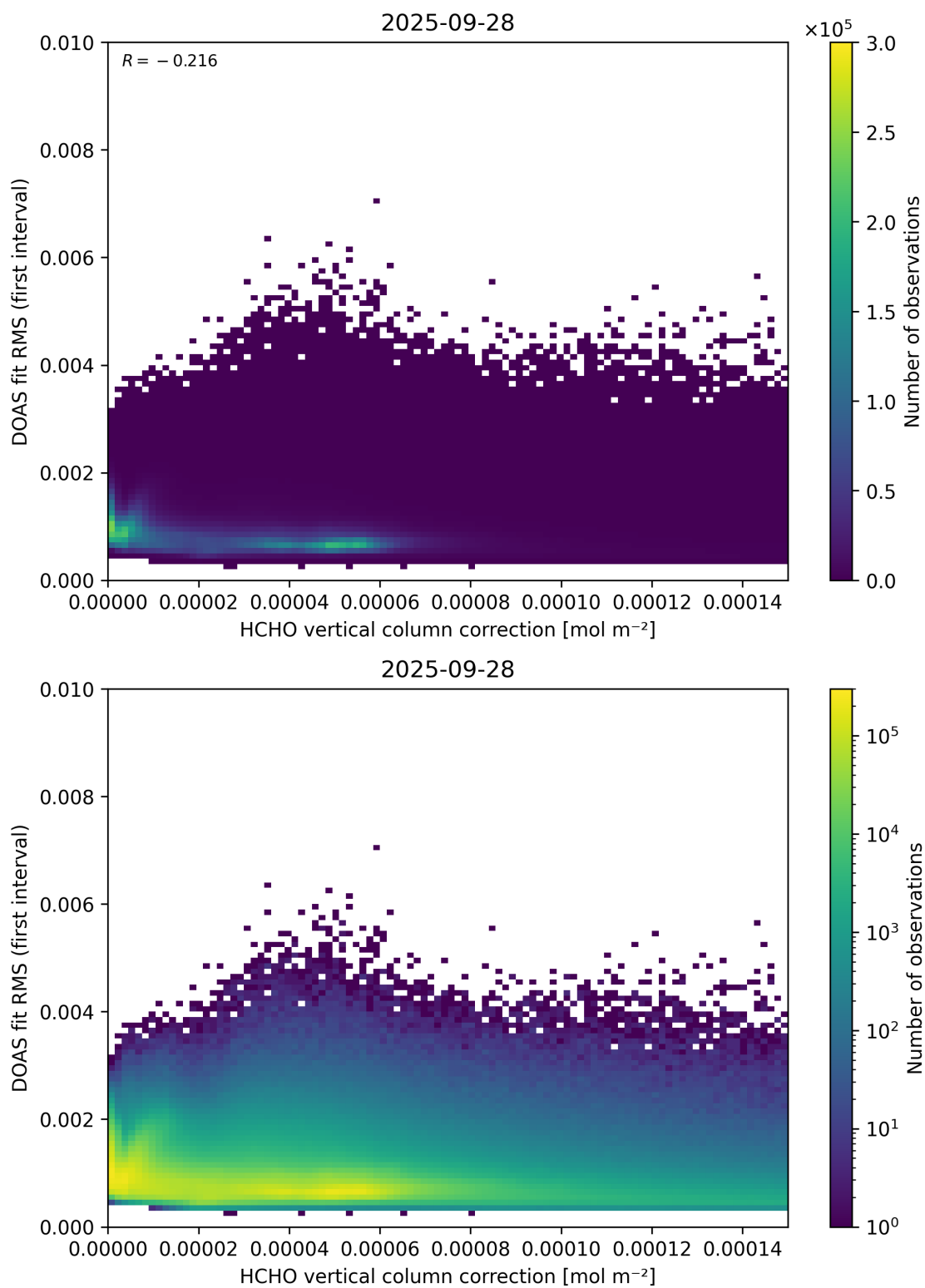
Figure 112: Scatter density plot of “HCHO vertical column correction” against “DOAS fit RMS (first interval)” for 2025-09-27 to 2025-09-29.
