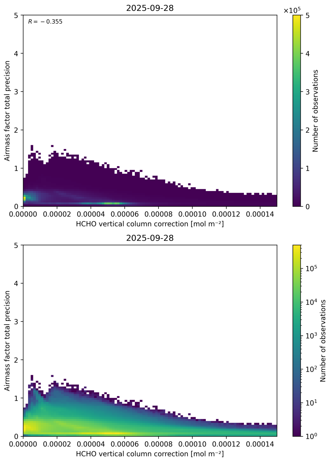
Figure 121: Scatter density plot of “HCHO vertical column correction” against “Airmass factor total precision” for 2025-09-27 to 2025-09-29.
