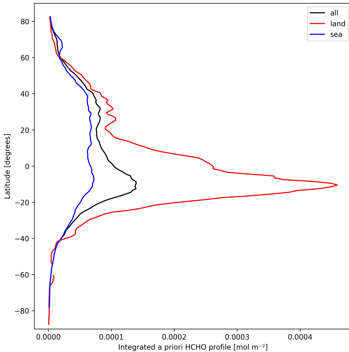
Figure 29: Zonal average of “Integrated a priori HCHO profile” for 2025-09-27 to 2025-09-29.
