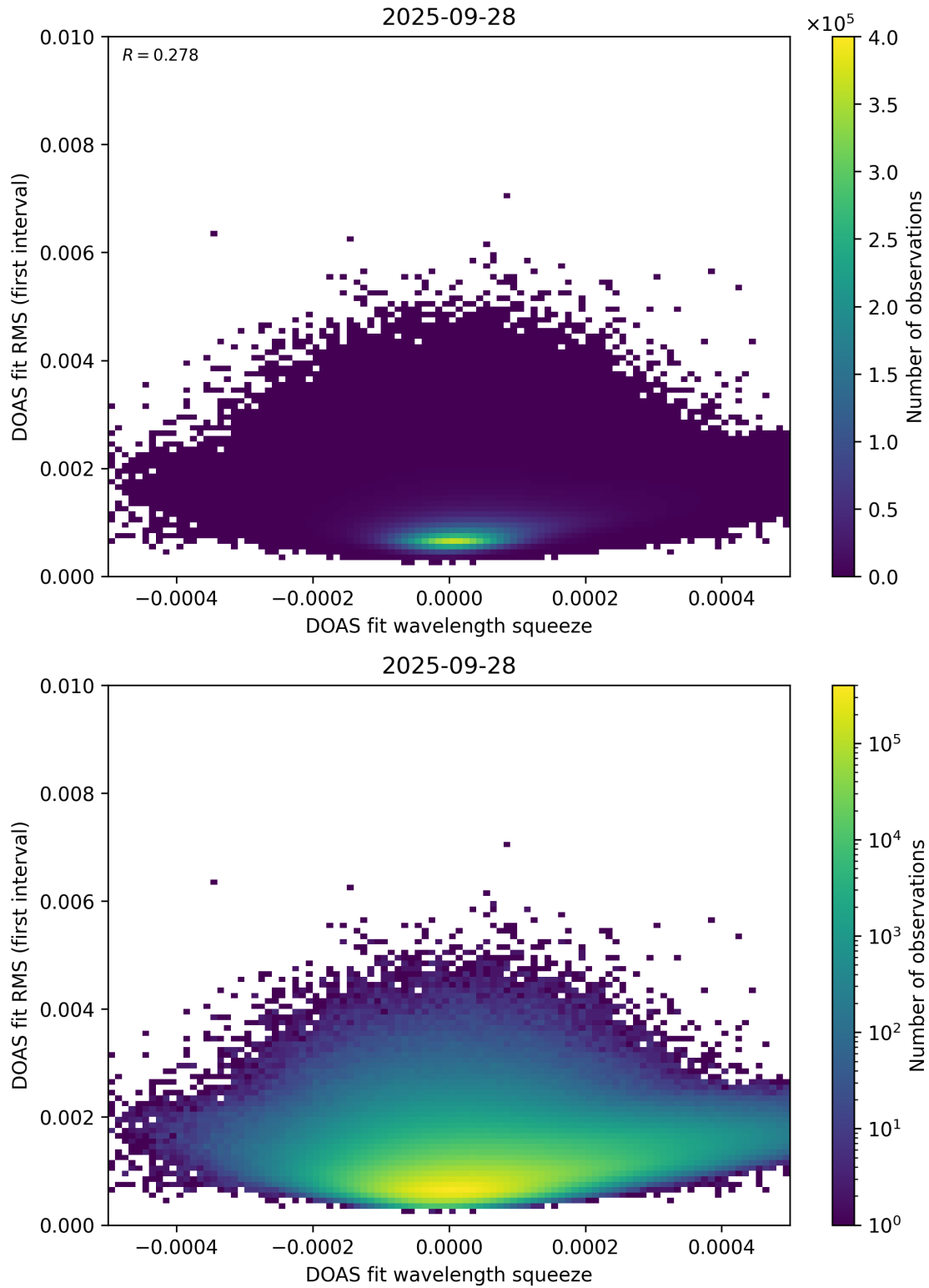
Figure 68: Scatter density plot of “DOAS fit wavelength squeeze” against “DOAS fit RMS (first interval)” for 2025-09-27 to 2025-09-29.
