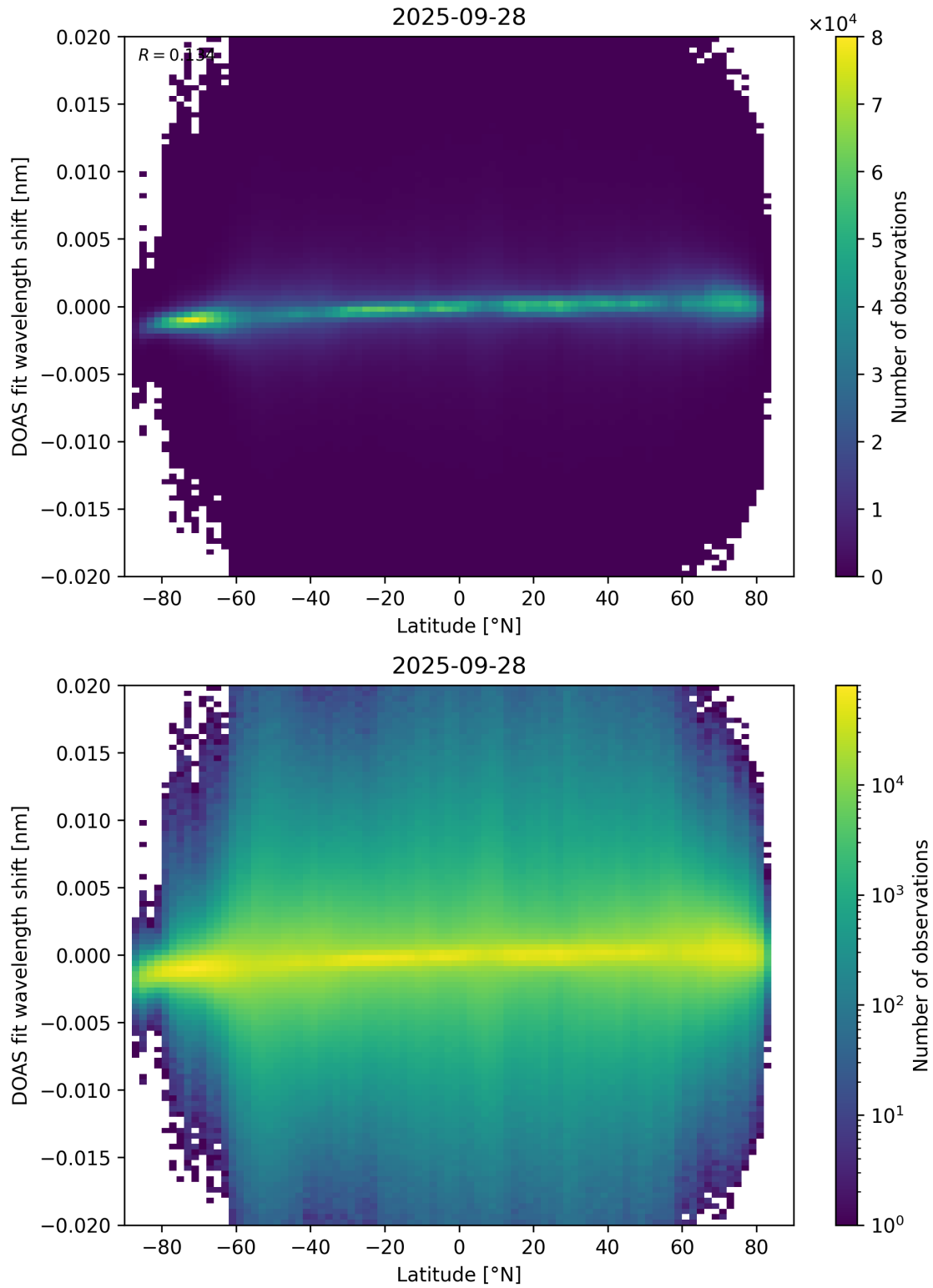
Figure 154: Scatter density plot of “Latitude” against “DOAS fit wavelength shift” for 2025-09-27 to 2025-09-29.
