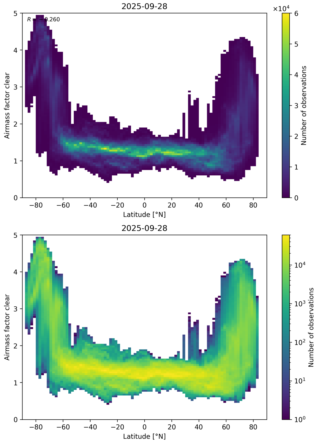
Figure 156: Scatter density plot of “Latitude” against “Airmass factor clear” for 2025-09-27 to 2025-09-29.
