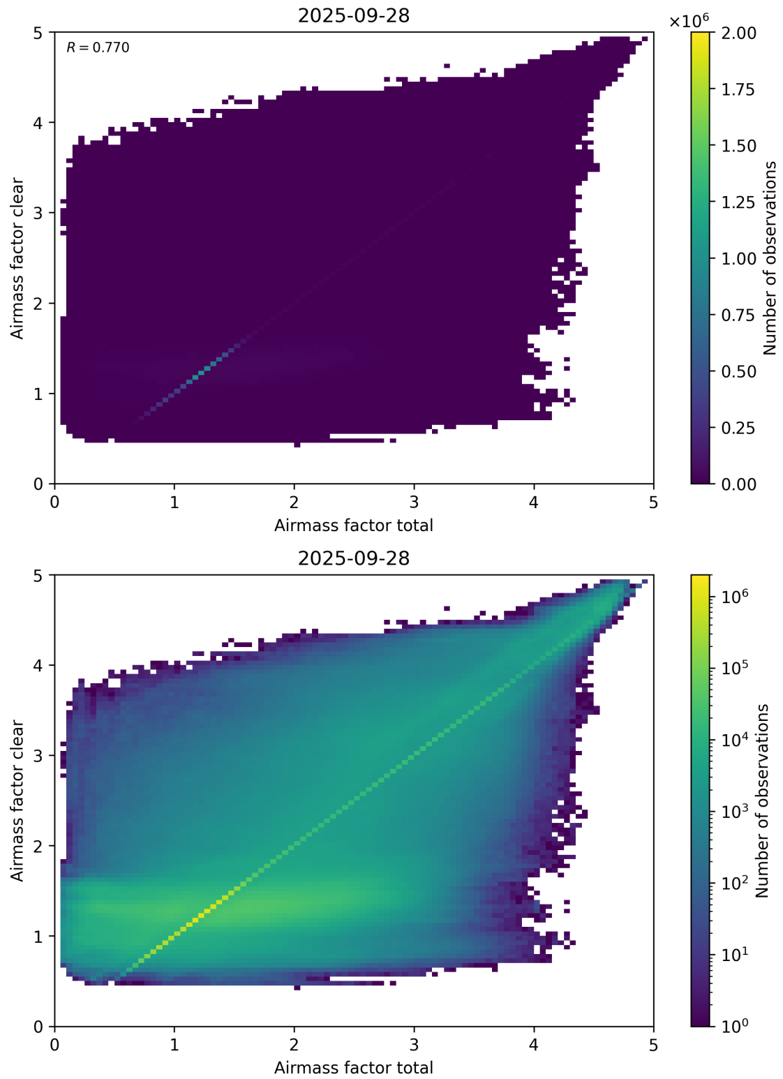
Figure 100: Scatter density plot of “Airmass factor total” against “Airmass factor clear” for 2025-09-27 to 2025-09-29.
