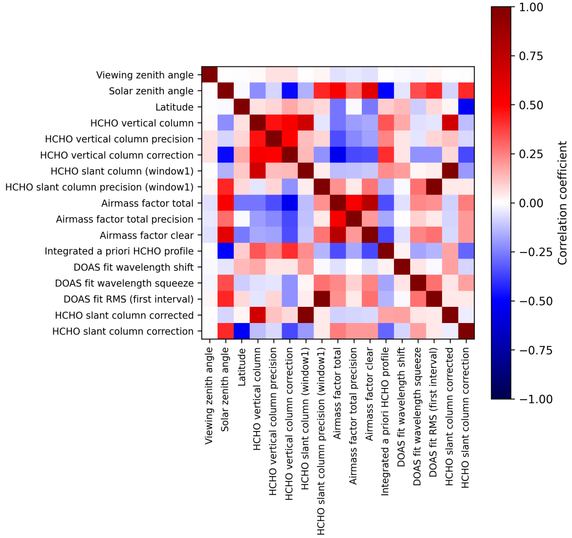
Figure 2: Map of correlation matrix for 2025-09-27 to 2025-09-29.
