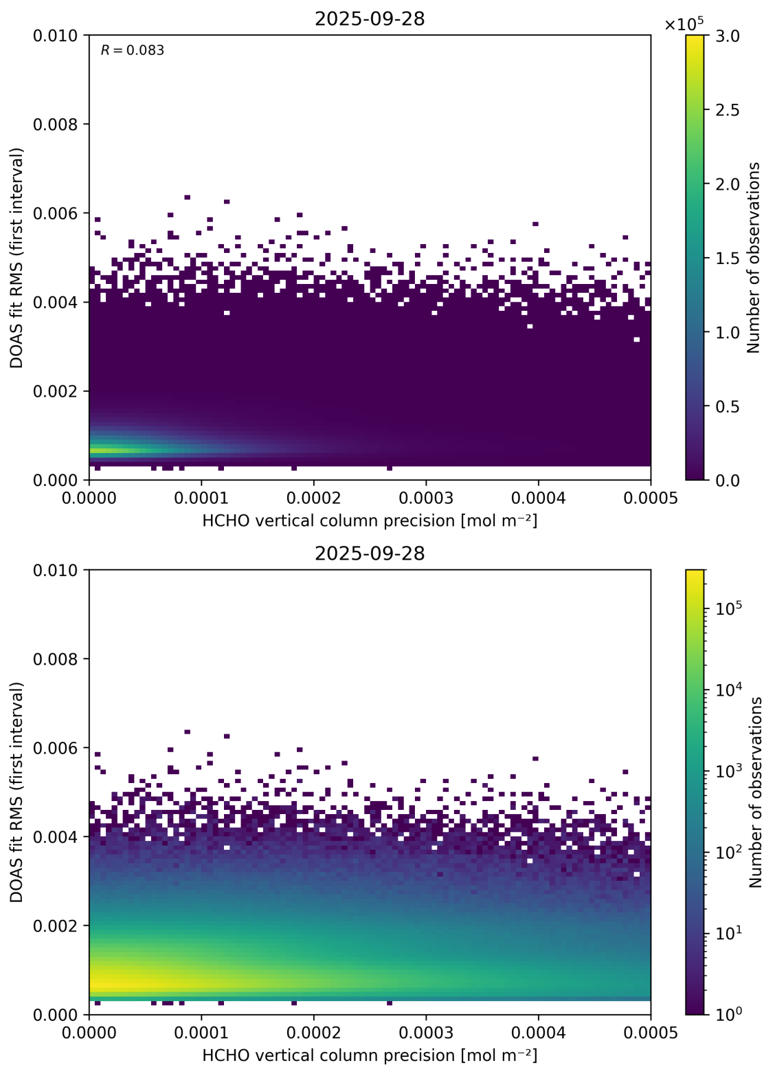
Figure 136: Scatter density plot of “HCHO vertical column precision” against “DOAS fit RMS (first interval)” for 2025-09-27 to 2025-09-29.
