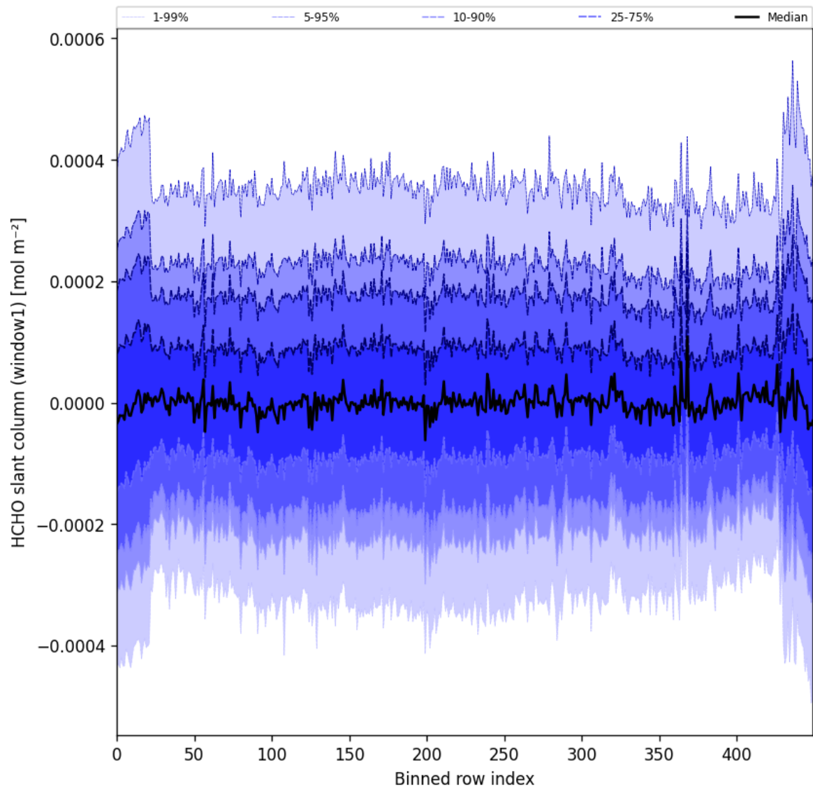
Figure 52: Along track statistics of “HCHO slant column (window1)” for 2025-09-27 to 2025-09-29
