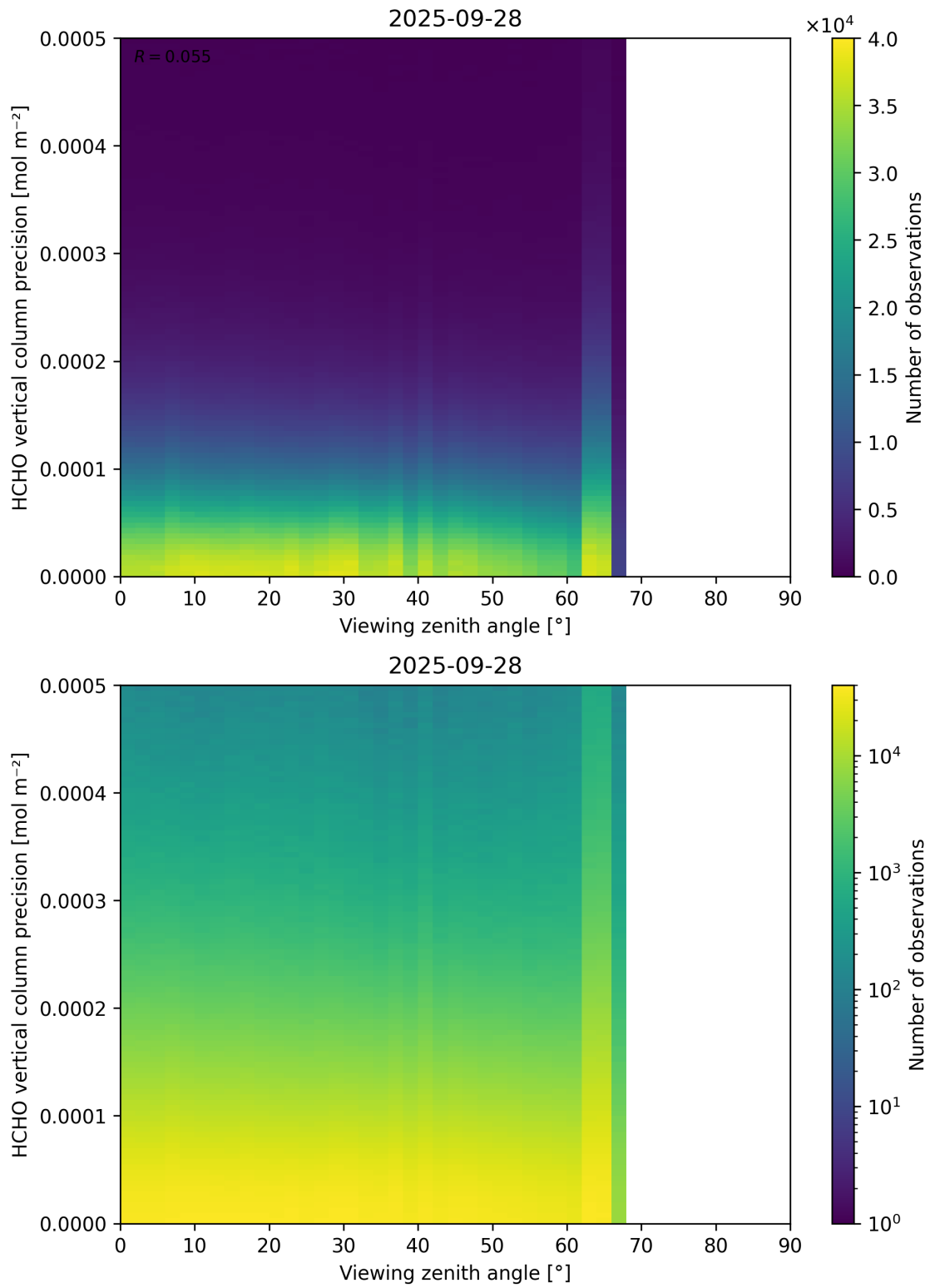
Figure 194: Scatter density plot of “Viewing zenith angle” against “HCHO vertical column precision” for 2025-09-27 to 2025-09-29.
