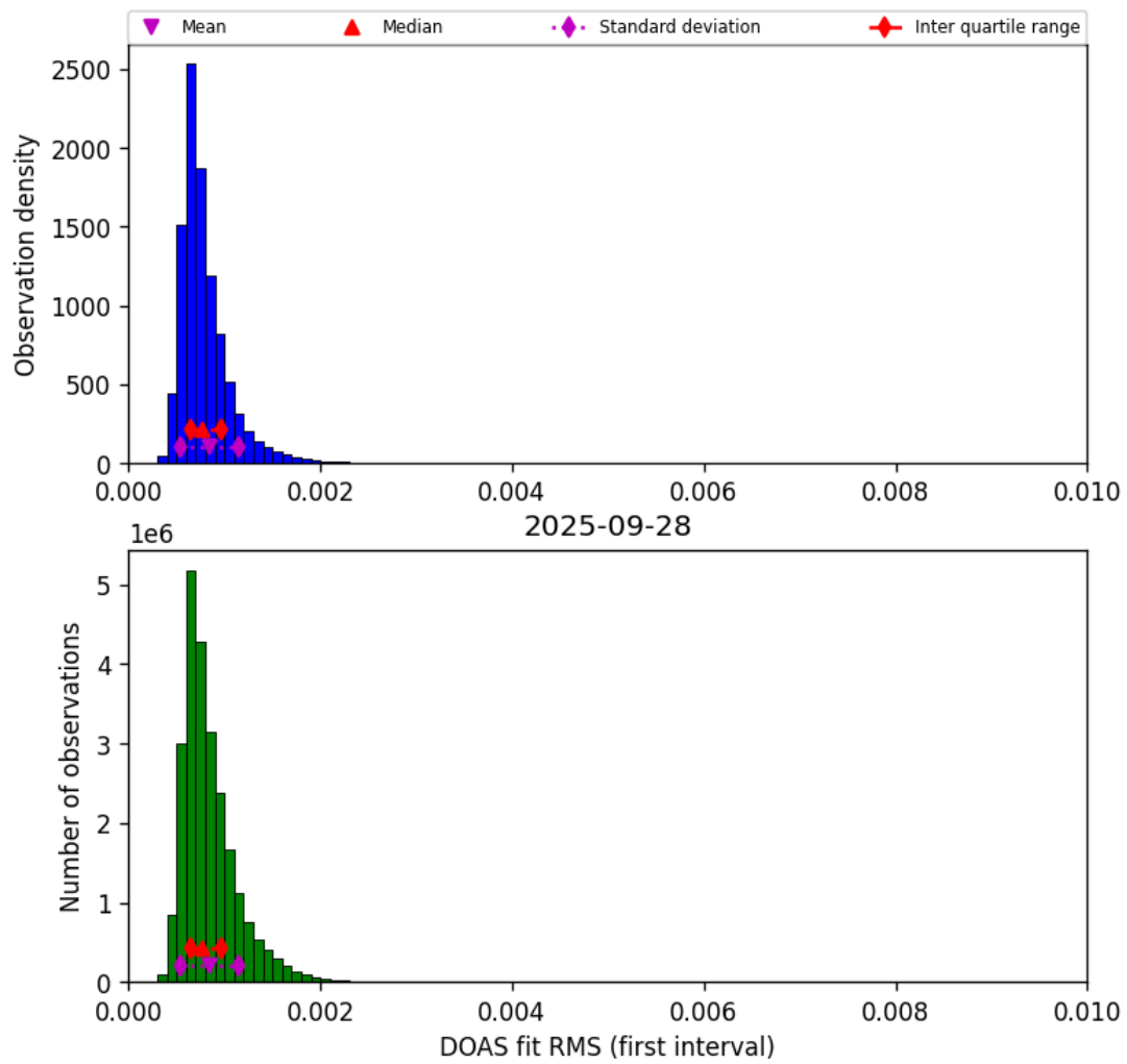
Figure 46: Histogram of “DOAS fit RMS (first interval)” for 2025-09-27 to 2025-09-29
