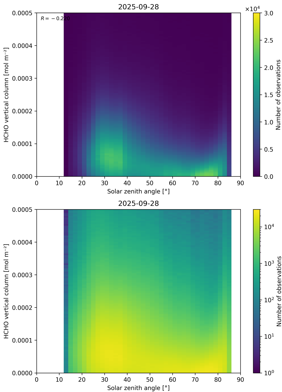
Figure 177: Scatter density plot of “Solar zenith angle” against “HCHO vertical column” for 2025-09-27 to 2025-09-29.
