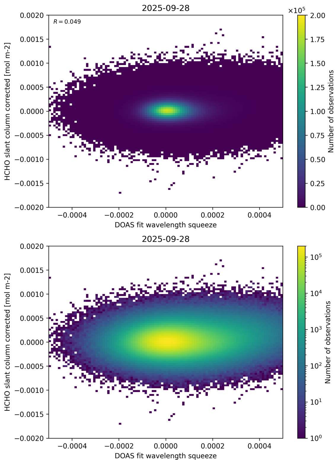
Figure 69: Scatter density plot of “DOAS fit wavelength squeeze” against “HCHO slant column corrected” for 2025-09-27 to 2025-09-29.
