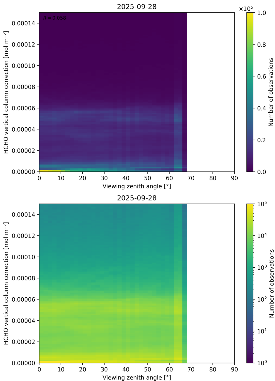
Figure 193: Scatter density plot of “Viewing zenith angle” against “HCHO vertical column correction” for 2025-09-27 to 2025-09-29.
