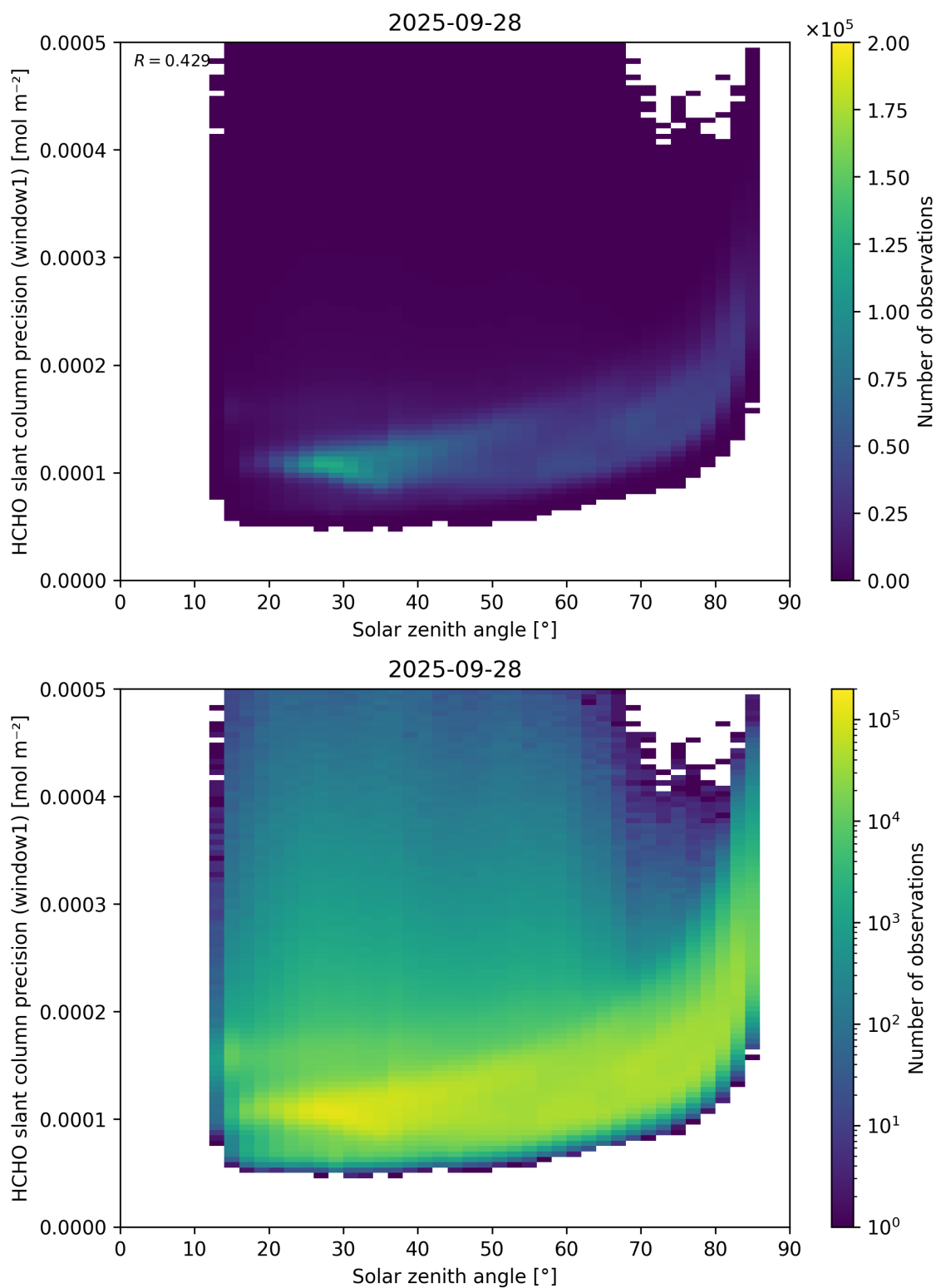
Figure 174: Scatter density plot of “Solar zenith angle” against “HCHO slant column precision (window1)” for 2025-09-27 to 2025-09-29.
