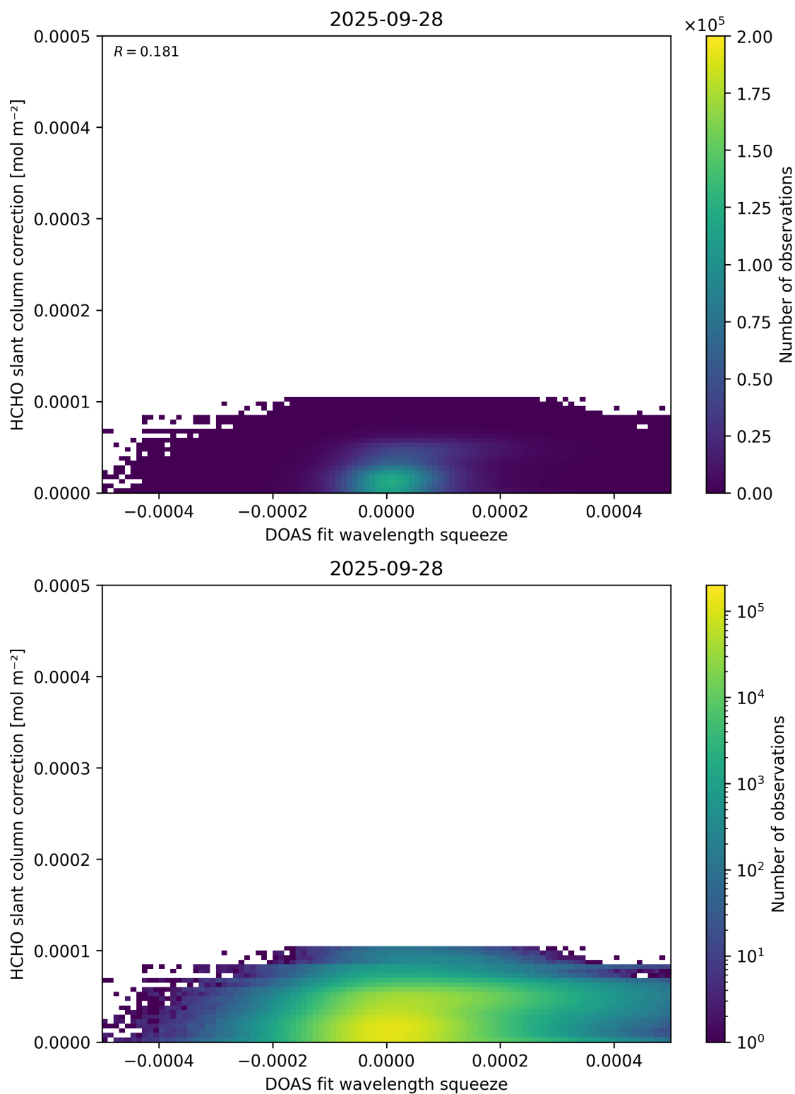
Figure 70: Scatter density plot of “DOAS fit wavelength squeeze” against “HCHO slant column correction” for 2025-09-27 to 2025-09-29.
