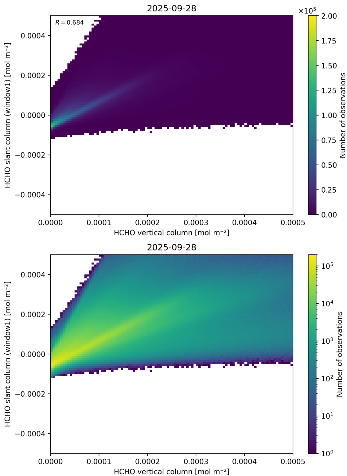
Figure 129: Scatter density plot of “HCHO vertical column” against “HCHO slant column (window1)” for 2025-09-27 to 2025-09-29.
