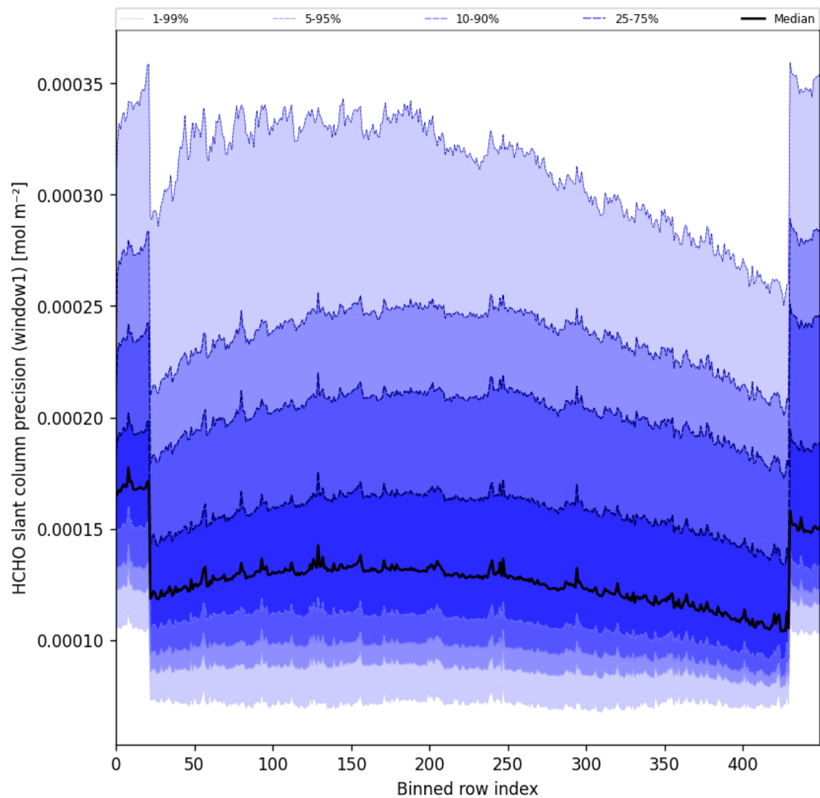
Figure 53: Along track statistics of “HCHO slant column precision (window1)” for 2025-09-27 to 2025-09-29
