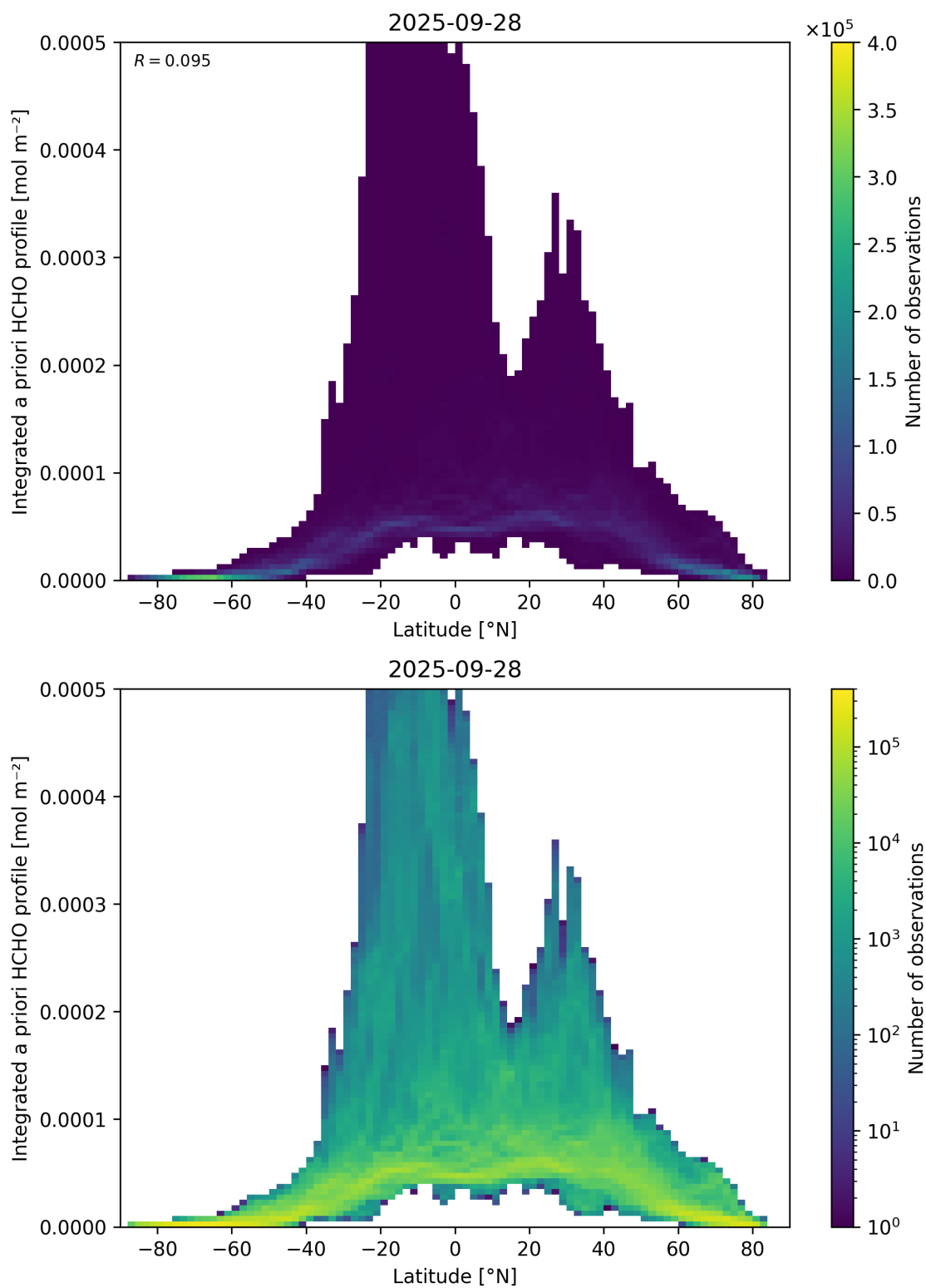
Figure 166: Scatter density plot of “Latitude” against “Integrated a priori HCHO profile” for 2025-09-27 to 2025-09-29.
