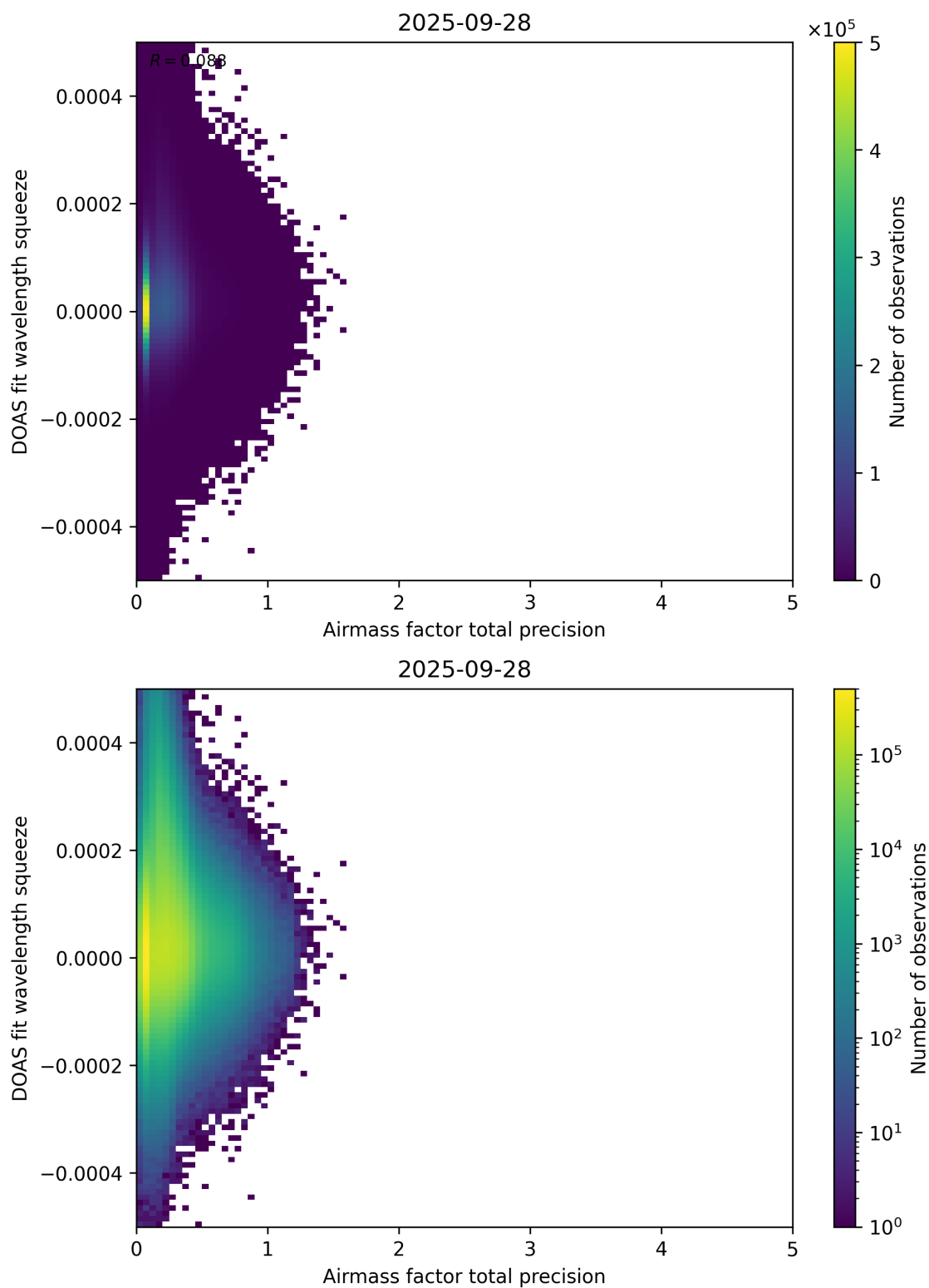
Figure 107: Scatter density plot of “Airmass factor total precision” against “DOAS fit wavelength squeeze” for 2025-09-27 to 2025-09-29.
