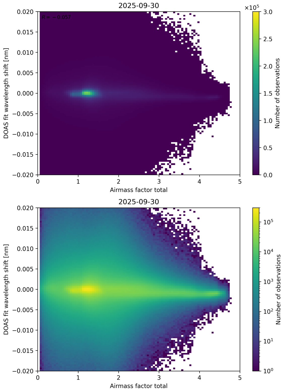
Figure 98: Scatter density plot of “Airmass factor total” against “DOAS fit wavelength shift” for 2025-09-29 to 2025-10-01.
