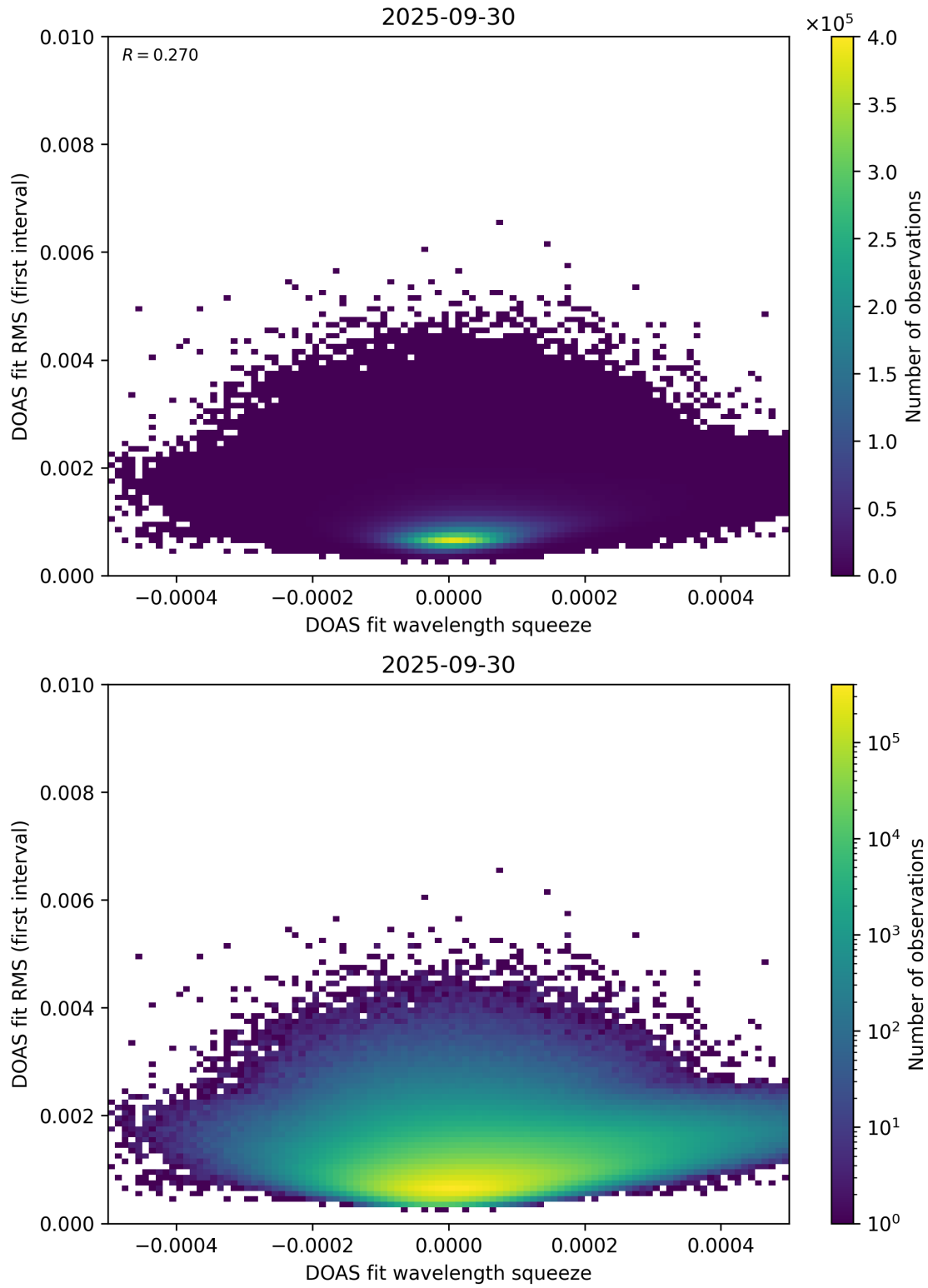
Figure 68: Scatter density plot of “DOAS fit wavelength squeeze” against “DOAS fit RMS (first interval)” for 2025-09-29 to 2025-10-01.
