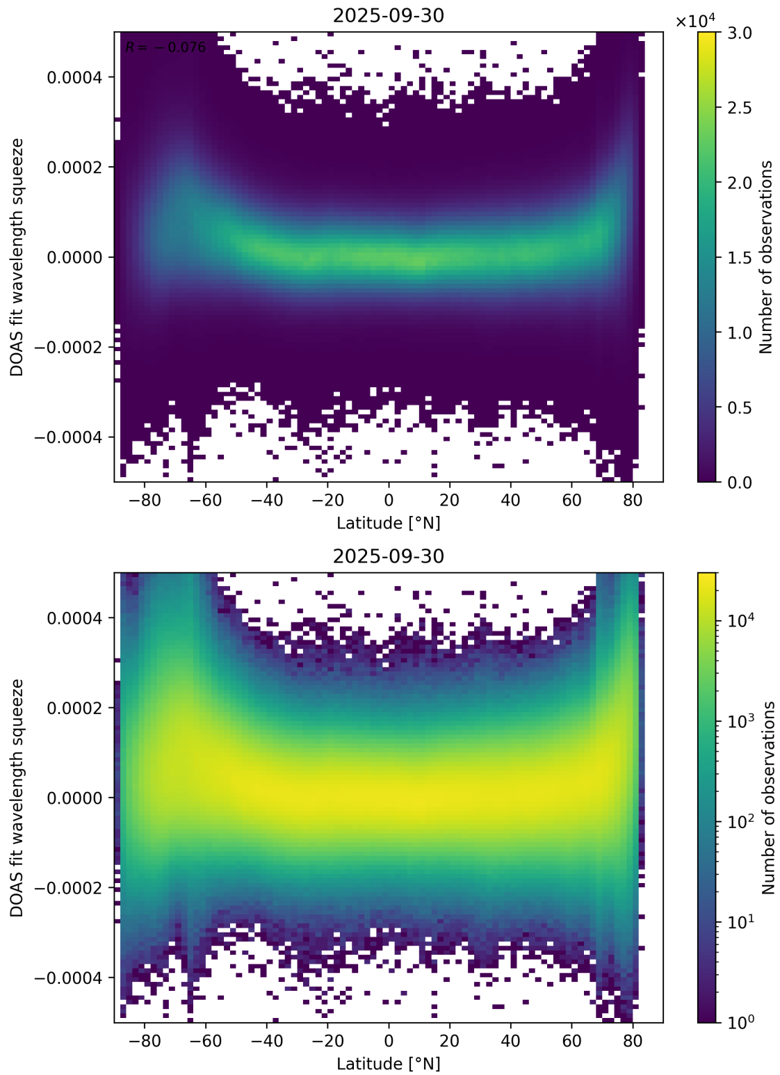
Figure 155: Scatter density plot of “Latitude” against “DOAS fit wavelength squeeze” for 2025-09-29 to 2025-10-01.
