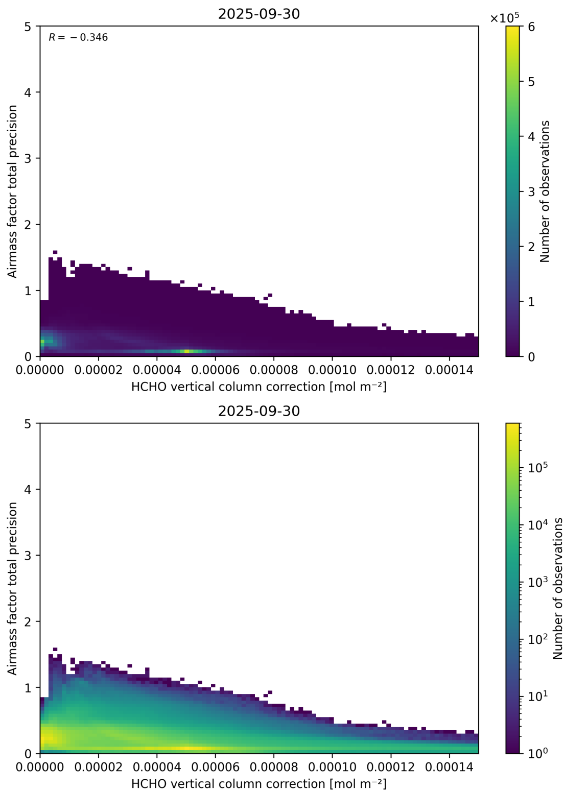
Figure 121: Scatter density plot of “HCHO vertical column correction” against “Airmass factor total precision” for 2025-09-29 to 2025-10-01.
