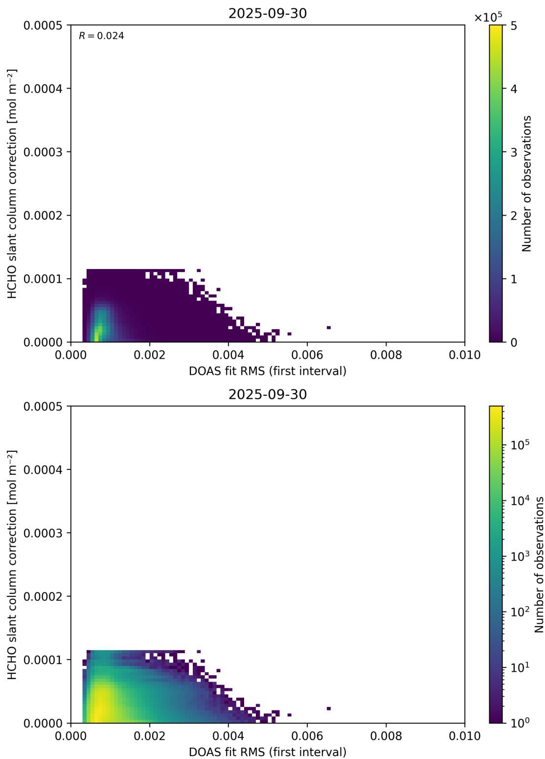
Figure 63: Scatter density plot of “DOAS fit RMS (first interval)” against “HCHO slant column correction” for 2025-09-29 to 2025-10-01.
