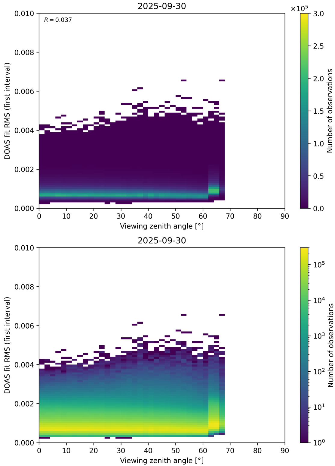
Figure 182: Scatter density plot of “Viewing zenith angle” against “DOAS fit RMS (first interval)” for 2025-09-29 to 2025-10-01.
