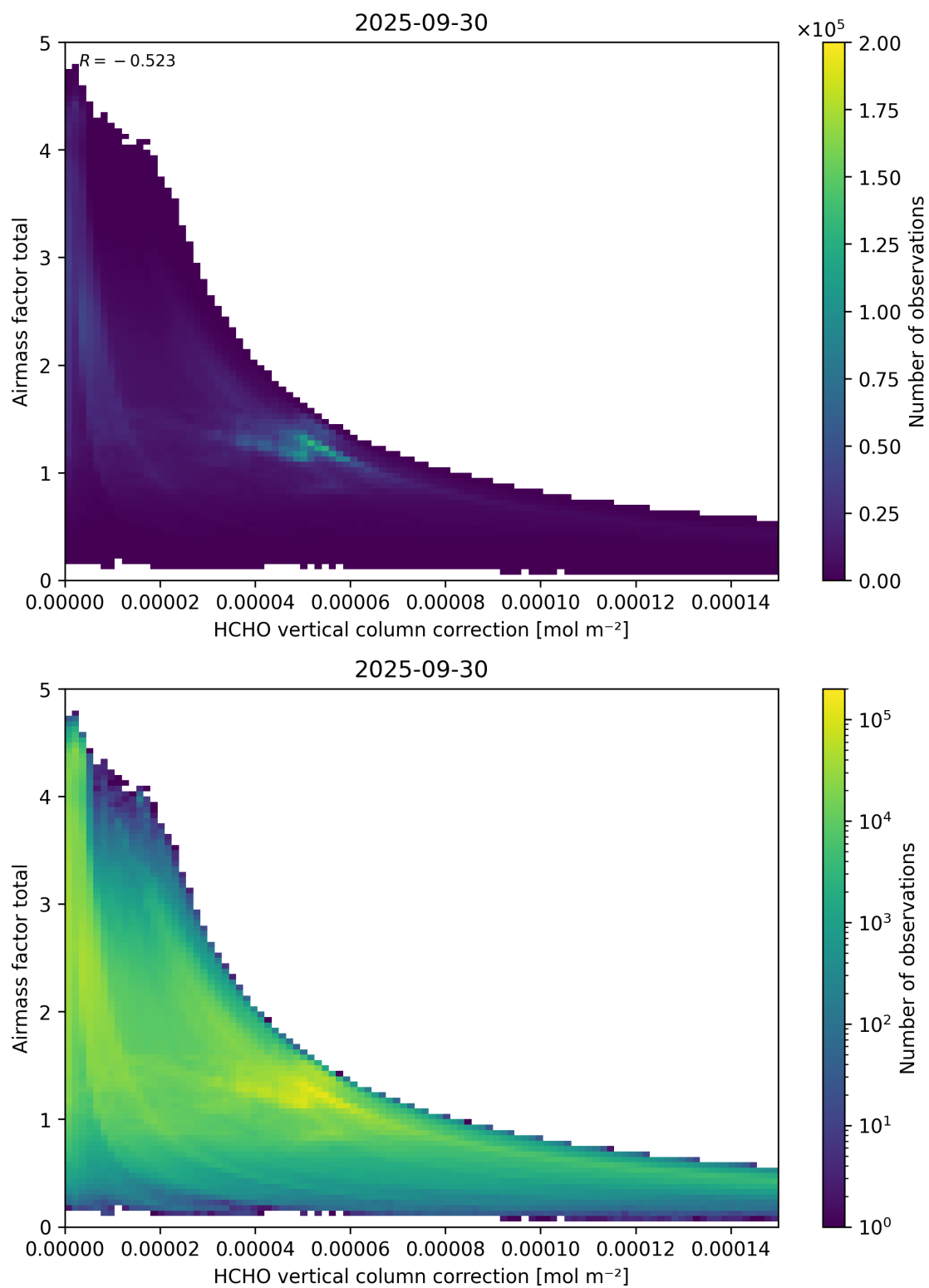
Figure 120: Scatter density plot of “HCHO vertical column correction” against “Airmass factor total” for 2025-09-29 to 2025-10-01.
