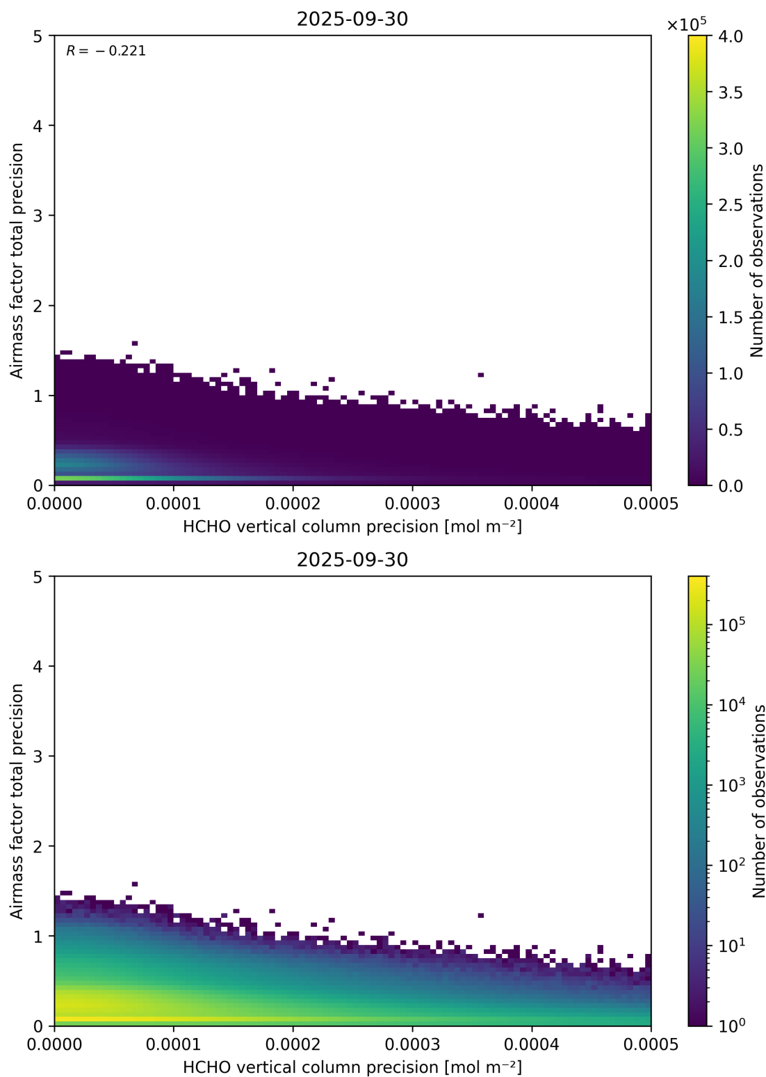
Figure 145: Scatter density plot of “HCHO vertical column precision” against “Airmass factor total precision” for 2025-09-29 to 2025-10-01.
