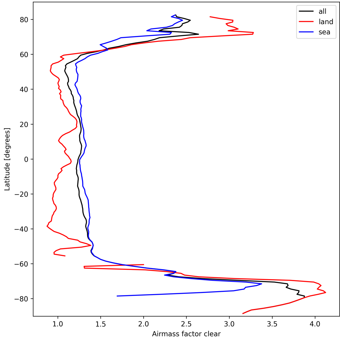
Figure 28: Zonal average of “Airmass factor clear” for 2025-09-29 to 2025-10-01.
