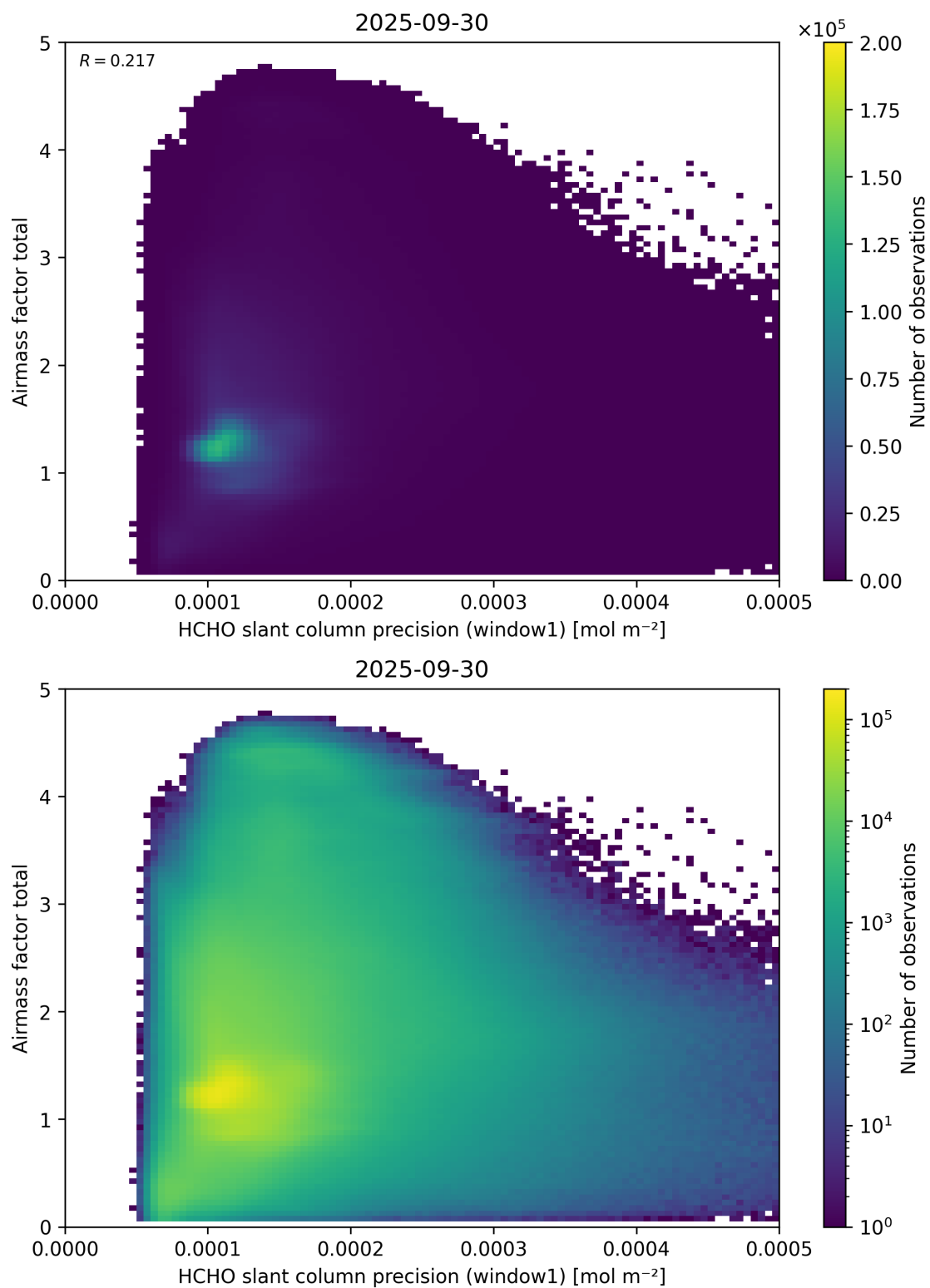
Figure 94: Scatter density plot of “HCHO slant column precision (window1)” against “Airmass factor total” for 2025-09-29 to 2025-10-01.
