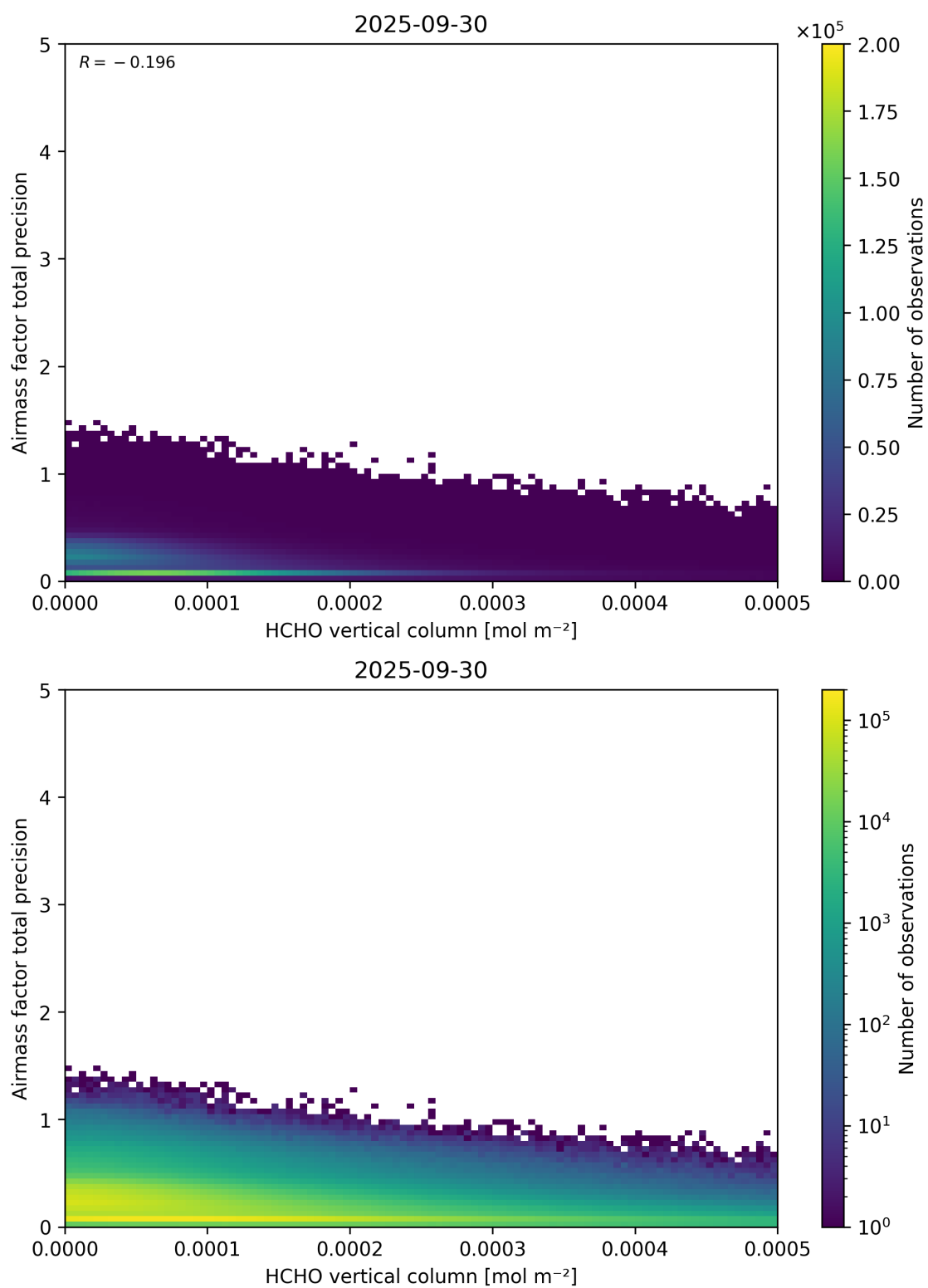
Figure 132: Scatter density plot of “HCHO vertical column” against “Airmass factor total precision” for 2025-09-29 to 2025-10-01.
