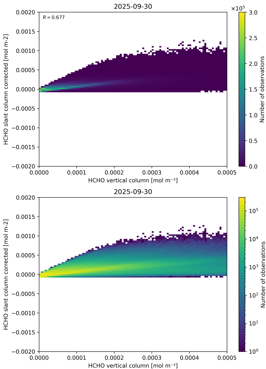
Figure 127: Scatter density plot of “HCHO vertical column” against “HCHO slant column corrected” for 2025-09-29 to 2025-10-01.
