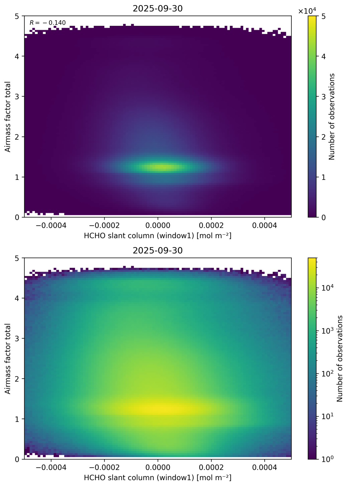
Figure 85: Scatter density plot of “HCHO slant column (window1)” against “Airmass factor total” for 2025-09-29 to 2025-10-01.
