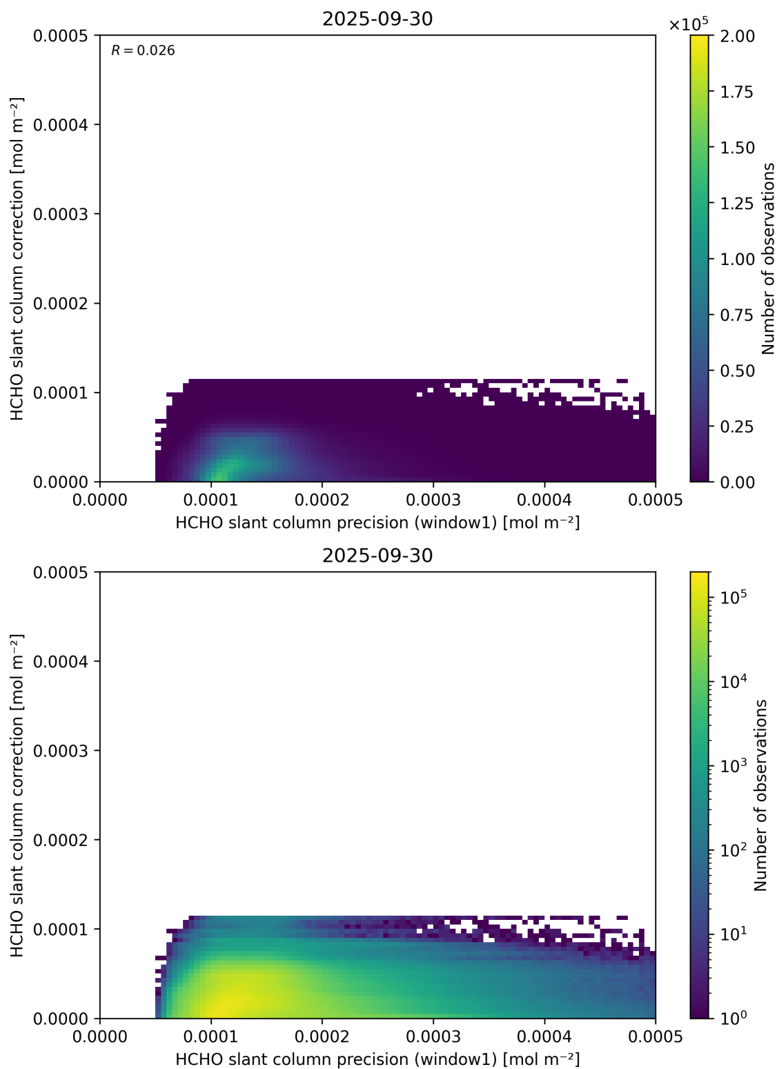
Figure 93: Scatter density plot of “HCHO slant column precision (window1)” against “HCHO slant column correction” for 2025-09-29 to 2025-10-01.
