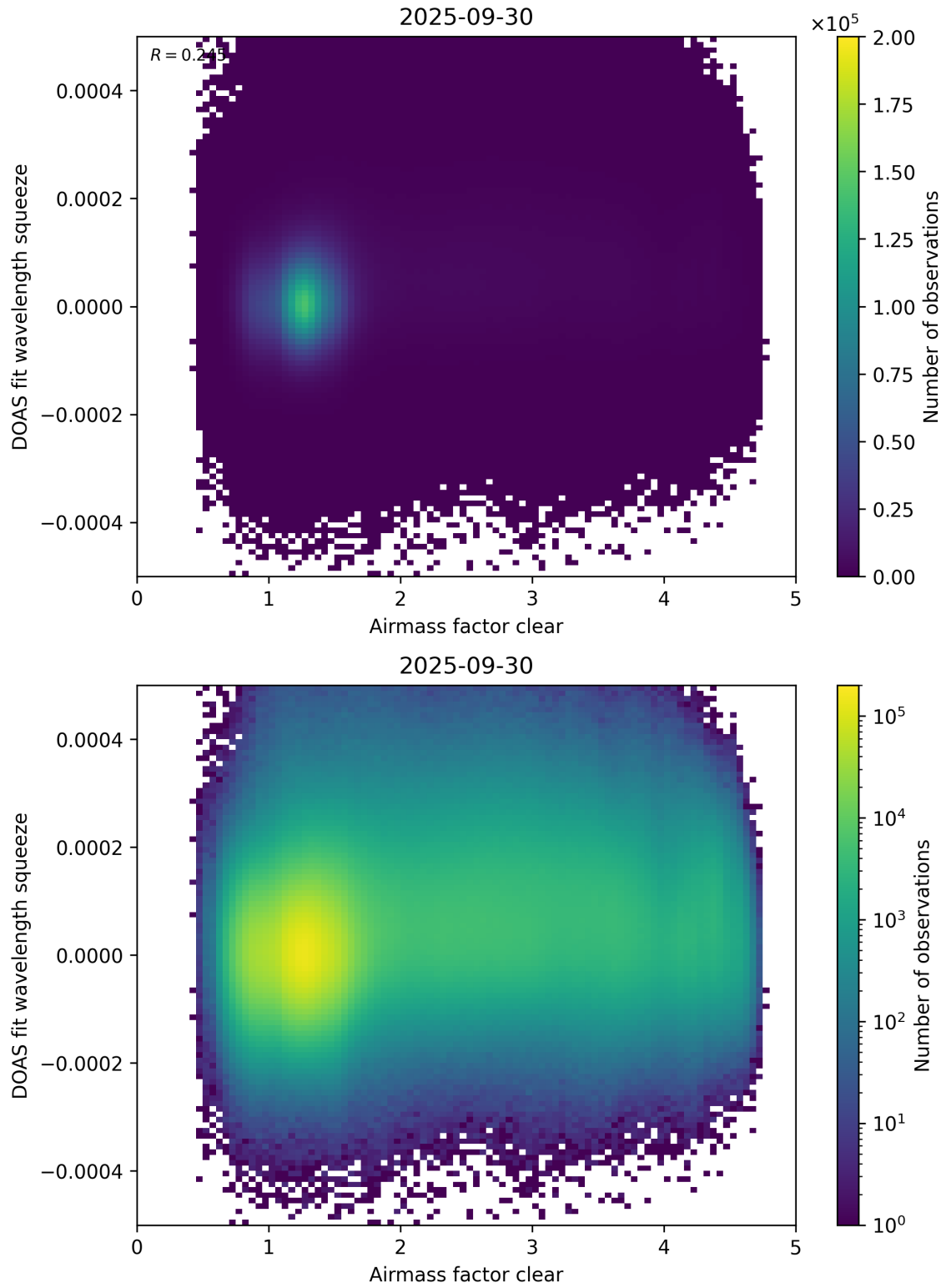
Figure 73: Scatter density plot of “Airmass factor clear” against “DOAS fit wavelength squeeze” for 2025-09-29 to 2025-10-01.
