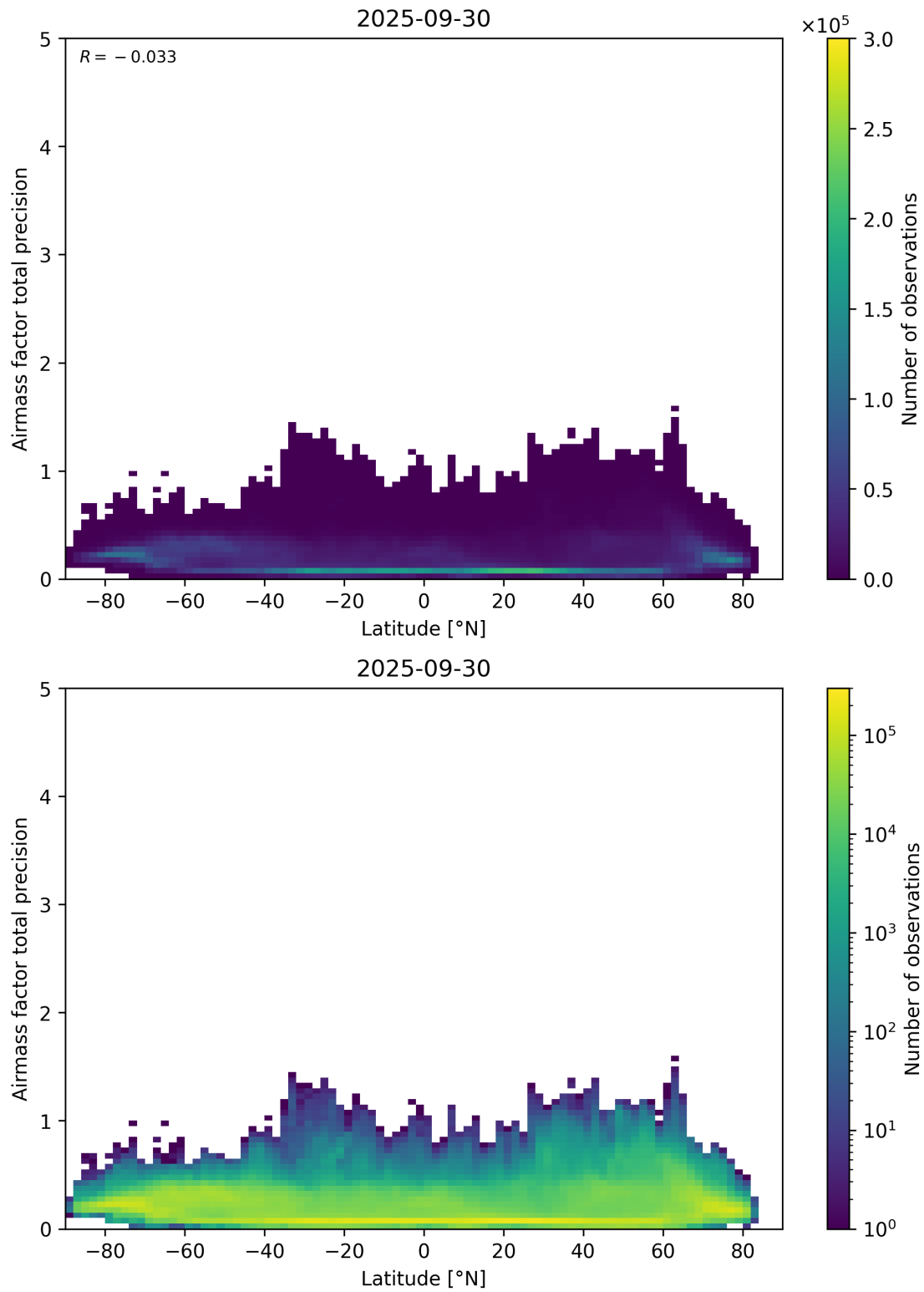
Figure 162: Scatter density plot of “Latitude” against “Airmass factor total precision” for 2025-09-29 to 2025-10-01.
