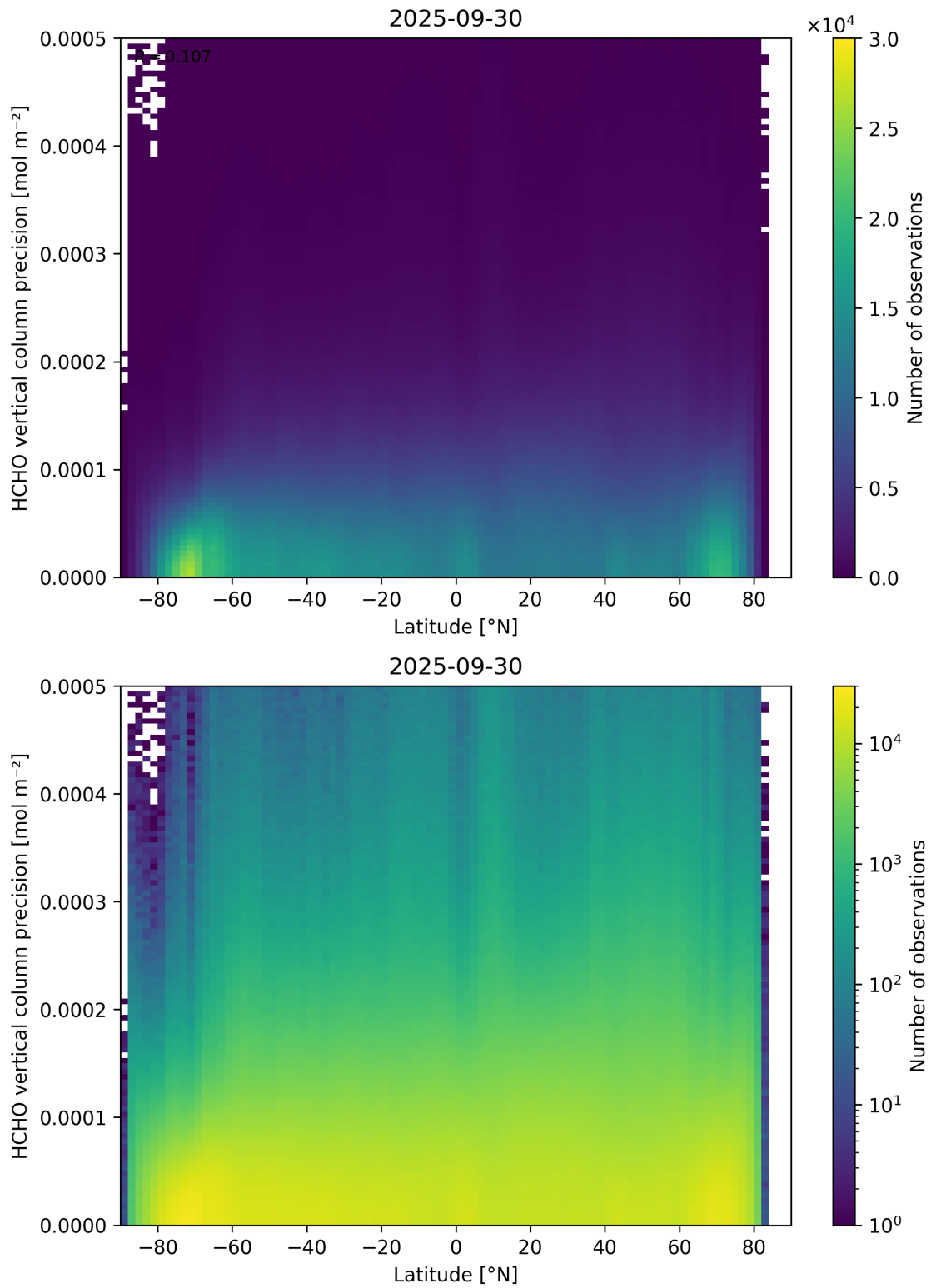
Figure 165: Scatter density plot of “Latitude” against “HCHO vertical column precision” for 2025-09-29 to 2025-10-01.
