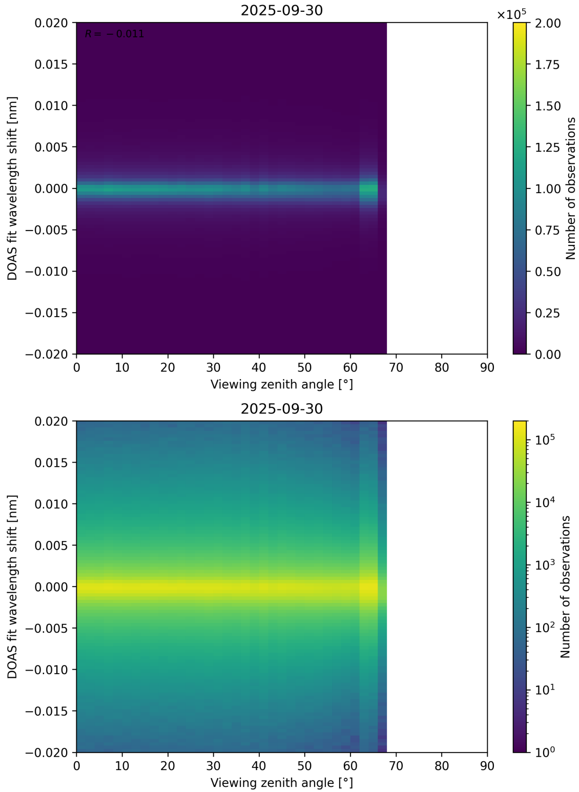
Figure 183: Scatter density plot of “Viewing zenith angle” against “DOAS fit wavelength shift” for 2025-09-29 to 2025-10-01.
