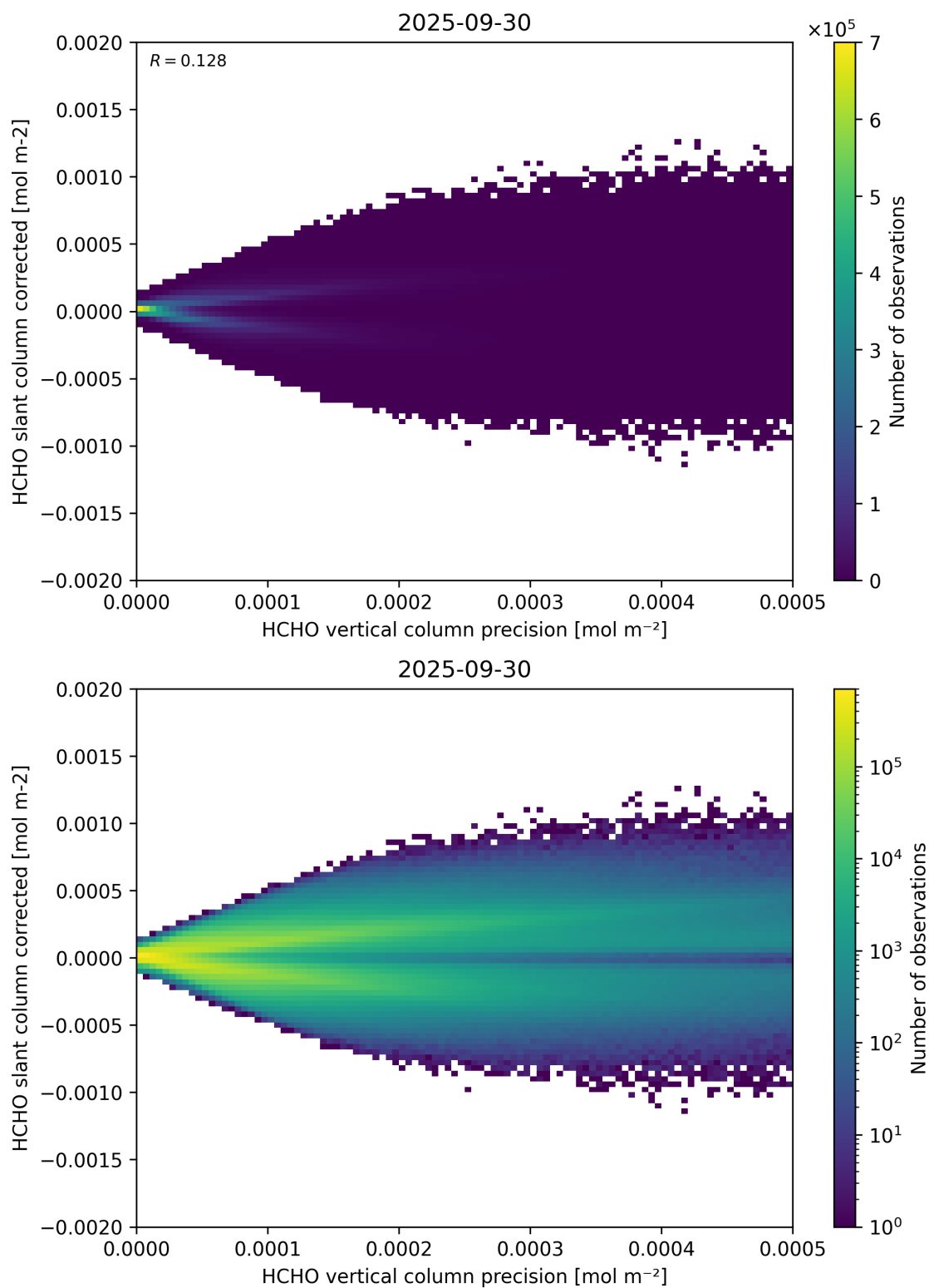
Figure 140: Scatter density plot of “HCHO vertical column precision” against “HCHO slant column corrected” for 2025-09-29 to 2025-10-01.
