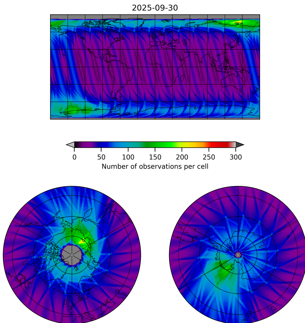
Figure 19: Map of the number of observations for 2025-09-29 to 2025-10-01
