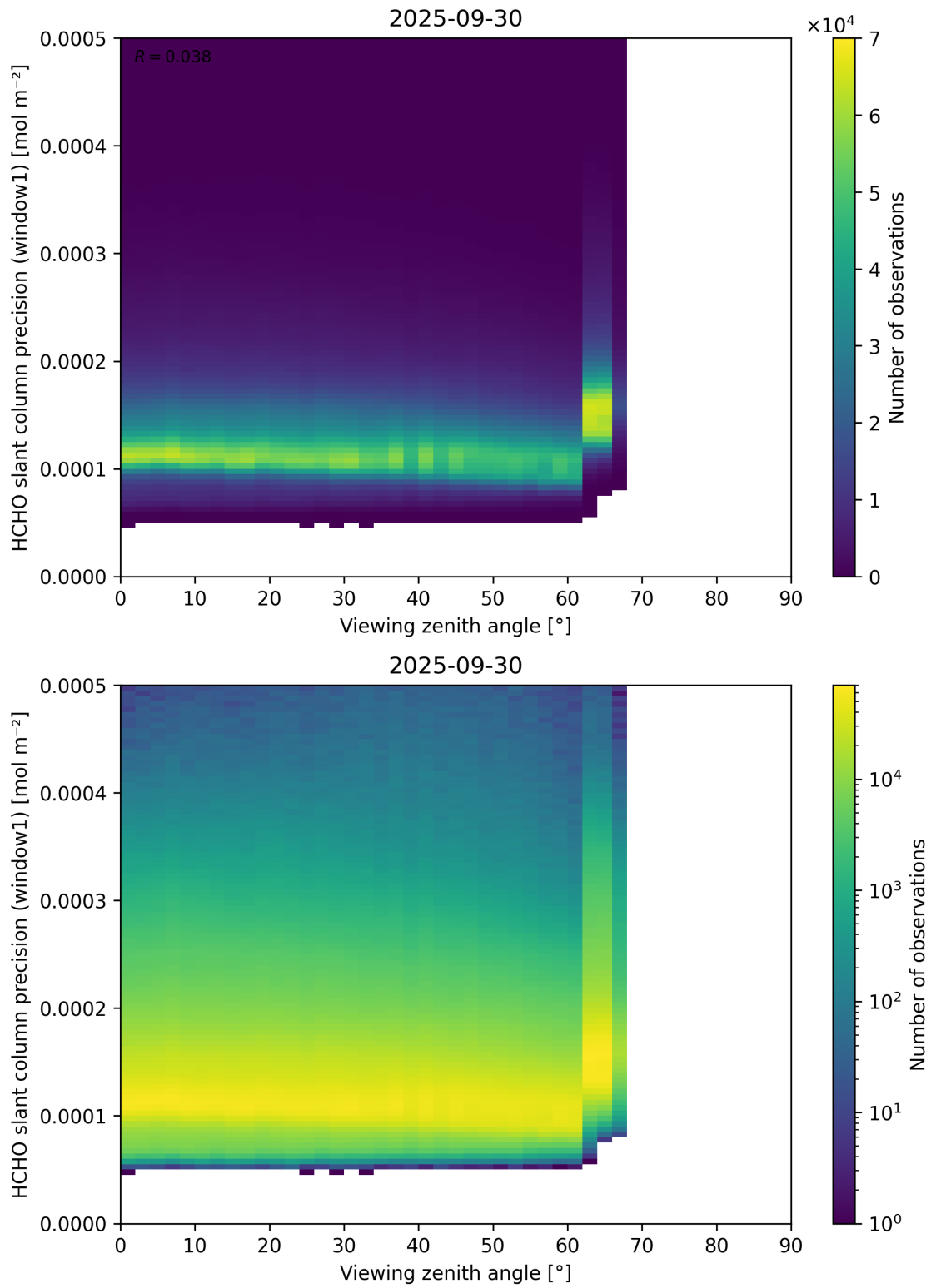
Figure 189: Scatter density plot of “Viewing zenith angle” against “HCHO slant column precision (window1)” for 2025-09-29 to 2025-10-01.
