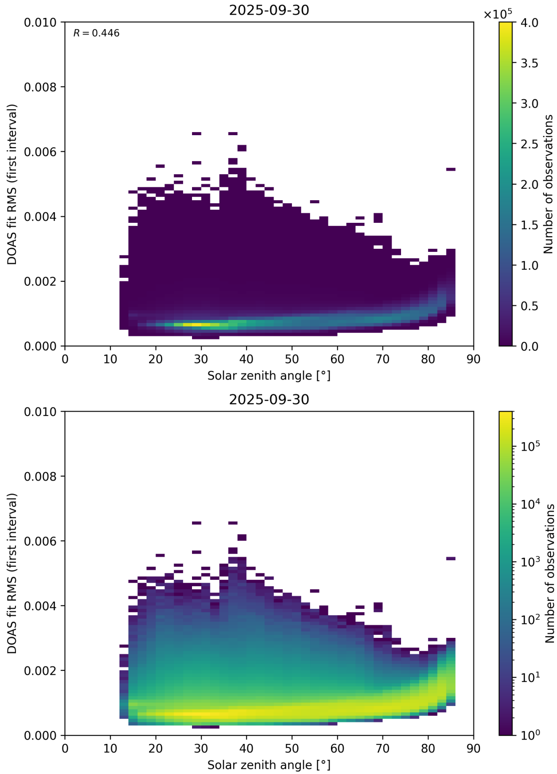
Figure 167: Scatter density plot of “Solar zenith angle” against “DOAS fit RMS (first interval)” for 2025-09-29 to 2025-10-01.
