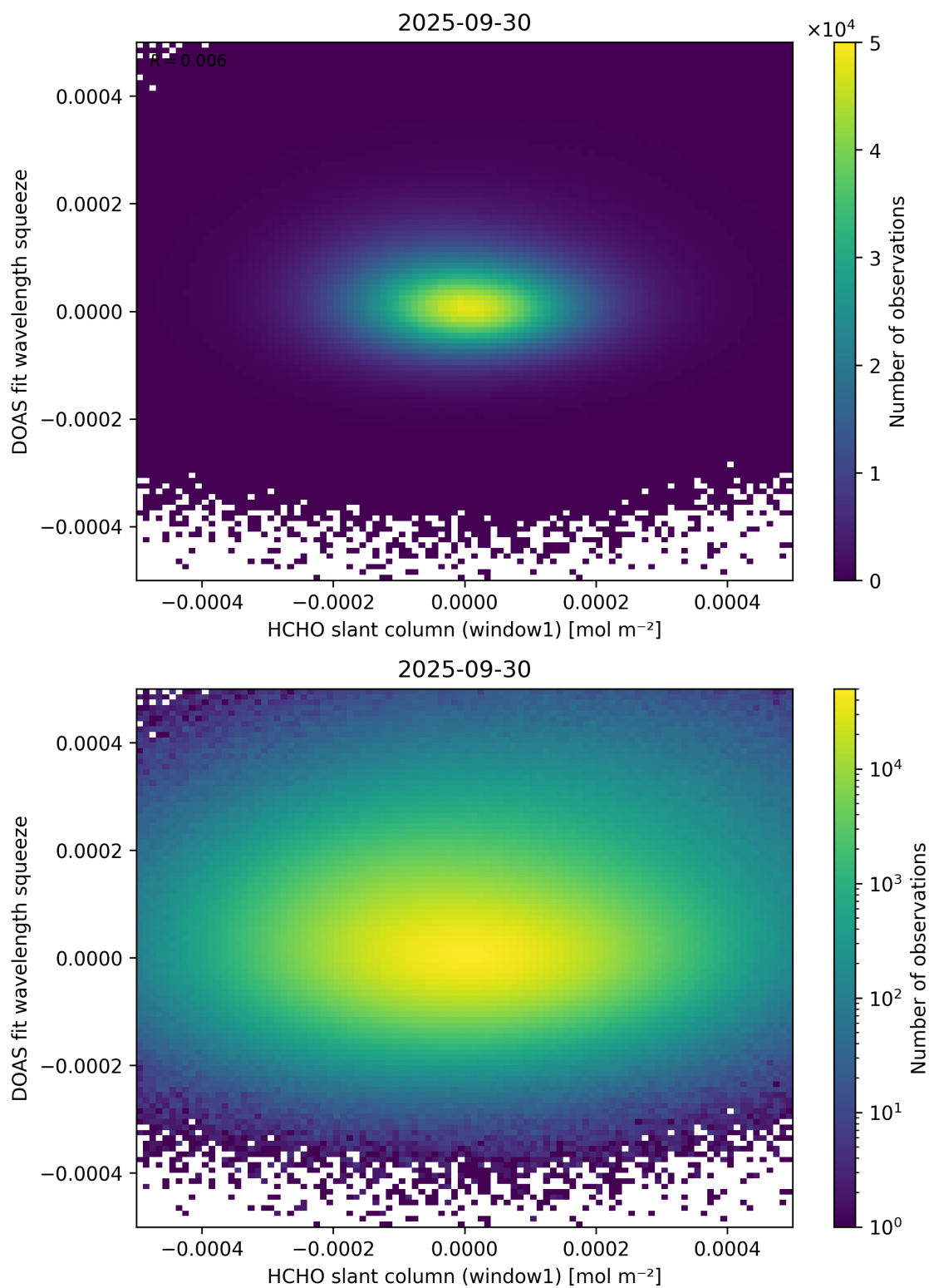
Figure 80: Scatter density plot of “HCHO slant column (window1)” against “DOAS fit wavelength squeeze” for 2025-09-29 to 2025-10-01.
