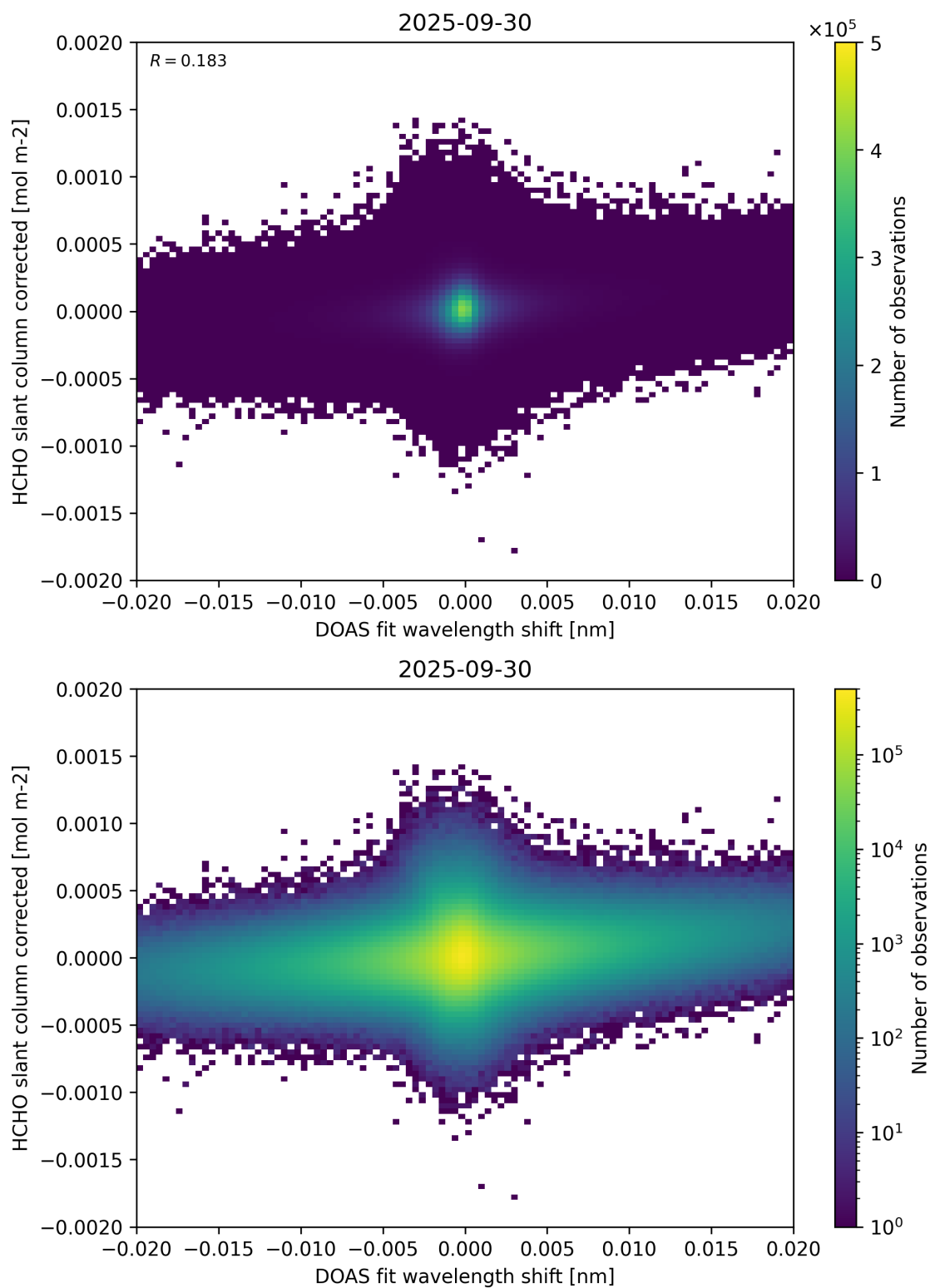
Figure 66: Scatter density plot of “DOAS fit wavelength shift” against “HCHO slant column corrected” for 2025-09-29 to 2025-10-01.
