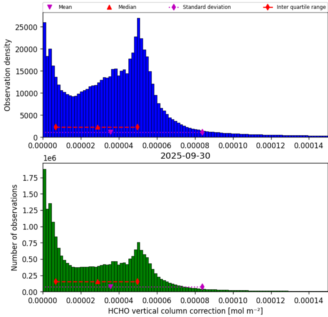
Figure 37: Histogram of “HCHO vertical column correction” for 2025-09-29 to 2025-10-01
