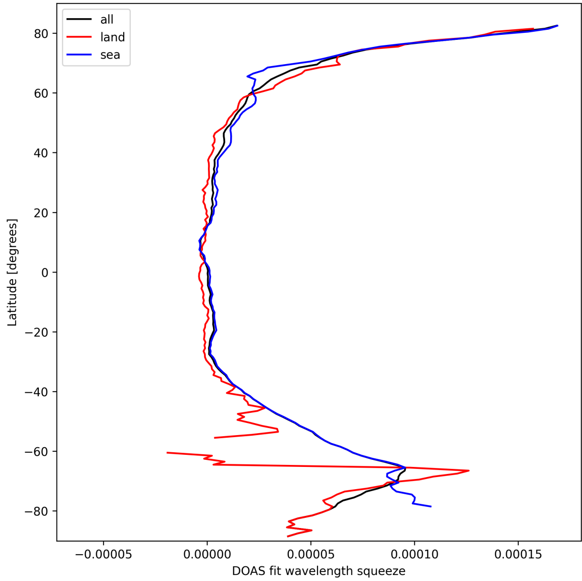
Figure 31: Zonal average of “DOAS fit wavelength squeeze” for 2025-09-29 to 2025-10-01.
