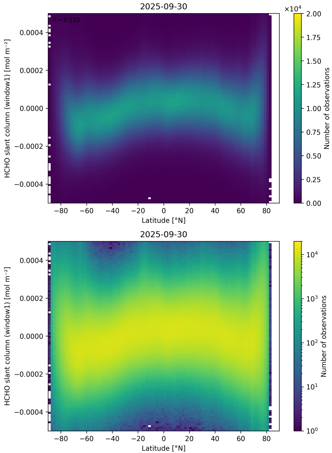
Figure 159: Scatter density plot of “Latitude” against “HCHO slant column (window1)” for 2025-09-29 to 2025-10-01.
