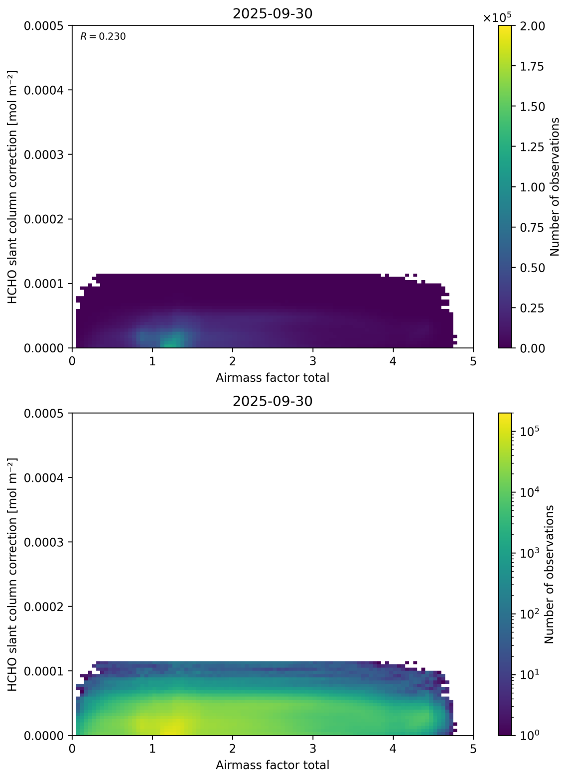
Figure 102: Scatter density plot of “Airmass factor total” against “HCHO slant column correction” for 2025-09-29 to 2025-10-01.
