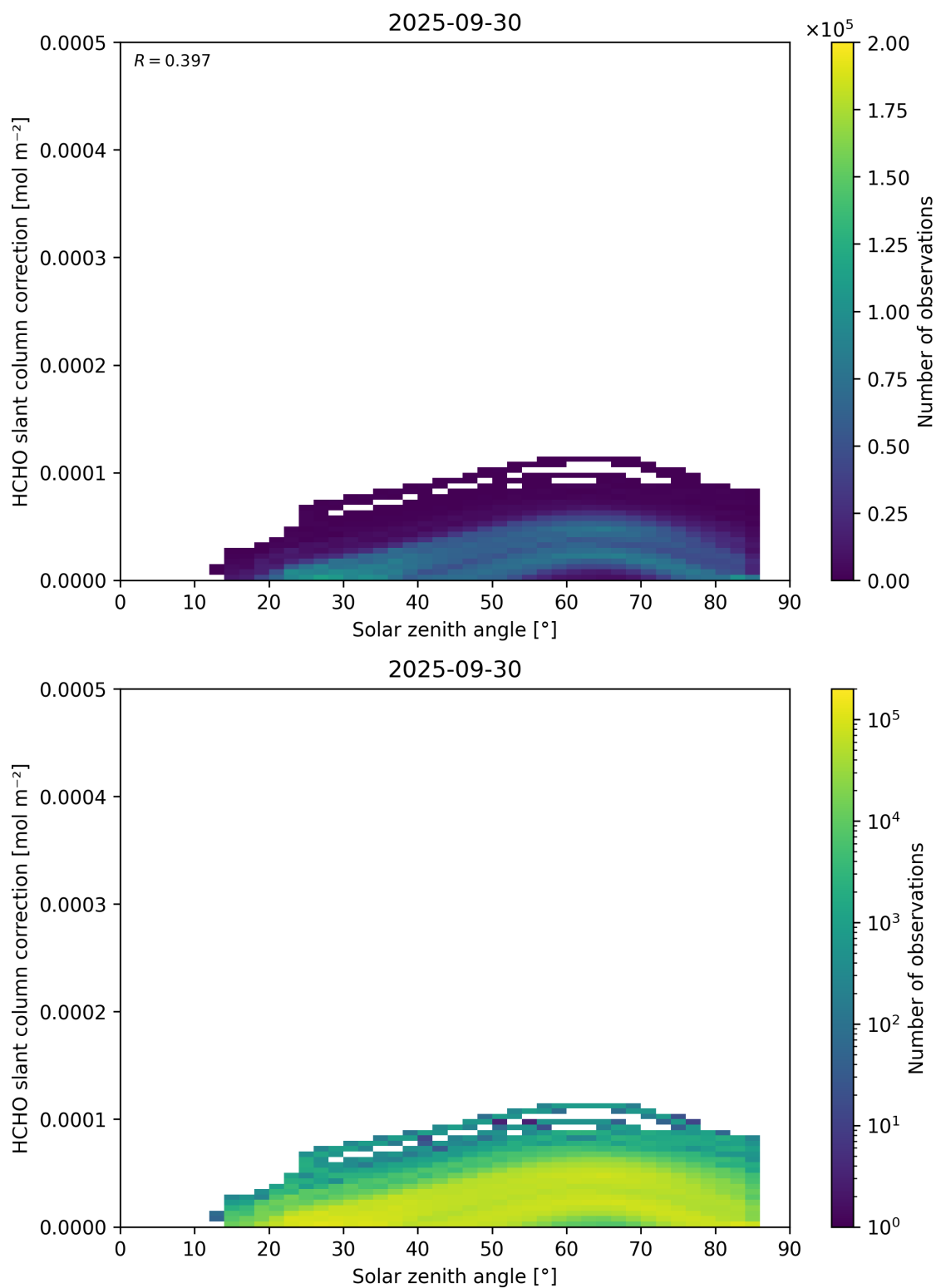
Figure 172: Scatter density plot of “Solar zenith angle” against “HCHO slant column correction” for 2025-09-29 to 2025-10-01.
