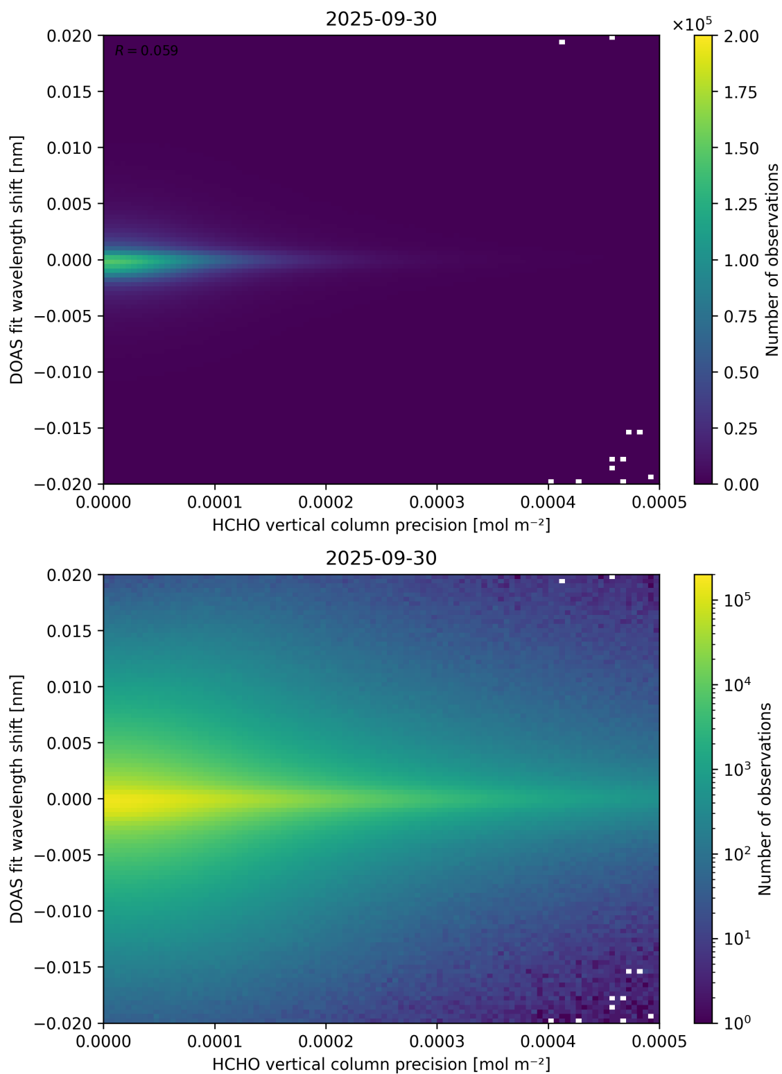
Figure 137: Scatter density plot of “HCHO vertical column precision” against “DOAS fit wavelength shift” for 2025-09-29 to 2025-10-01.
