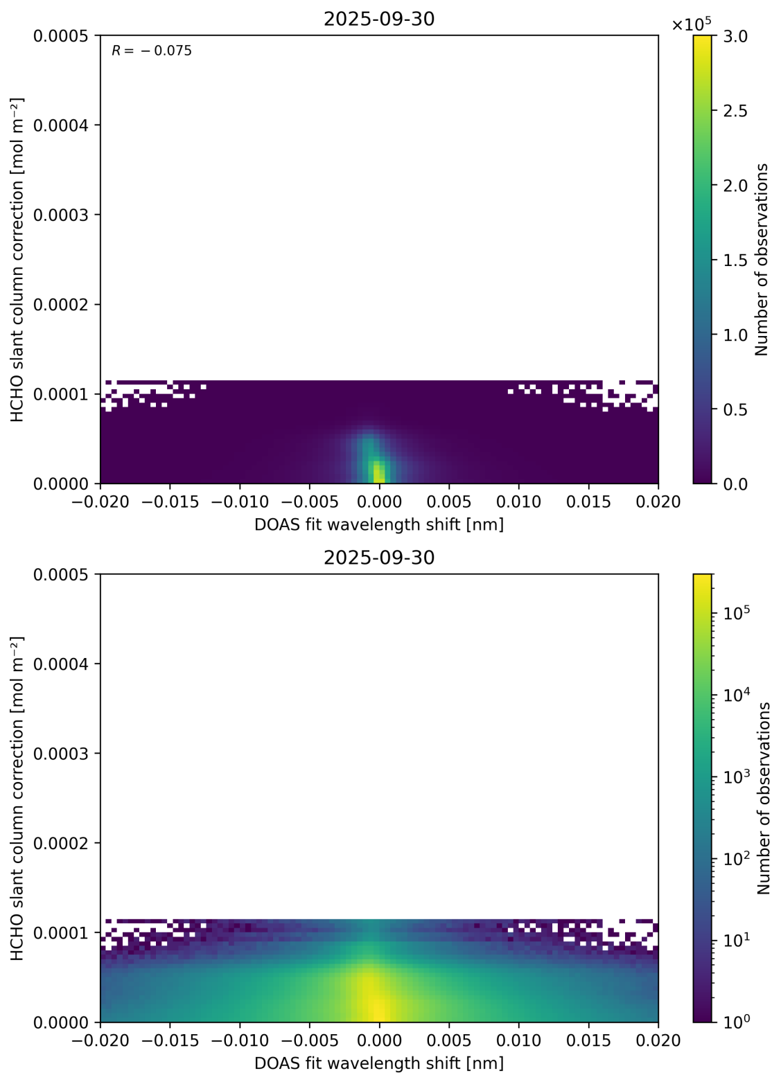
Figure 67: Scatter density plot of “DOAS fit wavelength shift” against “HCHO slant column correction” for 2025-09-29 to 2025-10-01.
