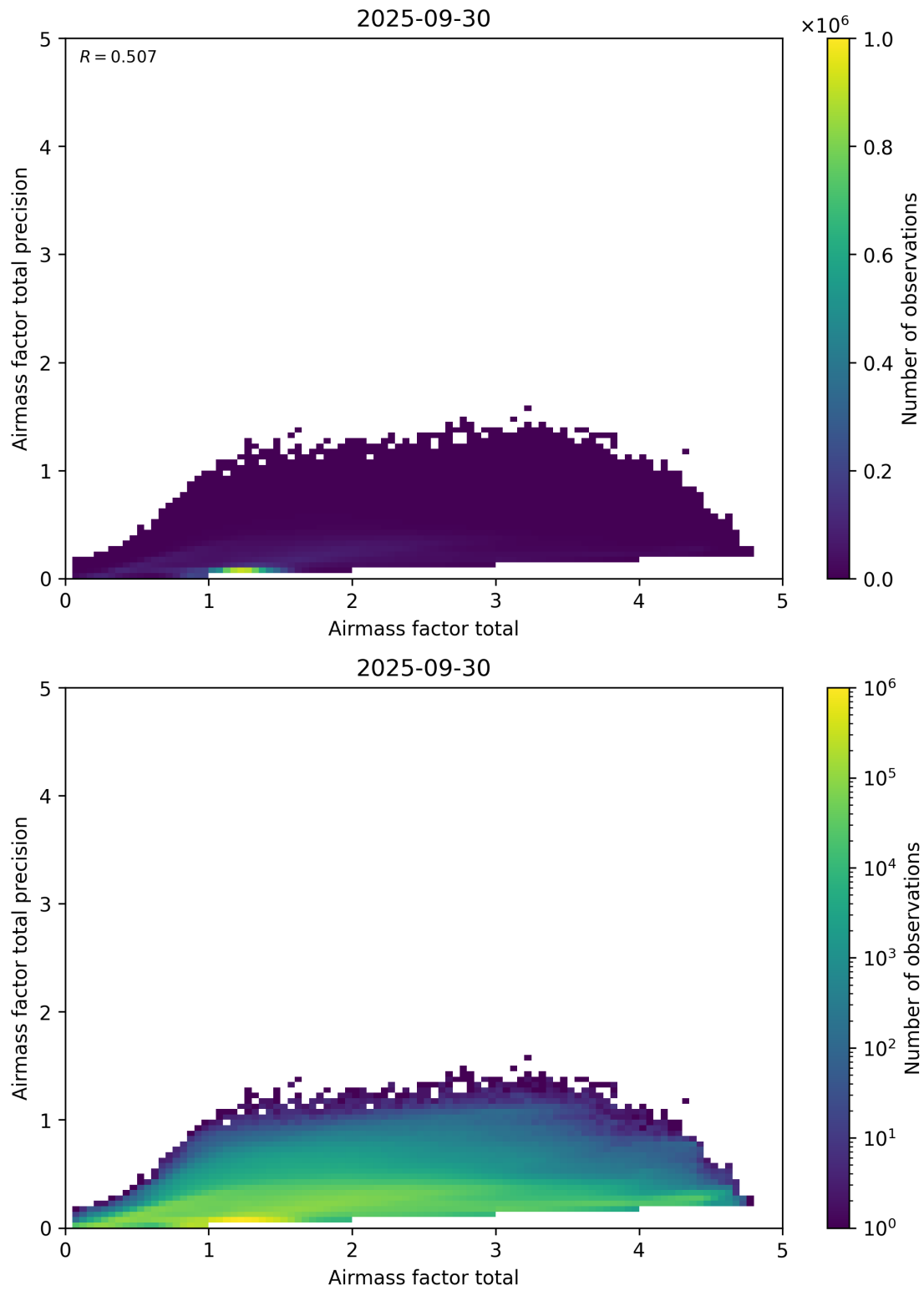
Figure 103: Scatter density plot of “Airmass factor total” against “Airmass factor total precision” for 2025-09-29 to 2025-10-01.
