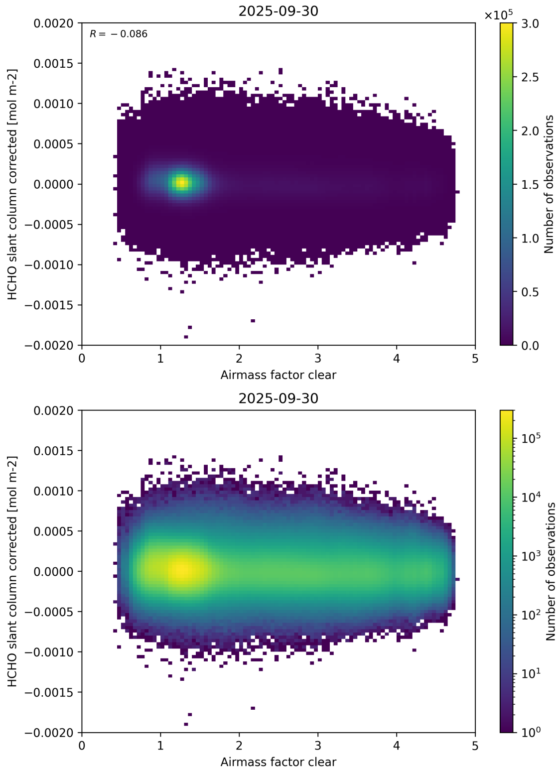
Figure 74: Scatter density plot of “Airmass factor clear” against “HCHO slant column corrected” for 2025-09-29 to 2025-10-01.
