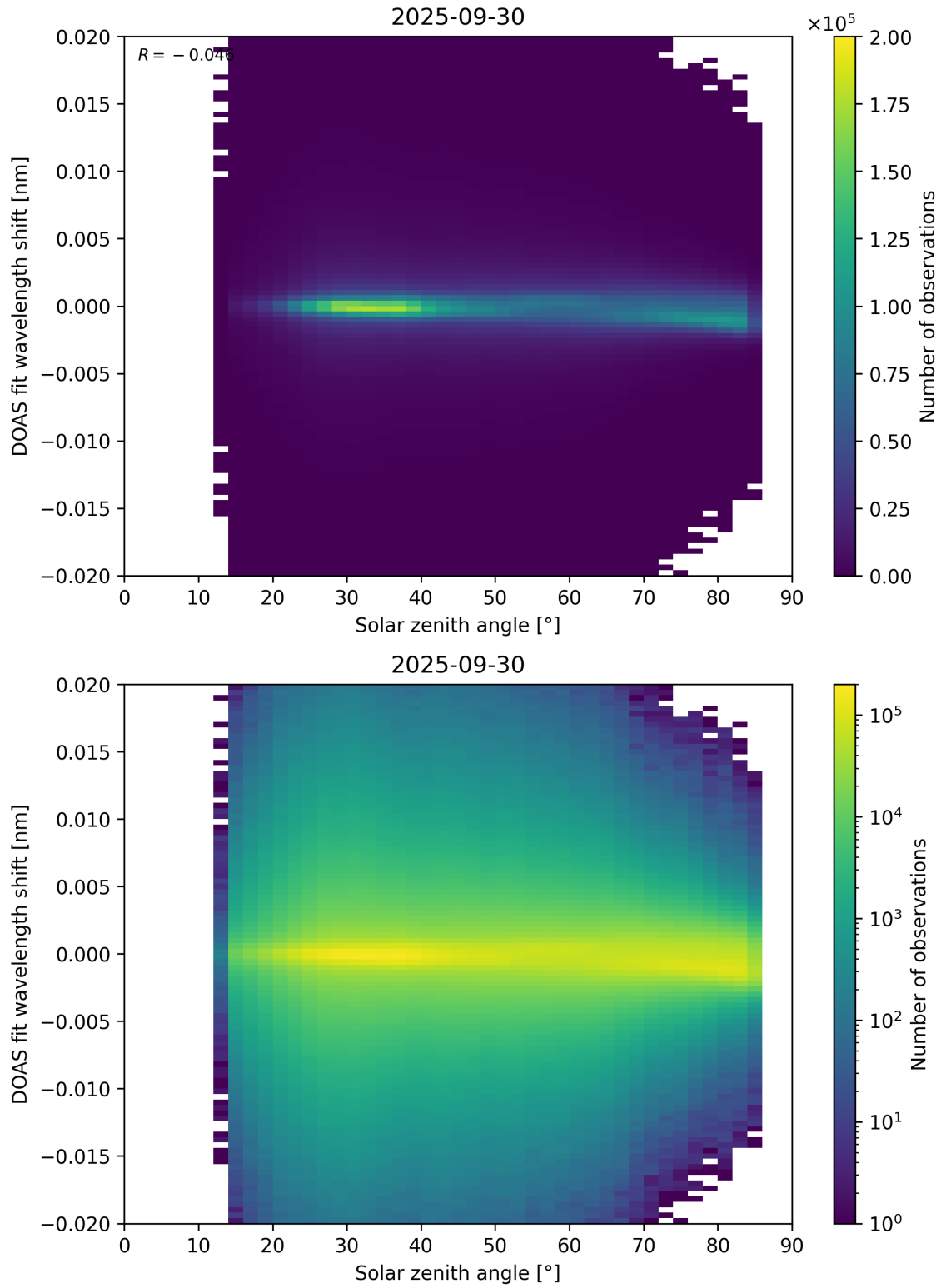
Figure 168: Scatter density plot of “Solar zenith angle” against “DOAS fit wavelength shift” for 2025-09-29 to 2025-10-01.
