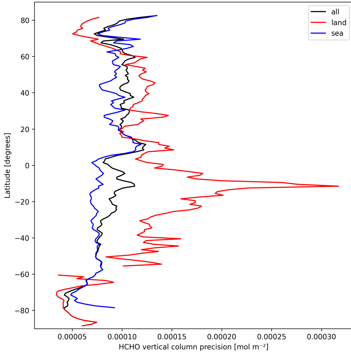
Figure 22: Zonal average of “HCHO vertical column precision” for 2025-09-29 to 2025-10-01.
