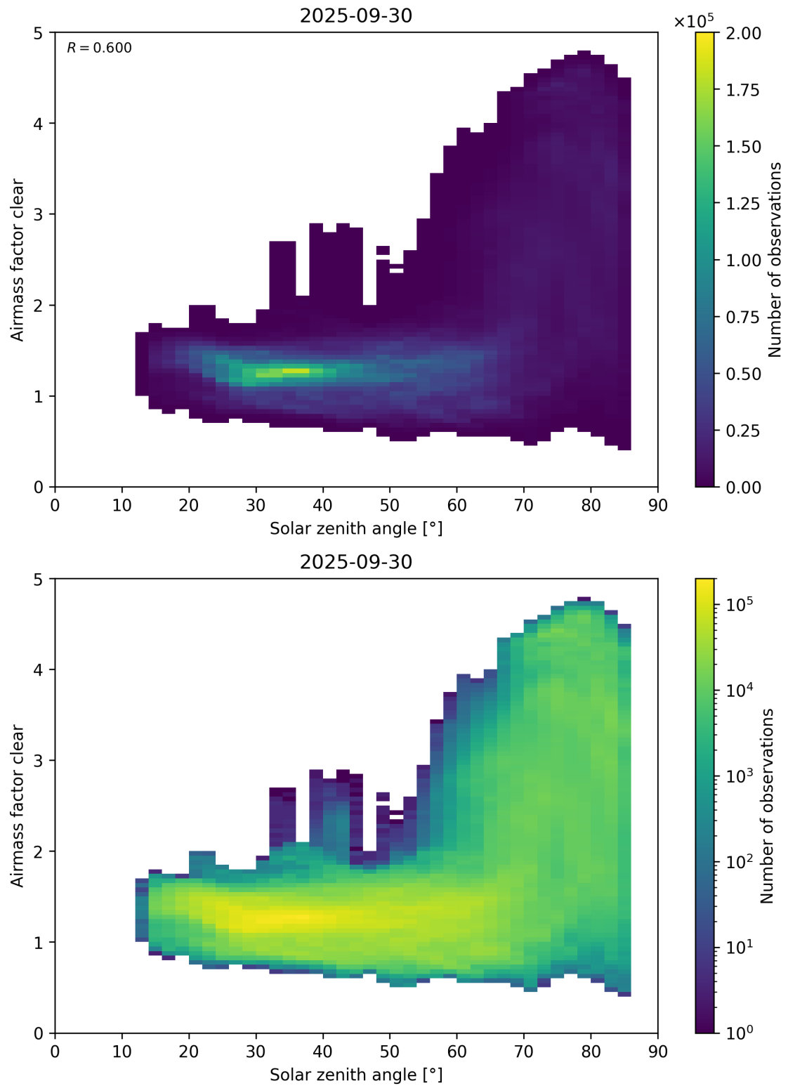
Figure 170: Scatter density plot of “Solar zenith angle” against “Airmass factor clear” for 2025-09-29 to 2025-10-01.
