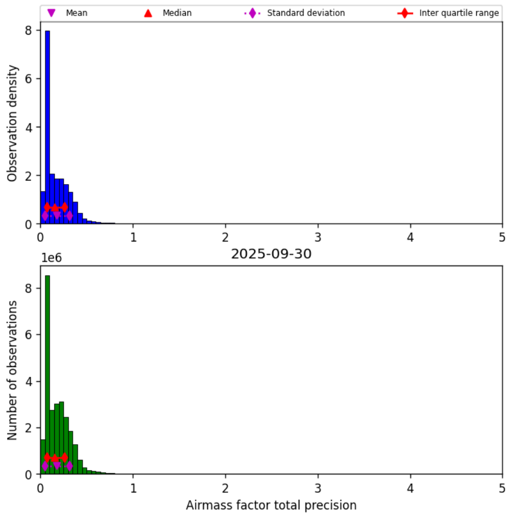
Figure 41: Histogram of “Airmass factor total precision” for 2025-09-29 to 2025-10-01
