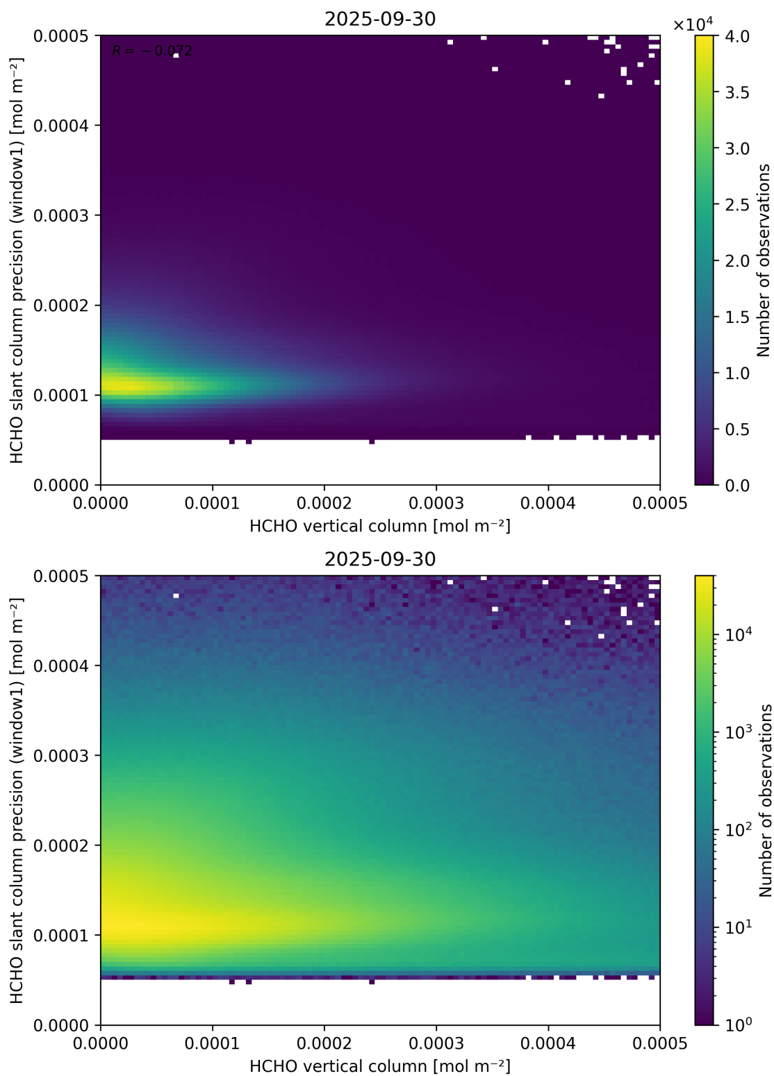
Figure 130: Scatter density plot of “HCHO vertical column” against “HCHO slant column precision (window1)” for 2025-09-29 to 2025-10-01.
