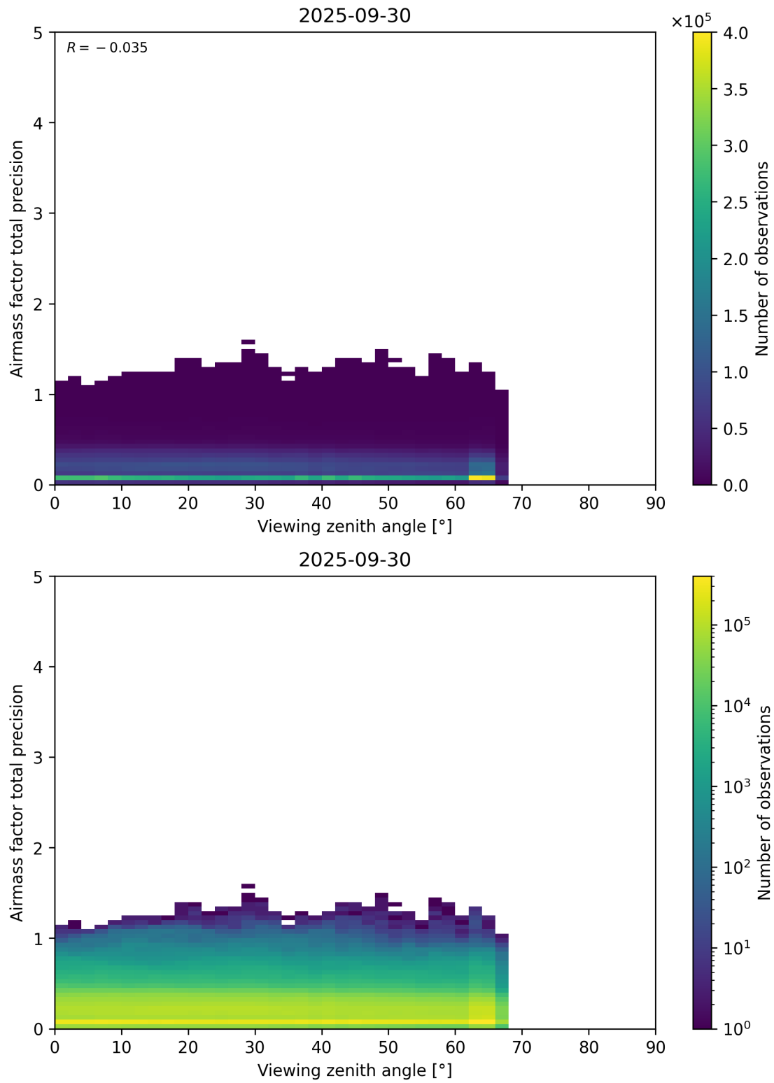
Figure 191: Scatter density plot of “Viewing zenith angle” against “Airmass factor total precision” for 2025-09-29 to 2025-10-01.
