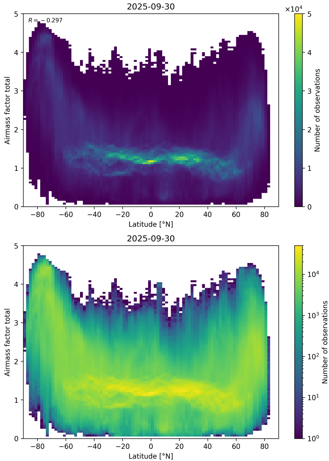
Figure 161: Scatter density plot of “Latitude” against “Airmass factor total” for 2025-09-29 to 2025-10-01.
