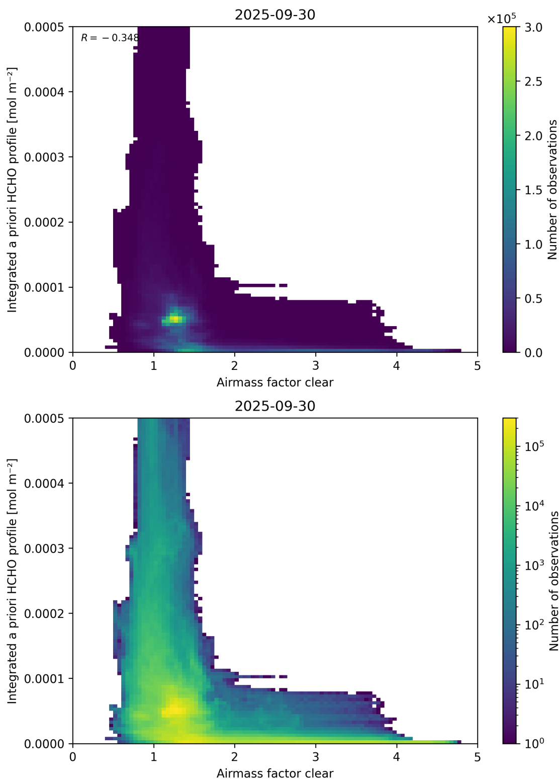
Figure 76: Scatter density plot of “Airmass factor clear” against “Integrated a priori HCHO profile” for 2025-09-29 to 2025-10-01.
