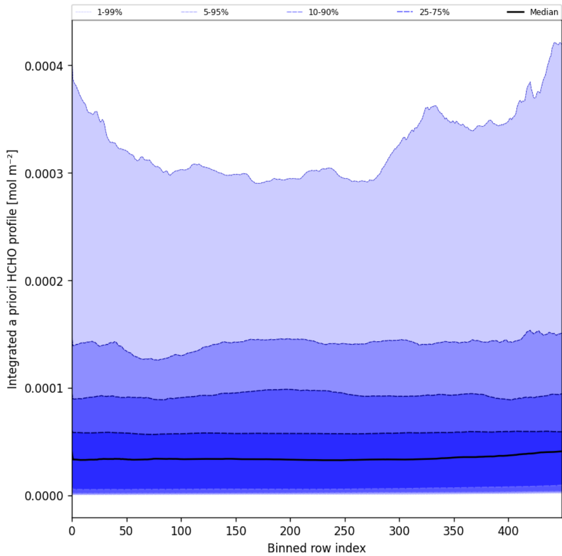
Figure 57: Along track statistics of "Integrated a priori HCHO profile" for 2025-09-29 to 2025-10-01
