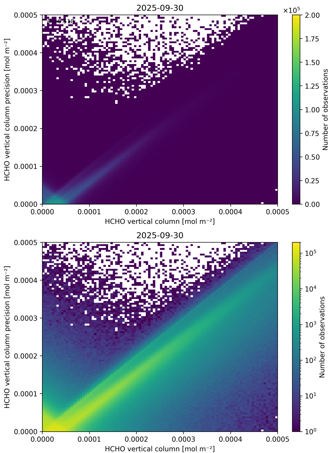
Figure 134: Scatter density plot of “HCHO vertical column” against “HCHO vertical column precision” for 2025-09-29 to 2025-10-01.
