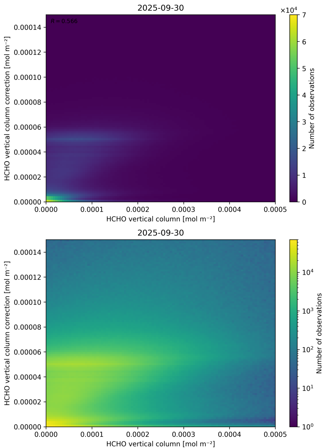
Figure 133: Scatter density plot of “HCHO vertical column” against “HCHO vertical column correction” for 2025-09-29 to 2025-10-01.
