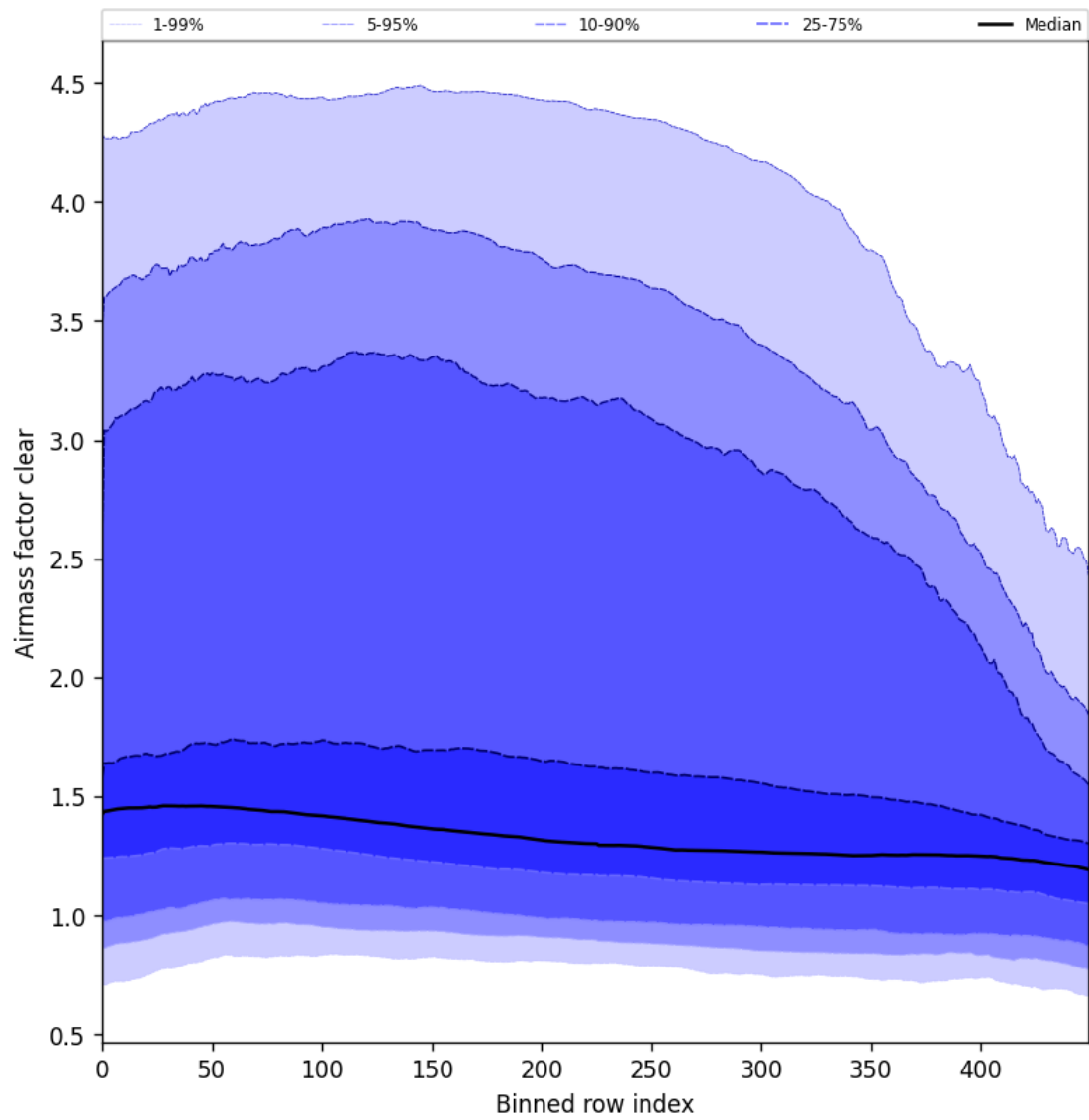
Figure 56: Along track statistics of “Air mass factor clear” for 2025-09-29 to 2025-10-01
