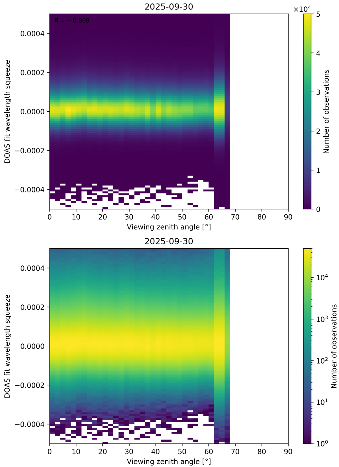
Figure 184: Scatter density plot of “Viewing zenith angle” against “DOAS fit wavelength squeeze” for 2025-09-29 to 2025-10-01.
