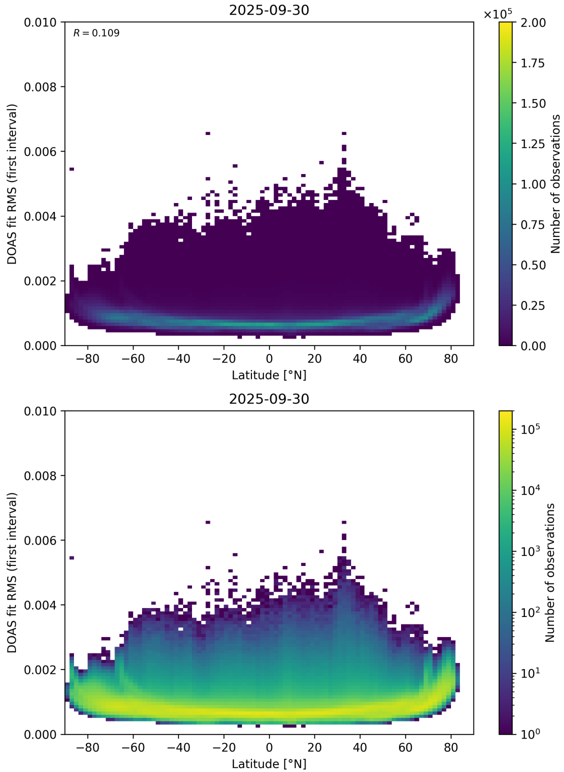
Figure 153: Scatter density plot of “Latitude” against “DOAS fit RMS (first interval)” for 2025-09-29 to 2025-10-01.
