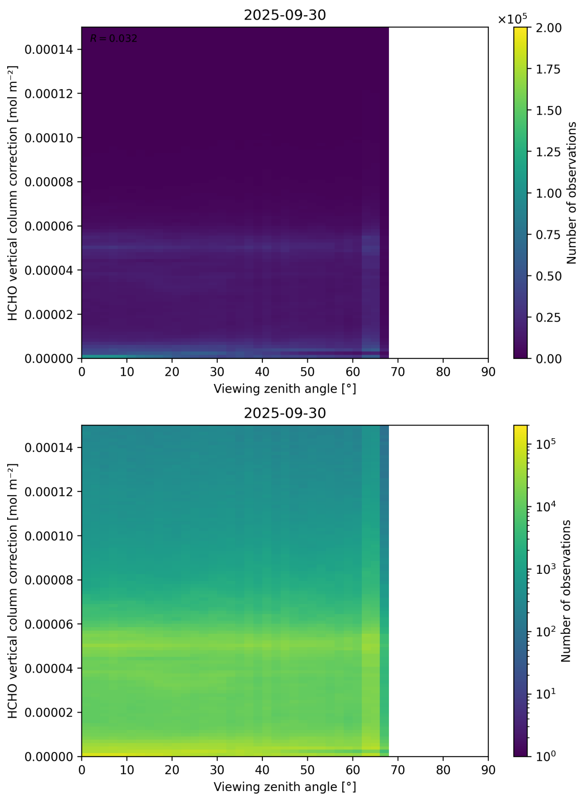
Figure 193: Scatter density plot of “Viewing zenith angle” against “HCHO vertical column correction” for 2025-09-29 to 2025-10-01.
