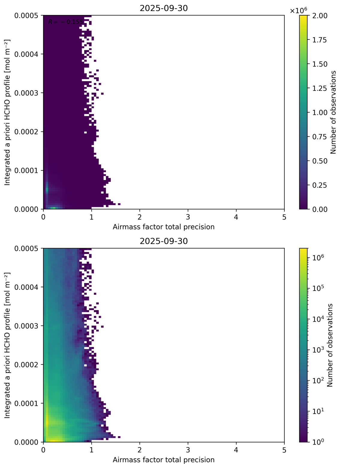
Figure 111: Scatter density plot of “Airmass factor total precision” against “Integrated a priori HCHO profile” for 2025-09-29 to 2025-10-01.
