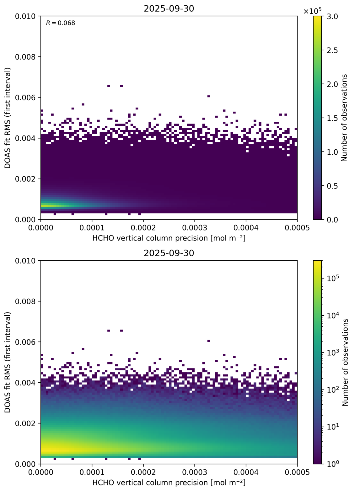
Figure 136: Scatter density plot of “HCHO vertical column precision” against “DOAS fit RMS (first interval)” for 2025-09-29 to 2025-10-01.
