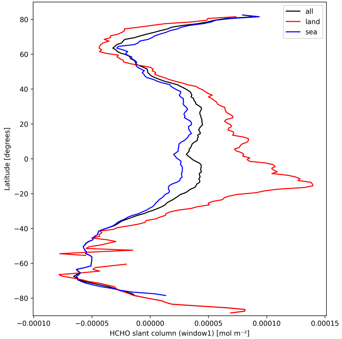
Figure 24: Zonal average of “HCHO slant column (window1)” for 2025-09-29 to 2025-10-01.
