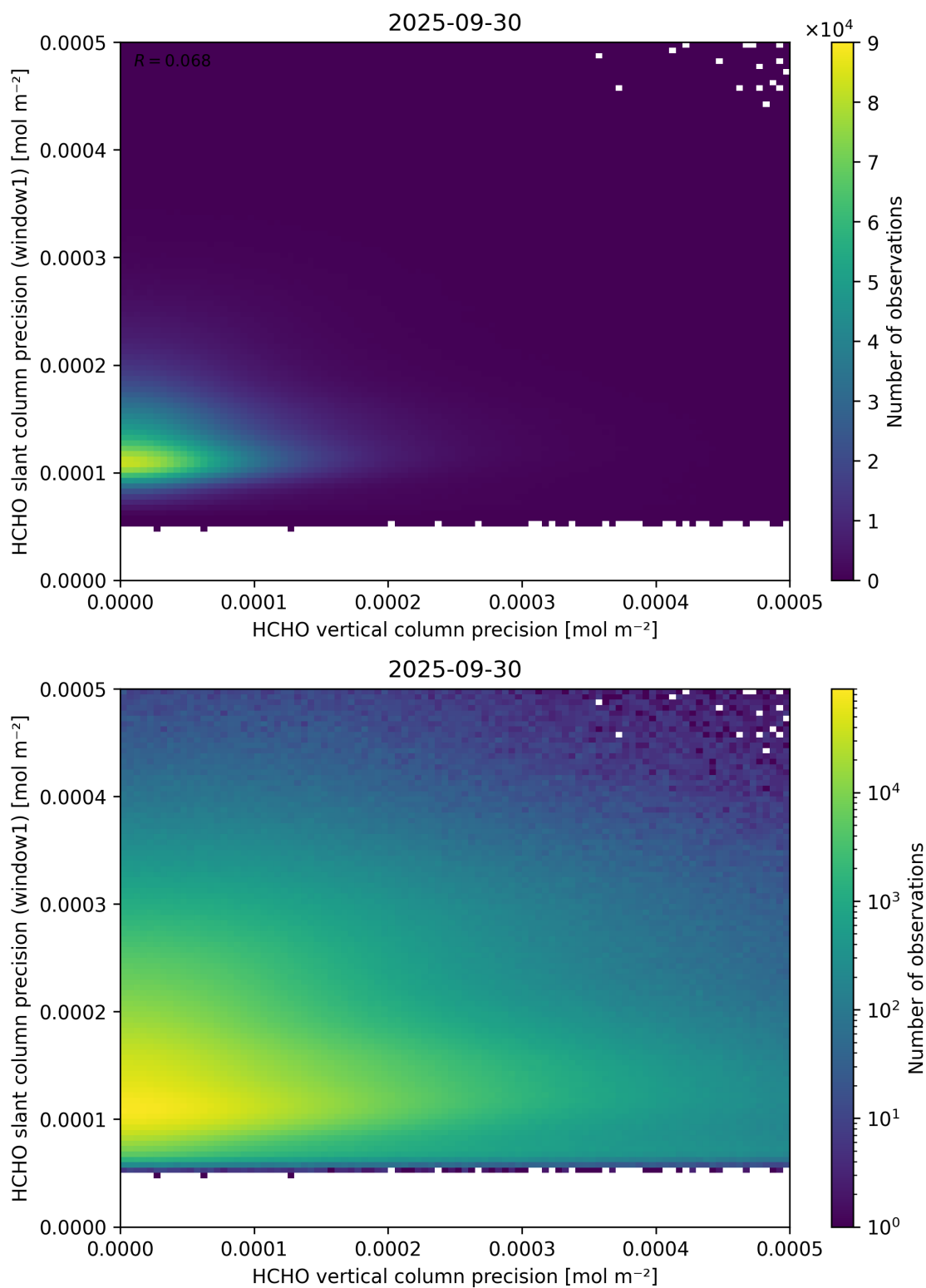
Figure 143: Scatter density plot of “HCHO vertical column precision” against “HCHO slant column precision (window1)” for 2025-09-29 to 2025-10-01.
