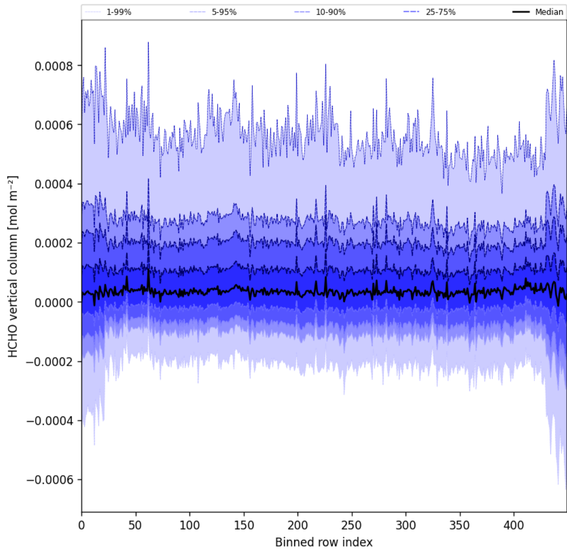
Figure 49: Along track statistics of “HCHO vertical column” for 2025-09-29 to 2025-10-01
