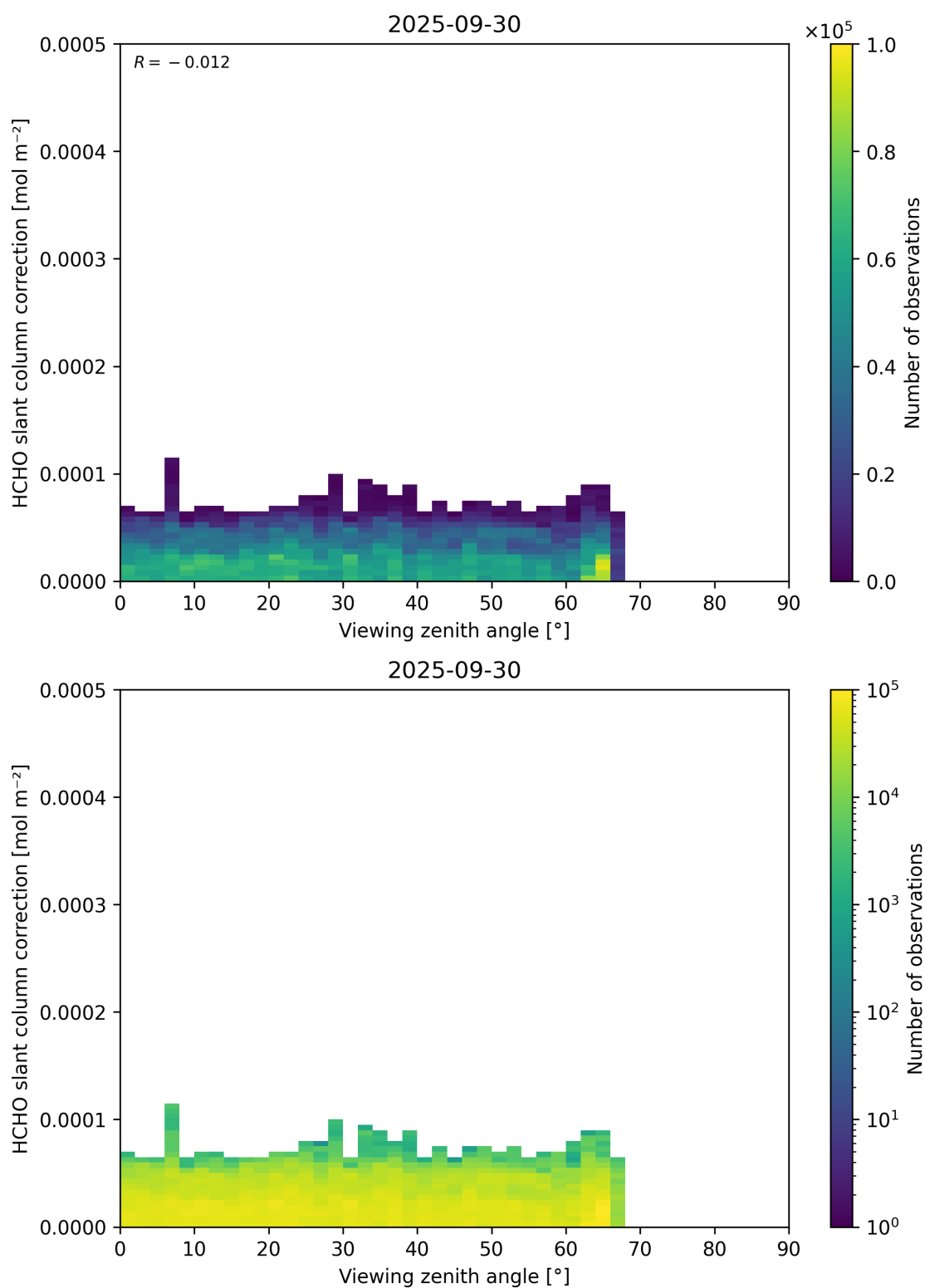
Figure 187: Scatter density plot of “Viewing zenith angle” against “HCHO slant column correction” for 2025-09-29 to 2025-10-01.
