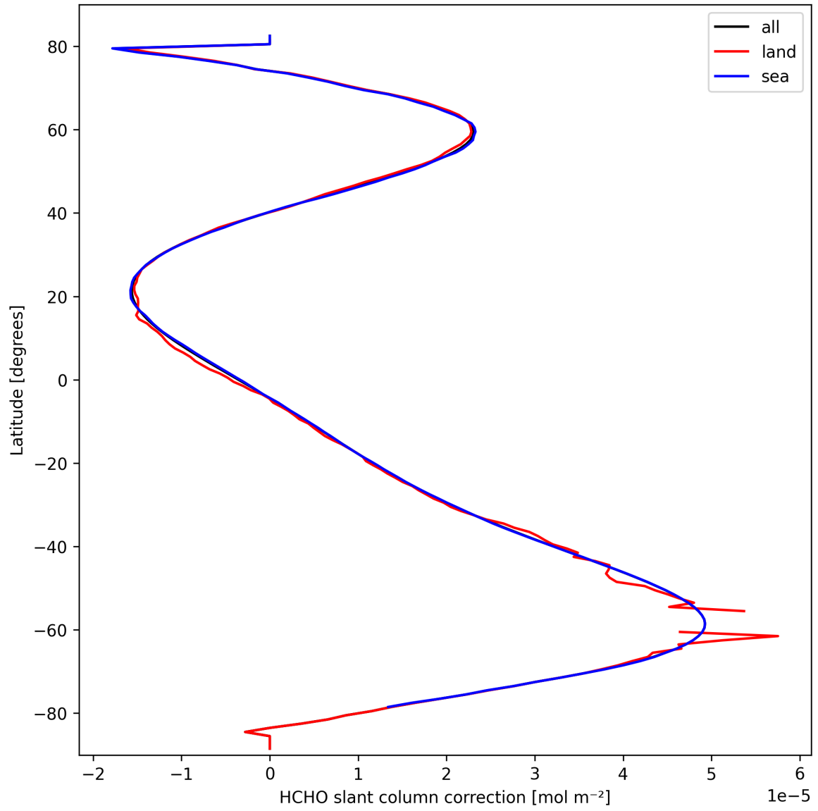
Figure 33: Zonal average of “HCHO slant column correction” for 2025-09-29 to 2025-10-01.
