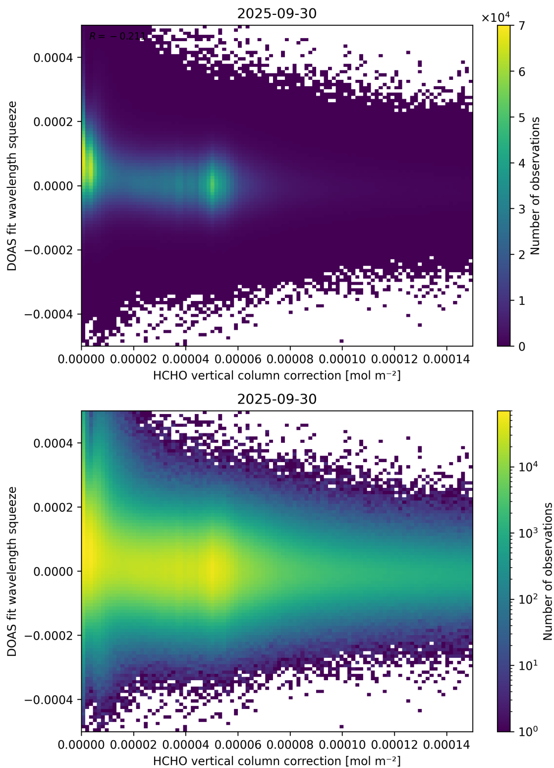
Figure 114: Scatter density plot of “HCHO vertical column correction” against “DOAS fit wavelength squeeze” for 2025-09-29 to 2025-10-01.
