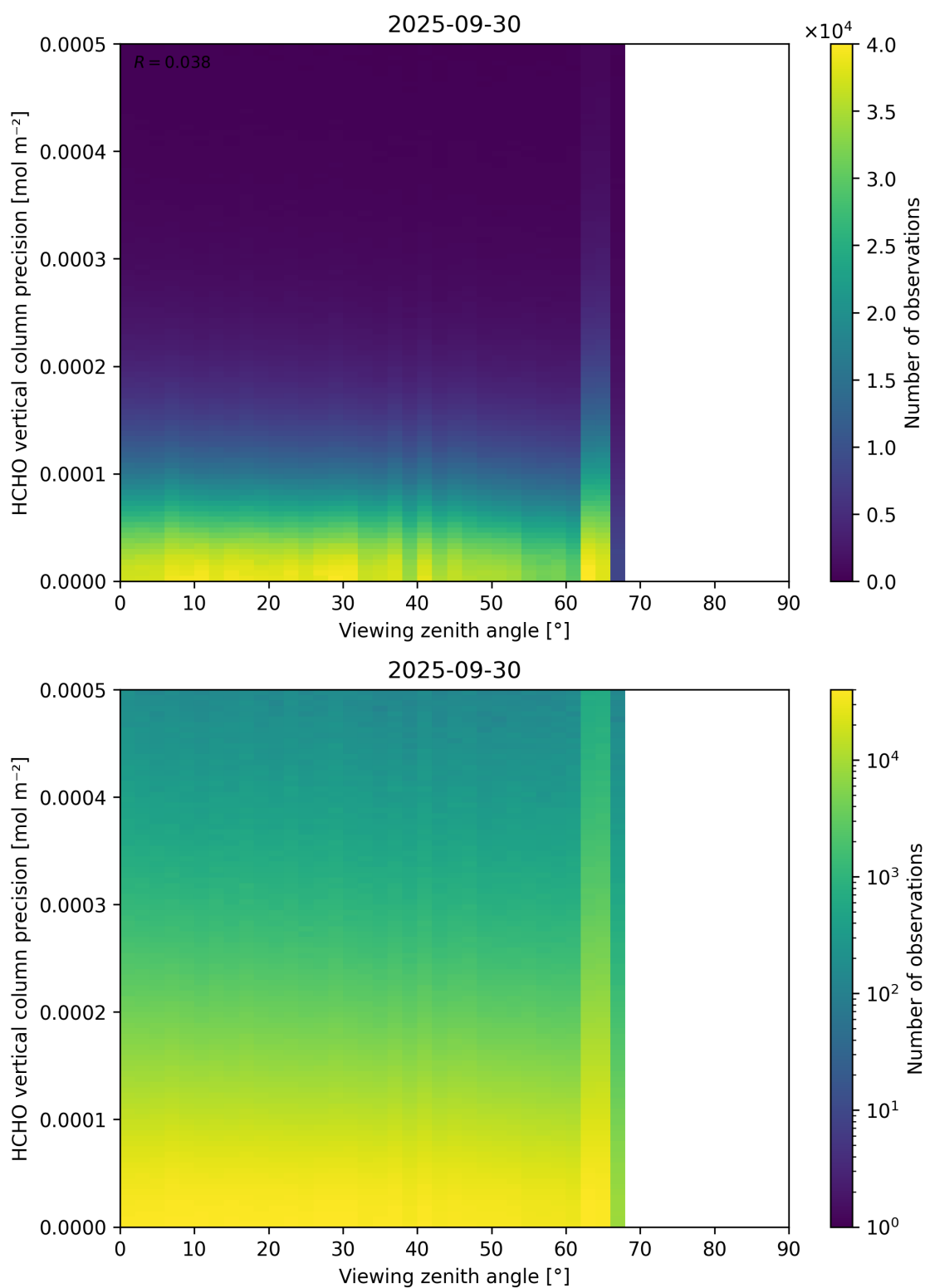
Figure 194: Scatter density plot of “Viewing zenith angle” against “HCHO vertical column precision” for 2025-09-29 to 2025-10-01.
