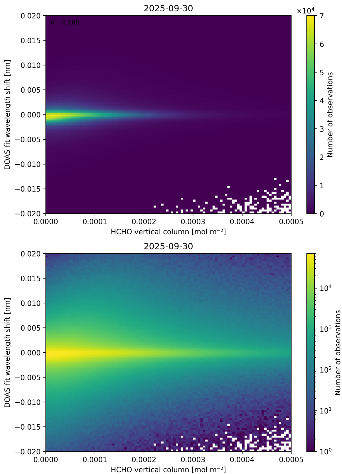
Figure 124: Scatter density plot of “HCHO vertical column” against “DOAS fit wavelength shift” for 2025-09-29 to 2025-10-01.
