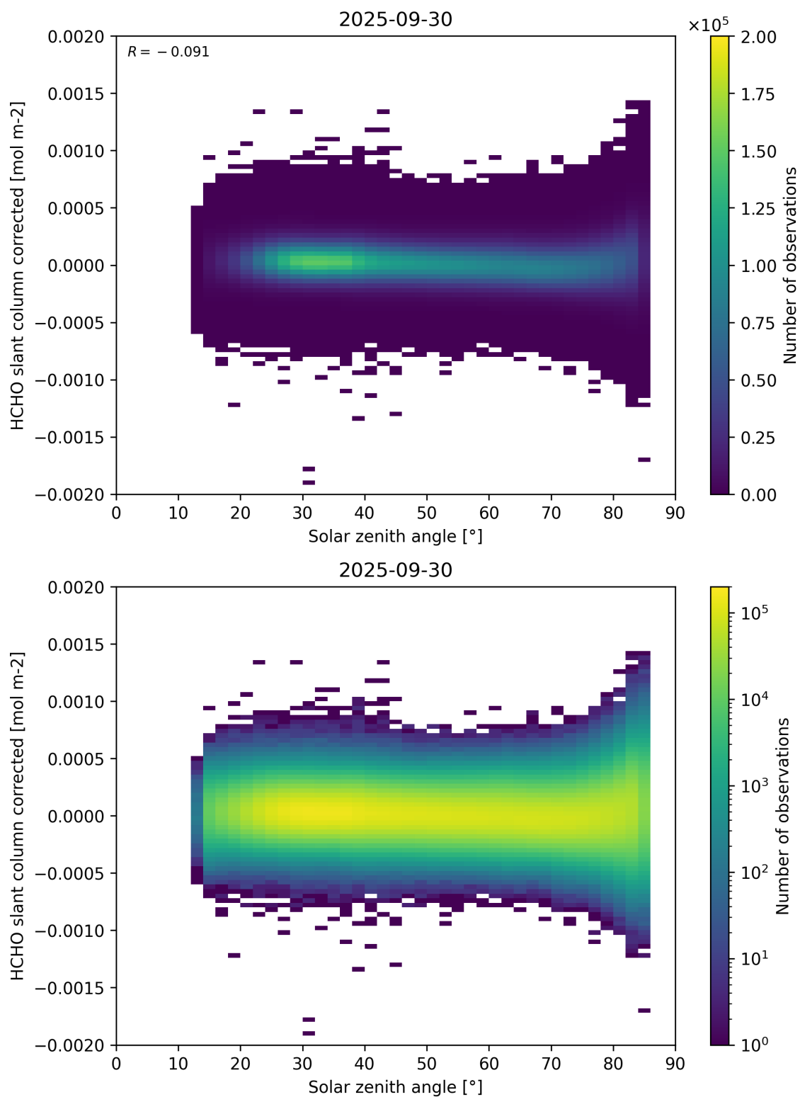
Figure 171: Scatter density plot of “Solar zenith angle” against “HCHO slant column corrected” for 2025-09-29 to 2025-10-01.
