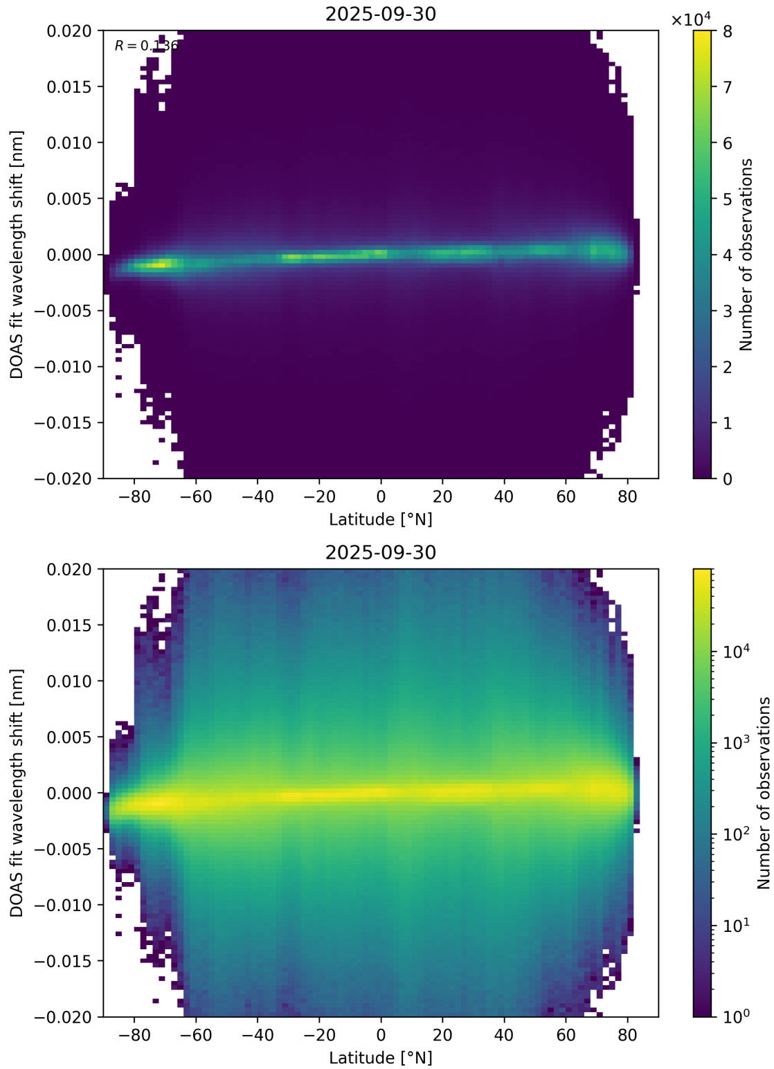
Figure 154: Scatter density plot of “Latitude” against “DOAS fit wavelength shift” for 2025-09-29 to 2025-10-01.
