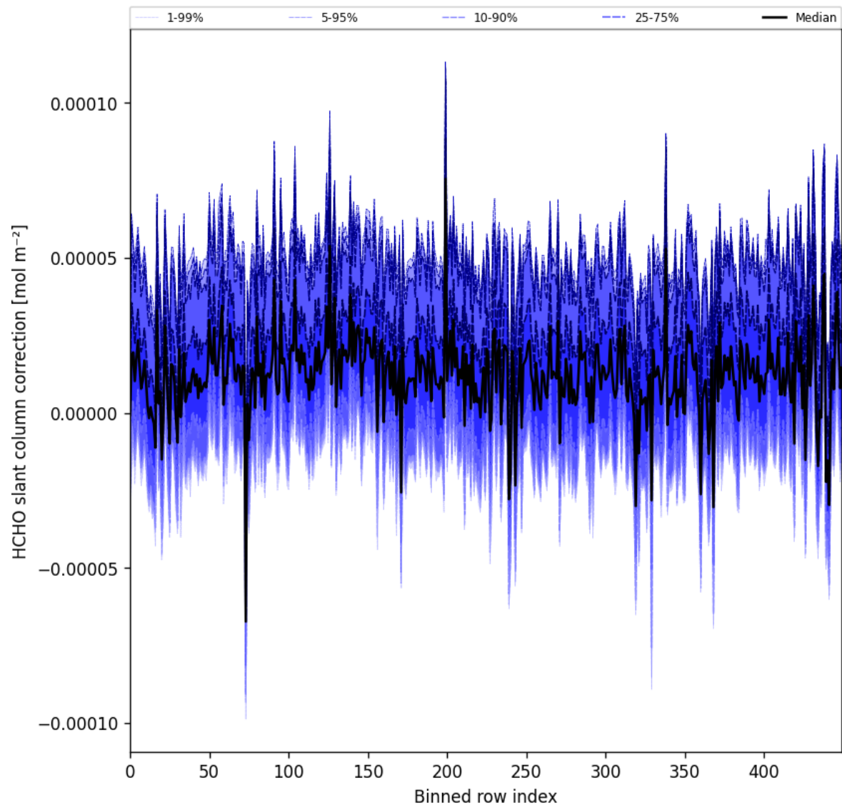
Figure 61: Along track statistics of “HCHO slant column correction” for 2025-09-29 to 2025-10-01
