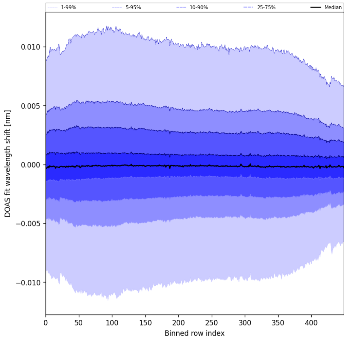
Figure 58: Along track statistics of “DOAS fit wavelength shift” for 2025-09-29 to 2025-10-01
