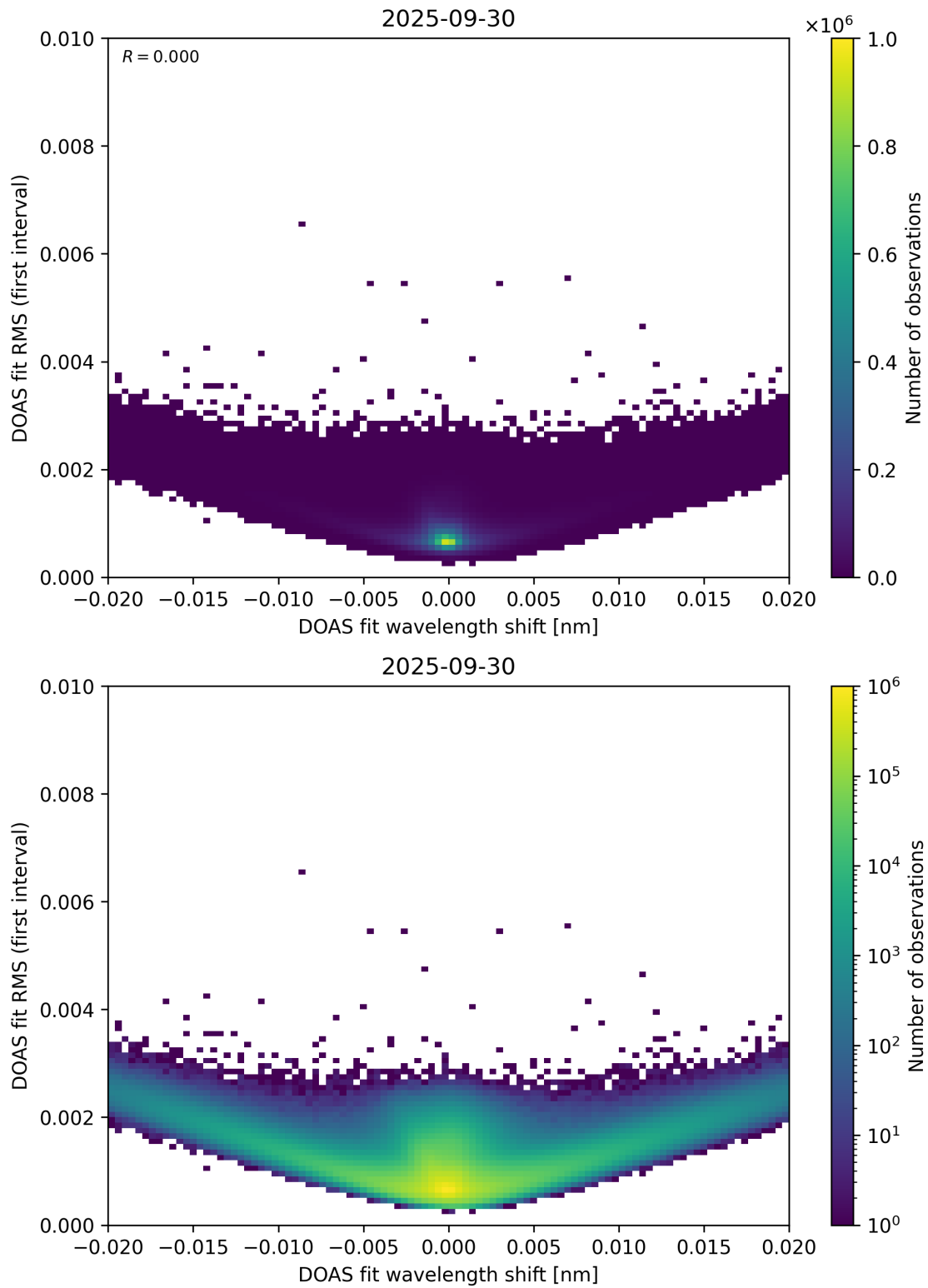
Figure 64: Scatter density plot of “DOAS fit wavelength shift” against “DOAS fit RMS (first interval)” for 2025-09-29 to 2025-10-01.
