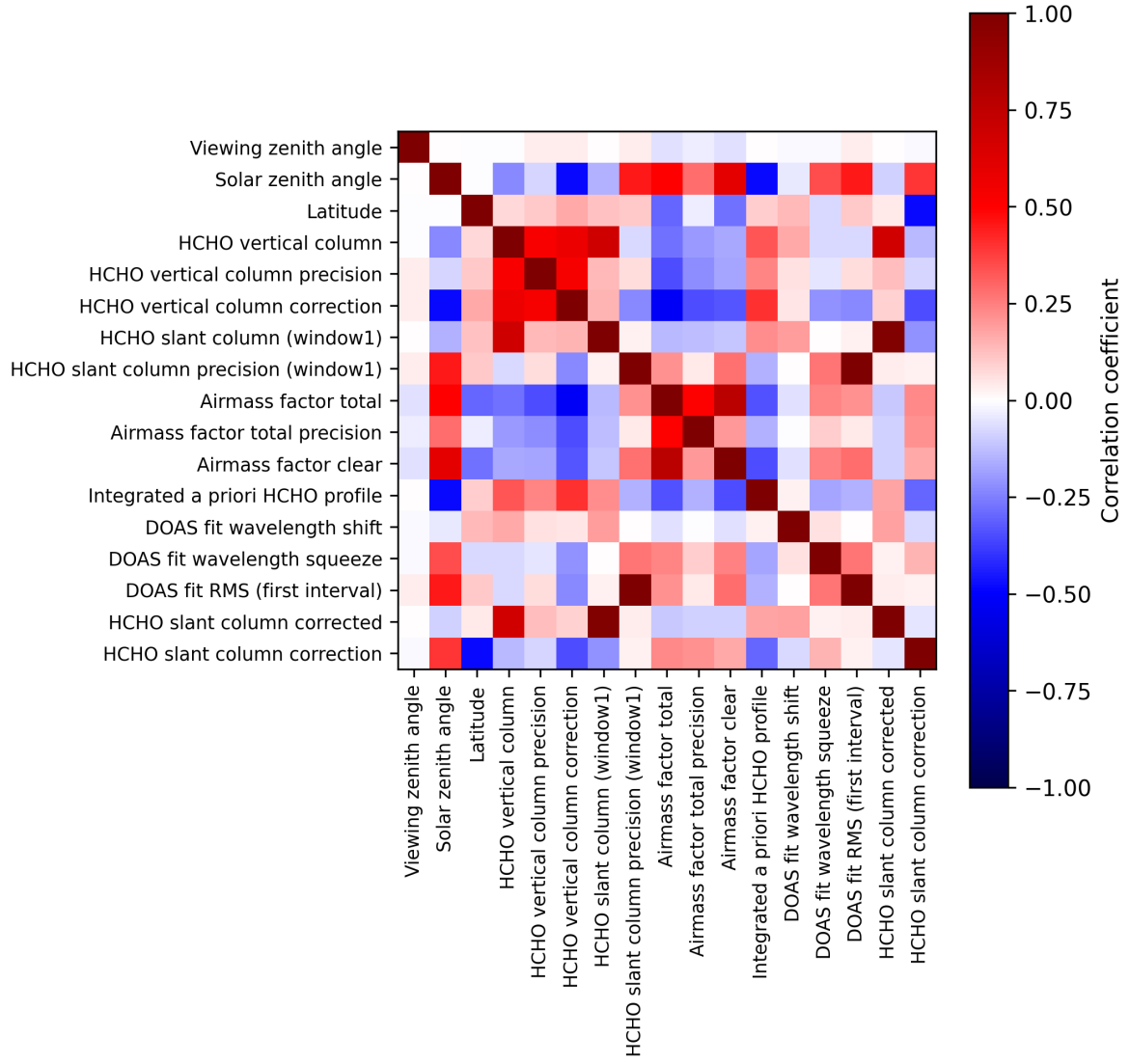
Figure 2: Map of correlation matrix for 2025-09-29 to 2025-10-01.
