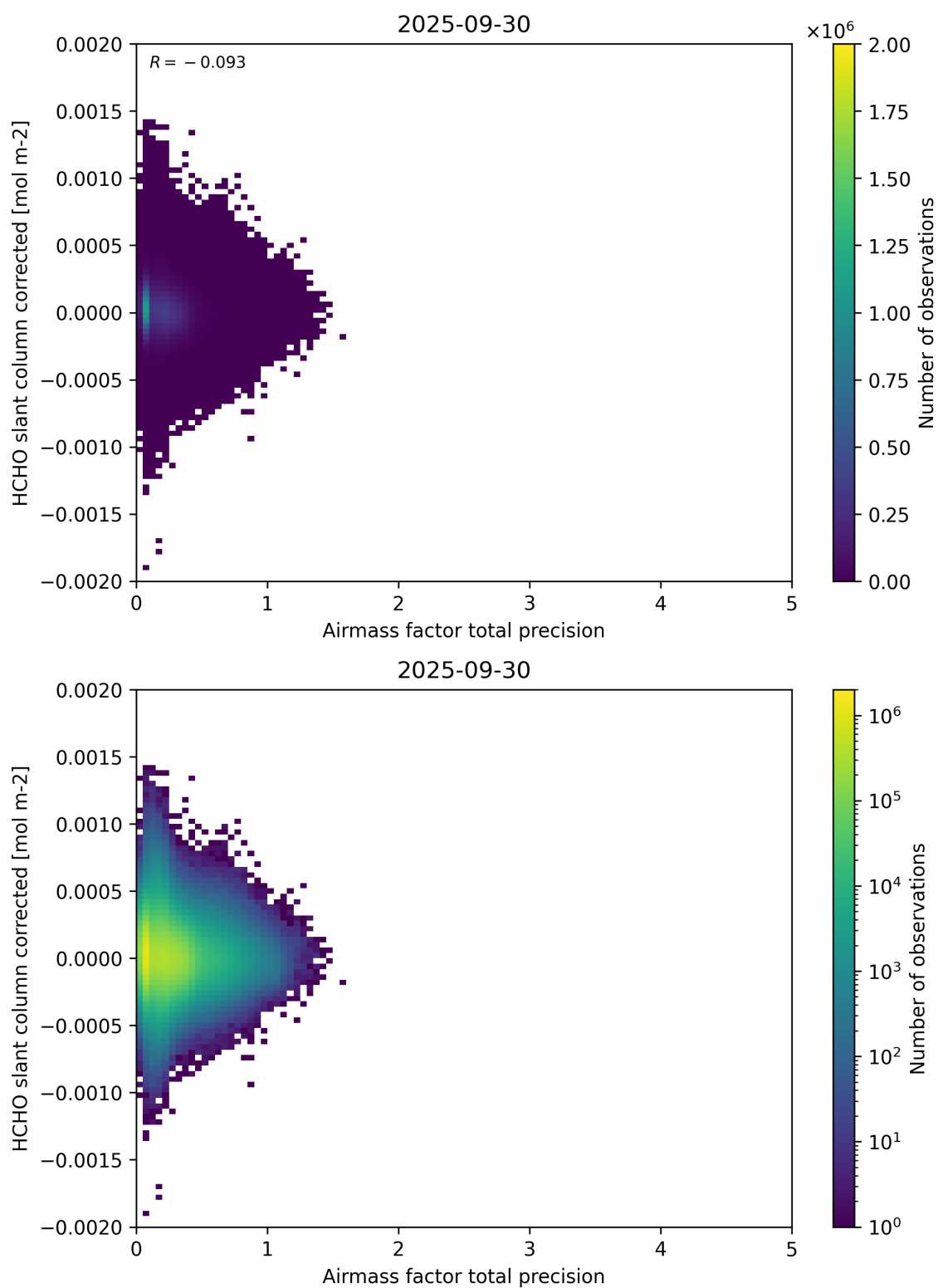
Figure 109: Scatter density plot of “Airmass factor total precision” against “HCHO slant column corrected” for 2025-09-29 to 2025-10-01.
