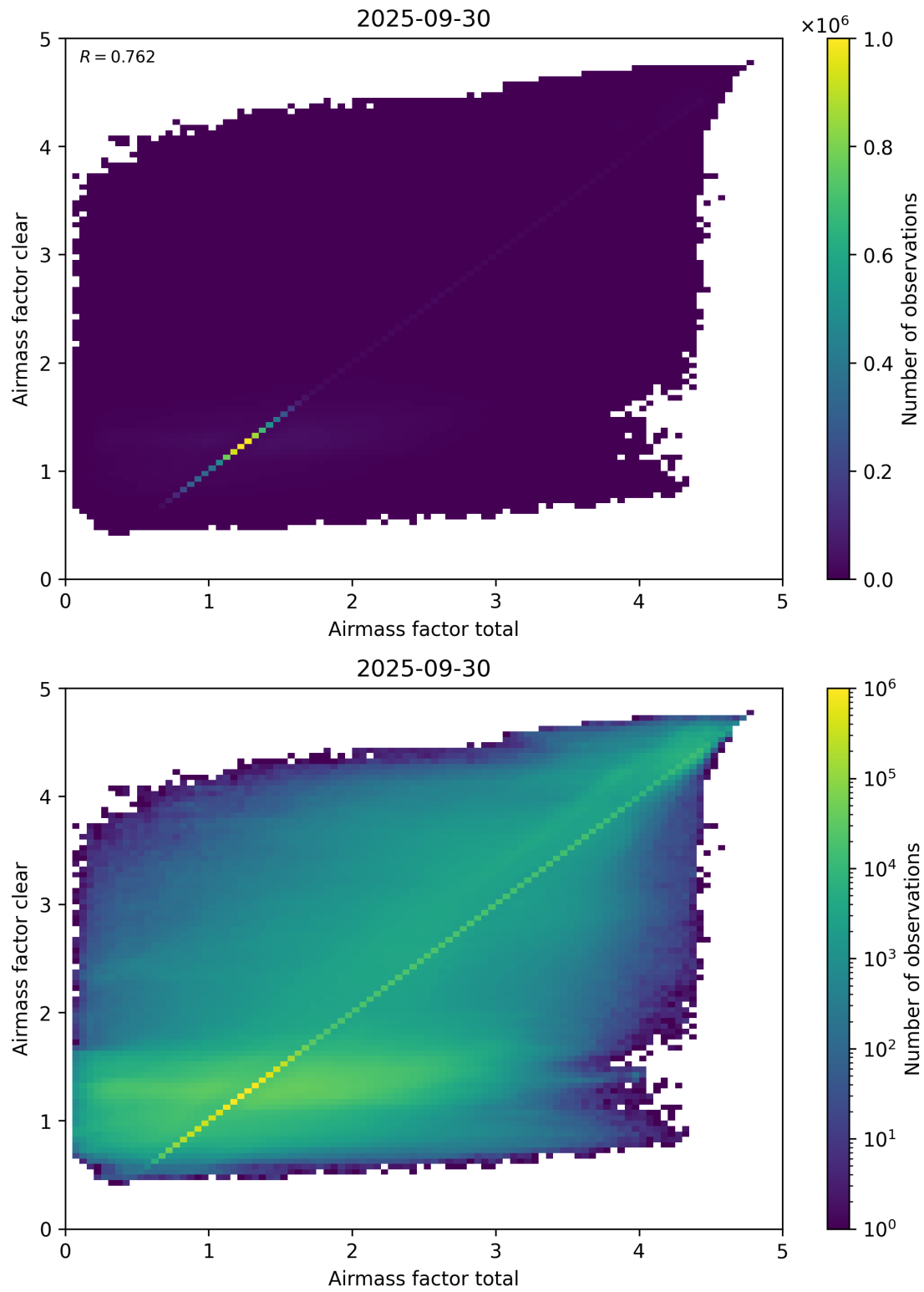
Figure 100: Scatter density plot of “Airmass factor total” against “Airmass factor clear” for 2025-09-29 to 2025-10-01.
