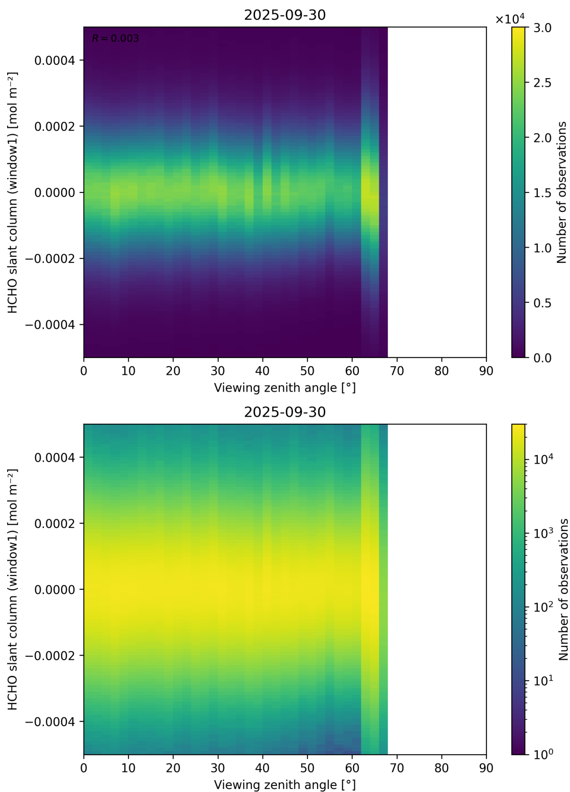
Figure 188: Scatter density plot of “Viewing zenith angle” against “HCHO slant column (window1)” for 2025-09-29 to 2025-10-01.
