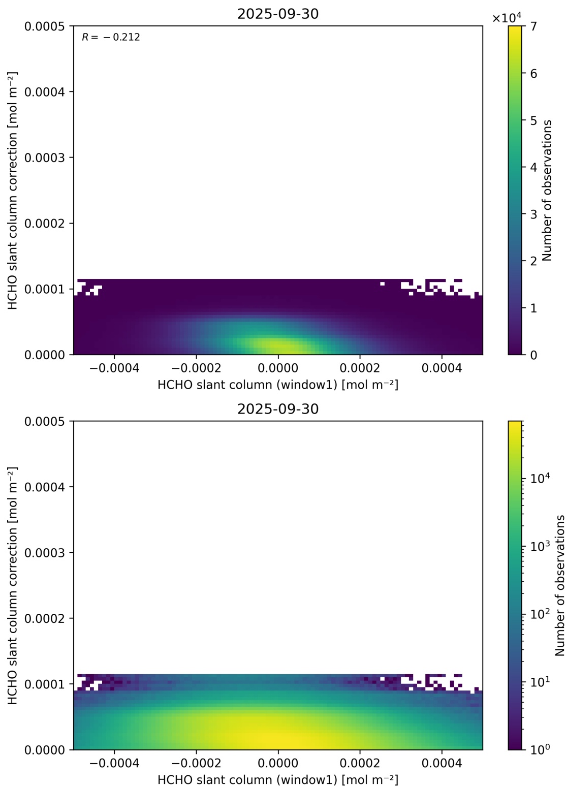
Figure 83: Scatter density plot of “HCHO slant column (window1)” against “HCHO slant column correction” for 2025-09-29 to 2025-10-01.
