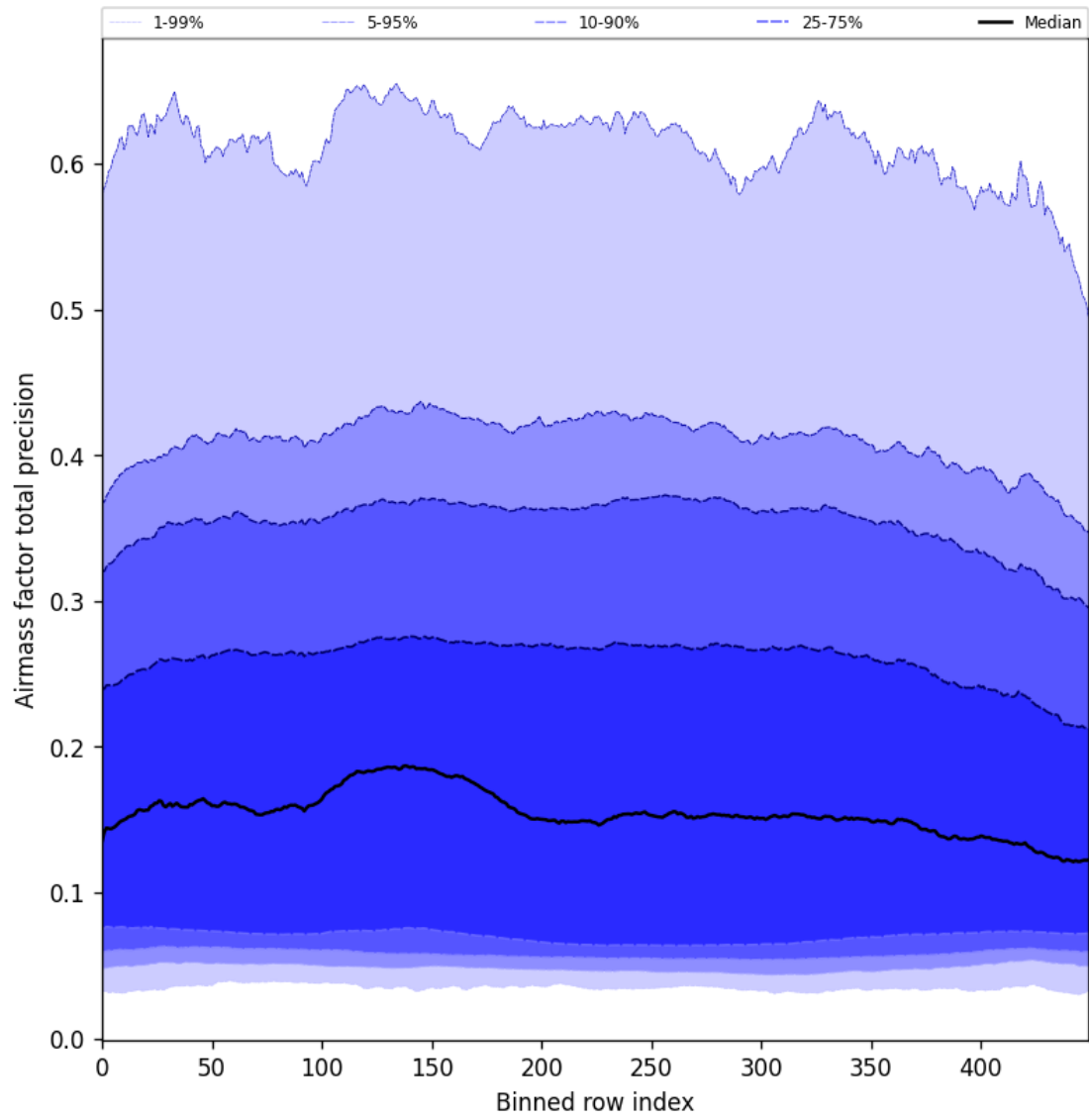
Figure 55: Along track statistics of “Airmass factor total precision” for 2025-09-29 to 2025-10-01
