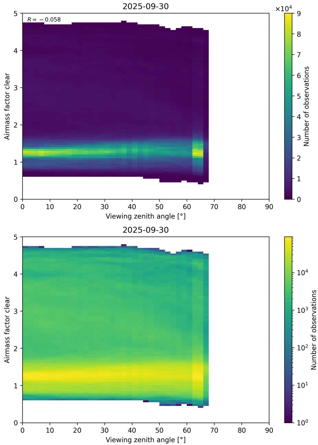
Figure 185: Scatter density plot of “Viewing zenith angle” against “Airmass factor clear” for 2025-09-29 to 2025-10-01.
