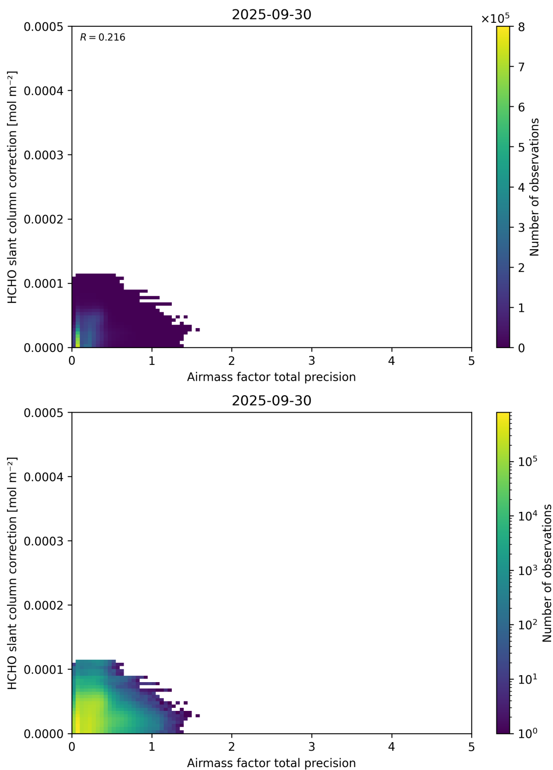
Figure 110: Scatter density plot of “Airmass factor total precision” against “HCHO slant column correction” for 2025-09-29 to 2025-10-01.
