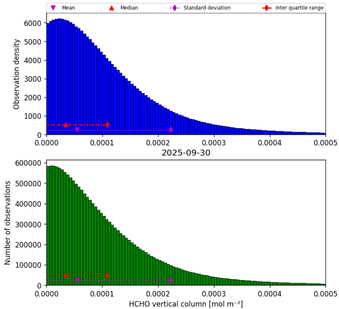
Figure 35: Histogram of “HCHO vertical column” for 2025-09-29 to 2025-10-01
