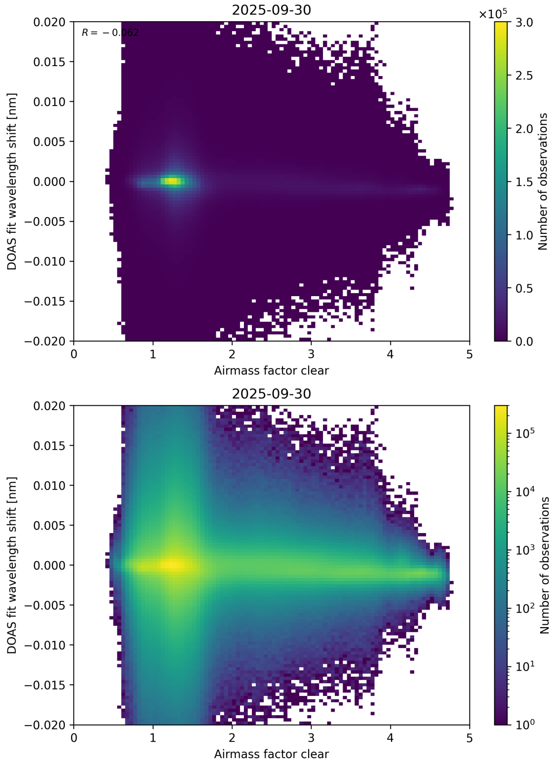
Figure 72: Scatter density plot of “Airmass factor clear” against “DOAS fit wavelength shift” for 2025-09-29 to 2025-10-01.
