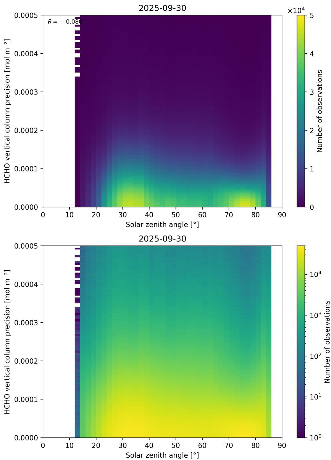
Figure 179: Scatter density plot of “Solar zenith angle” against “HCHO vertical column precision” for 2025-09-29 to 2025-10-01.
