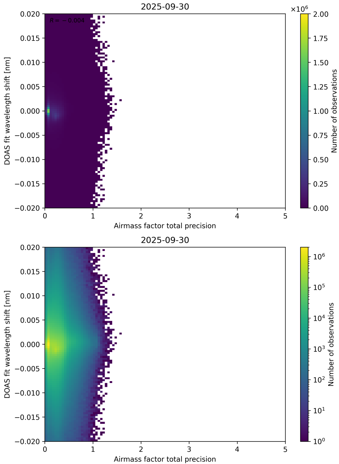
Figure 106: Scatter density plot of “Airmass factor total precision” against “DOAS fit wavelength shift” for 2025-09-29 to 2025-10-01.
