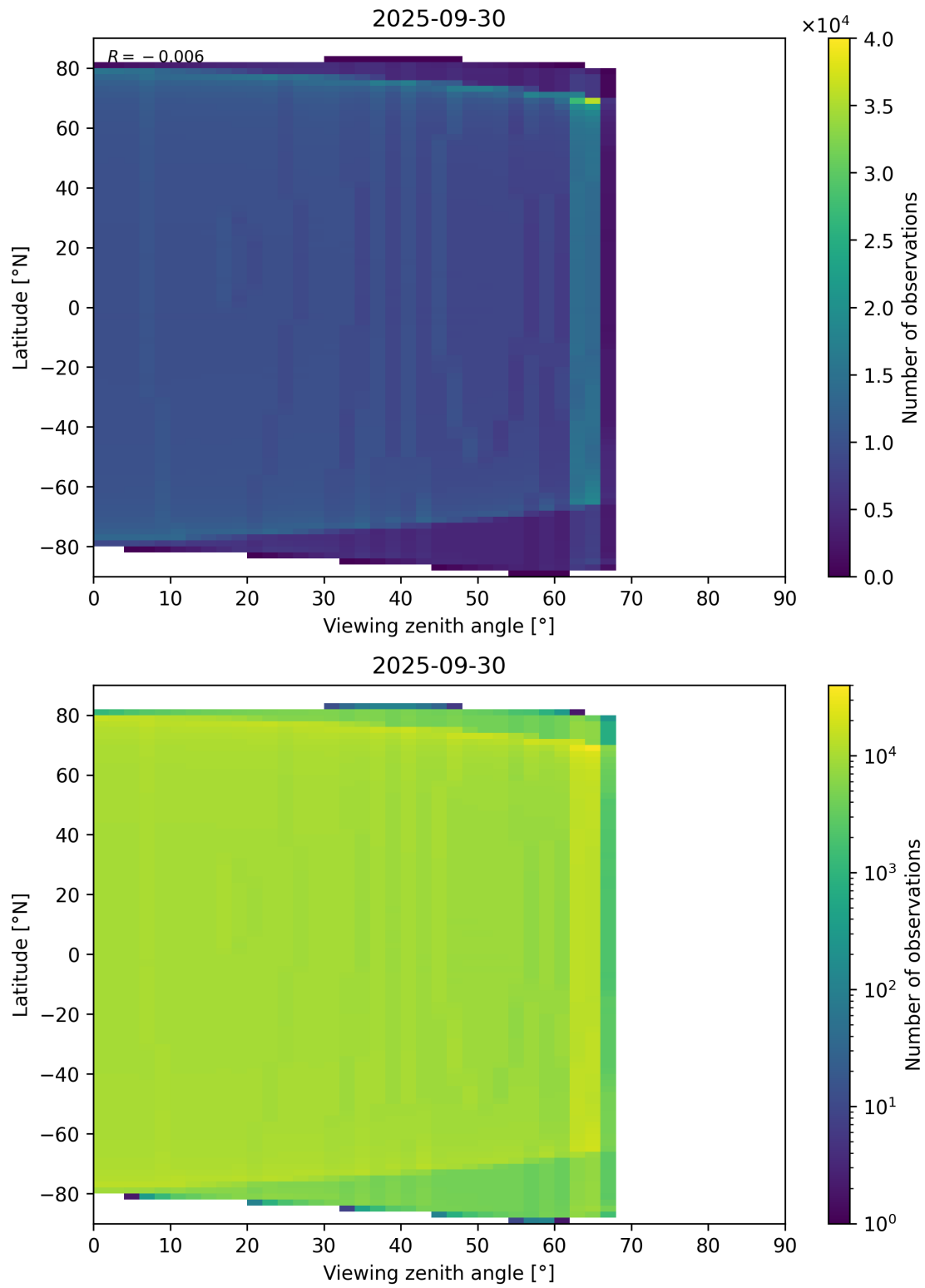
Figure 196: Scatter density plot of “Viewing zenith angle” against “Latitude” for 2025-09-29 to 2025-10-01.
