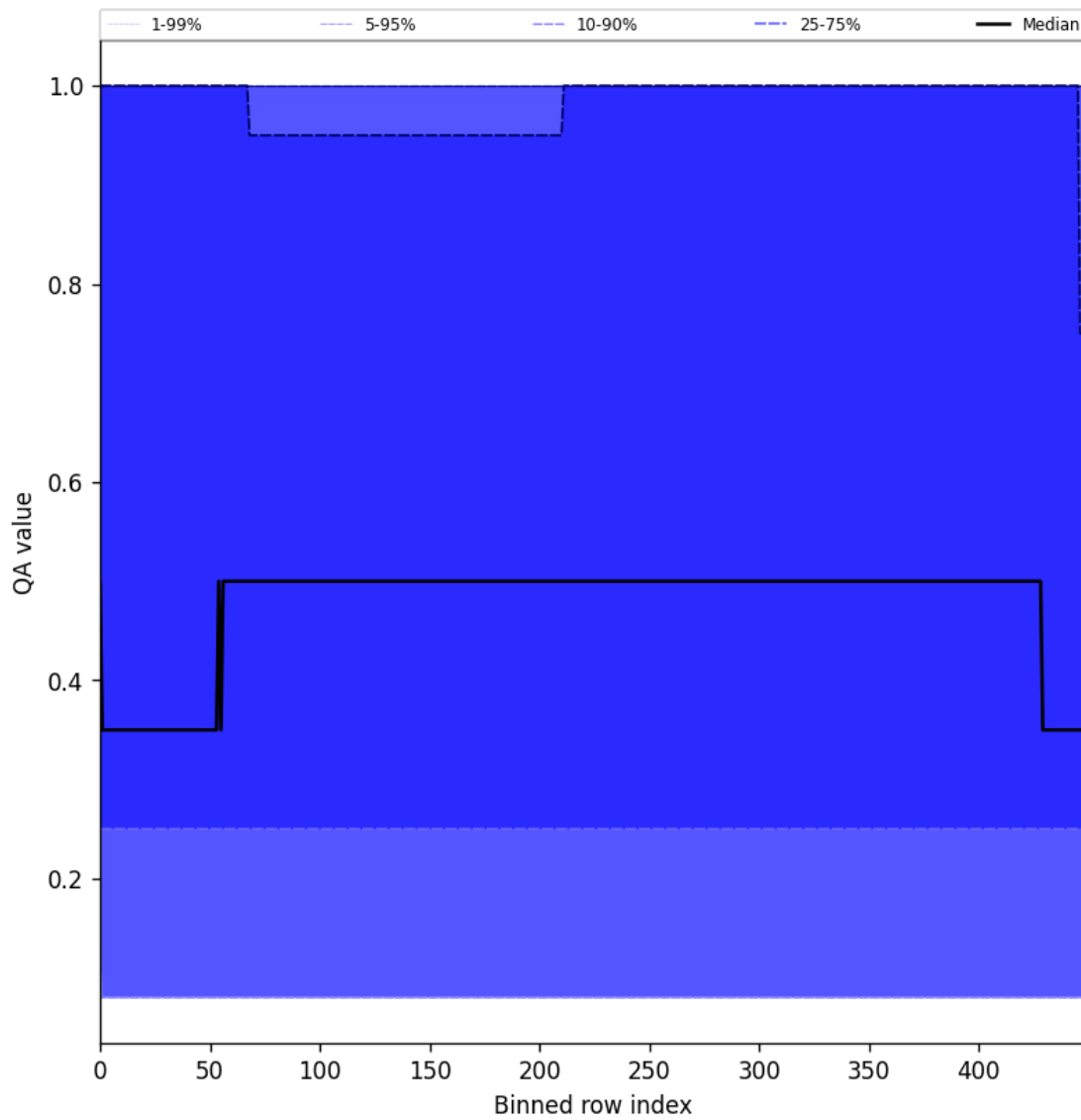
Figure 48: Along track statistics of “QA value” for 2025-09-29 to 2025-10-01
