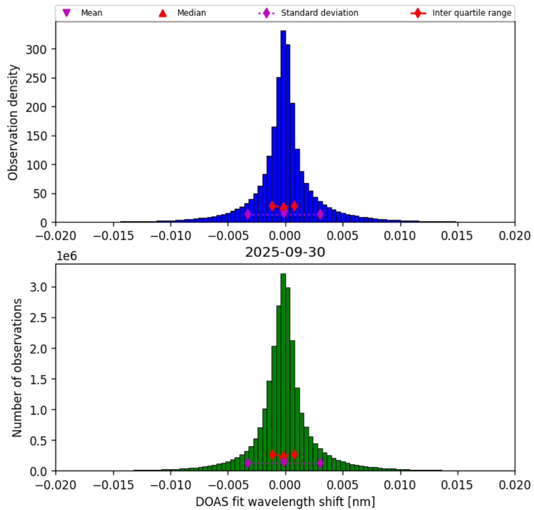
Figure 44: Histogram of “DOAS fit wavelength shift” for 2025-09-29 to 2025-10-01
