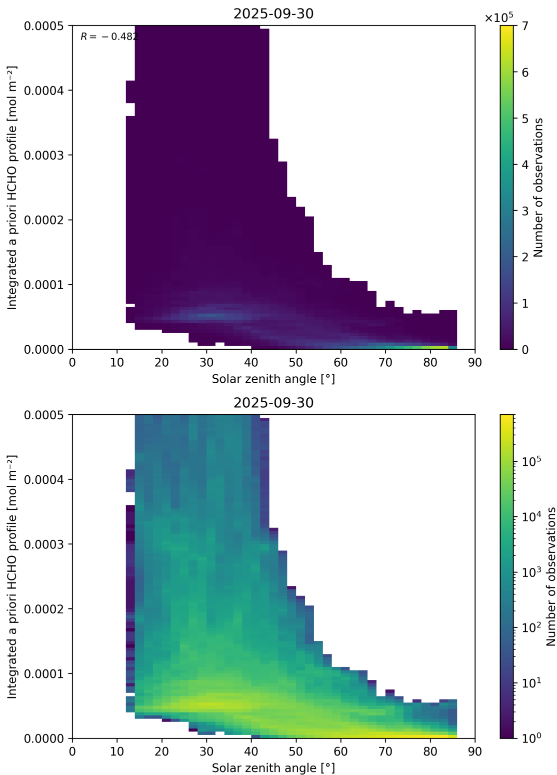
Figure 180: Scatter density plot of “Solar zenith angle” against “Integrated a priori HCHO profile” for 2025-09-29 to 2025-10-01.
