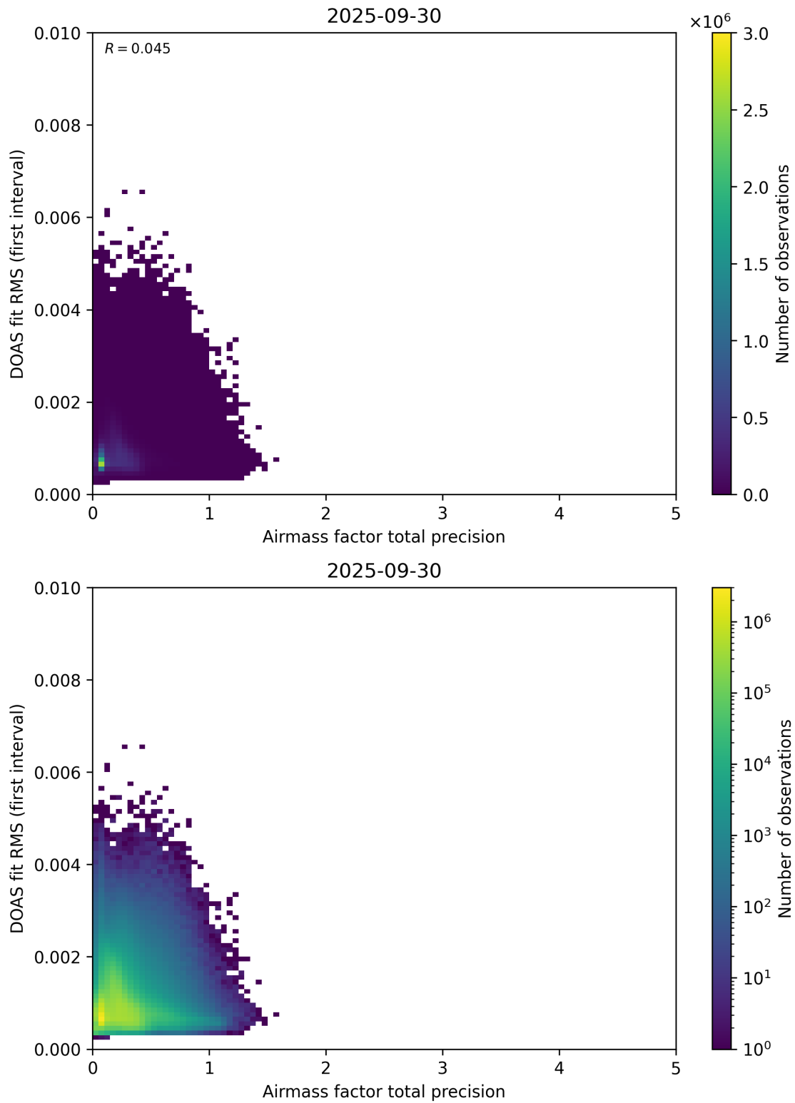
Figure 105: Scatter density plot of “Airmass factor total precision” against “DOAS fit RMS (first interval)” for 2025-09-29 to 2025-10-01.
