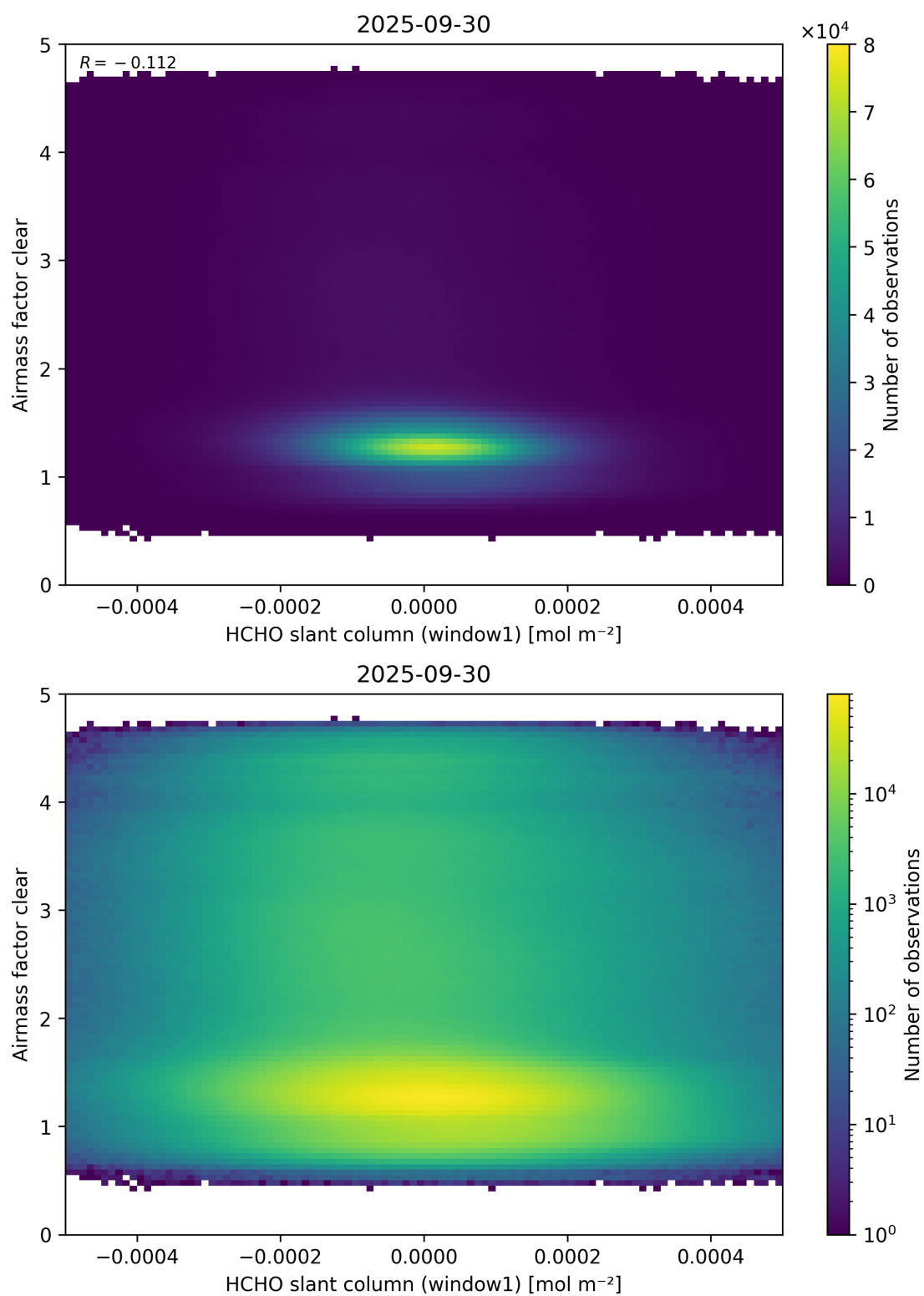
Figure 81: Scatter density plot of “HCHO slant column (window1)” against “Airmass factor clear” for 2025-09-29 to 2025-10-01.
