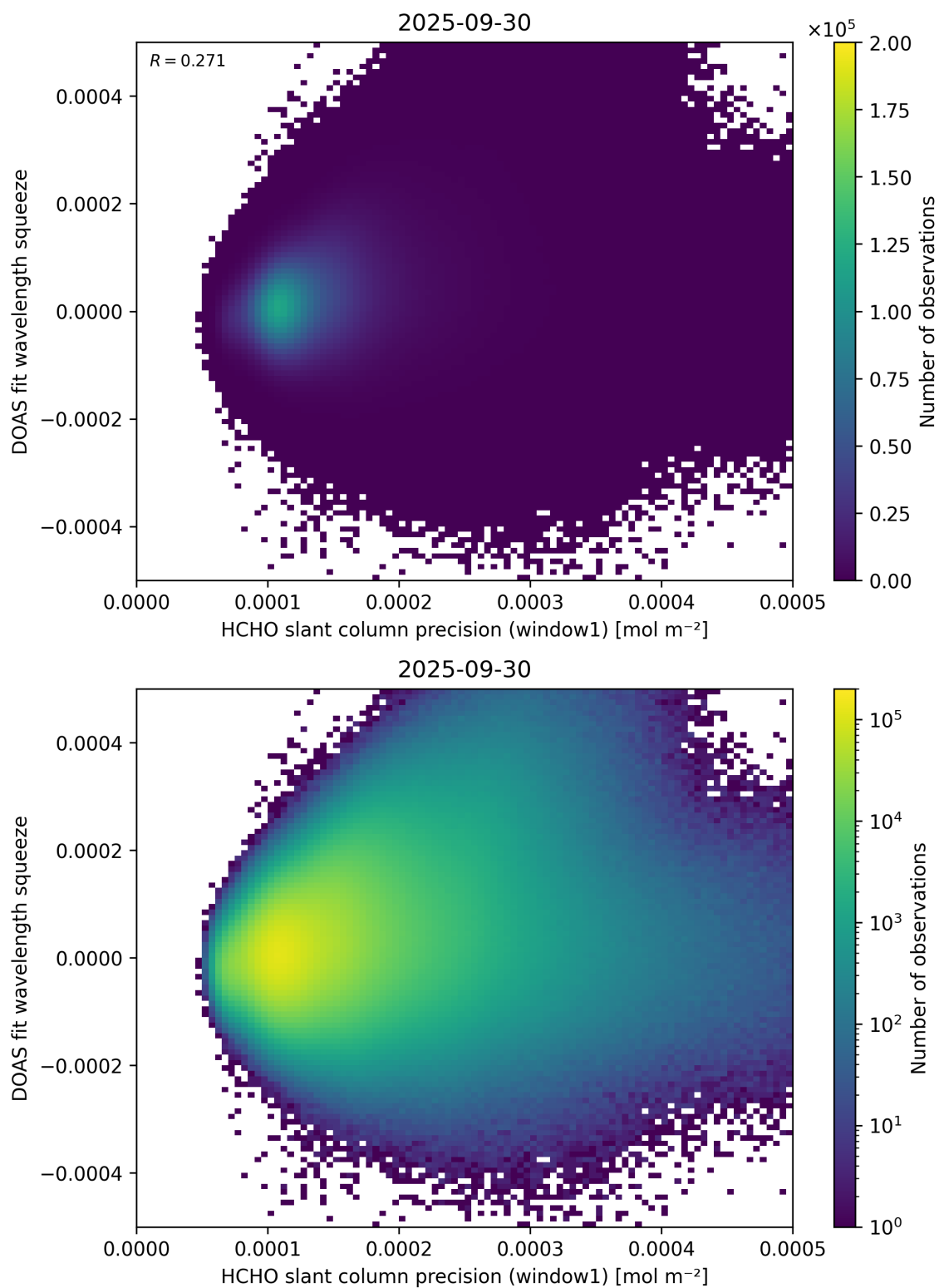
Figure 90: Scatter density plot of “HCHO slant column precision (window1)” against “DOAS fit wavelength squeeze” for 2025-09-29 to 2025-10-01.
