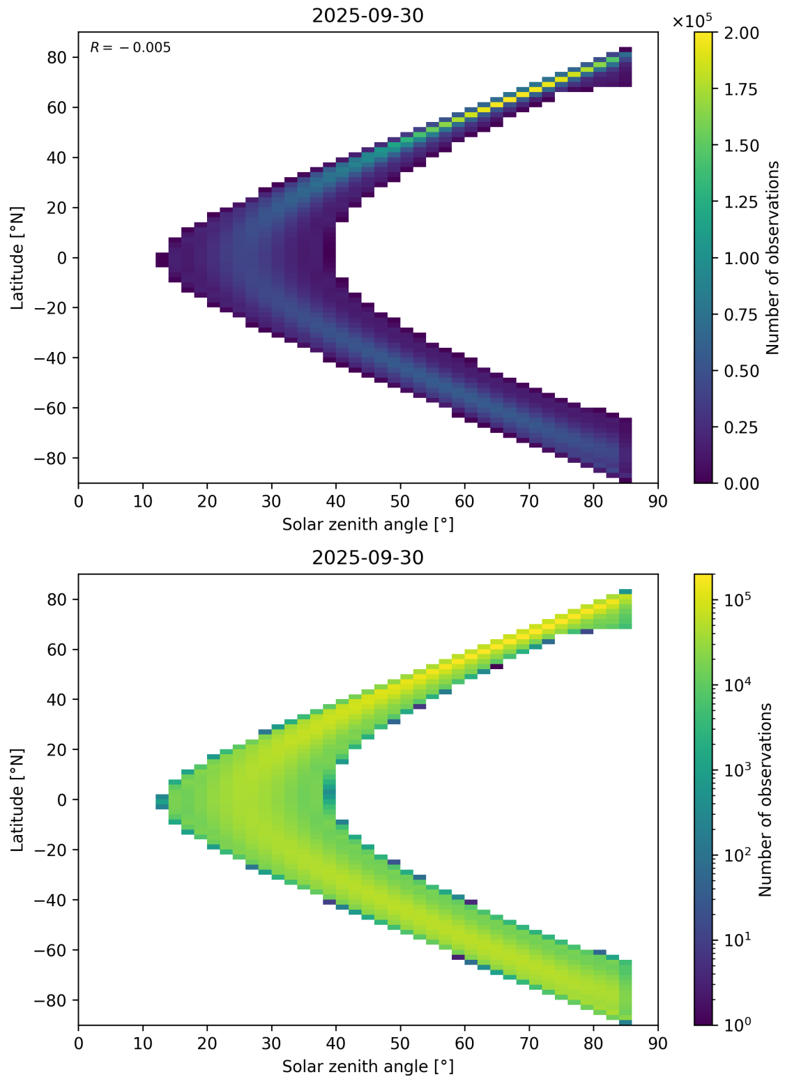
Figure 181: Scatter density plot of “Solar zenith angle” against “Latitude” for 2025-09-29 to 2025-10-01.
