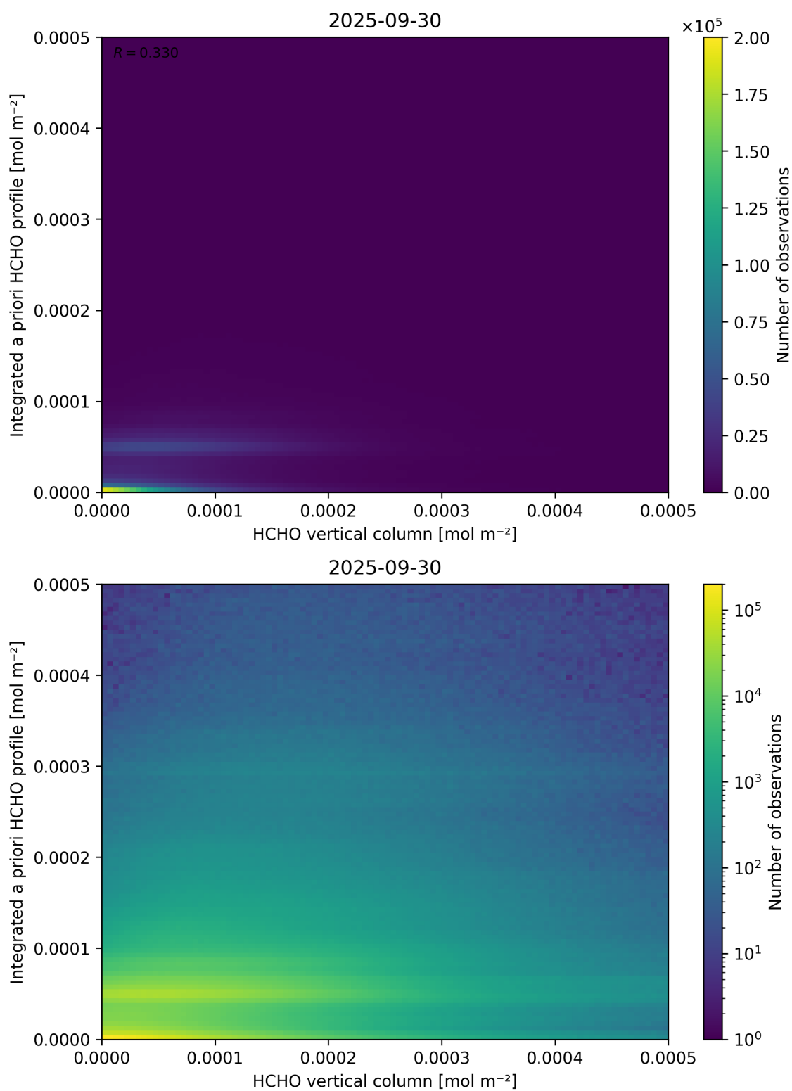
Figure 135: Scatter density plot of “HCHO vertical column” against “Integrated a priori HCHO profile” for 2025-09-29 to 2025-10-01.
