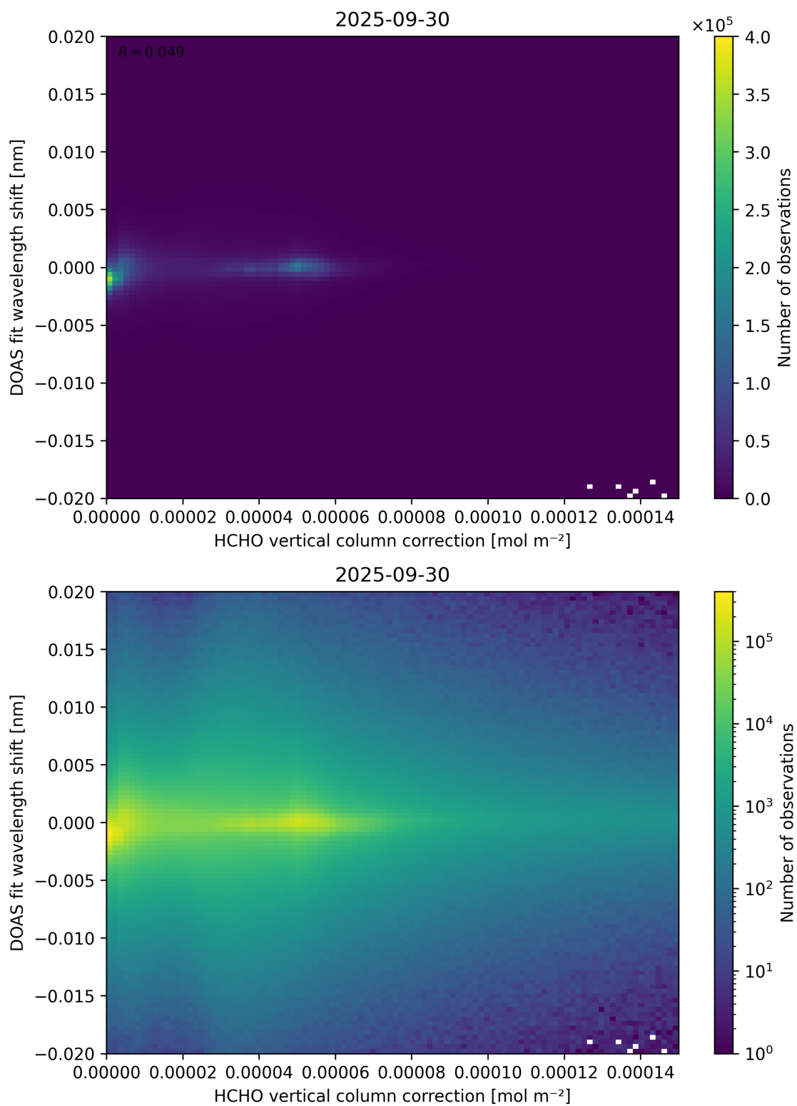
Figure 113: Scatter density plot of “HCHO vertical column correction” against “DOAS fit wavelength shift” for 2025-09-29 to 2025-10-01.
