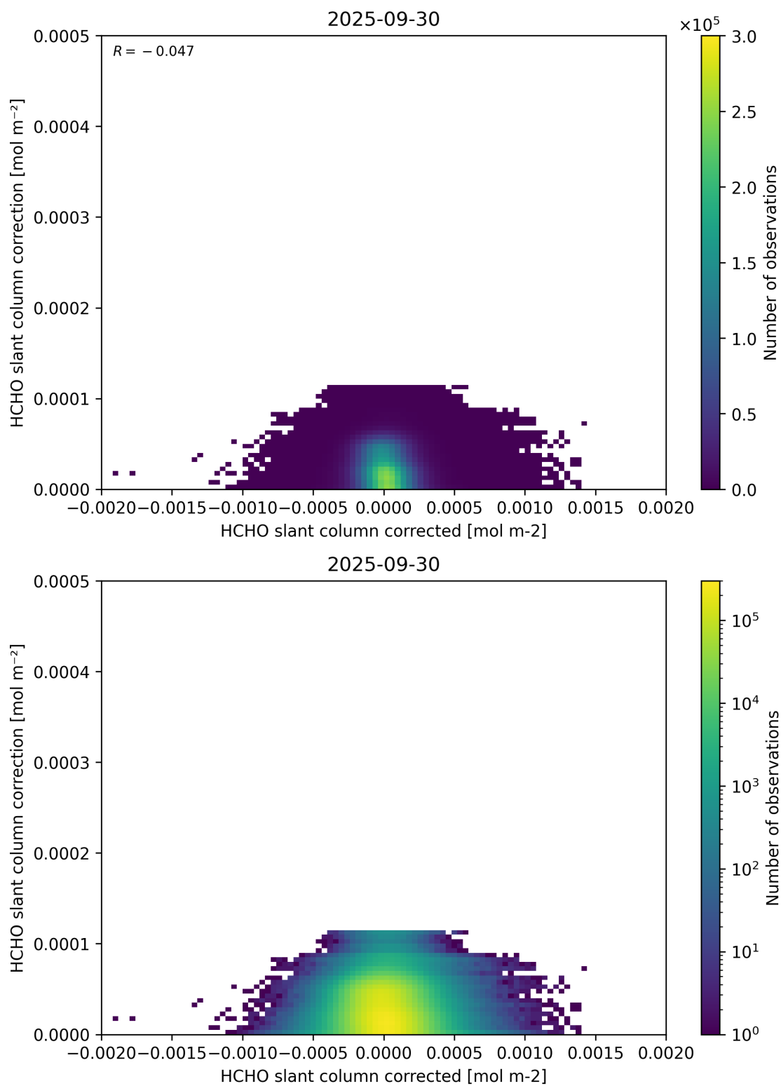
Figure 77: Scatter density plot of “HCHO slant column corrected” against “HCHO slant column correction” for 2025-09-29 to 2025-10-01.
