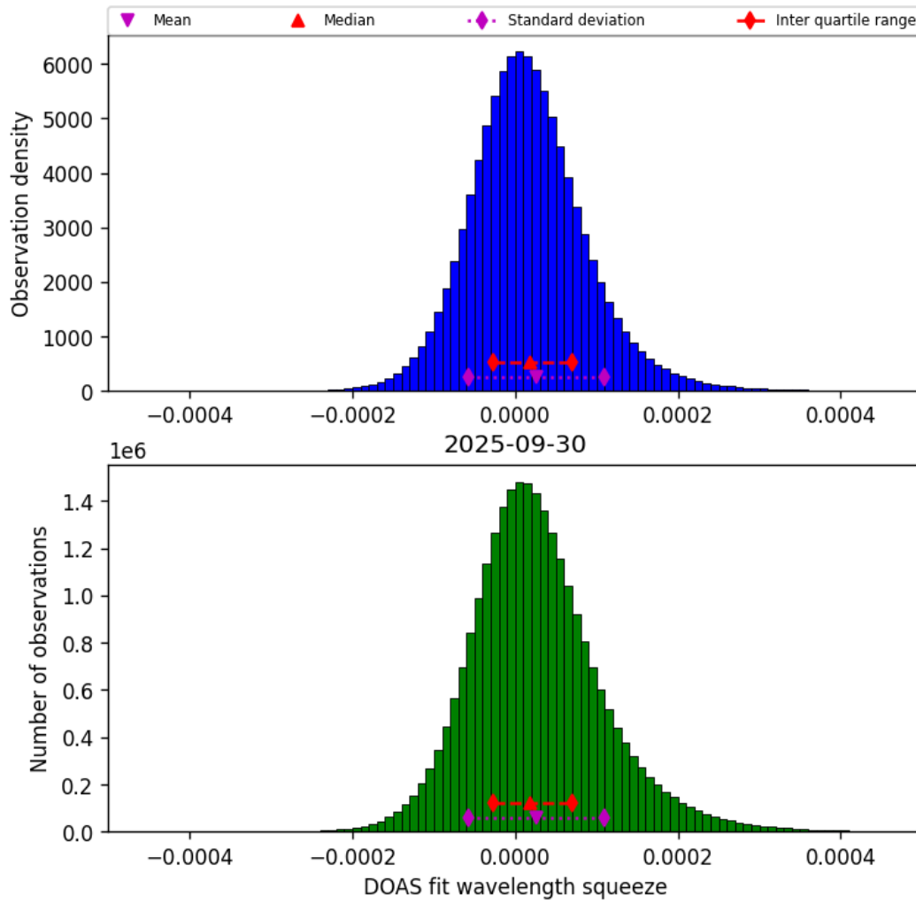
Figure 45: Histogram of “DOAS fit wavelength squeeze” for 2025-09-29 to 2025-10-01
