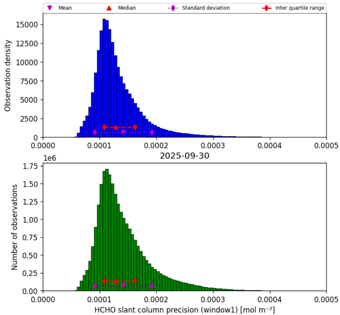
Figure 39: Histogram of “HCHO slant column precision (window1)” for 2025-09-29 to 2025-10-01
