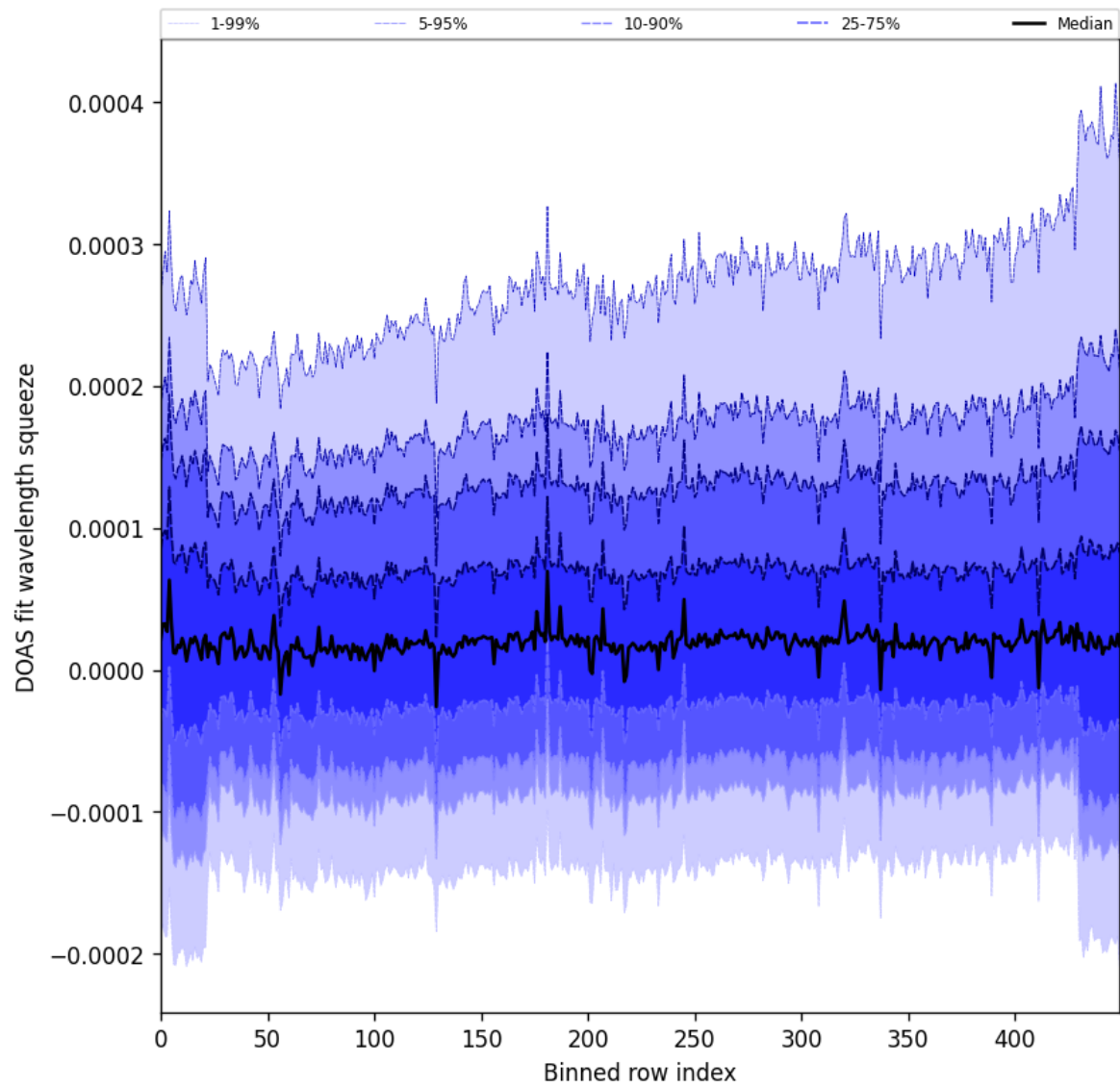
Figure 59: Along track statistics of “DOAS fit wavelength squeeze” for 2025-09-29 to 2025-10-01
