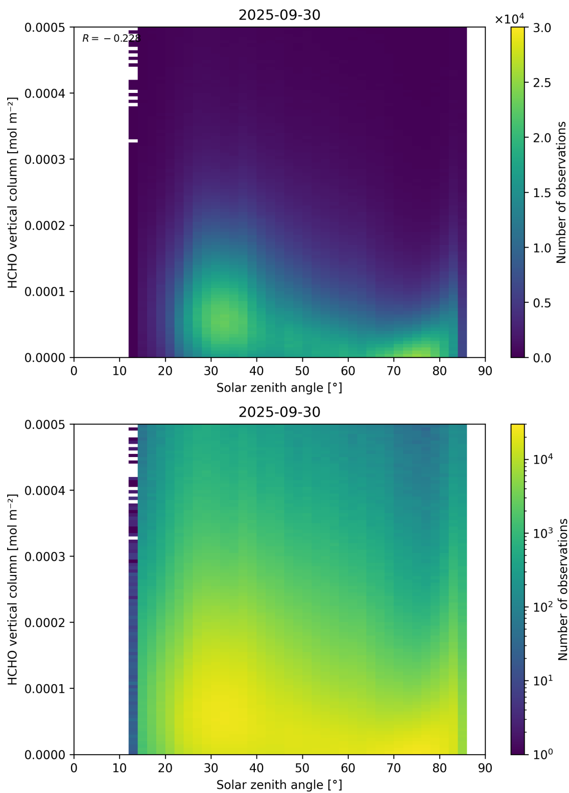
Figure 177: Scatter density plot of “Solar zenith angle” against “HCHO vertical column” for 2025-09-29 to 2025-10-01.
