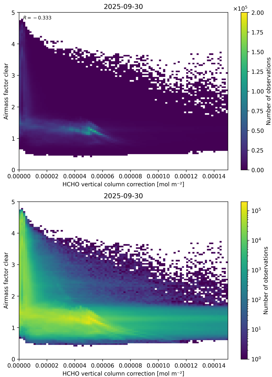
Figure 115: Scatter density plot of “HCHO vertical column correction” against “Airmass factor clear” for 2025-09-29 to 2025-10-01.
