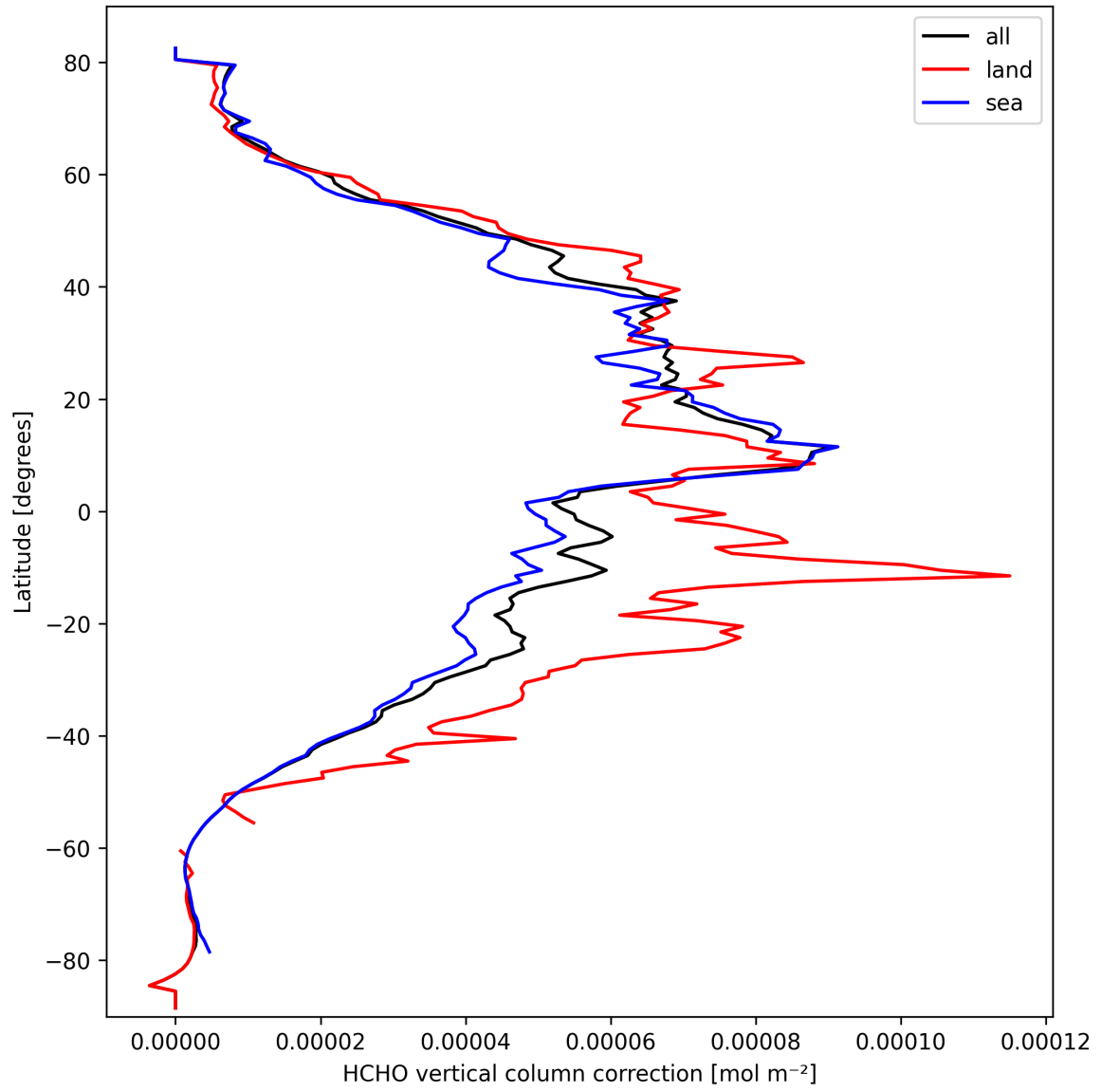
Figure 23: Zonal average of “HCHO vertical column correction” for 2025-09-29 to 2025-10-01.
