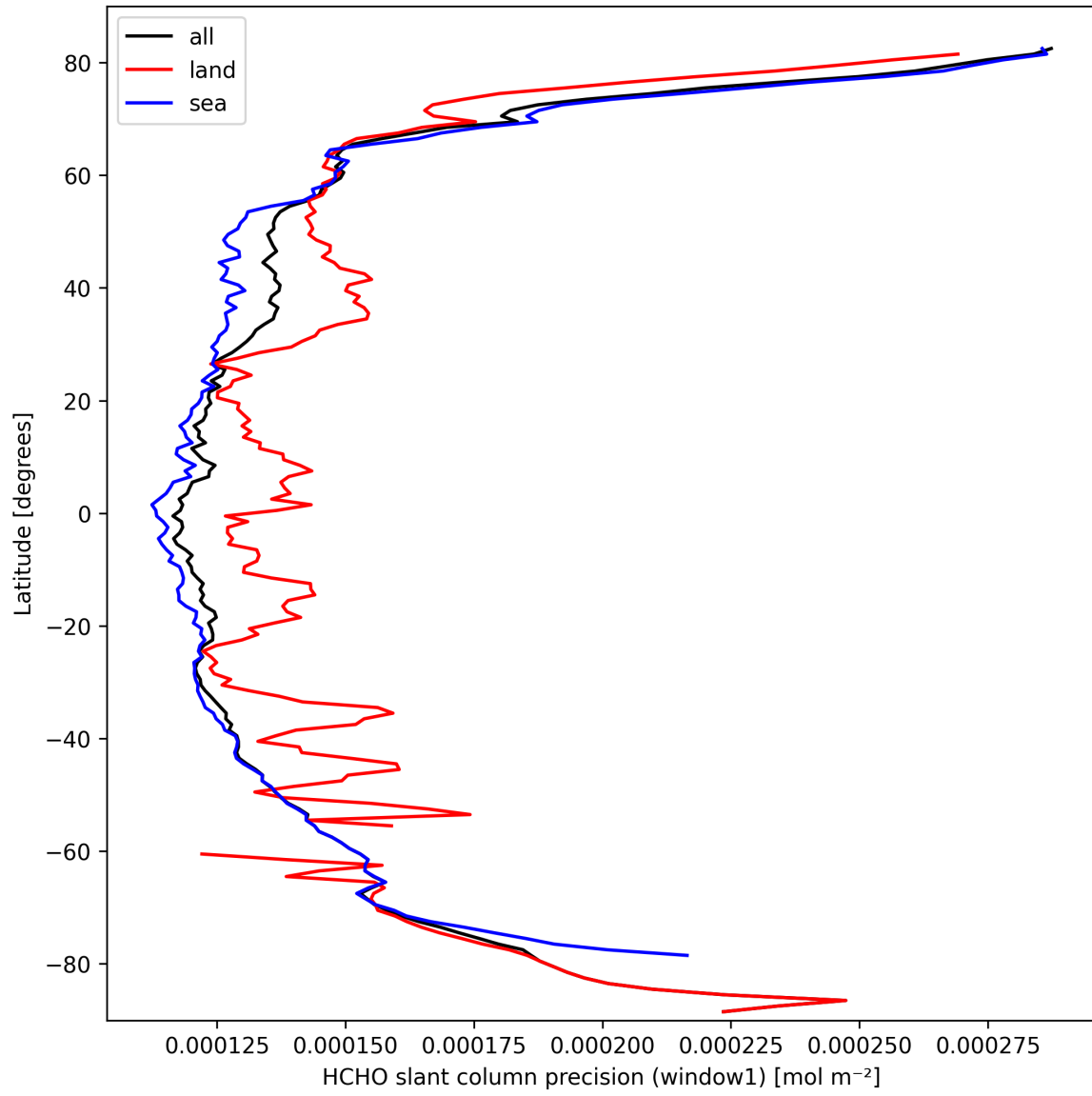
Figure 25: Zonal average of “HCHO slant column precision (window1)” for 2025-09-29 to 2025-10-01.
