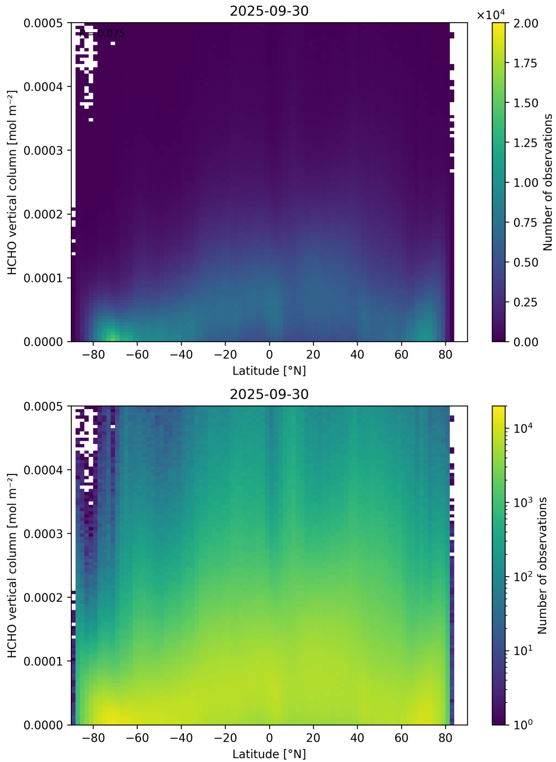
Figure 163: Scatter density plot of “Latitude” against “HCHO vertical column” for 2025-09-29 to 2025-10-01.
