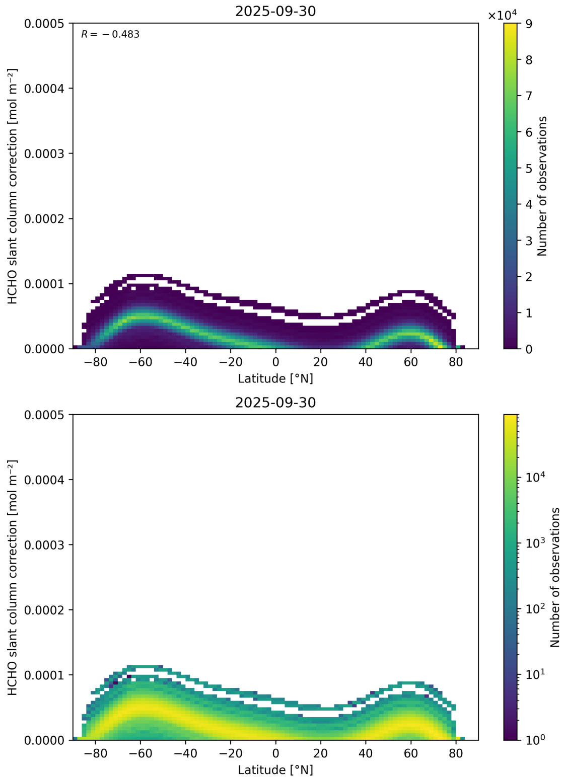
Figure 158: Scatter density plot of “Latitude” against “HCHO slant column correction” for 2025-09-29 to 2025-10-01.
