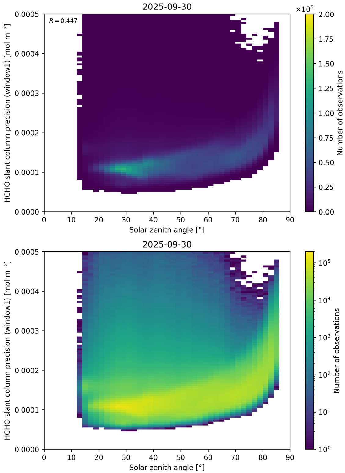
Figure 174: Scatter density plot of “Solar zenith angle” against “HCHO slant column precision (window1)” for 2025-09-29 to 2025-10-01.
