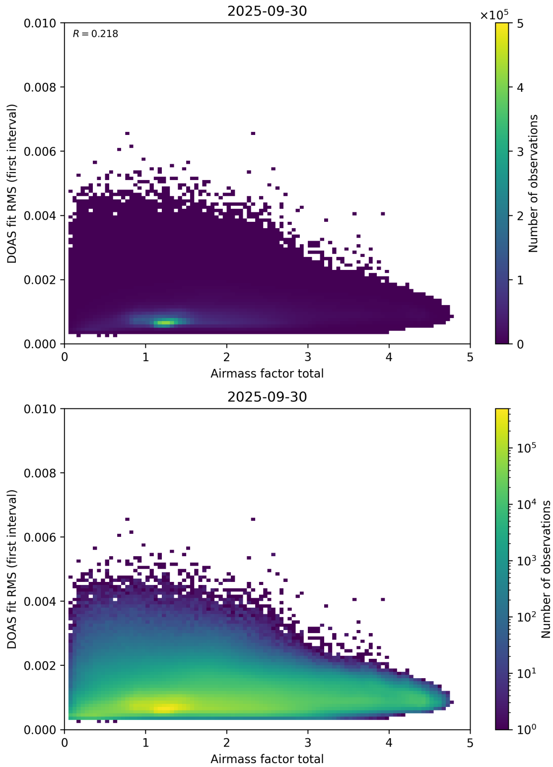
Figure 97: Scatter density plot of “Airmass factor total” against “DOAS fit RMS (first interval)” for 2025-09-29 to 2025-10-01.
