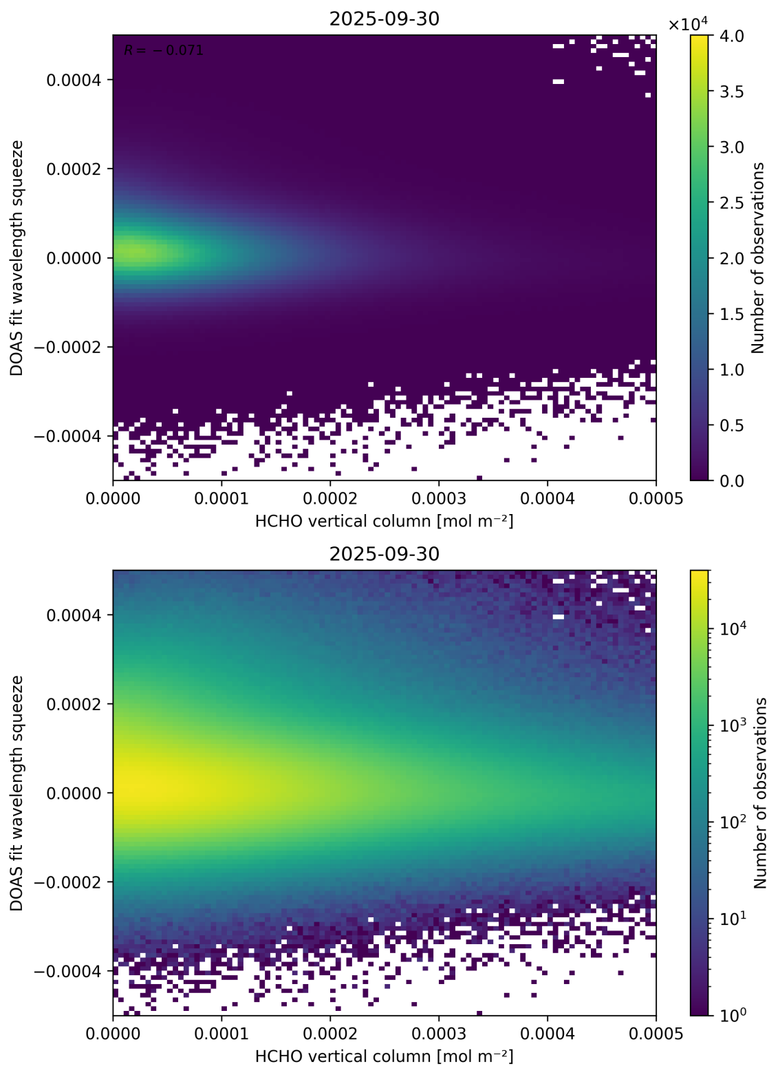
Figure 125: Scatter density plot of “HCHO vertical column” against “DOAS fit wavelength squeeze” for 2025-09-29 to 2025-10-01.
