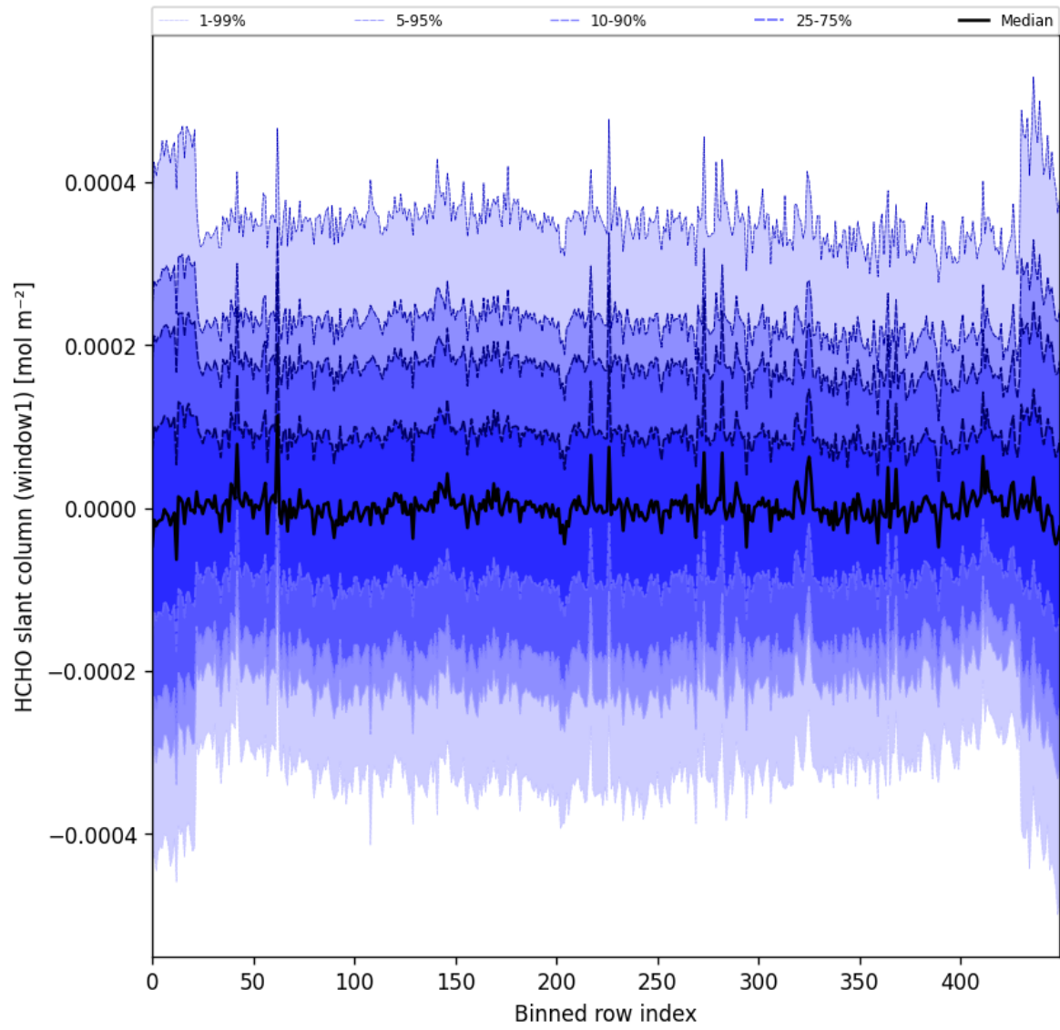
Figure 52: Along track statistics of “HCHO slant column (window1)” for 2025-09-29 to 2025-10-01
