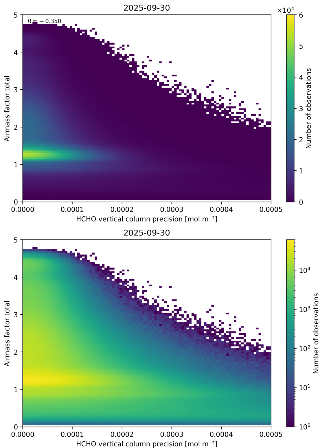
Figure 144: Scatter density plot of “HCHO vertical column precision” against “Airmass factor total” for 2025-09-29 to 2025-10-01.
