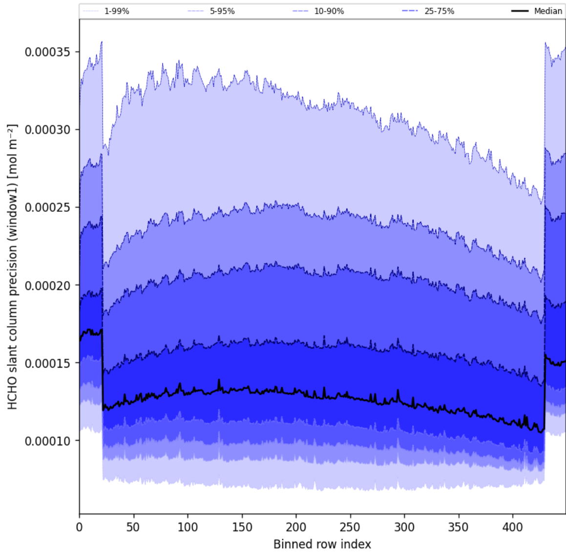
Figure 53: Along track statistics of "HCHO slant column precision (window1)" for 2025-09-29 to 2025-10-01
