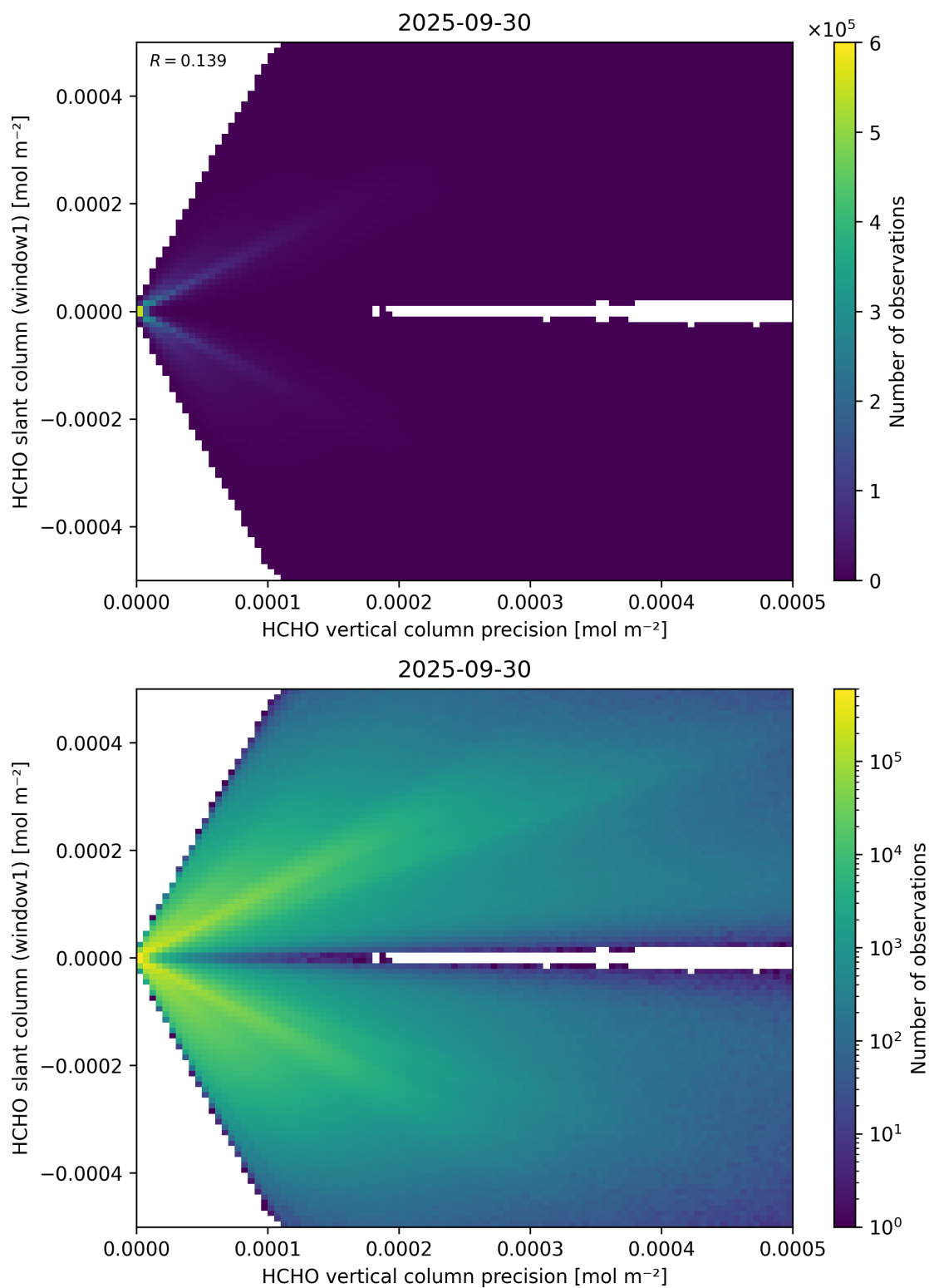
Figure 142: Scatter density plot of “HCHO vertical column precision” against “HCHO slant column (window1)” for 2025-09-29 to 2025-10-01.
