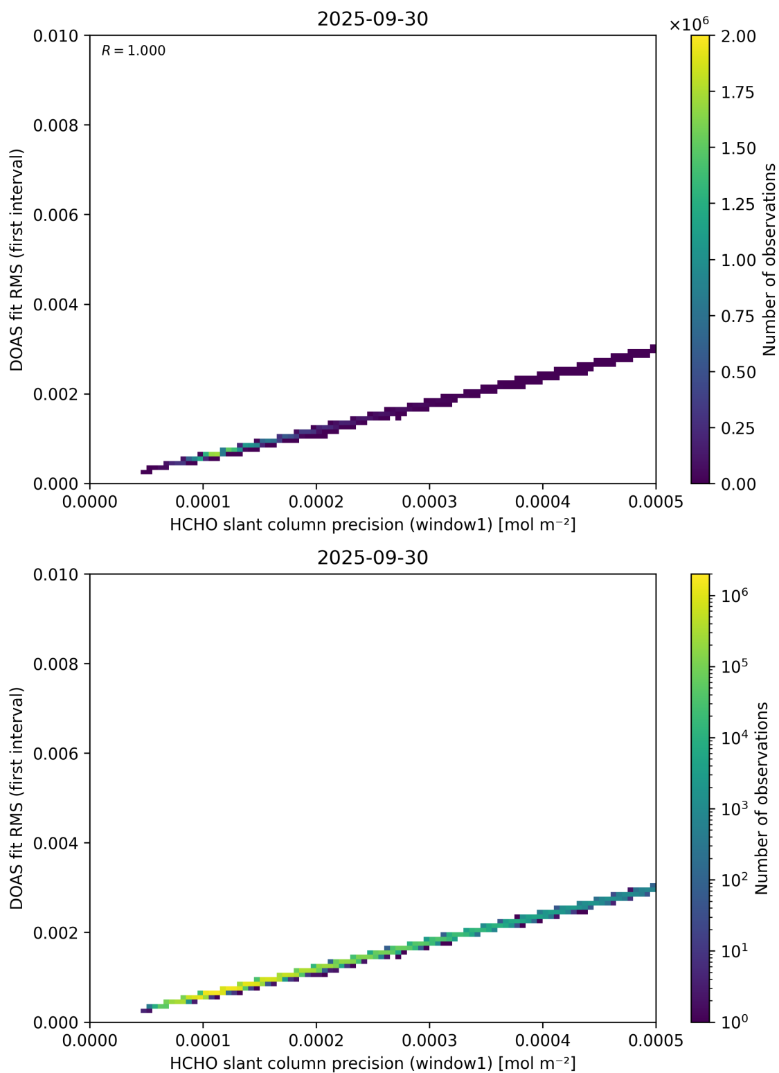
Figure 88: Scatter density plot of “HCHO slant column precision (window1)” against “DOAS fit RMS (first interval)” for 2025-09-29 to 2025-10-01.
