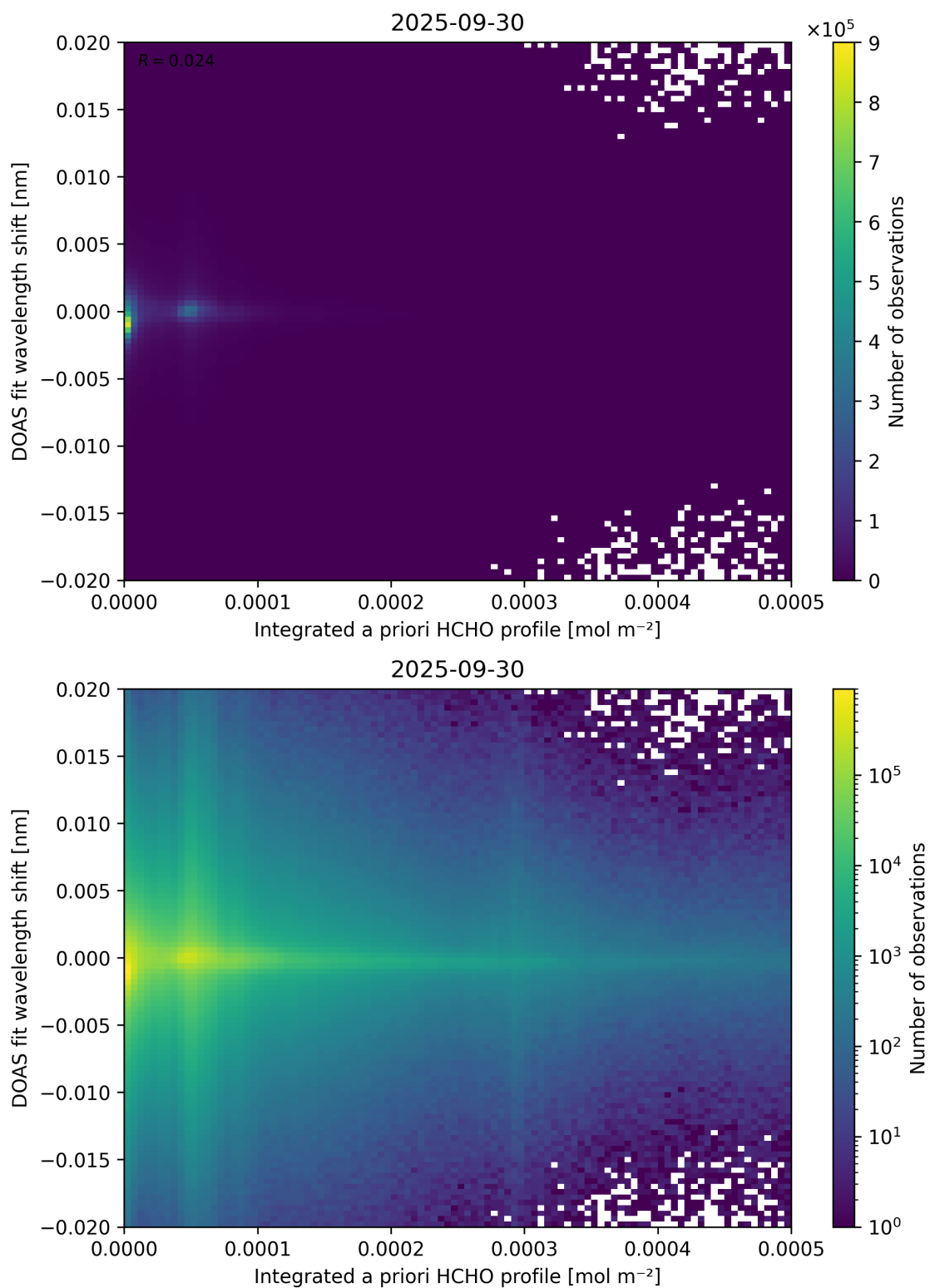
Figure 149: Scatter density plot of “Integrated a priori HCHO profile” against “DOAS fit wavelength shift” for 2025-09-29 to 2025-10-01.
