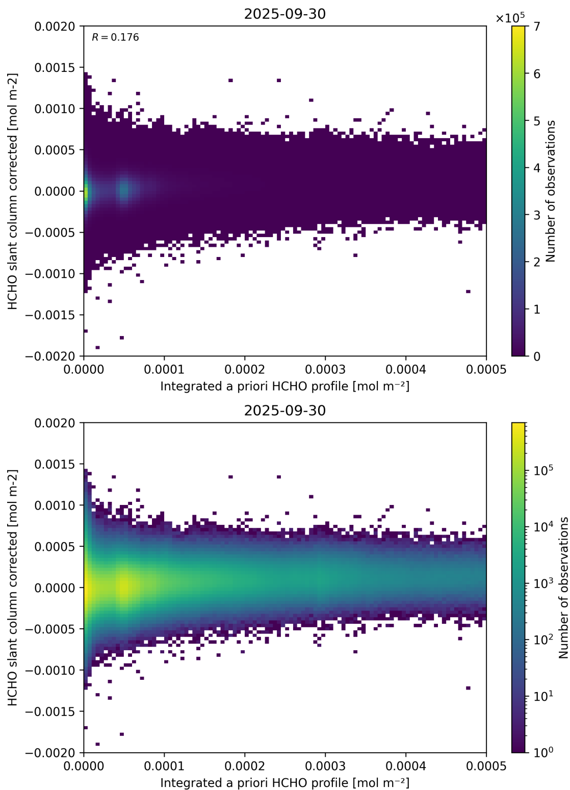
Figure 151: Scatter density plot of “Integrated a priori HCHO profile” against “HCHO slant column corrected” for 2025-09-29 to 2025-10-01.
