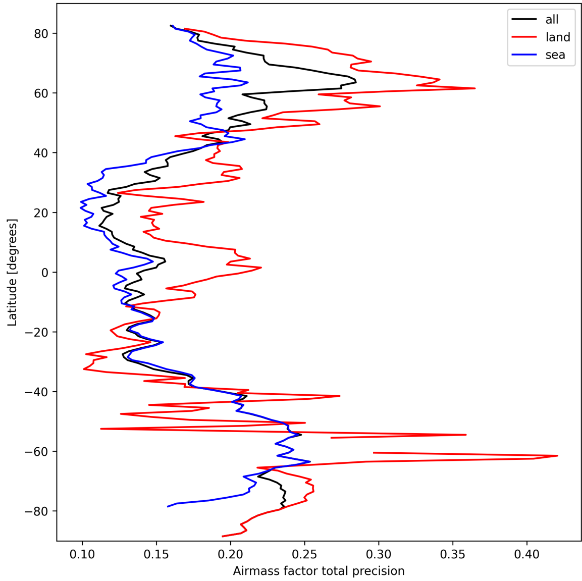
Figure 27: Zonal average of “Airmass factor total precision” for 2025-09-29 to 2025-10-01.
