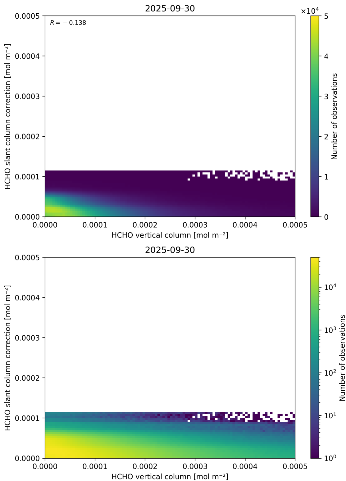
Figure 128: Scatter density plot of “HCHO vertical column” against “HCHO slant column correction” for 2025-09-29 to 2025-10-01.
