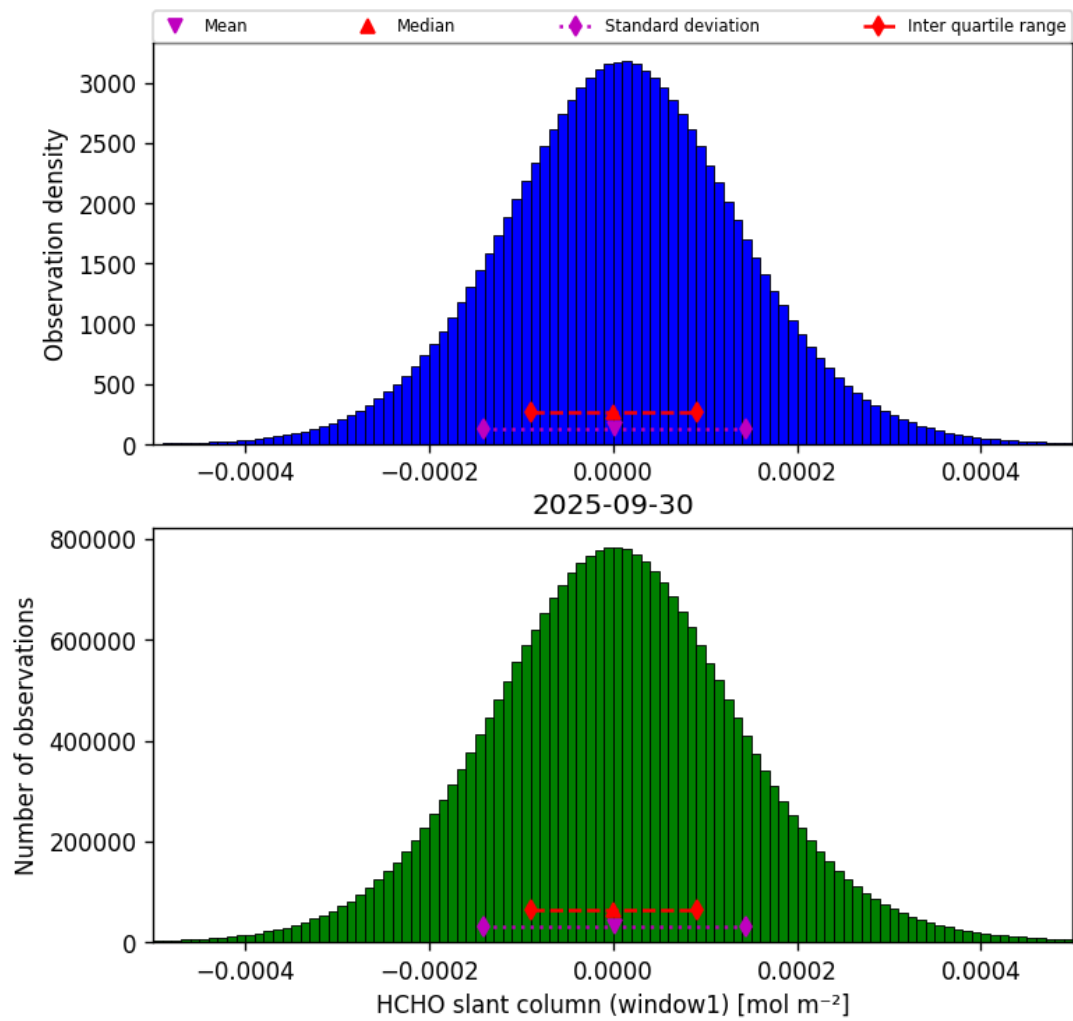
Figure 38: Histogram of “HCHO slant column (window1)” for 2025-09-29 to 2025-10-01
