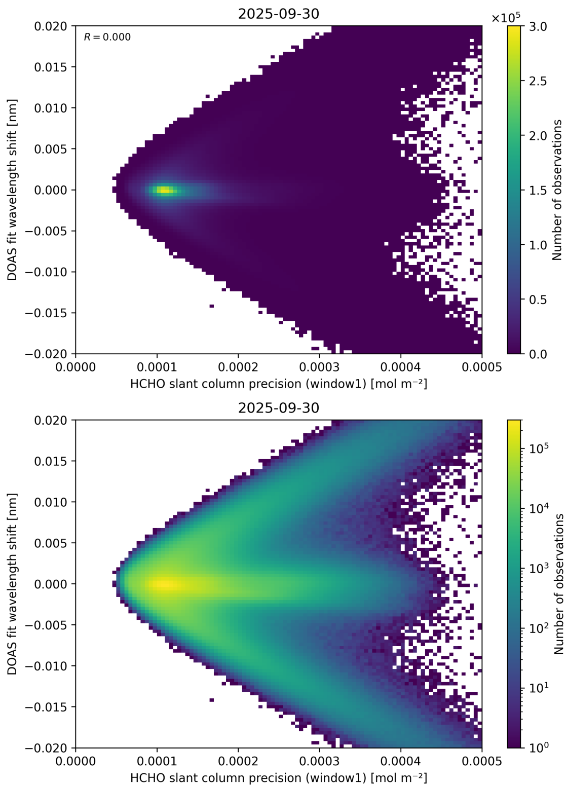
Figure 89: Scatter density plot of “HCHO slant column precision (window1)” against “DOAS fit wavelength shift” for 2025-09-29 to 2025-10-01.
