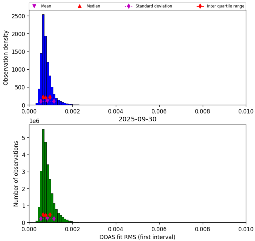
Figure 46: Histogram of “DOAS fit RMS (first interval)” for 2025-09-29 to 2025-10-01
