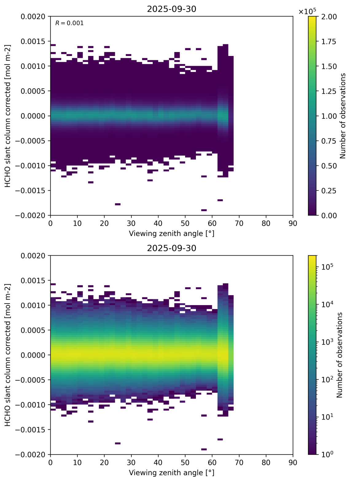
Figure 186: Scatter density plot of “Viewing zenith angle” against “HCHO slant column corrected” for 2025-09-29 to 2025-10-01.
