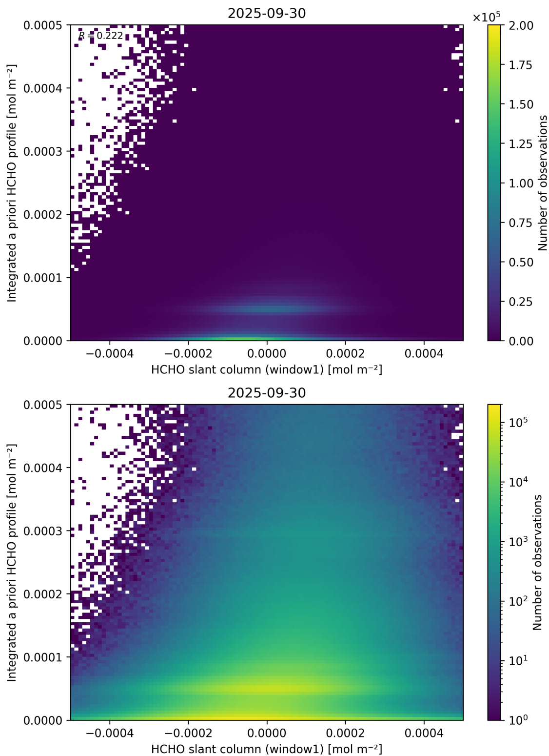
Figure 87: Scatter density plot of “HCHO slant column (window1)” against “Integrated a priori HCHO profile” for 2025-09-29 to 2025-10-01.
