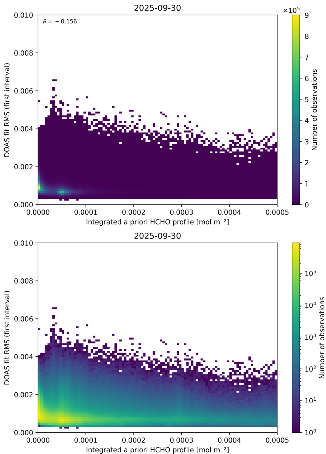
Figure 148: Scatter density plot of “Integrated a priori HCHO profile” against “DOAS fit RMS (first interval)” for 2025-09-29 to 2025-10-01.
