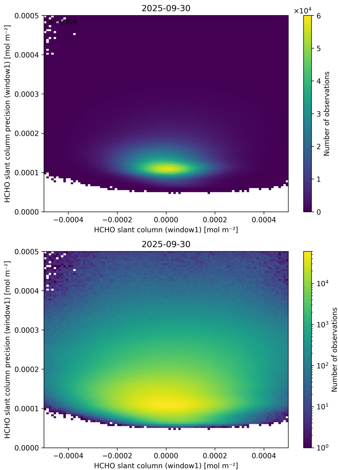
Figure 84: Scatter density plot of “HCHO slant column (window1)” against “HCHO slant column precision (window1)” for 2025-09-29 to 2025-10-01.
