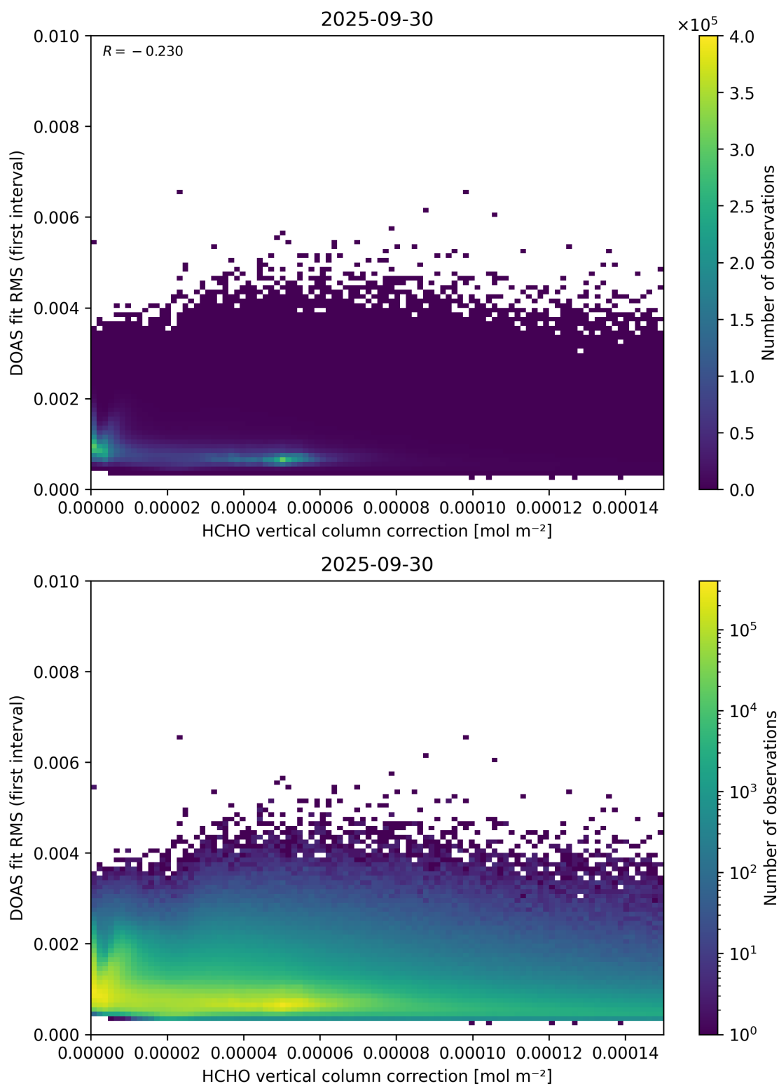
Figure 112: Scatter density plot of “HCHO vertical column correction” against “DOAS fit RMS (first interval)” for 2025-09-29 to 2025-10-01.
