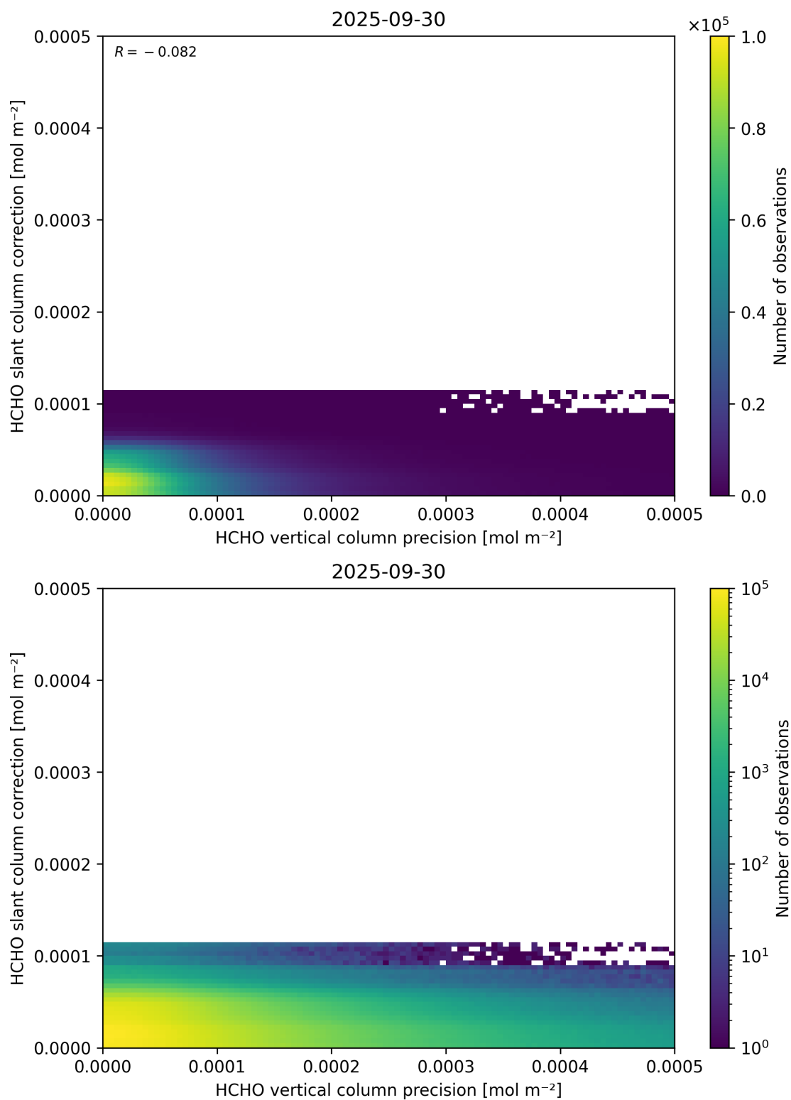
Figure 141: Scatter density plot of “HCHO vertical column precision” against “HCHO slant column correction” for 2025-09-29 to 2025-10-01.
