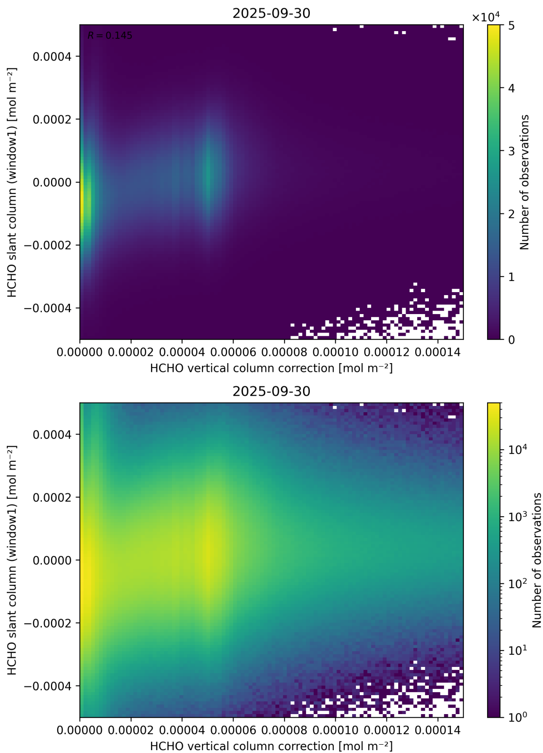
Figure 118: Scatter density plot of “HCHO vertical column correction” against “HCHO slant column (window1)” for 2025-09-29 to 2025-10-01.
