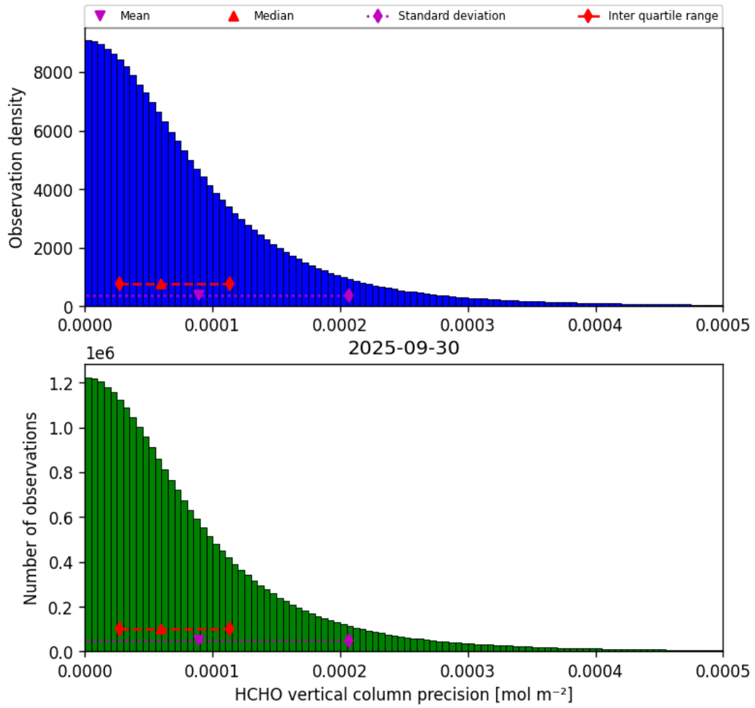
Figure 36: Histogram of “HCHO vertical column precision” for 2025-09-29 to 2025-10-01
