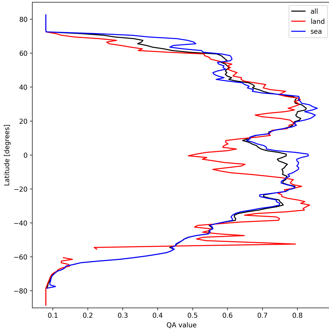
Figure 20: Zonal average of “QA value” for 2025-09-29 to 2025-10-01.
