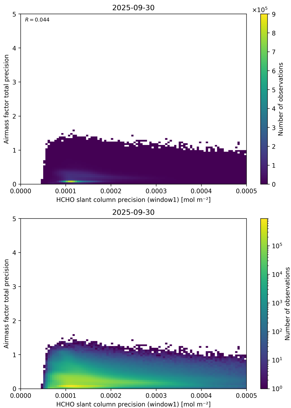
Figure 95: Scatter density plot of “HCHO slant column precision (window1)” against “Airmass factor total precision” for 2025-09-29 to 2025-10-01.
