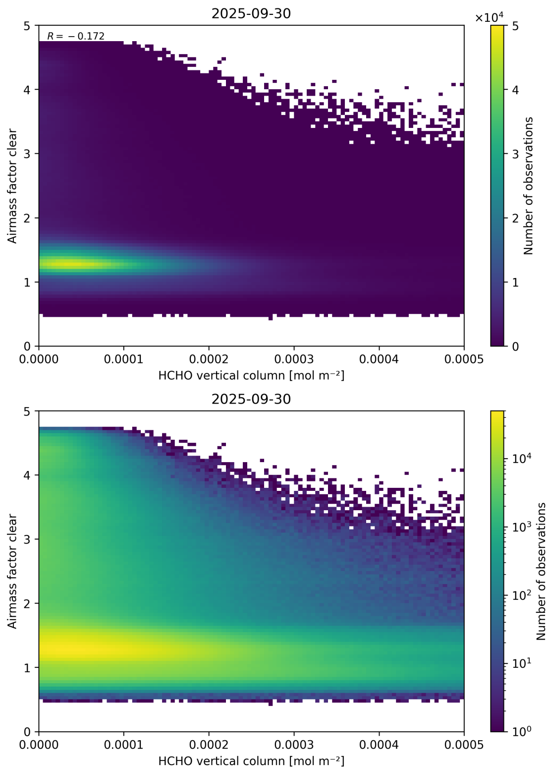
Figure 126: Scatter density plot of “HCHO vertical column” against “Airmass factor clear” for 2025-09-29 to 2025-10-01.
