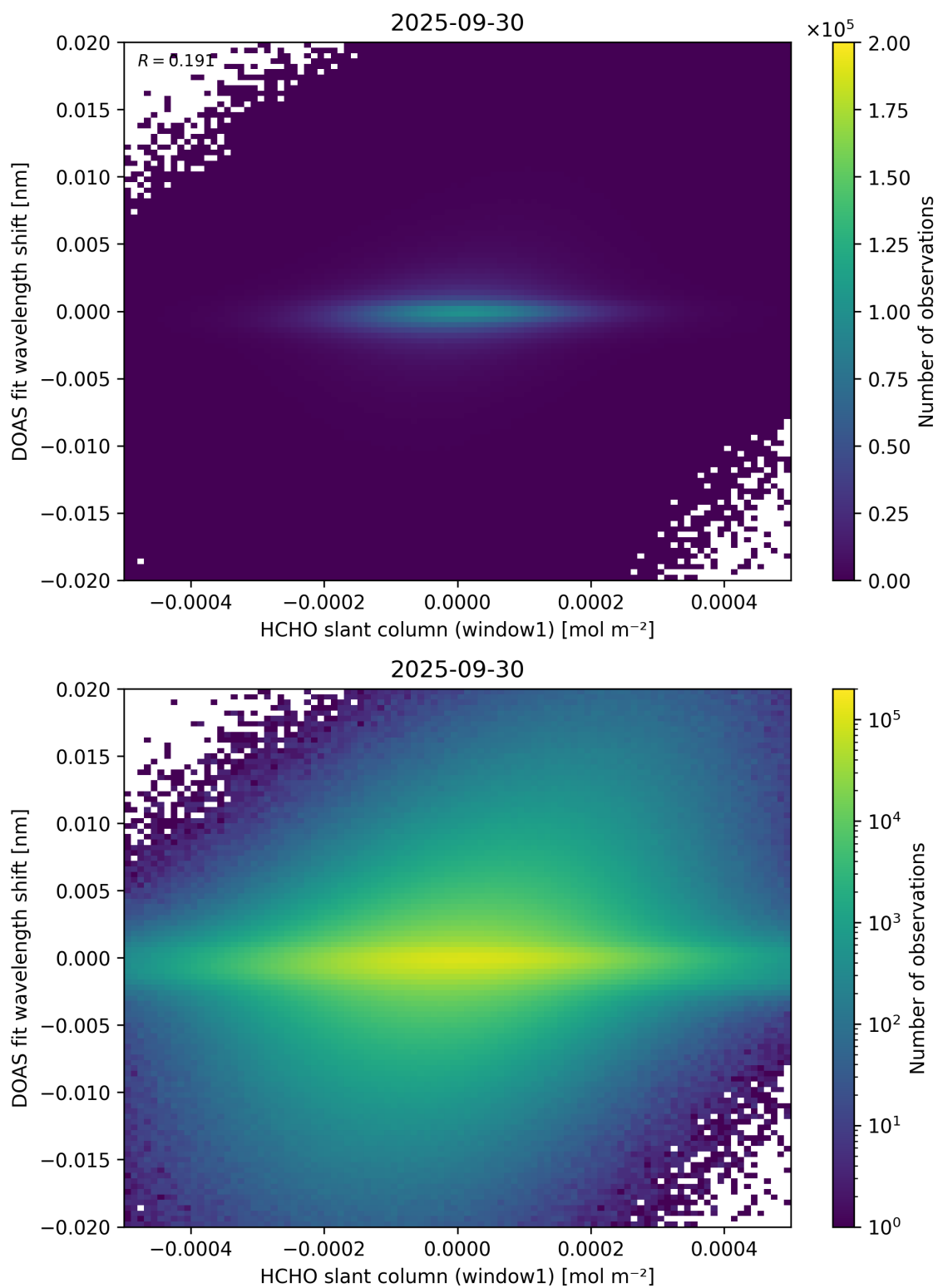
Figure 79: Scatter density plot of “HCHO slant column (window1)” against “DOAS fit wavelength shift” for 2025-09-29 to 2025-10-01.
