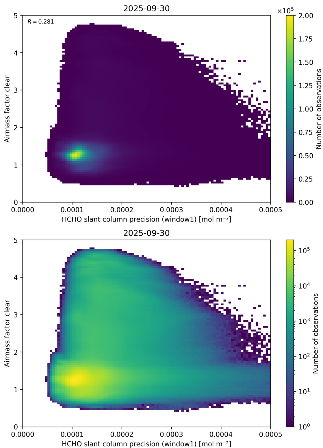
Figure 91: Scatter density plot of “HCHO slant column precision (window1)” against “Airmass factor clear” for 2025-09-29 to 2025-10-01.
