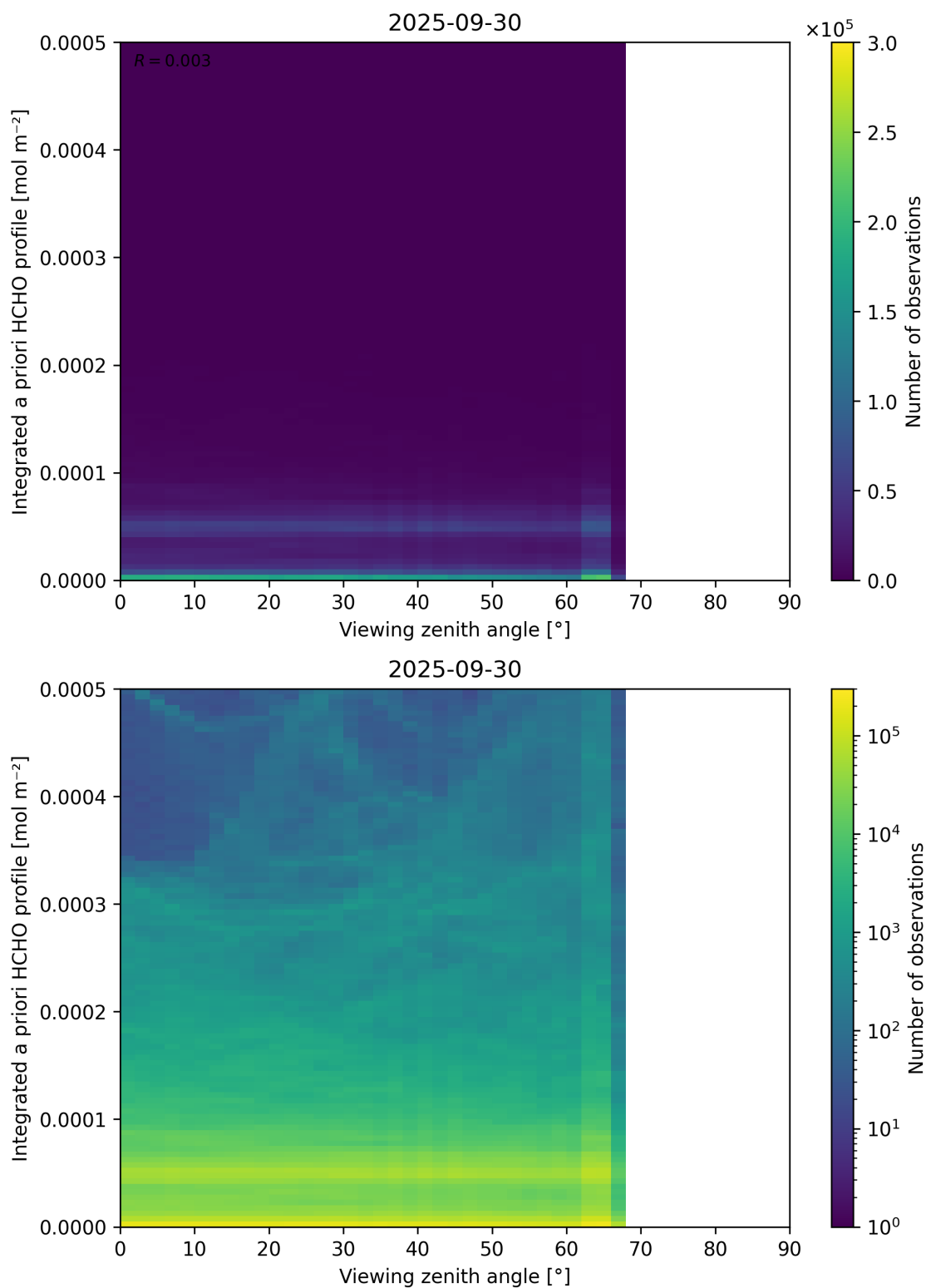
Figure 195: Scatter density plot of “Viewing zenith angle” against “Integrated a priori HCHO profile” for 2025-09-29 to 2025-10-01.
