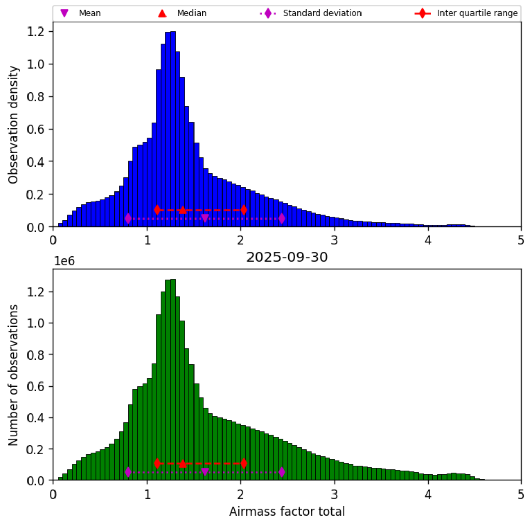
Figure 40: Histogram of “Airmass factor total” for 2025-09-29 to 2025-10-01
