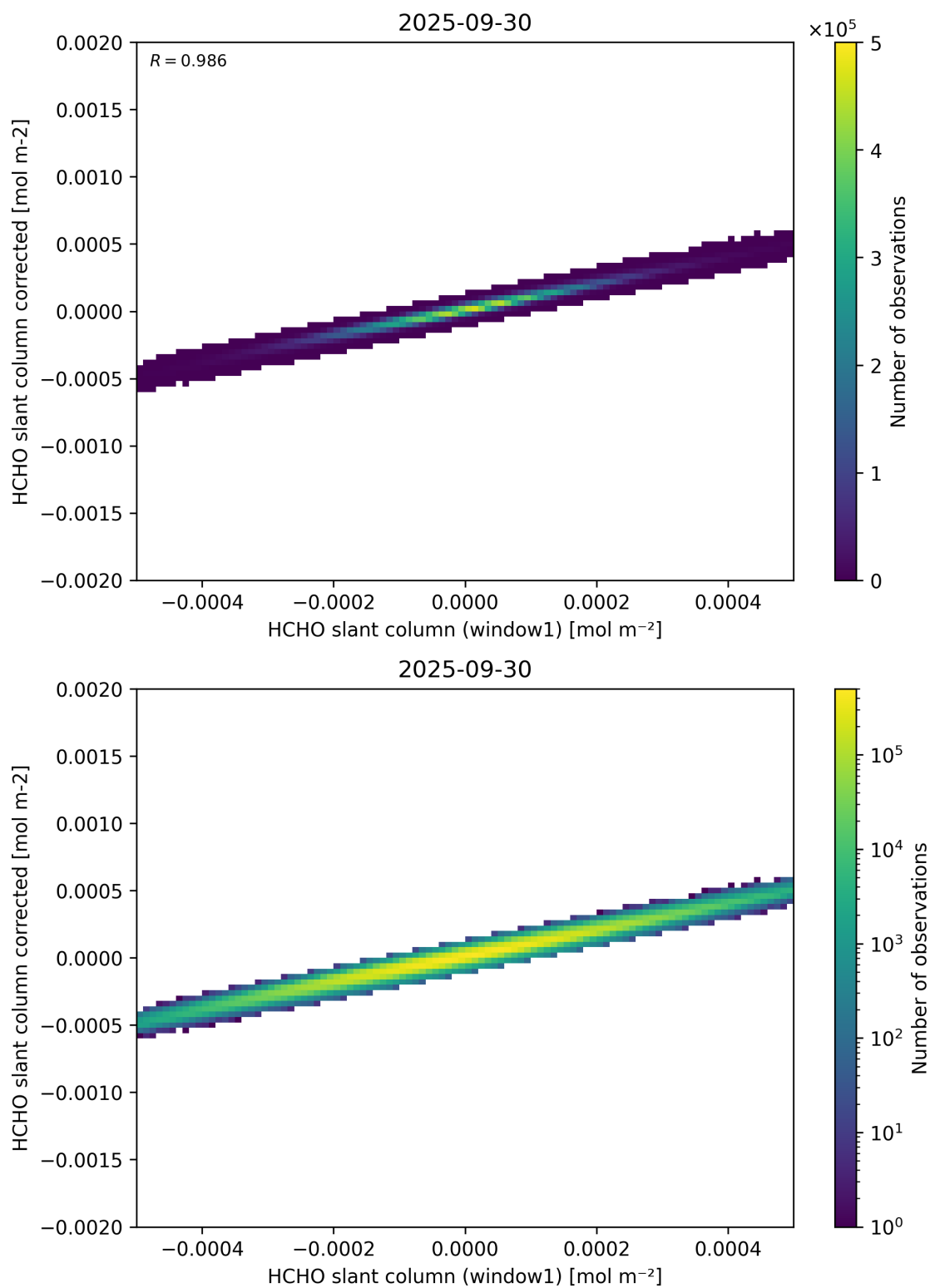
Figure 82: Scatter density plot of “HCHO slant column (window1)” against “HCHO slant column corrected” for 2025-09-29 to 2025-10-01.
