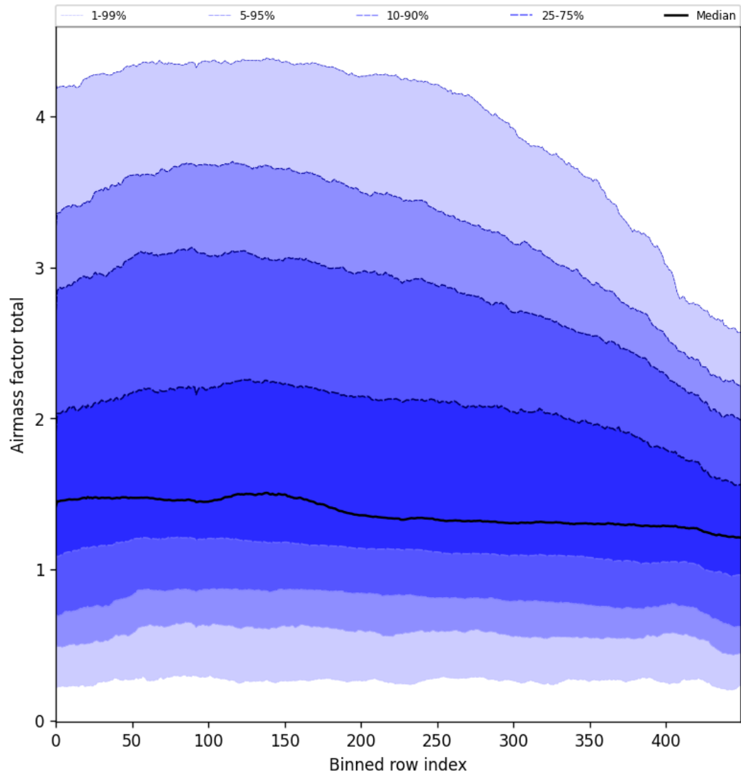
Figure 54: Along track statistics of “Airmass factor total” for 2025-09-29 to 2025-10-01
