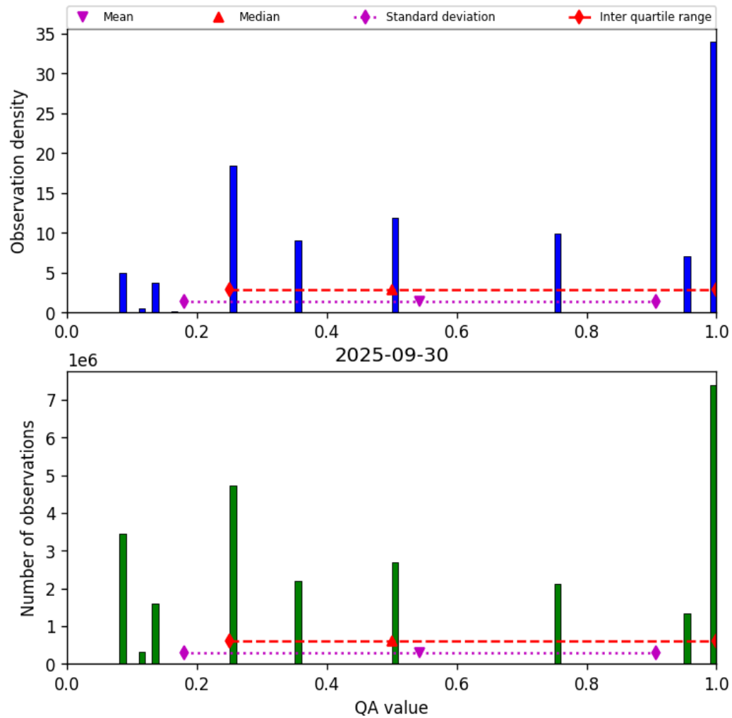
Figure 34: Histogram of “QA value” for 2025-09-29 to 2025-10-01
