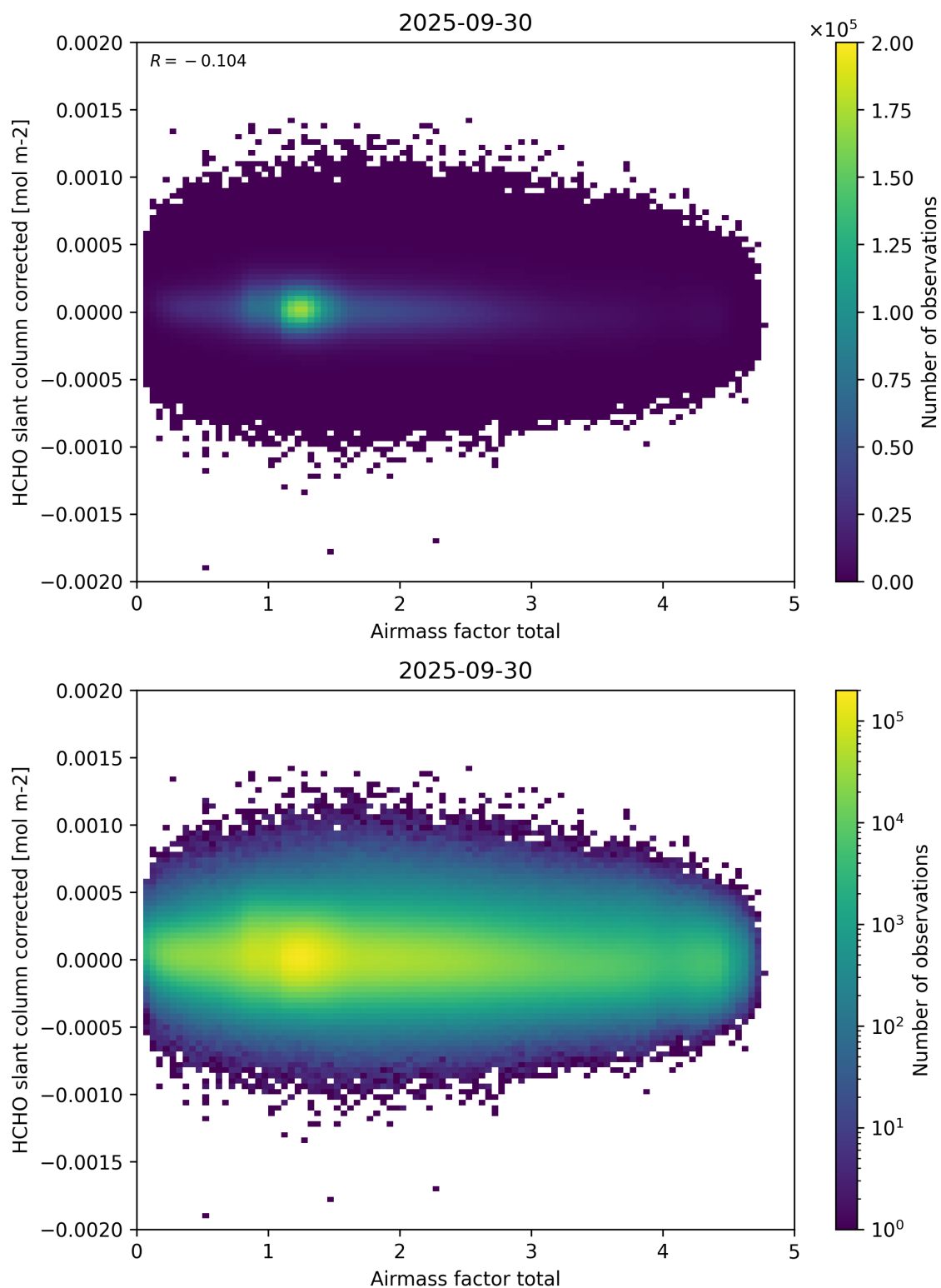
Figure 101: Scatter density plot of “Airmass factor total” against “HCHO slant column corrected” for 2025-09-29 to 2025-10-01.
