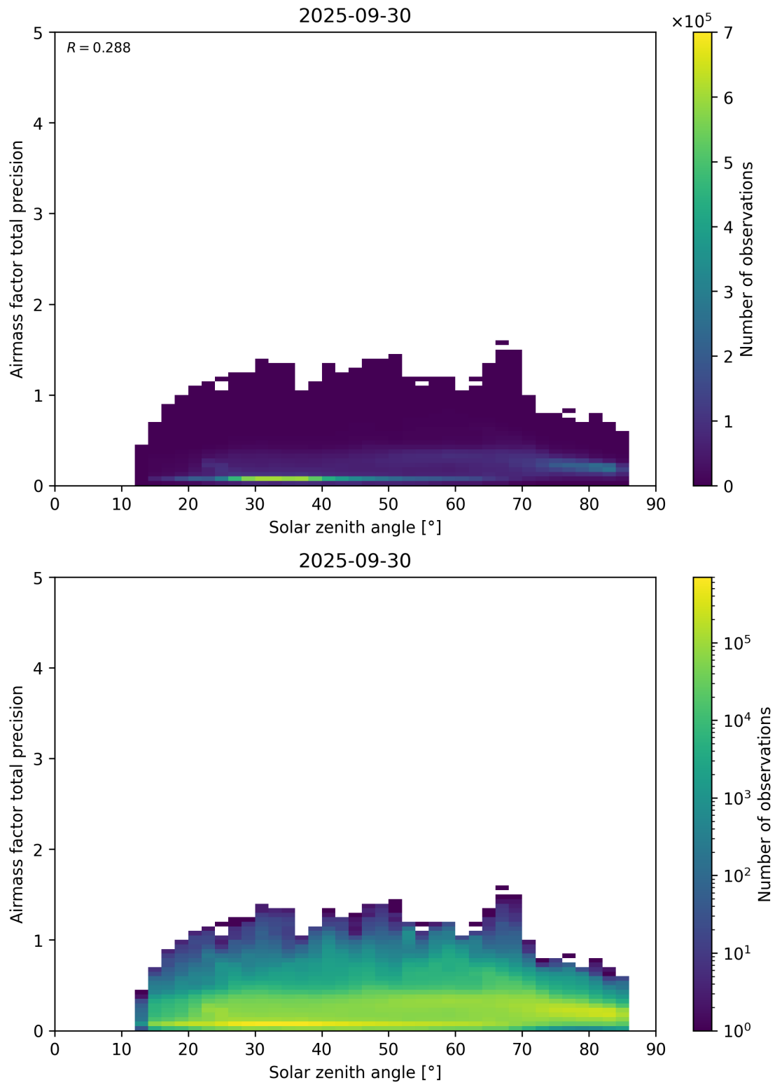
Figure 176: Scatter density plot of “Solar zenith angle” against “Airmass factor total precision” for 2025-09-29 to 2025-10-01.
