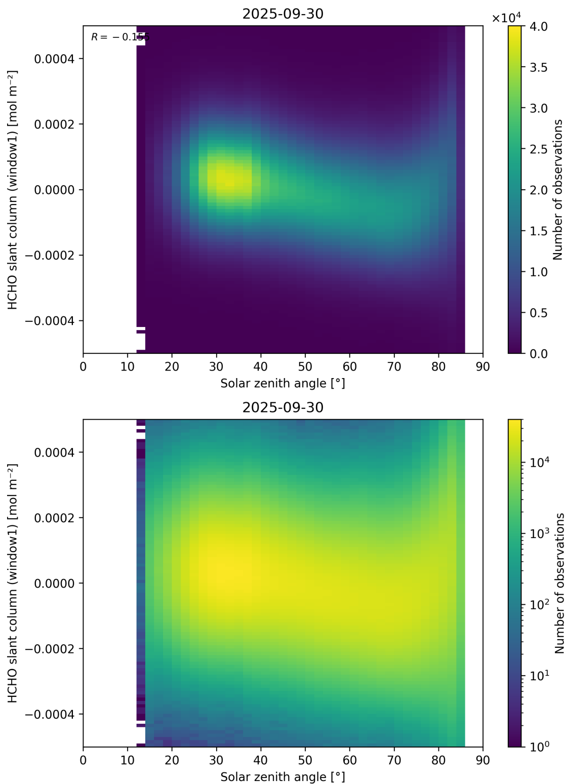
Figure 173: Scatter density plot of “Solar zenith angle” against “HCHO slant column (window1)” for 2025-09-29 to 2025-10-01.
