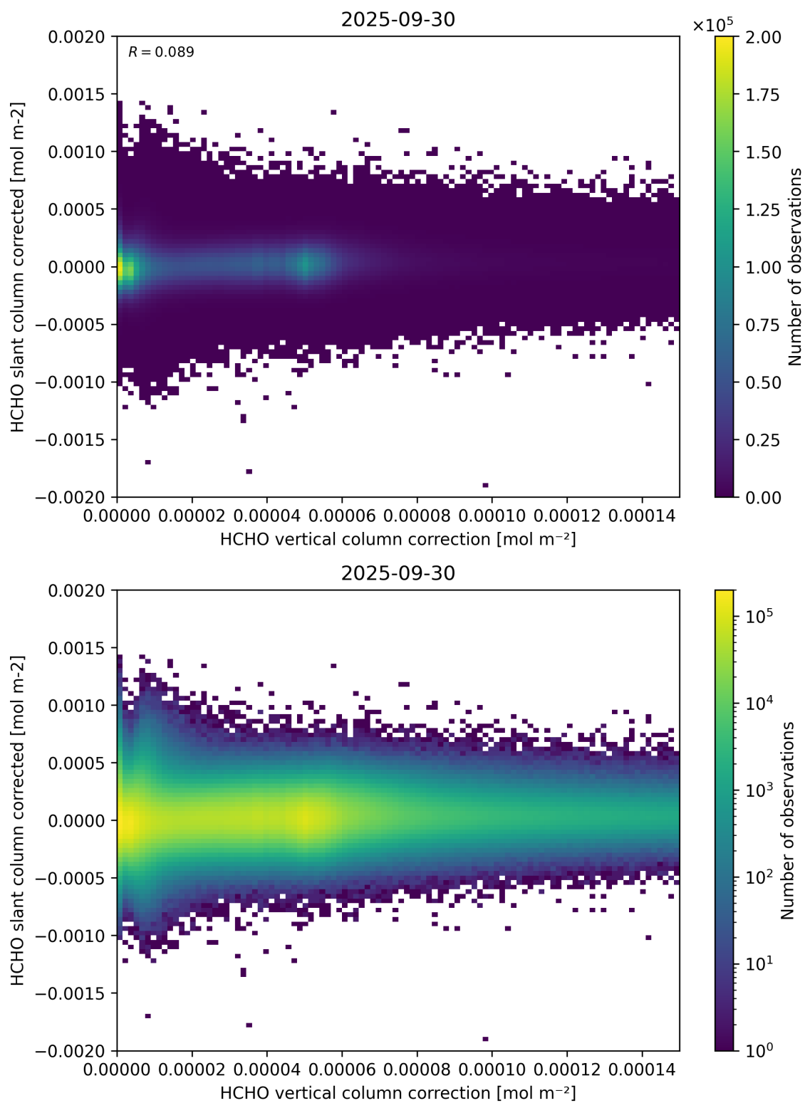
Figure 116: Scatter density plot of “HCHO vertical column correction” against “HCHO slant column corrected” for 2025-09-29 to 2025-10-01.
