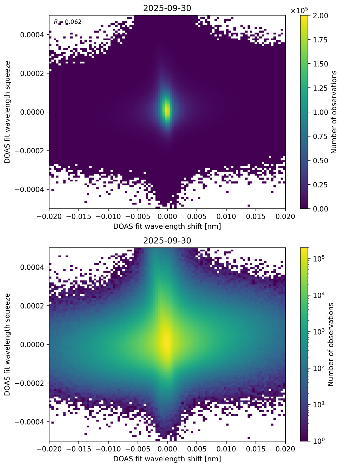
Figure 65: Scatter density plot of “DOAS fit wavelength shift” against “DOAS fit wavelength squeeze” for 2025-09-29 to 2025-10-01.
