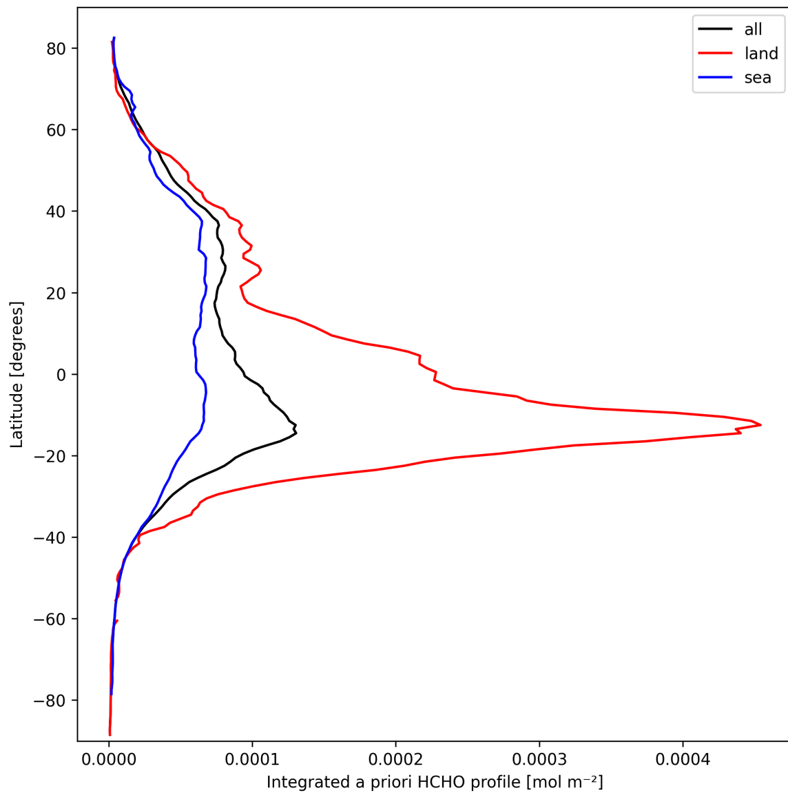
Figure 29: Zonal average of “Integrated a priori HCHO profile” for 2025-09-29 to 2025-10-01.
