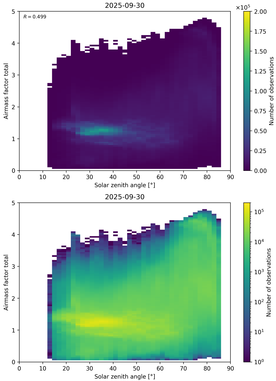
Figure 175: Scatter density plot of “Solar zenith angle” against “Airmass factor total” for 2025-09-29 to 2025-10-01.
