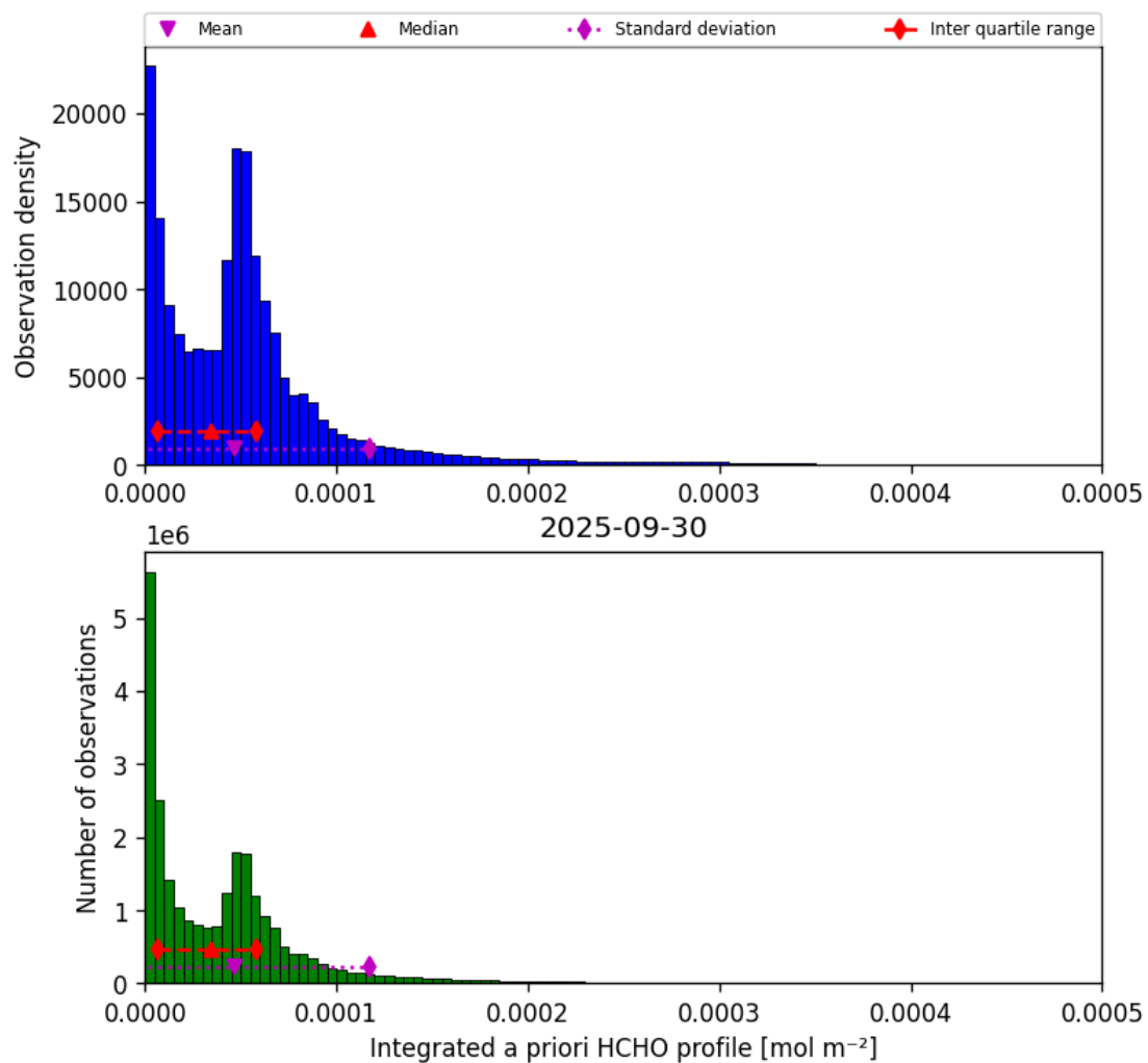
Figure 43: Histogram of “Integrated a priori HCHO profile” for 2025-09-29 to 2025-10-01
