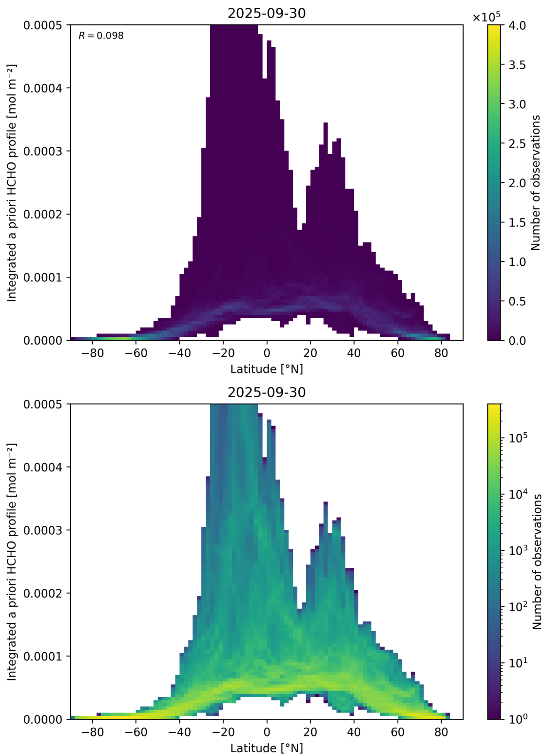
Figure 166: Scatter density plot of “Latitude” against “Integrated a priori HCHO profile” for 2025-09-29 to 2025-10-01.
