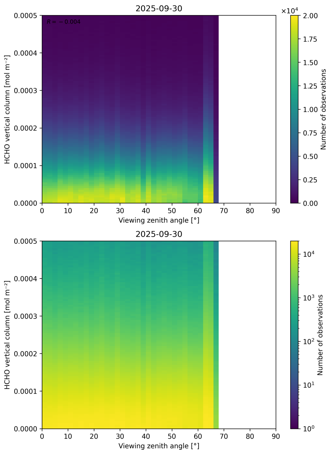
Figure 192: Scatter density plot of “Viewing zenith angle” against “HCHO vertical column” for 2025-09-29 to 2025-10-01.
