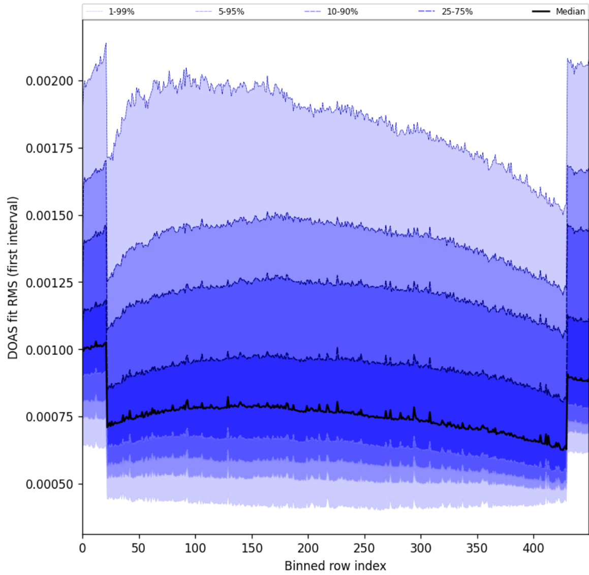
Figure 60: Along track statistics of “DOAS fit RMS (first interval)” for 2025-09-29 to 2025-10-01
