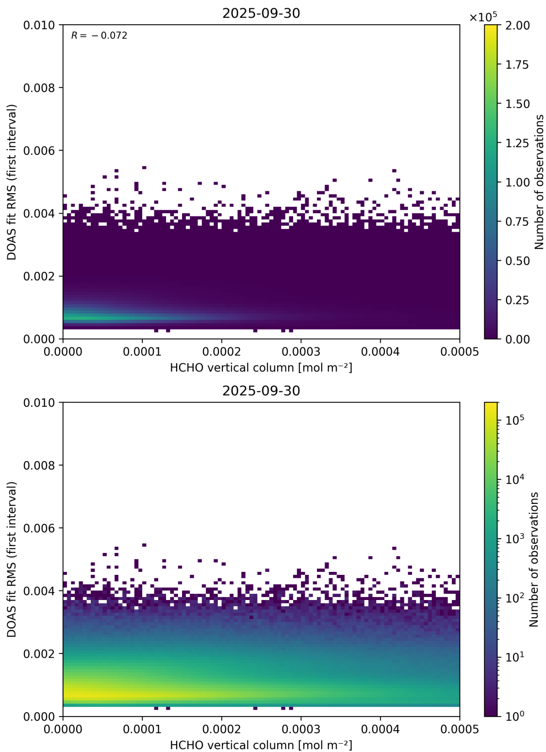
Figure 123: Scatter density plot of “HCHO vertical column” against “DOAS fit RMS (first interval)” for 2025-09-29 to 2025-10-01.
