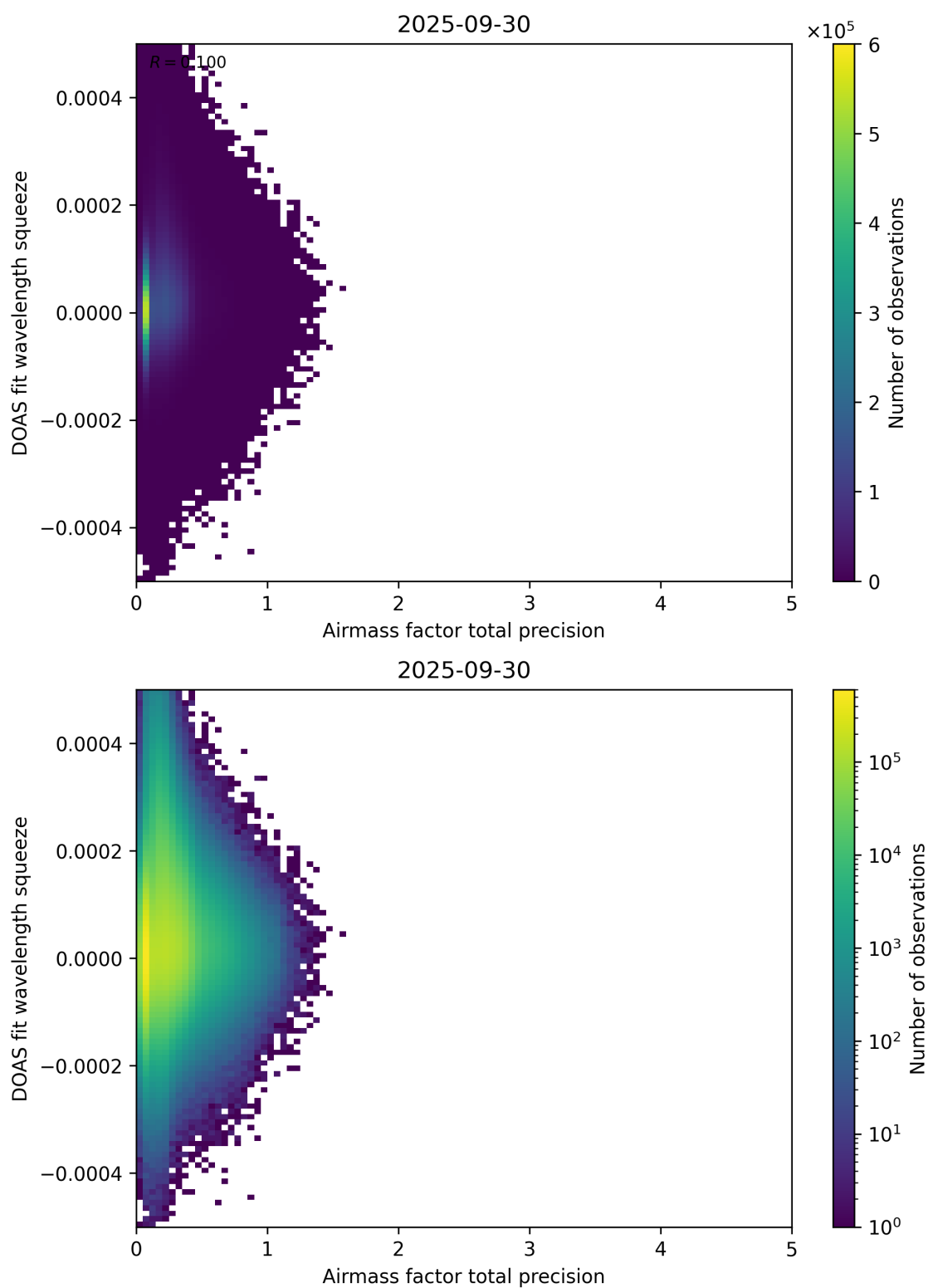
Figure 107: Scatter density plot of “Airmass factor total precision” against “DOAS fit wavelength squeeze” for 2025-09-29 to 2025-10-01.
