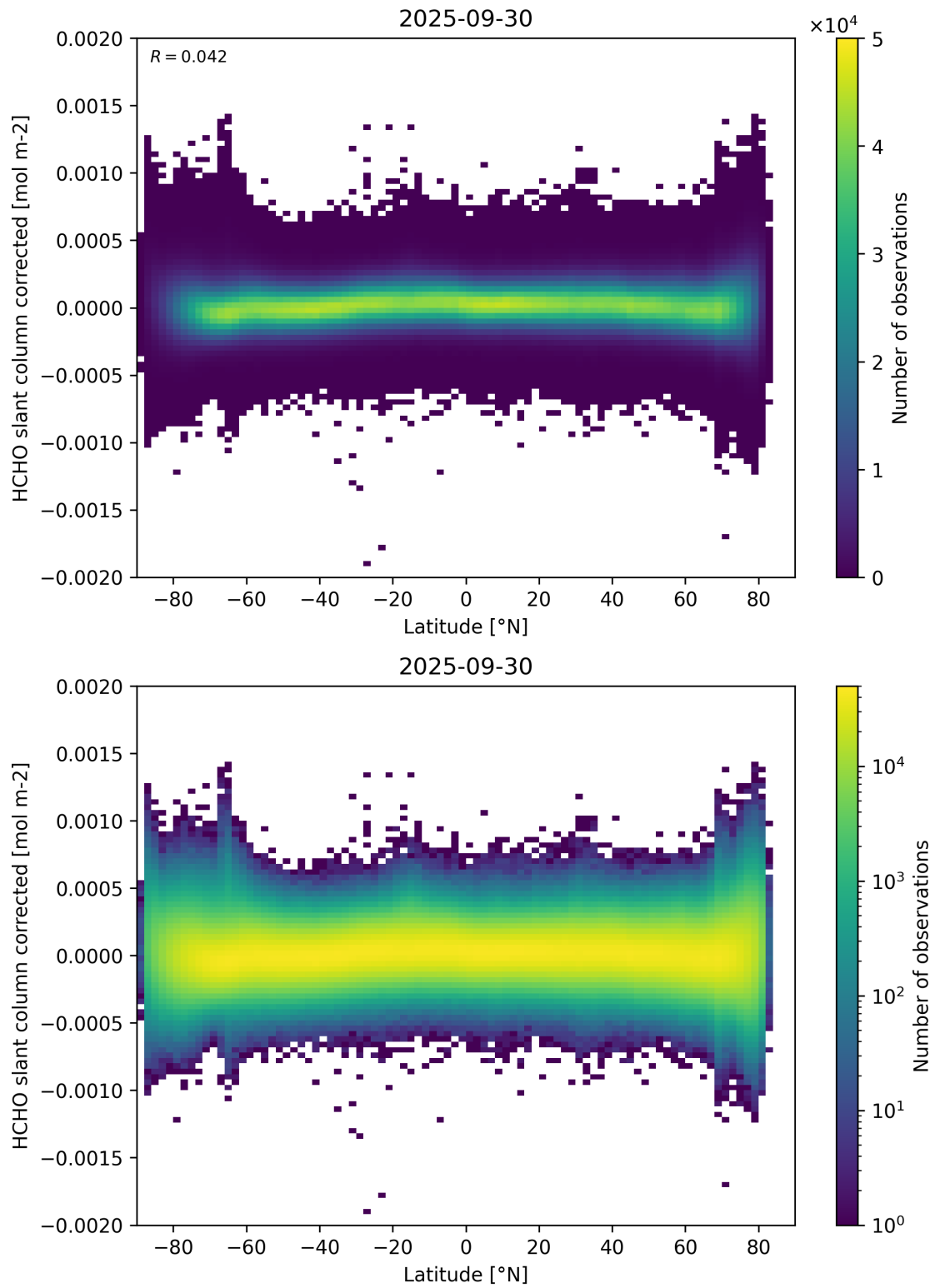
Figure 157: Scatter density plot of “Latitude” against “HCHO slant column corrected” for 2025-09-29 to 2025-10-01.
