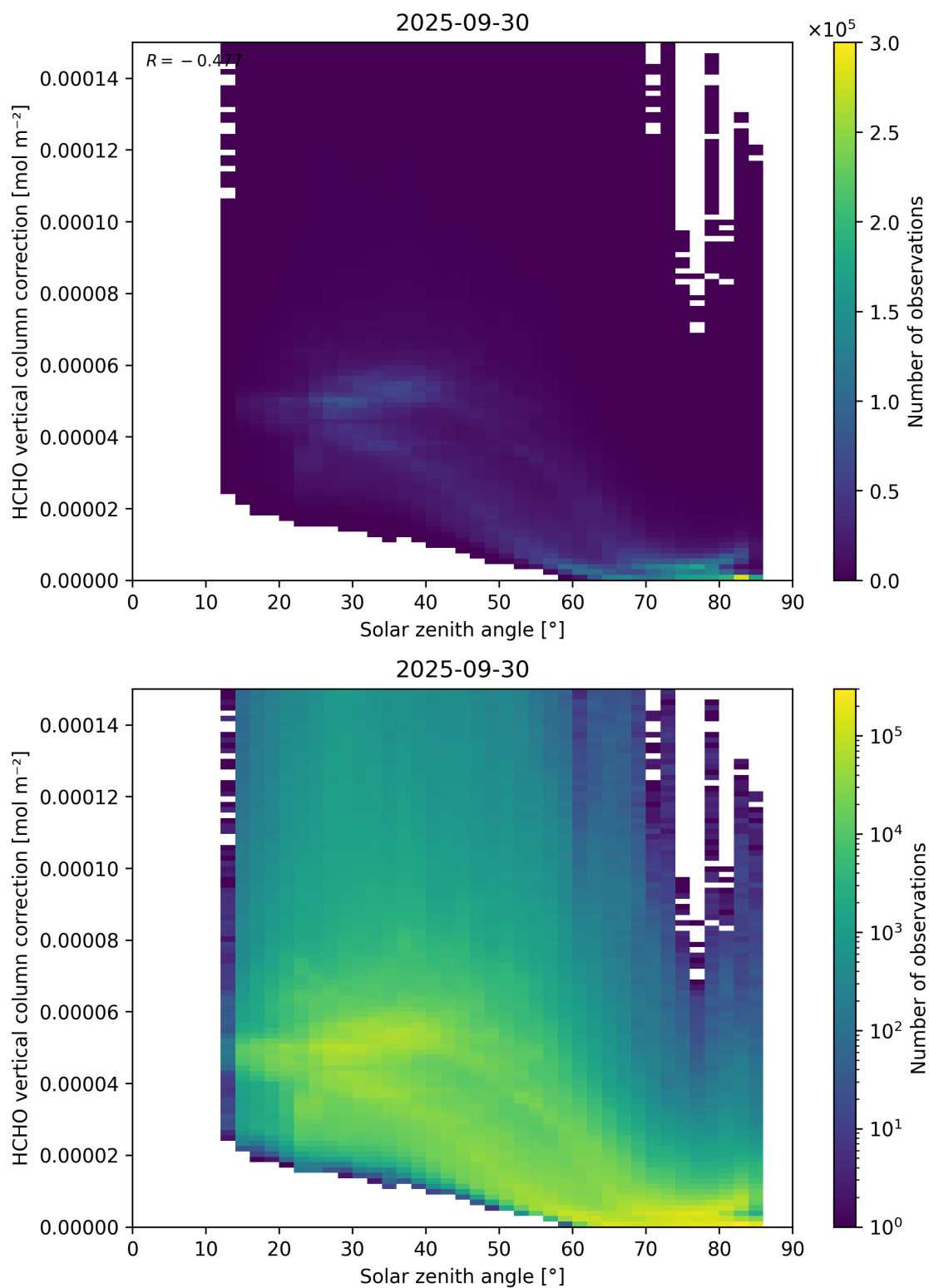
Figure 178: Scatter density plot of “Solar zenith angle” against “HCHO vertical column correction” for 2025-09-29 to 2025-10-01.
