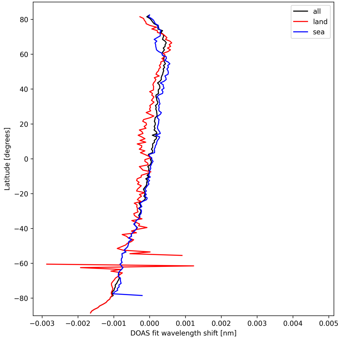
Figure 30: Zonal average of “DOAS fit wavelength shift” for 2025-09-29 to 2025-10-01.
