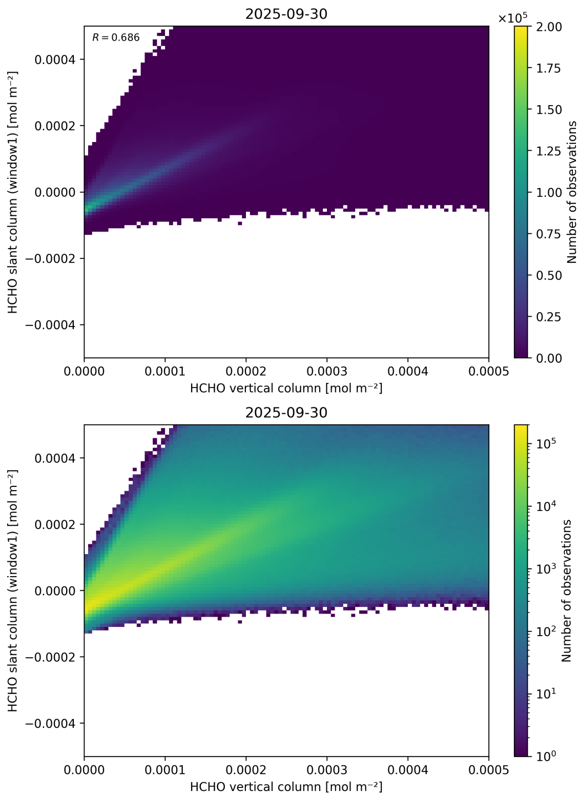
Figure 129: Scatter density plot of “HCHO vertical column” against “HCHO slant column (window1)” for 2025-09-29 to 2025-10-01.
