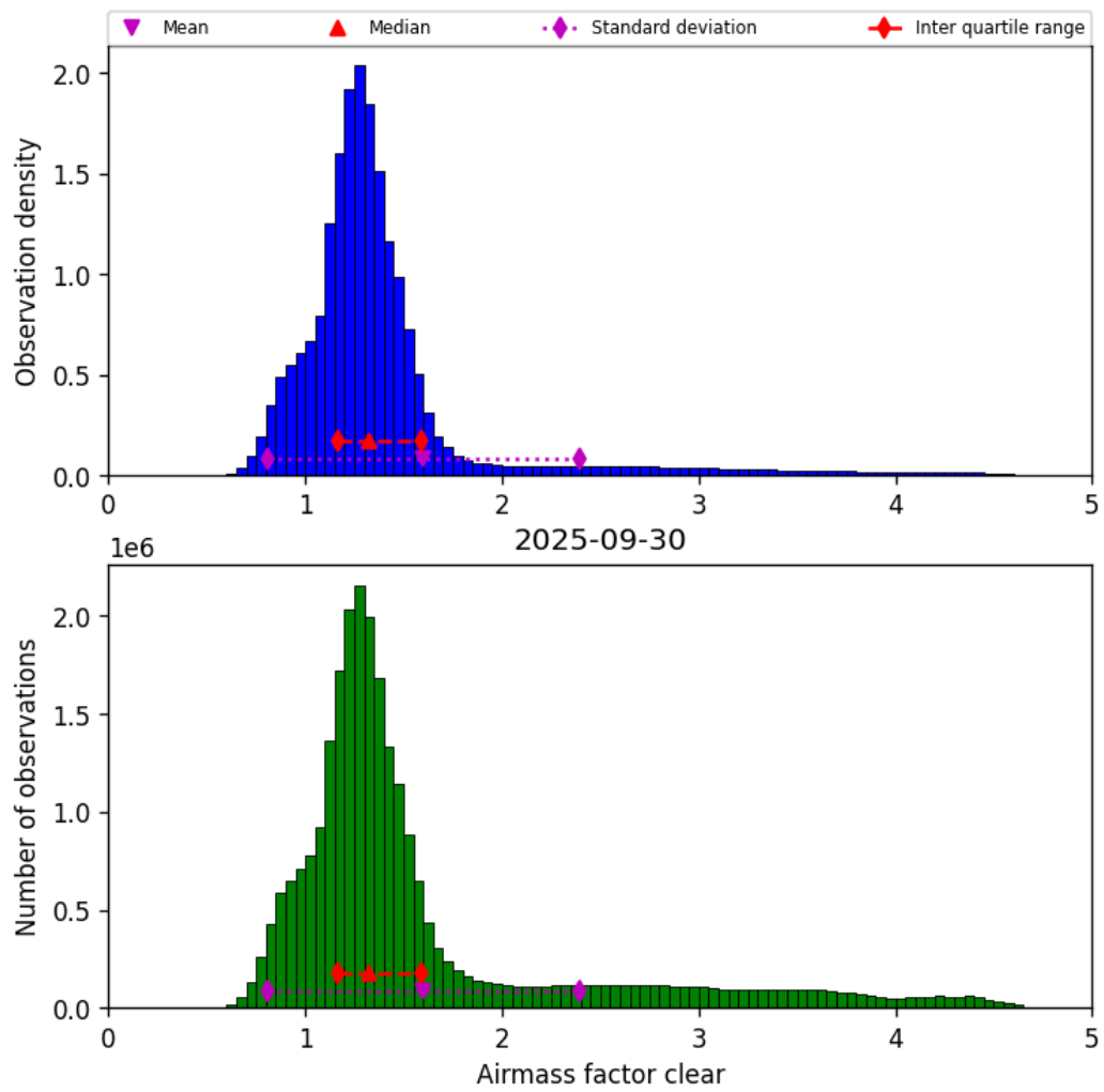
Figure 42: Histogram of “Airmass factor clear” for 2025-09-29 to 2025-10-01
