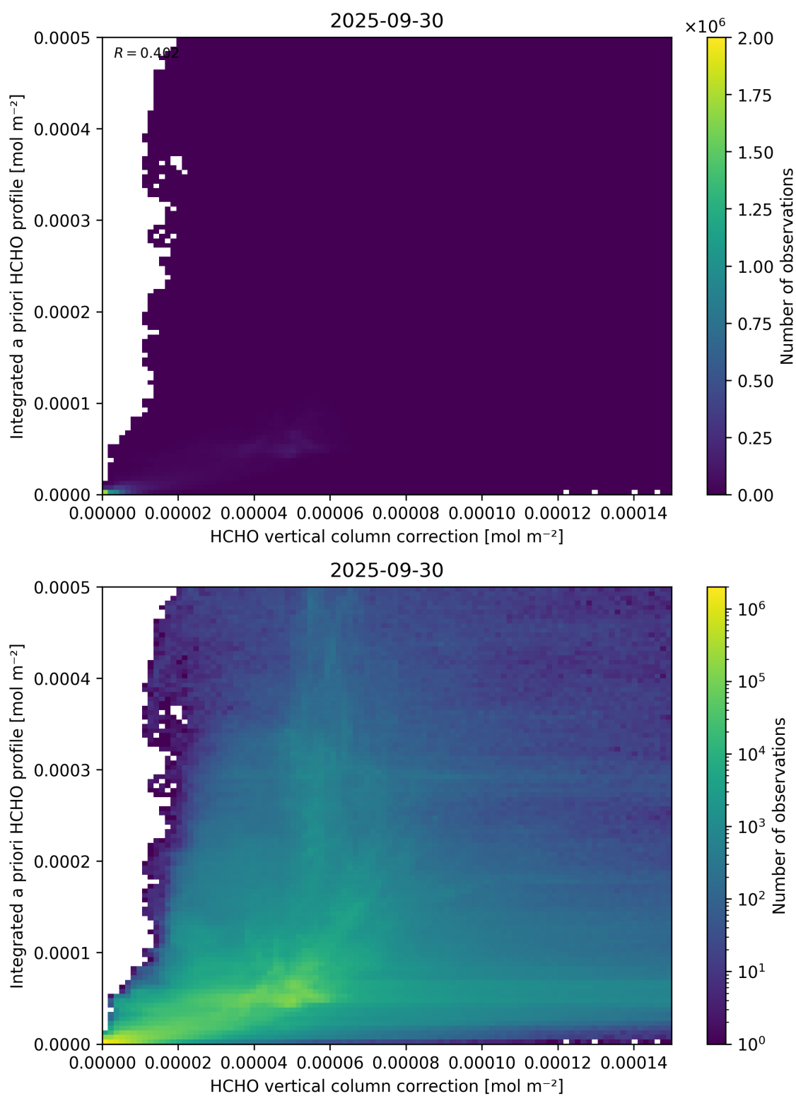
Figure 122: Scatter density plot of “HCHO vertical column correction” against “Integrated a priori HCHO profile” for 2025-09-29 to 2025-10-01.
