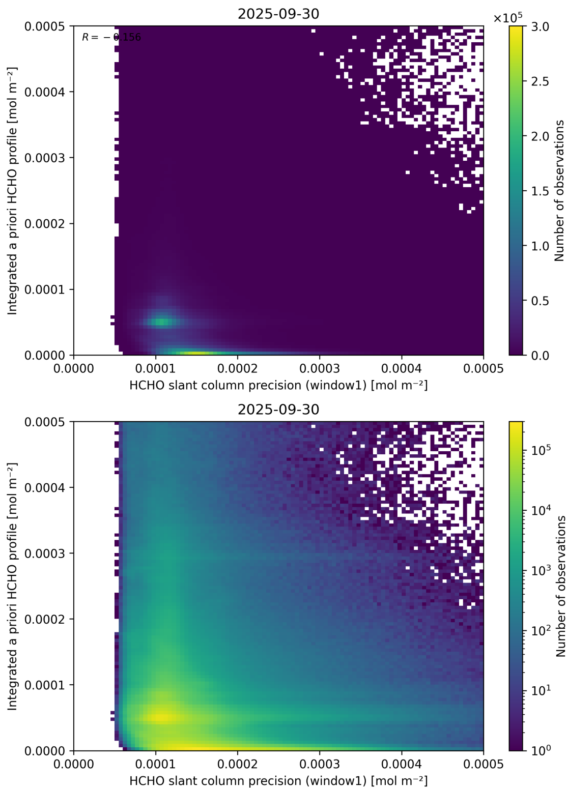
Figure 96: Scatter density plot of “HCHO slant column precision (window1)” against “Integrated a priori HCHO profile” for 2025-09-29 to 2025-10-01.
