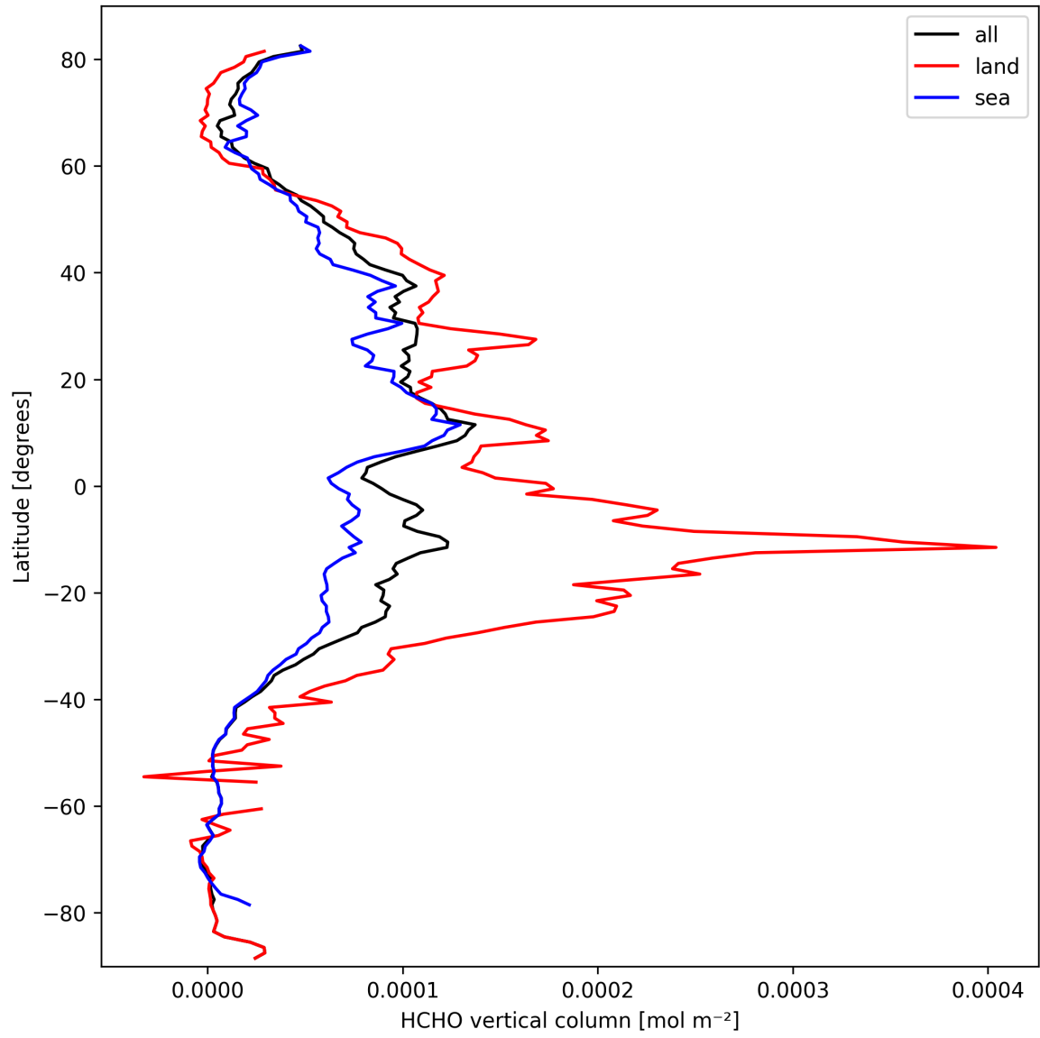
Figure 21: Zonal average of “HCHO vertical column” for 2025-09-29 to 2025-10-01.
