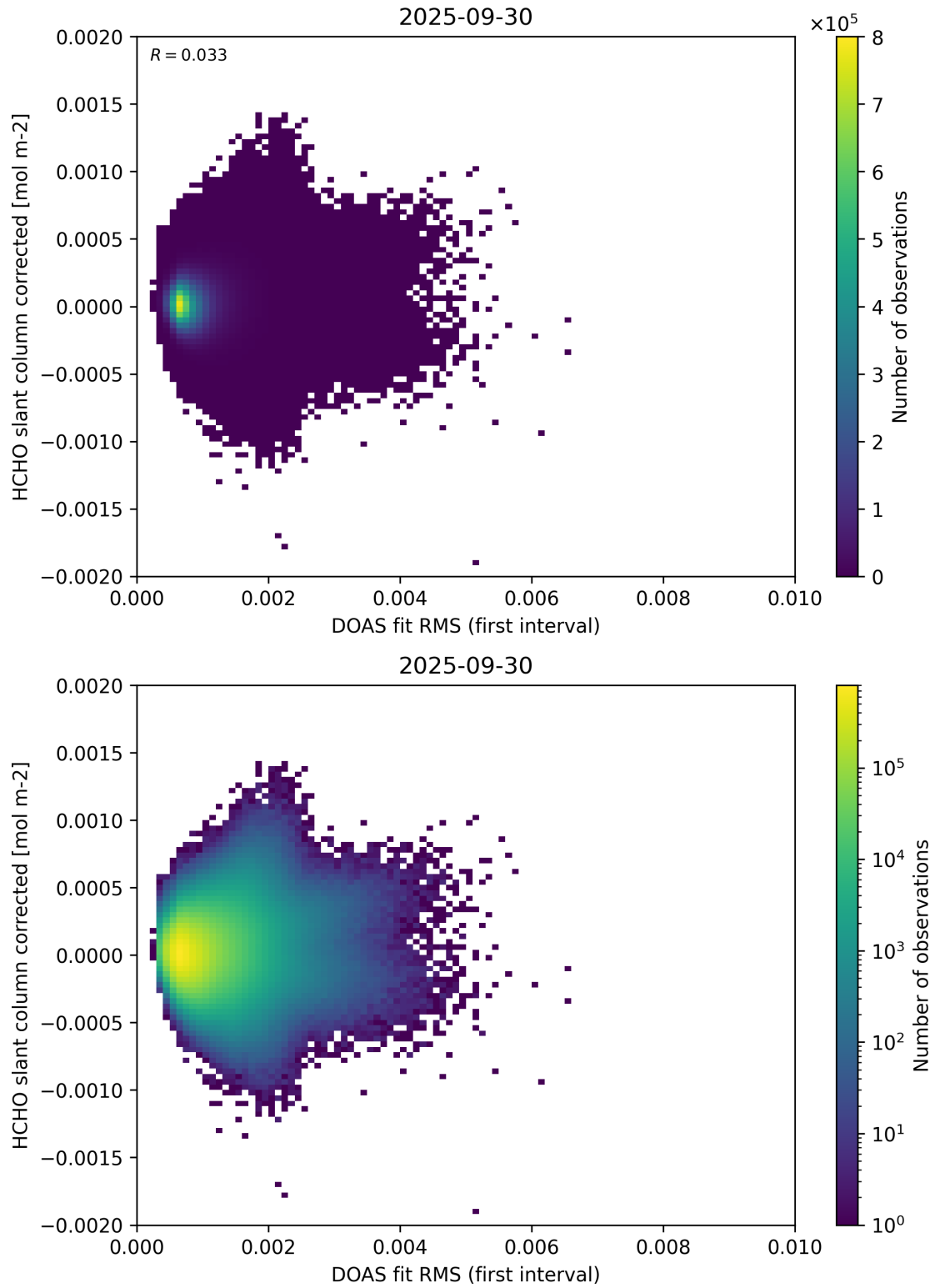
Figure 62: Scatter density plot of “DOAS fit RMS (first interval)” against “HCHO slant column corrected” for 2025-09-29 to 2025-10-01.
