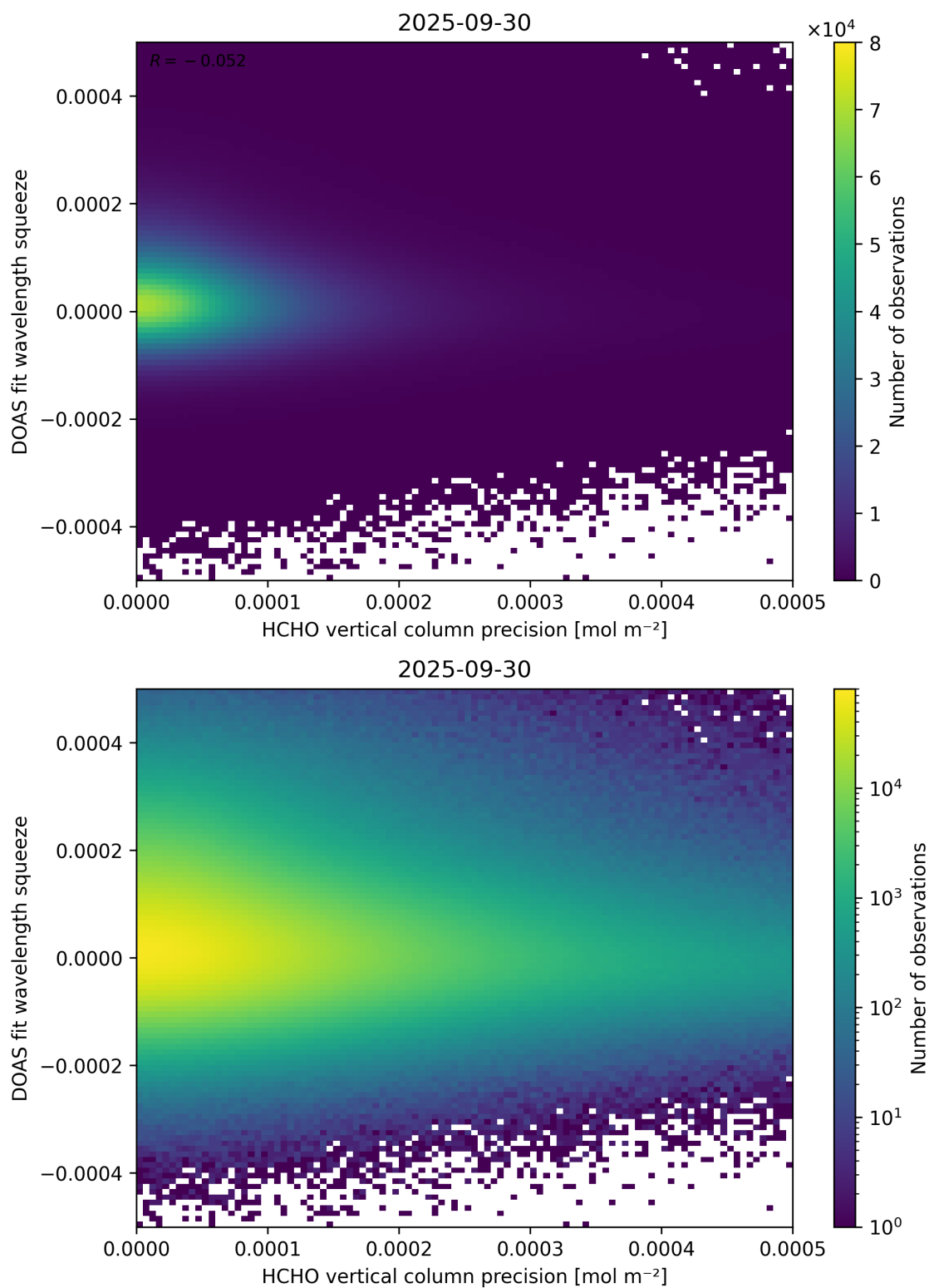
Figure 138: Scatter density plot of “HCHO vertical column precision” against “DOAS fit wavelength squeeze” for 2025-09-29 to 2025-10-01.
