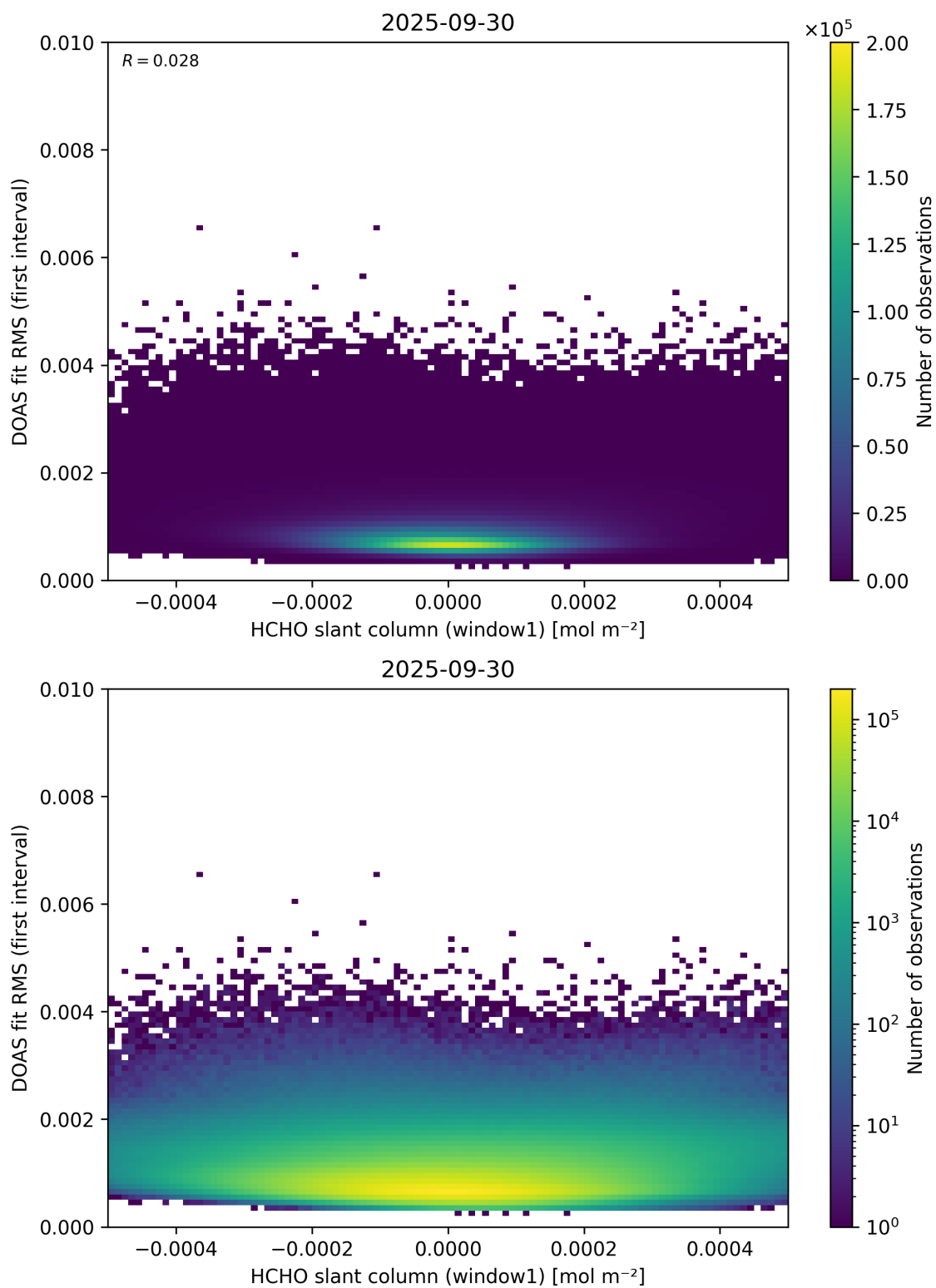
Figure 78: Scatter density plot of “HCHO slant column (window1)” against “DOAS fit RMS (first interval)” for 2025-09-29 to 2025-10-01.
