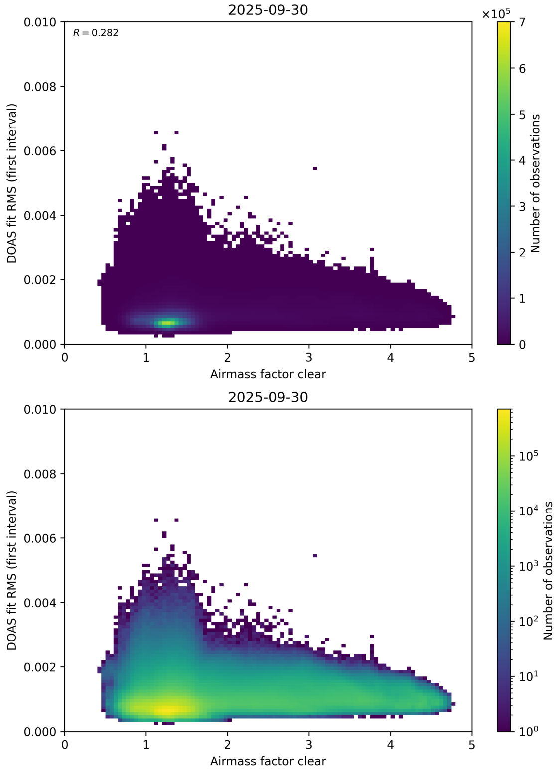
Figure 71: Scatter density plot of “Airmass factor clear” against “DOAS fit RMS (first interval)” for 2025-09-29 to 2025-10-01.
