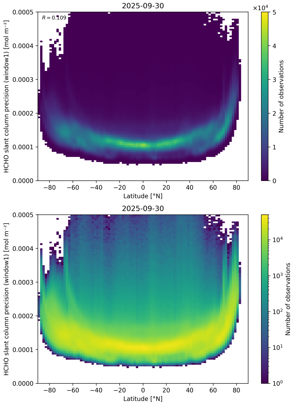
Figure 160: Scatter density plot of “Latitude” against “HCHO slant column precision (window1)” for 2025-09-29 to 2025-10-01.
