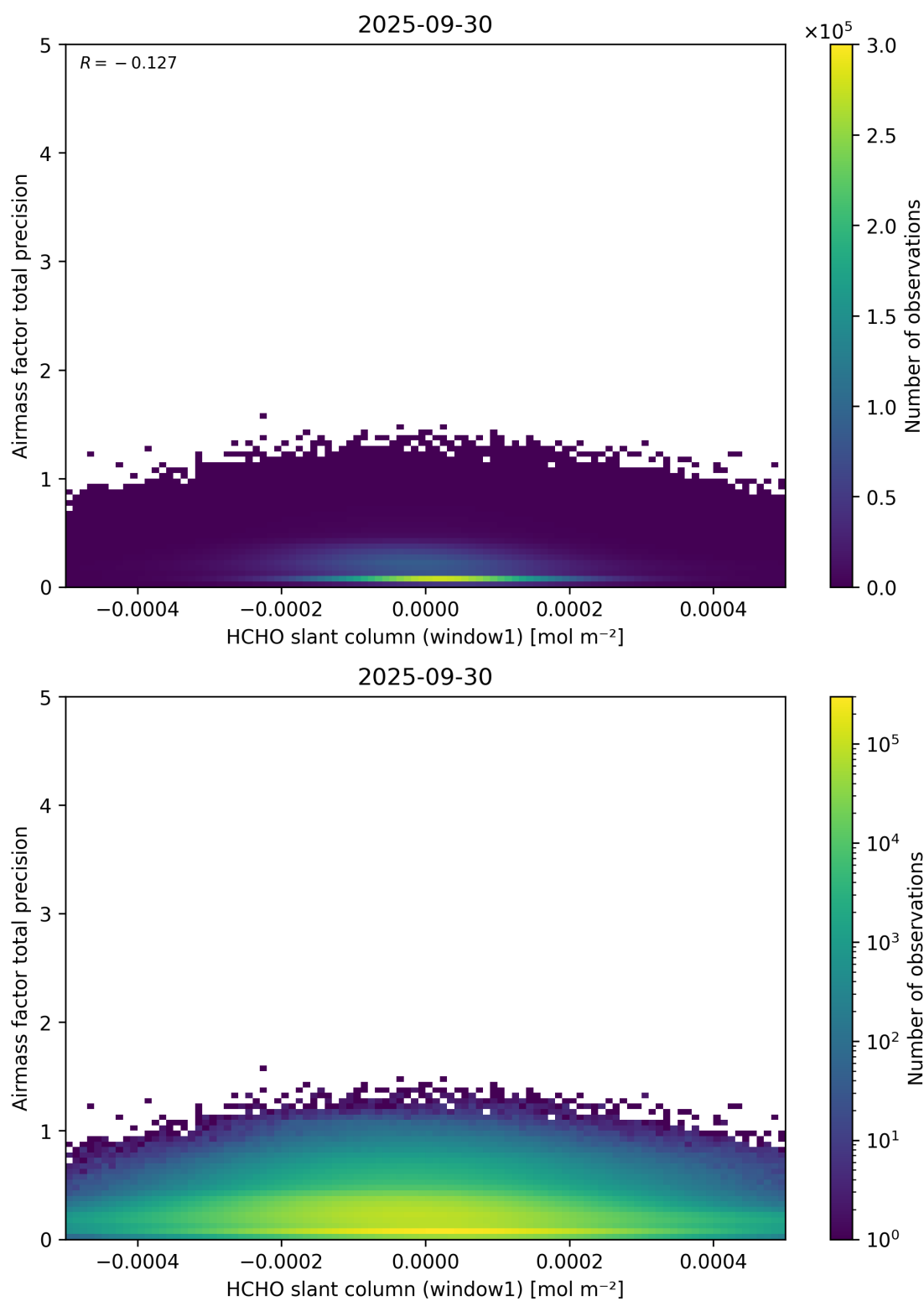
Figure 86: Scatter density plot of “HCHO slant column (window1)” against “Airmass factor total precision” for 2025-09-29 to 2025-10-01.
