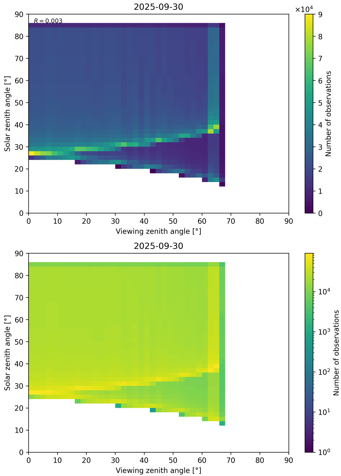
Figure 197: Scatter density plot of “Viewing zenith angle” against “Solar zenith angle” for 2025-09-29 to 2025-10-01.
