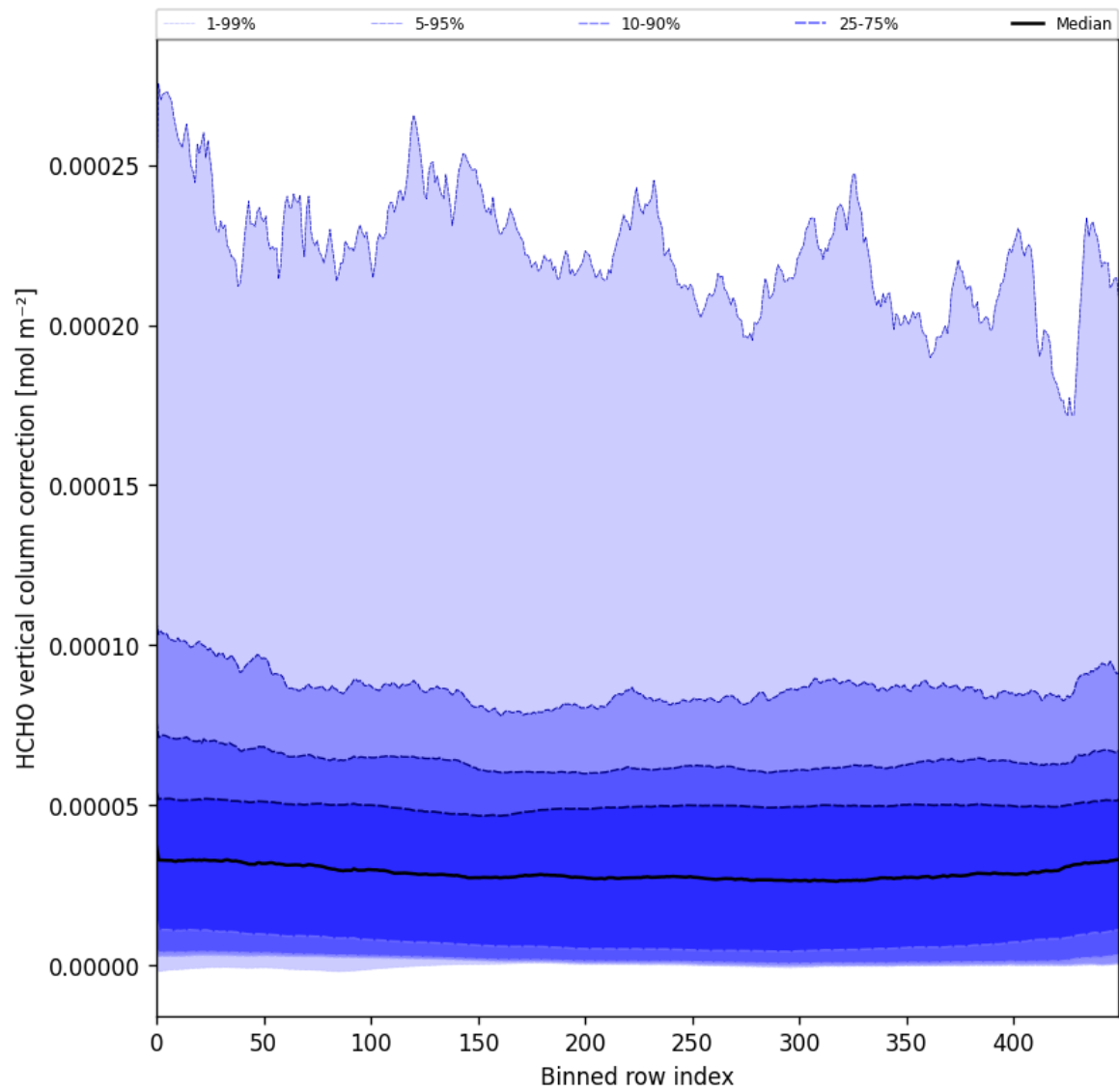
Figure 51: Along track statistics of “HCHO vertical column correction” for 2025-09-29 to 2025-10-01
