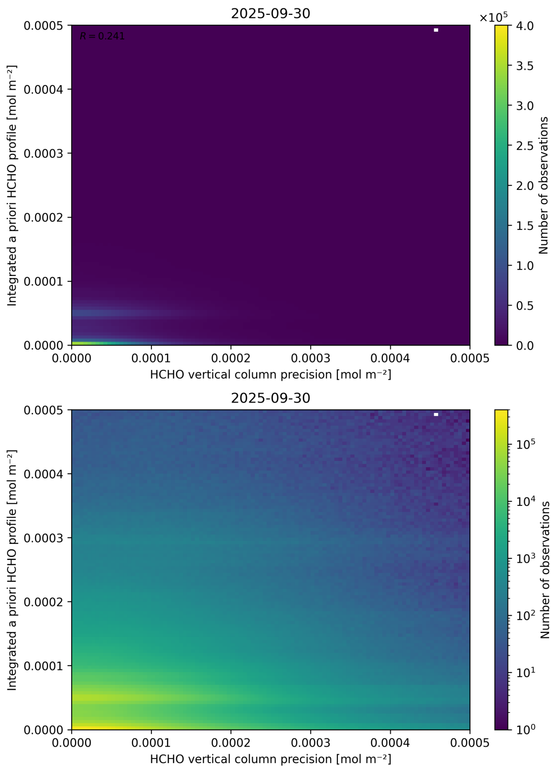
Figure 147: Scatter density plot of “HCHO vertical column precision” against “Integrated a priori HCHO profile” for 2025-09-29 to 2025-10-01.
