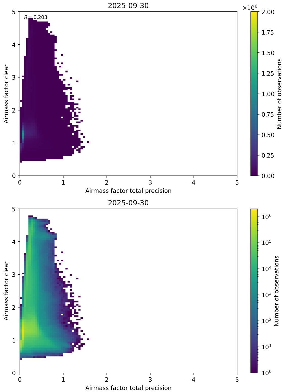
Figure 108: Scatter density plot of “Airmass factor total precision” against “Airmass factor clear” for 2025-09-29 to 2025-10-01.
