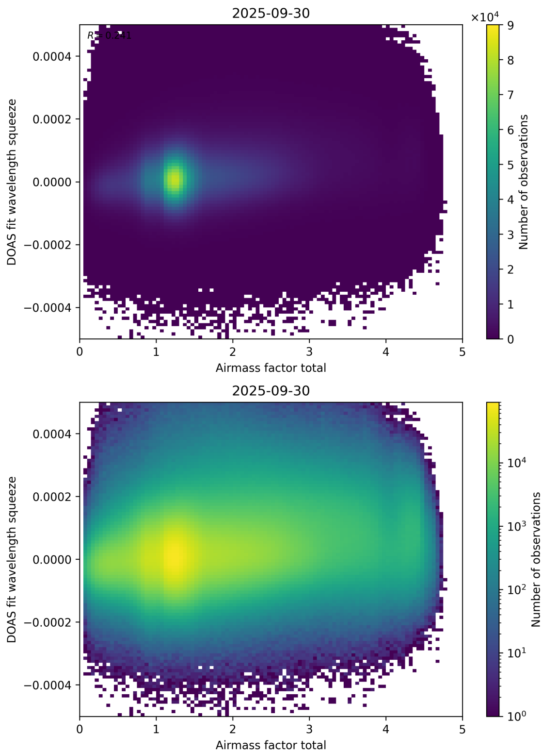
Figure 99: Scatter density plot of “Airmass factor total” against “DOAS fit wavelength squeeze” for 2025-09-29 to 2025-10-01.
