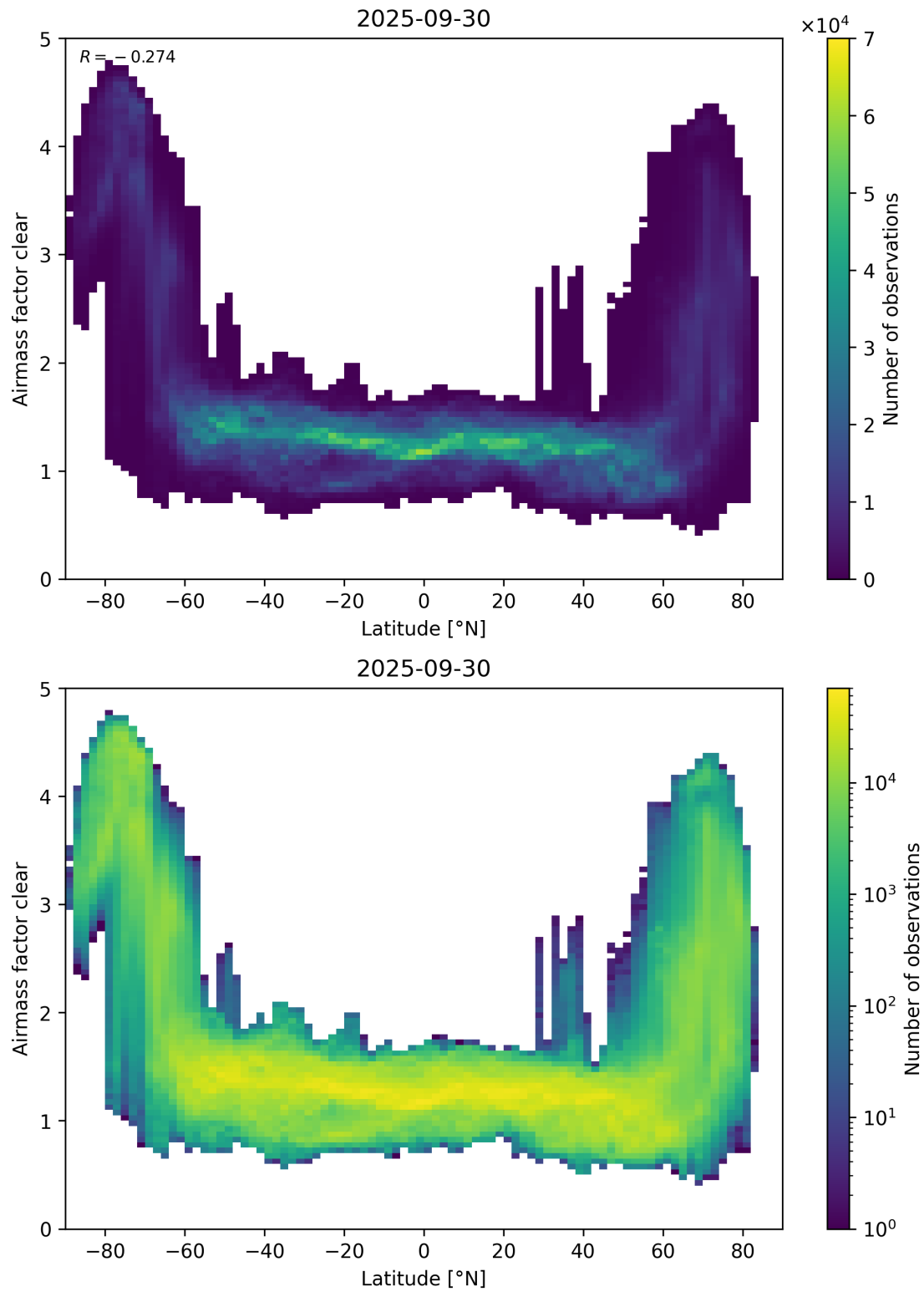
Figure 156: Scatter density plot of “Latitude” against “Airmass factor clear” for 2025-09-29 to 2025-10-01.
