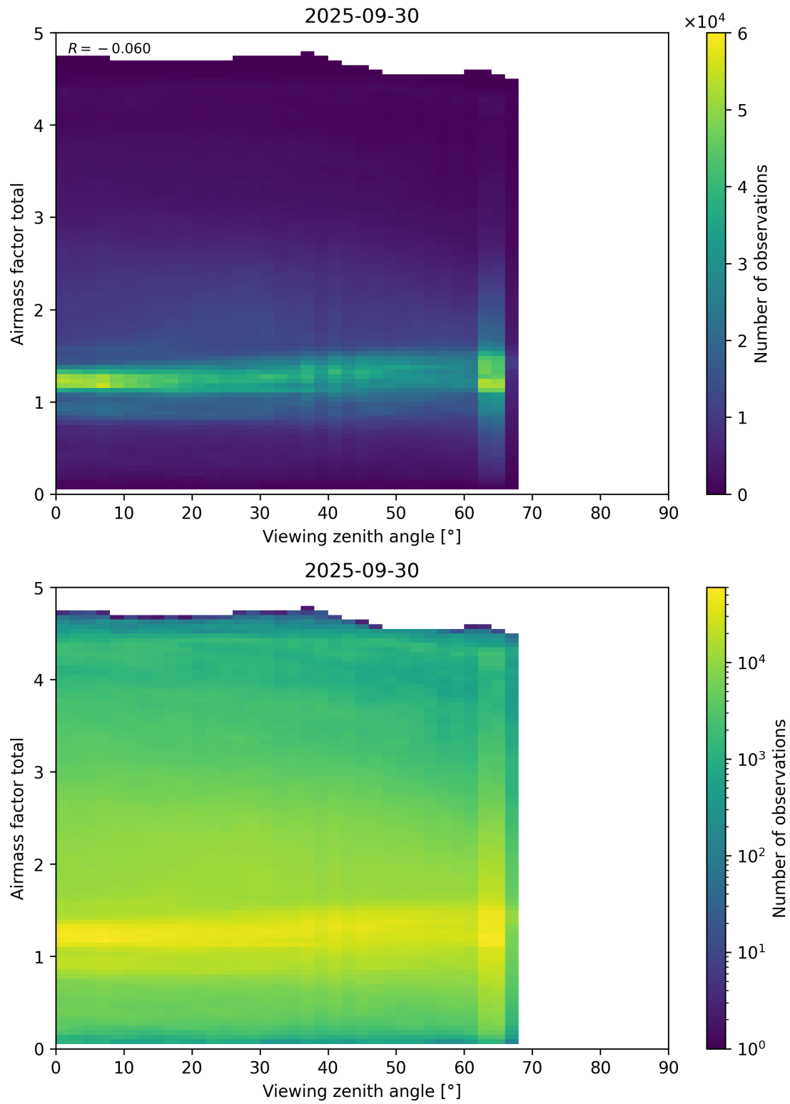
Figure 190: Scatter density plot of “Viewing zenith angle” against “Airmass factor total” for 2025-09-29 to 2025-10-01.
