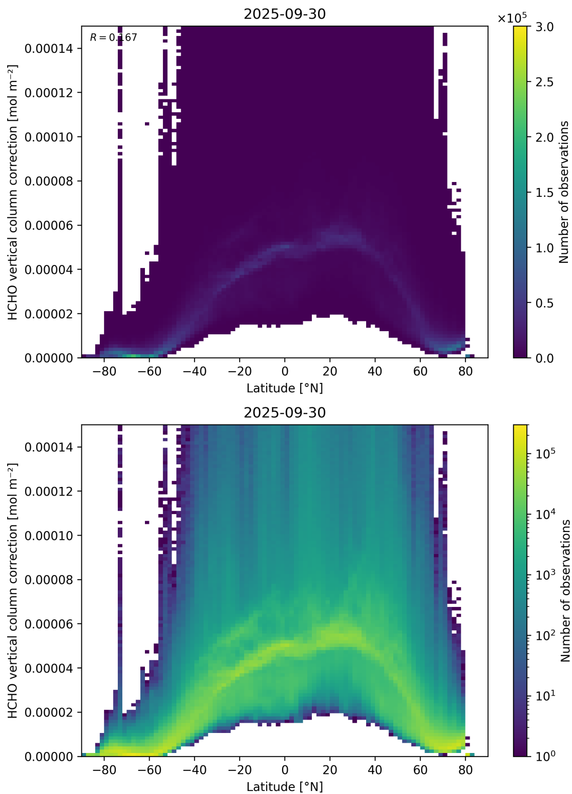
Figure 164: Scatter density plot of “Latitude” against “HCHO vertical column correction” for 2025-09-29 to 2025-10-01.
