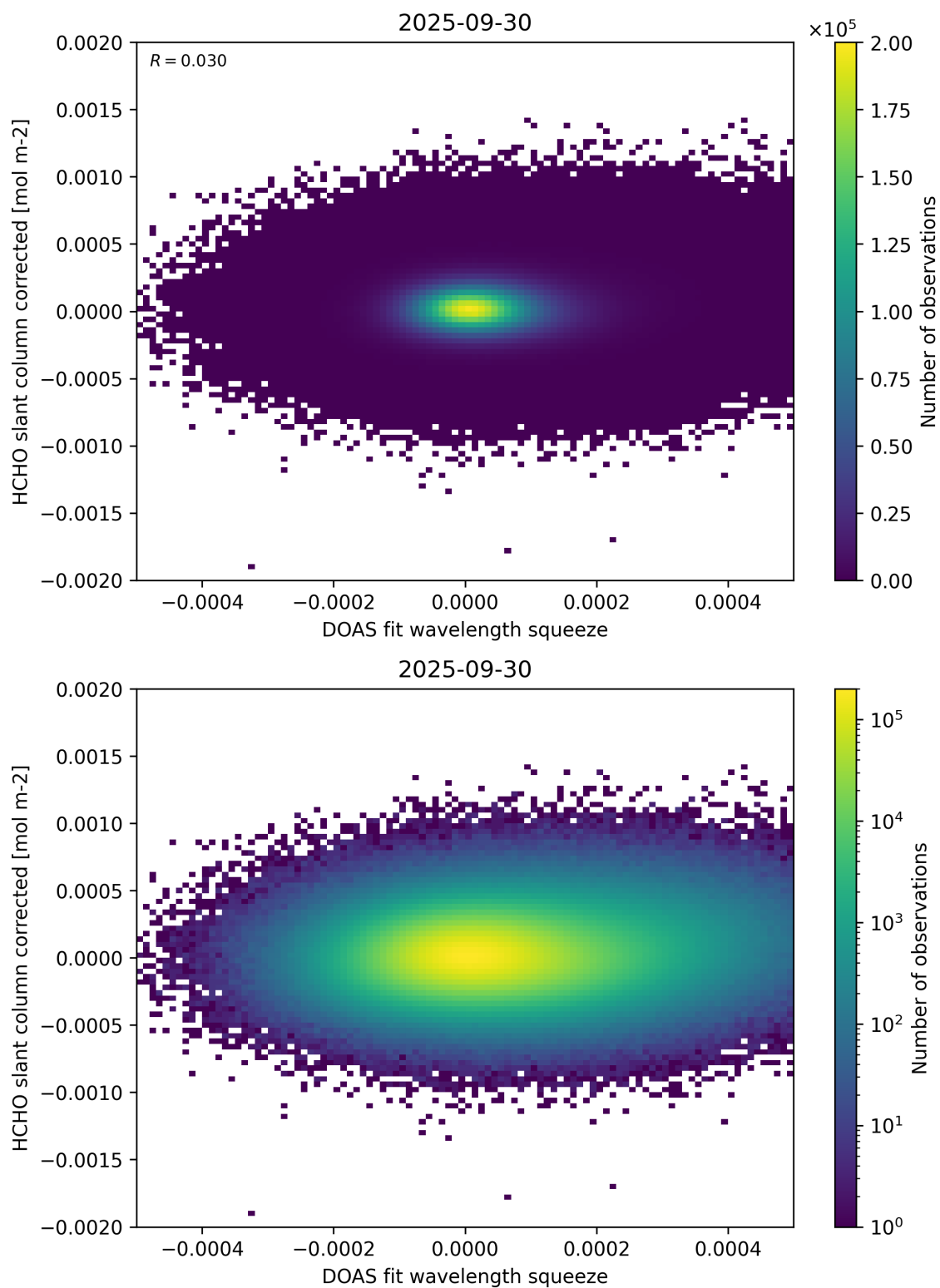
Figure 69: Scatter density plot of “DOAS fit wavelength squeeze” against “HCHO slant column corrected” for 2025-09-29 to 2025-10-01.
