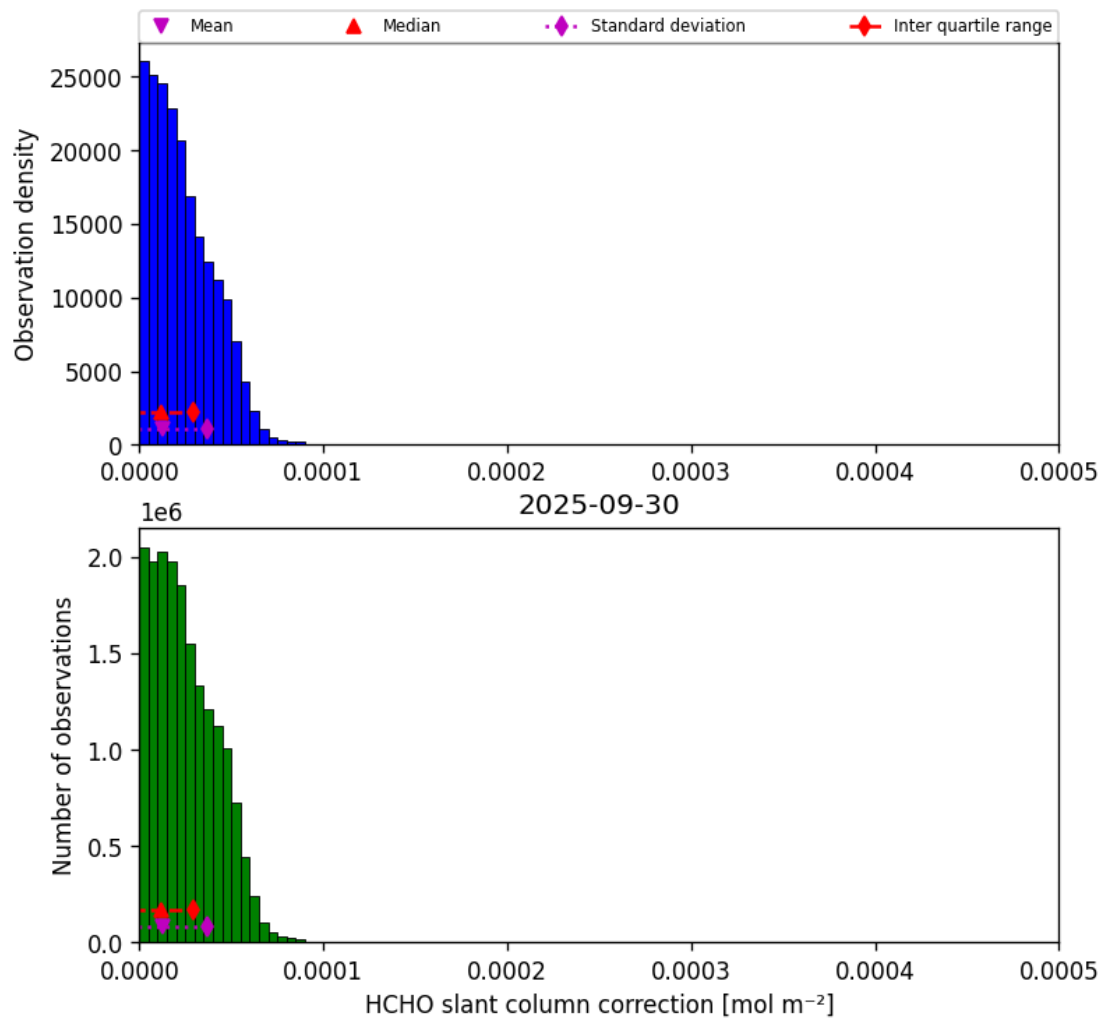
Figure 47: Histogram of “HCHO slant column correction” for 2025-09-29 to 2025-10-01
