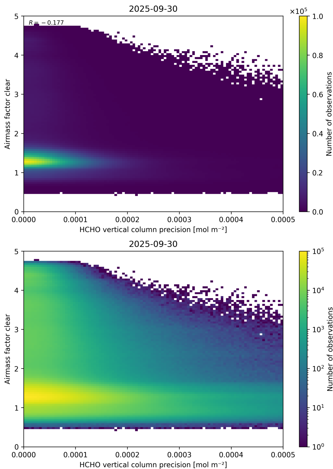
Figure 139: Scatter density plot of “HCHO vertical column precision” against “Airmass factor clear” for 2025-09-29 to 2025-10-01.
