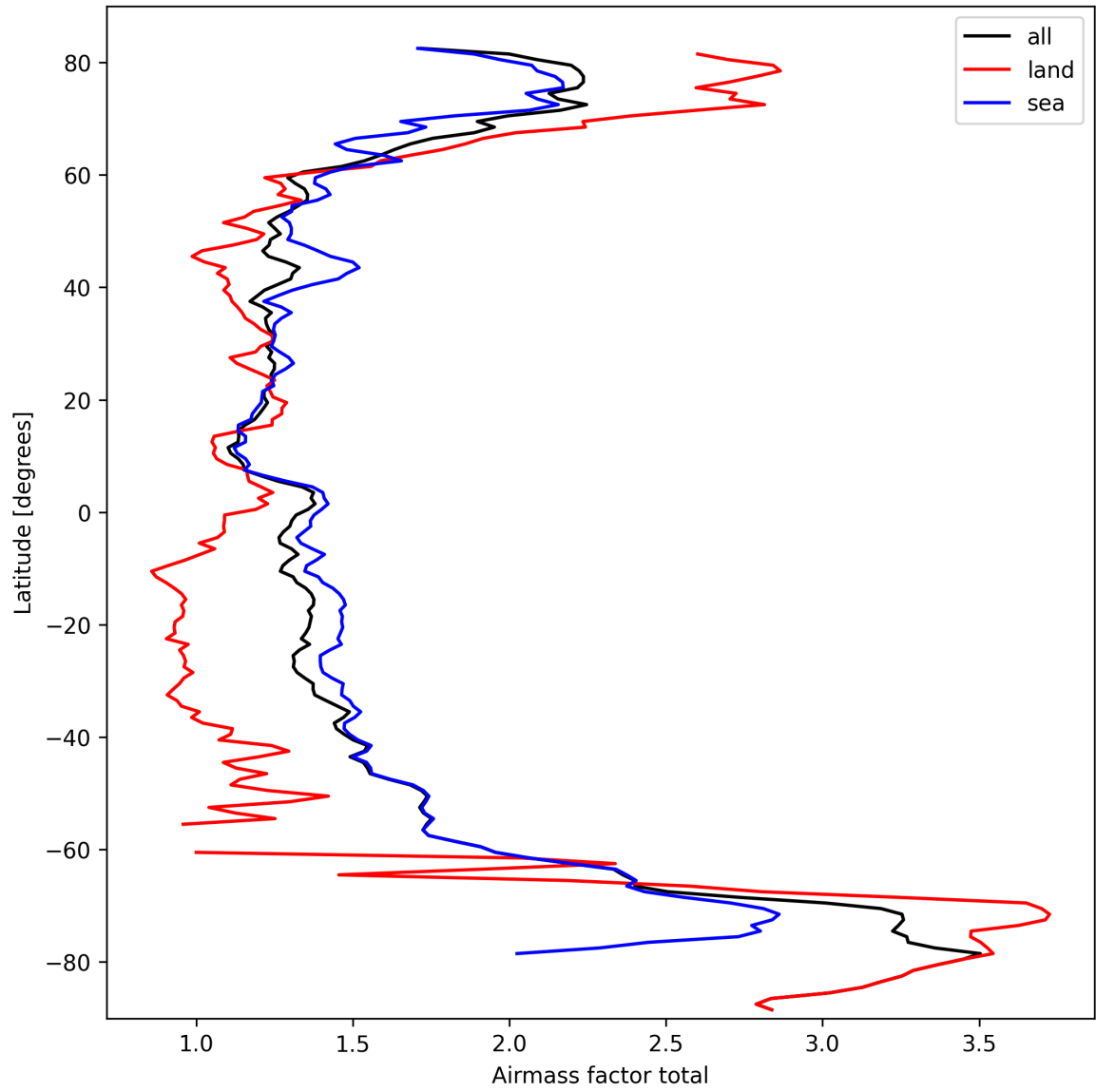
Figure 26: Zonal average of “Airmass factor total” for 2025-09-29 to 2025-10-01.
