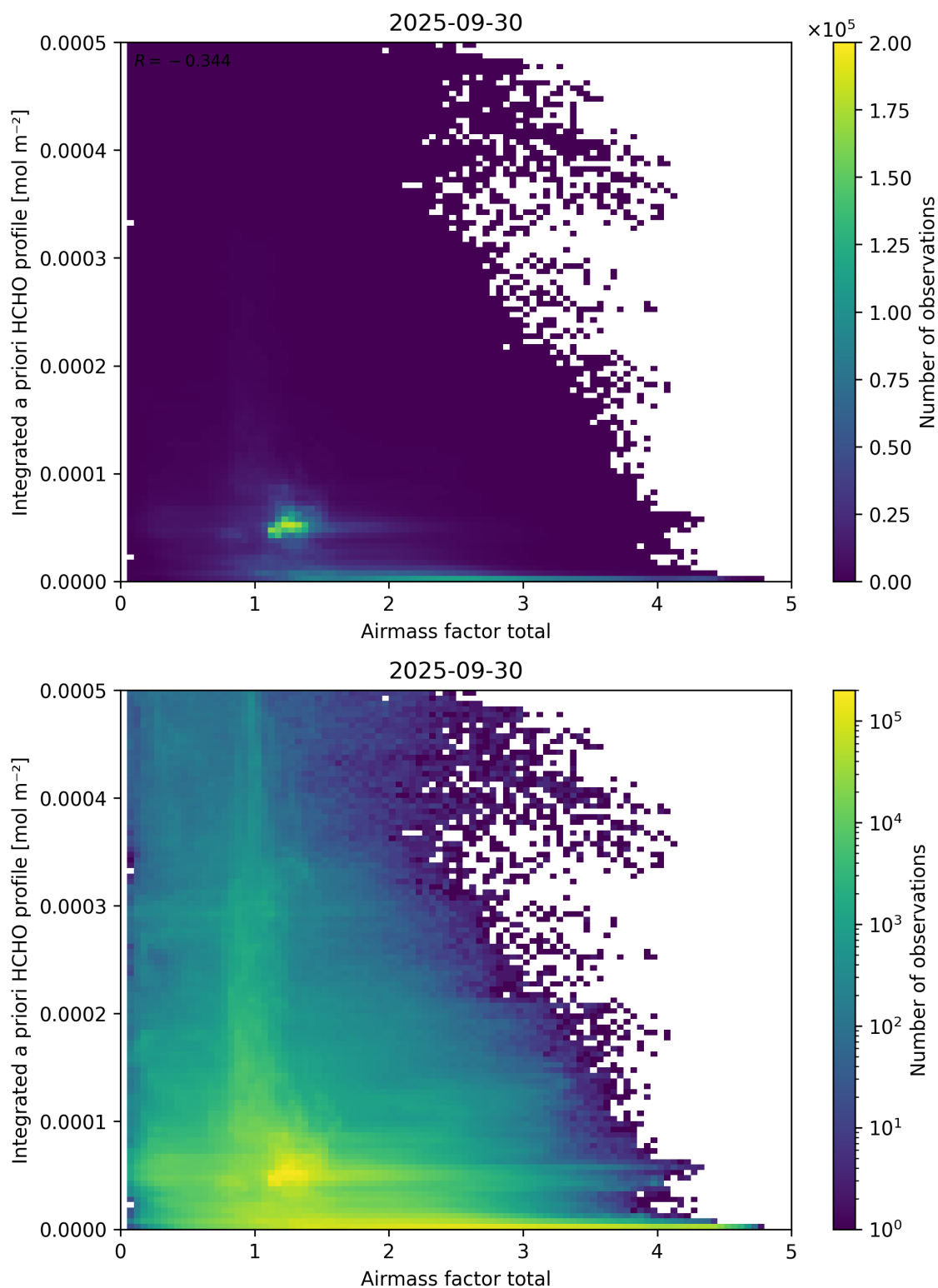
Figure 104: Scatter density plot of “Airmass factor total” against “Integrated a priori HCHO profile” for 2025-09-29 to 2025-10-01.
