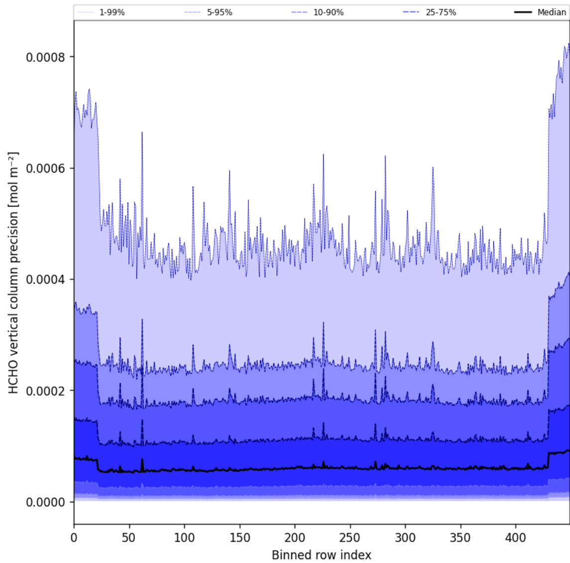
Figure 50: Along track statistics of “HCHO vertical column precision” for 2025-09-29 to 2025-10-01
