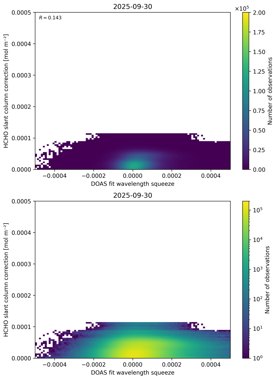
Figure 70: Scatter density plot of “DOAS fit wavelength squeeze” against “HCHO slant column correction” for 2025-09-29 to 2025-10-01.
