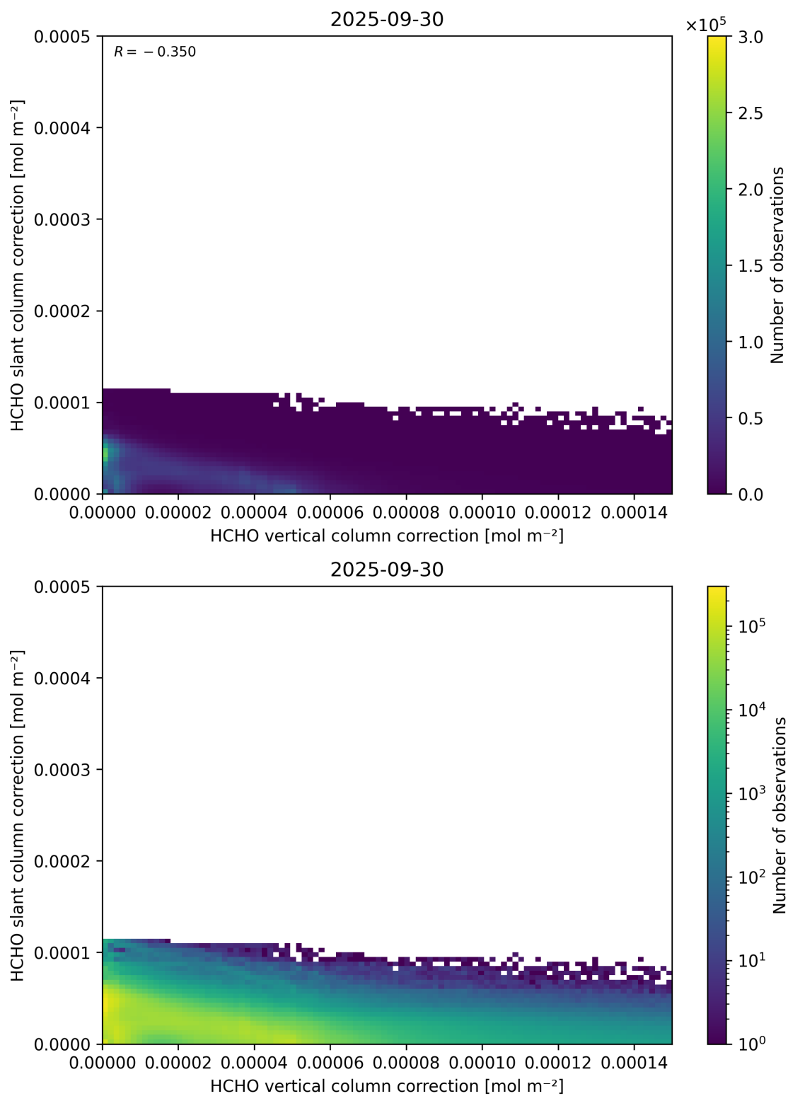
Figure 117: Scatter density plot of “HCHO vertical column correction” against “HCHO slant column correction” for 2025-09-29 to 2025-10-01.
