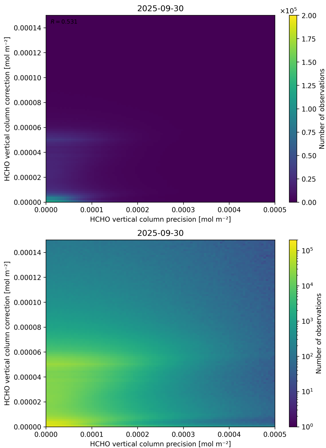
Figure 146: Scatter density plot of “HCHO vertical column precision” against “HCHO vertical column correction” for 2025-09-29 to 2025-10-01.
