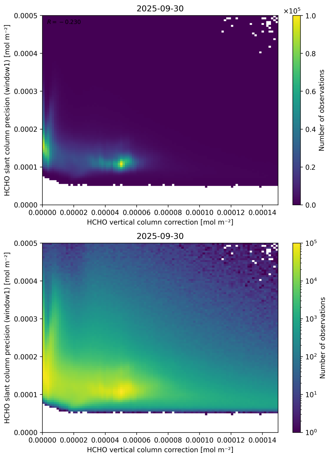
Figure 119: Scatter density plot of “HCHO vertical column correction” against “HCHO slant column precision (window1)” for 2025-09-29 to 2025-10-01.
