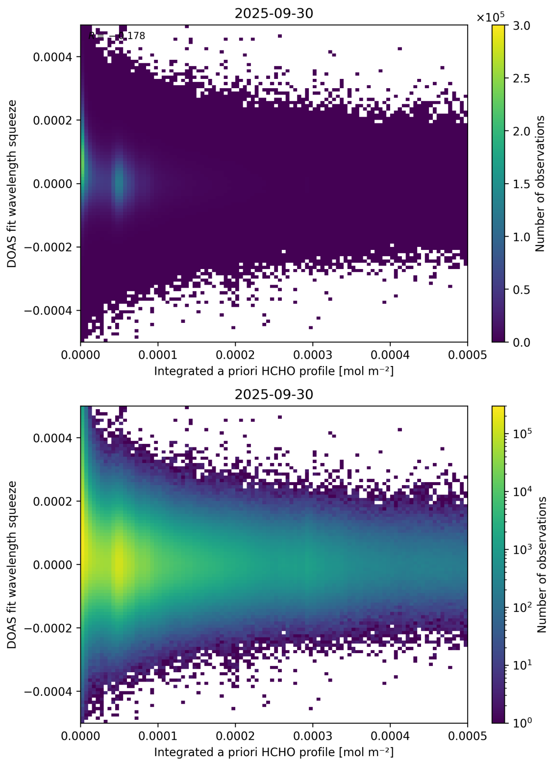
Figure 150: Scatter density plot of “Integrated a priori HCHO profile” against “DOAS fit wavelength squeeze” for 2025-09-29 to 2025-10-01.
