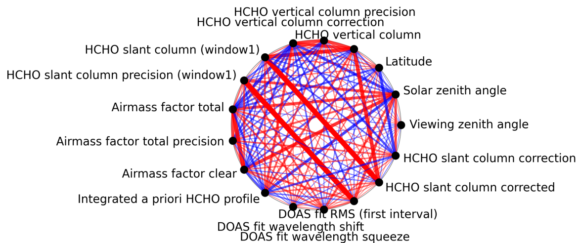
Figure 1: Map of correlation graph for 2025-09-29 to 2025-10-01.
