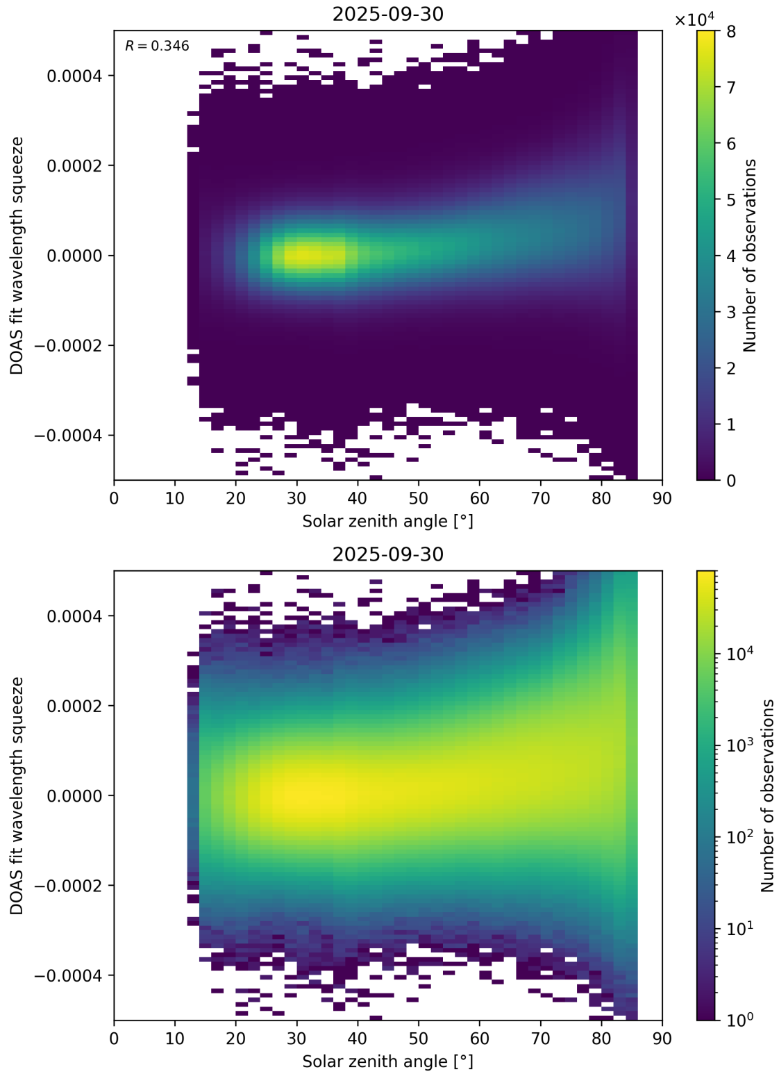
Figure 169: Scatter density plot of “Solar zenith angle” against “DOAS fit wavelength squeeze” for 2025-09-29 to 2025-10-01.
