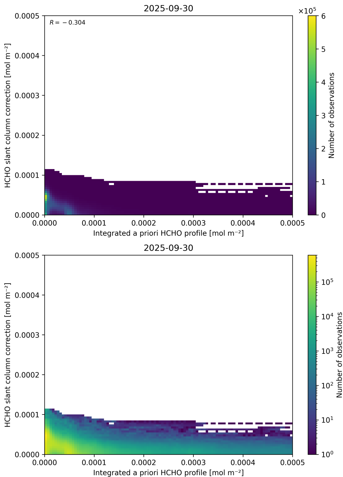
Figure 152: Scatter density plot of “Integrated a priori HCHO profile” against “HCHO slant column correction” for 2025-09-29 to 2025-10-01.
