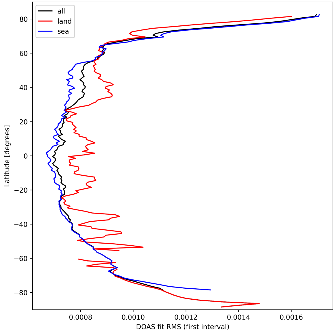
Figure 32: Zonal average of “DOAS fit RMS (first interval)” for 2025-09-29 to 2025-10-01.
