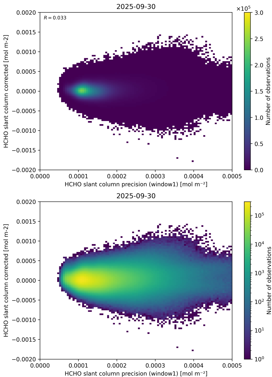
Figure 92: Scatter density plot of “HCHO slant column precision (window1)” against “HCHO slant column corrected” for 2025-09-29 to 2025-10-01.
