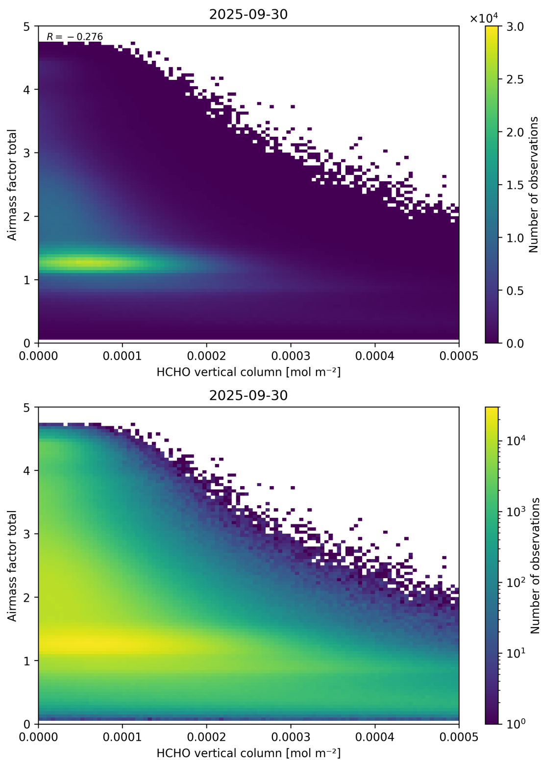
Figure 131: Scatter density plot of “HCHO vertical column” against “Airmass factor total” for 2025-09-29 to 2025-10-01.
