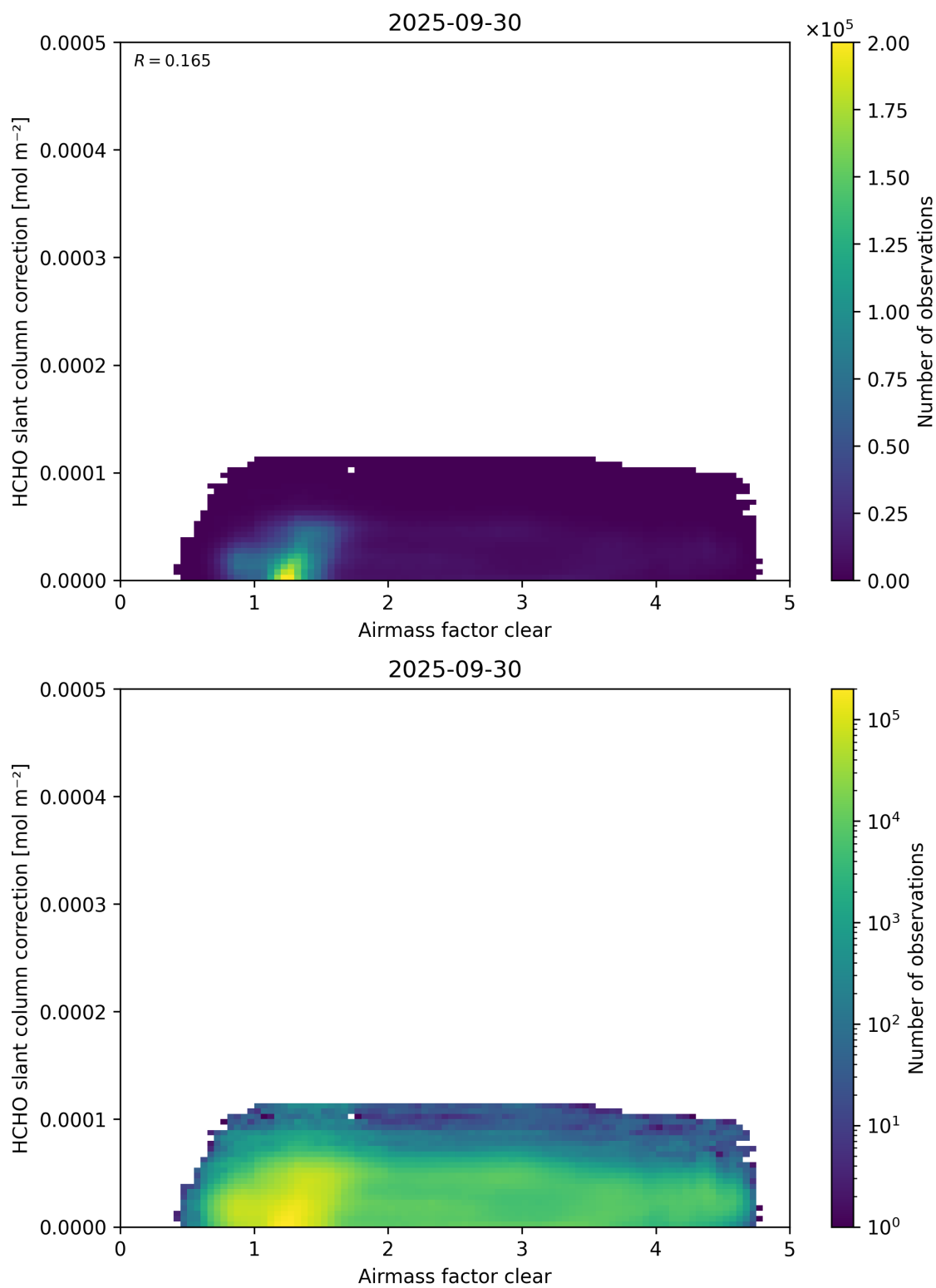
Figure 75: Scatter density plot of “Airmass factor clear” against “HCHO slant column correction” for 2025-09-29 to 2025-10-01.
