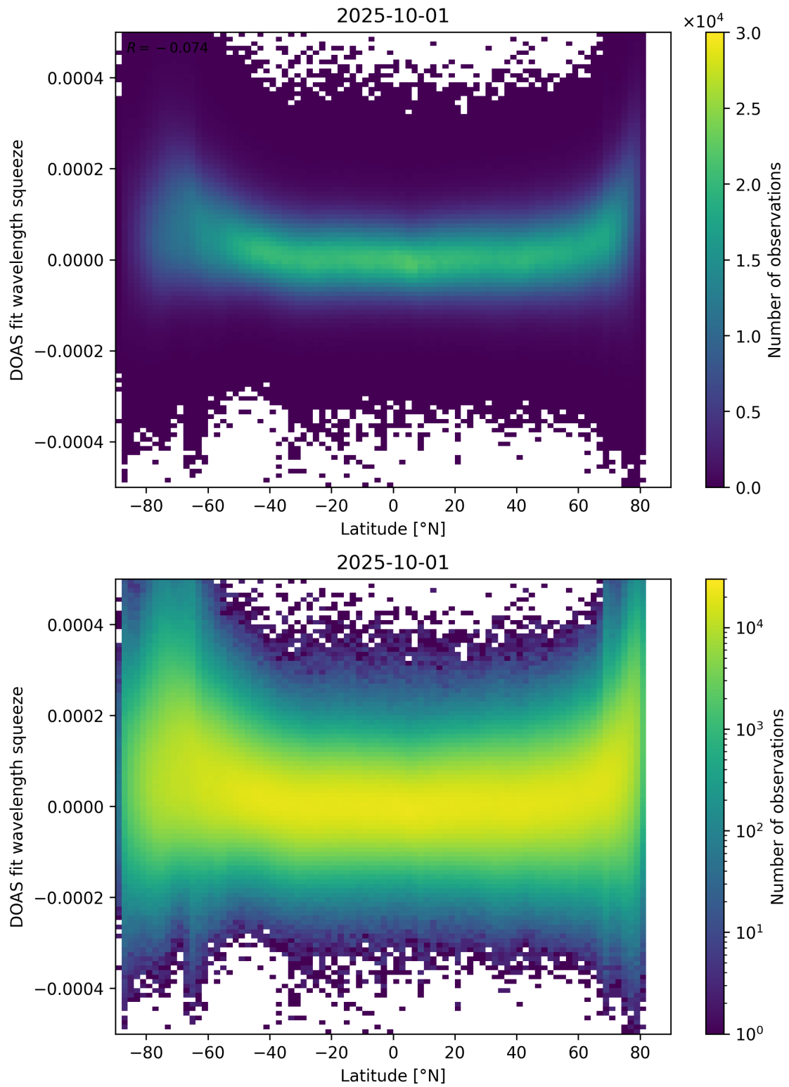
Figure 155: Scatter density plot of “Latitude” against “DOAS fit wavelength squeeze” for 2025-10-01 to 2025-10-02.
