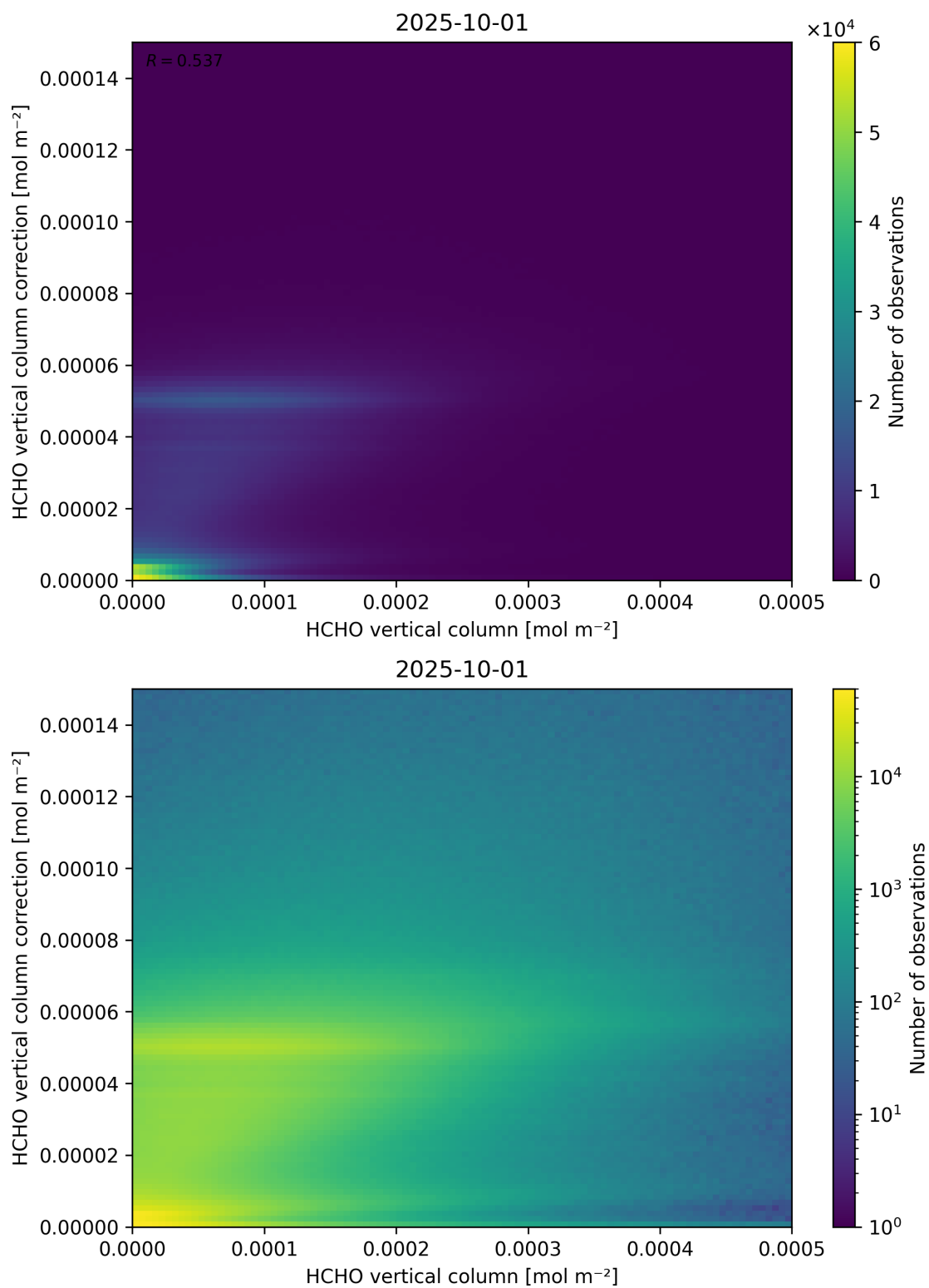
Figure 133: Scatter density plot of “HCHO vertical column” against “HCHO vertical column correction” for 2025-10-01 to 2025-10-02.
