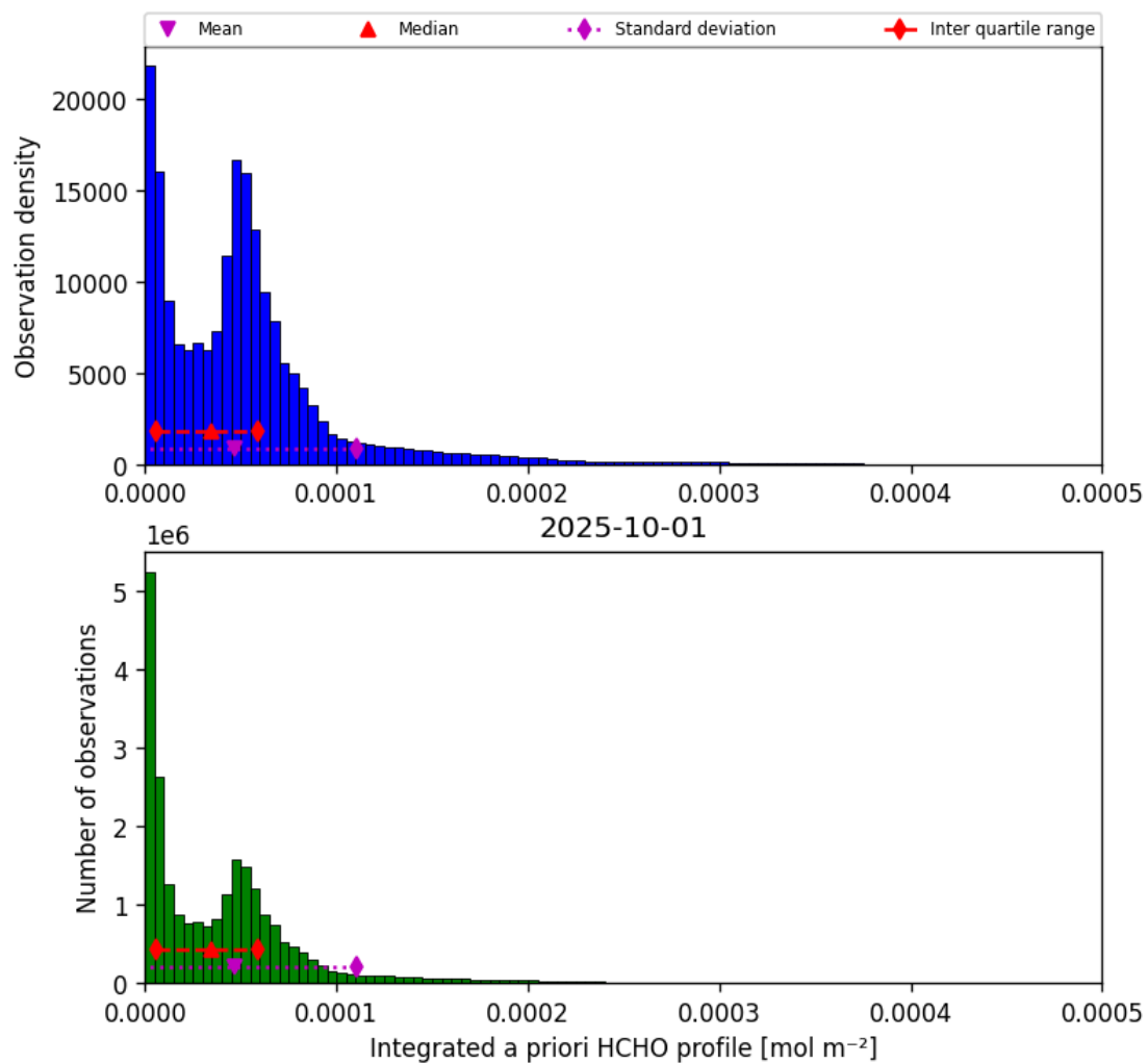
Figure 43: Histogram of “Integrated a priori HCHO profile” for 2025-10-01 to 2025-10-02
