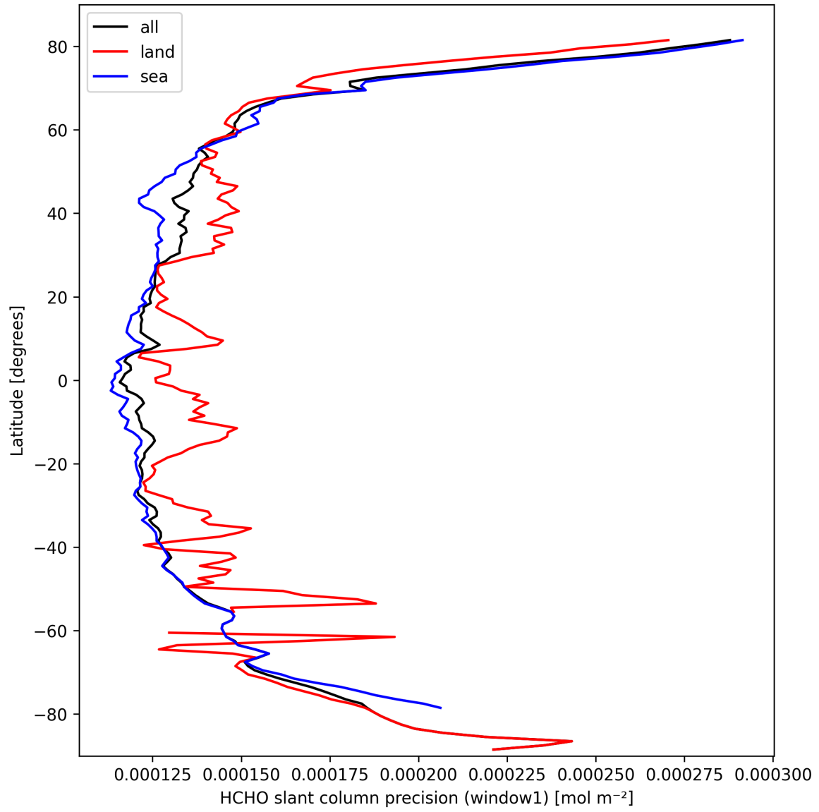
Figure 25: Zonal average of “HCHO slant column precision (window1)” for 2025-10-01 to 2025-10-02.
