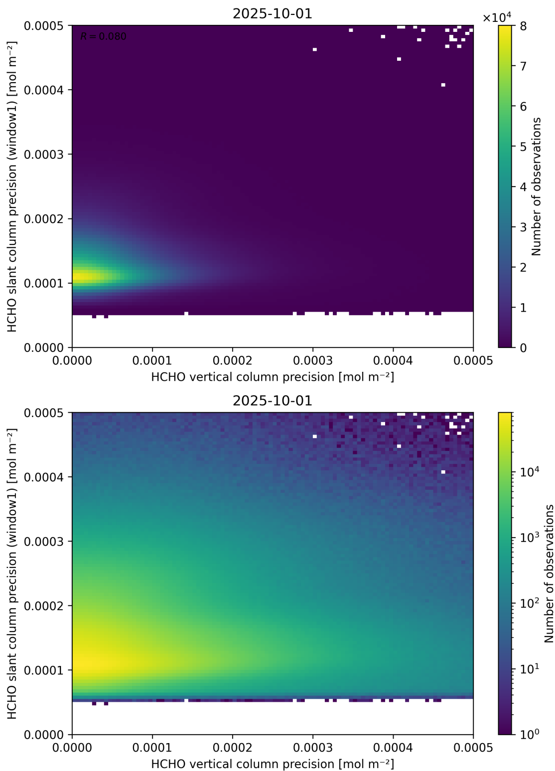
Figure 143: Scatter density plot of “HCHO vertical column precision” against “HCHO slant column precision (window1)” for 2025-10-01 to 2025-10-02.
