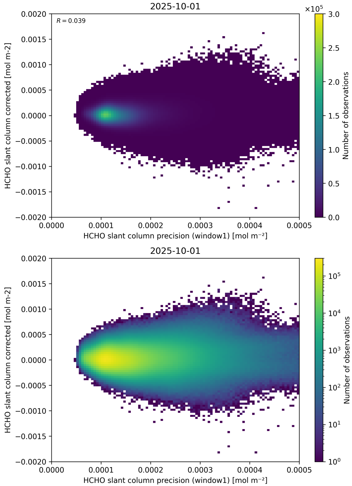
Figure 92: Scatter density plot of “HCHO slant column precision (window1)” against “HCHO slant column corrected” for 2025-10-01 to 2025-10-02.
