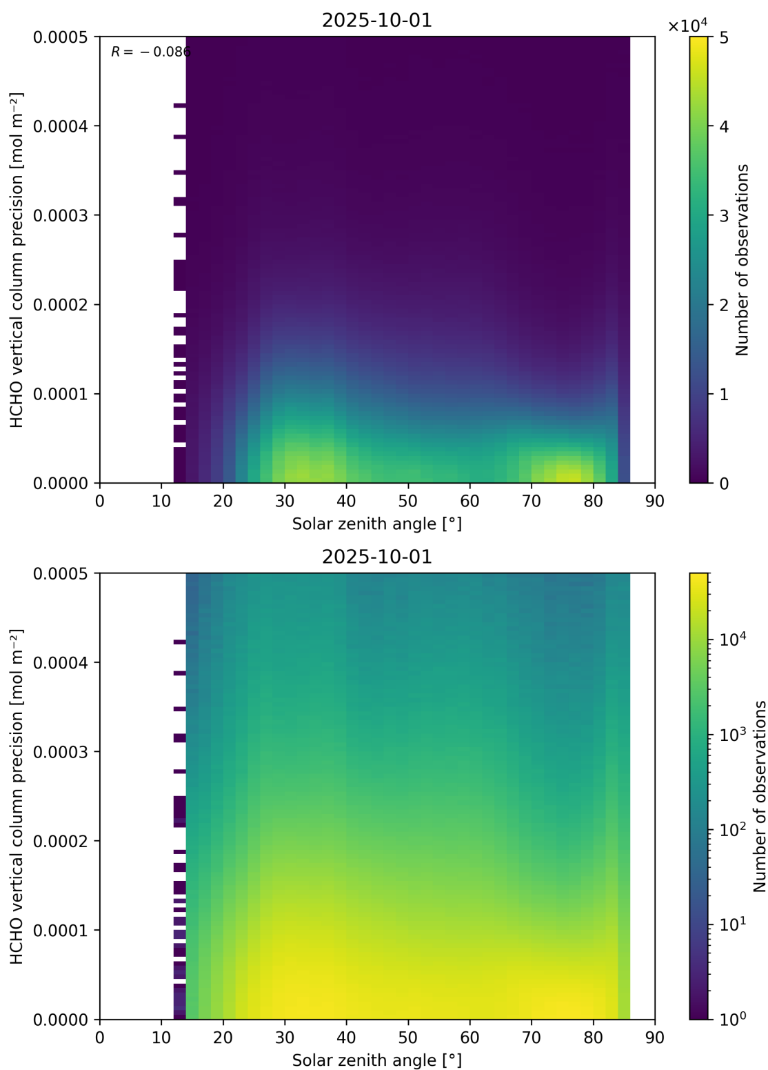
Figure 179: Scatter density plot of “Solar zenith angle” against “HCHO vertical column precision” for 2025-10-01 to 2025-10-02.
