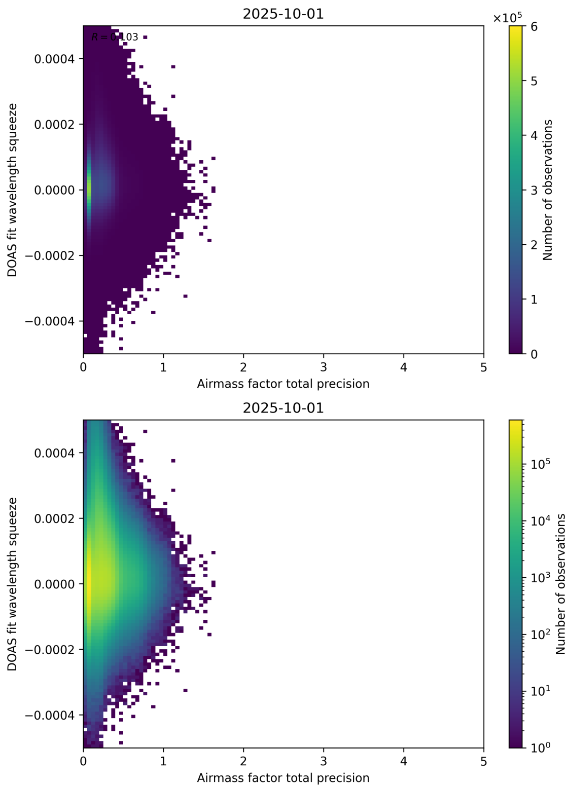
Figure 107: Scatter density plot of “Airmass factor total precision” against “DOAS fit wavelength squeeze” for 2025-10-01 to 2025-10-02.
