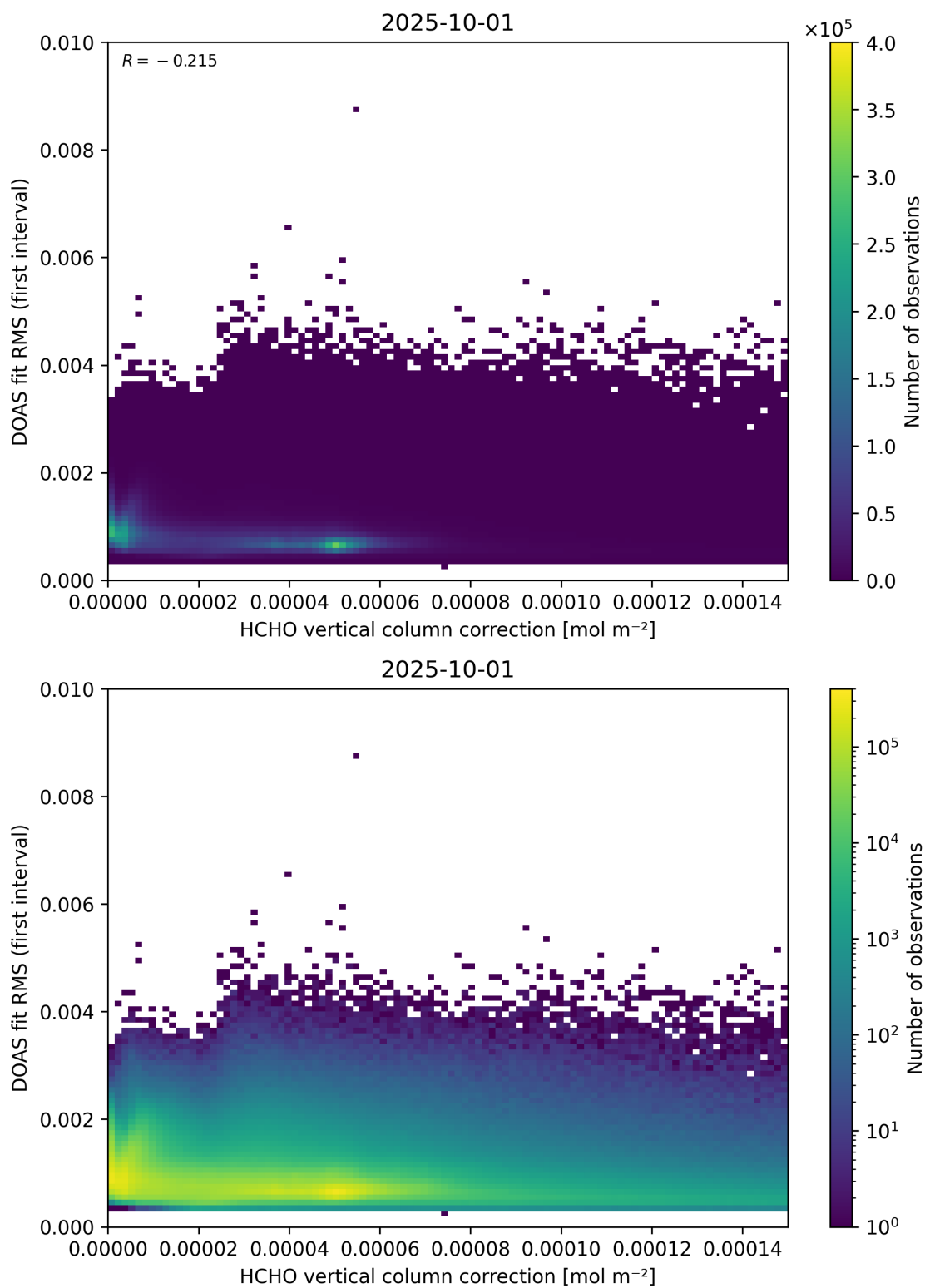
Figure 112: Scatter density plot of “HCHO vertical column correction” against “DOAS fit RMS (first interval)” for 2025-10-01 to 2025-10-02.
