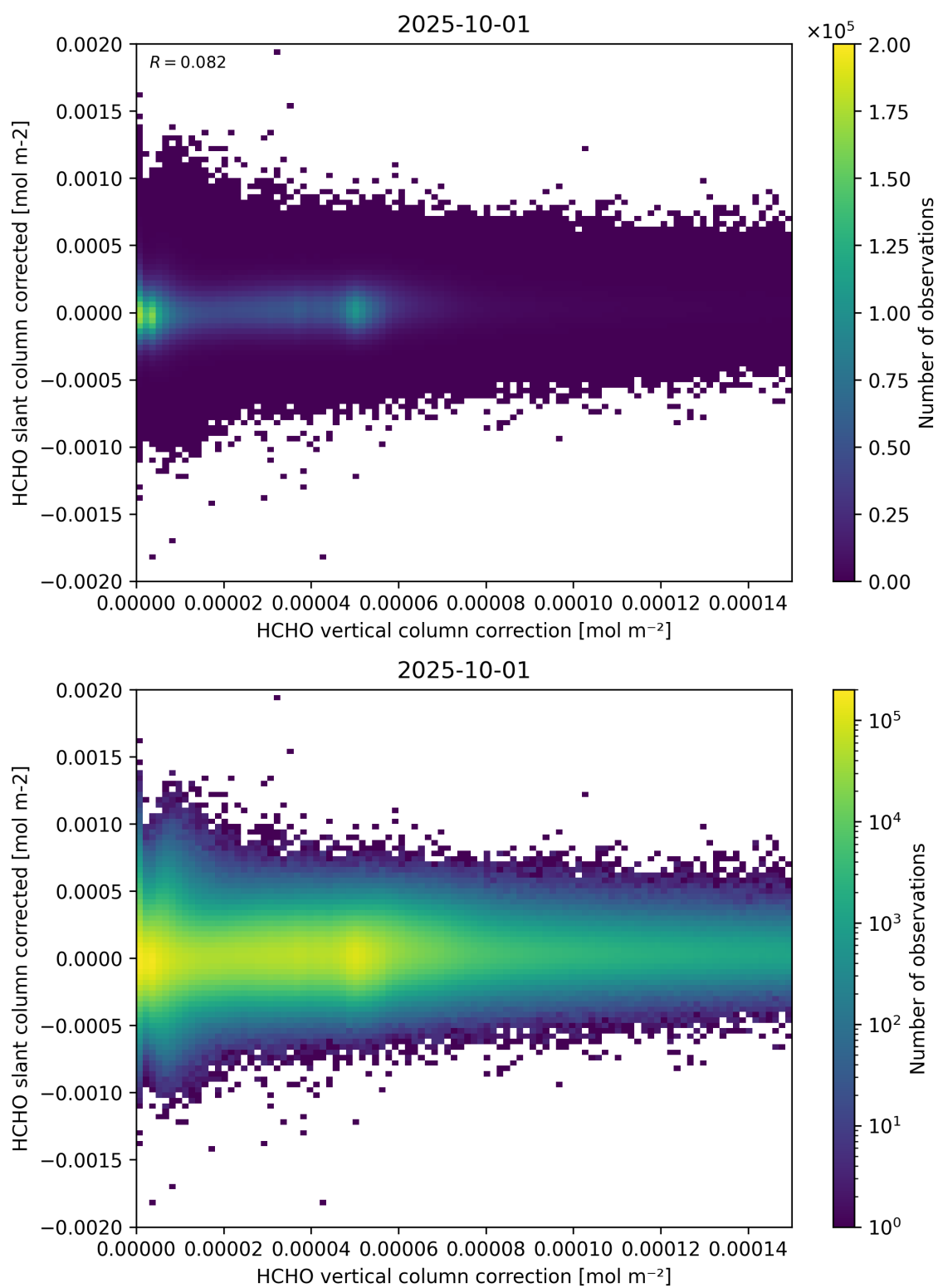
Figure 116: Scatter density plot of “HCHO vertical column correction” against “HCHO slant column corrected” for 2025-10-01 to 2025-10-02.
