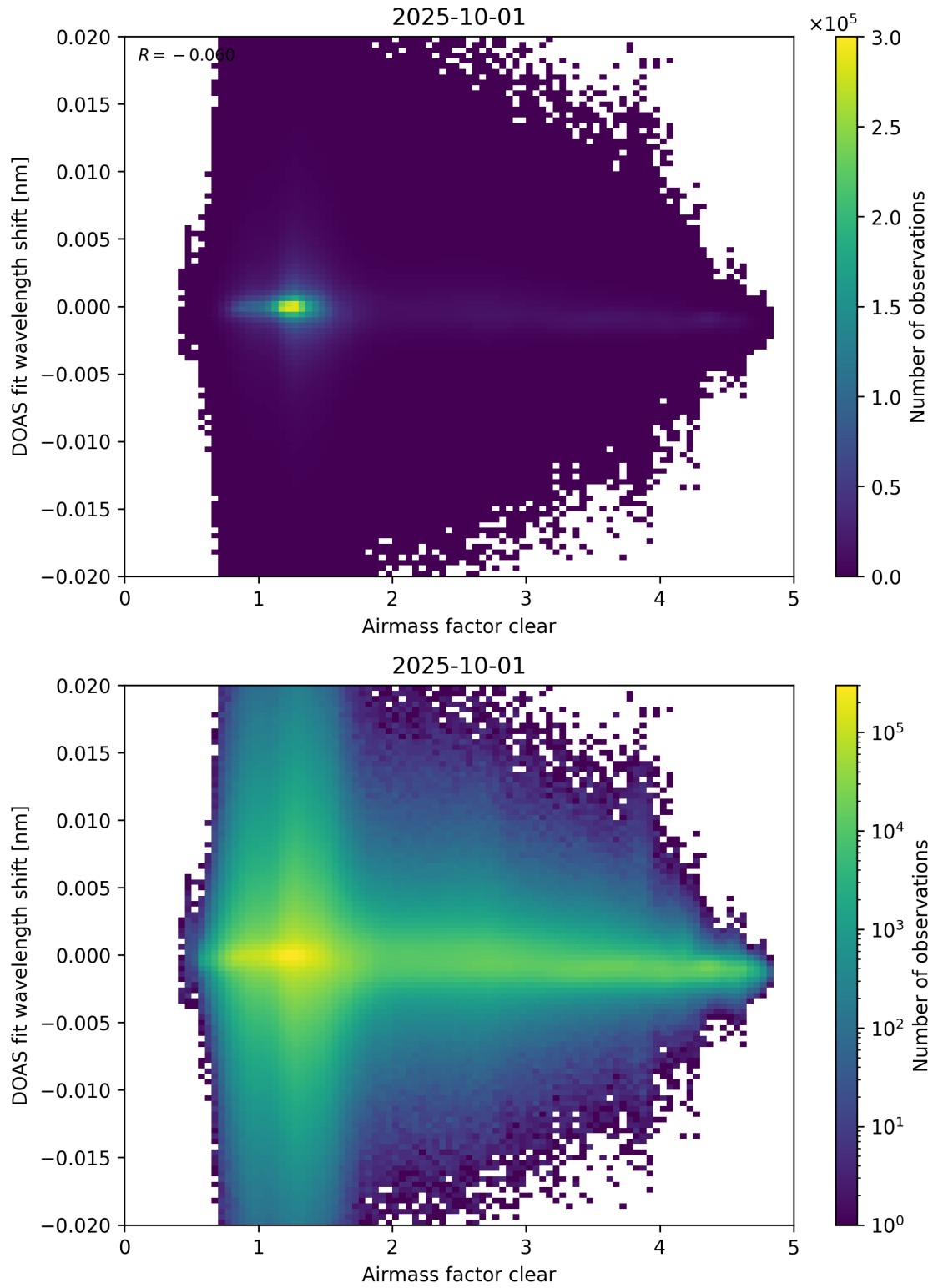
Figure 72: Scatter density plot of “Airmass factor clear” against “DOAS fit wavelength shift” for 2025-10-01 to 2025-10-02.
