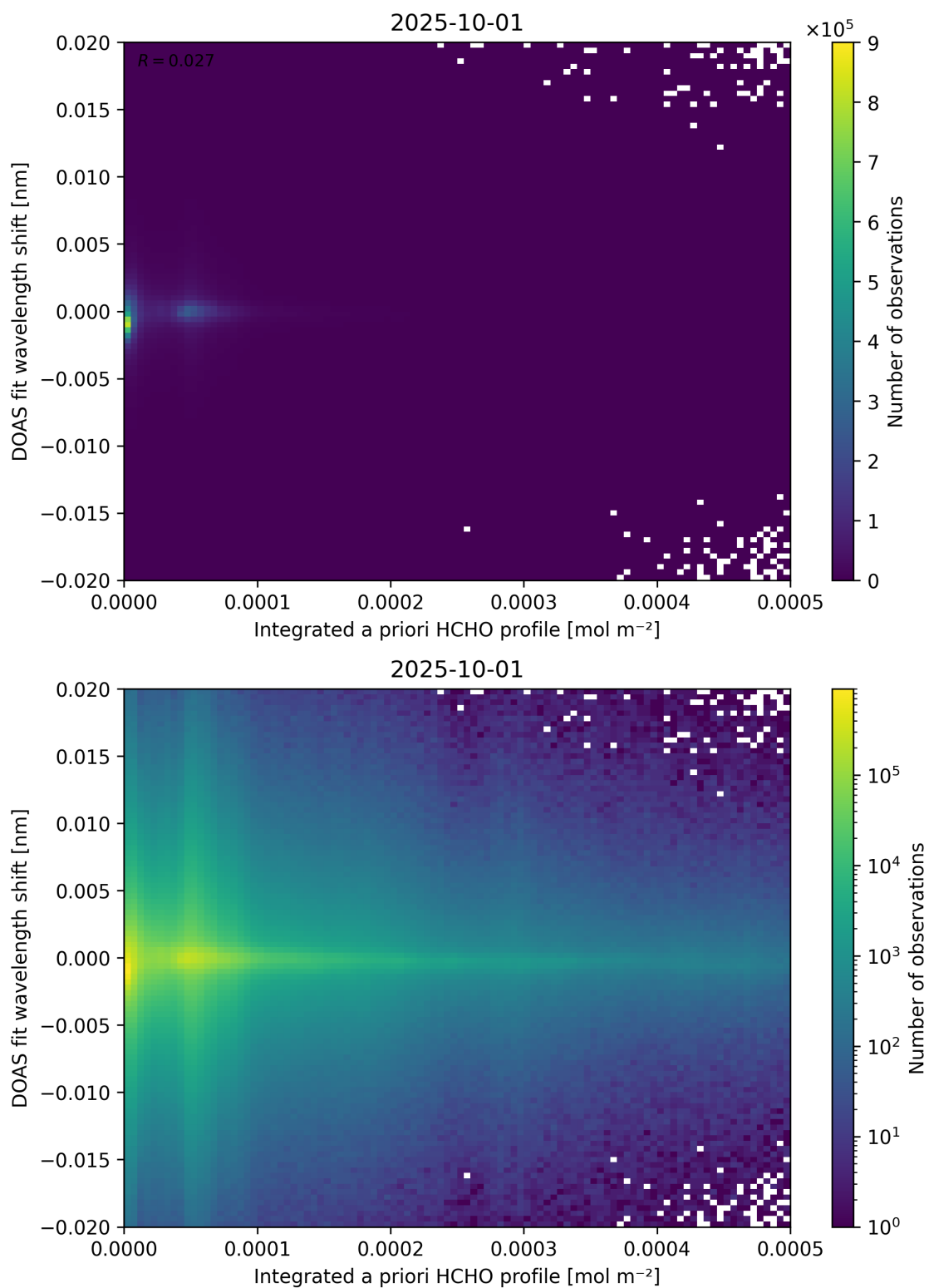
Figure 149: Scatter density plot of “Integrated a priori HCHO profile” against “DOAS fit wavelength shift” for 2025-10-01 to 2025-10-02.
