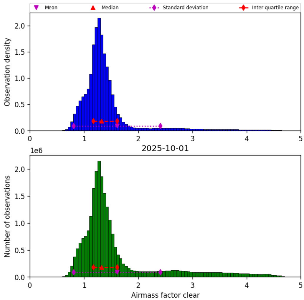
Figure 42: Histogram of “Airmass factor clear” for 2025-10-01 to 2025-10-02
