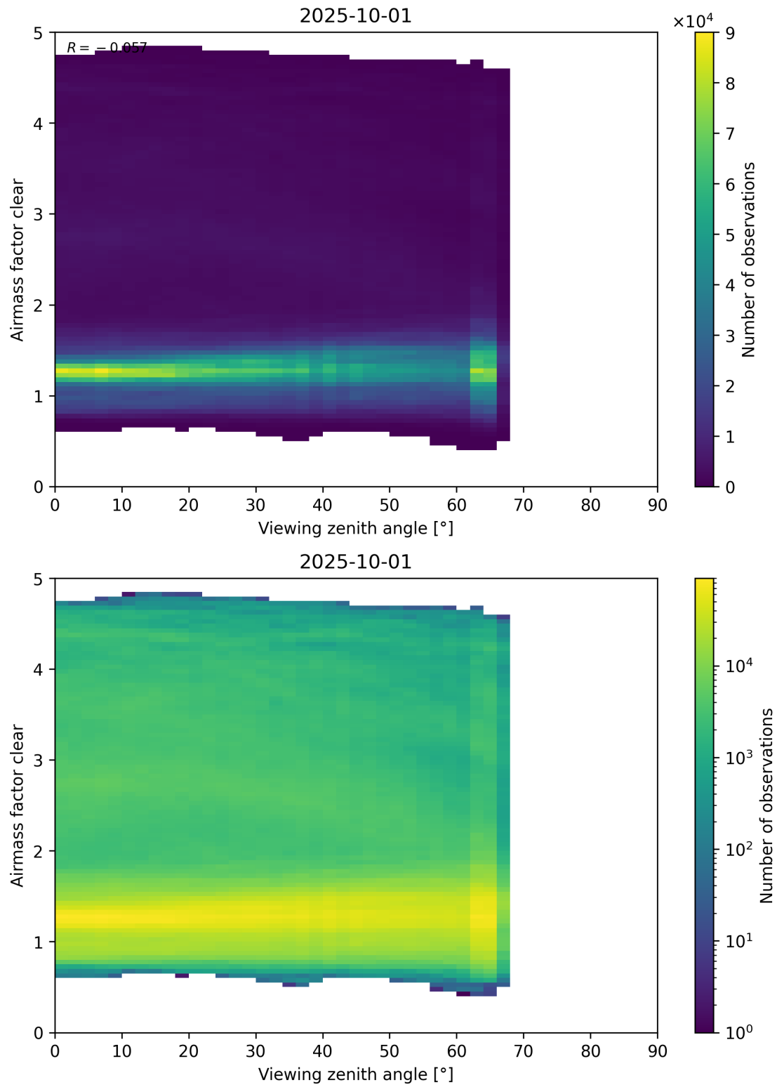
Figure 185: Scatter density plot of “Viewing zenith angle” against “Airmass factor clear” for 2025-10-01 to 2025-10-02.
