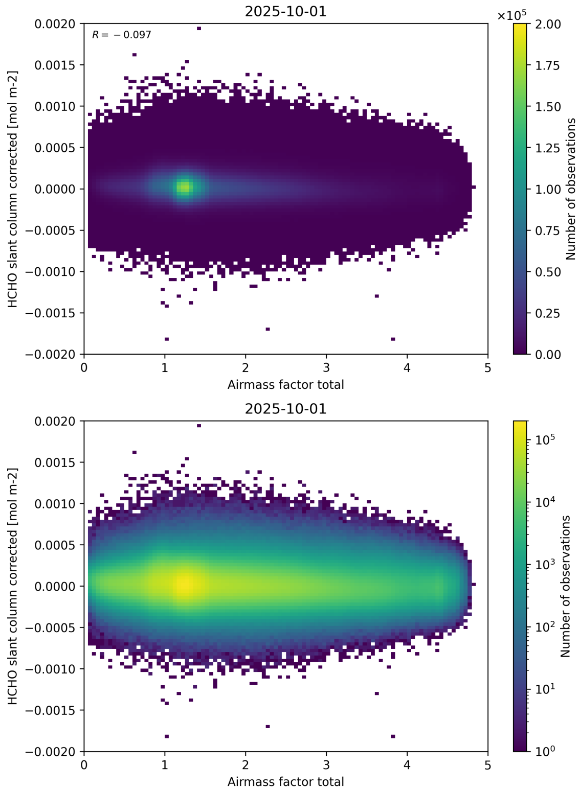
Figure 101: Scatter density plot of “Airmass factor total” against “HCHO slant column corrected” for 2025-10-01 to 2025-10-02.
