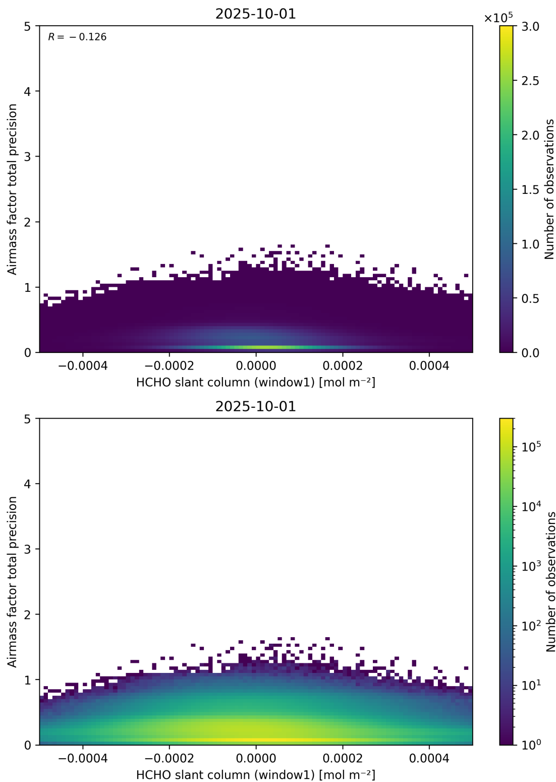
Figure 86: Scatter density plot of “HCHO slant column (window1)” against “Airmass factor total precision” for 2025-10-01 to 2025-10-02.
