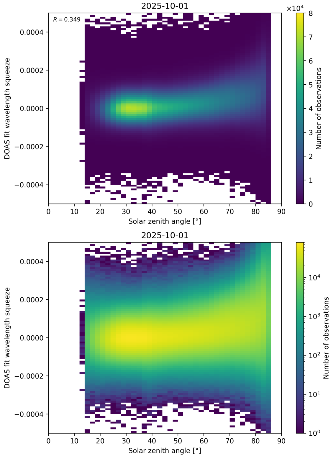
Figure 169: Scatter density plot of “Solar zenith angle” against “DOAS fit wavelength squeeze” for 2025-10-01 to 2025-10-02.
