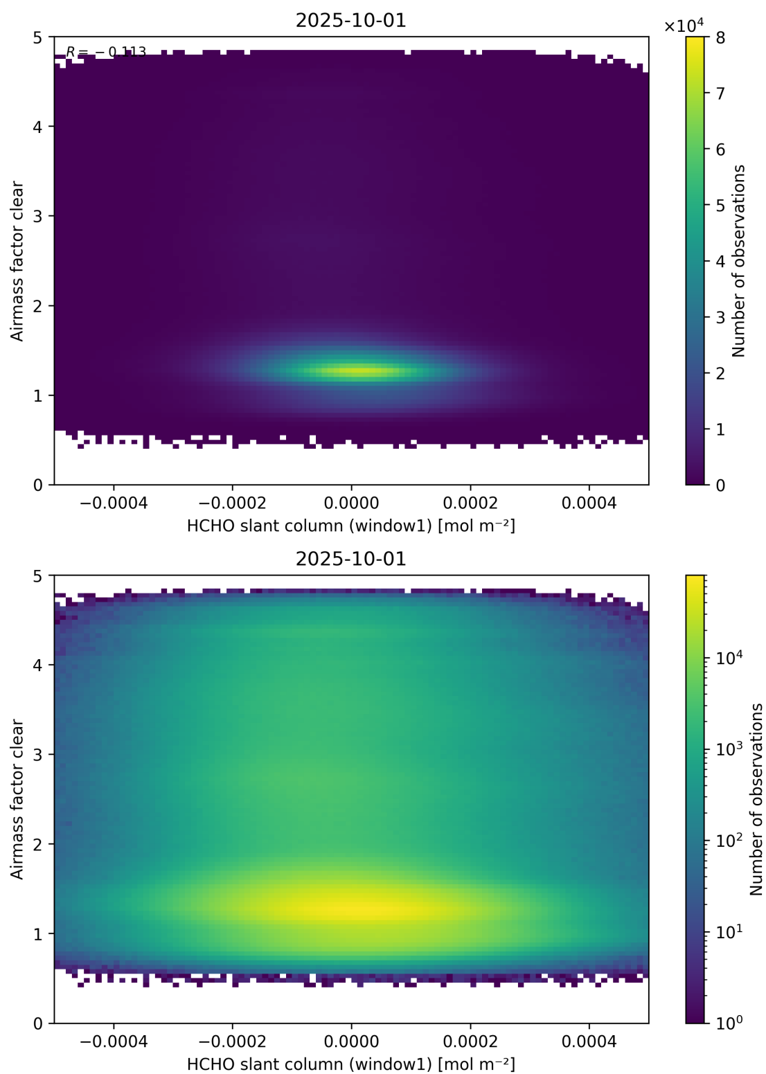
Figure 81: Scatter density plot of “HCHO slant column (window1)” against “Airmass factor clear” for 2025-10-01 to 2025-10-02.
