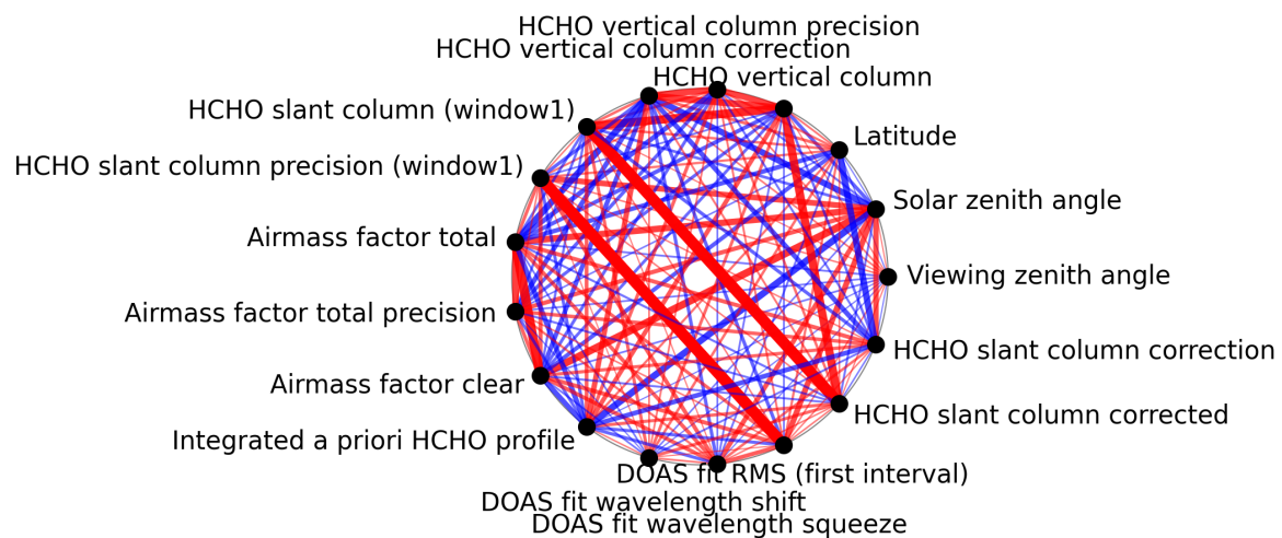
Figure 1: Map of correlation graph for 2025-10-01 to 2025-10-02.
