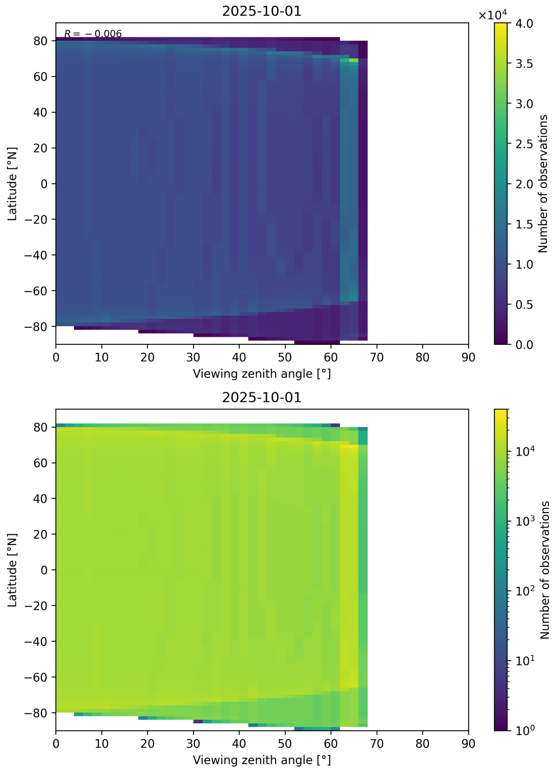
Figure 196: Scatter density plot of “Viewing zenith angle” against “Latitude” for 2025-10-01 to 2025-10-02.
