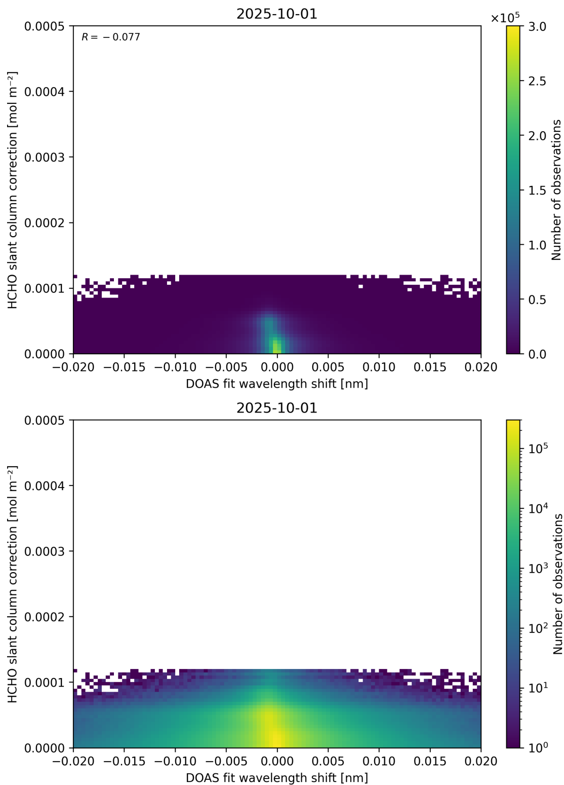
Figure 67: Scatter density plot of “DOAS fit wavelength shift” against “HCHO slant column correction” for 2025-10-01 to 2025-10-02.
