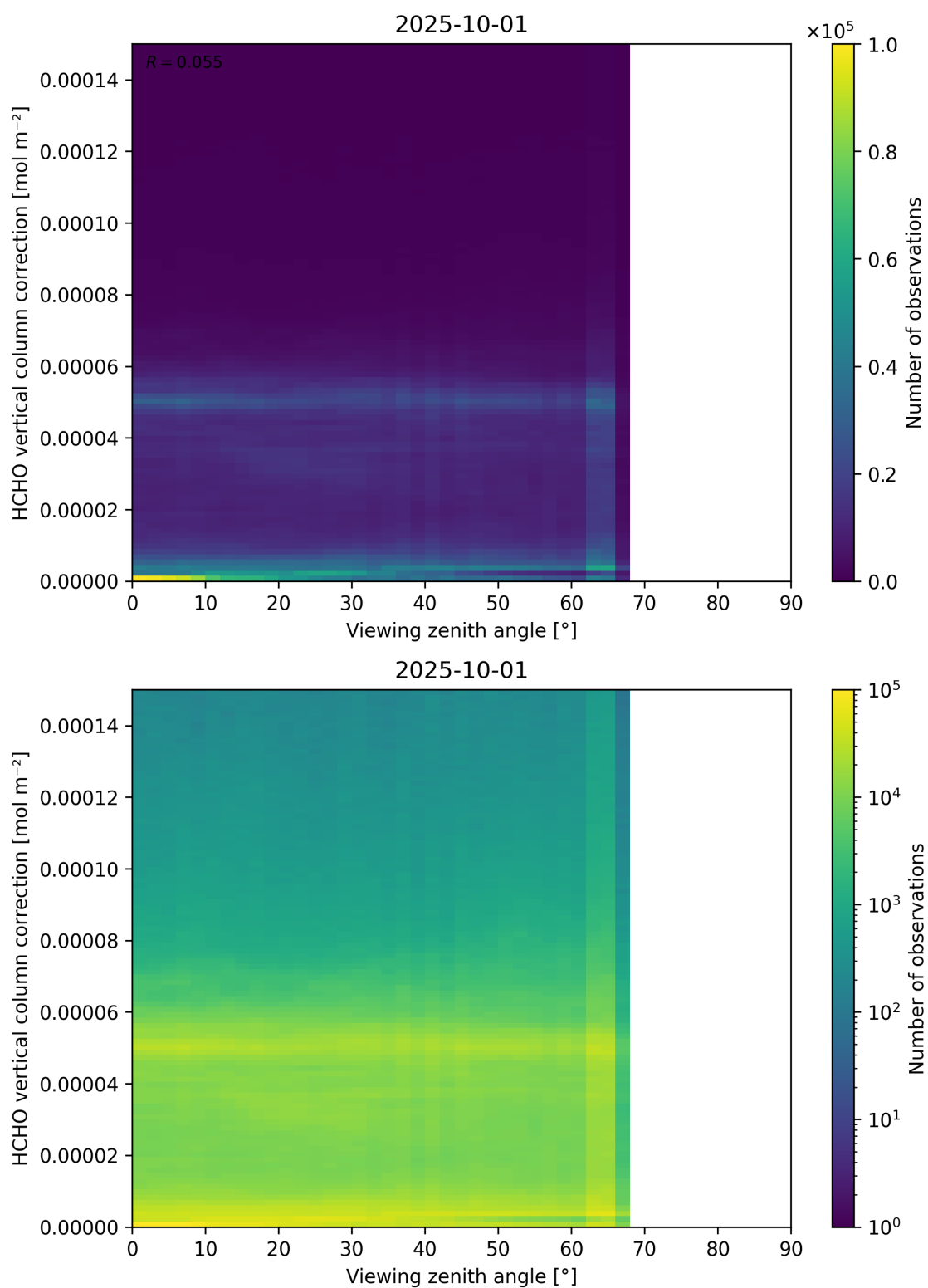
Figure 193: Scatter density plot of “Viewing zenith angle” against “HCHO vertical column correction” for 2025-10-01 to 2025-10-02.
