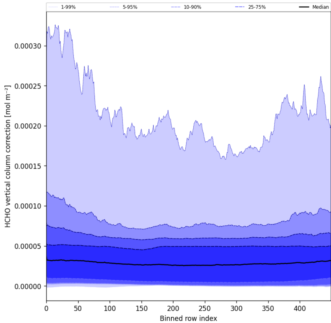
Figure 51: Along track statistics of “HCHO vertical column correction” for 2025-10-01 to 2025-10-02
