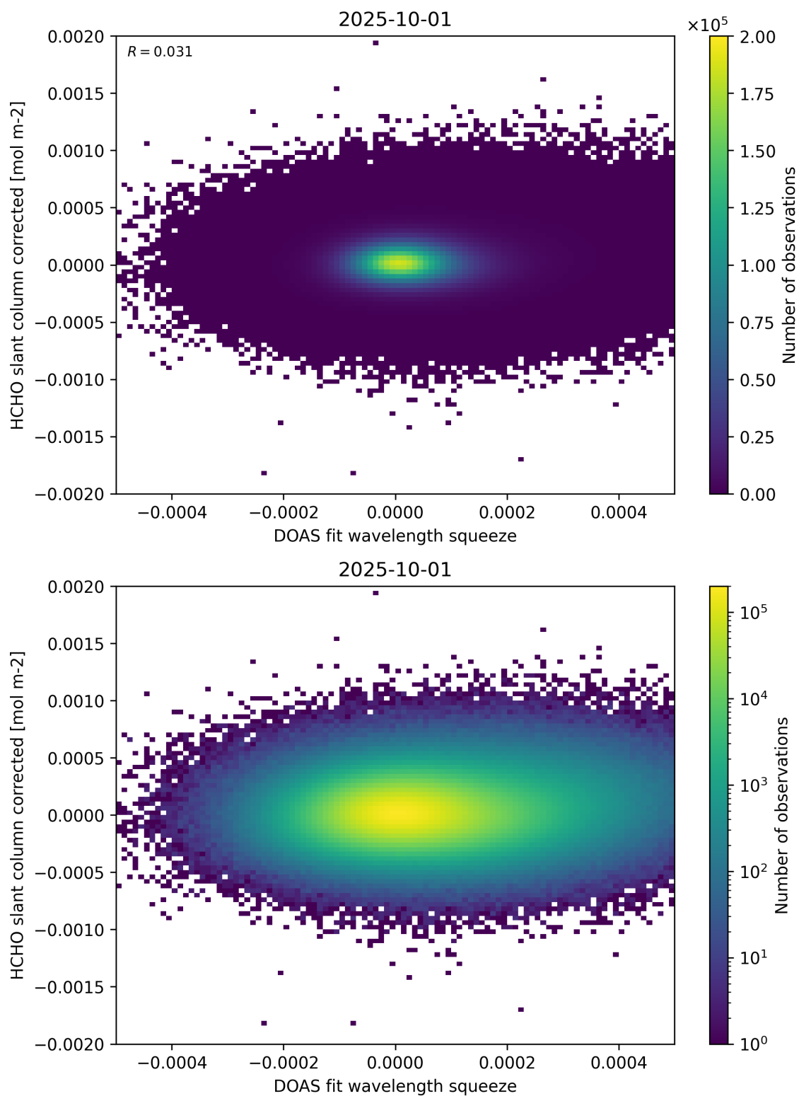
Figure 69: Scatter density plot of “DOAS fit wavelength squeeze” against “HCHO slant column corrected” for 2025-10-01 to 2025-10-02.
