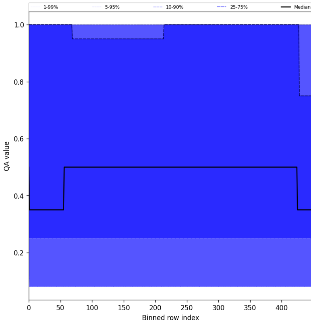
Figure 48: Along track statistics of “QA value” for 2025-10-01 to 2025-10-02
