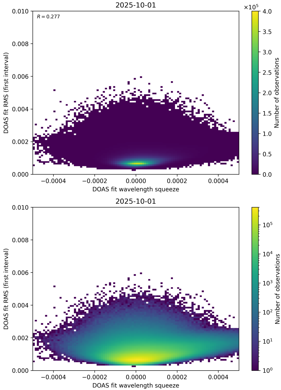
Figure 68: Scatter density plot of “DOAS fit wavelength squeeze” against “DOAS fit RMS (first interval)” for 2025-10-01 to 2025-10-02.
