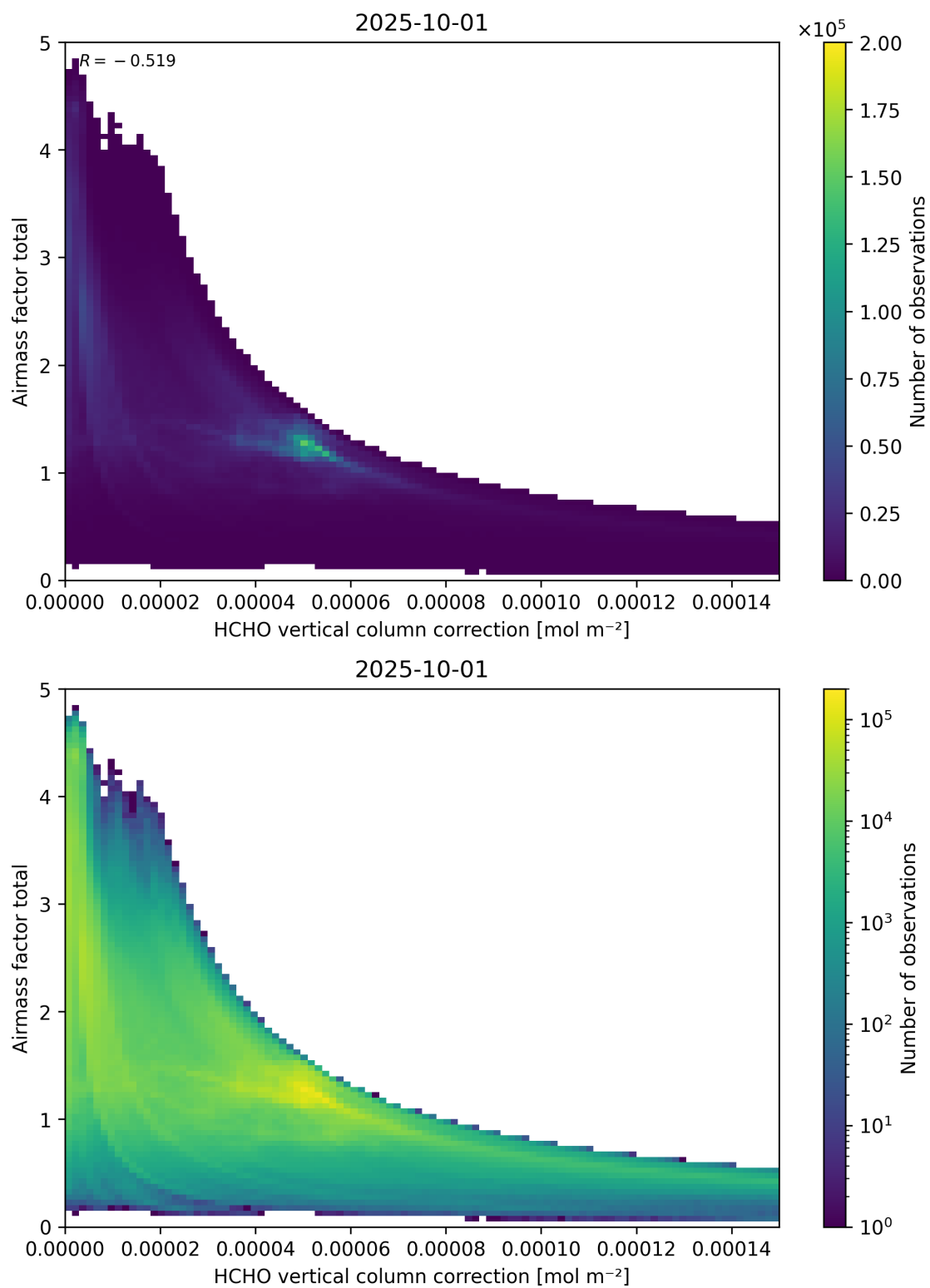
Figure 120: Scatter density plot of “HCHO vertical column correction” against “Airmass factor total” for 2025-10-01 to 2025-10-02.
