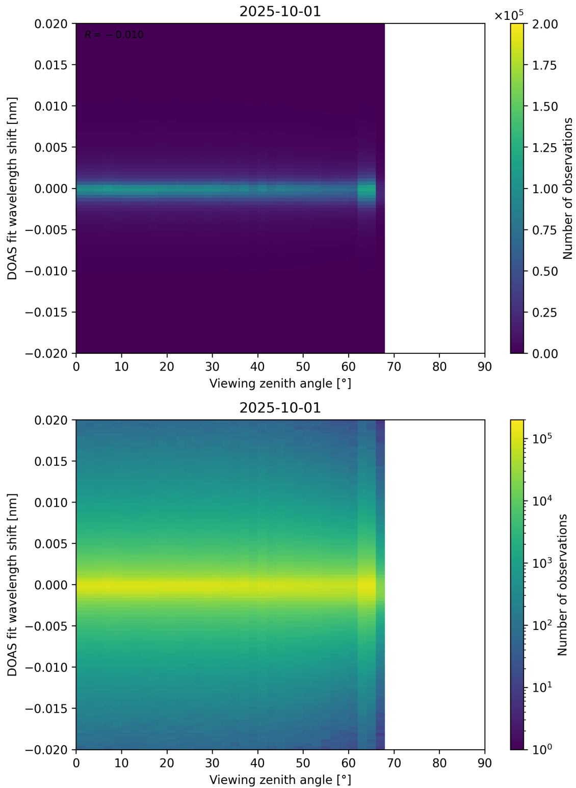
Figure 183: Scatter density plot of “Viewing zenith angle” against “DOAS fit wavelength shift” for 2025-10-01 to 2025-10-02.
