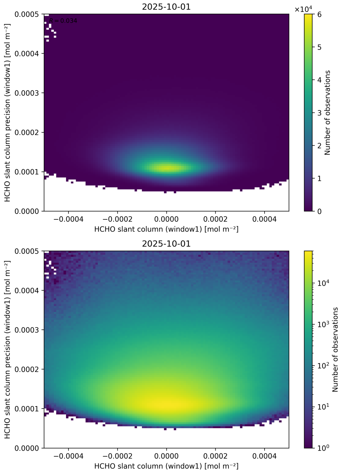
Figure 84: Scatter density plot of “HCHO slant column (window1)” against “HCHO slant column precision (window1)” for 2025-10-01 to 2025-10-02.
