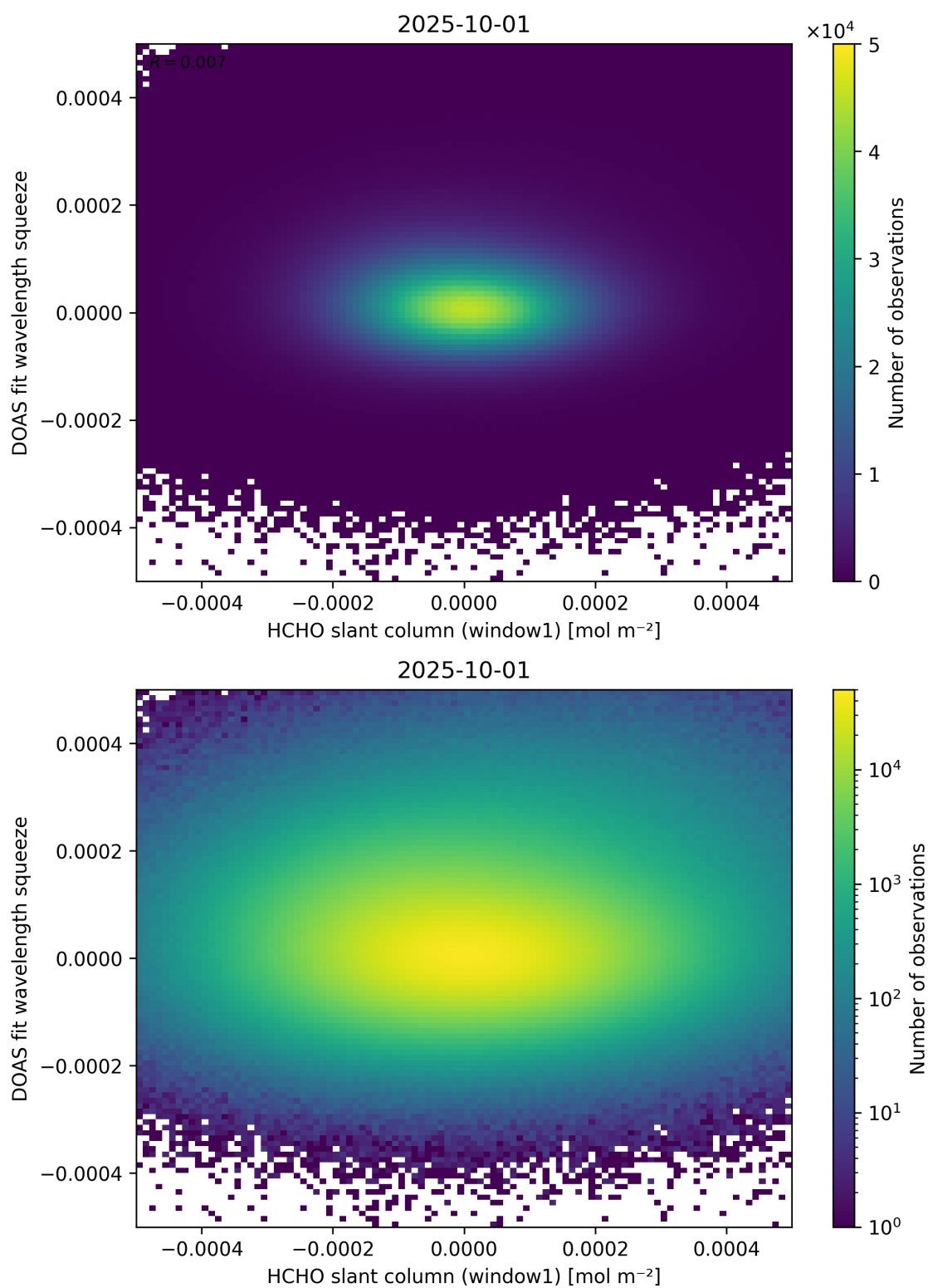
Figure 80: Scatter density plot of “HCHO slant column (window1)” against “DOAS fit wavelength squeeze” for 2025-10-01 to 2025-10-02.
