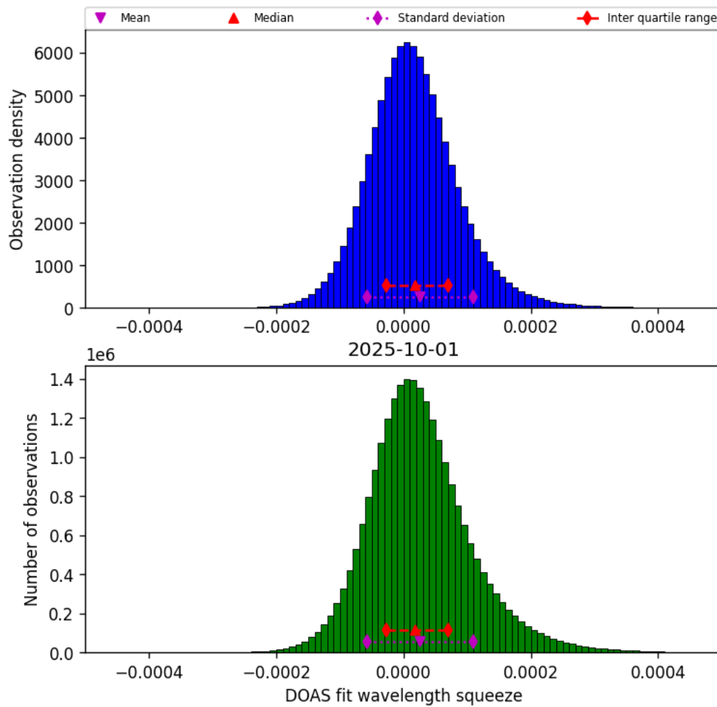
Figure 45: Histogram of “DOAS fit wavelength squeeze” for 2025-10-01 to 2025-10-02
