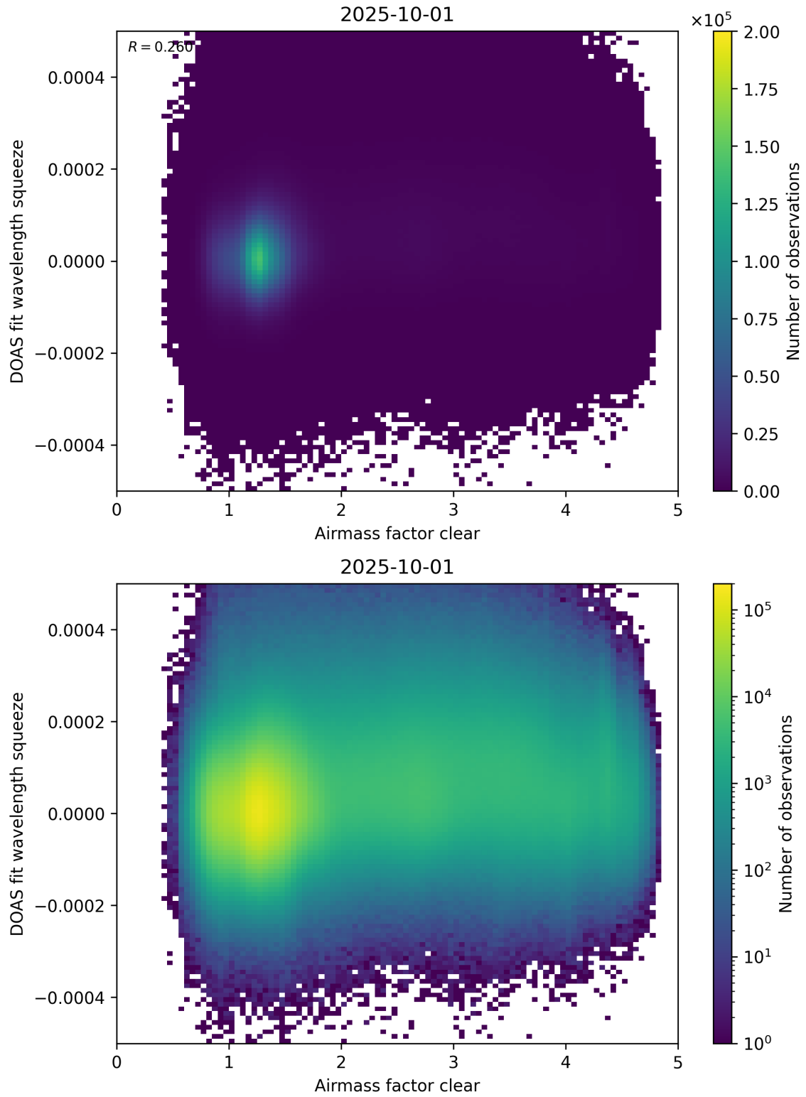
Figure 73: Scatter density plot of “Airmass factor clear” against “DOAS fit wavelength squeeze” for 2025-10-01 to 2025-10-02.
