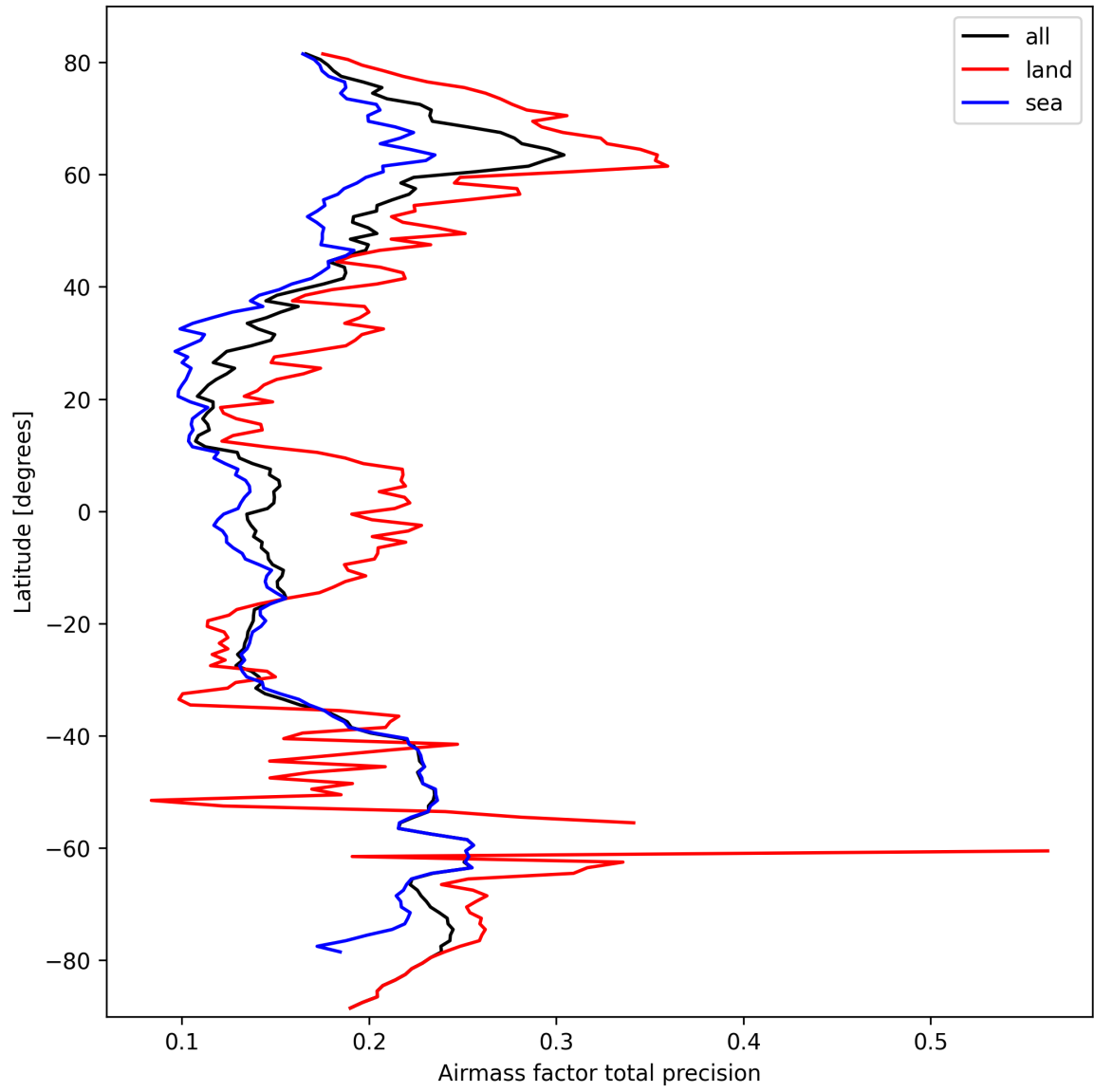
Figure 27: Zonal average of “Airmass factor total precision” for 2025-10-01 to 2025-10-02.
