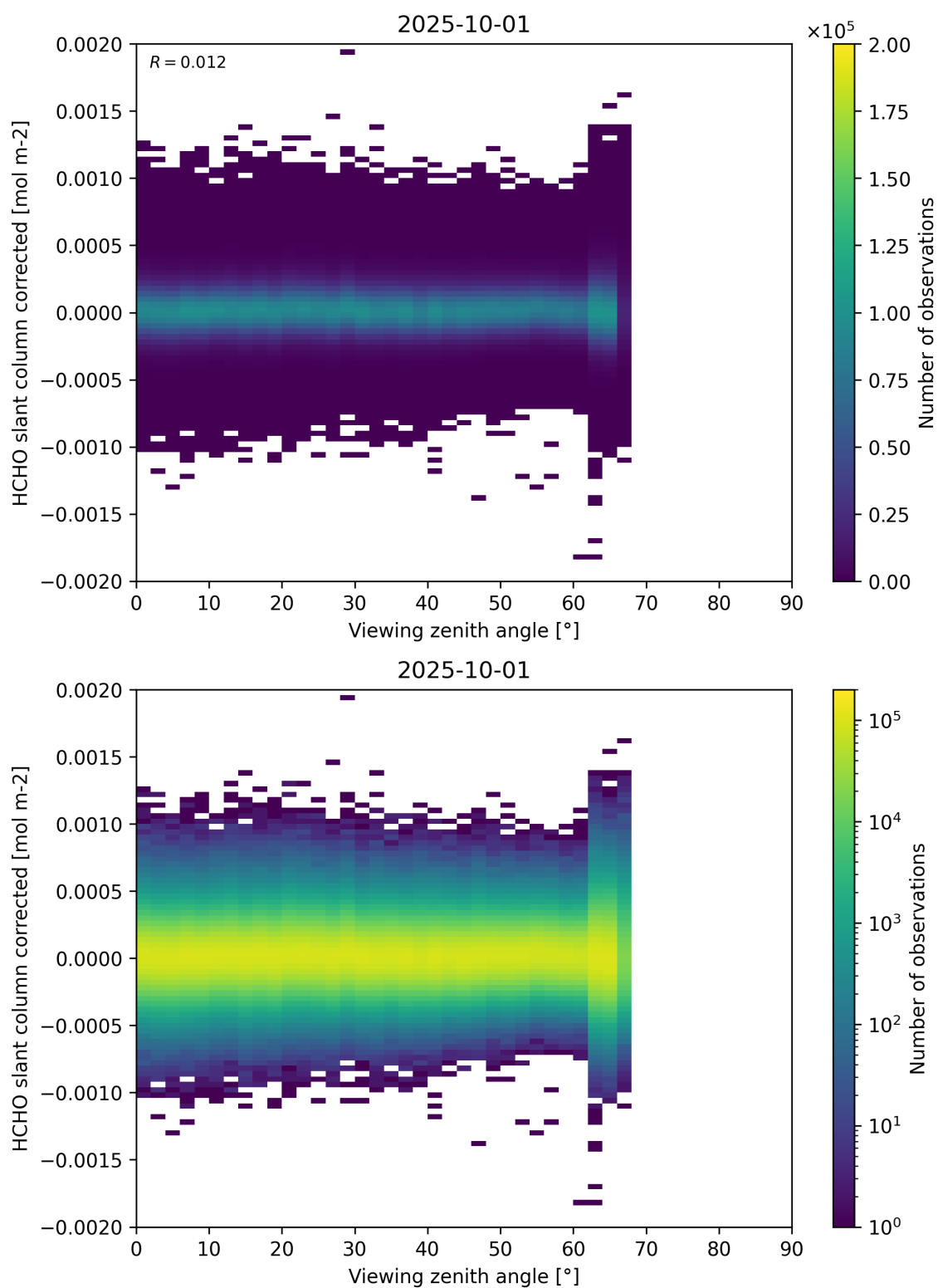
Figure 186: Scatter density plot of “Viewing zenith angle” against “HCHO slant column corrected” for 2025-10-01 to 2025-10-02.
