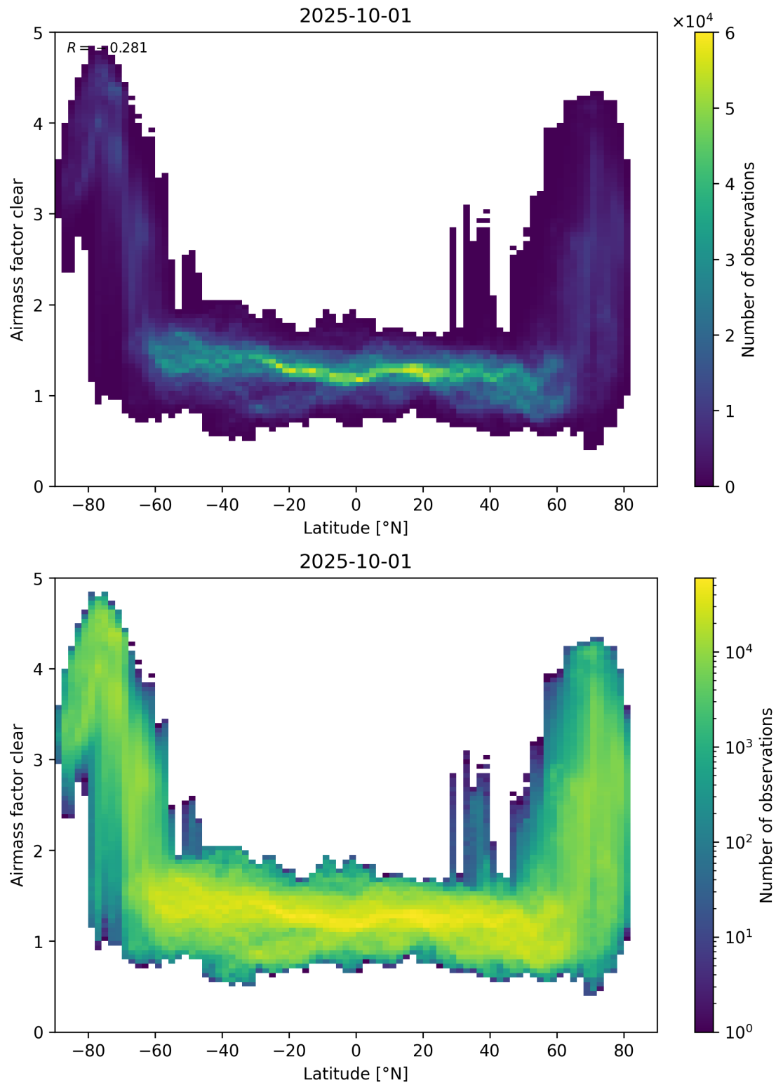
Figure 156: Scatter density plot of “Latitude” against “Airmass factor clear” for 2025-10-01 to 2025-10-02.
