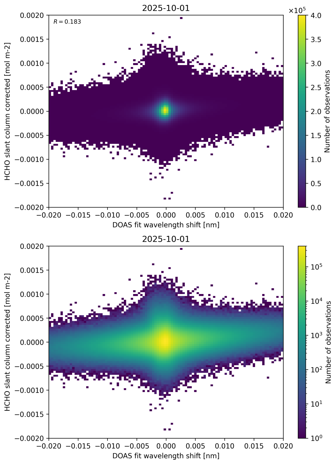
Figure 66: Scatter density plot of “DOAS fit wavelength shift” against “HCHO slant column corrected” for 2025-10-01 to 2025-10-02.
