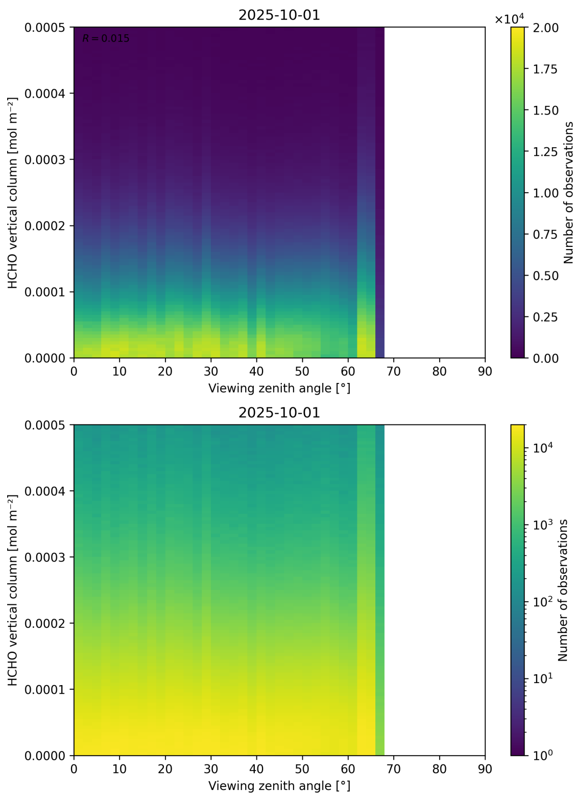
Figure 192: Scatter density plot of “Viewing zenith angle” against “HCHO vertical column” for 2025-10-01 to 2025-10-02.
