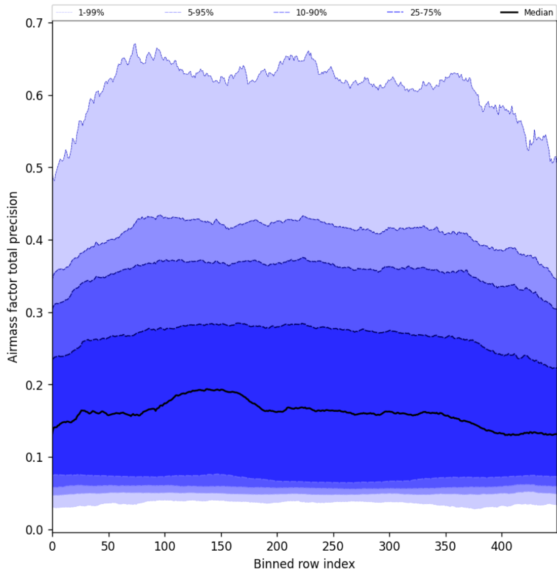
Figure 55: Along track statistics of “Airmass factor total precision” for 2025-10-01 to 2025-10-02
