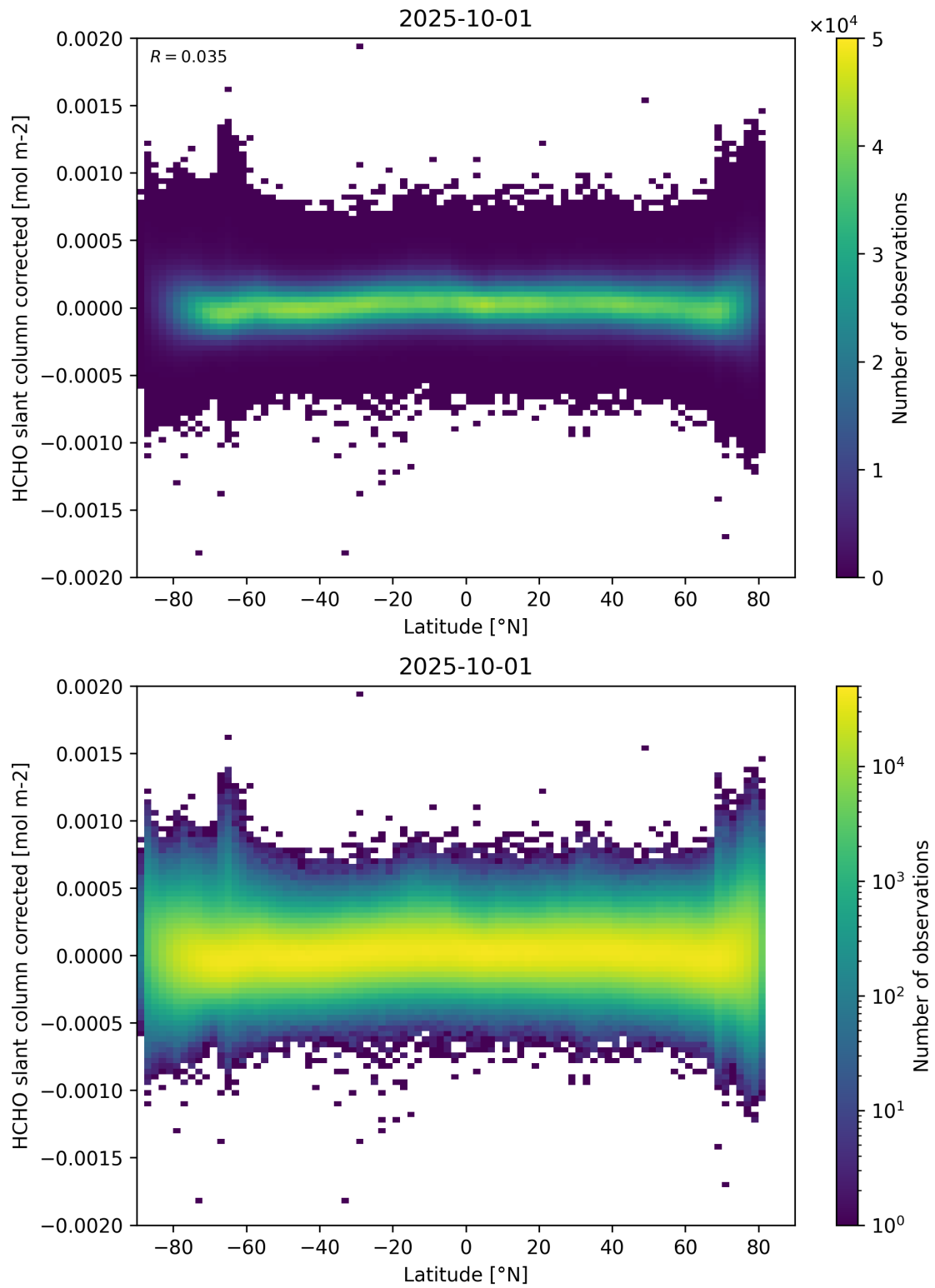
Figure 157: Scatter density plot of “Latitude” against “HCHO slant column corrected” for 2025-10-01 to 2025-10-02.
