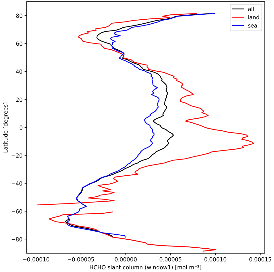
Figure 24: Zonal average of “HCHO slant column (window1)” for 2025-10-01 to 2025-10-02.
