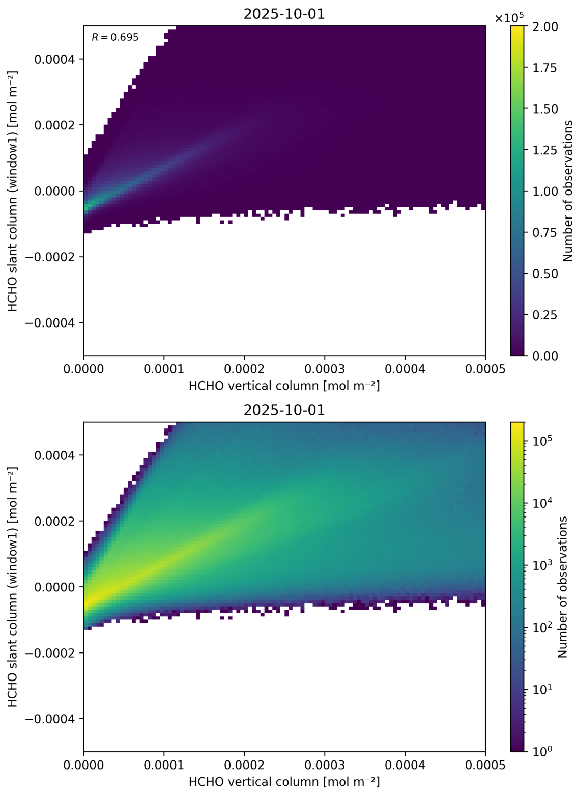
Figure 129: Scatter density plot of “HCHO vertical column” against “HCHO slant column (window1)” for 2025-10-01 to 2025-10-02.
