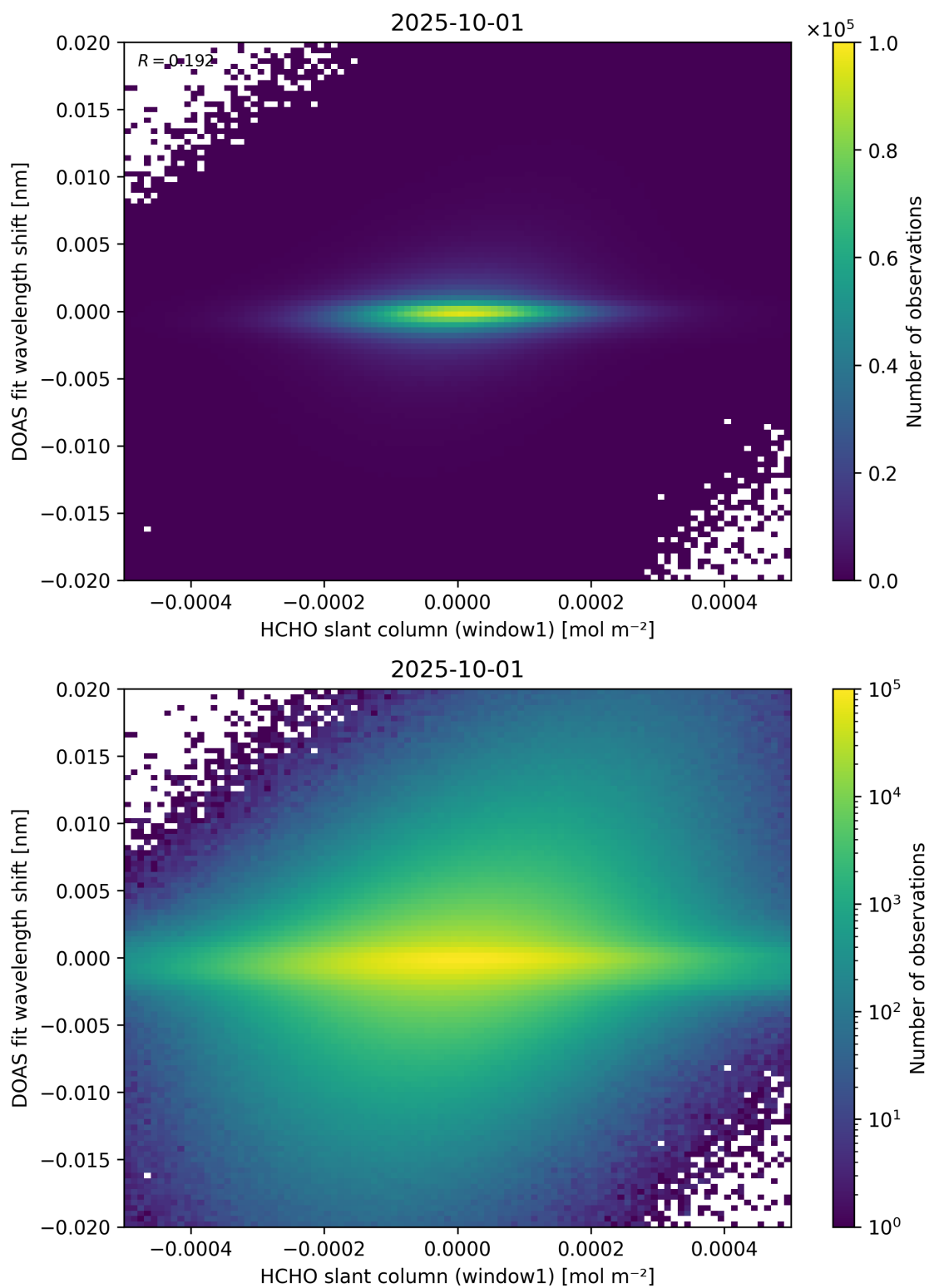
Figure 79: Scatter density plot of “HCHO slant column (window1)” against “DOAS fit wavelength shift” for 2025-10-01 to 2025-10-02.
