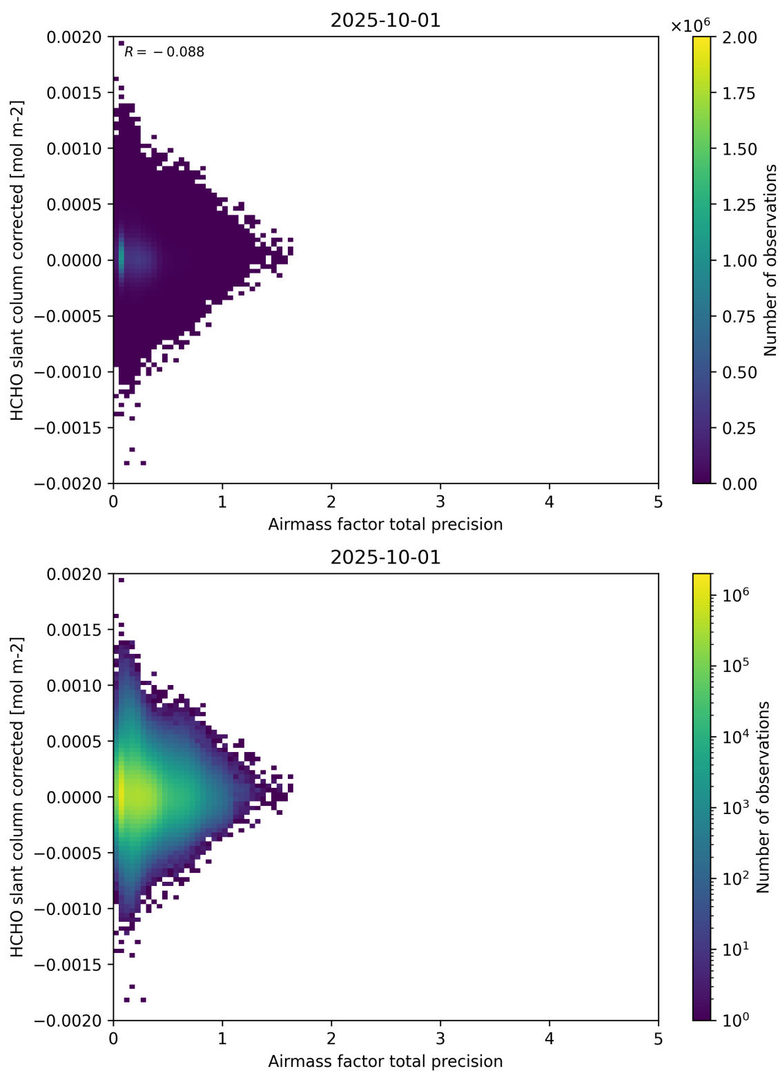
Figure 109: Scatter density plot of “Airmass factor total precision” against “HCHO slant column corrected” for 2025-10-01 to 2025-10-02.
