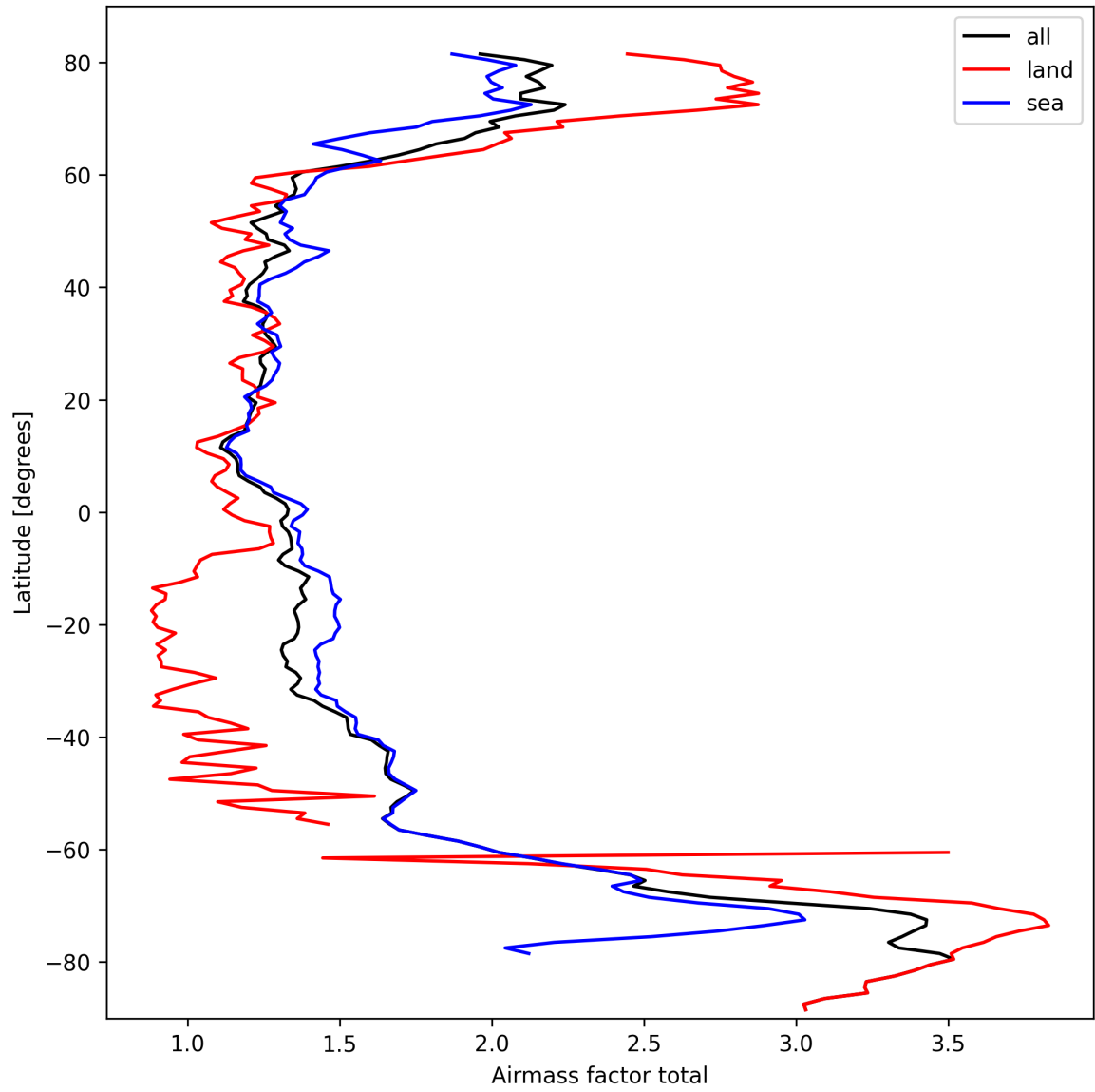
Figure 26: Zonal average of “Airmass factor total” for 2025-10-01 to 2025-10-02.
