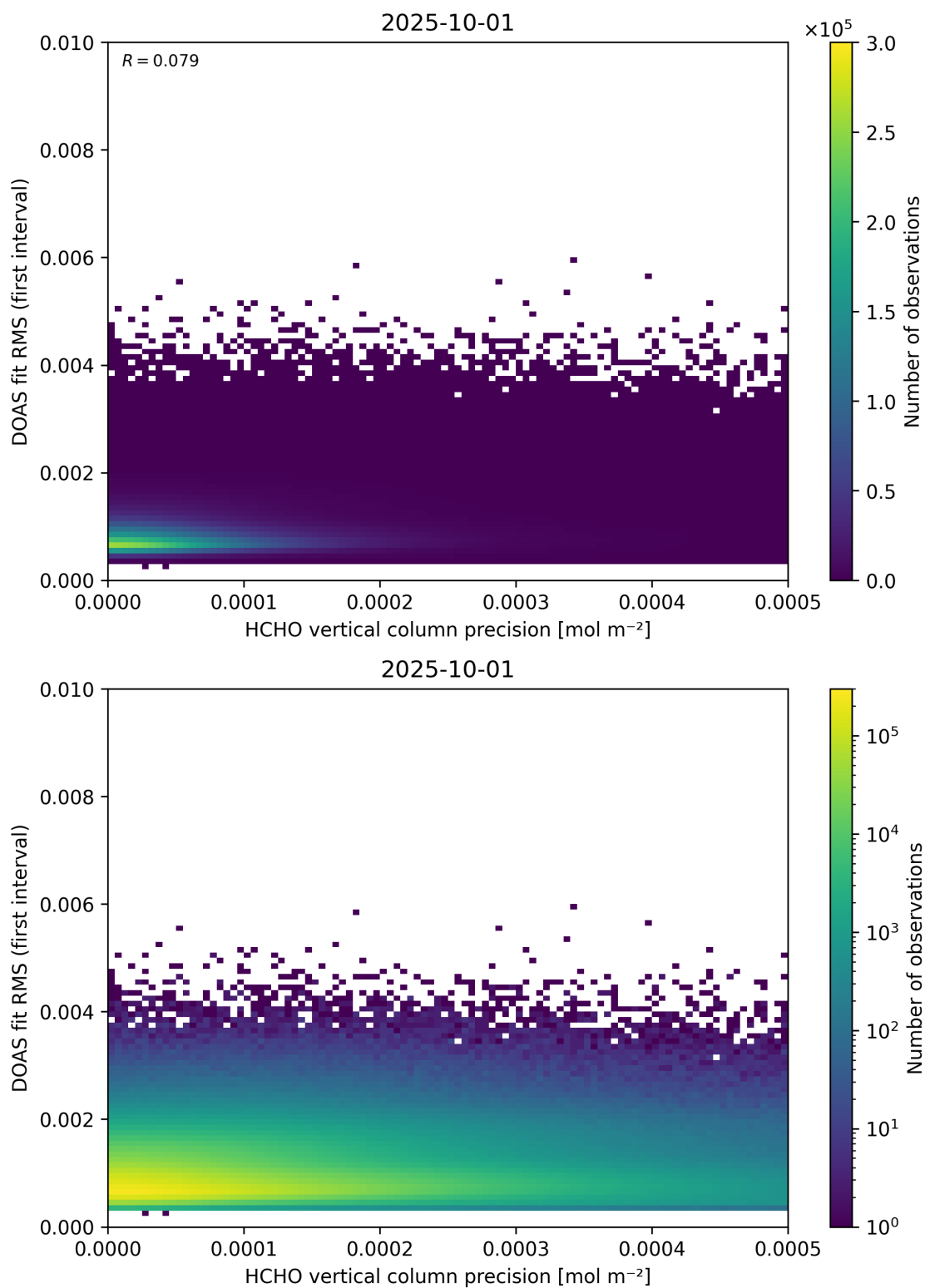
Figure 136: Scatter density plot of “HCHO vertical column precision” against “DOAS fit RMS (first interval)” for 2025-10-01 to 2025-10-02.
