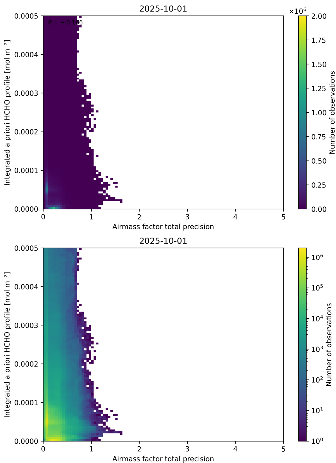
Figure 111: Scatter density plot of “Airmass factor total precision” against “Integrated a priori HCHO profile” for 2025-10-01 to 2025-10-02.
