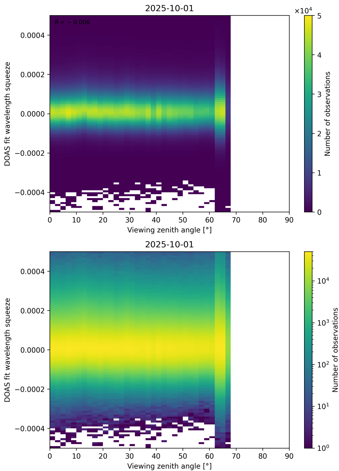
Figure 184: Scatter density plot of “Viewing zenith angle” against “DOAS fit wavelength squeeze” for 2025-10-01 to 2025-10-02.
