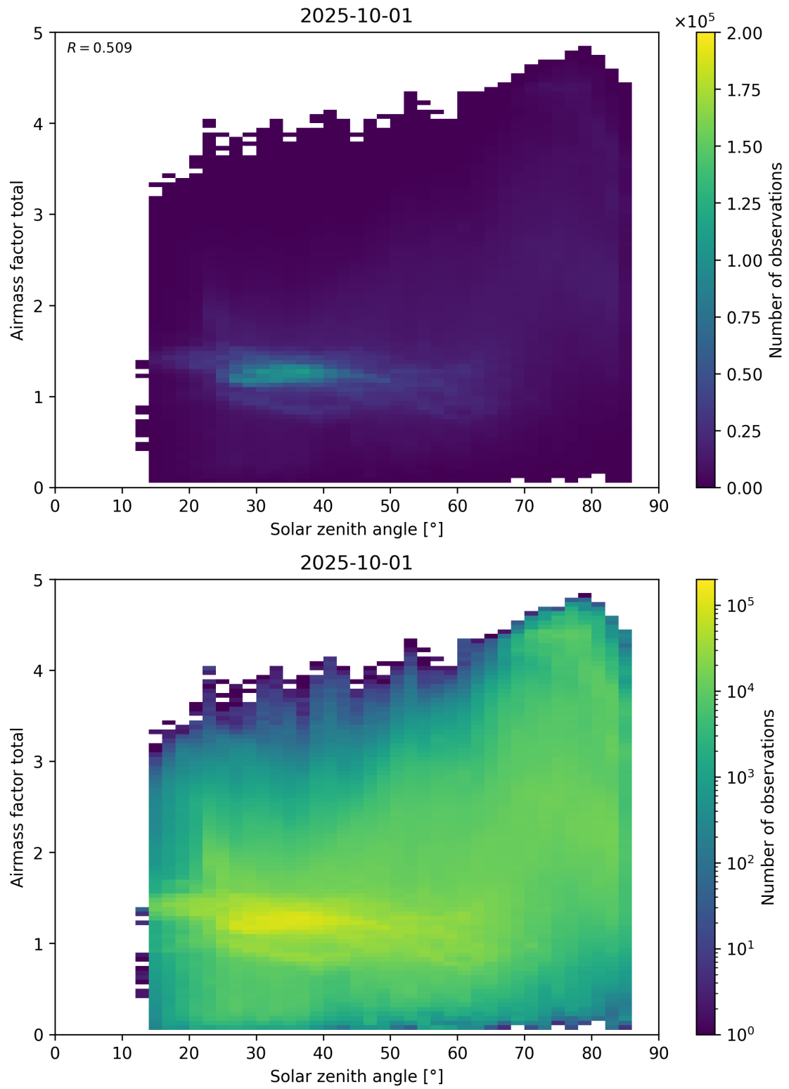
Figure 175: Scatter density plot of “Solar zenith angle” against “Airmass factor total” for 2025-10-01 to 2025-10-02.
