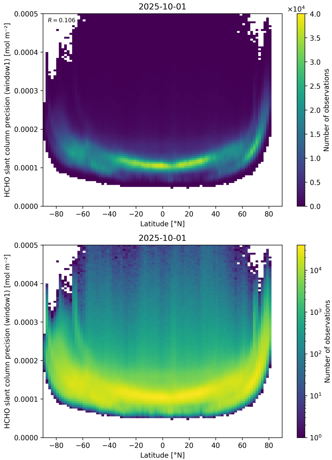
Figure 160: Scatter density plot of “Latitude” against “HCHO slant column precision (window1)” for 2025-10-01 to 2025-10-02.
