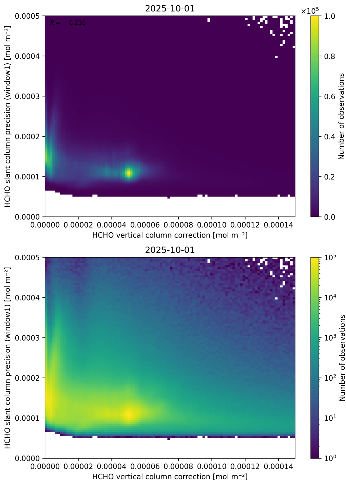
Figure 119: Scatter density plot of “HCHO vertical column correction” against “HCHO slant column precision (window1)” for 2025-10-01 to 2025-10-02.
