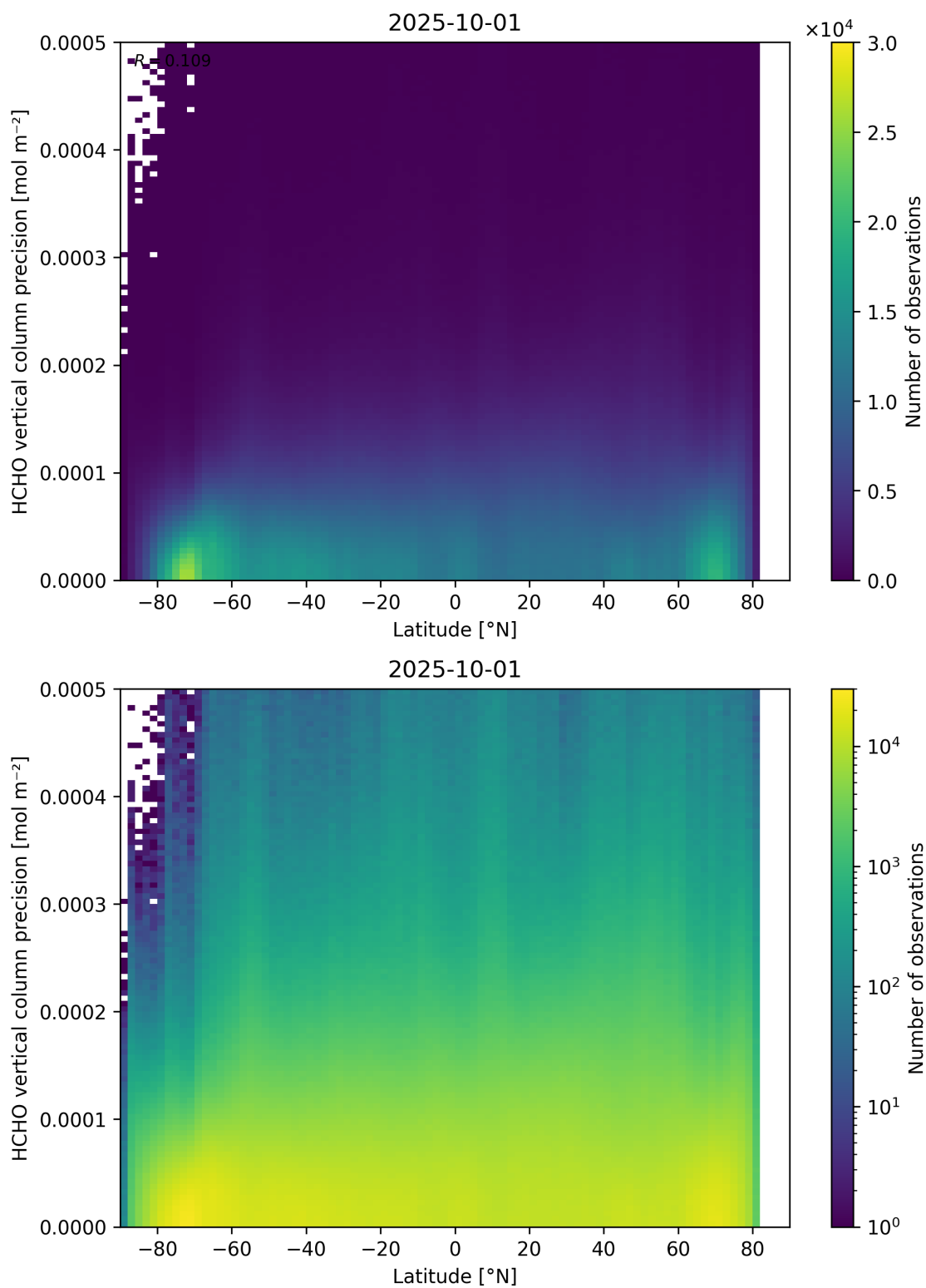
Figure 165: Scatter density plot of “Latitude” against “HCHO vertical column precision” for 2025-10-01 to 2025-10-02.
