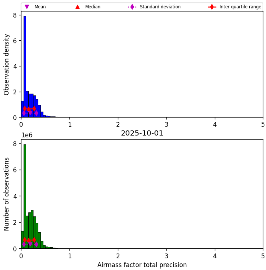
Figure 41: Histogram of “Airmass factor total precision” for 2025-10-01 to 2025-10-02
