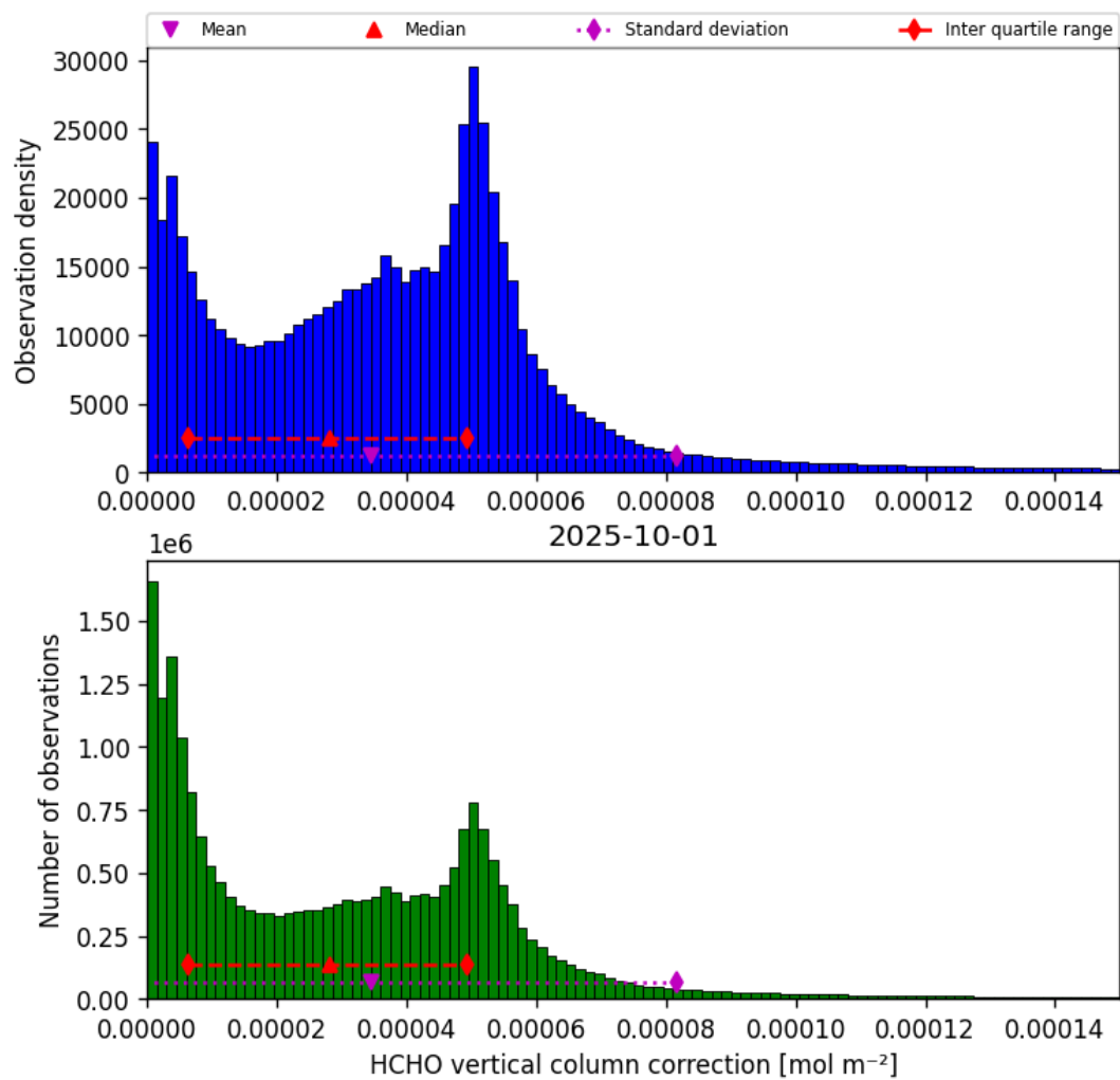
Figure 37: Histogram of “HCHO vertical column correction” for 2025-10-01 to 2025-10-02
