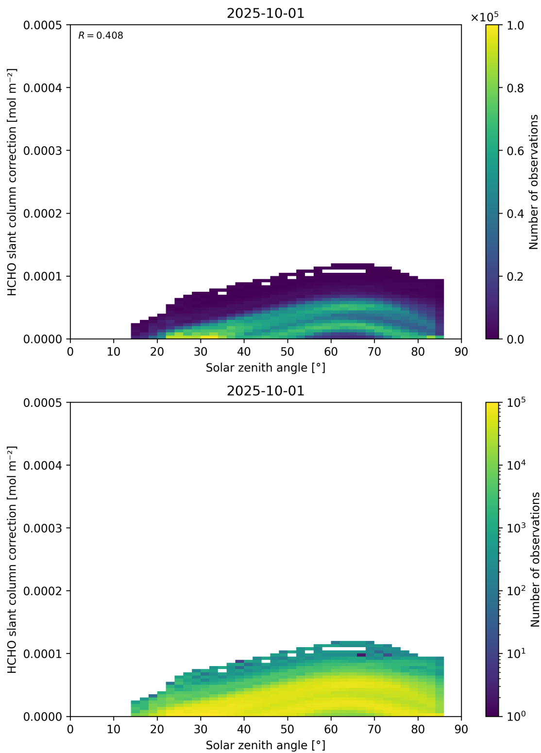
Figure 172: Scatter density plot of “Solar zenith angle” against “HCHO slant column correction” for 2025-10-01 to 2025-10-02.
