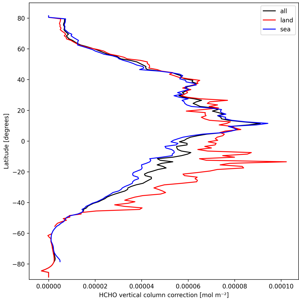
Figure 23: Zonal average of “HCHO vertical column correction” for 2025-10-01 to 2025-10-02.
