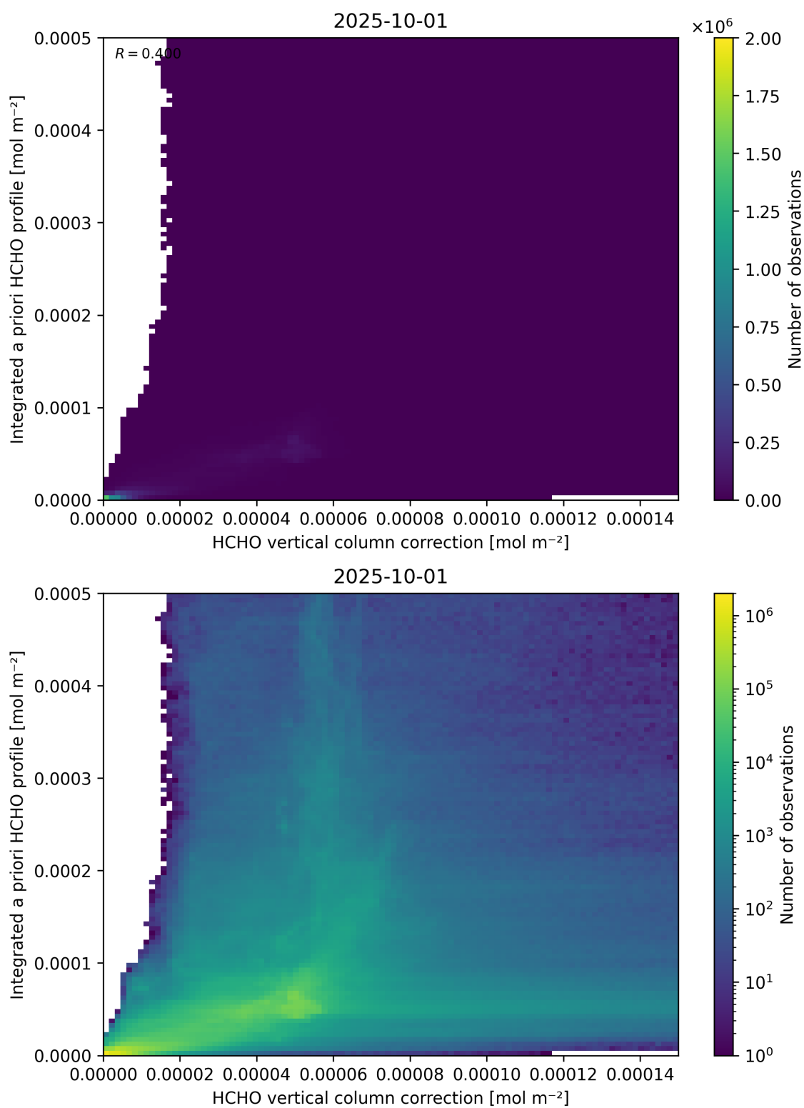
Figure 122: Scatter density plot of “HCHO vertical column correction” against “Integrated a priori HCHO profile” for 2025-10-01 to 2025-10-02.
