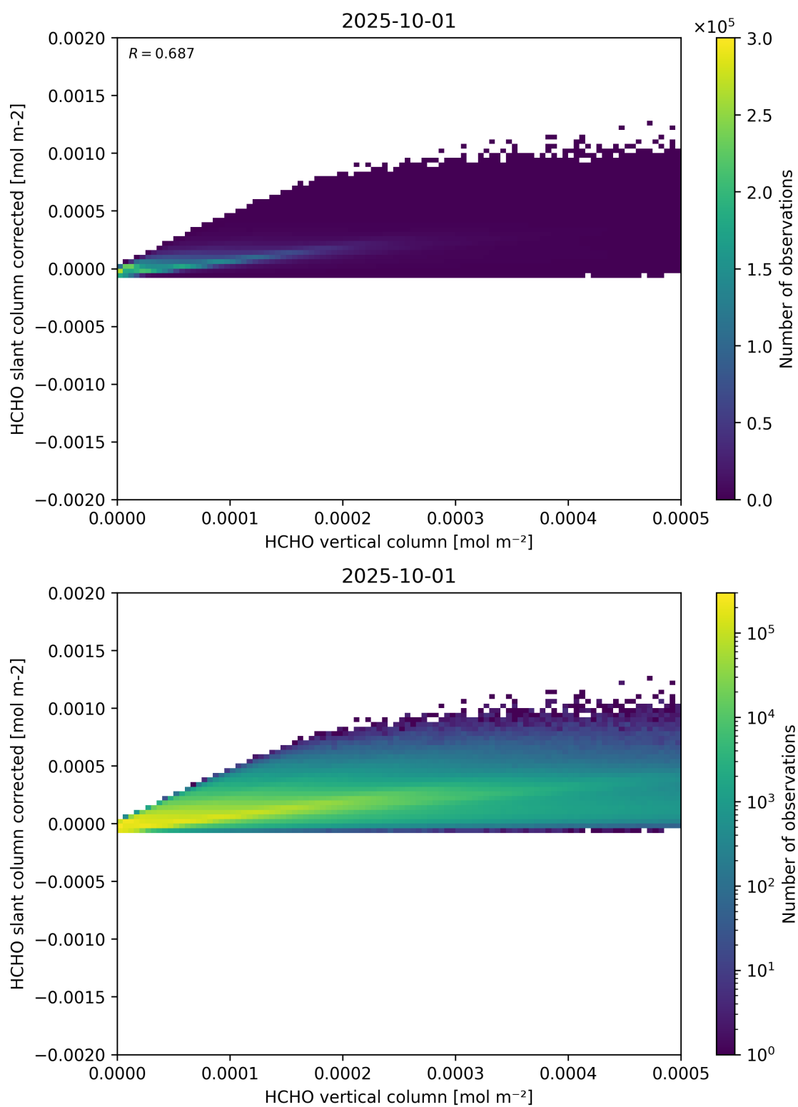
Figure 127: Scatter density plot of “HCHO vertical column” against “HCHO slant column corrected” for 2025-10-01 to 2025-10-02.
