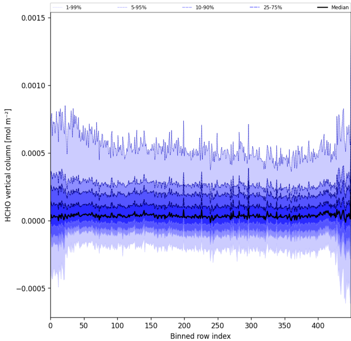
Figure 49: Along track statistics of “HCHO vertical column” for 2025-10-01 to 2025-10-02
