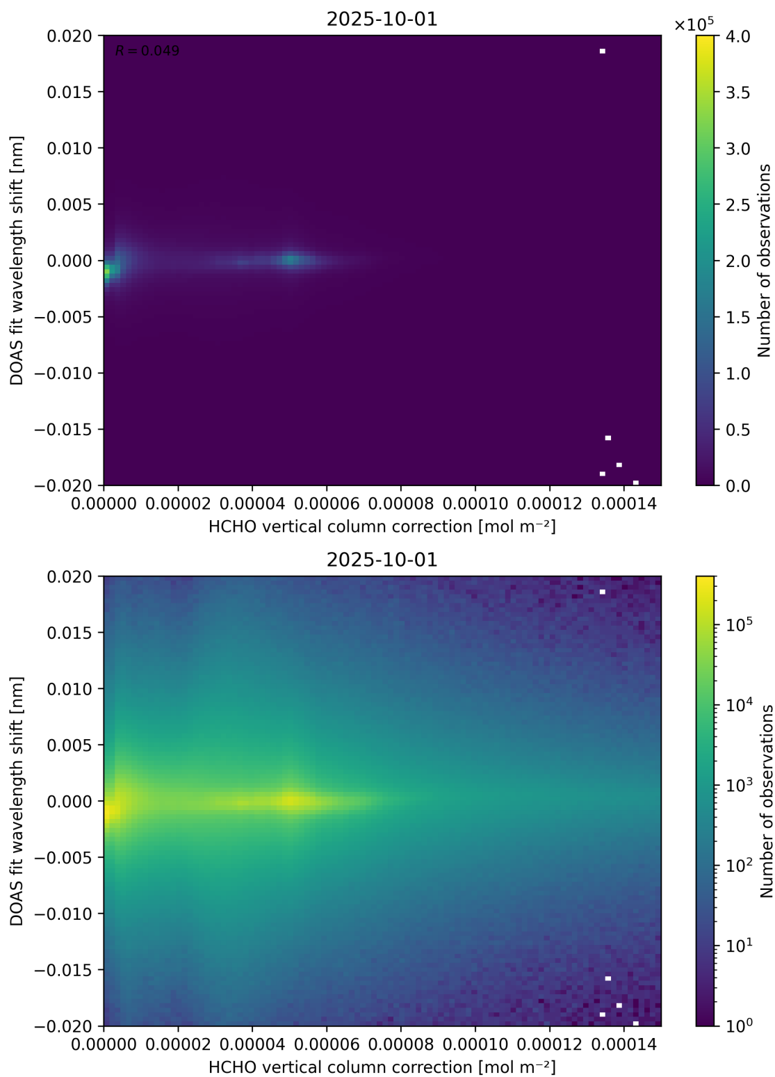
Figure 113: Scatter density plot of “HCHO vertical column correction” against “DOAS fit wavelength shift” for 2025-10-01 to 2025-10-02.
