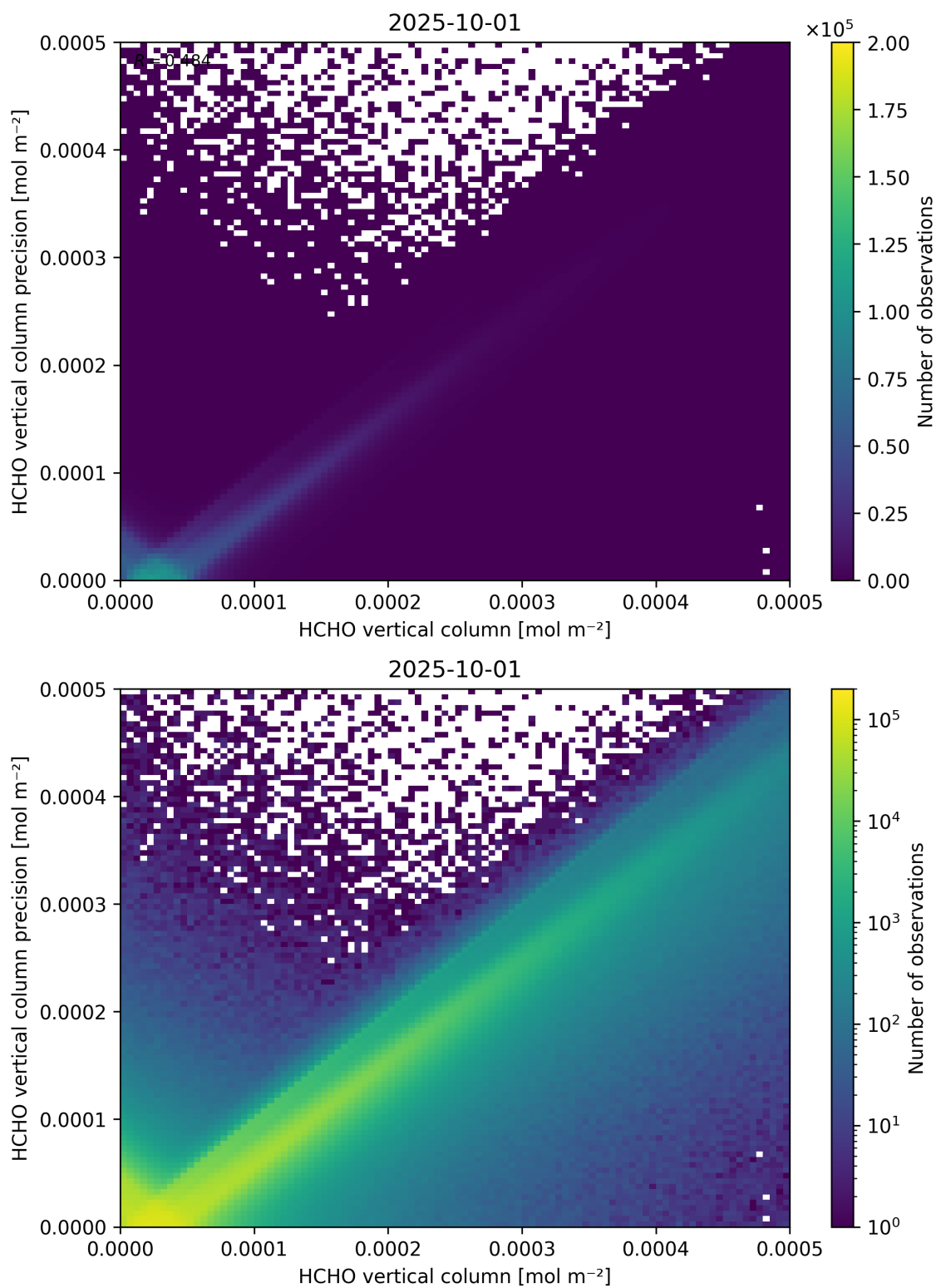
Figure 134: Scatter density plot of “HCHO vertical column” against “HCHO vertical column precision” for 2025-10-01 to 2025-10-02.
