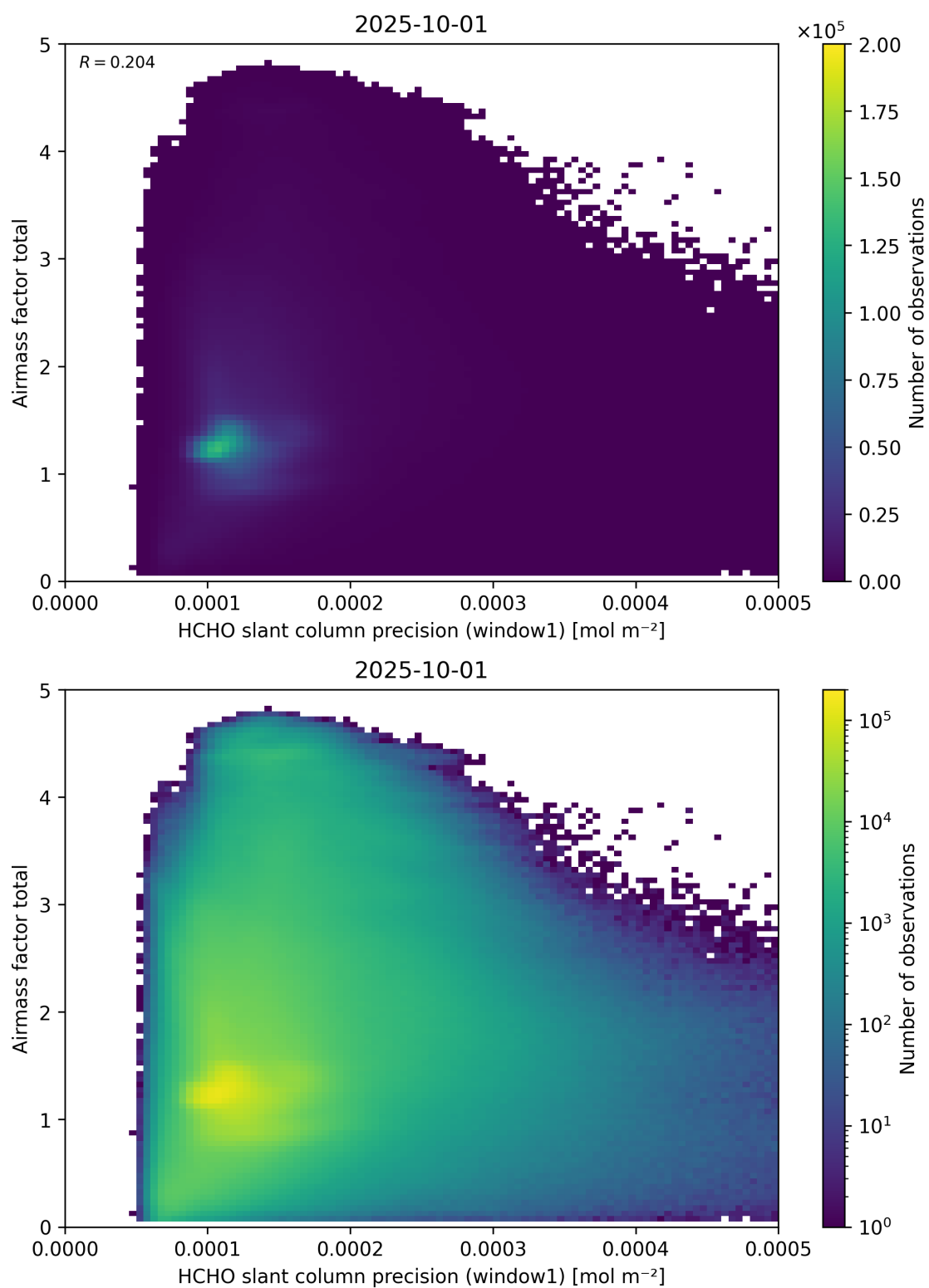
Figure 94: Scatter density plot of “HCHO slant column precision (window1)” against “Airmass factor total” for 2025-10-01 to 2025-10-02.
