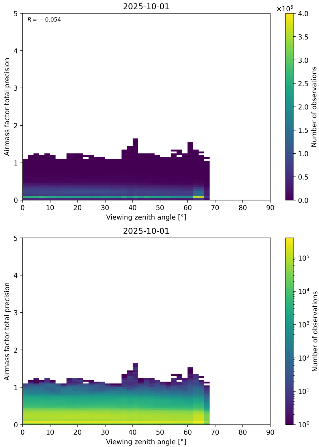
Figure 191: Scatter density plot of “Viewing zenith angle” against “Airmass factor total precision” for 2025-10-01 to 2025-10-02.
