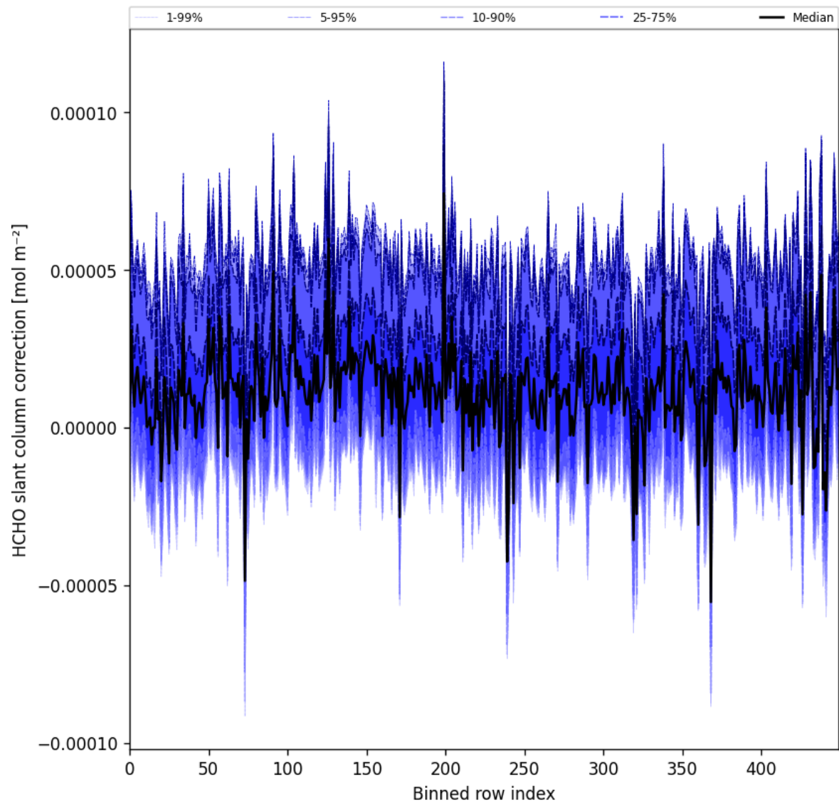
Figure 61: Along track statistics of “HCHO slant column correction” for 2025-10-01 to 2025-10-02
