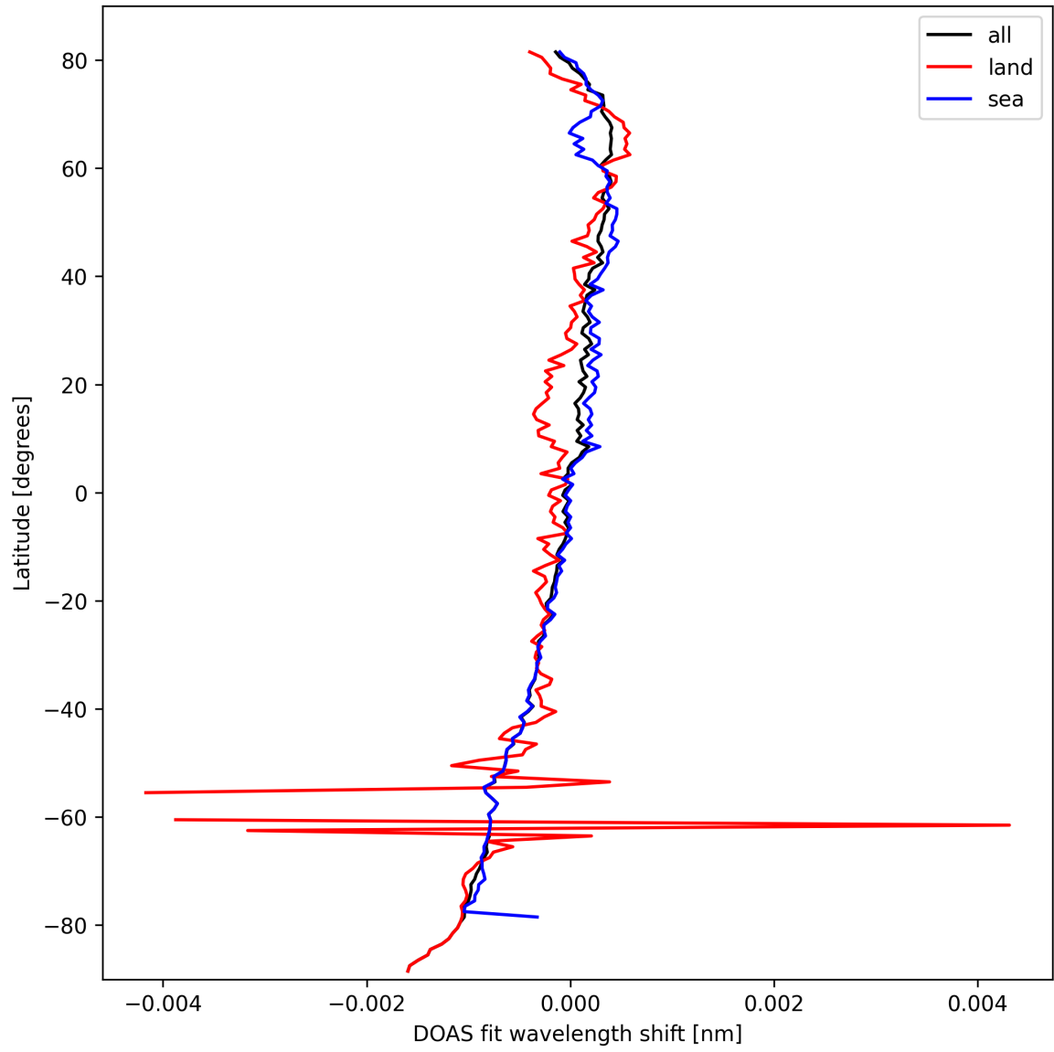
Figure 30: Zonal average of “DOAS fit wavelength shift” for 2025-10-01 to 2025-10-02.
