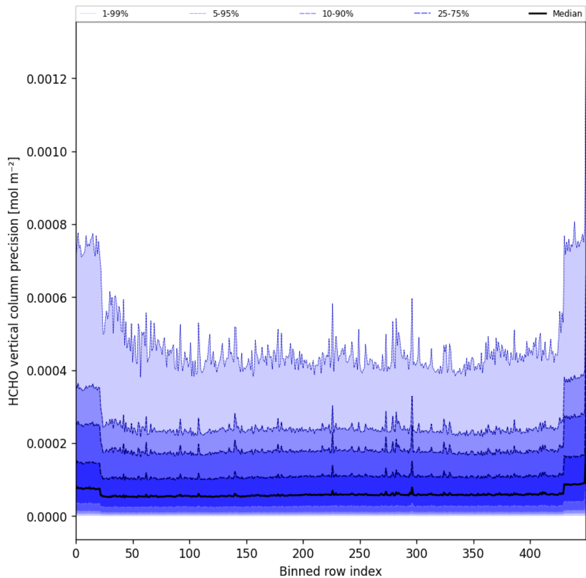
Figure 50: Along track statistics of “HCHO vertical column precision” for 2025-10-01 to 2025-10-02
