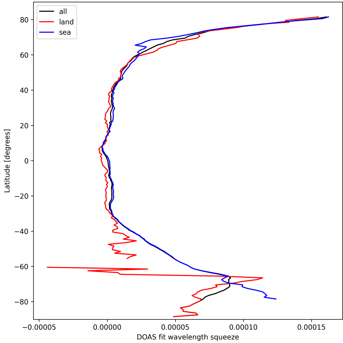
Figure 31: Zonal average of “DOAS fit wavelength squeeze” for 2025-10-01 to 2025-10-02.
