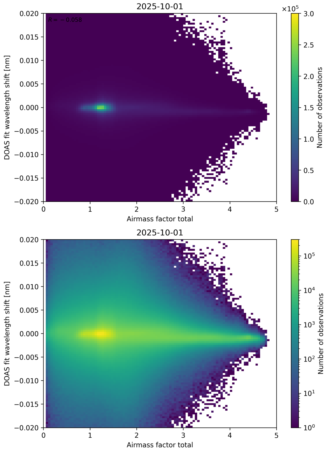
Figure 98: Scatter density plot of “Airmass factor total” against “DOAS fit wavelength shift” for 2025-10-01 to 2025-10-02.
