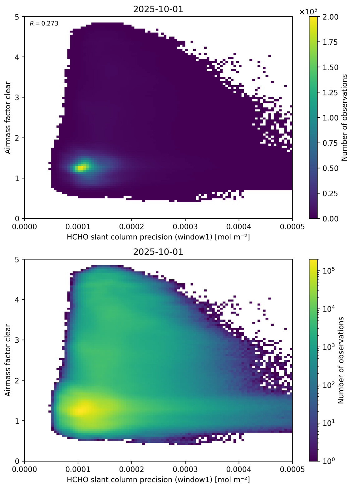
Figure 91: Scatter density plot of “HCHO slant column precision (window1)” against “Airmass factor clear” for 2025-10-01 to 2025-10-02.
