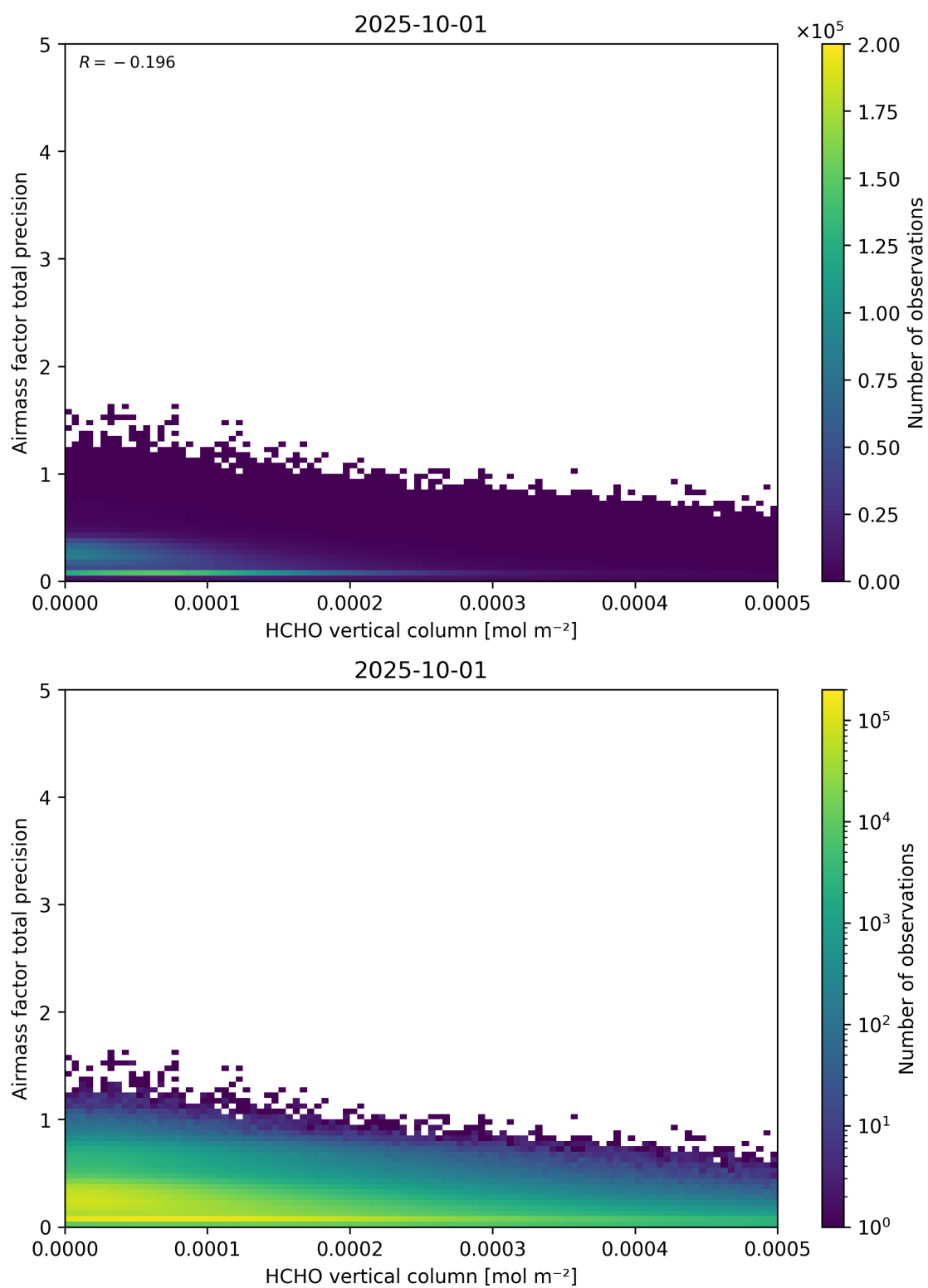
Figure 132: Scatter density plot of “HCHO vertical column” against “Airmass factor total precision” for 2025-10-01 to 2025-10-02.
