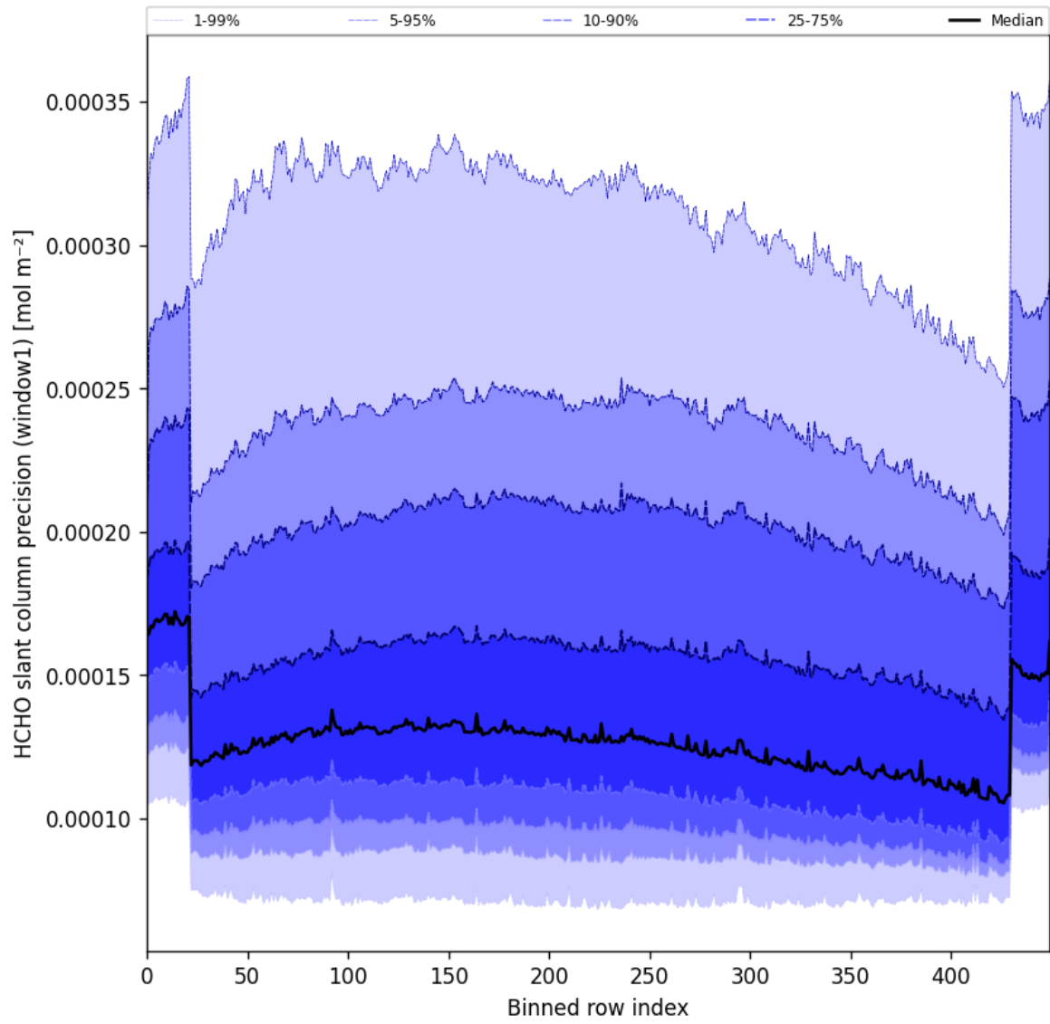
Figure 53: Along track statistics of “HCHO slant column precision (window1)” for 2025-10-01 to 2025-10-02
