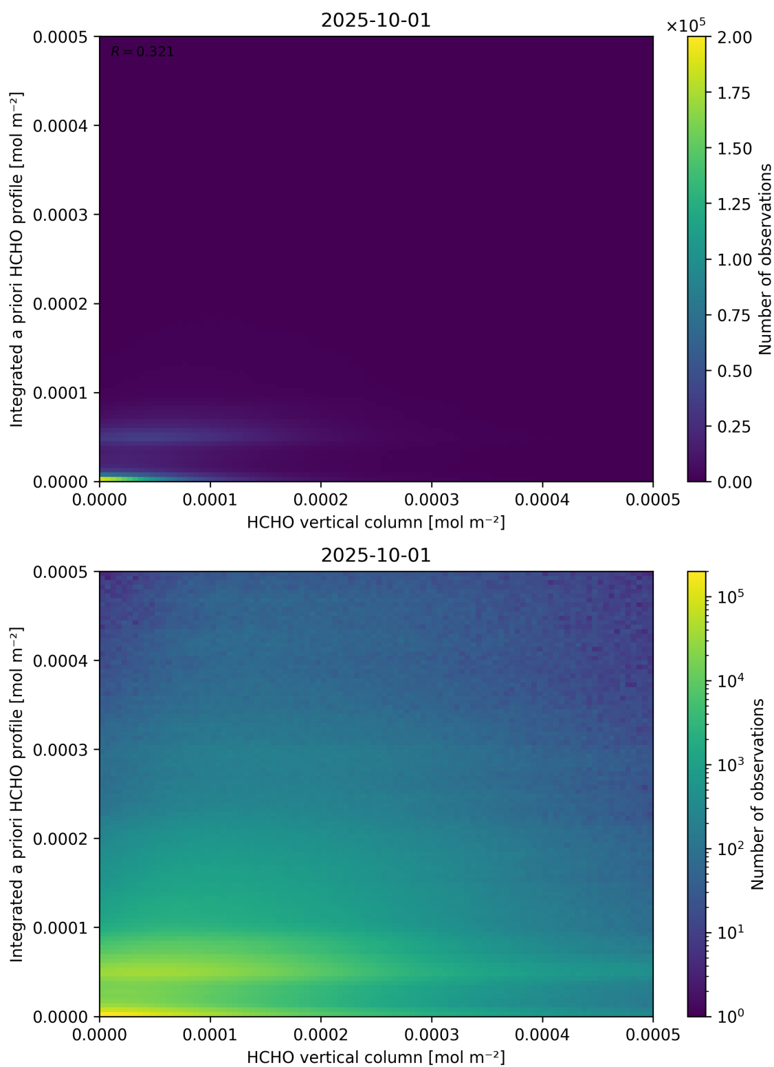
Figure 135: Scatter density plot of “HCHO vertical column” against “Integrated a priori HCHO profile” for 2025-10-01 to 2025-10-02.
