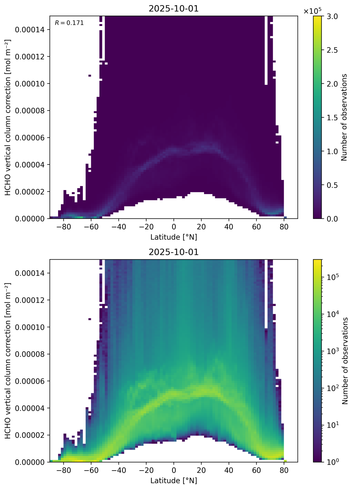
Figure 164: Scatter density plot of “Latitude” against “HCHO vertical column correction” for 2025-10-01 to 2025-10-02.
