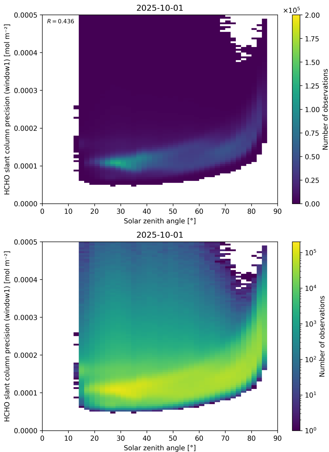
Figure 174: Scatter density plot of “Solar zenith angle” against “HCHO slant column precision (window1)” for 2025-10-01 to 2025-10-02.
