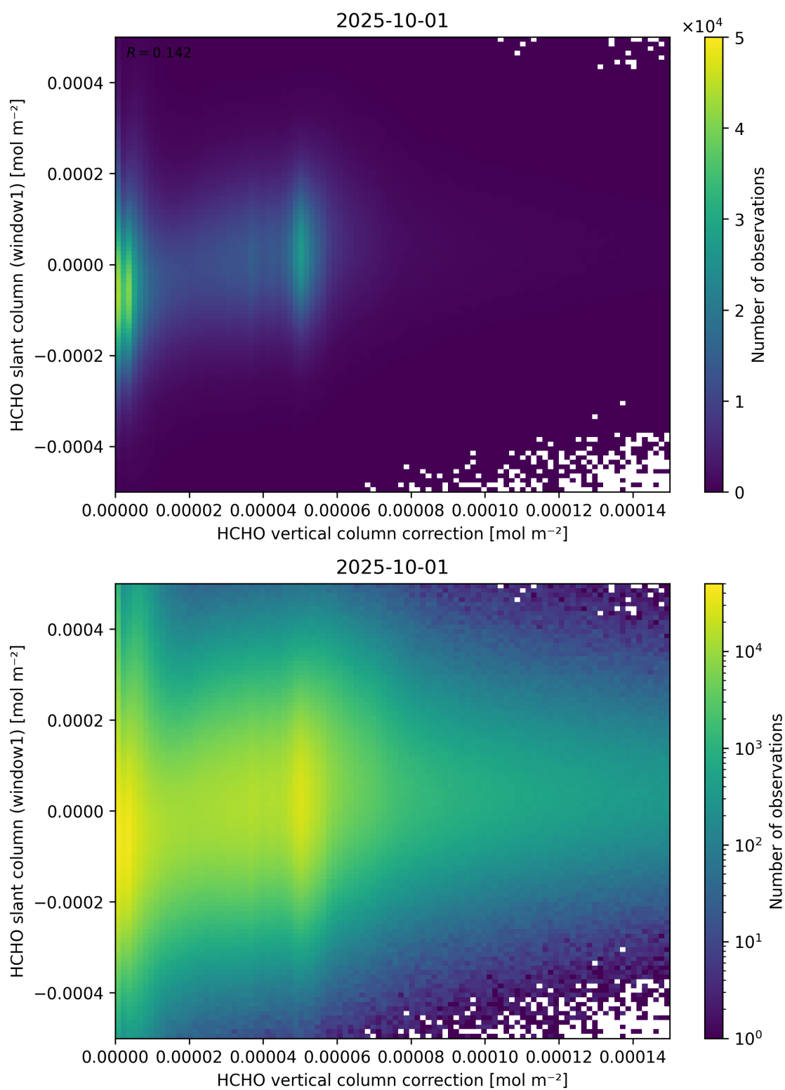
Figure 118: Scatter density plot of “HCHO vertical column correction” against “HCHO slant column (window1)” for 2025-10-01 to 2025-10-02.
