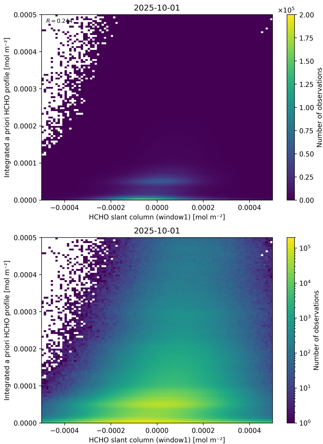
Figure 87: Scatter density plot of “HCHO slant column (window1)” against “Integrated a priori HCHO profile” for 2025-10-01 to 2025-10-02.
