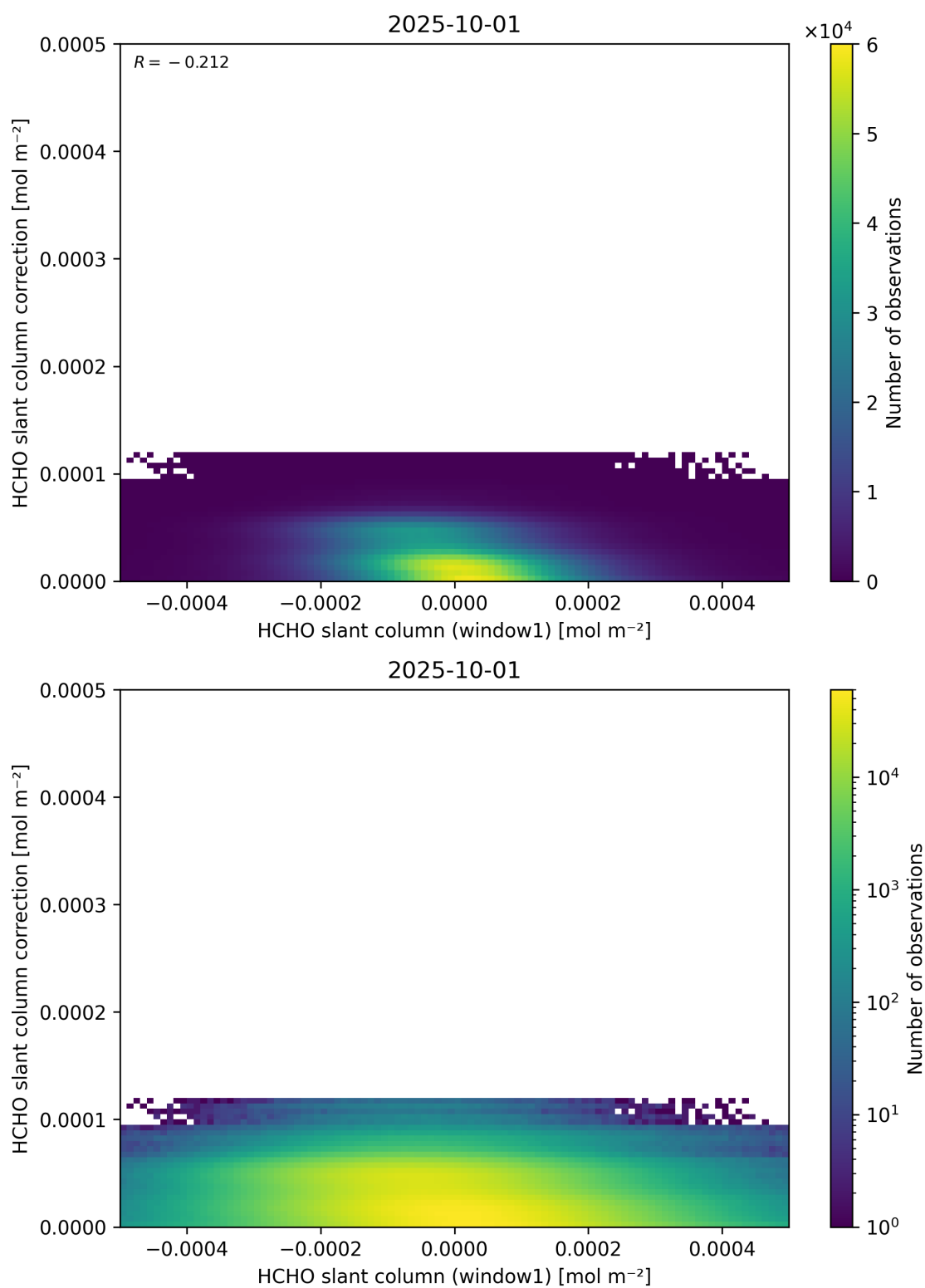
Figure 83: Scatter density plot of “HCHO slant column (window1)” against “HCHO slant column correction” for 2025-10-01 to 2025-10-02.
