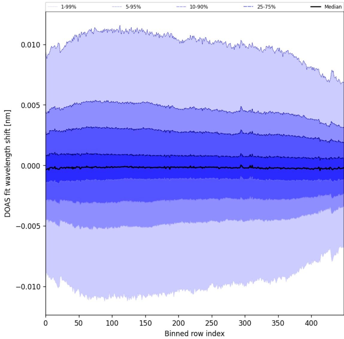
Figure 58: Along track statistics of “DOAS fit wavelength shift” for 2025-10-01 to 2025-10-02
