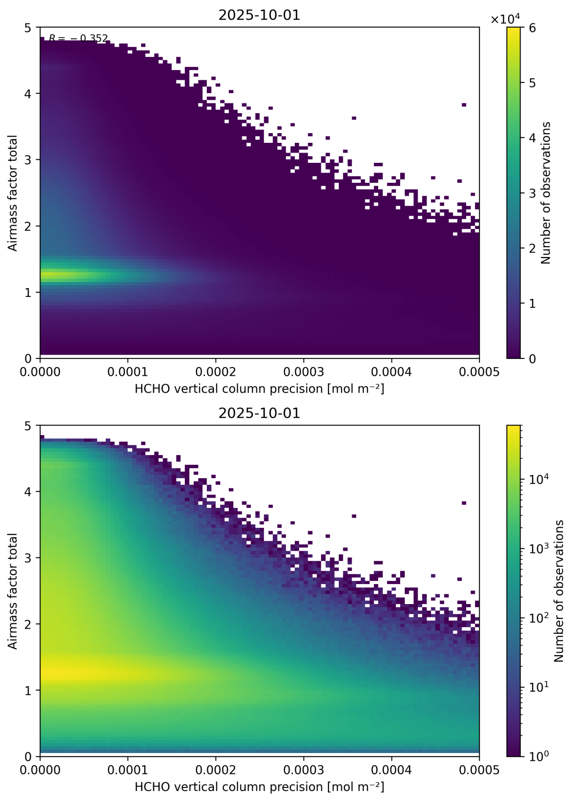
Figure 144: Scatter density plot of “HCHO vertical column precision” against “Airmass factor total” for 2025-10-01 to 2025-10-02.
