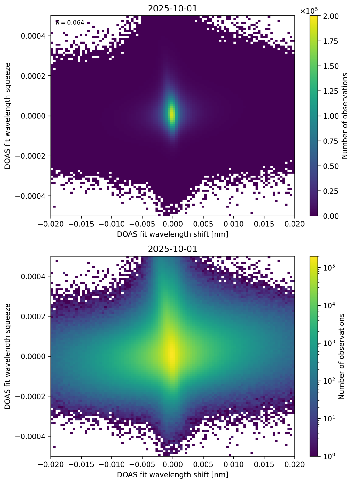
Figure 65: Scatter density plot of “DOAS fit wavelength shift” against “DOAS fit wavelength squeeze” for 2025-10-01 to 2025-10-02.
