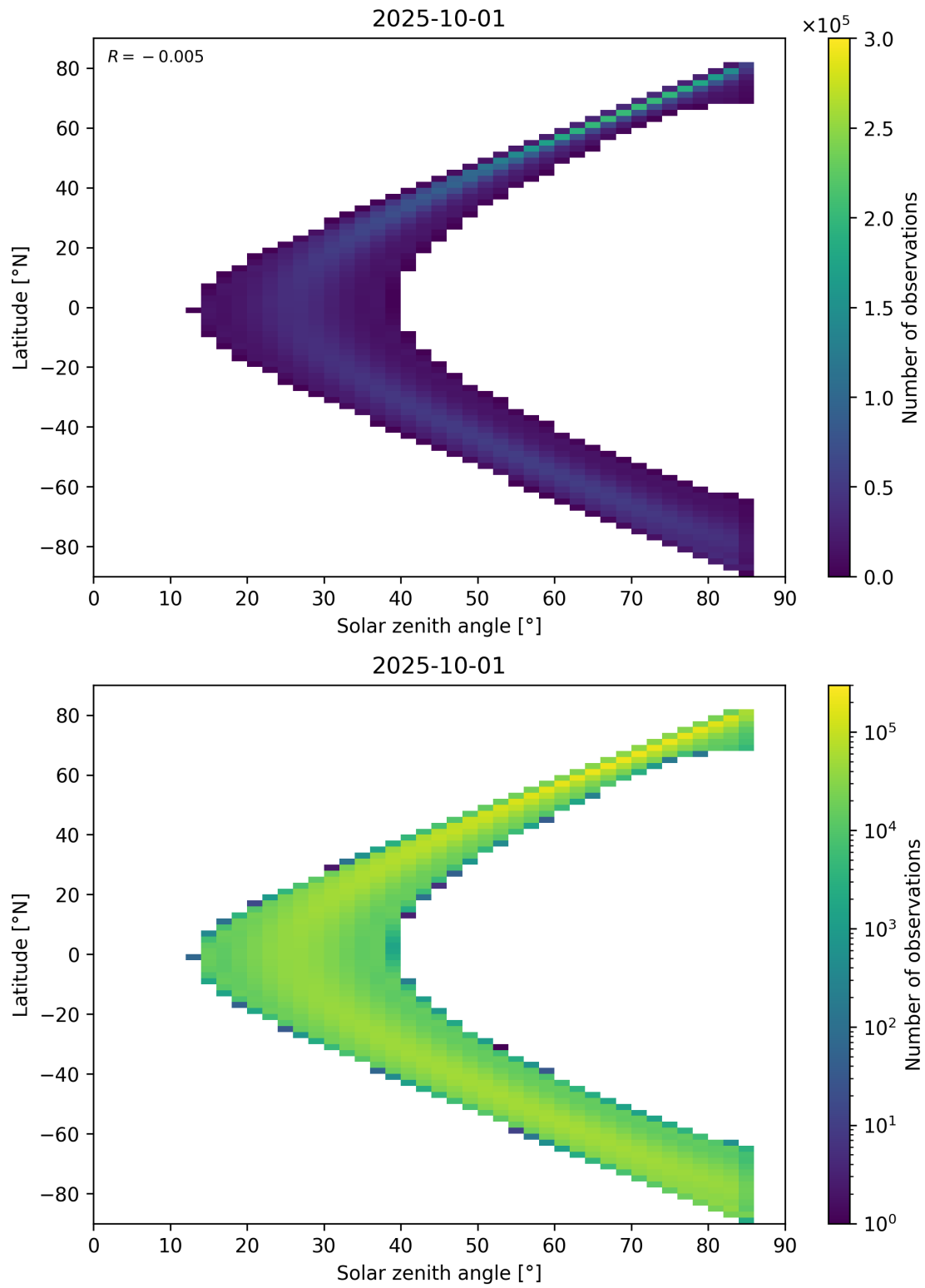
Figure 181: Scatter density plot of “Solar zenith angle” against “Latitude” for 2025-10-01 to 2025-10-02.
