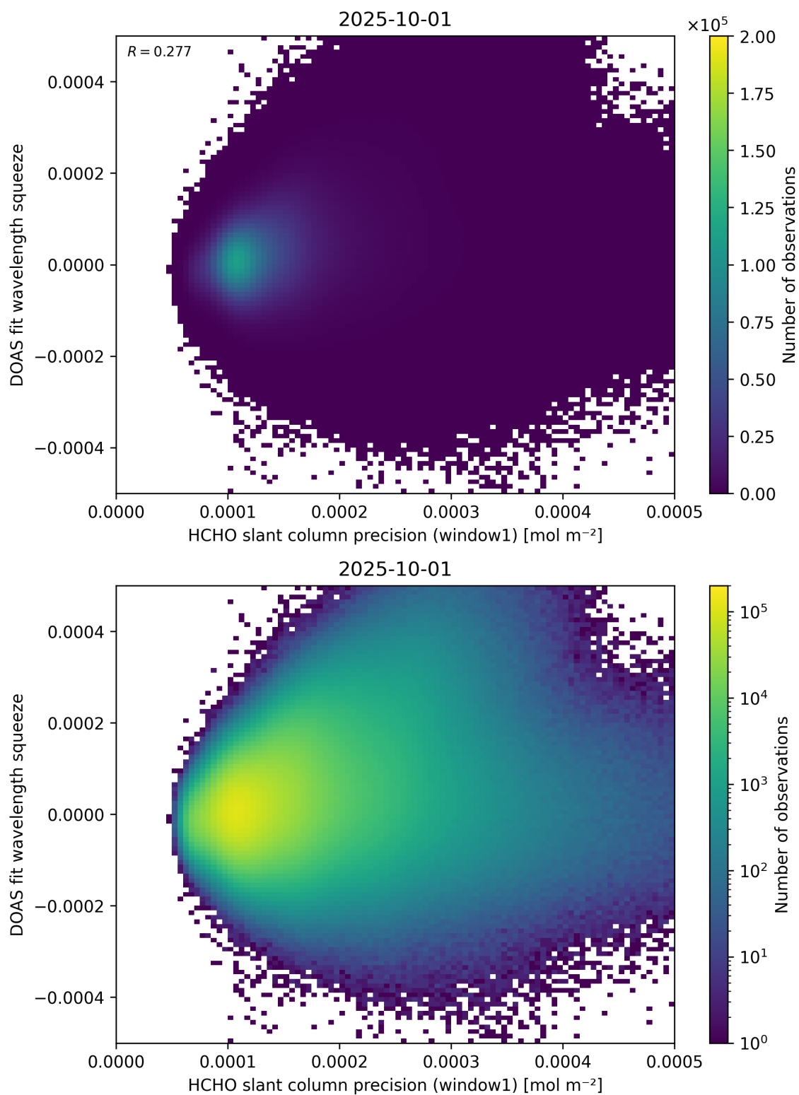
Figure 90: Scatter density plot of “HCHO slant column precision (window1)” against “DOAS fit wavelength squeeze” for 2025-10-01 to 2025-10-02.
