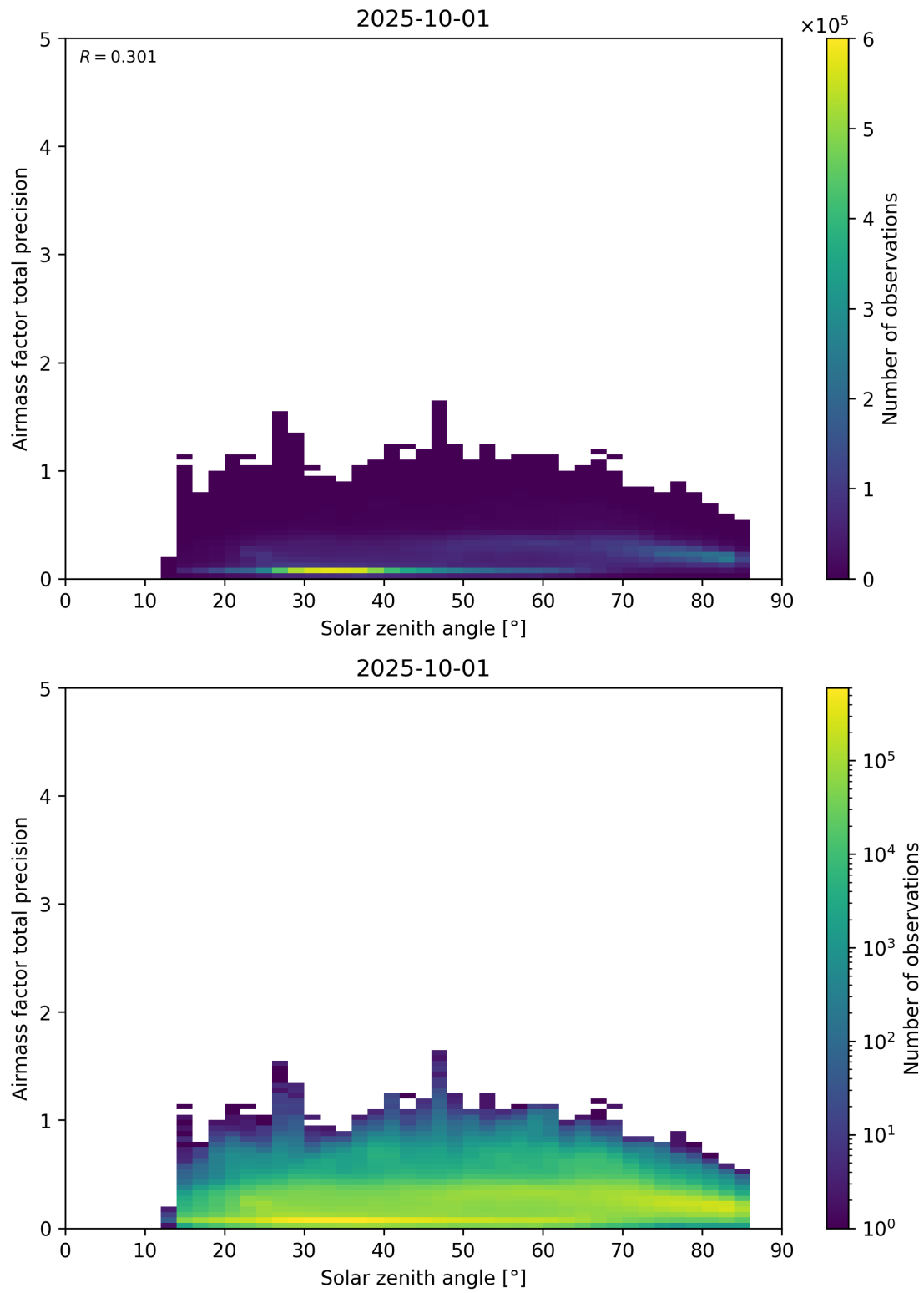
Figure 176: Scatter density plot of “Solar zenith angle” against “Airmass factor total precision” for 2025-10-01 to 2025-10-02.
