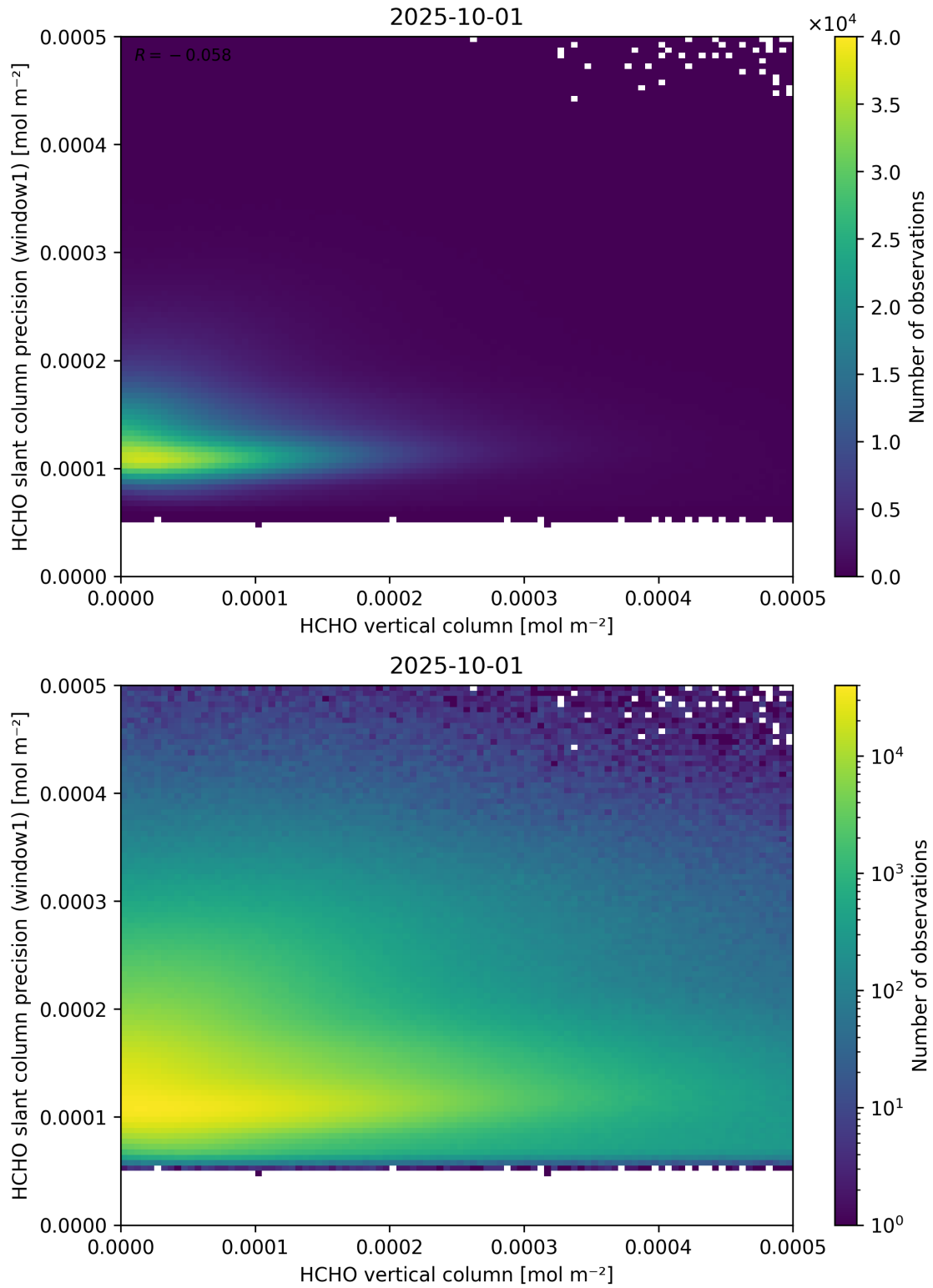
Figure 130: Scatter density plot of “HCHO vertical column” against “HCHO slant column precision (window1)” for 2025-10-01 to 2025-10-02.
