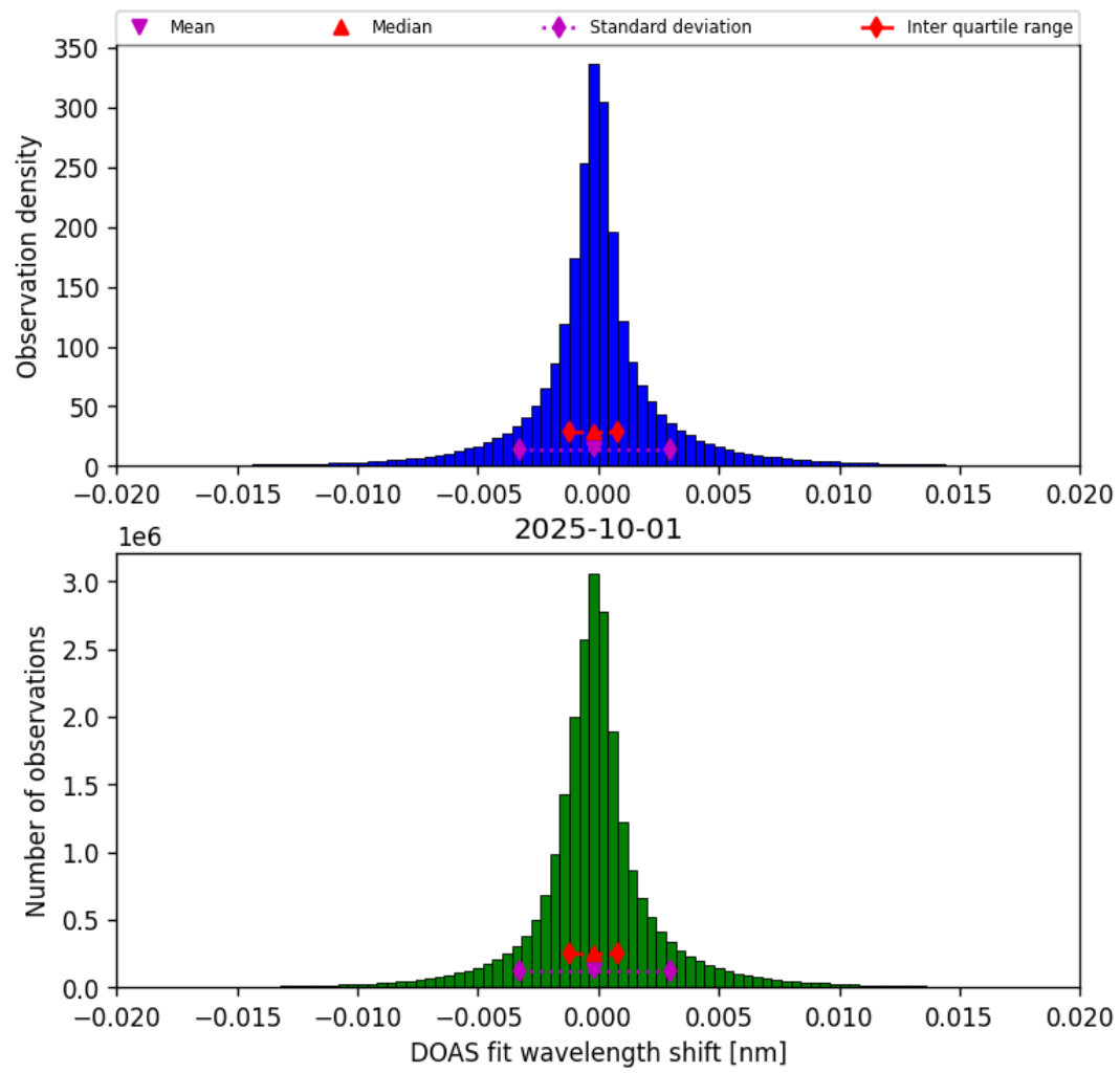
Figure 44: Histogram of “DOAS fit wavelength shift” for 2025-10-01 to 2025-10-02
