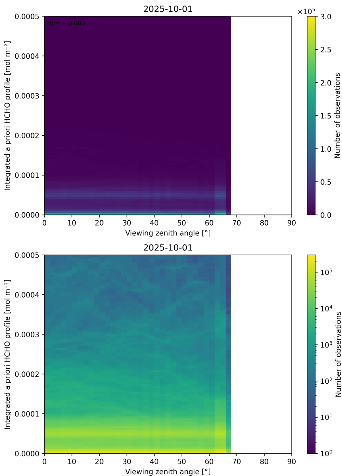
Figure 195: Scatter density plot of “Viewing zenith angle” against “Integrated a priori HCHO profile” for 2025-10-01 to 2025-10-02.
