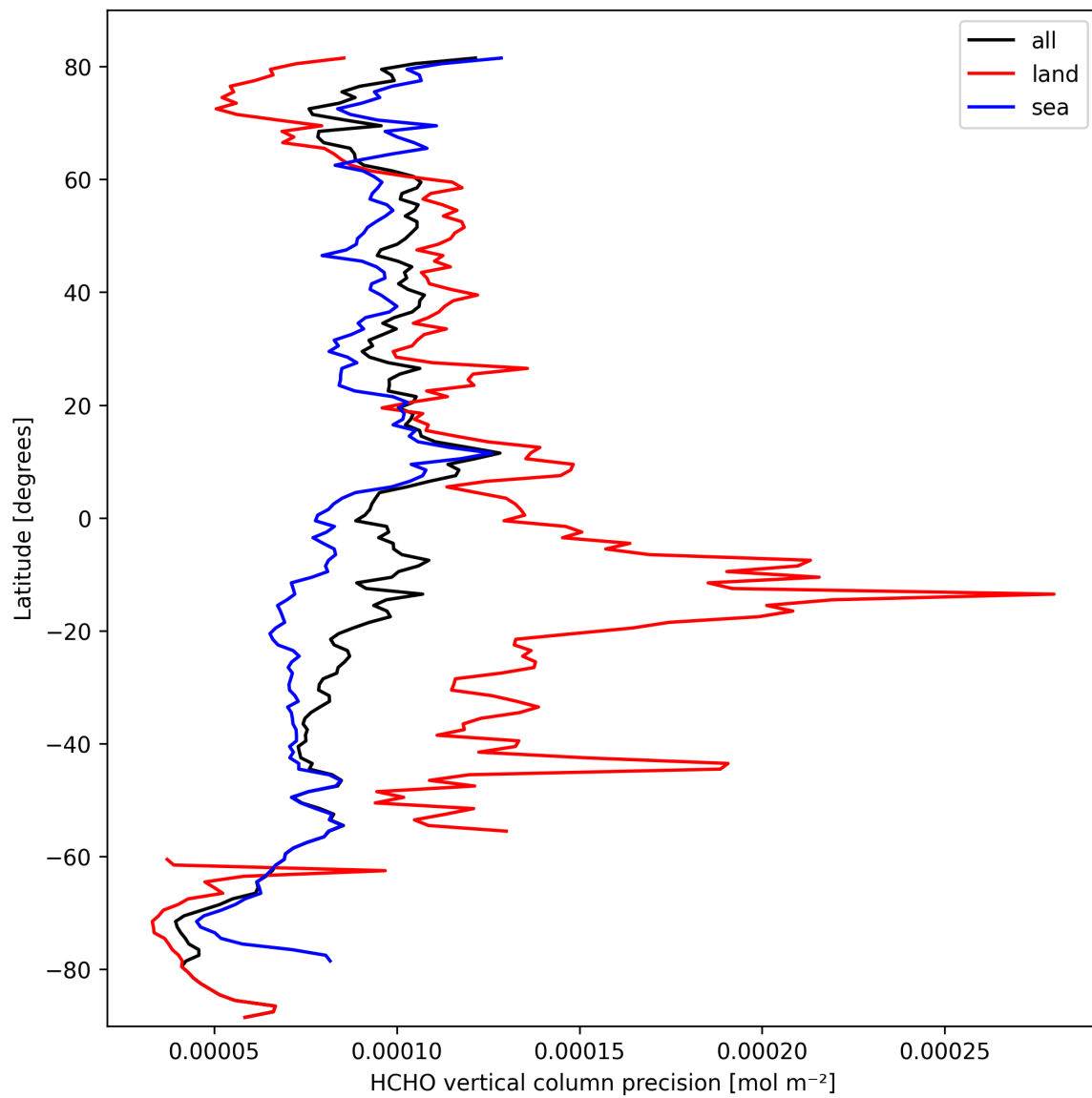
Figure 22: Zonal average of “HCHO vertical column precision” for 2025-10-01 to 2025-10-02.
