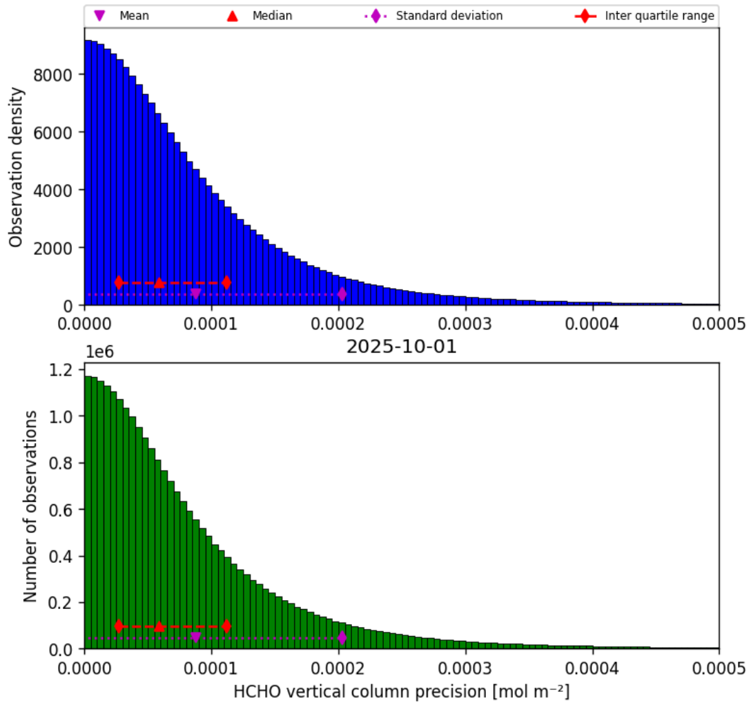
Figure 36: Histogram of “HCHO vertical column precision” for 2025-10-01 to 2025-10-02
