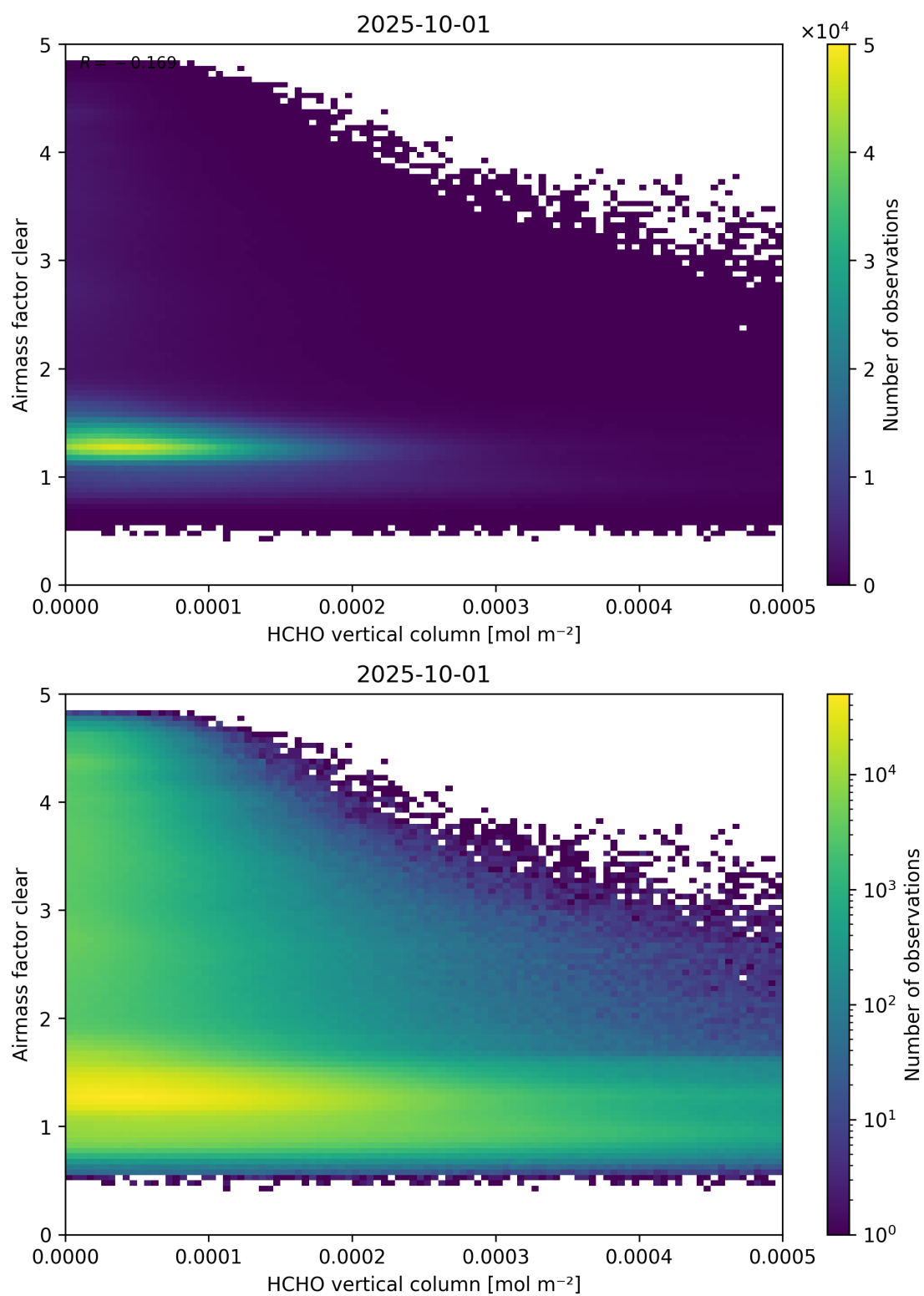
Figure 126: Scatter density plot of “HCHO vertical column” against “Airmass factor clear” for 2025-10-01 to 2025-10-02.
