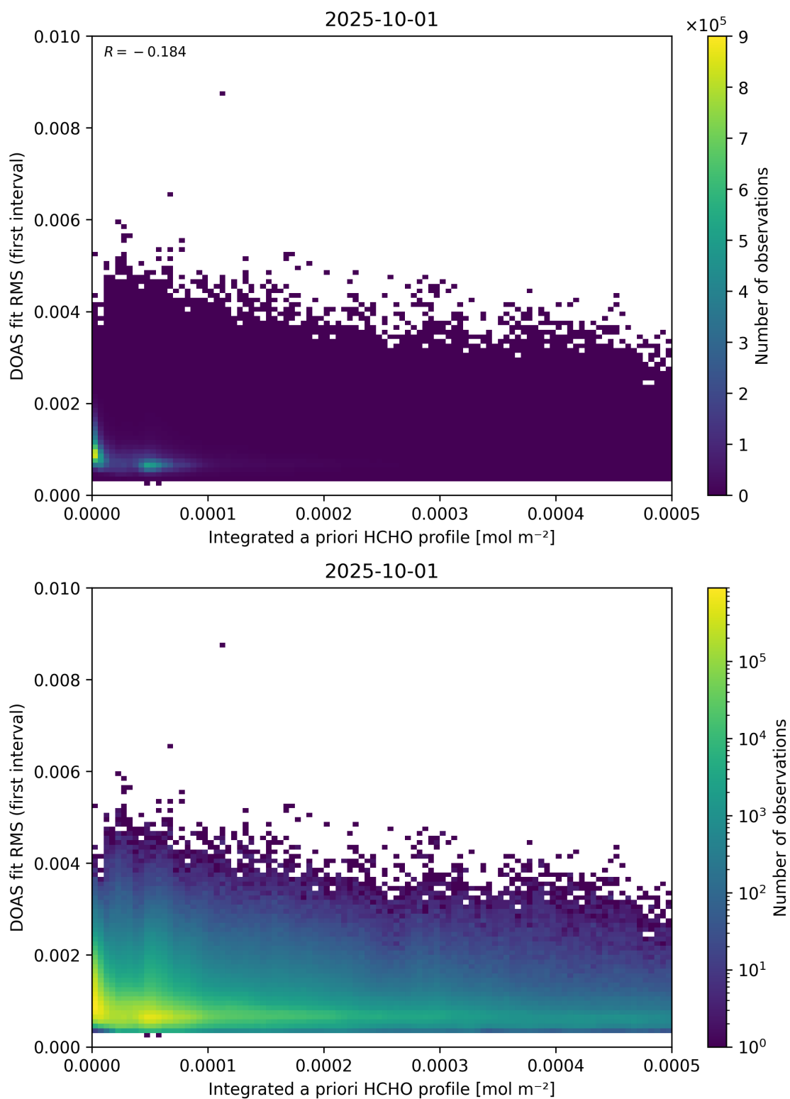
Figure 148: Scatter density plot of “Integrated a priori HCHO profile” against “DOAS fit RMS (first interval)” for 2025-10-01 to 2025-10-02.
