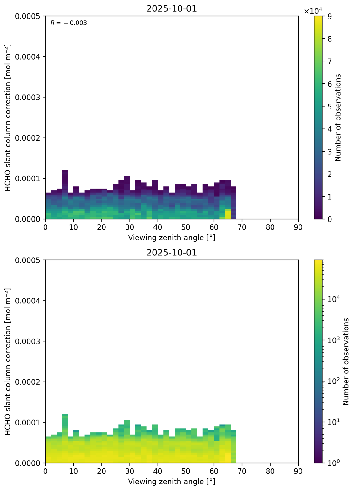
Figure 187: Scatter density plot of “Viewing zenith angle” against “HCHO slant column correction” for 2025-10-01 to 2025-10-02.
