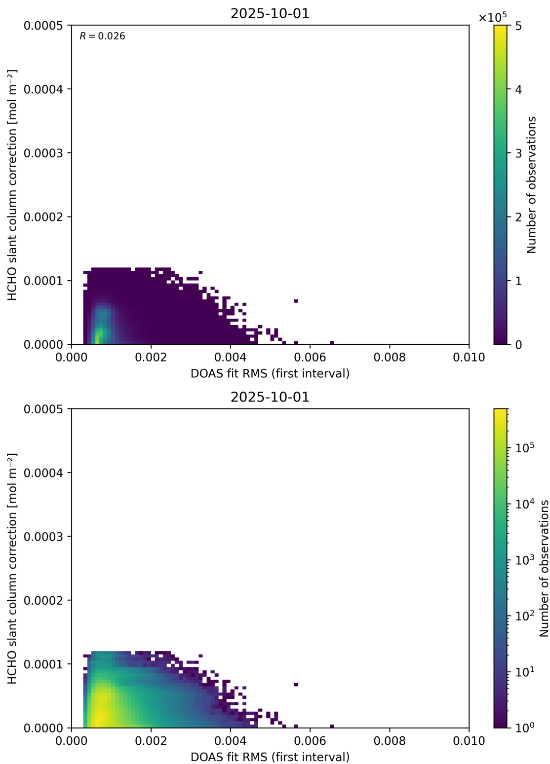
Figure 63: Scatter density plot of “DOAS fit RMS (first interval)” against “HCHO slant column correction” for 2025-10-01 to 2025-10-02.
