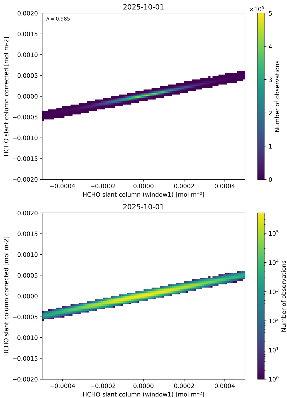
Figure 82: Scatter density plot of “HCHO slant column (window1)” against “HCHO slant column corrected” for 2025-10-01 to 2025-10-02.
