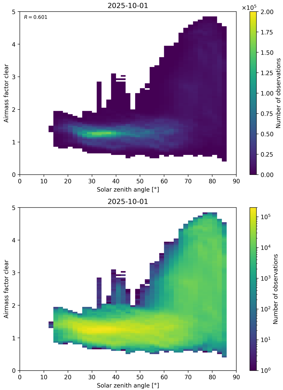
Figure 170: Scatter density plot of “Solar zenith angle” against “Airmass factor clear” for 2025-10-01 to 2025-10-02.
