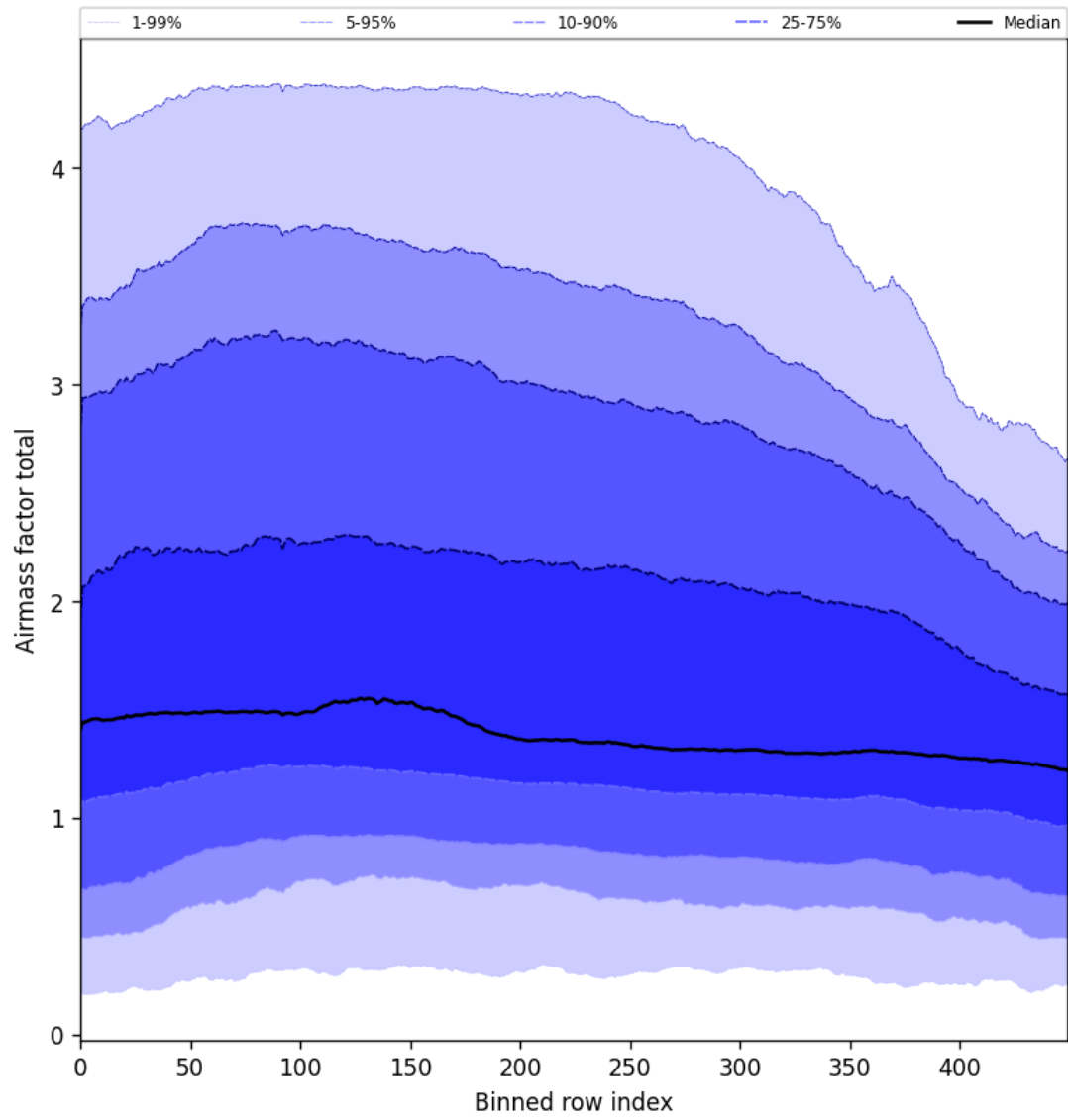
Figure 54: Along track statistics of “Airmass factor total” for 2025-10-01 to 2025-10-02
