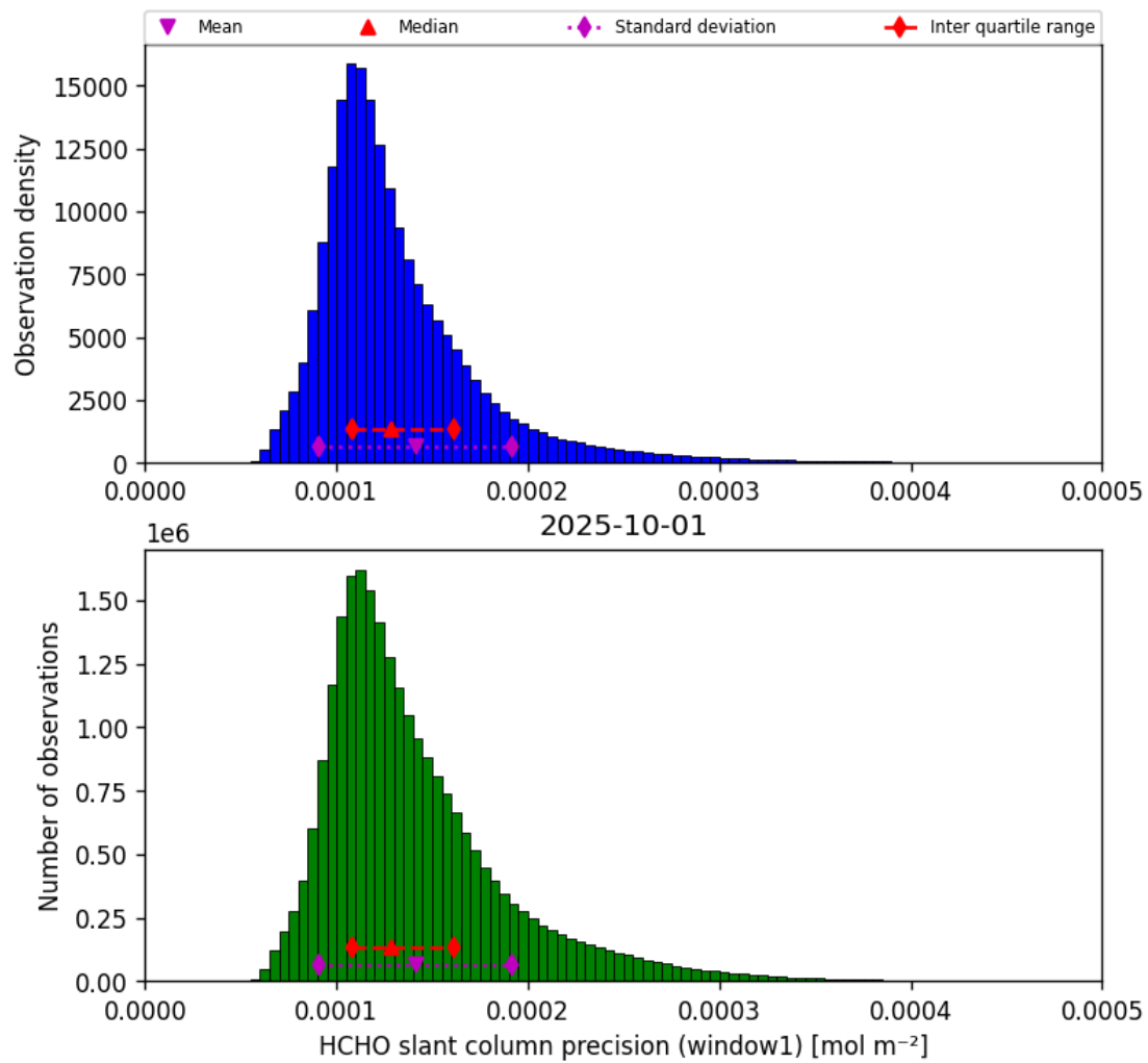
Figure 39: Histogram of “HCHO slant column precision (window1)” for 2025-10-01 to 2025-10-02
