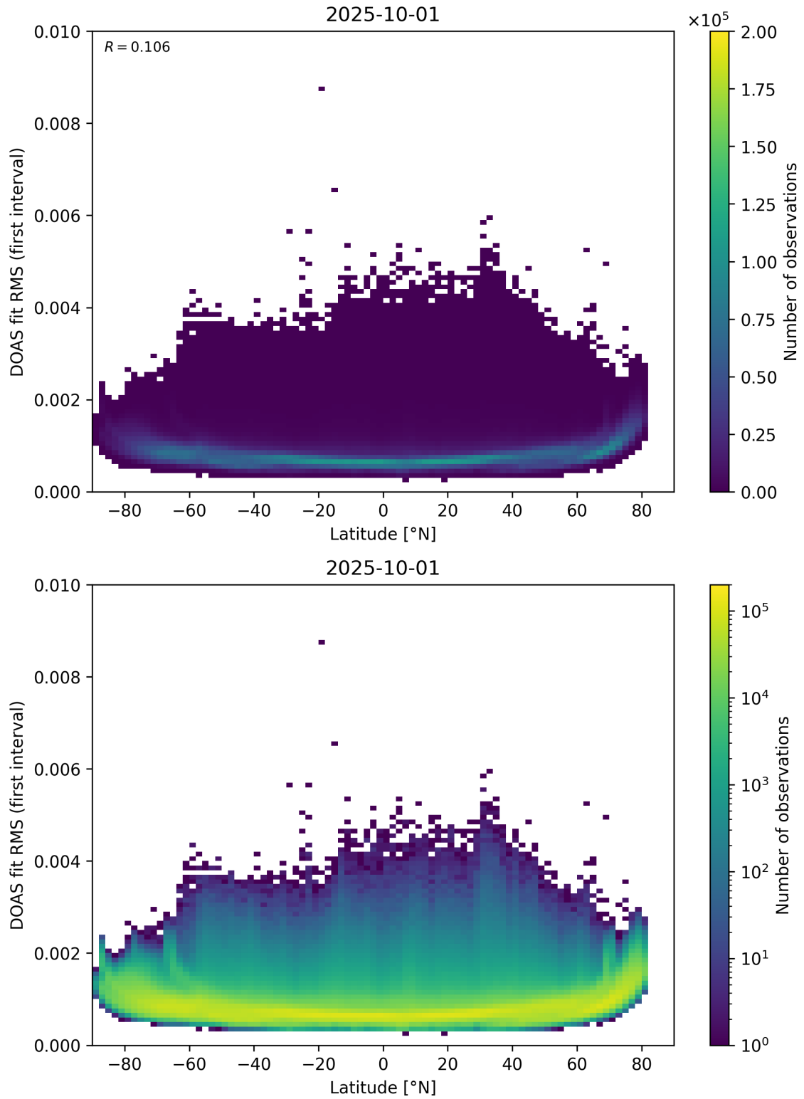
Figure 153: Scatter density plot of “Latitude” against “DOAS fit RMS (first interval)” for 2025-10-01 to 2025-10-02.
