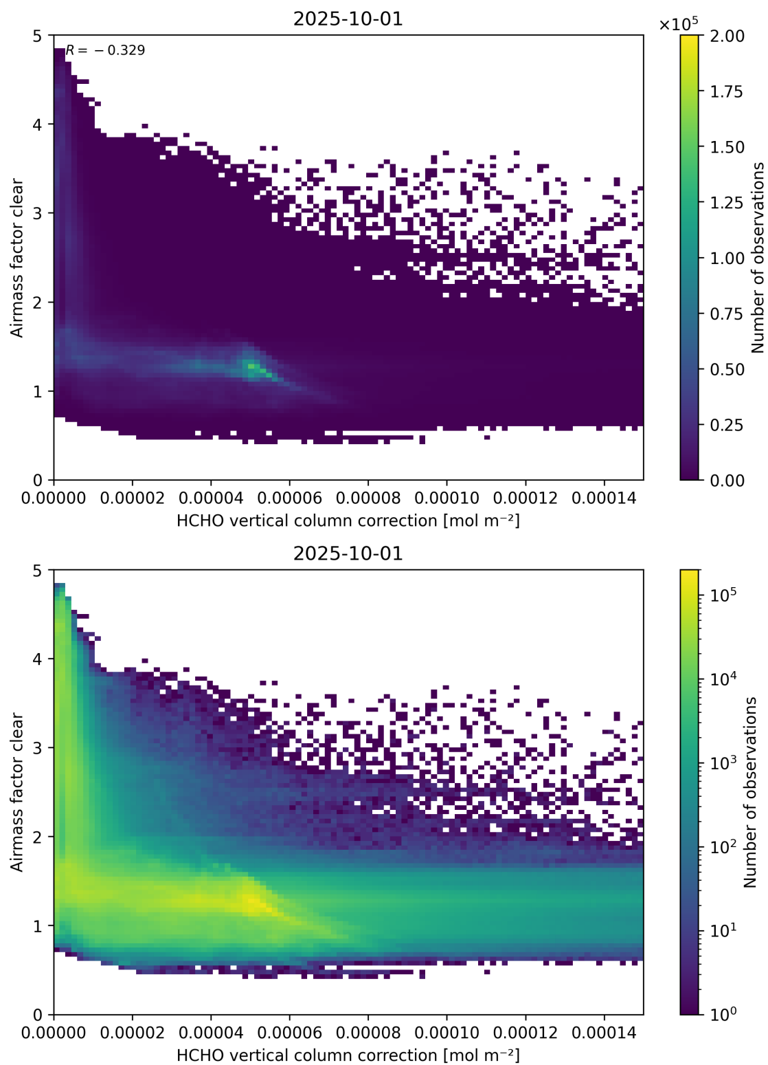
Figure 115: Scatter density plot of “HCHO vertical column correction” against “Airmass factor clear” for 2025-10-01 to 2025-10-02.
