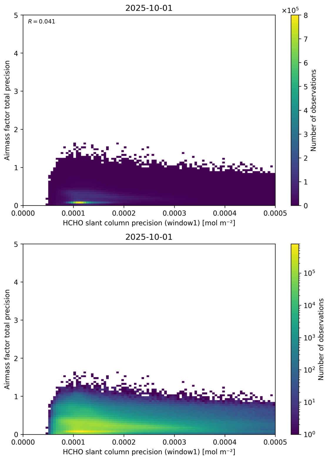
Figure 95: Scatter density plot of “HCHO slant column precision (window1)” against “Airmass factor total precision” for 2025-10-01 to 2025-10-02.
