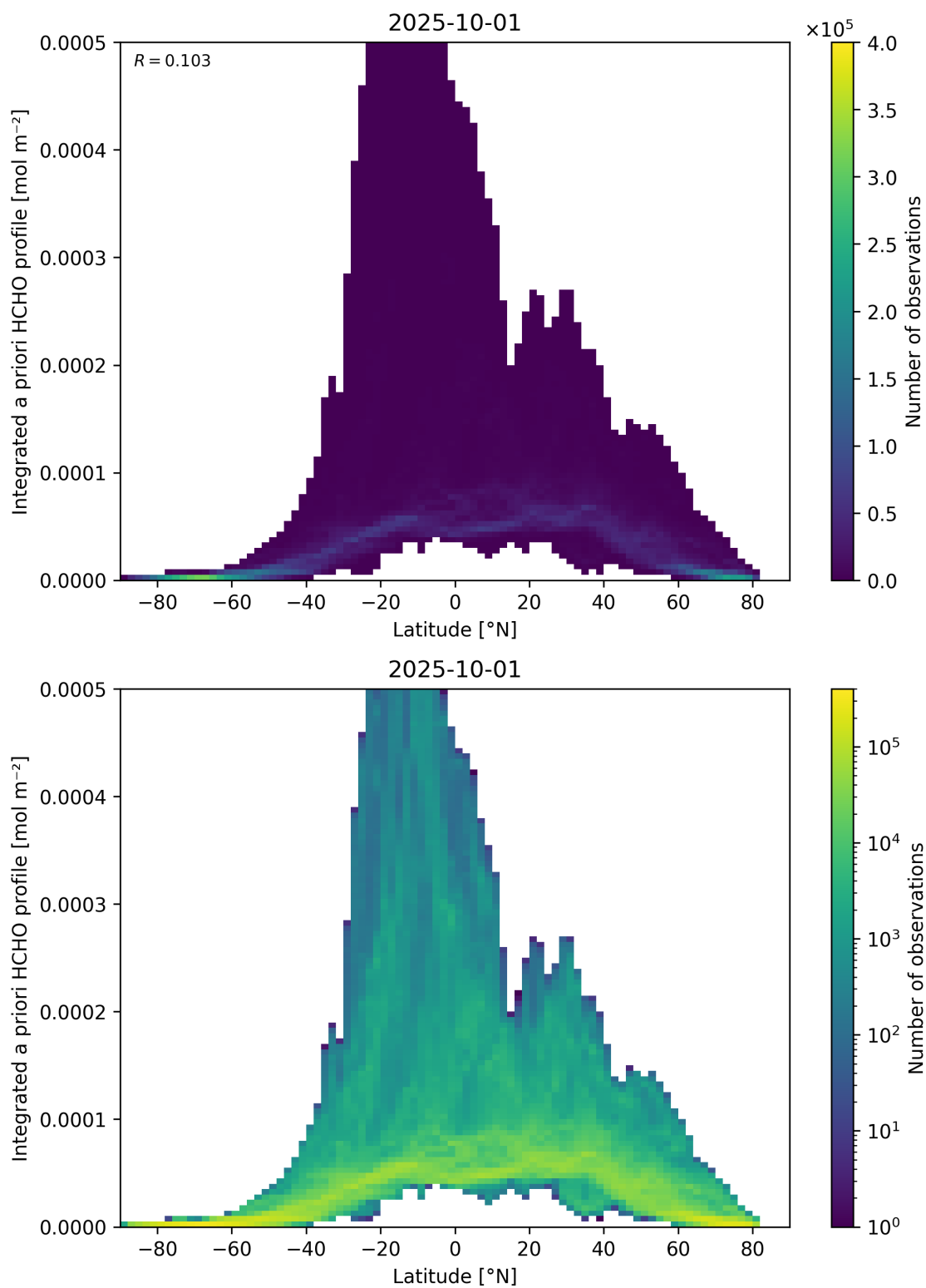
Figure 166: Scatter density plot of “Latitude” against “Integrated a priori HCHO profile” for 2025-10-01 to 2025-10-02.
