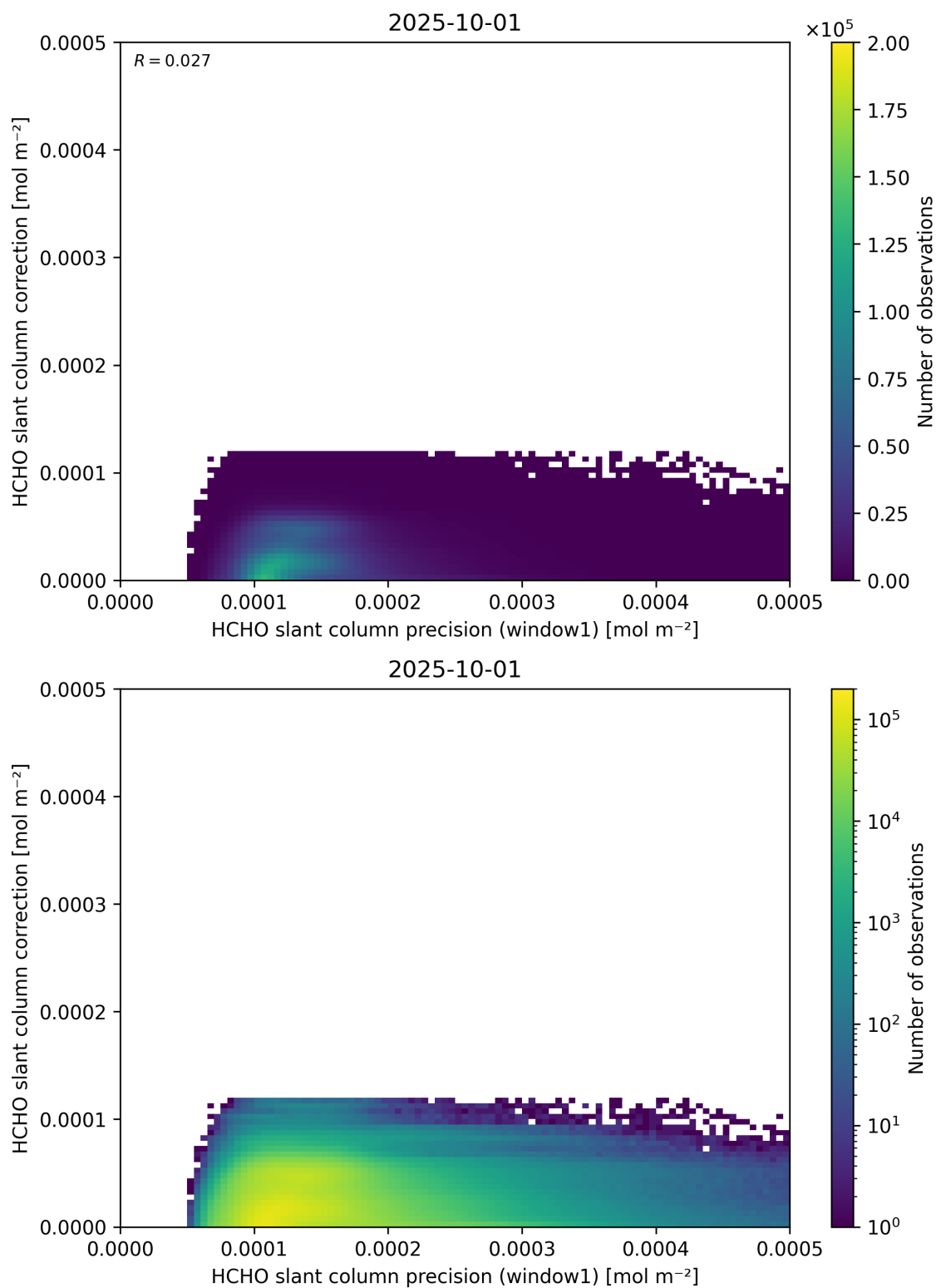
Figure 93: Scatter density plot of “HCHO slant column precision (window1)” against “HCHO slant column correction” for 2025-10-01 to 2025-10-02.
