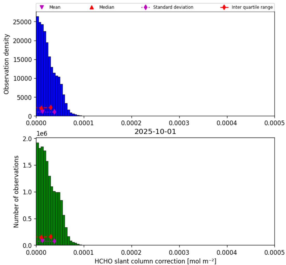
Figure 47: Histogram of “HCHO slant column correction” for 2025-10-01 to 2025-10-02
