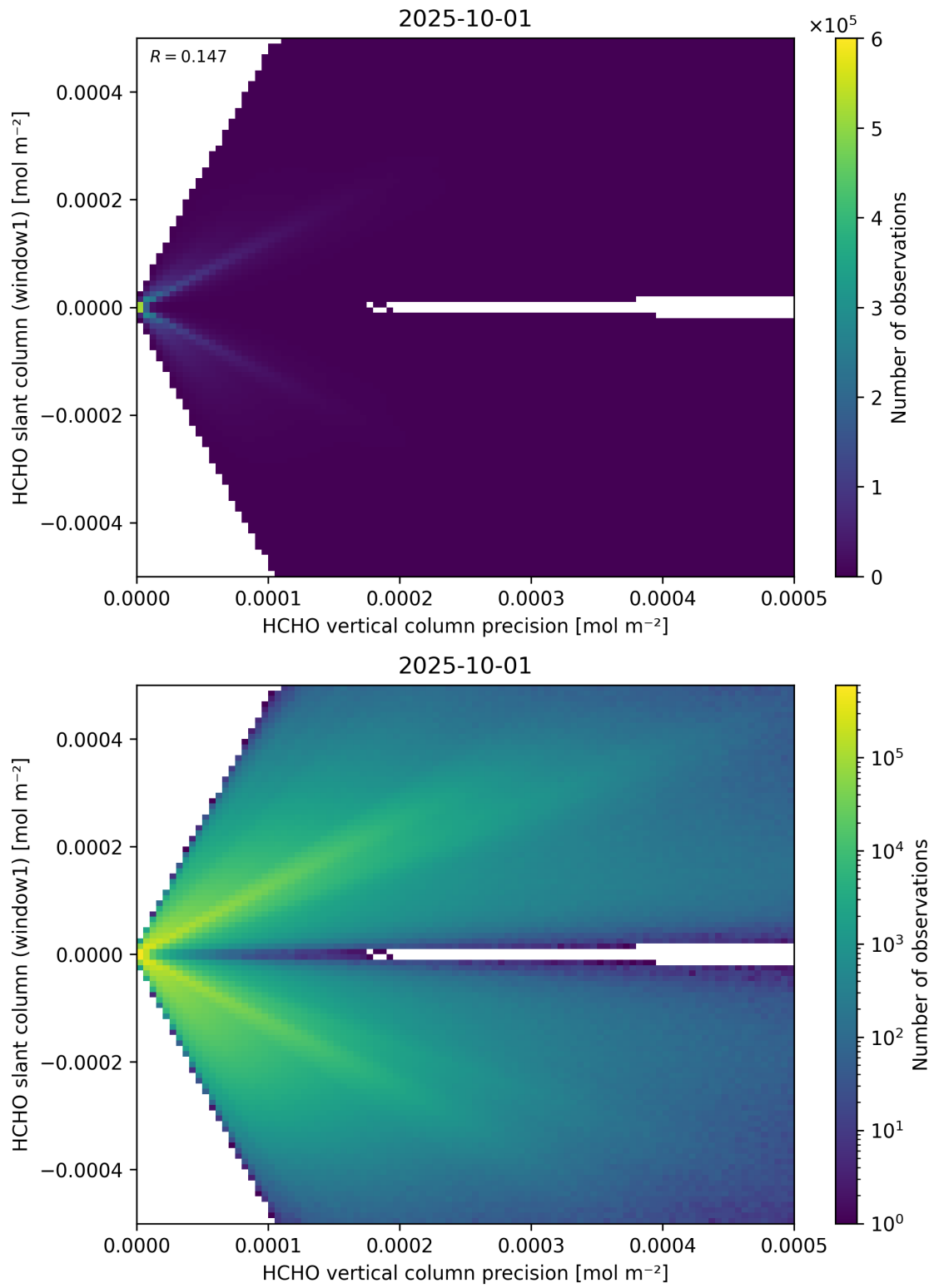
Figure 142: Scatter density plot of “HCHO vertical column precision” against “HCHO slant column (window1)” for 2025-10-01 to 2025-10-02.
