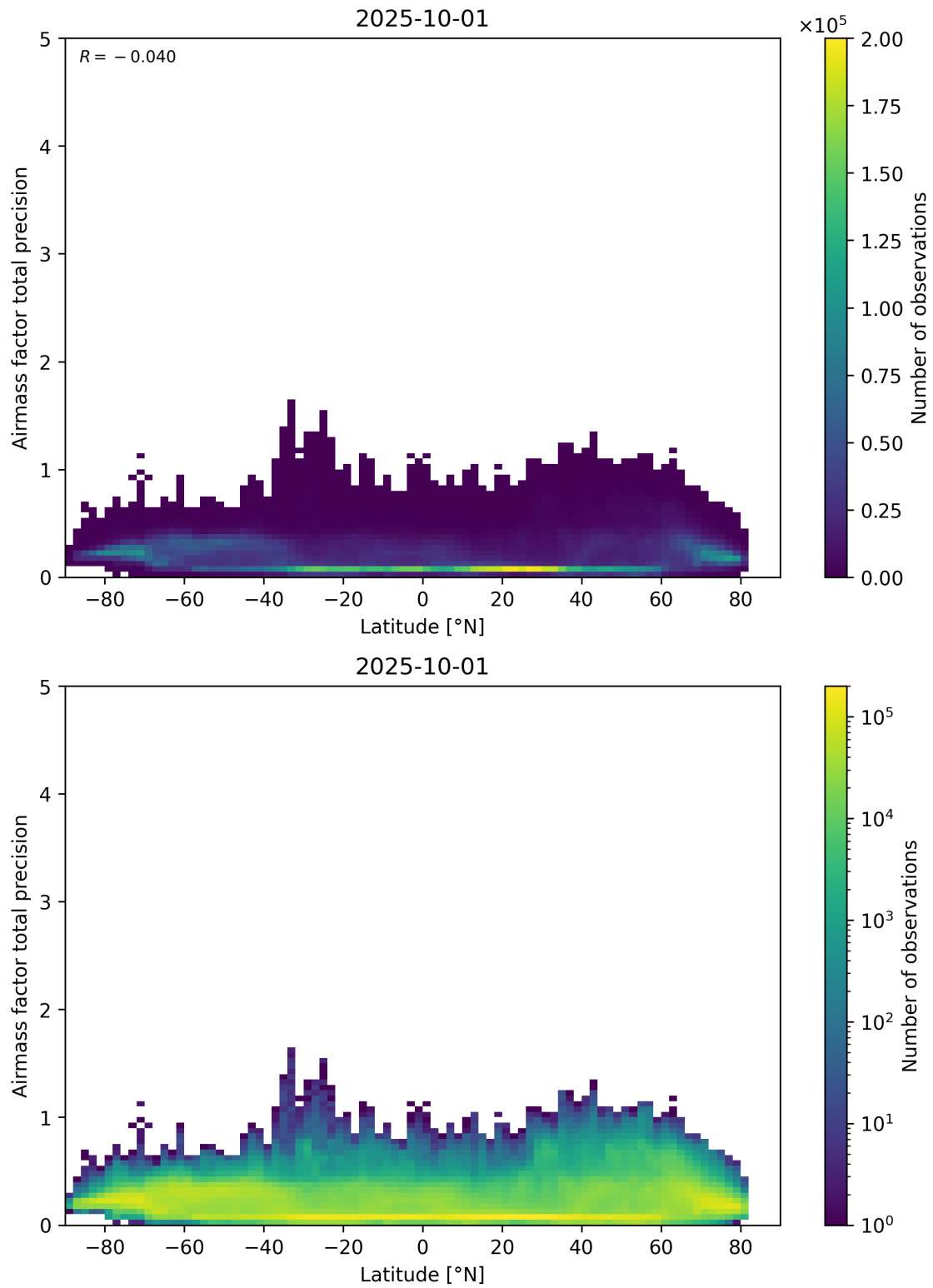
Figure 162: Scatter density plot of “Latitude” against “Airmass factor total precision” for 2025-10-01 to 2025-10-02.
