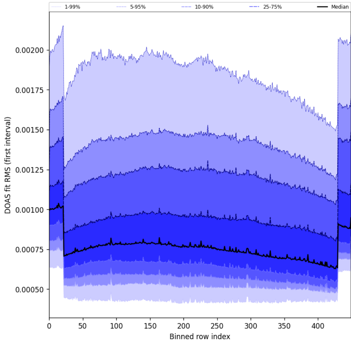
Figure 60: Along track statistics of “DOAS fit RMS (first interval)” for 2025-10-01 to 2025-10-02
