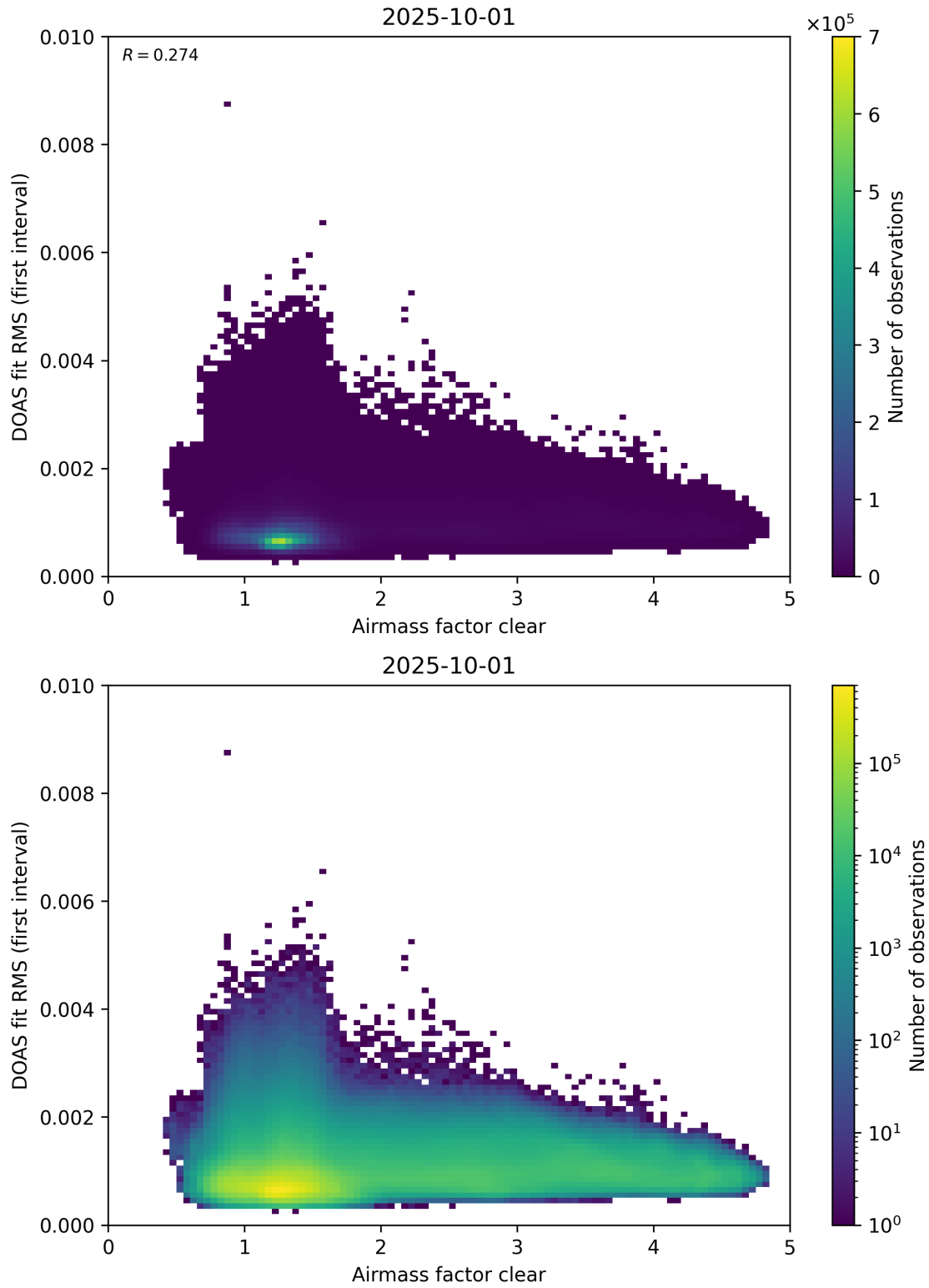
Figure 71: Scatter density plot of “Airmass factor clear” against “DOAS fit RMS (first interval)” for 2025-10-01 to 2025-10-02.
