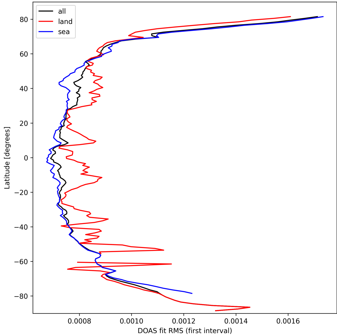
Figure 32: Zonal average of “DOAS fit RMS (first interval)” for 2025-10-01 to 2025-10-02.
