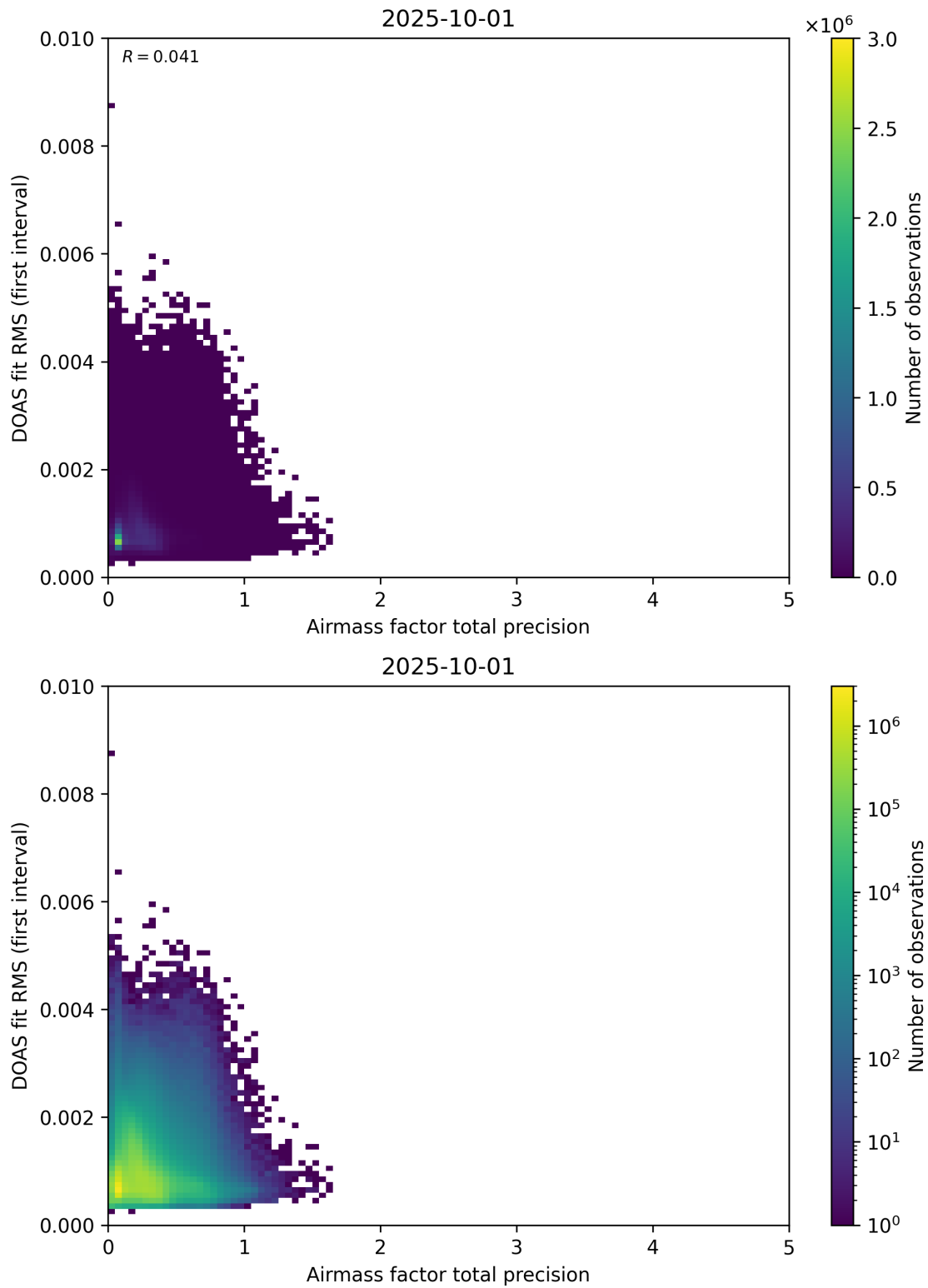
Figure 105: Scatter density plot of “Airmass factor total precision” against “DOAS fit RMS (first interval)” for 2025-10-01 to 2025-10-02.
