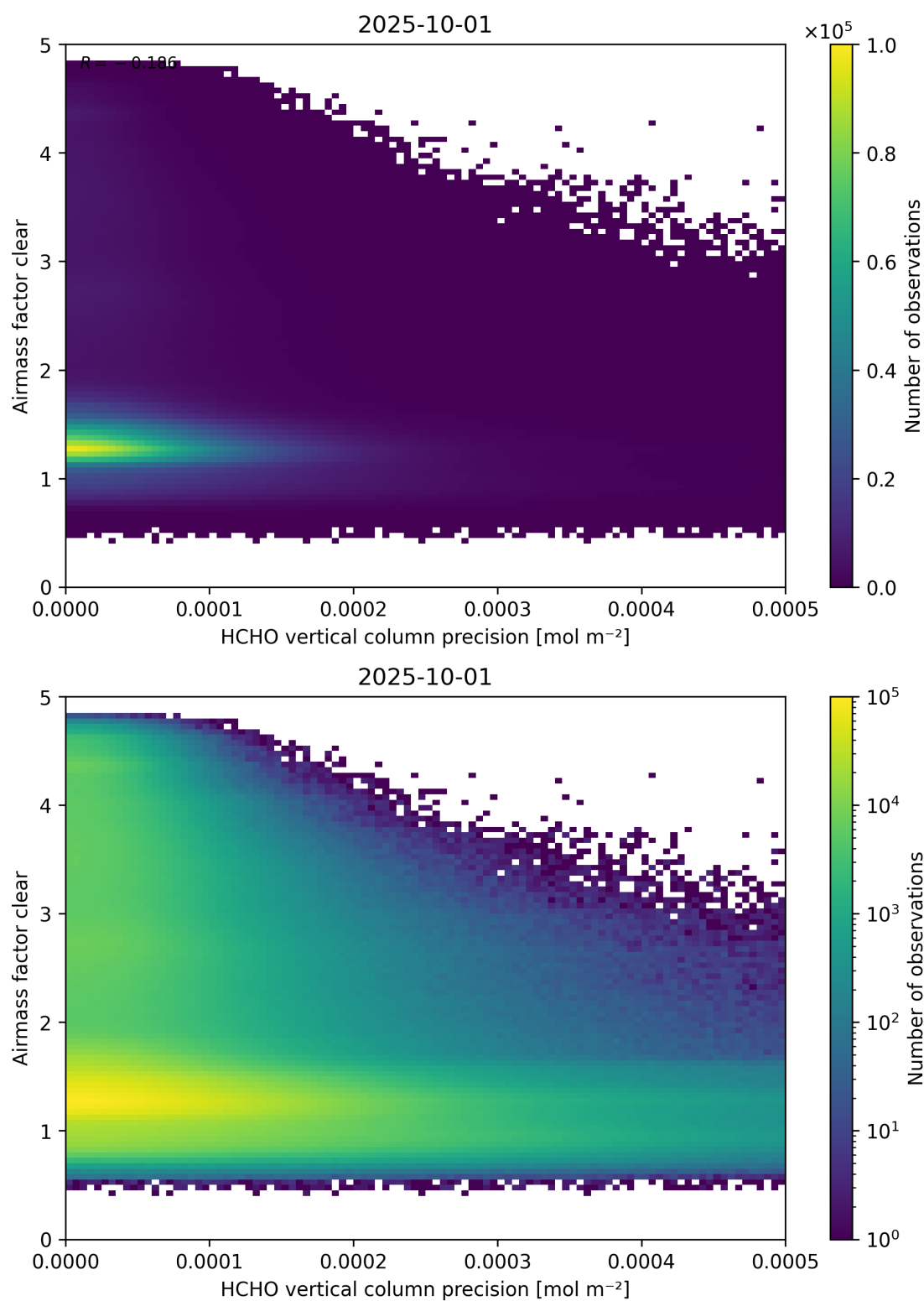
Figure 139: Scatter density plot of “HCHO vertical column precision” against “Airmass factor clear” for 2025-10-01 to 2025-10-02.
