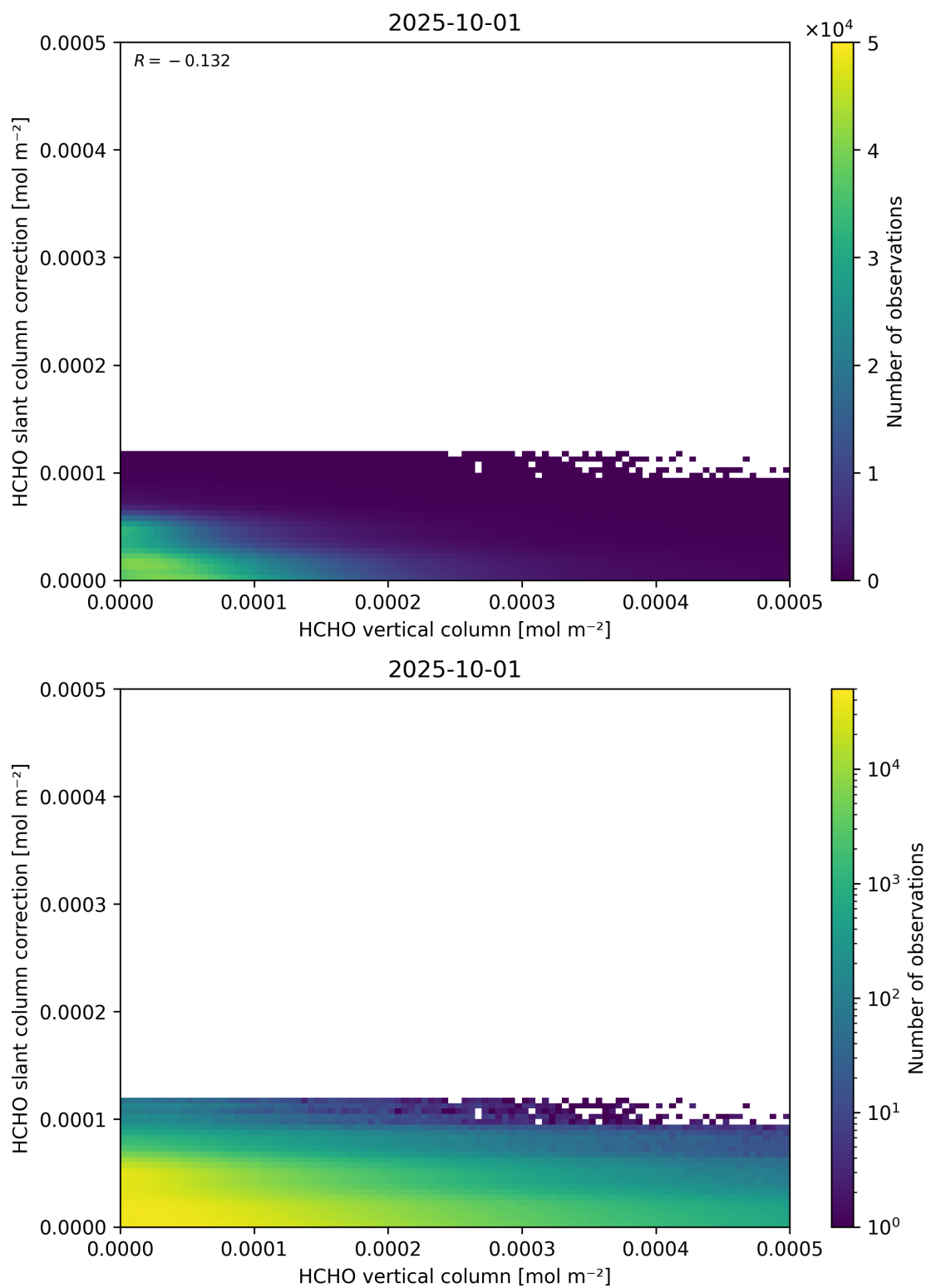
Figure 128: Scatter density plot of “HCHO vertical column” against “HCHO slant column correction” for 2025-10-01 to 2025-10-02.
