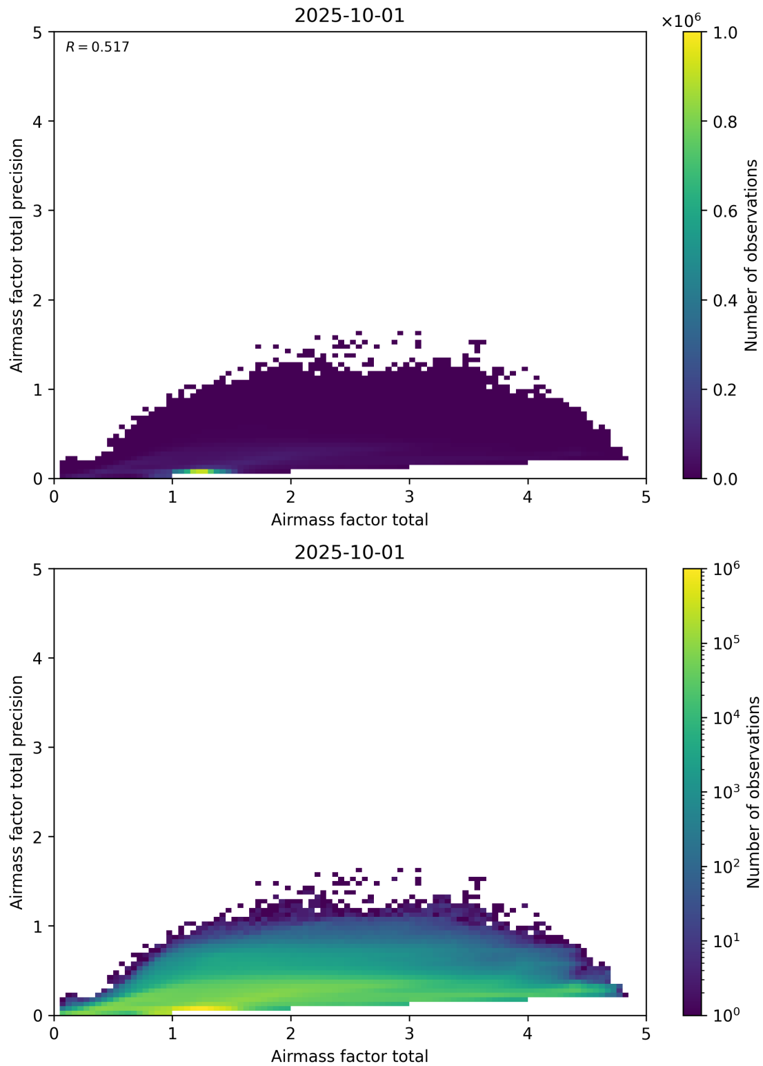
Figure 103: Scatter density plot of “Airmass factor total” against “Airmass factor total precision” for 2025-10-01 to 2025-10-02.
