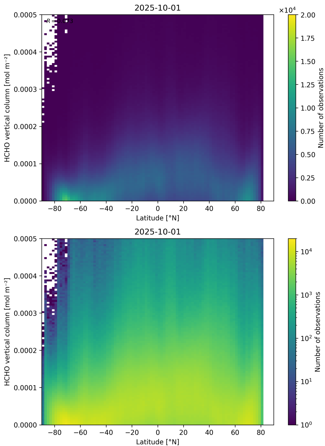
Figure 163: Scatter density plot of “Latitude” against “HCHO vertical column” for 2025-10-01 to 2025-10-02.
