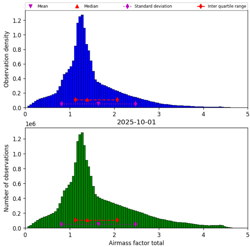
Figure 40: Histogram of “Airmass factor total” for 2025-10-01 to 2025-10-02
