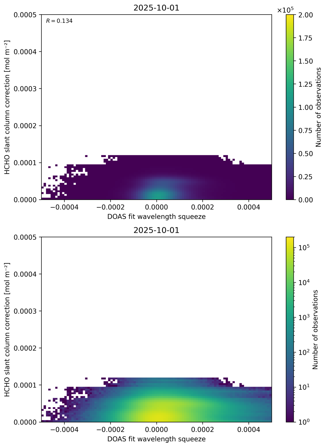
Figure 70: Scatter density plot of “DOAS fit wavelength squeeze” against “HCHO slant column correction” for 2025-10-01 to 2025-10-02.
