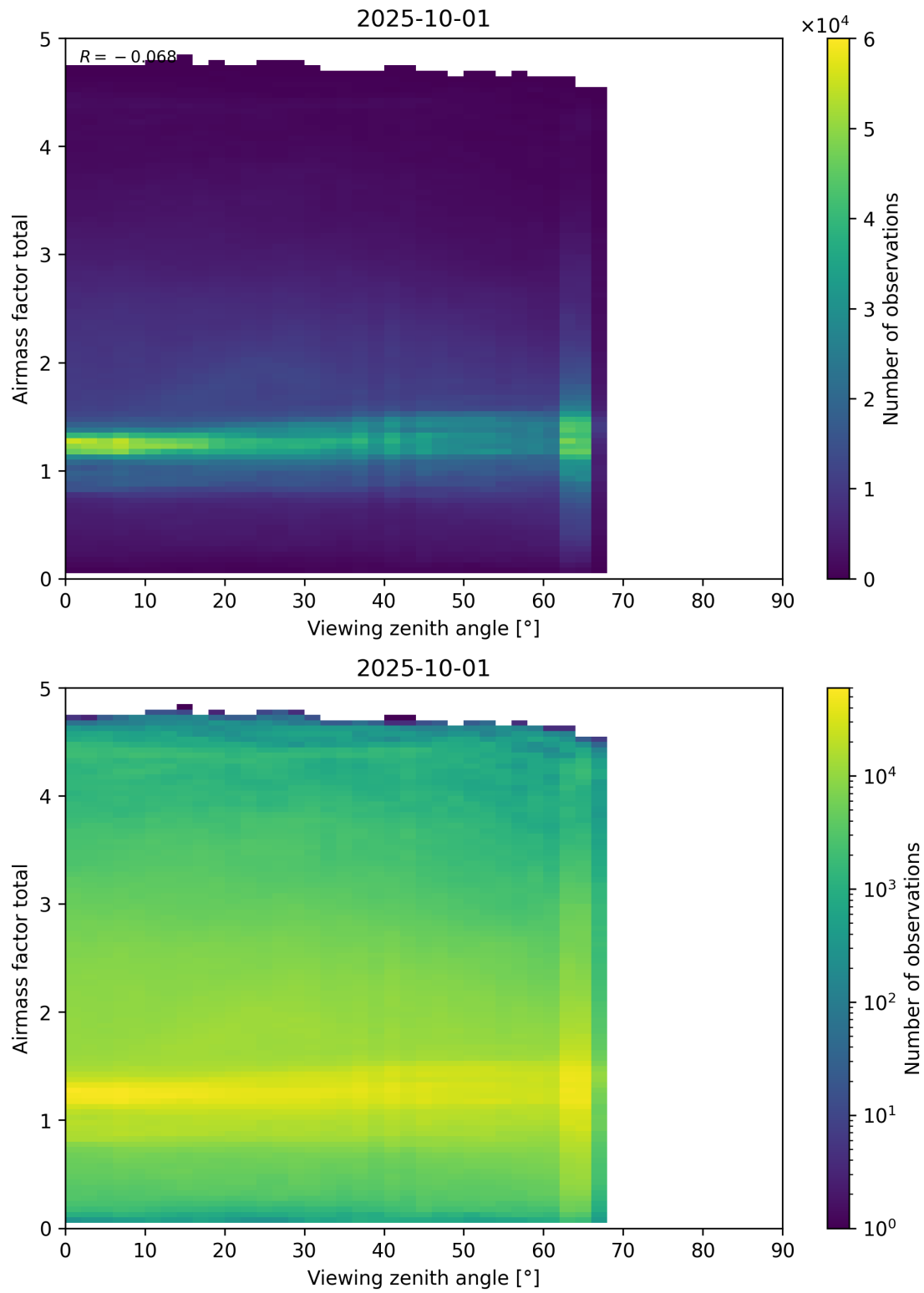
Figure 190: Scatter density plot of “Viewing zenith angle” against “Airmass factor total” for 2025-10-01 to 2025-10-02.
