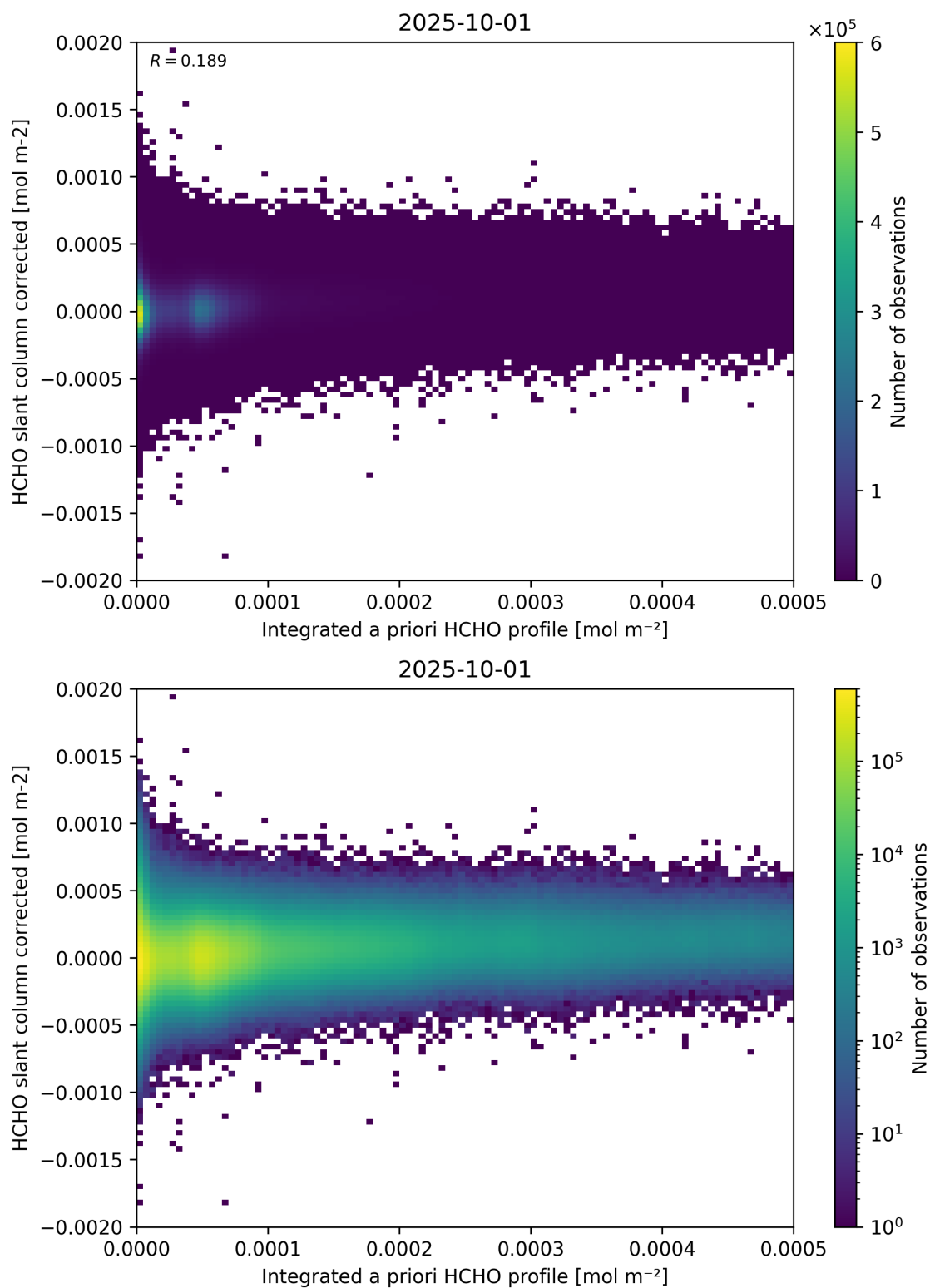
Figure 151: Scatter density plot of “Integrated a priori HCHO profile” against “HCHO slant column corrected” for 2025-10-01 to 2025-10-02.
