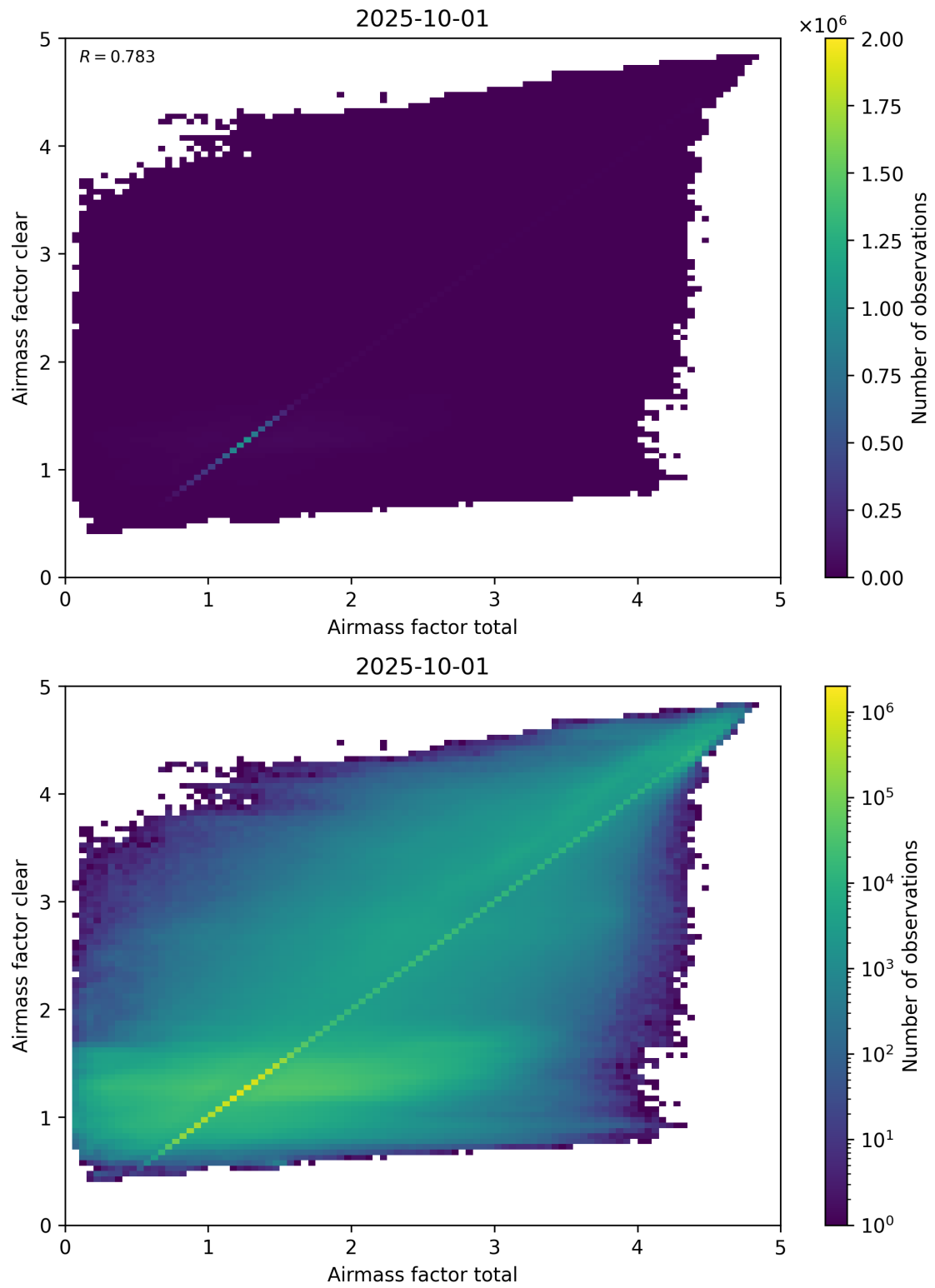
Figure 100: Scatter density plot of “Airmass factor total” against “Airmass factor clear” for 2025-10-01 to 2025-10-02.
