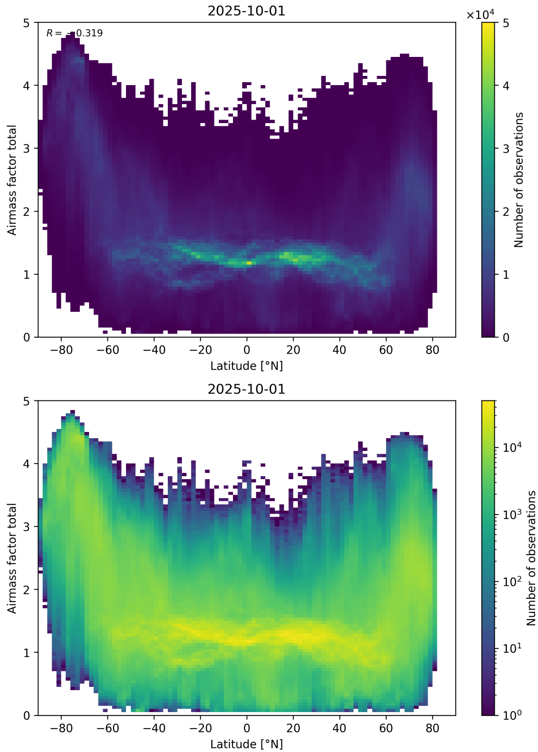
Figure 161: Scatter density plot of “Latitude” against “Airmass factor total” for 2025-10-01 to 2025-10-02.
