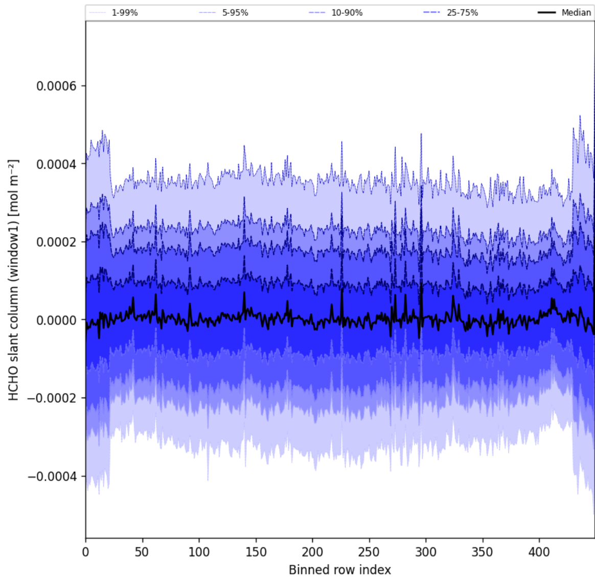
Figure 52: Along track statistics of “HCHO slant column (window1)” for 2025-10-01 to 2025-10-02
