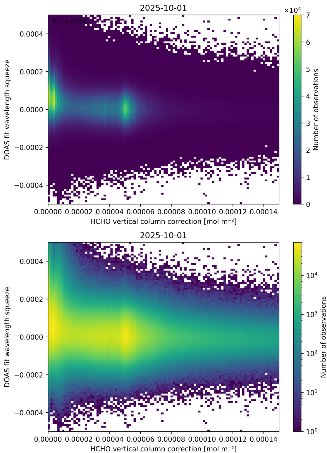
Figure 114: Scatter density plot of “HCHO vertical column correction” against “DOAS fit wavelength squeeze” for 2025-10-01 to 2025-10-02.
