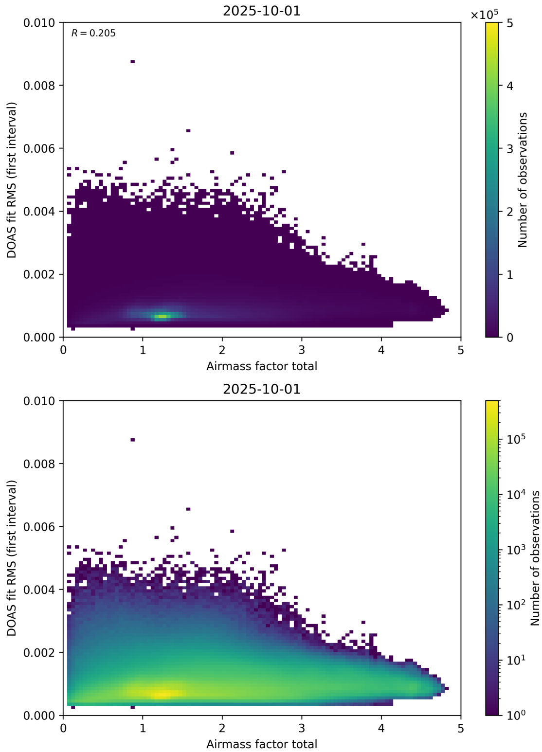
Figure 97: Scatter density plot of “Airmass factor total” against “DOAS fit RMS (first interval)” for 2025-10-01 to 2025-10-02.
