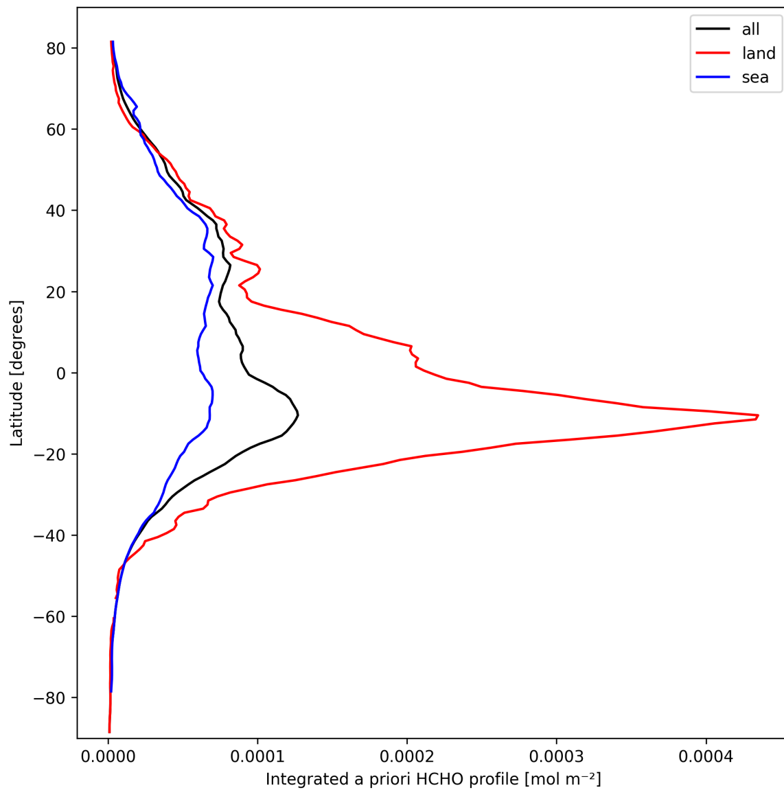
Figure 29: Zonal average of “Integrated a priori HCHO profile” for 2025-10-01 to 2025-10-02.
