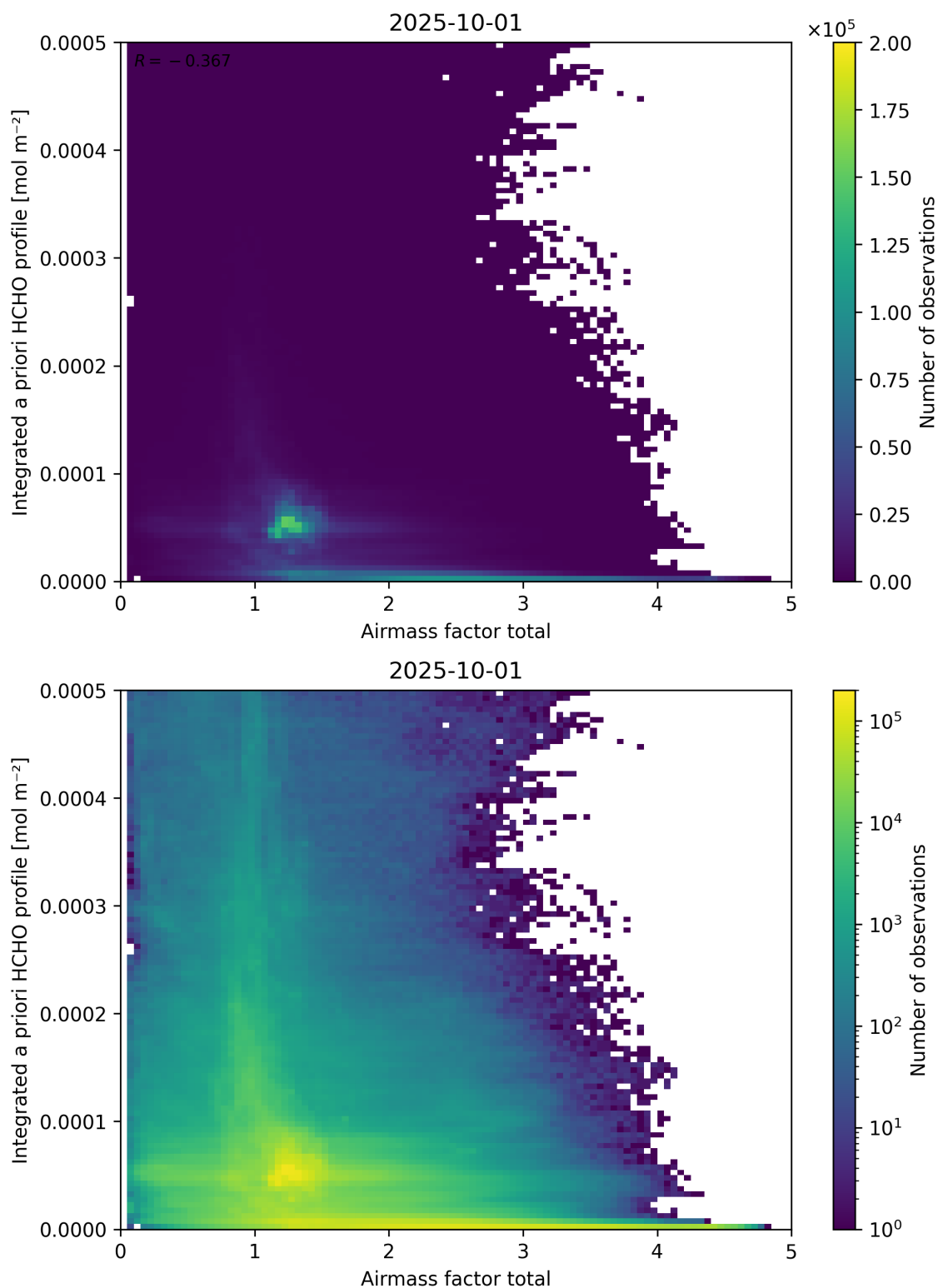
Figure 104: Scatter density plot of “Airmass factor total” against “Integrated a priori HCHO profile” for 2025-10-01 to 2025-10-02.
