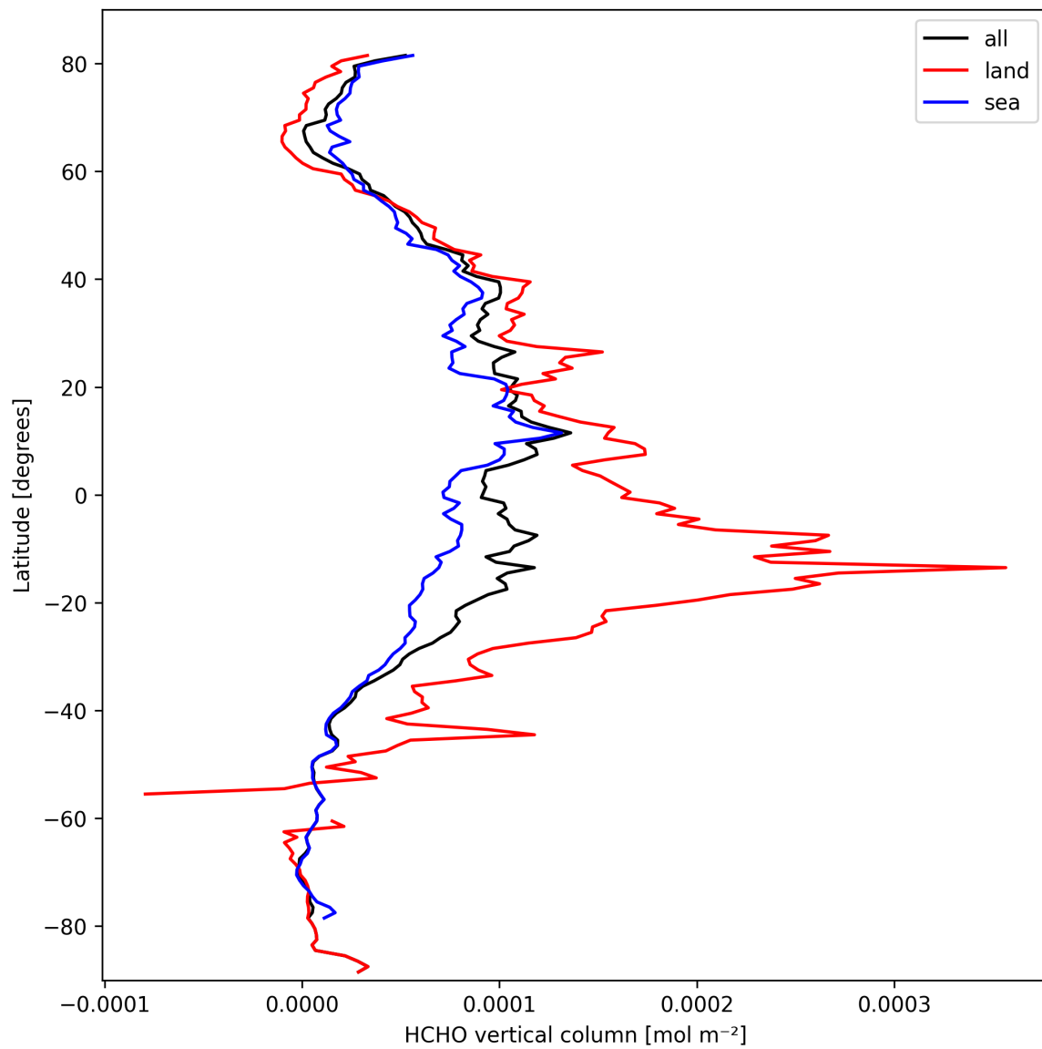
Figure 21: Zonal average of “HCHO vertical column” for 2025-10-01 to 2025-10-02.
