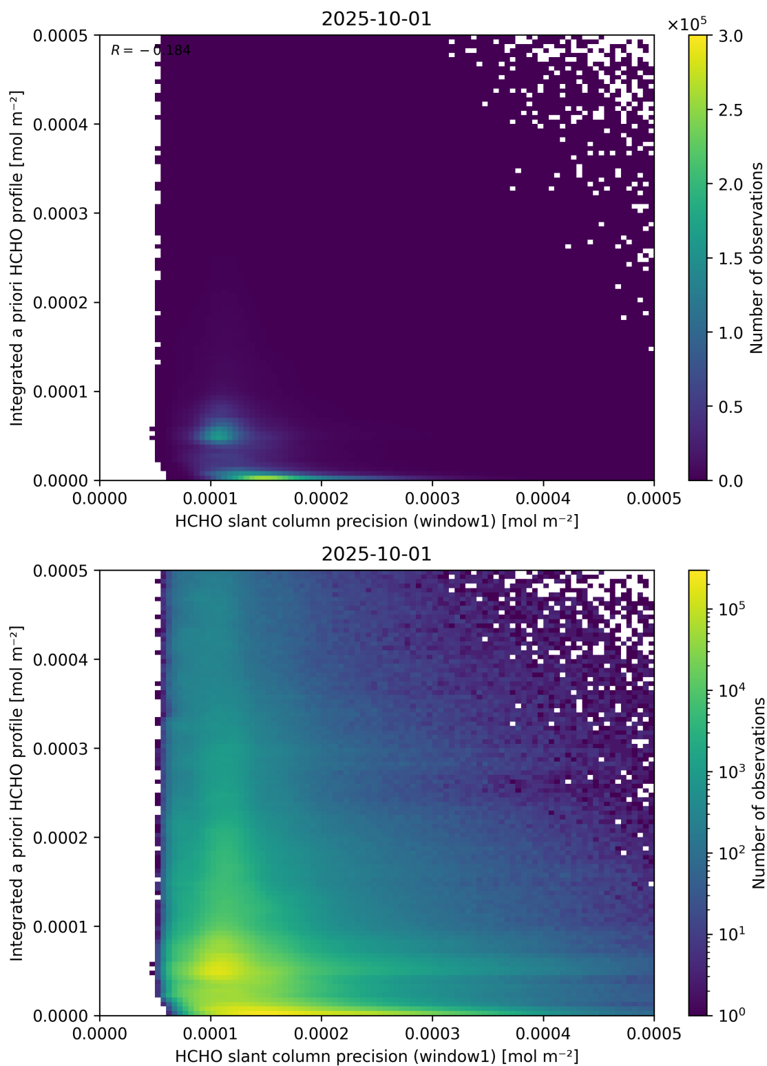
Figure 96: Scatter density plot of “HCHO slant column precision (window1)” against “Integrated a priori HCHO profile” for 2025-10-01 to 2025-10-02.
