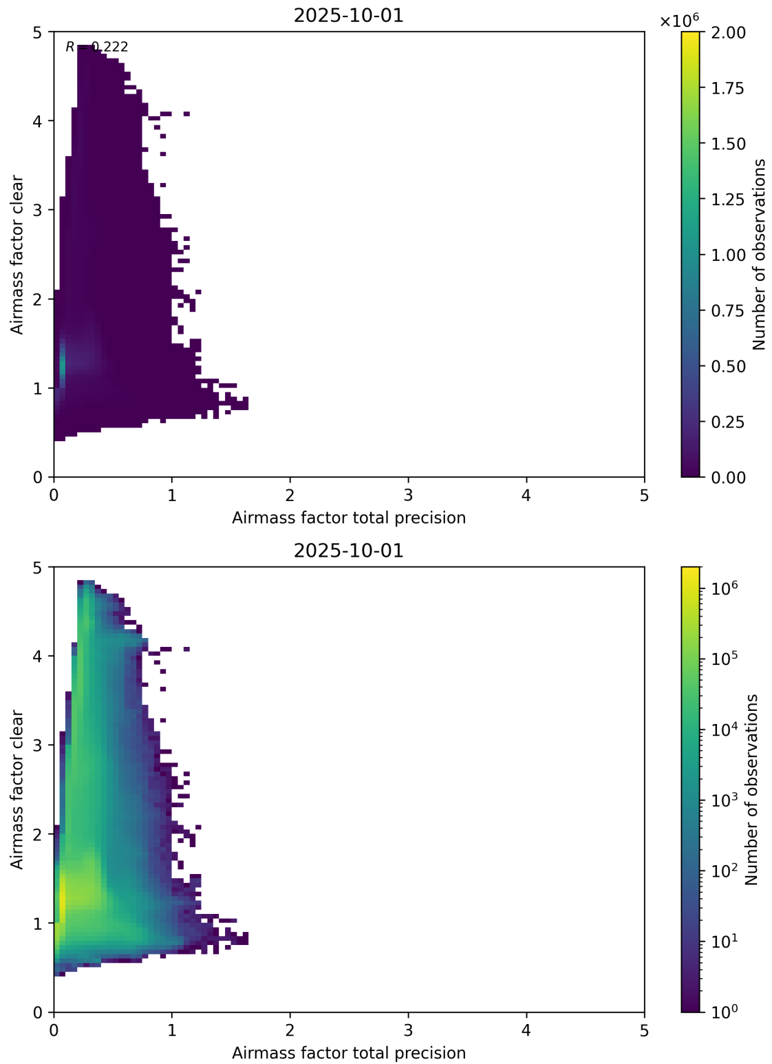
Figure 108: Scatter density plot of “Airmass factor total precision” against “Airmass factor clear” for 2025-10-01 to 2025-10-02.
