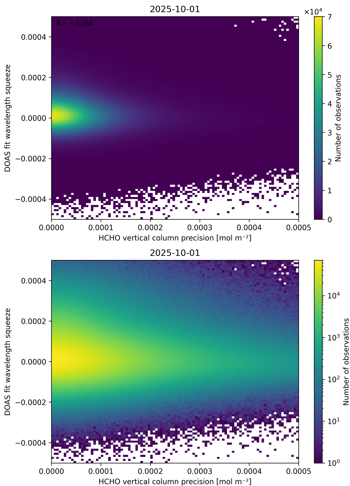
Figure 138: Scatter density plot of “HCHO vertical column precision” against “DOAS fit wavelength squeeze” for 2025-10-01 to 2025-10-02.
