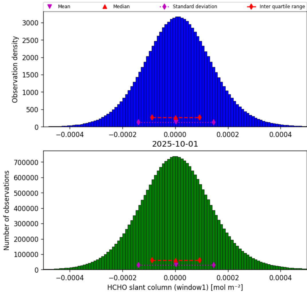
Figure 38: Histogram of "HCHO slant column (window1)" for 2025-10-01 to 2025-10-02
