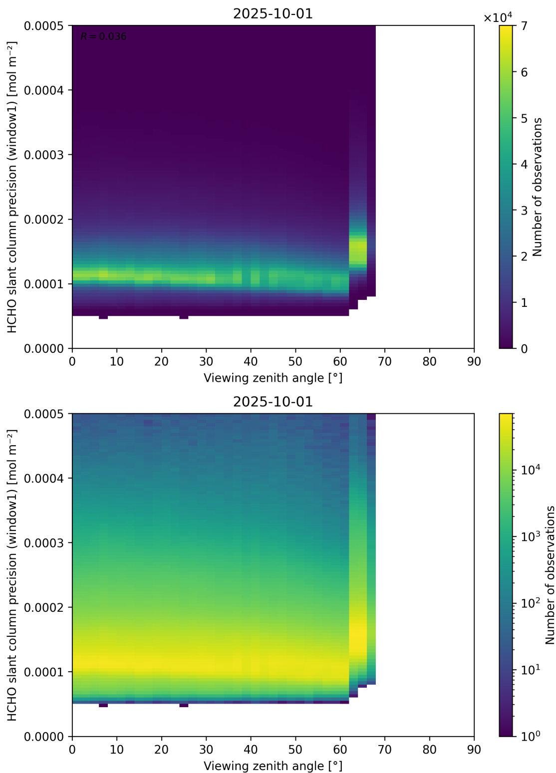
Figure 189: Scatter density plot of “Viewing zenith angle” against “HCHO slant column precision (window1)” for 2025-10-01 to 2025-10-02.
