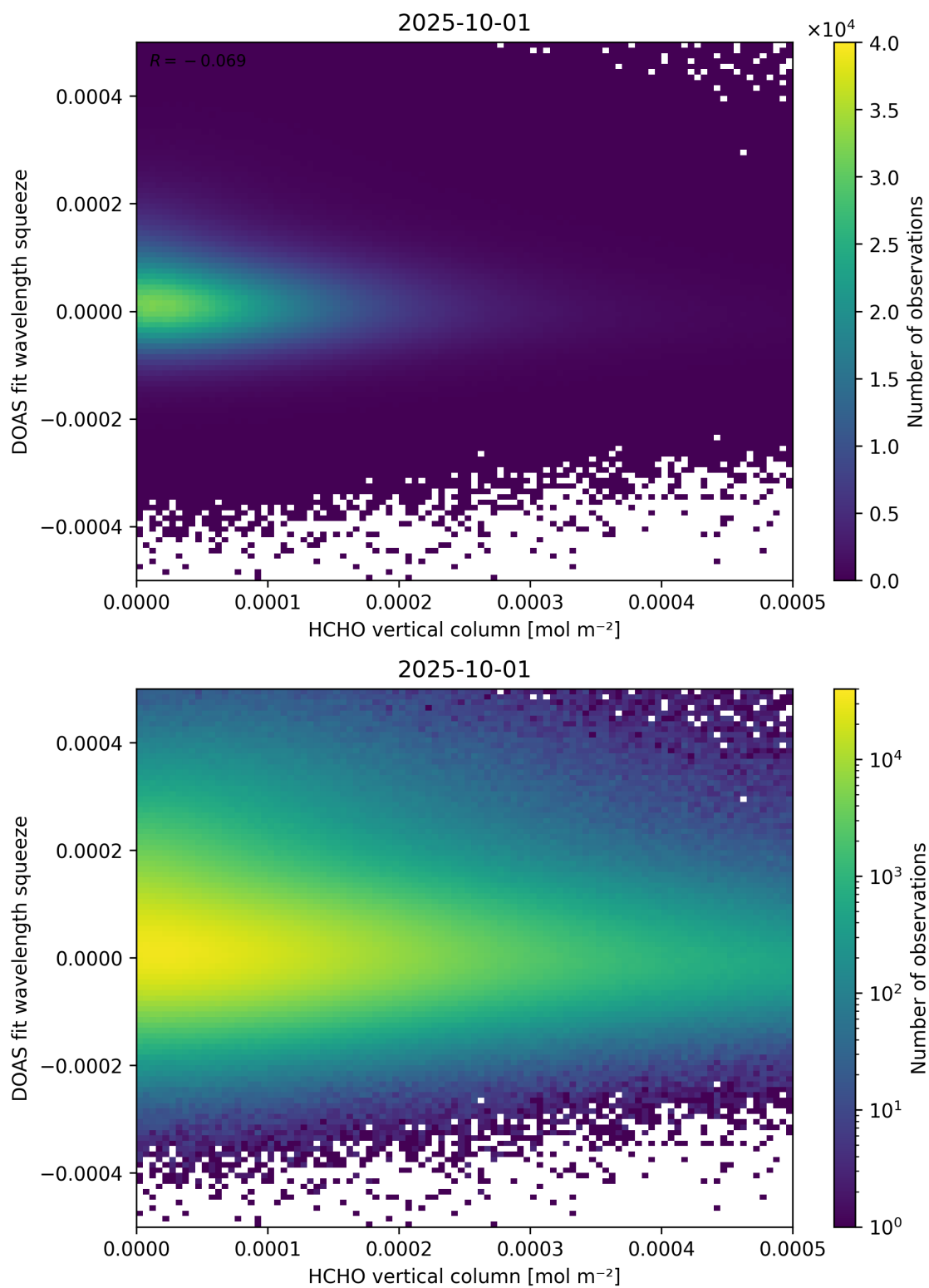
Figure 125: Scatter density plot of “HCHO vertical column” against “DOAS fit wavelength squeeze” for 2025-10-01 to 2025-10-02.
