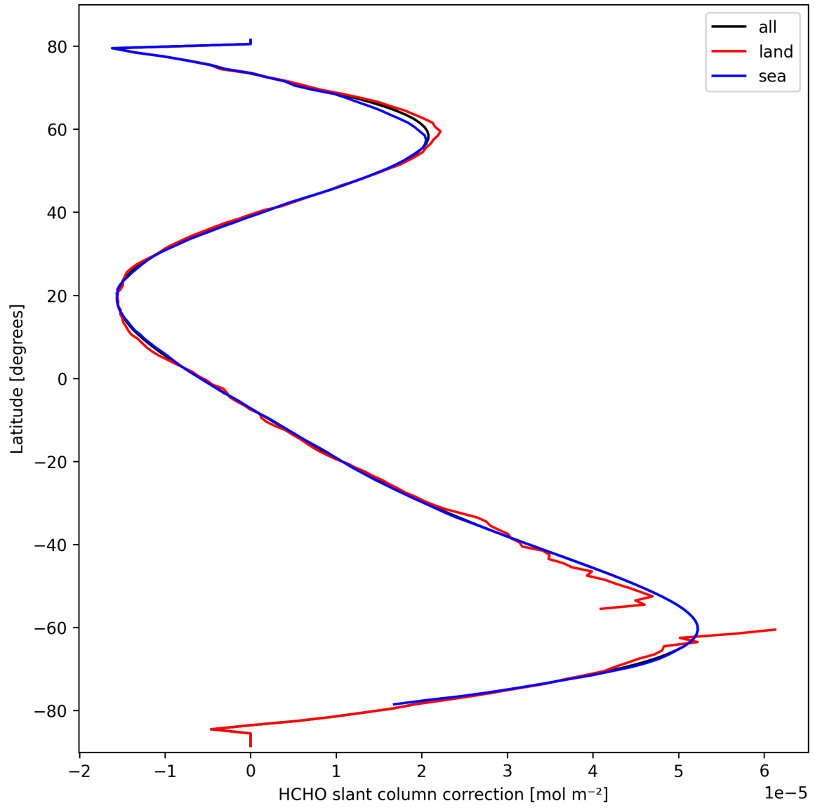
Figure 33: Zonal average of “HCHO slant column correction” for 2025-10-01 to 2025-10-02.
