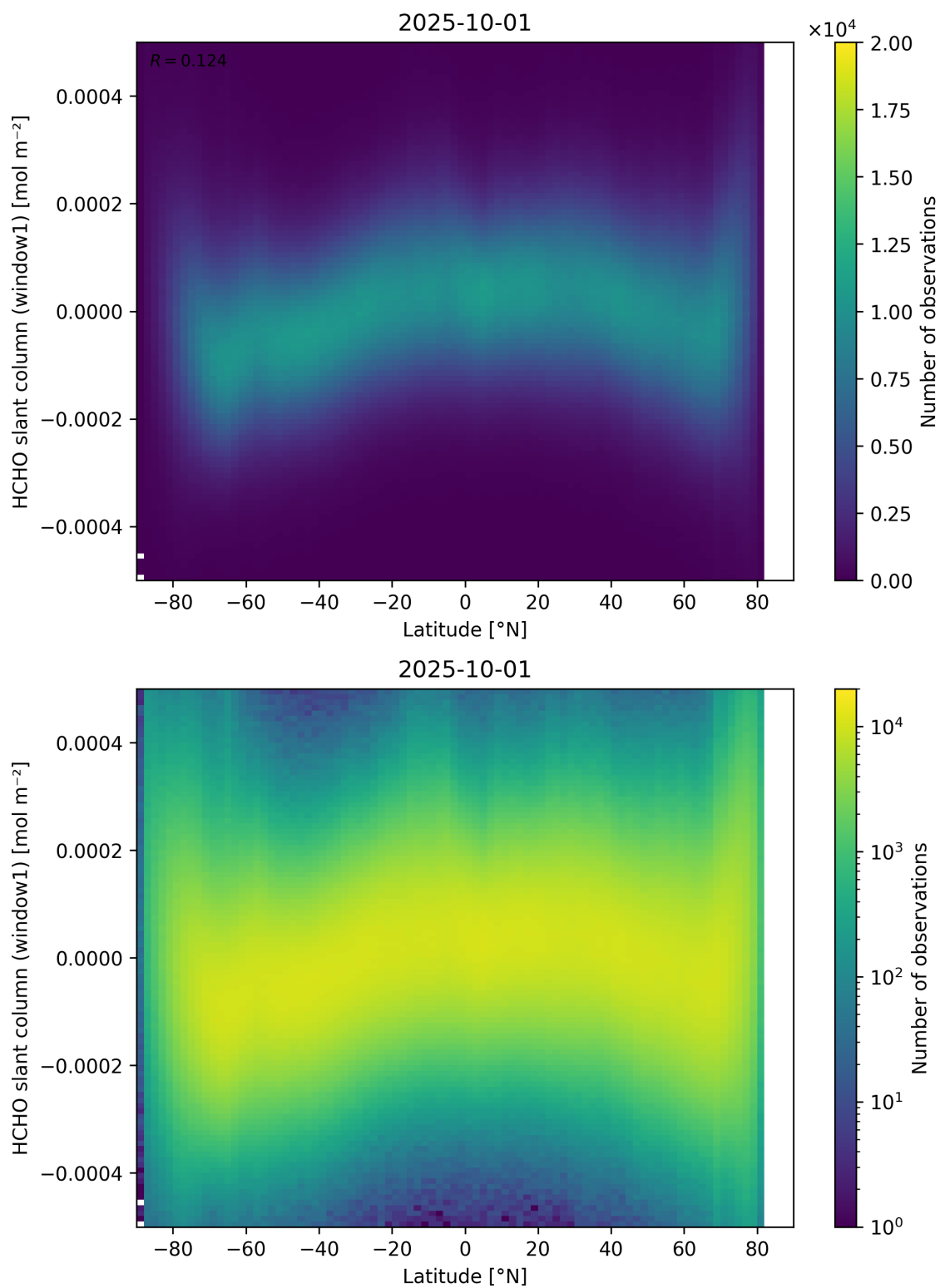
Figure 159: Scatter density plot of “Latitude” against “HCHO slant column (window1)” for 2025-10-01 to 2025-10-02.
