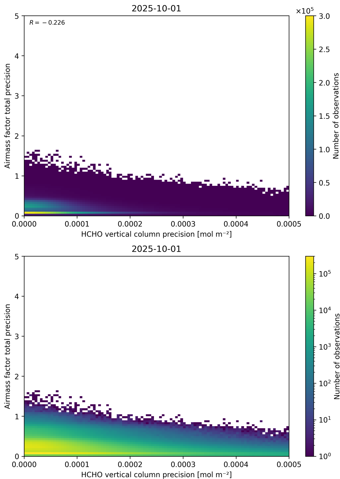
Figure 145: Scatter density plot of “HCHO vertical column precision” against “Airmass factor total precision” for 2025-10-01 to 2025-10-02.
