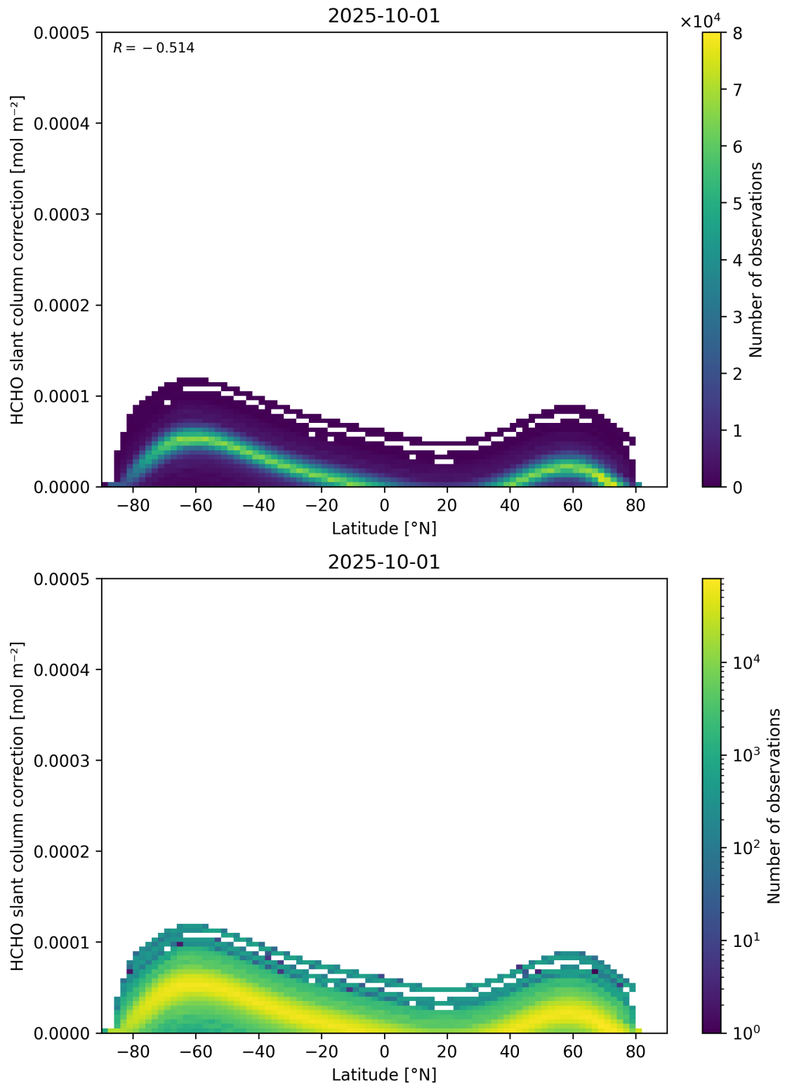
Figure 158: Scatter density plot of “Latitude” against “HCHO slant column correction” for 2025-10-01 to 2025-10-02.
