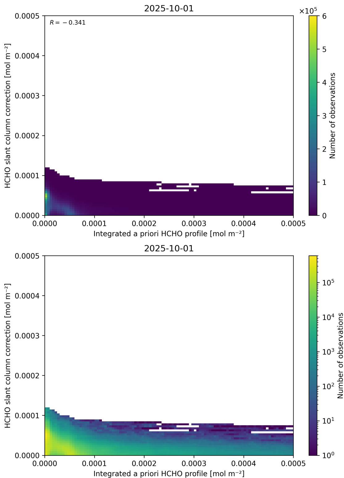
Figure 152: Scatter density plot of “Integrated a priori HCHO profile” against “HCHO slant column correction” for 2025-10-01 to 2025-10-02.
