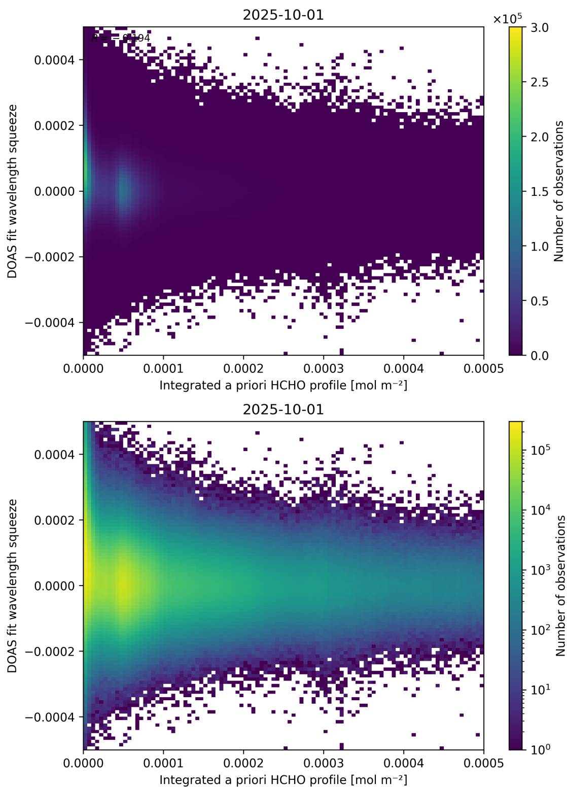
Figure 150: Scatter density plot of “Integrated a priori HCHO profile” against “DOAS fit wavelength squeeze” for 2025-10-01 to 2025-10-02.
