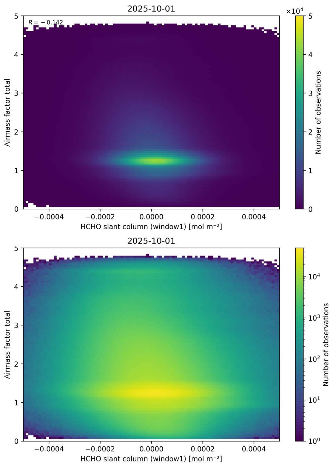
Figure 85: Scatter density plot of “HCHO slant column (window1)” against “Airmass factor total” for 2025-10-01 to 2025-10-02.
