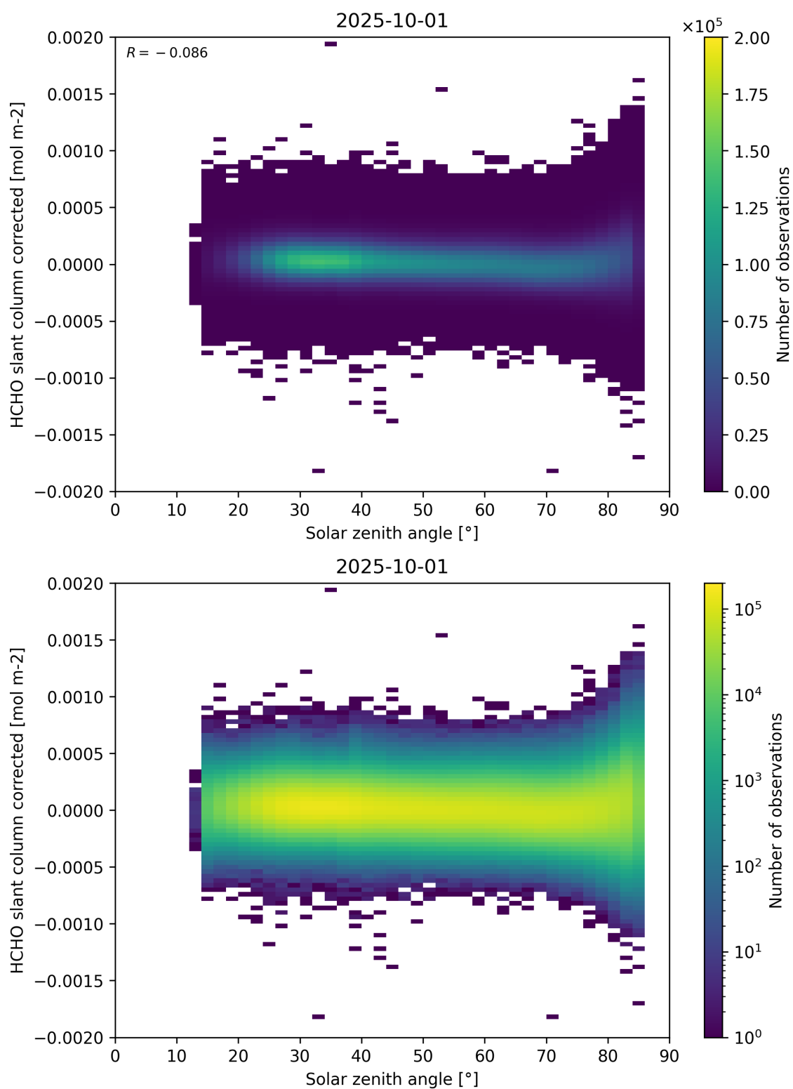
Figure 171: Scatter density plot of “Solar zenith angle” against “HCHO slant column corrected” for 2025-10-01 to 2025-10-02.
