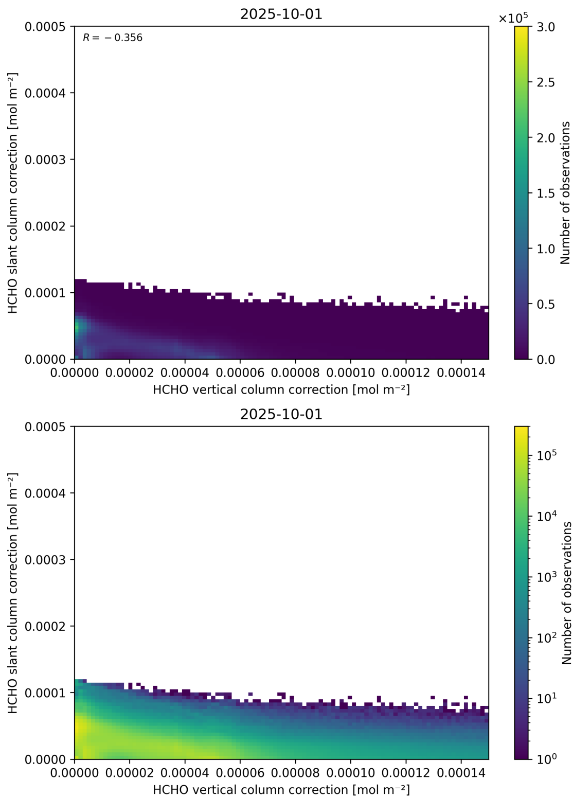
Figure 117: Scatter density plot of “HCHO vertical column correction” against “HCHO slant column correction” for 2025-10-01 to 2025-10-02.
