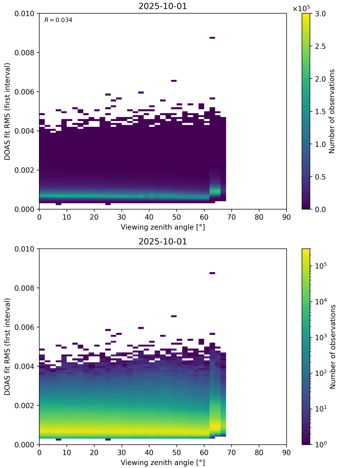
Figure 182: Scatter density plot of “Viewing zenith angle” against “DOAS fit RMS (first interval)” for 2025-10-01 to 2025-10-02.
