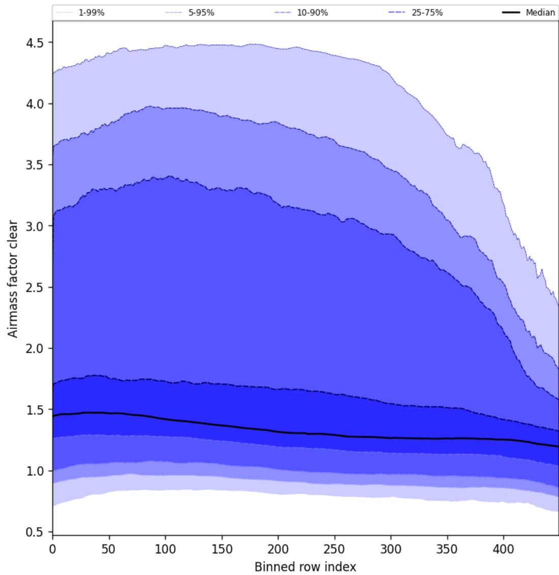
Figure 56: Along track statistics of “Air mass factor clear” for 2025-10-01 to 2025-10-02
