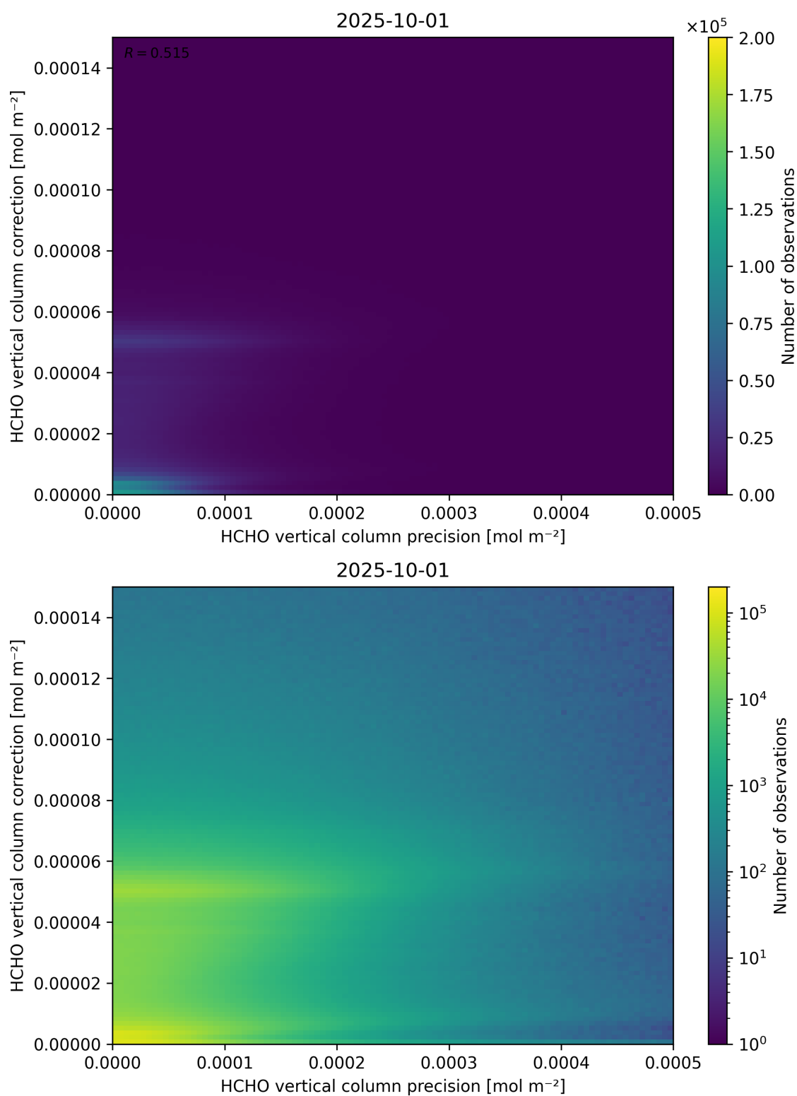
Figure 146: Scatter density plot of “HCHO vertical column precision” against “HCHO vertical column correction” for 2025-10-01 to 2025-10-02.
