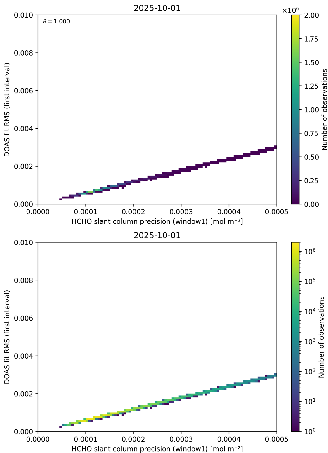
Figure 88: Scatter density plot of “HCHO slant column precision (window1)” against “DOAS fit RMS (first interval)” for 2025-10-01 to 2025-10-02.
