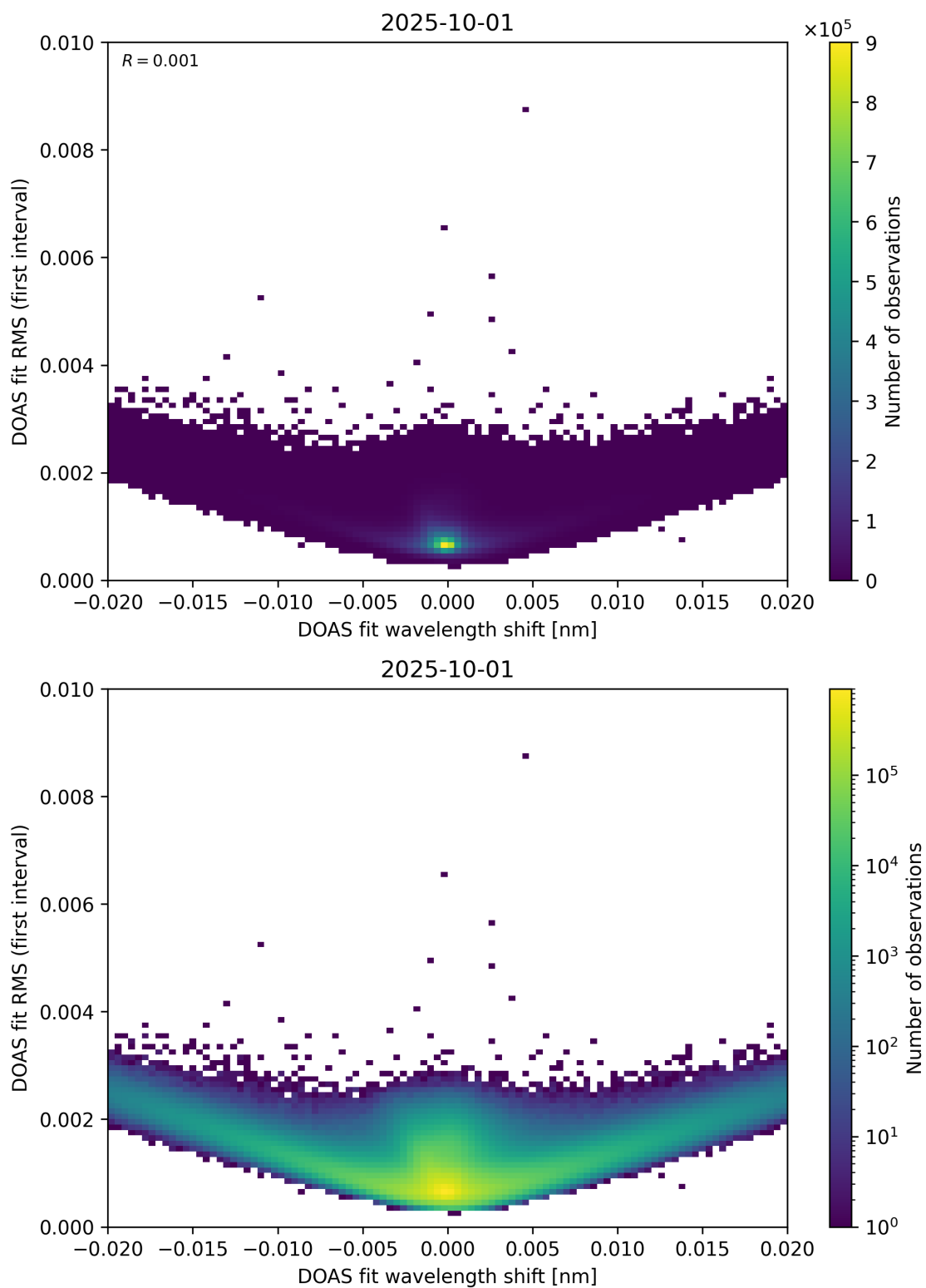
Figure 64: Scatter density plot of “DOAS fit wavelength shift” against “DOAS fit RMS (first interval)” for 2025-10-01 to 2025-10-02.
