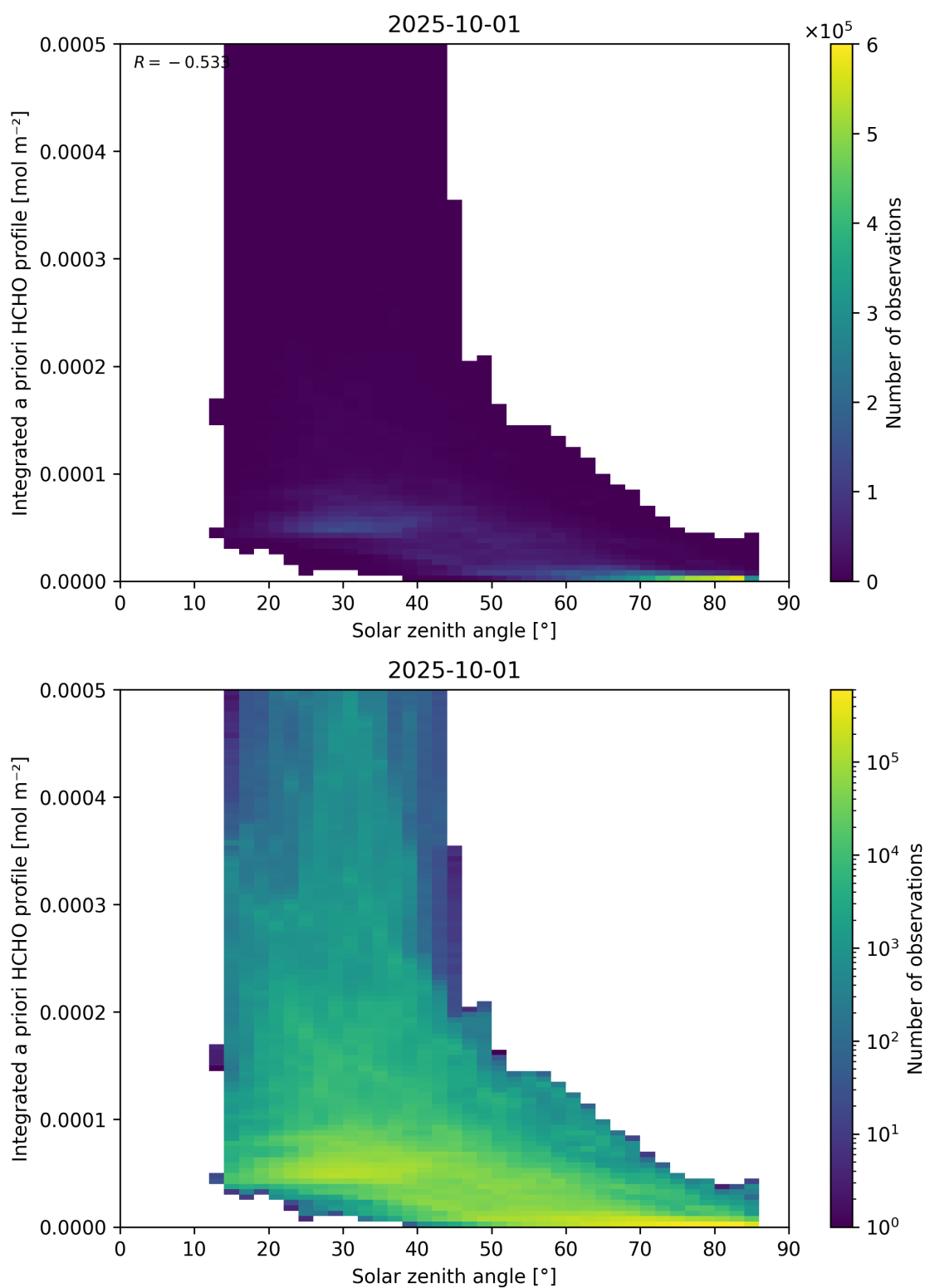
Figure 180: Scatter density plot of “Solar zenith angle” against “Integrated a priori HCHO profile” for 2025-10-01 to 2025-10-02.
