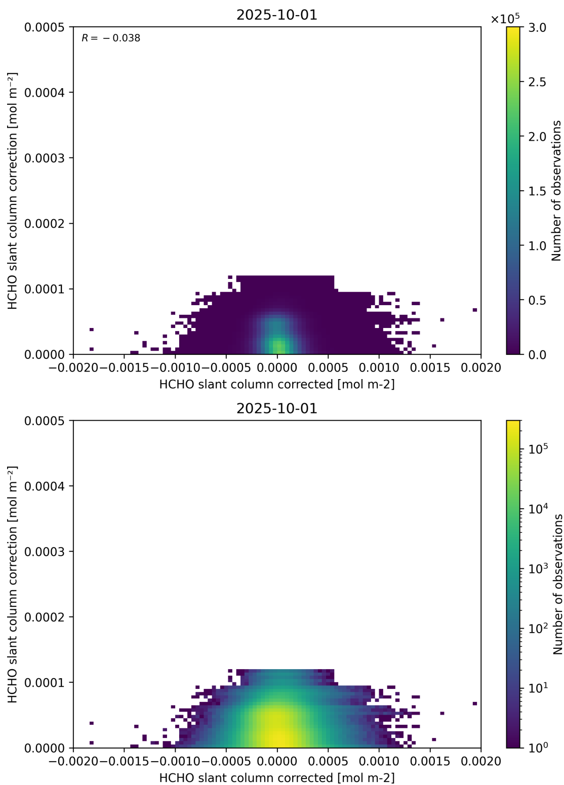
Figure 77: Scatter density plot of “HCHO slant column corrected” against “HCHO slant column correction” for 2025-10-01 to 2025-10-02.
