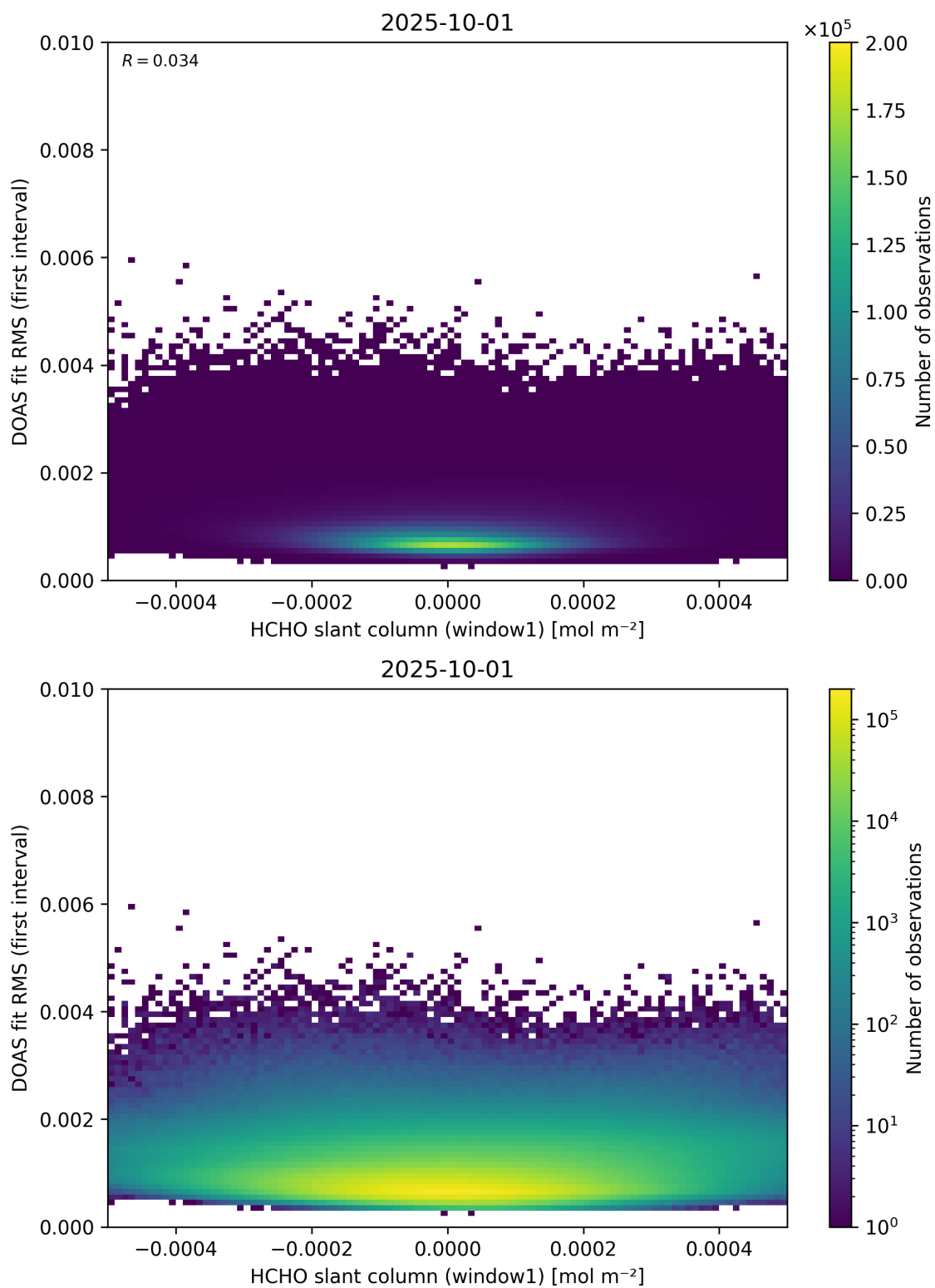
Figure 78: Scatter density plot of “HCHO slant column (window1)” against “DOAS fit RMS (first interval)” for 2025-10-01 to 2025-10-02.
