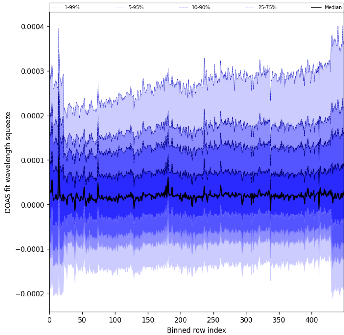
Figure 59: Along track statistics of “DOAS fit wavelength squeeze” for 2025-10-01 to 2025-10-02
