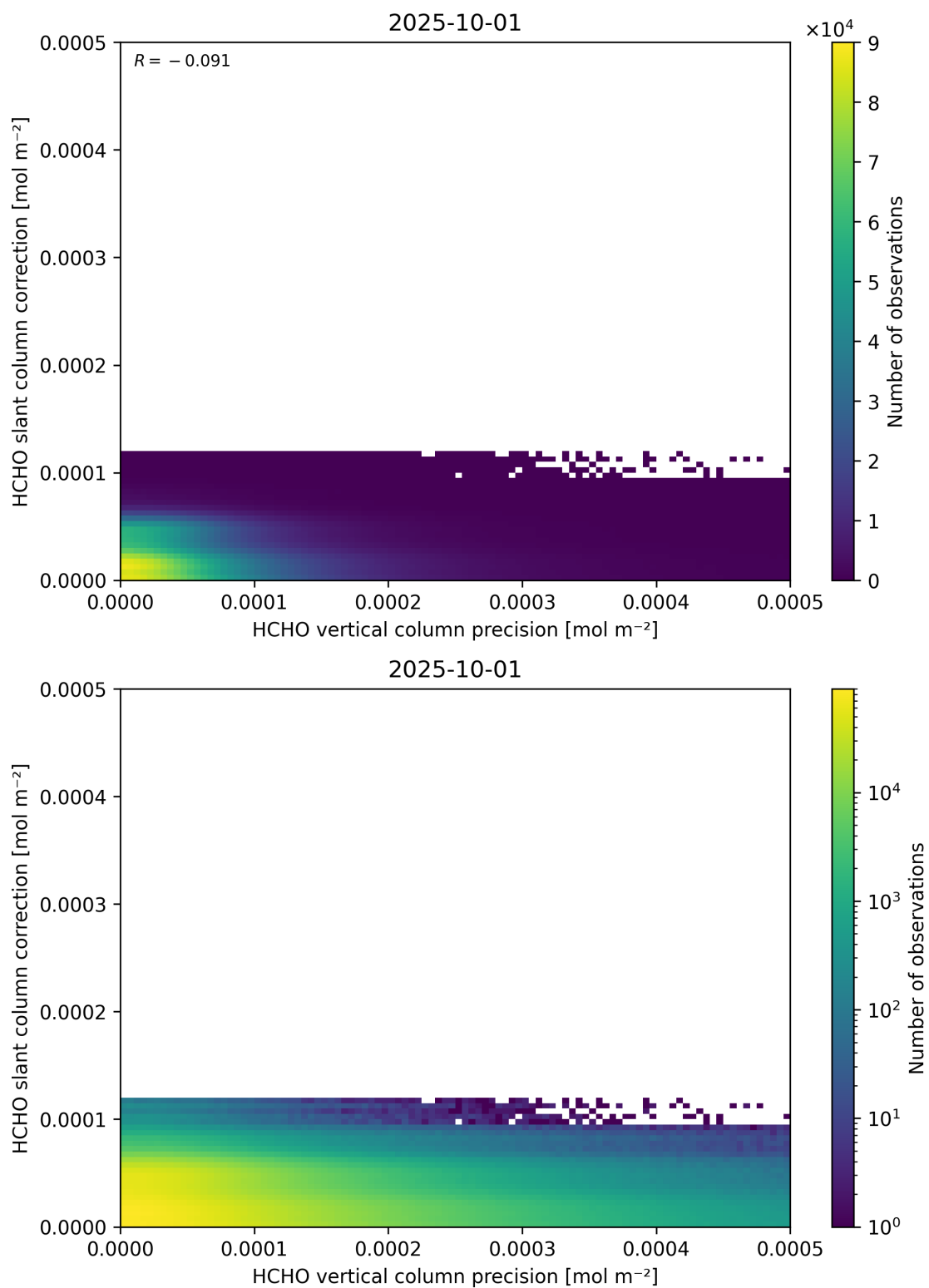
Figure 141: Scatter density plot of “HCHO vertical column precision” against “HCHO slant column correction” for 2025-10-01 to 2025-10-02.
