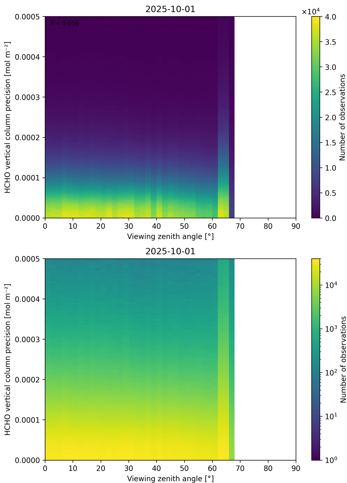
Figure 194: Scatter density plot of “Viewing zenith angle” against “HCHO vertical column precision” for 2025-10-01 to 2025-10-02.
