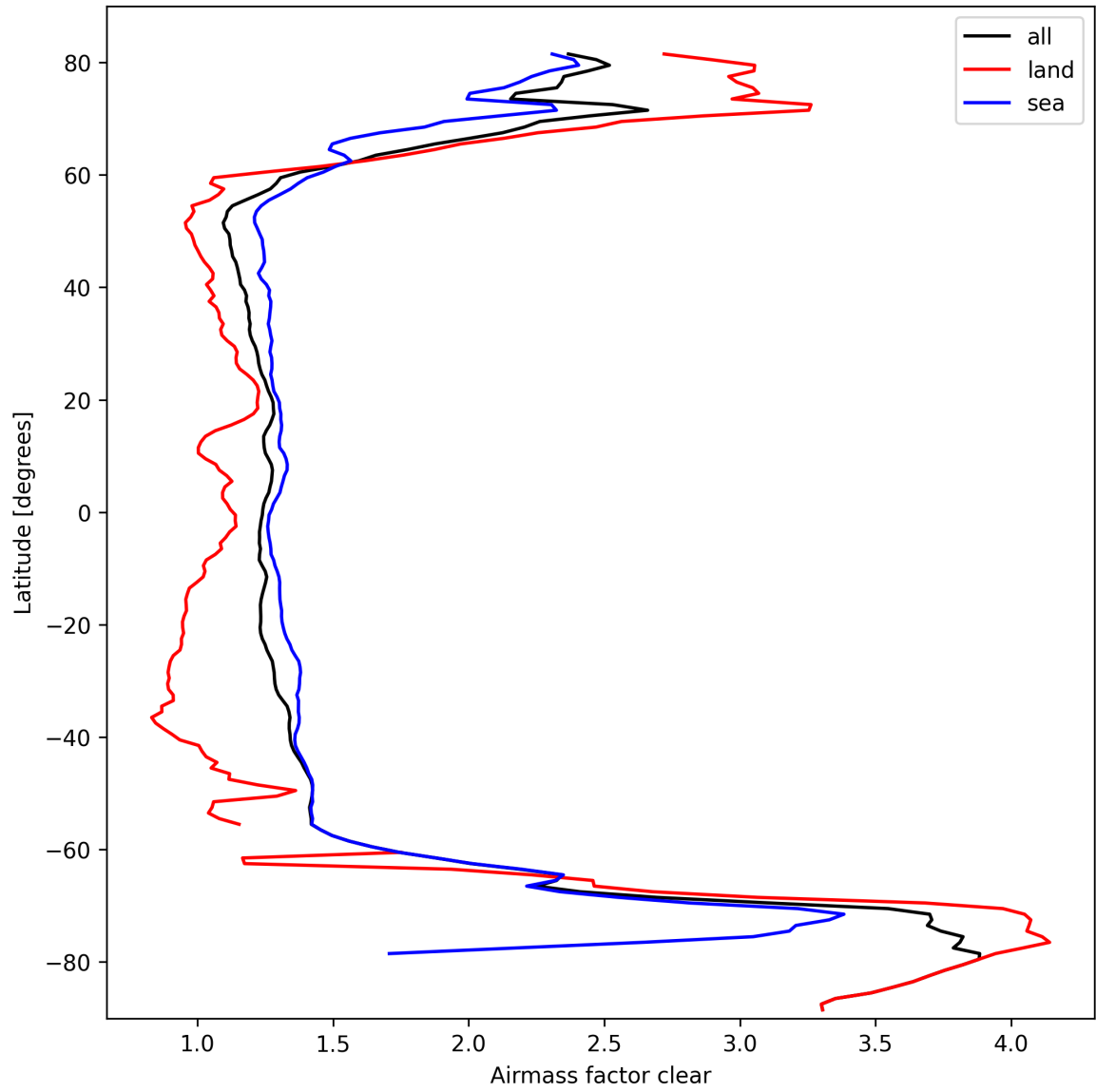
Figure 28: Zonal average of “Airmass factor clear” for 2025-10-01 to 2025-10-02.
