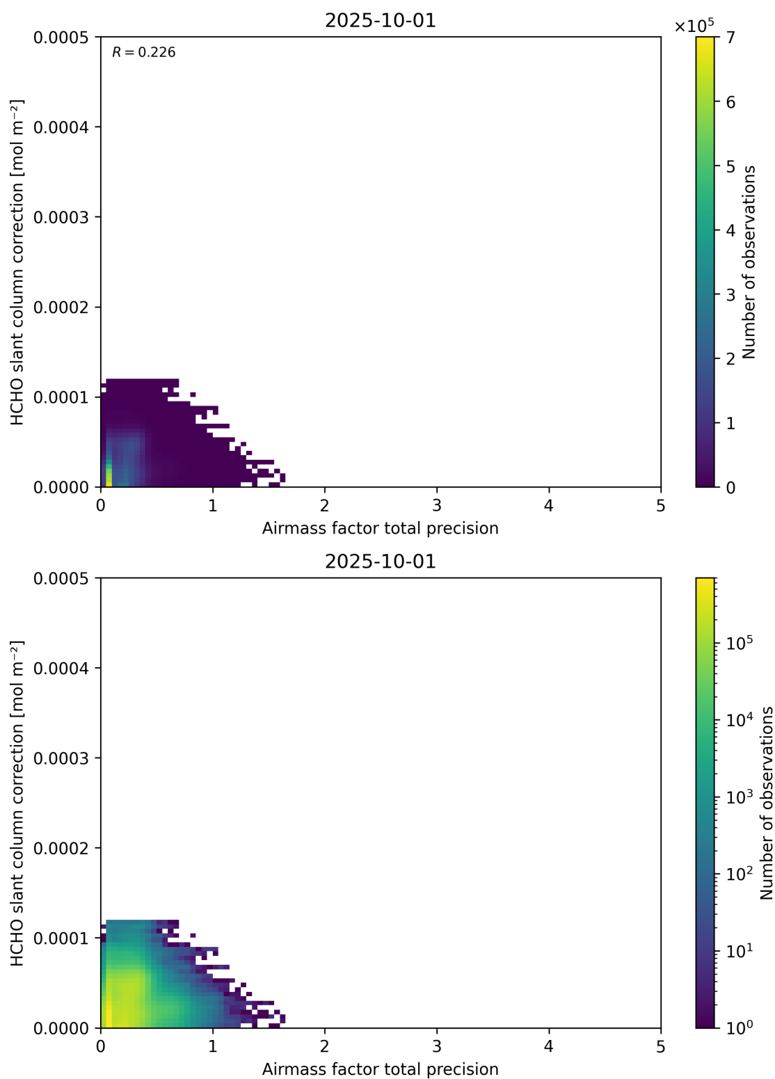
Figure 110: Scatter density plot of “Airmass factor total precision” against “HCHO slant column correction” for 2025-10-01 to 2025-10-02.
