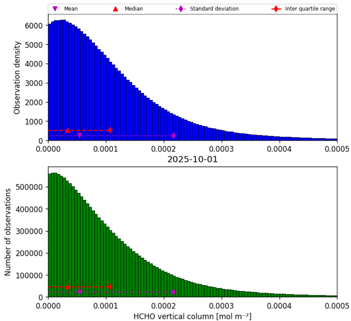
Figure 35: Histogram of “HCHO vertical column” for 2025-10-01 to 2025-10-02
