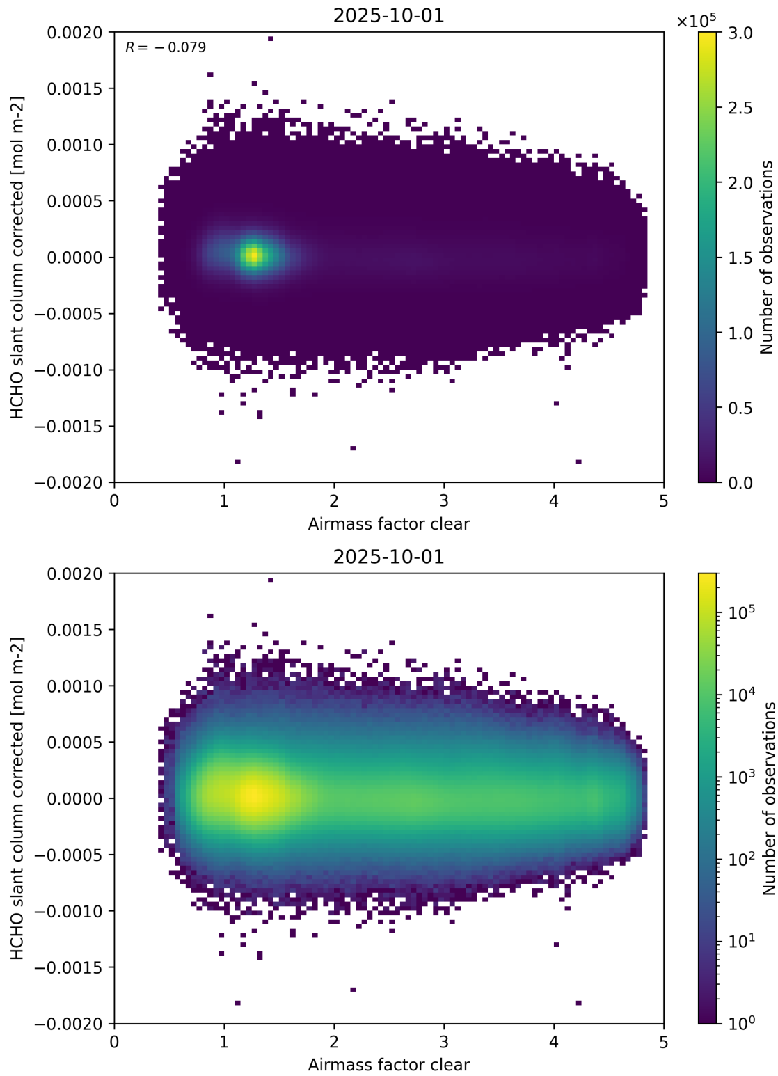
Figure 74: Scatter density plot of “Airmass factor clear” against “HCHO slant column corrected” for 2025-10-01 to 2025-10-02.
