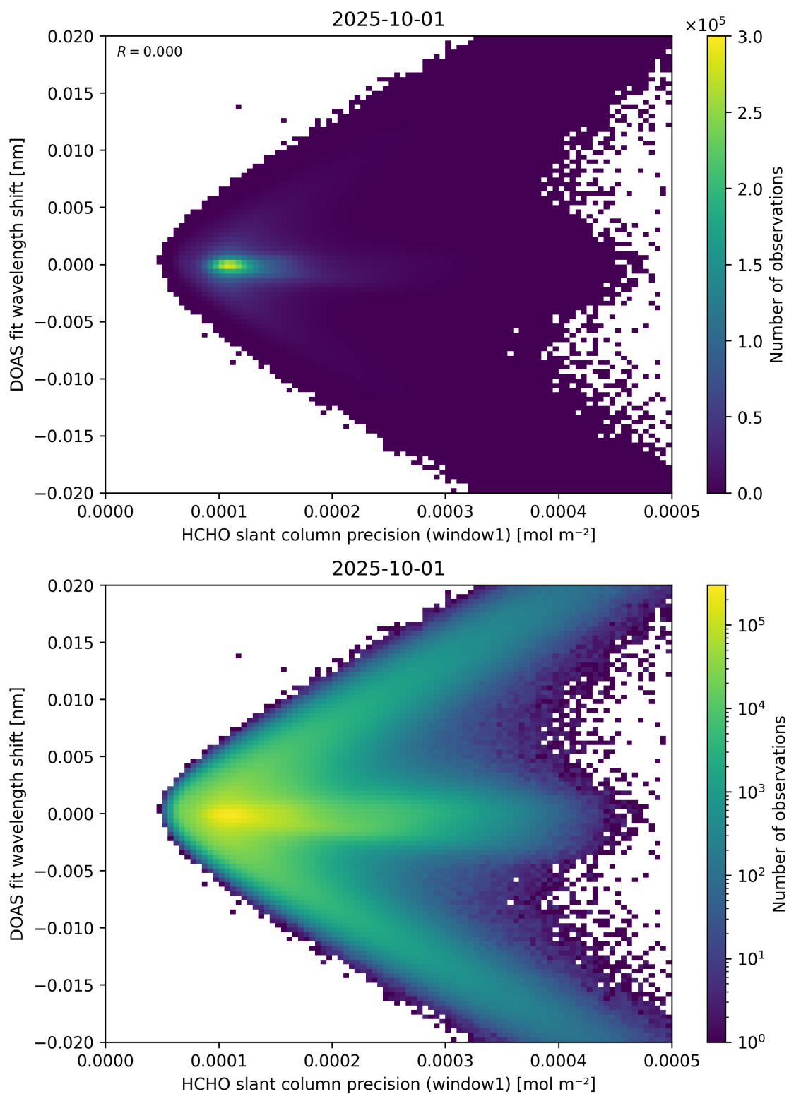
Figure 89: Scatter density plot of “HCHO slant column precision (window1)” against “DOAS fit wavelength shift” for 2025-10-01 to 2025-10-02.
