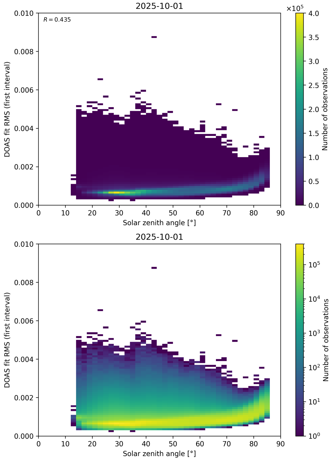
Figure 167: Scatter density plot of “Solar zenith angle” against “DOAS fit RMS (first interval)” for 2025-10-01 to 2025-10-02.
