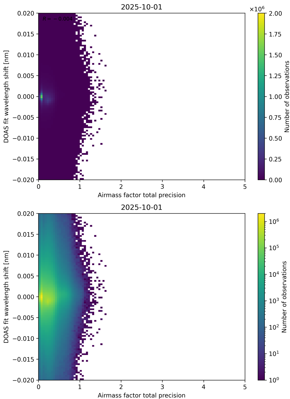
Figure 106: Scatter density plot of “Airmass factor total precision” against “DOAS fit wavelength shift” for 2025-10-01 to 2025-10-02.
