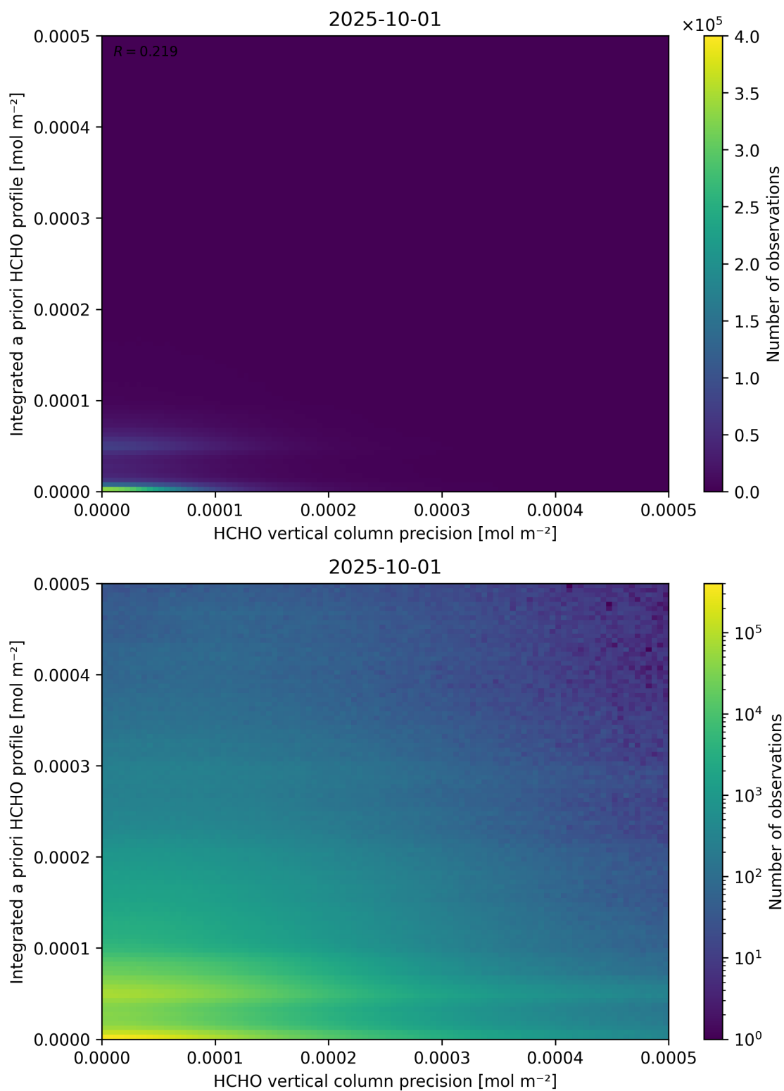
Figure 147: Scatter density plot of “HCHO vertical column precision” against “Integrated a priori HCHO profile” for 2025-10-01 to 2025-10-02.
