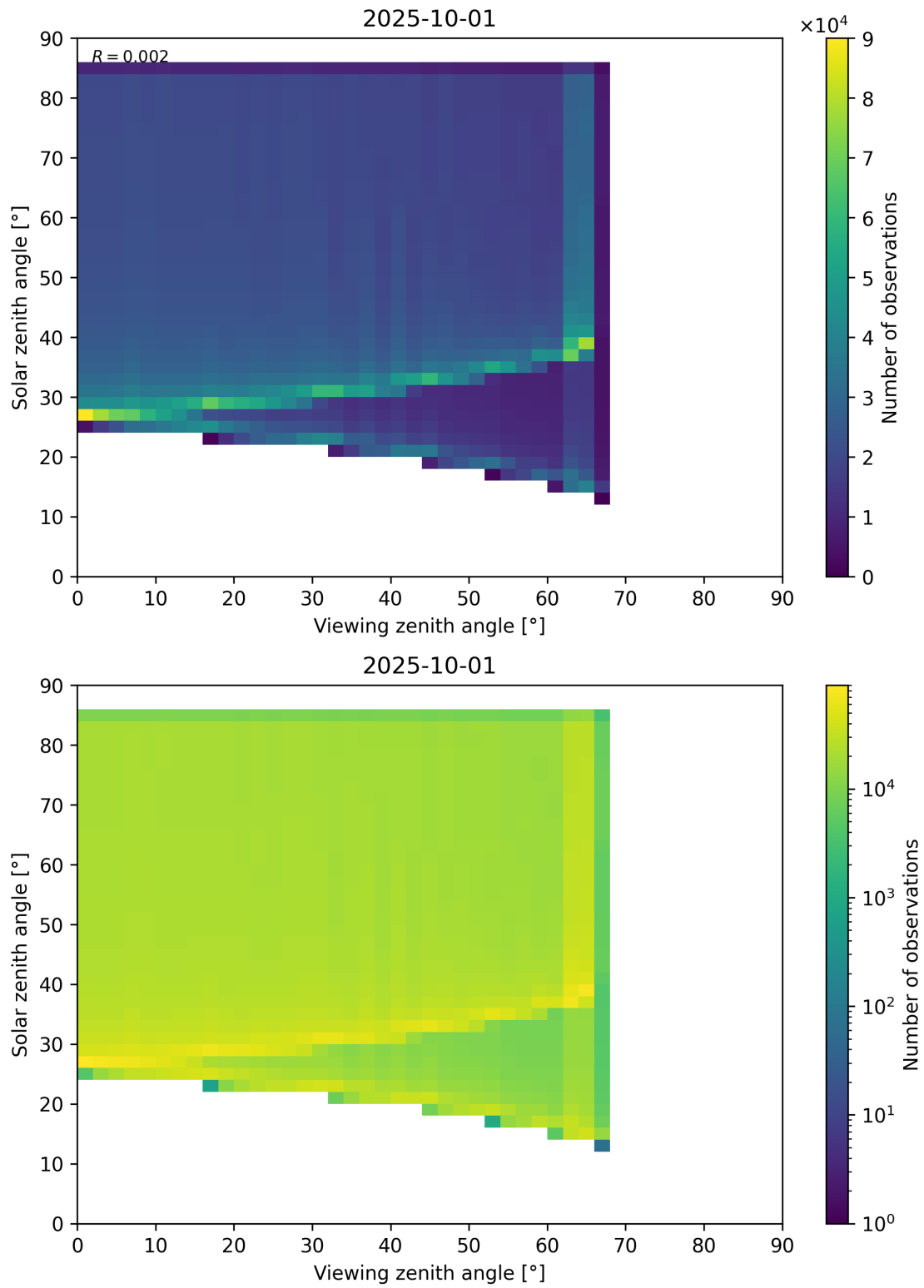
Figure 197: Scatter density plot of “Viewing zenith angle” against “Solar zenith angle” for 2025-10-01 to 2025-10-02.
