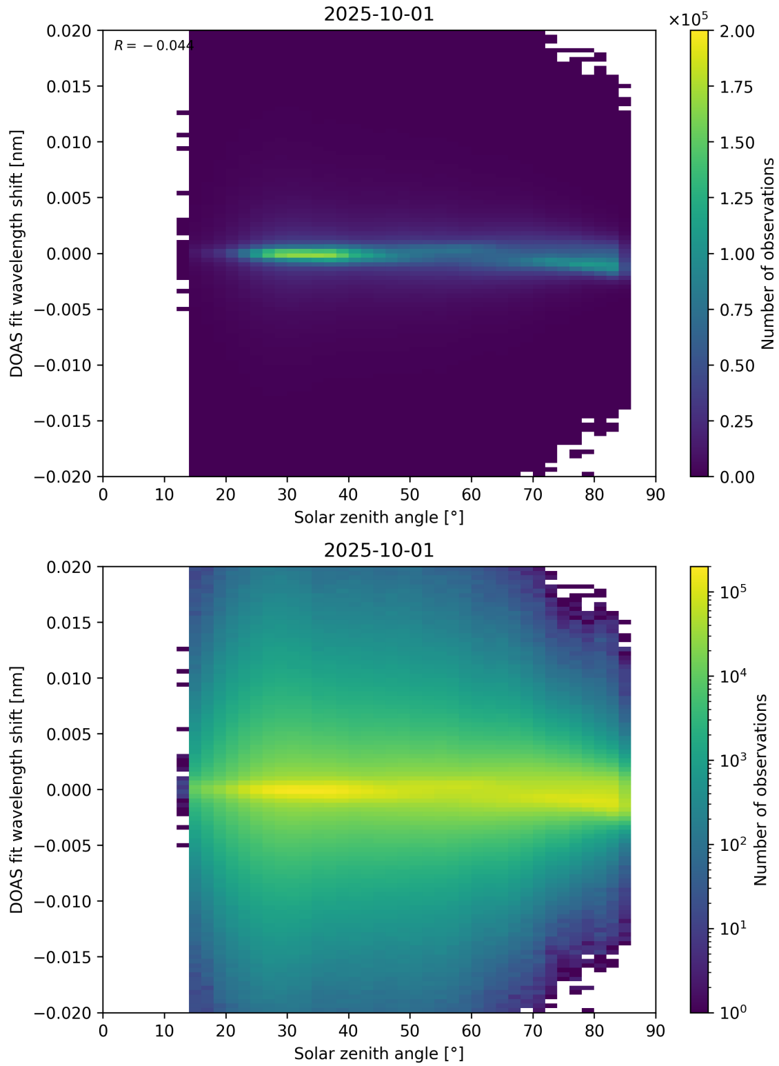
Figure 168: Scatter density plot of “Solar zenith angle” against “DOAS fit wavelength shift” for 2025-10-01 to 2025-10-02.
