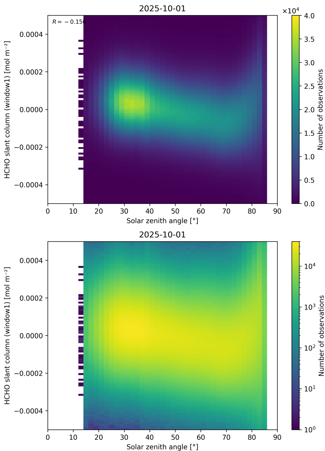
Figure 173: Scatter density plot of “Solar zenith angle” against “HCHO slant column (window1)” for 2025-10-01 to 2025-10-02.
