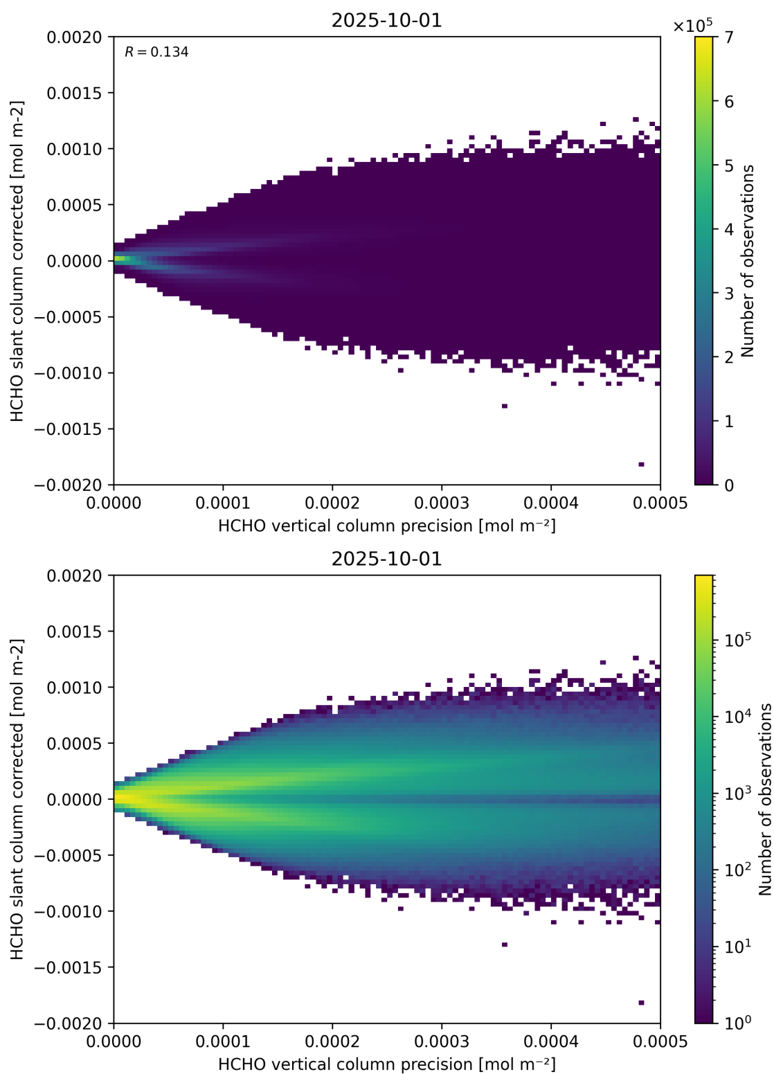
Figure 140: Scatter density plot of “HCHO vertical column precision” against “HCHO slant column corrected” for 2025-10-01 to 2025-10-02.
