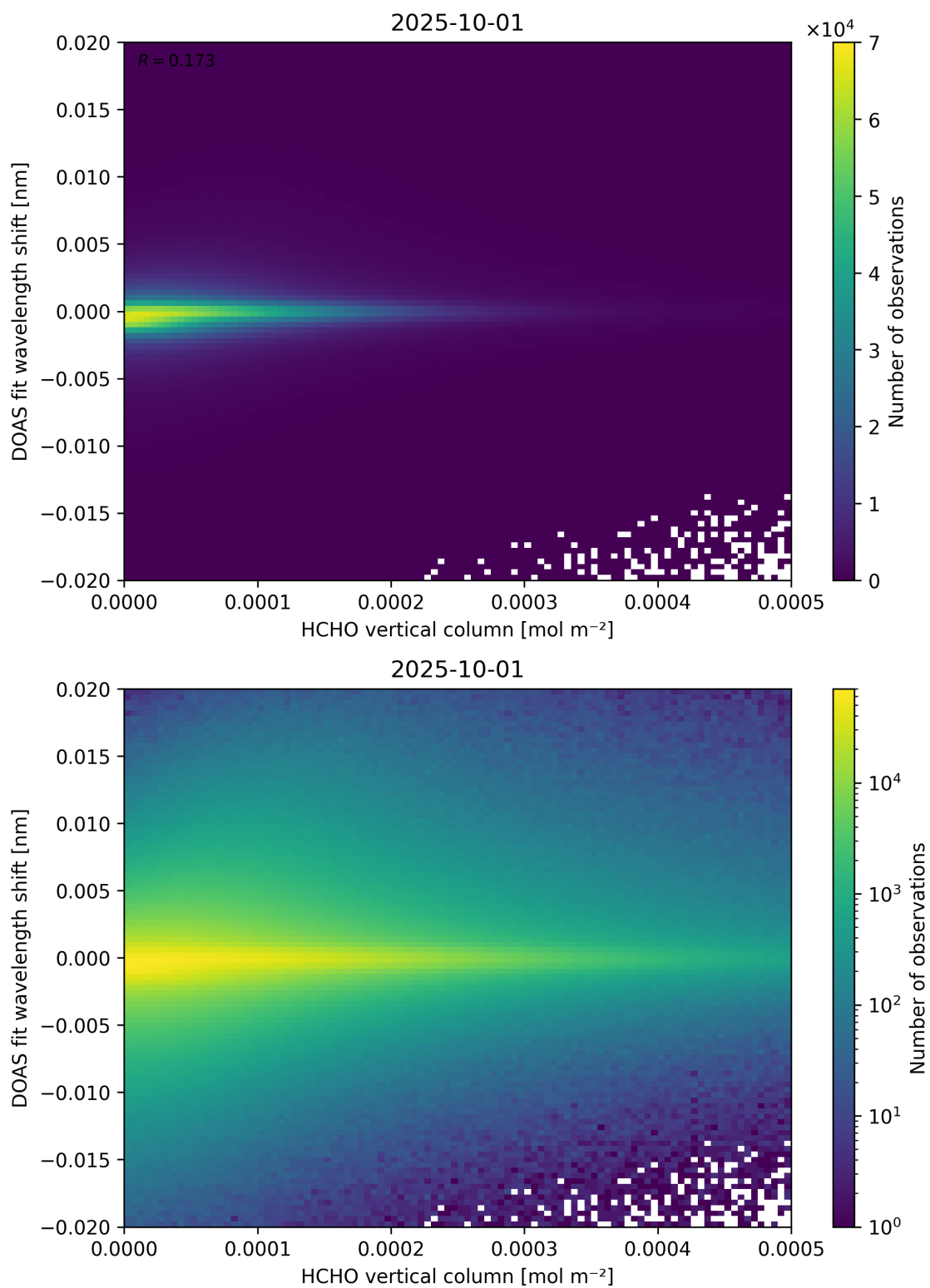
Figure 124: Scatter density plot of “HCHO vertical column” against “DOAS fit wavelength shift” for 2025-10-01 to 2025-10-02.
