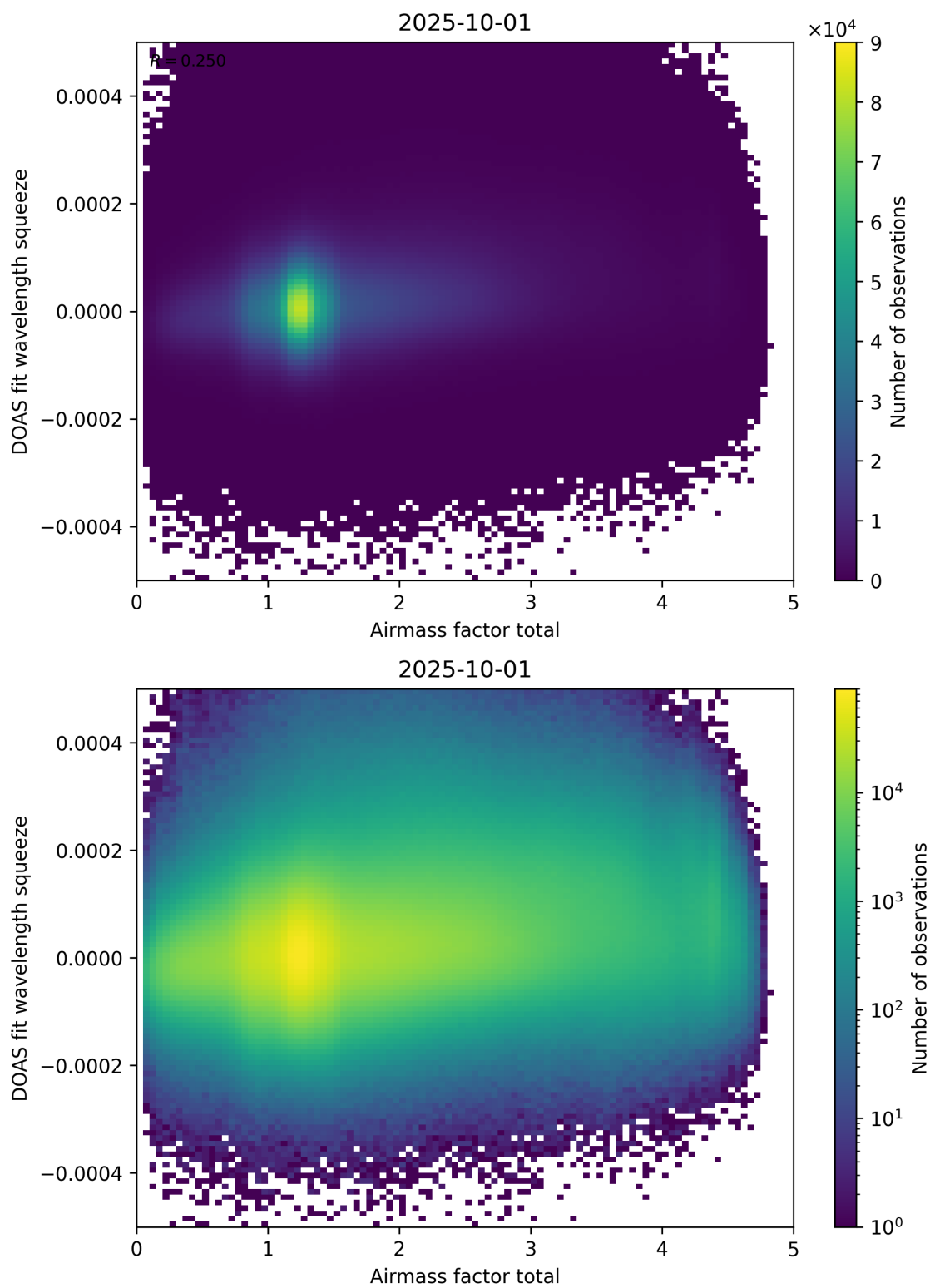
Figure 99: Scatter density plot of “Airmass factor total” against “DOAS fit wavelength squeeze” for 2025-10-01 to 2025-10-02.
