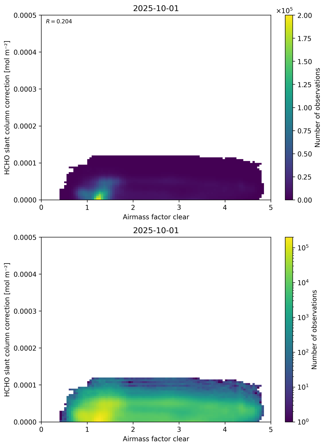
Figure 75: Scatter density plot of “Airmass factor clear” against “HCHO slant column correction” for 2025-10-01 to 2025-10-02.
