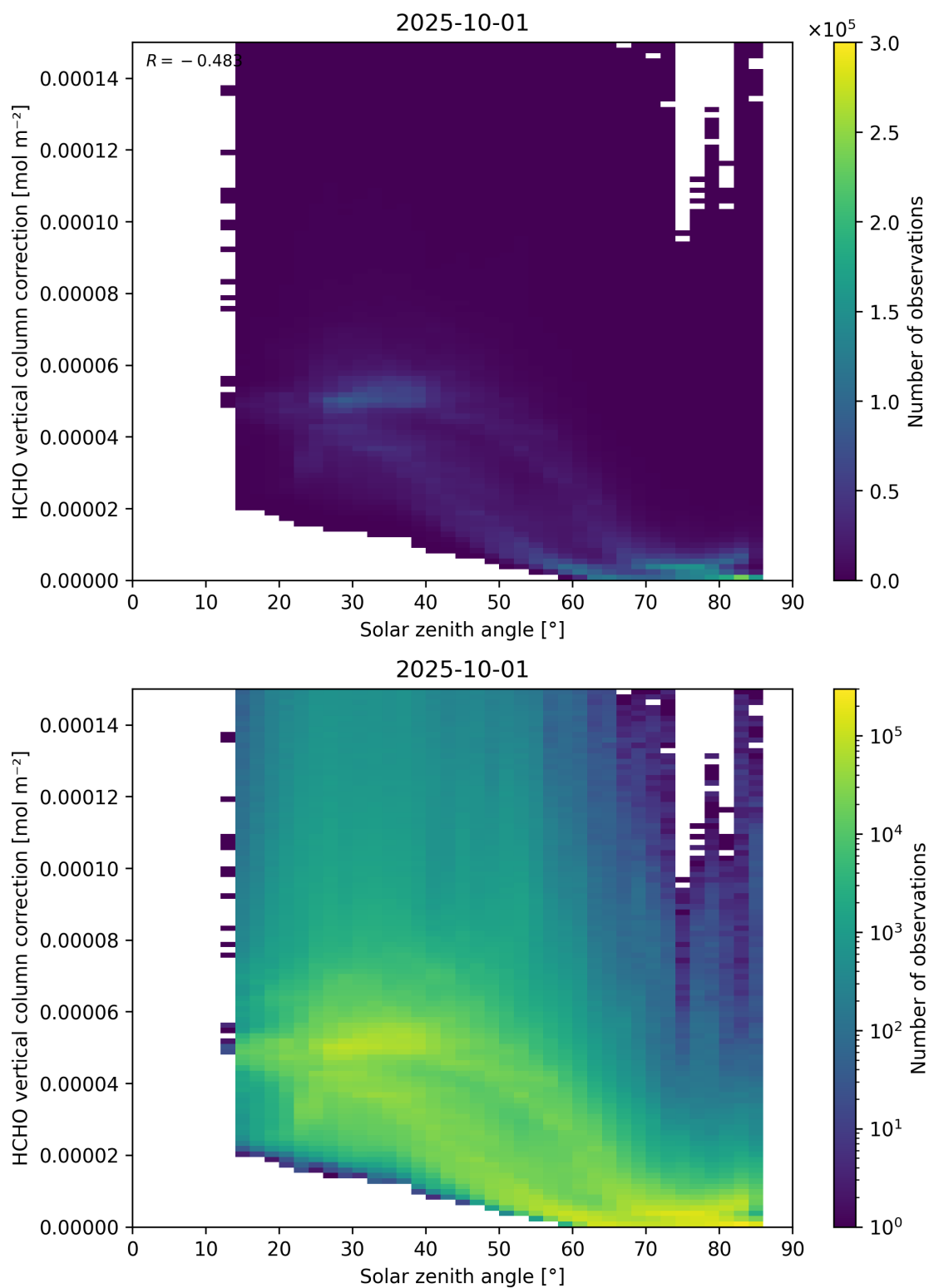
Figure 178: Scatter density plot of “Solar zenith angle” against “HCHO vertical column correction” for 2025-10-01 to 2025-10-02.
