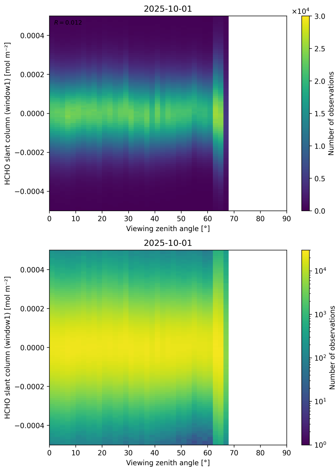
Figure 188: Scatter density plot of “Viewing zenith angle” against “HCHO slant column (window1)” for 2025-10-01 to 2025-10-02.
