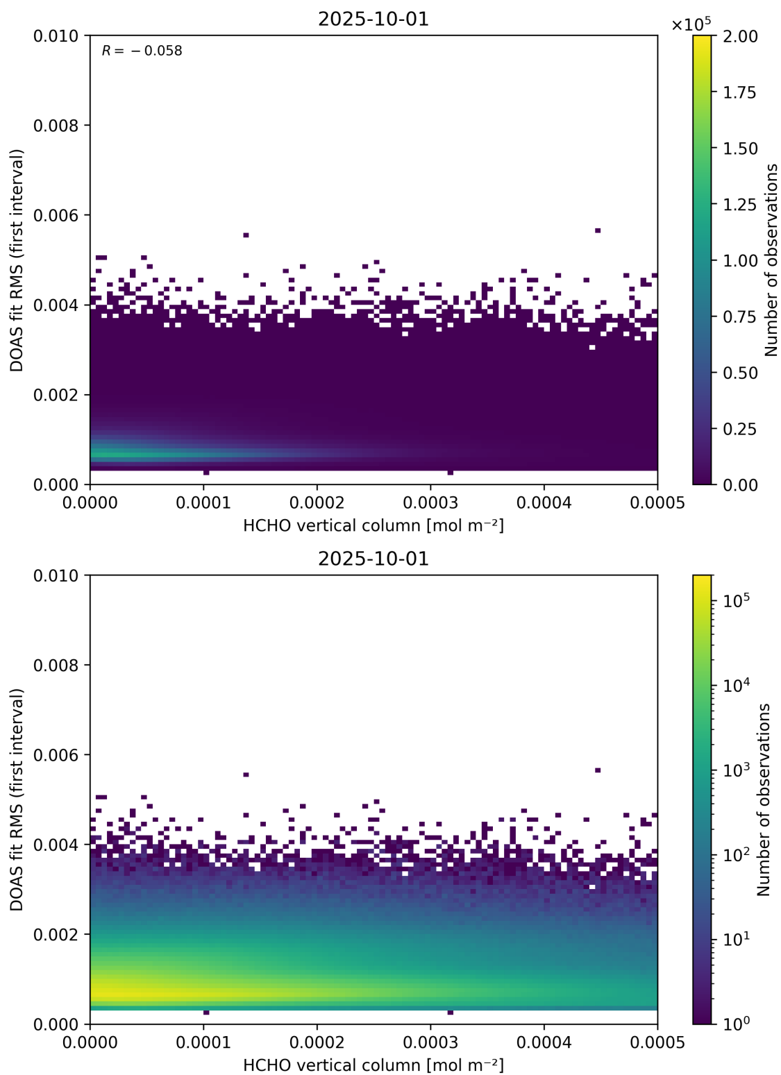
Figure 123: Scatter density plot of “HCHO vertical column” against “DOAS fit RMS (first interval)” for 2025-10-01 to 2025-10-02.
