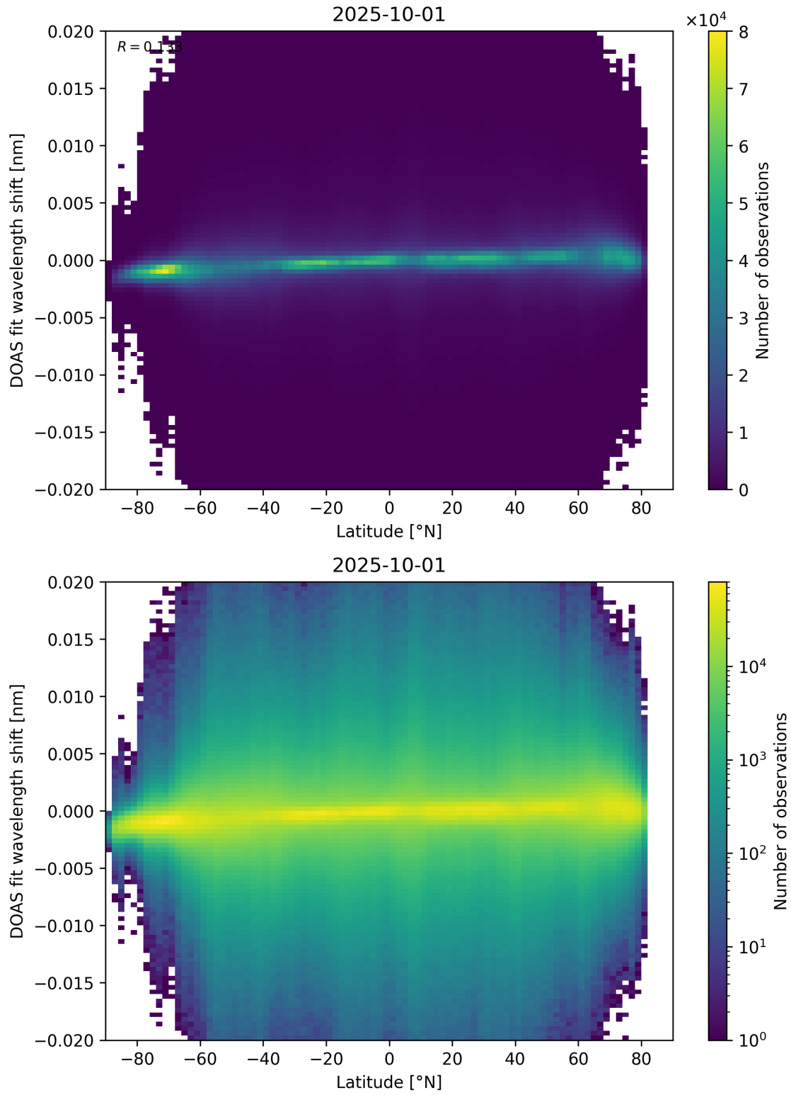
Figure 154: Scatter density plot of “Latitude” against “DOAS fit wavelength shift” for 2025-10-01 to 2025-10-02.
