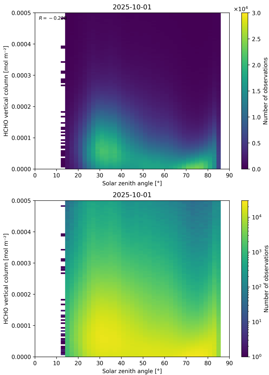
Figure 177: Scatter density plot of “Solar zenith angle” against “HCHO vertical column” for 2025-10-01 to 2025-10-02.
