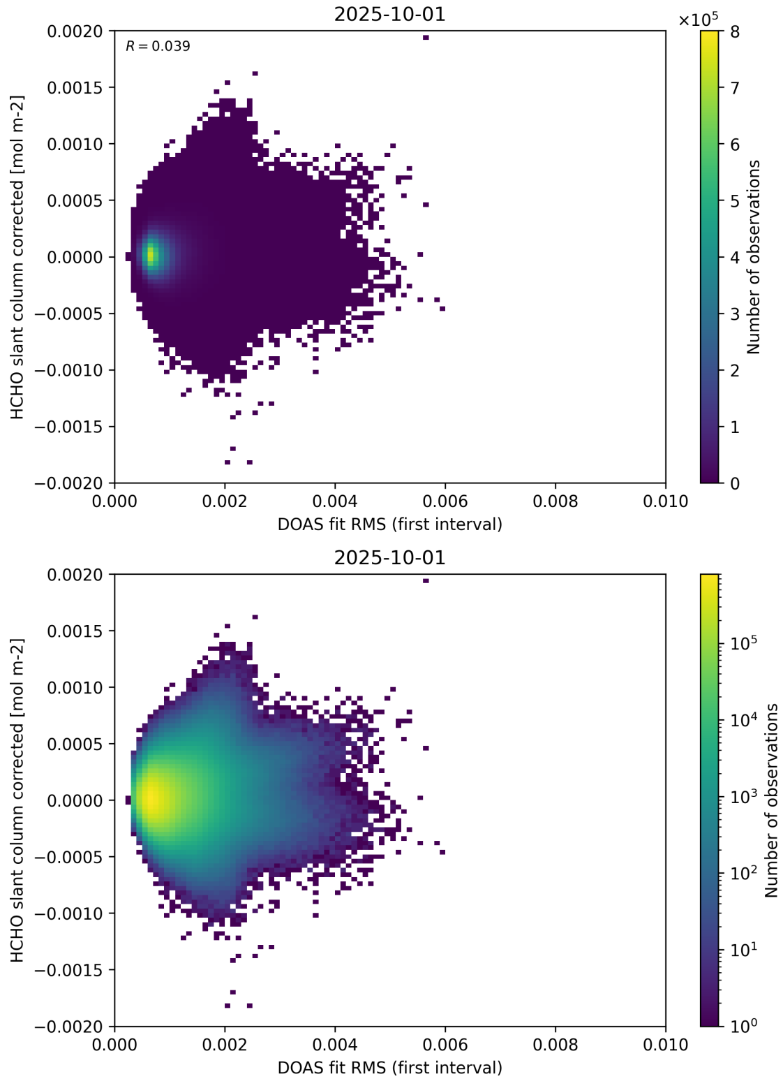
Figure 62: Scatter density plot of “DOAS fit RMS (first interval)” against “HCHO slant column corrected” for 2025-10-01 to 2025-10-02.
