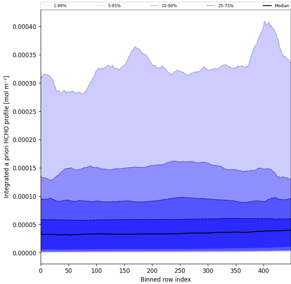
Figure 57: Along track statistics of "Integrated a priori HCHO profile" for 2025-10-01 to 2025-10-02
