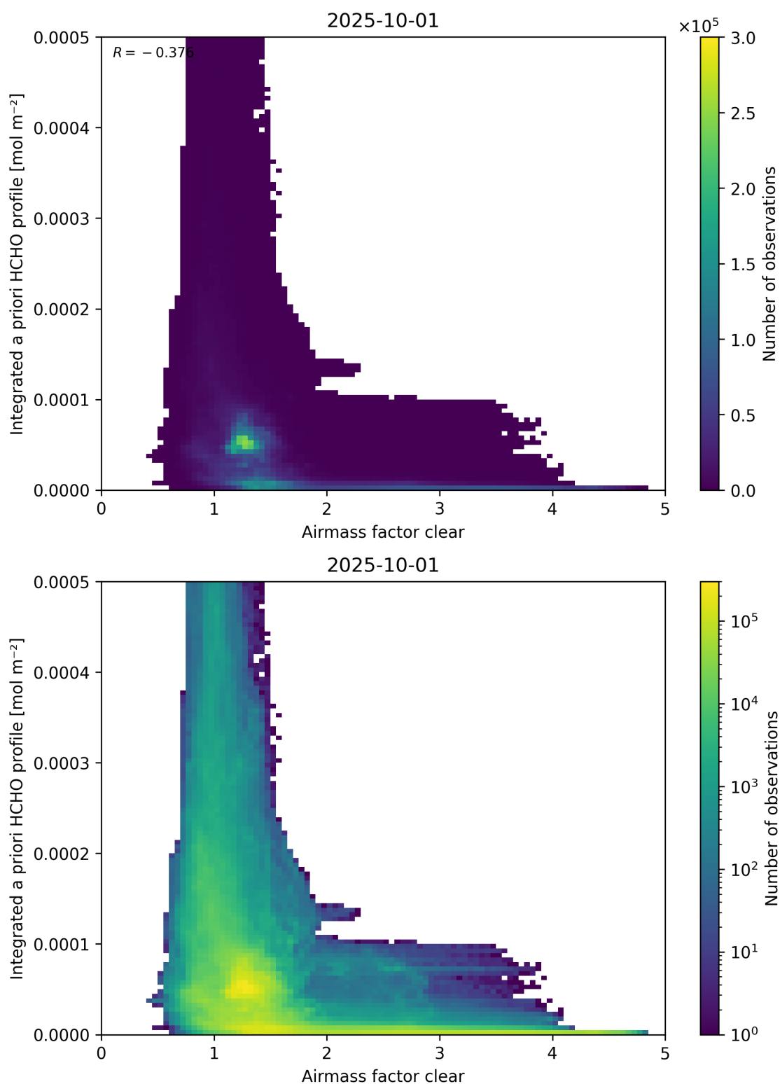
Figure 76: Scatter density plot of “Airmass factor clear” against “Integrated a priori HCHO profile” for 2025-10-01 to 2025-10-02.
