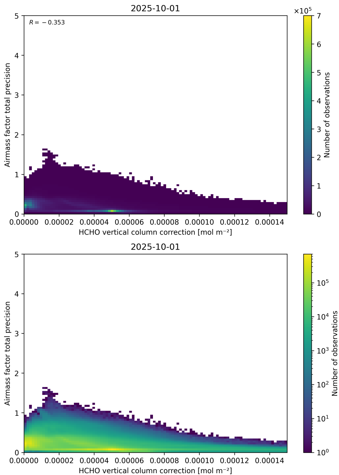
Figure 121: Scatter density plot of “HCHO vertical column correction” against “Airmass factor total precision” for 2025-10-01 to 2025-10-02.
