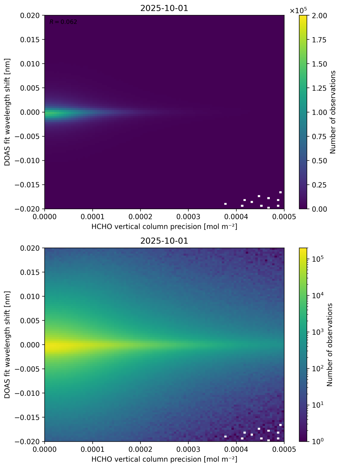
Figure 137: Scatter density plot of “HCHO vertical column precision” against “DOAS fit wavelength shift” for 2025-10-01 to 2025-10-02.
