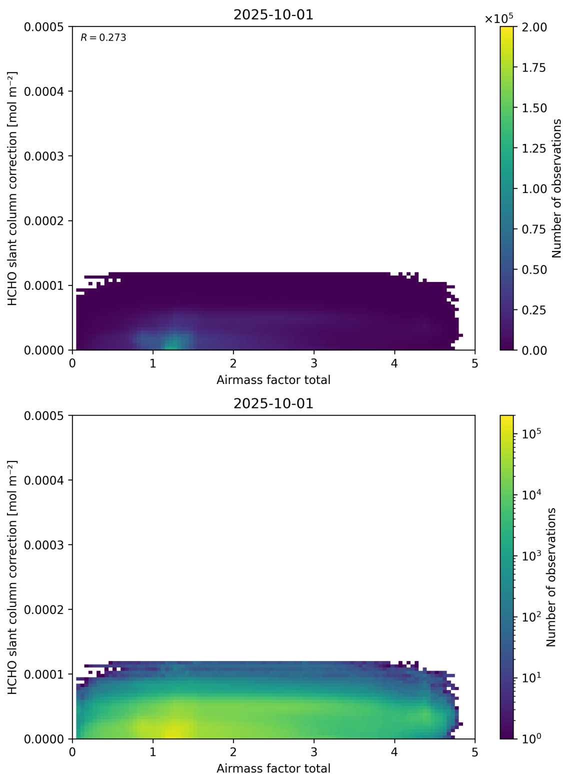
Figure 102: Scatter density plot of “Airmass factor total” against “HCHO slant column correction” for 2025-10-01 to 2025-10-02.
