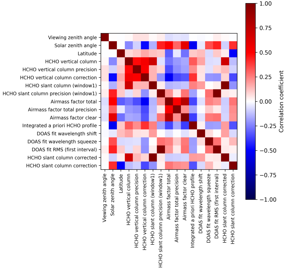
Figure 2: Map of correlation matrix for 2025-10-01 to 2025-10-02.
