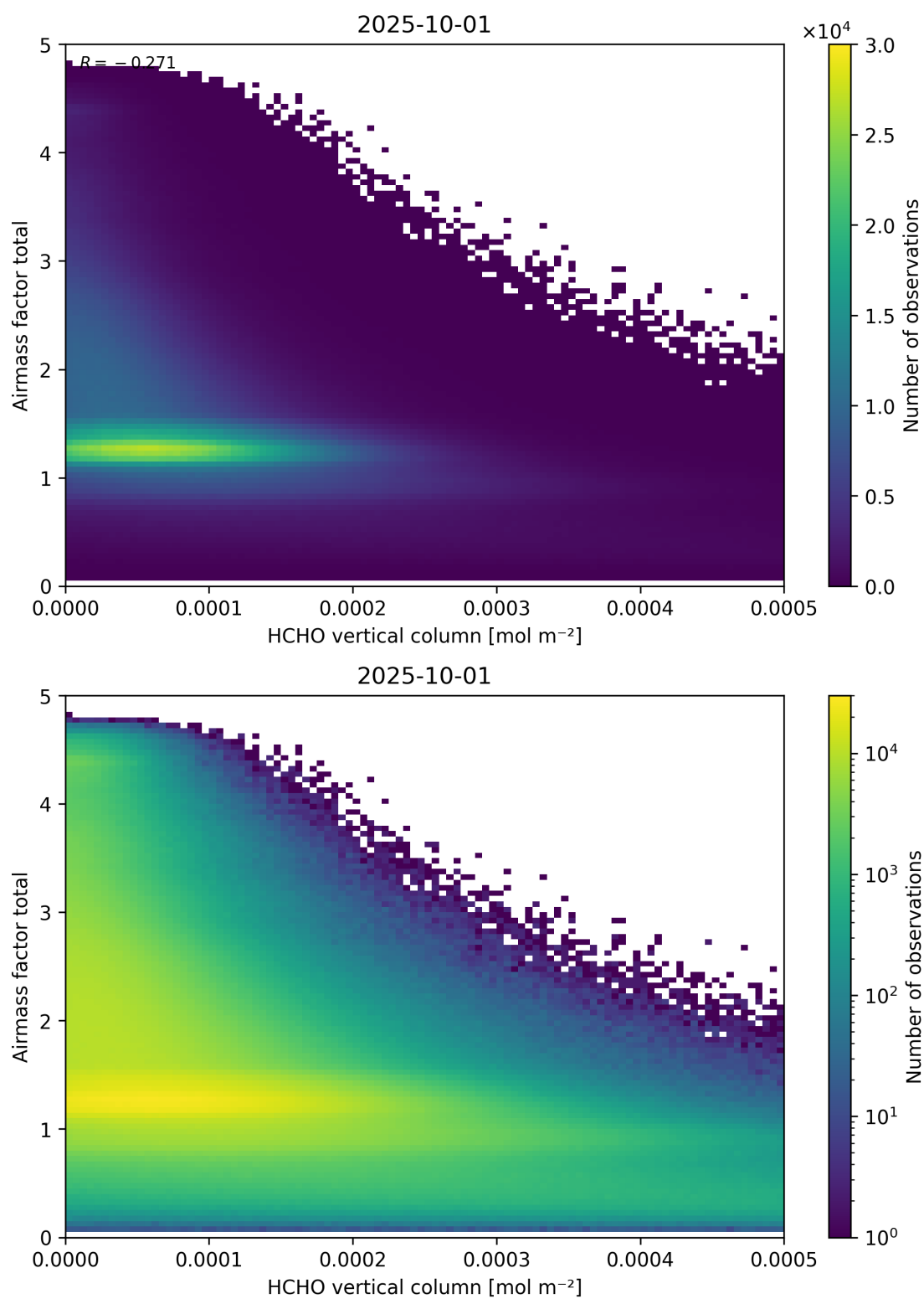
Figure 131: Scatter density plot of “HCHO vertical column” against “Airmass factor total” for 2025-10-01 to 2025-10-02.
