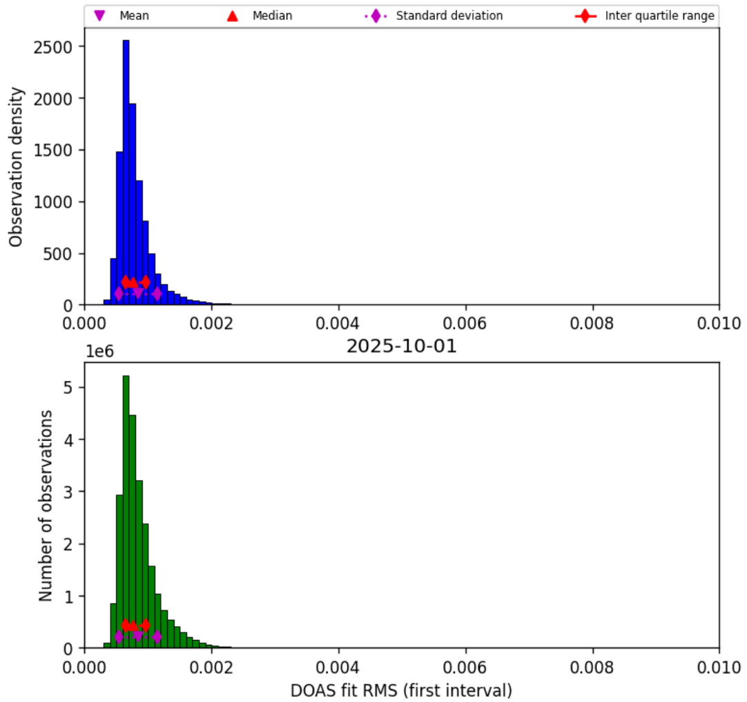
Figure 46: Histogram of “DOAS fit RMS (first interval)” for 2025-10-01 to 2025-10-02
