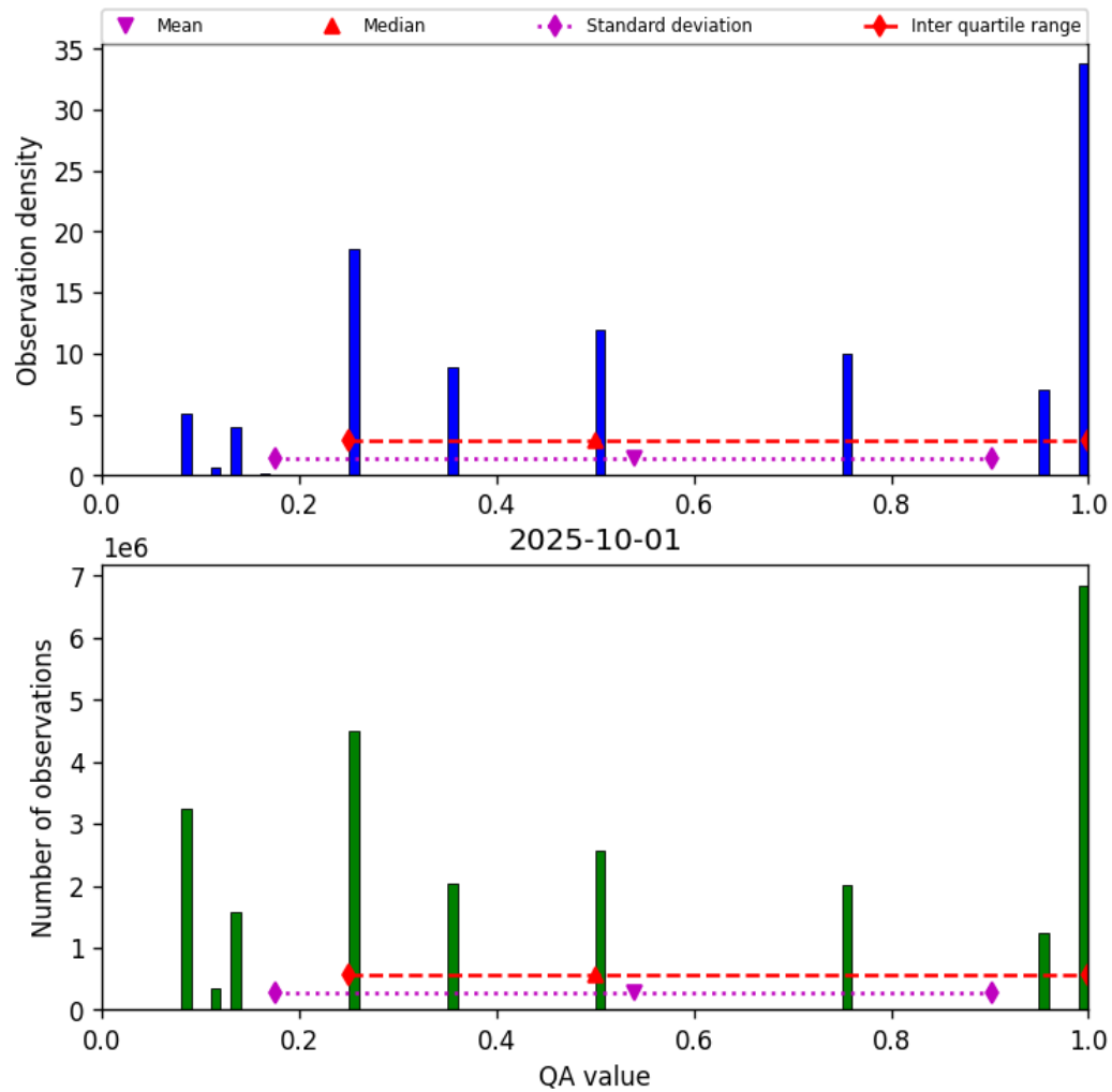
Figure 34: Histogram of “QA value” for 2025-10-01 to 2025-10-02
