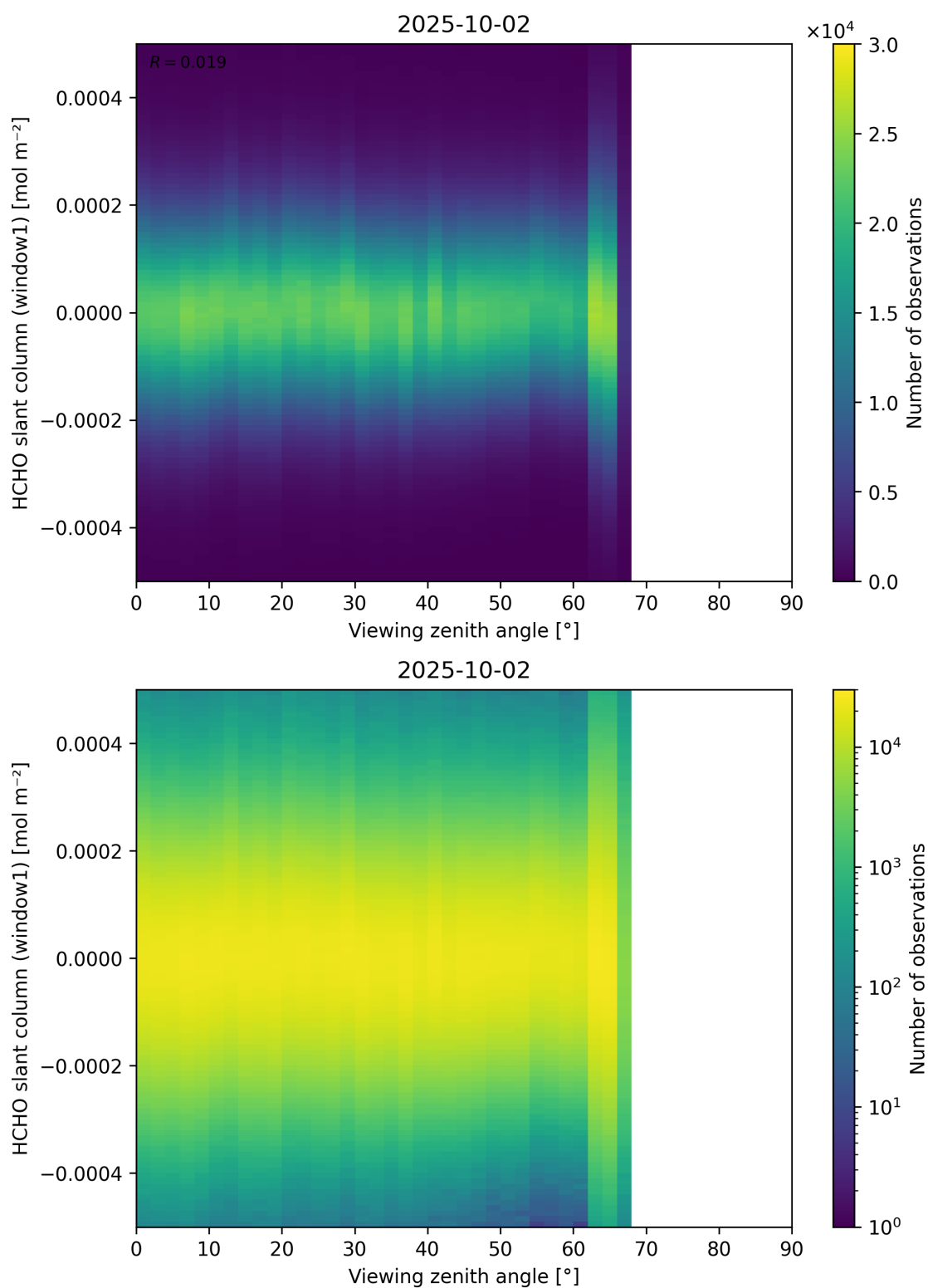
Figure 188: Scatter density plot of “Viewing zenith angle” against “HCHO slant column (window1)” for 2025-10-01 to 2025-10-03.
