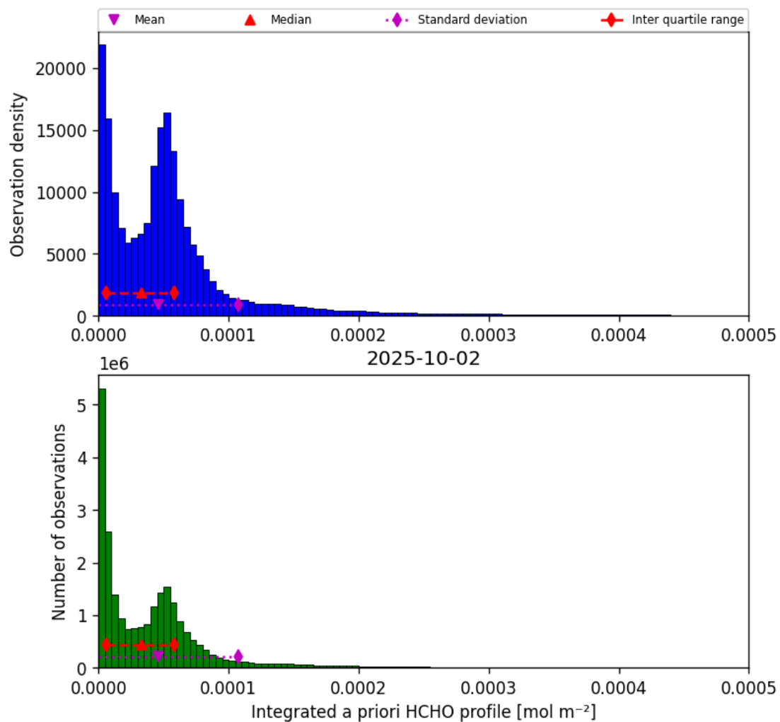
Figure 43: Histogram of “Integrated a priori HCHO profile” for 2025-10-01 to 2025-10-03
