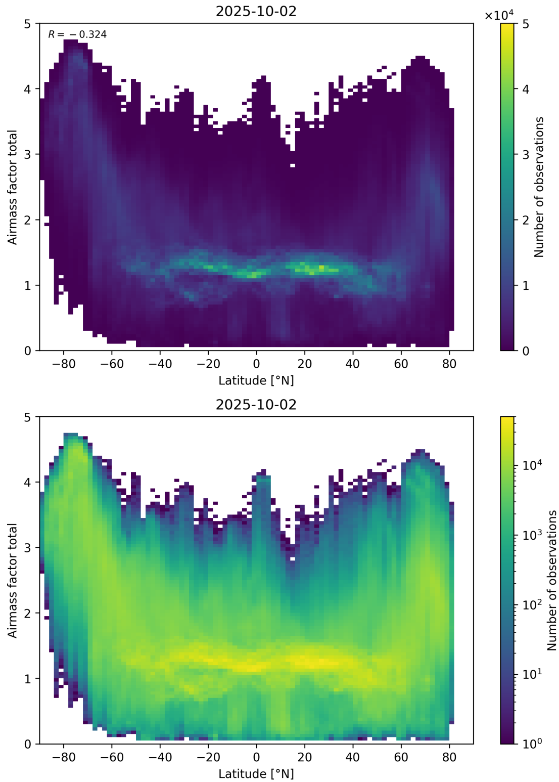
Figure 161: Scatter density plot of “Latitude” against “Airmass factor total” for 2025-10-01 to 2025-10-03.
