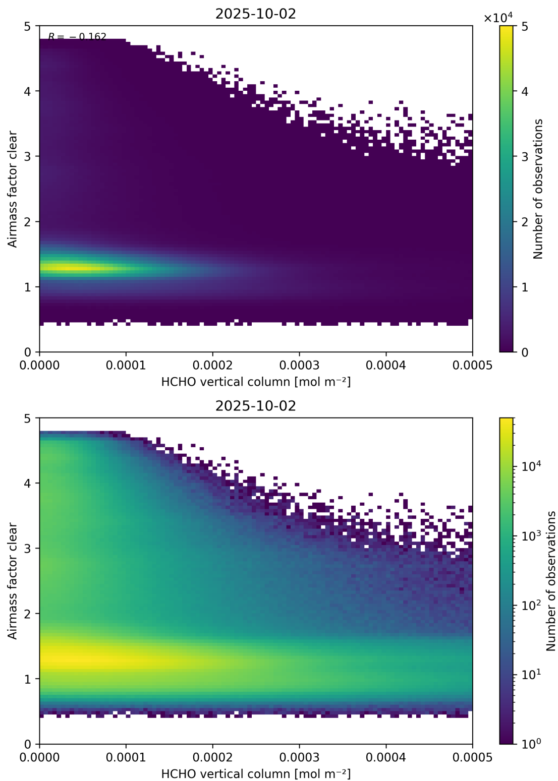
Figure 126: Scatter density plot of “HCHO vertical column” against “Airmass factor clear” for 2025-10-01 to 2025-10-03.
