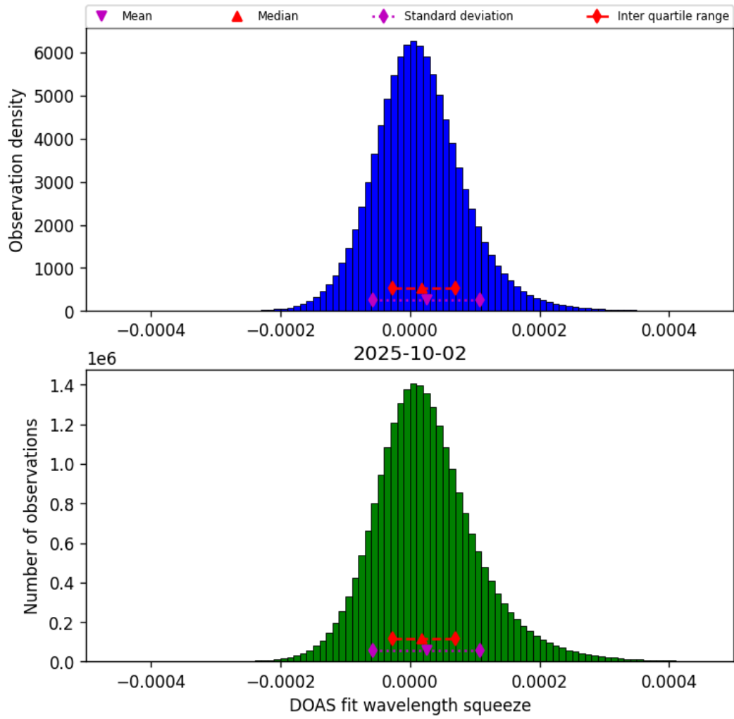
Figure 45: Histogram of “DOAS fit wavelength squeeze” for 2025-10-01 to 2025-10-03
