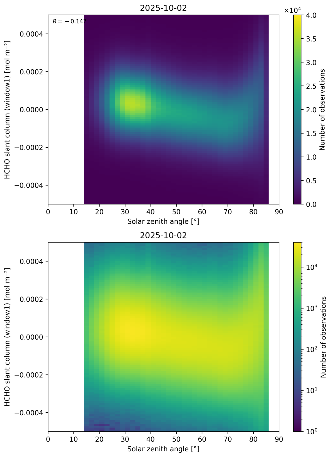
Figure 173: Scatter density plot of “Solar zenith angle” against “HCHO slant column (window1)” for 2025-10-01 to 2025-10-03.
