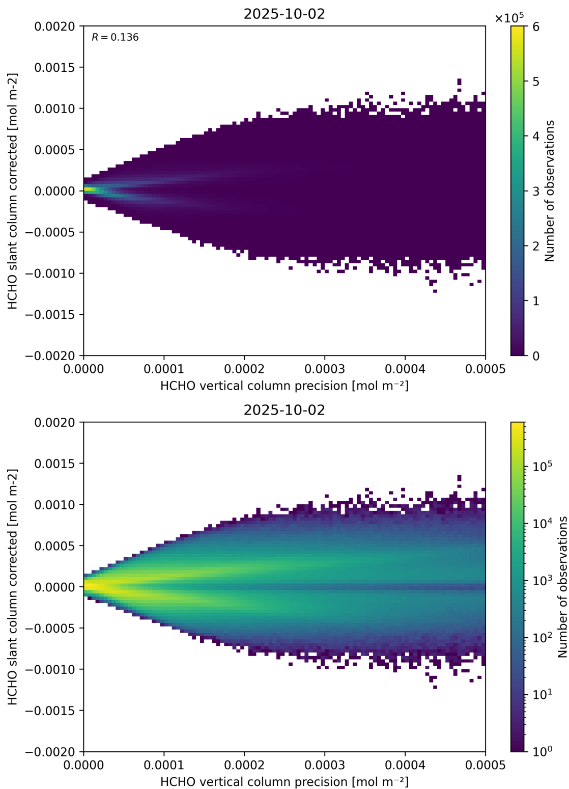
Figure 140: Scatter density plot of “HCHO vertical column precision” against “HCHO slant column corrected” for 2025-10-01 to 2025-10-03.
