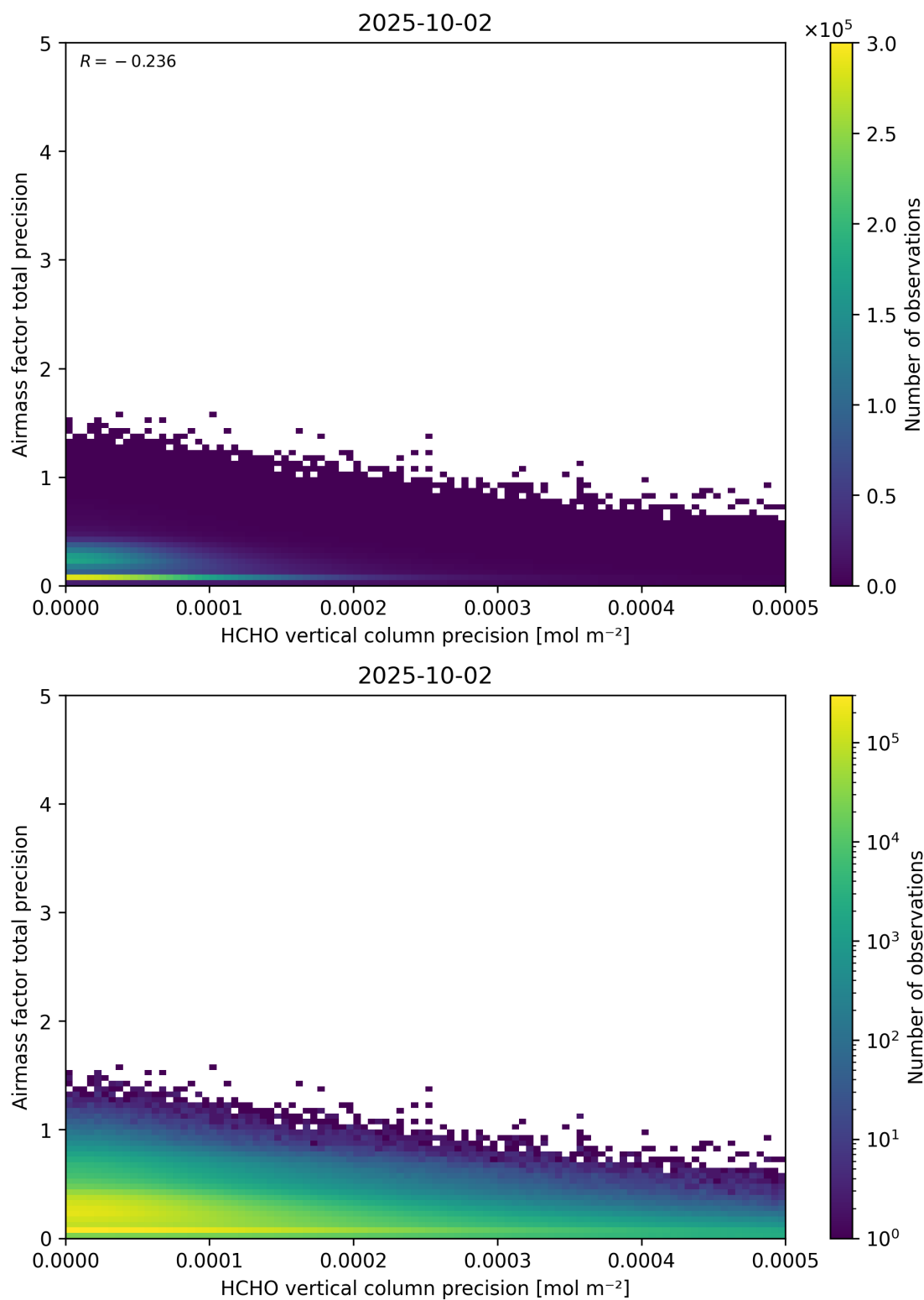
Figure 145: Scatter density plot of “HCHO vertical column precision” against “Airmass factor total precision” for 2025-10-01 to 2025-10-03.
