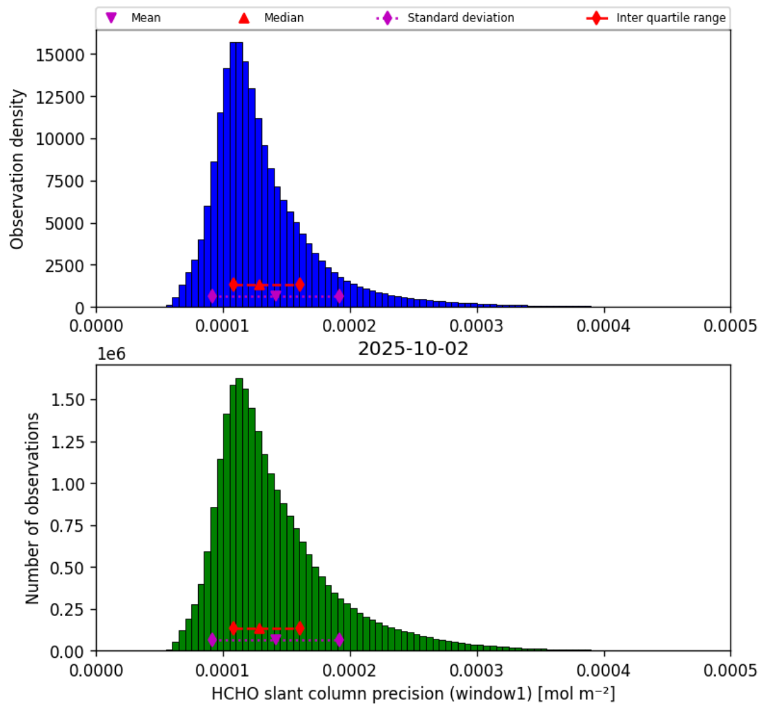
Figure 39: Histogram of “HCHO slant column precision (window1)” for 2025-10-01 to 2025-10-03
