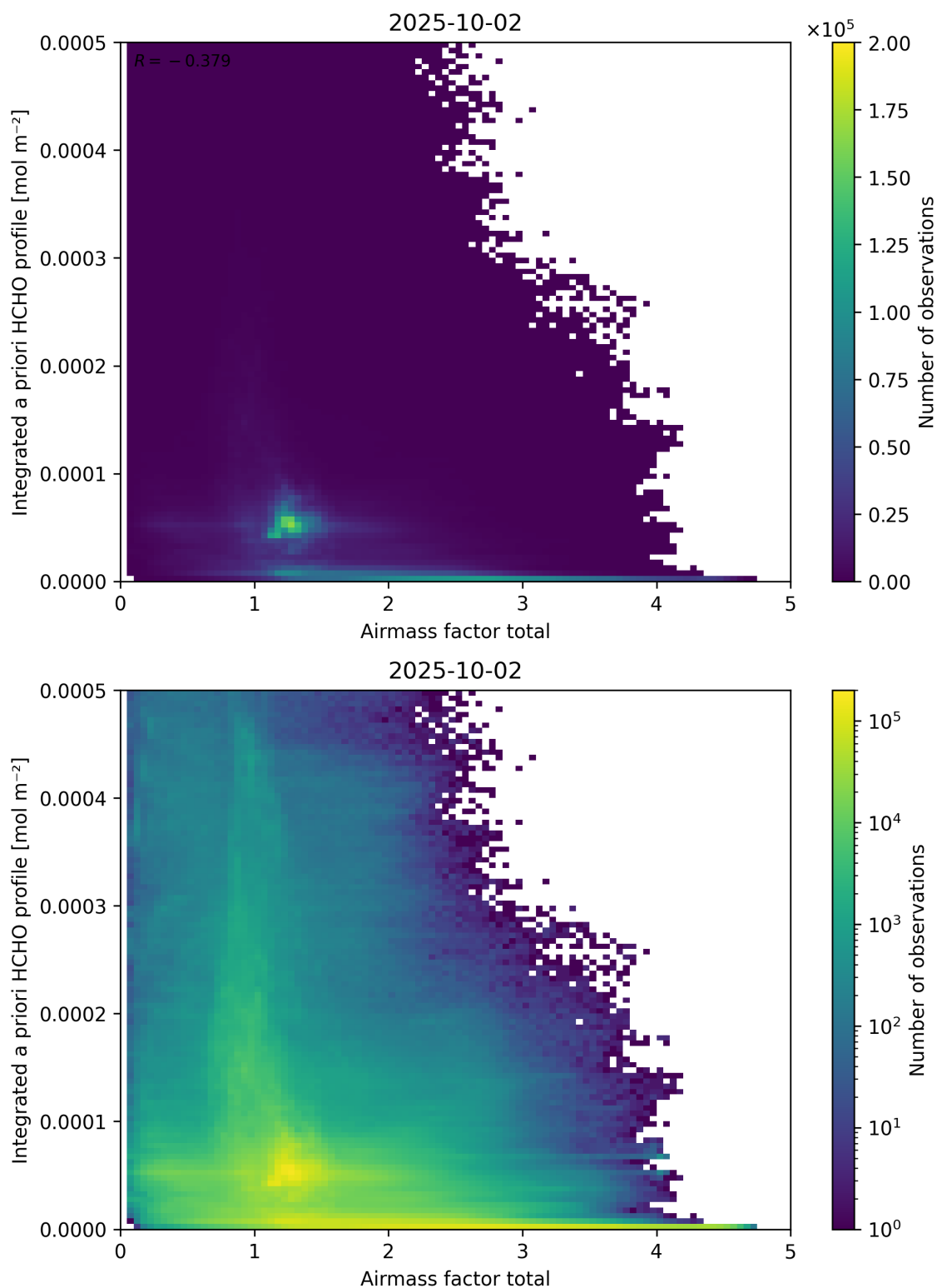
Figure 104: Scatter density plot of “Airmass factor total” against “Integrated a priori HCHO profile” for 2025-10-01 to 2025-10-03.
