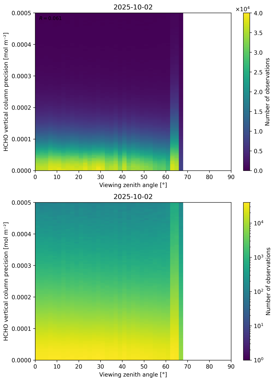
Figure 194: Scatter density plot of “Viewing zenith angle” against “HCHO vertical column precision” for 2025-10-01 to 2025-10-03.
