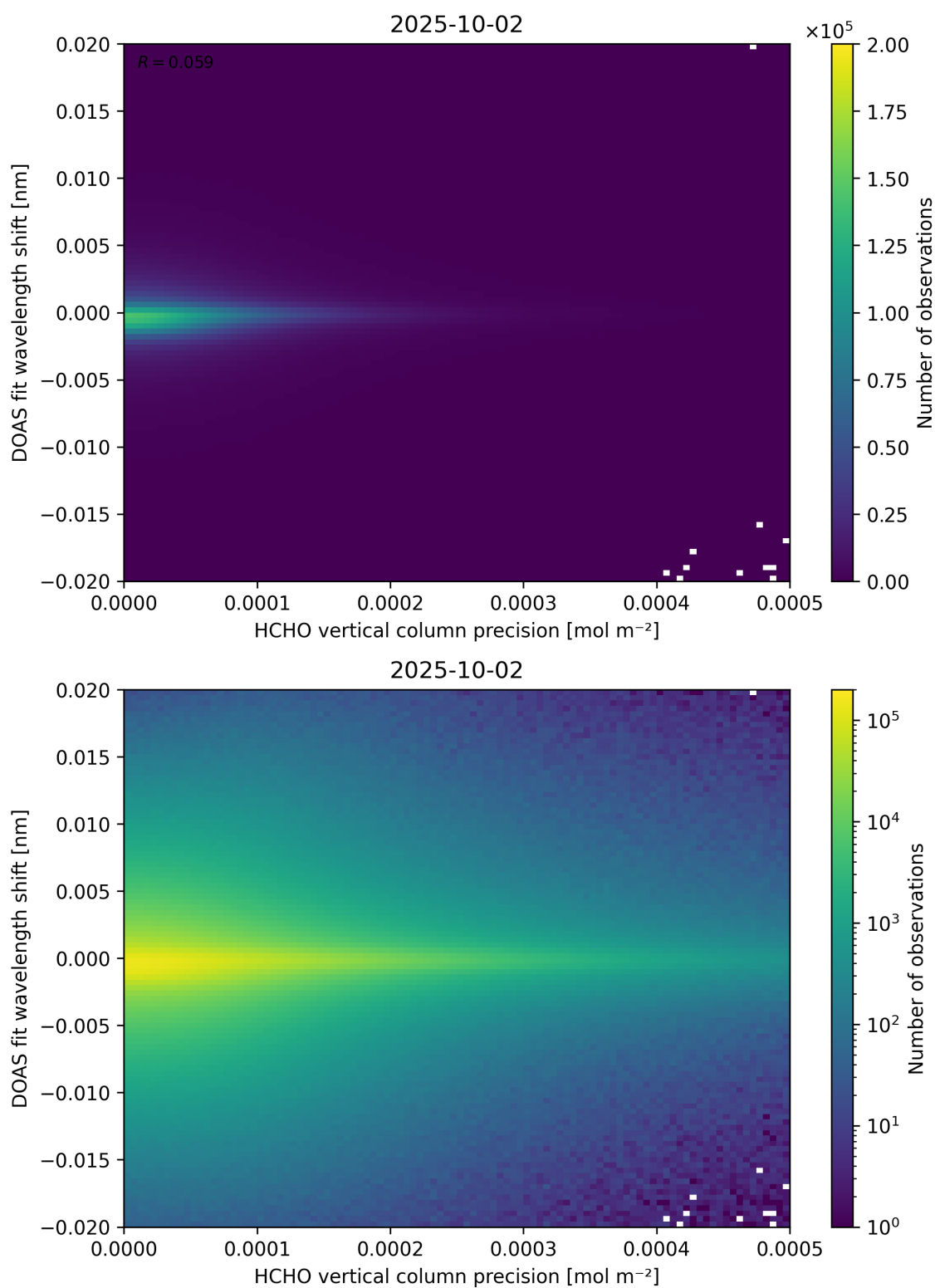
Figure 137: Scatter density plot of “HCHO vertical column precision” against “DOAS fit wavelength shift” for 2025-10-01 to 2025-10-03.
