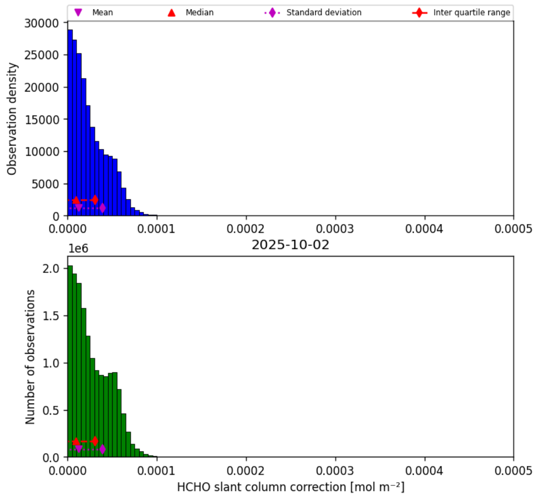
Figure 47: Histogram of “HCHO slant column correction” for 2025-10-01 to 2025-10-03
