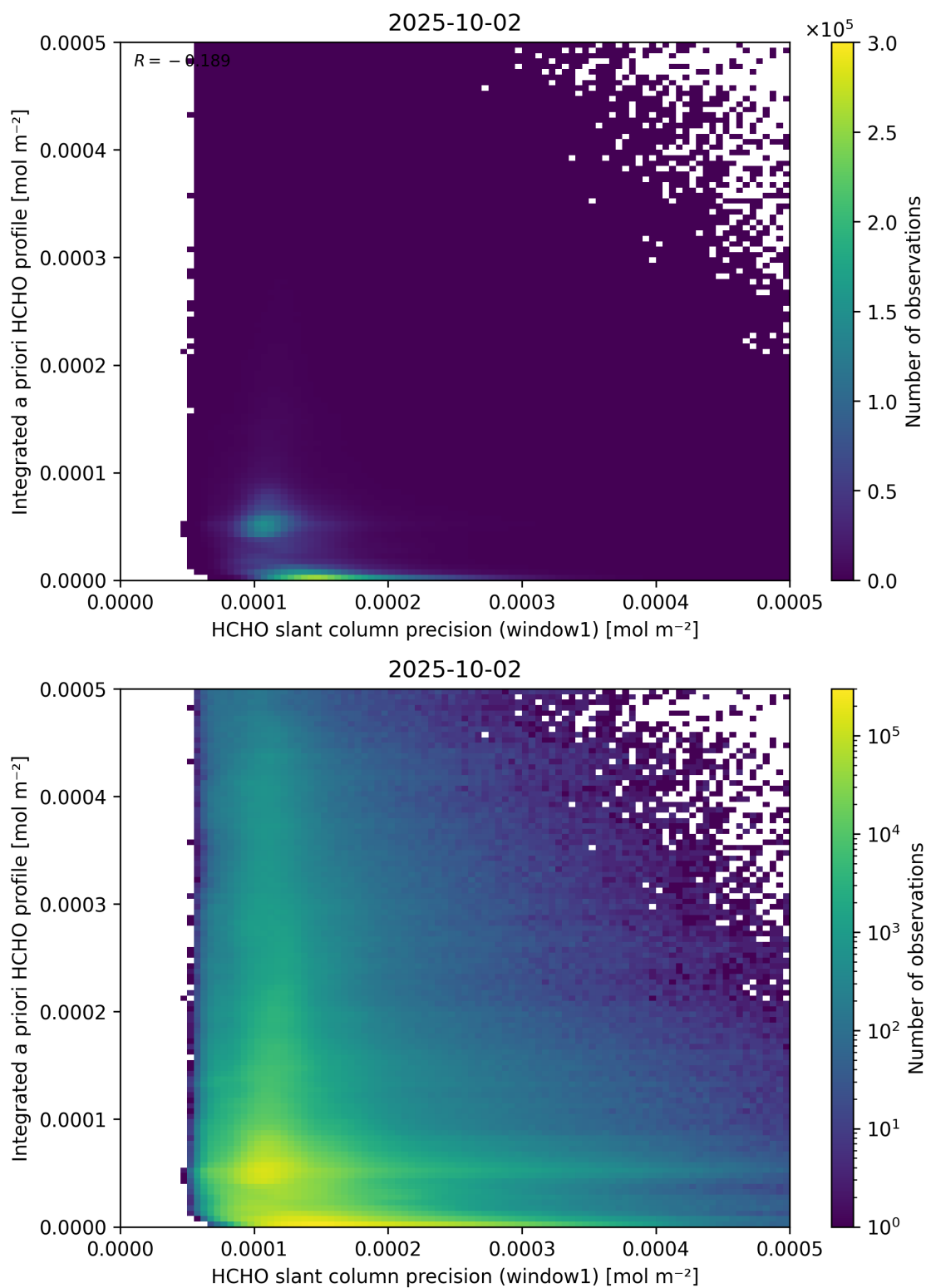
Figure 96: Scatter density plot of “HCHO slant column precision (window1)” against “Integrated a priori HCHO profile” for 2025-10-01 to 2025-10-03.
