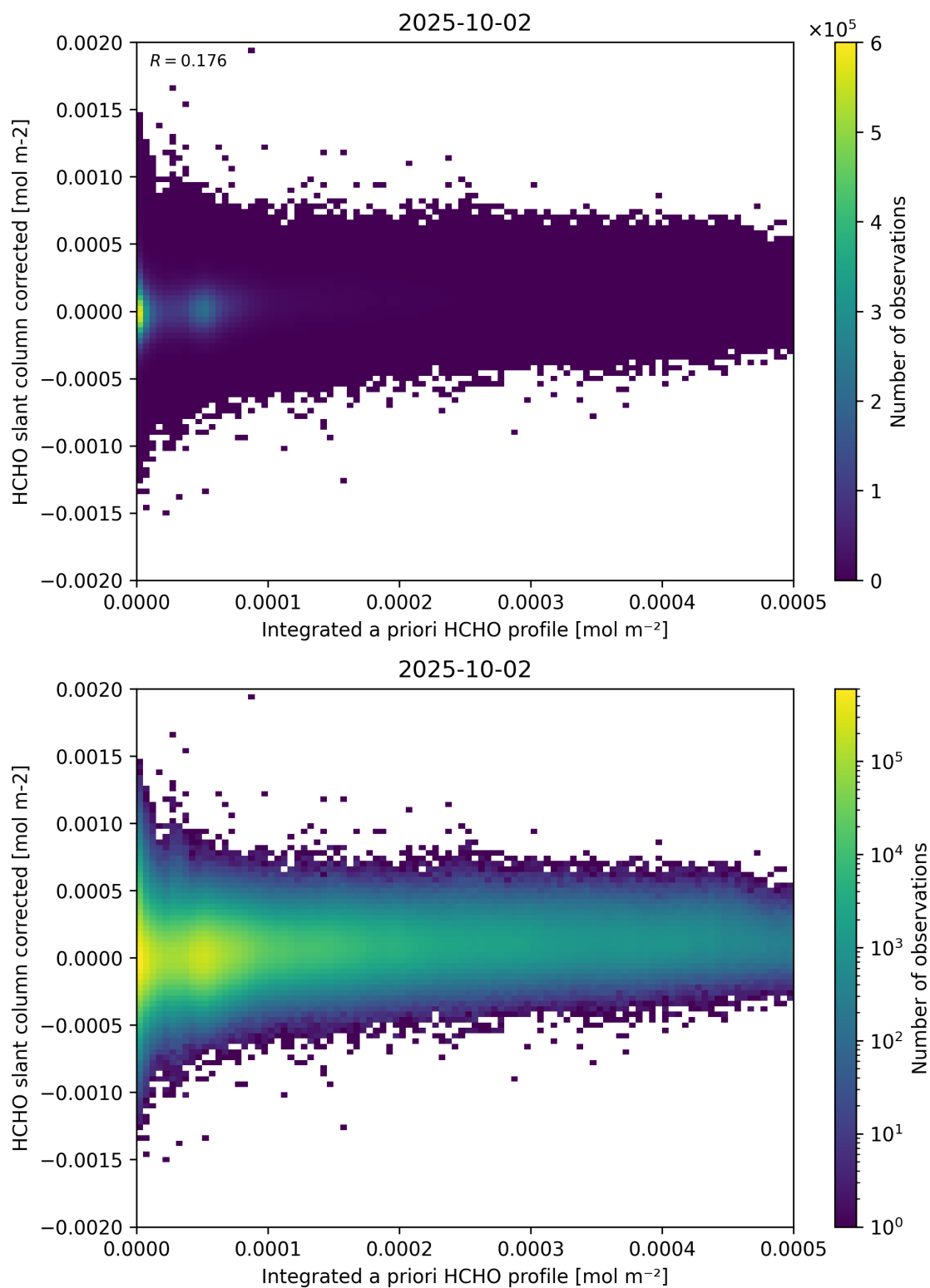
Figure 151: Scatter density plot of “Integrated a priori HCHO profile” against “HCHO slant column corrected” for 2025-10-01 to 2025-10-03.
