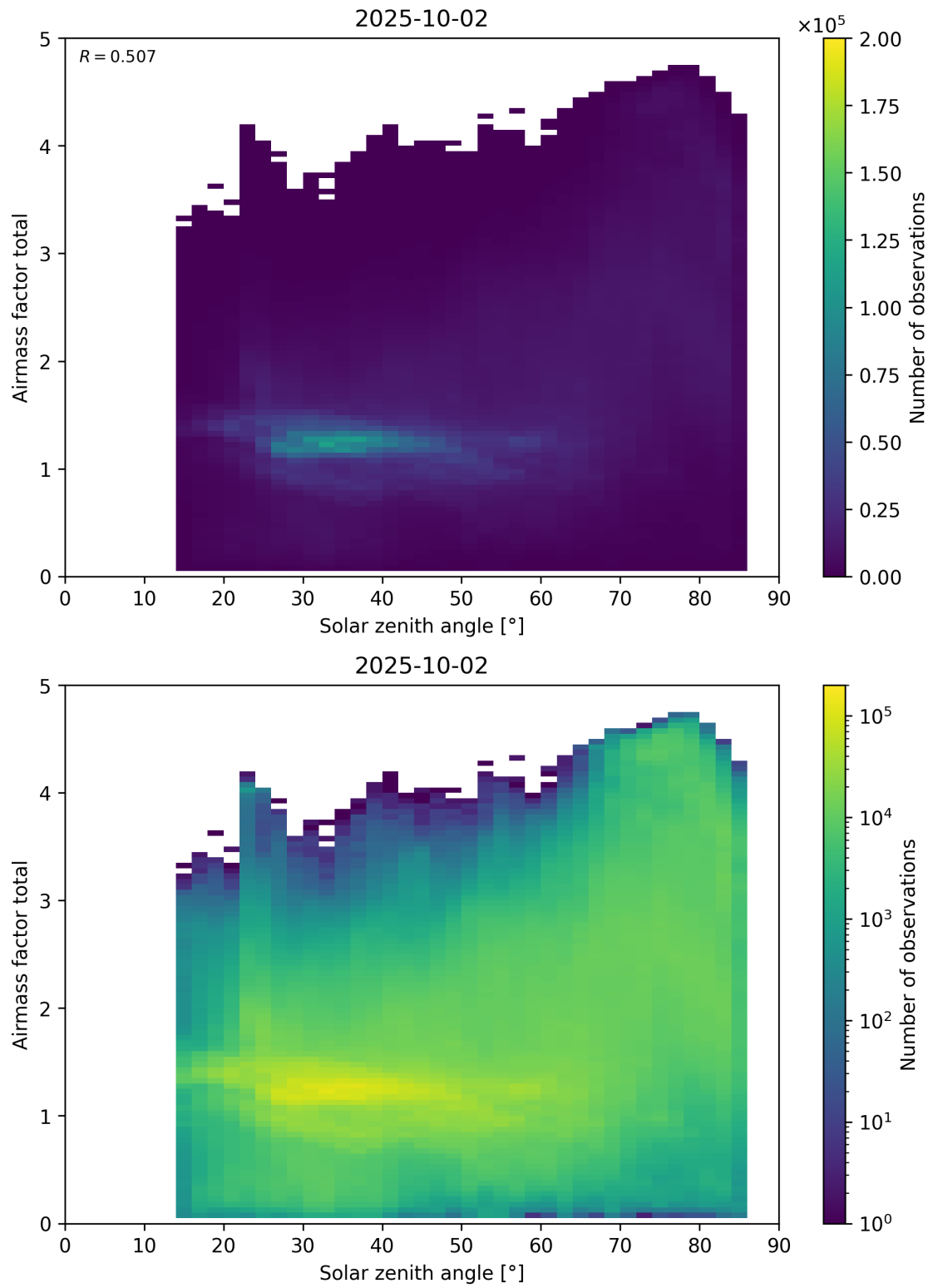
Figure 175: Scatter density plot of “Solar zenith angle” against “Airmass factor total” for 2025-10-01 to 2025-10-03.
