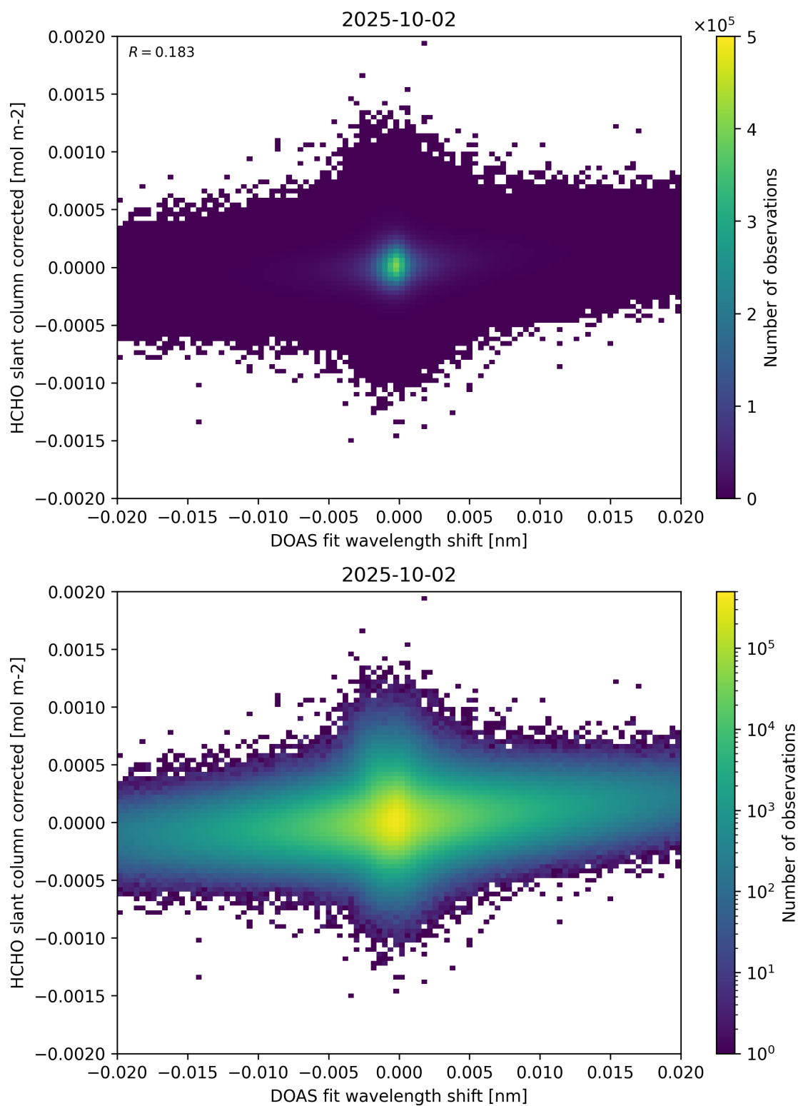
Figure 66: Scatter density plot of “DOAS fit wavelength shift” against “HCHO slant column corrected” for 2025-10-01 to 2025-10-03.
