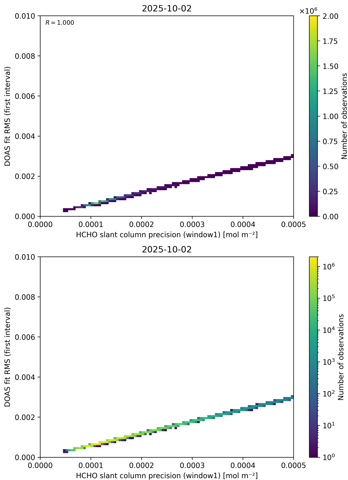
Figure 88: Scatter density plot of “HCHO slant column precision (window1)” against “DOAS fit RMS (first interval)” for 2025-10-01 to 2025-10-03.
