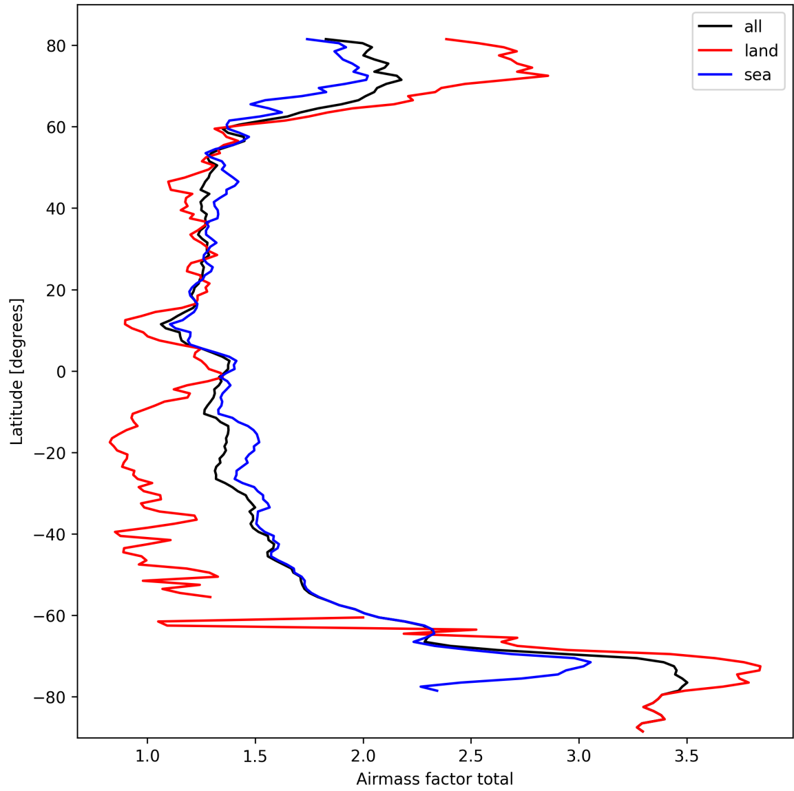
Figure 26: Zonal average of “Airmass factor total” for 2025-10-01 to 2025-10-03.
