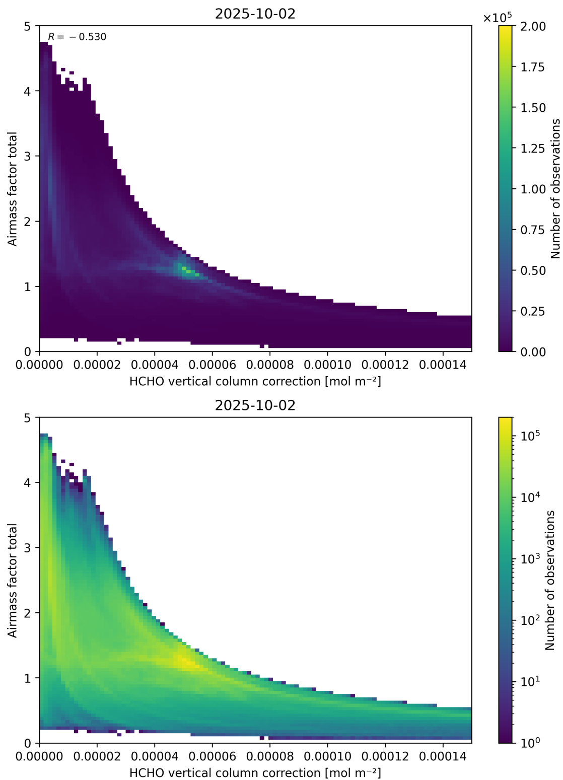
Figure 120: Scatter density plot of “HCHO vertical column correction” against “Airmass factor total” for 2025-10-01 to 2025-10-03.
