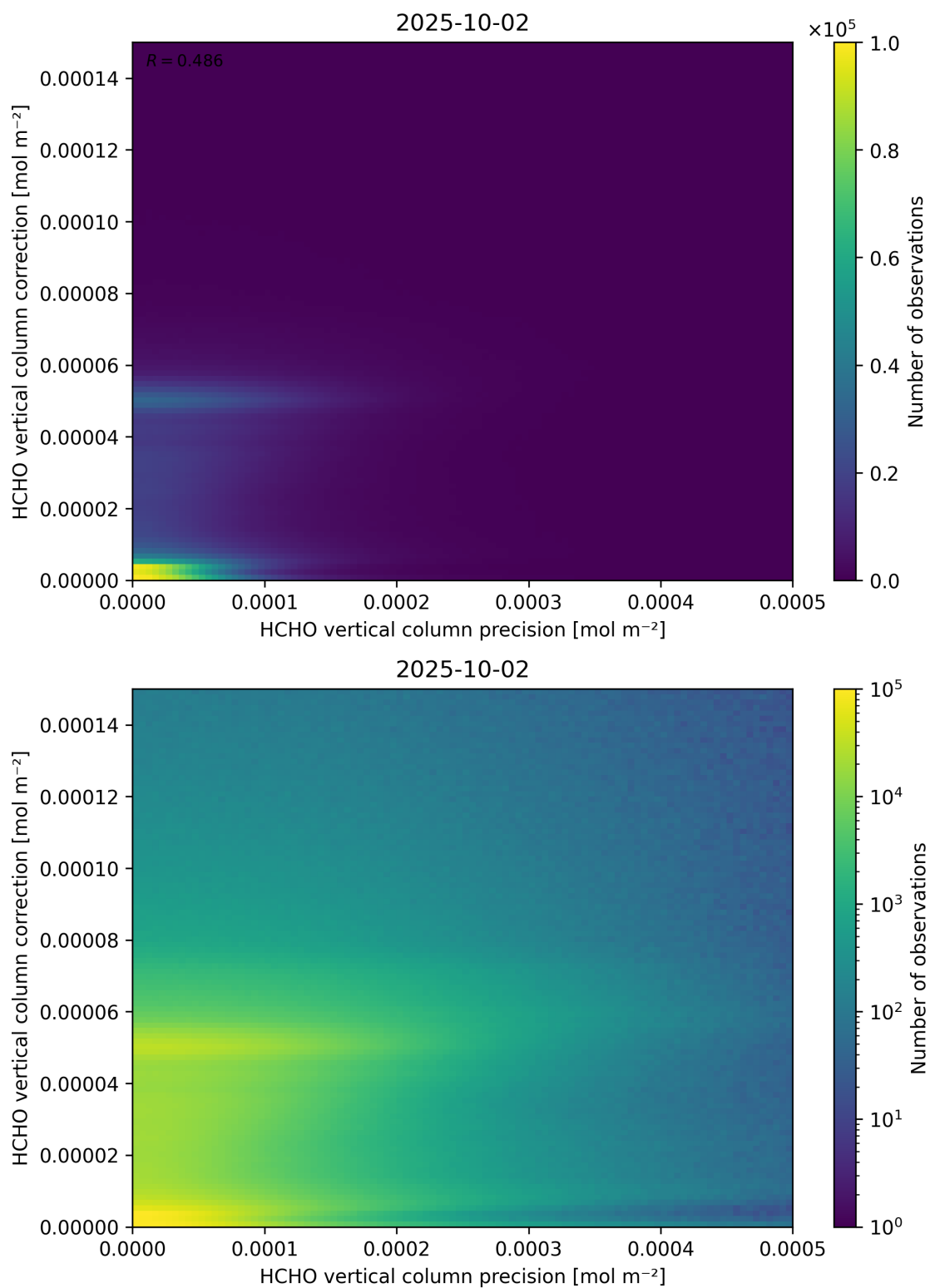
Figure 146: Scatter density plot of “HCHO vertical column precision” against “HCHO vertical column correction” for 2025-10-01 to 2025-10-03.
