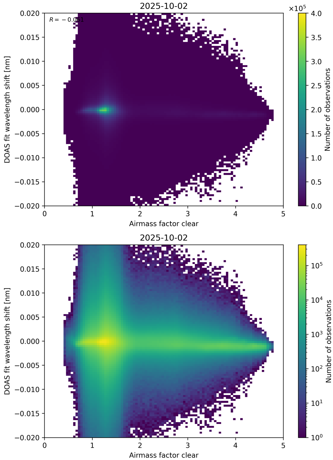
Figure 72: Scatter density plot of “Airmass factor clear” against “DOAS fit wavelength shift” for 2025-10-01 to 2025-10-03.
