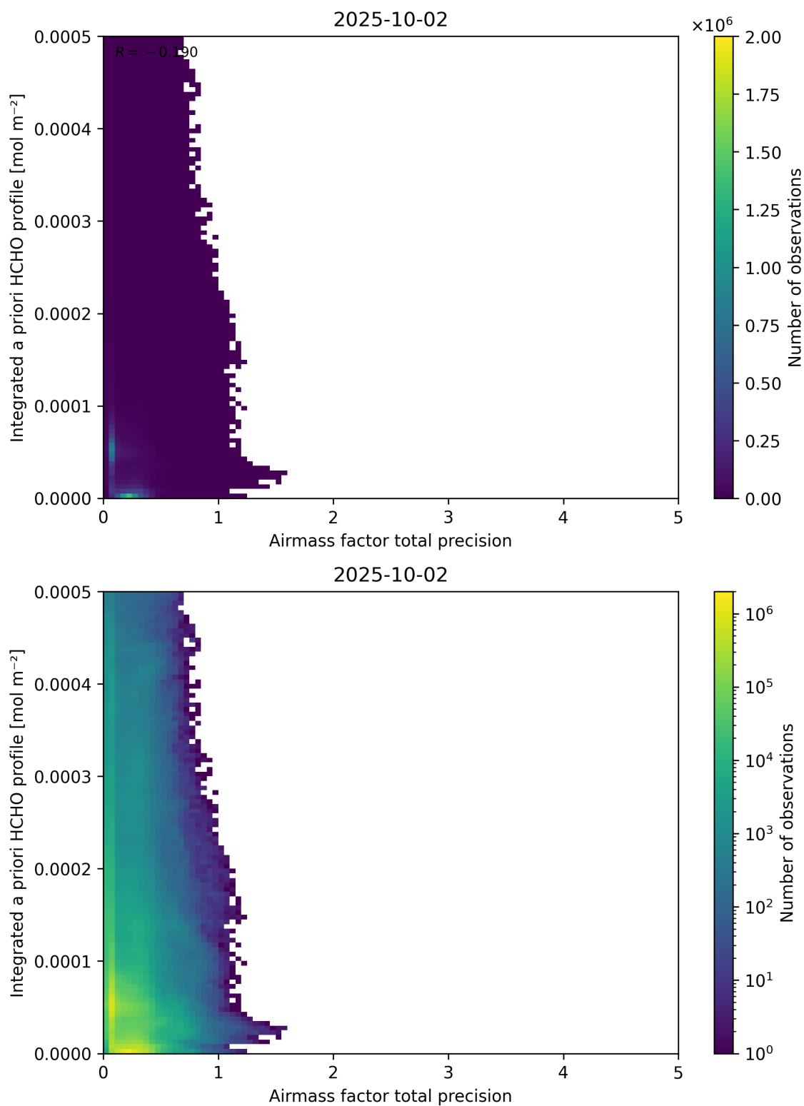
Figure 111: Scatter density plot of “Airmass factor total precision” against “Integrated a priori HCHO profile” for 2025-10-01 to 2025-10-03.
