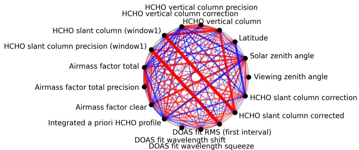
Figure 1: Map of correlation graph for 2025-10-01 to 2025-10-03.
