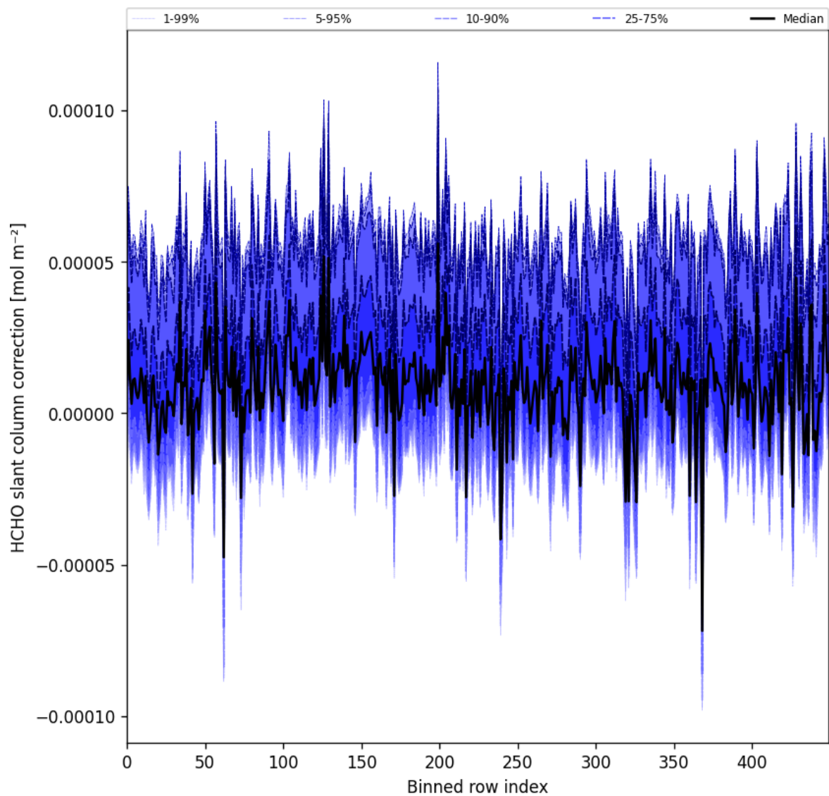
Figure 61: Along track statistics of “HCHO slant column correction” for 2025-10-01 to 2025-10-03
