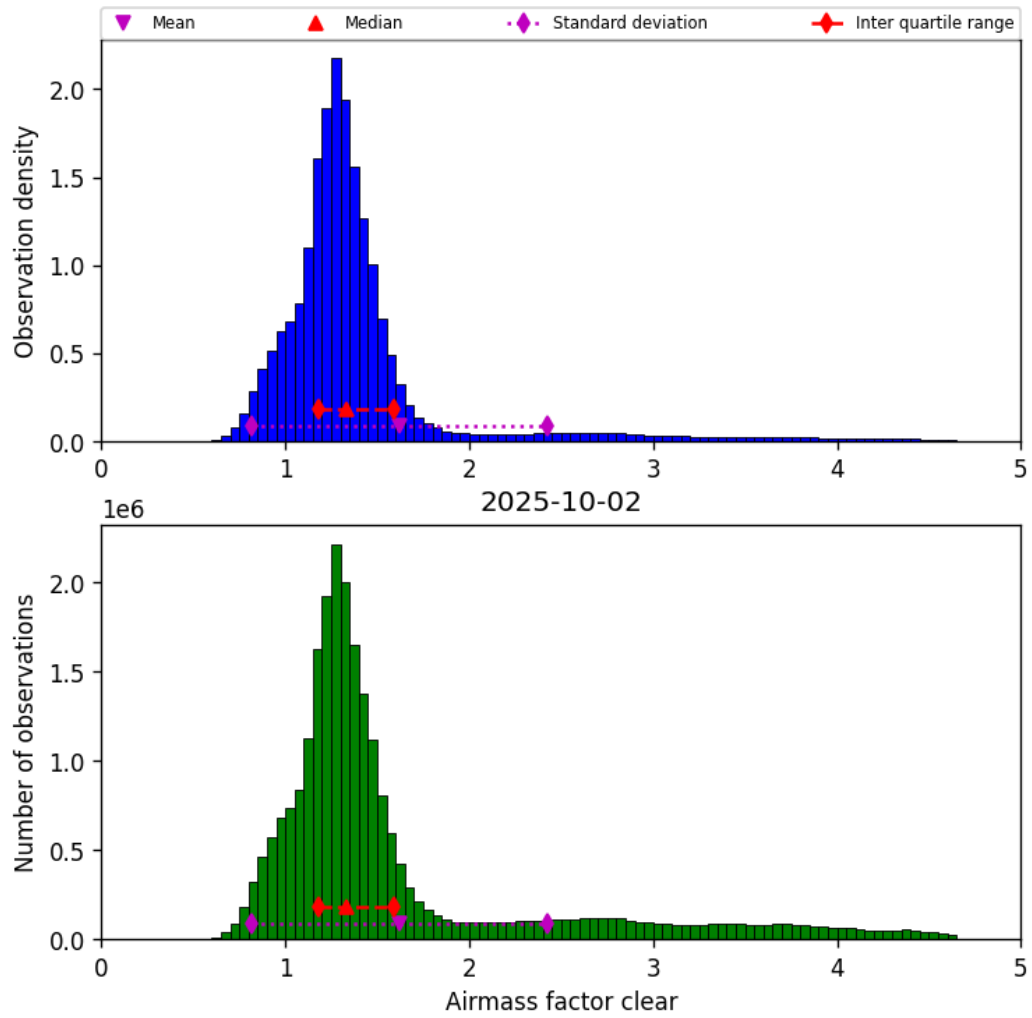
Figure 42: Histogram of “Airmass factor clear” for 2025-10-01 to 2025-10-03
