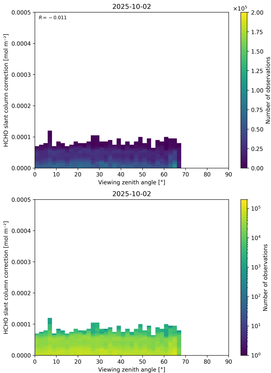
Figure 187: Scatter density plot of “Viewing zenith angle” against “HCHO slant column correction” for 2025-10-01 to 2025-10-03.
