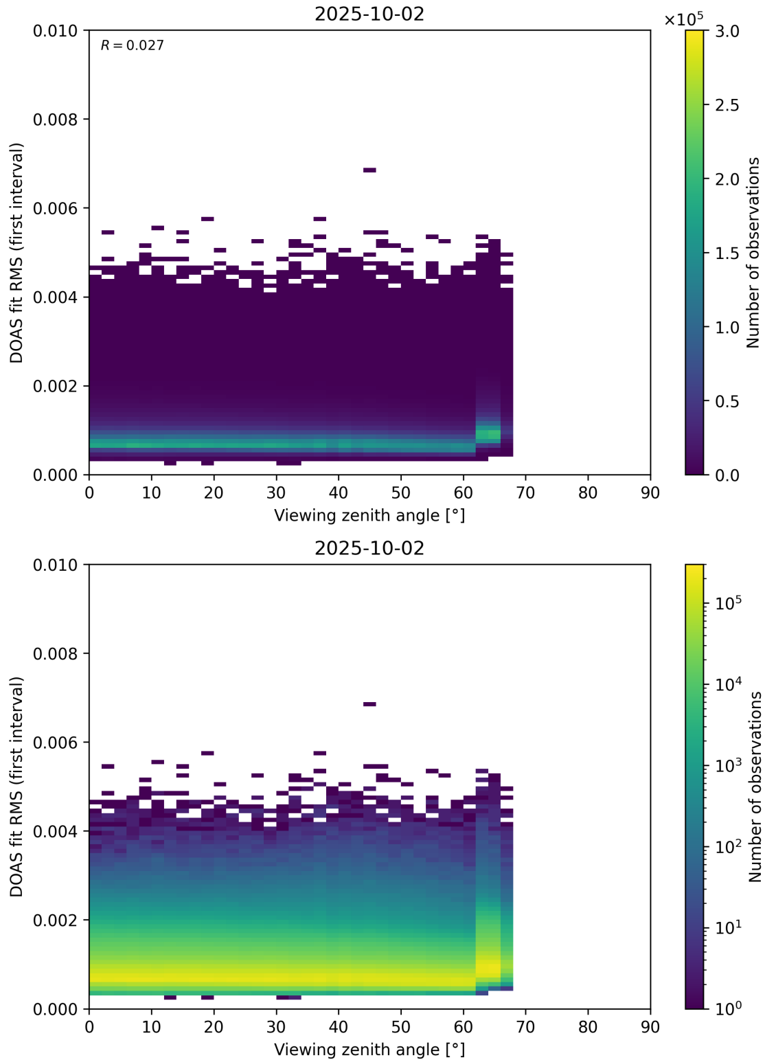
Figure 182: Scatter density plot of “Viewing zenith angle” against “DOAS fit RMS (first interval)” for 2025-10-01 to 2025-10-03.
