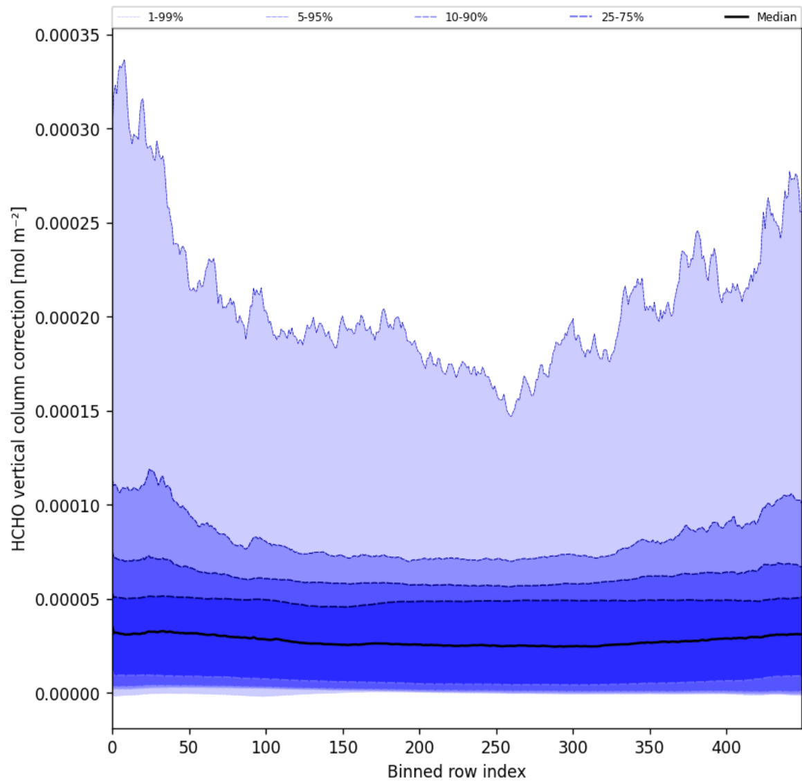
Figure 51: Along track statistics of “HCHO vertical column correction” for 2025-10-01 to 2025-10-03
