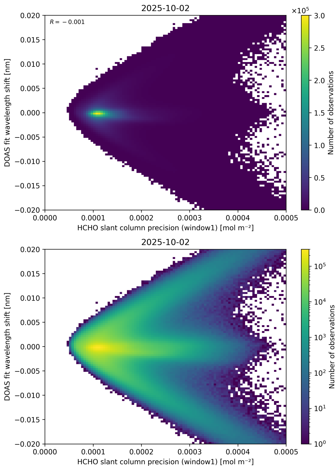
Figure 89: Scatter density plot of “HCHO slant column precision (window1)” against “DOAS fit wavelength shift” for 2025-10-01 to 2025-10-03.
