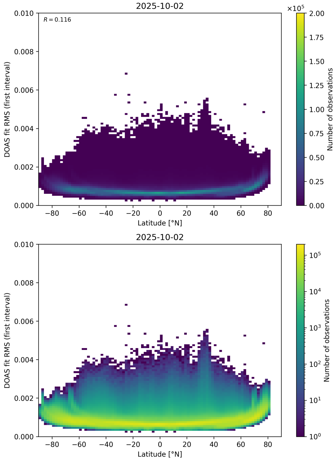
Figure 153: Scatter density plot of “Latitude” against “DOAS fit RMS (first interval)” for 2025-10-01 to 2025-10-03.
