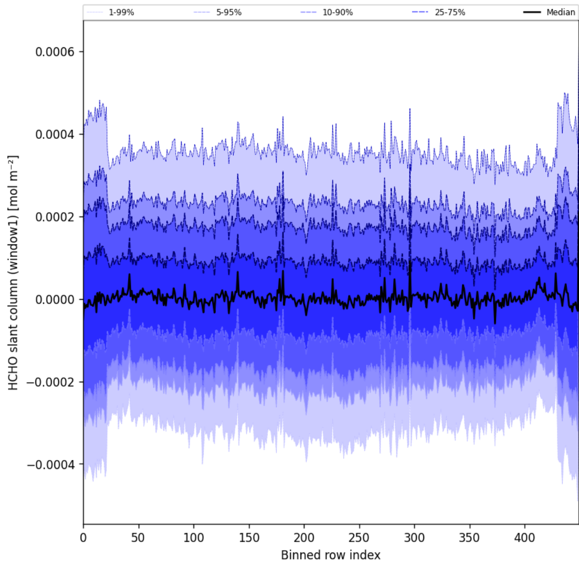
Figure 52: Along track statistics of “HCHO slant column (window1)” for 2025-10-01 to 2025-10-03
