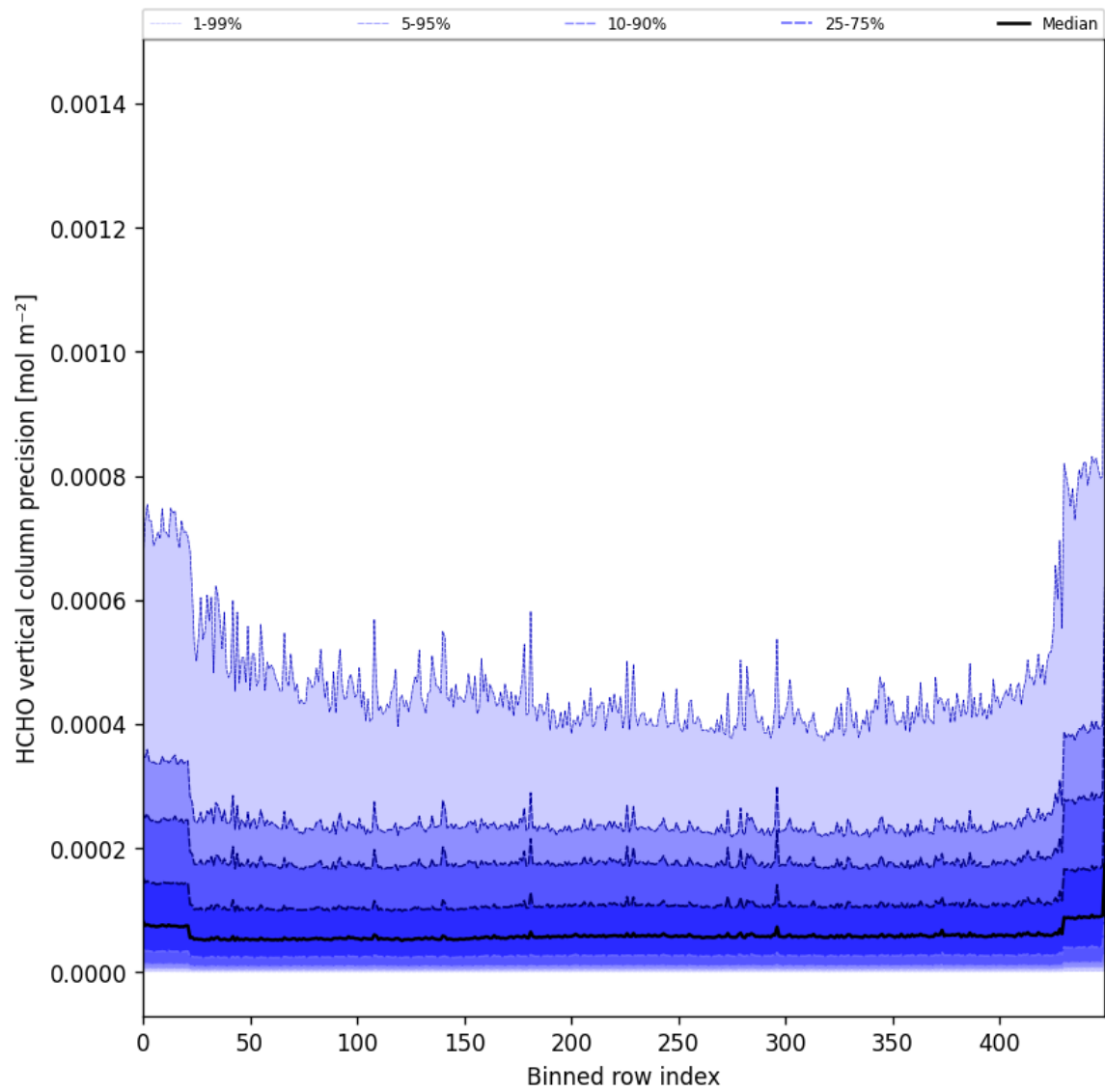
Figure 50: Along track statistics of “HCHO vertical column precision” for 2025-10-01 to 2025-10-03
