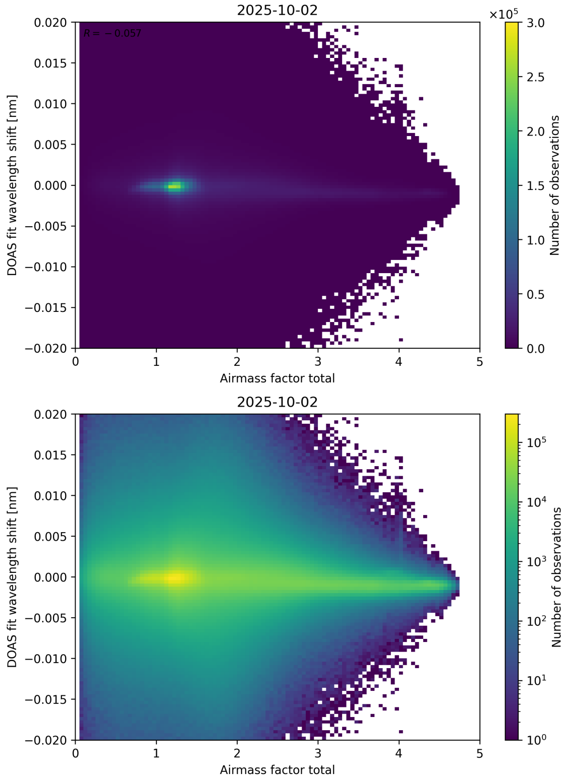
Figure 98: Scatter density plot of “Airmass factor total” against “DOAS fit wavelength shift” for 2025-10-01 to 2025-10-03.
