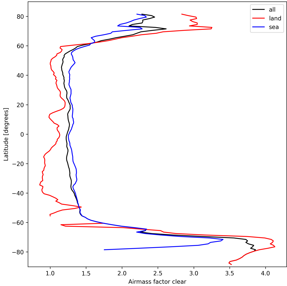
Figure 28: Zonal average of “Airmass factor clear” for 2025-10-01 to 2025-10-03.
