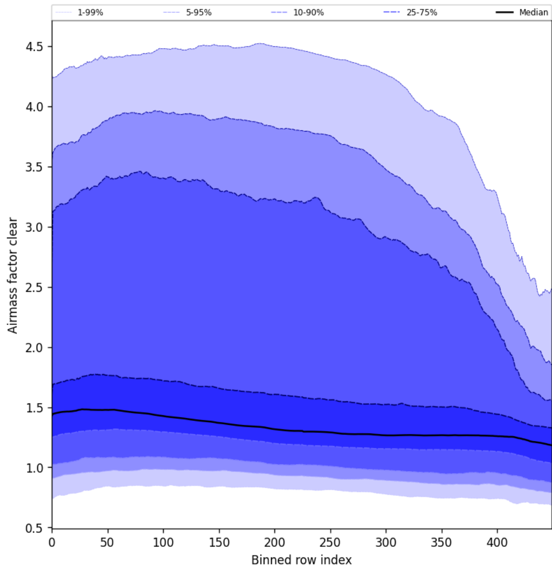
Figure 56: Along track statistics of “Air mass factor clear” for 2025-10-01 to 2025-10-03
