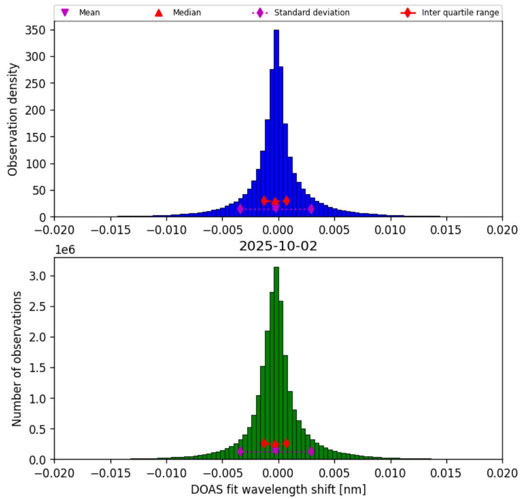
Figure 44: Histogram of “DOAS fit wavelength shift” for 2025-10-01 to 2025-10-03
