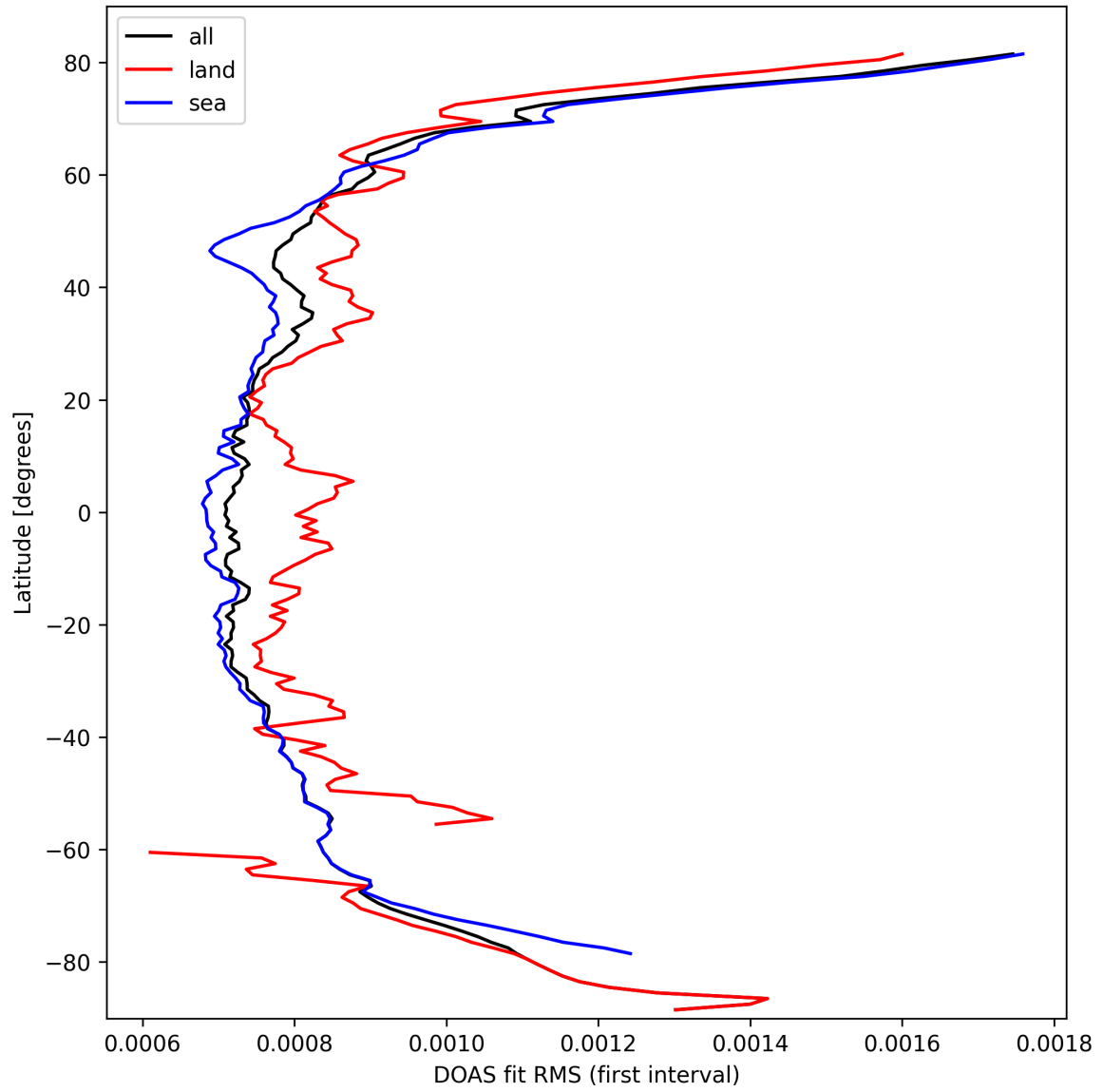
Figure 32: Zonal average of “DOAS fit RMS (first interval)” for 2025-10-01 to 2025-10-03.
