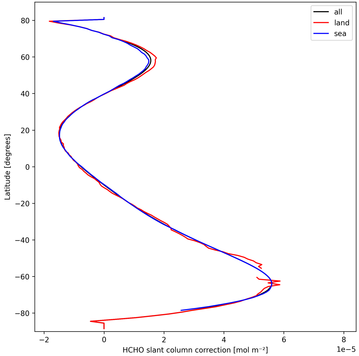
Figure 33: Zonal average of “HCHO slant column correction” for 2025-10-01 to 2025-10-03.
