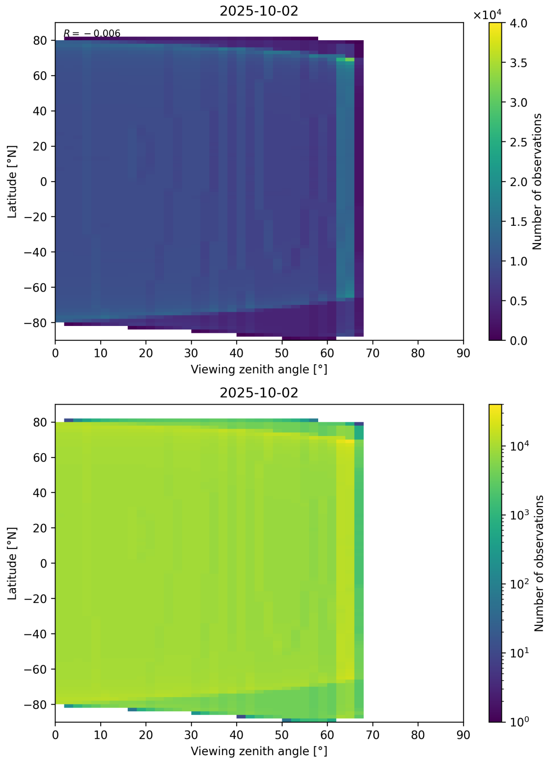
Figure 196: Scatter density plot of “Viewing zenith angle” against “Latitude” for 2025-10-01 to 2025-10-03.
