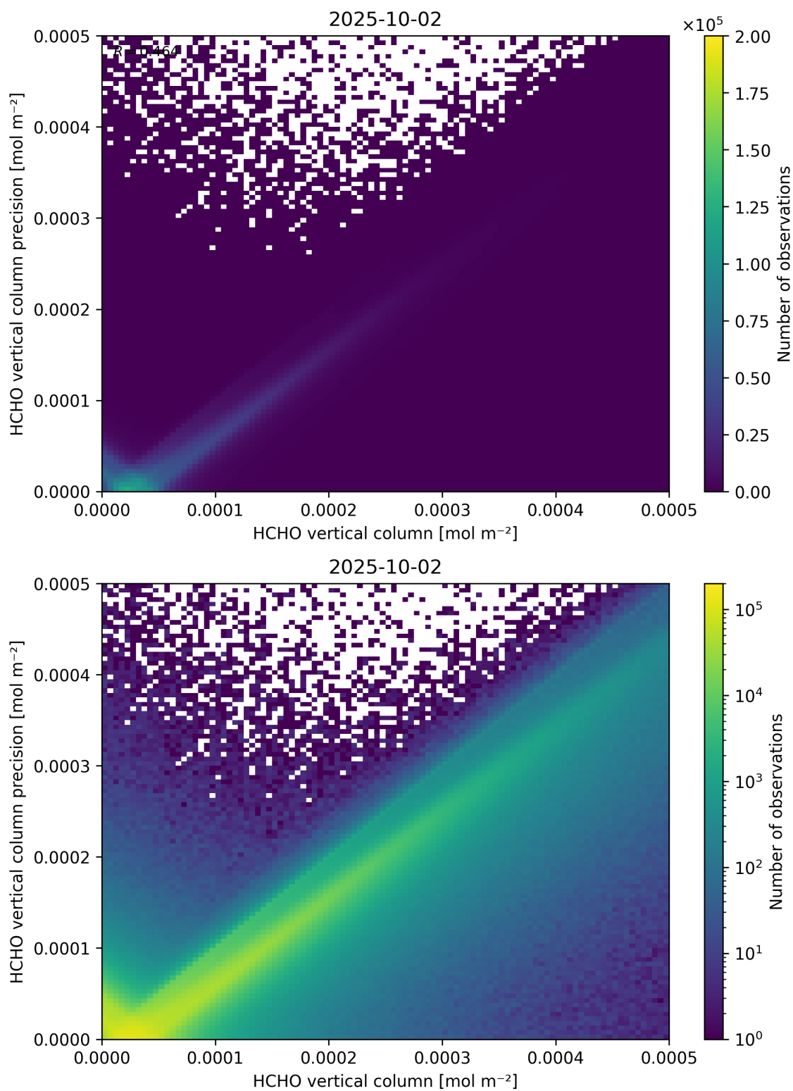
Figure 134: Scatter density plot of “HCHO vertical column” against “HCHO vertical column precision” for 2025-10-01 to 2025-10-03.
