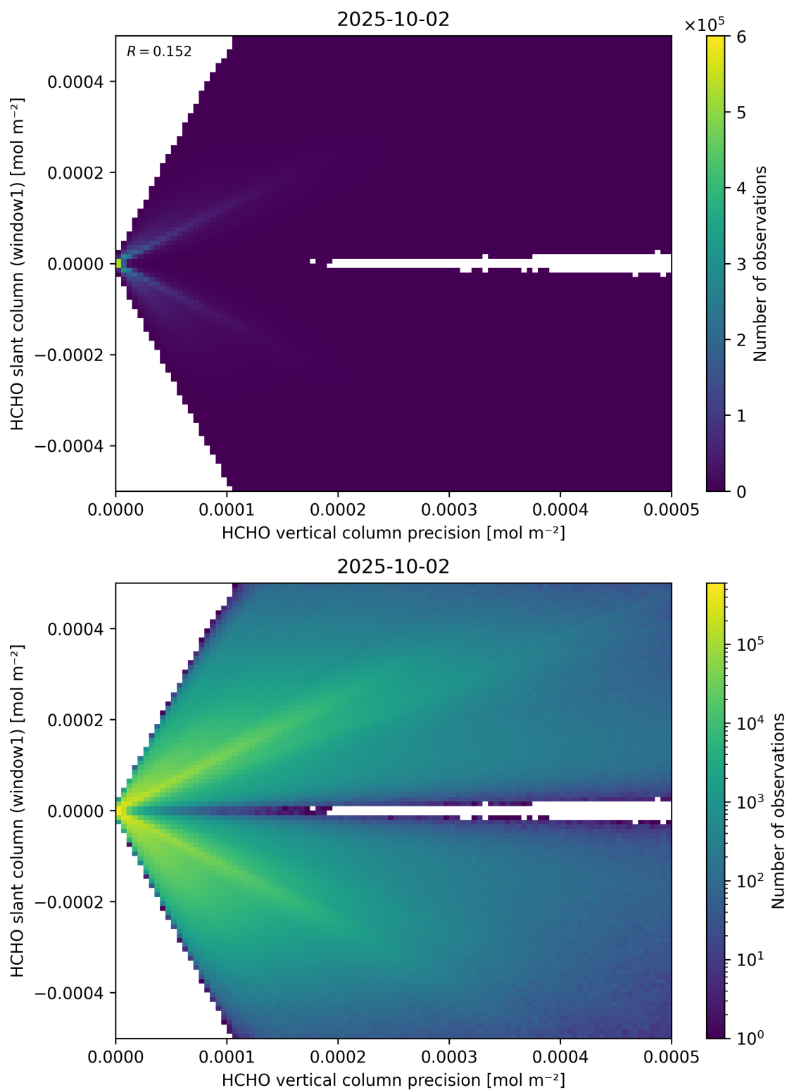
Figure 142: Scatter density plot of “HCHO vertical column precision” against “HCHO slant column (window1)” for 2025-10-01 to 2025-10-03.
