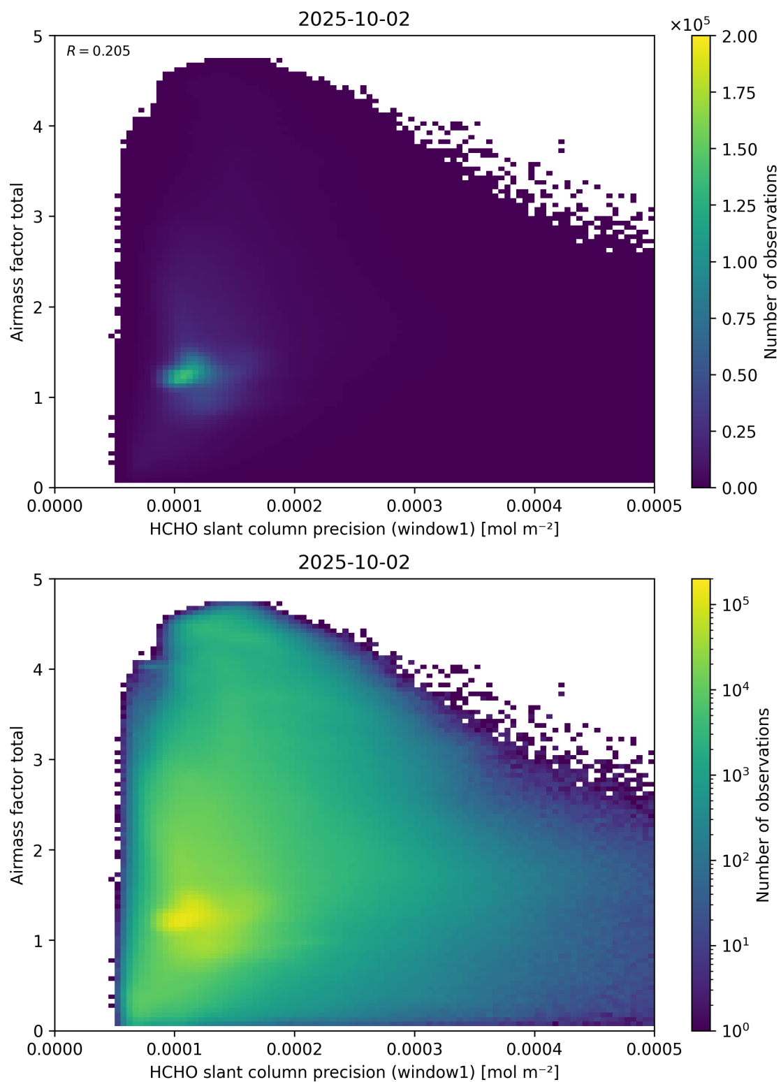
Figure 94: Scatter density plot of “HCHO slant column precision (window1)” against “Airmass factor total” for 2025-10-01 to 2025-10-03.
