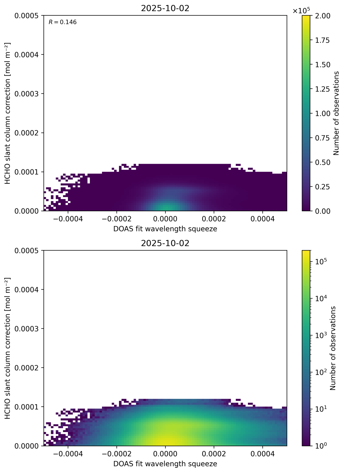
Figure 70: Scatter density plot of “DOAS fit wavelength squeeze” against “HCHO slant column correction” for 2025-10-01 to 2025-10-03.
