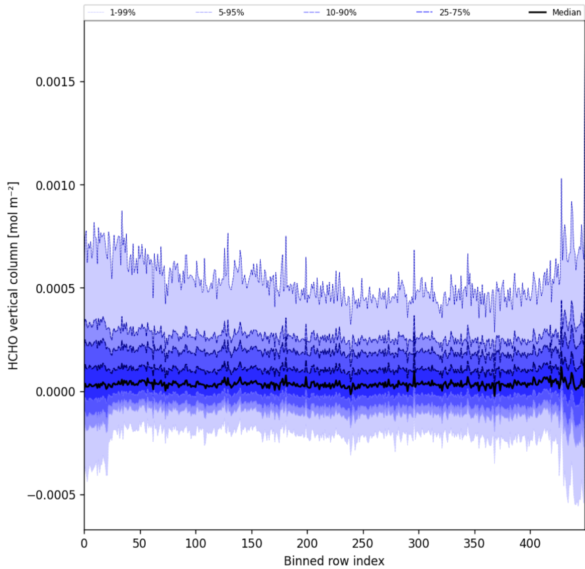
Figure 49: Along track statistics of “HCHO vertical column” for 2025-10-01 to 2025-10-03
