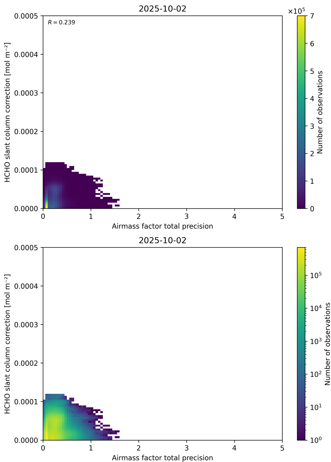
Figure 110: Scatter density plot of “Airmass factor total precision” against “HCHO slant column correction” for 2025-10-01 to 2025-10-03.
