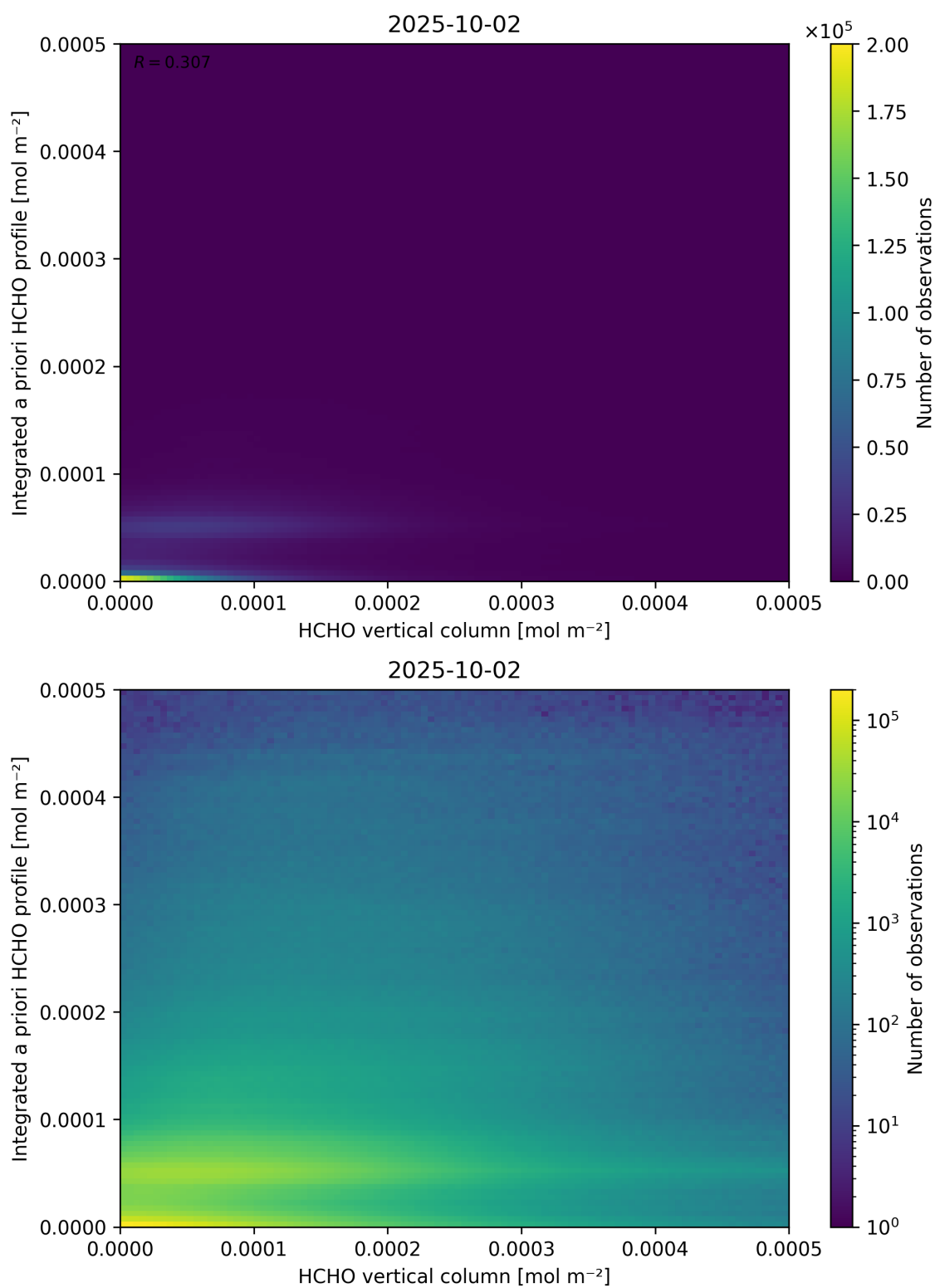
Figure 135: Scatter density plot of “HCHO vertical column” against “Integrated a priori HCHO profile” for 2025-10-01 to 2025-10-03.
