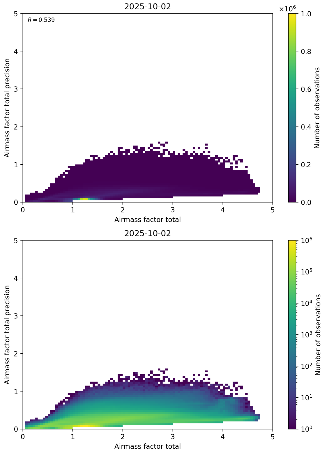
Figure 103: Scatter density plot of “Airmass factor total” against “Airmass factor total precision” for 2025-10-01 to 2025-10-03.
