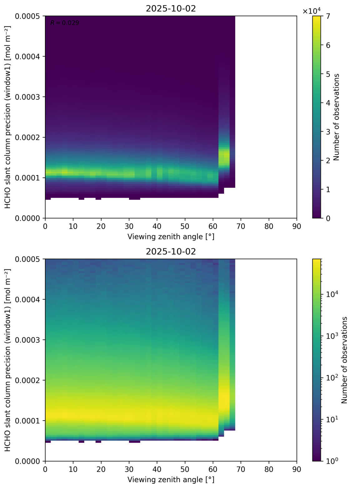
Figure 189: Scatter density plot of “Viewing zenith angle” against “HCHO slant column precision (window1)” for 2025-10-01 to 2025-10-03.
