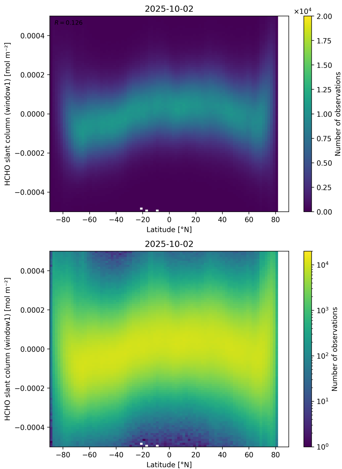
Figure 159: Scatter density plot of “Latitude” against “HCHO slant column (window1)” for 2025-10-01 to 2025-10-03.
