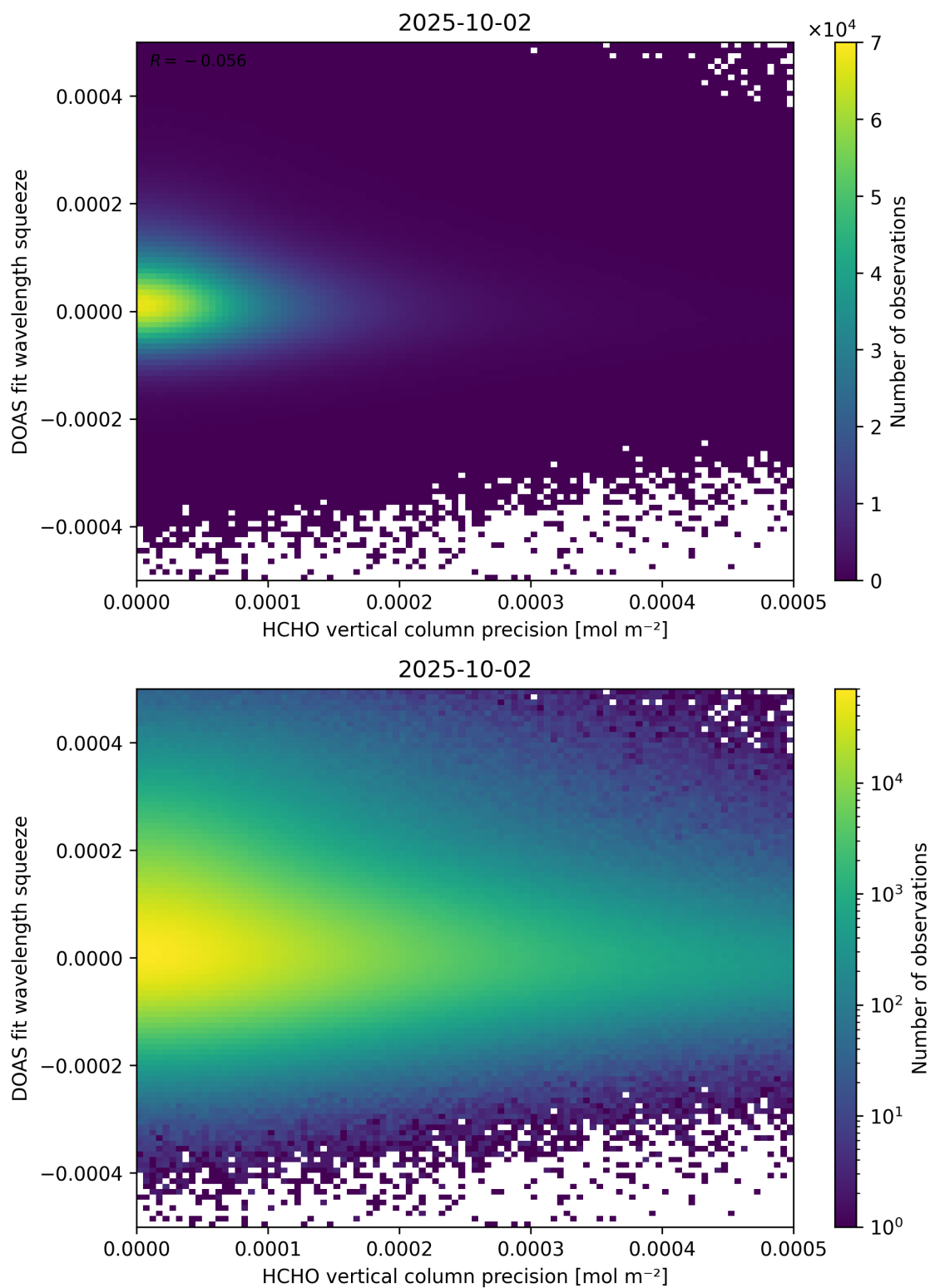
Figure 138: Scatter density plot of “HCHO vertical column precision” against “DOAS fit wavelength squeeze” for 2025-10-01 to 2025-10-03.
