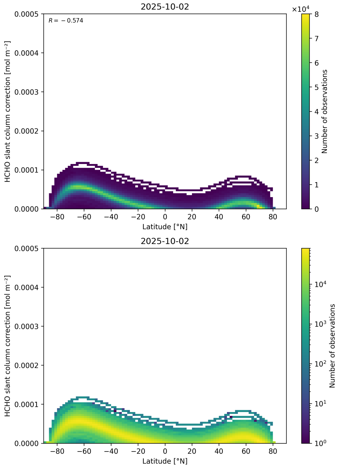
Figure 158: Scatter density plot of “Latitude” against “HCHO slant column correction” for 2025-10-01 to 2025-10-03.
