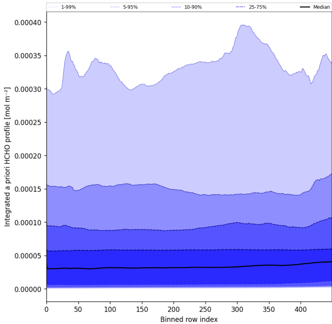
Figure 57: Along track statistics of “Integrated a priori HCHO profile” for 2025-10-01 to 2025-10-03
