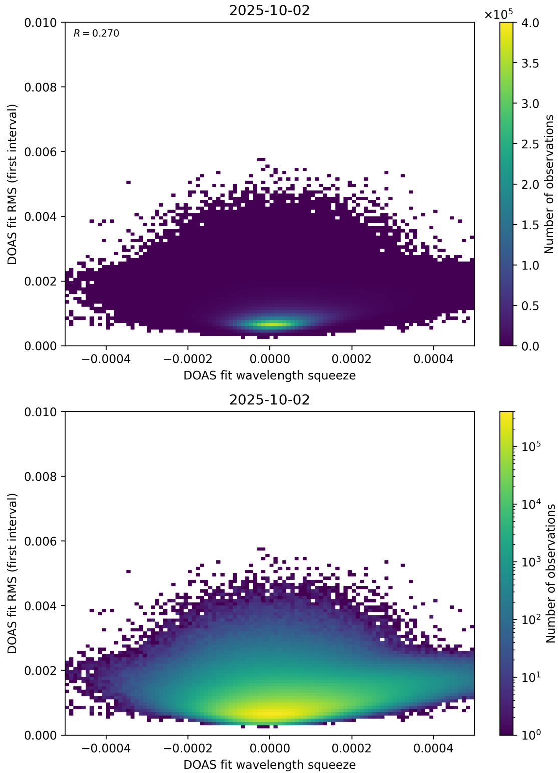
Figure 68: Scatter density plot of “DOAS fit wavelength squeeze” against “DOAS fit RMS (first interval)” for 2025-10-01 to 2025-10-03.
