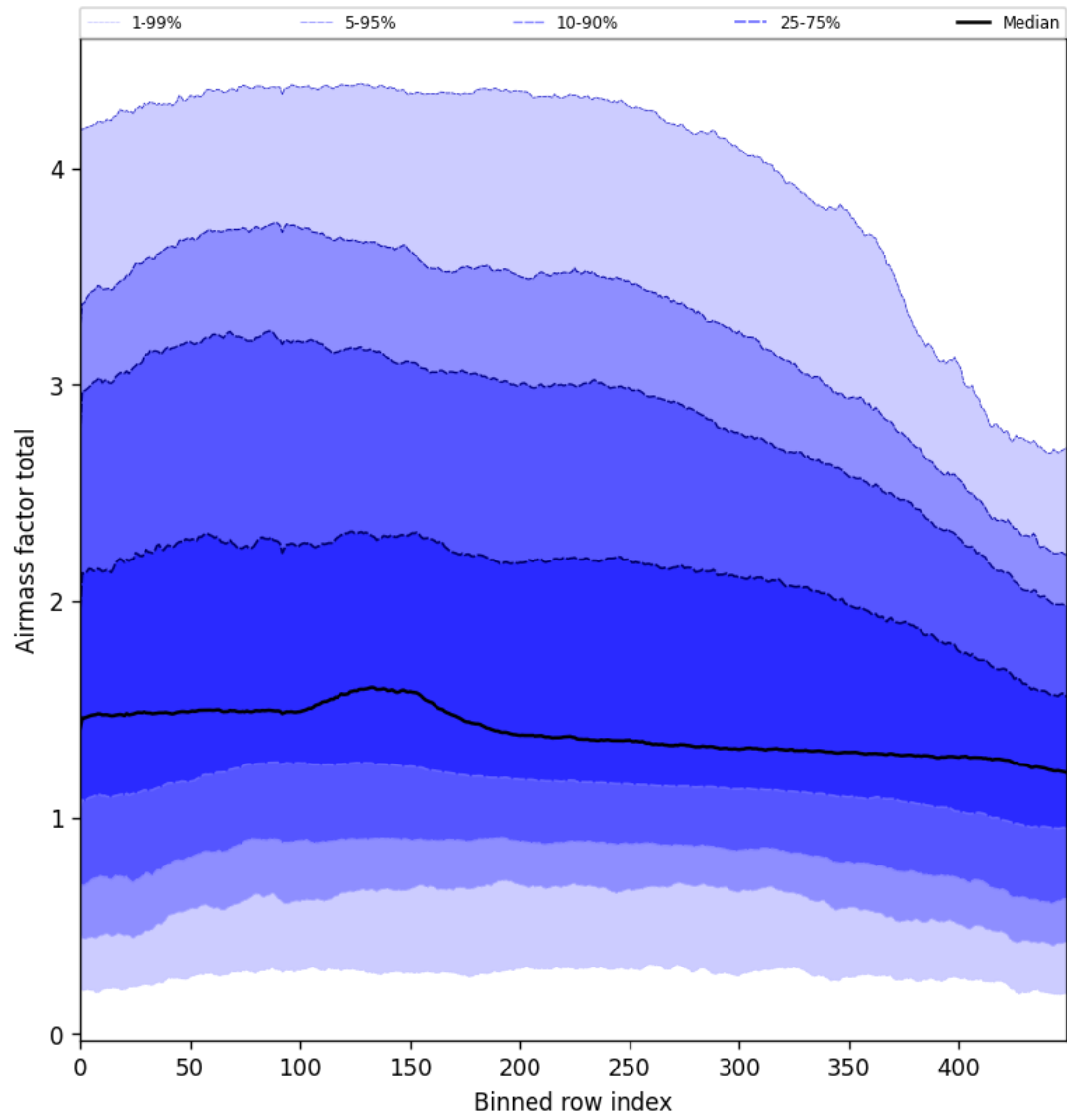
Figure 54: Along track statistics of “Airmass factor total” for 2025-10-01 to 2025-10-03
