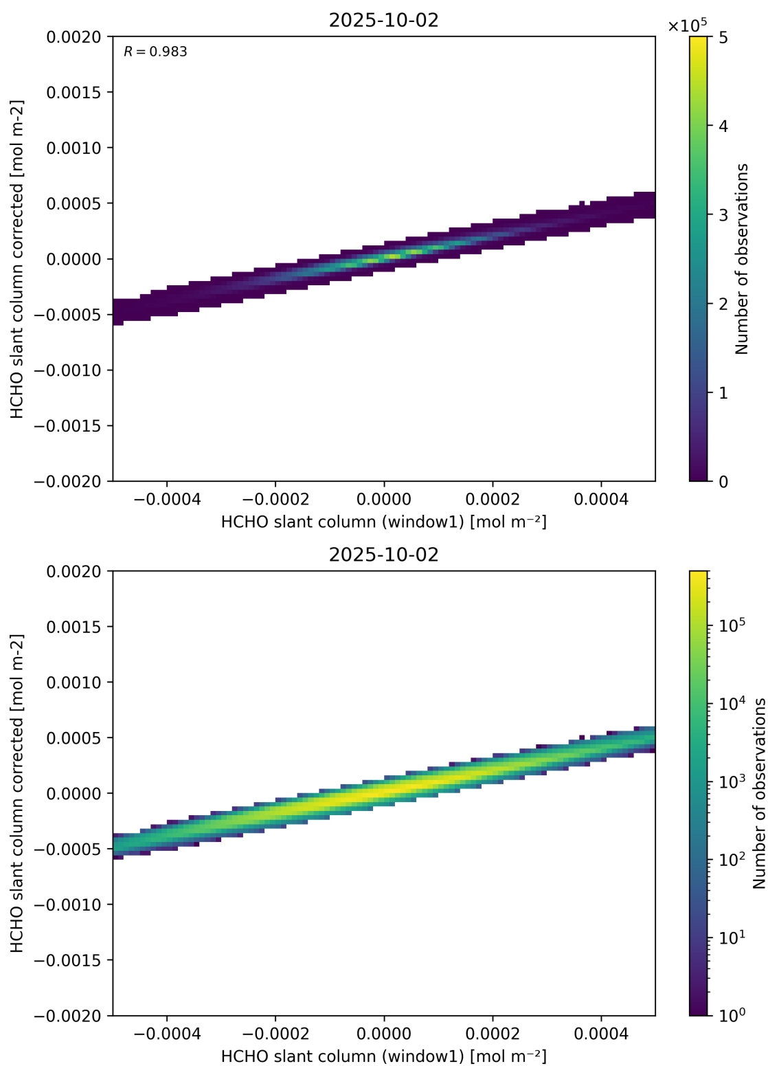
Figure 82: Scatter density plot of “HCHO slant column (window1)” against “HCHO slant column corrected” for 2025-10-01 to 2025-10-03.
