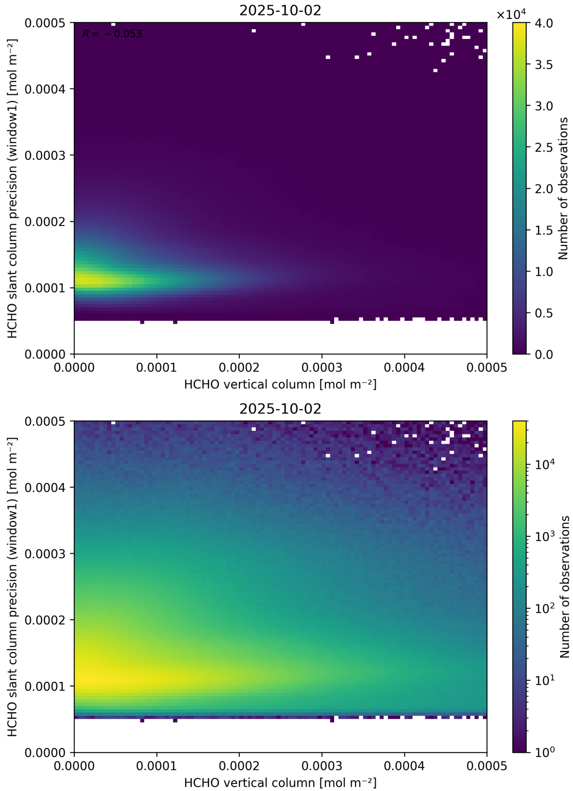
Figure 130: Scatter density plot of “HCHO vertical column” against “HCHO slant column precision (window1)” for 2025-10-01 to 2025-10-03.
