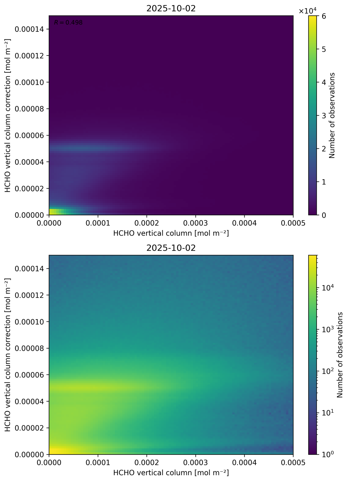
Figure 133: Scatter density plot of “HCHO vertical column” against “HCHO vertical column correction” for 2025-10-01 to 2025-10-03.
