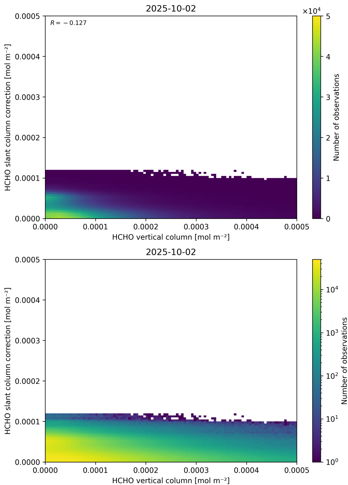
Figure 128: Scatter density plot of “HCHO vertical column” against “HCHO slant column correction” for 2025-10-01 to 2025-10-03.
