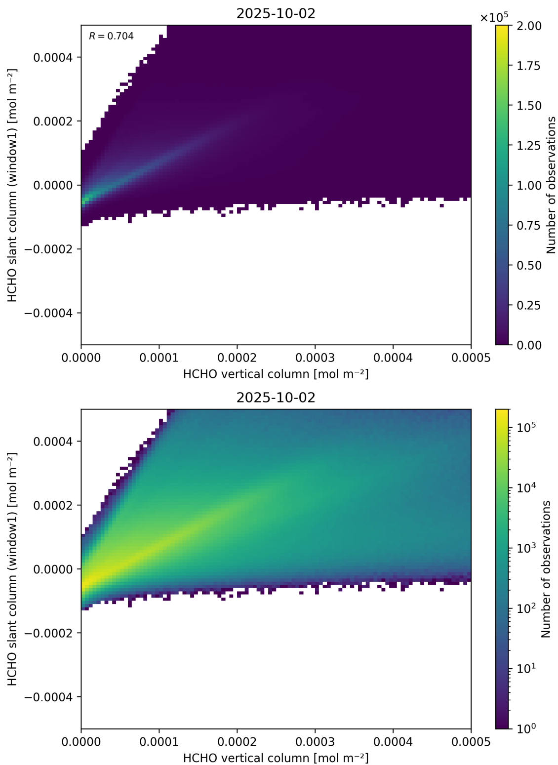
Figure 129: Scatter density plot of “HCHO vertical column” against “HCHO slant column (window1)” for 2025-10-01 to 2025-10-03.
