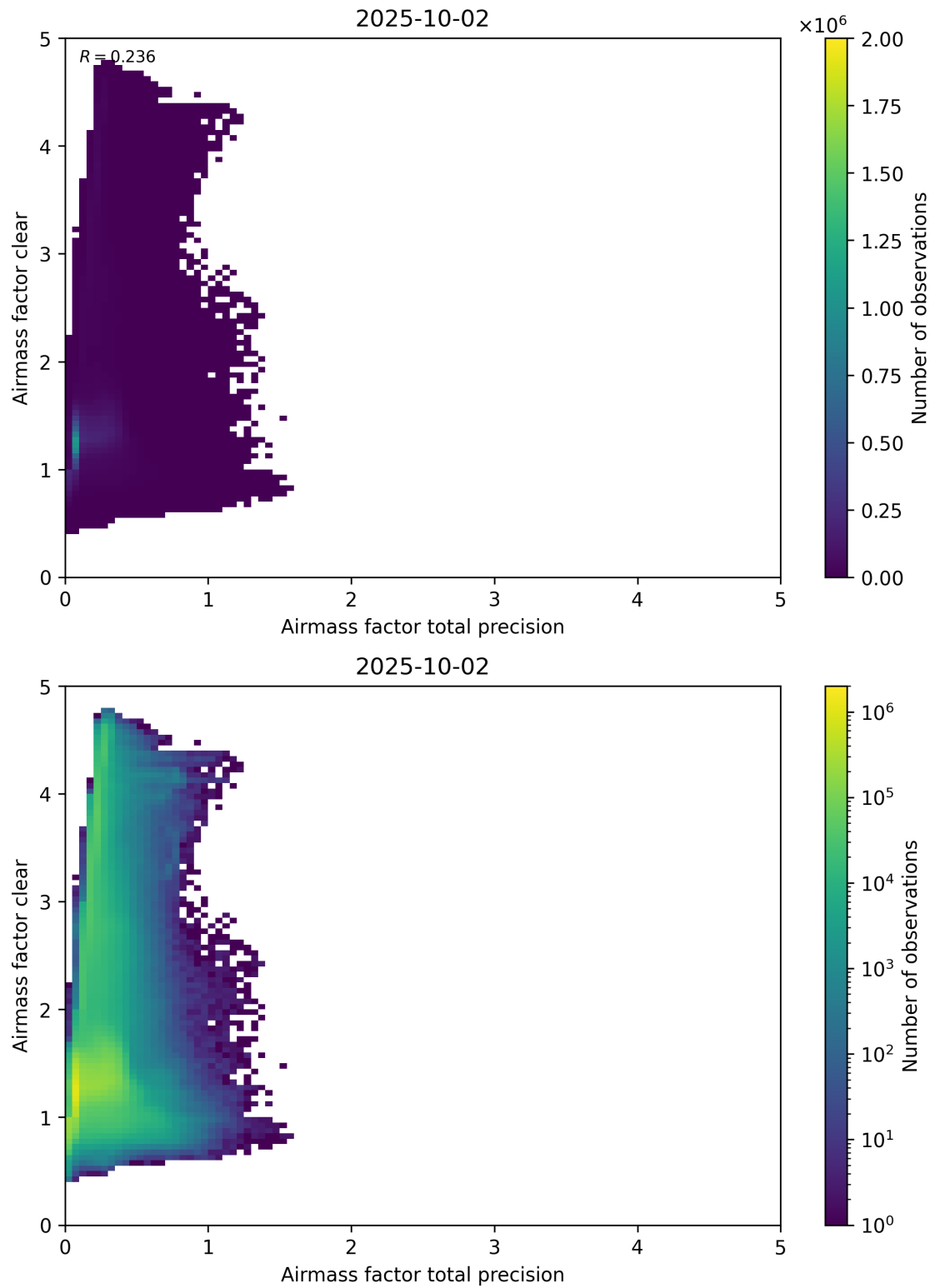
Figure 108: Scatter density plot of “Airmass factor total precision” against “Airmass factor clear” for 2025-10-01 to 2025-10-03.
