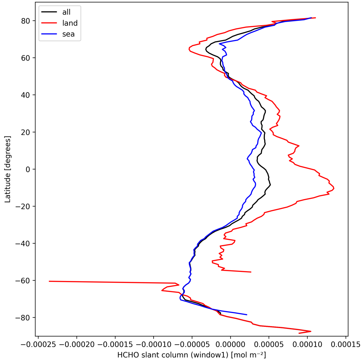
Figure 24: Zonal average of “HCHO slant column (window1)” for 2025-10-01 to 2025-10-03.
