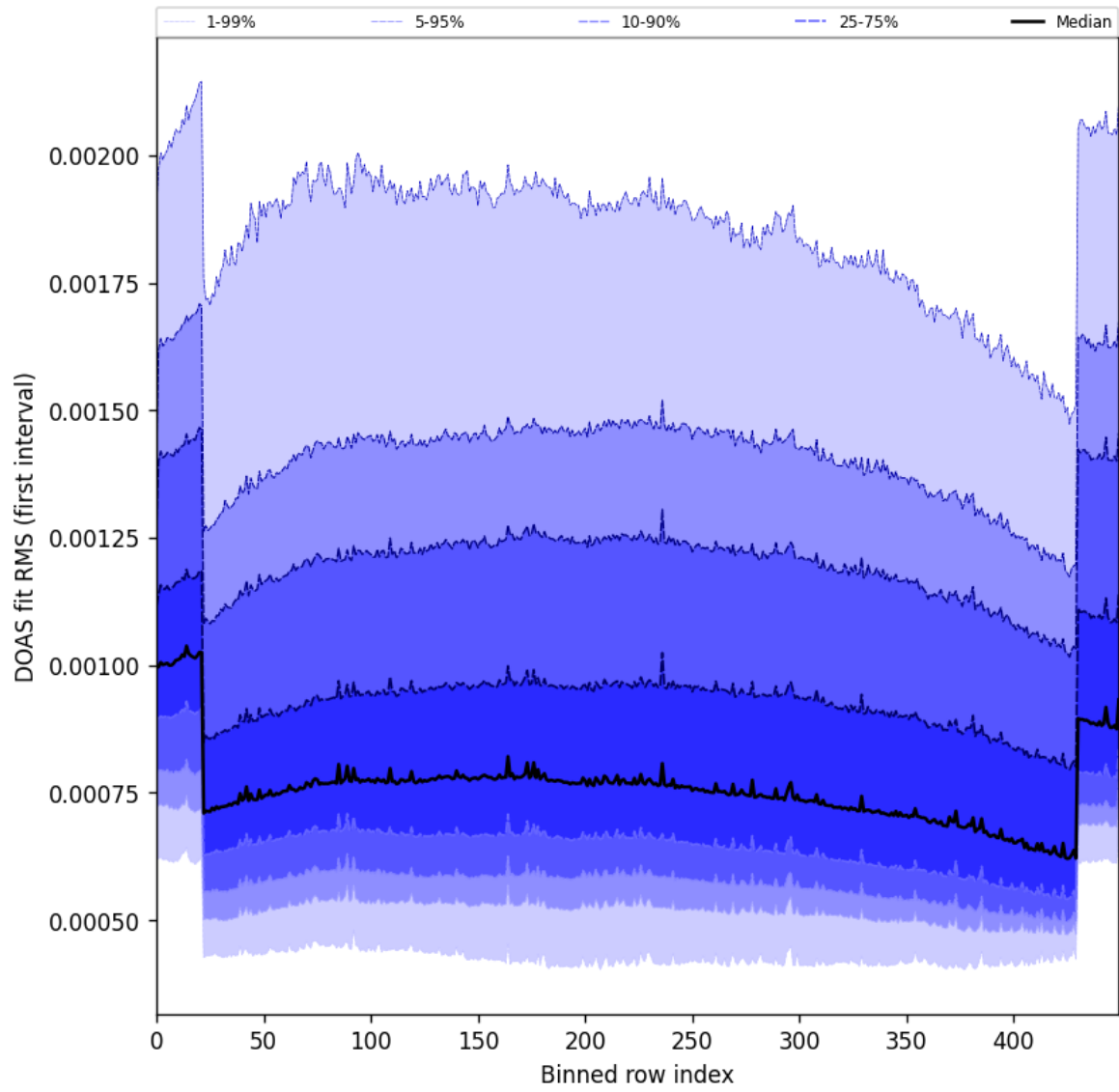
Figure 60: Along track statistics of “DOAS fit RMS (first interval)” for 2025-10-01 to 2025-10-03
