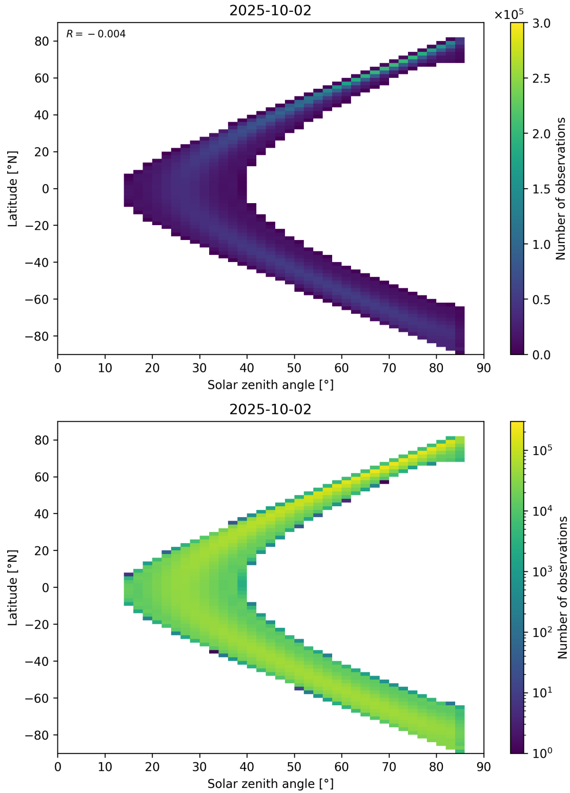
Figure 181: Scatter density plot of “Solar zenith angle” against “Latitude” for 2025-10-01 to 2025-10-03.
