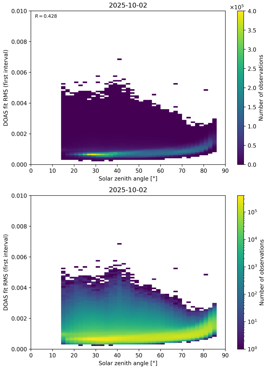
Figure 167: Scatter density plot of “Solar zenith angle” against “DOAS fit RMS (first interval)” for 2025-10-01 to 2025-10-03.
