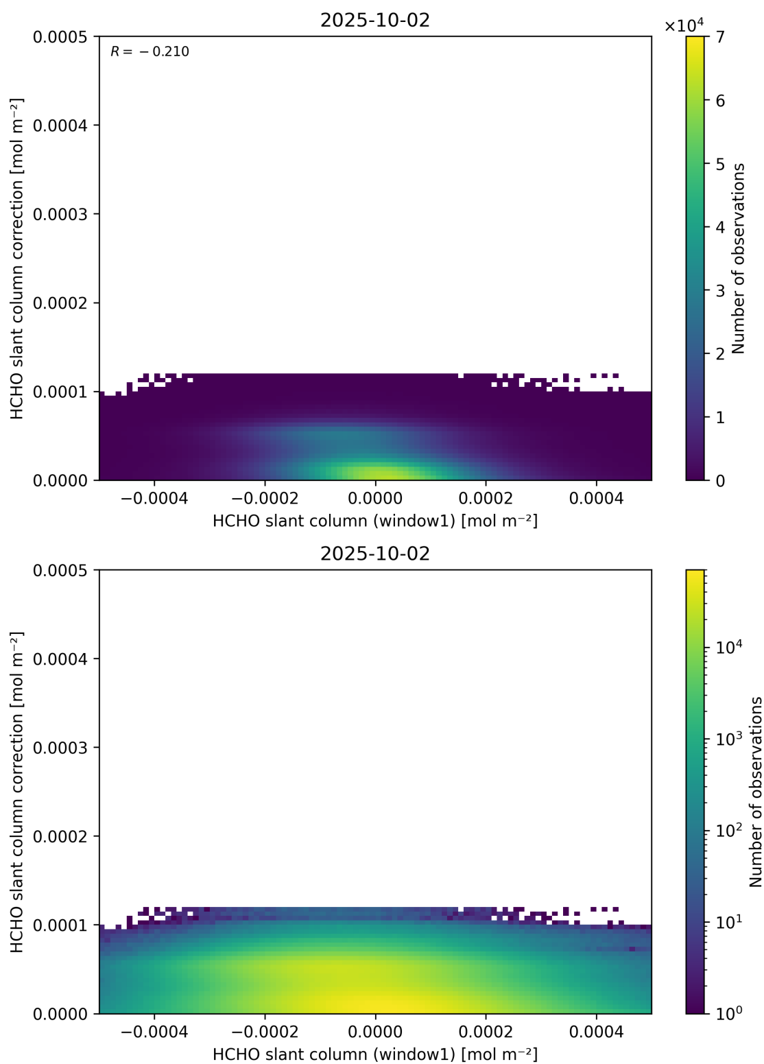
Figure 83: Scatter density plot of “HCHO slant column (window1)” against “HCHO slant column correction” for 2025-10-01 to 2025-10-03.
