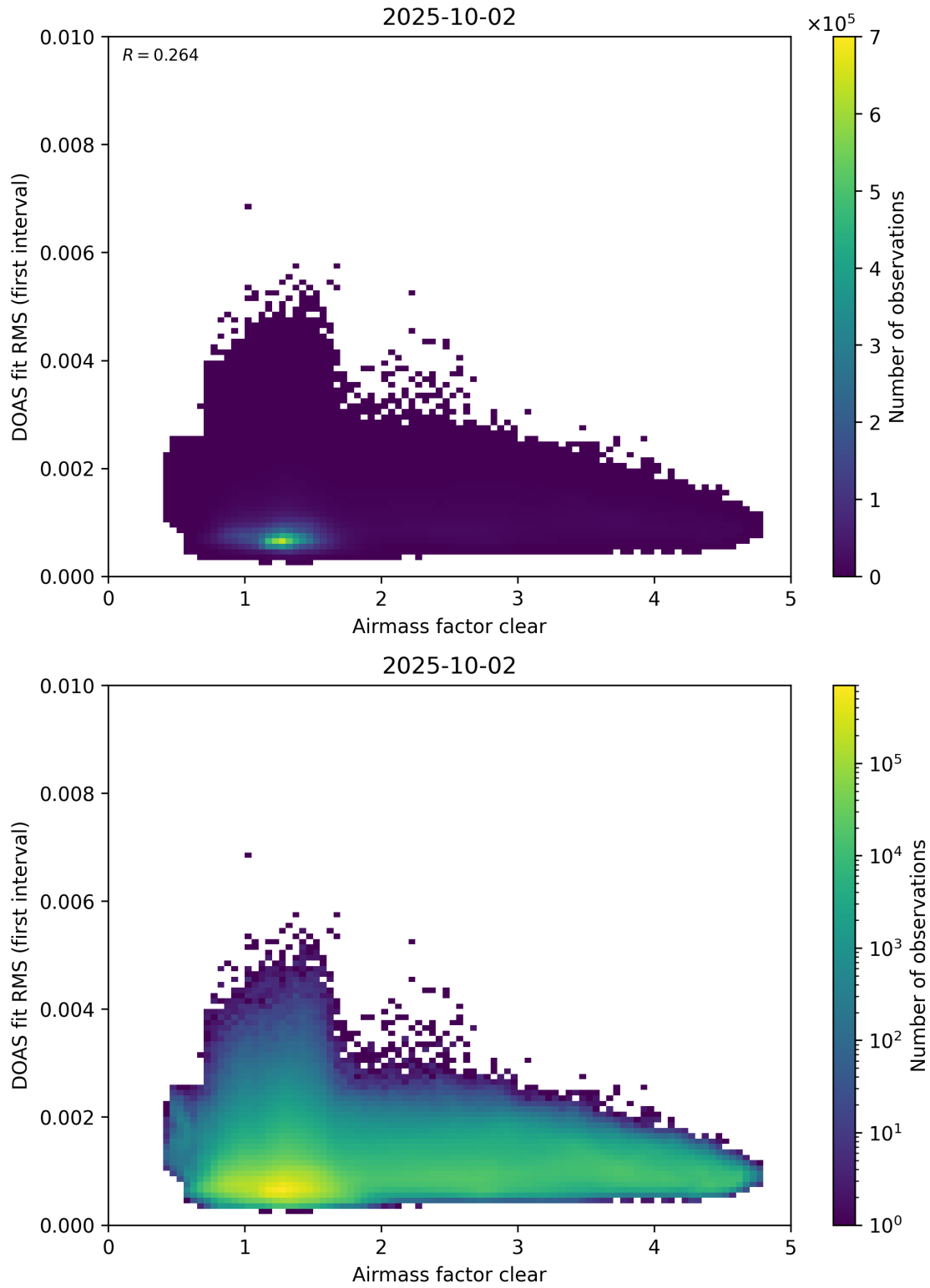
Figure 71: Scatter density plot of “Airmass factor clear” against “DOAS fit RMS (first interval)” for 2025-10-01 to 2025-10-03.
