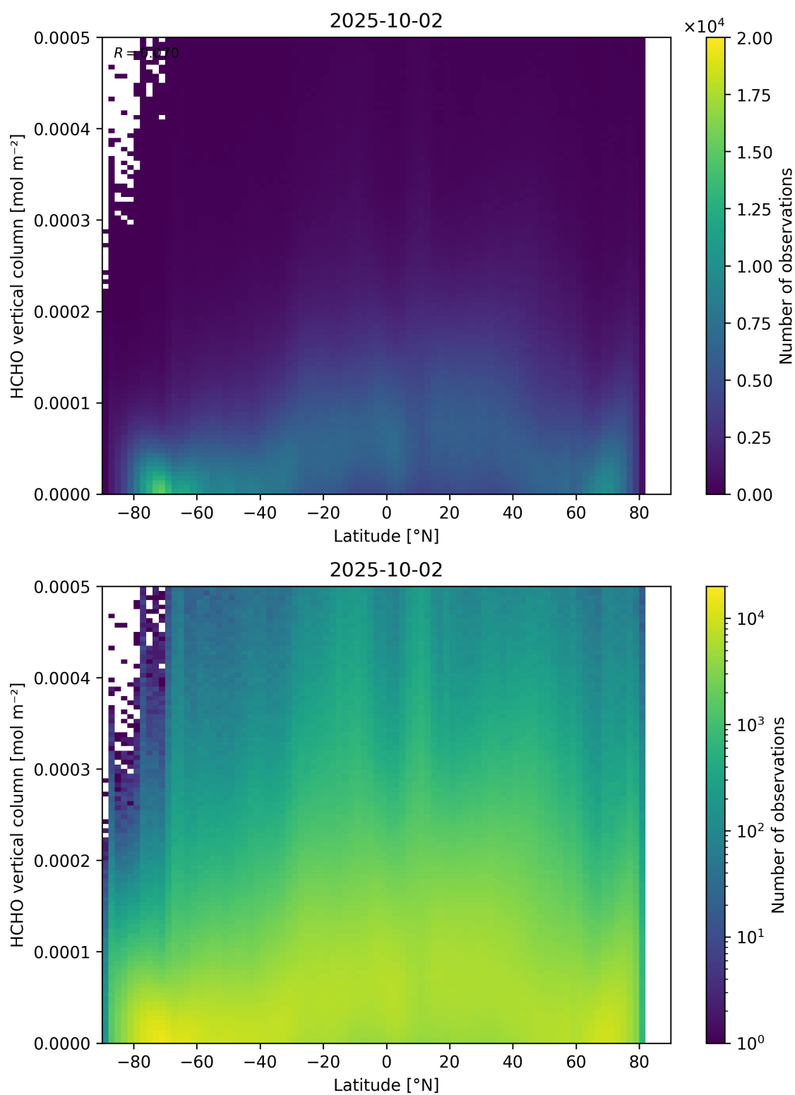
Figure 163: Scatter density plot of “Latitude” against “HCHO vertical column” for 2025-10-01 to 2025-10-03.
