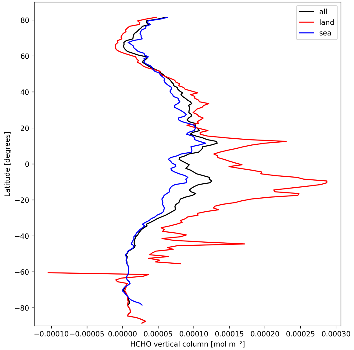
Figure 21: Zonal average of “HCHO vertical column” for 2025-10-01 to 2025-10-03.
