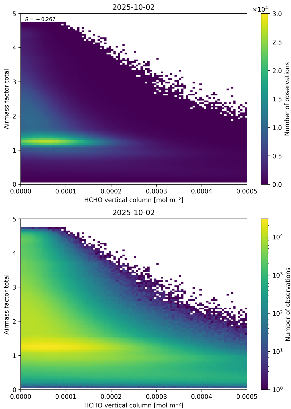
Figure 131: Scatter density plot of “HCHO vertical column” against “Airmass factor total” for 2025-10-01 to 2025-10-03.
