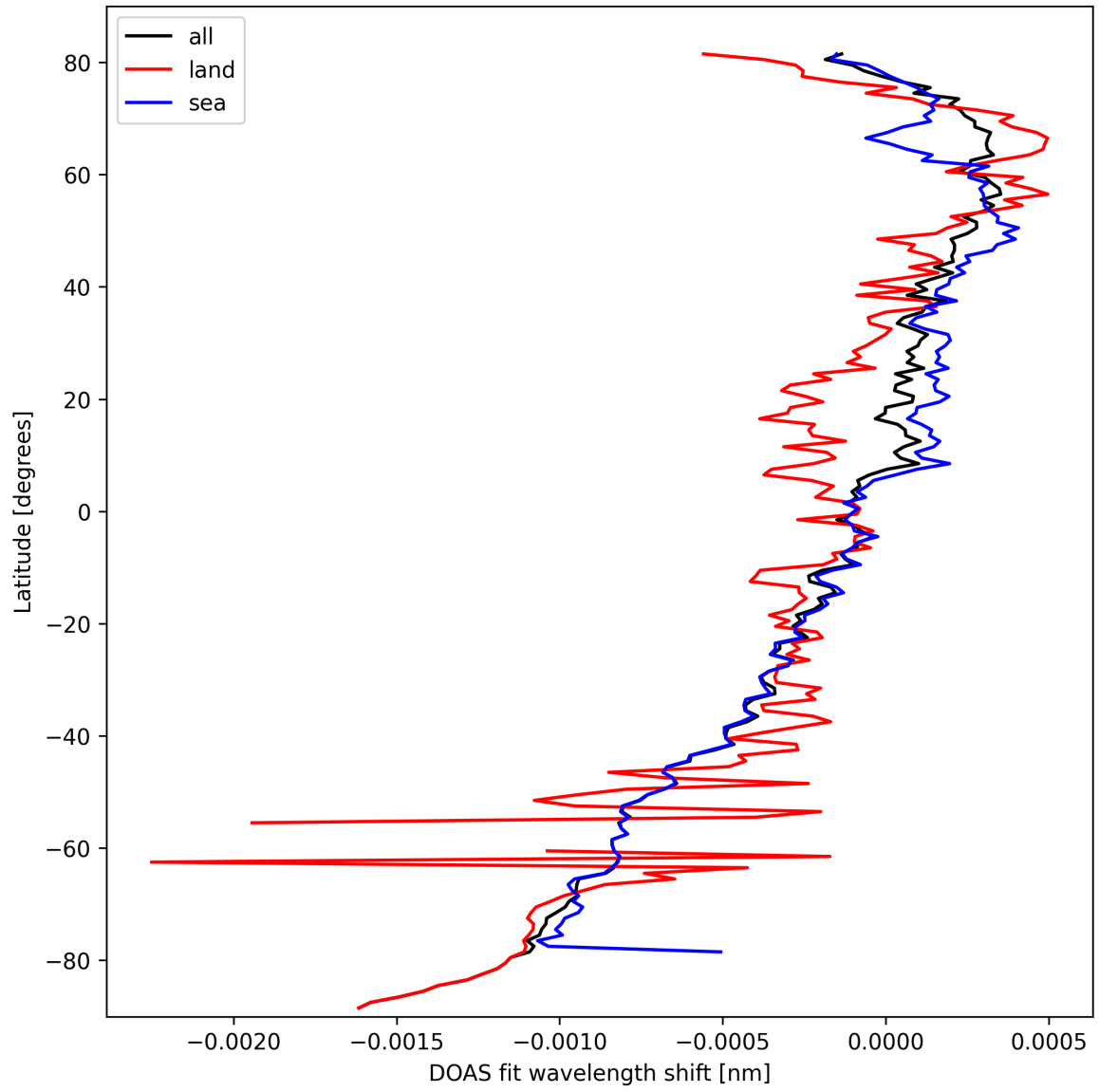
Figure 30: Zonal average of "DOAS fit wavelength shift" for 2025-10-01 to 2025-10-03.
