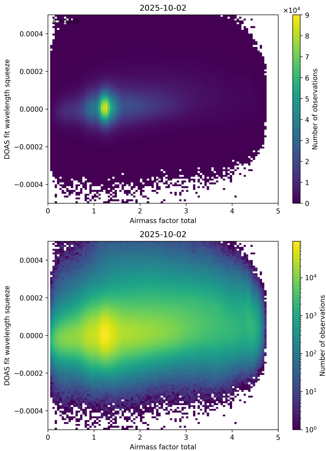
Figure 99: Scatter density plot of “Airmass factor total” against “DOAS fit wavelength squeeze” for 2025-10-01 to 2025-10-03.
