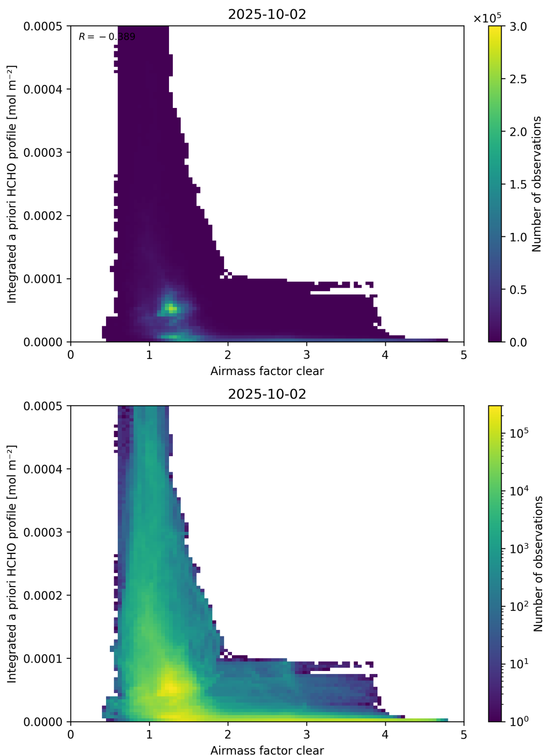
Figure 76: Scatter density plot of “Airmass factor clear” against “Integrated a priori HCHO profile” for 2025-10-01 to 2025-10-03.
