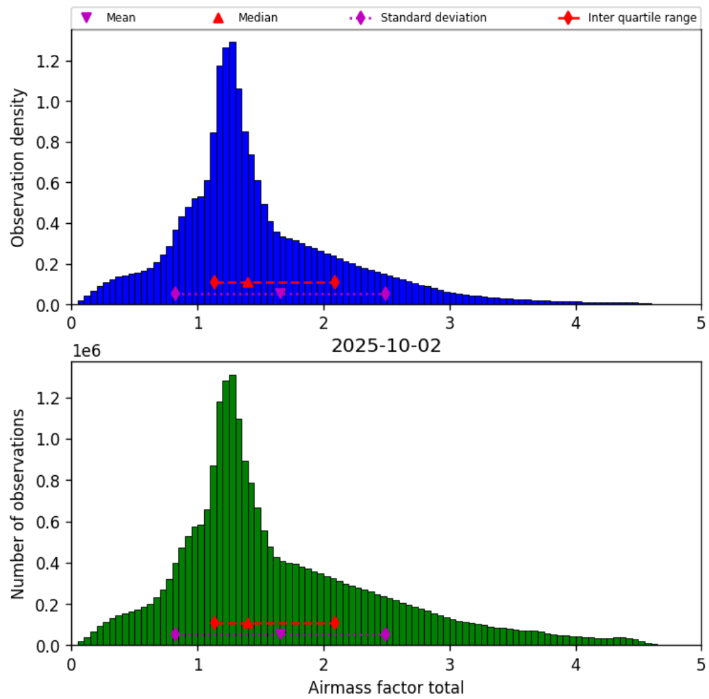
Figure 40: Histogram of “Airmass factor total” for 2025-10-01 to 2025-10-03
