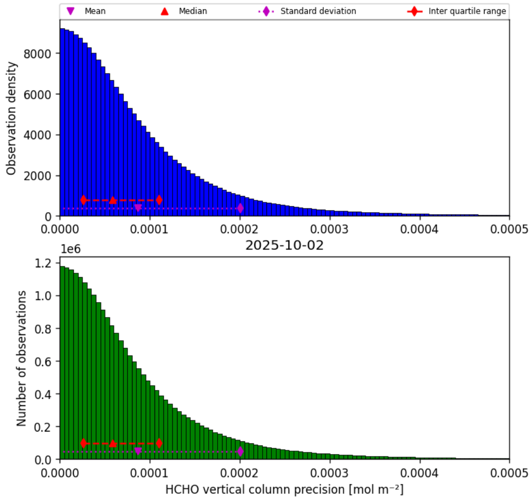
Figure 36: Histogram of “HCHO vertical column precision” for 2025-10-01 to 2025-10-03
