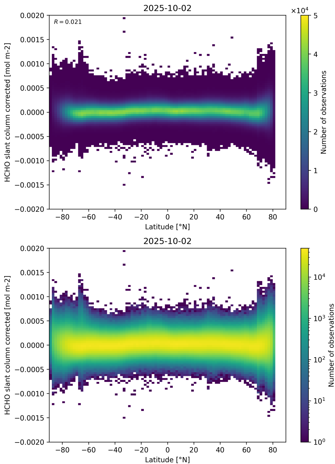
Figure 157: Scatter density plot of “Latitude” against “HCHO slant column corrected” for 2025-10-01 to 2025-10-03.
