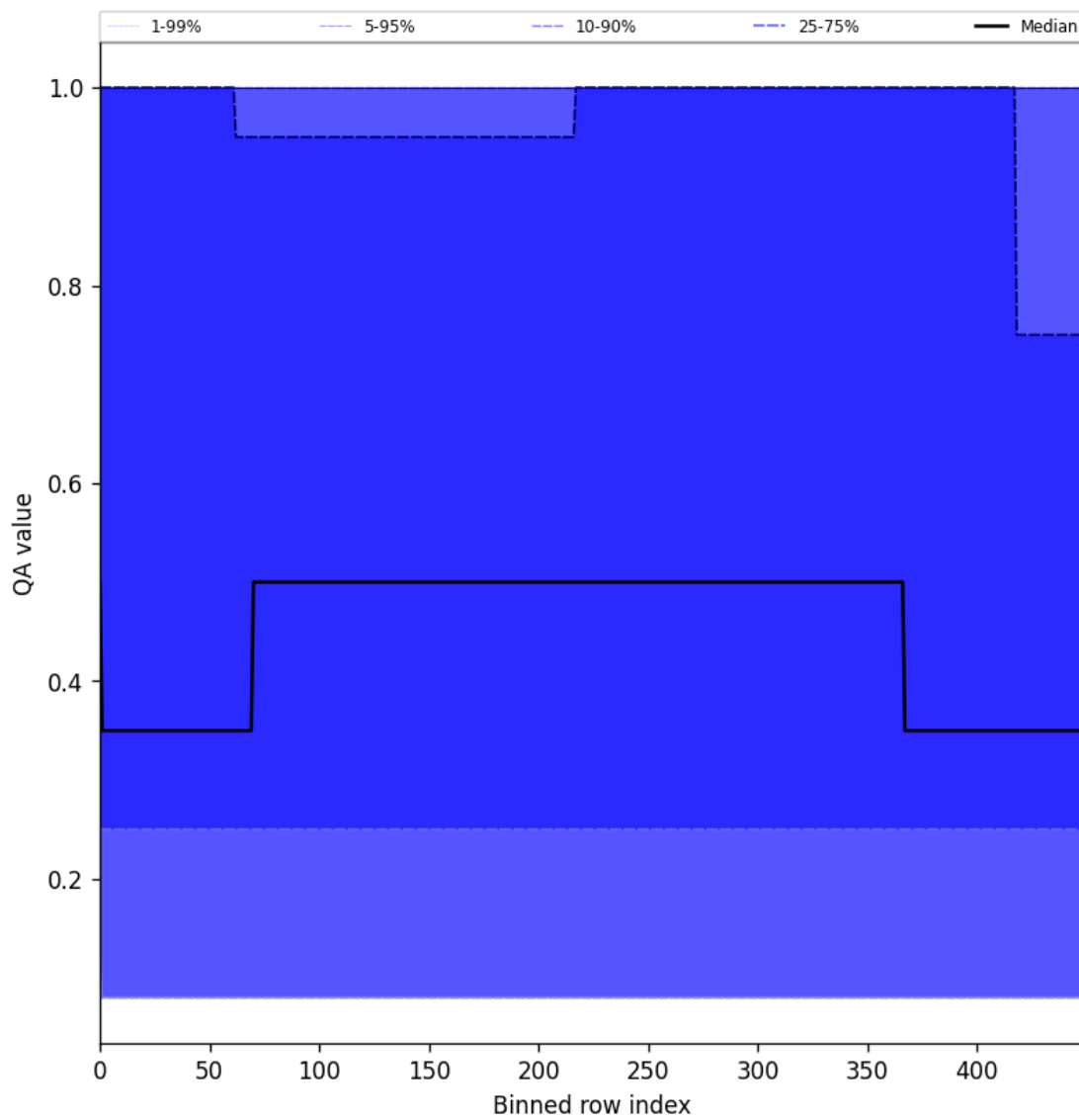
Figure 48: Along track statistics of “QA value” for 2025-10-01 to 2025-10-03
