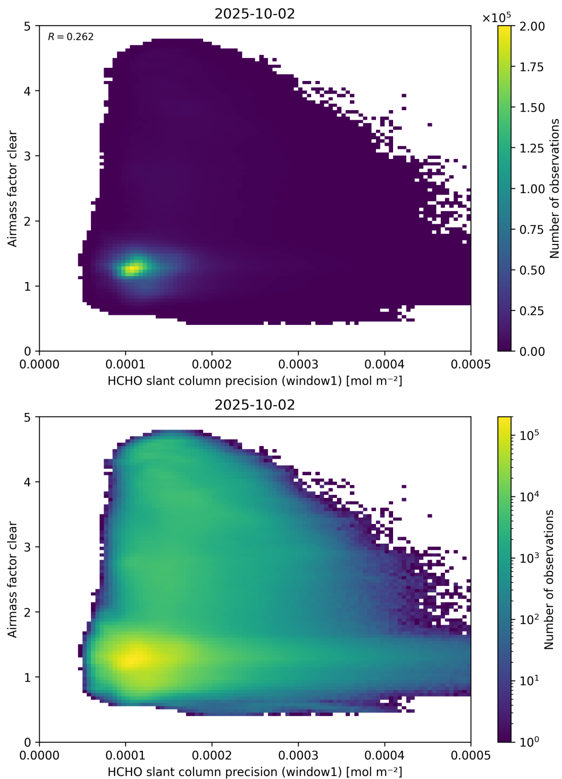
Figure 91: Scatter density plot of “HCHO slant column precision (window1)” against “Airmass factor clear” for 2025-10-01 to 2025-10-03.
