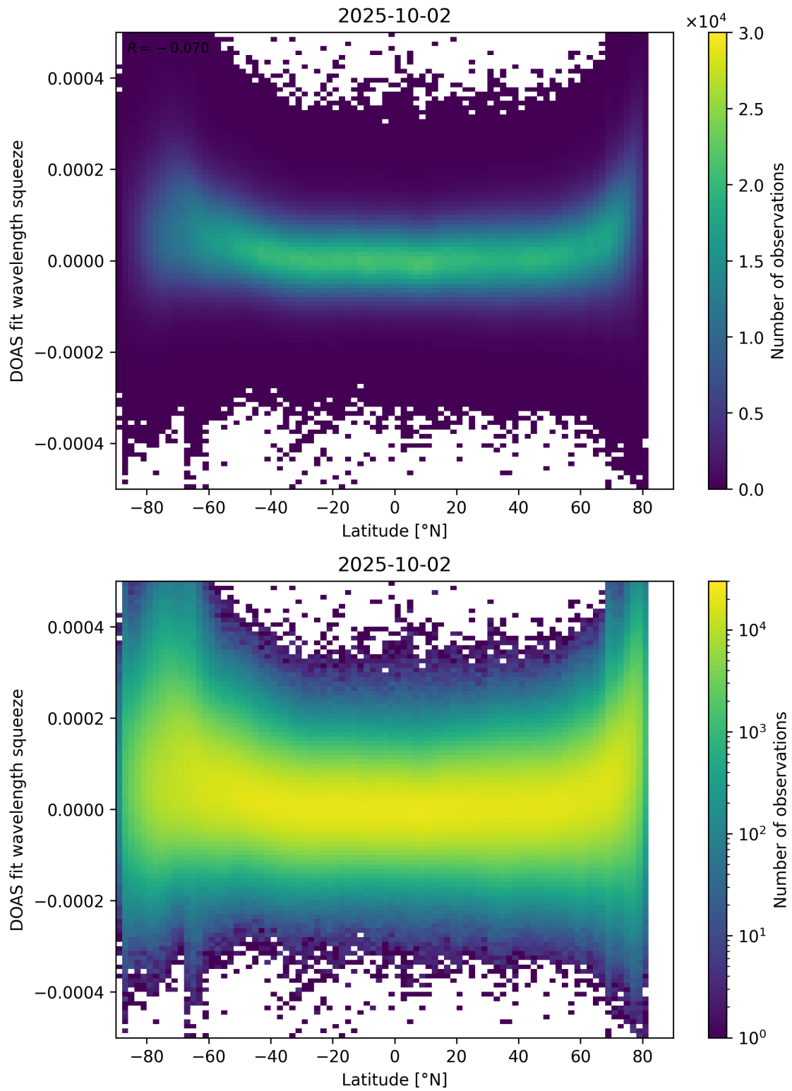
Figure 155: Scatter density plot of “Latitude” against “DOAS fit wavelength squeeze” for 2025-10-01 to 2025-10-03.
