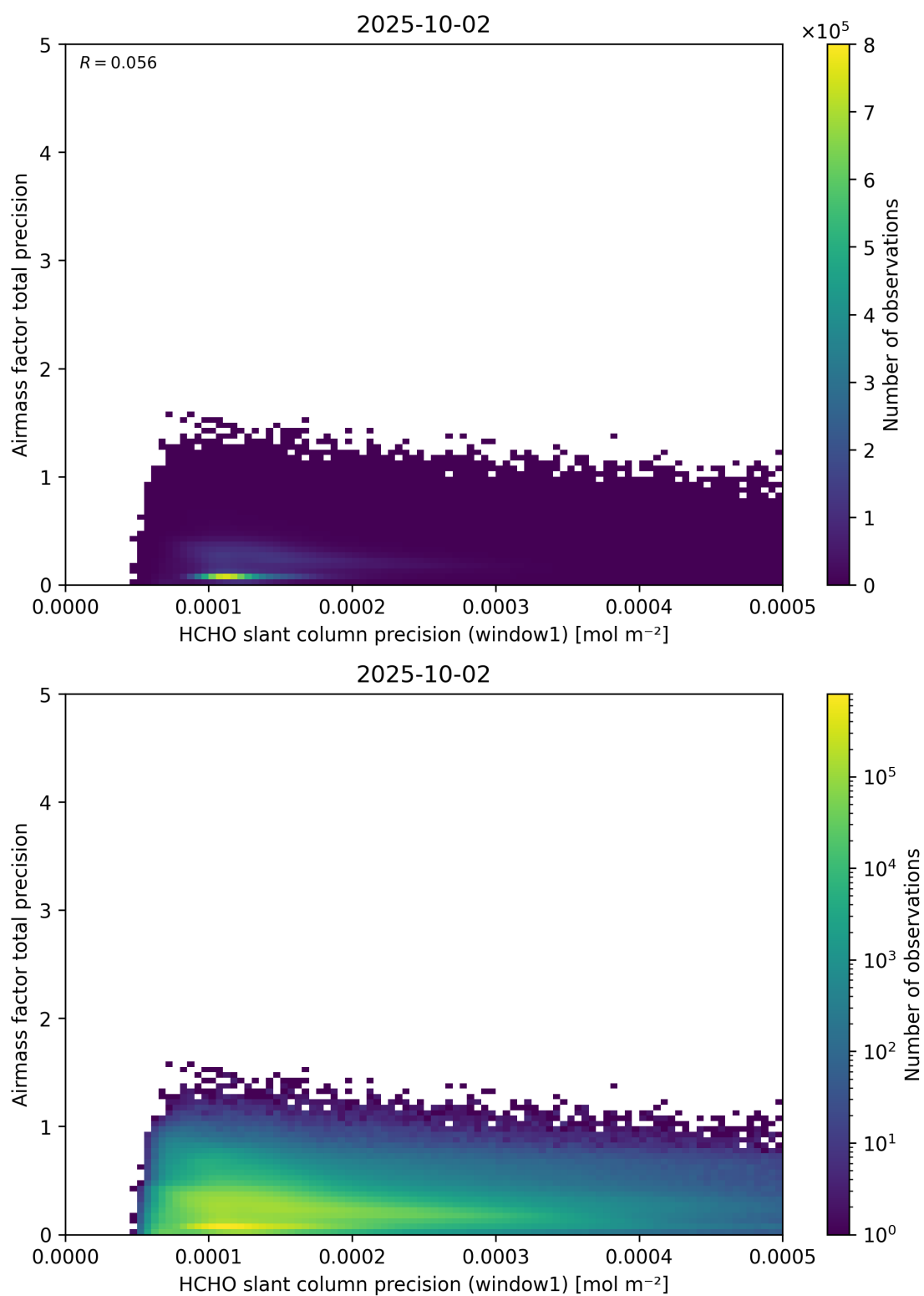
Figure 95: Scatter density plot of “HCHO slant column precision (window1)” against “Airmass factor total precision” for 2025-10-01 to 2025-10-03.
