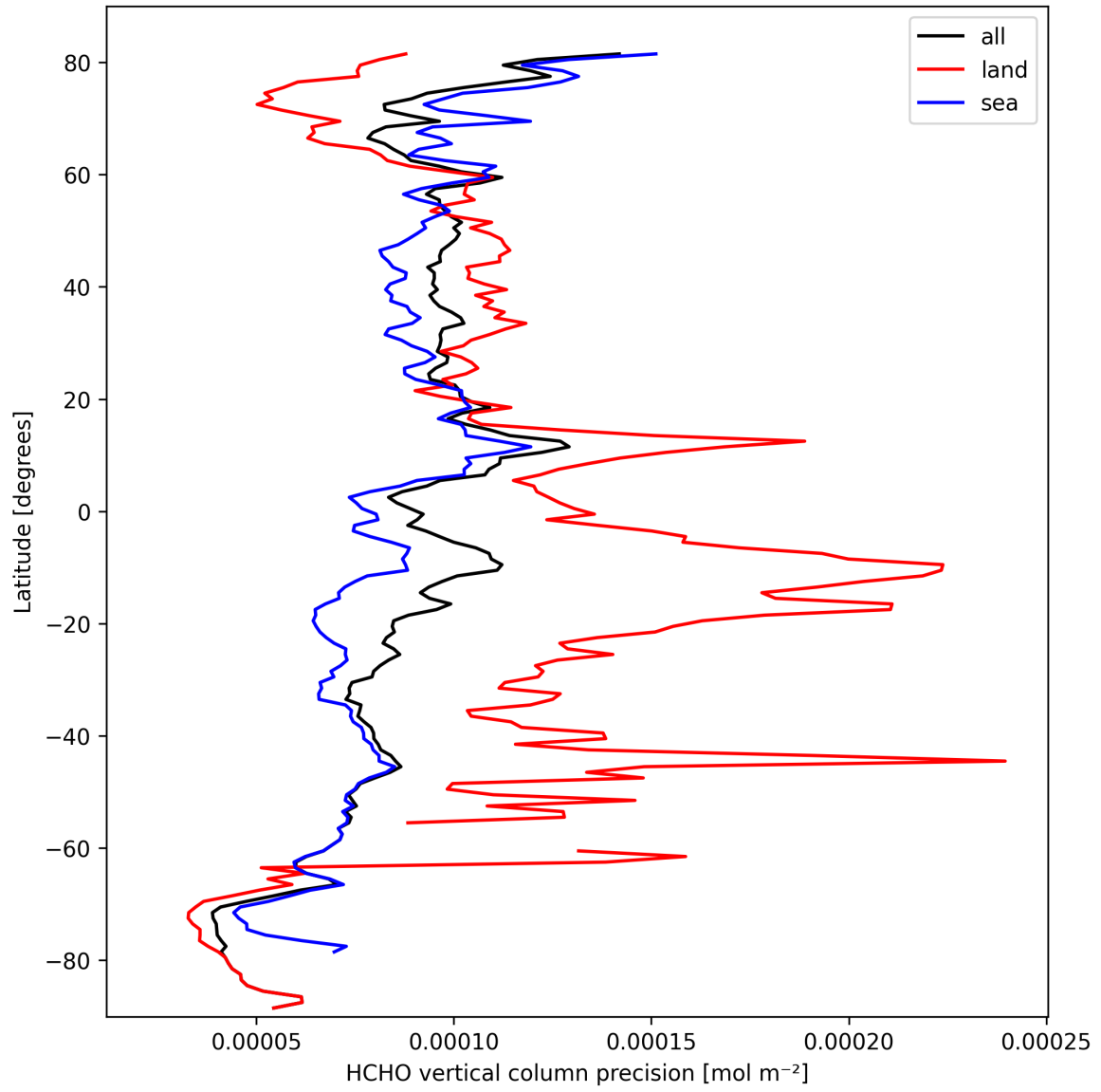
Figure 22: Zonal average of "HCHO vertical column precision" for 2025-10-01 to 2025-10-03.
