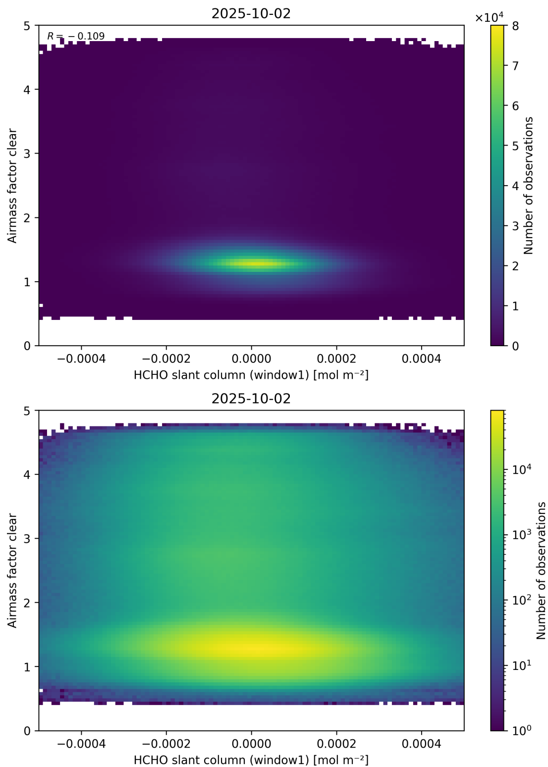
Figure 81: Scatter density plot of “HCHO slant column (window1)” against “Airmass factor clear” for 2025-10-01 to 2025-10-03.
