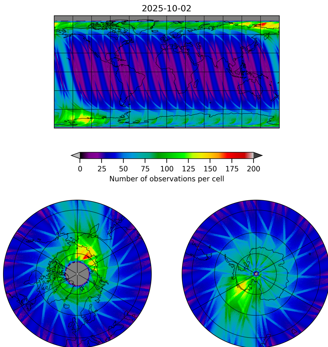
Figure 19: Map of the number of observations for 2025-10-01 to 2025-10-03
