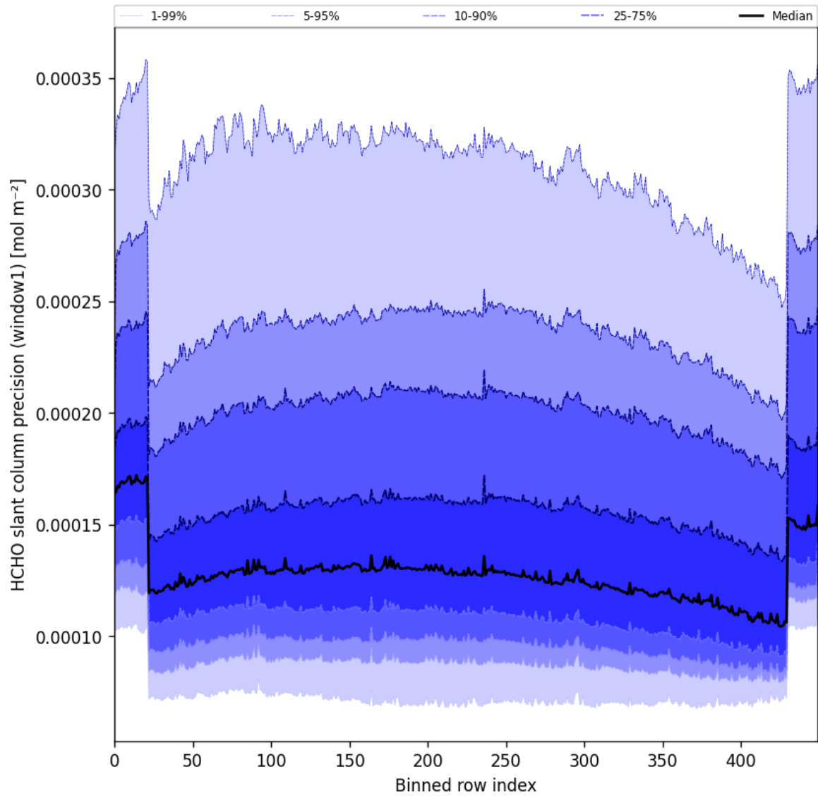
Figure 53: Along track statistics of “HCHO slant column precision (window1)” for 2025-10-01 to 2025-10-03
