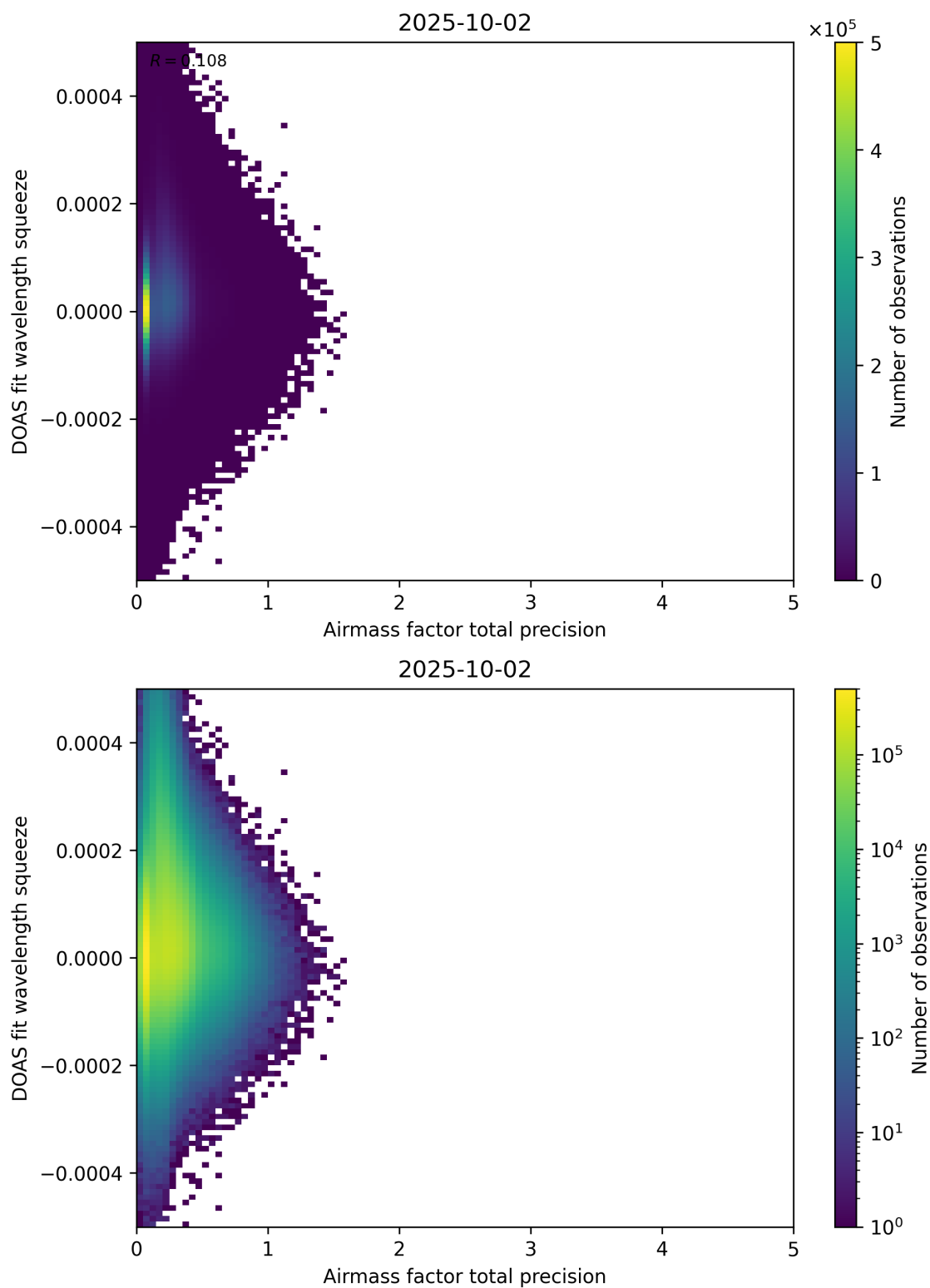
Figure 107: Scatter density plot of “Airmass factor total precision” against “DOAS fit wavelength squeeze” for 2025-10-01 to 2025-10-03.
