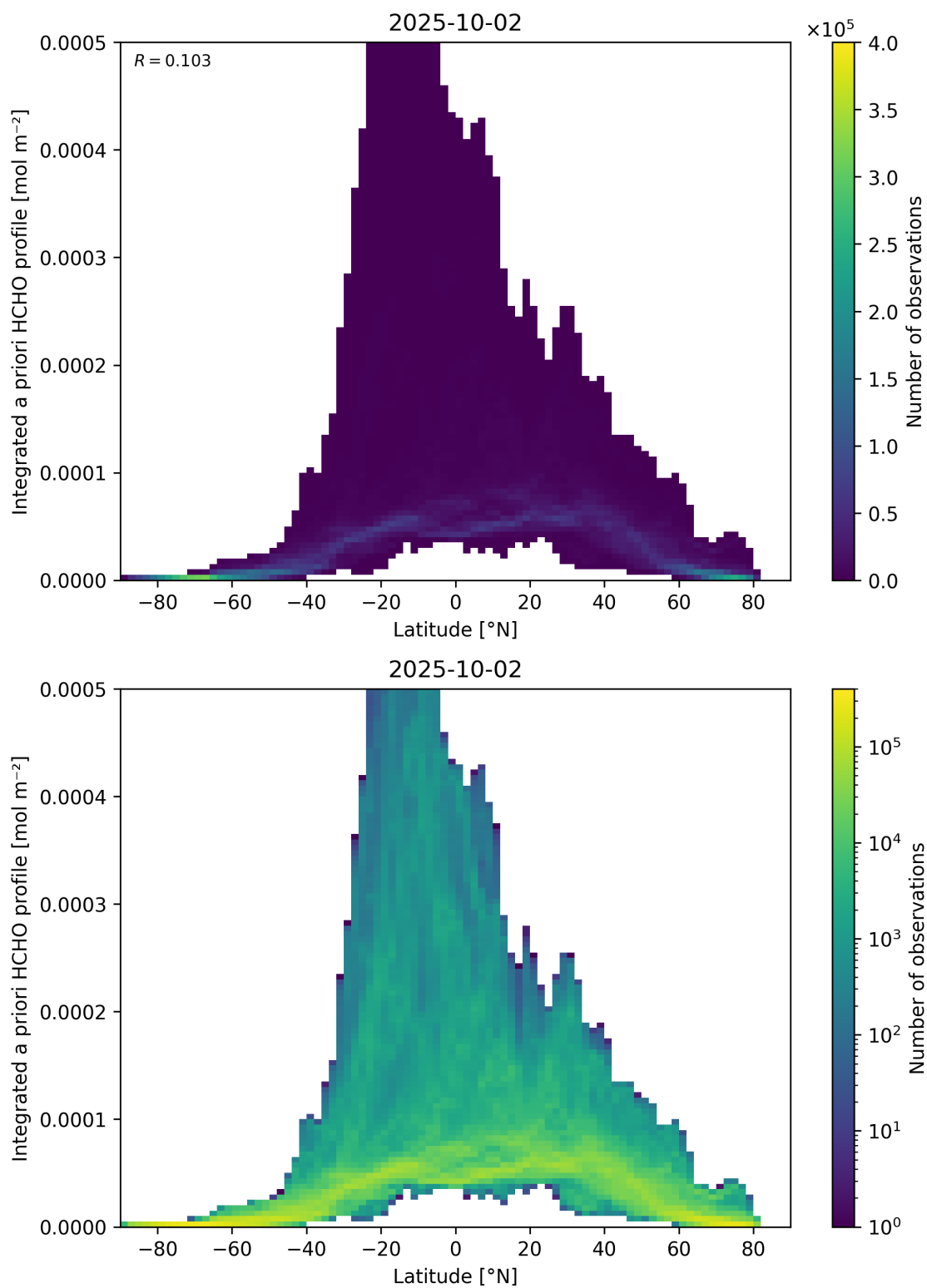
Figure 166: Scatter density plot of “Latitude” against “Integrated a priori HCHO profile” for 2025-10-01 to 2025-10-03.
