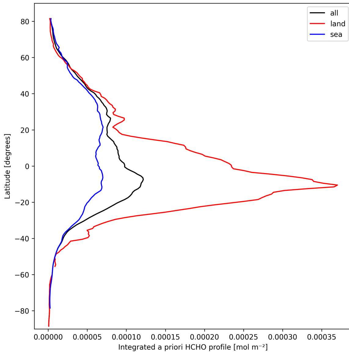
Figure 29: Zonal average of “Integrated a priori HCHO profile” for 2025-10-01 to 2025-10-03.
