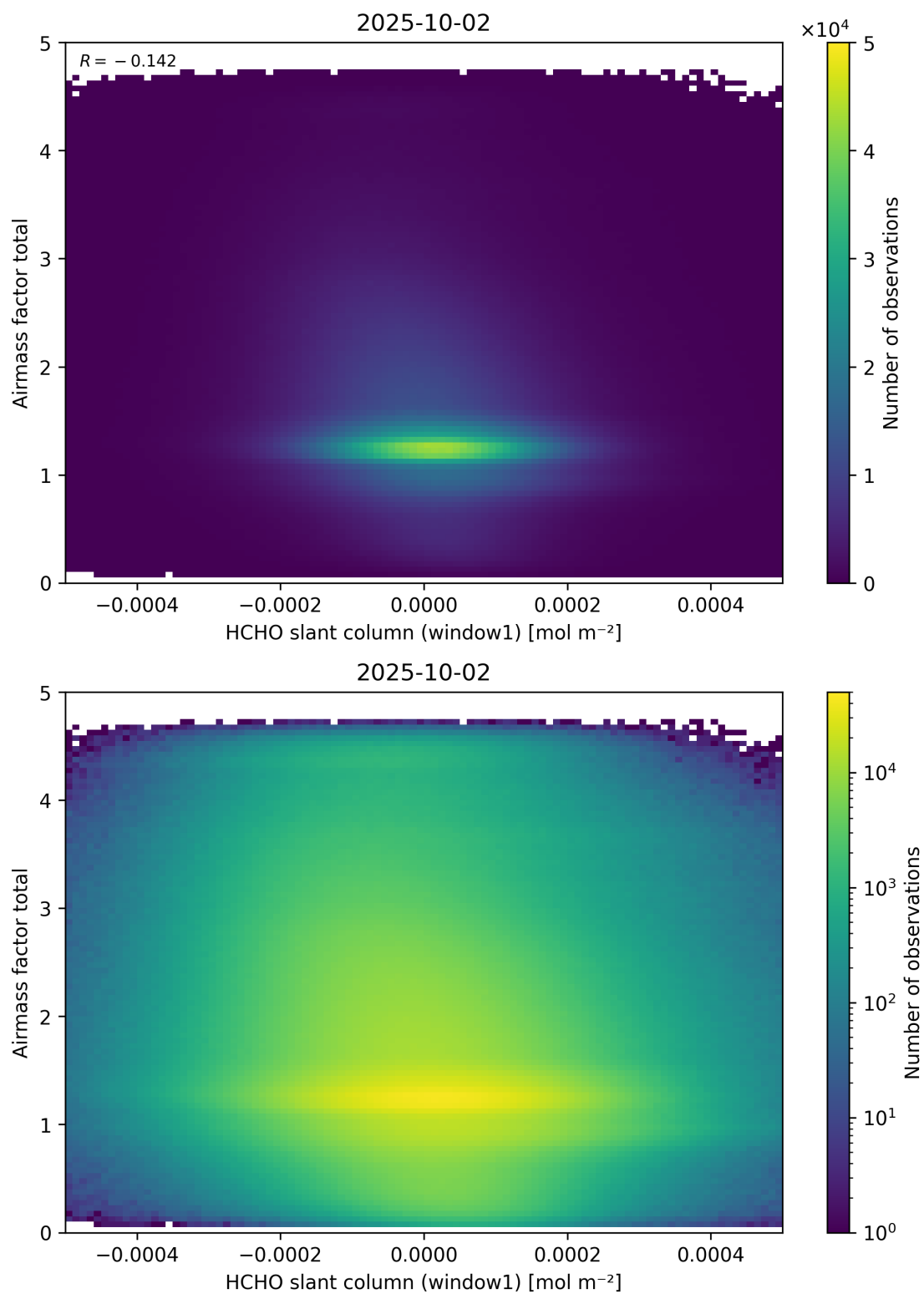
Figure 85: Scatter density plot of “HCHO slant column (window1)” against “Airmass factor total” for 2025-10-01 to 2025-10-03.
