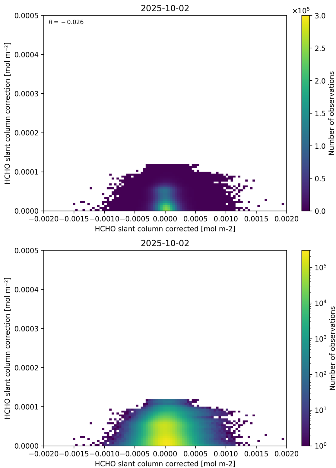
Figure 77: Scatter density plot of “HCHO slant column corrected” against “HCHO slant column correction” for 2025-10-01 to 2025-10-03.
