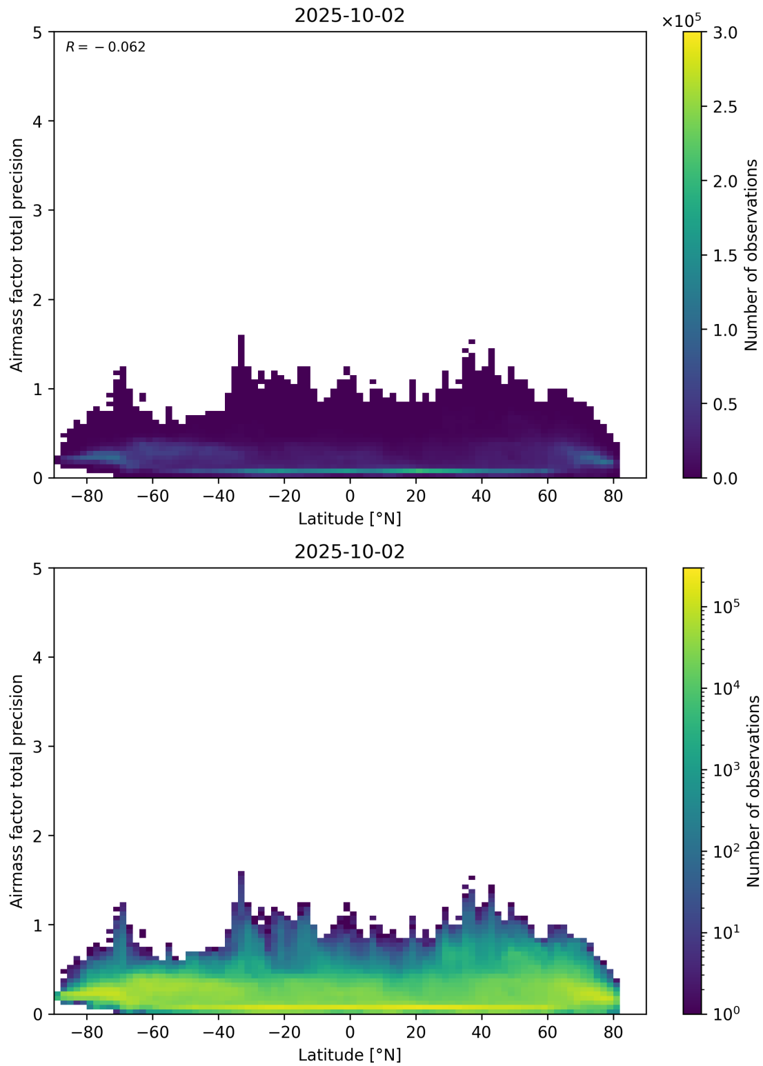
Figure 162: Scatter density plot of “Latitude” against “Airmass factor total precision” for 2025-10-01 to 2025-10-03.
