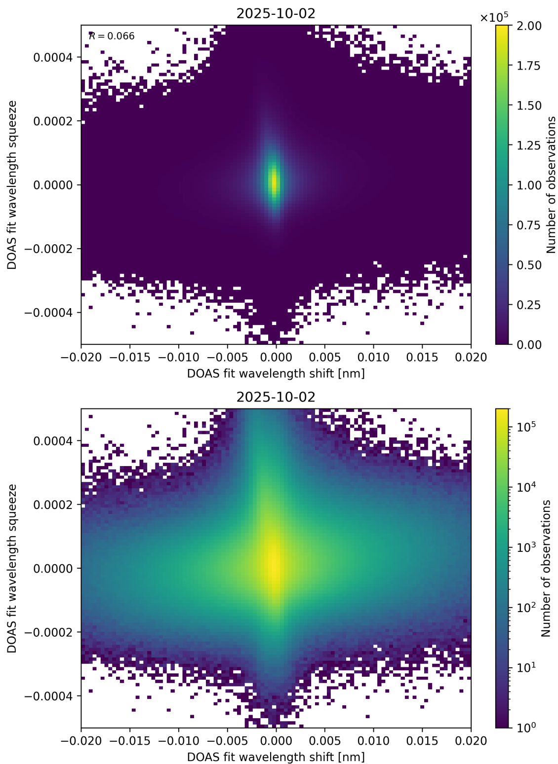
Figure 65: Scatter density plot of “DOAS fit wavelength shift” against “DOAS fit wavelength squeeze” for 2025-10-01 to 2025-10-03.
