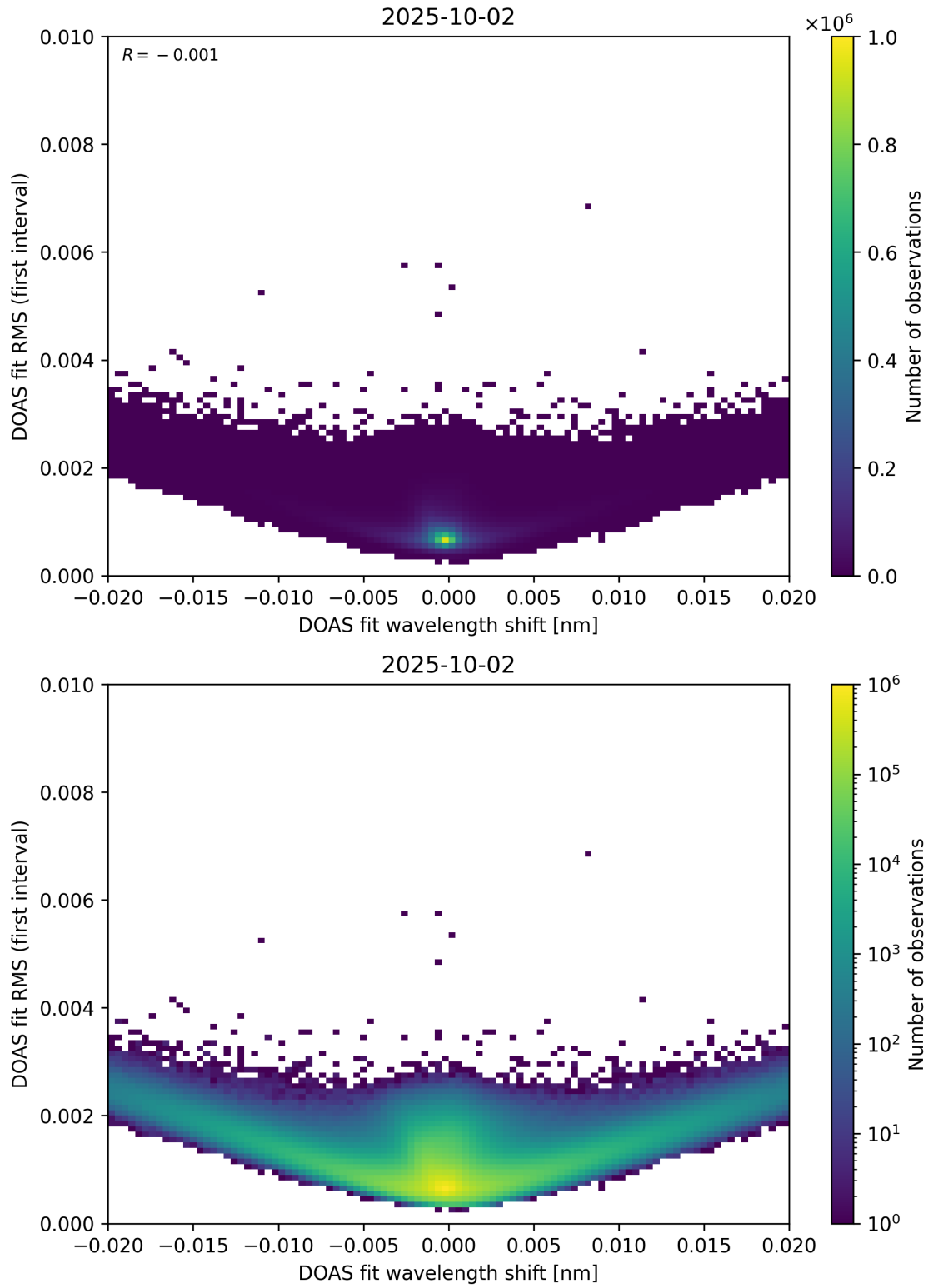
Figure 64: Scatter density plot of “DOAS fit wavelength shift” against “DOAS fit RMS (first interval)” for 2025-10-01 to 2025-10-03.
