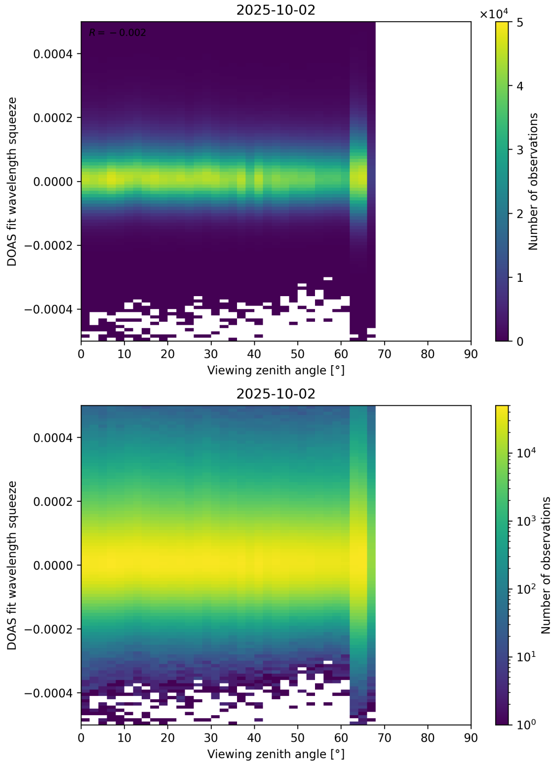
Figure 184: Scatter density plot of “Viewing zenith angle” against “DOAS fit wavelength squeeze” for 2025-10-01 to 2025-10-03.
