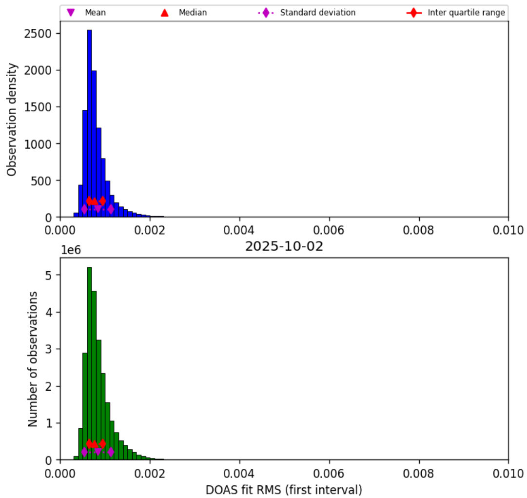
Figure 46: Histogram of “DOAS fit RMS (first interval)” for 2025-10-01 to 2025-10-03
