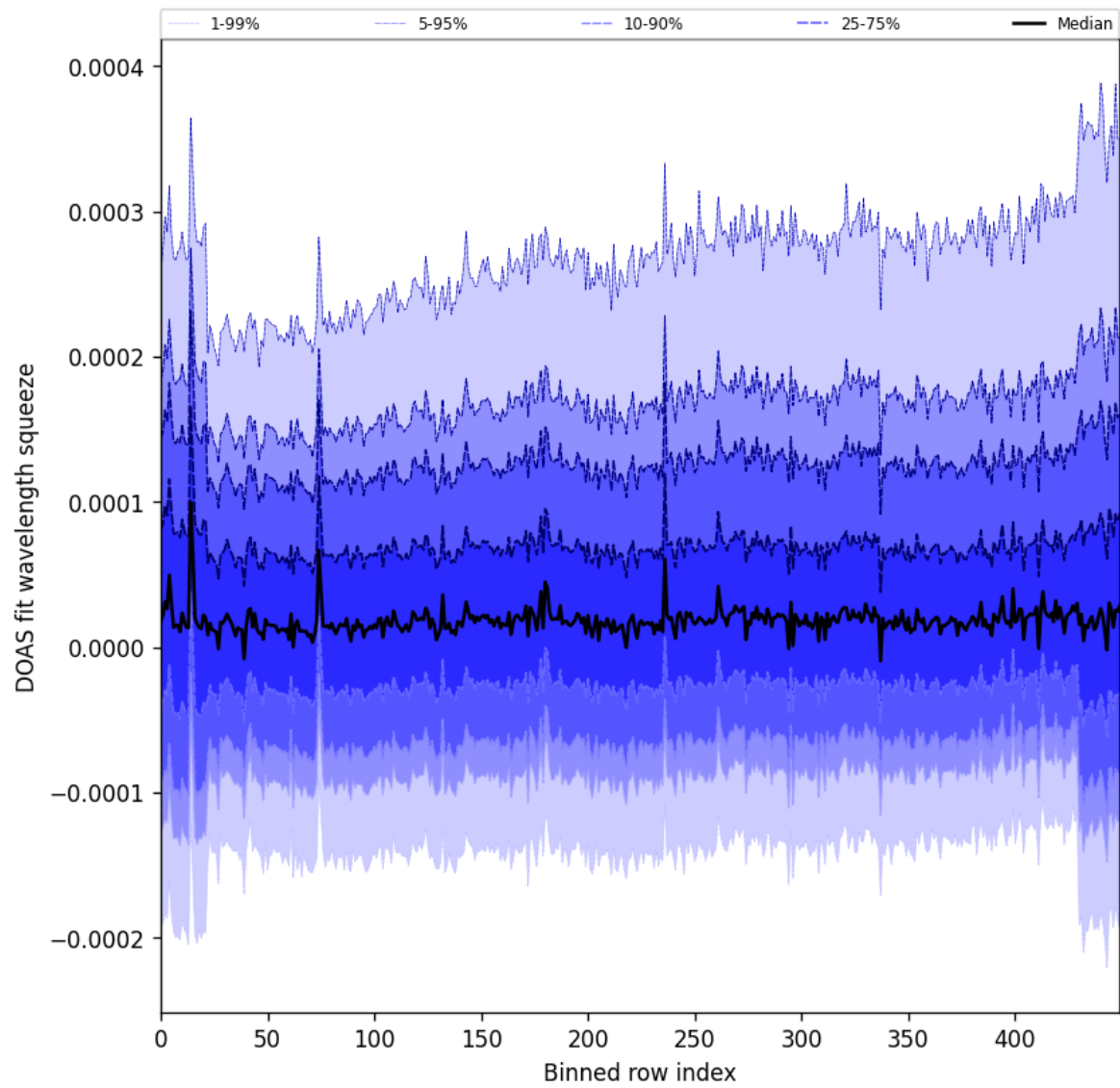
Figure 59: Along track statistics of “DOAS fit wavelength squeeze” for 2025-10-01 to 2025-10-03
