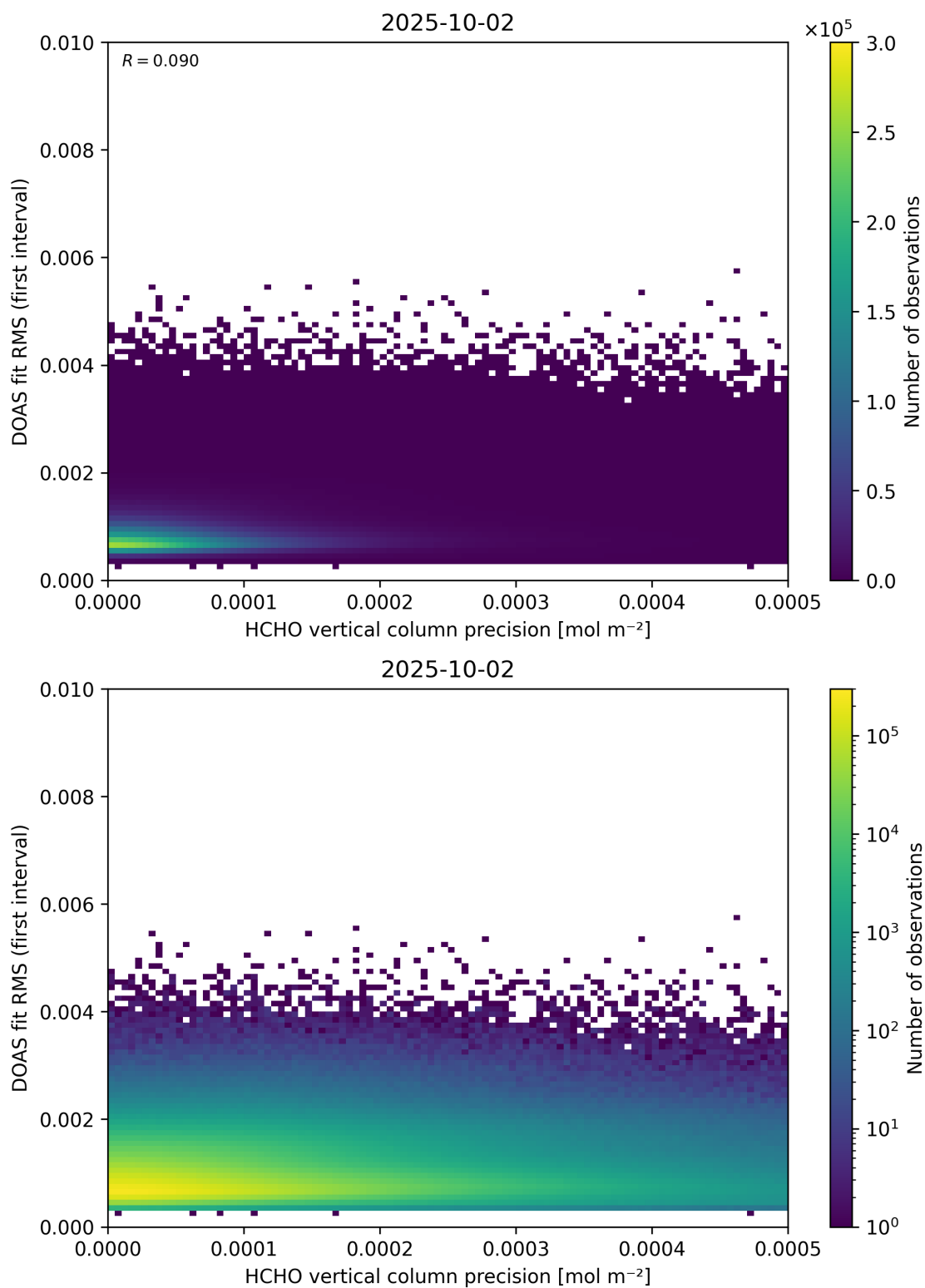
Figure 136: Scatter density plot of “HCHO vertical column precision” against “DOAS fit RMS (first interval)” for 2025-10-01 to 2025-10-03.
