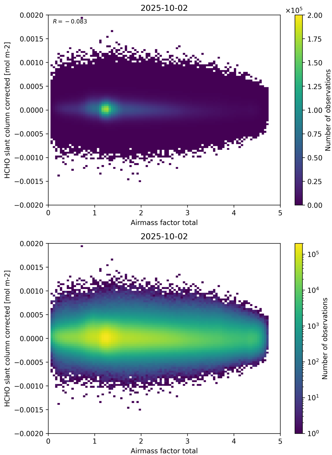
Figure 101: Scatter density plot of “Airmass factor total” against “HCHO slant column corrected” for 2025-10-01 to 2025-10-03.
