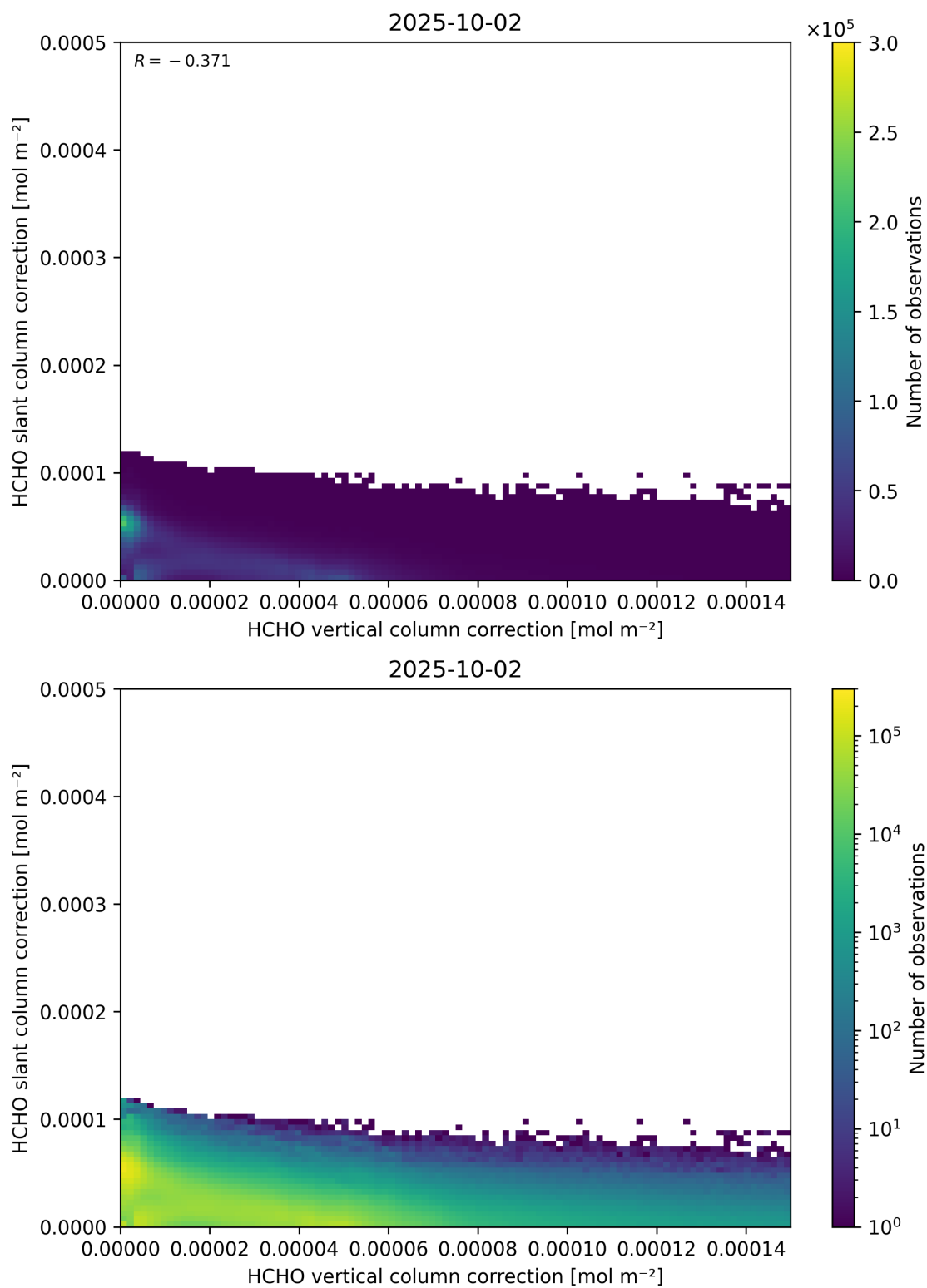
Figure 117: Scatter density plot of “HCHO vertical column correction” against “HCHO slant column correction” for 2025-10-01 to 2025-10-03.
