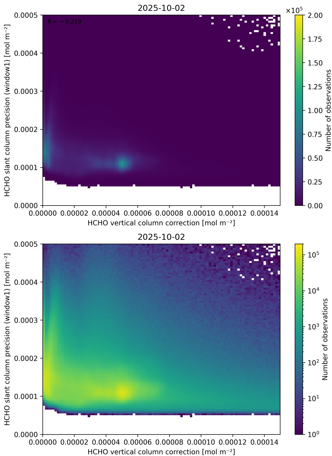
Figure 119: Scatter density plot of “HCHO vertical column correction” against “HCHO slant column precision (window1)” for 2025-10-01 to 2025-10-03.
