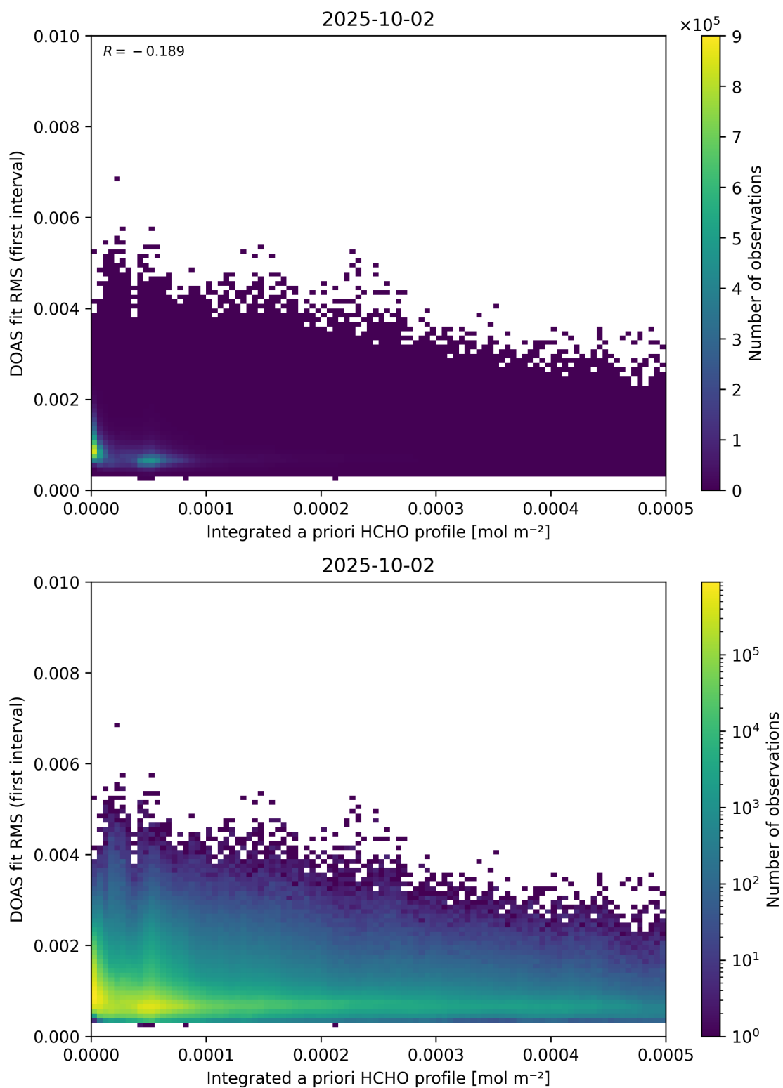
Figure 148: Scatter density plot of “Integrated a priori HCHO profile” against “DOAS fit RMS (first interval)” for 2025-10-01 to 2025-10-03.
