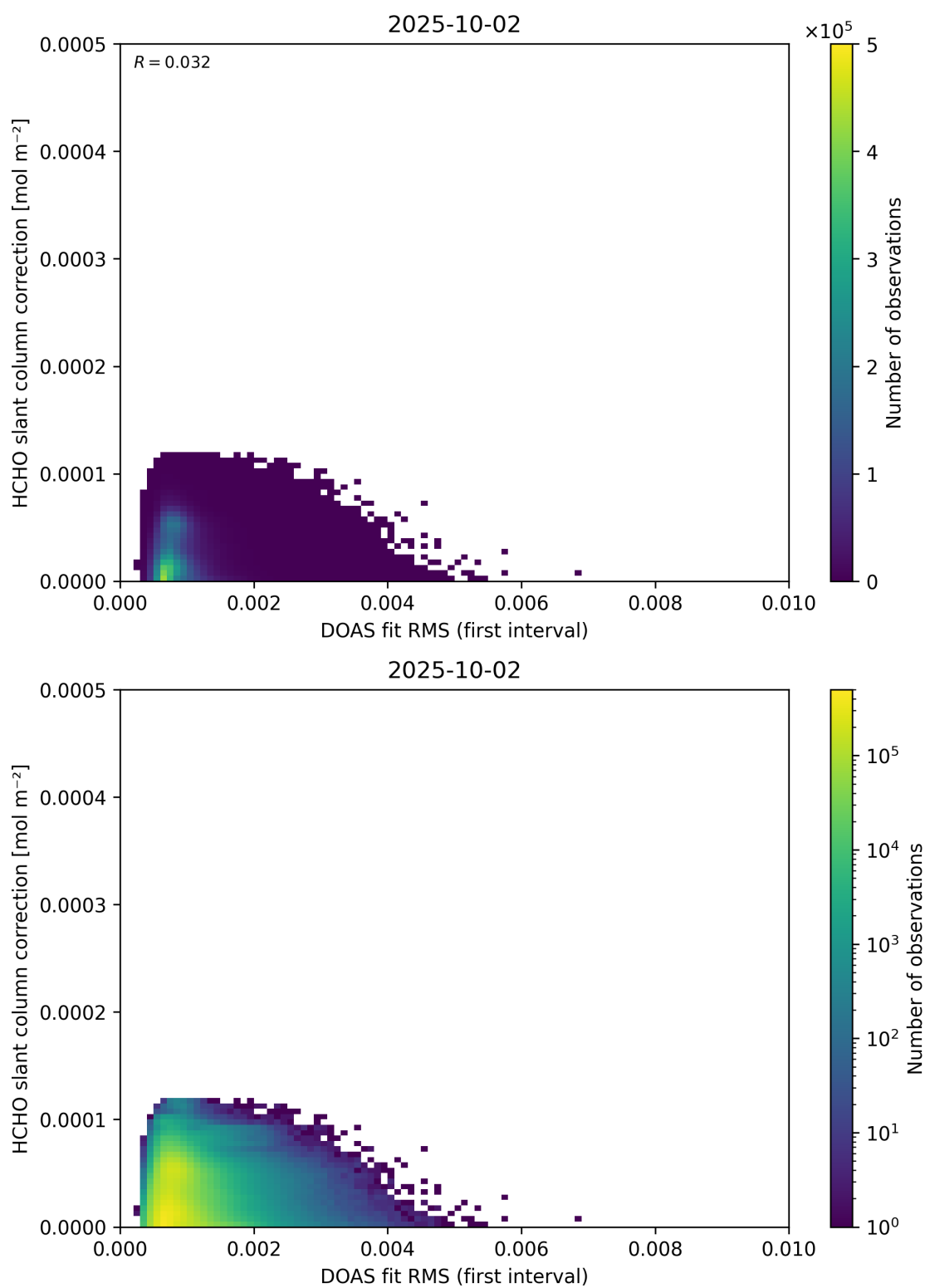
Figure 63: Scatter density plot of “DOAS fit RMS (first interval)” against “HCHO slant column correction” for 2025-10-01 to 2025-10-03.
