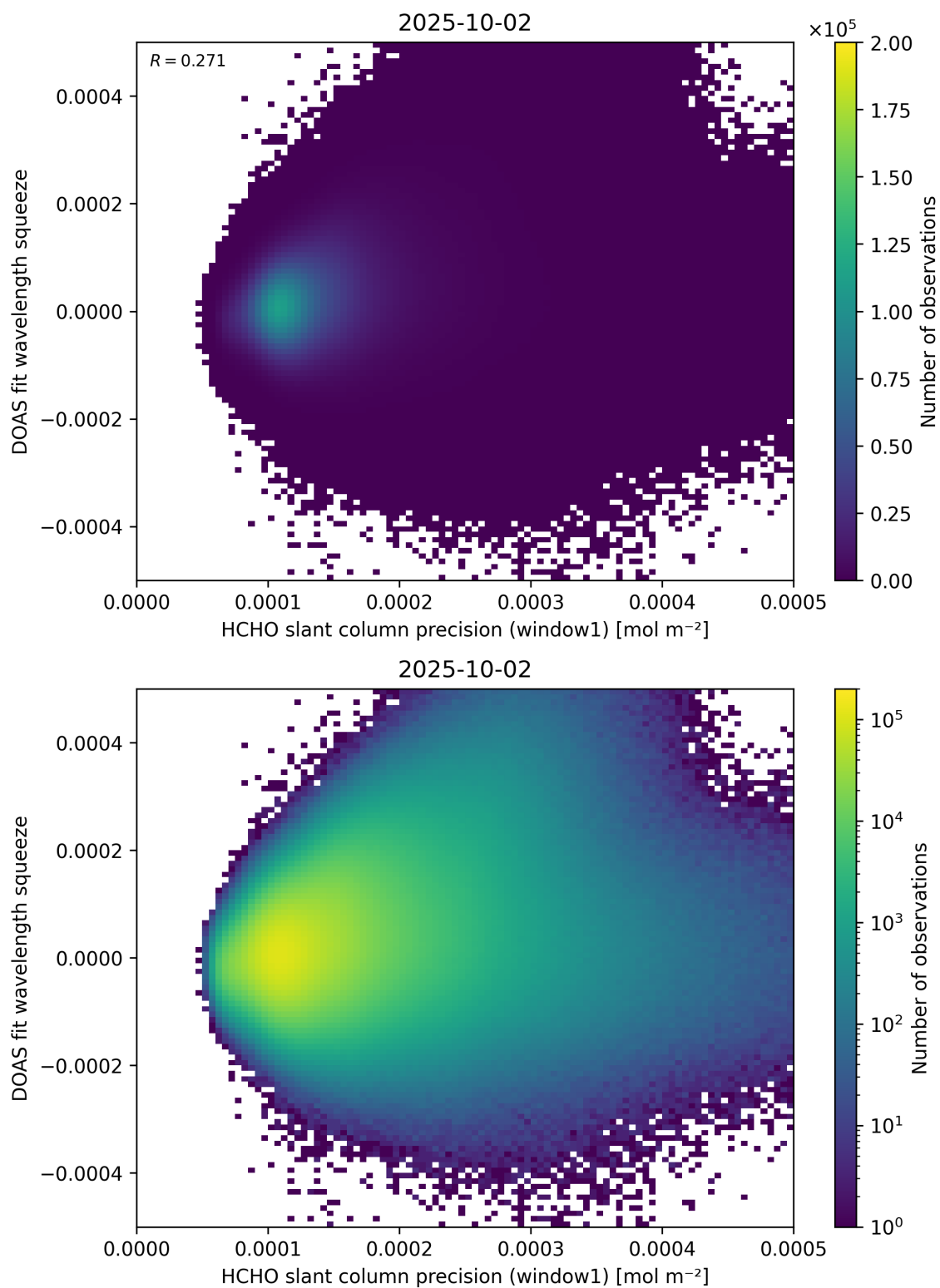
Figure 90: Scatter density plot of “HCHO slant column precision (window1)” against “DOAS fit wavelength squeeze” for 2025-10-01 to 2025-10-03.
