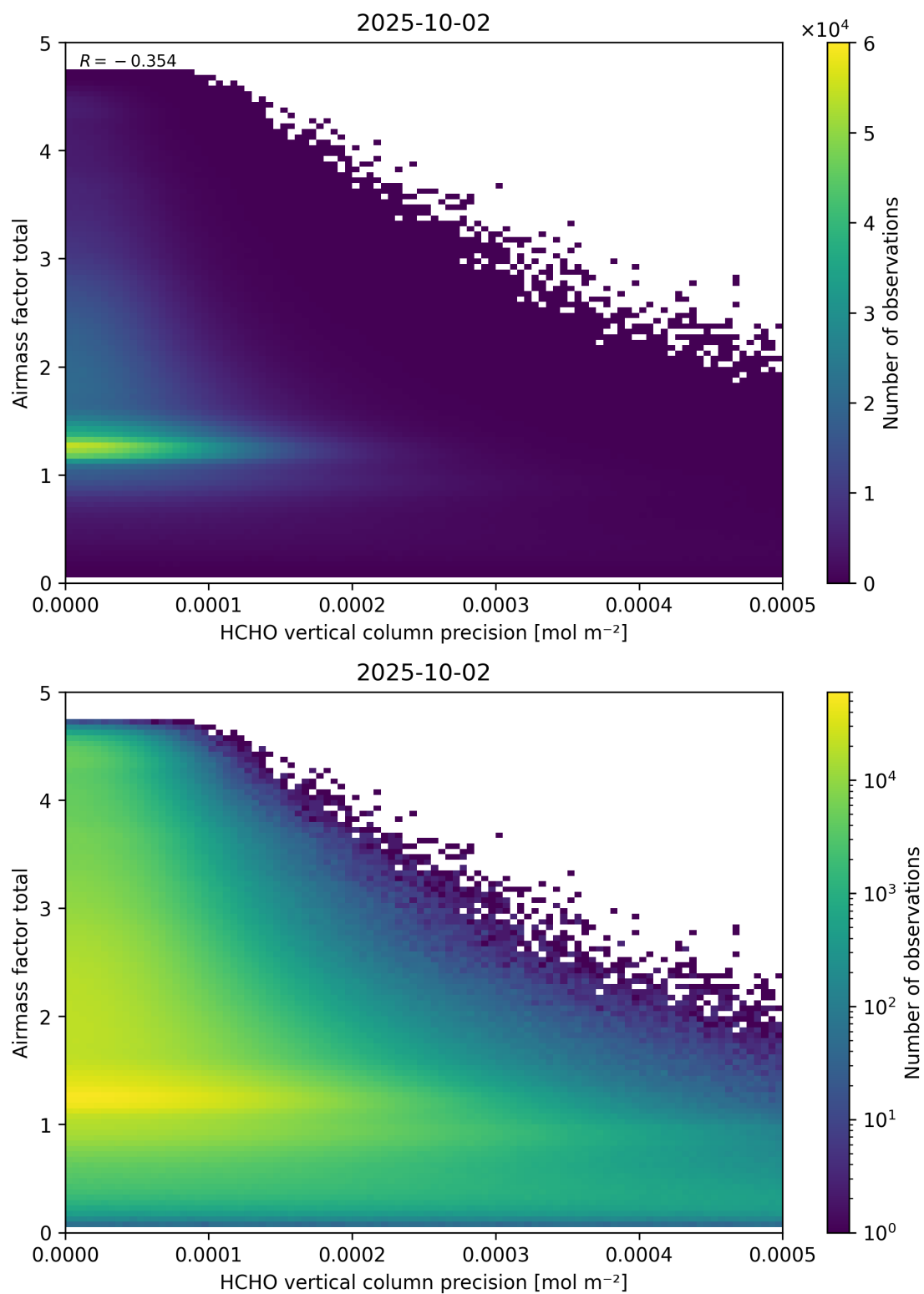
Figure 144: Scatter density plot of “HCHO vertical column precision” against “Airmass factor total” for 2025-10-01 to 2025-10-03.
