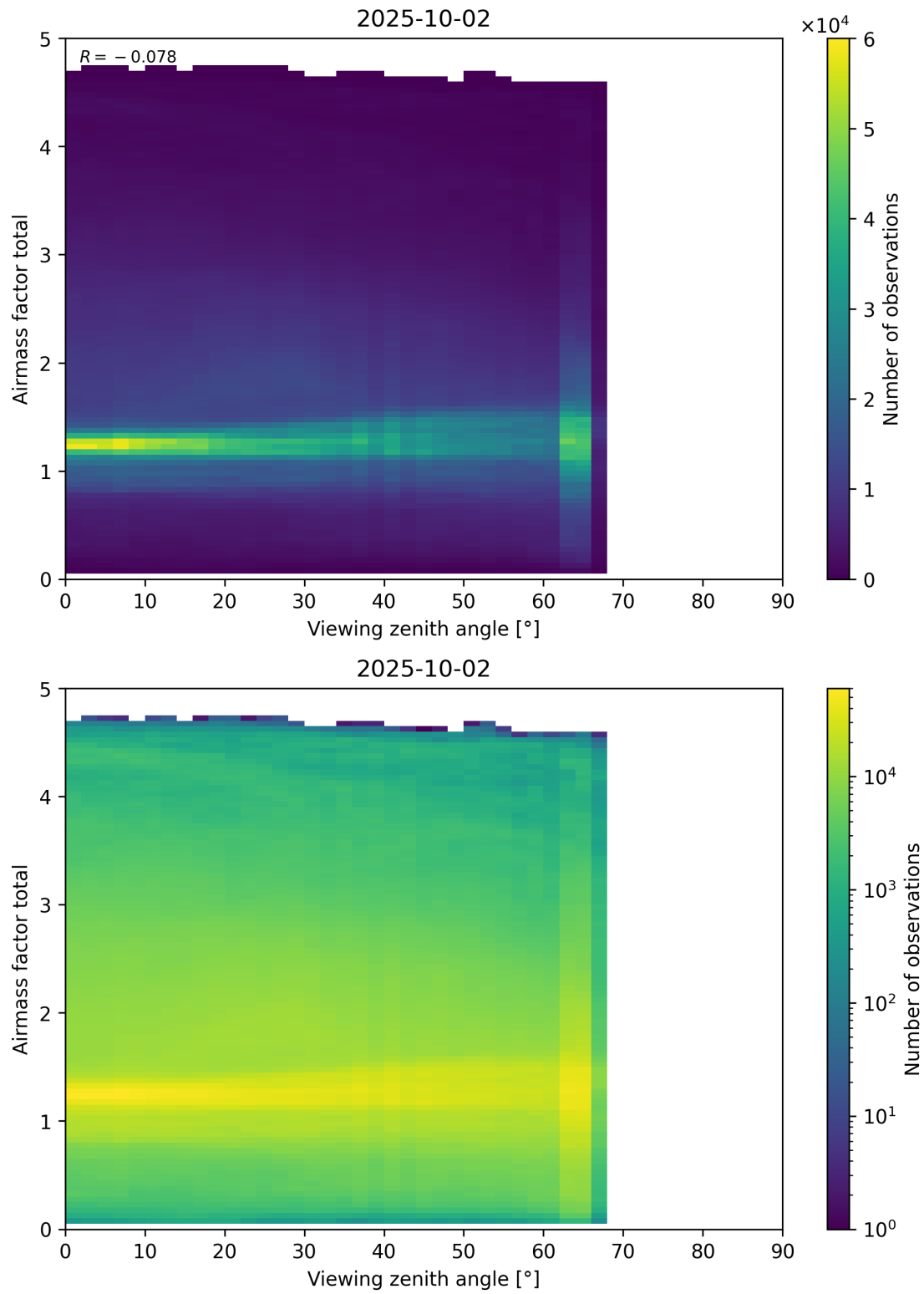
Figure 190: Scatter density plot of “Viewing zenith angle” against “Airmass factor total” for 2025-10-01 to 2025-10-03.
