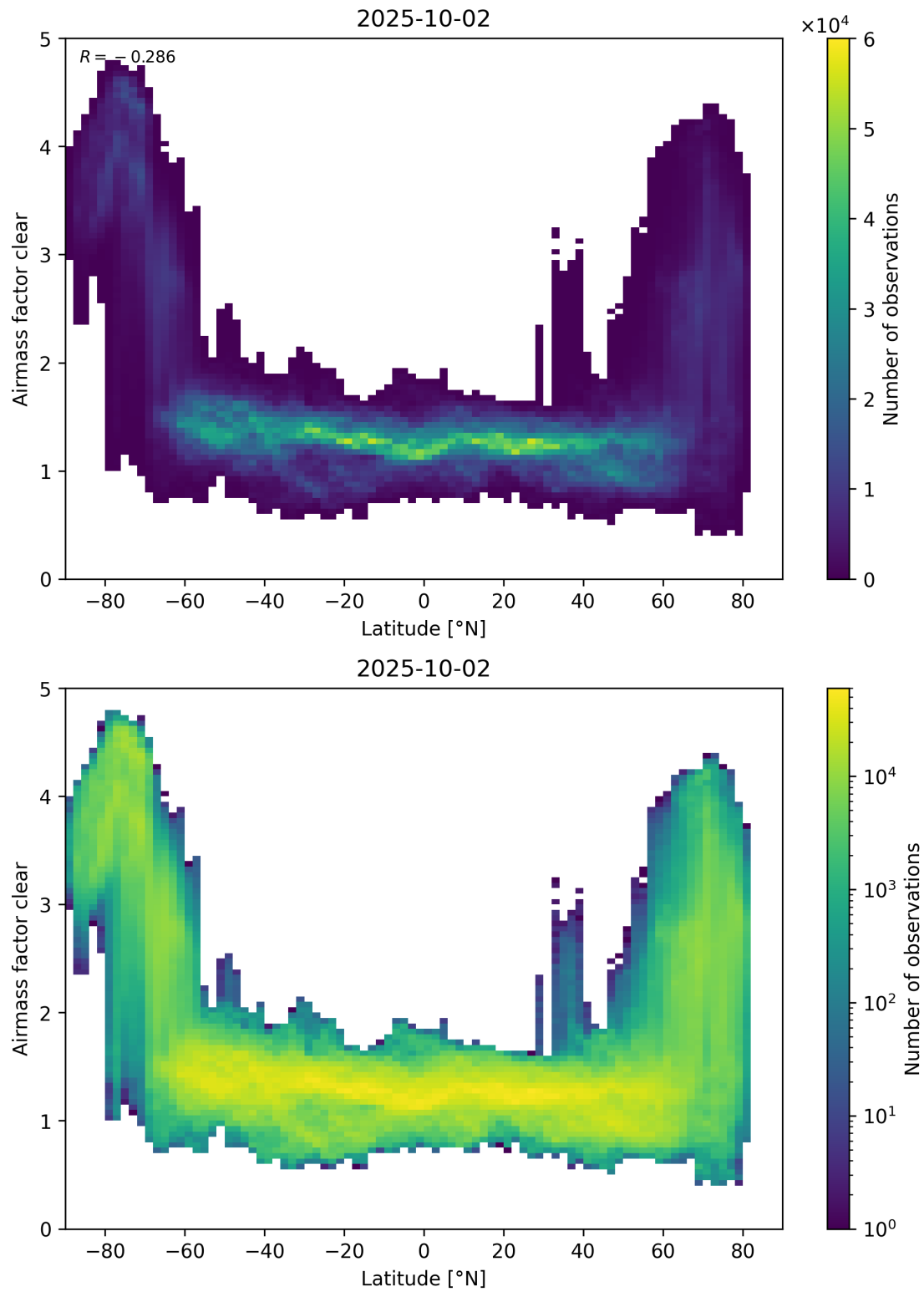
Figure 156: Scatter density plot of “Latitude” against “Airmass factor clear” for 2025-10-01 to 2025-10-03.
