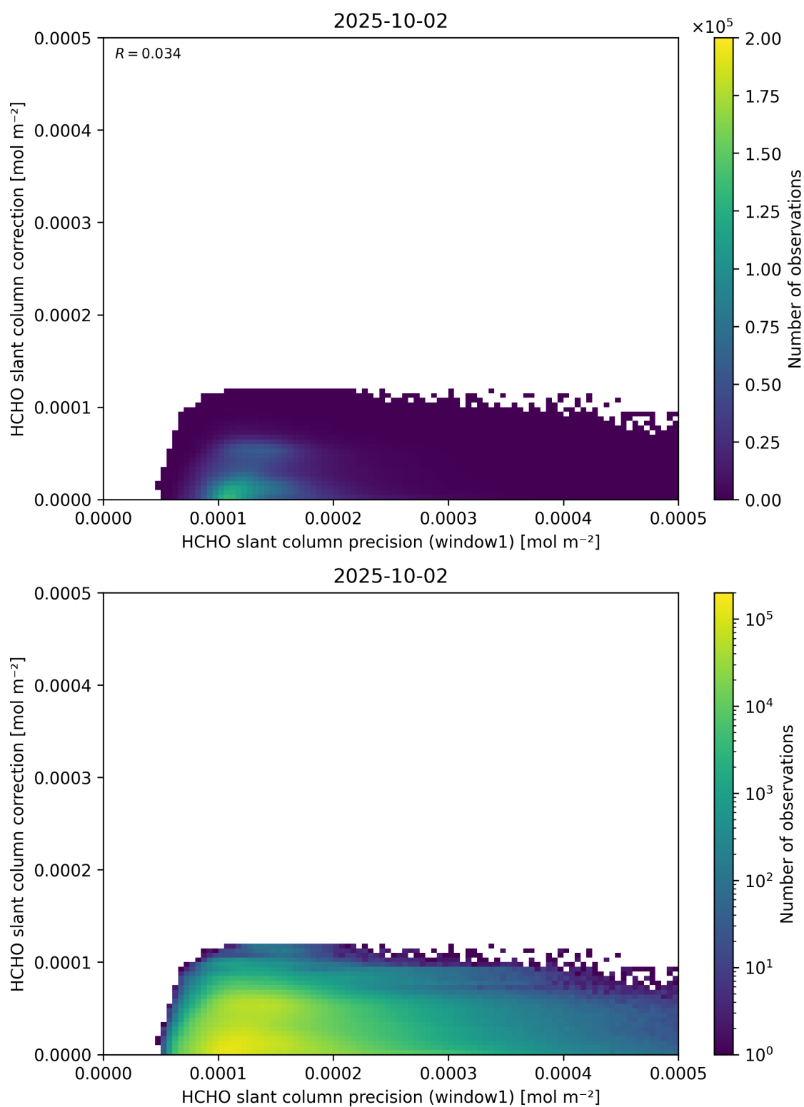
Figure 93: Scatter density plot of “HCHO slant column precision (window1)” against “HCHO slant column correction” for 2025-10-01 to 2025-10-03.
