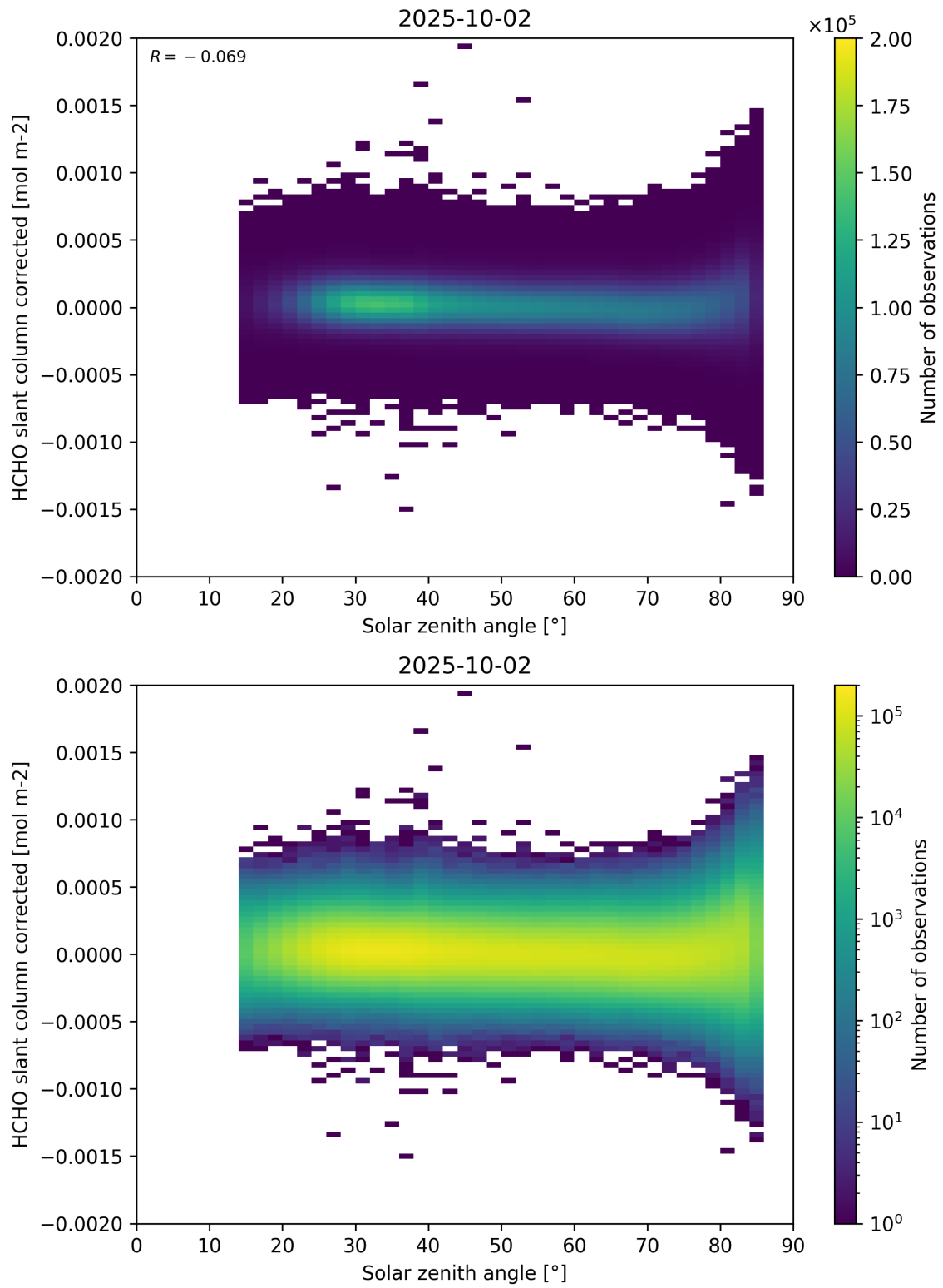
Figure 171: Scatter density plot of “Solar zenith angle” against “HCHO slant column corrected” for 2025-10-01 to 2025-10-03.
