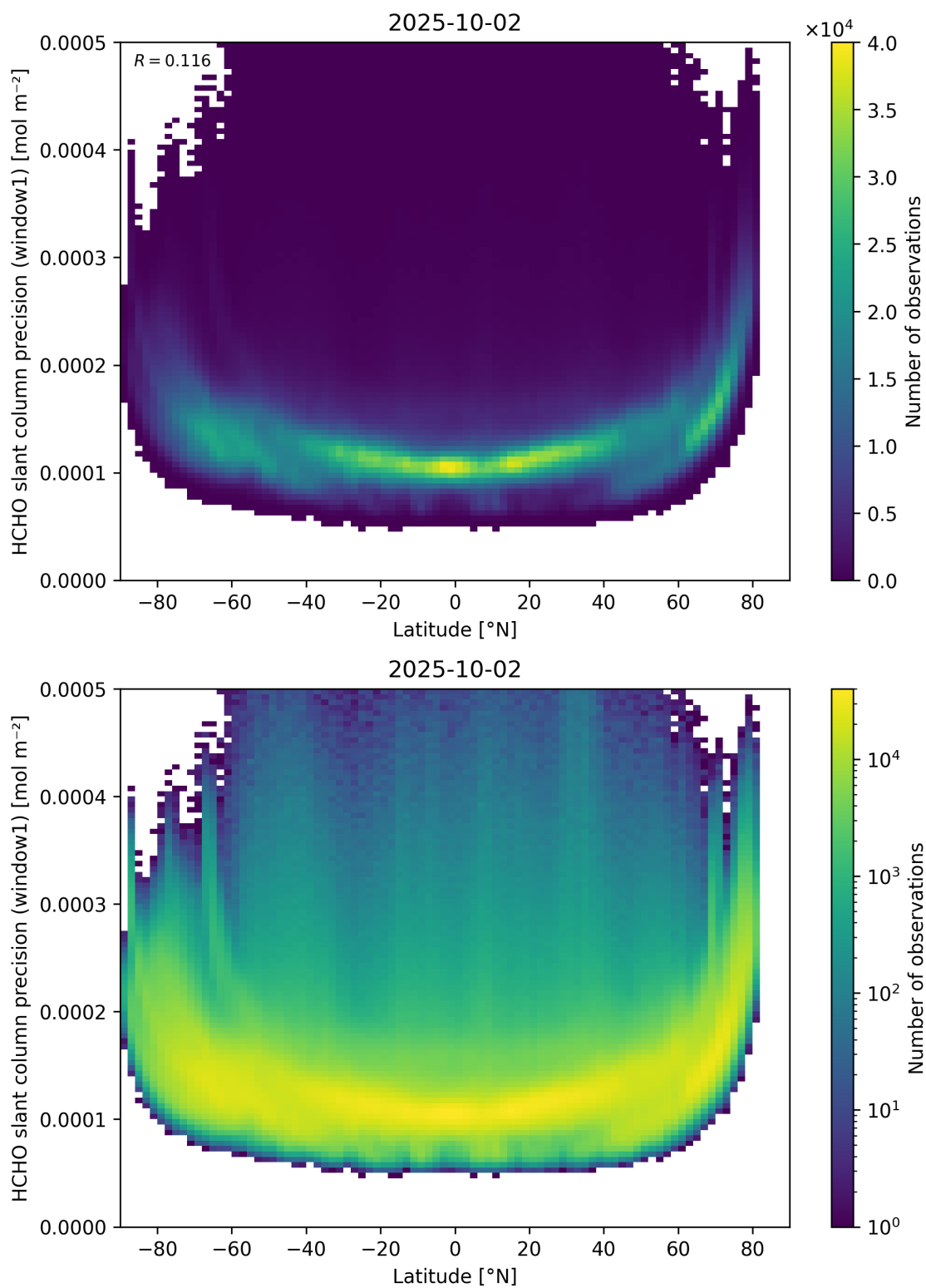
Figure 160: Scatter density plot of “Latitude” against “HCHO slant column precision (window1)” for 2025-10-01 to 2025-10-03.
