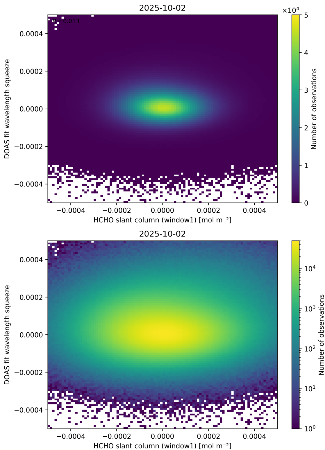
Figure 80: Scatter density plot of “HCHO slant column (window1)” against “DOAS fit wavelength squeeze” for 2025-10-01 to 2025-10-03.
