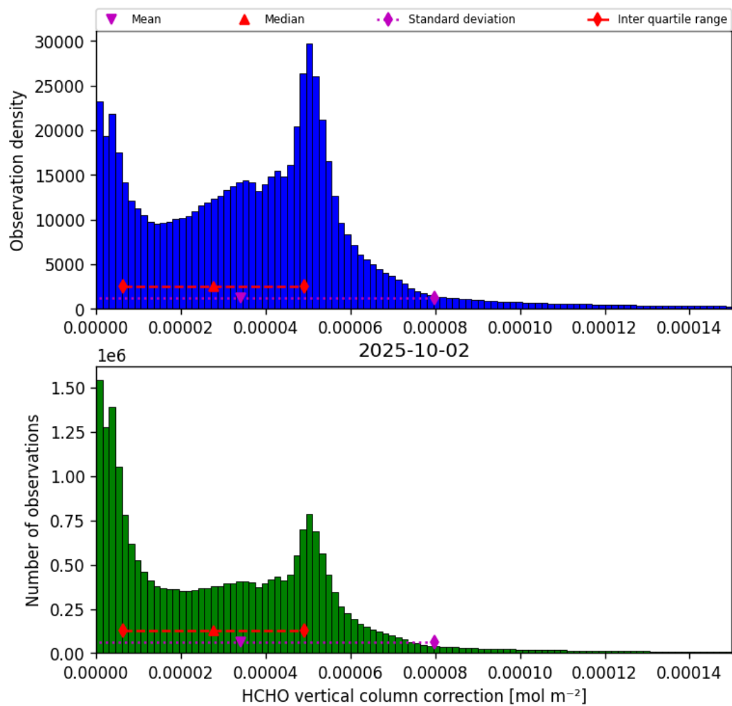
Figure 37: Histogram of “HCHO vertical column correction” for 2025-10-01 to 2025-10-03
