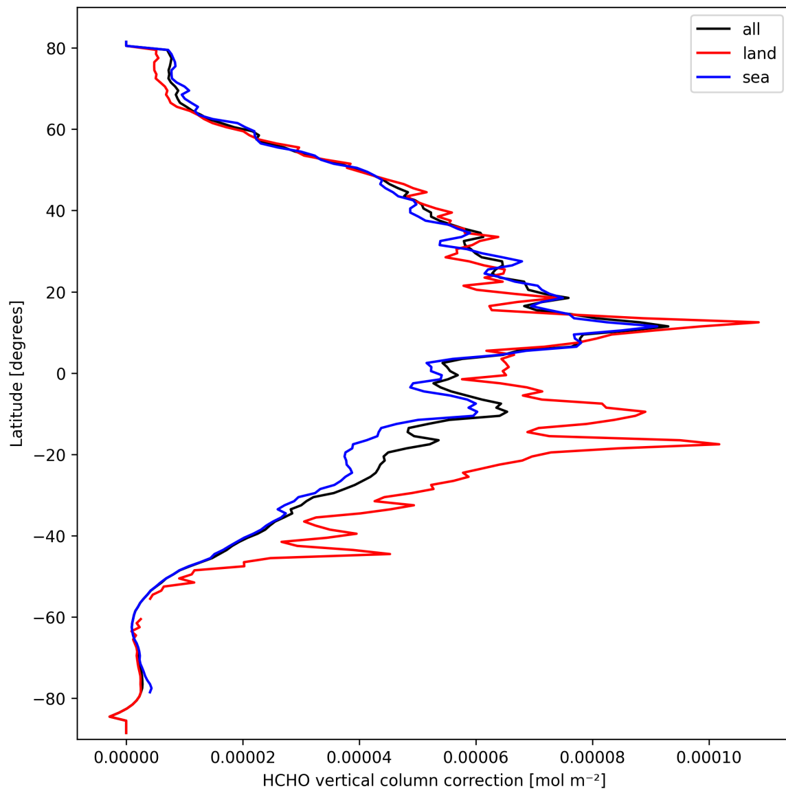
Figure 23: Zonal average of “HCHO vertical column correction” for 2025-10-01 to 2025-10-03.
