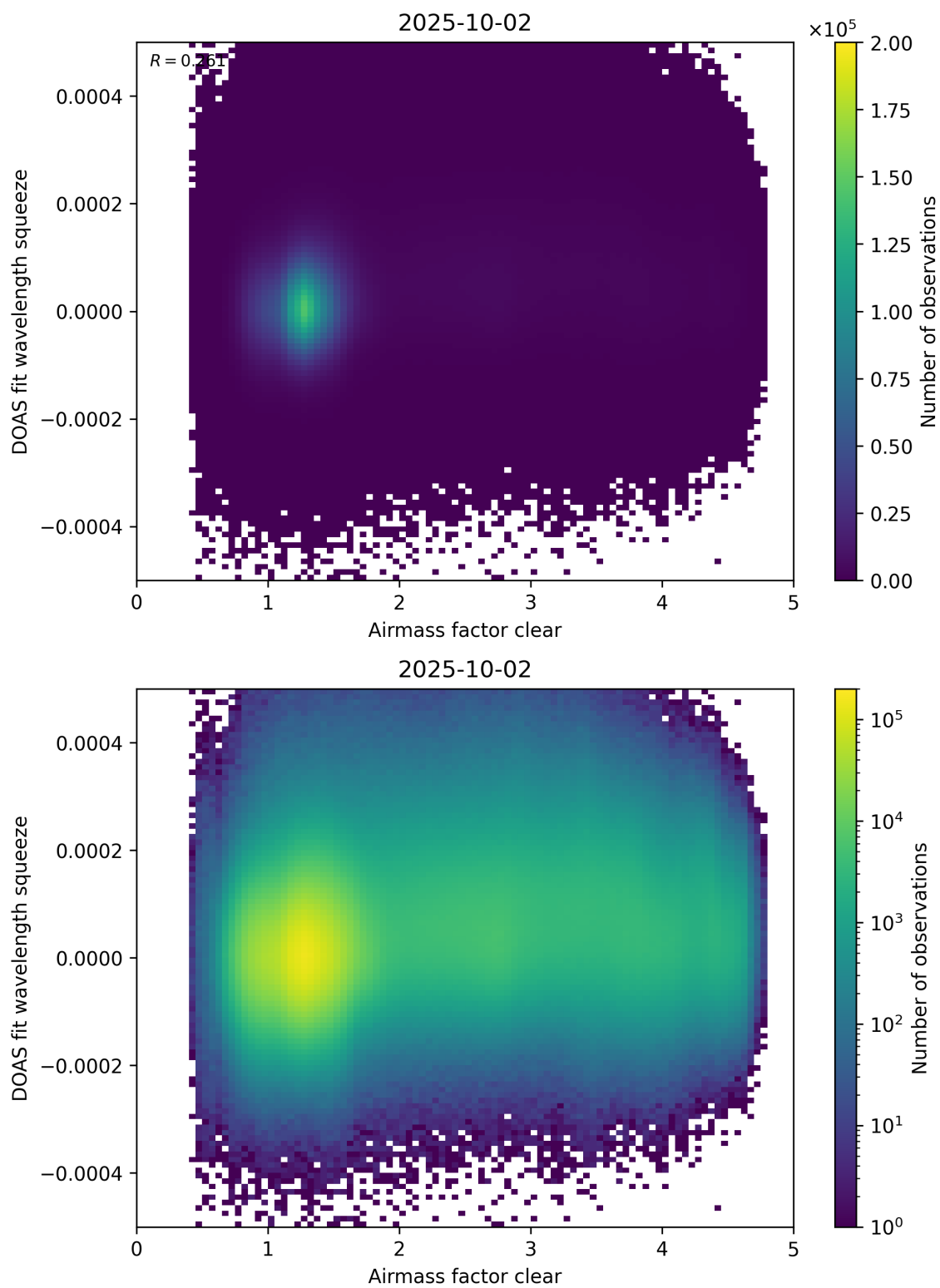
Figure 73: Scatter density plot of “Airmass factor clear” against “DOAS fit wavelength squeeze” for 2025-10-01 to 2025-10-03.
