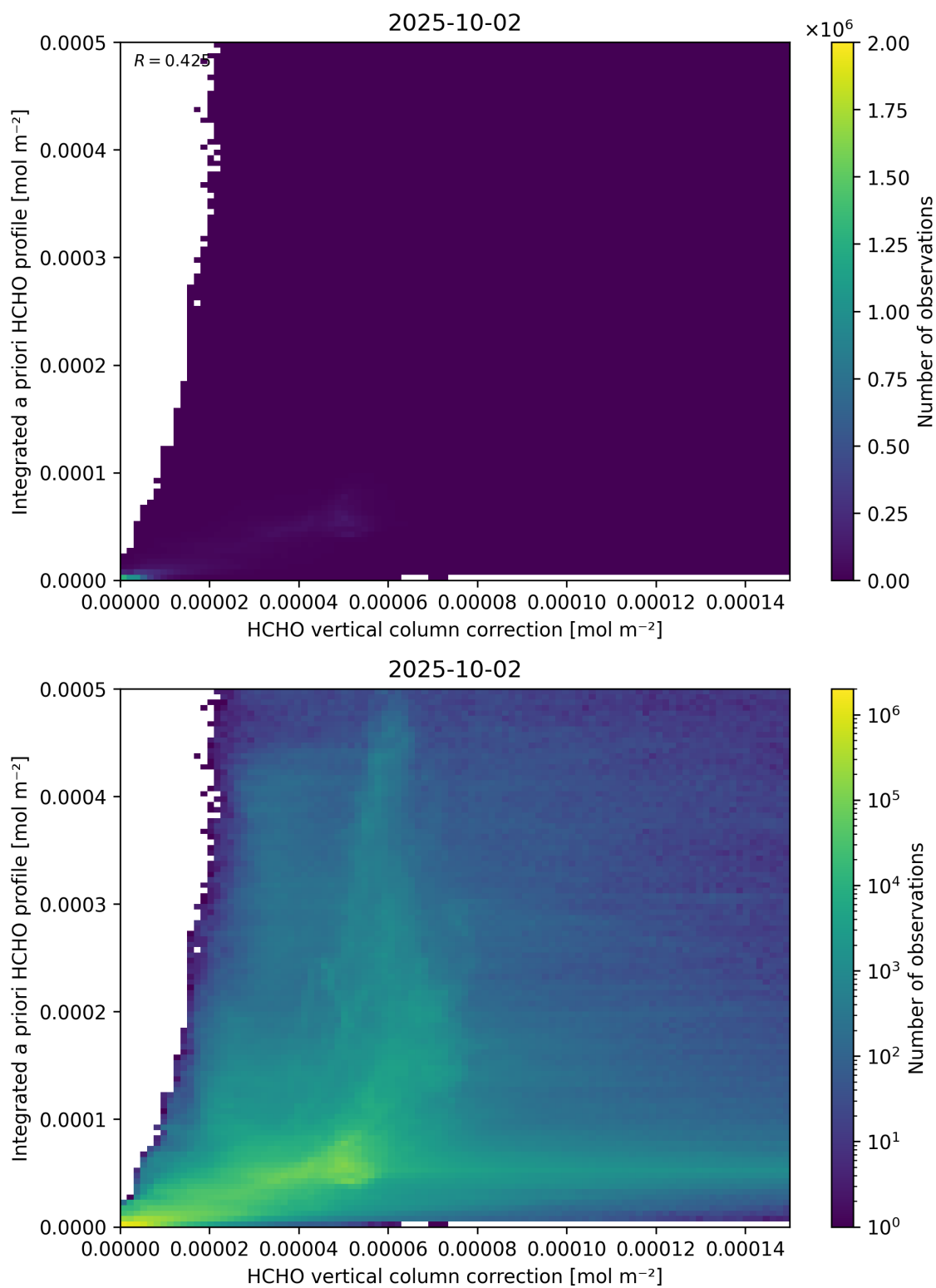
Figure 122: Scatter density plot of “HCHO vertical column correction” against “Integrated a priori HCHO profile” for 2025-10-01 to 2025-10-03.
