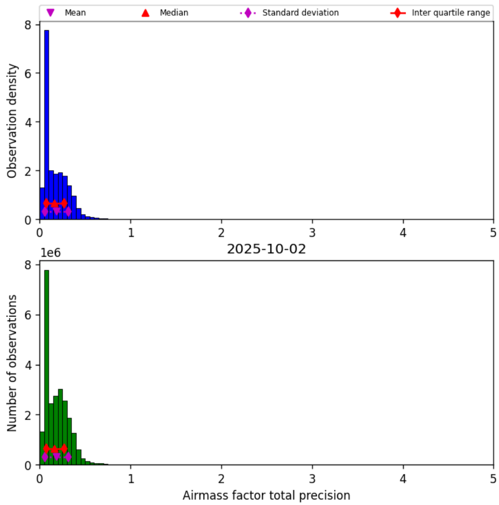
Figure 41: Histogram of “Airmass factor total precision” for 2025-10-01 to 2025-10-03
