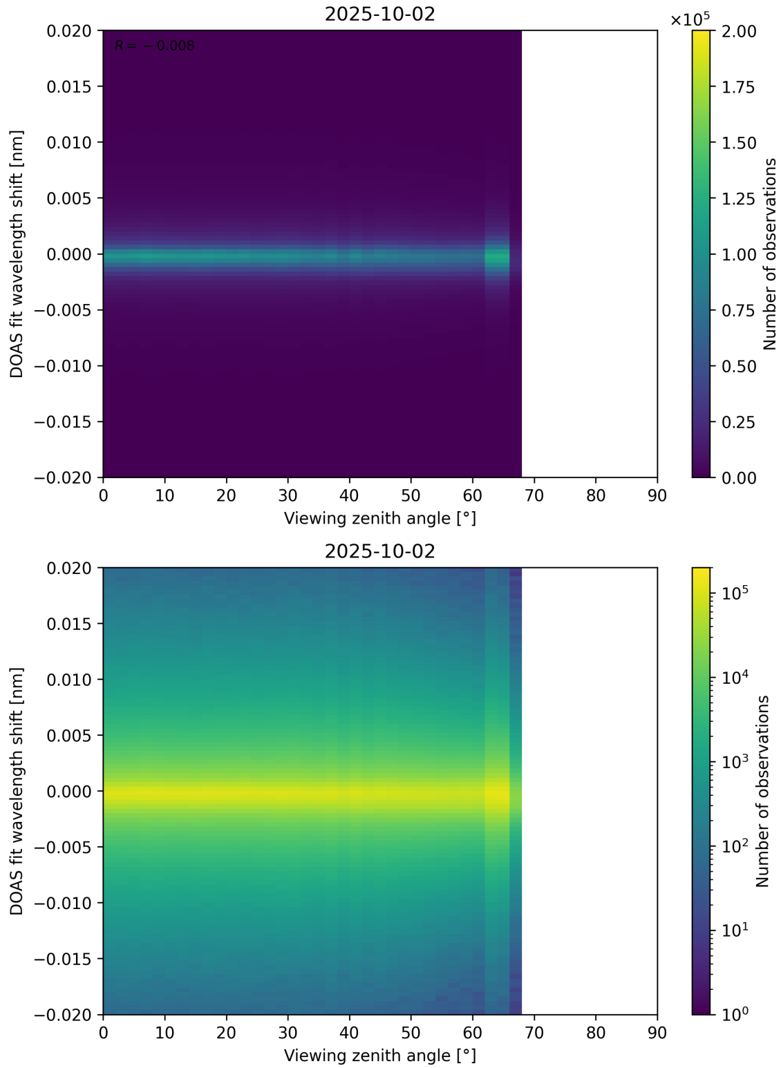
Figure 183: Scatter density plot of “Viewing zenith angle” against “DOAS fit wavelength shift” for 2025-10-01 to 2025-10-03.
