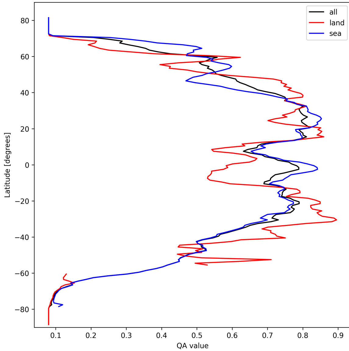
Figure 20: Zonal average of “QA value” for 2025-10-01 to 2025-10-03.
