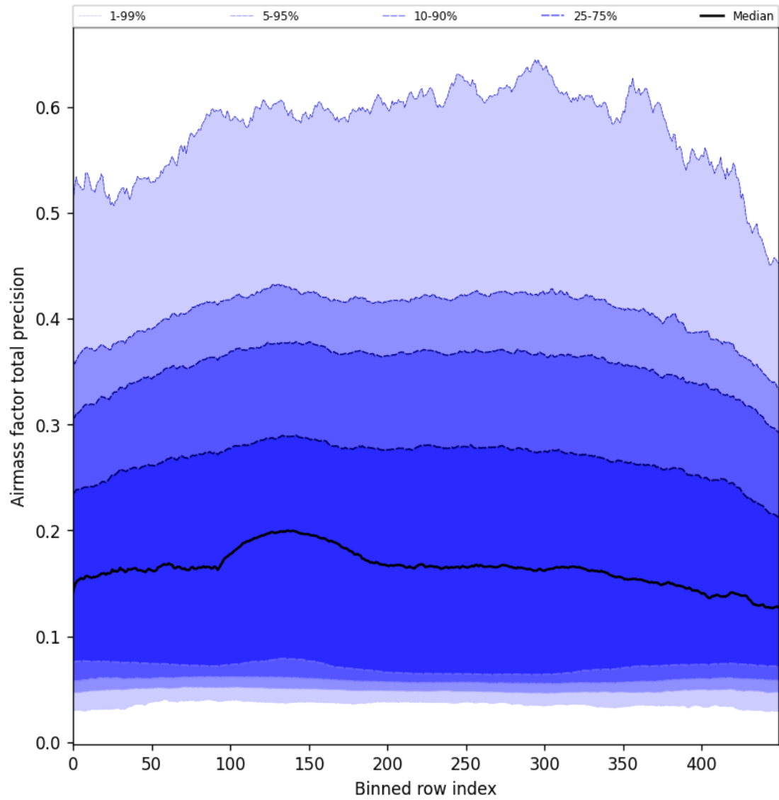
Figure 55: Along track statistics of “Airmass factor total precision” for 2025-10-01 to 2025-10-03
