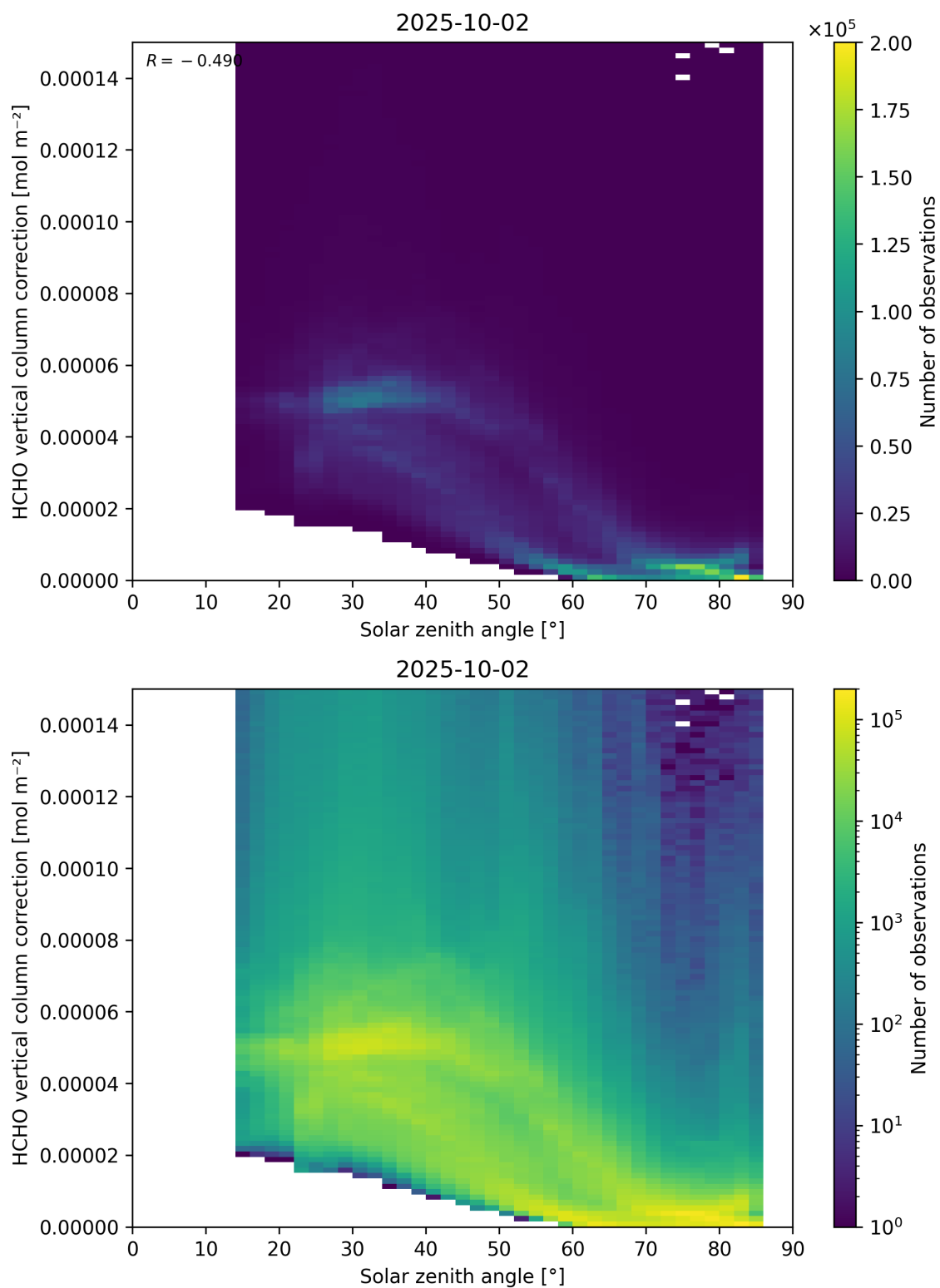
Figure 178: Scatter density plot of “Solar zenith angle” against “HCHO vertical column correction” for 2025-10-01 to 2025-10-03.
