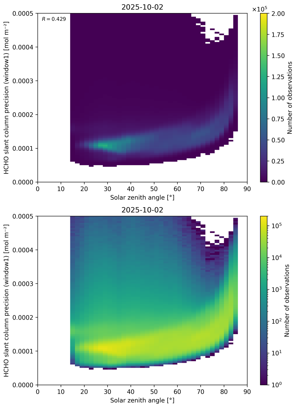
Figure 174: Scatter density plot of “Solar zenith angle” against “HCHO slant column precision (window1)” for 2025-10-01 to 2025-10-03.
