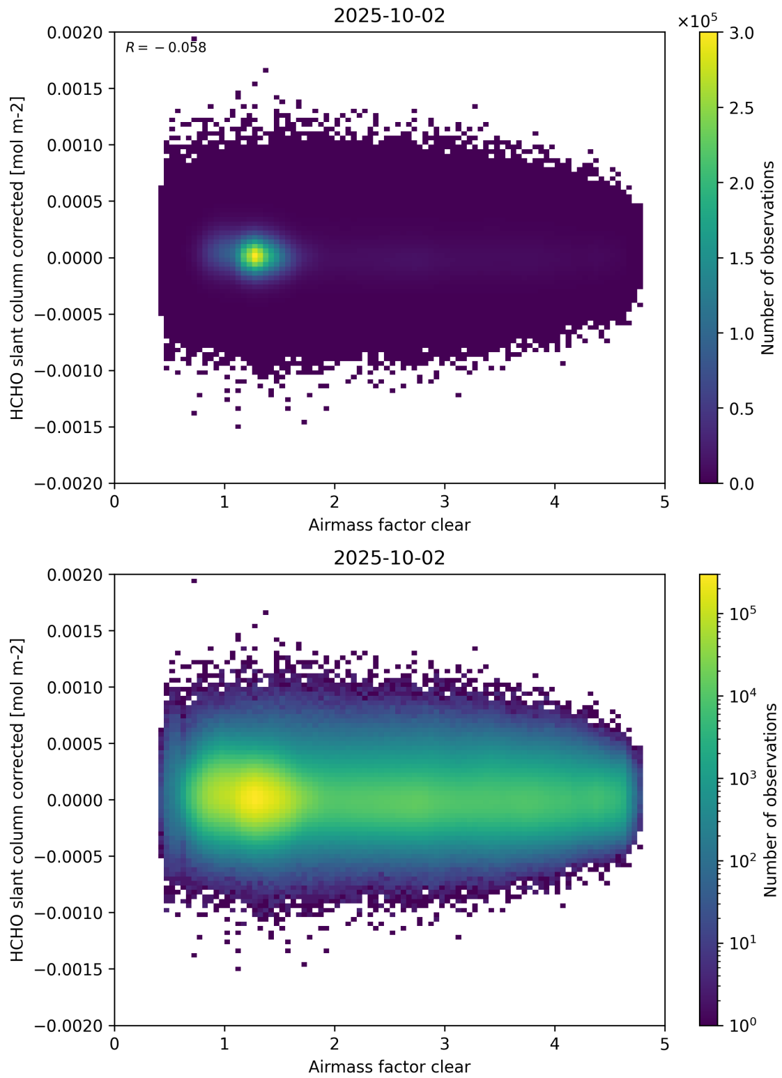
Figure 74: Scatter density plot of “Airmass factor clear” against “HCHO slant column corrected” for 2025-10-01 to 2025-10-03.
