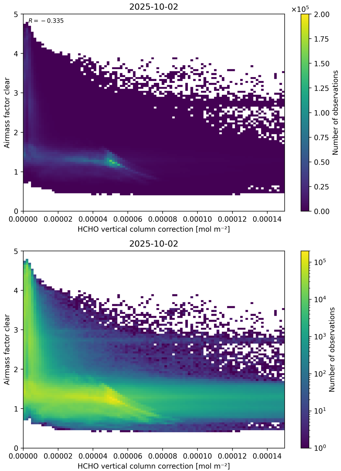
Figure 115: Scatter density plot of “HCHO vertical column correction” against “Airmass factor clear” for 2025-10-01 to 2025-10-03.
