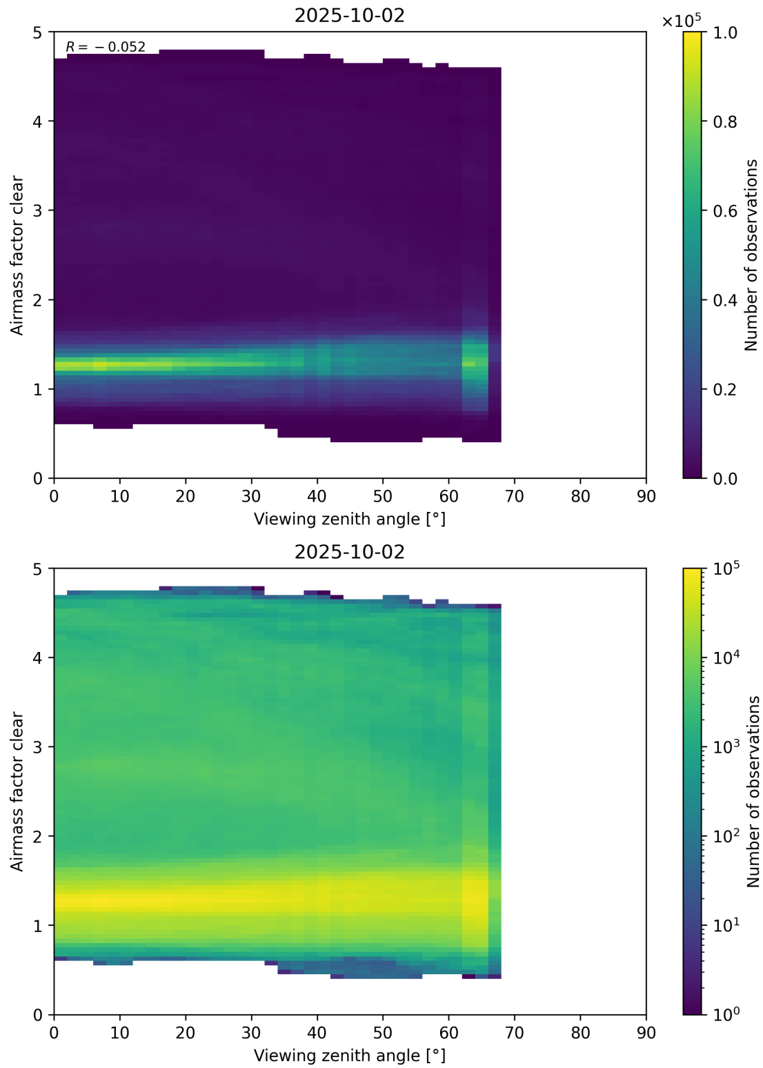
Figure 185: Scatter density plot of “Viewing zenith angle” against “Airmass factor clear” for 2025-10-01 to 2025-10-03.
