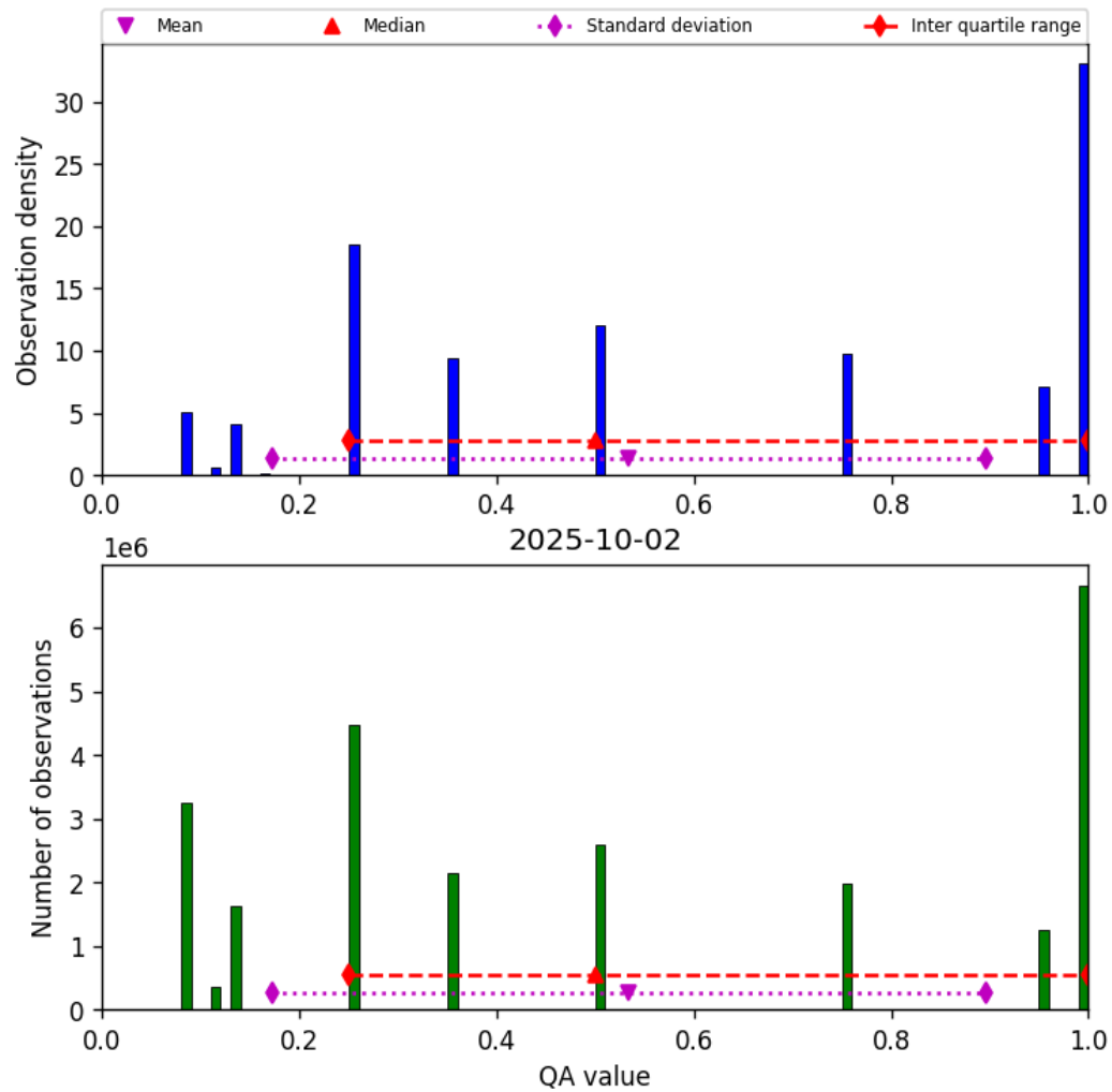
Figure 34: Histogram of “QA value” for 2025-10-01 to 2025-10-03
