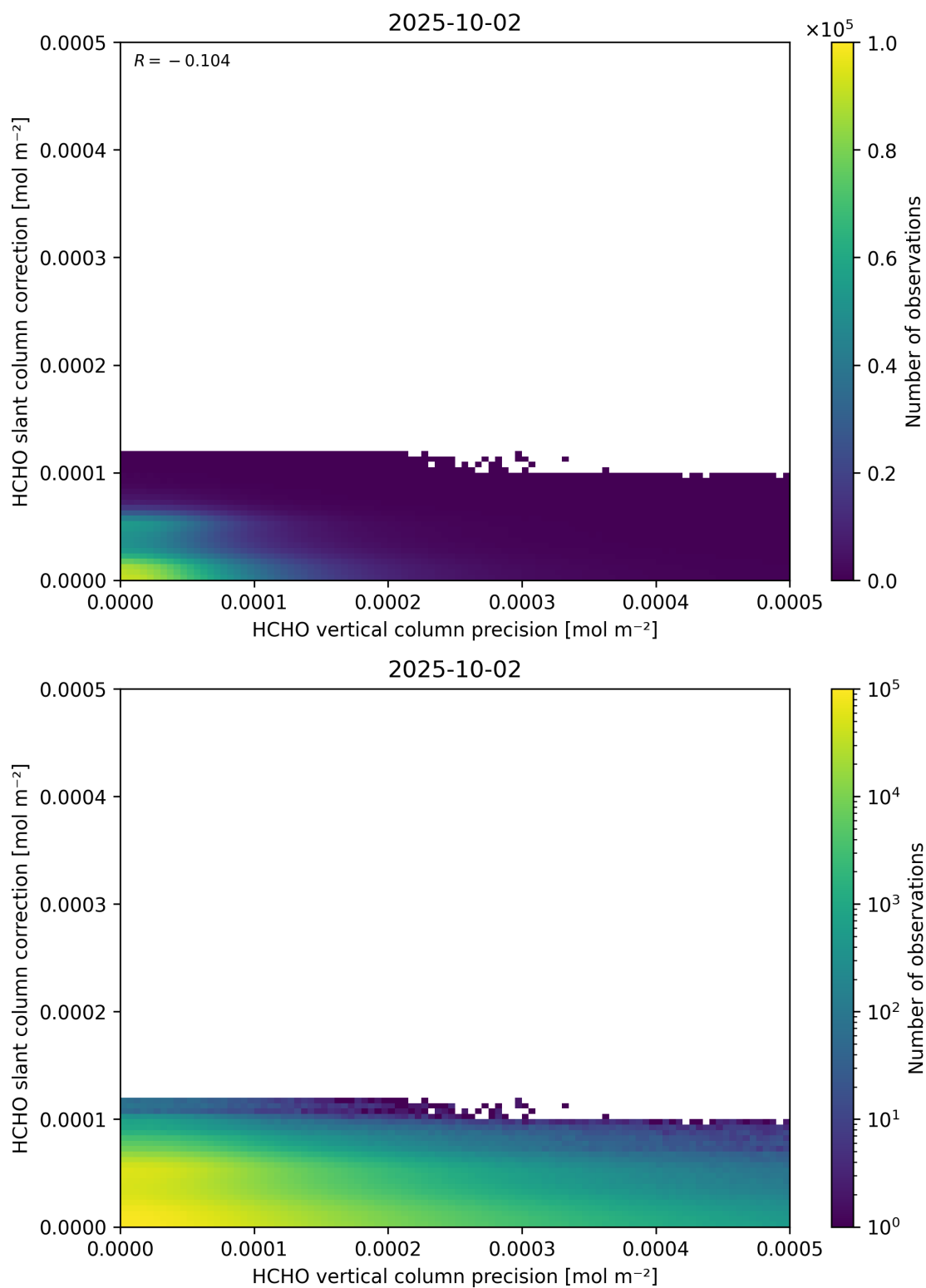
Figure 141: Scatter density plot of “HCHO vertical column precision” against “HCHO slant column correction” for 2025-10-01 to 2025-10-03.
