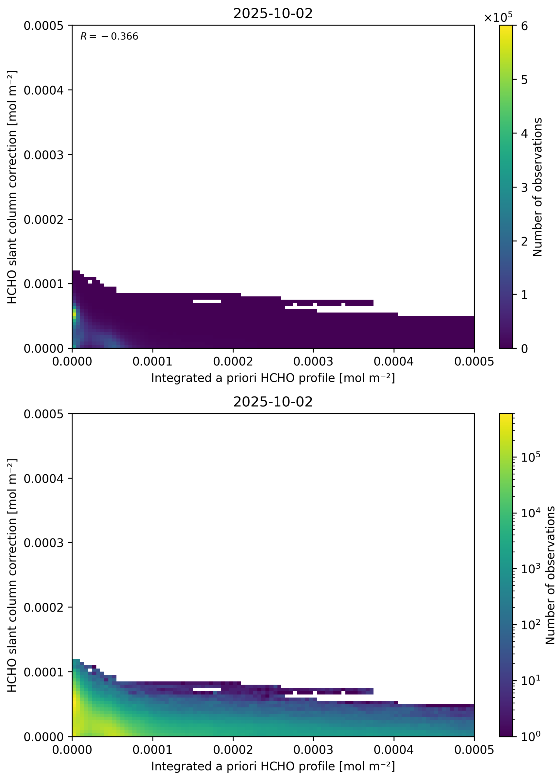
Figure 152: Scatter density plot of “Integrated a priori HCHO profile” against “HCHO slant column correction” for 2025-10-01 to 2025-10-03.
