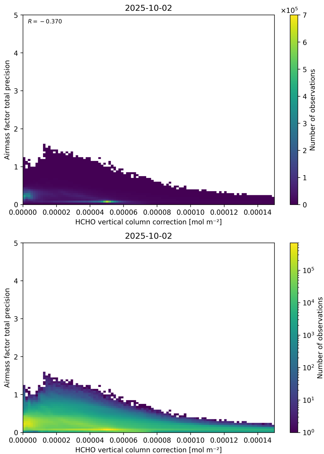
Figure 121: Scatter density plot of “HCHO vertical column correction” against “Airmass factor total precision” for 2025-10-01 to 2025-10-03.
