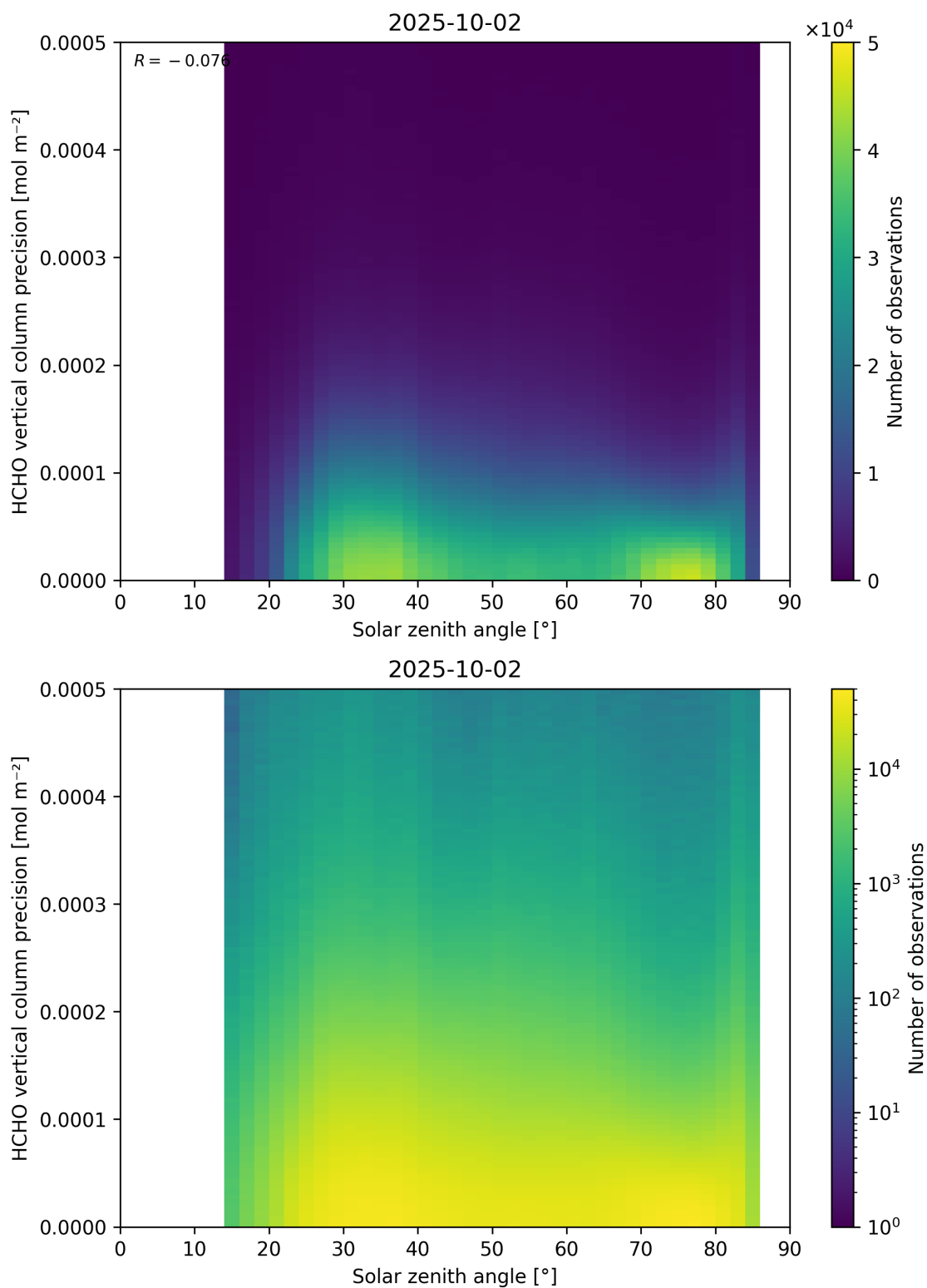
Figure 179: Scatter density plot of “Solar zenith angle” against “HCHO vertical column precision” for 2025-10-01 to 2025-10-03.
