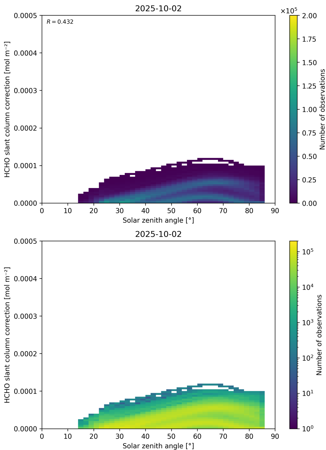
Figure 172: Scatter density plot of “Solar zenith angle” against “HCHO slant column correction” for 2025-10-01 to 2025-10-03.
