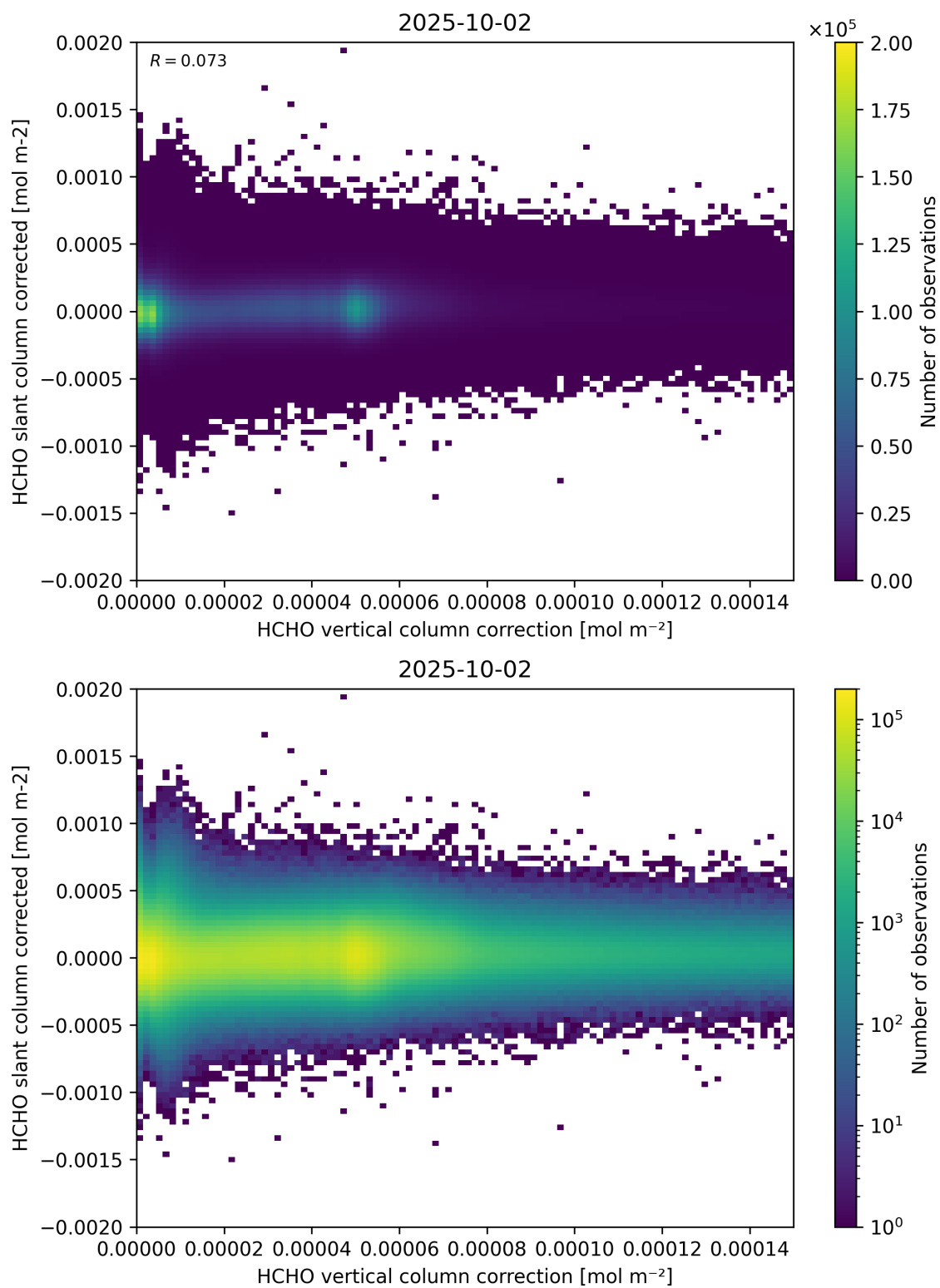
Figure 116: Scatter density plot of “HCHO vertical column correction” against “HCHO slant column corrected” for 2025-10-01 to 2025-10-03.
