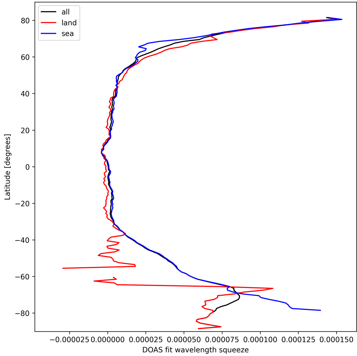
Figure 31: Zonal average of “DOAS fit wavelength squeeze” for 2025-10-01 to 2025-10-03.
