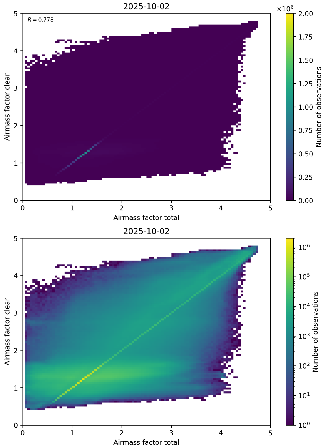
Figure 100: Scatter density plot of “Airmass factor total” against “Airmass factor clear” for 2025-10-01 to 2025-10-03.
