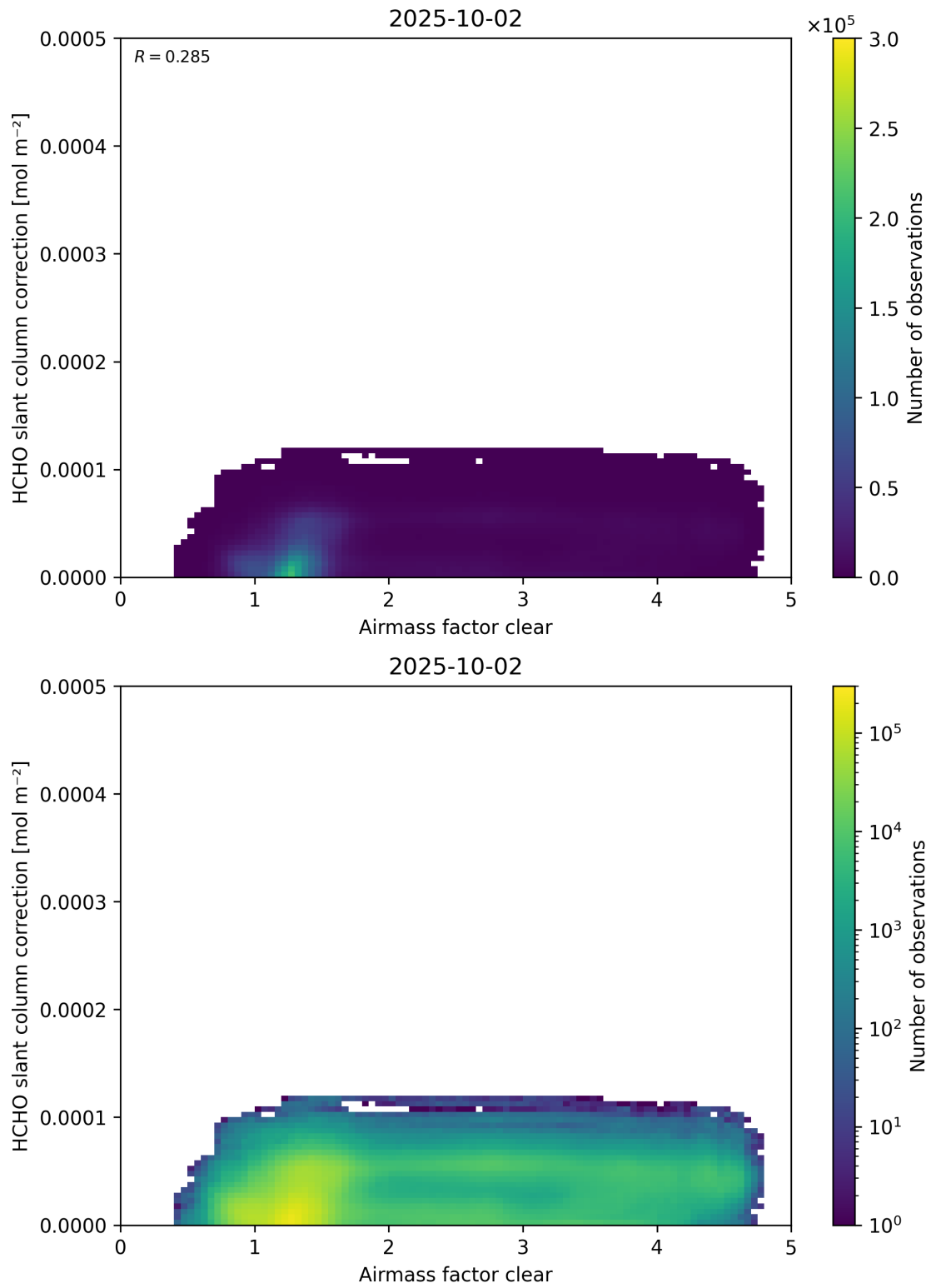
Figure 75: Scatter density plot of “Airmass factor clear” against “HCHO slant column correction” for 2025-10-01 to 2025-10-03.
