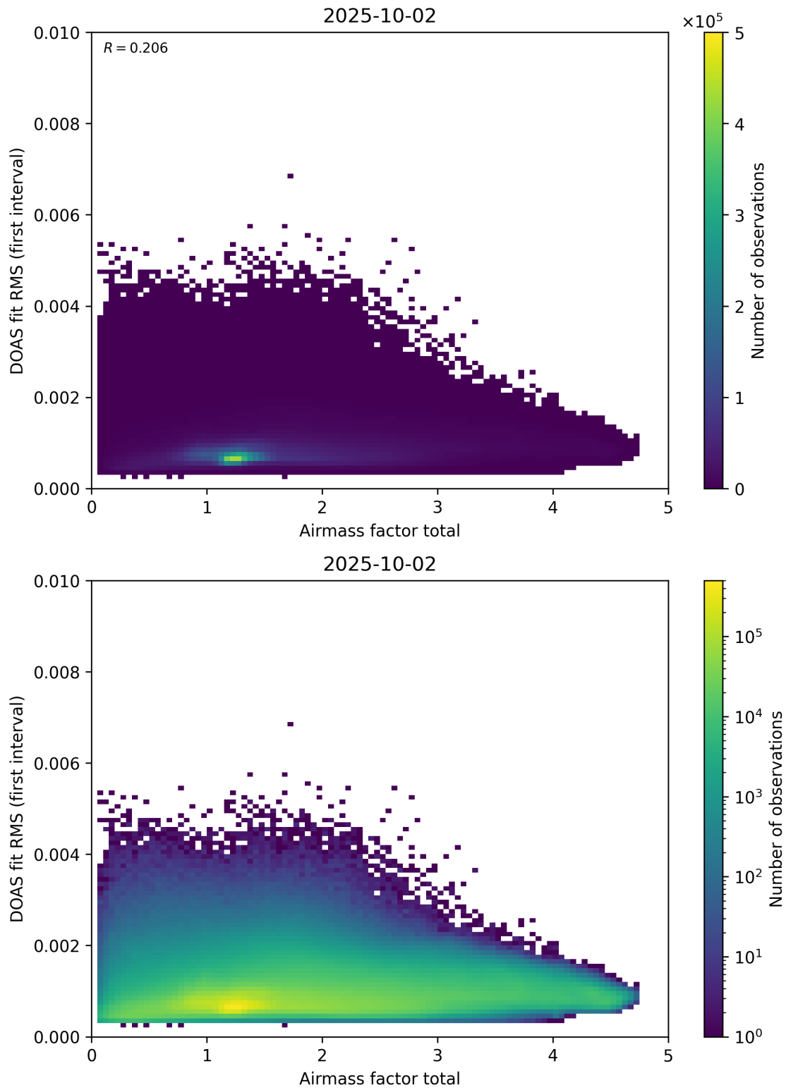
Figure 97: Scatter density plot of “Airmass factor total” against “DOAS fit RMS (first interval)” for 2025-10-01 to 2025-10-03.
