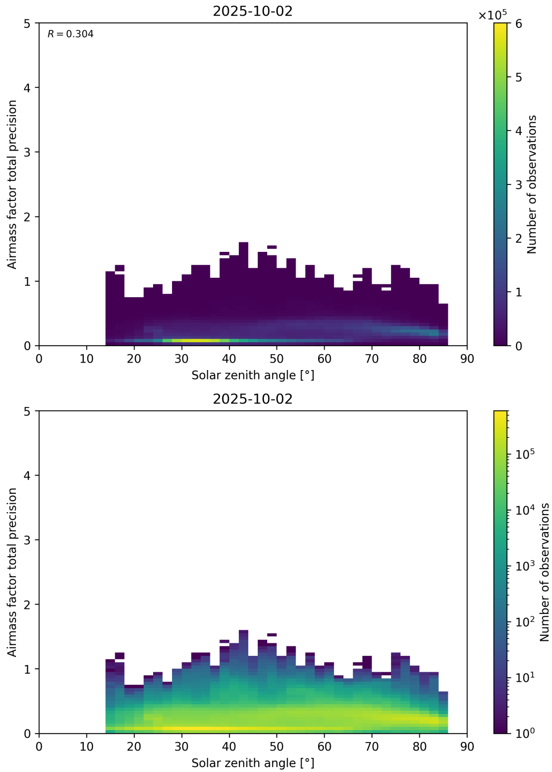
Figure 176: Scatter density plot of “Solar zenith angle” against “Airmass factor total precision” for 2025-10-01 to 2025-10-03.
