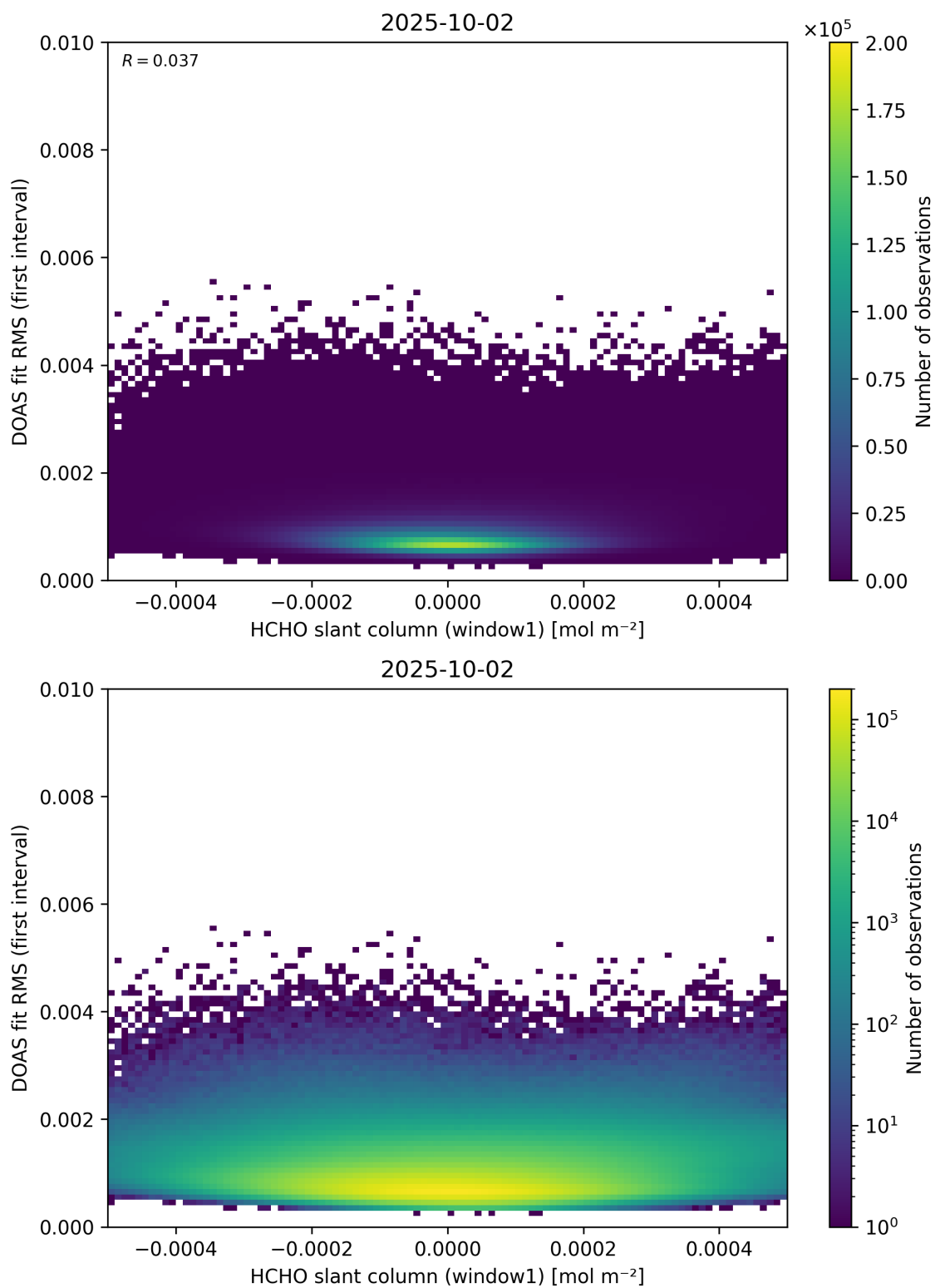
Figure 78: Scatter density plot of “HCHO slant column (window1)” against “DOAS fit RMS (first interval)” for 2025-10-01 to 2025-10-03.
