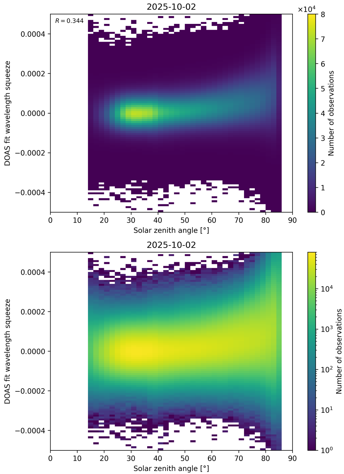
Figure 169: Scatter density plot of “Solar zenith angle” against “DOAS fit wavelength squeeze” for 2025-10-01 to 2025-10-03.
