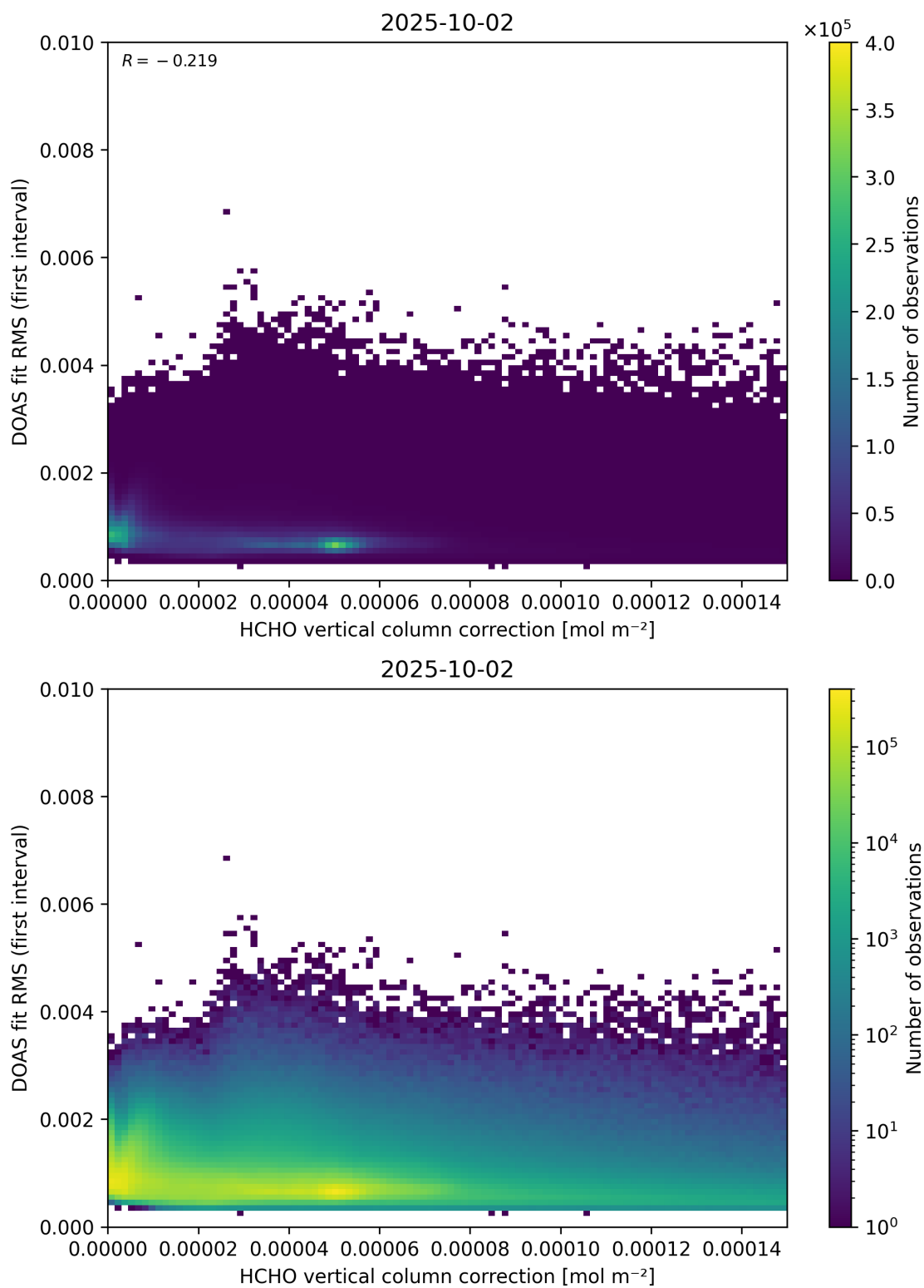
Figure 112: Scatter density plot of “HCHO vertical column correction” against “DOAS fit RMS (first interval)” for 2025-10-01 to 2025-10-03.
