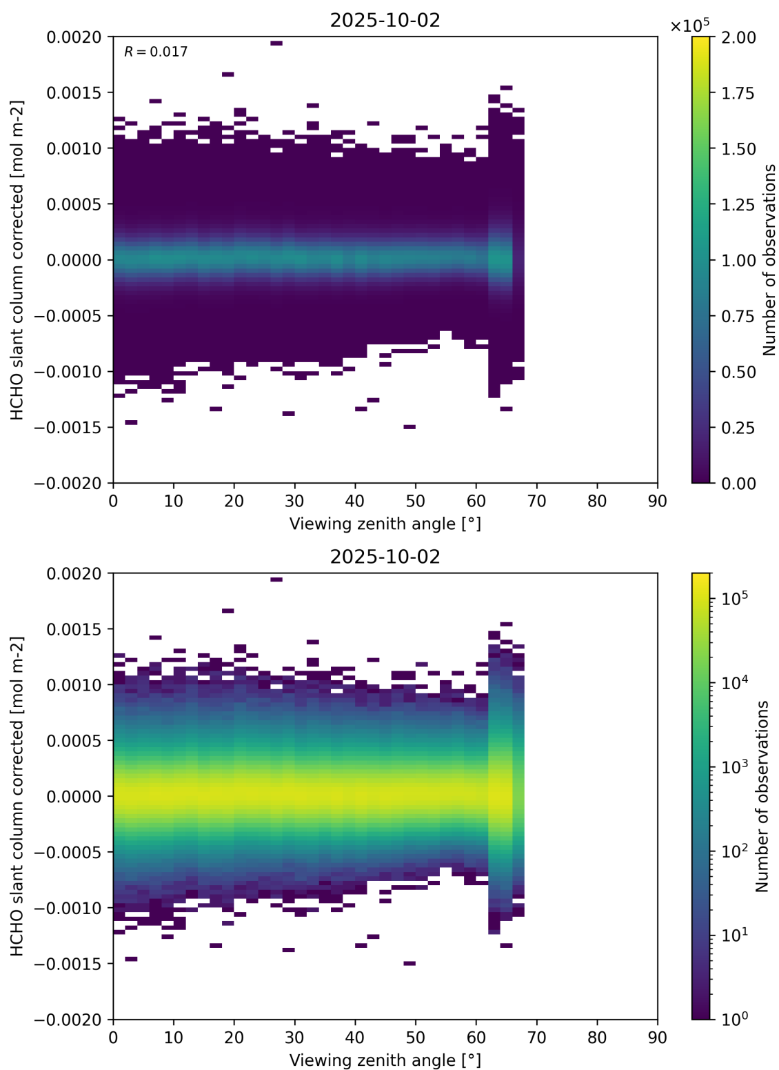
Figure 186: Scatter density plot of “Viewing zenith angle” against “HCHO slant column corrected” for 2025-10-01 to 2025-10-03.
