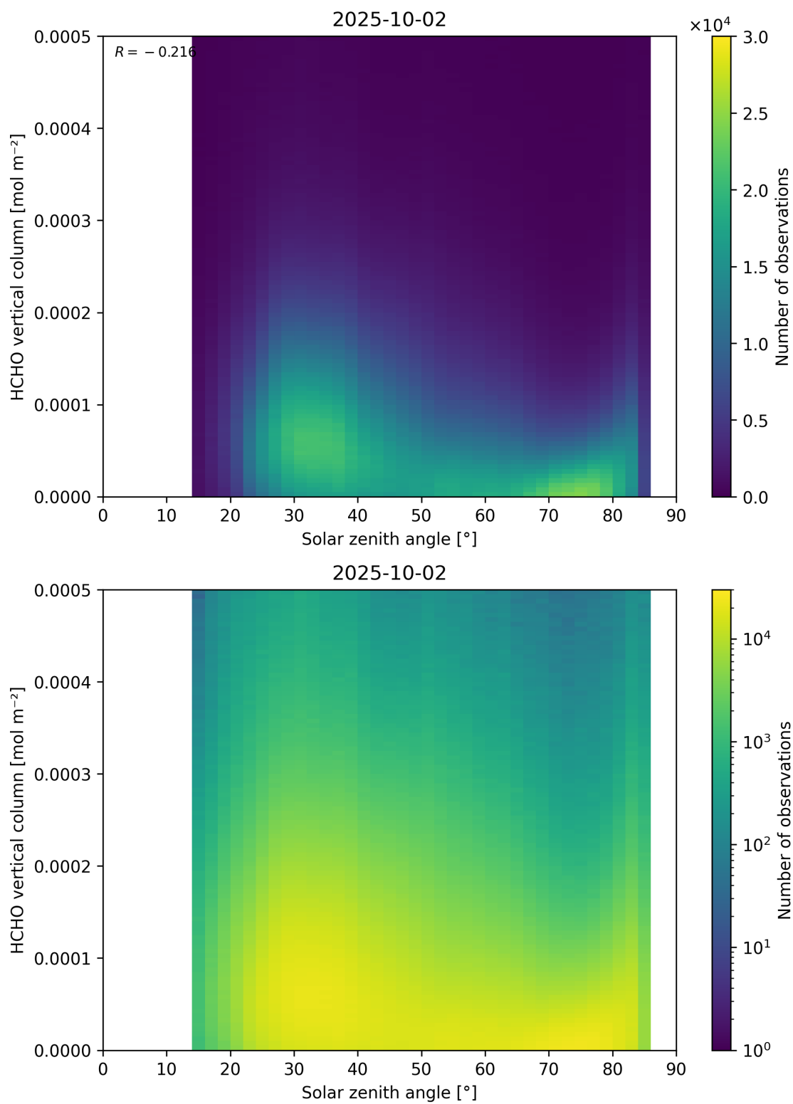
Figure 177: Scatter density plot of “Solar zenith angle” against “HCHO vertical column” for 2025-10-01 to 2025-10-03.
