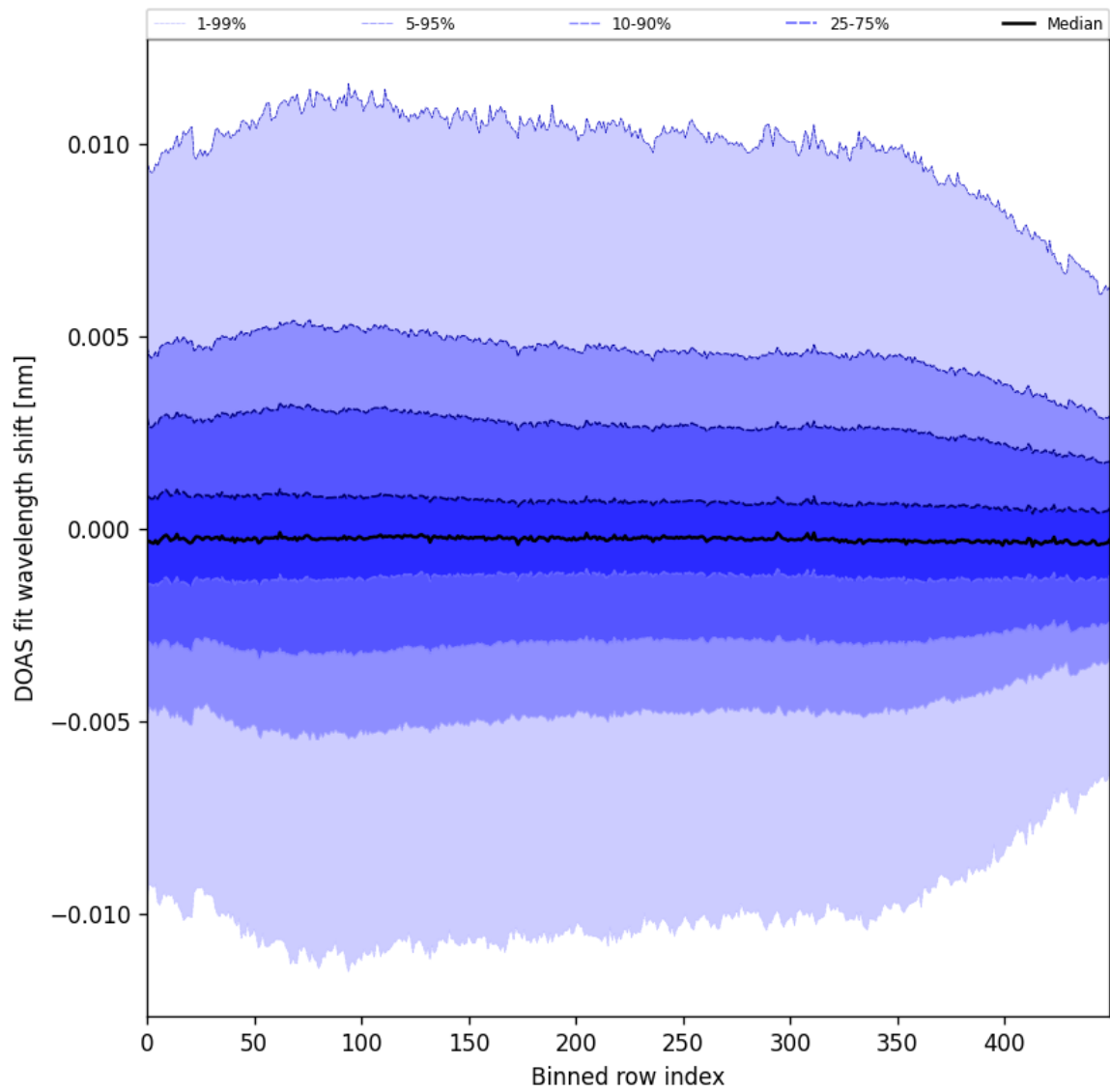
Figure 58: Along track statistics of “DOAS fit wavelength shift” for 2025-10-01 to 2025-10-03
