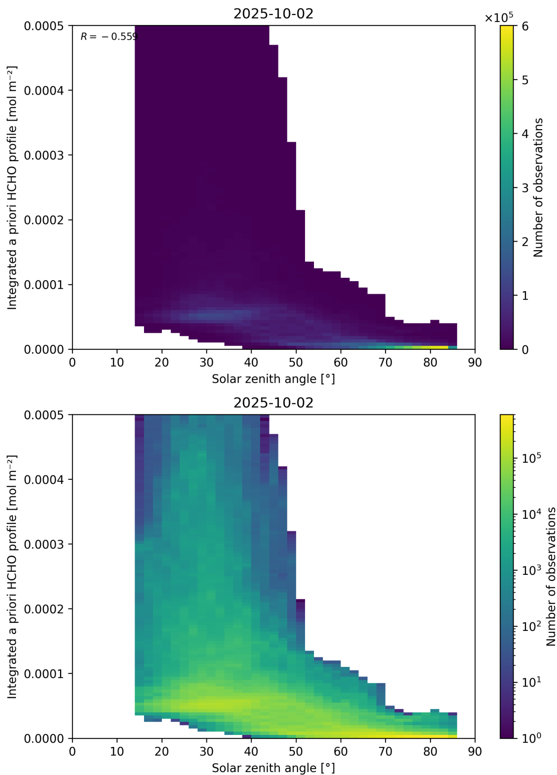
Figure 180: Scatter density plot of “Solar zenith angle” against “Integrated a priori HCHO profile” for 2025-10-01 to 2025-10-03.
