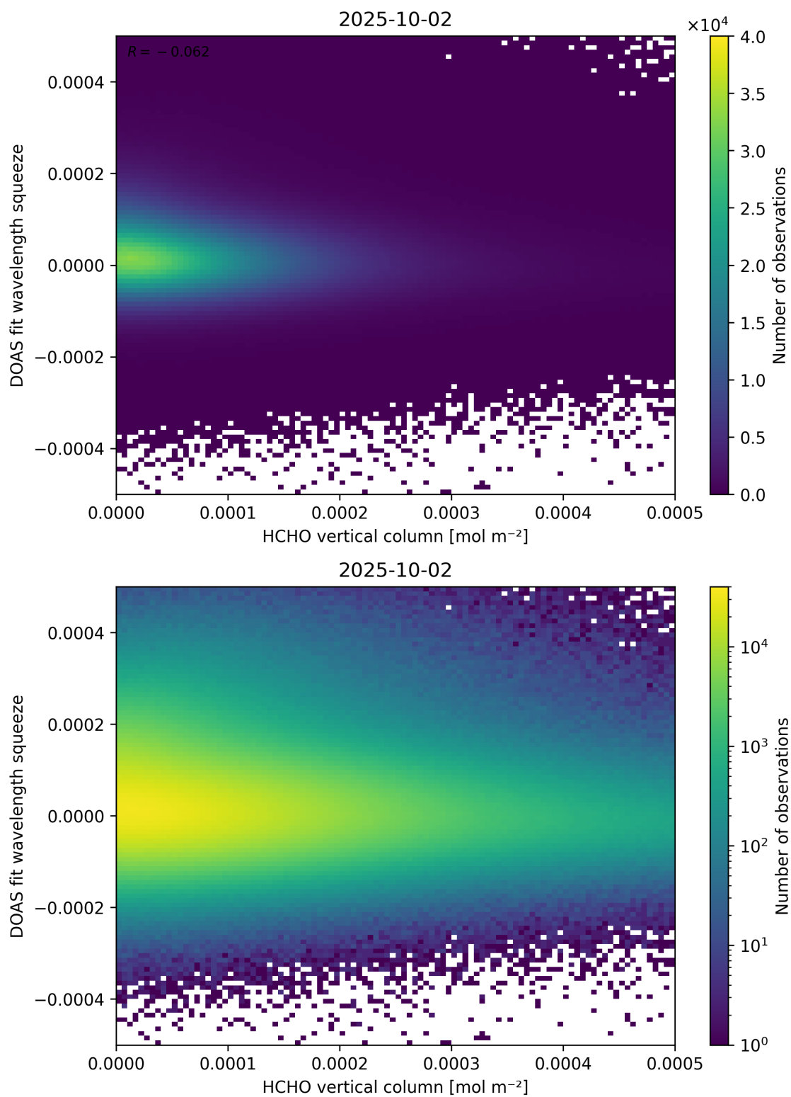
Figure 125: Scatter density plot of “HCHO vertical column” against “DOAS fit wavelength squeeze” for 2025-10-01 to 2025-10-03.
