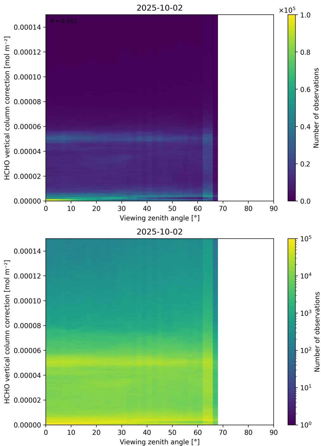
Figure 193: Scatter density plot of “Viewing zenith angle” against “HCHO vertical column correction” for 2025-10-01 to 2025-10-03.
