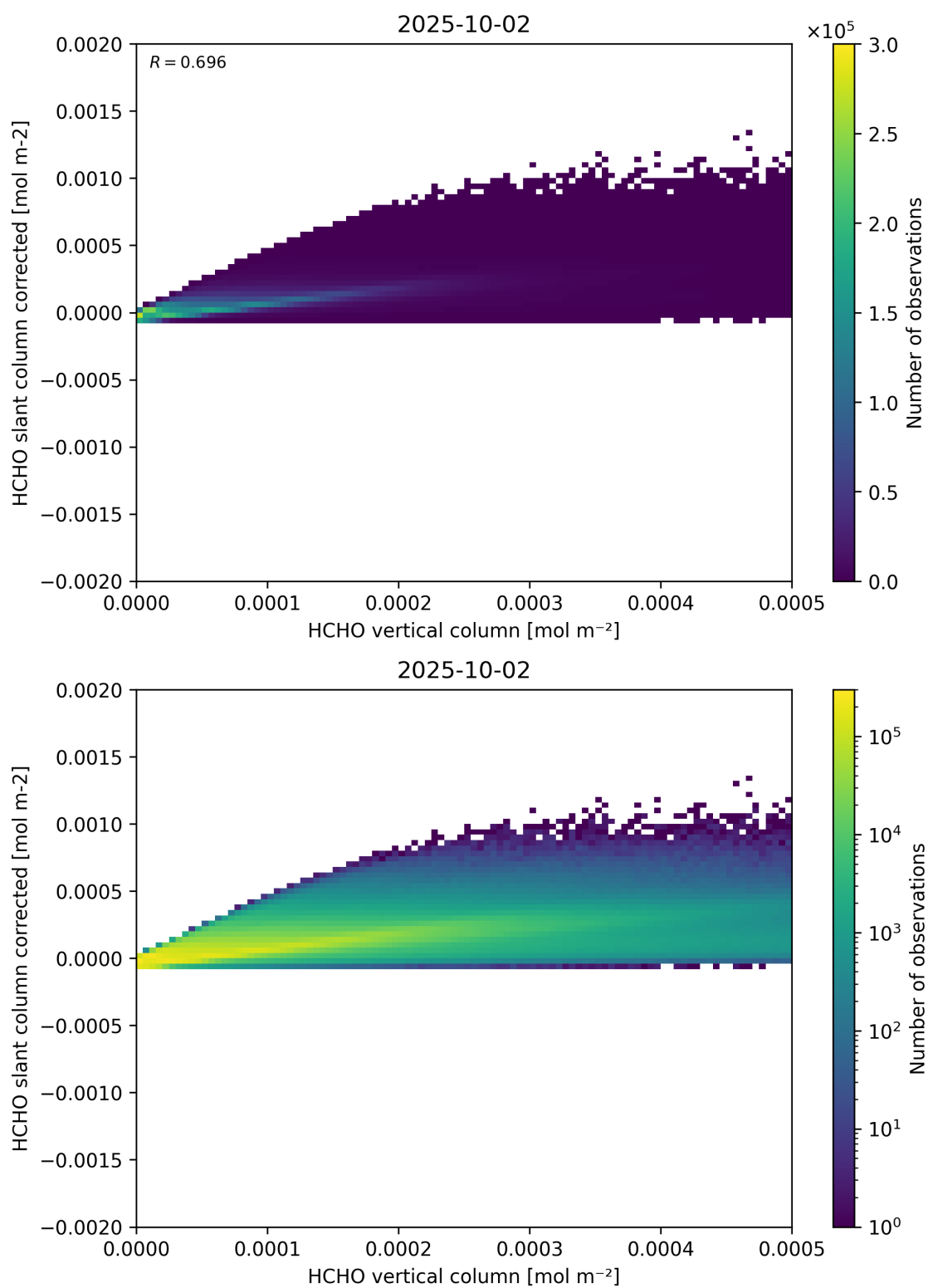
Figure 127: Scatter density plot of “HCHO vertical column” against “HCHO slant column corrected” for 2025-10-01 to 2025-10-03.
