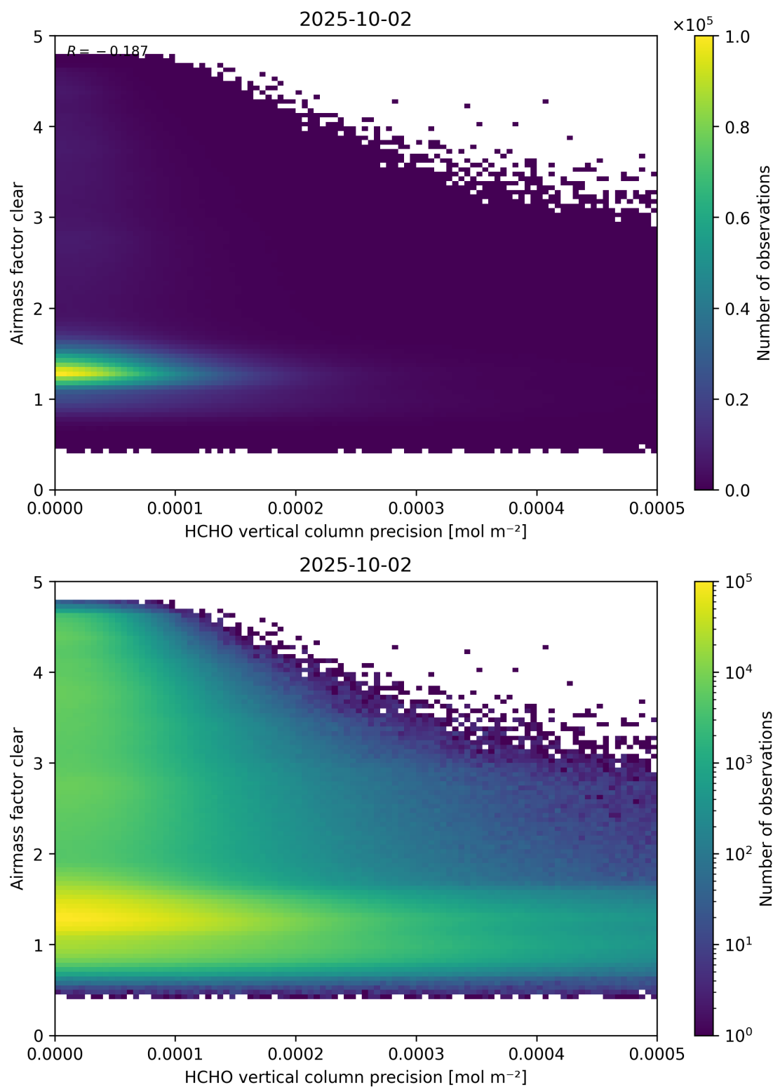
Figure 139: Scatter density plot of “HCHO vertical column precision” against “Airmass factor clear” for 2025-10-01 to 2025-10-03.
