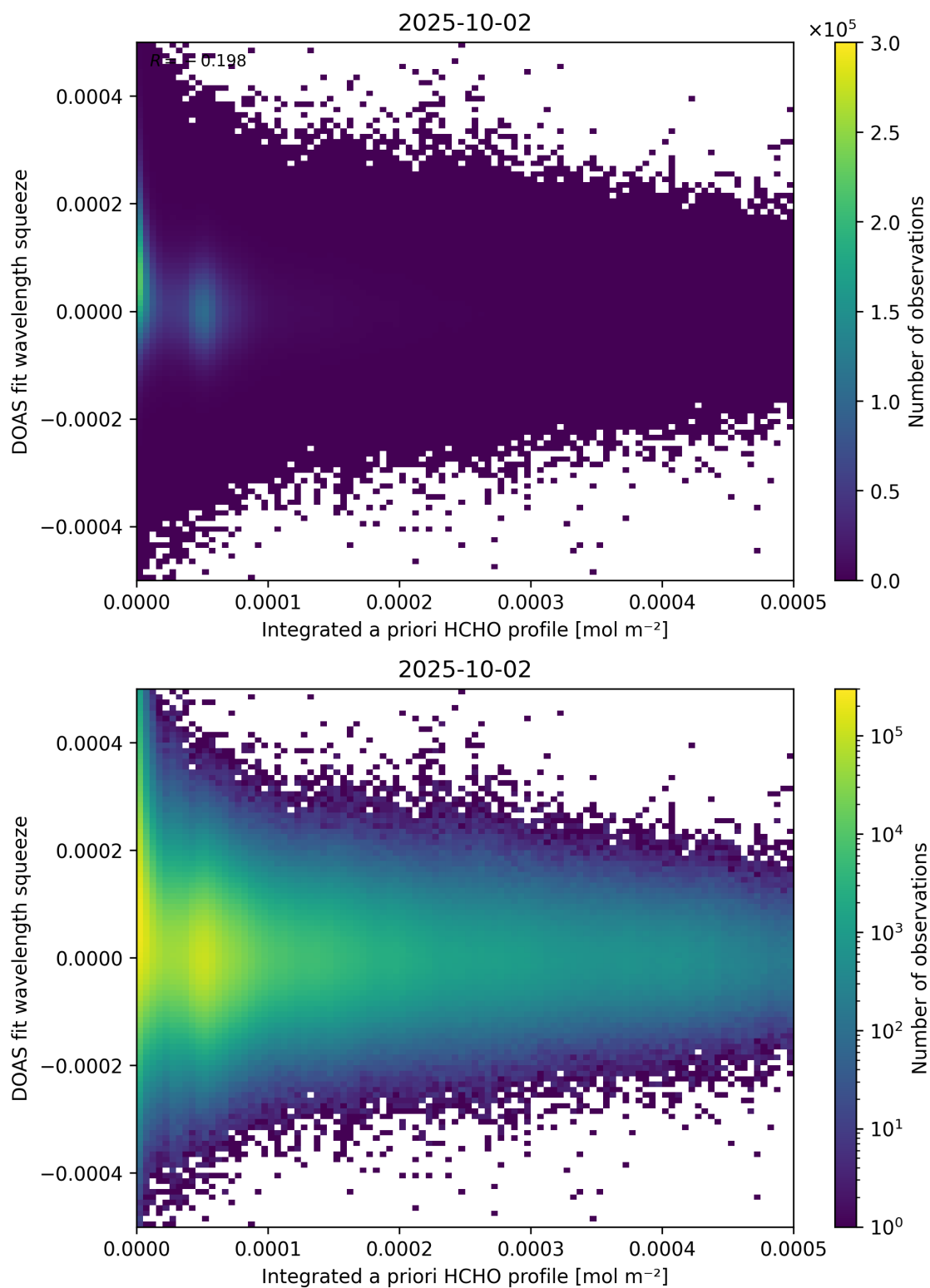
Figure 150: Scatter density plot of “Integrated a priori HCHO profile” against “DOAS fit wavelength squeeze” for 2025-10-01 to 2025-10-03.
