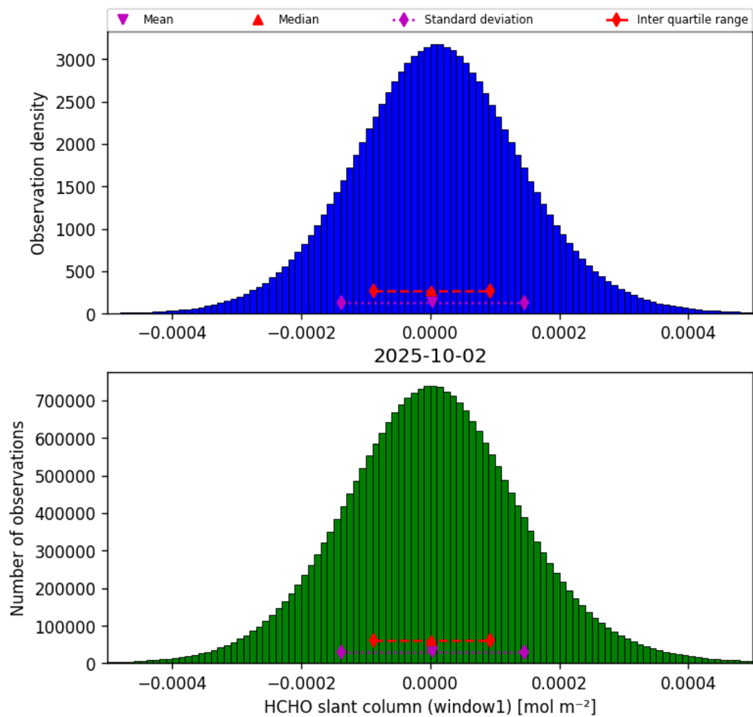
Figure 38: Histogram of “HCHO slant column (window1)” for 2025-10-01 to 2025-10-03
