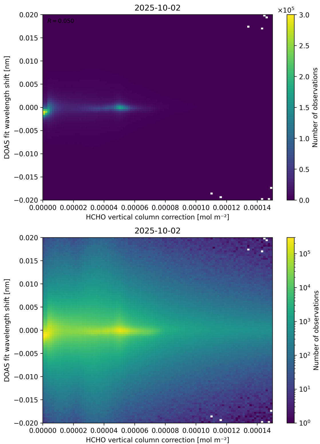
Figure 113: Scatter density plot of “HCHO vertical column correction” against “DOAS fit wavelength shift” for 2025-10-01 to 2025-10-03.
