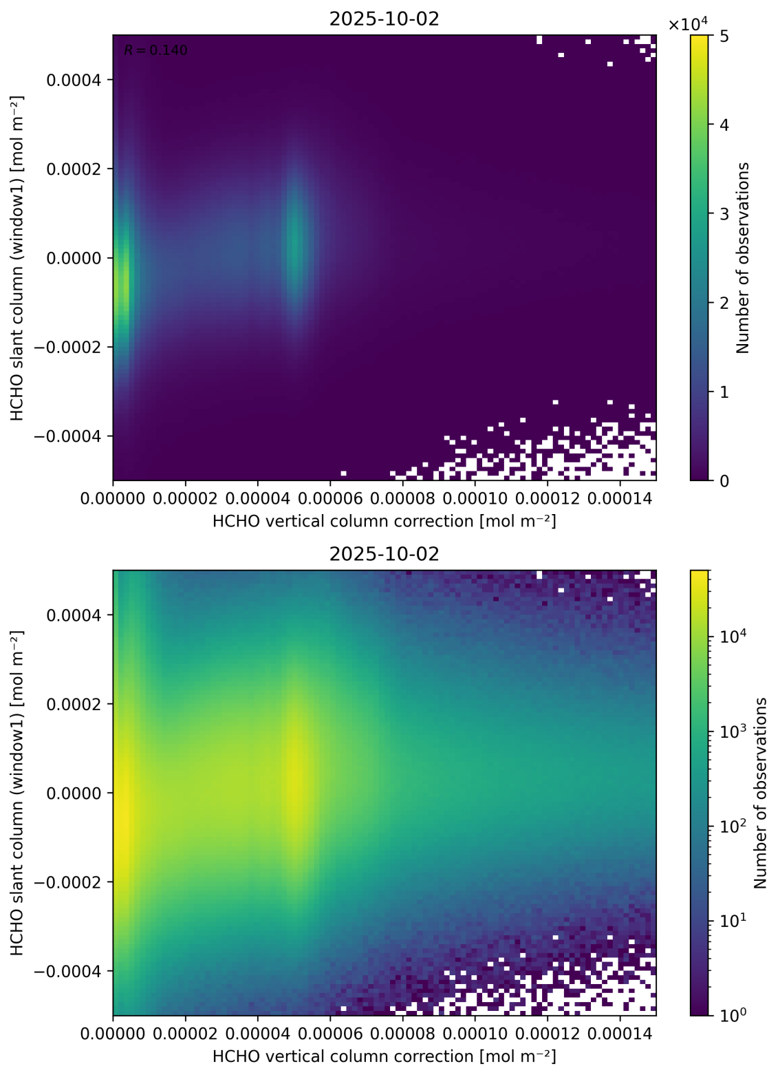
Figure 118: Scatter density plot of “HCHO vertical column correction” against “HCHO slant column (window1)” for 2025-10-01 to 2025-10-03.
