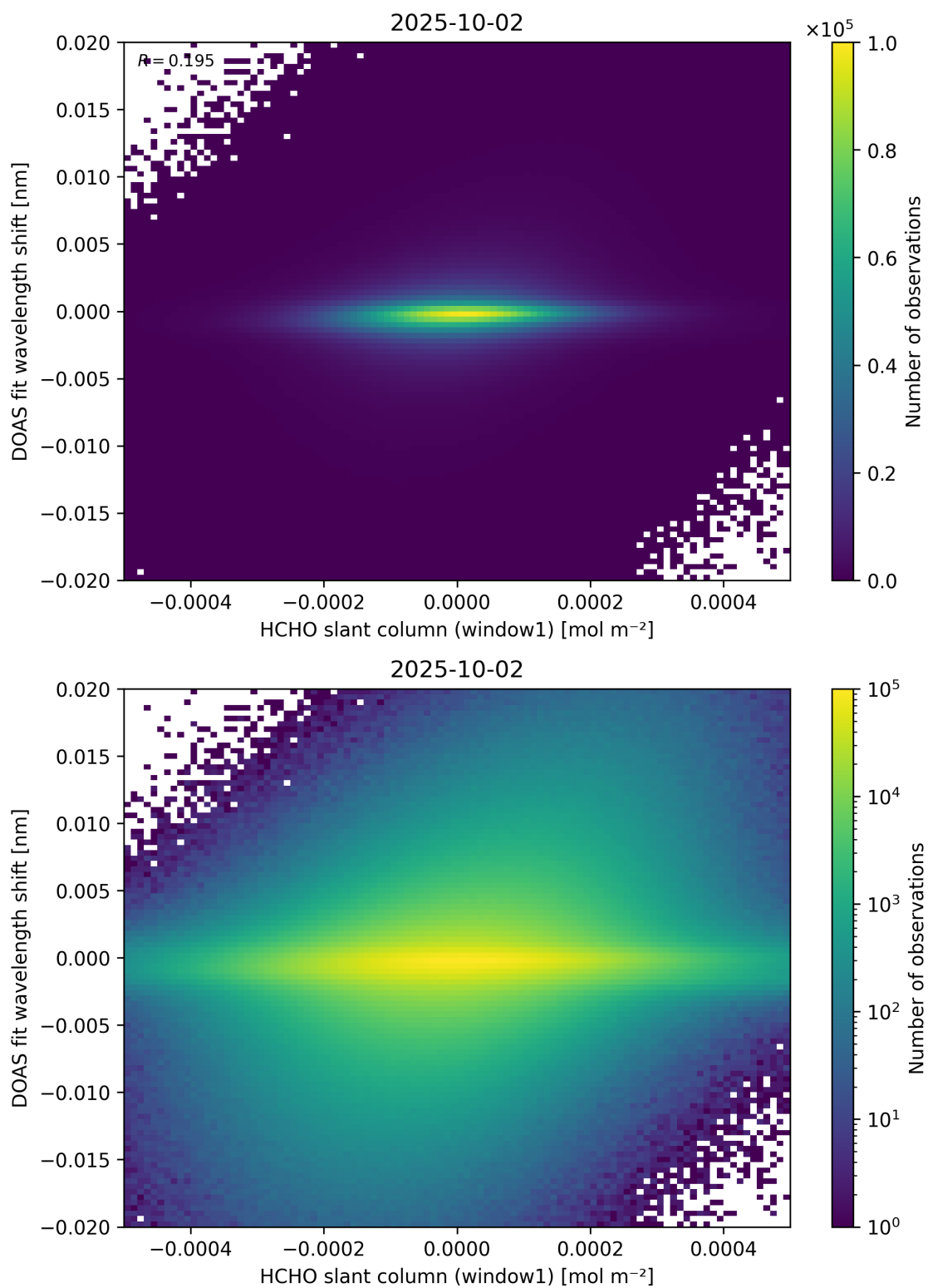
Figure 79: Scatter density plot of “HCHO slant column (window1)” against “DOAS fit wavelength shift” for 2025-10-01 to 2025-10-03.
