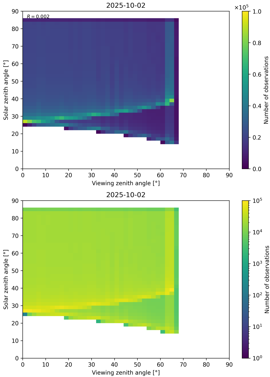
Figure 197: Scatter density plot of “Viewing zenith angle” against “Solar zenith angle” for 2025-10-01 to 2025-10-03.
