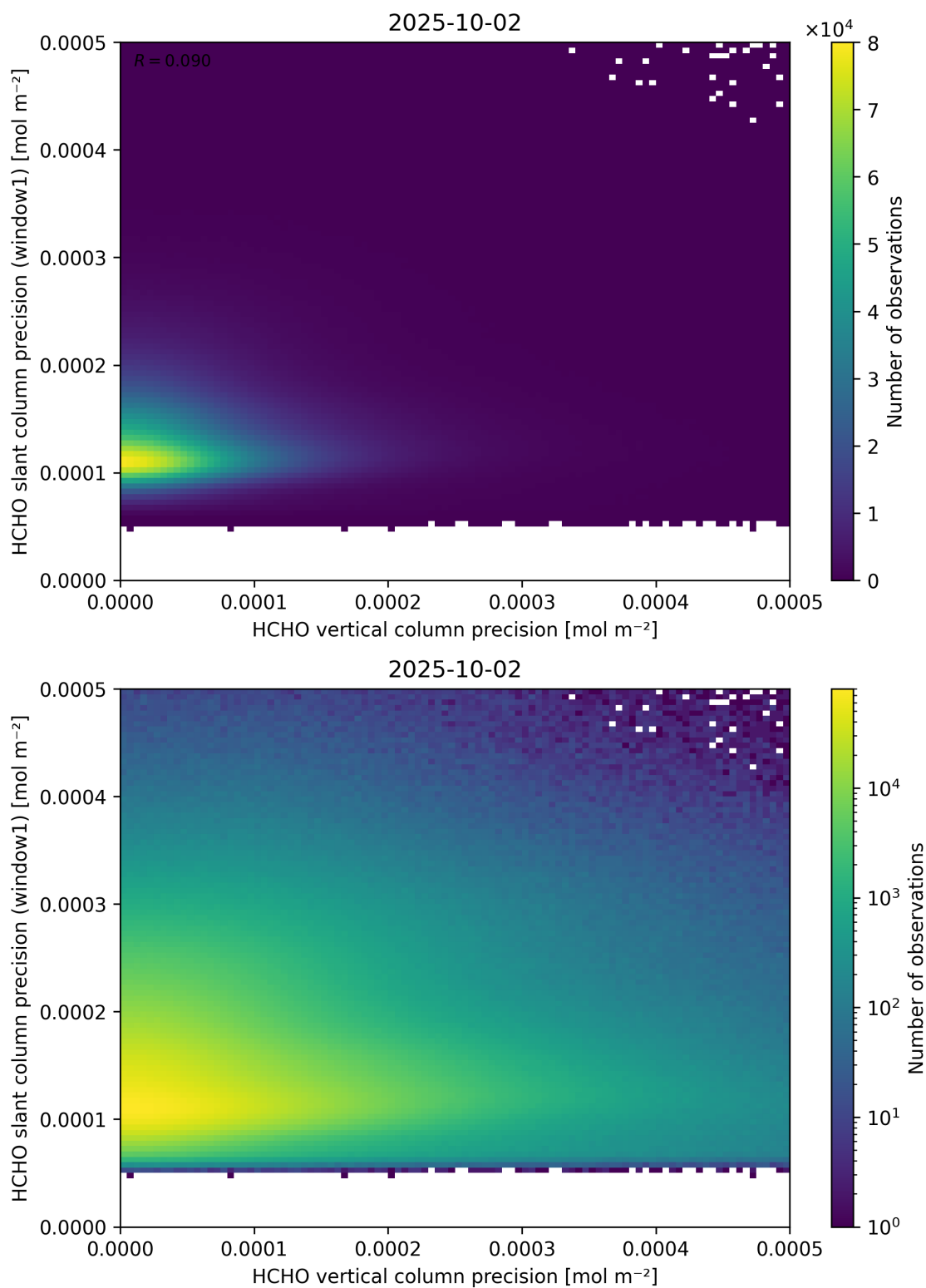
Figure 143: Scatter density plot of “HCHO vertical column precision” against “HCHO slant column precision (window1)” for 2025-10-01 to 2025-10-03.
