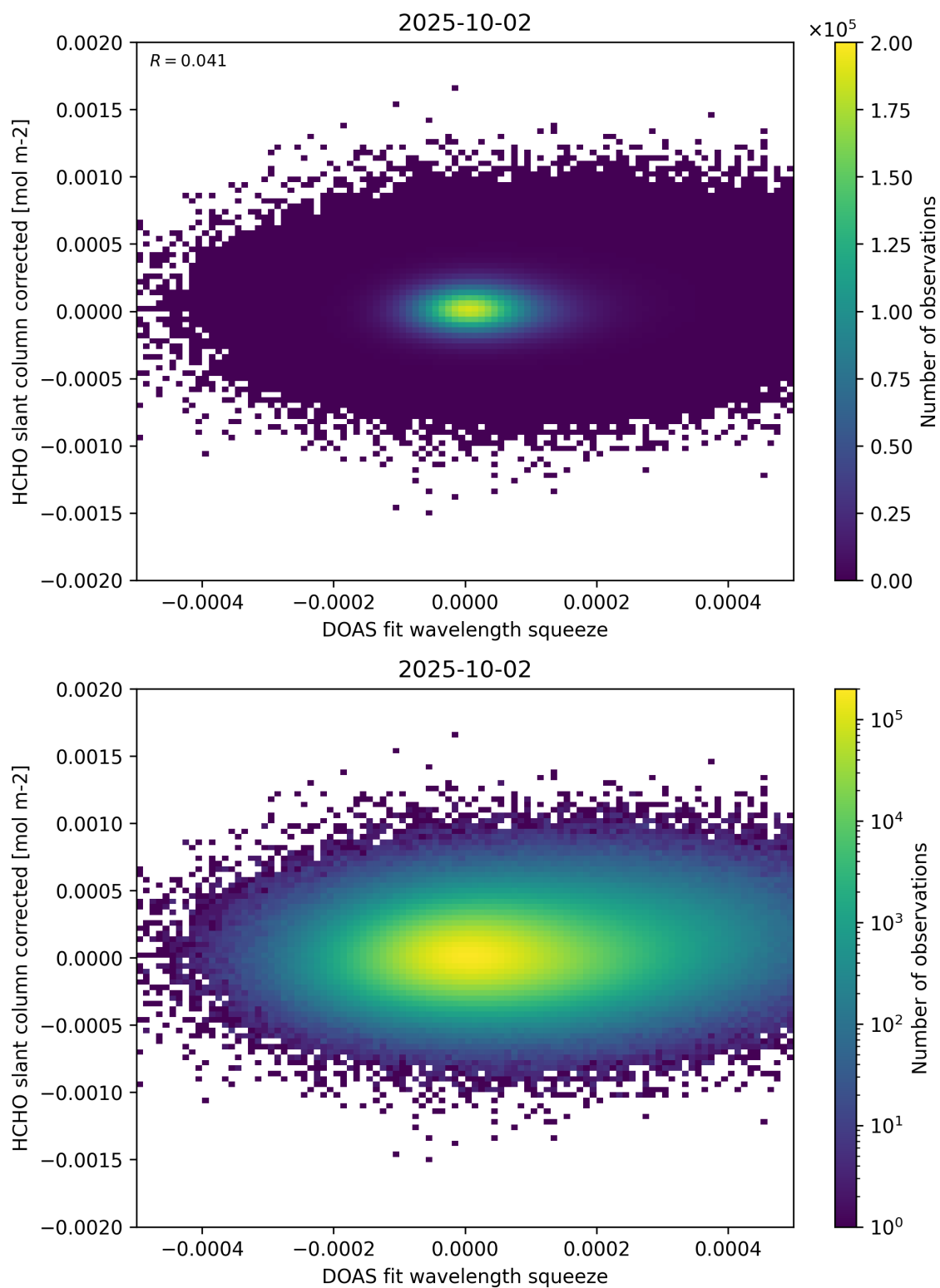
Figure 69: Scatter density plot of “DOAS fit wavelength squeeze” against “HCHO slant column corrected” for 2025-10-01 to 2025-10-03.
