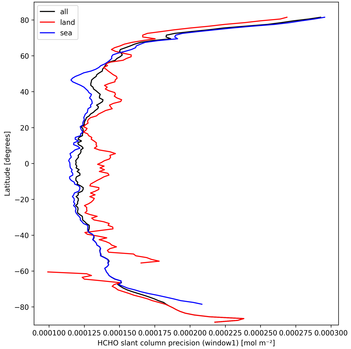
Figure 25: Zonal average of “HCHO slant column precision (window1)” for 2025-10-01 to 2025-10-03.
