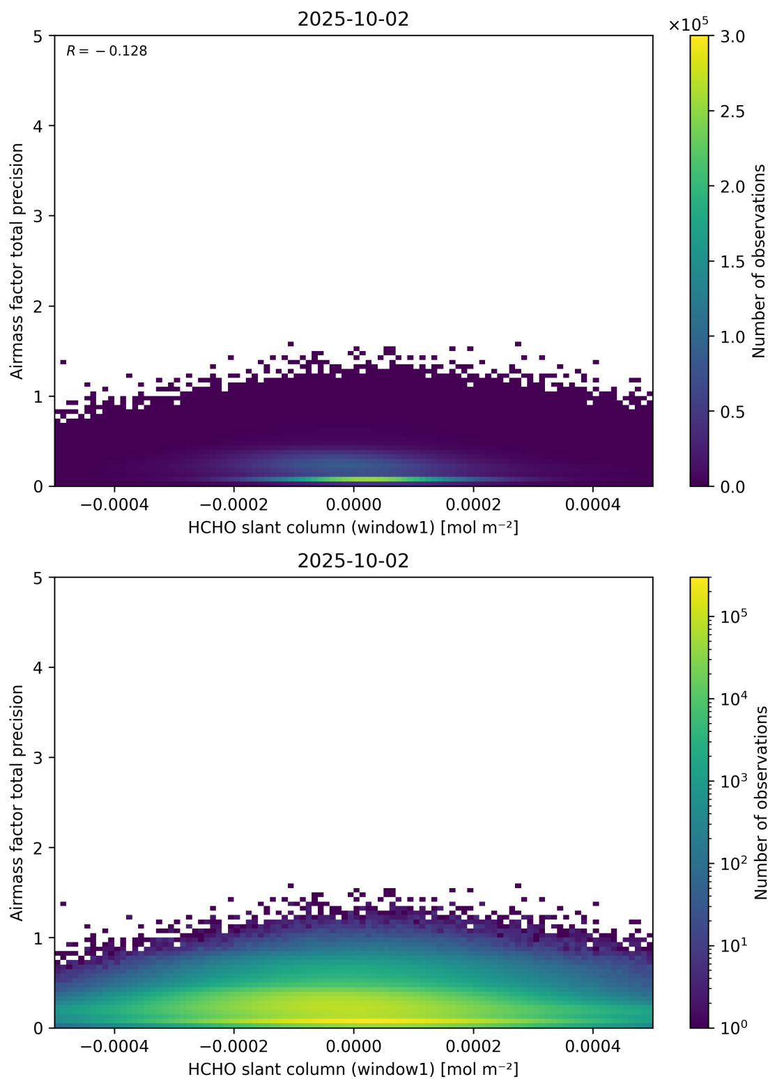
Figure 86: Scatter density plot of “HCHO slant column (window1)” against “Airmass factor total precision” for 2025-10-01 to 2025-10-03.
