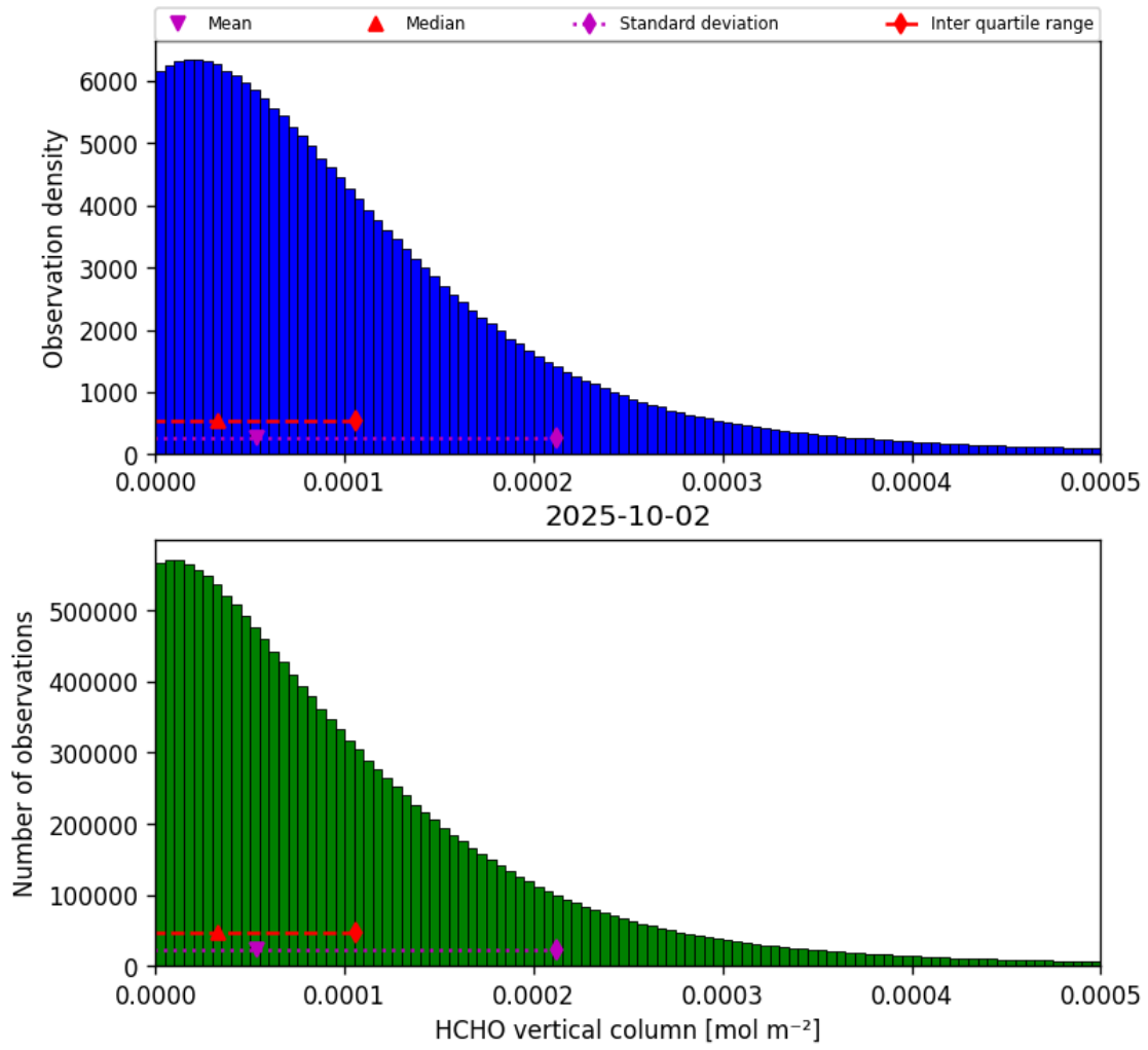
Figure 35: Histogram of “HCHO vertical column” for 2025-10-01 to 2025-10-03
