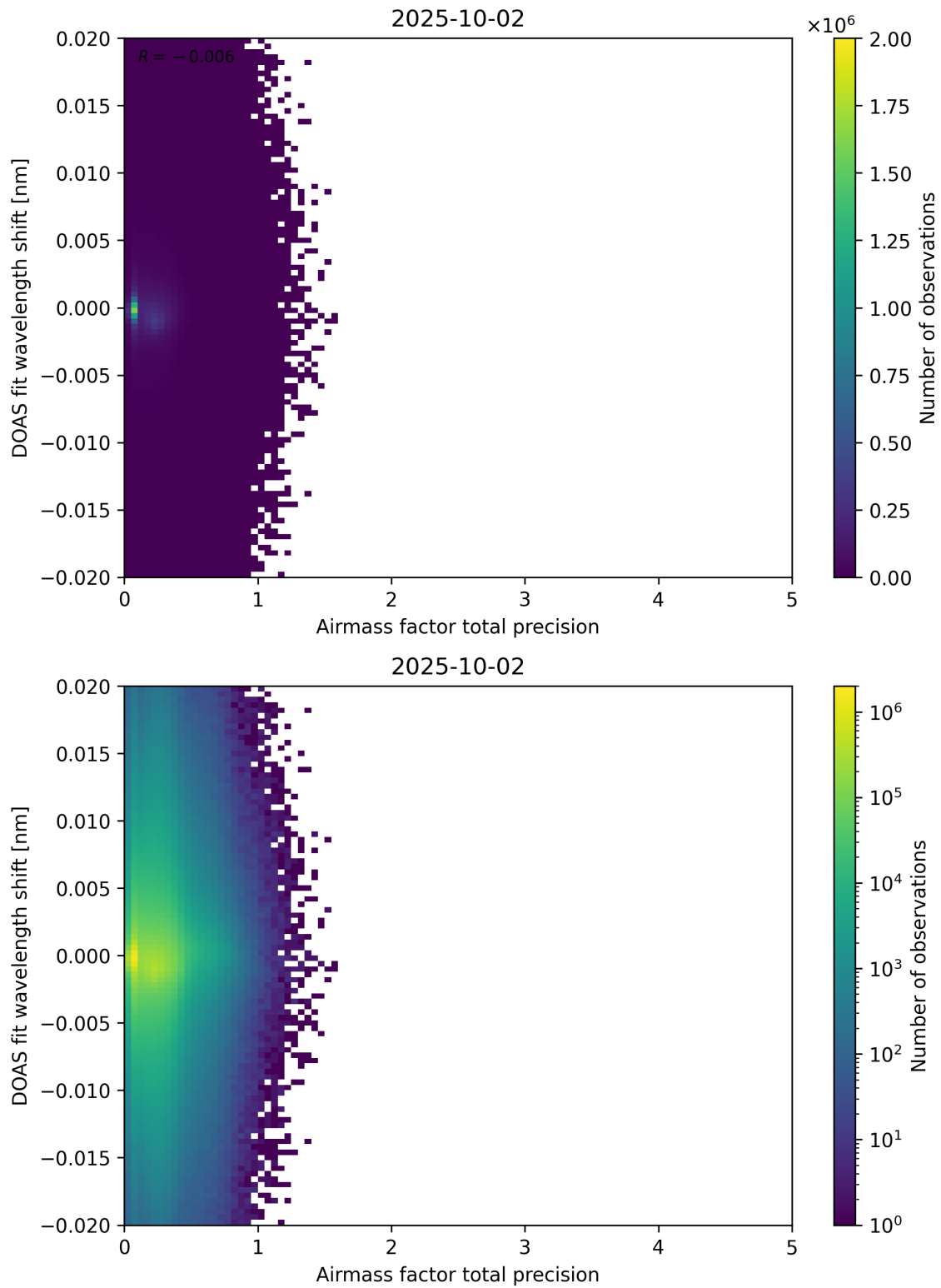
Figure 106: Scatter density plot of “Airmass factor total precision” against “DOAS fit wavelength shift” for 2025-10-01 to 2025-10-03.
