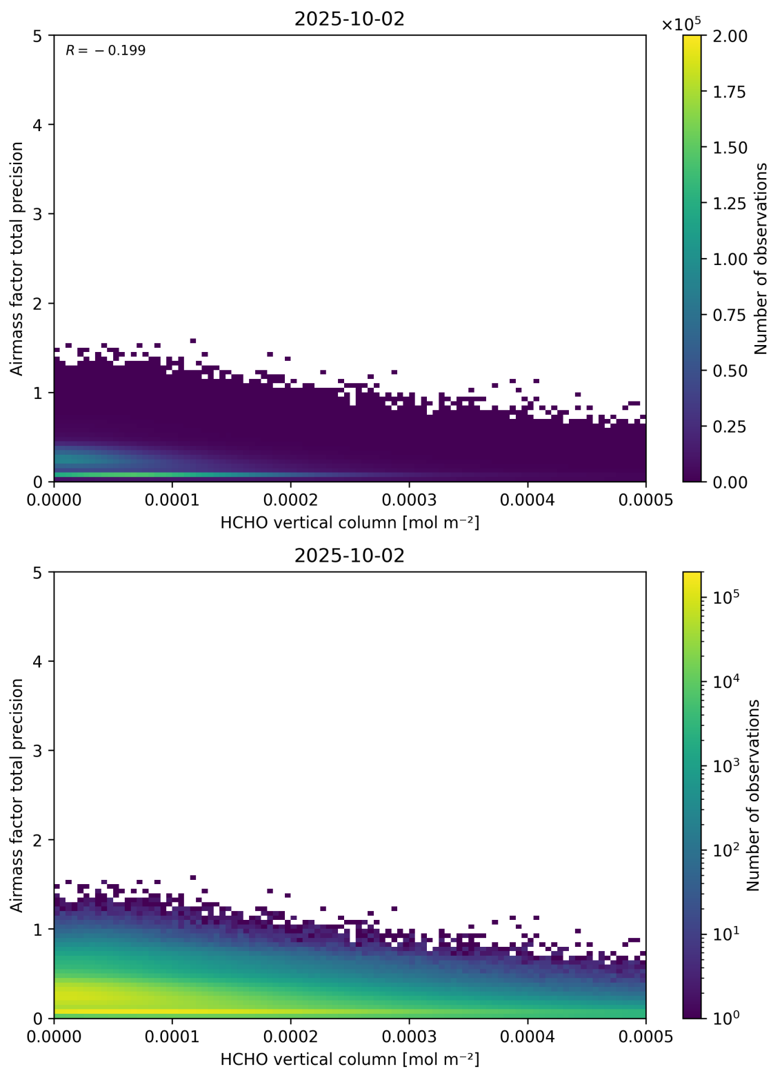
Figure 132: Scatter density plot of “HCHO vertical column” against “Airmass factor total precision” for 2025-10-01 to 2025-10-03.
