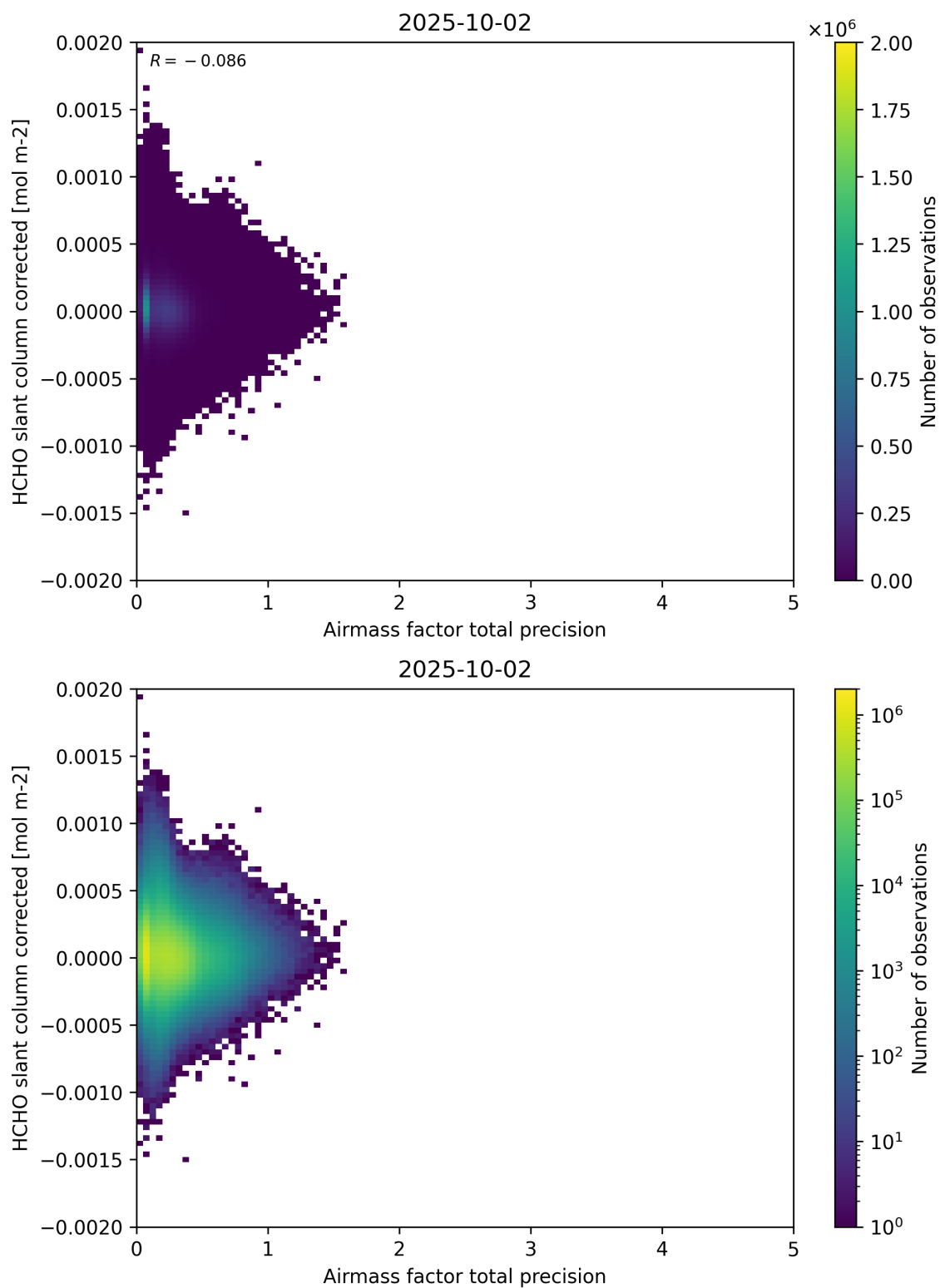
Figure 109: Scatter density plot of “Airmass factor total precision” against “HCHO slant column corrected” for 2025-10-01 to 2025-10-03.
