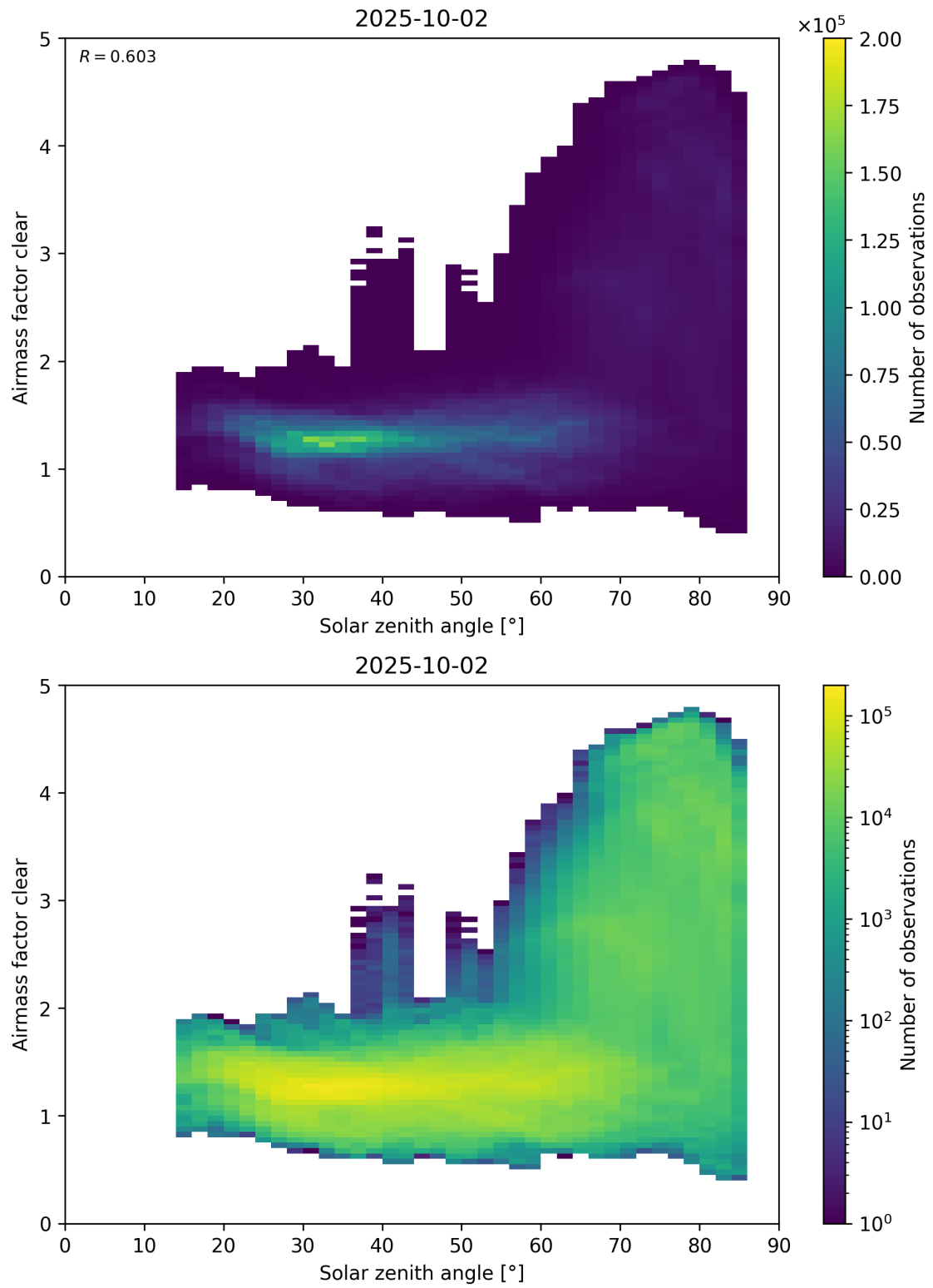
Figure 170: Scatter density plot of “Solar zenith angle” against “Airmass factor clear” for 2025-10-01 to 2025-10-03.
