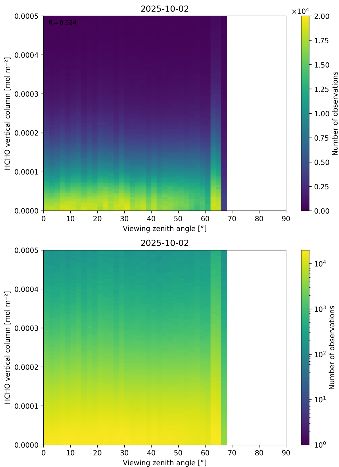
Figure 192: Scatter density plot of “Viewing zenith angle” against “HCHO vertical column” for 2025-10-01 to 2025-10-03.
