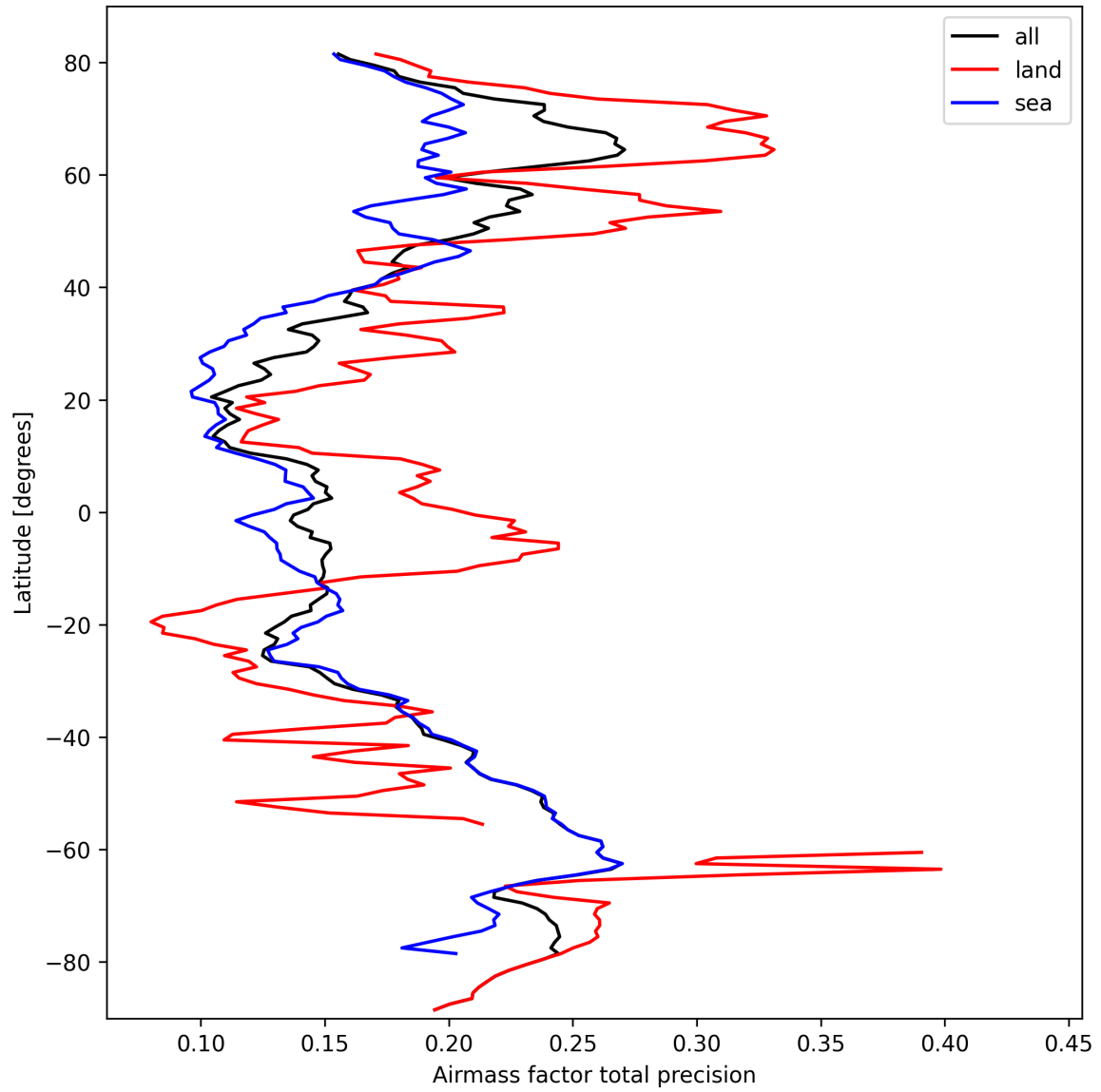
Figure 27: Zonal average of “Airmass factor total precision” for 2025-10-01 to 2025-10-03.
