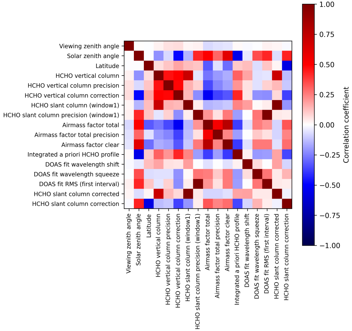
Figure 2: Map of correlation matrix for 2025-10-01 to 2025-10-03.
