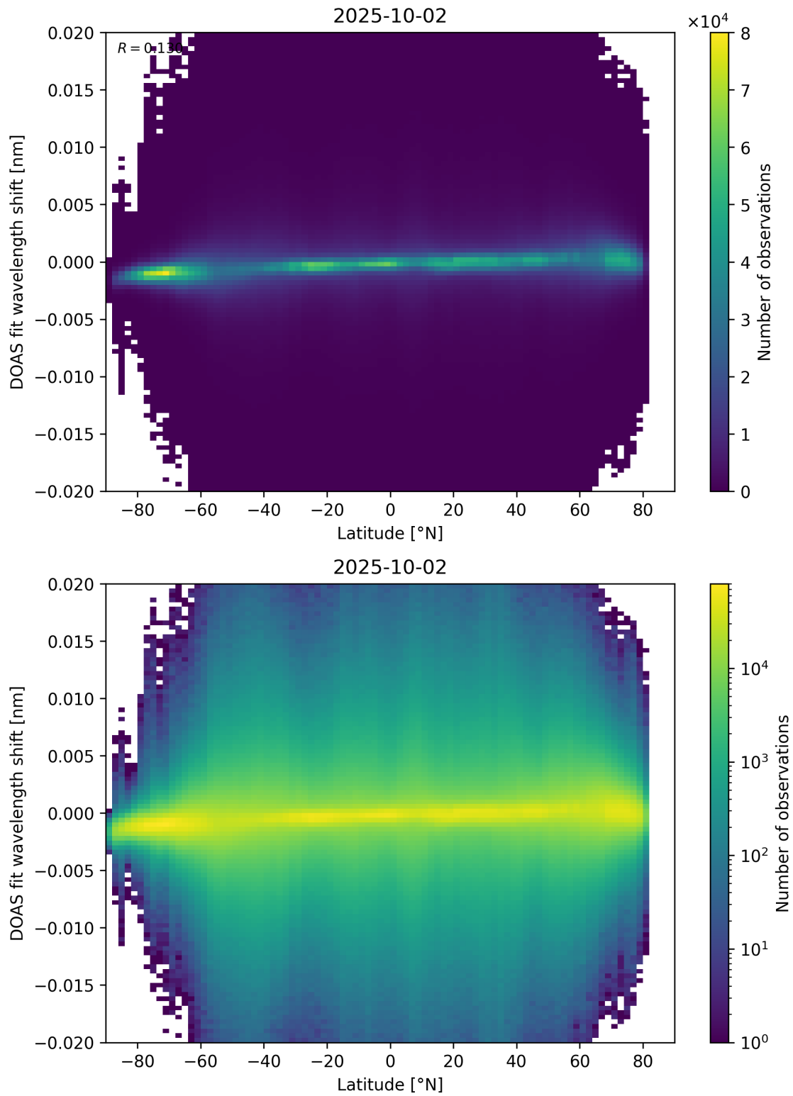
Figure 154: Scatter density plot of “Latitude” against “DOAS fit wavelength shift” for 2025-10-01 to 2025-10-03.
