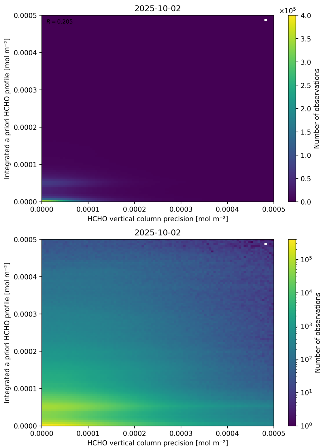
Figure 147: Scatter density plot of “HCHO vertical column precision” against “Integrated a priori HCHO profile” for 2025-10-01 to 2025-10-03.
