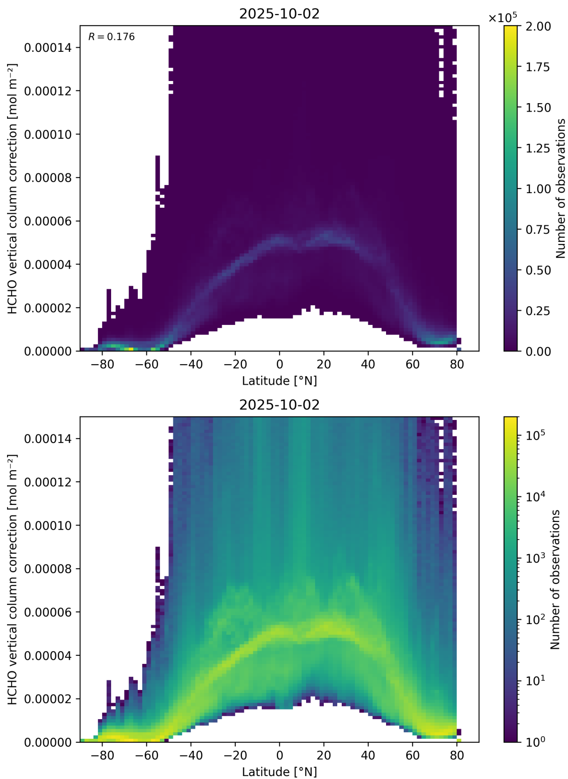
Figure 164: Scatter density plot of “Latitude” against “HCHO vertical column correction” for 2025-10-01 to 2025-10-03.
