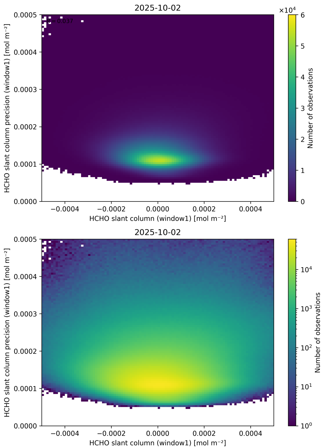
Figure 84: Scatter density plot of “HCHO slant column (window1)” against “HCHO slant column precision (window1)” for 2025-10-01 to 2025-10-03.
