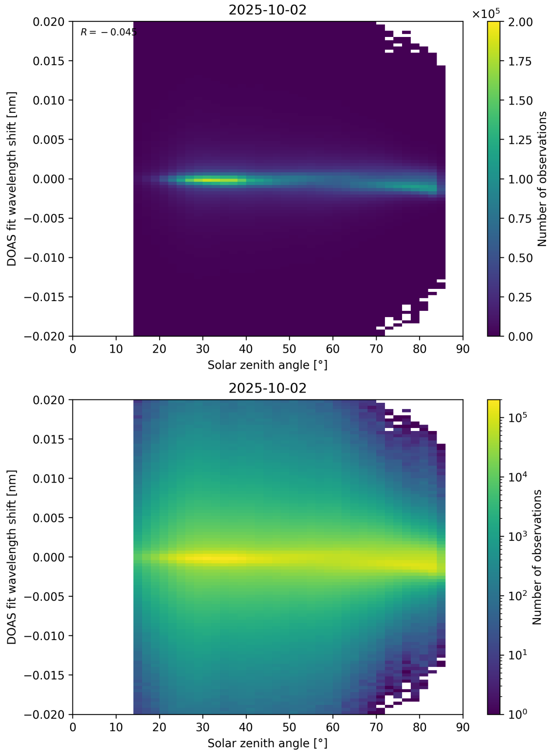
Figure 168: Scatter density plot of “Solar zenith angle” against “DOAS fit wavelength shift” for 2025-10-01 to 2025-10-03.
