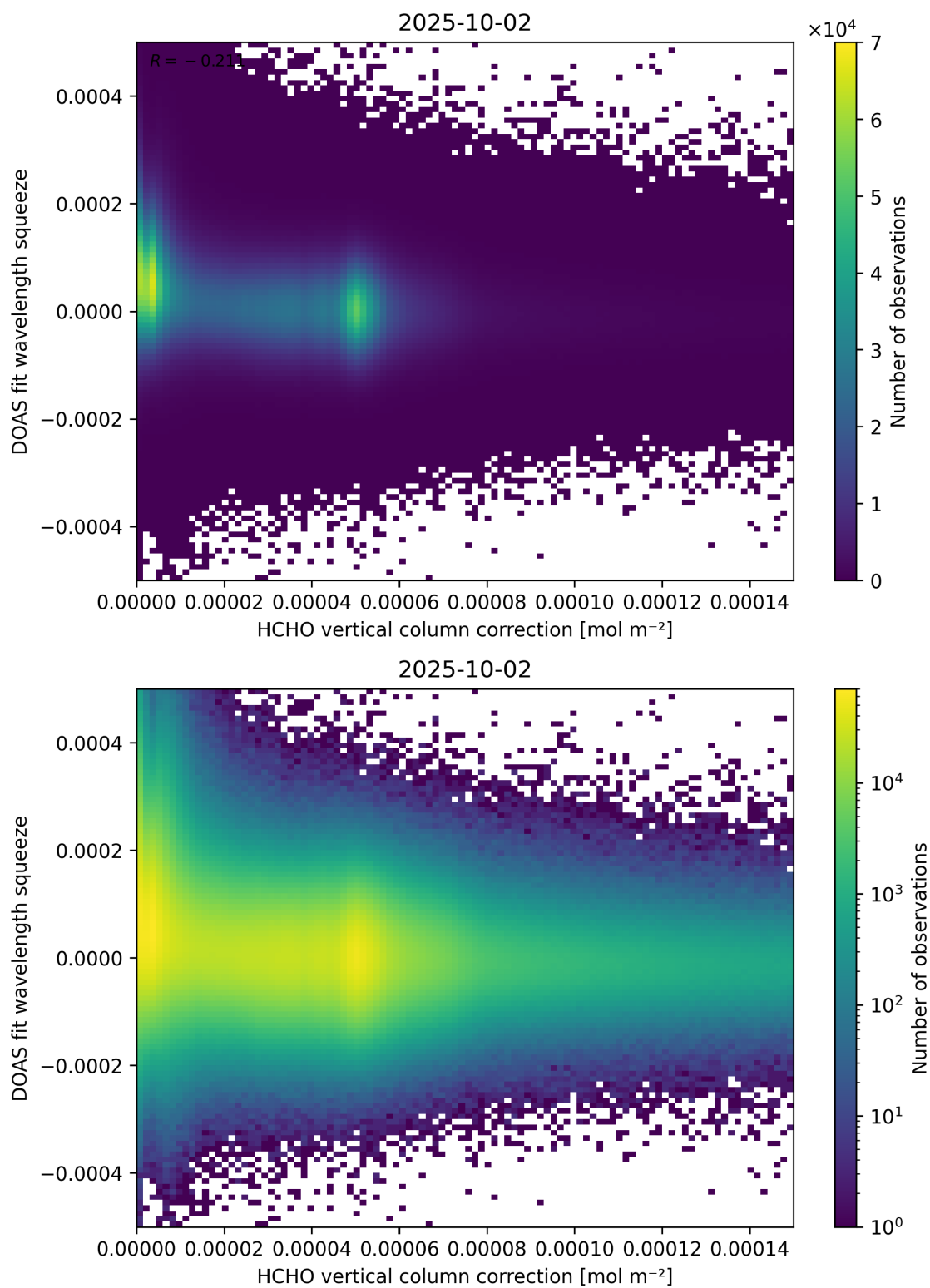
Figure 114: Scatter density plot of “HCHO vertical column correction” against “DOAS fit wavelength squeeze” for 2025-10-01 to 2025-10-03.
