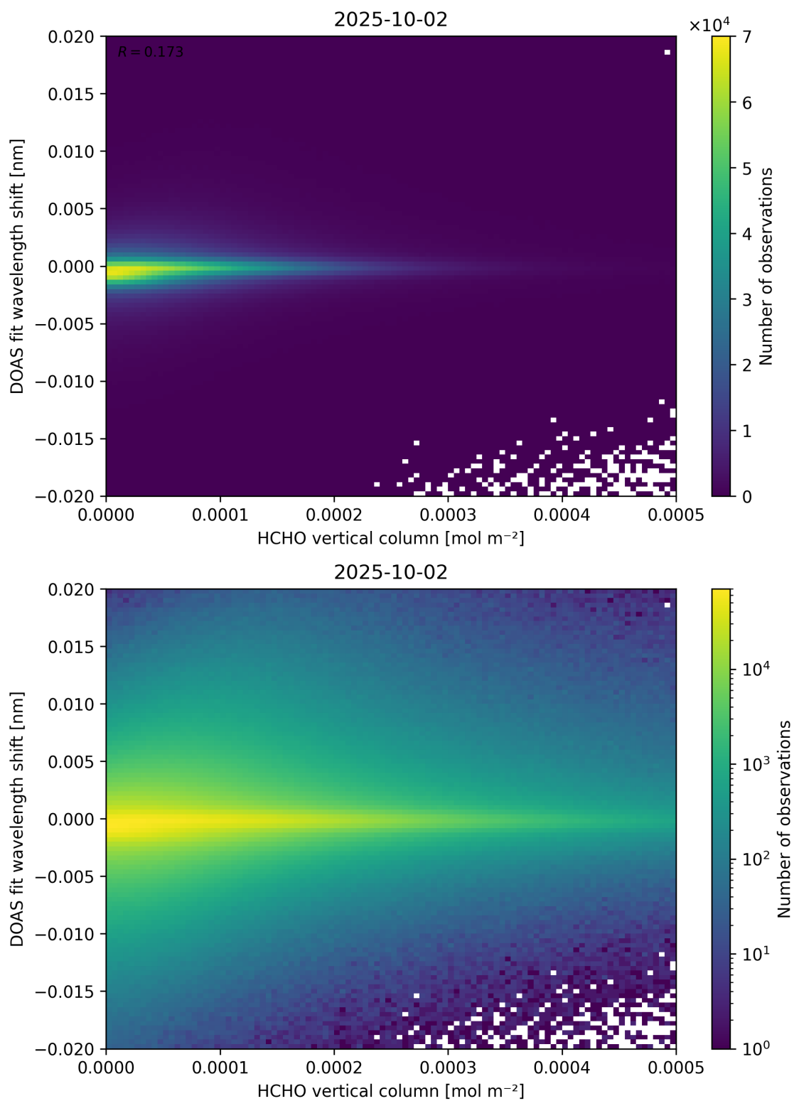
Figure 124: Scatter density plot of “HCHO vertical column” against “DOAS fit wavelength shift” for 2025-10-01 to 2025-10-03.
