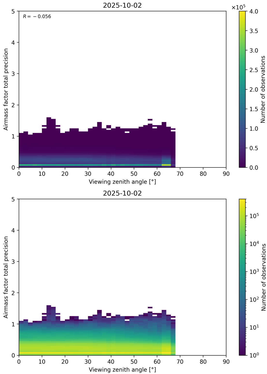
Figure 191: Scatter density plot of “Viewing zenith angle” against “Airmass factor total precision” for 2025-10-01 to 2025-10-03.
