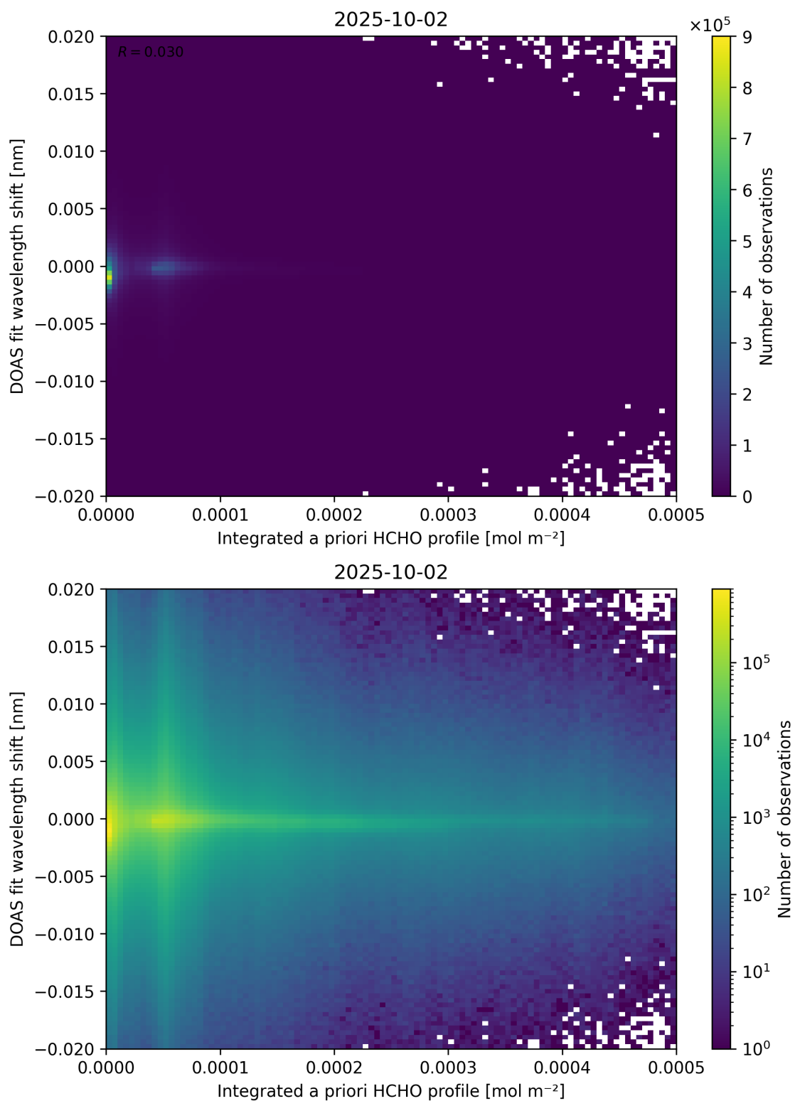
Figure 149: Scatter density plot of “Integrated a priori HCHO profile” against “DOAS fit wavelength shift” for 2025-10-01 to 2025-10-03.
