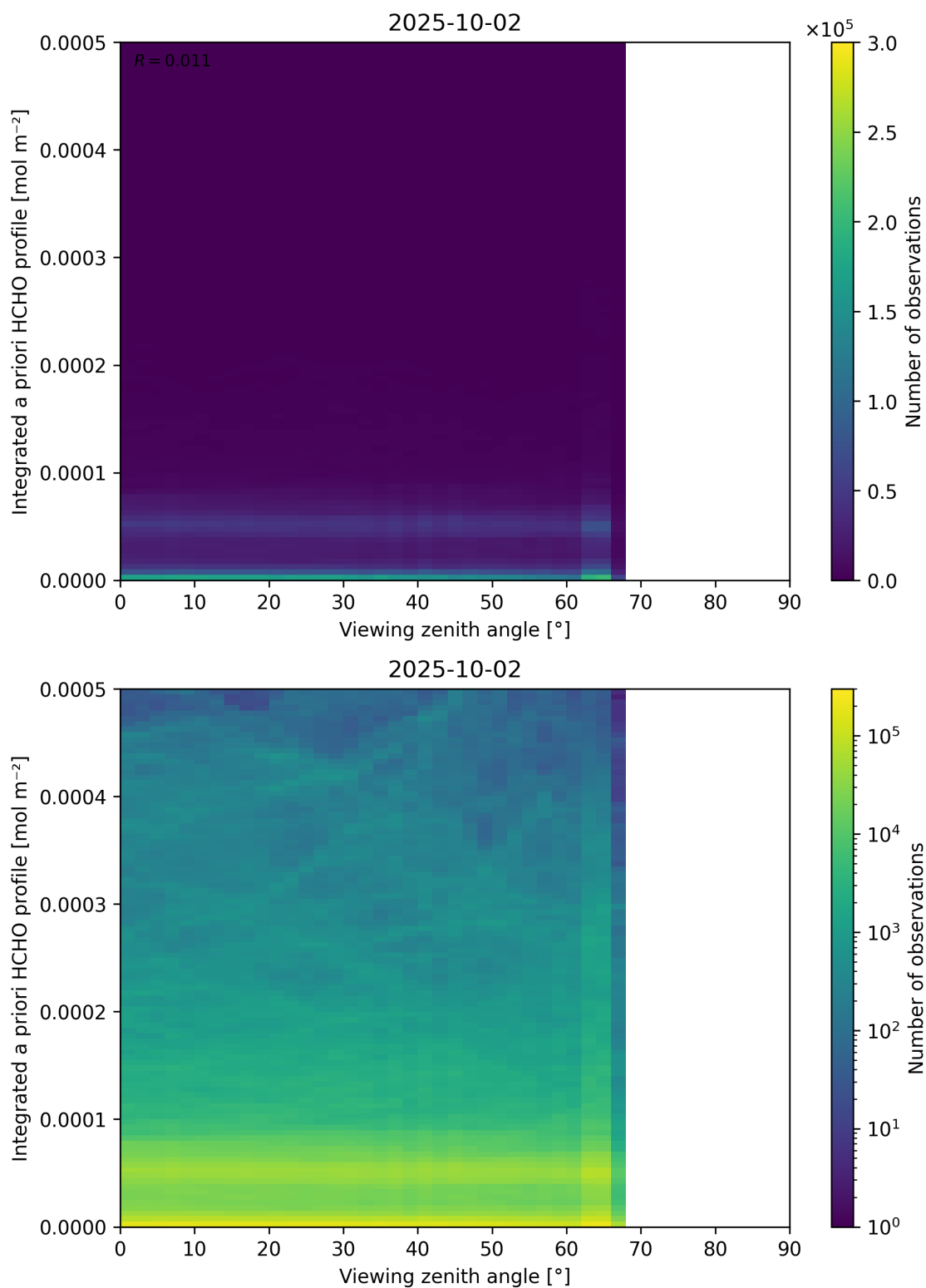
Figure 195: Scatter density plot of “Viewing zenith angle” against “Integrated a priori HCHO profile” for 2025-10-01 to 2025-10-03.
