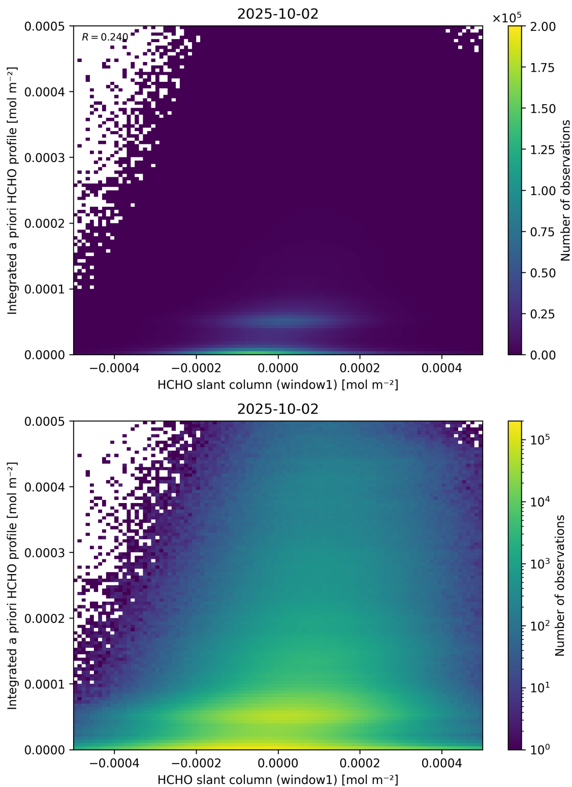
Figure 87: Scatter density plot of “HCHO slant column (window1)” against “Integrated a priori HCHO profile” for 2025-10-01 to 2025-10-03.
