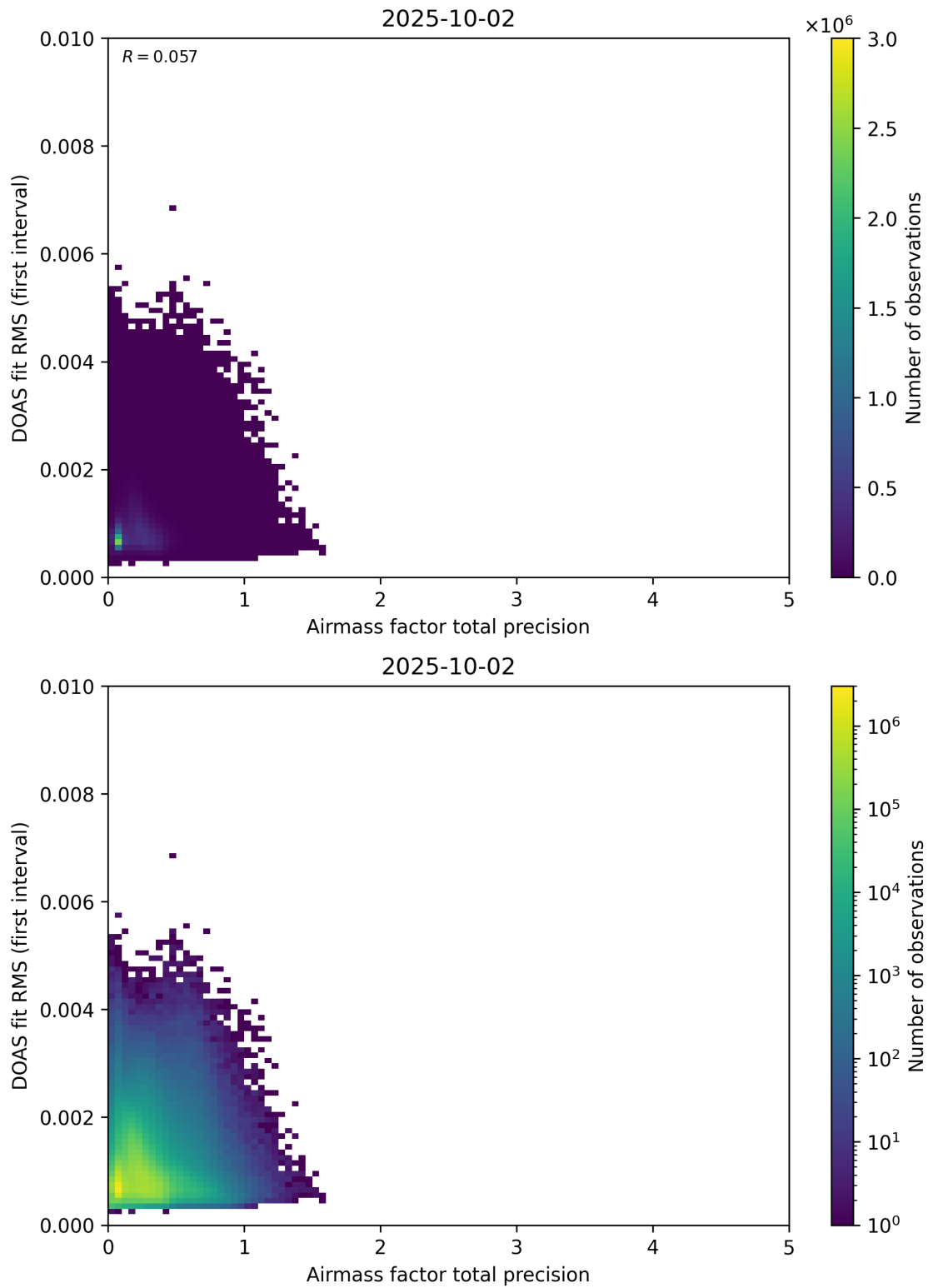
Figure 105: Scatter density plot of “Airmass factor total precision” against “DOAS fit RMS (first interval)” for 2025-10-01 to 2025-10-03.
