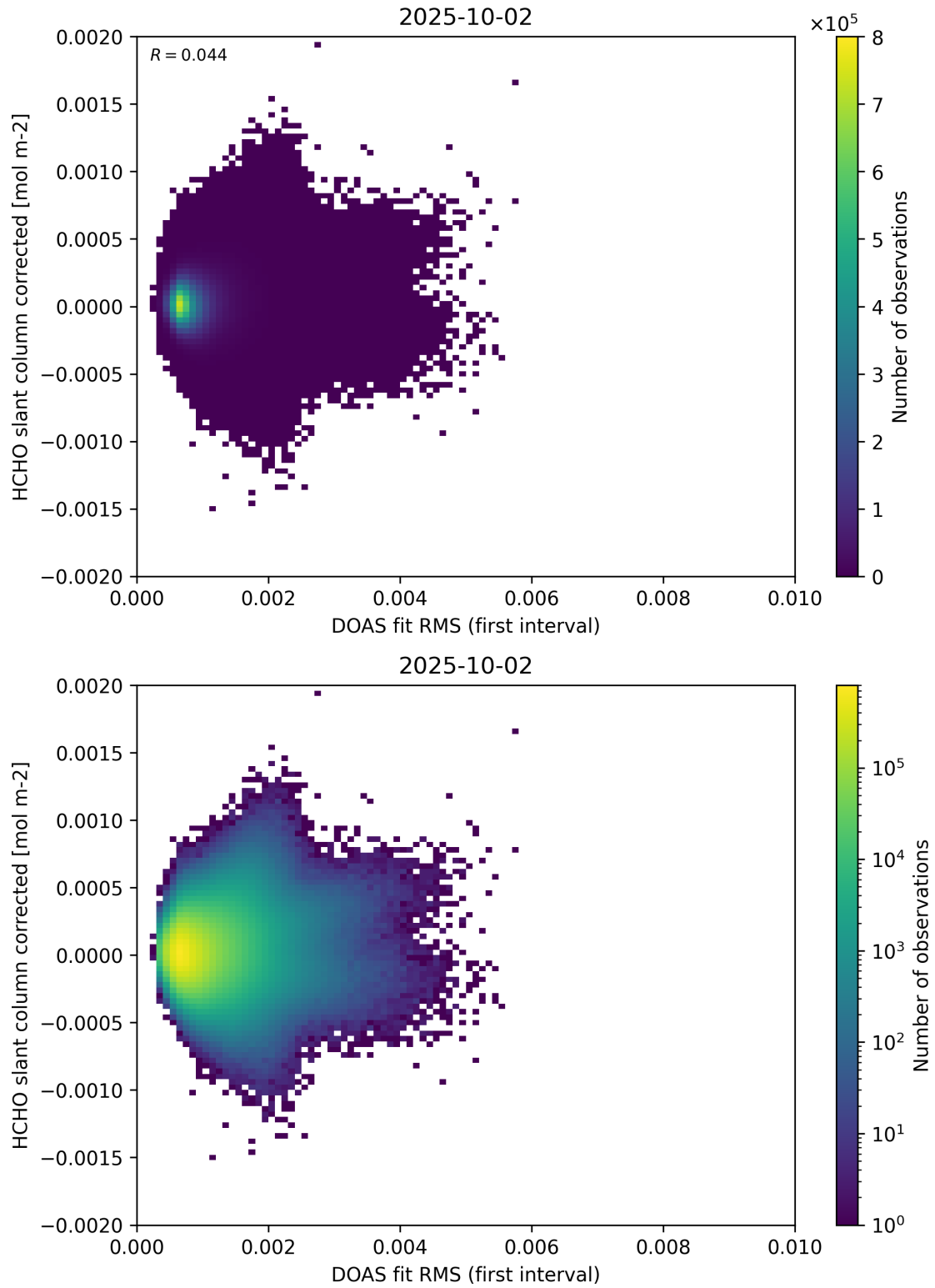
Figure 62: Scatter density plot of “DOAS fit RMS (first interval)” against “HCHO slant column corrected” for 2025-10-01 to 2025-10-03.
