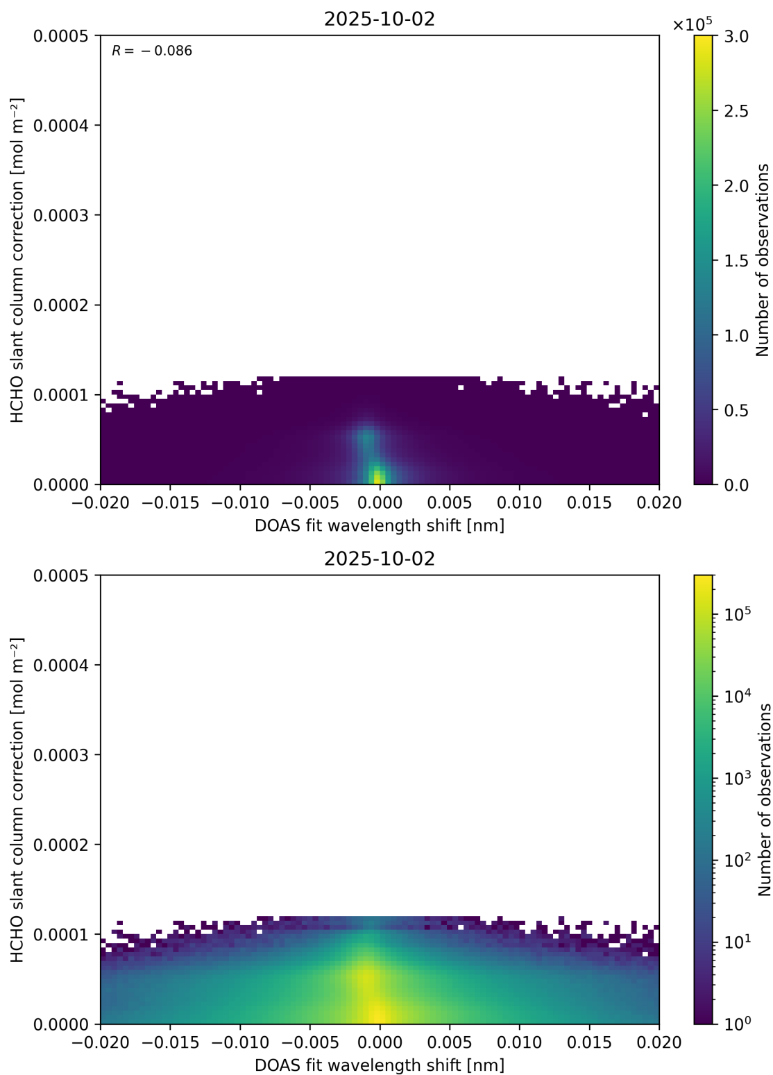
Figure 67: Scatter density plot of “DOAS fit wavelength shift” against “HCHO slant column correction” for 2025-10-01 to 2025-10-03.
