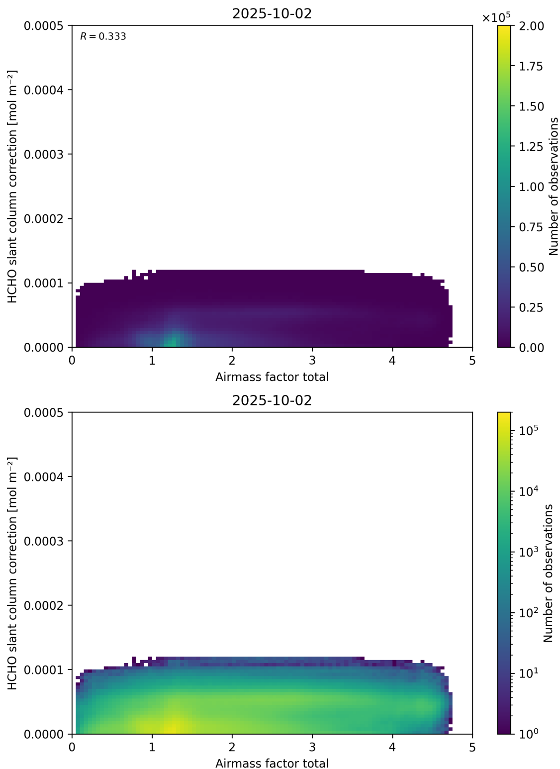
Figure 102: Scatter density plot of “Airmass factor total” against “HCHO slant column correction” for 2025-10-01 to 2025-10-03.
