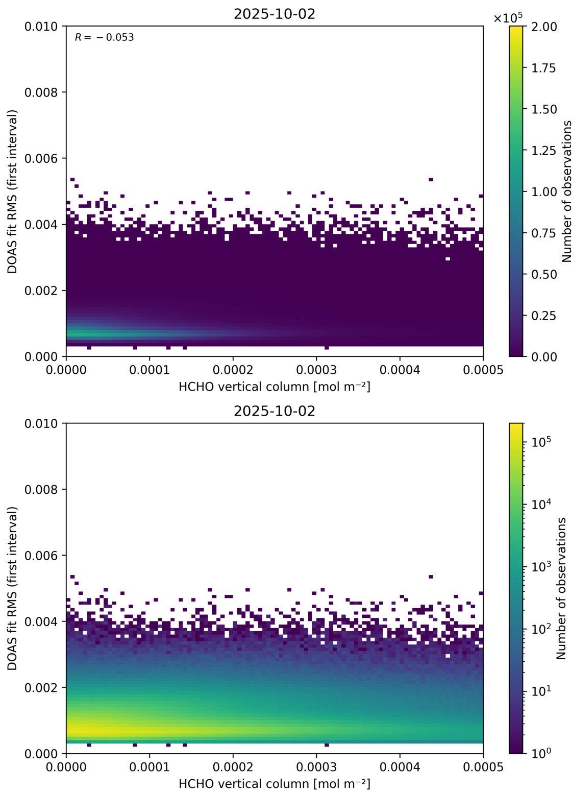
Figure 123: Scatter density plot of “HCHO vertical column” against “DOAS fit RMS (first interval)” for 2025-10-01 to 2025-10-03.
