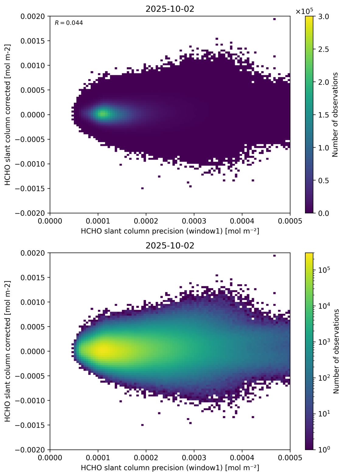
Figure 92: Scatter density plot of “HCHO slant column precision (window1)” against “HCHO slant column corrected” for 2025-10-01 to 2025-10-03.
