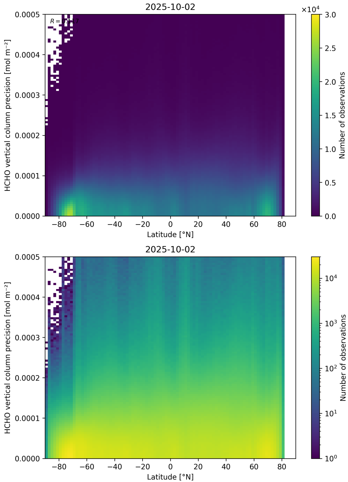
Figure 165: Scatter density plot of “Latitude” against “HCHO vertical column precision” for 2025-10-01 to 2025-10-03.
