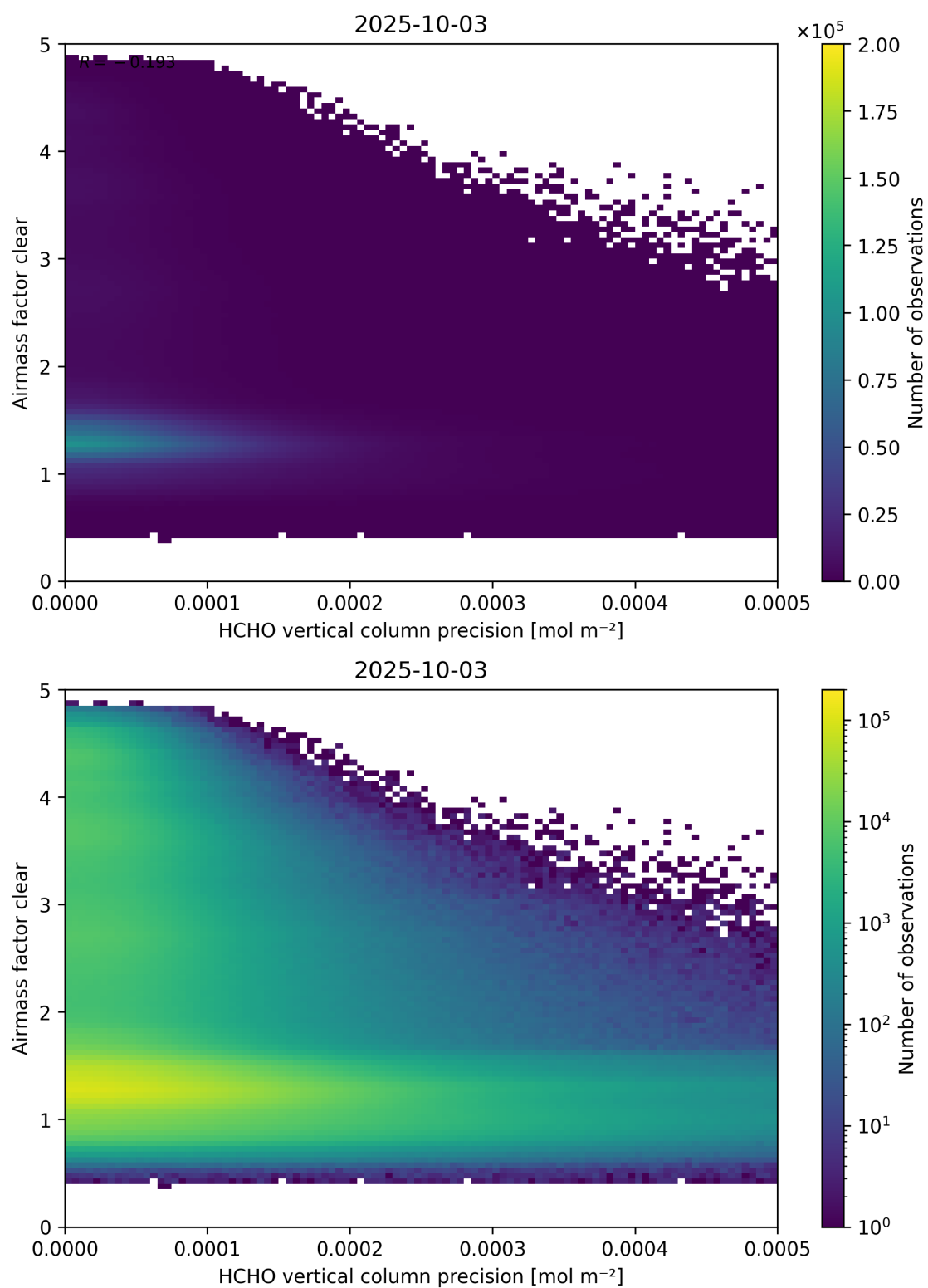
Figure 139: Scatter density plot of “HCHO vertical column precision” against “Airmass factor clear” for 2025-10-02 to 2025-10-04.
