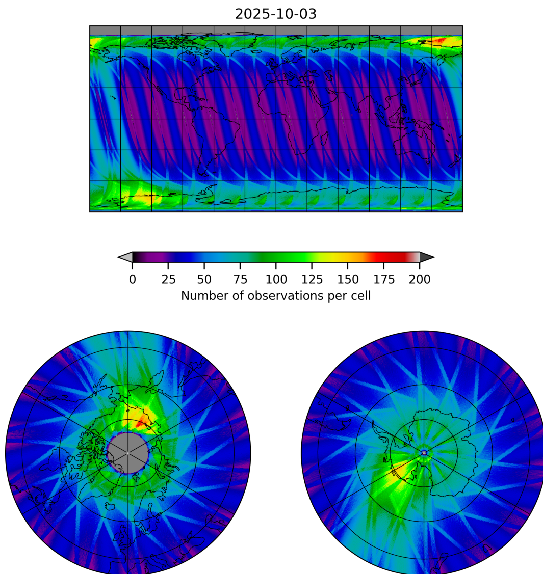
Figure 19: Map of the number of observations for 2025-10-02 to 2025-10-04
