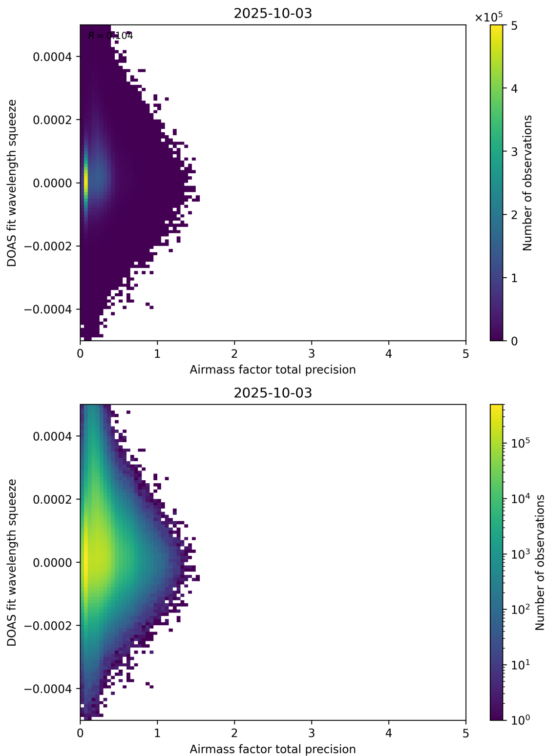
Figure 107: Scatter density plot of “Airmass factor total precision” against “DOAS fit wavelength squeeze” for 2025-10-02 to 2025-10-04.
