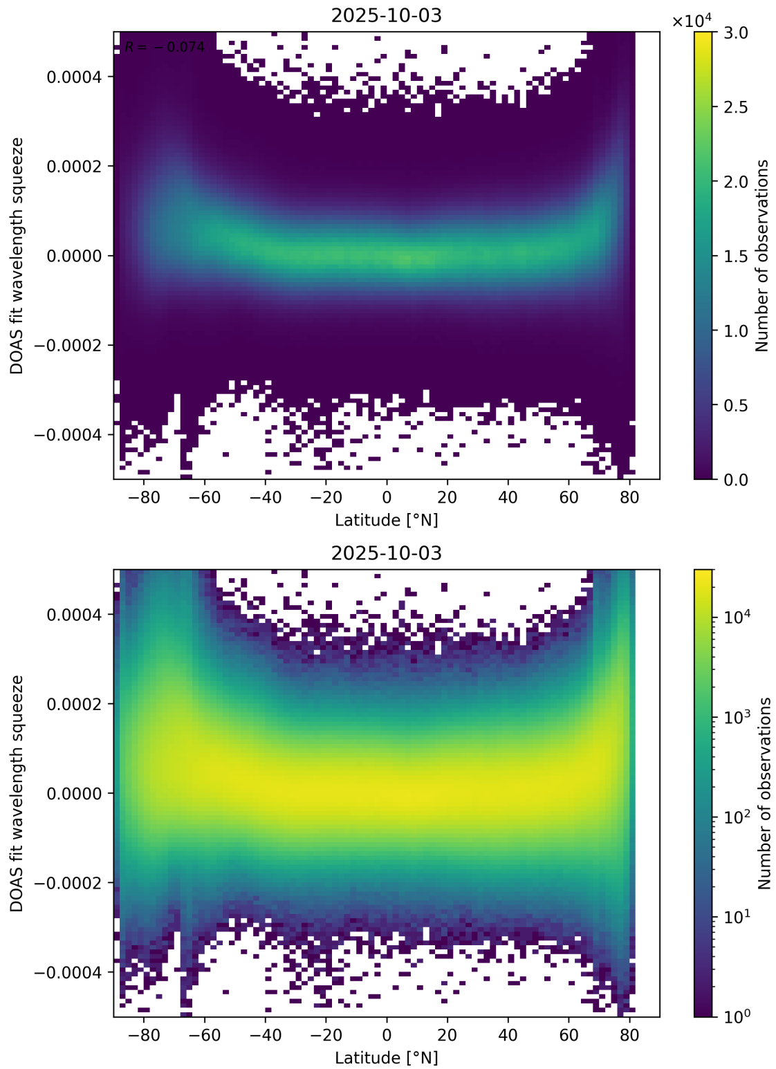
Figure 155: Scatter density plot of “Latitude” against “DOAS fit wavelength squeeze” for 2025-10-02 to 2025-10-04.
