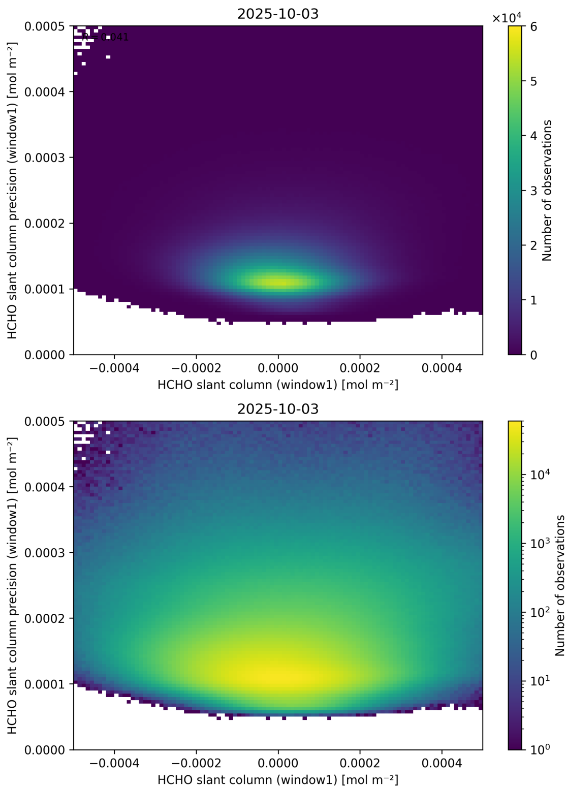
Figure 84: Scatter density plot of “HCHO slant column (window1)” against “HCHO slant column precision (window1)” for 2025-10-02 to 2025-10-04.
