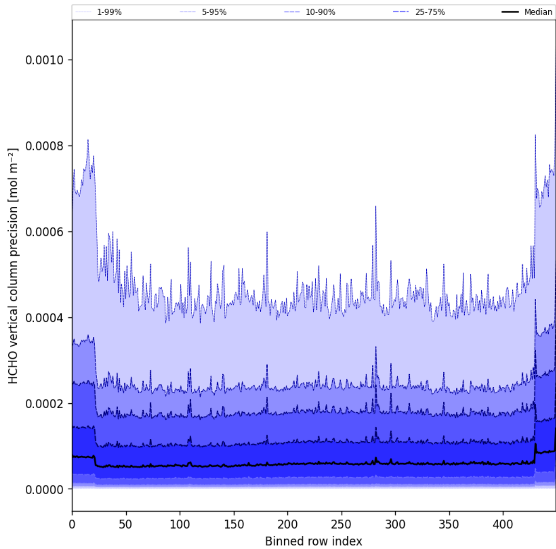
Figure 50: Along track statistics of “HCHO vertical column precision” for 2025-10-02 to 2025-10-04
