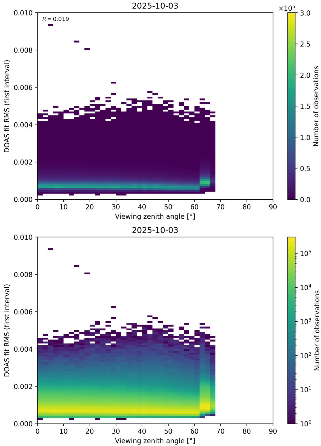
Figure 182: Scatter density plot of “Viewing zenith angle” against “DOAS fit RMS (first interval)” for 2025-10-02 to 2025-10-04.
