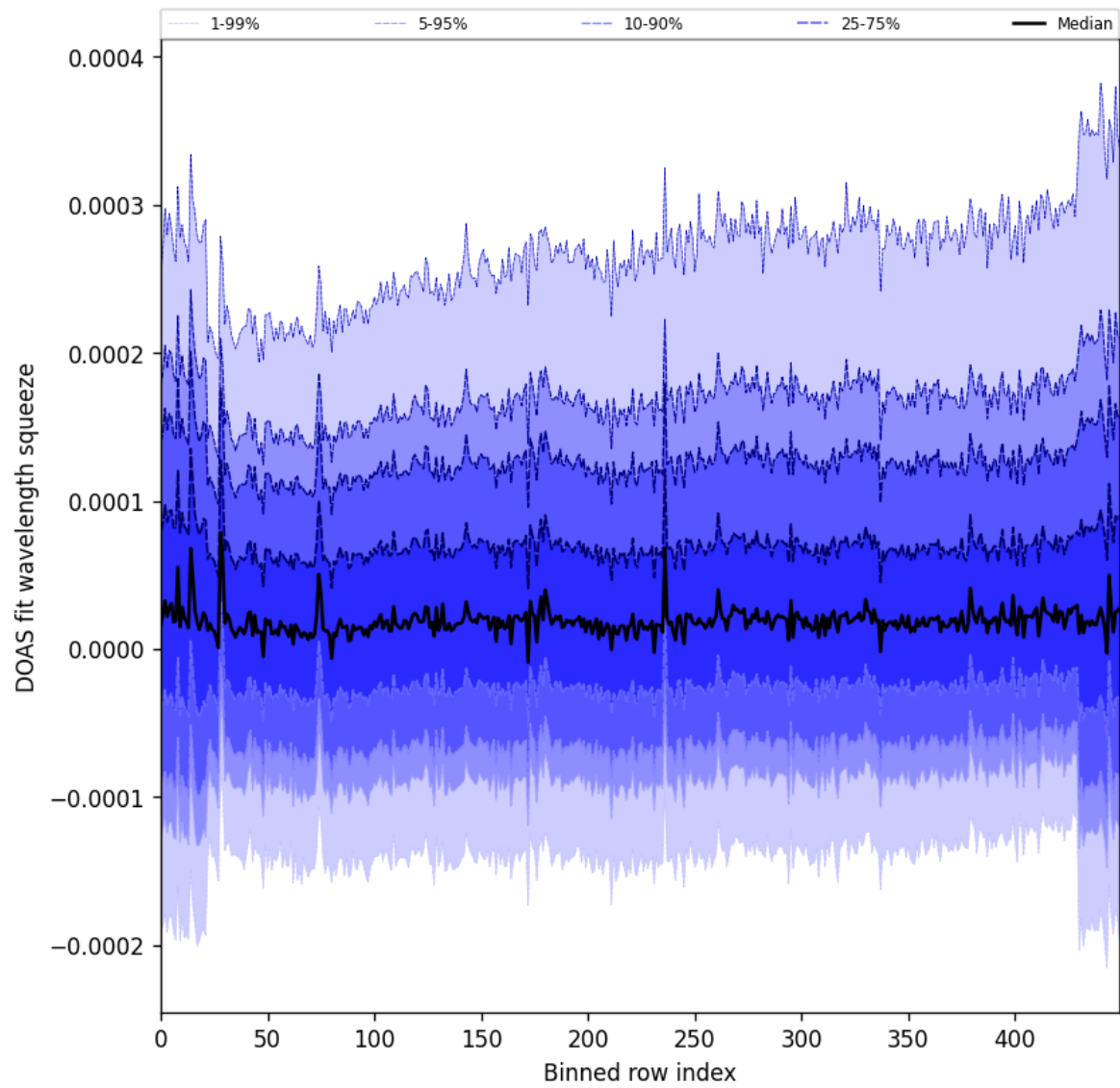
Figure 59: Along track statistics of “DOAS fit wavelength squeeze” for 2025-10-02 to 2025-10-04
