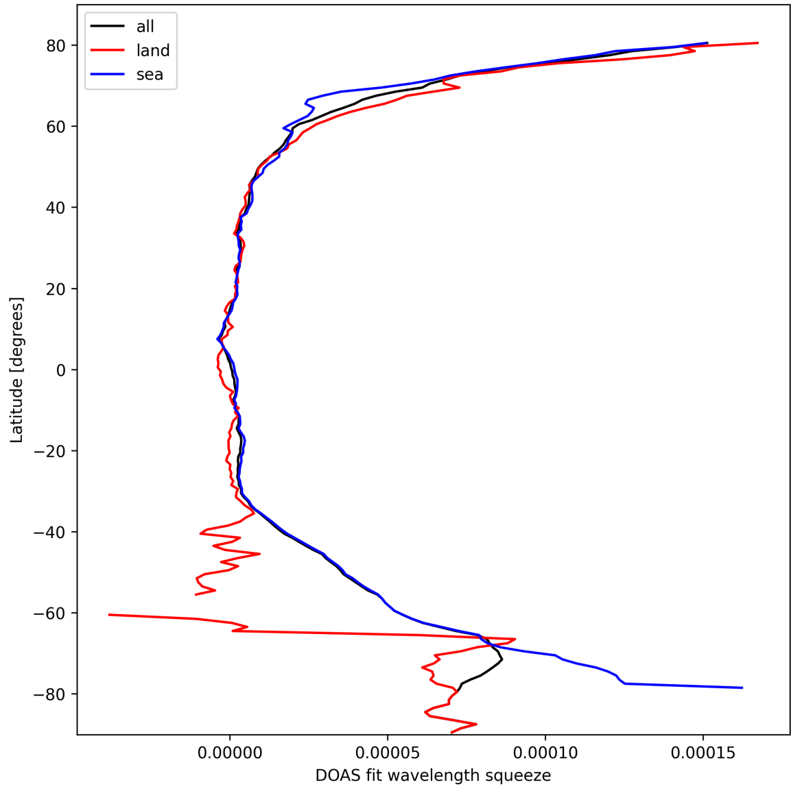
Figure 31: Zonal average of “DOAS fit wavelength squeeze” for 2025-10-02 to 2025-10-04.
