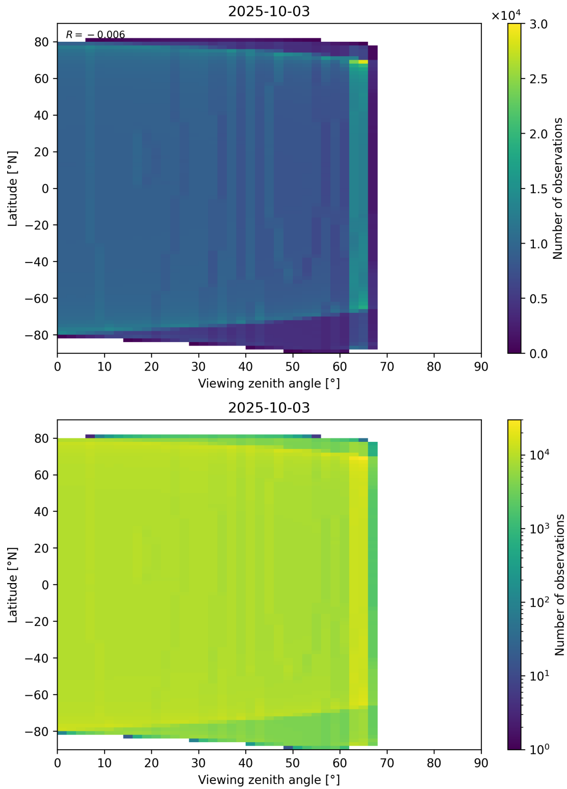
Figure 196: Scatter density plot of “Viewing zenith angle” against “Latitude” for 2025-10-02 to 2025-10-04.
