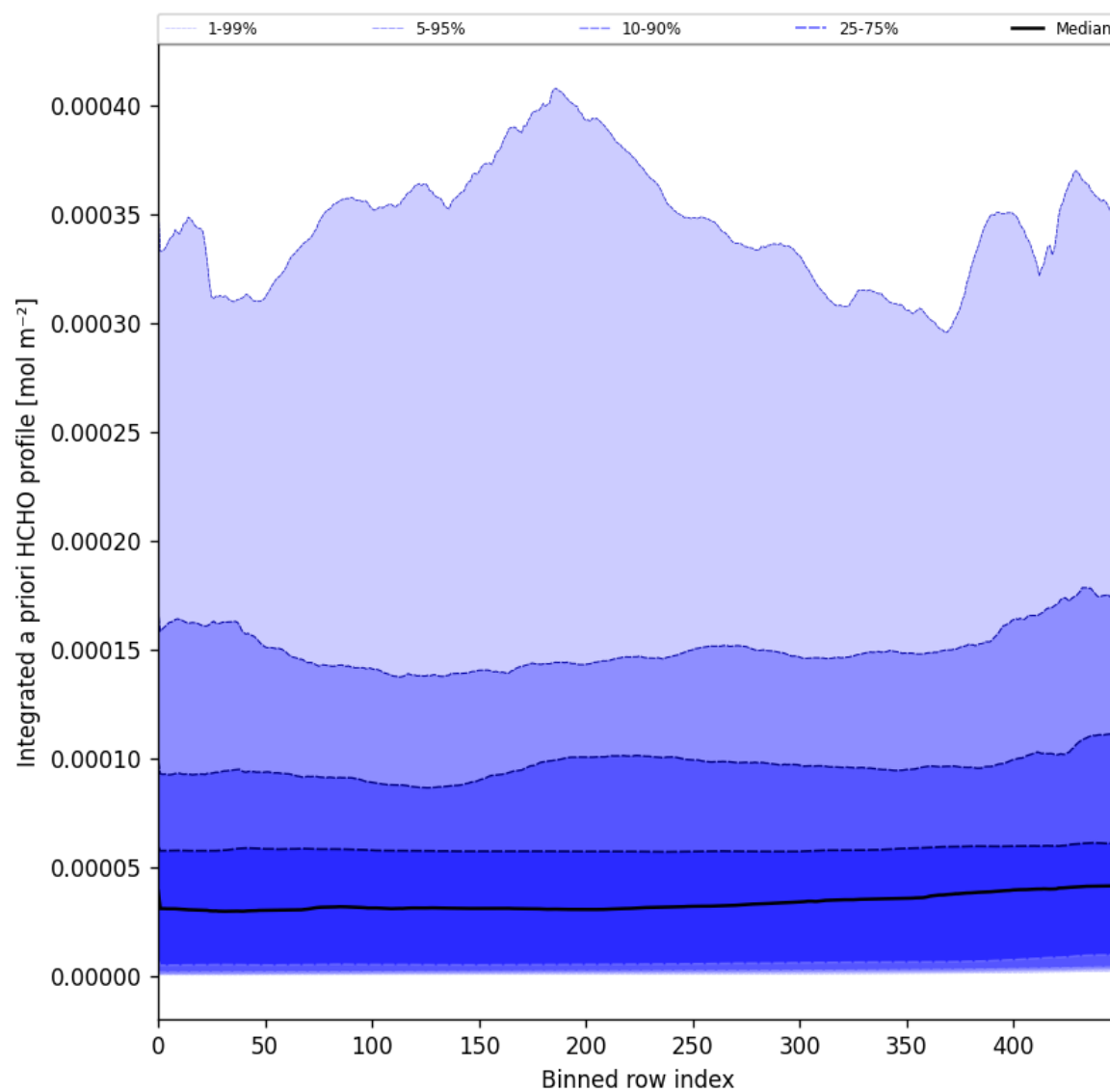
Figure 57: Along track statistics of “Integrated a priori HCHO profile” for 2025-10-02 to 2025-10-04
