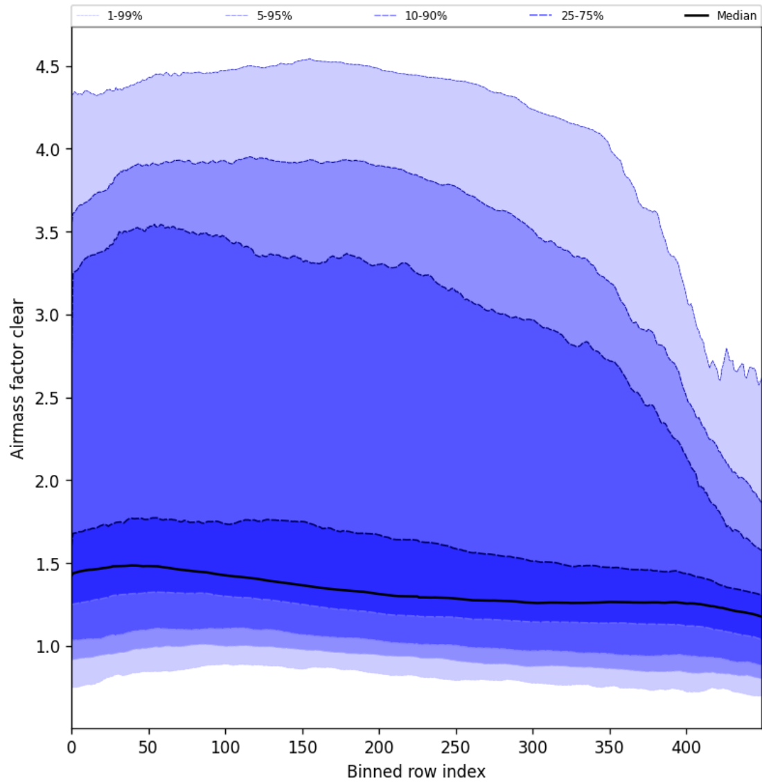
Figure 56: Along track statistics of “Air mass factor clear” for 2025-10-02 to 2025-10-04
