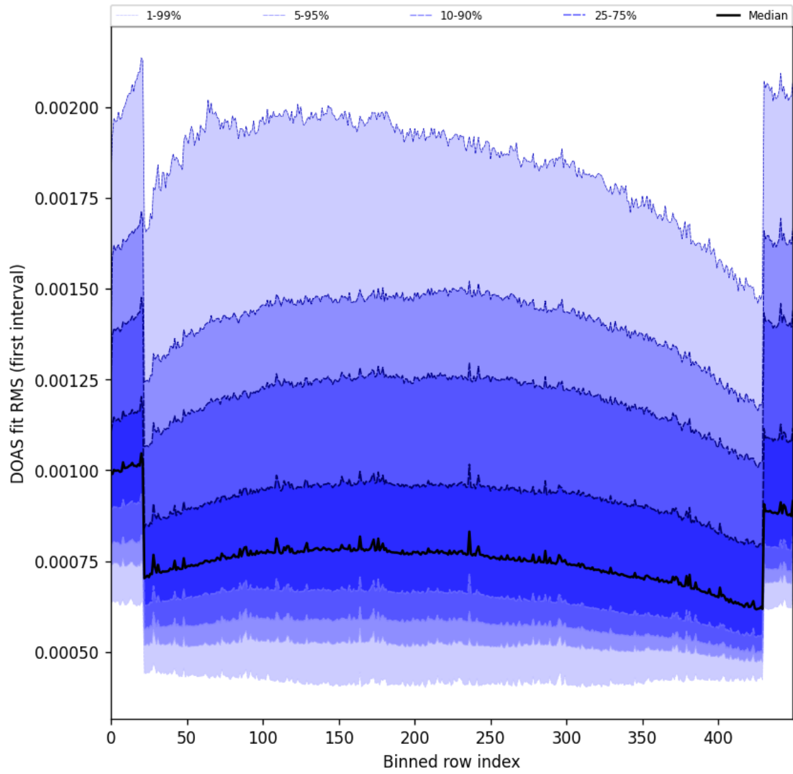
Figure 60: Along track statistics of “DOAS fit RMS (first interval)” for 2025-10-02 to 2025-10-04
