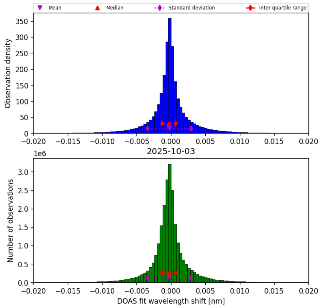
Figure 44: Histogram of “DOAS fit wavelength shift” for 2025-10-02 to 2025-10-04
