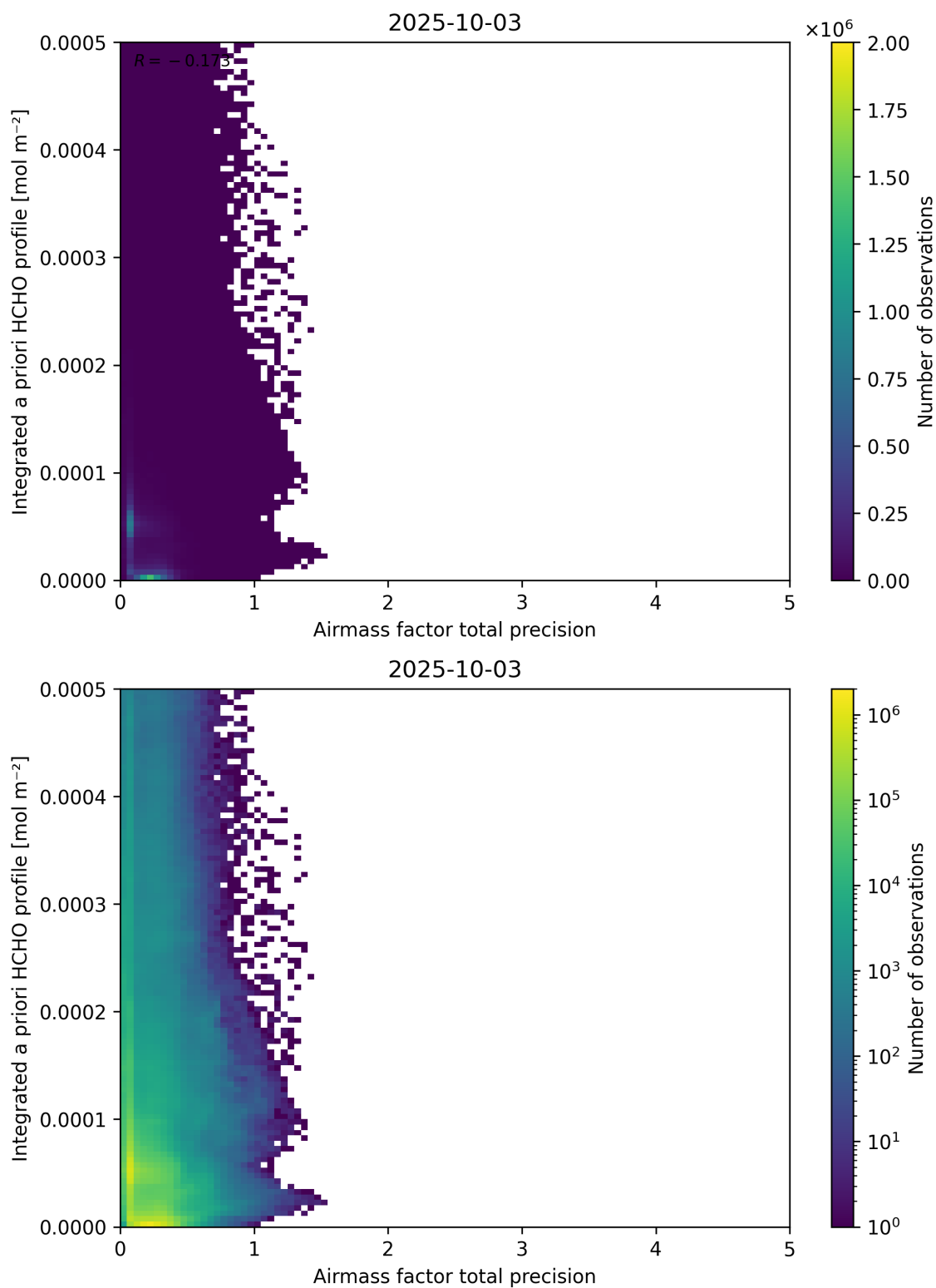
Figure 111: Scatter density plot of “Airmass factor total precision” against “Integrated a priori HCHO profile” for 2025-10-02 to 2025-10-04.
