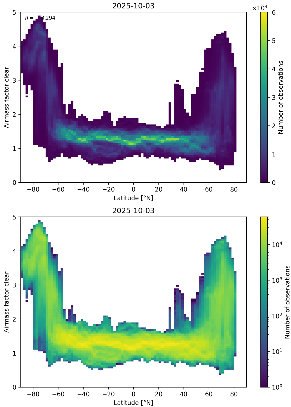
Figure 156: Scatter density plot of “Latitude” against “Airmass factor clear” for 2025-10-02 to 2025-10-04.
