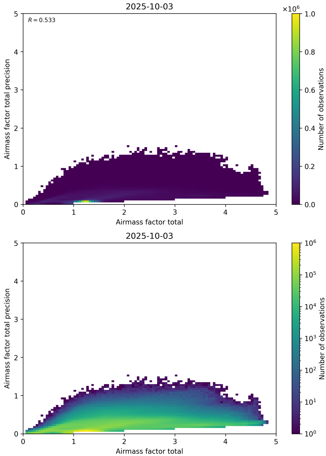
Figure 103: Scatter density plot of “Airmass factor total” against “Airmass factor total precision” for 2025-10-02 to 2025-10-04.
