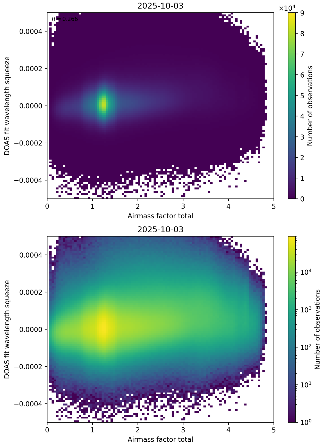
Figure 99: Scatter density plot of “Airmass factor total” against “DOAS fit wavelength squeeze” for 2025-10-02 to 2025-10-04.
