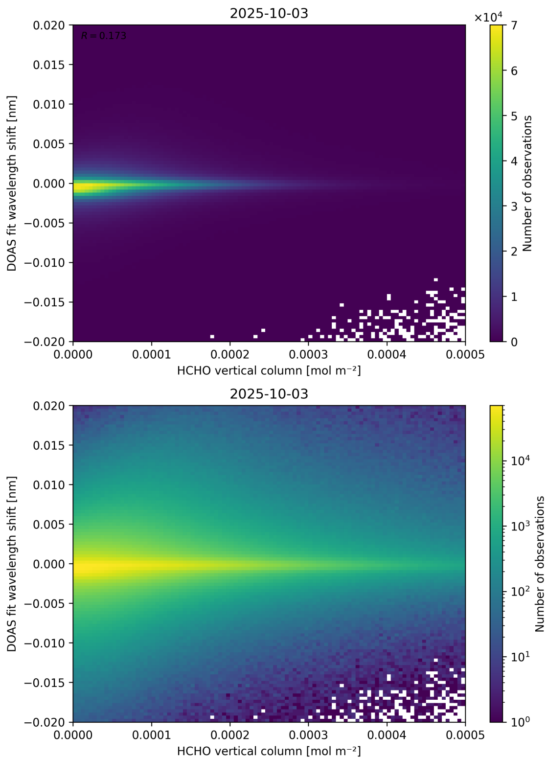
Figure 124: Scatter density plot of “HCHO vertical column” against “DOAS fit wavelength shift” for 2025-10-02 to 2025-10-04.
