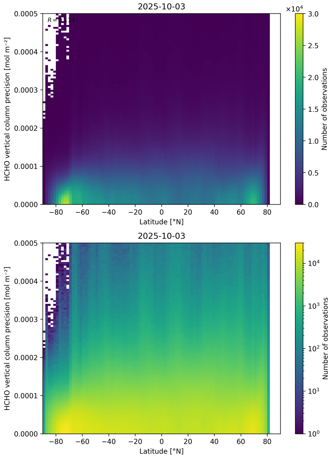
Figure 165: Scatter density plot of “Latitude” against “HCHO vertical column precision” for 2025-10-02 to 2025-10-04.
