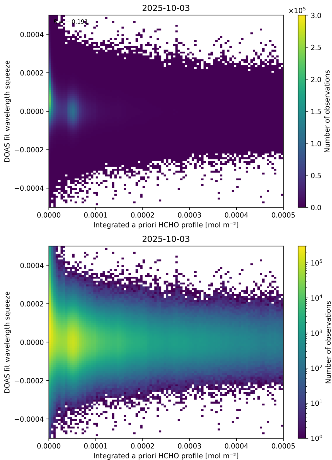
Figure 150: Scatter density plot of “Integrated a priori HCHO profile” against “DOAS fit wavelength squeeze” for 2025-10-02 to 2025-10-04.
