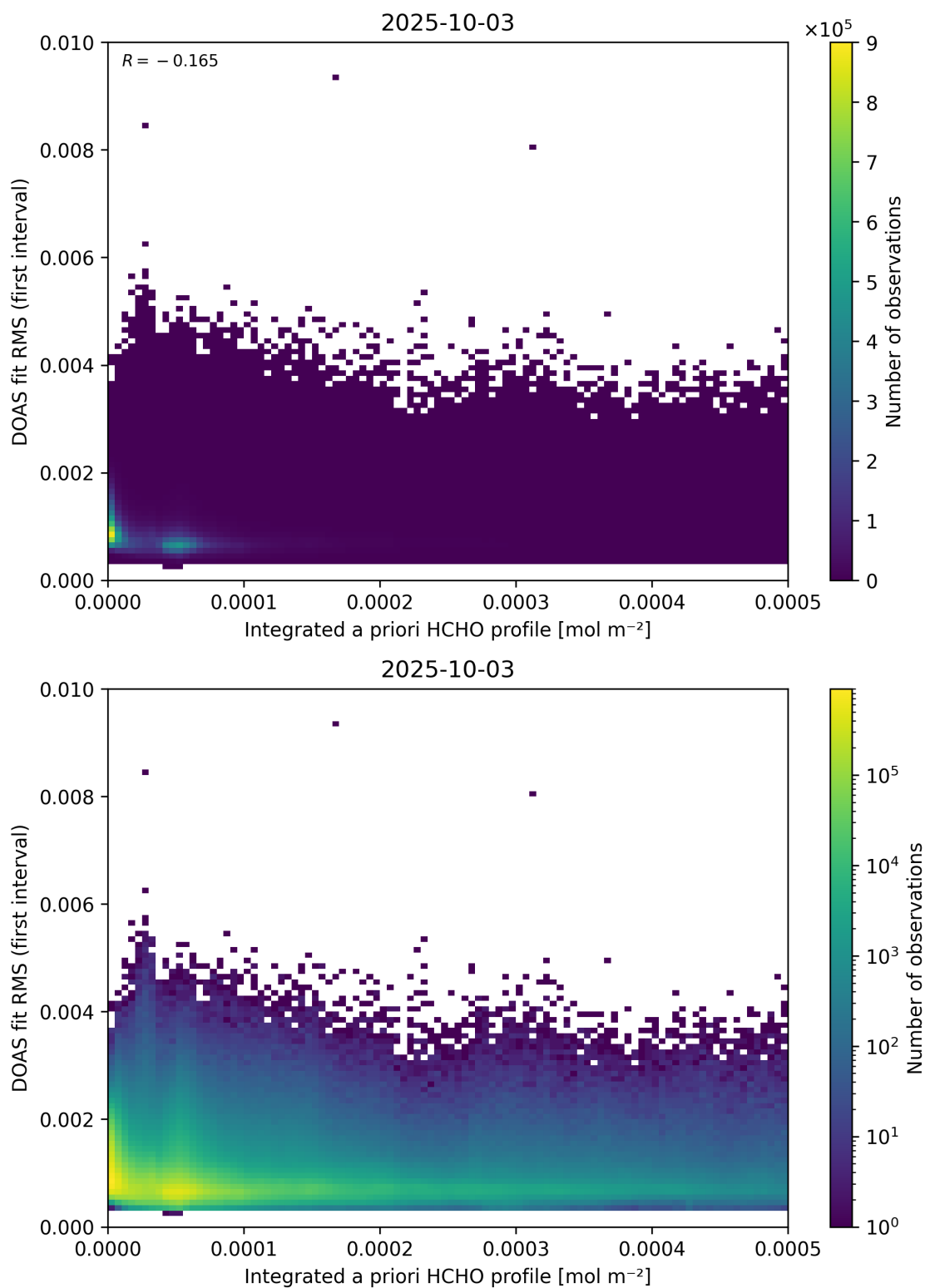
Figure 148: Scatter density plot of “Integrated a priori HCHO profile” against “DOAS fit RMS (first interval)” for 2025-10-02 to 2025-10-04.
