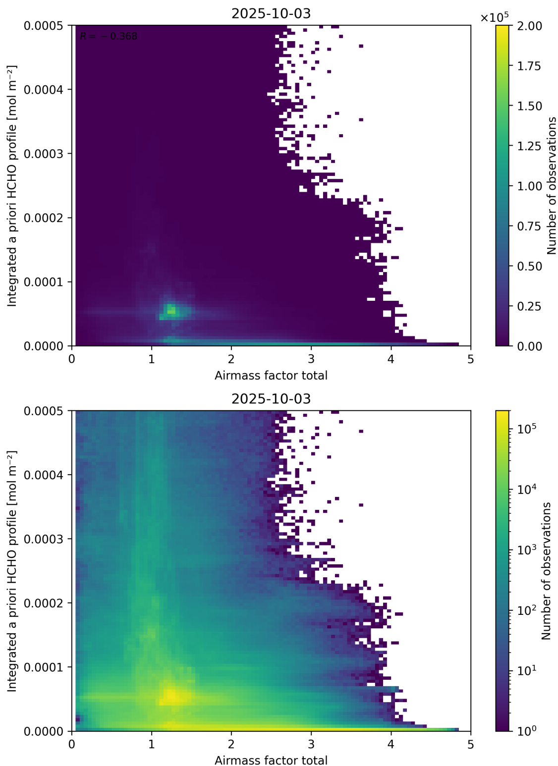
Figure 104: Scatter density plot of “Airmass factor total” against “Integrated a priori HCHO profile” for 2025-10-02 to 2025-10-04.
