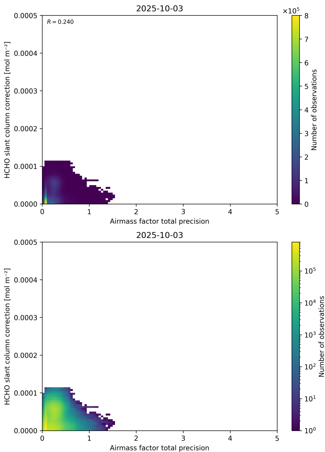
Figure 110: Scatter density plot of “Airmass factor total precision” against “HCHO slant column correction” for 2025-10-02 to 2025-10-04.
