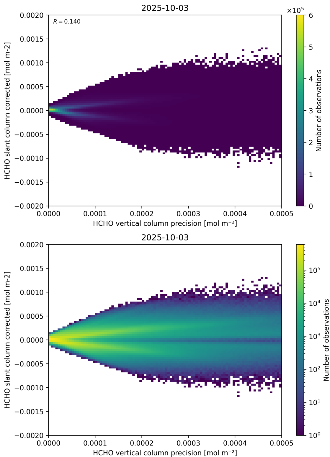
Figure 140: Scatter density plot of “HCHO vertical column precision” against “HCHO slant column corrected” for 2025-10-02 to 2025-10-04.
