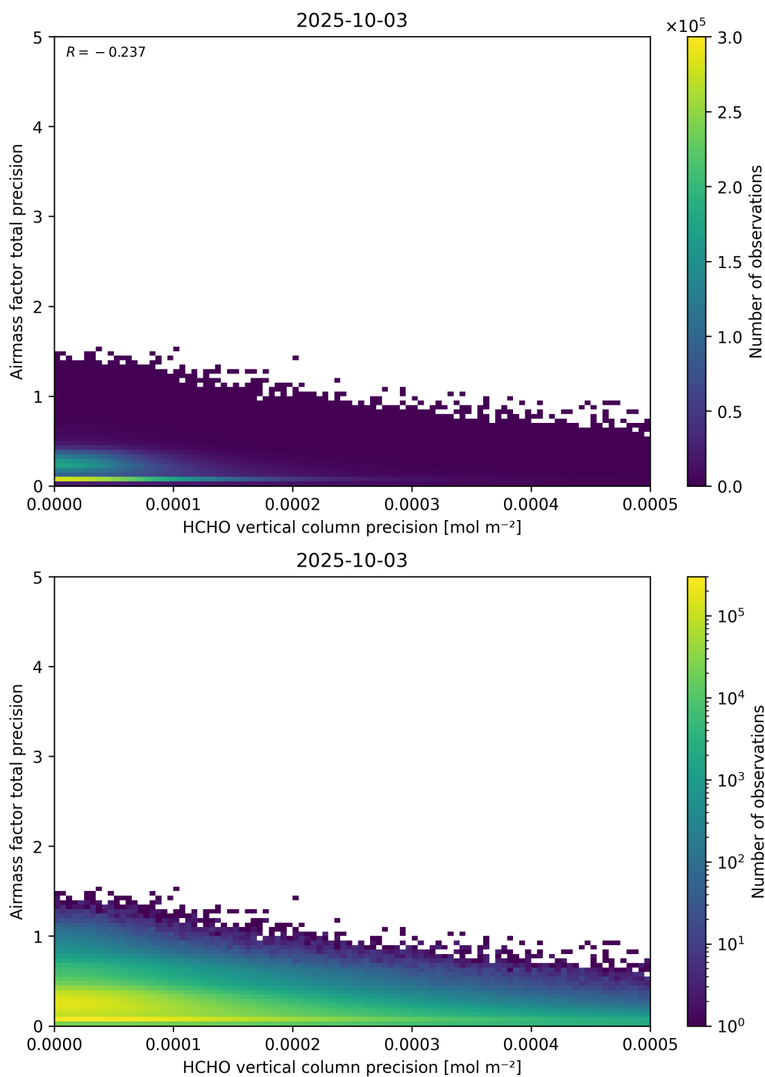
Figure 145: Scatter density plot of “HCHO vertical column precision” against “Airmass factor total precision” for 2025-10-02 to 2025-10-04.
