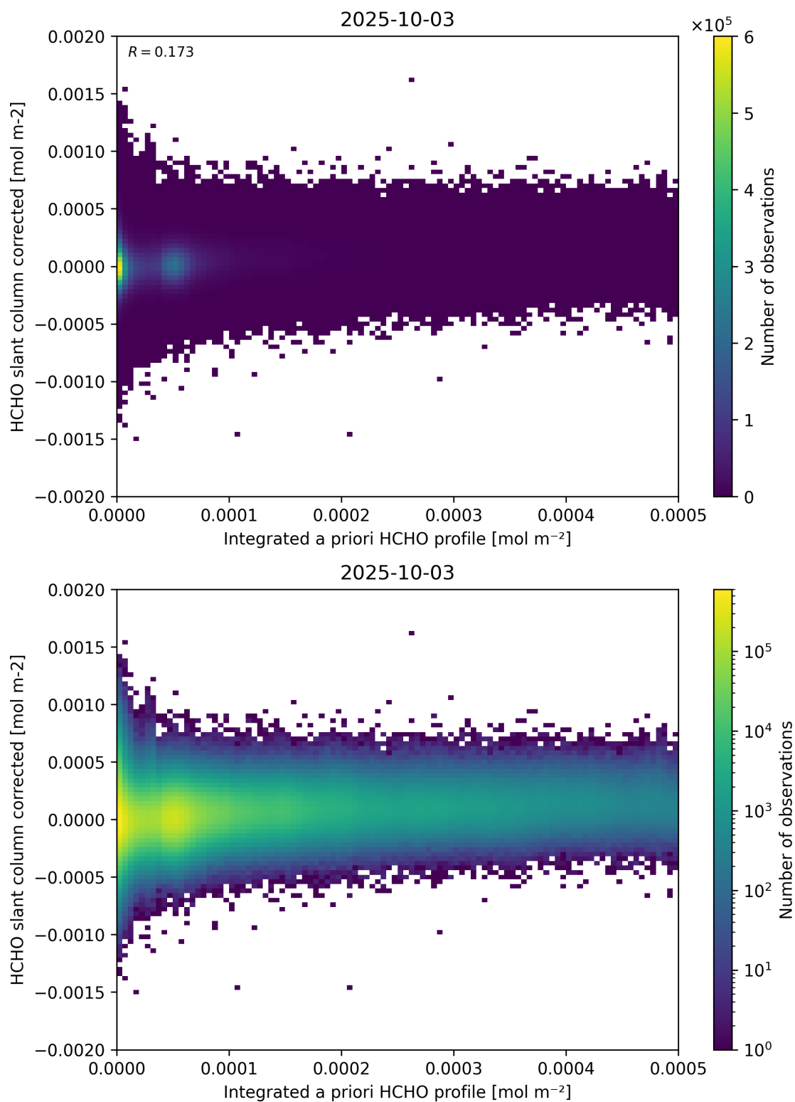
Figure 151: Scatter density plot of “Integrated a priori HCHO profile” against “HCHO slant column corrected” for 2025-10-02 to 2025-10-04.
