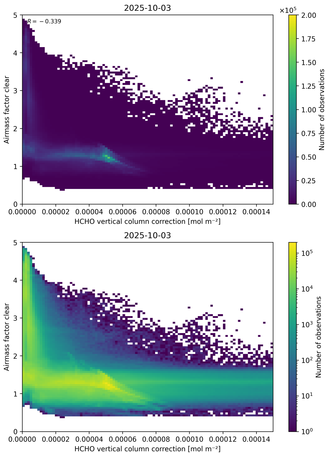
Figure 115: Scatter density plot of “HCHO vertical column correction” against “Airmass factor clear” for 2025-10-02 to 2025-10-04.
