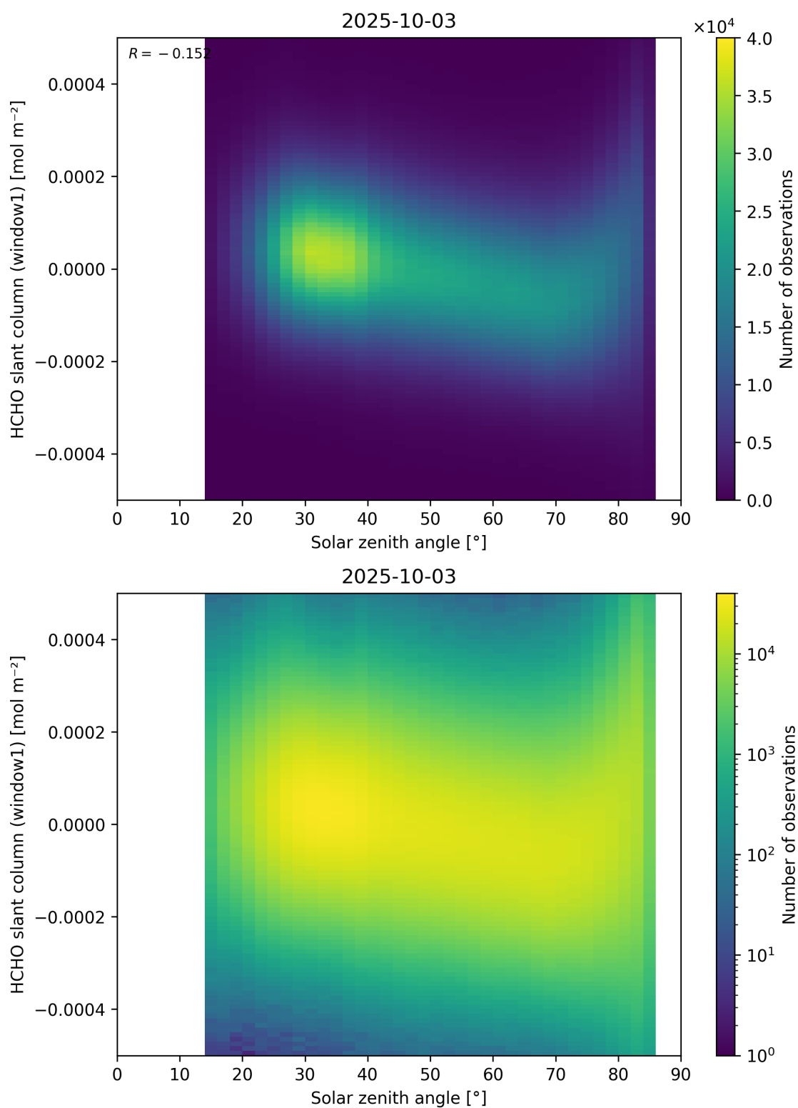
Figure 173: Scatter density plot of “Solar zenith angle” against “HCHO slant column (window1)” for 2025-10-02 to 2025-10-04.
