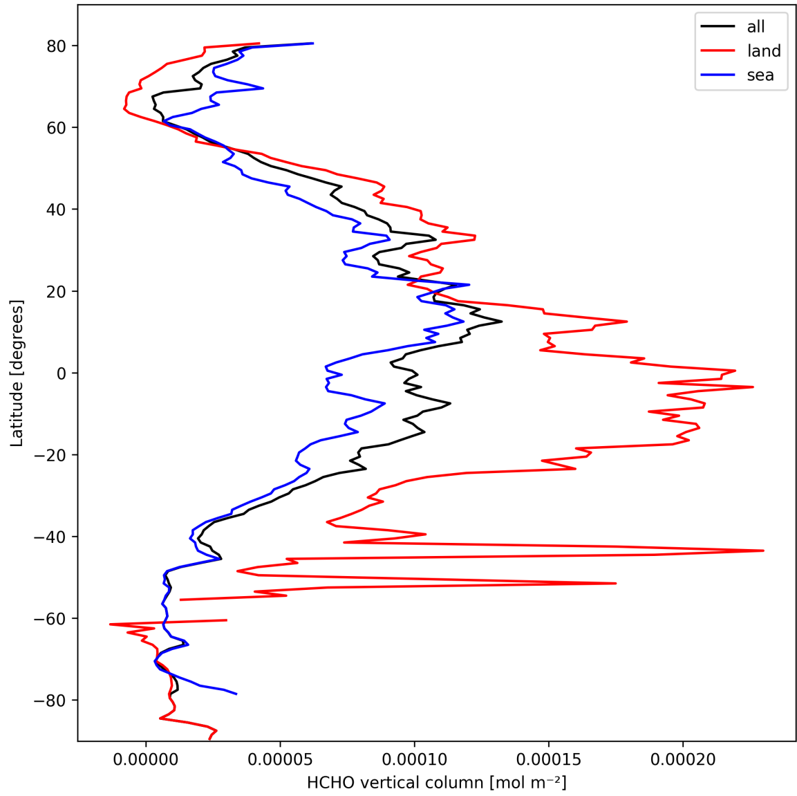
Figure 21: Zonal average of “HCHO vertical column” for 2025-10-02 to 2025-10-04.
