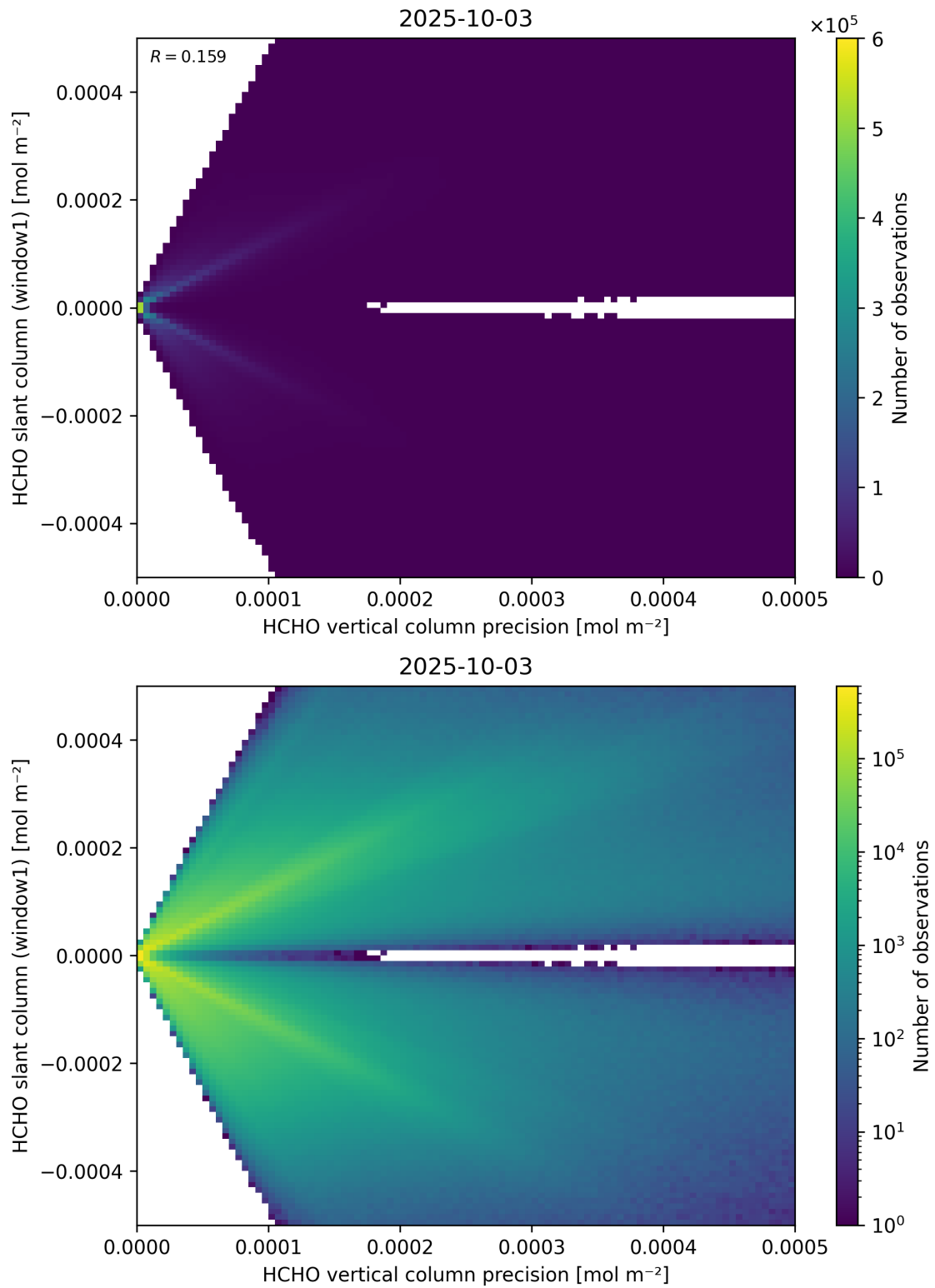
Figure 142: Scatter density plot of “HCHO vertical column precision” against “HCHO slant column (window1)” for 2025-10-02 to 2025-10-04.
