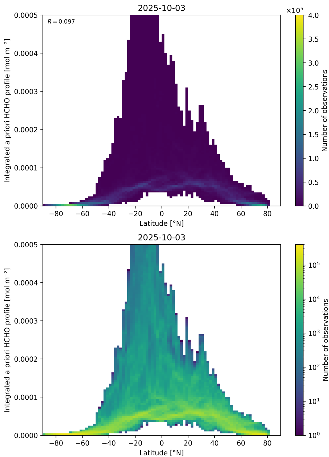
Figure 166: Scatter density plot of “Latitude” against “Integrated a priori HCHO profile” for 2025-10-02 to 2025-10-04.
