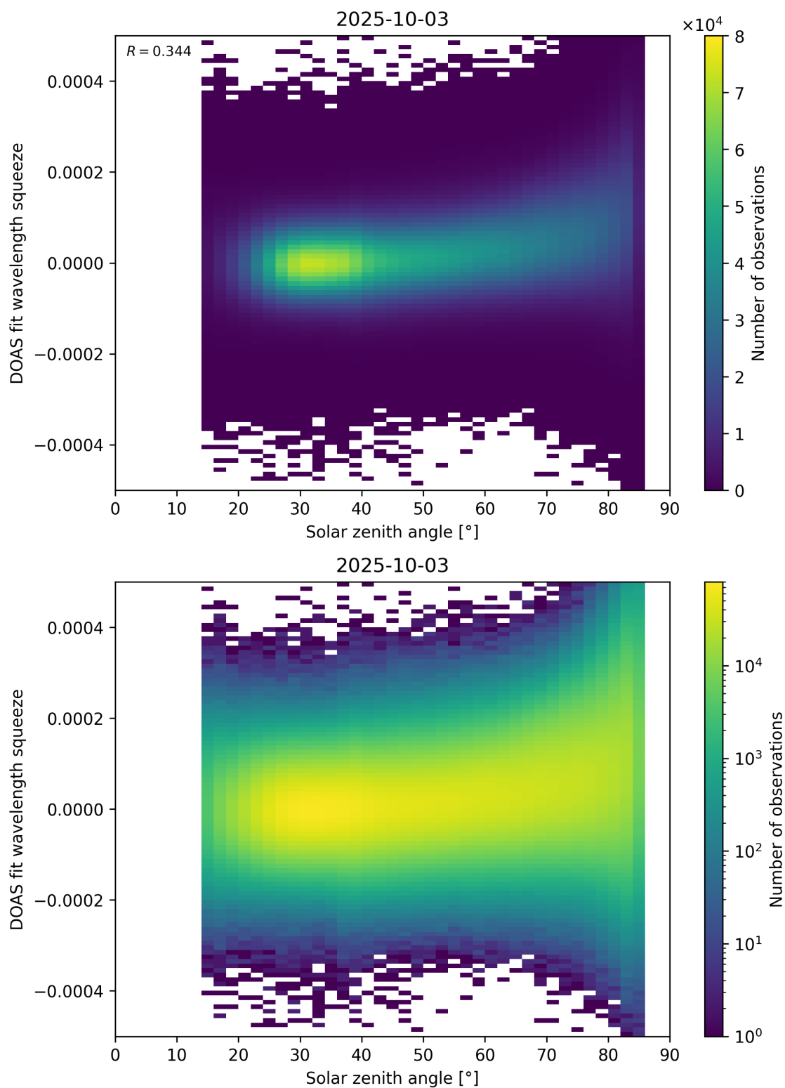
Figure 169: Scatter density plot of “Solar zenith angle” against “DOAS fit wavelength squeeze” for 2025-10-02 to 2025-10-04.
