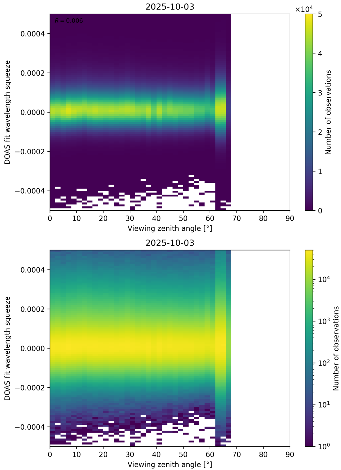
Figure 184: Scatter density plot of “Viewing zenith angle” against “DOAS fit wavelength squeeze” for 2025-10-02 to 2025-10-04.
