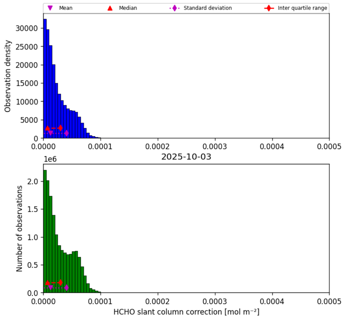
Figure 47: Histogram of “HCHO slant column correction” for 2025-10-02 to 2025-10-04
