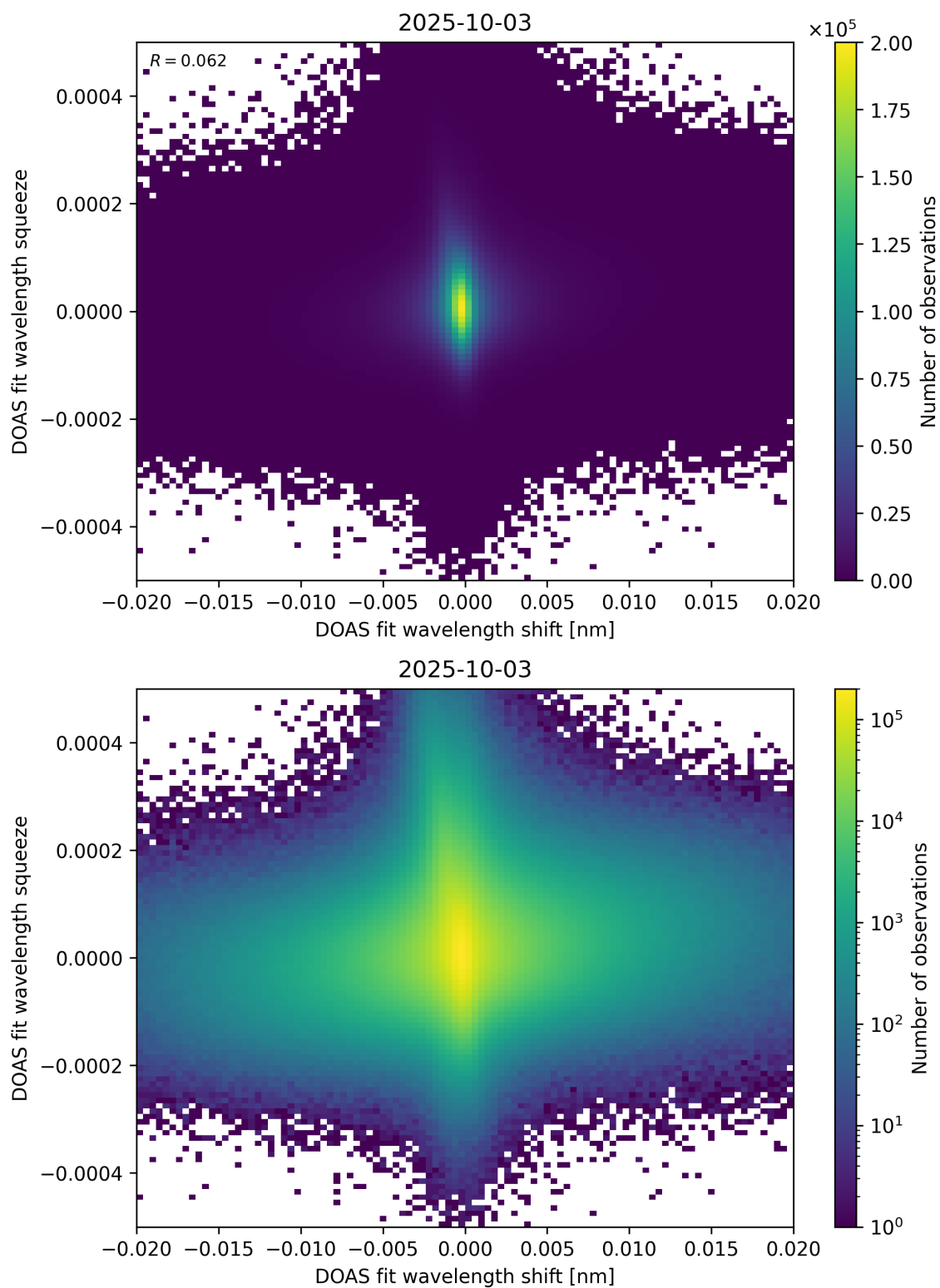
Figure 65: Scatter density plot of “DOAS fit wavelength shift” against “DOAS fit wavelength squeeze” for 2025-10-02 to 2025-10-04.
