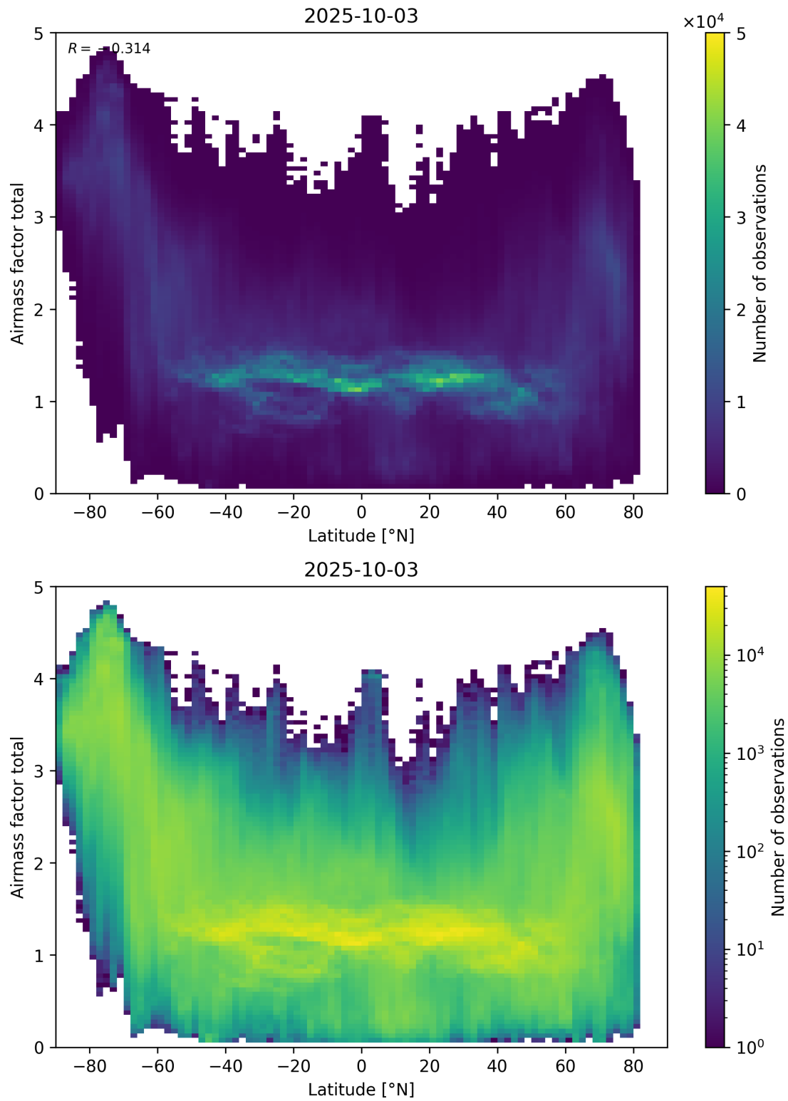
Figure 161: Scatter density plot of “Latitude” against “Airmass factor total” for 2025-10-02 to 2025-10-04.
