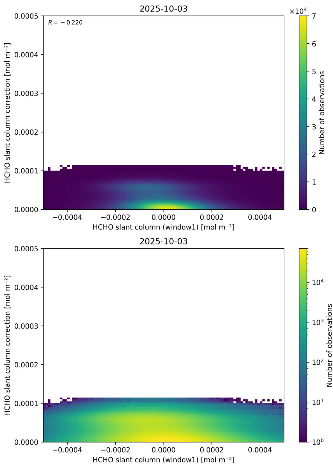
Figure 83: Scatter density plot of “HCHO slant column (window1)” against “HCHO slant column correction” for 2025-10-02 to 2025-10-04.
