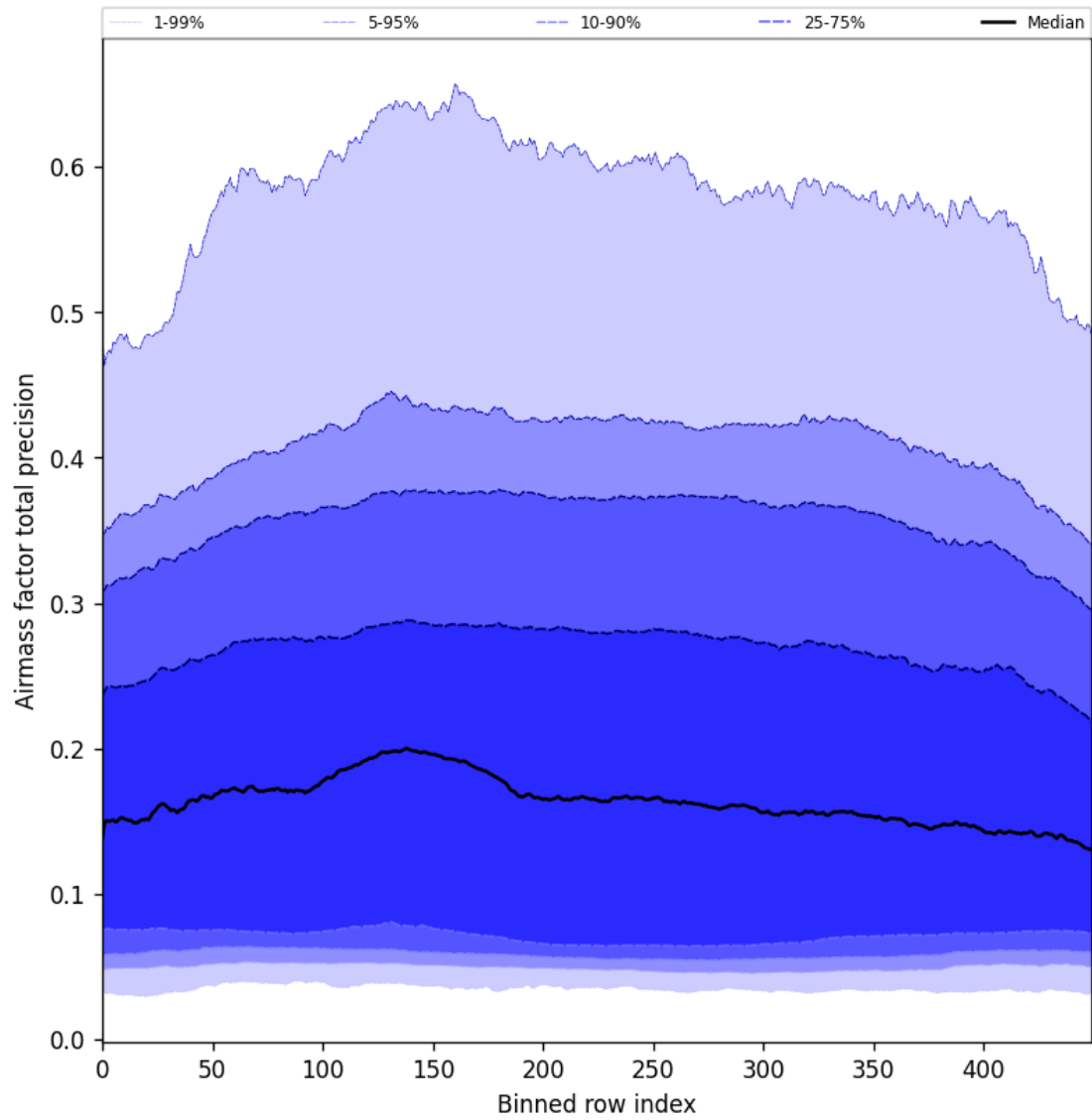
Figure 55: Along track statistics of “Airmass factor total precision” for 2025-10-02 to 2025-10-04
