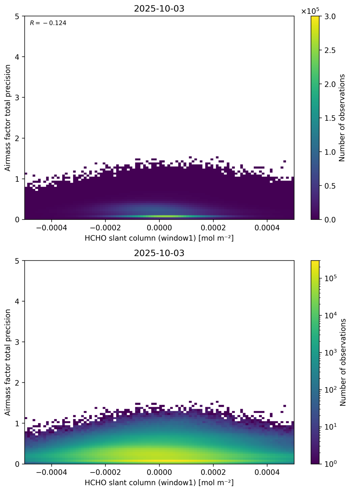
Figure 86: Scatter density plot of “HCHO slant column (window1)” against “Airmass factor total precision” for 2025-10-02 to 2025-10-04.
