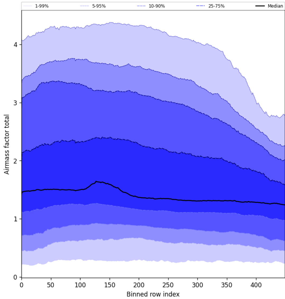
Figure 54: Along track statistics of “Airmass factor total” for 2025-10-02 to 2025-10-04
