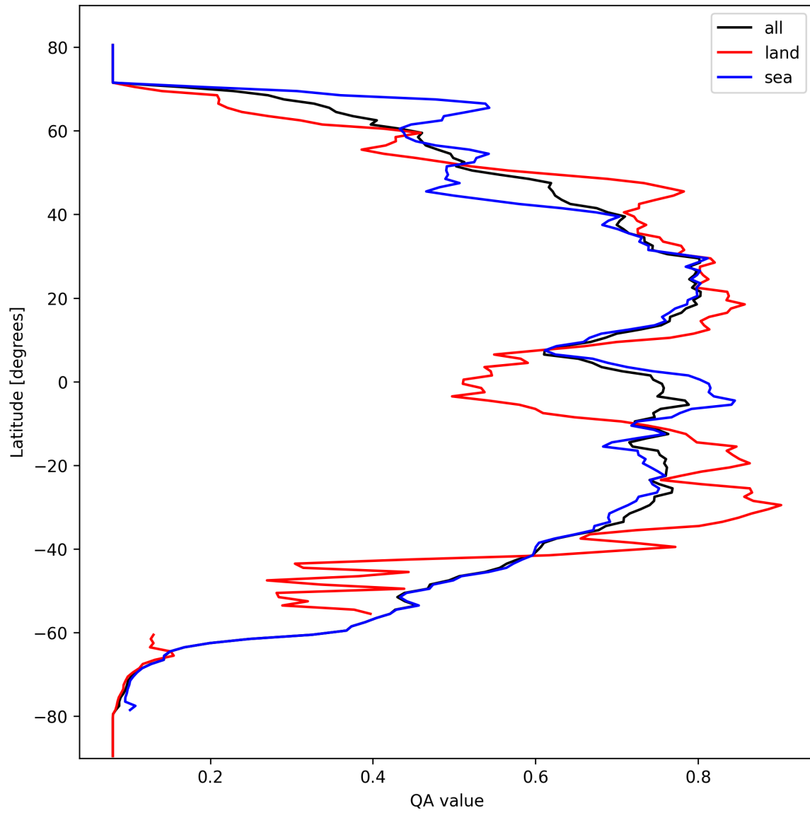
Figure 20: Zonal average of “QA value” for 2025-10-02 to 2025-10-04.
