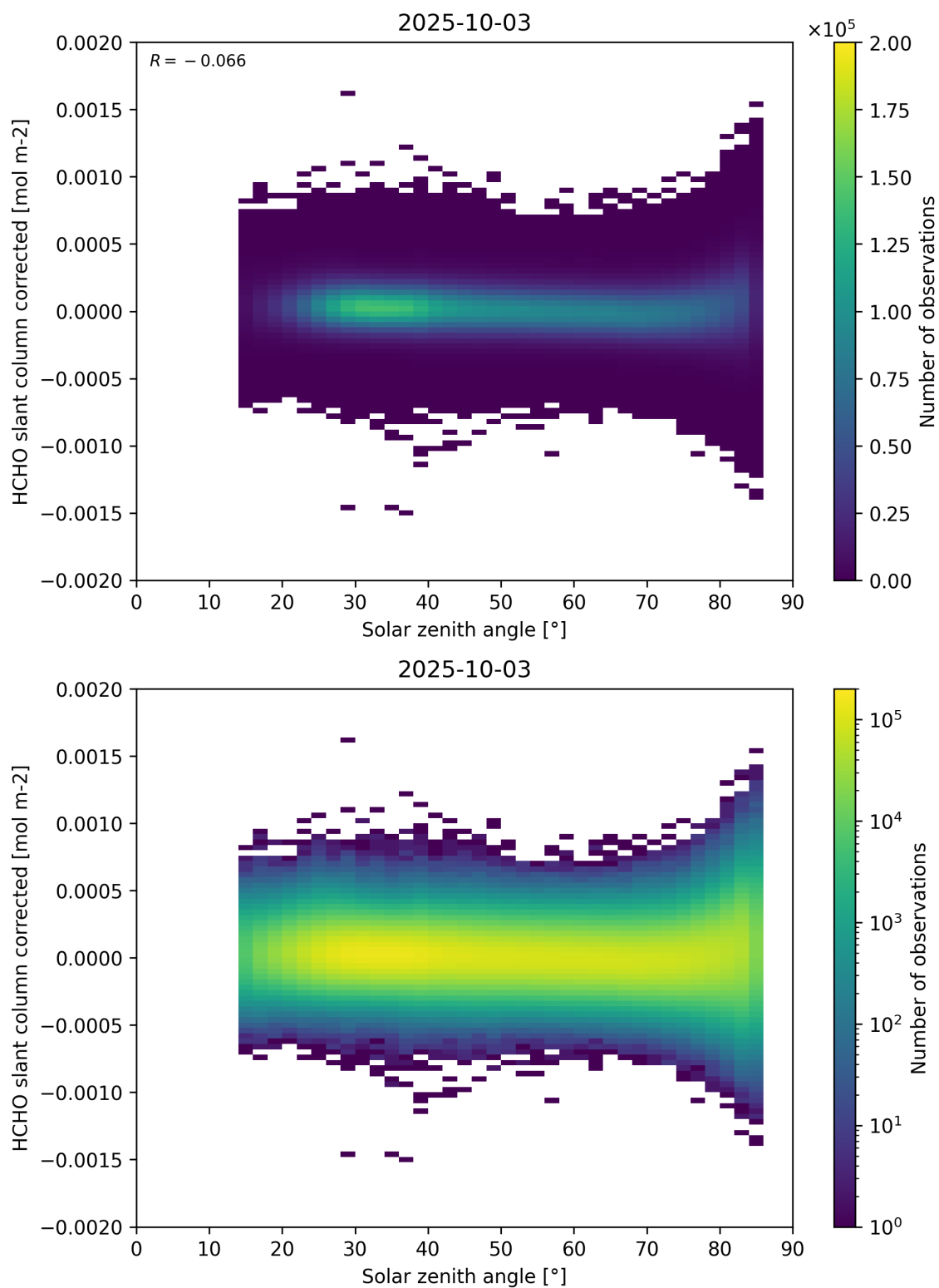
Figure 171: Scatter density plot of “Solar zenith angle” against “HCHO slant column corrected” for 2025-10-02 to 2025-10-04.
