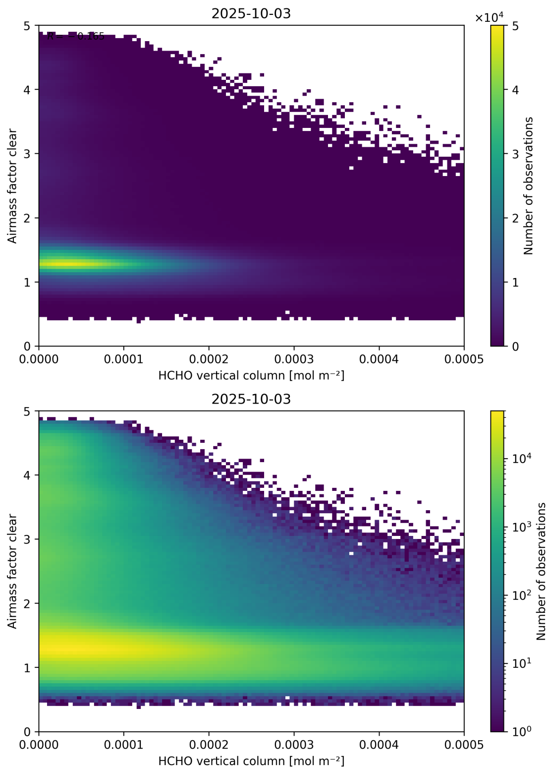
Figure 126: Scatter density plot of “HCHO vertical column” against “Airmass factor clear” for 2025-10-02 to 2025-10-04.
