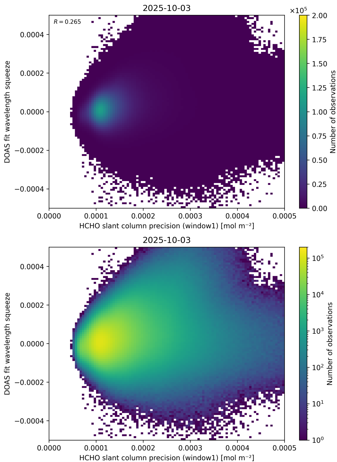
Figure 90: Scatter density plot of “HCHO slant column precision (window1)” against “DOAS fit wavelength squeeze” for 2025-10-02 to 2025-10-04.
