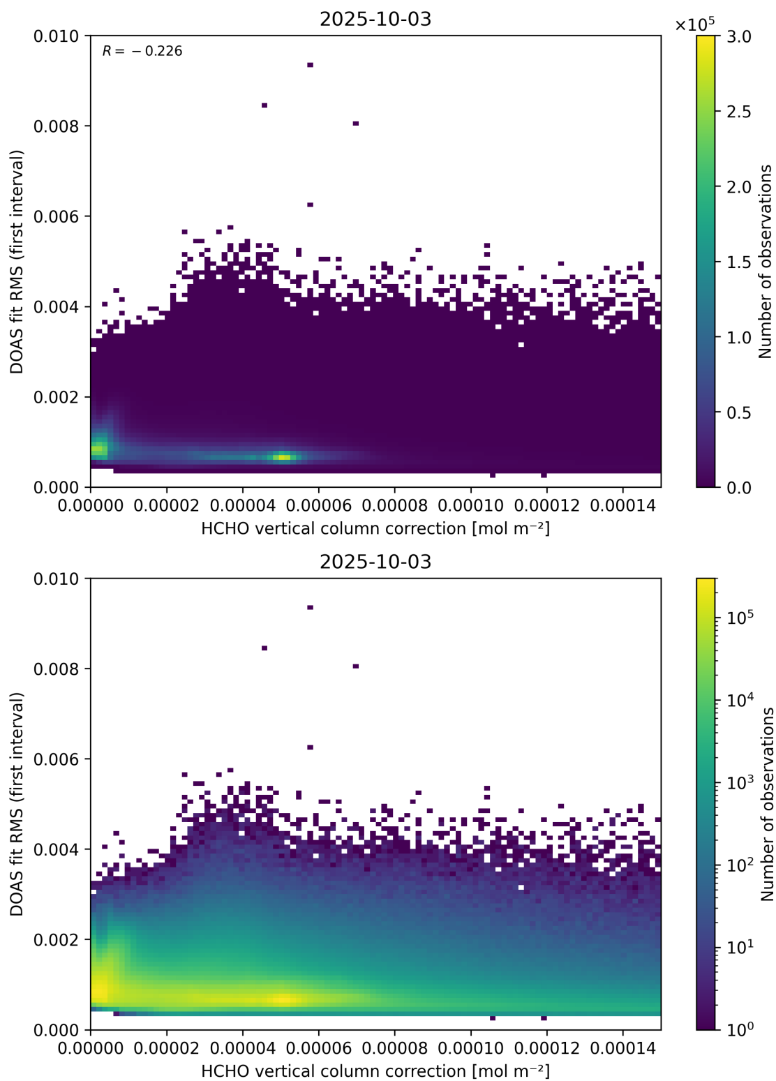
Figure 112: Scatter density plot of “HCHO vertical column correction” against “DOAS fit RMS (first interval)” for 2025-10-02 to 2025-10-04.
