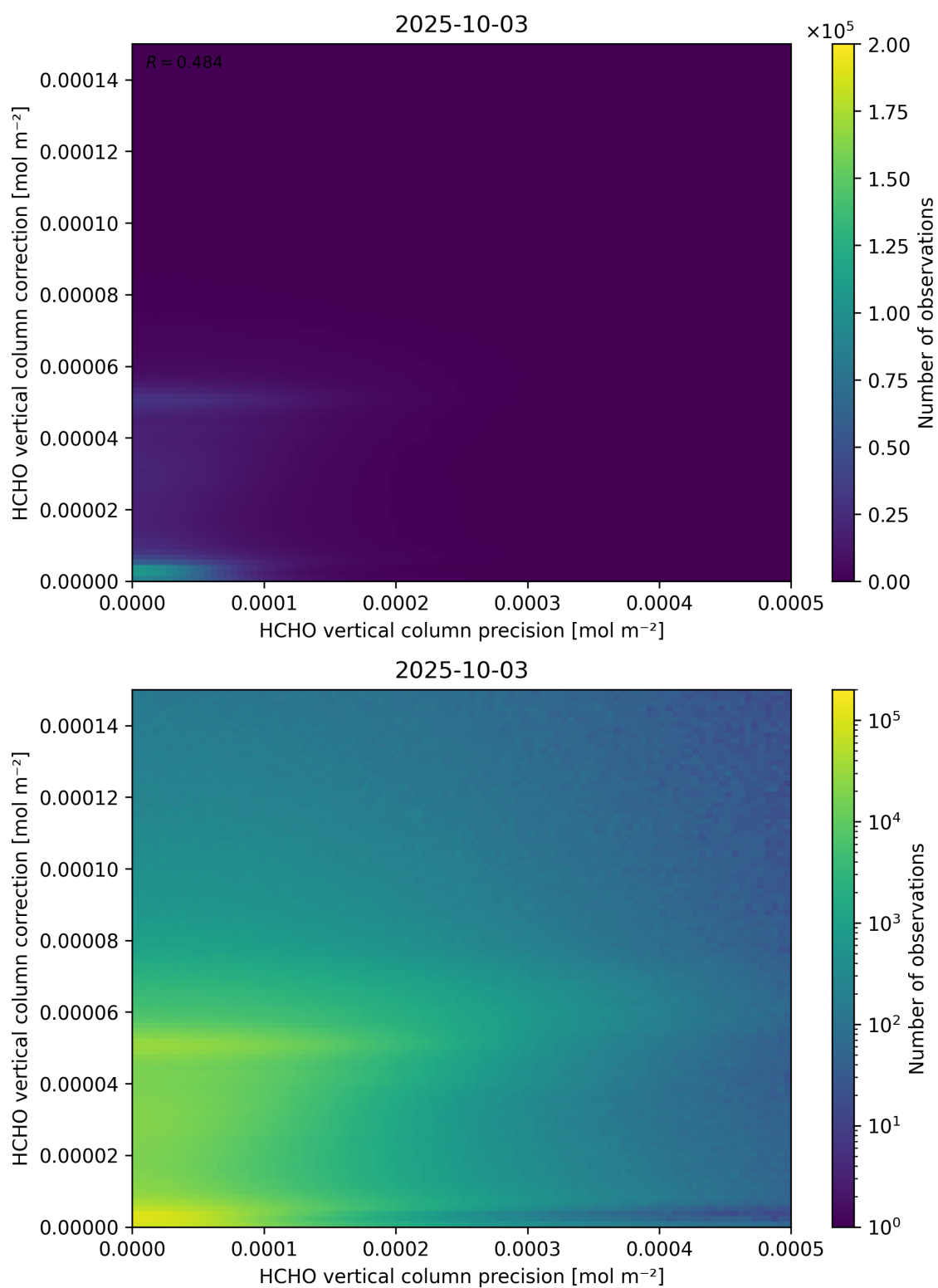
Figure 146: Scatter density plot of “HCHO vertical column precision” against “HCHO vertical column correction” for 2025-10-02 to 2025-10-04.
