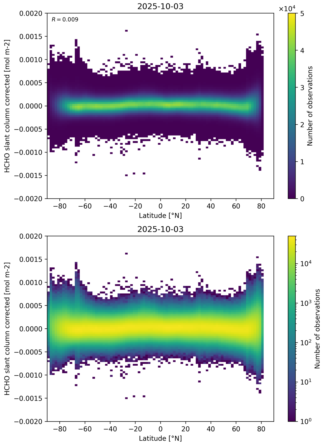
Figure 157: Scatter density plot of “Latitude” against “HCHO slant column corrected” for 2025-10-02 to 2025-10-04.
