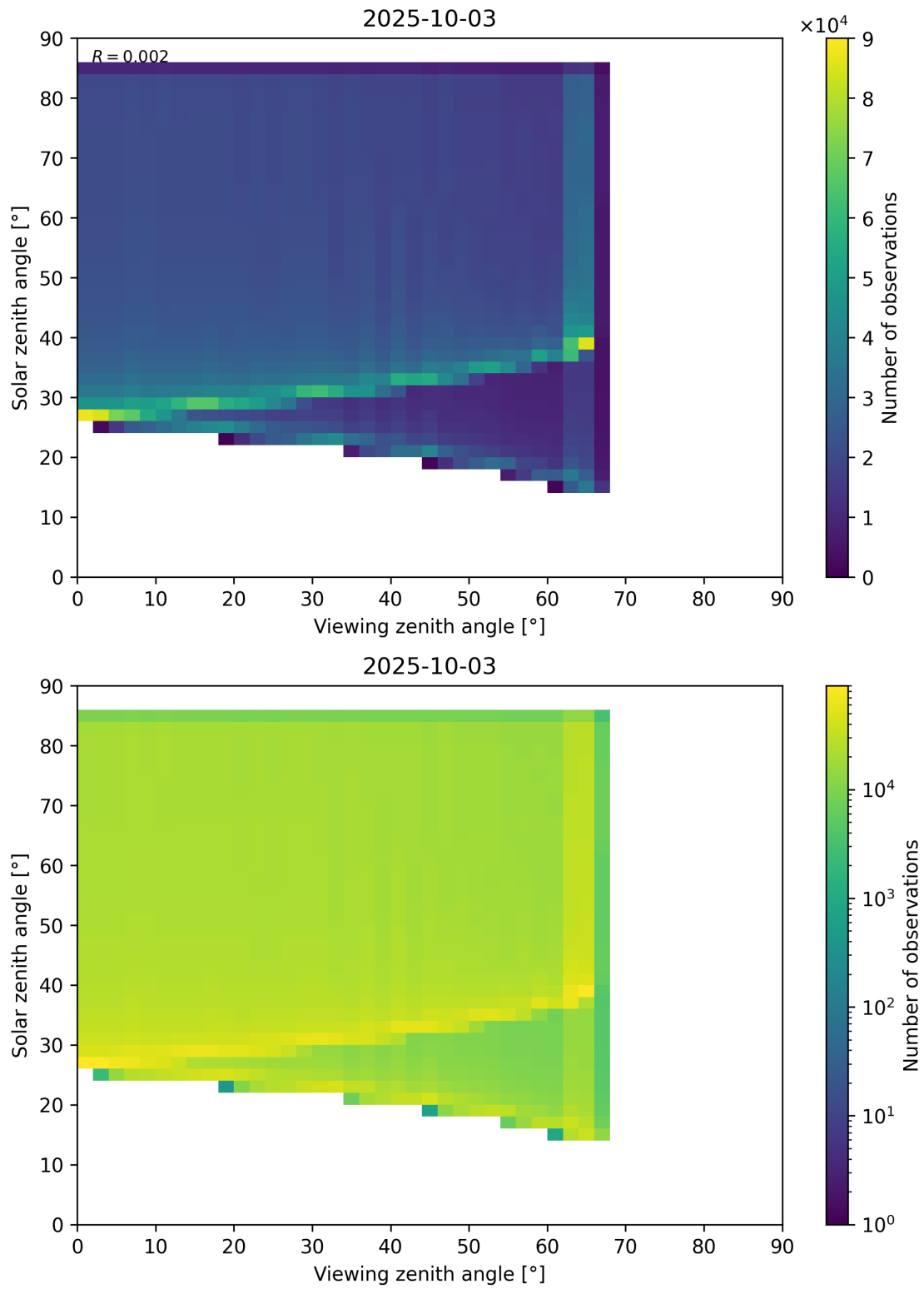
Figure 197: Scatter density plot of “Viewing zenith angle” against “Solar zenith angle” for 2025-10-02 to 2025-10-04.
