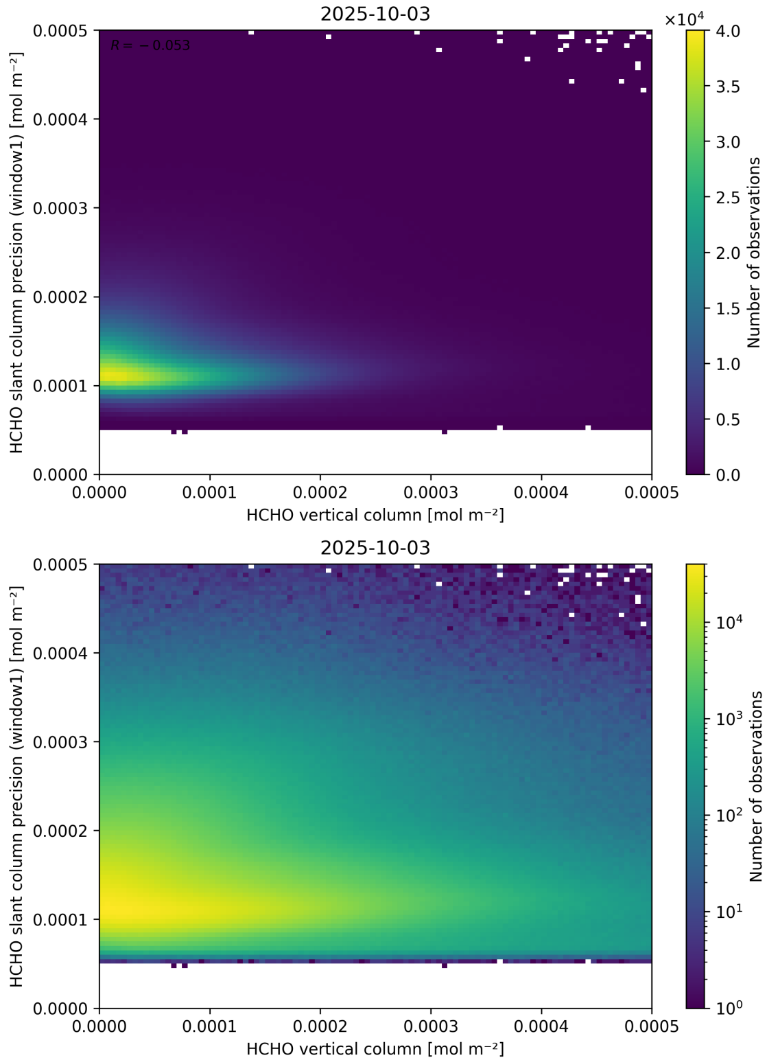
Figure 130: Scatter density plot of “HCHO vertical column” against “HCHO slant column precision (window1)” for 2025-10-02 to 2025-10-04.
