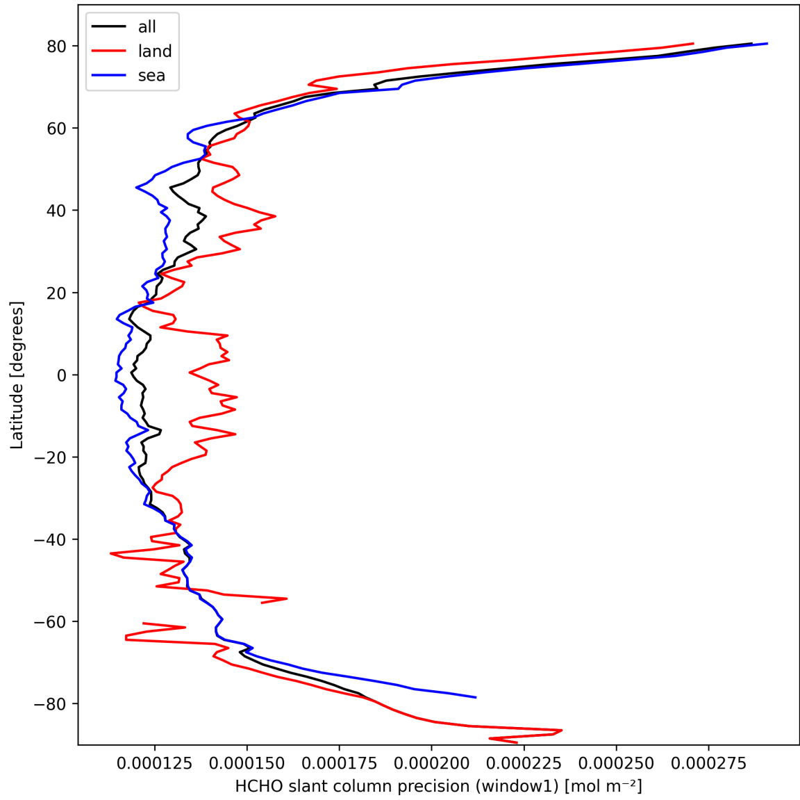
Figure 25: Zonal average of “HCHO slant column precision (window1)” for 2025-10-02 to 2025-10-04.
