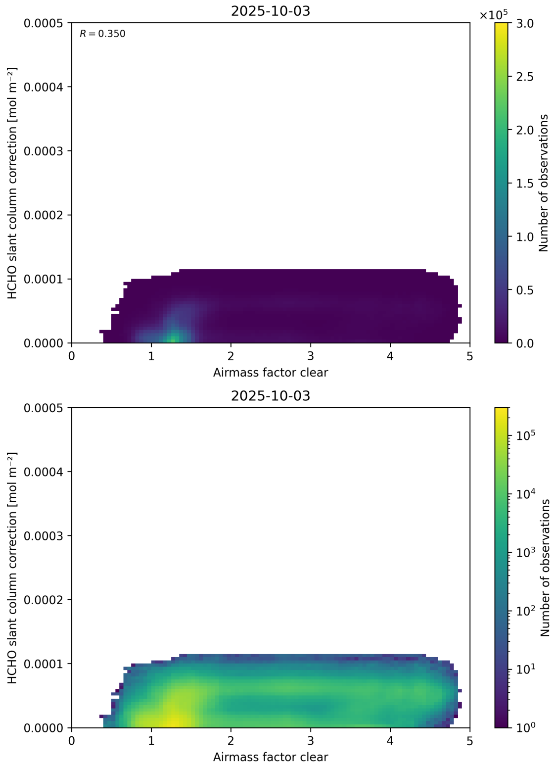
Figure 75: Scatter density plot of “Airmass factor clear” against “HCHO slant column correction” for 2025-10-02 to 2025-10-04.
