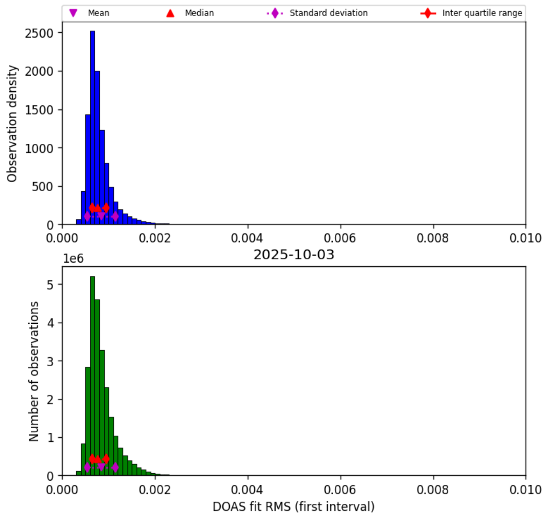
Figure 46: Histogram of “DOAS fit RMS (first interval)” for 2025-10-02 to 2025-10-04
