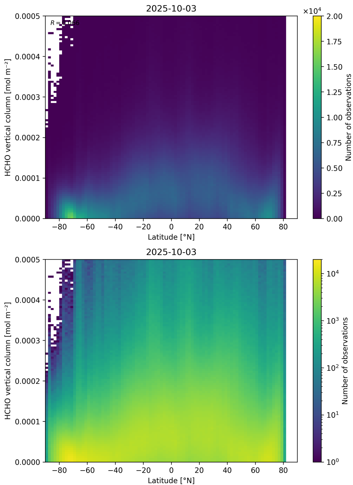
Figure 163: Scatter density plot of “Latitude” against “HCHO vertical column” for 2025-10-02 to 2025-10-04.
