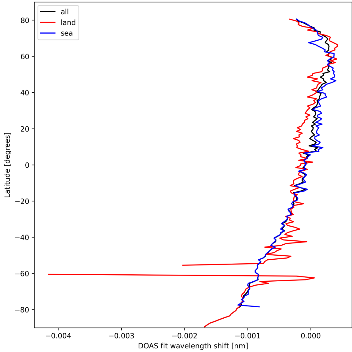
Figure 30: Zonal average of “DOAS fit wavelength shift” for 2025-10-02 to 2025-10-04.
