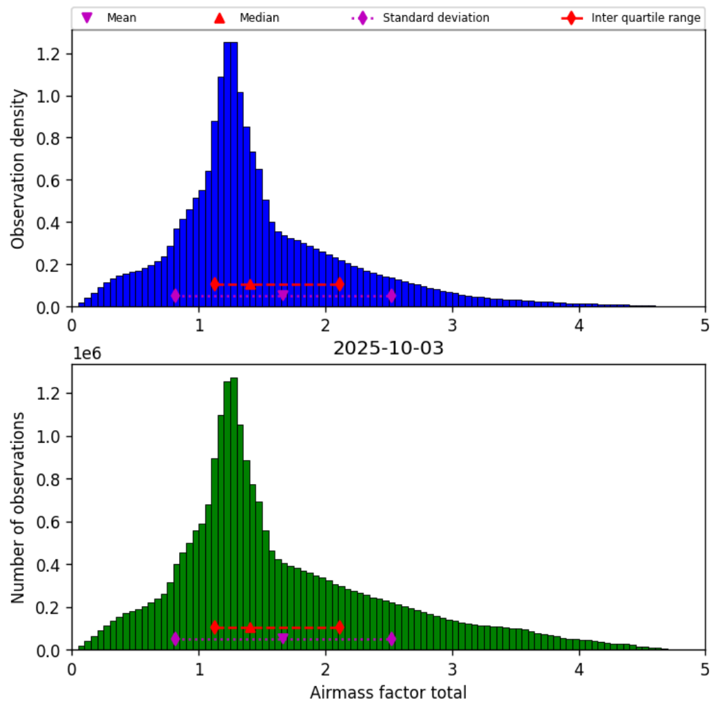
Figure 40: Histogram of “Airmass factor total” for 2025-10-02 to 2025-10-04
