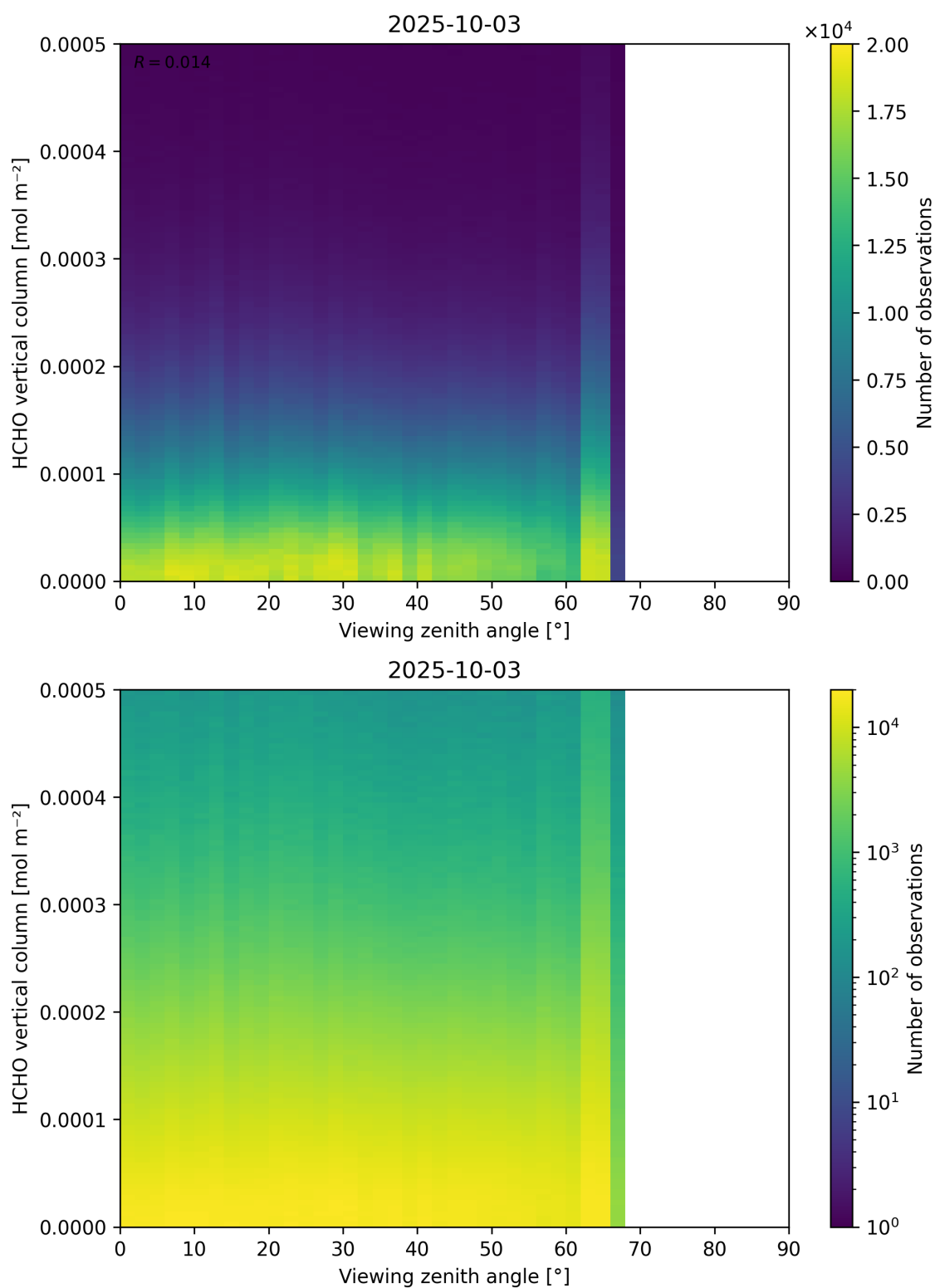
Figure 192: Scatter density plot of “Viewing zenith angle” against “HCHO vertical column” for 2025-10-02 to 2025-10-04.
