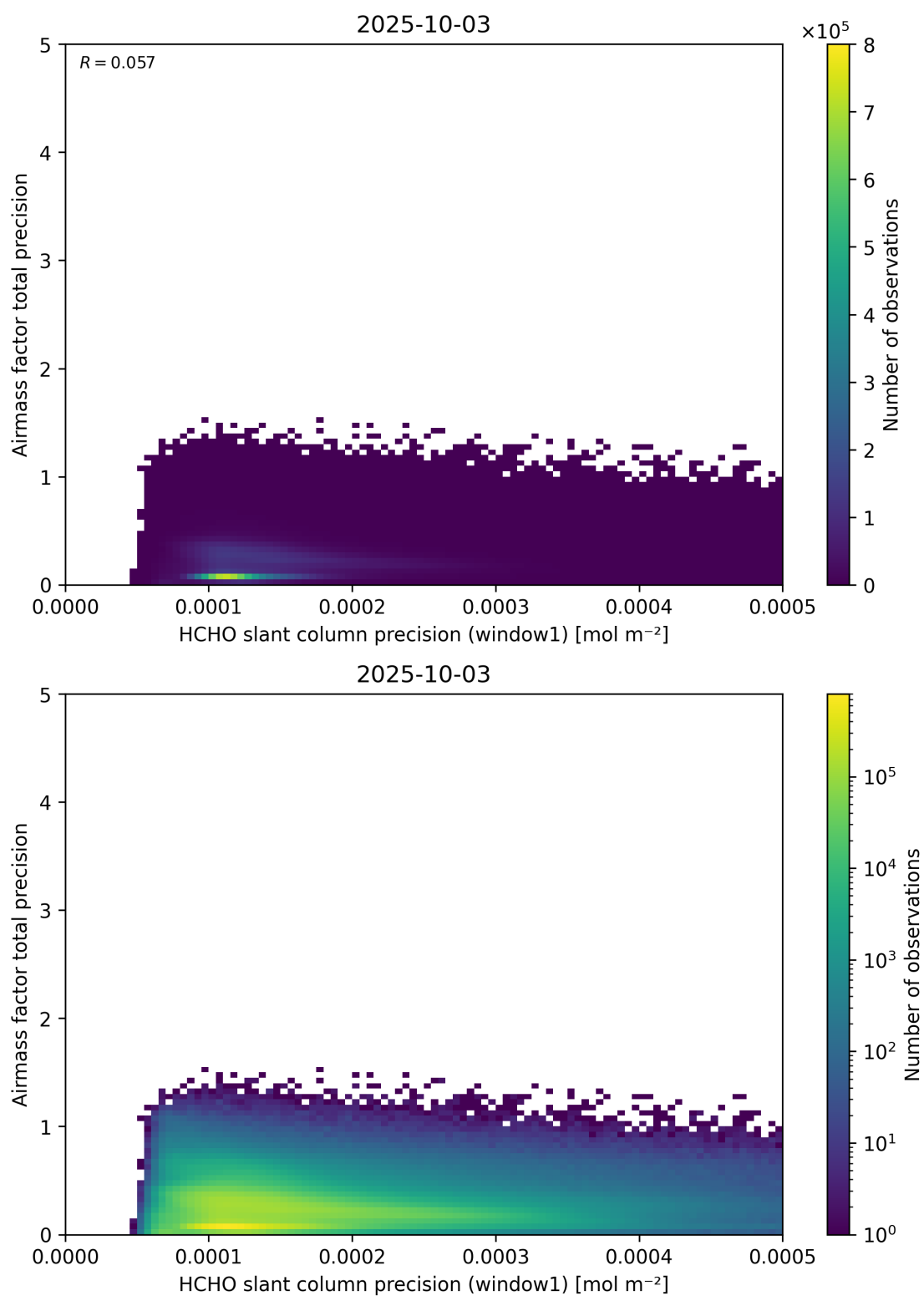
Figure 95: Scatter density plot of “HCHO slant column precision (window1)” against “Airmass factor total precision” for 2025-10-02 to 2025-10-04.
