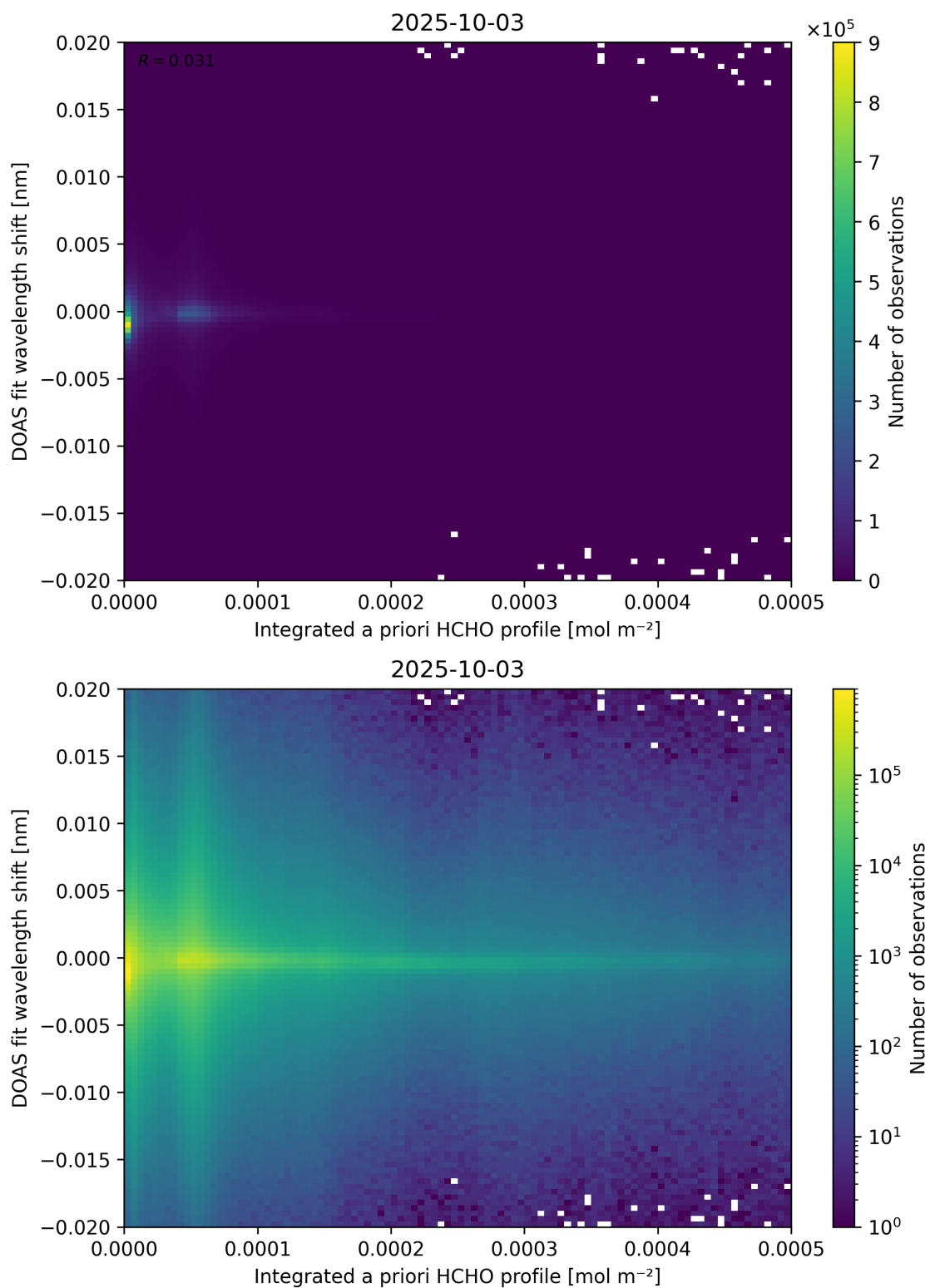
Figure 149: Scatter density plot of “Integrated a priori HCHO profile” against “DOAS fit wavelength shift” for 2025-10-02 to 2025-10-04.
