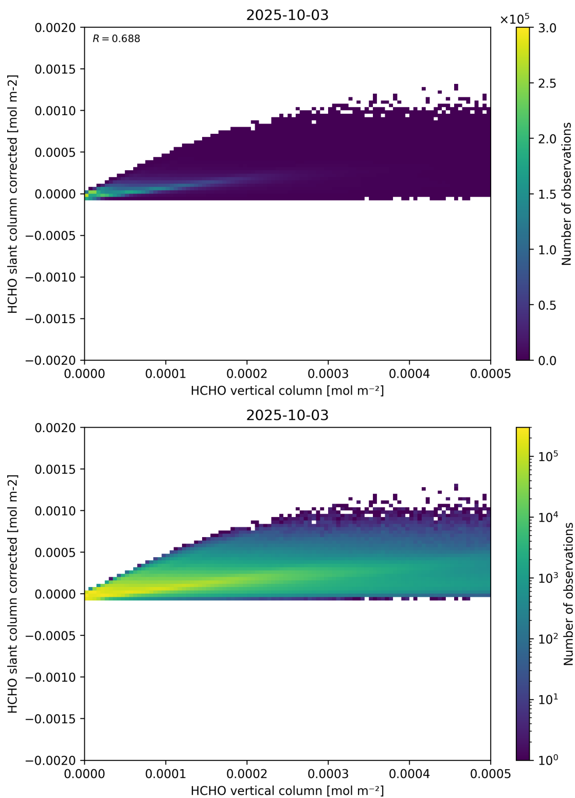
Figure 127: Scatter density plot of “HCHO vertical column” against “HCHO slant column corrected” for 2025-10-02 to 2025-10-04.
