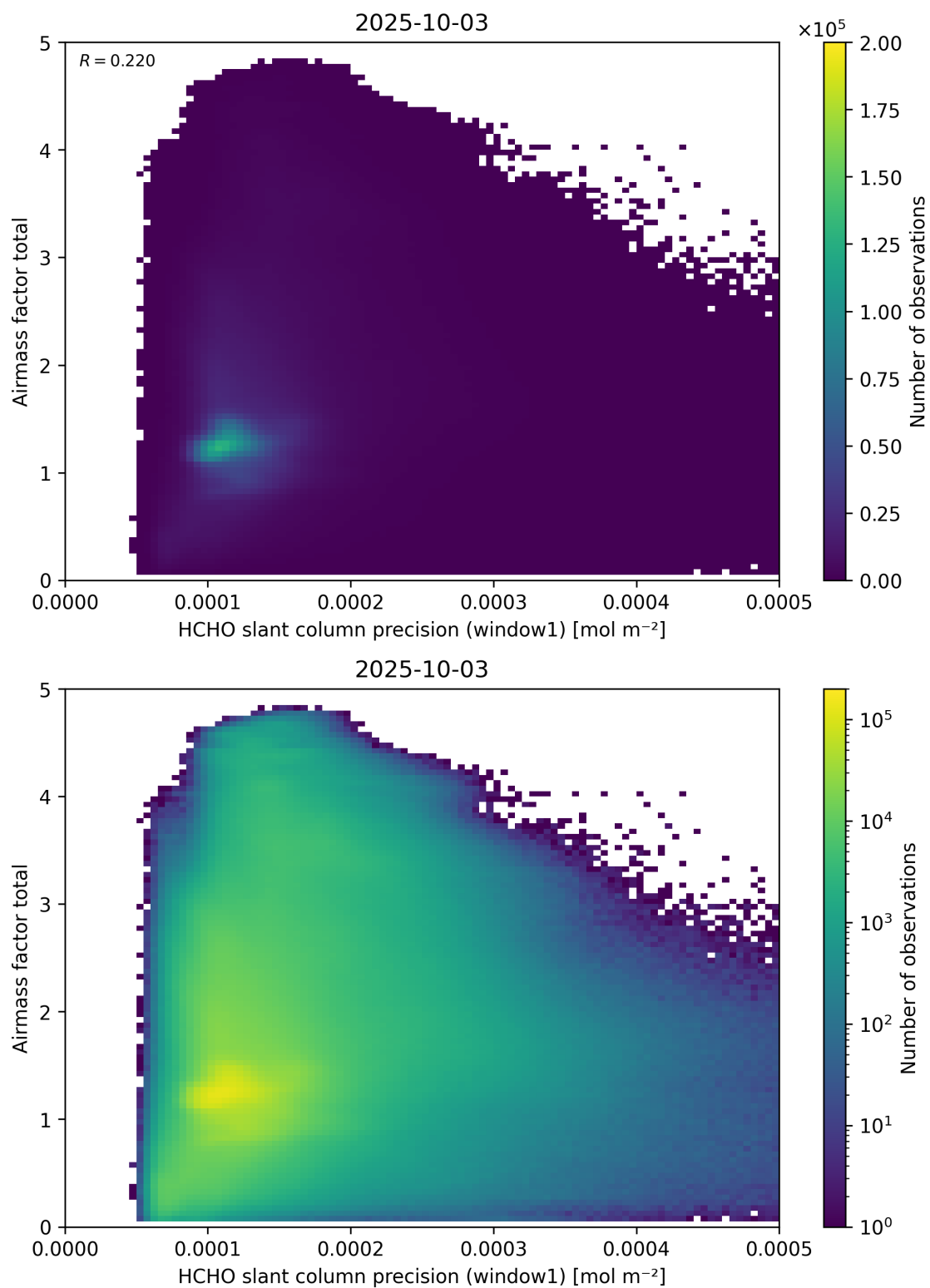
Figure 94: Scatter density plot of “HCHO slant column precision (window1)” against “Airmass factor total” for 2025-10-02 to 2025-10-04.
