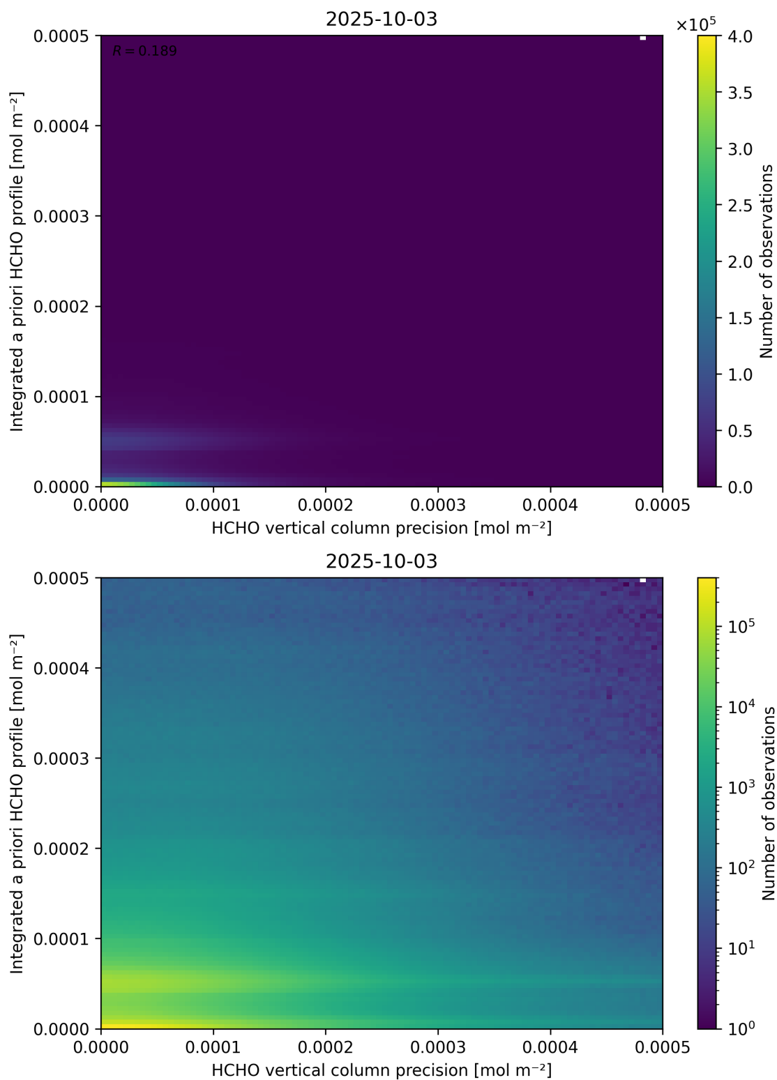
Figure 147: Scatter density plot of “HCHO vertical column precision” against “Integrated a priori HCHO profile” for 2025-10-02 to 2025-10-04.
