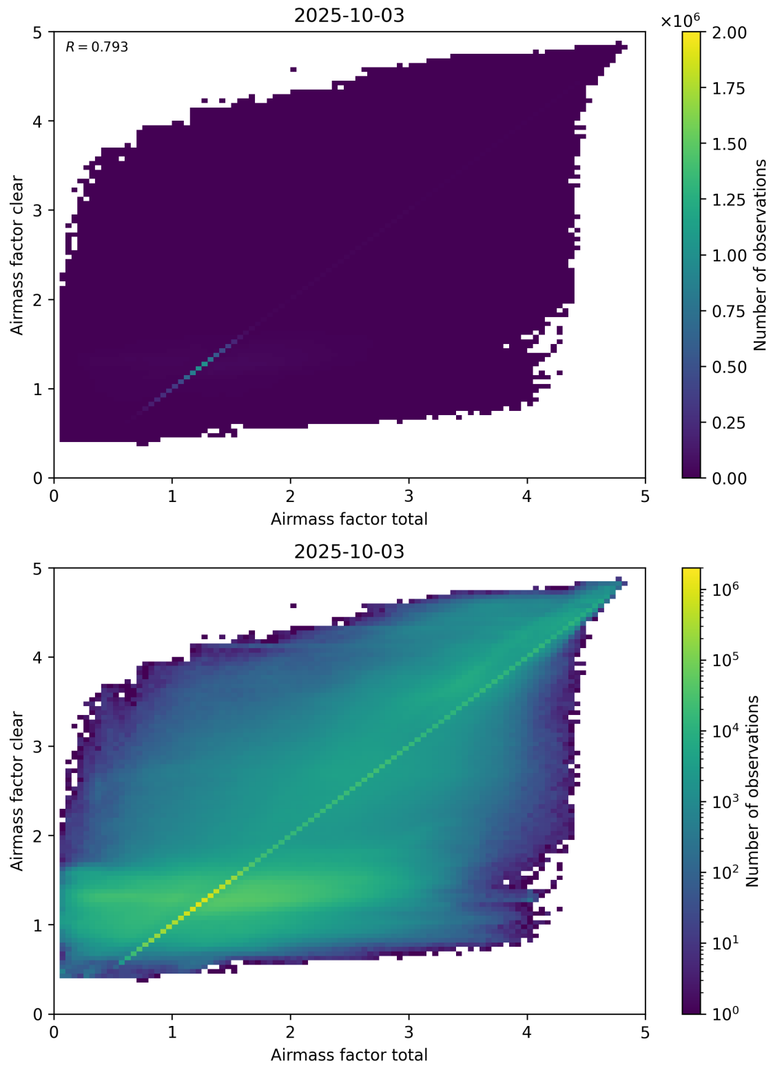
Figure 100: Scatter density plot of “Airmass factor total” against “Airmass factor clear” for 2025-10-02 to 2025-10-04.
