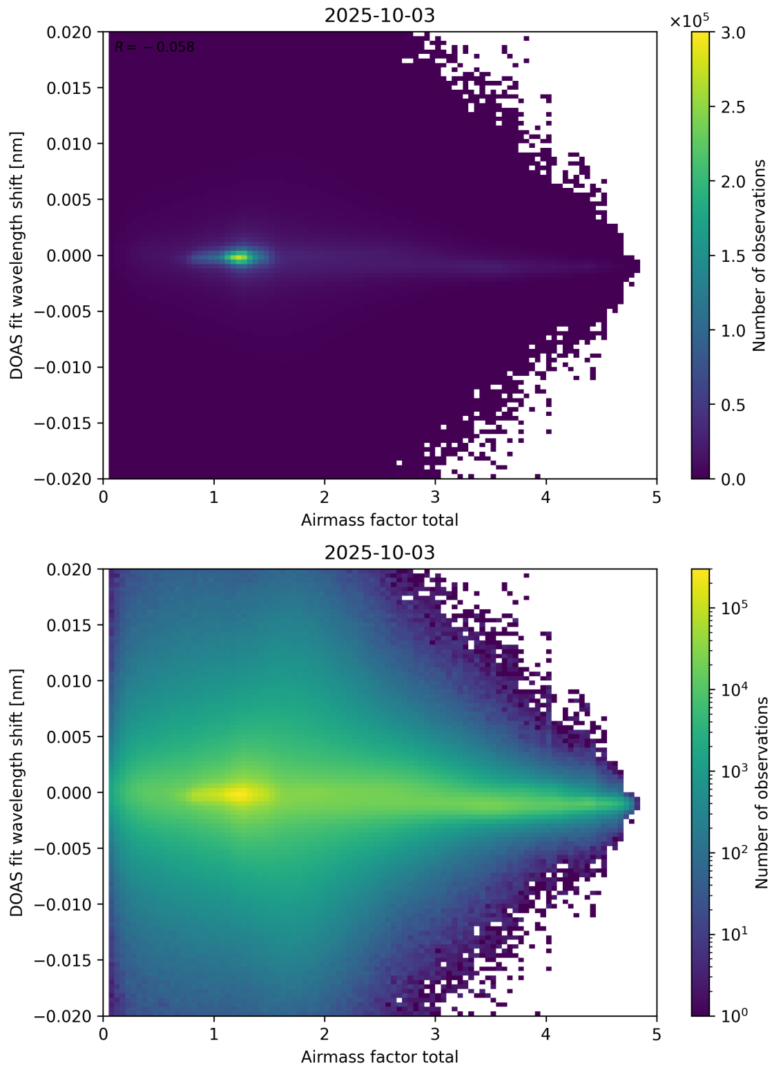
Figure 98: Scatter density plot of “Airmass factor total” against “DOAS fit wavelength shift” for 2025-10-02 to 2025-10-04.
