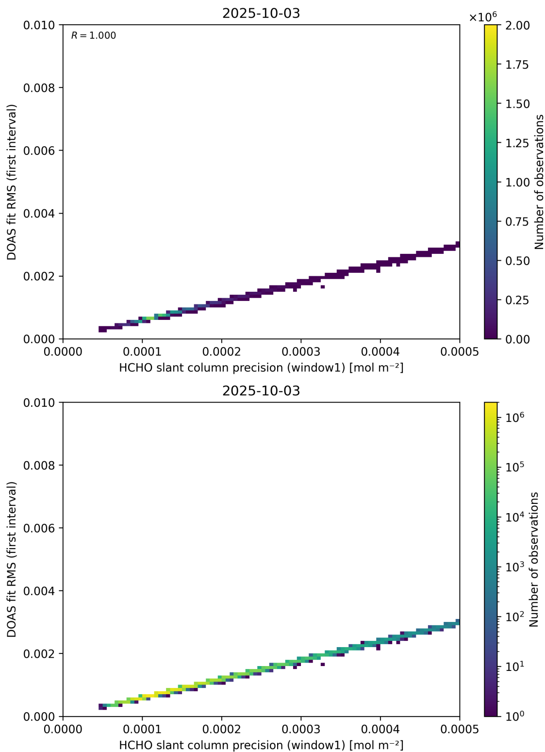
Figure 88: Scatter density plot of “HCHO slant column precision (window1)” against “DOAS fit RMS (first interval)” for 2025-10-02 to 2025-10-04.
