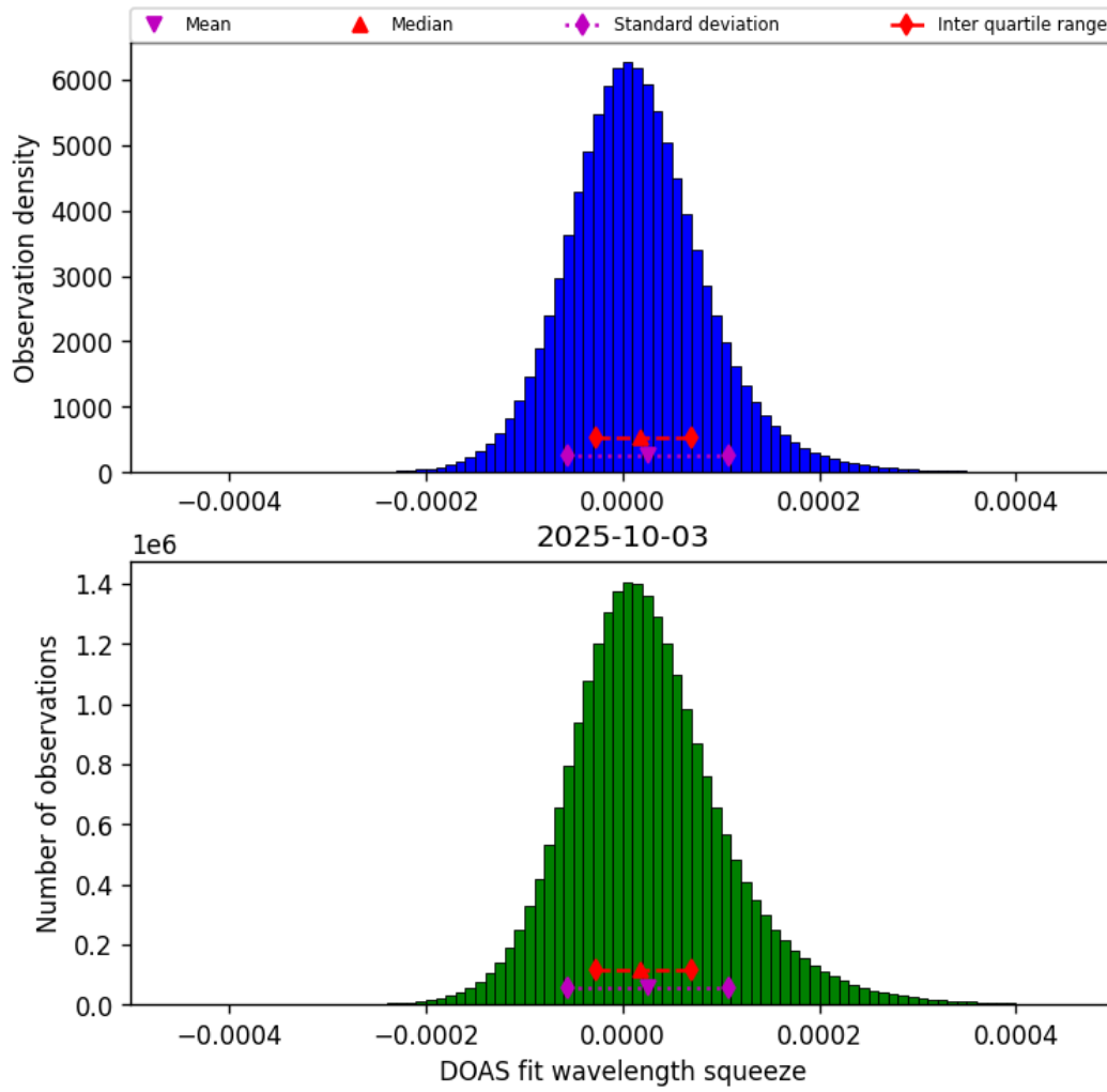
Figure 45: Histogram of “DOAS fit wavelength squeeze” for 2025-10-02 to 2025-10-04
