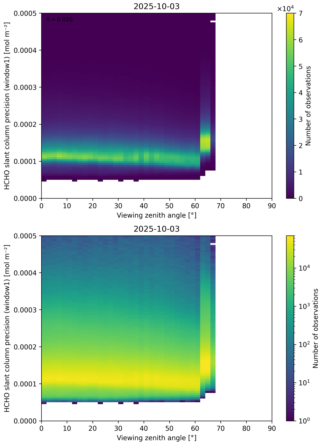
Figure 189: Scatter density plot of “Viewing zenith angle” against “HCHO slant column precision (window1)” for 2025-10-02 to 2025-10-04.
