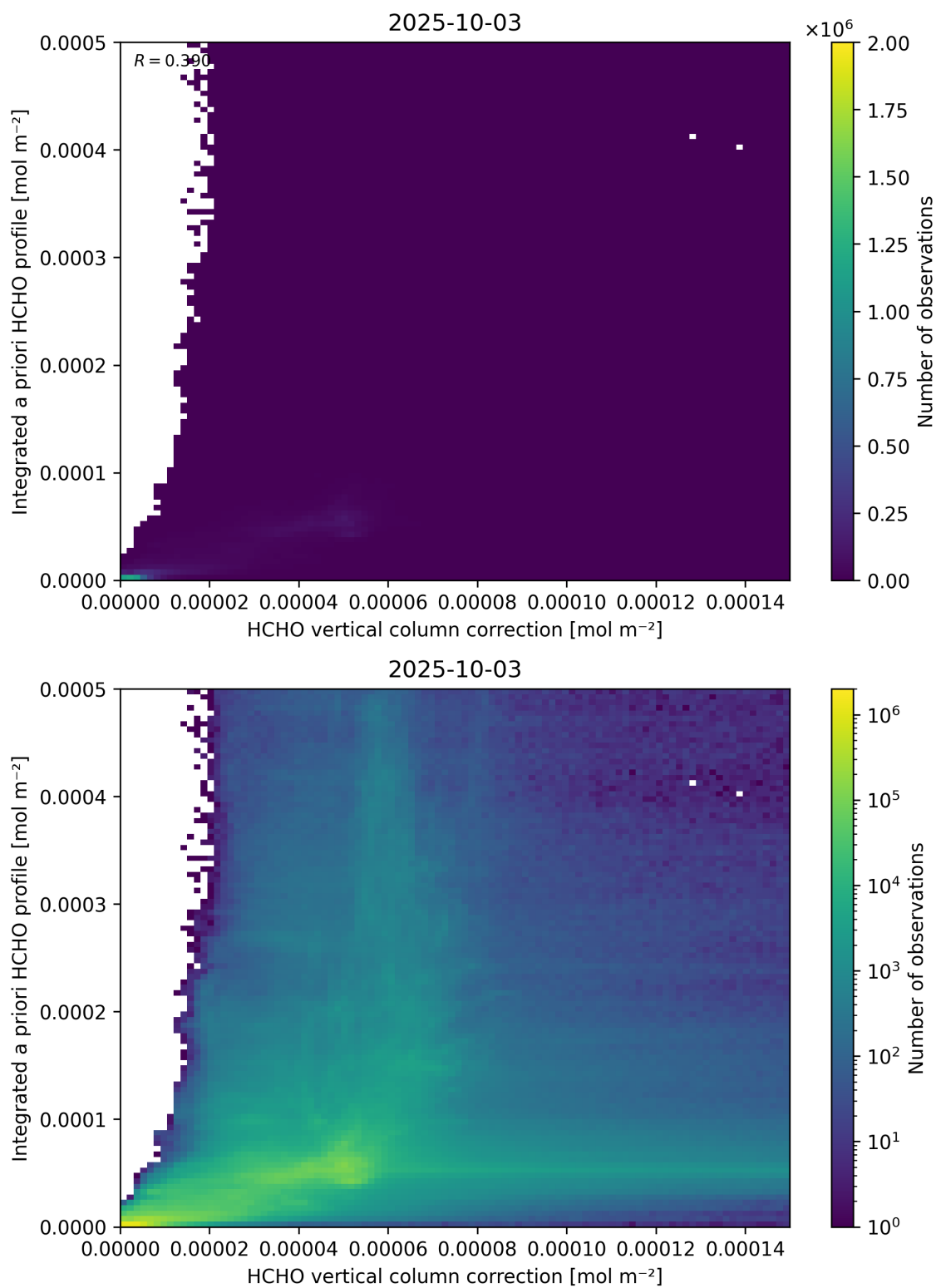
Figure 122: Scatter density plot of “HCHO vertical column correction” against “Integrated a priori HCHO profile” for 2025-10-02 to 2025-10-04.
