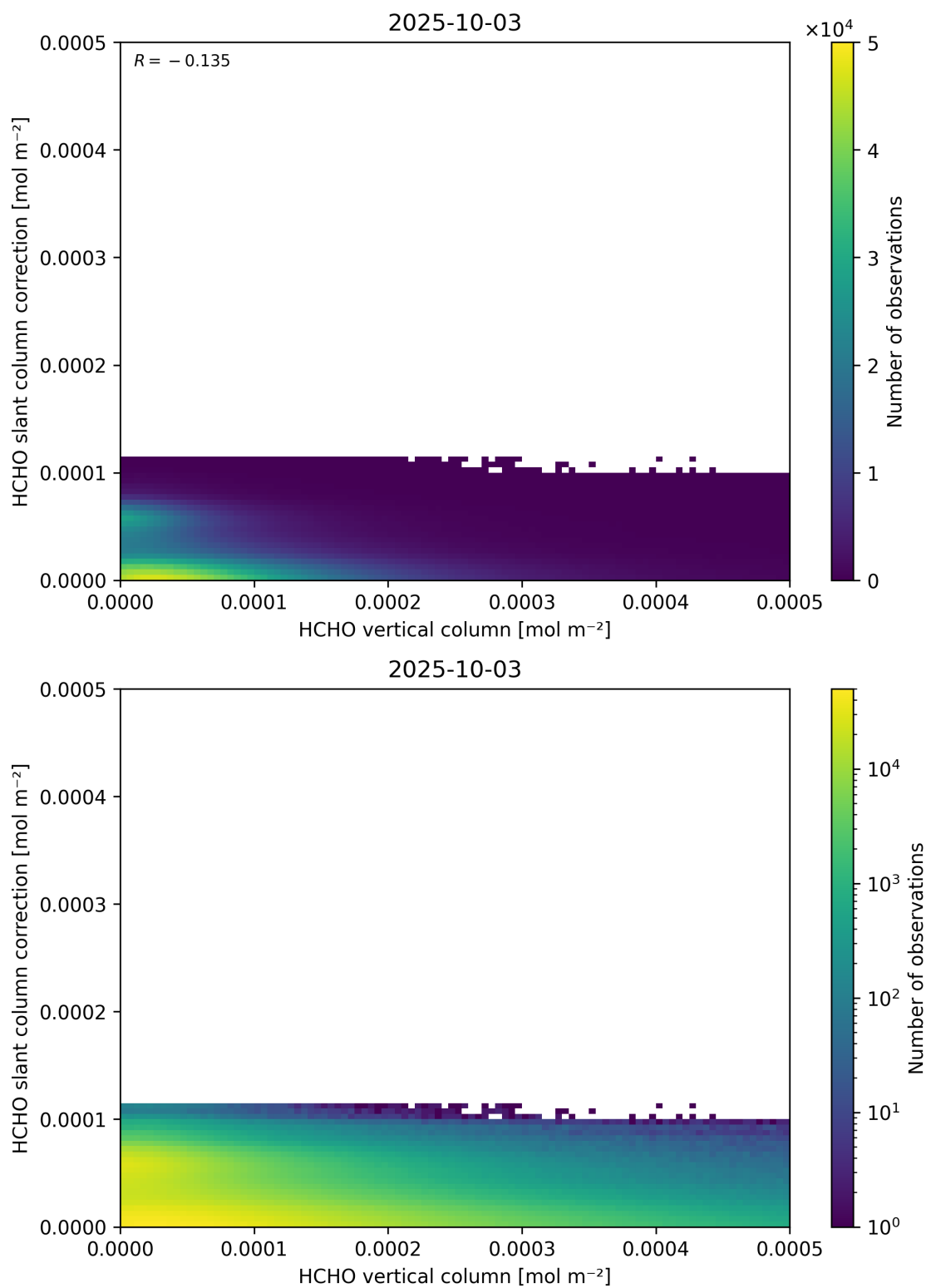
Figure 128: Scatter density plot of “HCHO vertical column” against “HCHO slant column correction” for 2025-10-02 to 2025-10-04.
