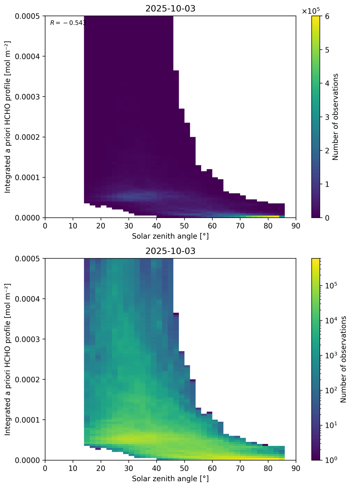
Figure 180: Scatter density plot of “Solar zenith angle” against “Integrated a priori HCHO profile” for 2025-10-02 to 2025-10-04.
