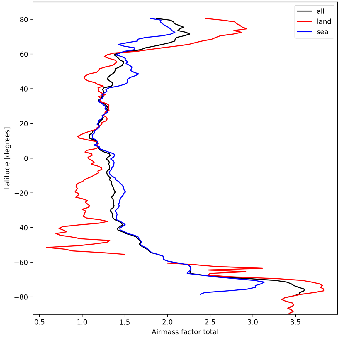
Figure 26: Zonal average of “Airmass factor total” for 2025-10-02 to 2025-10-04.
