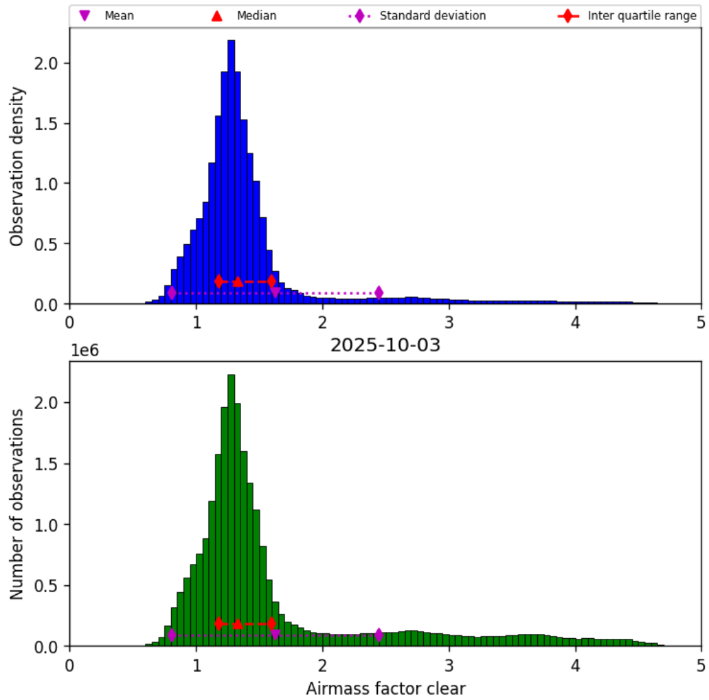
Figure 42: Histogram of “Airmass factor clear” for 2025-10-02 to 2025-10-04
