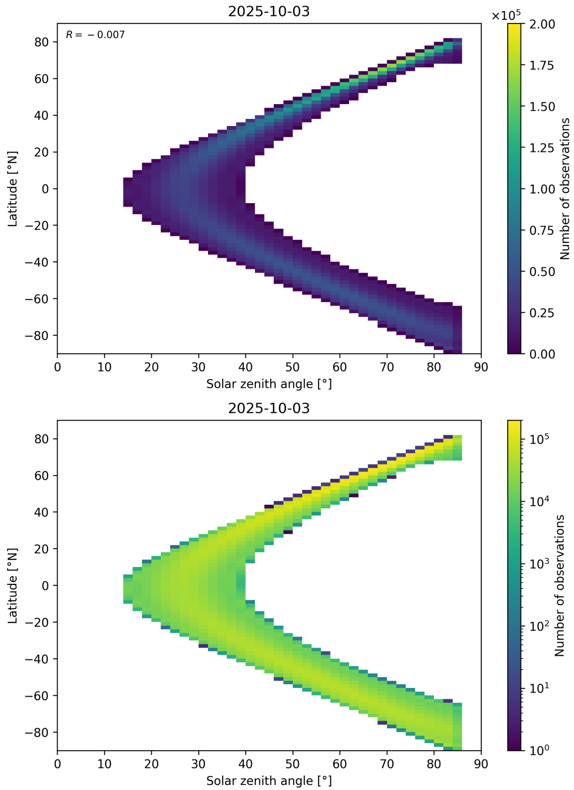
Figure 181: Scatter density plot of “Solar zenith angle” against “Latitude” for 2025-10-02 to 2025-10-04.
