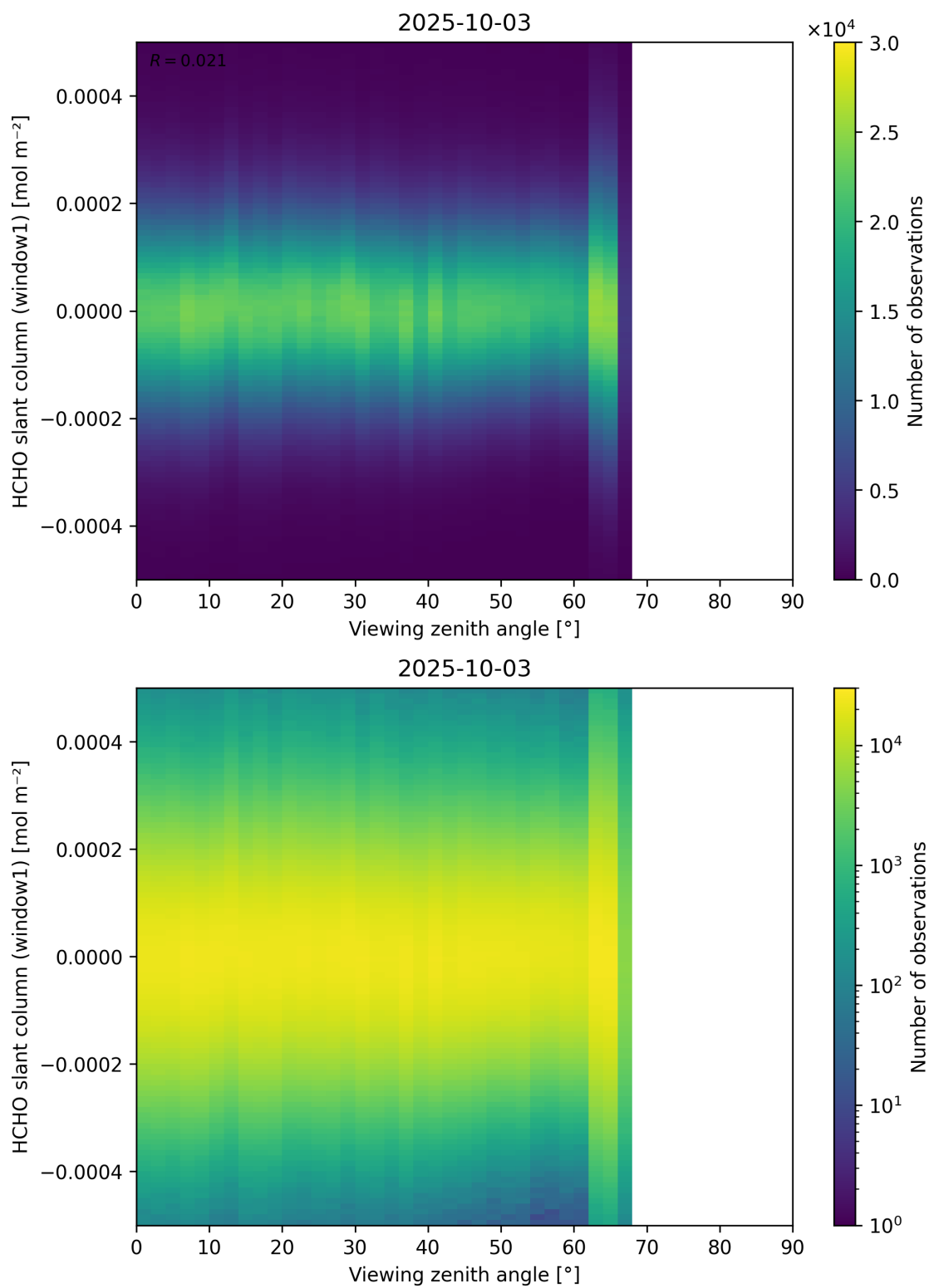
Figure 188: Scatter density plot of “Viewing zenith angle” against “HCHO slant column (window1)” for 2025-10-02 to 2025-10-04.
