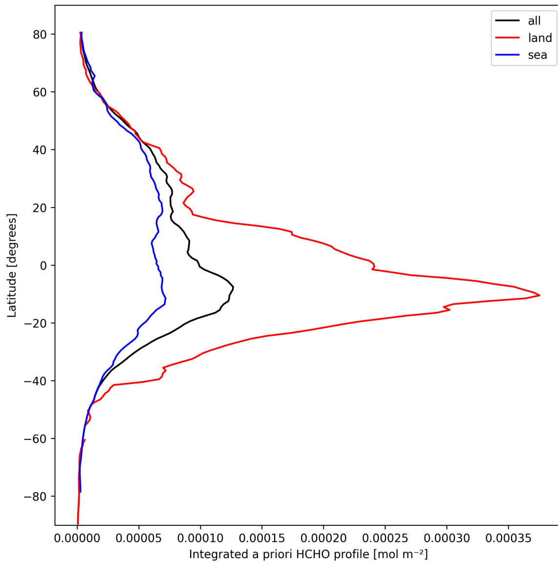
Figure 29: Zonal average of “Integrated a priori HCHO profile” for 2025-10-02 to 2025-10-04.
