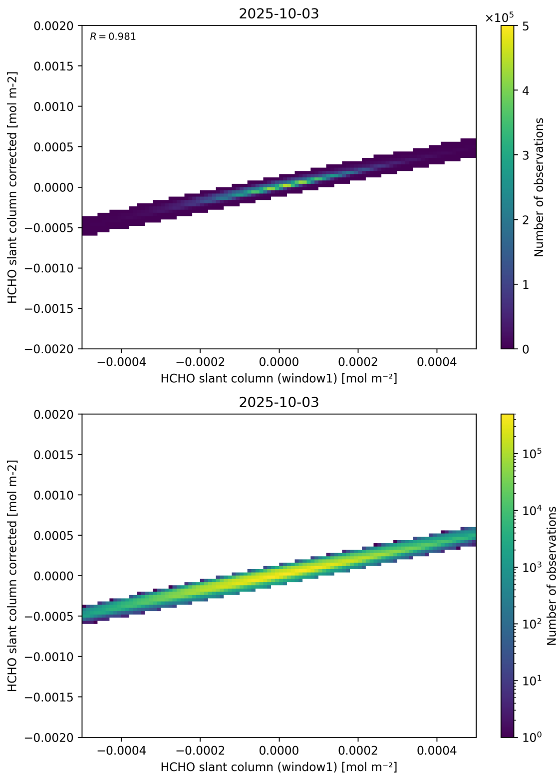
Figure 82: Scatter density plot of “HCHO slant column (window1)” against “HCHO slant column corrected” for 2025-10-02 to 2025-10-04.
