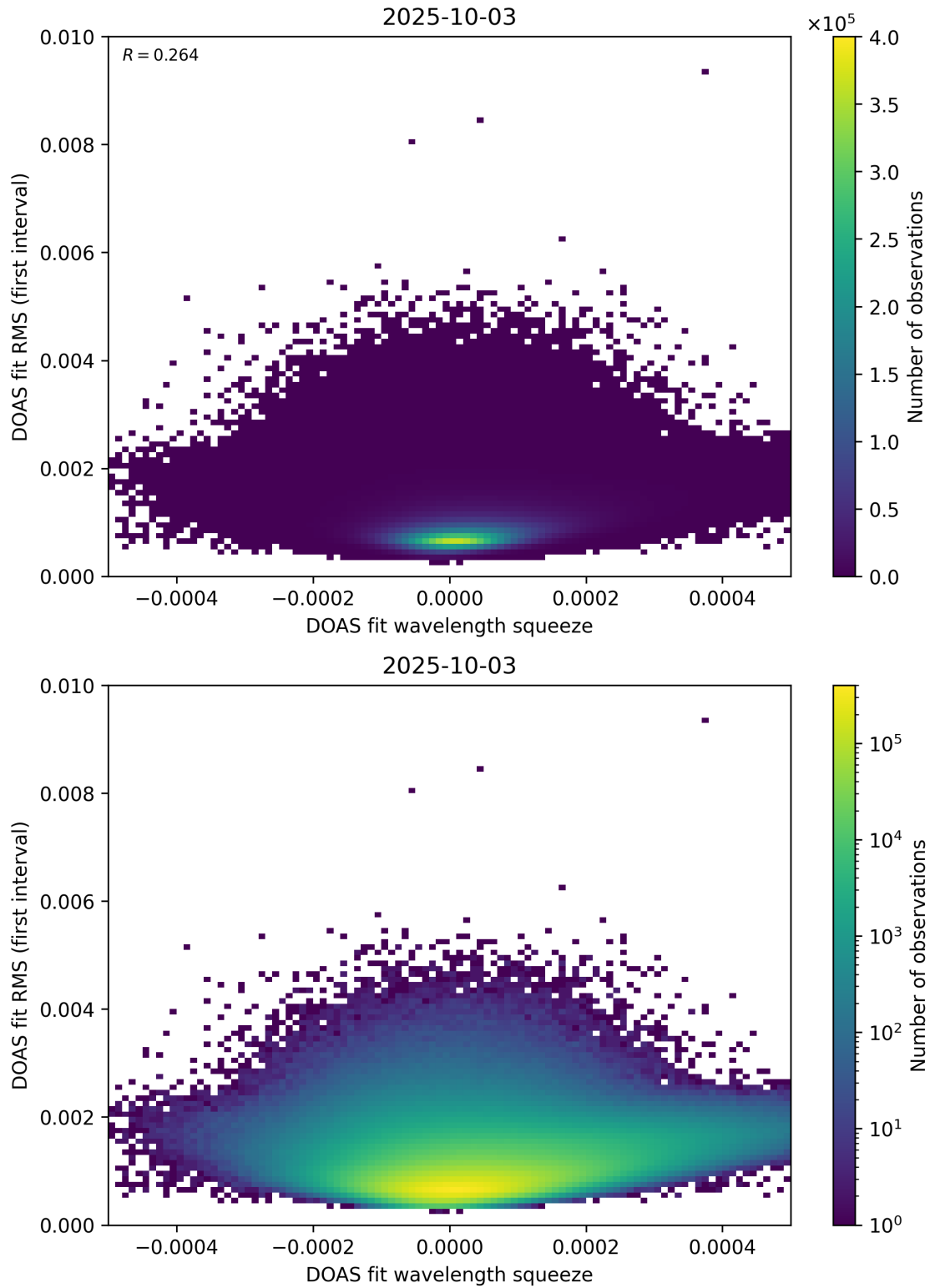
Figure 68: Scatter density plot of “DOAS fit wavelength squeeze” against “DOAS fit RMS (first interval)” for 2025-10-02 to 2025-10-04.
