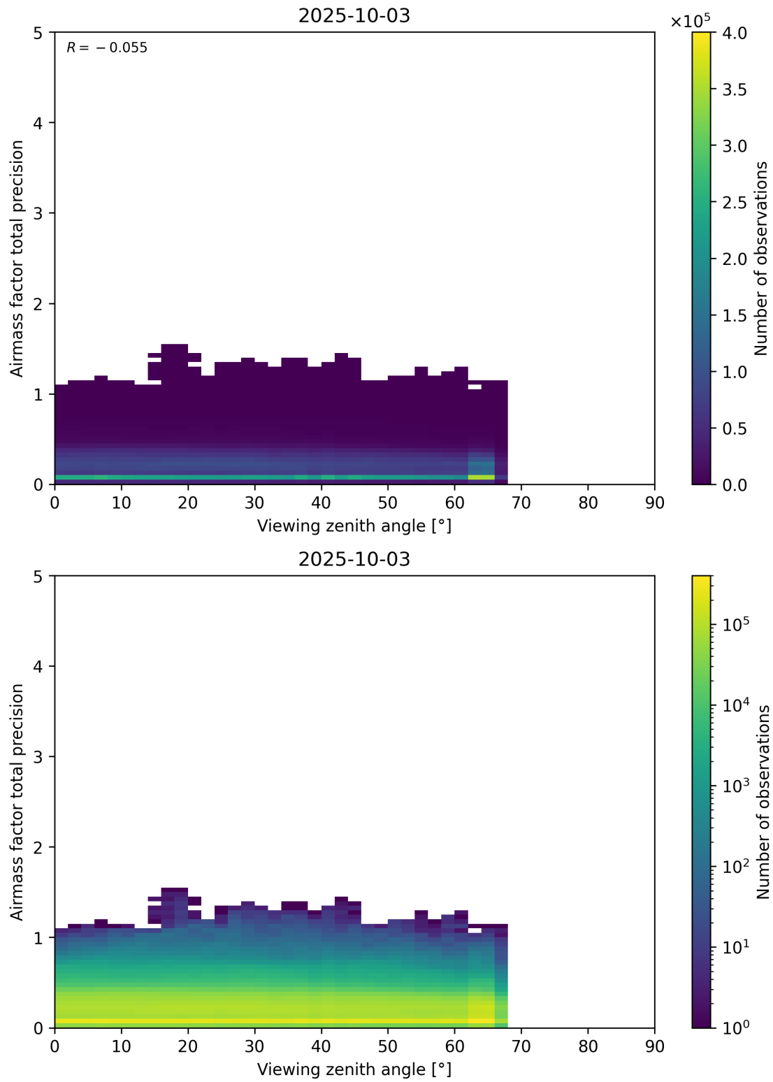
Figure 191: Scatter density plot of “Viewing zenith angle” against “Airmass factor total precision” for 2025-10-02 to 2025-10-04.
