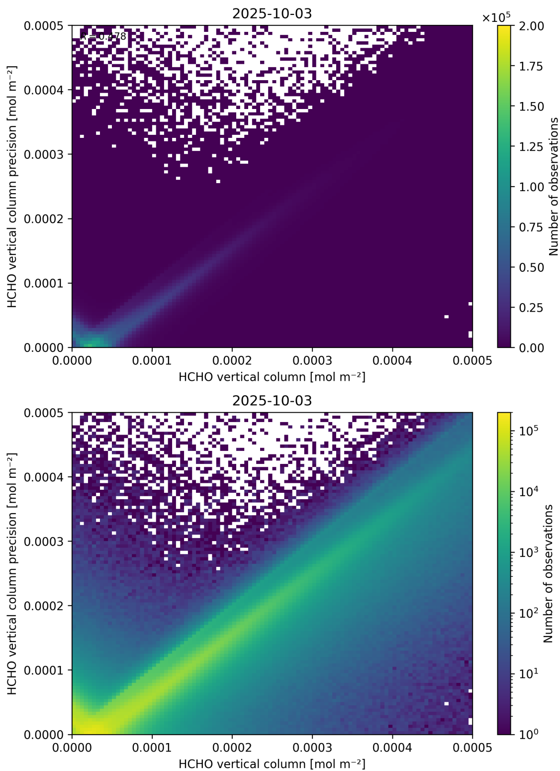
Figure 134: Scatter density plot of “HCHO vertical column” against “HCHO vertical column precision” for 2025-10-02 to 2025-10-04.
