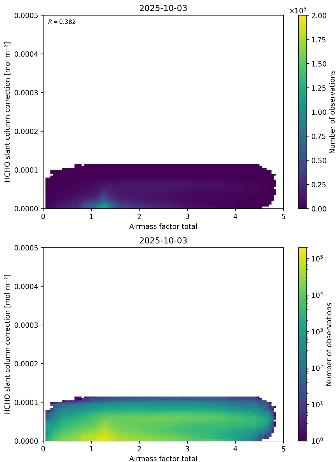
Figure 102: Scatter density plot of “Airmass factor total” against “HCHO slant column correction” for 2025-10-02 to 2025-10-04.
