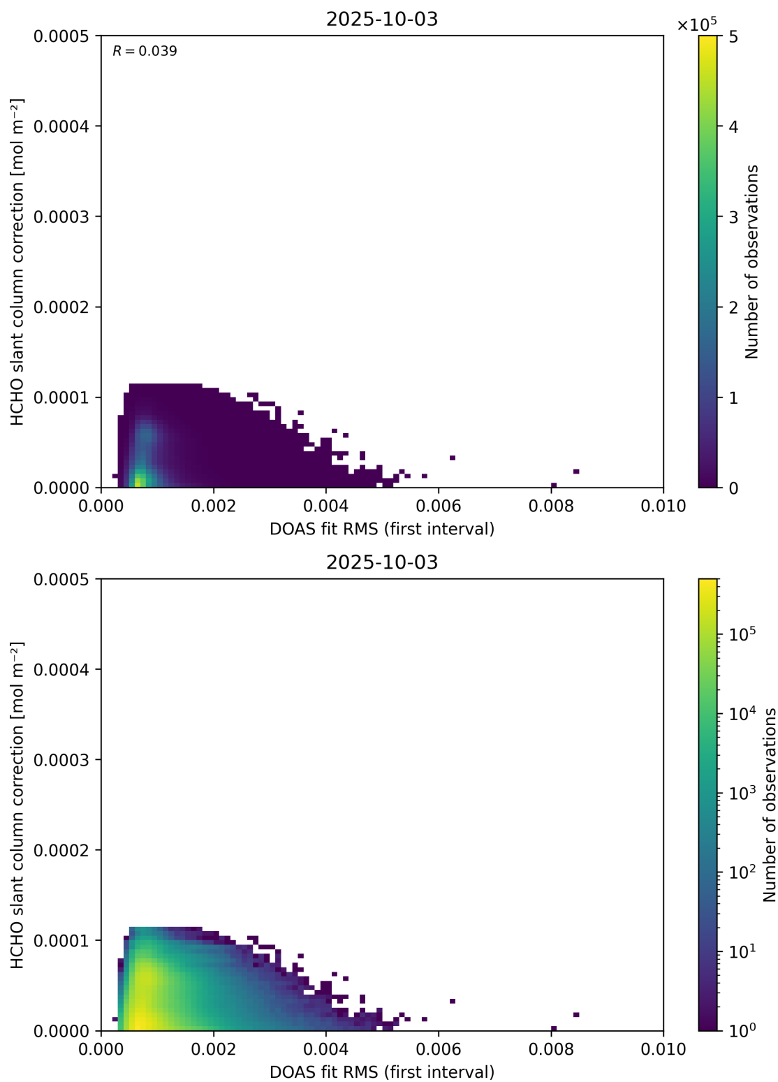
Figure 63: Scatter density plot of “DOAS fit RMS (first interval)” against “HCHO slant column correction” for 2025-10-02 to 2025-10-04.
