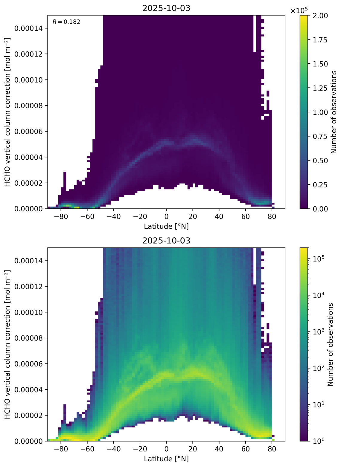
Figure 164: Scatter density plot of “Latitude” against “HCHO vertical column correction” for 2025-10-02 to 2025-10-04.
