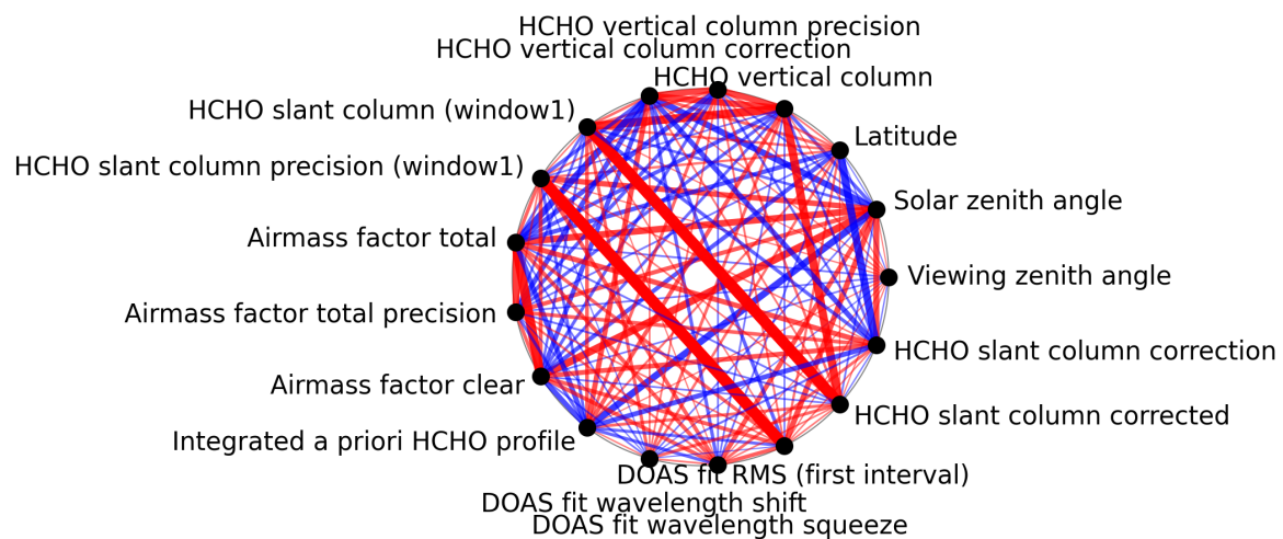
Figure 1: Map of correlation graph for 2025-10-02 to 2025-10-04.
