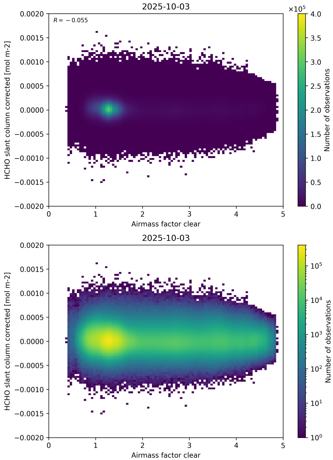
Figure 74: Scatter density plot of “Airmass factor clear” against “HCHO slant column corrected” for 2025-10-02 to 2025-10-04.
