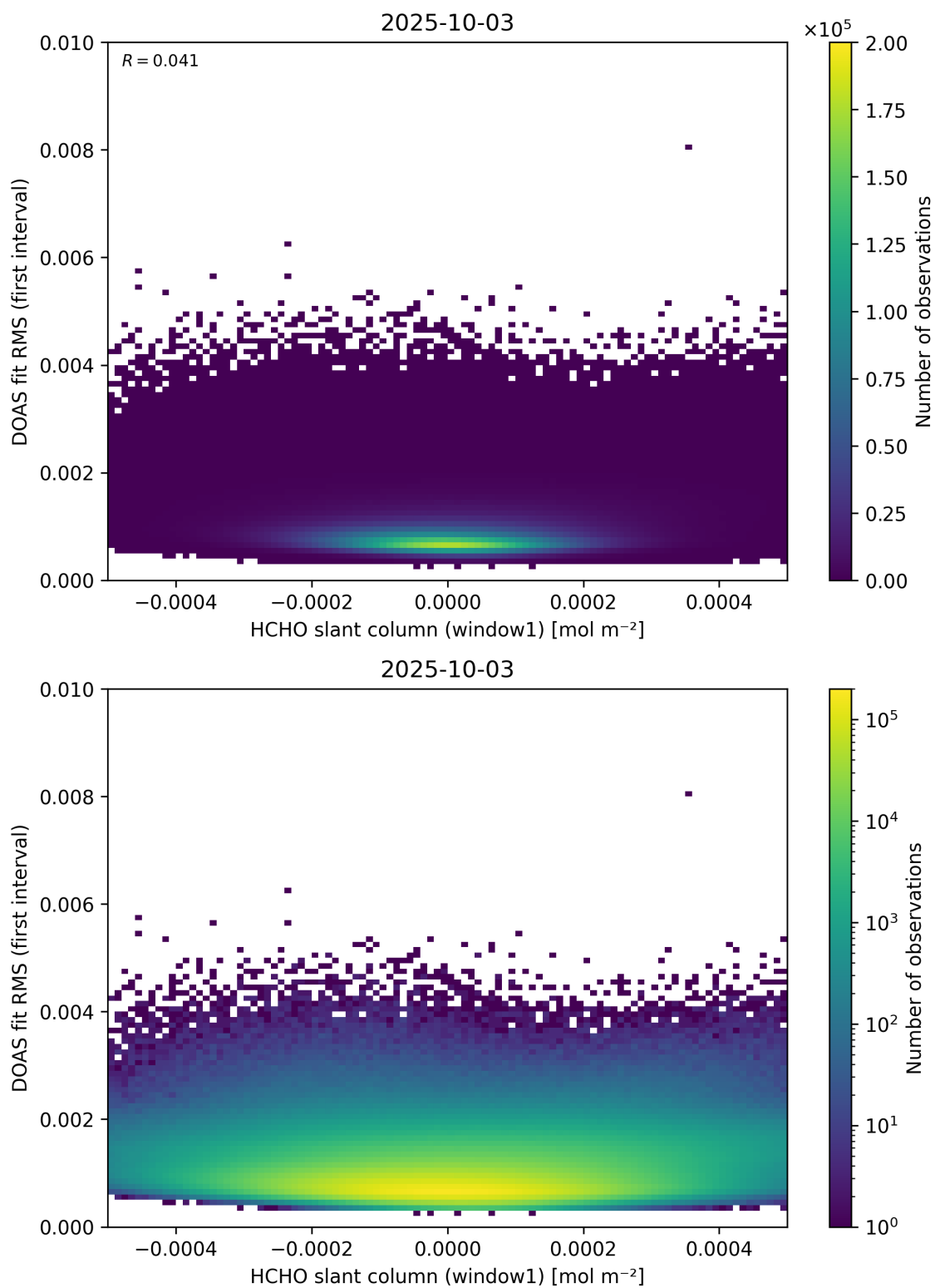
Figure 78: Scatter density plot of “HCHO slant column (window1)” against “DOAS fit RMS (first interval)” for 2025-10-02 to 2025-10-04.
