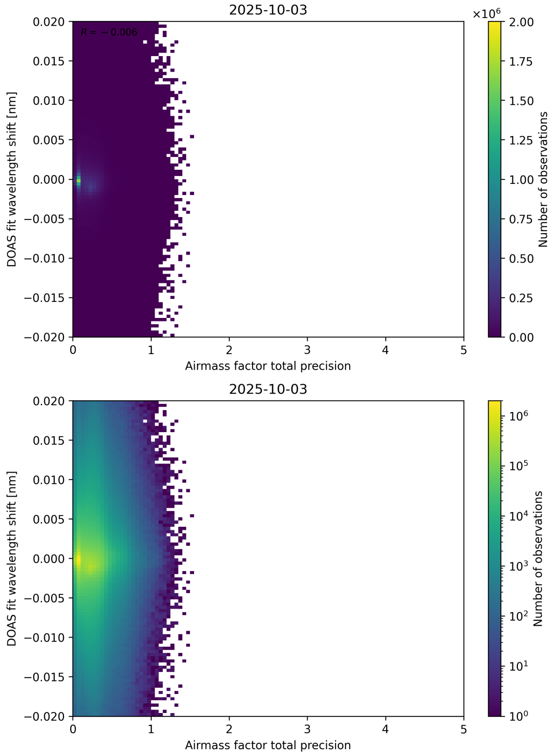
Figure 106: Scatter density plot of “Airmass factor total precision” against “DOAS fit wavelength shift” for 2025-10-02 to 2025-10-04.
