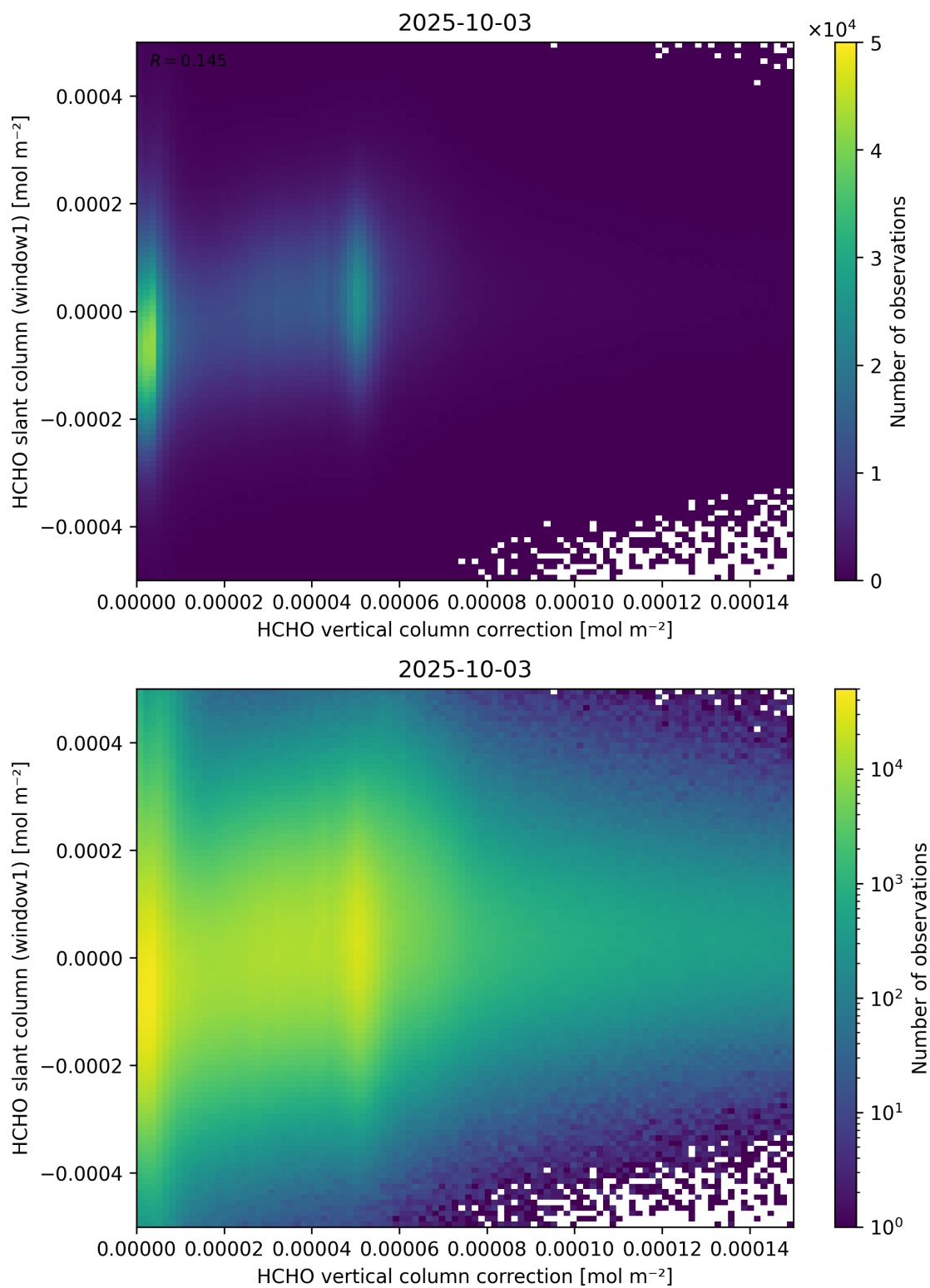
Figure 118: Scatter density plot of “HCHO vertical column correction” against “HCHO slant column (window1)” for 2025-10-02 to 2025-10-04.
