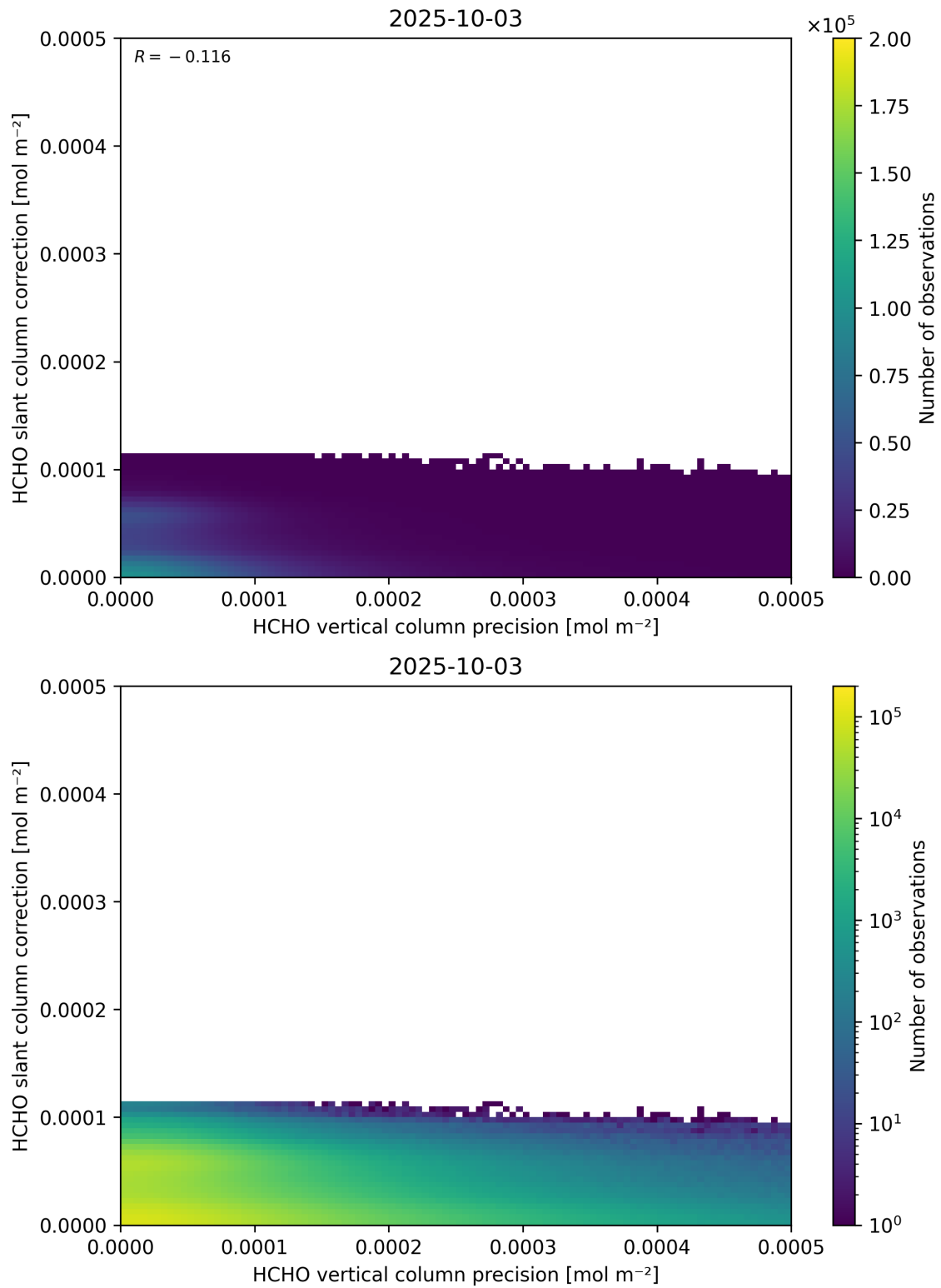
Figure 141: Scatter density plot of “HCHO vertical column precision” against “HCHO slant column correction” for 2025-10-02 to 2025-10-04.
