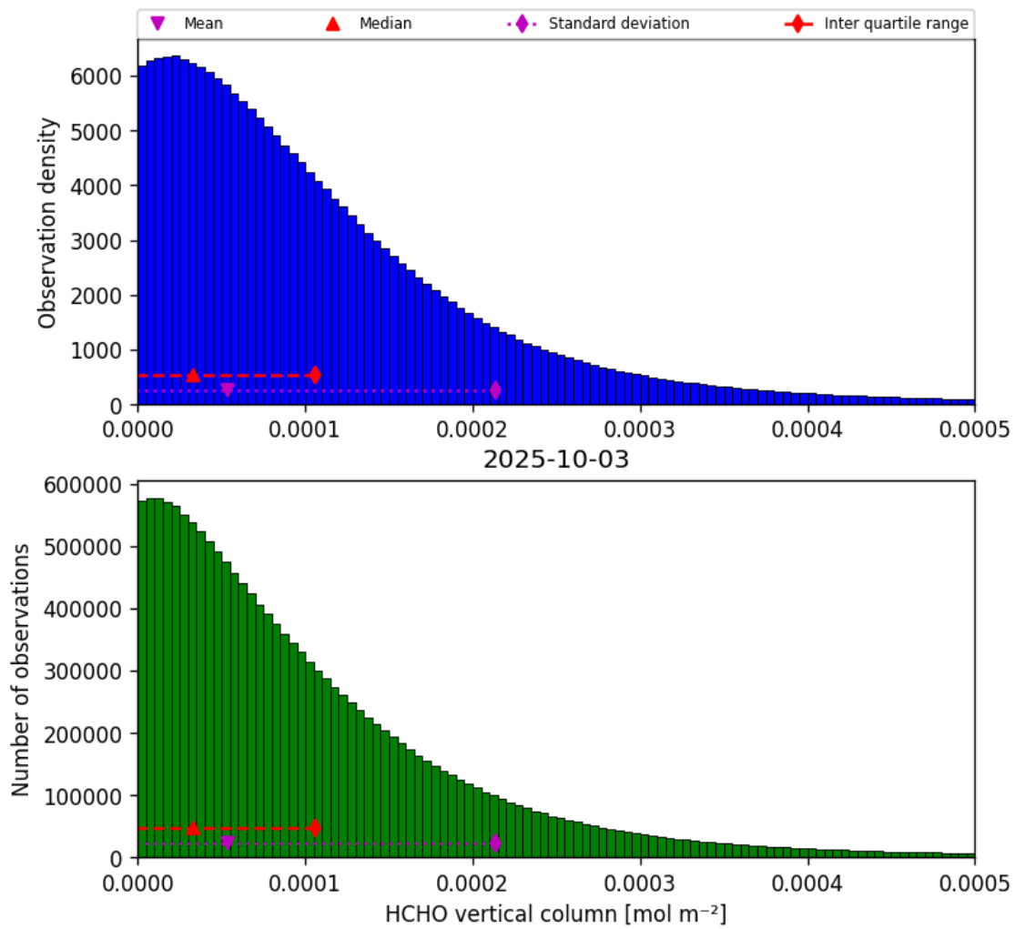
Figure 35: Histogram of “HCHO vertical column” for 2025-10-02 to 2025-10-04
