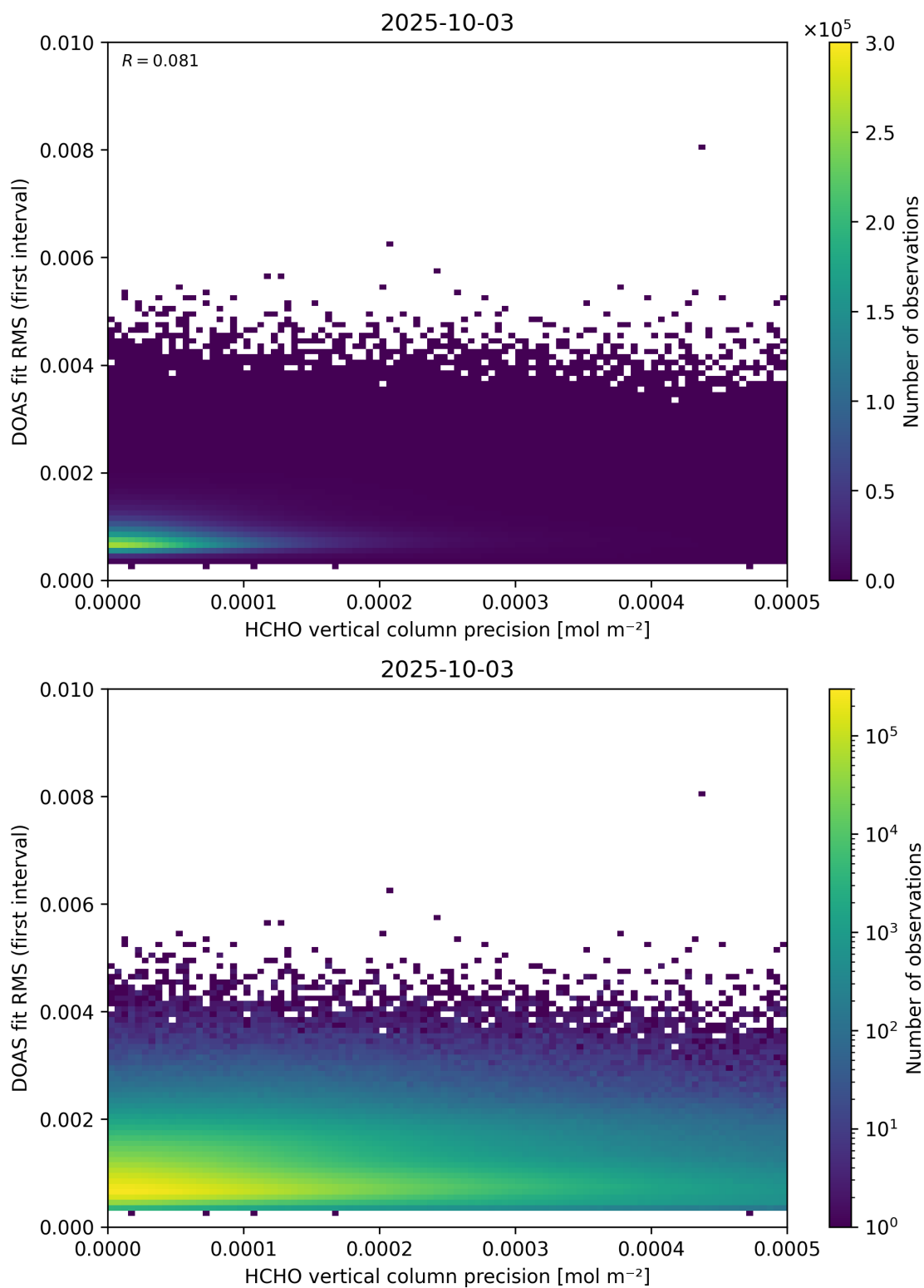
Figure 136: Scatter density plot of “HCHO vertical column precision” against “DOAS fit RMS (first interval)” for 2025-10-02 to 2025-10-04.
