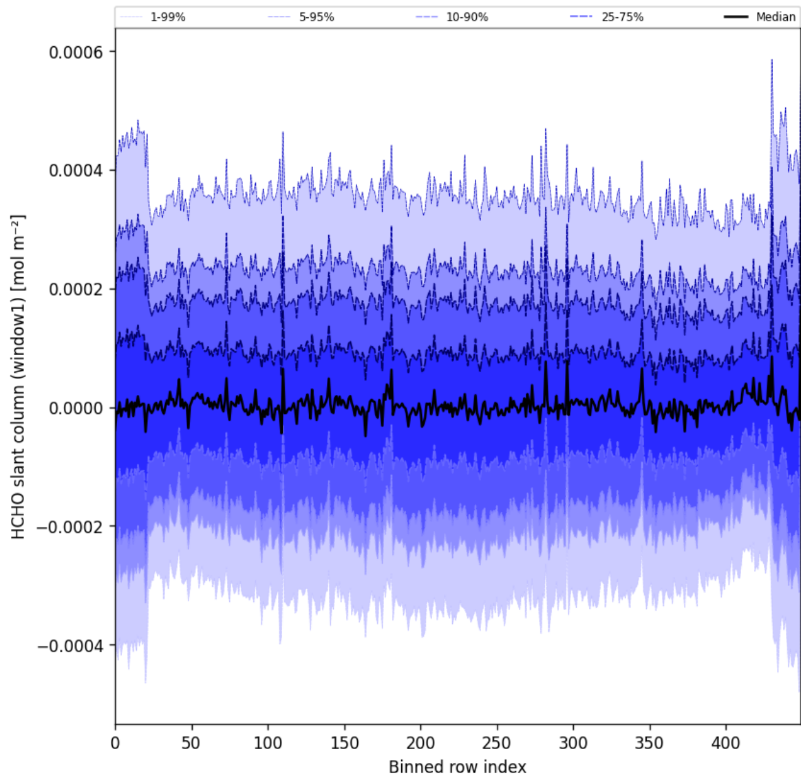
Figure 52: Along track statistics of “HCHO slant column (window1)” for 2025-10-02 to 2025-10-04
