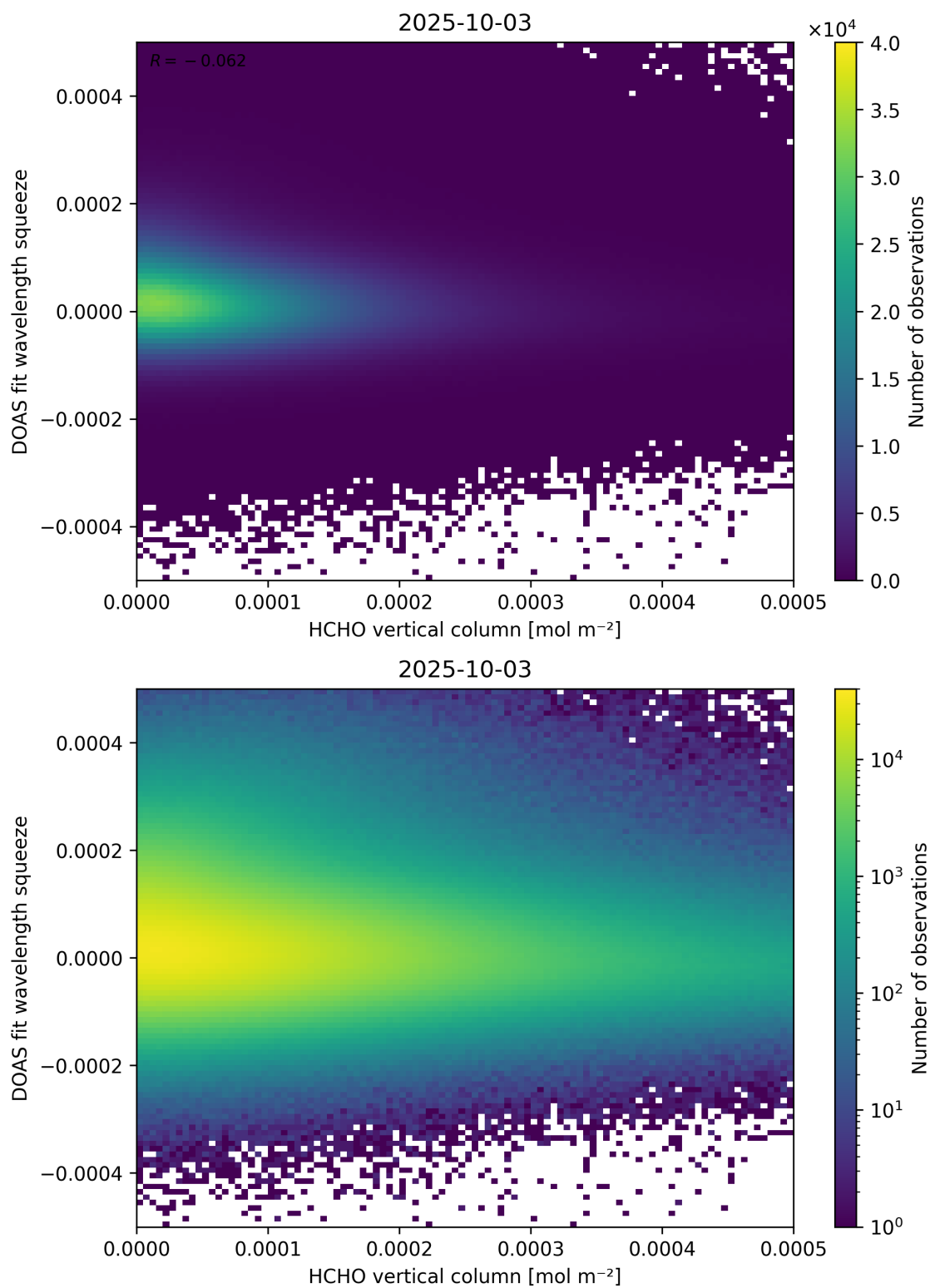
Figure 125: Scatter density plot of “HCHO vertical column” against “DOAS fit wavelength squeeze” for 2025-10-02 to 2025-10-04.
