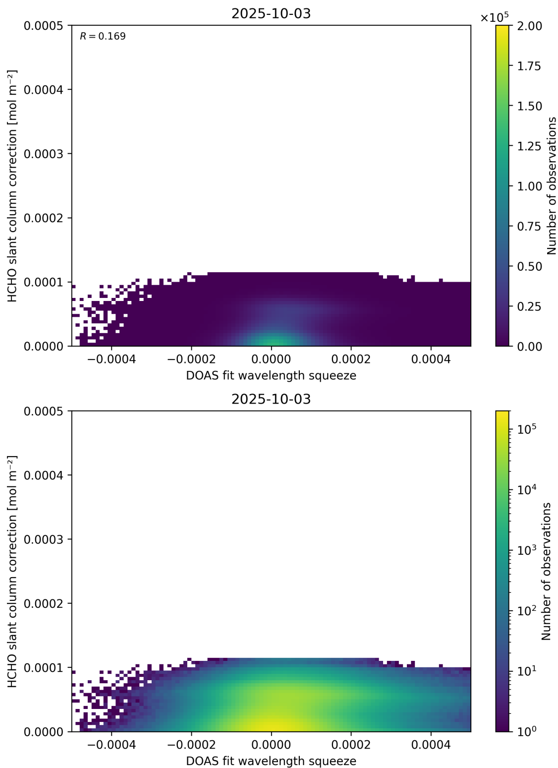
Figure 70: Scatter density plot of “DOAS fit wavelength squeeze” against “HCHO slant column correction” for 2025-10-02 to 2025-10-04.
