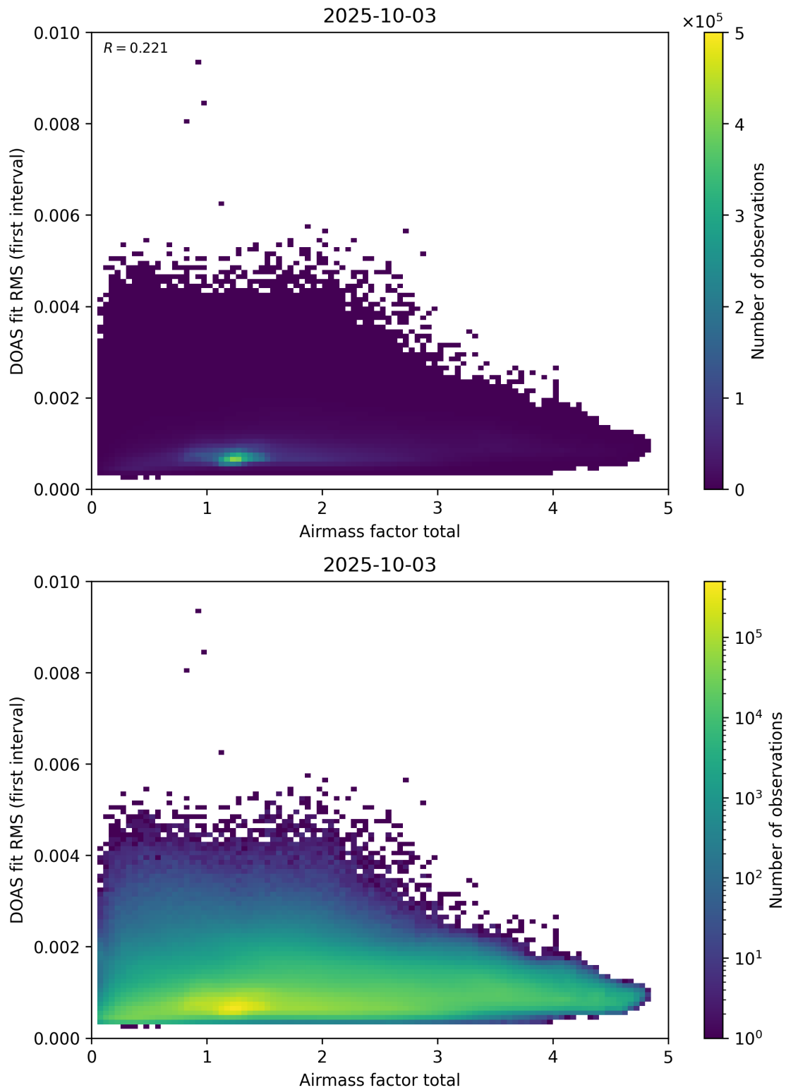
Figure 97: Scatter density plot of “Airmass factor total” against “DOAS fit RMS (first interval)” for 2025-10-02 to 2025-10-04.
