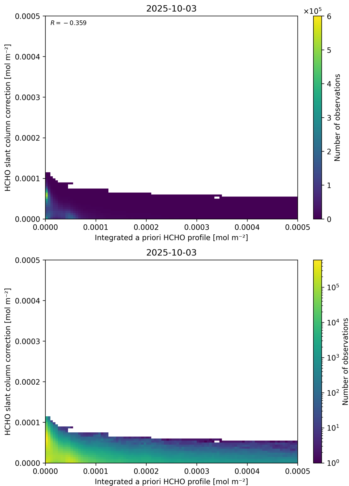
Figure 152: Scatter density plot of “Integrated a priori HCHO profile” against “HCHO slant column correction” for 2025-10-02 to 2025-10-04.
