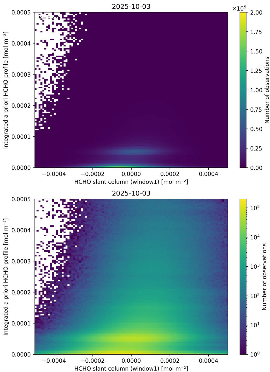
Figure 87: Scatter density plot of “HCHO slant column (window1)” against “Integrated a priori HCHO profile” for 2025-10-02 to 2025-10-04.
