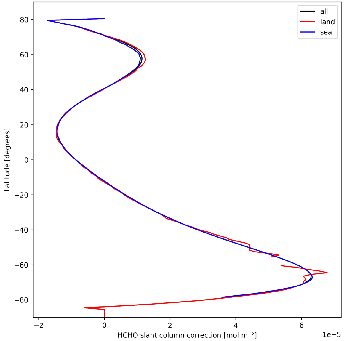
Figure 33: Zonal average of “HCHO slant column correction” for 2025-10-02 to 2025-10-04.
