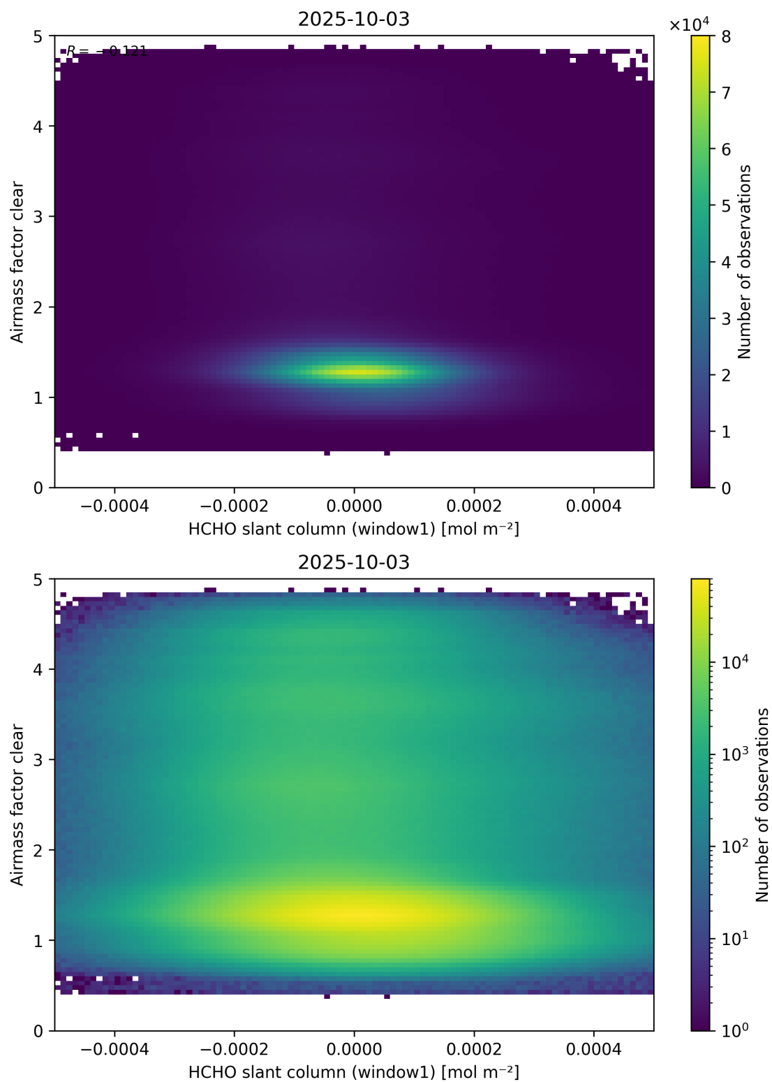
Figure 81: Scatter density plot of “HCHO slant column (window1)” against “Airmass factor clear” for 2025-10-02 to 2025-10-04.
