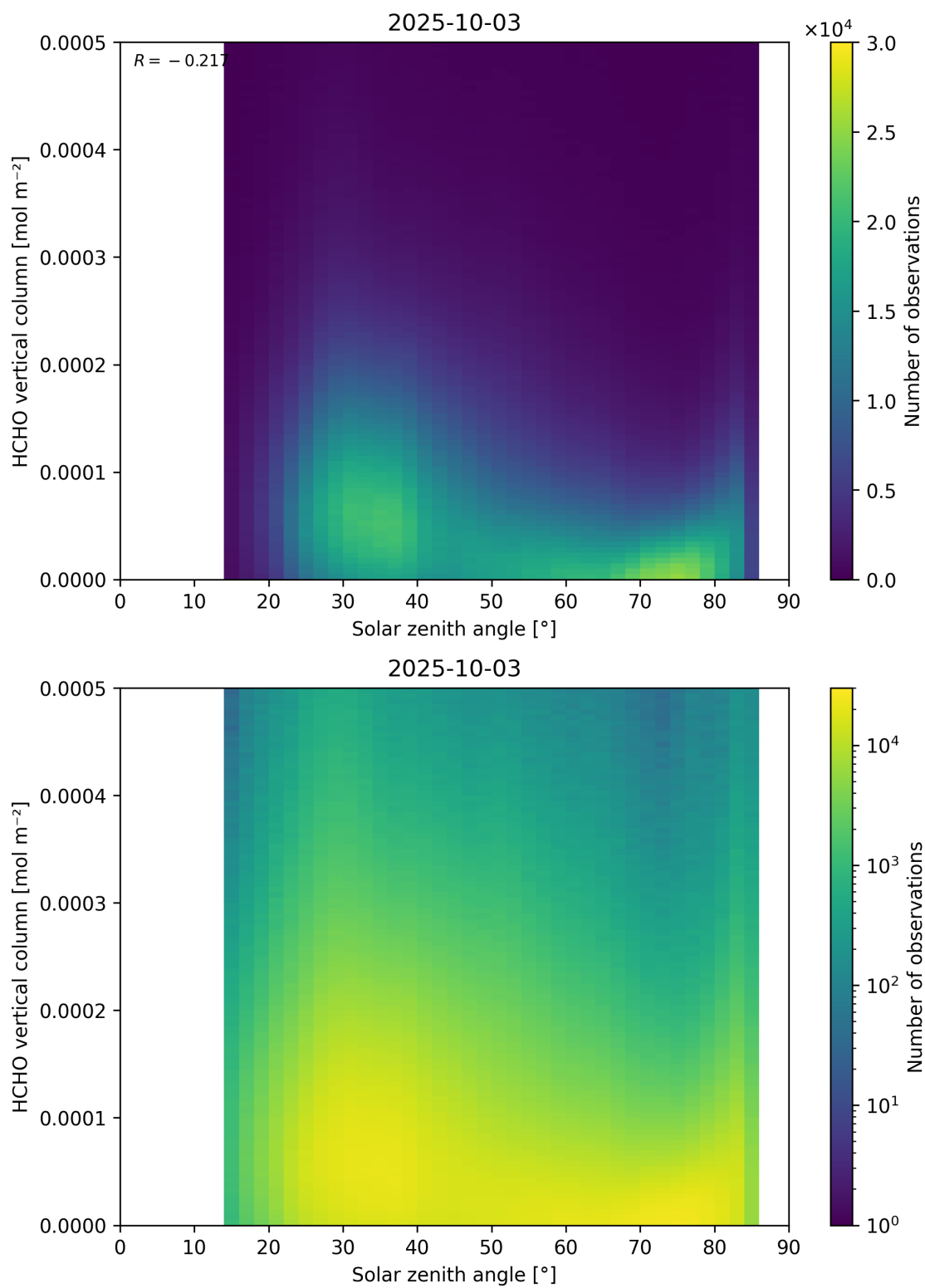
Figure 177: Scatter density plot of “Solar zenith angle” against “HCHO vertical column” for 2025-10-02 to 2025-10-04.
