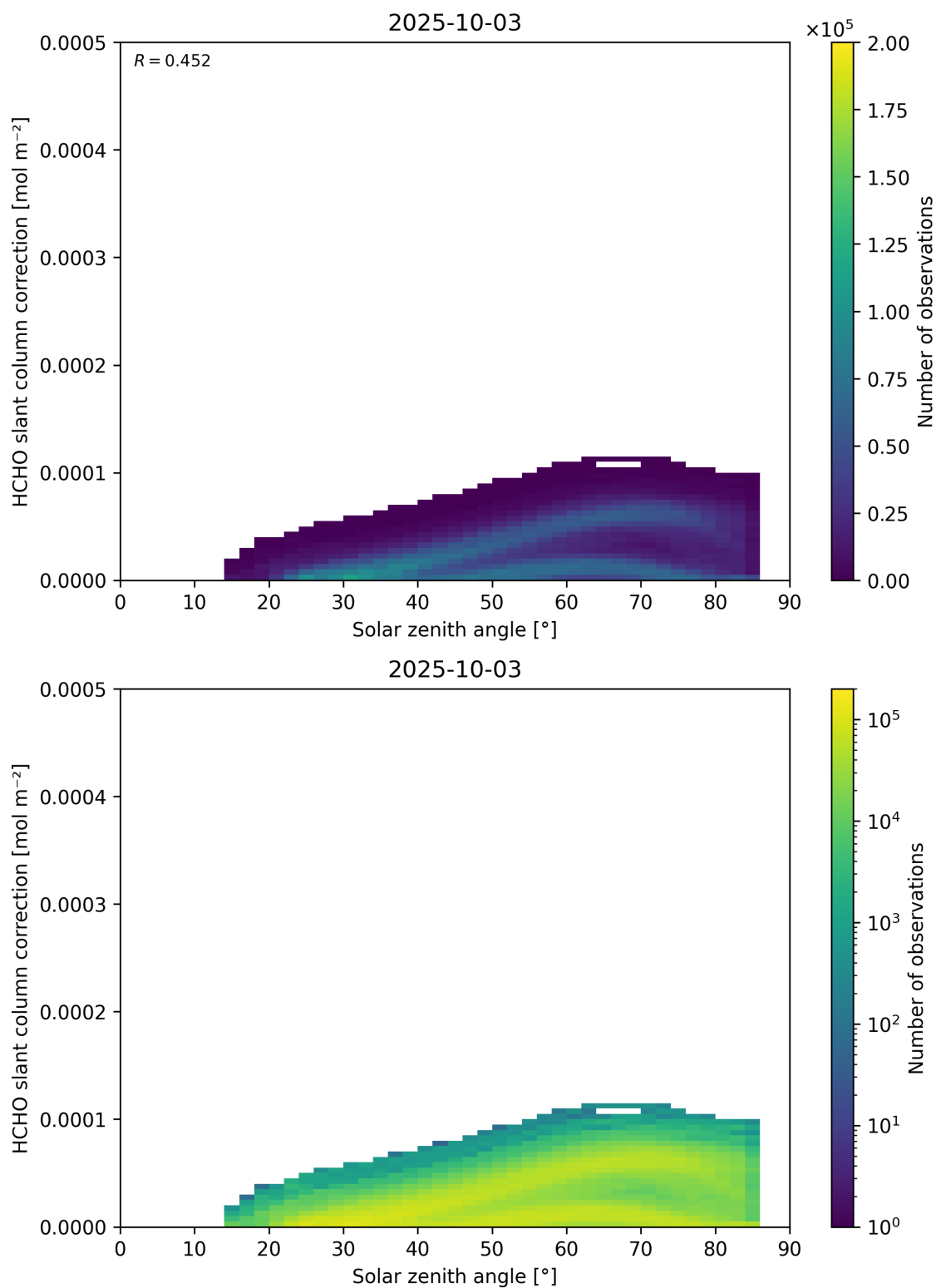
Figure 172: Scatter density plot of “Solar zenith angle” against “HCHO slant column correction” for 2025-10-02 to 2025-10-04.
