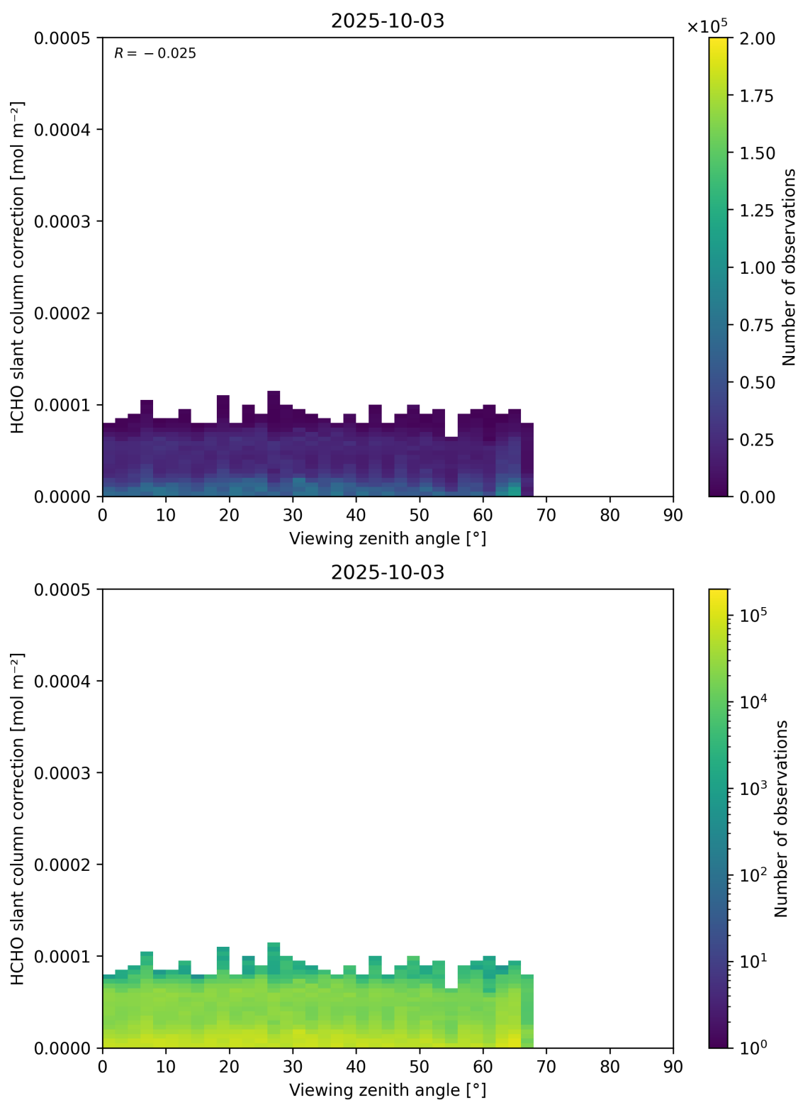
Figure 187: Scatter density plot of “Viewing zenith angle” against “HCHO slant column correction” for 2025-10-02 to 2025-10-04.
