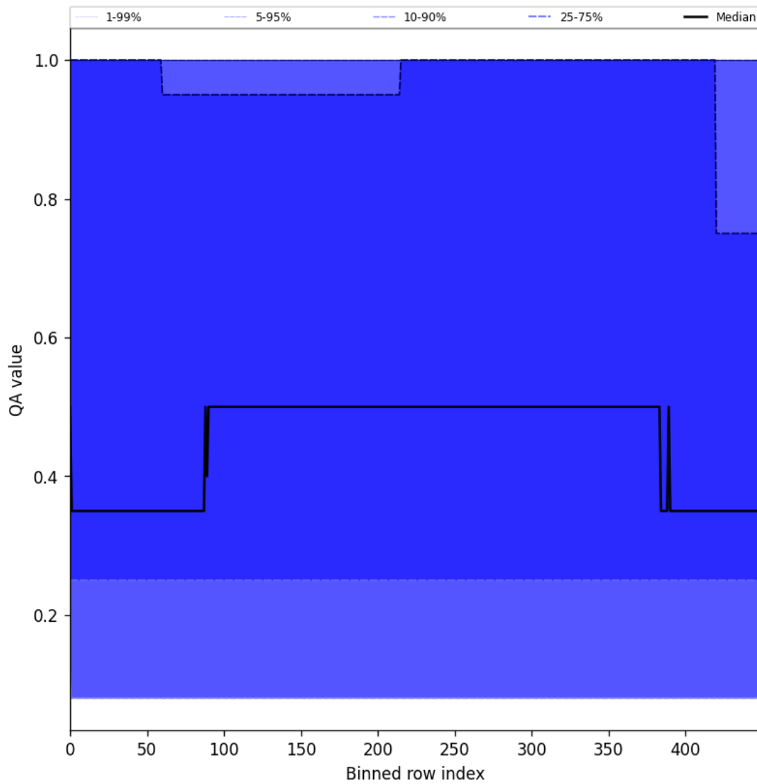
Figure 48: Along track statistics of “QA value” for 2025-10-02 to 2025-10-04
