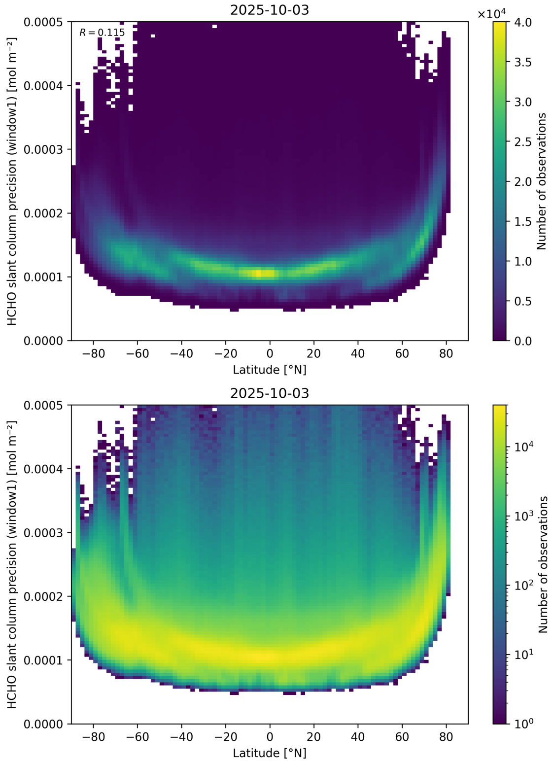
Figure 160: Scatter density plot of “Latitude” against “HCHO slant column precision (window1)” for 2025-10-02 to 2025-10-04.
