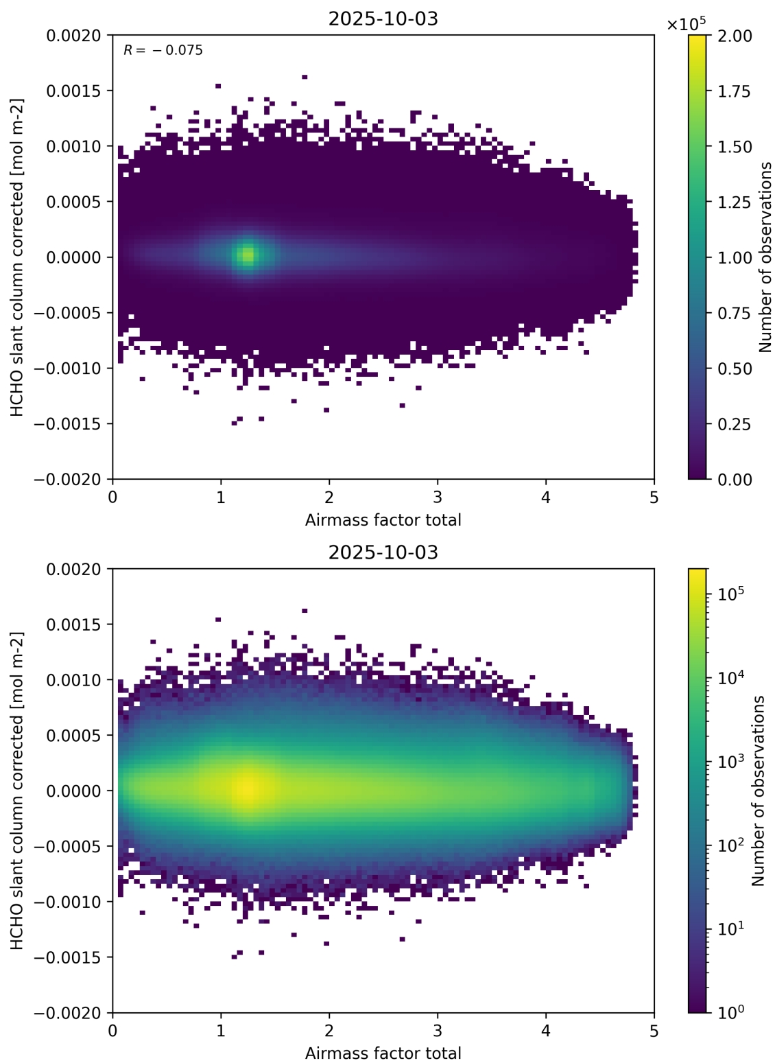
Figure 101: Scatter density plot of “Airmass factor total” against “HCHO slant column corrected” for 2025-10-02 to 2025-10-04.
