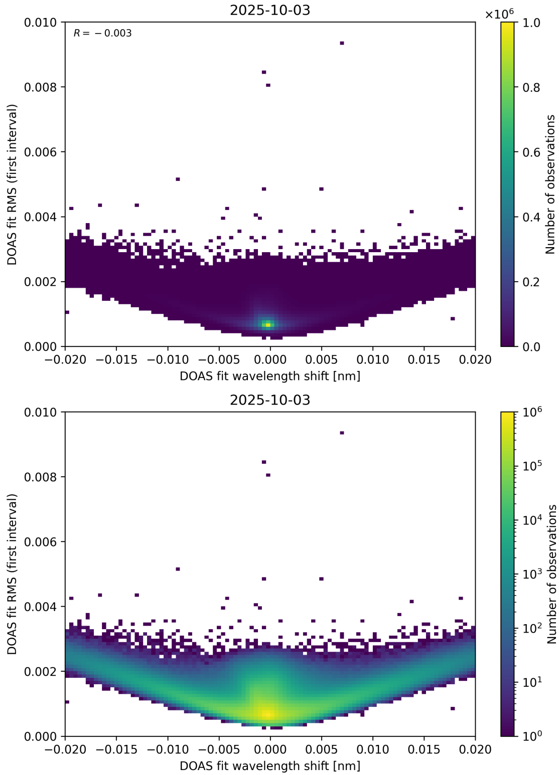
Figure 64: Scatter density plot of “DOAS fit wavelength shift” against “DOAS fit RMS (first interval)” for 2025-10-02 to 2025-10-04.
