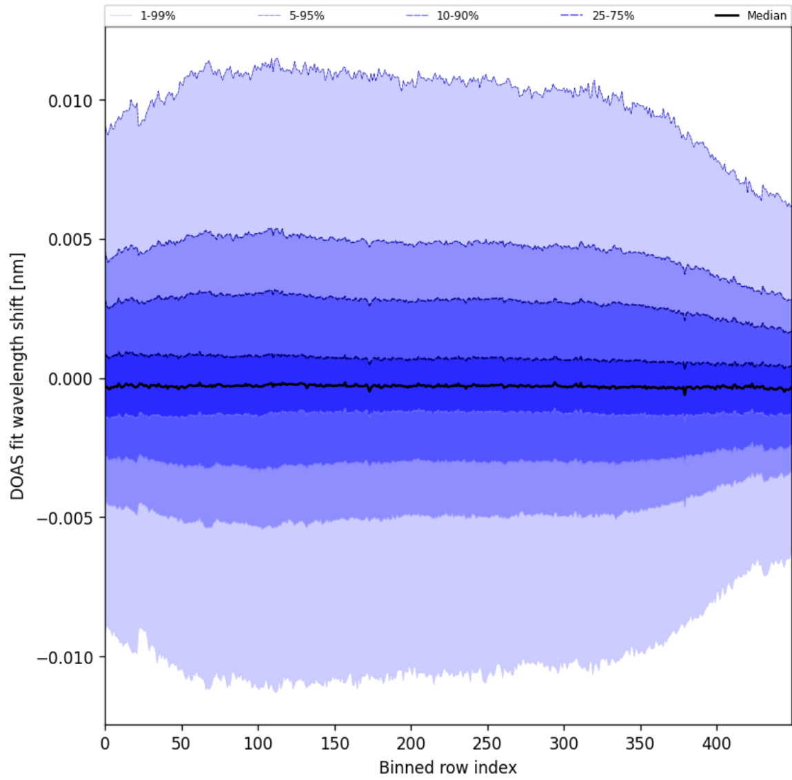
Figure 58: Along track statistics of “DOAS fit wavelength shift” for 2025-10-02 to 2025-10-04
