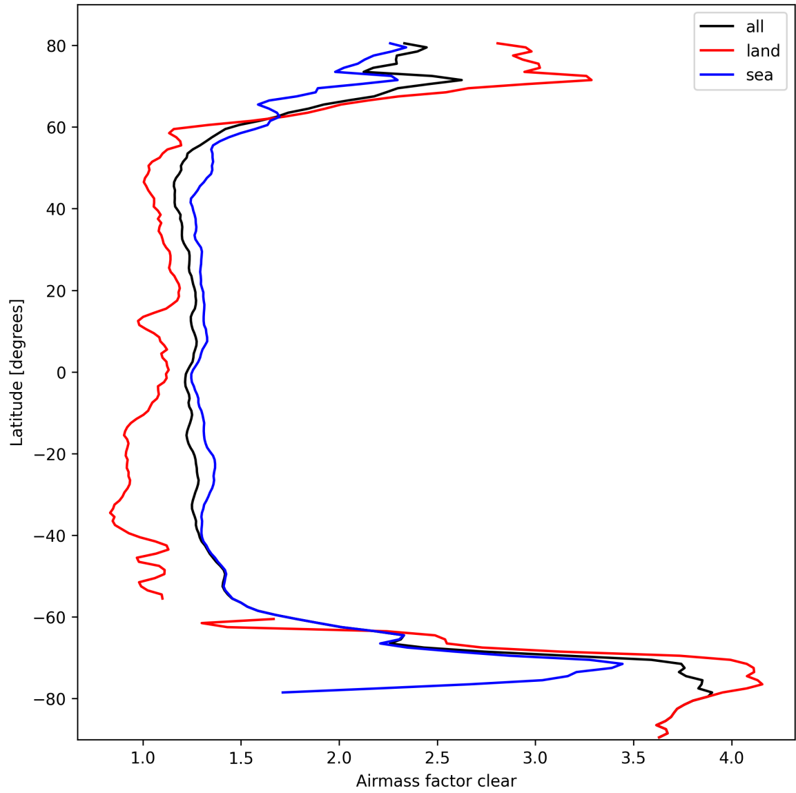
Figure 28: Zonal average of “Airmass factor clear” for 2025-10-02 to 2025-10-04.
