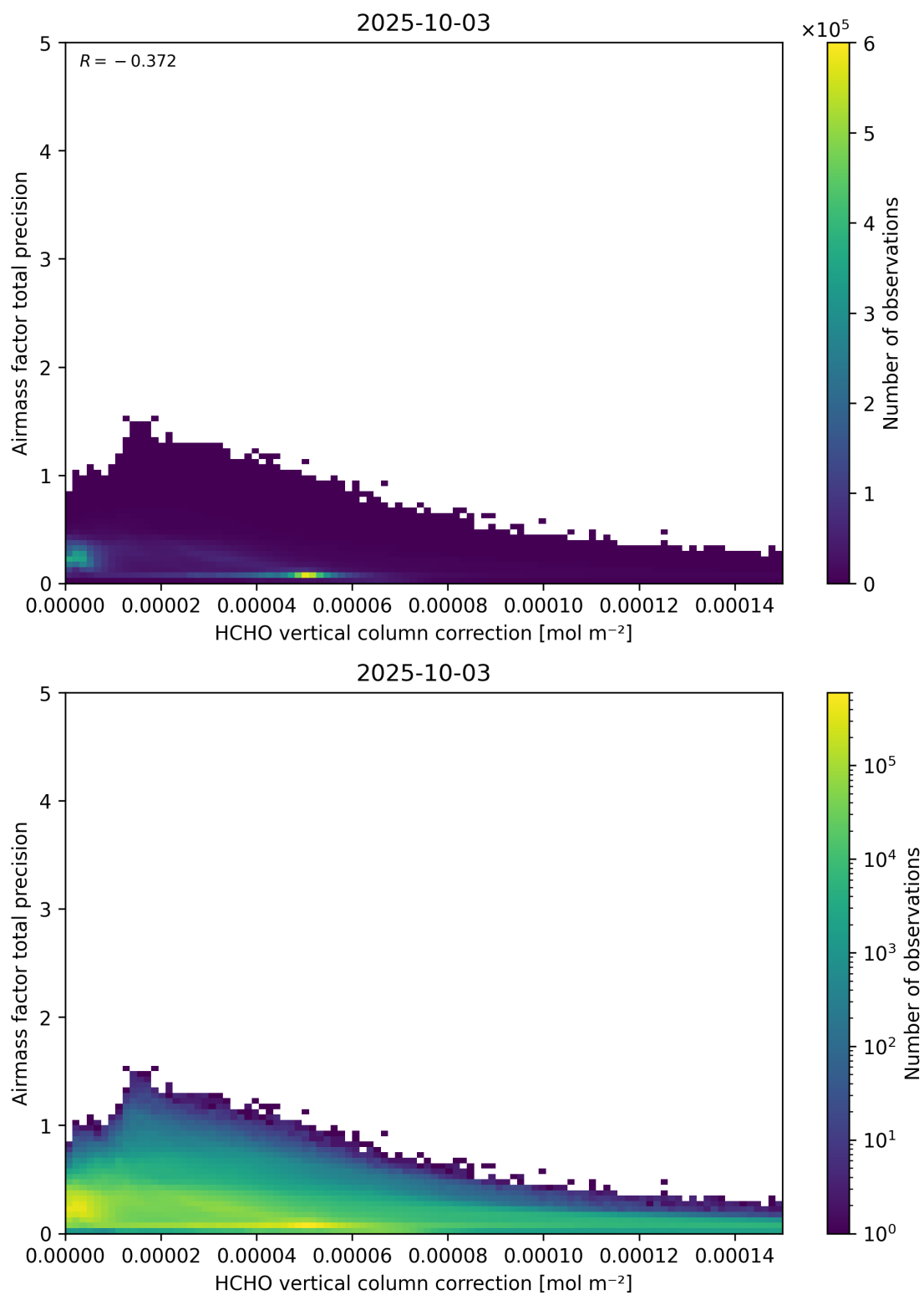
Figure 121: Scatter density plot of “HCHO vertical column correction” against “Airmass factor total precision” for 2025-10-02 to 2025-10-04.
