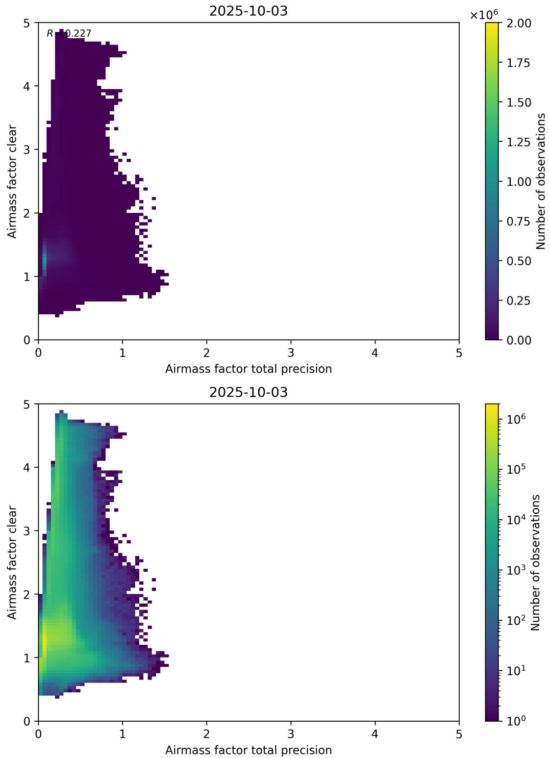
Figure 108: Scatter density plot of “Airmass factor total precision” against “Airmass factor clear” for 2025-10-02 to 2025-10-04.
