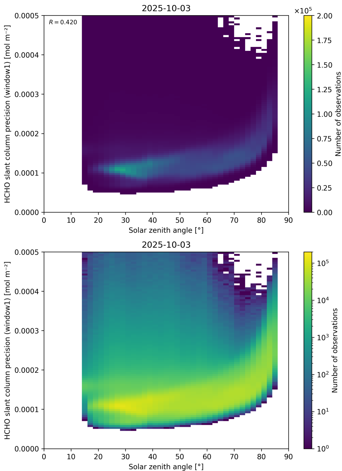
Figure 174: Scatter density plot of “Solar zenith angle” against “HCHO slant column precision (window1)” for 2025-10-02 to 2025-10-04.
