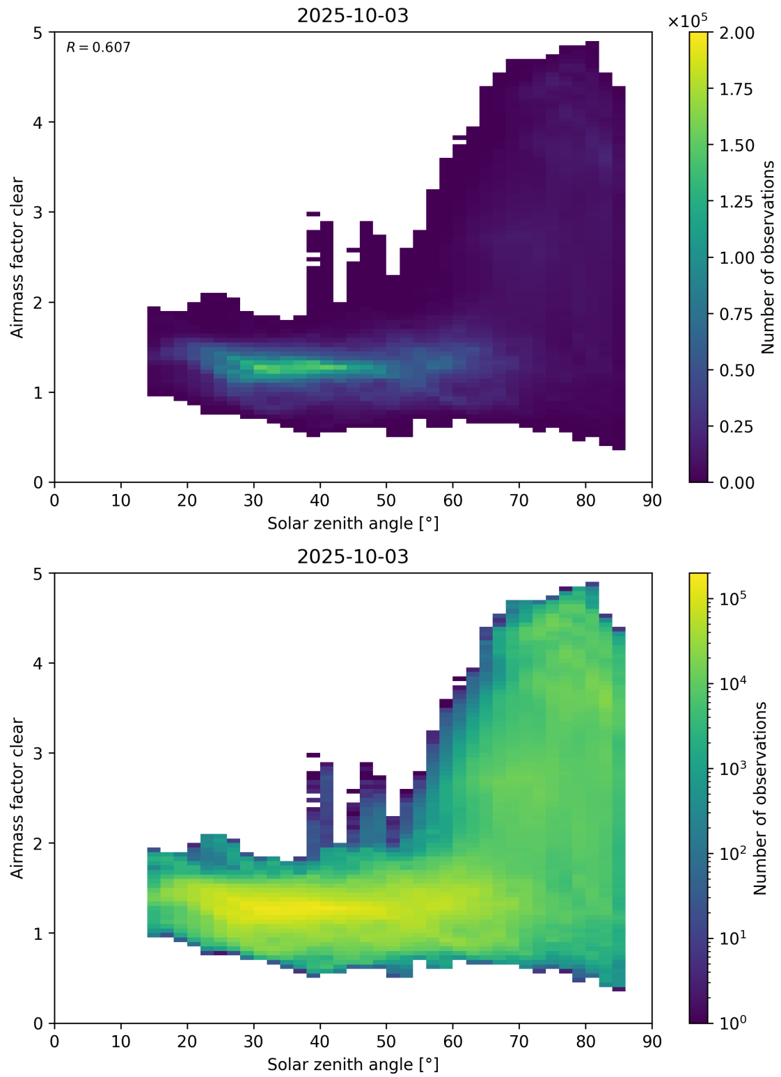
Figure 170: Scatter density plot of “Solar zenith angle” against “Airmass factor clear” for 2025-10-02 to 2025-10-04.
