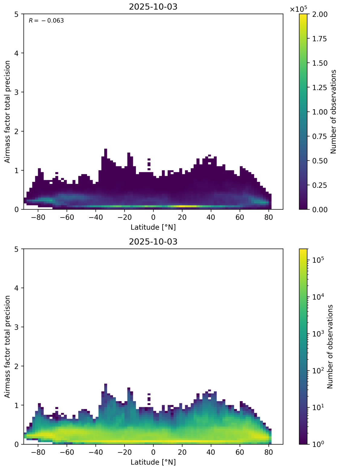
Figure 162: Scatter density plot of “Latitude” against “Airmass factor total precision” for 2025-10-02 to 2025-10-04.
