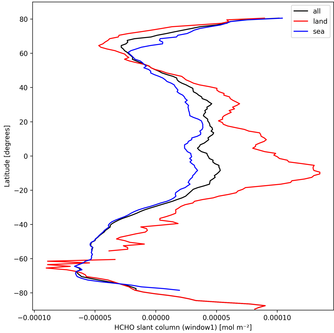
Figure 24: Zonal average of “HCHO slant column (window1)” for 2025-10-02 to 2025-10-04.
