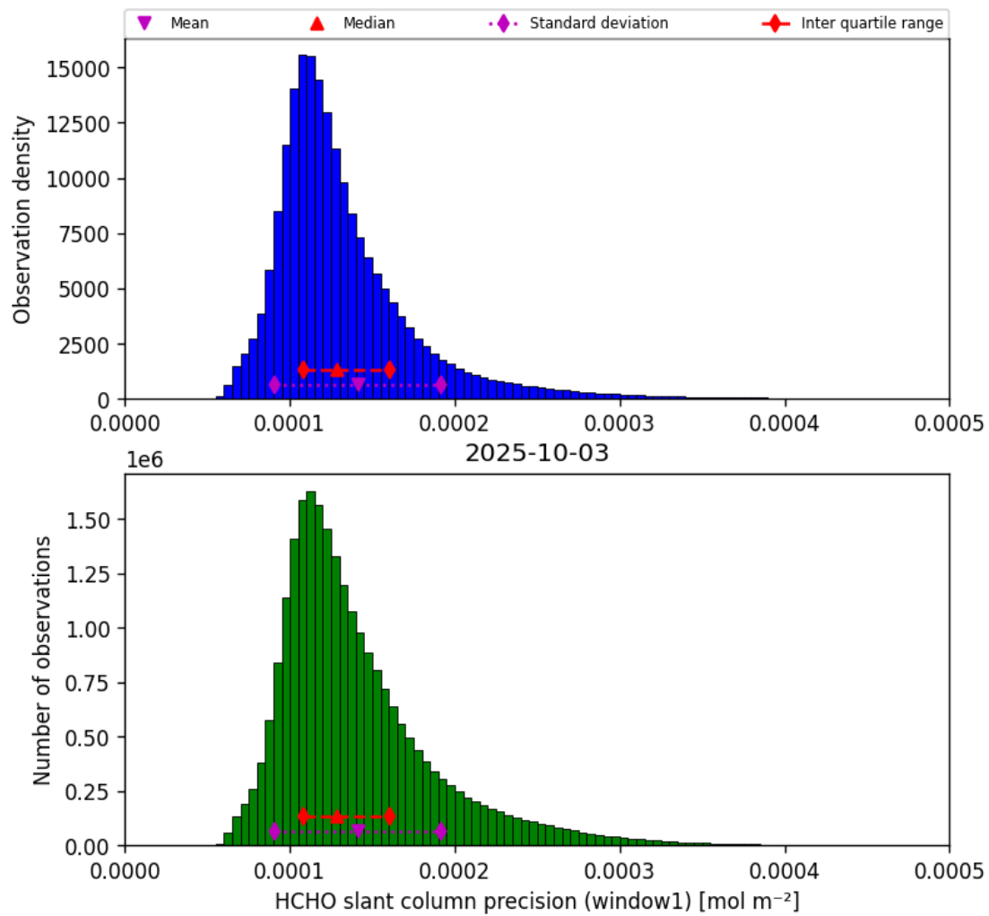
Figure 39: Histogram of “HCHO slant column precision (window1)” for 2025-10-02 to 2025-10-04
