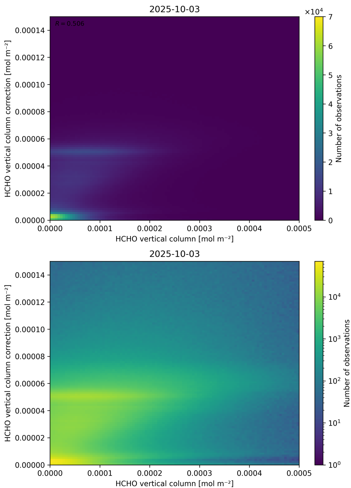
Figure 133: Scatter density plot of “HCHO vertical column” against “HCHO vertical column correction” for 2025-10-02 to 2025-10-04.
