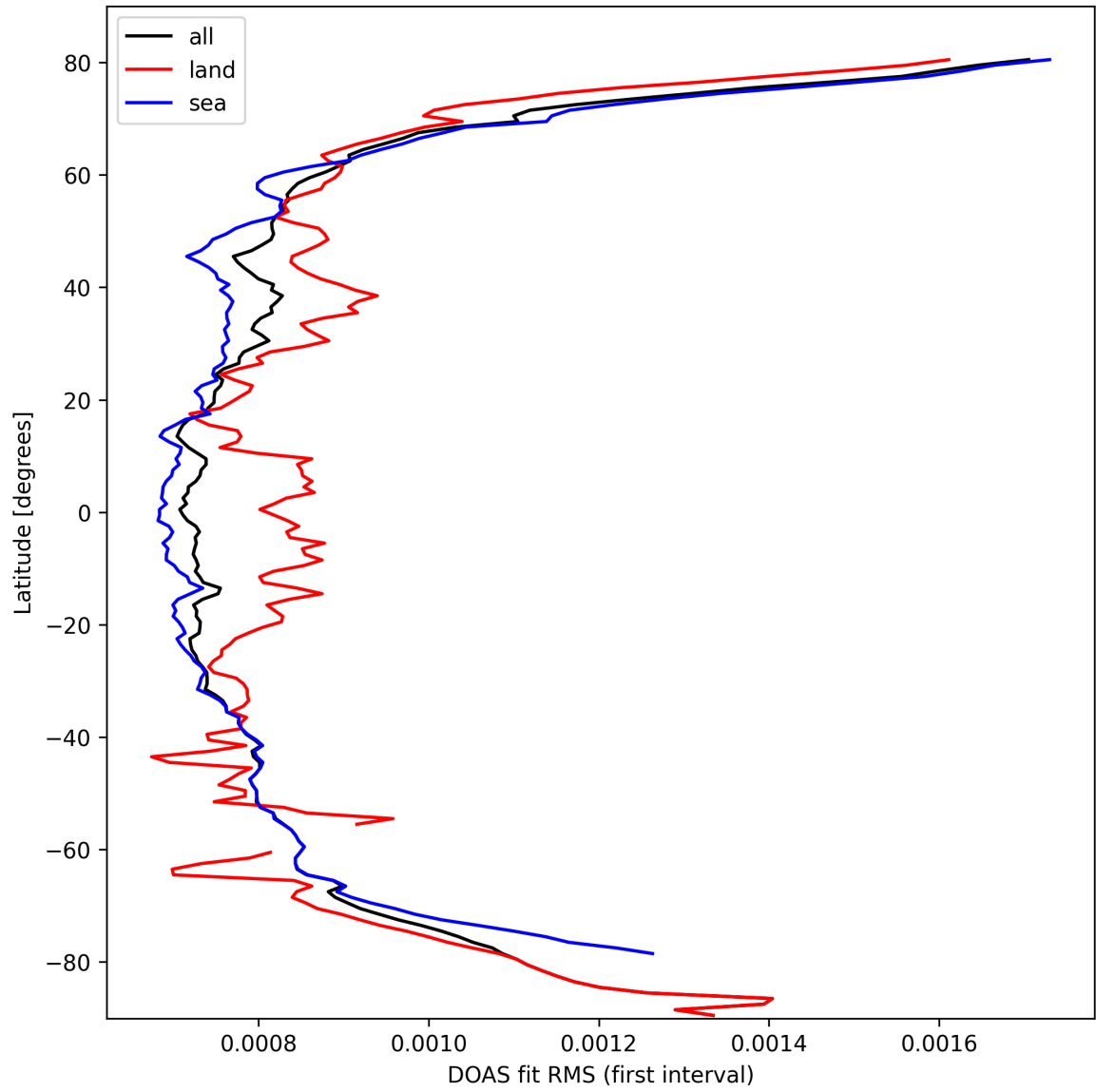
Figure 32: Zonal average of “DOAS fit RMS (first interval)” for 2025-10-02 to 2025-10-04.
