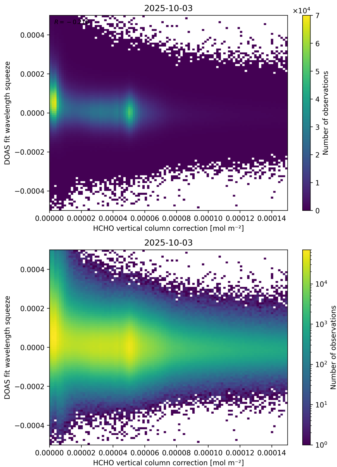
Figure 114: Scatter density plot of “HCHO vertical column correction” against “DOAS fit wavelength squeeze” for 2025-10-02 to 2025-10-04.
