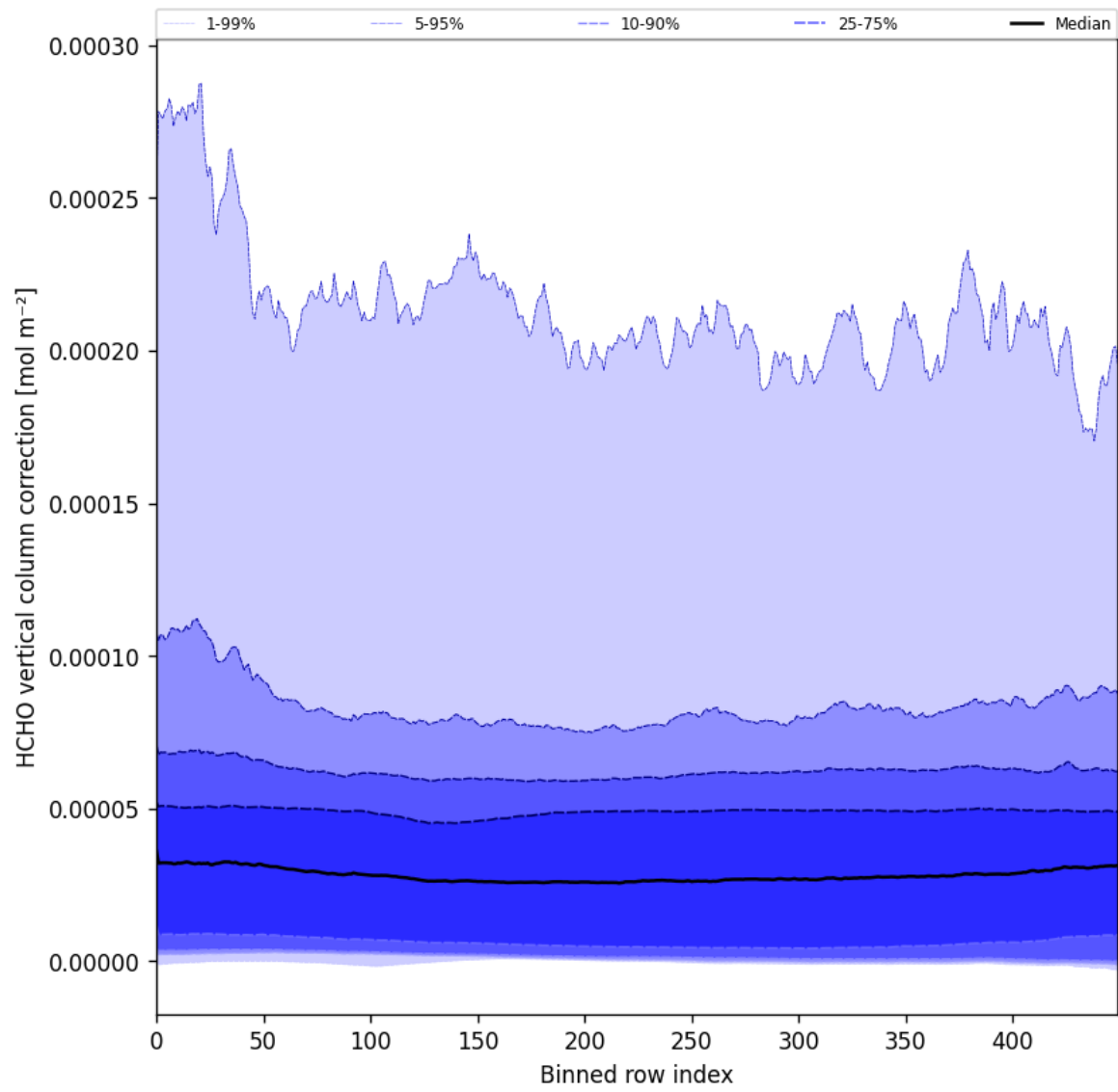
Figure 51: Along track statistics of “HCHO vertical column correction” for 2025-10-02 to 2025-10-04
