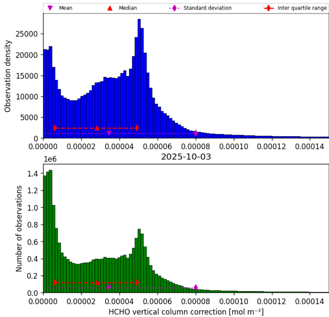
Figure 37: Histogram of “HCHO vertical column correction” for 2025-10-02 to 2025-10-04
