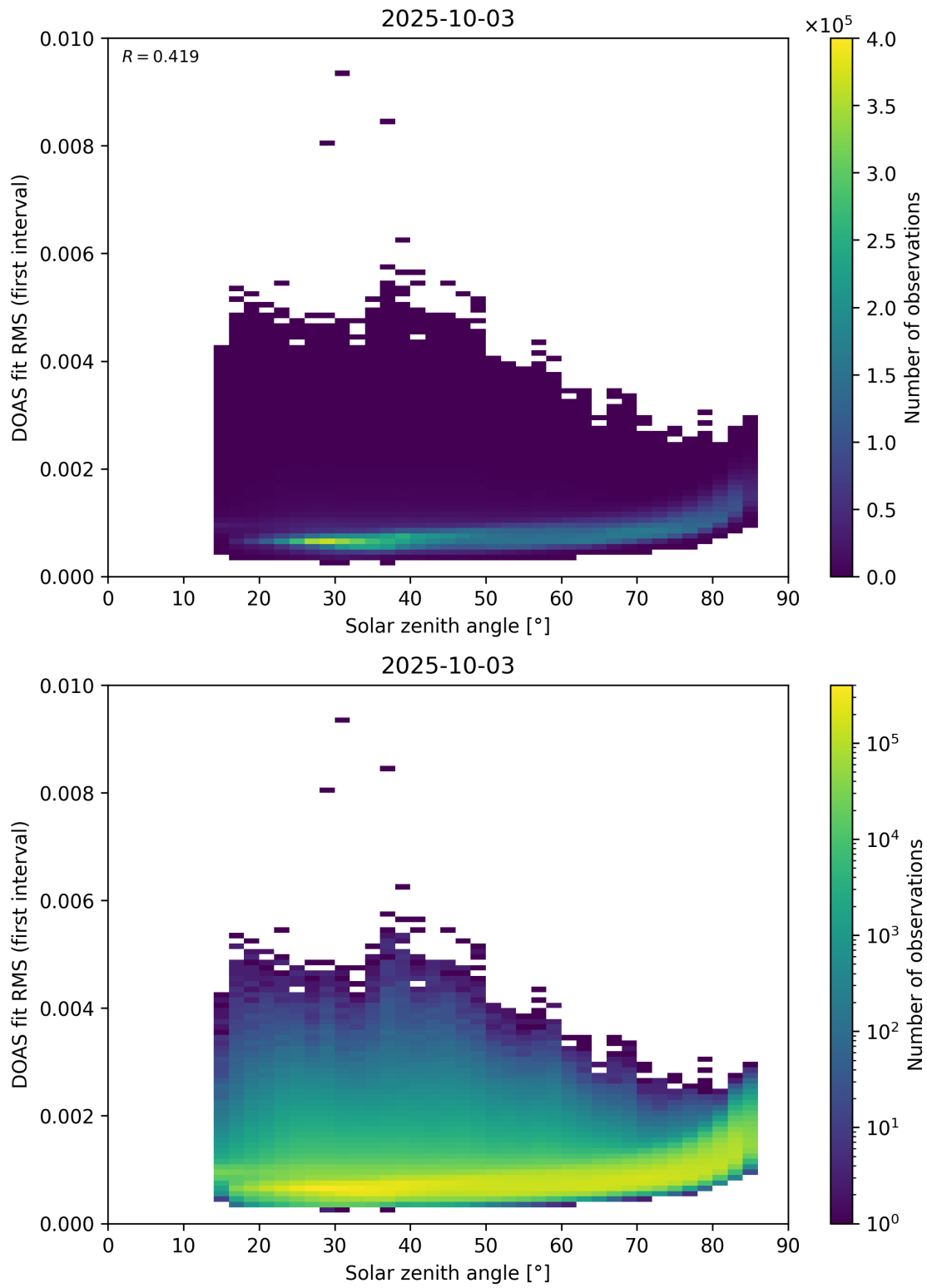
Figure 167: Scatter density plot of “Solar zenith angle” against “DOAS fit RMS (first interval)” for 2025-10-02 to 2025-10-04.
