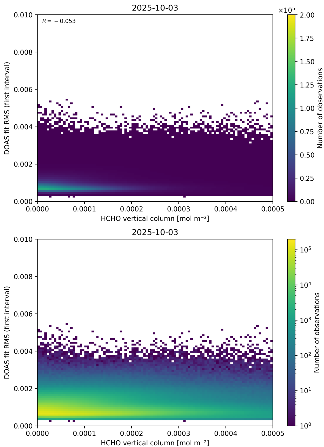
Figure 123: Scatter density plot of “HCHO vertical column” against “DOAS fit RMS (first interval)” for 2025-10-02 to 2025-10-04.
