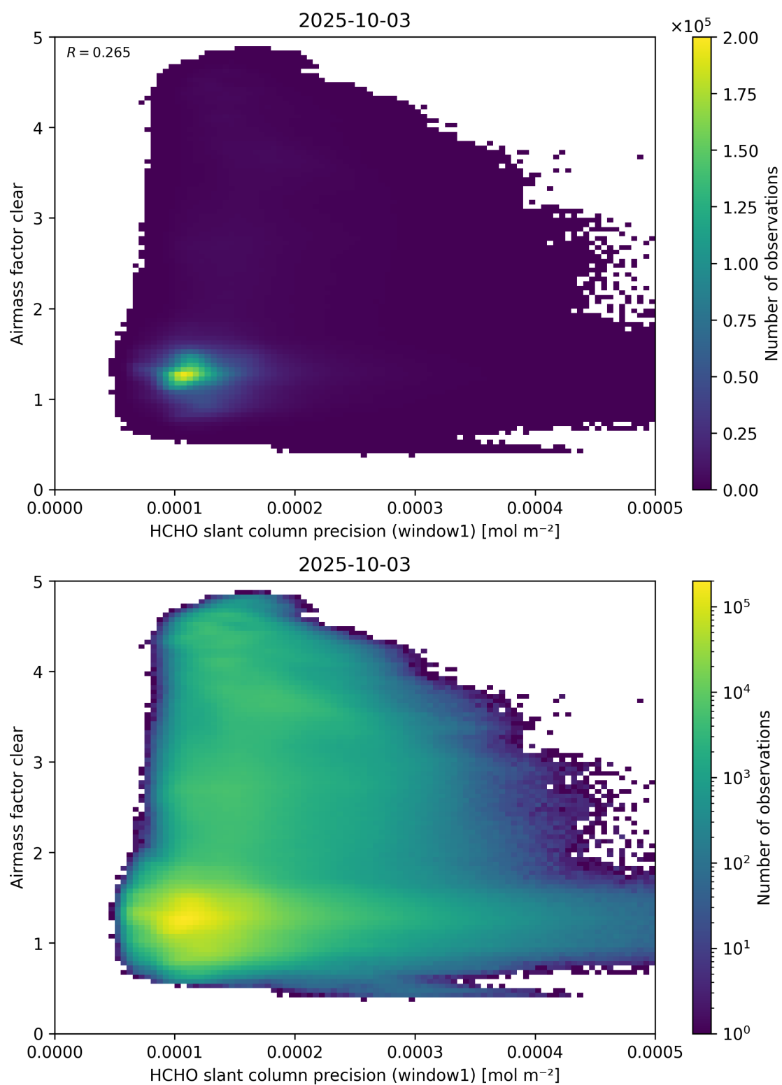
Figure 91: Scatter density plot of “HCHO slant column precision (window1)” against “Airmass factor clear” for 2025-10-02 to 2025-10-04.
