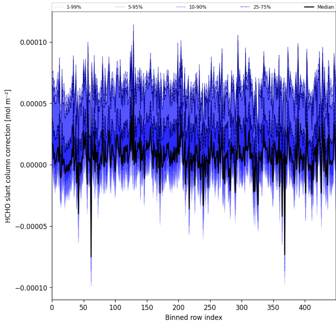
Figure 61: Along track statistics of “HCHO slant column correction” for 2025-10-02 to 2025-10-04
