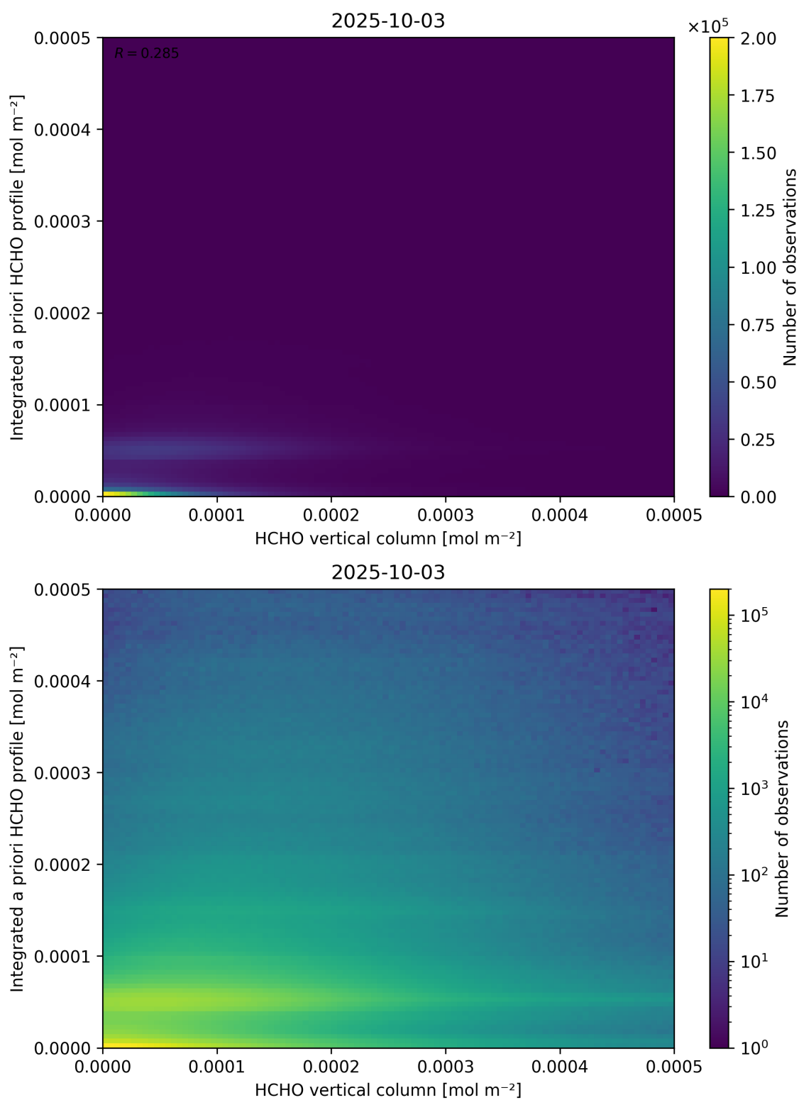
Figure 135: Scatter density plot of “HCHO vertical column” against “Integrated a priori HCHO profile” for 2025-10-02 to 2025-10-04.
