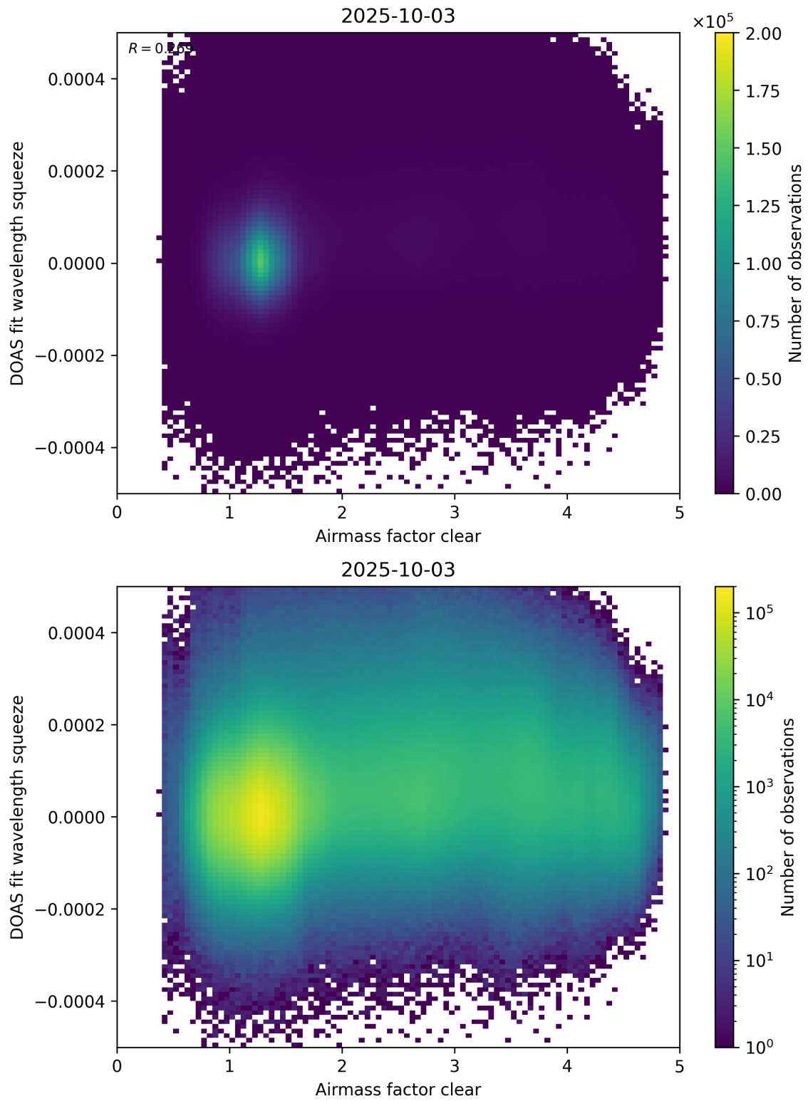
Figure 73: Scatter density plot of “Airmass factor clear” against “DOAS fit wavelength squeeze” for 2025-10-02 to 2025-10-04.
