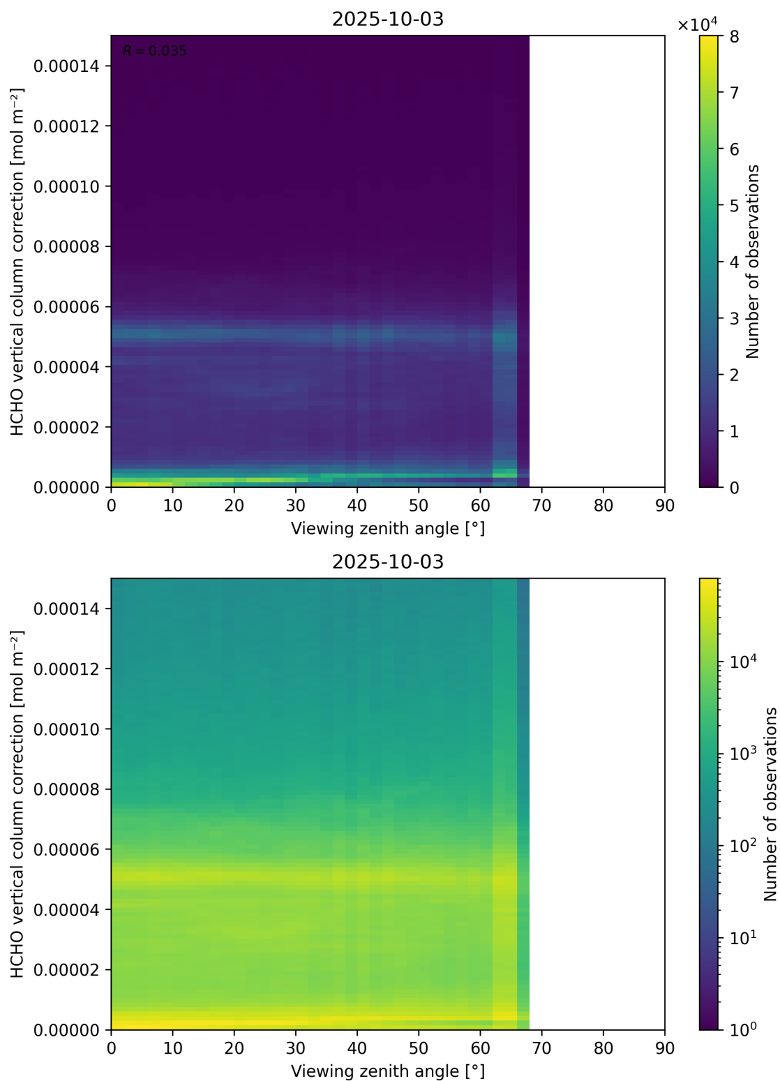
Figure 193: Scatter density plot of “Viewing zenith angle” against “HCHO vertical column correction” for 2025-10-02 to 2025-10-04.
