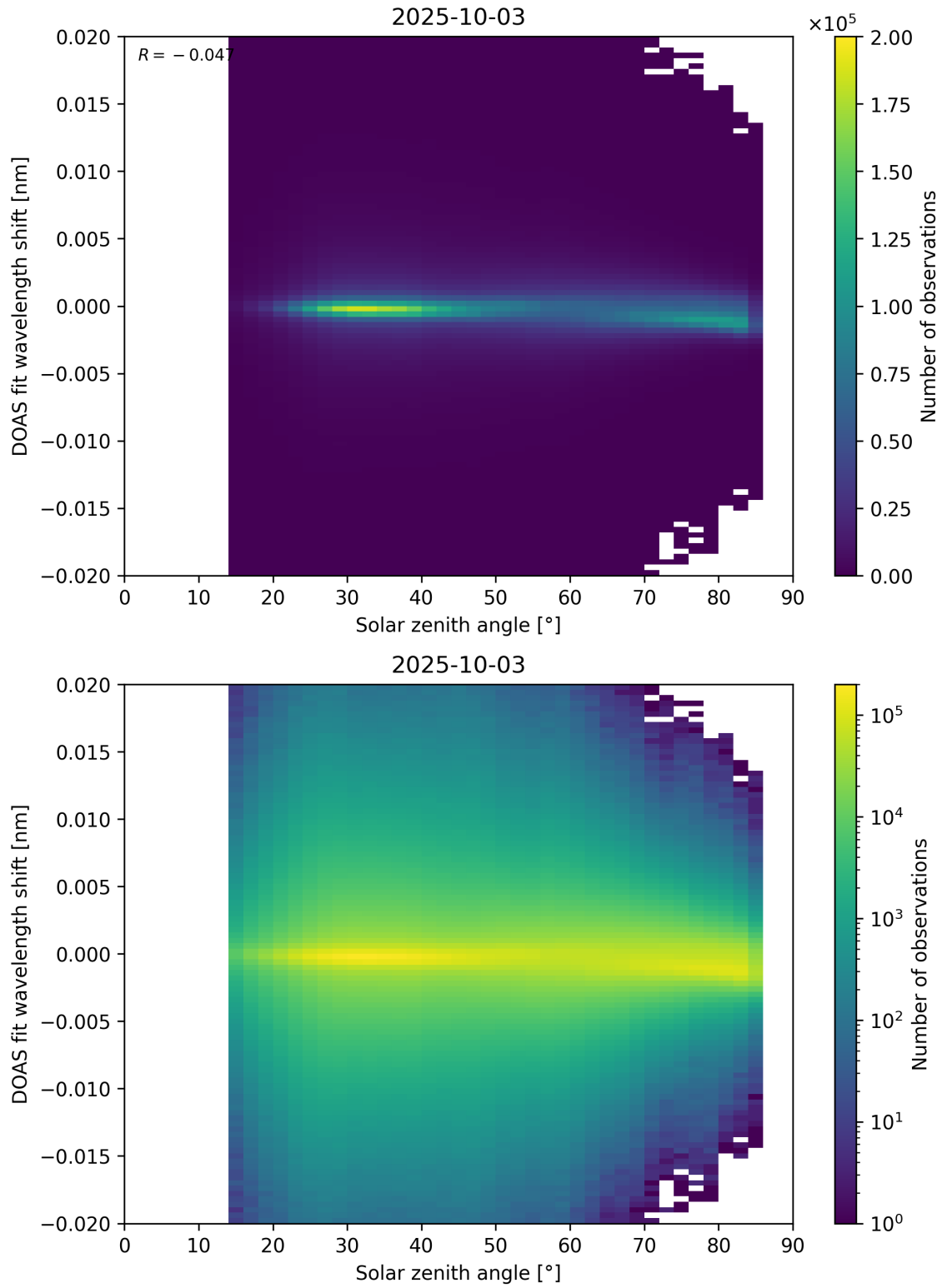
Figure 168: Scatter density plot of “Solar zenith angle” against “DOAS fit wavelength shift” for 2025-10-02 to 2025-10-04.
