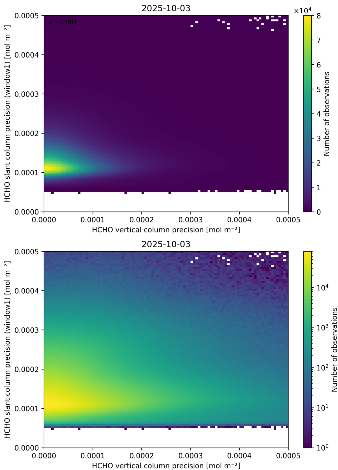
Figure 143: Scatter density plot of “HCHO vertical column precision” against “HCHO slant column precision (window1)” for 2025-10-02 to 2025-10-04.
