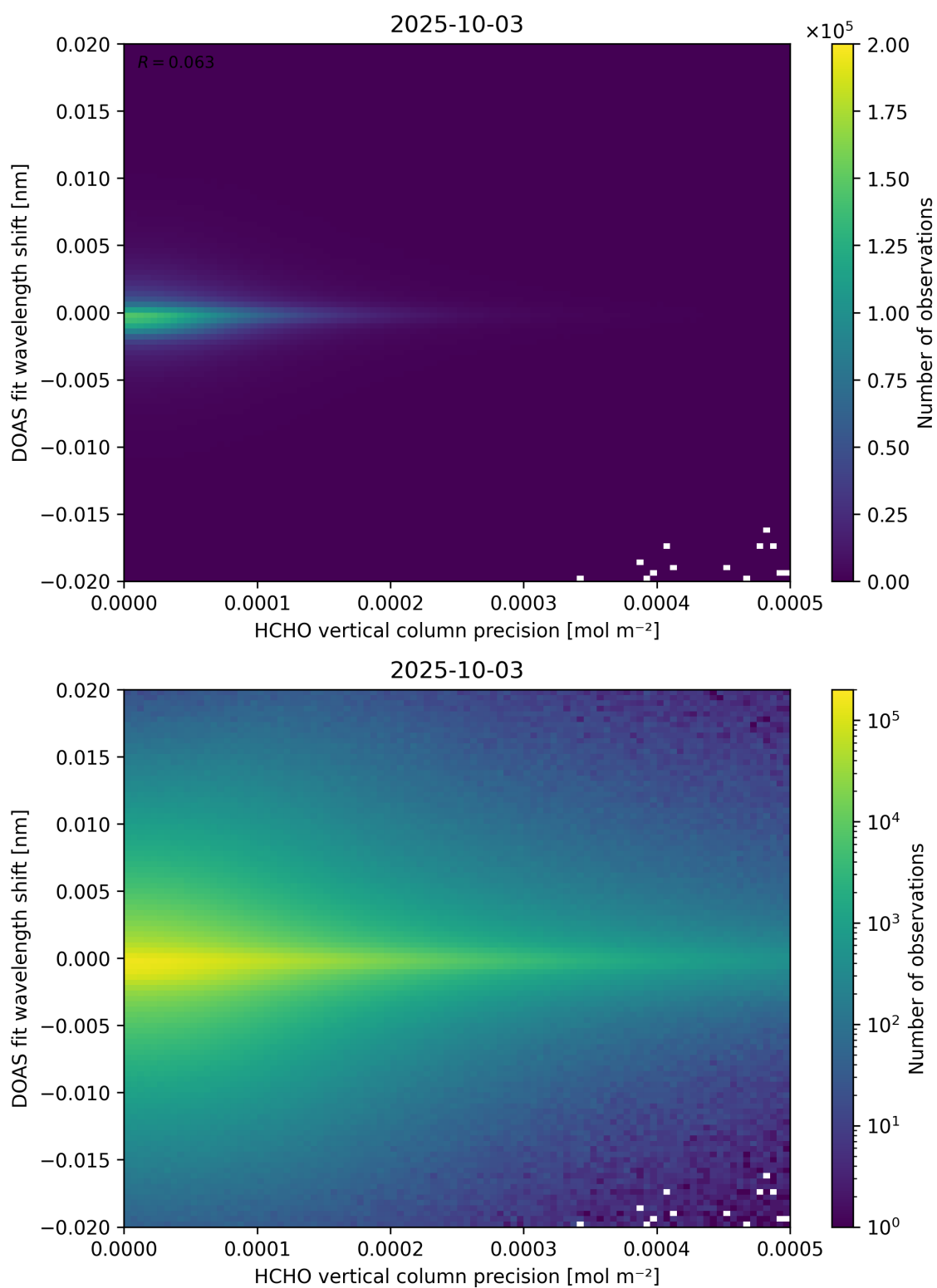
Figure 137: Scatter density plot of “HCHO vertical column precision” against “DOAS fit wavelength shift” for 2025-10-02 to 2025-10-04.
