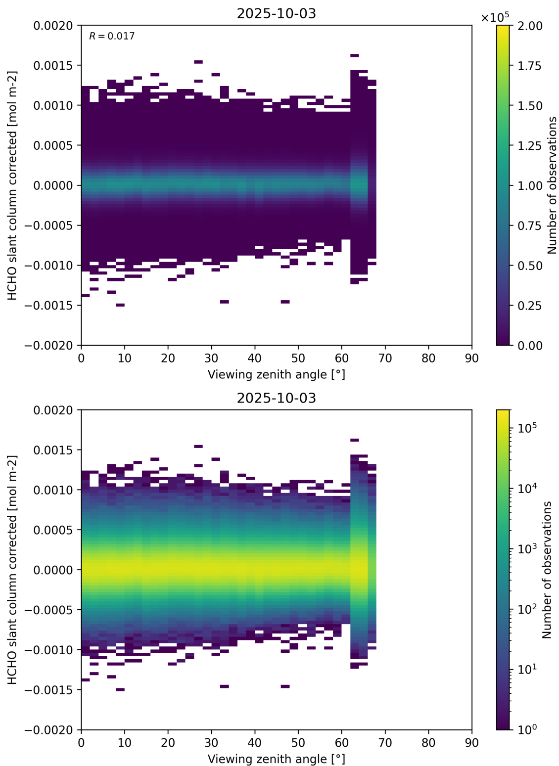
Figure 186: Scatter density plot of “Viewing zenith angle” against “HCHO slant column corrected” for 2025-10-02 to 2025-10-04.
