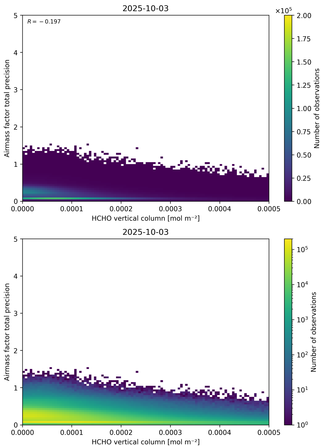
Figure 132: Scatter density plot of “HCHO vertical column” against “Airmass factor total precision” for 2025-10-02 to 2025-10-04.
