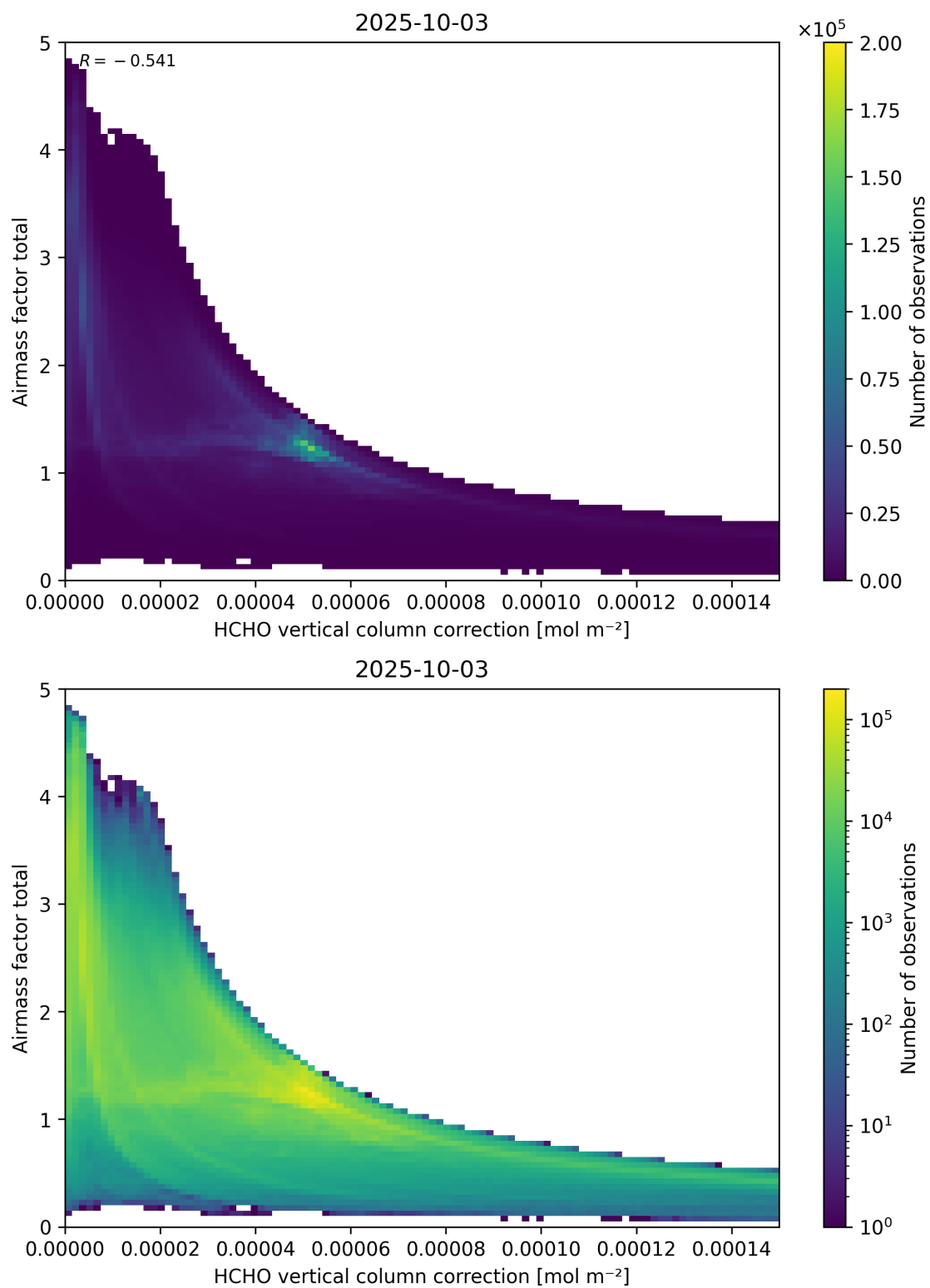
Figure 120: Scatter density plot of “HCHO vertical column correction” against “Airmass factor total” for 2025-10-02 to 2025-10-04.
