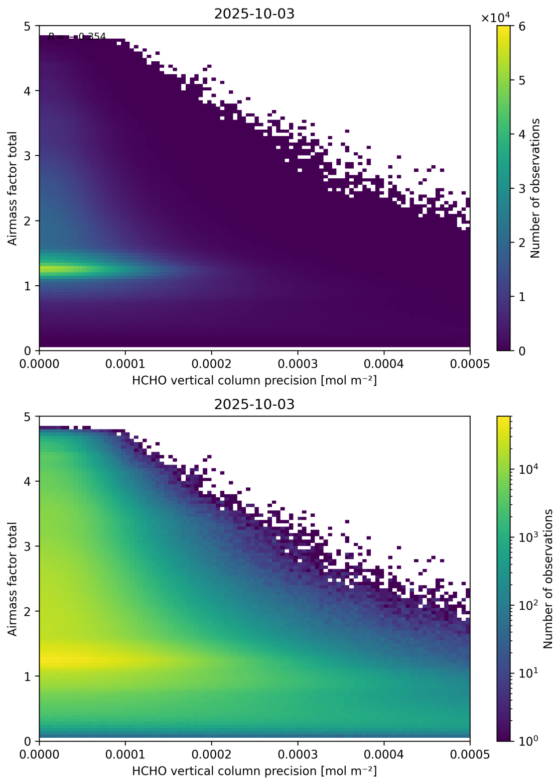
Figure 144: Scatter density plot of “HCHO vertical column precision” against “Airmass factor total” for 2025-10-02 to 2025-10-04.
