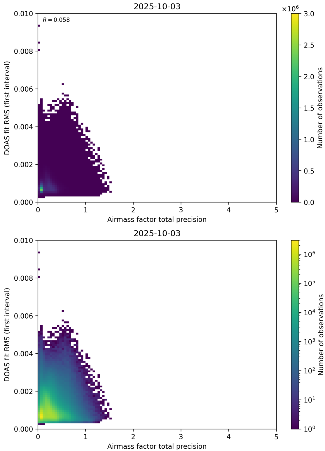
Figure 105: Scatter density plot of “Airmass factor total precision” against “DOAS fit RMS (first interval)” for 2025-10-02 to 2025-10-04.
