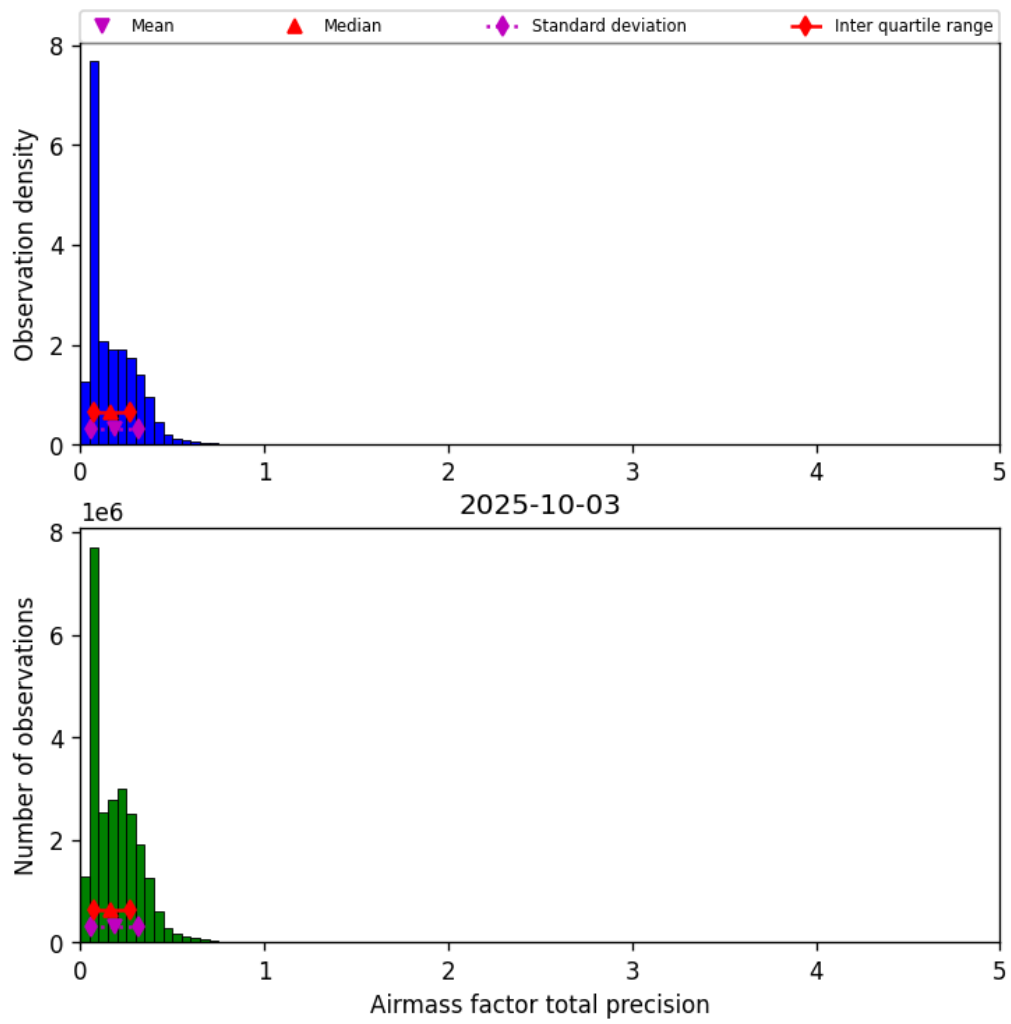
Figure 41: Histogram of “Airmass factor total precision” for 2025-10-02 to 2025-10-04
