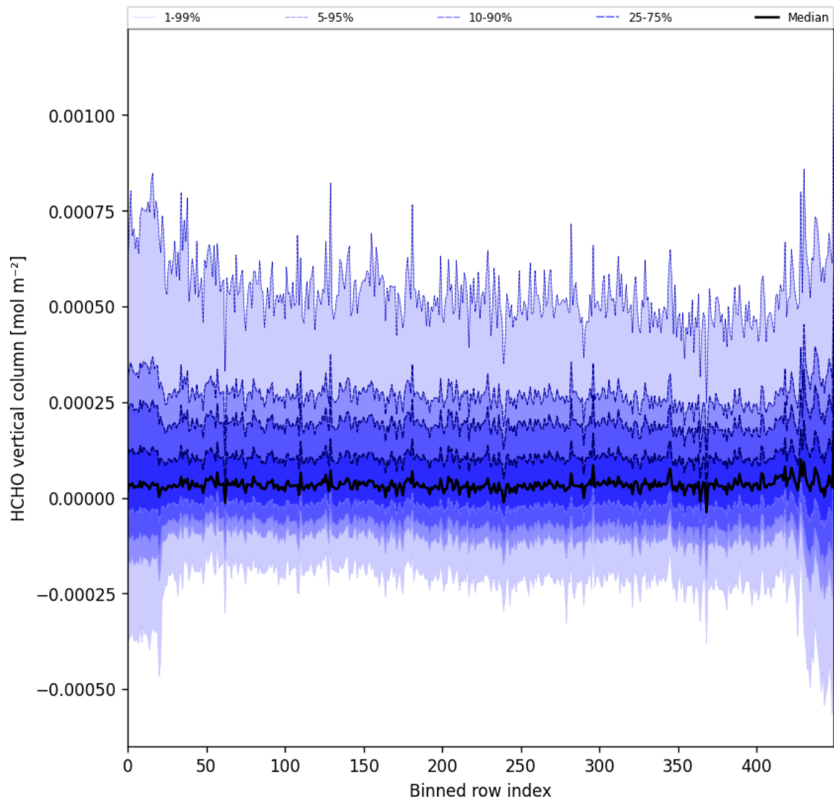
Figure 49: Along track statistics of “HCHO vertical column” for 2025-10-02 to 2025-10-04
