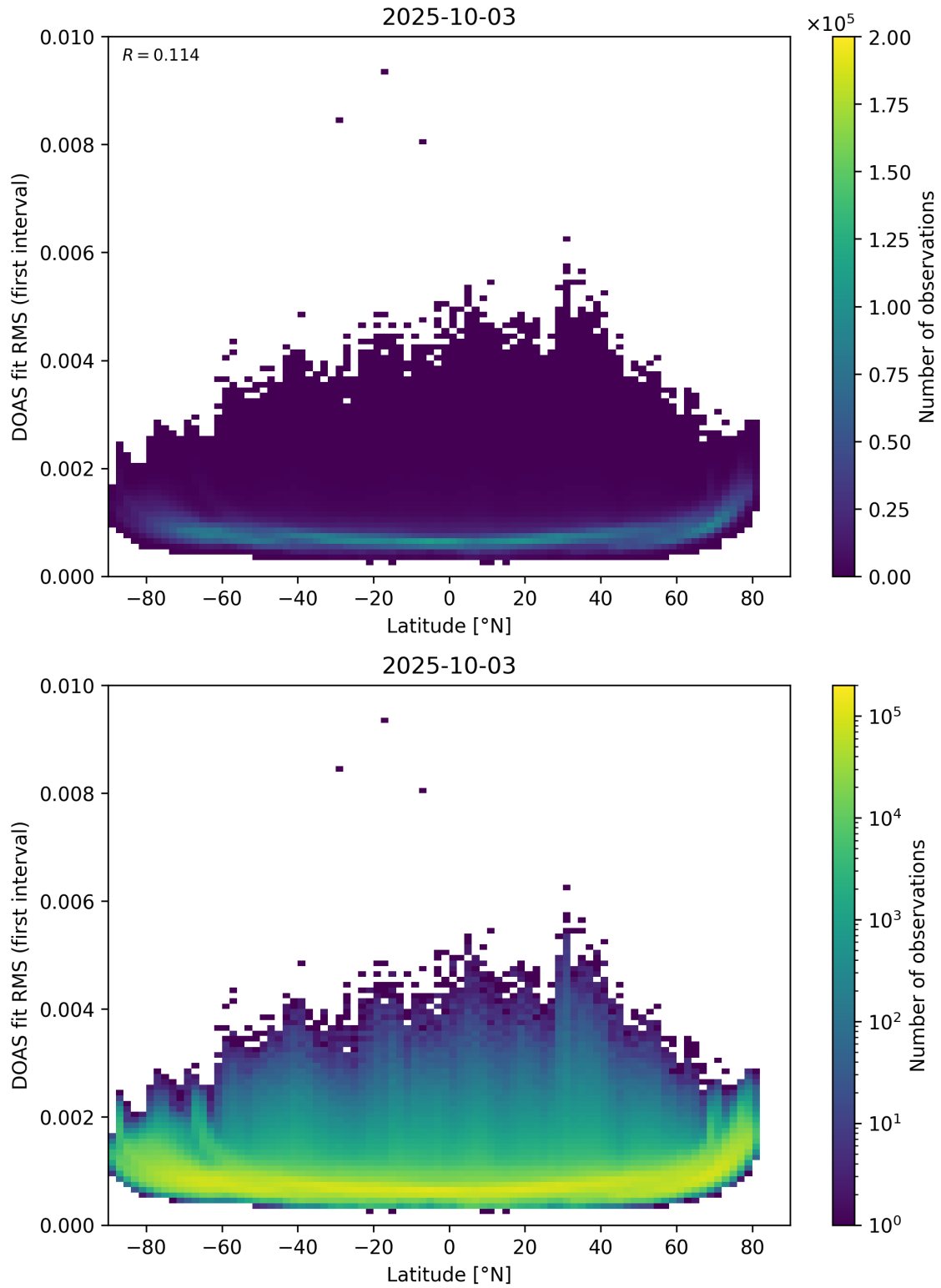
Figure 153: Scatter density plot of “Latitude” against “DOAS fit RMS (first interval)” for 2025-10-02 to 2025-10-04.
