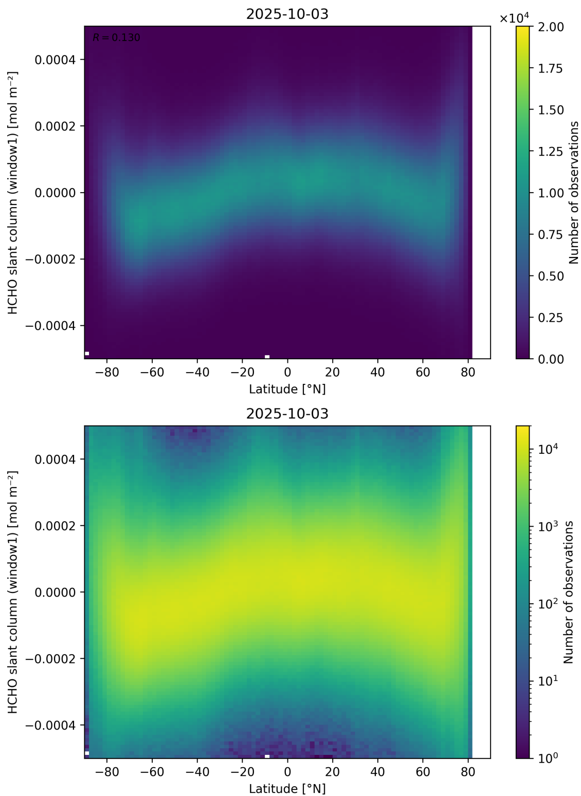
Figure 159: Scatter density plot of “Latitude” against “HCHO slant column (window1)” for 2025-10-02 to 2025-10-04.
