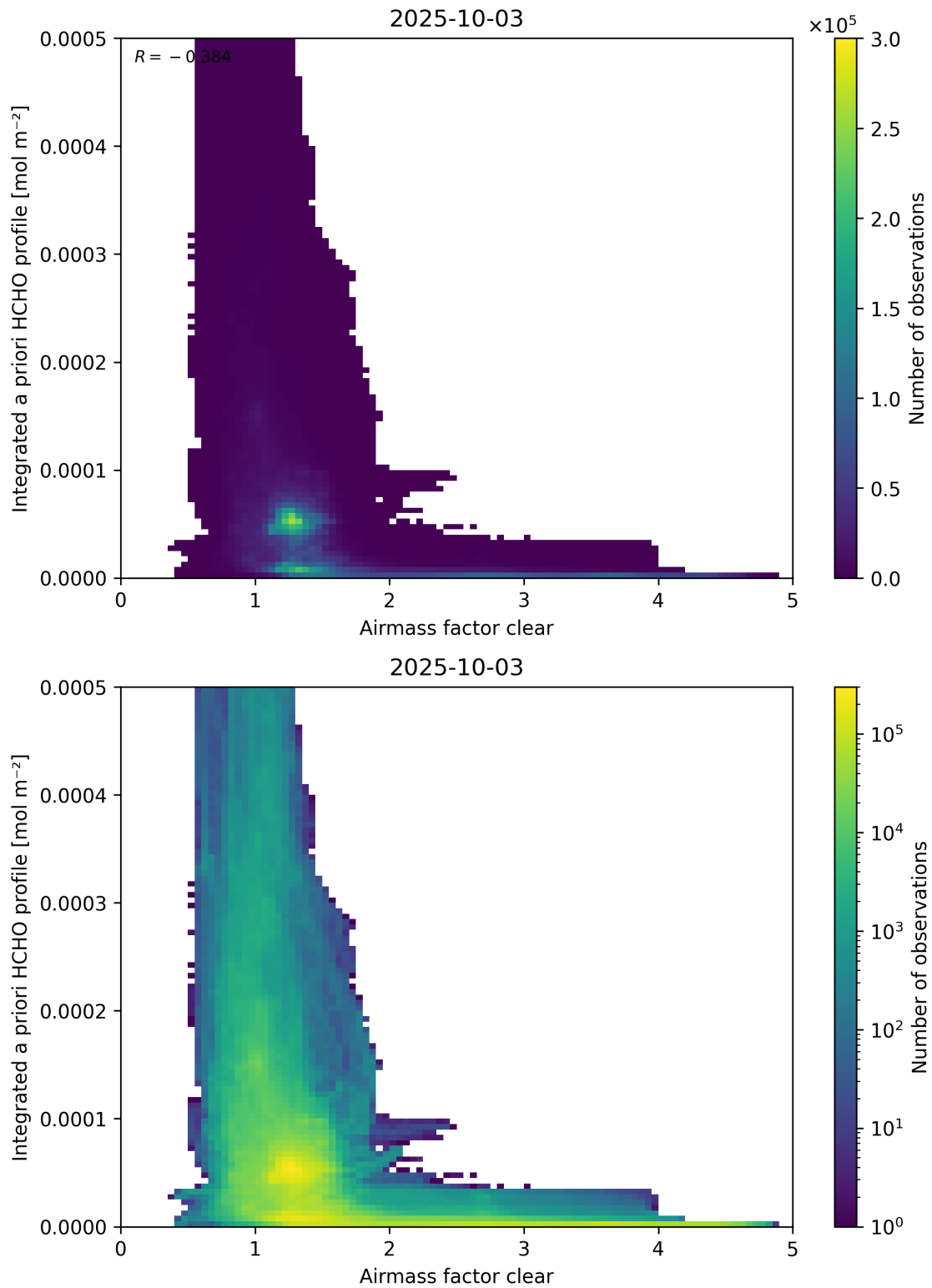
Figure 76: Scatter density plot of “Airmass factor clear” against “Integrated a priori HCHO profile” for 2025-10-02 to 2025-10-04.
