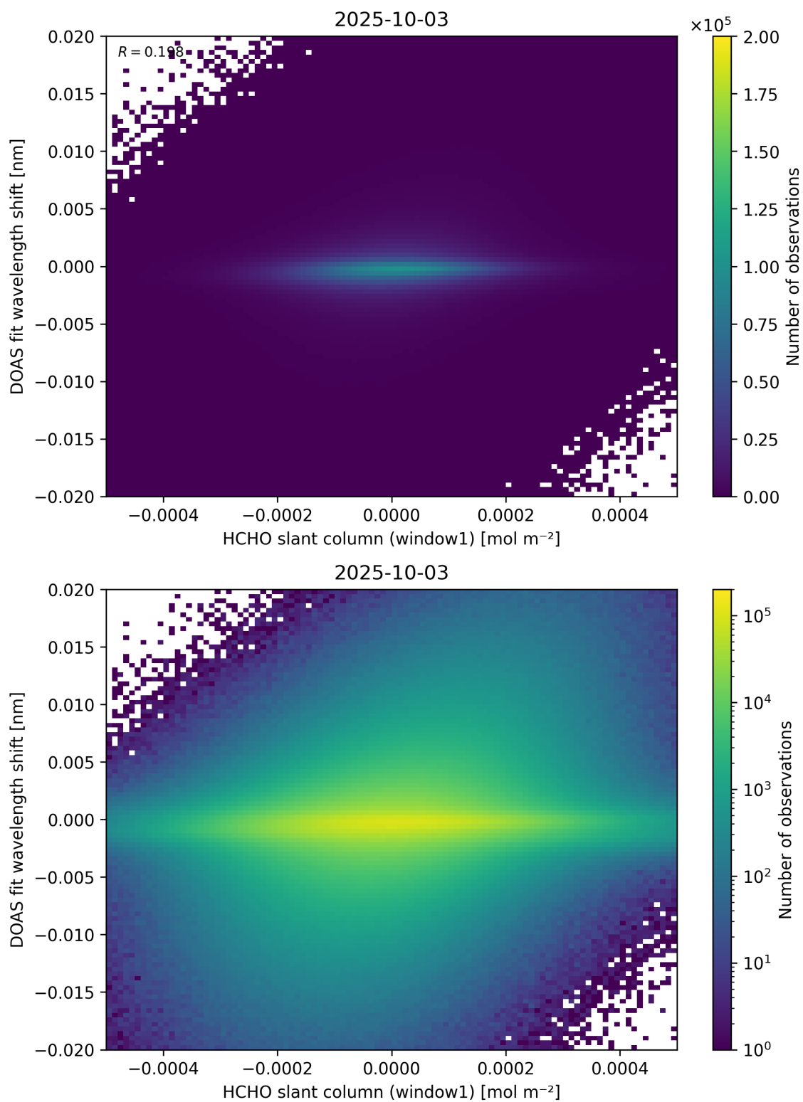
Figure 79: Scatter density plot of “HCHO slant column (window1)” against “DOAS fit wavelength shift” for 2025-10-02 to 2025-10-04.
