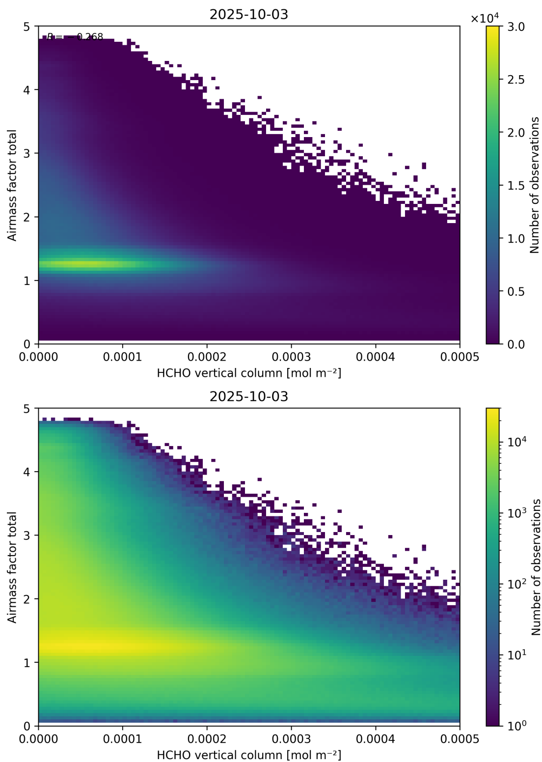
Figure 131: Scatter density plot of “HCHO vertical column” against “Airmass factor total” for 2025-10-02 to 2025-10-04.
