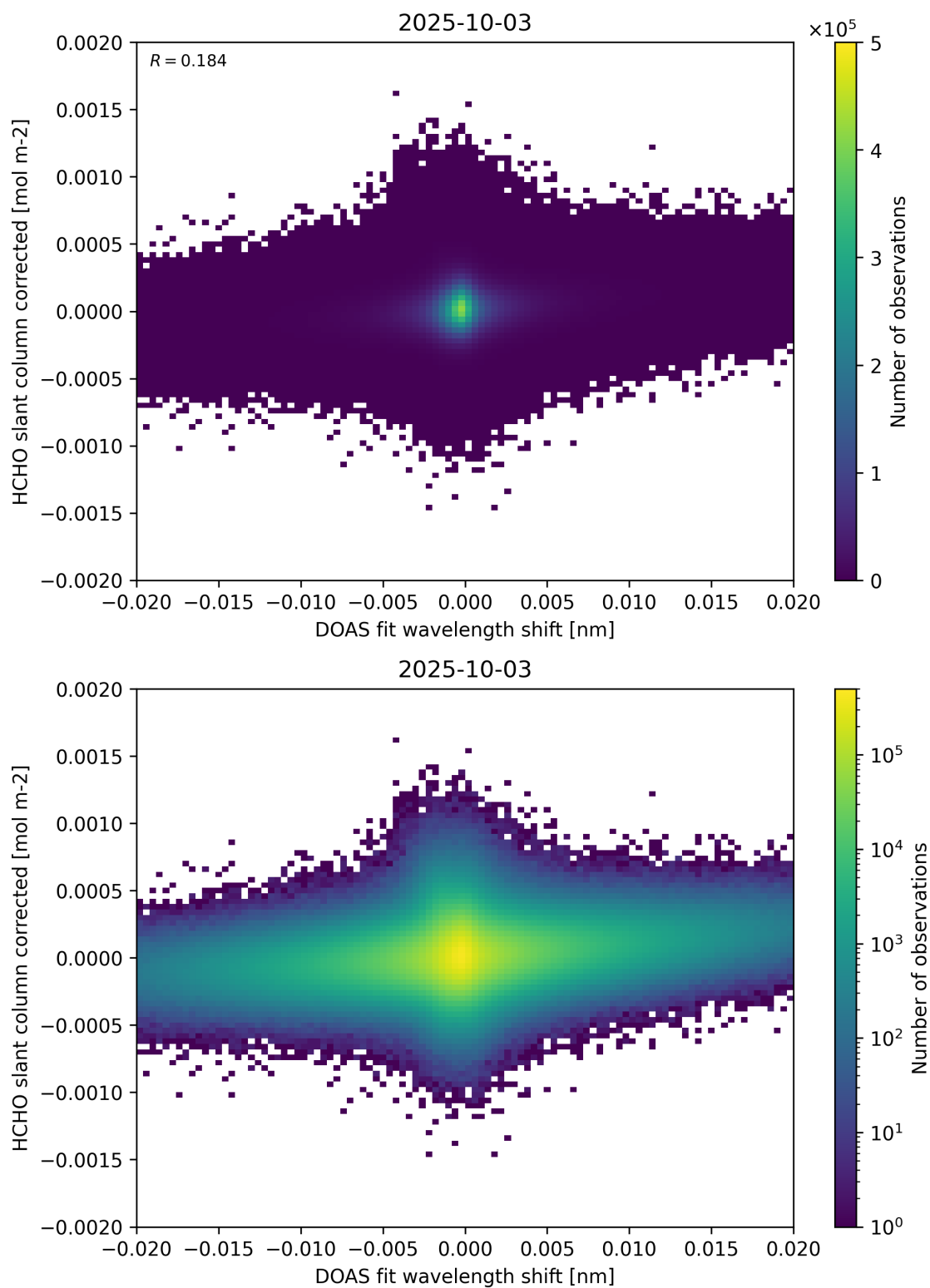
Figure 66: Scatter density plot of “DOAS fit wavelength shift” against “HCHO slant column corrected” for 2025-10-02 to 2025-10-04.
