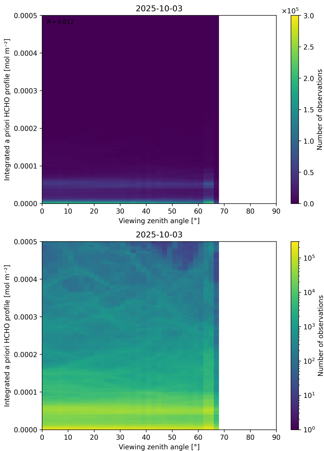
Figure 195: Scatter density plot of “Viewing zenith angle” against “Integrated a priori HCHO profile” for 2025-10-02 to 2025-10-04.
