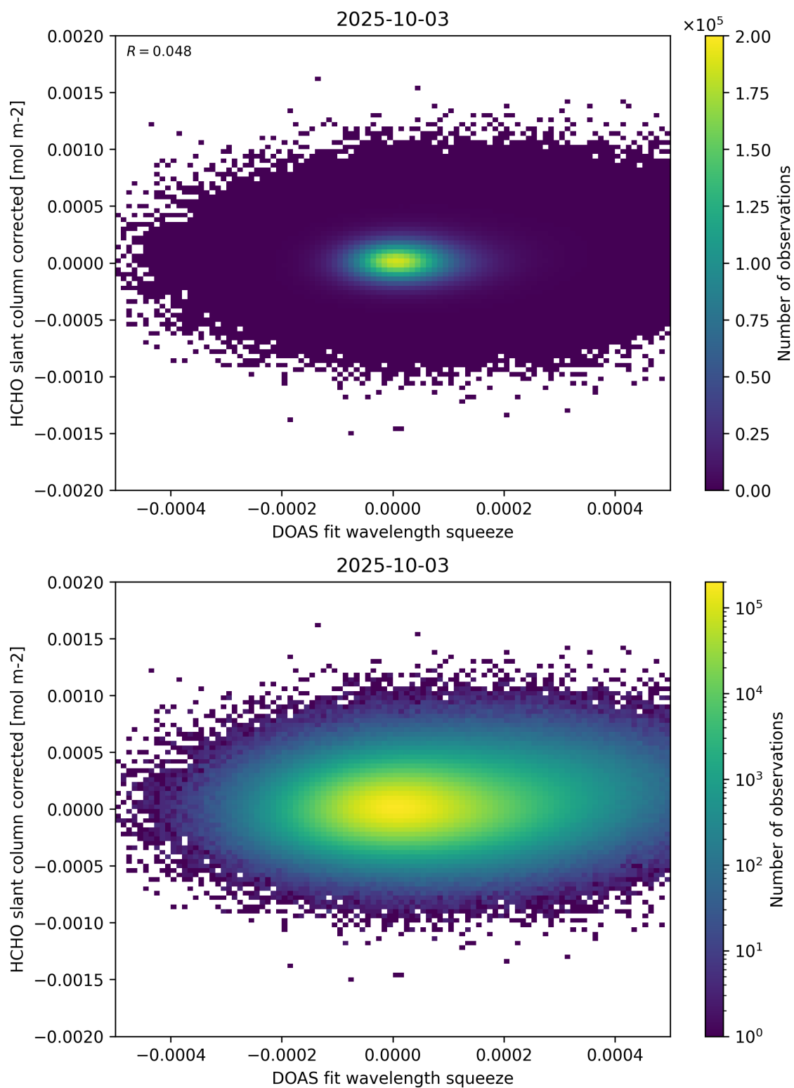
Figure 69: Scatter density plot of “DOAS fit wavelength squeeze” against “HCHO slant column corrected” for 2025-10-02 to 2025-10-04.
