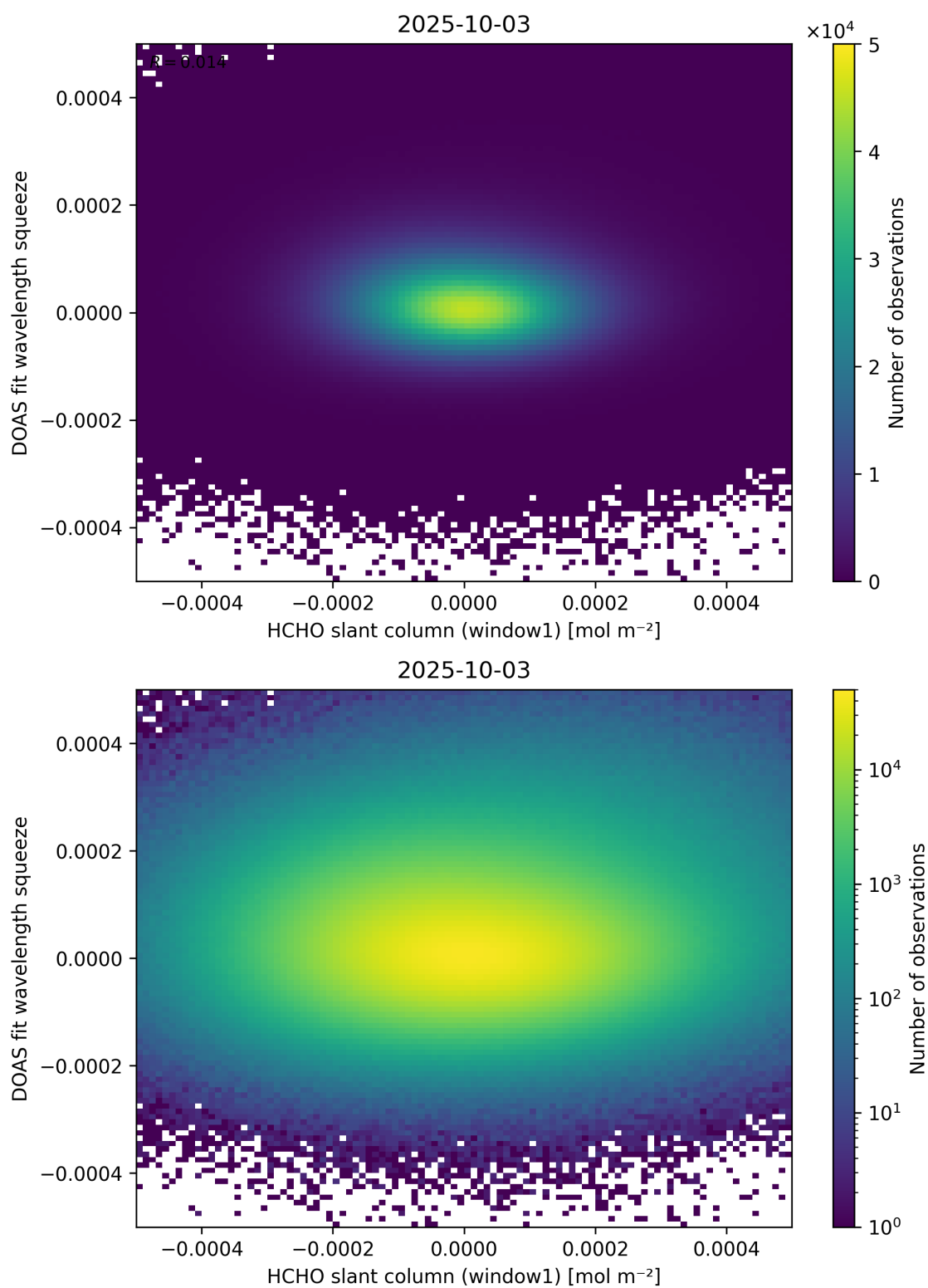
Figure 80: Scatter density plot of “HCHO slant column (window1)” against “DOAS fit wavelength squeeze” for 2025-10-02 to 2025-10-04.
