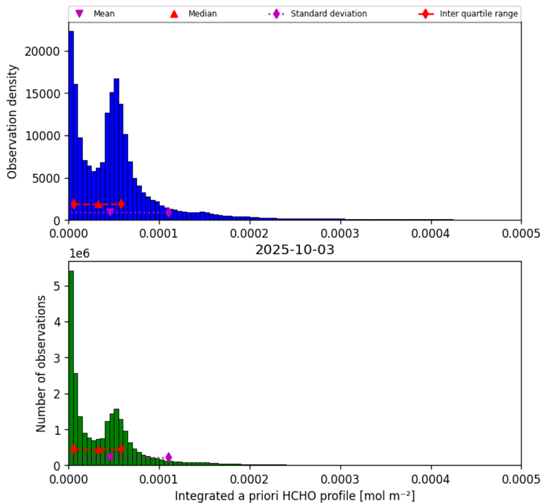
Figure 43: Histogram of “Integrated a priori HCHO profile” for 2025-10-02 to 2025-10-04
