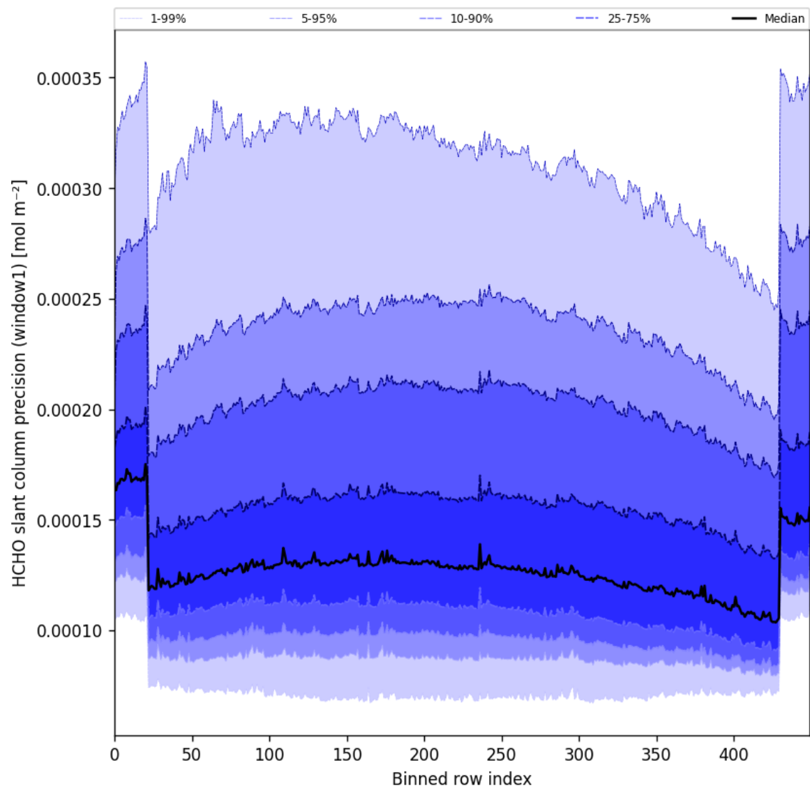
Figure 53: Along track statistics of “HCHO slant column precision (window1)” for 2025-10-02 to 2025-10-04
