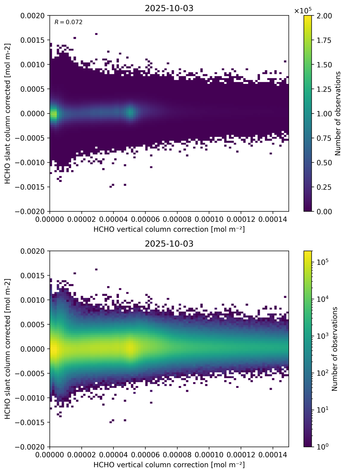
Figure 116: Scatter density plot of “HCHO vertical column correction” against “HCHO slant column corrected” for 2025-10-02 to 2025-10-04.
