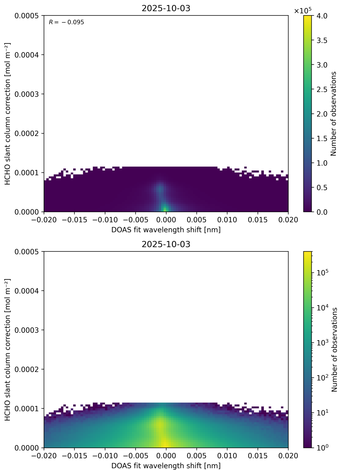
Figure 67: Scatter density plot of “DOAS fit wavelength shift” against “HCHO slant column correction” for 2025-10-02 to 2025-10-04.
