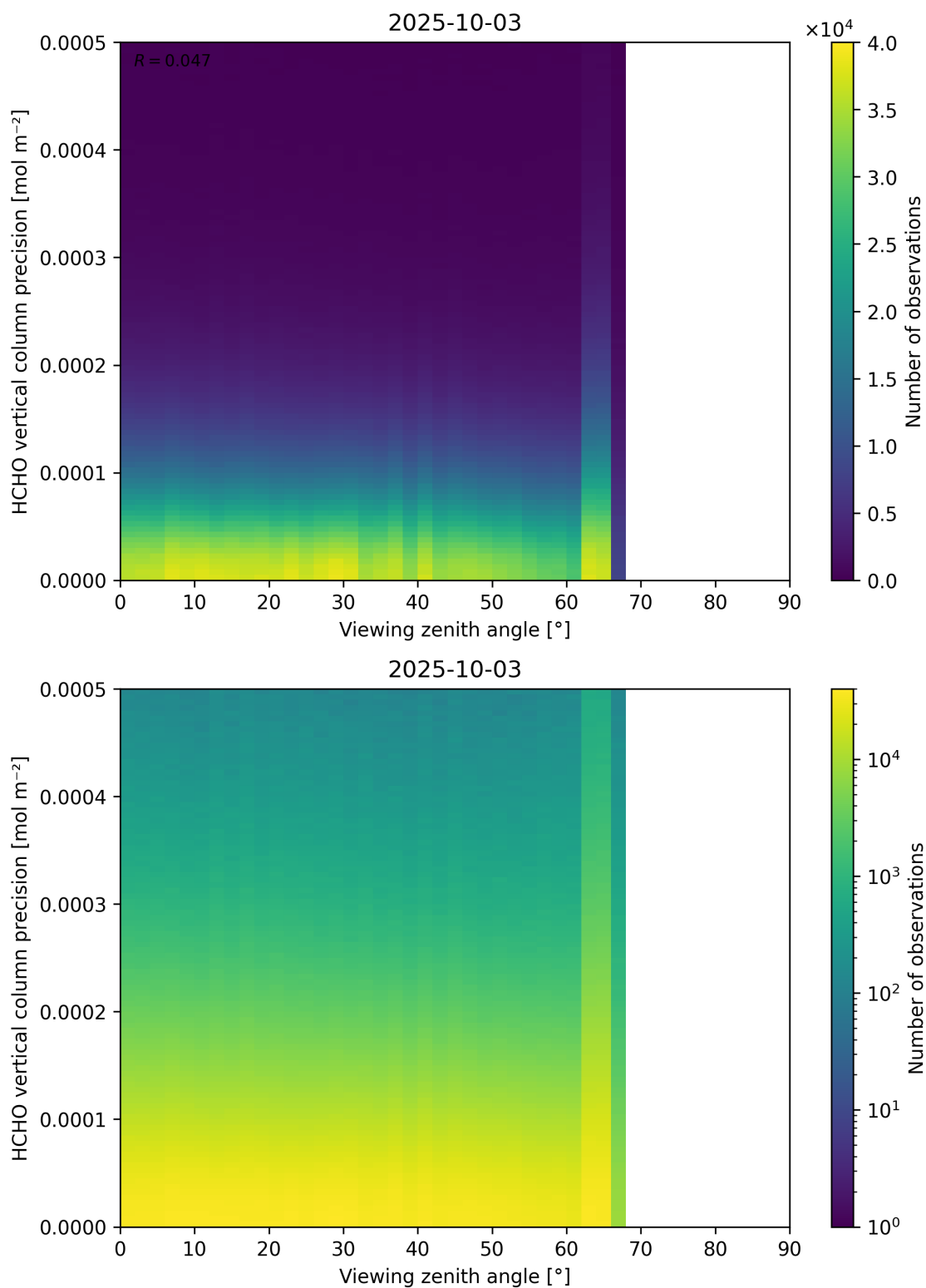
Figure 194: Scatter density plot of “Viewing zenith angle” against “HCHO vertical column precision” for 2025-10-02 to 2025-10-04.
