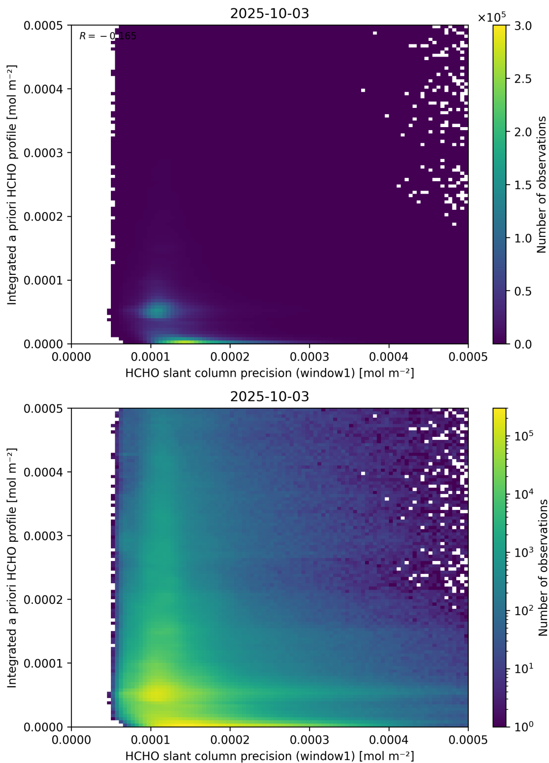
Figure 96: Scatter density plot of “HCHO slant column precision (window1)” against “Integrated a priori HCHO profile” for 2025-10-02 to 2025-10-04.
