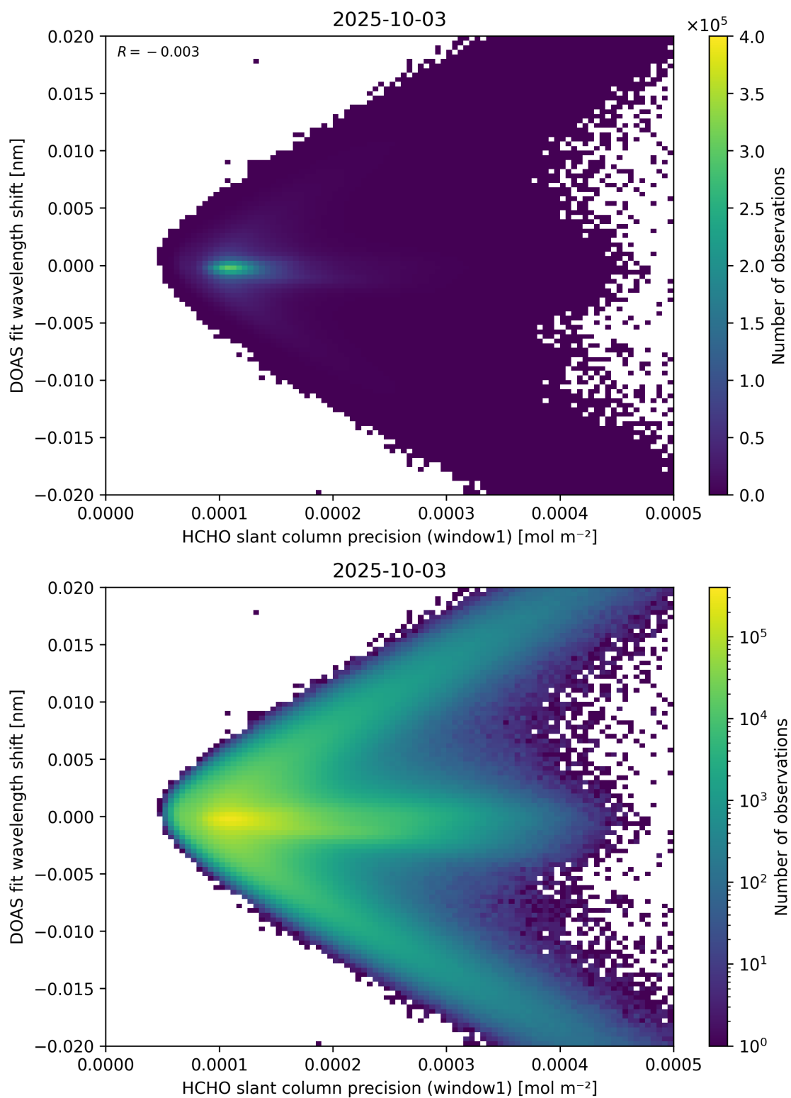
Figure 89: Scatter density plot of “HCHO slant column precision (window1)” against “DOAS fit wavelength shift” for 2025-10-02 to 2025-10-04.
