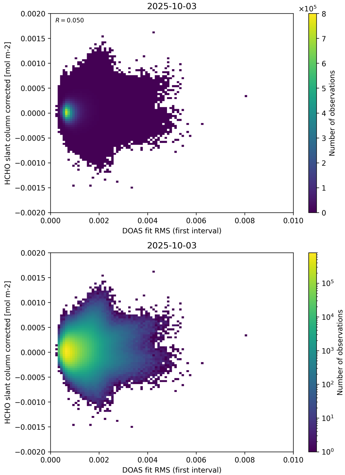
Figure 62: Scatter density plot of “DOAS fit RMS (first interval)” against “HCHO slant column corrected” for 2025-10-02 to 2025-10-04.
