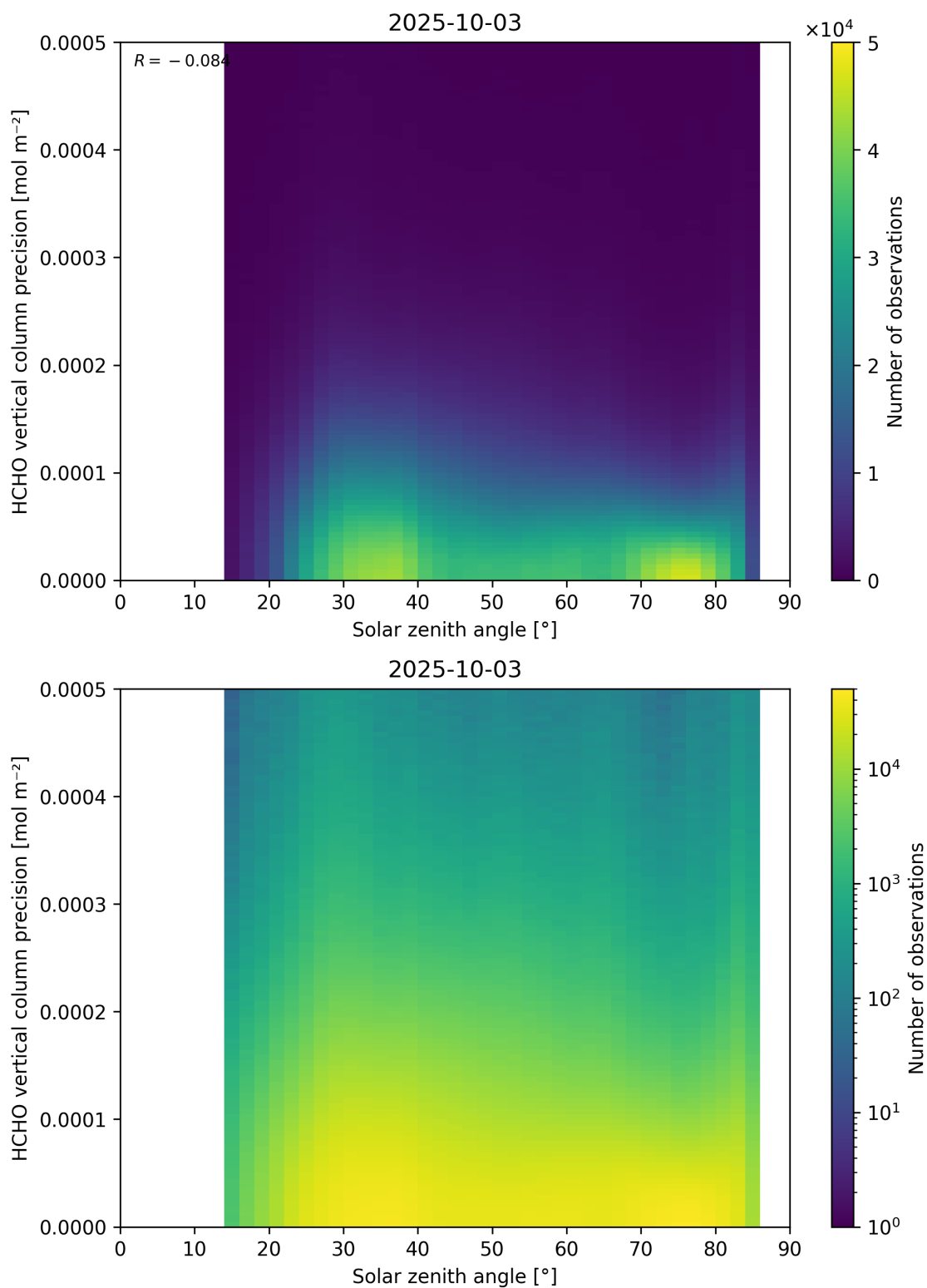
Figure 179: Scatter density plot of “Solar zenith angle” against “HCHO vertical column precision” for 2025-10-02 to 2025-10-04.
