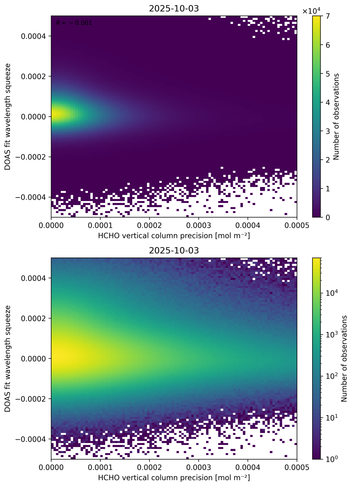
Figure 138: Scatter density plot of “HCHO vertical column precision” against “DOAS fit wavelength squeeze” for 2025-10-02 to 2025-10-04.
