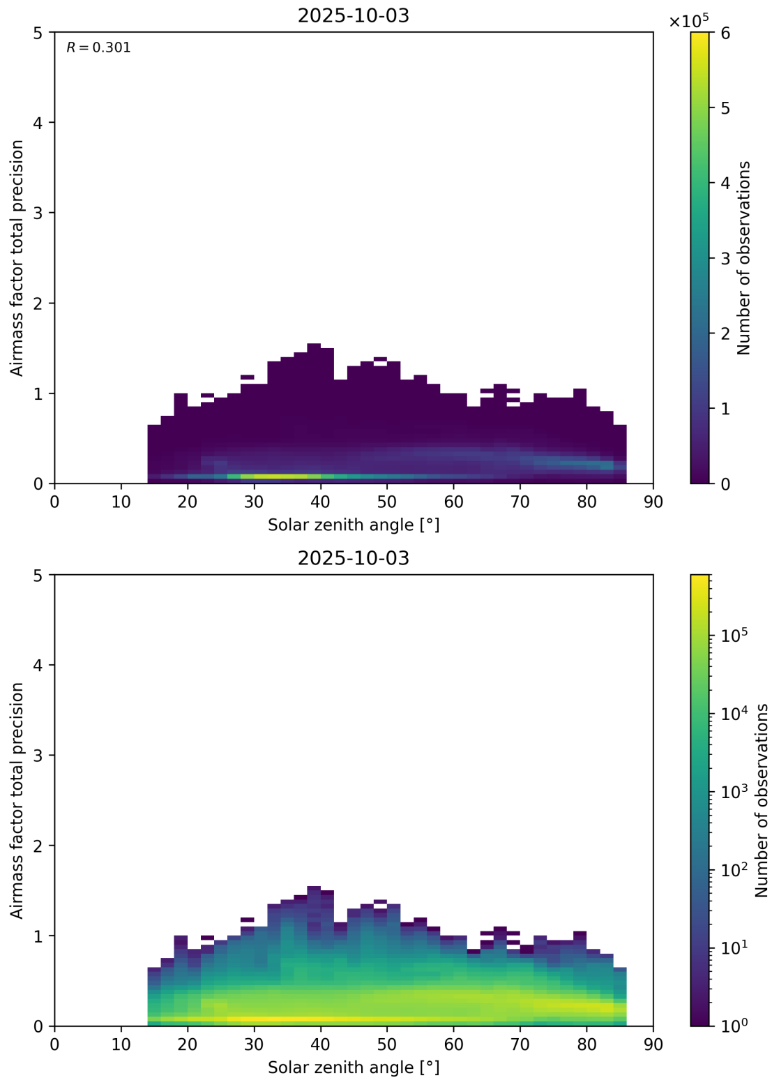
Figure 176: Scatter density plot of “Solar zenith angle” against “Airmass factor total precision” for 2025-10-02 to 2025-10-04.
