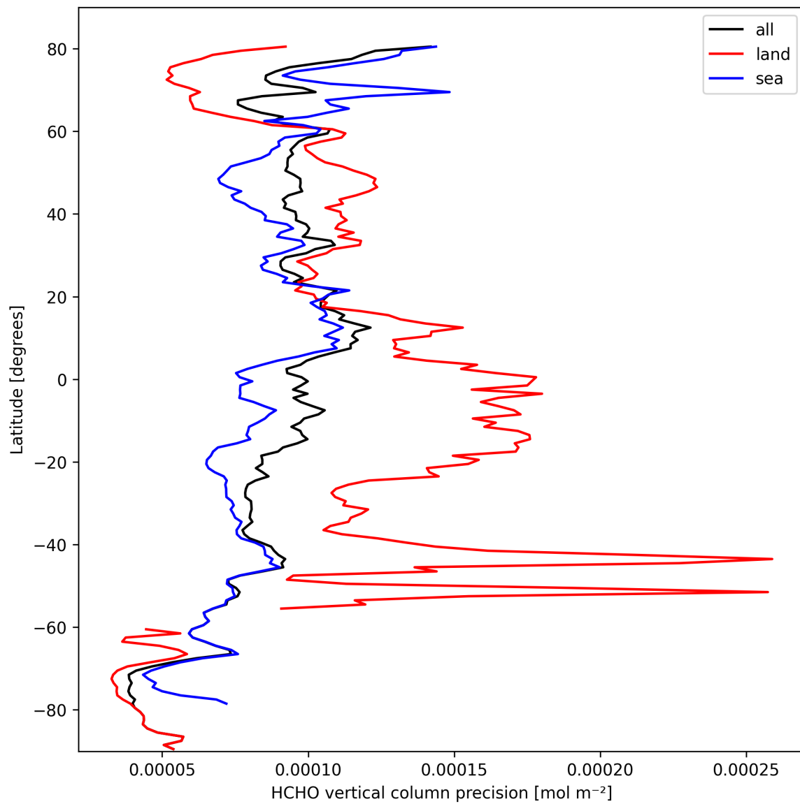
Figure 22: Zonal average of “HCHO vertical column precision” for 2025-10-02 to 2025-10-04.
