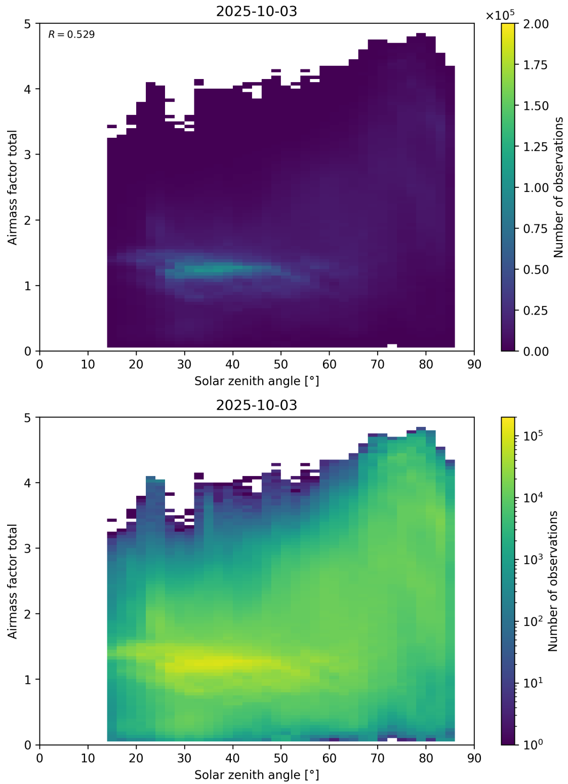
Figure 175: Scatter density plot of “Solar zenith angle” against “Airmass factor total” for 2025-10-02 to 2025-10-04.
