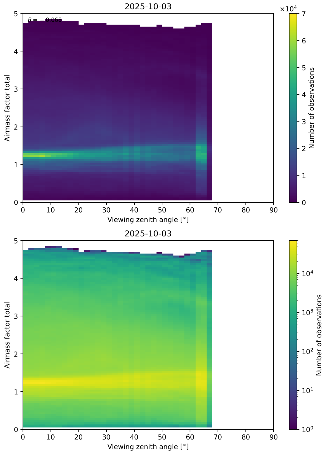
Figure 190: Scatter density plot of “Viewing zenith angle” against “Airmass factor total” for 2025-10-02 to 2025-10-04.
