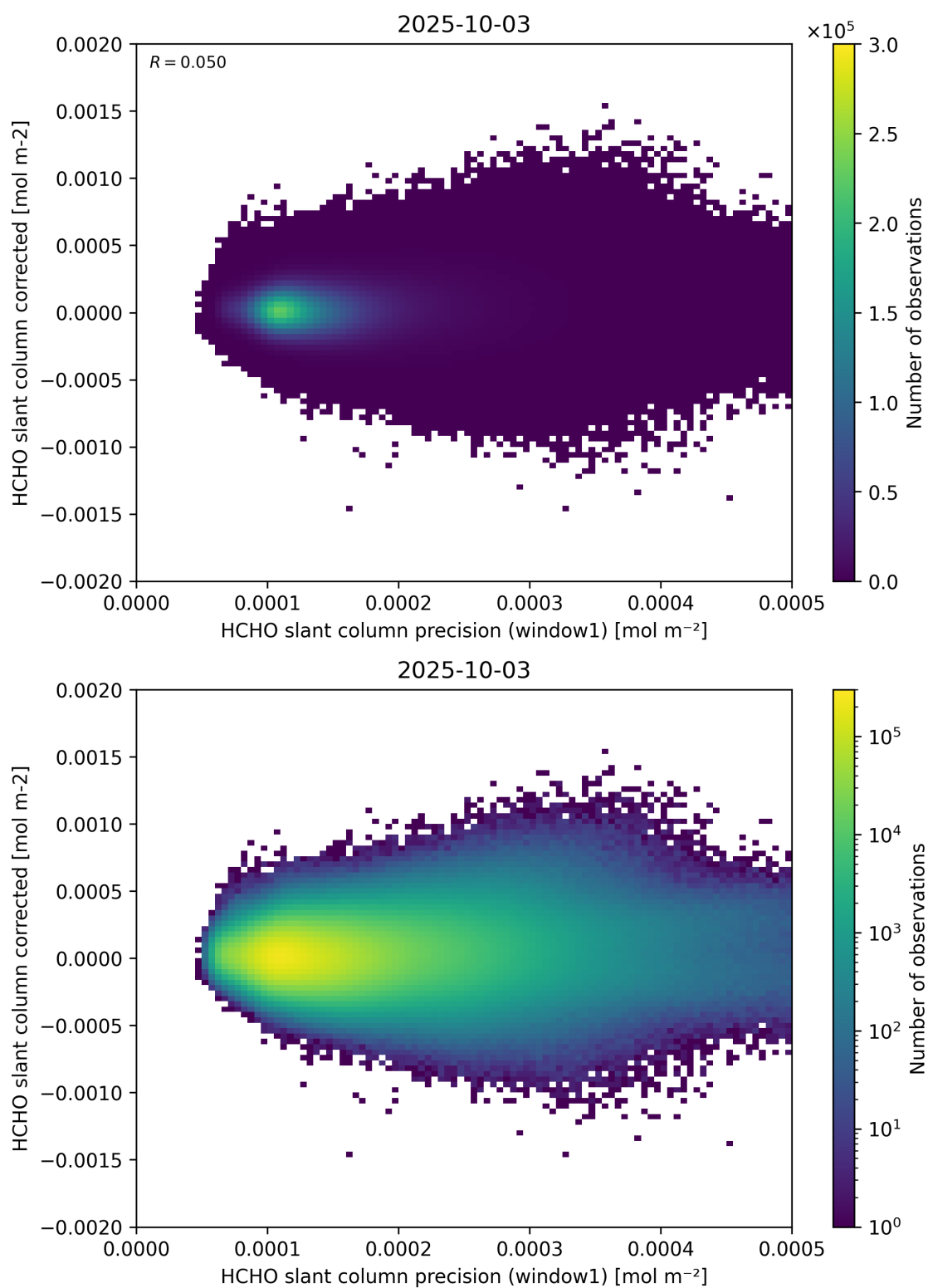
Figure 92: Scatter density plot of “HCHO slant column precision (window1)” against “HCHO slant column corrected” for 2025-10-02 to 2025-10-04.
