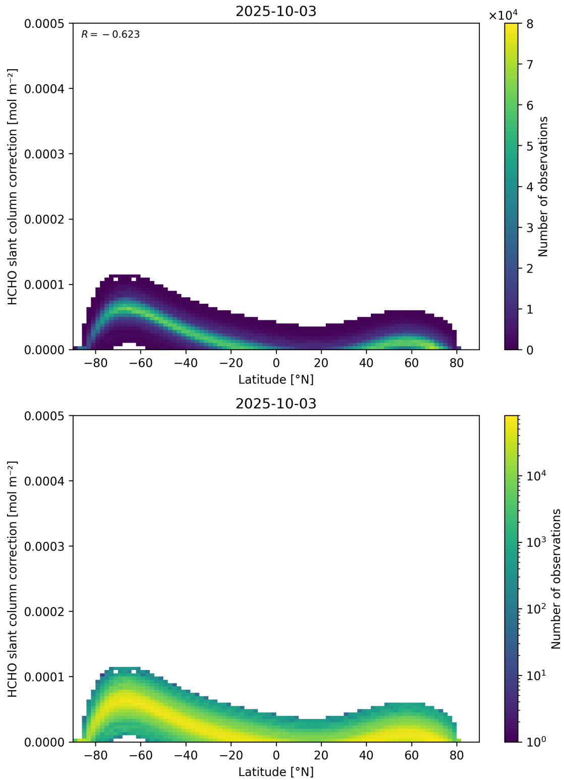
Figure 158: Scatter density plot of “Latitude” against “HCHO slant column correction” for 2025-10-02 to 2025-10-04.
