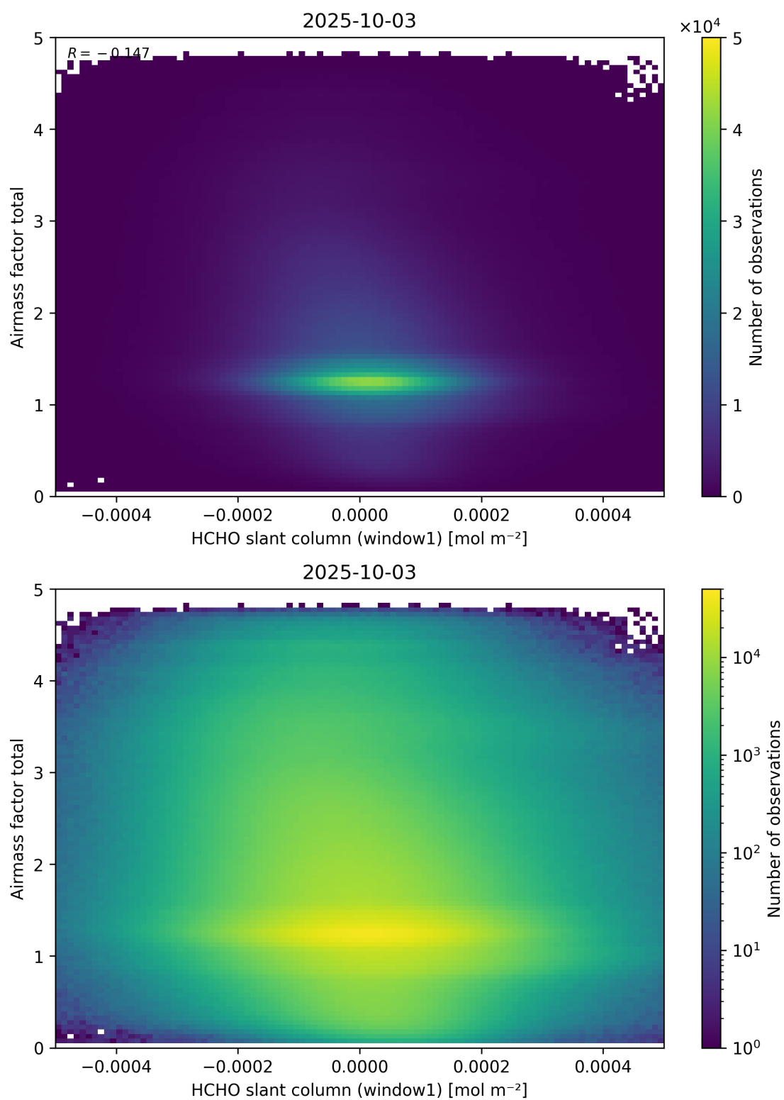
Figure 85: Scatter density plot of “HCHO slant column (window1)” against “Airmass factor total” for 2025-10-02 to 2025-10-04.
