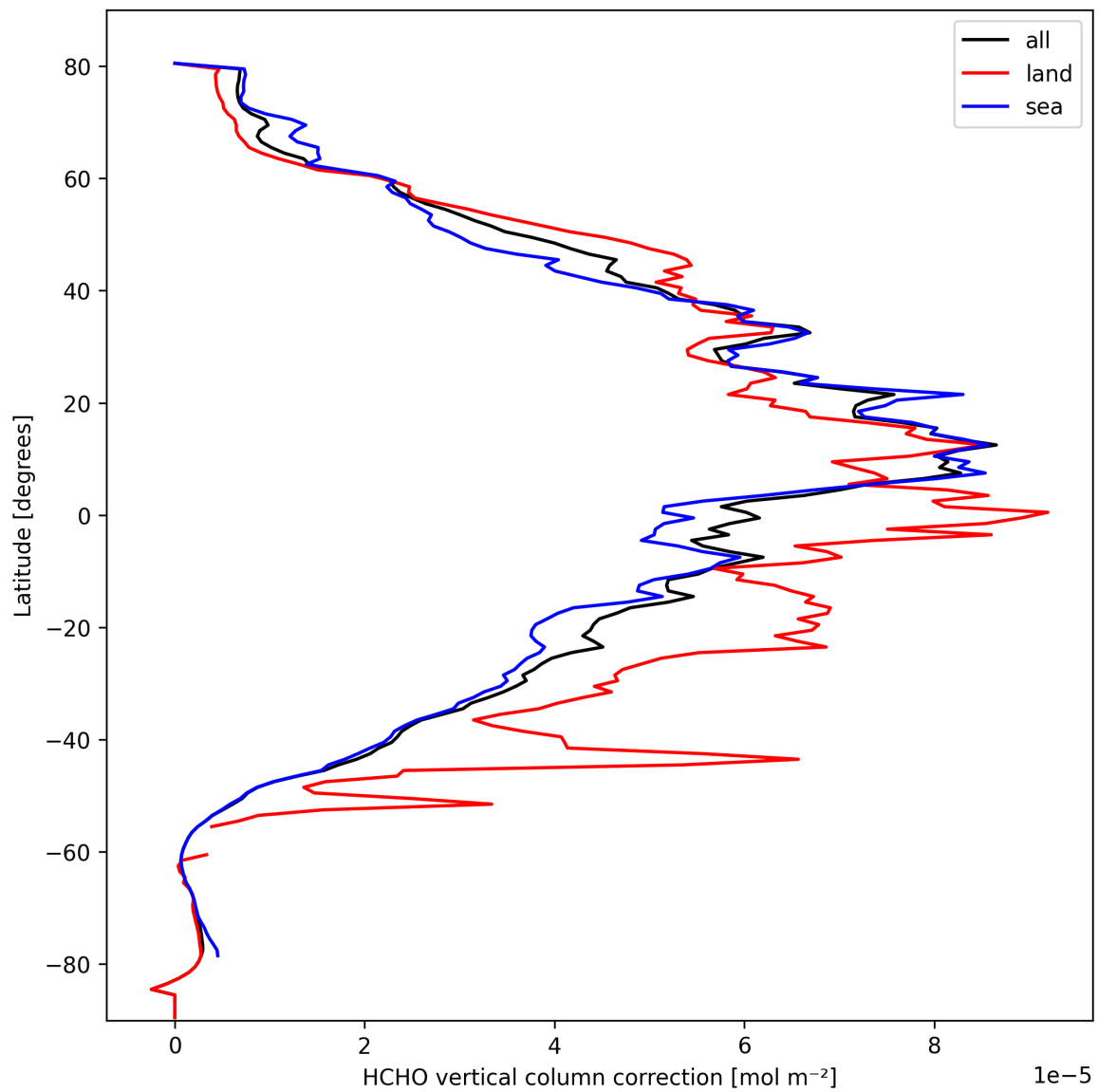
Figure 23: Zonal average of "HCHO vertical column correction" for 2025-10-02 to 2025-10-04.
