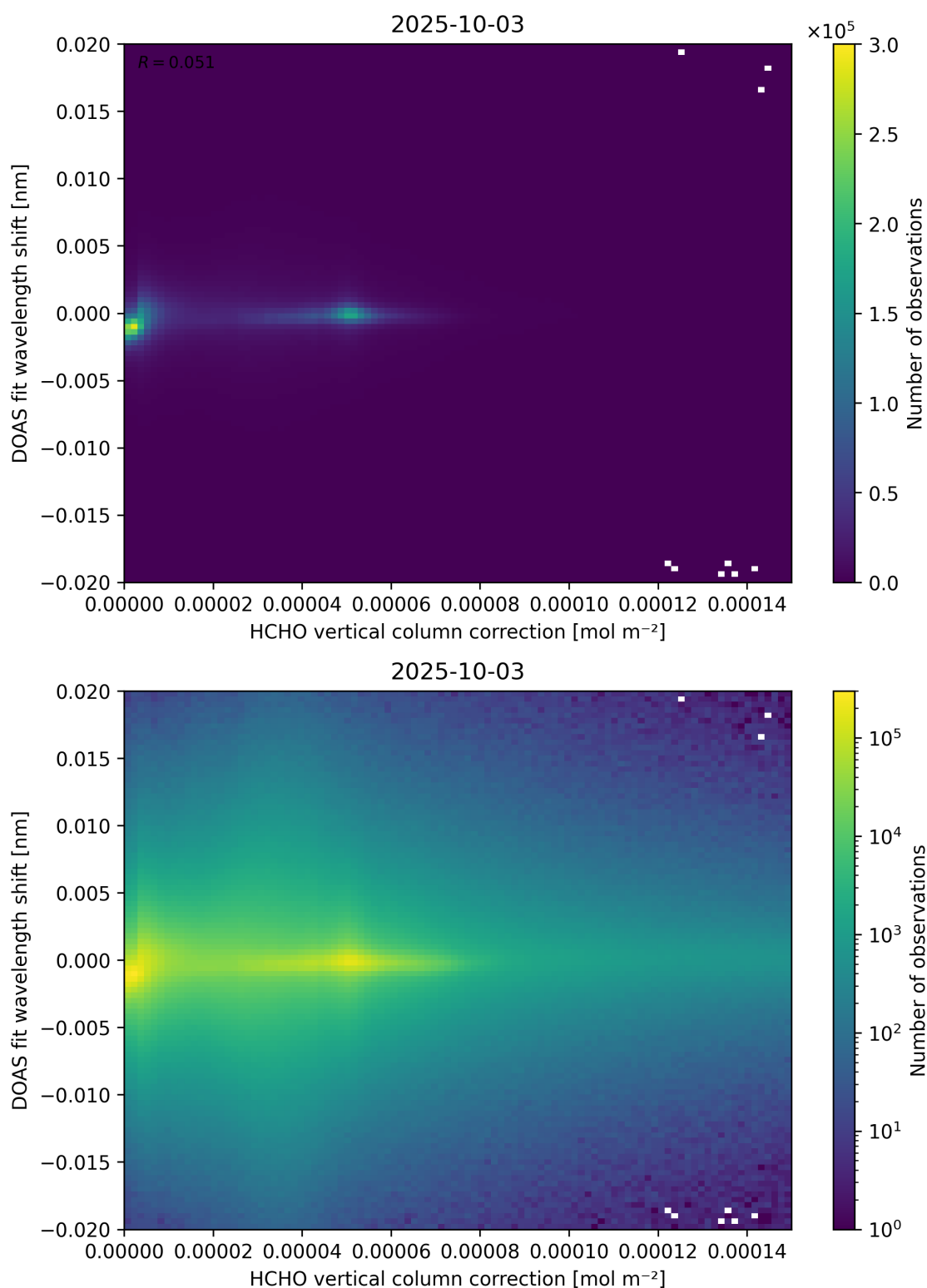
Figure 113: Scatter density plot of “HCHO vertical column correction” against “DOAS fit wavelength shift” for 2025-10-02 to 2025-10-04.
