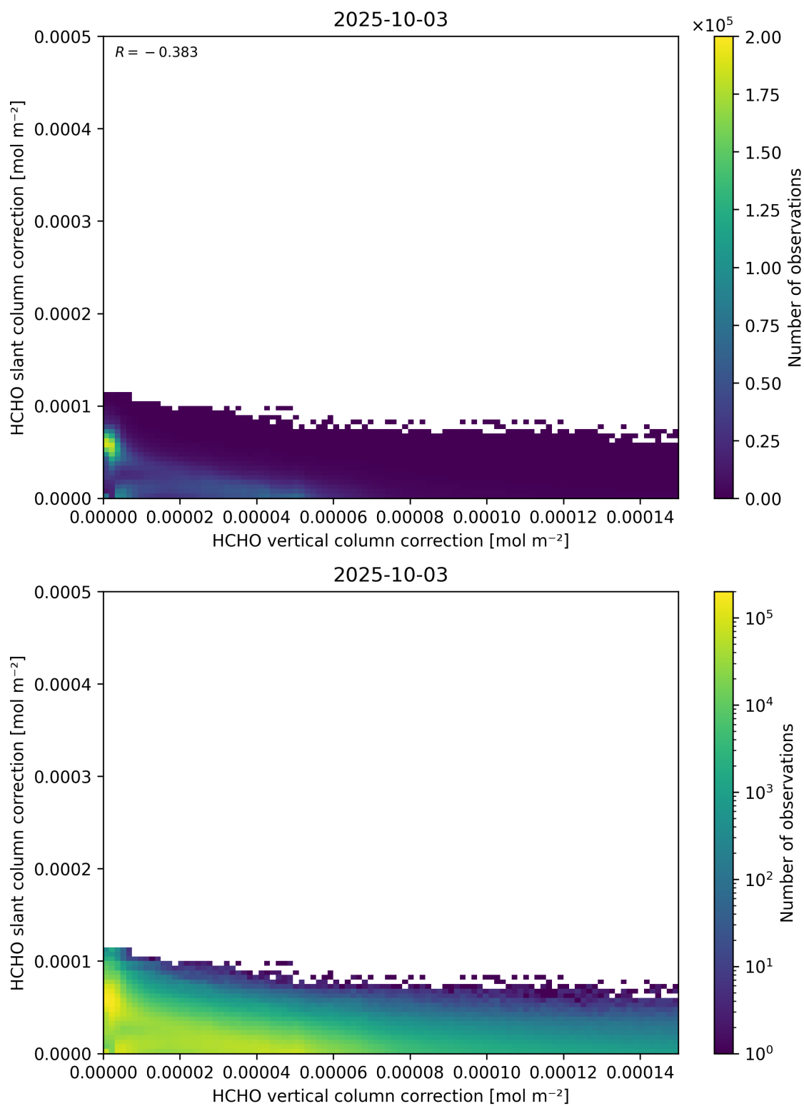
Figure 117: Scatter density plot of “HCHO vertical column correction” against “HCHO slant column correction” for 2025-10-02 to 2025-10-04.
