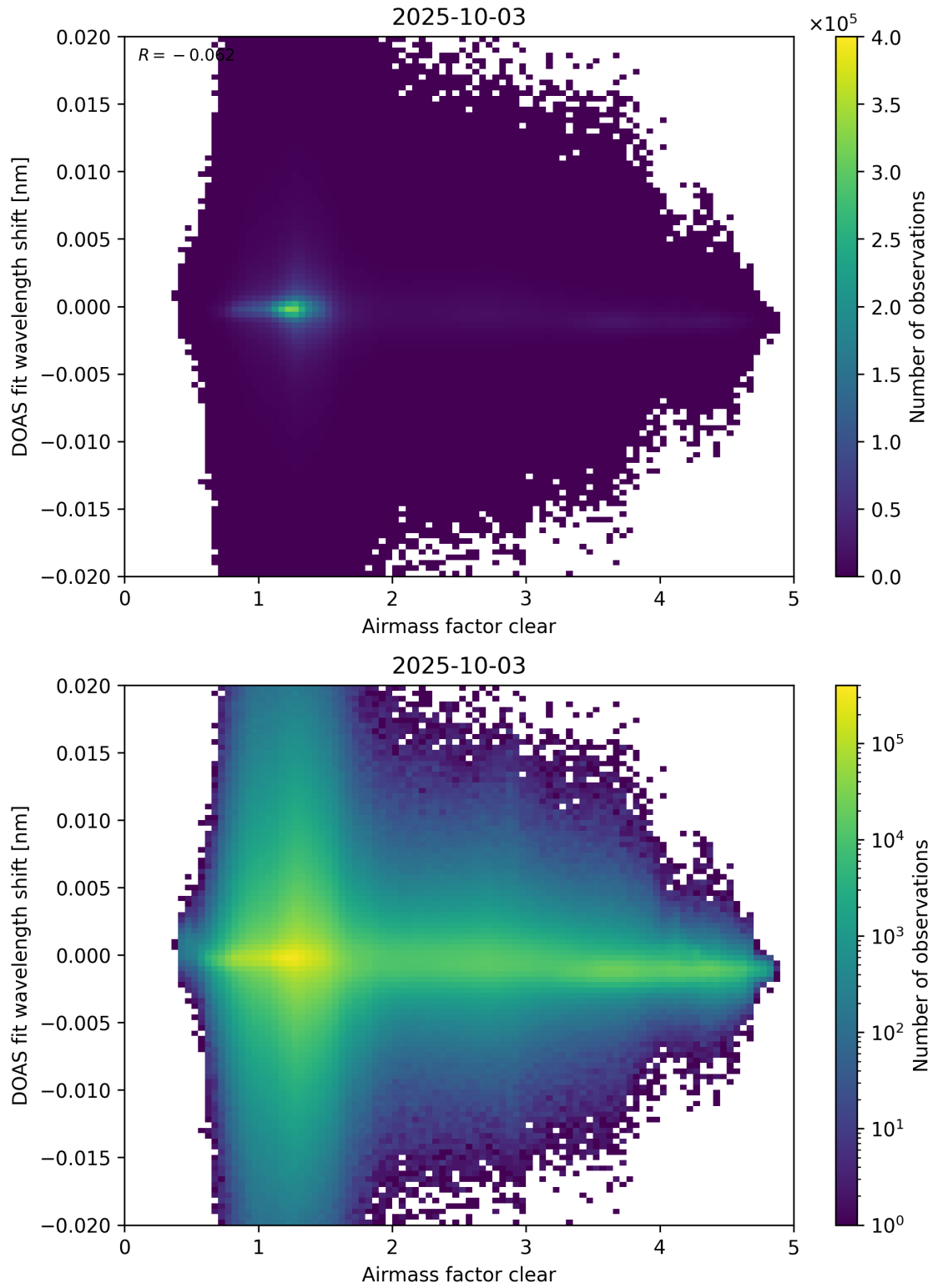
Figure 72: Scatter density plot of “Airmass factor clear” against “DOAS fit wavelength shift” for 2025-10-02 to 2025-10-04.
