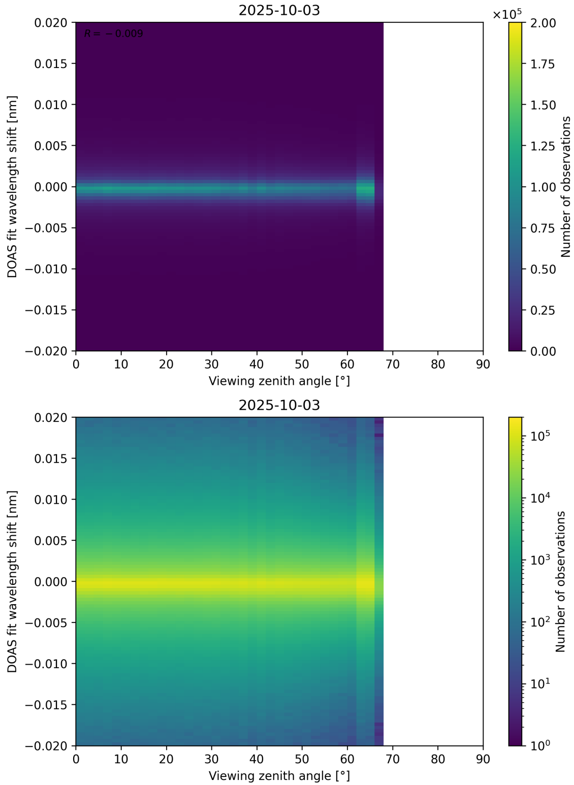
Figure 183: Scatter density plot of “Viewing zenith angle” against “DOAS fit wavelength shift” for 2025-10-02 to 2025-10-04.
