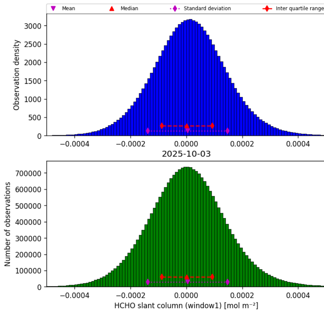
Figure 38: Histogram of “HCHO slant column (window1)” for 2025-10-02 to 2025-10-04
