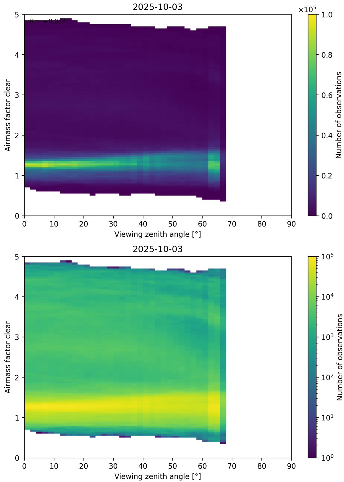
Figure 185: Scatter density plot of “Viewing zenith angle” against “Airmass factor clear” for 2025-10-02 to 2025-10-04.
