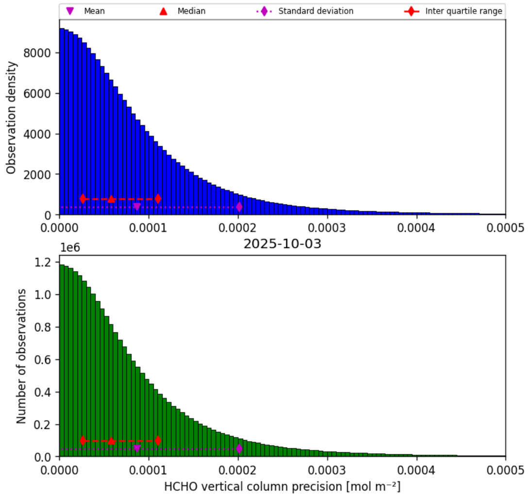
Figure 36: Histogram of “HCHO vertical column precision” for 2025-10-02 to 2025-10-04
