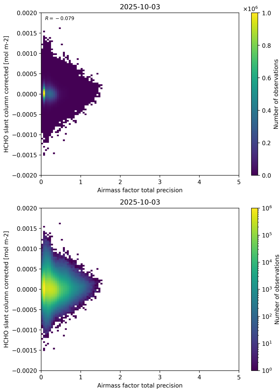
Figure 109: Scatter density plot of “Airmass factor total precision” against “HCHO slant column corrected” for 2025-10-02 to 2025-10-04.
