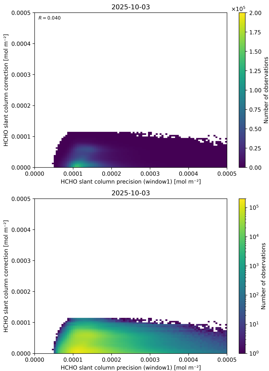
Figure 93: Scatter density plot of “HCHO slant column precision (window1)” against “HCHO slant column correction” for 2025-10-02 to 2025-10-04.
