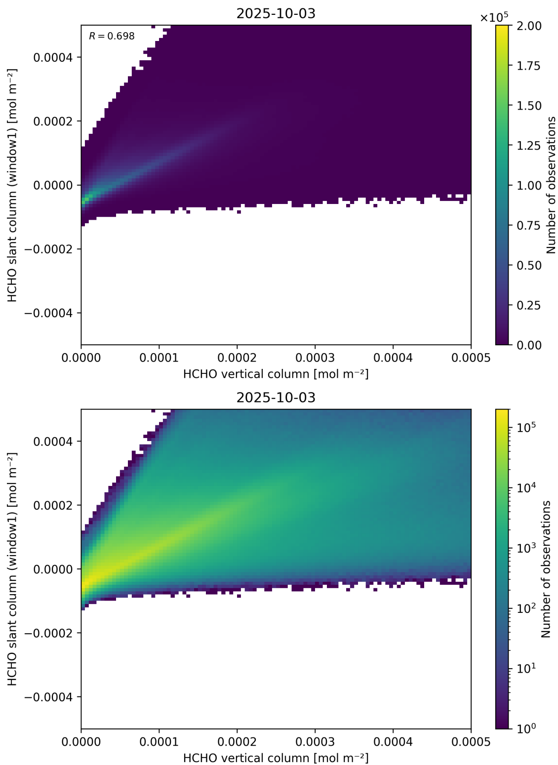
Figure 129: Scatter density plot of “HCHO vertical column” against “HCHO slant column (window1)” for 2025-10-02 to 2025-10-04.
