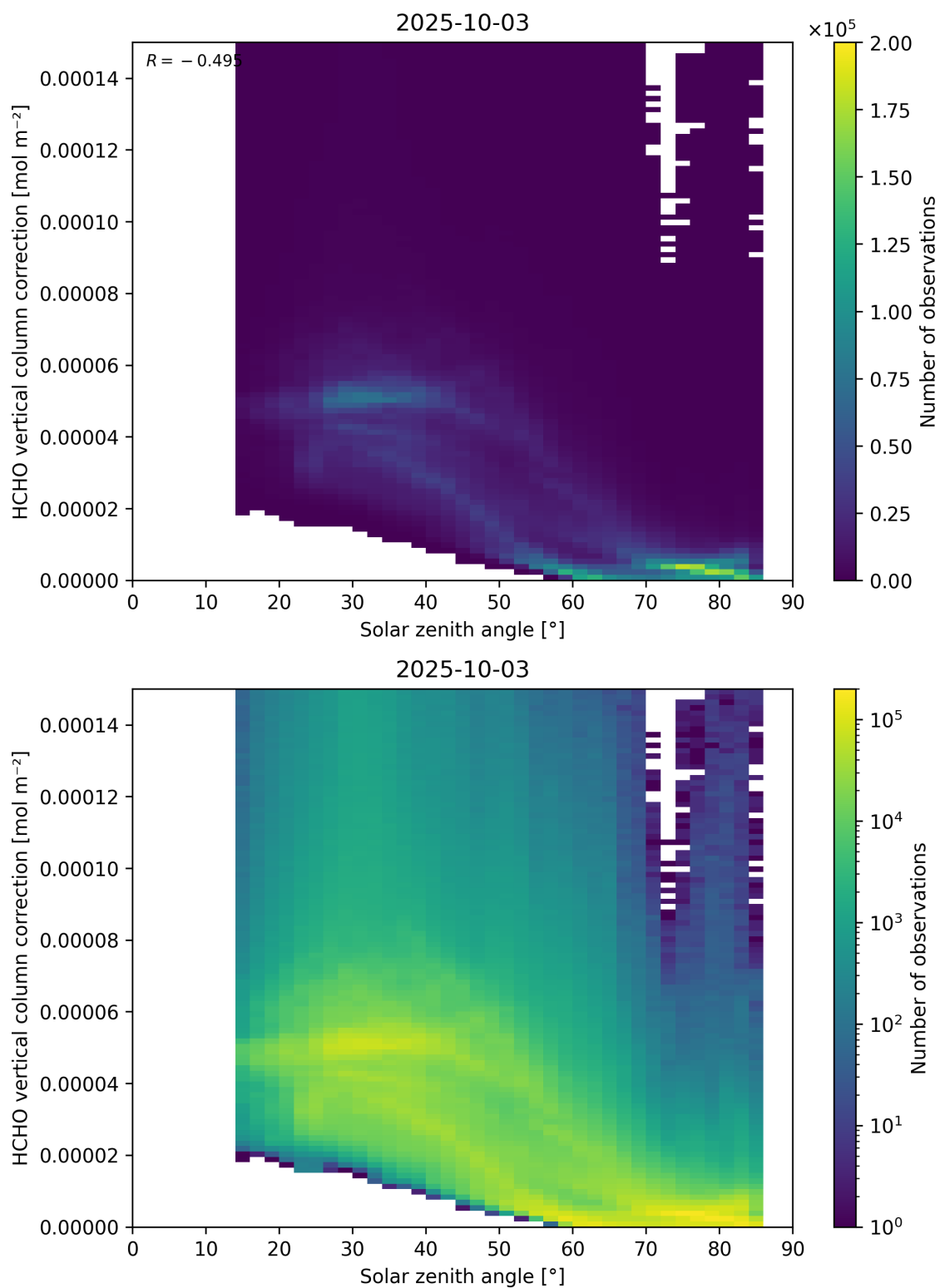
Figure 178: Scatter density plot of “Solar zenith angle” against “HCHO vertical column correction” for 2025-10-02 to 2025-10-04.
