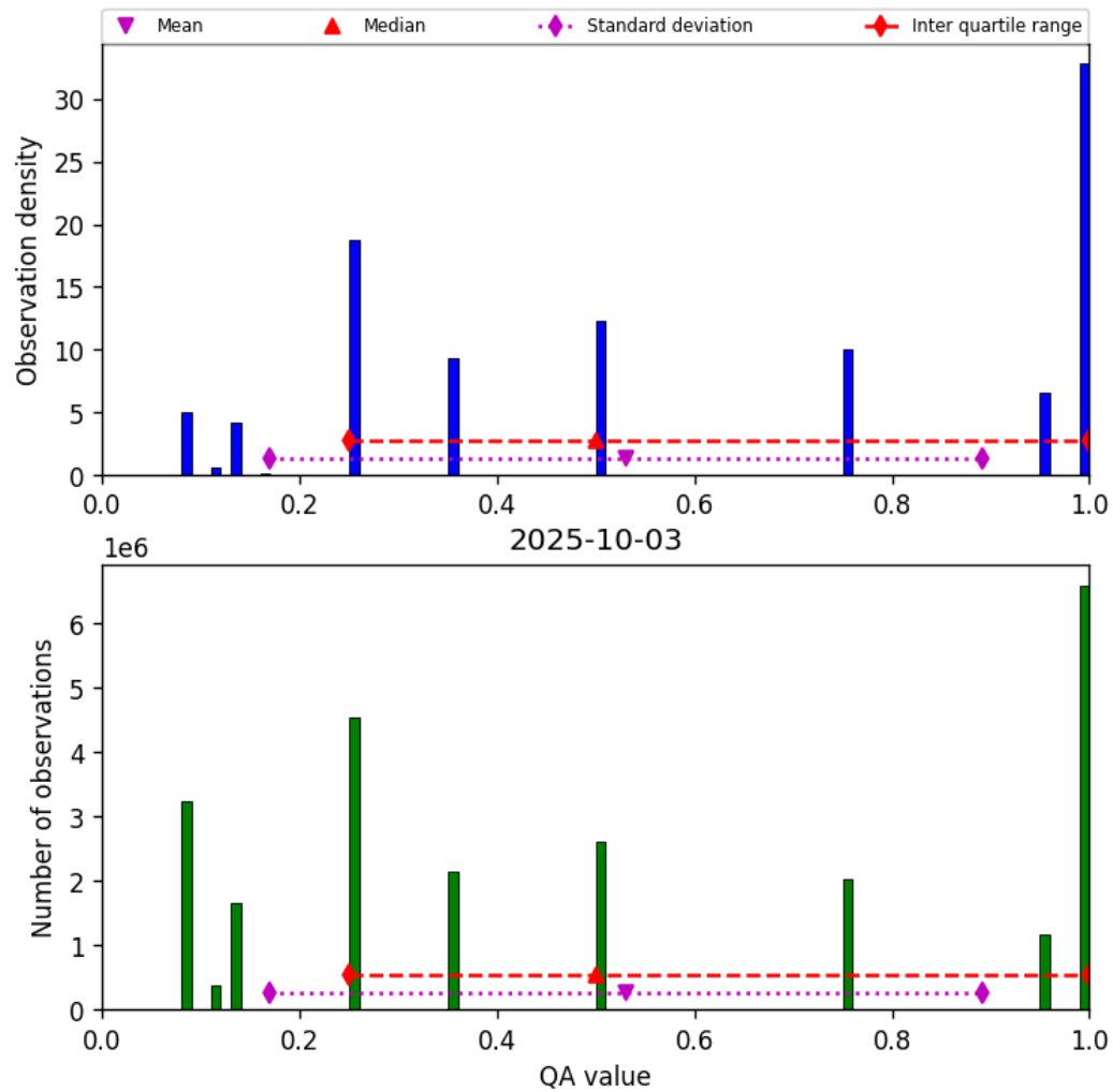
Figure 34: Histogram of “QA value” for 2025-10-02 to 2025-10-04
