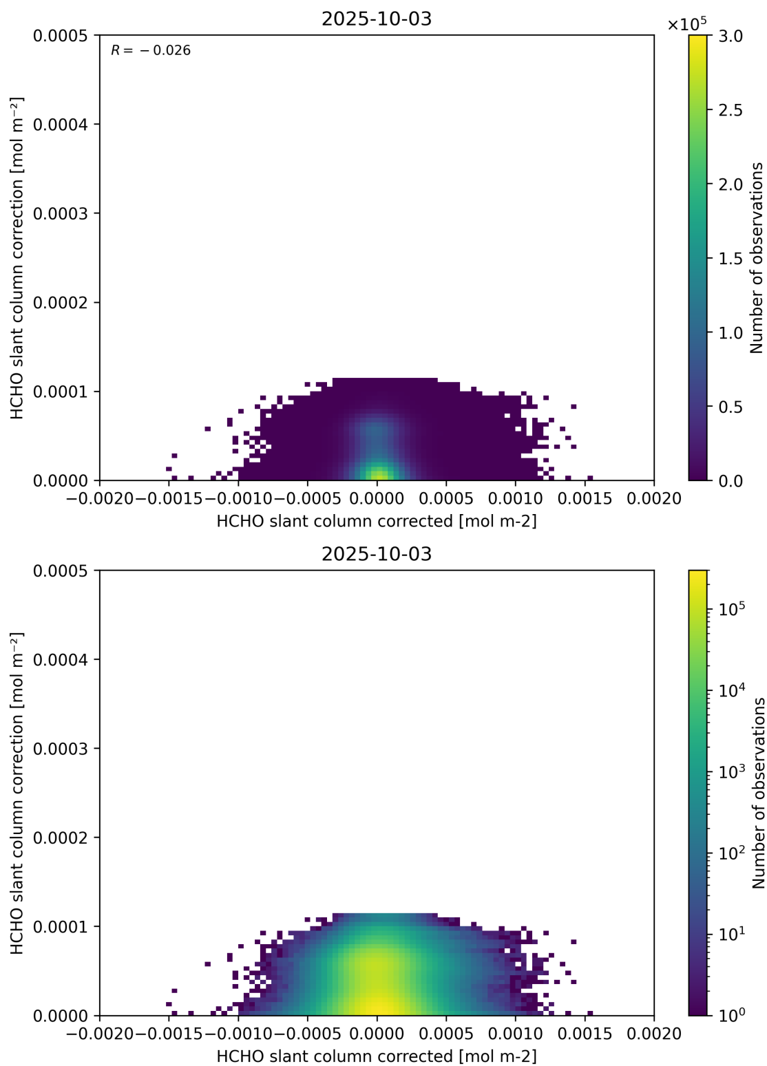
Figure 77: Scatter density plot of “HCHO slant column corrected” against “HCHO slant column correction” for 2025-10-02 to 2025-10-04.
