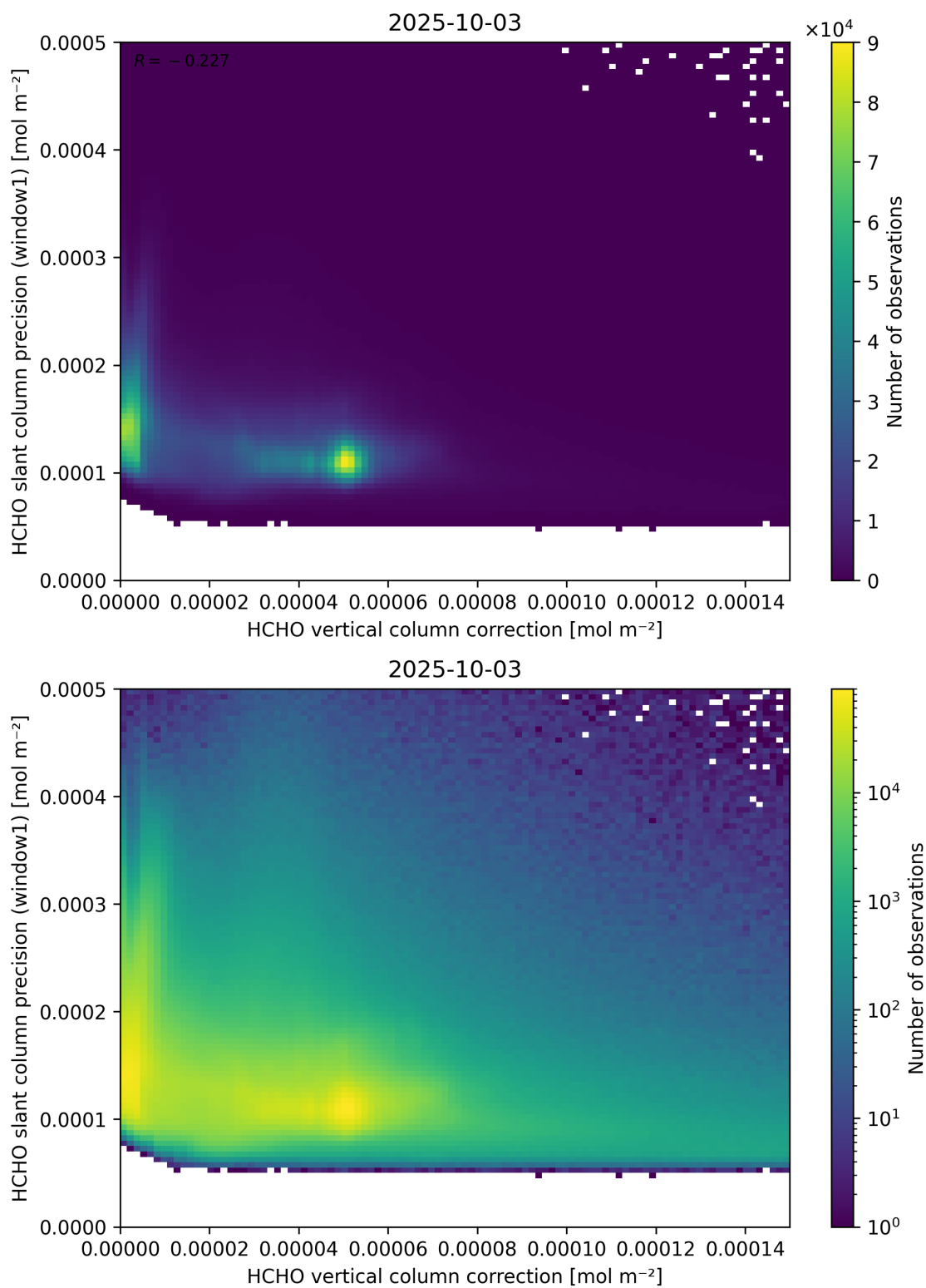
Figure 119: Scatter density plot of “HCHO vertical column correction” against “HCHO slant column precision (window1)” for 2025-10-02 to 2025-10-04.
