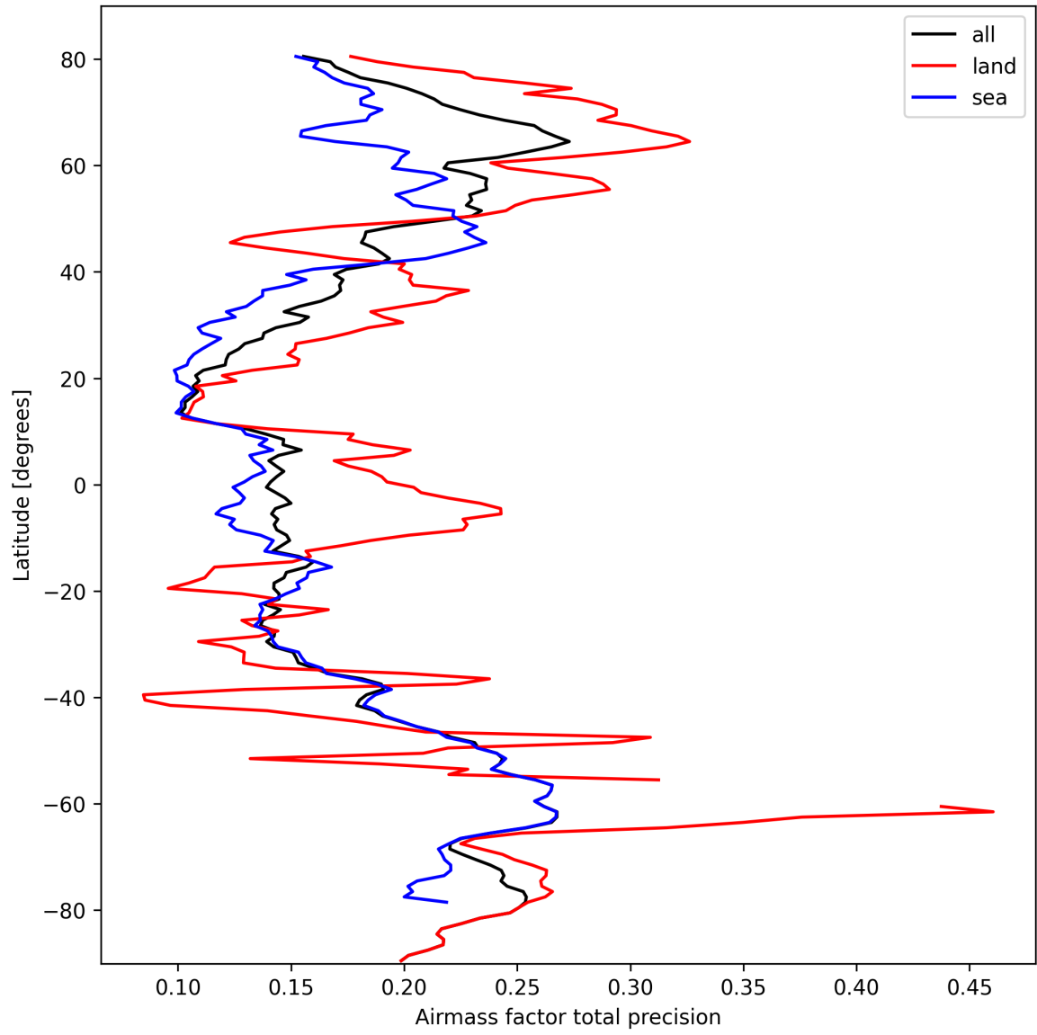
Figure 27: Zonal average of “Airmass factor total precision” for 2025-10-02 to 2025-10-04.
