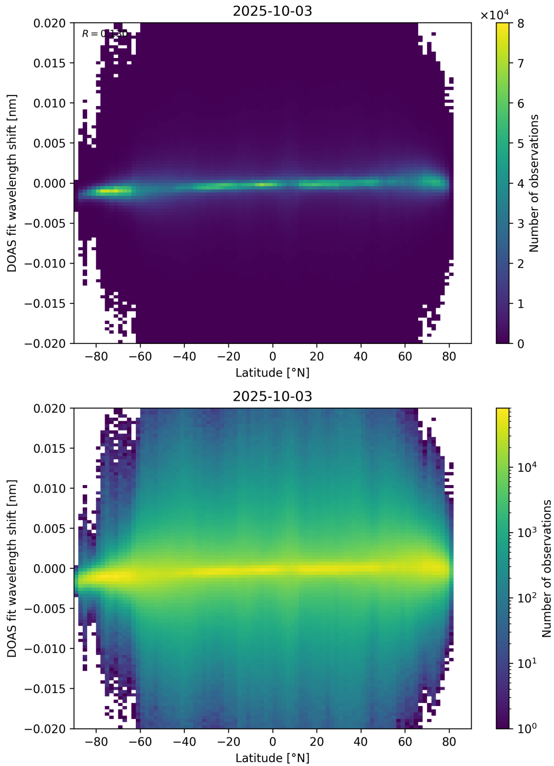
Figure 154: Scatter density plot of “Latitude” against “DOAS fit wavelength shift” for 2025-10-02 to 2025-10-04.
