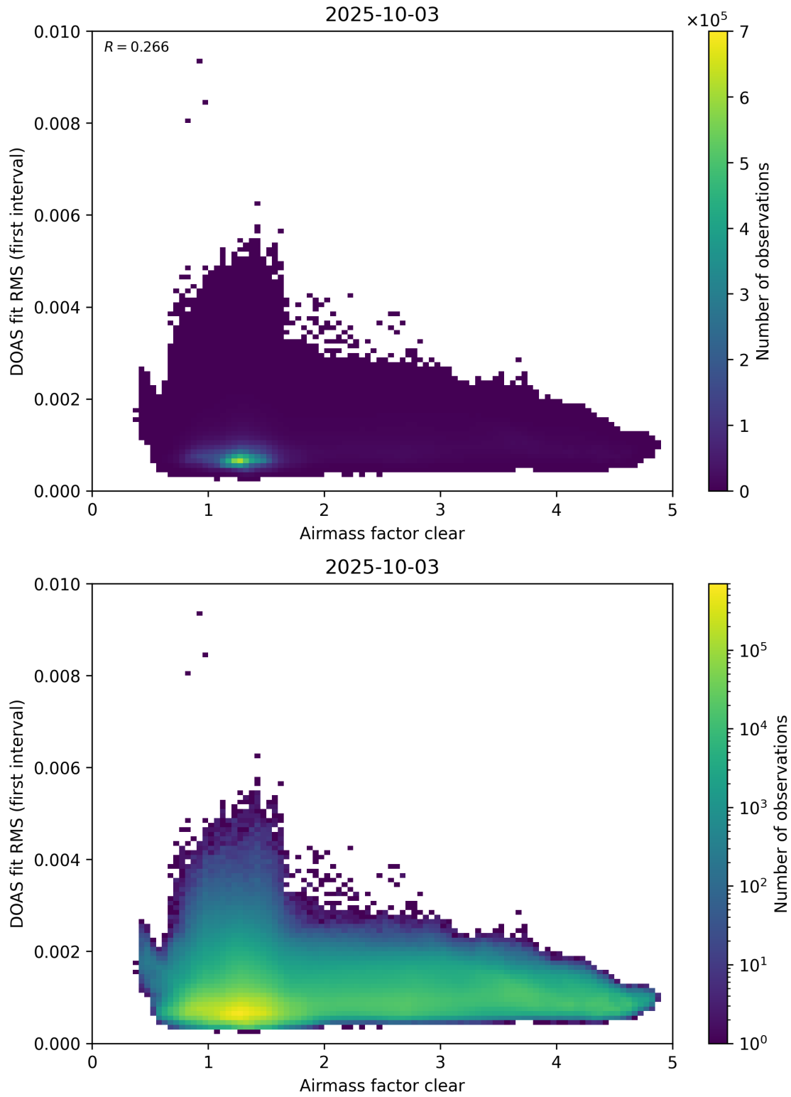
Figure 71: Scatter density plot of “Airmass factor clear” against “DOAS fit RMS (first interval)” for 2025-10-02 to 2025-10-04.
