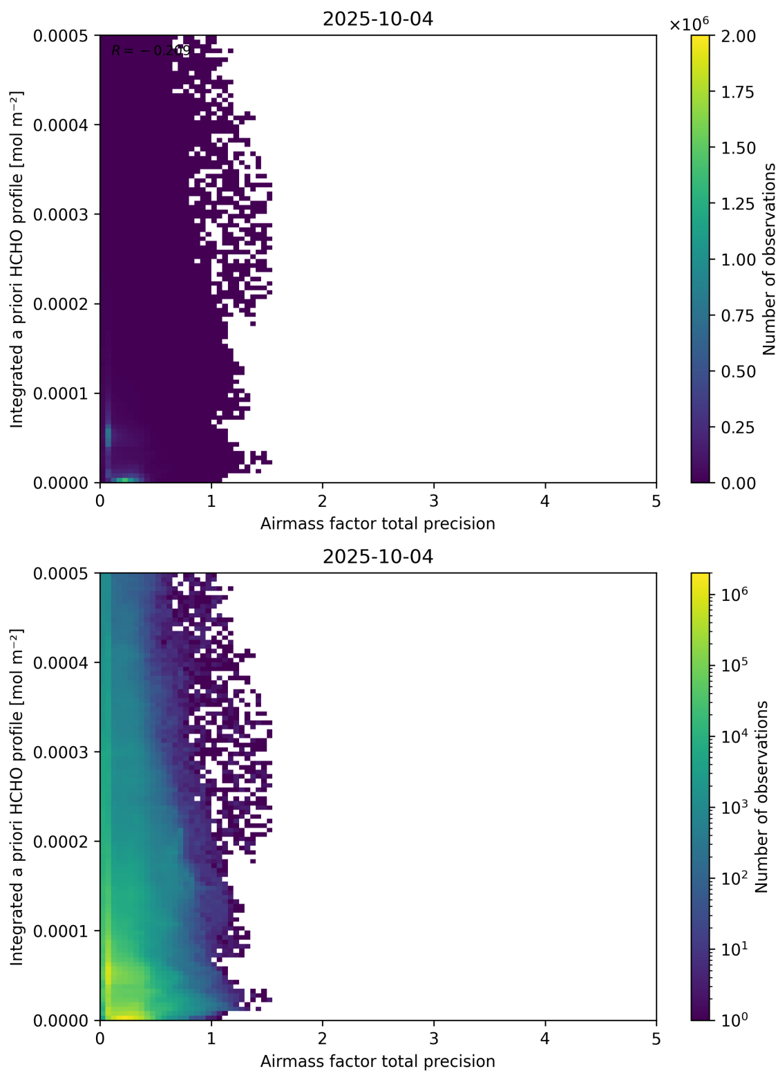
Figure 111: Scatter density plot of “Airmass factor total precision” against “Integrated a priori HCHO profile” for 2025-10-03 to 2025-10-05.
