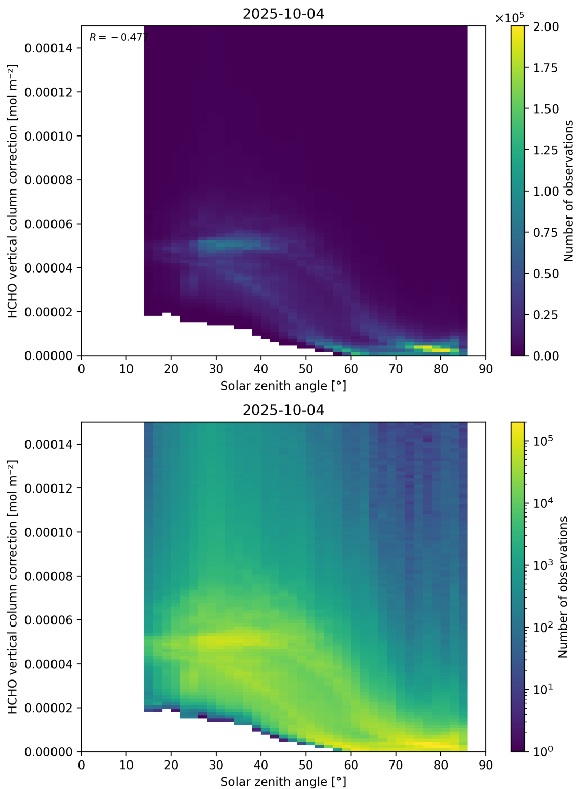
Figure 178: Scatter density plot of “Solar zenith angle” against “HCHO vertical column correction” for 2025-10-03 to 2025-10-05.
