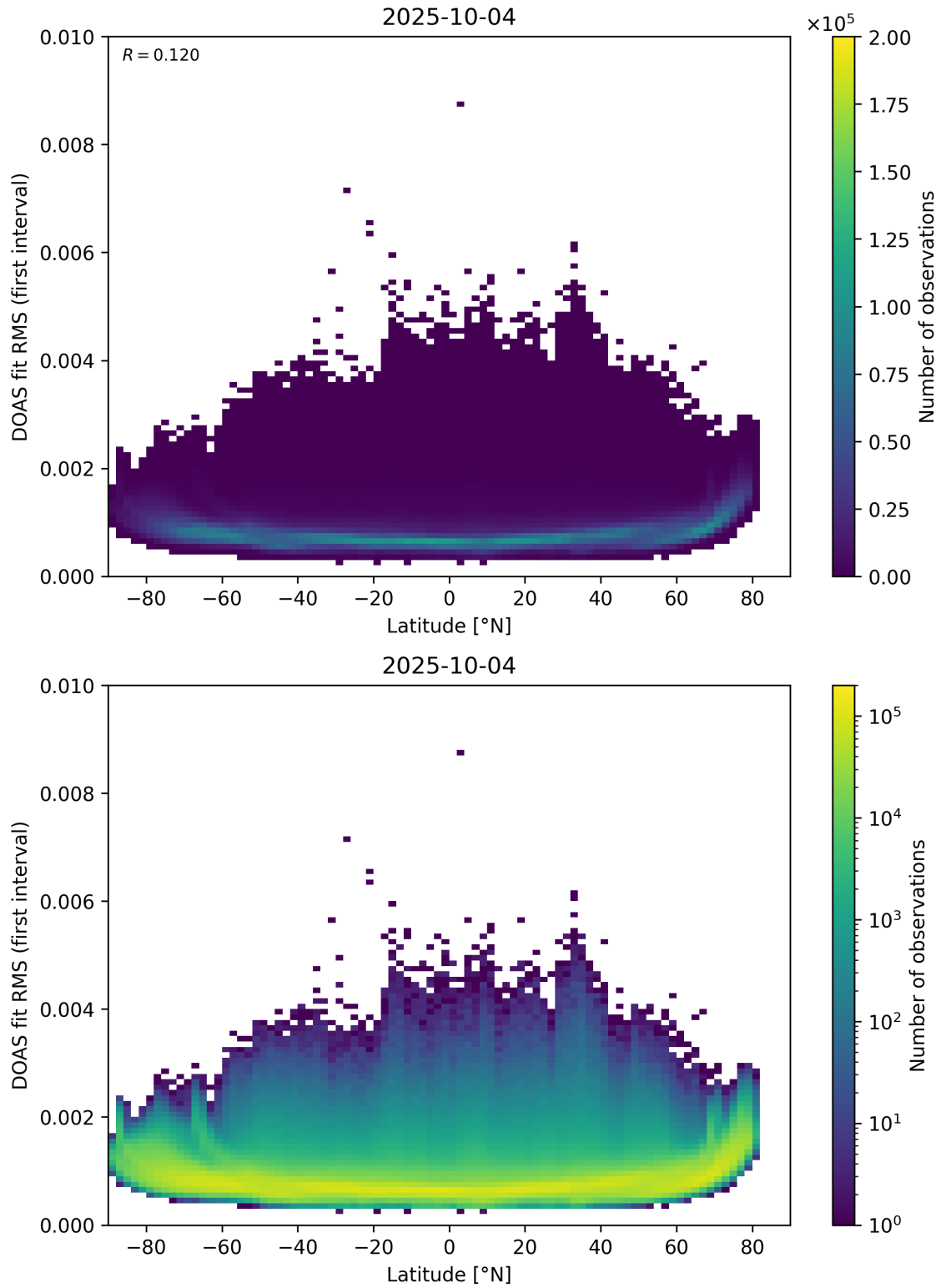
Figure 153: Scatter density plot of “Latitude” against “DOAS fit RMS (first interval)” for 2025-10-03 to 2025-10-05.
