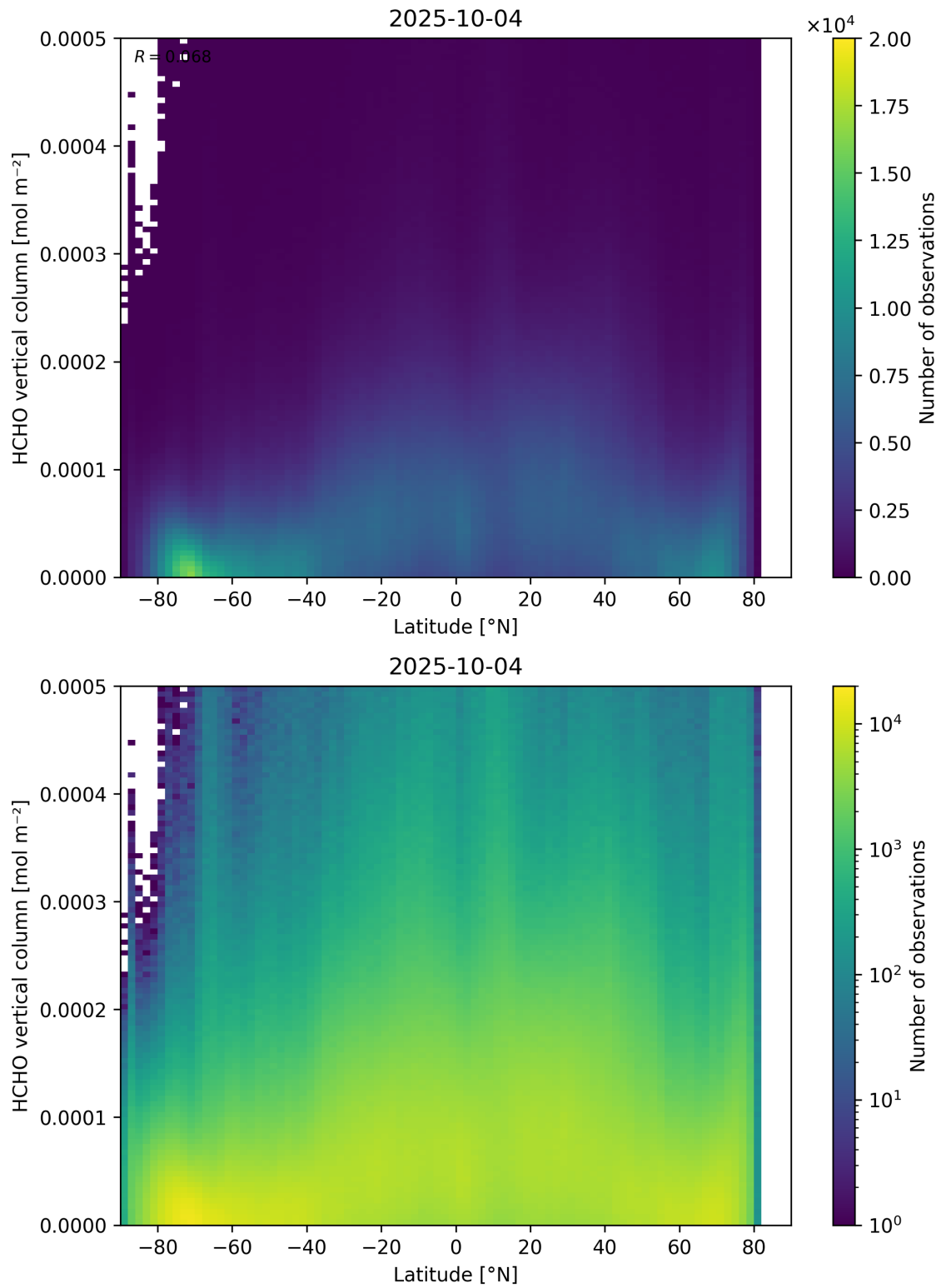
Figure 163: Scatter density plot of “Latitude” against “HCHO vertical column” for 2025-10-03 to 2025-10-05.
