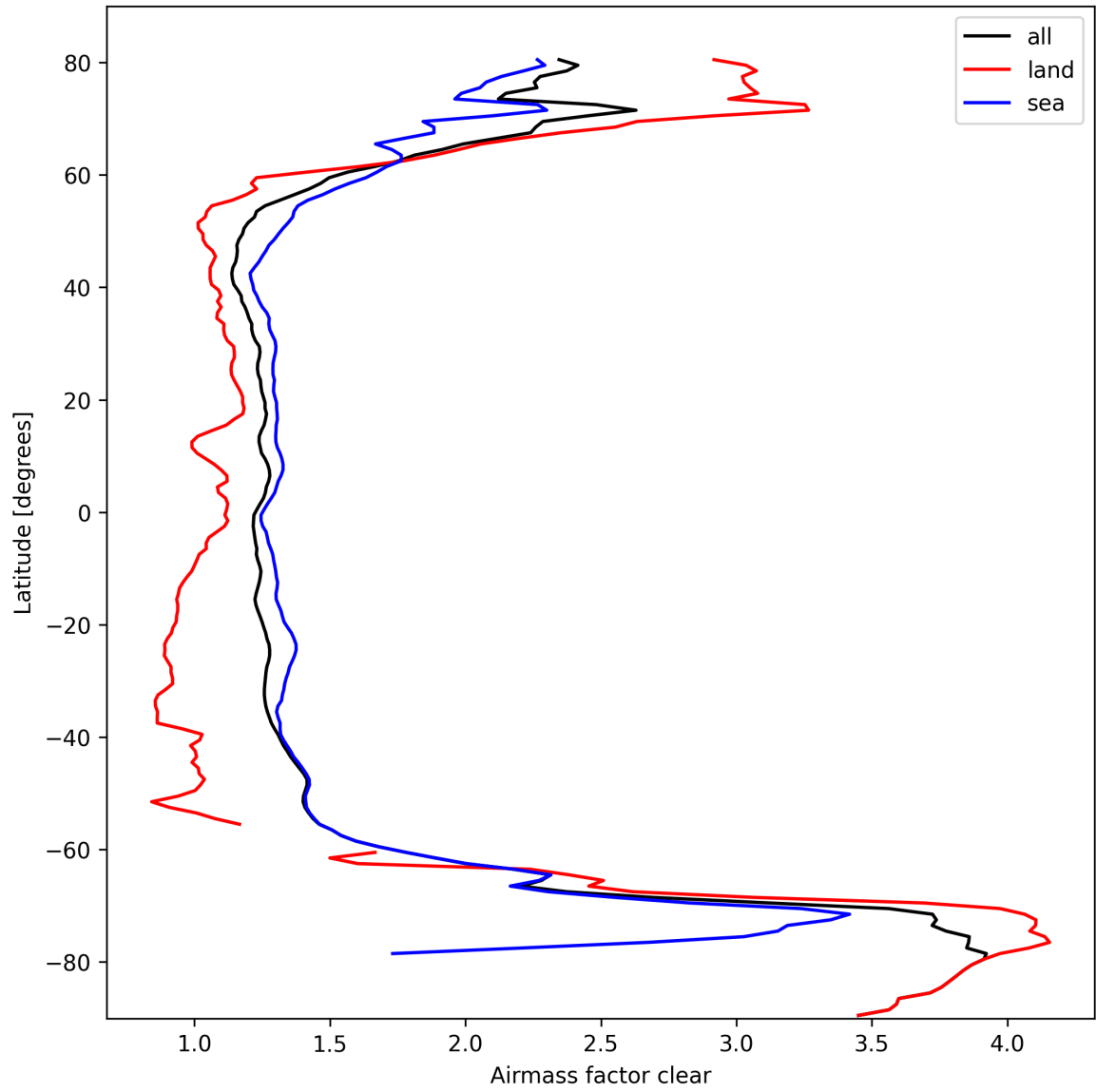
Figure 28: Zonal average of “Airmass factor clear” for 2025-10-03 to 2025-10-05.
