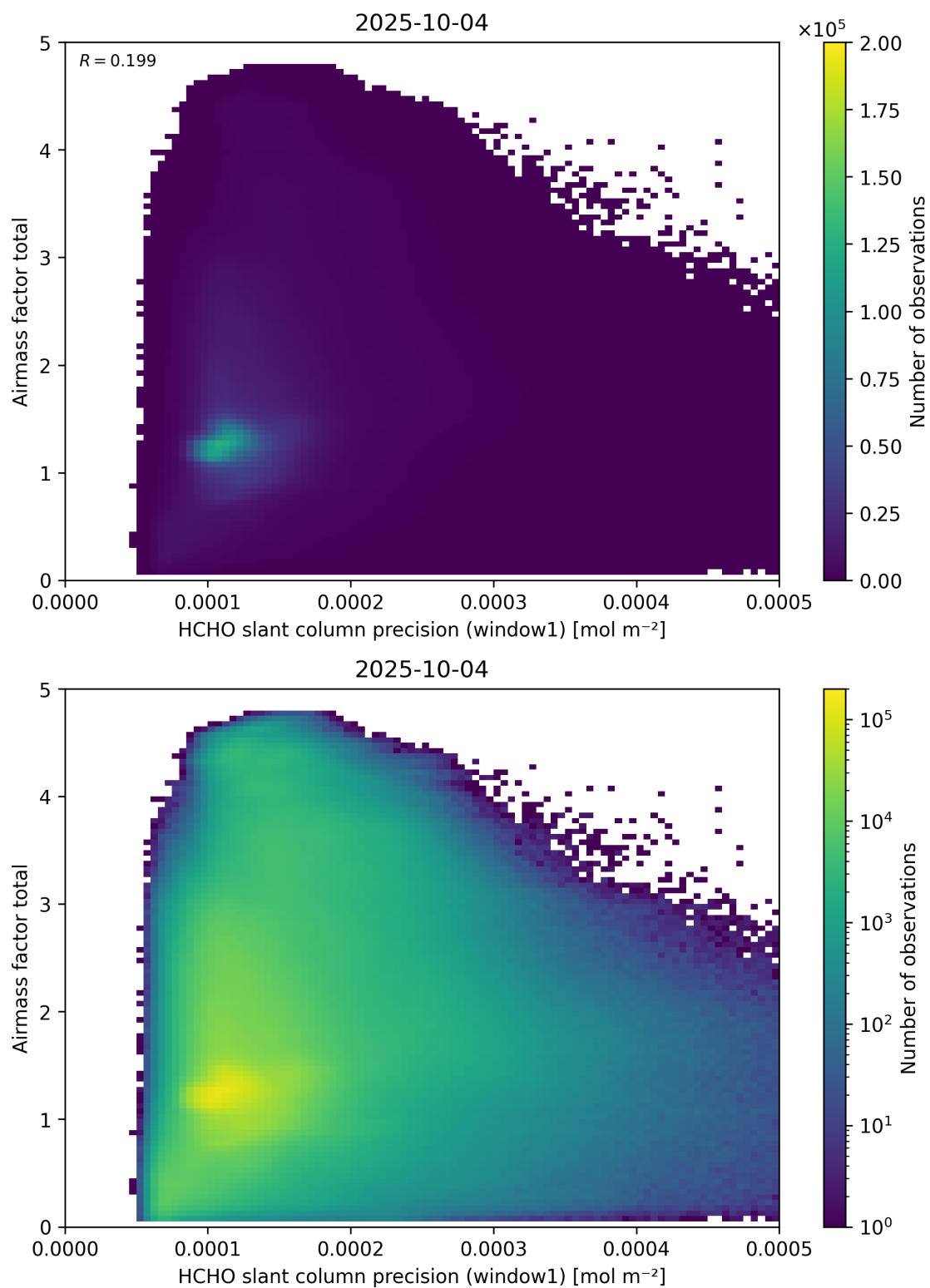
Figure 94: Scatter density plot of “HCHO slant column precision (window1)” against “Airmass factor total” for 2025-10-03 to 2025-10-05.
