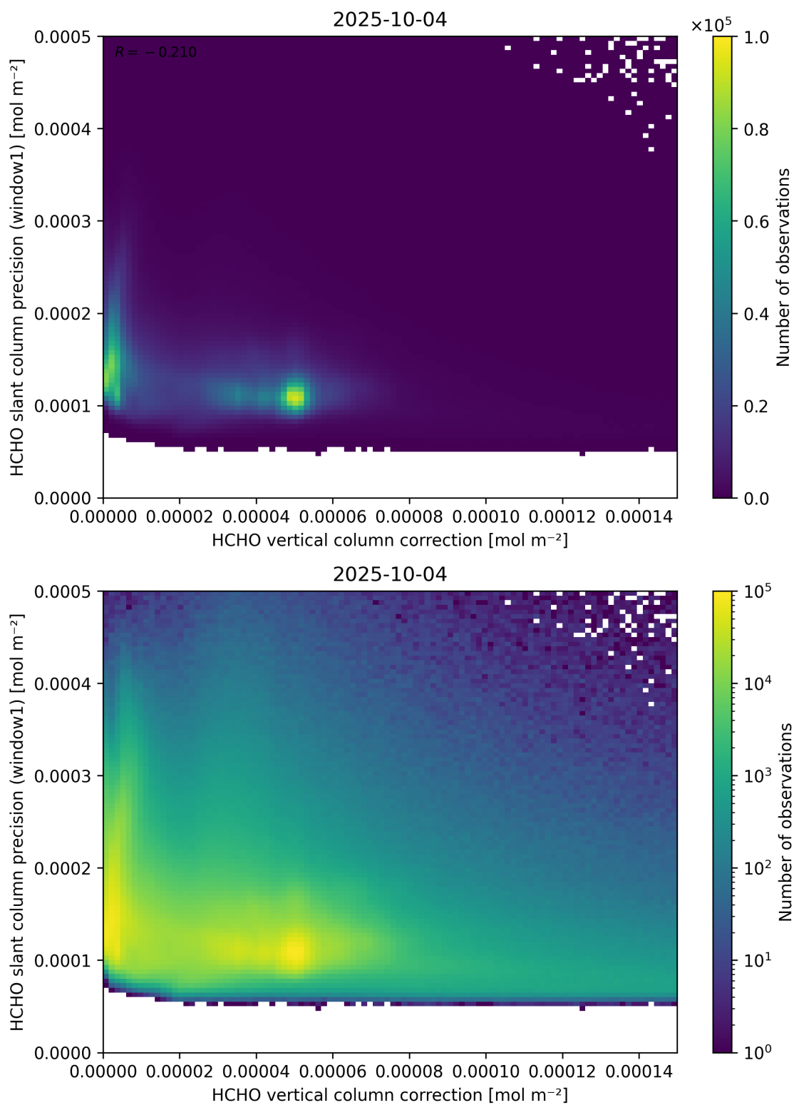
Figure 119: Scatter density plot of “HCHO vertical column correction” against “HCHO slant column precision (window1)” for 2025-10-03 to 2025-10-05.
