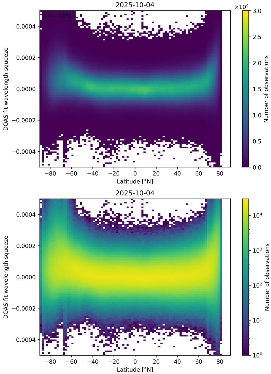
Figure 155: Scatter density plot of “Latitude” against “DOAS fit wavelength squeeze” for 2025-10-03 to 2025-10-05.
