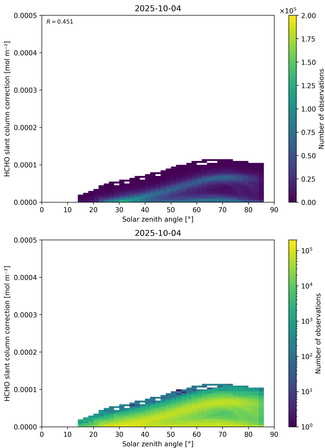
Figure 172: Scatter density plot of “Solar zenith angle” against “HCHO slant column correction” for 2025-10-03 to 2025-10-05.
