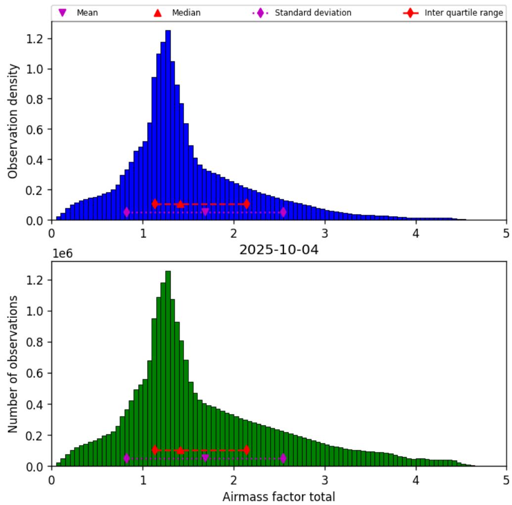
Figure 40: Histogram of “Airmass factor total” for 2025-10-03 to 2025-10-05
