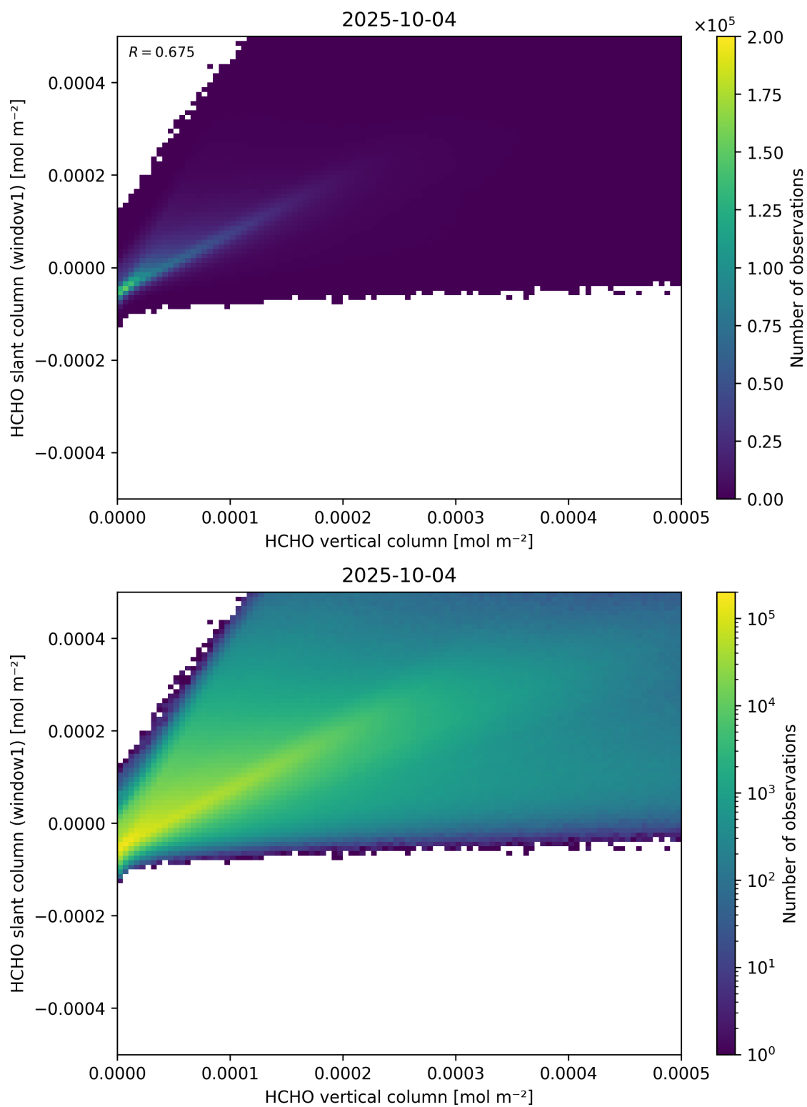
Figure 129: Scatter density plot of “HCHO vertical column” against “HCHO slant column (window1)” for 2025-10-03 to 2025-10-05.
