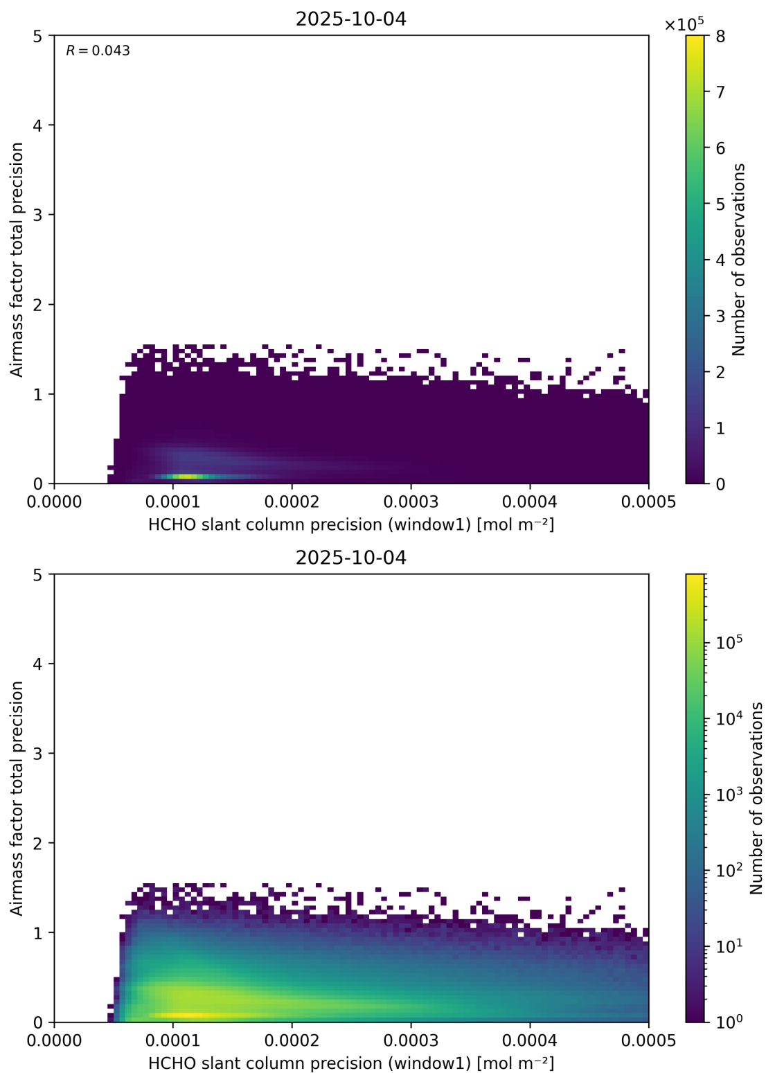
Figure 95: Scatter density plot of “HCHO slant column precision (window1)” against “Airmass factor total precision” for 2025-10-03 to 2025-10-05.
