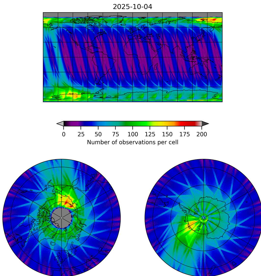
Figure 19: Map of the number of observations for 2025-10-03 to 2025-10-05
