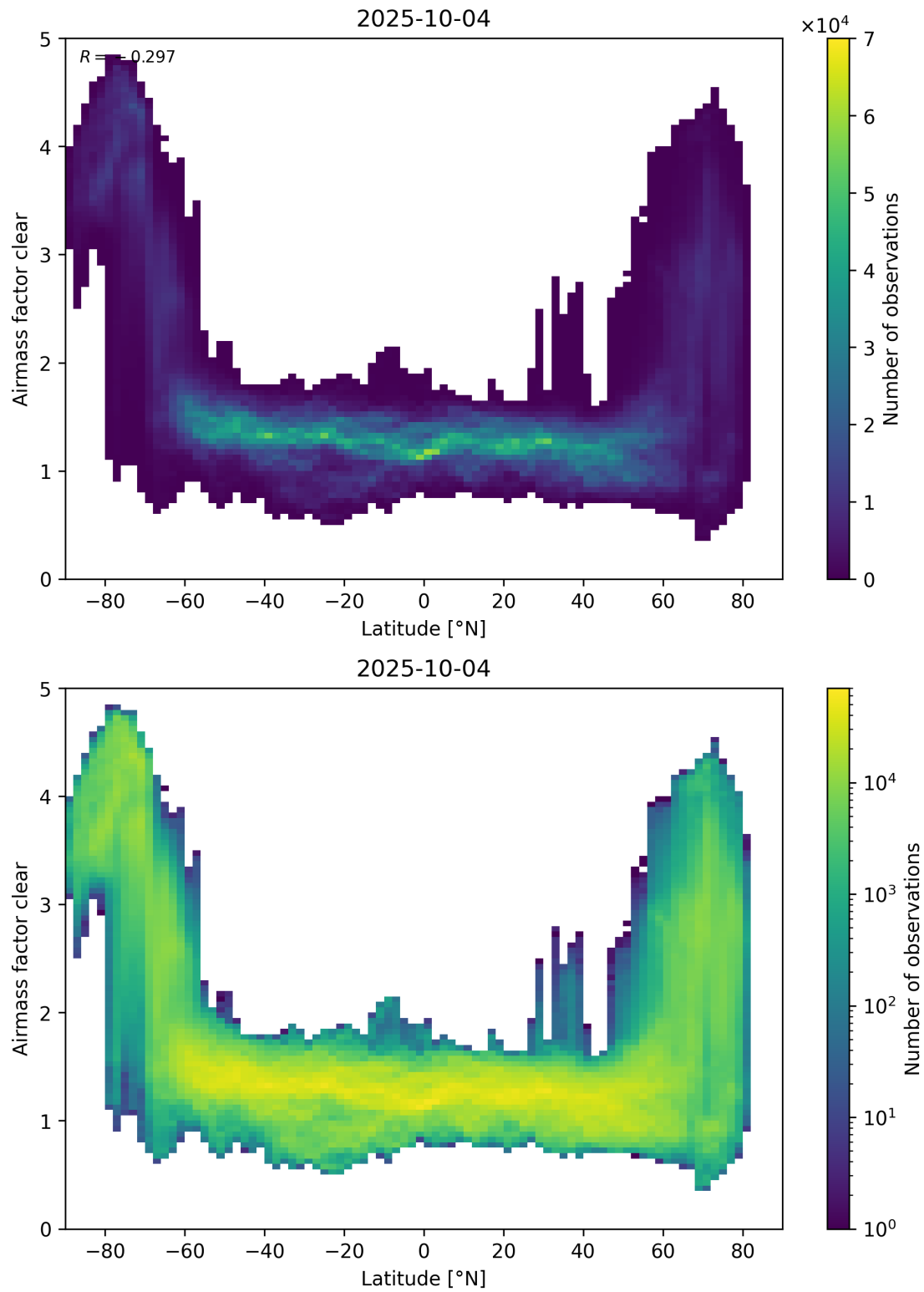
Figure 156: Scatter density plot of “Latitude” against “Airmass factor clear” for 2025-10-03 to 2025-10-05.
