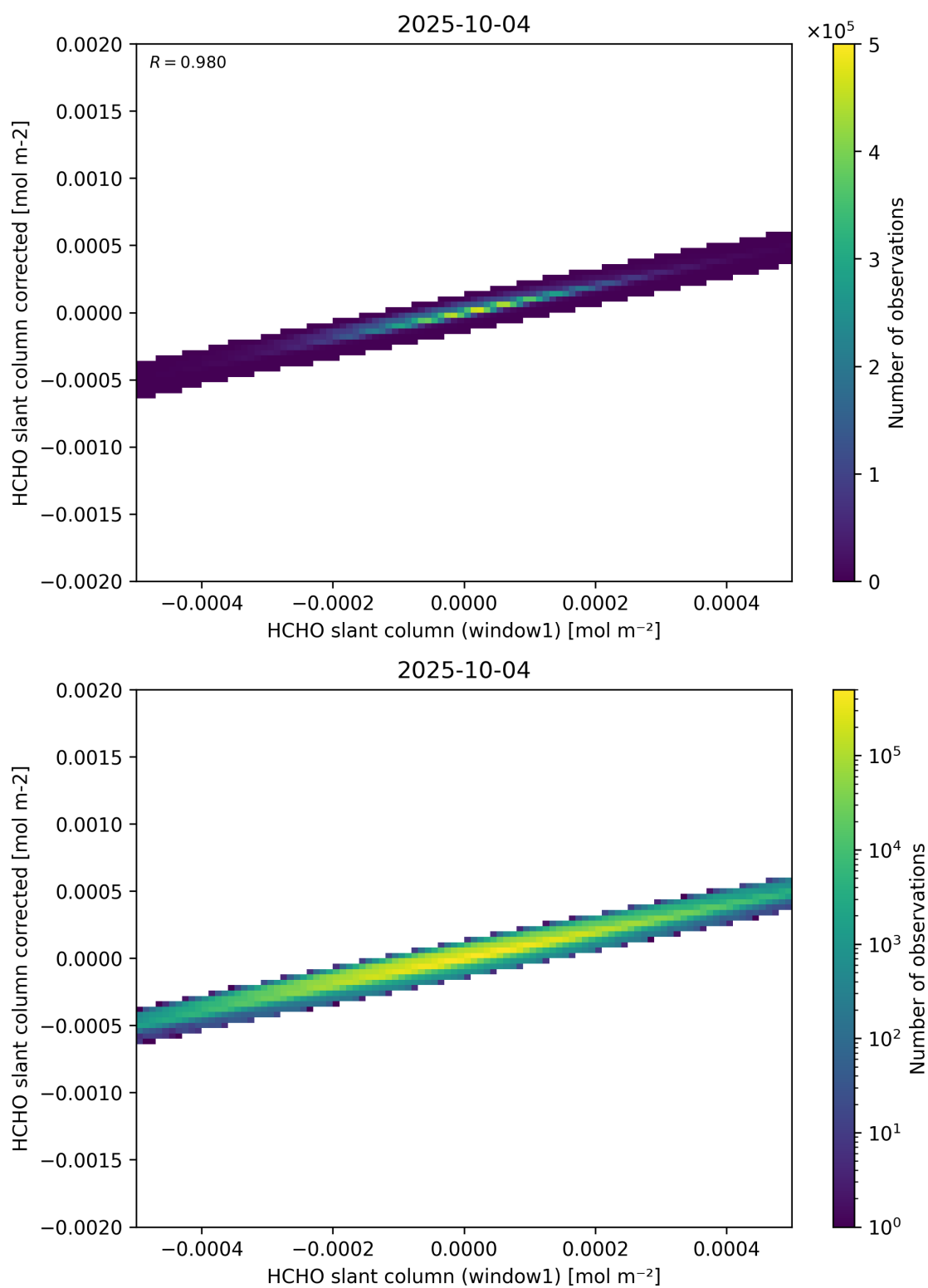
Figure 82: Scatter density plot of “HCHO slant column (window1)” against “HCHO slant column corrected” for 2025-10-03 to 2025-10-05.
