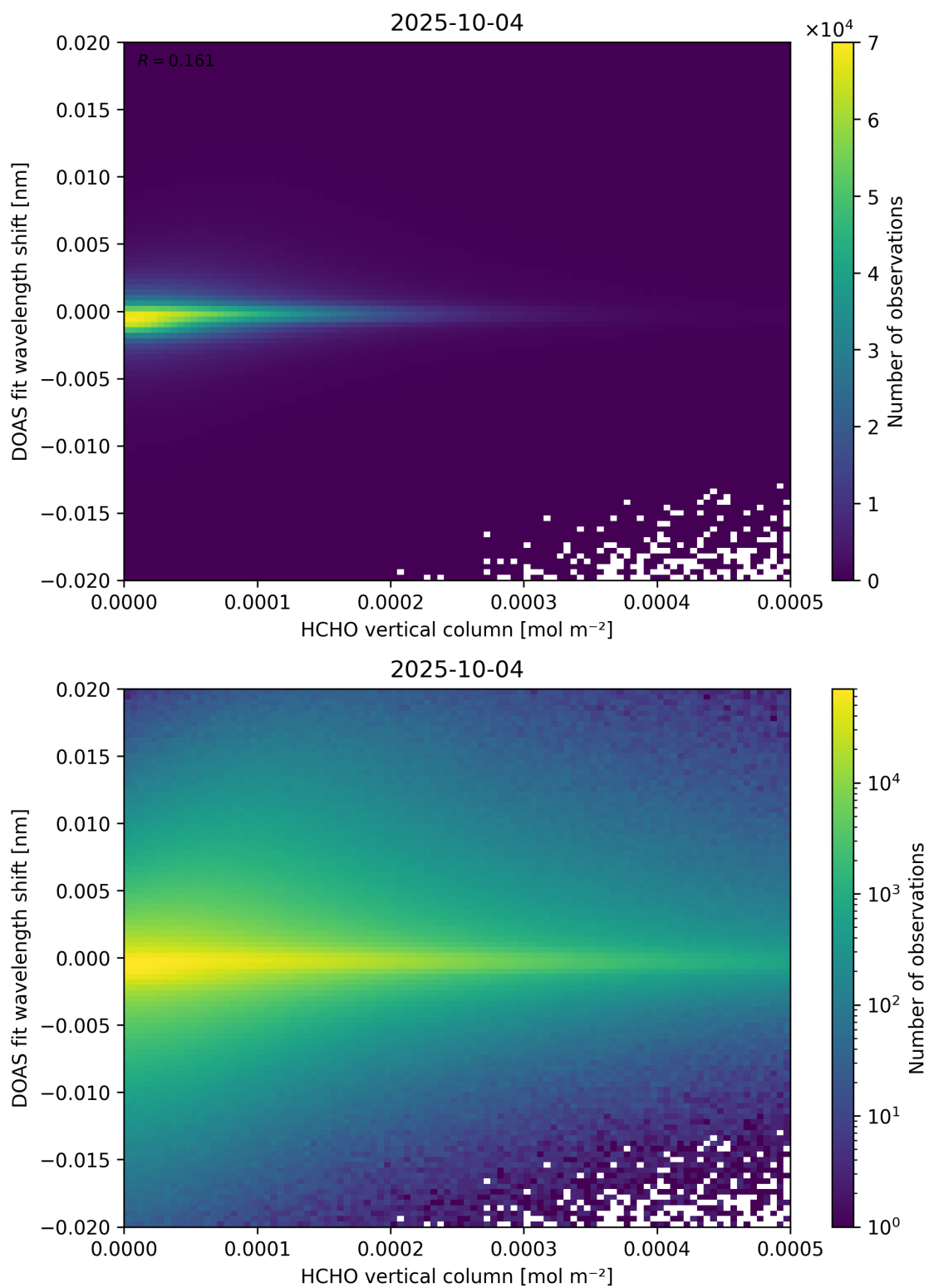
Figure 124: Scatter density plot of “HCHO vertical column” against “DOAS fit wavelength shift” for 2025-10-03 to 2025-10-05.
