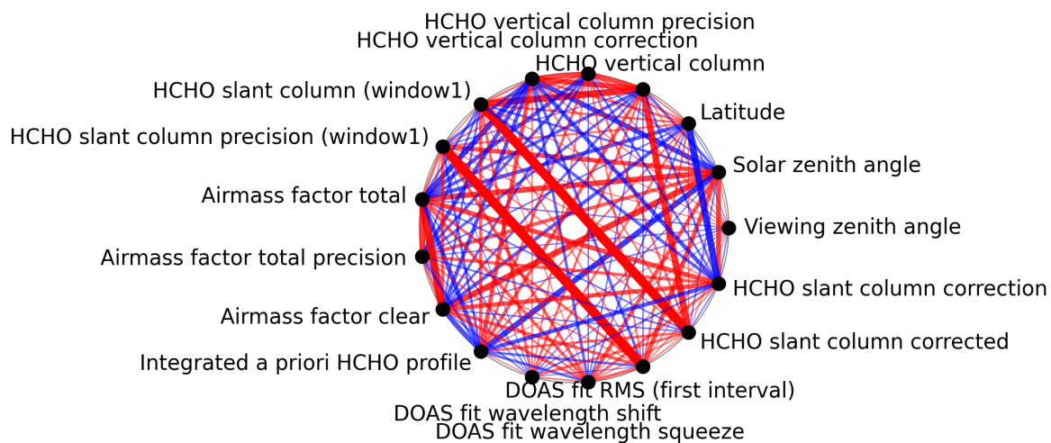
Figure 1: Map of correlation graph for 2025-10-03 to 2025-10-05.
