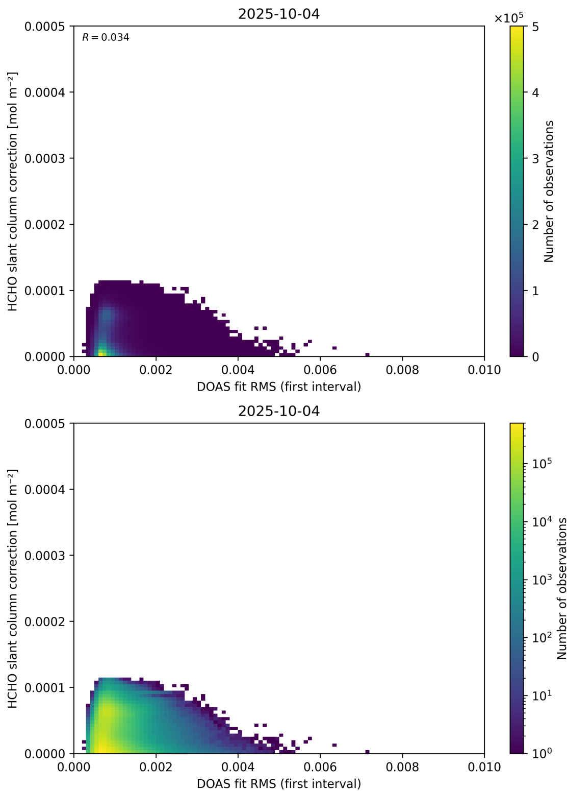
Figure 63: Scatter density plot of “DOAS fit RMS (first interval)” against “HCHO slant column correction” for 2025-10-03 to 2025-10-05.
