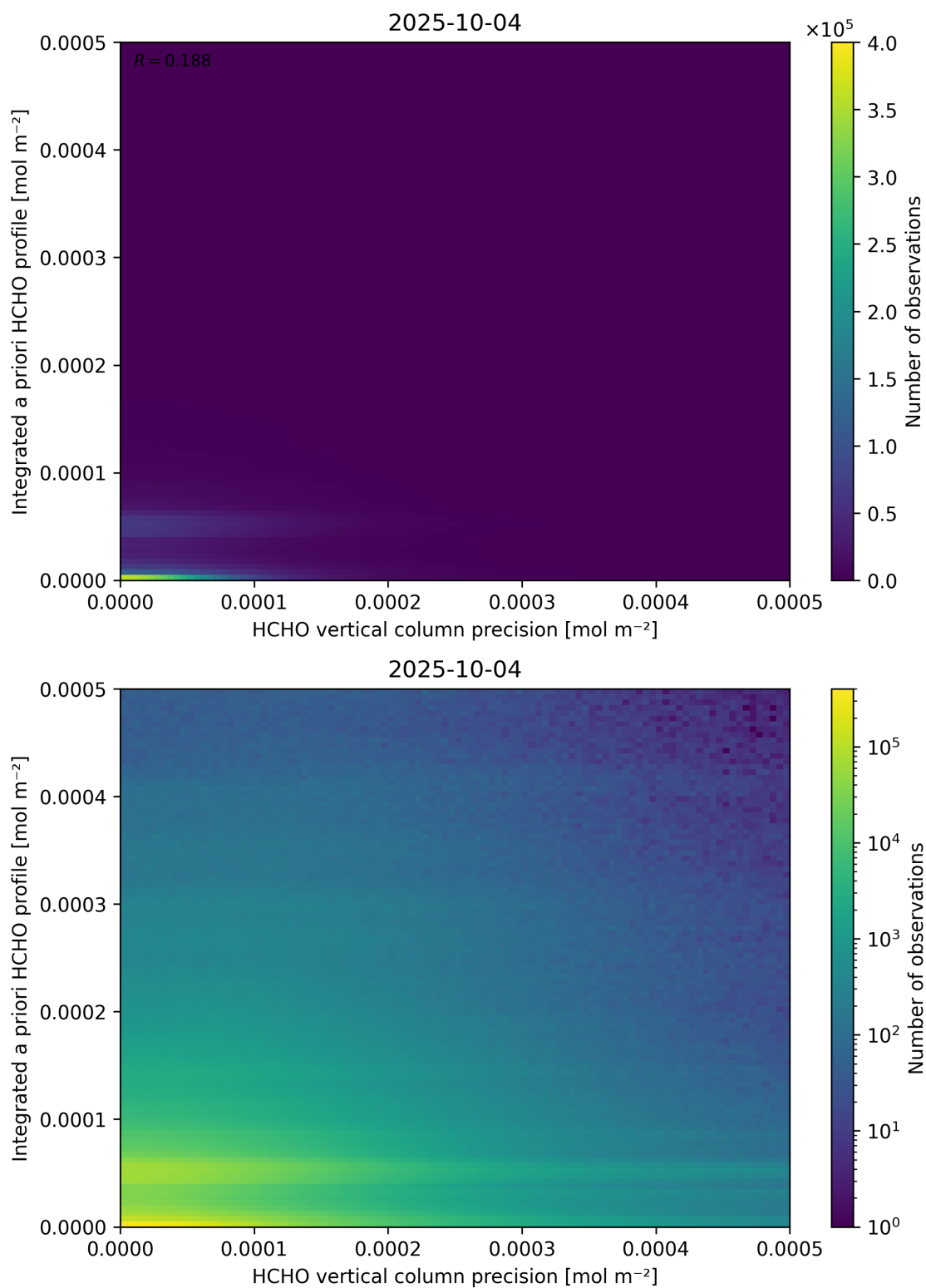
Figure 147: Scatter density plot of “HCHO vertical column precision” against “Integrated a priori HCHO profile” for 2025-10-03 to 2025-10-05.
