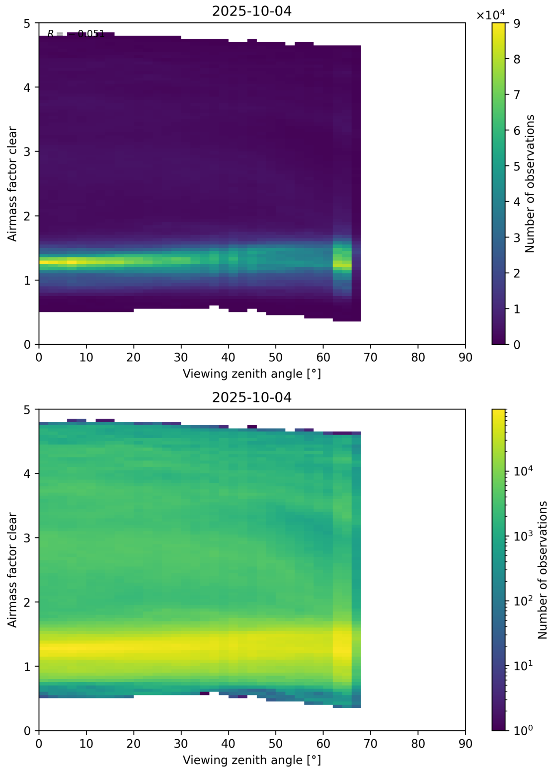
Figure 185: Scatter density plot of “Viewing zenith angle” against “Airmass factor clear” for 2025-10-03 to 2025-10-05.
