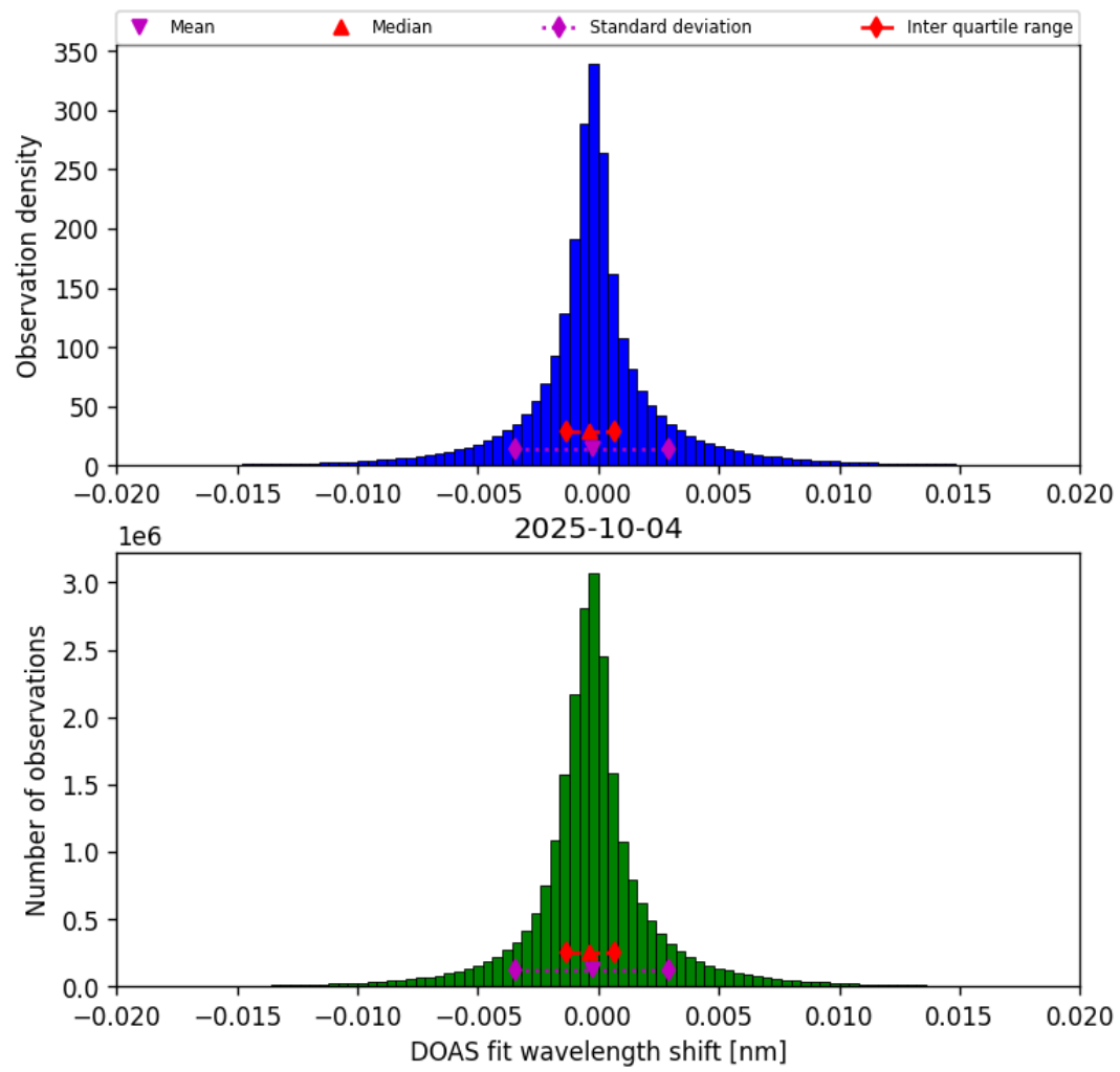
Figure 44: Histogram of “DOAS fit wavelength shift” for 2025-10-03 to 2025-10-05
