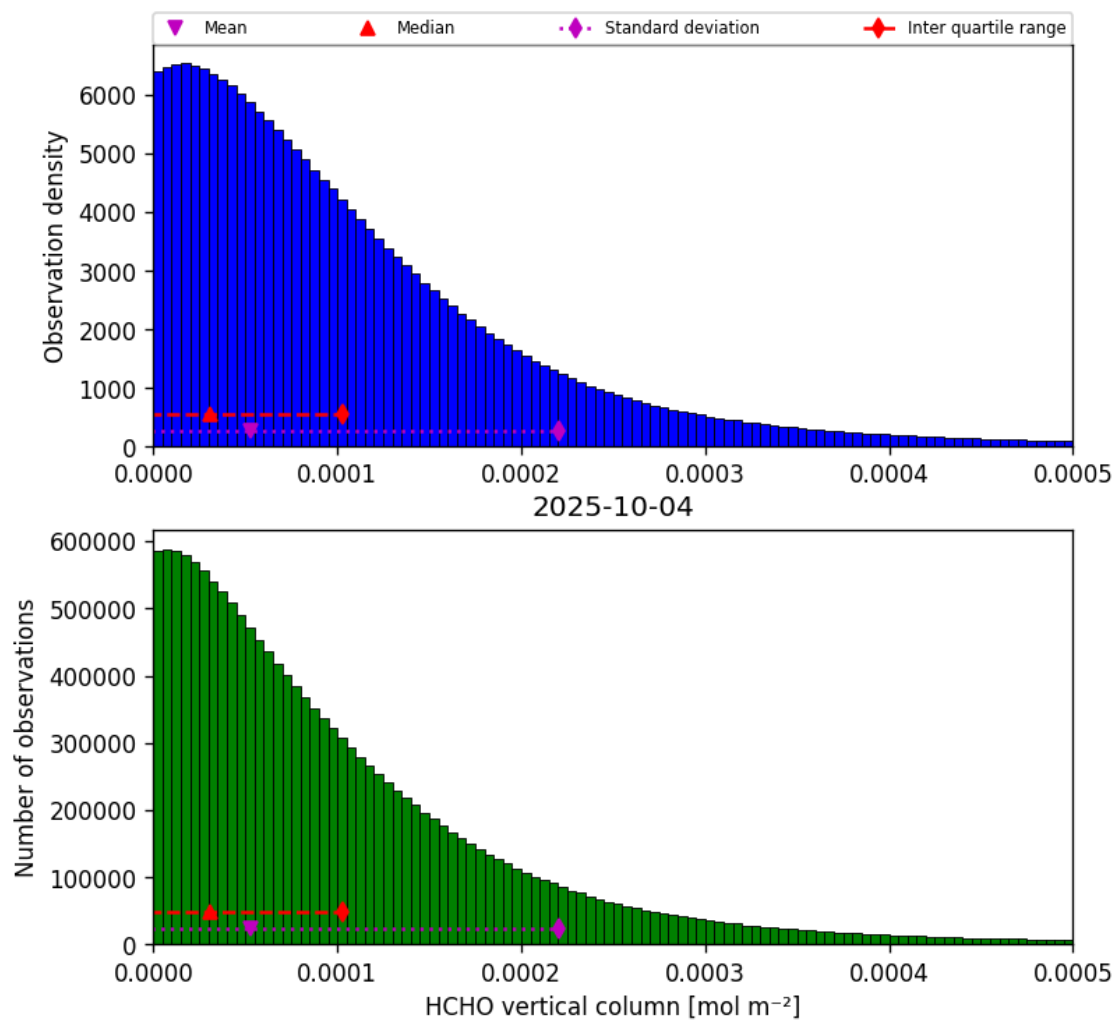
Figure 35: Histogram of “HCHO vertical column” for 2025-10-03 to 2025-10-05
