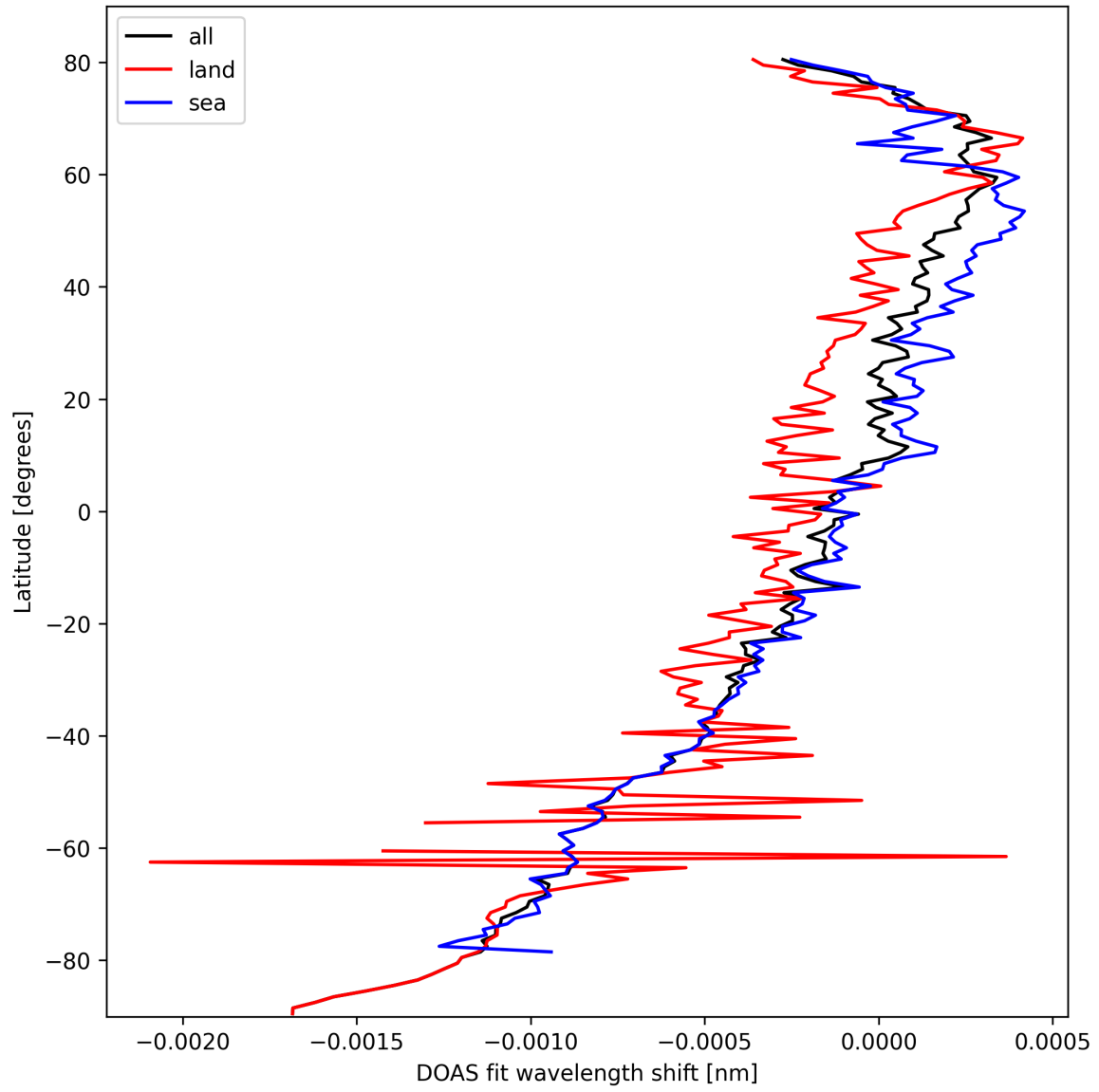
Figure 30: Zonal average of “DOAS fit wavelength shift” for 2025-10-03 to 2025-10-05.
