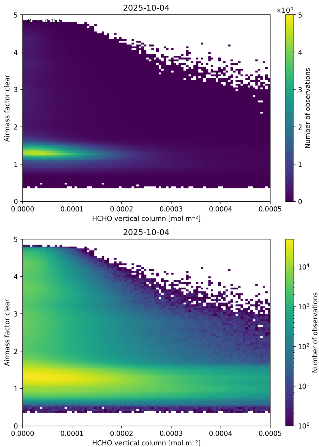
Figure 126: Scatter density plot of “HCHO vertical column” against “Airmass factor clear” for 2025-10-03 to 2025-10-05.
