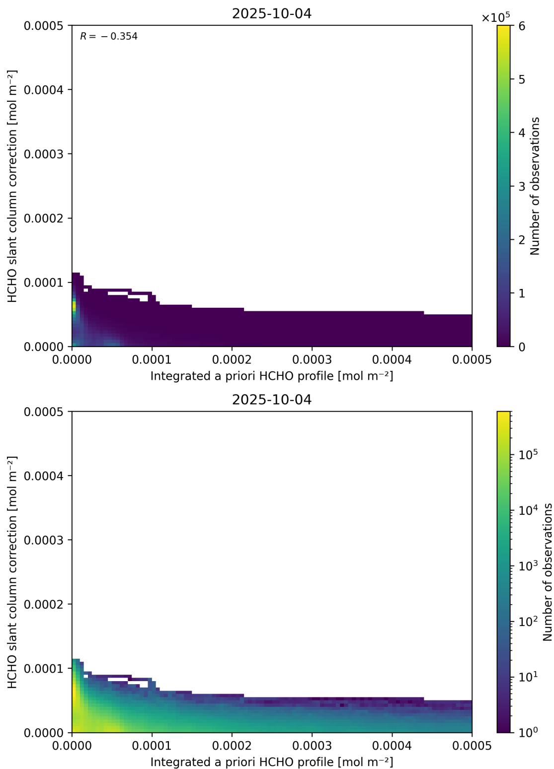
Figure 152: Scatter density plot of “Integrated a priori HCHO profile” against “HCHO slant column correction” for 2025-10-03 to 2025-10-05.
