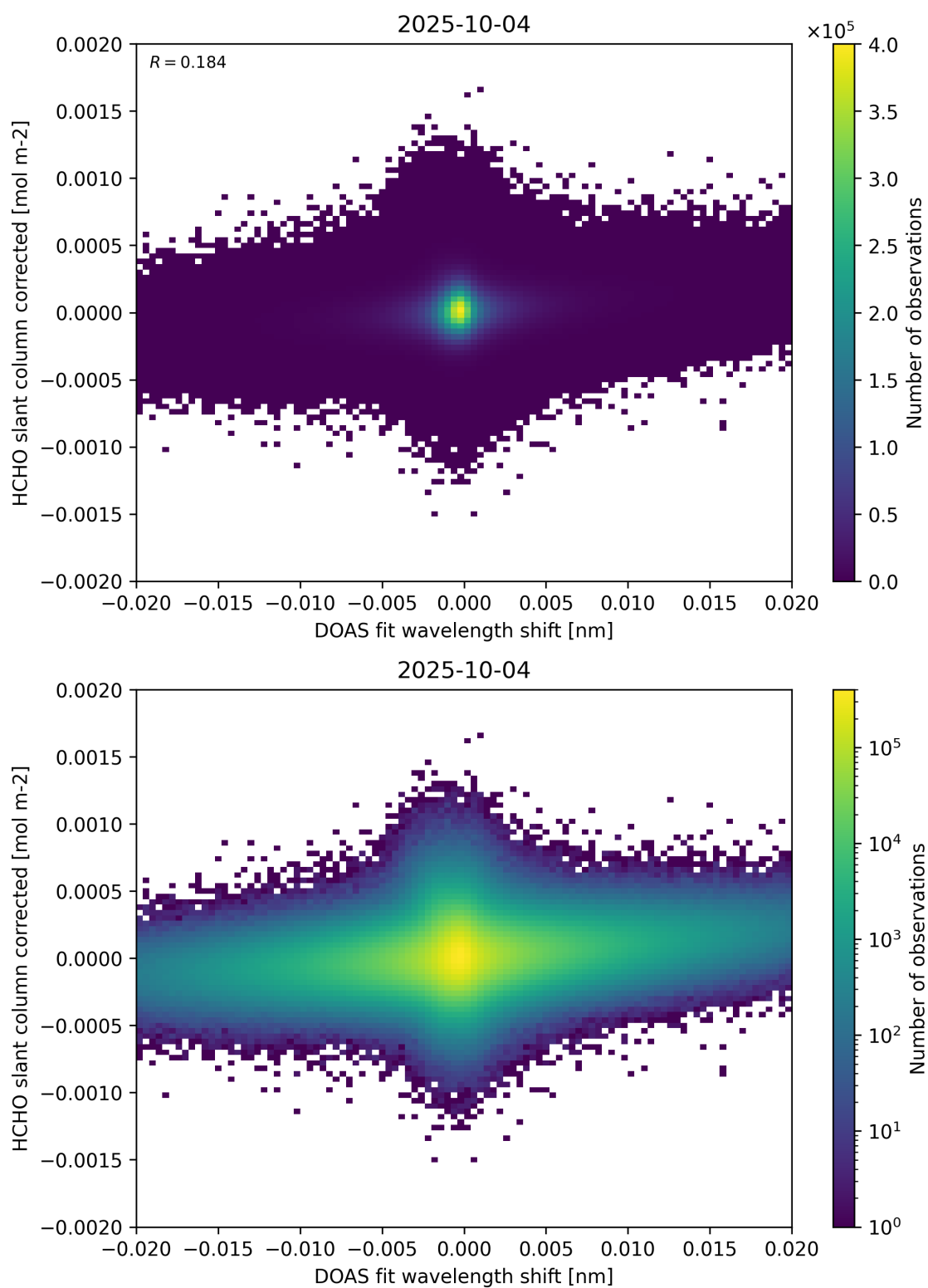
Figure 66: Scatter density plot of “DOAS fit wavelength shift” against “HCHO slant column corrected” for 2025-10-03 to 2025-10-05.
