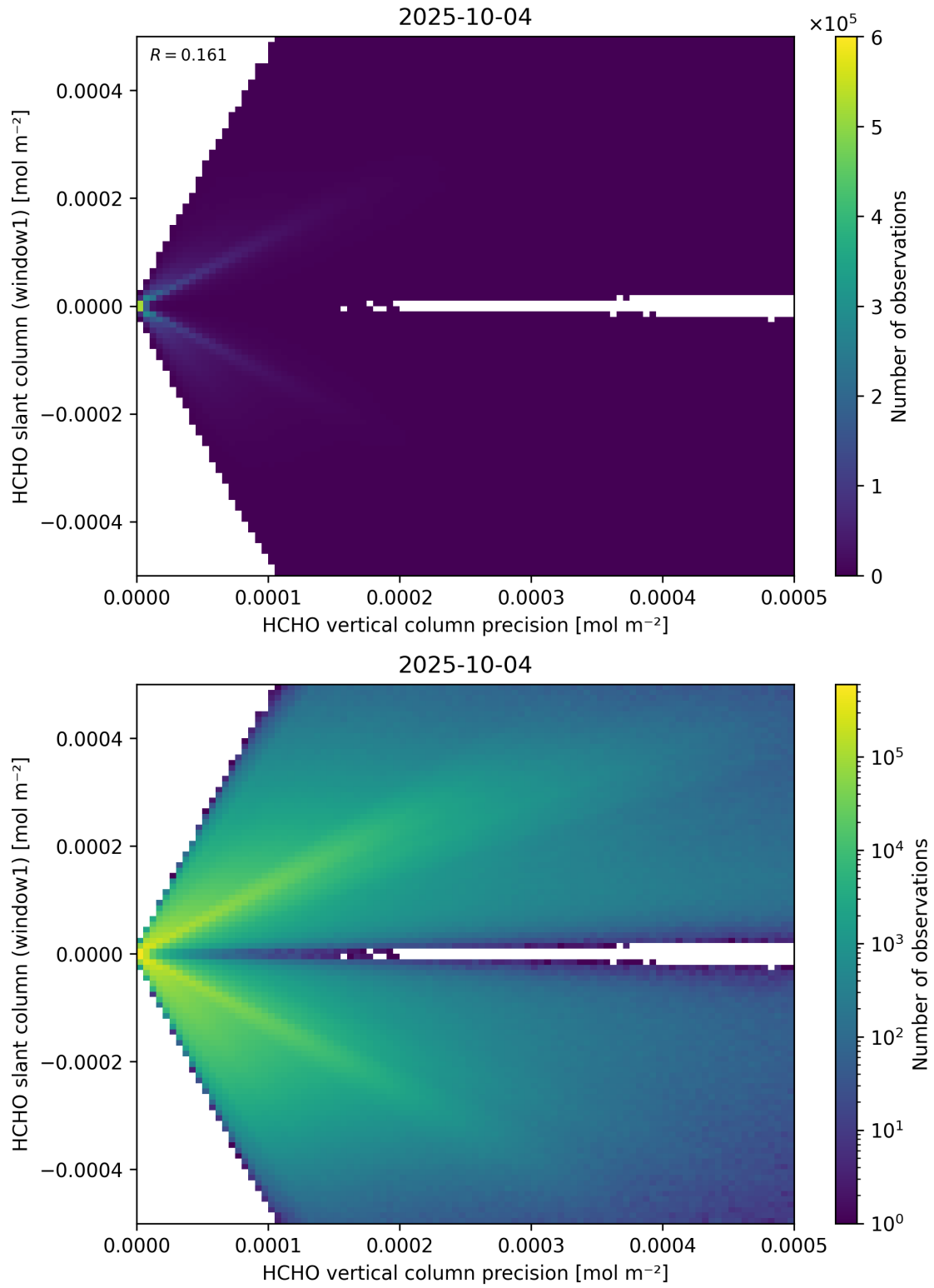
Figure 142: Scatter density plot of “HCHO vertical column precision” against “HCHO slant column (window1)” for 2025-10-03 to 2025-10-05.
