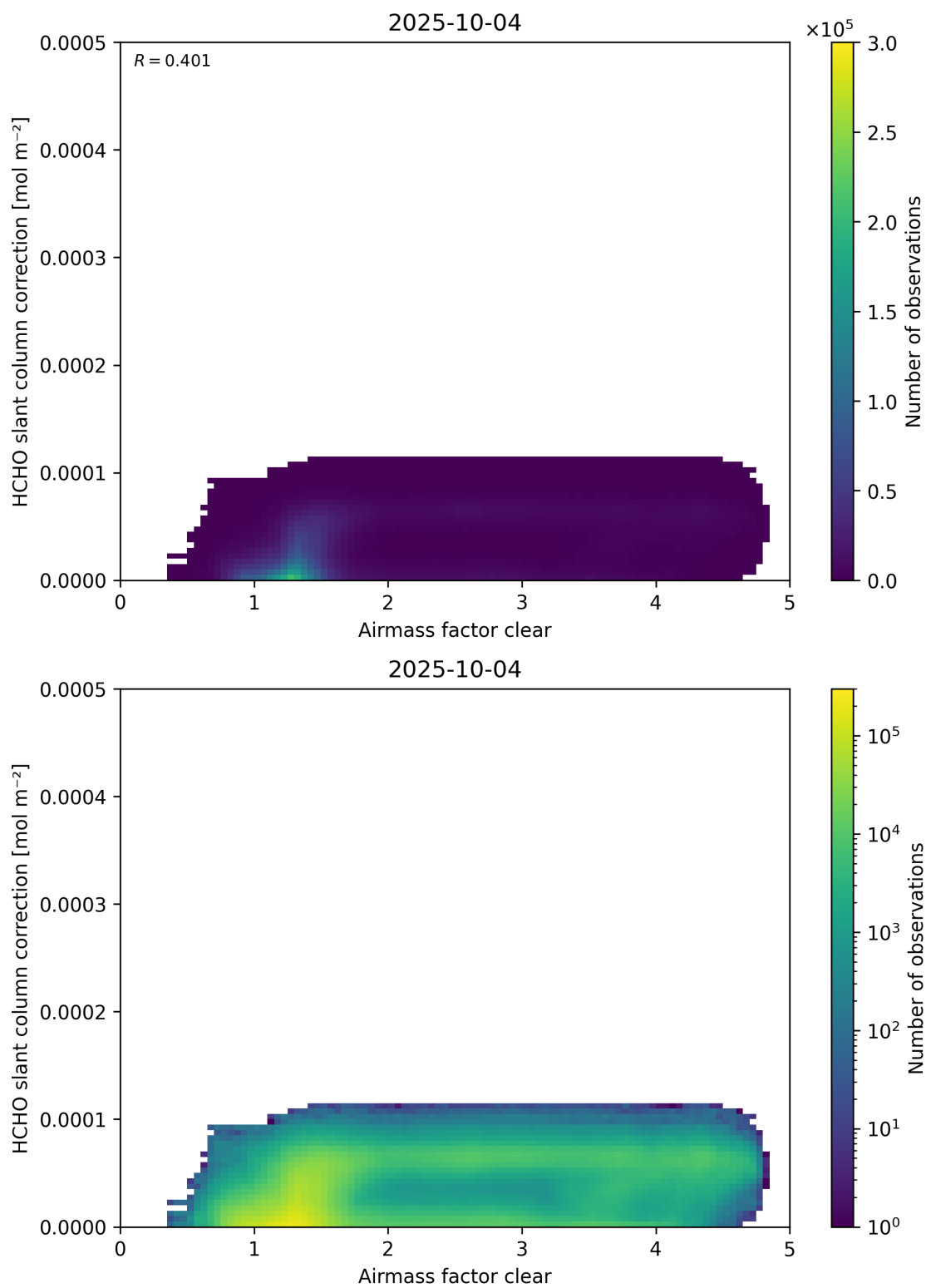
Figure 75: Scatter density plot of “Airmass factor clear” against “HCHO slant column correction” for 2025-10-03 to 2025-10-05.
