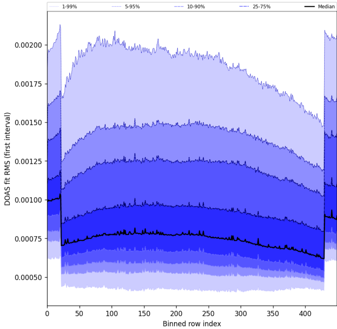
Figure 60: Along track statistics of “DOAS fit RMS (first interval)” for 2025-10-03 to 2025-10-05
