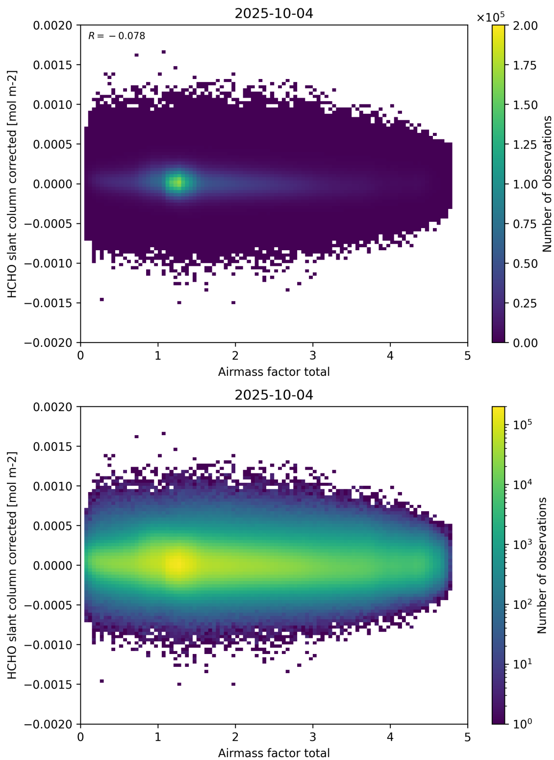
Figure 101: Scatter density plot of “Airmass factor total” against “HCHO slant column corrected” for 2025-10-03 to 2025-10-05.
