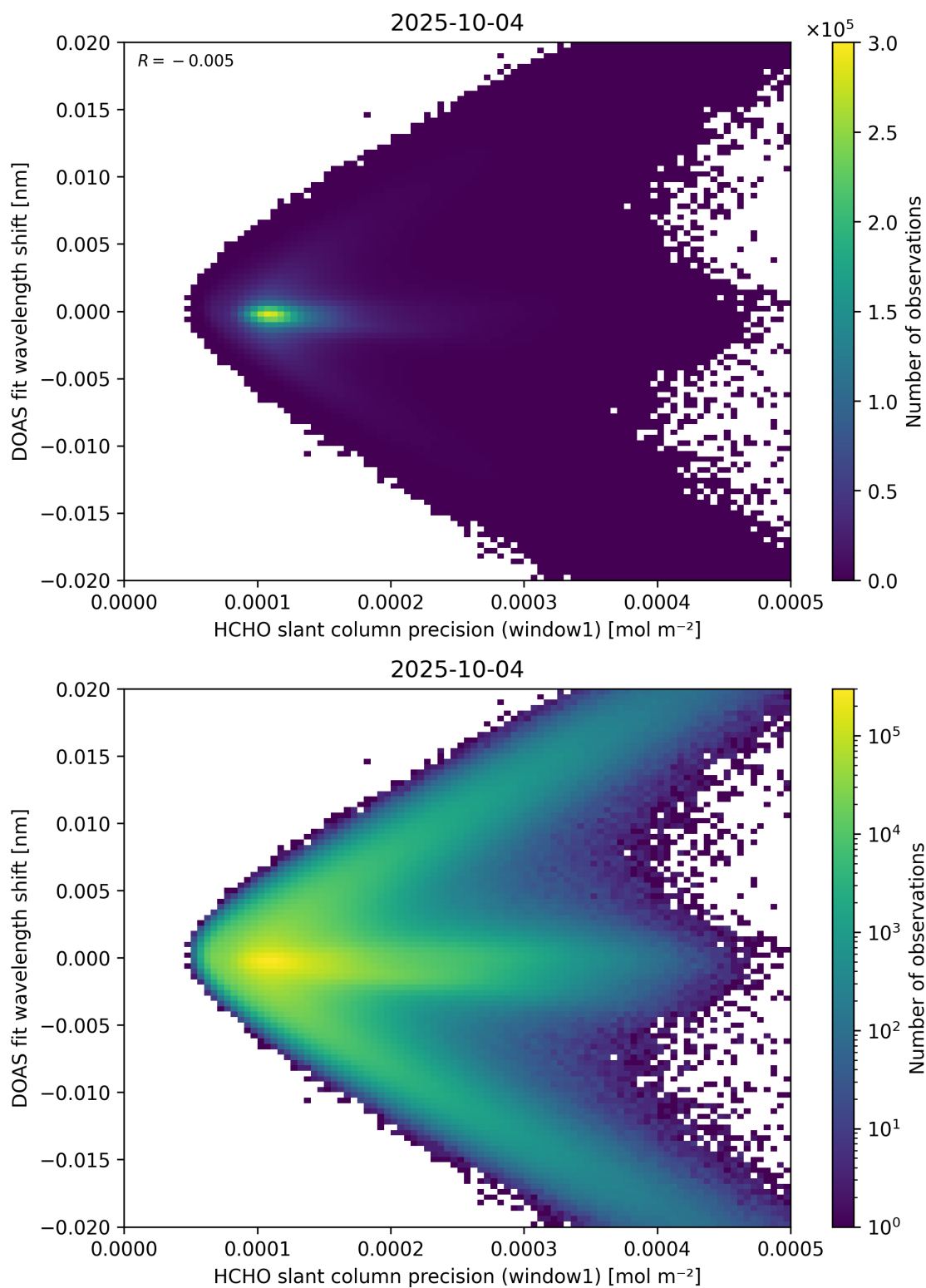
Figure 89: Scatter density plot of “HCHO slant column precision (window1)” against “DOAS fit wavelength shift” for 2025-10-03 to 2025-10-05.
