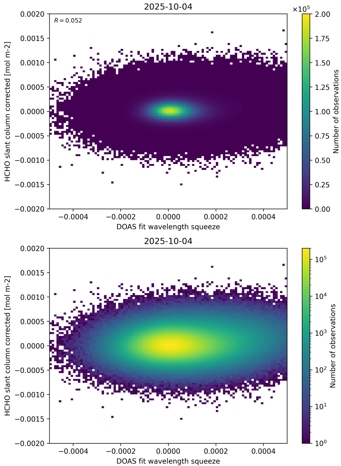
Figure 69: Scatter density plot of “DOAS fit wavelength squeeze” against “HCHO slant column corrected” for 2025-10-03 to 2025-10-05.
