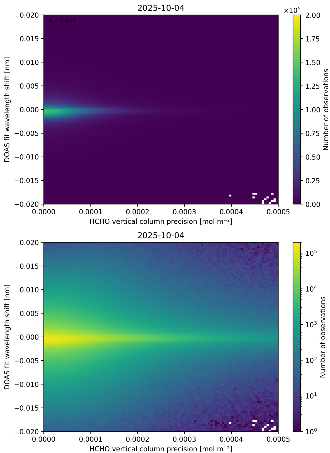
Figure 137: Scatter density plot of “HCHO vertical column precision” against “DOAS fit wavelength shift” for 2025-10-03 to 2025-10-05.
