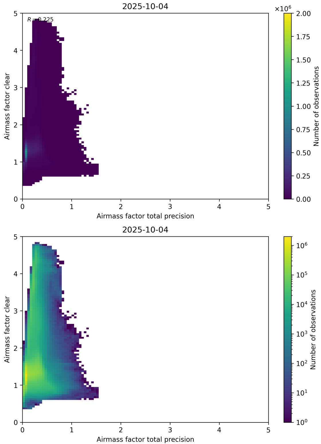
Figure 108: Scatter density plot of “Airmass factor total precision” against “Airmass factor clear” for 2025-10-03 to 2025-10-05.
