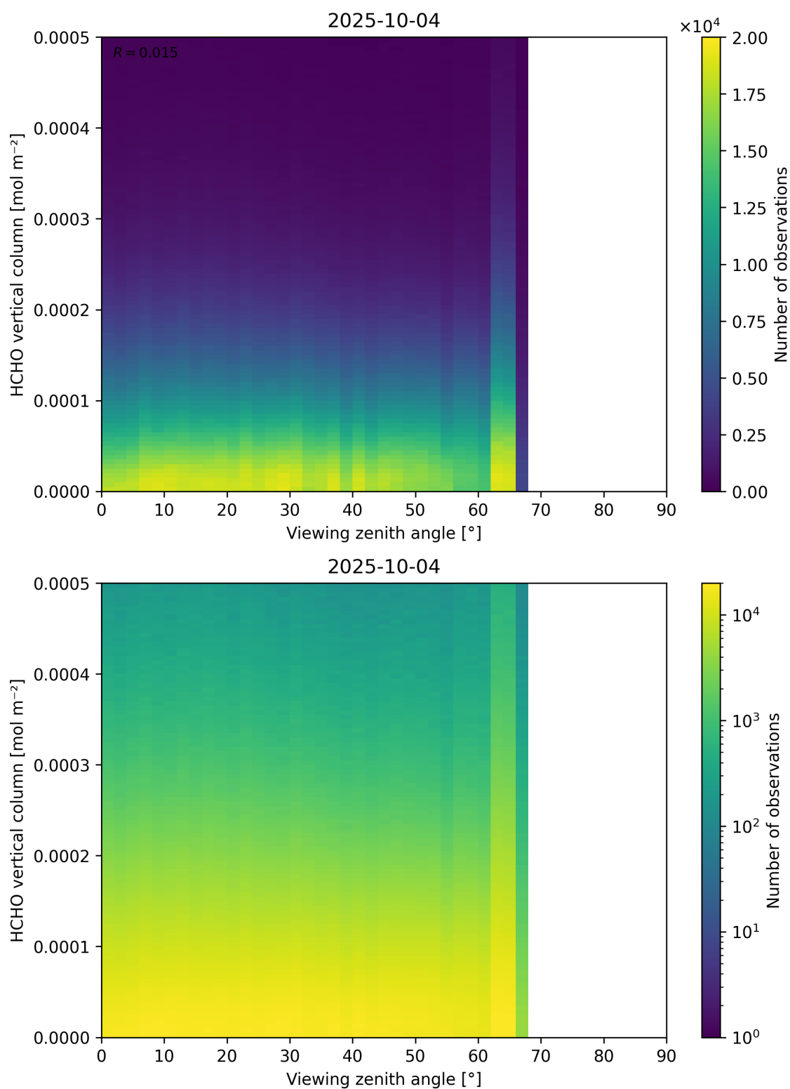
Figure 192: Scatter density plot of “Viewing zenith angle” against “HCHO vertical column” for 2025-10-03 to 2025-10-05.
