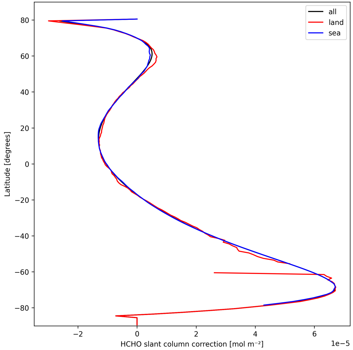
Figure 33: Zonal average of “HCHO slant column correction” for 2025-10-03 to 2025-10-05.
