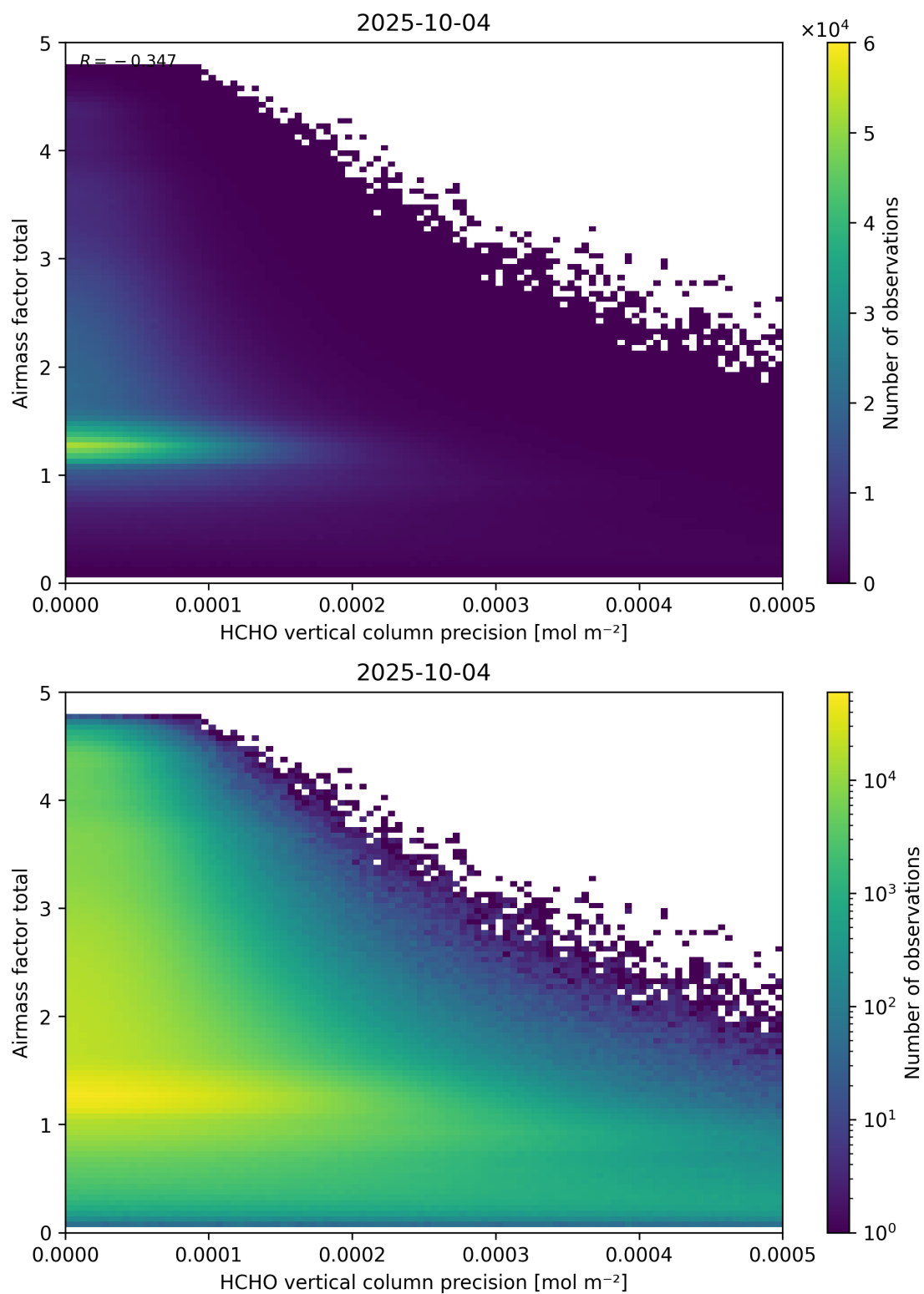
Figure 144: Scatter density plot of “HCHO vertical column precision” against “Airmass factor total” for 2025-10-03 to 2025-10-05.
