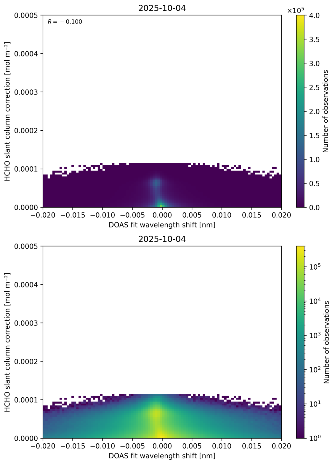
Figure 67: Scatter density plot of “DOAS fit wavelength shift” against “HCHO slant column correction” for 2025-10-03 to 2025-10-05.
