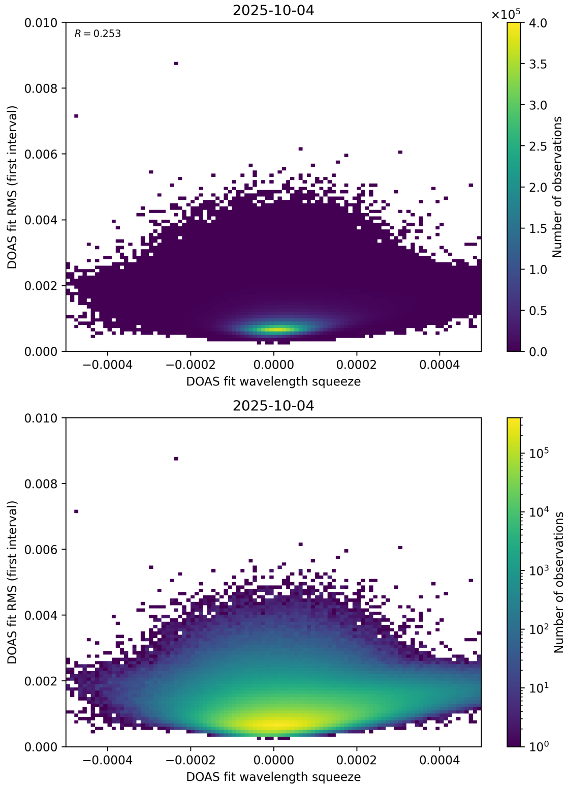
Figure 68: Scatter density plot of “DOAS fit wavelength squeeze” against “DOAS fit RMS (first interval)” for 2025-10-03 to 2025-10-05.
