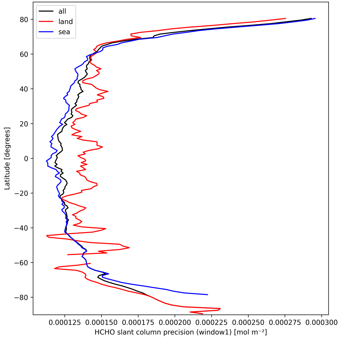
Figure 25: Zonal average of "HCHO slant column precision (window1)" for 2025-10-03 to 2025-10-05.
