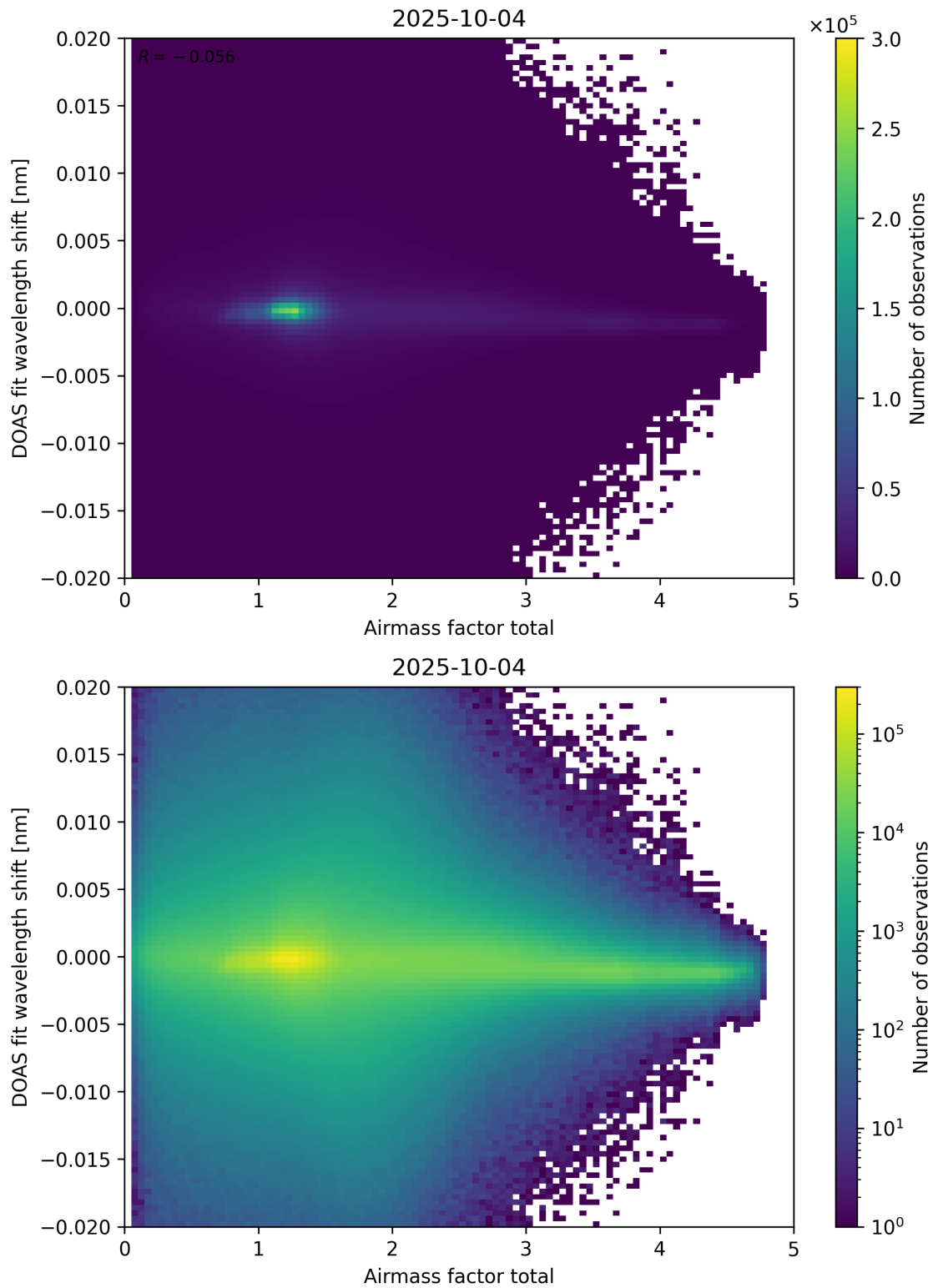
Figure 98: Scatter density plot of “Airmass factor total” against “DOAS fit wavelength shift” for 2025-10-03 to 2025-10-05.
