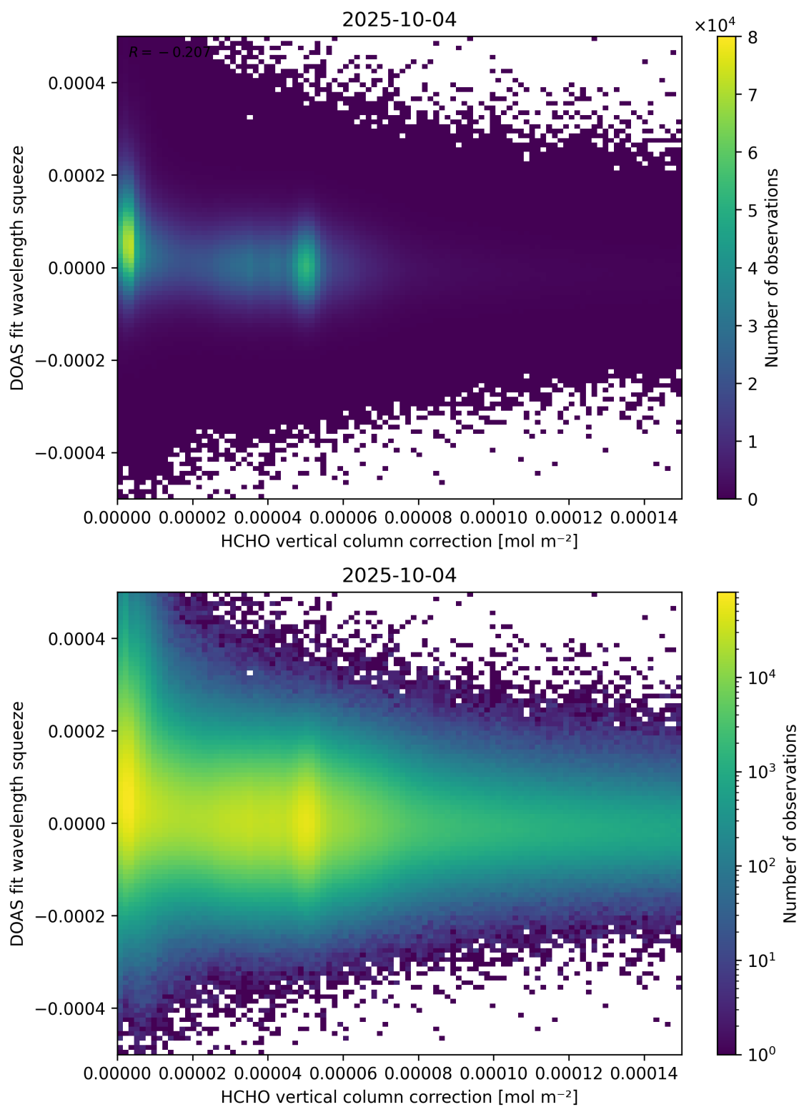
Figure 114: Scatter density plot of “HCHO vertical column correction” against “DOAS fit wavelength squeeze” for 2025-10-03 to 2025-10-05.
