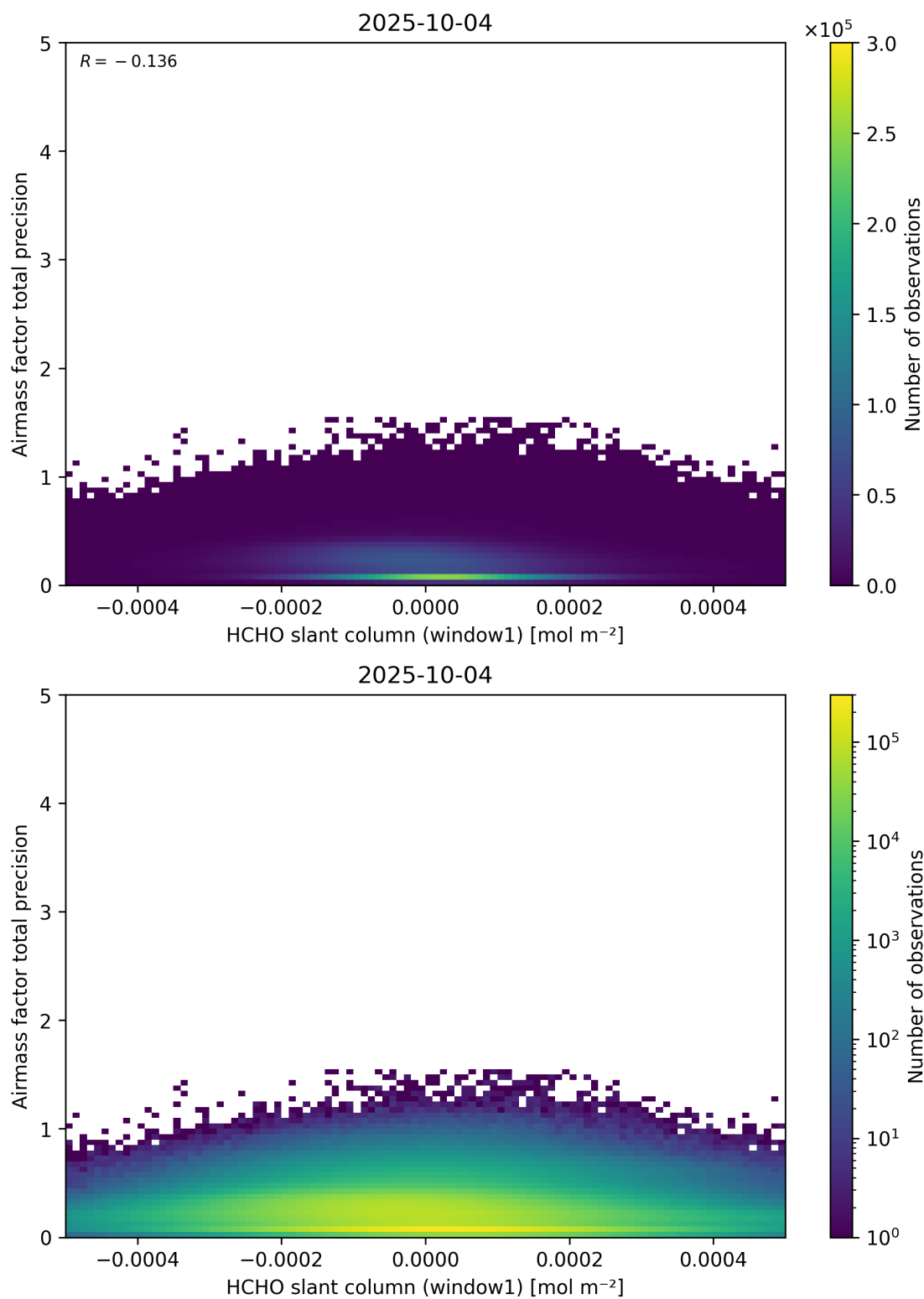
Figure 86: Scatter density plot of “HCHO slant column (window1)” against “Airmass factor total precision” for 2025-10-03 to 2025-10-05.
