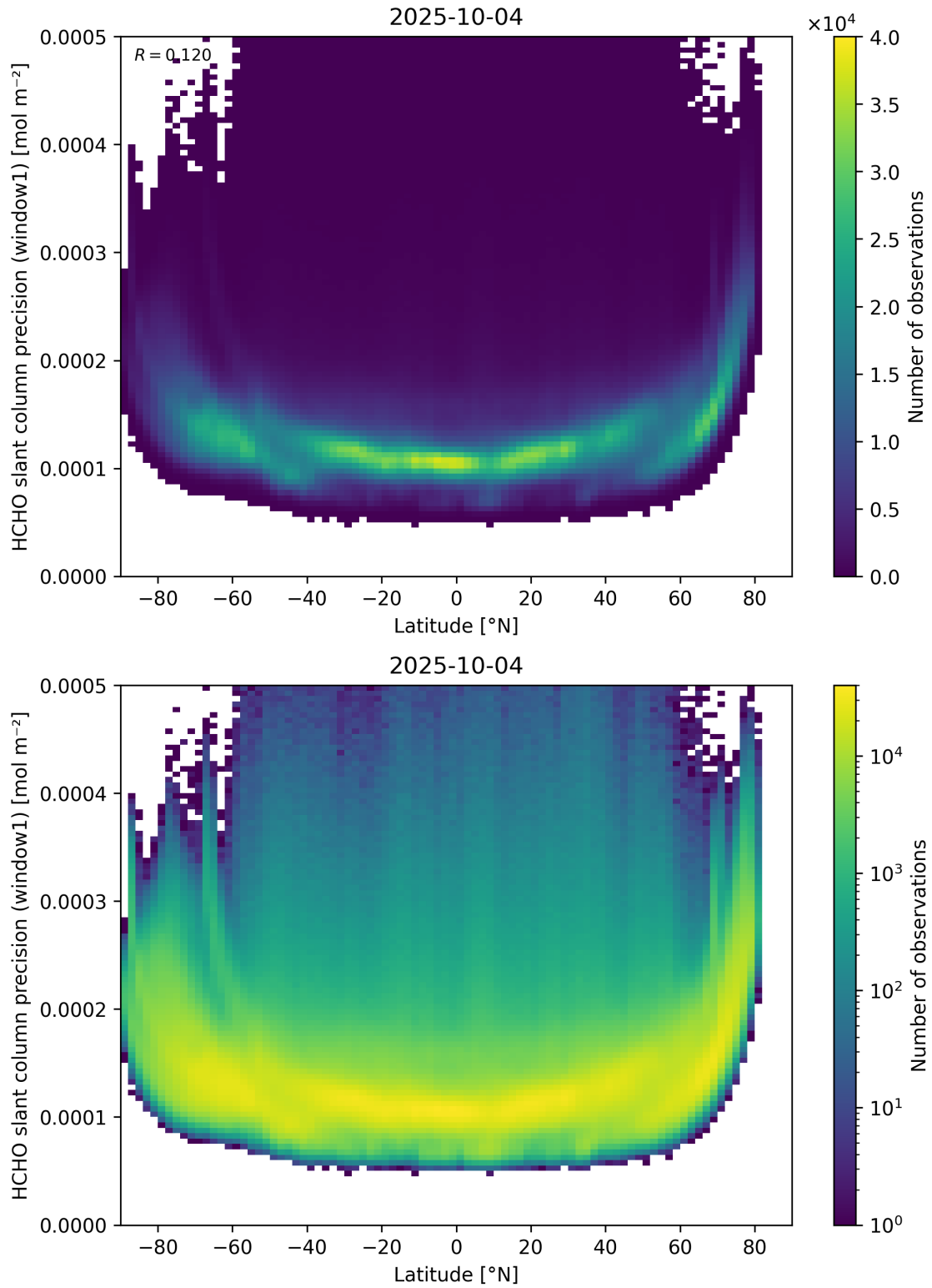
Figure 160: Scatter density plot of “Latitude” against “HCHO slant column precision (window1)” for 2025-10-03 to 2025-10-05.
