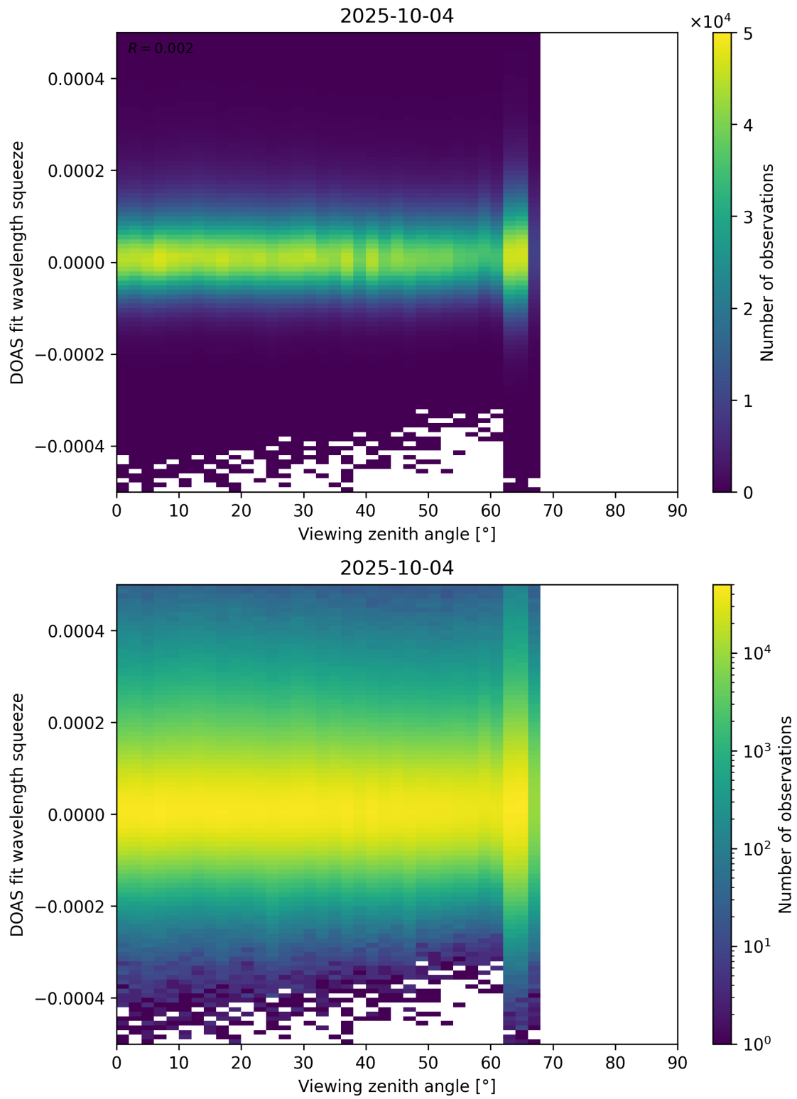
Figure 184: Scatter density plot of “Viewing zenith angle” against “DOAS fit wavelength squeeze” for 2025-10-03 to 2025-10-05.
