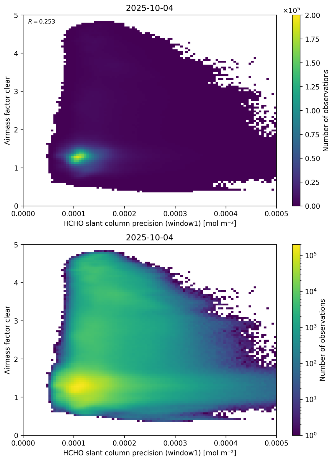
Figure 91: Scatter density plot of “HCHO slant column precision (window1)” against “Airmass factor clear” for 2025-10-03 to 2025-10-05.
