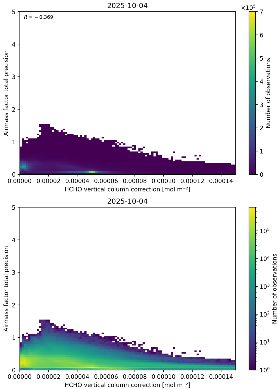
Figure 121: Scatter density plot of “HCHO vertical column correction” against “Airmass factor total precision” for 2025-10-03 to 2025-10-05.
