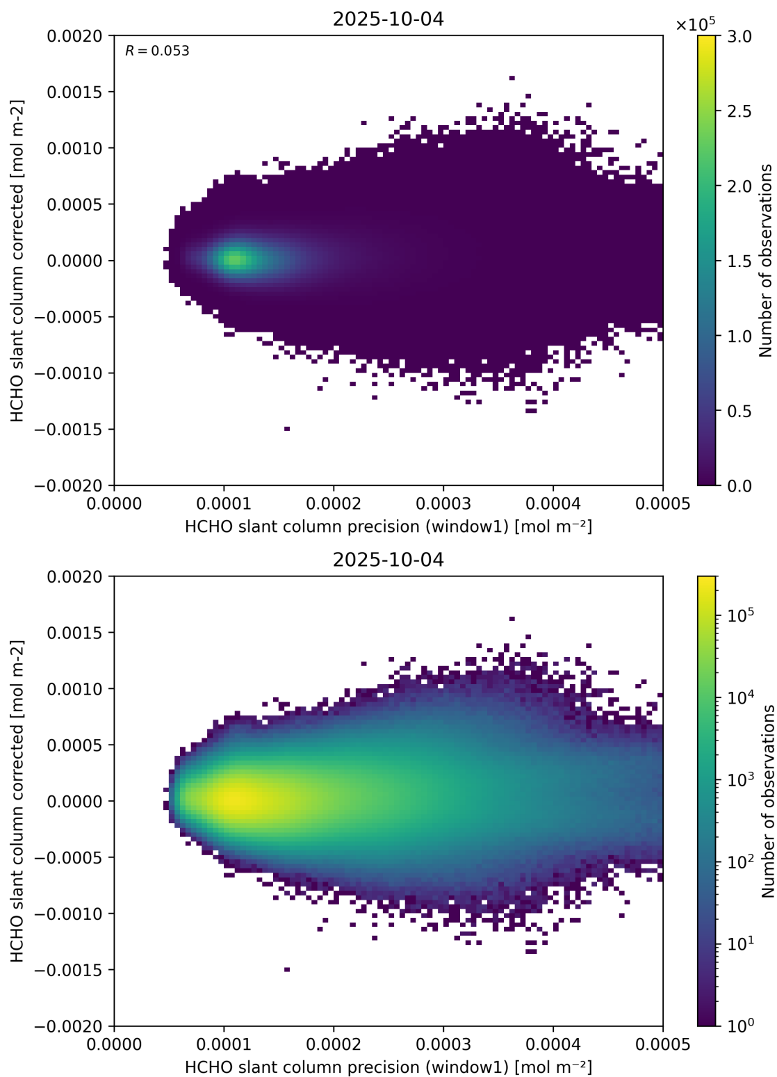
Figure 92: Scatter density plot of “HCHO slant column precision (window1)” against “HCHO slant column corrected” for 2025-10-03 to 2025-10-05.
