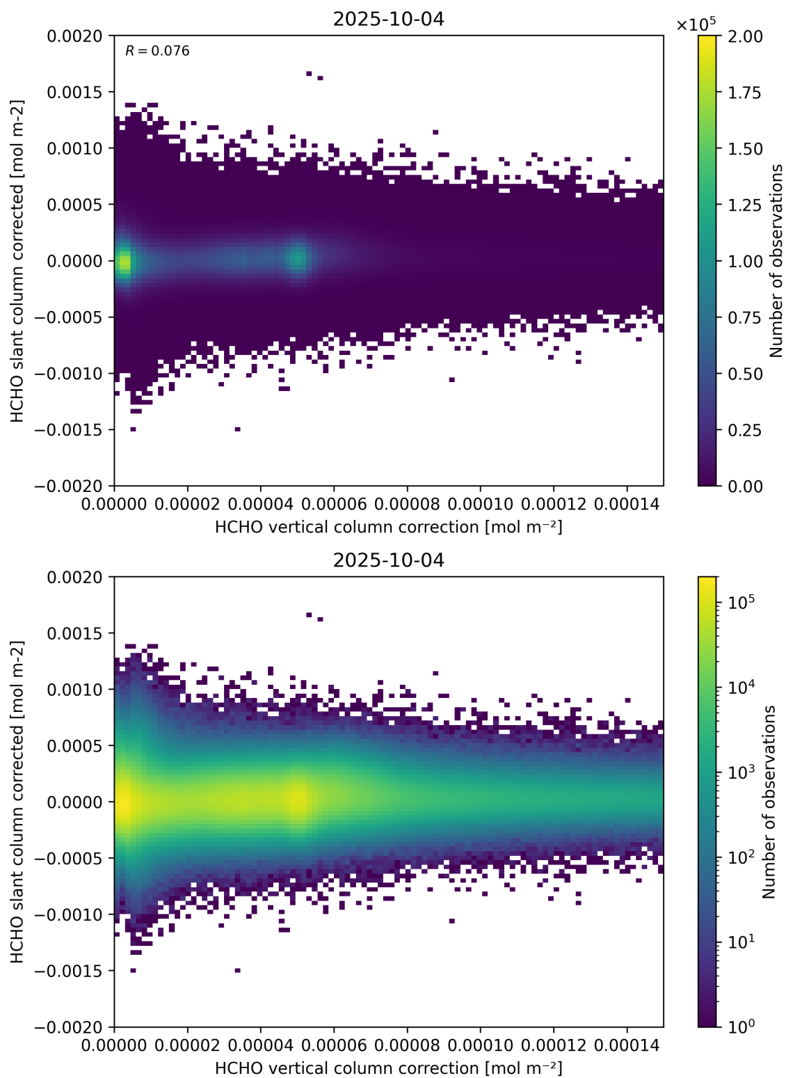
Figure 116: Scatter density plot of “HCHO vertical column correction” against “HCHO slant column corrected” for 2025-10-03 to 2025-10-05.
