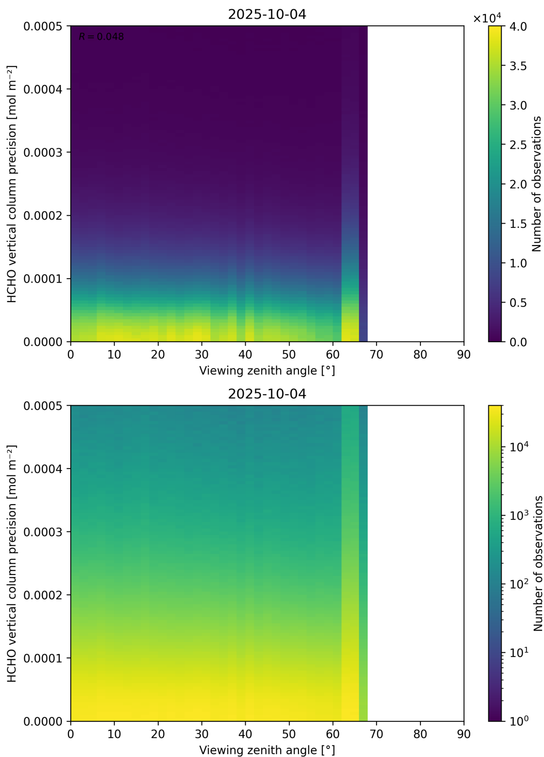
Figure 194: Scatter density plot of “Viewing zenith angle” against “HCHO vertical column precision” for 2025-10-03 to 2025-10-05.
