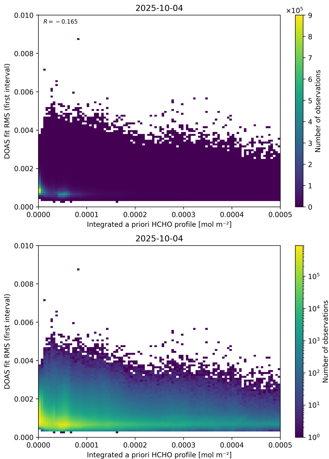
Figure 148: Scatter density plot of “Integrated a priori HCHO profile” against “DOAS fit RMS (first interval)” for 2025-10-03 to 2025-10-05.
