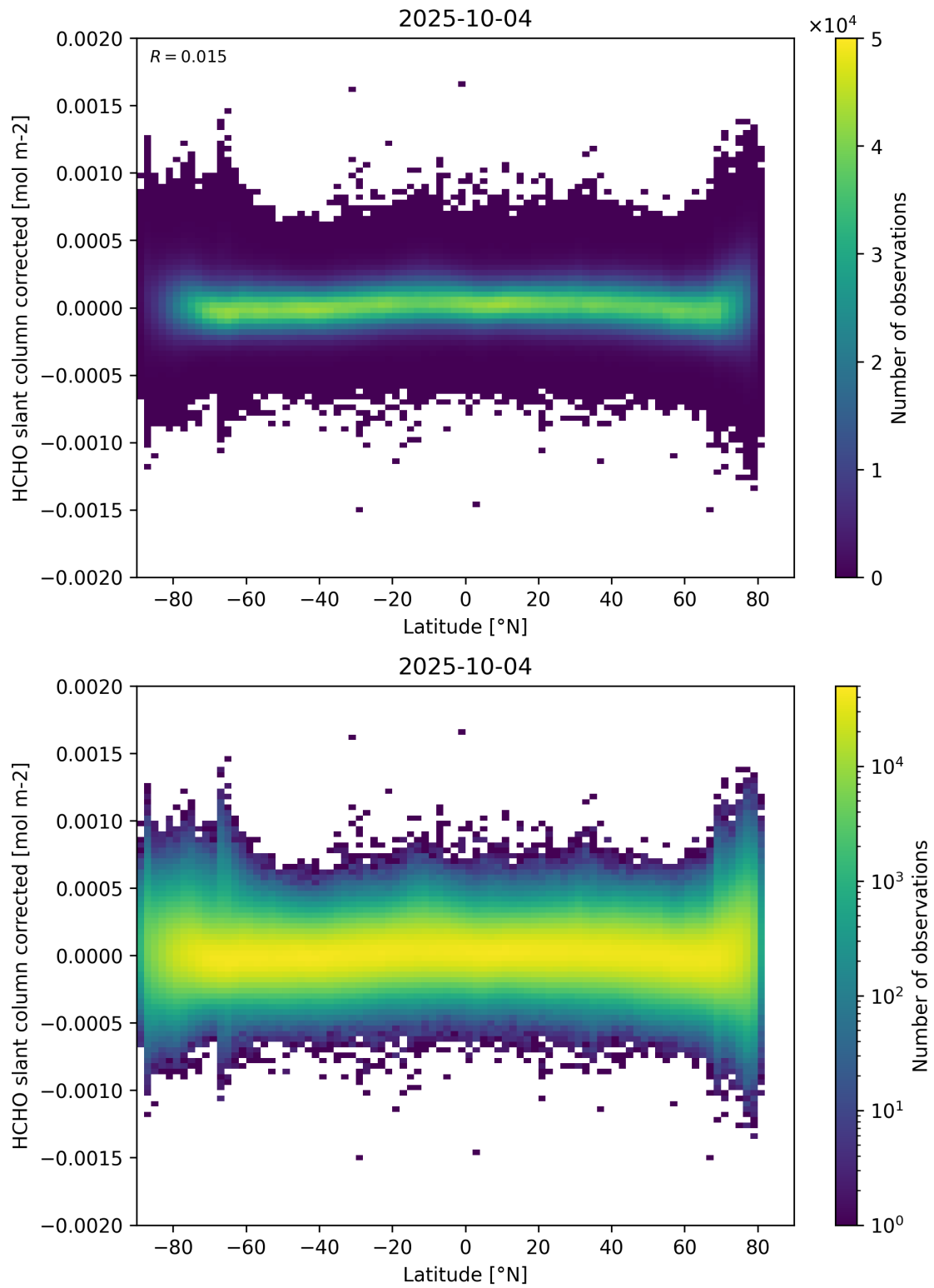
Figure 157: Scatter density plot of “Latitude” against “HCHO slant column corrected” for 2025-10-03 to 2025-10-05.
