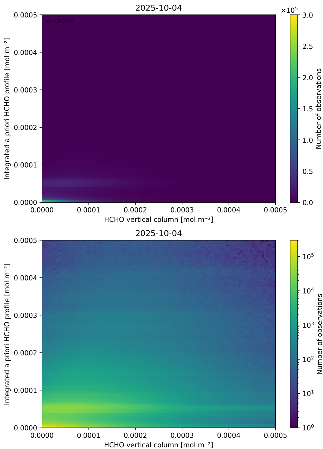
Figure 135: Scatter density plot of “HCHO vertical column” against “Integrated a priori HCHO profile” for 2025-10-03 to 2025-10-05.
