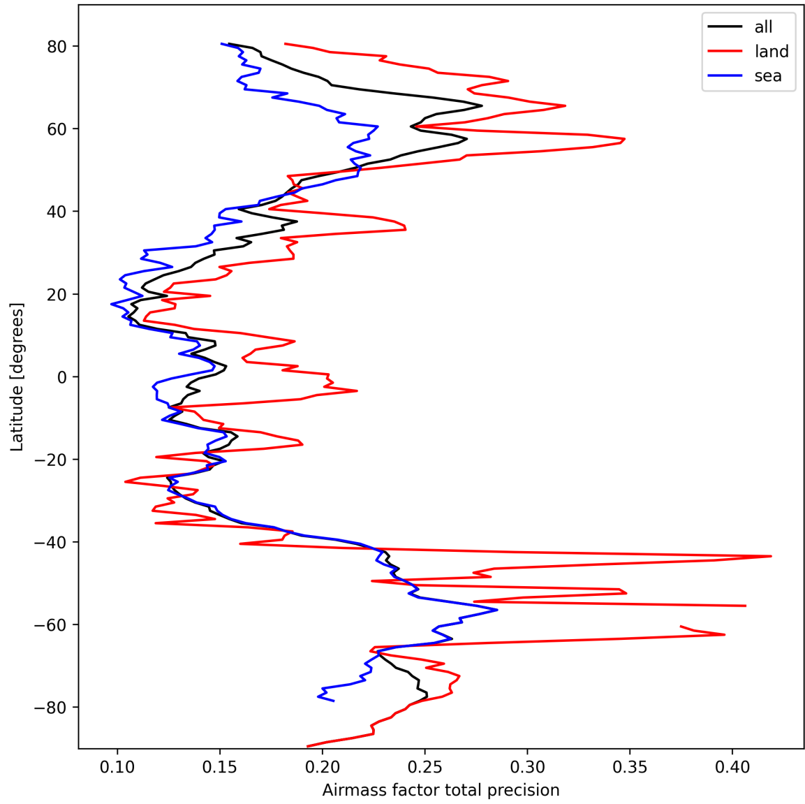
Figure 27: Zonal average of “Airmass factor total precision” for 2025-10-03 to 2025-10-05.
