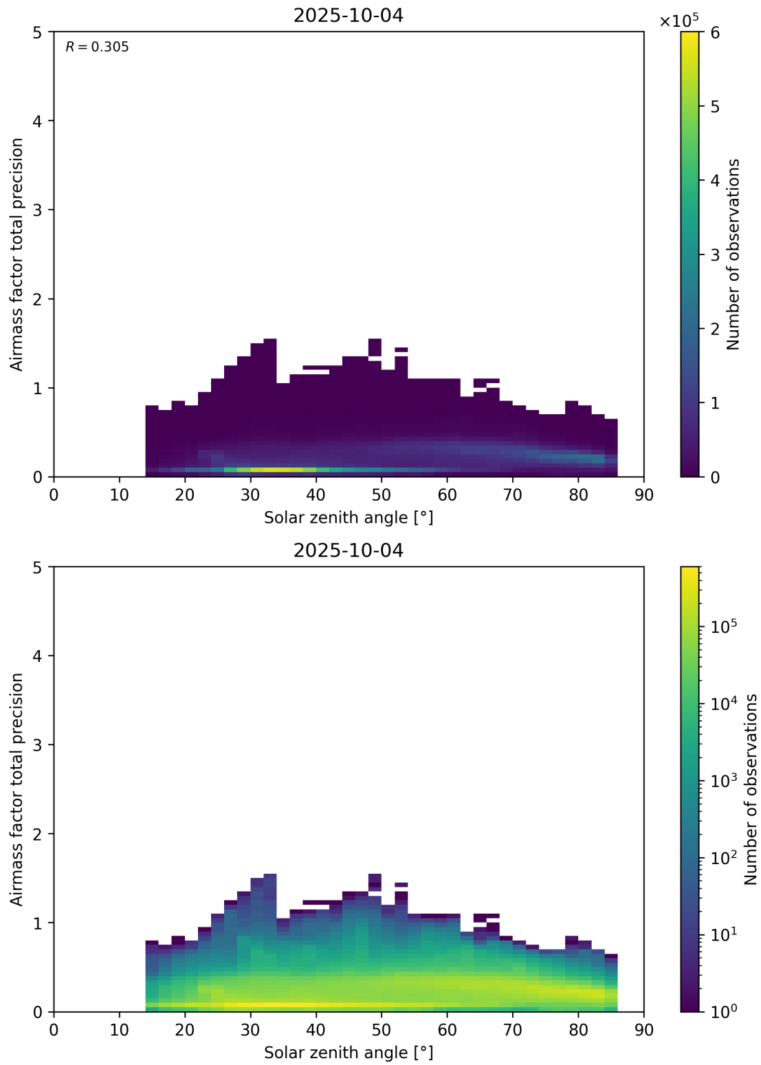
Figure 176: Scatter density plot of “Solar zenith angle” against “Airmass factor total precision” for 2025-10-03 to 2025-10-05.
