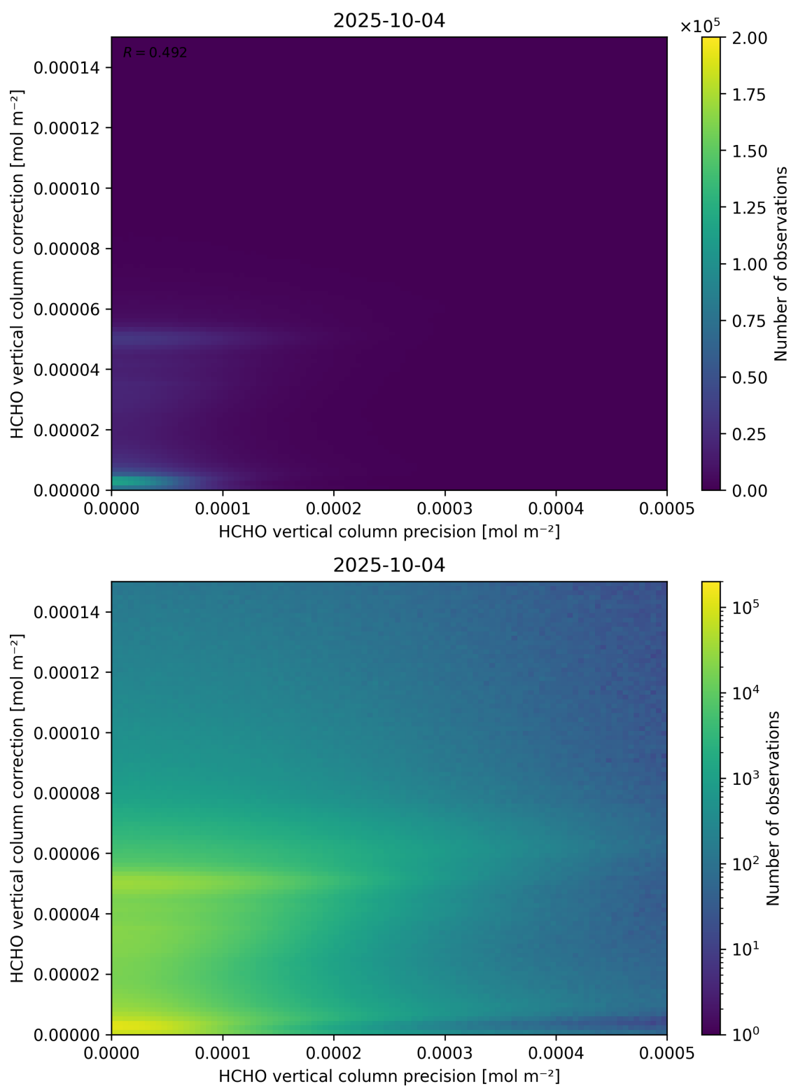
Figure 146: Scatter density plot of “HCHO vertical column precision” against “HCHO vertical column correction” for 2025-10-03 to 2025-10-05.
