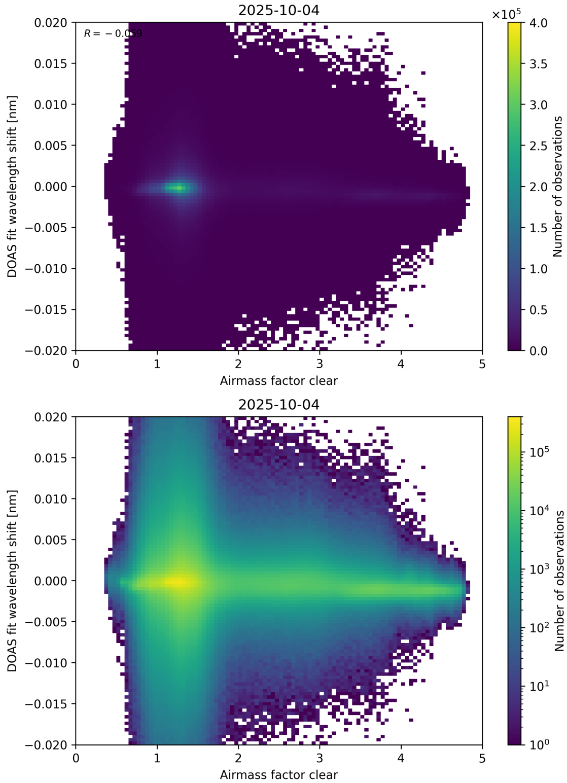
Figure 72: Scatter density plot of “Airmass factor clear” against “DOAS fit wavelength shift” for 2025-10-03 to 2025-10-05.
