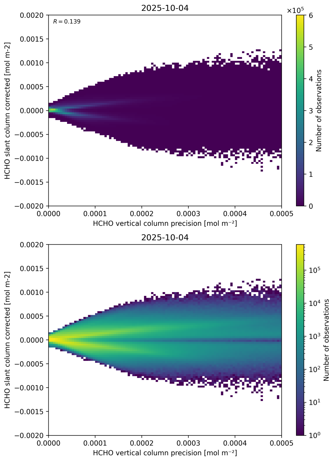
Figure 140: Scatter density plot of “HCHO vertical column precision” against “HCHO slant column corrected” for 2025-10-03 to 2025-10-05.
