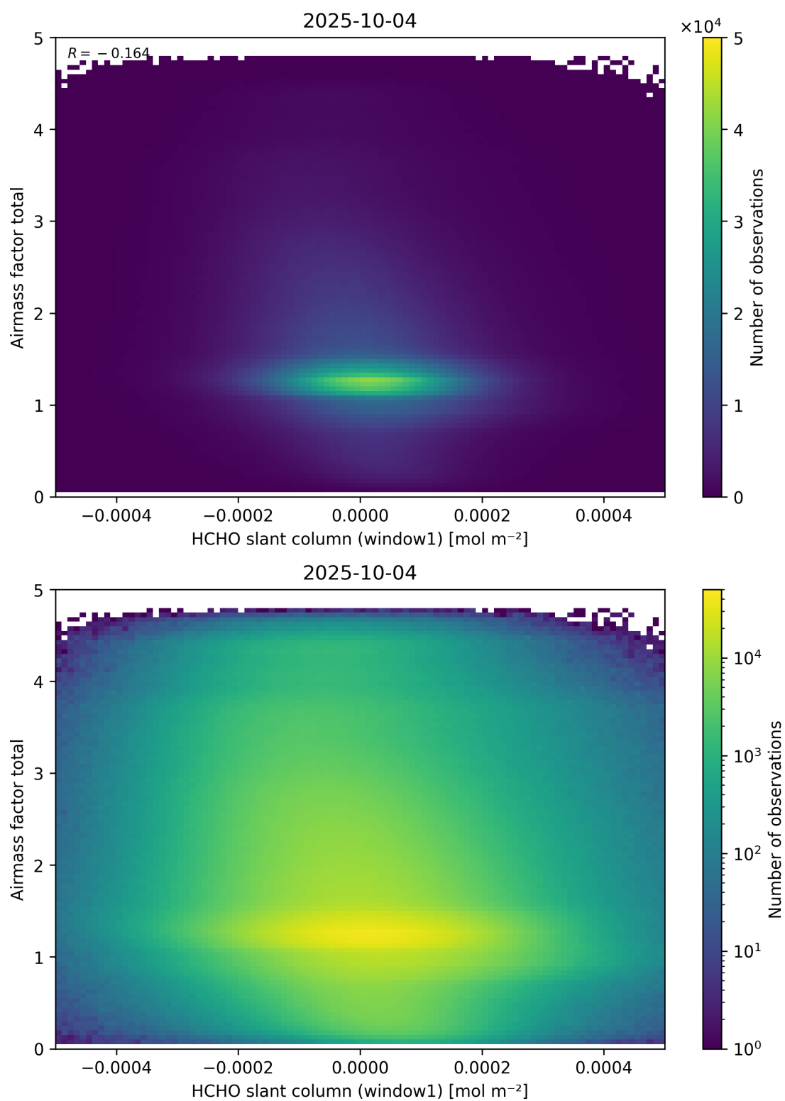
Figure 85: Scatter density plot of “HCHO slant column (window1)” against “Airmass factor total” for 2025-10-03 to 2025-10-05.
