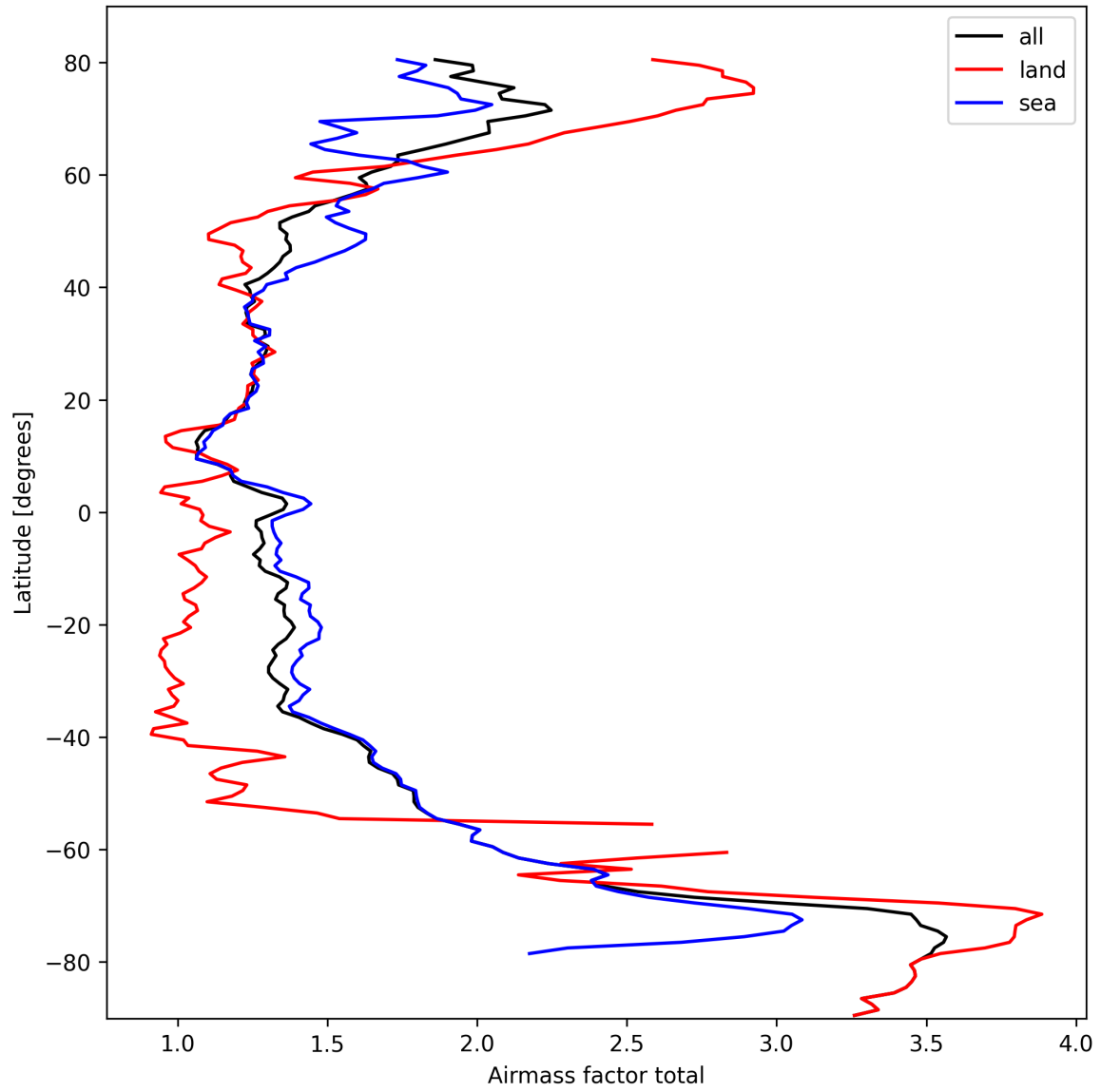
Figure 26: Zonal average of “Airmass factor total” for 2025-10-03 to 2025-10-05.
