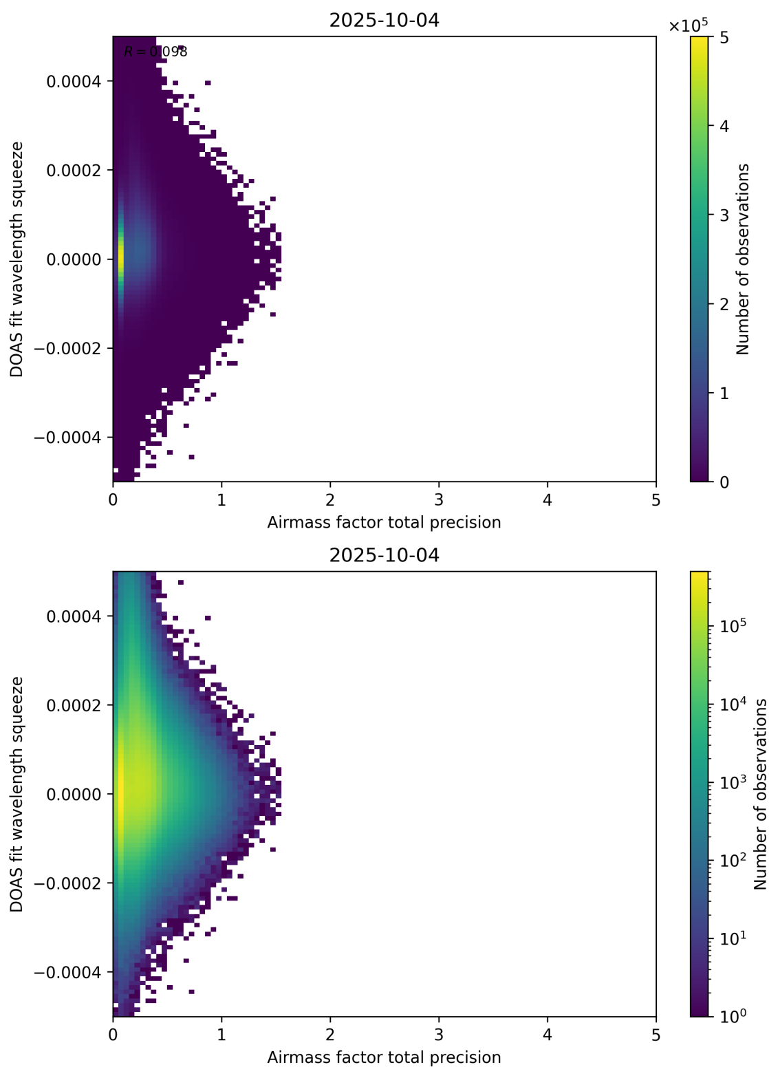
Figure 107: Scatter density plot of “Airmass factor total precision” against “DOAS fit wavelength squeeze” for 2025-10-03 to 2025-10-05.
