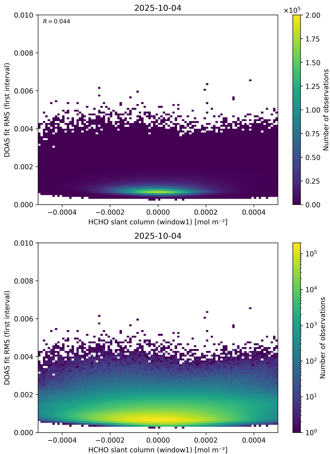
Figure 78: Scatter density plot of “HCHO slant column (window1)” against “DOAS fit RMS (first interval)” for 2025-10-03 to 2025-10-05.
