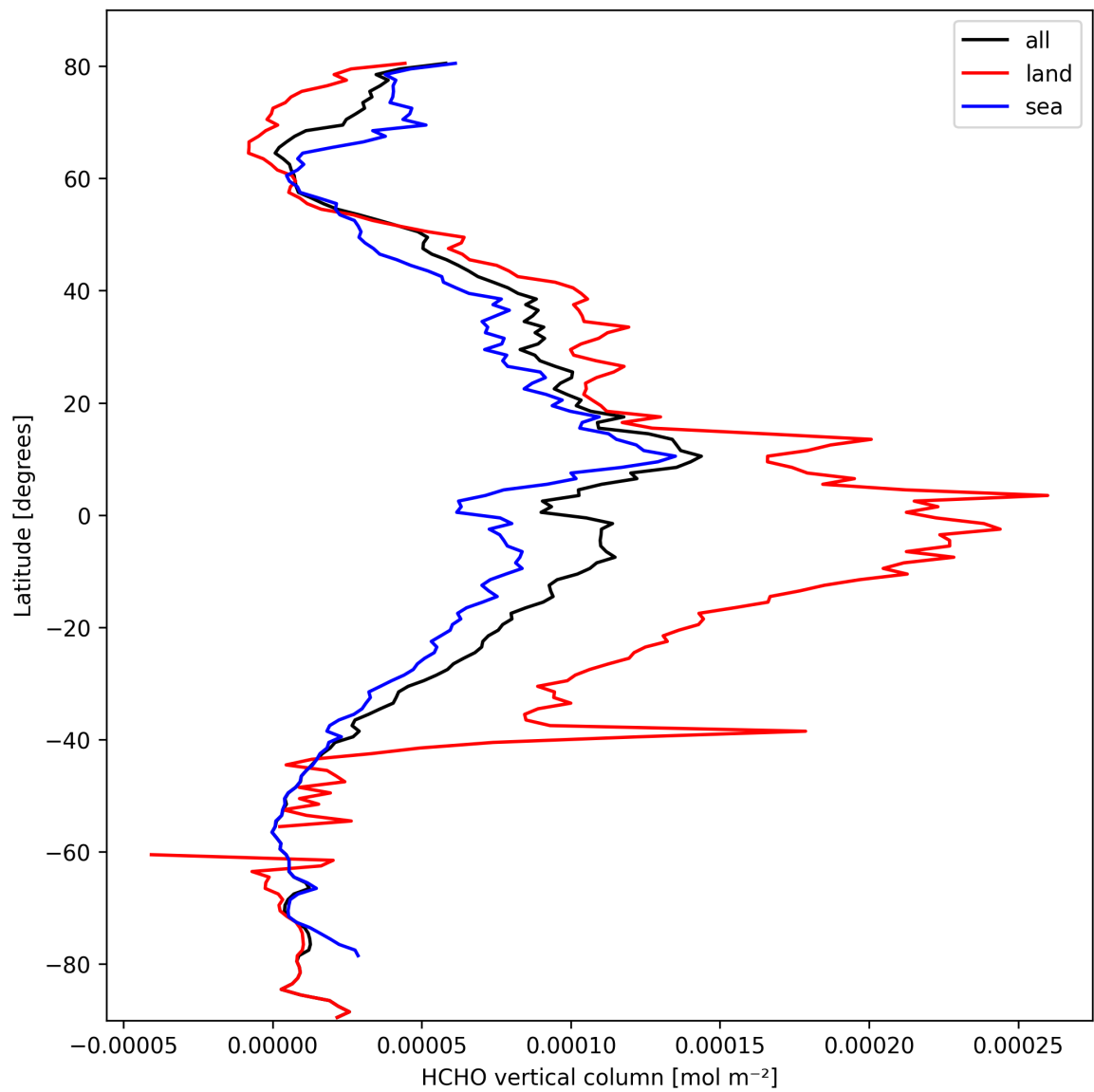
Figure 21: Zonal average of “HCHO vertical column” for 2025-10-03 to 2025-10-05.
