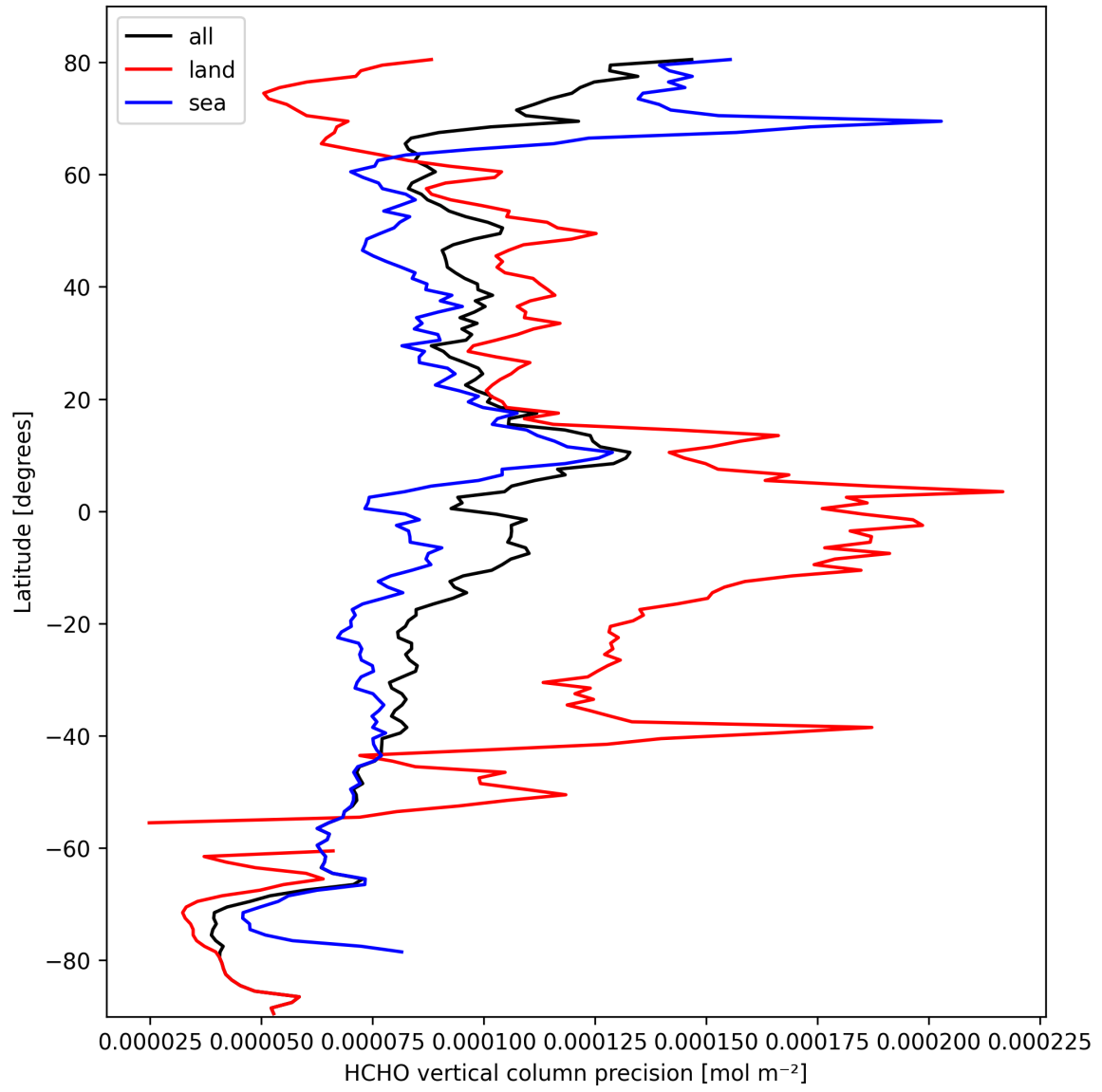
Figure 22: Zonal average of “HCHO vertical column precision” for 2025-10-03 to 2025-10-05.
