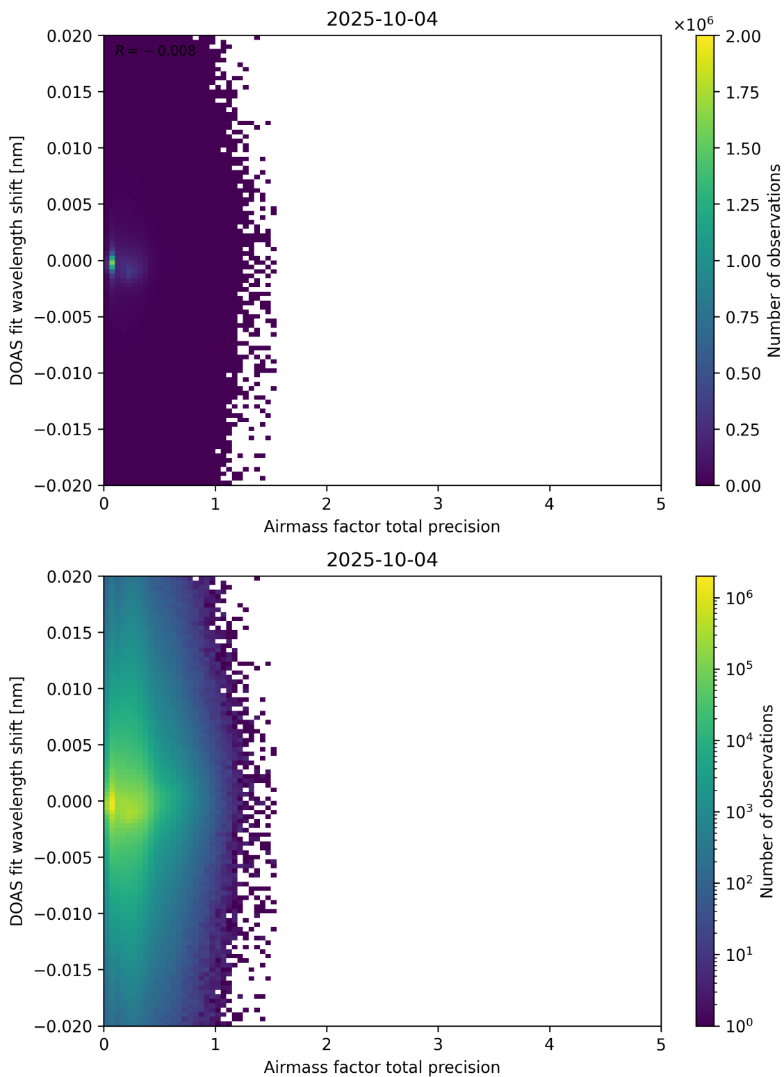
Figure 106: Scatter density plot of “Airmass factor total precision” against “DOAS fit wavelength shift” for 2025-10-03 to 2025-10-05.
