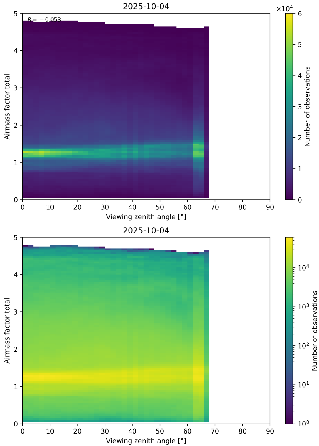
Figure 190: Scatter density plot of “Viewing zenith angle” against “Airmass factor total” for 2025-10-03 to 2025-10-05.
