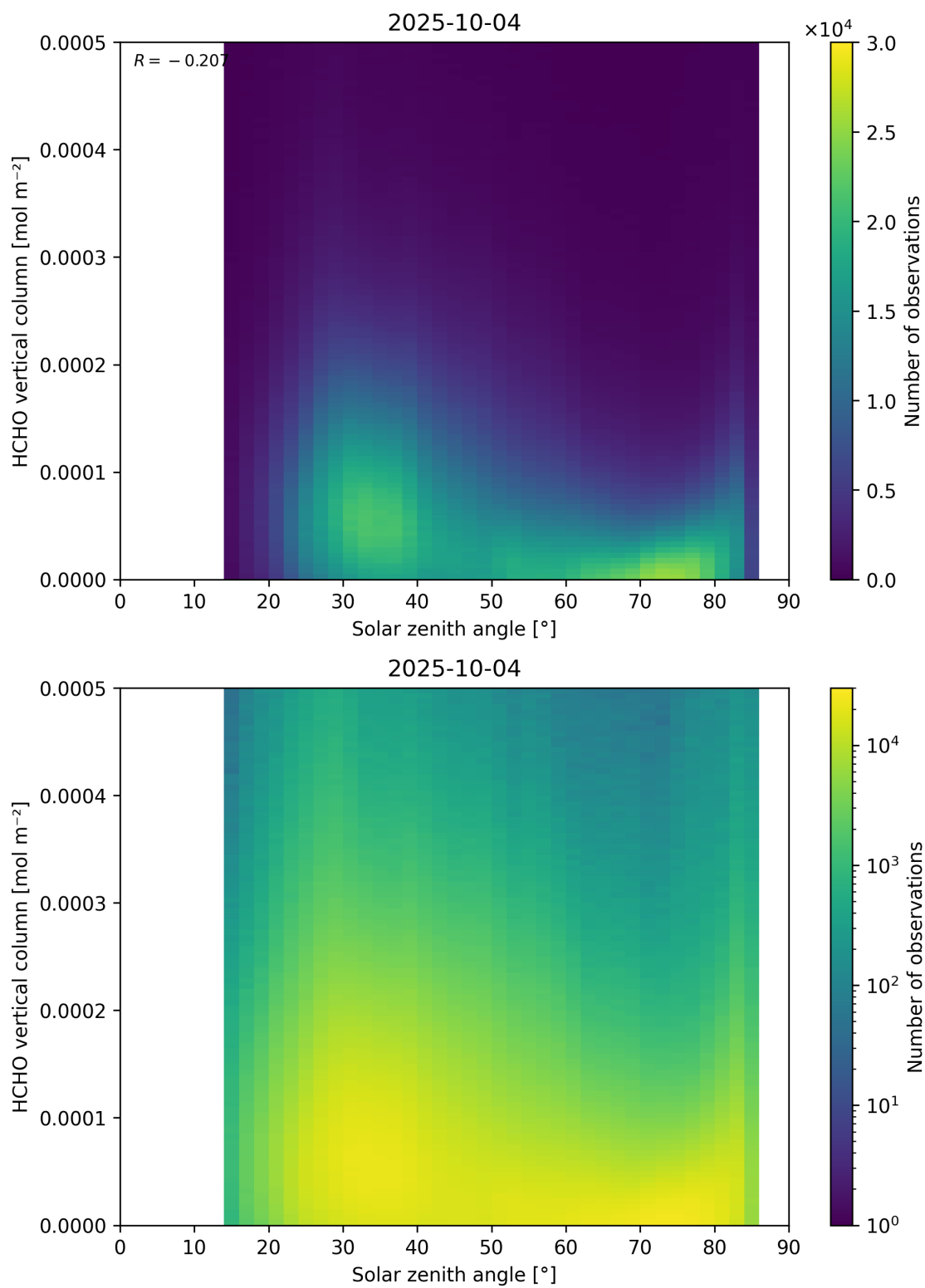
Figure 177: Scatter density plot of “Solar zenith angle” against “HCHO vertical column” for 2025-10-03 to 2025-10-05.
