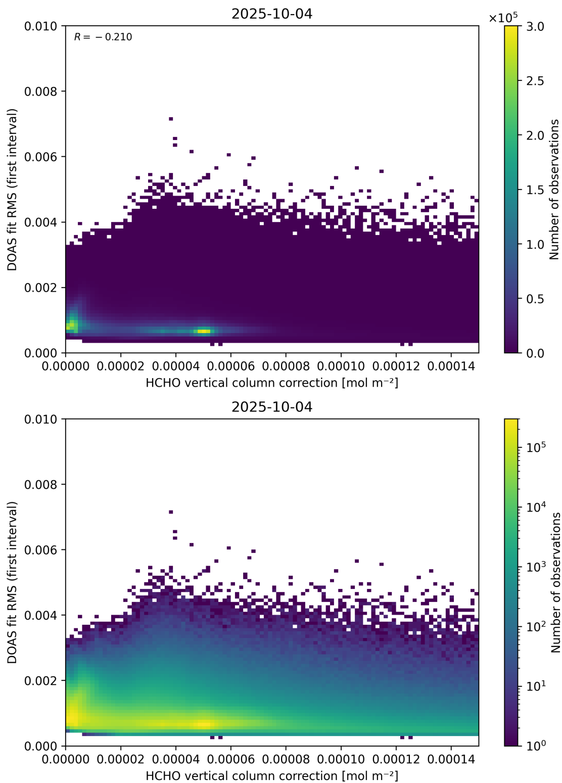
Figure 112: Scatter density plot of “HCHO vertical column correction” against “DOAS fit RMS (first interval)” for 2025-10-03 to 2025-10-05.
