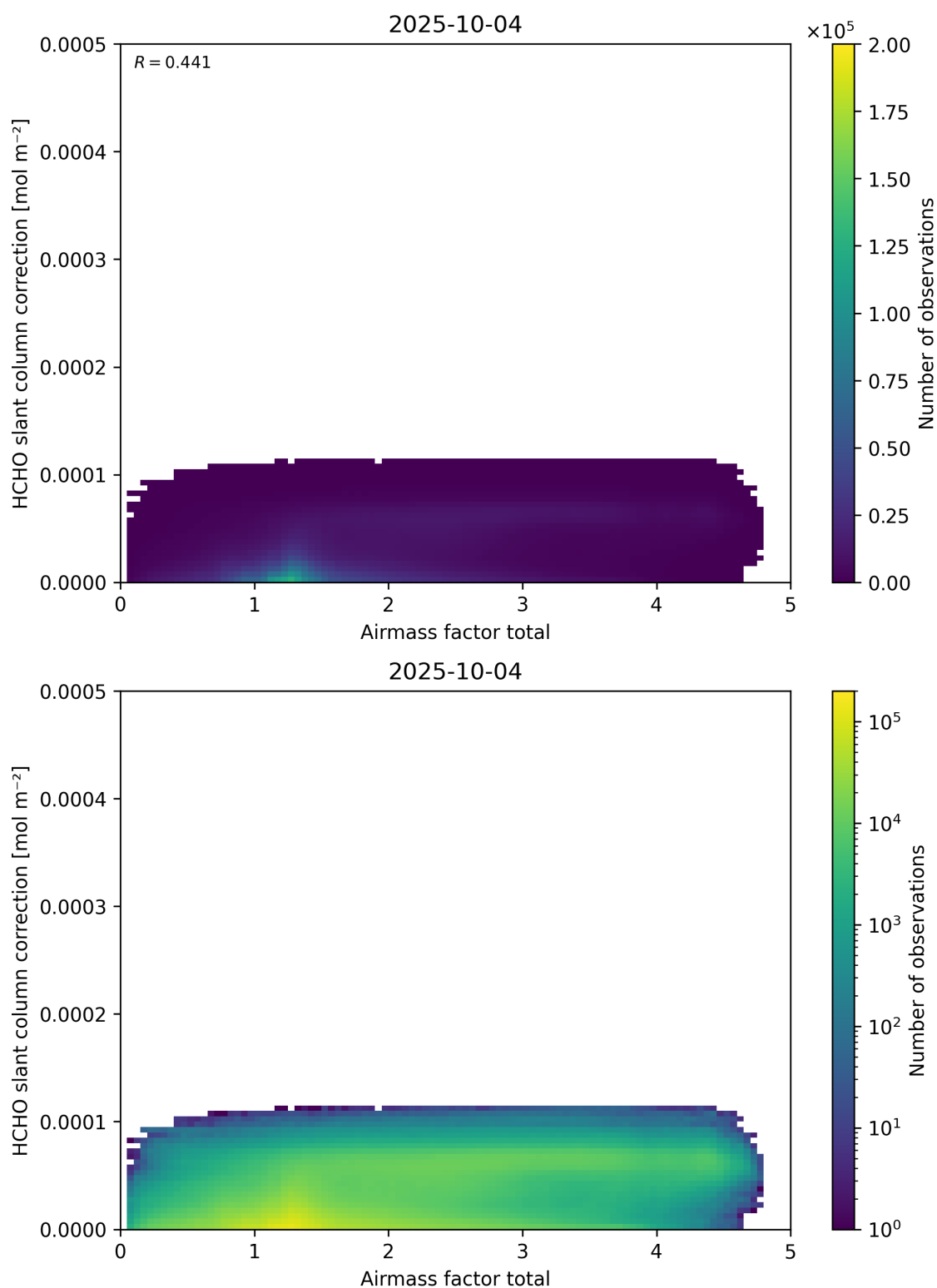
Figure 102: Scatter density plot of “Airmass factor total” against “HCHO slant column correction” for 2025-10-03 to 2025-10-05.
