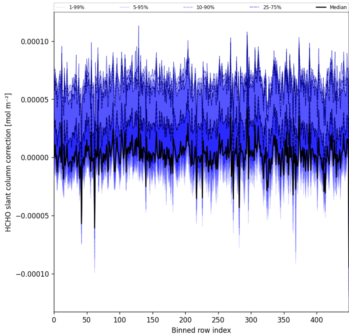
Figure 61: Along track statistics of "HCHO slant column correction" for 2025-10-03 to 2025-10-05
