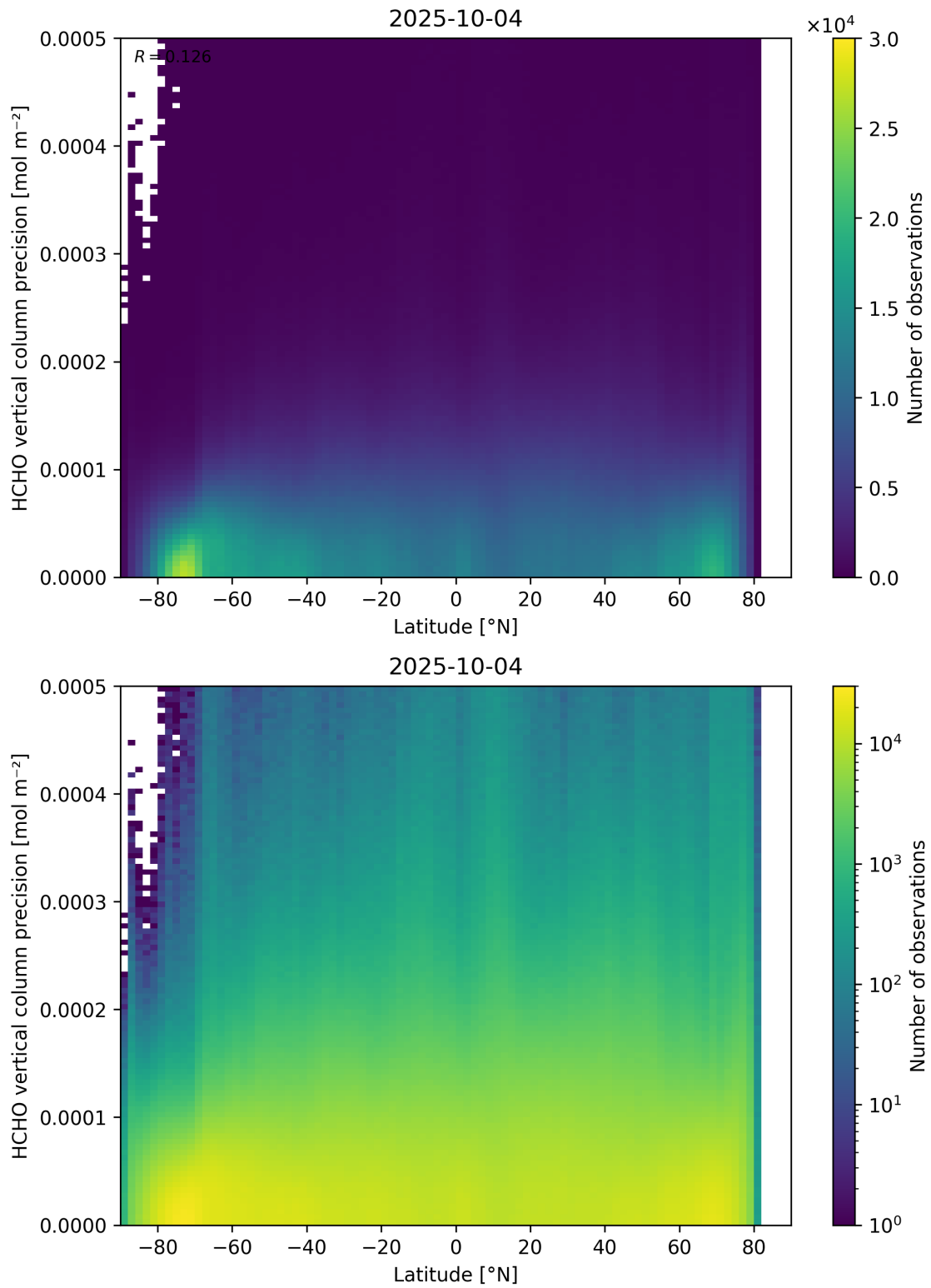
Figure 165: Scatter density plot of “Latitude” against “HCHO vertical column precision” for 2025-10-03 to 2025-10-05.
