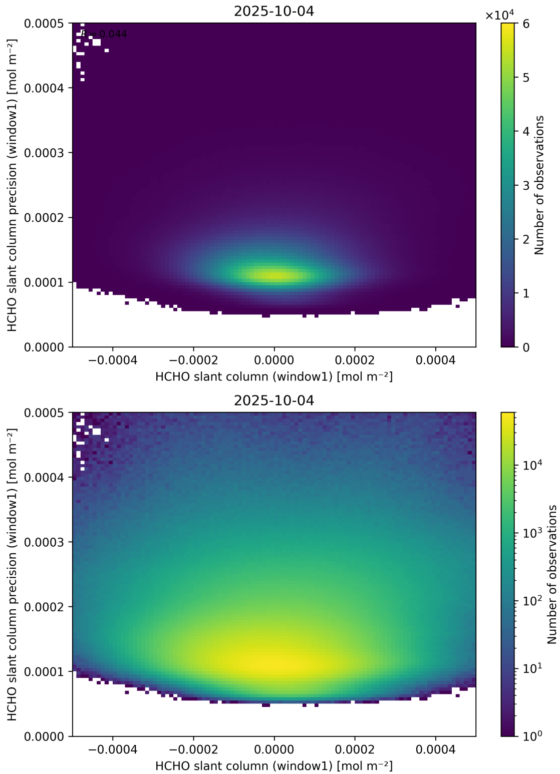
Figure 84: Scatter density plot of “HCHO slant column (window1)” against “HCHO slant column precision (window1)” for 2025-10-03 to 2025-10-05.
