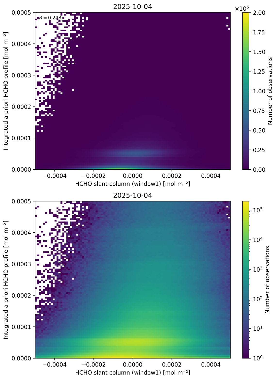
Figure 87: Scatter density plot of “HCHO slant column (window1)” against “Integrated a priori HCHO profile” for 2025-10-03 to 2025-10-05.
