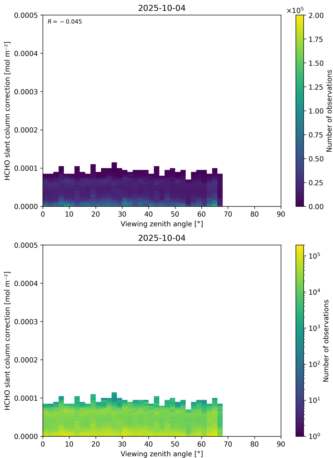
Figure 187: Scatter density plot of “Viewing zenith angle” against “HCHO slant column correction” for 2025-10-03 to 2025-10-05.
