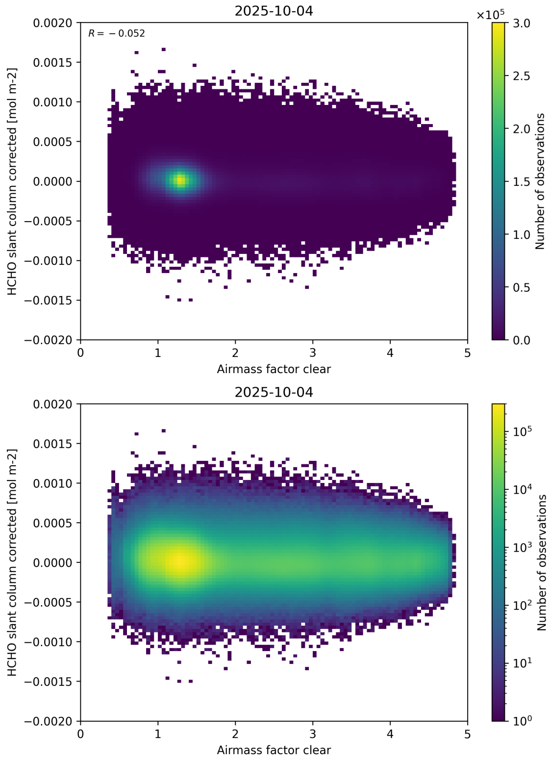
Figure 74: Scatter density plot of “Airmass factor clear” against “HCHO slant column corrected” for 2025-10-03 to 2025-10-05.
