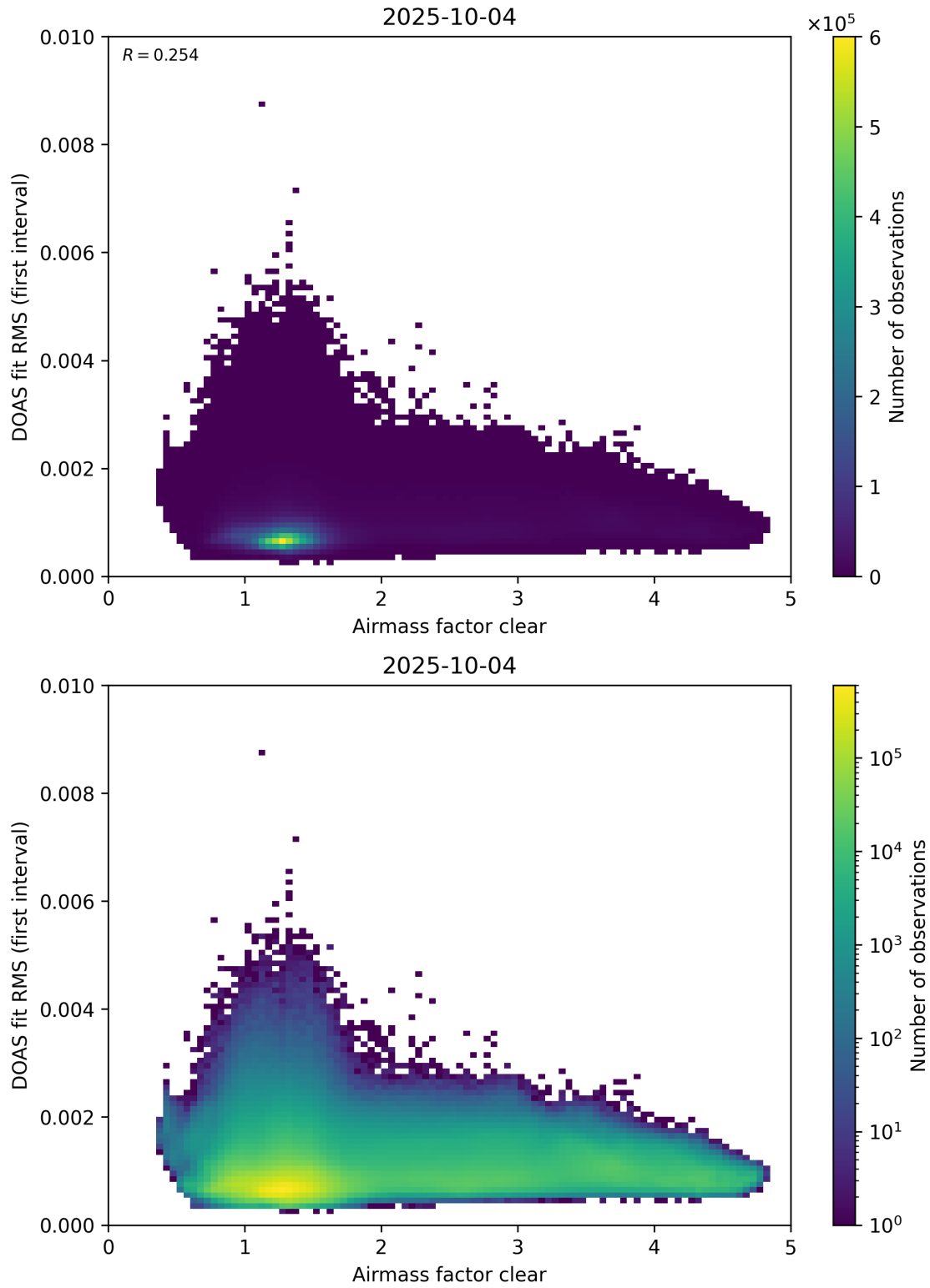
Figure 71: Scatter density plot of “Airmass factor clear” against “DOAS fit RMS (first interval)” for 2025-10-03 to 2025-10-05.
