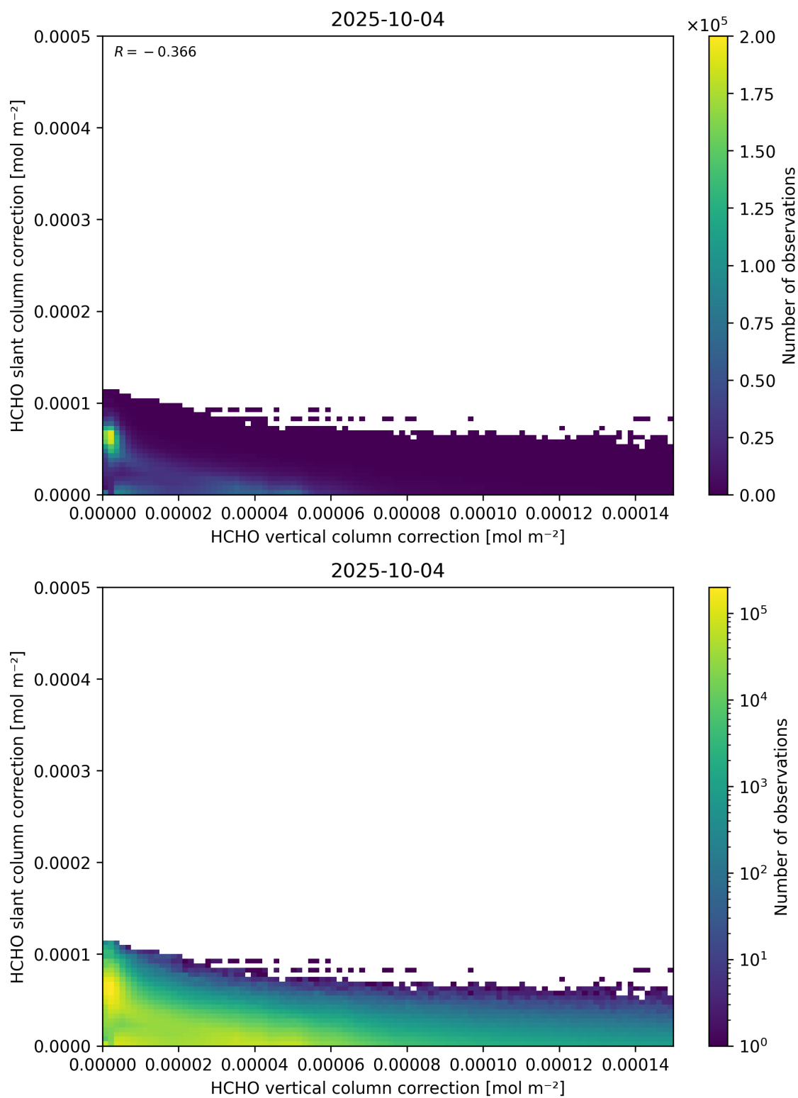
Figure 117: Scatter density plot of “HCHO vertical column correction” against “HCHO slant column correction” for 2025-10-03 to 2025-10-05.
