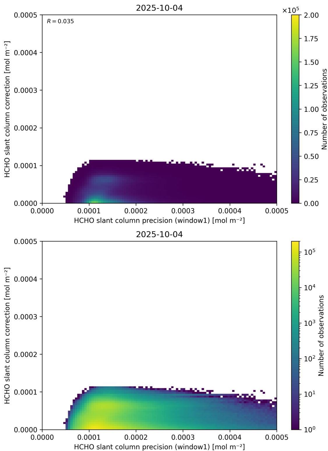
Figure 93: Scatter density plot of “HCHO slant column precision (window1)” against “HCHO slant column correction” for 2025-10-03 to 2025-10-05.
