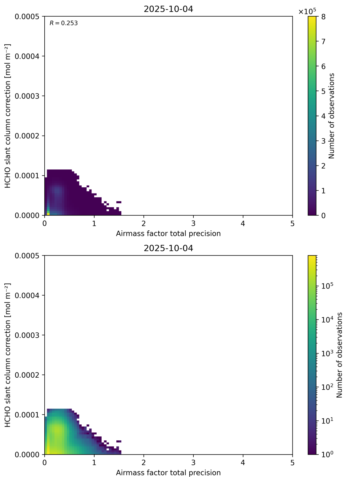
Figure 110: Scatter density plot of “Airmass factor total precision” against “HCHO slant column correction” for 2025-10-03 to 2025-10-05.
