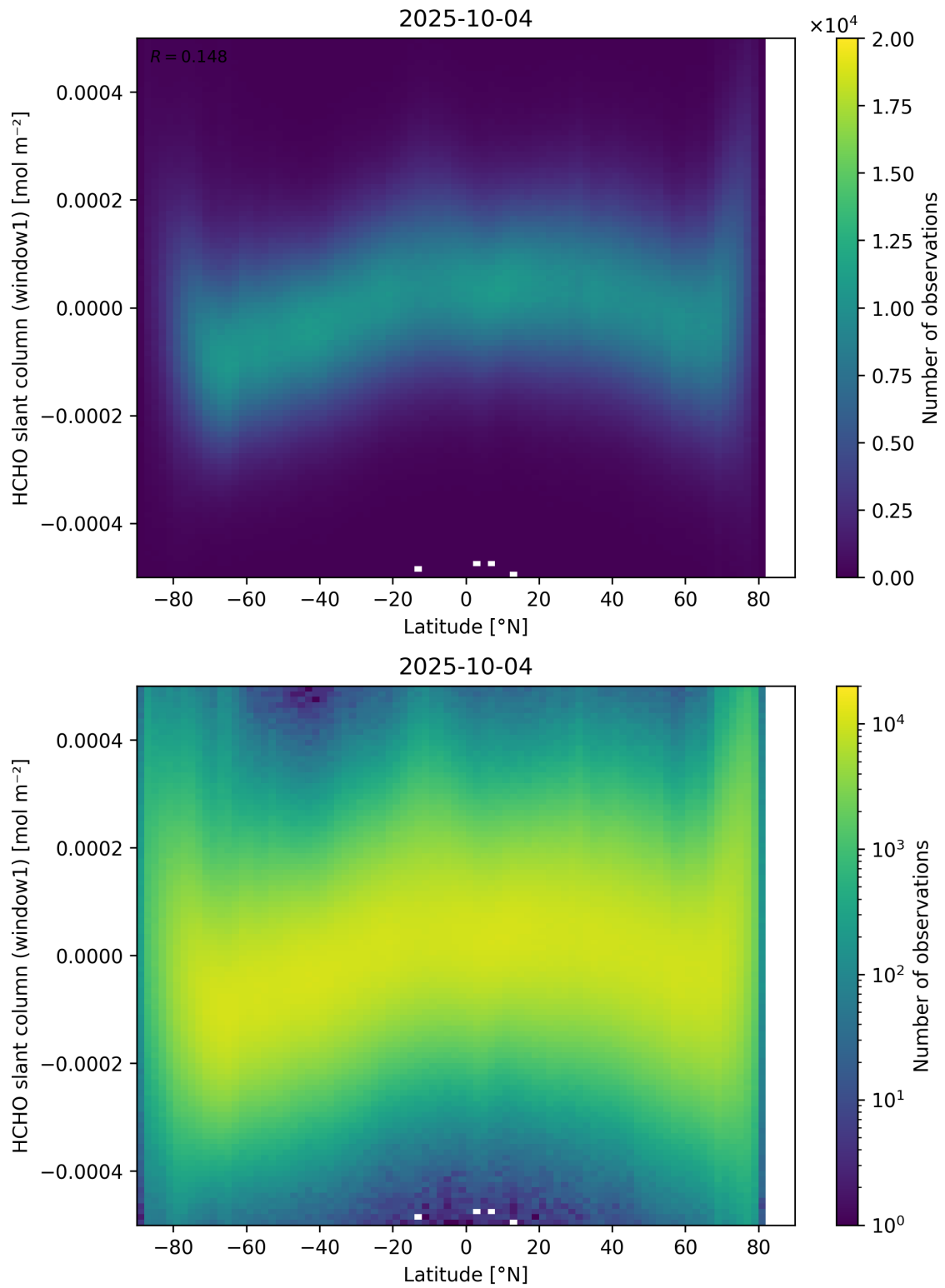
Figure 159: Scatter density plot of “Latitude” against “HCHO slant column (window1)” for 2025-10-03 to 2025-10-05.
