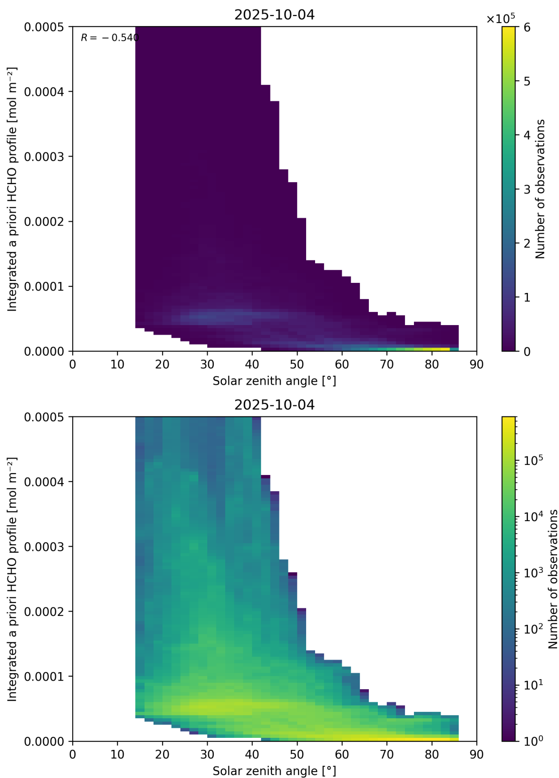
Figure 180: Scatter density plot of “Solar zenith angle” against “Integrated a priori HCHO profile” for 2025-10-03 to 2025-10-05.
