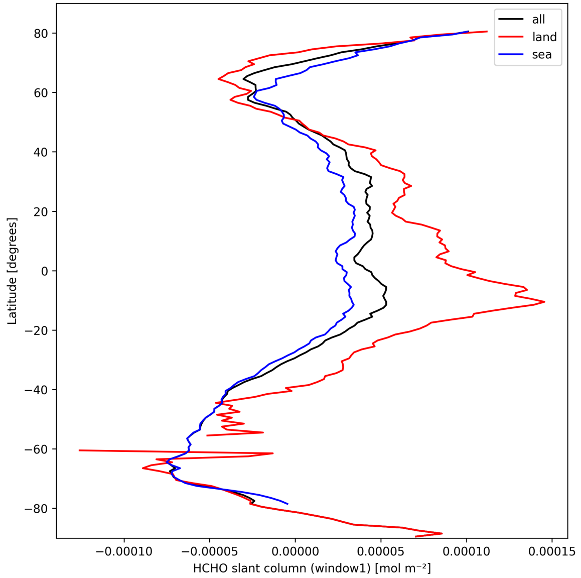
Figure 24: Zonal average of “HCHO slant column (window1)” for 2025-10-03 to 2025-10-05.
