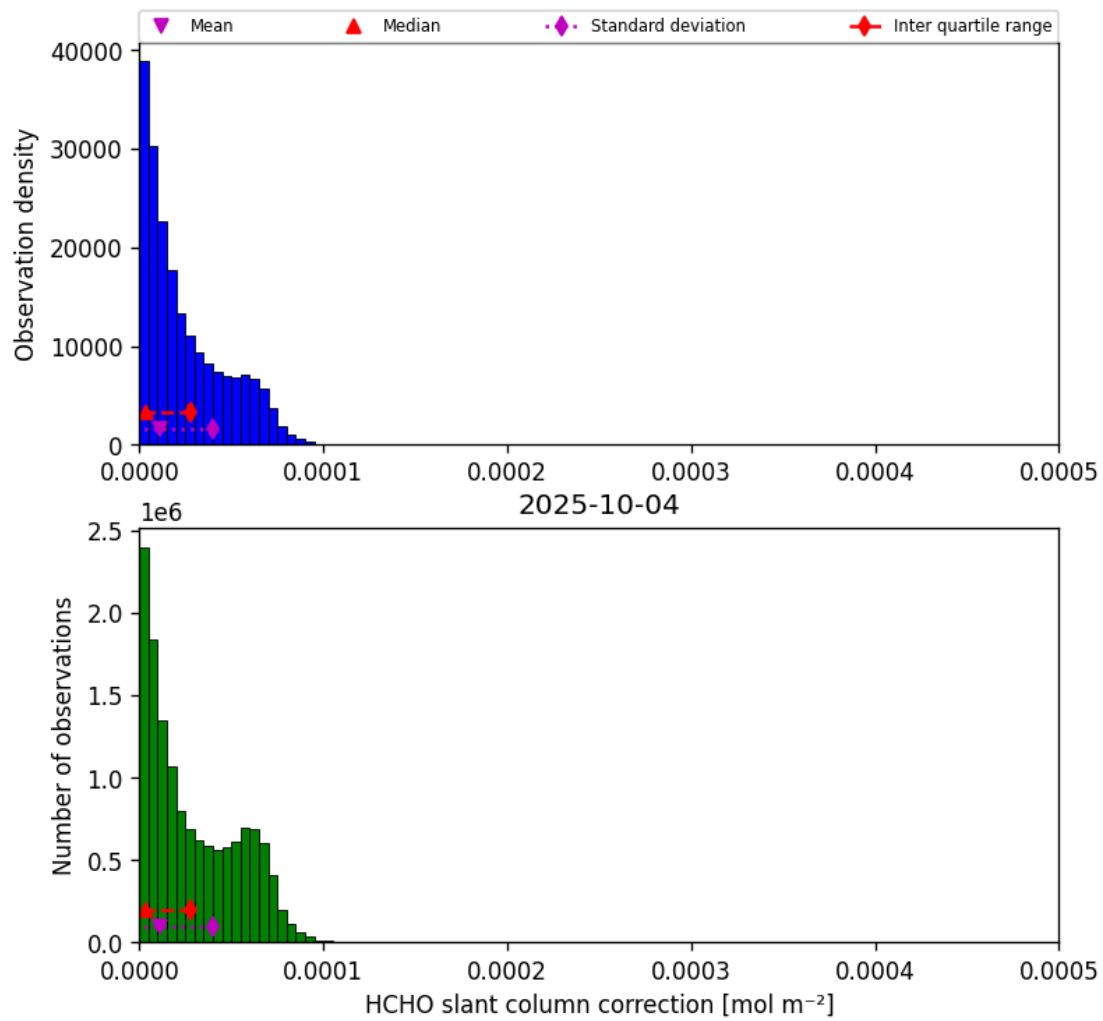
Figure 47: Histogram of “HCHO slant column correction” for 2025-10-03 to 2025-10-05
