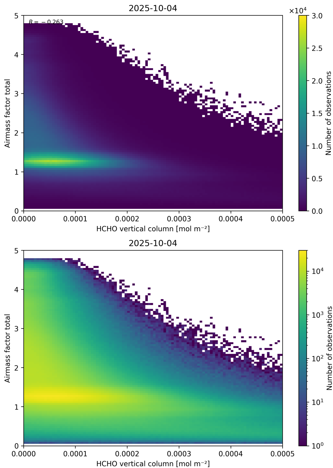
Figure 131: Scatter density plot of “HCHO vertical column” against “Airmass factor total” for 2025-10-03 to 2025-10-05.
