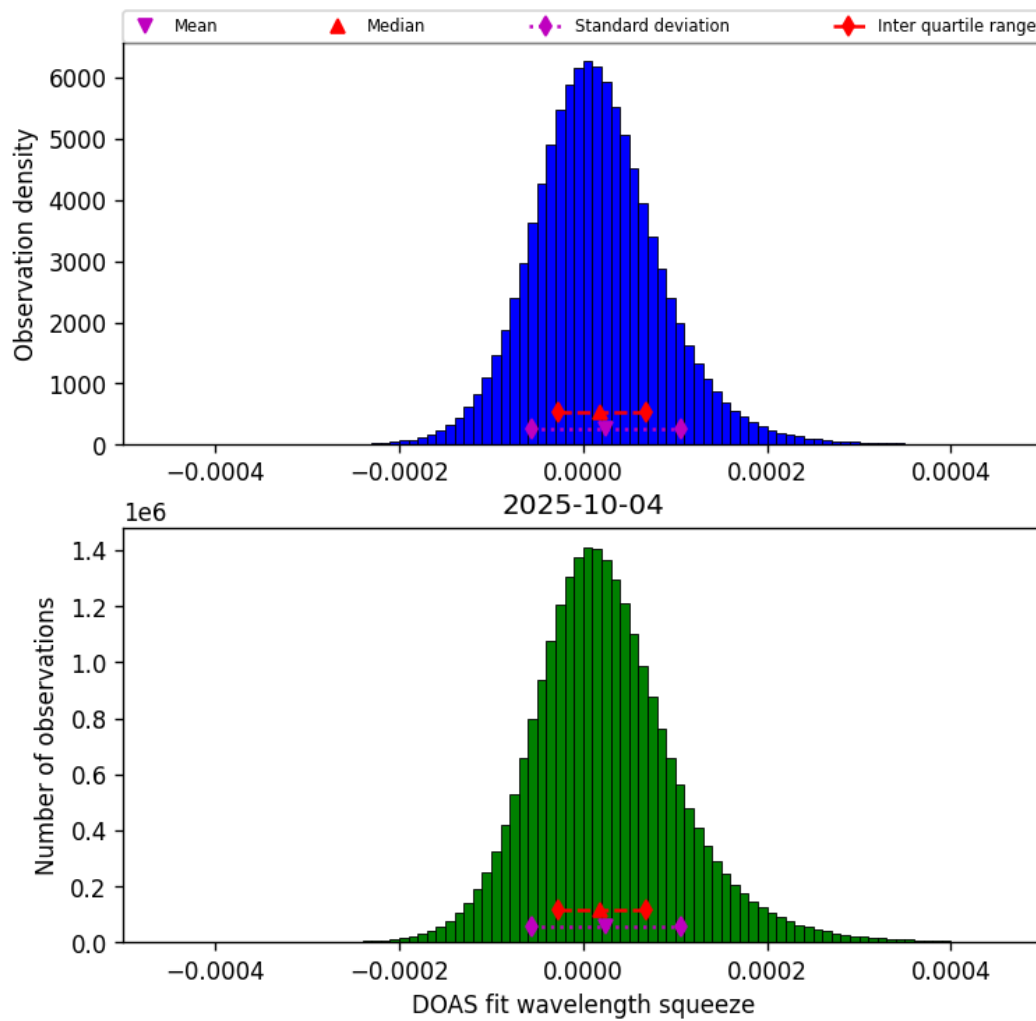
Figure 45: Histogram of “DOAS fit wavelength squeeze” for 2025-10-03 to 2025-10-05
