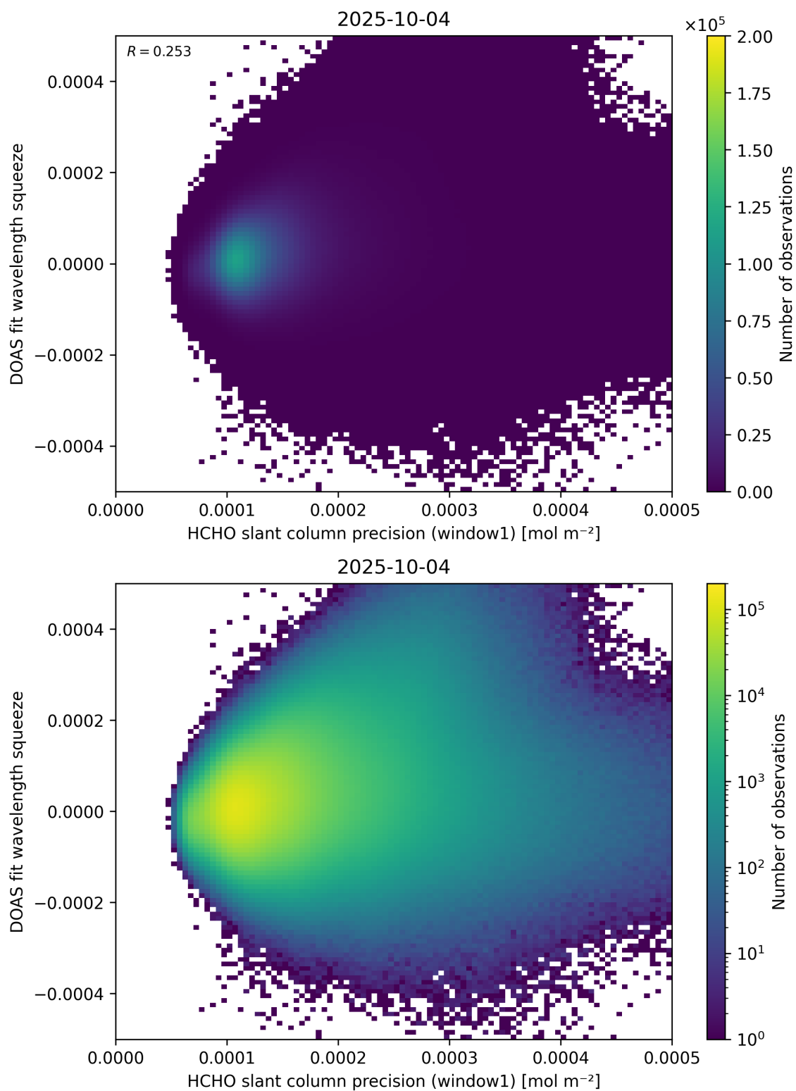
Figure 90: Scatter density plot of “HCHO slant column precision (window1)” against “DOAS fit wavelength squeeze” for 2025-10-03 to 2025-10-05.
