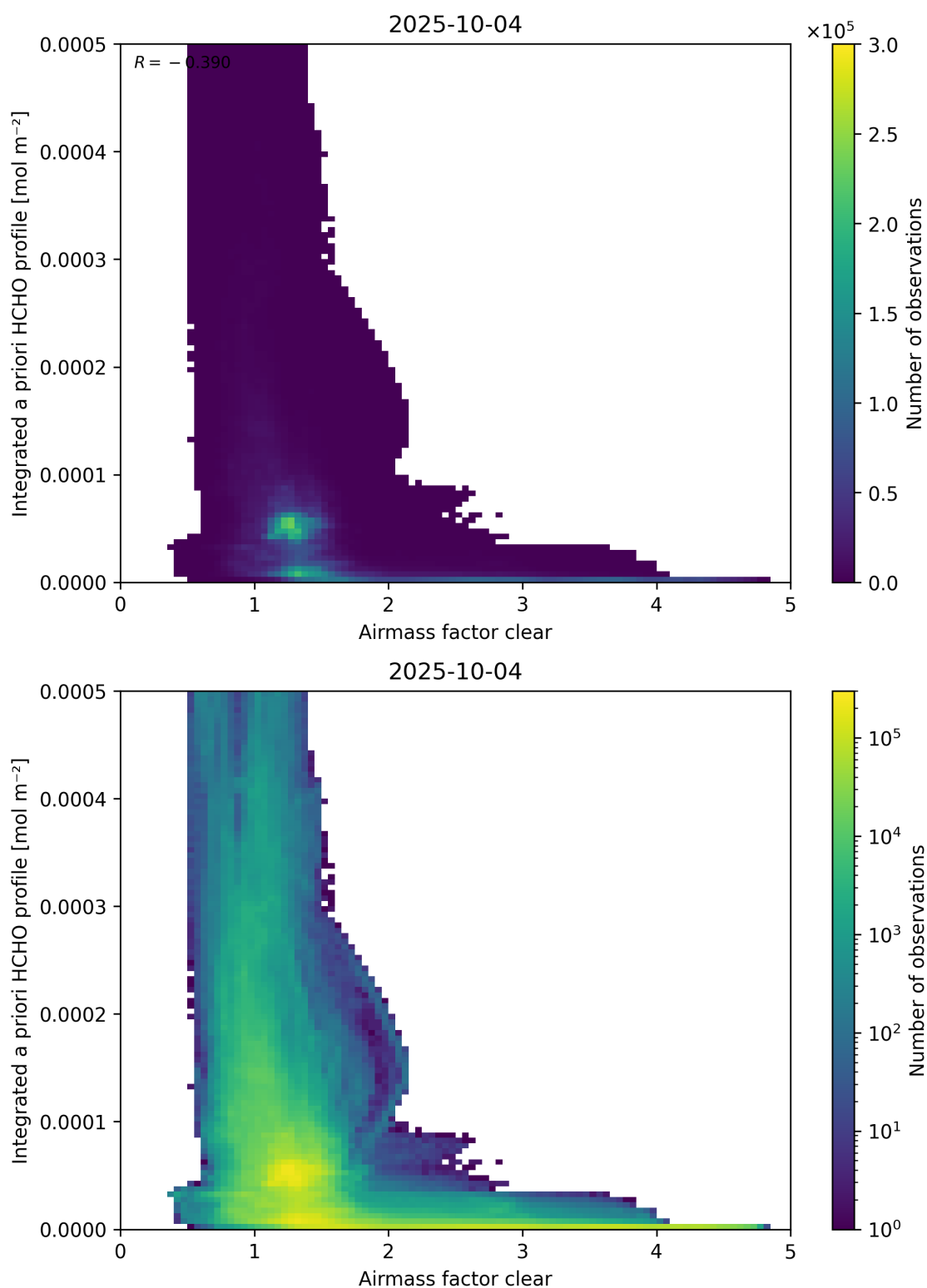
Figure 76: Scatter density plot of “Airmass factor clear” against “Integrated a priori HCHO profile” for 2025-10-03 to 2025-10-05.
