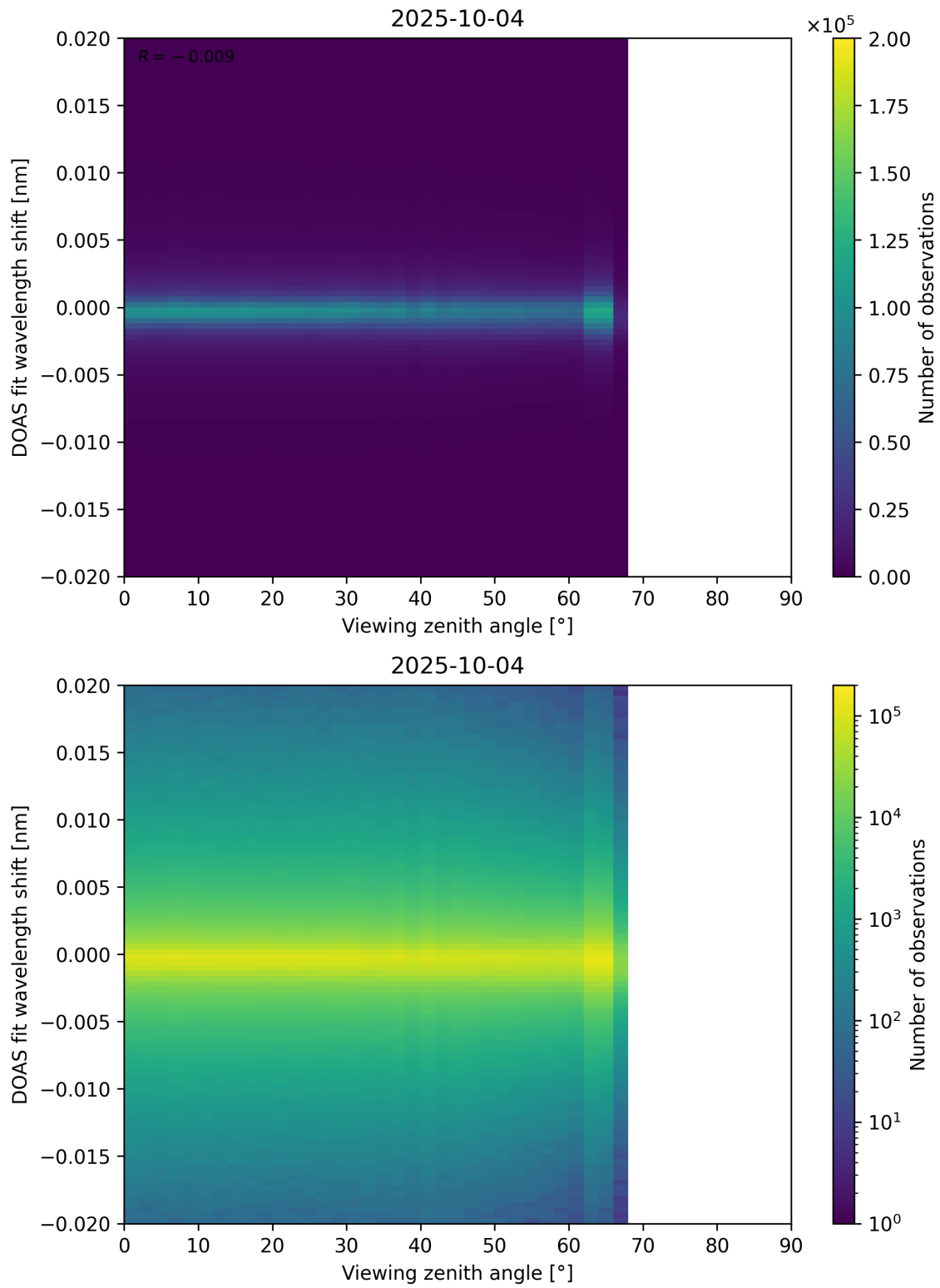
Figure 183: Scatter density plot of “Viewing zenith angle” against “DOAS fit wavelength shift” for 2025-10-03 to 2025-10-05.
