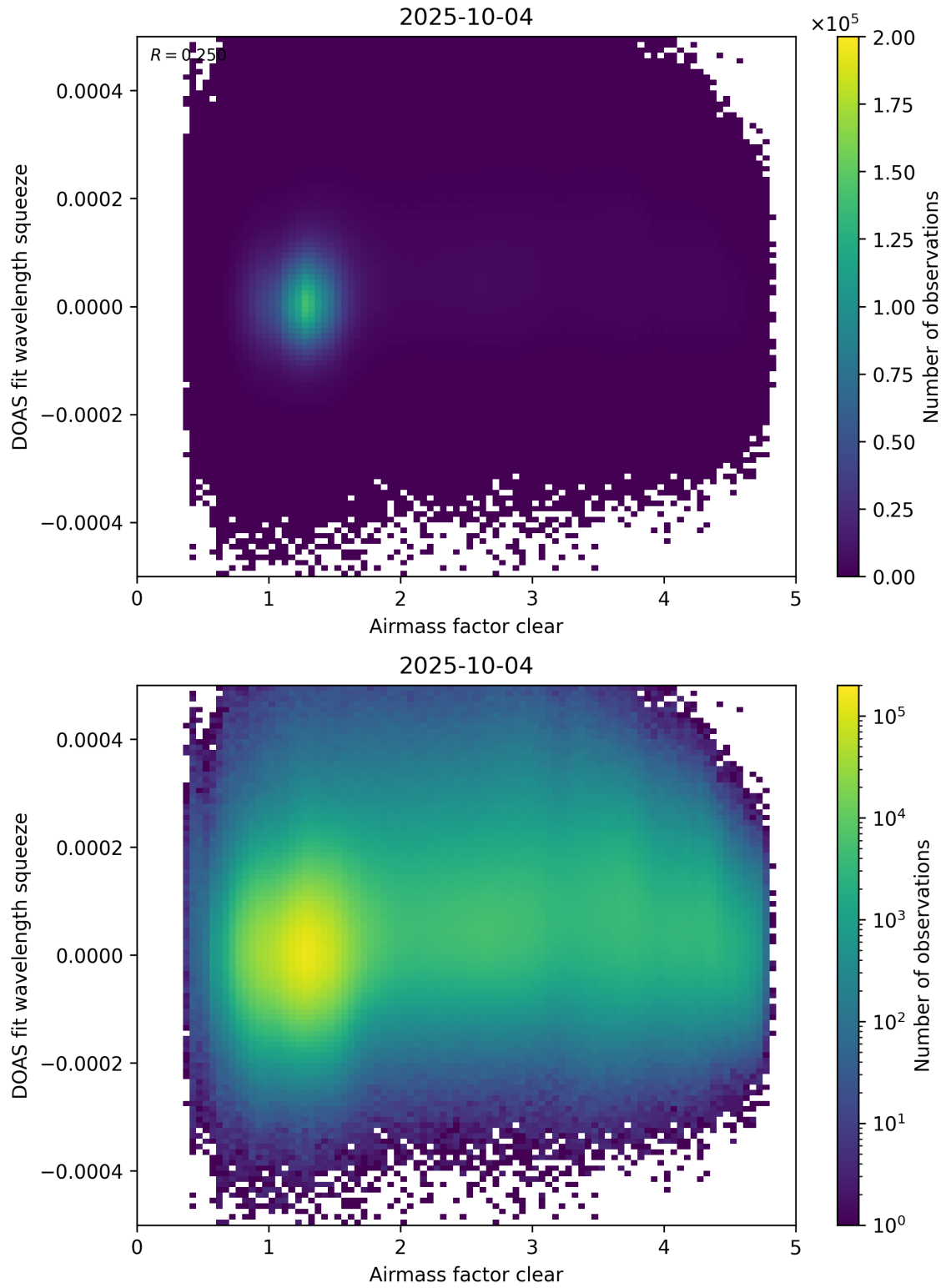
Figure 73: Scatter density plot of “Airmass factor clear” against “DOAS fit wavelength squeeze” for 2025-10-03 to 2025-10-05.
