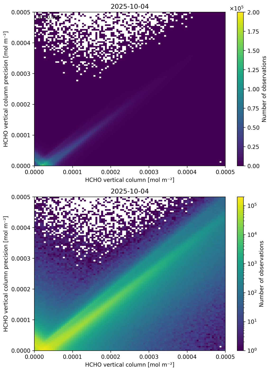
Figure 134: Scatter density plot of “HCHO vertical column” against “HCHO vertical column precision” for 2025-10-03 to 2025-10-05.
