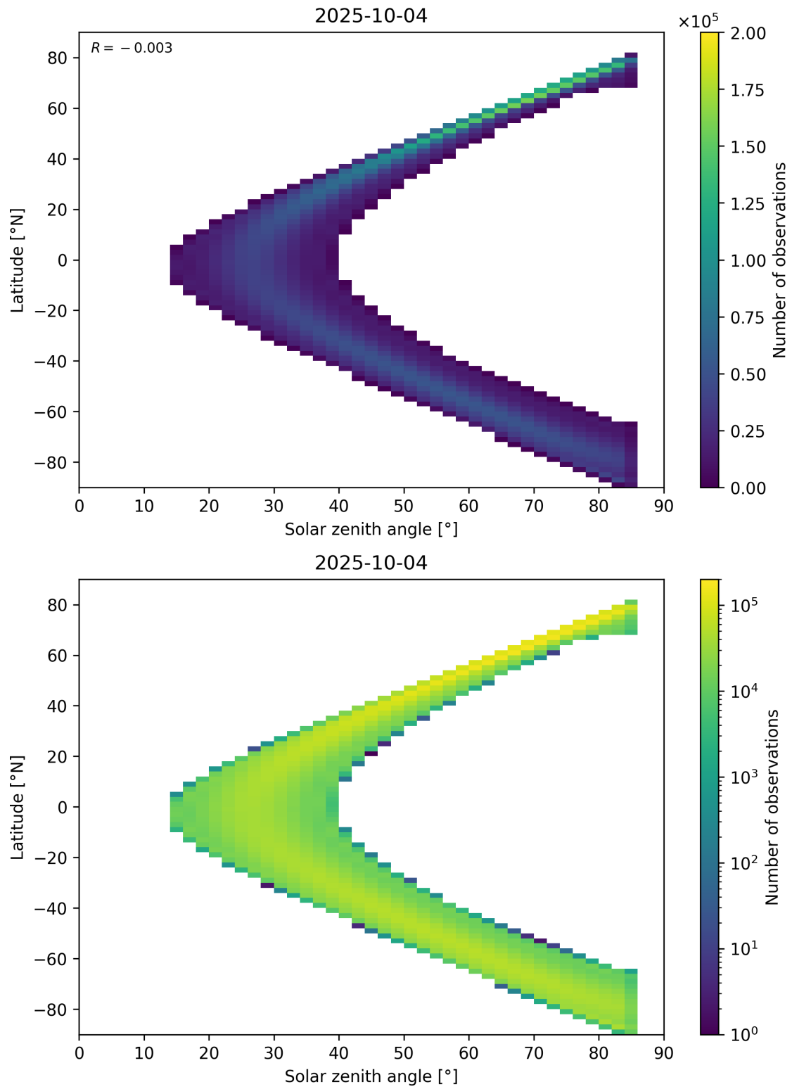
Figure 181: Scatter density plot of “Solar zenith angle” against “Latitude” for 2025-10-03 to 2025-10-05.
