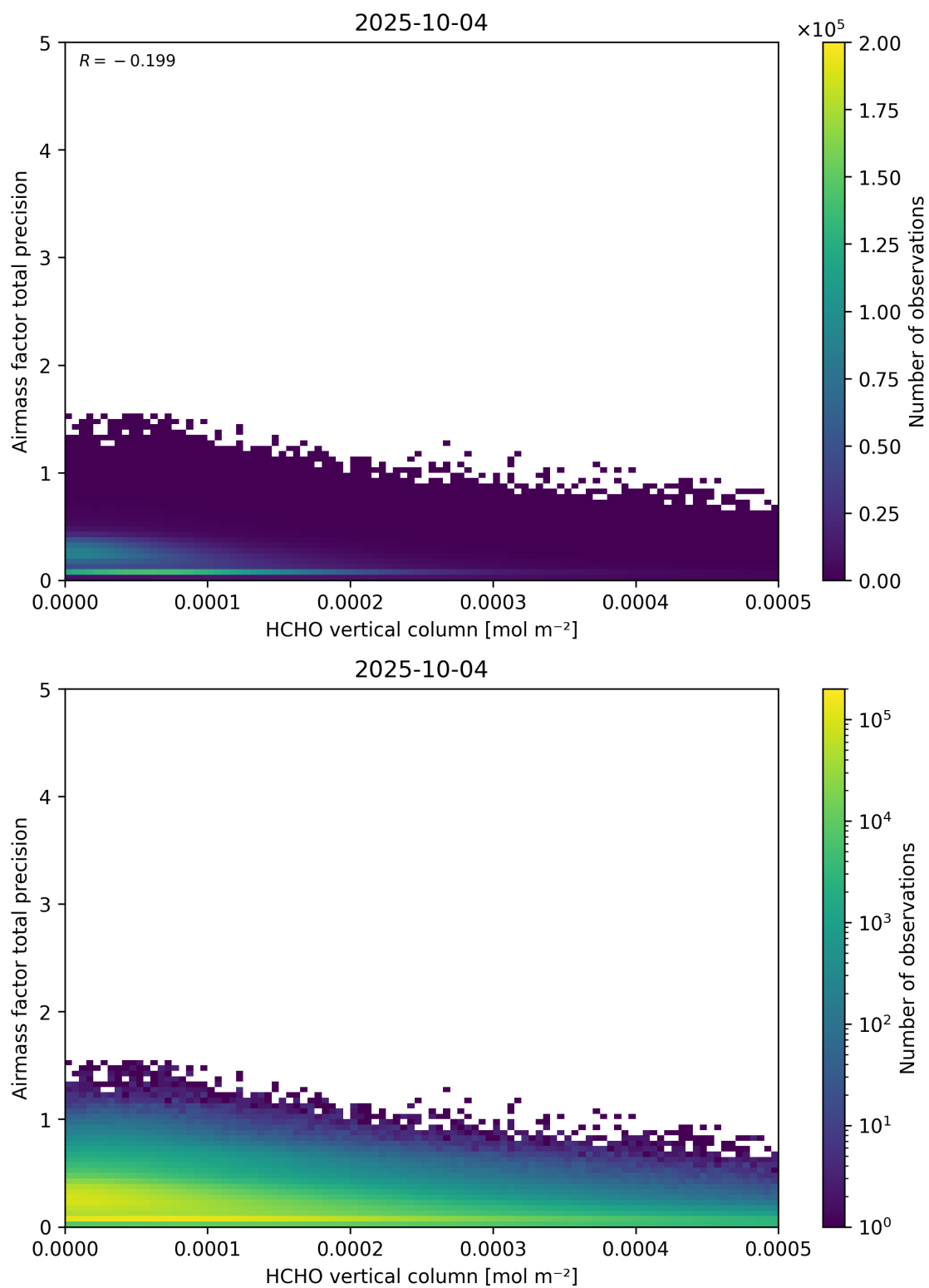
Figure 132: Scatter density plot of “HCHO vertical column” against “Airmass factor total precision” for 2025-10-03 to 2025-10-05.
