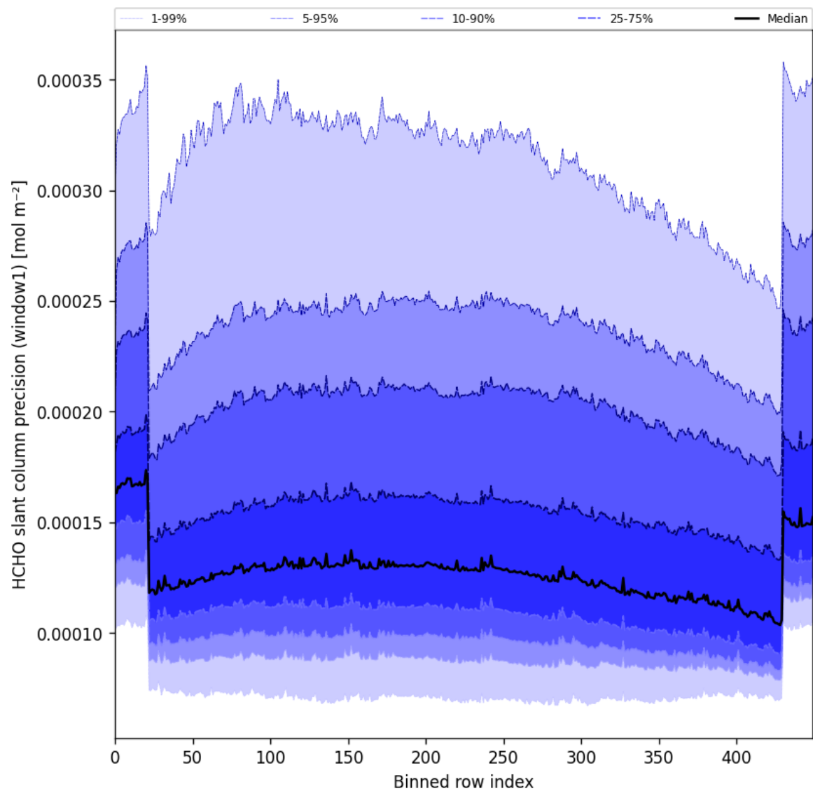
Figure 53: Along track statistics of “HCHO slant column precision (window1)” for 2025-10-03 to 2025-10-05
