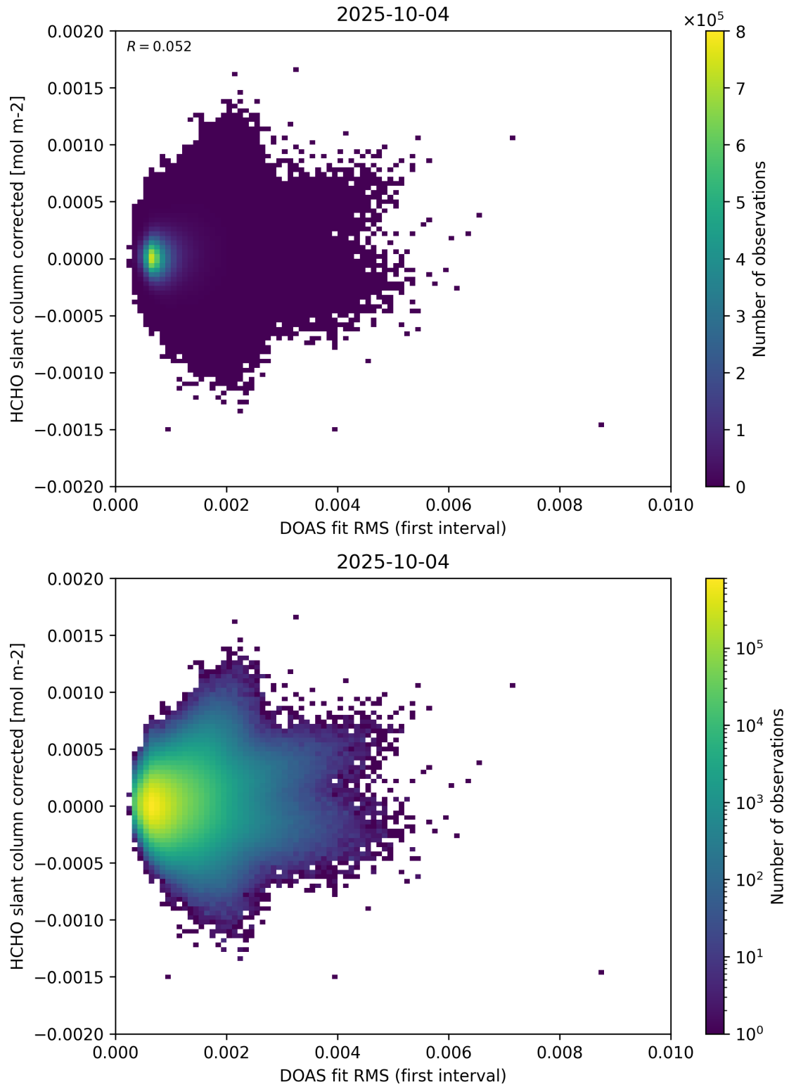
Figure 62: Scatter density plot of “DOAS fit RMS (first interval)” against “HCHO slant column corrected” for 2025-10-03 to 2025-10-05.
