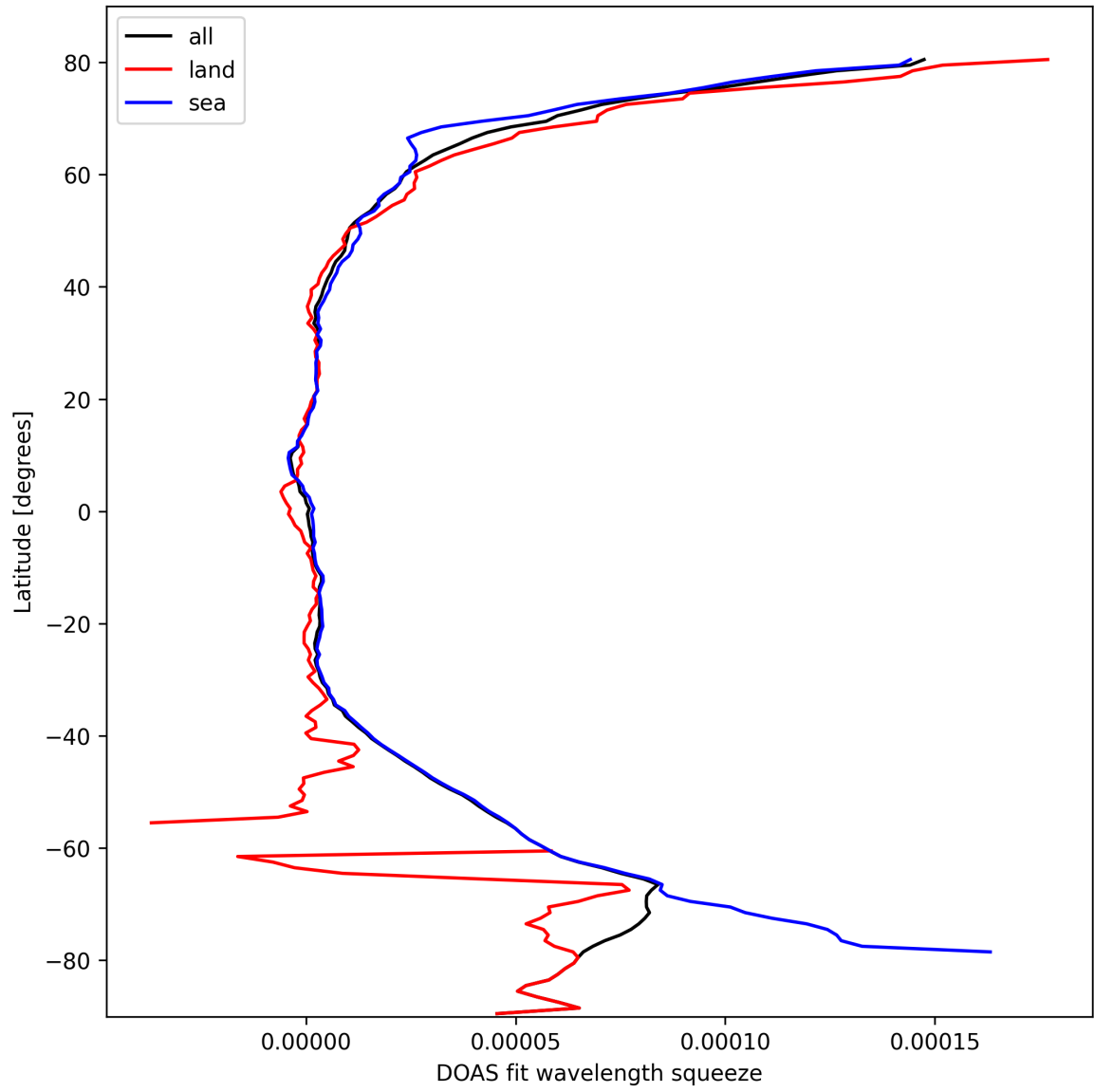
Figure 31: Zonal average of “DOAS fit wavelength squeeze” for 2025-10-03 to 2025-10-05.
