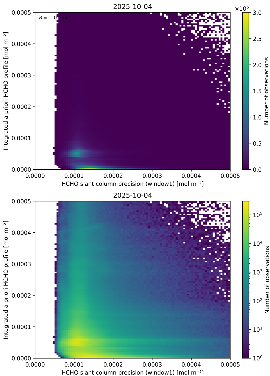
Figure 96: Scatter density plot of “HCHO slant column precision (window1)” against “Integrated a priori HCHO profile” for 2025-10-03 to 2025-10-05.
