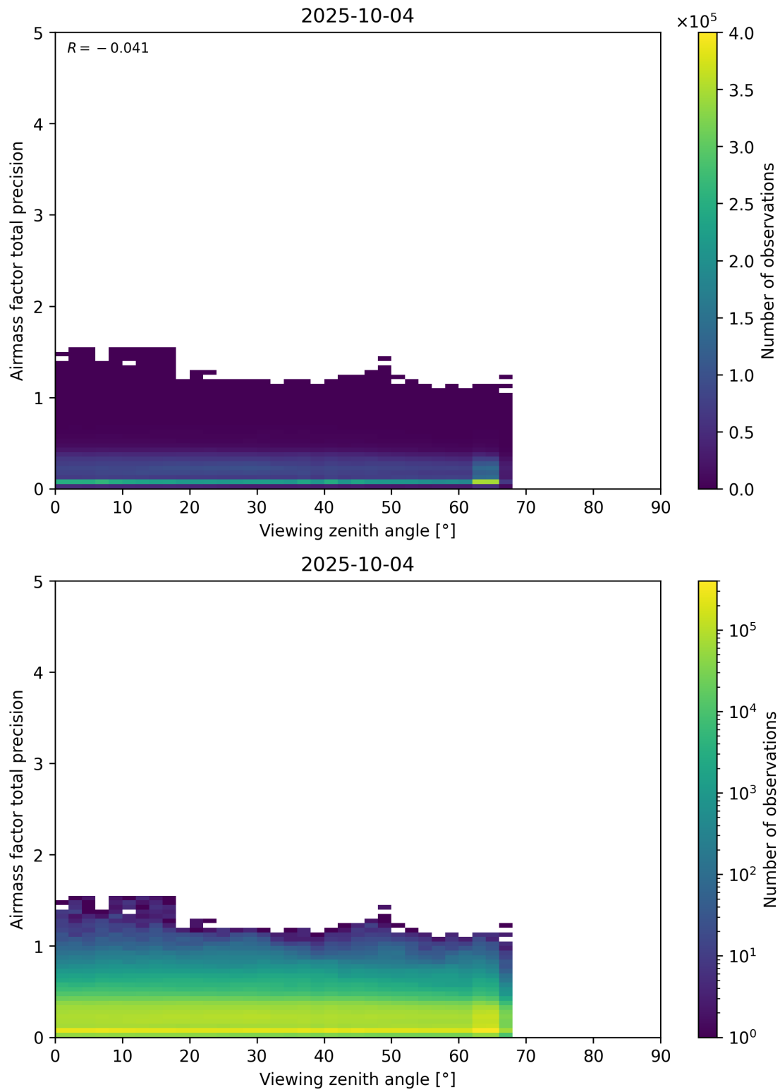
Figure 191: Scatter density plot of “Viewing zenith angle” against “Airmass factor total precision” for 2025-10-03 to 2025-10-05.
