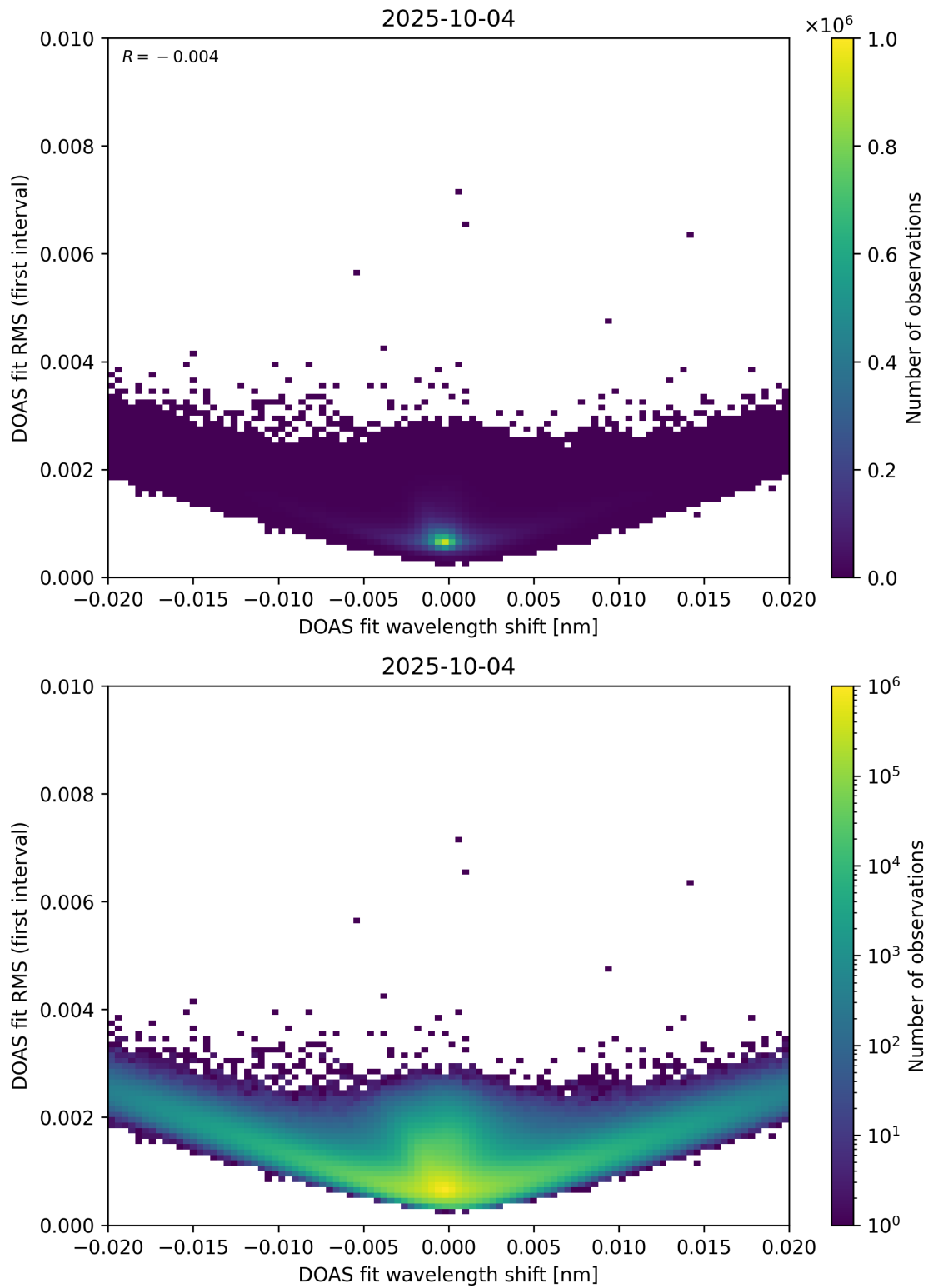
Figure 64: Scatter density plot of “DOAS fit wavelength shift” against “DOAS fit RMS (first interval)” for 2025-10-03 to 2025-10-05.
