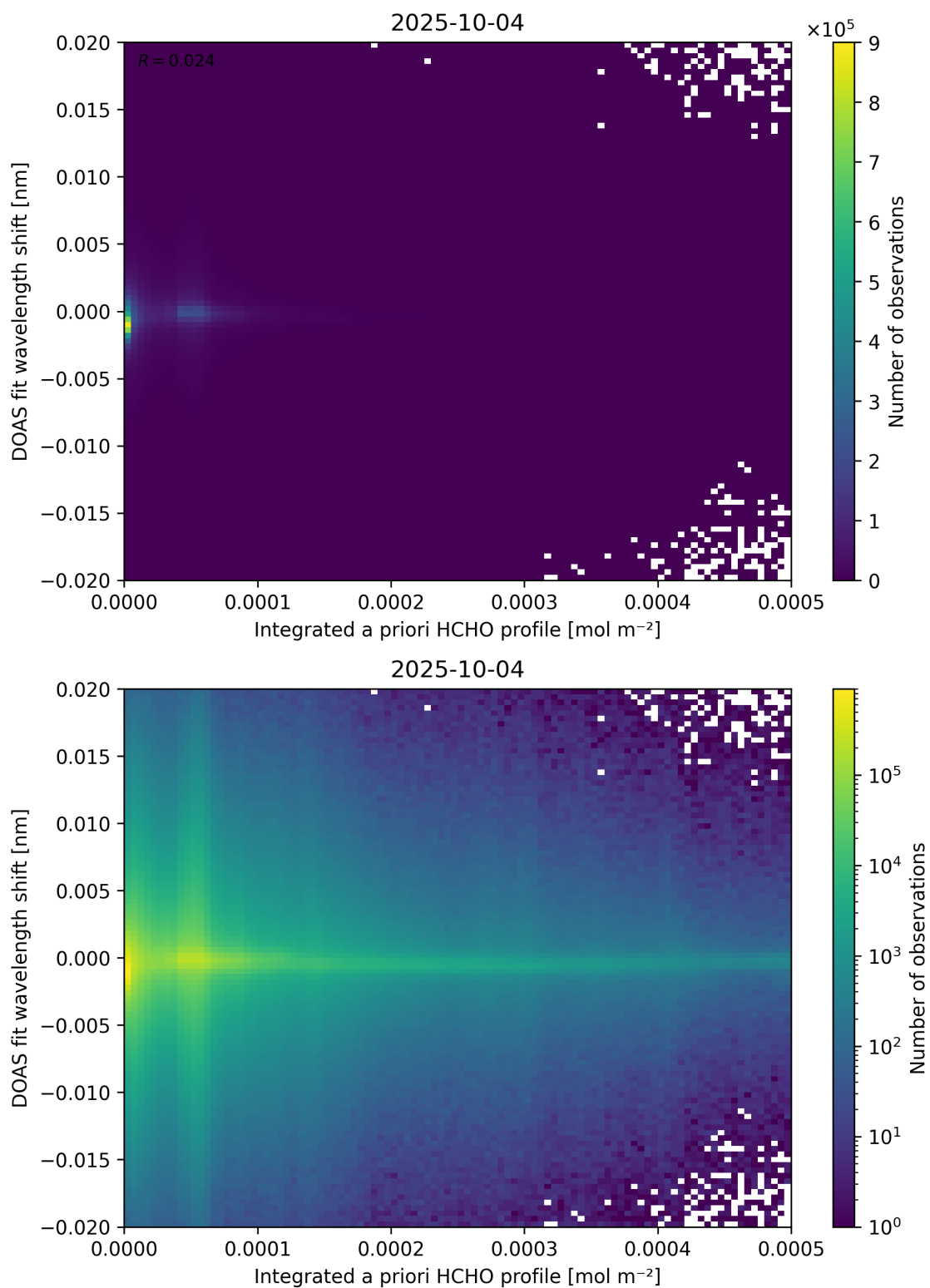
Figure 149: Scatter density plot of “Integrated a priori HCHO profile” against “DOAS fit wavelength shift” for 2025-10-03 to 2025-10-05.
