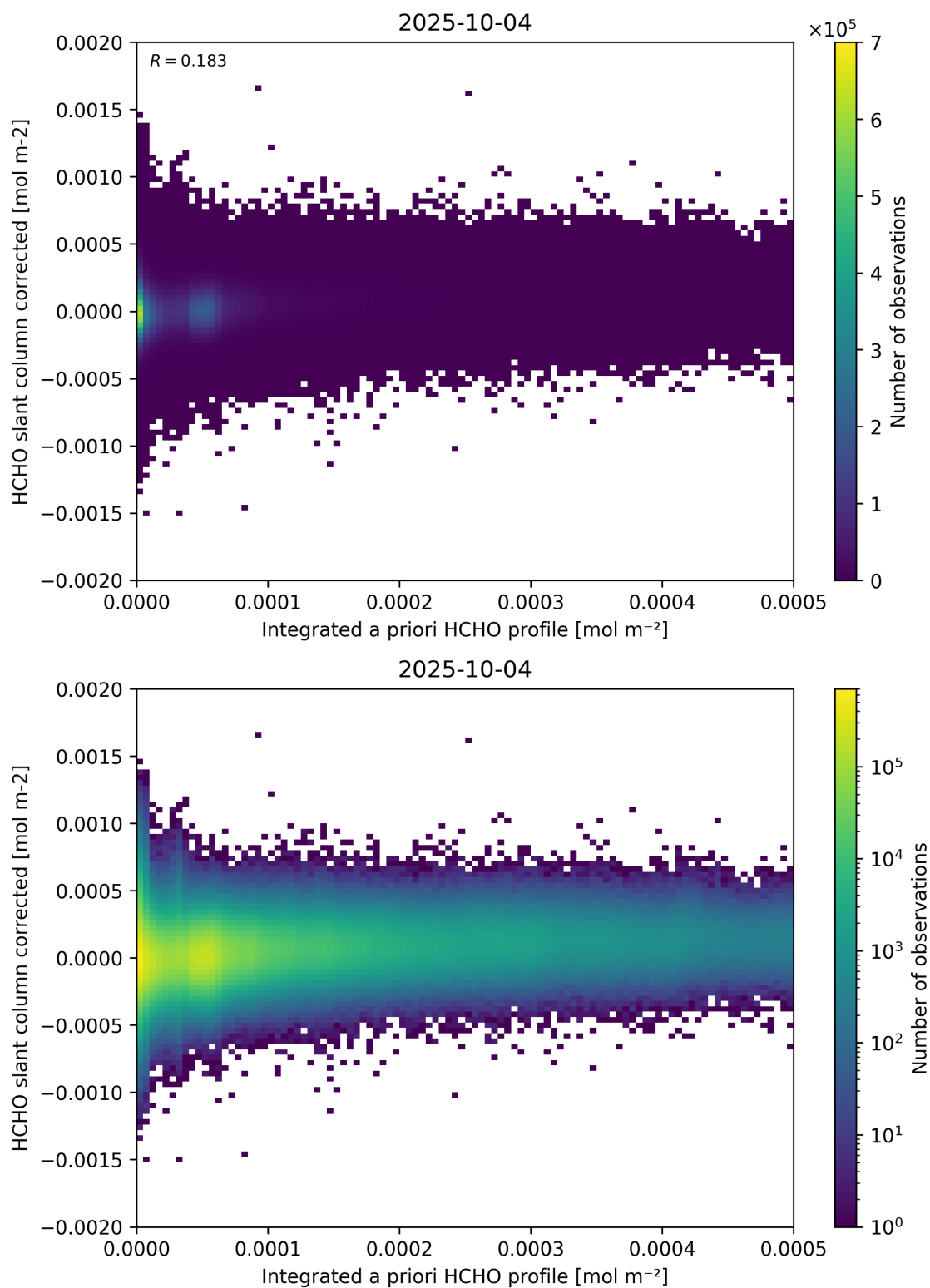
Figure 151: Scatter density plot of “Integrated a priori HCHO profile” against “HCHO slant column corrected” for 2025-10-03 to 2025-10-05.
