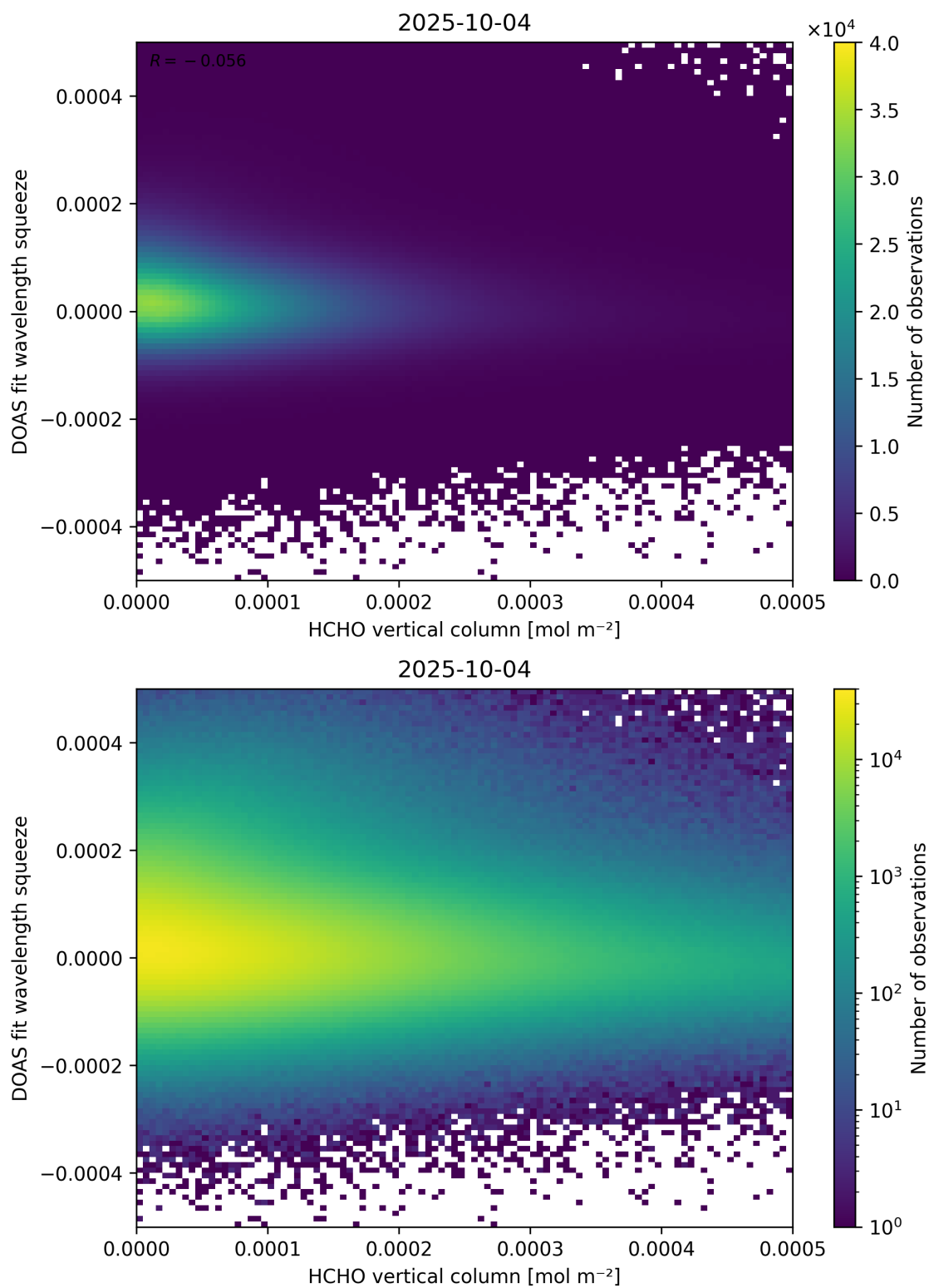
Figure 125: Scatter density plot of “HCHO vertical column” against “DOAS fit wavelength squeeze” for 2025-10-03 to 2025-10-05.
