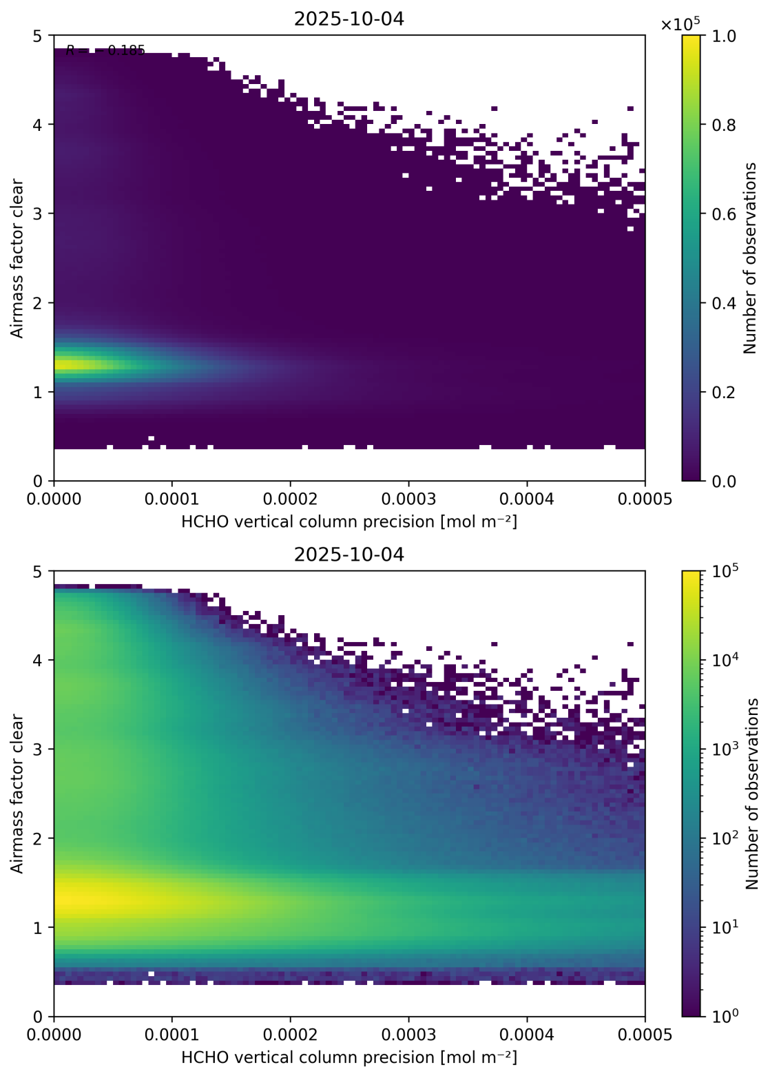
Figure 139: Scatter density plot of “HCHO vertical column precision” against “Airmass factor clear” for 2025-10-03 to 2025-10-05.
