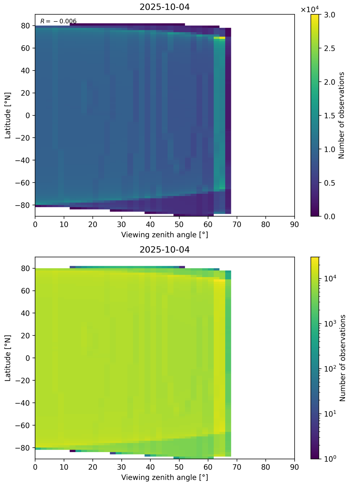
Figure 196: Scatter density plot of “Viewing zenith angle” against “Latitude” for 2025-10-03 to 2025-10-05.
