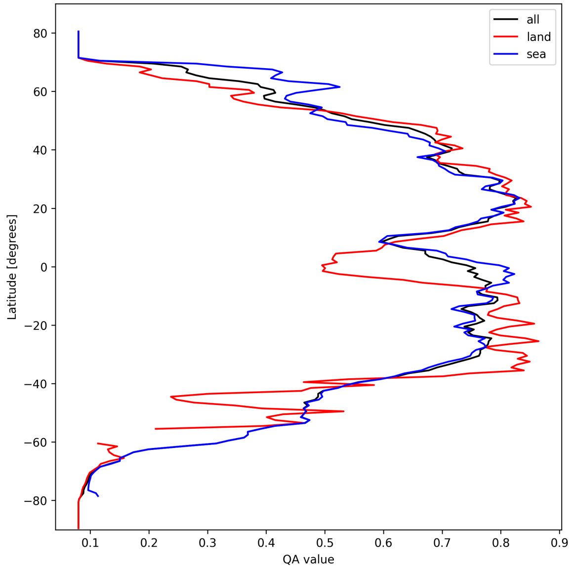
Figure 20: Zonal average of “QA value” for 2025-10-03 to 2025-10-05.
