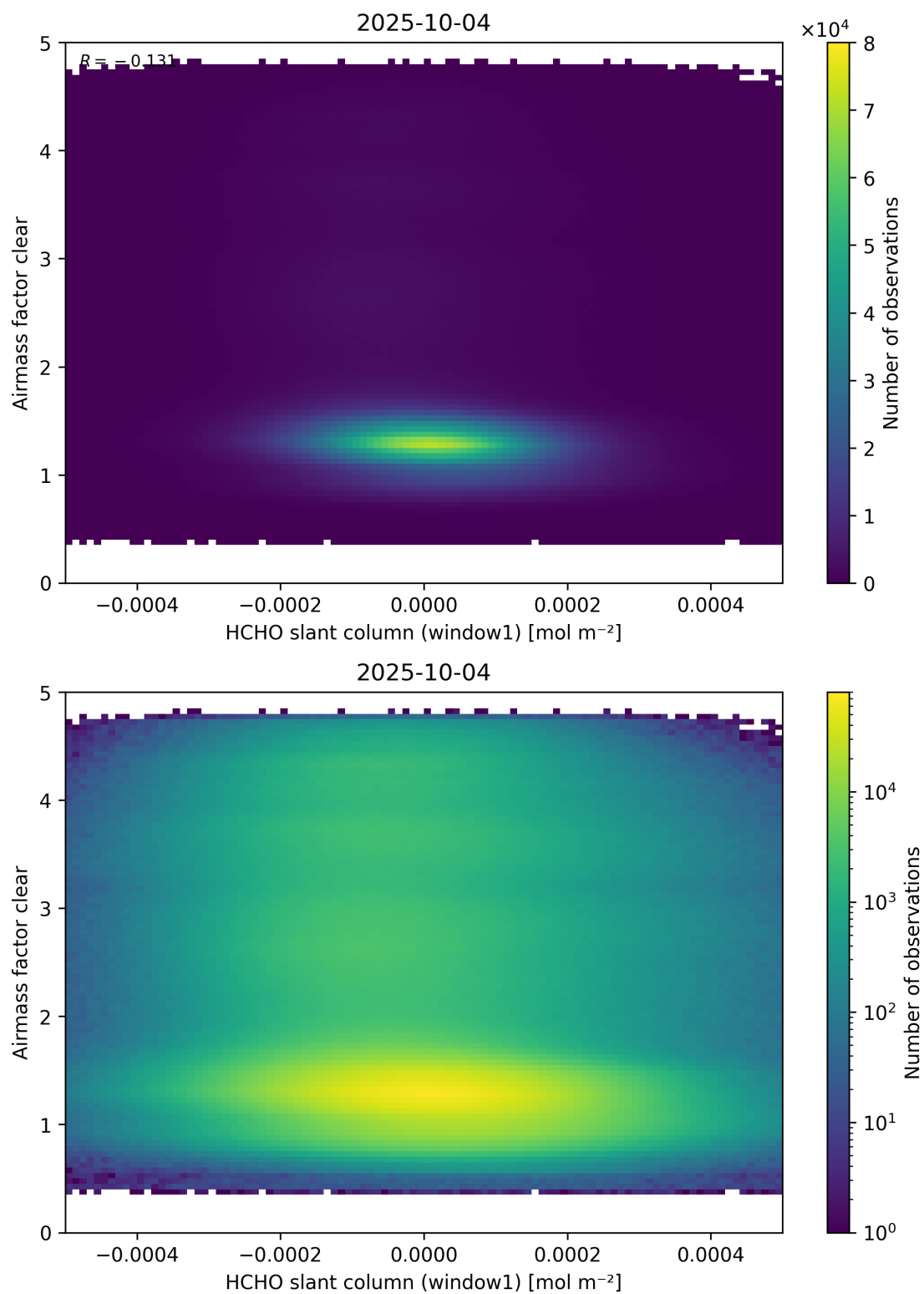
Figure 81: Scatter density plot of “HCHO slant column (window1)” against “Airmass factor clear” for 2025-10-03 to 2025-10-05.
