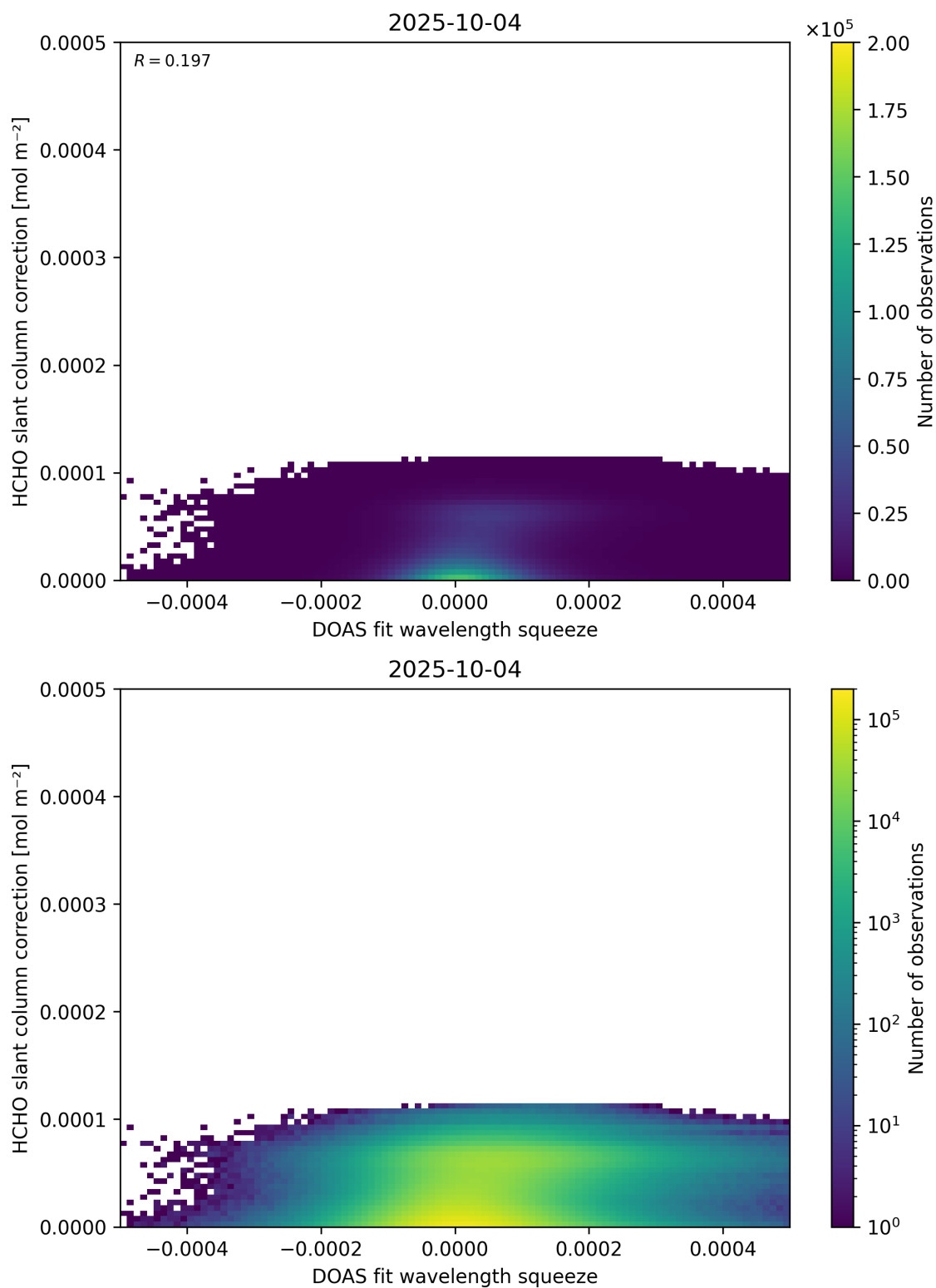
Figure 70: Scatter density plot of “DOAS fit wavelength squeeze” against “HCHO slant column correction” for 2025-10-03 to 2025-10-05.
