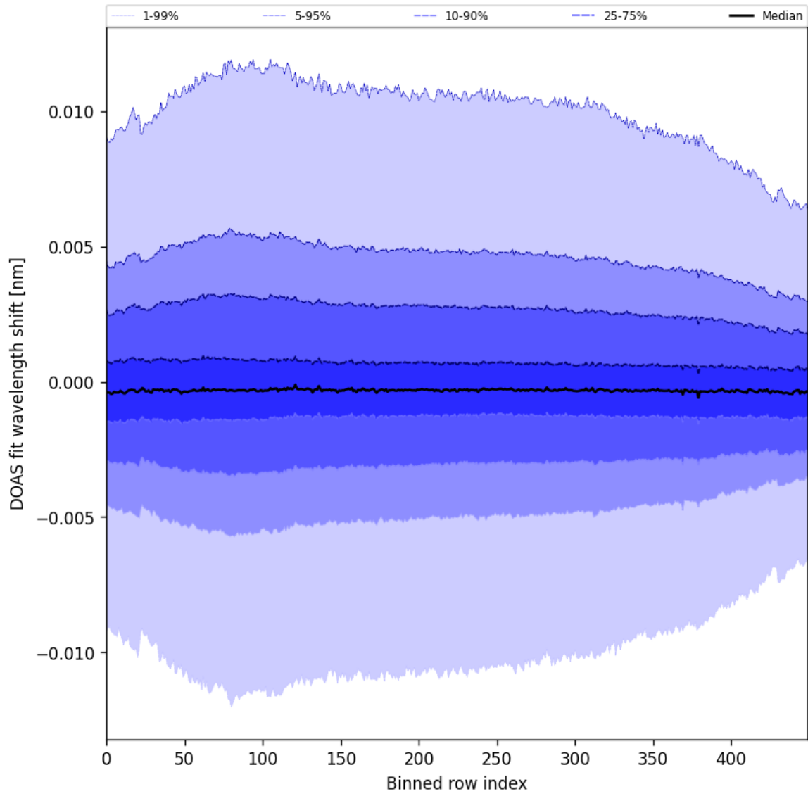
Figure 58: Along track statistics of “DOAS fit wavelength shift” for 2025-10-03 to 2025-10-05
