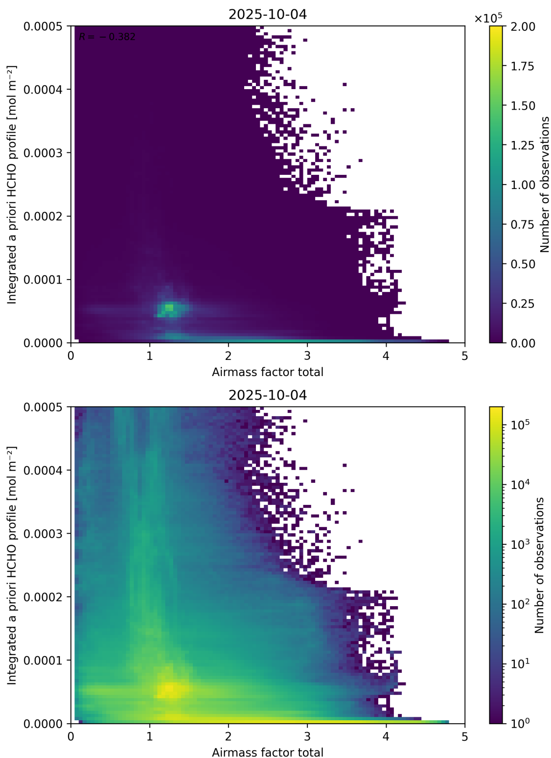
Figure 104: Scatter density plot of “Airmass factor total” against “Integrated a priori HCHO profile” for 2025-10-03 to 2025-10-05.
