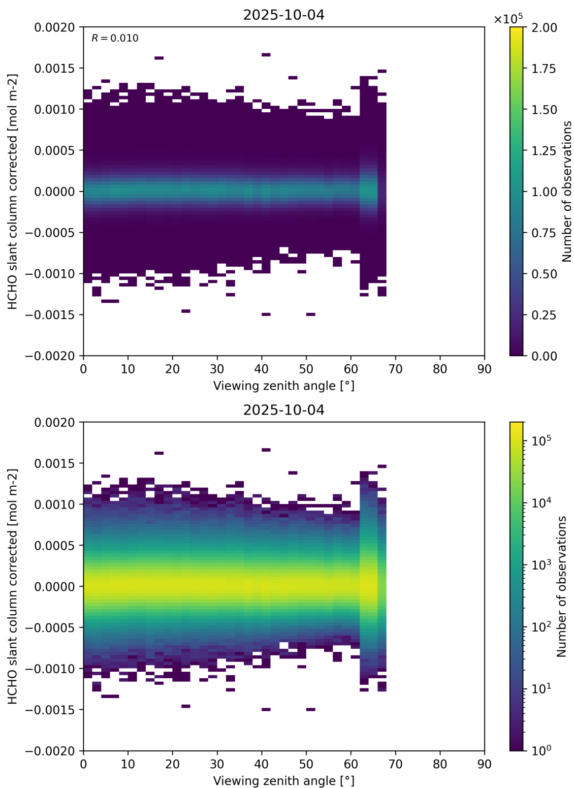
Figure 186: Scatter density plot of “Viewing zenith angle” against “HCHO slant column corrected” for 2025-10-03 to 2025-10-05.
