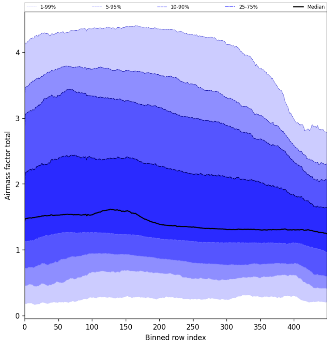
Figure 54: Along track statistics of “Airmass factor total” for 2025-10-03 to 2025-10-05
