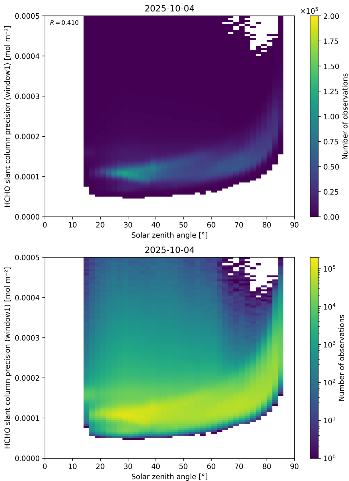
Figure 174: Scatter density plot of “Solar zenith angle” against “HCHO slant column precision (window1)” for 2025-10-03 to 2025-10-05.
