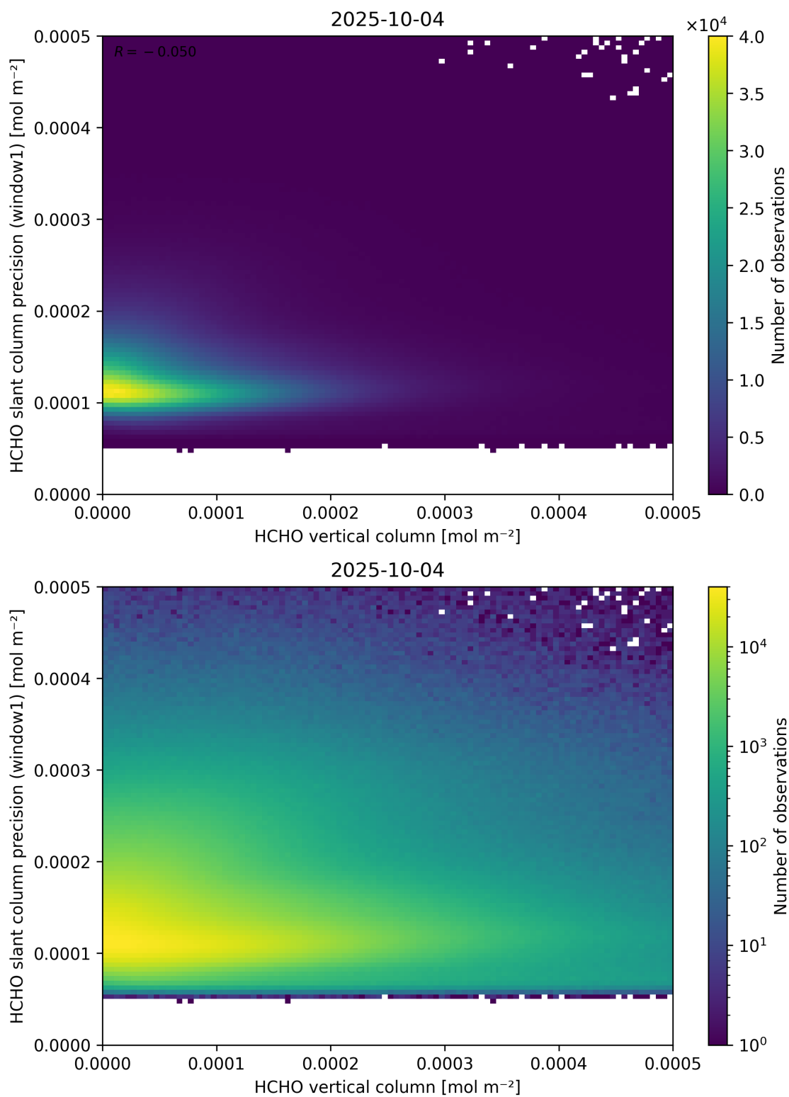
Figure 130: Scatter density plot of “HCHO vertical column” against “HCHO slant column precision (window1)” for 2025-10-03 to 2025-10-05.
