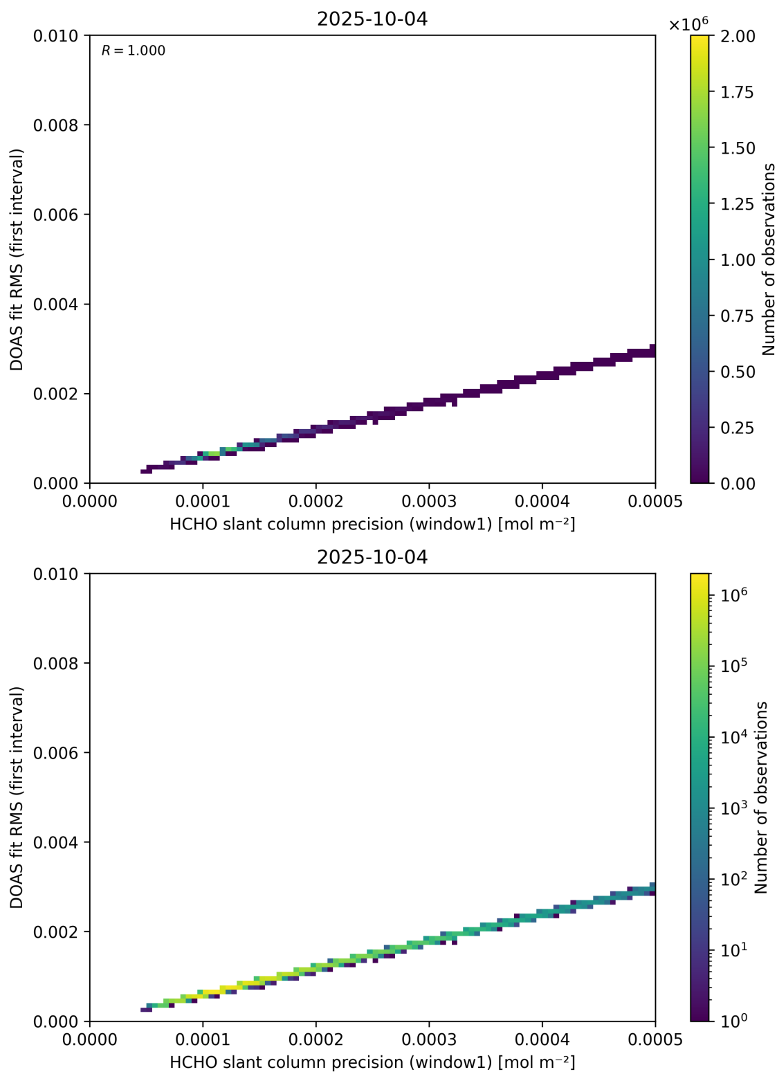
Figure 88: Scatter density plot of “HCHO slant column precision (window1)” against “DOAS fit RMS (first interval)” for 2025-10-03 to 2025-10-05.
