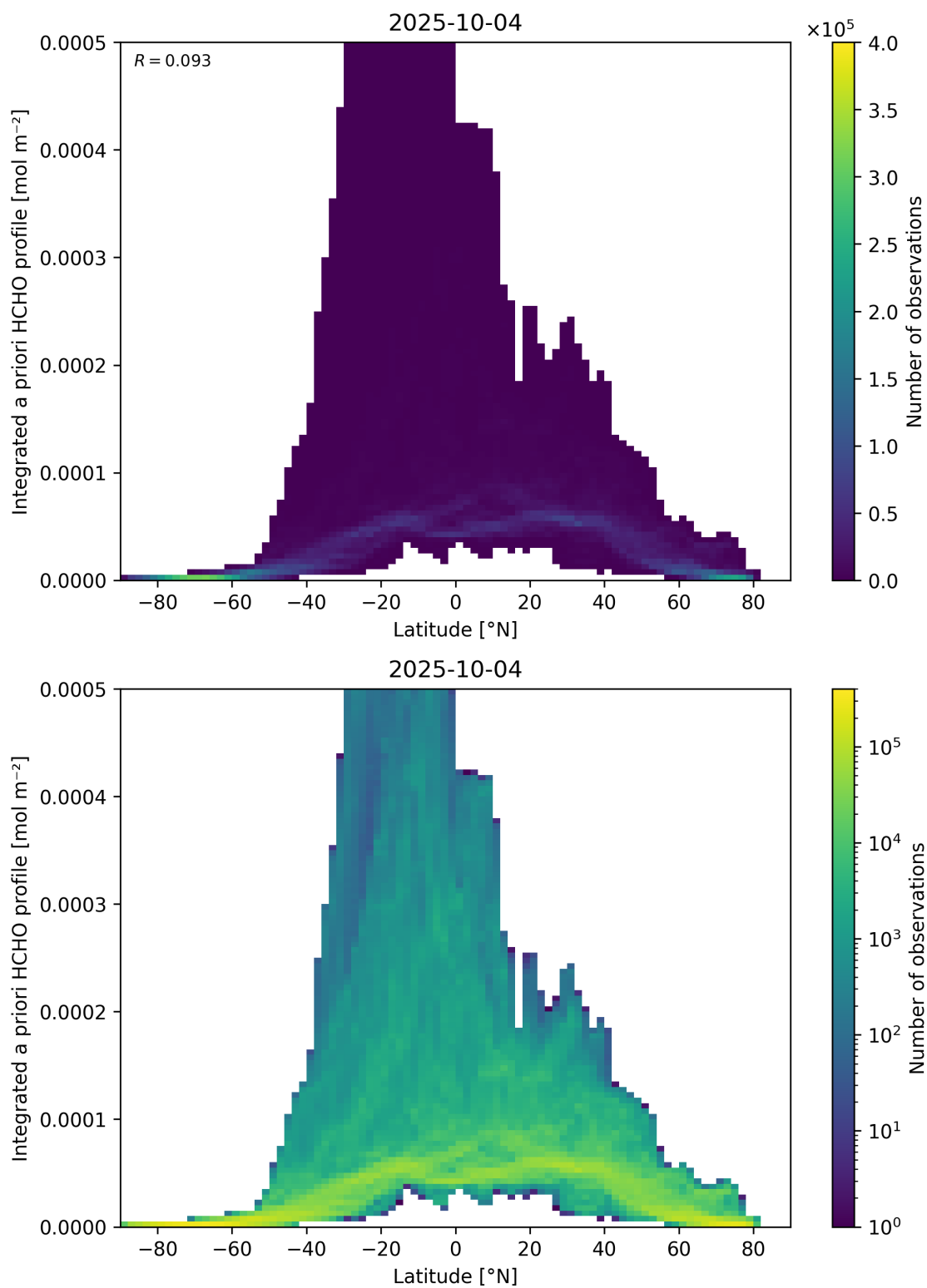
Figure 166: Scatter density plot of “Latitude” against “Integrated a priori HCHO profile” for 2025-10-03 to 2025-10-05.
