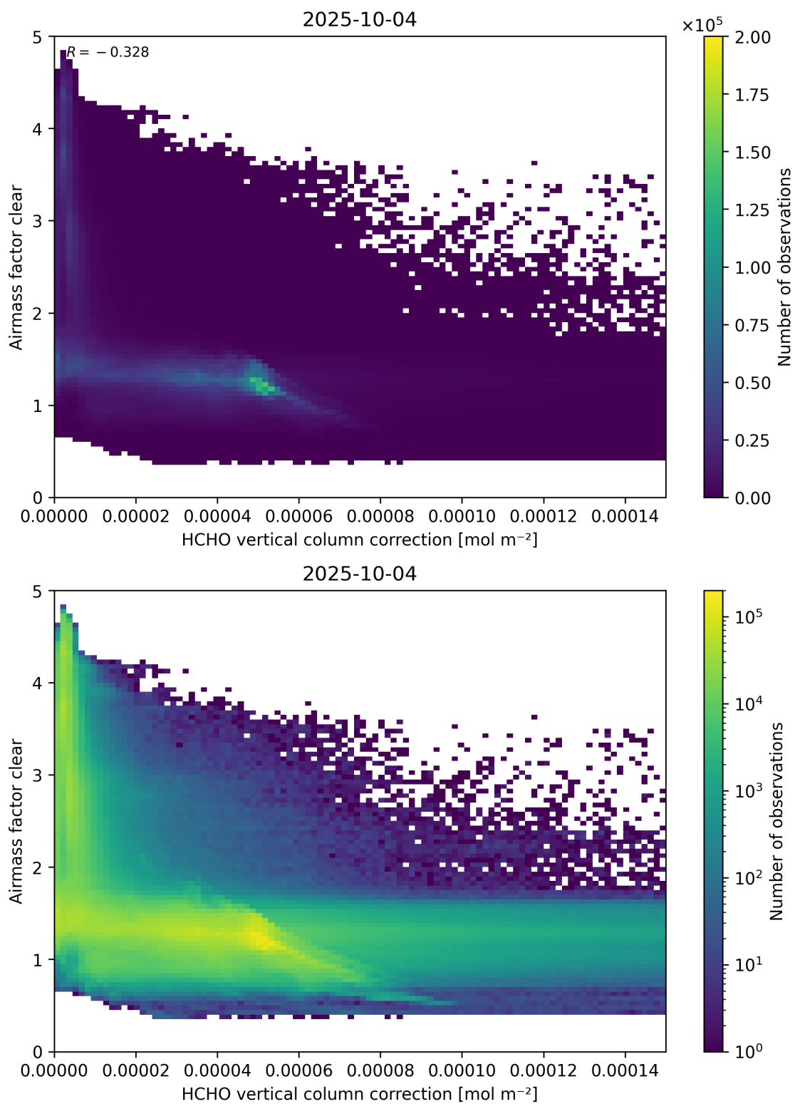
Figure 115: Scatter density plot of “HCHO vertical column correction” against “Airmass factor clear” for 2025-10-03 to 2025-10-05.
