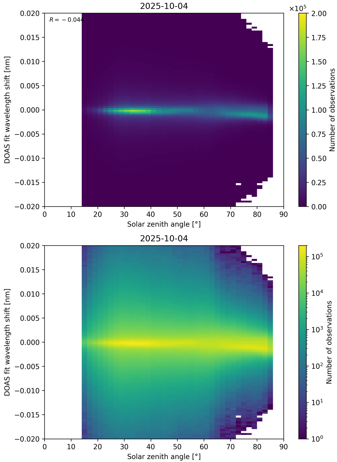
Figure 168: Scatter density plot of “Solar zenith angle” against “DOAS fit wavelength shift” for 2025-10-03 to 2025-10-05.
