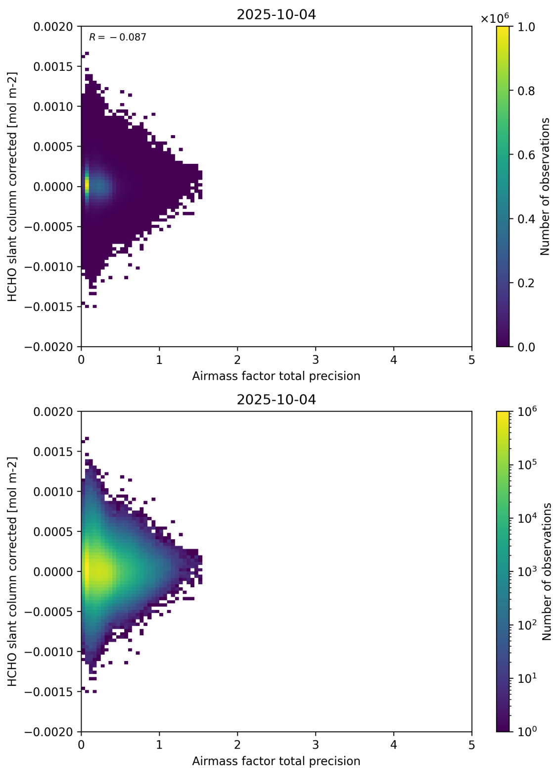
Figure 109: Scatter density plot of “Airmass factor total precision” against “HCHO slant column corrected” for 2025-10-03 to 2025-10-05.
