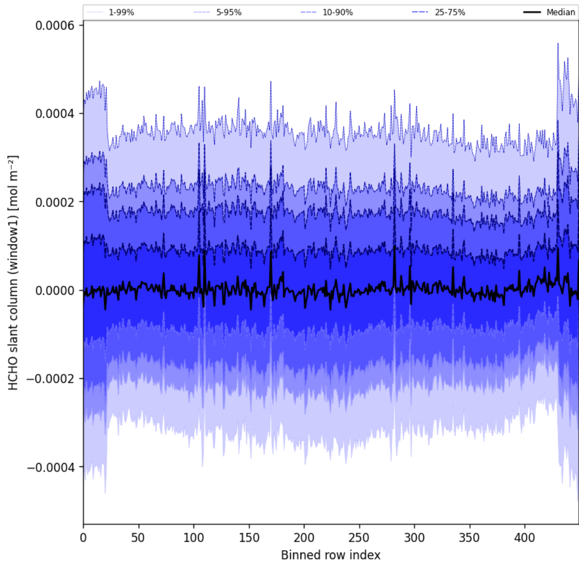
Figure 52: Along track statistics of “HCHO slant column (window1)” for 2025-10-03 to 2025-10-05
