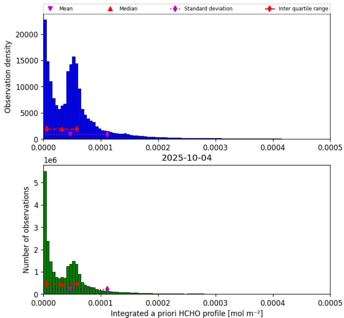
Figure 43: Histogram of “Integrated a priori HCHO profile” for 2025-10-03 to 2025-10-05
