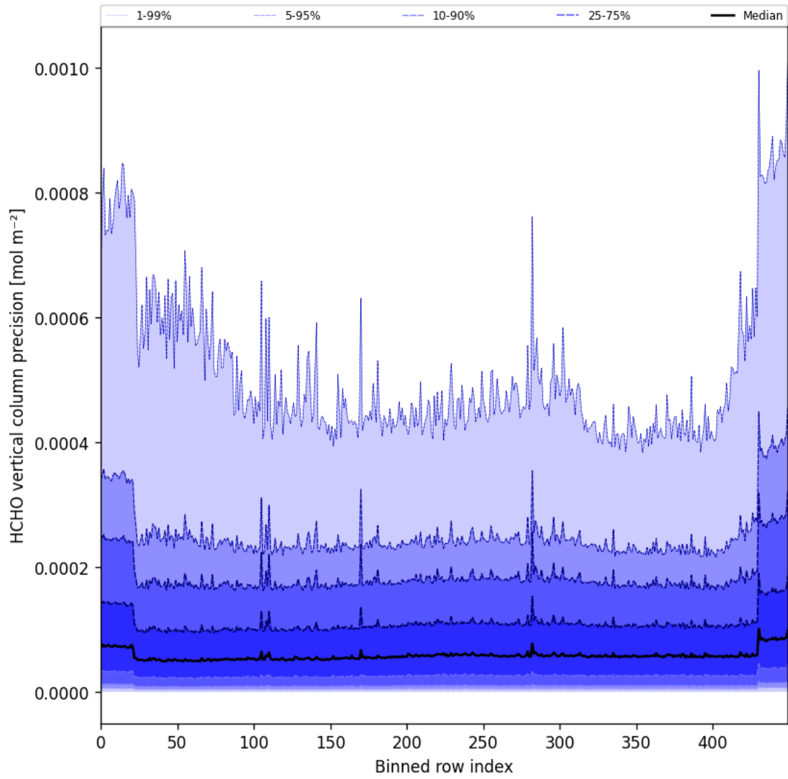
Figure 50: Along track statistics of “HCHO vertical column precision” for 2025-10-03 to 2025-10-05
