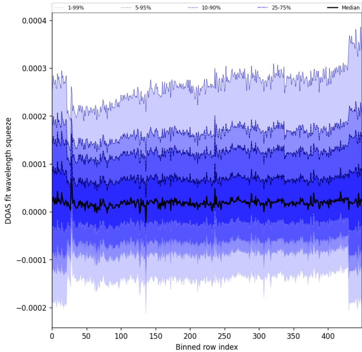
Figure 59: Along track statistics of “DOAS fit wavelength squeeze” for 2025-10-03 to 2025-10-05
