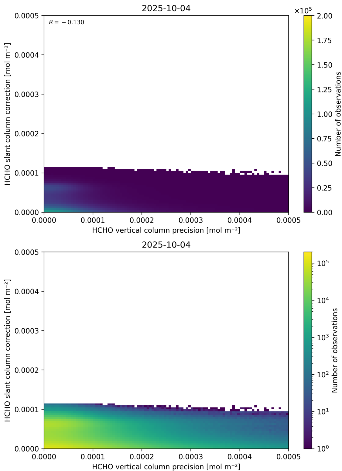
Figure 141: Scatter density plot of “HCHO vertical column precision” against “HCHO slant column correction” for 2025-10-03 to 2025-10-05.
