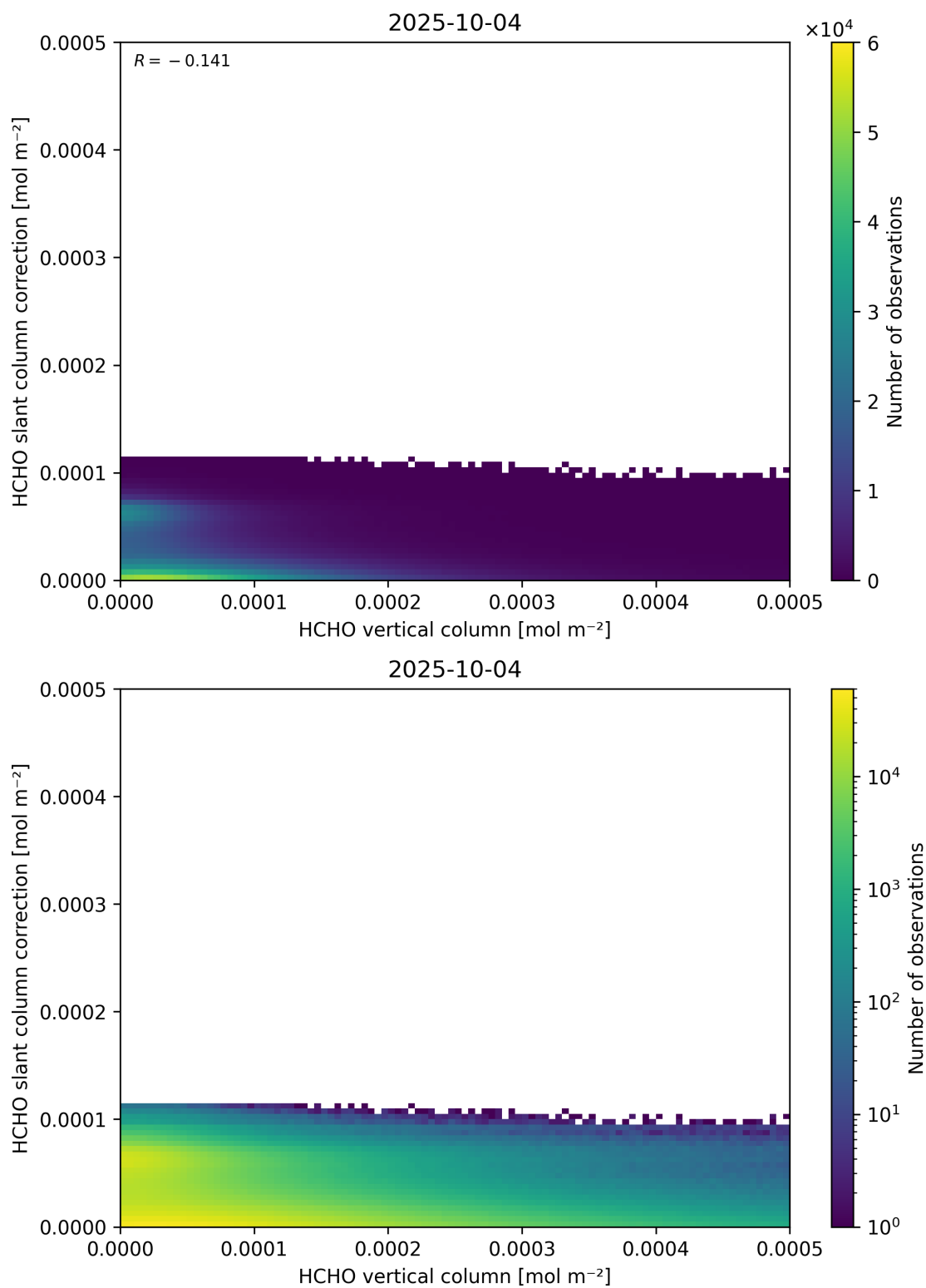
Figure 128: Scatter density plot of “HCHO vertical column” against “HCHO slant column correction” for 2025-10-03 to 2025-10-05.
