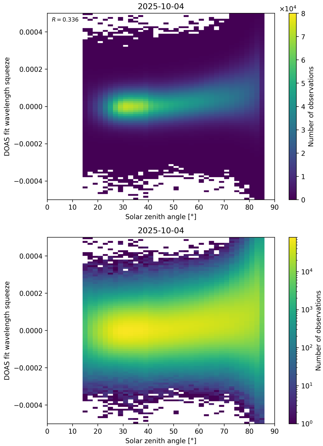
Figure 169: Scatter density plot of “Solar zenith angle” against “DOAS fit wavelength squeeze” for 2025-10-03 to 2025-10-05.
