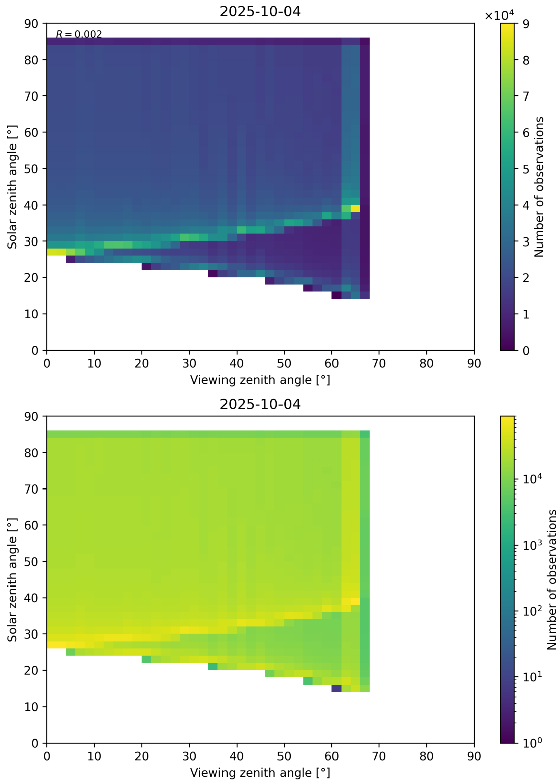
Figure 197: Scatter density plot of “Viewing zenith angle” against “Solar zenith angle” for 2025-10-03 to 2025-10-05.
