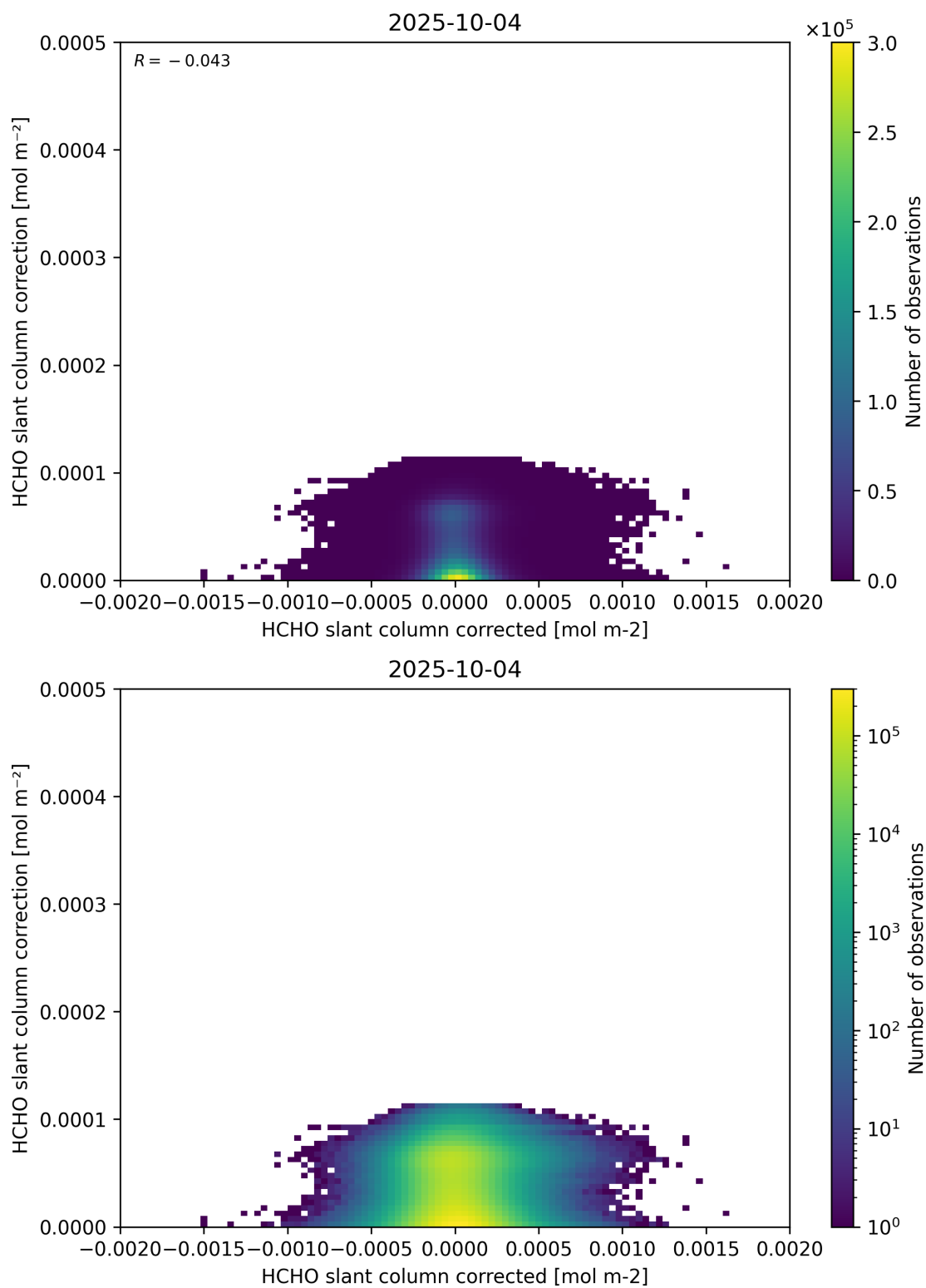
Figure 77: Scatter density plot of “HCHO slant column corrected” against “HCHO slant column correction” for 2025-10-03 to 2025-10-05.
