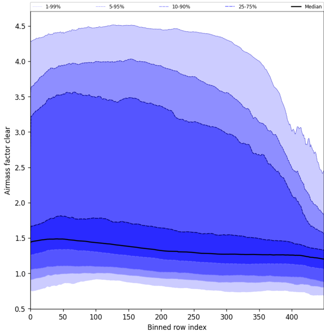
Figure 56: Along track statistics of “Airmass factor clear” for 2025-10-03 to 2025-10-05
