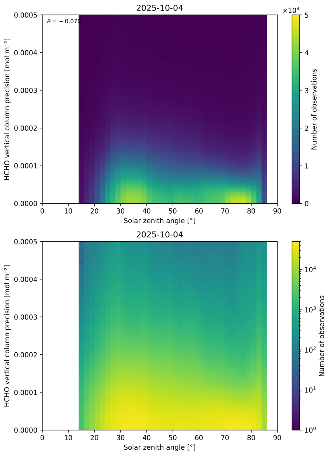
Figure 179: Scatter density plot of “Solar zenith angle” against “HCHO vertical column precision” for 2025-10-03 to 2025-10-05.
