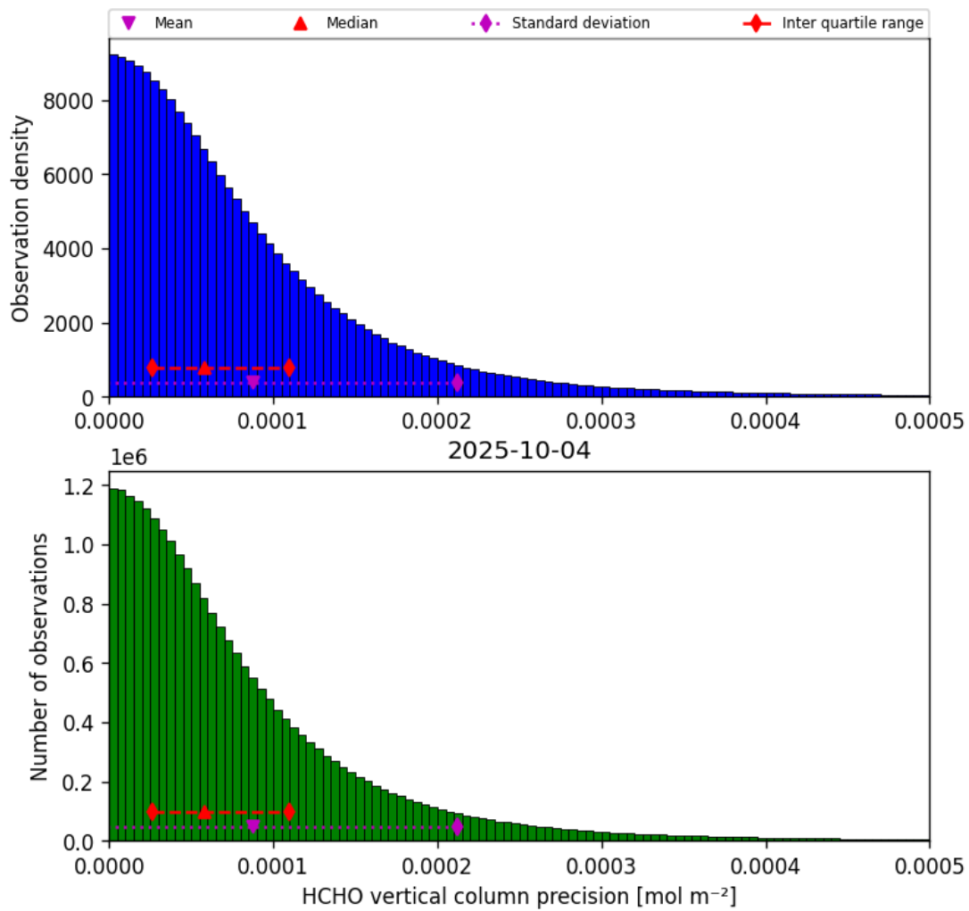
Figure 36: Histogram of “HCHO vertical column precision” for 2025-10-03 to 2025-10-05
