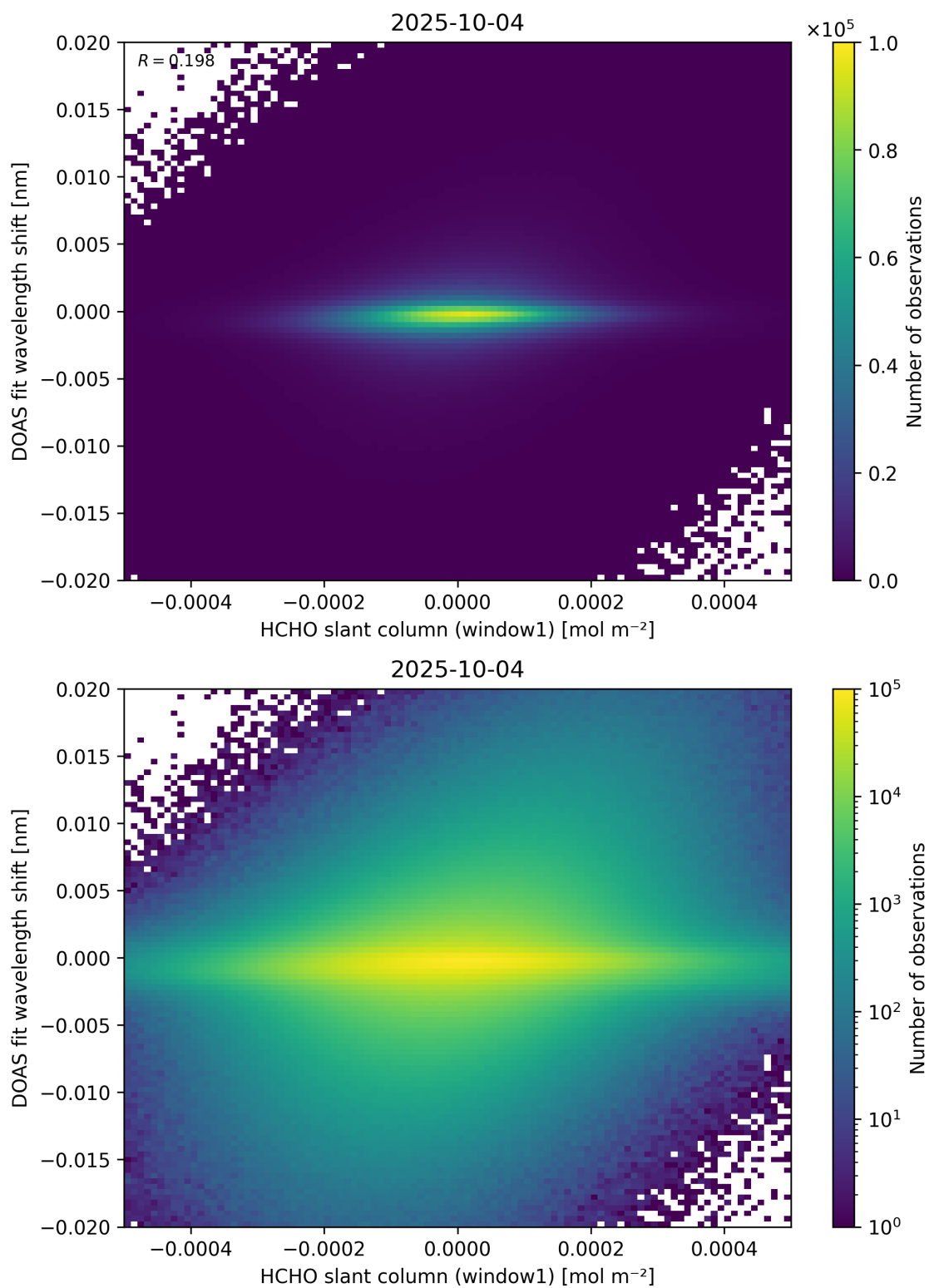
Figure 79: Scatter density plot of “HCHO slant column (window1)” against “DOAS fit wavelength shift” for 2025-10-03 to 2025-10-05.
