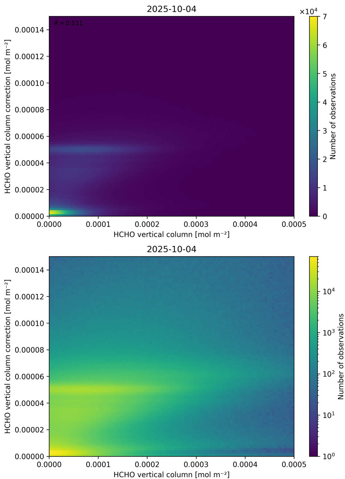
Figure 133: Scatter density plot of “HCHO vertical column” against “HCHO vertical column correction” for 2025-10-03 to 2025-10-05.
