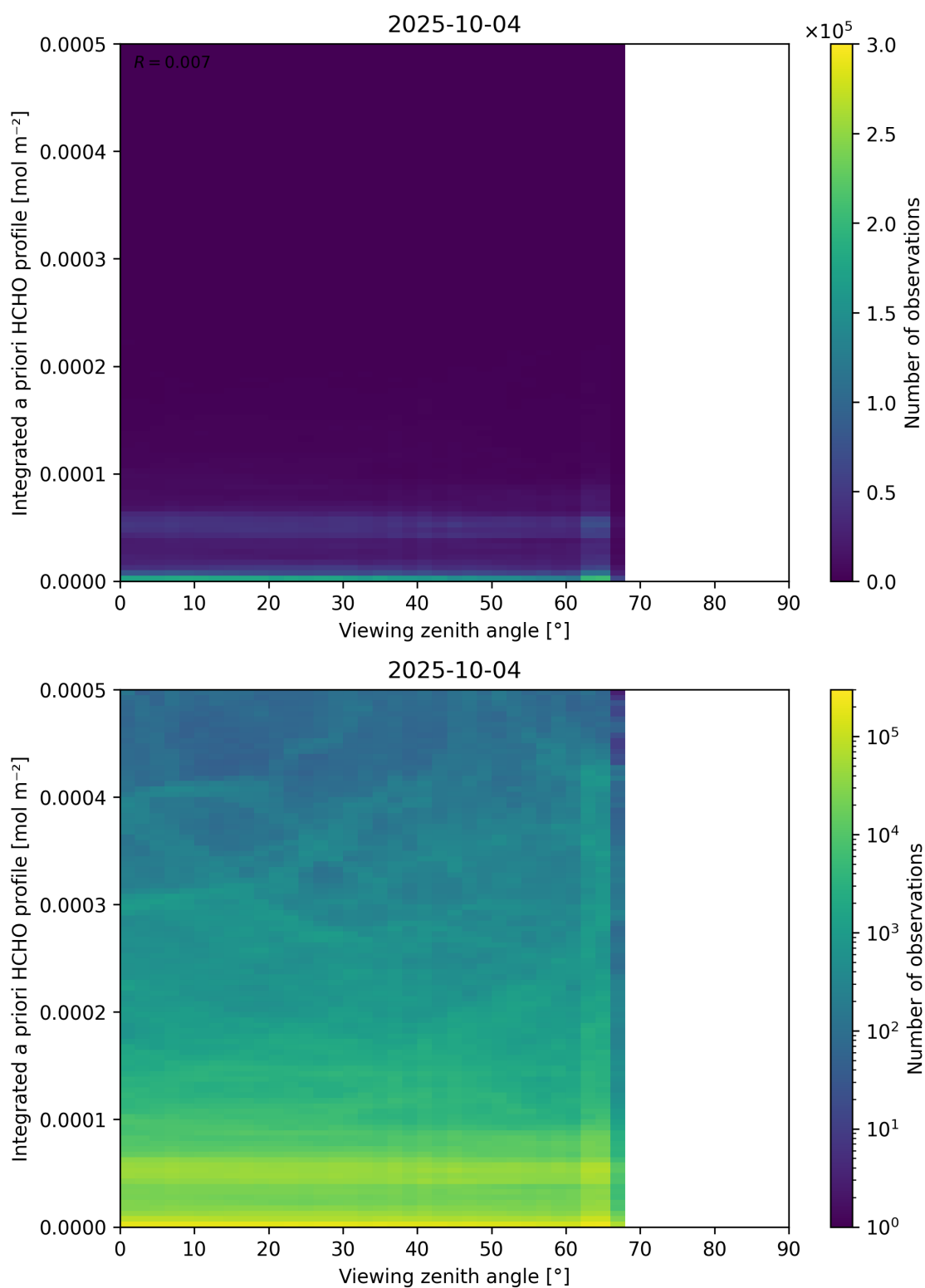
Figure 195: Scatter density plot of “Viewing zenith angle” against “Integrated a priori HCHO profile” for 2025-10-03 to 2025-10-05.
