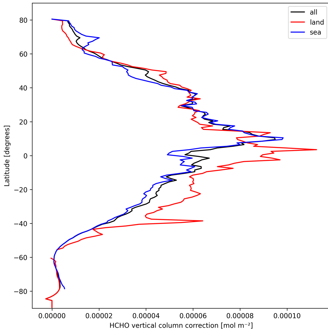
Figure 23: Zonal average of “HCHO vertical column correction” for 2025-10-03 to 2025-10-05.
