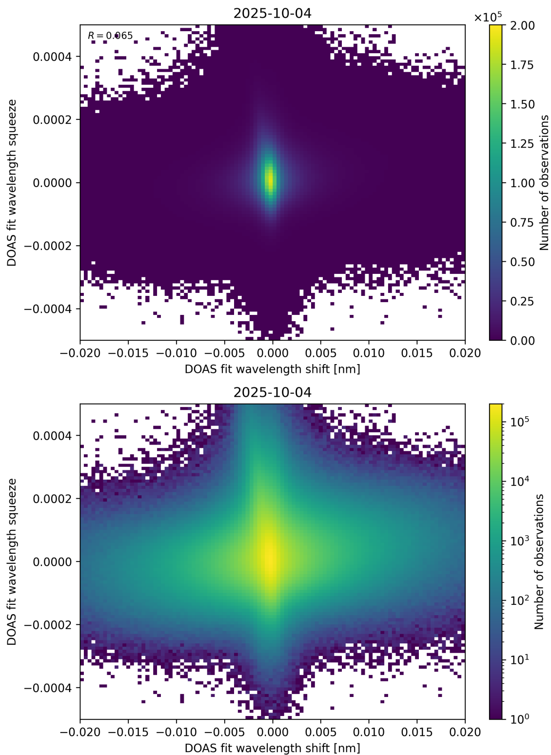
Figure 65: Scatter density plot of “DOAS fit wavelength shift” against “DOAS fit wavelength squeeze” for 2025-10-03 to 2025-10-05.
