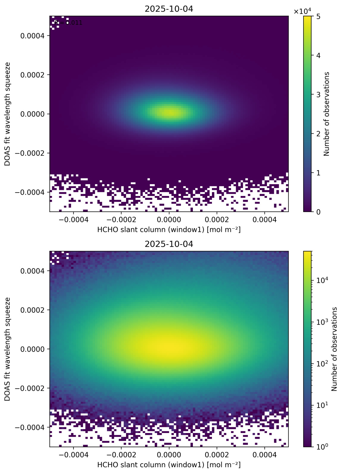
Figure 80: Scatter density plot of “HCHO slant column (window1)” against “DOAS fit wavelength squeeze” for 2025-10-03 to 2025-10-05.
