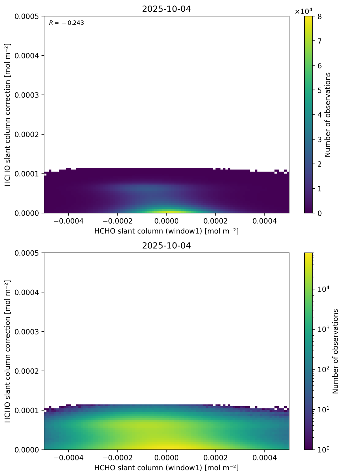
Figure 83: Scatter density plot of “HCHO slant column (window1)” against “HCHO slant column correction” for 2025-10-03 to 2025-10-05.
