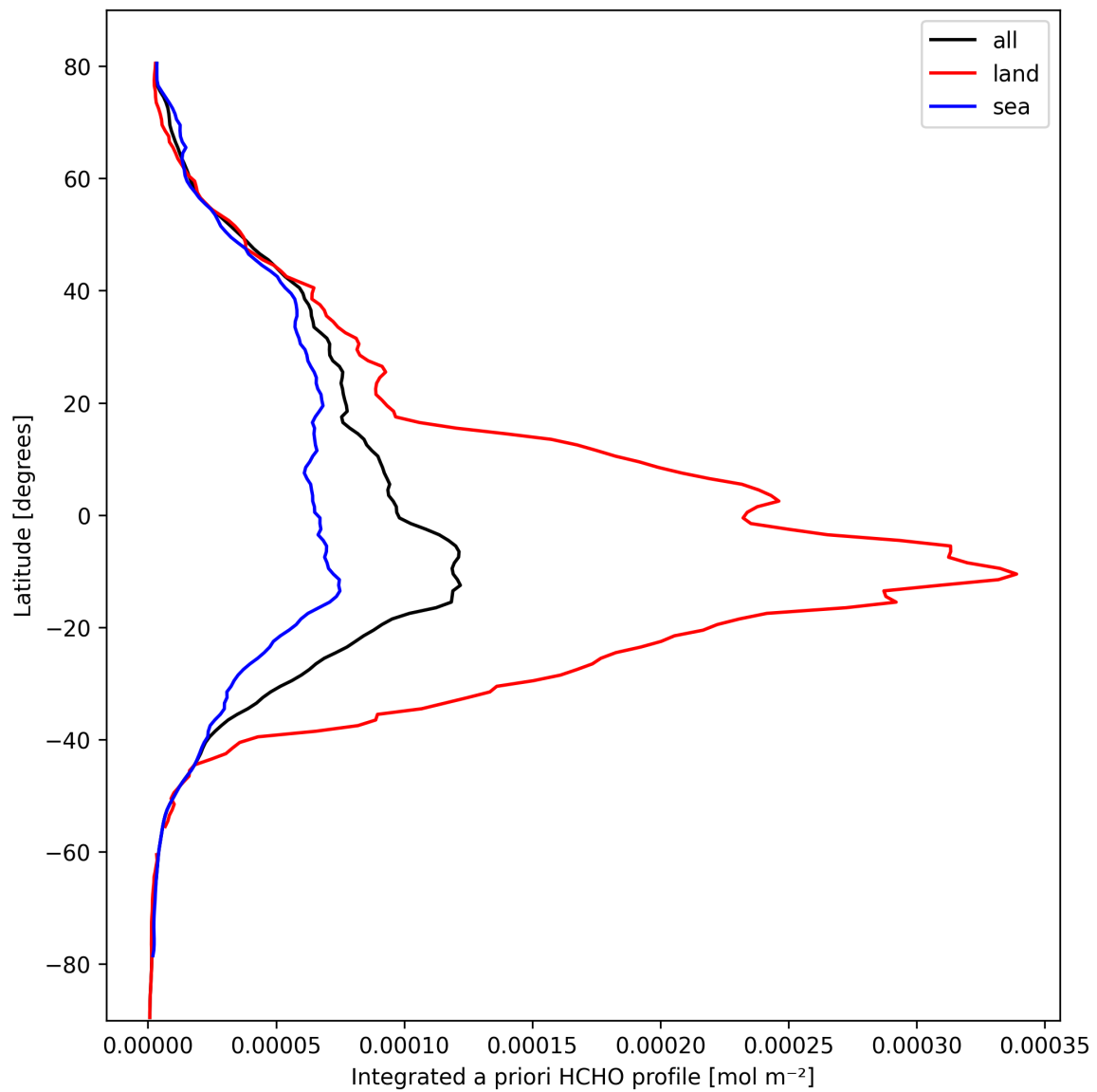
Figure 29: Zonal average of “Integrated a priori HCHO profile” for 2025-10-03 to 2025-10-05.
