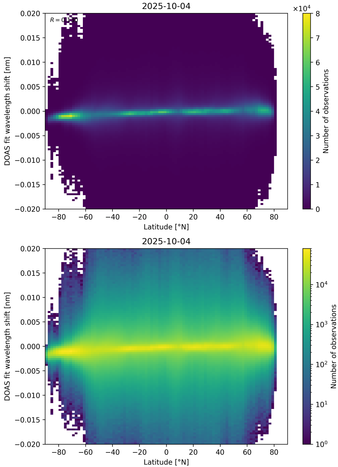
Figure 154: Scatter density plot of “Latitude” against “DOAS fit wavelength shift” for 2025-10-03 to 2025-10-05.
