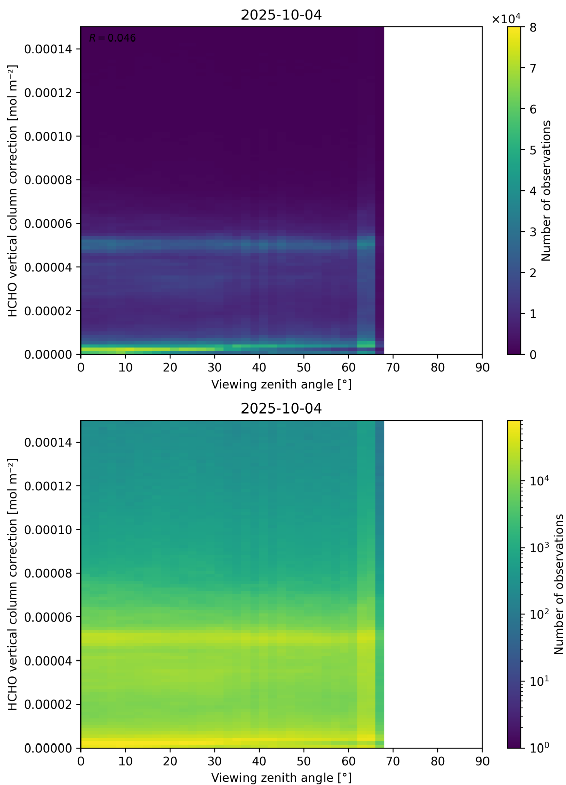
Figure 193: Scatter density plot of “Viewing zenith angle” against “HCHO vertical column correction” for 2025-10-03 to 2025-10-05.
