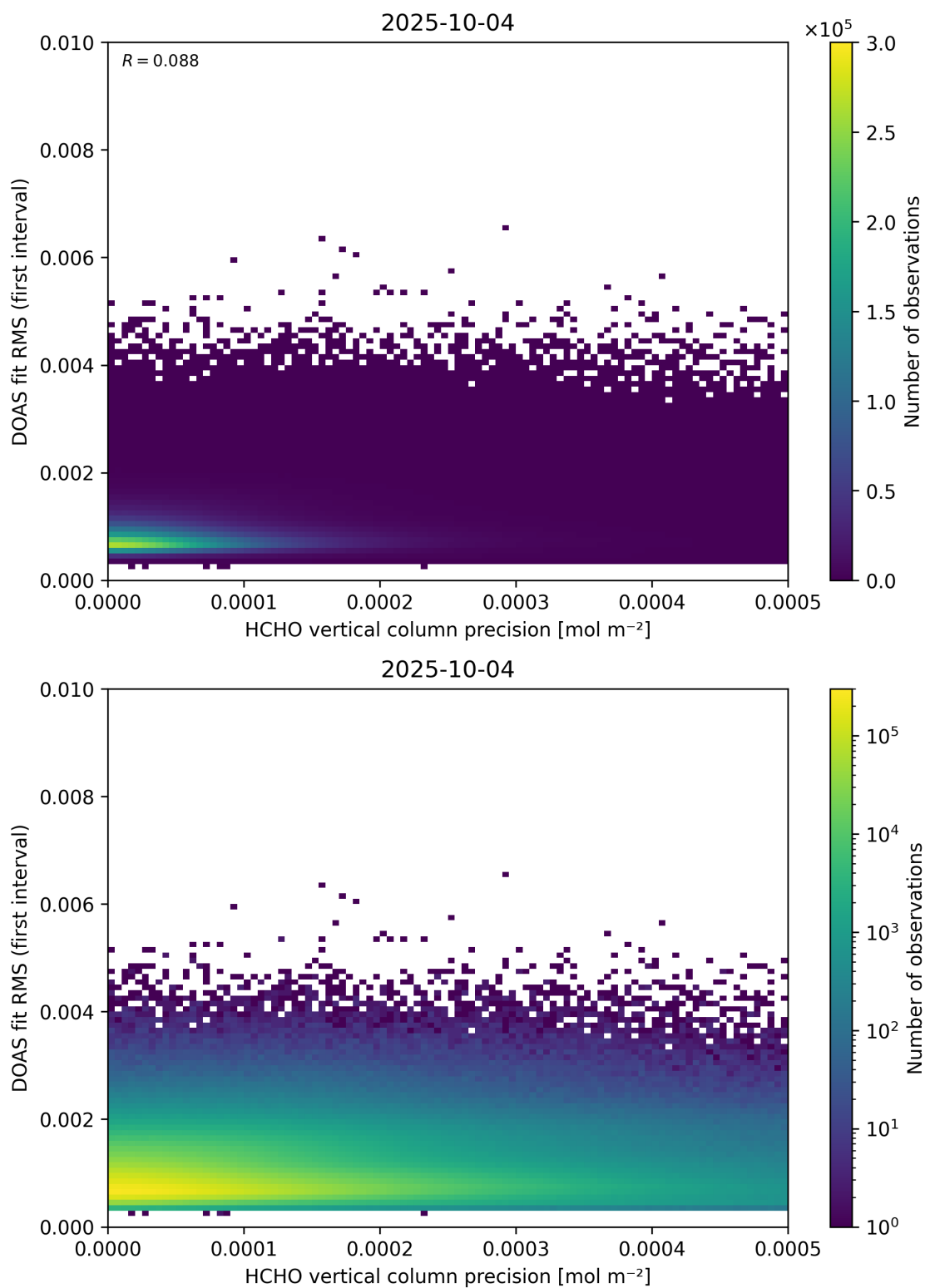
Figure 136: Scatter density plot of “HCHO vertical column precision” against “DOAS fit RMS (first interval)” for 2025-10-03 to 2025-10-05.
