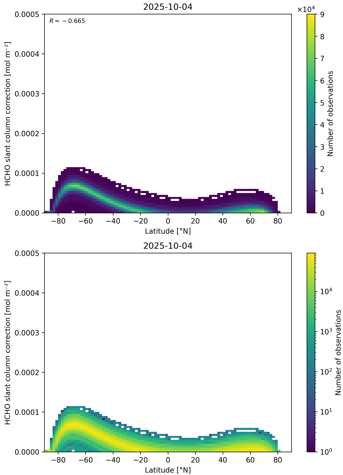
Figure 158: Scatter density plot of “Latitude” against “HCHO slant column correction” for 2025-10-03 to 2025-10-05.
