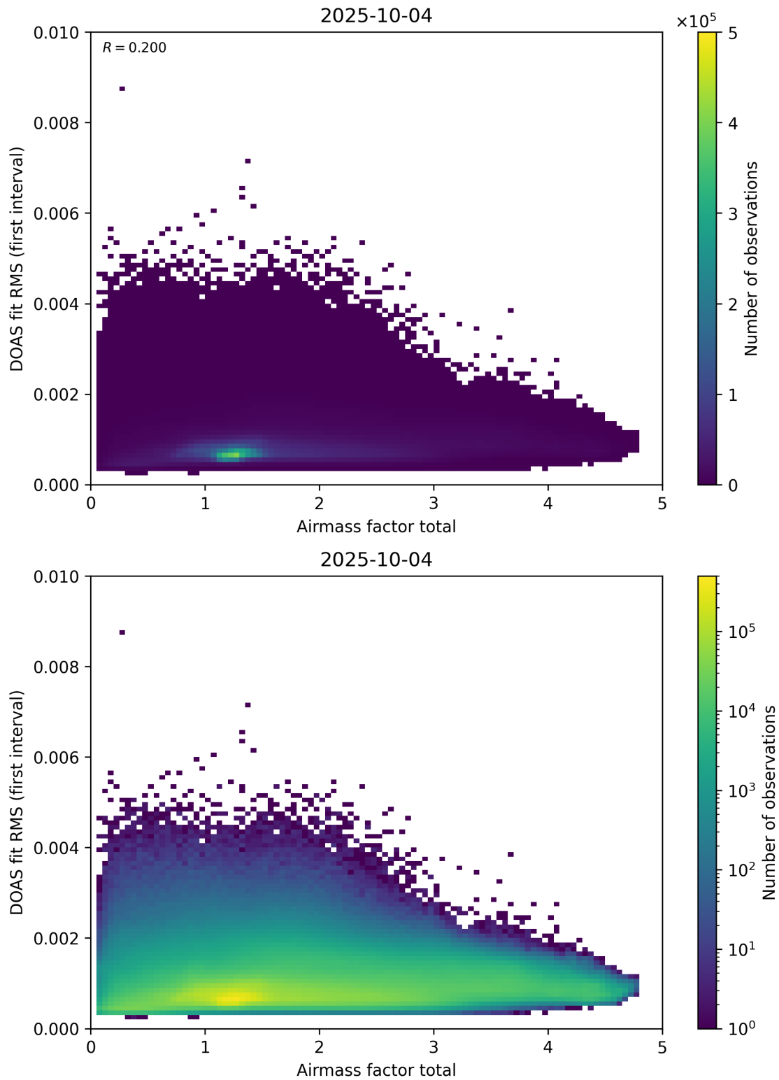
Figure 97: Scatter density plot of “Airmass factor total” against “DOAS fit RMS (first interval)” for 2025-10-03 to 2025-10-05.
