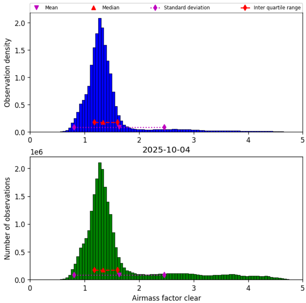
Figure 42: Histogram of “Airmass factor clear” for 2025-10-03 to 2025-10-05
