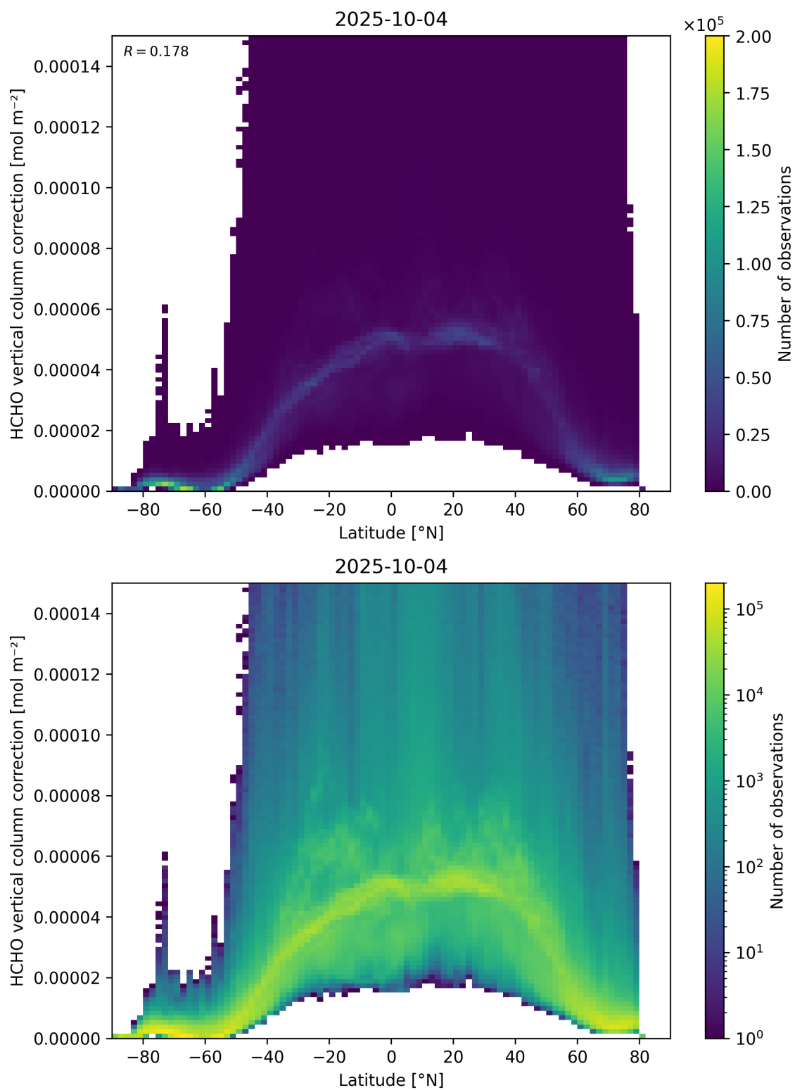
Figure 164: Scatter density plot of “Latitude” against “HCHO vertical column correction” for 2025-10-03 to 2025-10-05.
