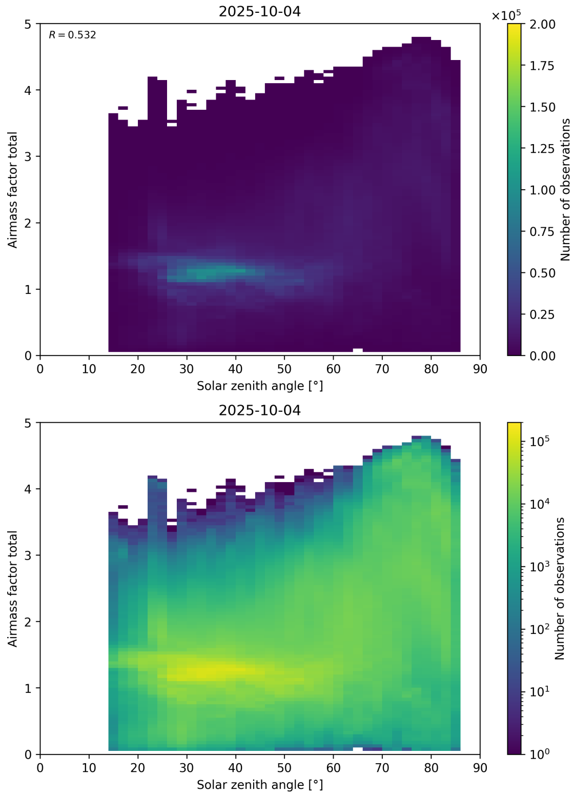
Figure 175: Scatter density plot of “Solar zenith angle” against “Airmass factor total” for 2025-10-03 to 2025-10-05.
