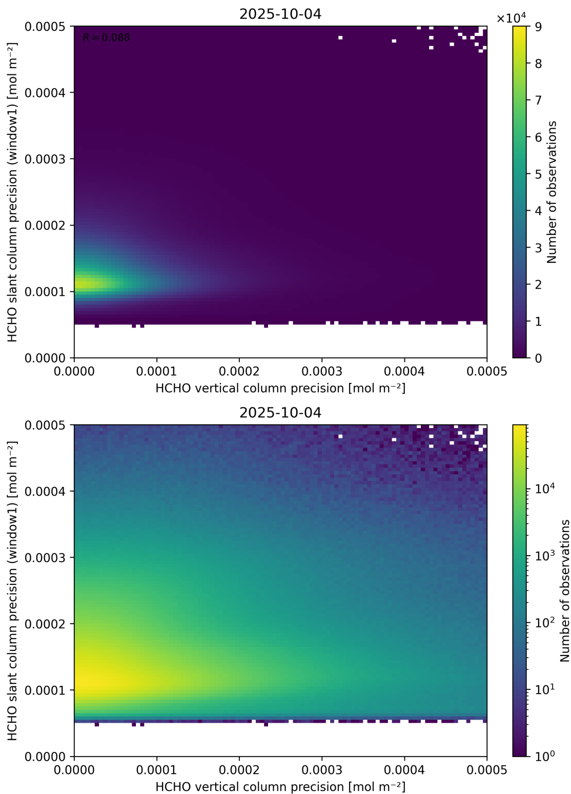
Figure 143: Scatter density plot of “HCHO vertical column precision” against “HCHO slant column precision (window1)” for 2025-10-03 to 2025-10-05.
