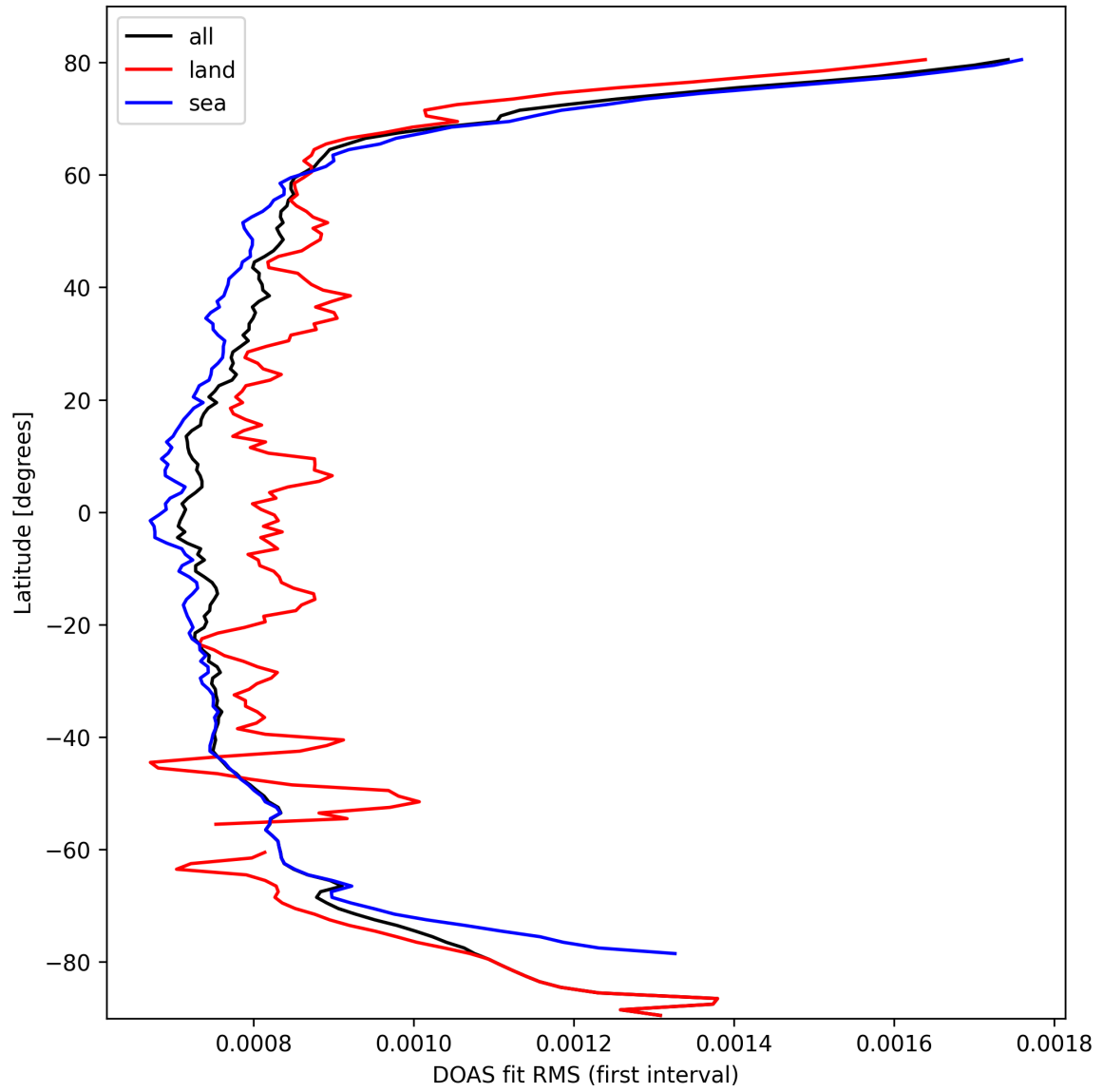
Figure 32: Zonal average of “DOAS fit RMS (first interval)” for 2025-10-03 to 2025-10-05.
