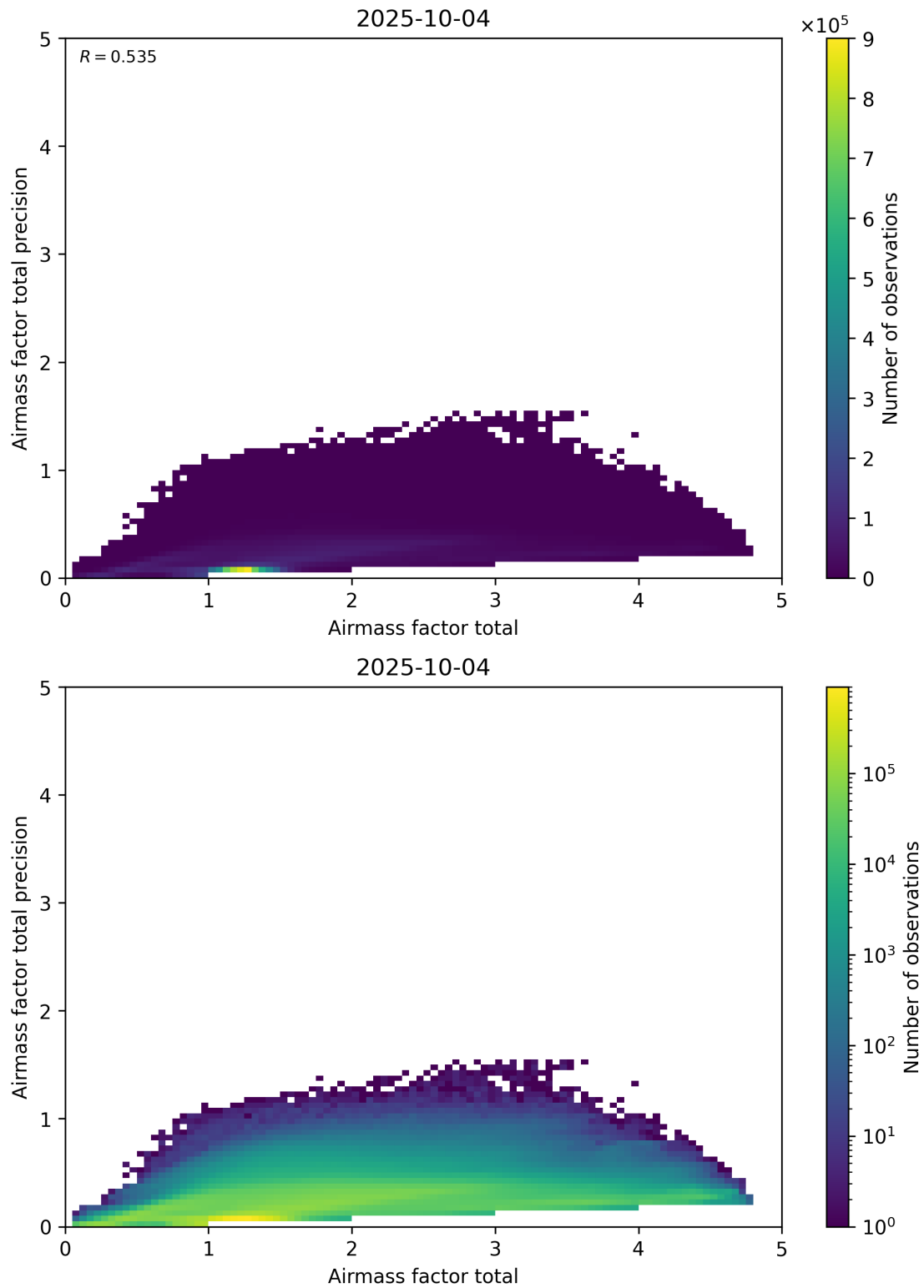
Figure 103: Scatter density plot of “Airmass factor total” against “Airmass factor total precision” for 2025-10-03 to 2025-10-05.
