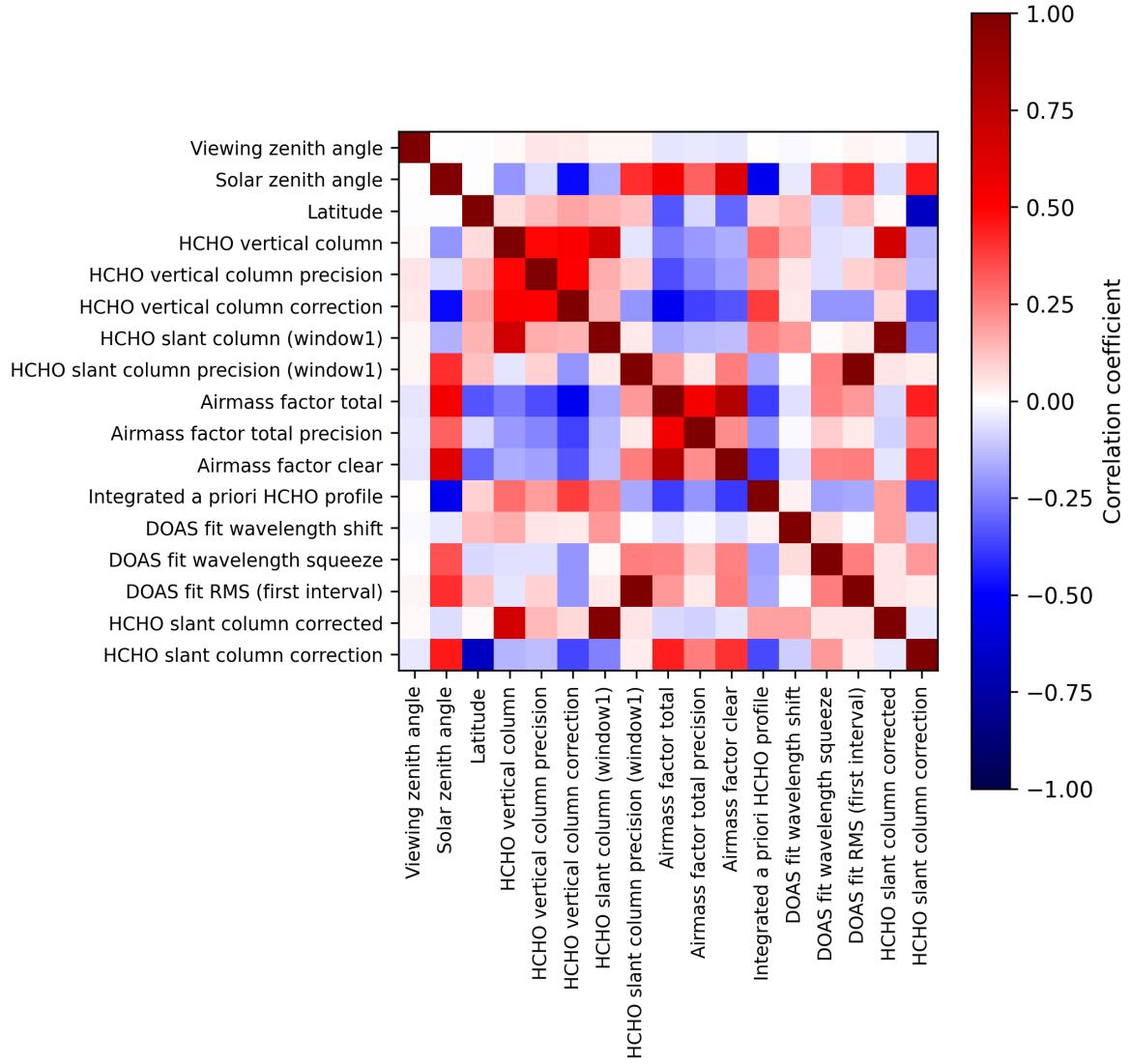
Figure 2: Map of correlation matrix for 2025-10-03 to 2025-10-05.
