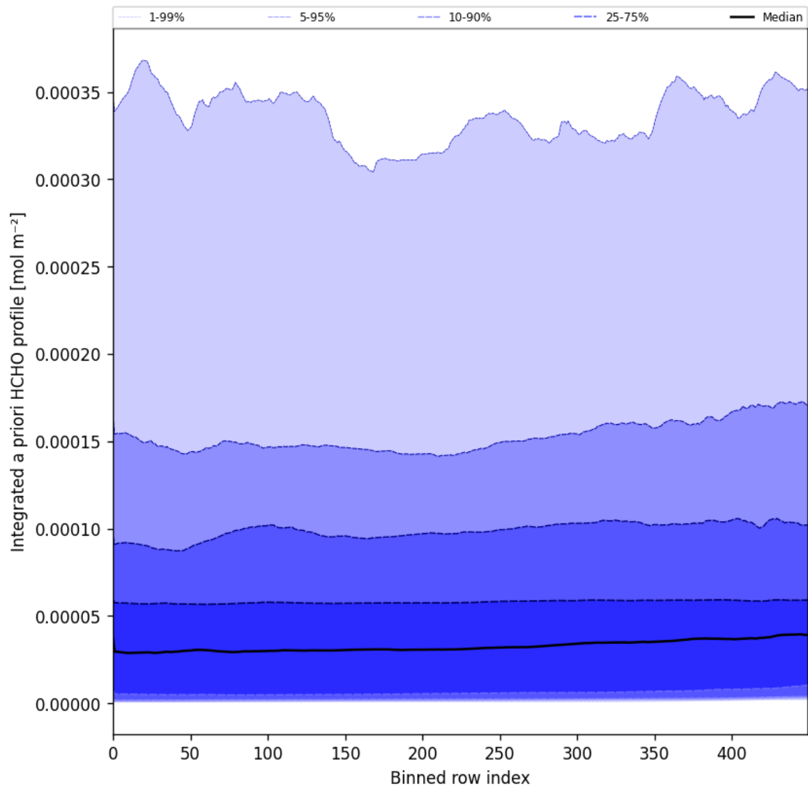
Figure 57: Along track statistics of “Integrated a priori HCHO profile” for 2025-10-03 to 2025-10-05
