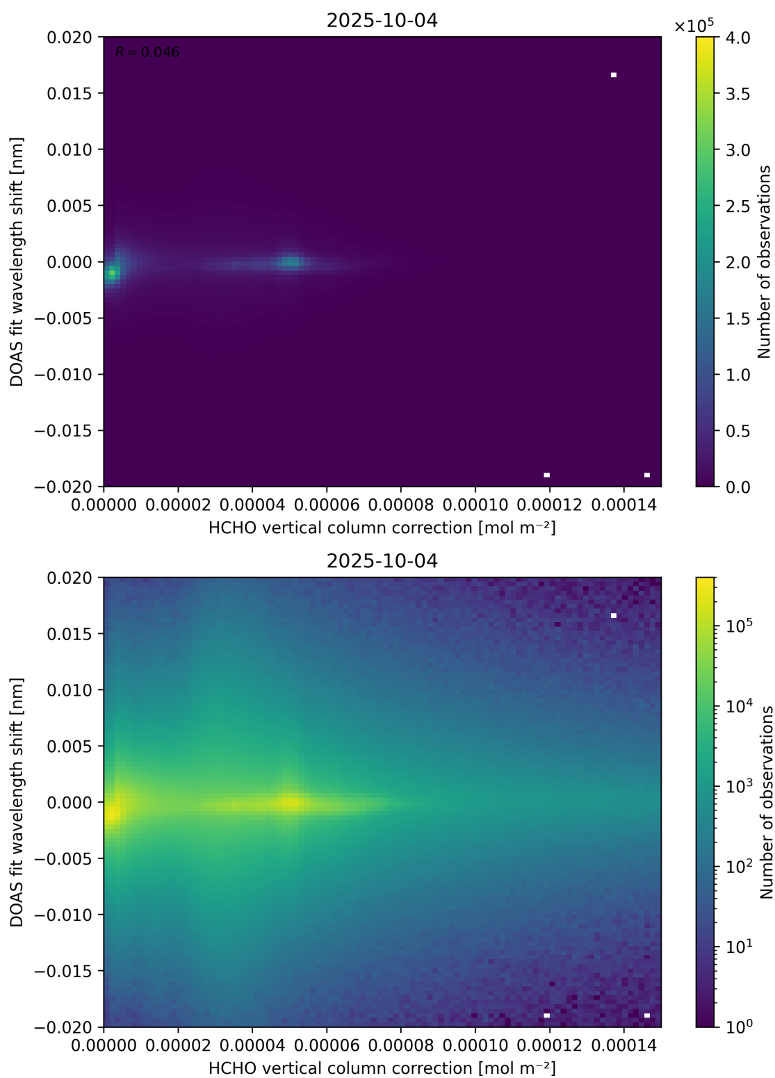
Figure 113: Scatter density plot of “HCHO vertical column correction” against “DOAS fit wavelength shift” for 2025-10-03 to 2025-10-05.
