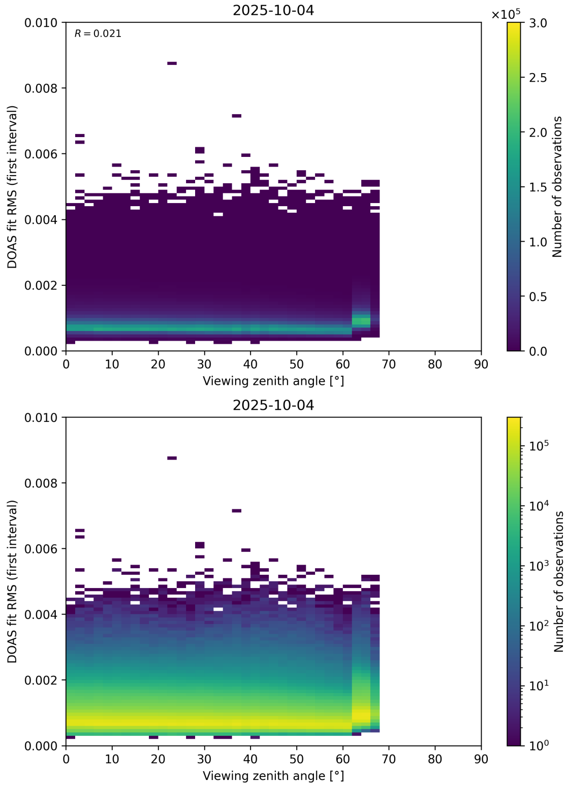
Figure 182: Scatter density plot of “Viewing zenith angle” against “DOAS fit RMS (first interval)” for 2025-10-03 to 2025-10-05.
