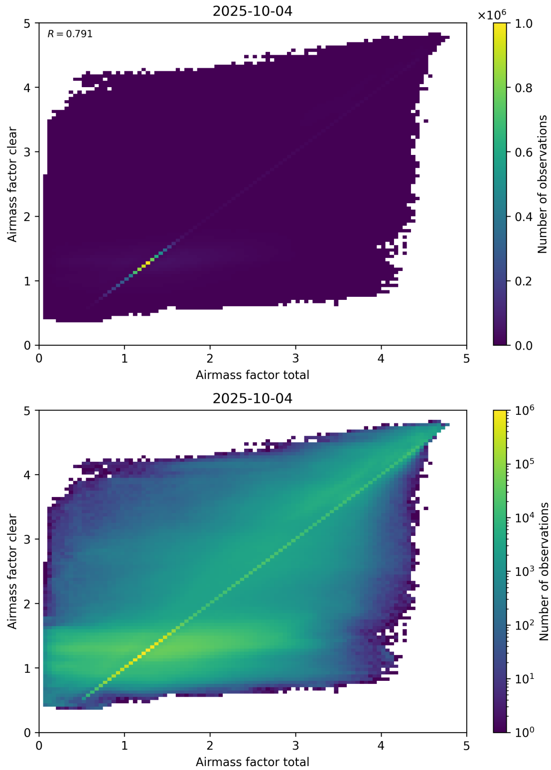
Figure 100: Scatter density plot of “Airmass factor total” against “Airmass factor clear” for 2025-10-03 to 2025-10-05.
