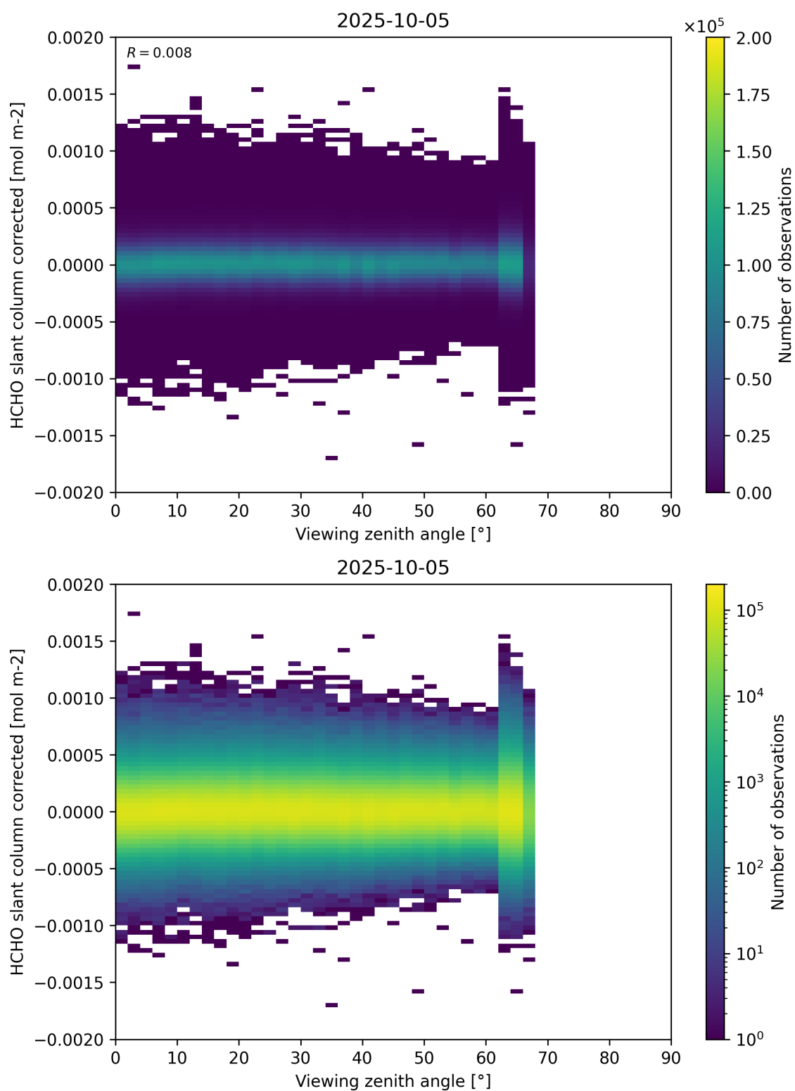
Figure 186: Scatter density plot of “Viewing zenith angle” against “HCHO slant column corrected” for 2025-10-04 to 2025-10-06.
