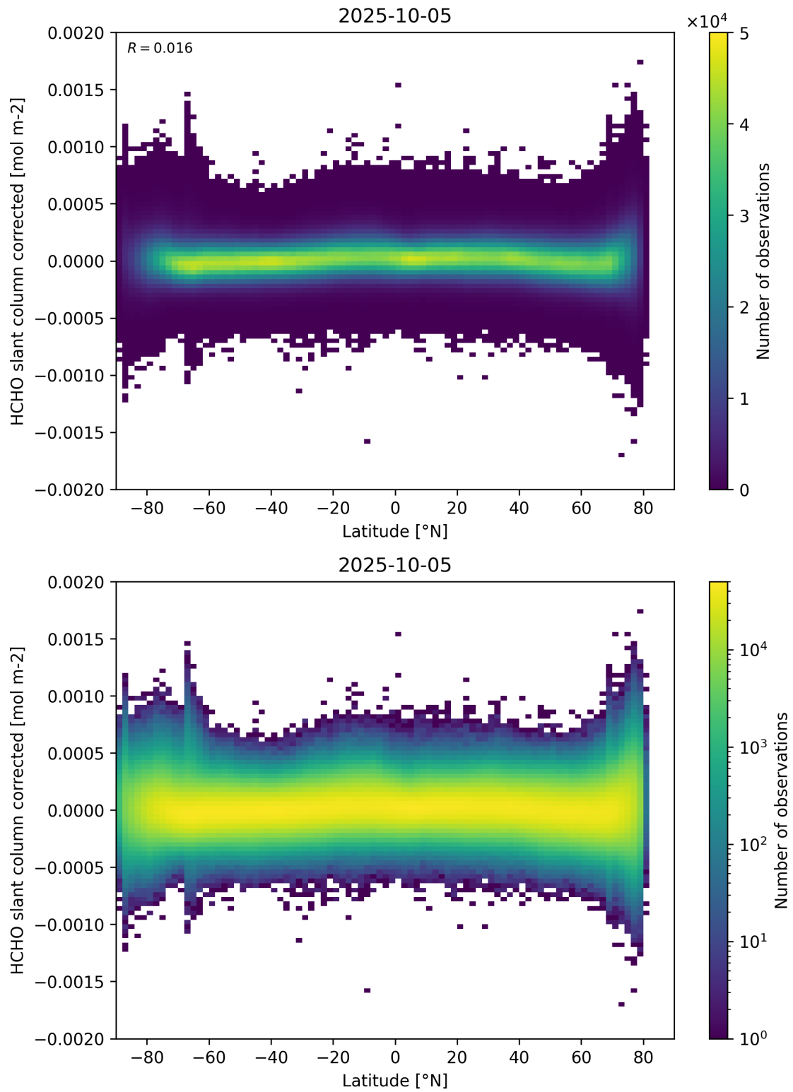
Figure 157: Scatter density plot of “Latitude” against “HCHO slant column corrected” for 2025-10-04 to 2025-10-06.
