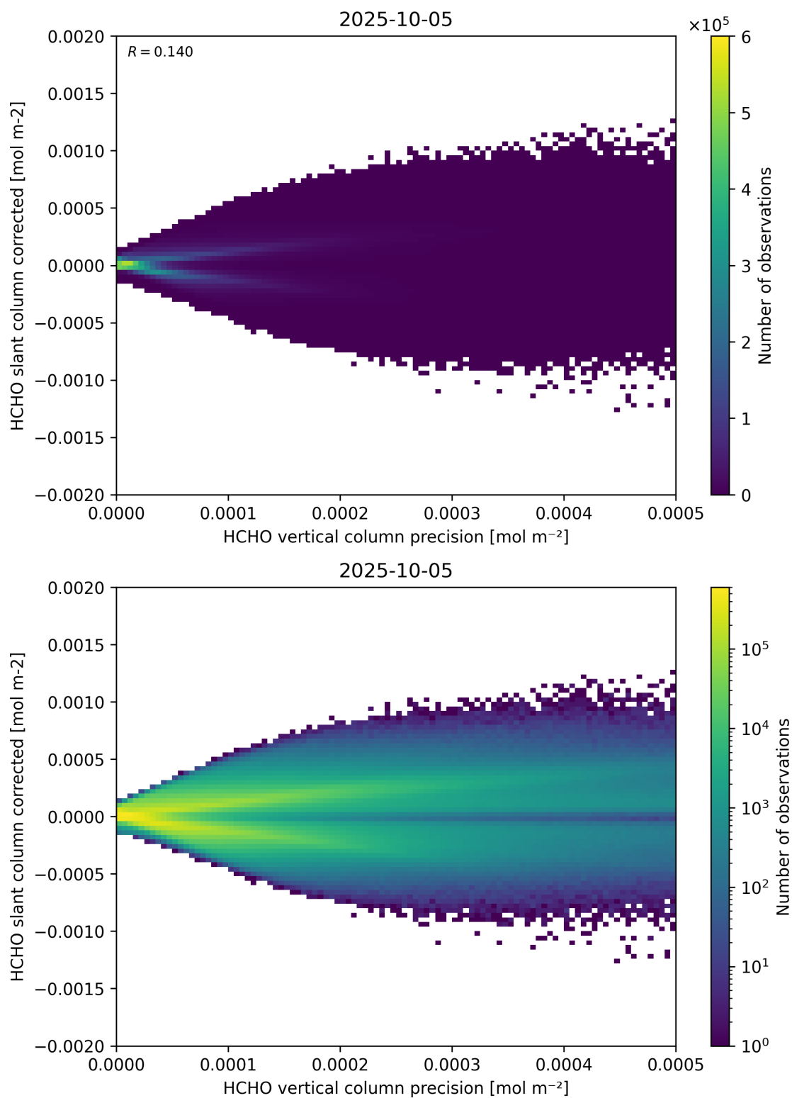
Figure 140: Scatter density plot of “HCHO vertical column precision” against “HCHO slant column corrected” for 2025-10-04 to 2025-10-06.
