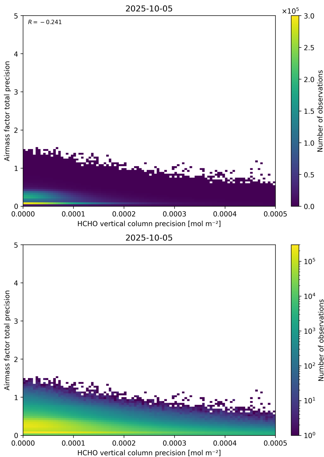
Figure 145: Scatter density plot of “HCHO vertical column precision” against “Airmass factor total precision” for 2025-10-04 to 2025-10-06.
