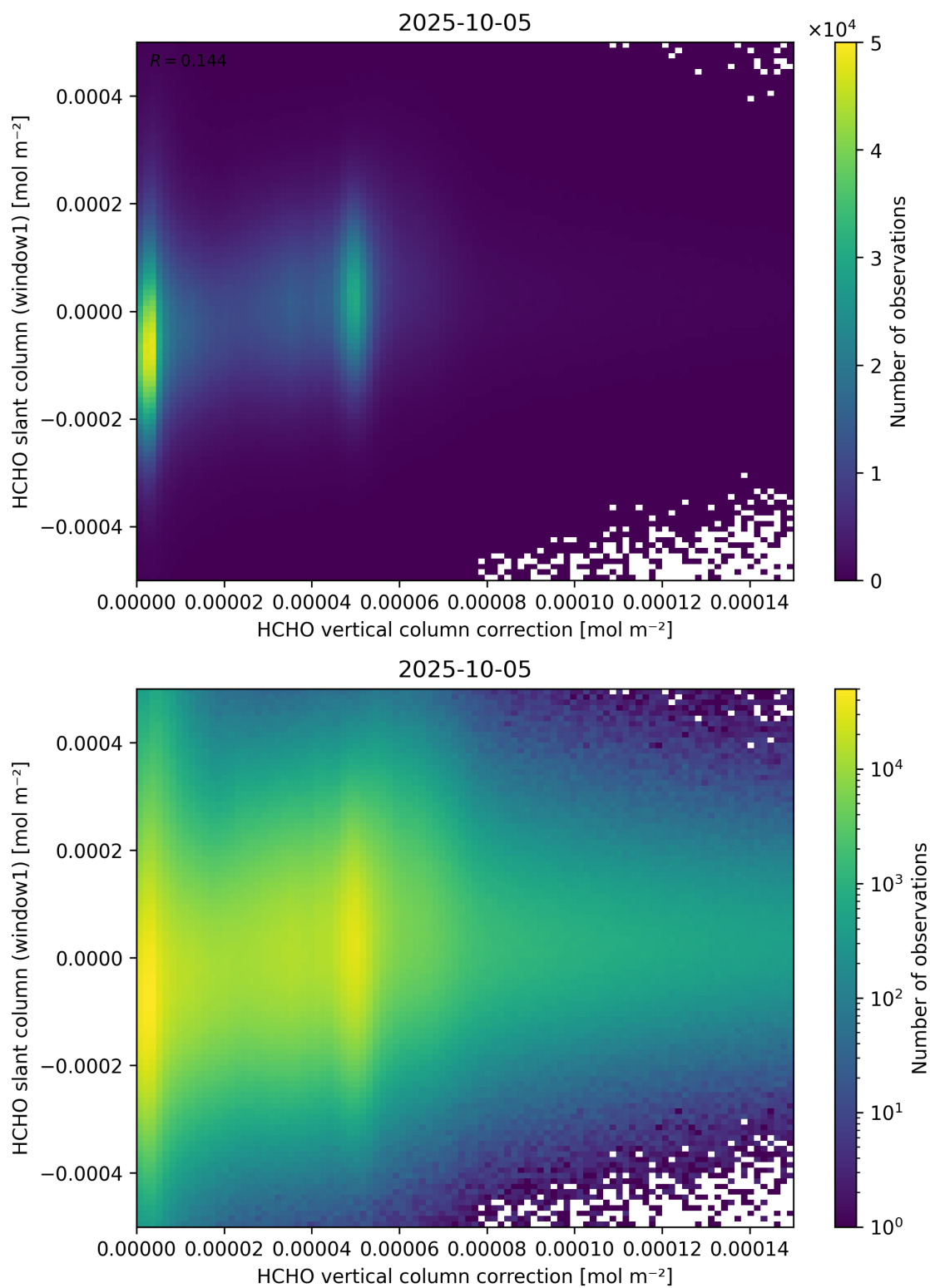
Figure 118: Scatter density plot of “HCHO vertical column correction” against “HCHO slant column (window1)” for 2025-10-04 to 2025-10-06.
