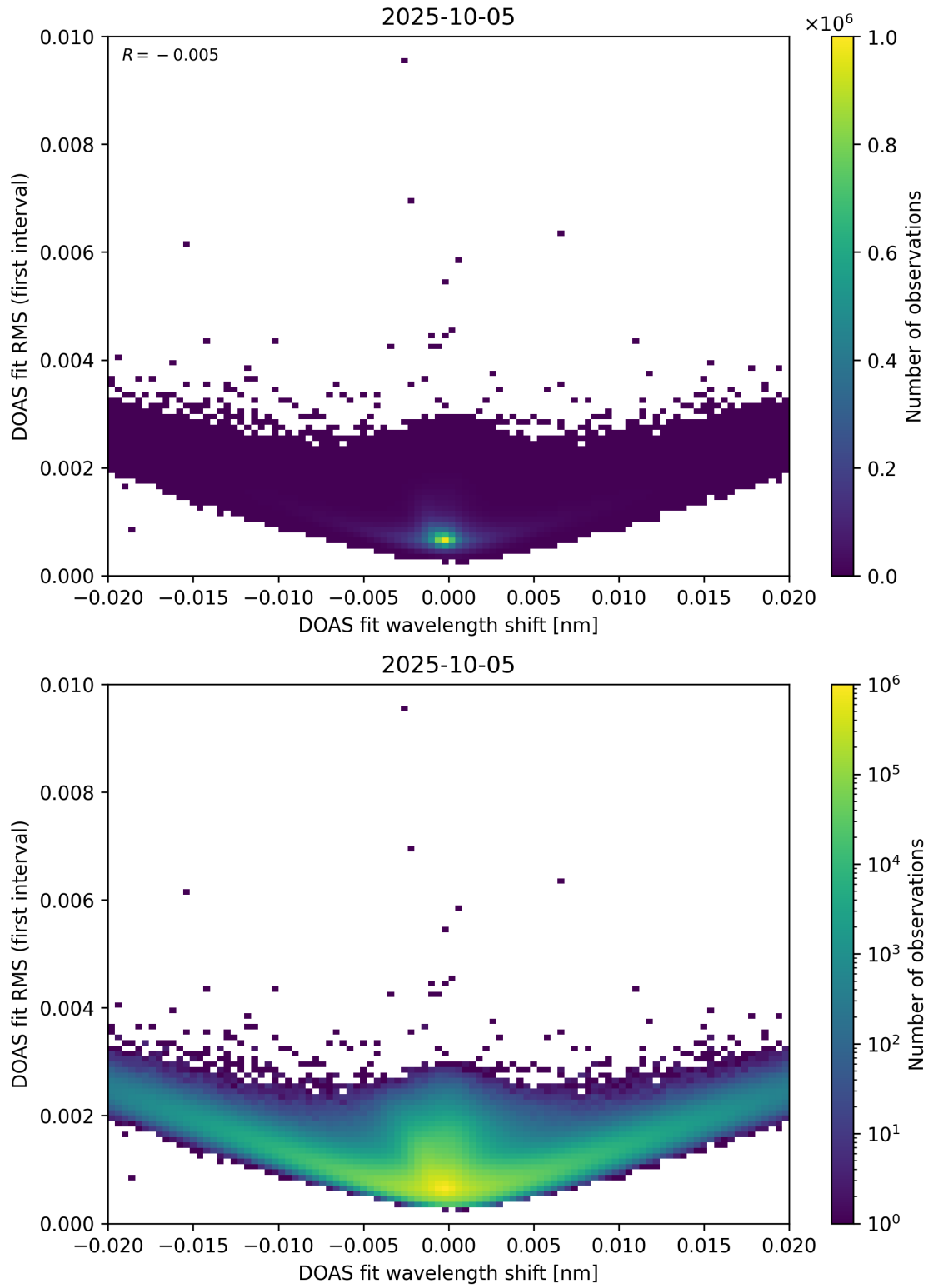
Figure 64: Scatter density plot of “DOAS fit wavelength shift” against “DOAS fit RMS (first interval)” for 2025-10-04 to 2025-10-06.
