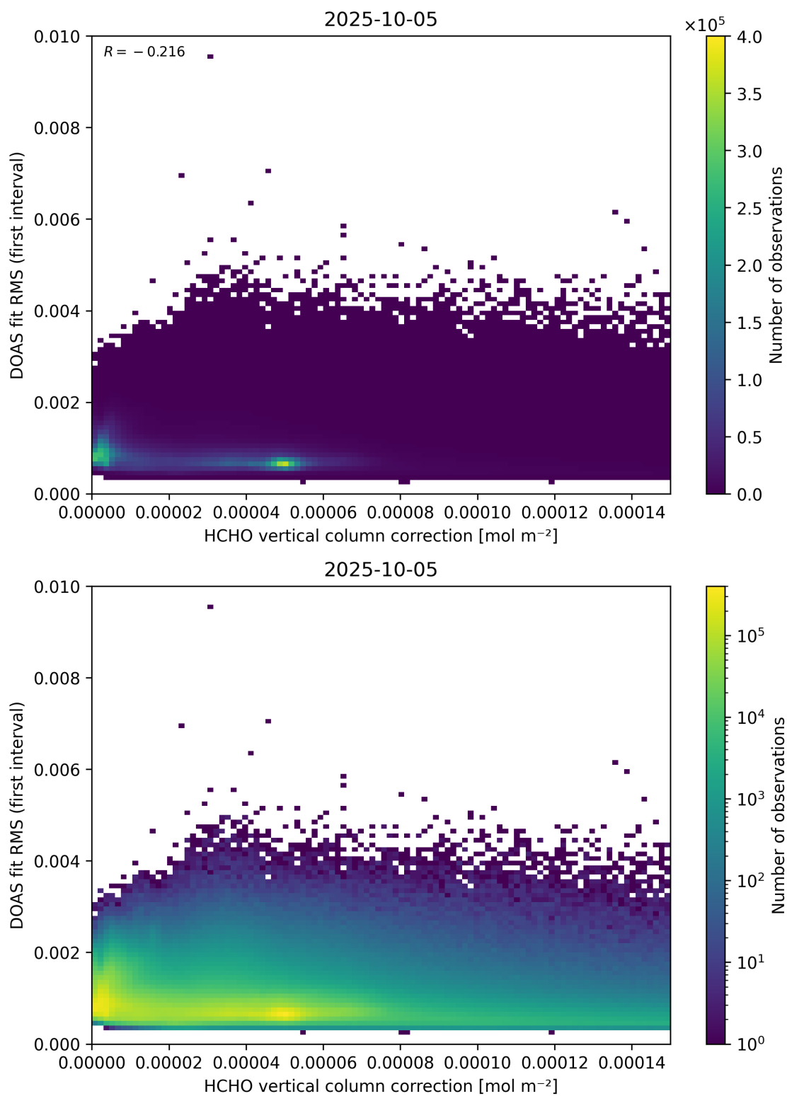
Figure 112: Scatter density plot of “HCHO vertical column correction” against “DOAS fit RMS (first interval)” for 2025-10-04 to 2025-10-06.
