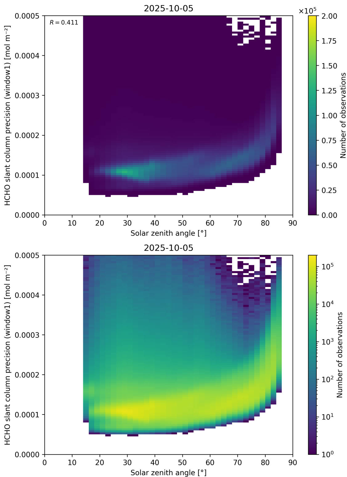
Figure 174: Scatter density plot of “Solar zenith angle” against “HCHO slant column precision (window1)” for 2025-10-04 to 2025-10-06.
