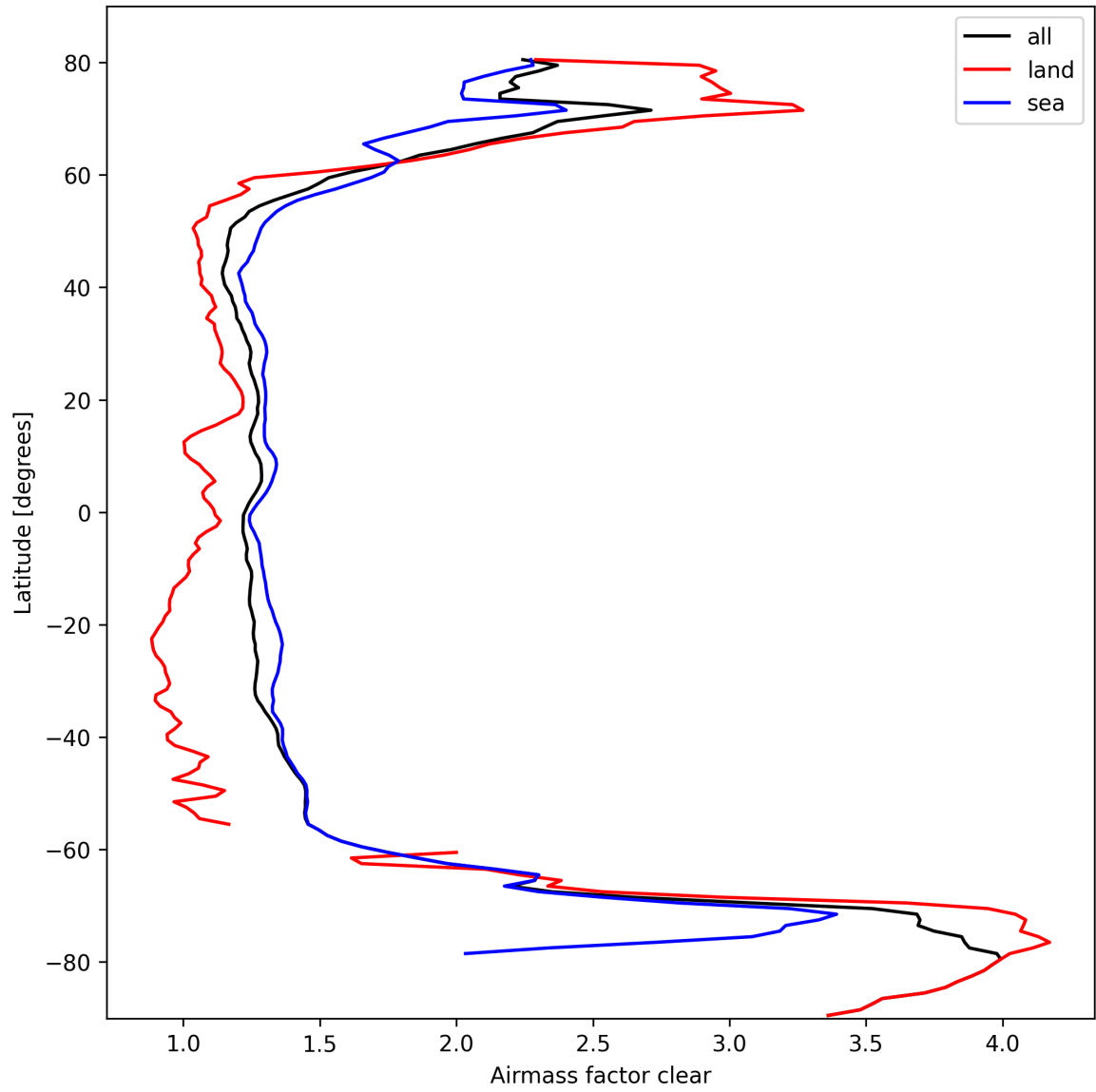
Figure 28: Zonal average of “Airmass factor clear” for 2025-10-04 to 2025-10-06.
