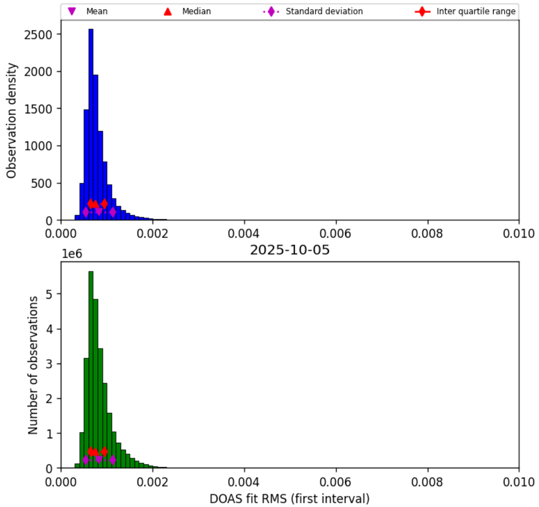
Figure 46: Histogram of “DOAS fit RMS (first interval)” for 2025-10-04 to 2025-10-06
