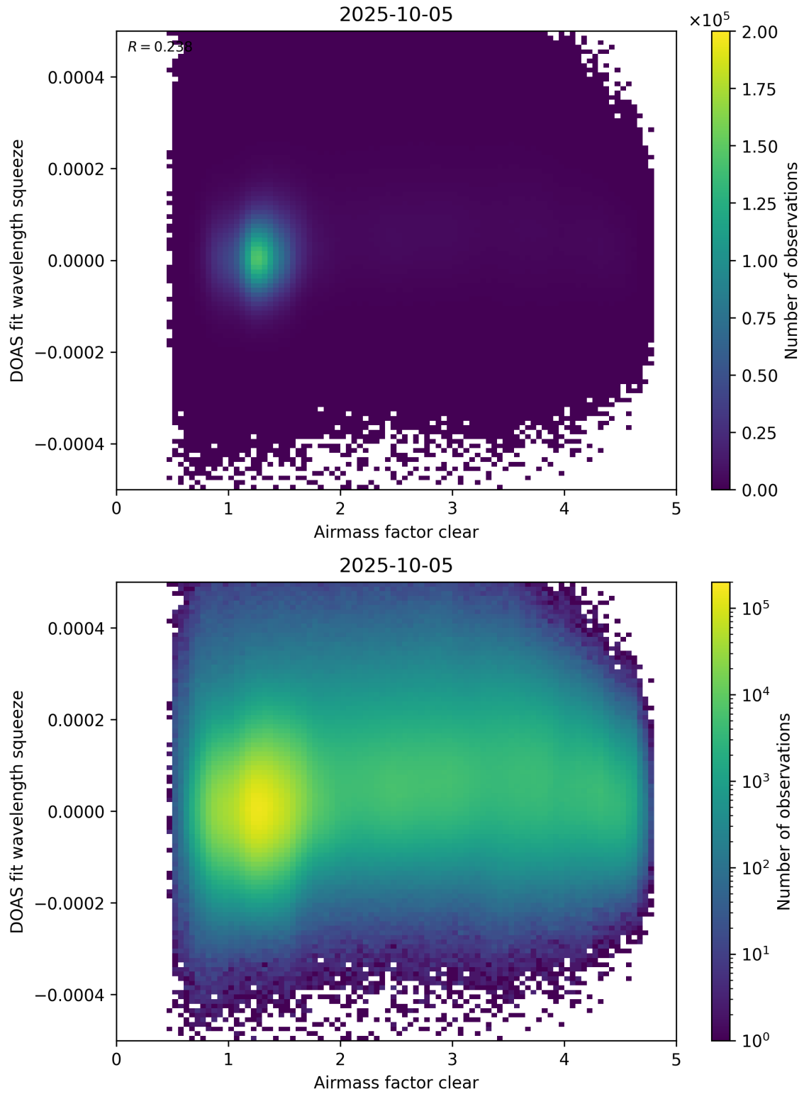
Figure 73: Scatter density plot of “Airmass factor clear” against “DOAS fit wavelength squeeze” for 2025-10-04 to 2025-10-06.
