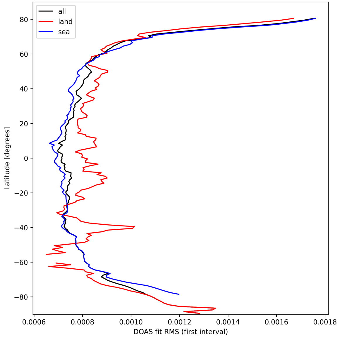
Figure 32: Zonal average of “DOAS fit RMS (first interval)” for 2025-10-04 to 2025-10-06.
