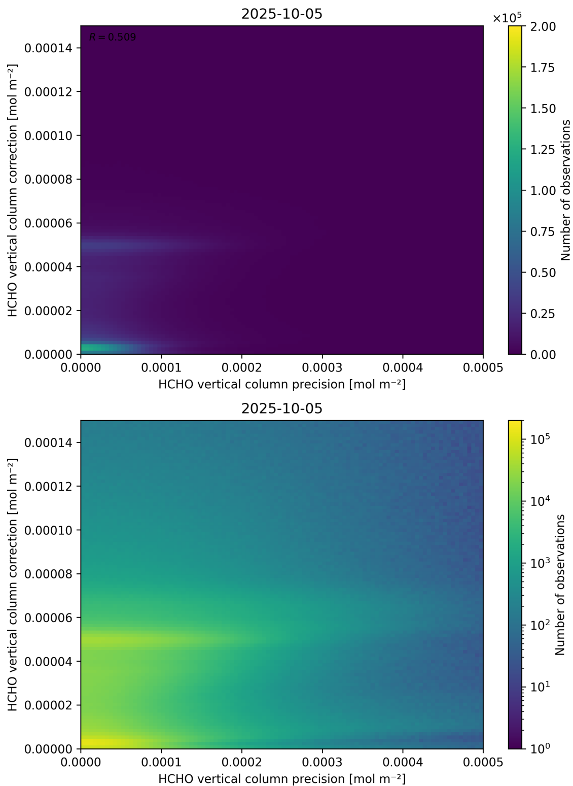
Figure 146: Scatter density plot of “HCHO vertical column precision” against “HCHO vertical column correction” for 2025-10-04 to 2025-10-06.
