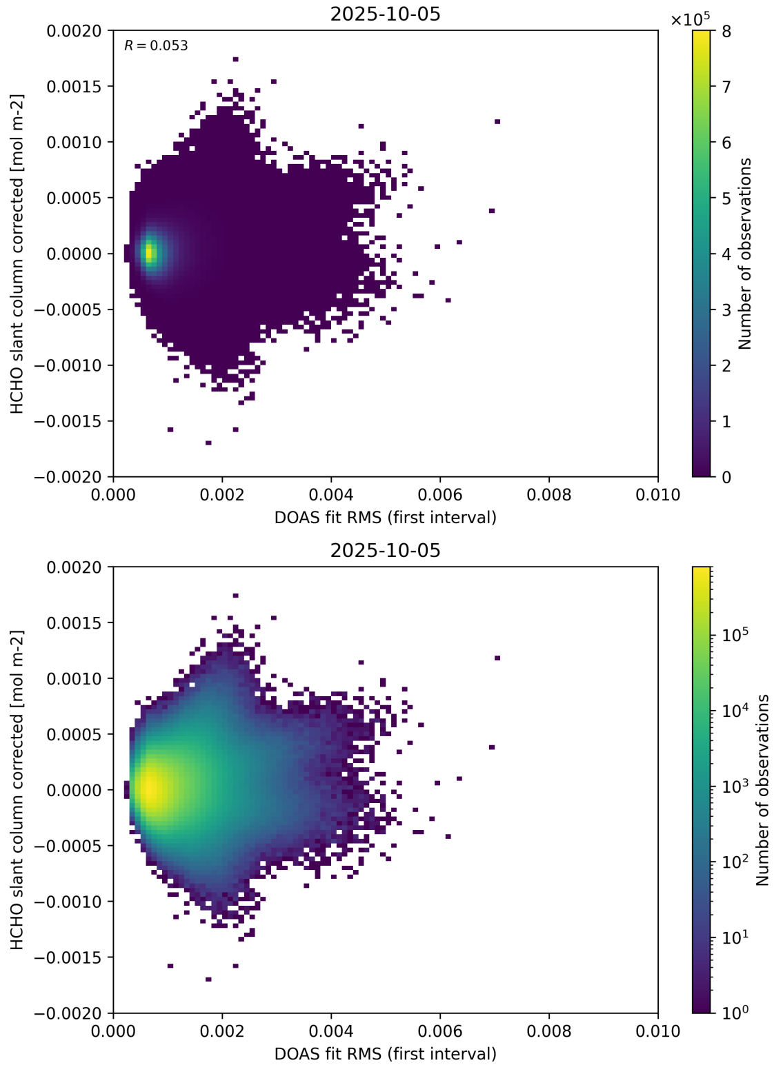
Figure 62: Scatter density plot of “DOAS fit RMS (first interval)” against “HCHO slant column corrected” for 2025-10-04 to 2025-10-06.
