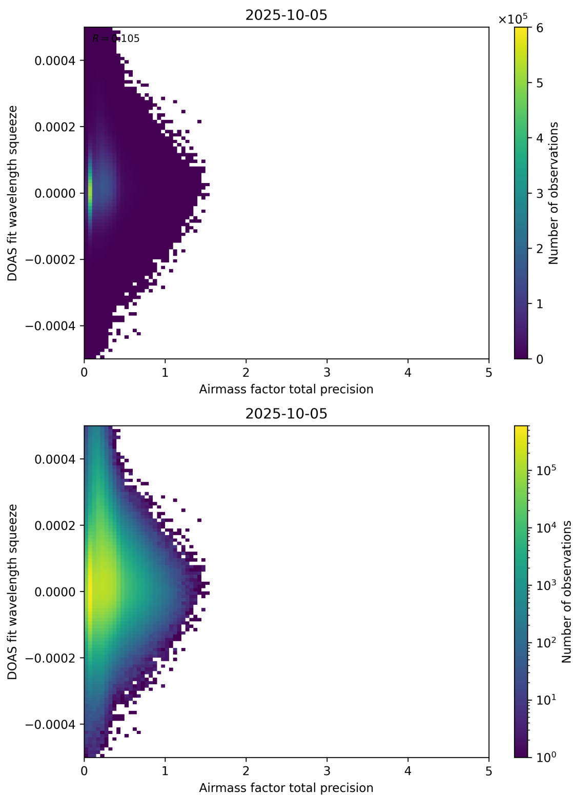
Figure 107: Scatter density plot of “Airmass factor total precision” against “DOAS fit wavelength squeeze” for 2025-10-04 to 2025-10-06.
