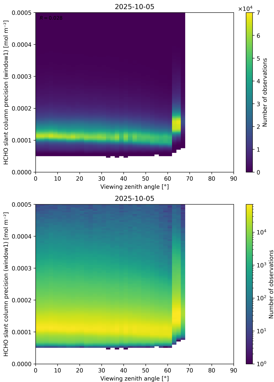
Figure 189: Scatter density plot of “Viewing zenith angle” against “HCHO slant column precision (window1)” for 2025-10-04 to 2025-10-06.
