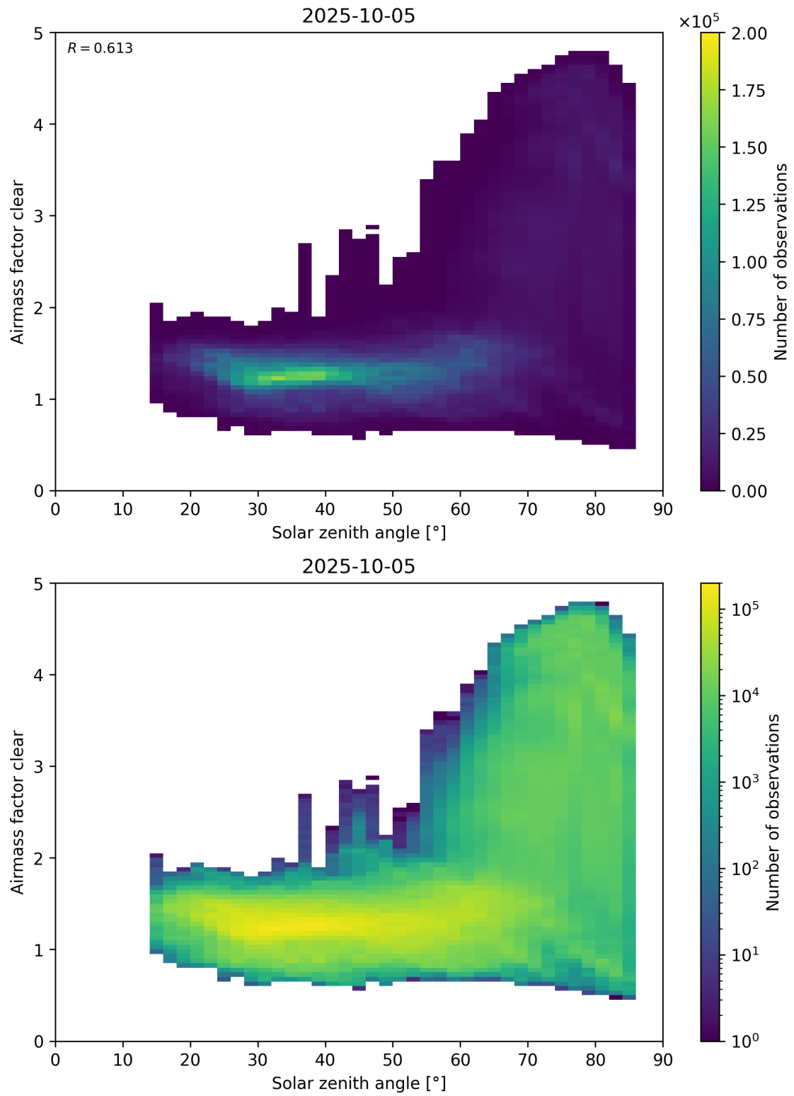
Figure 170: Scatter density plot of “Solar zenith angle” against “Airmass factor clear” for 2025-10-04 to 2025-10-06.
