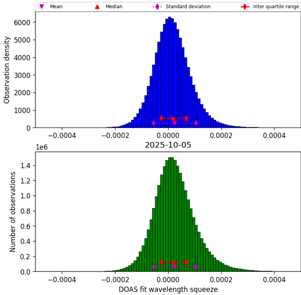
Figure 45: Histogram of “DOAS fit wavelength squeeze” for 2025-10-04 to 2025-10-06
