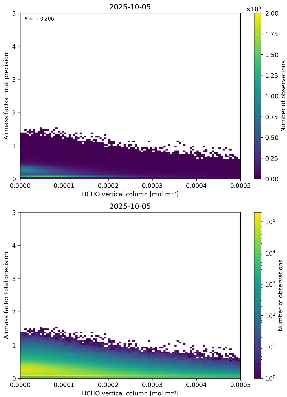
Figure 132: Scatter density plot of “HCHO vertical column” against “Airmass factor total precision” for 2025-10-04 to 2025-10-06.
