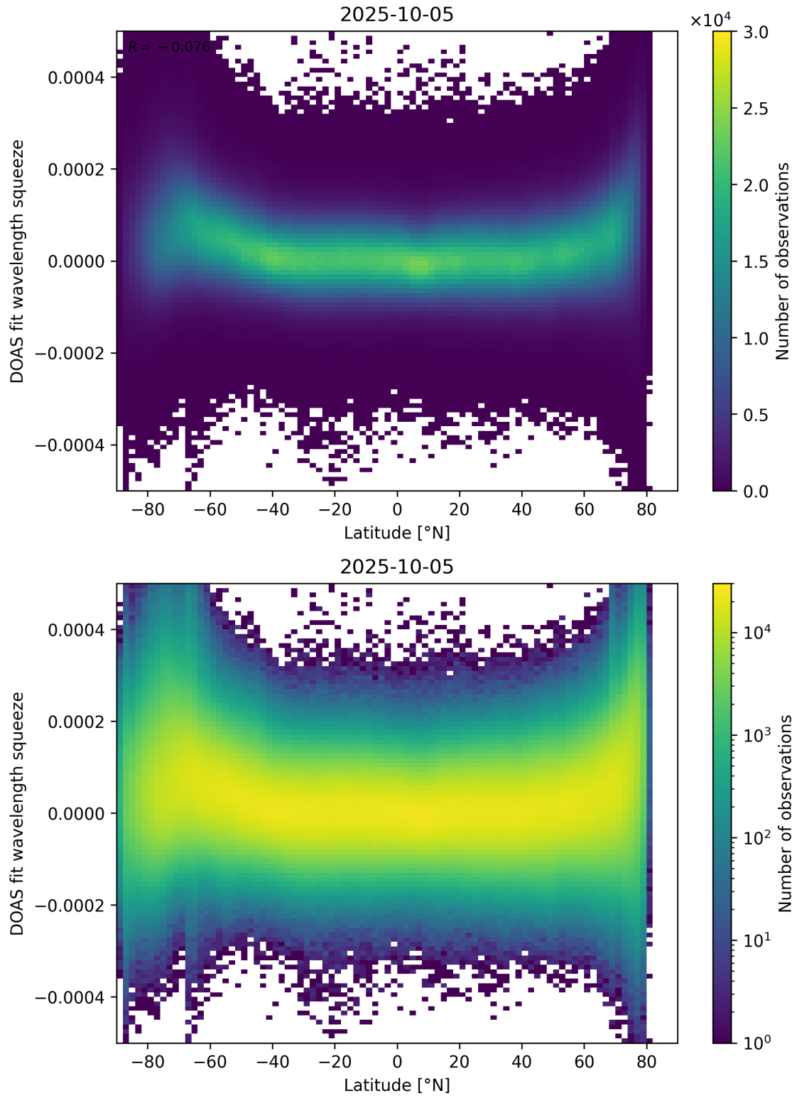
Figure 155: Scatter density plot of “Latitude” against “DOAS fit wavelength squeeze” for 2025-10-04 to 2025-10-06.
