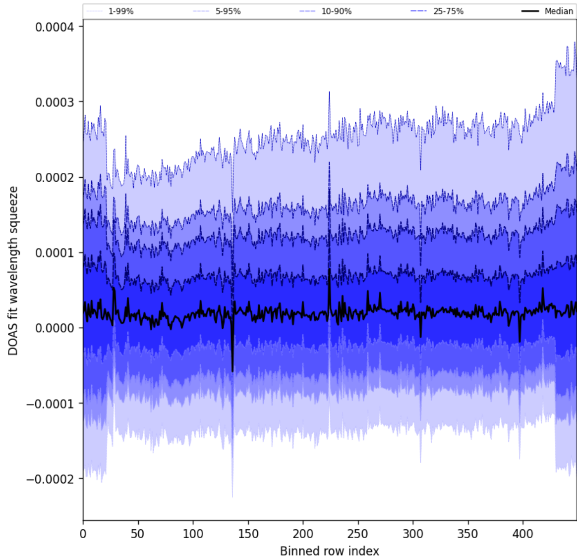
Figure 59: Along track statistics of “DOAS fit wavelength squeeze” for 2025-10-04 to 2025-10-06
