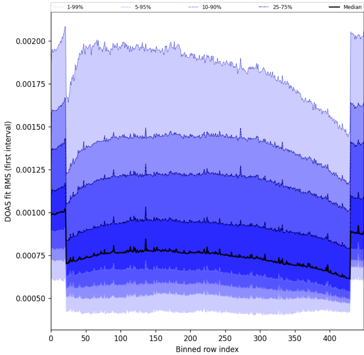
Figure 60: Along track statistics of “DOAS fit RMS (first interval)” for 2025-10-04 to 2025-10-06
