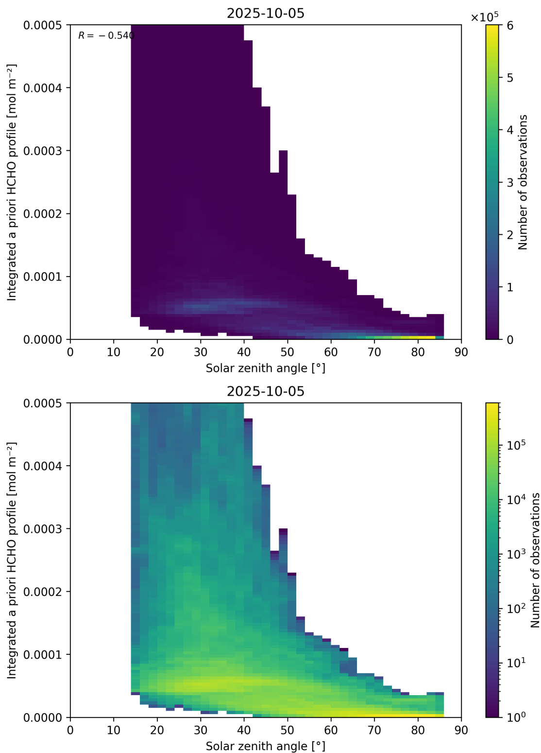
Figure 180: Scatter density plot of “Solar zenith angle” against “Integrated a priori HCHO profile” for 2025-10-04 to 2025-10-06.
