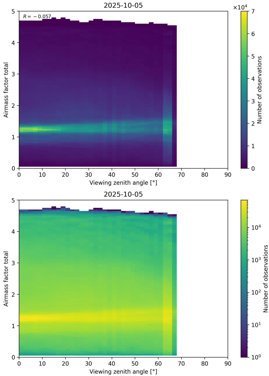
Figure 190: Scatter density plot of “Viewing zenith angle” against “Airmass factor total” for 2025-10-04 to 2025-10-06.
