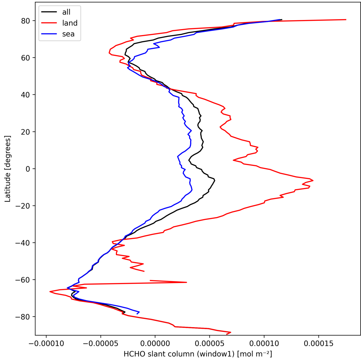
Figure 24: Zonal average of “HCHO slant column (window1)” for 2025-10-04 to 2025-10-06.
