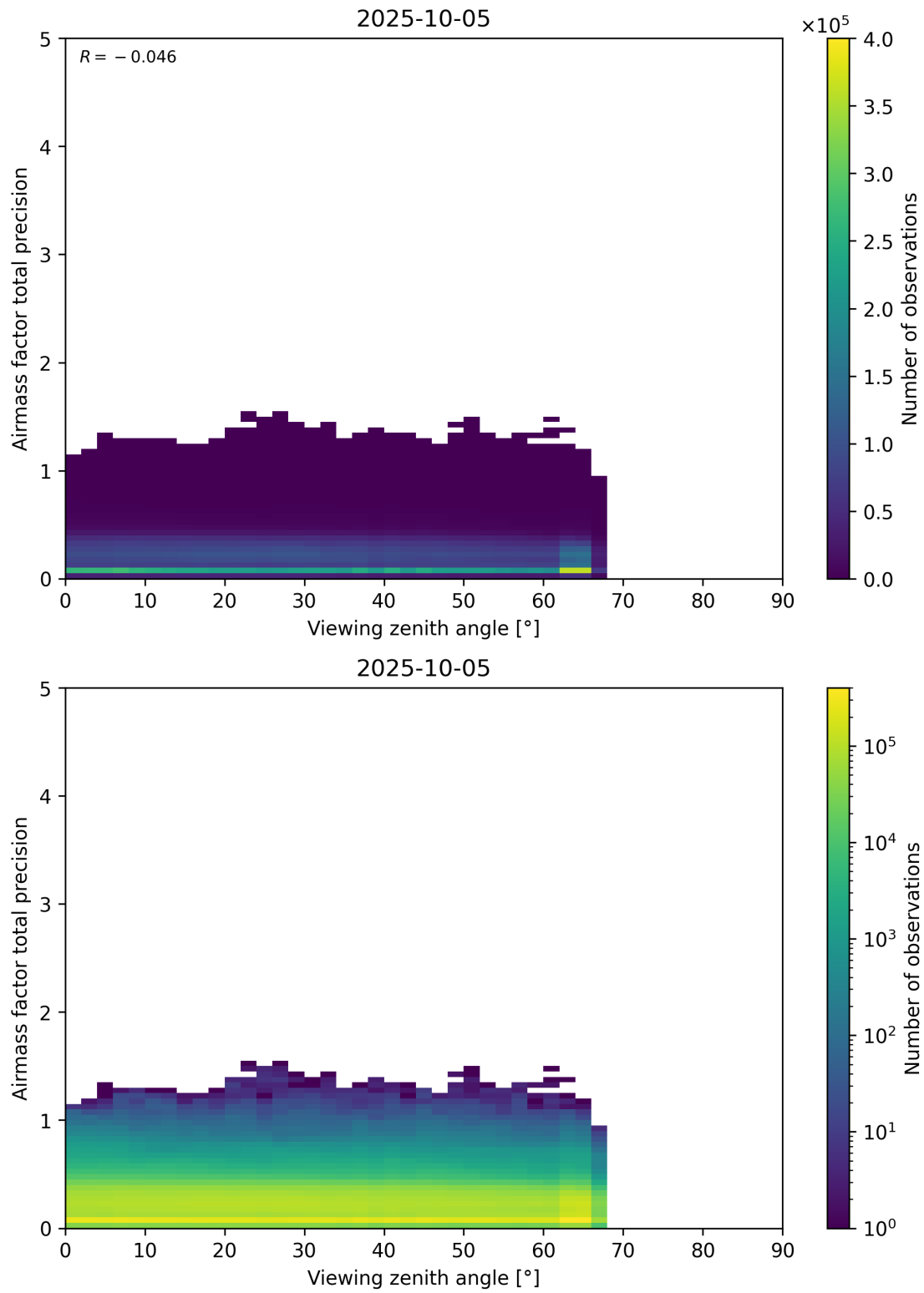
Figure 191: Scatter density plot of “Viewing zenith angle” against “Airmass factor total precision” for 2025-10-04 to 2025-10-06.
