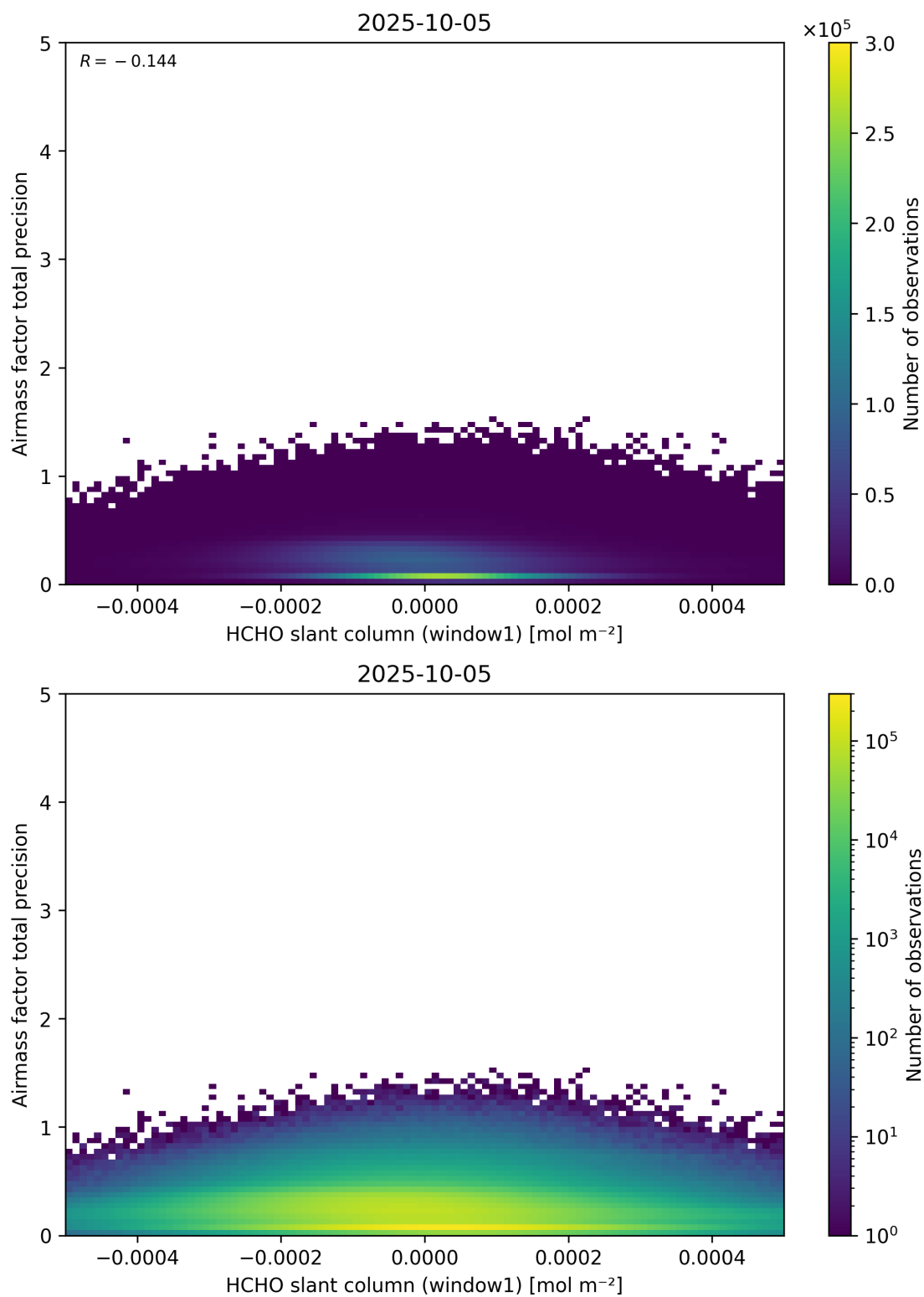
Figure 86: Scatter density plot of “HCHO slant column (window1)” against “Airmass factor total precision” for 2025-10-04 to 2025-10-06.
