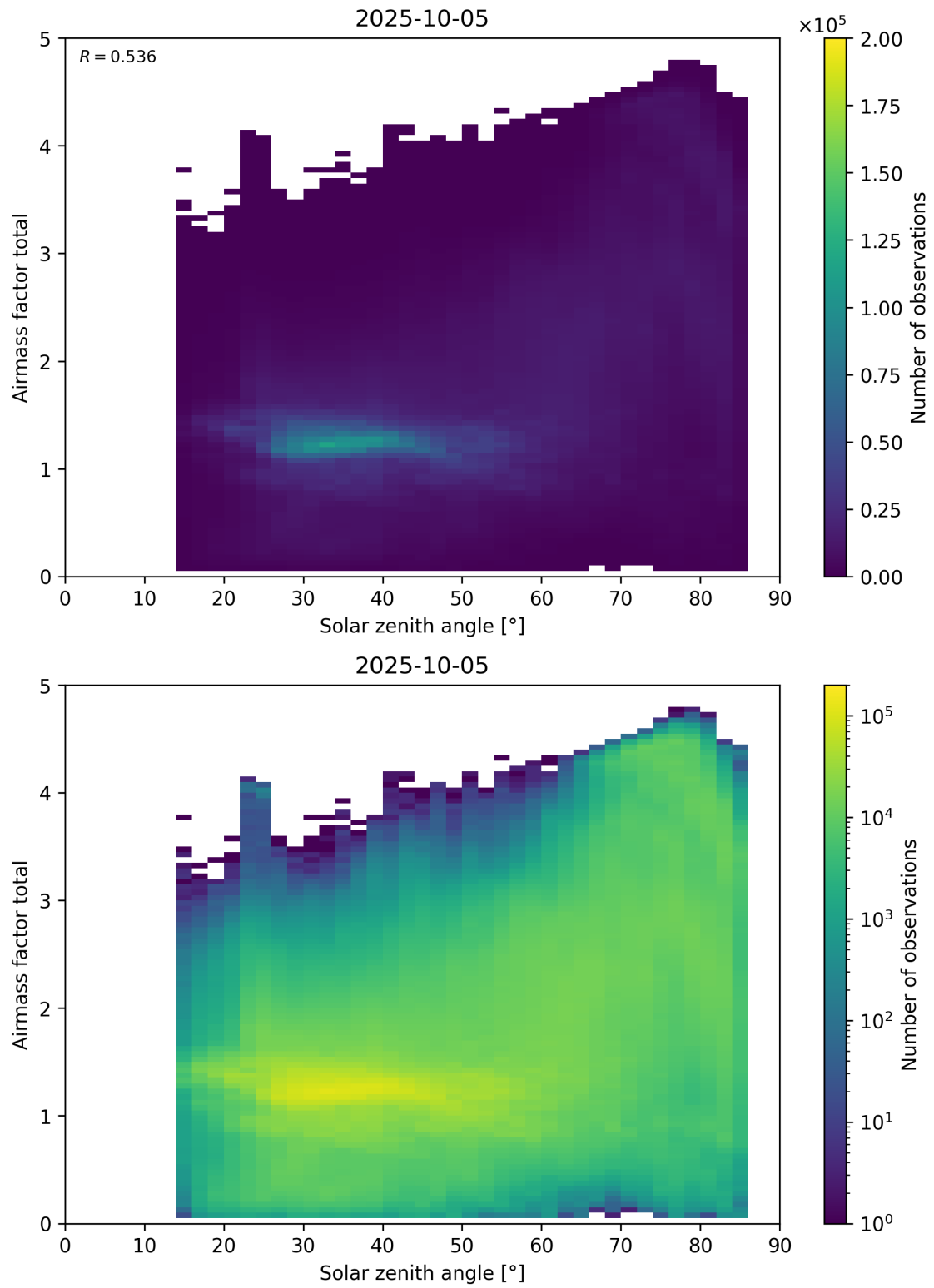
Figure 175: Scatter density plot of “Solar zenith angle” against “Airmass factor total” for 2025-10-04 to 2025-10-06.
