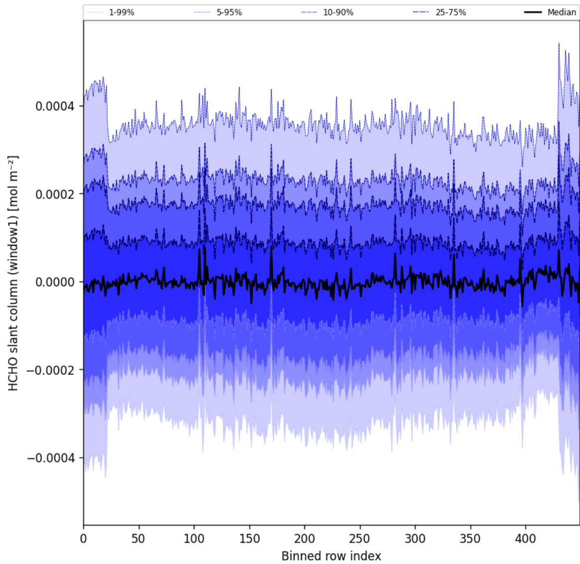
Figure 52: Along track statistics of “HCHO slant column (window1)” for 2025-10-04 to 2025-10-06
