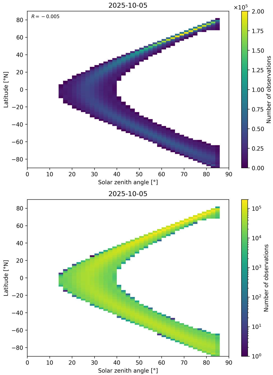
Figure 181: Scatter density plot of “Solar zenith angle” against “Latitude” for 2025-10-04 to 2025-10-06.
