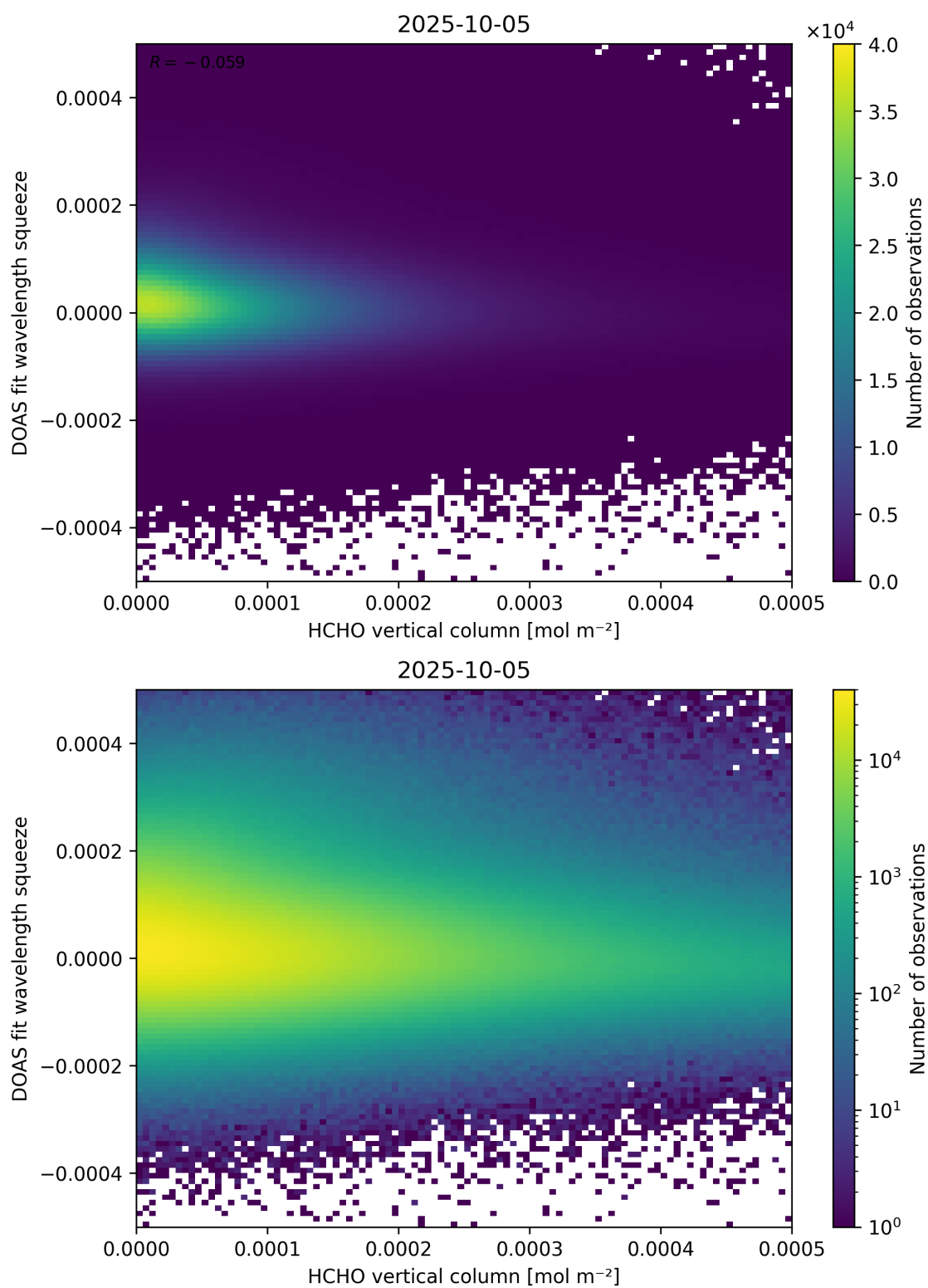
Figure 125: Scatter density plot of “HCHO vertical column” against “DOAS fit wavelength squeeze” for 2025-10-04 to 2025-10-06.
