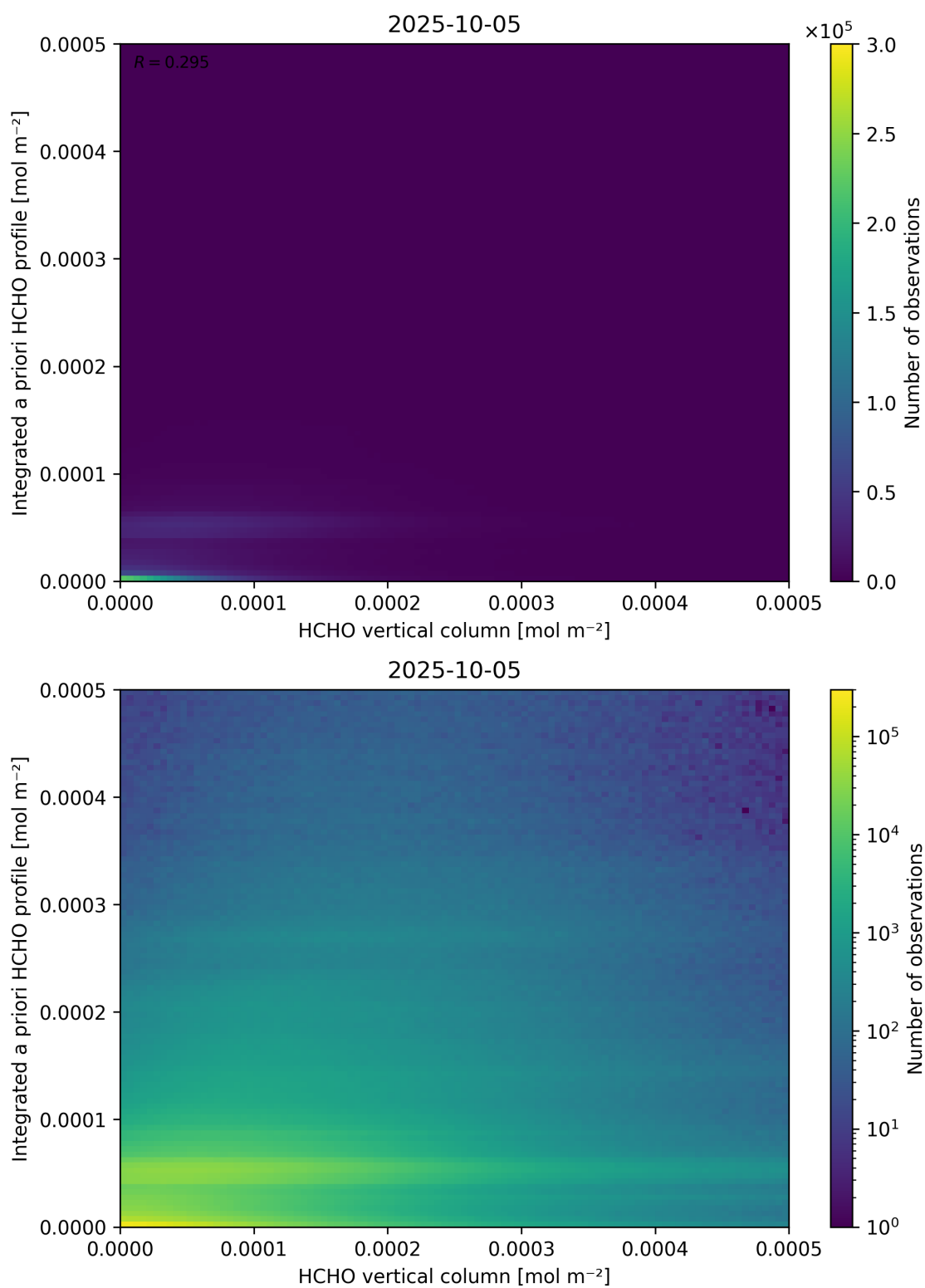
Figure 135: Scatter density plot of “HCHO vertical column” against “Integrated a priori HCHO profile” for 2025-10-04 to 2025-10-06.
