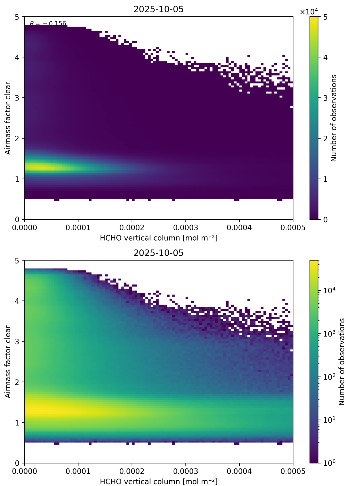
Figure 126: Scatter density plot of “HCHO vertical column” against “Airmass factor clear” for 2025-10-04 to 2025-10-06.
