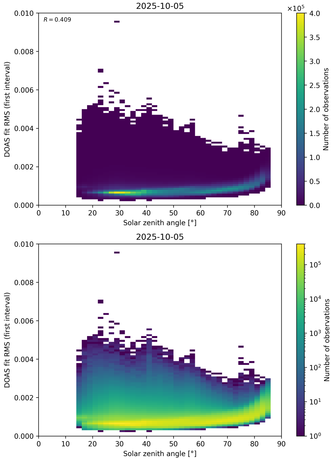
Figure 167: Scatter density plot of “Solar zenith angle” against “DOAS fit RMS (first interval)” for 2025-10-04 to 2025-10-06.
