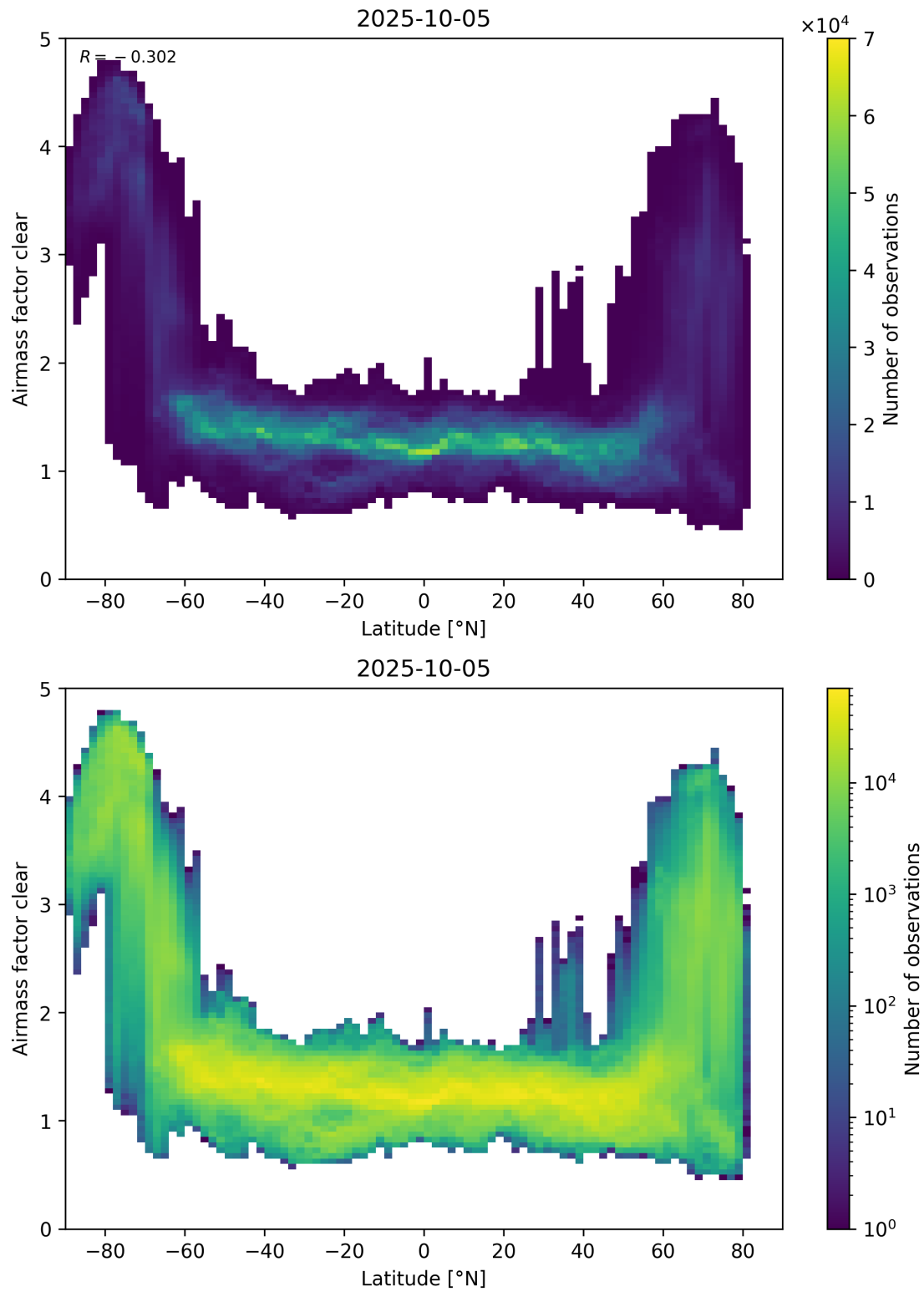
Figure 156: Scatter density plot of “Latitude” against “Airmass factor clear” for 2025-10-04 to 2025-10-06.
