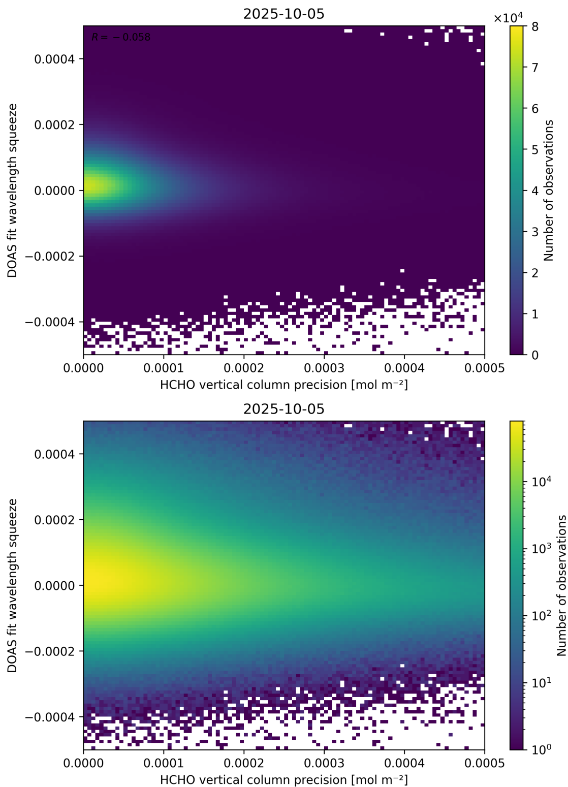
Figure 138: Scatter density plot of “HCHO vertical column precision” against “DOAS fit wavelength squeeze” for 2025-10-04 to 2025-10-06.
