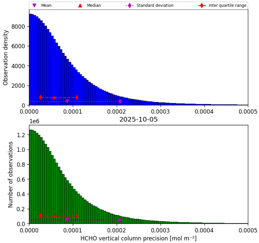
Figure 36: Histogram of “HCHO vertical column precision” for 2025-10-04 to 2025-10-06
