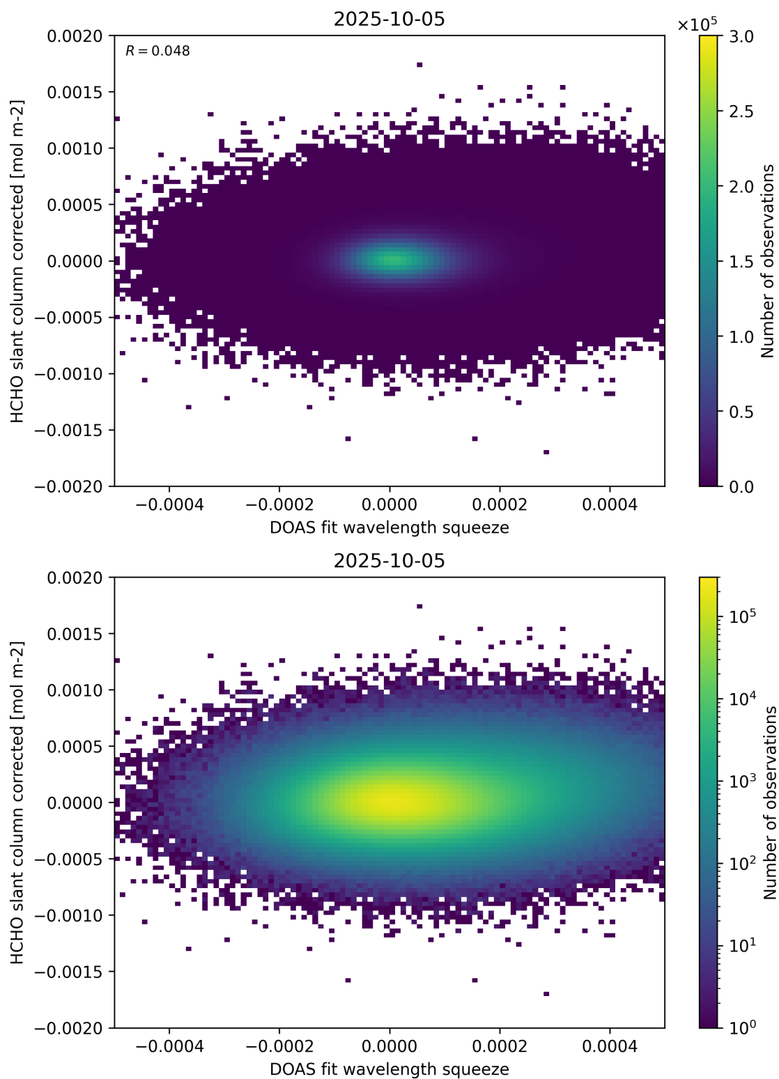
Figure 69: Scatter density plot of “DOAS fit wavelength squeeze” against “HCHO slant column corrected” for 2025-10-04 to 2025-10-06.
