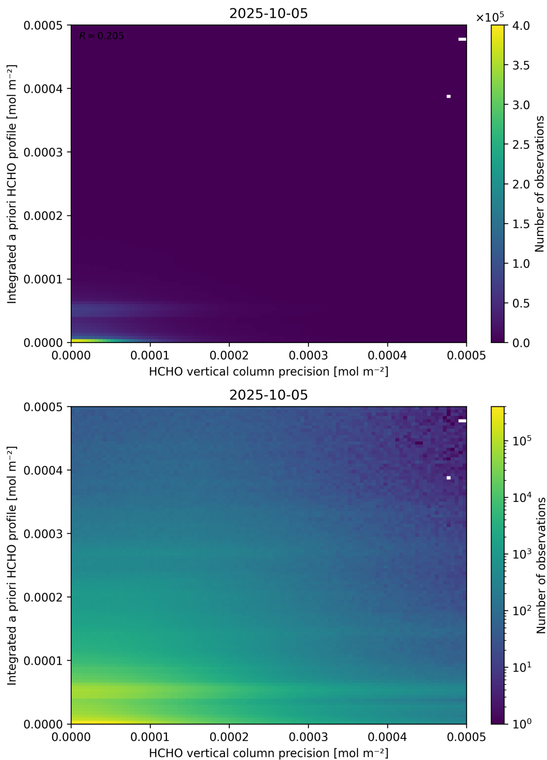
Figure 147: Scatter density plot of “HCHO vertical column precision” against “Integrated a priori HCHO profile” for 2025-10-04 to 2025-10-06.
