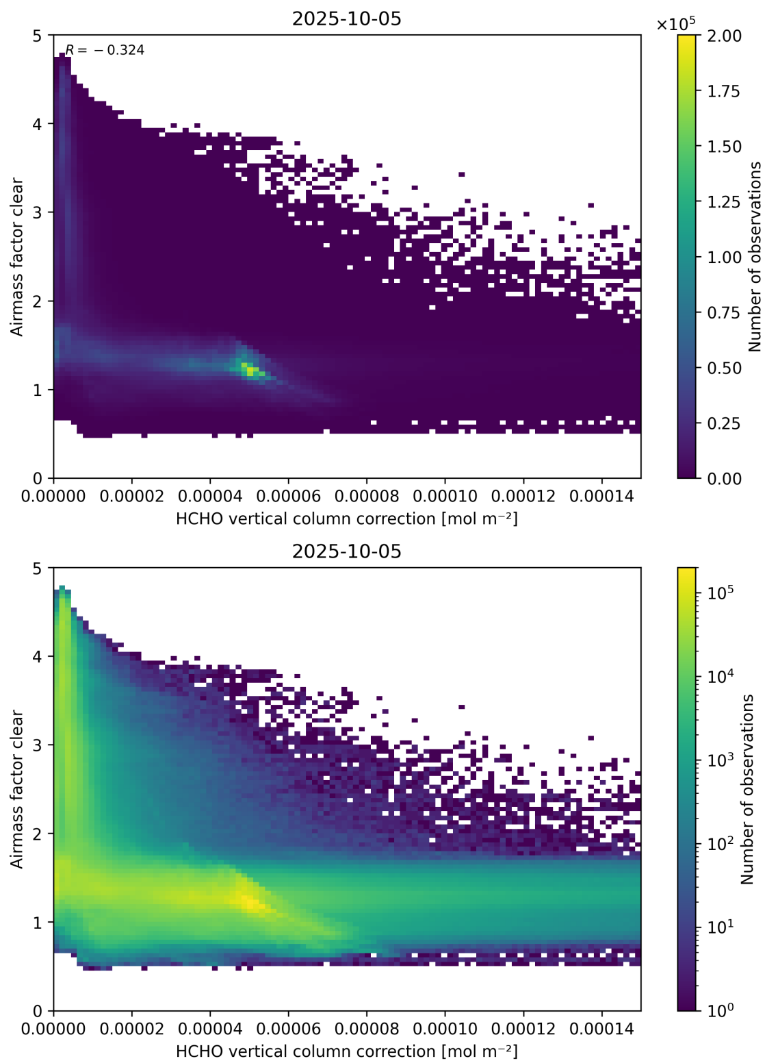
Figure 115: Scatter density plot of “HCHO vertical column correction” against “Airmass factor clear” for 2025-10-04 to 2025-10-06.
