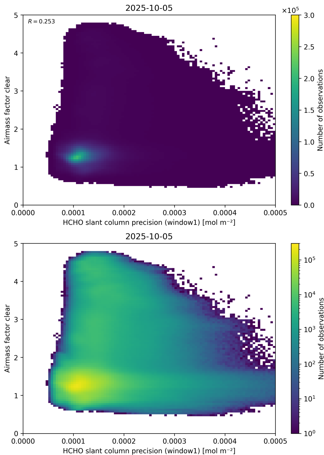
Figure 91: Scatter density plot of “HCHO slant column precision (window1)” against “Airmass factor clear” for 2025-10-04 to 2025-10-06.
