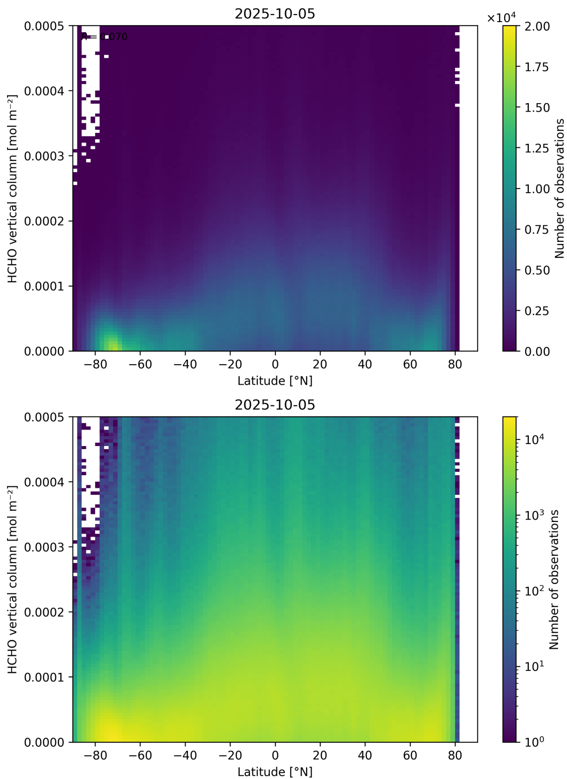
Figure 163: Scatter density plot of “Latitude” against “HCHO vertical column” for 2025-10-04 to 2025-10-06.
