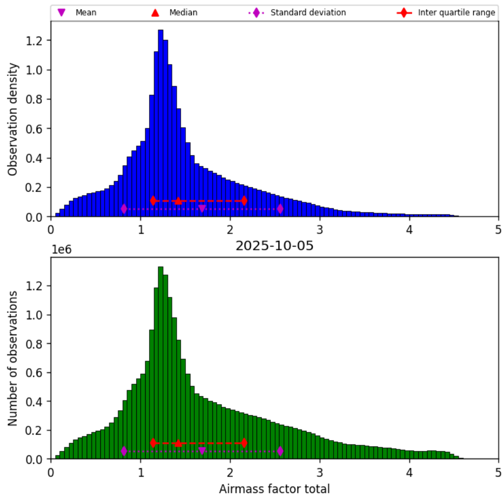
Figure 40: Histogram of “Airmass factor total” for 2025-10-04 to 2025-10-06
