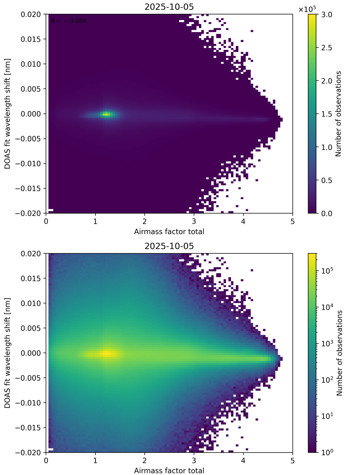
Figure 98: Scatter density plot of “Airmass factor total” against “DOAS fit wavelength shift” for 2025-10-04 to 2025-10-06.
