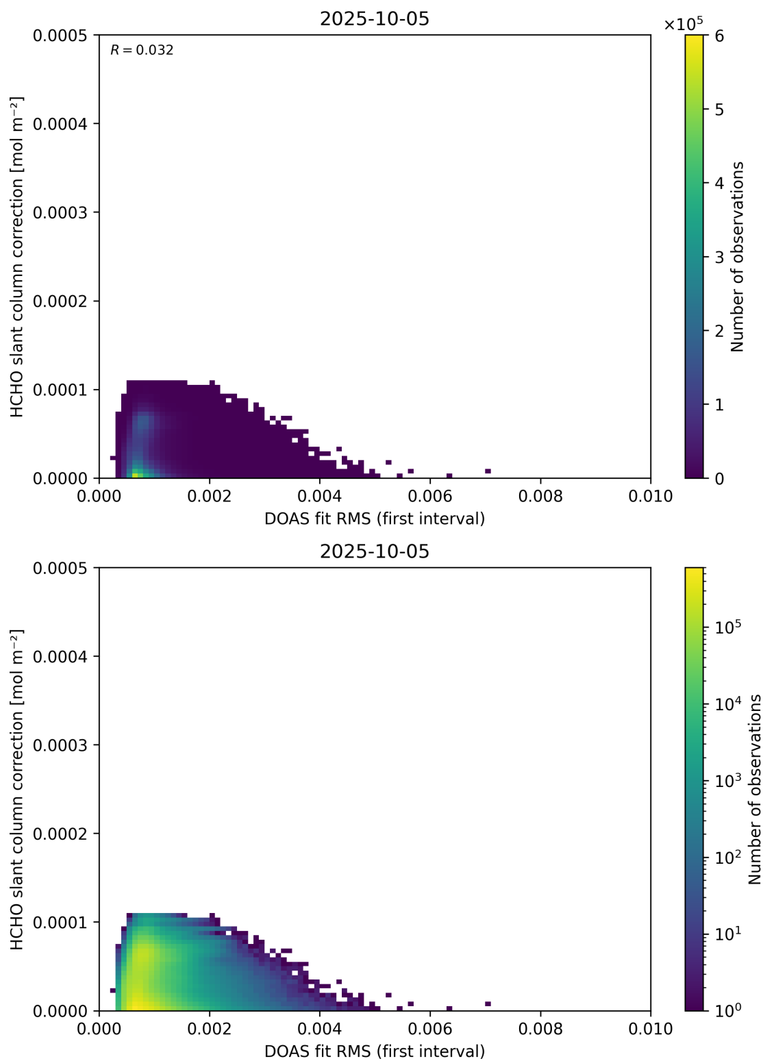
Figure 63: Scatter density plot of “DOAS fit RMS (first interval)” against “HCHO slant column correction” for 2025-10-04 to 2025-10-06.
