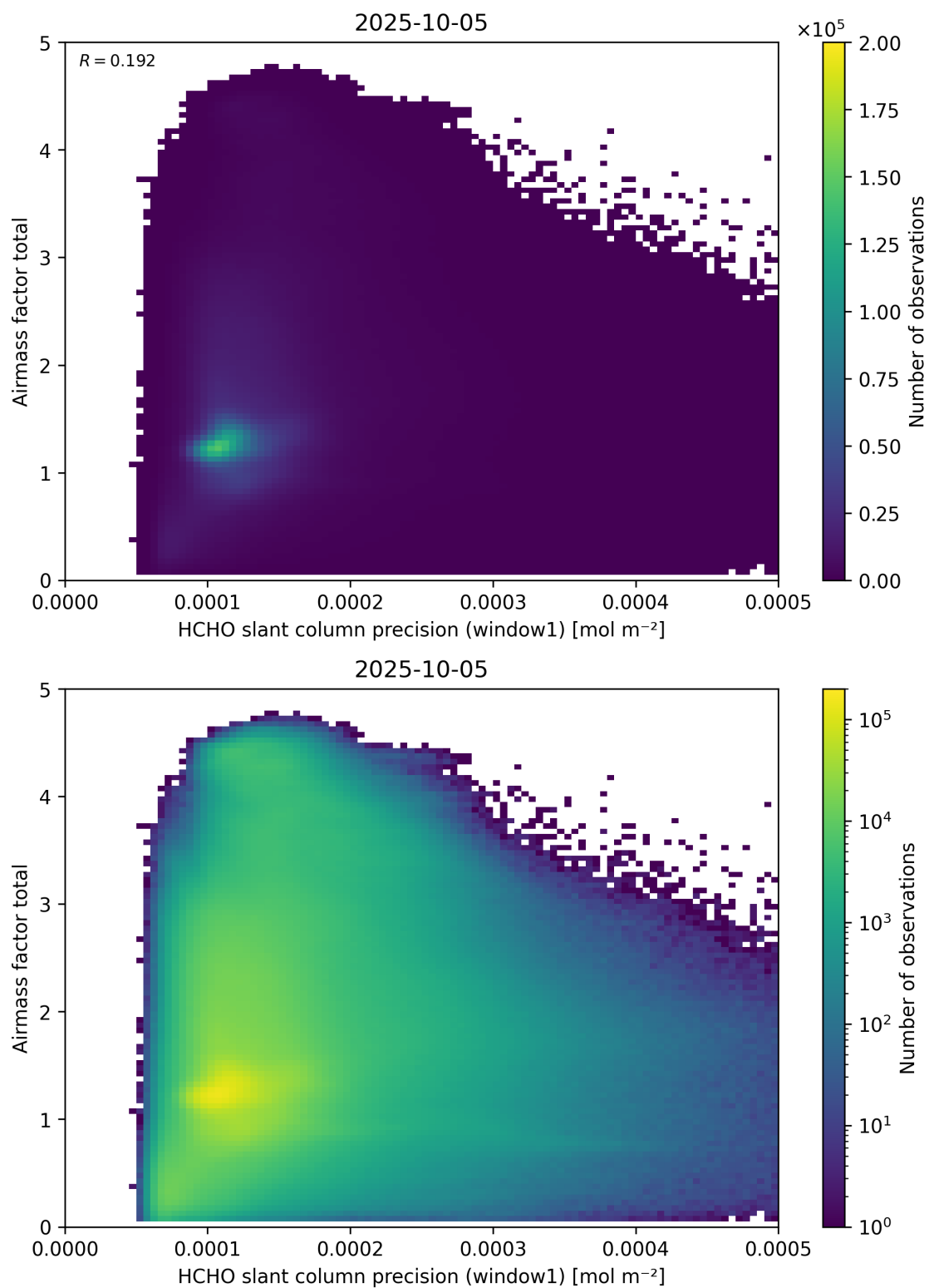
Figure 94: Scatter density plot of “HCHO slant column precision (window1)” against “Airmass factor total” for 2025-10-04 to 2025-10-06.
