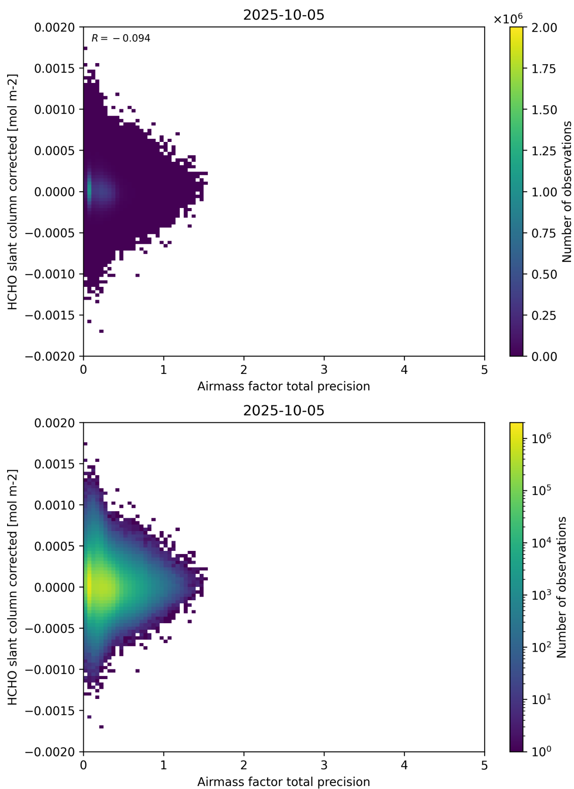
Figure 109: Scatter density plot of “Airmass factor total precision” against “HCHO slant column corrected” for 2025-10-04 to 2025-10-06.
