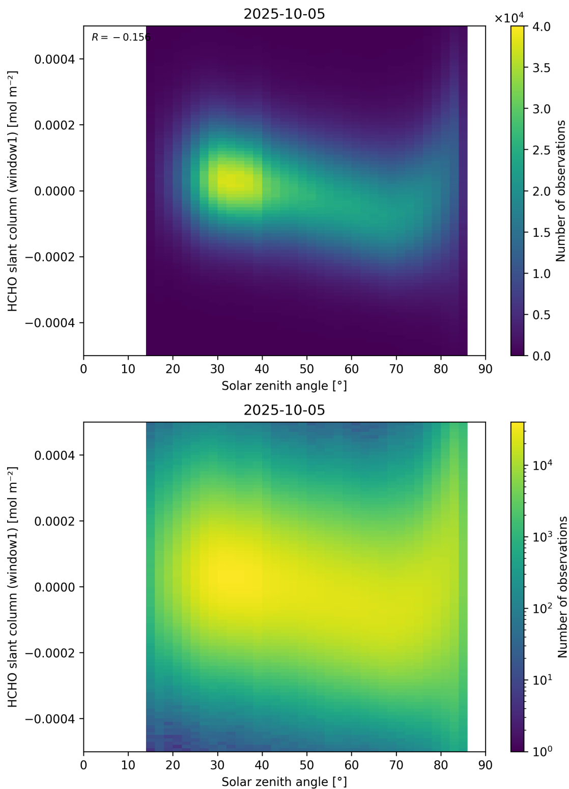
Figure 173: Scatter density plot of “Solar zenith angle” against “HCHO slant column (window1)” for 2025-10-04 to 2025-10-06.
