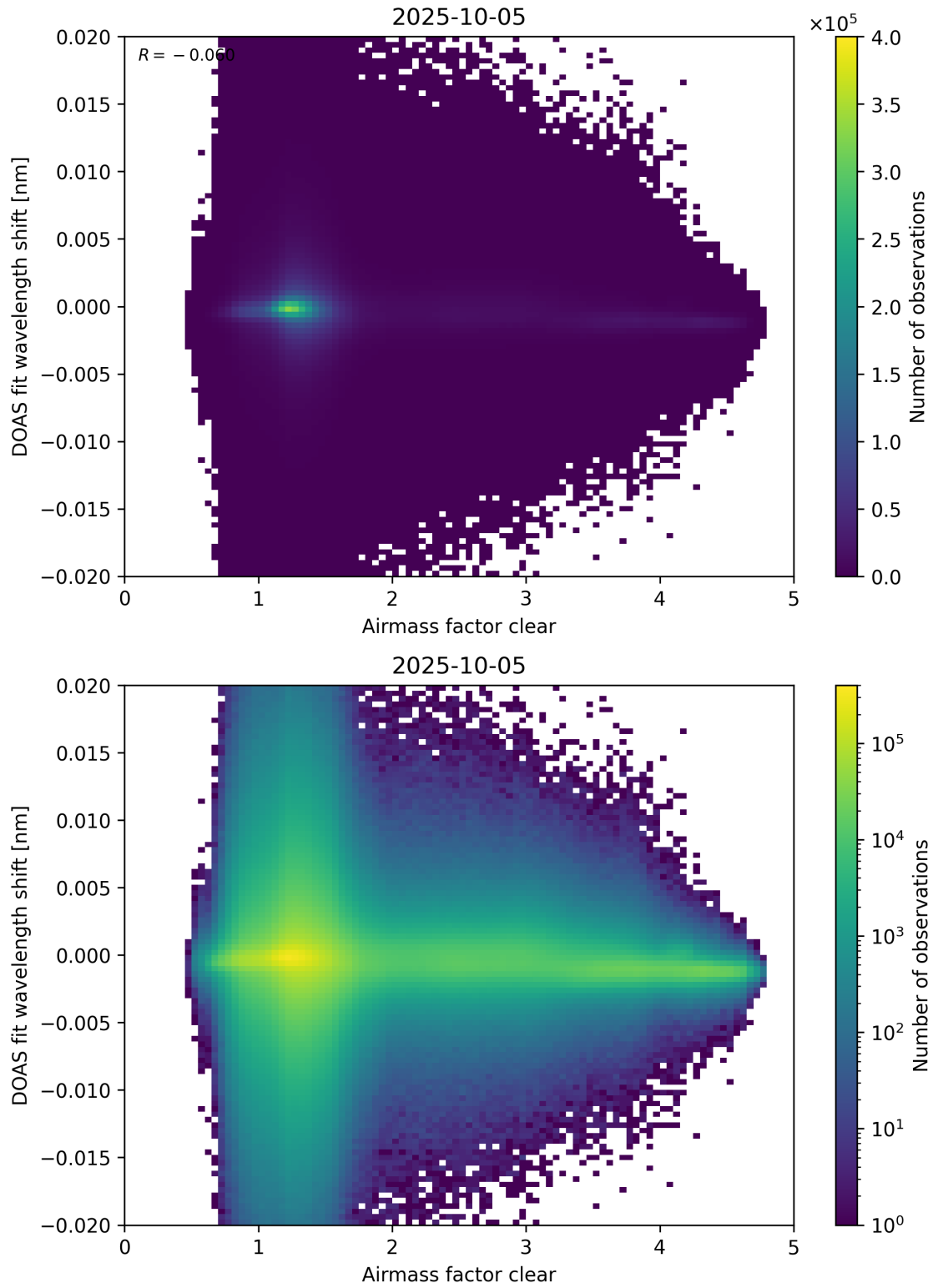
Figure 72: Scatter density plot of “Airmass factor clear” against “DOAS fit wavelength shift” for 2025-10-04 to 2025-10-06.
