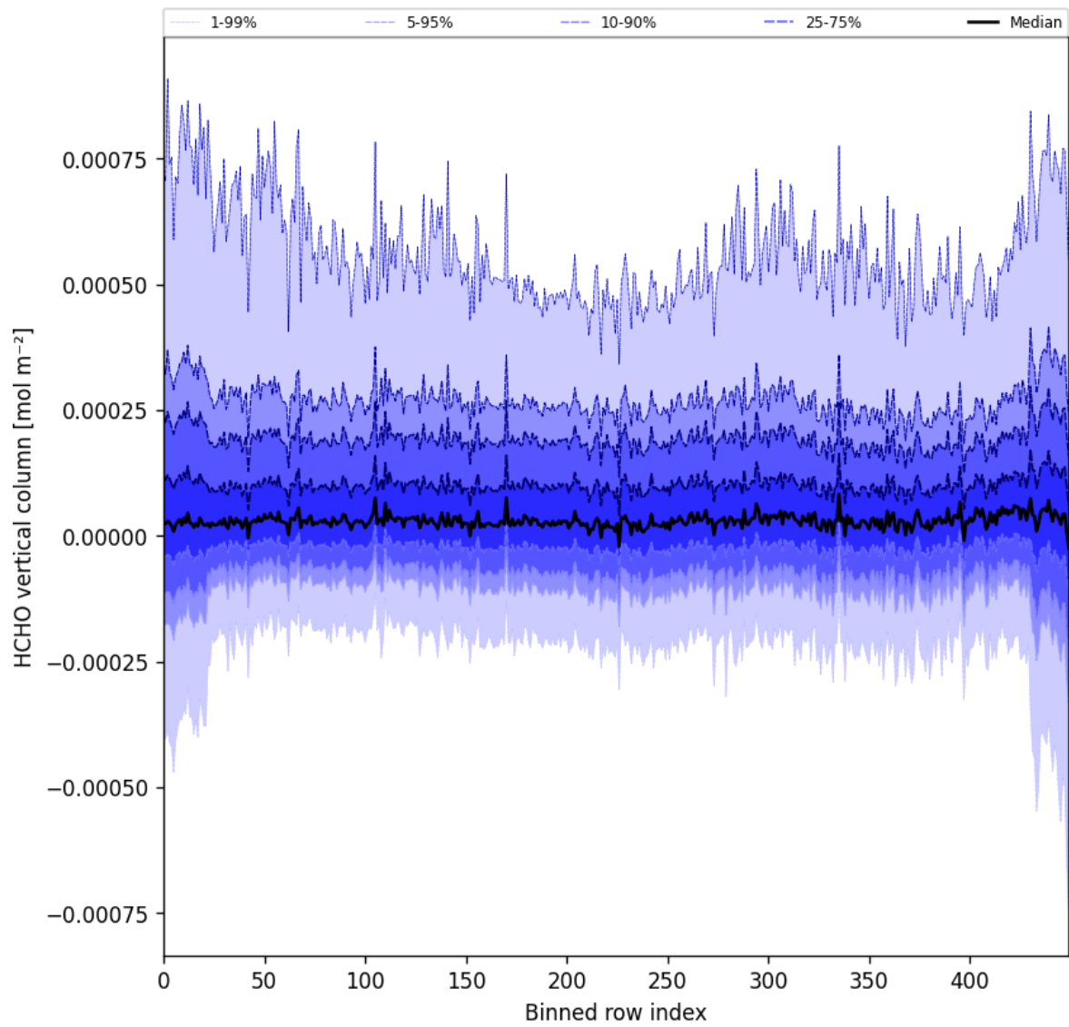
Figure 49: Along track statistics of “HCHO vertical column” for 2025-10-04 to 2025-10-06
