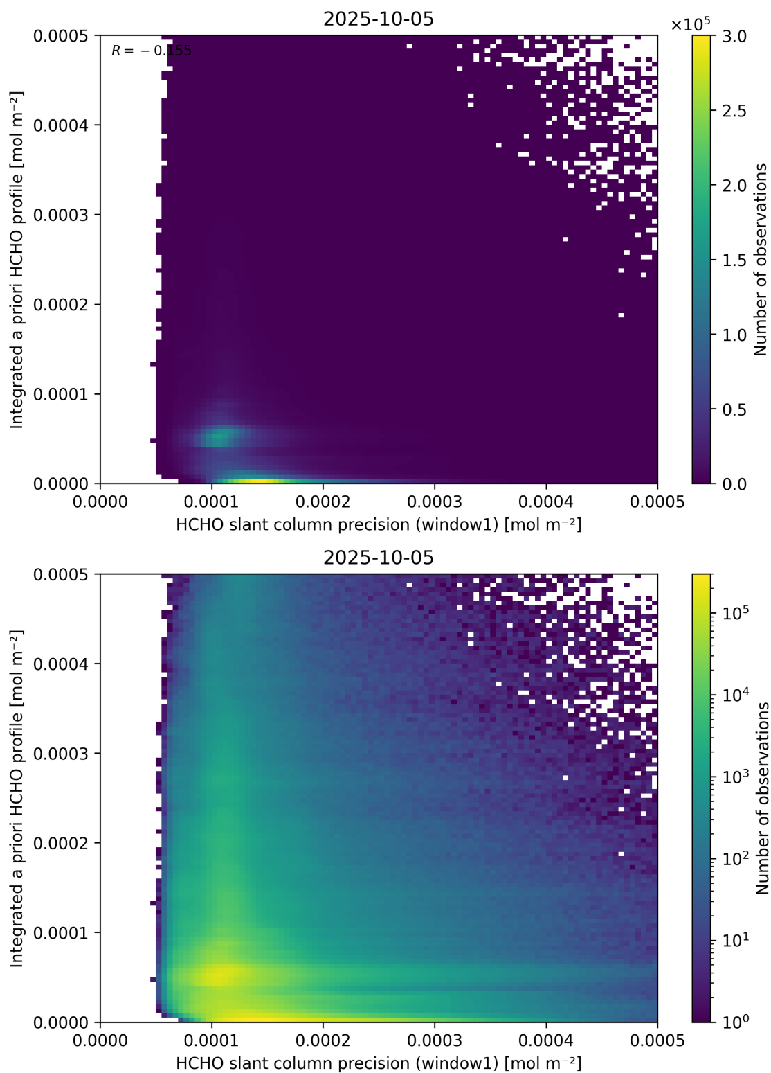
Figure 96: Scatter density plot of “HCHO slant column precision (window1)” against “Integrated a priori HCHO profile” for 2025-10-04 to 2025-10-06.
