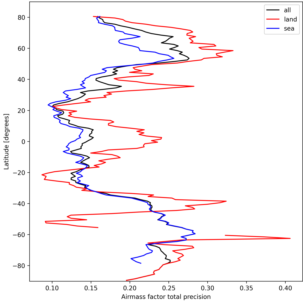
Figure 27: Zonal average of “Airmass factor total precision” for 2025-10-04 to 2025-10-06.
