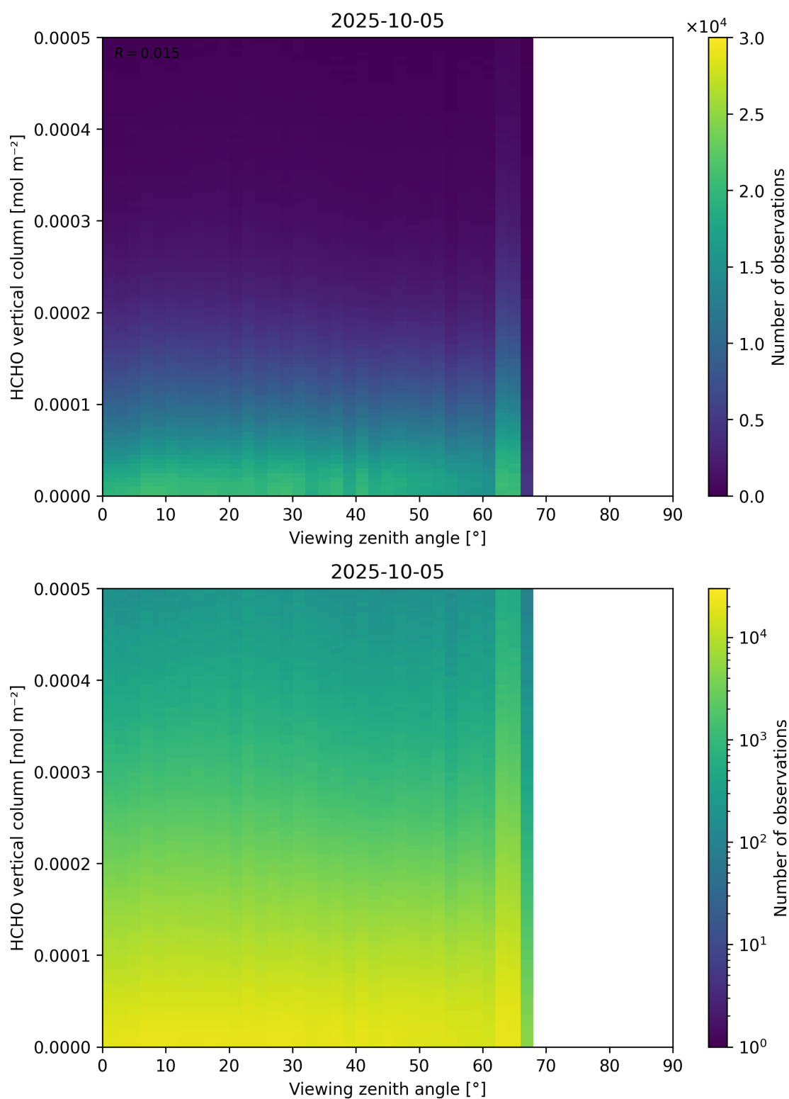
Figure 192: Scatter density plot of “Viewing zenith angle” against “HCHO vertical column” for 2025-10-04 to 2025-10-06.
