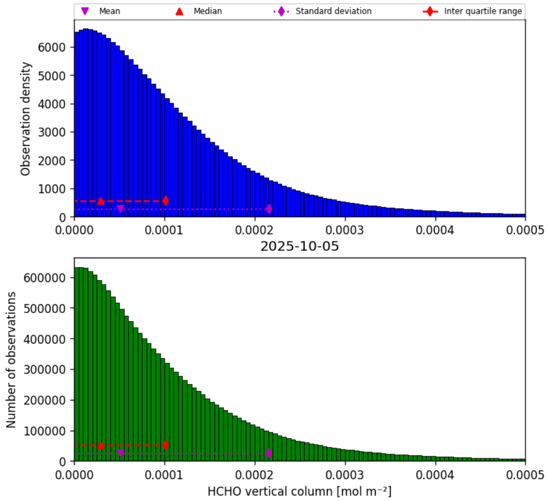
Figure 35: Histogram of “HCHO vertical column” for 2025-10-04 to 2025-10-06
