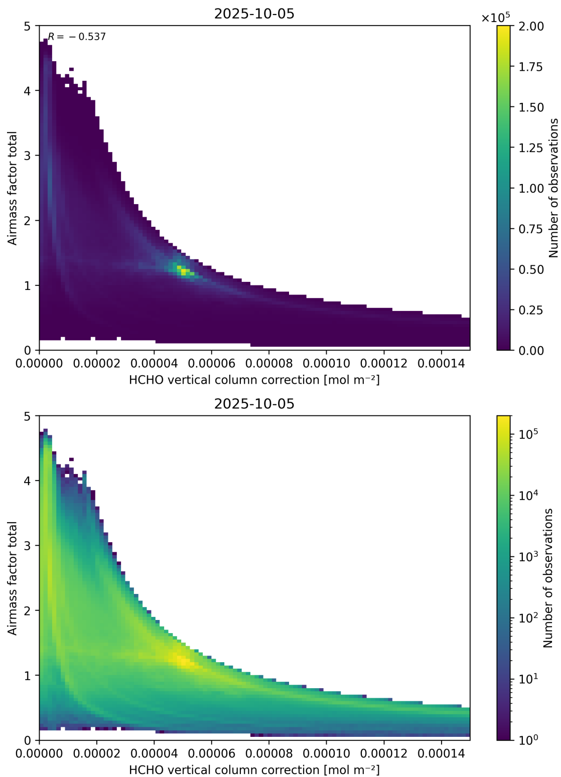
Figure 120: Scatter density plot of “HCHO vertical column correction” against “Airmass factor total” for 2025-10-04 to 2025-10-06.
