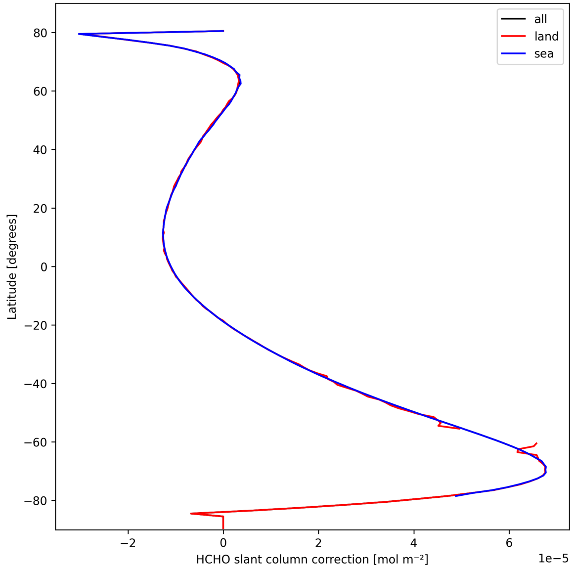
Figure 33: Zonal average of "HCHO slant column correction" for 2025-10-04 to 2025-10-06.
