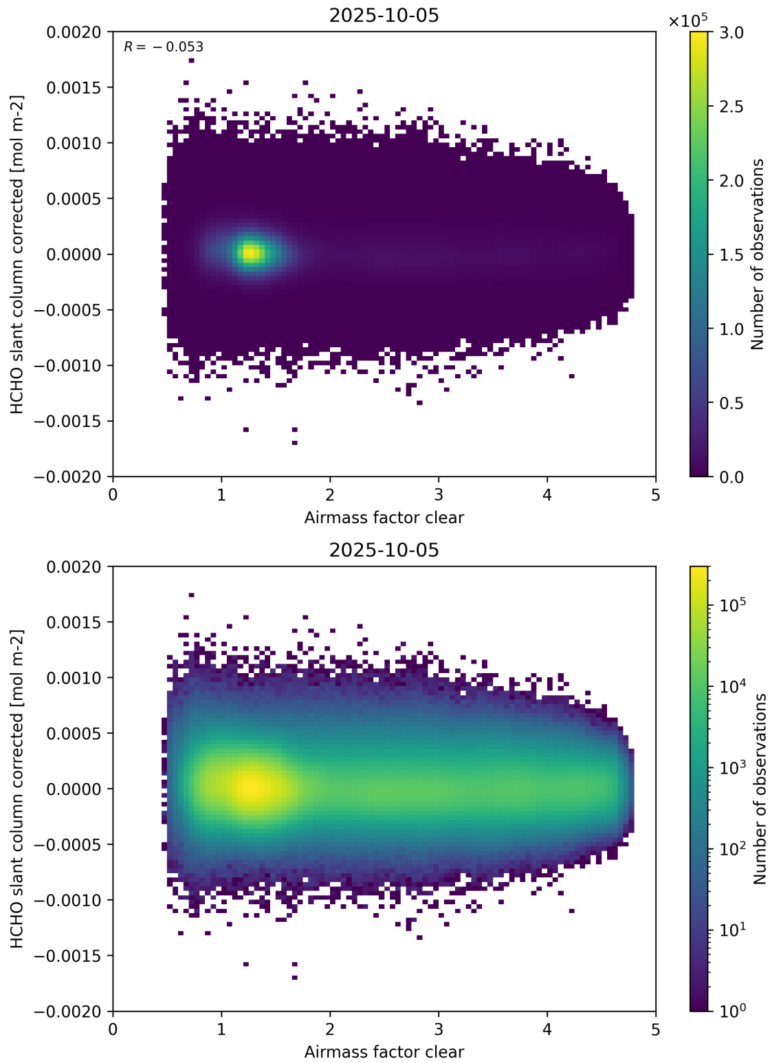
Figure 74: Scatter density plot of “Airmass factor clear” against “HCHO slant column corrected” for 2025-10-04 to 2025-10-06.
