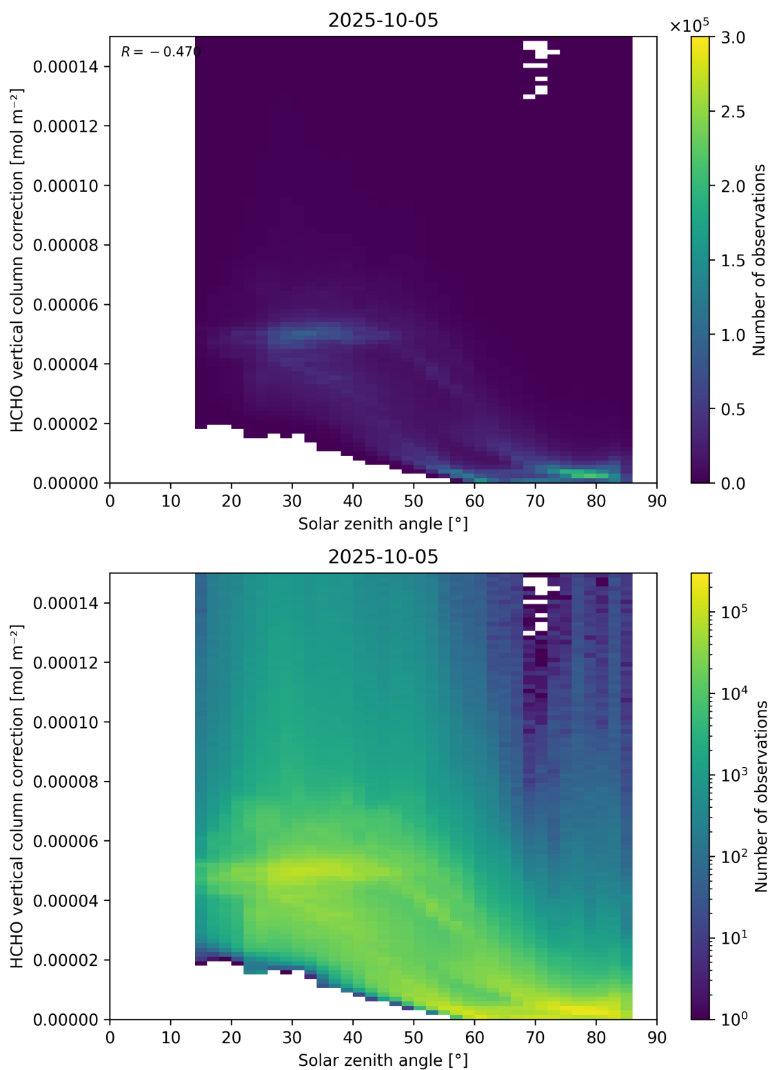
Figure 178: Scatter density plot of “Solar zenith angle” against “HCHO vertical column correction” for 2025-10-04 to 2025-10-06.
