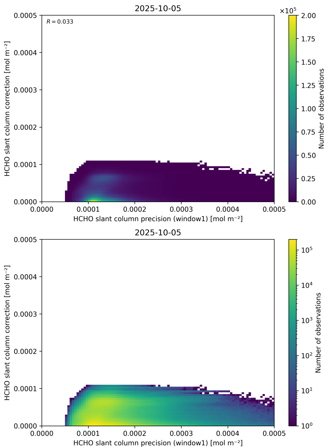
Figure 93: Scatter density plot of “HCHO slant column precision (window1)” against “HCHO slant column correction” for 2025-10-04 to 2025-10-06.
