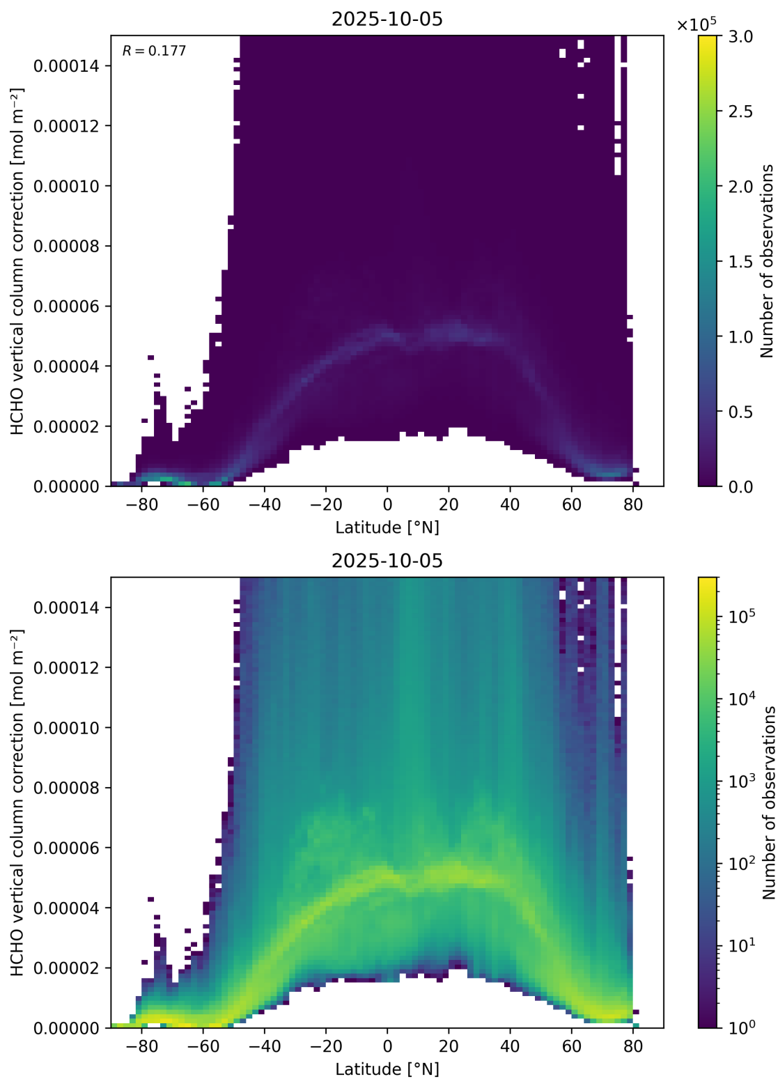
Figure 164: Scatter density plot of “Latitude” against “HCHO vertical column correction” for 2025-10-04 to 2025-10-06.
