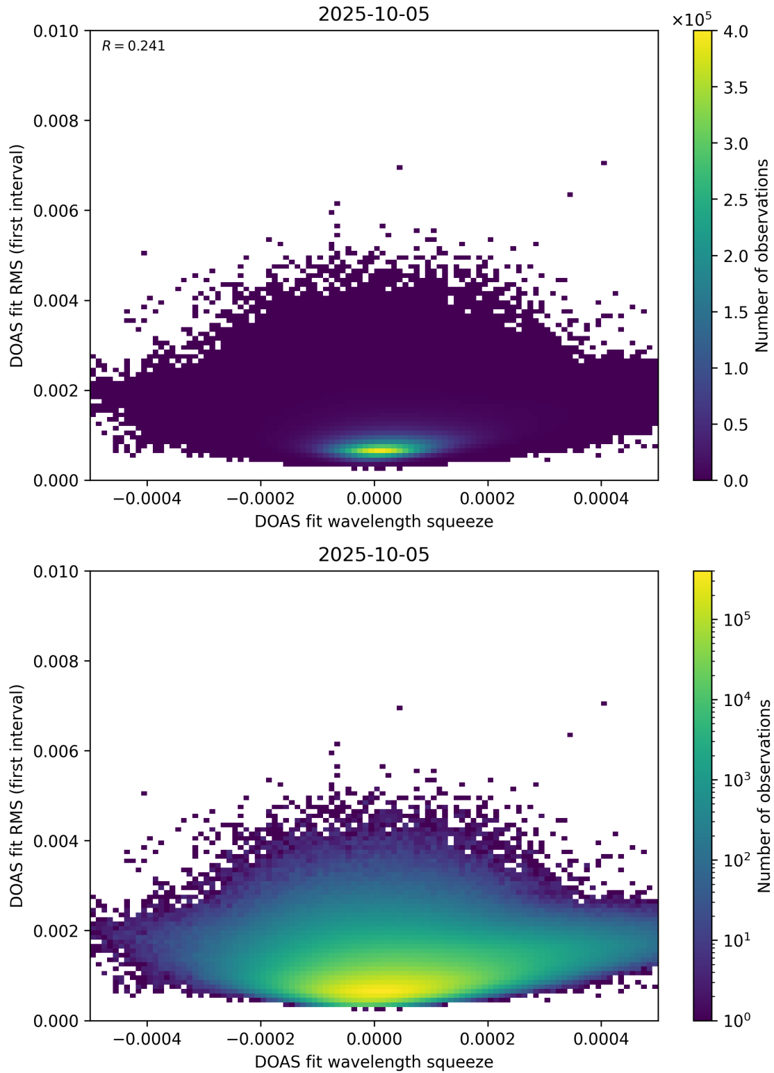
Figure 68: Scatter density plot of “DOAS fit wavelength squeeze” against “DOAS fit RMS (first interval)” for 2025-10-04 to 2025-10-06.
