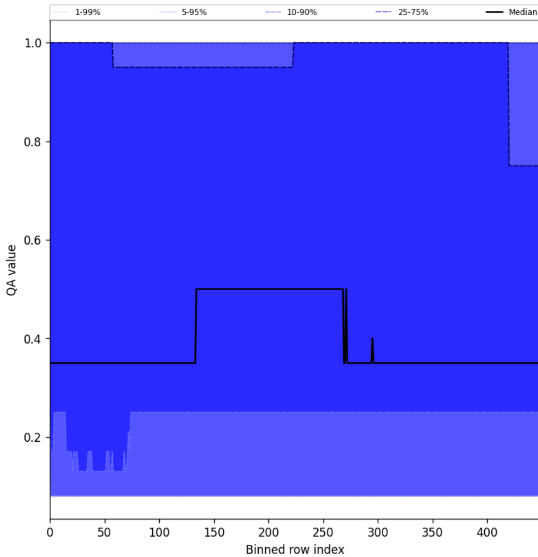
Figure 48: Along track statistics of “QA value” for 2025-10-04 to 2025-10-06
