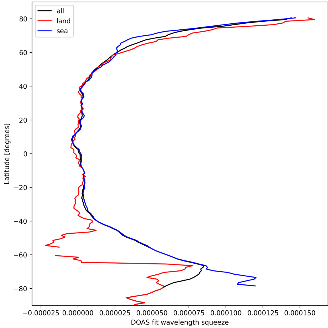
Figure 31: Zonal average of “DOAS fit wavelength squeeze” for 2025-10-04 to 2025-10-06.
