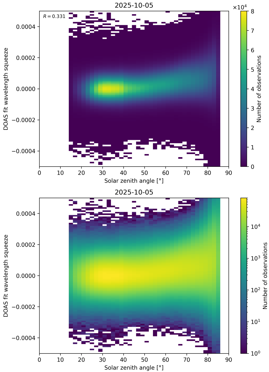
Figure 169: Scatter density plot of “Solar zenith angle” against “DOAS fit wavelength squeeze” for 2025-10-04 to 2025-10-06.
