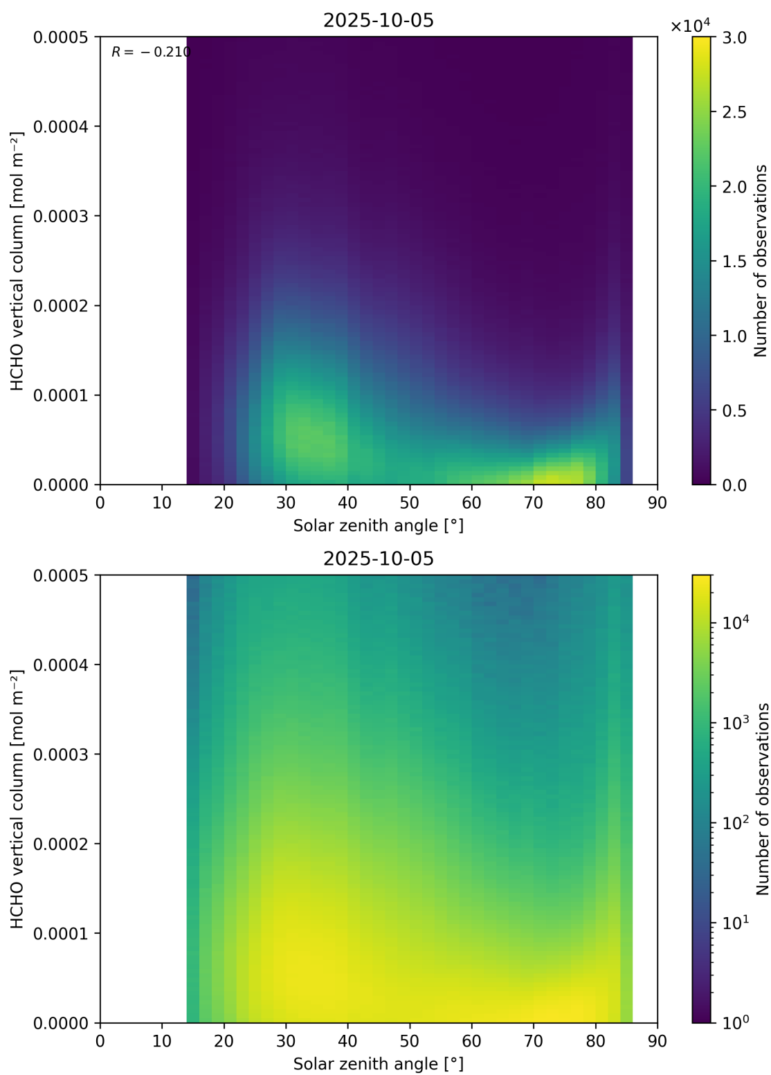
Figure 177: Scatter density plot of “Solar zenith angle” against “HCHO vertical column” for 2025-10-04 to 2025-10-06.
