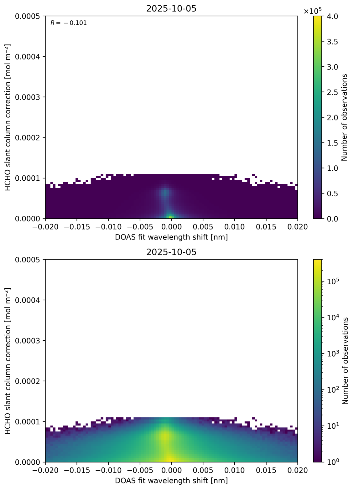
Figure 67: Scatter density plot of “DOAS fit wavelength shift” against “HCHO slant column correction” for 2025-10-04 to 2025-10-06.
