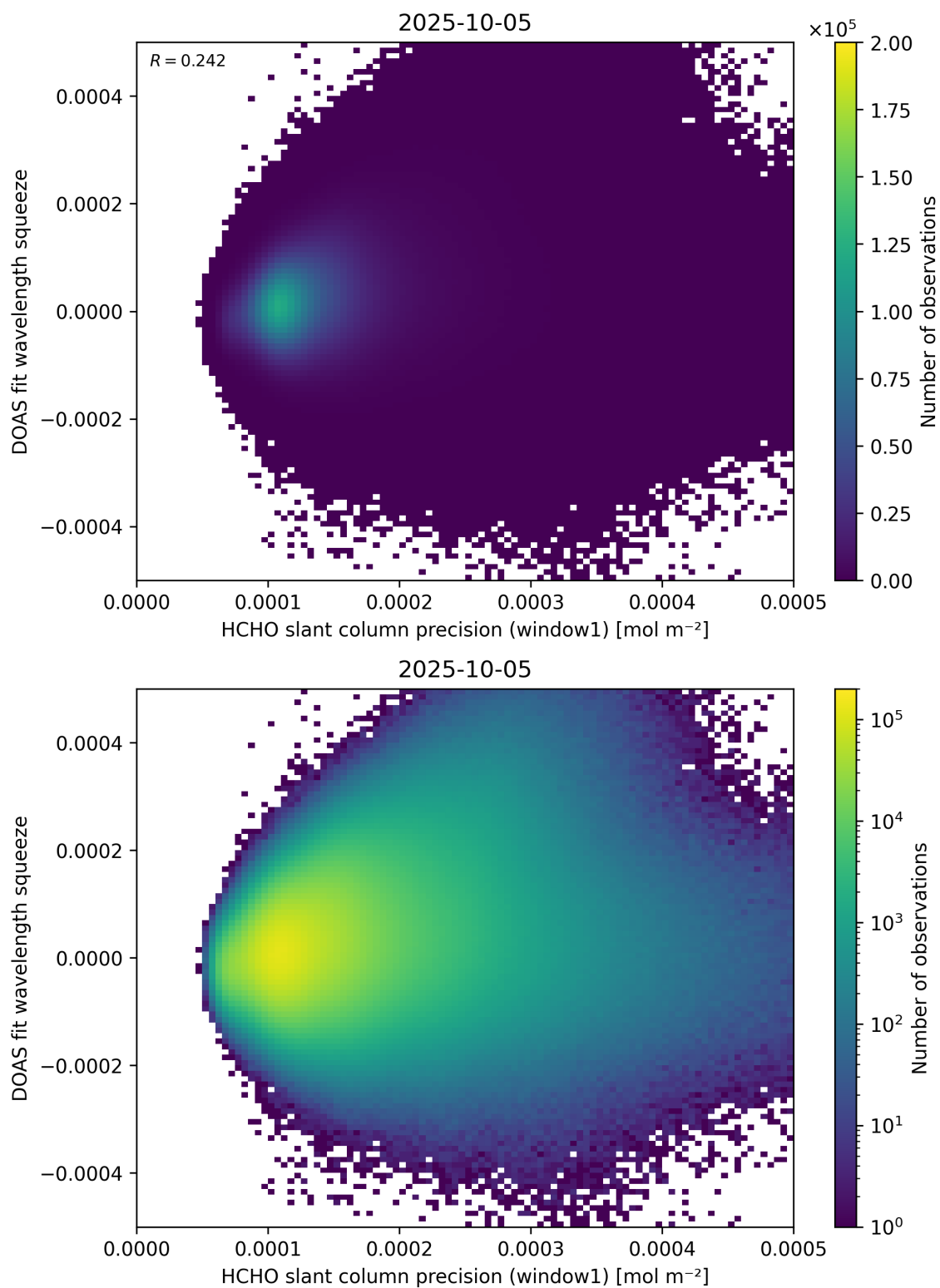
Figure 90: Scatter density plot of “HCHO slant column precision (window1)” against “DOAS fit wavelength squeeze” for 2025-10-04 to 2025-10-06.
