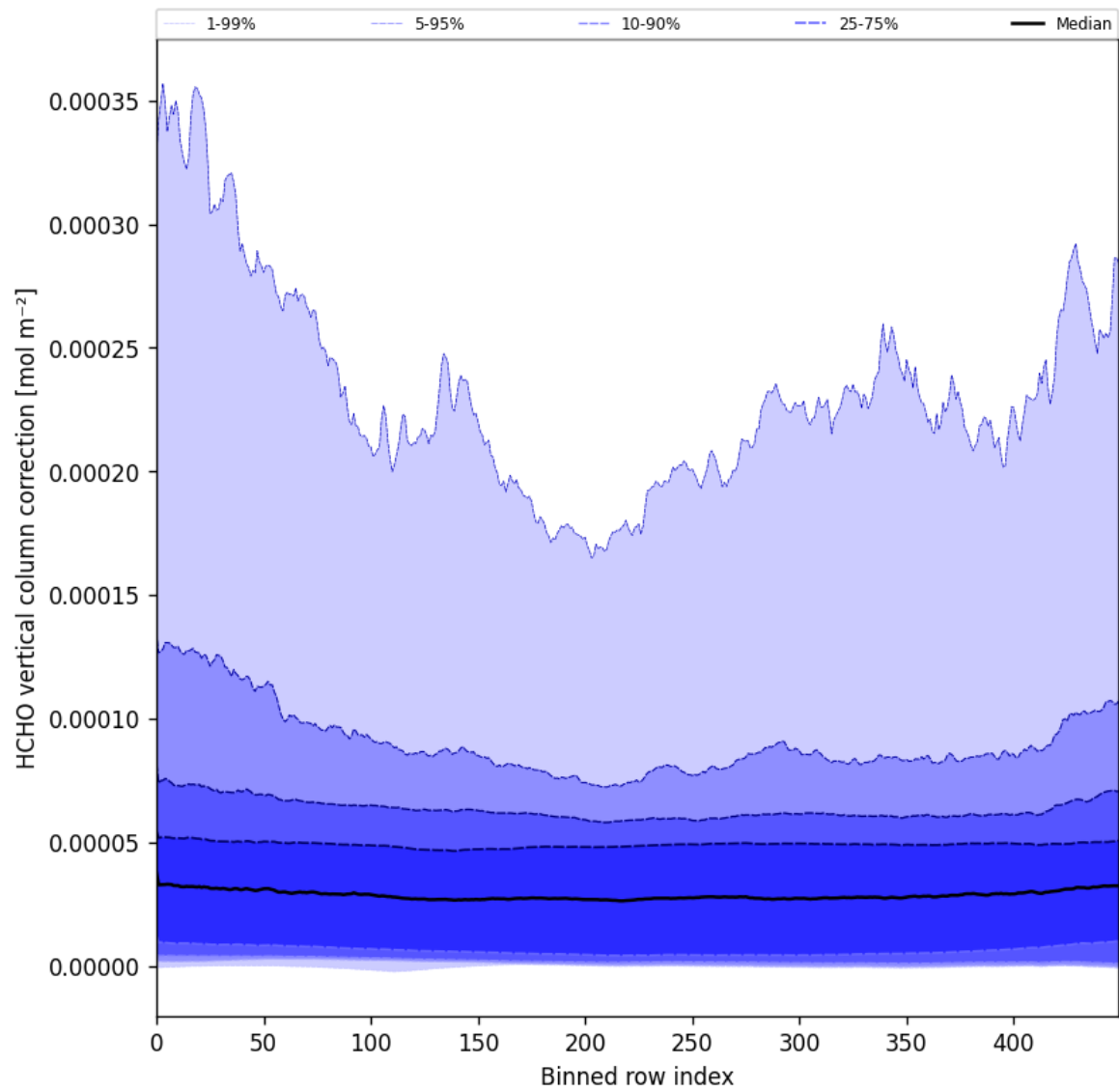
Figure 51: Along track statistics of “HCHO vertical column correction” for 2025-10-04 to 2025-10-06
