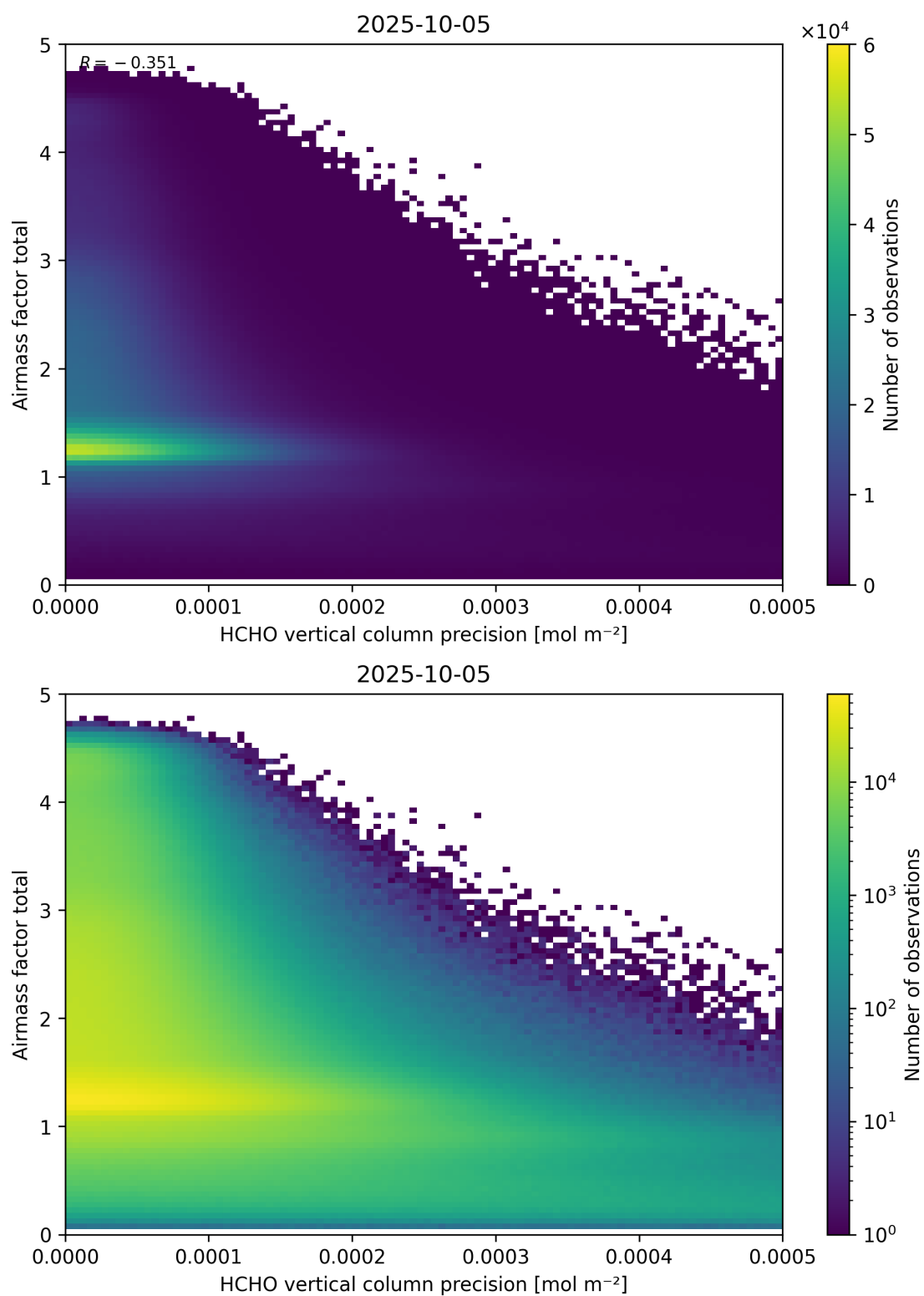
Figure 144: Scatter density plot of “HCHO vertical column precision” against “Airmass factor total” for 2025-10-04 to 2025-10-06.
