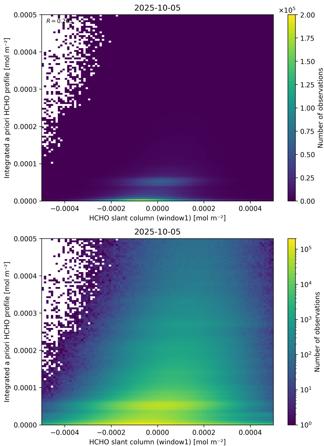
Figure 87: Scatter density plot of “HCHO slant column (window1)” against “Integrated a priori HCHO profile” for 2025-10-04 to 2025-10-06.
