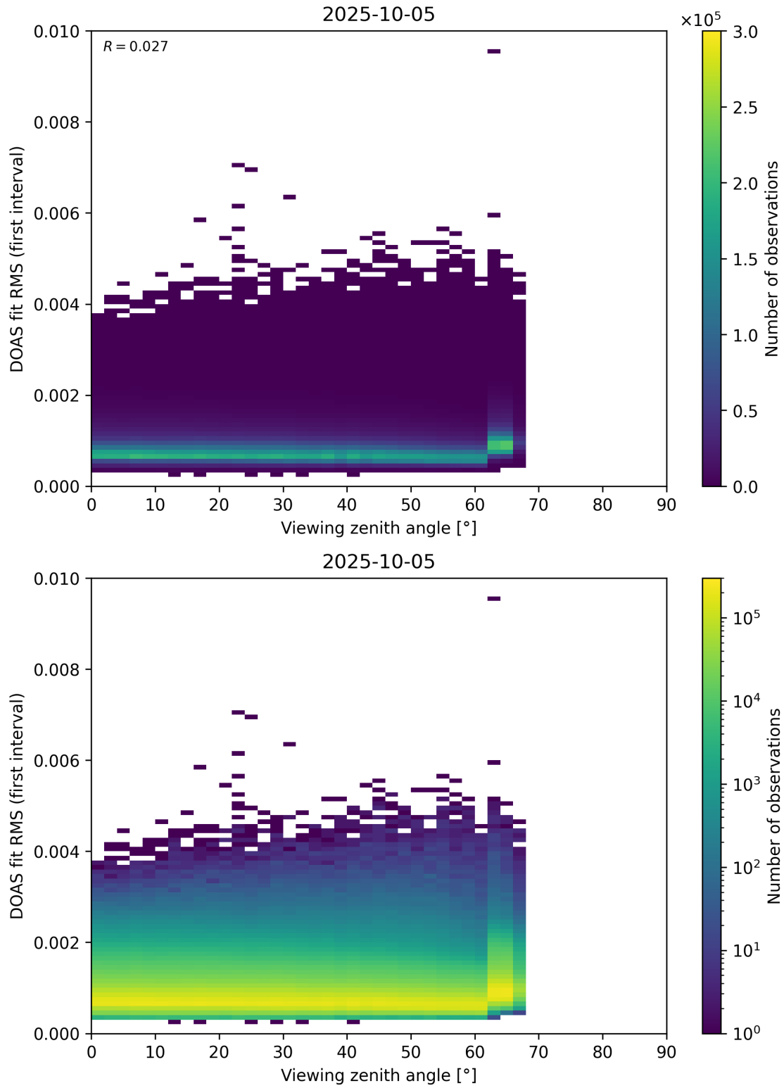
Figure 182: Scatter density plot of “Viewing zenith angle” against “DOAS fit RMS (first interval)” for 2025-10-04 to 2025-10-06.
