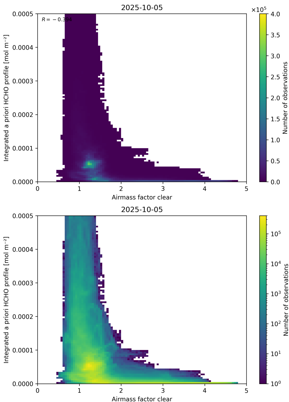
Figure 76: Scatter density plot of “Airmass factor clear” against “Integrated a priori HCHO profile” for 2025-10-04 to 2025-10-06.
