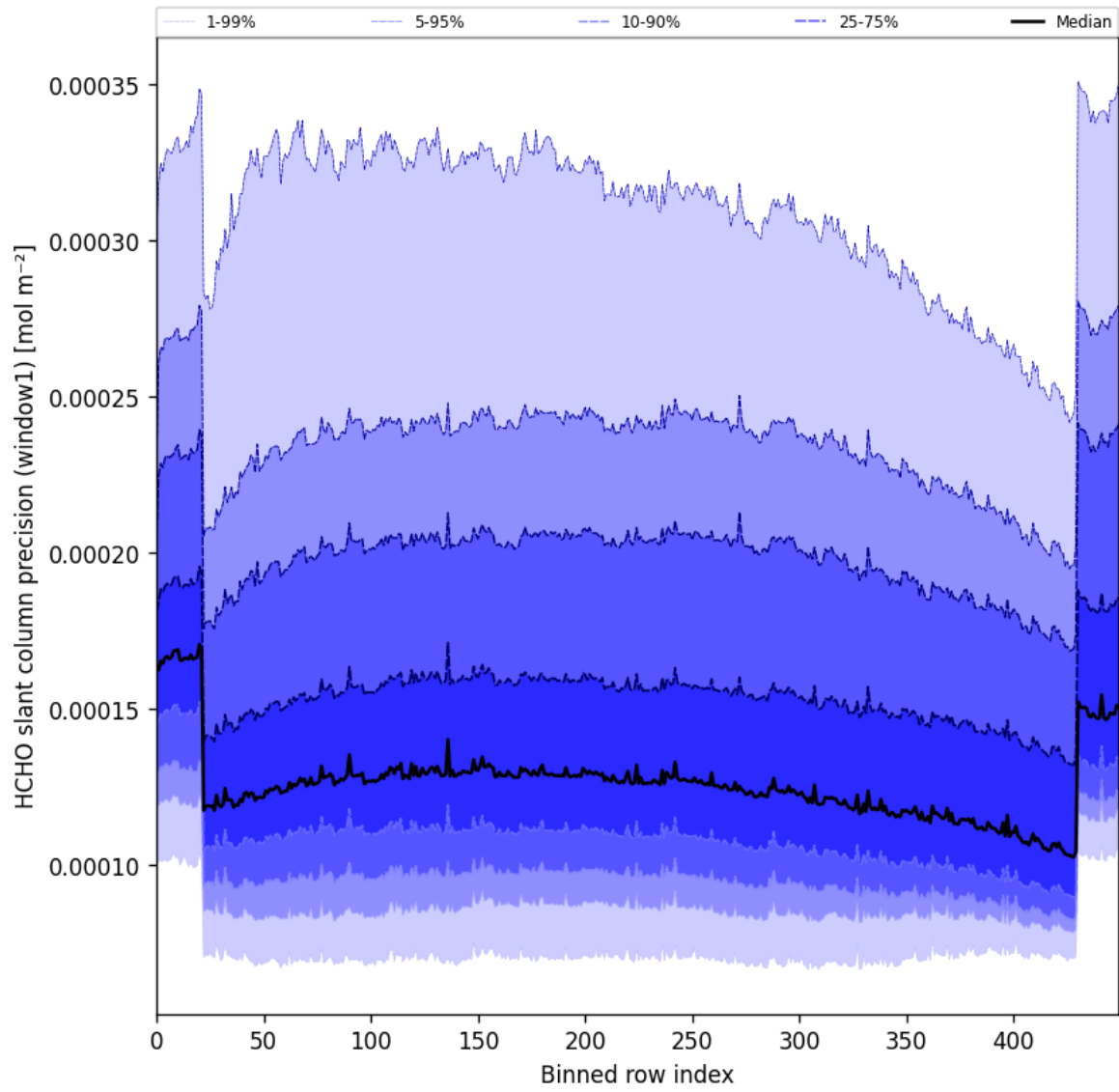
Figure 53: Along track statistics of “HCHO slant column precision (window1)” for 2025-10-04 to 2025-10-06
