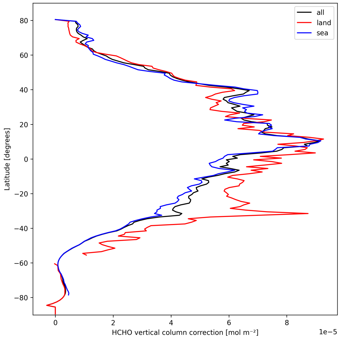
Figure 23: Zonal average of “HCHO vertical column correction” for 2025-10-04 to 2025-10-06.
