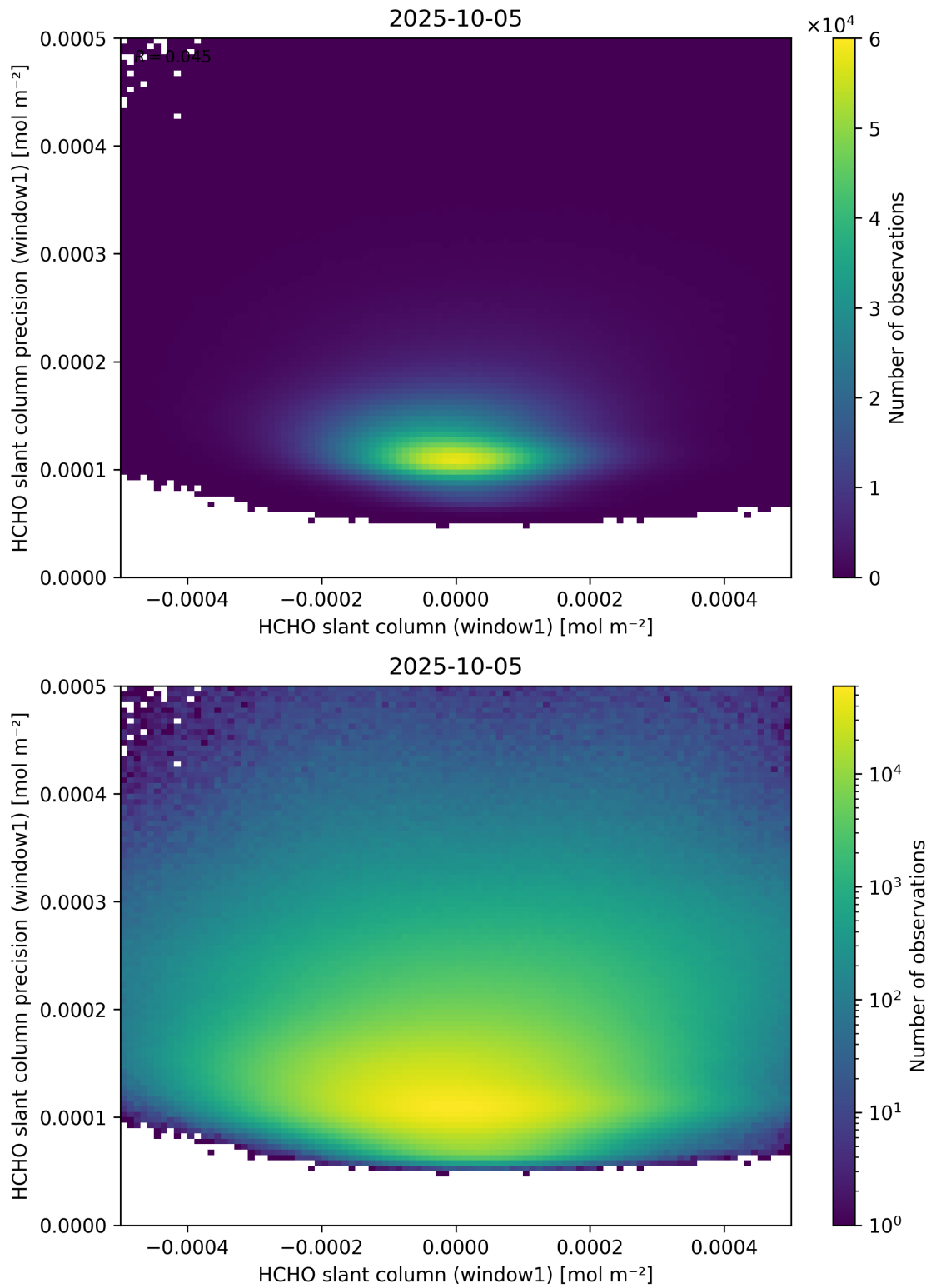
Figure 84: Scatter density plot of “HCHO slant column (window1)” against “HCHO slant column precision (window1)” for 2025-10-04 to 2025-10-06.
