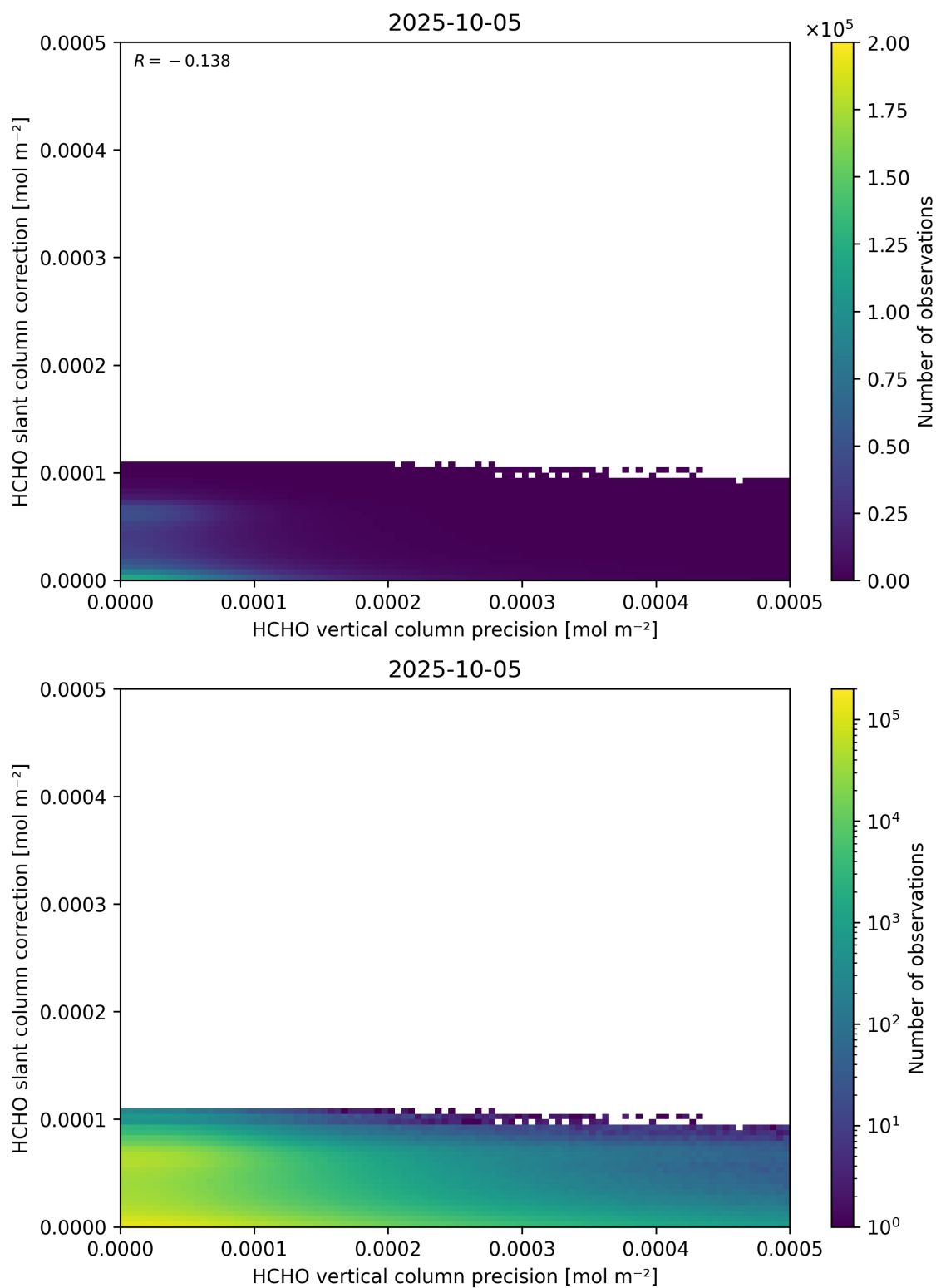
Figure 141: Scatter density plot of “HCHO vertical column precision” against “HCHO slant column correction” for 2025-10-04 to 2025-10-06.
