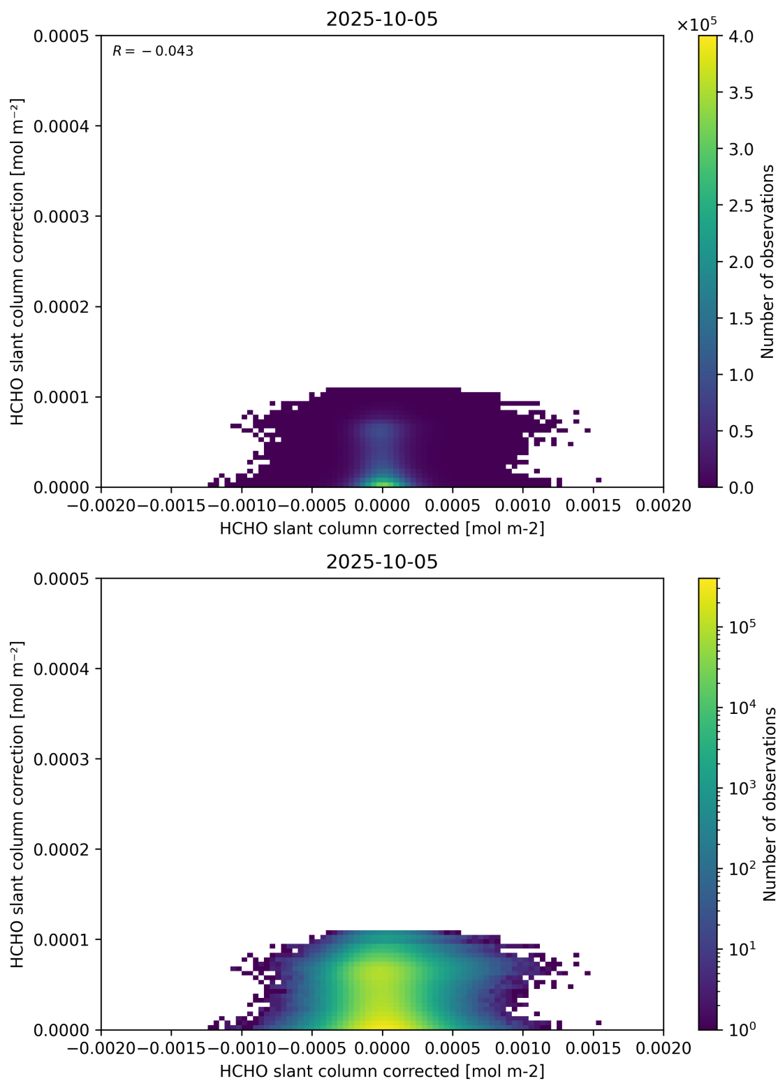
Figure 77: Scatter density plot of “HCHO slant column corrected” against “HCHO slant column correction” for 2025-10-04 to 2025-10-06.
