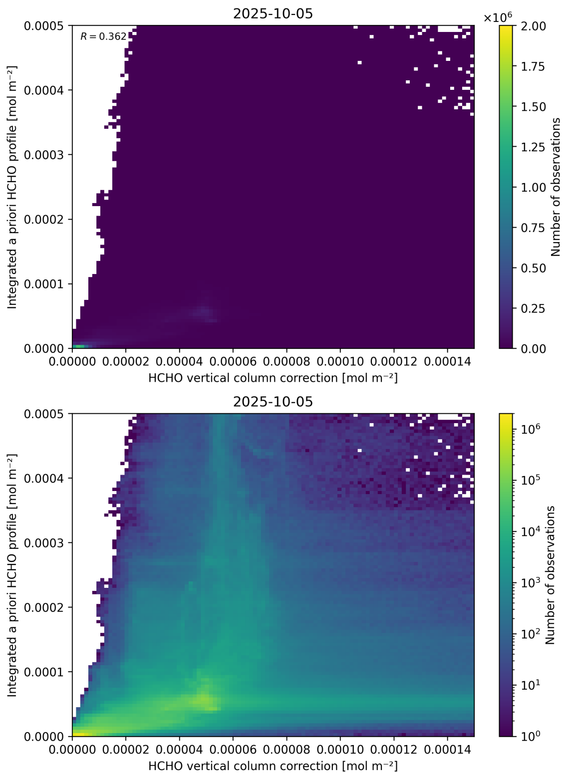
Figure 122: Scatter density plot of “HCHO vertical column correction” against “Integrated a priori HCHO profile” for 2025-10-04 to 2025-10-06.
