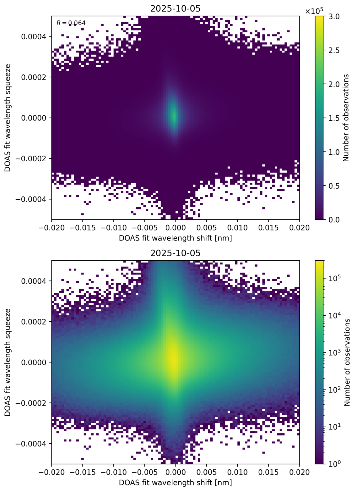
Figure 65: Scatter density plot of “DOAS fit wavelength shift” against “DOAS fit wavelength squeeze” for 2025-10-04 to 2025-10-06.
