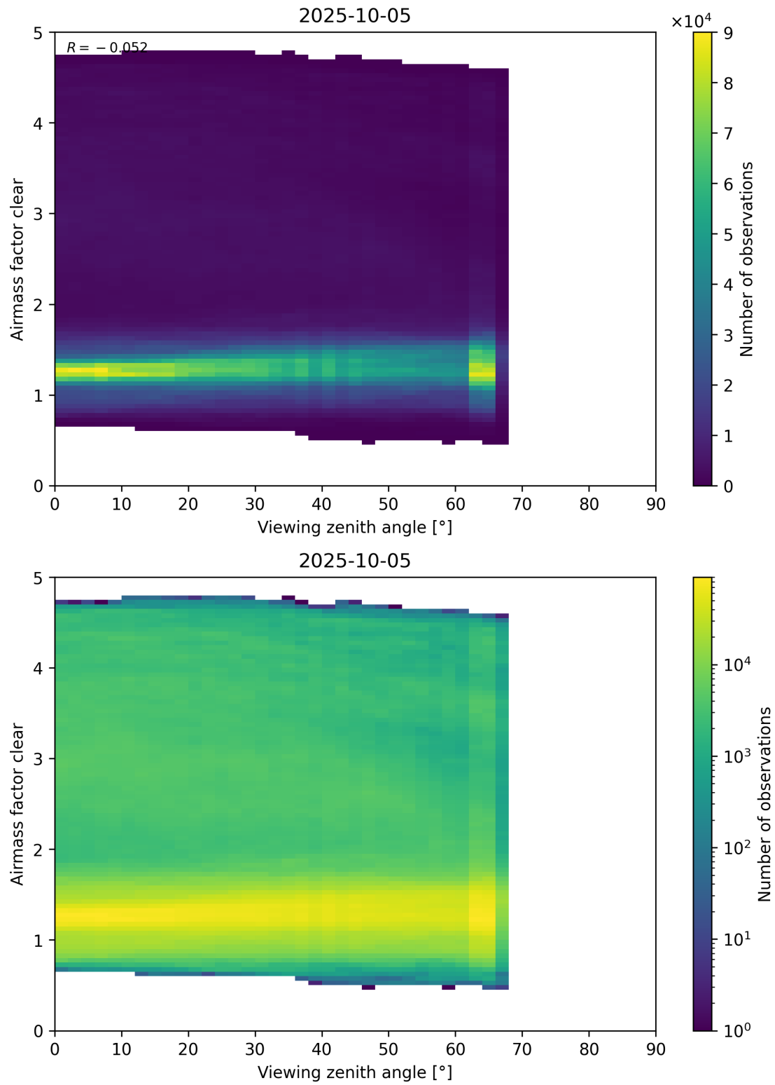
Figure 185: Scatter density plot of “Viewing zenith angle” against “Airmass factor clear” for 2025-10-04 to 2025-10-06.
