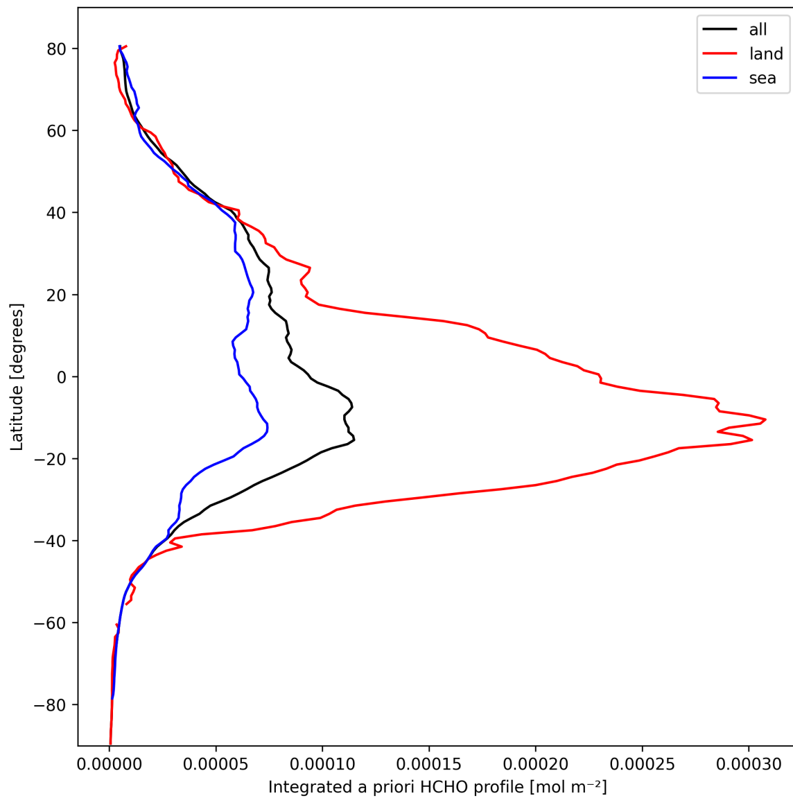
Figure 29: Zonal average of “Integrated a priori HCHO profile” for 2025-10-04 to 2025-10-06.
