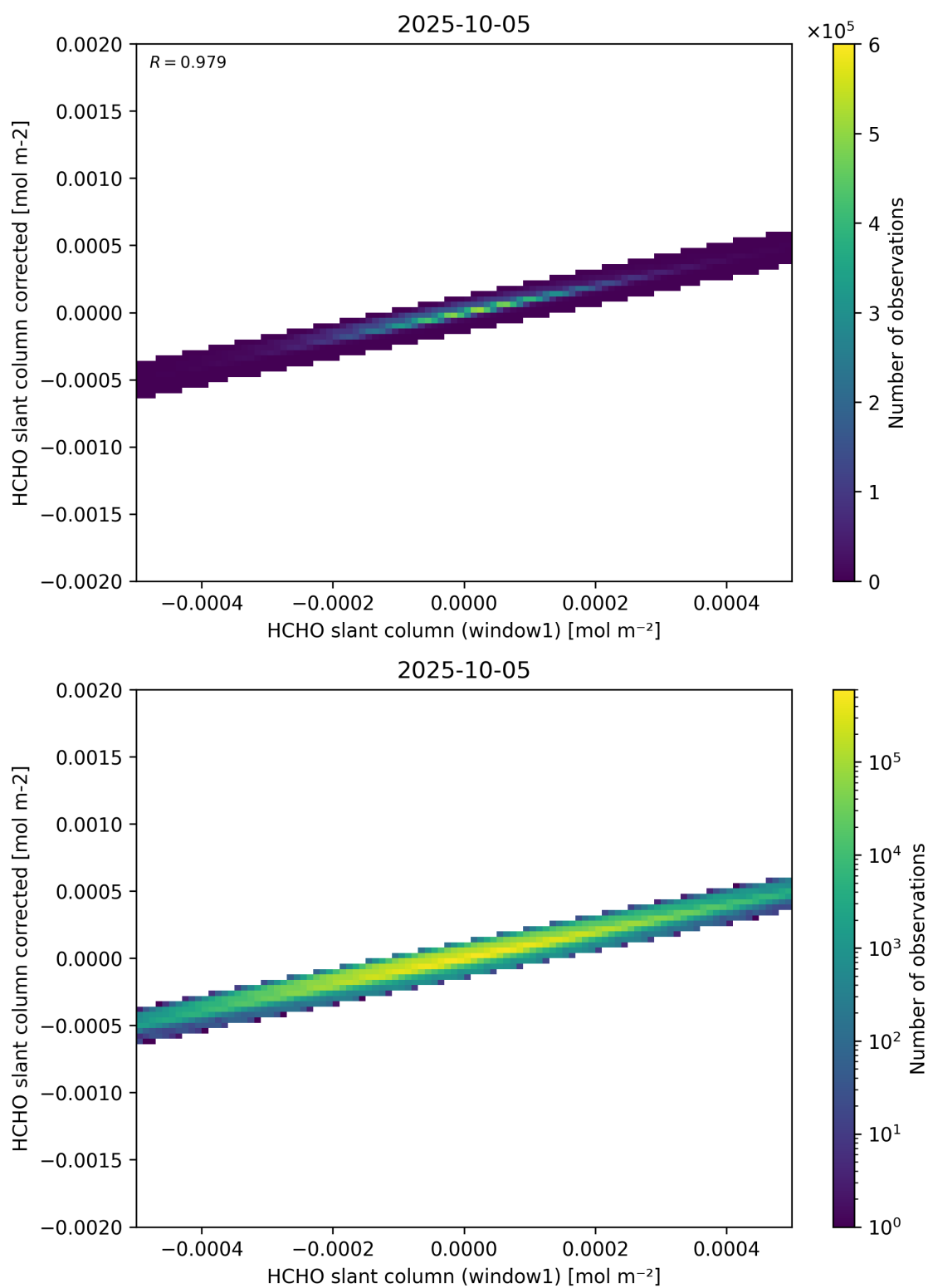
Figure 82: Scatter density plot of “HCHO slant column (window1)” against “HCHO slant column corrected” for 2025-10-04 to 2025-10-06.
