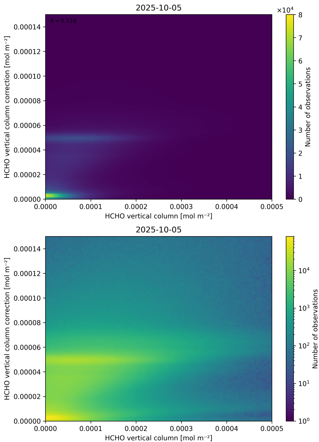
Figure 133: Scatter density plot of “HCHO vertical column” against “HCHO vertical column correction” for 2025-10-04 to 2025-10-06.
