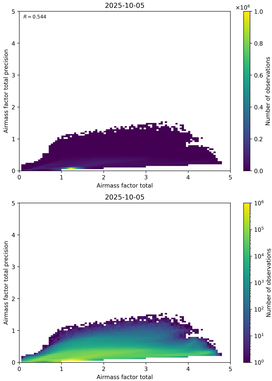
Figure 103: Scatter density plot of “Airmass factor total” against “Airmass factor total precision” for 2025-10-04 to 2025-10-06.
