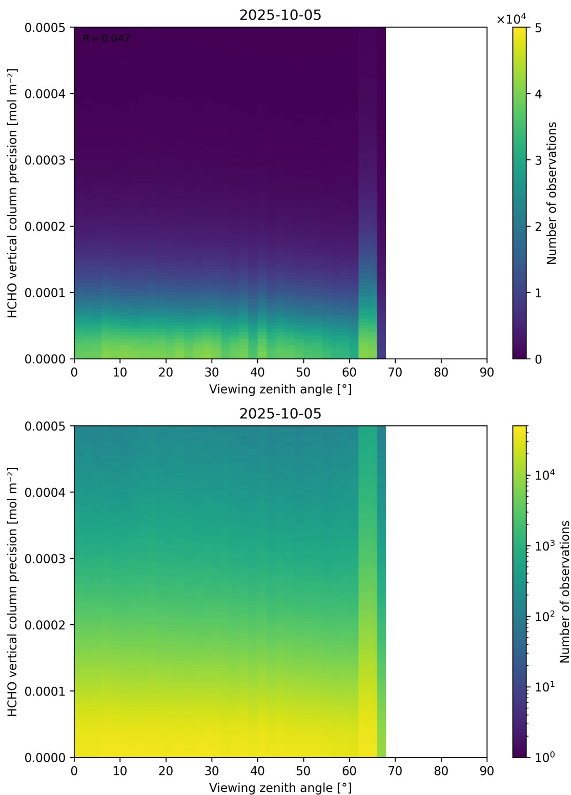
Figure 194: Scatter density plot of “Viewing zenith angle” against “HCHO vertical column precision” for 2025-10-04 to 2025-10-06.
