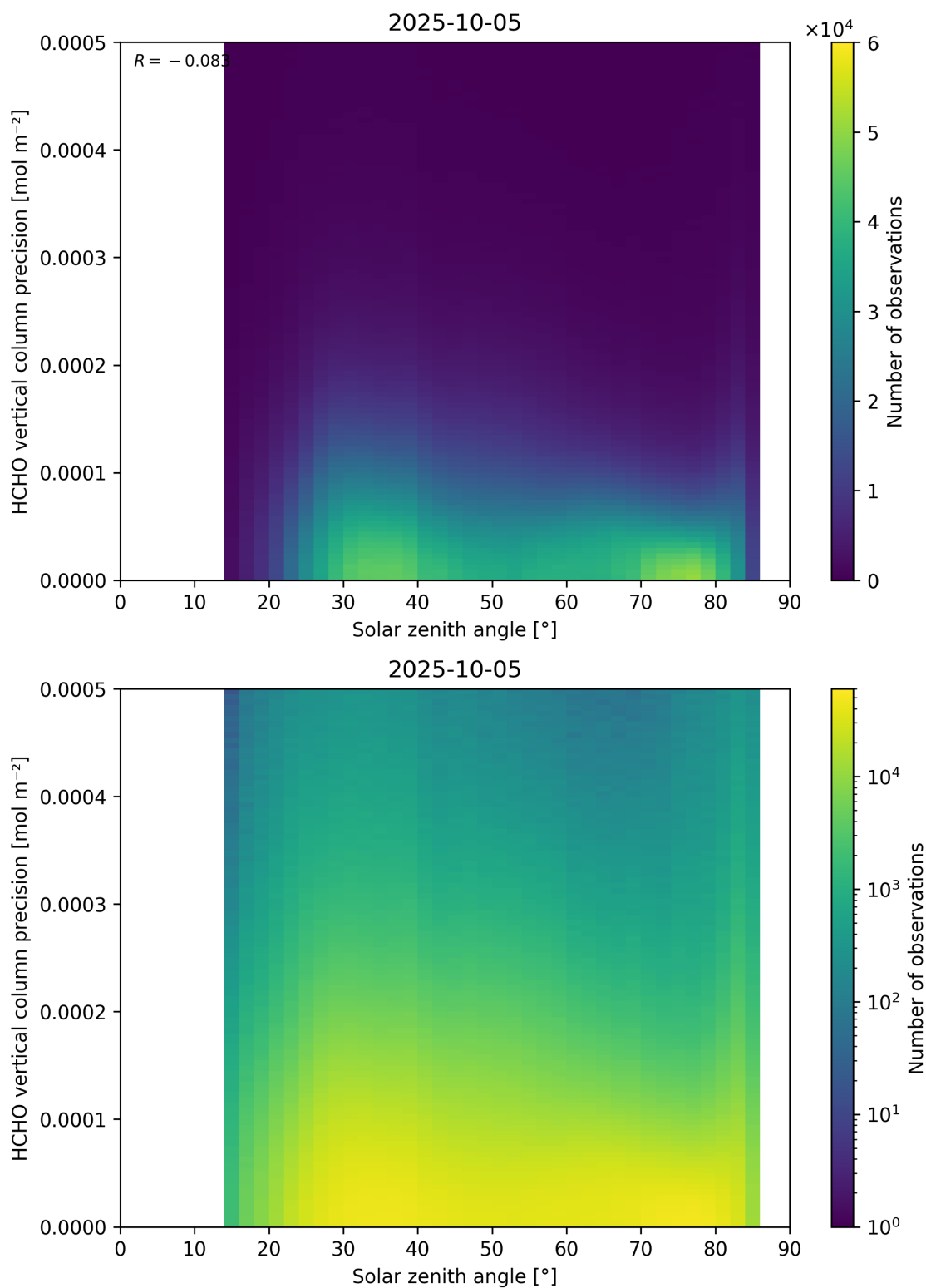
Figure 179: Scatter density plot of “Solar zenith angle” against “HCHO vertical column precision” for 2025-10-04 to 2025-10-06.
