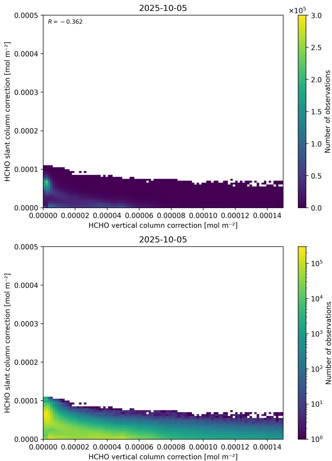
Figure 117: Scatter density plot of “HCHO vertical column correction” against “HCHO slant column correction” for 2025-10-04 to 2025-10-06.
