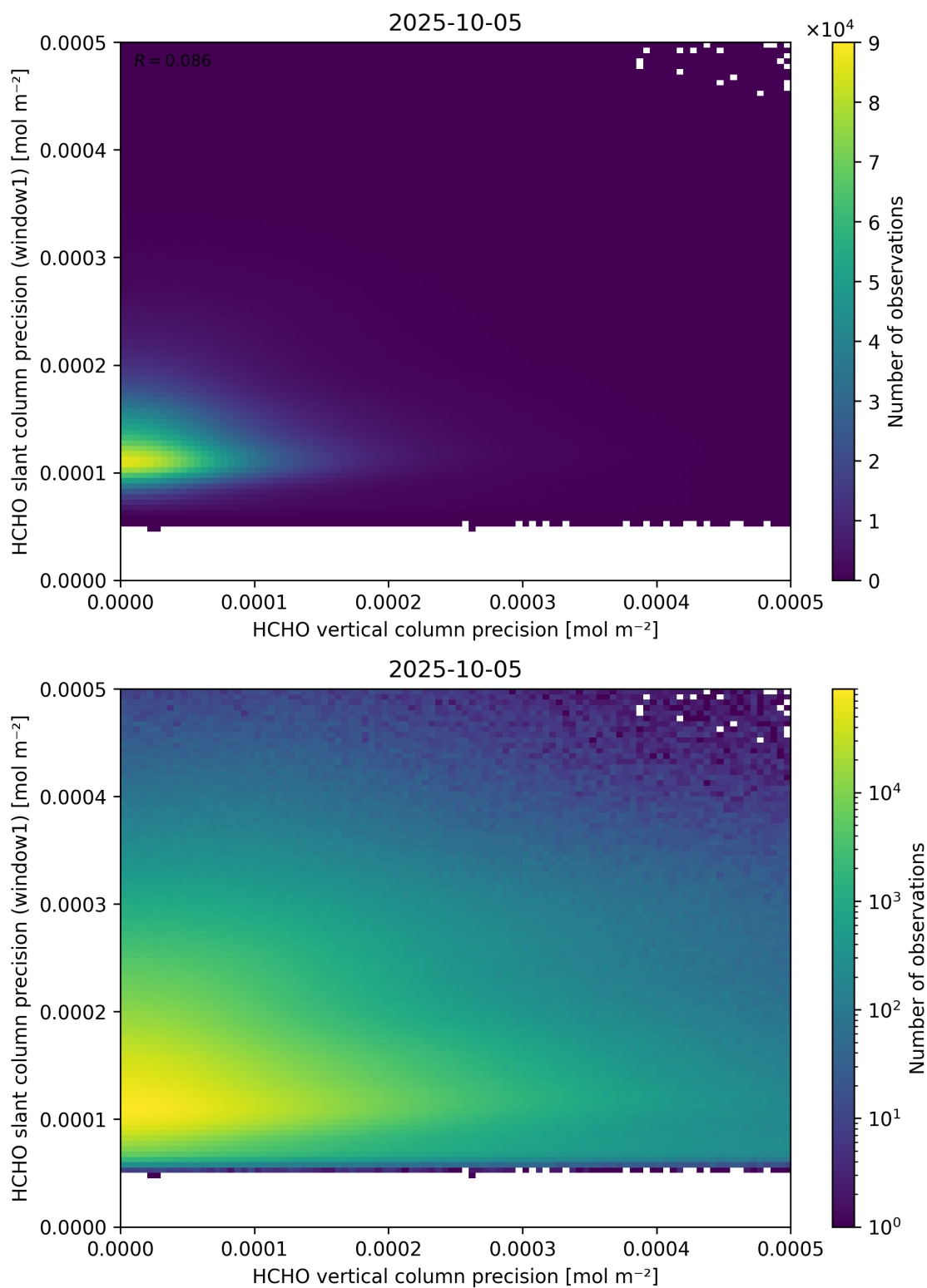
Figure 143: Scatter density plot of “HCHO vertical column precision” against “HCHO slant column precision (window1)” for 2025-10-04 to 2025-10-06.
