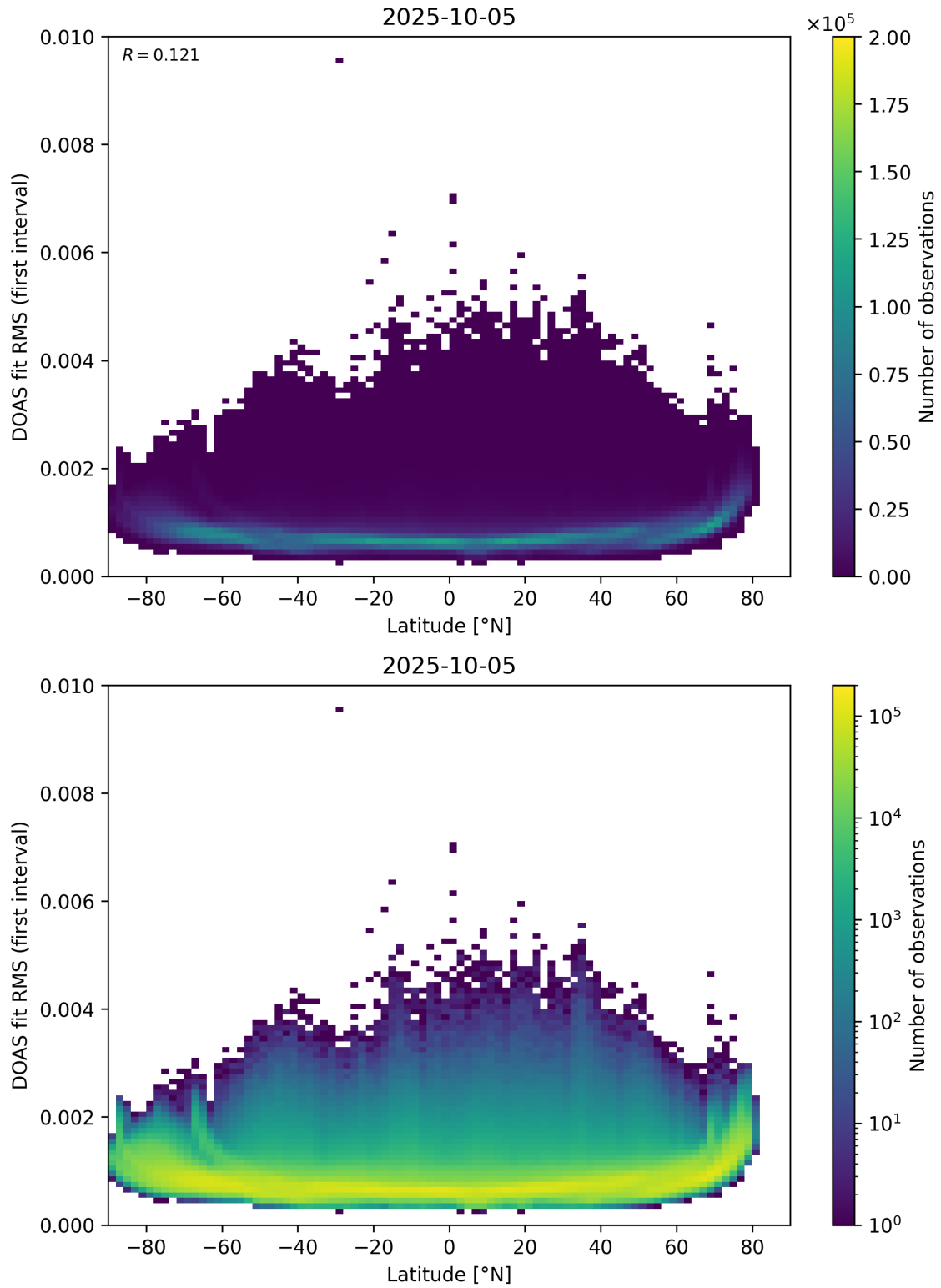
Figure 153: Scatter density plot of “Latitude” against “DOAS fit RMS (first interval)” for 2025-10-04 to 2025-10-06.
