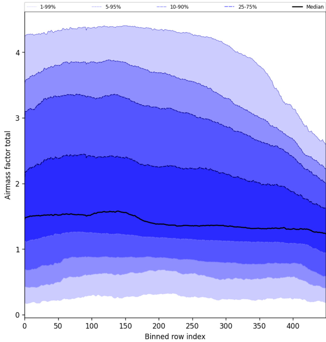
Figure 54: Along track statistics of “Airmass factor total” for 2025-10-04 to 2025-10-06
