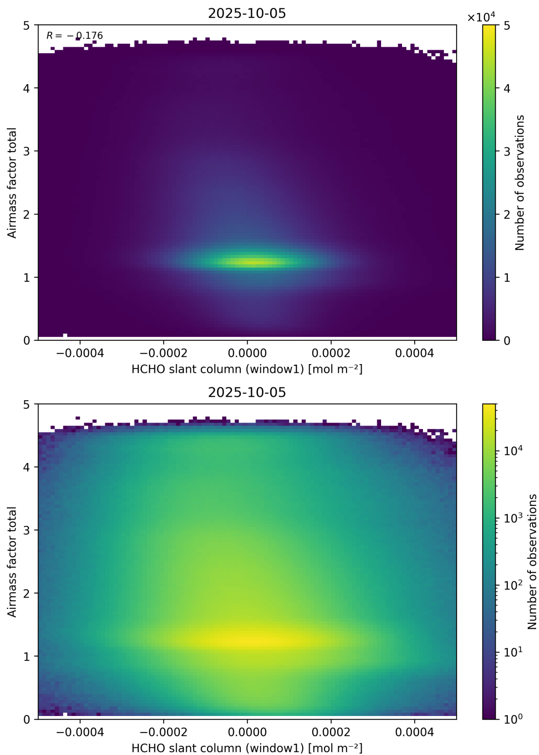
Figure 85: Scatter density plot of “HCHO slant column (window1)” against “Airmass factor total” for 2025-10-04 to 2025-10-06.
