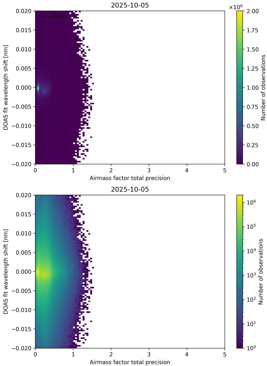
Figure 106: Scatter density plot of “Airmass factor total precision” against “DOAS fit wavelength shift” for 2025-10-04 to 2025-10-06.
