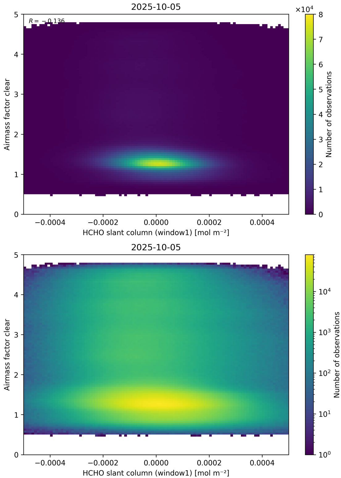
Figure 81: Scatter density plot of “HCHO slant column (window1)” against “Airmass factor clear” for 2025-10-04 to 2025-10-06.
