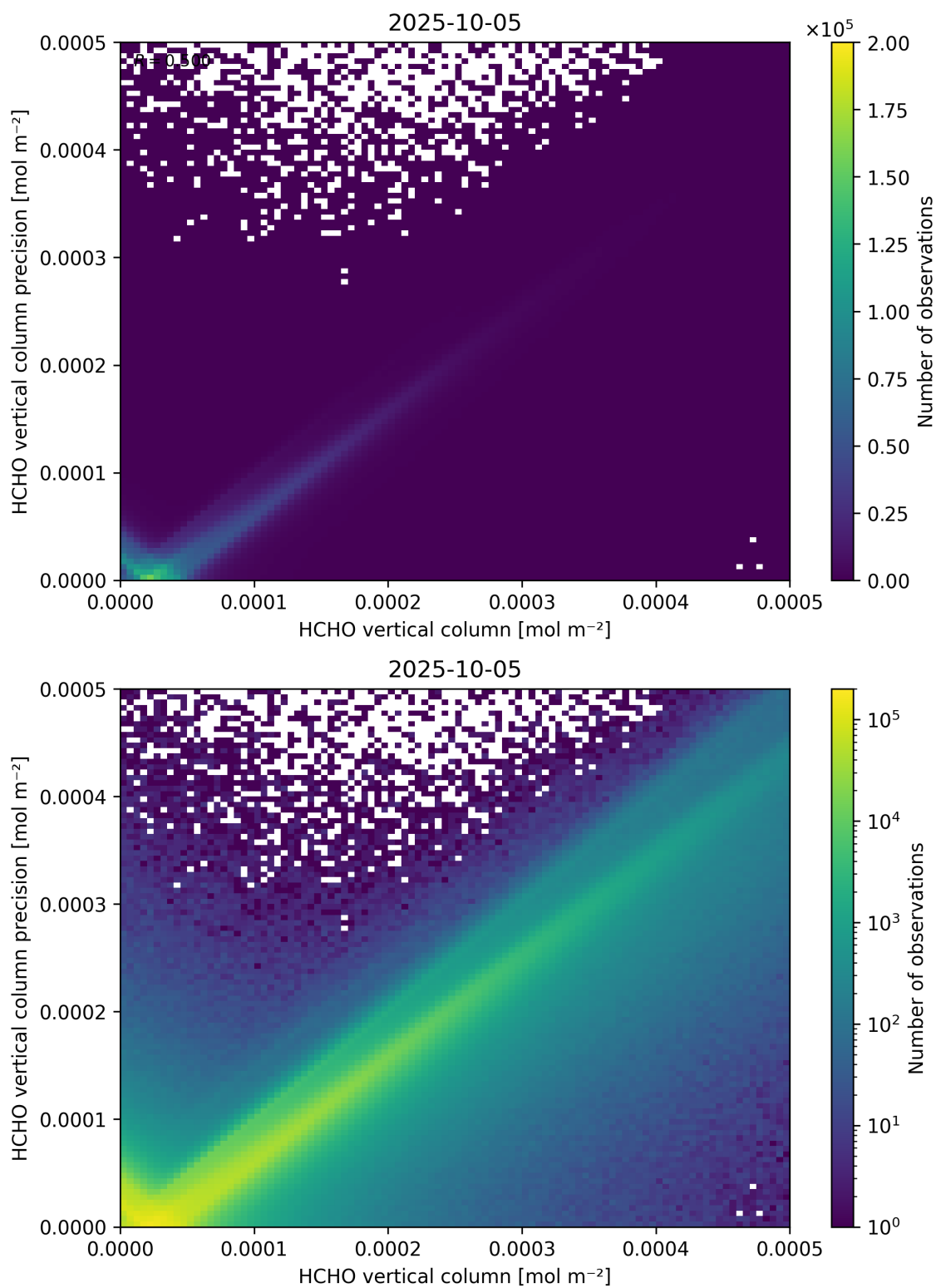
Figure 134: Scatter density plot of “HCHO vertical column” against “HCHO vertical column precision” for 2025-10-04 to 2025-10-06.
