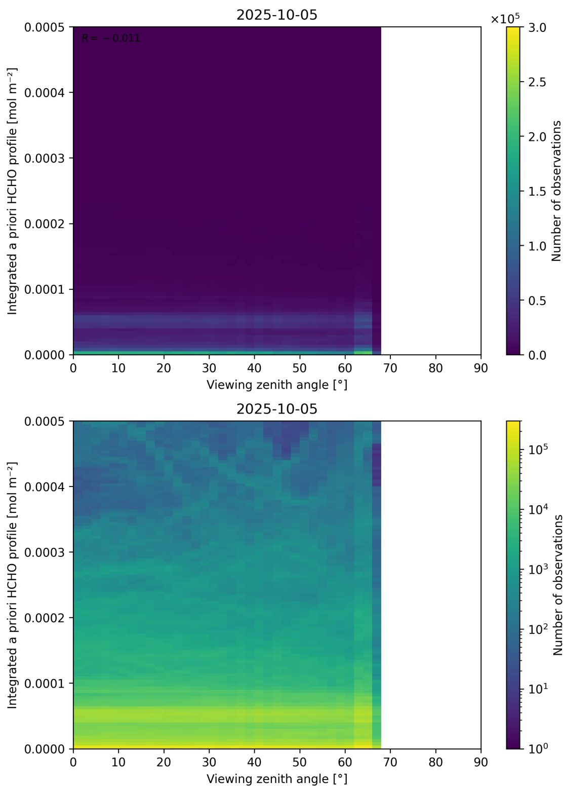
Figure 195: Scatter density plot of “Viewing zenith angle” against “Integrated a priori HCHO profile” for 2025-10-04 to 2025-10-06.
