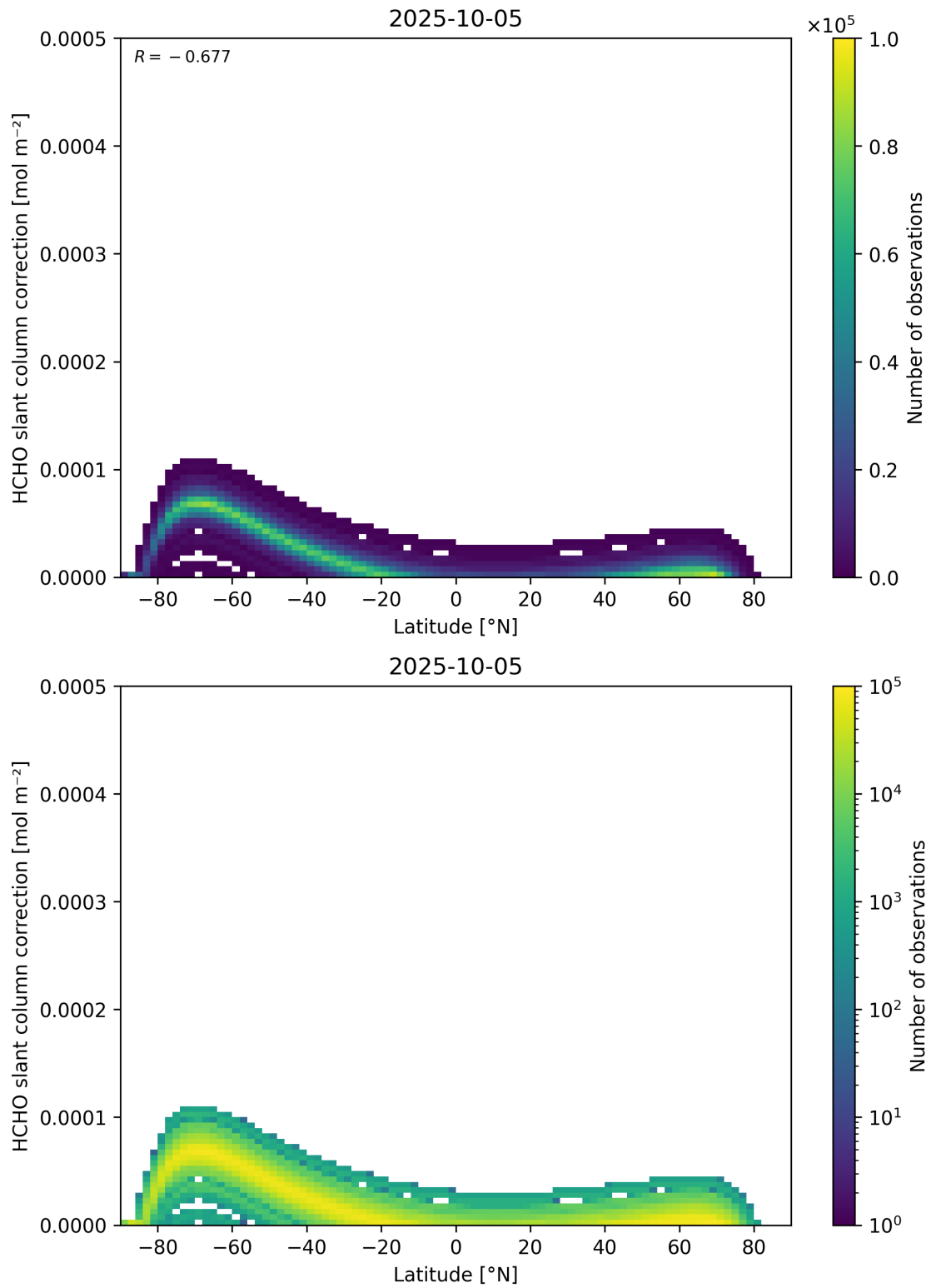
Figure 158: Scatter density plot of “Latitude” against “HCHO slant column correction” for 2025-10-04 to 2025-10-06.
