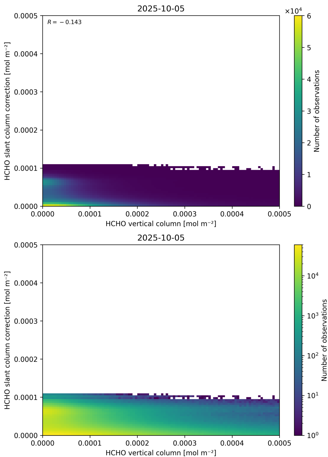
Figure 128: Scatter density plot of “HCHO vertical column” against “HCHO slant column correction” for 2025-10-04 to 2025-10-06.
