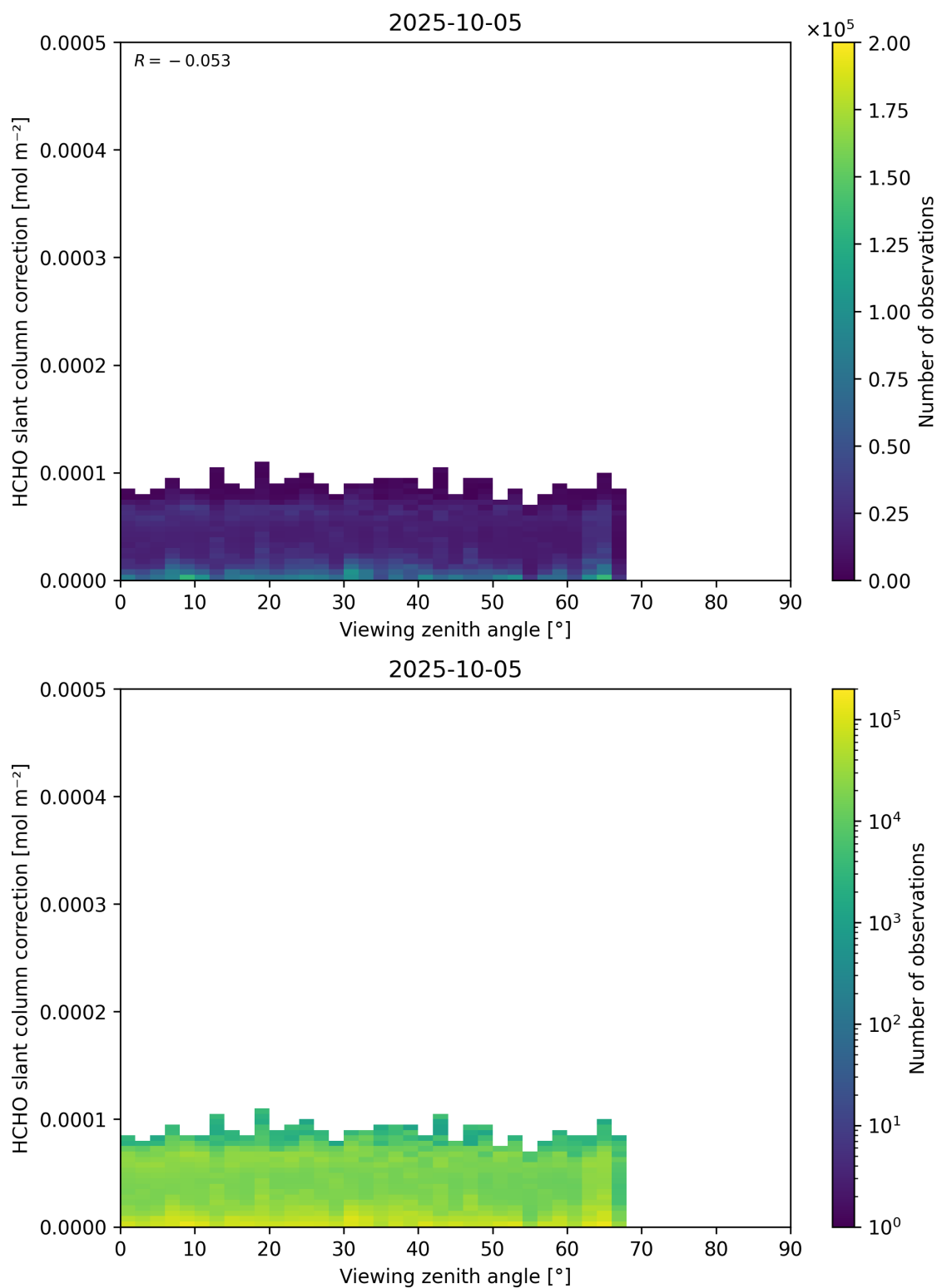
Figure 187: Scatter density plot of “Viewing zenith angle” against “HCHO slant column correction” for 2025-10-04 to 2025-10-06.
