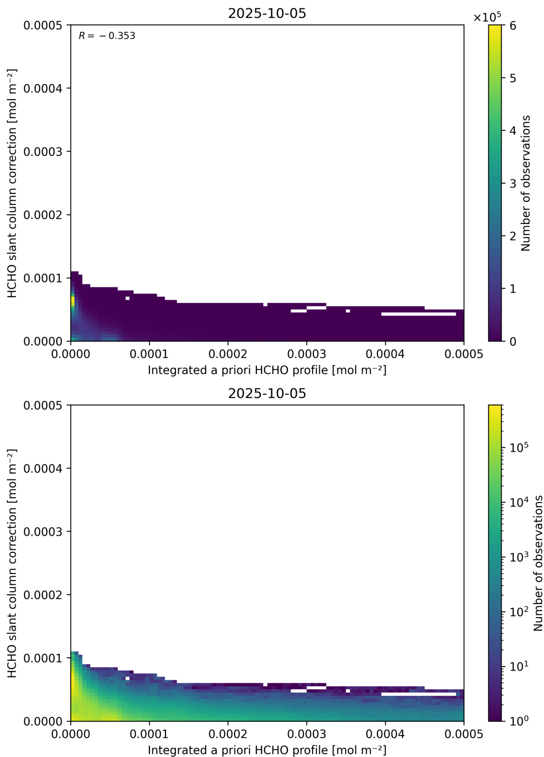
Figure 152: Scatter density plot of “Integrated a priori HCHO profile” against “HCHO slant column correction” for 2025-10-04 to 2025-10-06.
