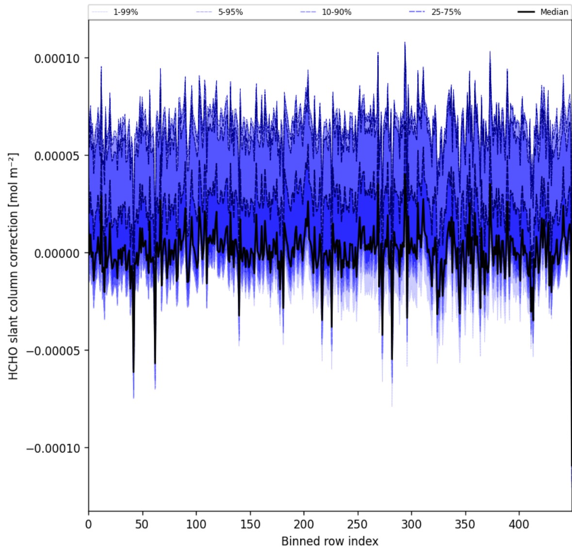
Figure 61: Along track statistics of “HCHO slant column correction” for 2025-10-04 to 2025-10-06
