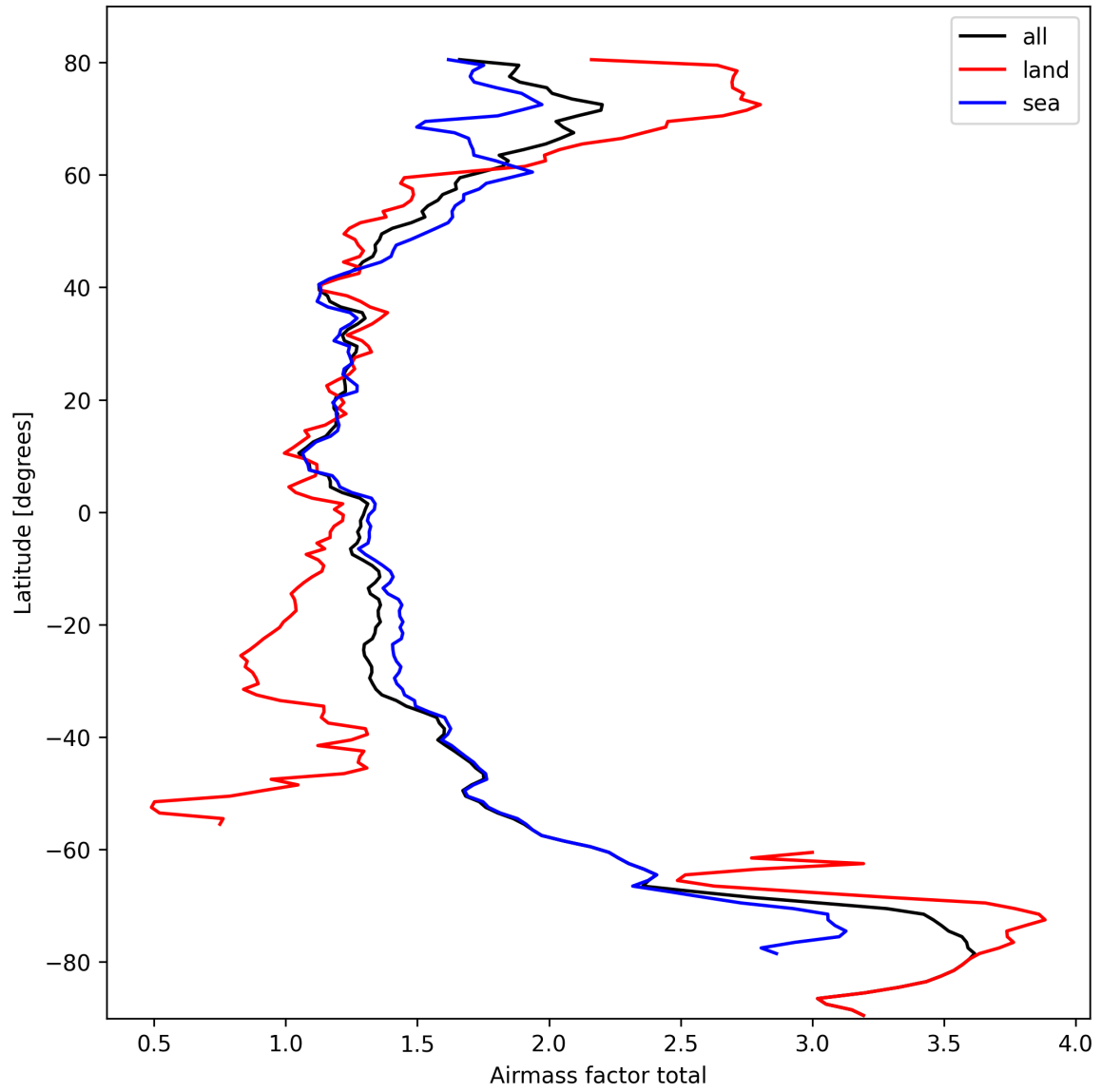
Figure 26: Zonal average of “Airmass factor total” for 2025-10-04 to 2025-10-06.
