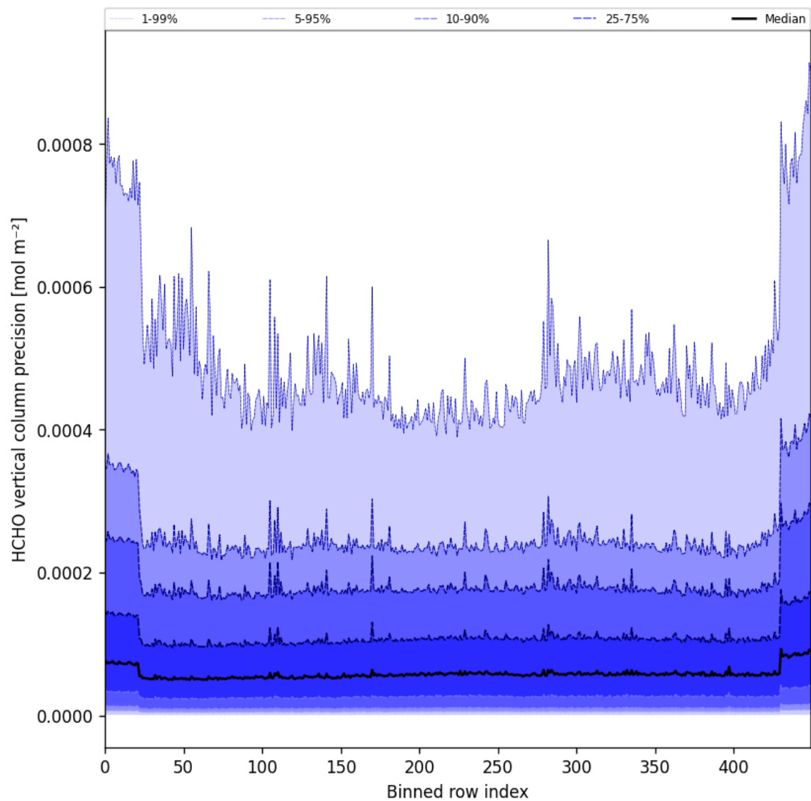
Figure 50: Along track statistics of “HCHO vertical column precision” for 2025-10-04 to 2025-10-06
