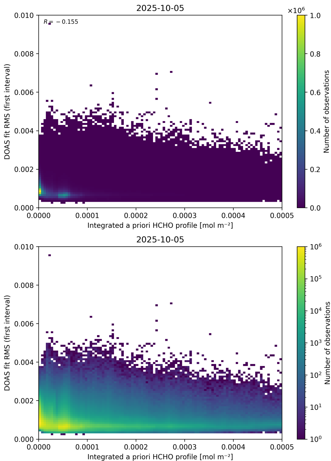
Figure 148: Scatter density plot of “Integrated a priori HCHO profile” against “DOAS fit RMS (first interval)” for 2025-10-04 to 2025-10-06.
