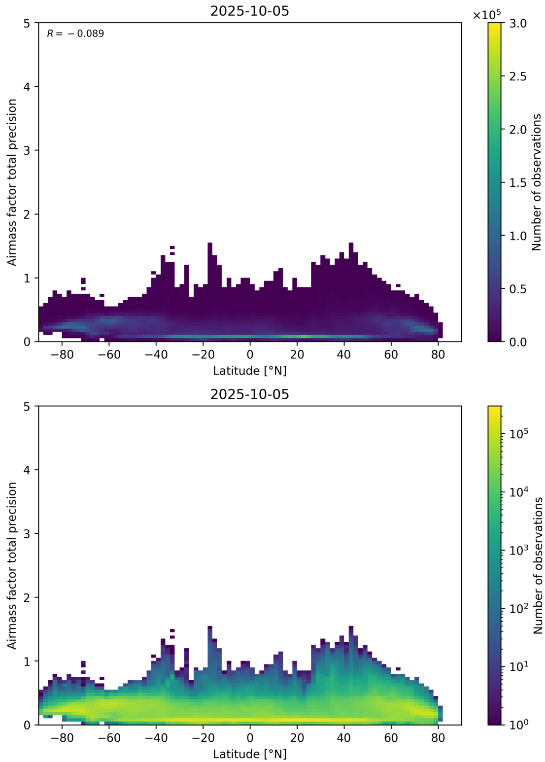
Figure 162: Scatter density plot of “Latitude” against “Airmass factor total precision” for 2025-10-04 to 2025-10-06.
