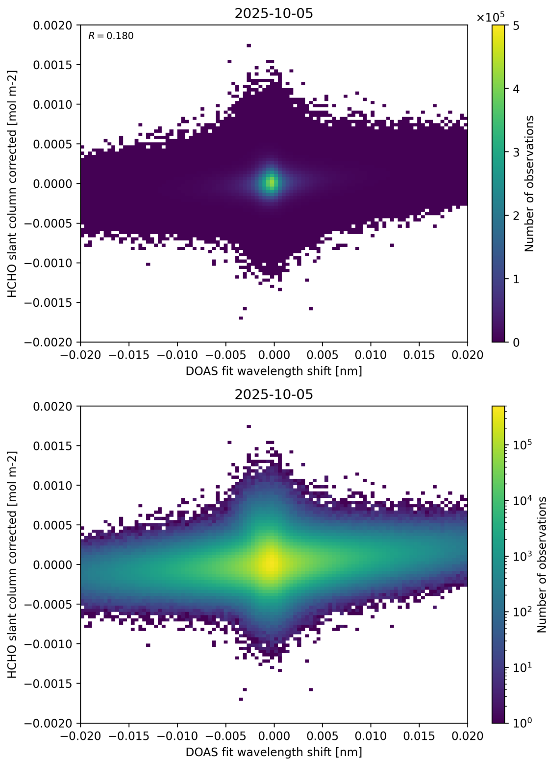
Figure 66: Scatter density plot of “DOAS fit wavelength shift” against “HCHO slant column corrected” for 2025-10-04 to 2025-10-06.
