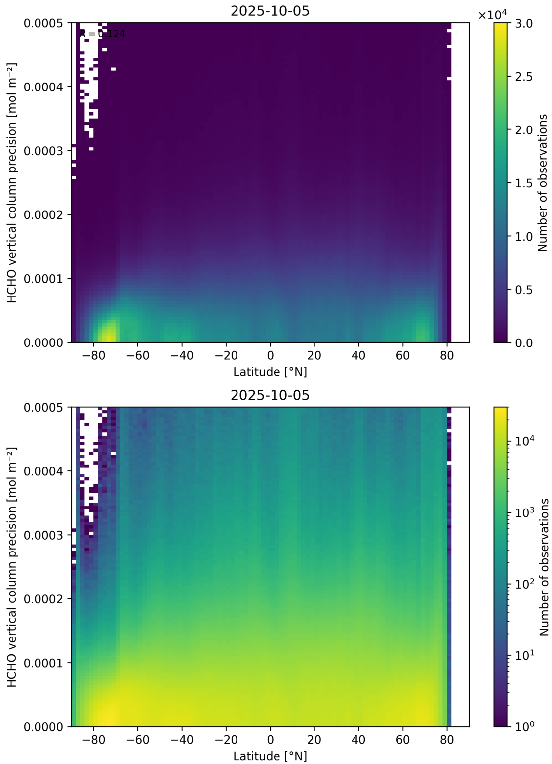
Figure 165: Scatter density plot of “Latitude” against “HCHO vertical column precision” for 2025-10-04 to 2025-10-06.
