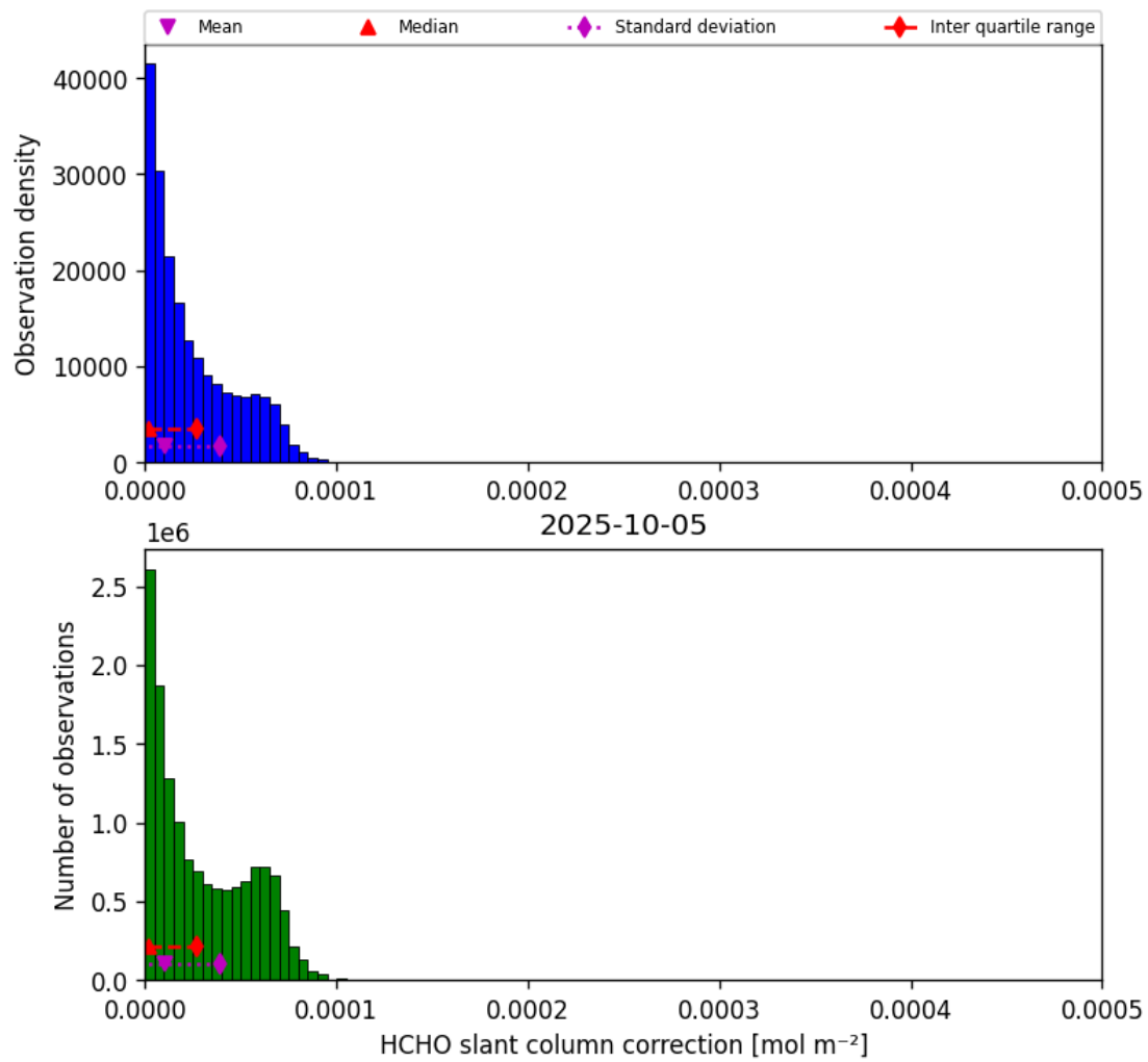
Figure 47: Histogram of “HCHO slant column correction” for 2025-10-04 to 2025-10-06
