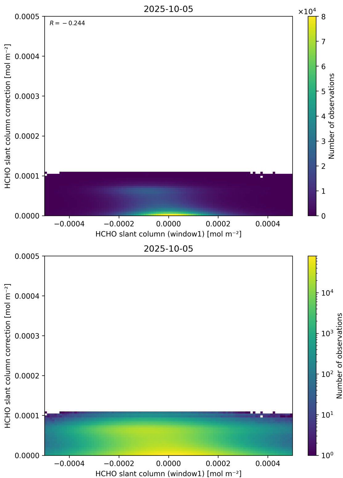
Figure 83: Scatter density plot of “HCHO slant column (window1)” against “HCHO slant column correction” for 2025-10-04 to 2025-10-06.
