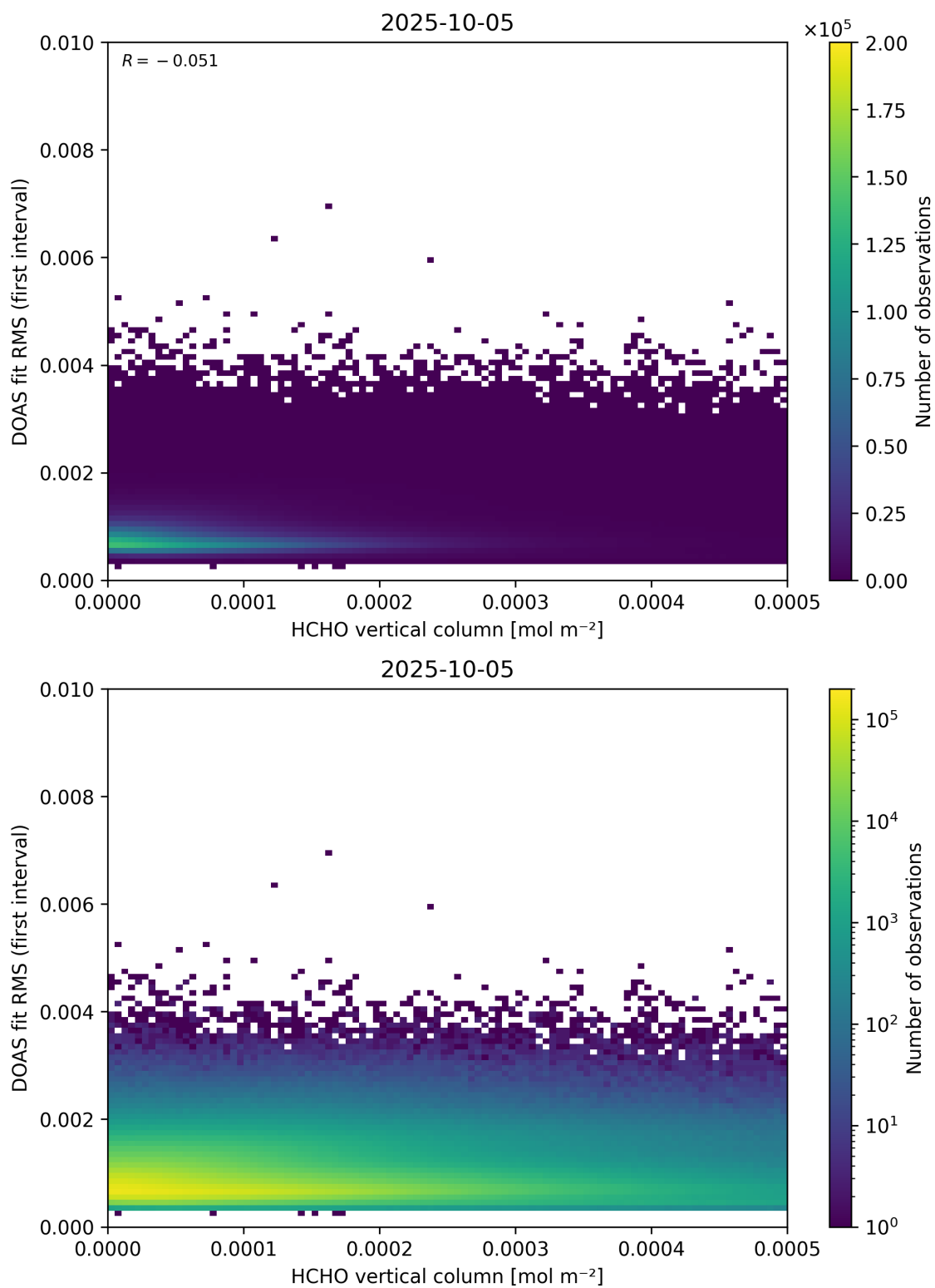
Figure 123: Scatter density plot of “HCHO vertical column” against “DOAS fit RMS (first interval)” for 2025-10-04 to 2025-10-06.
