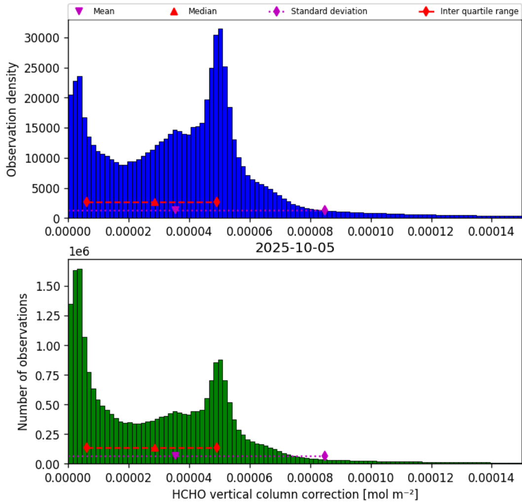
Figure 37: Histogram of “HCHO vertical column correction” for 2025-10-04 to 2025-10-06
