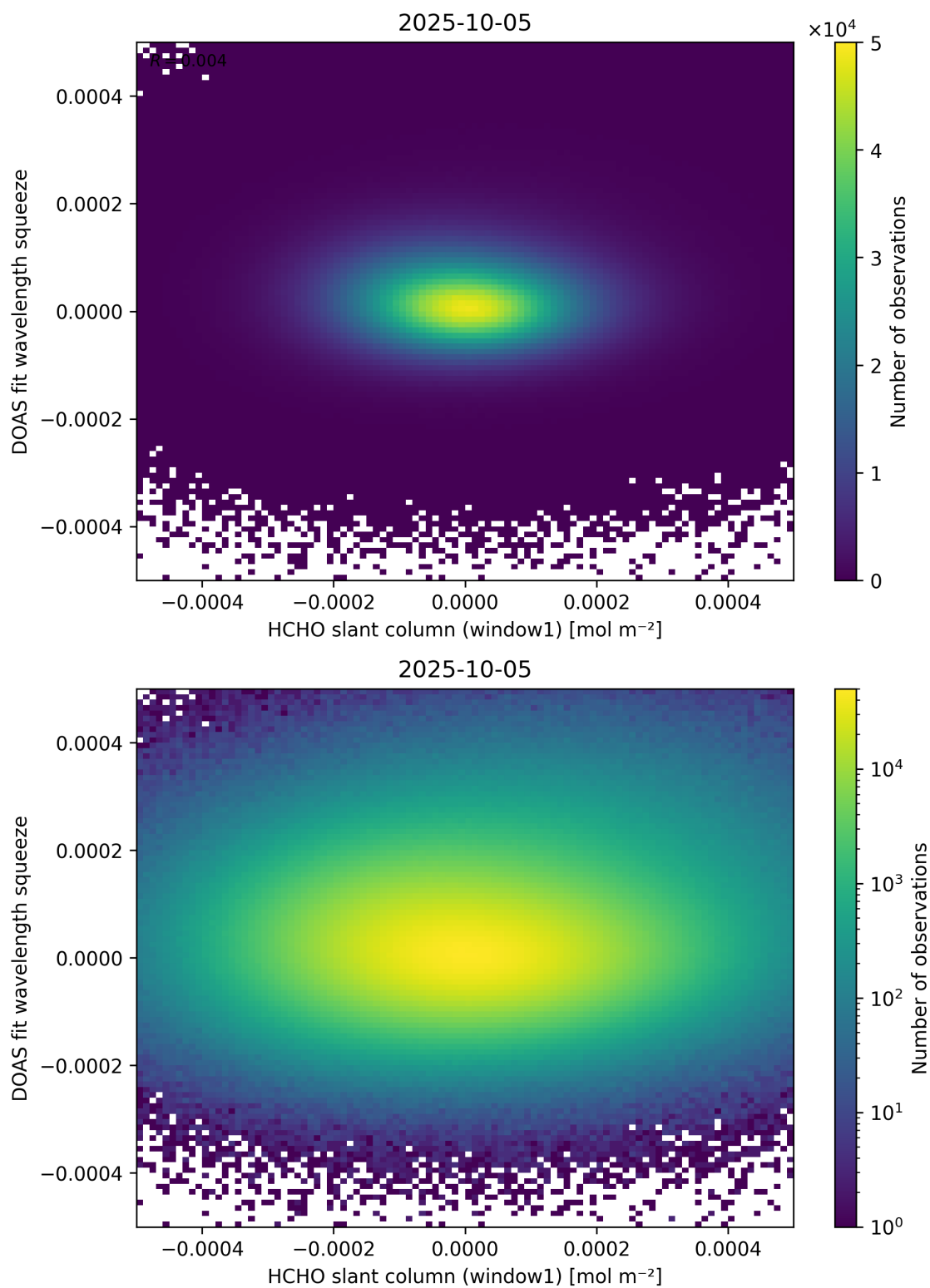
Figure 80: Scatter density plot of “HCHO slant column (window1)” against “DOAS fit wavelength squeeze” for 2025-10-04 to 2025-10-06.
