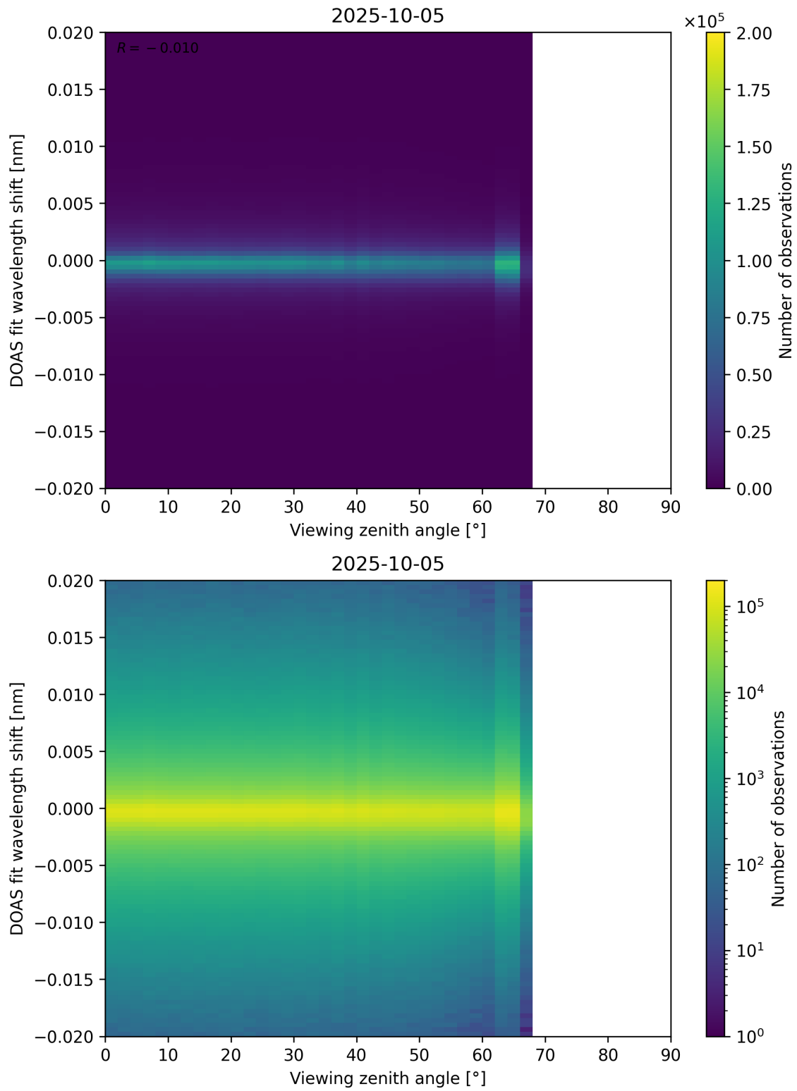
Figure 183: Scatter density plot of “Viewing zenith angle” against “DOAS fit wavelength shift” for 2025-10-04 to 2025-10-06.
