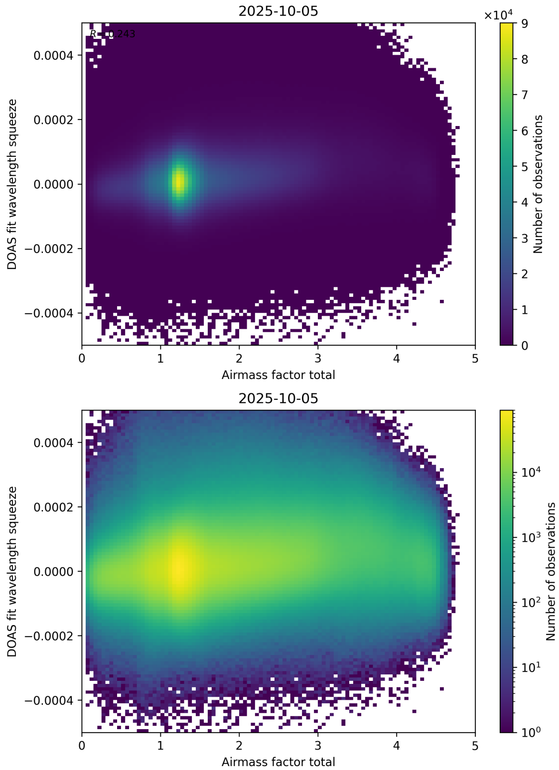
Figure 99: Scatter density plot of “Airmass factor total” against “DOAS fit wavelength squeeze” for 2025-10-04 to 2025-10-06.
