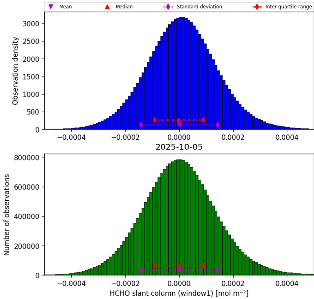
Figure 38: Histogram of “HCHO slant column (window1)” for 2025-10-04 to 2025-10-06
