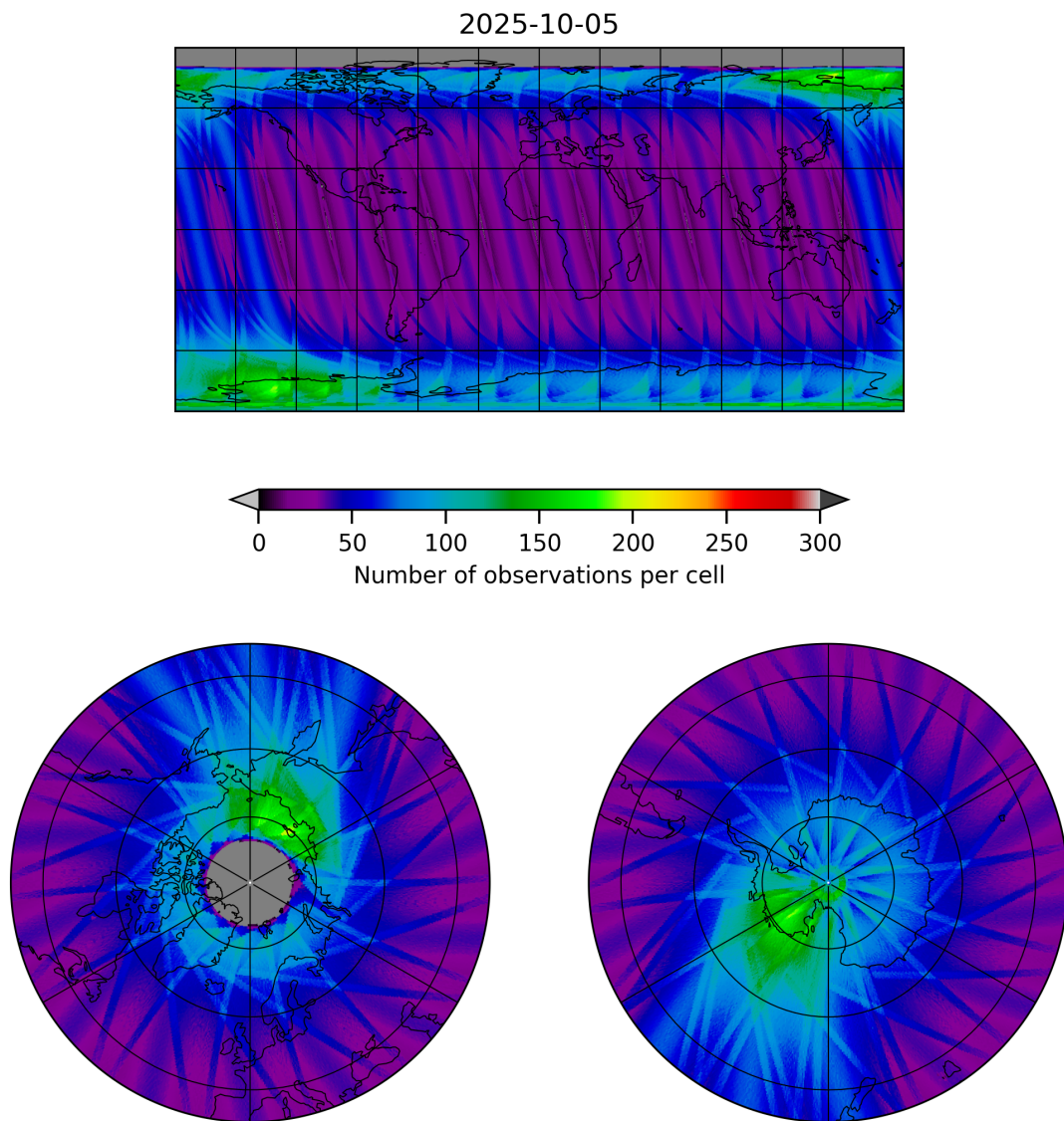
Figure 19: Map of the number of observations for 2025-10-04 to 2025-10-06
