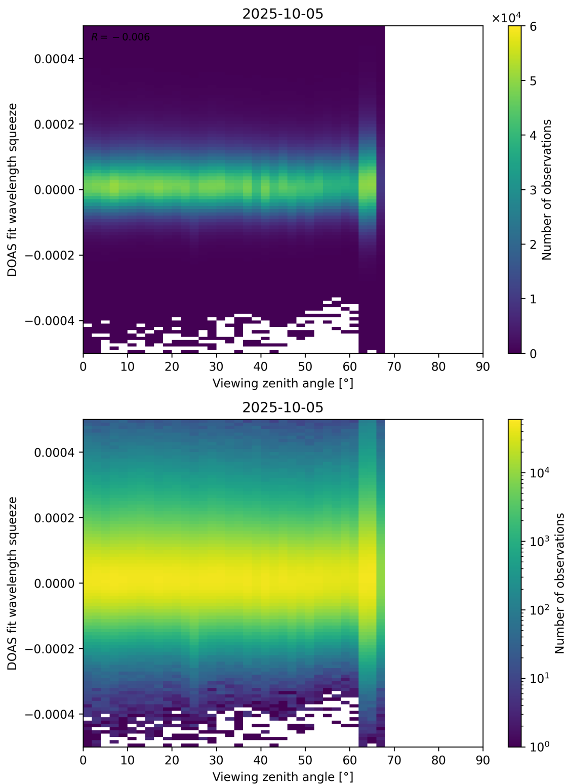
Figure 184: Scatter density plot of “Viewing zenith angle” against “DOAS fit wavelength squeeze” for 2025-10-04 to 2025-10-06.
