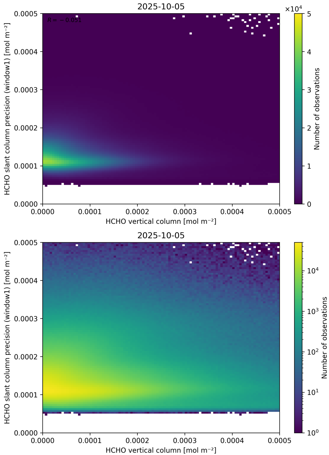
Figure 130: Scatter density plot of “HCHO vertical column” against “HCHO slant column precision (window1)” for 2025-10-04 to 2025-10-06.
