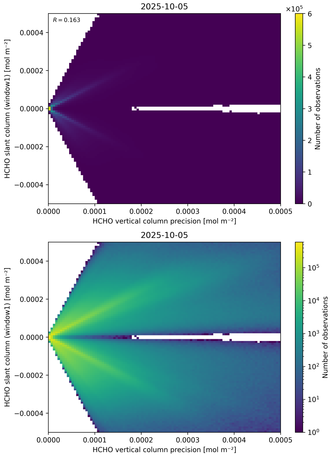
Figure 142: Scatter density plot of “HCHO vertical column precision” against “HCHO slant column (window1)” for 2025-10-04 to 2025-10-06.
