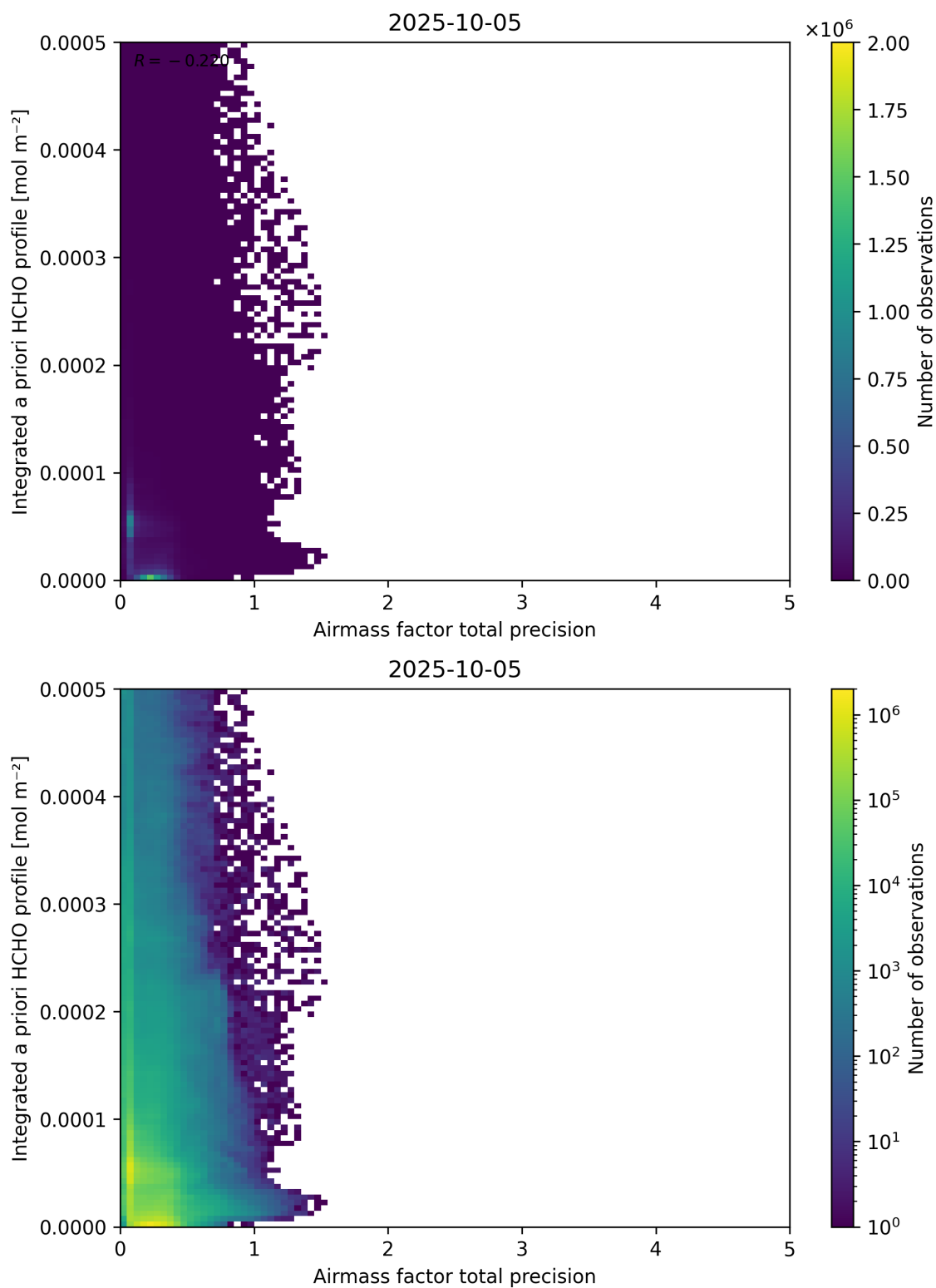
Figure 111: Scatter density plot of “Airmass factor total precision” against “Integrated a priori HCHO profile” for 2025-10-04 to 2025-10-06.
