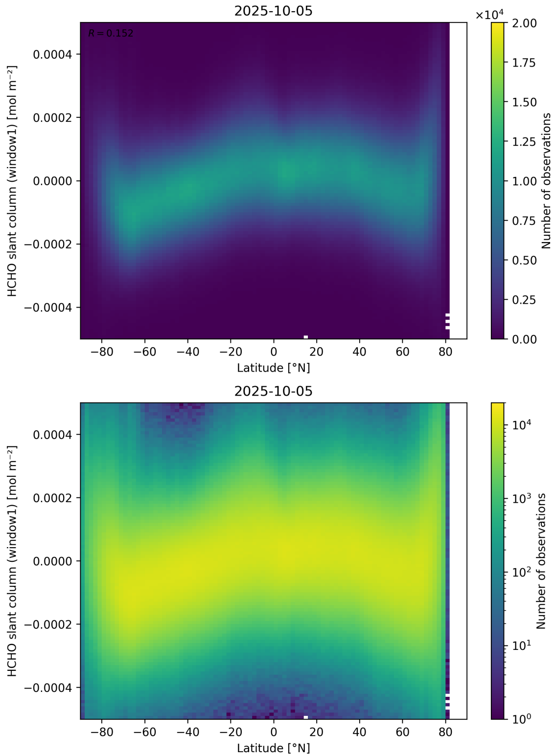
Figure 159: Scatter density plot of “Latitude” against “HCHO slant column (window1)” for 2025-10-04 to 2025-10-06.
