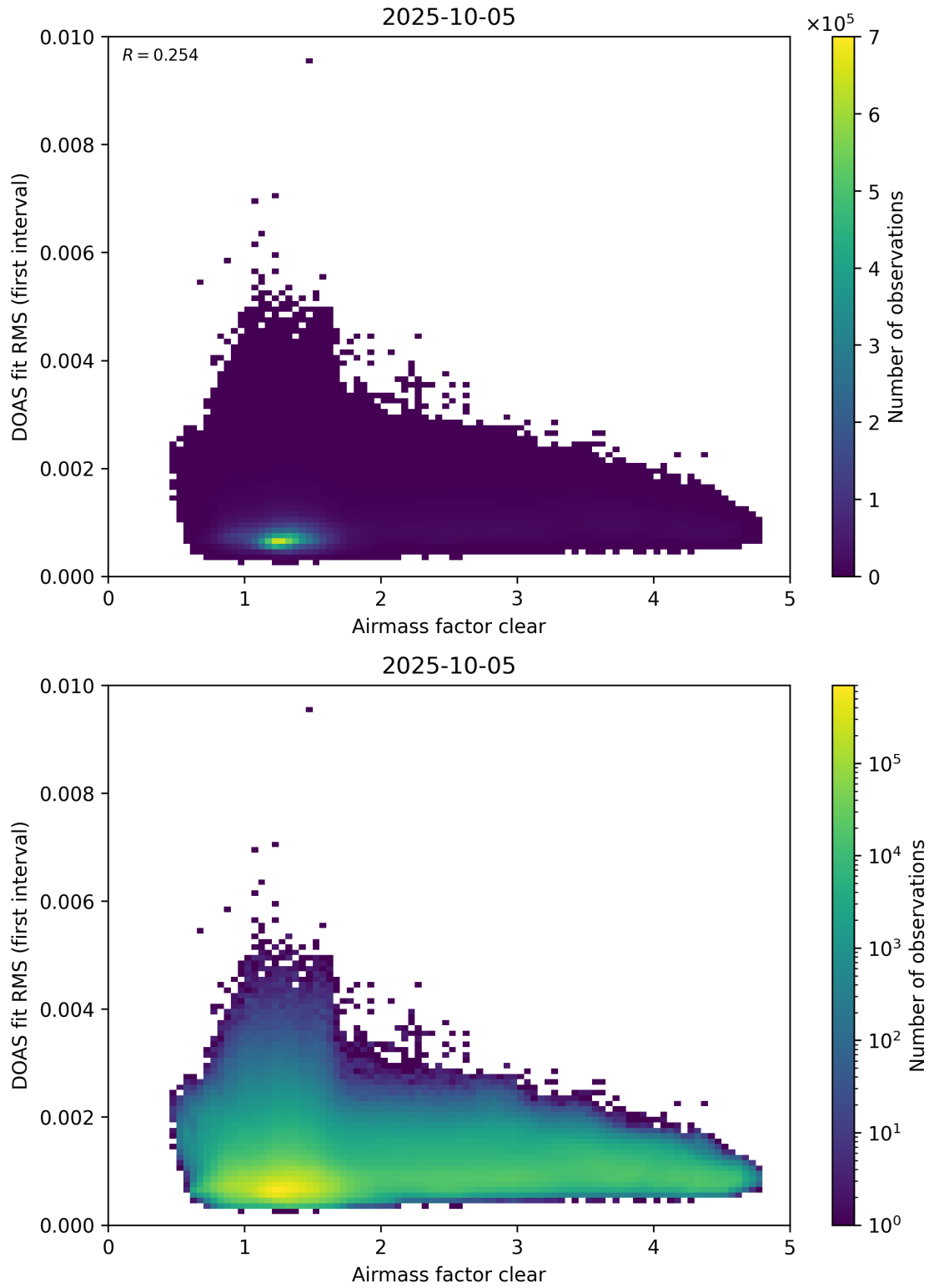
Figure 71: Scatter density plot of “Airmass factor clear” against “DOAS fit RMS (first interval)” for 2025-10-04 to 2025-10-06.
