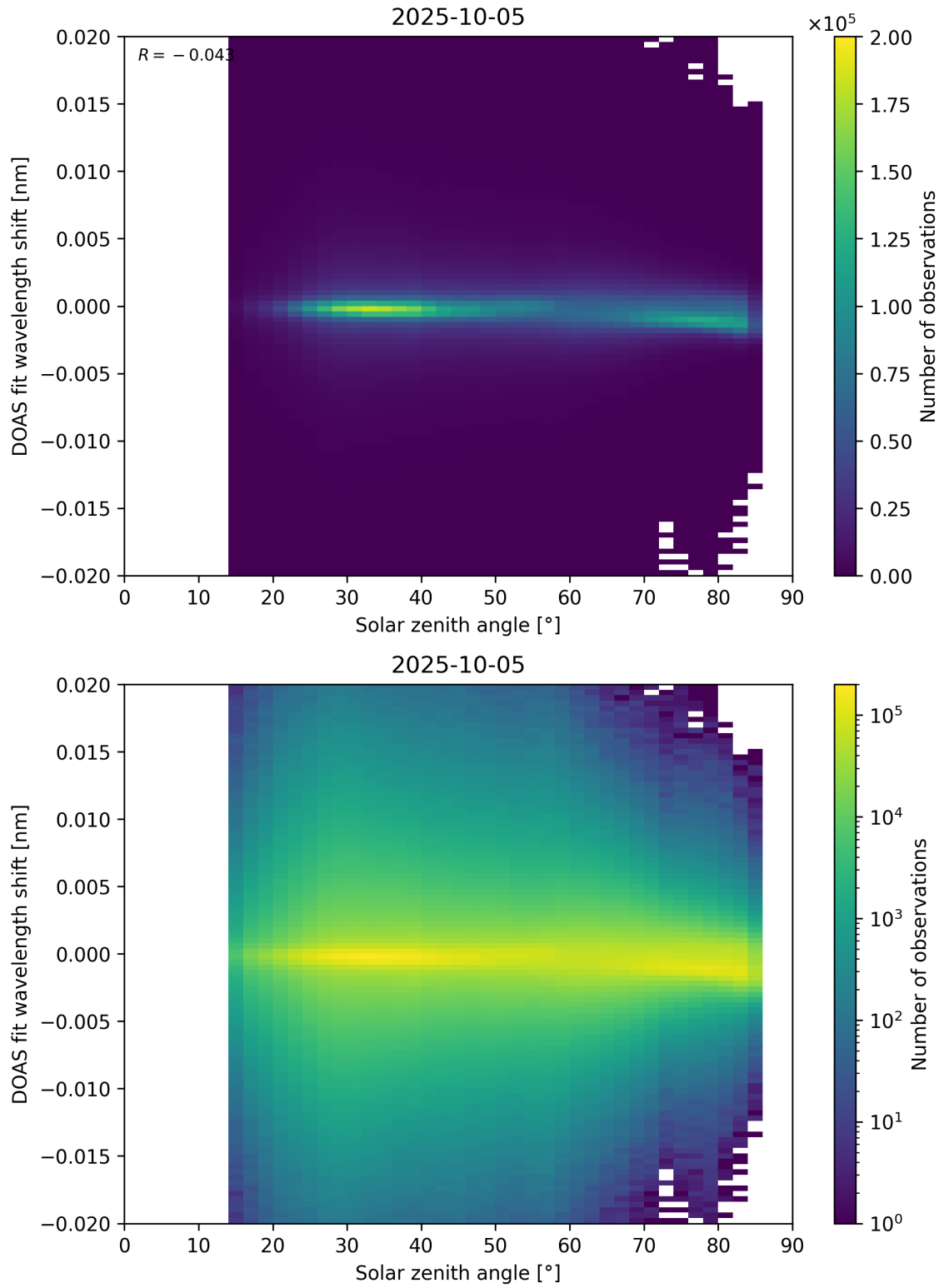
Figure 168: Scatter density plot of “Solar zenith angle” against “DOAS fit wavelength shift” for 2025-10-04 to 2025-10-06.
