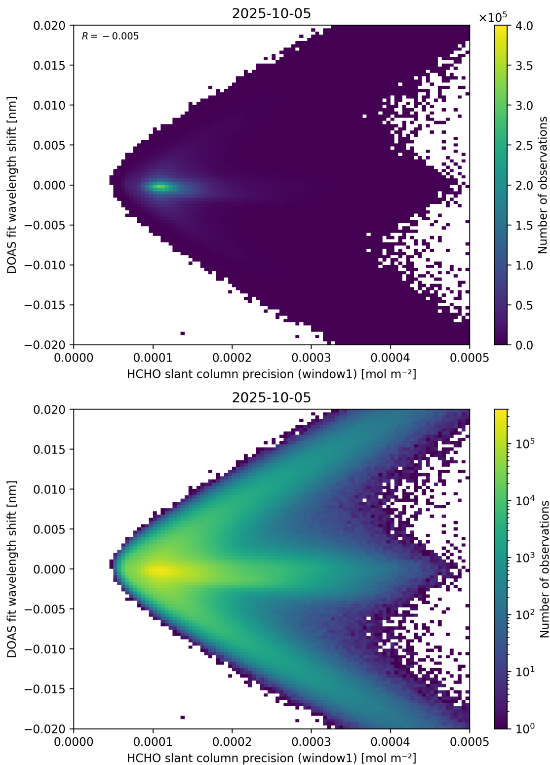
Figure 89: Scatter density plot of “HCHO slant column precision (window1)” against “DOAS fit wavelength shift” for 2025-10-04 to 2025-10-06.
