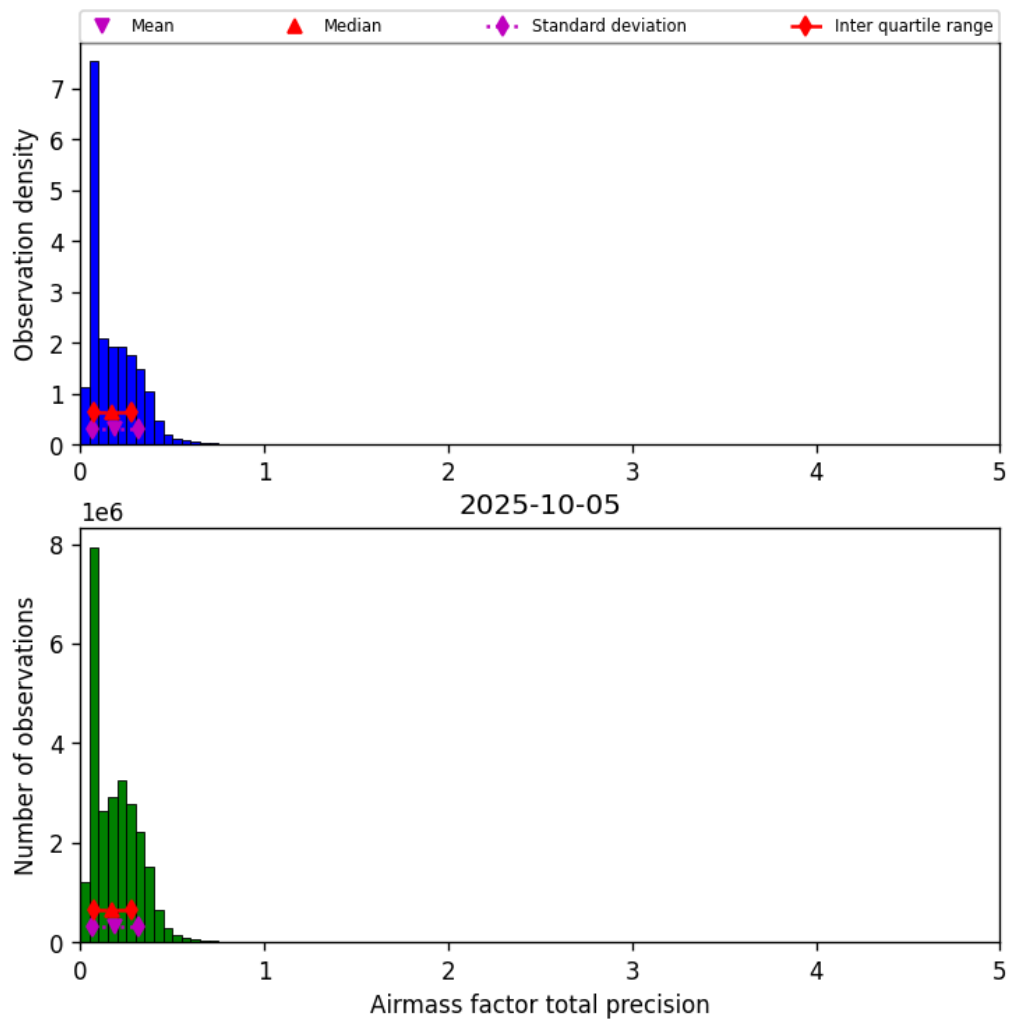
Figure 41: Histogram of “Airmass factor total precision” for 2025-10-04 to 2025-10-06
