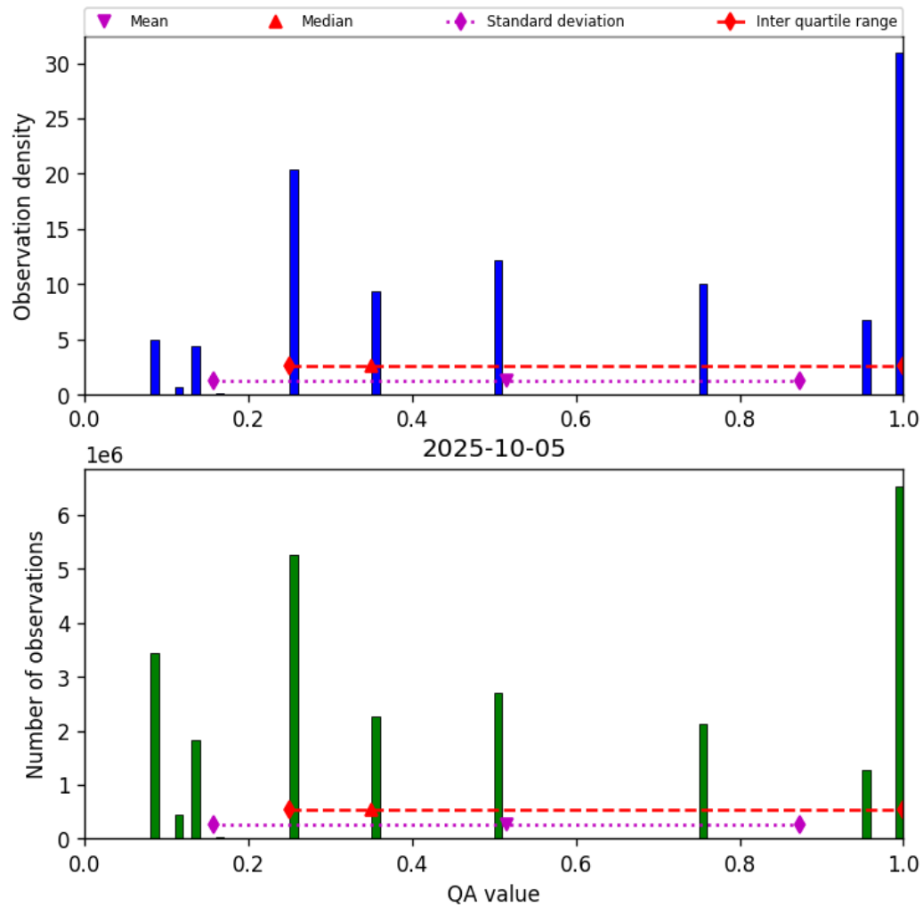
Figure 34: Histogram of “QA value” for 2025-10-04 to 2025-10-06
