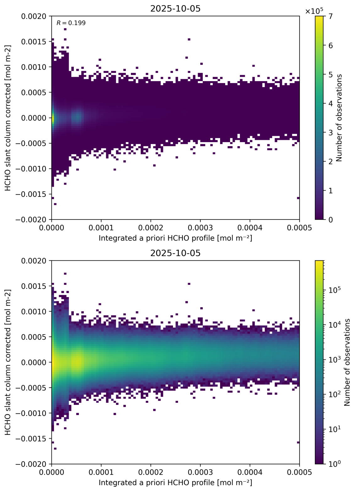
Figure 151: Scatter density plot of “Integrated a priori HCHO profile” against “HCHO slant column corrected” for 2025-10-04 to 2025-10-06.
