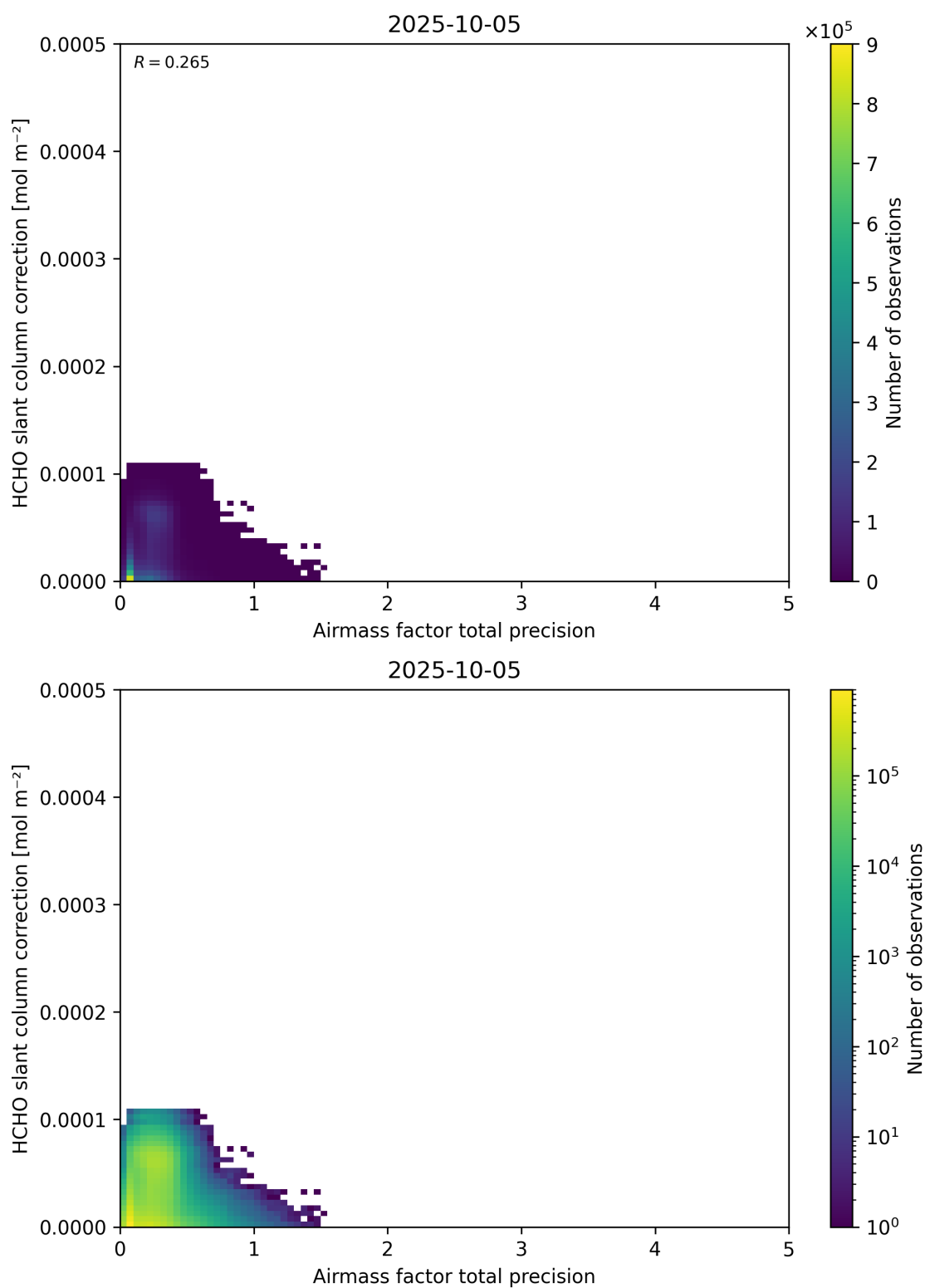
Figure 110: Scatter density plot of “Airmass factor total precision” against “HCHO slant column correction” for 2025-10-04 to 2025-10-06.
