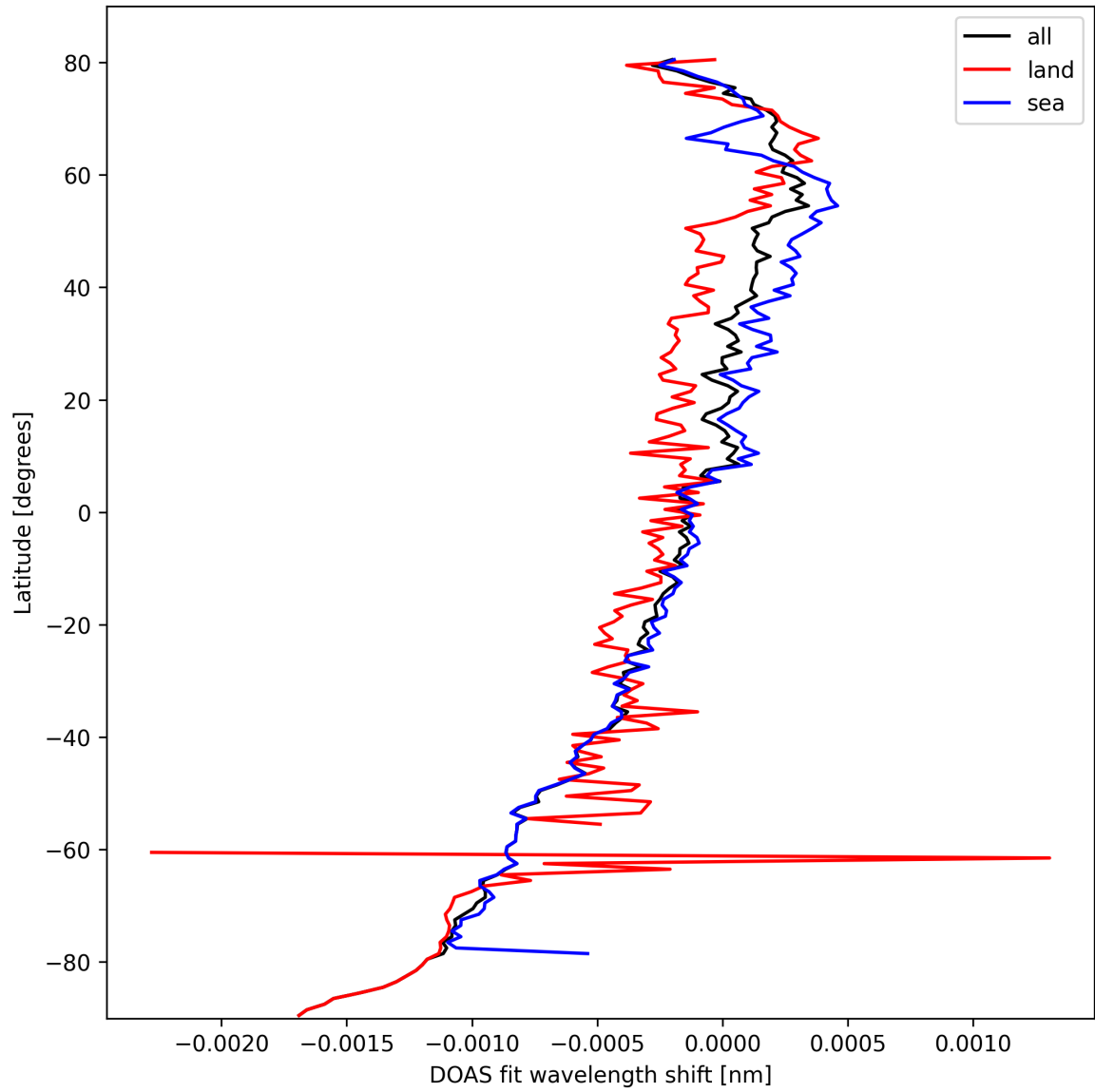
Figure 30: Zonal average of “DOAS fit wavelength shift” for 2025-10-04 to 2025-10-06.
