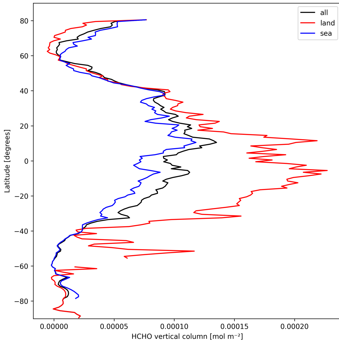
Figure 21: Zonal average of “HCHO vertical column” for 2025-10-04 to 2025-10-06.
