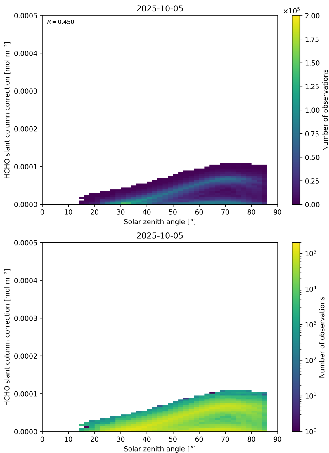
Figure 172: Scatter density plot of “Solar zenith angle” against “HCHO slant column correction” for 2025-10-04 to 2025-10-06.
