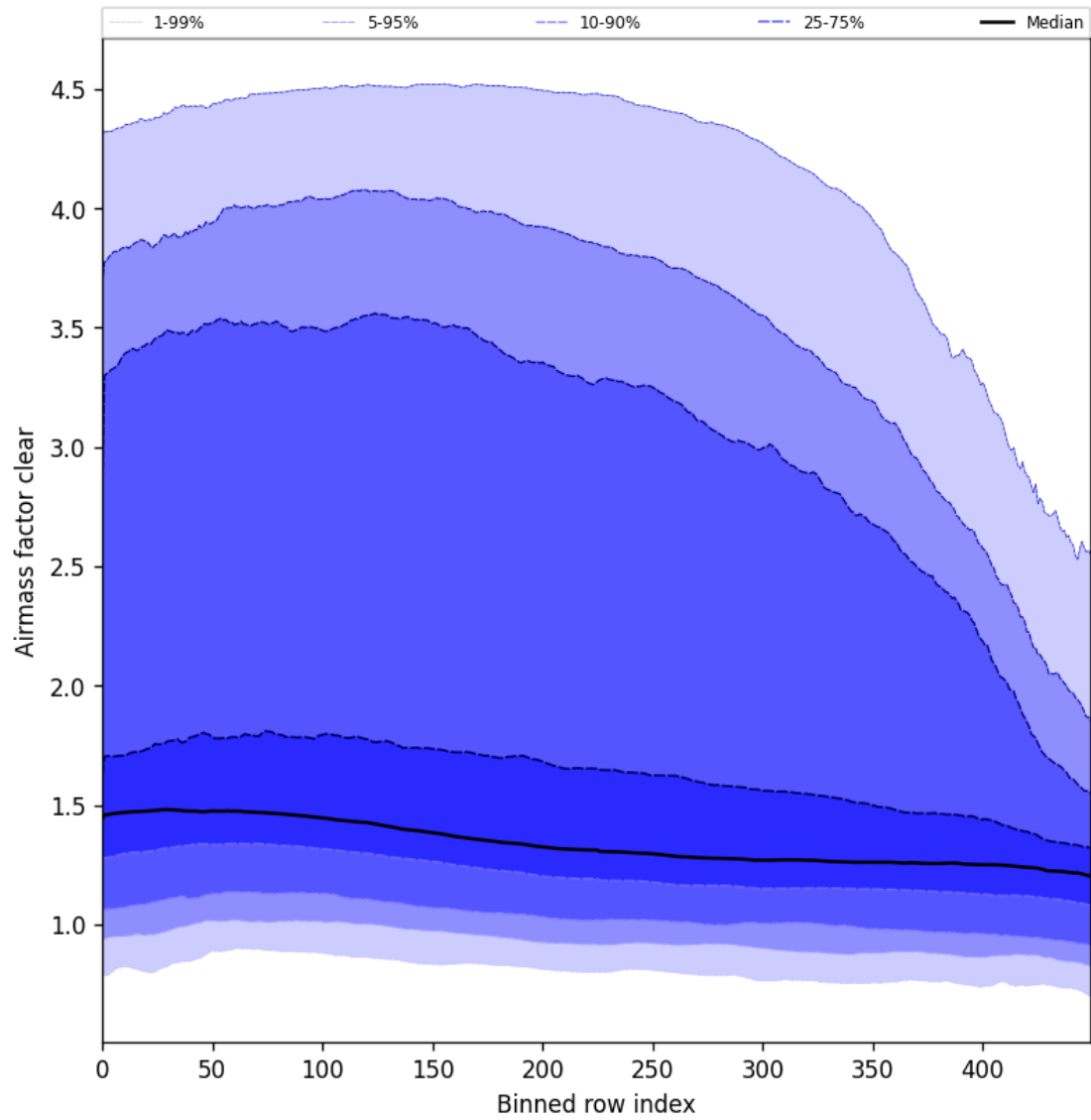
Figure 56: Along track statistics of “Airmass factor clear” for 2025-10-04 to 2025-10-06
