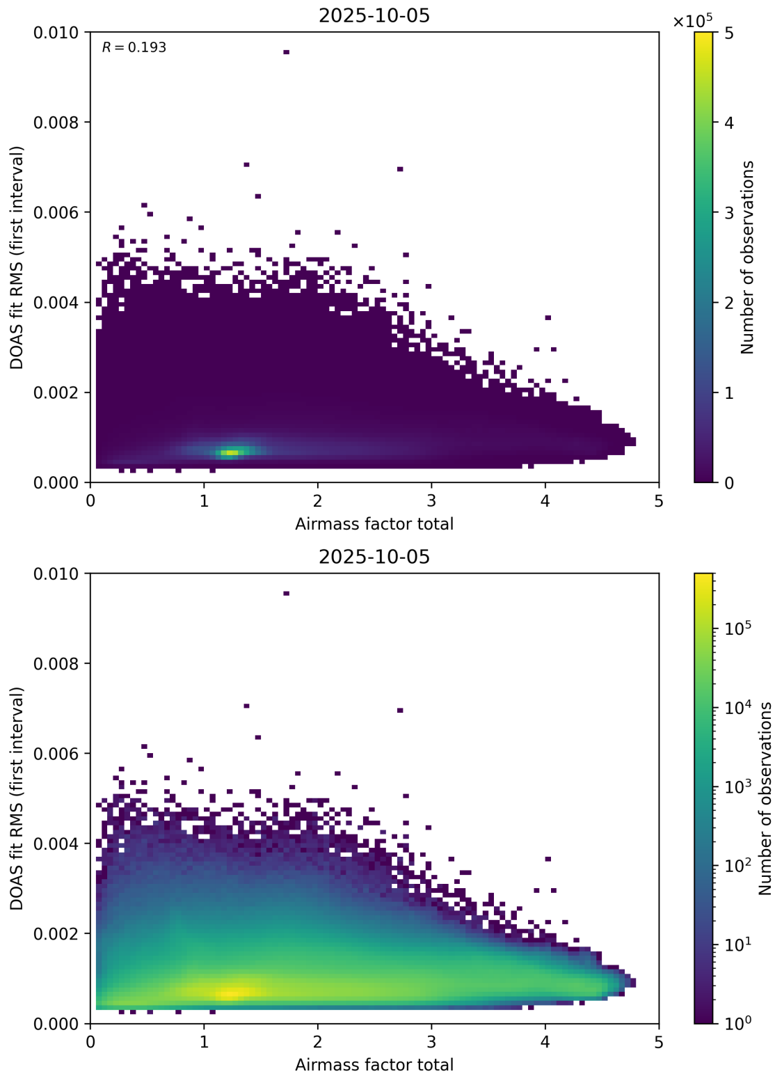
Figure 97: Scatter density plot of “Airmass factor total” against “DOAS fit RMS (first interval)” for 2025-10-04 to 2025-10-06.
