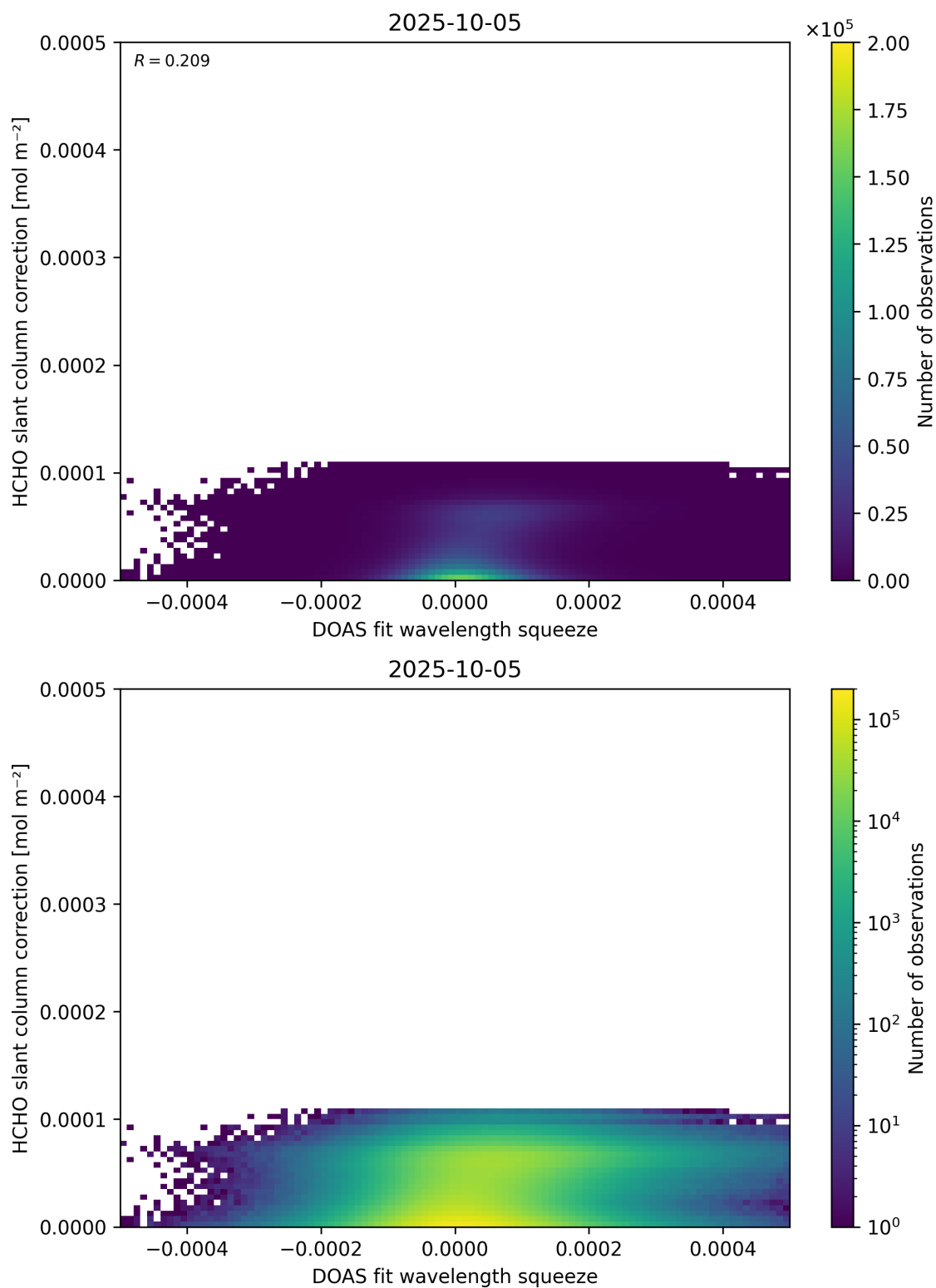
Figure 70: Scatter density plot of “DOAS fit wavelength squeeze” against “HCHO slant column correction” for 2025-10-04 to 2025-10-06.
