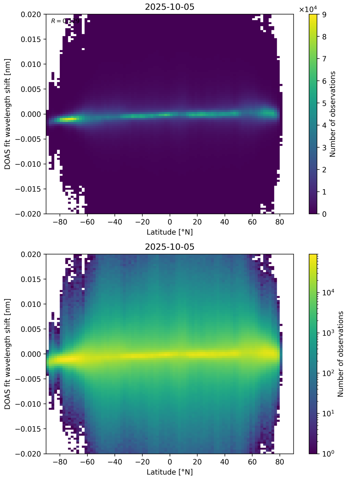
Figure 154: Scatter density plot of “Latitude” against “DOAS fit wavelength shift” for 2025-10-04 to 2025-10-06.
