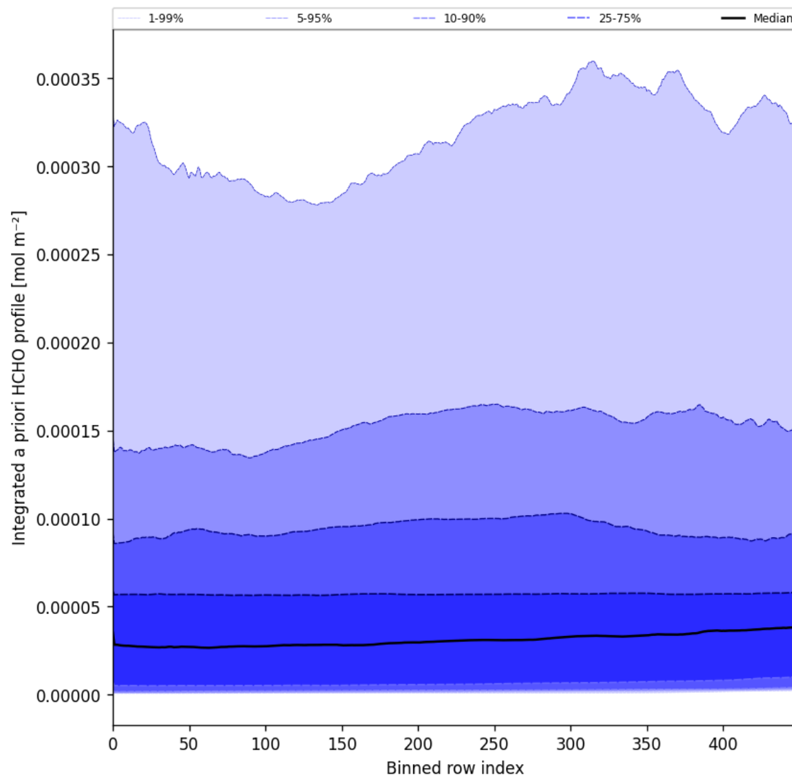
Figure 57: Along track statistics of “Integrated a priori HCHO profile” for 2025-10-04 to 2025-10-06
