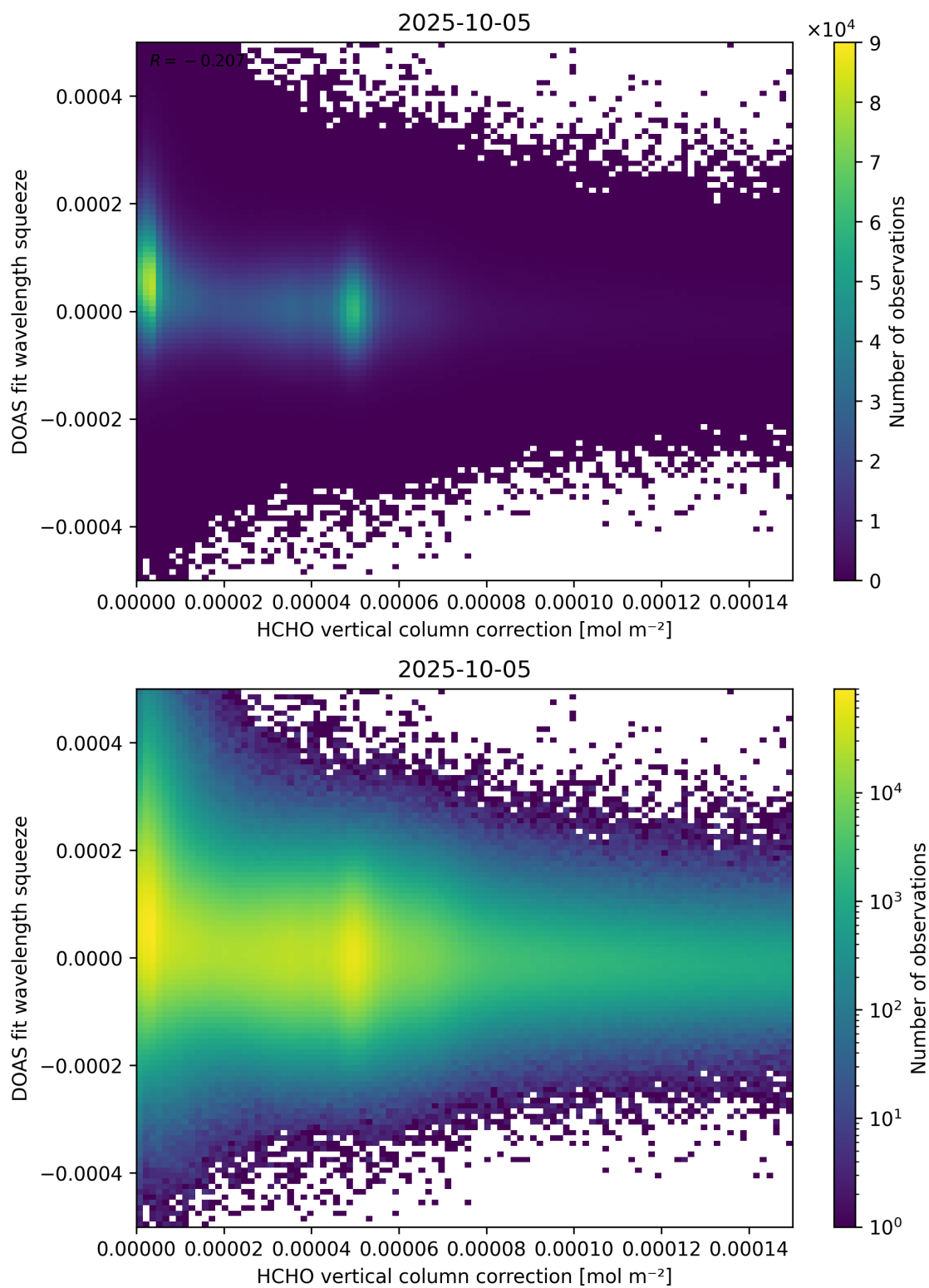
Figure 114: Scatter density plot of “HCHO vertical column correction” against “DOAS fit wavelength squeeze” for 2025-10-04 to 2025-10-06.
