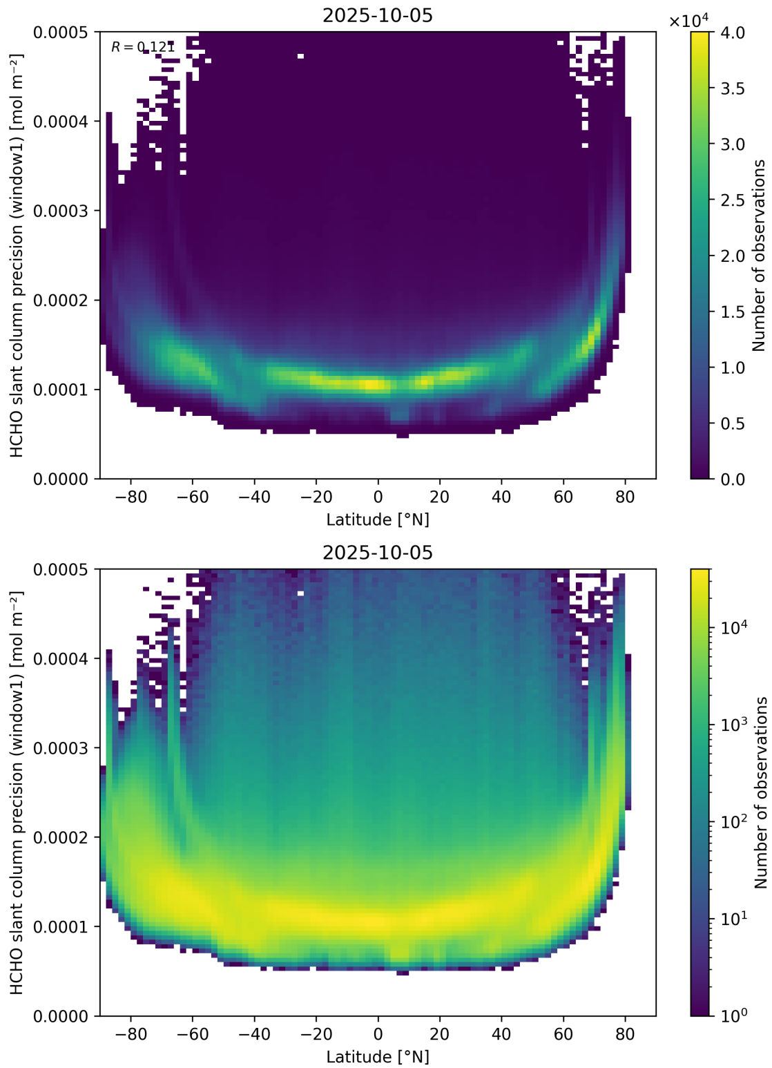
Figure 160: Scatter density plot of “Latitude” against “HCHO slant column precision (window1)” for 2025-10-04 to 2025-10-06.
