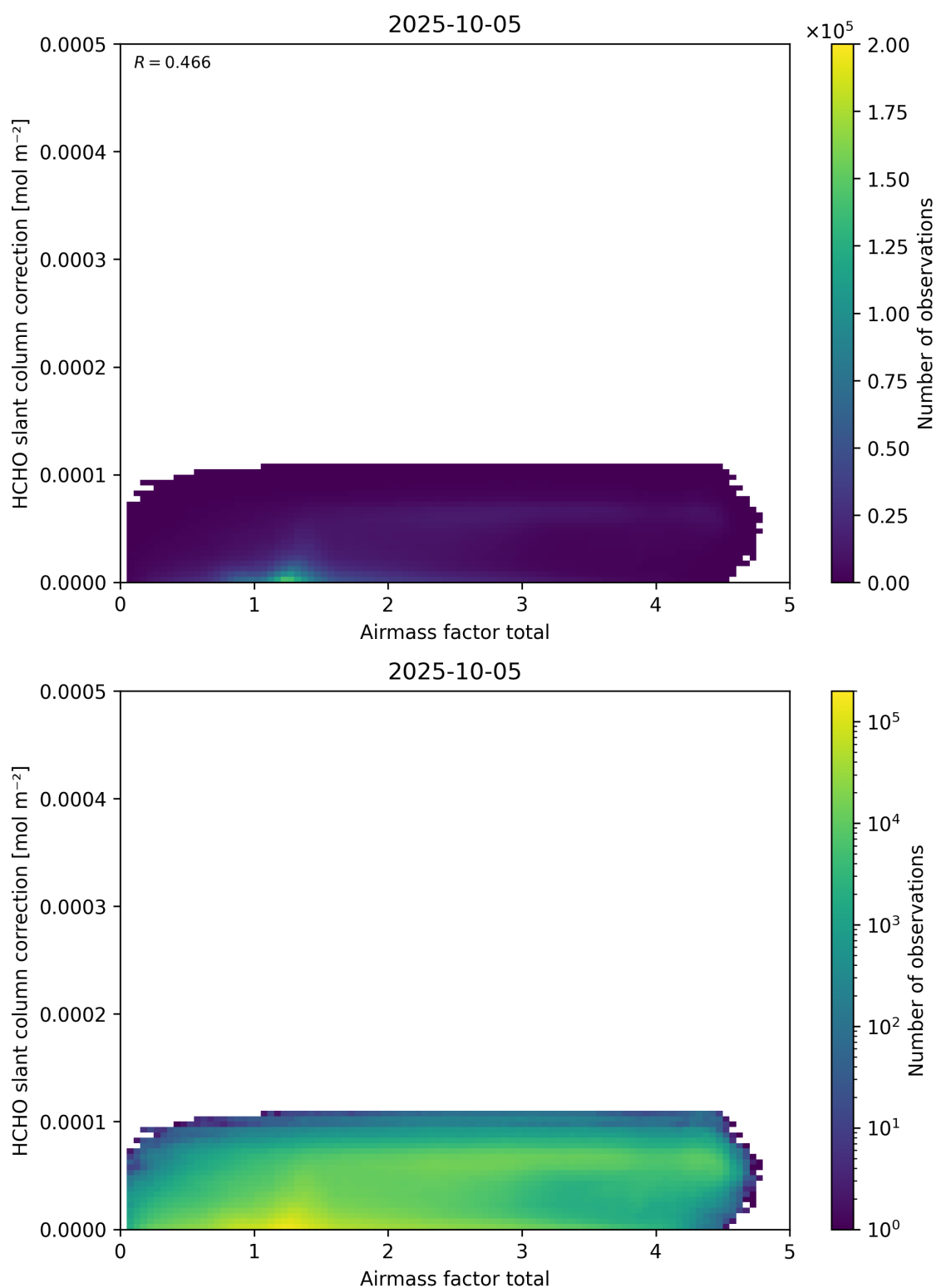
Figure 102: Scatter density plot of “Airmass factor total” against “HCHO slant column correction” for 2025-10-04 to 2025-10-06.
