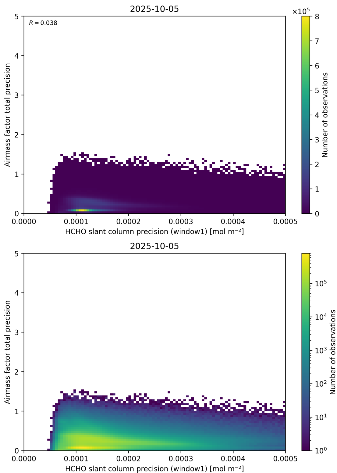
Figure 95: Scatter density plot of “HCHO slant column precision (window1)” against “Airmass factor total precision” for 2025-10-04 to 2025-10-06.
