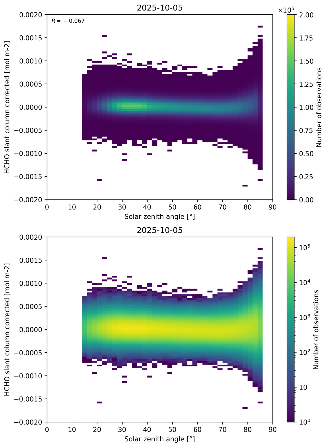
Figure 171: Scatter density plot of “Solar zenith angle” against “HCHO slant column corrected” for 2025-10-04 to 2025-10-06.
