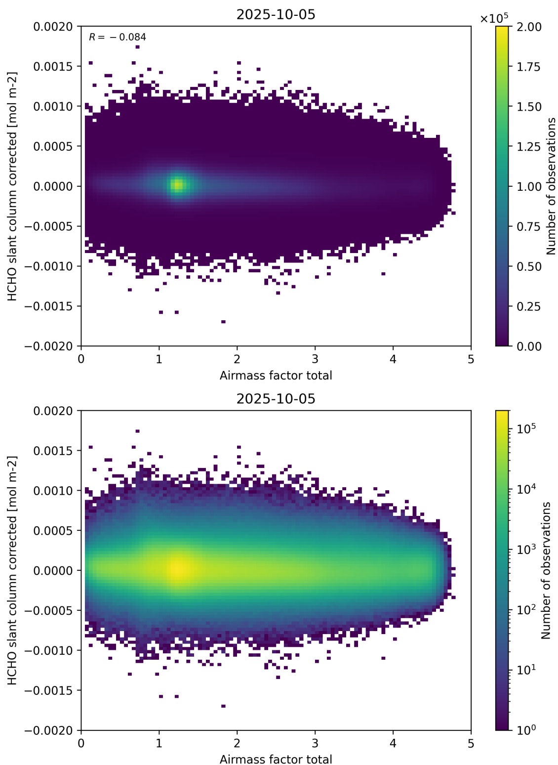
Figure 101: Scatter density plot of “Airmass factor total” against “HCHO slant column corrected” for 2025-10-04 to 2025-10-06.
