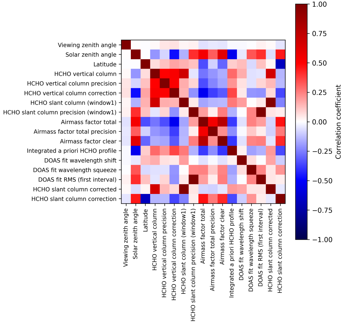
Figure 2: Map of correlation matrix for 2025-10-04 to 2025-10-06.
