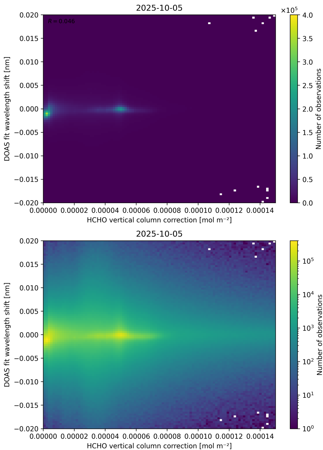
Figure 113: Scatter density plot of “HCHO vertical column correction” against “DOAS fit wavelength shift” for 2025-10-04 to 2025-10-06.
