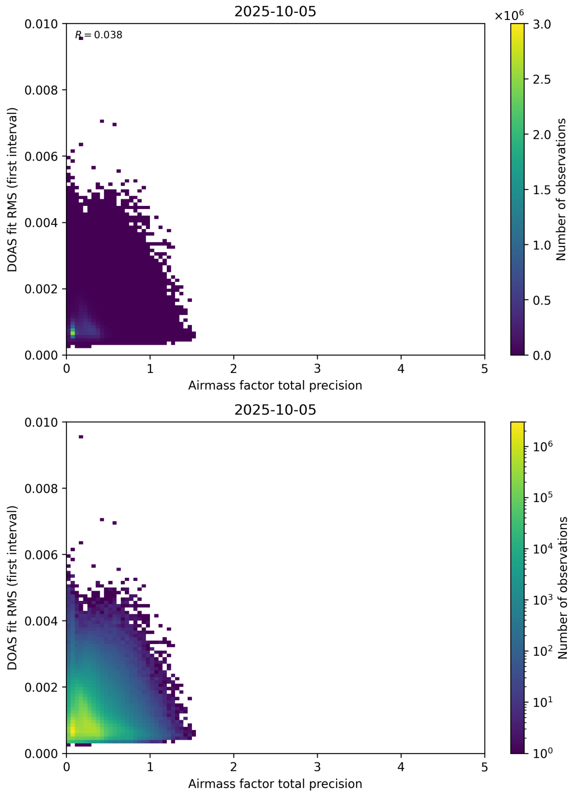
Figure 105: Scatter density plot of “Airmass factor total precision” against “DOAS fit RMS (first interval)” for 2025-10-04 to 2025-10-06.
