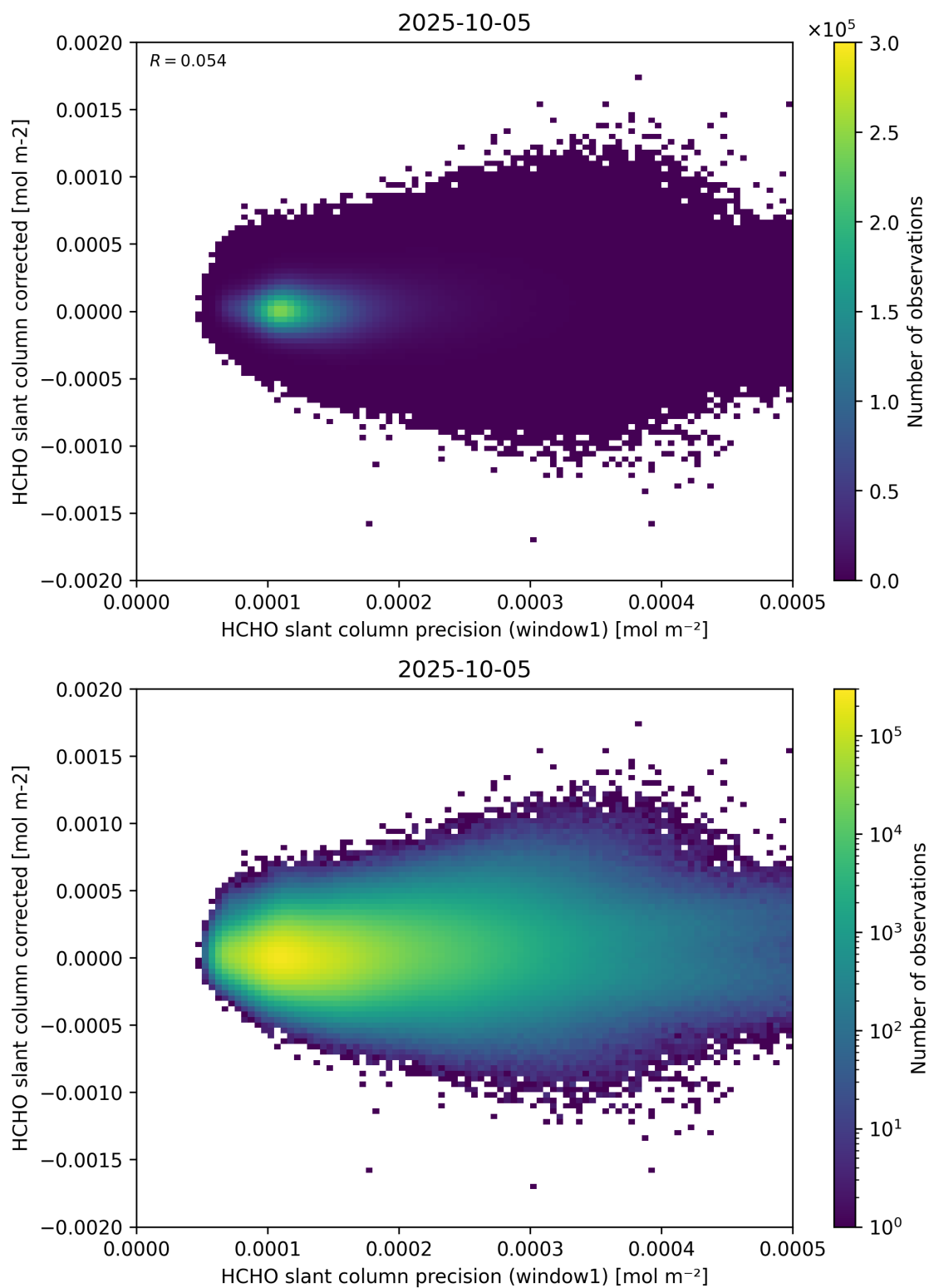
Figure 92: Scatter density plot of “HCHO slant column precision (window1)” against “HCHO slant column corrected” for 2025-10-04 to 2025-10-06.
