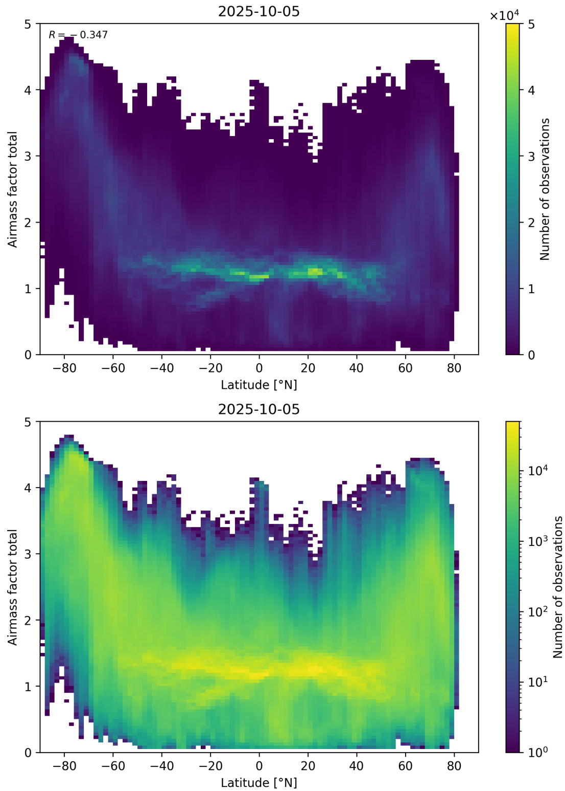
Figure 161: Scatter density plot of “Latitude” against “Airmass factor total” for 2025-10-04 to 2025-10-06.
