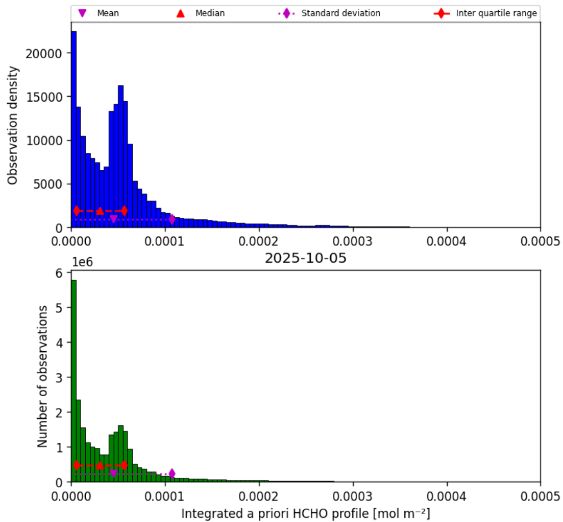
Figure 43: Histogram of “Integrated a priori HCHO profile” for 2025-10-04 to 2025-10-06
