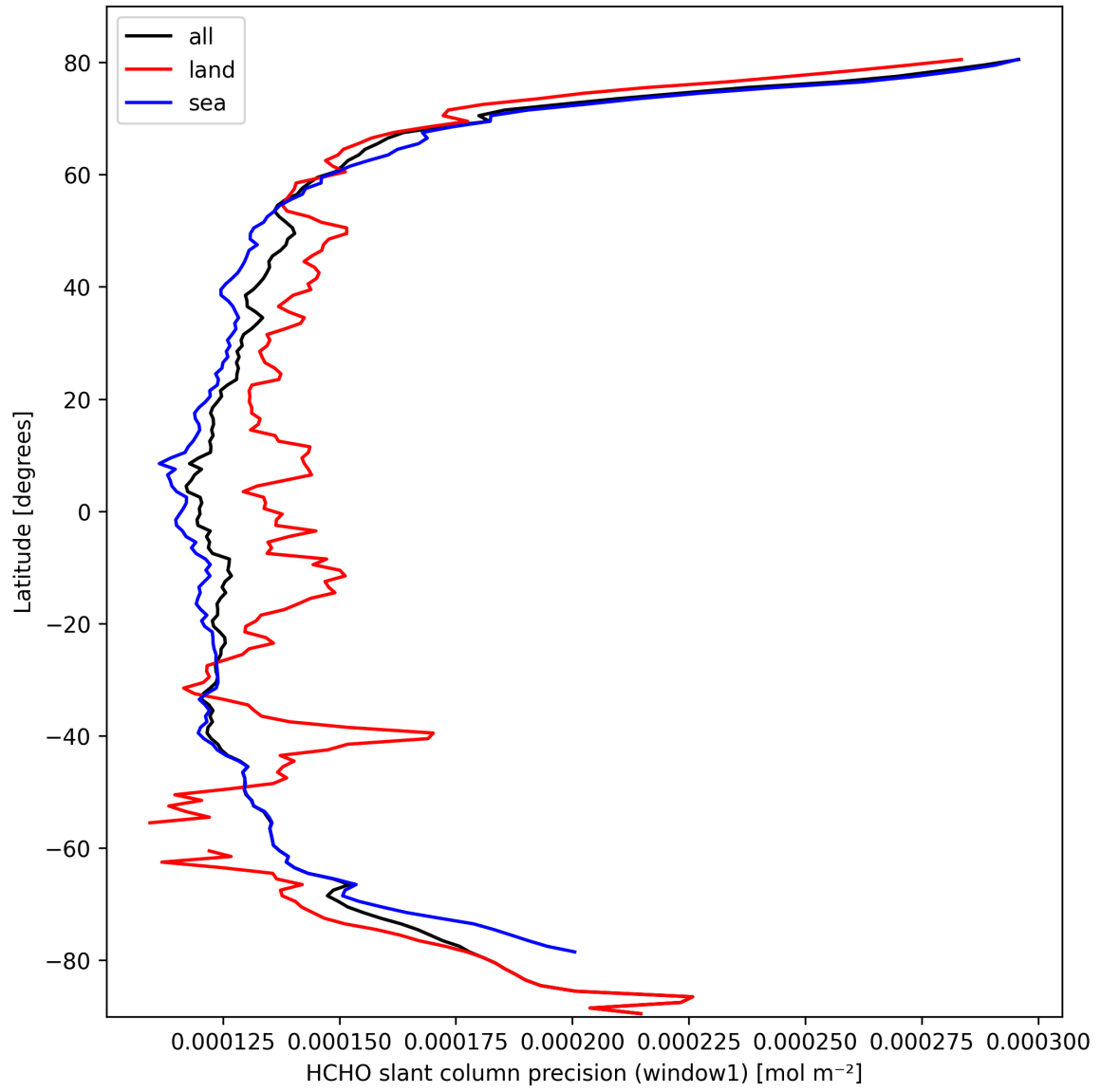
Figure 25: Zonal average of “HCHO slant column precision (window1)” for 2025-10-04 to 2025-10-06.
