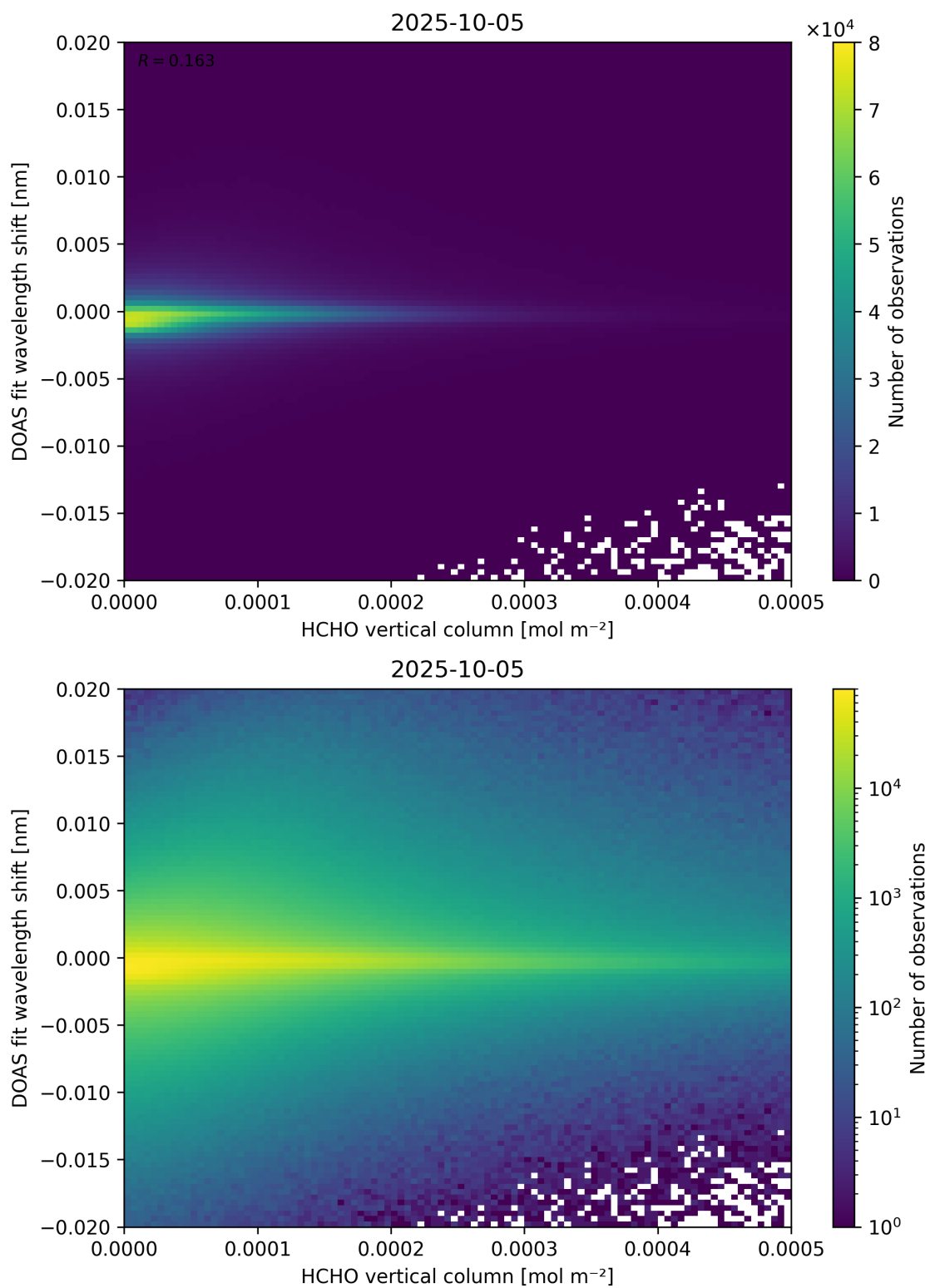
Figure 124: Scatter density plot of “HCHO vertical column” against “DOAS fit wavelength shift” for 2025-10-04 to 2025-10-06.
