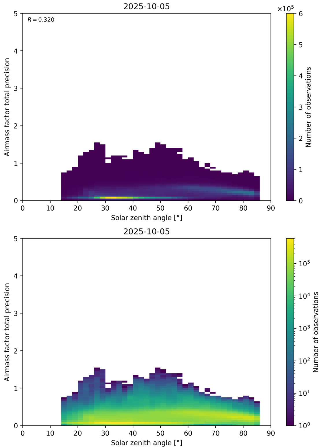
Figure 176: Scatter density plot of “Solar zenith angle” against “Airmass factor total precision” for 2025-10-04 to 2025-10-06.
