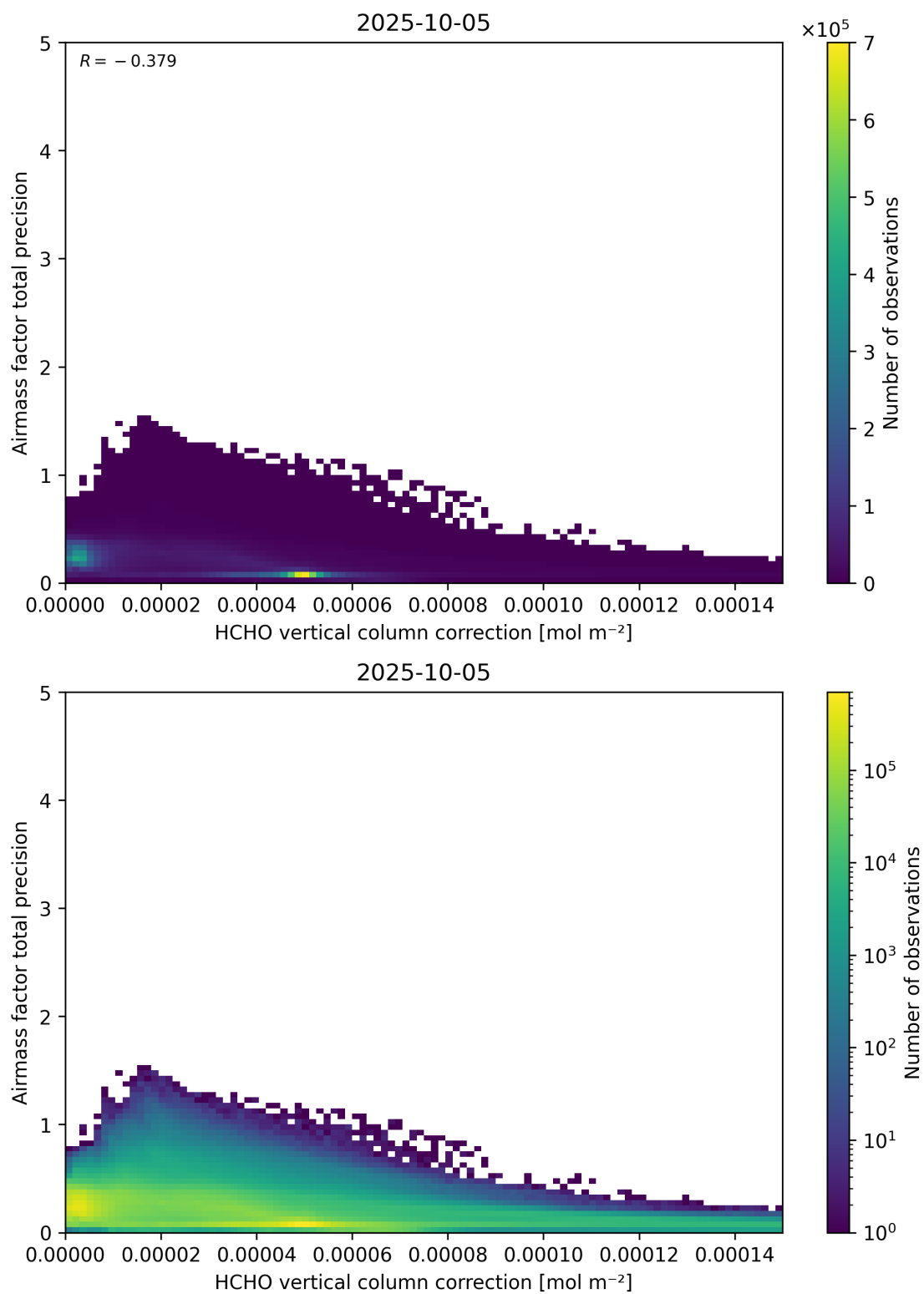
Figure 121: Scatter density plot of “HCHO vertical column correction” against “Airmass factor total precision” for 2025-10-04 to 2025-10-06.
