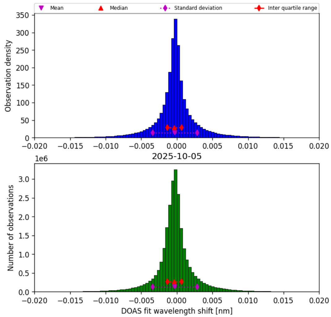
Figure 44: Histogram of “DOAS fit wavelength shift” for 2025-10-04 to 2025-10-06
