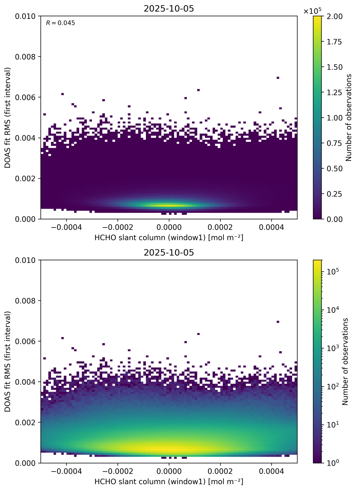
Figure 78: Scatter density plot of “HCHO slant column (window1)” against “DOAS fit RMS (first interval)” for 2025-10-04 to 2025-10-06.
