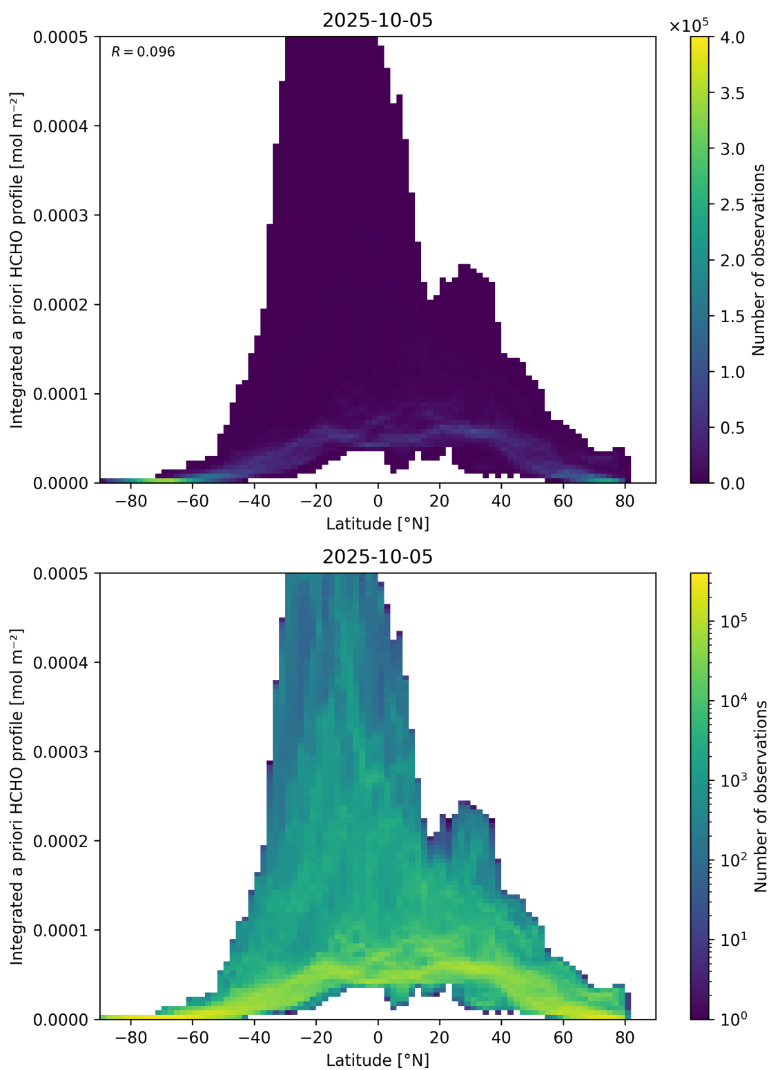
Figure 166: Scatter density plot of “Latitude” against “Integrated a priori HCHO profile” for 2025-10-04 to 2025-10-06.
