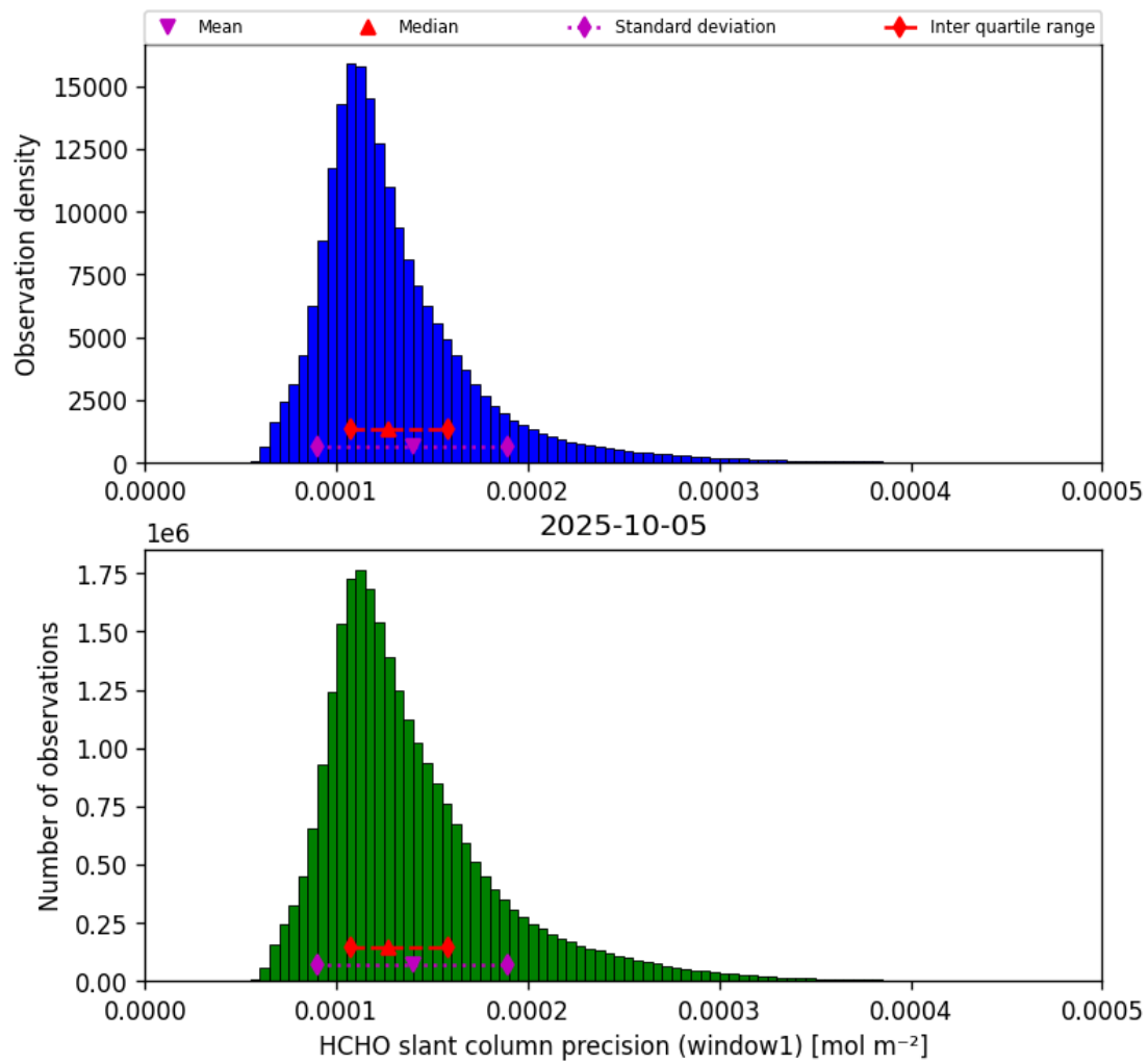
Figure 39: Histogram of “HCHO slant column precision (window1)” for 2025-10-04 to 2025-10-06
