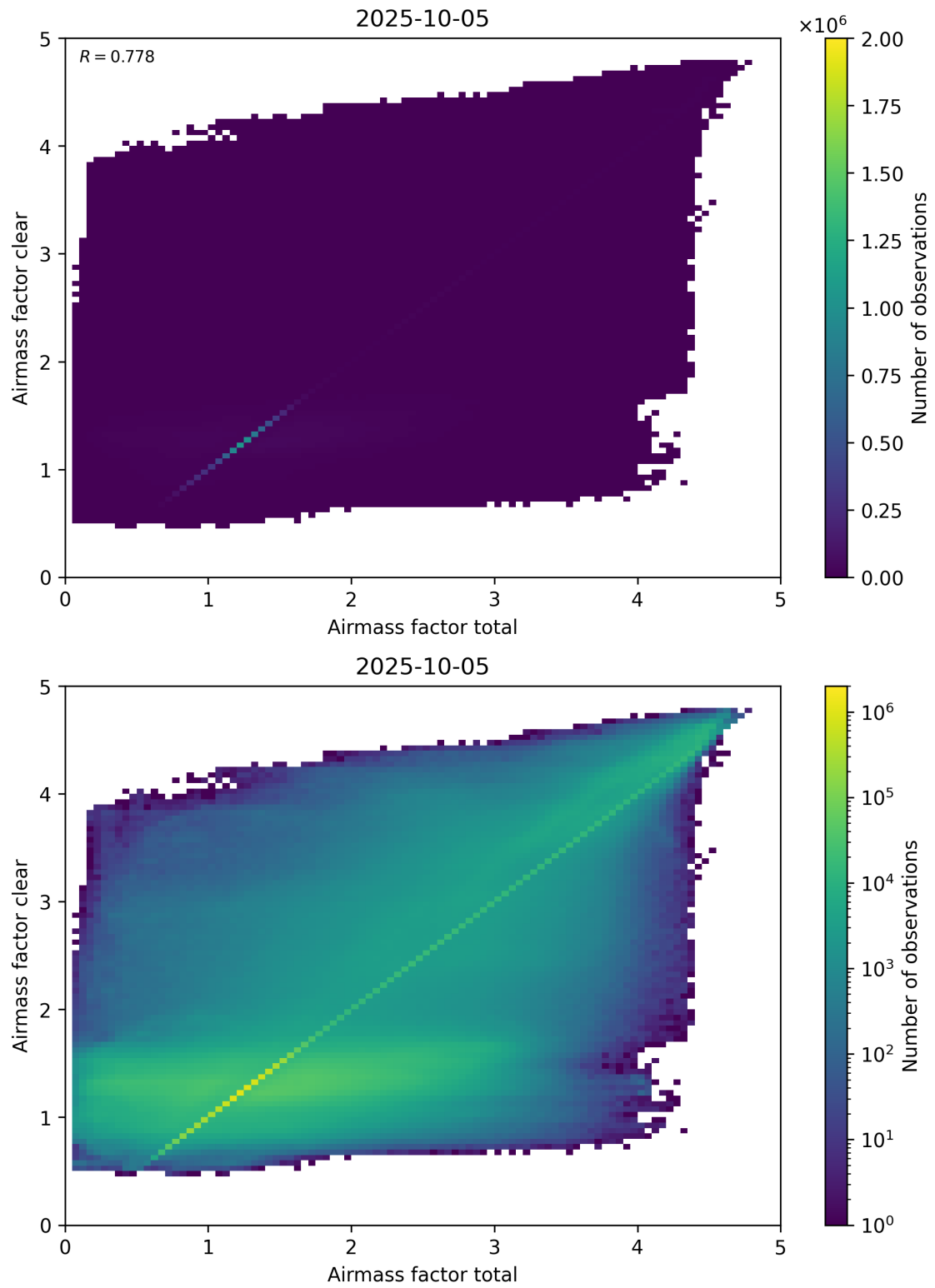
Figure 100: Scatter density plot of “Airmass factor total” against “Airmass factor clear” for 2025-10-04 to 2025-10-06.
