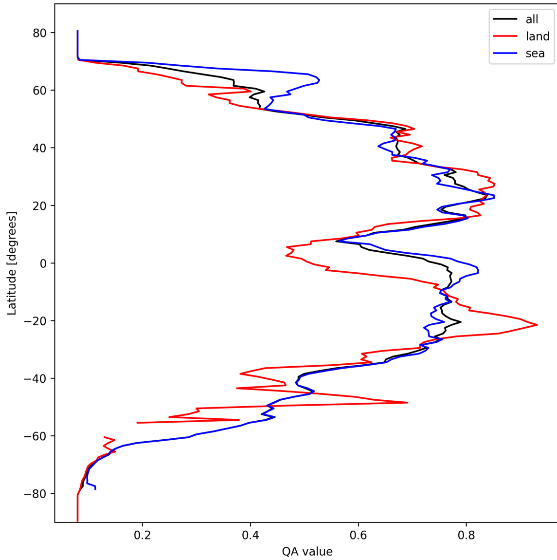
Figure 20: Zonal average of “QA value” for 2025-10-04 to 2025-10-06.
