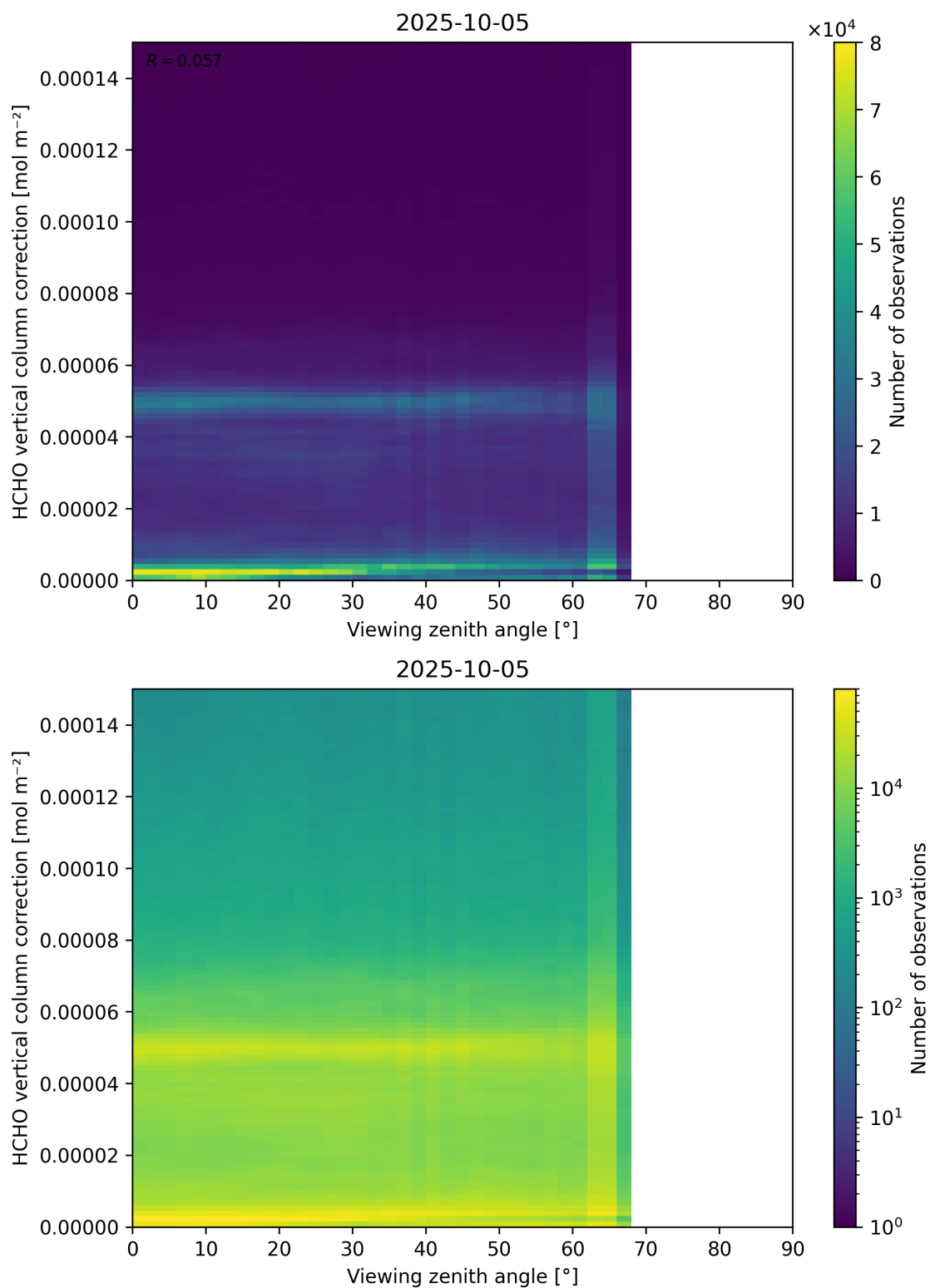
Figure 193: Scatter density plot of “Viewing zenith angle” against “HCHO vertical column correction” for 2025-10-04 to 2025-10-06.
