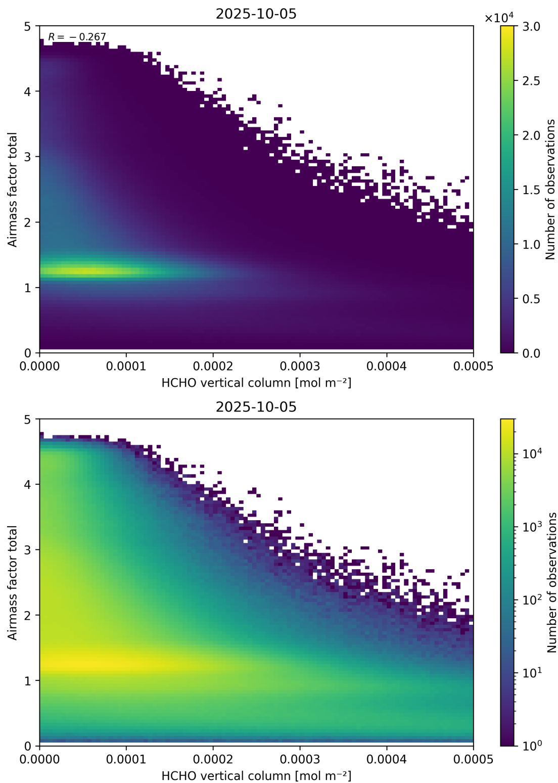
Figure 131: Scatter density plot of “HCHO vertical column” against “Airmass factor total” for 2025-10-04 to 2025-10-06.
