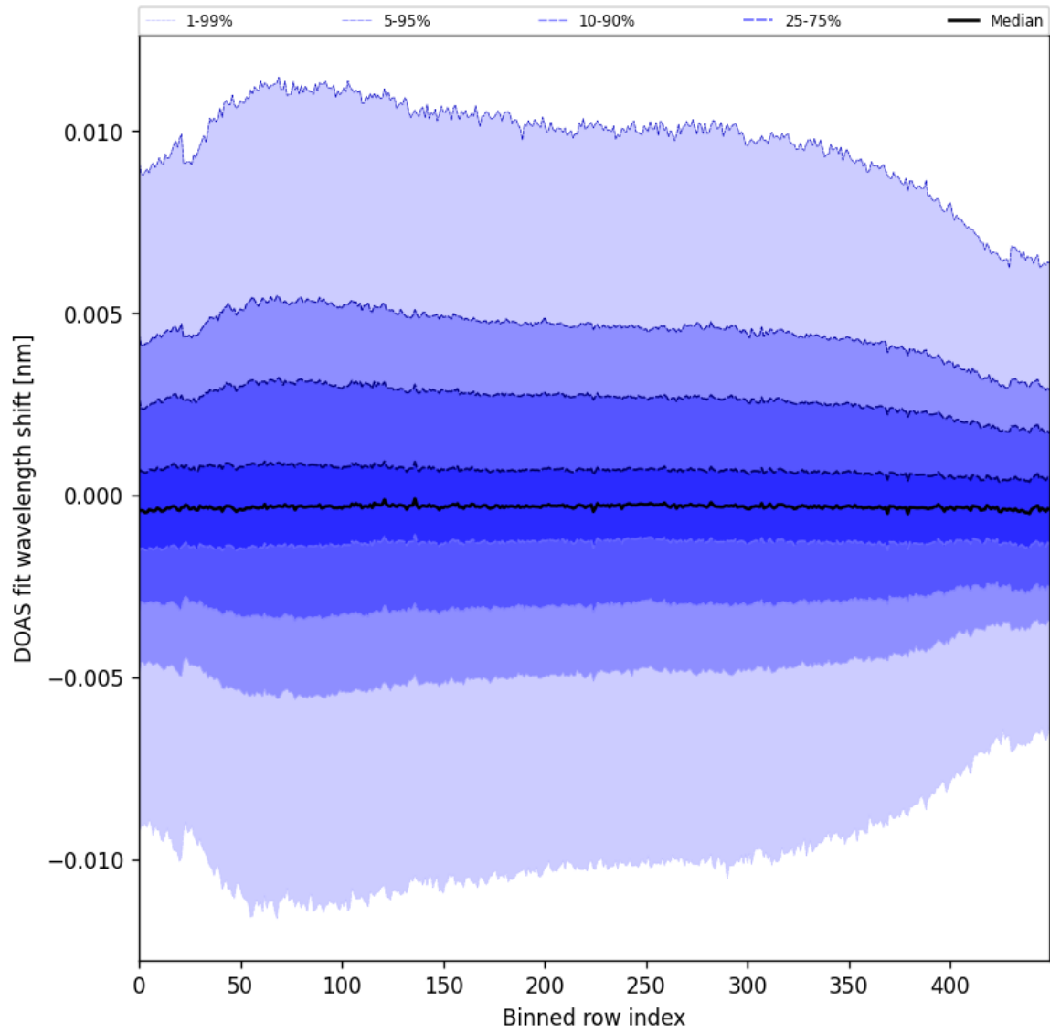
Figure 58: Along track statistics of “DOAS fit wavelength shift” for 2025-10-04 to 2025-10-06
