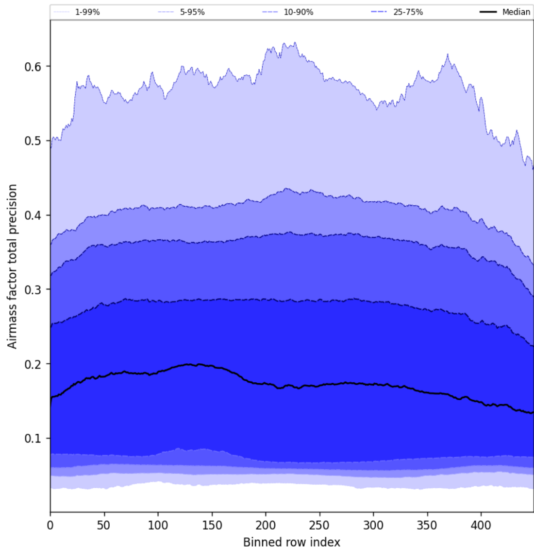
Figure 55: Along track statistics of “Airmass factor total precision” for 2025-10-04 to 2025-10-06
