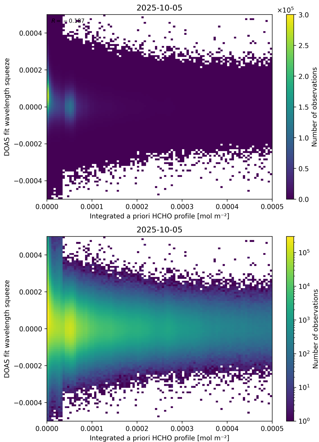
Figure 150: Scatter density plot of “Integrated a priori HCHO profile” against “DOAS fit wavelength squeeze” for 2025-10-04 to 2025-10-06.
