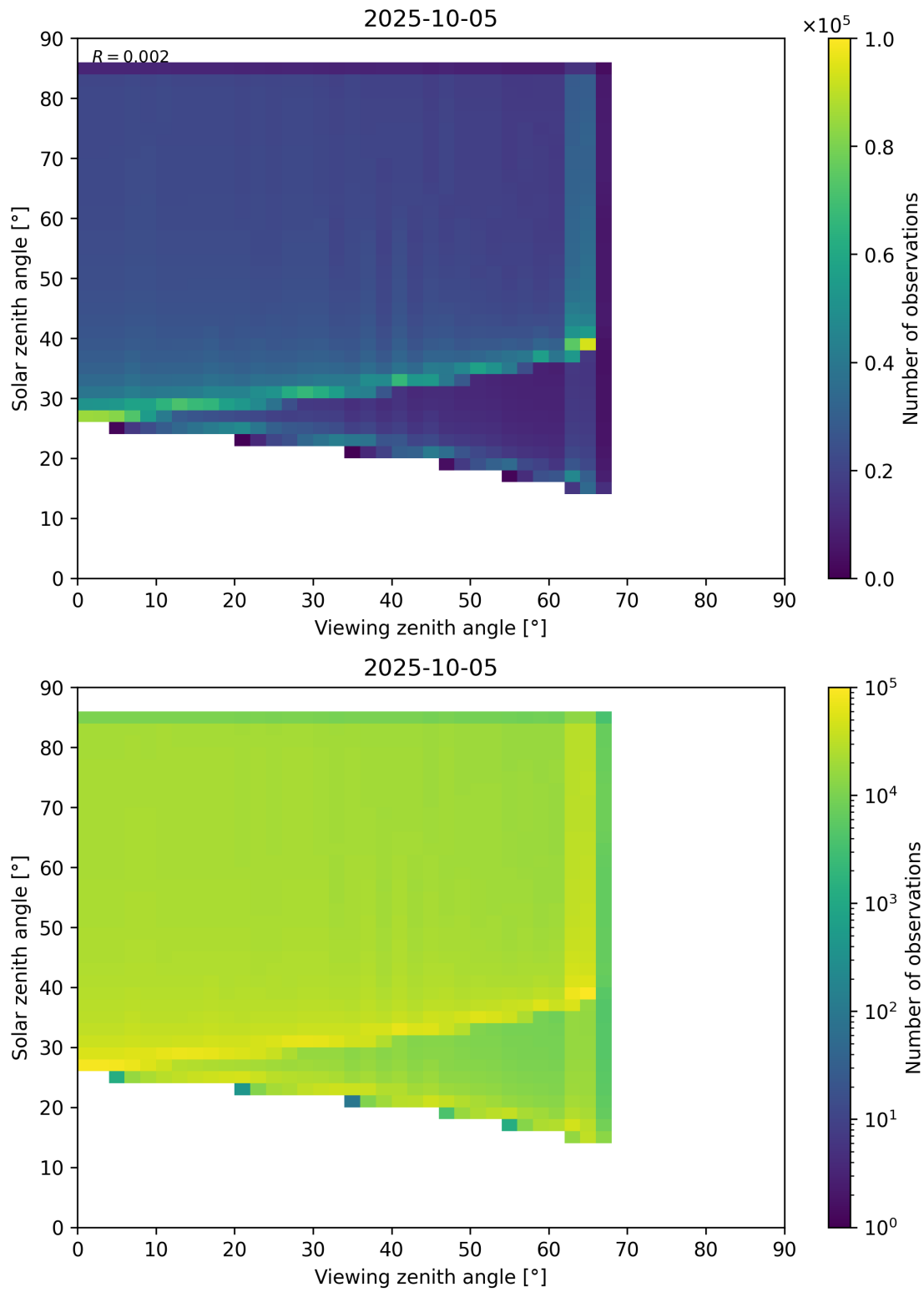
Figure 197: Scatter density plot of “Viewing zenith angle” against “Solar zenith angle” for 2025-10-04 to 2025-10-06.
