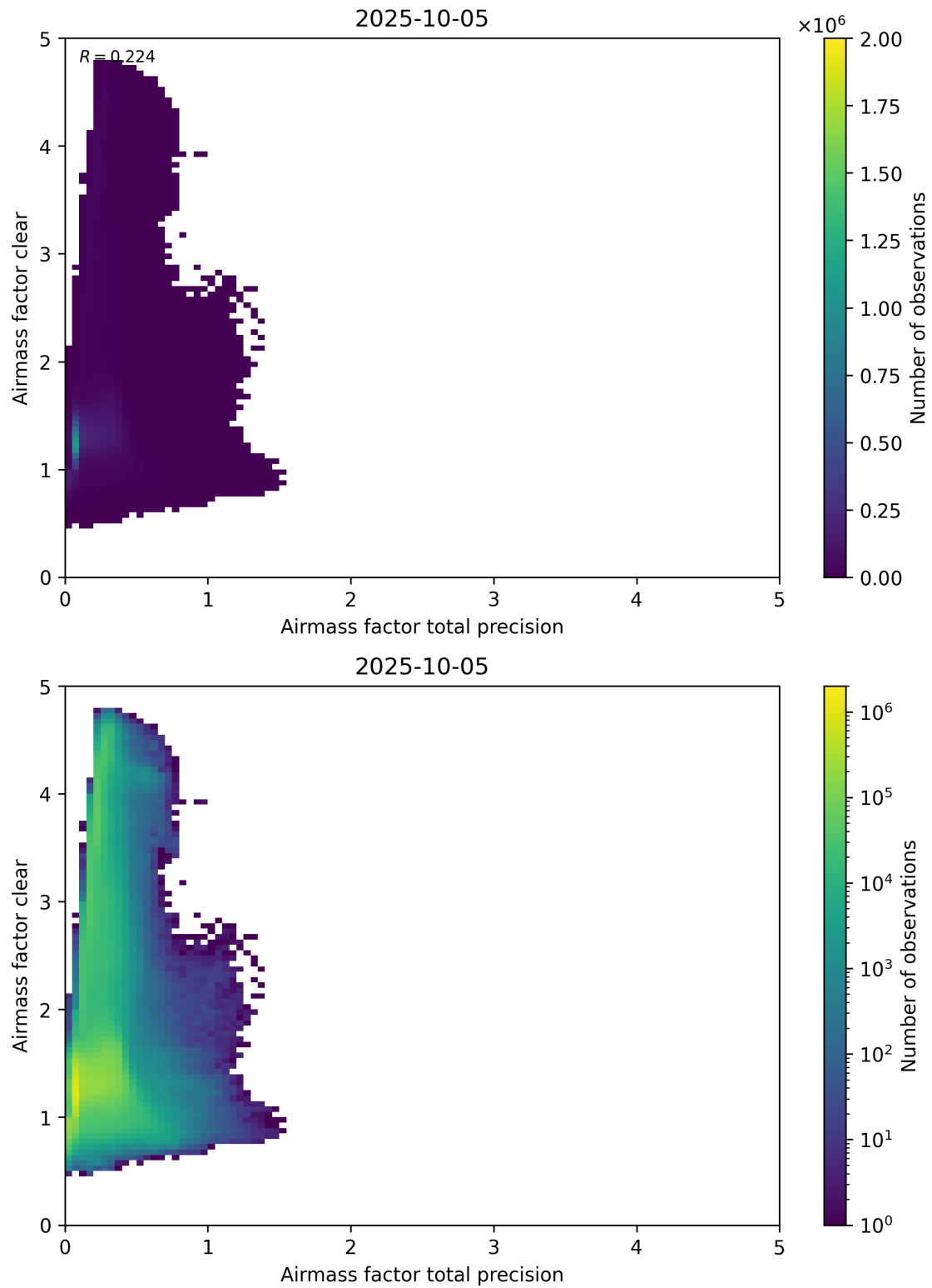
Figure 108: Scatter density plot of “Airmass factor total precision” against “Airmass factor clear” for 2025-10-04 to 2025-10-06.
