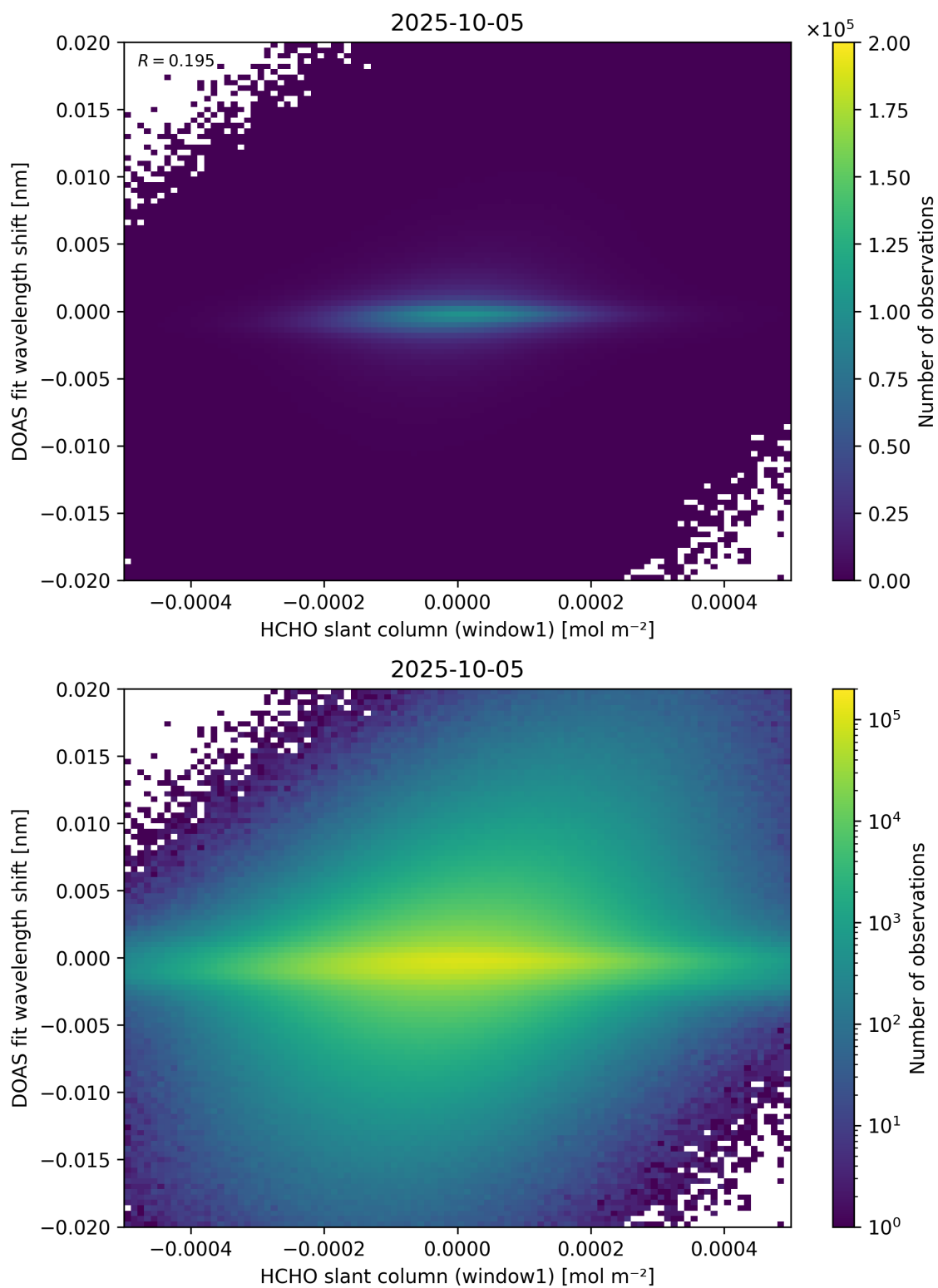
Figure 79: Scatter density plot of “HCHO slant column (window1)” against “DOAS fit wavelength shift” for 2025-10-04 to 2025-10-06.
