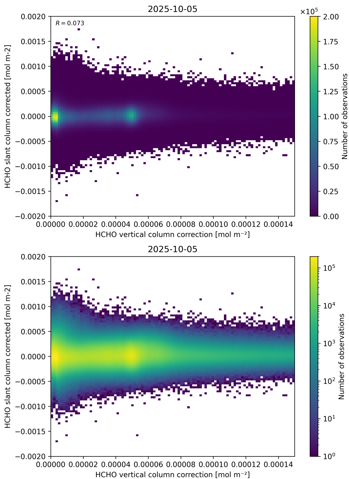
Figure 116: Scatter density plot of “HCHO vertical column correction” against “HCHO slant column corrected” for 2025-10-04 to 2025-10-06.
