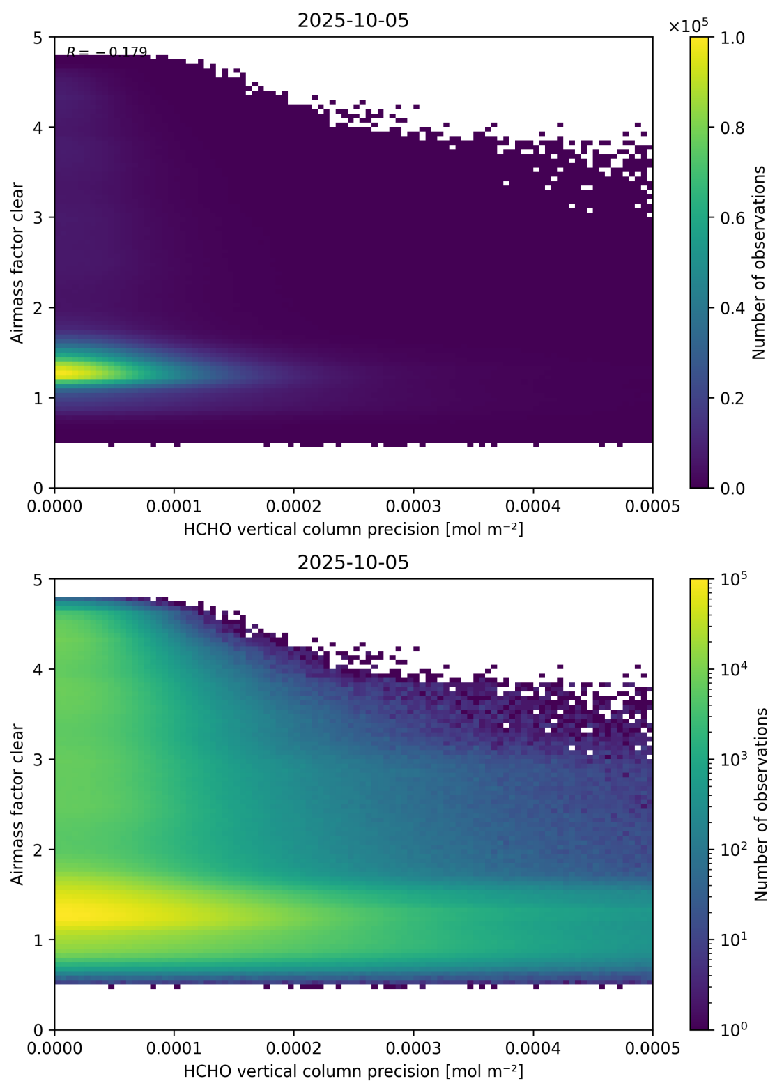
Figure 139: Scatter density plot of “HCHO vertical column precision” against “Airmass factor clear” for 2025-10-04 to 2025-10-06.
