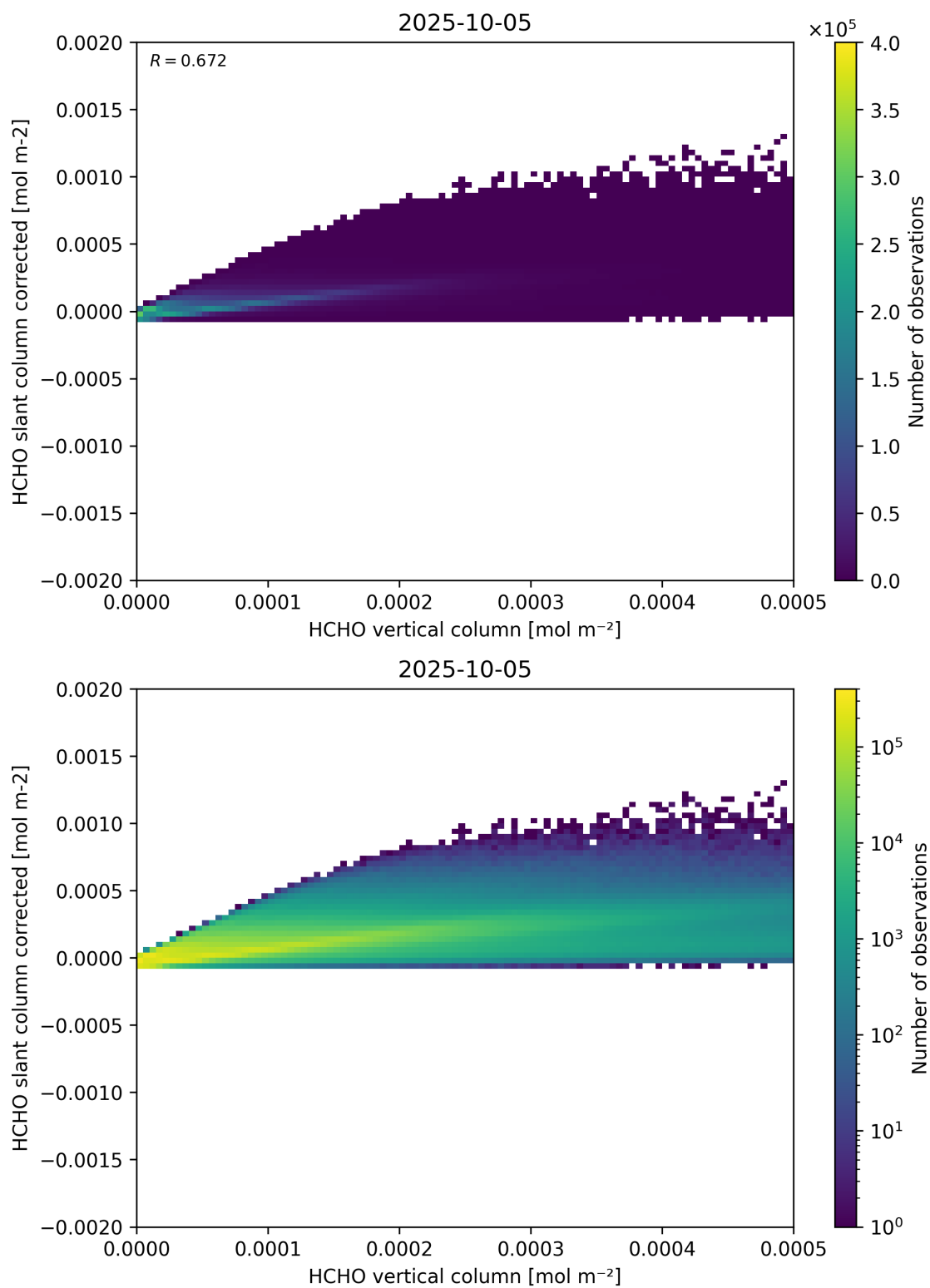
Figure 127: Scatter density plot of “HCHO vertical column” against “HCHO slant column corrected” for 2025-10-04 to 2025-10-06.
