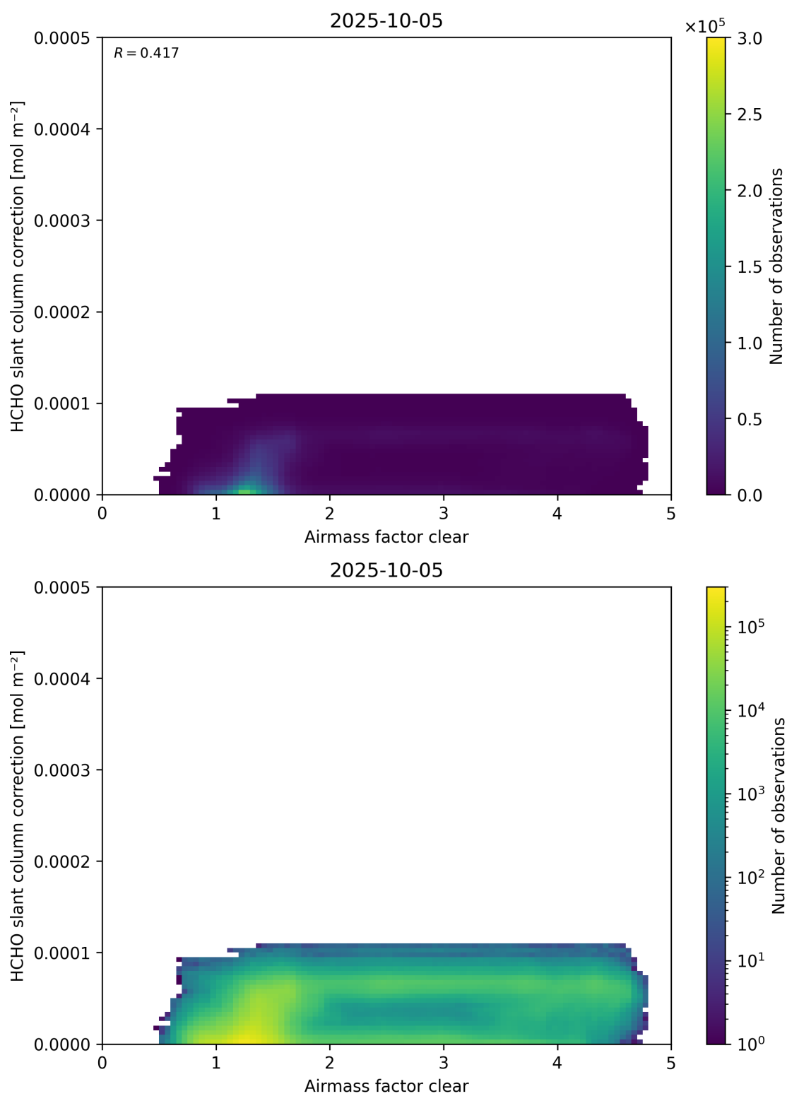
Figure 75: Scatter density plot of “Airmass factor clear” against “HCHO slant column correction” for 2025-10-04 to 2025-10-06.
