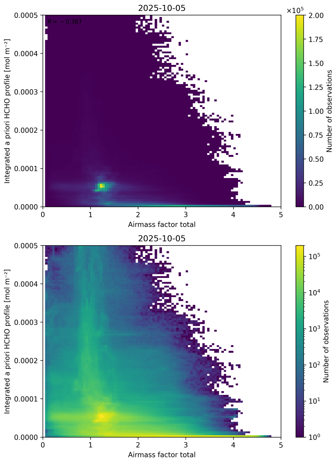
Figure 104: Scatter density plot of “Airmass factor total” against “Integrated a priori HCHO profile” for 2025-10-04 to 2025-10-06.
