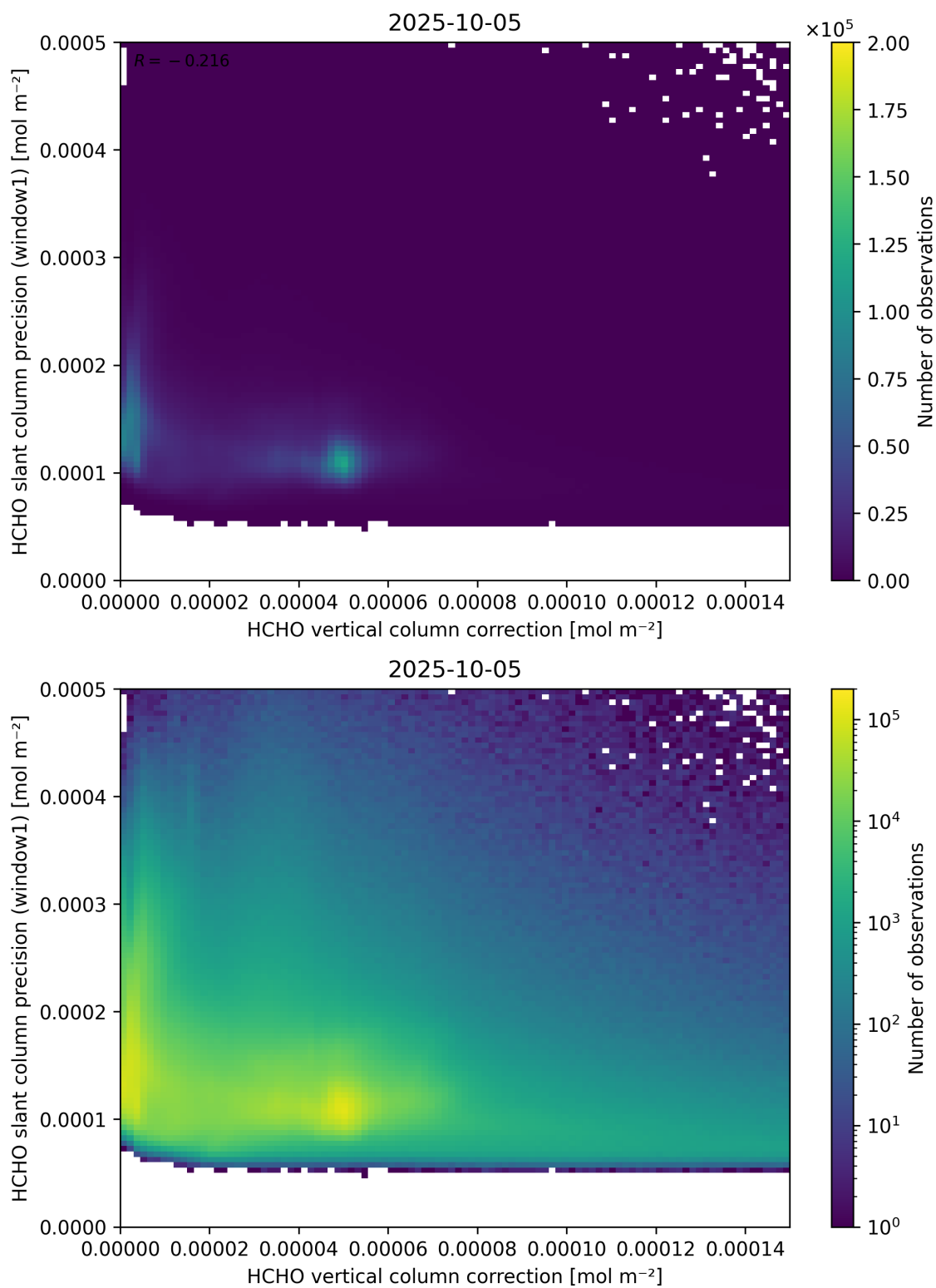
Figure 119: Scatter density plot of “HCHO vertical column correction” against “HCHO slant column precision (window1)” for 2025-10-04 to 2025-10-06.
