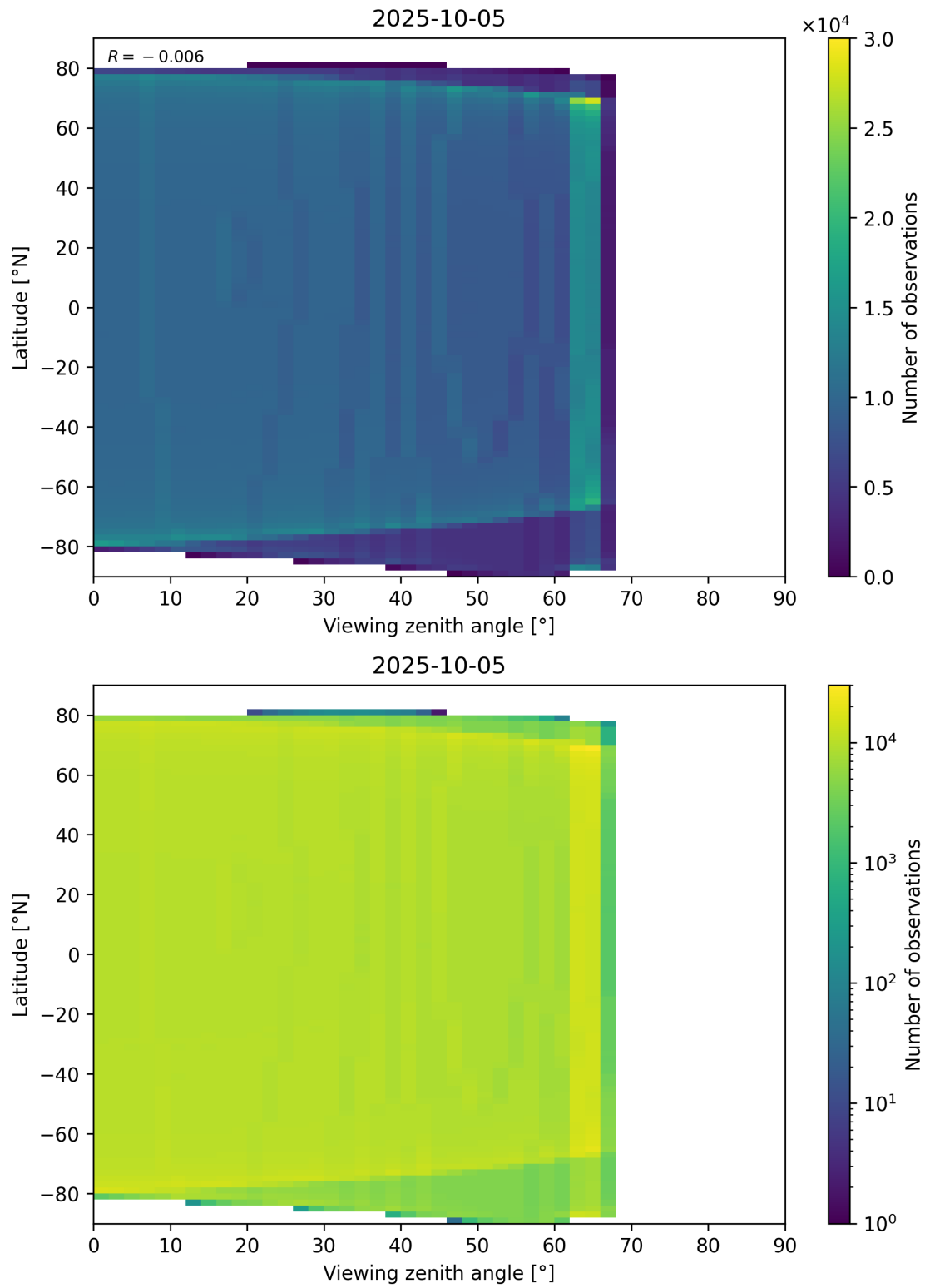
Figure 196: Scatter density plot of “Viewing zenith angle” against “Latitude” for 2025-10-04 to 2025-10-06.
