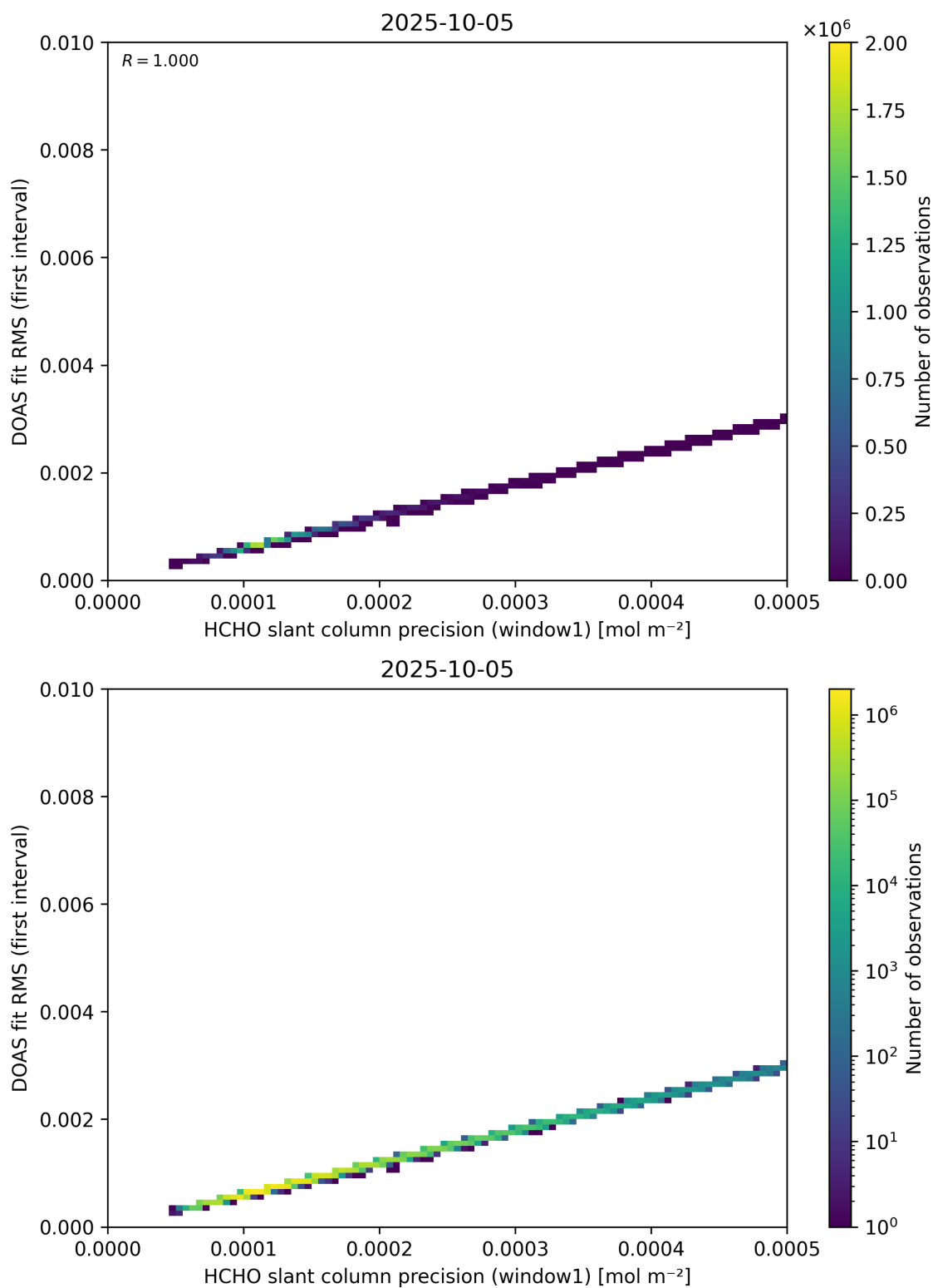
Figure 88: Scatter density plot of “HCHO slant column precision (window1)” against “DOAS fit RMS (first interval)” for 2025-10-04 to 2025-10-06.
