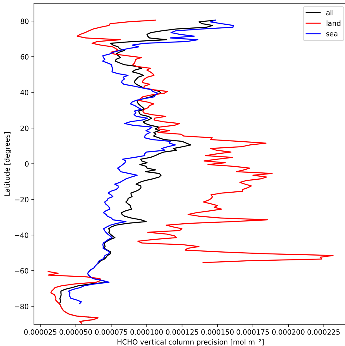
Figure 22: Zonal average of “HCHO vertical column precision” for 2025-10-04 to 2025-10-06.
