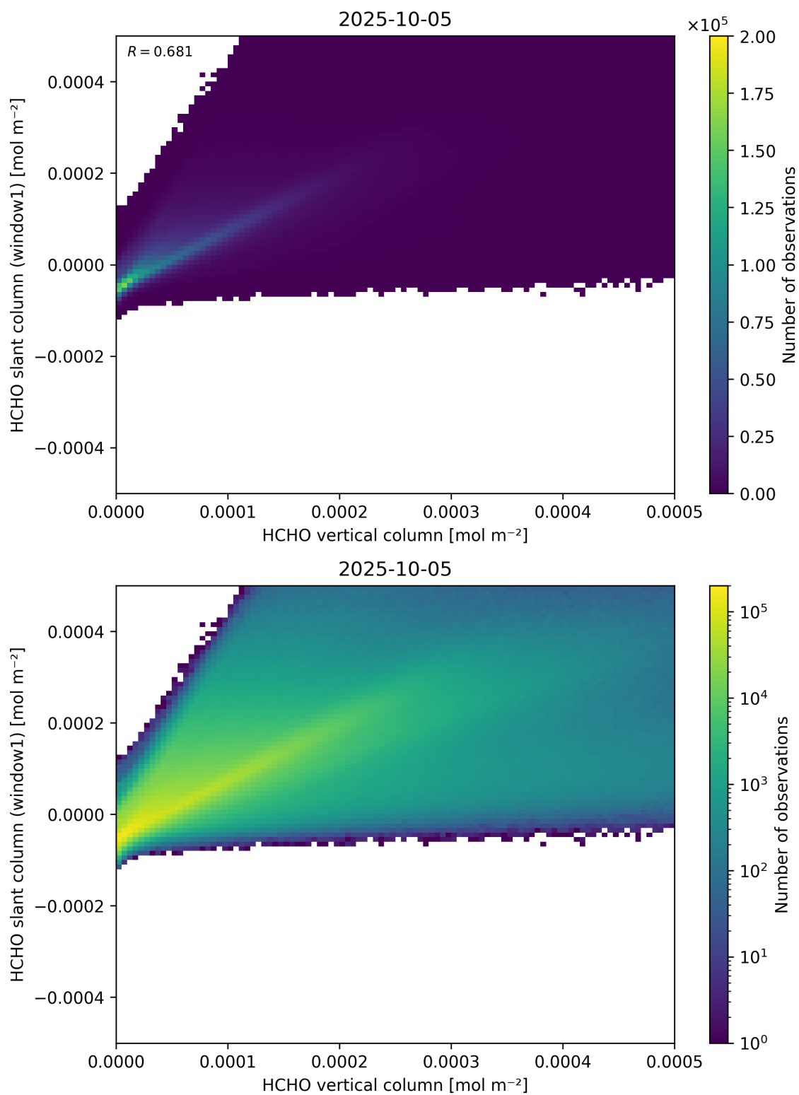
Figure 129: Scatter density plot of “HCHO vertical column” against “HCHO slant column (window1)” for 2025-10-04 to 2025-10-06.
