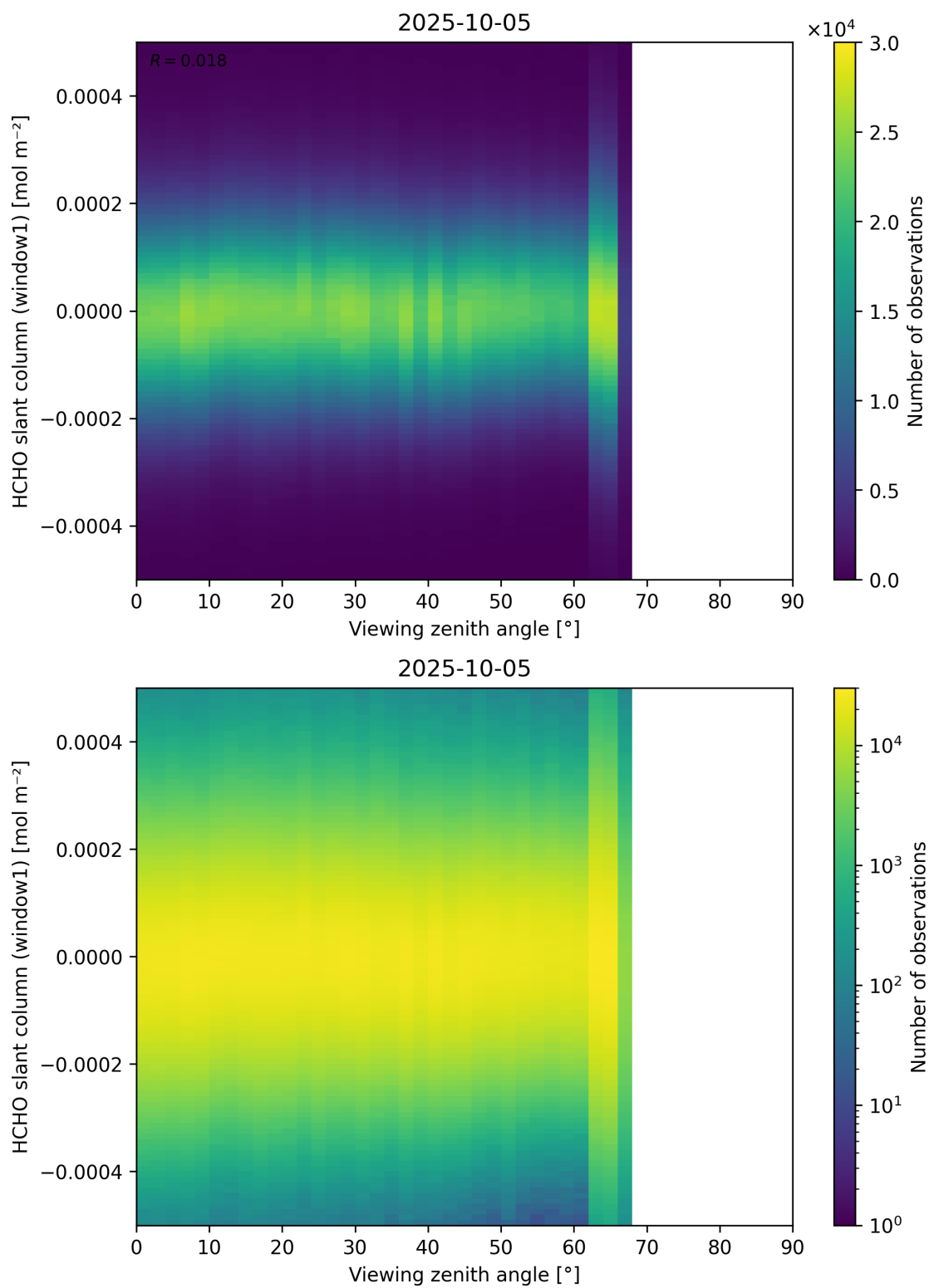
Figure 188: Scatter density plot of “Viewing zenith angle” against “HCHO slant column (window1)” for 2025-10-04 to 2025-10-06.
