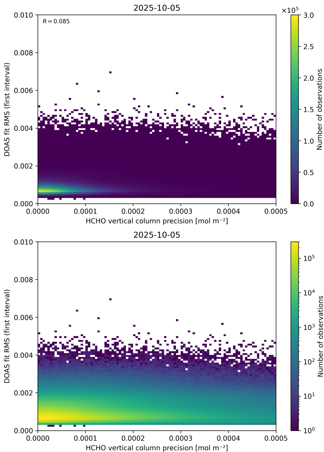
Figure 136: Scatter density plot of “HCHO vertical column precision” against “DOAS fit RMS (first interval)” for 2025-10-04 to 2025-10-06.
