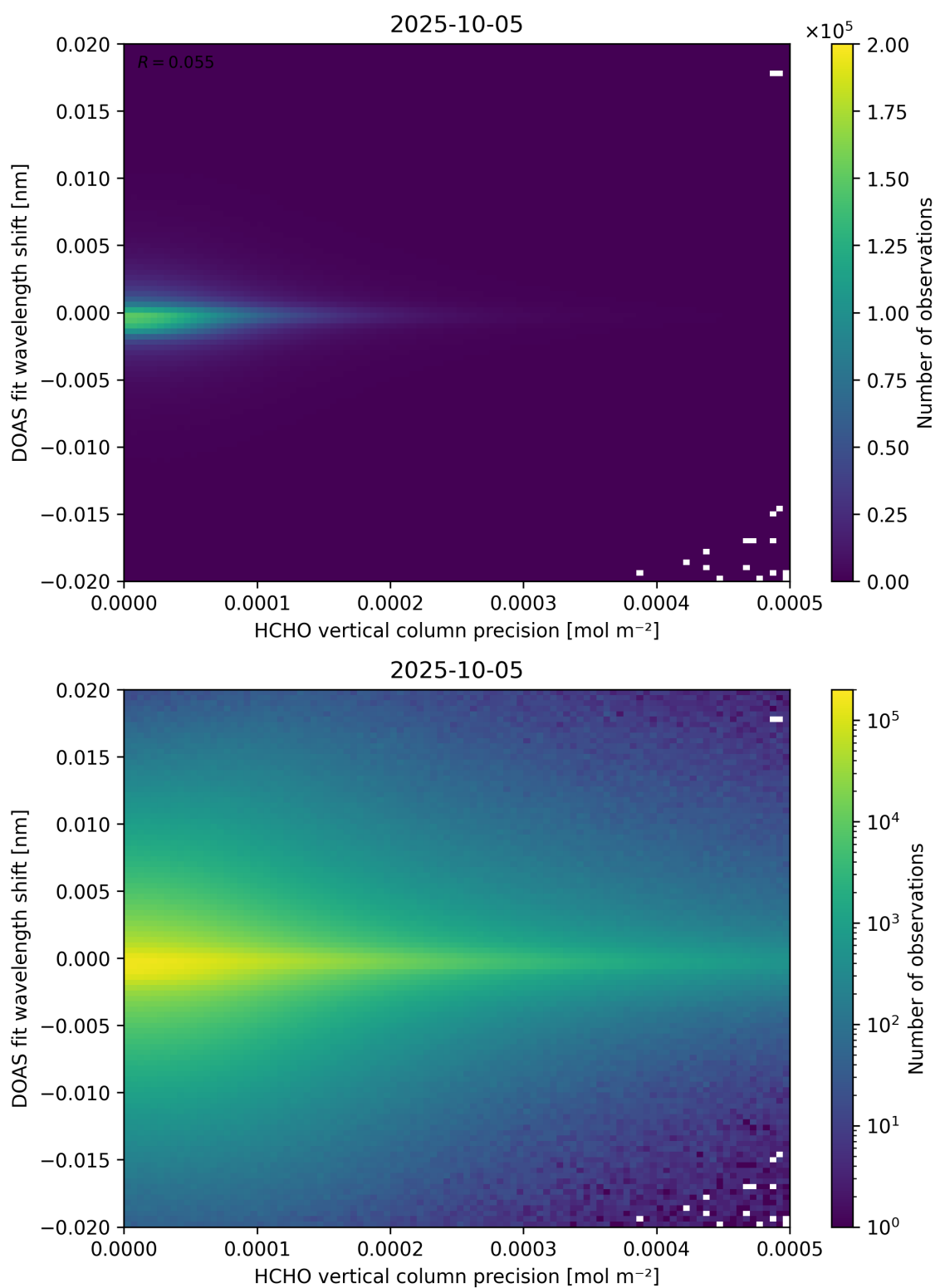
Figure 137: Scatter density plot of “HCHO vertical column precision” against “DOAS fit wavelength shift” for 2025-10-04 to 2025-10-06.
