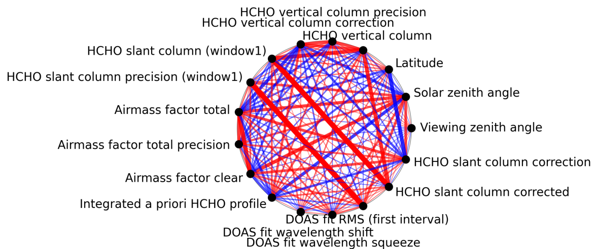
Figure 1: Map of correlation graph for 2025-10-04 to 2025-10-06.
