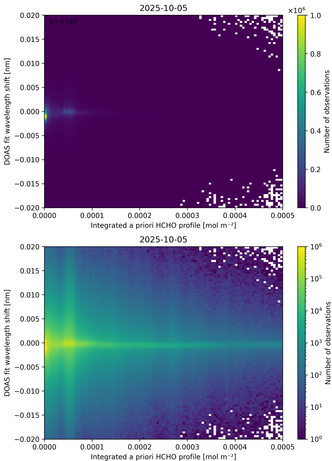
Figure 149: Scatter density plot of “Integrated a priori HCHO profile” against “DOAS fit wavelength shift” for 2025-10-04 to 2025-10-06.
