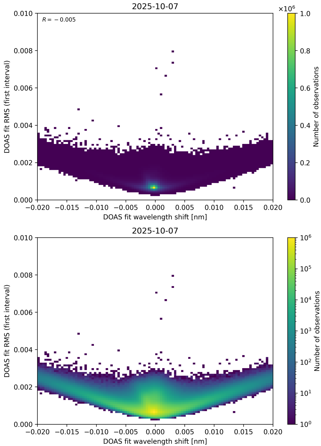
Figure 64: Scatter density plot of “DOAS fit wavelength shift” against “DOAS fit RMS (first interval)” for 2025-10-06 to 2025-10-08.
