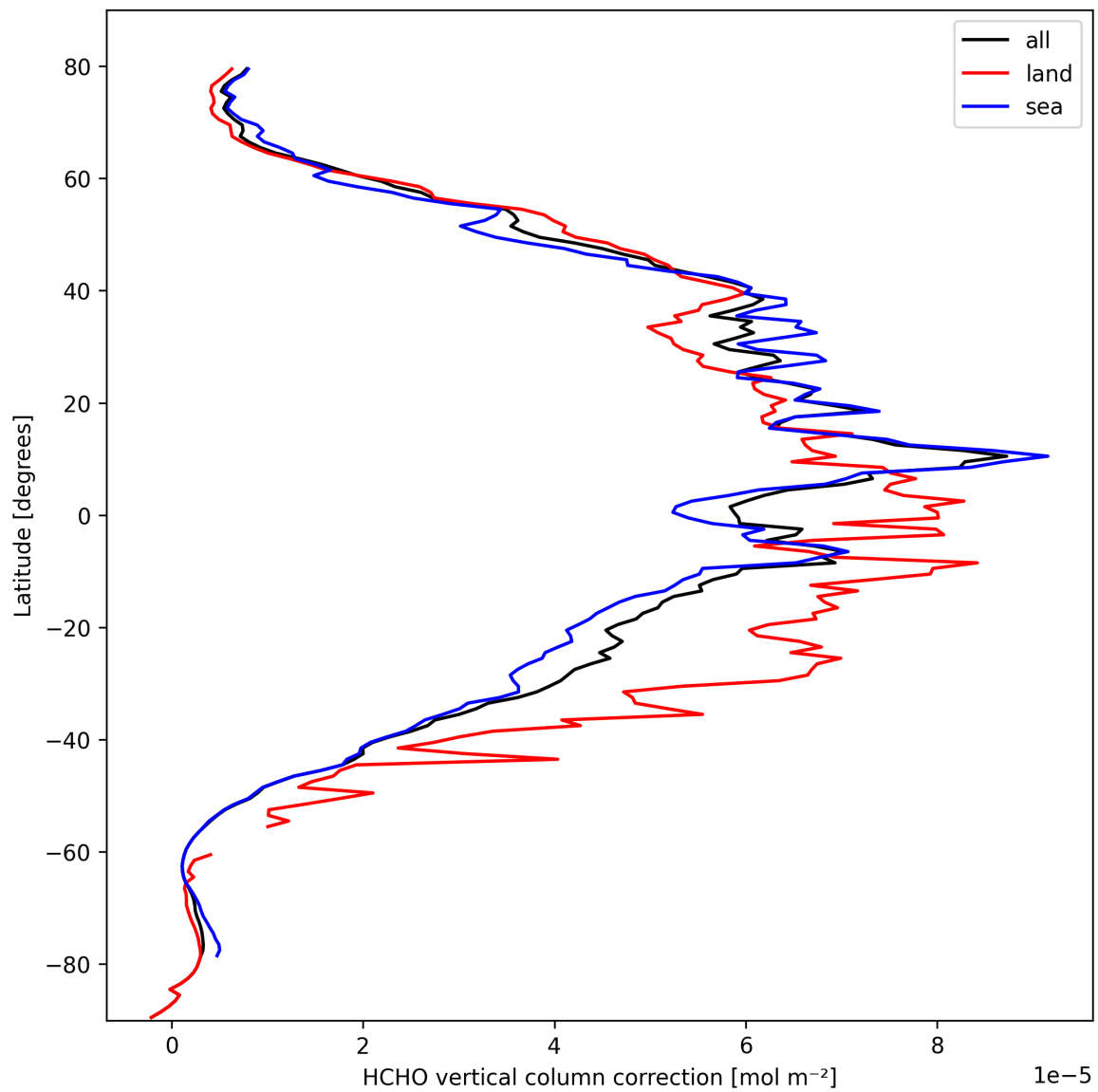
Figure 23: Zonal average of “HCHO vertical column correction” for 2025-10-06 to 2025-10-08.
