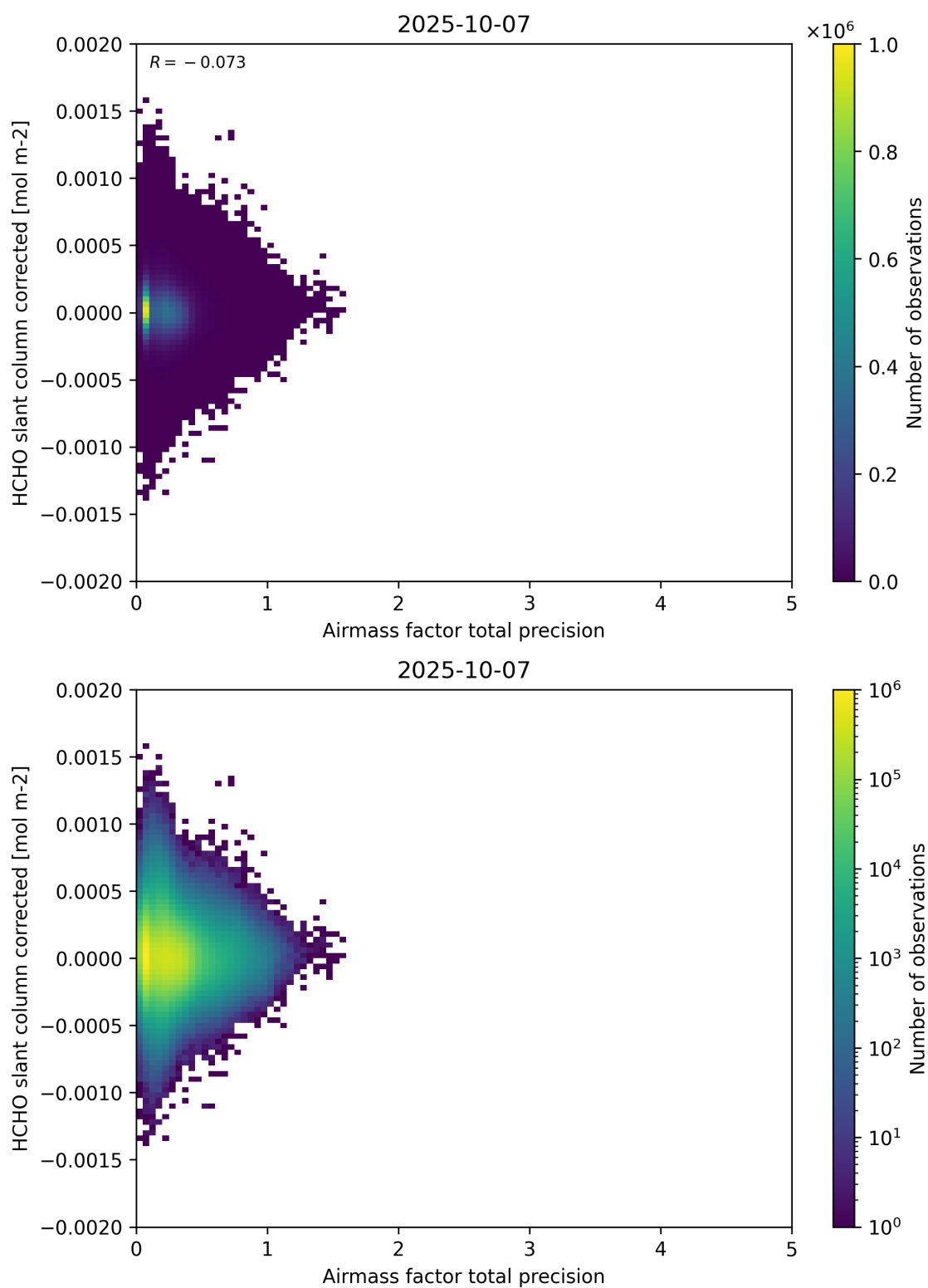
Figure 109: Scatter density plot of “Airmass factor total precision” against “HCHO slant column corrected” for 2025-10-06 to 2025-10-08.
