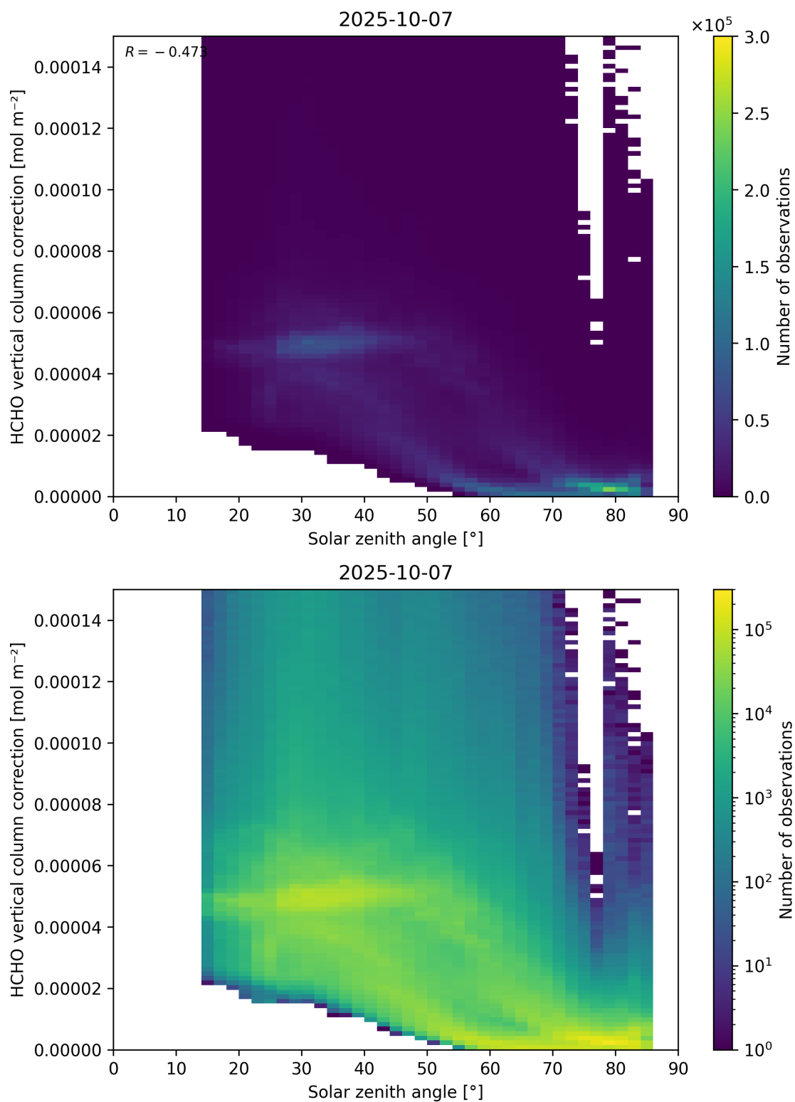
Figure 178: Scatter density plot of “Solar zenith angle” against “HCHO vertical column correction” for 2025-10-06 to 2025-10-08.
