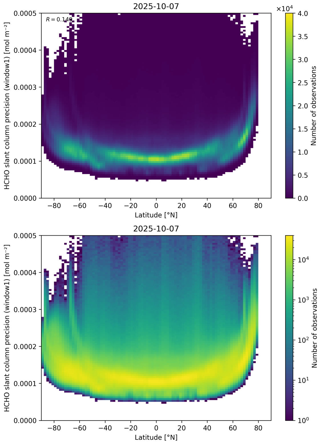
Figure 160: Scatter density plot of “Latitude” against “HCHO slant column precision (window1)” for 2025-10-06 to 2025-10-08.
