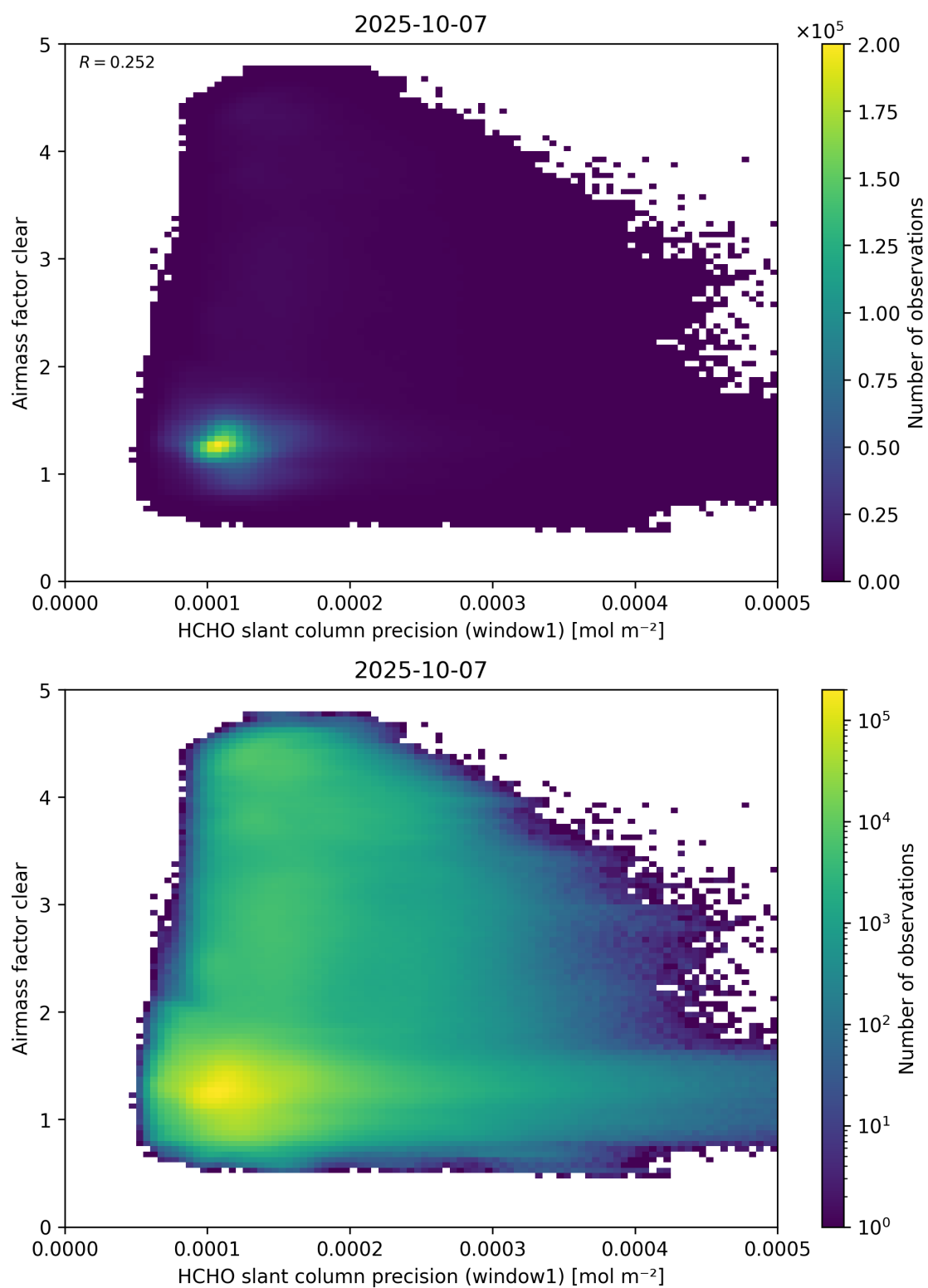
Figure 91: Scatter density plot of “HCHO slant column precision (window1)” against “Airmass factor clear” for 2025-10-06 to 2025-10-08.
