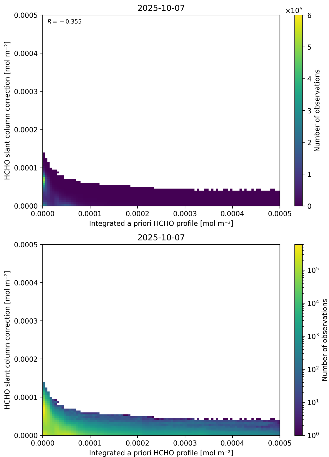
Figure 152: Scatter density plot of “Integrated a priori HCHO profile” against “HCHO slant column correction” for 2025-10-06 to 2025-10-08.
