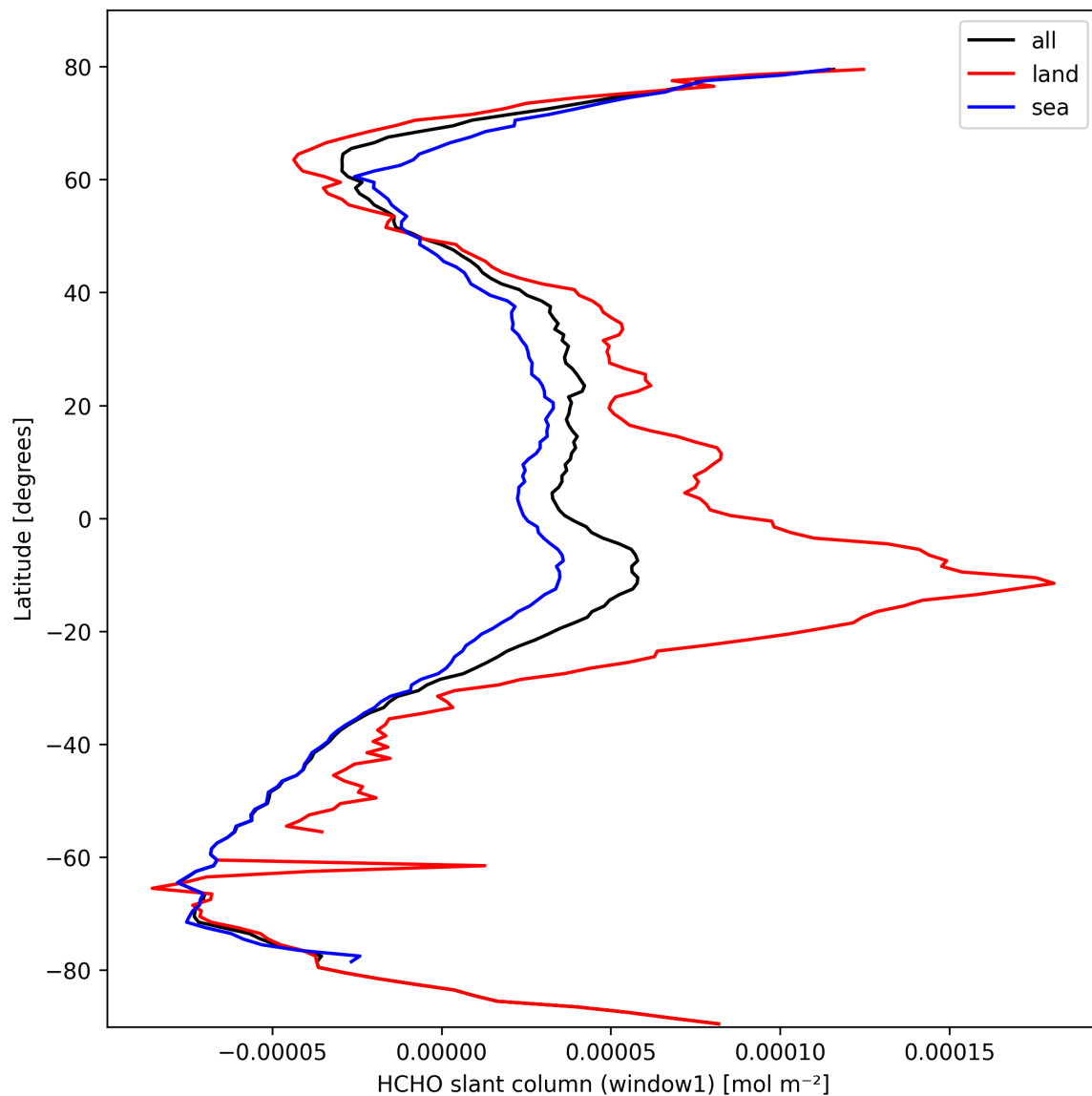
Figure 24: Zonal average of “HCHO slant column (window1)” for 2025-10-06 to 2025-10-08.
