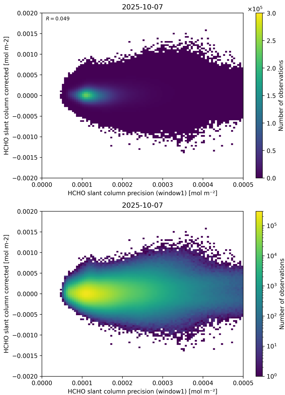
Figure 92: Scatter density plot of “HCHO slant column precision (window1)” against “HCHO slant column corrected” for 2025-10-06 to 2025-10-08.
