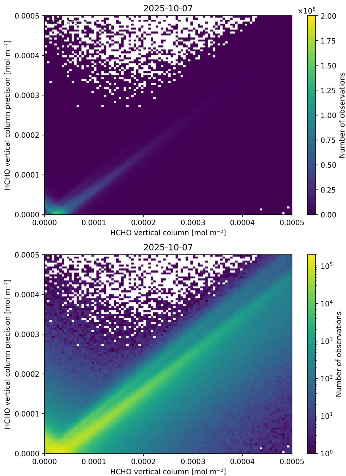
Figure 134: Scatter density plot of “HCHO vertical column” against “HCHO vertical column precision” for 2025-10-06 to 2025-10-08.
