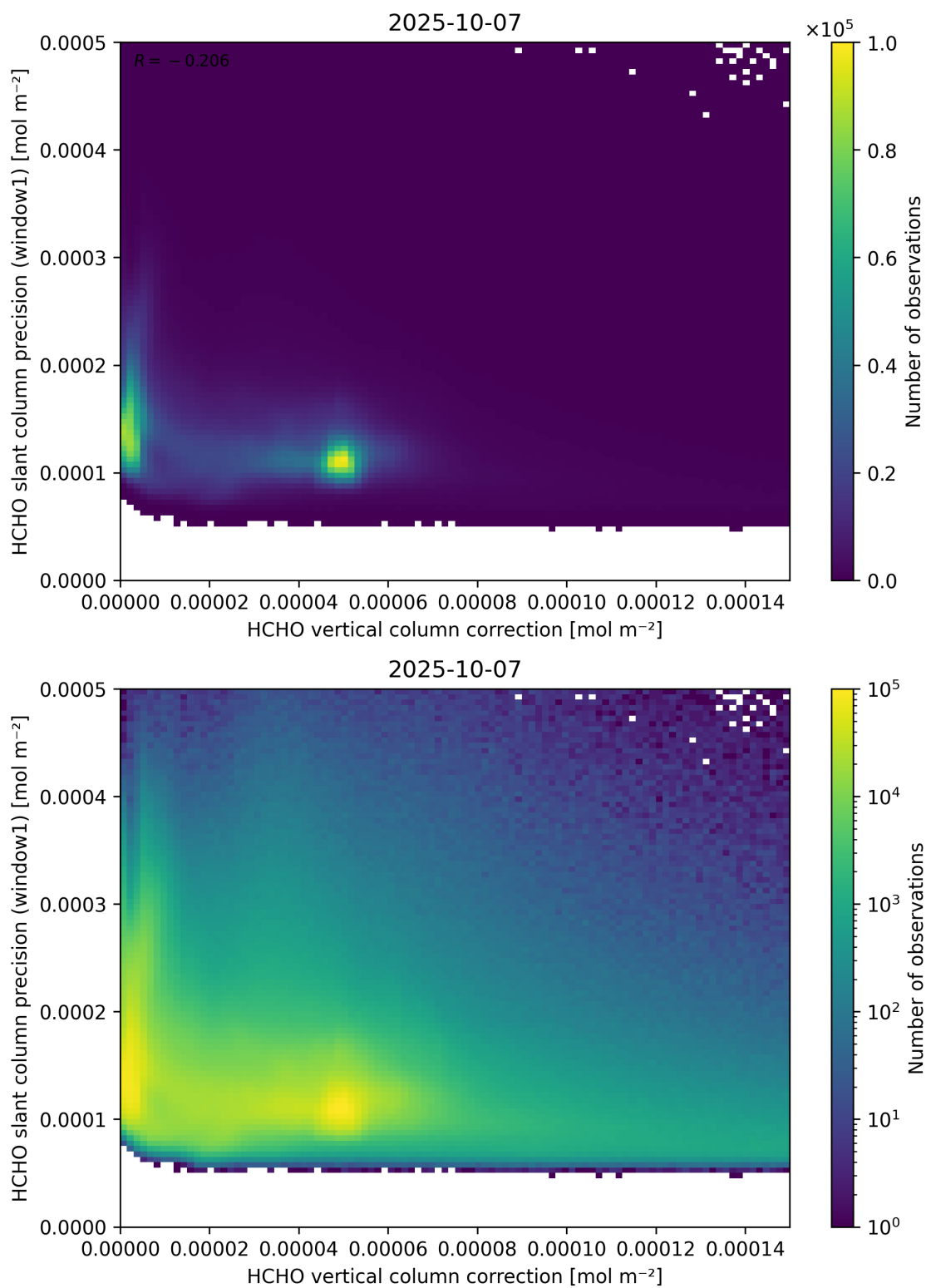
Figure 119: Scatter density plot of “HCHO vertical column correction” against “HCHO slant column precision (window1)” for 2025-10-06 to 2025-10-08.
