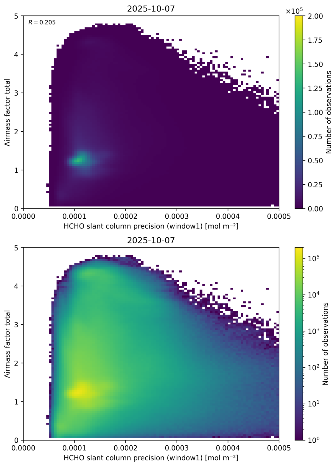
Figure 94: Scatter density plot of “HCHO slant column precision (window1)” against “Airmass factor total” for 2025-10-06 to 2025-10-08.
