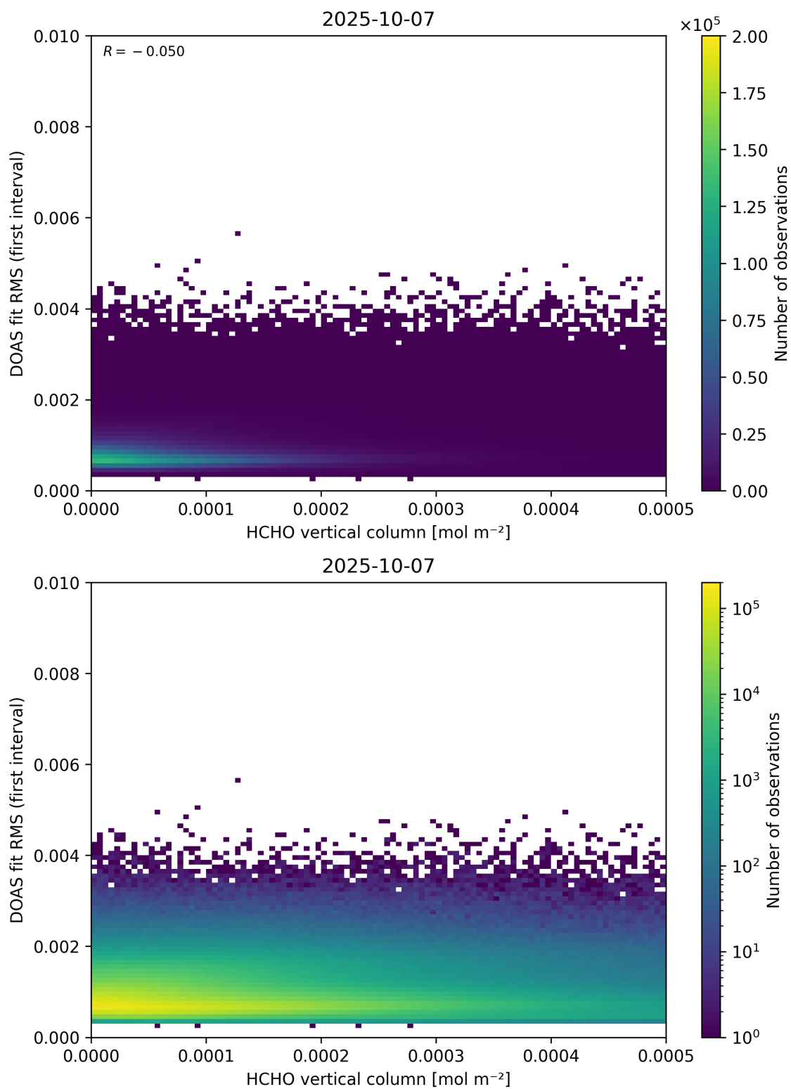
Figure 123: Scatter density plot of “HCHO vertical column” against “DOAS fit RMS (first interval)” for 2025-10-06 to 2025-10-08.
