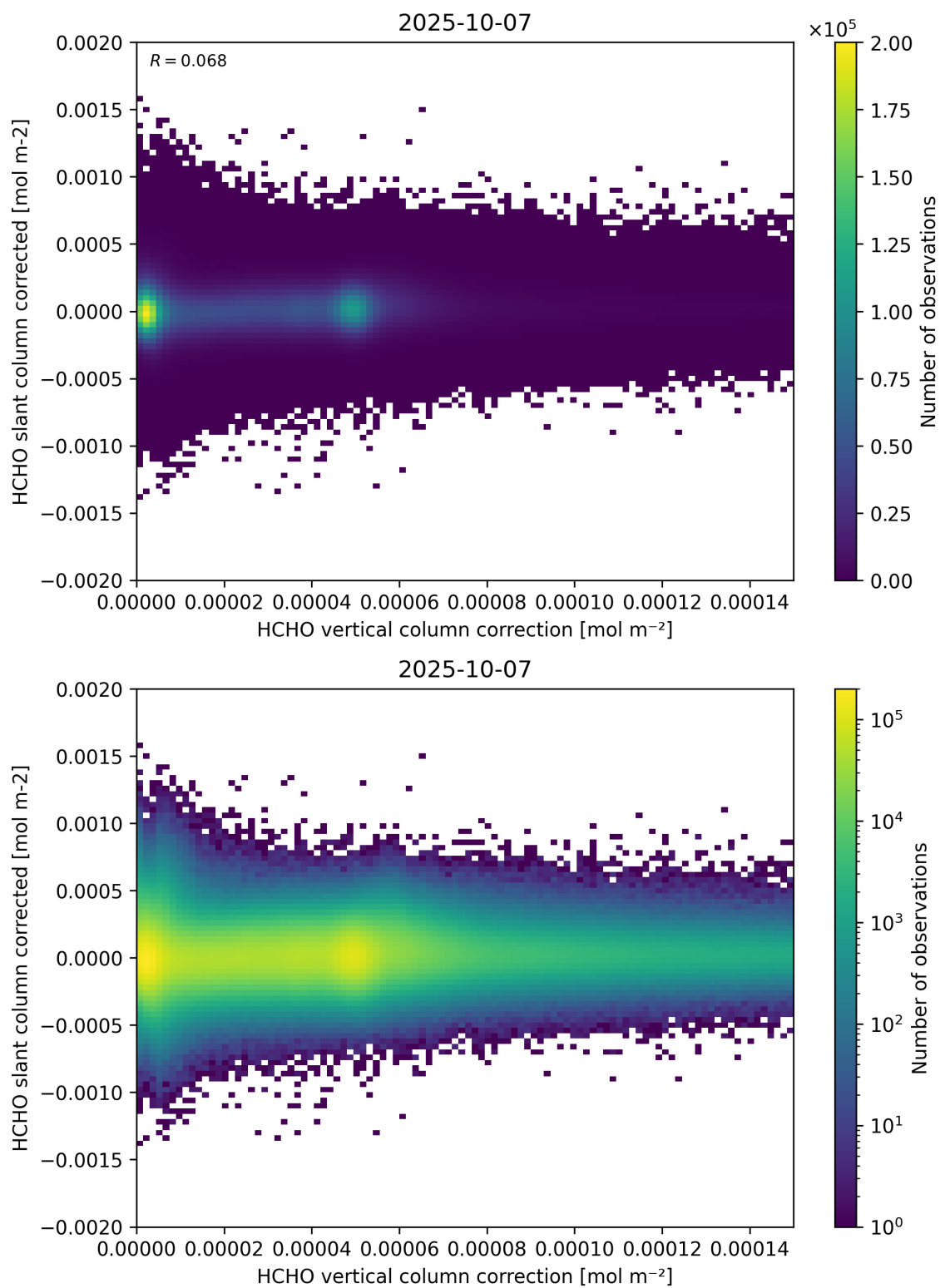
Figure 116: Scatter density plot of “HCHO vertical column correction” against “HCHO slant column corrected” for 2025-10-06 to 2025-10-08.
