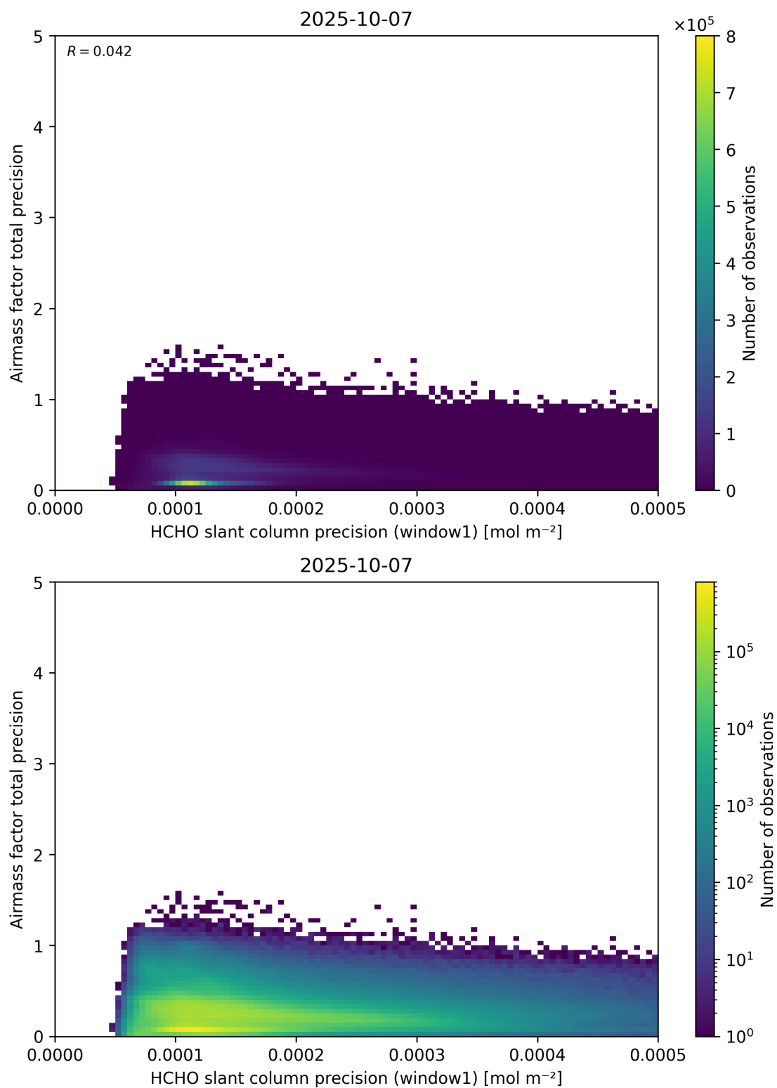
Figure 95: Scatter density plot of “HCHO slant column precision (window1)” against “Airmass factor total precision” for 2025-10-06 to 2025-10-08.
