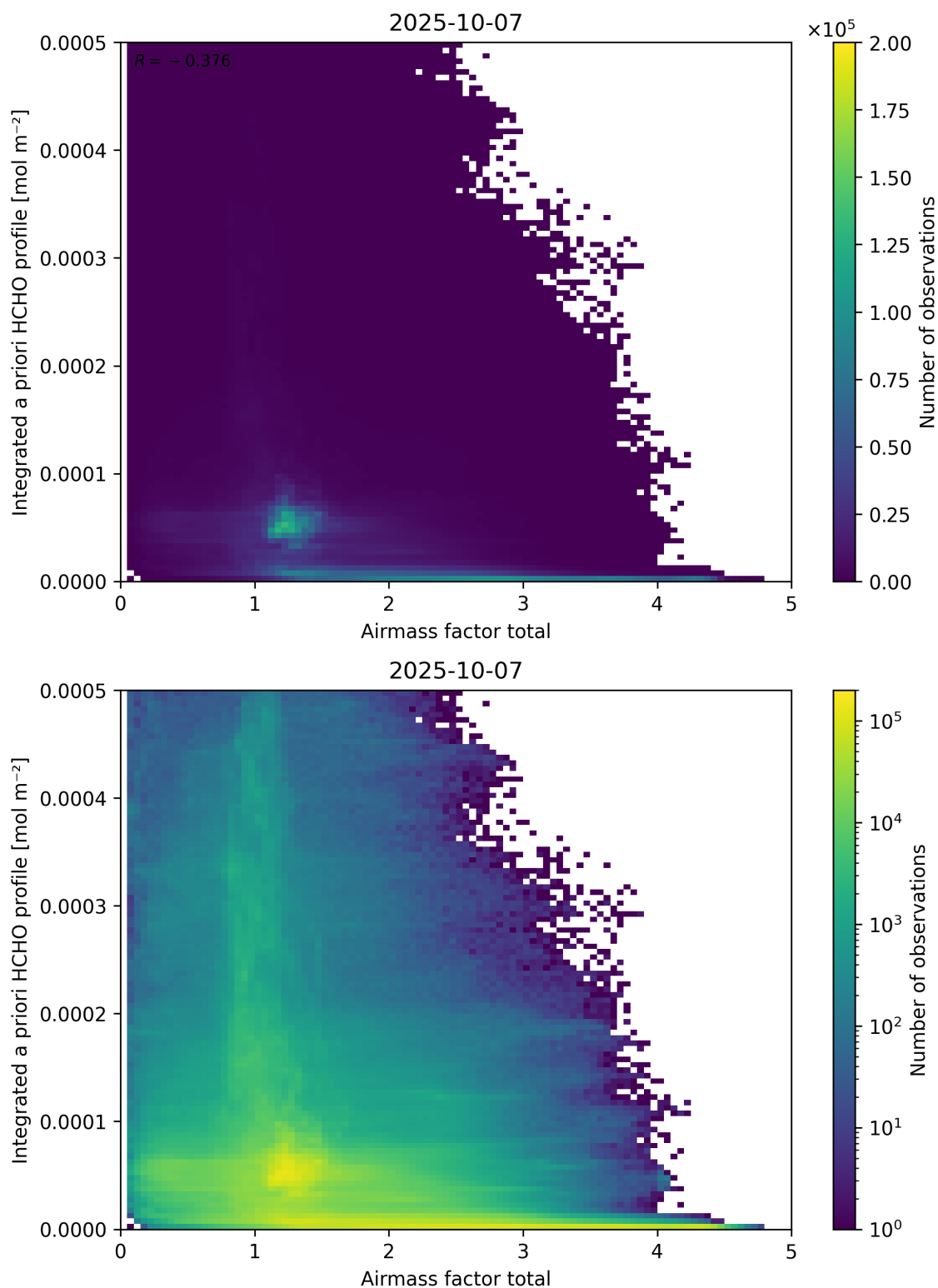
Figure 104: Scatter density plot of “Airmass factor total” against “Integrated a priori HCHO profile” for 2025-10-06 to 2025-10-08.
