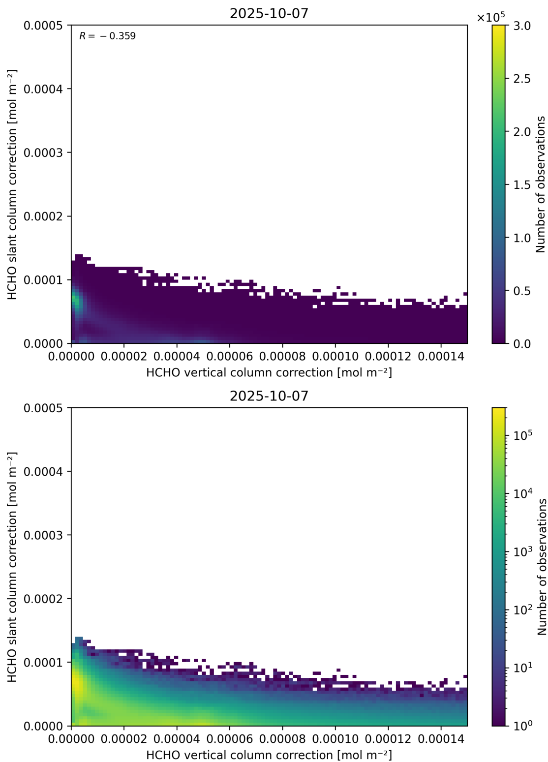
Figure 117: Scatter density plot of “HCHO vertical column correction” against “HCHO slant column correction” for 2025-10-06 to 2025-10-08.
