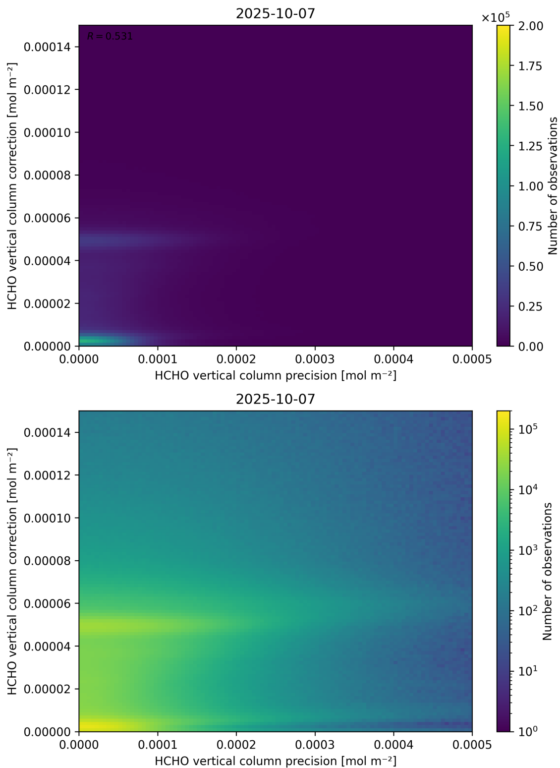
Figure 146: Scatter density plot of “HCHO vertical column precision” against “HCHO vertical column correction” for 2025-10-06 to 2025-10-08.
