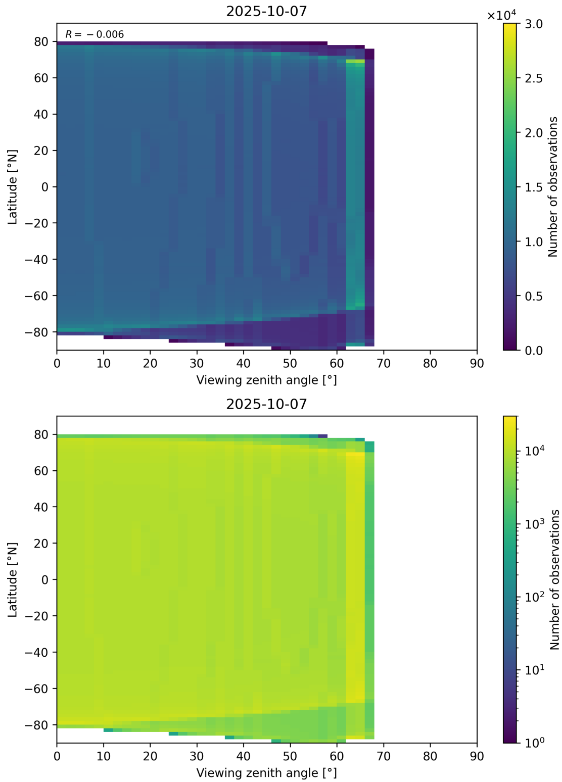
Figure 196: Scatter density plot of “Viewing zenith angle” against “Latitude” for 2025-10-06 to 2025-10-08.
