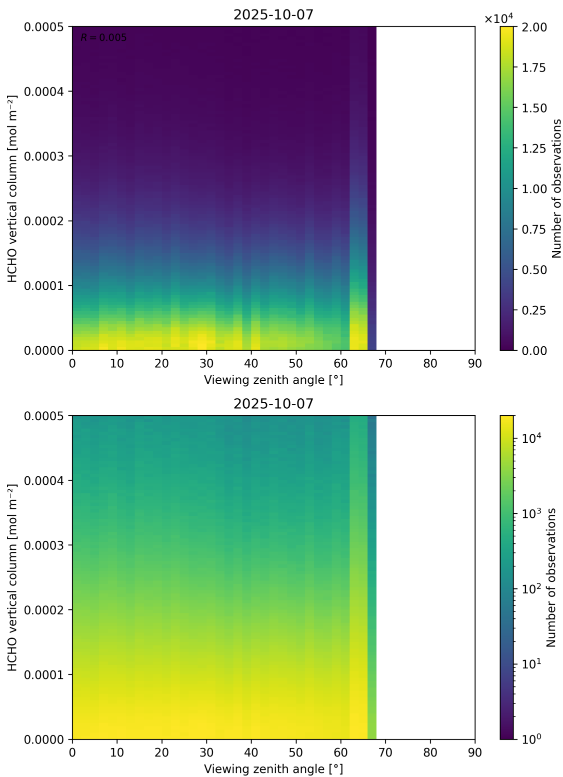
Figure 192: Scatter density plot of “Viewing zenith angle” against “HCHO vertical column” for 2025-10-06 to 2025-10-08.
