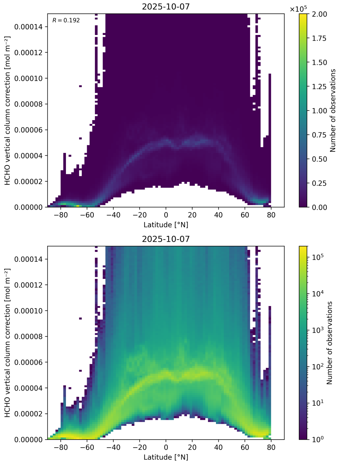
Figure 164: Scatter density plot of “Latitude” against “HCHO vertical column correction” for 2025-10-06 to 2025-10-08.
