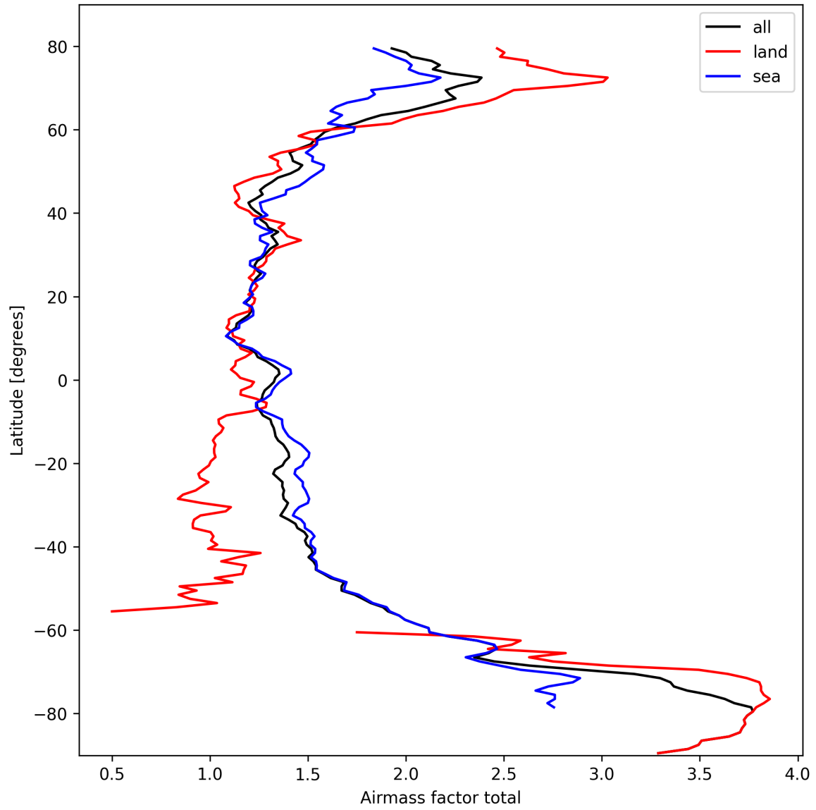
Figure 26: Zonal average of “Airmass factor total” for 2025-10-06 to 2025-10-08.
