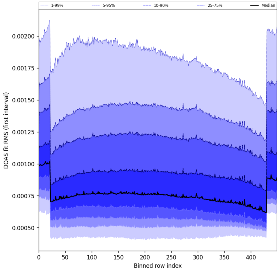
Figure 60: Along track statistics of “DOAS fit RMS (first interval)” for 2025-10-06 to 2025-10-08
