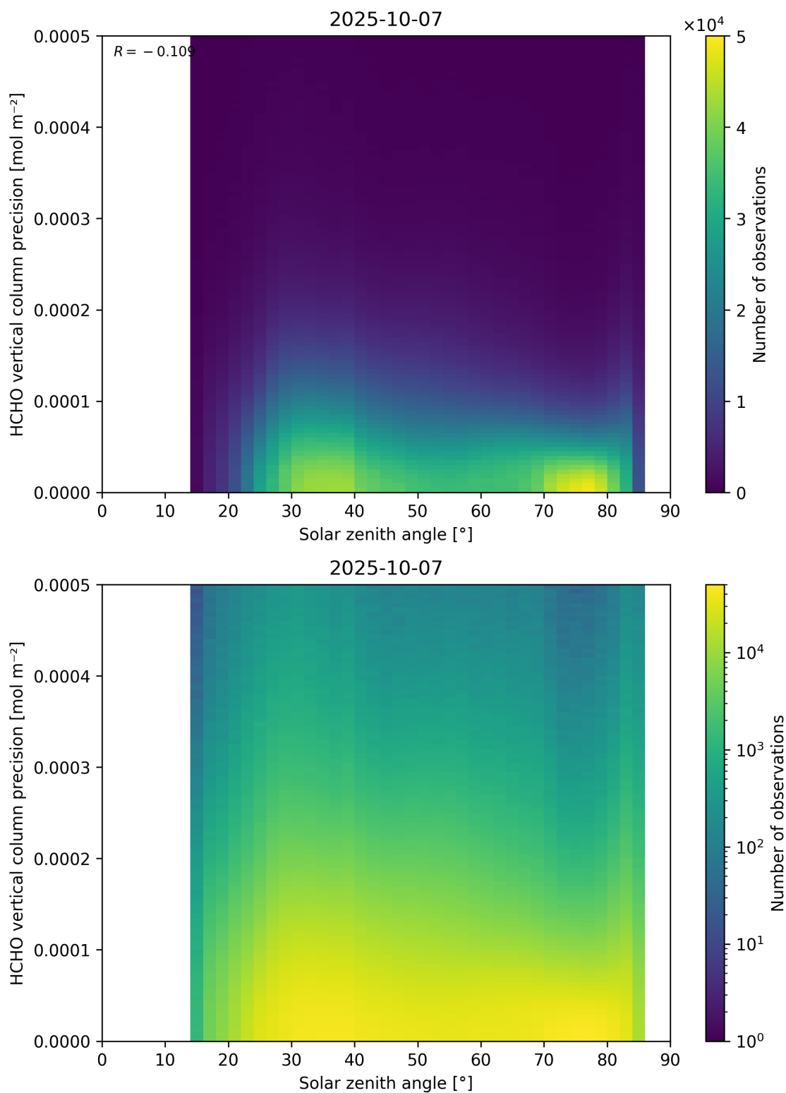
Figure 179: Scatter density plot of “Solar zenith angle” against “HCHO vertical column precision” for 2025-10-06 to 2025-10-08.
