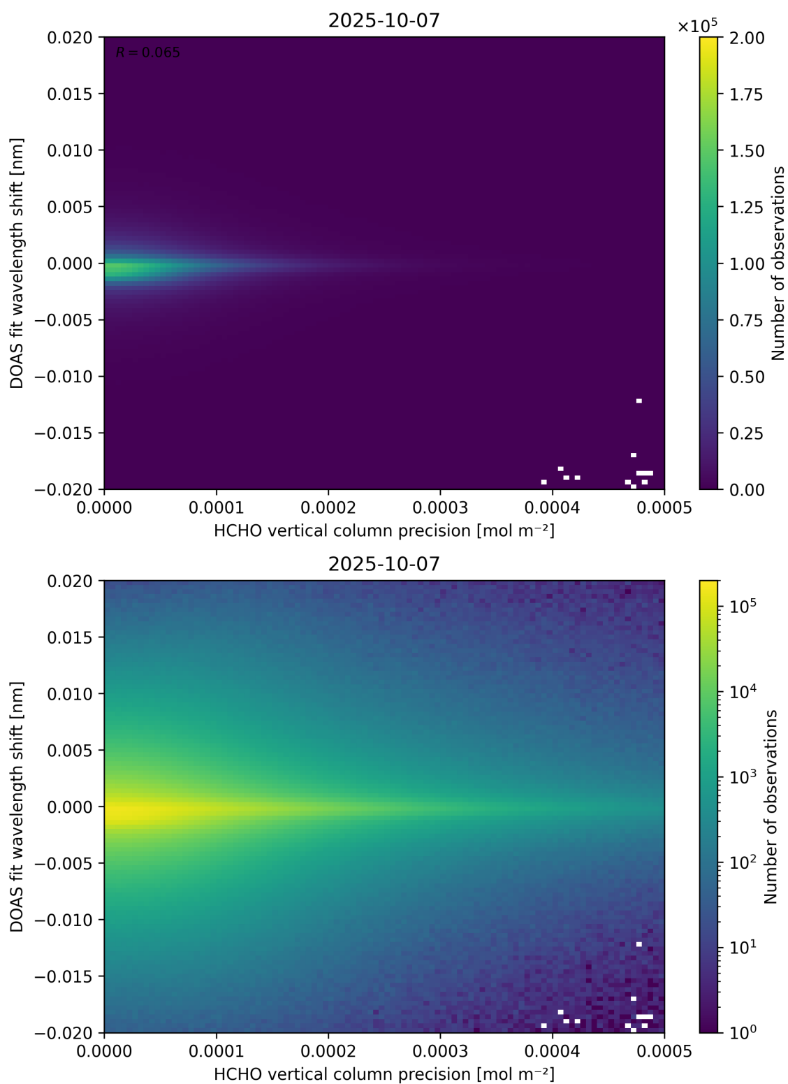
Figure 137: Scatter density plot of “HCHO vertical column precision” against “DOAS fit wavelength shift” for 2025-10-06 to 2025-10-08.
