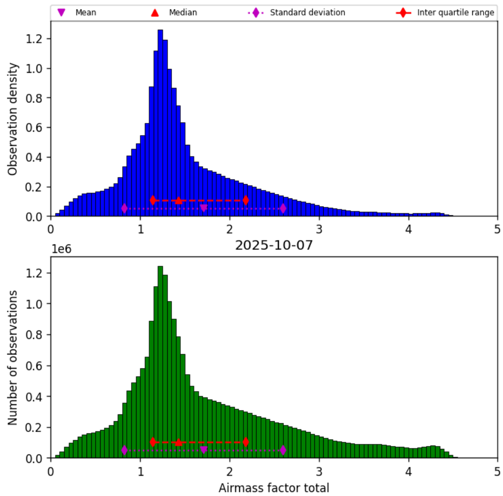
Figure 40: Histogram of “Airmass factor total” for 2025-10-06 to 2025-10-08
