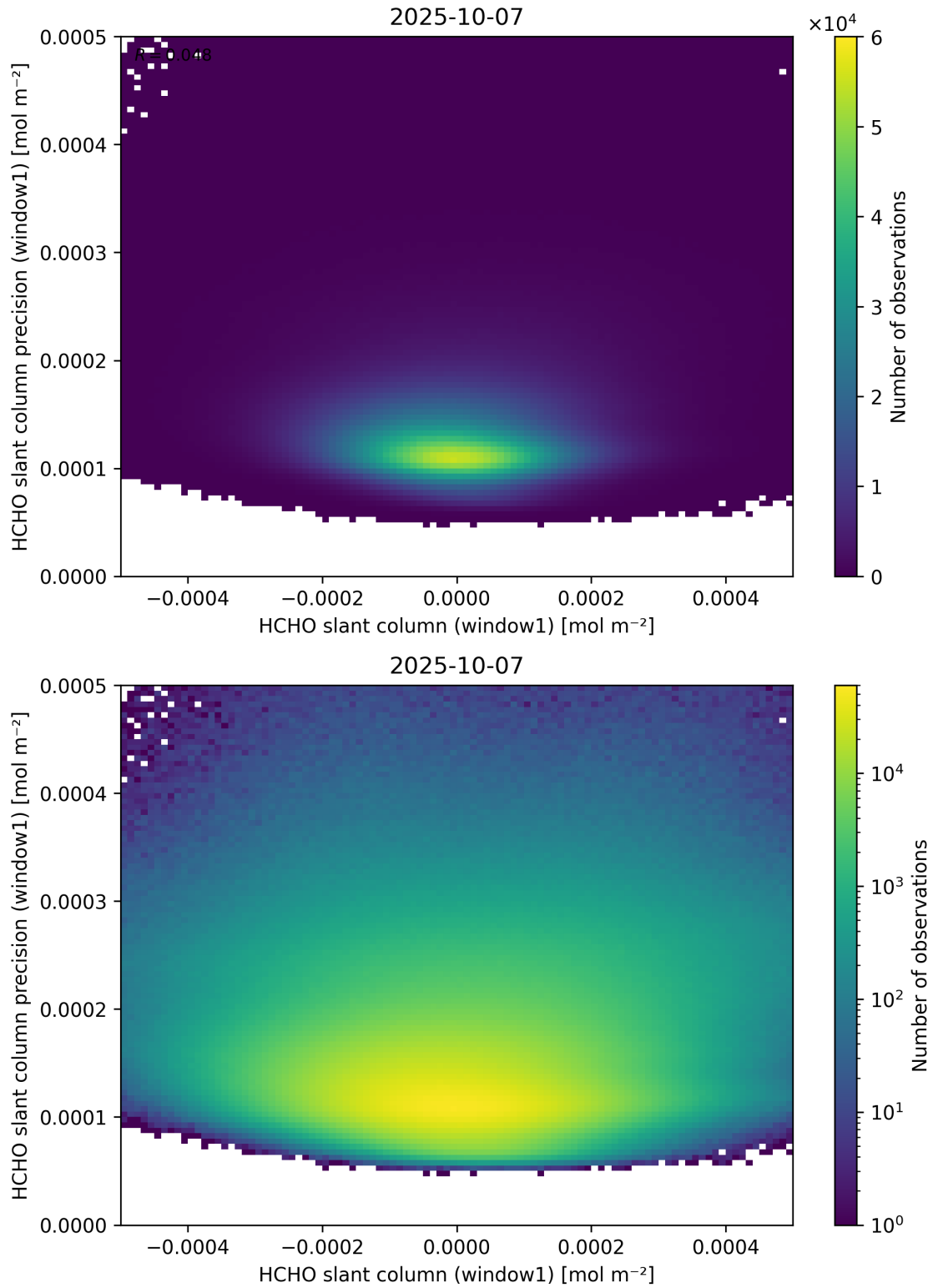
Figure 84: Scatter density plot of “HCHO slant column (window1)” against “HCHO slant column precision (window1)” for 2025-10-06 to 2025-10-08.
