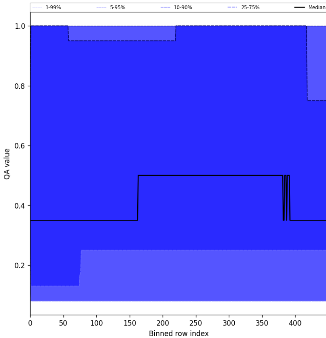
Figure 48: Along track statistics of “QA value” for 2025-10-06 to 2025-10-08
