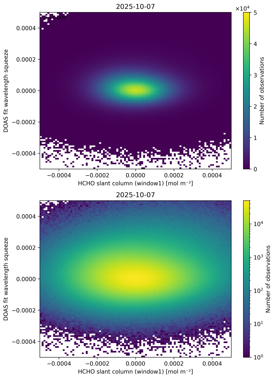
Figure 80: Scatter density plot of “HCHO slant column (window1)” against “DOAS fit wavelength squeeze” for 2025-10-06 to 2025-10-08.
