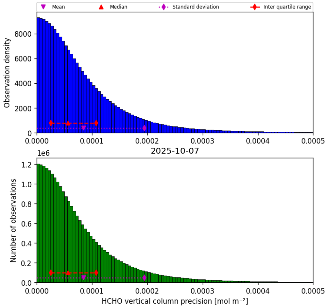
Figure 36: Histogram of “HCHO vertical column precision” for 2025-10-06 to 2025-10-08
