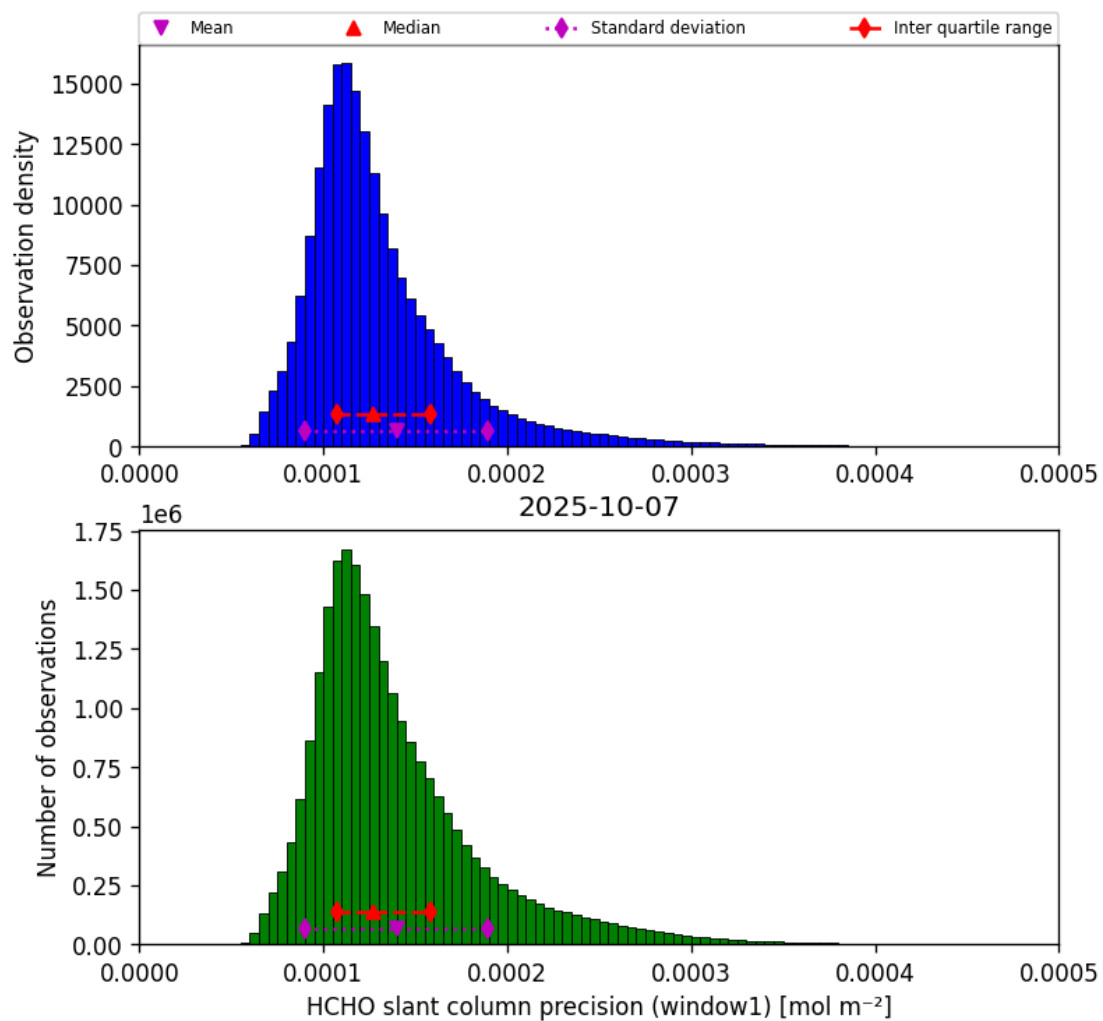
Figure 39: Histogram of “HCHO slant column precision (window1)” for 2025-10-06 to 2025-10-08
