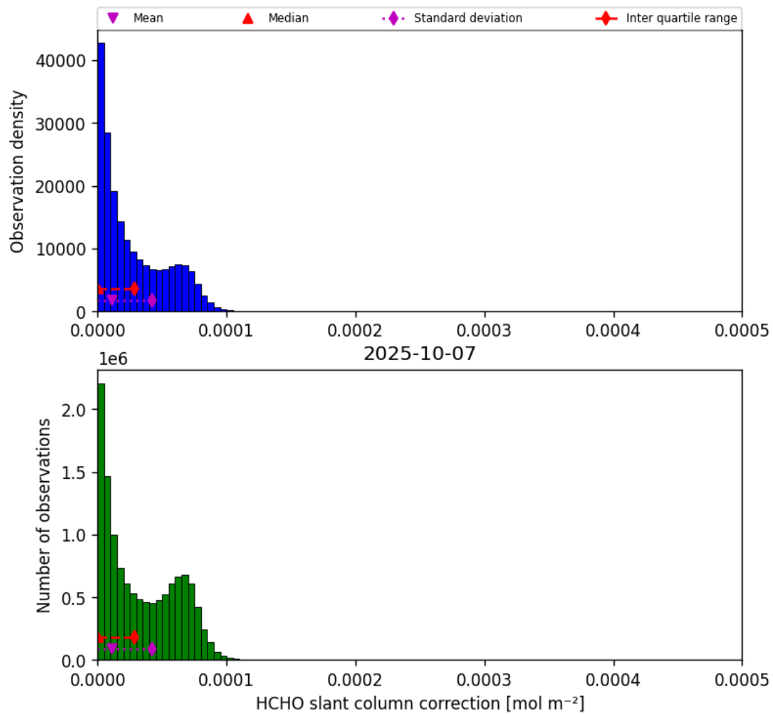
Figure 47: Histogram of “HCHO slant column correction” for 2025-10-06 to 2025-10-08
