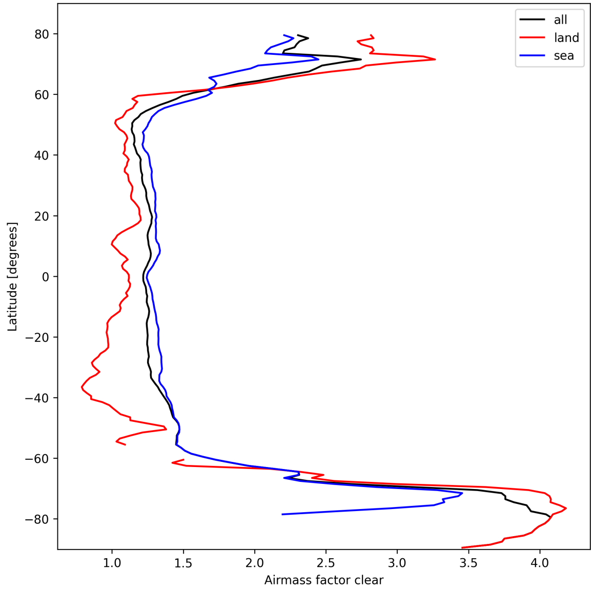
Figure 28: Zonal average of “Airmass factor clear” for 2025-10-06 to 2025-10-08.
