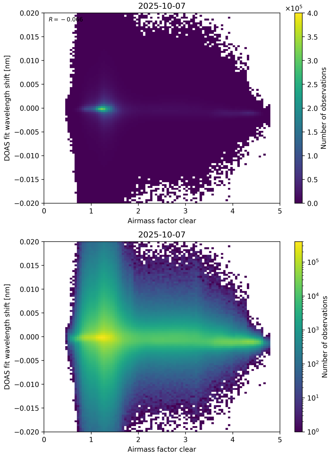
Figure 72: Scatter density plot of “Airmass factor clear” against “DOAS fit wavelength shift” for 2025-10-06 to 2025-10-08.
