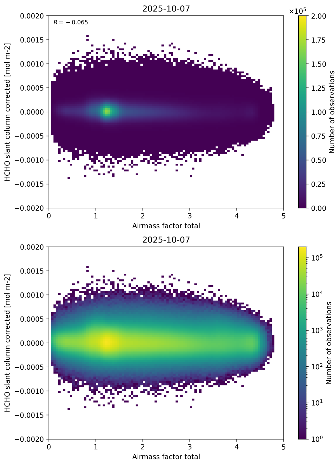
Figure 101: Scatter density plot of “Airmass factor total” against “HCHO slant column corrected” for 2025-10-06 to 2025-10-08.
