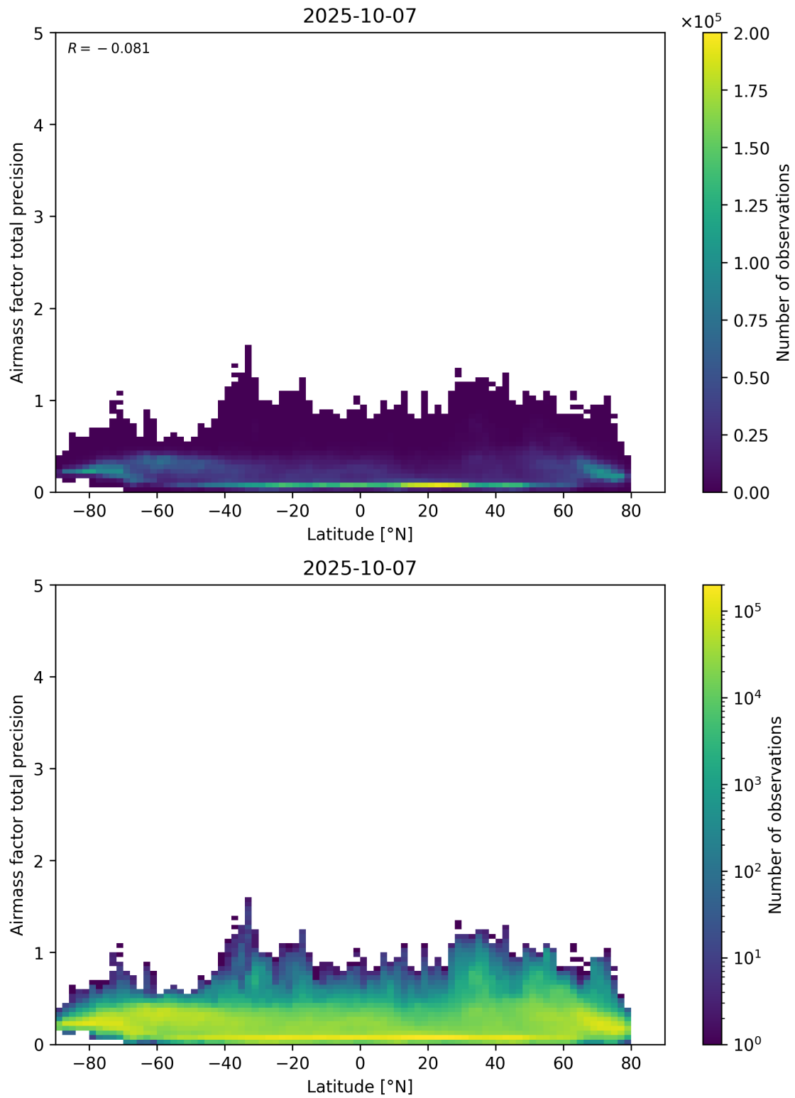
Figure 162: Scatter density plot of “Latitude” against “Airmass factor total precision” for 2025-10-06 to 2025-10-08.
