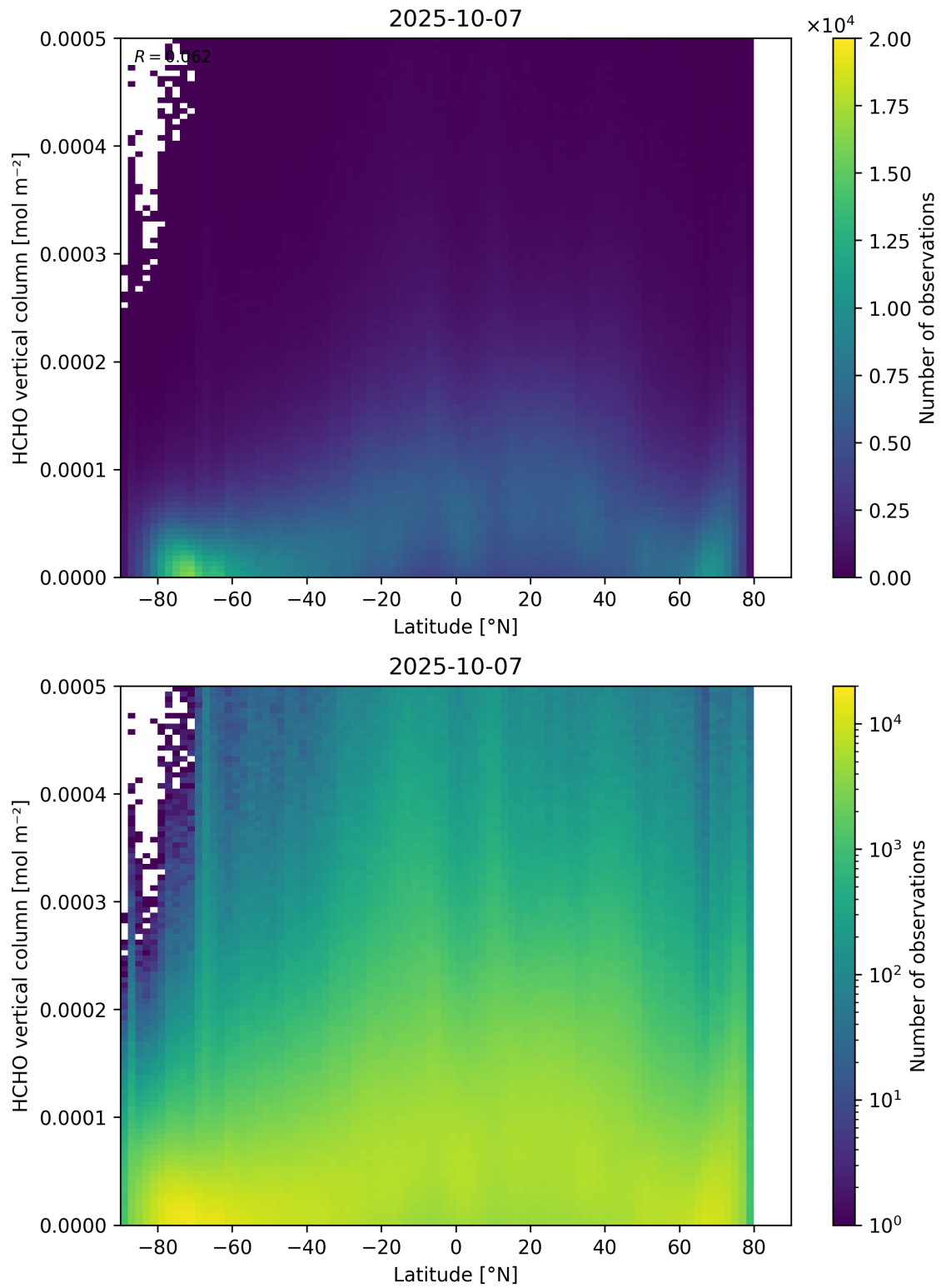
Figure 163: Scatter density plot of “Latitude” against “HCHO vertical column” for 2025-10-06 to 2025-10-08.
