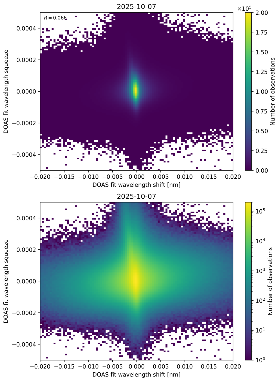
Figure 65: Scatter density plot of “DOAS fit wavelength shift” against “DOAS fit wavelength squeeze” for 2025-10-06 to 2025-10-08.
