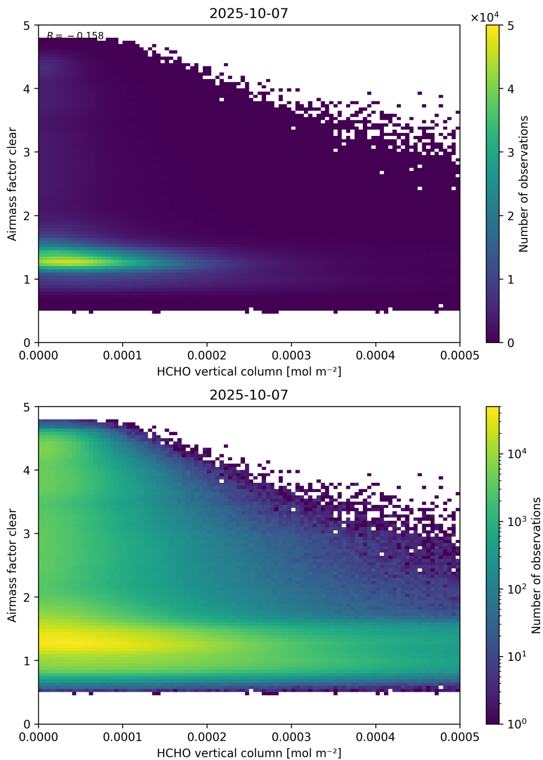
Figure 126: Scatter density plot of “HCHO vertical column” against “Airmass factor clear” for 2025-10-06 to 2025-10-08.
