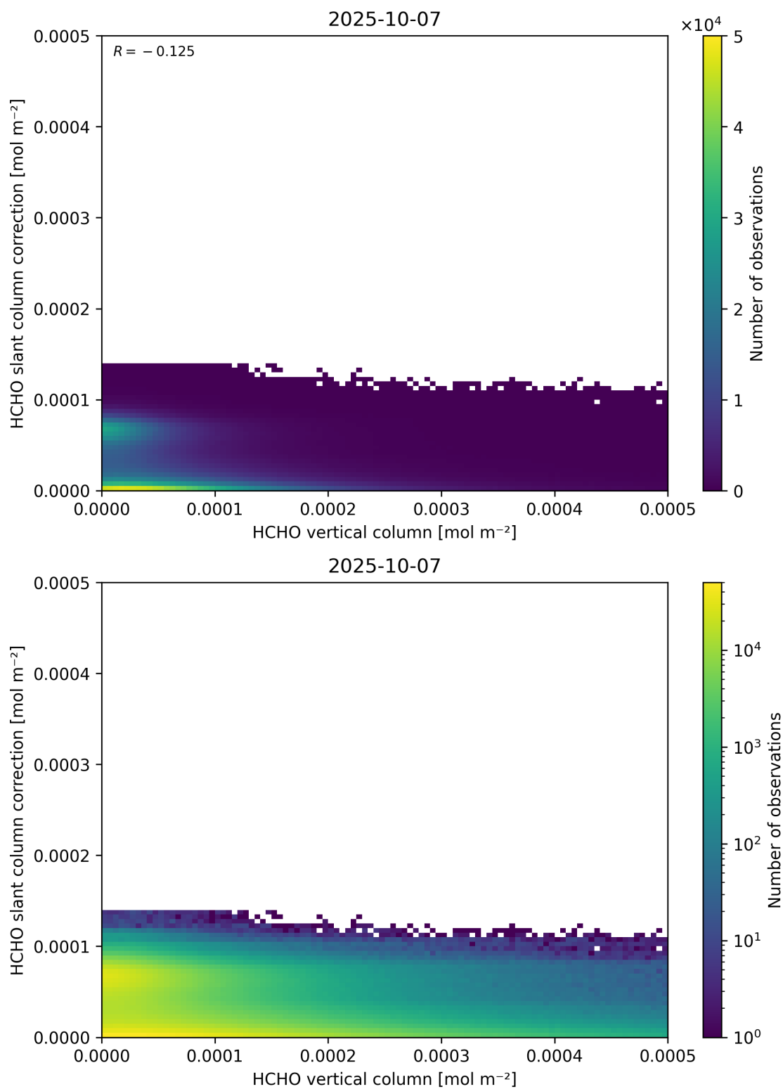
Figure 128: Scatter density plot of “HCHO vertical column” against “HCHO slant column correction” for 2025-10-06 to 2025-10-08.
