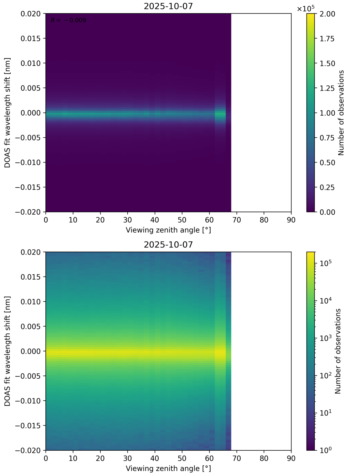
Figure 183: Scatter density plot of “Viewing zenith angle” against “DOAS fit wavelength shift” for 2025-10-06 to 2025-10-08.
