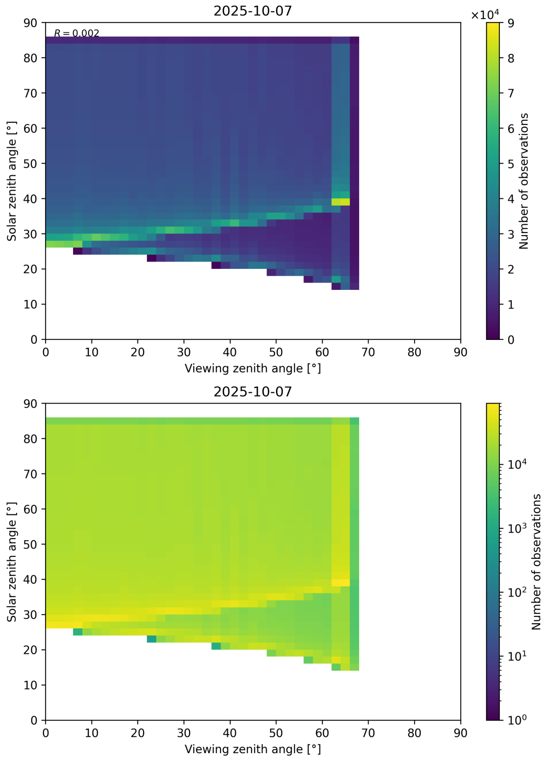
Figure 197: Scatter density plot of “Viewing zenith angle” against “Solar zenith angle” for 2025-10-06 to 2025-10-08.
