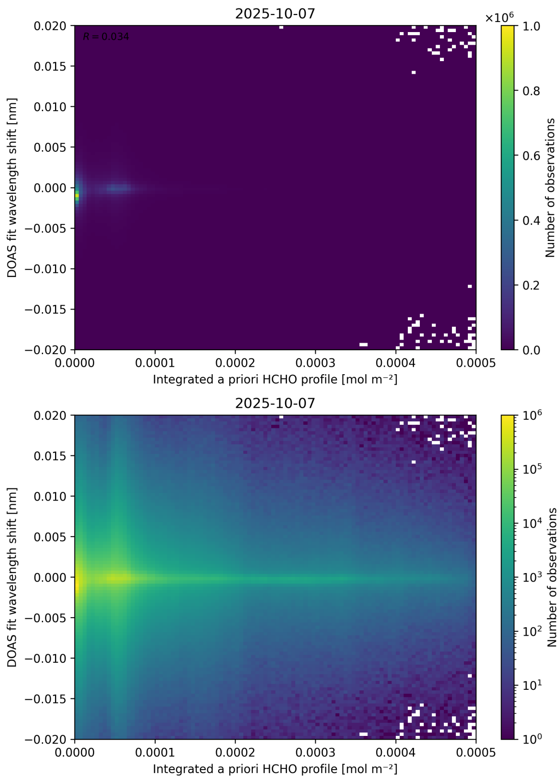
Figure 149: Scatter density plot of “Integrated a priori HCHO profile” against “DOAS fit wavelength shift” for 2025-10-06 to 2025-10-08.
