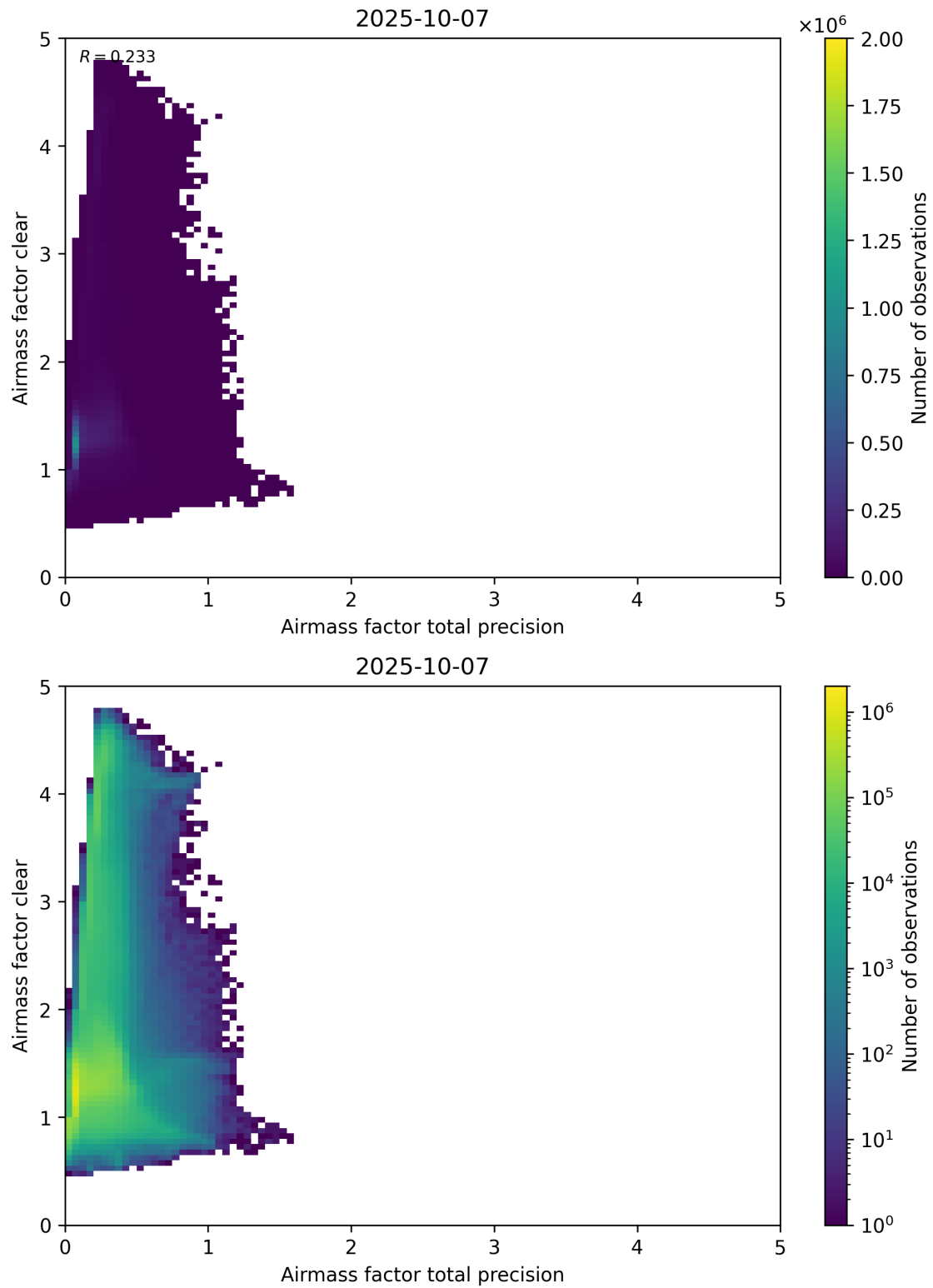
Figure 108: Scatter density plot of “Airmass factor total precision” against “Airmass factor clear” for 2025-10-06 to 2025-10-08.
