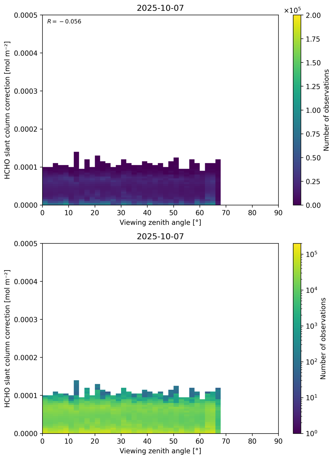
Figure 187: Scatter density plot of “Viewing zenith angle” against “HCHO slant column correction” for 2025-10-06 to 2025-10-08.
