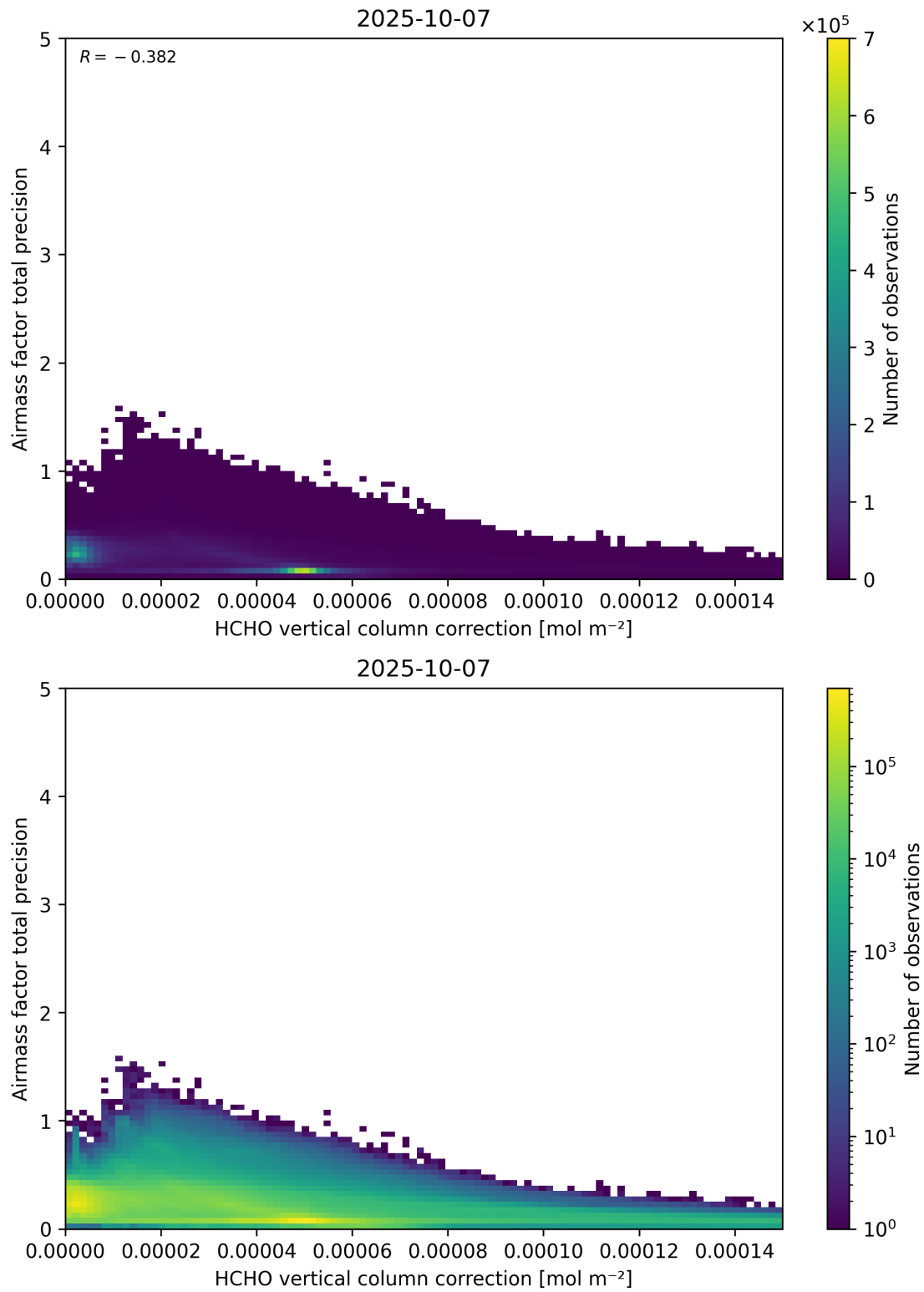
Figure 121: Scatter density plot of “HCHO vertical column correction” against “Airmass factor total precision” for 2025-10-06 to 2025-10-08.
