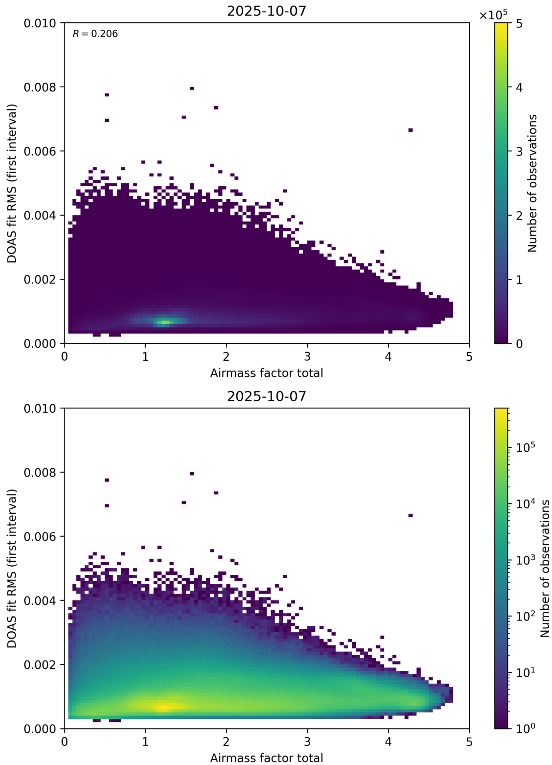
Figure 97: Scatter density plot of “Airmass factor total” against “DOAS fit RMS (first interval)” for 2025-10-06 to 2025-10-08.
