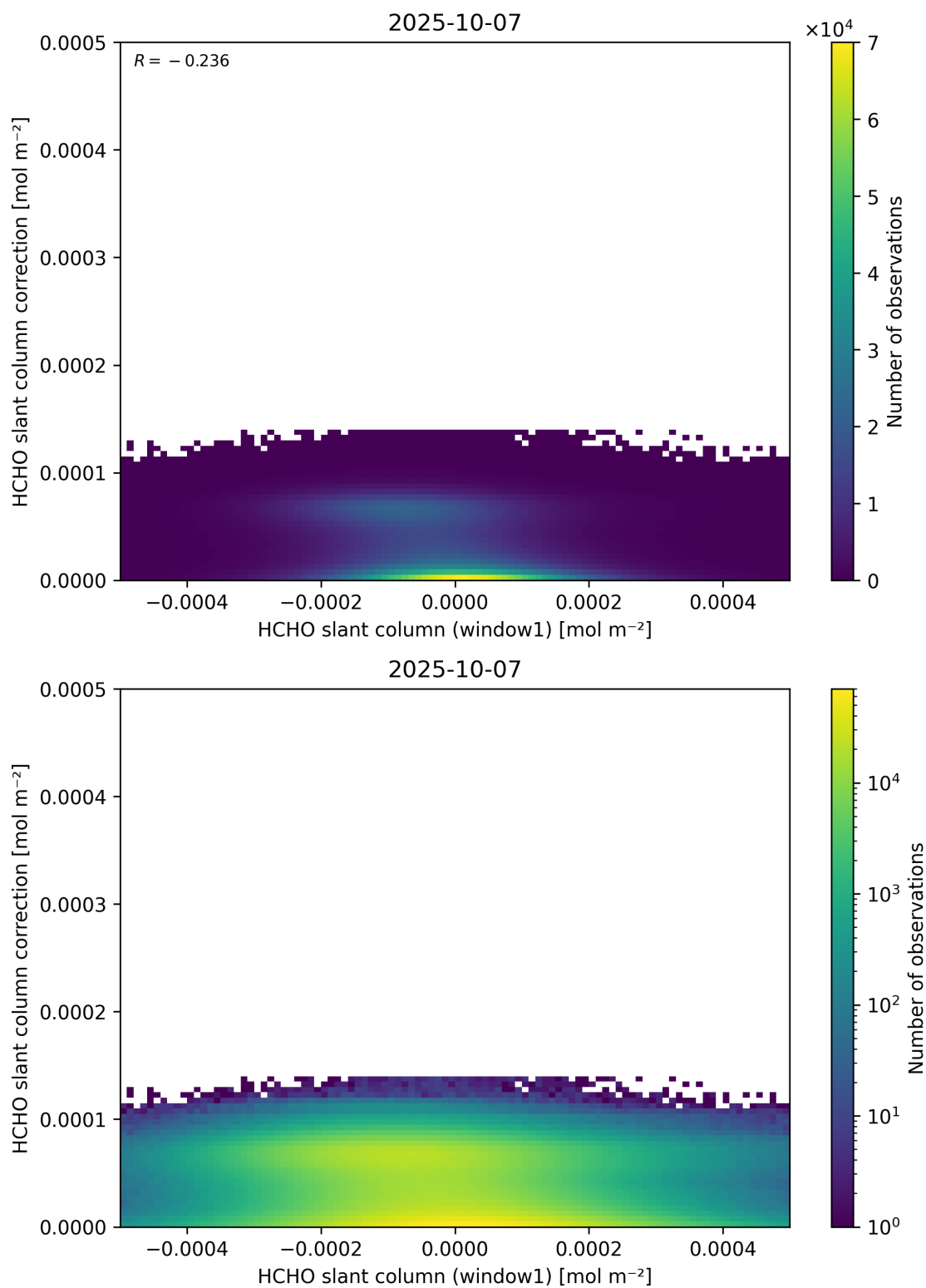
Figure 83: Scatter density plot of “HCHO slant column (window1)” against “HCHO slant column correction” for 2025-10-06 to 2025-10-08.
