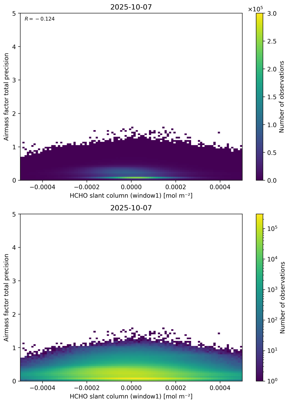
Figure 86: Scatter density plot of “HCHO slant column (window1)” against “Airmass factor total precision” for 2025-10-06 to 2025-10-08.
