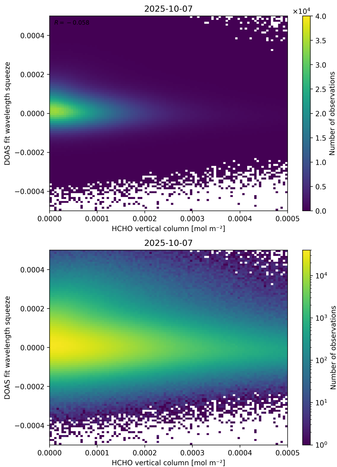
Figure 125: Scatter density plot of “HCHO vertical column” against “DOAS fit wavelength squeeze” for 2025-10-06 to 2025-10-08.
