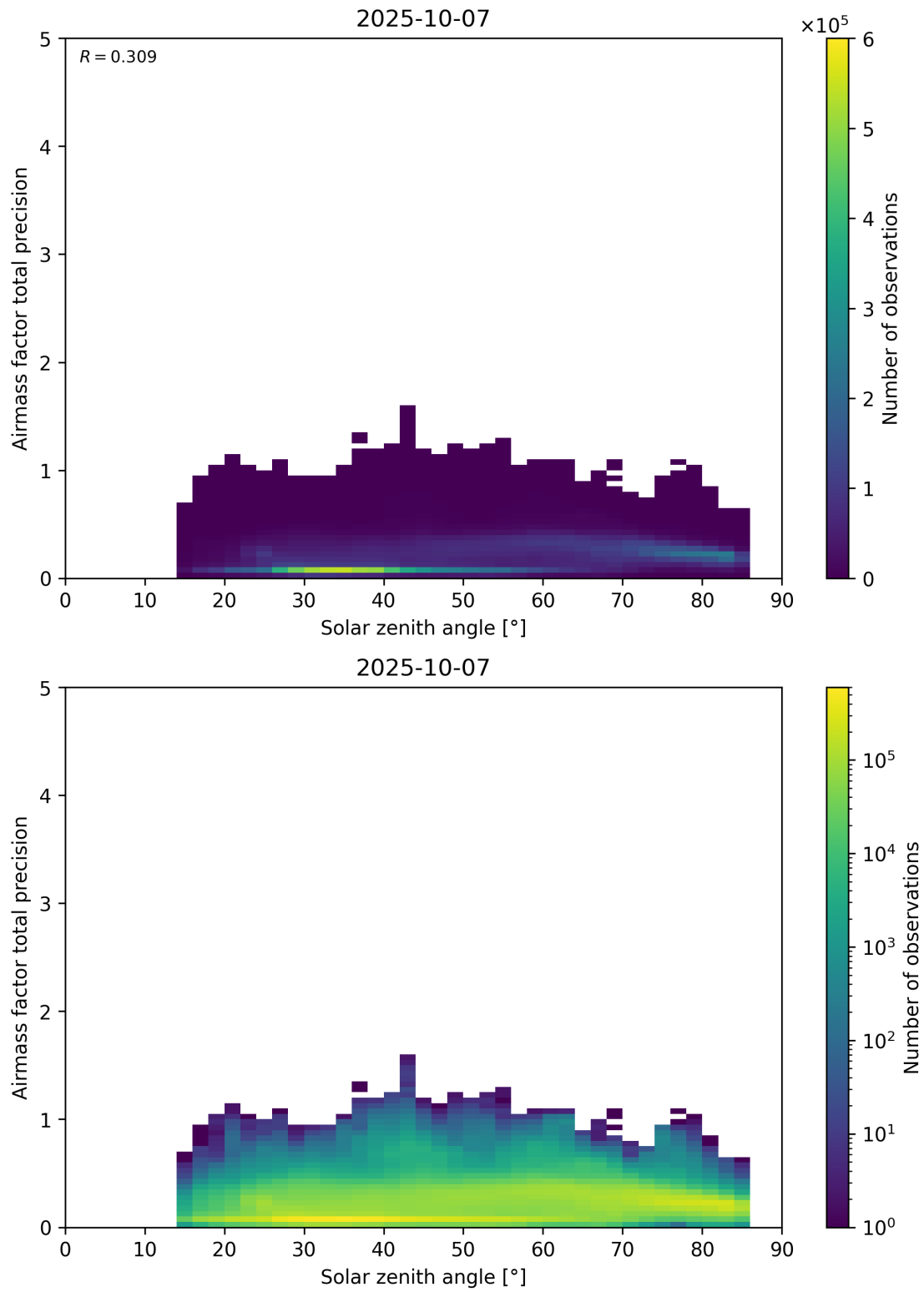
Figure 176: Scatter density plot of “Solar zenith angle” against “Airmass factor total precision” for 2025-10-06 to 2025-10-08.
