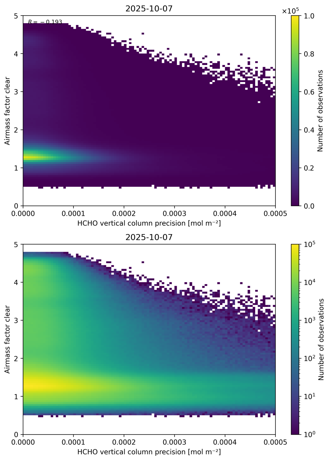
Figure 139: Scatter density plot of “HCHO vertical column precision” against “Airmass factor clear” for 2025-10-06 to 2025-10-08.
