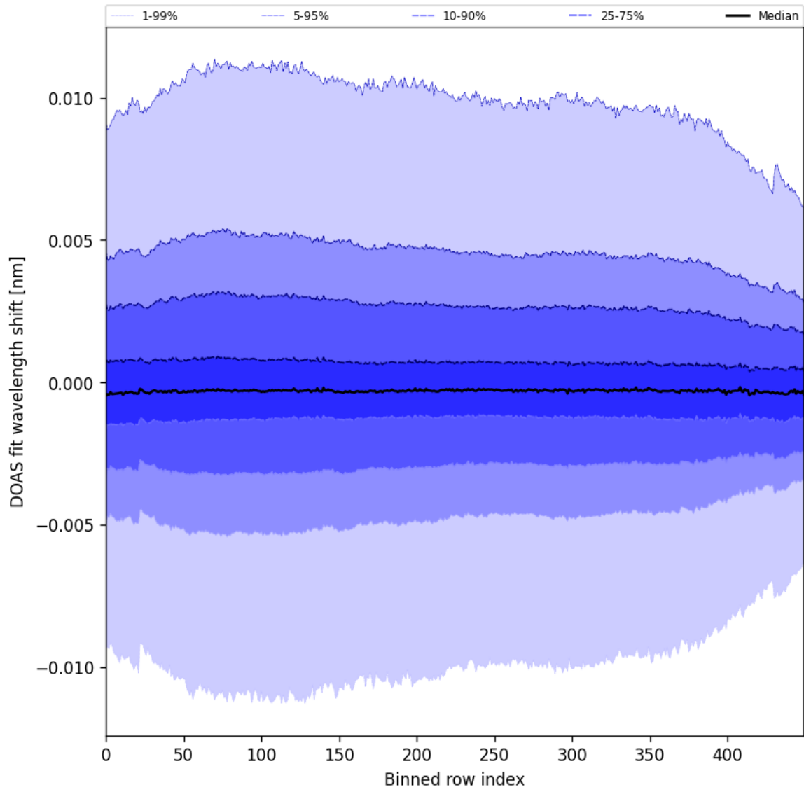
Figure 58: Along track statistics of “DOAS fit wavelength shift” for 2025-10-06 to 2025-10-08
