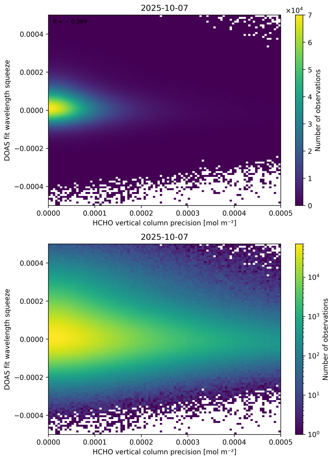
Figure 138: Scatter density plot of “HCHO vertical column precision” against “DOAS fit wavelength squeeze” for 2025-10-06 to 2025-10-08.
