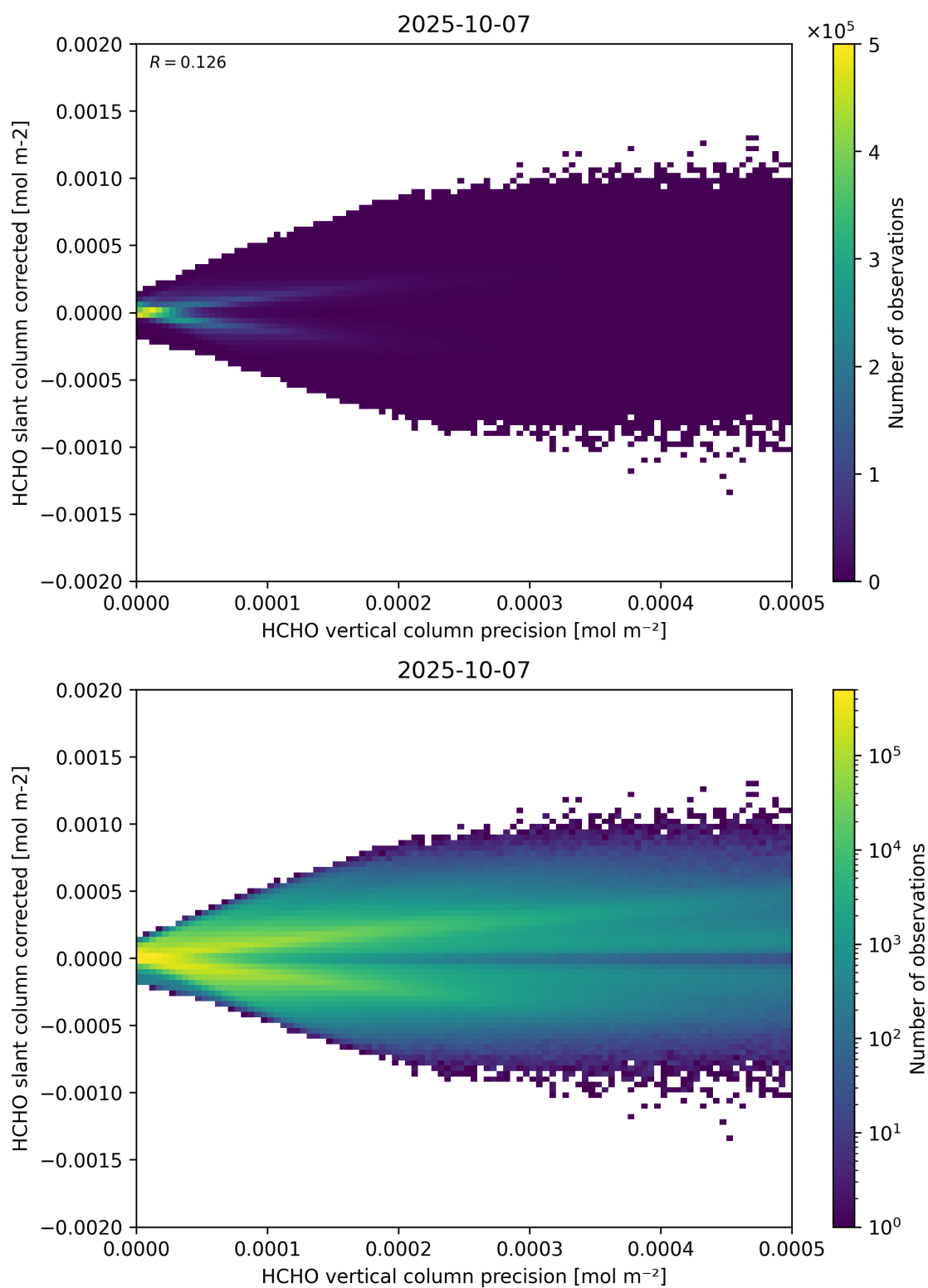
Figure 140: Scatter density plot of “HCHO vertical column precision” against “HCHO slant column corrected” for 2025-10-06 to 2025-10-08.
