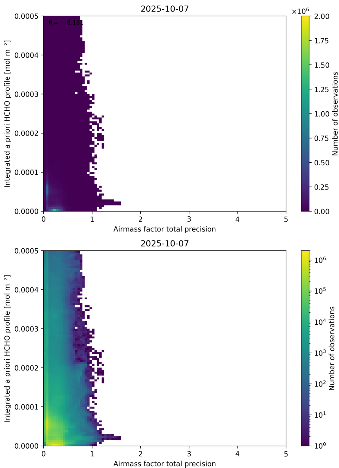
Figure 111: Scatter density plot of “Airmass factor total precision” against “Integrated a priori HCHO profile” for 2025-10-06 to 2025-10-08.
