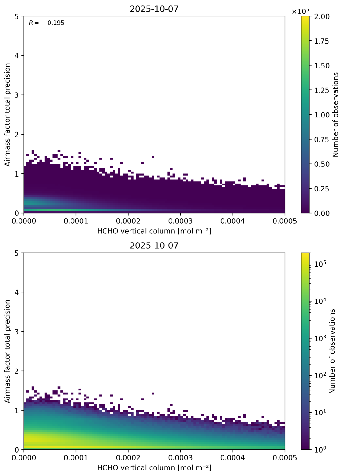
Figure 132: Scatter density plot of “HCHO vertical column” against “Airmass factor total precision” for 2025-10-06 to 2025-10-08.
