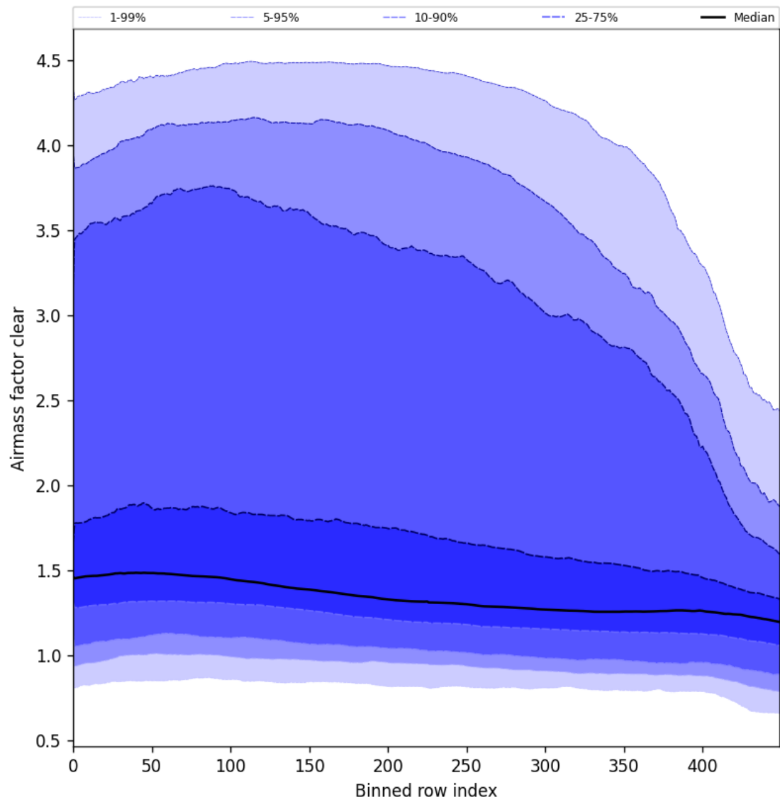
Figure 56: Along track statistics of “Airmass factor clear” for 2025-10-06 to 2025-10-08
