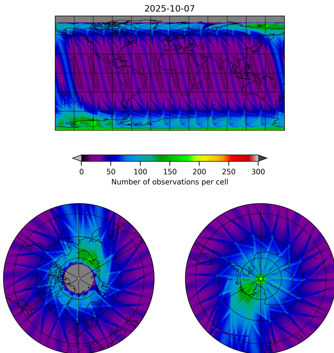
Figure 19: Map of the number of observations for 2025-10-06 to 2025-10-08
