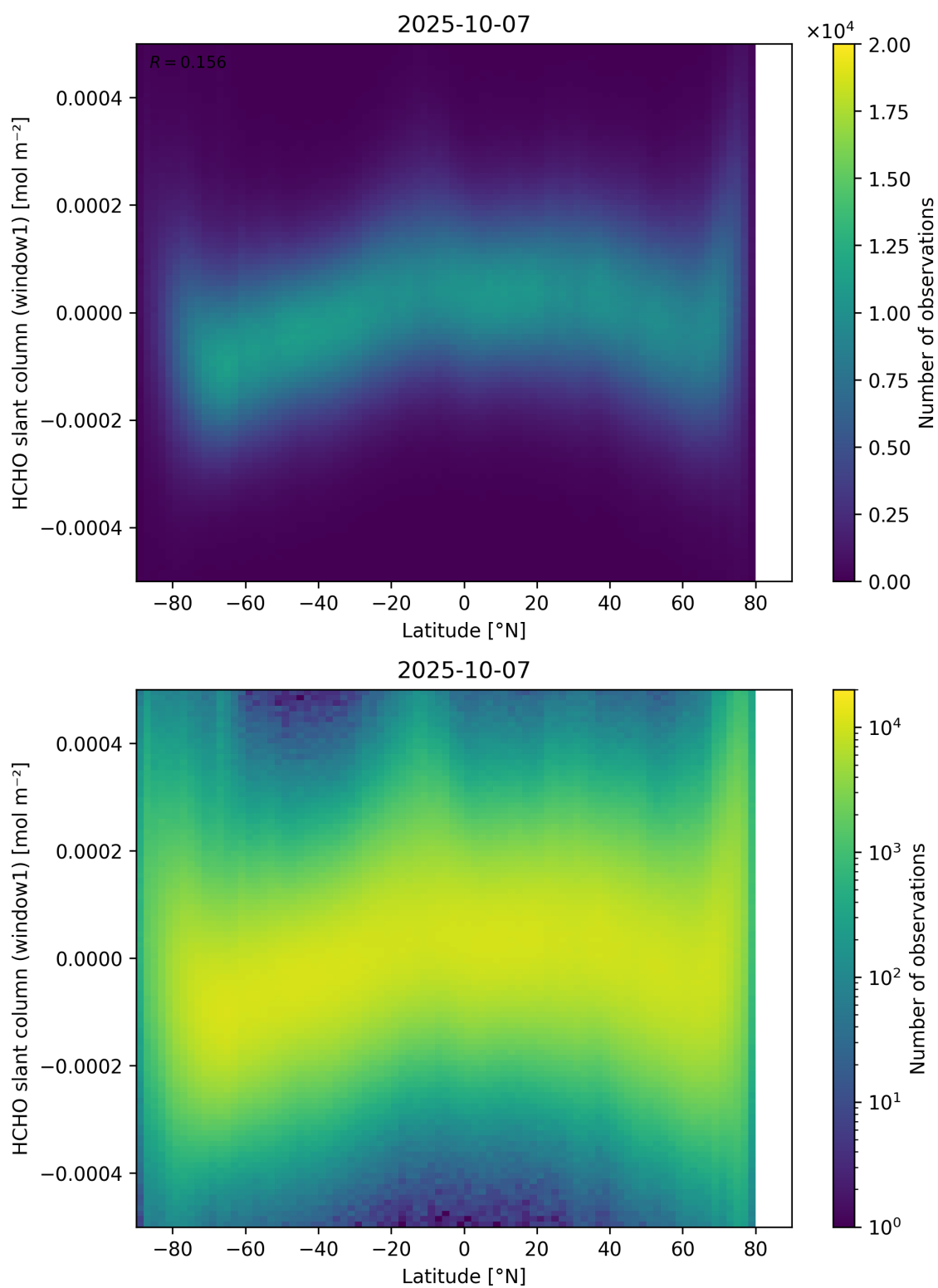
Figure 159: Scatter density plot of “Latitude” against “HCHO slant column (window1)” for 2025-10-06 to 2025-10-08.
