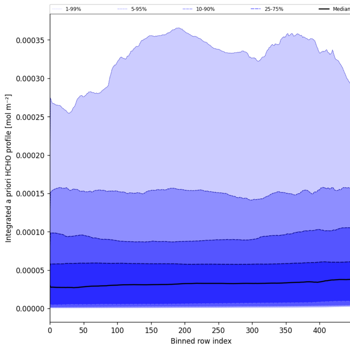
Figure 57: Along track statistics of "Integrated a priori HCHO profile" for 2025-10-06 to 2025-10-08
