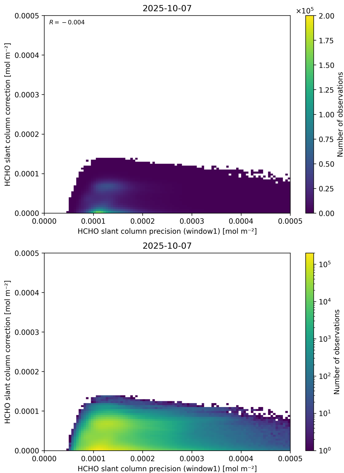
Figure 93: Scatter density plot of “HCHO slant column precision (window1)” against “HCHO slant column correction” for 2025-10-06 to 2025-10-08.
