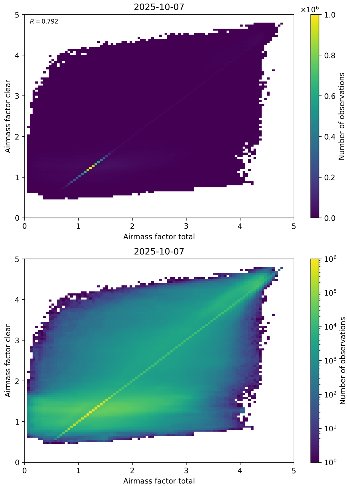
Figure 100: Scatter density plot of “Airmass factor total” against “Airmass factor clear” for 2025-10-06 to 2025-10-08.
