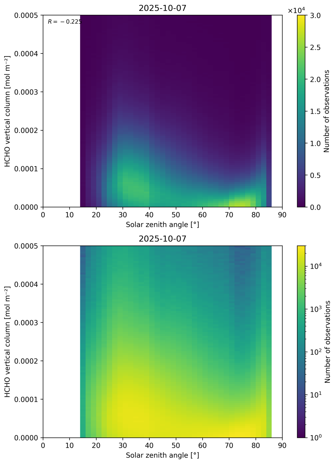
Figure 177: Scatter density plot of “Solar zenith angle” against “HCHO vertical column” for 2025-10-06 to 2025-10-08.
