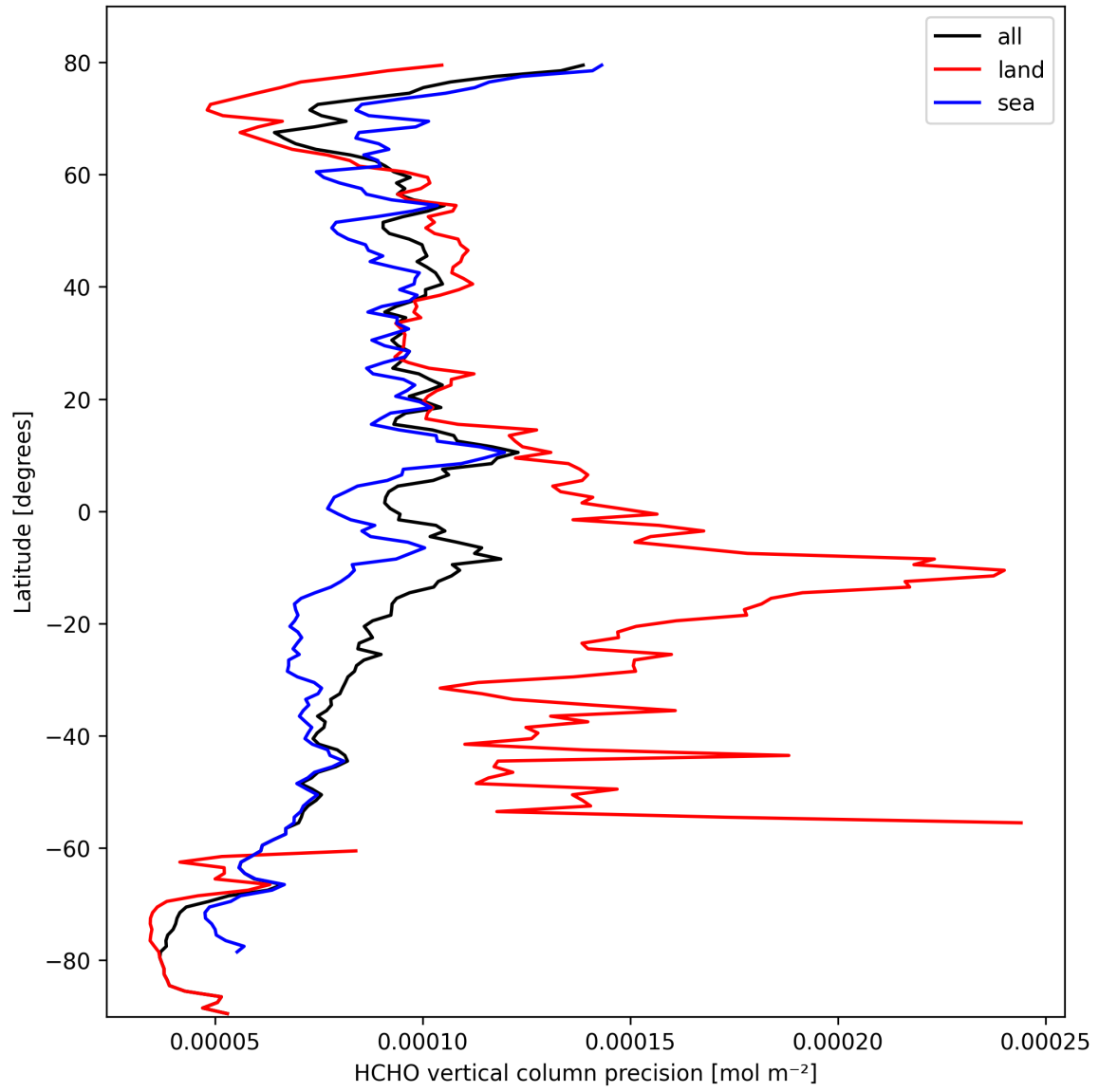
Figure 22: Zonal average of “HCHO vertical column precision” for 2025-10-06 to 2025-10-08.
