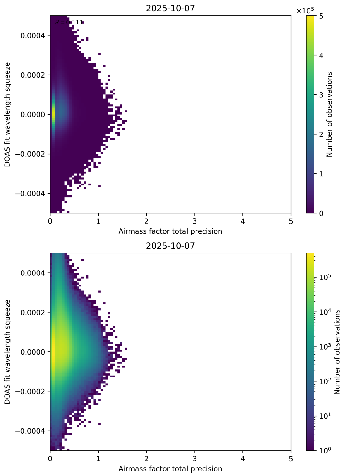
Figure 107: Scatter density plot of “Airmass factor total precision” against “DOAS fit wavelength squeeze” for 2025-10-06 to 2025-10-08.
