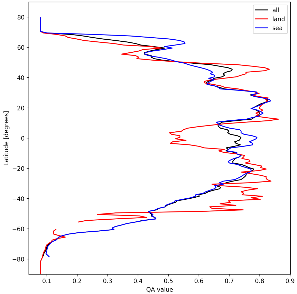
Figure 20: Zonal average of “QA value” for 2025-10-06 to 2025-10-08.
