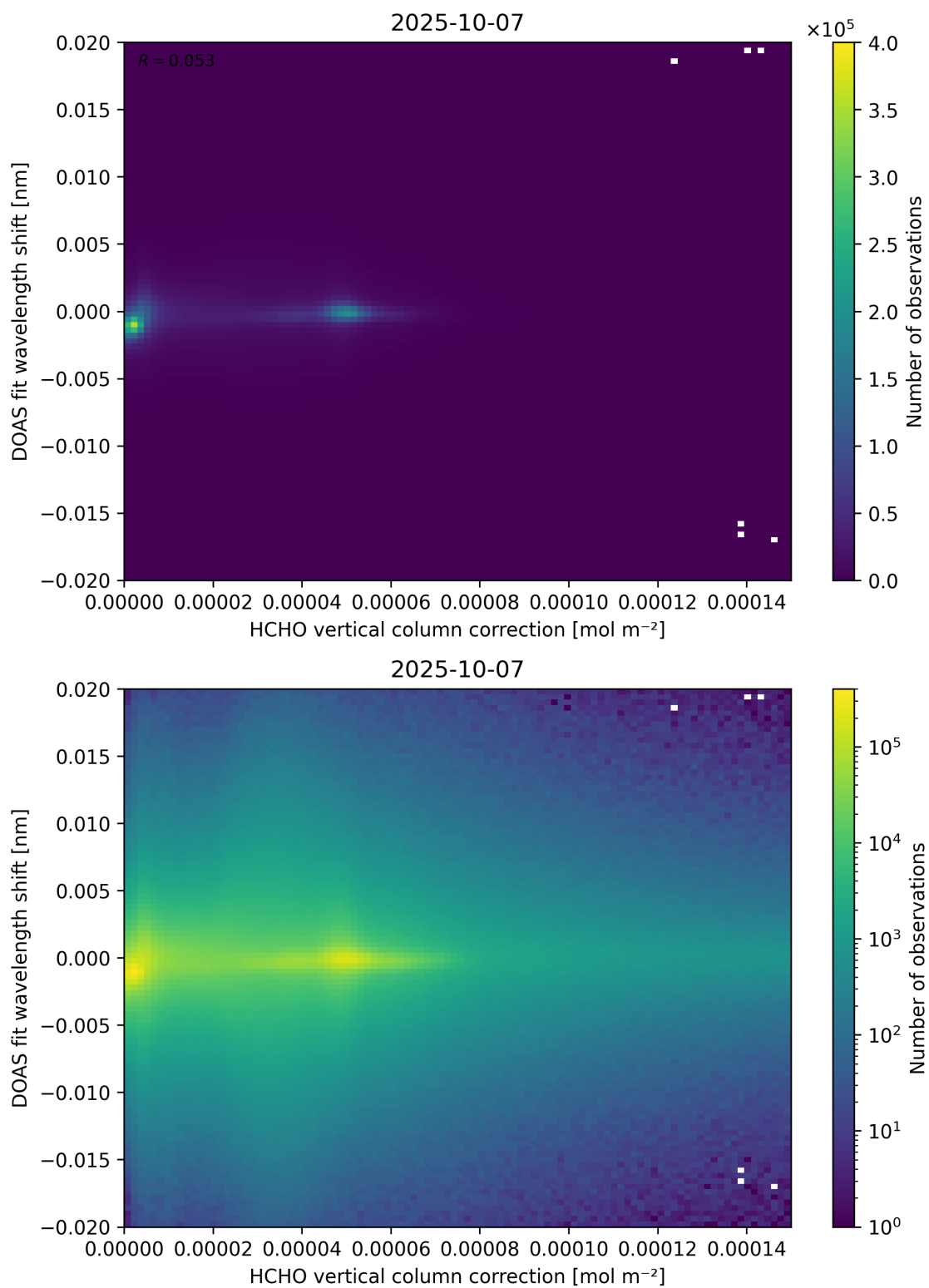
Figure 113: Scatter density plot of “HCHO vertical column correction” against “DOAS fit wavelength shift” for 2025-10-06 to 2025-10-08.
