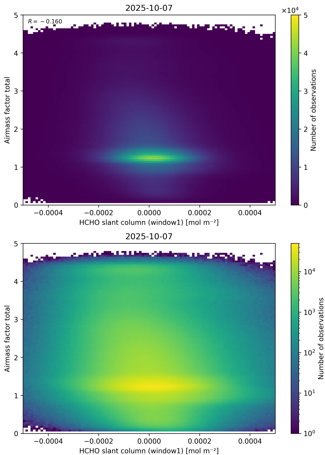
Figure 85: Scatter density plot of “HCHO slant column (window1)” against “Airmass factor total” for 2025-10-06 to 2025-10-08.
