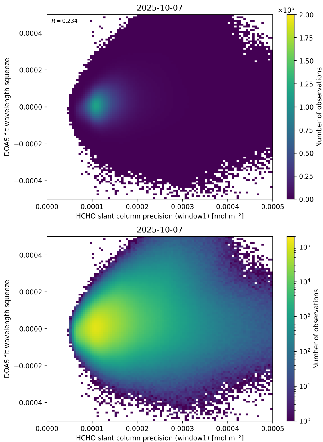
Figure 90: Scatter density plot of “HCHO slant column precision (window1)” against “DOAS fit wavelength squeeze” for 2025-10-06 to 2025-10-08.
