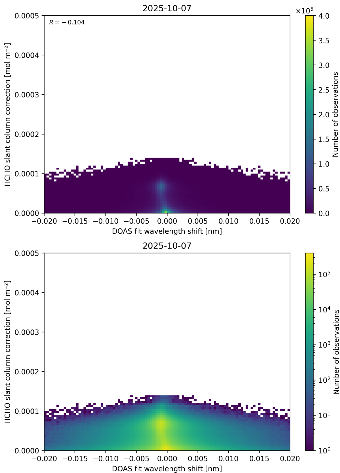
Figure 67: Scatter density plot of “DOAS fit wavelength shift” against “HCHO slant column correction” for 2025-10-06 to 2025-10-08.
