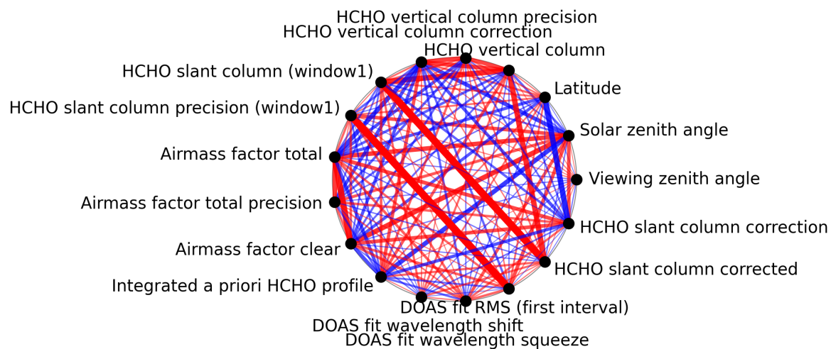
Figure 1: Map of correlation graph for 2025-10-06 to 2025-10-08.
