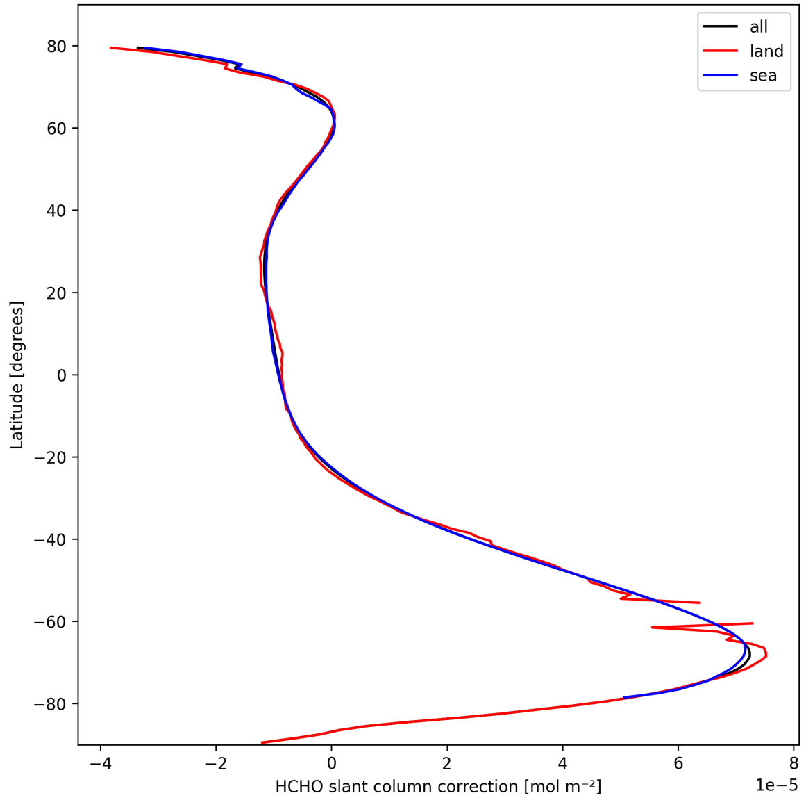
Figure 33: Zonal average of "HCHO slant column correction" for 2025-10-06 to 2025-10-08.
