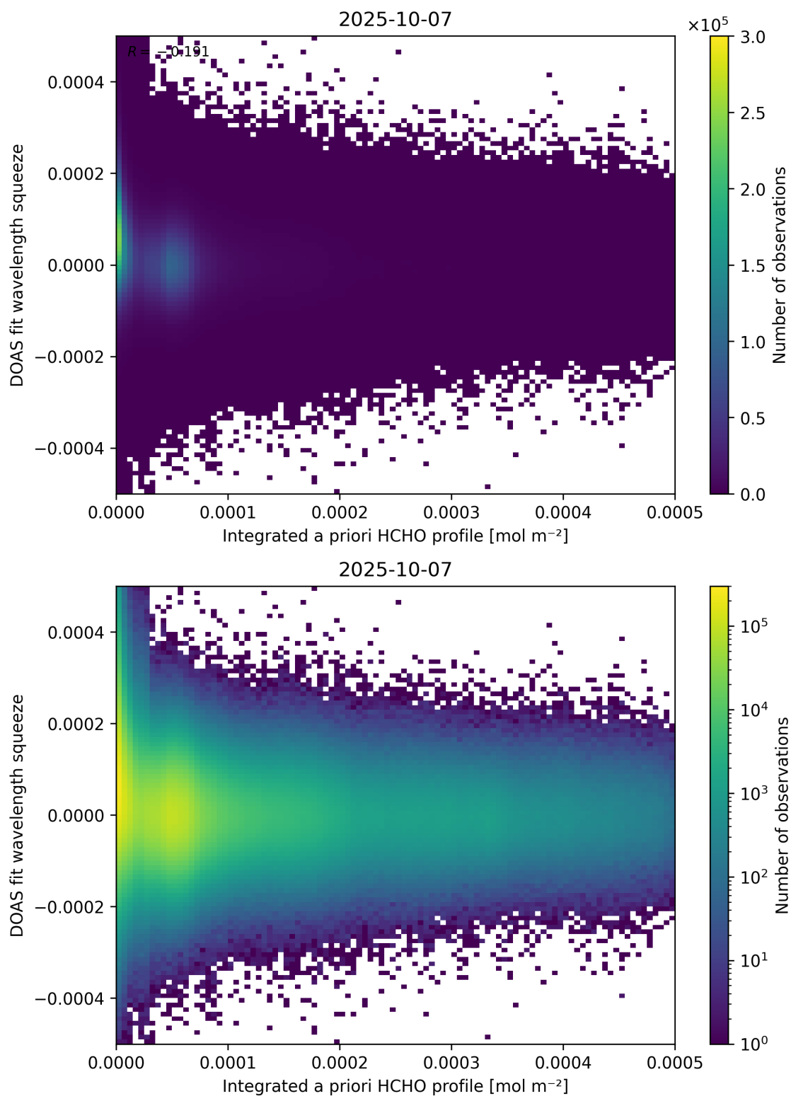
Figure 150: Scatter density plot of “Integrated a priori HCHO profile” against “DOAS fit wavelength squeeze” for 2025-10-06 to 2025-10-08.
