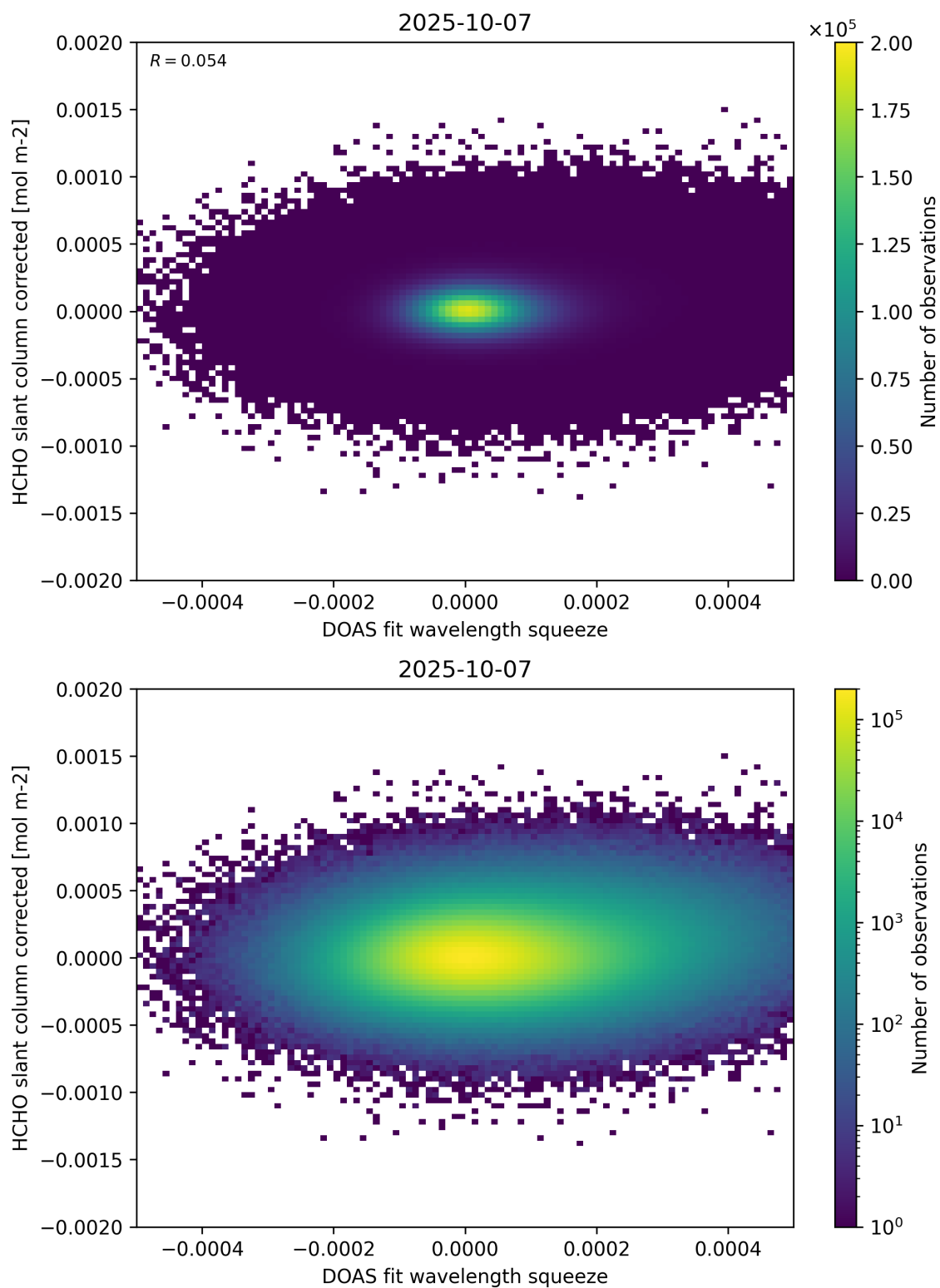
Figure 69: Scatter density plot of “DOAS fit wavelength squeeze” against “HCHO slant column corrected” for 2025-10-06 to 2025-10-08.
