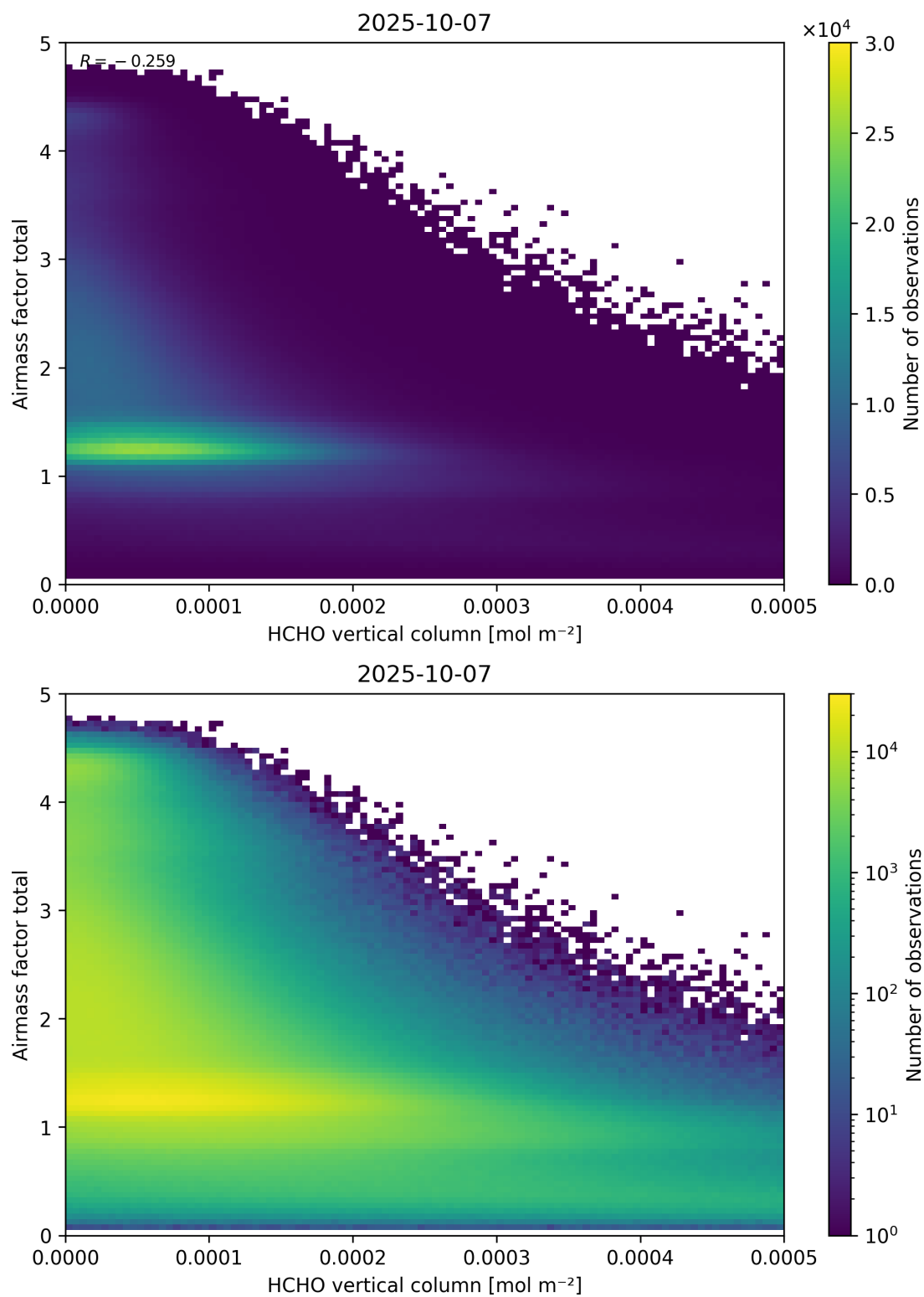
Figure 131: Scatter density plot of “HCHO vertical column” against “Airmass factor total” for 2025-10-06 to 2025-10-08.
