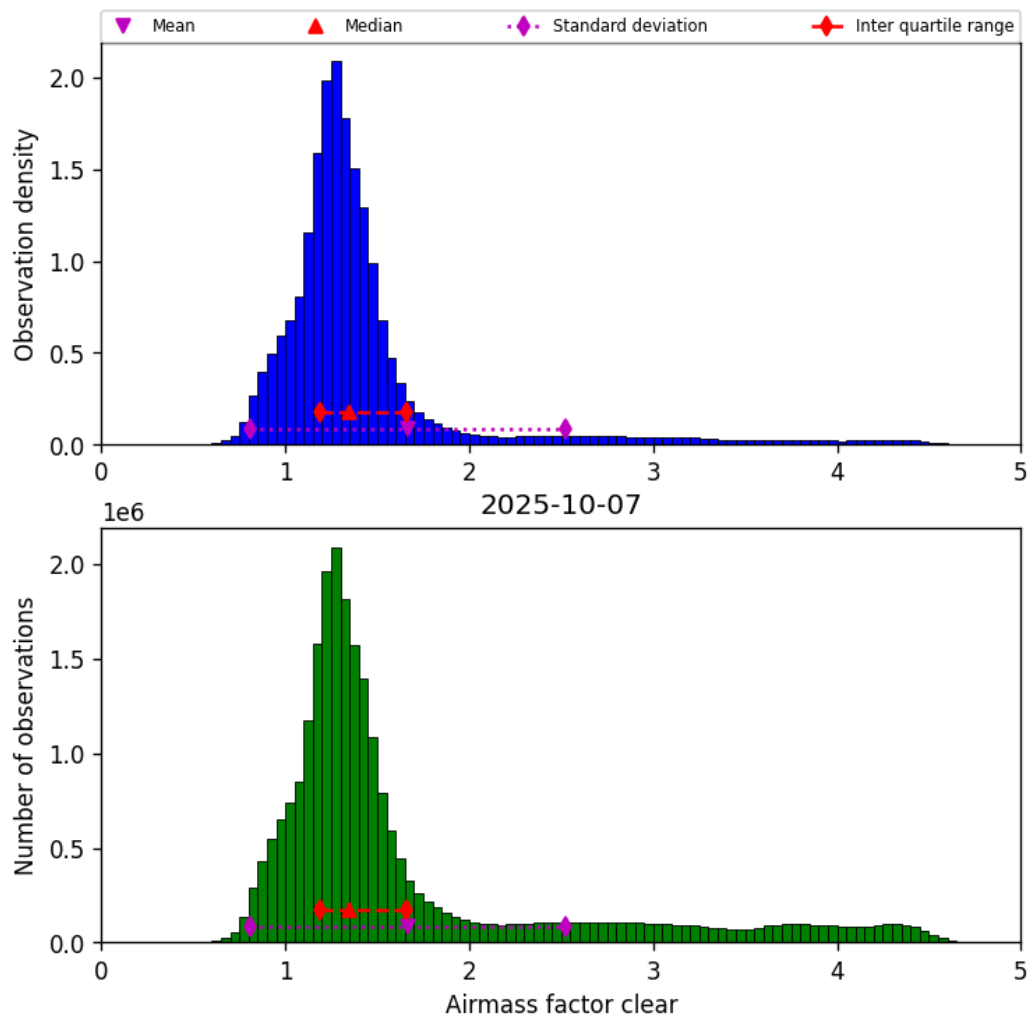
Figure 42: Histogram of “Airmass factor clear” for 2025-10-06 to 2025-10-08
