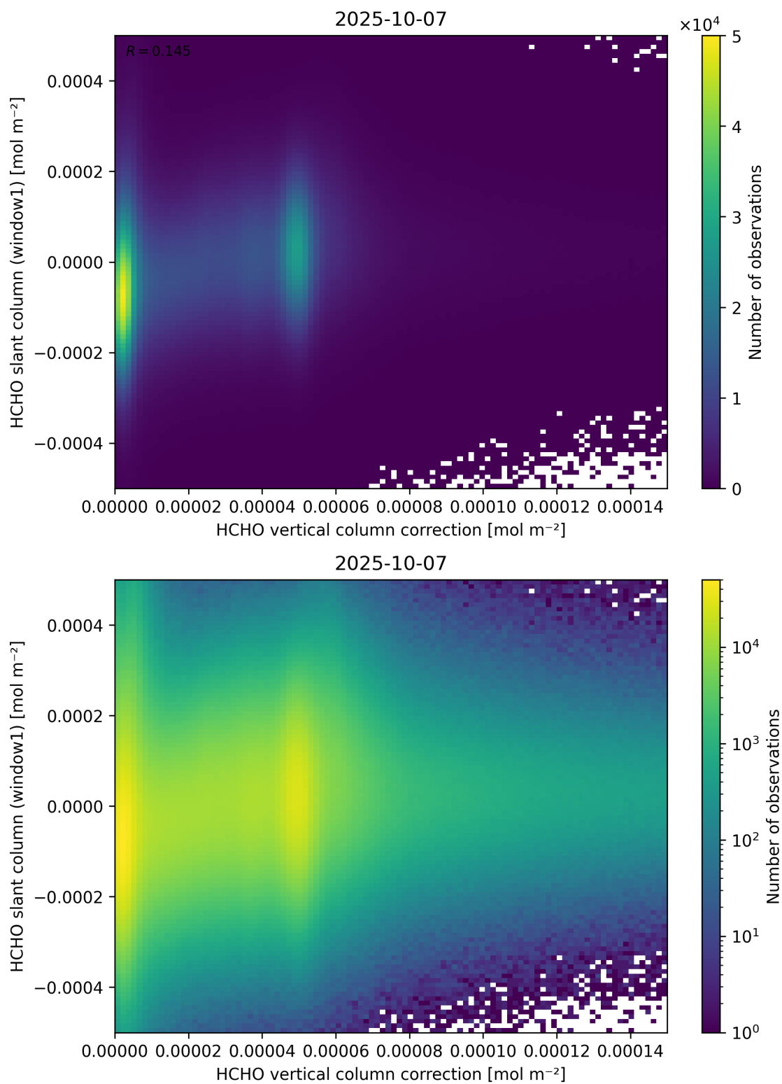
Figure 118: Scatter density plot of “HCHO vertical column correction” against “HCHO slant column (window1)” for 2025-10-06 to 2025-10-08.
