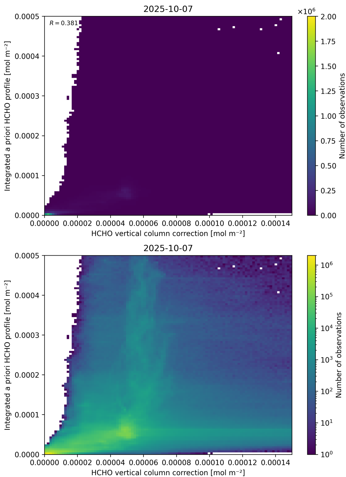
Figure 122: Scatter density plot of “HCHO vertical column correction” against “Integrated a priori HCHO profile” for 2025-10-06 to 2025-10-08.
