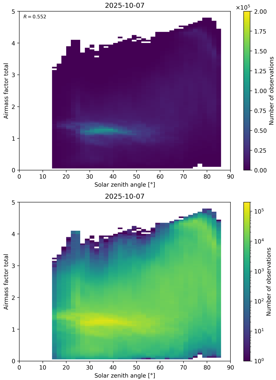
Figure 175: Scatter density plot of “Solar zenith angle” against “Airmass factor total” for 2025-10-06 to 2025-10-08.
