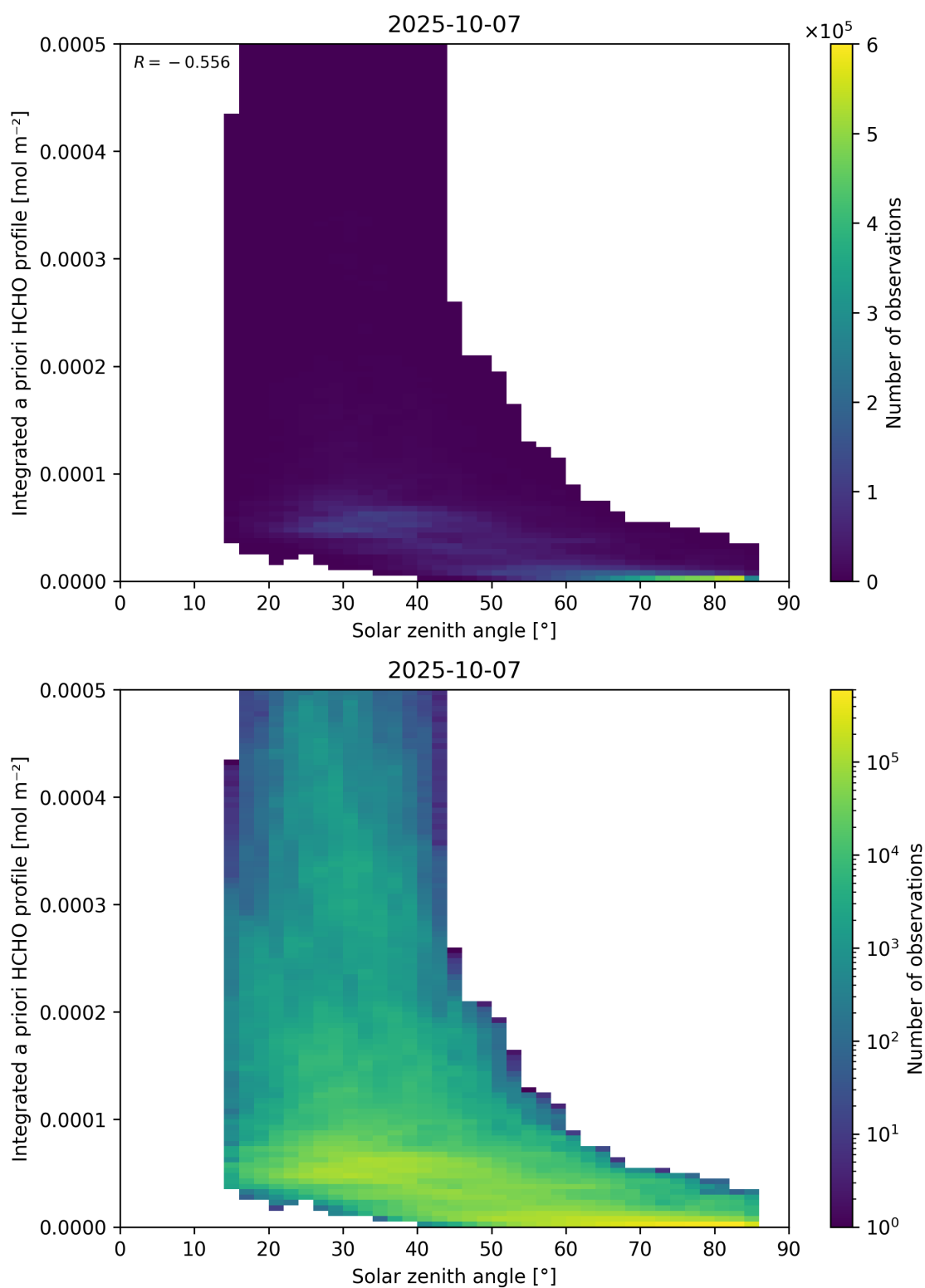
Figure 180: Scatter density plot of “Solar zenith angle” against “Integrated a priori HCHO profile” for 2025-10-06 to 2025-10-08.
