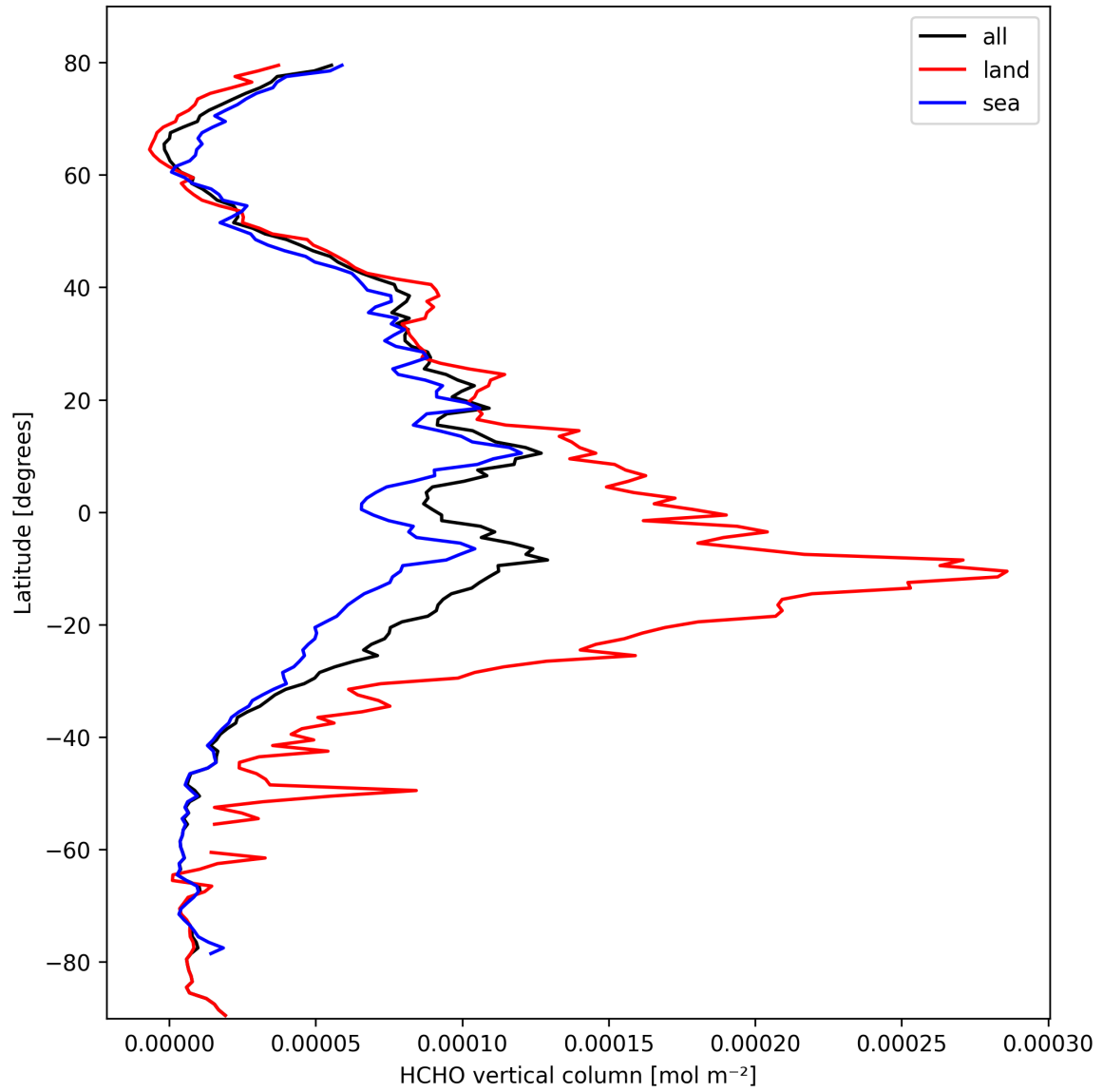
Figure 21: Zonal average of “HCHO vertical column” for 2025-10-06 to 2025-10-08.
