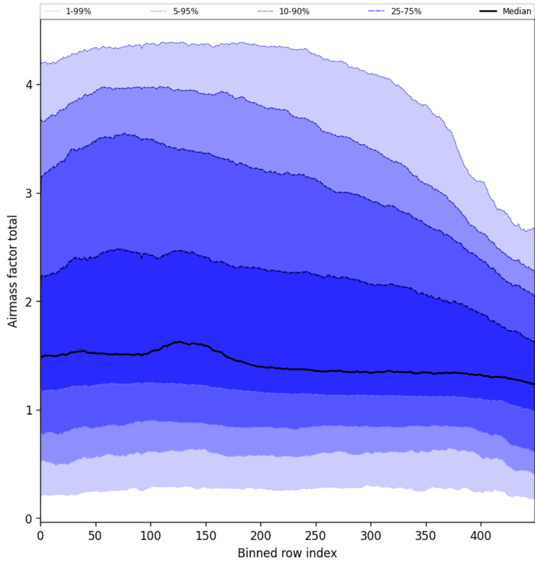
Figure 54: Along track statistics of “Airmass factor total” for 2025-10-06 to 2025-10-08
