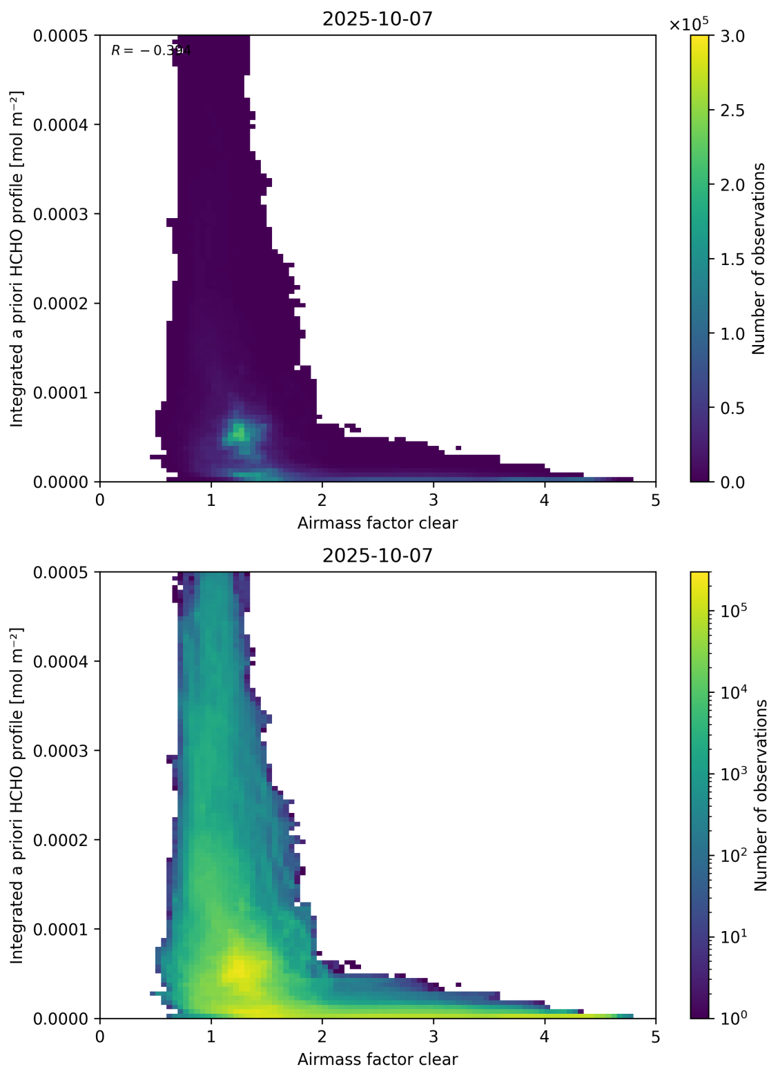
Figure 76: Scatter density plot of “Airmass factor clear” against “Integrated a priori HCHO profile” for 2025-10-06 to 2025-10-08.
