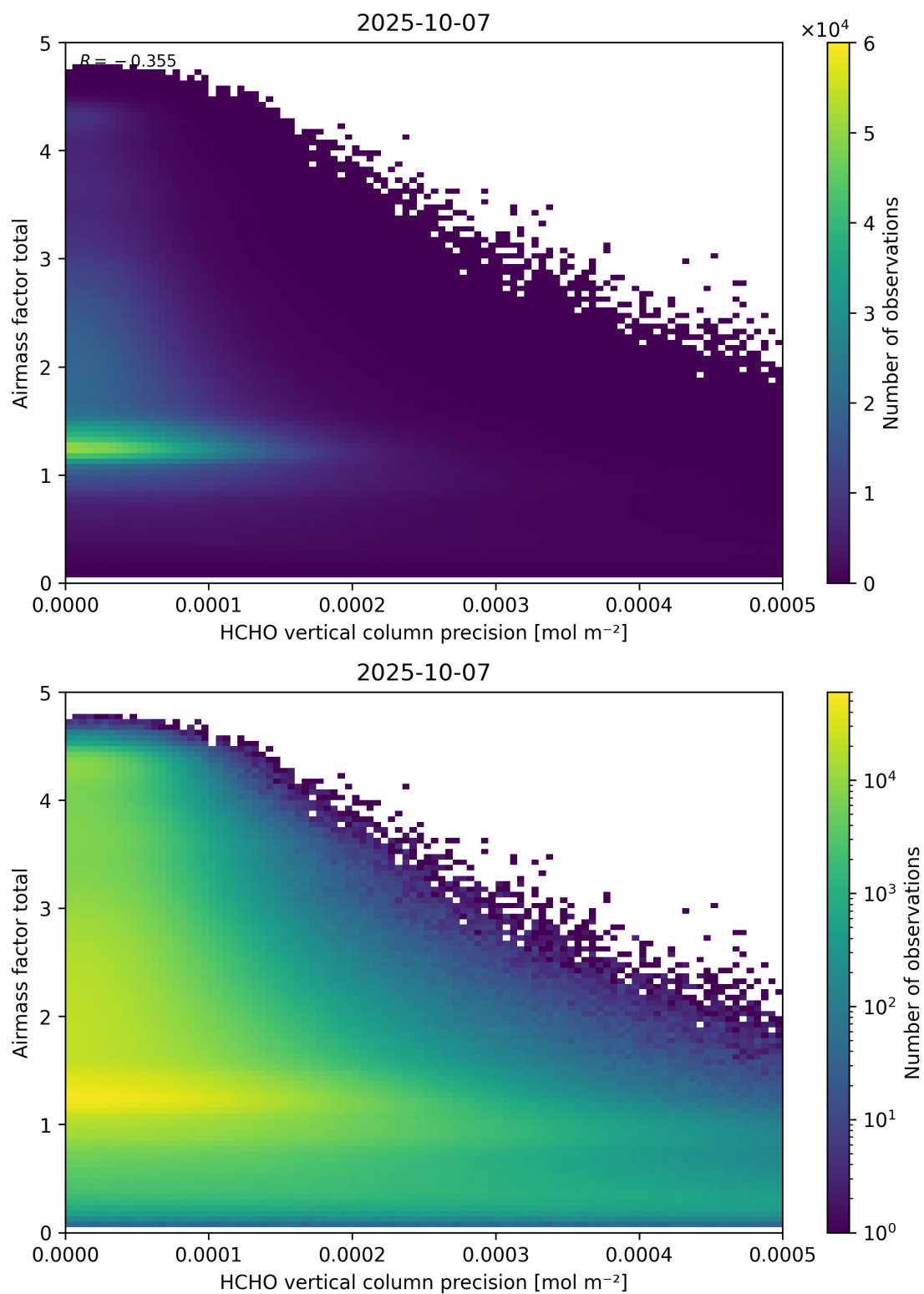
Figure 144: Scatter density plot of “HCHO vertical column precision” against “Airmass factor total” for 2025-10-06 to 2025-10-08.
