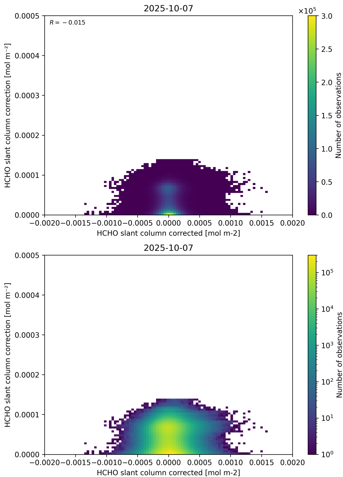
Figure 77: Scatter density plot of “HCHO slant column corrected” against “HCHO slant column correction” for 2025-10-06 to 2025-10-08.
