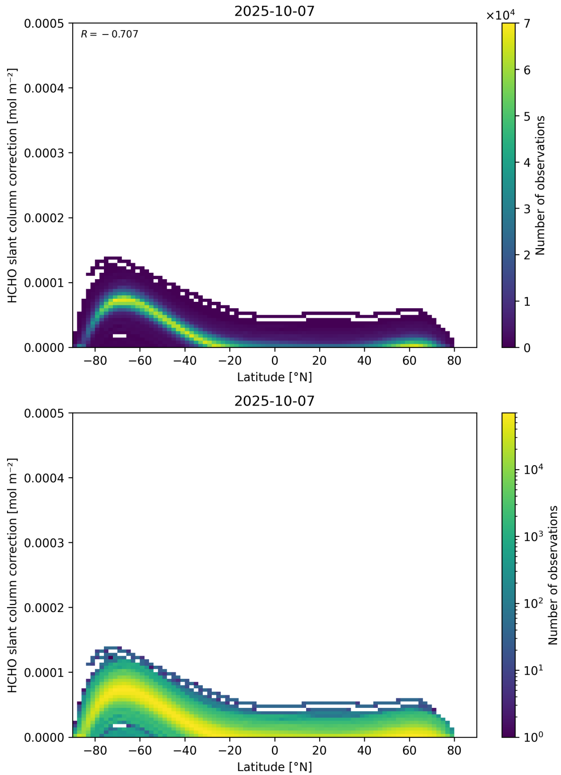
Figure 158: Scatter density plot of “Latitude” against “HCHO slant column correction” for 2025-10-06 to 2025-10-08.
