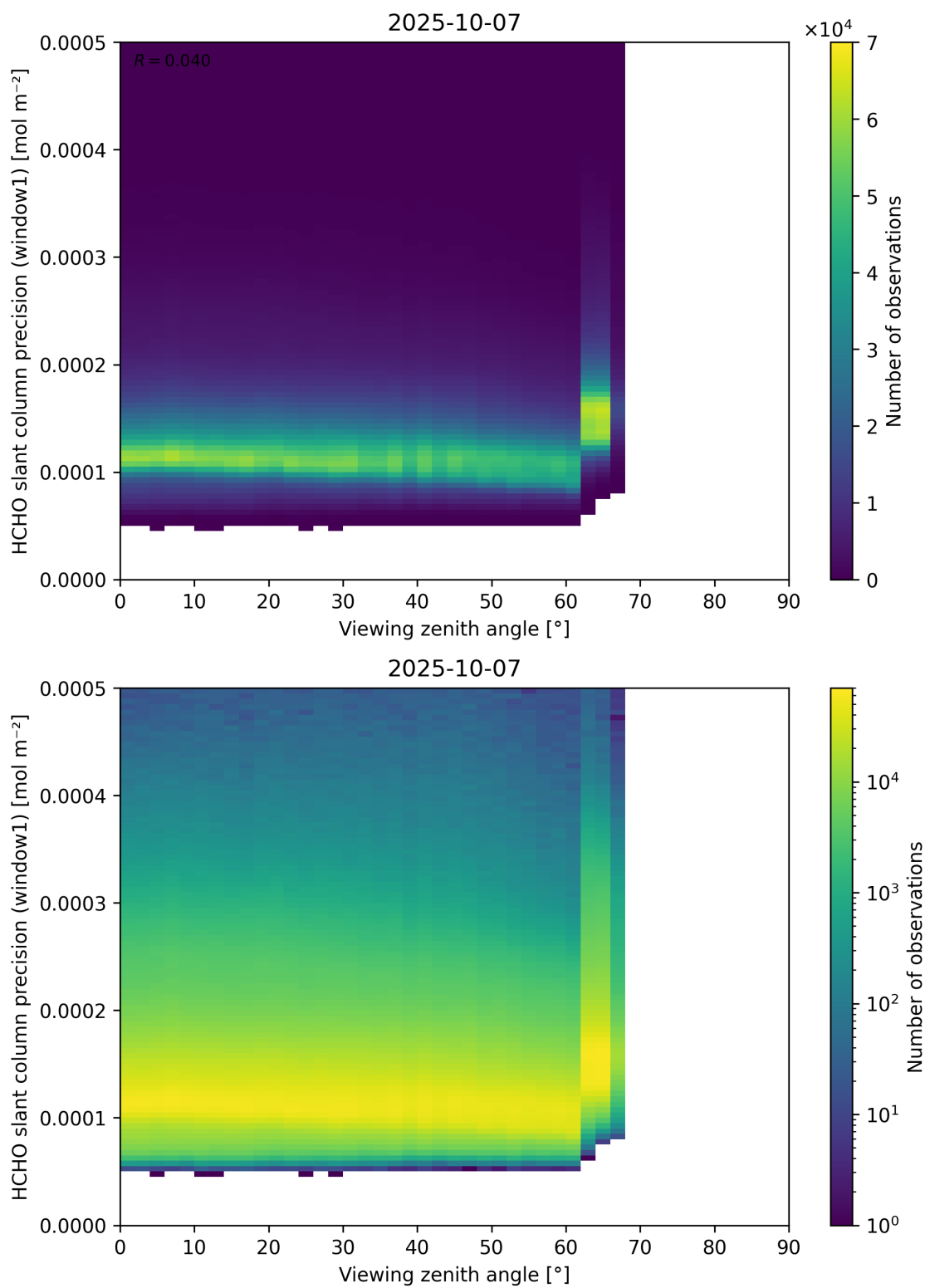
Figure 189: Scatter density plot of “Viewing zenith angle” against “HCHO slant column precision (window1)” for 2025-10-06 to 2025-10-08.
