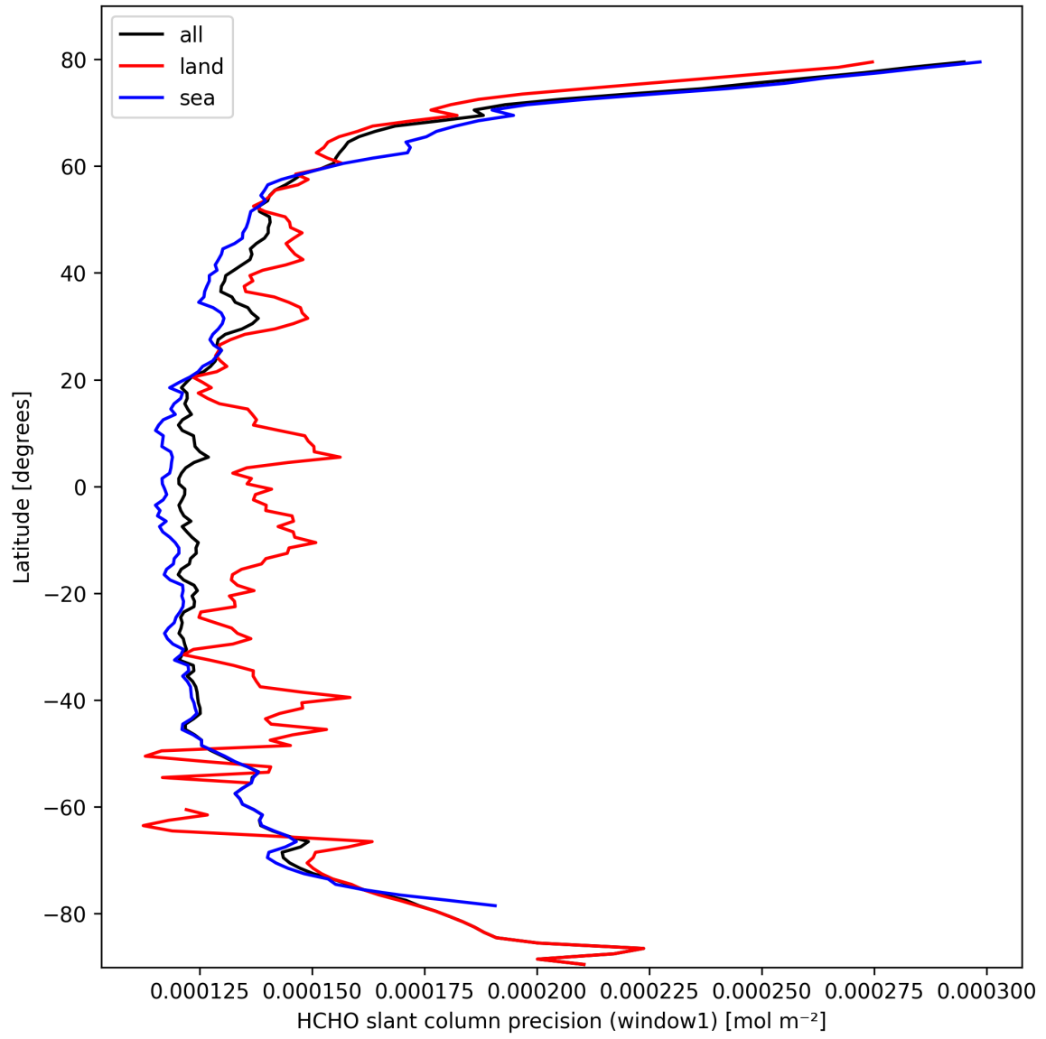
Figure 25: Zonal average of “HCHO slant column precision (window1)” for 2025-10-06 to 2025-10-08.
