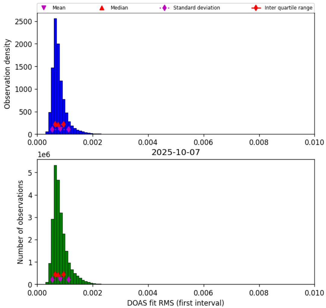
Figure 46: Histogram of “DOAS fit RMS (first interval)” for 2025-10-06 to 2025-10-08
