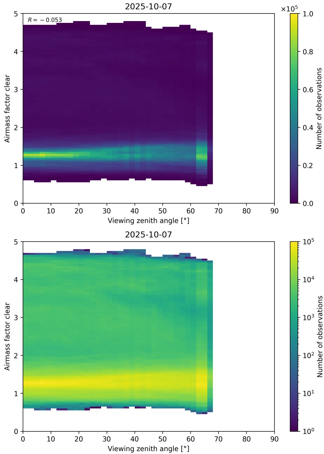
Figure 185: Scatter density plot of “Viewing zenith angle” against “Airmass factor clear” for 2025-10-06 to 2025-10-08.
