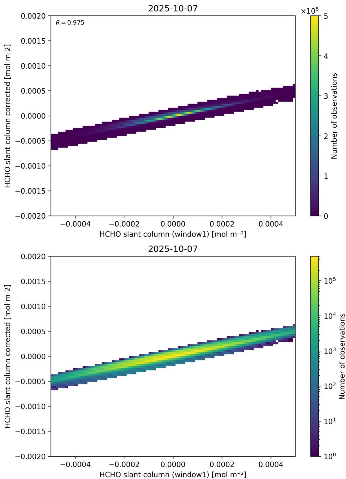
Figure 82: Scatter density plot of “HCHO slant column (window1)” against “HCHO slant column corrected” for 2025-10-06 to 2025-10-08.
