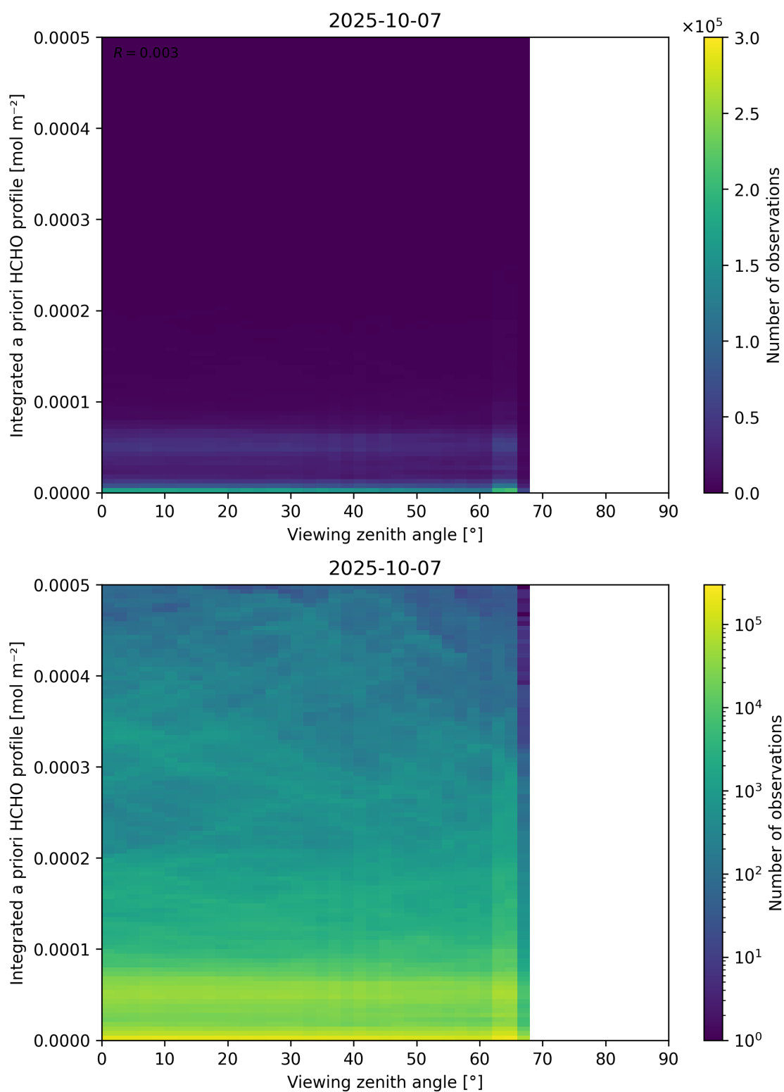
Figure 195: Scatter density plot of “Viewing zenith angle” against “Integrated a priori HCHO profile” for 2025-10-06 to 2025-10-08.
