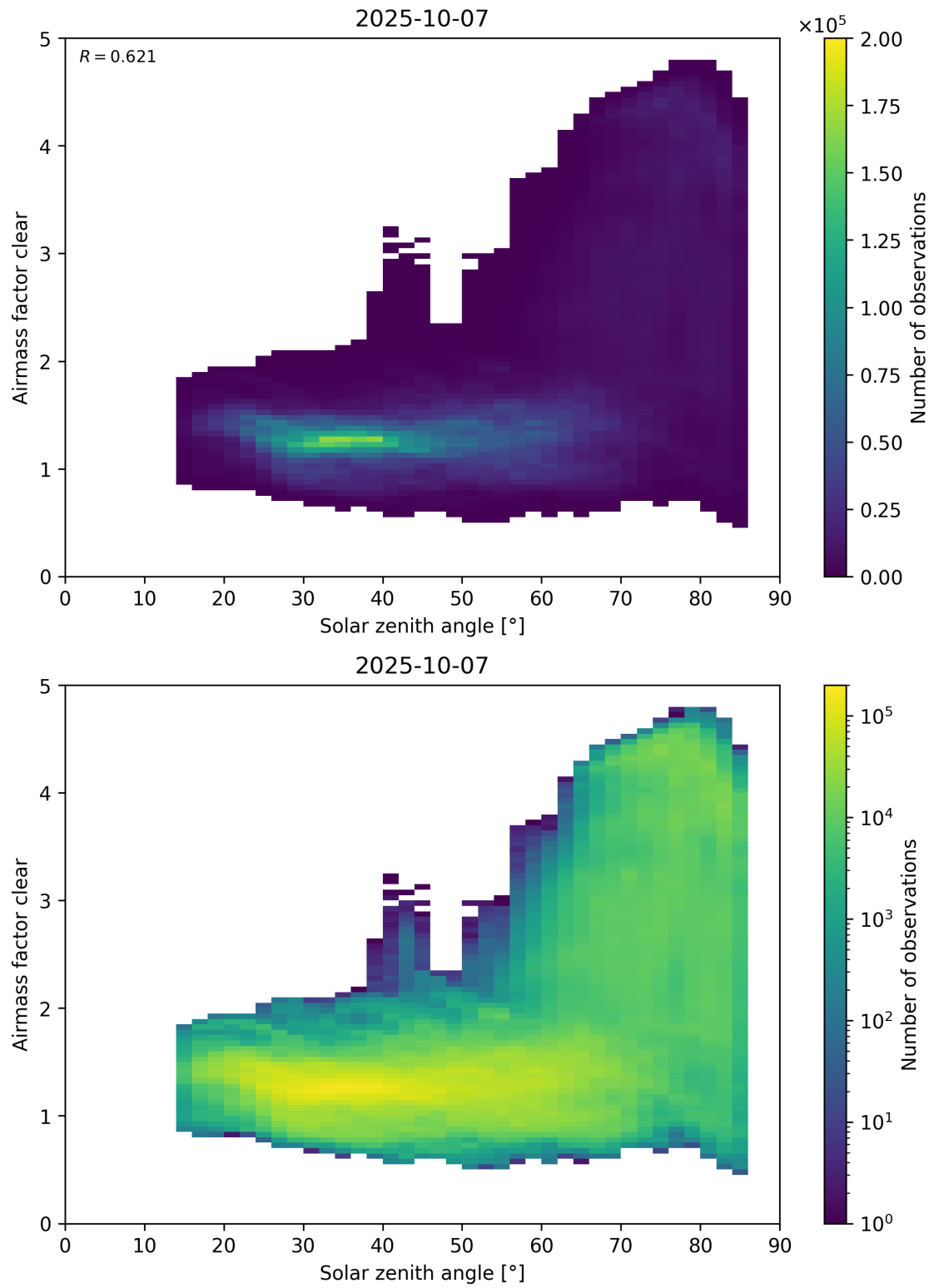
Figure 170: Scatter density plot of “Solar zenith angle” against “Airmass factor clear” for 2025-10-06 to 2025-10-08.
