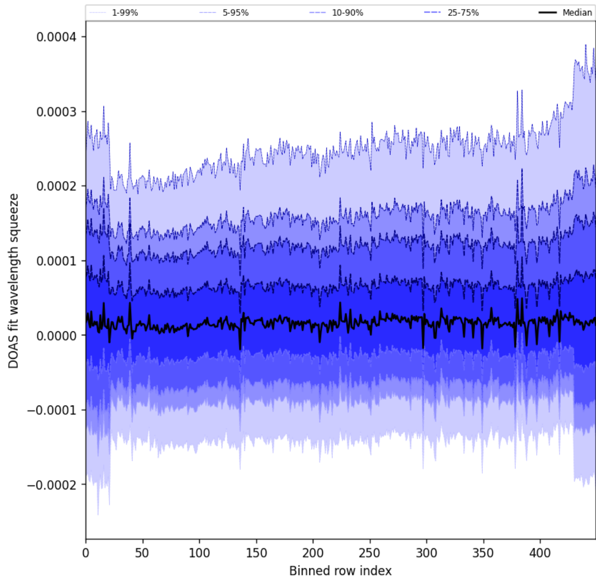
Figure 59: Along track statistics of “DOAS fit wavelength squeeze” for 2025-10-06 to 2025-10-08
