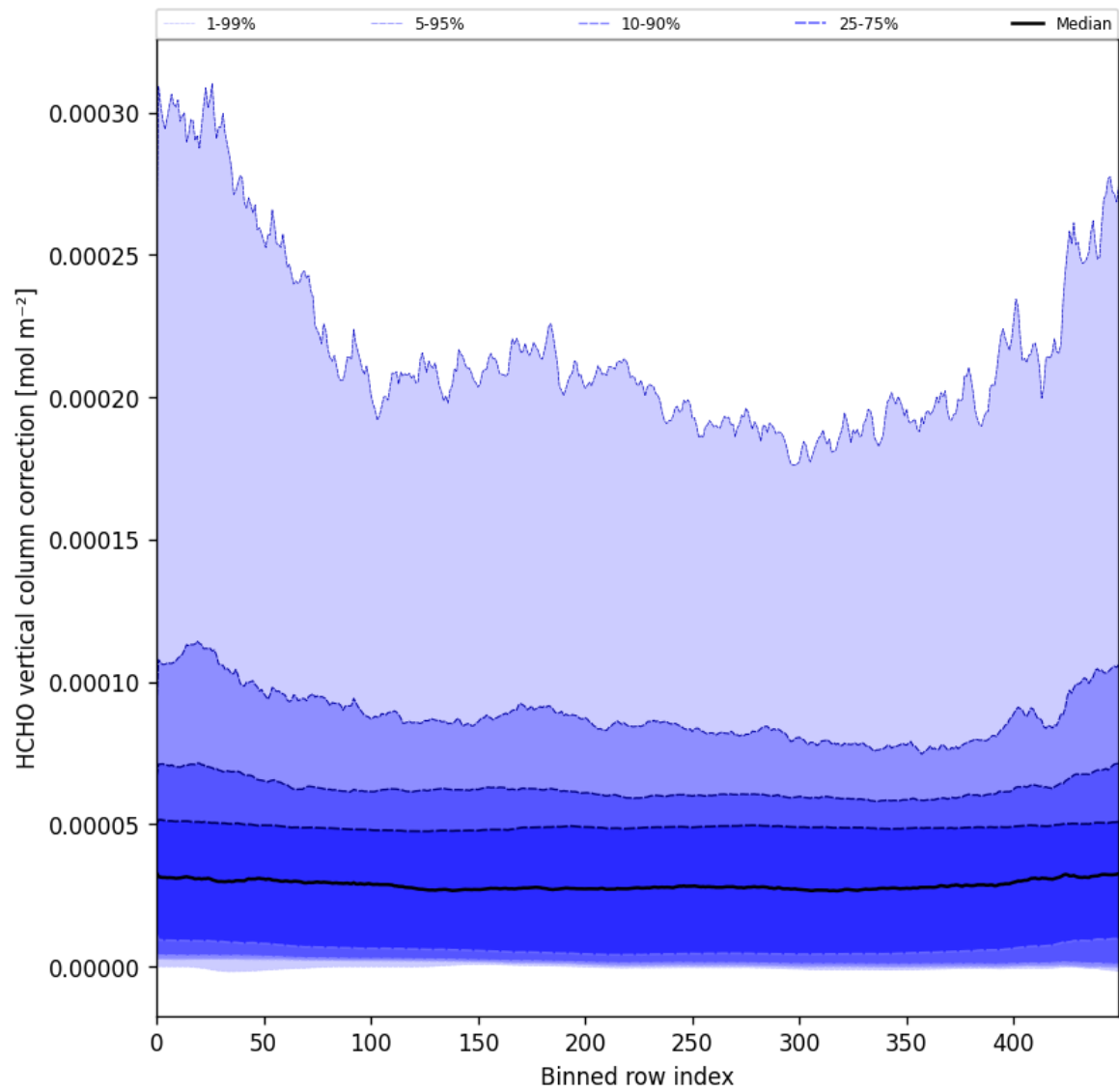
Figure 51: Along track statistics of “HCHO vertical column correction” for 2025-10-06 to 2025-10-08
