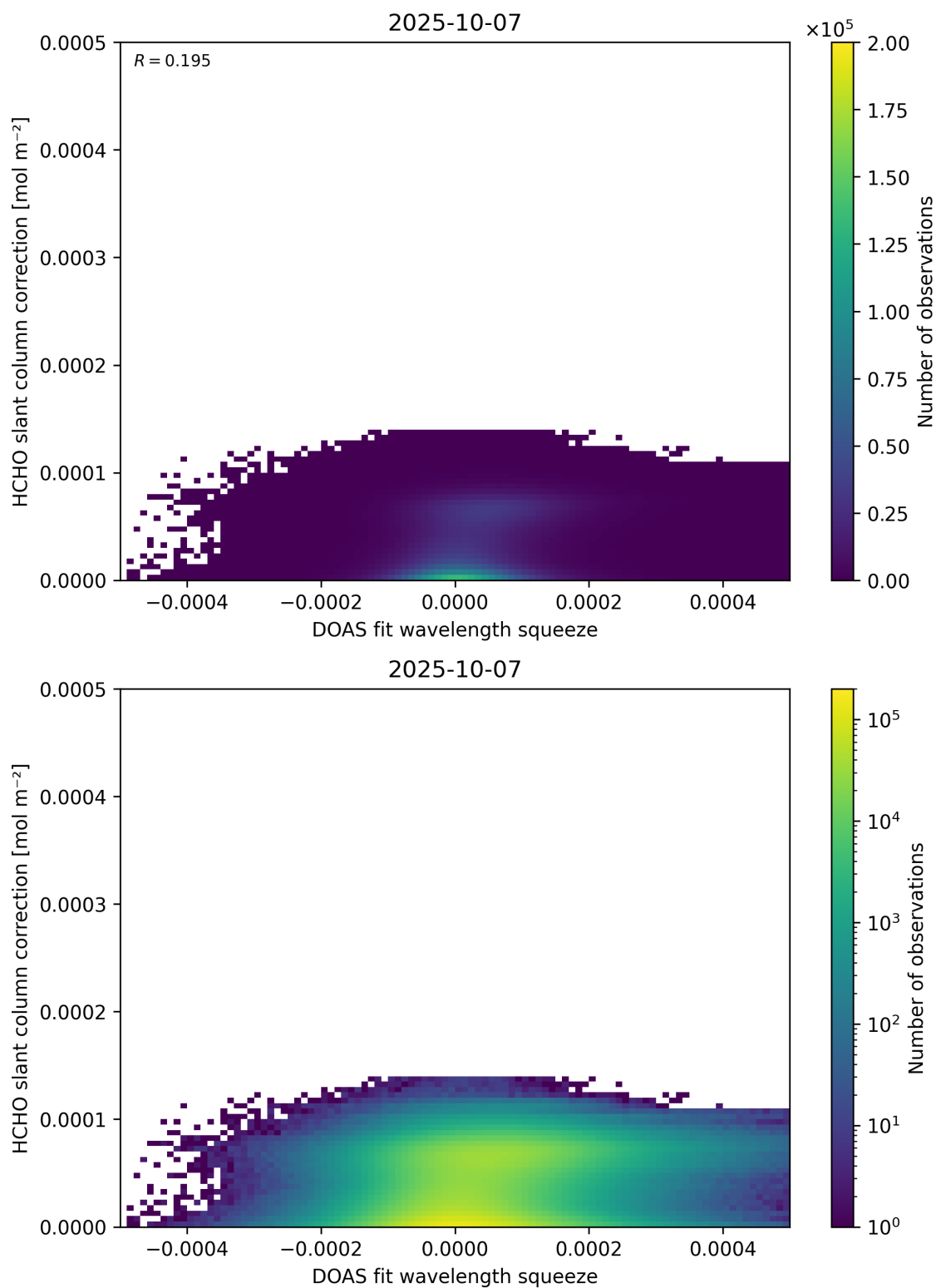
Figure 70: Scatter density plot of “DOAS fit wavelength squeeze” against “HCHO slant column correction” for 2025-10-06 to 2025-10-08.
