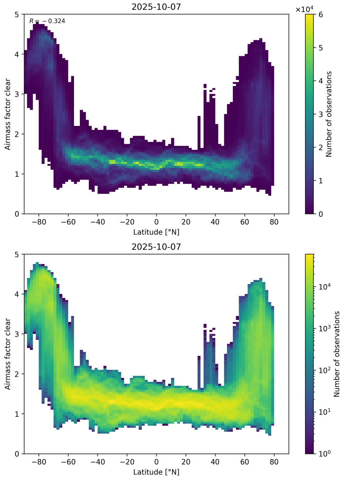
Figure 156: Scatter density plot of “Latitude” against “Airmass factor clear” for 2025-10-06 to 2025-10-08.
