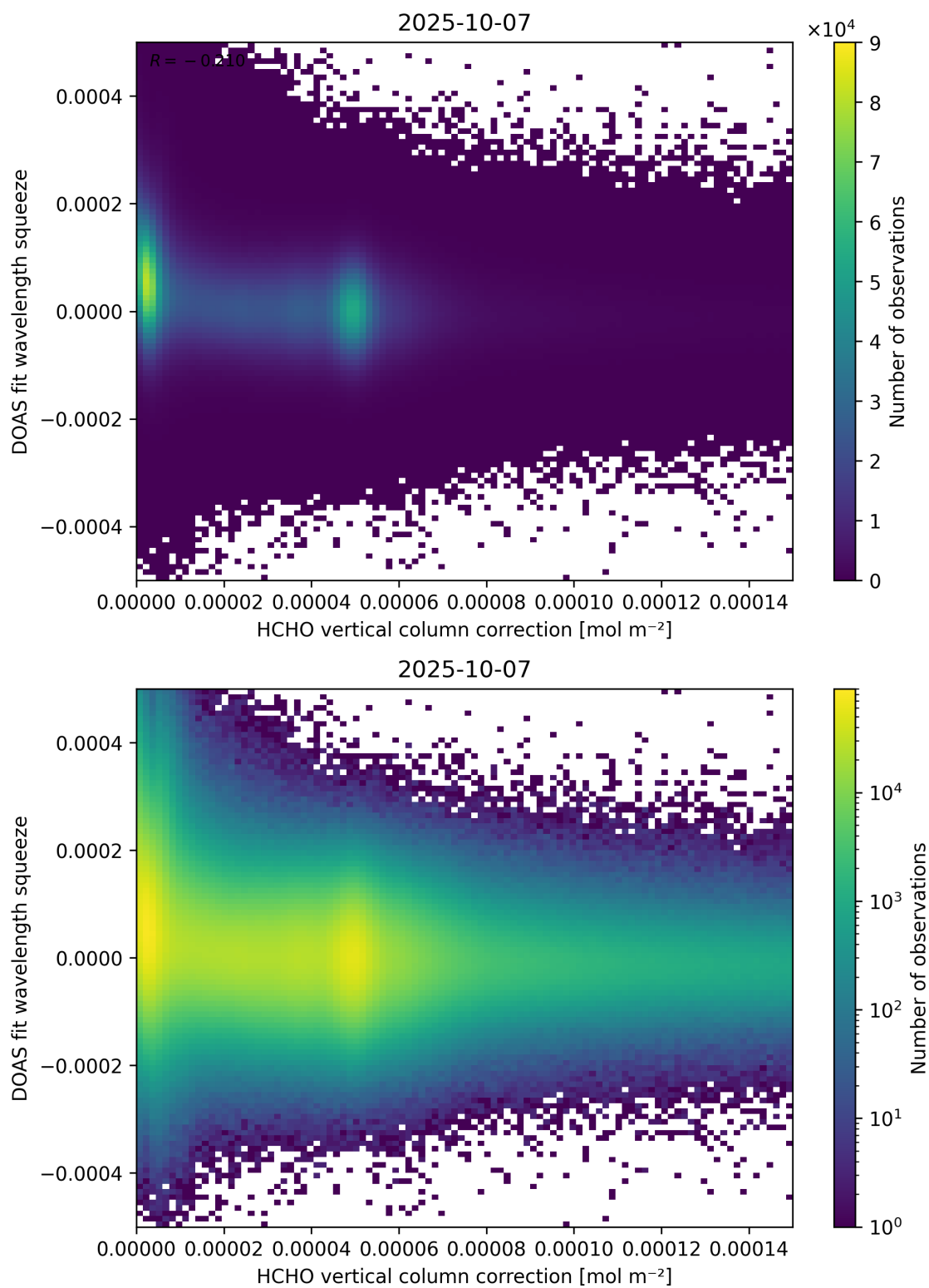
Figure 114: Scatter density plot of “HCHO vertical column correction” against “DOAS fit wavelength squeeze” for 2025-10-06 to 2025-10-08.
