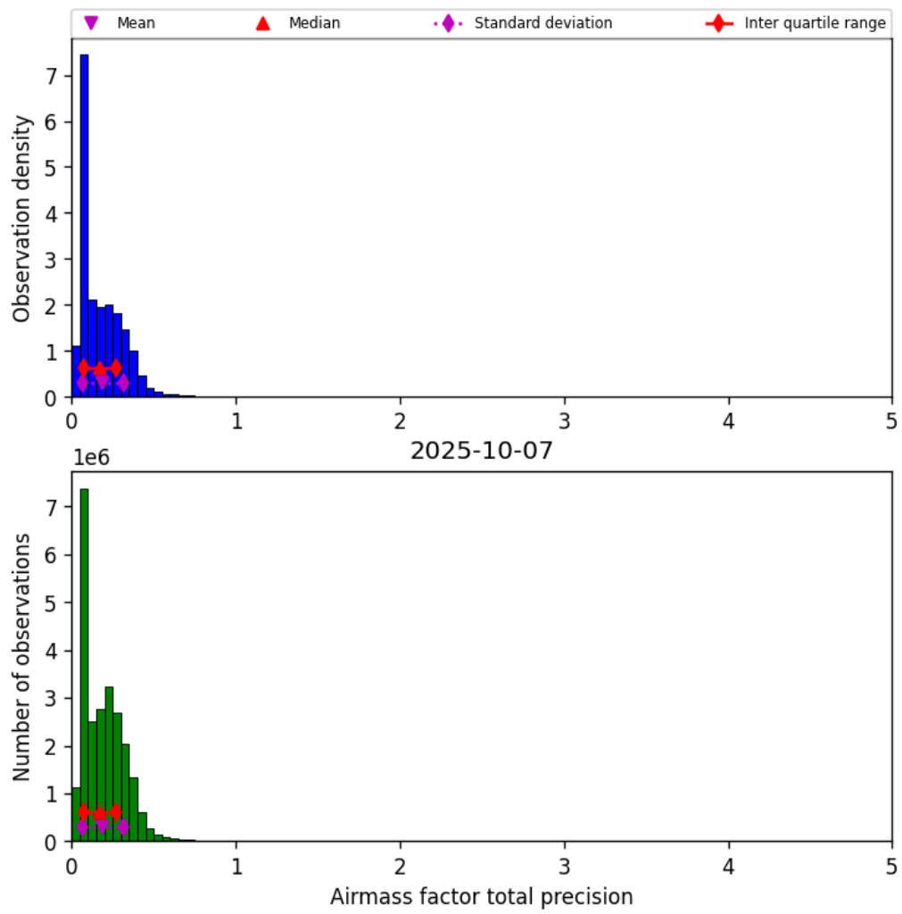
Figure 41: Histogram of “Airmass factor total precision” for 2025-10-06 to 2025-10-08
