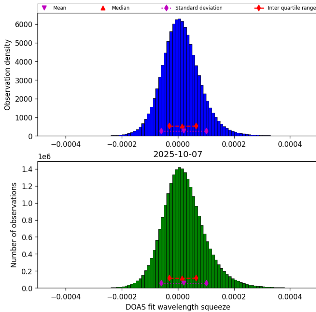
Figure 45: Histogram of “DOAS fit wavelength squeeze” for 2025-10-06 to 2025-10-08
