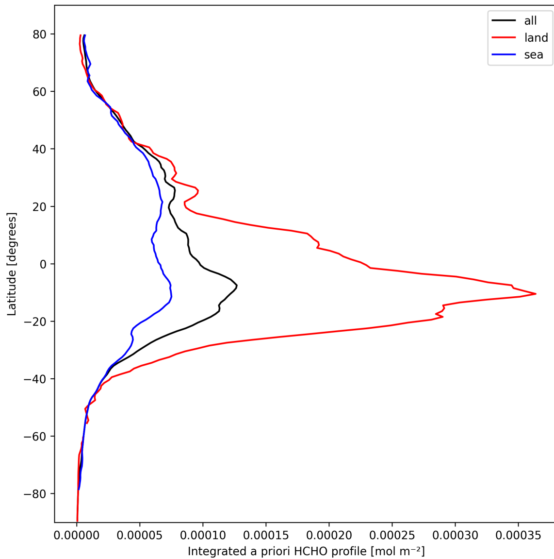
Figure 29: Zonal average of “Integrated a priori HCHO profile” for 2025-10-06 to 2025-10-08.
