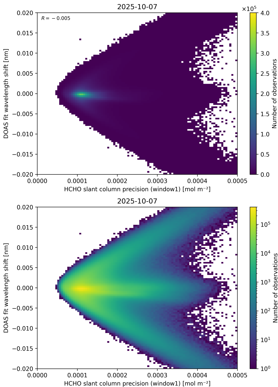
Figure 89: Scatter density plot of “HCHO slant column precision (window1)” against “DOAS fit wavelength shift” for 2025-10-06 to 2025-10-08.
