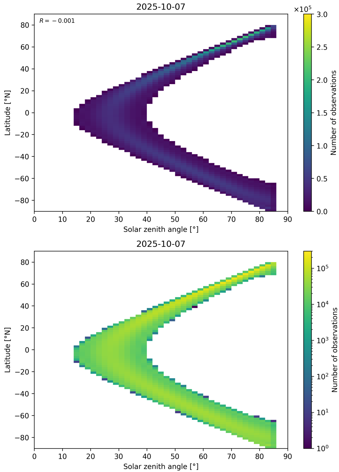
Figure 181: Scatter density plot of “Solar zenith angle” against “Latitude” for 2025-10-06 to 2025-10-08.
