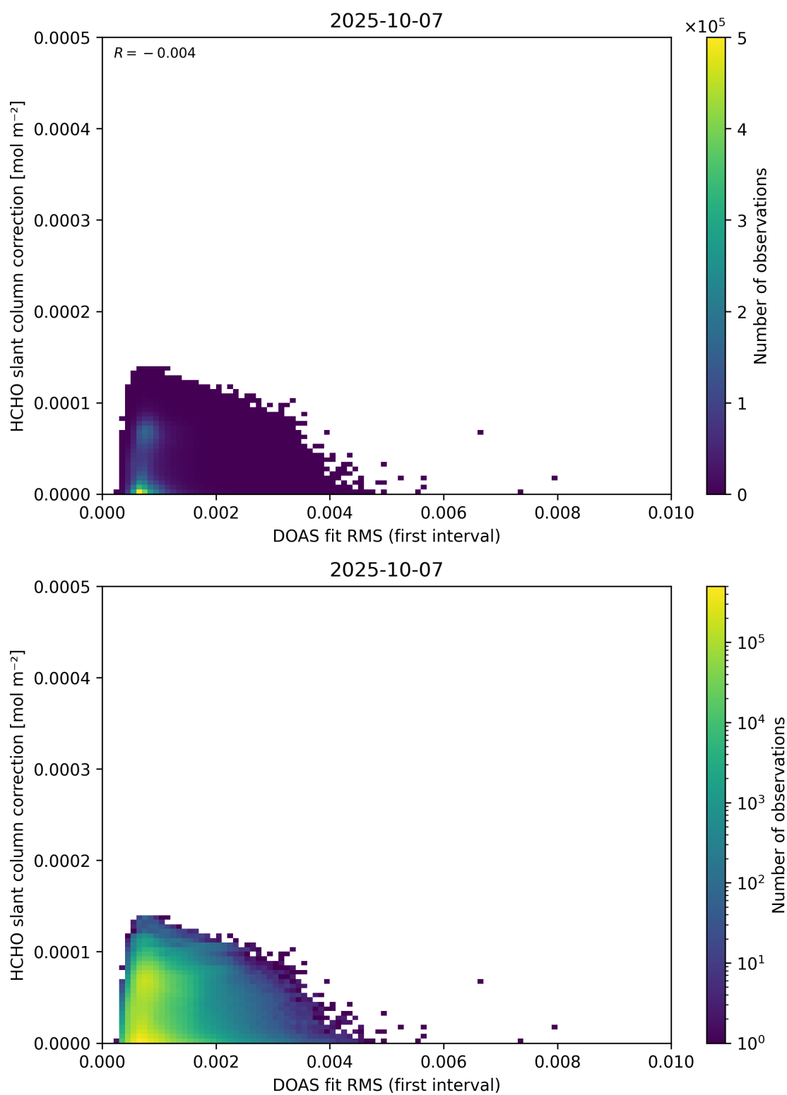
Figure 63: Scatter density plot of “DOAS fit RMS (first interval)” against “HCHO slant column correction” for 2025-10-06 to 2025-10-08.
