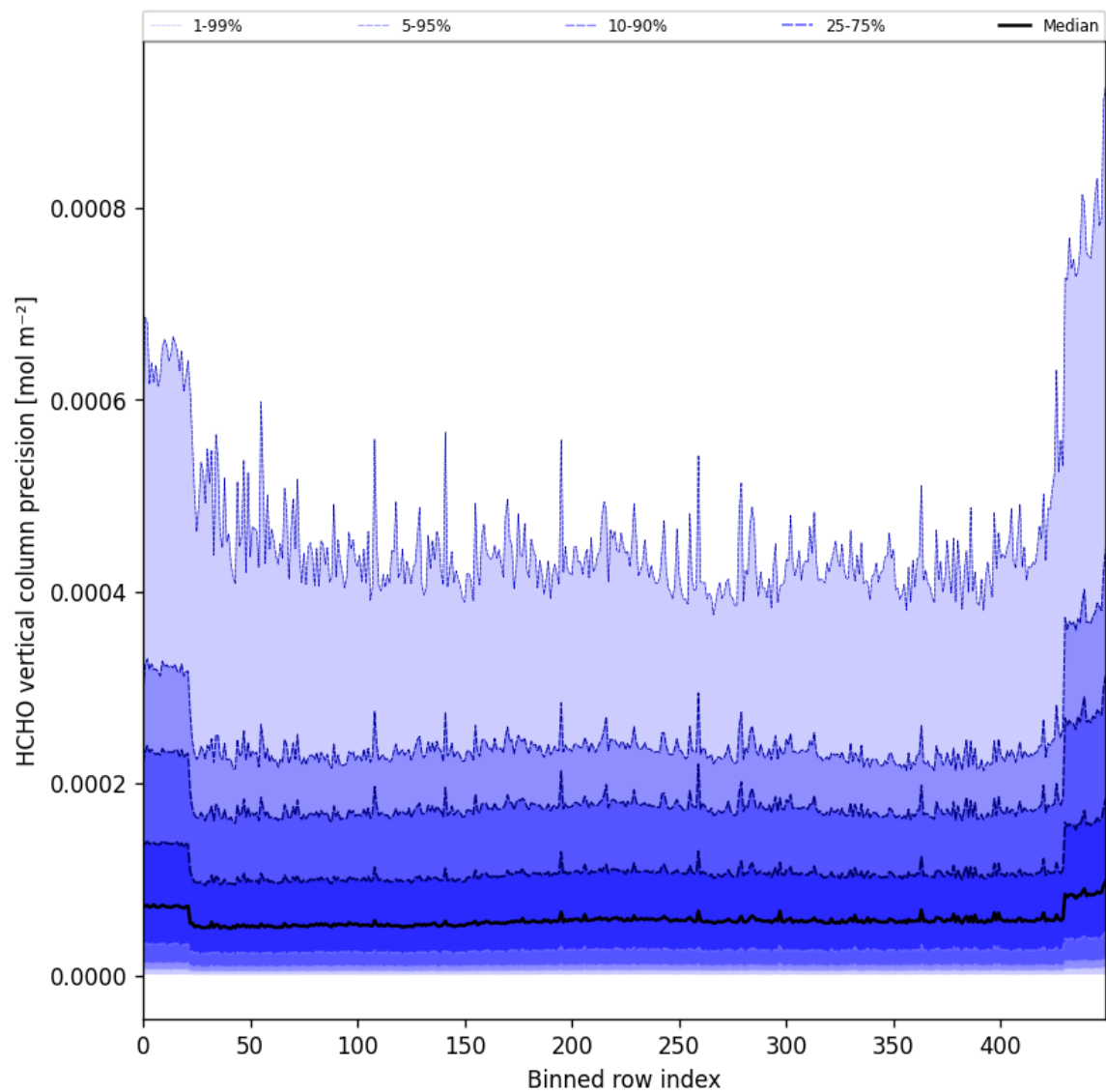
Figure 50: Along track statistics of “HCHO vertical column precision” for 2025-10-06 to 2025-10-08
