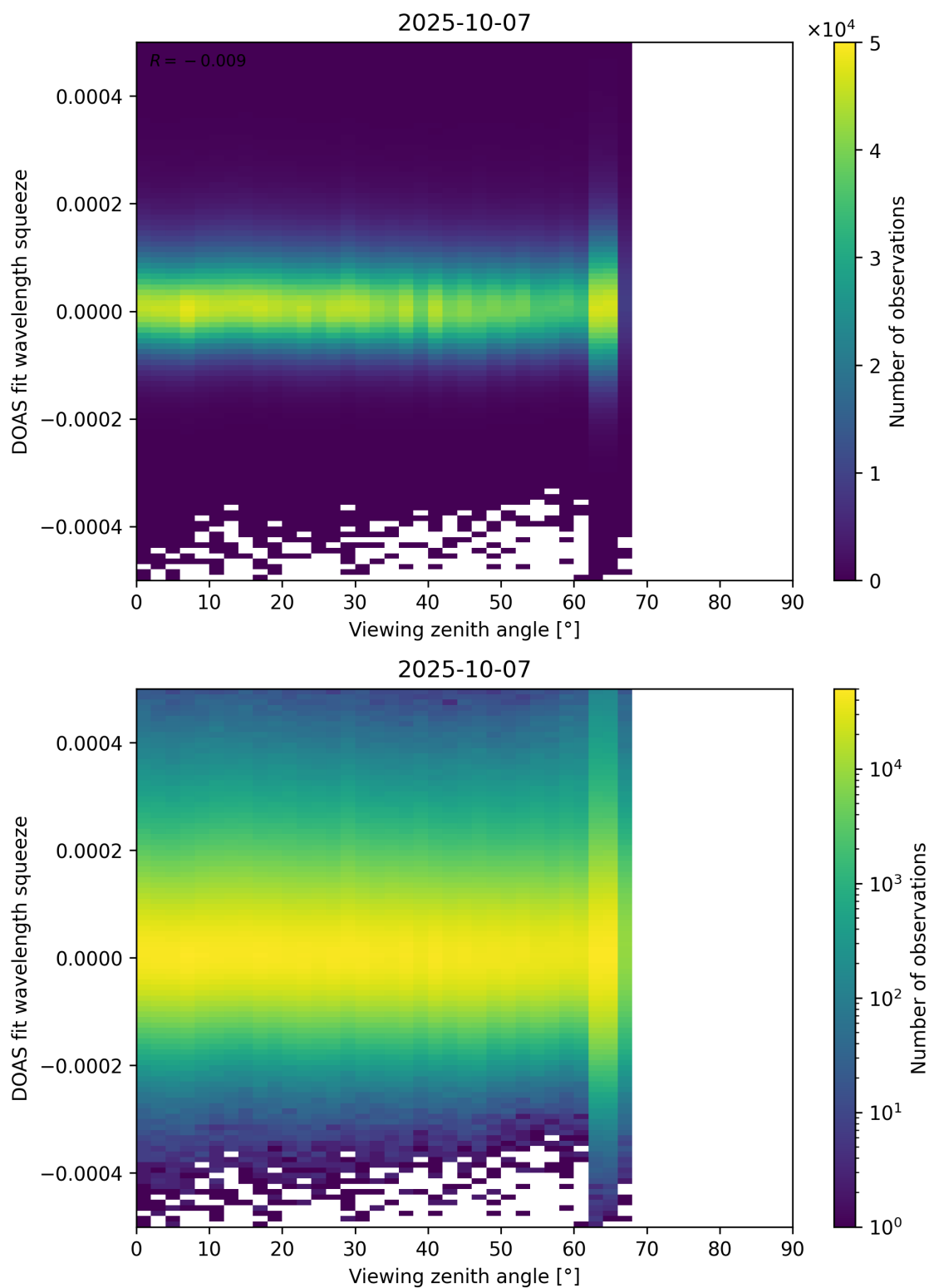
Figure 184: Scatter density plot of “Viewing zenith angle” against “DOAS fit wavelength squeeze” for 2025-10-06 to 2025-10-08.
