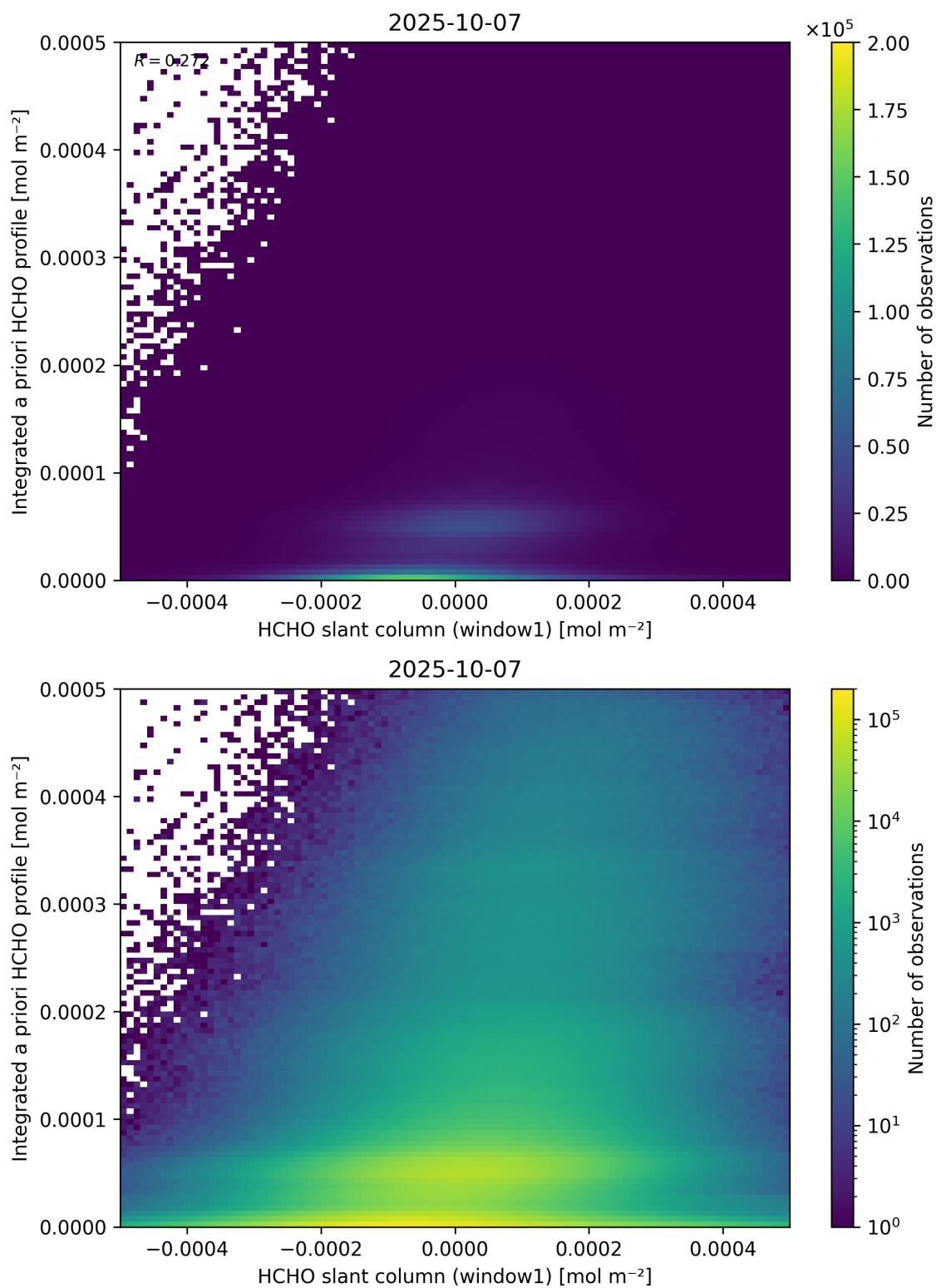
Figure 87: Scatter density plot of “HCHO slant column (window1)” against “Integrated a priori HCHO profile” for 2025-10-06 to 2025-10-08.
