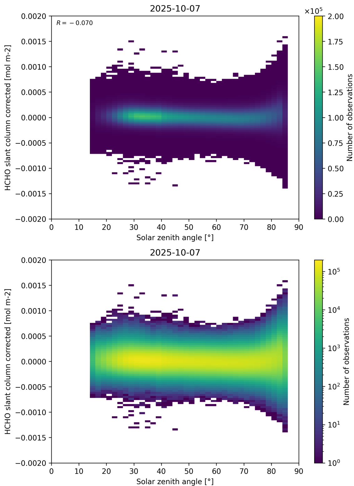
Figure 171: Scatter density plot of “Solar zenith angle” against “HCHO slant column corrected” for 2025-10-06 to 2025-10-08.
