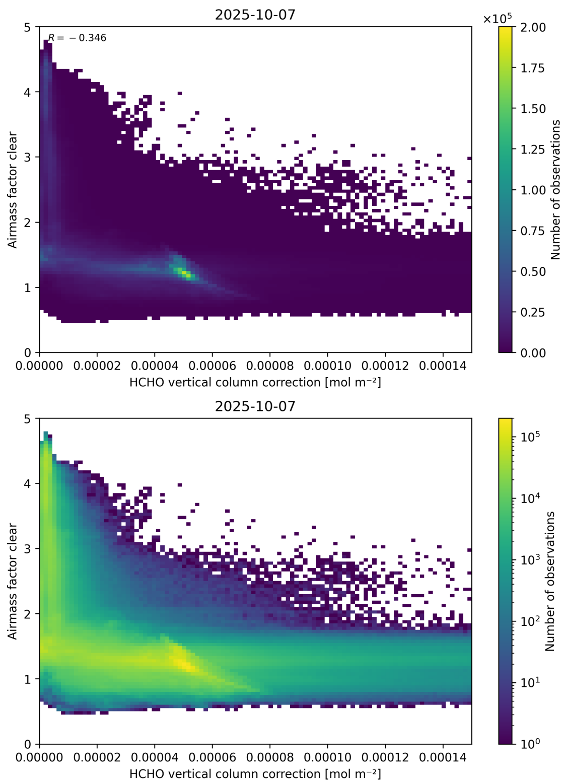
Figure 115: Scatter density plot of “HCHO vertical column correction” against “Airmass factor clear” for 2025-10-06 to 2025-10-08.
