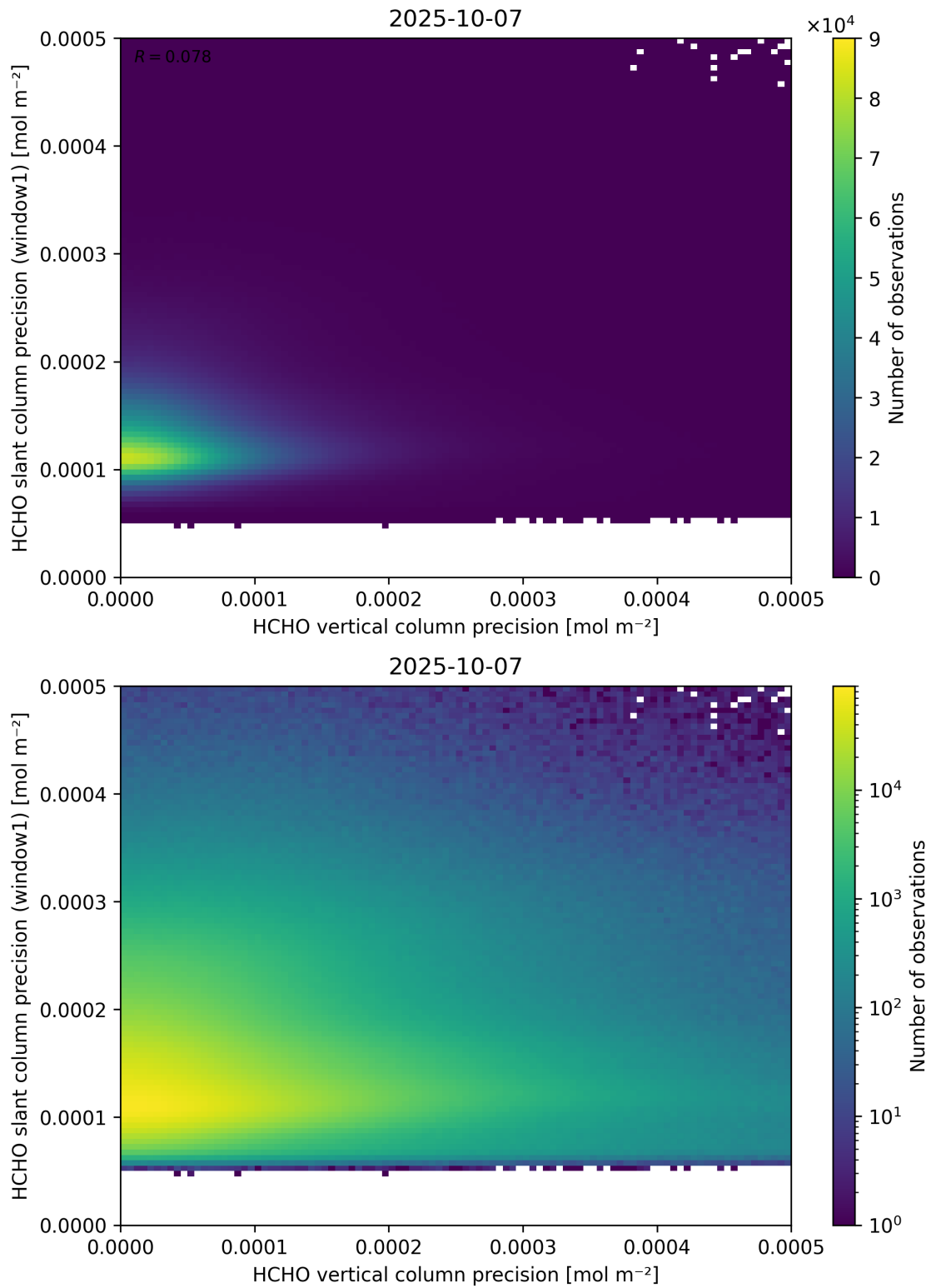
Figure 143: Scatter density plot of “HCHO vertical column precision” against “HCHO slant column precision (window1)” for 2025-10-06 to 2025-10-08.
