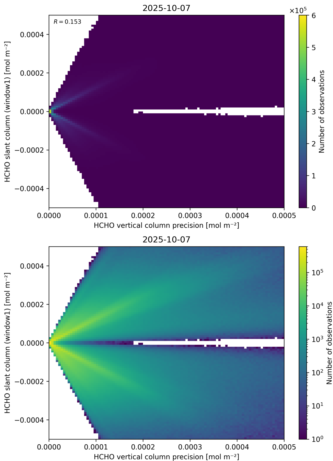
Figure 142: Scatter density plot of “HCHO vertical column precision” against “HCHO slant column (window1)” for 2025-10-06 to 2025-10-08.
