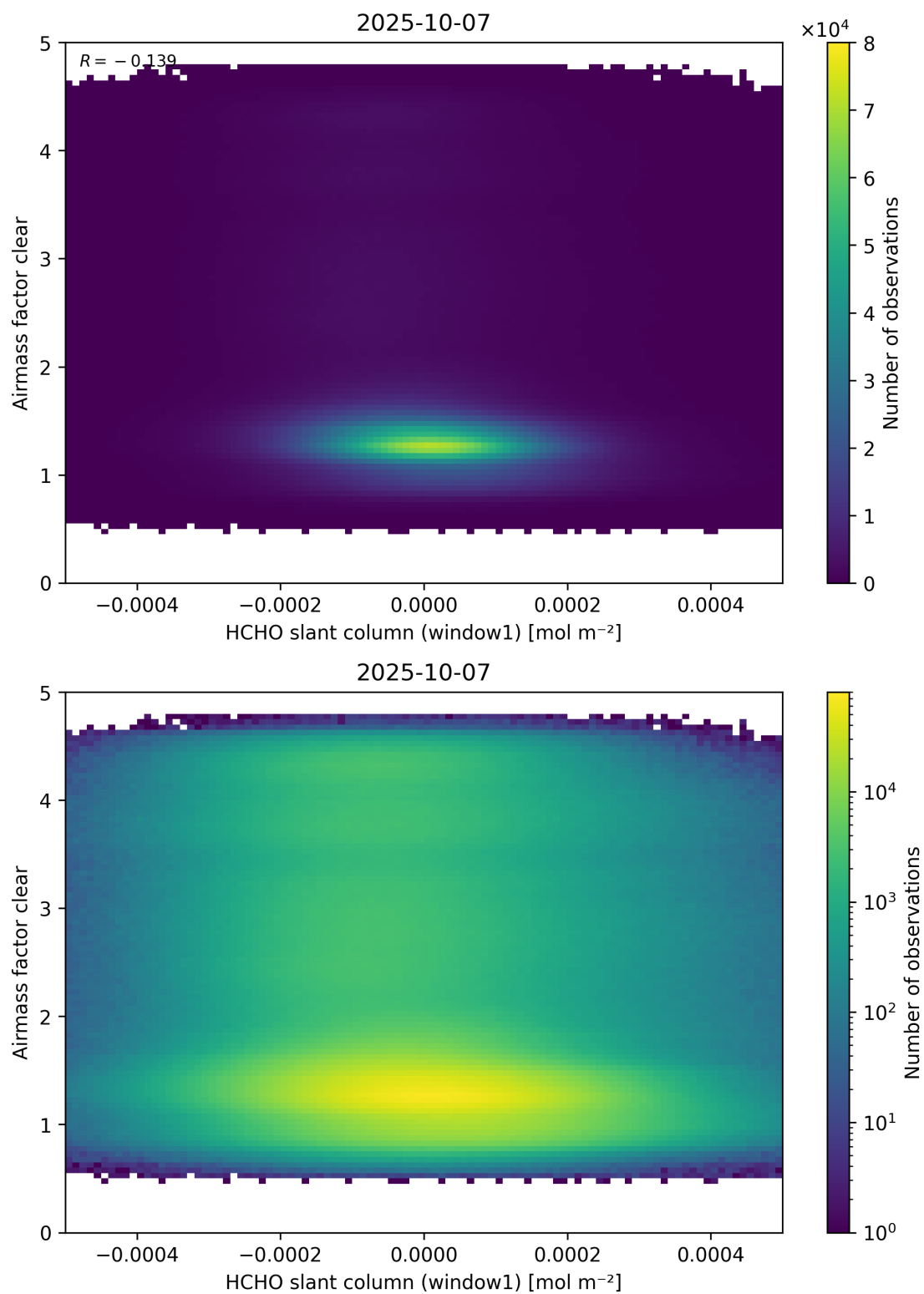
Figure 81: Scatter density plot of “HCHO slant column (window1)” against “Airmass factor clear” for 2025-10-06 to 2025-10-08.
