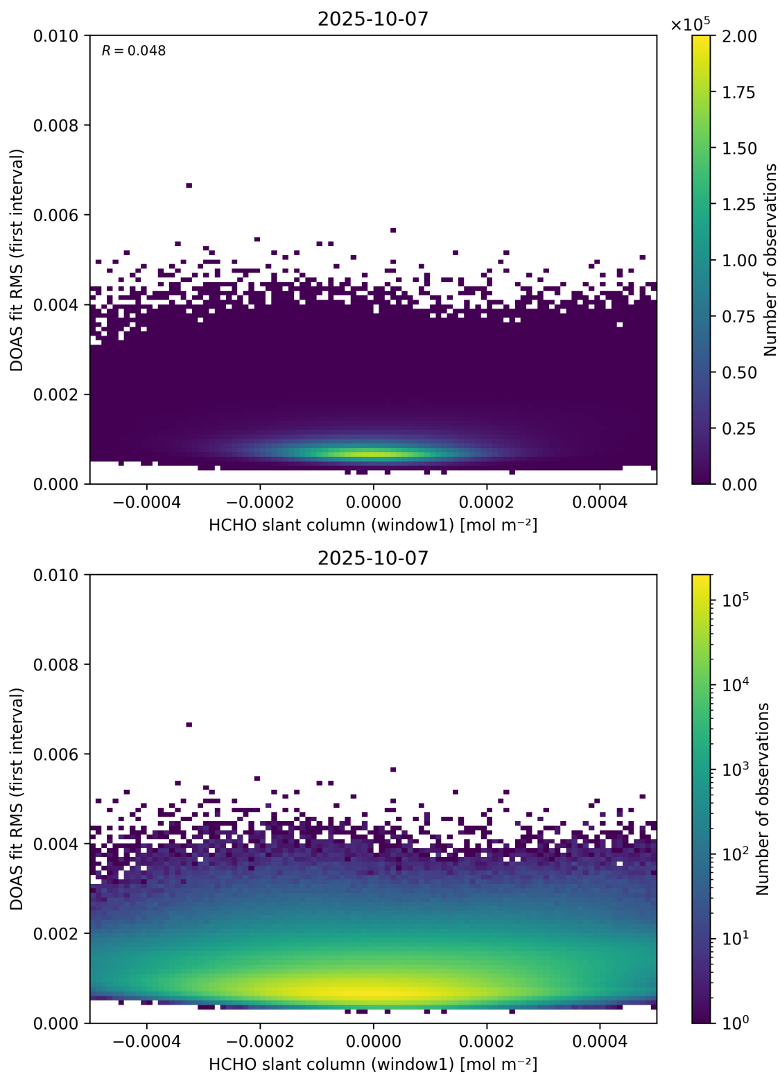
Figure 78: Scatter density plot of “HCHO slant column (window1)” against “DOAS fit RMS (first interval)” for 2025-10-06 to 2025-10-08.
