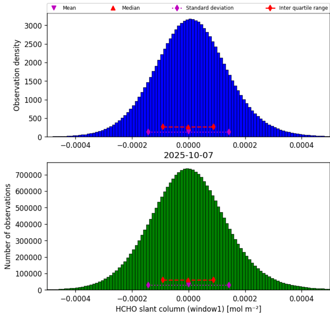
Figure 38: Histogram of “HCHO slant column (window1)” for 2025-10-06 to 2025-10-08
