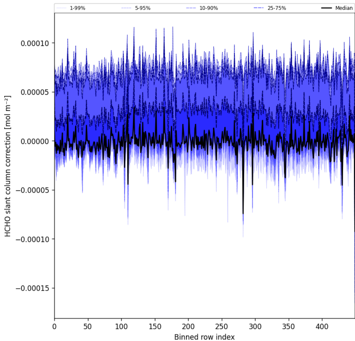
Figure 61: Along track statistics of “HCHO slant column correction” for 2025-10-06 to 2025-10-08
