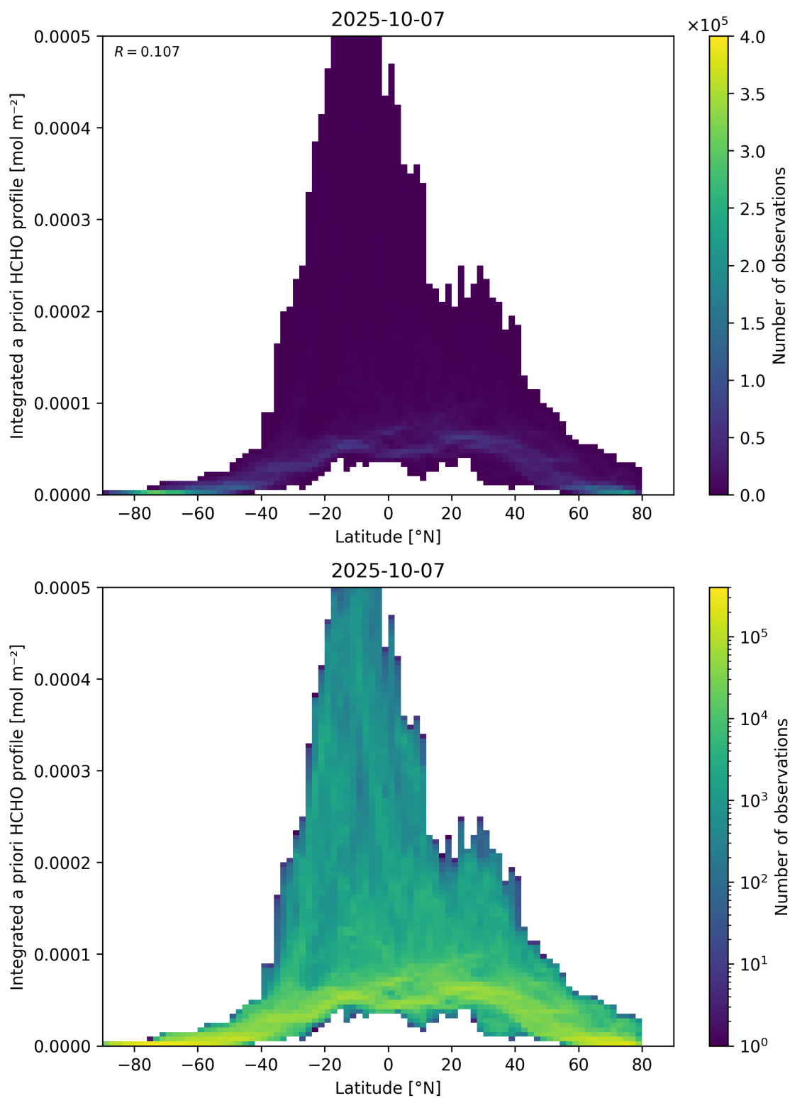
Figure 166: Scatter density plot of “Latitude” against “Integrated a priori HCHO profile” for 2025-10-06 to 2025-10-08.
