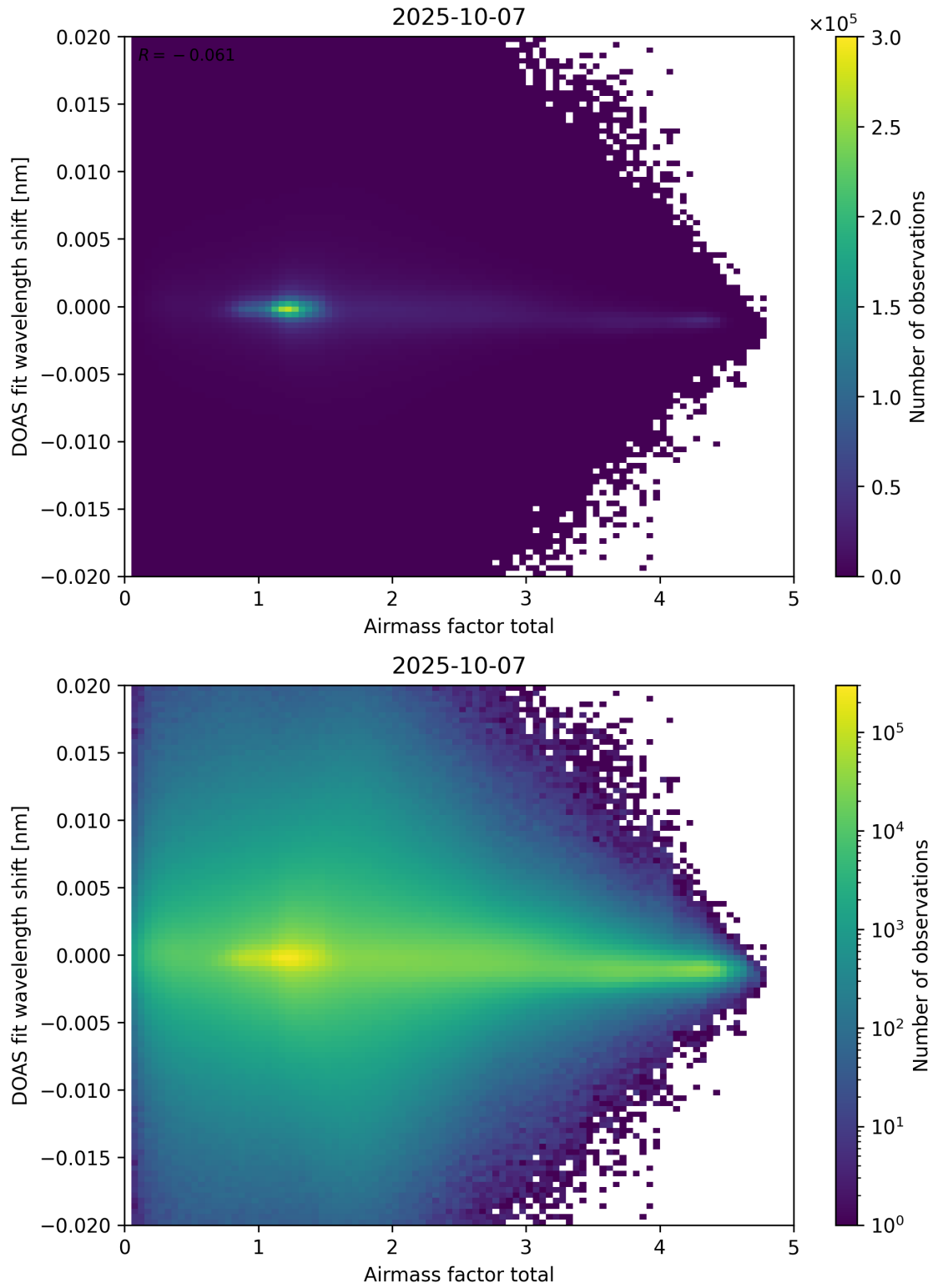
Figure 98: Scatter density plot of “Airmass factor total” against “DOAS fit wavelength shift” for 2025-10-06 to 2025-10-08.
