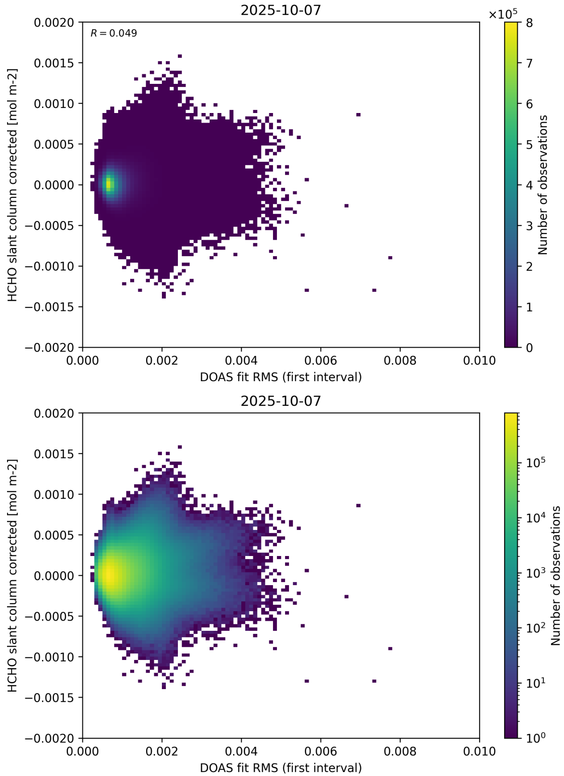
Figure 62: Scatter density plot of “DOAS fit RMS (first interval)” against “HCHO slant column corrected” for 2025-10-06 to 2025-10-08.
