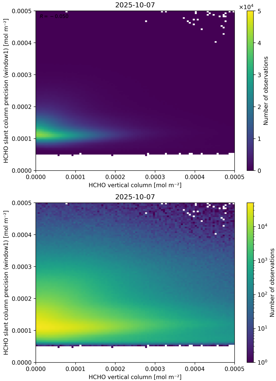
Figure 130: Scatter density plot of “HCHO vertical column” against “HCHO slant column precision (window1)” for 2025-10-06 to 2025-10-08.
