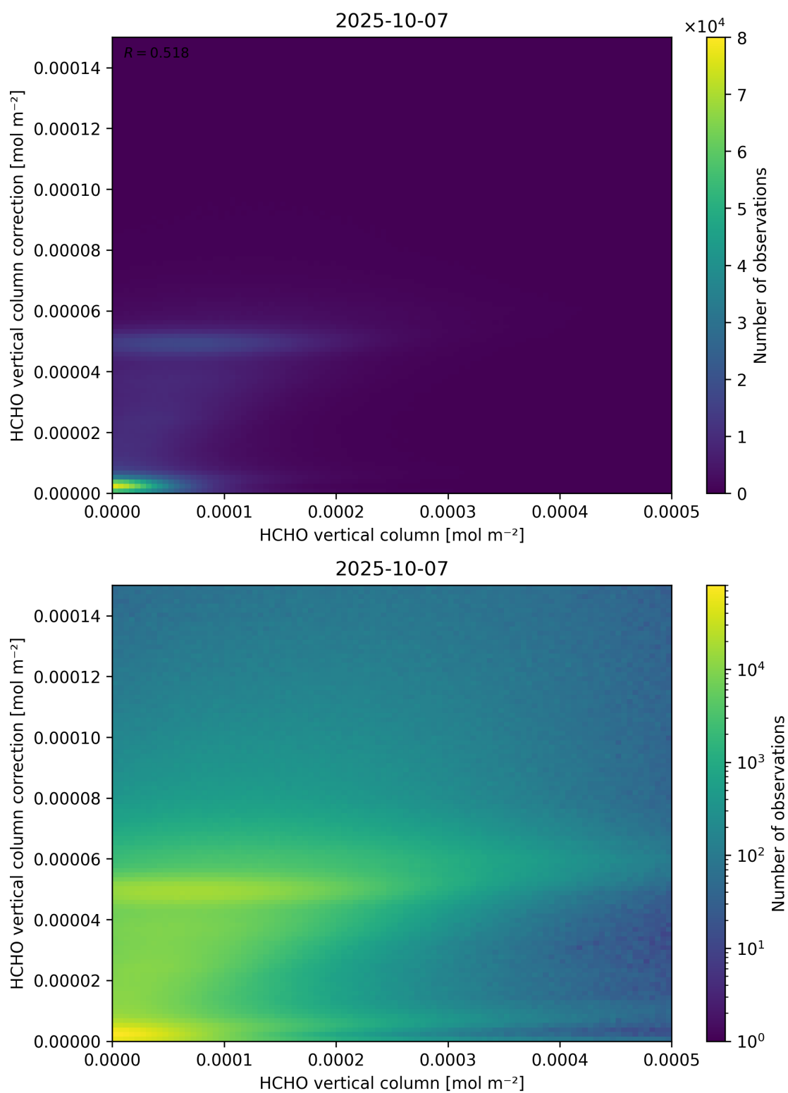
Figure 133: Scatter density plot of “HCHO vertical column” against “HCHO vertical column correction” for 2025-10-06 to 2025-10-08.
