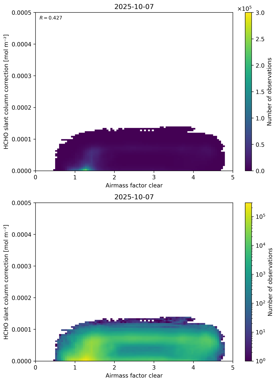
Figure 75: Scatter density plot of “Airmass factor clear” against “HCHO slant column correction” for 2025-10-06 to 2025-10-08.
