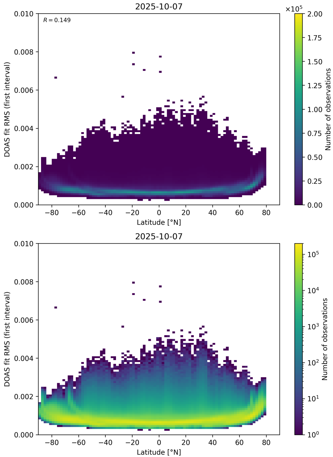
Figure 153: Scatter density plot of “Latitude” against “DOAS fit RMS (first interval)” for 2025-10-06 to 2025-10-08.
