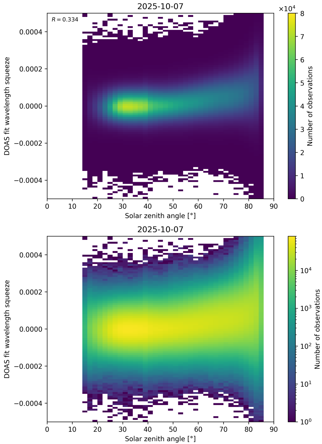
Figure 169: Scatter density plot of “Solar zenith angle” against “DOAS fit wavelength squeeze” for 2025-10-06 to 2025-10-08.
