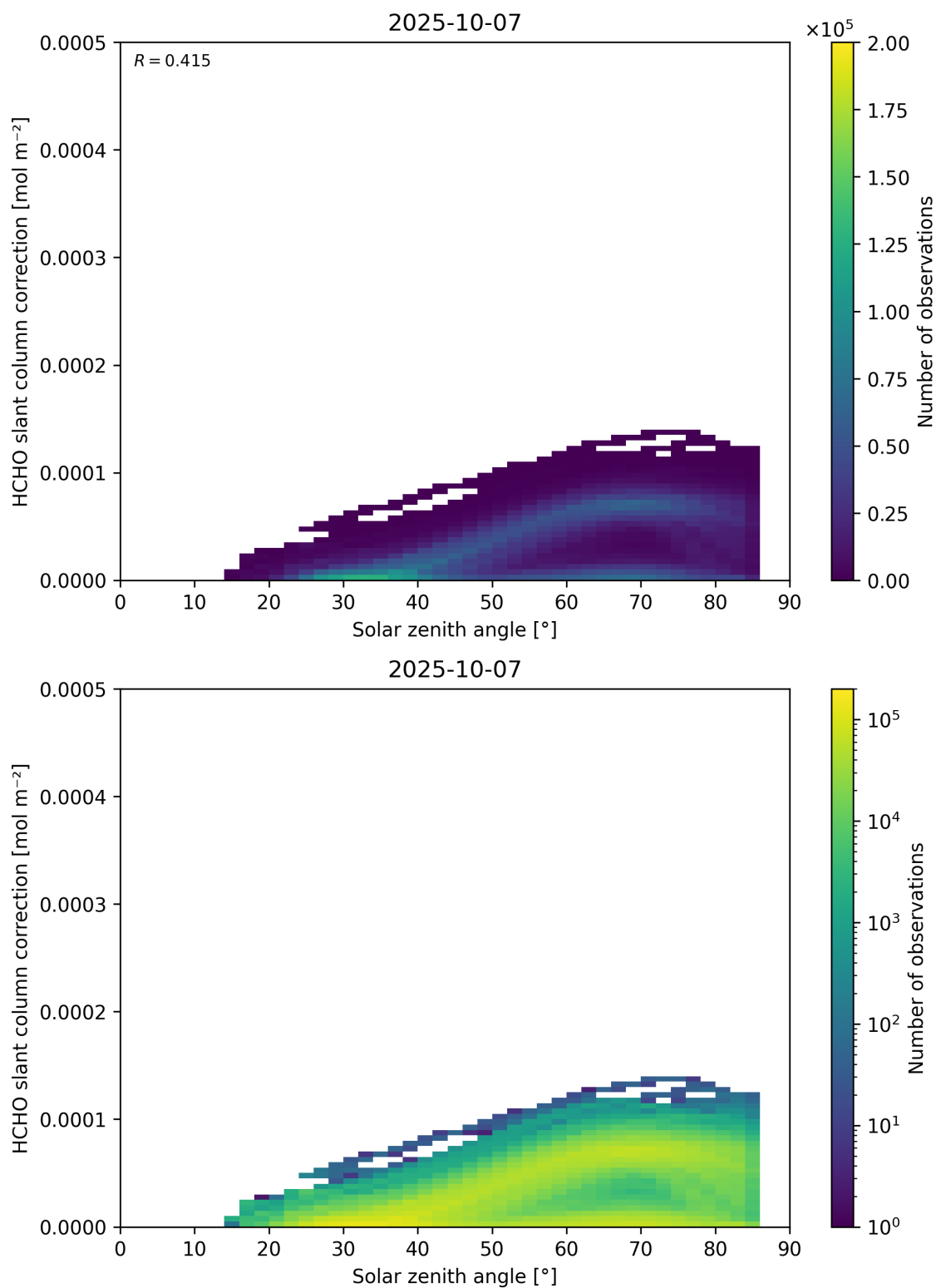
Figure 172: Scatter density plot of “Solar zenith angle” against “HCHO slant column correction” for 2025-10-06 to 2025-10-08.
