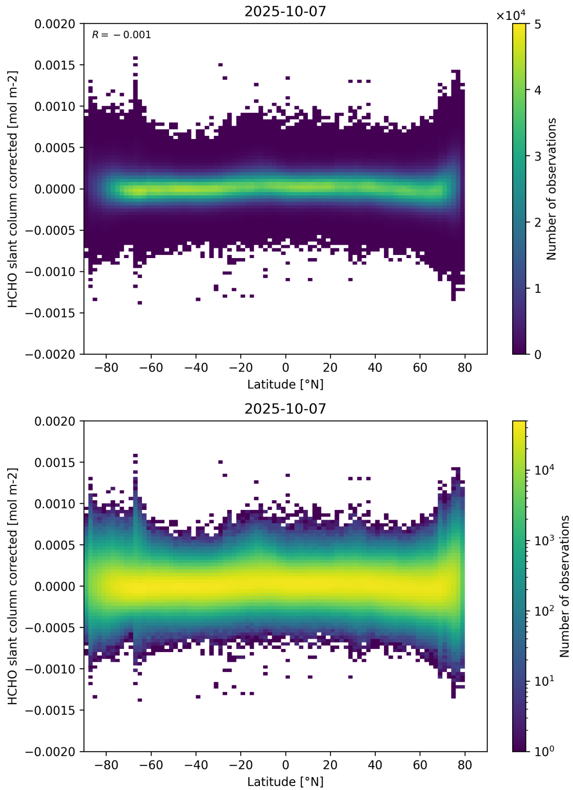
Figure 157: Scatter density plot of “Latitude” against “HCHO slant column corrected” for 2025-10-06 to 2025-10-08.
