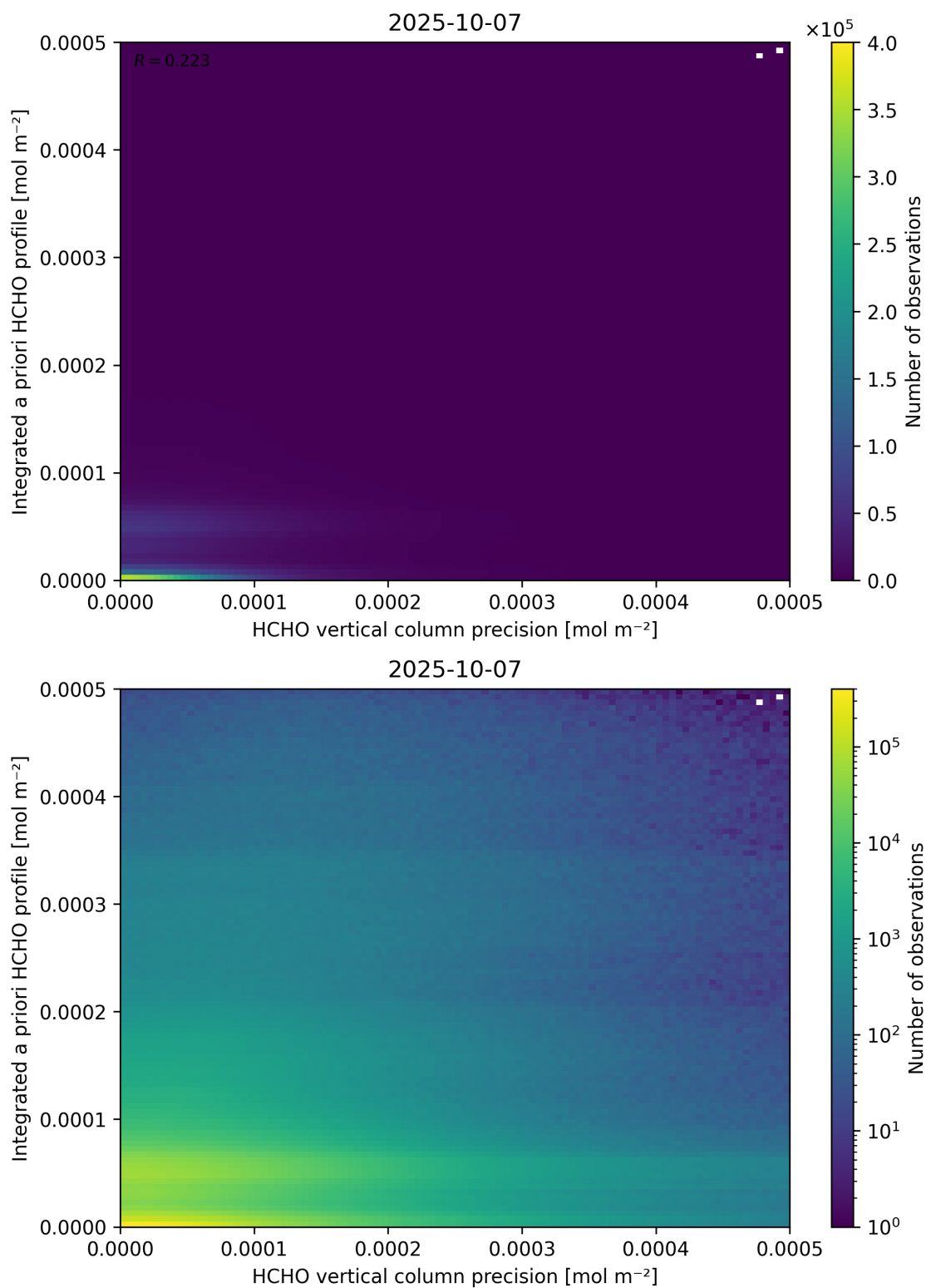
Figure 147: Scatter density plot of “HCHO vertical column precision” against “Integrated a priori HCHO profile” for 2025-10-06 to 2025-10-08.
