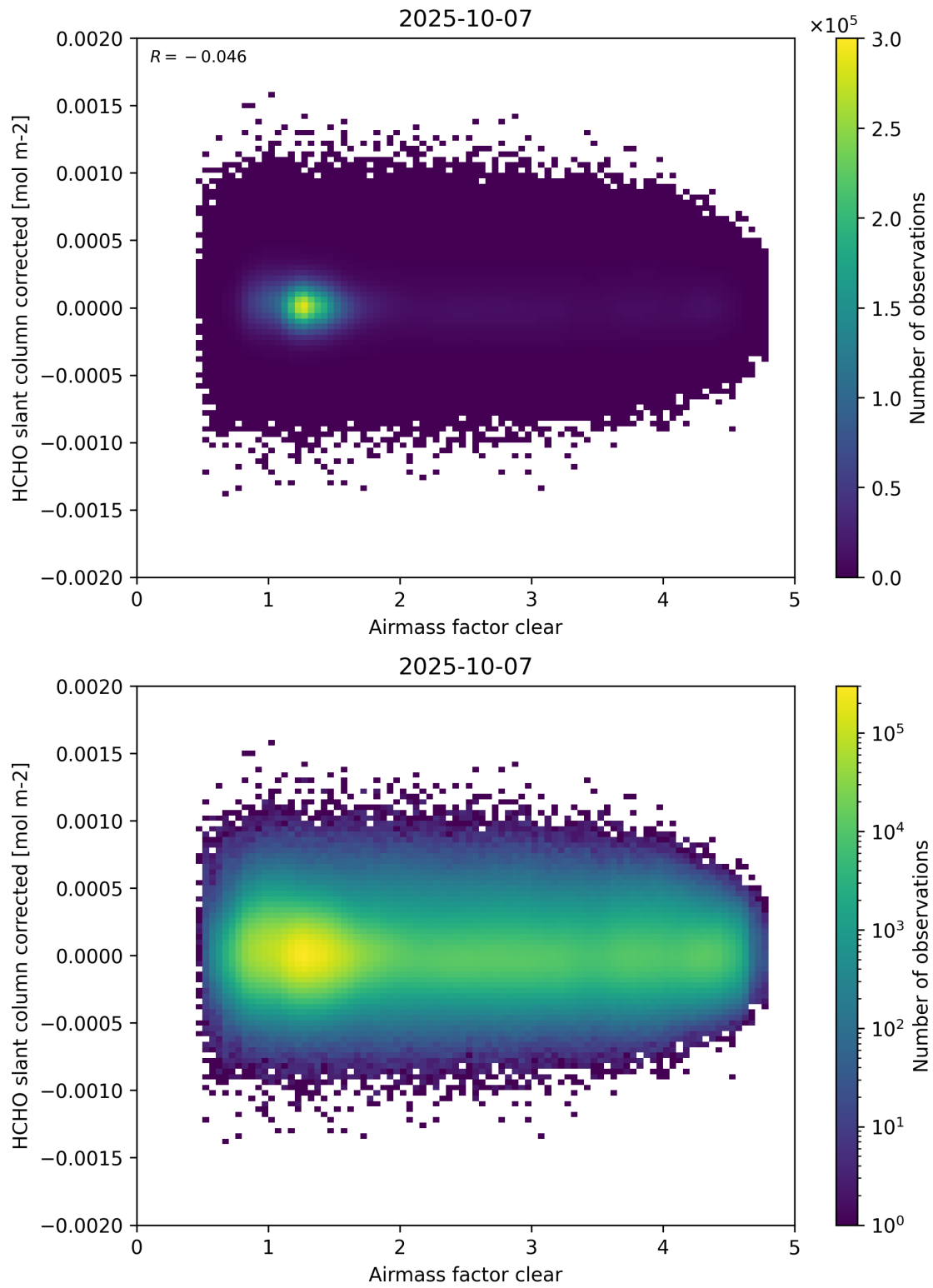
Figure 74: Scatter density plot of “Airmass factor clear” against “HCHO slant column corrected” for 2025-10-06 to 2025-10-08.
