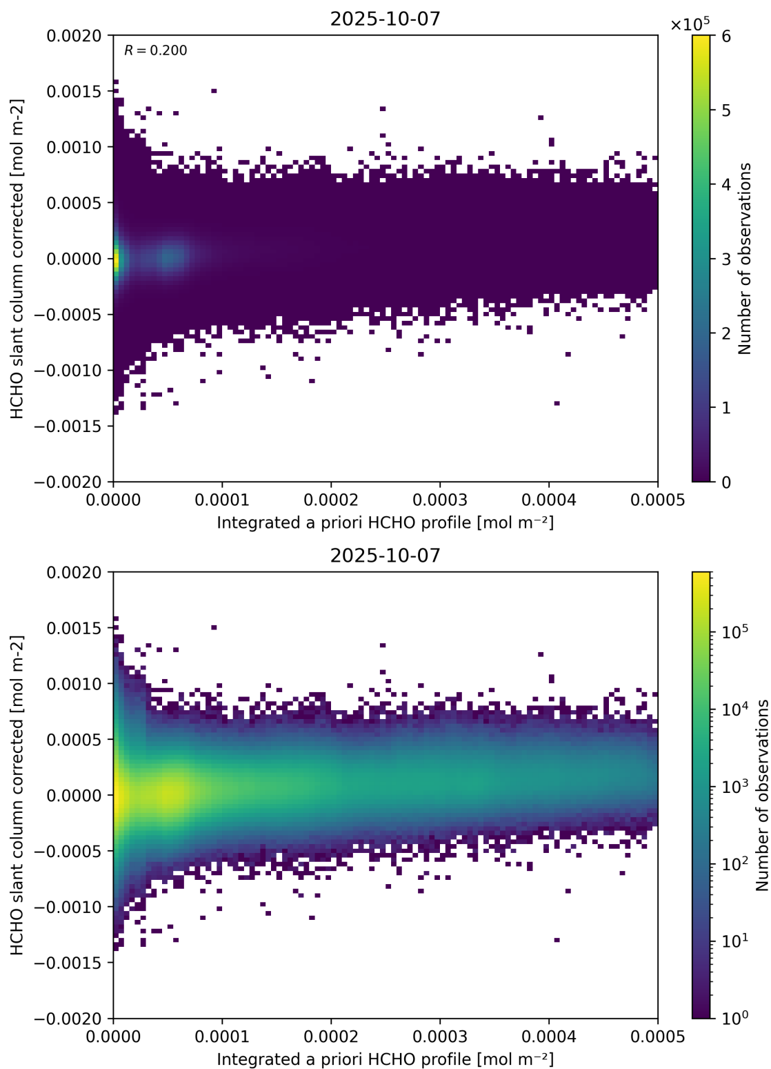
Figure 151: Scatter density plot of “Integrated a priori HCHO profile” against “HCHO slant column corrected” for 2025-10-06 to 2025-10-08.
