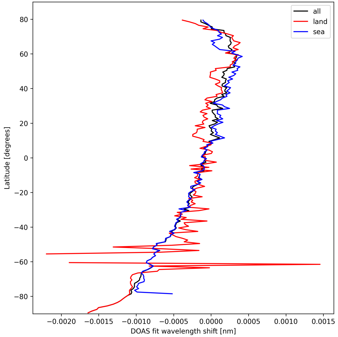
Figure 30: Zonal average of “DOAS fit wavelength shift” for 2025-10-06 to 2025-10-08.
