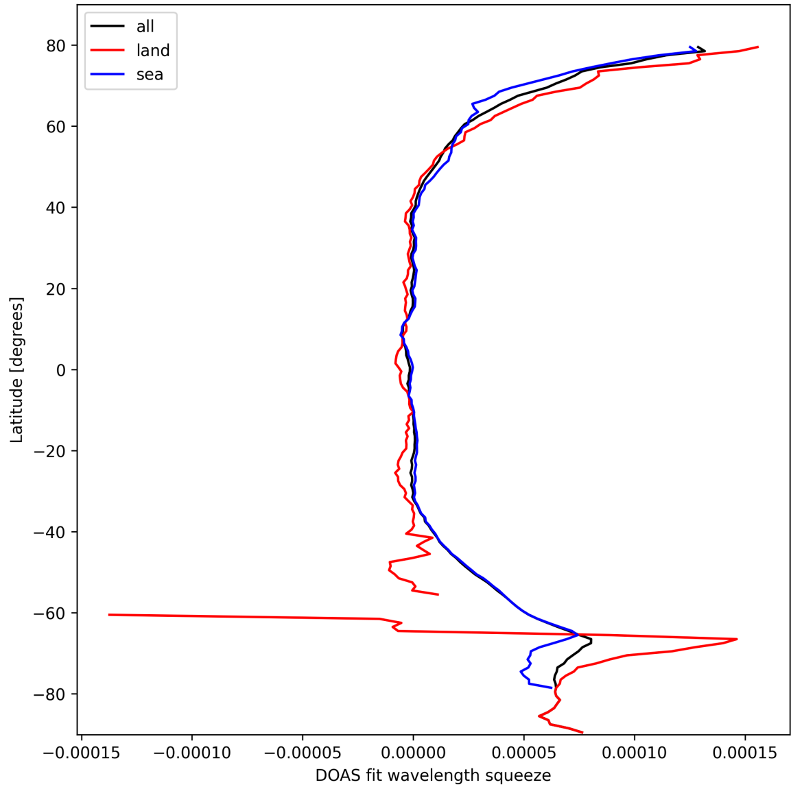
Figure 31: Zonal average of “DOAS fit wavelength squeeze” for 2025-10-06 to 2025-10-08.
