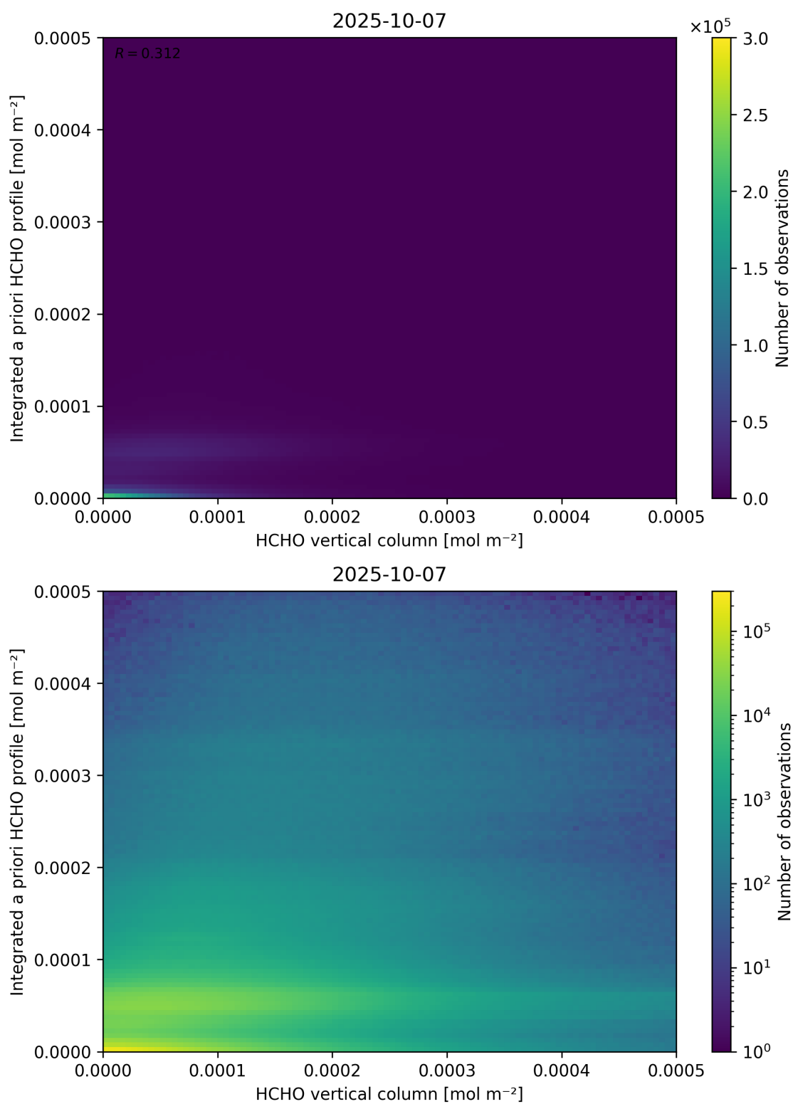
Figure 135: Scatter density plot of “HCHO vertical column” against “Integrated a priori HCHO profile” for 2025-10-06 to 2025-10-08.
