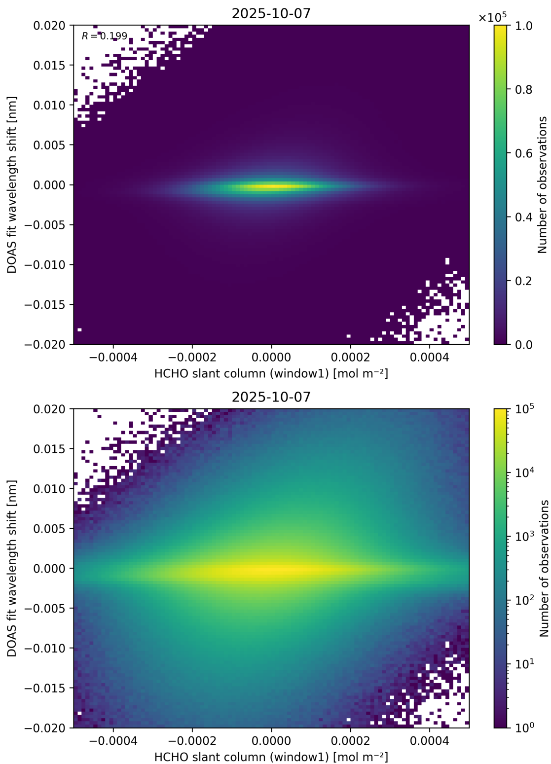
Figure 79: Scatter density plot of “HCHO slant column (window1)” against “DOAS fit wavelength shift” for 2025-10-06 to 2025-10-08.
