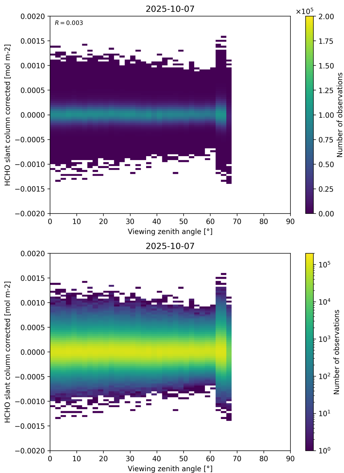
Figure 186: Scatter density plot of “Viewing zenith angle” against “HCHO slant column corrected” for 2025-10-06 to 2025-10-08.
