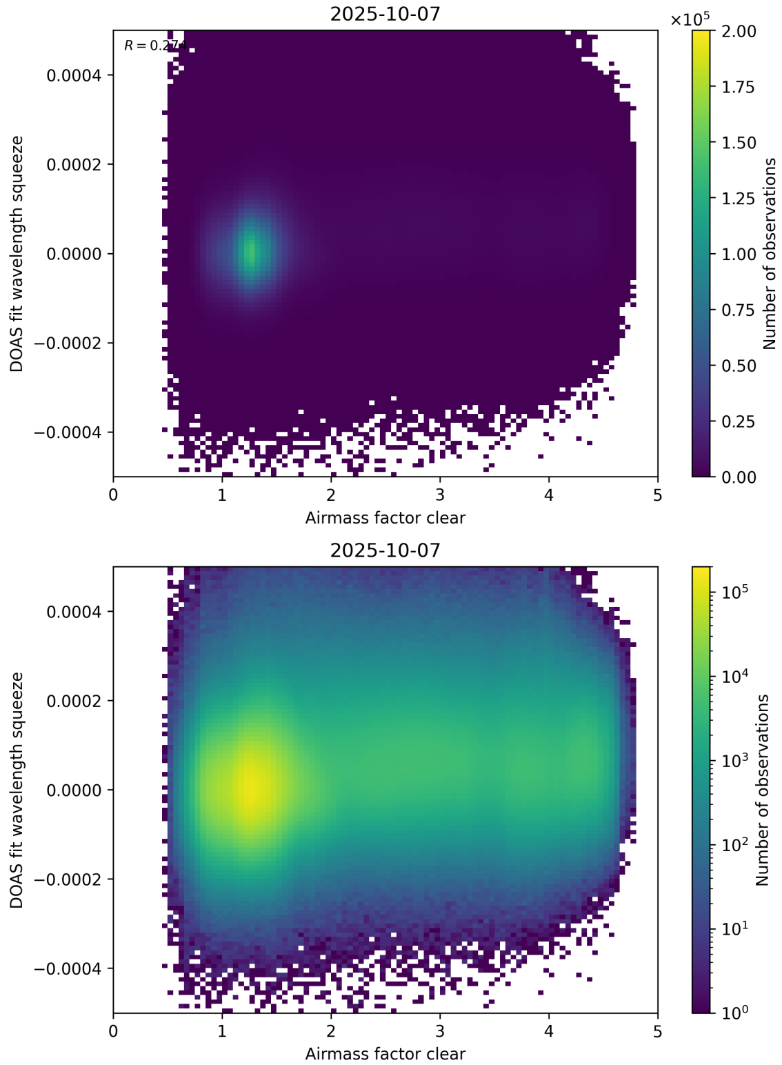
Figure 73: Scatter density plot of “Airmass factor clear” against “DOAS fit wavelength squeeze” for 2025-10-06 to 2025-10-08.
