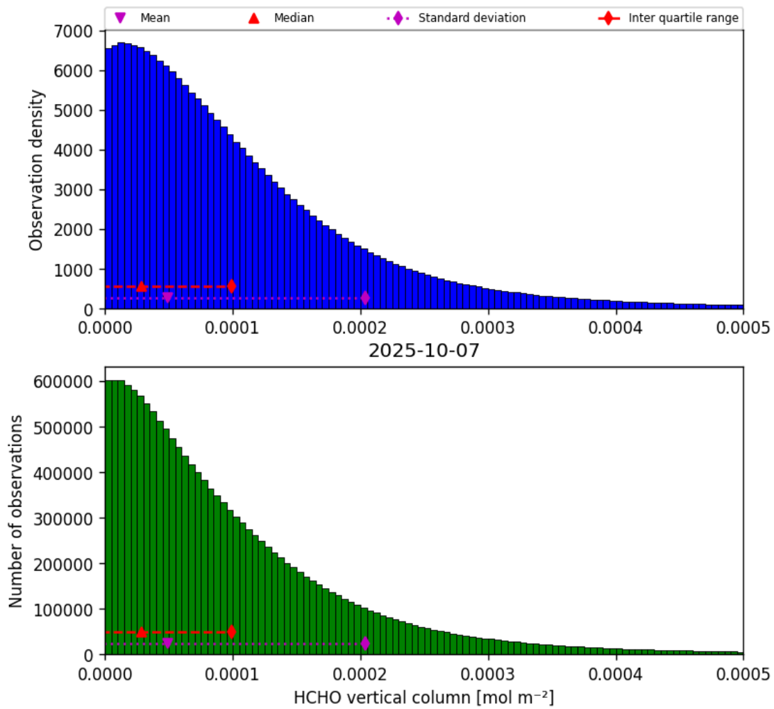
Figure 35: Histogram of “HCHO vertical column” for 2025-10-06 to 2025-10-08
