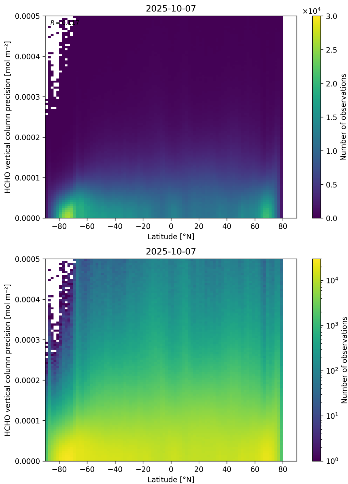
Figure 165: Scatter density plot of “Latitude” against “HCHO vertical column precision” for 2025-10-06 to 2025-10-08.
