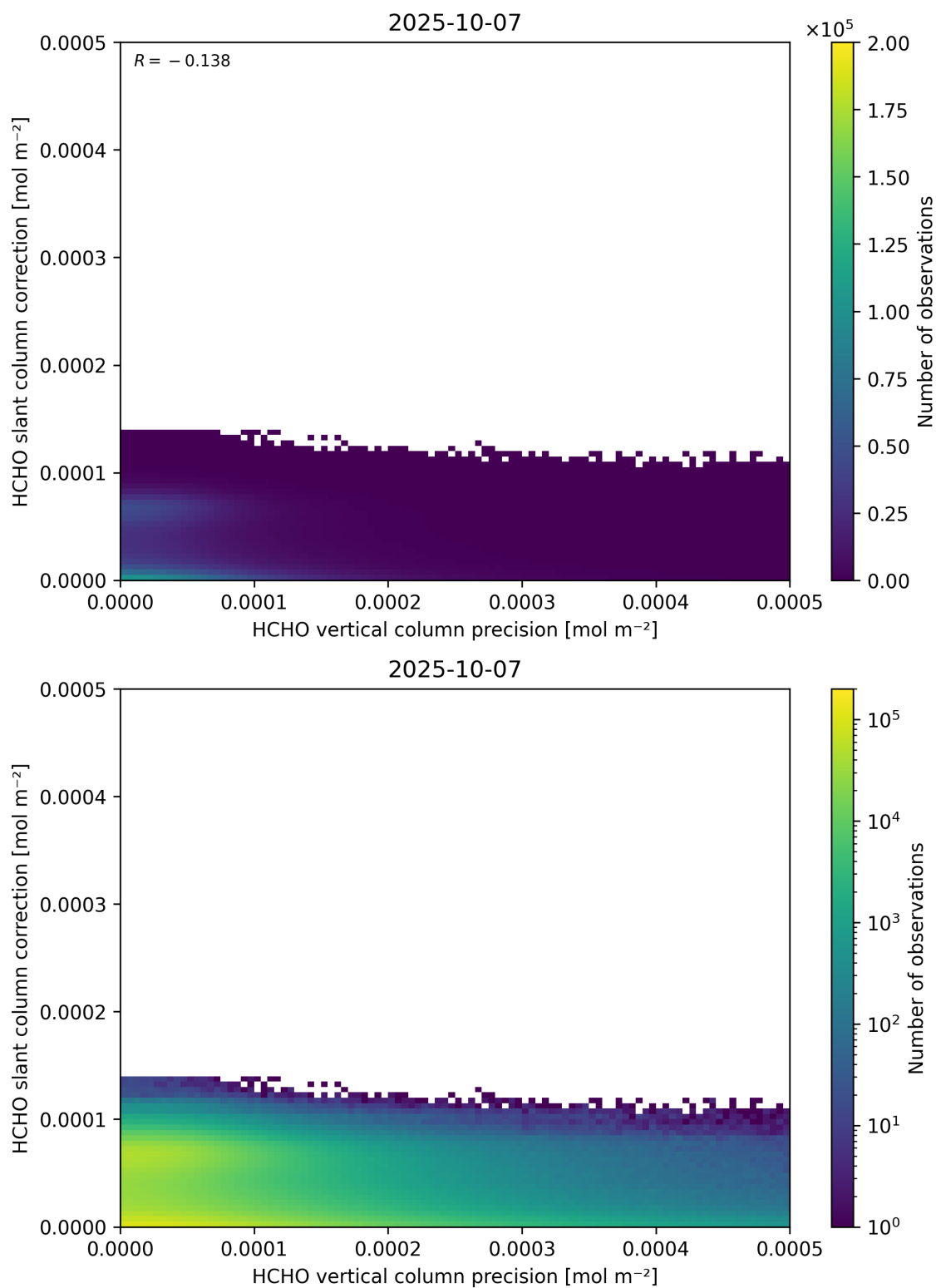
Figure 141: Scatter density plot of “HCHO vertical column precision” against “HCHO slant column correction” for 2025-10-06 to 2025-10-08.
