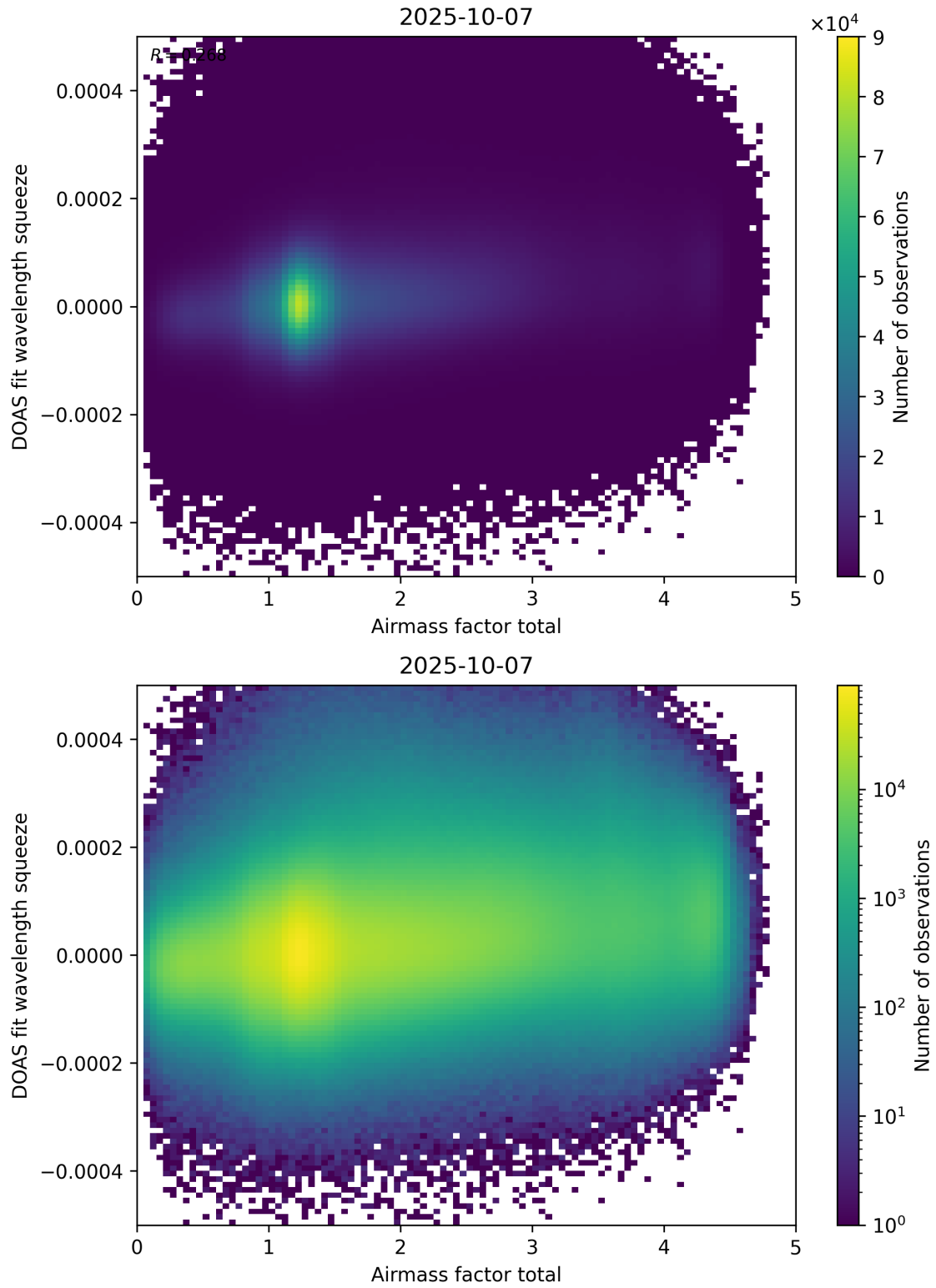
Figure 99: Scatter density plot of “Airmass factor total” against “DOAS fit wavelength squeeze” for 2025-10-06 to 2025-10-08.
