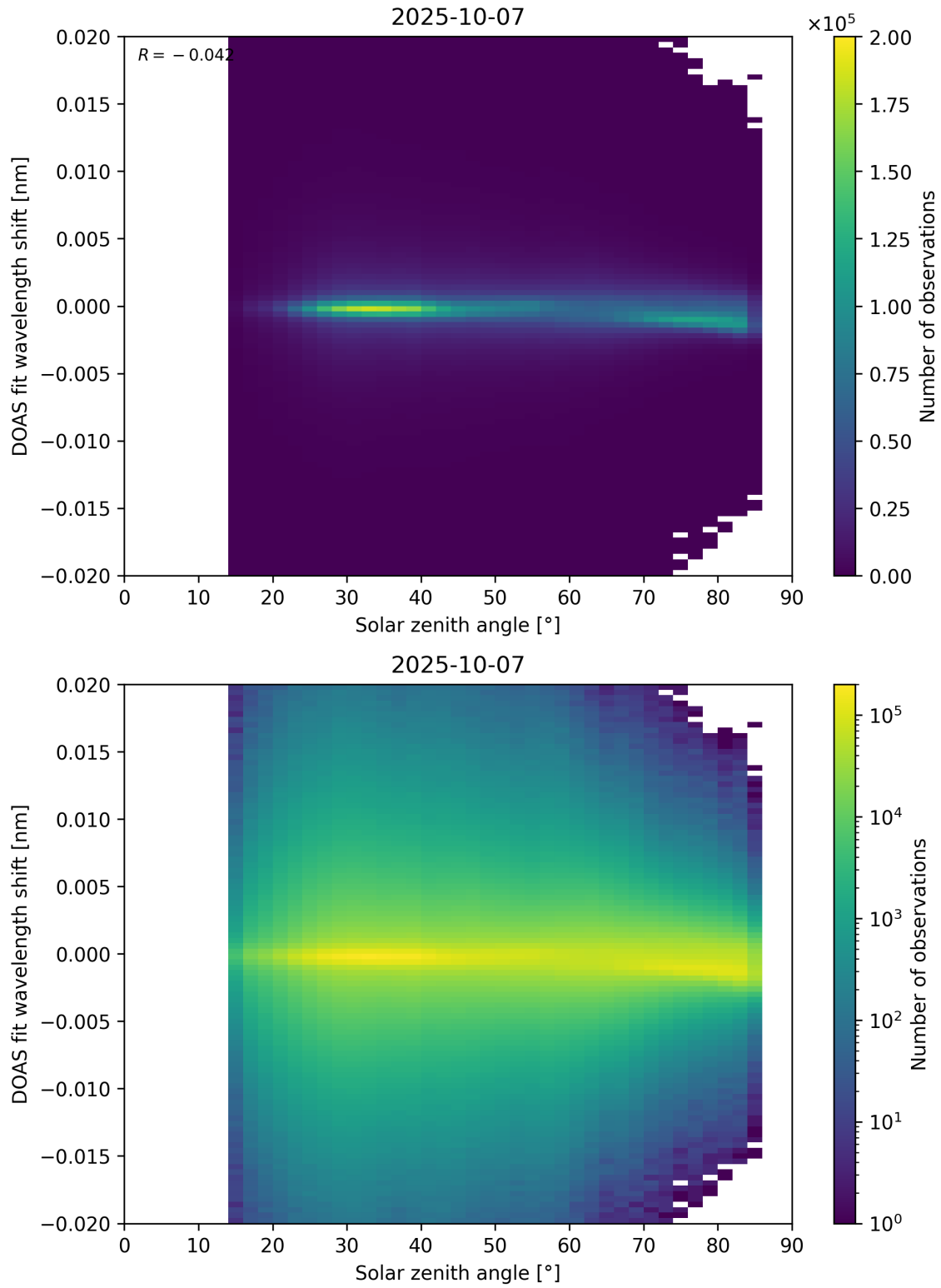
Figure 168: Scatter density plot of “Solar zenith angle” against “DOAS fit wavelength shift” for 2025-10-06 to 2025-10-08.
