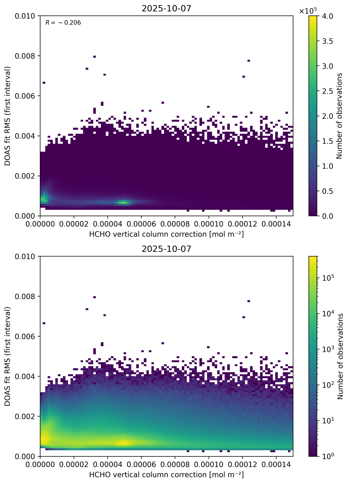
Figure 112: Scatter density plot of “HCHO vertical column correction” against “DOAS fit RMS (first interval)” for 2025-10-06 to 2025-10-08.
