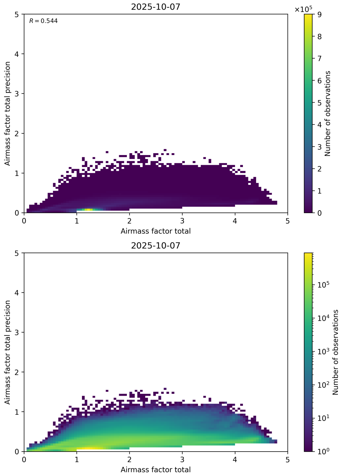
Figure 103: Scatter density plot of “Airmass factor total” against “Airmass factor total precision” for 2025-10-06 to 2025-10-08.
