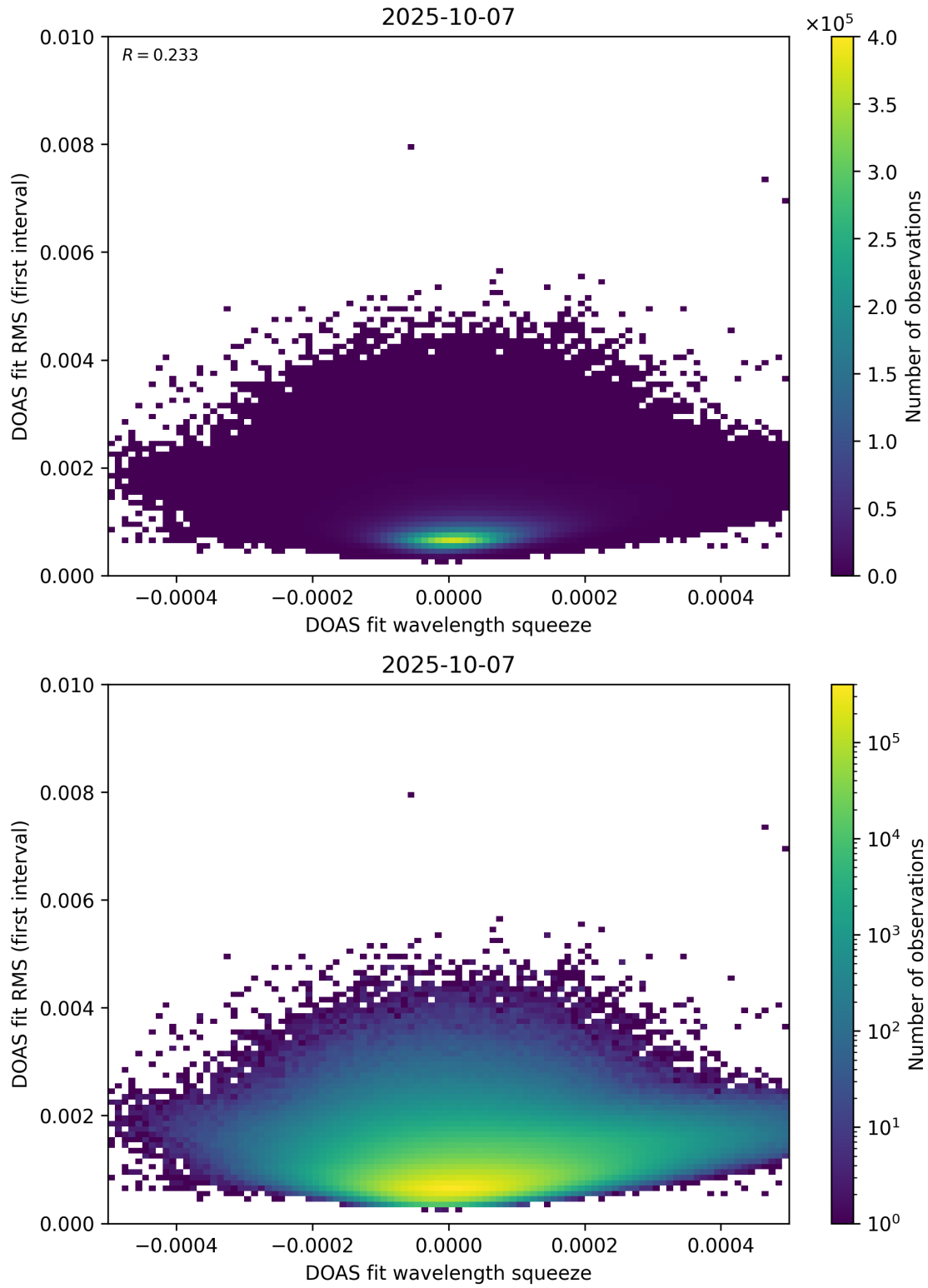
Figure 68: Scatter density plot of “DOAS fit wavelength squeeze” against “DOAS fit RMS (first interval)” for 2025-10-06 to 2025-10-08.
