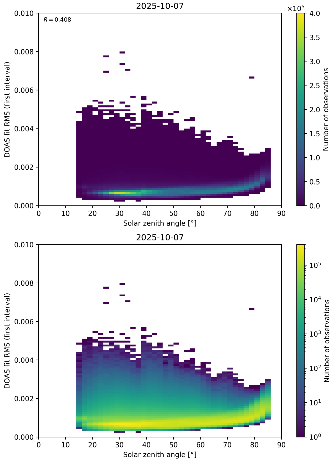
Figure 167: Scatter density plot of “Solar zenith angle” against “DOAS fit RMS (first interval)” for 2025-10-06 to 2025-10-08.
