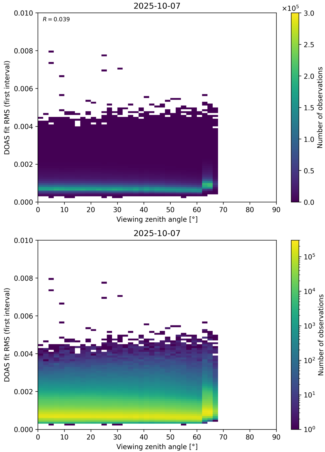
Figure 182: Scatter density plot of “Viewing zenith angle” against “DOAS fit RMS (first interval)” for 2025-10-06 to 2025-10-08.
