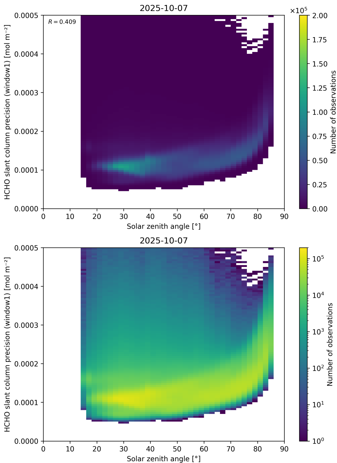
Figure 174: Scatter density plot of “Solar zenith angle” against “HCHO slant column precision (window1)” for 2025-10-06 to 2025-10-08.
