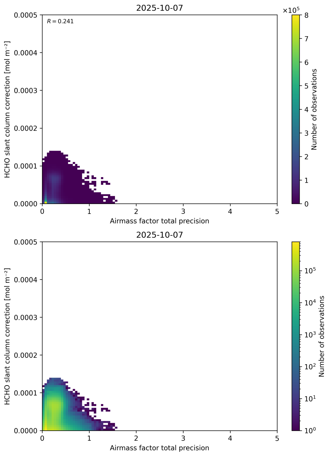
Figure 110: Scatter density plot of “Airmass factor total precision” against “HCHO slant column correction” for 2025-10-06 to 2025-10-08.
