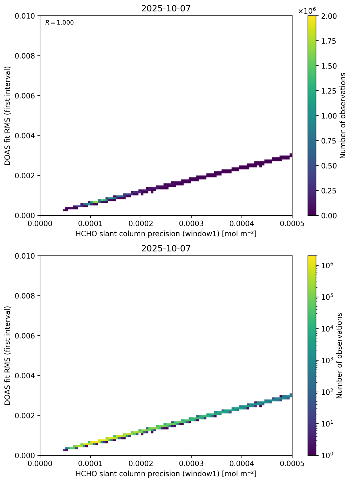
Figure 88: Scatter density plot of “HCHO slant column precision (window1)” against “DOAS fit RMS (first interval)” for 2025-10-06 to 2025-10-08.
