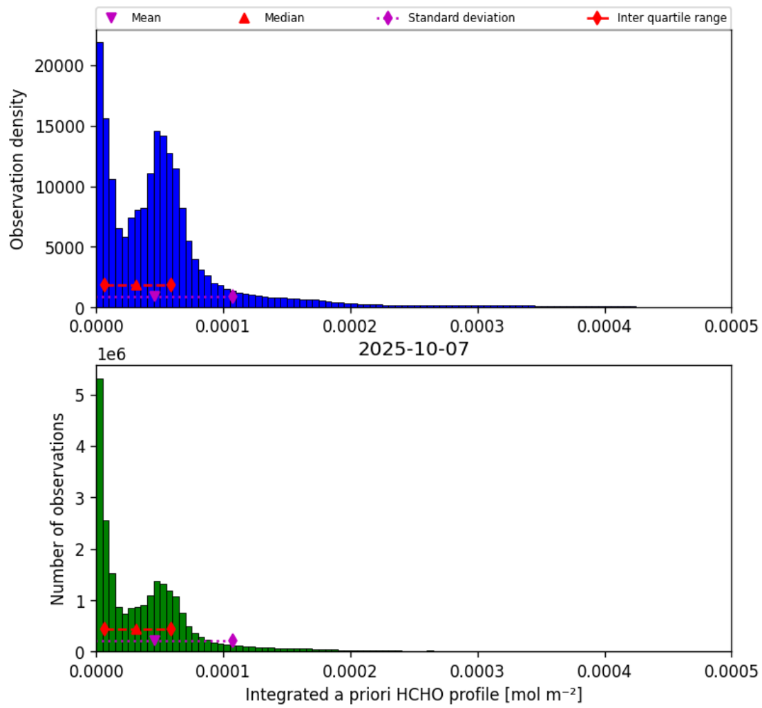
Figure 43: Histogram of “Integrated a priori HCHO profile” for 2025-10-06 to 2025-10-08
