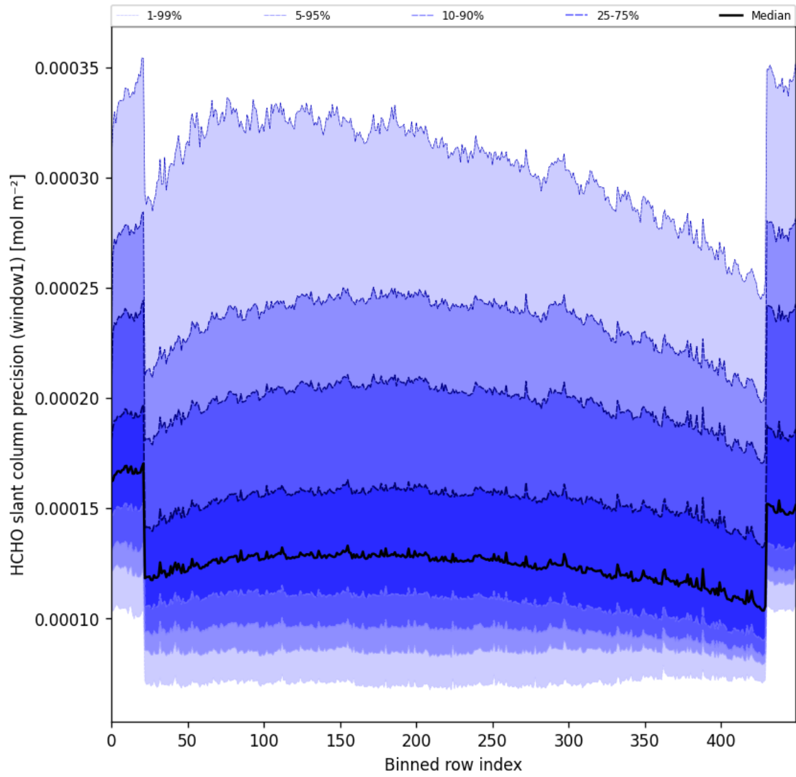
Figure 53: Along track statistics of “HCHO slant column precision (window1)” for 2025-10-06 to 2025-10-08
