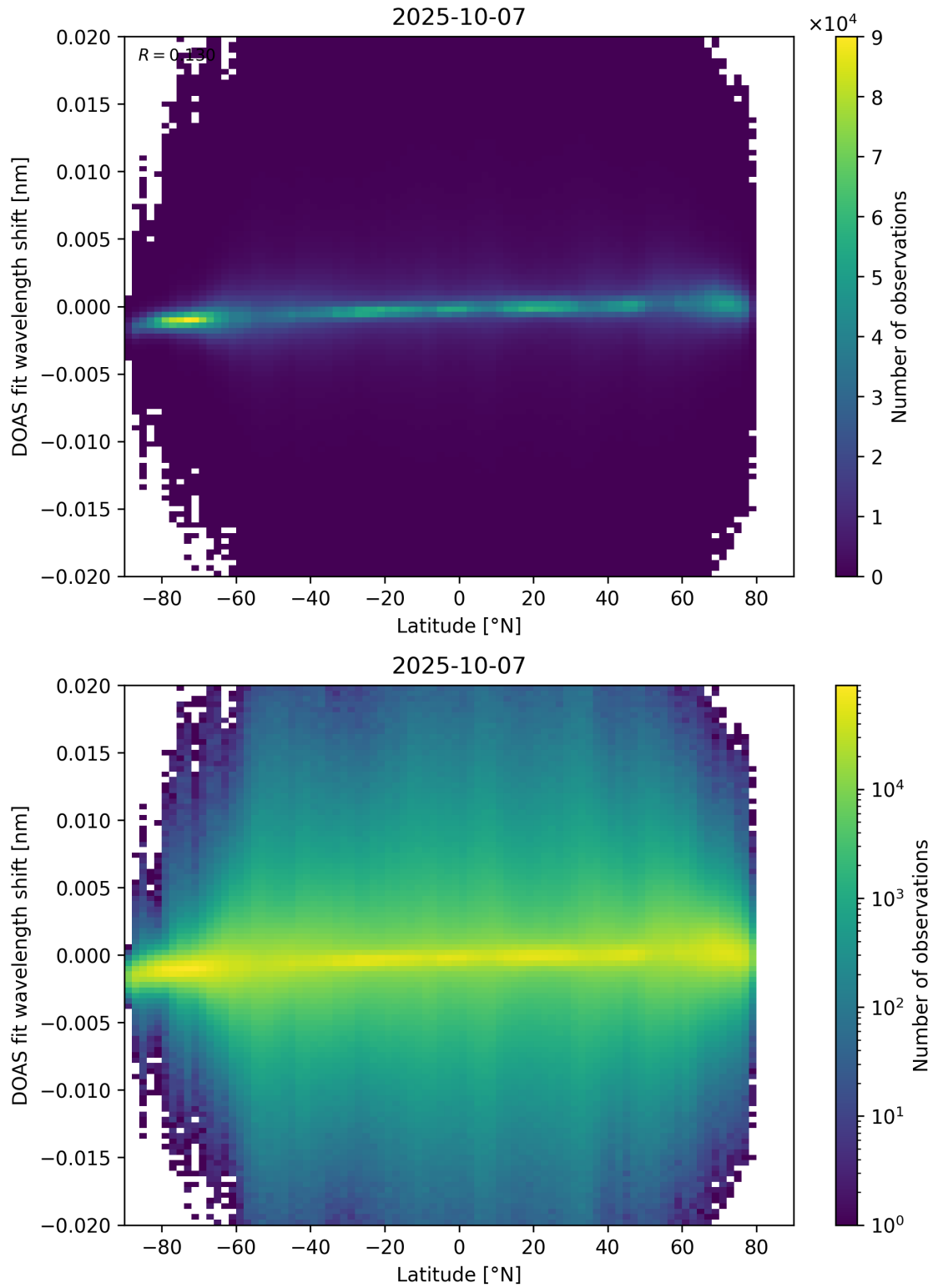
Figure 154: Scatter density plot of “Latitude” against “DOAS fit wavelength shift” for 2025-10-06 to 2025-10-08.
