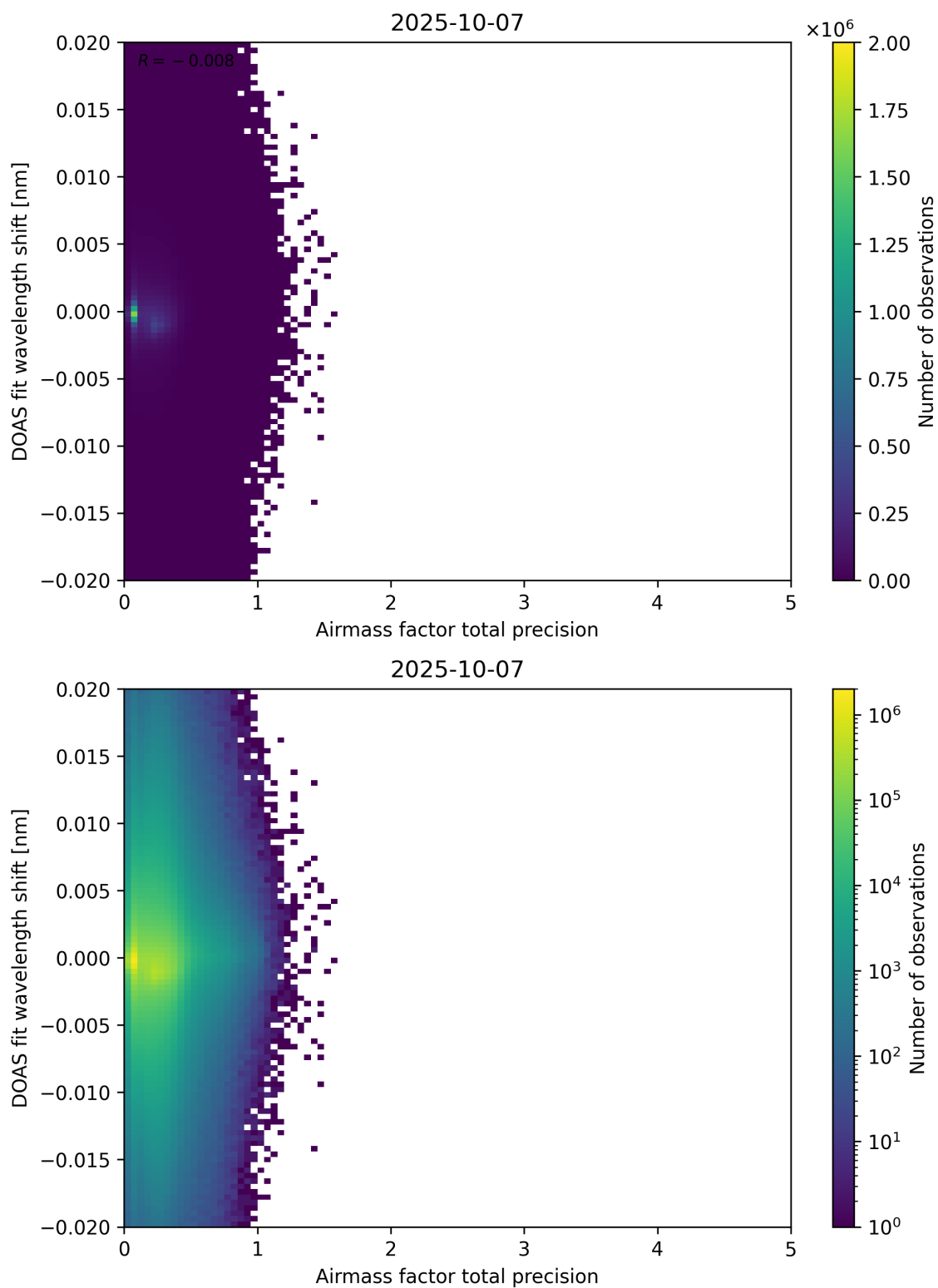
Figure 106: Scatter density plot of “Airmass factor total precision” against “DOAS fit wavelength shift” for 2025-10-06 to 2025-10-08.
