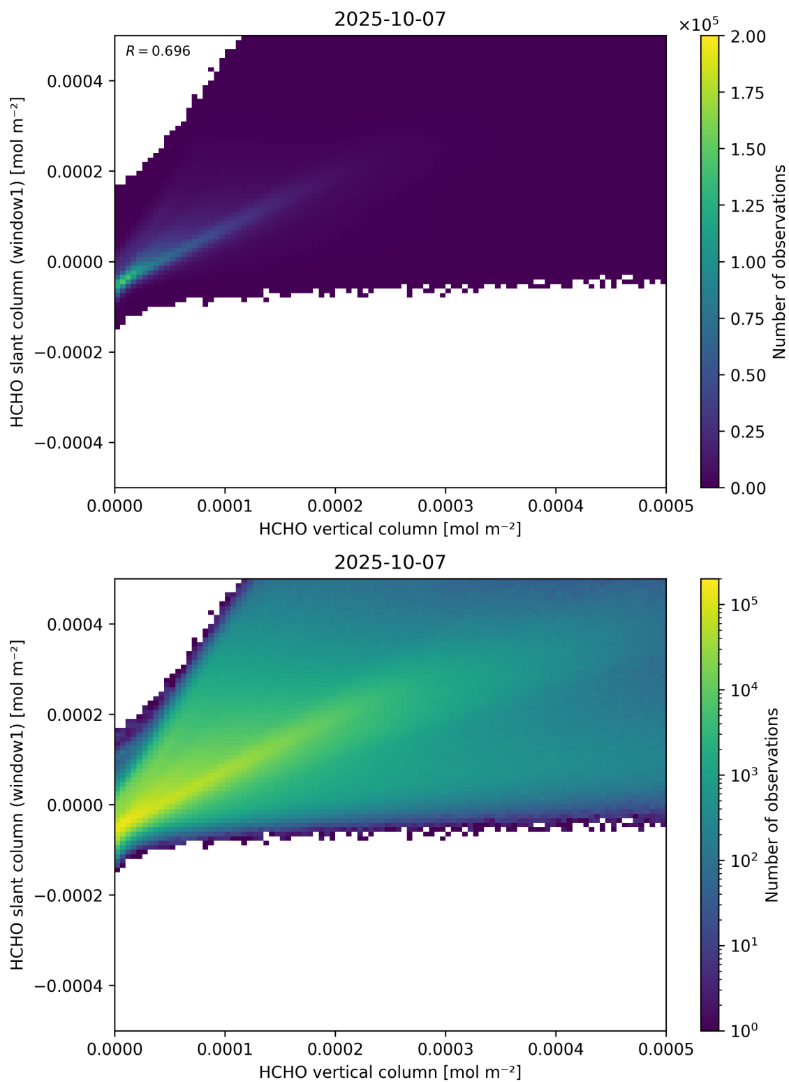
Figure 129: Scatter density plot of “HCHO vertical column” against “HCHO slant column (window1)” for 2025-10-06 to 2025-10-08.
