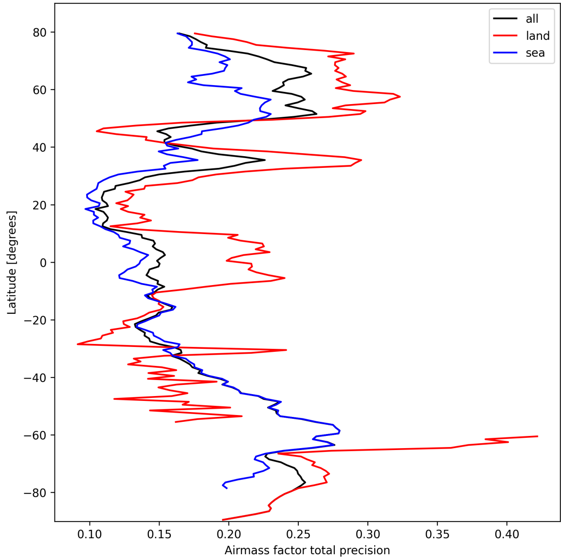
Figure 27: Zonal average of “Airmass factor total precision” for 2025-10-06 to 2025-10-08.
