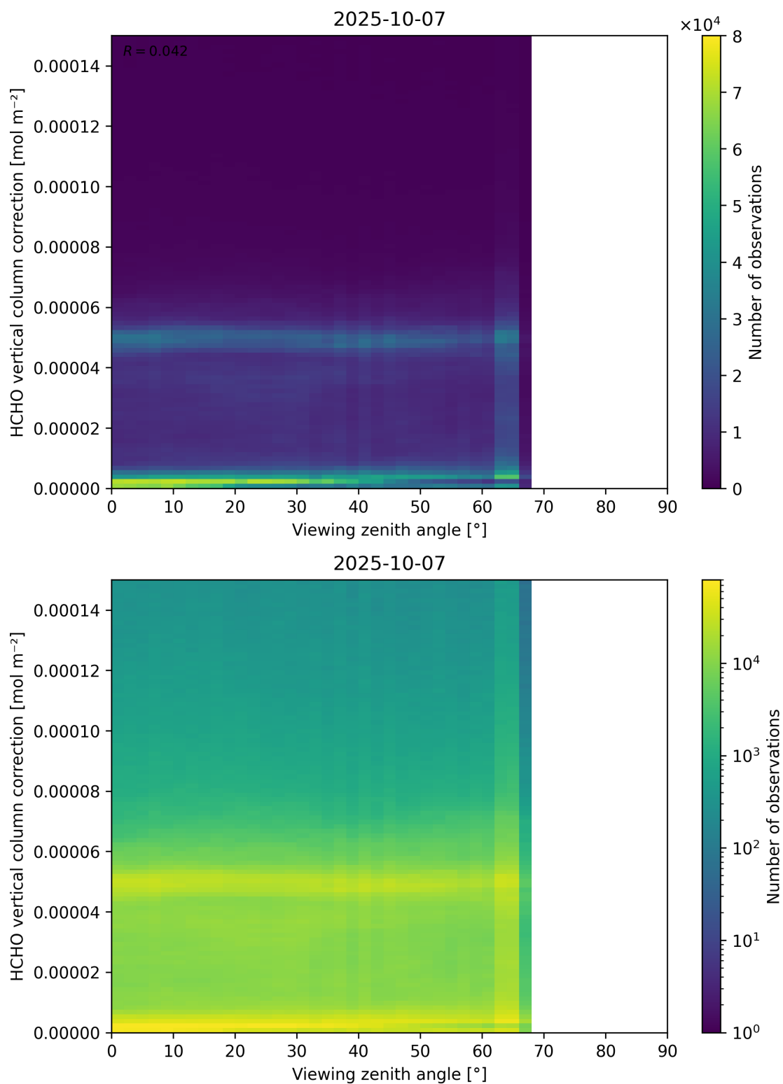
Figure 193: Scatter density plot of “Viewing zenith angle” against “HCHO vertical column correction” for 2025-10-06 to 2025-10-08.
