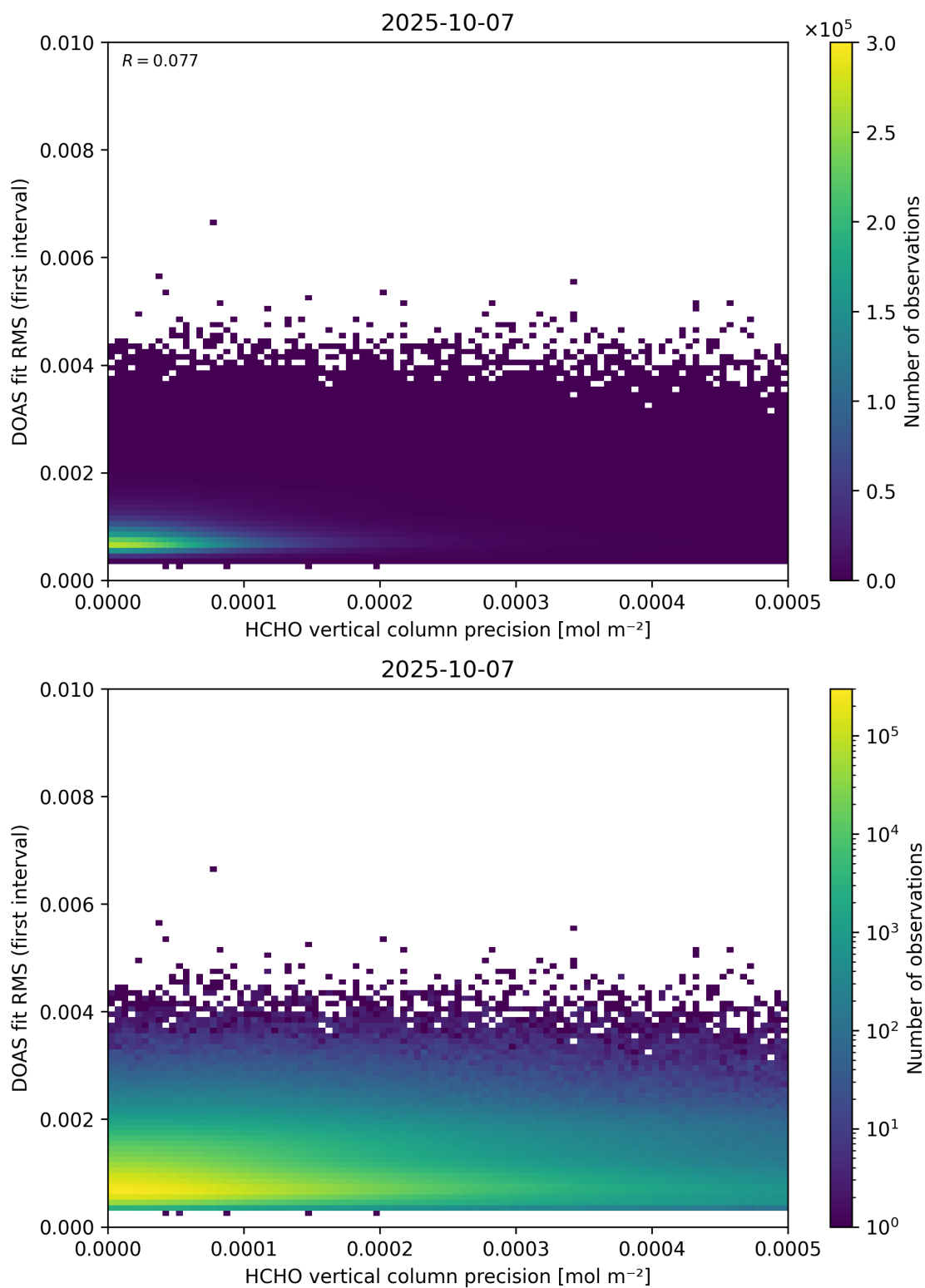
Figure 136: Scatter density plot of “HCHO vertical column precision” against “DOAS fit RMS (first interval)” for 2025-10-06 to 2025-10-08.
