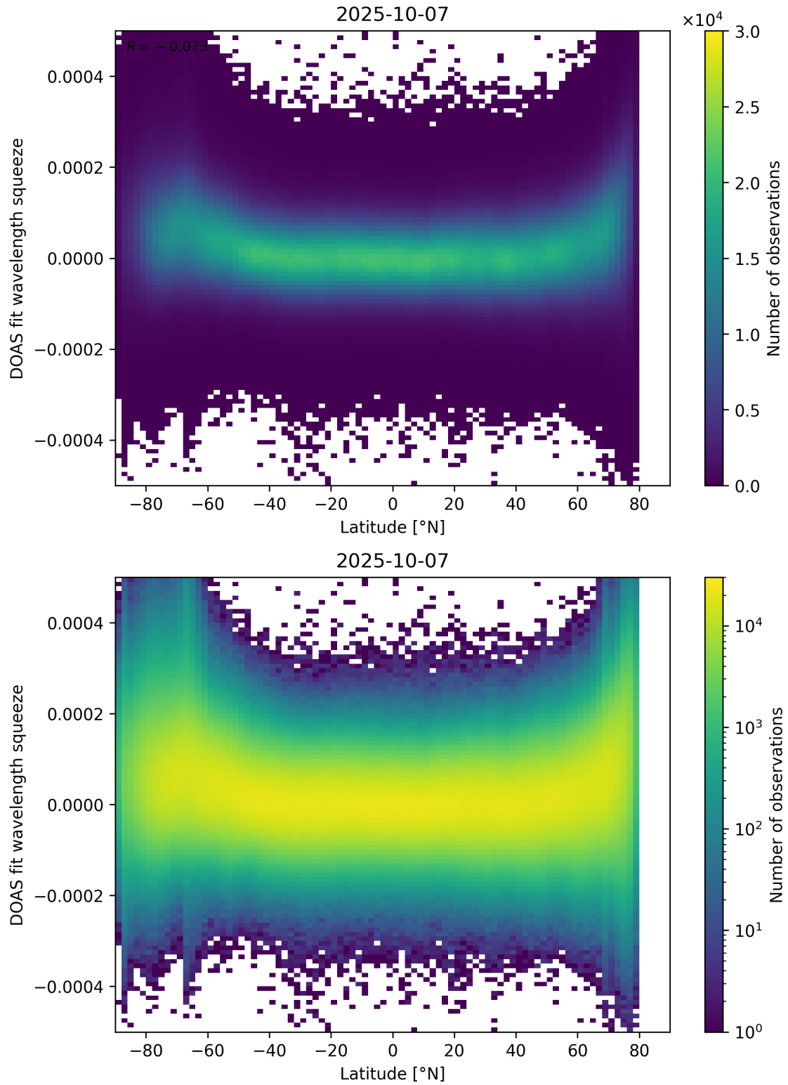
Figure 155: Scatter density plot of “Latitude” against “DOAS fit wavelength squeeze” for 2025-10-06 to 2025-10-08.
