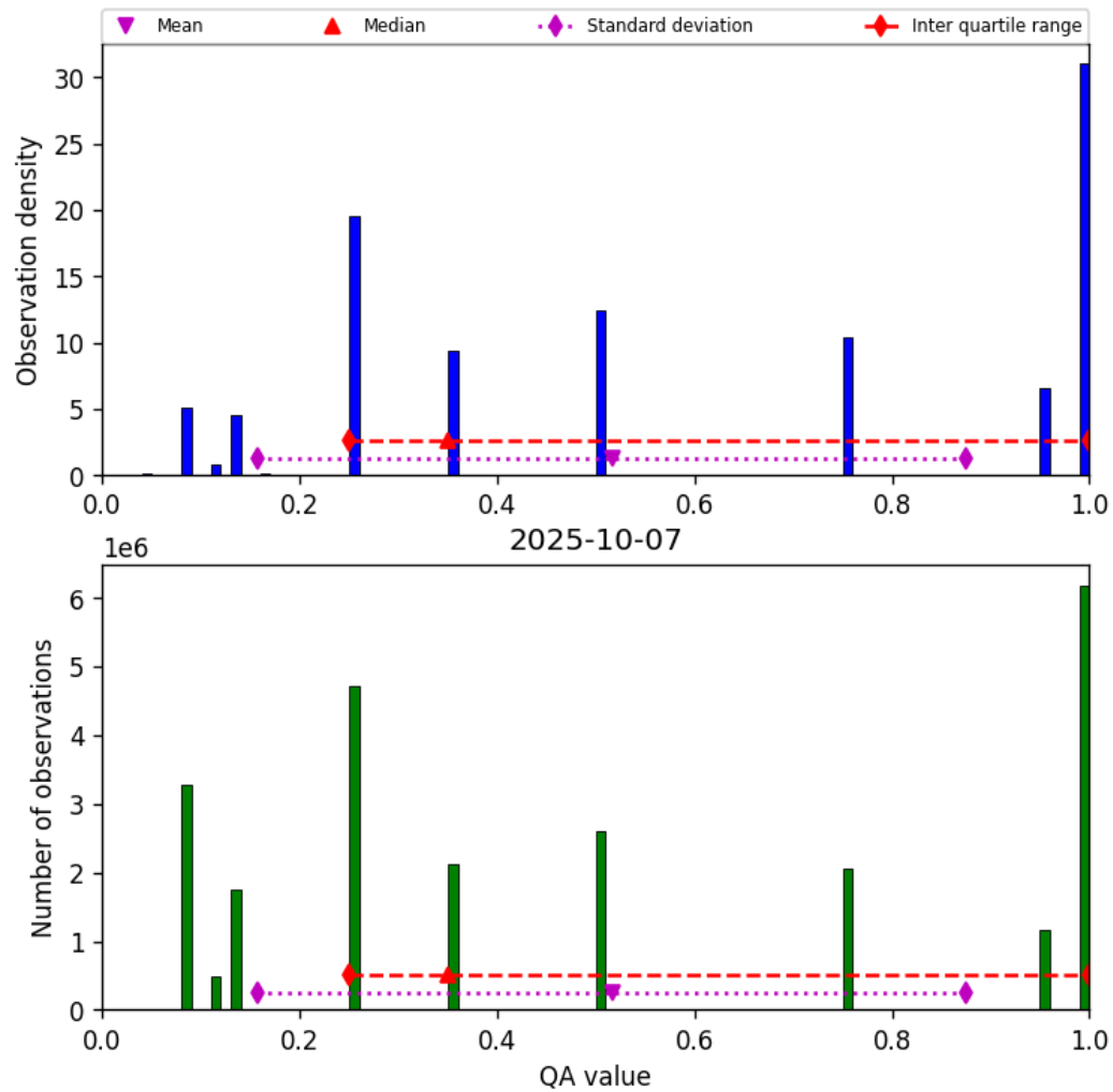
Figure 34: Histogram of “QA value” for 2025-10-06 to 2025-10-08
