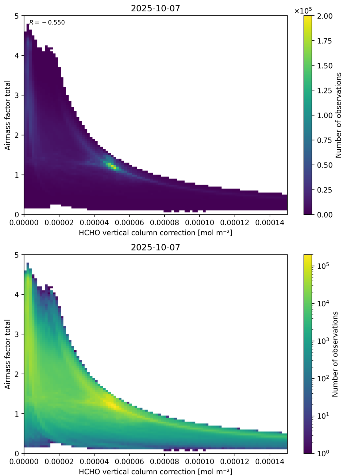
Figure 120: Scatter density plot of “HCHO vertical column correction” against “Airmass factor total” for 2025-10-06 to 2025-10-08.
