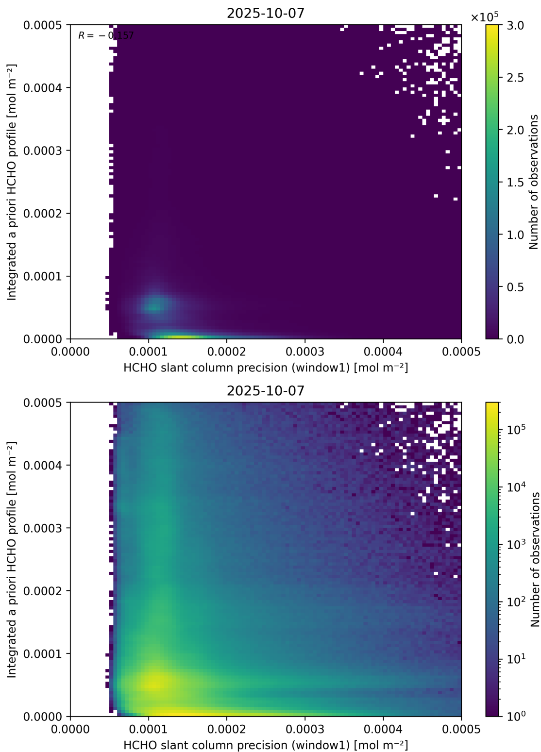
Figure 96: Scatter density plot of “HCHO slant column precision (window1)” against “Integrated a priori HCHO profile” for 2025-10-06 to 2025-10-08.
