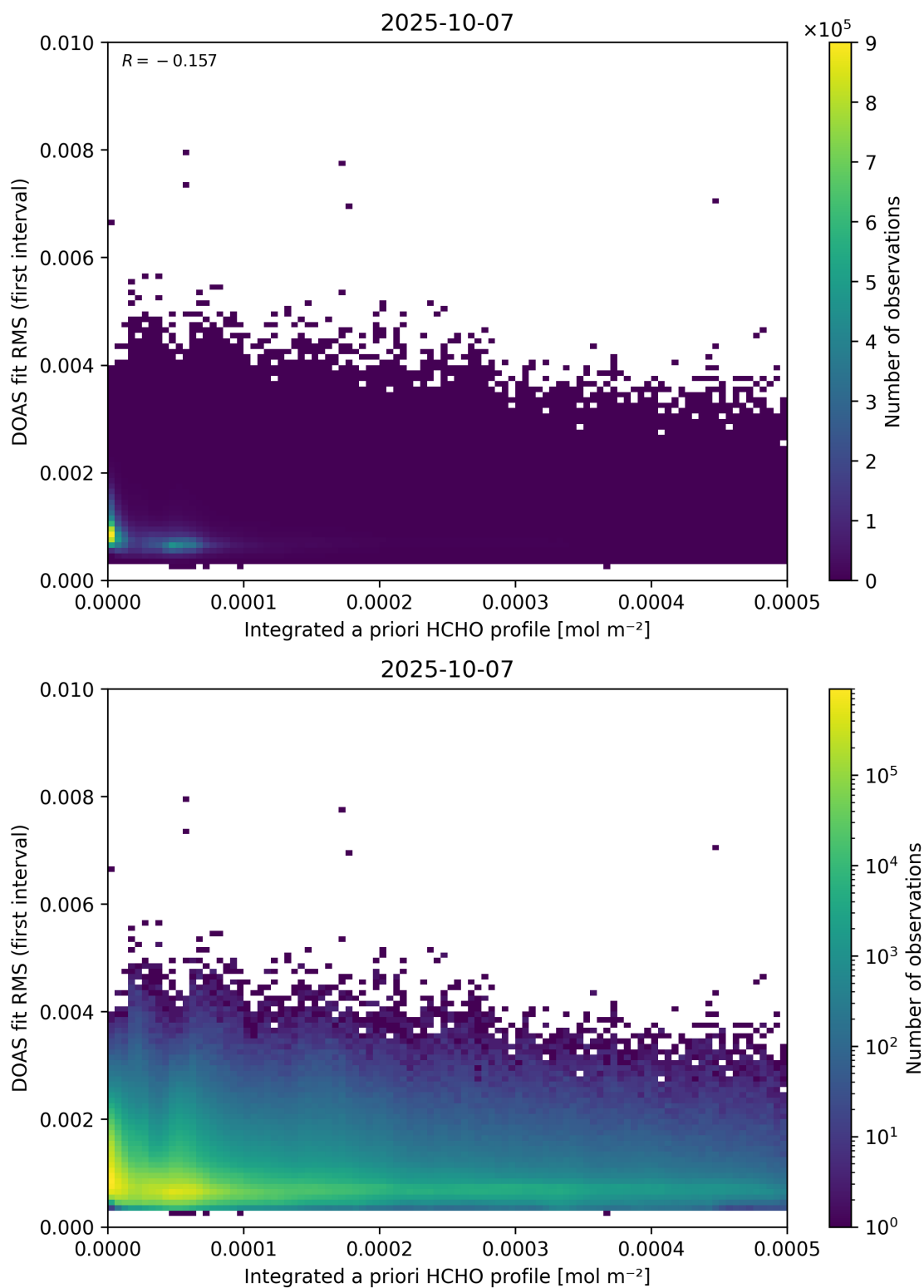
Figure 148: Scatter density plot of “Integrated a priori HCHO profile” against “DOAS fit RMS (first interval)” for 2025-10-06 to 2025-10-08.
