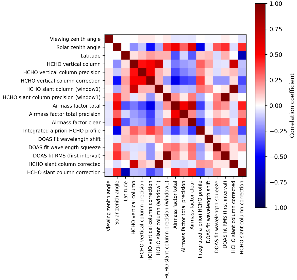
Figure 2: Map of correlation matrix for 2025-10-06 to 2025-10-08.
