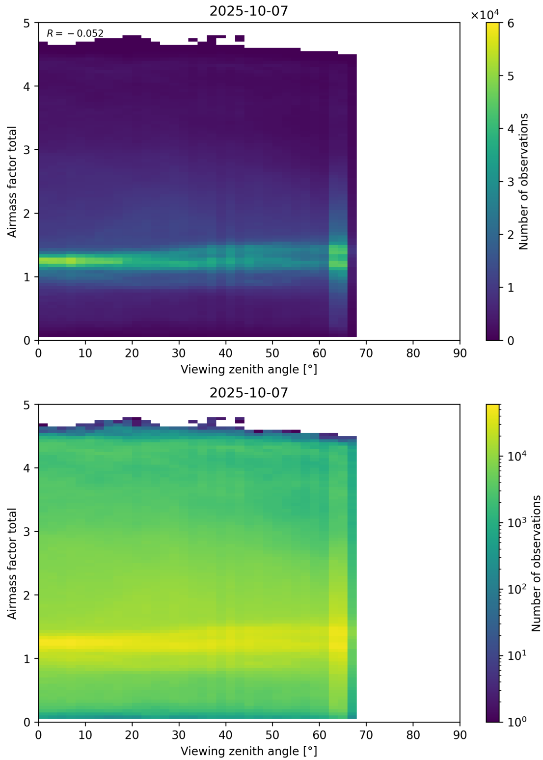
Figure 190: Scatter density plot of “Viewing zenith angle” against “Airmass factor total” for 2025-10-06 to 2025-10-08.
