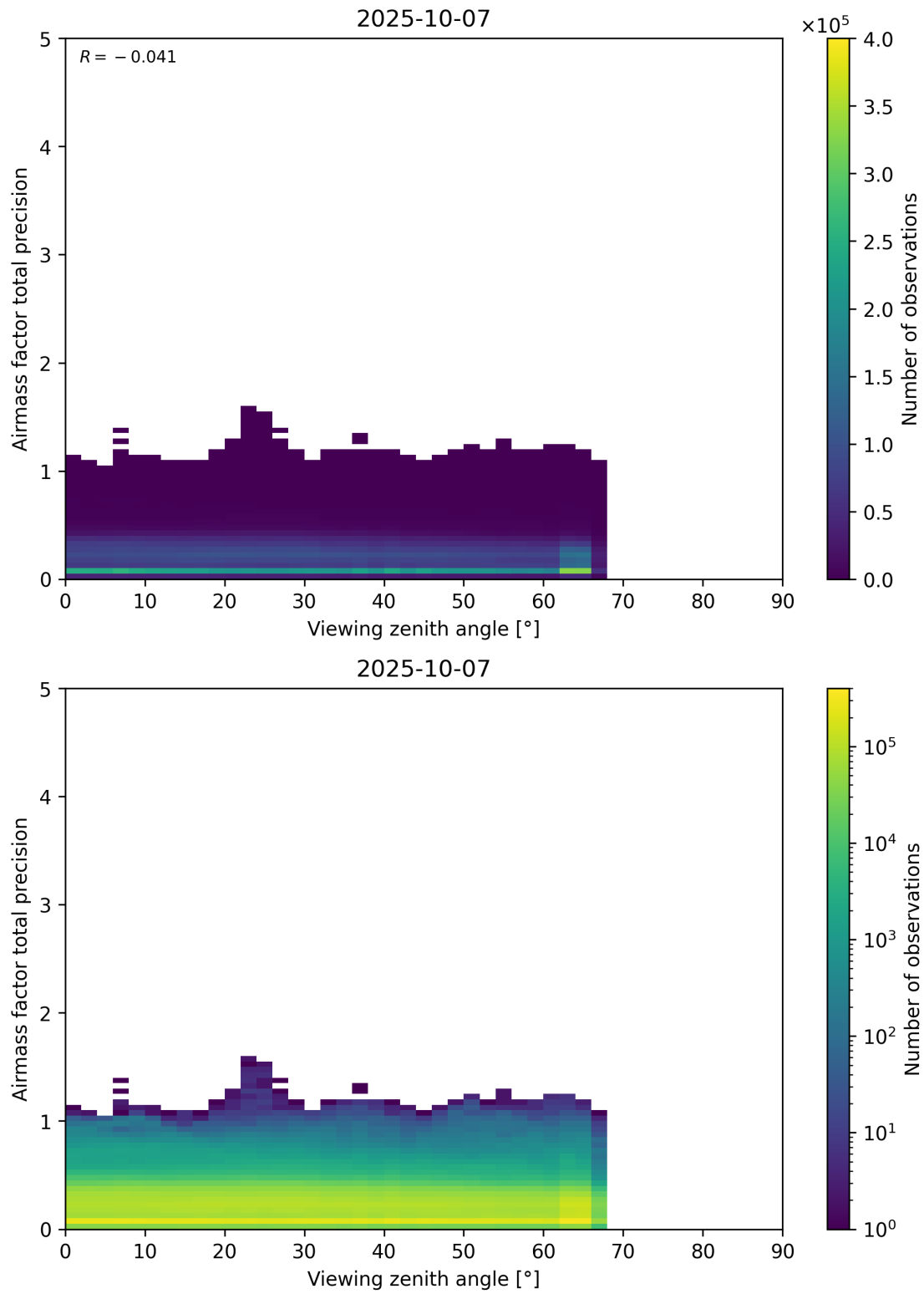
Figure 191: Scatter density plot of “Viewing zenith angle” against “Airmass factor total precision” for 2025-10-06 to 2025-10-08.
