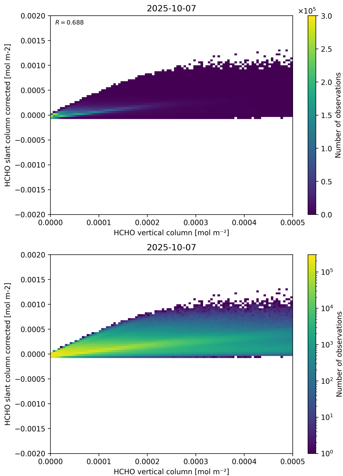
Figure 127: Scatter density plot of “HCHO vertical column” against “HCHO slant column corrected” for 2025-10-06 to 2025-10-08.
