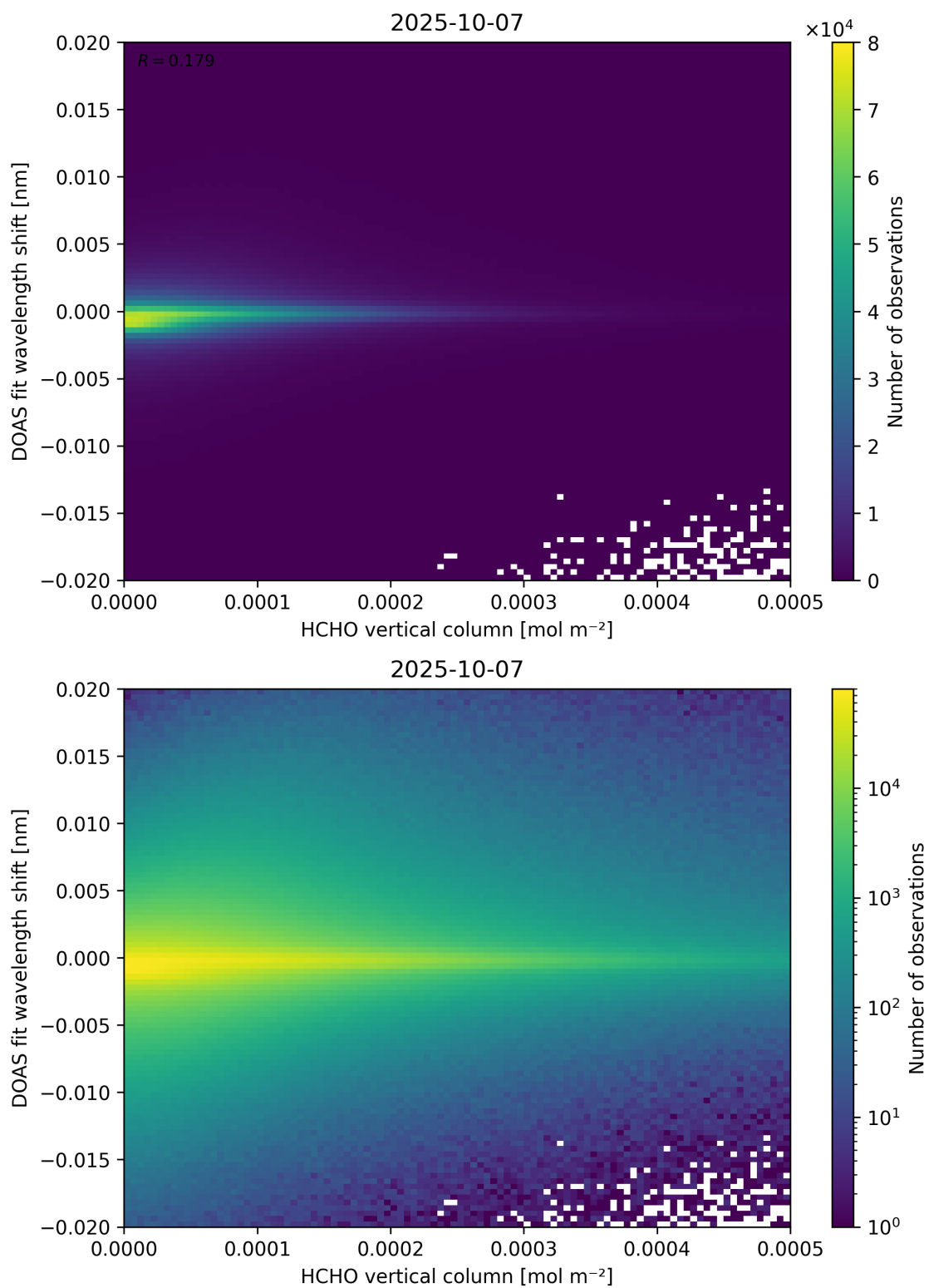
Figure 124: Scatter density plot of “HCHO vertical column” against “DOAS fit wavelength shift” for 2025-10-06 to 2025-10-08.
