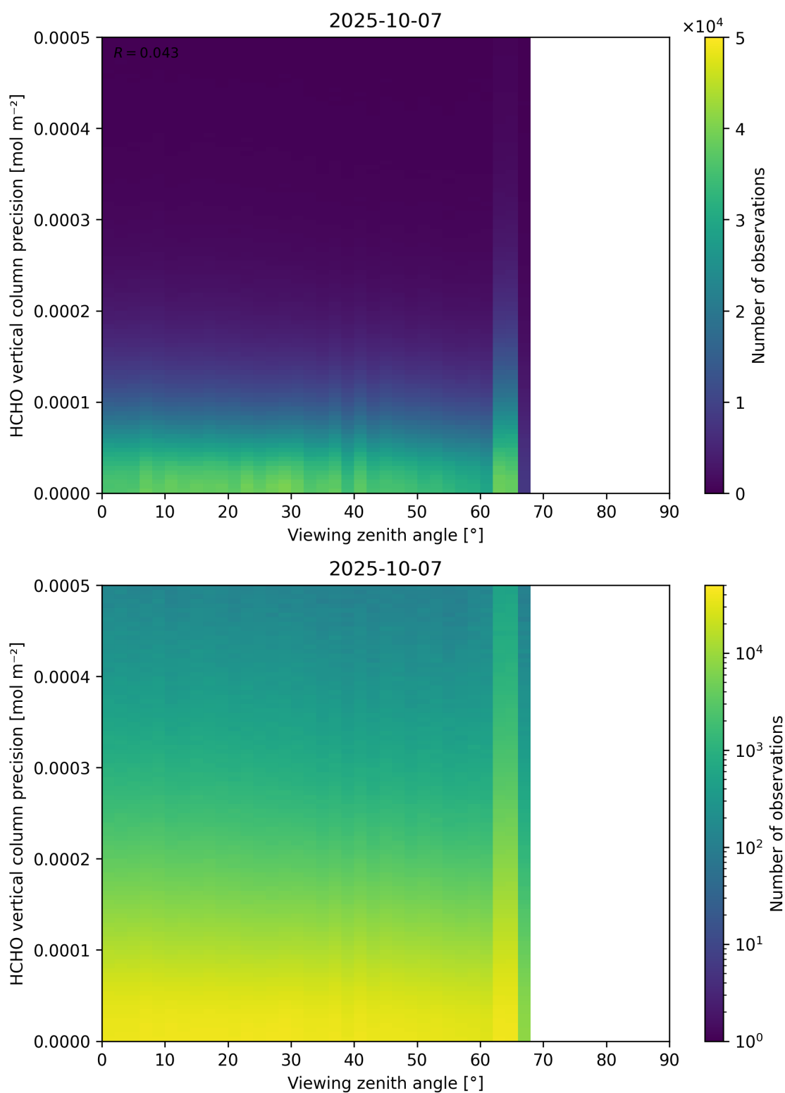
Figure 194: Scatter density plot of “Viewing zenith angle” against “HCHO vertical column precision” for 2025-10-06 to 2025-10-08.
