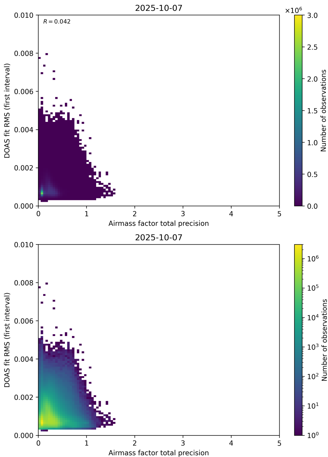
Figure 105: Scatter density plot of “Airmass factor total precision” against “DOAS fit RMS (first interval)” for 2025-10-06 to 2025-10-08.
