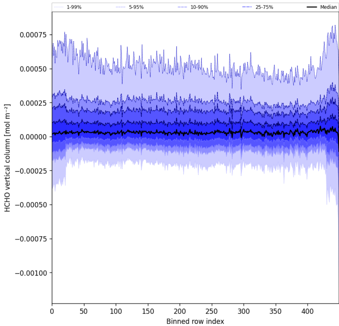
Figure 49: Along track statistics of “HCHO vertical column” for 2025-10-06 to 2025-10-08
