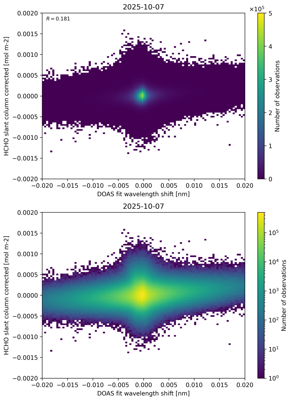
Figure 66: Scatter density plot of “DOAS fit wavelength shift” against “HCHO slant column corrected” for 2025-10-06 to 2025-10-08.
