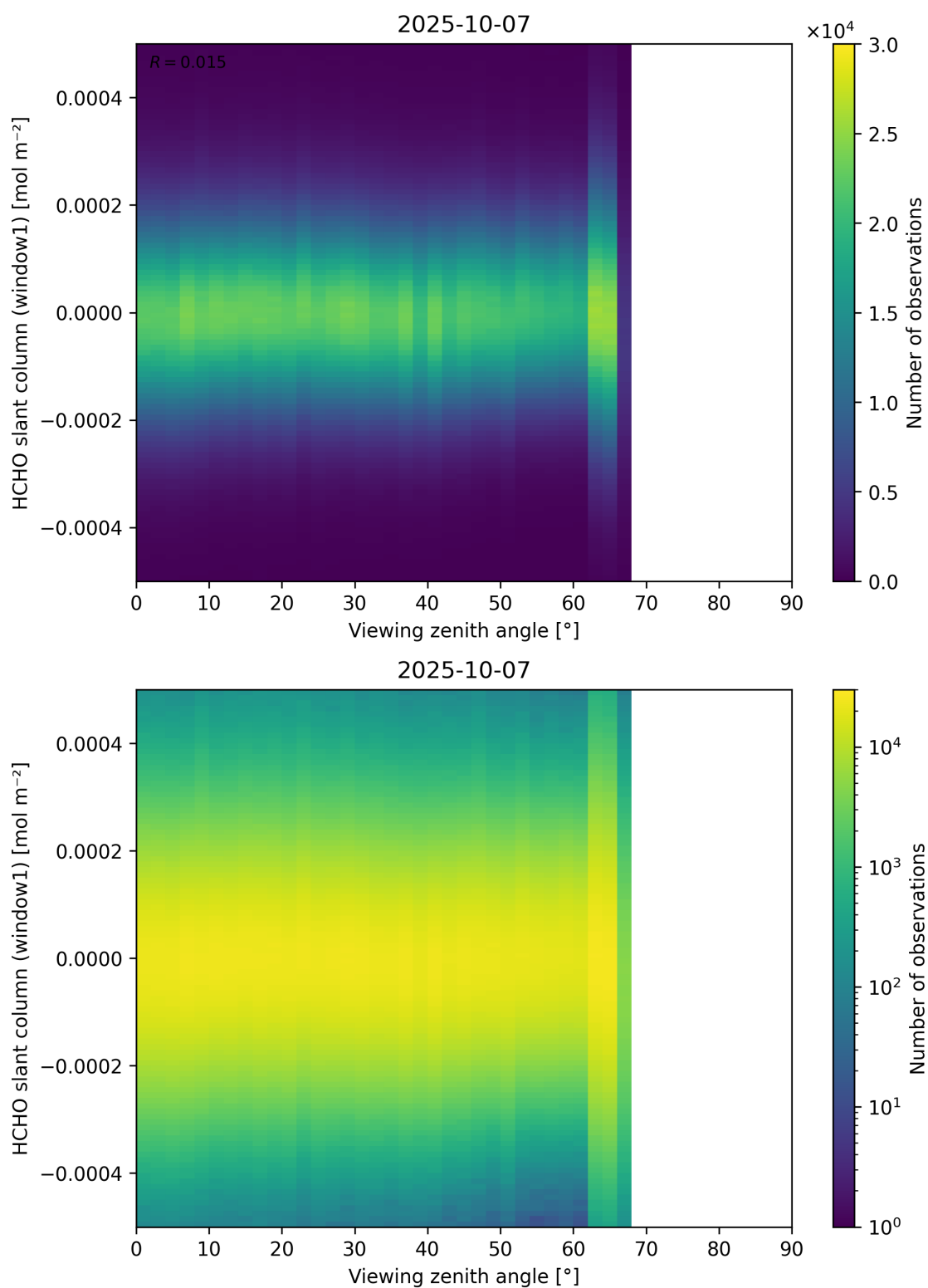
Figure 188: Scatter density plot of “Viewing zenith angle” against “HCHO slant column (window1)” for 2025-10-06 to 2025-10-08.
