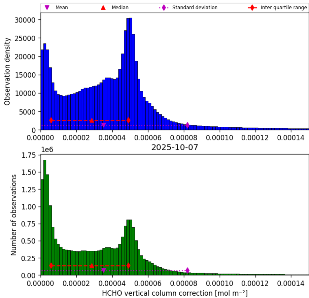
Figure 37: Histogram of “HCHO vertical column correction” for 2025-10-06 to 2025-10-08
