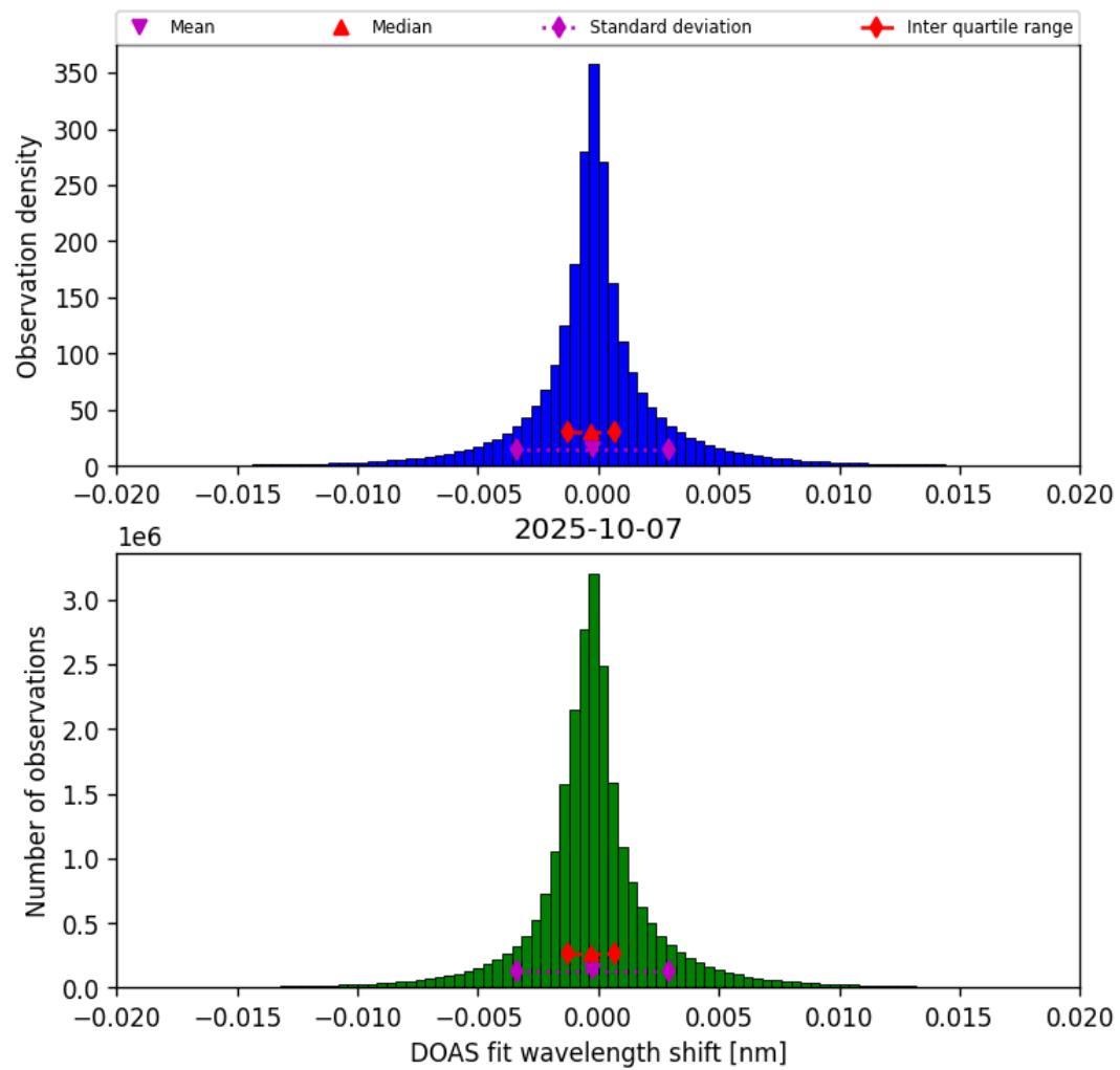
Figure 44: Histogram of “DOAS fit wavelength shift” for 2025-10-06 to 2025-10-08
