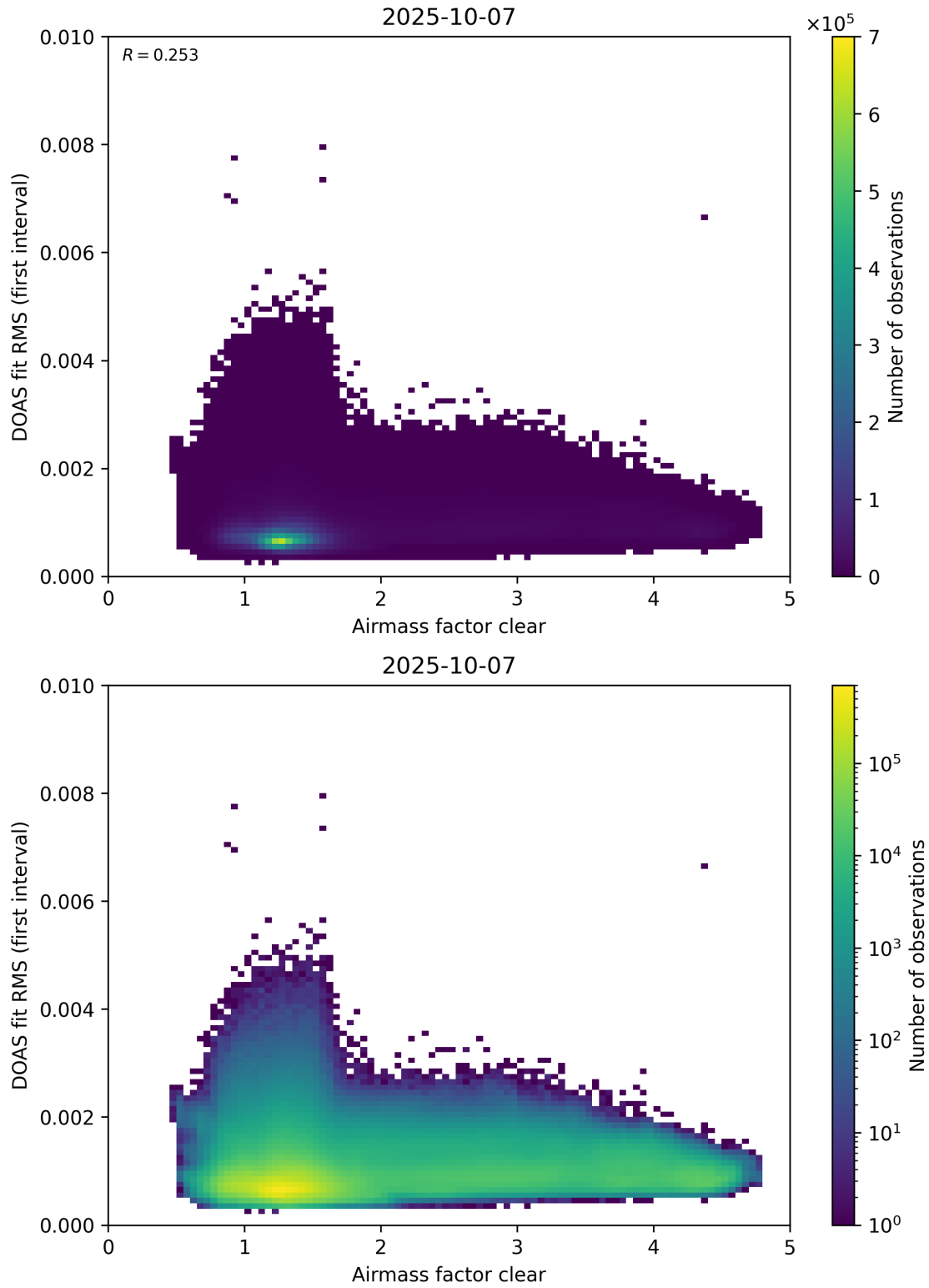
Figure 71: Scatter density plot of “Airmass factor clear” against “DOAS fit RMS (first interval)” for 2025-10-06 to 2025-10-08.
