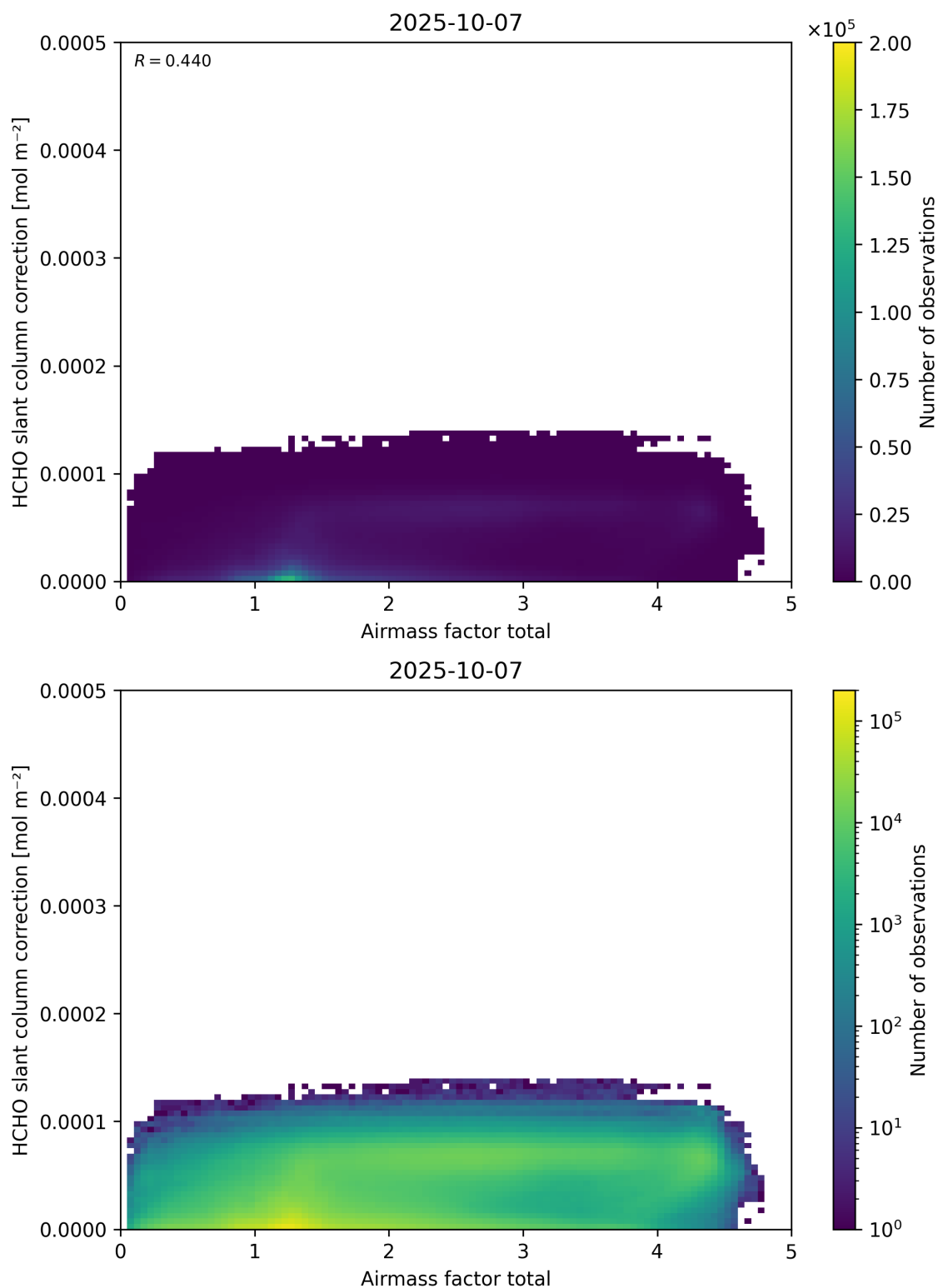
Figure 102: Scatter density plot of “Airmass factor total” against “HCHO slant column correction” for 2025-10-06 to 2025-10-08.
