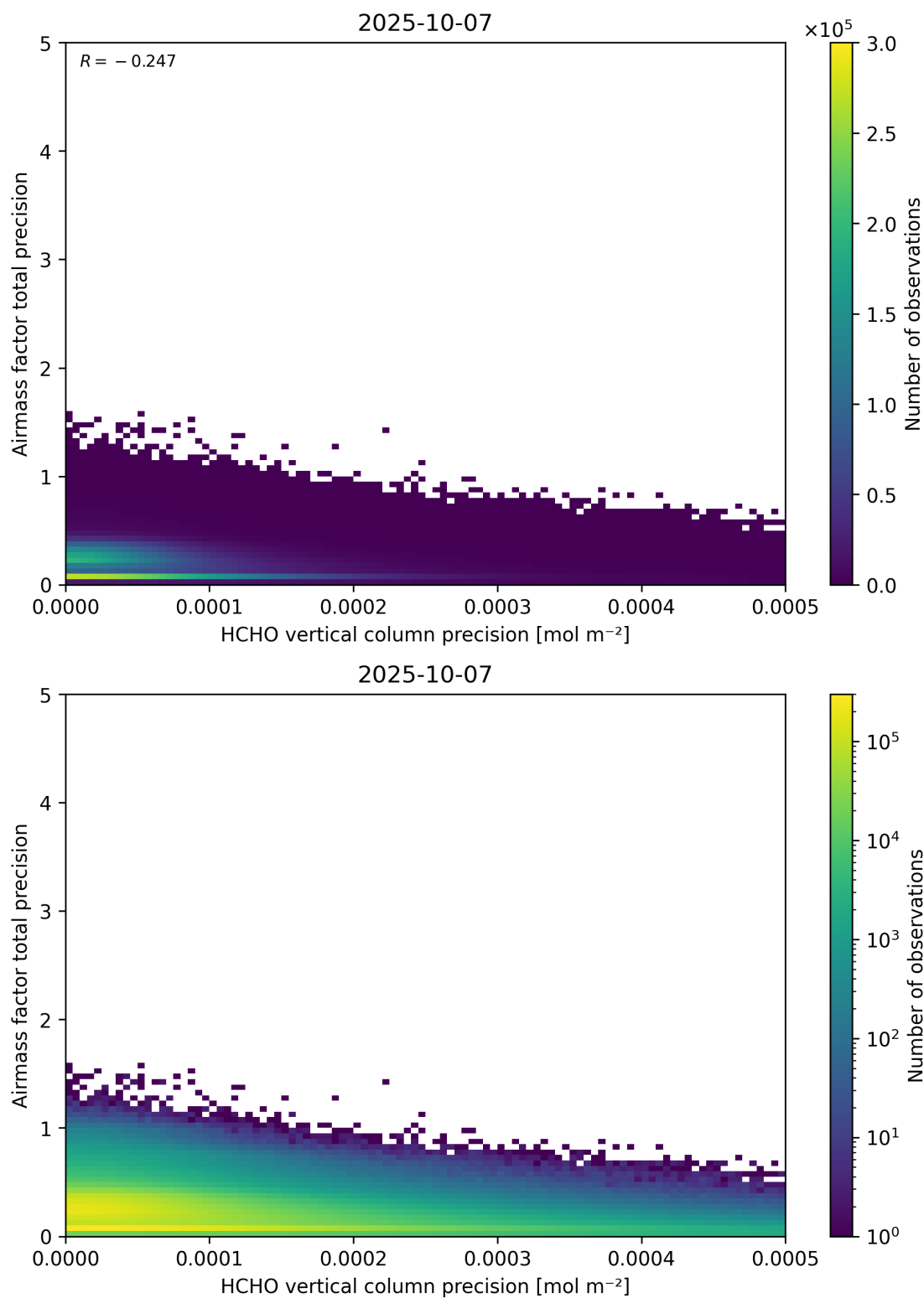
Figure 145: Scatter density plot of “HCHO vertical column precision” against “Airmass factor total precision” for 2025-10-06 to 2025-10-08.
