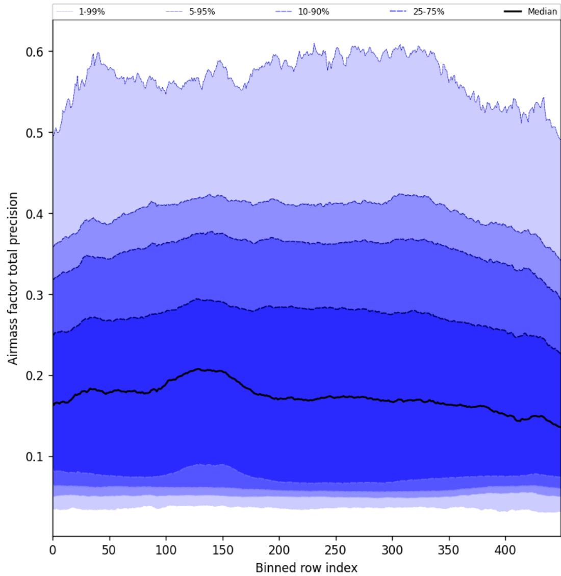
Figure 55: Along track statistics of “Airmass factor total precision” for 2025-10-06 to 2025-10-08
