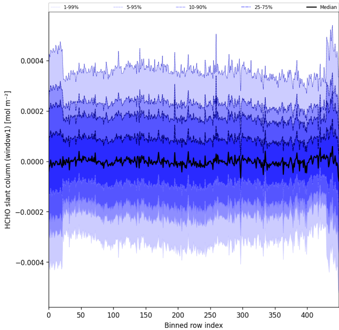
Figure 52: Along track statistics of “HCHO slant column (window1)” for 2025-10-06 to 2025-10-08
