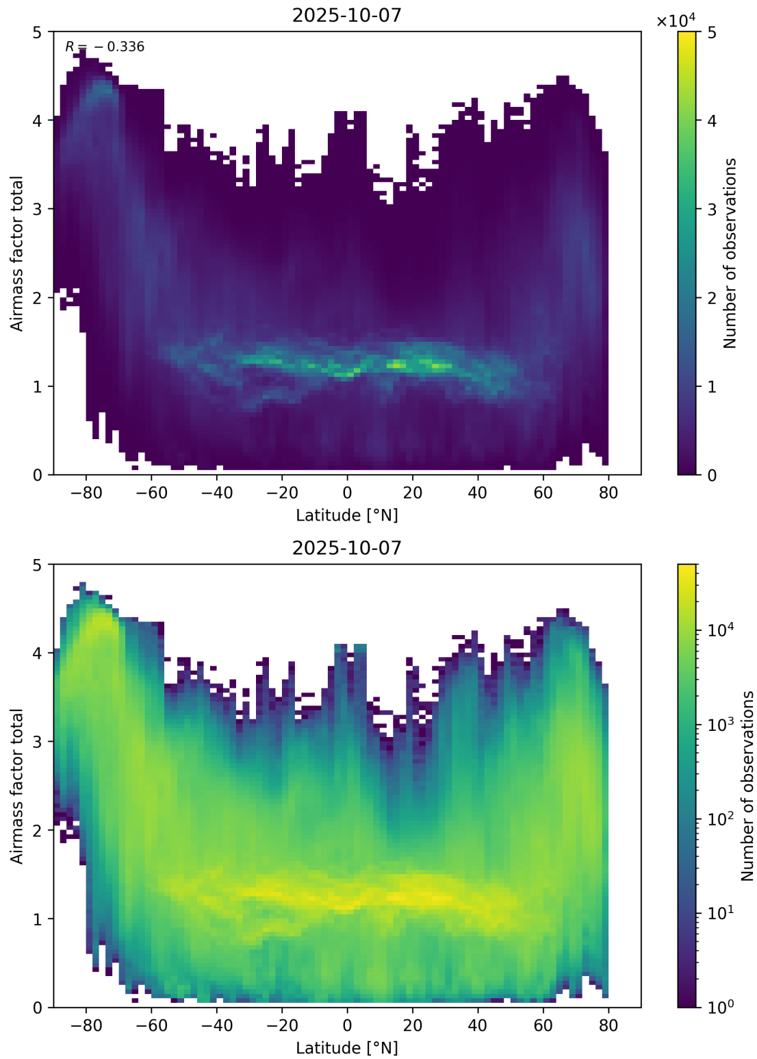
Figure 161: Scatter density plot of “Latitude” against “Airmass factor total” for 2025-10-06 to 2025-10-08.
