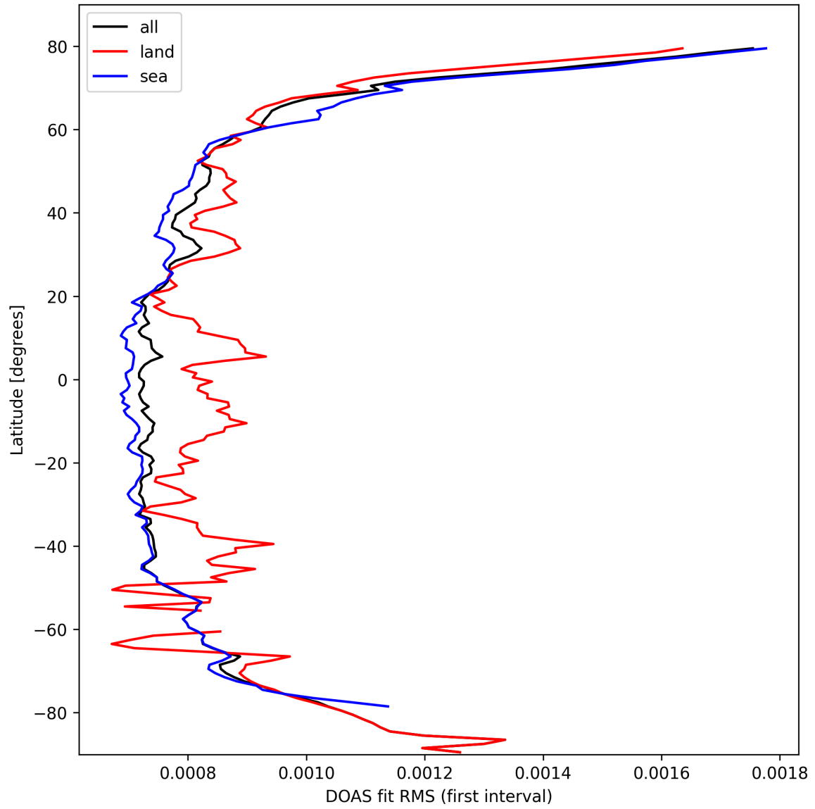
Figure 32: Zonal average of “DOAS fit RMS (first interval)” for 2025-10-06 to 2025-10-08.
