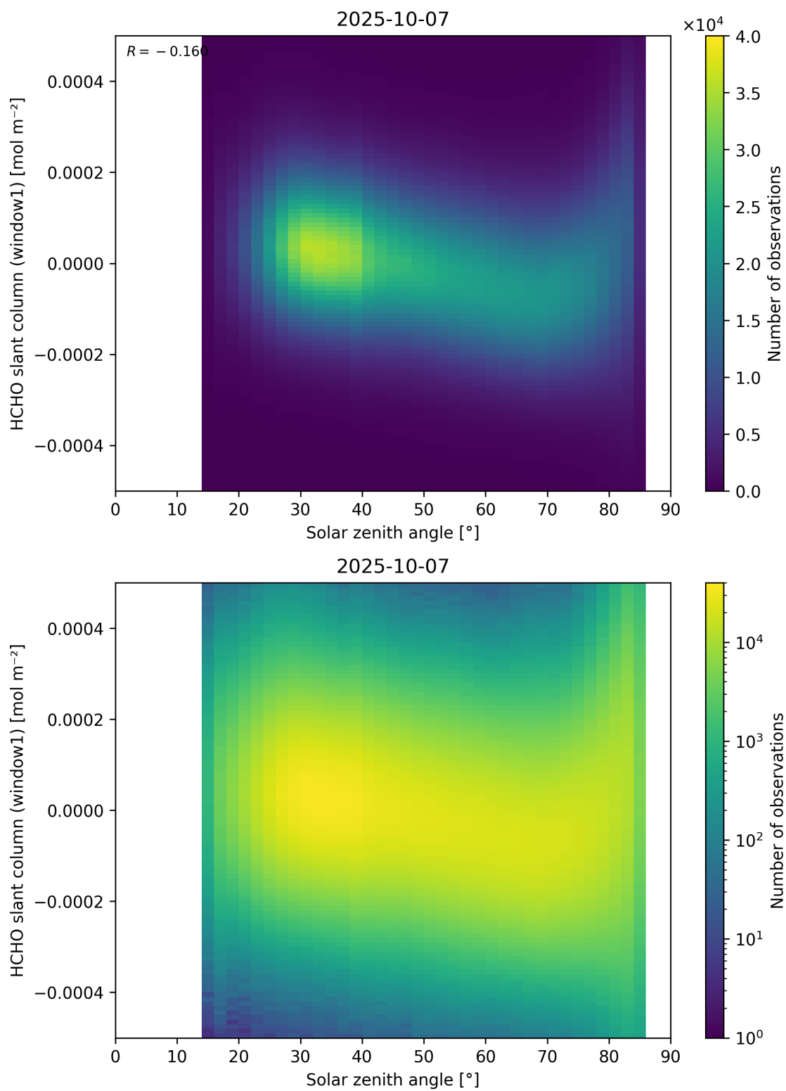
Figure 173: Scatter density plot of “Solar zenith angle” against “HCHO slant column (window1)” for 2025-10-06 to 2025-10-08.
