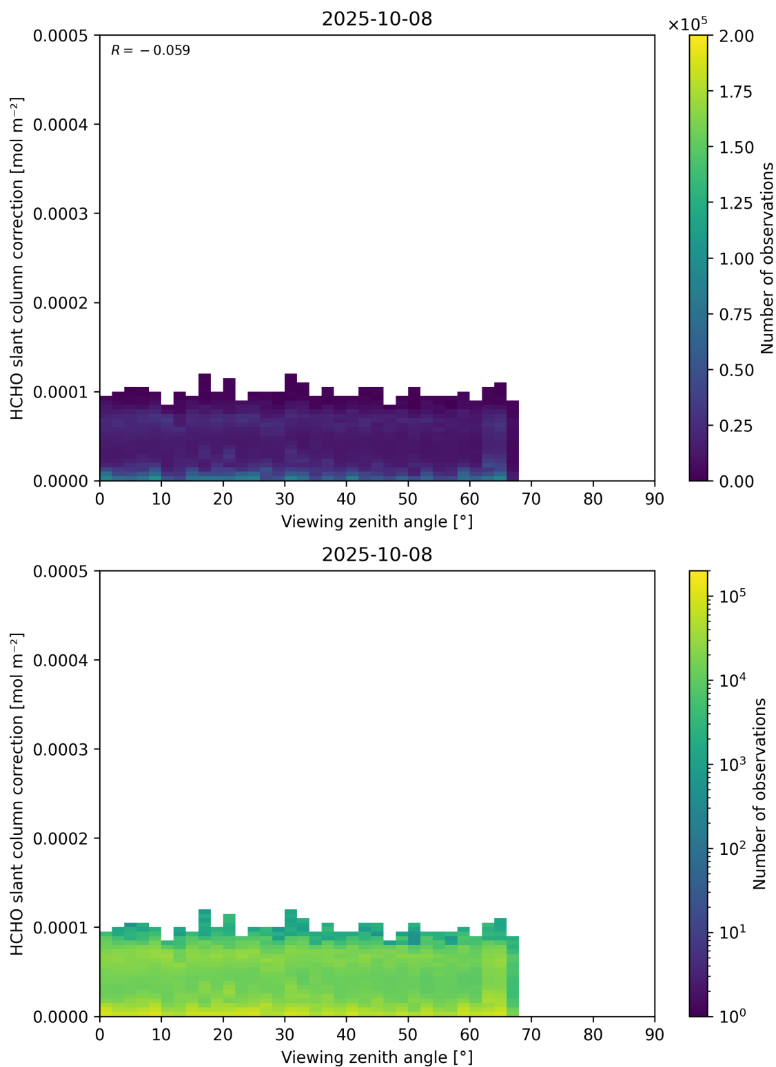
Figure 187: Scatter density plot of “Viewing zenith angle” against “HCHO slant column correction” for 2025-10-07 to 2025-10-09.
