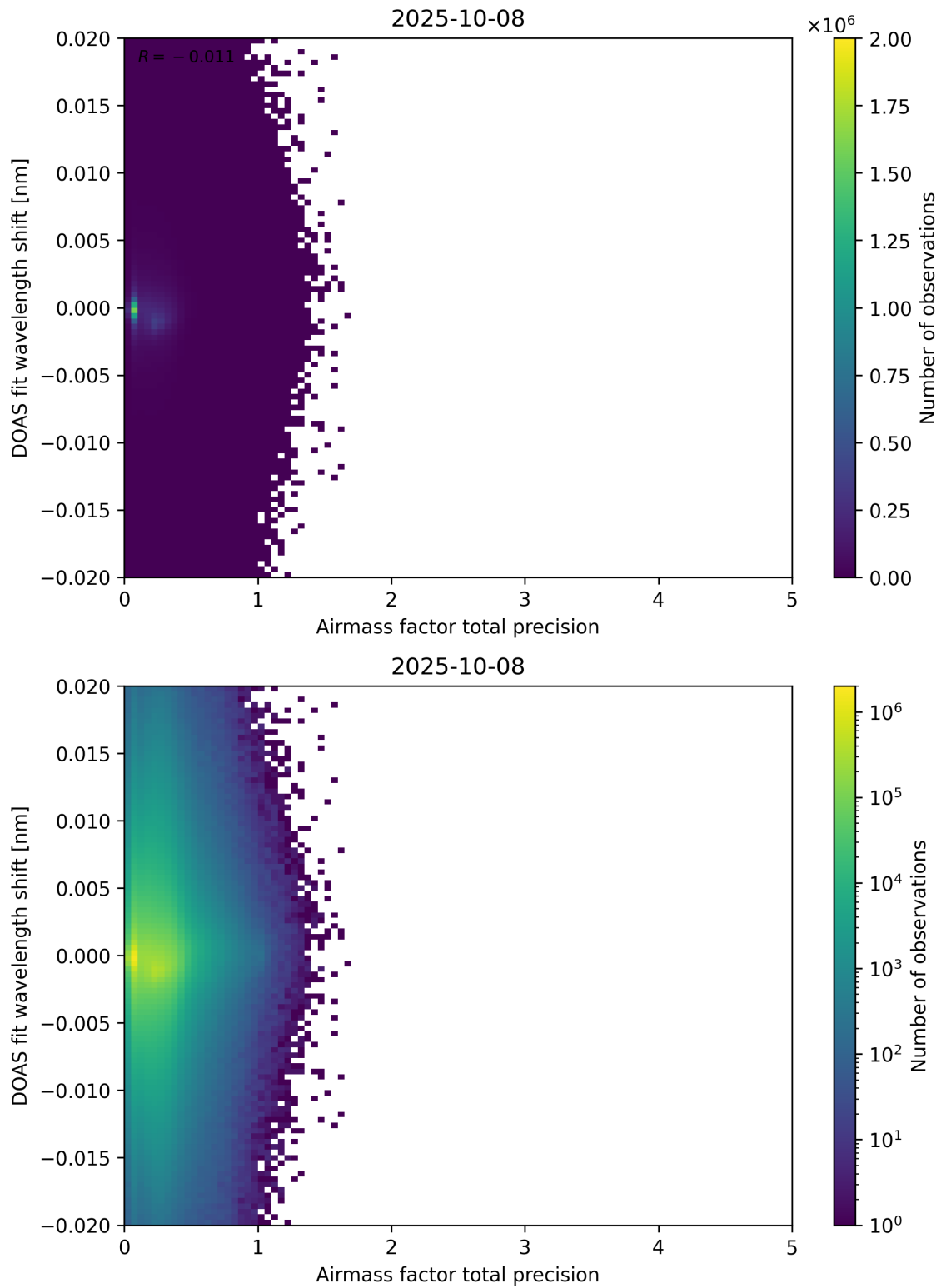
Figure 106: Scatter density plot of “Airmass factor total precision” against “DOAS fit wavelength shift” for 2025-10-07 to 2025-10-09.
