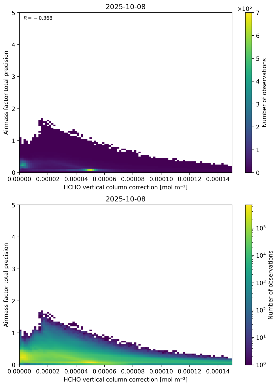
Figure 121: Scatter density plot of “HCHO vertical column correction” against “Airmass factor total precision” for 2025-10-07 to 2025-10-09.
