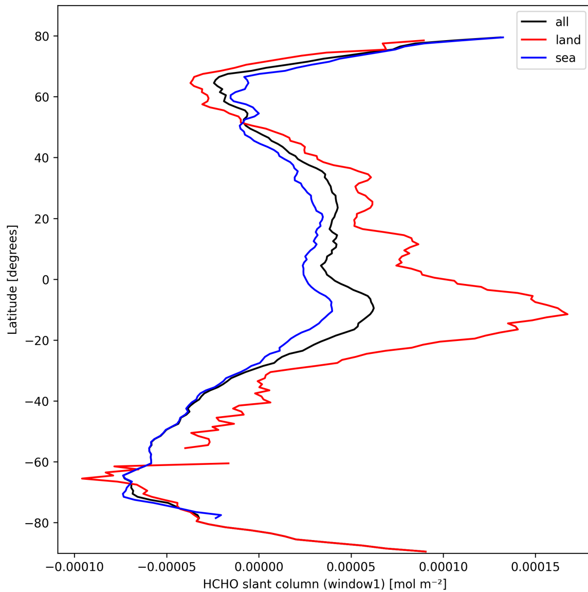
Figure 24: Zonal average of “HCHO slant column (window1)” for 2025-10-07 to 2025-10-09.
