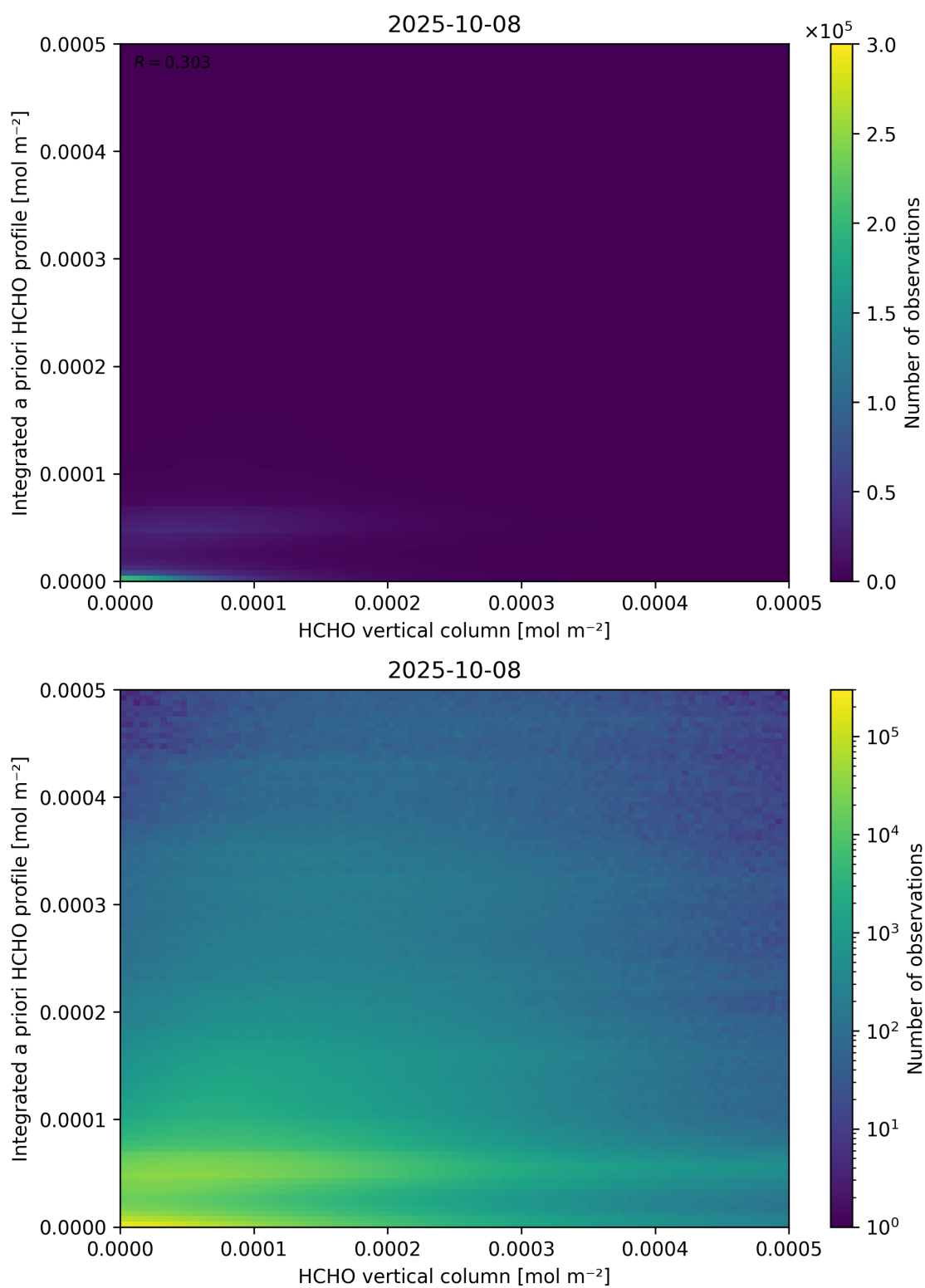
Figure 135: Scatter density plot of “HCHO vertical column” against “Integrated a priori HCHO profile” for 2025-10-07 to 2025-10-09.
