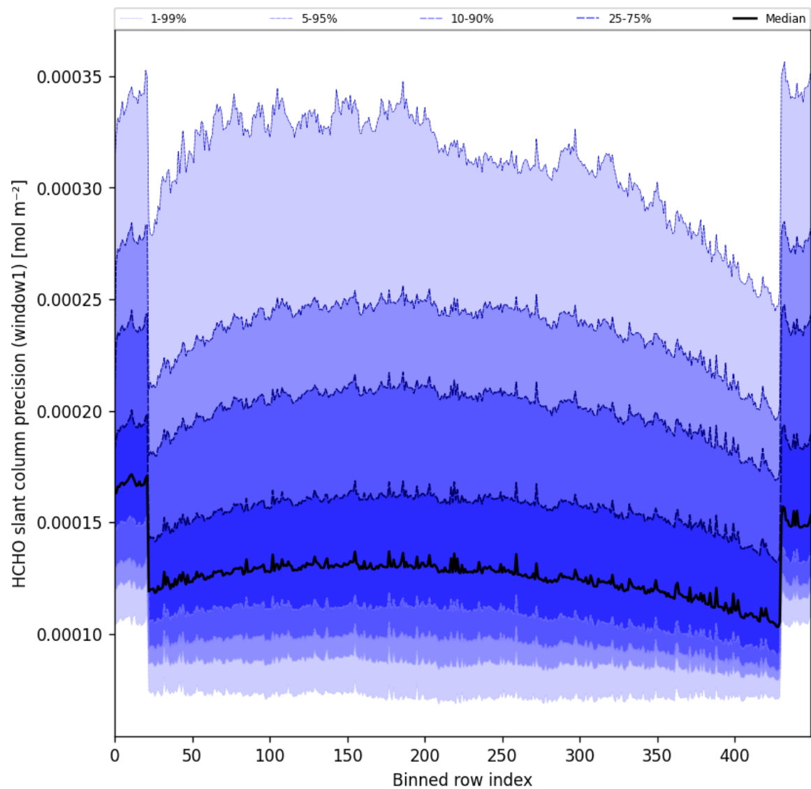
Figure 53: Along track statistics of “HCHO slant column precision (window1)” for 2025-10-07 to 2025-10-09
