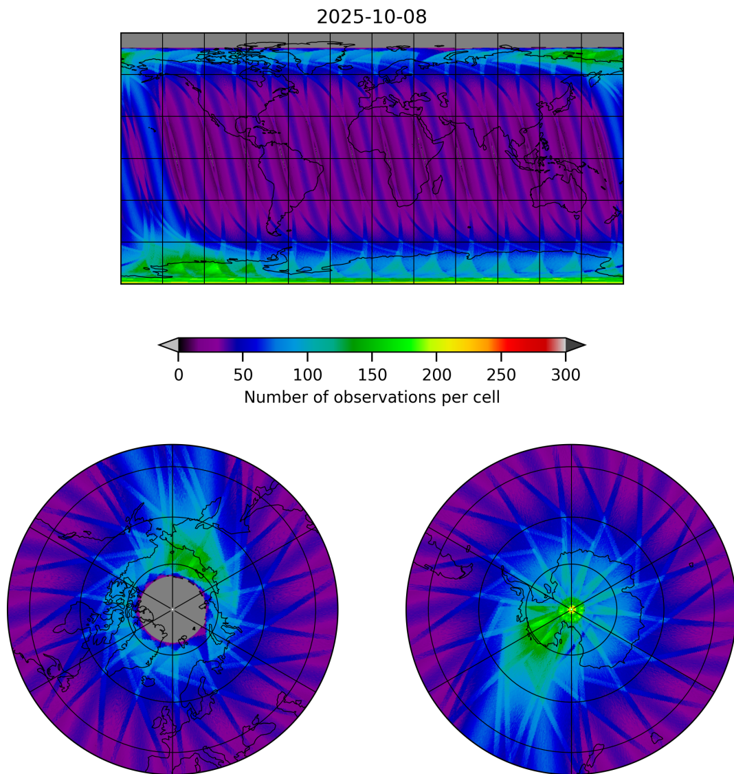
Figure 19: Map of the number of observations for 2025-10-07 to 2025-10-09
