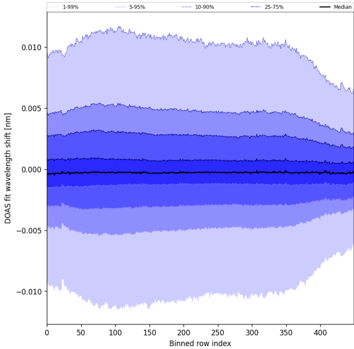
Figure 58: Along track statistics of “DOAS fit wavelength shift” for 2025-10-07 to 2025-10-09
