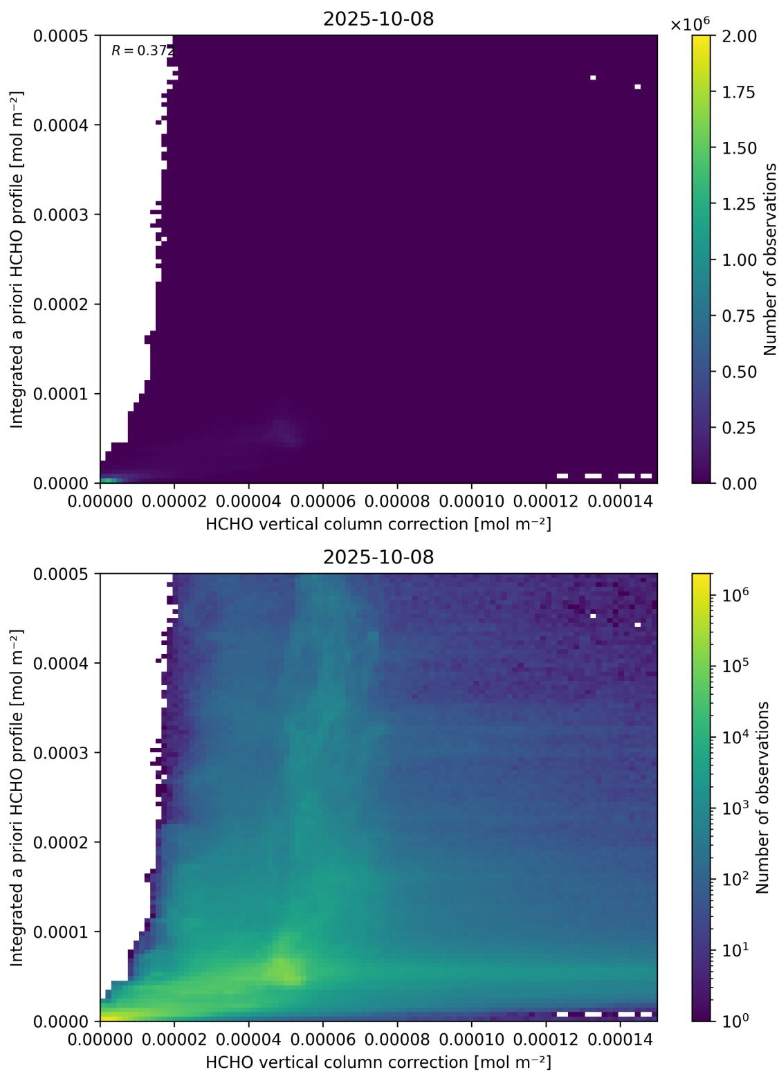
Figure 122: Scatter density plot of “HCHO vertical column correction” against “Integrated a priori HCHO profile” for 2025-10-07 to 2025-10-09.
