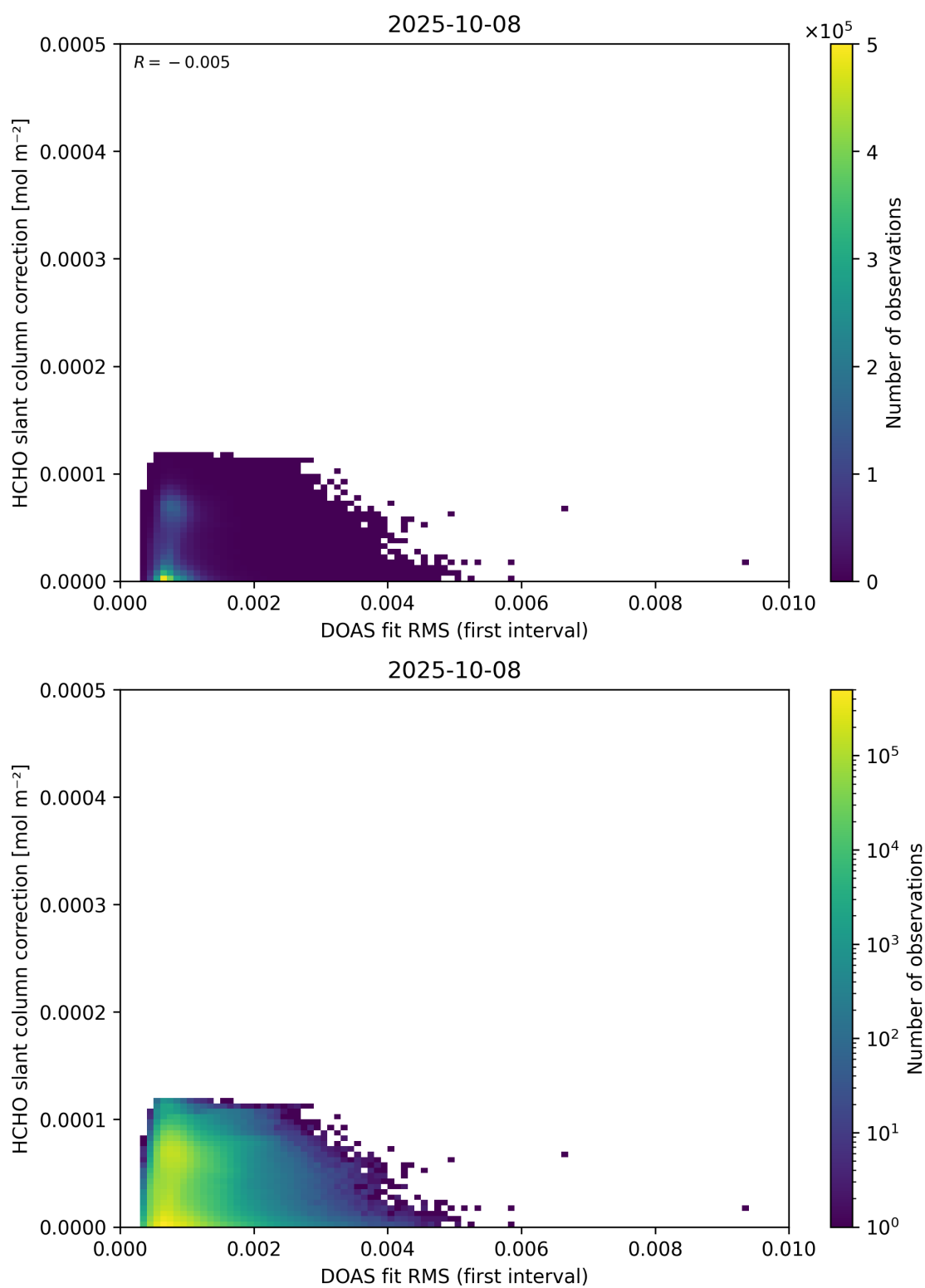
Figure 63: Scatter density plot of “DOAS fit RMS (first interval)” against “HCHO slant column correction” for 2025-10-07 to 2025-10-09.
