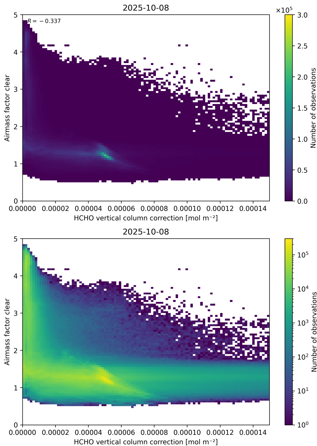
Figure 115: Scatter density plot of “HCHO vertical column correction” against “Airmass factor clear” for 2025-10-07 to 2025-10-09.
