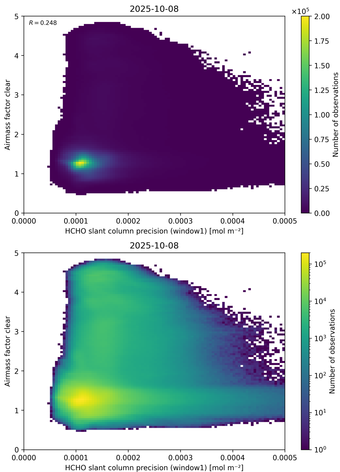
Figure 91: Scatter density plot of “HCHO slant column precision (window1)” against “Airmass factor clear” for 2025-10-07 to 2025-10-09.
