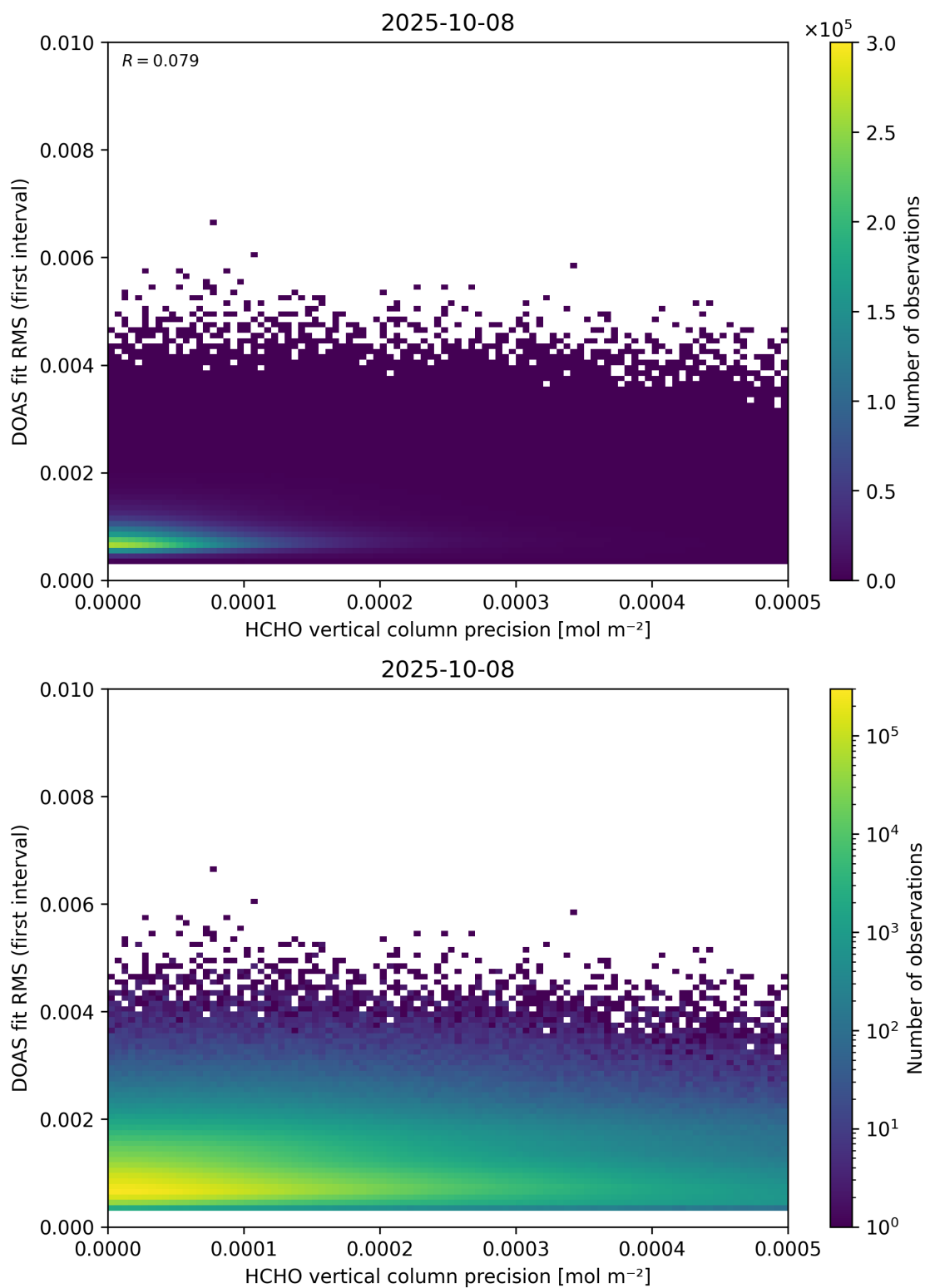
Figure 136: Scatter density plot of “HCHO vertical column precision” against “DOAS fit RMS (first interval)” for 2025-10-07 to 2025-10-09.
