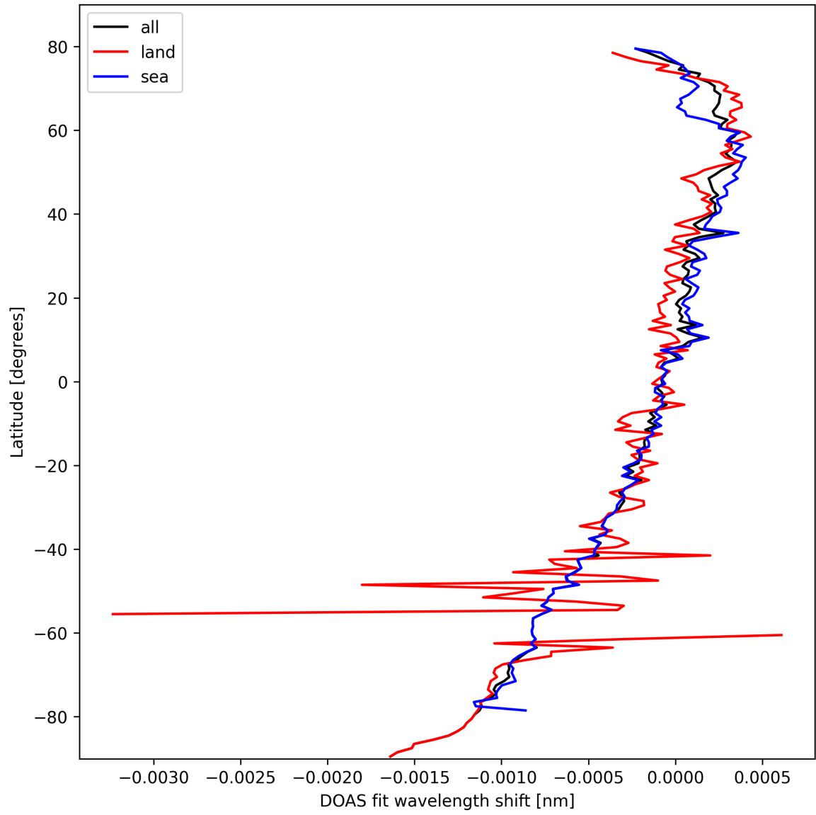
Figure 30: Zonal average of “DOAS fit wavelength shift” for 2025-10-07 to 2025-10-09.
