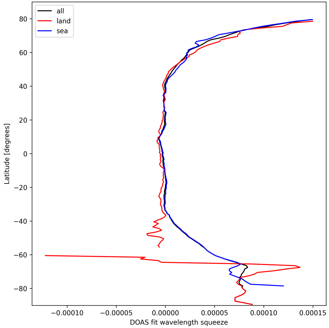
Figure 31: Zonal average of “DOAS fit wavelength squeeze” for 2025-10-07 to 2025-10-09.
