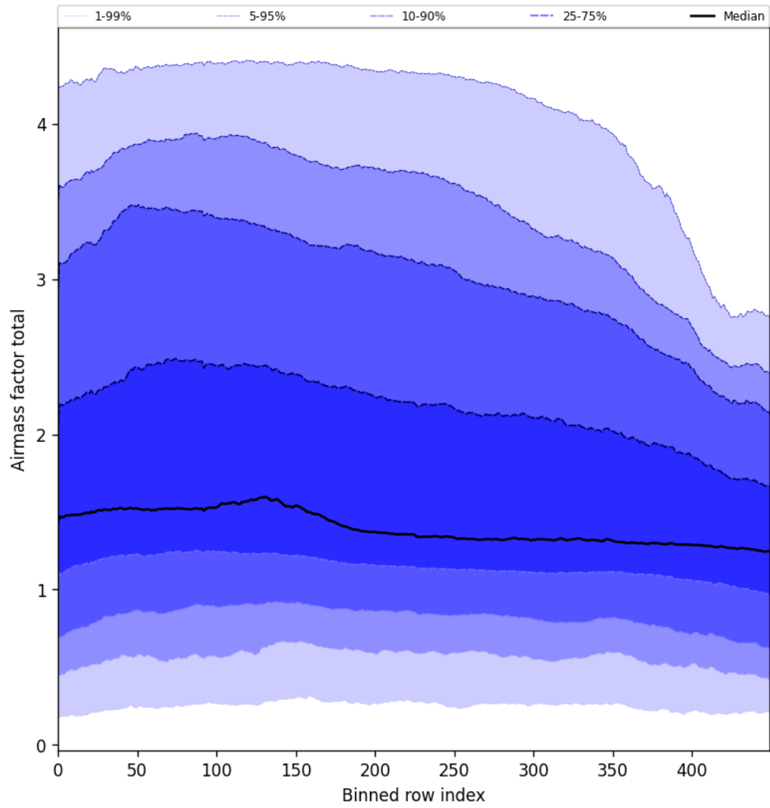
Figure 54: Along track statistics of “Airmass factor total” for 2025-10-07 to 2025-10-09
