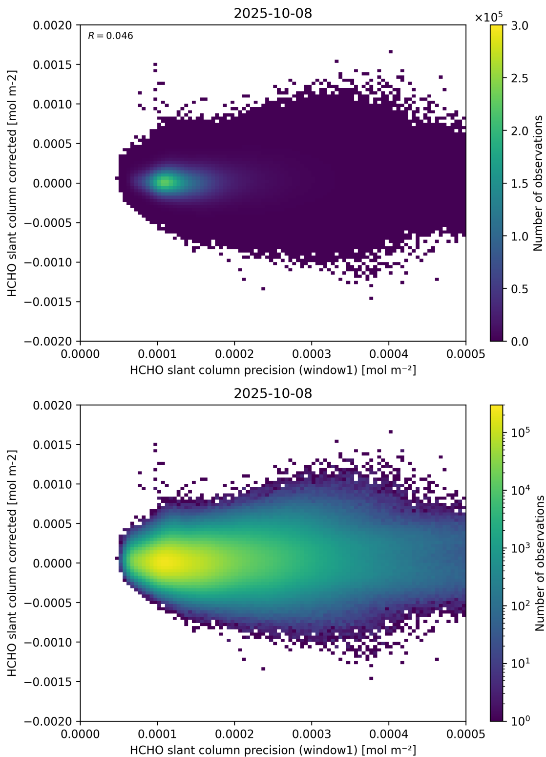
Figure 92: Scatter density plot of “HCHO slant column precision (window1)” against “HCHO slant column corrected” for 2025-10-07 to 2025-10-09.
