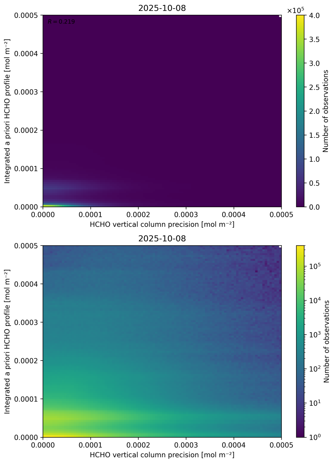
Figure 147: Scatter density plot of “HCHO vertical column precision” against “Integrated a priori HCHO profile” for 2025-10-07 to 2025-10-09.
