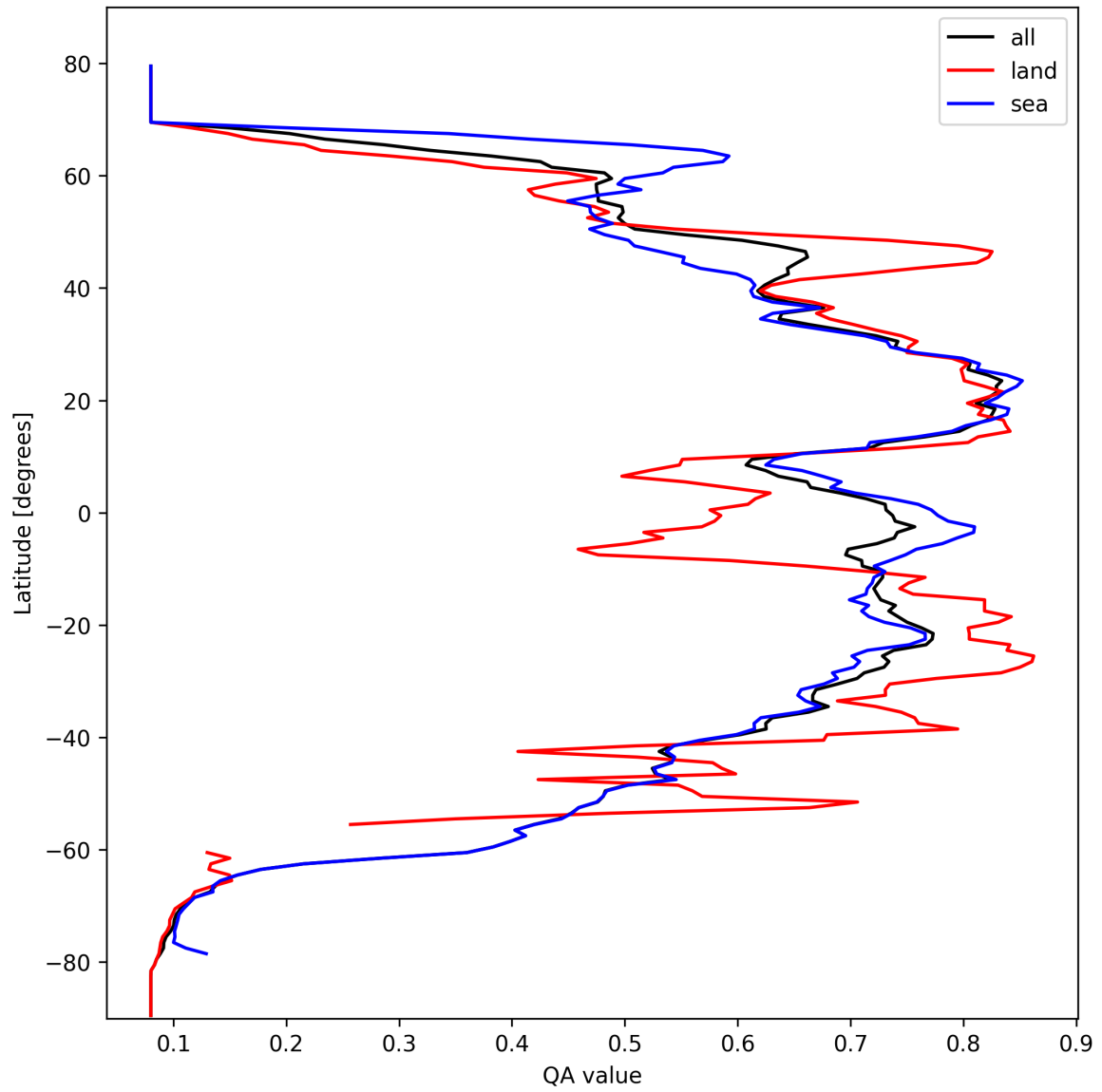
Figure 20: Zonal average of “QA value” for 2025-10-07 to 2025-10-09.
