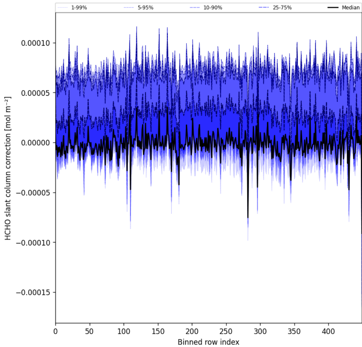
Figure 61: Along track statistics of “HCHO slant column correction” for 2025-10-07 to 2025-10-09
