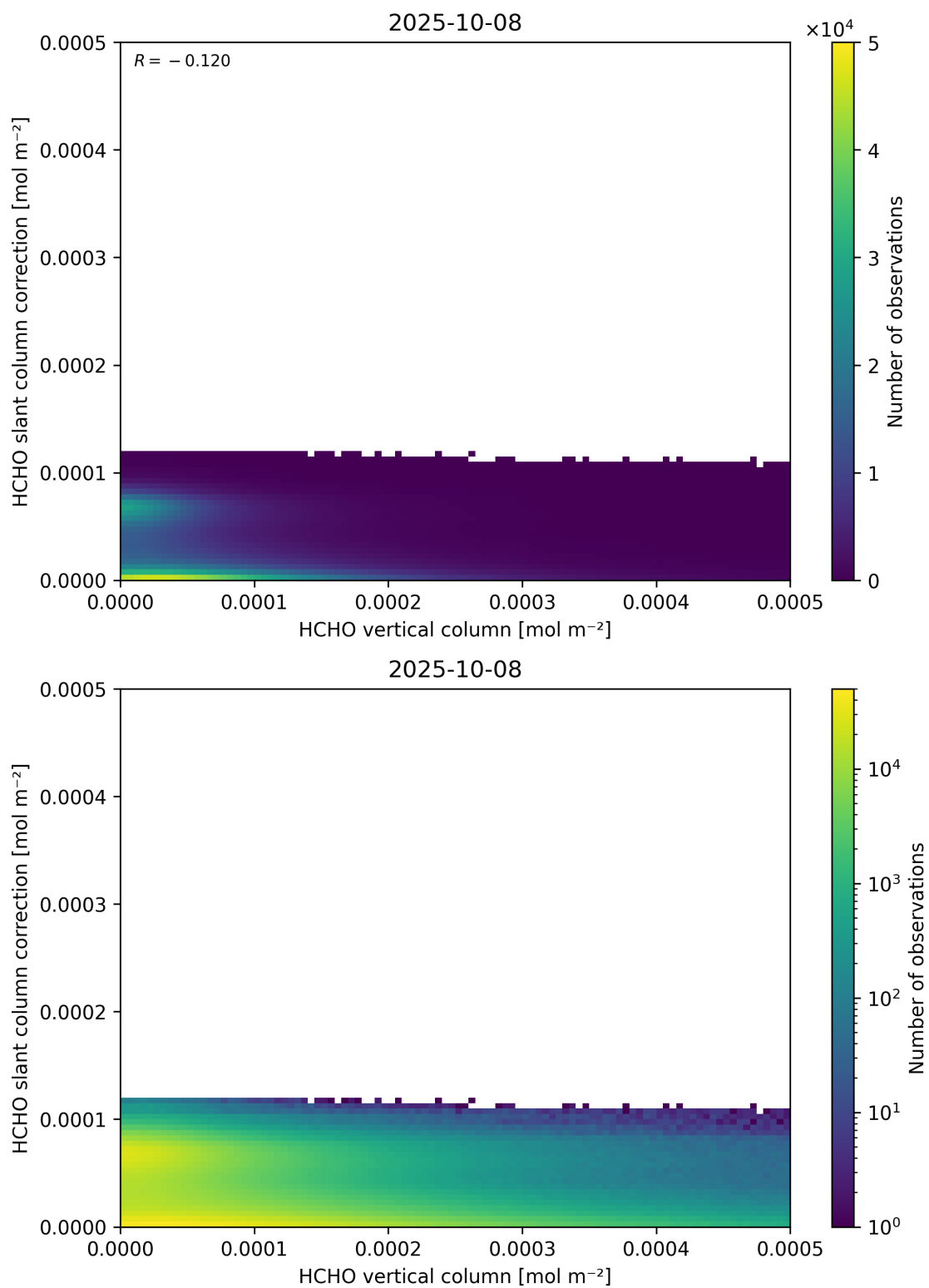
Figure 128: Scatter density plot of “HCHO vertical column” against “HCHO slant column correction” for 2025-10-07 to 2025-10-09.
