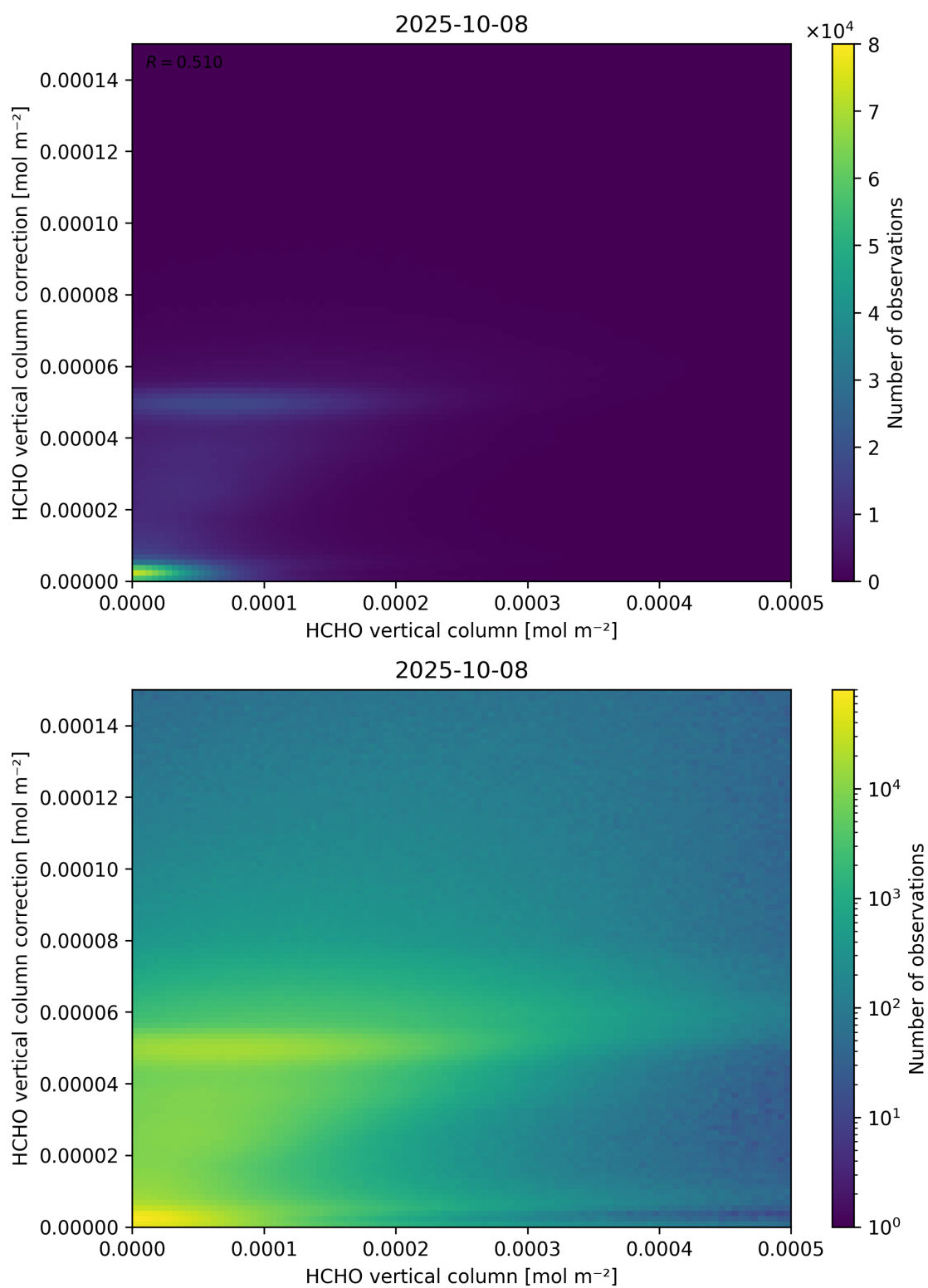
Figure 133: Scatter density plot of “HCHO vertical column” against “HCHO vertical column correction” for 2025-10-07 to 2025-10-09.
