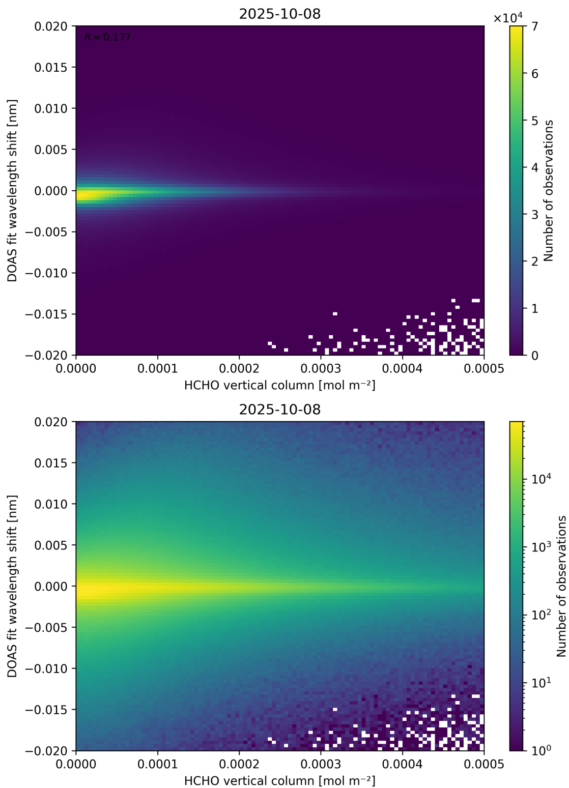
Figure 124: Scatter density plot of “HCHO vertical column” against “DOAS fit wavelength shift” for 2025-10-07 to 2025-10-09.
