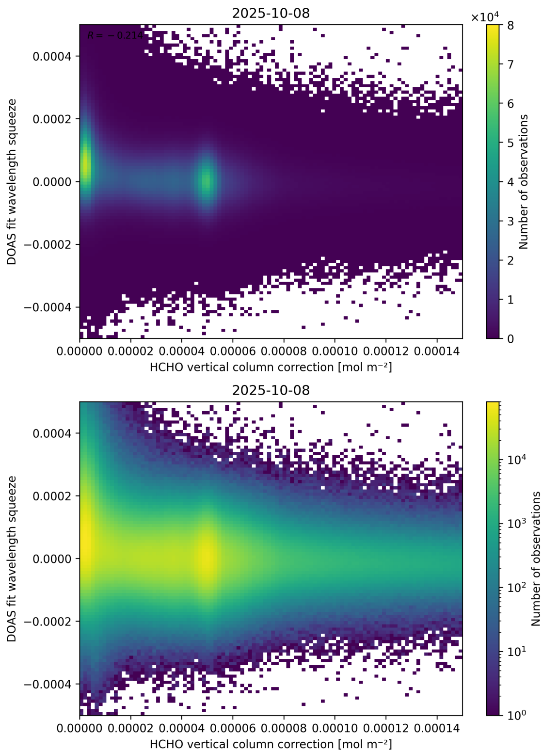
Figure 114: Scatter density plot of “HCHO vertical column correction” against “DOAS fit wavelength squeeze” for 2025-10-07 to 2025-10-09.
