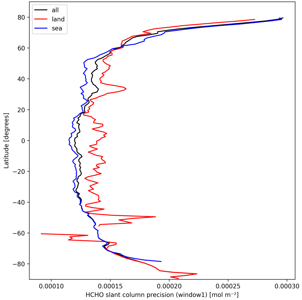
Figure 25: Zonal average of "HCHO slant column precision (window1)" for 2025-10-07 to 2025-10-09.
