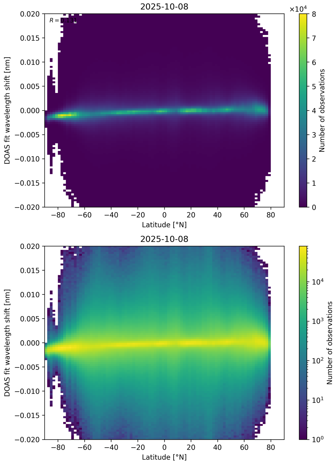
Figure 154: Scatter density plot of “Latitude” against “DOAS fit wavelength shift” for 2025-10-07 to 2025-10-09.
