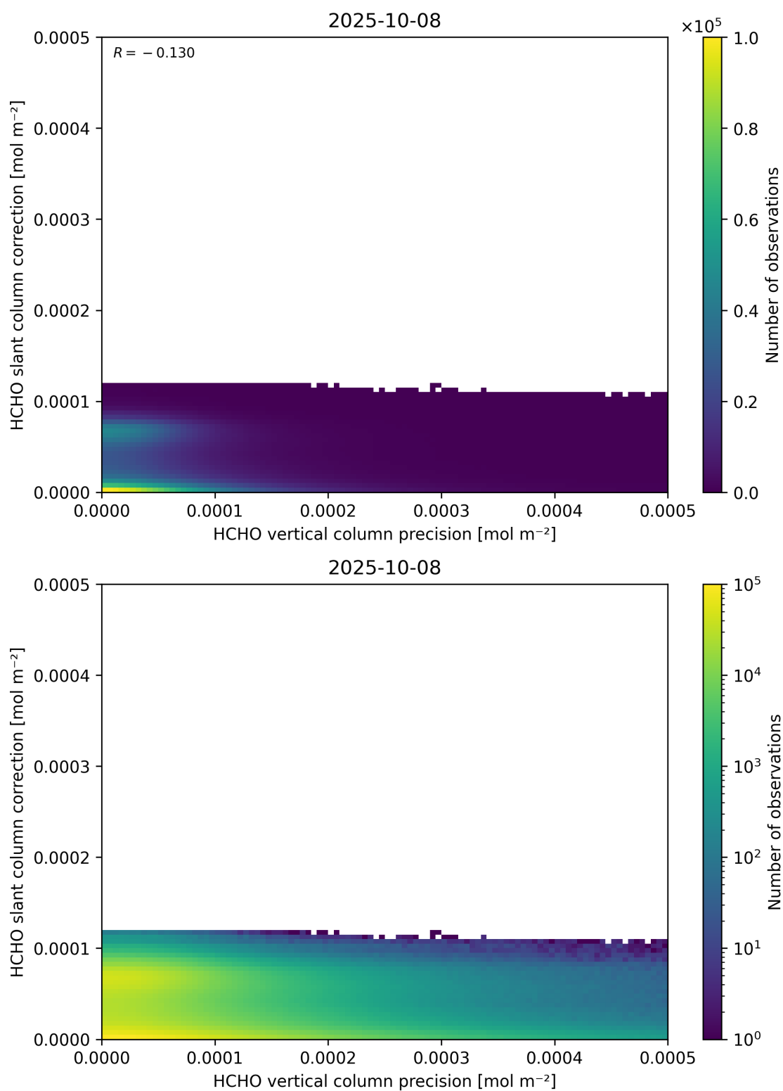
Figure 141: Scatter density plot of “HCHO vertical column precision” against “HCHO slant column correction” for 2025-10-07 to 2025-10-09.
