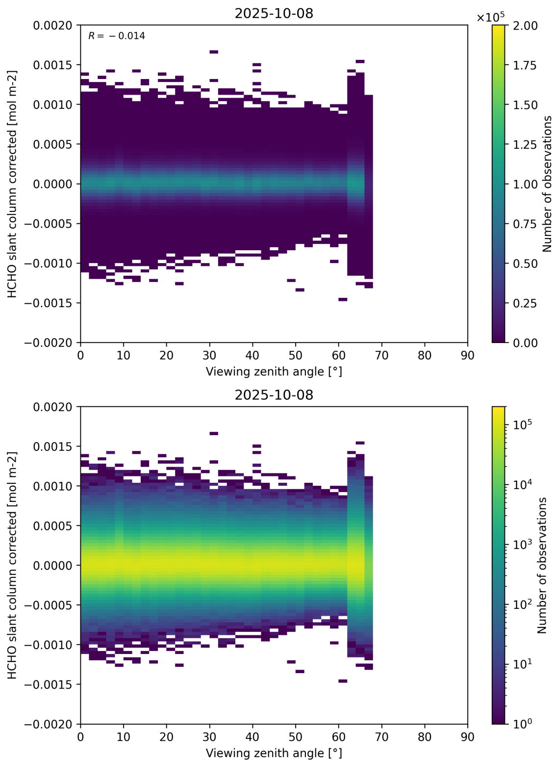
Figure 186: Scatter density plot of “Viewing zenith angle” against “HCHO slant column corrected” for 2025-10-07 to 2025-10-09.
