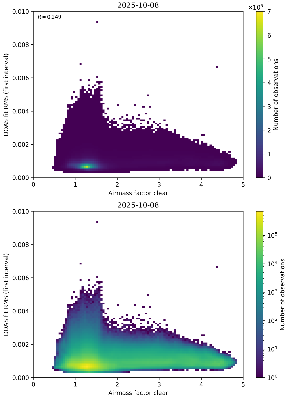
Figure 71: Scatter density plot of “Airmass factor clear” against “DOAS fit RMS (first interval)” for 2025-10-07 to 2025-10-09.
