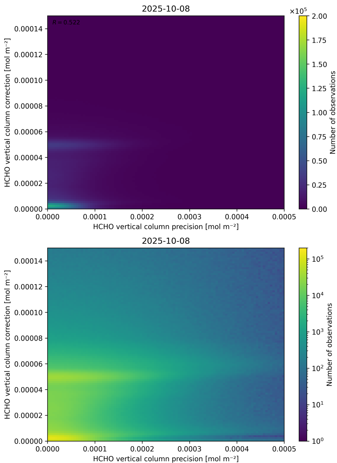
Figure 146: Scatter density plot of “HCHO vertical column precision” against “HCHO vertical column correction” for 2025-10-07 to 2025-10-09.
