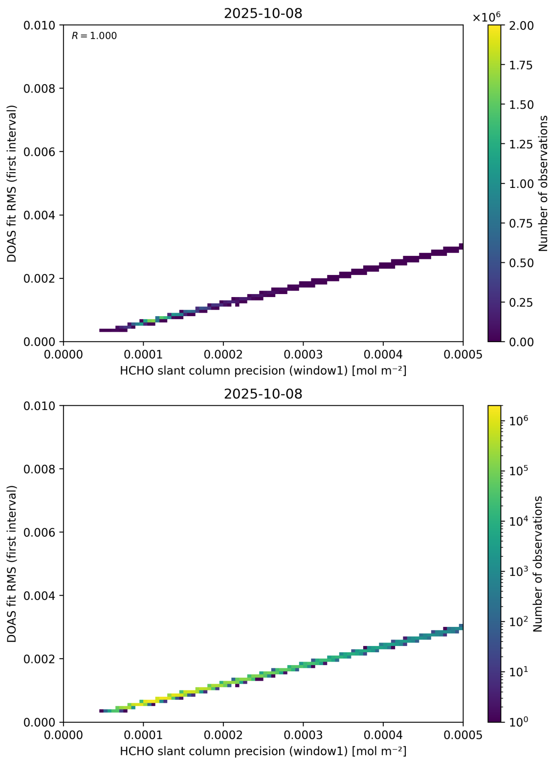
Figure 88: Scatter density plot of “HCHO slant column precision (window1)” against “DOAS fit RMS (first interval)” for 2025-10-07 to 2025-10-09.
