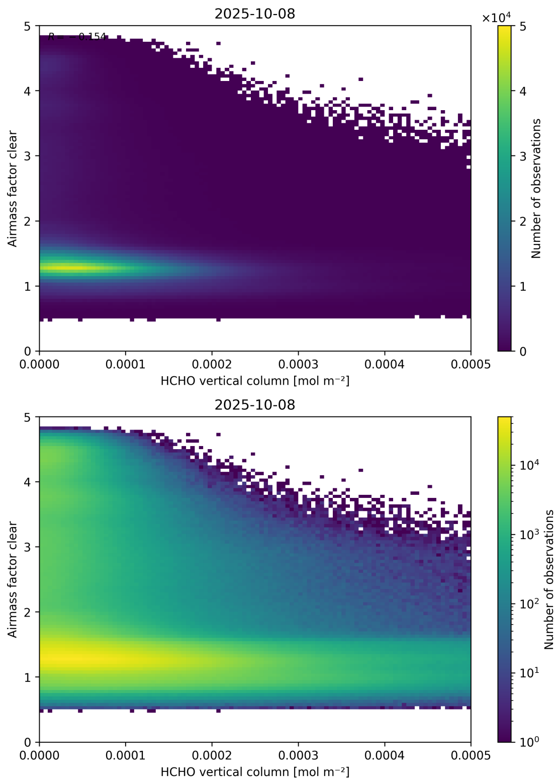
Figure 126: Scatter density plot of “HCHO vertical column” against “Airmass factor clear” for 2025-10-07 to 2025-10-09.
