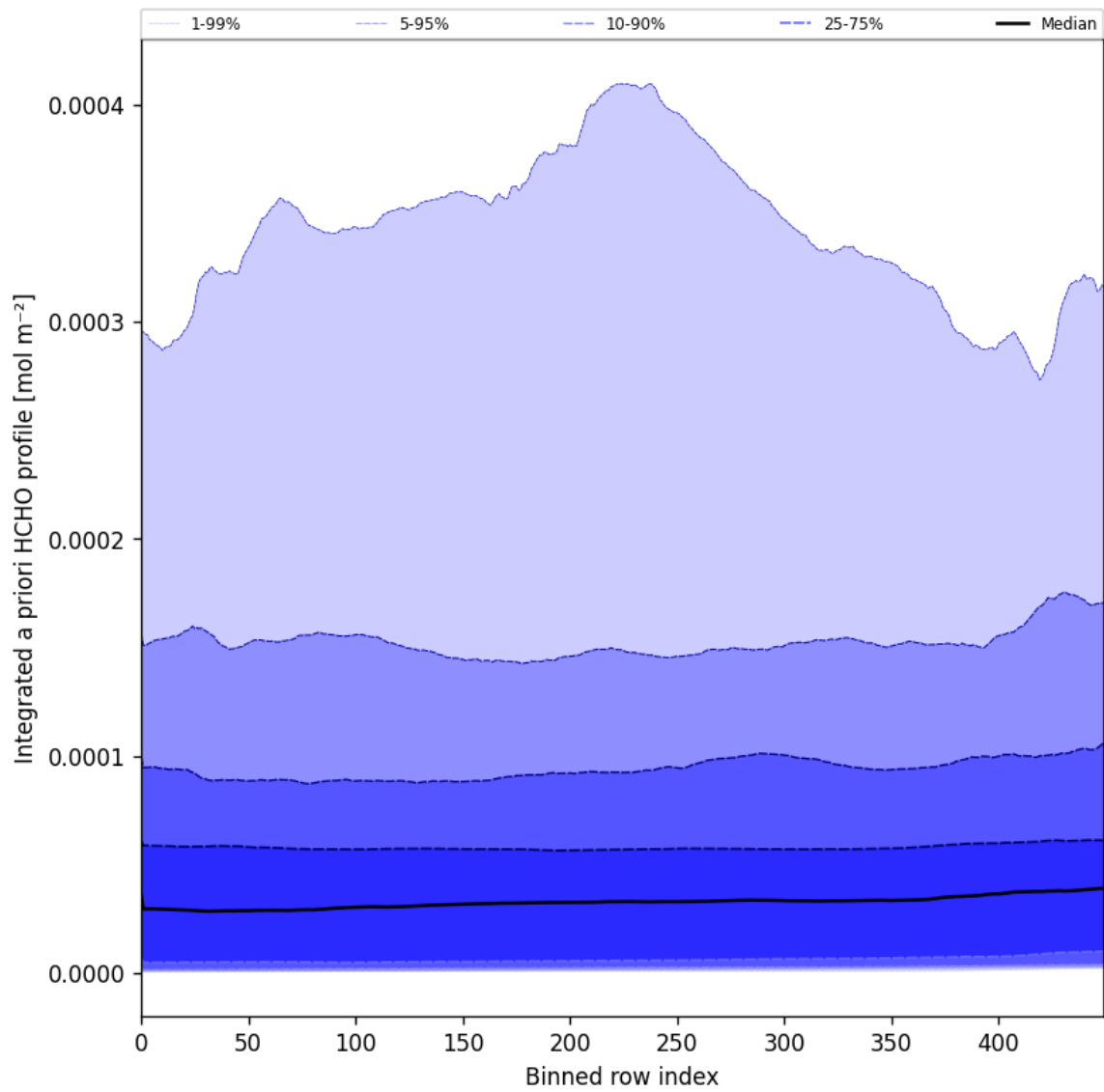
Figure 57: Along track statistics of “Integrated a priori HCHO profile” for 2025-10-07 to 2025-10-09
