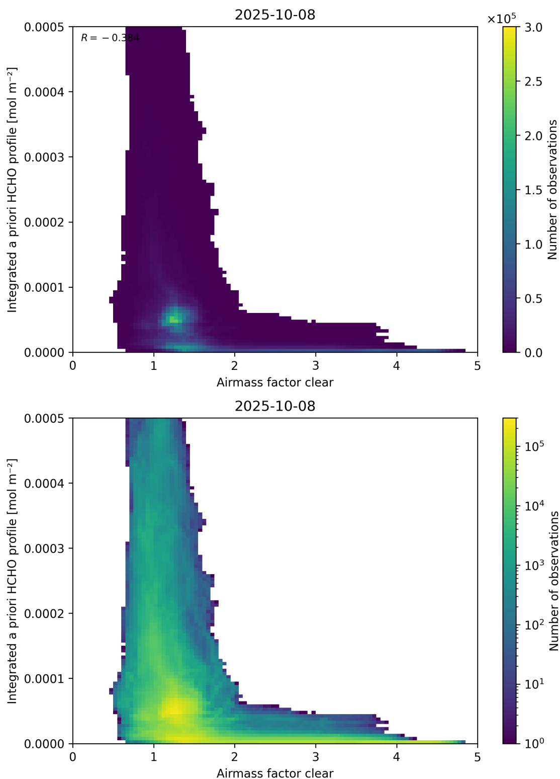
Figure 76: Scatter density plot of “Airmass factor clear” against “Integrated a priori HCHO profile” for 2025-10-07 to 2025-10-09.
