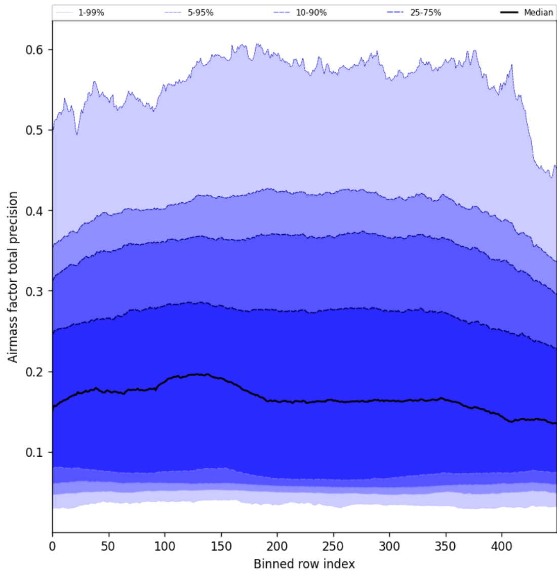
Figure 55: Along track statistics of “Airmass factor total precision” for 2025-10-07 to 2025-10-09
