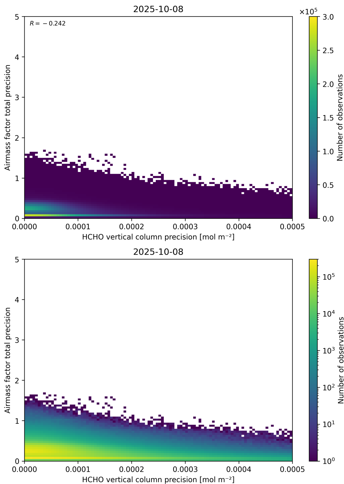
Figure 145: Scatter density plot of “HCHO vertical column precision” against “Airmass factor total precision” for 2025-10-07 to 2025-10-09.
