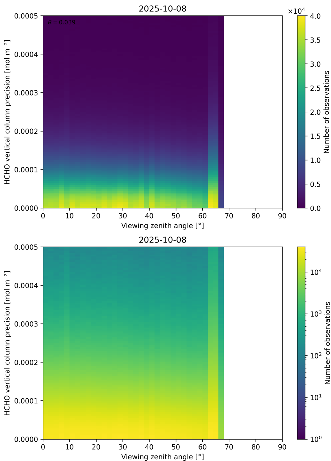
Figure 194: Scatter density plot of “Viewing zenith angle” against “HCHO vertical column precision” for 2025-10-07 to 2025-10-09.
