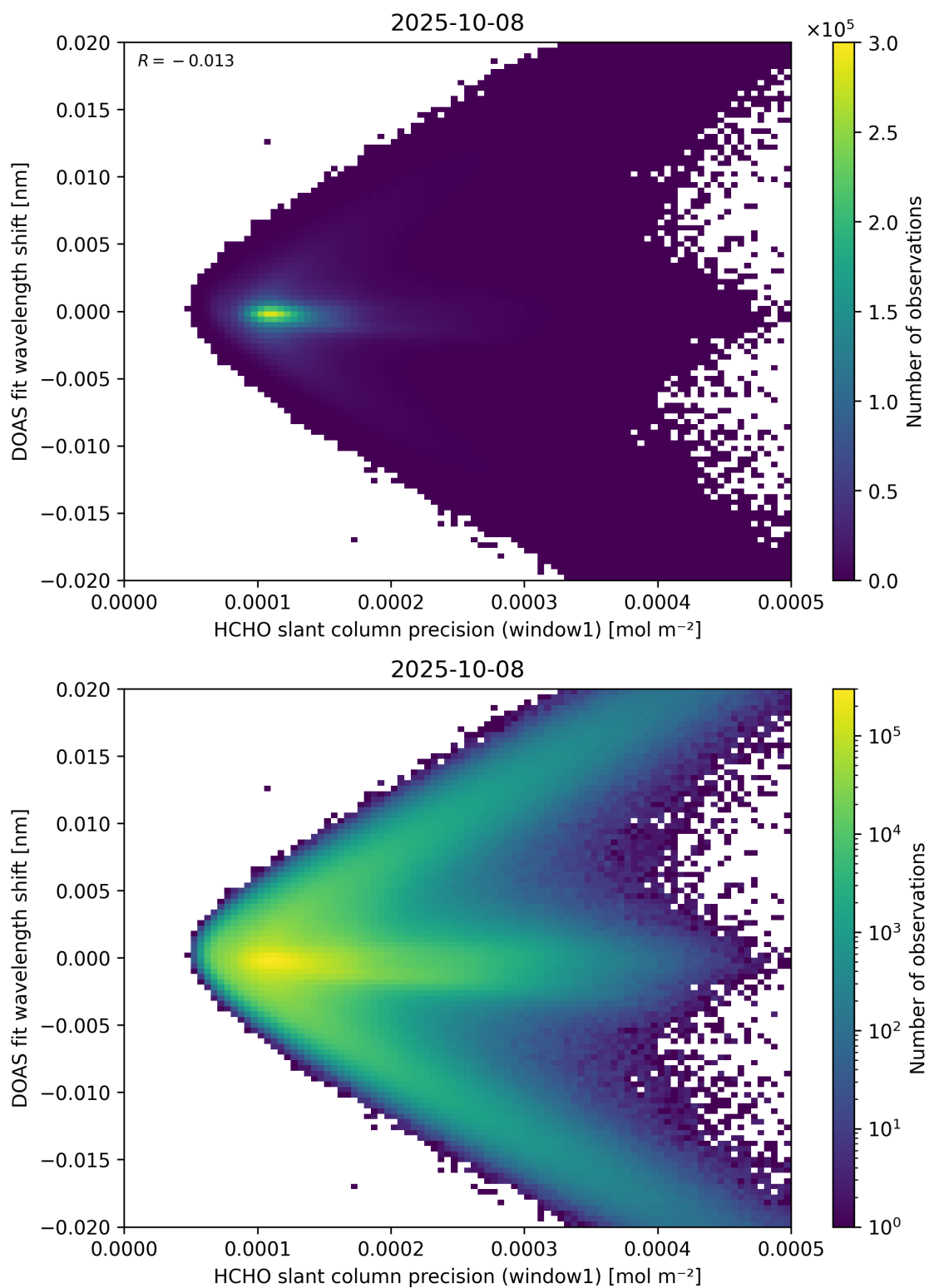
Figure 89: Scatter density plot of “HCHO slant column precision (window1)” against “DOAS fit wavelength shift” for 2025-10-07 to 2025-10-09.
