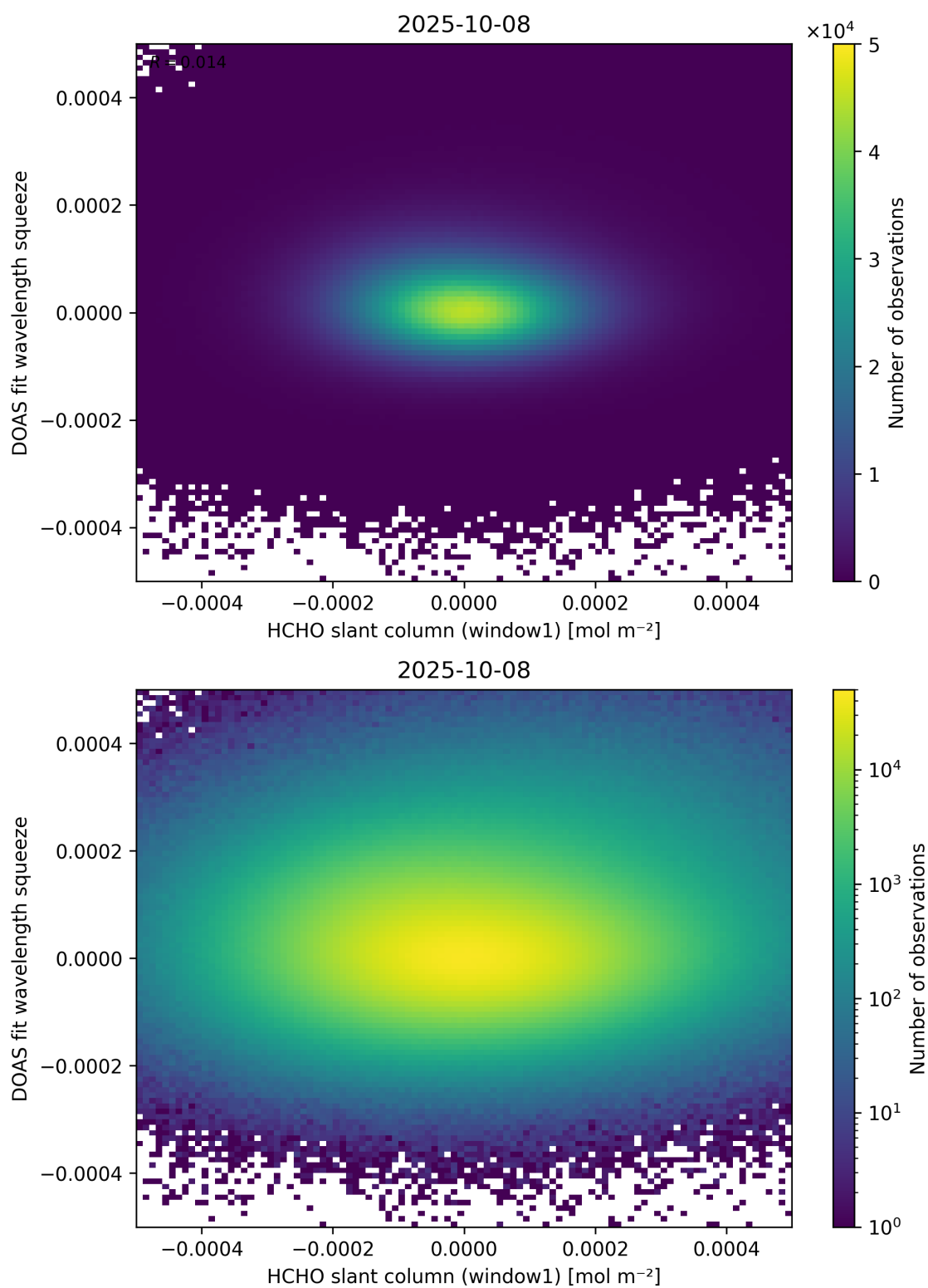
Figure 80: Scatter density plot of “HCHO slant column (window1)” against “DOAS fit wavelength squeeze” for 2025-10-07 to 2025-10-09.
