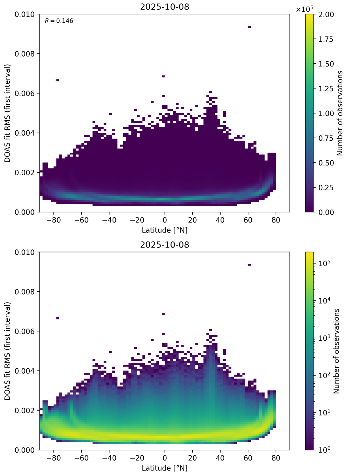
Figure 153: Scatter density plot of “Latitude” against “DOAS fit RMS (first interval)” for 2025-10-07 to 2025-10-09.
