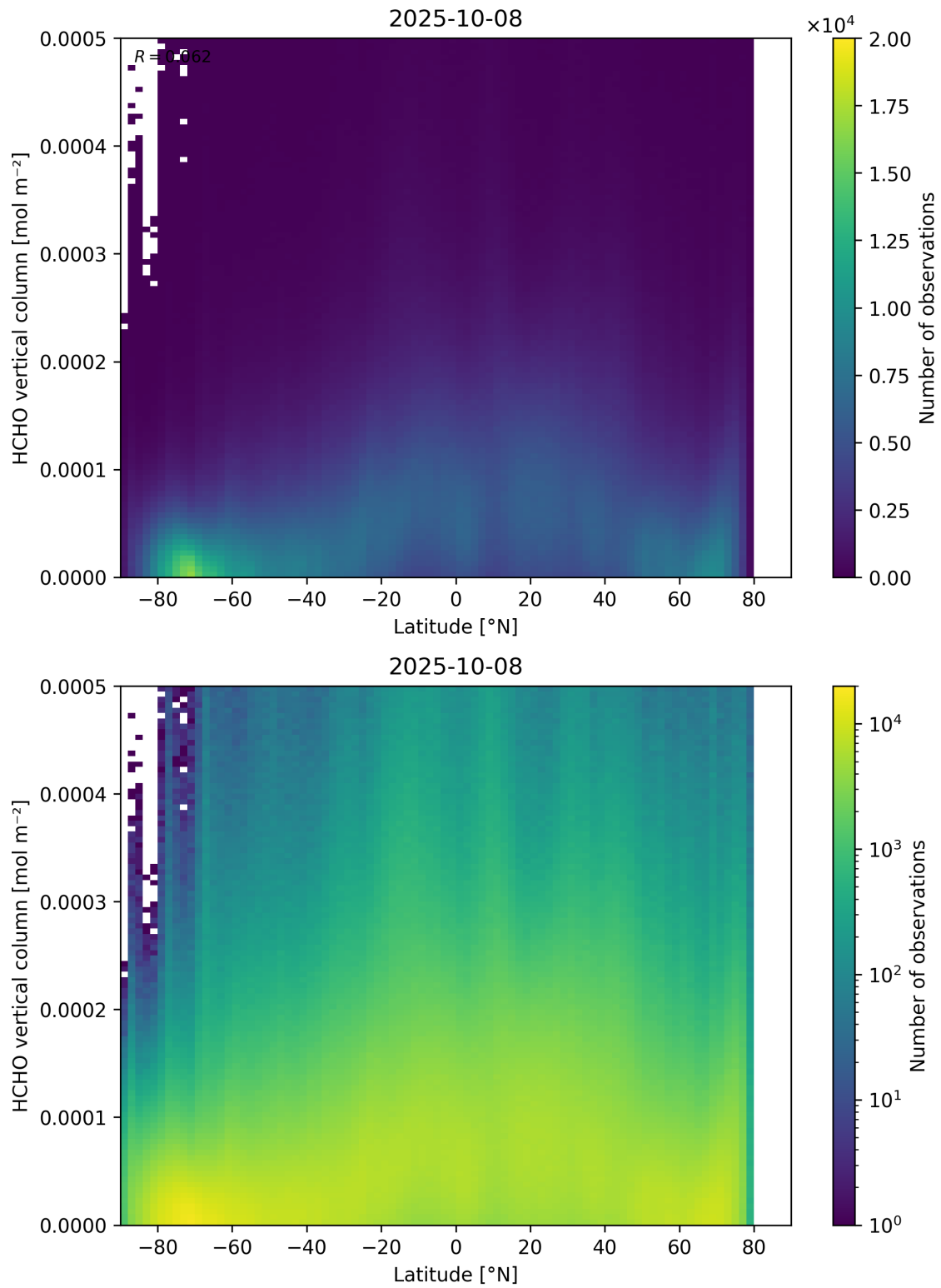
Figure 163: Scatter density plot of “Latitude” against “HCHO vertical column” for 2025-10-07 to 2025-10-09.
