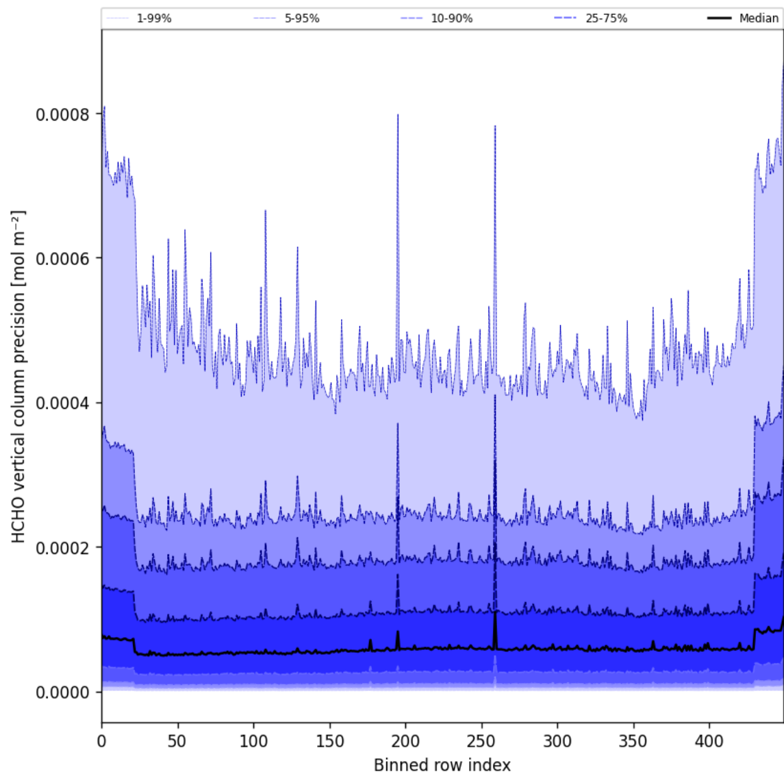
Figure 50: Along track statistics of “HCHO vertical column precision” for 2025-10-07 to 2025-10-09
