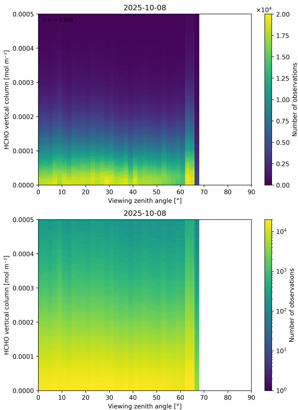
Figure 192: Scatter density plot of “Viewing zenith angle” against “HCHO vertical column” for 2025-10-07 to 2025-10-09.
