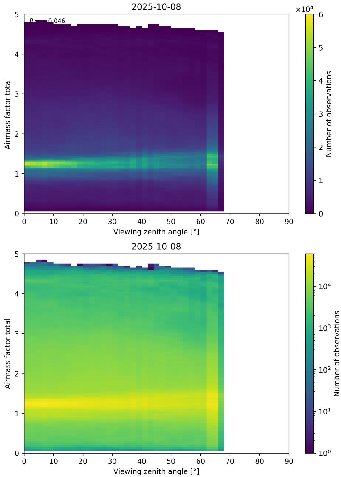
Figure 190: Scatter density plot of “Viewing zenith angle” against “Airmass factor total” for 2025-10-07 to 2025-10-09.
