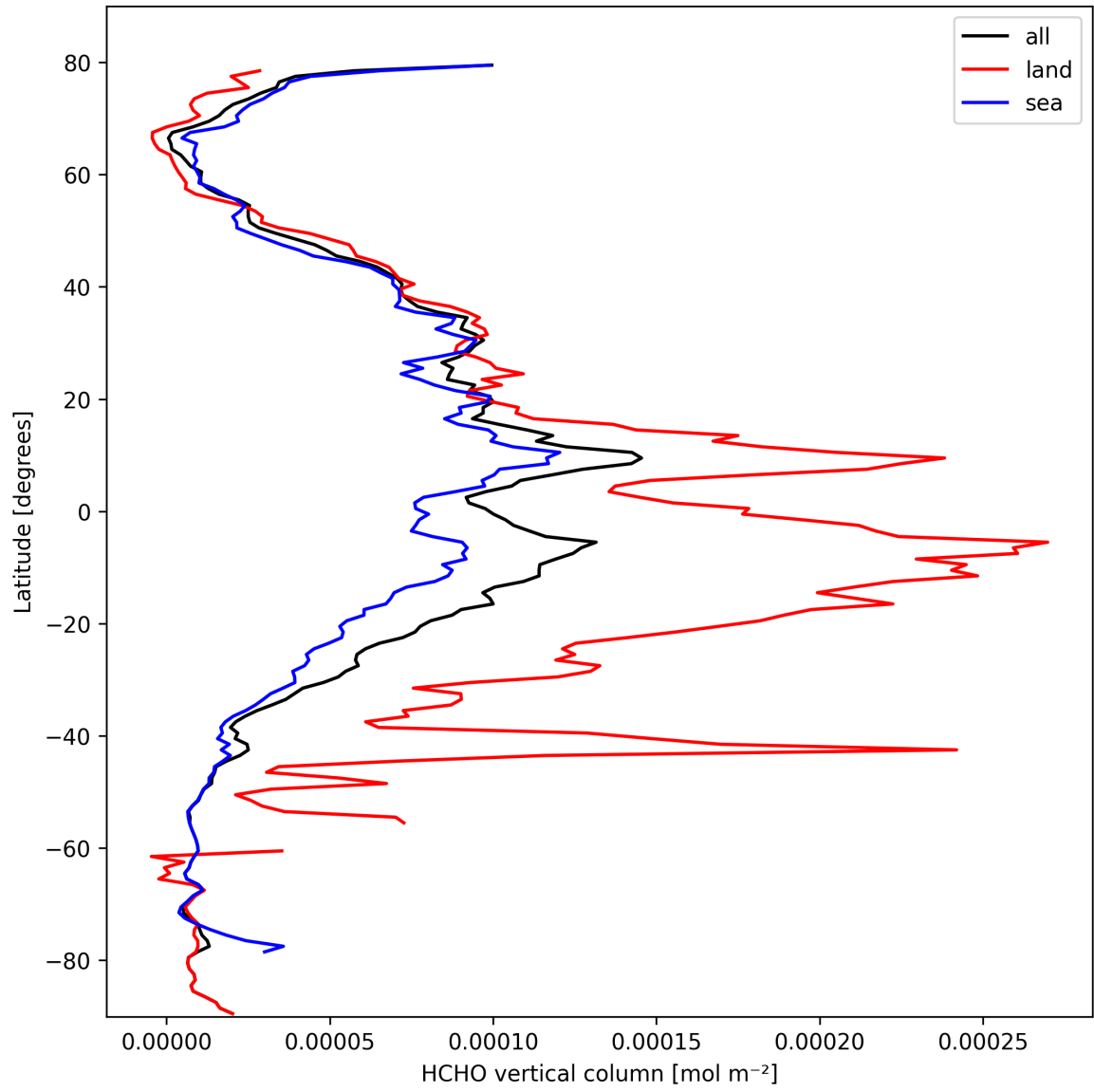
Figure 21: Zonal average of “HCHO vertical column” for 2025-10-07 to 2025-10-09.
