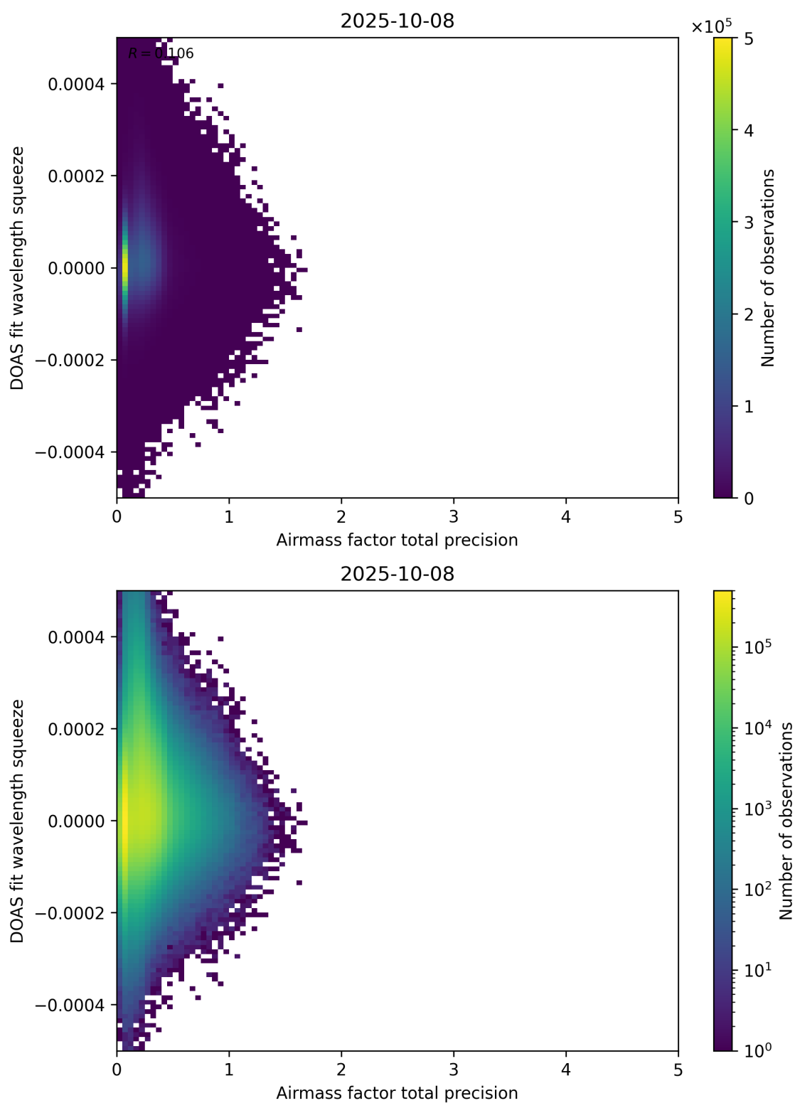
Figure 107: Scatter density plot of “Airmass factor total precision” against “DOAS fit wavelength squeeze” for 2025-10-07 to 2025-10-09.
