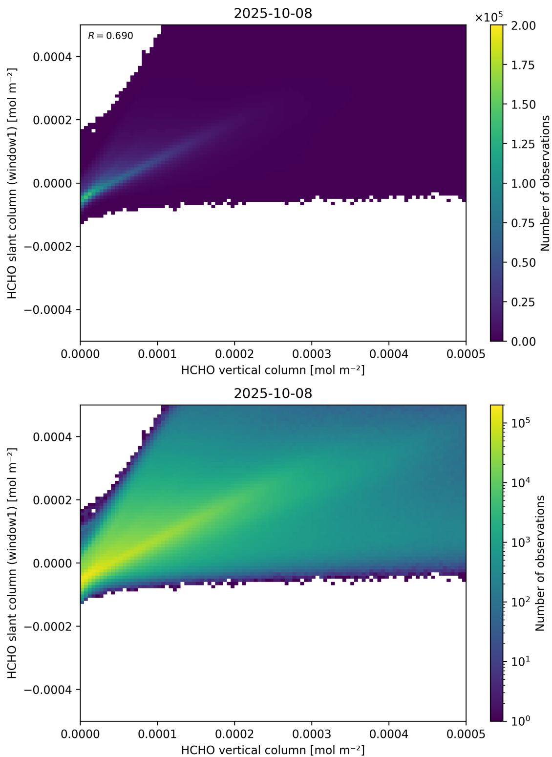
Figure 129: Scatter density plot of “HCHO vertical column” against “HCHO slant column (window1)” for 2025-10-07 to 2025-10-09.
