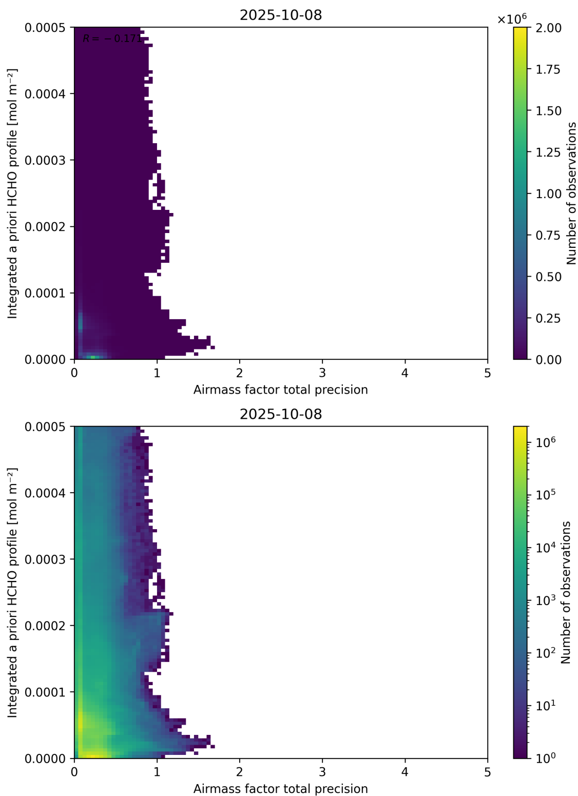
Figure 111: Scatter density plot of “Airmass factor total precision” against “Integrated a priori HCHO profile” for 2025-10-07 to 2025-10-09.
