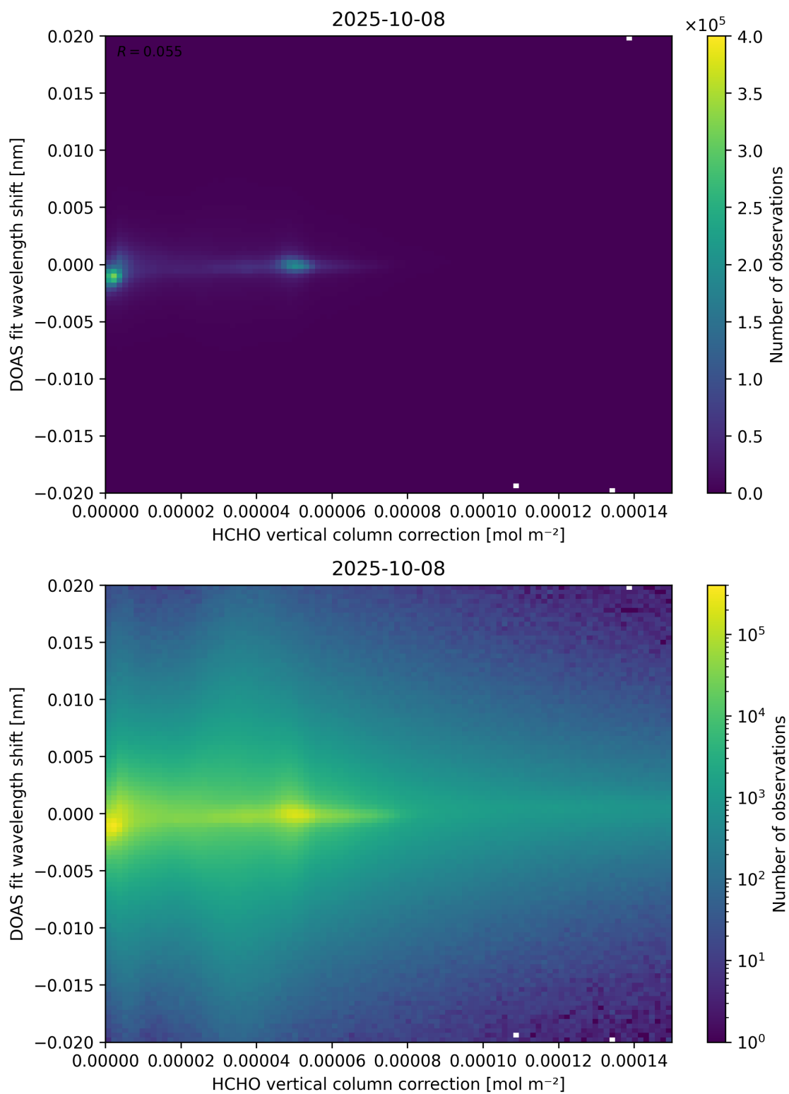
Figure 113: Scatter density plot of “HCHO vertical column correction” against “DOAS fit wavelength shift” for 2025-10-07 to 2025-10-09.
