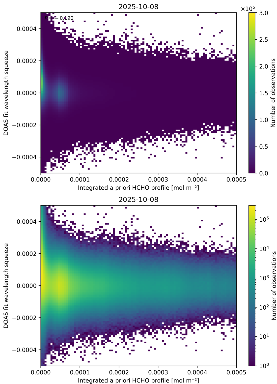
Figure 150: Scatter density plot of “Integrated a priori HCHO profile” against “DOAS fit wavelength squeeze” for 2025-10-07 to 2025-10-09.
