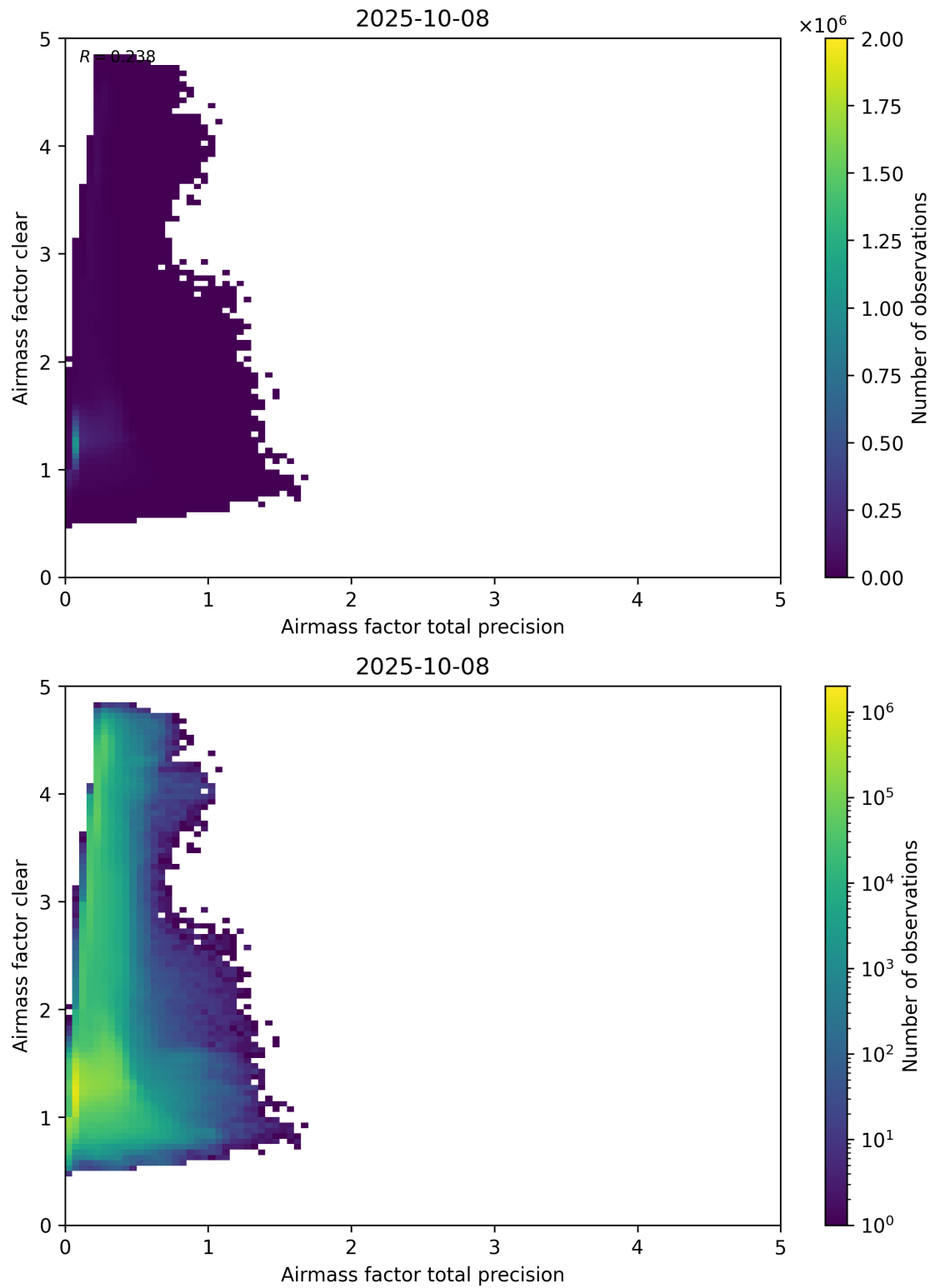
Figure 108: Scatter density plot of “Airmass factor total precision” against “Airmass factor clear” for 2025-10-07 to 2025-10-09.
