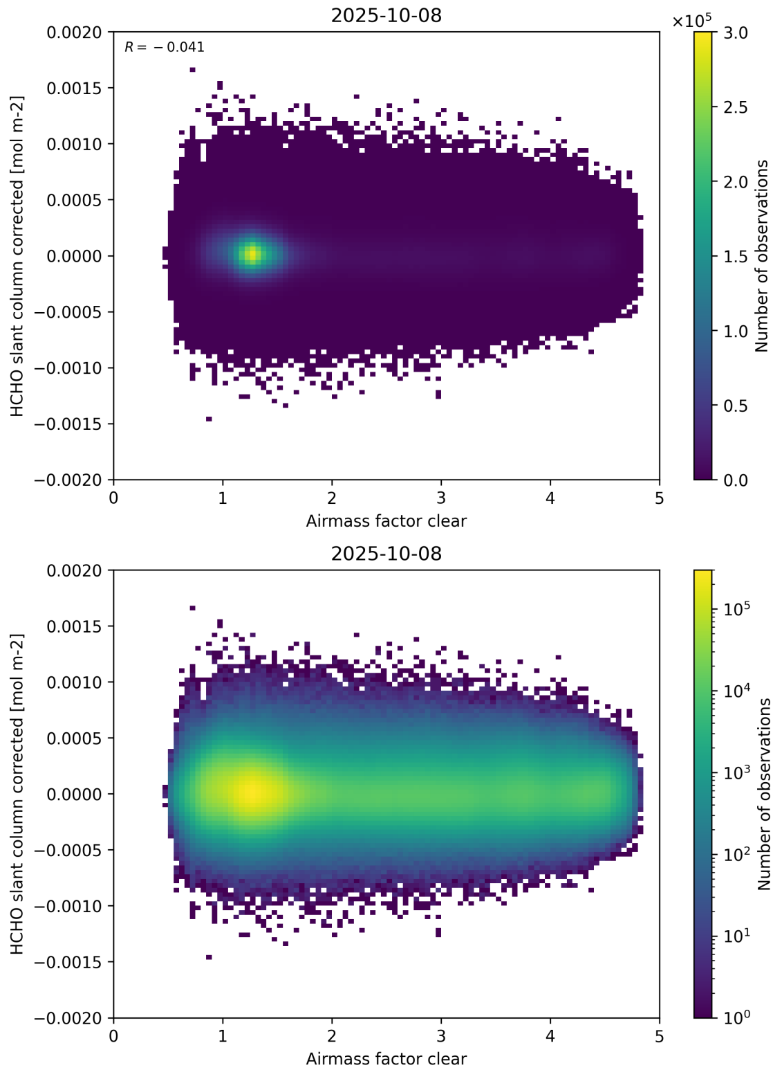
Figure 74: Scatter density plot of “Airmass factor clear” against “HCHO slant column corrected” for 2025-10-07 to 2025-10-09.
