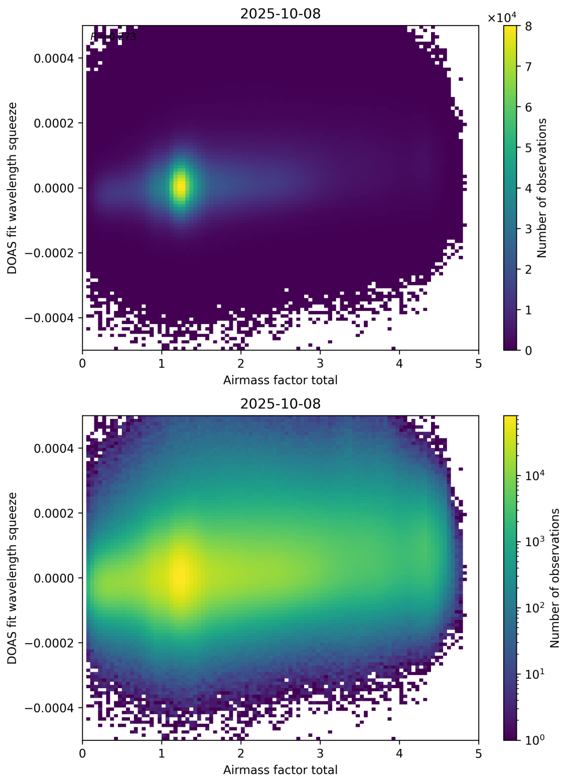
Figure 99: Scatter density plot of “Airmass factor total” against “DOAS fit wavelength squeeze” for 2025-10-07 to 2025-10-09.
