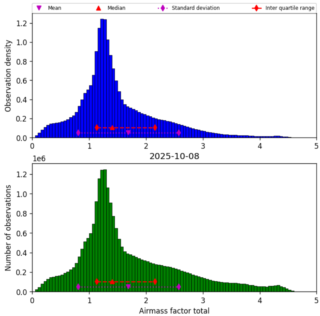
Figure 40: Histogram of “Airmass factor total” for 2025-10-07 to 2025-10-09
