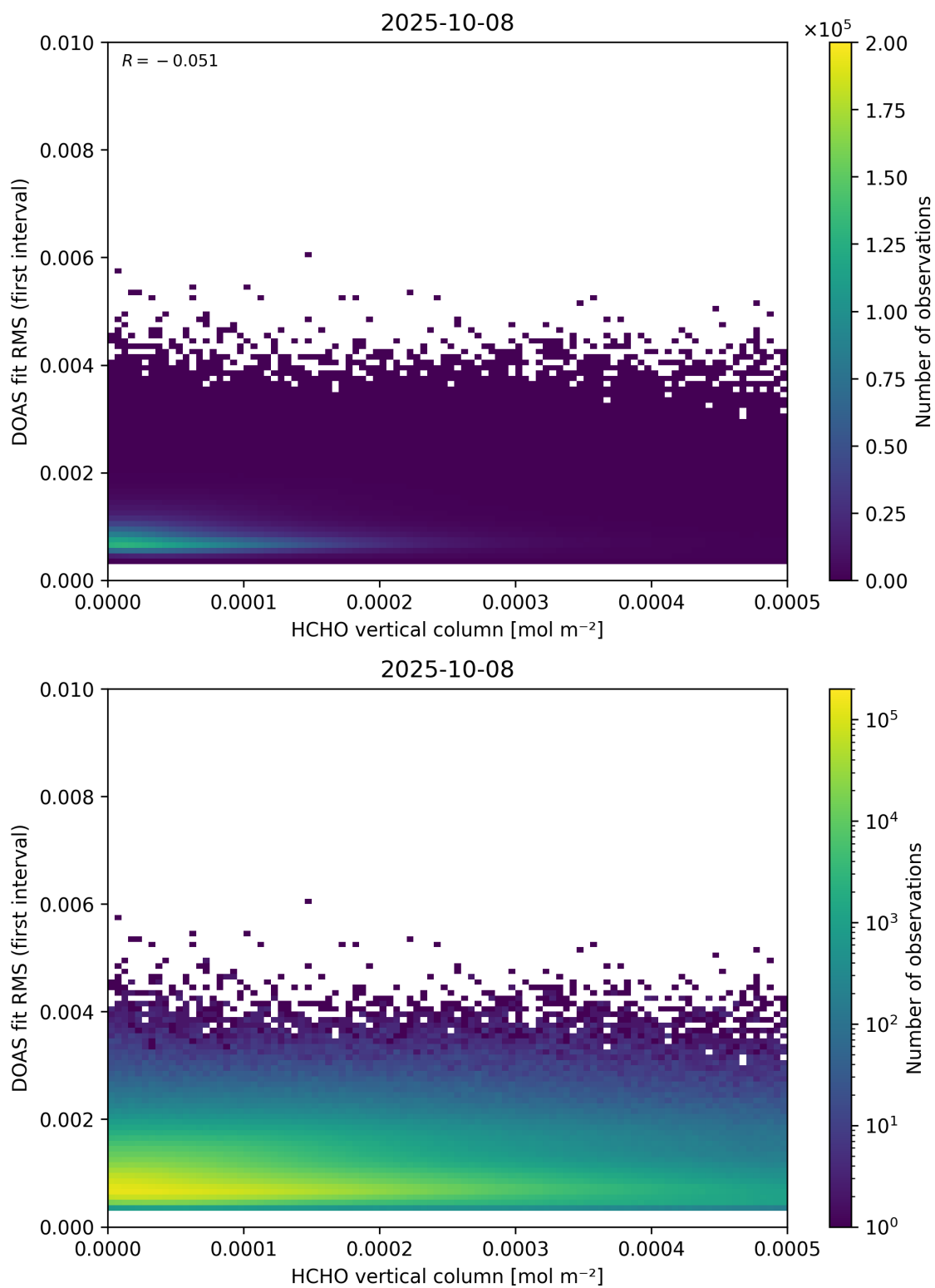
Figure 123: Scatter density plot of “HCHO vertical column” against “DOAS fit RMS (first interval)” for 2025-10-07 to 2025-10-09.
