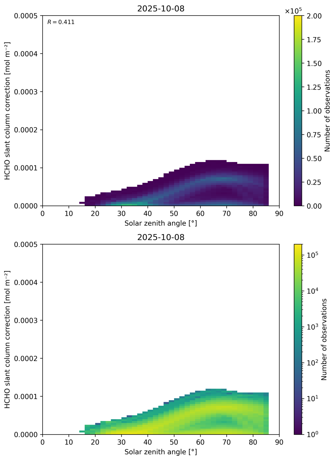
Figure 172: Scatter density plot of “Solar zenith angle” against “HCHO slant column correction” for 2025-10-07 to 2025-10-09.
