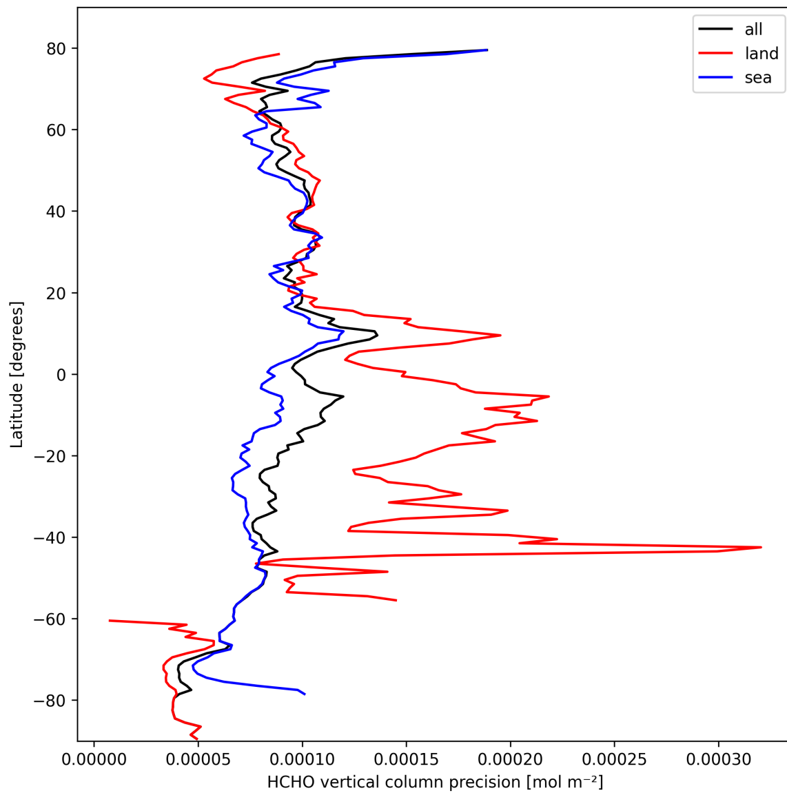
Figure 22: Zonal average of “HCHO vertical column precision” for 2025-10-07 to 2025-10-09.
