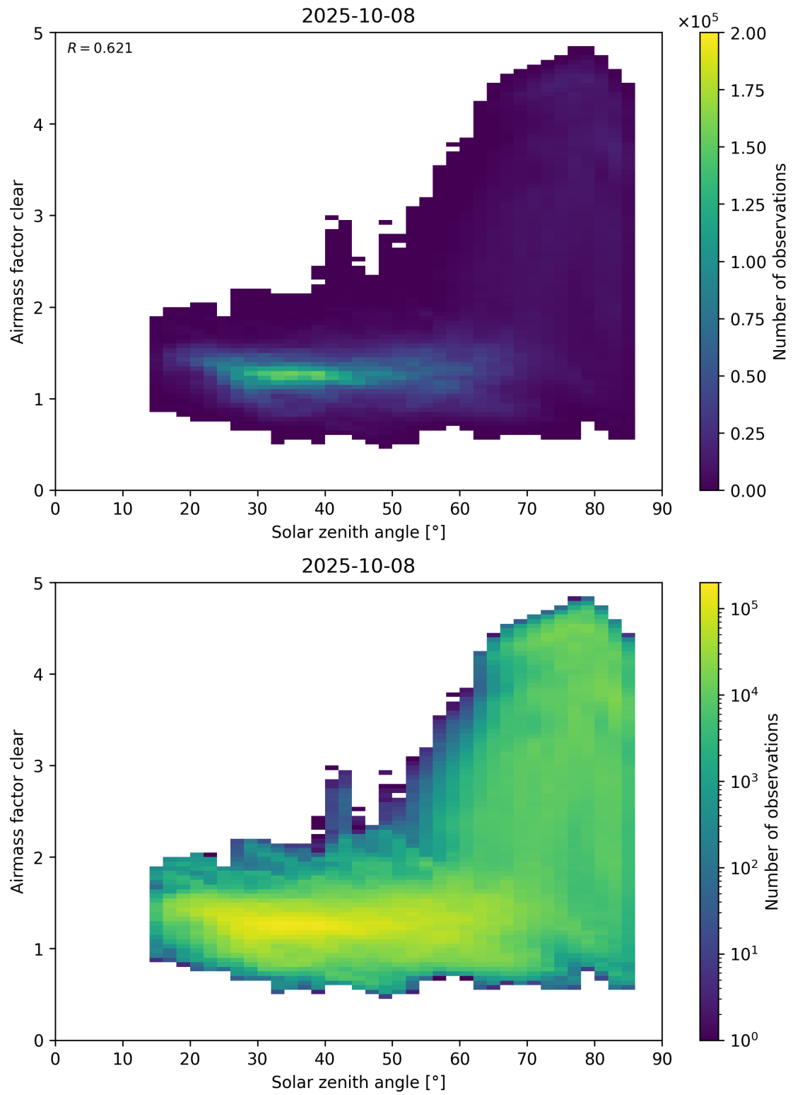
Figure 170: Scatter density plot of “Solar zenith angle” against “Airmass factor clear” for 2025-10-07 to 2025-10-09.
