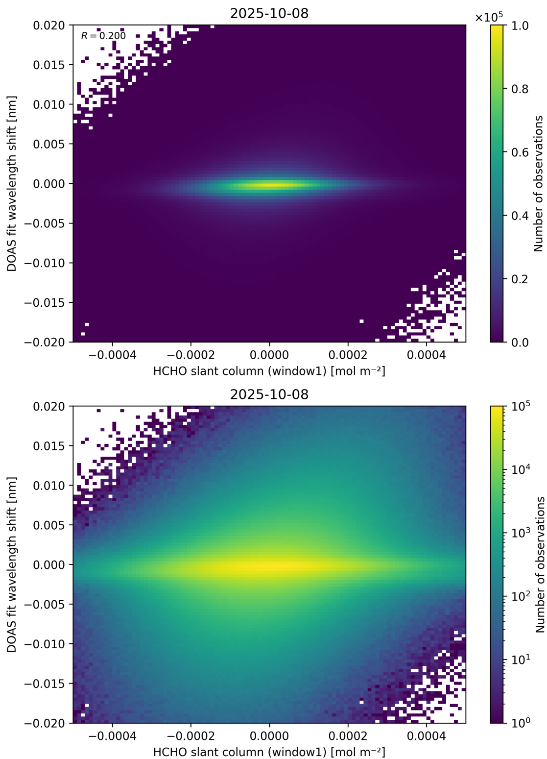
Figure 79: Scatter density plot of “HCHO slant column (window1)” against “DOAS fit wavelength shift” for 2025-10-07 to 2025-10-09.
