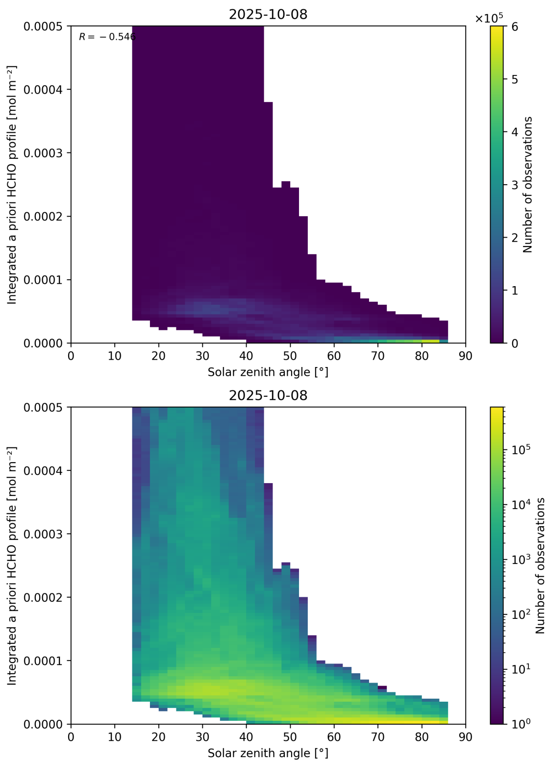
Figure 180: Scatter density plot of “Solar zenith angle” against “Integrated a priori HCHO profile” for 2025-10-07 to 2025-10-09.
