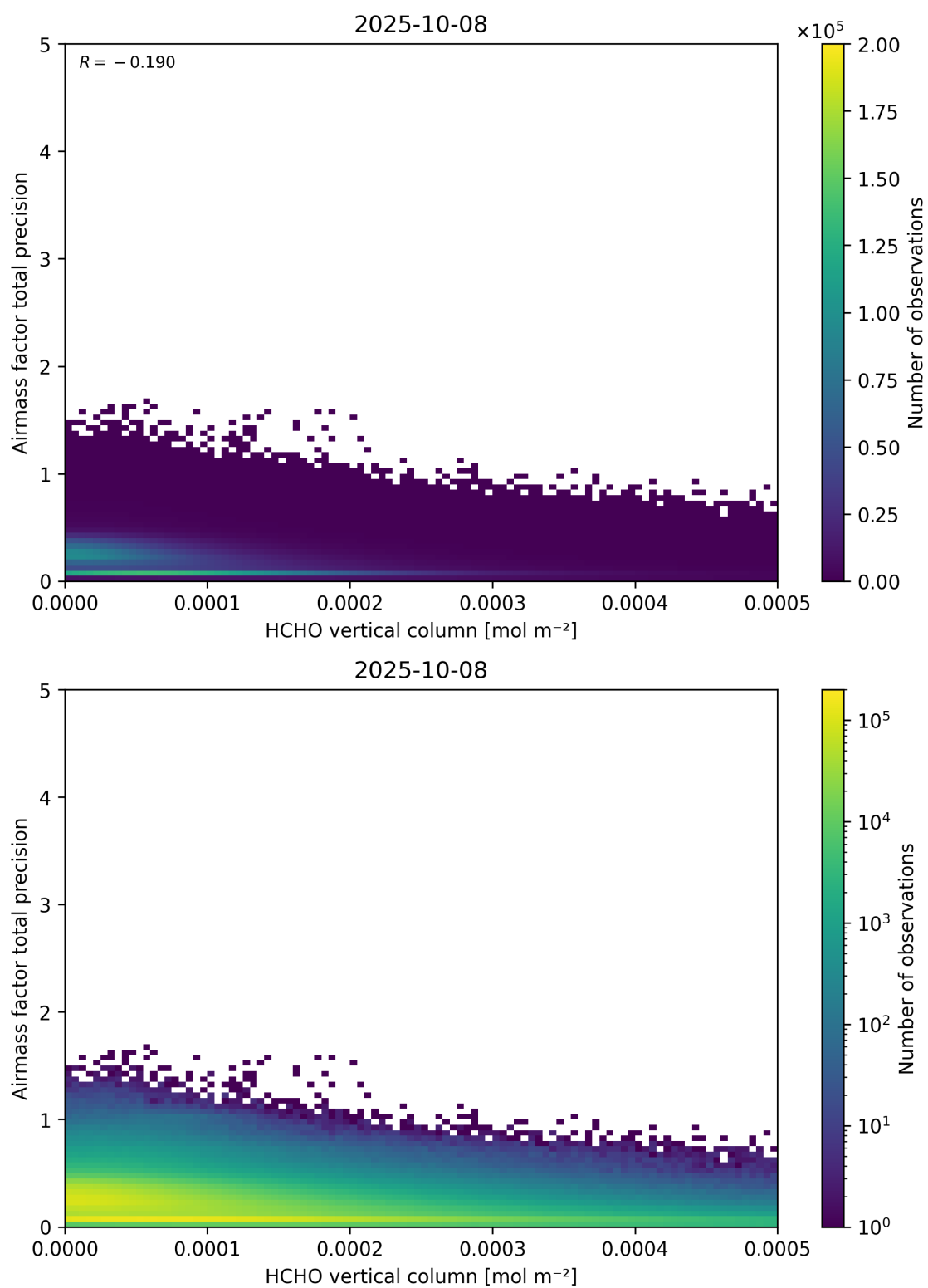
Figure 132: Scatter density plot of “HCHO vertical column” against “Airmass factor total precision” for 2025-10-07 to 2025-10-09.
