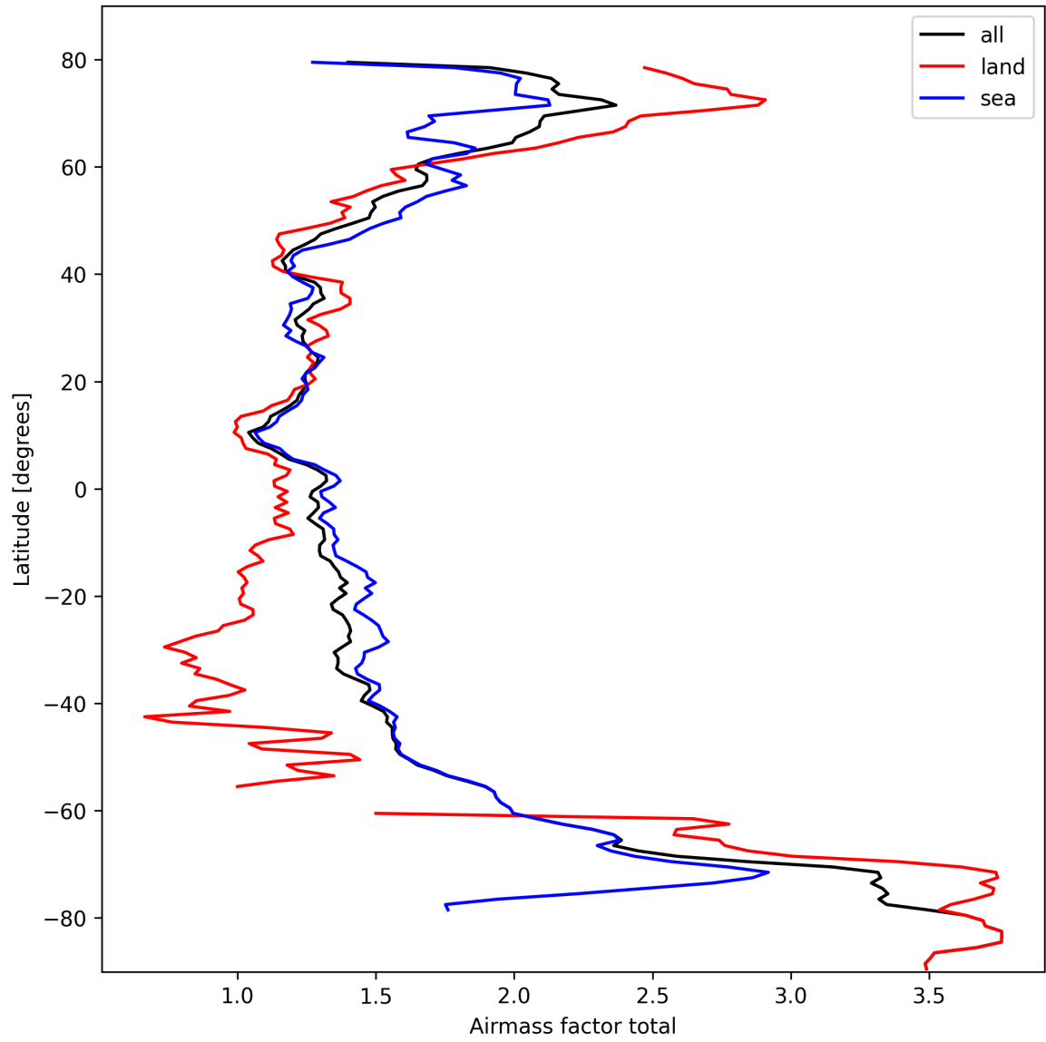
Figure 26: Zonal average of “Airmass factor total” for 2025-10-07 to 2025-10-09.
