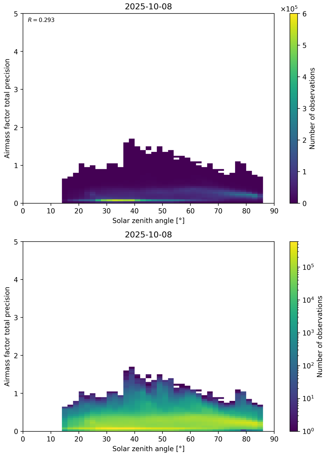
Figure 176: Scatter density plot of “Solar zenith angle” against “Airmass factor total precision” for 2025-10-07 to 2025-10-09.
