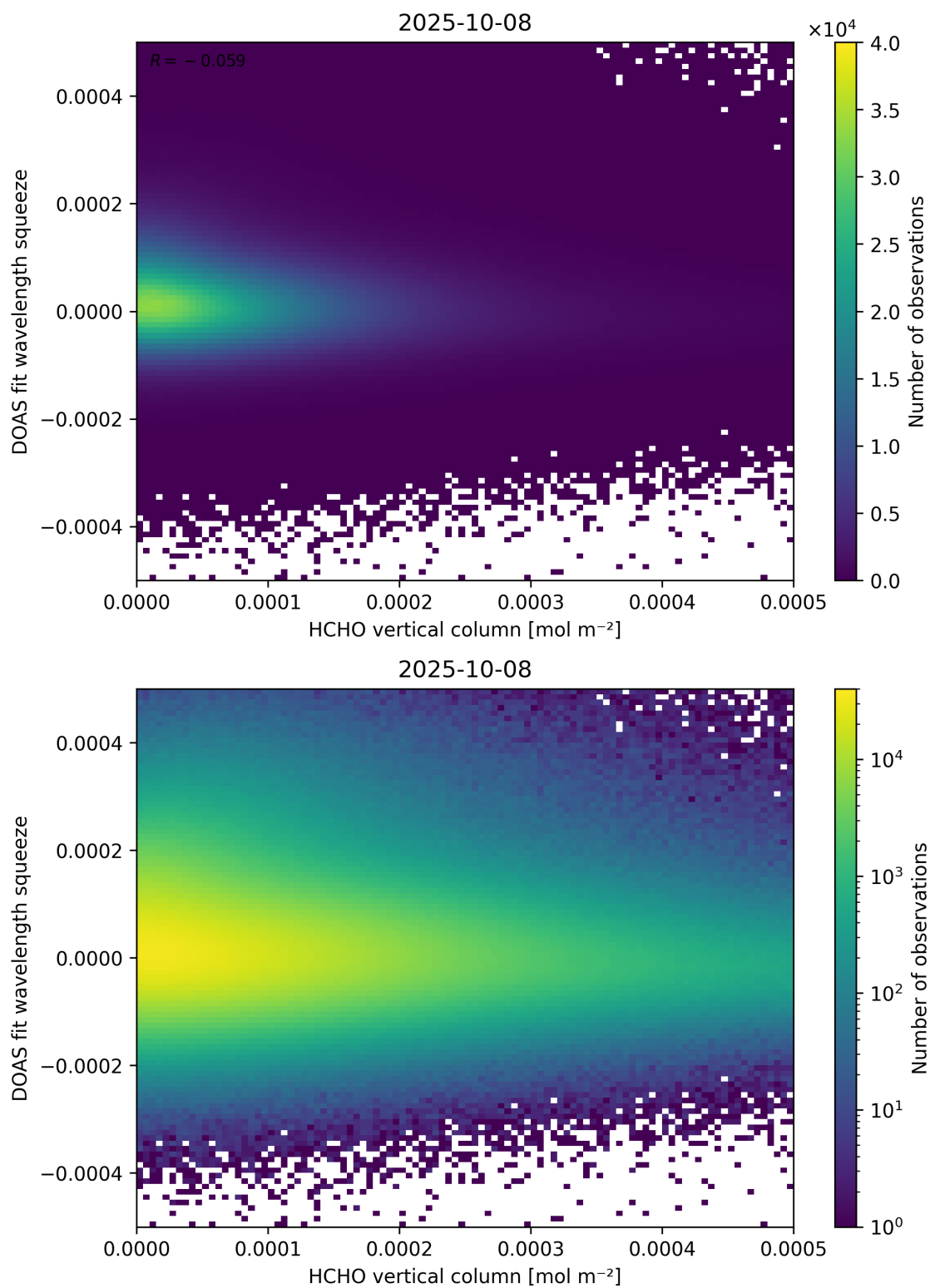
Figure 125: Scatter density plot of “HCHO vertical column” against “DOAS fit wavelength squeeze” for 2025-10-07 to 2025-10-09.
