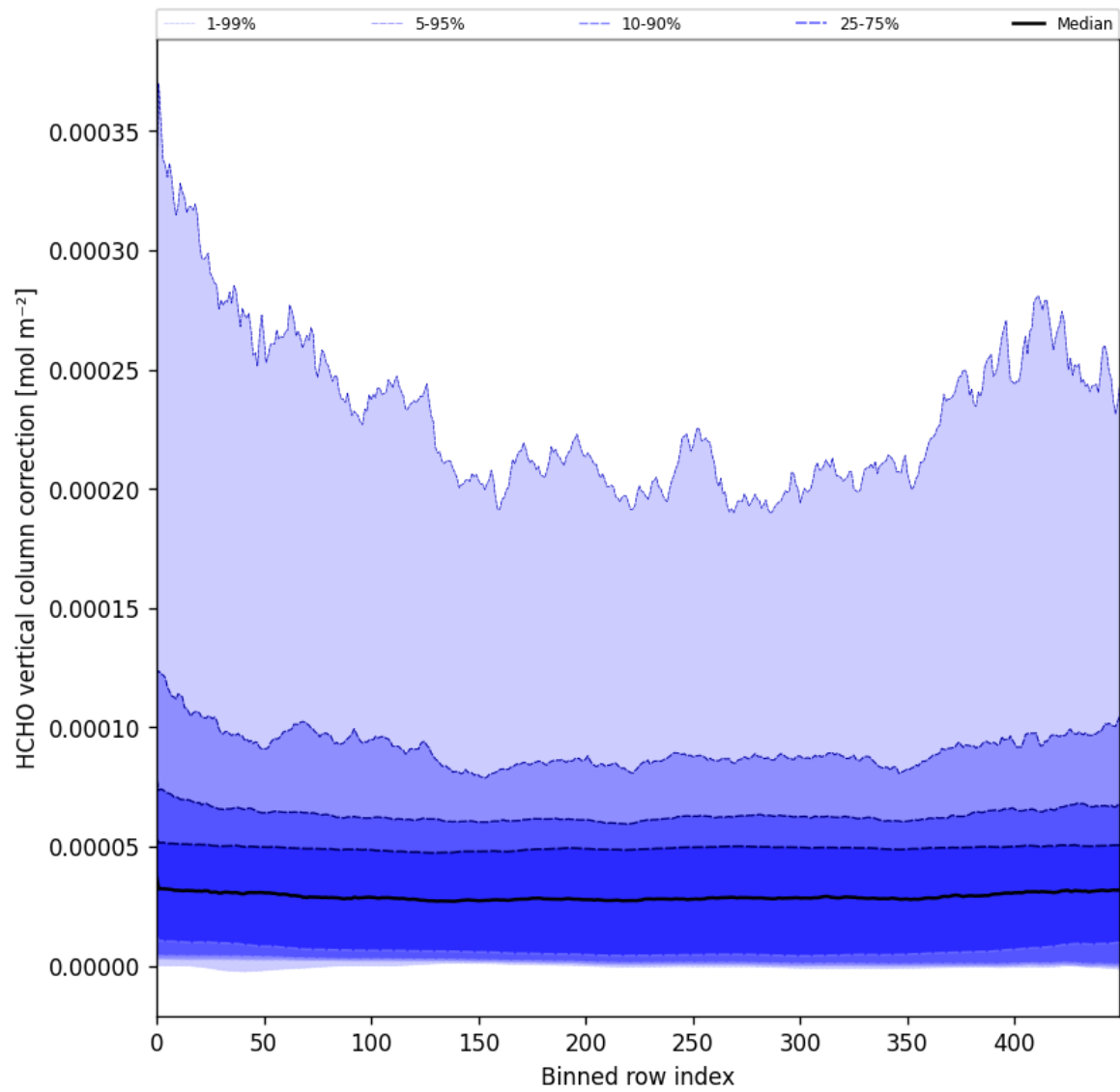
Figure 51: Along track statistics of “HCHO vertical column correction” for 2025-10-07 to 2025-10-09
