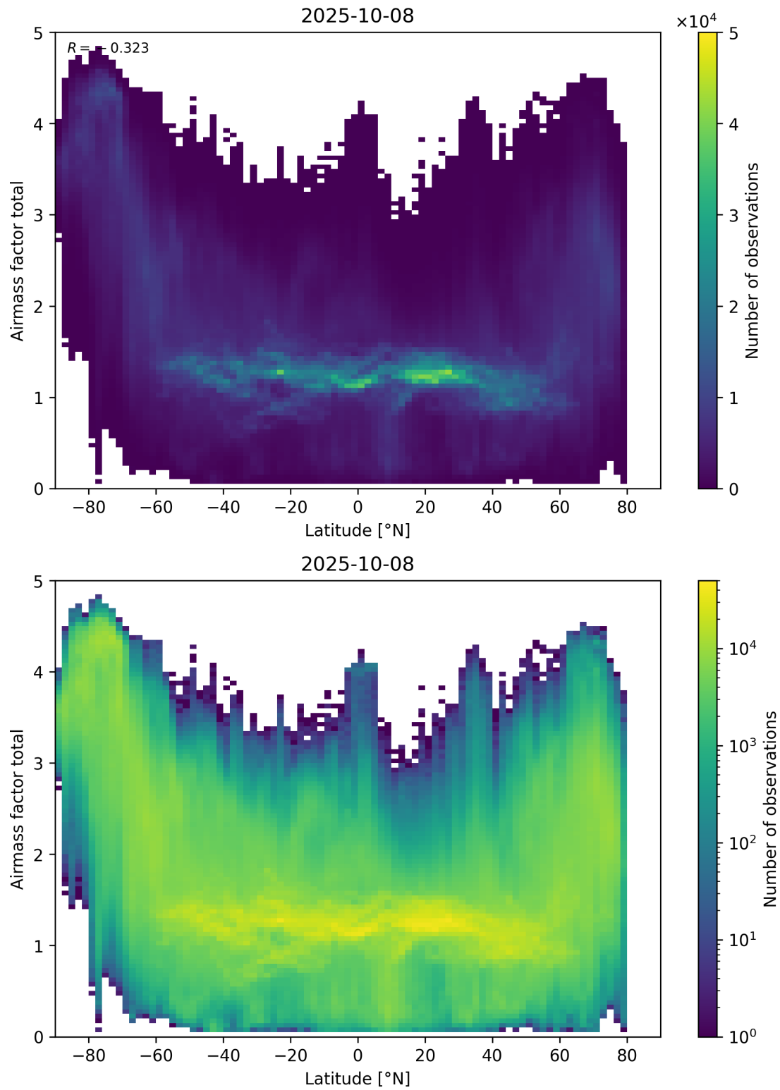
Figure 161: Scatter density plot of “Latitude” against “Airmass factor total” for 2025-10-07 to 2025-10-09.
