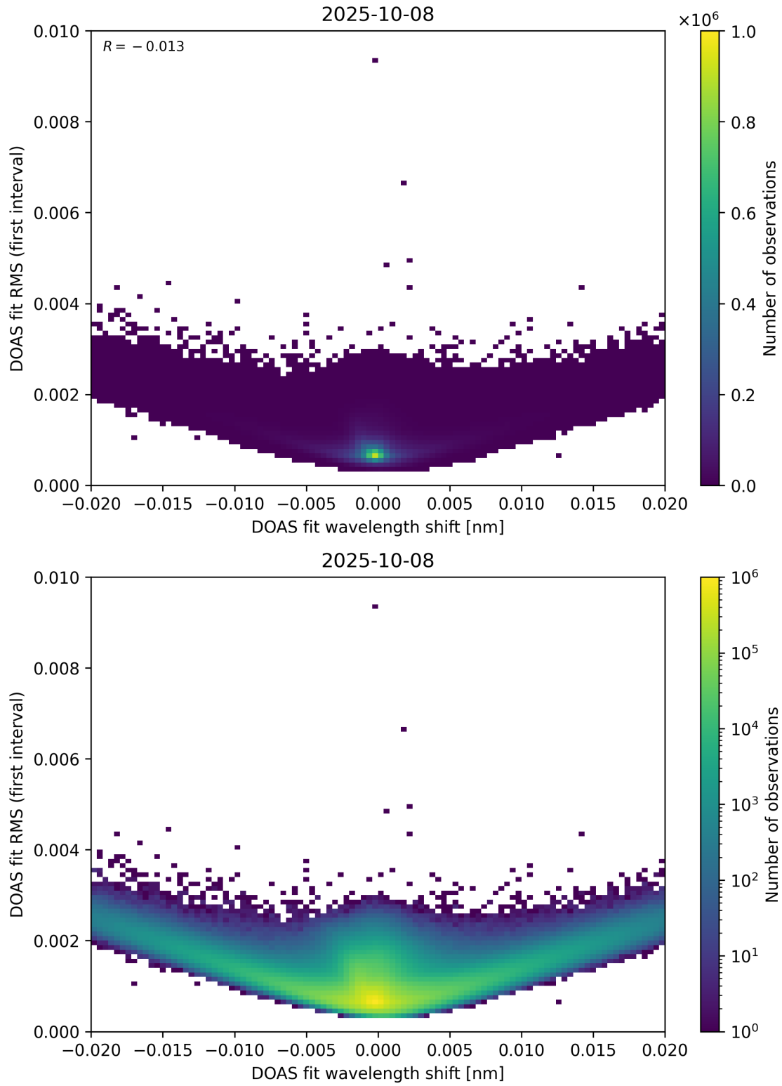
Figure 64: Scatter density plot of “DOAS fit wavelength shift” against “DOAS fit RMS (first interval)” for 2025-10-07 to 2025-10-09.
