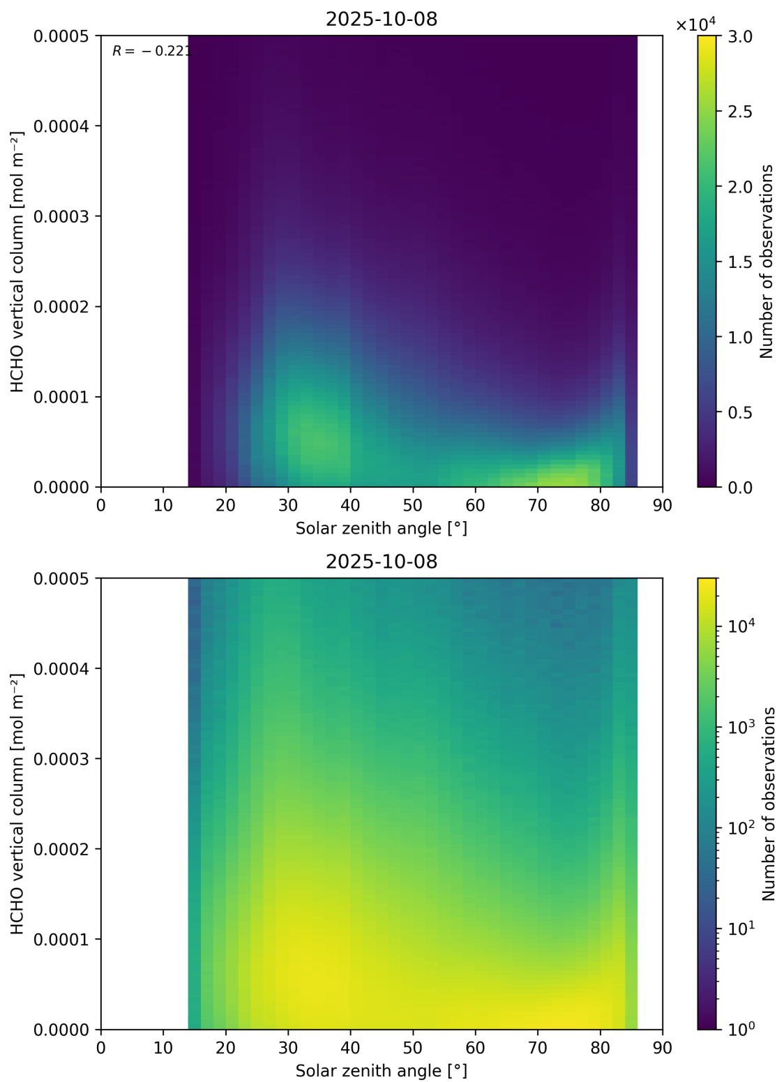
Figure 177: Scatter density plot of “Solar zenith angle” against “HCHO vertical column” for 2025-10-07 to 2025-10-09.
