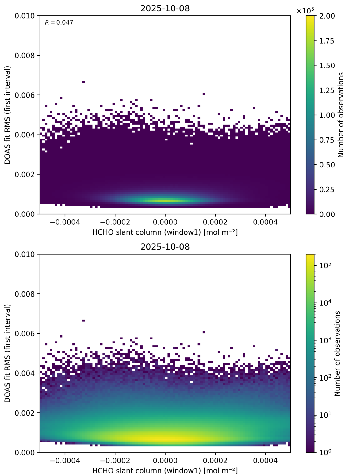
Figure 78: Scatter density plot of “HCHO slant column (window1)” against “DOAS fit RMS (first interval)” for 2025-10-07 to 2025-10-09.
