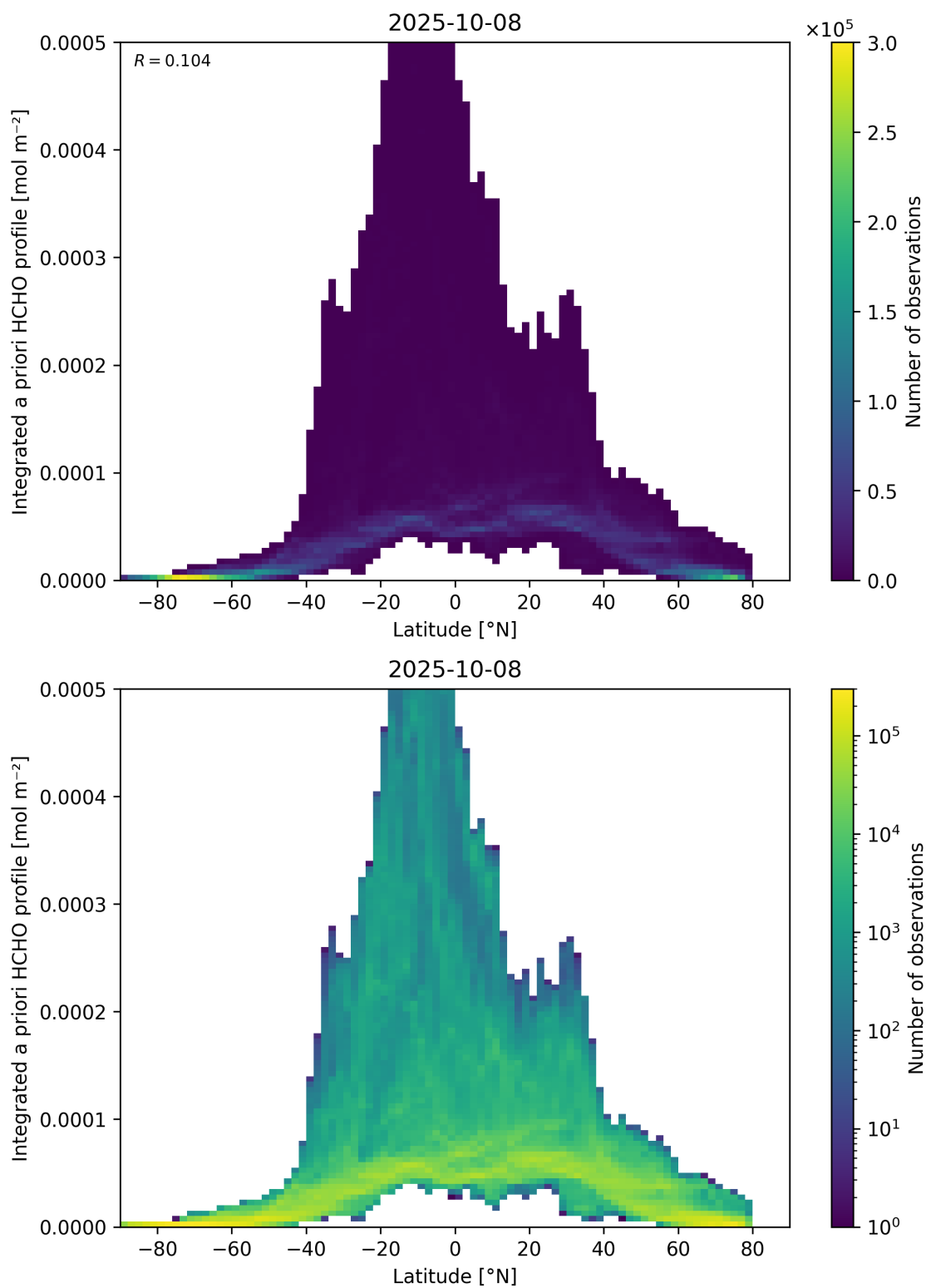
Figure 166: Scatter density plot of “Latitude” against “Integrated a priori HCHO profile” for 2025-10-07 to 2025-10-09.
