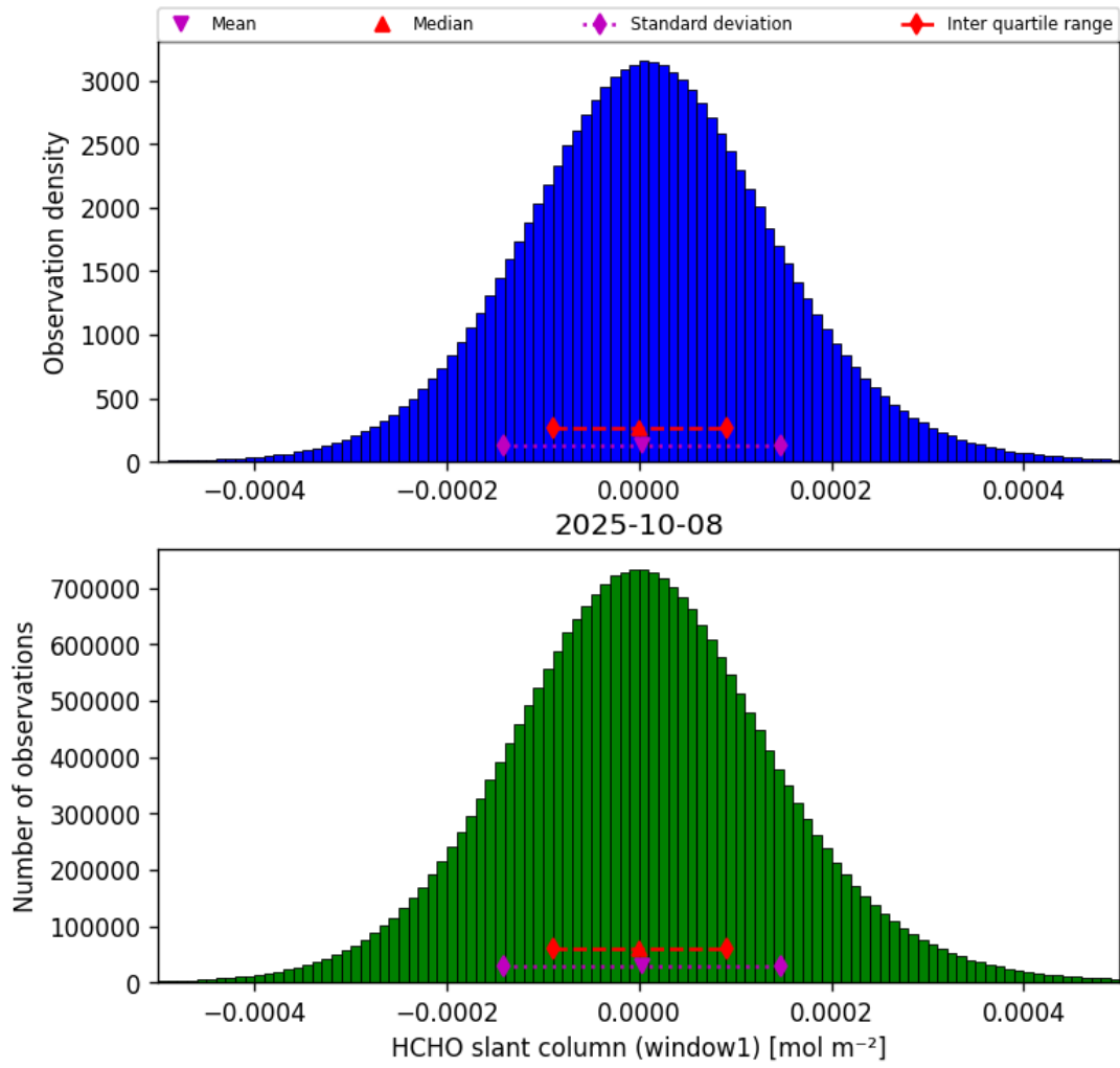
Figure 38: Histogram of “HCHO slant column (window1)” for 2025-10-07 to 2025-10-09
