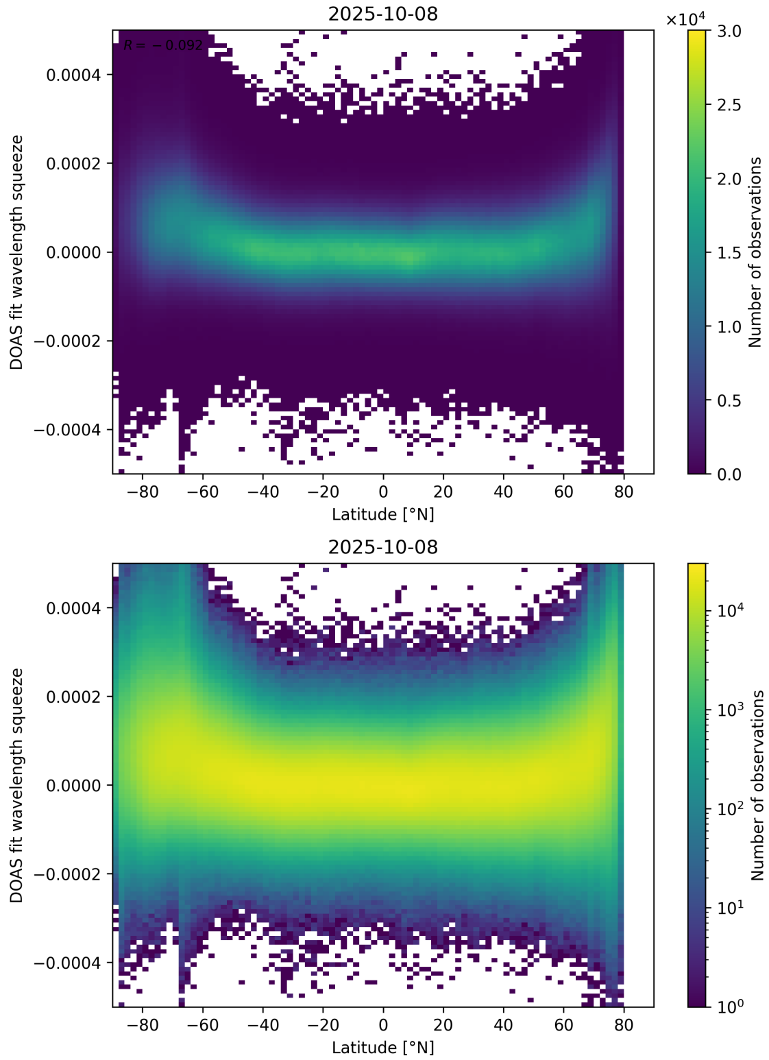
Figure 155: Scatter density plot of “Latitude” against “DOAS fit wavelength squeeze” for 2025-10-07 to 2025-10-09.
