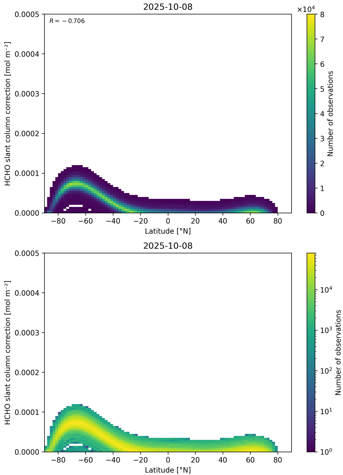
Figure 158: Scatter density plot of “Latitude” against “HCHO slant column correction” for 2025-10-07 to 2025-10-09.
