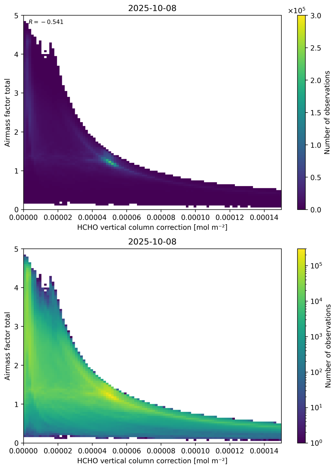
Figure 120: Scatter density plot of “HCHO vertical column correction” against “Airmass factor total” for 2025-10-07 to 2025-10-09.
