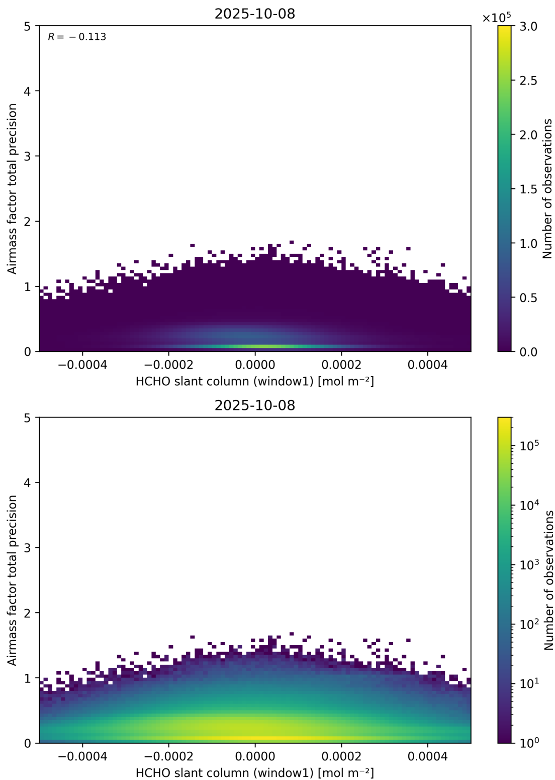
Figure 86: Scatter density plot of “HCHO slant column (window1)” against “Airmass factor total precision” for 2025-10-07 to 2025-10-09.
