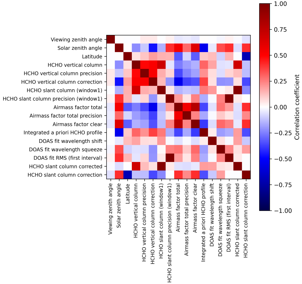
Figure 2: Map of correlation matrix for 2025-10-07 to 2025-10-09.
