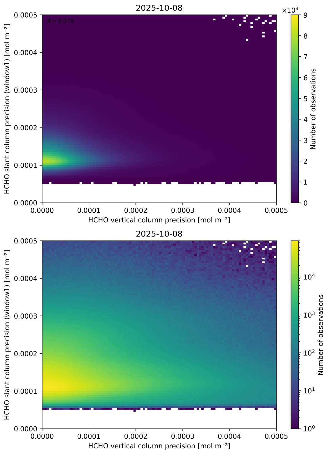
Figure 143: Scatter density plot of “HCHO vertical column precision” against “HCHO slant column precision (window1)” for 2025-10-07 to 2025-10-09.
