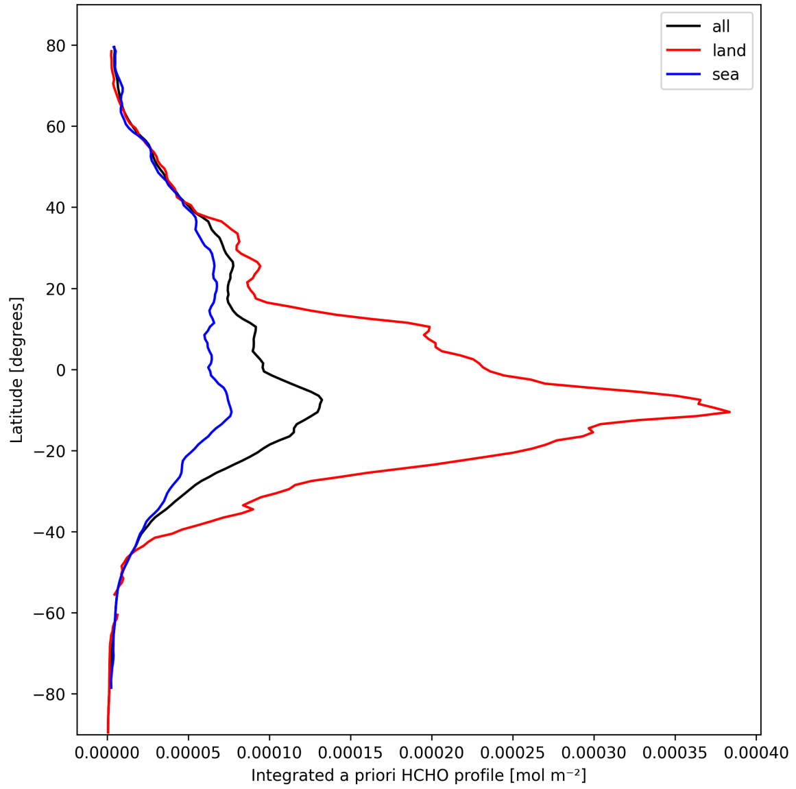
Figure 29: Zonal average of “Integrated a priori HCHO profile” for 2025-10-07 to 2025-10-09.
