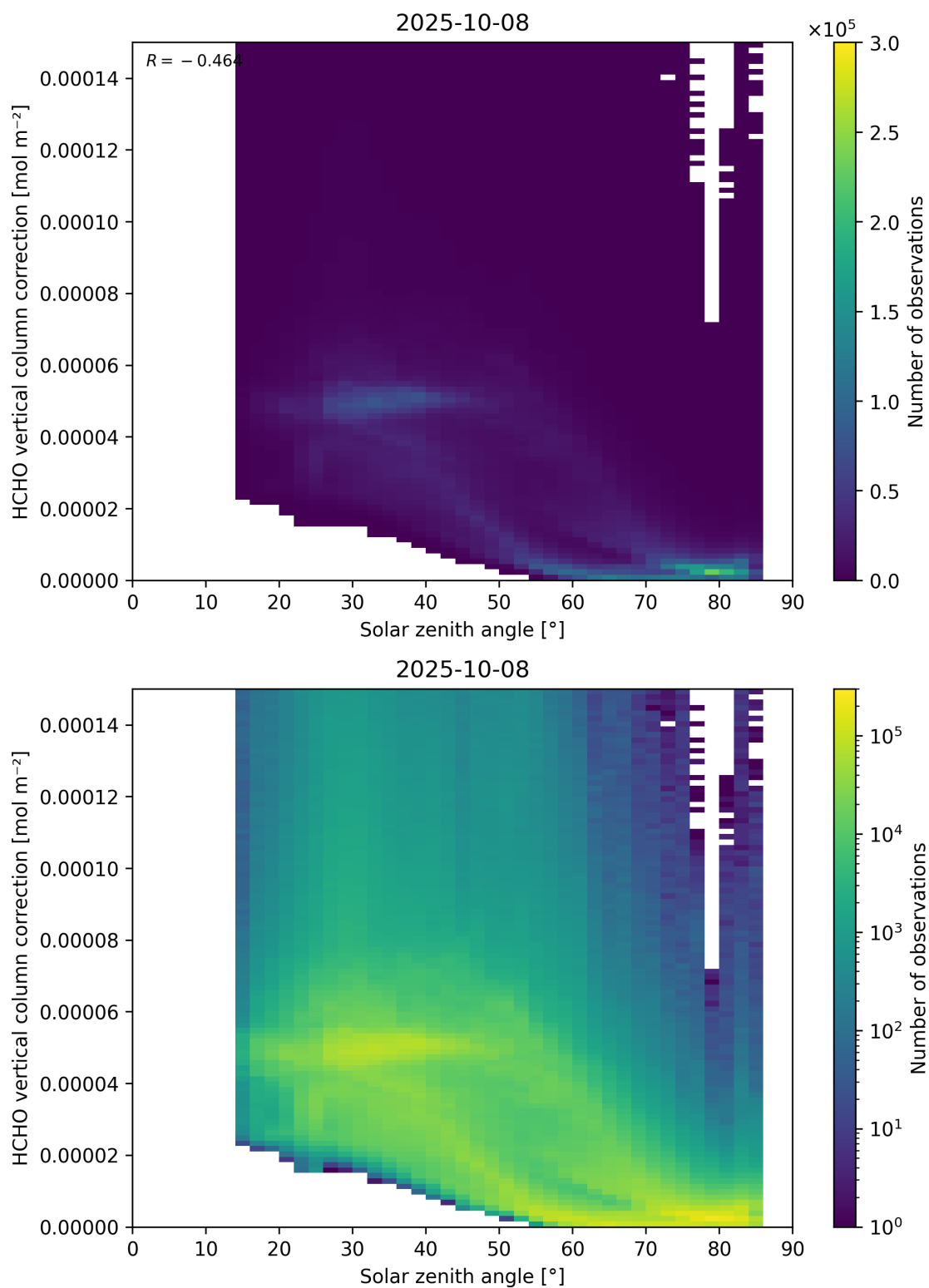
Figure 178: Scatter density plot of “Solar zenith angle” against “HCHO vertical column correction” for 2025-10-07 to 2025-10-09.
