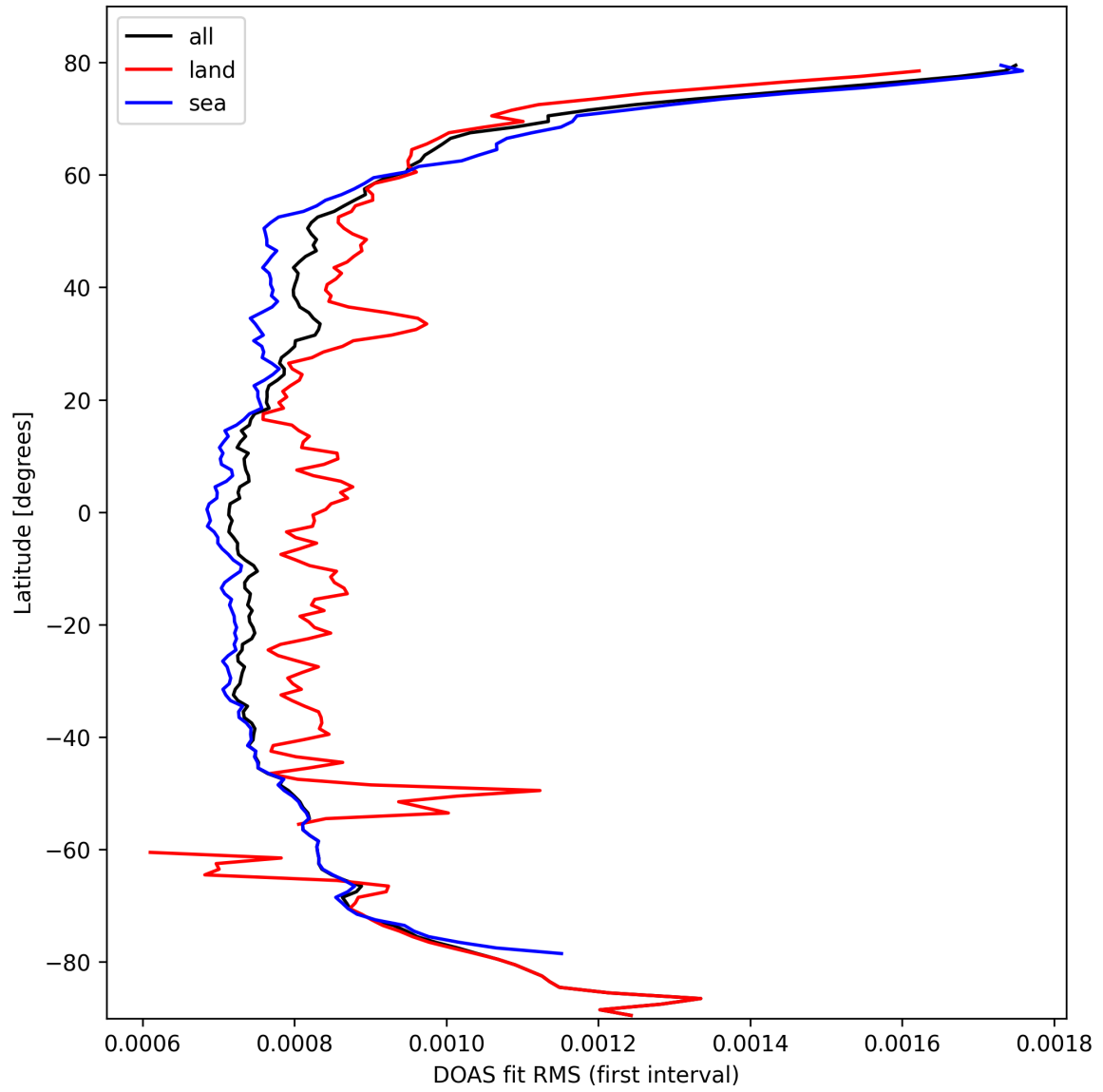
Figure 32: Zonal average of “DOAS fit RMS (first interval)” for 2025-10-07 to 2025-10-09.
