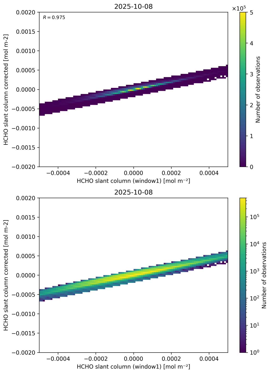
Figure 82: Scatter density plot of “HCHO slant column (window1)” against “HCHO slant column corrected” for 2025-10-07 to 2025-10-09.
