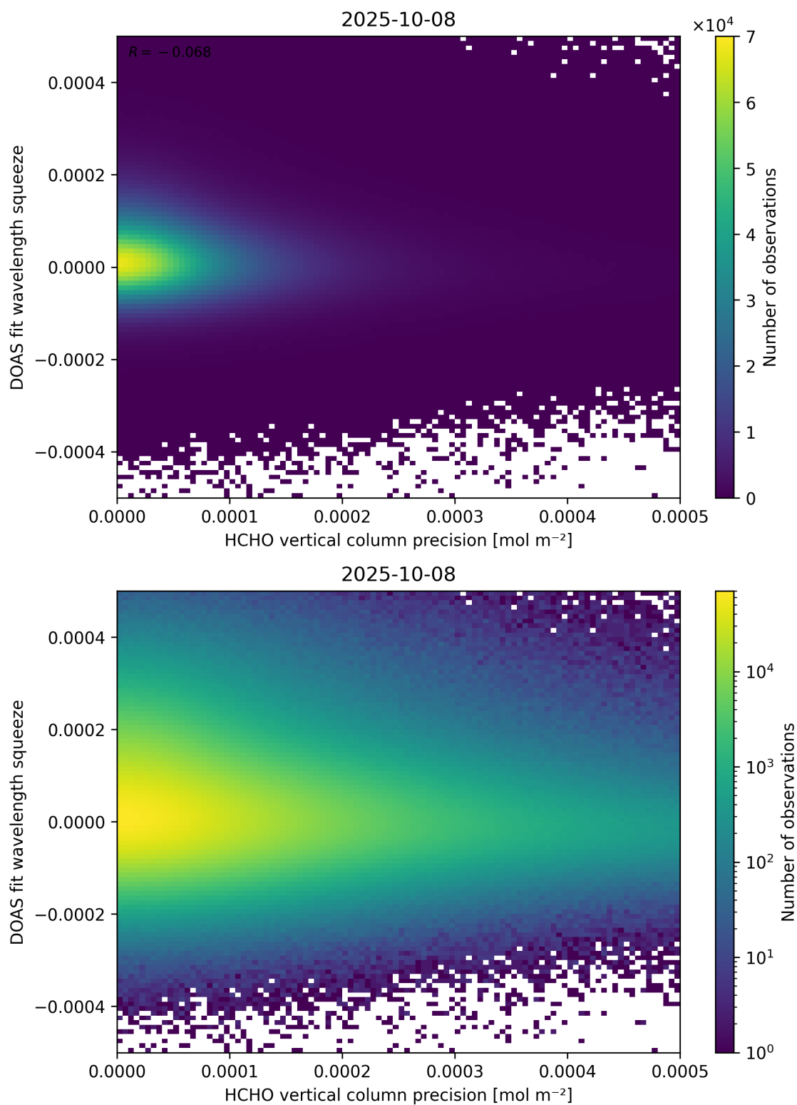
Figure 138: Scatter density plot of “HCHO vertical column precision” against “DOAS fit wavelength squeeze” for 2025-10-07 to 2025-10-09.
