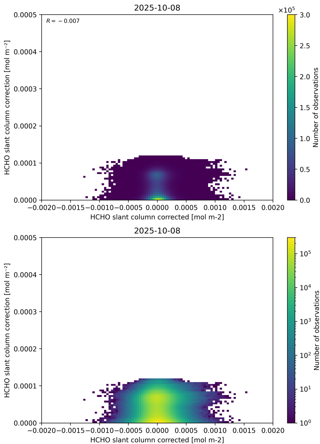
Figure 77: Scatter density plot of “HCHO slant column corrected” against “HCHO slant column correction” for 2025-10-07 to 2025-10-09.
