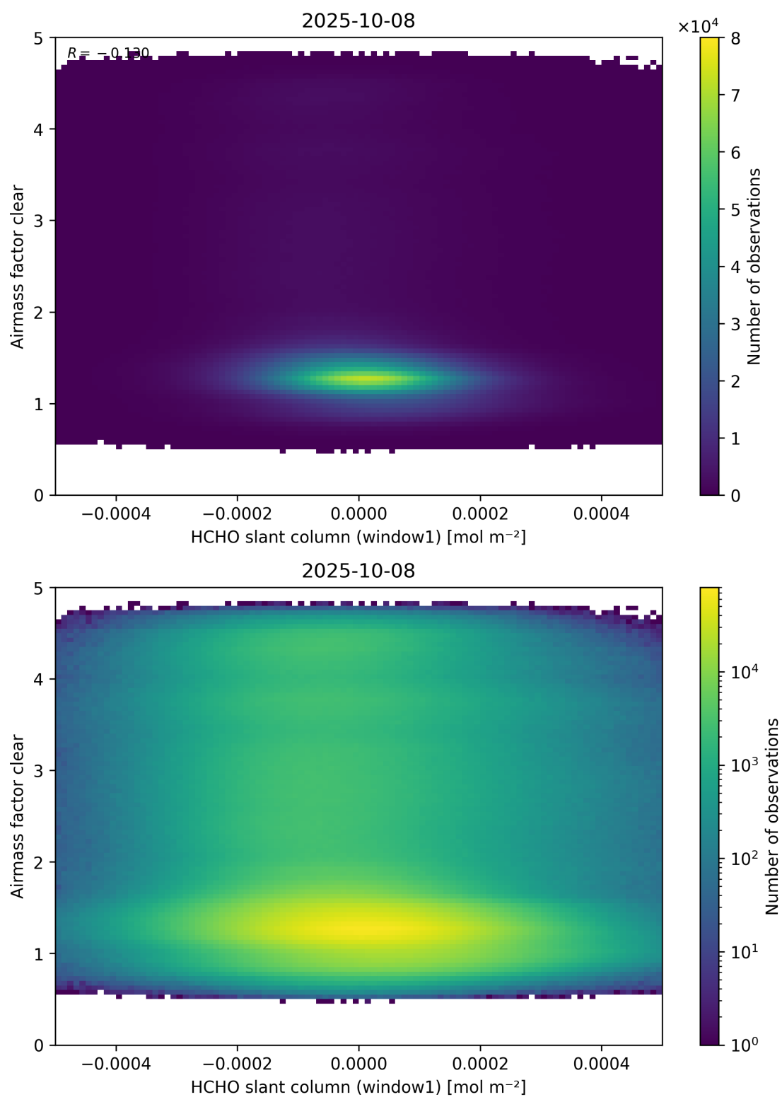
Figure 81: Scatter density plot of “HCHO slant column (window1)” against “Airmass factor clear” for 2025-10-07 to 2025-10-09.
