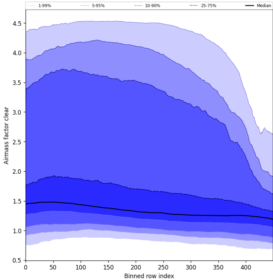
Figure 56: Along track statistics of “Airmass factor clear” for 2025-10-07 to 2025-10-09
