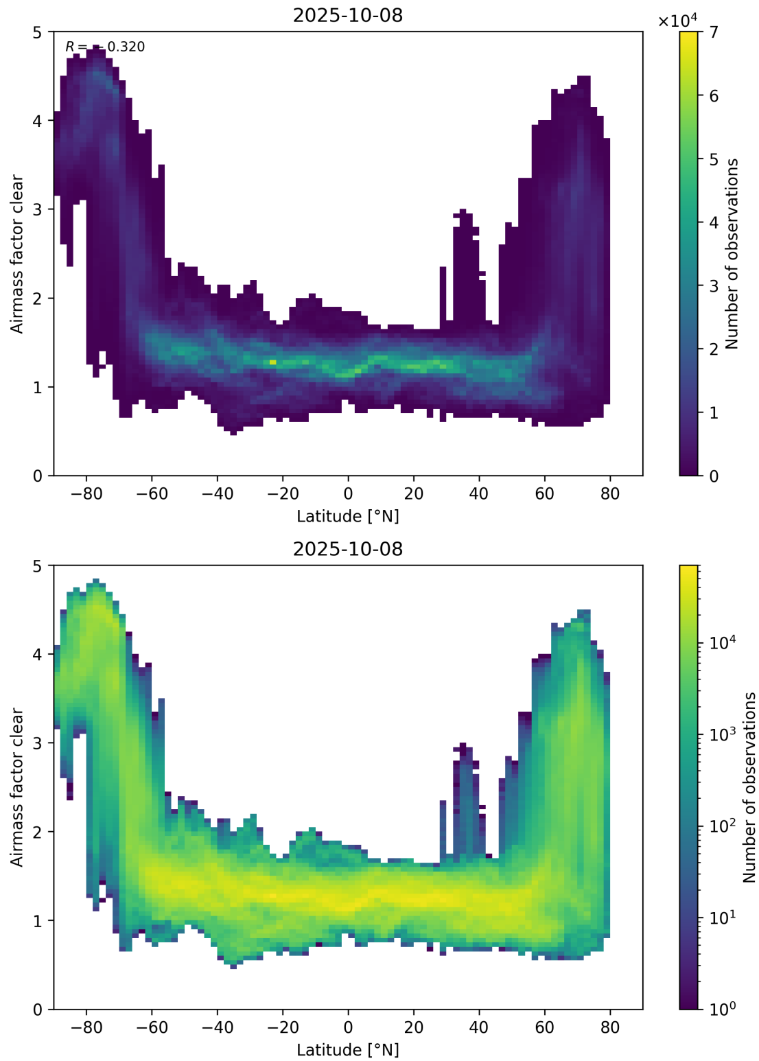
Figure 156: Scatter density plot of “Latitude” against “Airmass factor clear” for 2025-10-07 to 2025-10-09.
