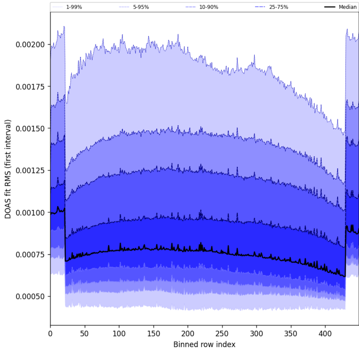
Figure 60: Along track statistics of “DOAS fit RMS (first interval)” for 2025-10-07 to 2025-10-09
