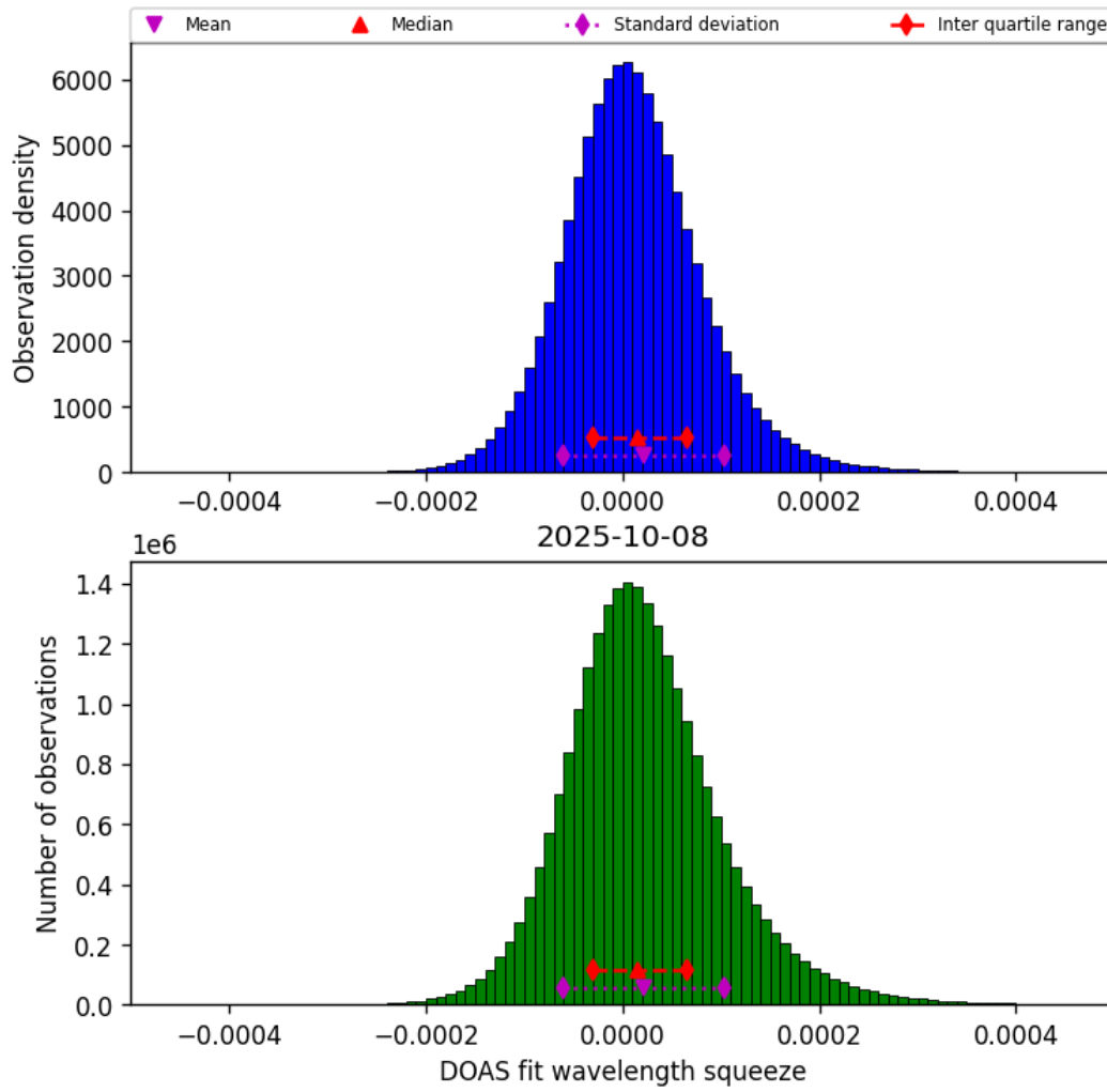
Figure 45: Histogram of “DOAS fit wavelength squeeze” for 2025-10-07 to 2025-10-09
