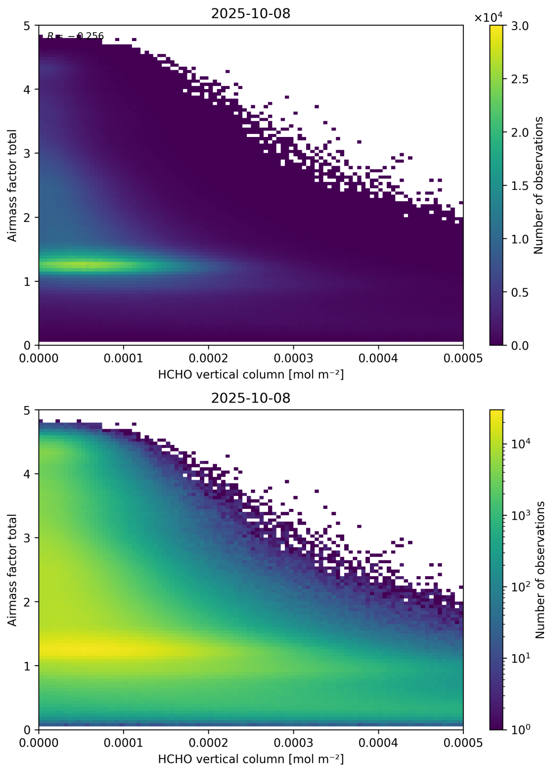
Figure 131: Scatter density plot of “HCHO vertical column” against “Airmass factor total” for 2025-10-07 to 2025-10-09.
