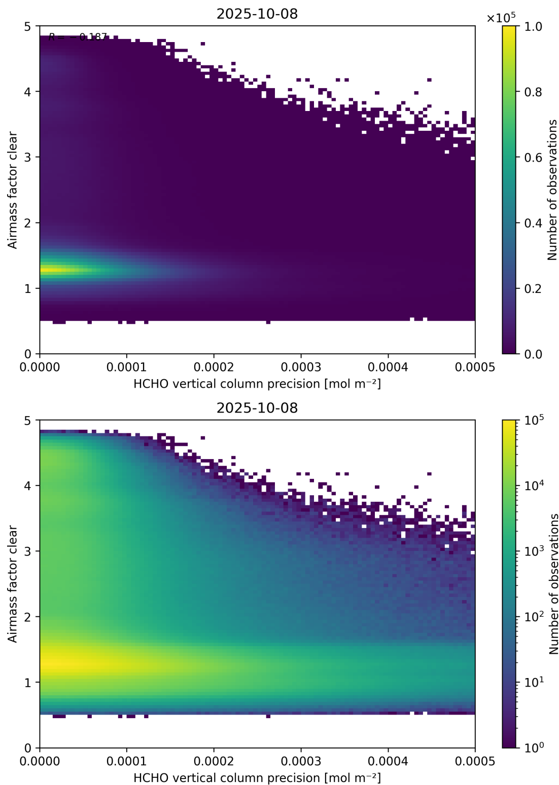
Figure 139: Scatter density plot of “HCHO vertical column precision” against “Airmass factor clear” for 2025-10-07 to 2025-10-09.
