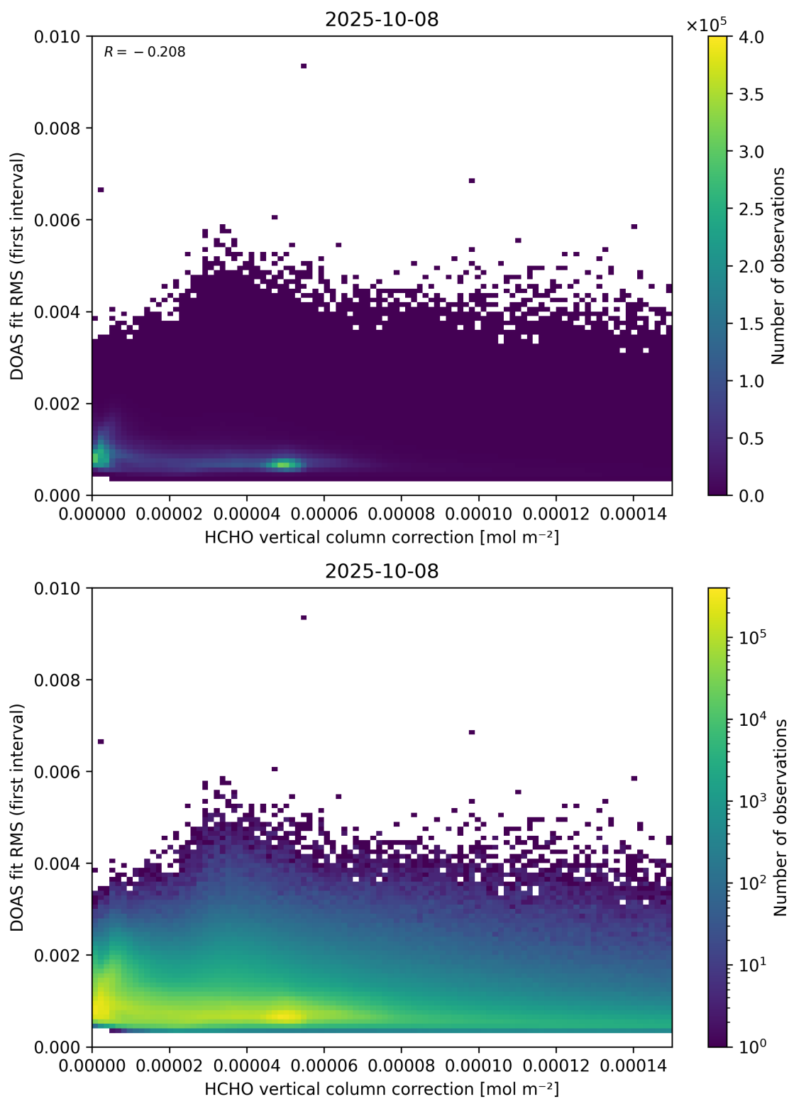
Figure 112: Scatter density plot of “HCHO vertical column correction” against “DOAS fit RMS (first interval)” for 2025-10-07 to 2025-10-09.
