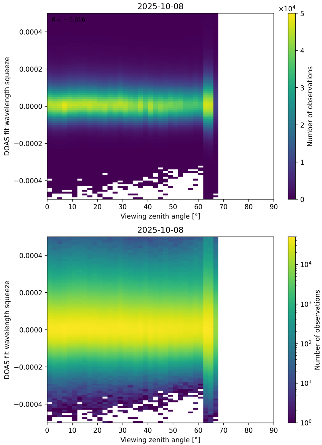
Figure 184: Scatter density plot of “Viewing zenith angle” against “DOAS fit wavelength squeeze” for 2025-10-07 to 2025-10-09.
