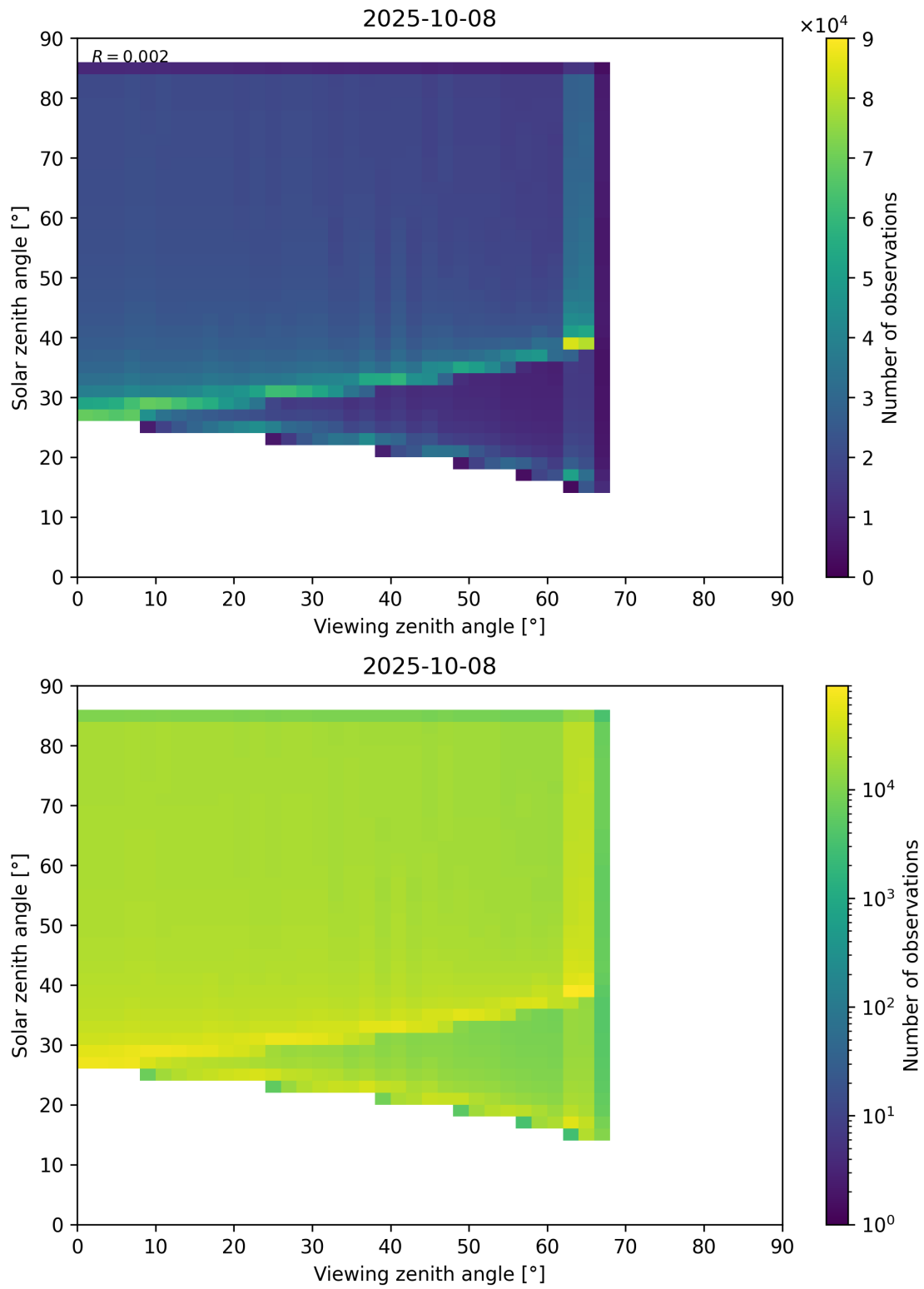
Figure 197: Scatter density plot of “Viewing zenith angle” against “Solar zenith angle” for 2025-10-07 to 2025-10-09.
