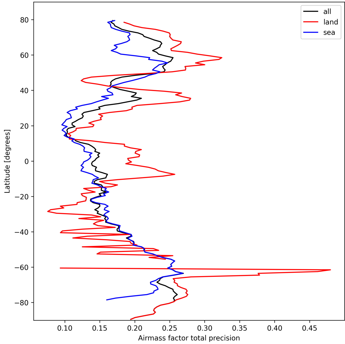
Figure 27: Zonal average of “Airmass factor total precision” for 2025-10-07 to 2025-10-09.
