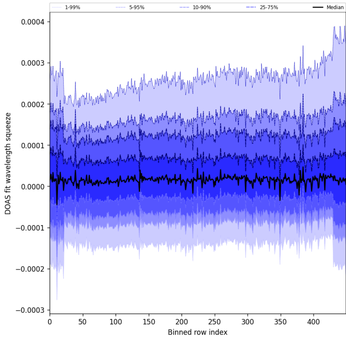
Figure 59: Along track statistics of “DOAS fit wavelength squeeze” for 2025-10-07 to 2025-10-09
