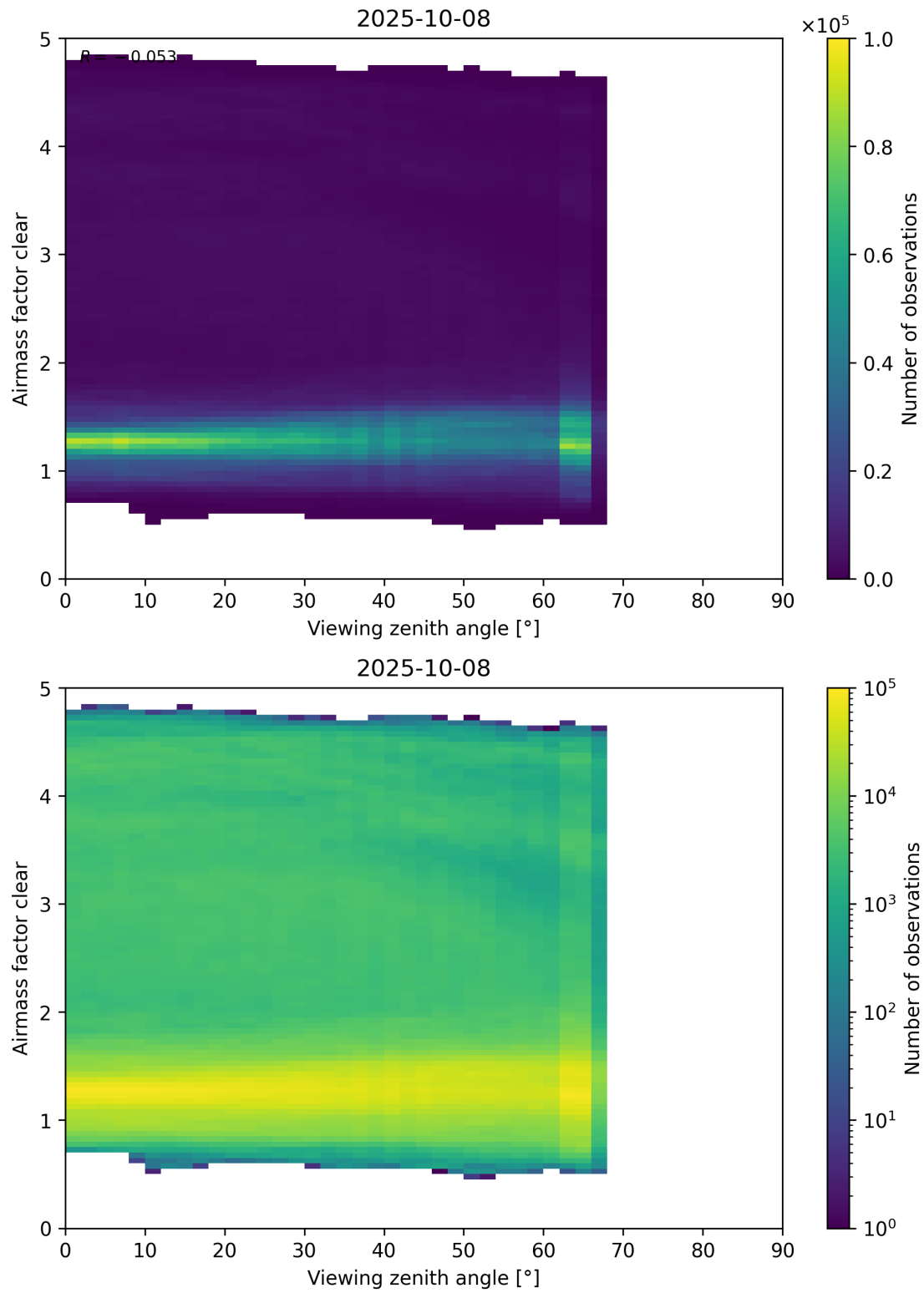
Figure 185: Scatter density plot of “Viewing zenith angle” against “Airmass factor clear” for 2025-10-07 to 2025-10-09.
