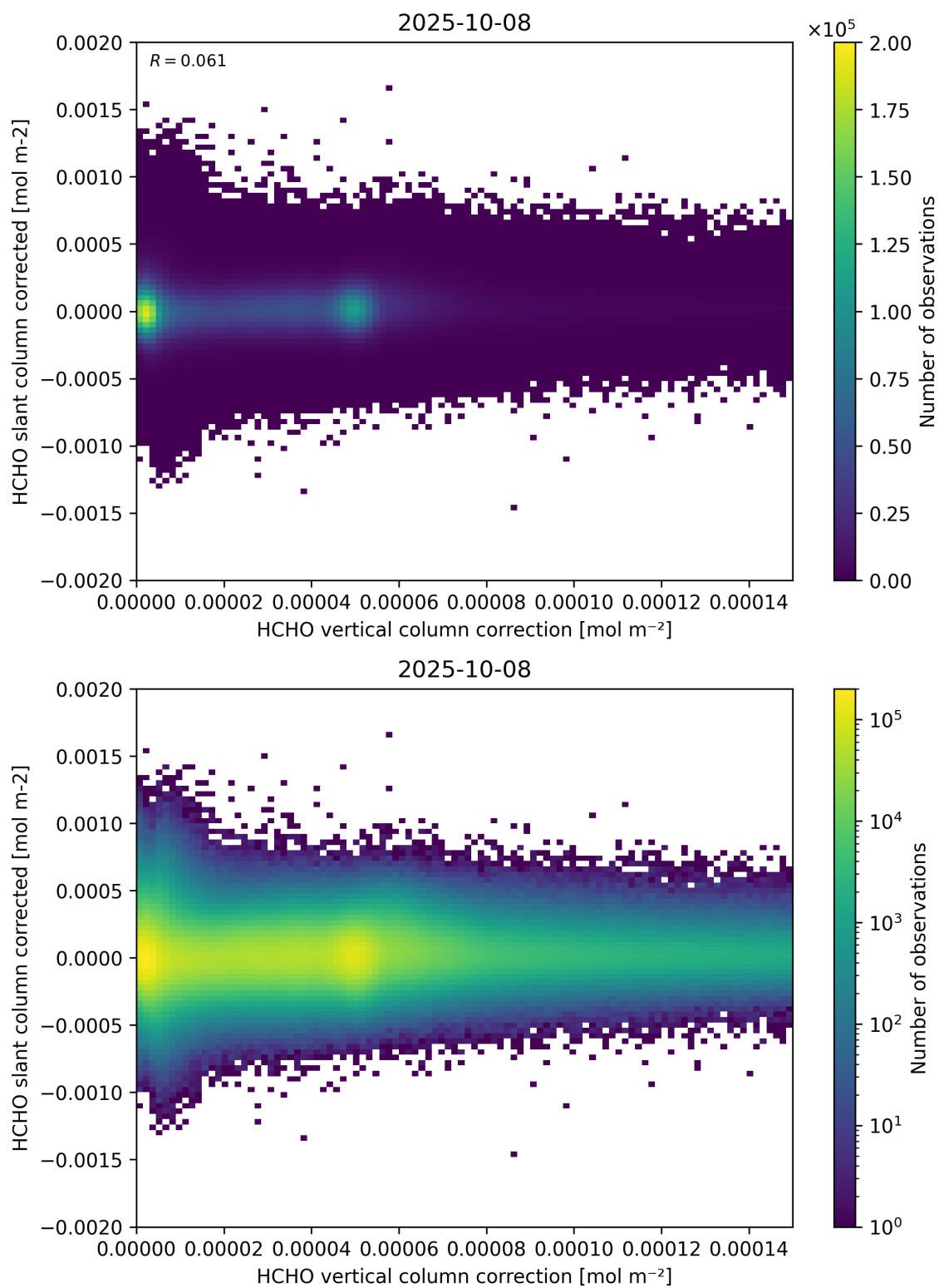
Figure 116: Scatter density plot of “HCHO vertical column correction” against “HCHO slant column corrected” for 2025-10-07 to 2025-10-09.
