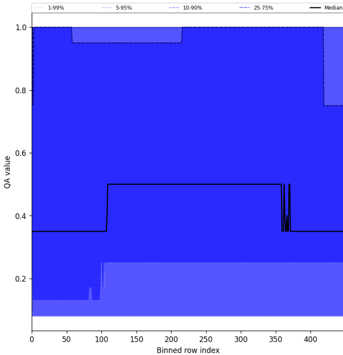
Figure 48: Along track statistics of “QA value” for 2025-10-07 to 2025-10-09
