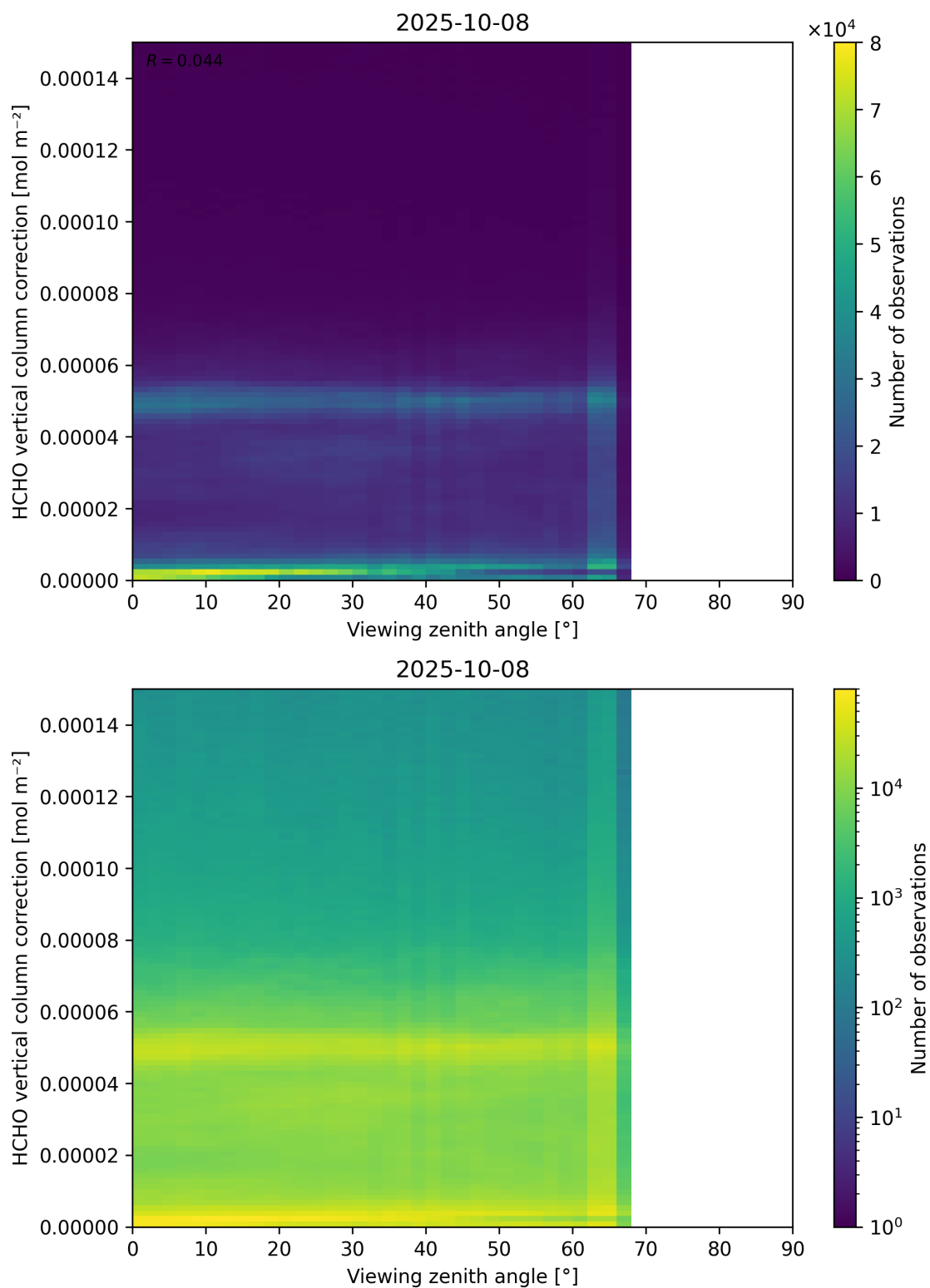
Figure 193: Scatter density plot of “Viewing zenith angle” against “HCHO vertical column correction” for 2025-10-07 to 2025-10-09.
