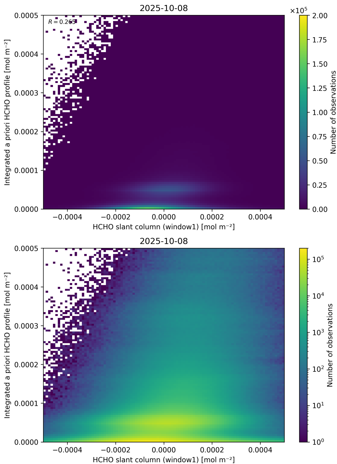
Figure 87: Scatter density plot of “HCHO slant column (window1)” against “Integrated a priori HCHO profile” for 2025-10-07 to 2025-10-09.
