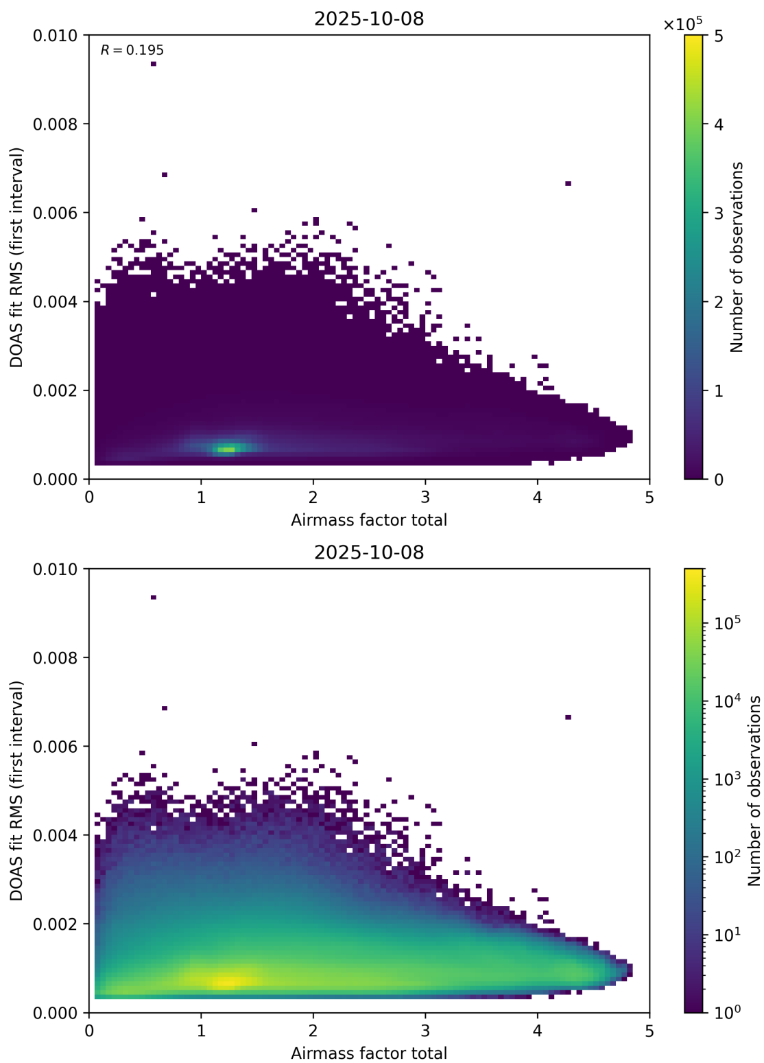
Figure 97: Scatter density plot of “Airmass factor total” against “DOAS fit RMS (first interval)” for 2025-10-07 to 2025-10-09.
