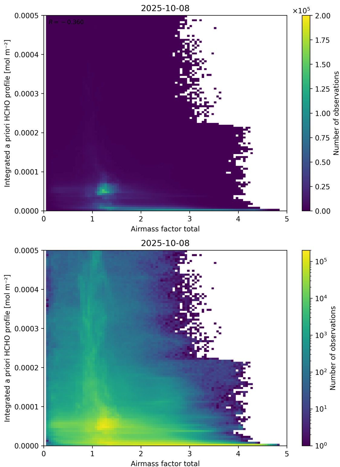
Figure 104: Scatter density plot of “Airmass factor total” against “Integrated a priori HCHO profile” for 2025-10-07 to 2025-10-09.
