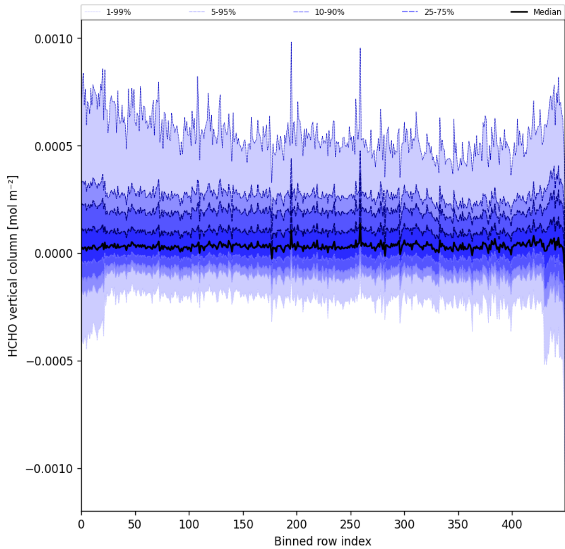
Figure 49: Along track statistics of “HCHO vertical column” for 2025-10-07 to 2025-10-09
