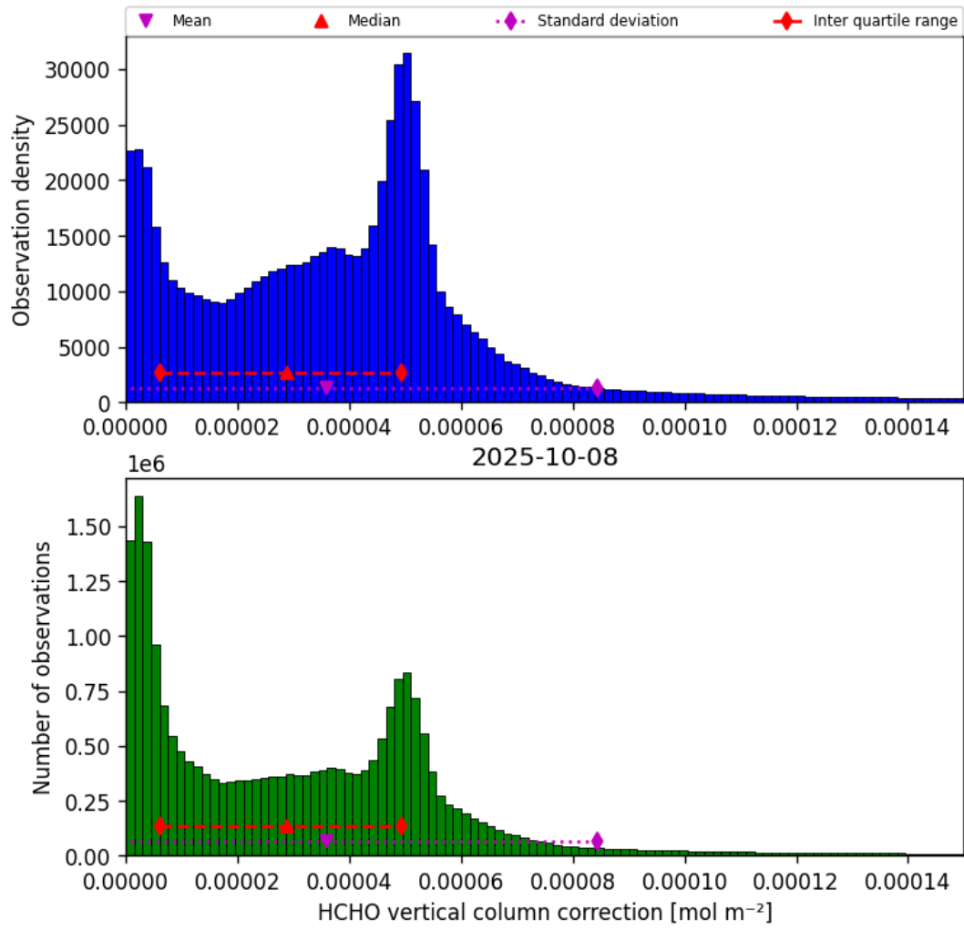
Figure 37: Histogram of “HCHO vertical column correction” for 2025-10-07 to 2025-10-09
