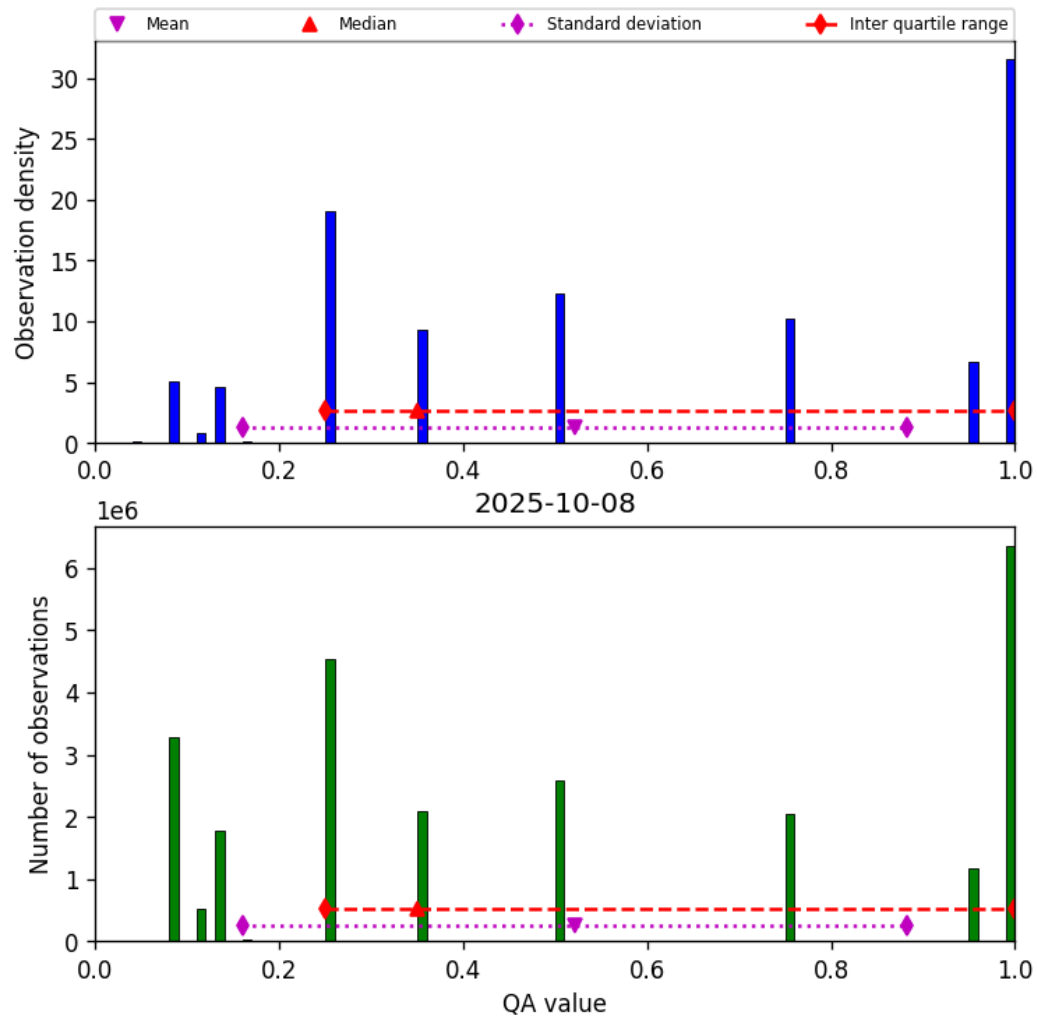
Figure 34: Histogram of “QA value” for 2025-10-07 to 2025-10-09
