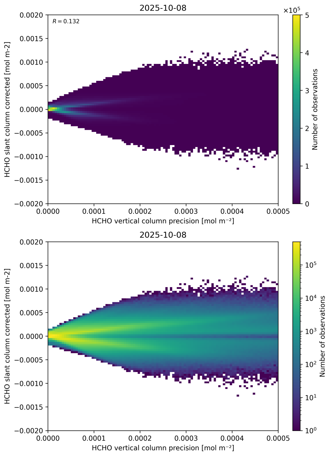
Figure 140: Scatter density plot of “HCHO vertical column precision” against “HCHO slant column corrected” for 2025-10-07 to 2025-10-09.
