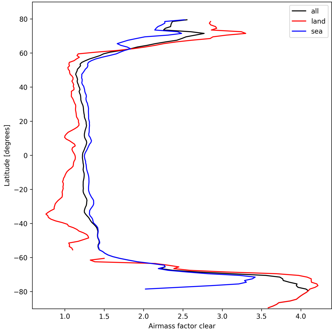
Figure 28: Zonal average of “Airmass factor clear” for 2025-10-07 to 2025-10-09.
