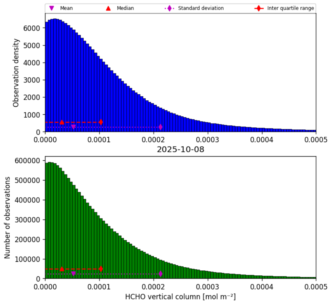
Figure 35: Histogram of “HCHO vertical column” for 2025-10-07 to 2025-10-09
