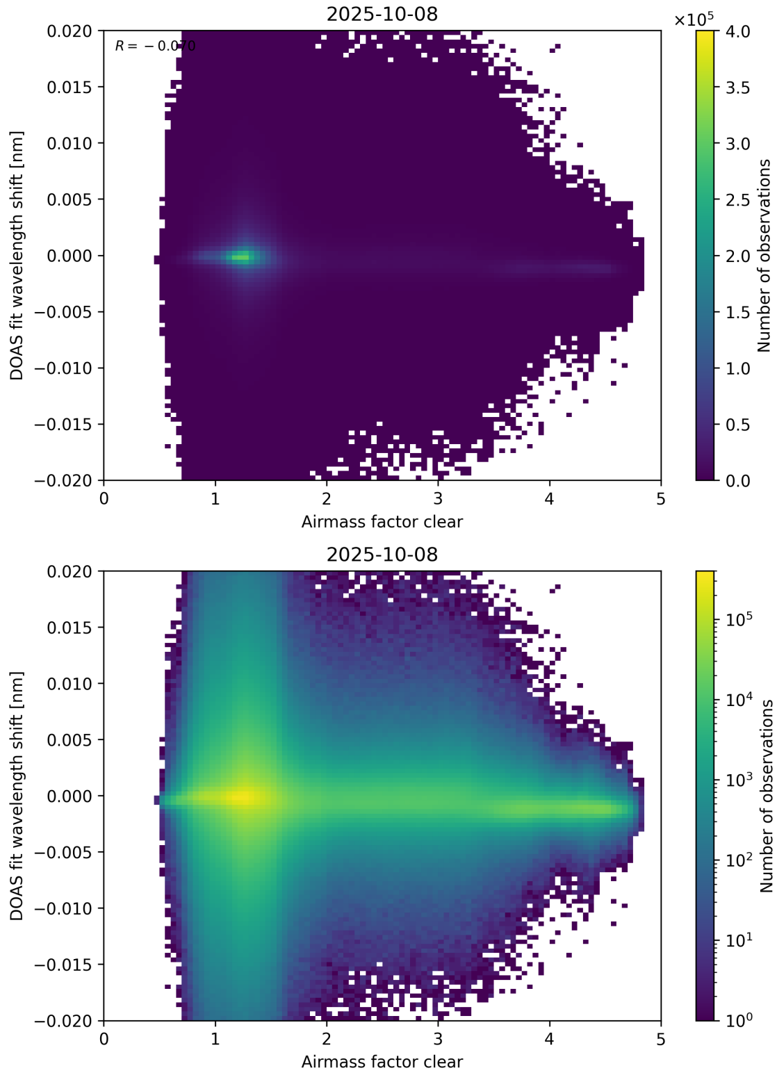
Figure 72: Scatter density plot of “Airmass factor clear” against “DOAS fit wavelength shift” for 2025-10-07 to 2025-10-09.
