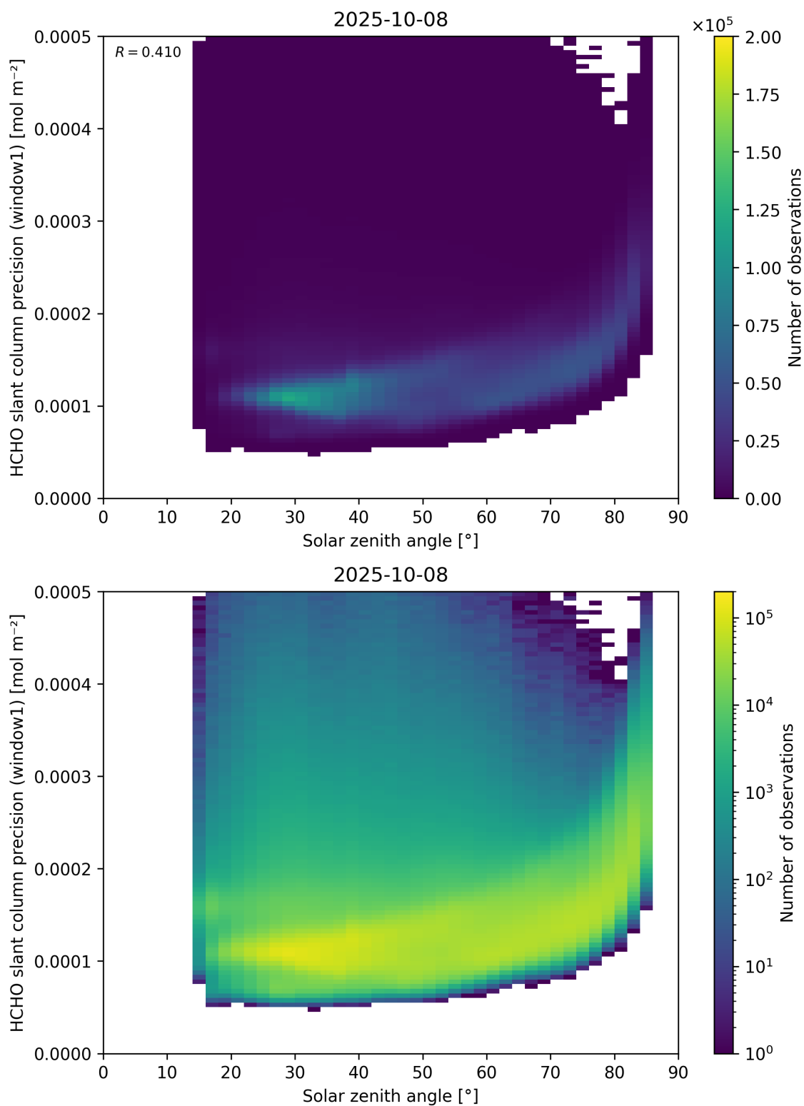
Figure 174: Scatter density plot of “Solar zenith angle” against “HCHO slant column precision (window1)” for 2025-10-07 to 2025-10-09.
