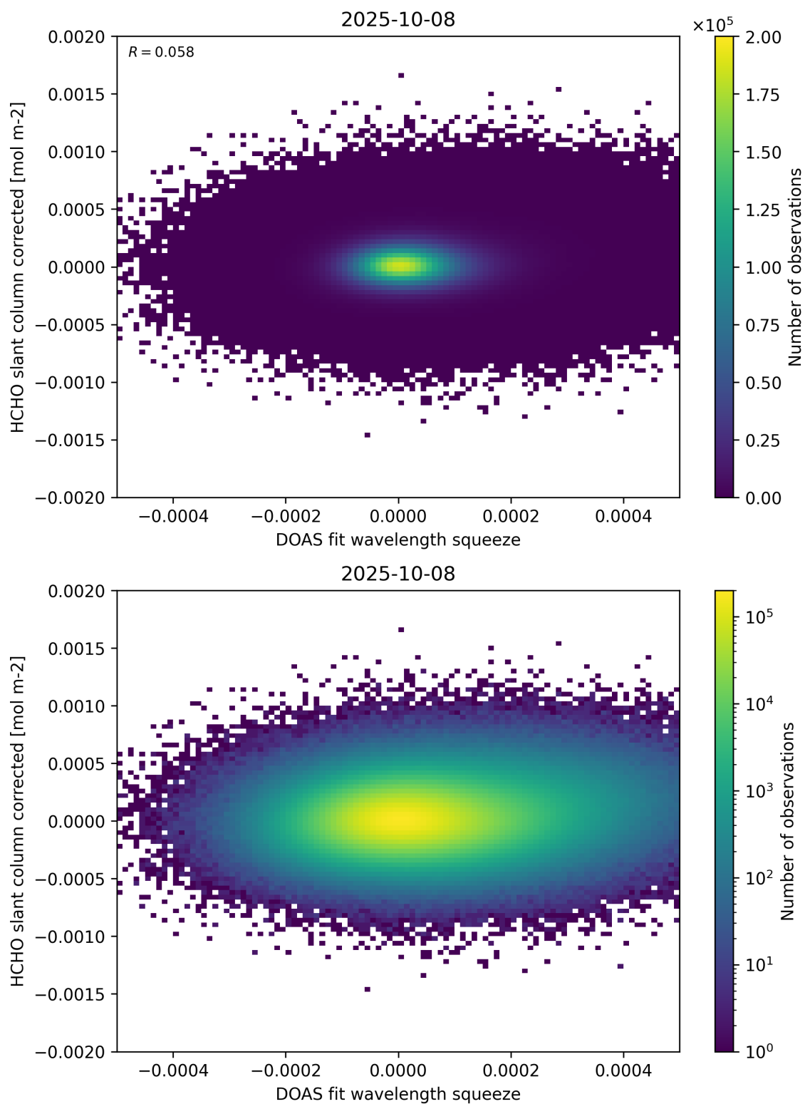
Figure 69: Scatter density plot of “DOAS fit wavelength squeeze” against “HCHO slant column corrected” for 2025-10-07 to 2025-10-09.
