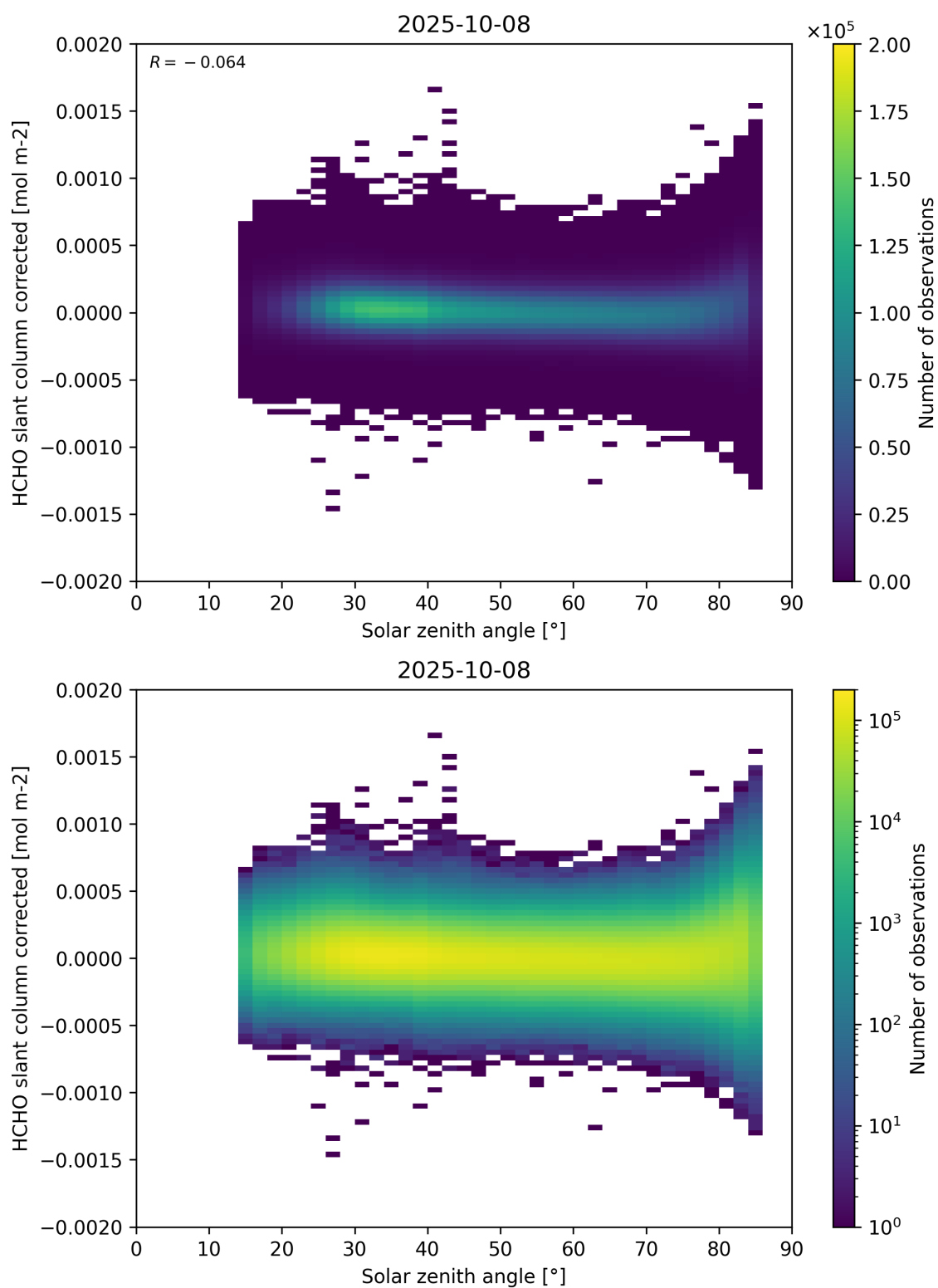
Figure 171: Scatter density plot of “Solar zenith angle” against “HCHO slant column corrected” for 2025-10-07 to 2025-10-09.
