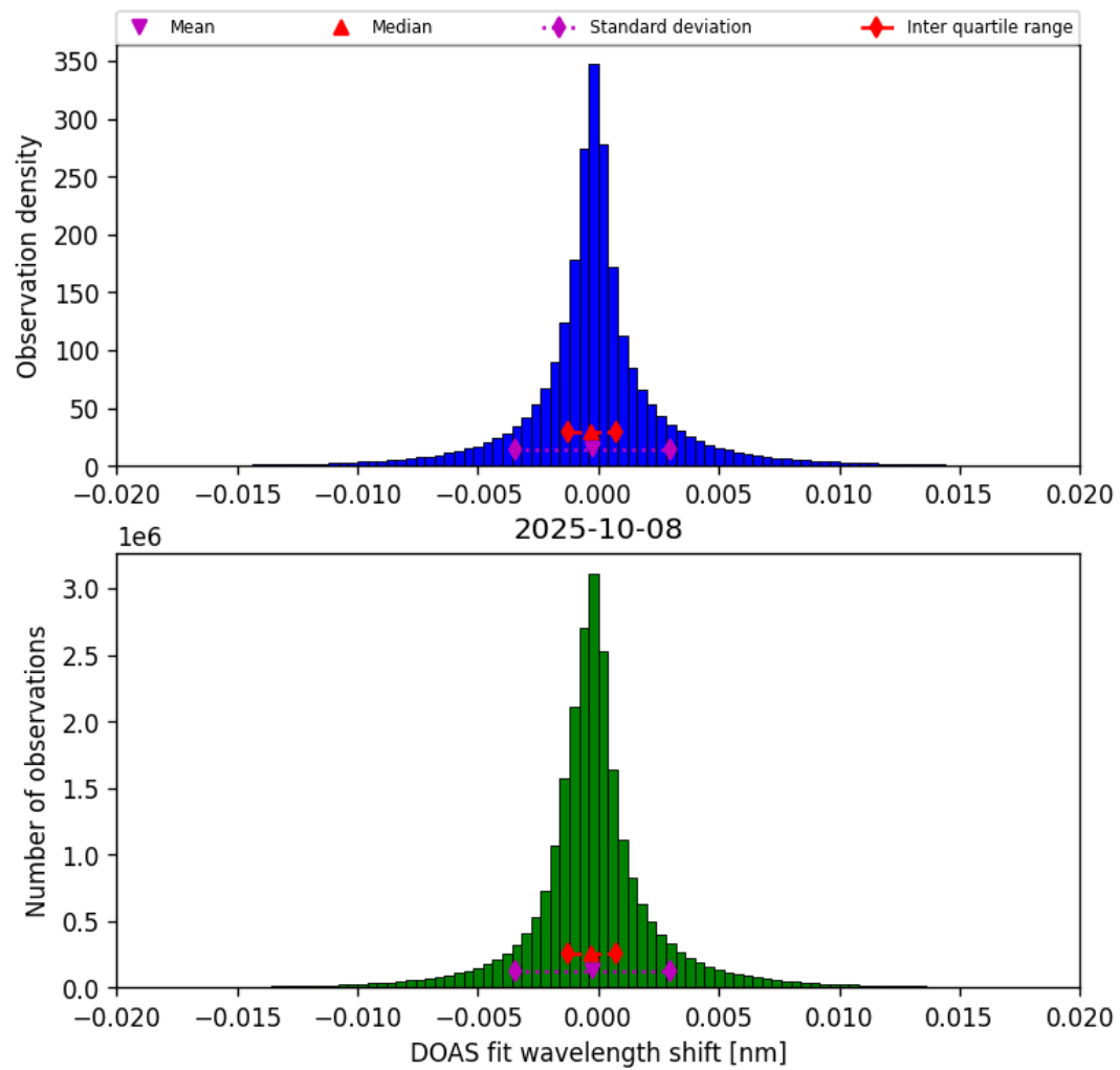
Figure 44: Histogram of “DOAS fit wavelength shift” for 2025-10-07 to 2025-10-09
