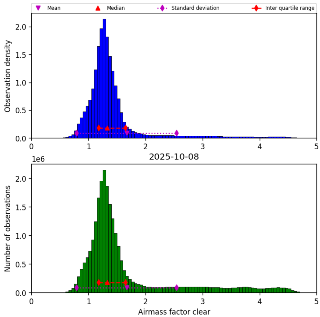
Figure 42: Histogram of “Airmass factor clear” for 2025-10-07 to 2025-10-09
