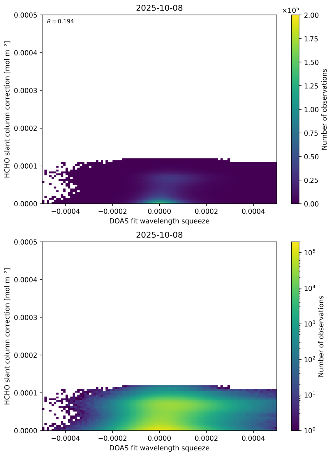
Figure 70: Scatter density plot of “DOAS fit wavelength squeeze” against “HCHO slant column correction” for 2025-10-07 to 2025-10-09.
