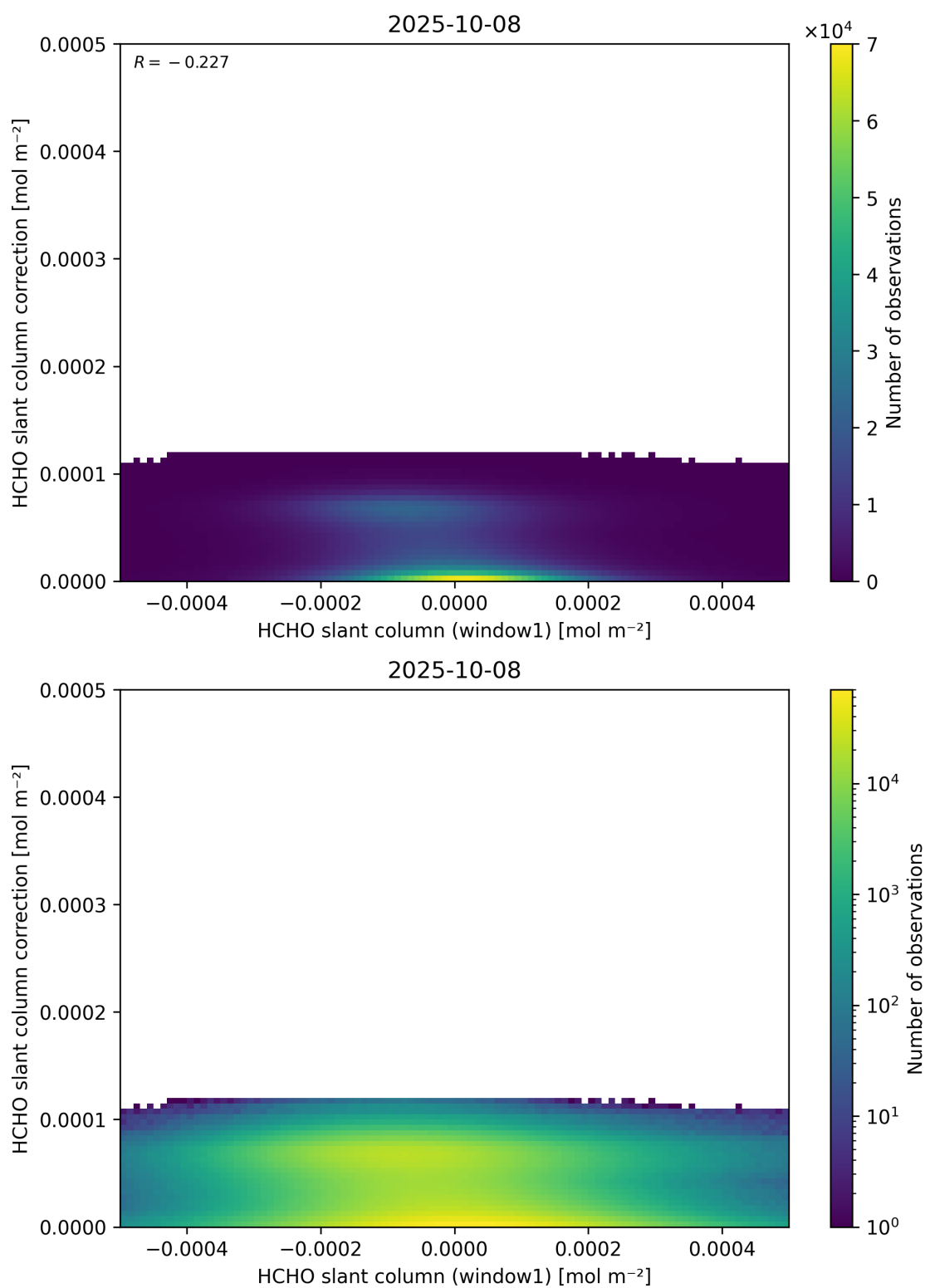
Figure 83: Scatter density plot of “HCHO slant column (window1)” against “HCHO slant column correction” for 2025-10-07 to 2025-10-09.
