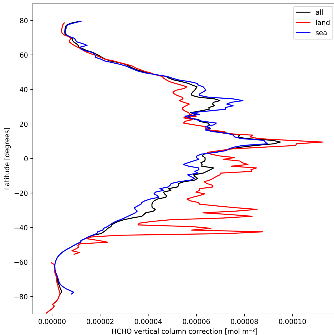
Figure 23: Zonal average of “HCHO vertical column correction” for 2025-10-07 to 2025-10-09.
