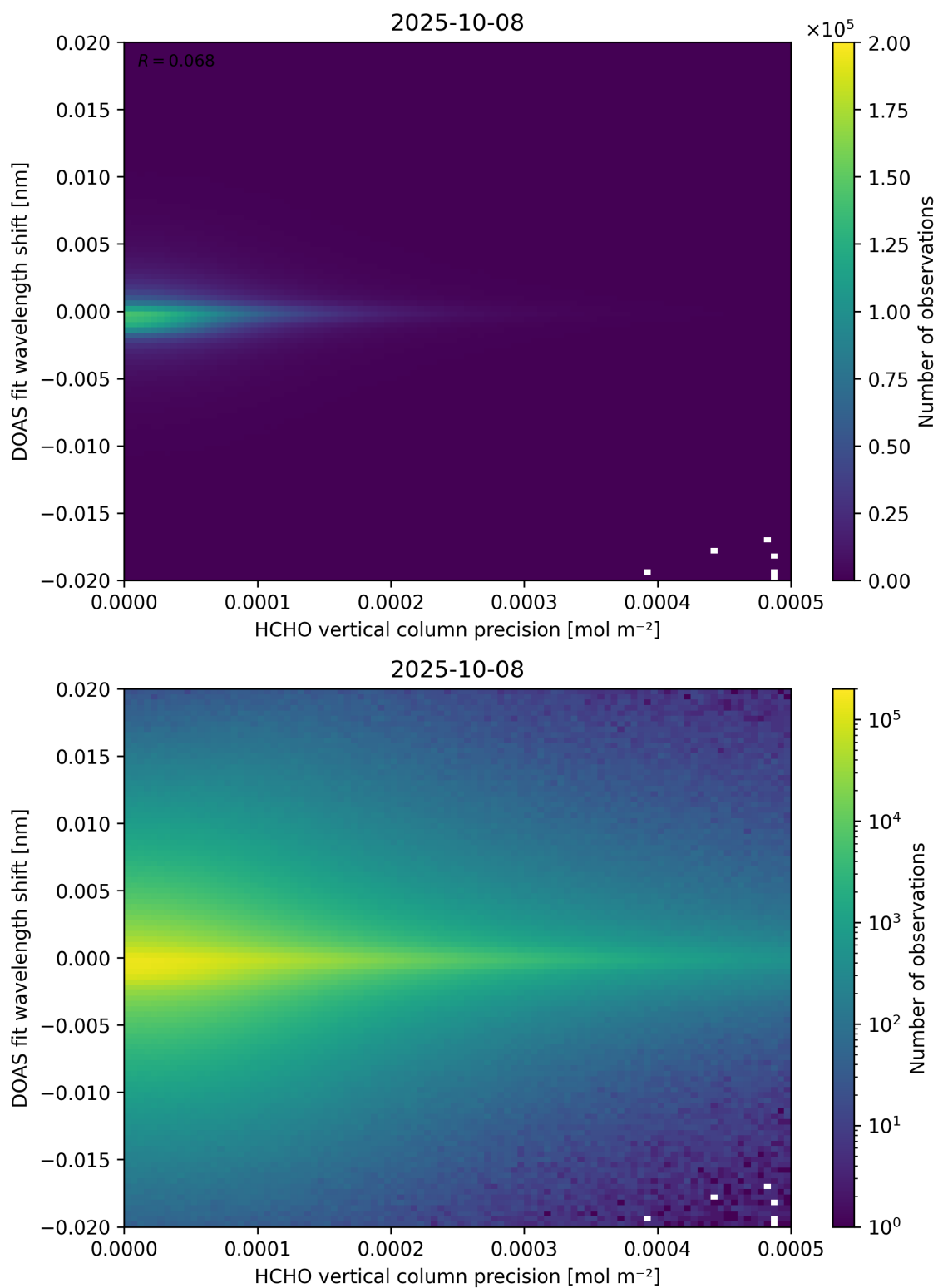
Figure 137: Scatter density plot of “HCHO vertical column precision” against “DOAS fit wavelength shift” for 2025-10-07 to 2025-10-09.
