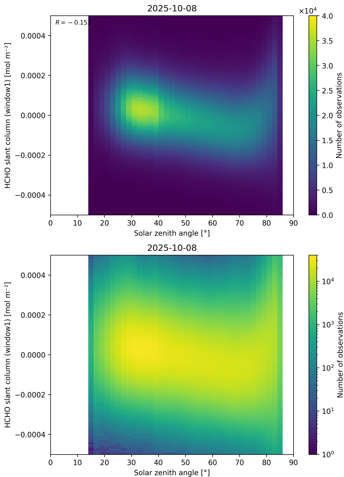
Figure 173: Scatter density plot of “Solar zenith angle” against “HCHO slant column (window1)” for 2025-10-07 to 2025-10-09.
