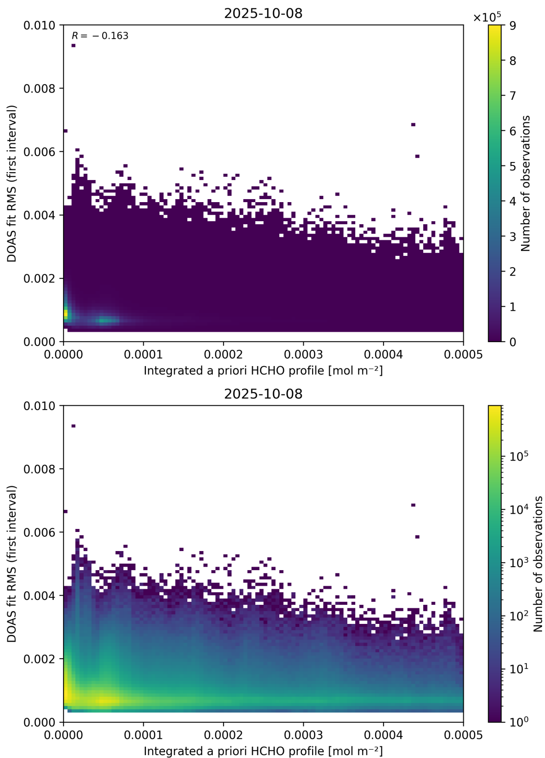
Figure 148: Scatter density plot of “Integrated a priori HCHO profile” against “DOAS fit RMS (first interval)” for 2025-10-07 to 2025-10-09.
