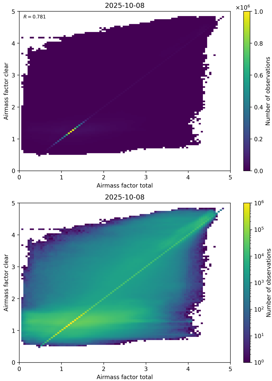
Figure 100: Scatter density plot of “Airmass factor total” against “Airmass factor clear” for 2025-10-07 to 2025-10-09.
