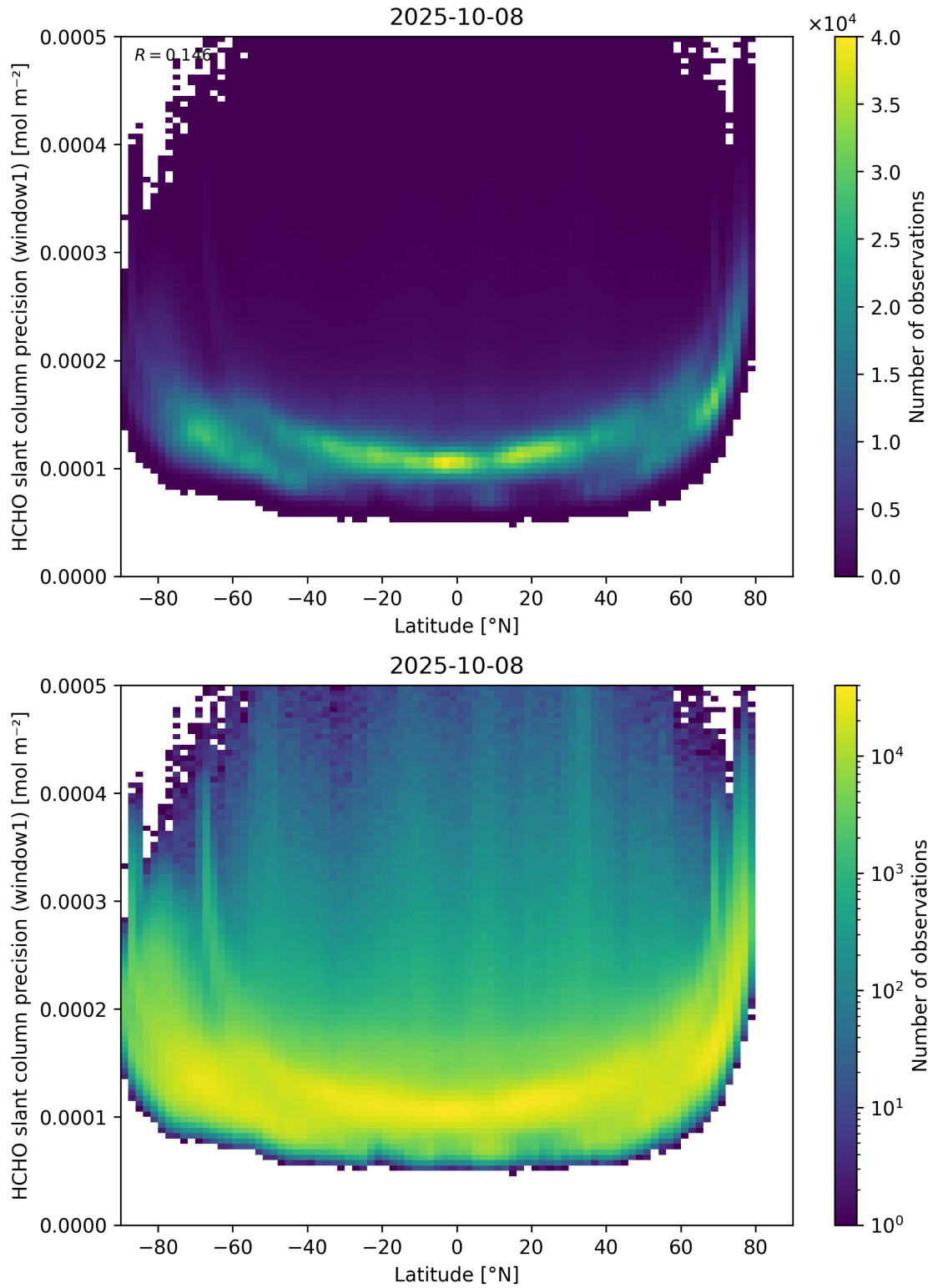
Figure 160: Scatter density plot of “Latitude” against “HCHO slant column precision (window1)” for 2025-10-07 to 2025-10-09.
