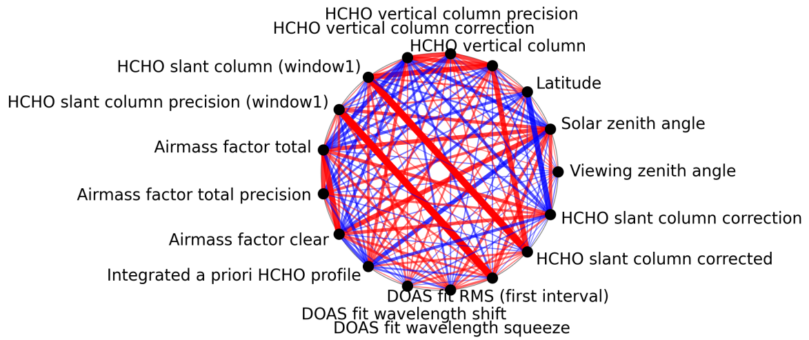
Figure 1: Map of correlation graph for 2025-10-07 to 2025-10-09.
