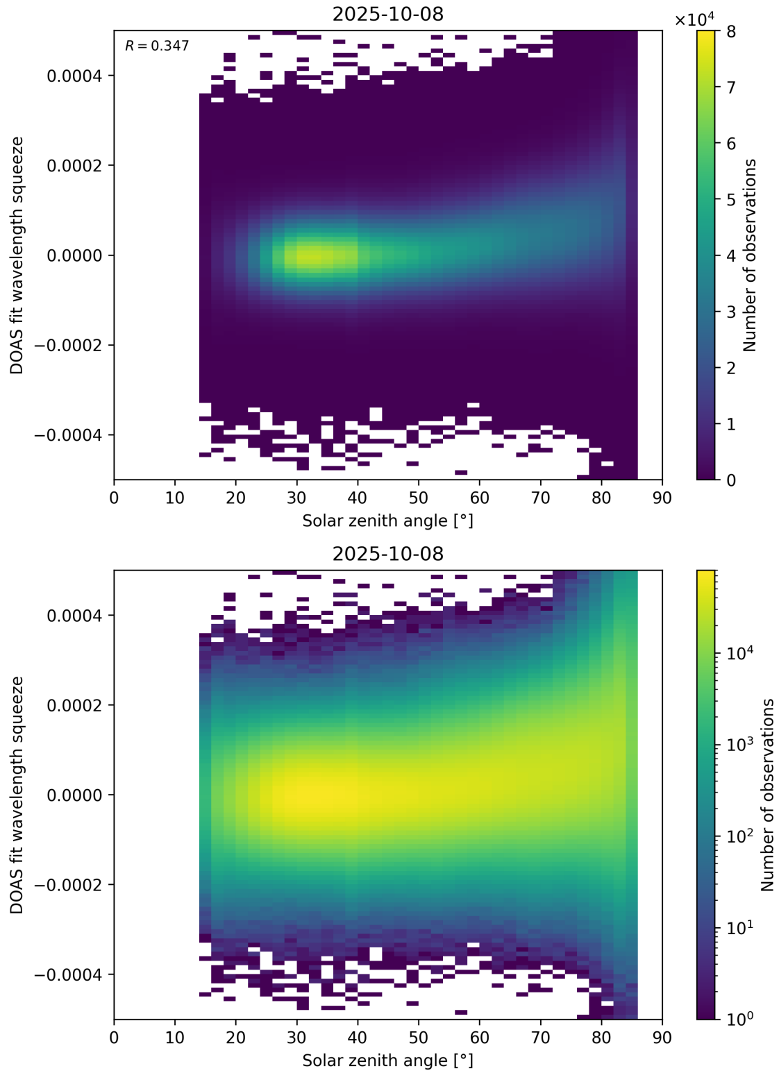
Figure 169: Scatter density plot of “Solar zenith angle” against “DOAS fit wavelength squeeze” for 2025-10-07 to 2025-10-09.
