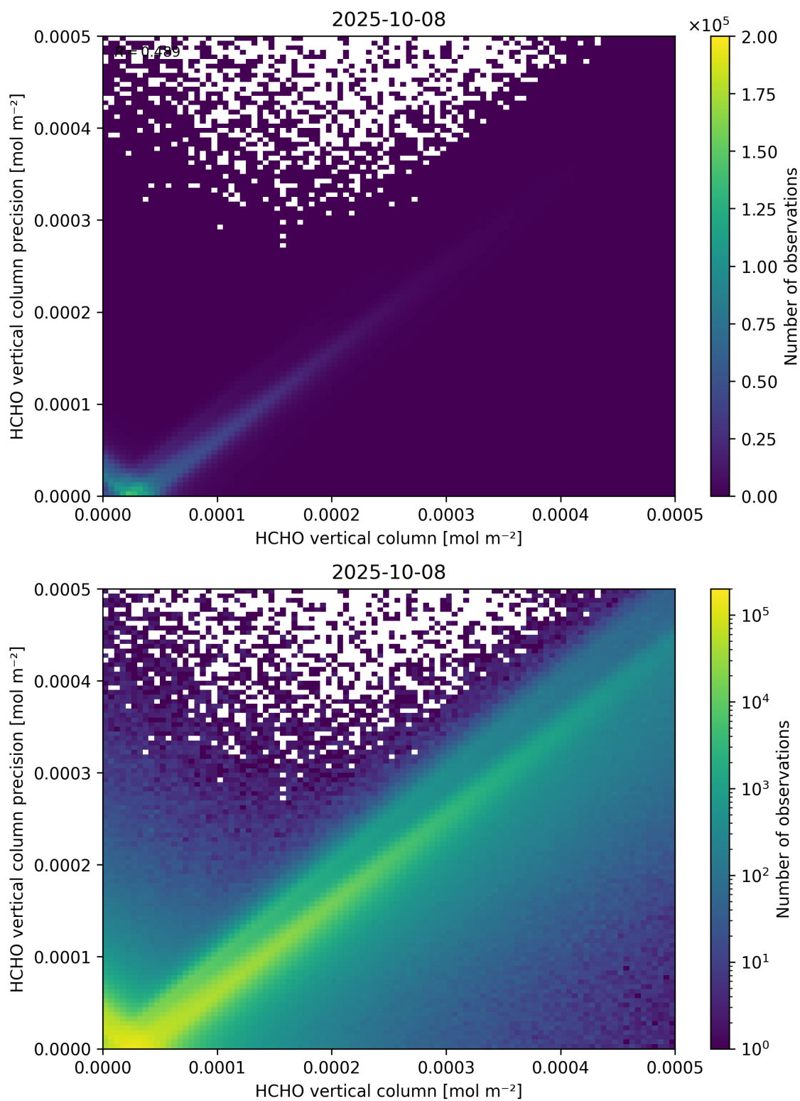
Figure 134: Scatter density plot of “HCHO vertical column” against “HCHO vertical column precision” for 2025-10-07 to 2025-10-09.
