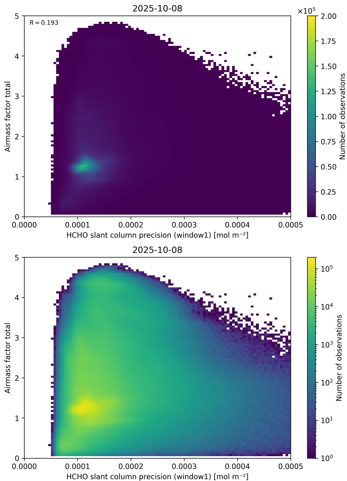
Figure 94: Scatter density plot of “HCHO slant column precision (window1)” against “Airmass factor total” for 2025-10-07 to 2025-10-09.
