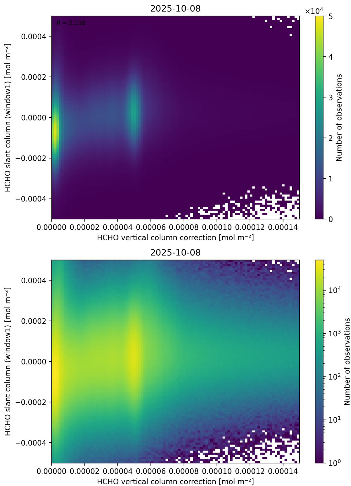
Figure 118: Scatter density plot of “HCHO vertical column correction” against “HCHO slant column (window1)” for 2025-10-07 to 2025-10-09.
