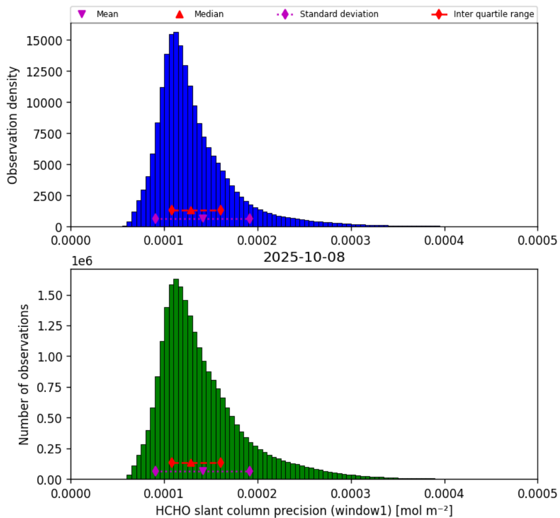
Figure 39: Histogram of “HCHO slant column precision (window1)” for 2025-10-07 to 2025-10-09
