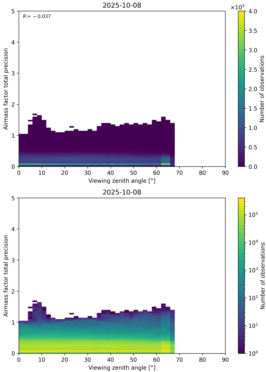
Figure 191: Scatter density plot of “Viewing zenith angle” against “Airmass factor total precision” for 2025-10-07 to 2025-10-09.
