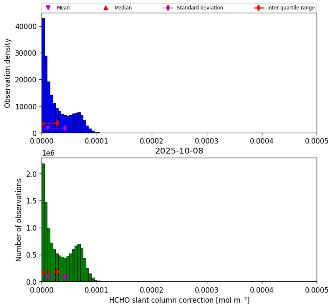
Figure 47: Histogram of “HCHO slant column correction” for 2025-10-07 to 2025-10-09
