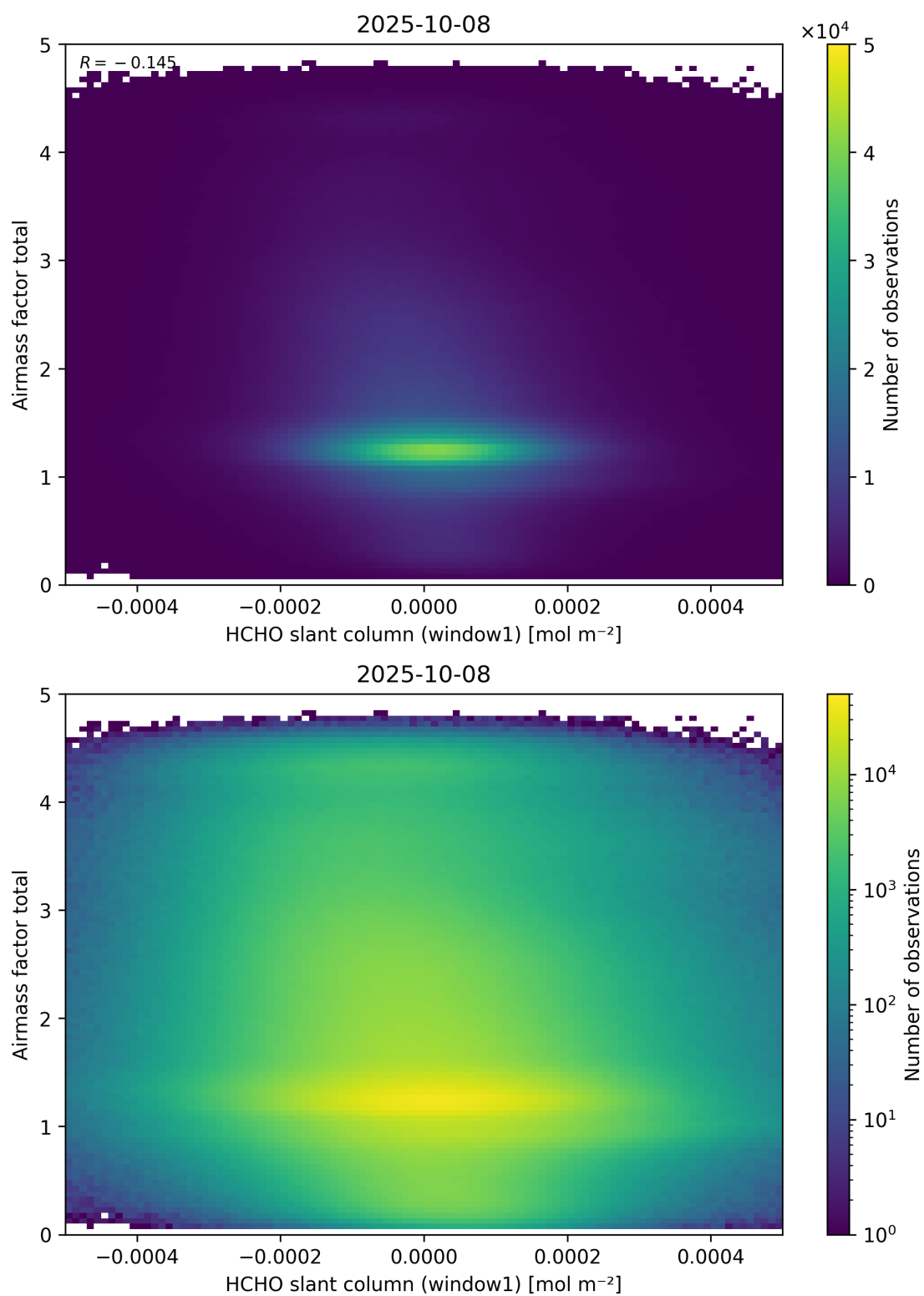
Figure 85: Scatter density plot of “HCHO slant column (window1)” against “Airmass factor total” for 2025-10-07 to 2025-10-09.
