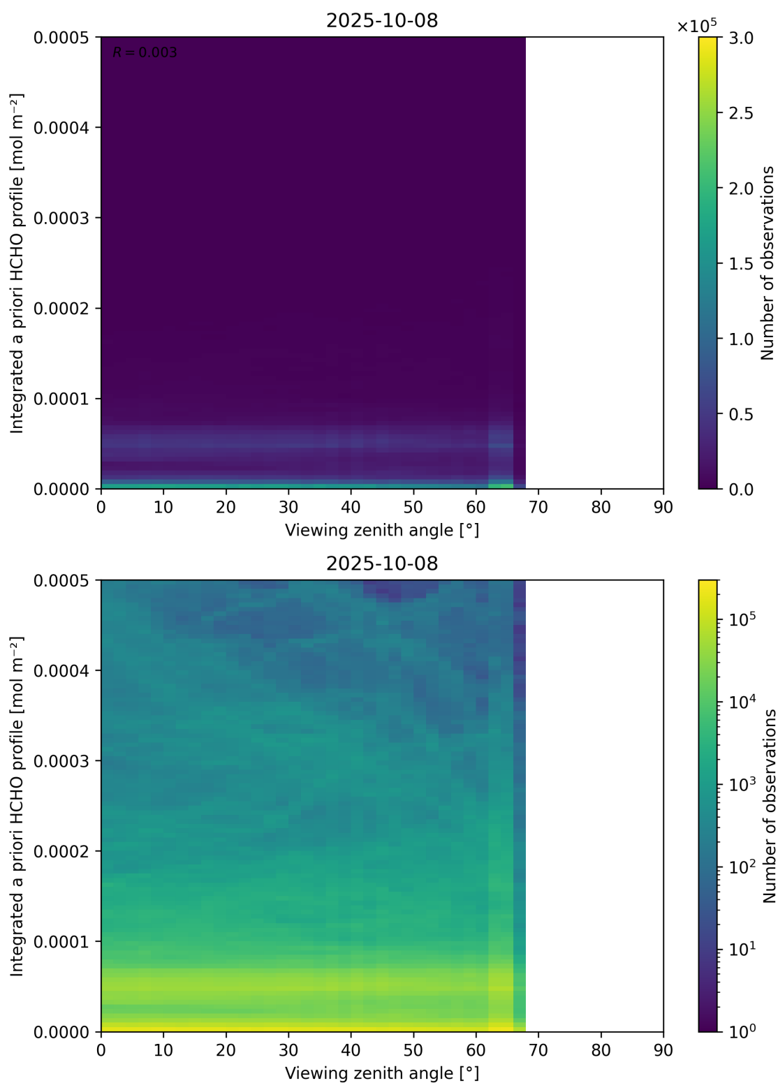
Figure 195: Scatter density plot of “Viewing zenith angle” against “Integrated a priori HCHO profile” for 2025-10-07 to 2025-10-09.
