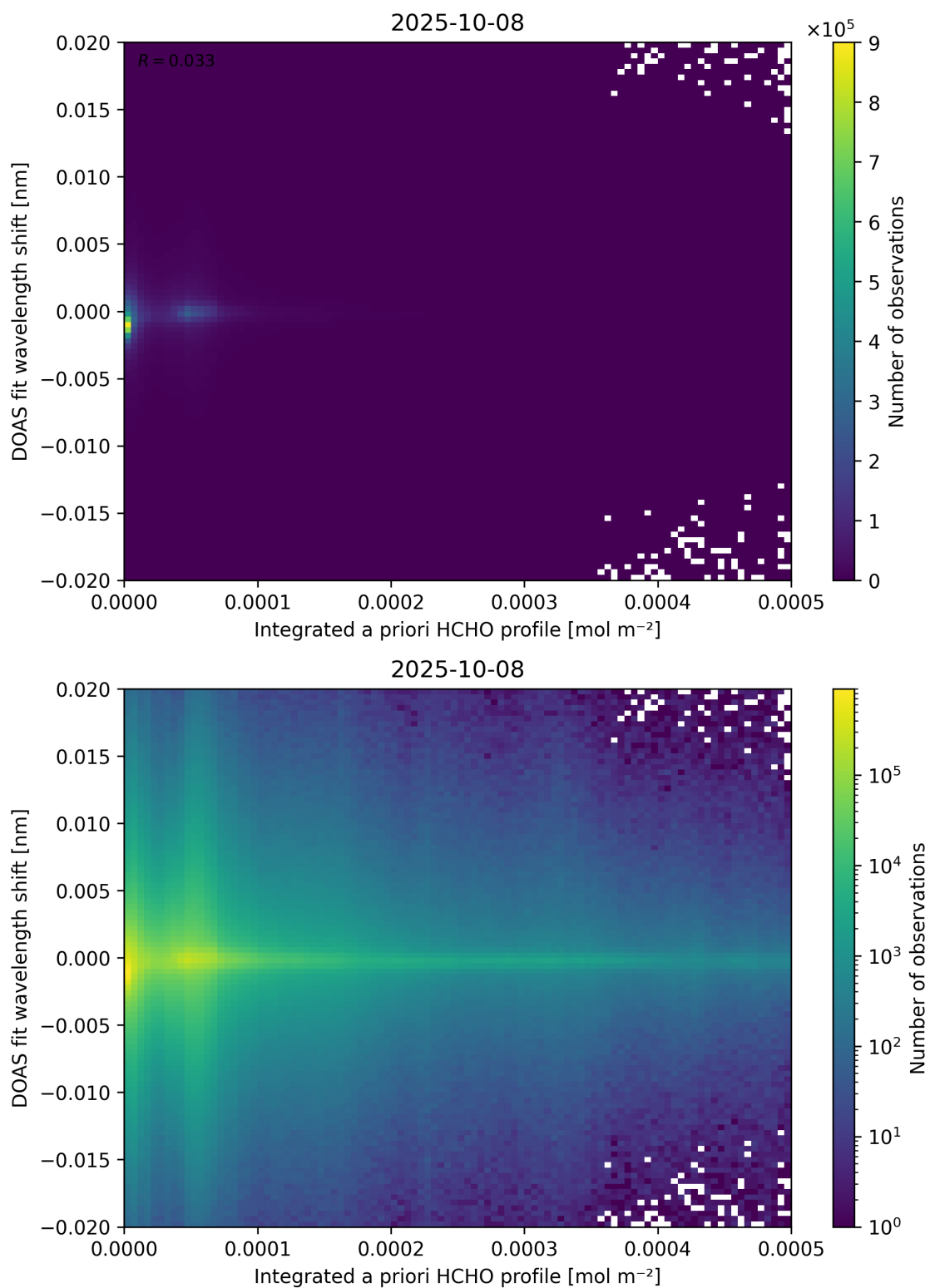
Figure 149: Scatter density plot of “Integrated a priori HCHO profile” against “DOAS fit wavelength shift” for 2025-10-07 to 2025-10-09.
