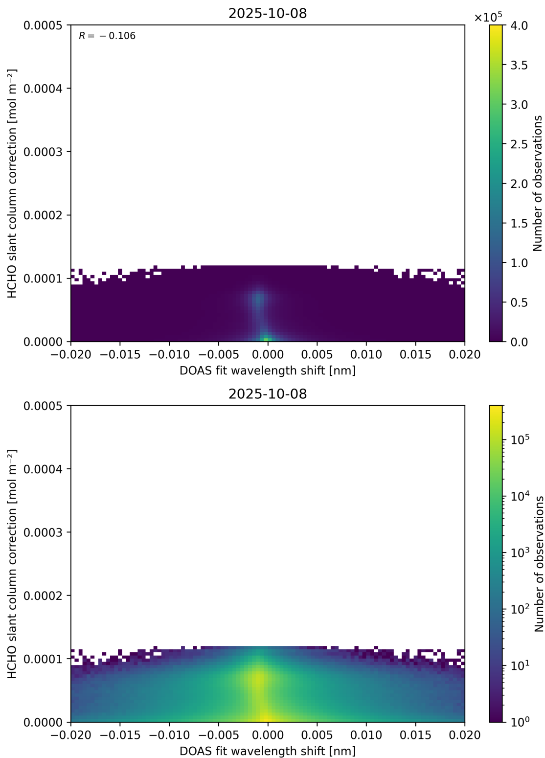
Figure 67: Scatter density plot of “DOAS fit wavelength shift” against “HCHO slant column correction” for 2025-10-07 to 2025-10-09.
