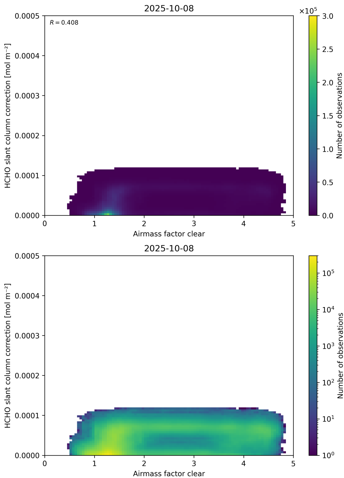
Figure 75: Scatter density plot of “Airmass factor clear” against “HCHO slant column correction” for 2025-10-07 to 2025-10-09.
