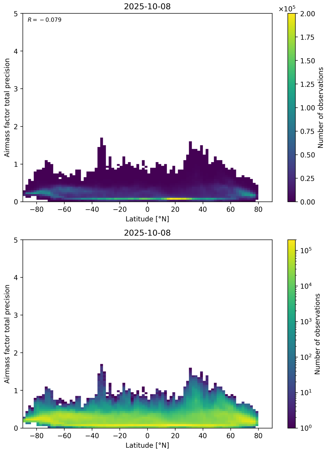
Figure 162: Scatter density plot of “Latitude” against “Airmass factor total precision” for 2025-10-07 to 2025-10-09.
