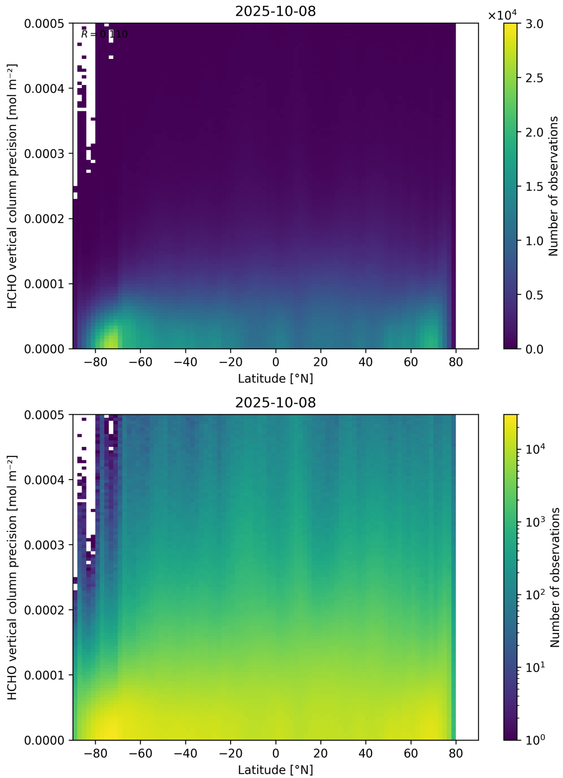
Figure 165: Scatter density plot of “Latitude” against “HCHO vertical column precision” for 2025-10-07 to 2025-10-09.
