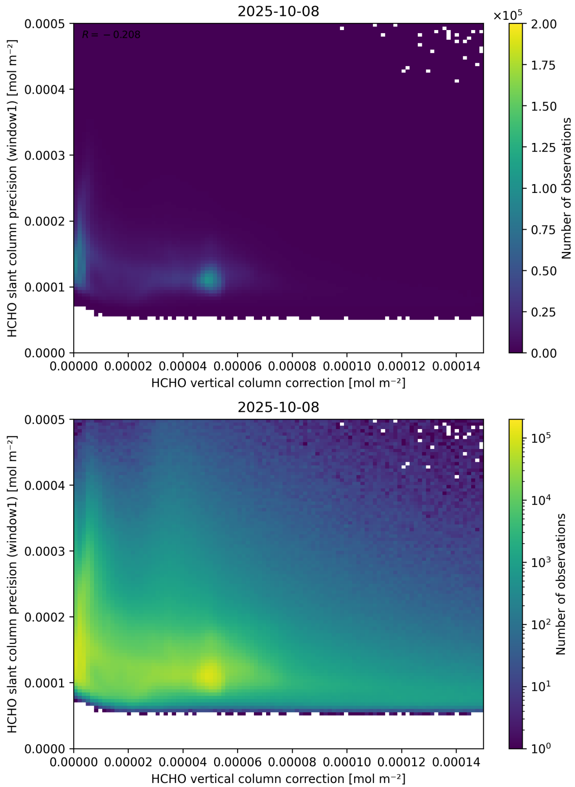
Figure 119: Scatter density plot of “HCHO vertical column correction” against “HCHO slant column precision (window1)” for 2025-10-07 to 2025-10-09.
