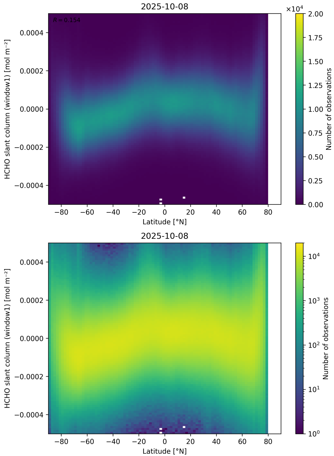
Figure 159: Scatter density plot of “Latitude” against “HCHO slant column (window1)” for 2025-10-07 to 2025-10-09.
