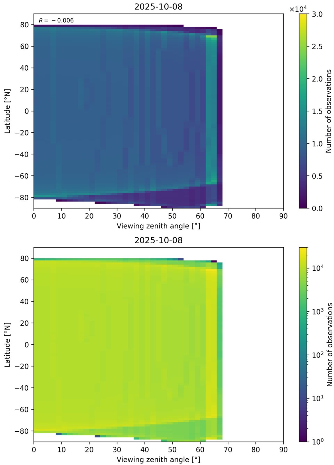
Figure 196: Scatter density plot of “Viewing zenith angle” against “Latitude” for 2025-10-07 to 2025-10-09.
