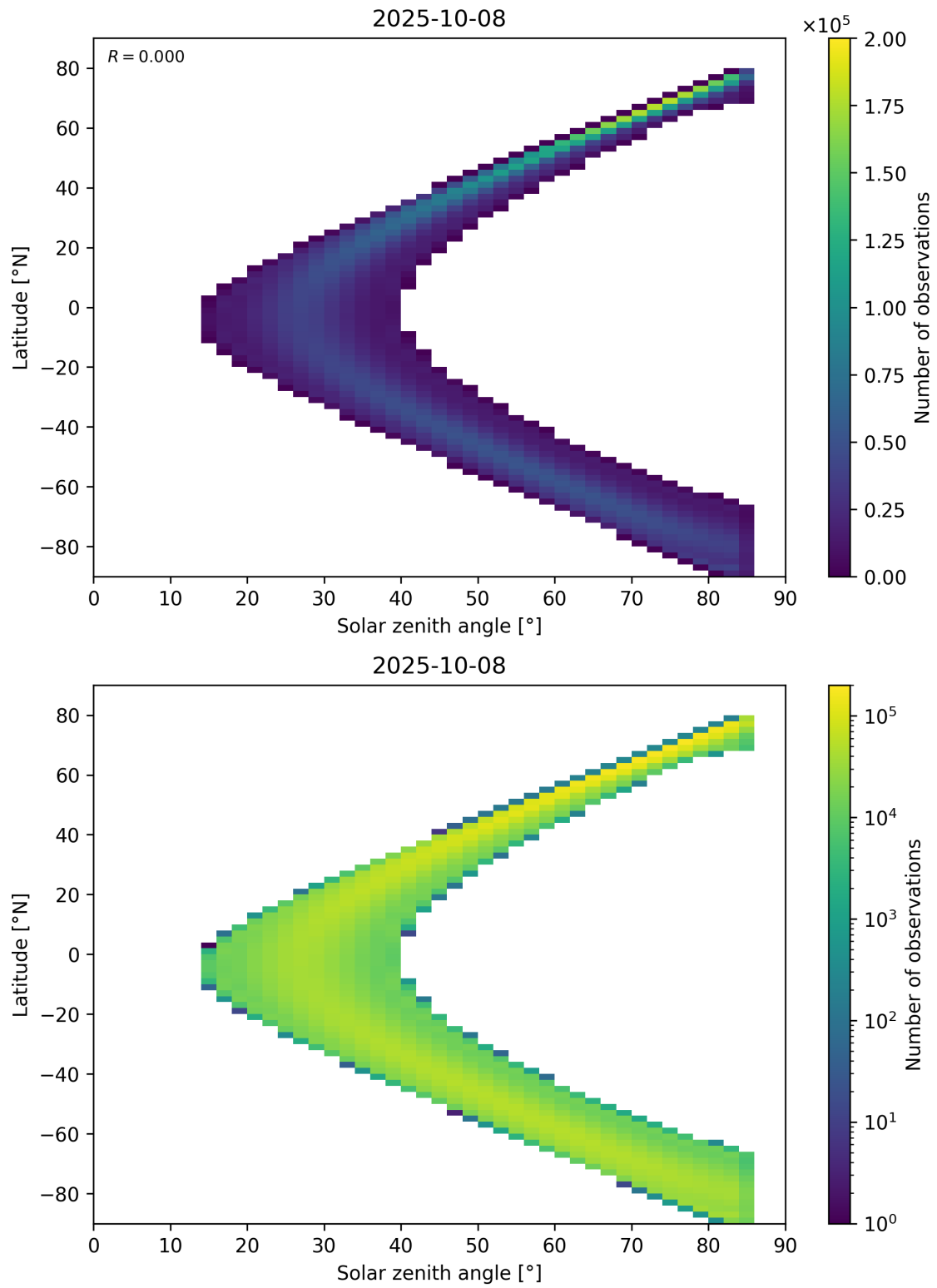
Figure 181: Scatter density plot of “Solar zenith angle” against “Latitude” for 2025-10-07 to 2025-10-09.
