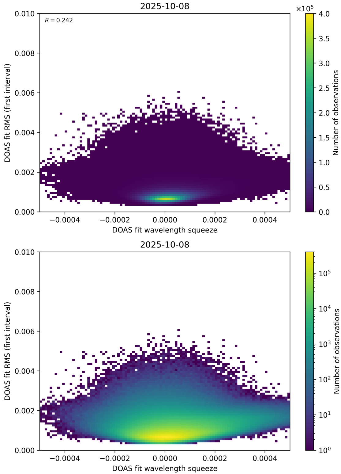
Figure 68: Scatter density plot of “DOAS fit wavelength squeeze” against “DOAS fit RMS (first interval)” for 2025-10-07 to 2025-10-09.
