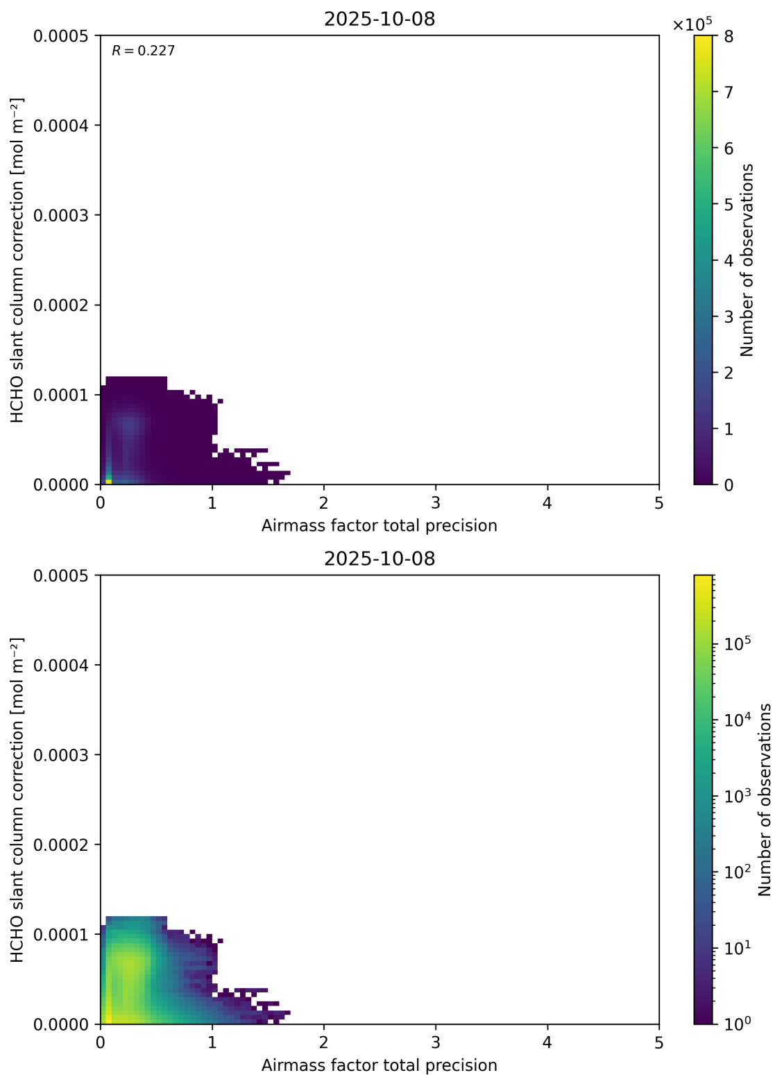
Figure 110: Scatter density plot of “Airmass factor total precision” against “HCHO slant column correction” for 2025-10-07 to 2025-10-09.
