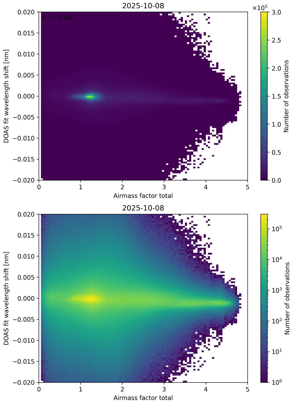
Figure 98: Scatter density plot of “Airmass factor total” against “DOAS fit wavelength shift” for 2025-10-07 to 2025-10-09.
