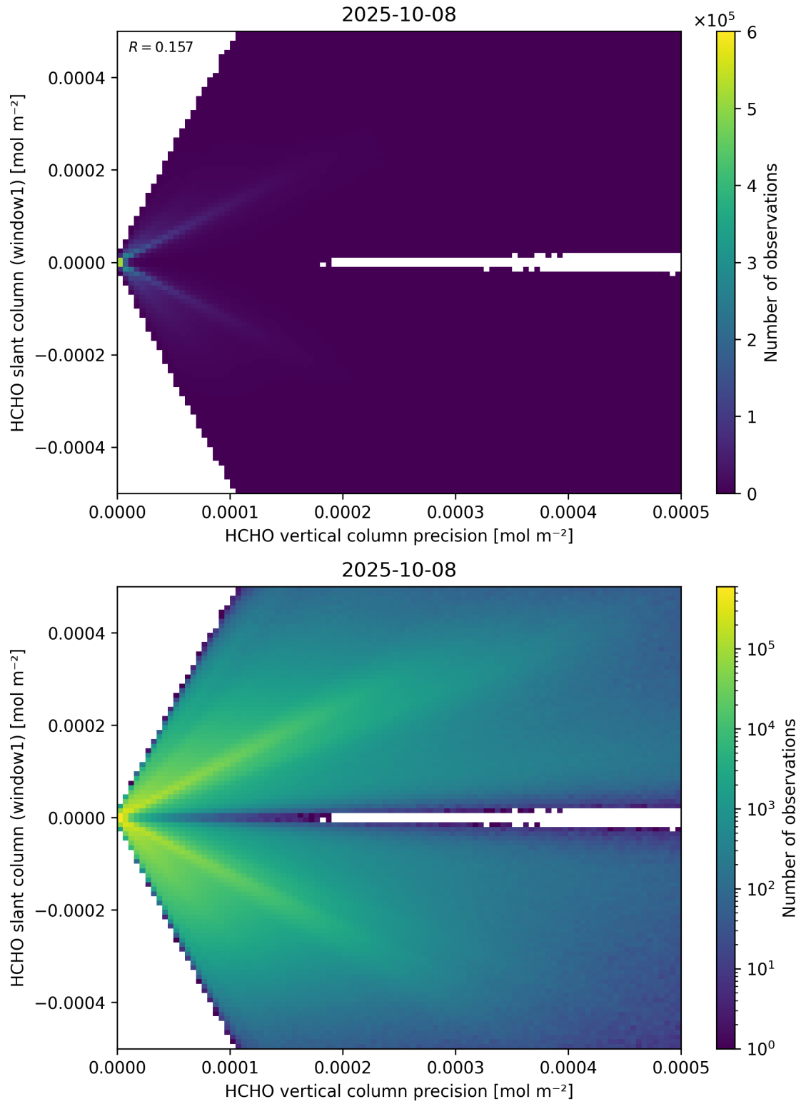
Figure 142: Scatter density plot of “HCHO vertical column precision” against “HCHO slant column (window1)” for 2025-10-07 to 2025-10-09.
