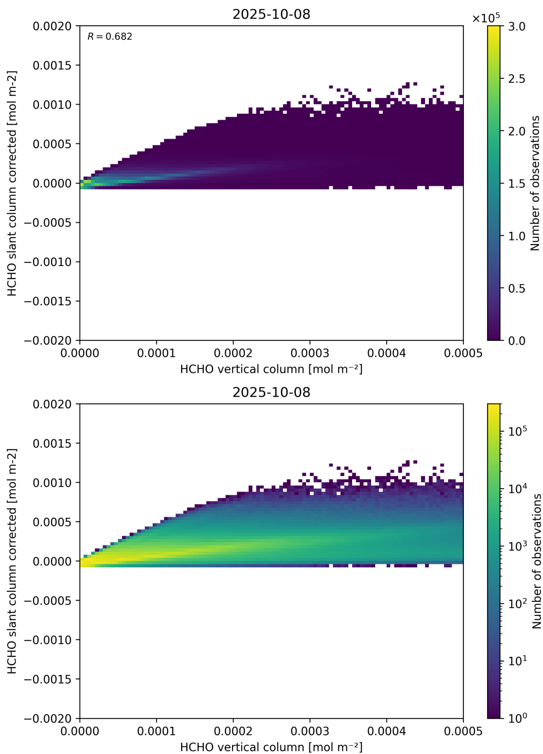
Figure 127: Scatter density plot of “HCHO vertical column” against “HCHO slant column corrected” for 2025-10-07 to 2025-10-09.
