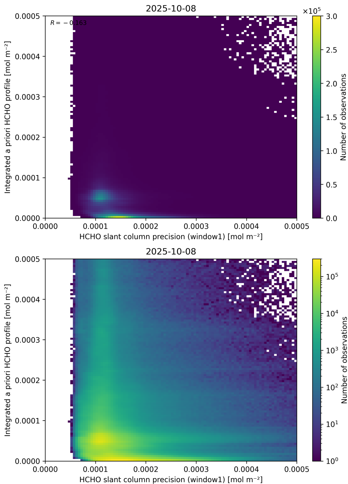
Figure 96: Scatter density plot of “HCHO slant column precision (window1)” against “Integrated a priori HCHO profile” for 2025-10-07 to 2025-10-09.
