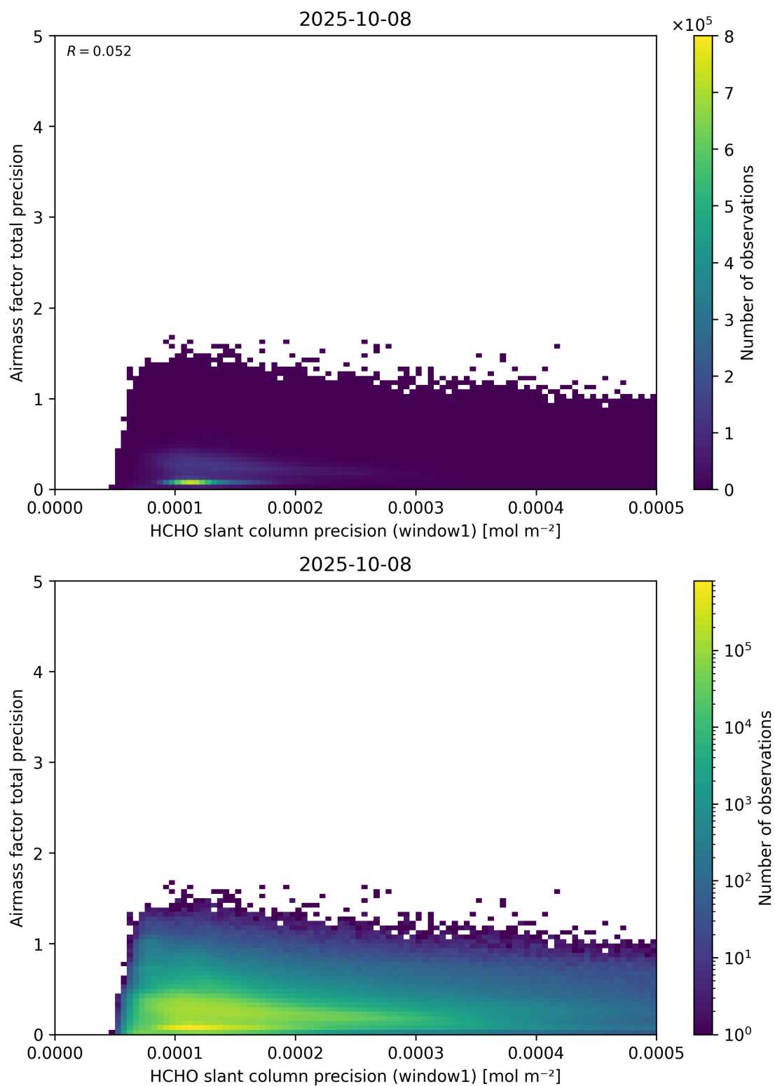
Figure 95: Scatter density plot of “HCHO slant column precision (window1)” against “Airmass factor total precision” for 2025-10-07 to 2025-10-09.
