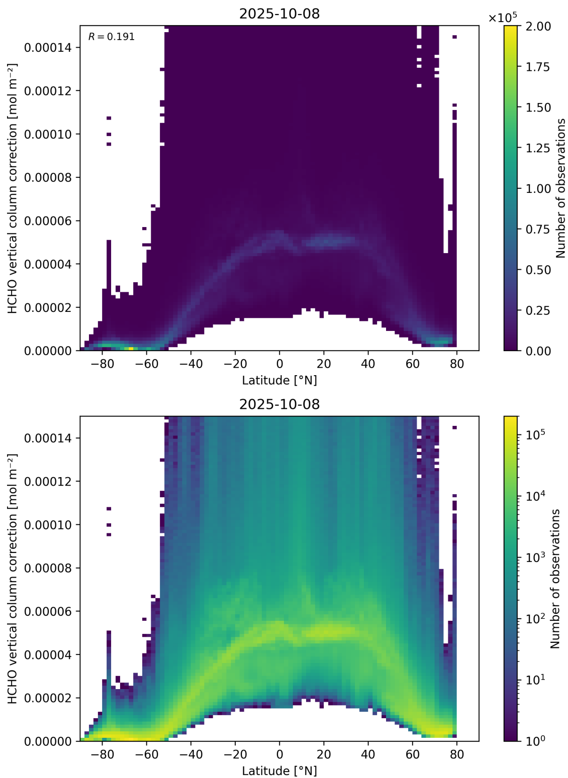
Figure 164: Scatter density plot of “Latitude” against “HCHO vertical column correction” for 2025-10-07 to 2025-10-09.
