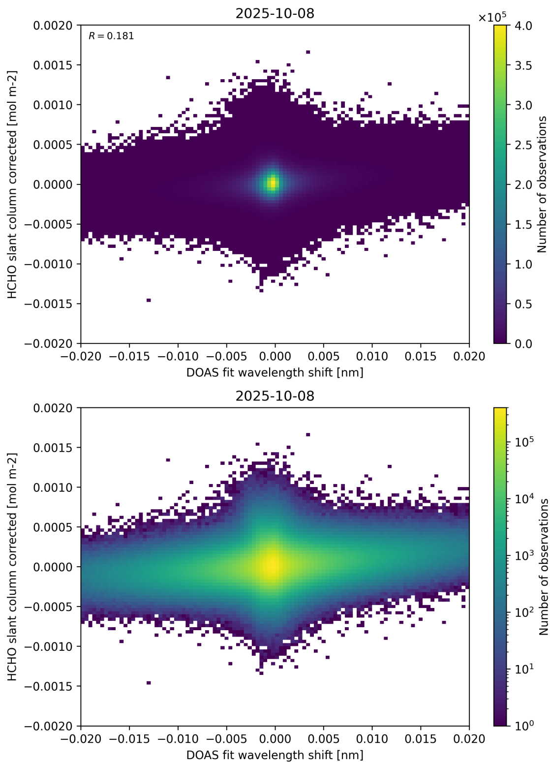
Figure 66: Scatter density plot of “DOAS fit wavelength shift” against “HCHO slant column corrected” for 2025-10-07 to 2025-10-09.
