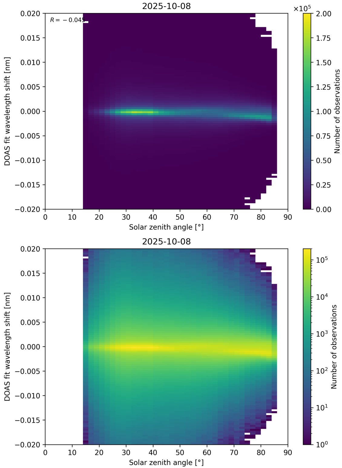
Figure 168: Scatter density plot of “Solar zenith angle” against “DOAS fit wavelength shift” for 2025-10-07 to 2025-10-09.
