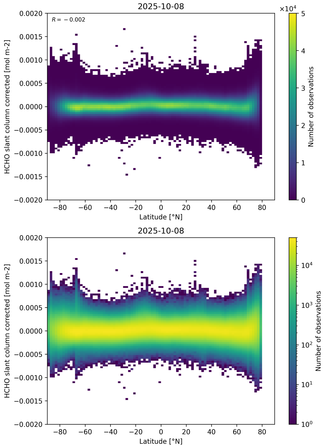
Figure 157: Scatter density plot of “Latitude” against “HCHO slant column corrected” for 2025-10-07 to 2025-10-09.
