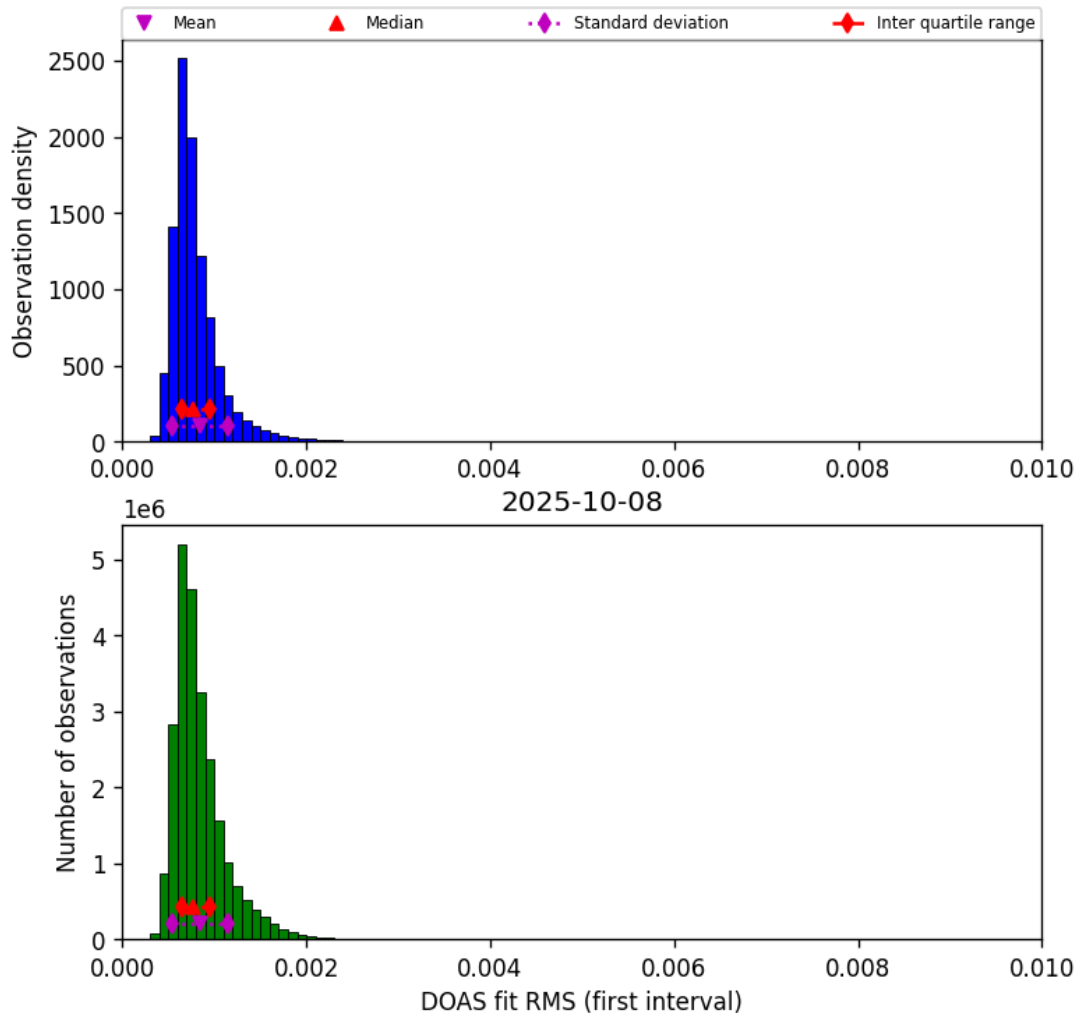
Figure 46: Histogram of “DOAS fit RMS (first interval)” for 2025-10-07 to 2025-10-09
