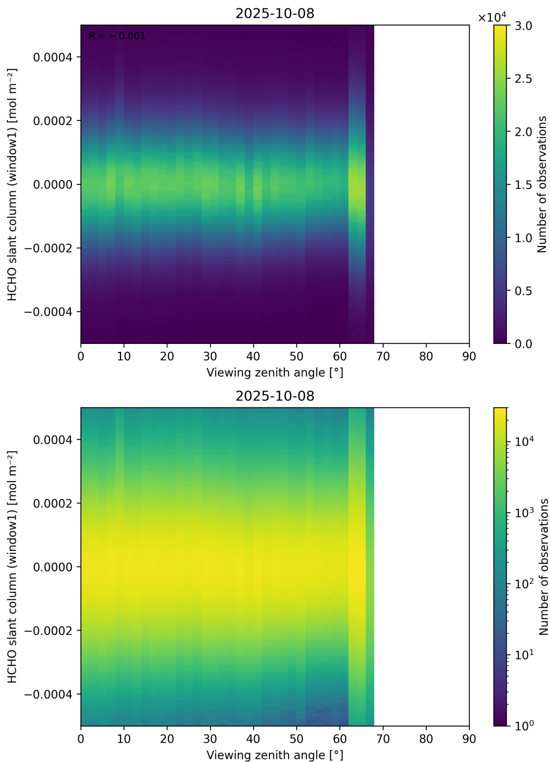
Figure 188: Scatter density plot of “Viewing zenith angle” against “HCHO slant column (window1)” for 2025-10-07 to 2025-10-09.
