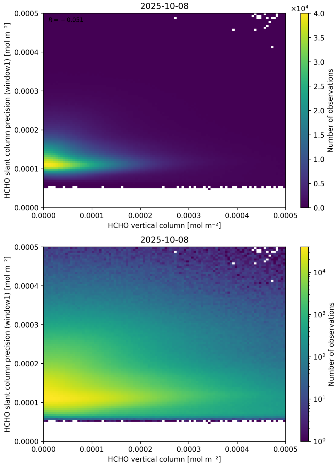
Figure 130: Scatter density plot of “HCHO vertical column” against “HCHO slant column precision (window1)” for 2025-10-07 to 2025-10-09.
