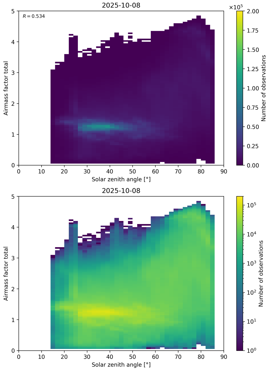
Figure 175: Scatter density plot of “Solar zenith angle” against “Airmass factor total” for 2025-10-07 to 2025-10-09.
