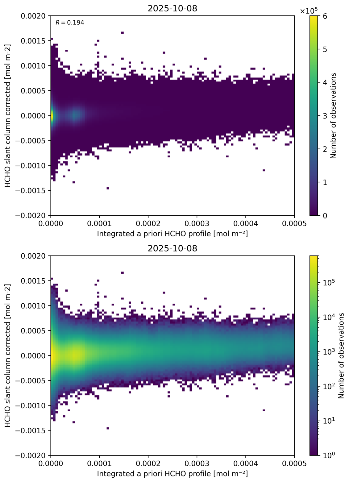
Figure 151: Scatter density plot of “Integrated a priori HCHO profile” against “HCHO slant column corrected” for 2025-10-07 to 2025-10-09.
