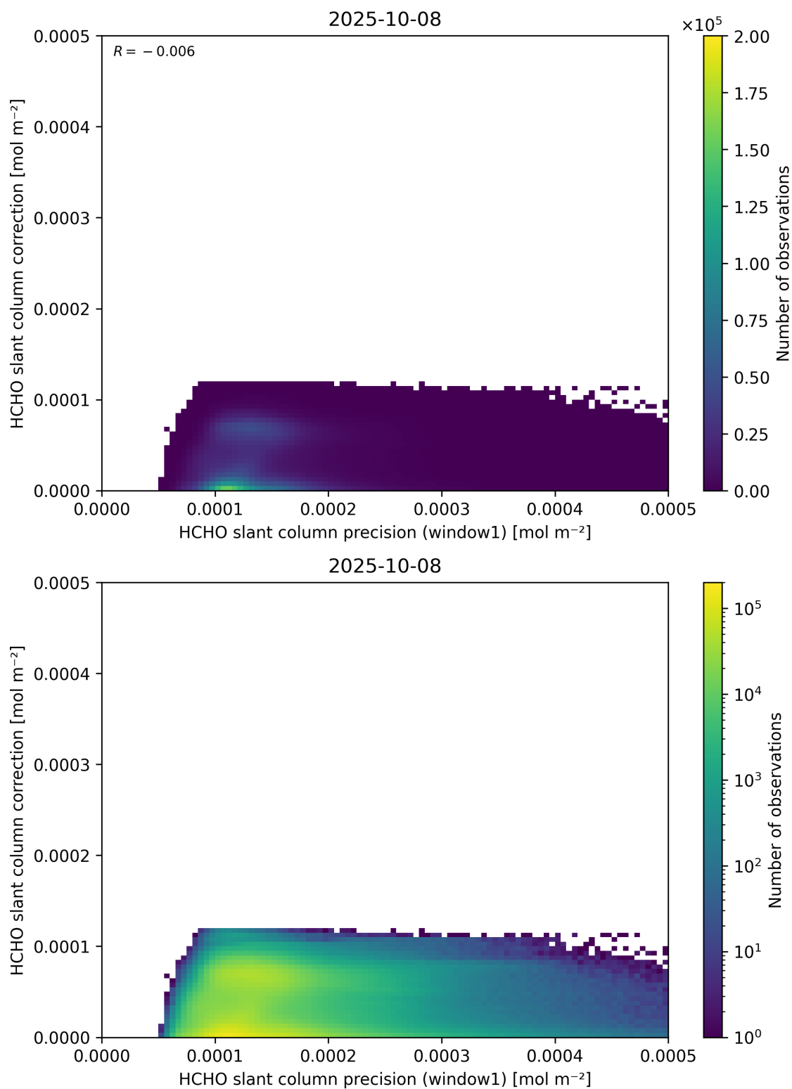
Figure 93: Scatter density plot of “HCHO slant column precision (window1)” against “HCHO slant column correction” for 2025-10-07 to 2025-10-09.
