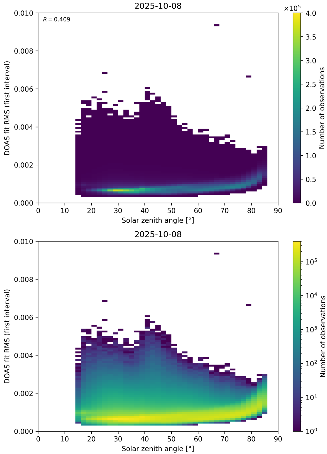
Figure 167: Scatter density plot of “Solar zenith angle” against “DOAS fit RMS (first interval)” for 2025-10-07 to 2025-10-09.
