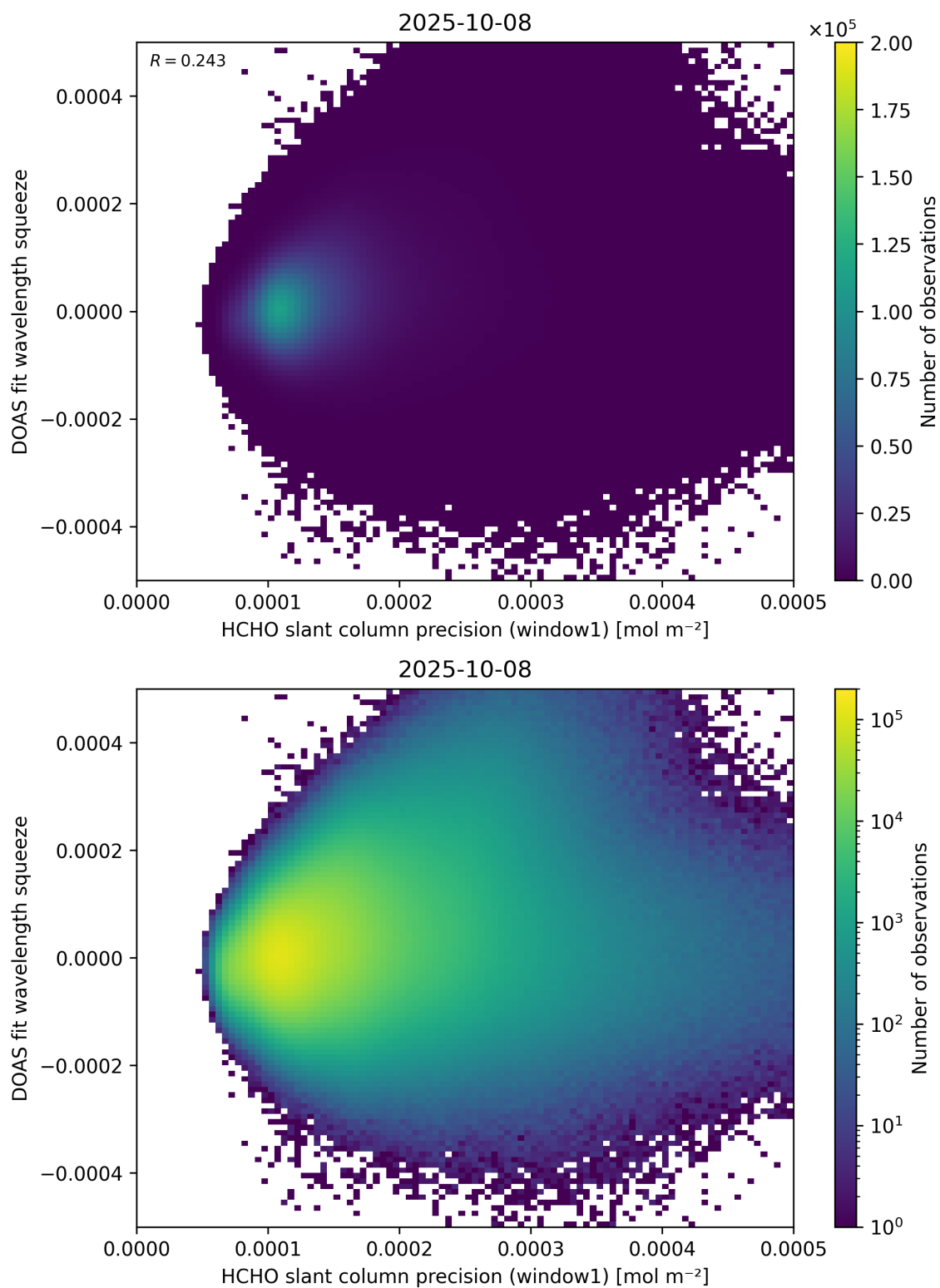
Figure 90: Scatter density plot of “HCHO slant column precision (window1)” against “DOAS fit wavelength squeeze” for 2025-10-07 to 2025-10-09.
