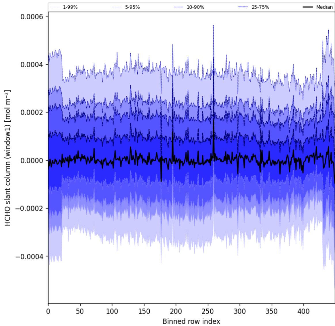
Figure 52: Along track statistics of “HCHO slant column (window1)” for 2025-10-07 to 2025-10-09
