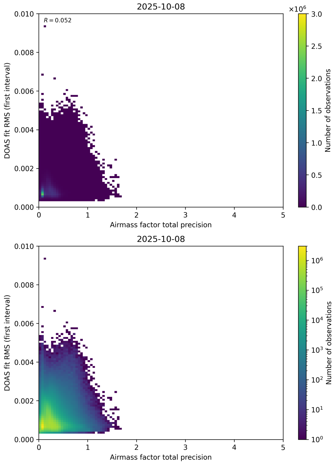
Figure 105: Scatter density plot of “Airmass factor total precision” against “DOAS fit RMS (first interval)” for 2025-10-07 to 2025-10-09.
