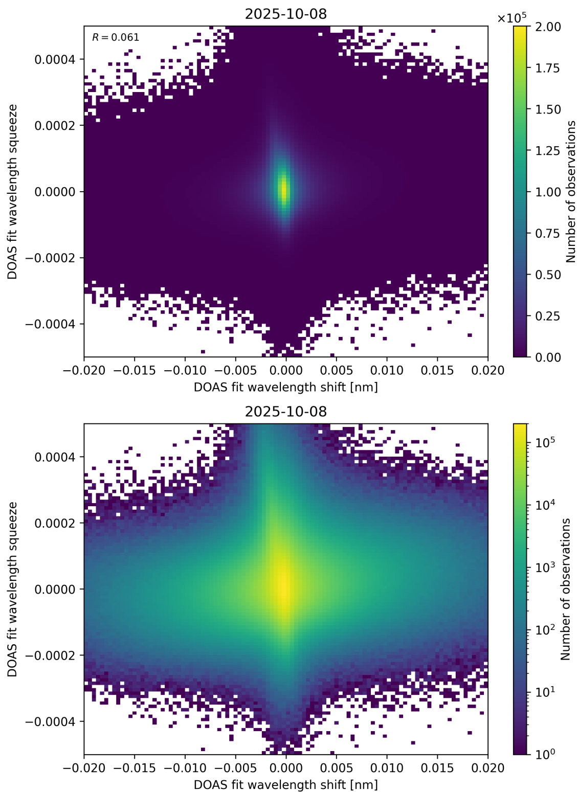
Figure 65: Scatter density plot of “DOAS fit wavelength shift” against “DOAS fit wavelength squeeze” for 2025-10-07 to 2025-10-09.
