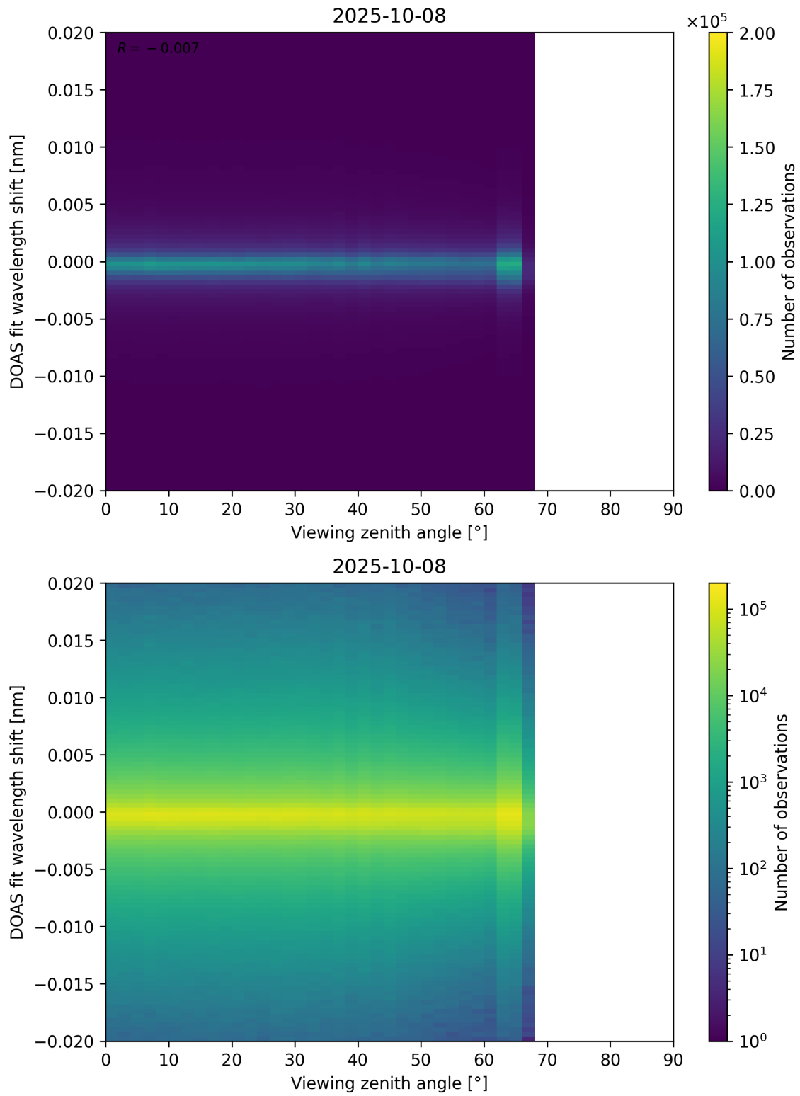
Figure 183: Scatter density plot of “Viewing zenith angle” against “DOAS fit wavelength shift” for 2025-10-07 to 2025-10-09.
