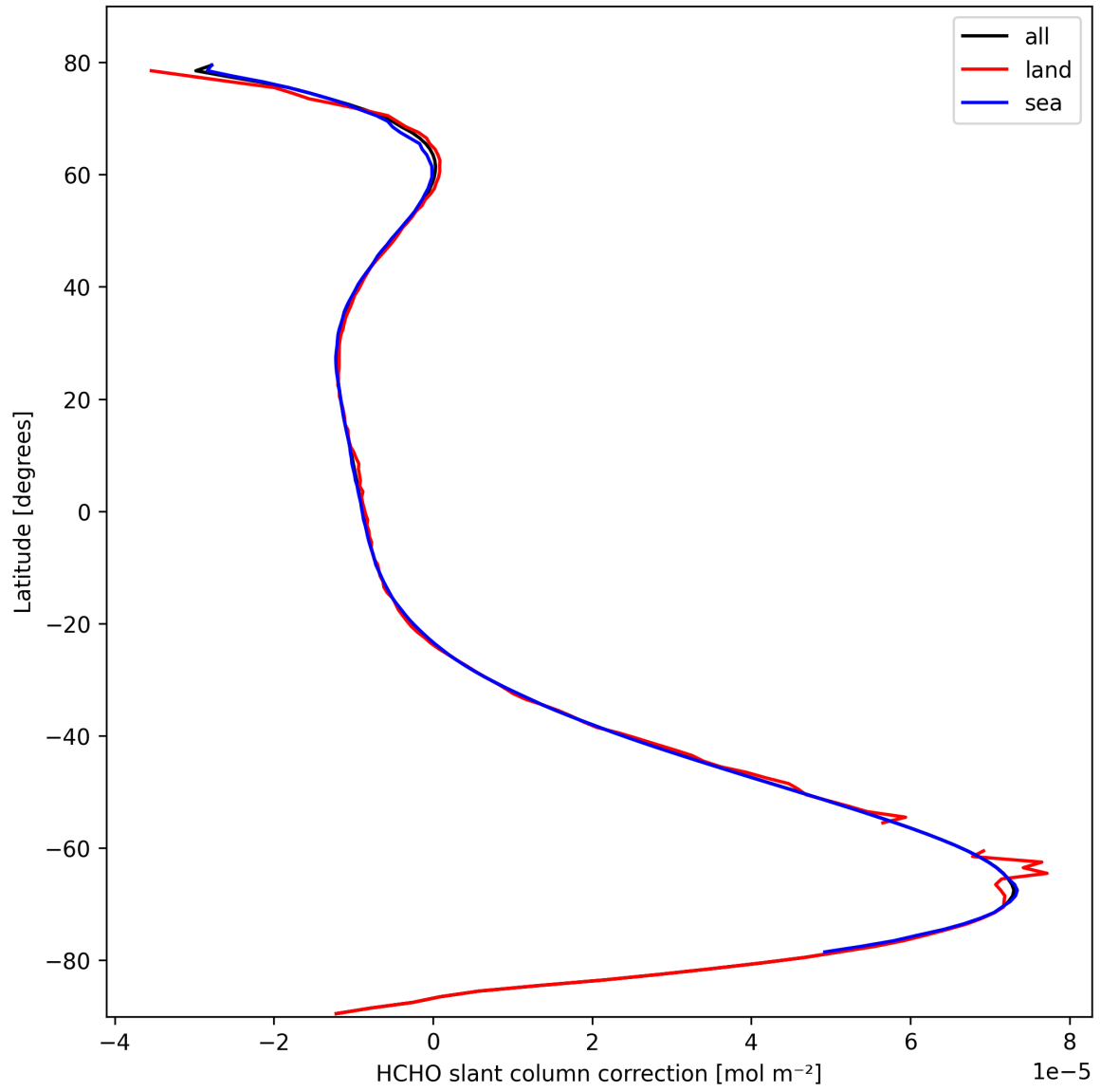
Figure 33: Zonal average of “HCHO slant column correction” for 2025-10-07 to 2025-10-09.
