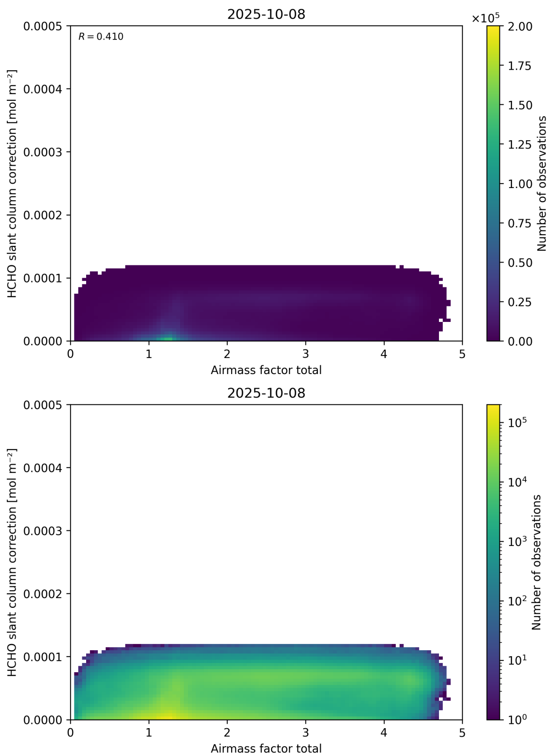
Figure 102: Scatter density plot of “Airmass factor total” against “HCHO slant column correction” for 2025-10-07 to 2025-10-09.
