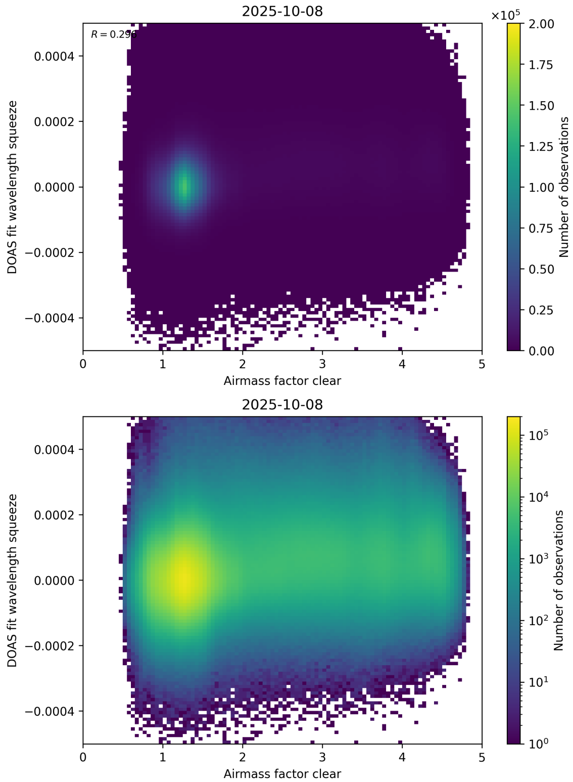
Figure 73: Scatter density plot of “Airmass factor clear” against “DOAS fit wavelength squeeze” for 2025-10-07 to 2025-10-09.
