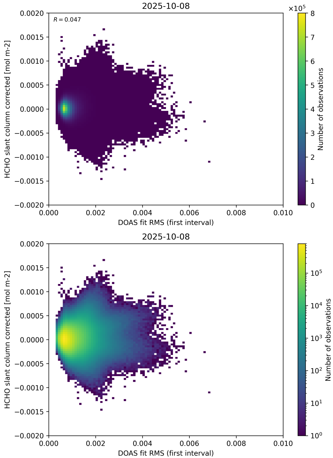
Figure 62: Scatter density plot of “DOAS fit RMS (first interval)” against “HCHO slant column corrected” for 2025-10-07 to 2025-10-09.
