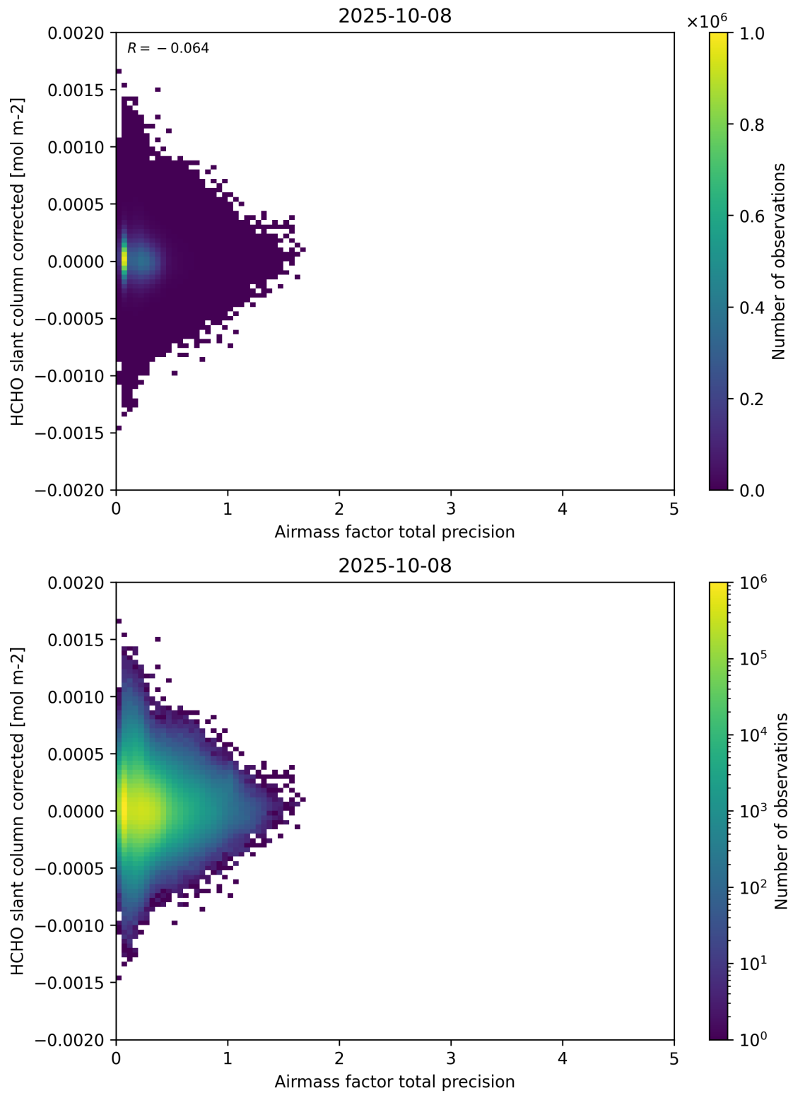
Figure 109: Scatter density plot of “Airmass factor total precision” against “HCHO slant column corrected” for 2025-10-07 to 2025-10-09.
