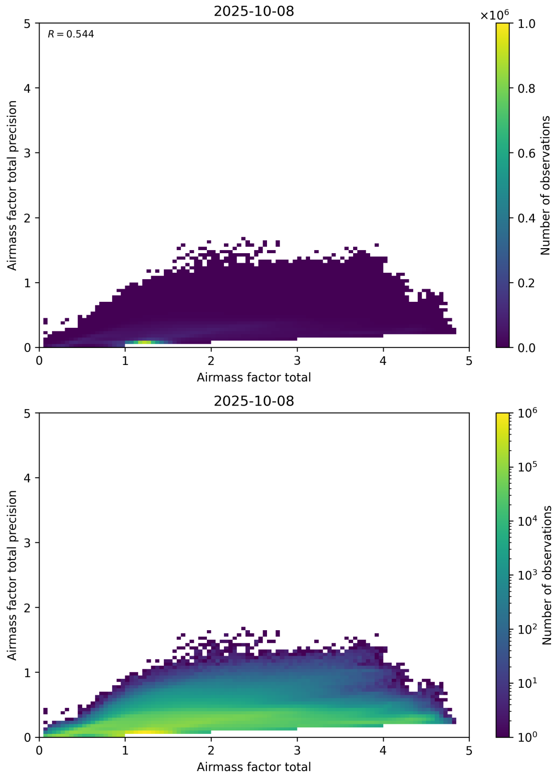
Figure 103: Scatter density plot of “Airmass factor total” against “Airmass factor total precision” for 2025-10-07 to 2025-10-09.
