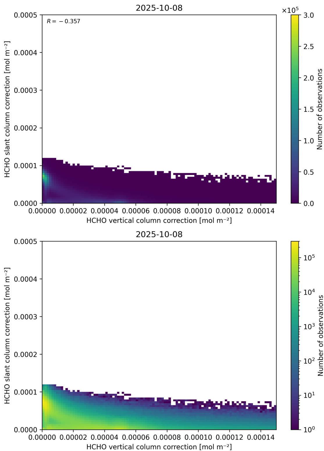
Figure 117: Scatter density plot of “HCHO vertical column correction” against “HCHO slant column correction” for 2025-10-07 to 2025-10-09.
