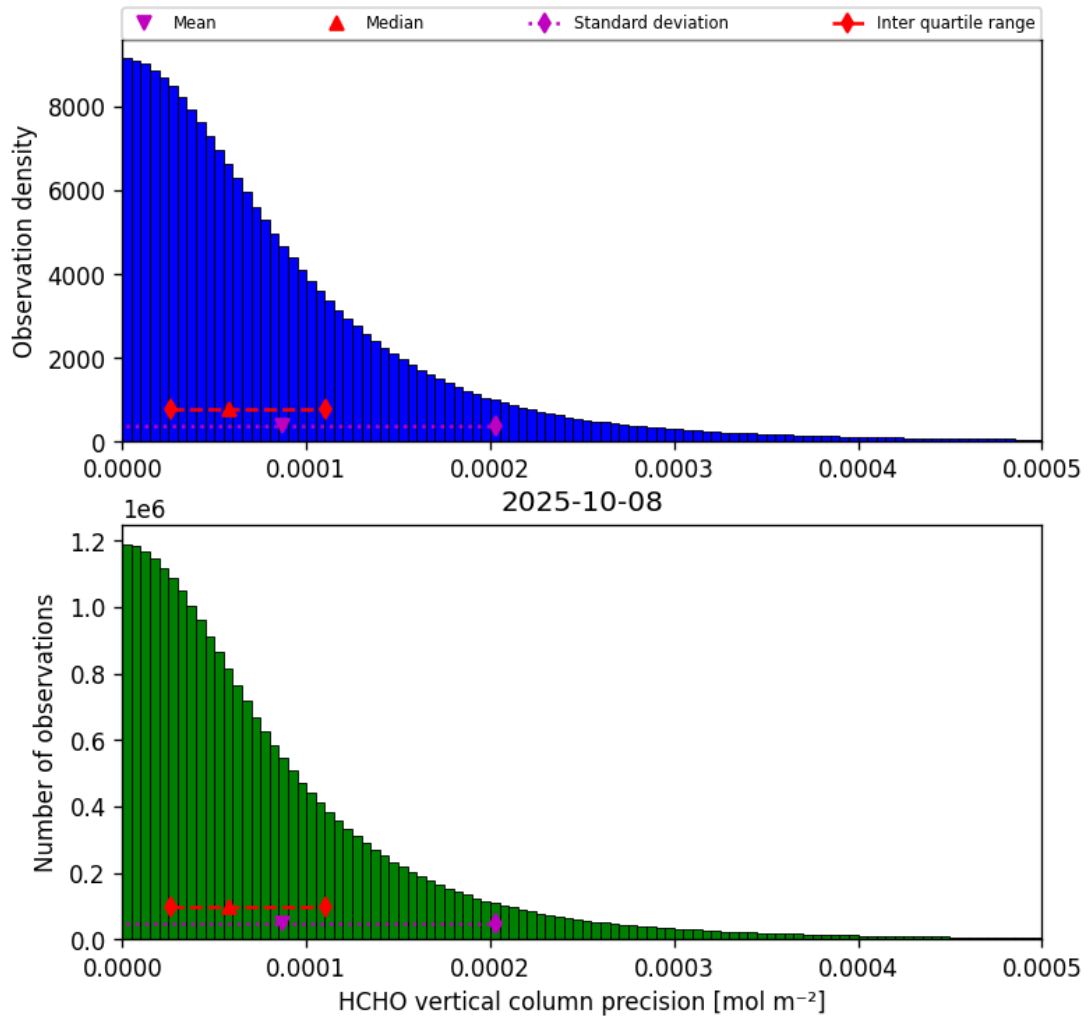
Figure 36: Histogram of “HCHO vertical column precision” for 2025-10-07 to 2025-10-09
