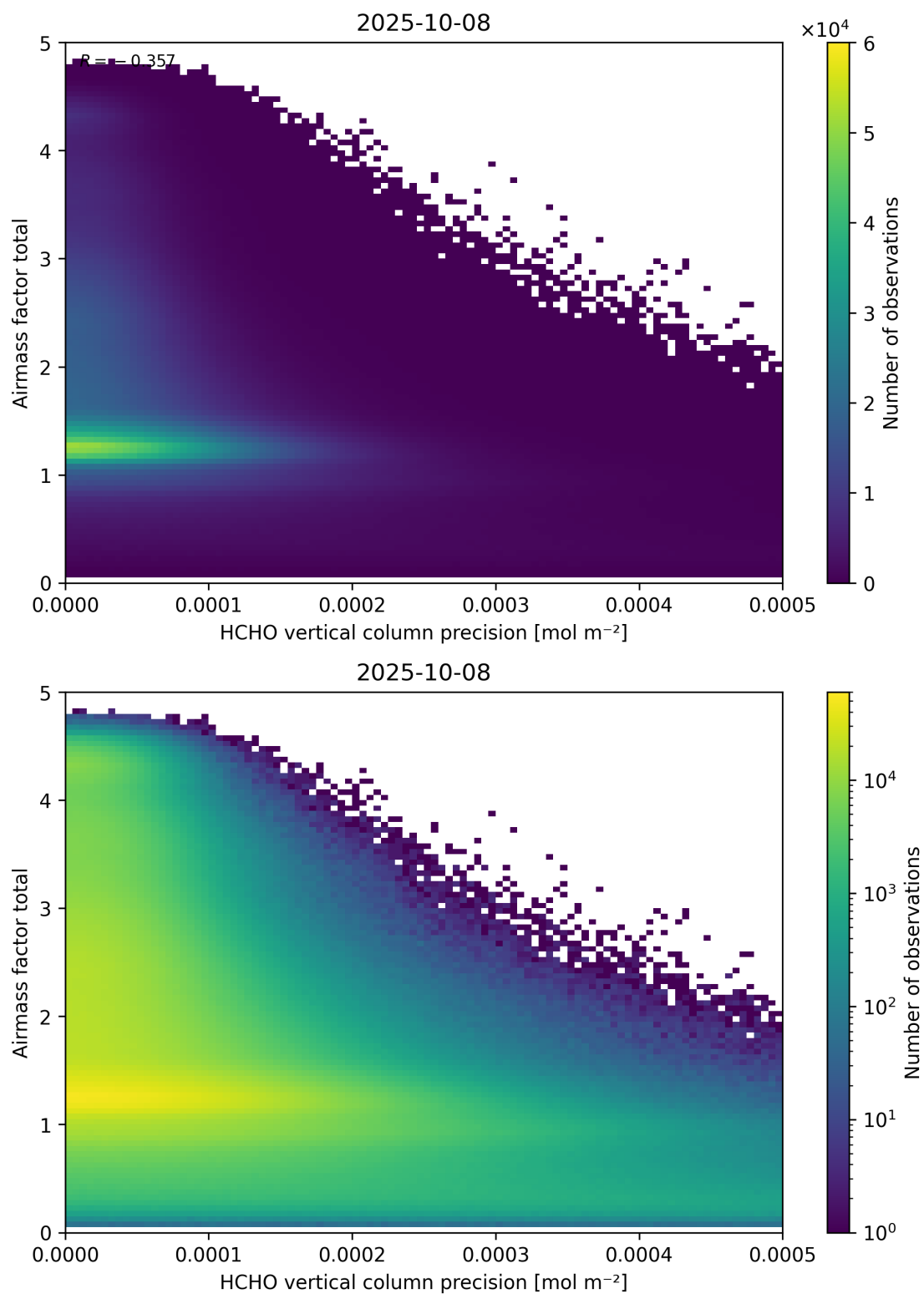
Figure 144: Scatter density plot of “HCHO vertical column precision” against “Airmass factor total” for 2025-10-07 to 2025-10-09.
