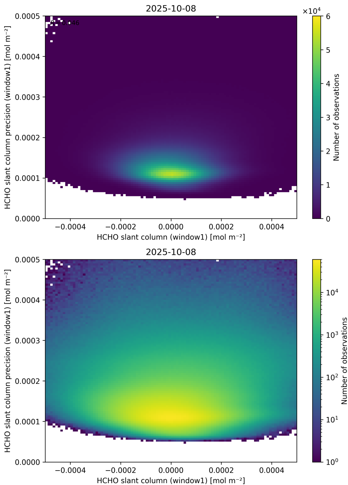
Figure 84: Scatter density plot of “HCHO slant column (window1)” against “HCHO slant column precision (window1)” for 2025-10-07 to 2025-10-09.
