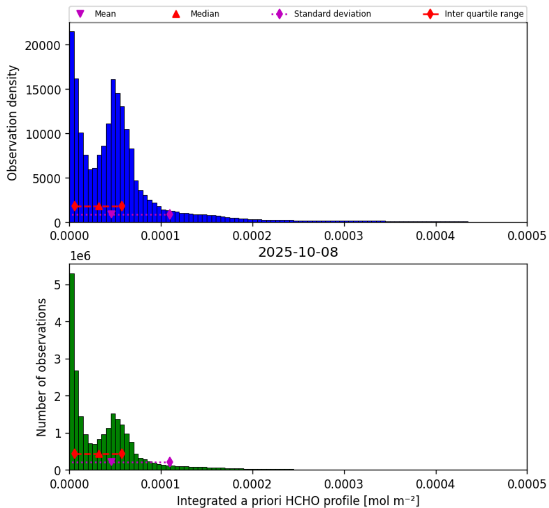
Figure 43: Histogram of “Integrated a priori HCHO profile” for 2025-10-07 to 2025-10-09
