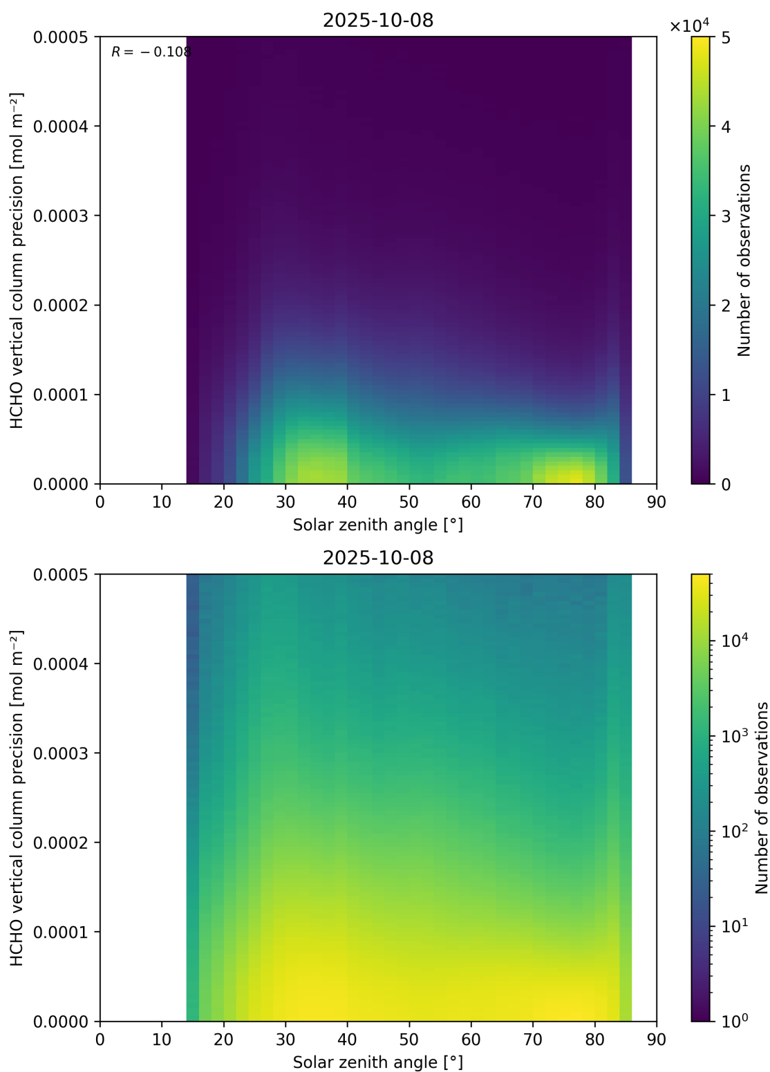
Figure 179: Scatter density plot of “Solar zenith angle” against “HCHO vertical column precision” for 2025-10-07 to 2025-10-09.
