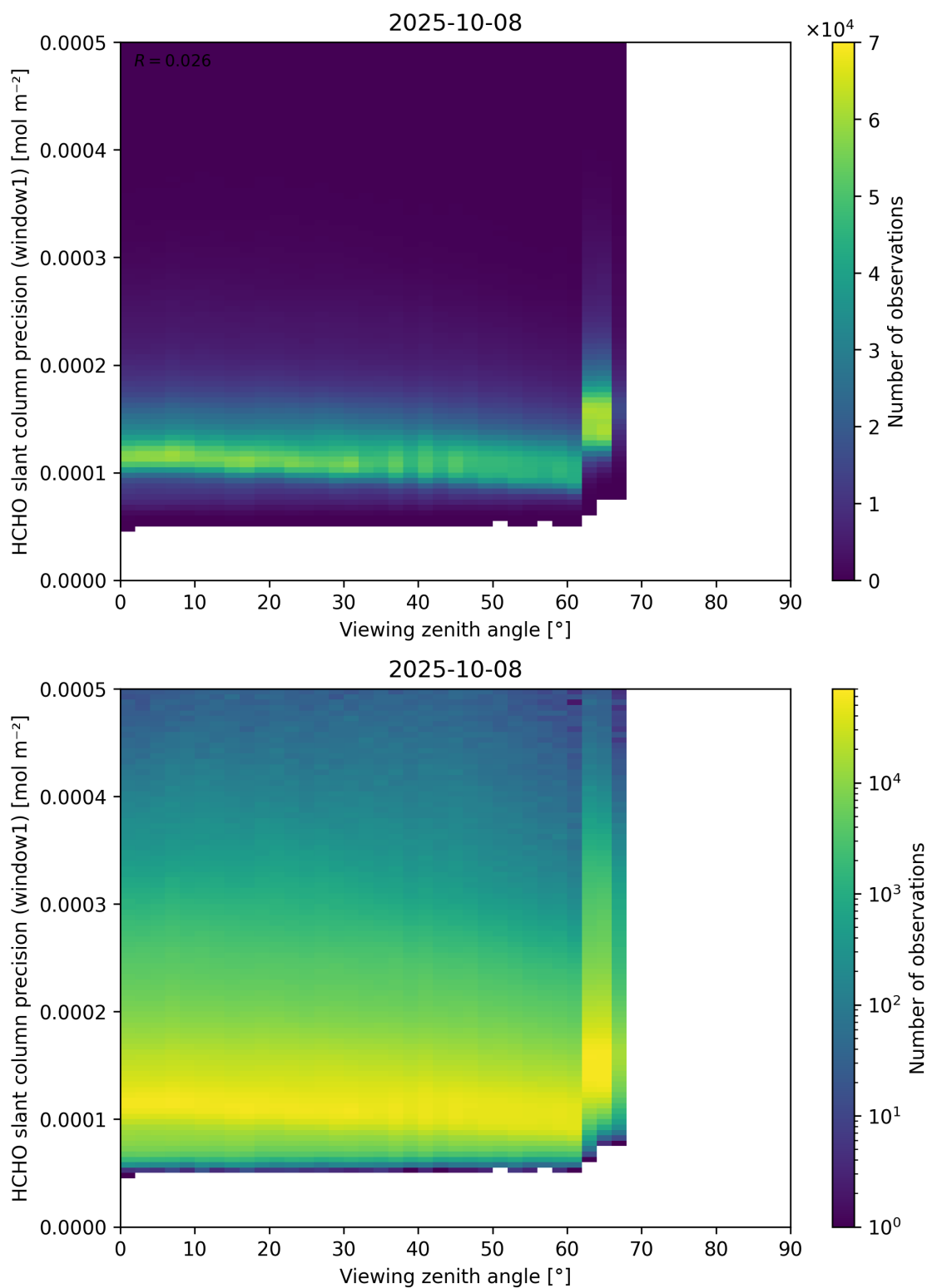
Figure 189: Scatter density plot of “Viewing zenith angle” against “HCHO slant column precision (window1)” for 2025-10-07 to 2025-10-09.
