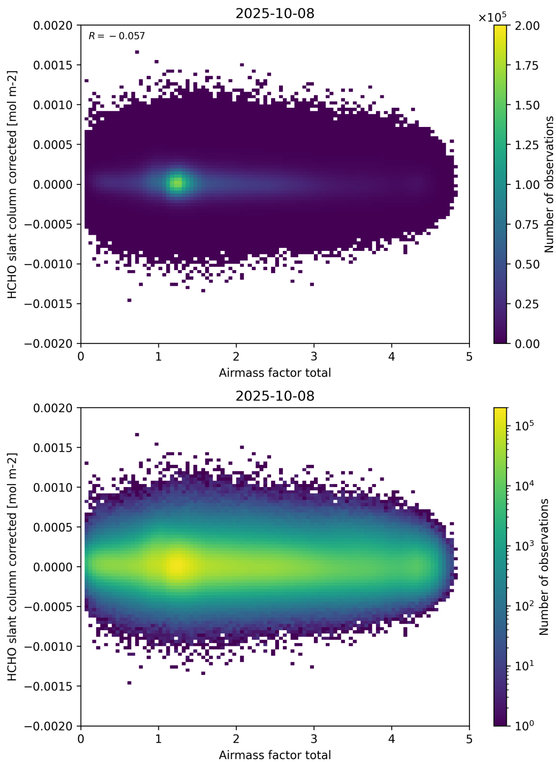
Figure 101: Scatter density plot of “Airmass factor total” against “HCHO slant column corrected” for 2025-10-07 to 2025-10-09.
