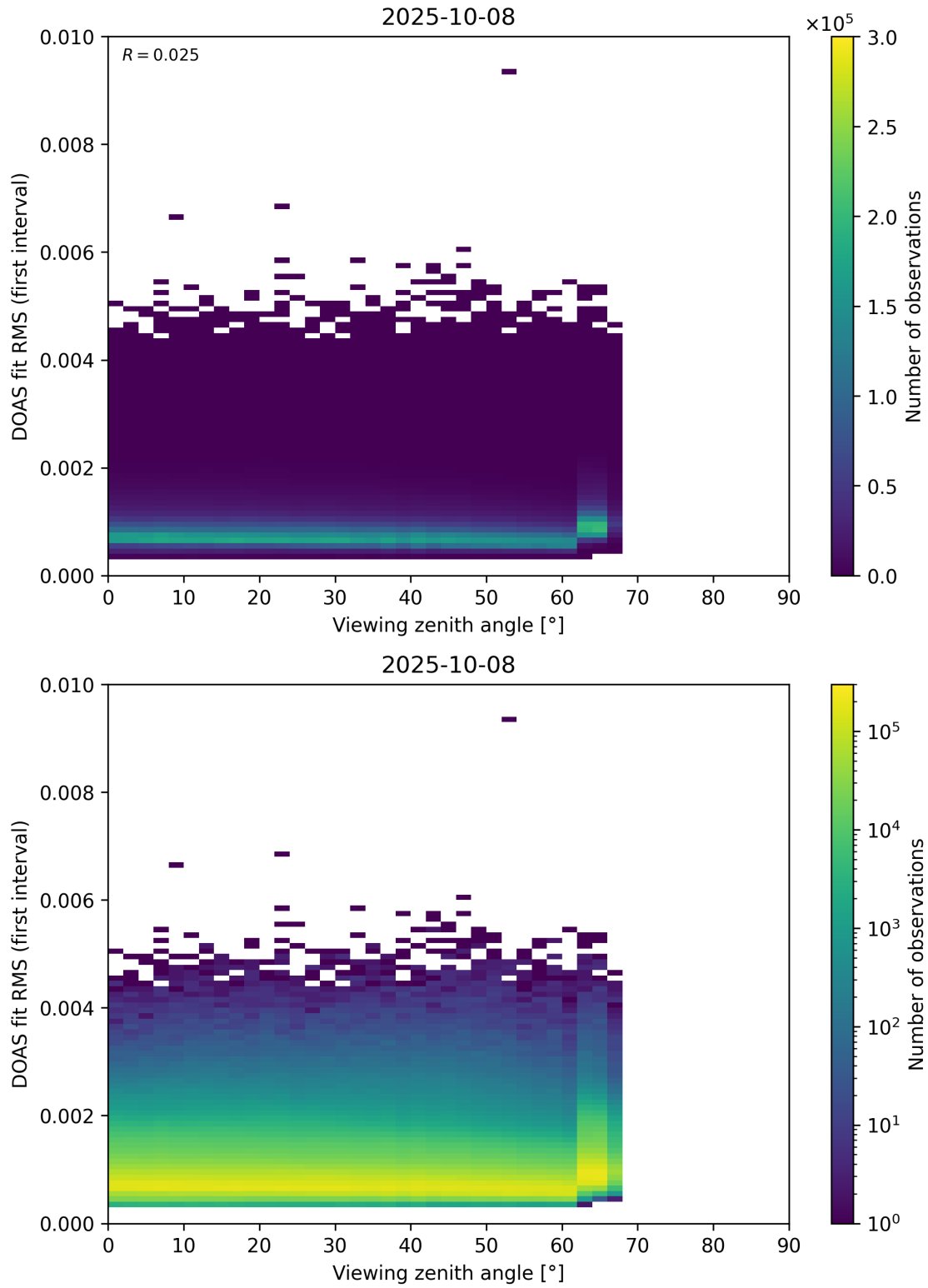
Figure 182: Scatter density plot of “Viewing zenith angle” against “DOAS fit RMS (first interval)” for 2025-10-07 to 2025-10-09.
