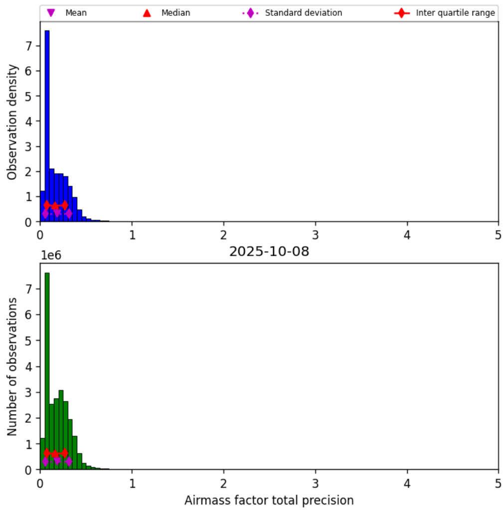
Figure 41: Histogram of “Airmass factor total precision” for 2025-10-07 to 2025-10-09
