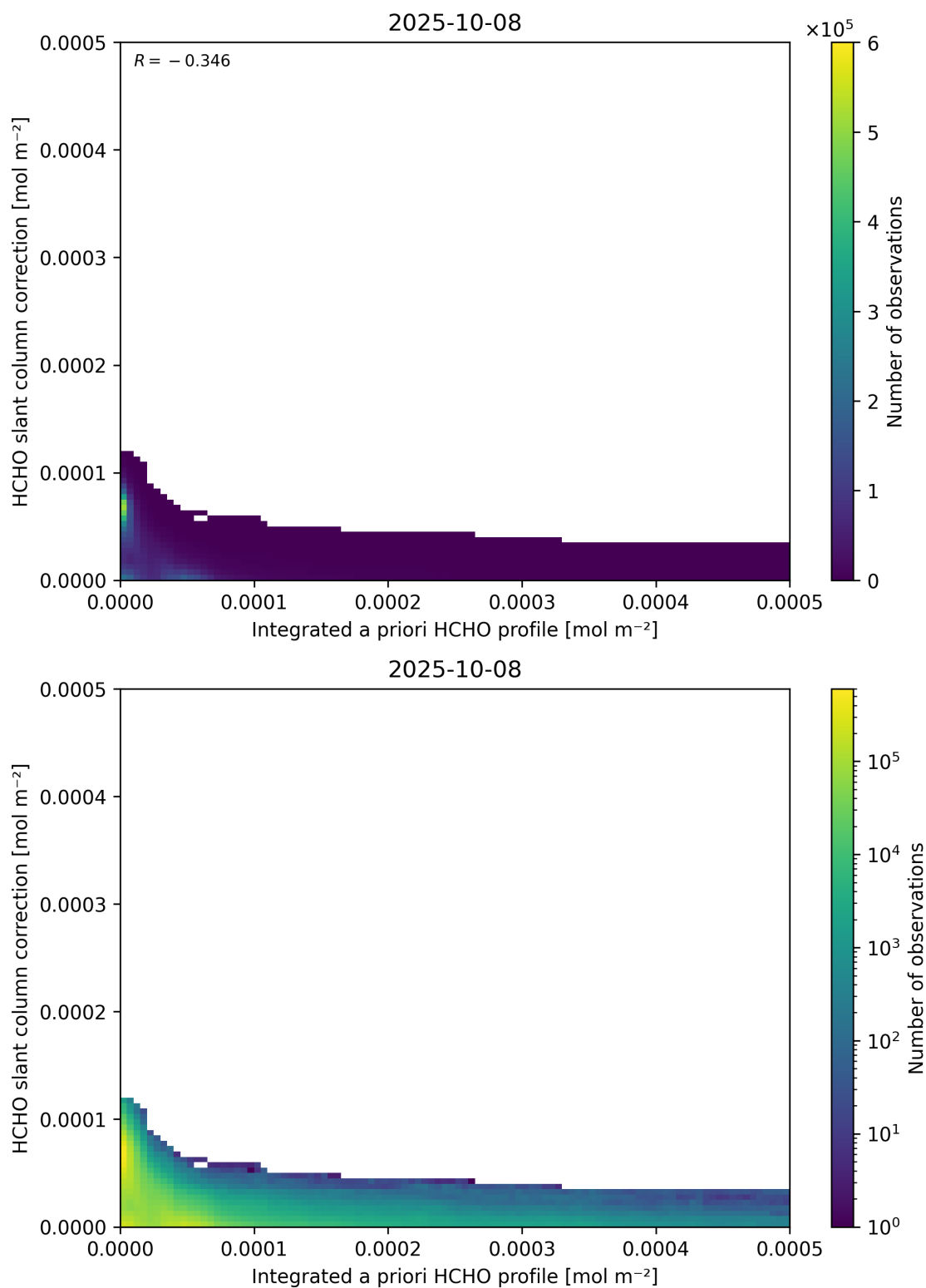
Figure 152: Scatter density plot of “Integrated a priori HCHO profile” against “HCHO slant column correction” for 2025-10-07 to 2025-10-09.
