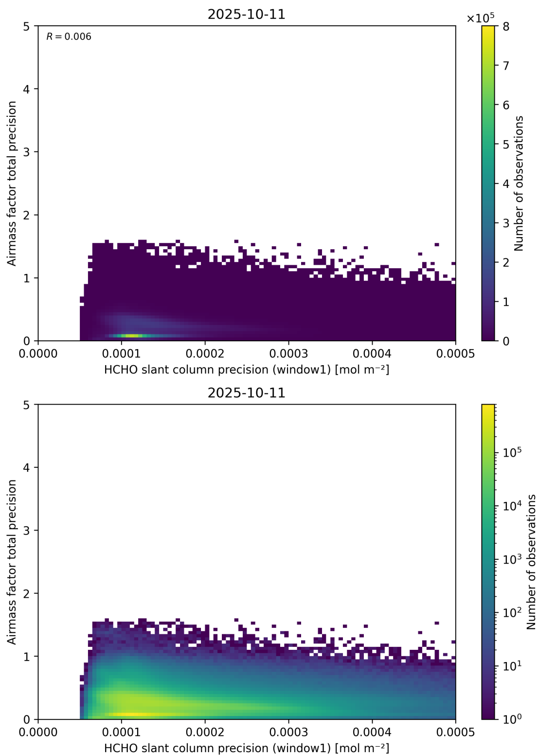
Figure 95: Scatter density plot of “HCHO slant column precision (window1)” against “Airmass factor total precision” for 2025-10-11 to 2025-10-12.
