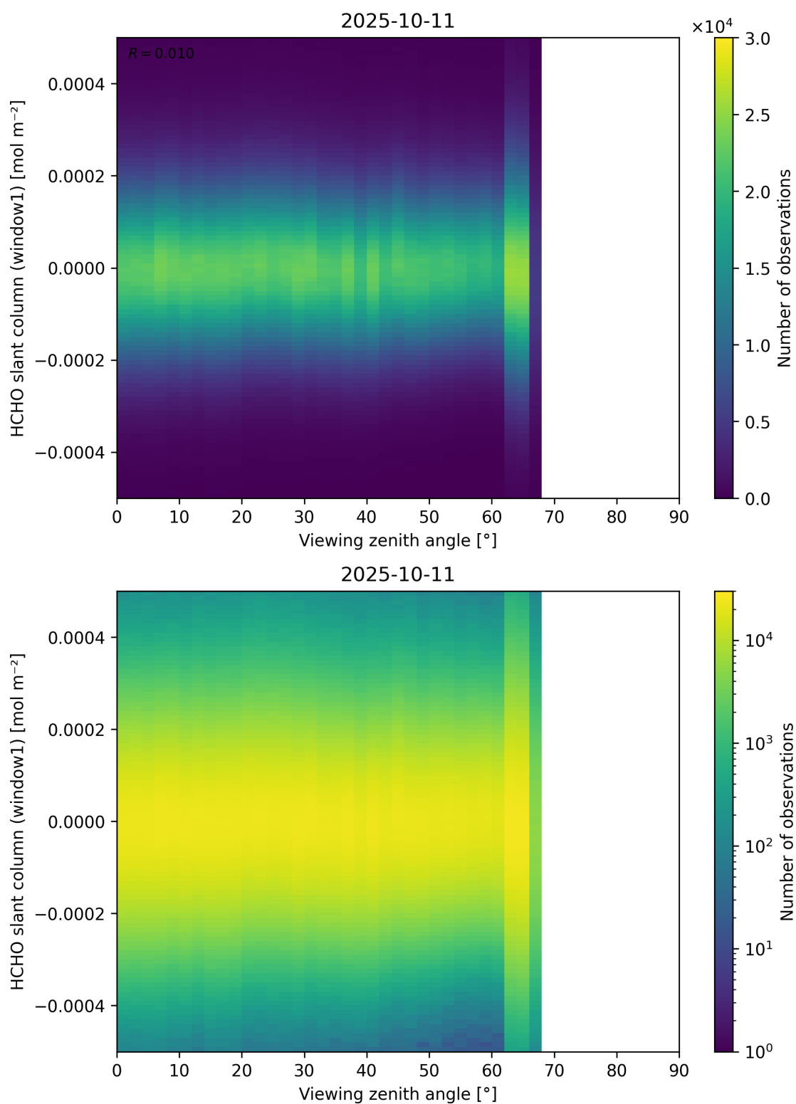
Figure 188: Scatter density plot of “Viewing zenith angle” against “HCHO slant column (window1)” for 2025-10-11 to 2025-10-12.
