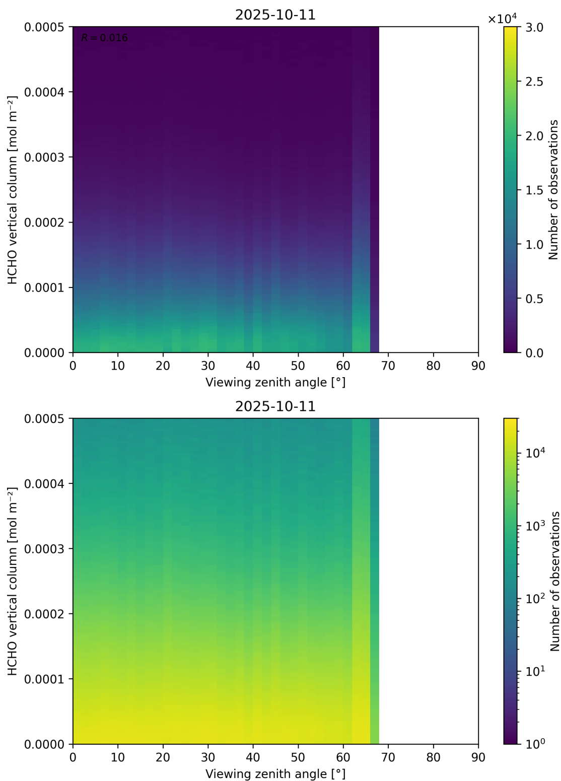
Figure 192: Scatter density plot of “Viewing zenith angle” against “HCHO vertical column” for 2025-10-11 to 2025-10-12.
