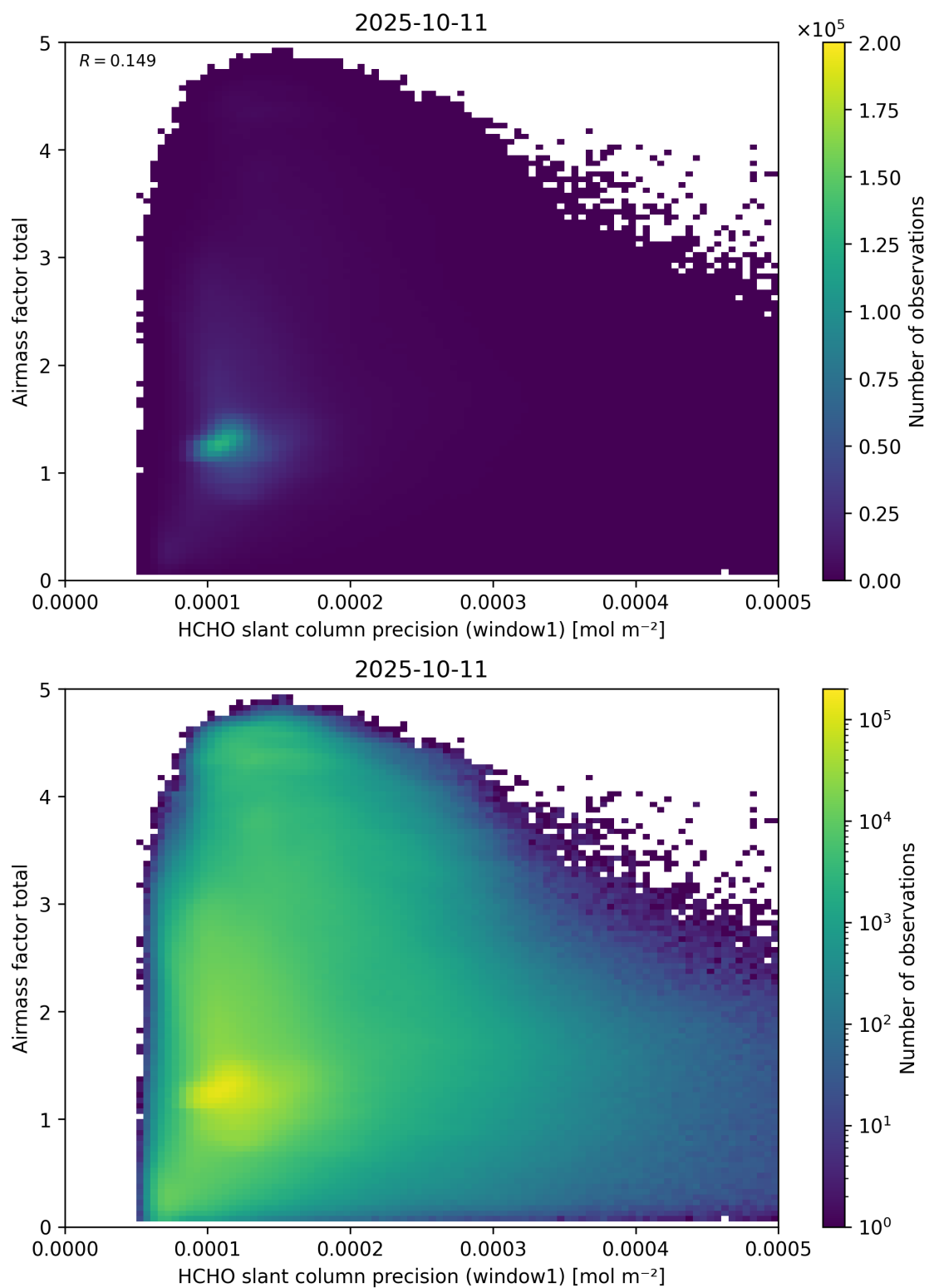
Figure 94: Scatter density plot of “HCHO slant column precision (window1)” against “Airmass factor total” for 2025-10-11 to 2025-10-12.
