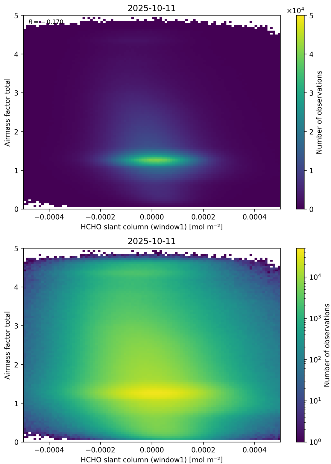
Figure 85: Scatter density plot of “HCHO slant column (window1)” against “Airmass factor total” for 2025-10-11 to 2025-10-12.
