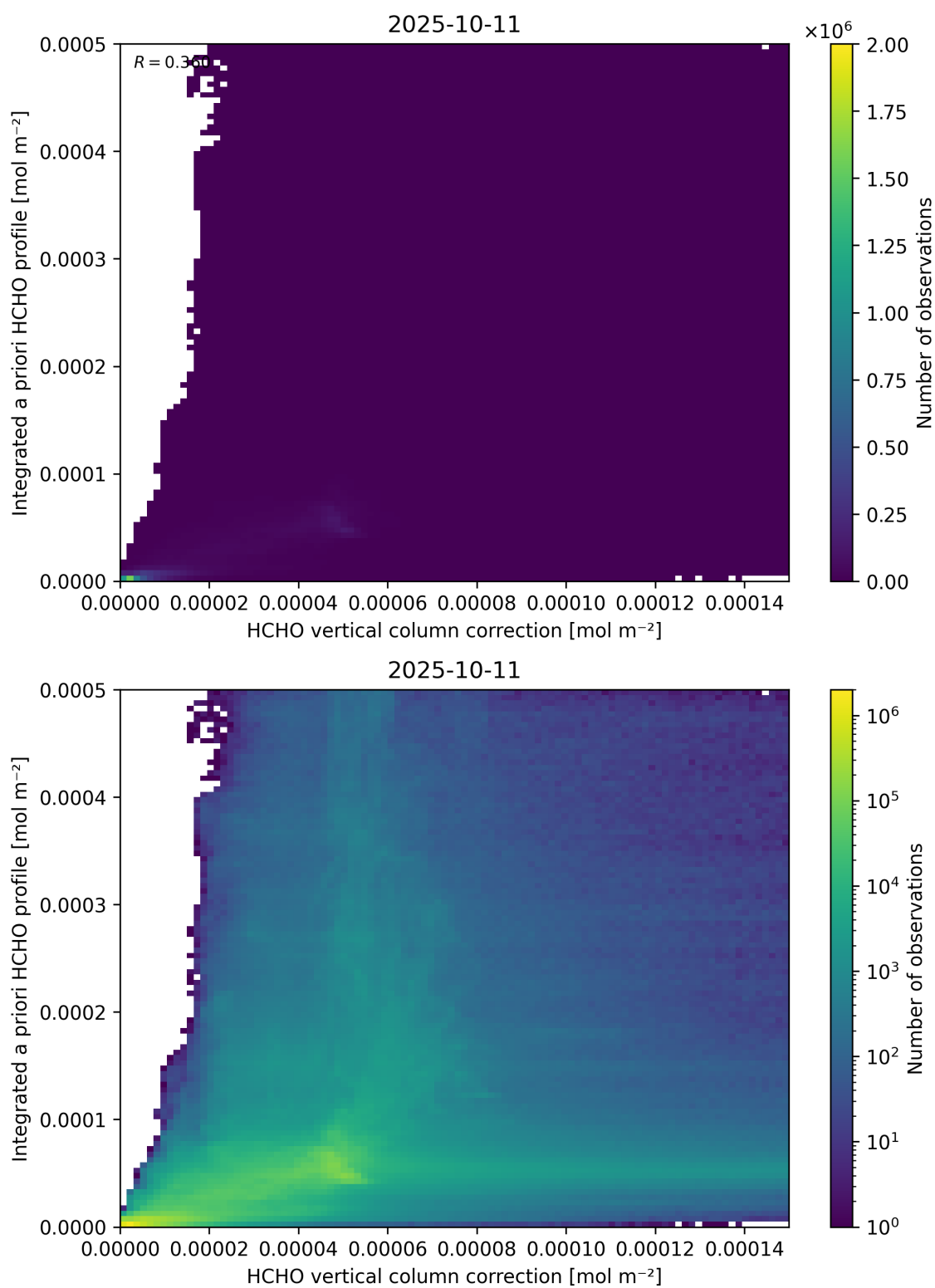
Figure 122: Scatter density plot of “HCHO vertical column correction” against “Integrated a priori HCHO profile” for 2025-10-11 to 2025-10-12.
