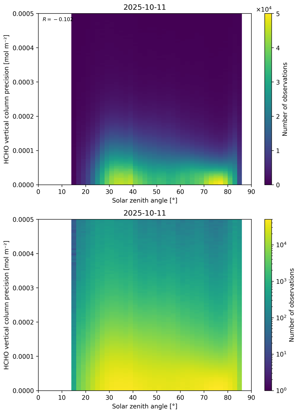
Figure 179: Scatter density plot of “Solar zenith angle” against “HCHO vertical column precision” for 2025-10-11 to 2025-10-12.
