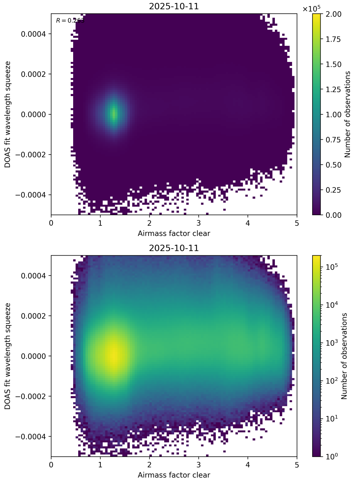
Figure 73: Scatter density plot of “Airmass factor clear” against “DOAS fit wavelength squeeze” for 2025-10-11 to 2025-10-12.
