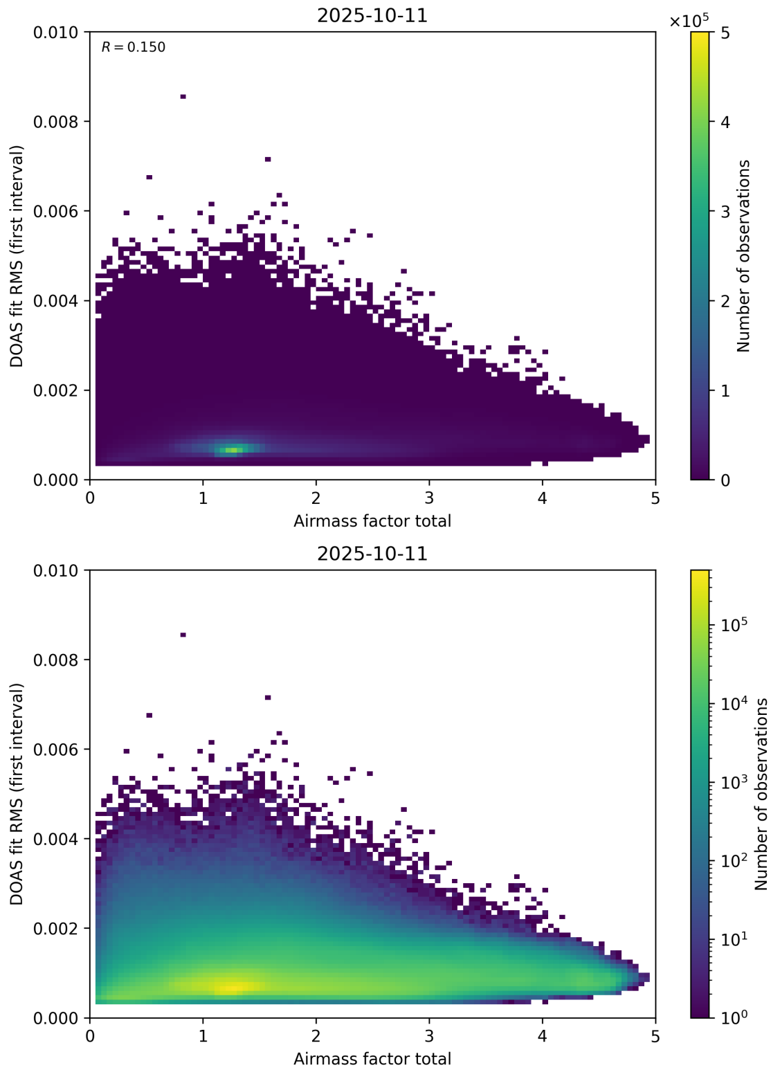
Figure 97: Scatter density plot of “Airmass factor total” against “DOAS fit RMS (first interval)” for 2025-10-11 to 2025-10-12.
