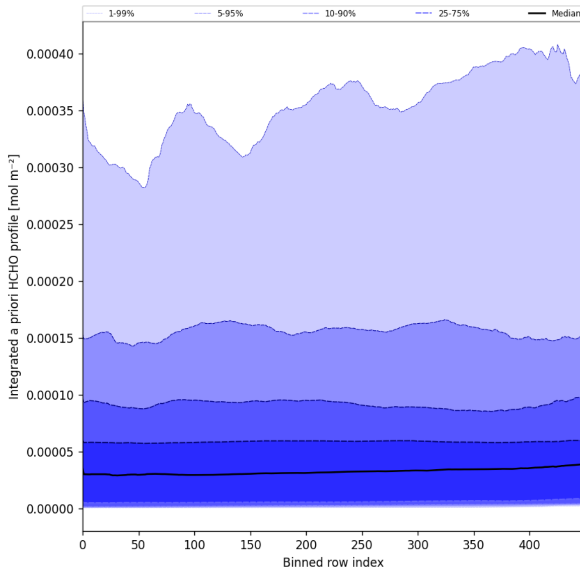
Figure 57: Along track statistics of "Integrated a priori HCHO profile" for 2025-10-11 to 2025-10-12
