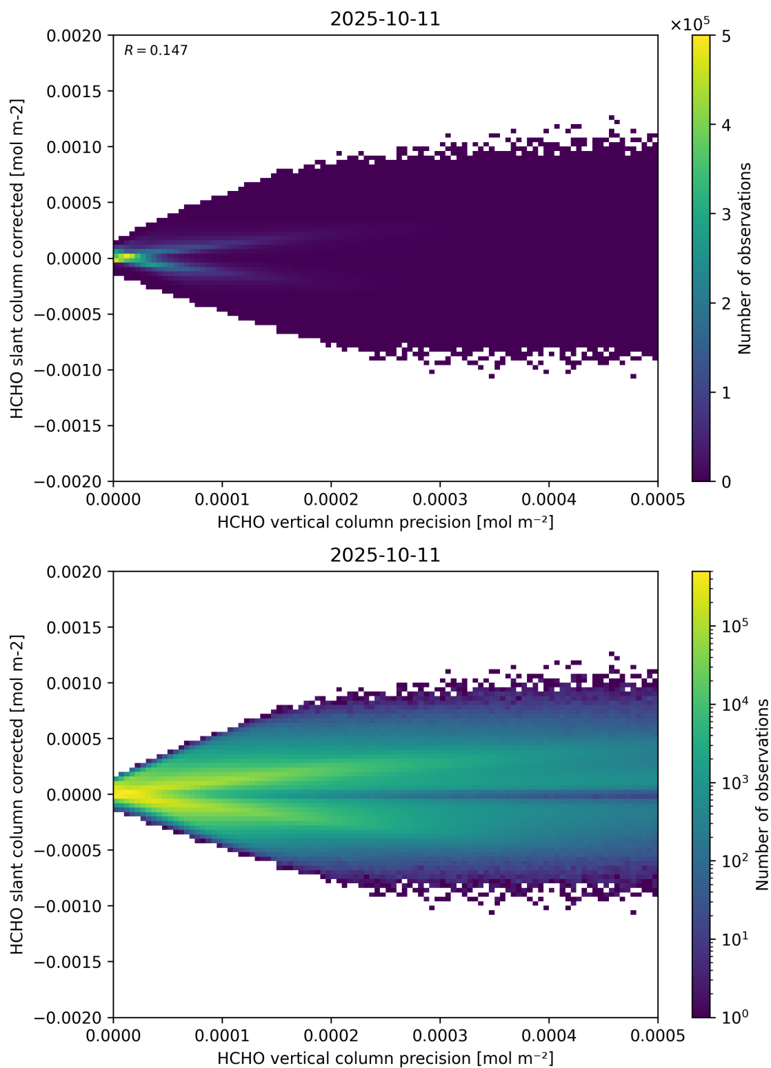
Figure 140: Scatter density plot of “HCHO vertical column precision” against “HCHO slant column corrected” for 2025-10-11 to 2025-10-12.
