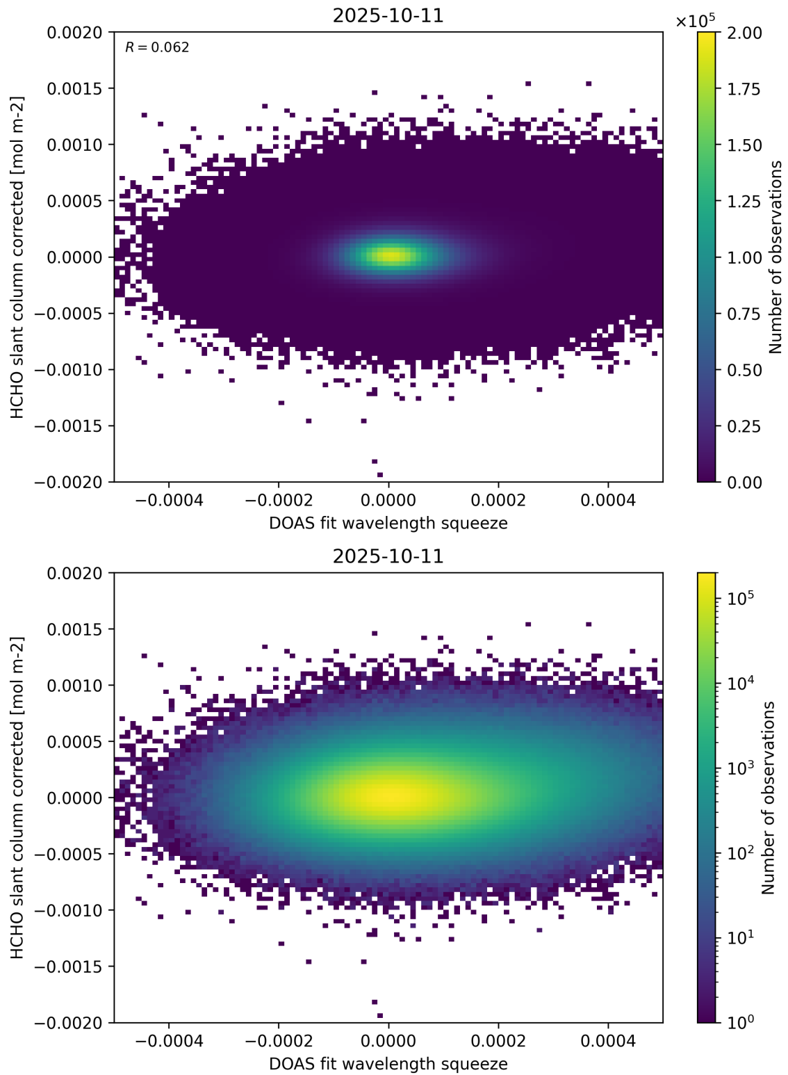
Figure 69: Scatter density plot of “DOAS fit wavelength squeeze” against “HCHO slant column corrected” for 2025-10-11 to 2025-10-12.
