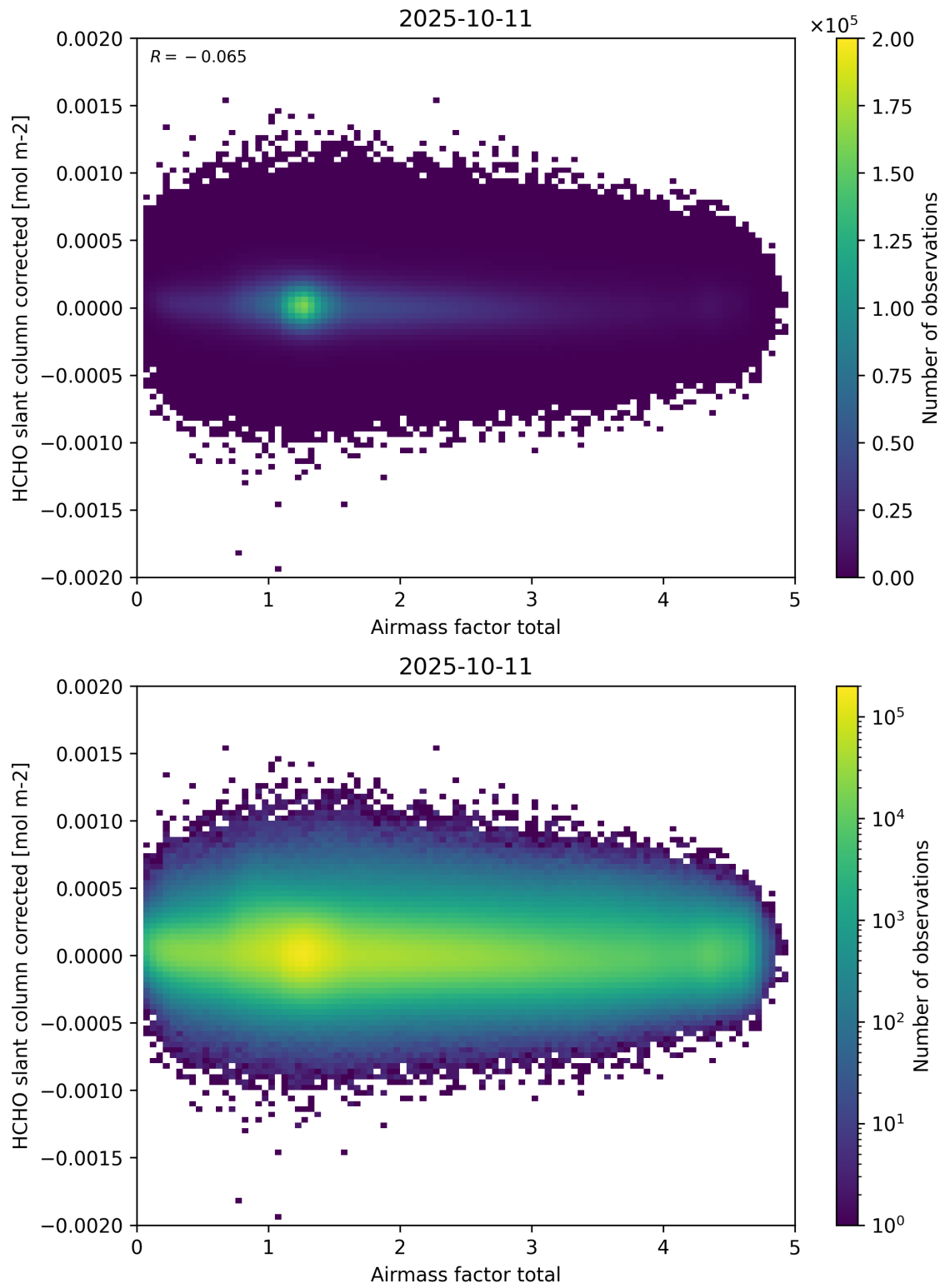
Figure 101: Scatter density plot of “Airmass factor total” against “HCHO slant column corrected” for 2025-10-11 to 2025-10-12.
