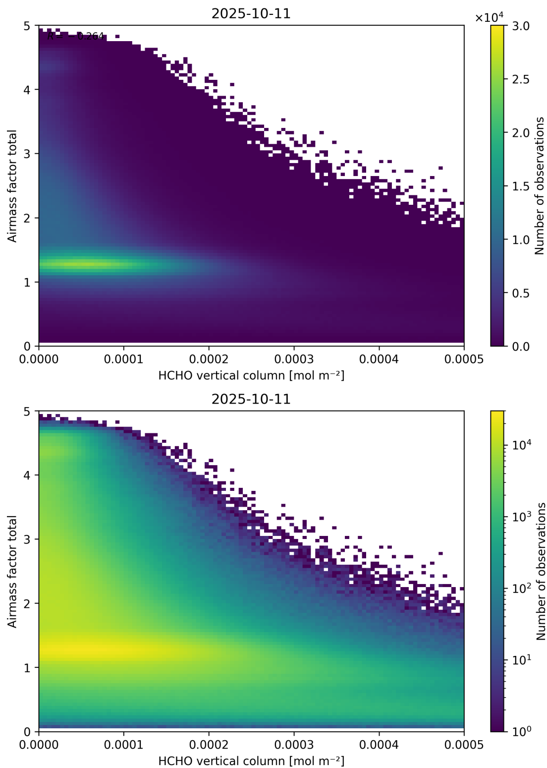
Figure 131: Scatter density plot of “HCHO vertical column” against “Airmass factor total” for 2025-10-11 to 2025-10-12.
