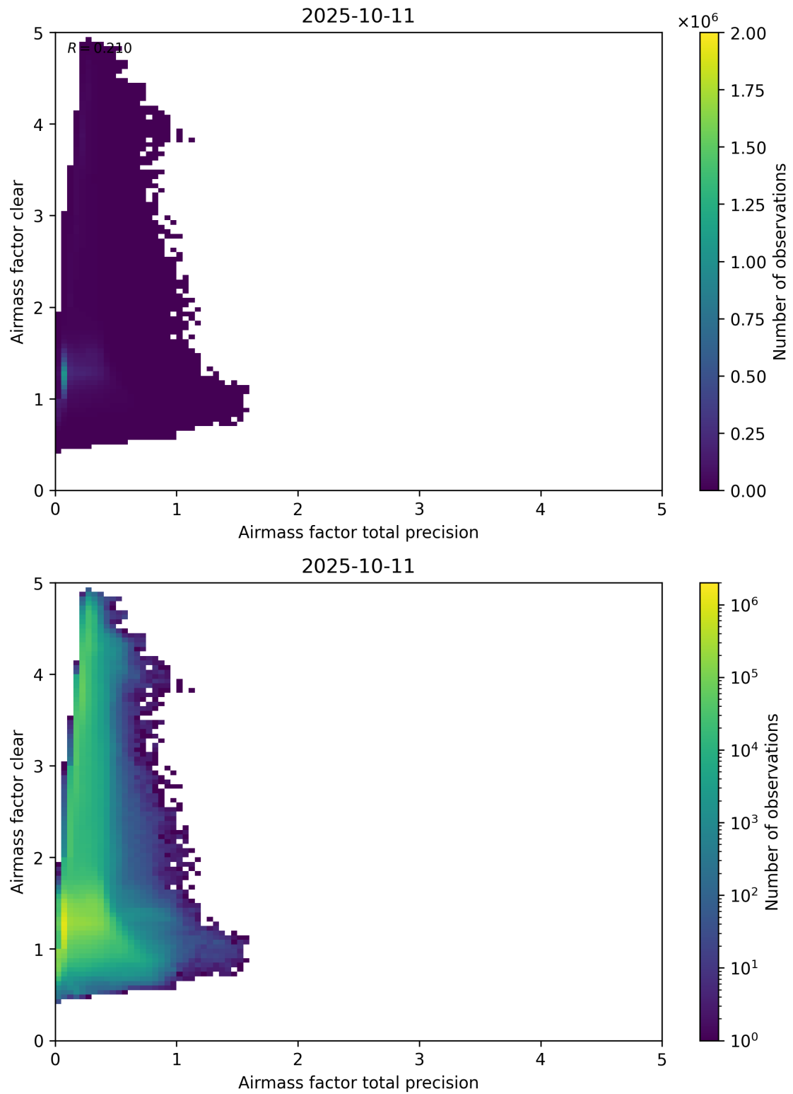
Figure 108: Scatter density plot of “Airmass factor total precision” against “Airmass factor clear” for 2025-10-11 to 2025-10-12.
