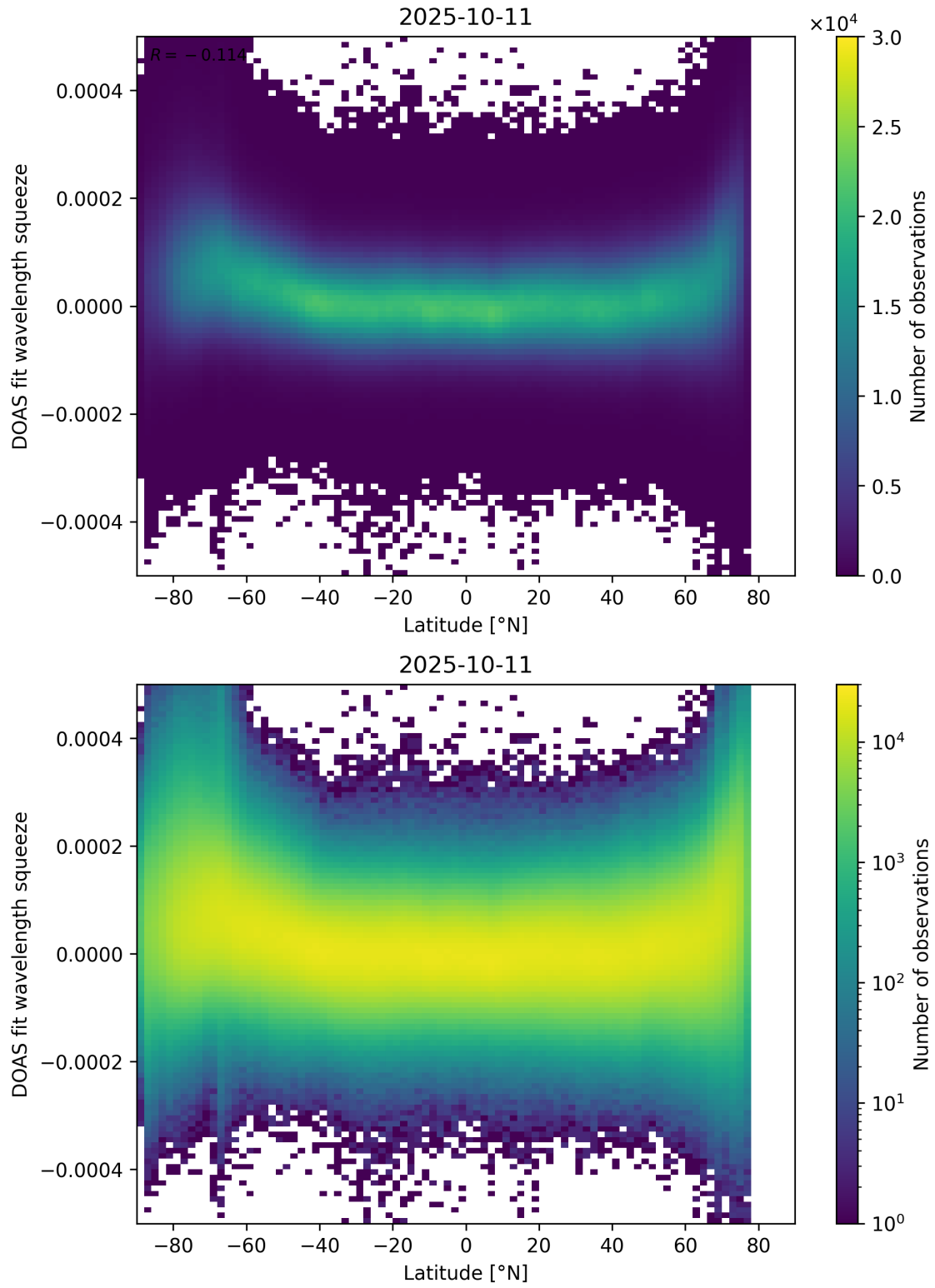
Figure 155: Scatter density plot of “Latitude” against “DOAS fit wavelength squeeze” for 2025-10-11 to 2025-10-12.
