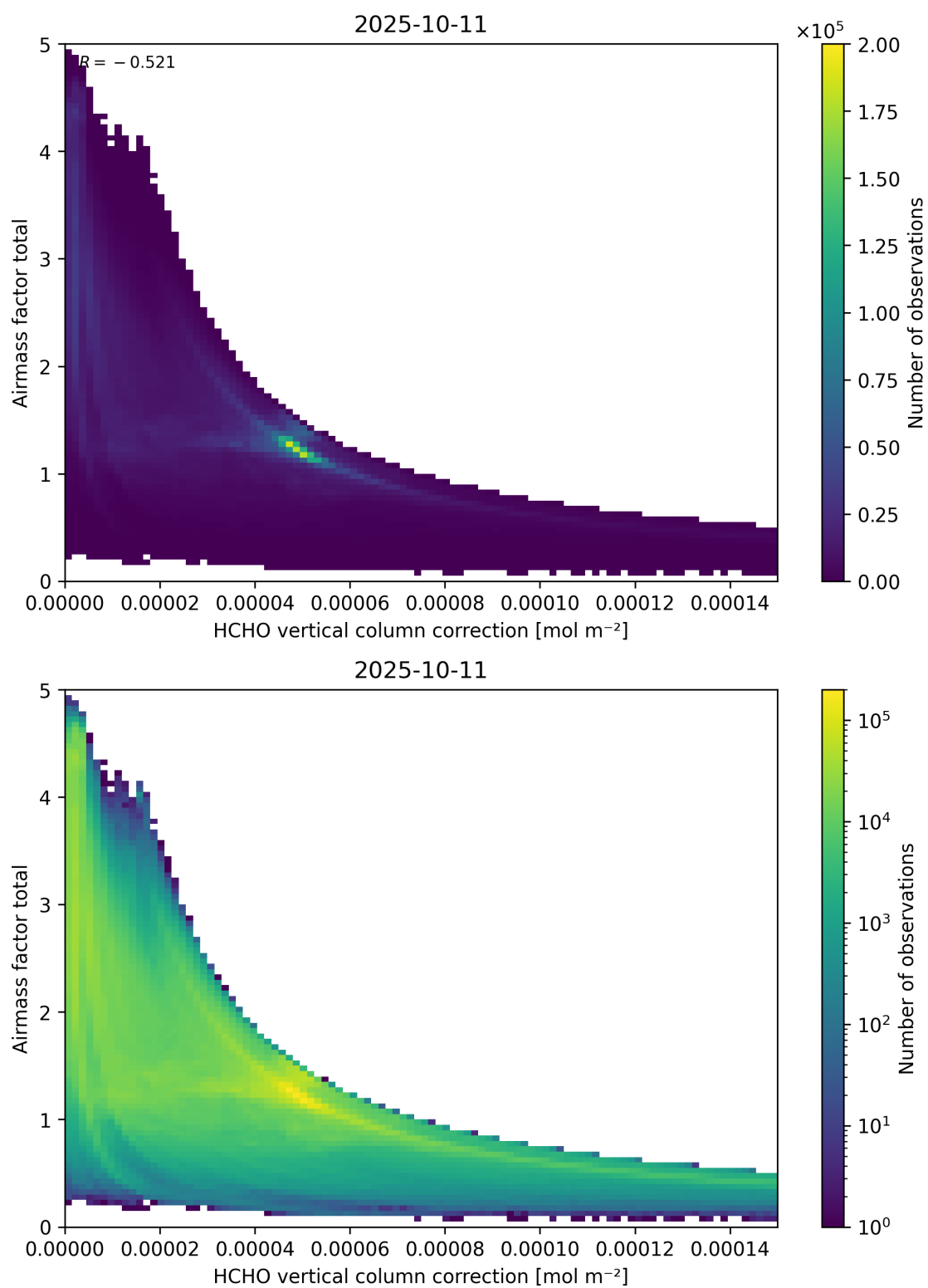
Figure 120: Scatter density plot of “HCHO vertical column correction” against “Airmass factor total” for 2025-10-11 to 2025-10-12.
