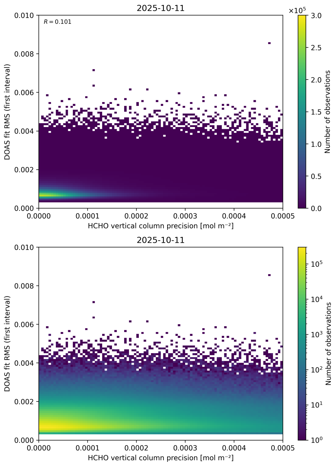
Figure 136: Scatter density plot of “HCHO vertical column precision” against “DOAS fit RMS (first interval)” for 2025-10-11 to 2025-10-12.
