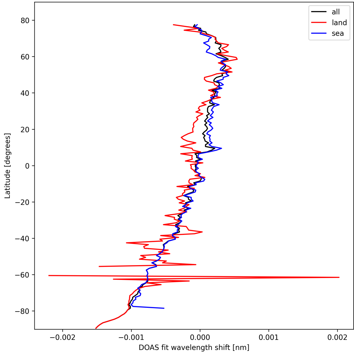
Figure 30: Zonal average of "DOAS fit wavelength shift" for 2025-10-11 to 2025-10-12.
