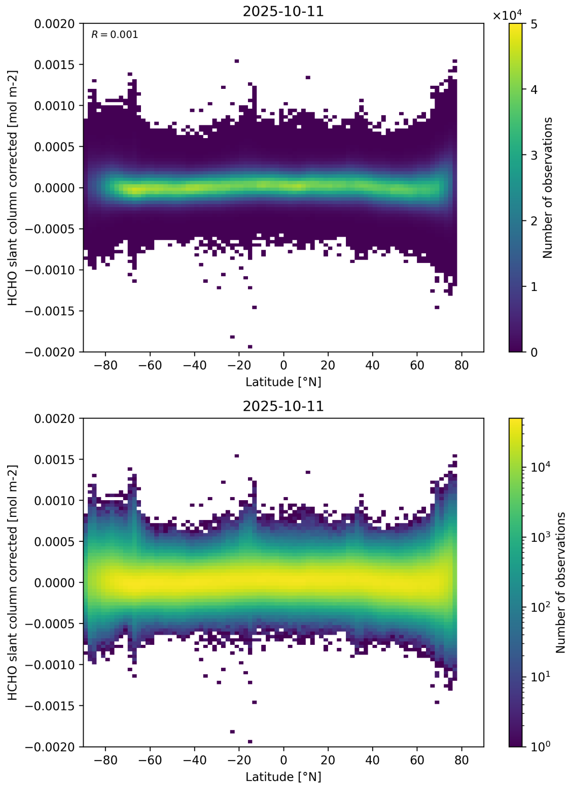
Figure 157: Scatter density plot of “Latitude” against “HCHO slant column corrected” for 2025-10-11 to 2025-10-12.
