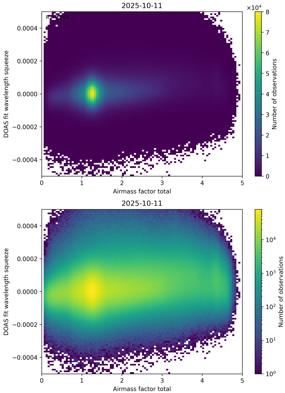
Figure 99: Scatter density plot of “Airmass factor total” against “DOAS fit wavelength squeeze” for 2025-10-11 to 2025-10-12.
