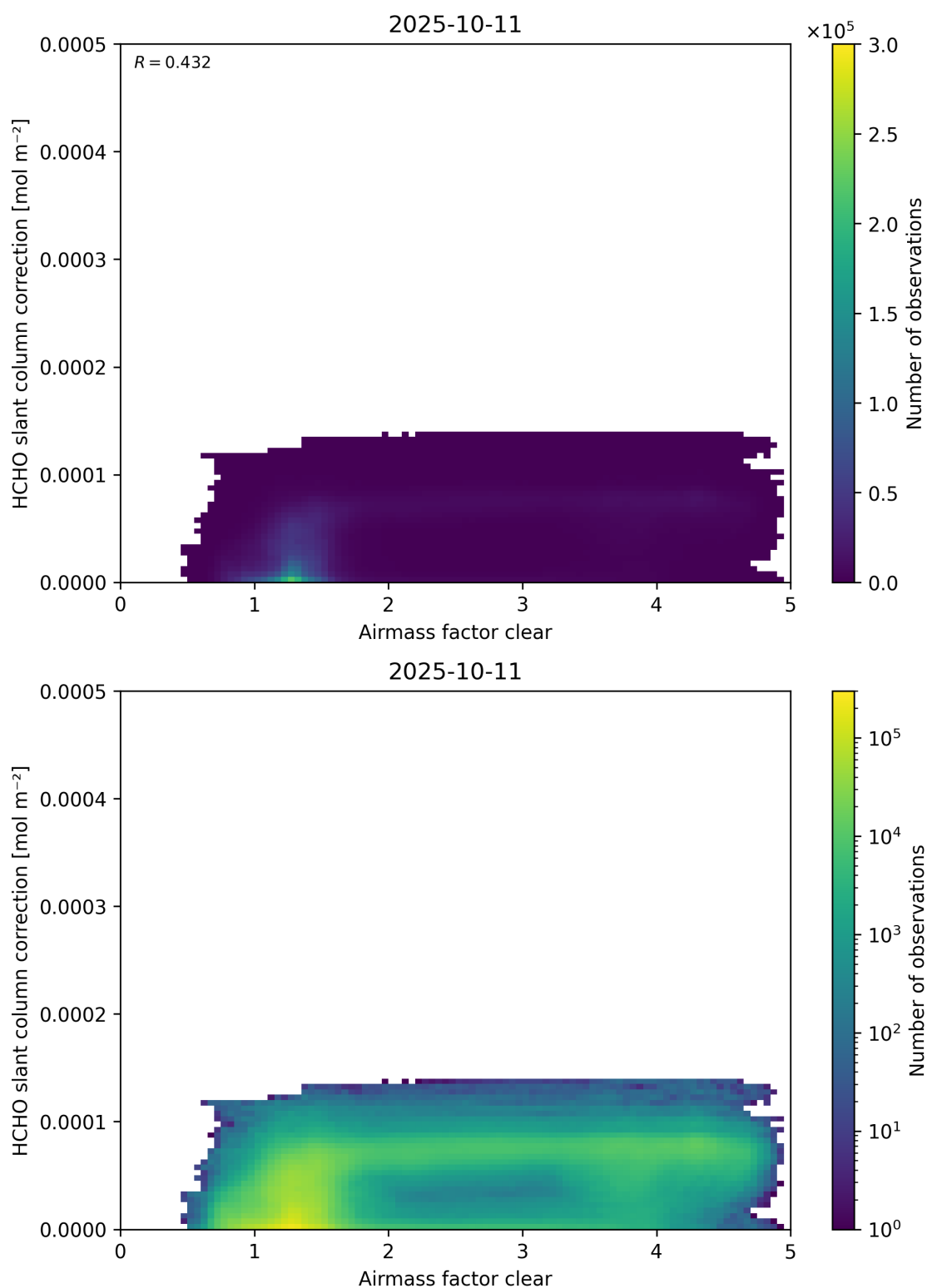
Figure 75: Scatter density plot of “Airmass factor clear” against “HCHO slant column correction” for 2025-10-11 to 2025-10-12.
