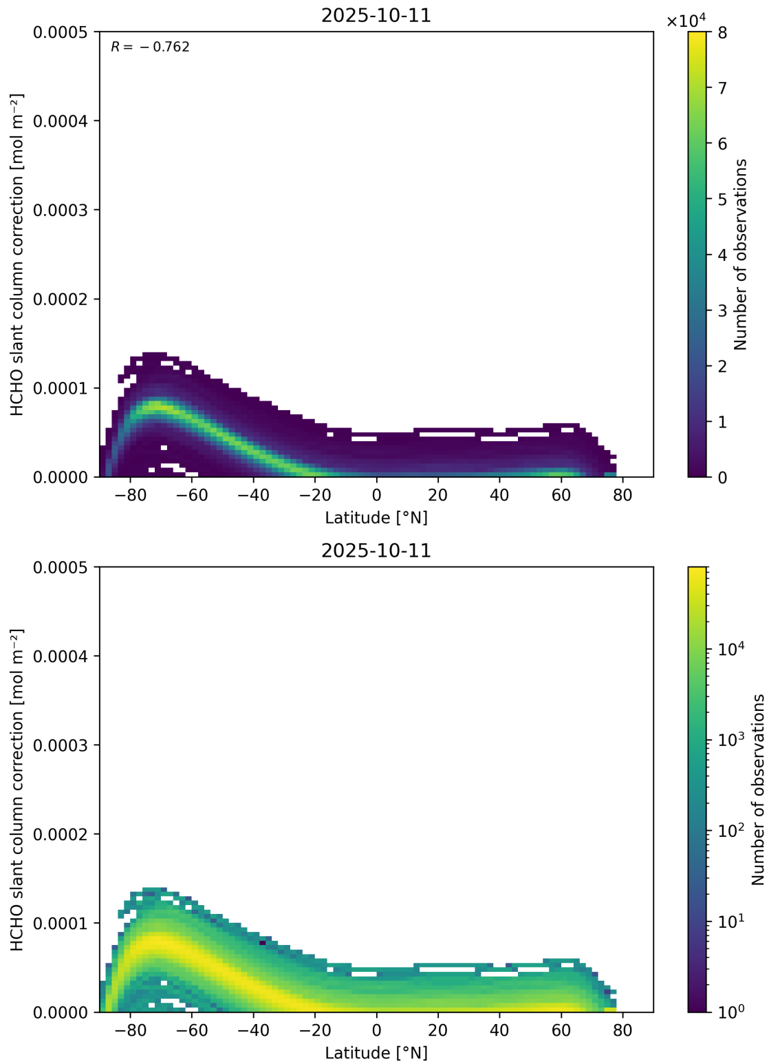
Figure 158: Scatter density plot of “Latitude” against “HCHO slant column correction” for 2025-10-11 to 2025-10-12.
