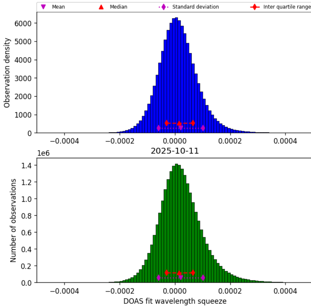
Figure 45: Histogram of “DOAS fit wavelength squeeze” for 2025-10-11 to 2025-10-12
