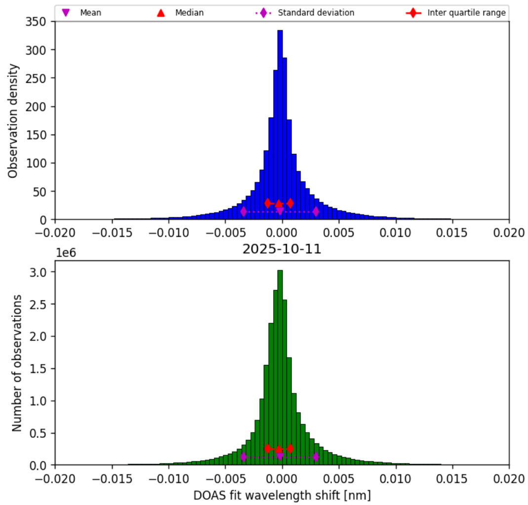
Figure 44: Histogram of “DOAS fit wavelength shift” for 2025-10-11 to 2025-10-12
