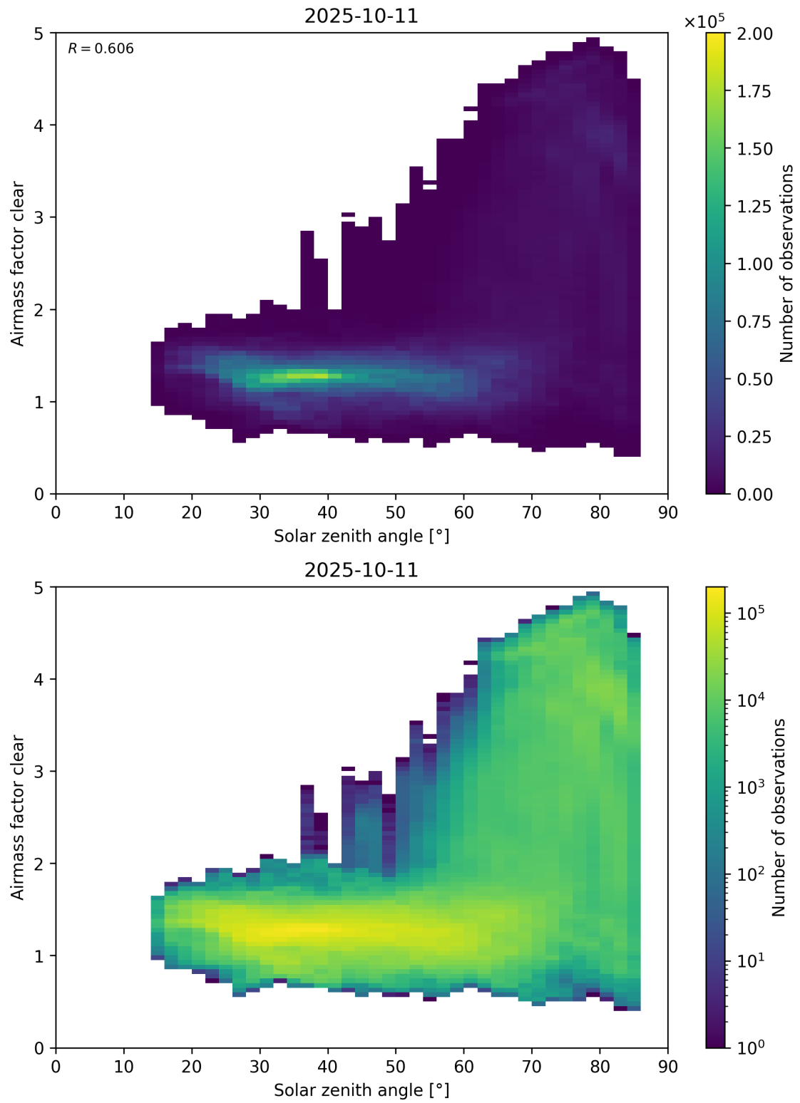
Figure 170: Scatter density plot of “Solar zenith angle” against “Airmass factor clear” for 2025-10-11 to 2025-10-12.
