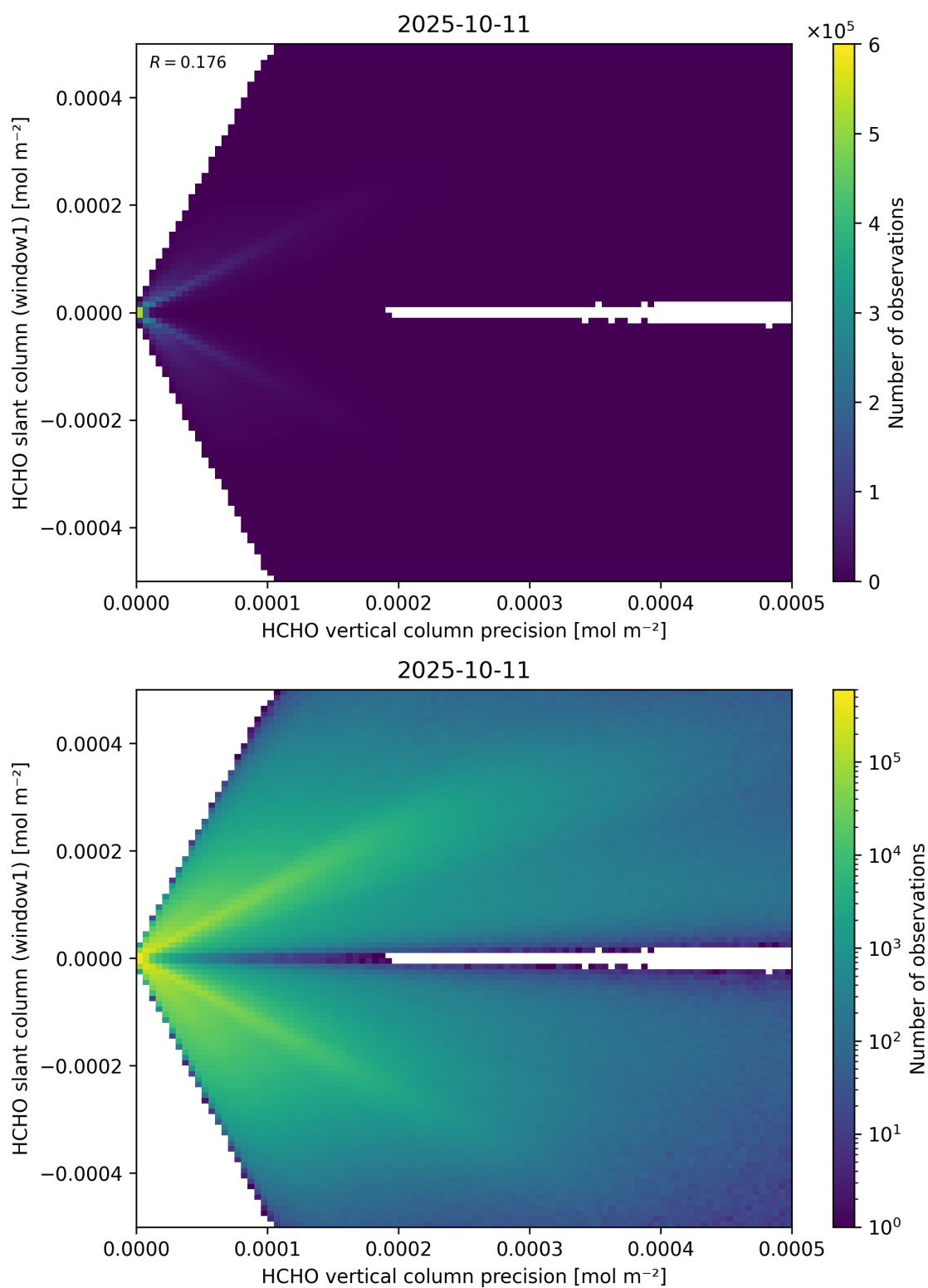
Figure 142: Scatter density plot of “HCHO vertical column precision” against “HCHO slant column (window1)” for 2025-10-11 to 2025-10-12.
