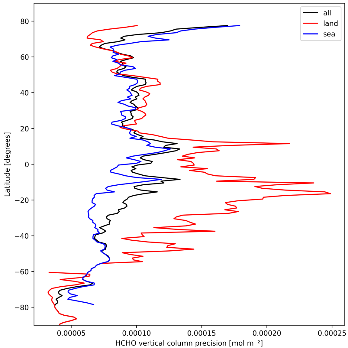
Figure 22: Zonal average of “HCHO vertical column precision” for 2025-10-11 to 2025-10-12.
