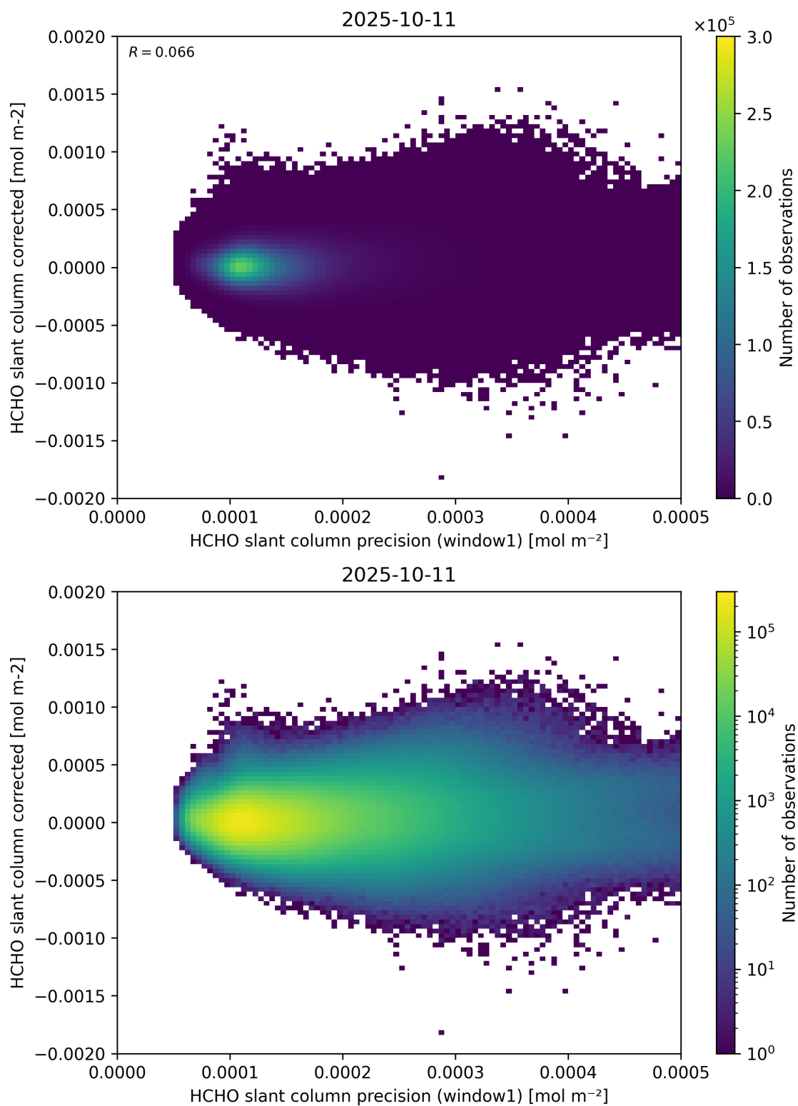
Figure 92: Scatter density plot of “HCHO slant column precision (window1)” against “HCHO slant column corrected” for 2025-10-11 to 2025-10-12.
