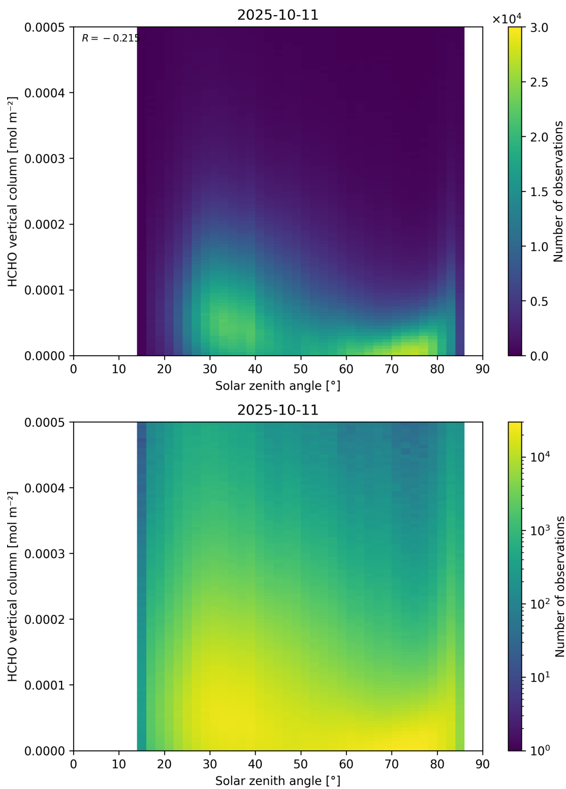
Figure 177: Scatter density plot of “Solar zenith angle” against “HCHO vertical column” for 2025-10-11 to 2025-10-12.
