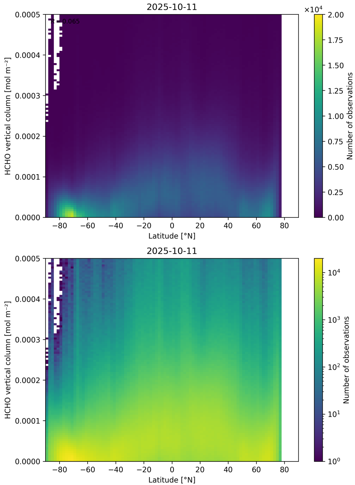
Figure 163: Scatter density plot of “Latitude” against “HCHO vertical column” for 2025-10-11 to 2025-10-12.
