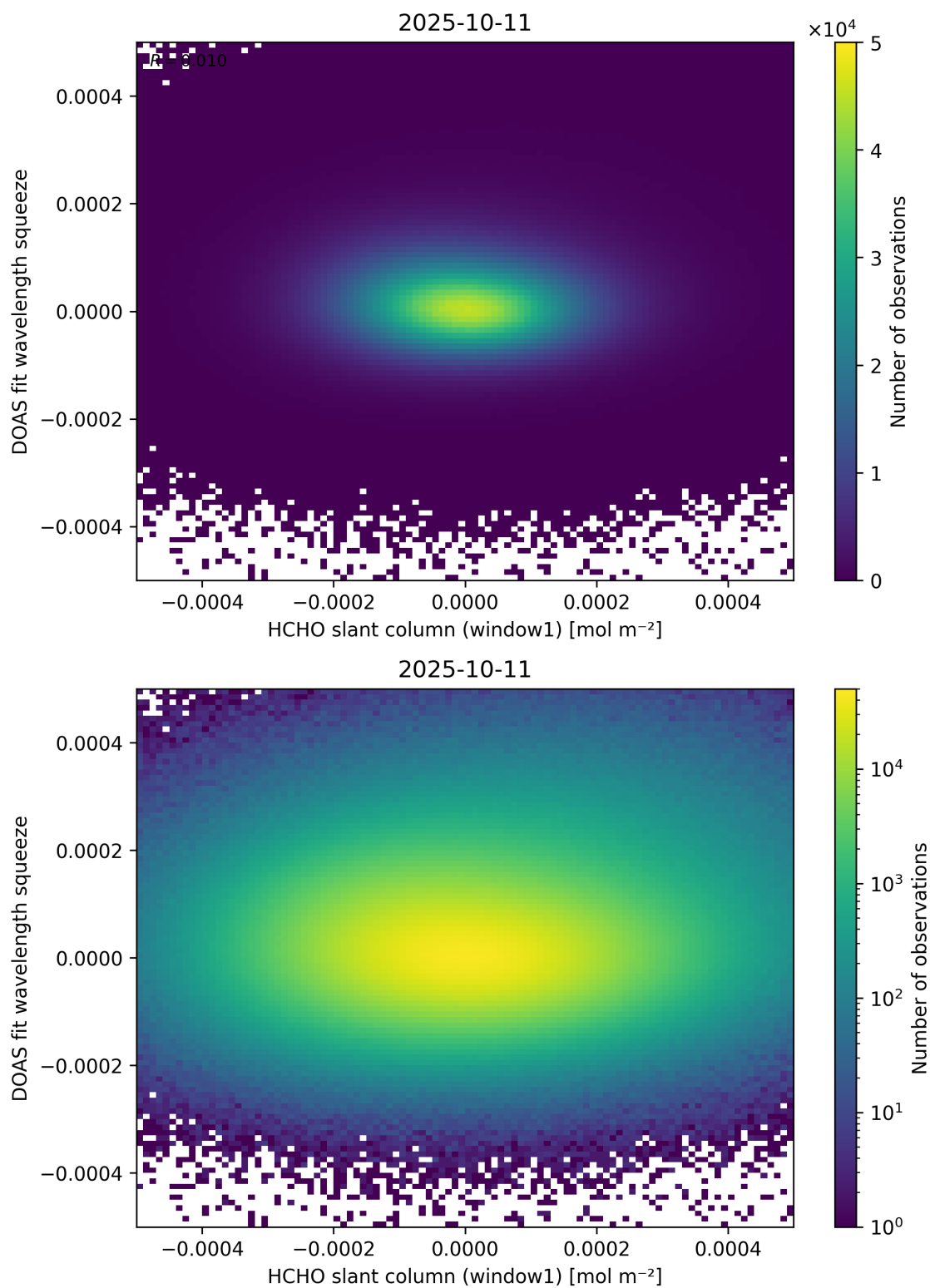
Figure 80: Scatter density plot of “HCHO slant column (window1)” against “DOAS fit wavelength squeeze” for 2025-10-11 to 2025-10-12.
