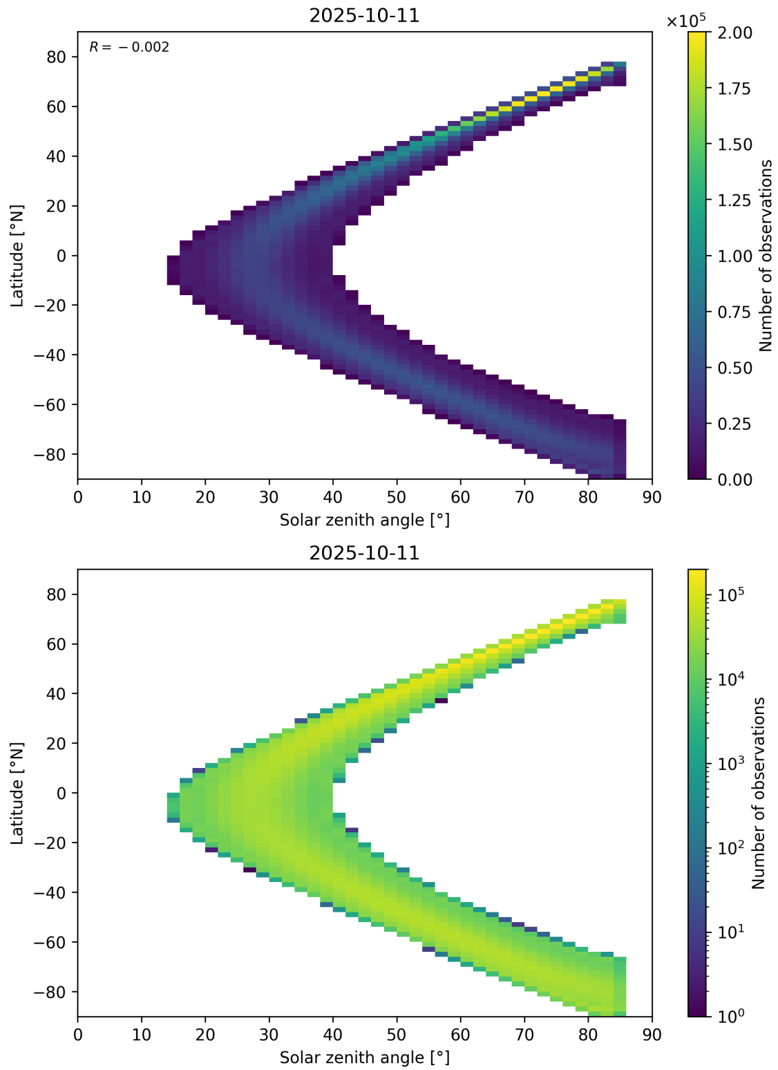
Figure 181: Scatter density plot of “Solar zenith angle” against “Latitude” for 2025-10-11 to 2025-10-12.
