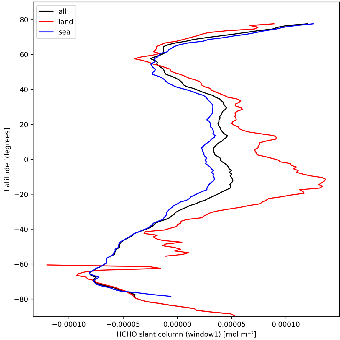
Figure 24: Zonal average of “HCHO slant column (window1)” for 2025-10-11 to 2025-10-12.
