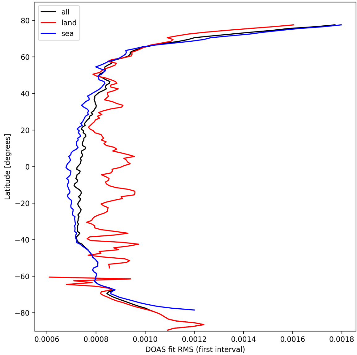
Figure 32: Zonal average of “DOAS fit RMS (first interval)” for 2025-10-11 to 2025-10-12.
