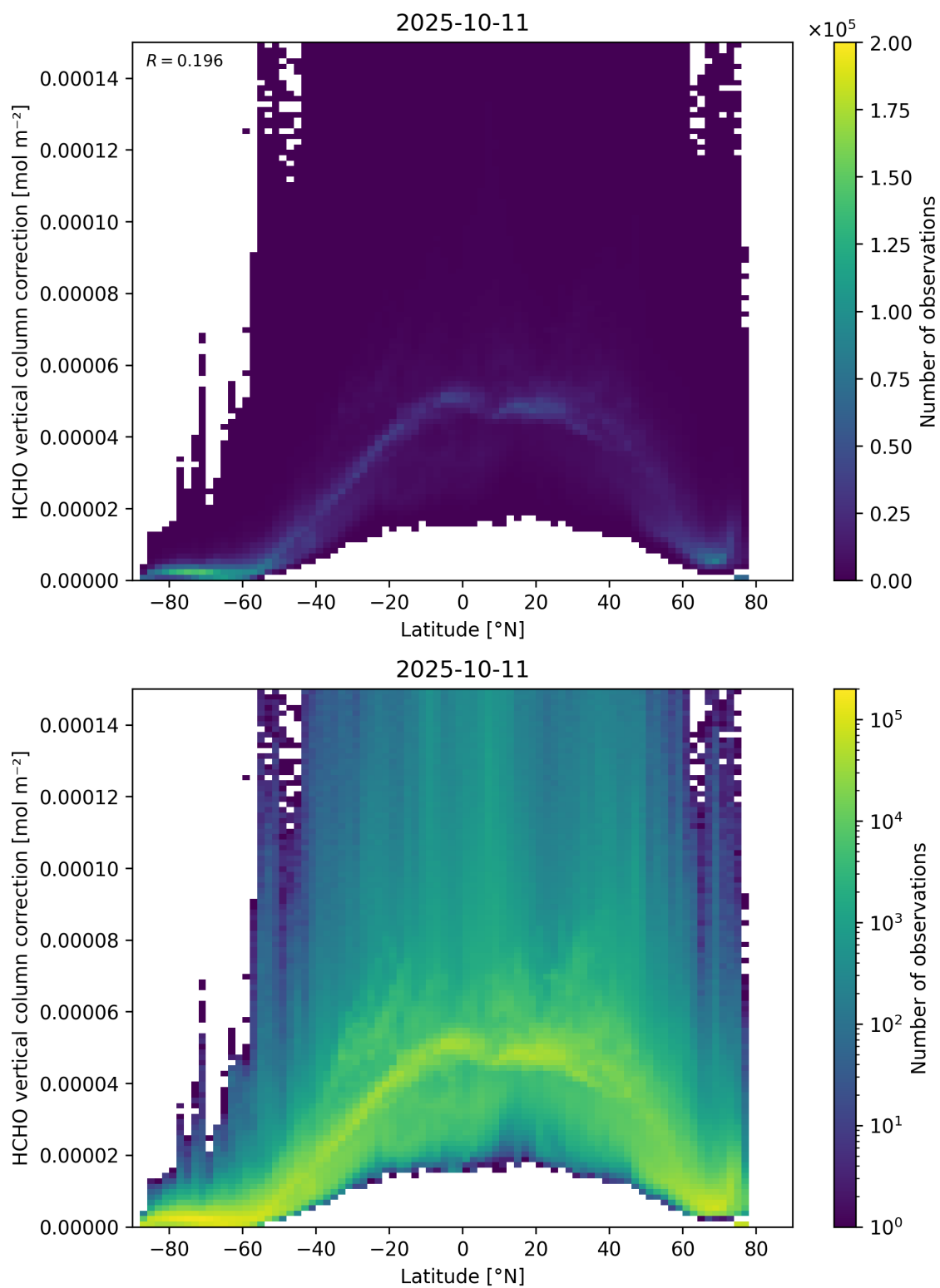
Figure 164: Scatter density plot of “Latitude” against “HCHO vertical column correction” for 2025-10-11 to 2025-10-12.
