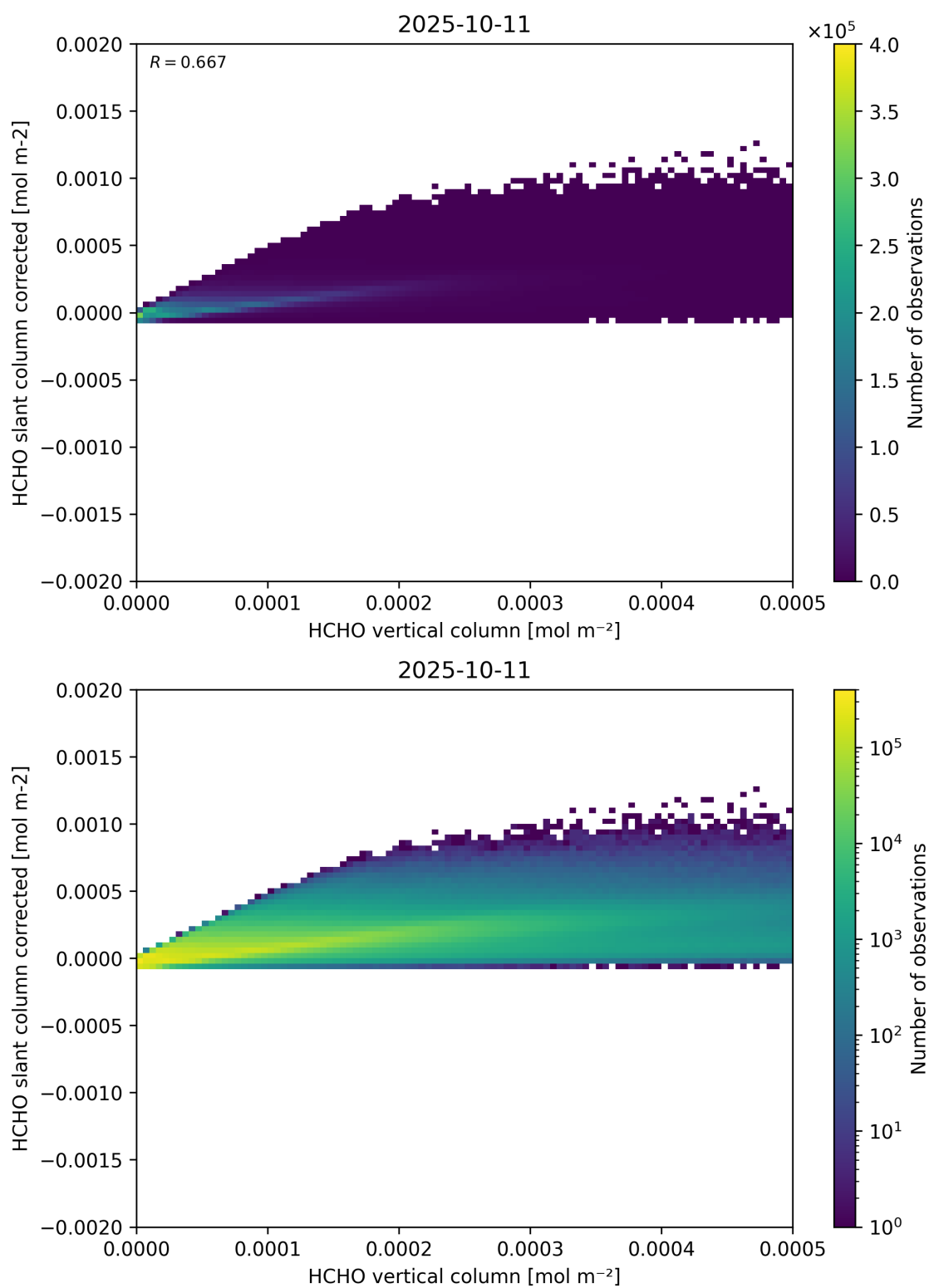
Figure 127: Scatter density plot of “HCHO vertical column” against “HCHO slant column corrected” for 2025-10-11 to 2025-10-12.
