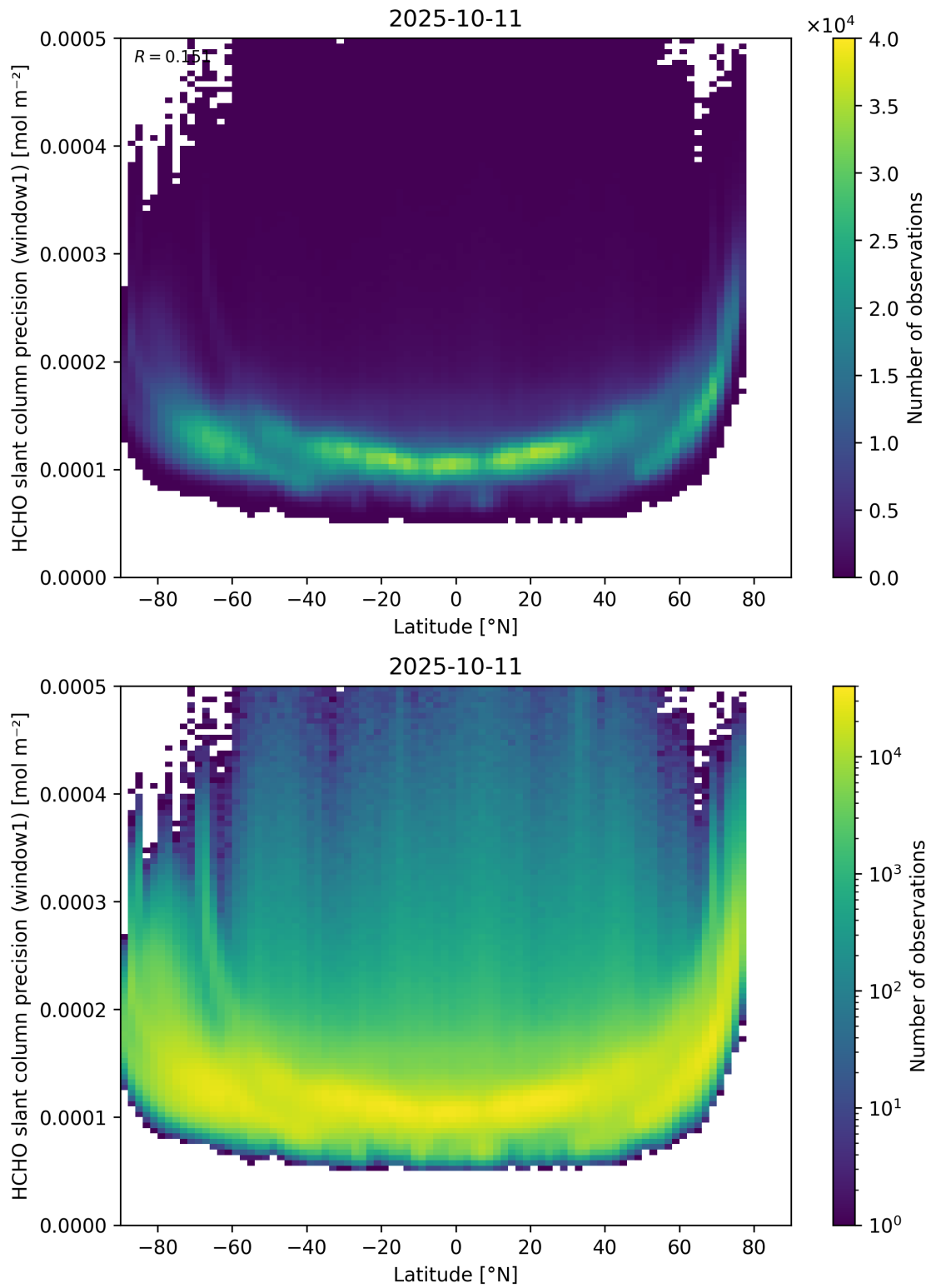
Figure 160: Scatter density plot of “Latitude” against “HCHO slant column precision (window1)” for 2025-10-11 to 2025-10-12.
