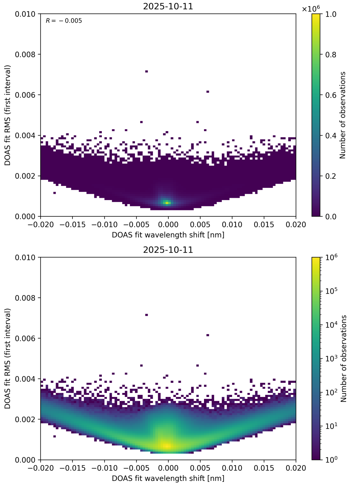
Figure 64: Scatter density plot of “DOAS fit wavelength shift” against “DOAS fit RMS (first interval)” for 2025-10-11 to 2025-10-12.
