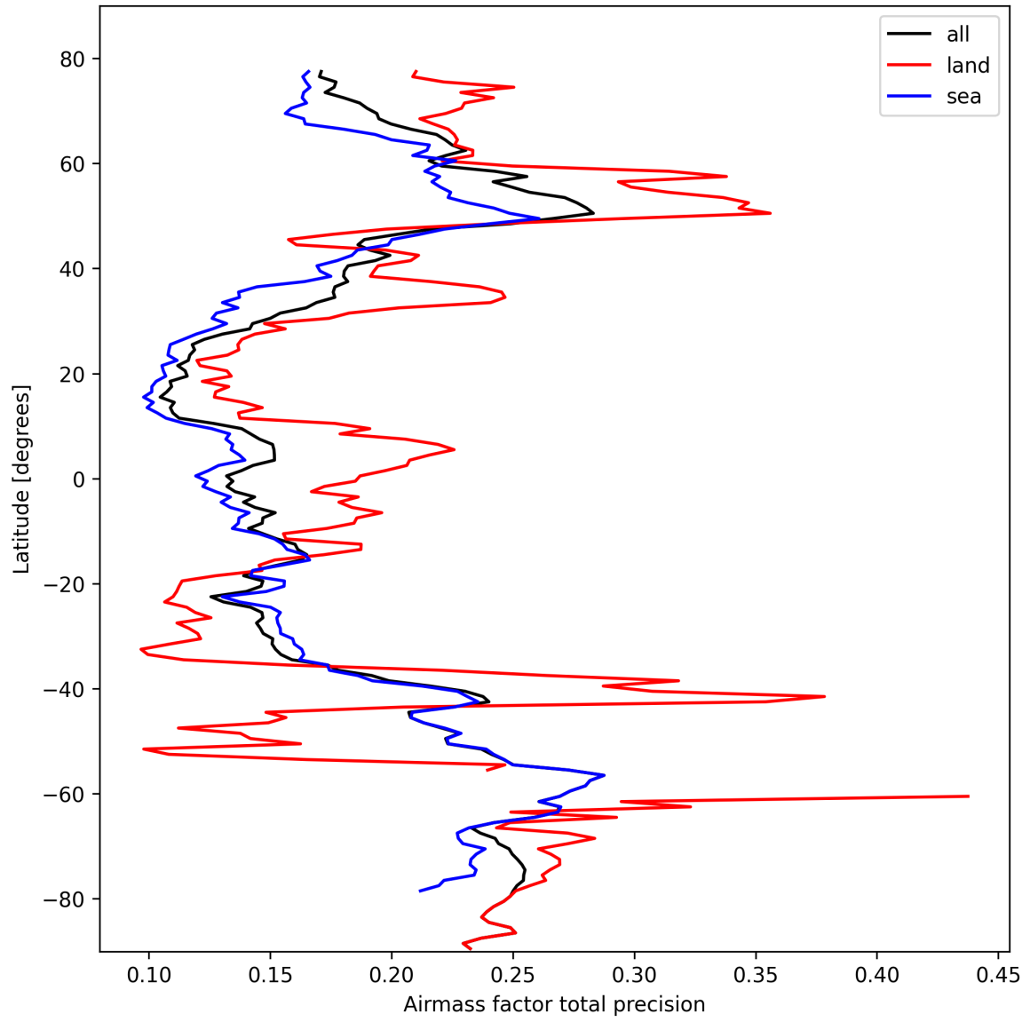
Figure 27: Zonal average of “Airmass factor total precision” for 2025-10-11 to 2025-10-12.
