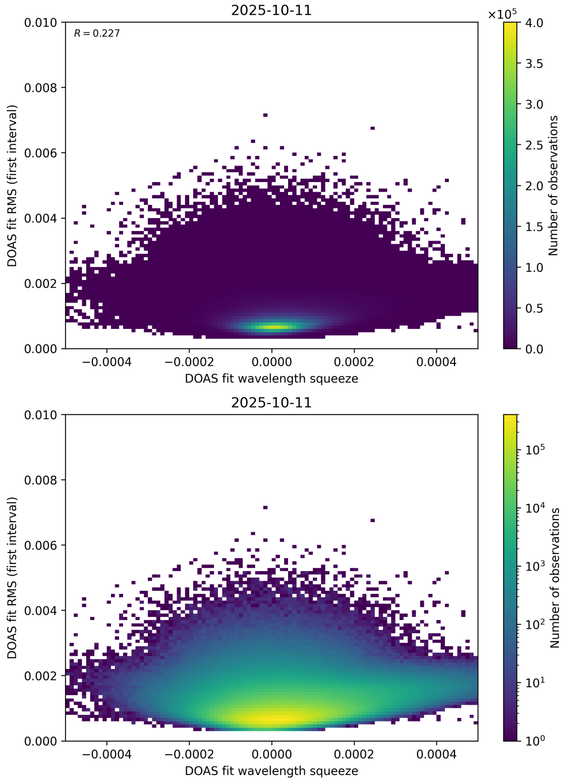
Figure 68: Scatter density plot of “DOAS fit wavelength squeeze” against “DOAS fit RMS (first interval)” for 2025-10-11 to 2025-10-12.
