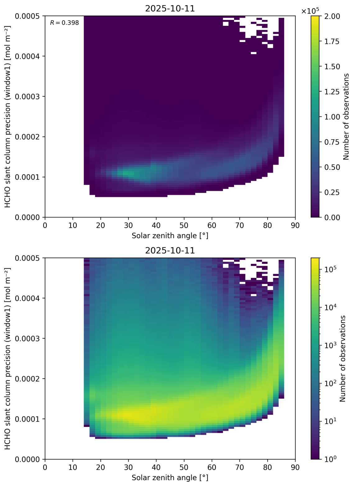
Figure 174: Scatter density plot of “Solar zenith angle” against “HCHO slant column precision (window1)” for 2025-10-11 to 2025-10-12.
