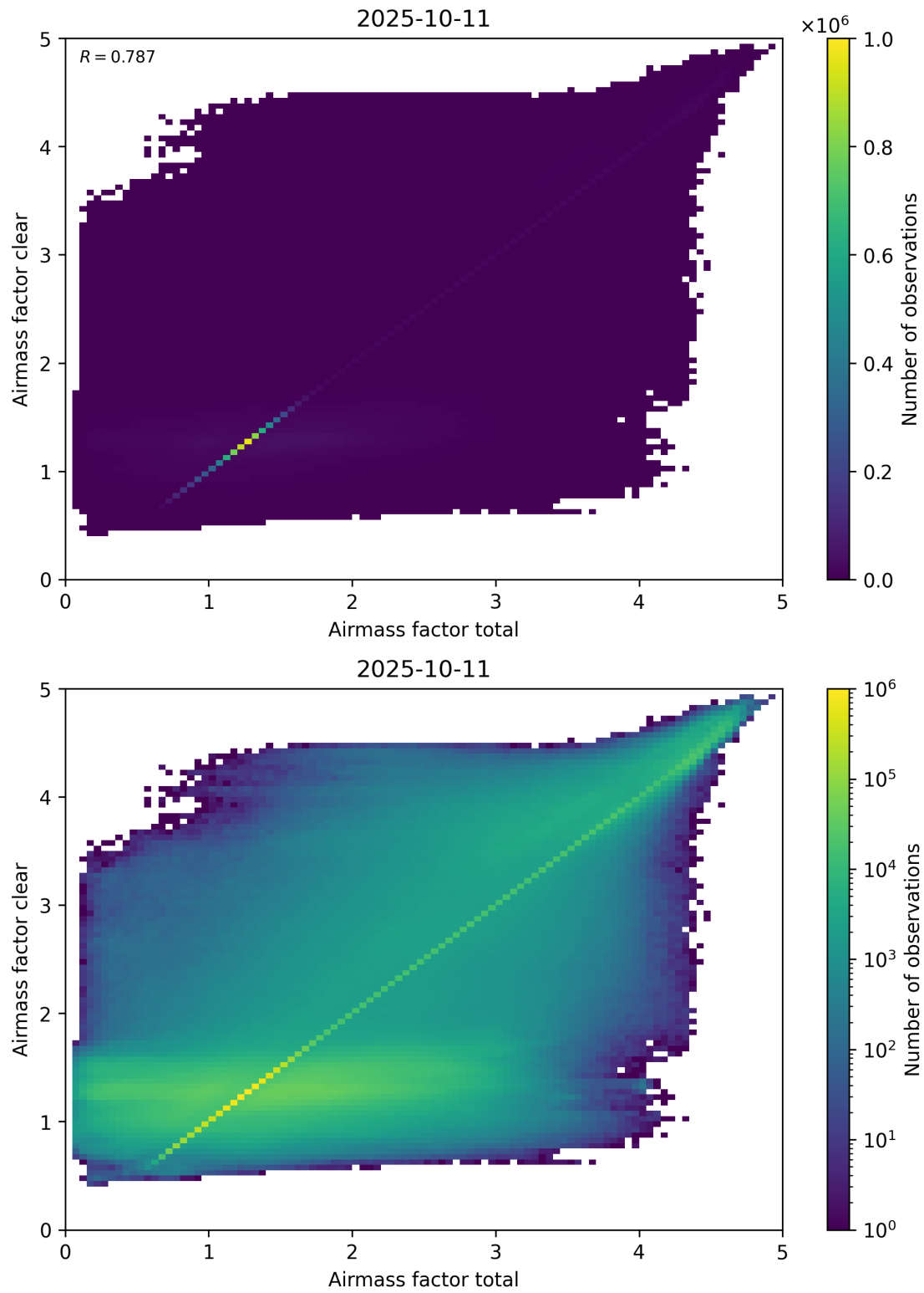
Figure 100: Scatter density plot of “Airmass factor total” against “Airmass factor clear” for 2025-10-11 to 2025-10-12.
