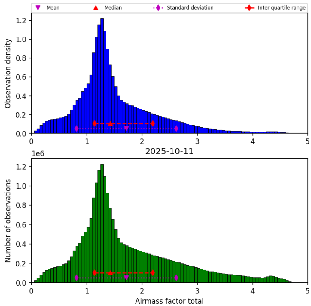
Figure 40: Histogram of “Airmass factor total” for 2025-10-11 to 2025-10-12
