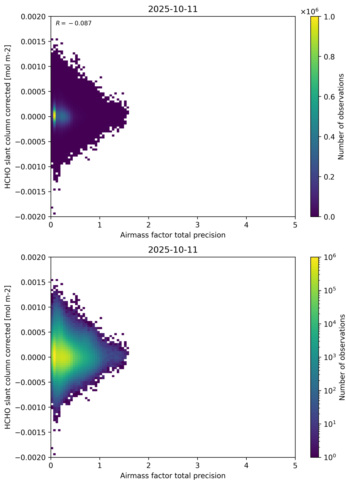
Figure 109: Scatter density plot of “Airmass factor total precision” against “HCHO slant column corrected” for 2025-10-11 to 2025-10-12.
