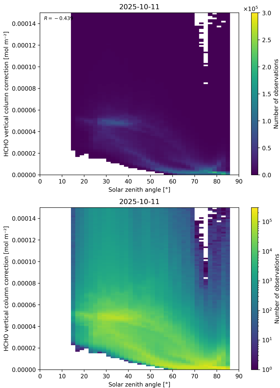
Figure 178: Scatter density plot of “Solar zenith angle” against “HCHO vertical column correction” for 2025-10-11 to 2025-10-12.
