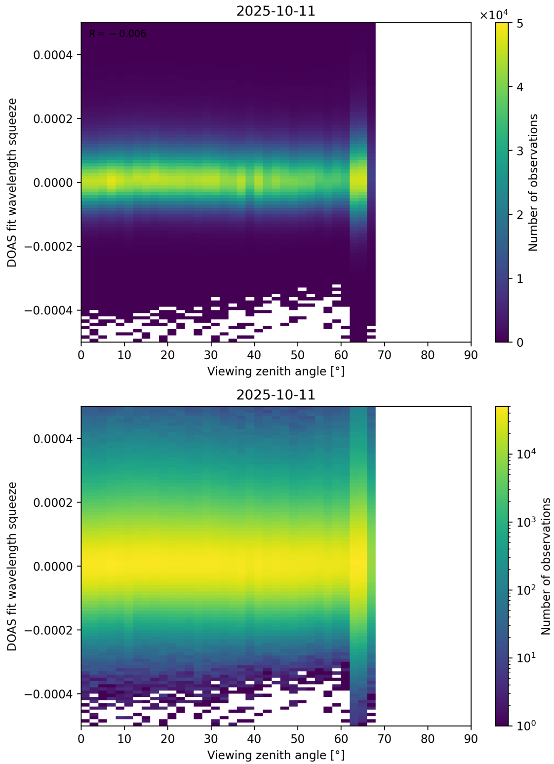
Figure 184: Scatter density plot of “Viewing zenith angle” against “DOAS fit wavelength squeeze” for 2025-10-11 to 2025-10-12.
