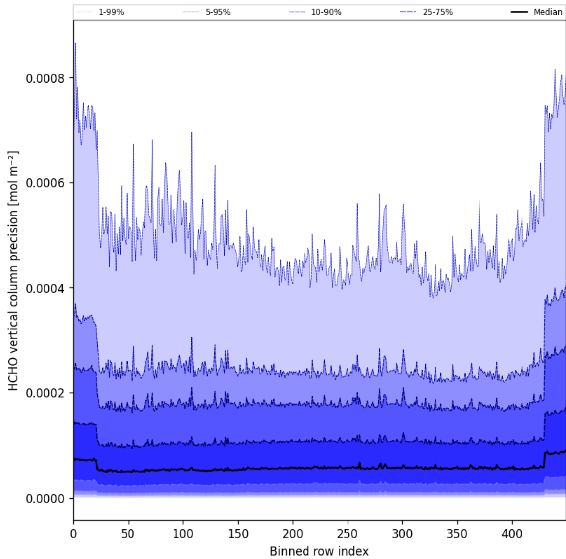
Figure 50: Along track statistics of “HCHO vertical column precision” for 2025-10-11 to 2025-10-12
