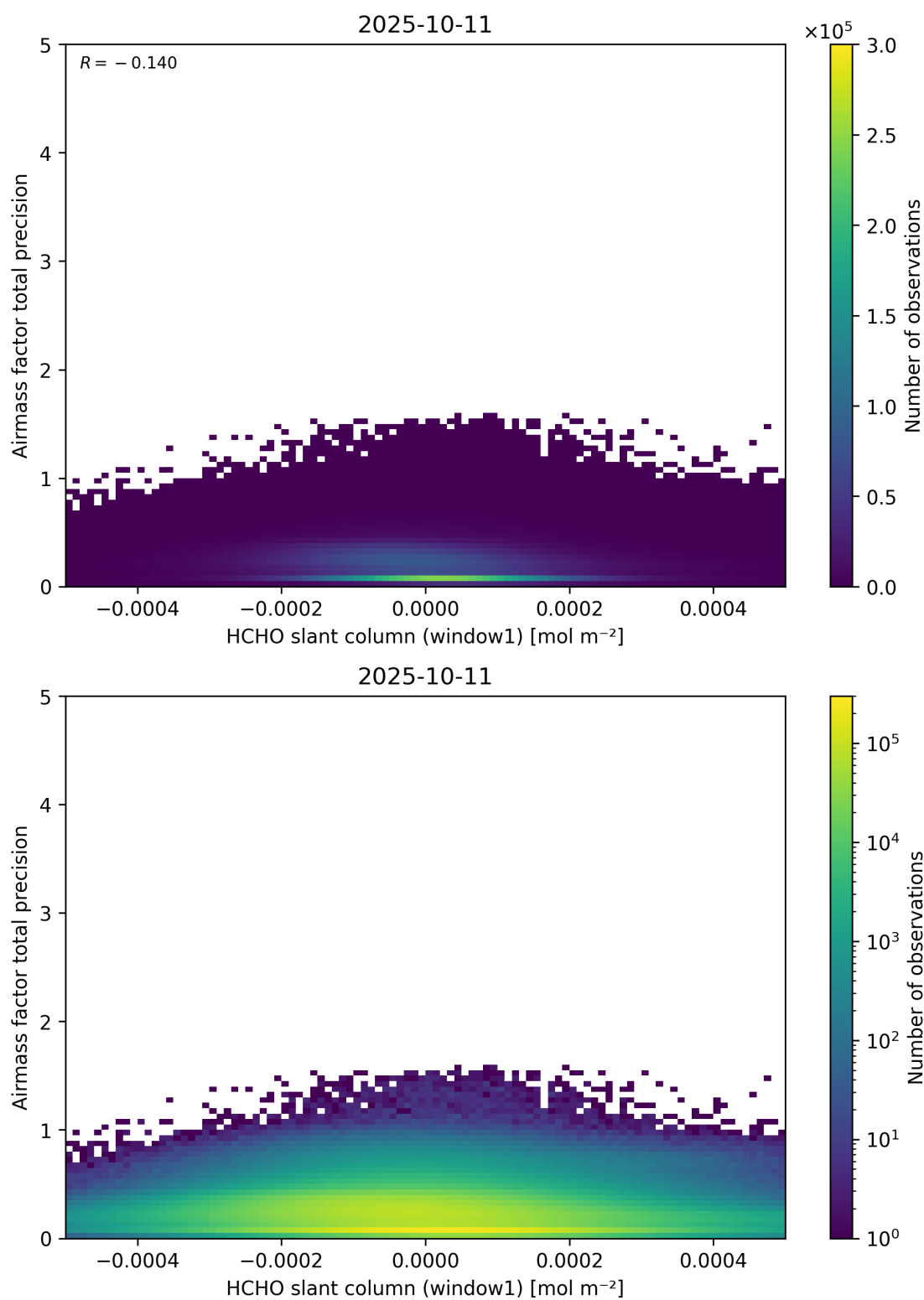
Figure 86: Scatter density plot of “HCHO slant column (window1)” against “Airmass factor total precision” for 2025-10-11 to 2025-10-12.
