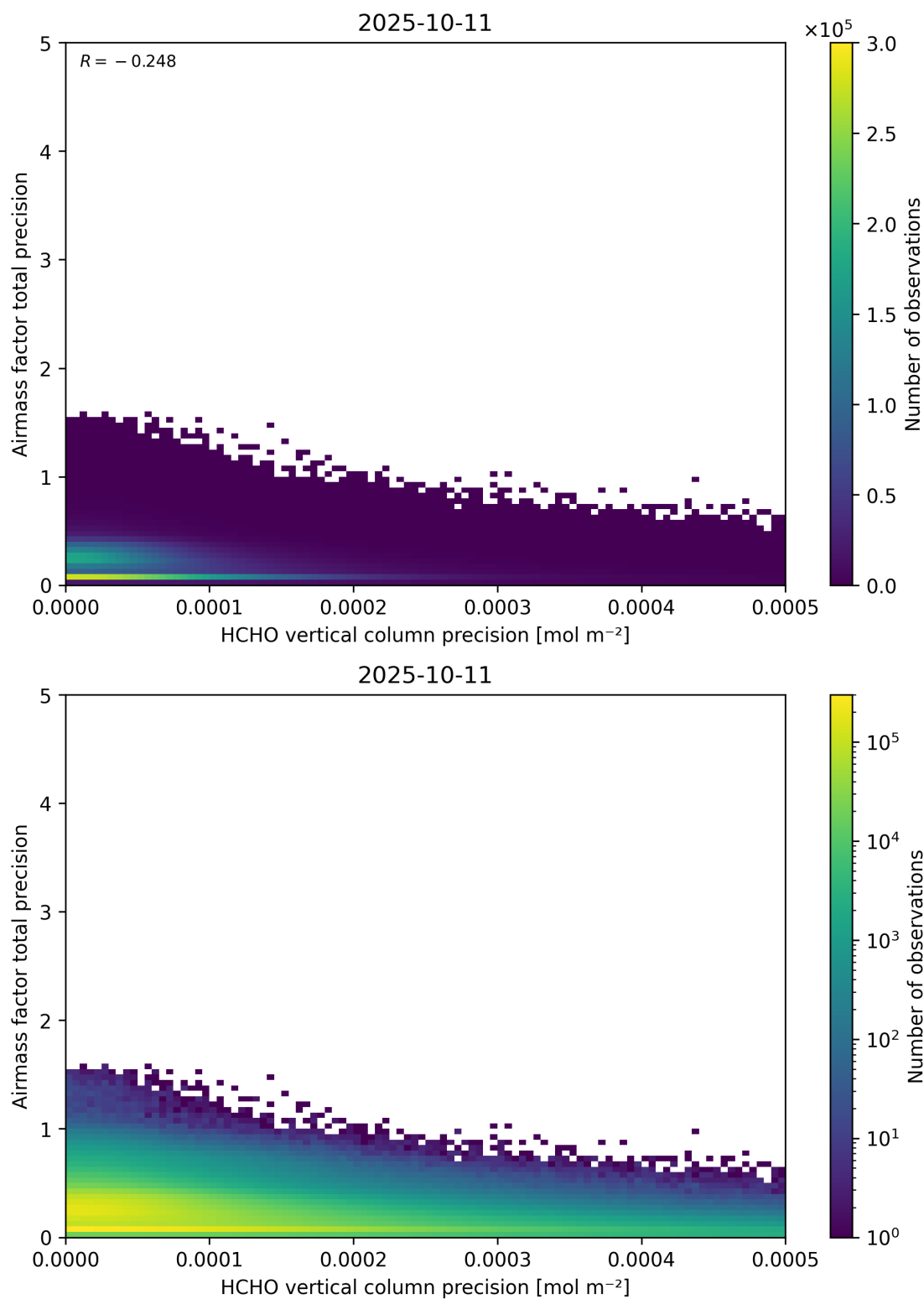
Figure 145: Scatter density plot of “HCHO vertical column precision” against “Airmass factor total precision” for 2025-10-11 to 2025-10-12.
