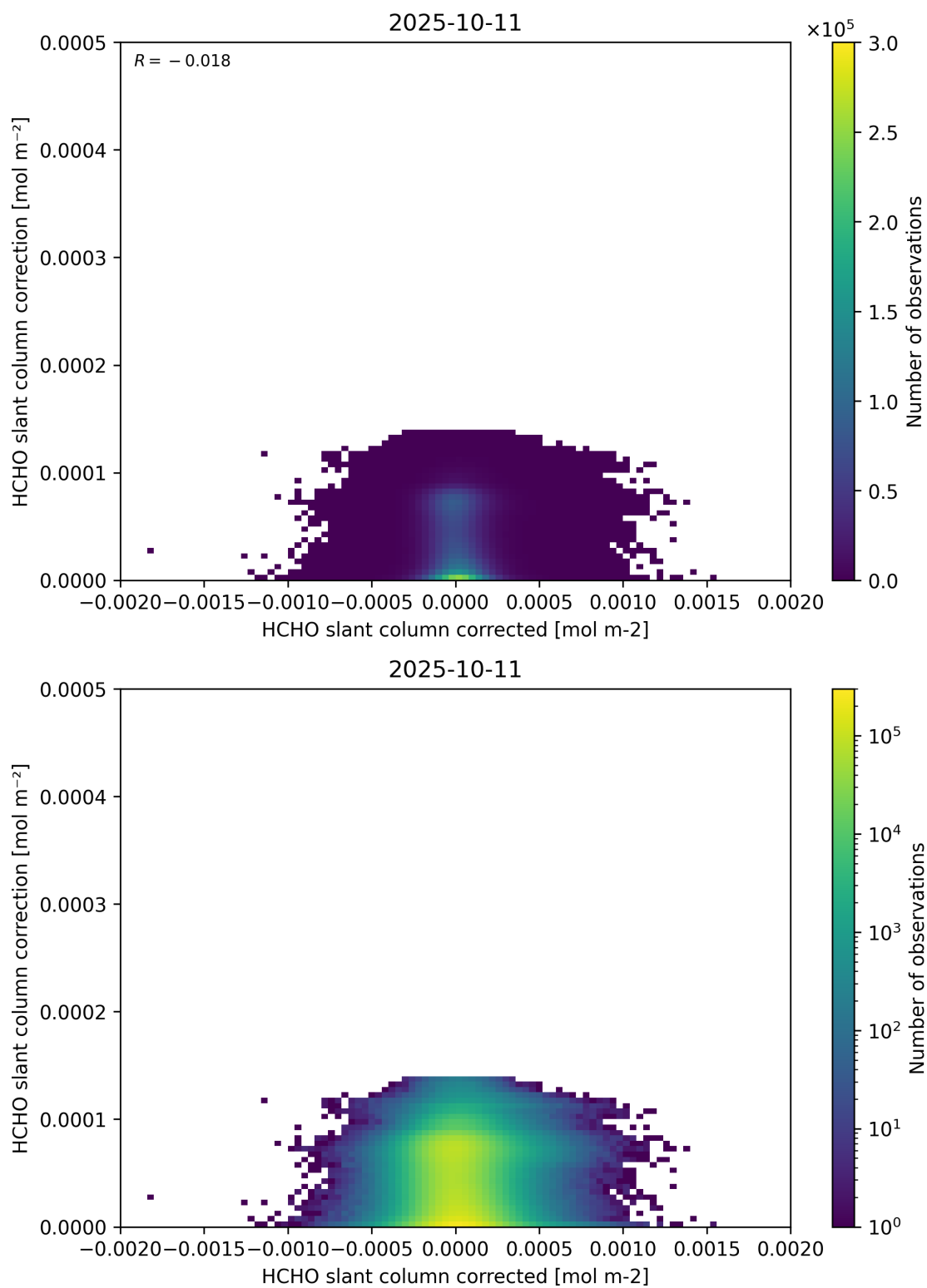
Figure 77: Scatter density plot of “HCHO slant column corrected” against “HCHO slant column correction” for 2025-10-11 to 2025-10-12.
