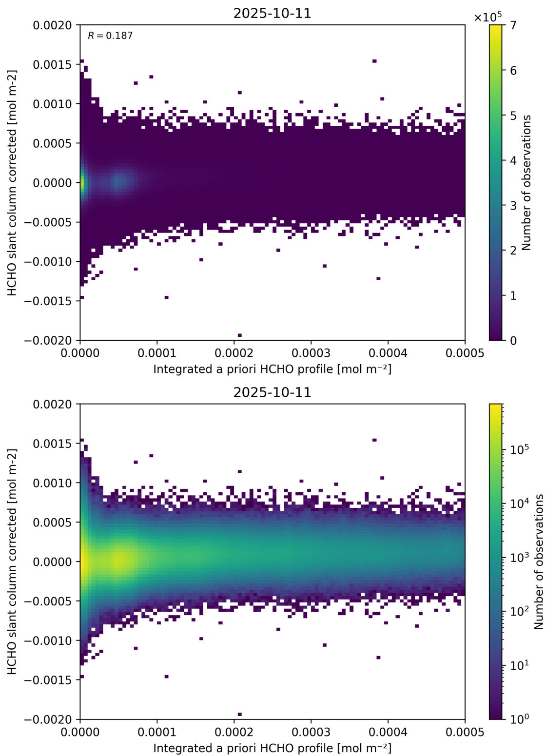
Figure 151: Scatter density plot of “Integrated a priori HCHO profile” against “HCHO slant column corrected” for 2025-10-11 to 2025-10-12.
