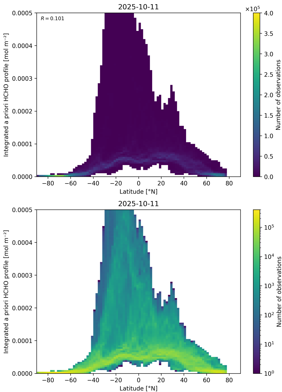
Figure 166: Scatter density plot of “Latitude” against “Integrated a priori HCHO profile” for 2025-10-11 to 2025-10-12.
