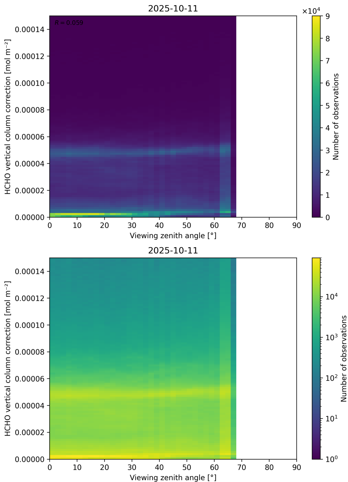
Figure 193: Scatter density plot of “Viewing zenith angle” against “HCHO vertical column correction” for 2025-10-11 to 2025-10-12.
