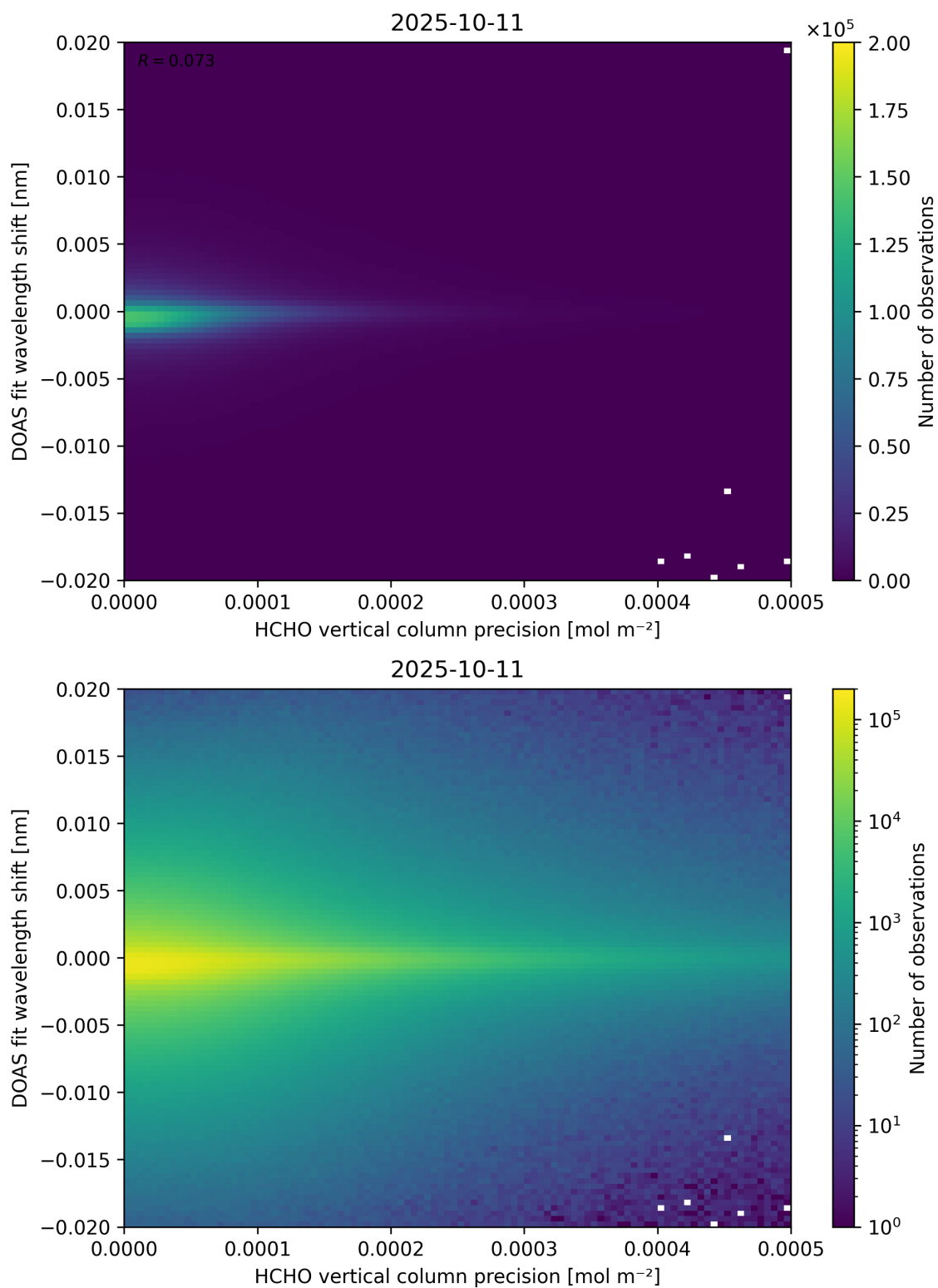
Figure 137: Scatter density plot of “HCHO vertical column precision” against “DOAS fit wavelength shift” for 2025-10-11 to 2025-10-12.
