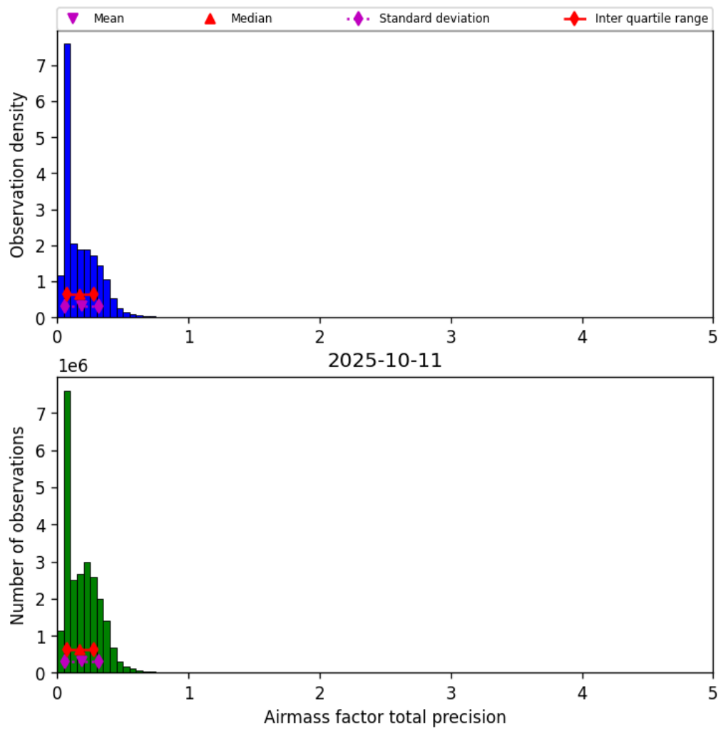
Figure 41: Histogram of “Airmass factor total precision” for 2025-10-11 to 2025-10-12
