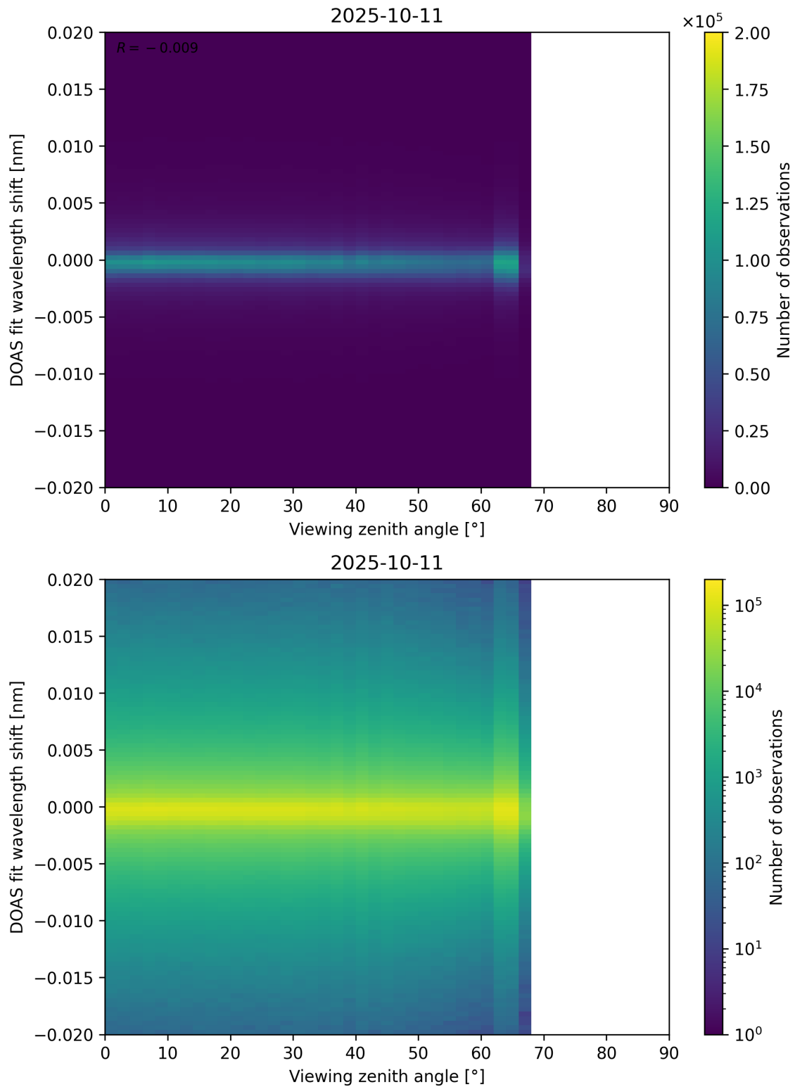
Figure 183: Scatter density plot of “Viewing zenith angle” against “DOAS fit wavelength shift” for 2025-10-11 to 2025-10-12.
