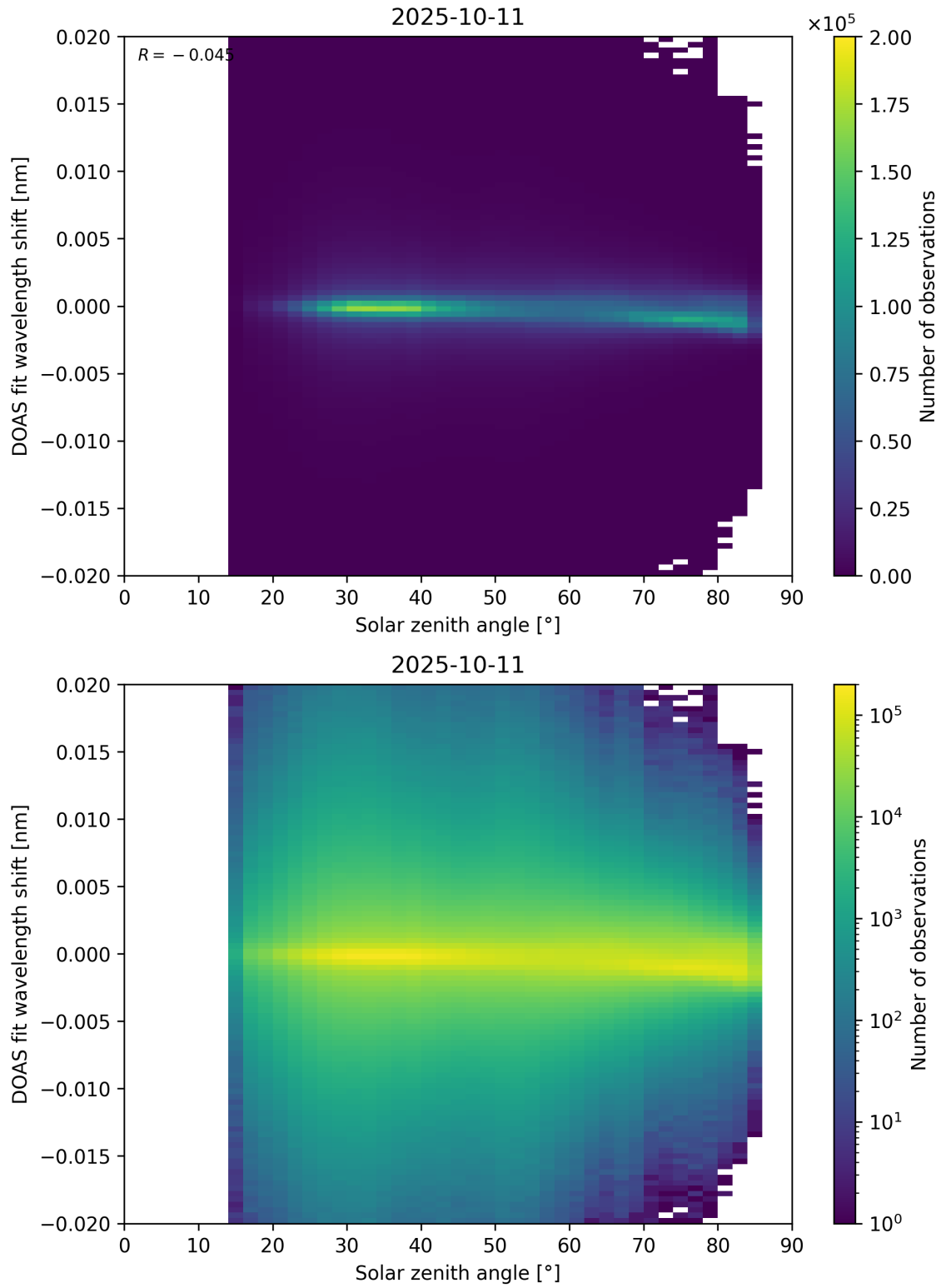
Figure 168: Scatter density plot of “Solar zenith angle” against “DOAS fit wavelength shift” for 2025-10-11 to 2025-10-12.
