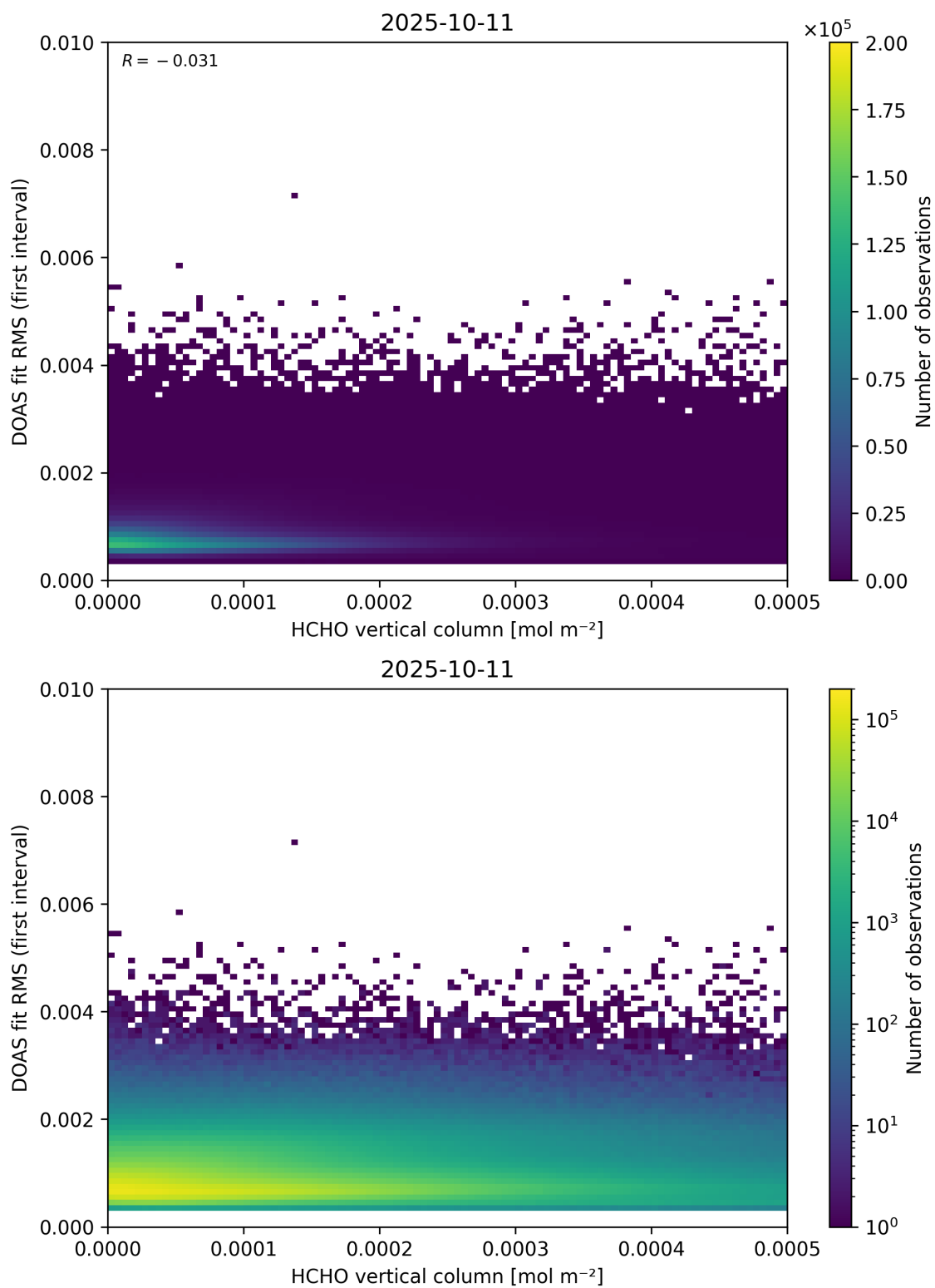
Figure 123: Scatter density plot of “HCHO vertical column” against “DOAS fit RMS (first interval)” for 2025-10-11 to 2025-10-12.
