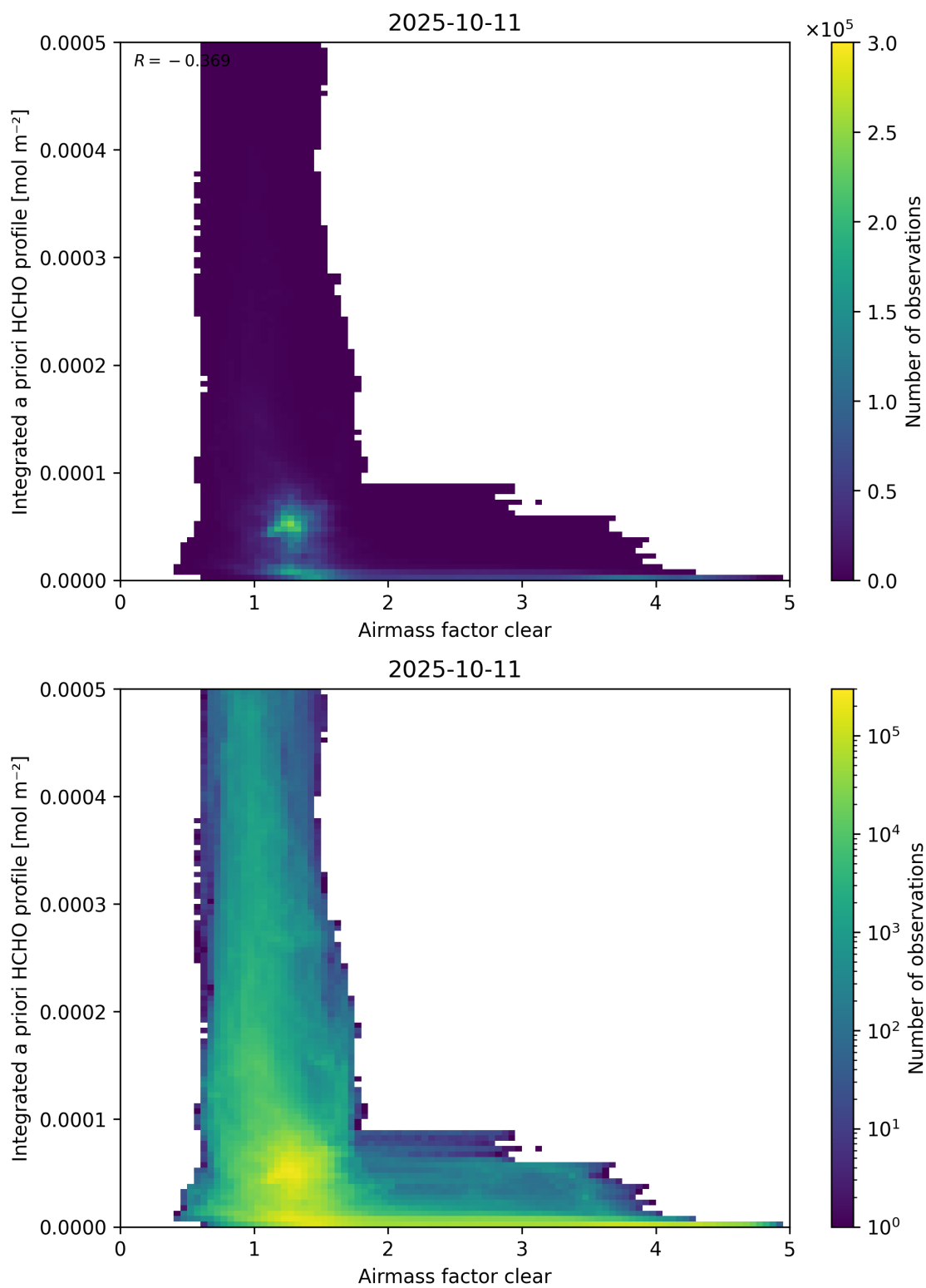
Figure 76: Scatter density plot of “Airmass factor clear” against “Integrated a priori HCHO profile” for 2025-10-11 to 2025-10-12.
