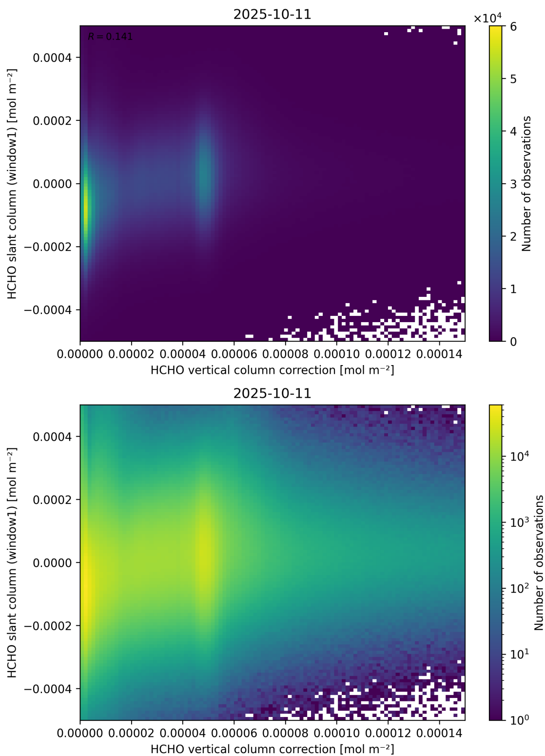
Figure 118: Scatter density plot of “HCHO vertical column correction” against “HCHO slant column (window1)” for 2025-10-11 to 2025-10-12.
