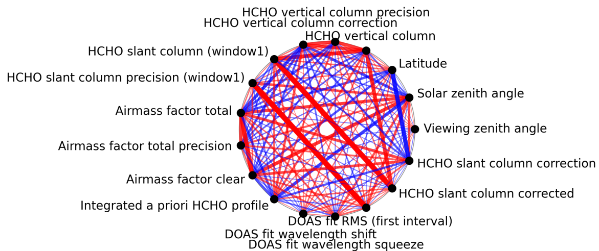
Figure 1: Map of correlation graph for 2025-10-11 to 2025-10-12.
