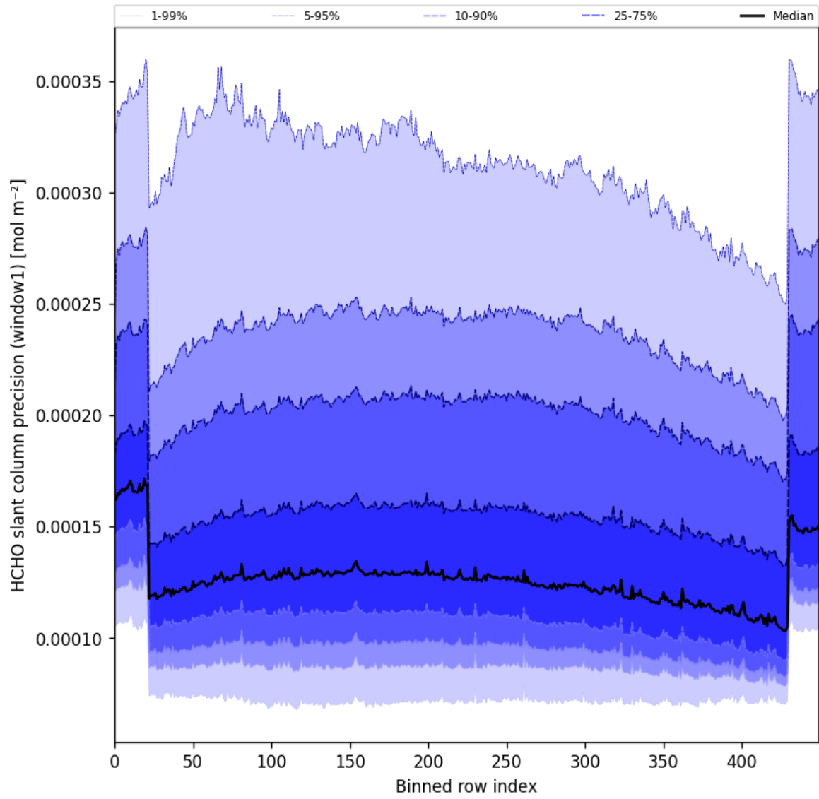
Figure 53: Along track statistics of “HCHO slant column precision (window1)” for 2025-10-11 to 2025-10-12
