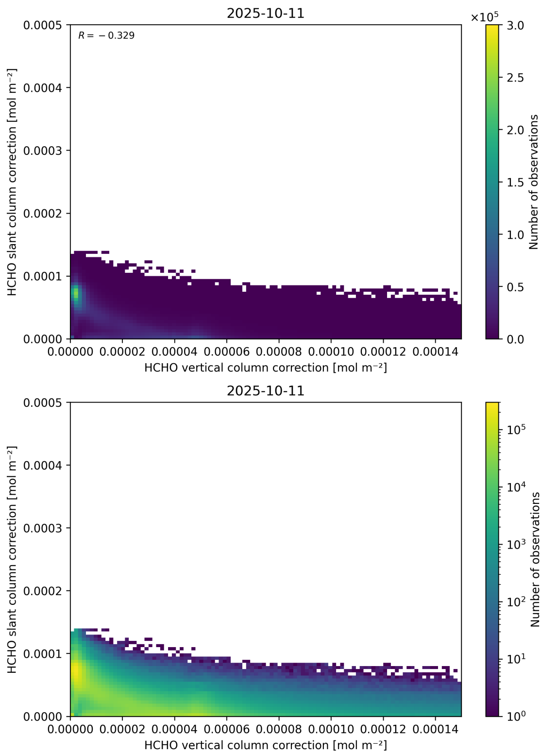
Figure 117: Scatter density plot of “HCHO vertical column correction” against “HCHO slant column correction” for 2025-10-11 to 2025-10-12.
