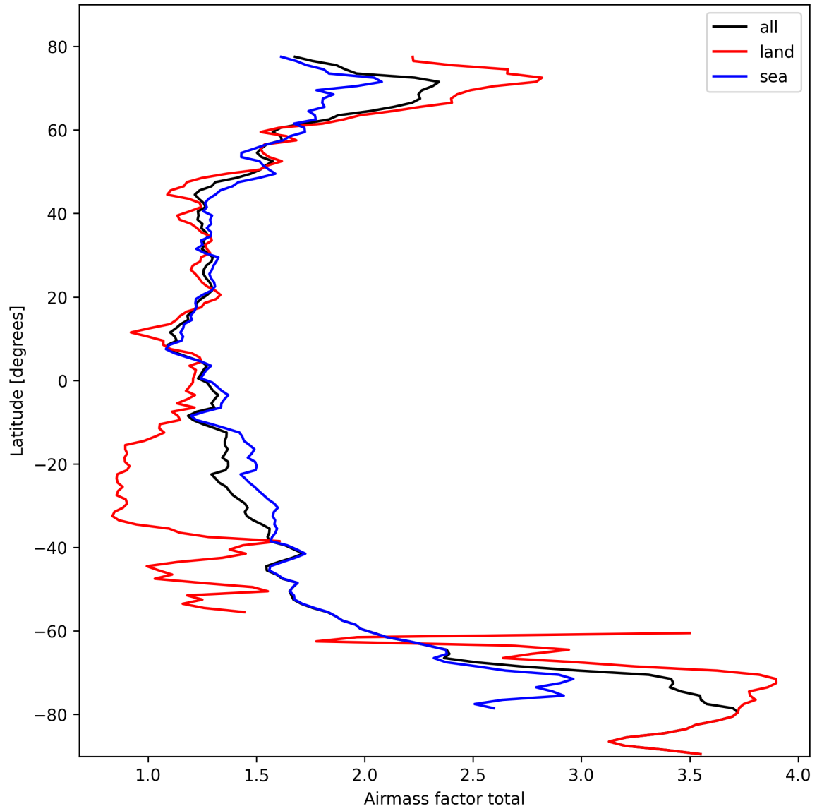
Figure 26: Zonal average of “Airmass factor total” for 2025-10-11 to 2025-10-12.
