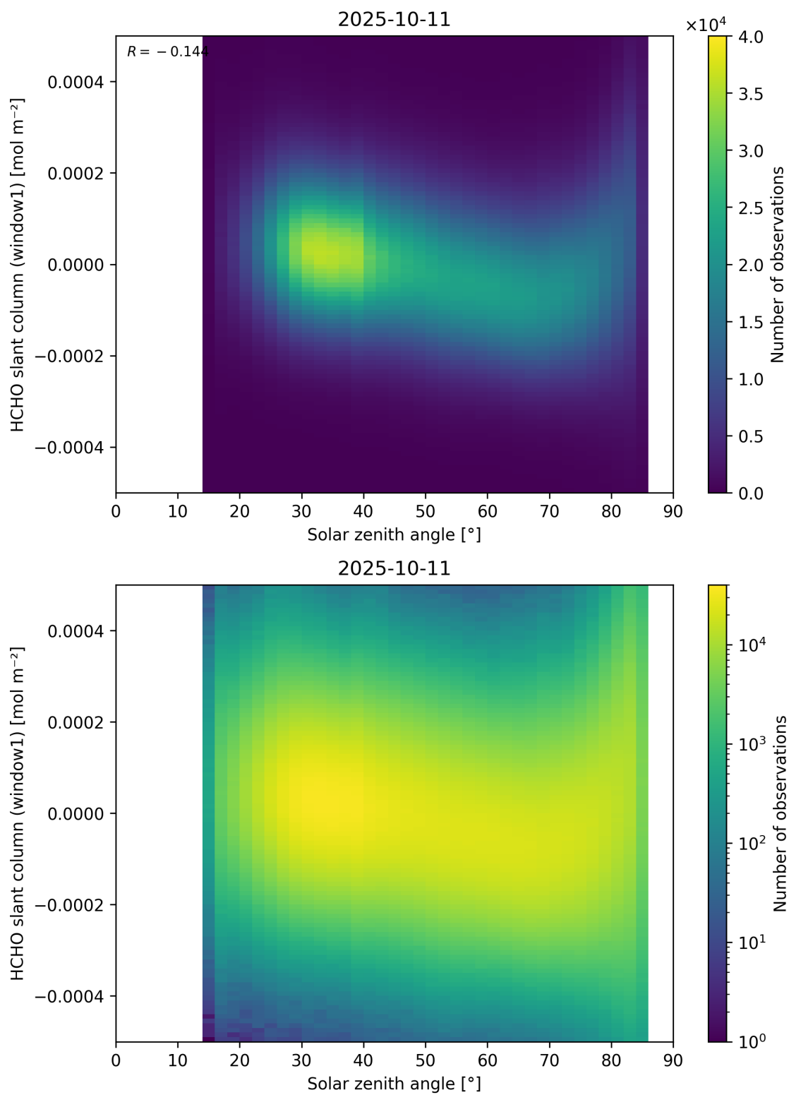
Figure 173: Scatter density plot of “Solar zenith angle” against “HCHO slant column (window1)” for 2025-10-11 to 2025-10-12.
