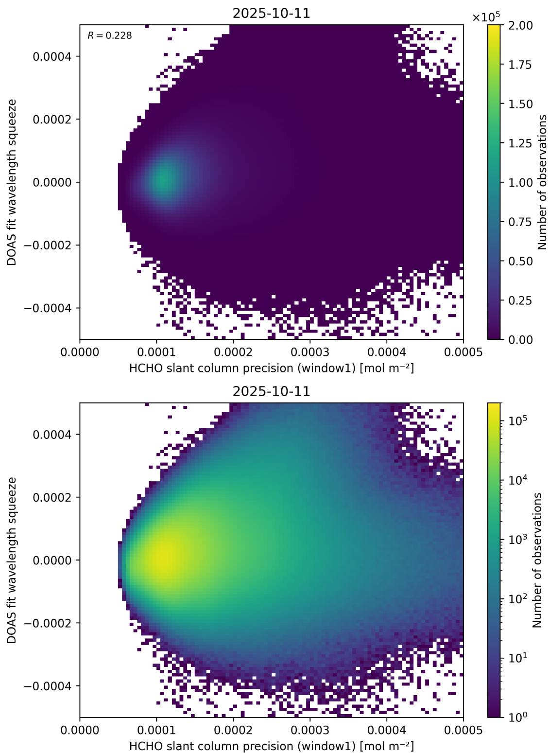
Figure 90: Scatter density plot of “HCHO slant column precision (window1)” against “DOAS fit wavelength squeeze” for 2025-10-11 to 2025-10-12.
