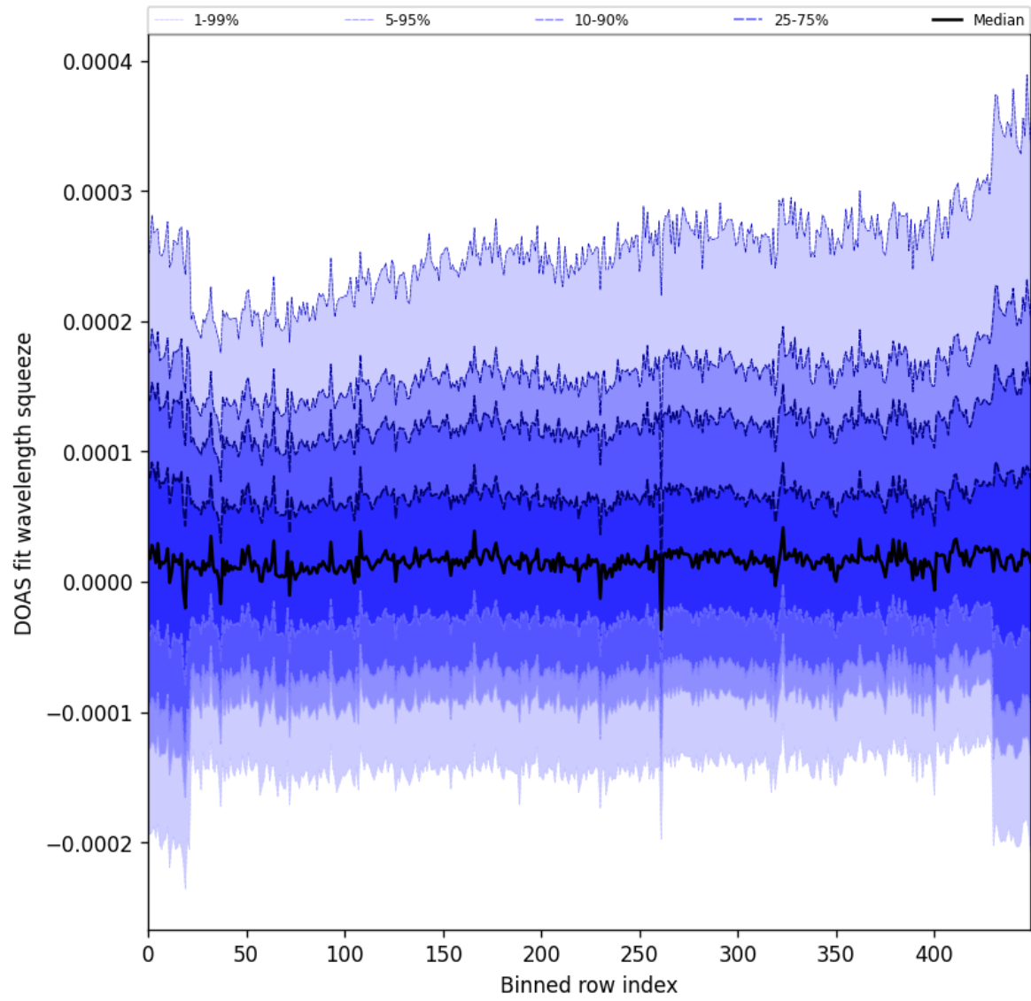
Figure 59: Along track statistics of “DOAS fit wavelength squeeze” for 2025-10-11 to 2025-10-12
