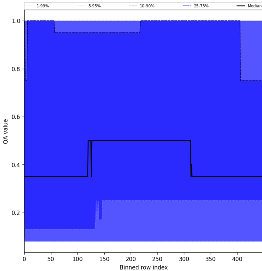
Figure 48: Along track statistics of “QA value” for 2025-10-11 to 2025-10-12
