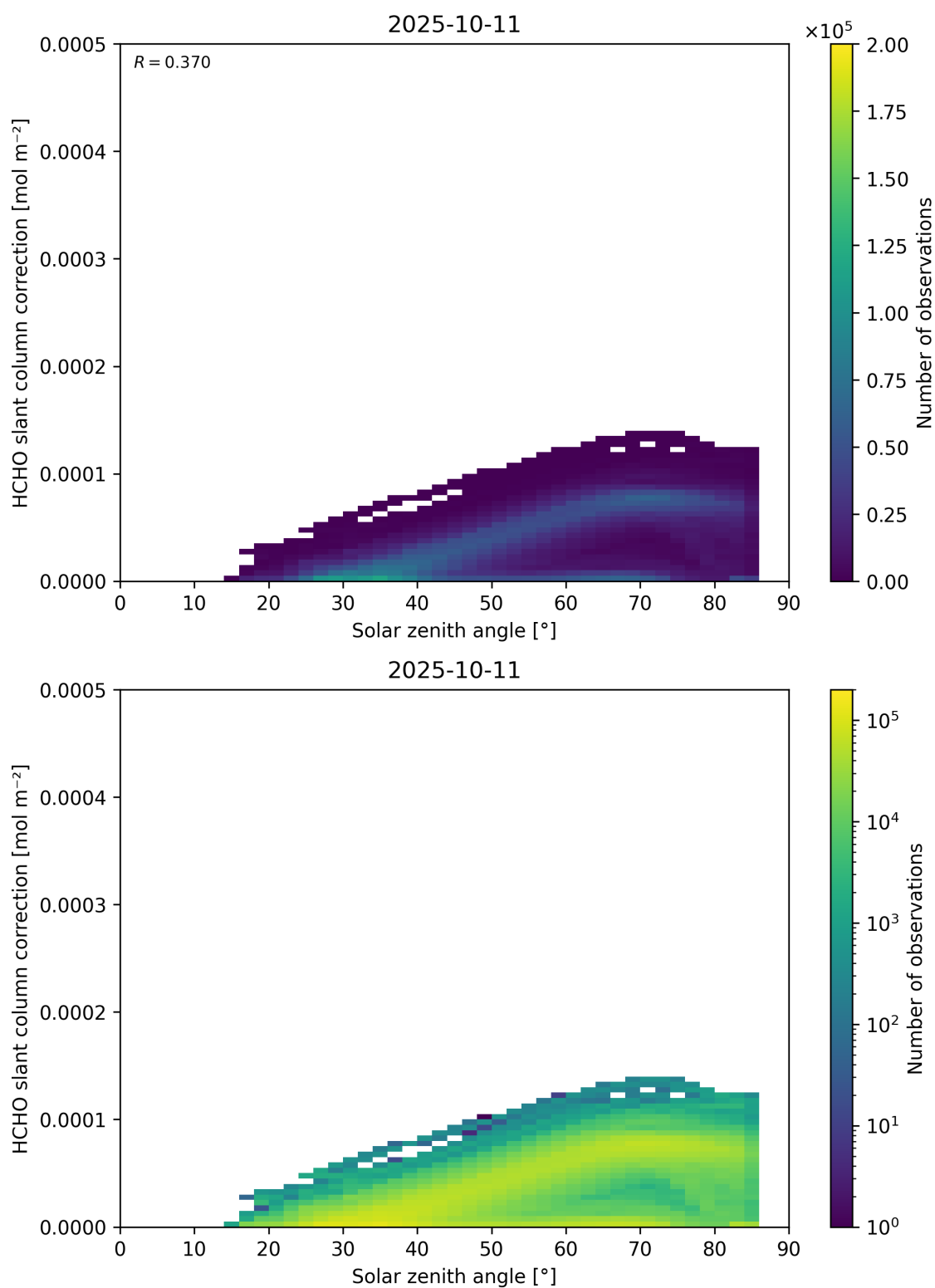
Figure 172: Scatter density plot of “Solar zenith angle” against “HCHO slant column correction” for 2025-10-11 to 2025-10-12.
