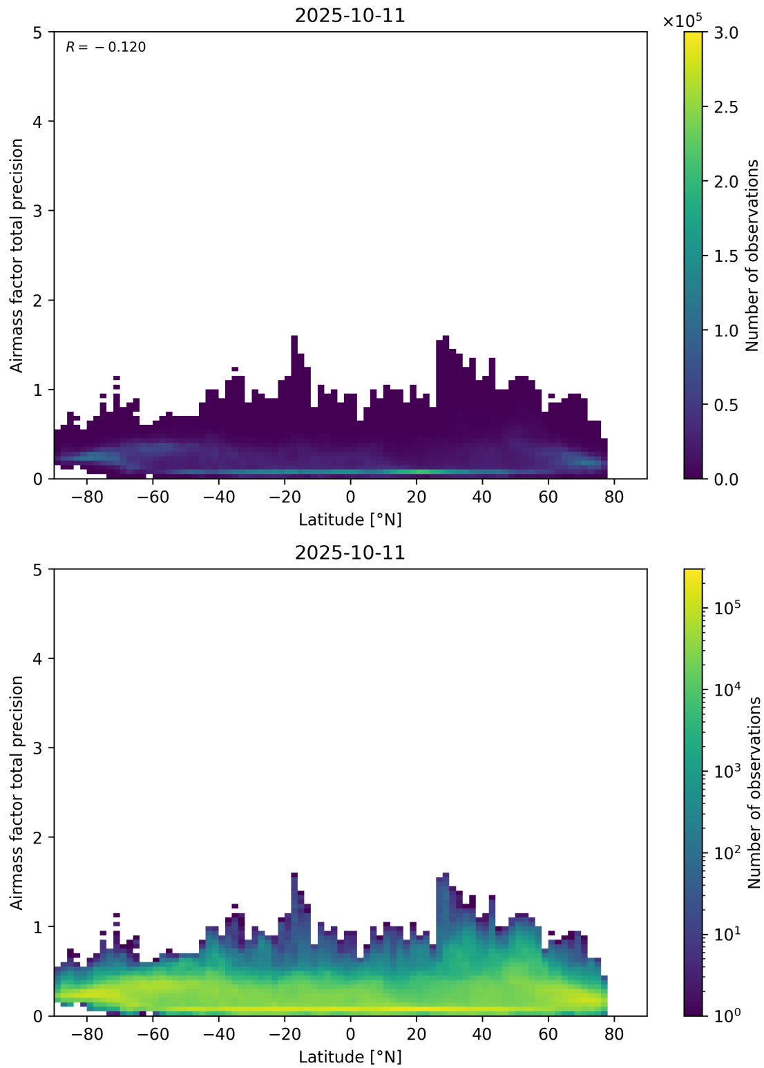
Figure 162: Scatter density plot of “Latitude” against “Airmass factor total precision” for 2025-10-11 to 2025-10-12.
