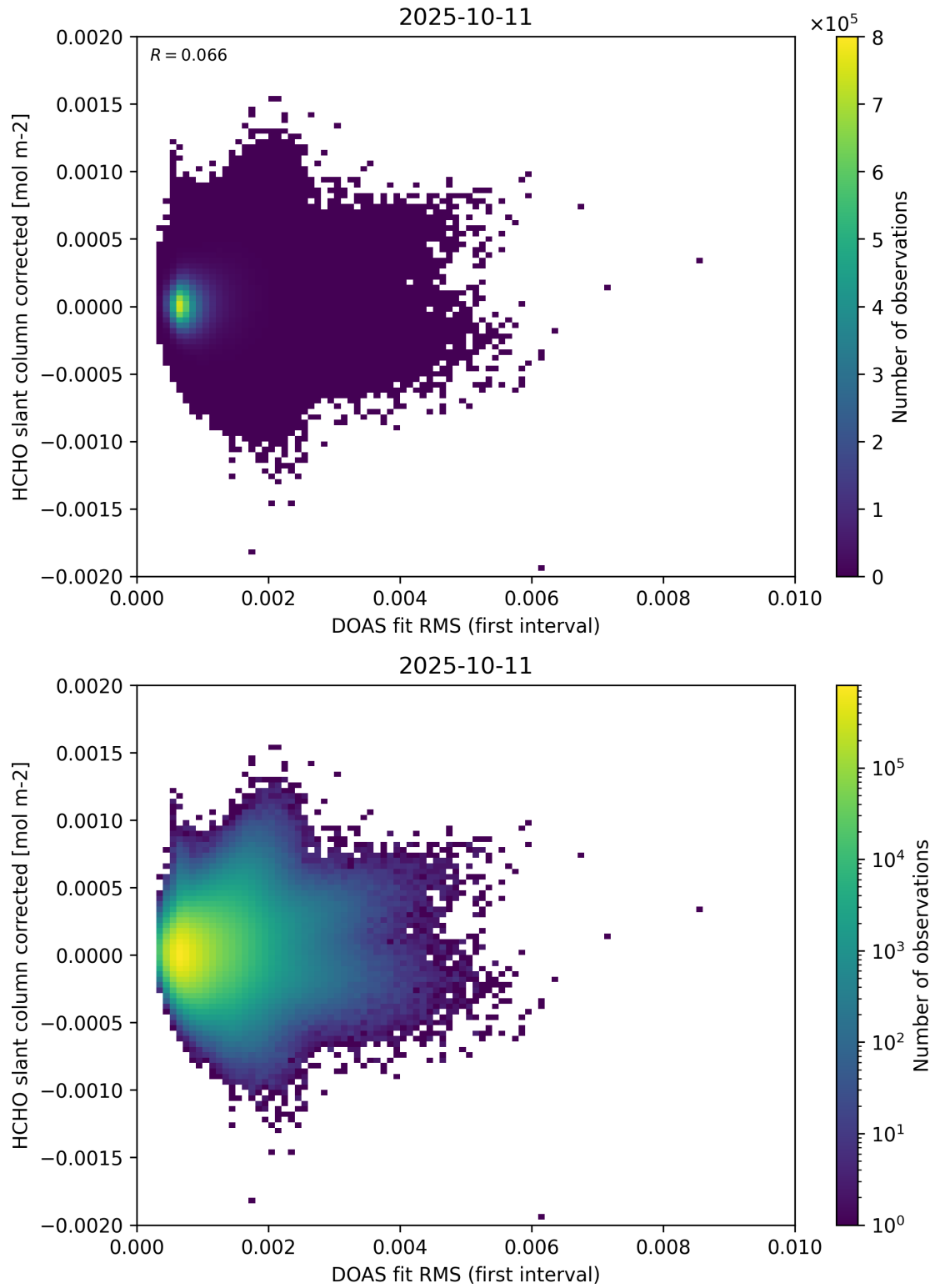
Figure 62: Scatter density plot of “DOAS fit RMS (first interval)” against “HCHO slant column corrected” for 2025-10-11 to 2025-10-12.
