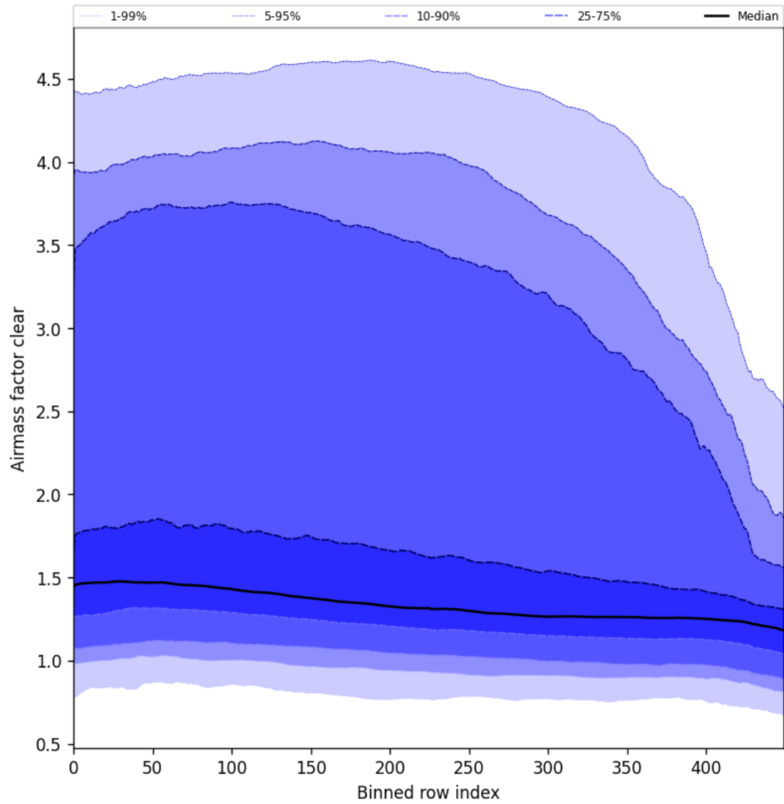
Figure 56: Along track statistics of “Airmass factor clear” for 2025-10-11 to 2025-10-12
