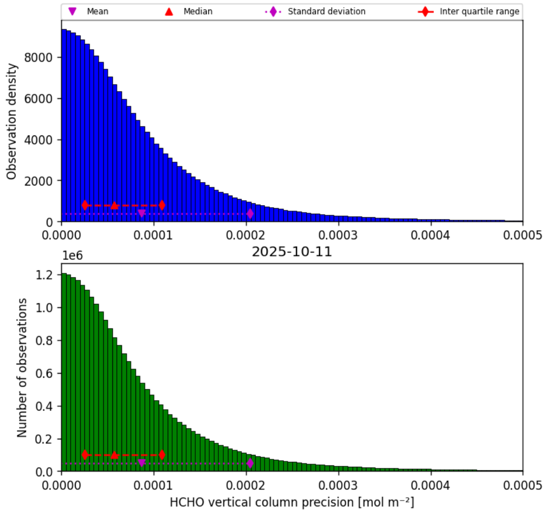
Figure 36: Histogram of “HCHO vertical column precision” for 2025-10-11 to 2025-10-12
