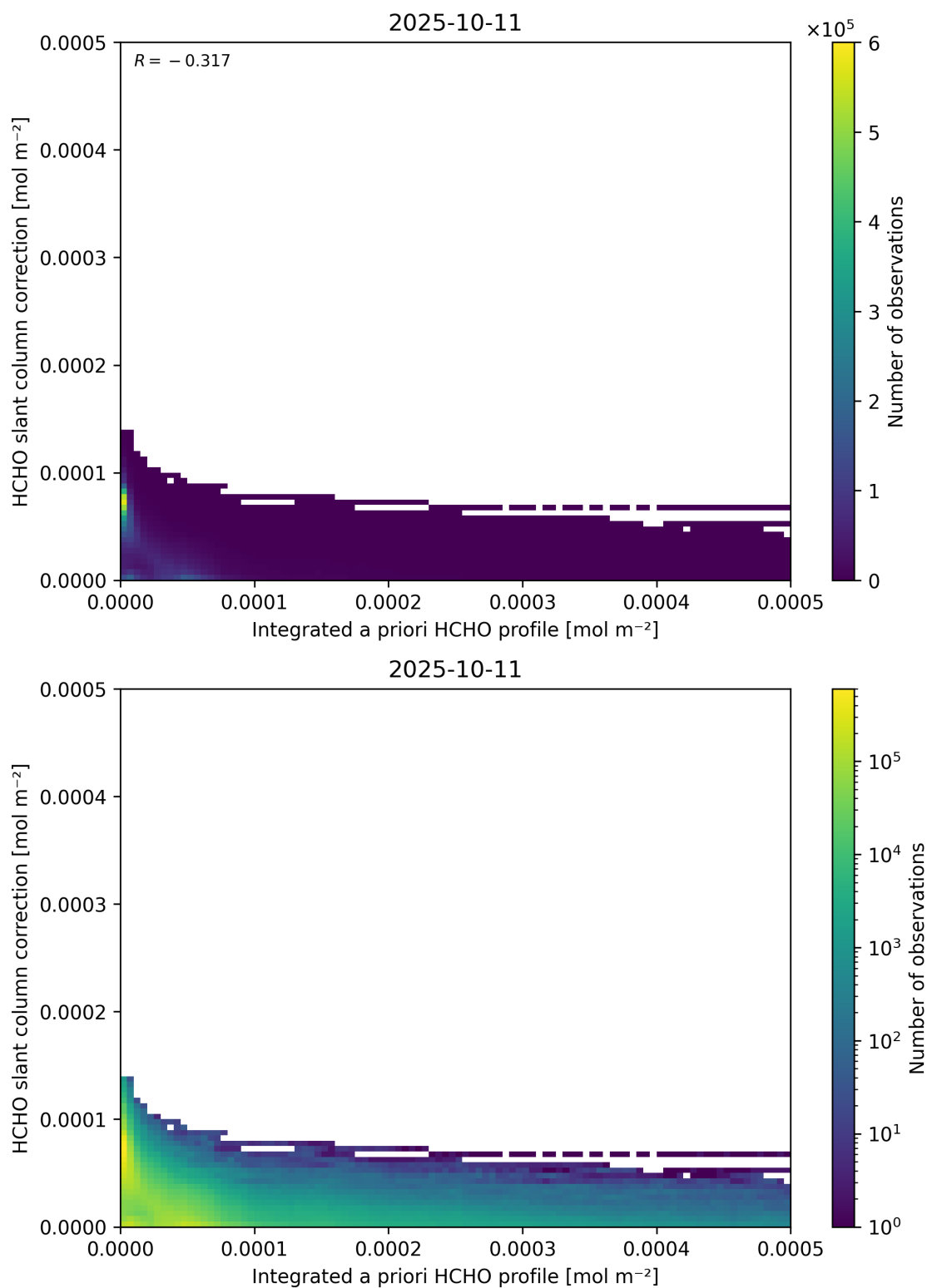
Figure 152: Scatter density plot of “Integrated a priori HCHO profile” against “HCHO slant column correction” for 2025-10-11 to 2025-10-12.
