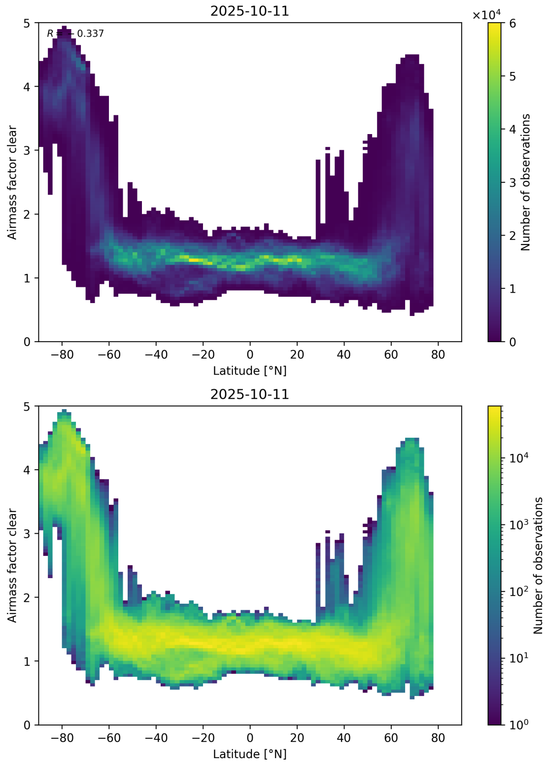
Figure 156: Scatter density plot of “Latitude” against “Airmass factor clear” for 2025-10-11 to 2025-10-12.
