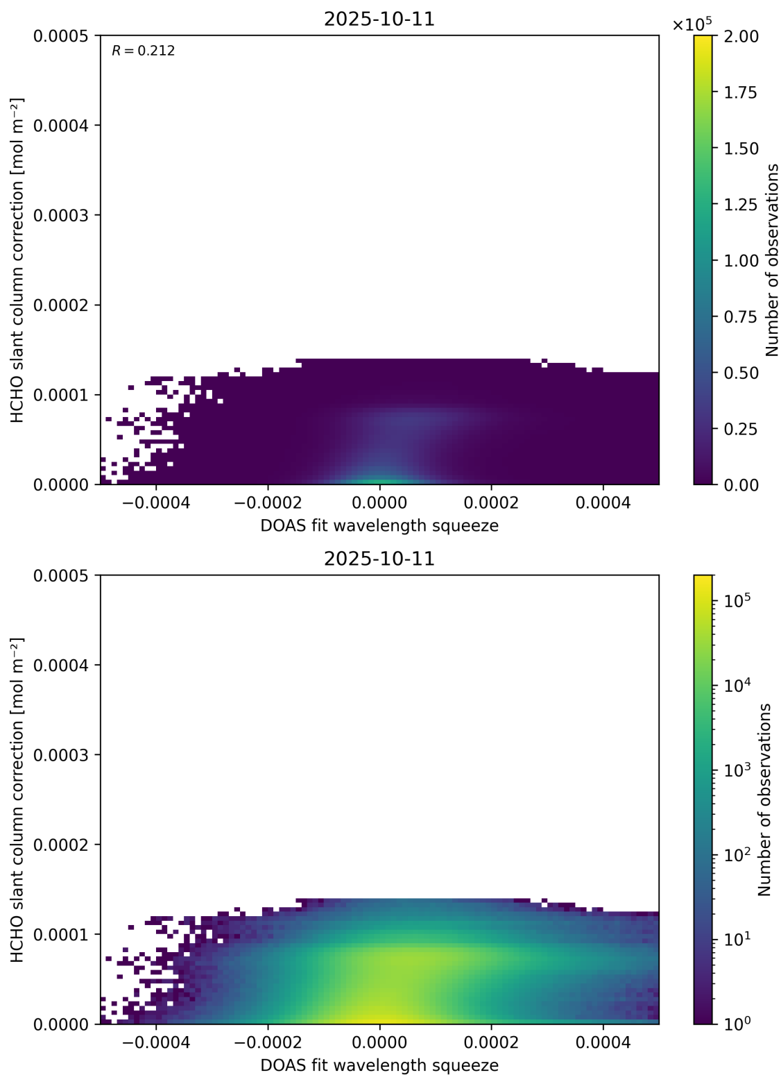
Figure 70: Scatter density plot of “DOAS fit wavelength squeeze” against “HCHO slant column correction” for 2025-10-11 to 2025-10-12.
