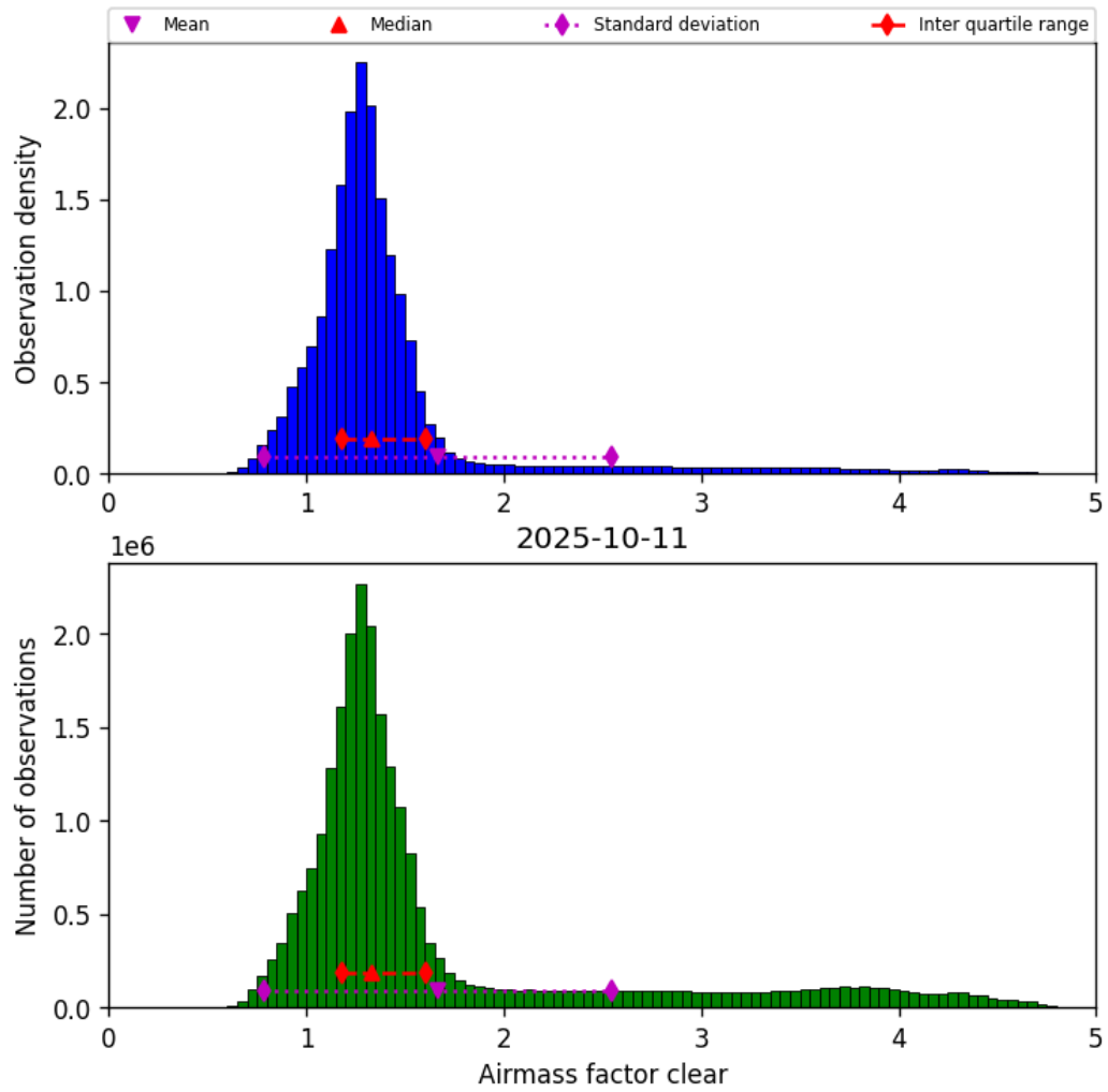
Figure 42: Histogram of “Airmass factor clear” for 2025-10-11 to 2025-10-12
