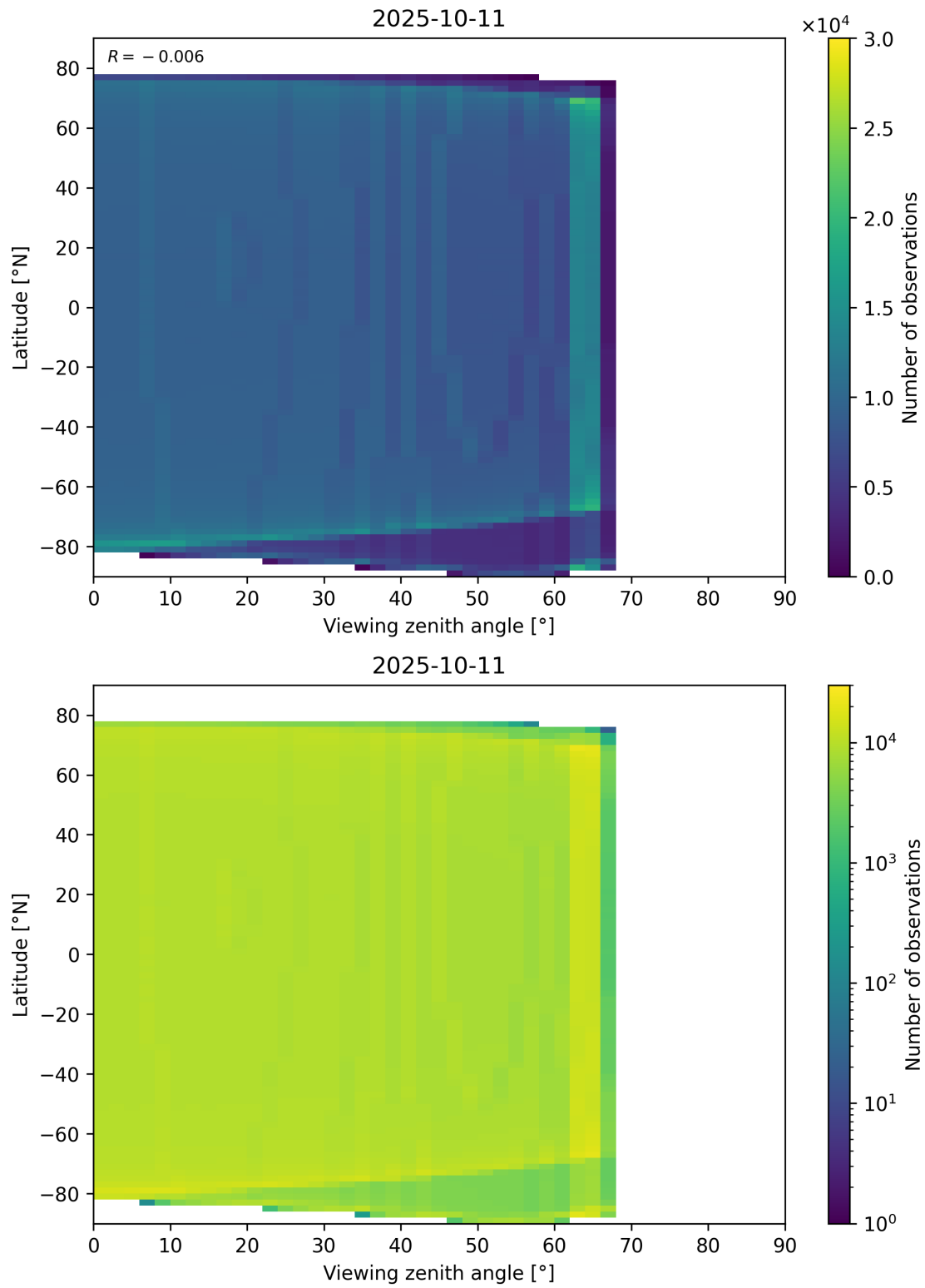
Figure 196: Scatter density plot of “Viewing zenith angle” against “Latitude” for 2025-10-11 to 2025-10-12.
