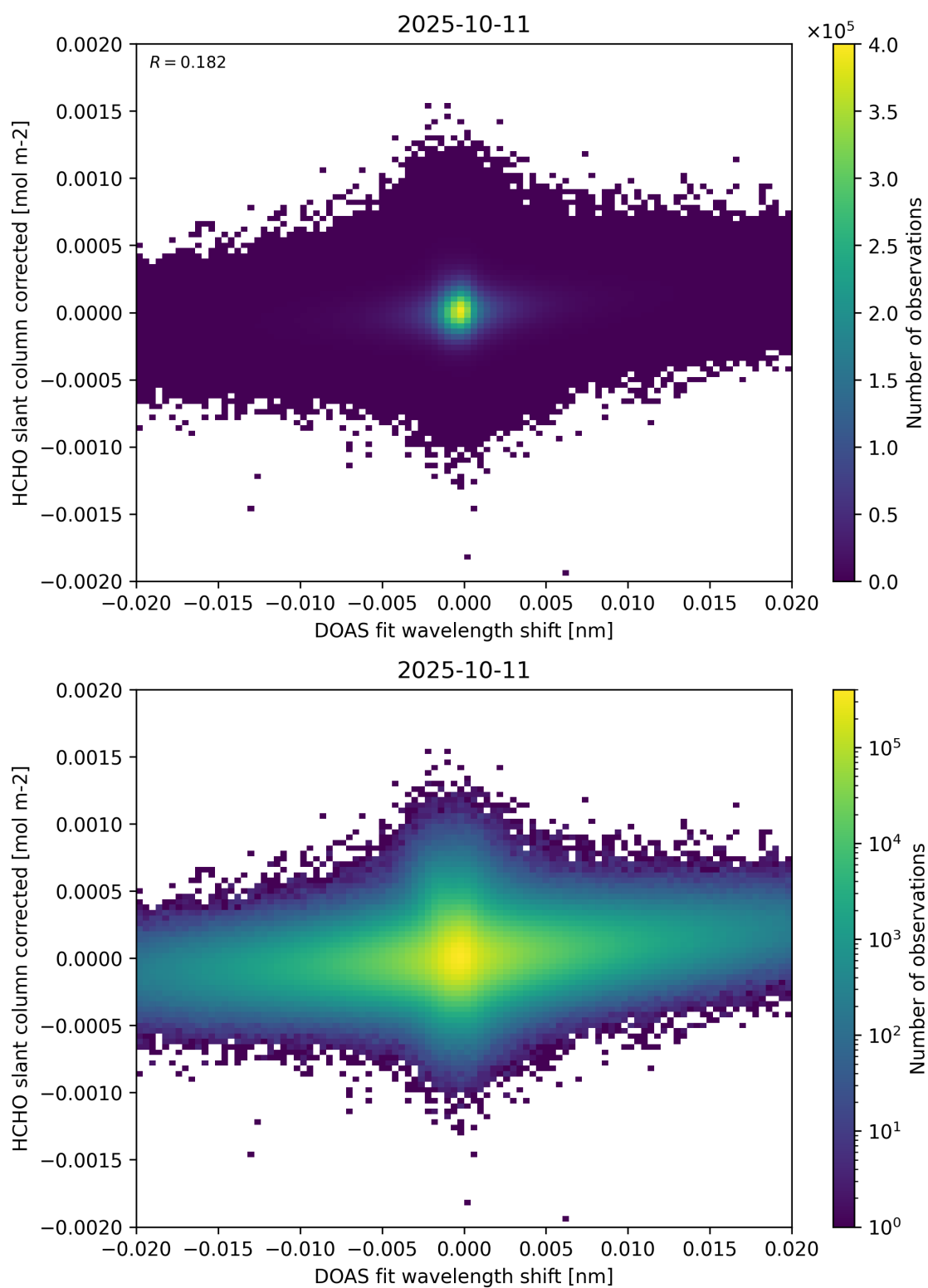
Figure 66: Scatter density plot of “DOAS fit wavelength shift” against “HCHO slant column corrected” for 2025-10-11 to 2025-10-12.
