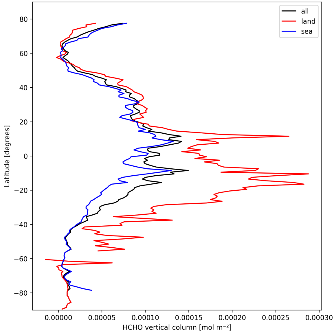
Figure 21: Zonal average of “HCHO vertical column” for 2025-10-11 to 2025-10-12.
