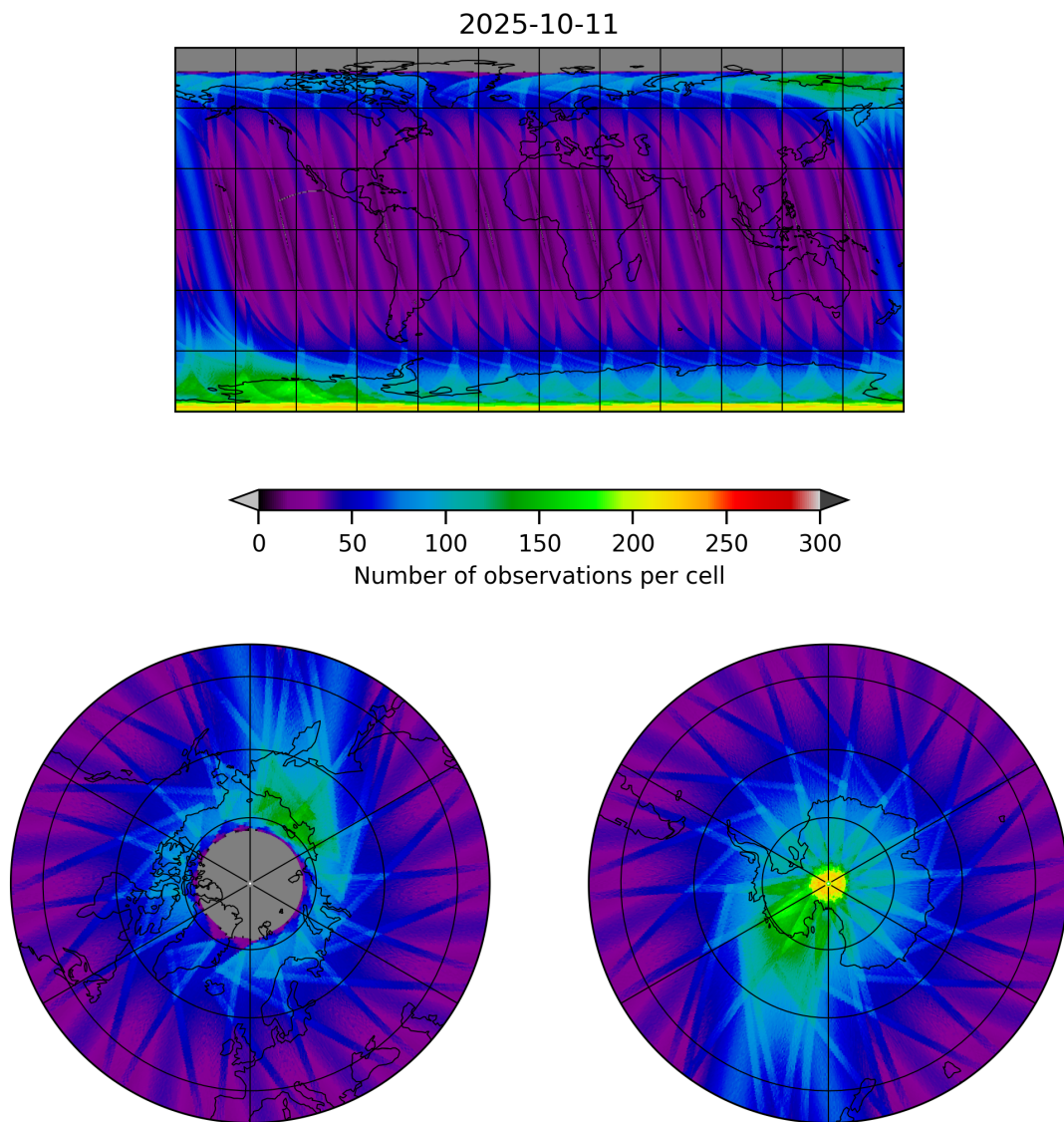
Figure 19: Map of the number of observations for 2025-10-11 to 2025-10-12
