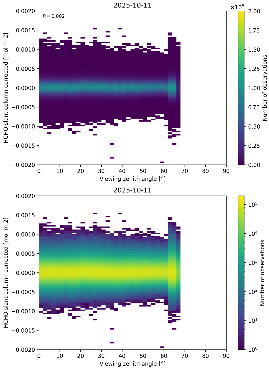
Figure 186: Scatter density plot of “Viewing zenith angle” against “HCHO slant column corrected” for 2025-10-11 to 2025-10-12.
