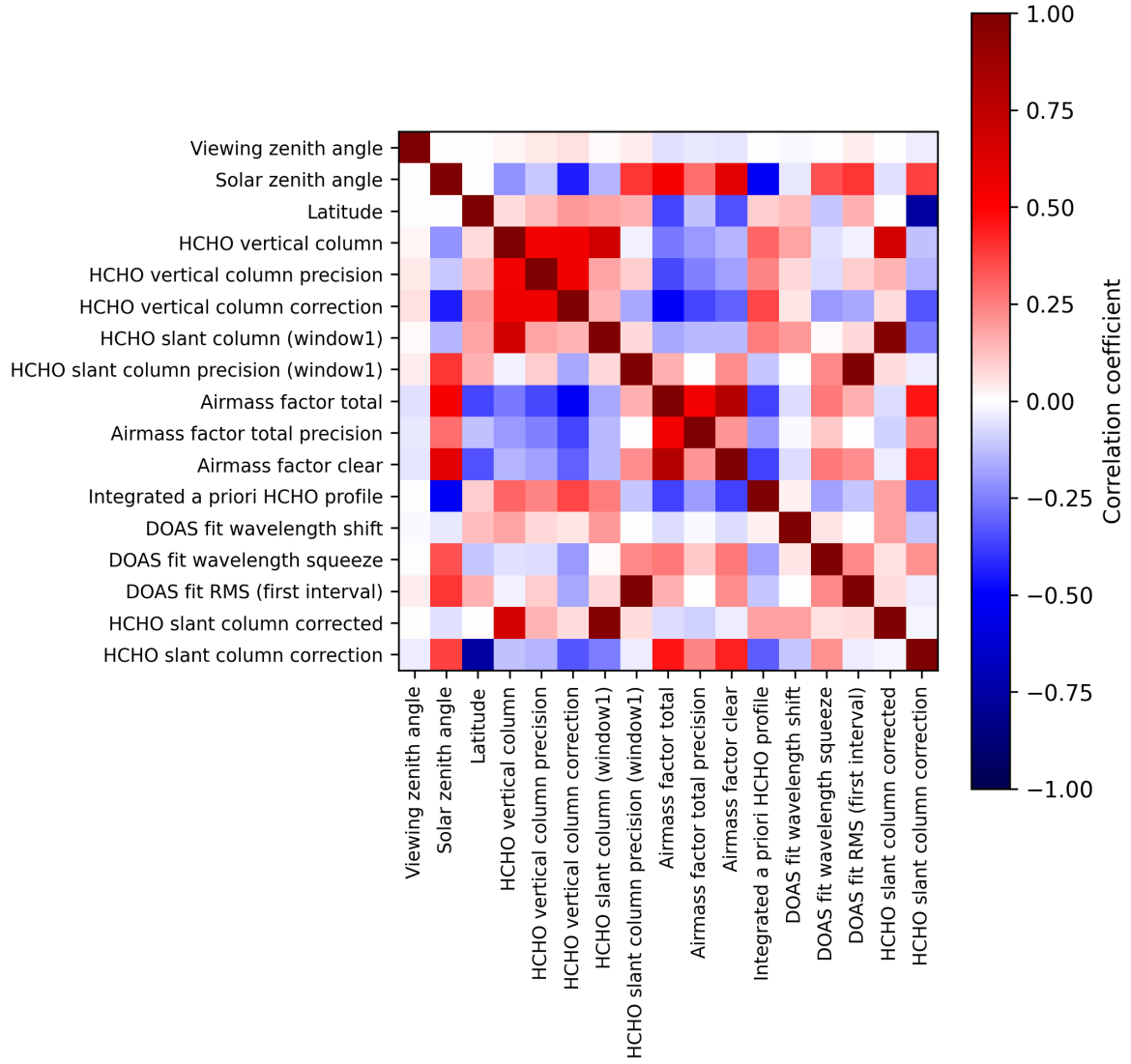
Figure 2: Map of correlation matrix for 2025-10-11 to 2025-10-12.
