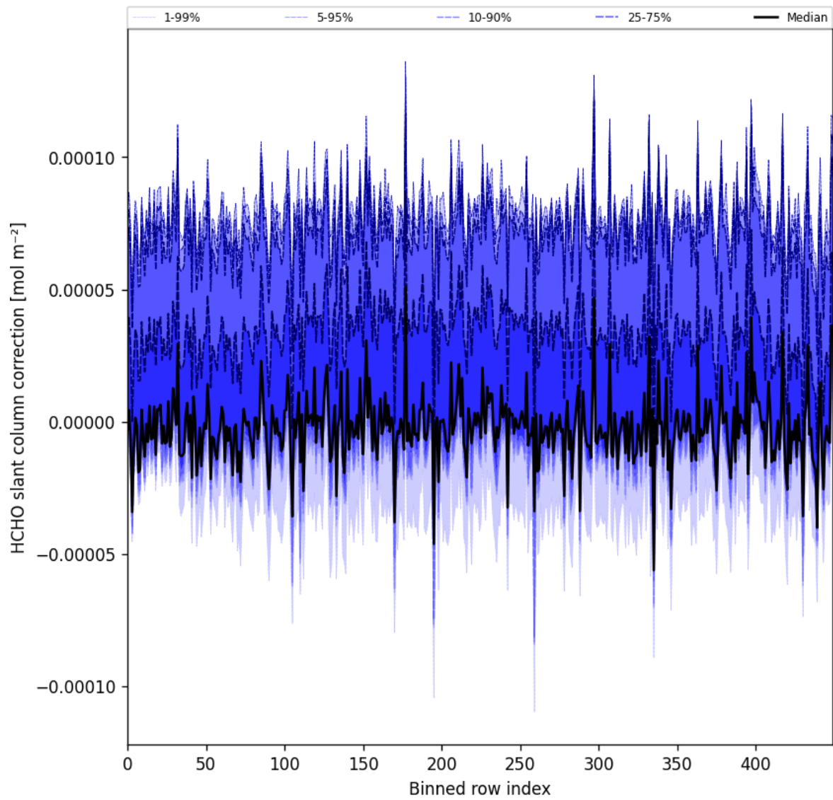
Figure 61: Along track statistics of “HCHO slant column correction” for 2025-10-11 to 2025-10-12
