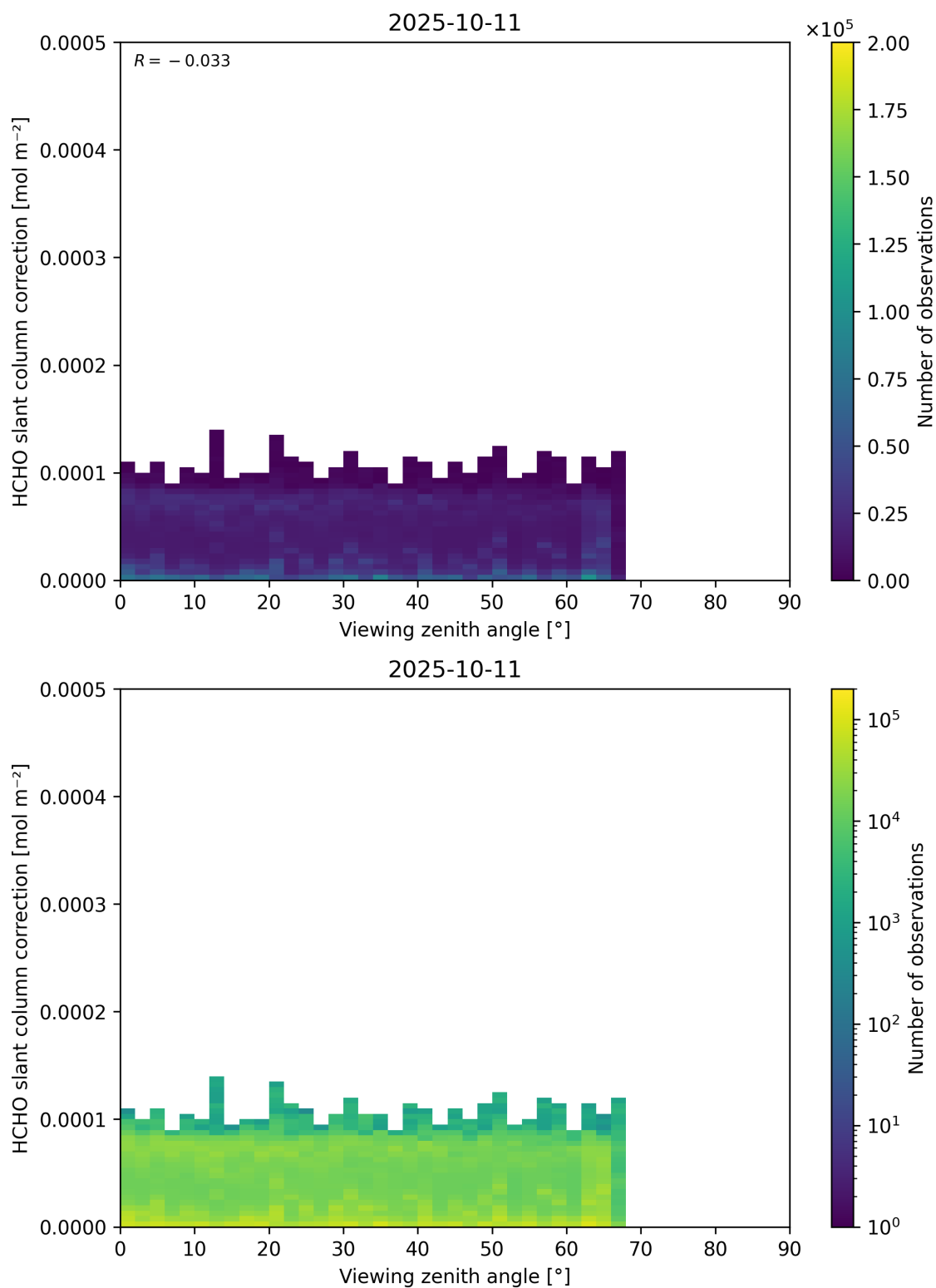
Figure 187: Scatter density plot of “Viewing zenith angle” against “HCHO slant column correction” for 2025-10-11 to 2025-10-12.
