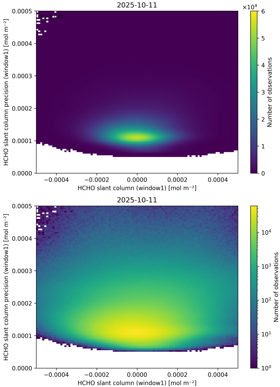
Figure 84: Scatter density plot of “HCHO slant column (window1)” against “HCHO slant column precision (window1)” for 2025-10-11 to 2025-10-12.
