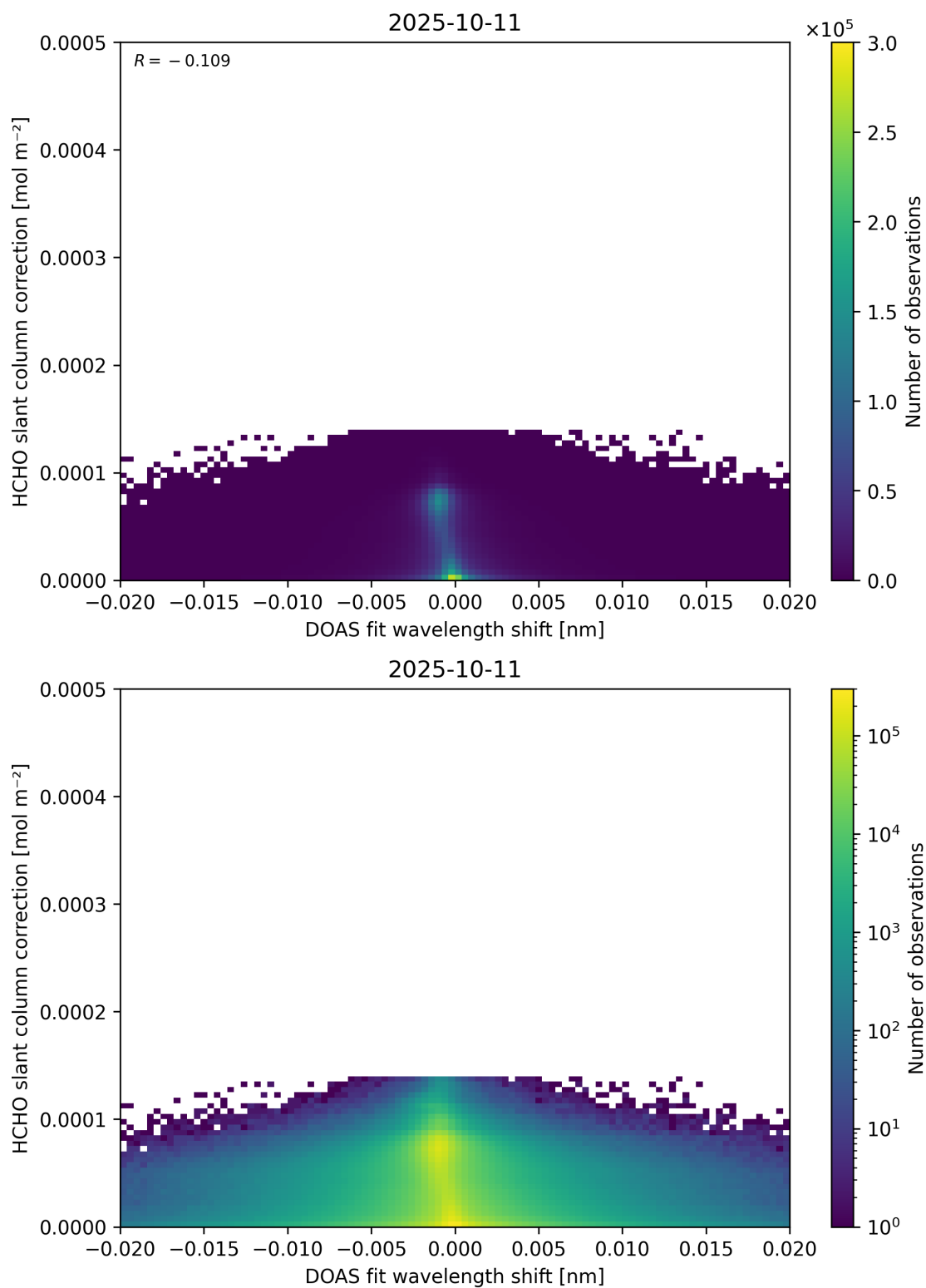
Figure 67: Scatter density plot of “DOAS fit wavelength shift” against “HCHO slant column correction” for 2025-10-11 to 2025-10-12.
