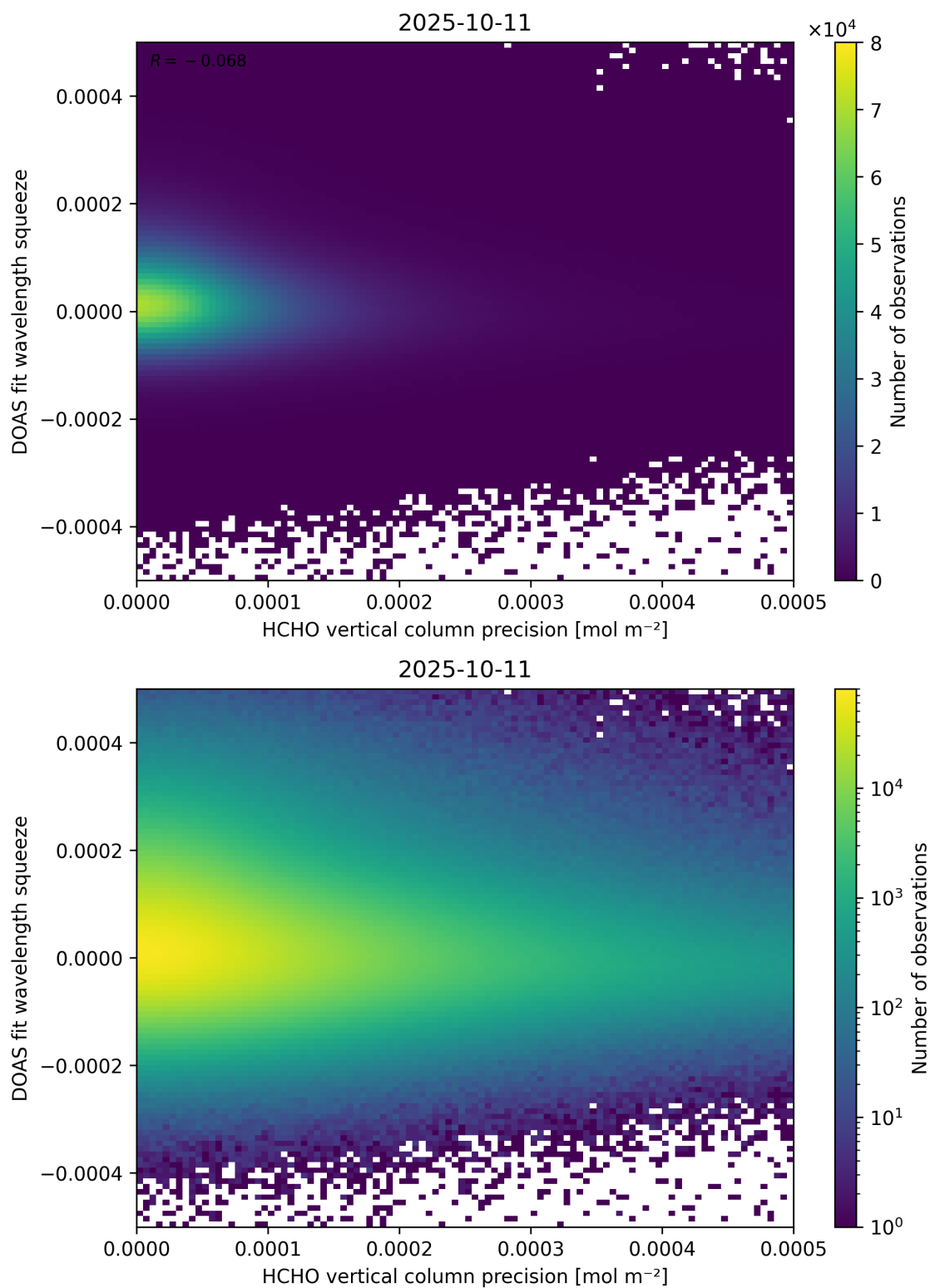
Figure 138: Scatter density plot of “HCHO vertical column precision” against “DOAS fit wavelength squeeze” for 2025-10-11 to 2025-10-12.
