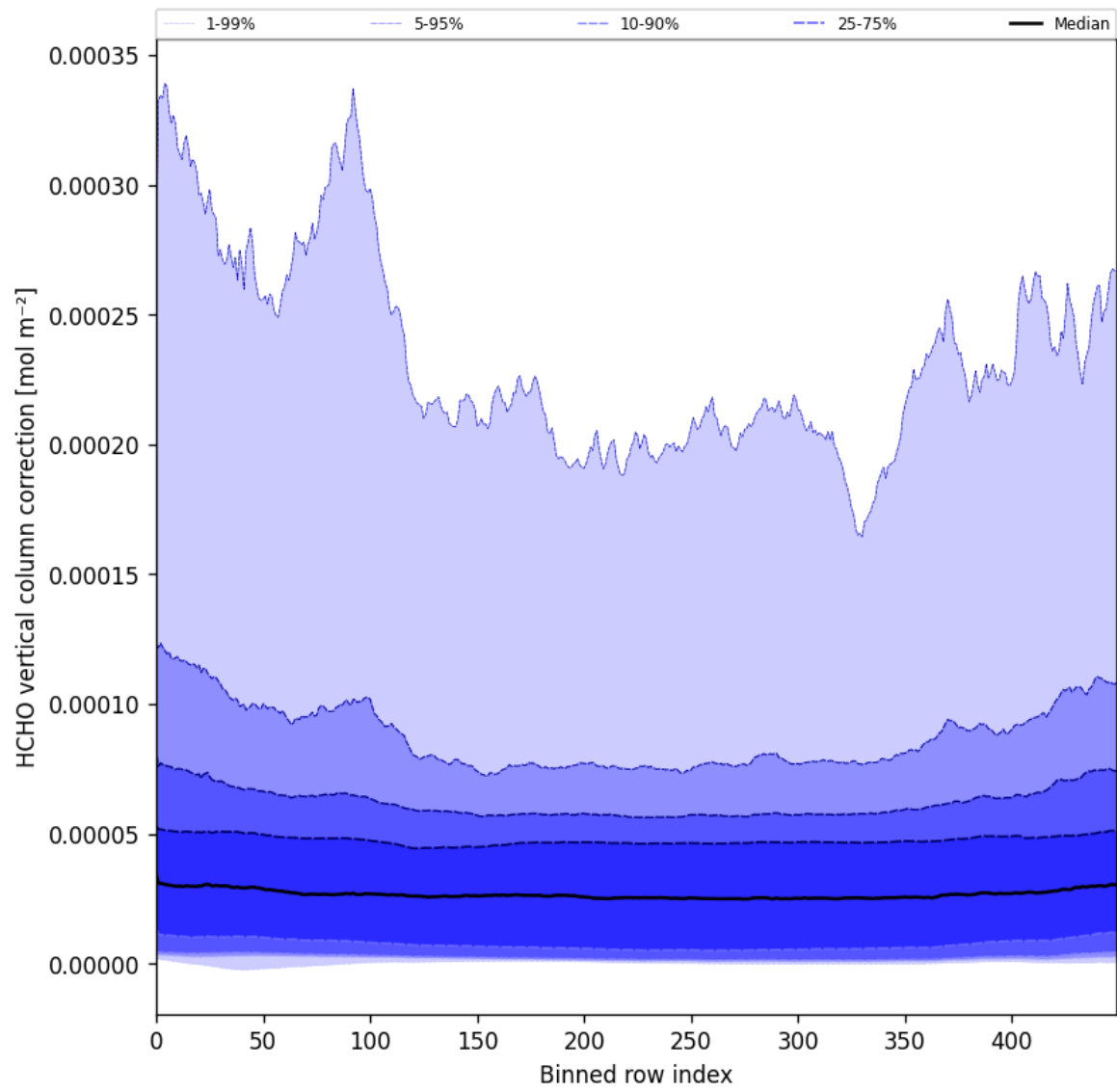
Figure 51: Along track statistics of “HCHO vertical column correction” for 2025-10-11 to 2025-10-12
