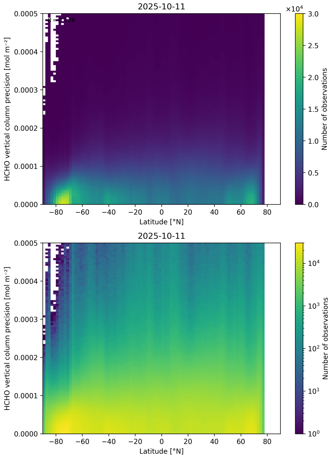
Figure 165: Scatter density plot of “Latitude” against “HCHO vertical column precision” for 2025-10-11 to 2025-10-12.
