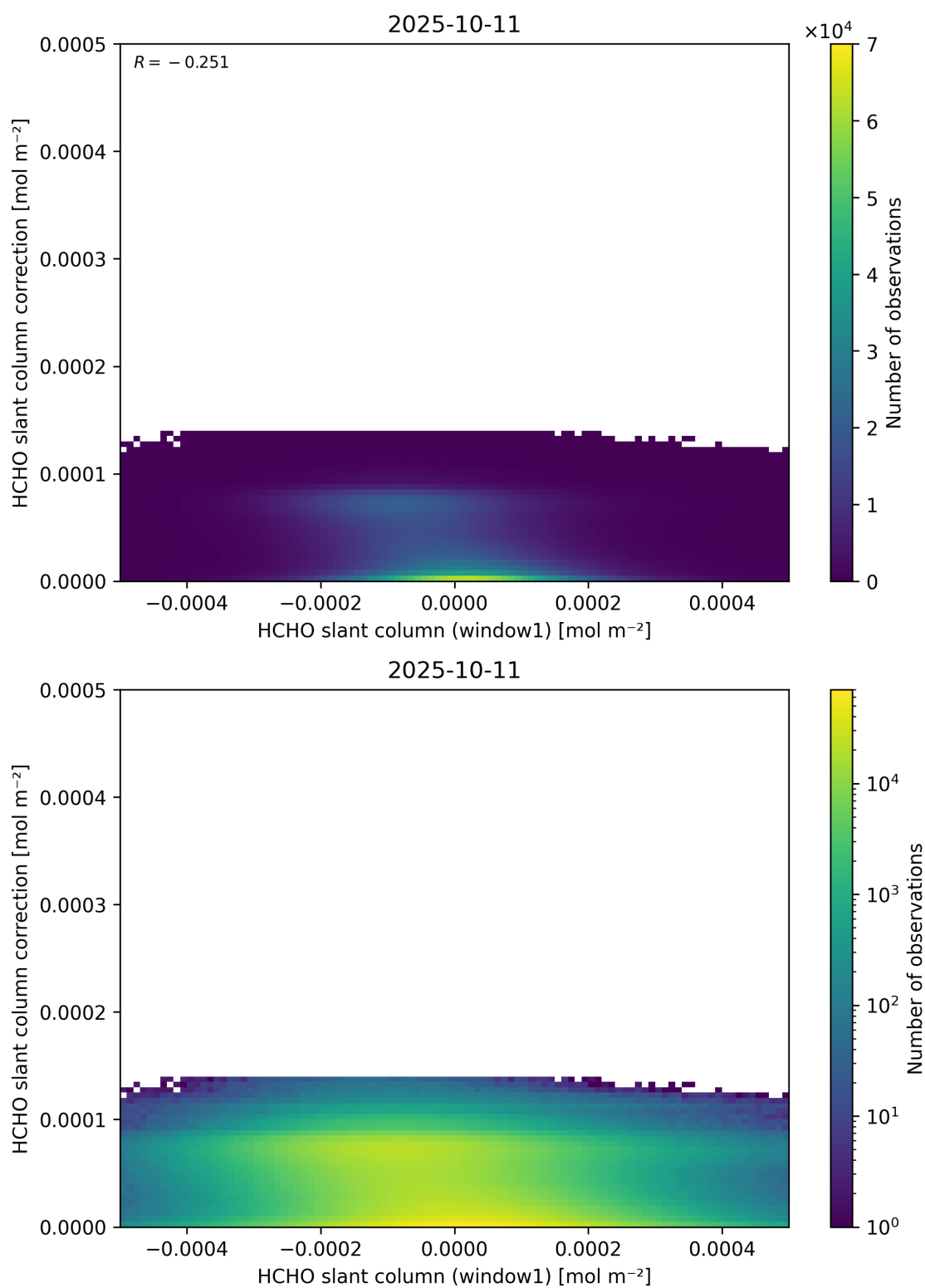
Figure 83: Scatter density plot of “HCHO slant column (window1)” against “HCHO slant column correction” for 2025-10-11 to 2025-10-12.
