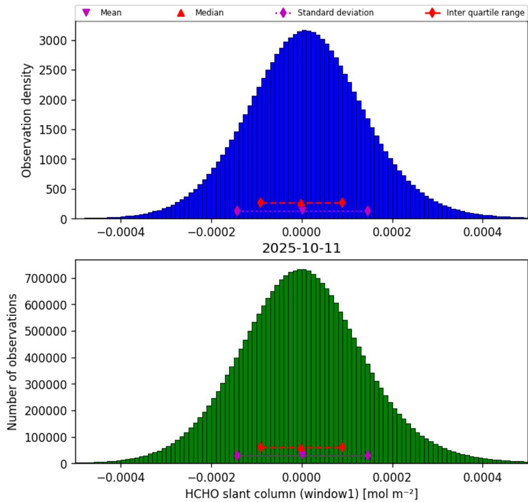
Figure 38: Histogram of “HCHO slant column (window1)” for 2025-10-11 to 2025-10-12
