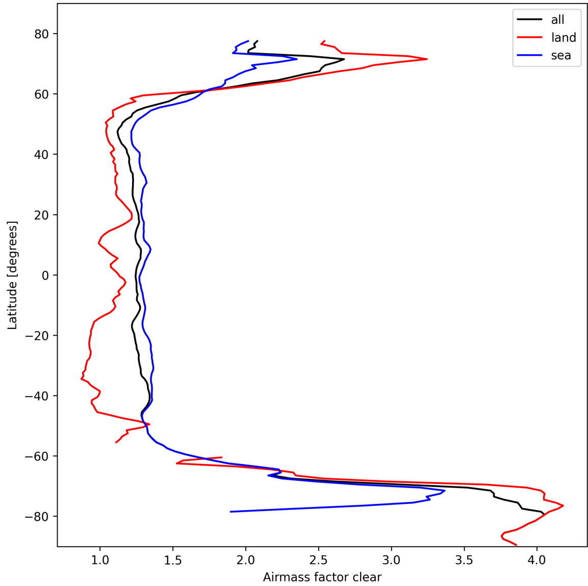
Figure 28: Zonal average of “Airmass factor clear” for 2025-10-11 to 2025-10-12.
