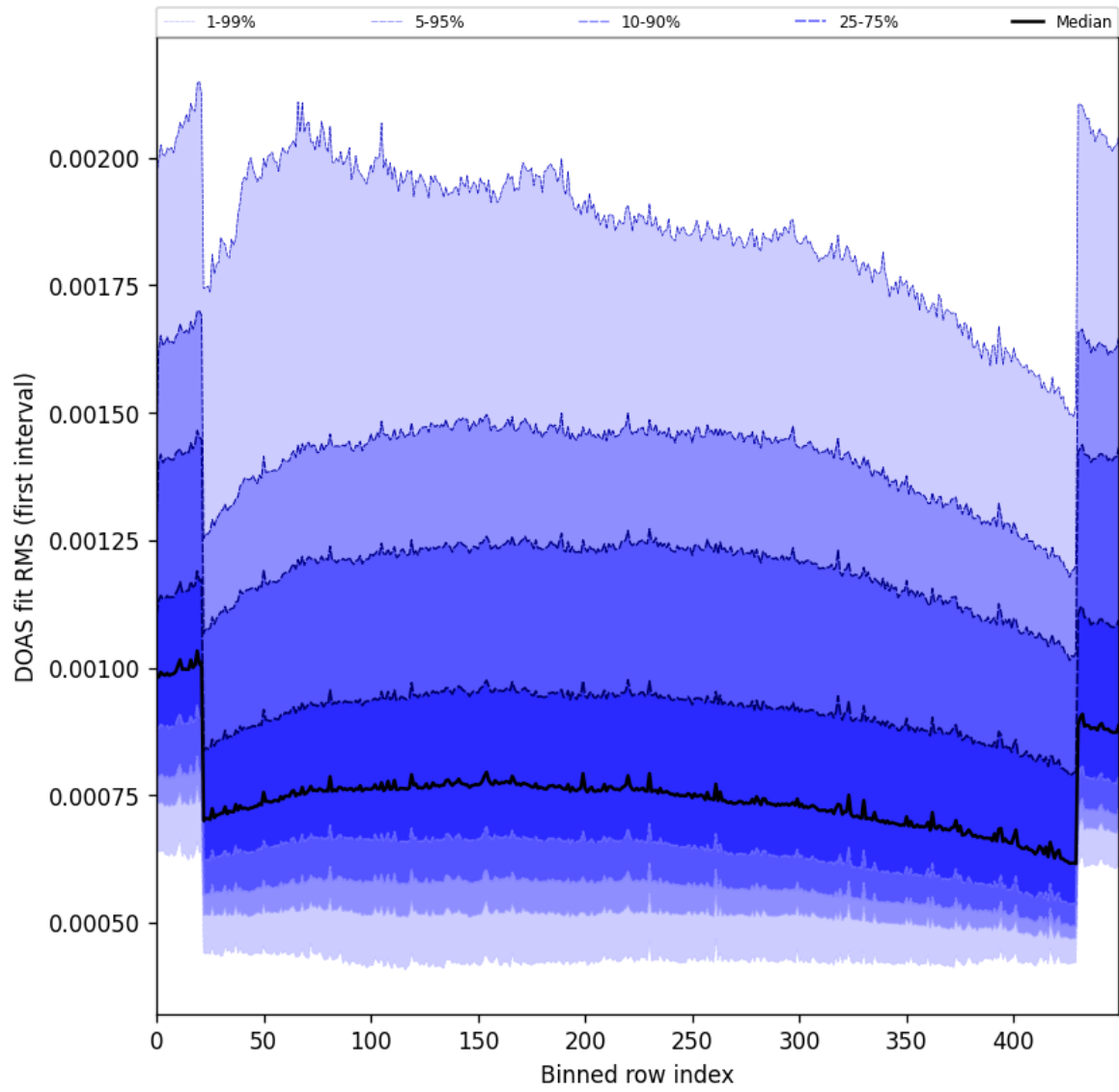
Figure 60: Along track statistics of “DOAS fit RMS (first interval)” for 2025-10-11 to 2025-10-12
