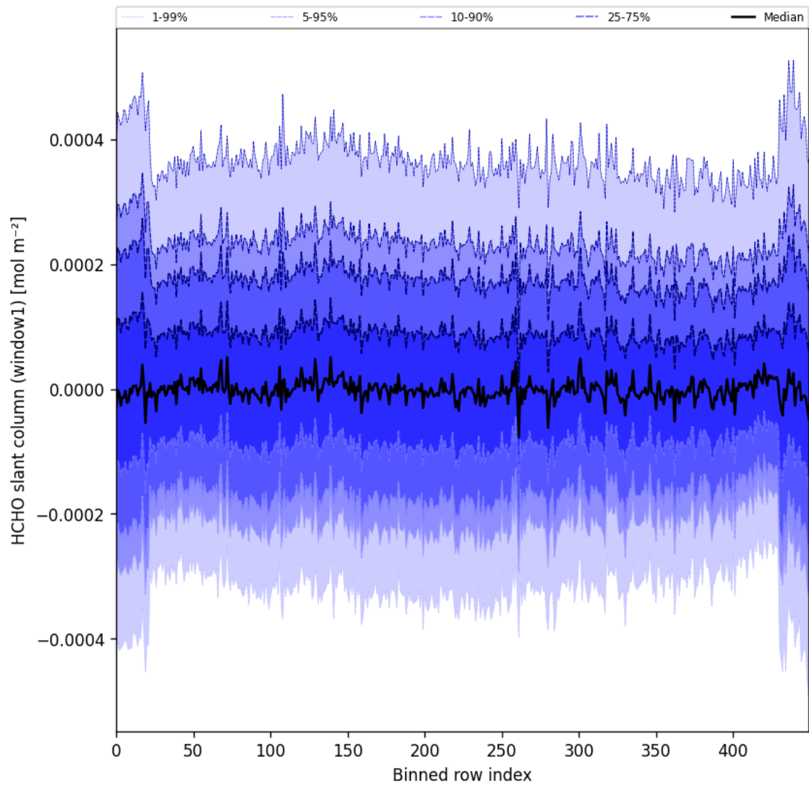
Figure 52: Along track statistics of “HCHO slant column (window1)” for 2025-10-11 to 2025-10-12
