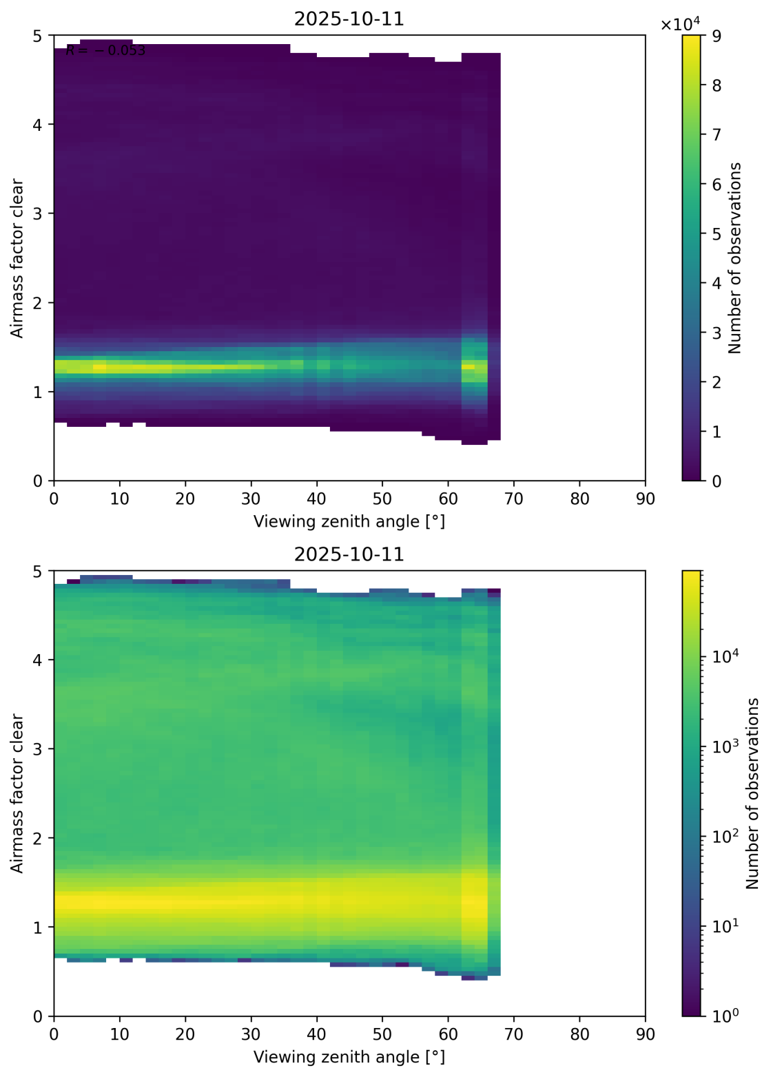
Figure 185: Scatter density plot of “Viewing zenith angle” against “Airmass factor clear” for 2025-10-11 to 2025-10-12.
