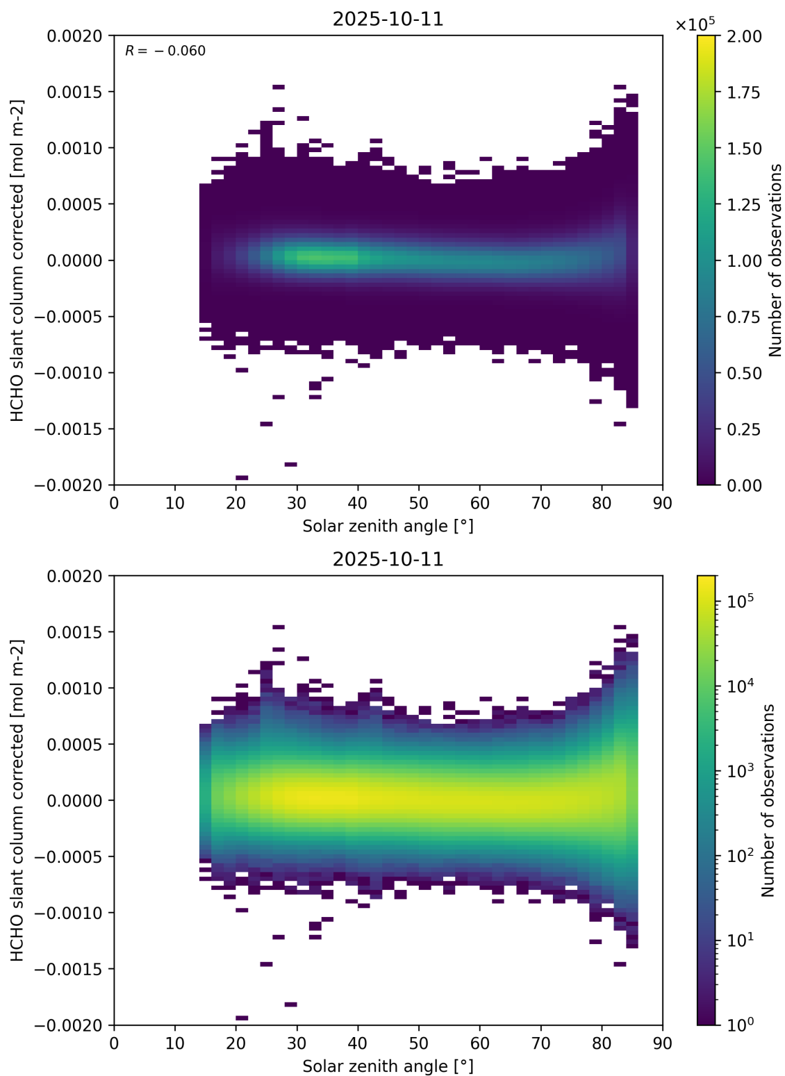
Figure 171: Scatter density plot of “Solar zenith angle” against “HCHO slant column corrected” for 2025-10-11 to 2025-10-12.
