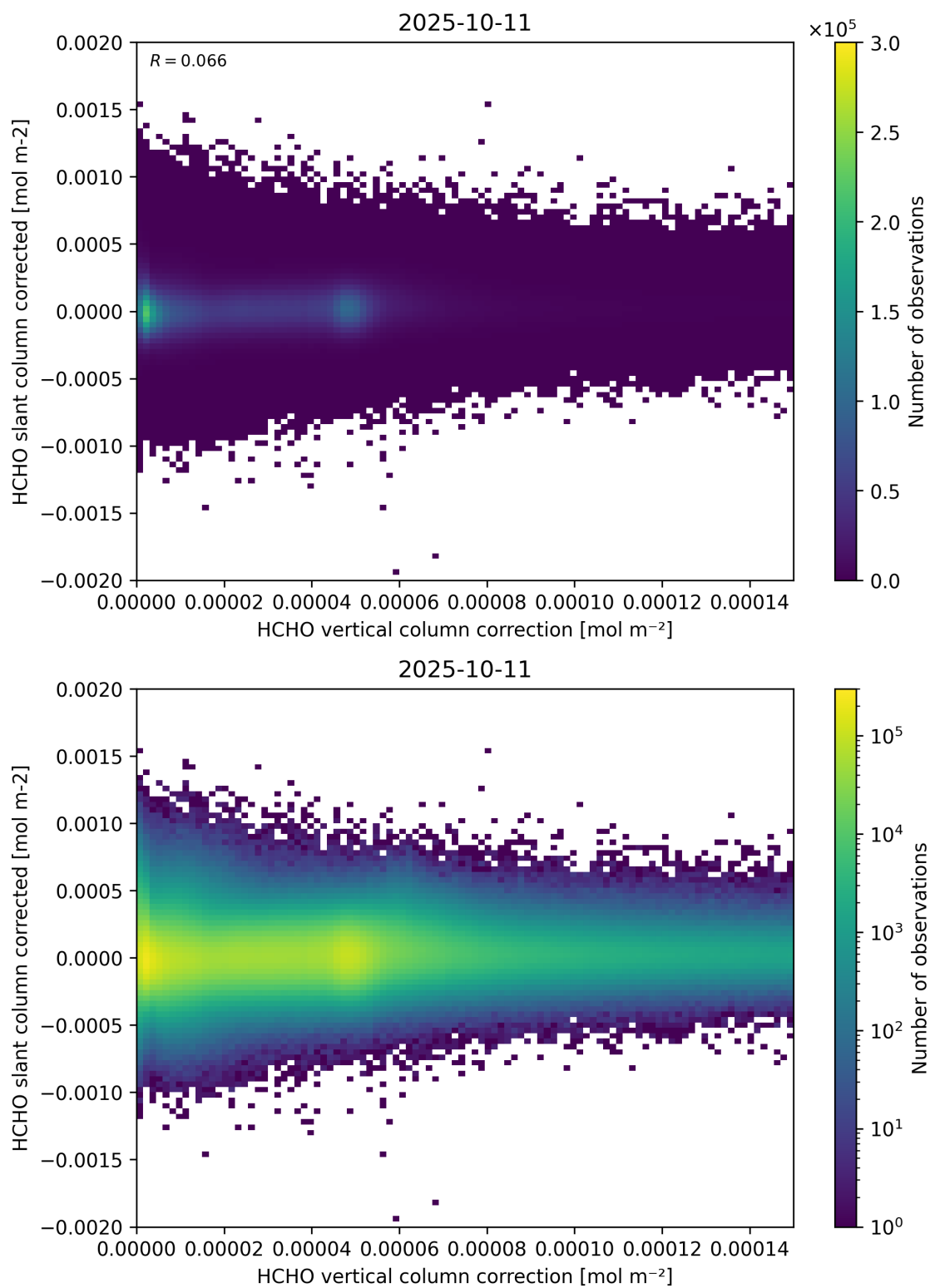
Figure 116: Scatter density plot of “HCHO vertical column correction” against “HCHO slant column corrected” for 2025-10-11 to 2025-10-12.
