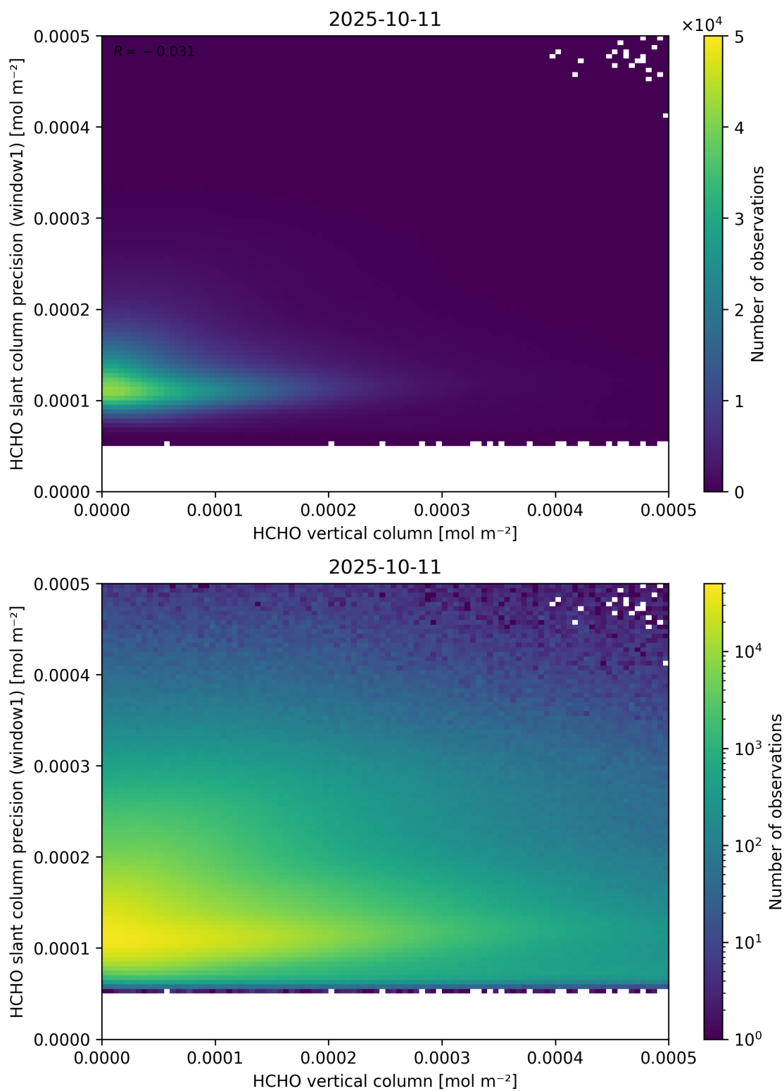
Figure 130: Scatter density plot of “HCHO vertical column” against “HCHO slant column precision (window1)” for 2025-10-11 to 2025-10-12.
