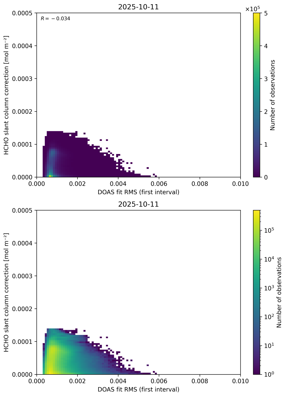
Figure 63: Scatter density plot of “DOAS fit RMS (first interval)” against “HCHO slant column correction” for 2025-10-11 to 2025-10-12.
