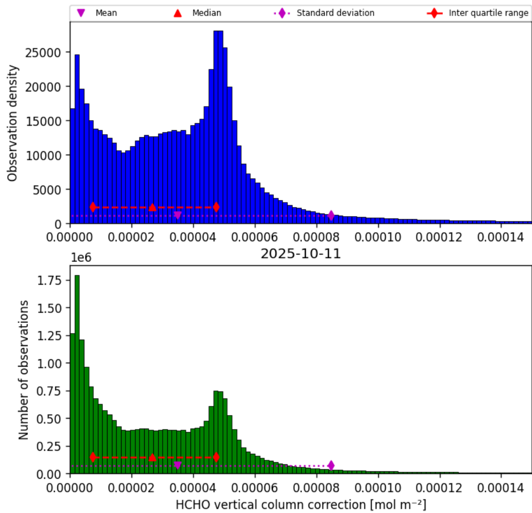
Figure 37: Histogram of “HCHO vertical column correction” for 2025-10-11 to 2025-10-12
