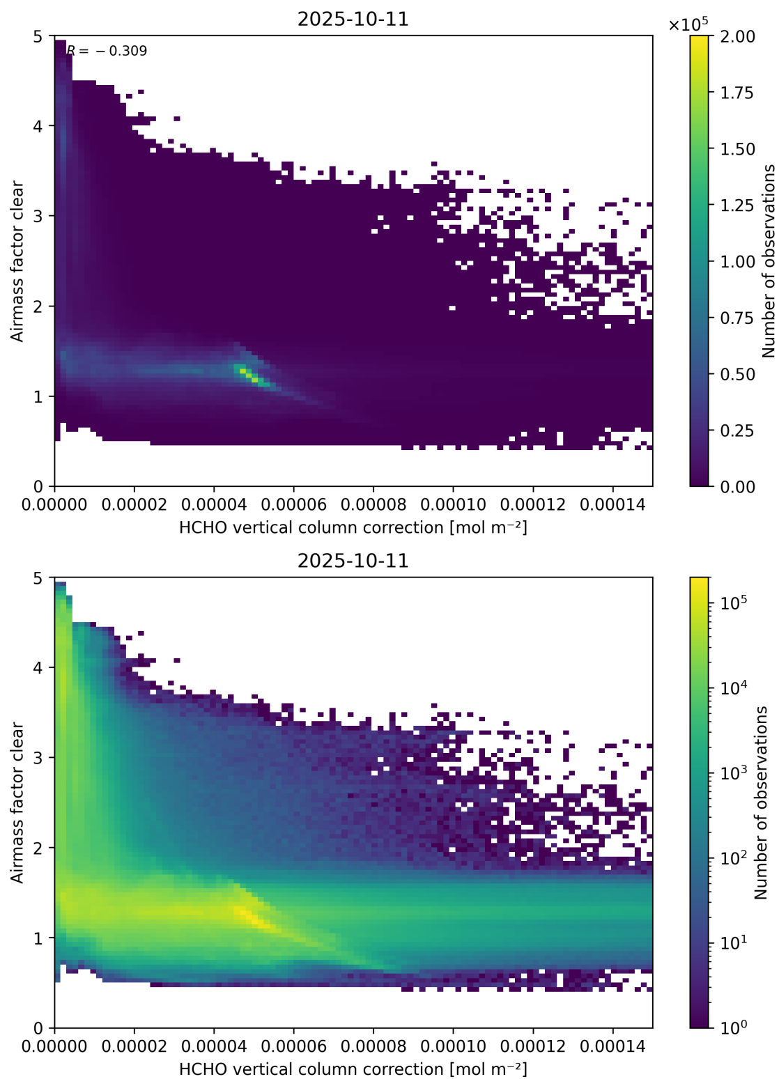
Figure 115: Scatter density plot of “HCHO vertical column correction” against “Airmass factor clear” for 2025-10-11 to 2025-10-12.
