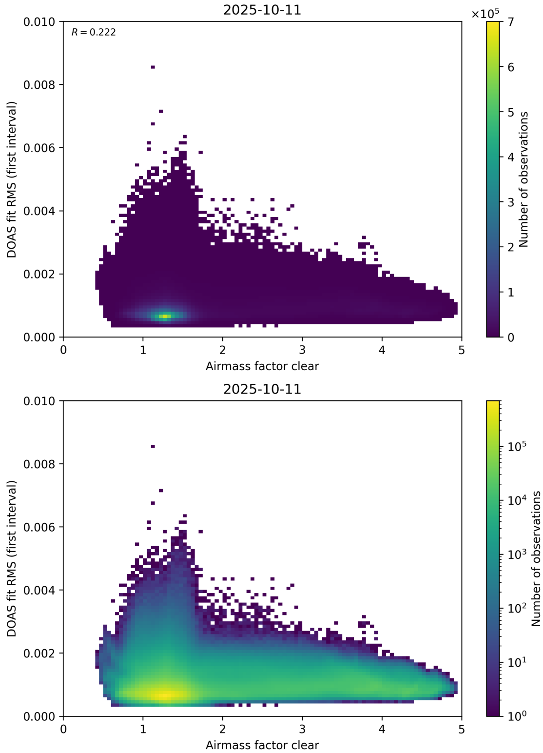
Figure 71: Scatter density plot of “Airmass factor clear” against “DOAS fit RMS (first interval)” for 2025-10-11 to 2025-10-12.
