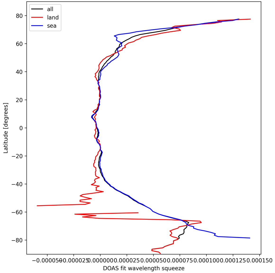
Figure 31: Zonal average of “DOAS fit wavelength squeeze” for 2025-10-11 to 2025-10-12.
