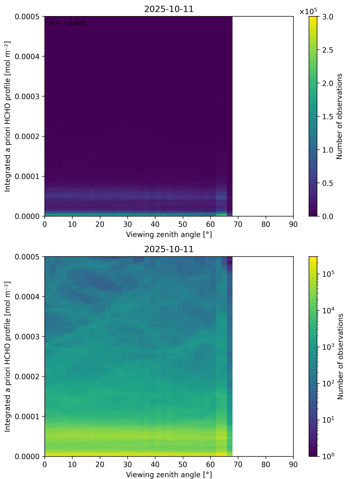
Figure 195: Scatter density plot of “Viewing zenith angle” against “Integrated a priori HCHO profile” for 2025-10-11 to 2025-10-12.
