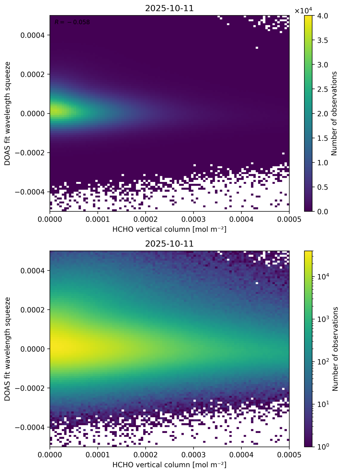
Figure 125: Scatter density plot of “HCHO vertical column” against “DOAS fit wavelength squeeze” for 2025-10-11 to 2025-10-12.
