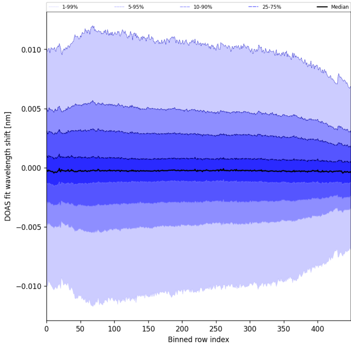
Figure 58: Along track statistics of “DOAS fit wavelength shift” for 2025-10-11 to 2025-10-12
