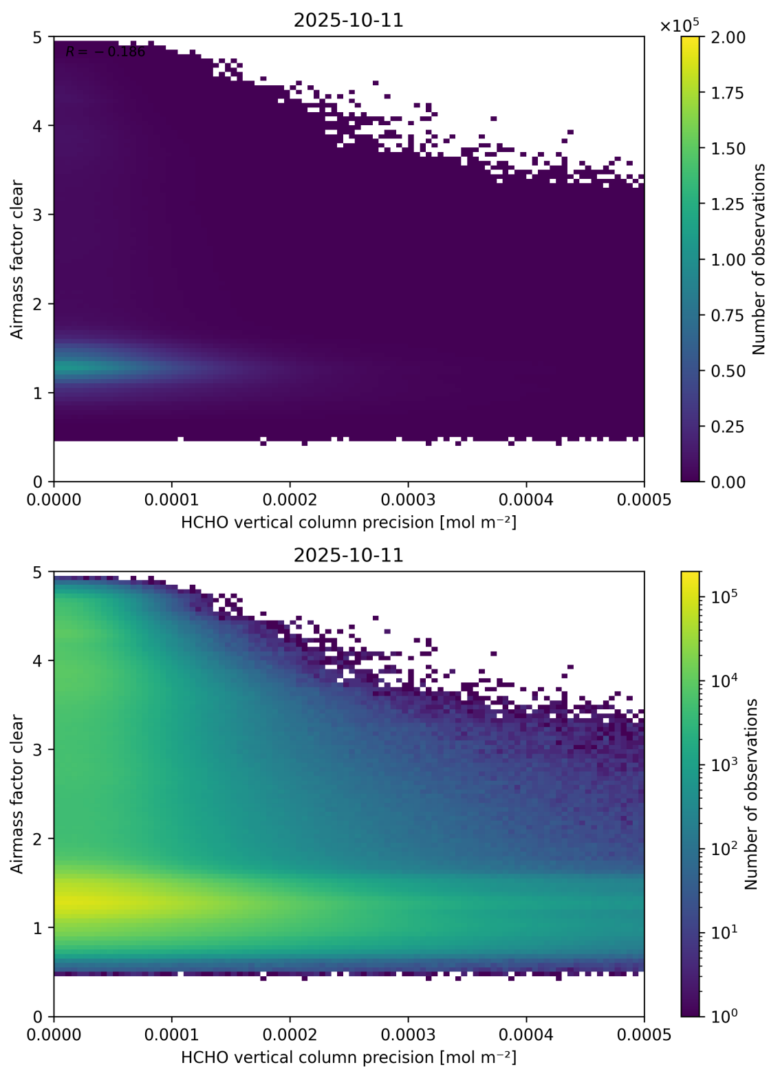
Figure 139: Scatter density plot of “HCHO vertical column precision” against “Airmass factor clear” for 2025-10-11 to 2025-10-12.
