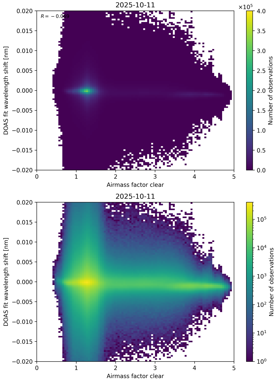
Figure 72: Scatter density plot of “Airmass factor clear” against “DOAS fit wavelength shift” for 2025-10-11 to 2025-10-12.
