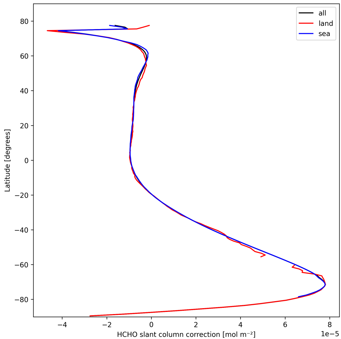
Figure 33: Zonal average of "HCHO slant column correction" for 2025-10-11 to 2025-10-12.
