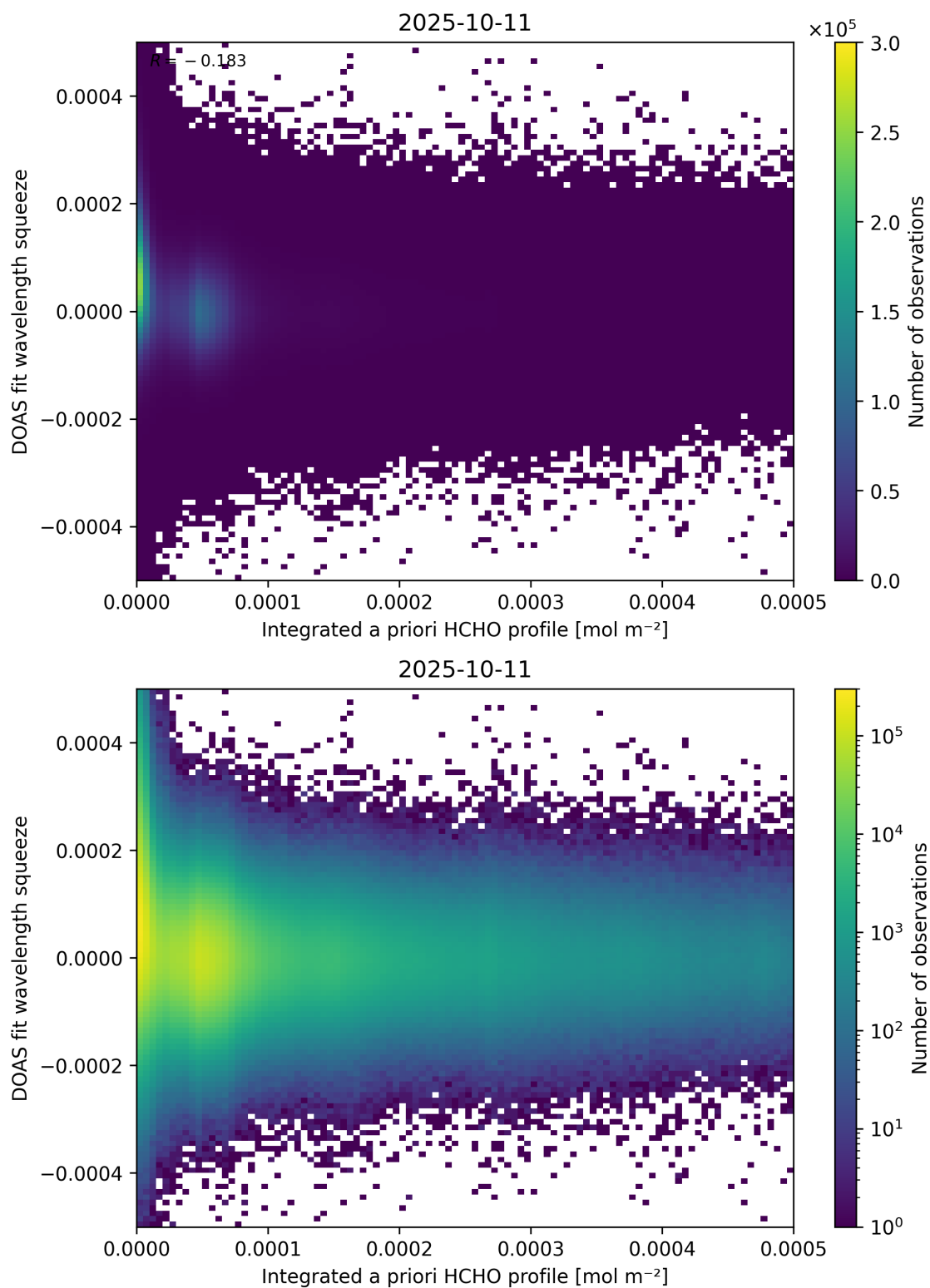
Figure 150: Scatter density plot of “Integrated a priori HCHO profile” against “DOAS fit wavelength squeeze” for 2025-10-11 to 2025-10-12.
