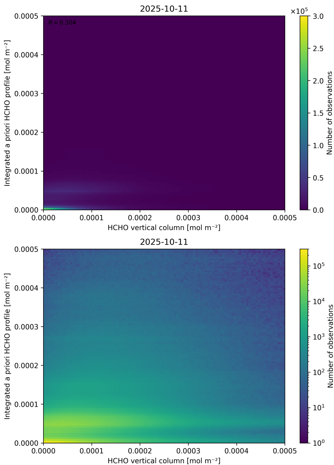
Figure 135: Scatter density plot of “HCHO vertical column” against “Integrated a priori HCHO profile” for 2025-10-11 to 2025-10-12.
