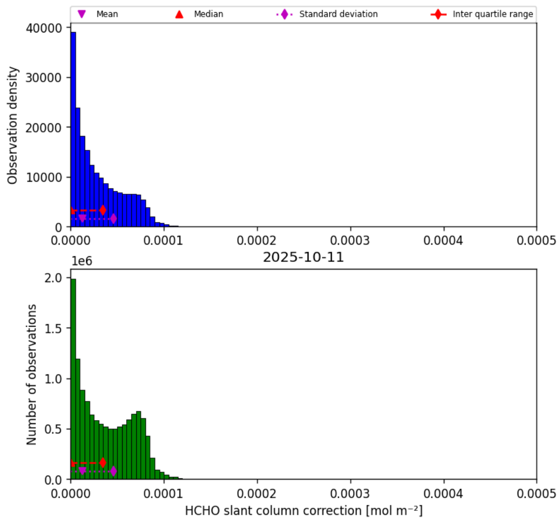
Figure 47: Histogram of “HCHO slant column correction” for 2025-10-11 to 2025-10-12
