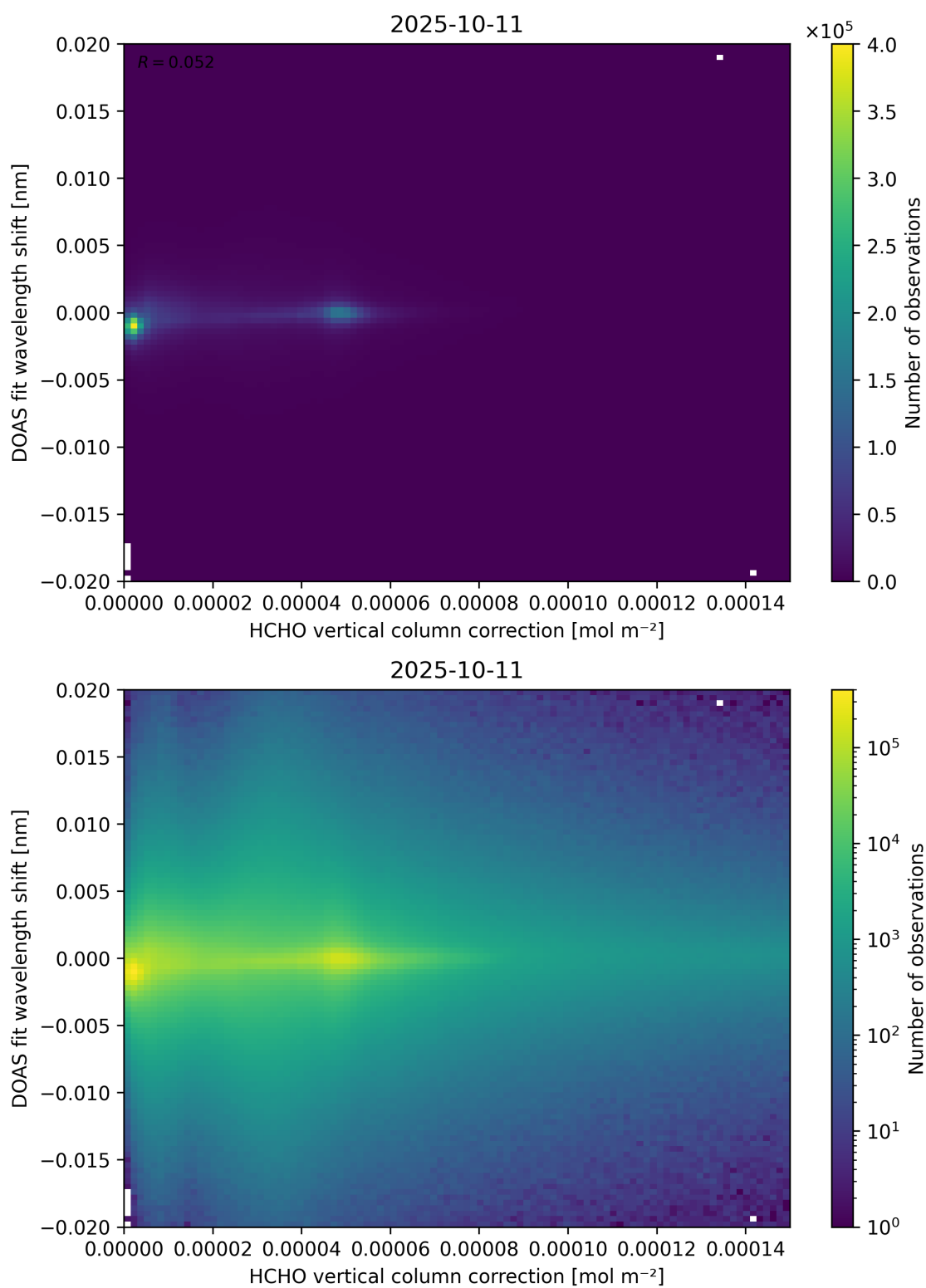
Figure 113: Scatter density plot of “HCHO vertical column correction” against “DOAS fit wavelength shift” for 2025-10-11 to 2025-10-12.
