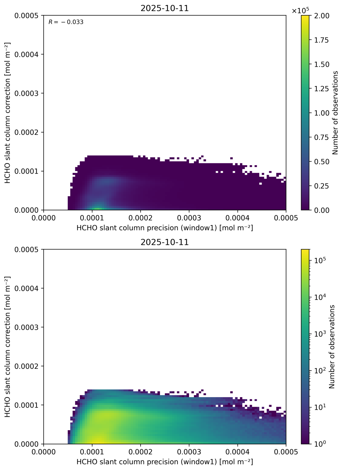
Figure 93: Scatter density plot of “HCHO slant column precision (window1)” against “HCHO slant column correction” for 2025-10-11 to 2025-10-12.
