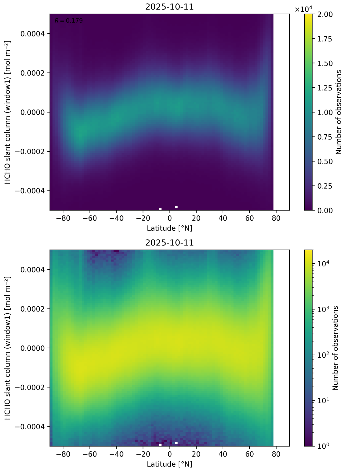
Figure 159: Scatter density plot of “Latitude” against “HCHO slant column (window1)” for 2025-10-11 to 2025-10-12.
