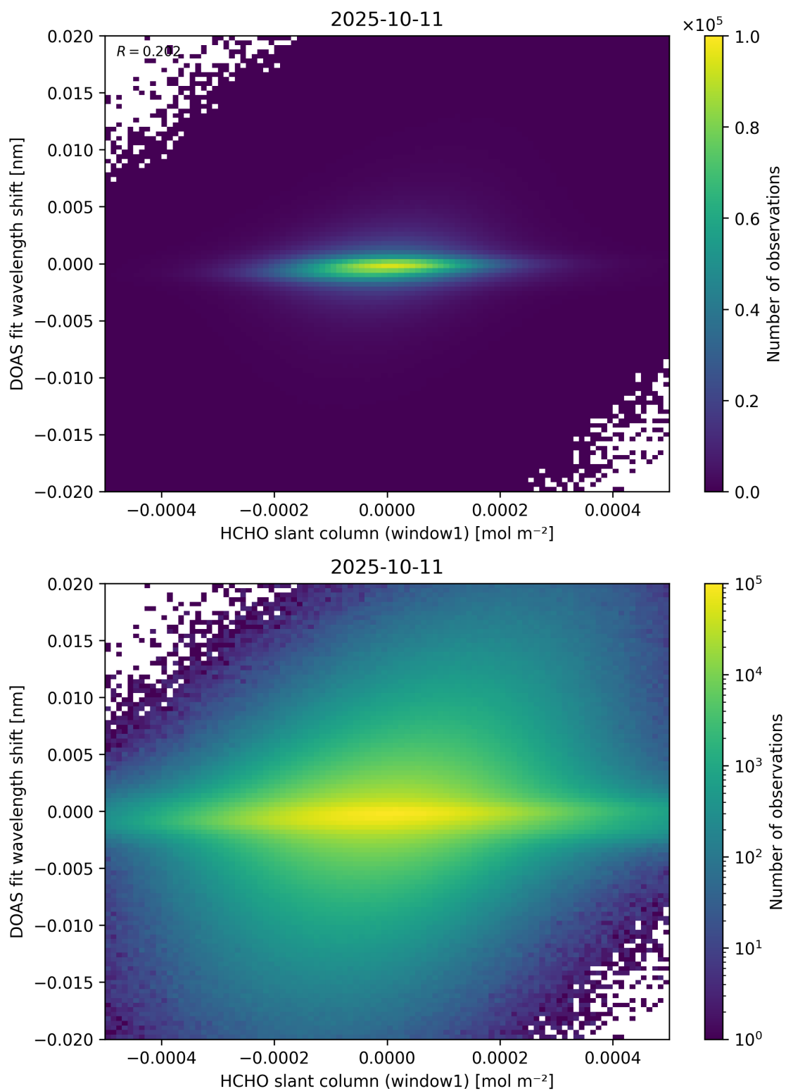
Figure 79: Scatter density plot of “HCHO slant column (window1)” against “DOAS fit wavelength shift” for 2025-10-11 to 2025-10-12.
