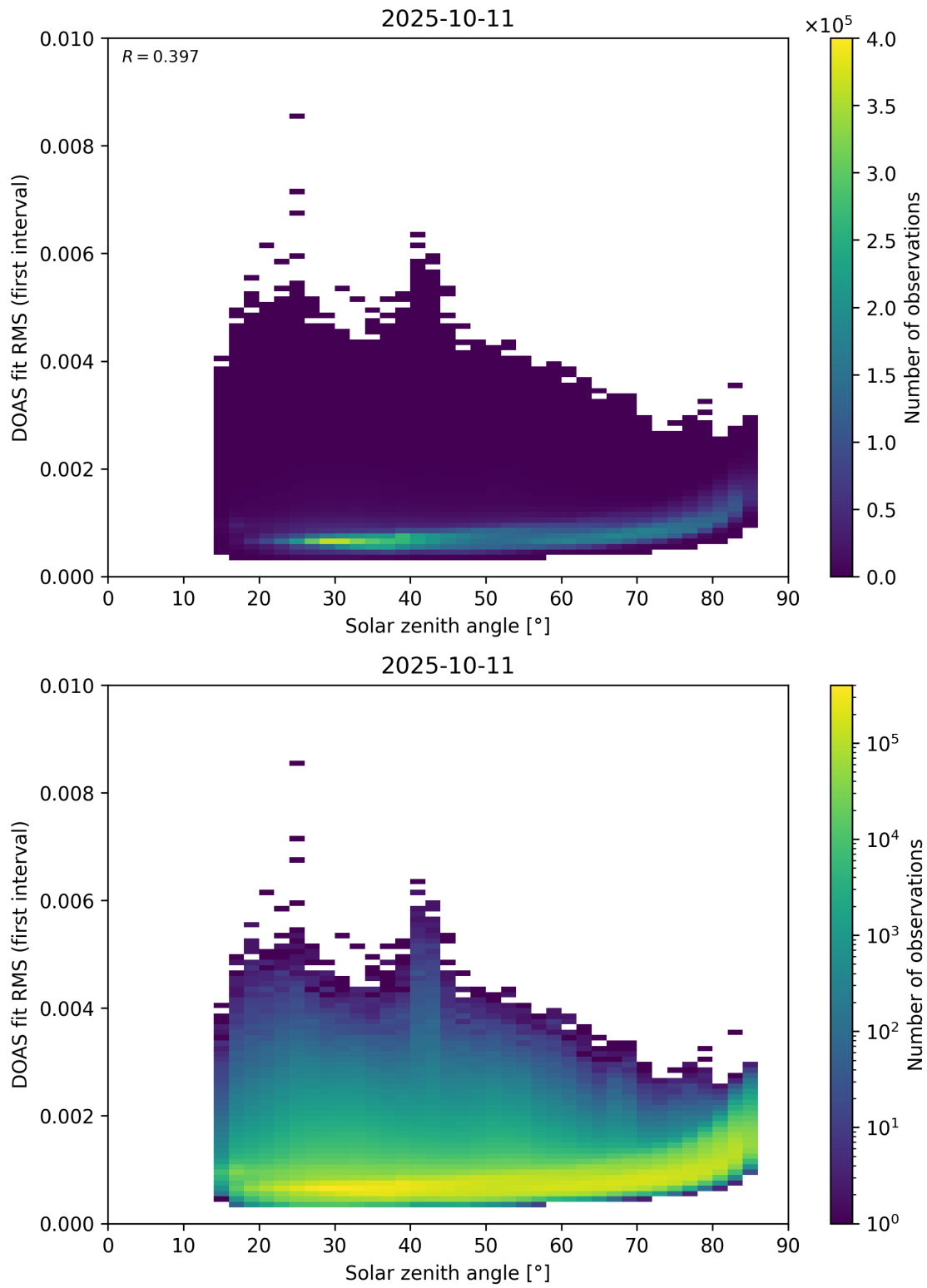
Figure 167: Scatter density plot of “Solar zenith angle” against “DOAS fit RMS (first interval)” for 2025-10-11 to 2025-10-12.
