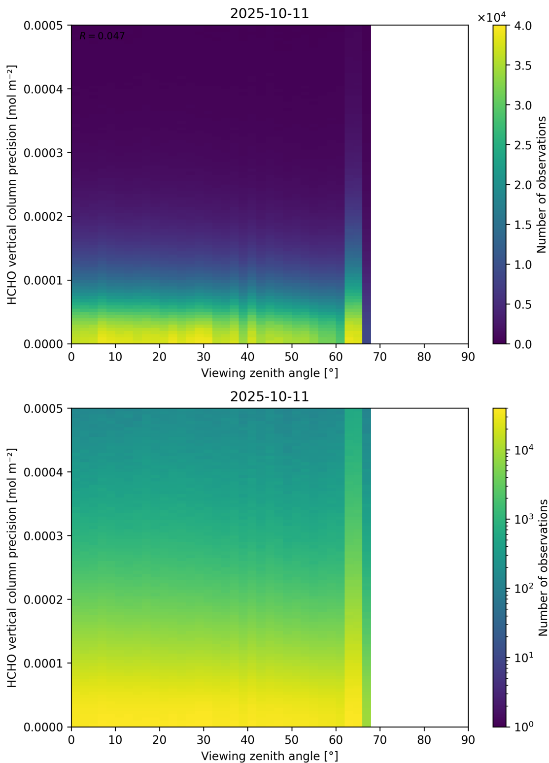
Figure 194: Scatter density plot of “Viewing zenith angle” against “HCHO vertical column precision” for 2025-10-11 to 2025-10-12.
