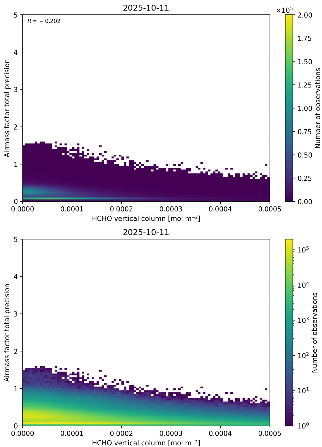
Figure 132: Scatter density plot of “HCHO vertical column” against “Airmass factor total precision” for 2025-10-11 to 2025-10-12.
