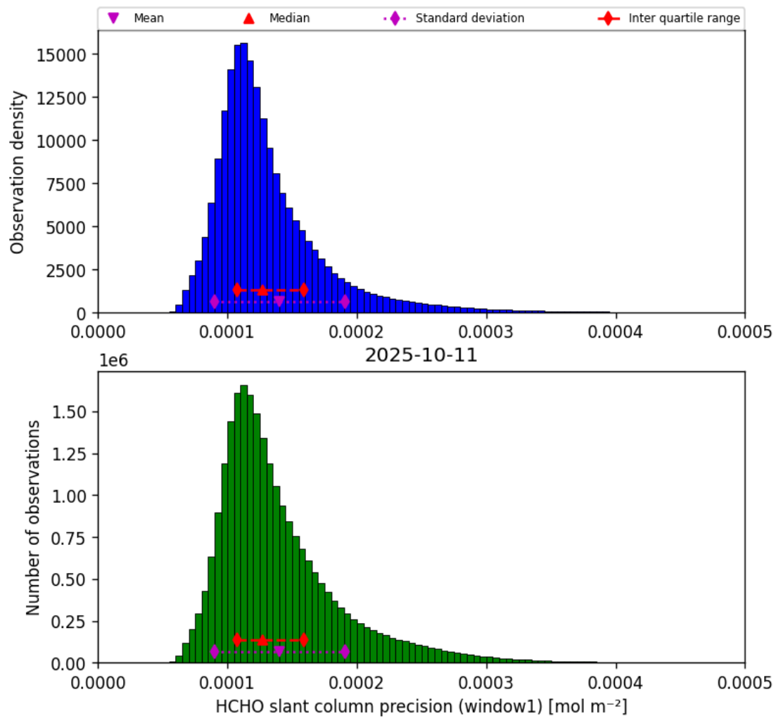
Figure 39: Histogram of “HCHO slant column precision (window1)” for 2025-10-11 to 2025-10-12
