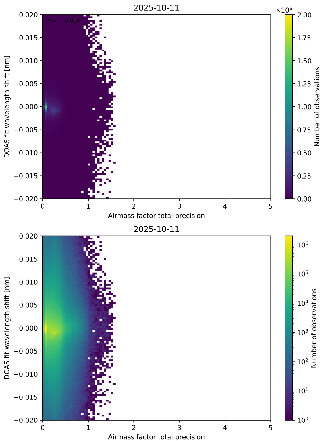
Figure 106: Scatter density plot of “Airmass factor total precision” against “DOAS fit wavelength shift” for 2025-10-11 to 2025-10-12.
