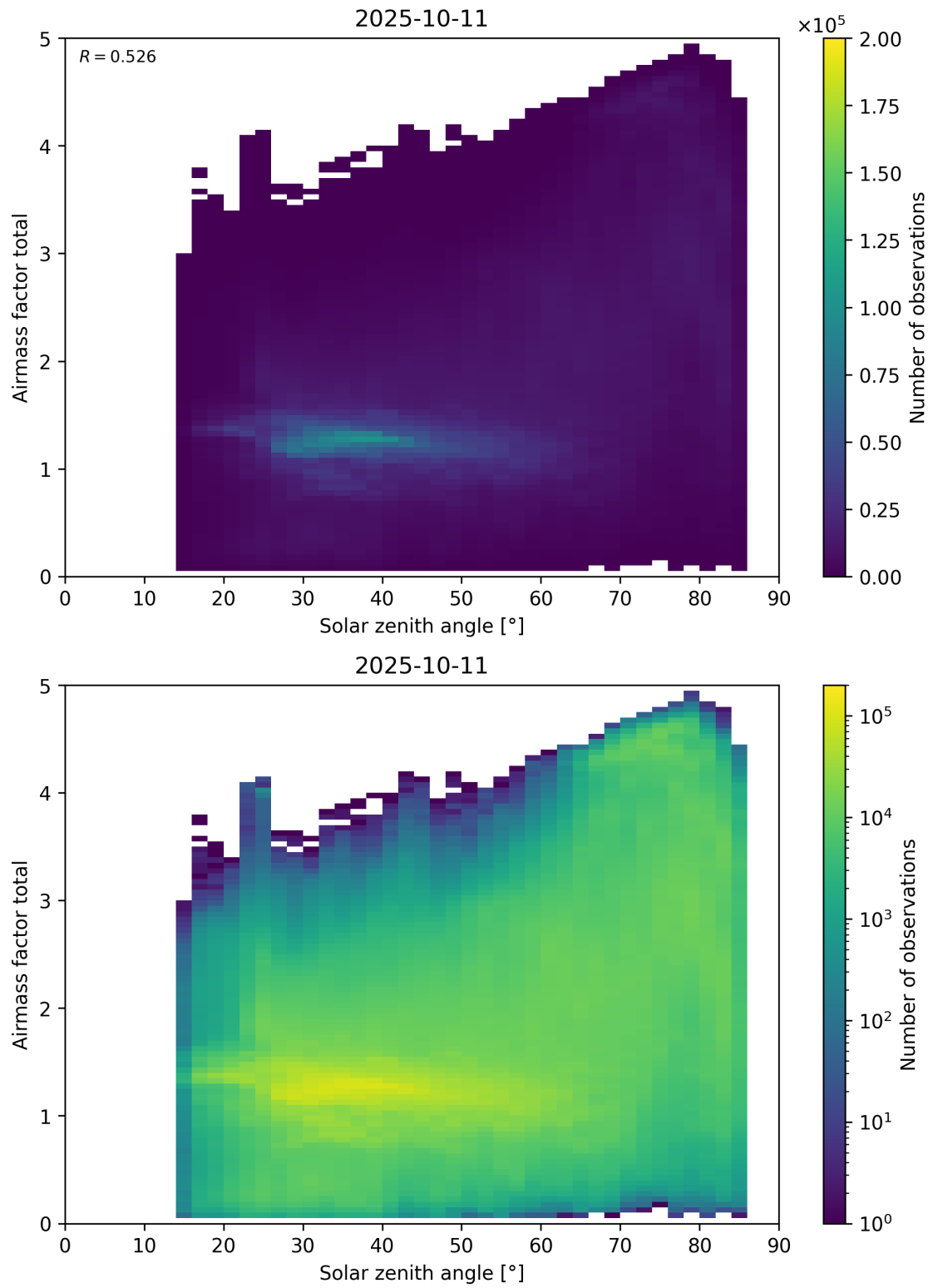
Figure 175: Scatter density plot of “Solar zenith angle” against “Airmass factor total” for 2025-10-11 to 2025-10-12.
