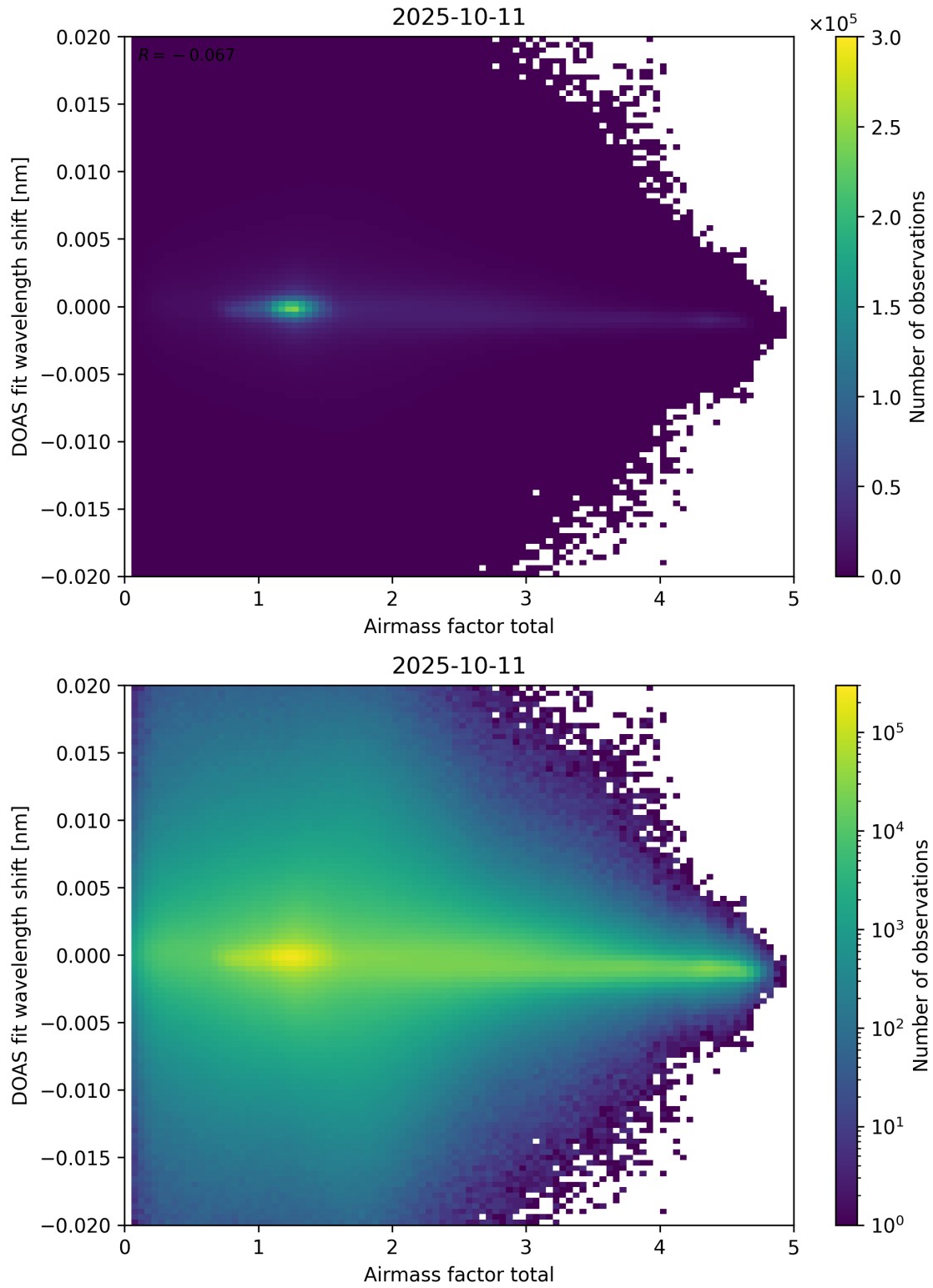
Figure 98: Scatter density plot of “Airmass factor total” against “DOAS fit wavelength shift” for 2025-10-11 to 2025-10-12.
