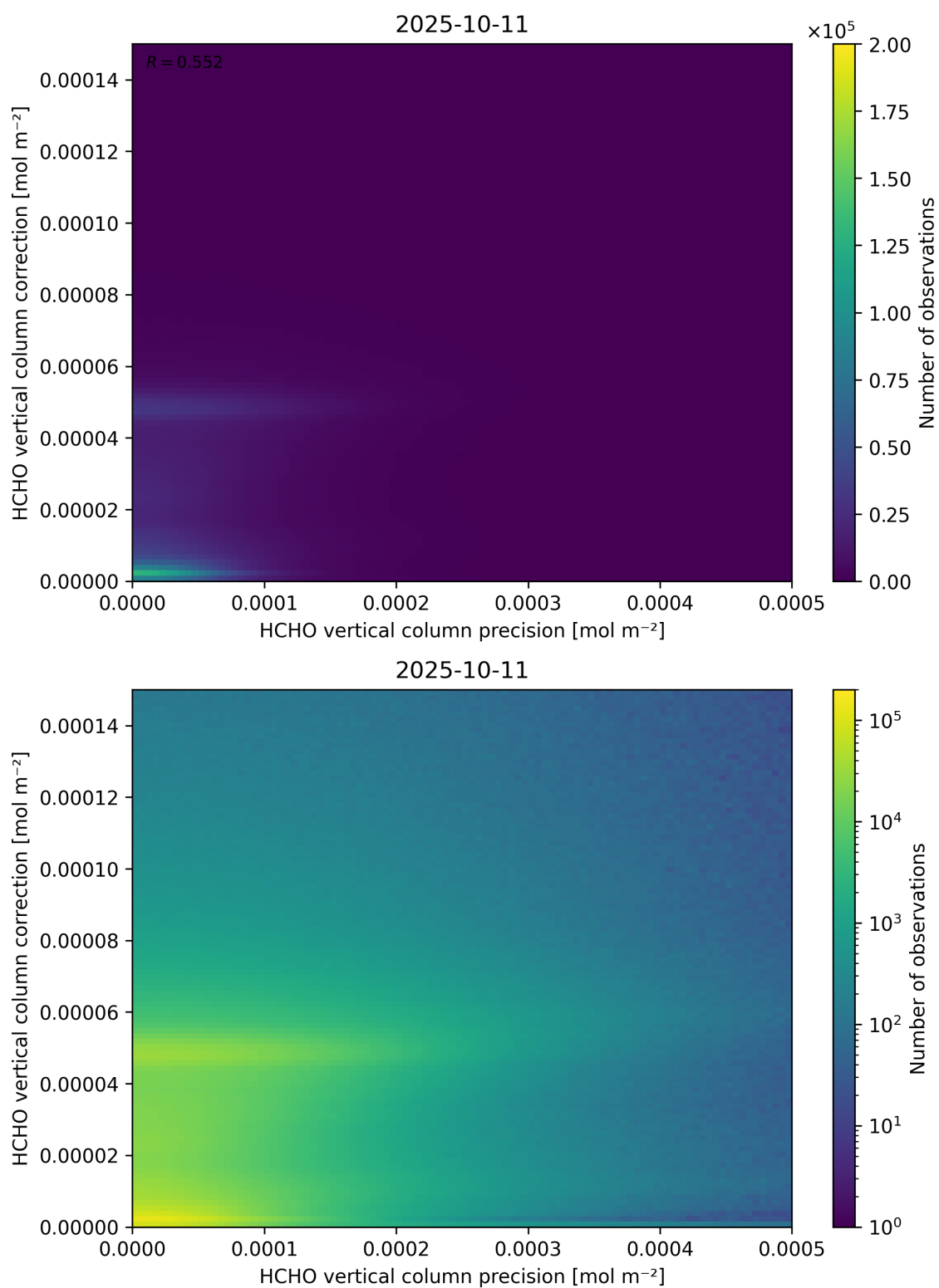
Figure 146: Scatter density plot of “HCHO vertical column precision” against “HCHO vertical column correction” for 2025-10-11 to 2025-10-12.
