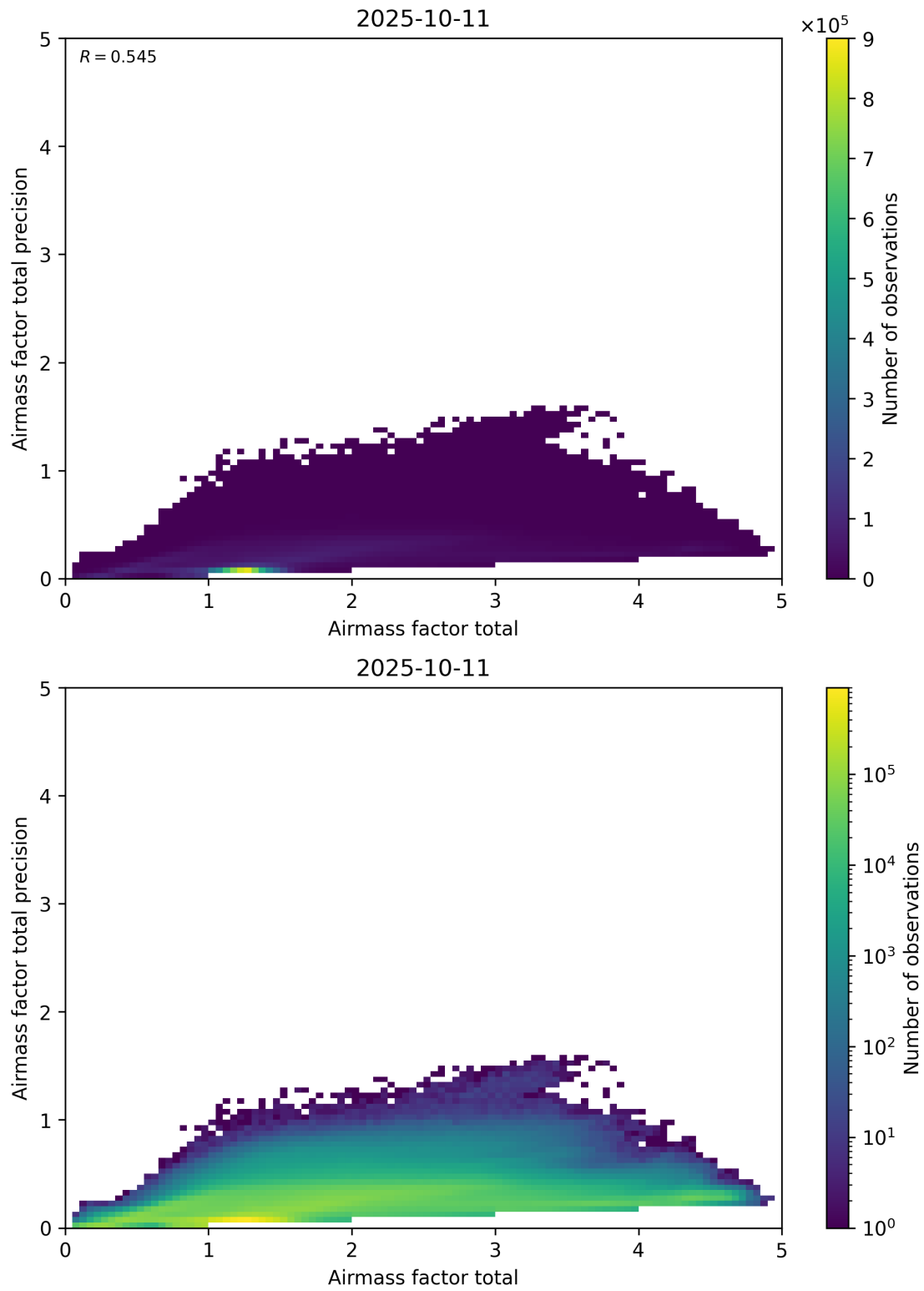
Figure 103: Scatter density plot of “Airmass factor total” against “Airmass factor total precision” for 2025-10-11 to 2025-10-12.
