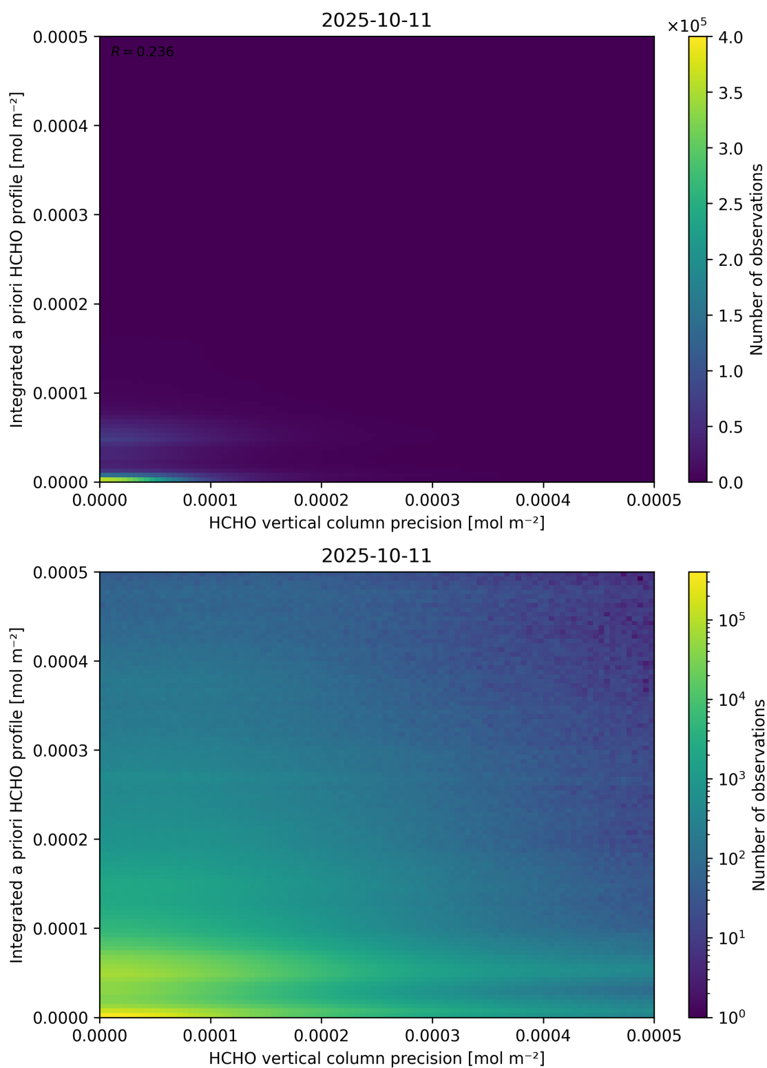
Figure 147: Scatter density plot of “HCHO vertical column precision” against “Integrated a priori HCHO profile” for 2025-10-11 to 2025-10-12.
