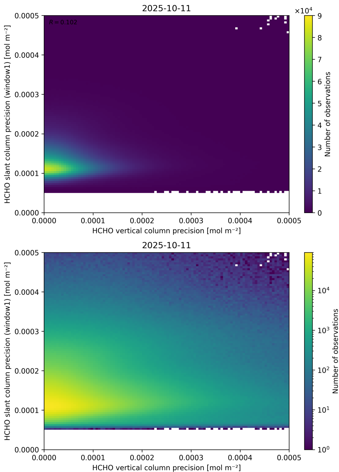
Figure 143: Scatter density plot of “HCHO vertical column precision” against “HCHO slant column precision (window1)” for 2025-10-11 to 2025-10-12.
