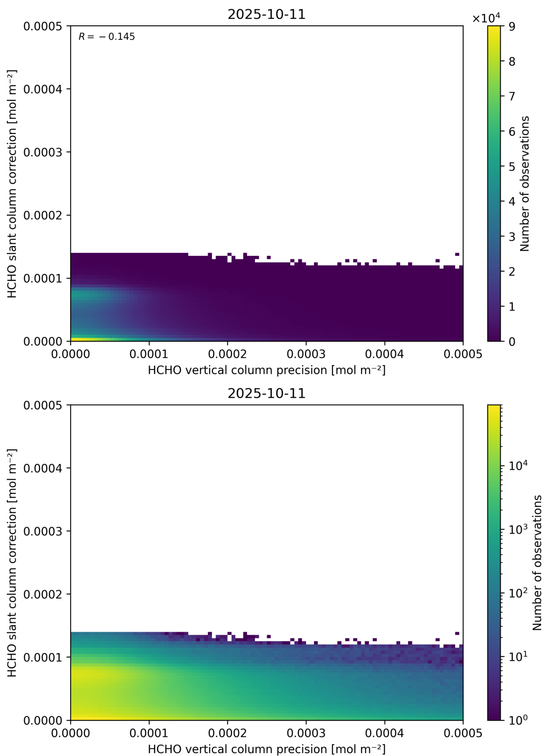
Figure 141: Scatter density plot of “HCHO vertical column precision” against “HCHO slant column correction” for 2025-10-11 to 2025-10-12.
