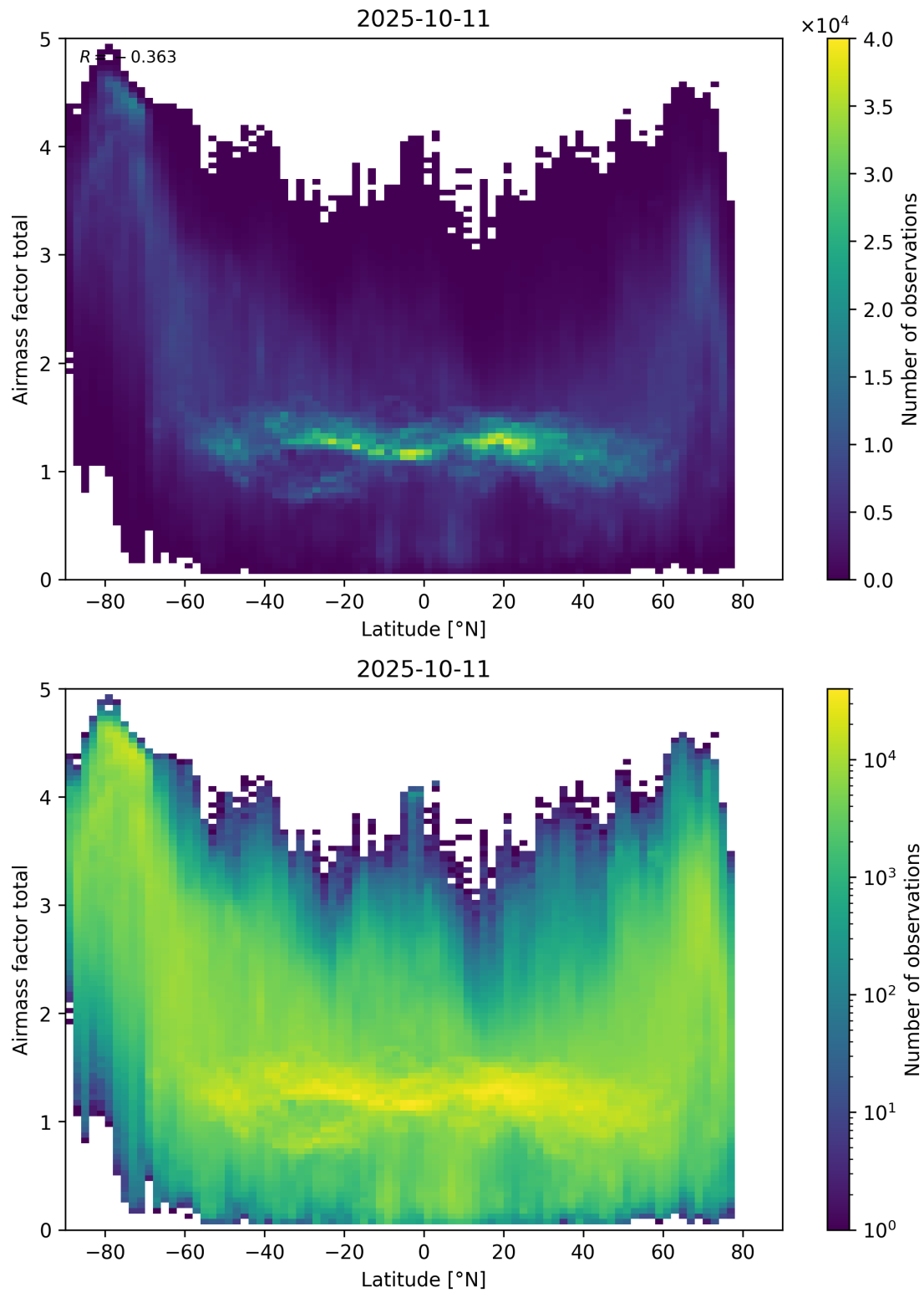
Figure 161: Scatter density plot of “Latitude” against “Airmass factor total” for 2025-10-11 to 2025-10-12.
