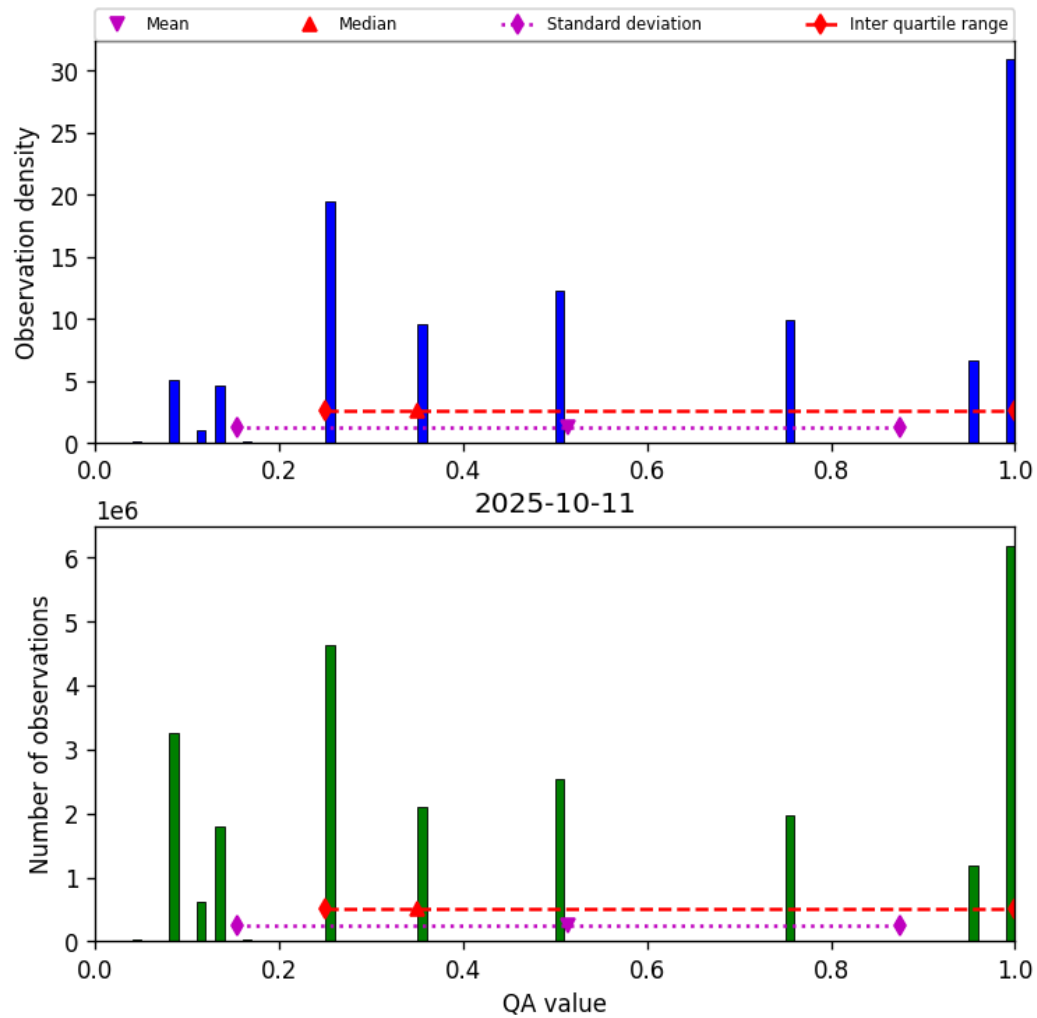
Figure 34: Histogram of “QA value” for 2025-10-11 to 2025-10-12
