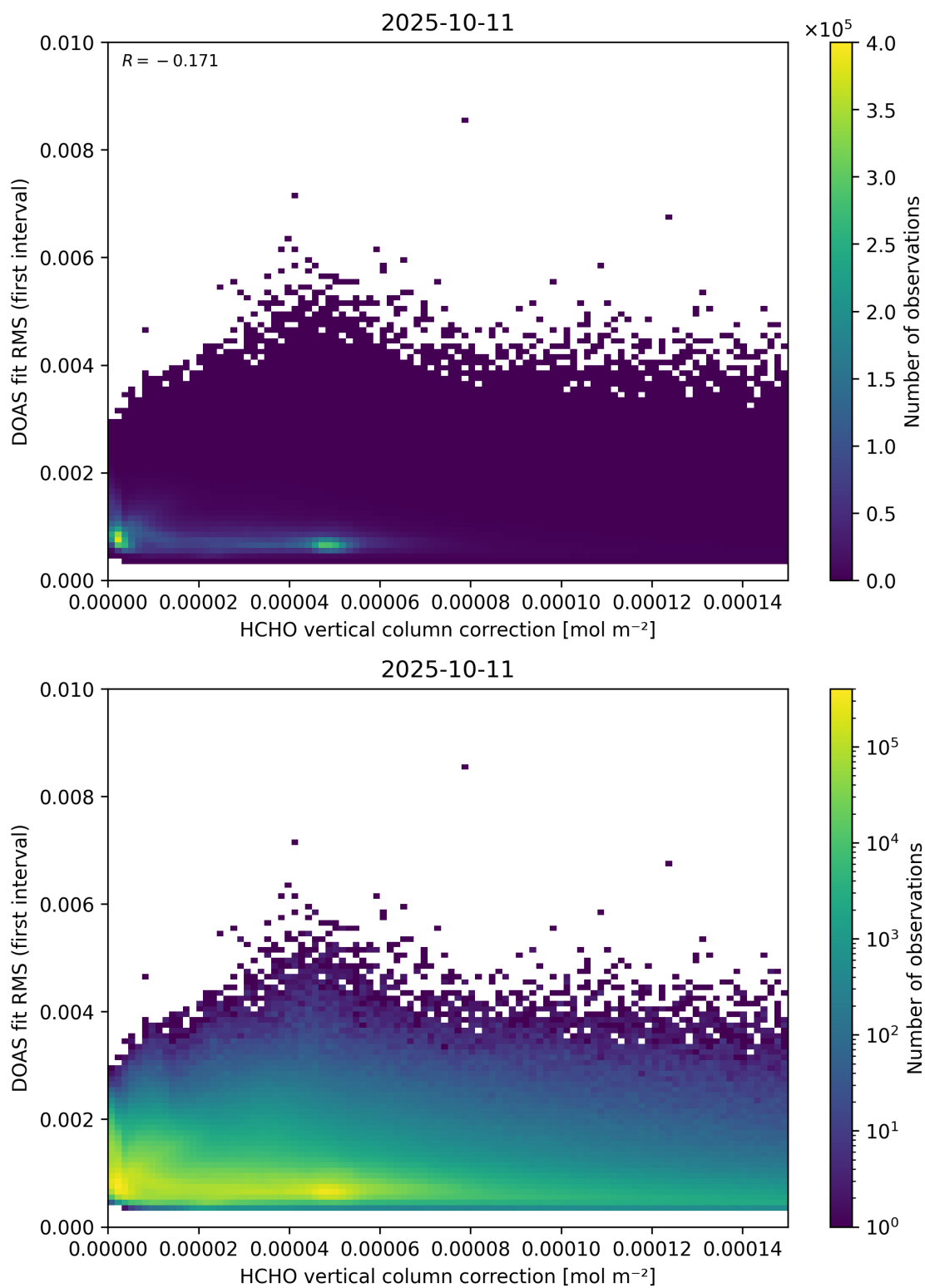
Figure 112: Scatter density plot of “HCHO vertical column correction” against “DOAS fit RMS (first interval)” for 2025-10-11 to 2025-10-12.
