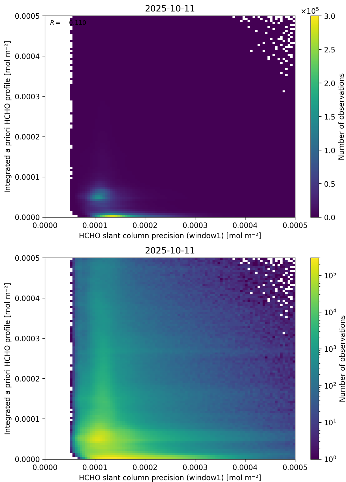
Figure 96: Scatter density plot of “HCHO slant column precision (window1)” against “Integrated a priori HCHO profile” for 2025-10-11 to 2025-10-12.
