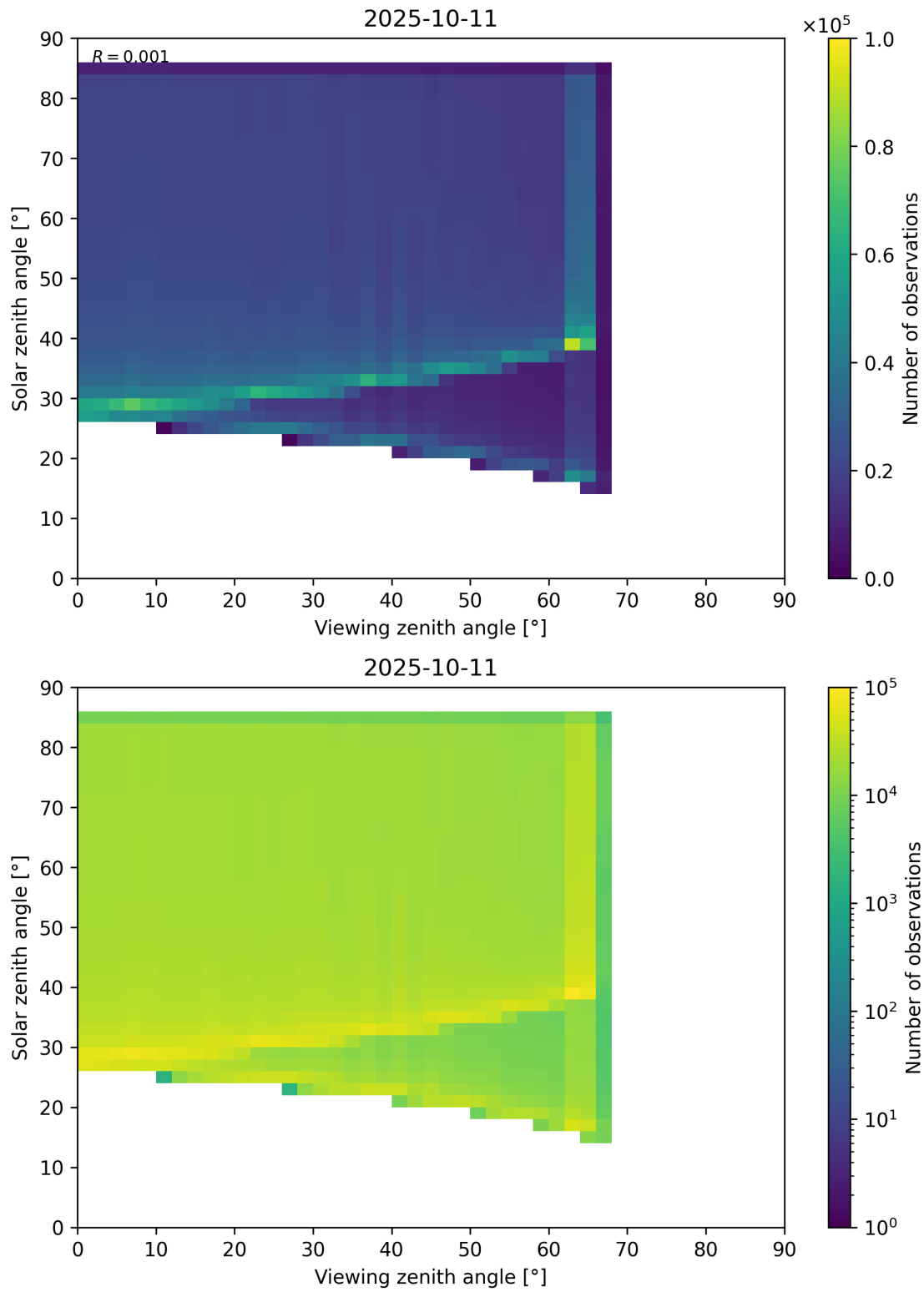
Figure 197: Scatter density plot of “Viewing zenith angle” against “Solar zenith angle” for 2025-10-11 to 2025-10-12.
