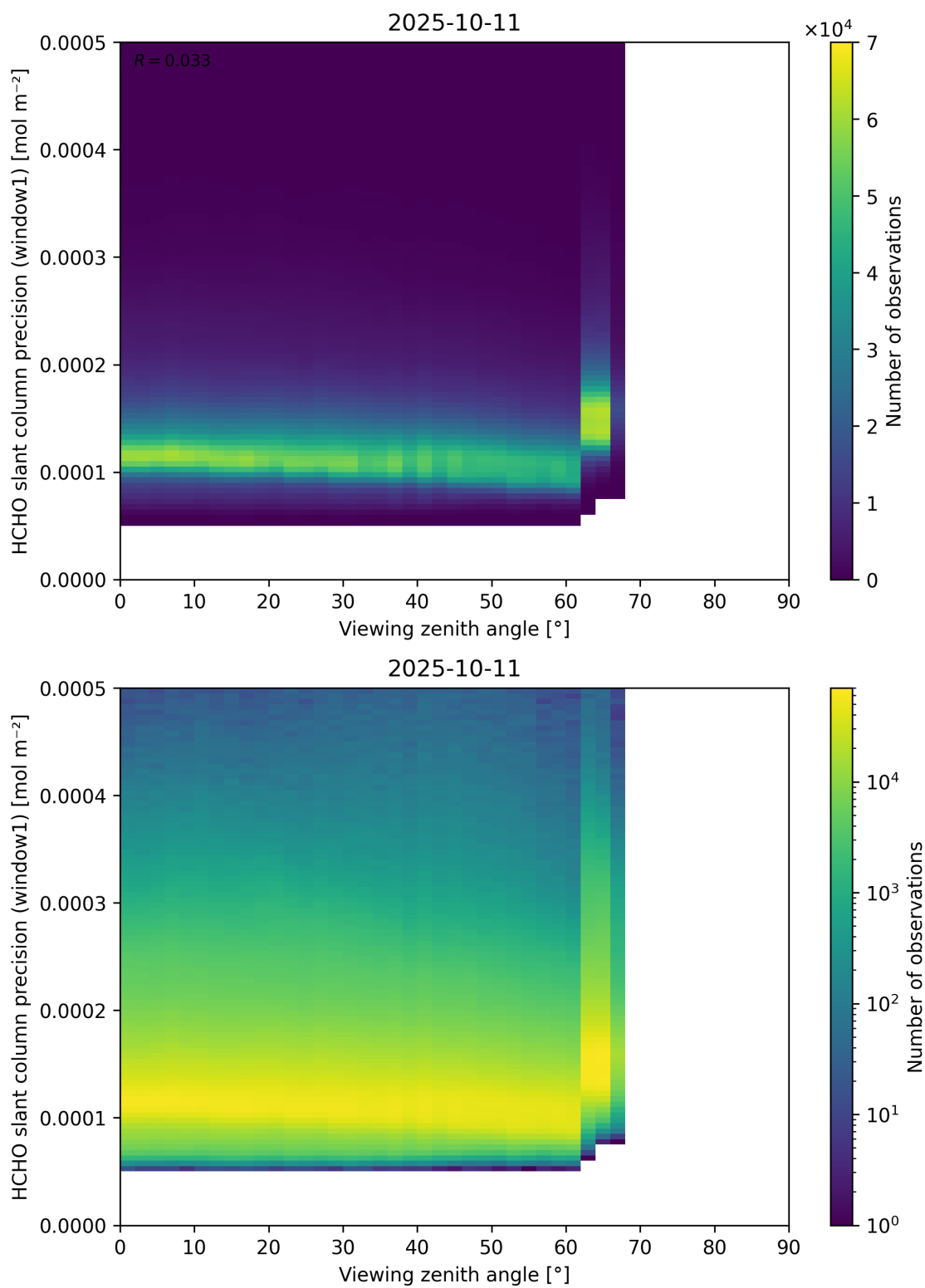
Figure 189: Scatter density plot of “Viewing zenith angle” against “HCHO slant column precision (window1)” for 2025-10-11 to 2025-10-12.
