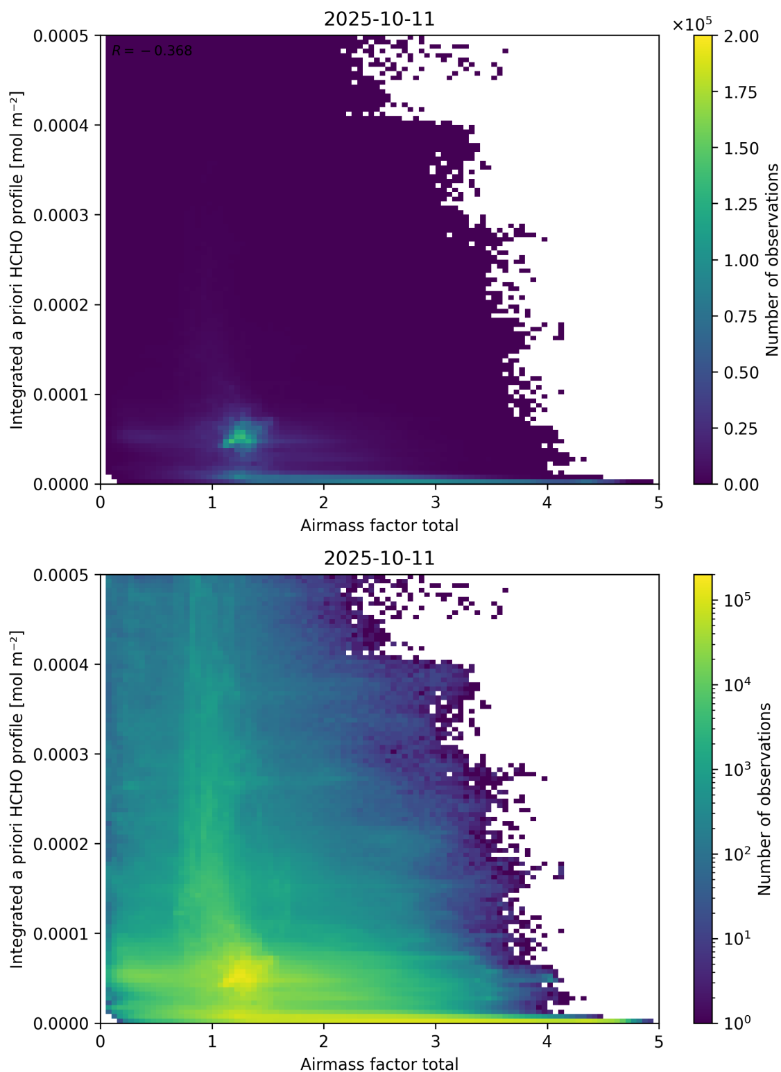
Figure 104: Scatter density plot of “Airmass factor total” against “Integrated a priori HCHO profile” for 2025-10-11 to 2025-10-12.
