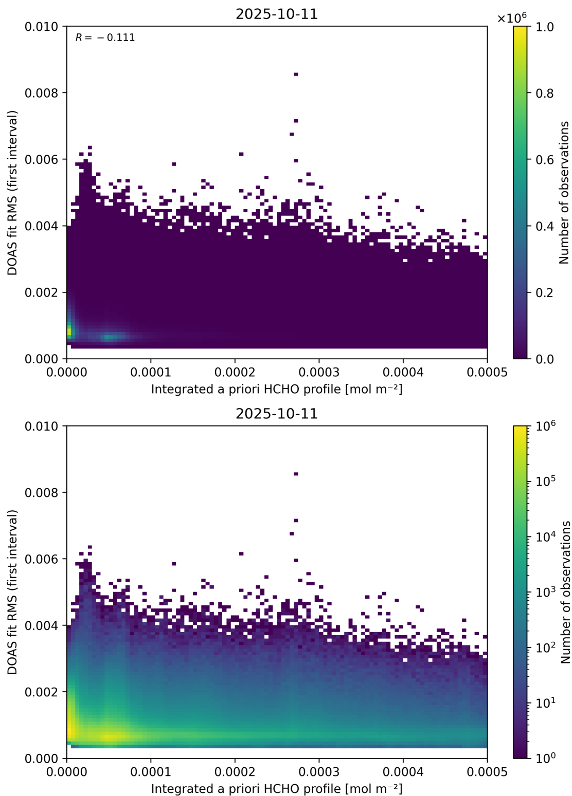
Figure 148: Scatter density plot of “Integrated a priori HCHO profile” against “DOAS fit RMS (first interval)” for 2025-10-11 to 2025-10-12.
