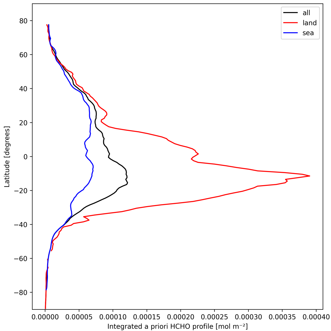
Figure 29: Zonal average of “Integrated a priori HCHO profile” for 2025-10-11 to 2025-10-12.
