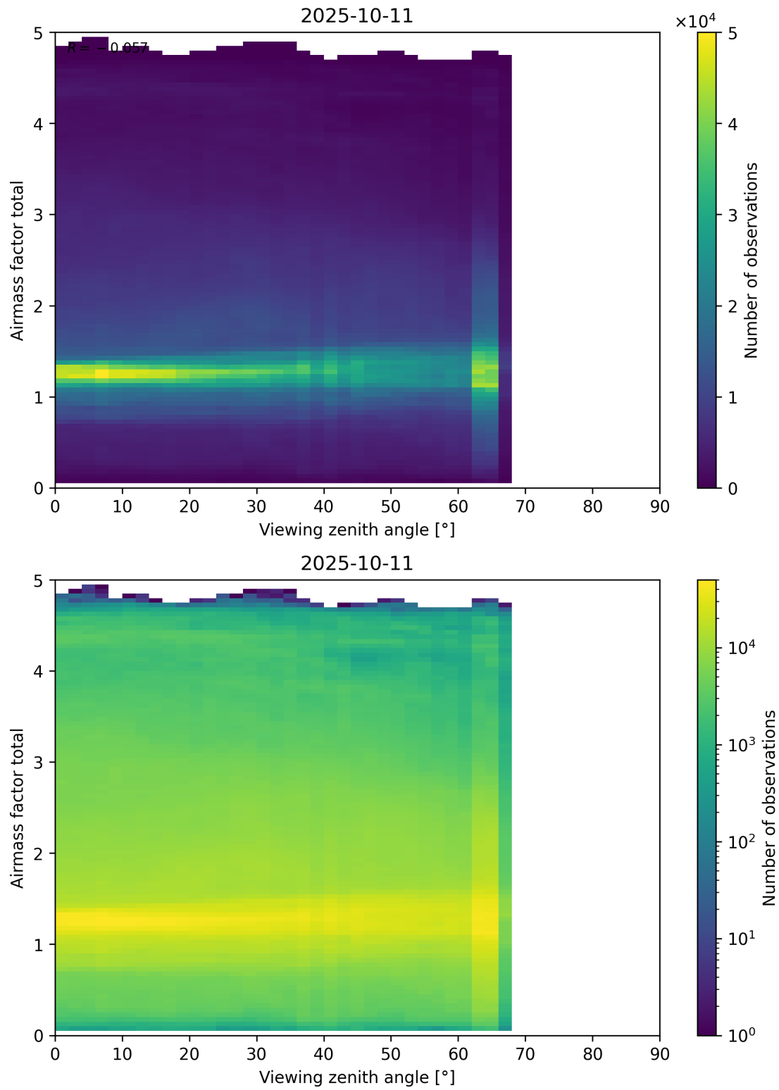
Figure 190: Scatter density plot of “Viewing zenith angle” against “Airmass factor total” for 2025-10-11 to 2025-10-12.
