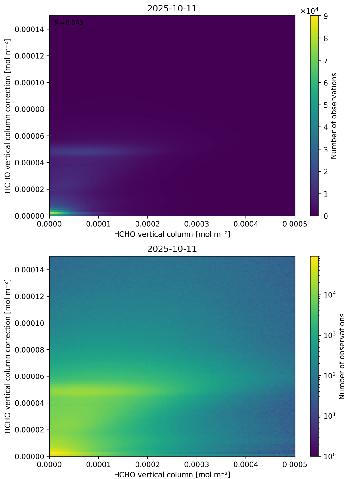
Figure 133: Scatter density plot of “HCHO vertical column” against “HCHO vertical column correction” for 2025-10-11 to 2025-10-12.
