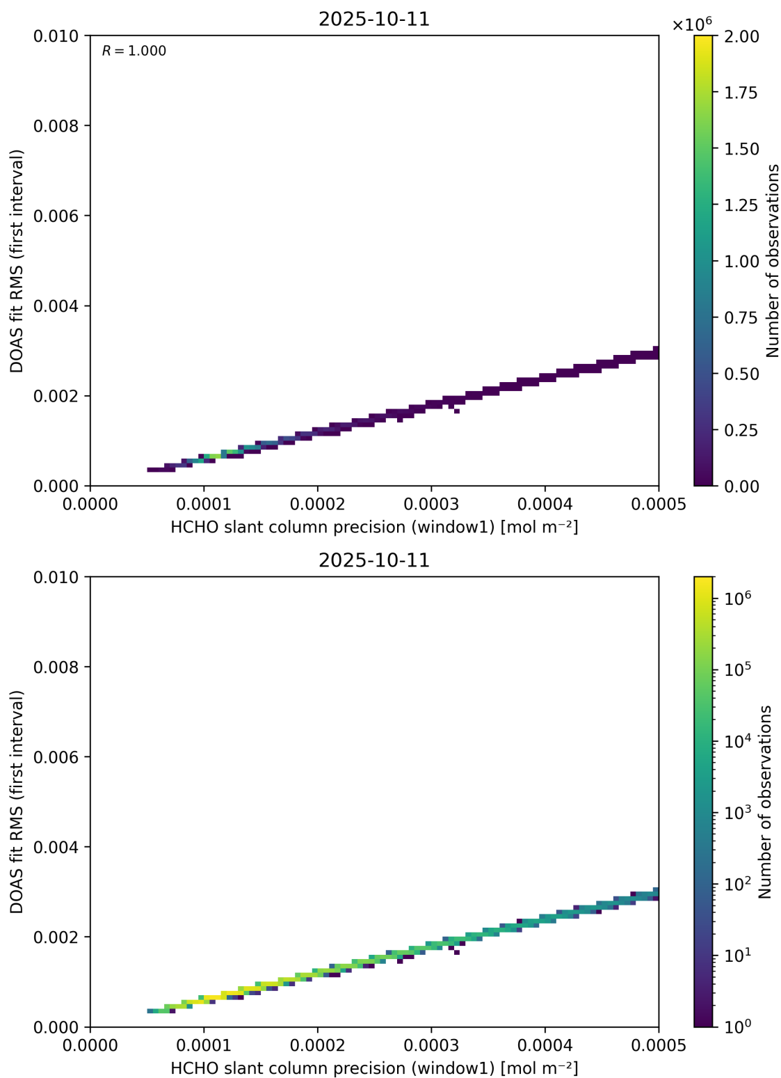
Figure 88: Scatter density plot of “HCHO slant column precision (window1)” against “DOAS fit RMS (first interval)” for 2025-10-11 to 2025-10-12.
