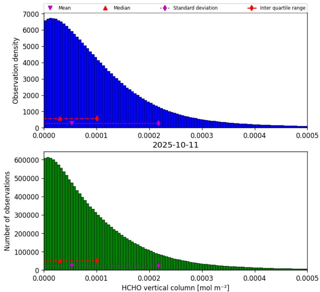
Figure 35: Histogram of “HCHO vertical column” for 2025-10-11 to 2025-10-12
