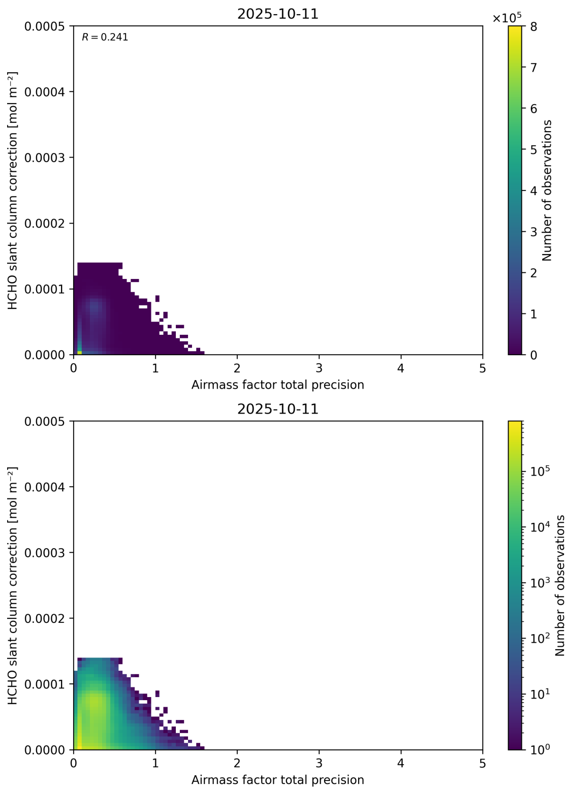
Figure 110: Scatter density plot of “Airmass factor total precision” against “HCHO slant column correction” for 2025-10-11 to 2025-10-12.
