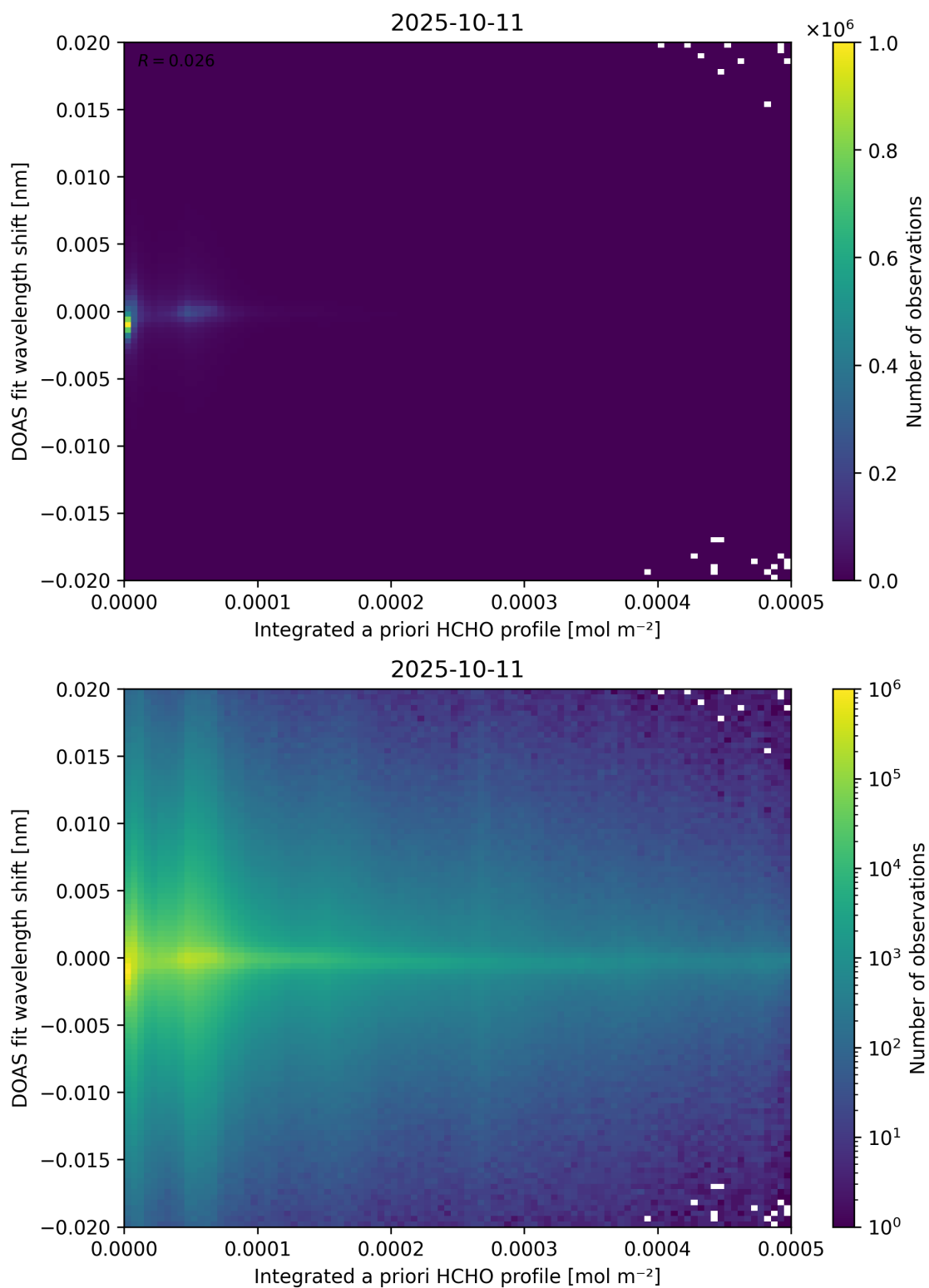
Figure 149: Scatter density plot of “Integrated a priori HCHO profile” against “DOAS fit wavelength shift” for 2025-10-11 to 2025-10-12.
