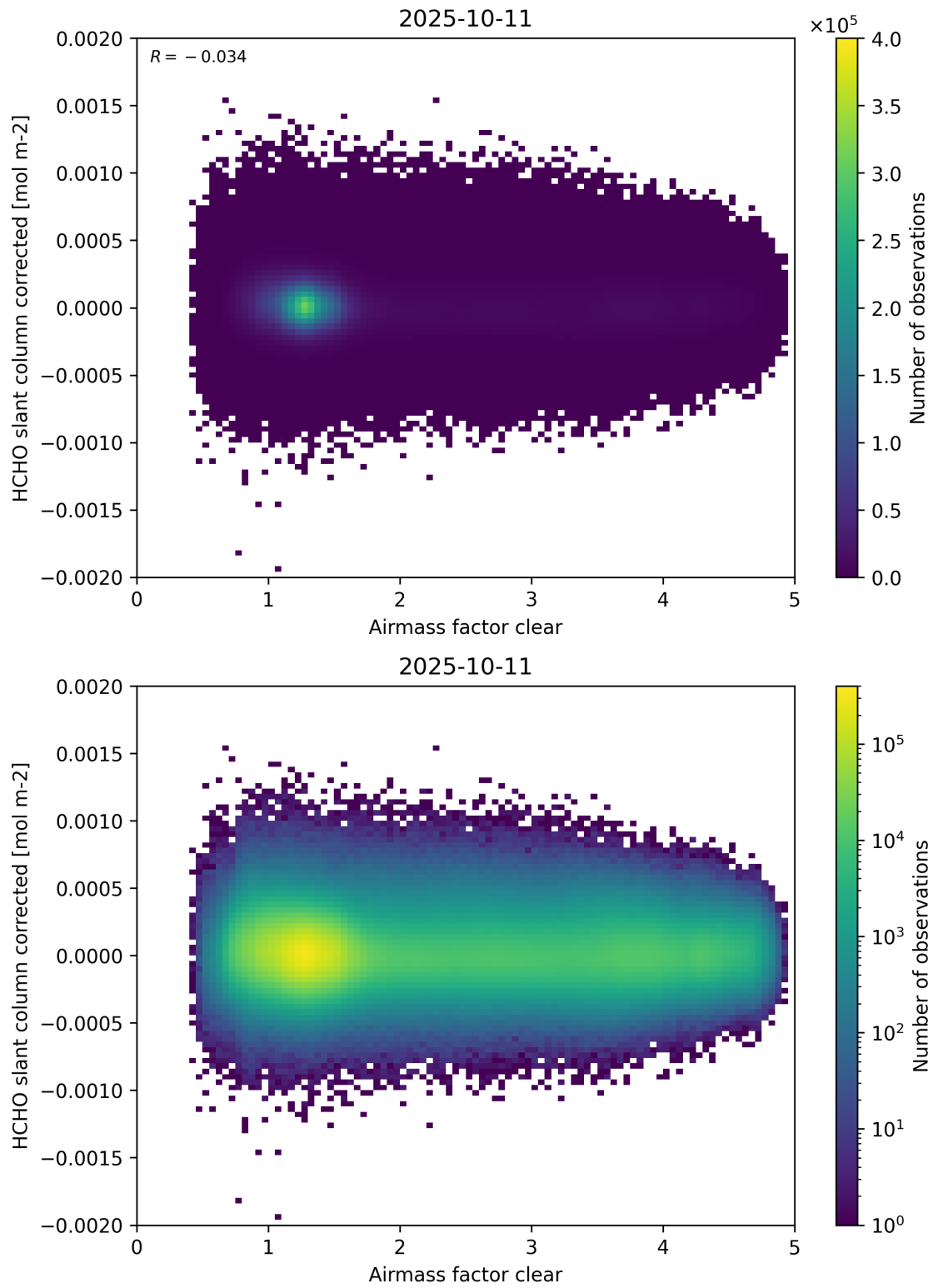
Figure 74: Scatter density plot of “Airmass factor clear” against “HCHO slant column corrected” for 2025-10-11 to 2025-10-12.
