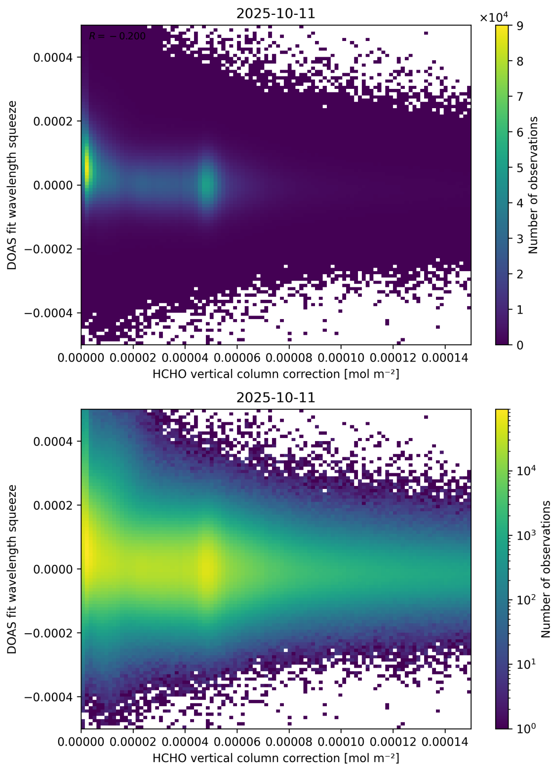
Figure 114: Scatter density plot of “HCHO vertical column correction” against “DOAS fit wavelength squeeze” for 2025-10-11 to 2025-10-12.
