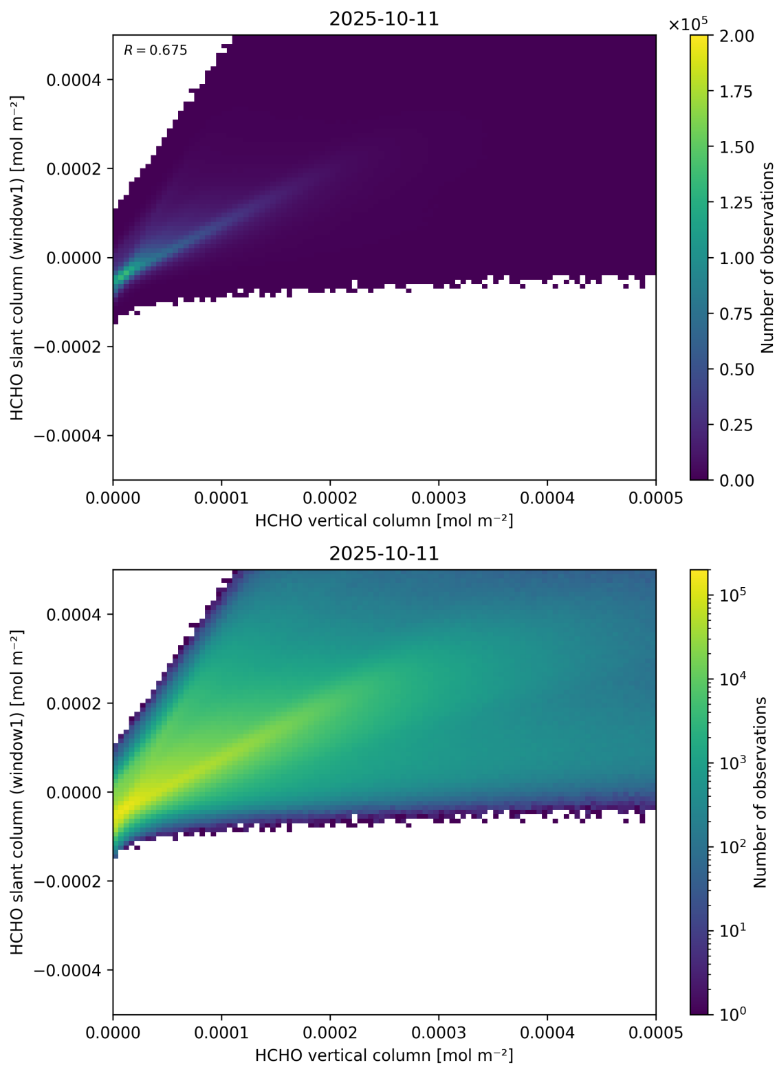
Figure 129: Scatter density plot of “HCHO vertical column” against “HCHO slant column (window1)” for 2025-10-11 to 2025-10-12.
