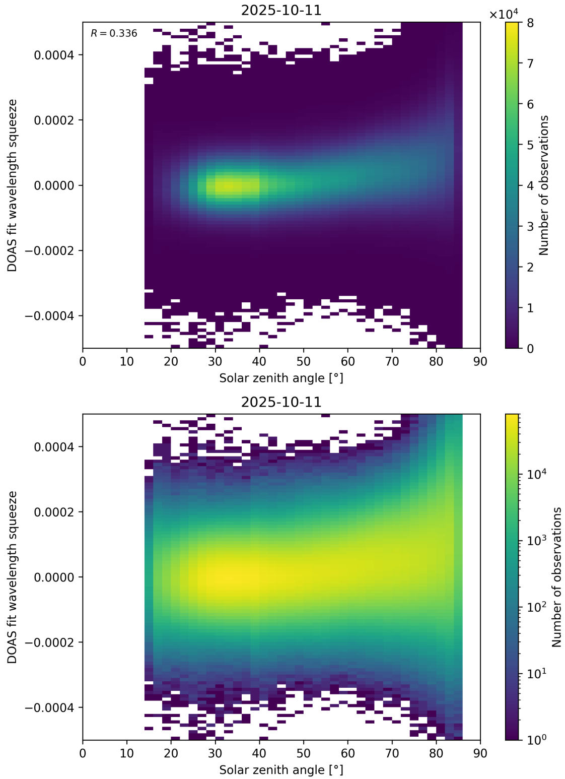
Figure 169: Scatter density plot of “Solar zenith angle” against “DOAS fit wavelength squeeze” for 2025-10-11 to 2025-10-12.
