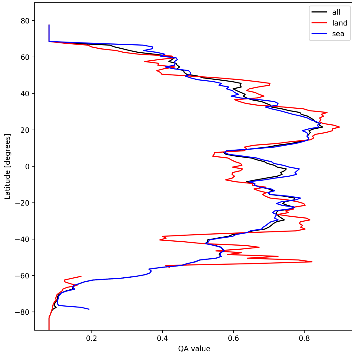
Figure 20: Zonal average of “QA value” for 2025-10-11 to 2025-10-12.
