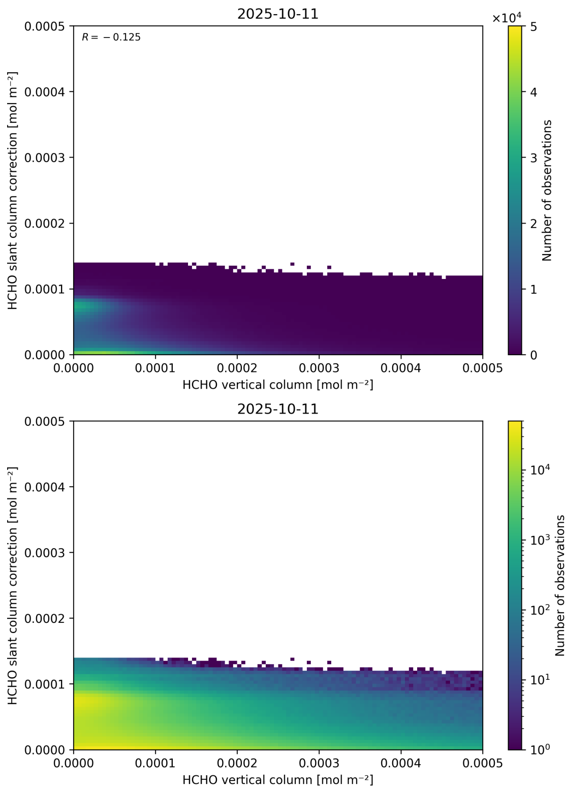
Figure 128: Scatter density plot of “HCHO vertical column” against “HCHO slant column correction” for 2025-10-11 to 2025-10-12.
