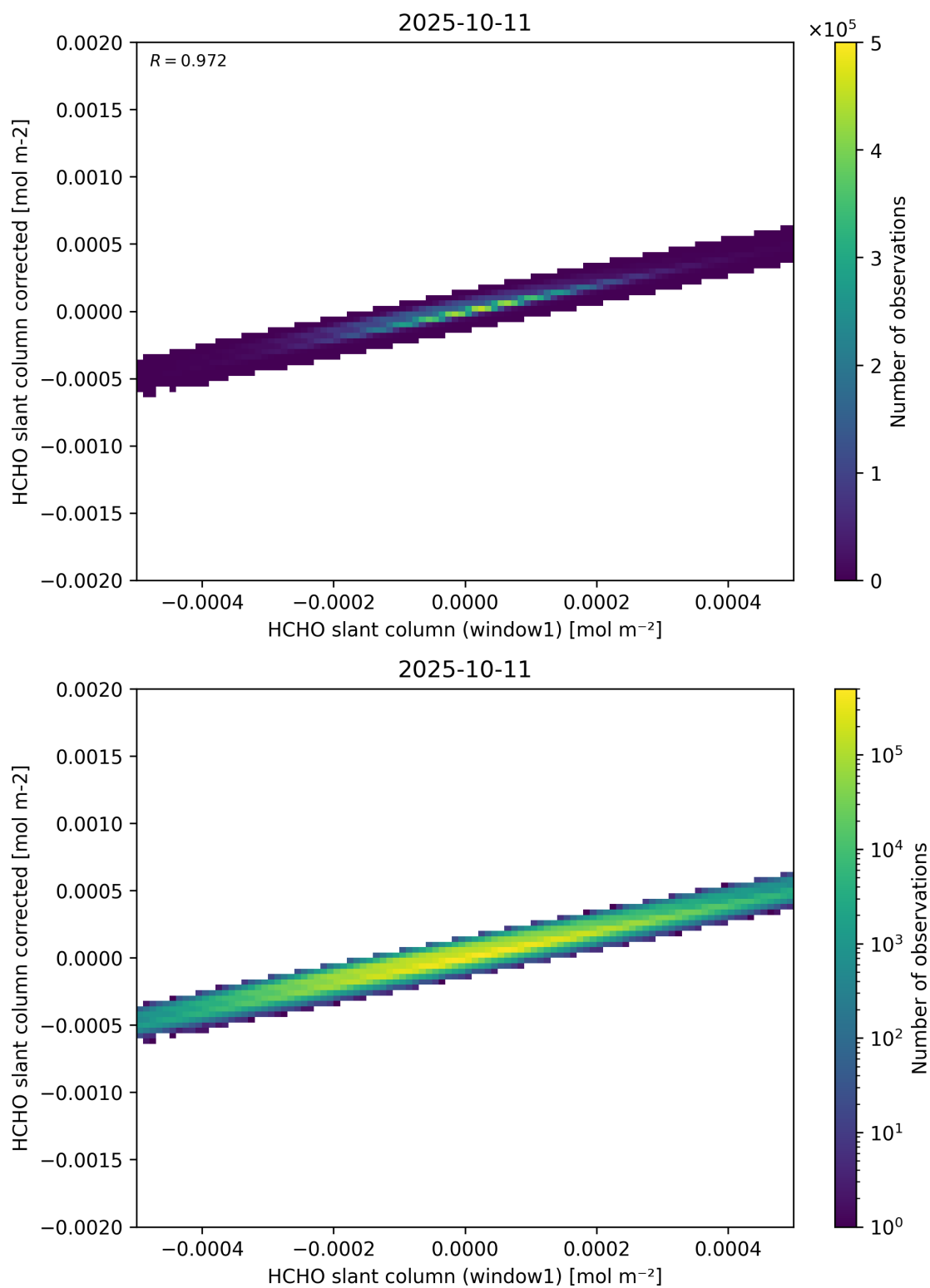
Figure 82: Scatter density plot of “HCHO slant column (window1)” against “HCHO slant column corrected” for 2025-10-11 to 2025-10-12.
