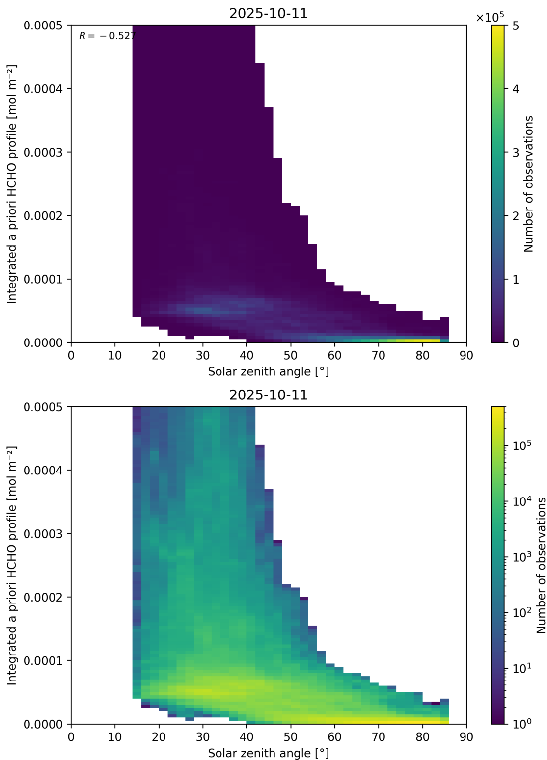
Figure 180: Scatter density plot of “Solar zenith angle” against “Integrated a priori HCHO profile” for 2025-10-11 to 2025-10-12.
