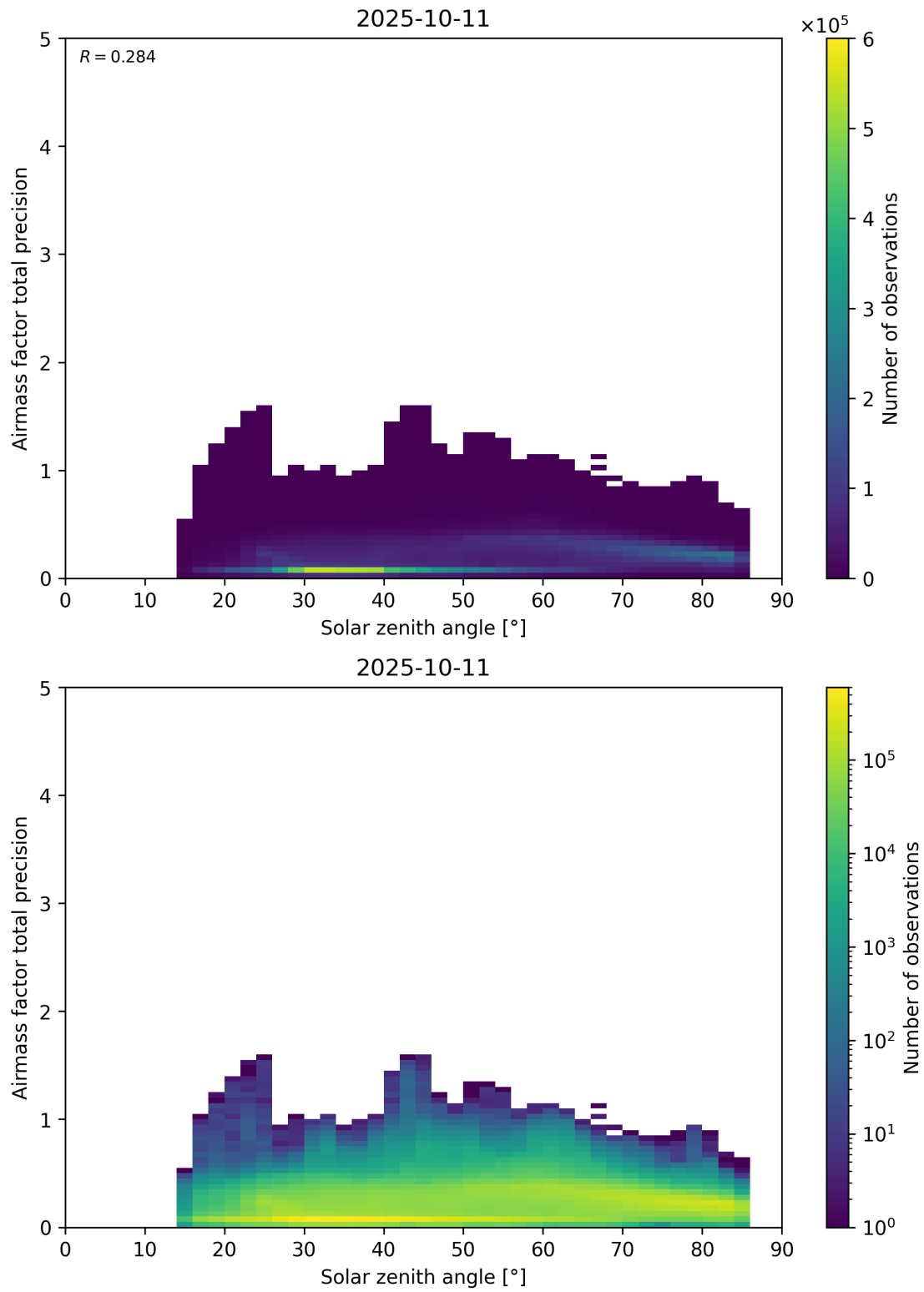
Figure 176: Scatter density plot of “Solar zenith angle” against “Airmass factor total precision” for 2025-10-11 to 2025-10-12.
