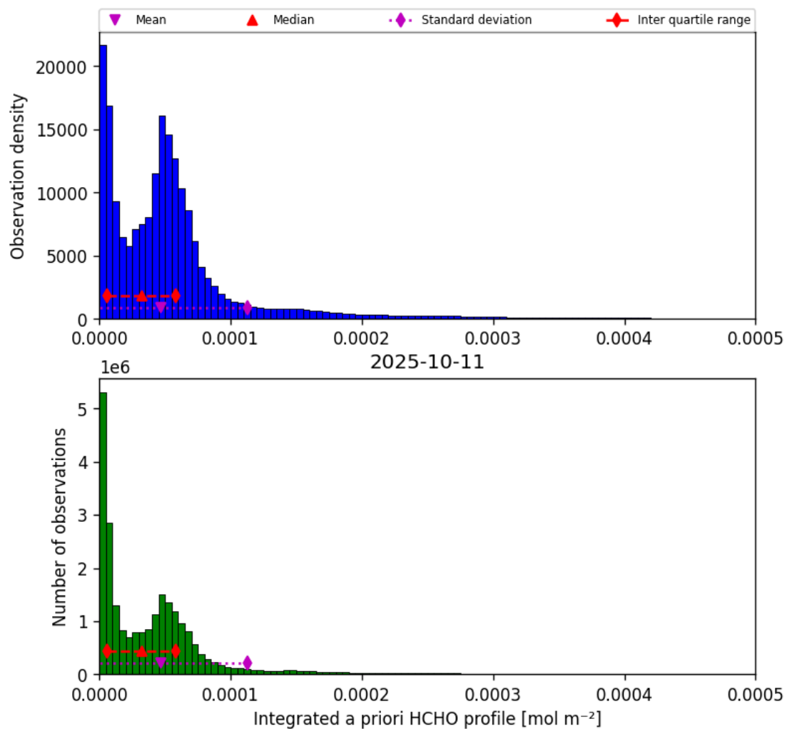
Figure 43: Histogram of “Integrated a priori HCHO profile” for 2025-10-11 to 2025-10-12
