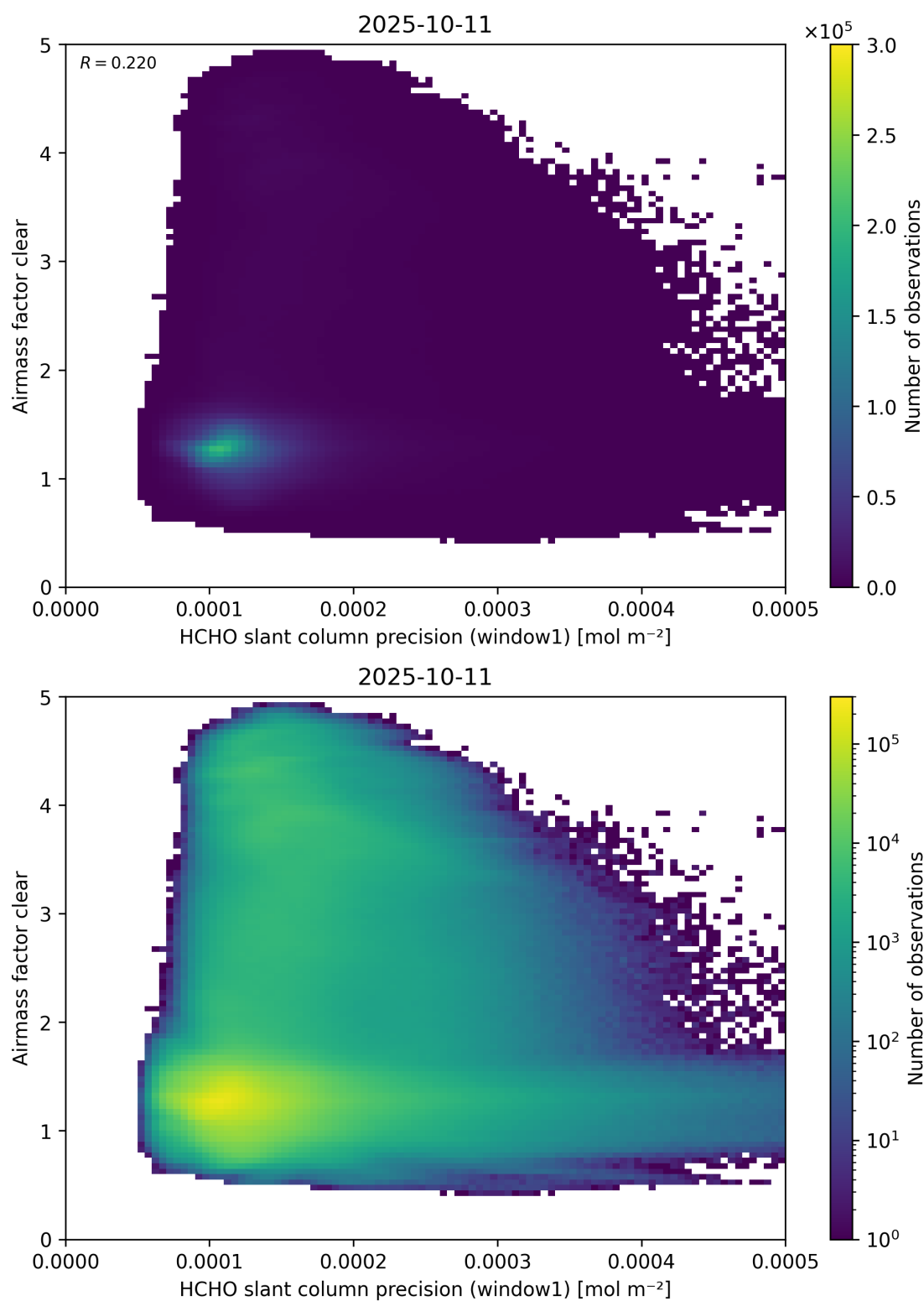
Figure 91: Scatter density plot of “HCHO slant column precision (window1)” against “Airmass factor clear” for 2025-10-11 to 2025-10-12.
