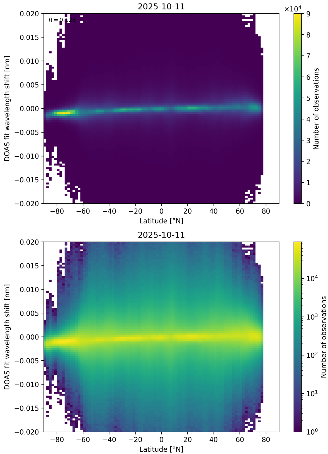
Figure 154: Scatter density plot of “Latitude” against “DOAS fit wavelength shift” for 2025-10-11 to 2025-10-12.
