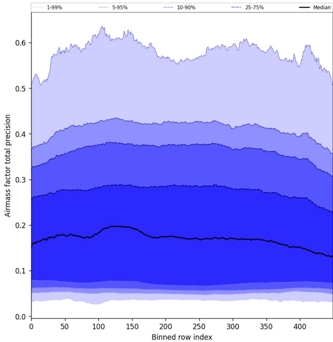
Figure 55: Along track statistics of “Airmass factor total precision” for 2025-10-11 to 2025-10-12
