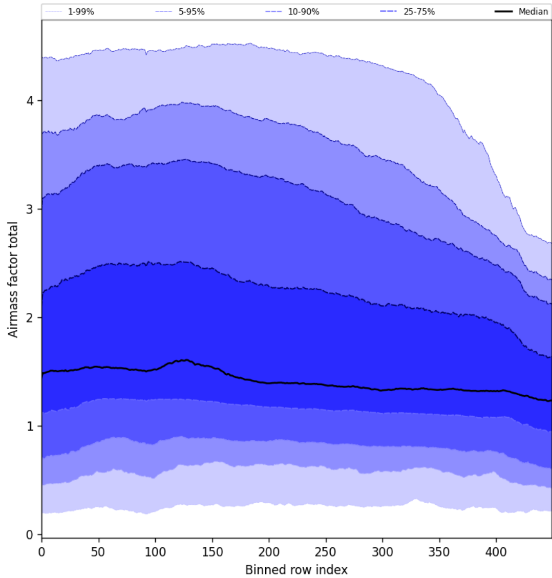
Figure 54: Along track statistics of “Airmass factor total” for 2025-10-11 to 2025-10-12
