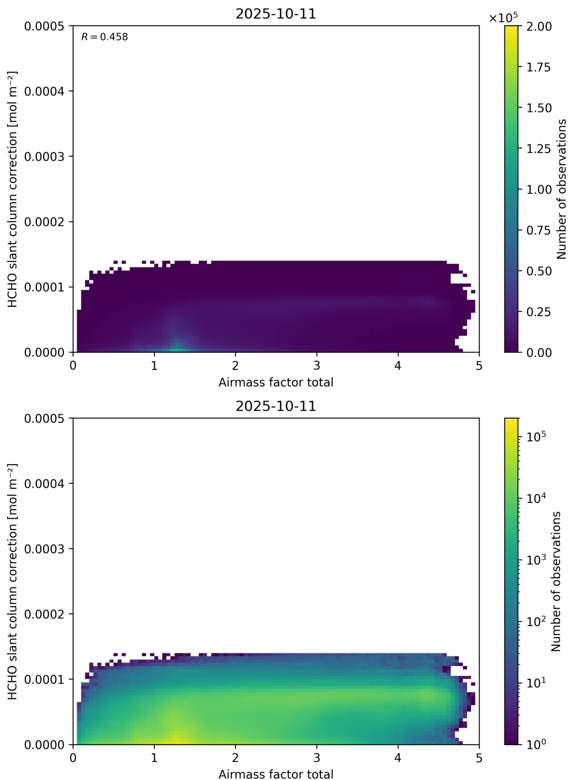
Figure 102: Scatter density plot of “Airmass factor total” against “HCHO slant column correction” for 2025-10-11 to 2025-10-12.
