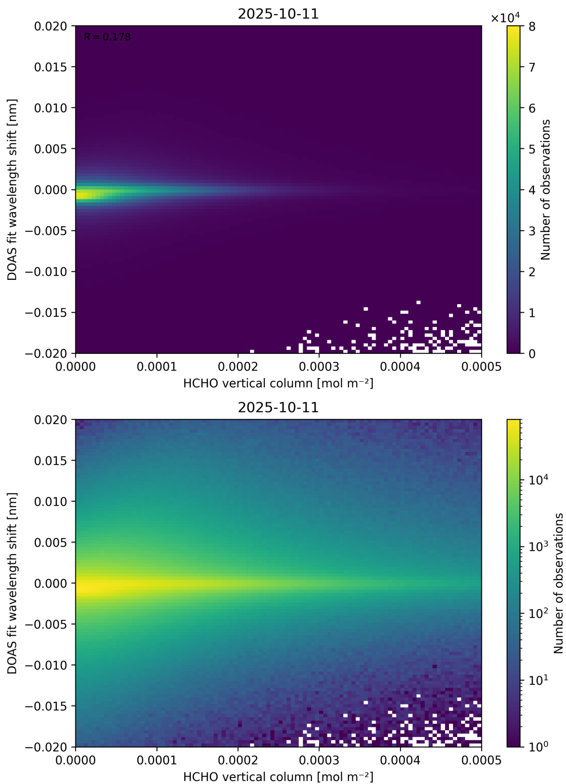
Figure 124: Scatter density plot of “HCHO vertical column” against “DOAS fit wavelength shift” for 2025-10-11 to 2025-10-12.
