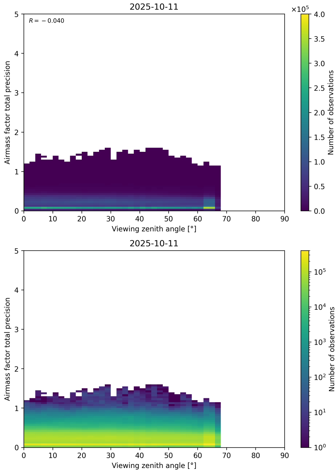
Figure 191: Scatter density plot of “Viewing zenith angle” against “Airmass factor total precision” for 2025-10-11 to 2025-10-12.
