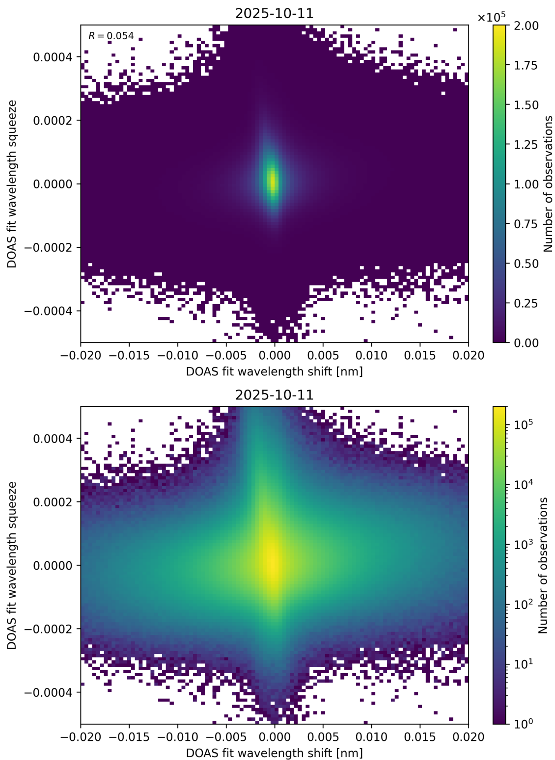
Figure 65: Scatter density plot of “DOAS fit wavelength shift” against “DOAS fit wavelength squeeze” for 2025-10-11 to 2025-10-12.
