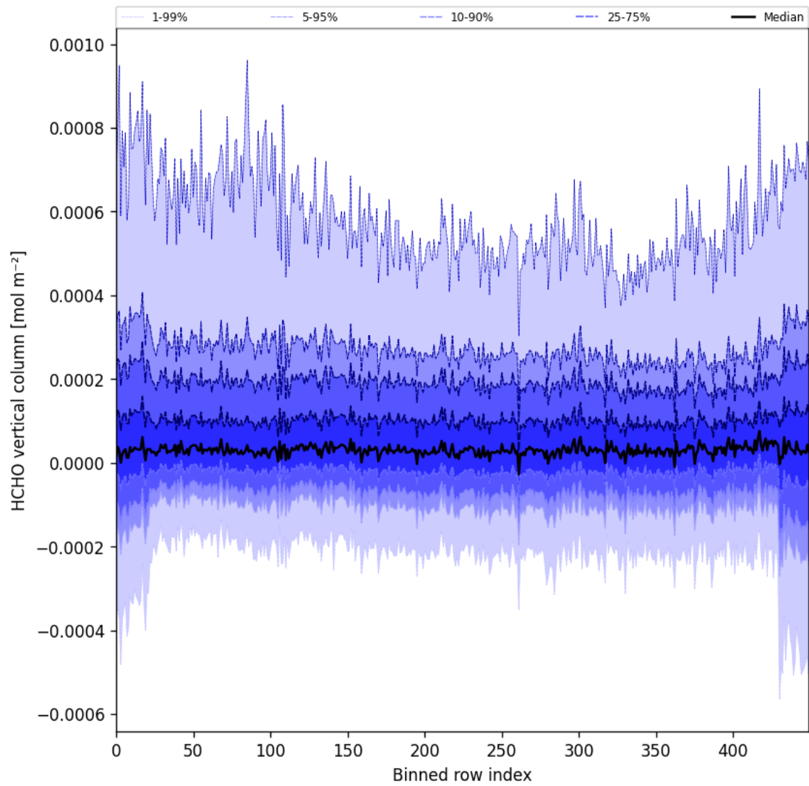
Figure 49: Along track statistics of “HCHO vertical column” for 2025-10-11 to 2025-10-12
