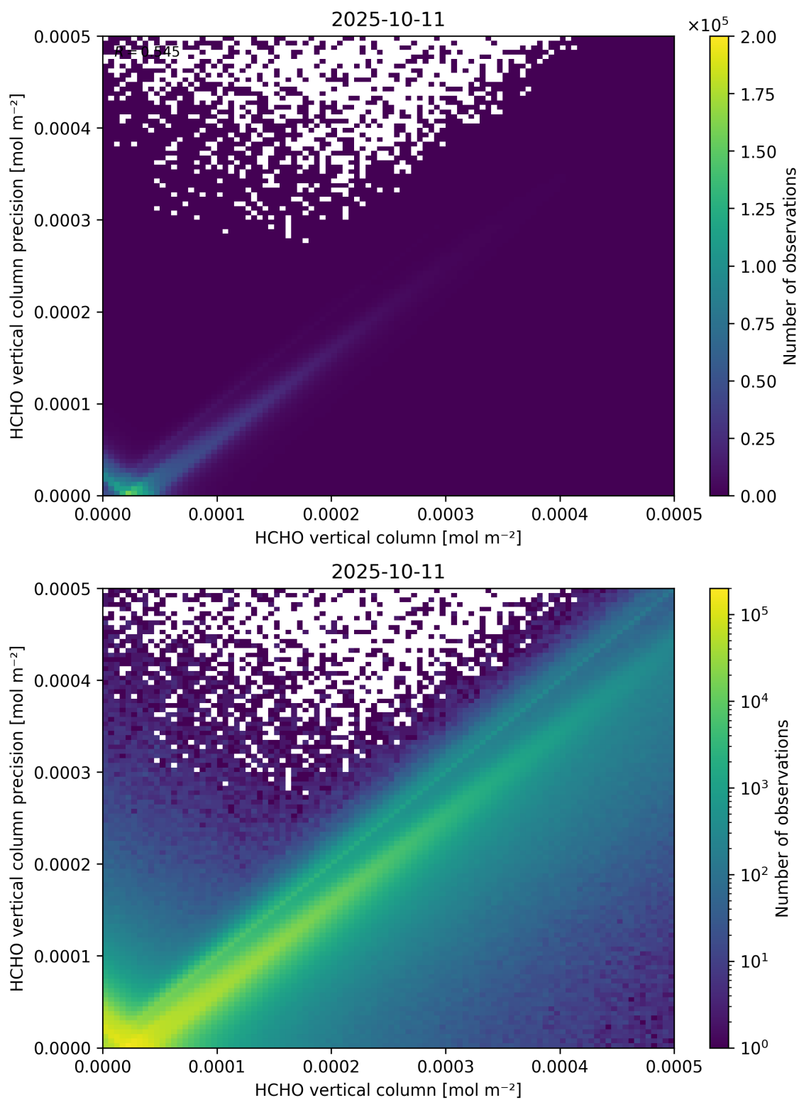
Figure 134: Scatter density plot of “HCHO vertical column” against “HCHO vertical column precision” for 2025-10-11 to 2025-10-12.
