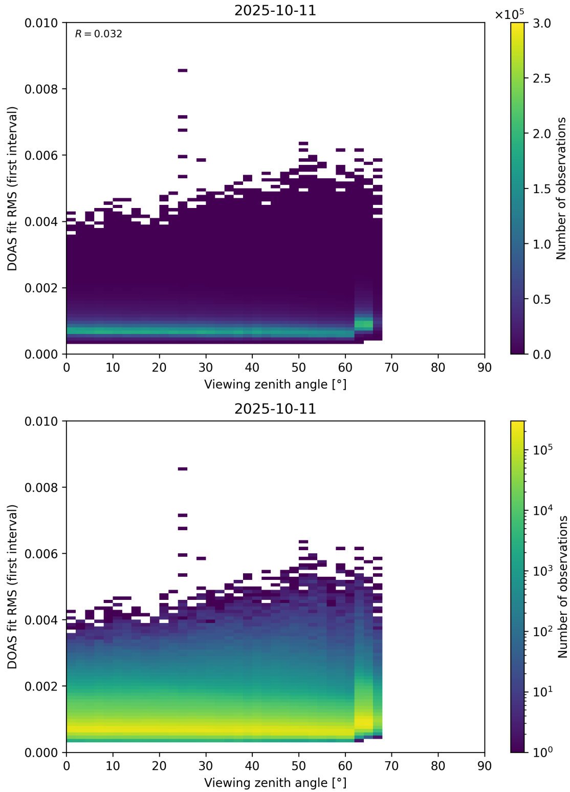
Figure 182: Scatter density plot of “Viewing zenith angle” against “DOAS fit RMS (first interval)” for 2025-10-11 to 2025-10-12.
