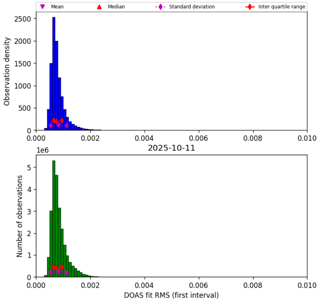
Figure 46: Histogram of “DOAS fit RMS (first interval)” for 2025-10-11 to 2025-10-12
