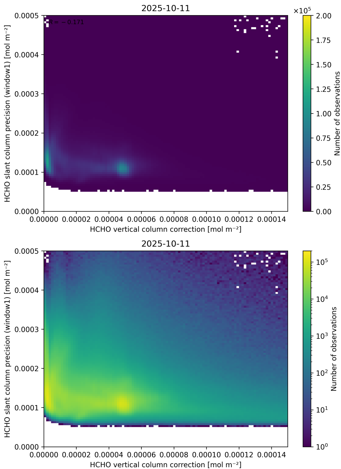
Figure 119: Scatter density plot of “HCHO vertical column correction” against “HCHO slant column precision (window1)” for 2025-10-11 to 2025-10-12.
