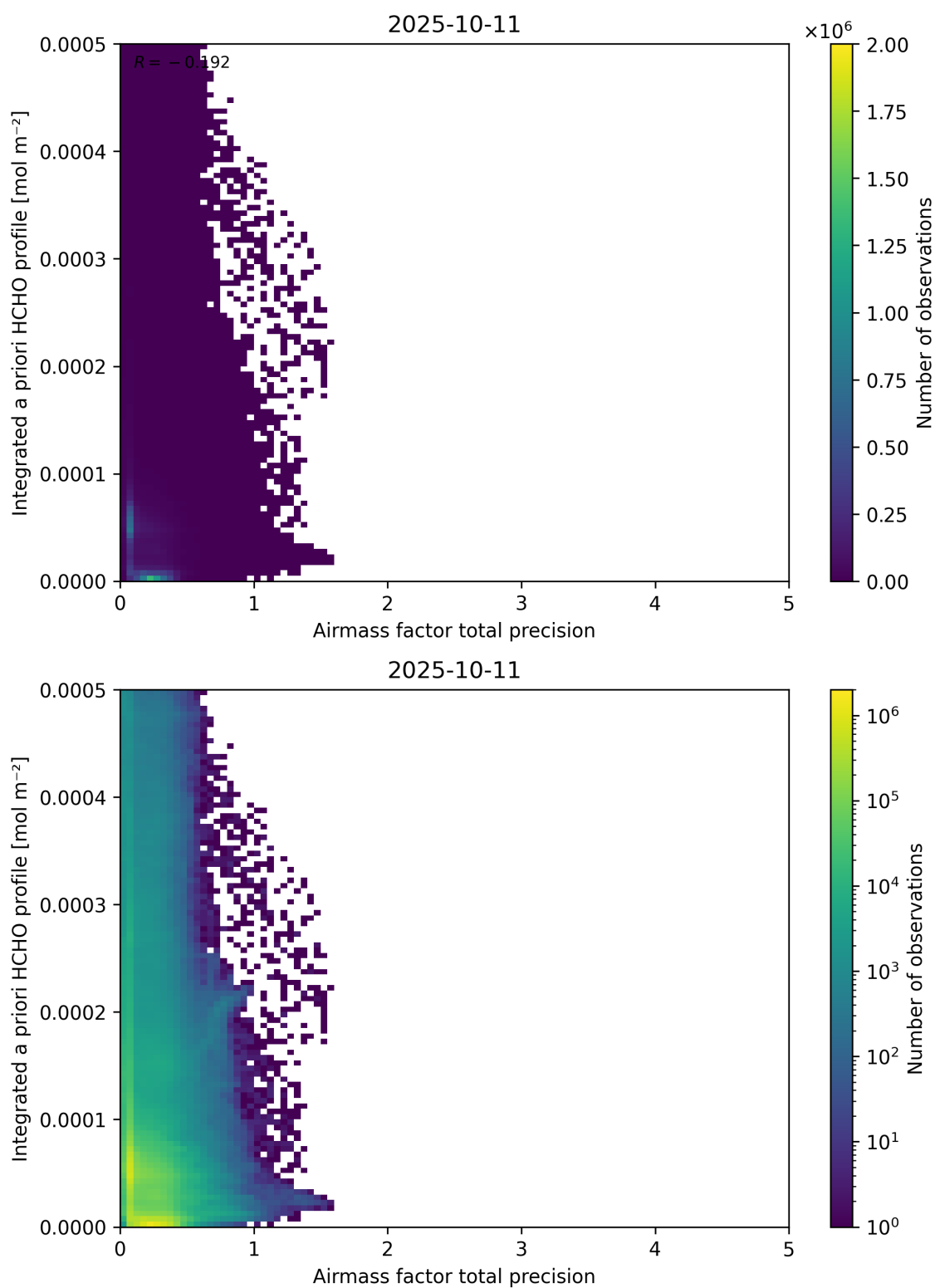
Figure 111: Scatter density plot of “Airmass factor total precision” against “Integrated a priori HCHO profile” for 2025-10-11 to 2025-10-12.
