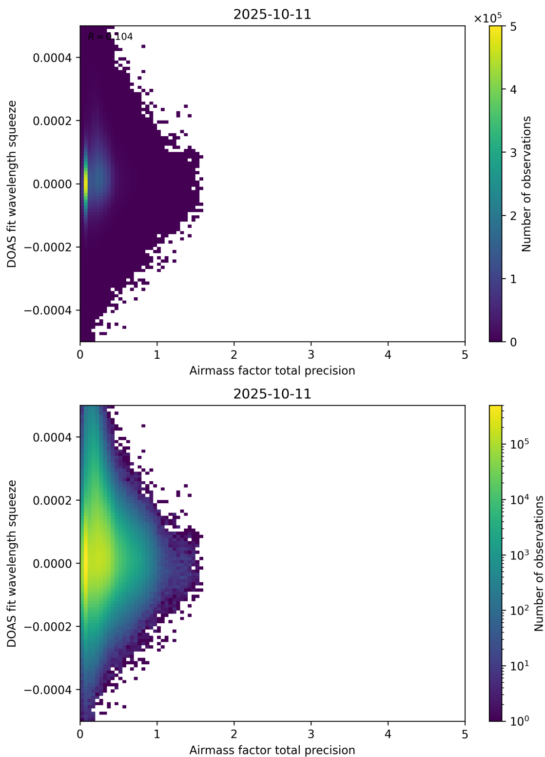
Figure 107: Scatter density plot of “Airmass factor total precision” against “DOAS fit wavelength squeeze” for 2025-10-11 to 2025-10-12.
