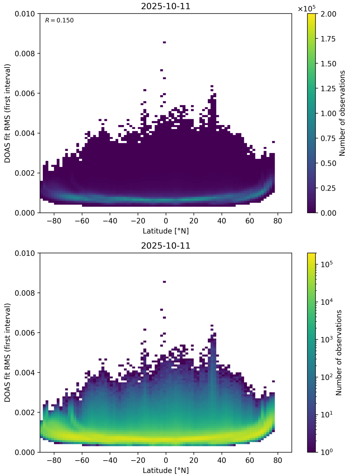
Figure 153: Scatter density plot of “Latitude” against “DOAS fit RMS (first interval)” for 2025-10-11 to 2025-10-12.
