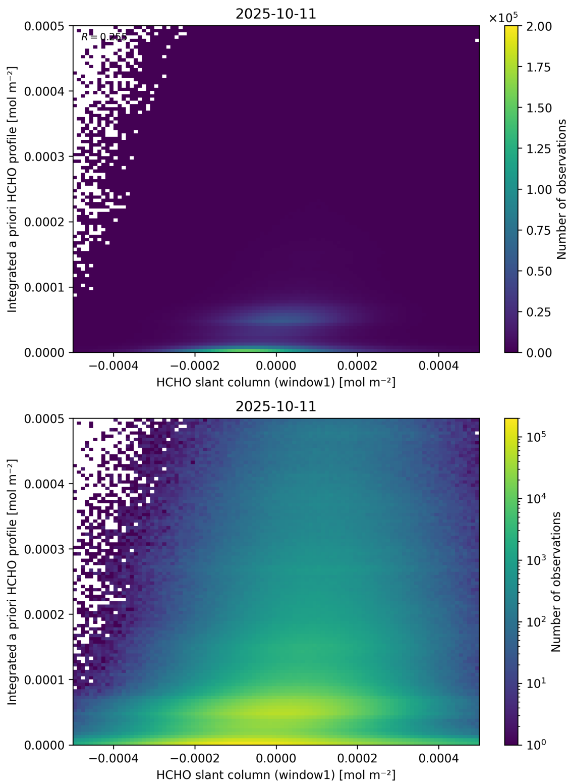
Figure 87: Scatter density plot of “HCHO slant column (window1)” against “Integrated a priori HCHO profile” for 2025-10-11 to 2025-10-12.
