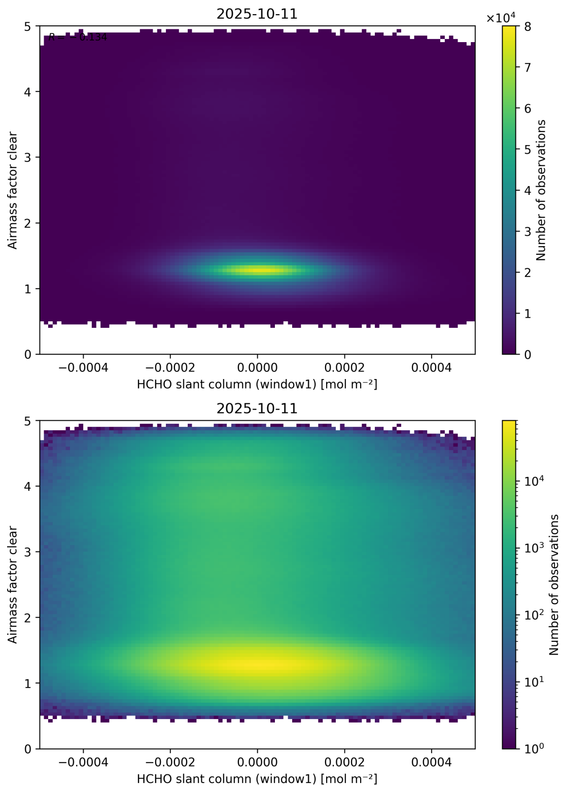
Figure 81: Scatter density plot of “HCHO slant column (window1)” against “Airmass factor clear” for 2025-10-11 to 2025-10-12.
