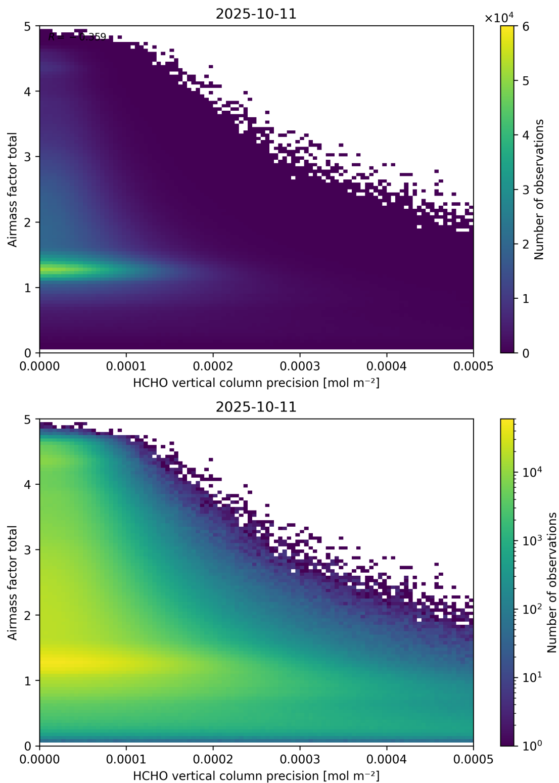
Figure 144: Scatter density plot of “HCHO vertical column precision” against “Airmass factor total” for 2025-10-11 to 2025-10-12.
