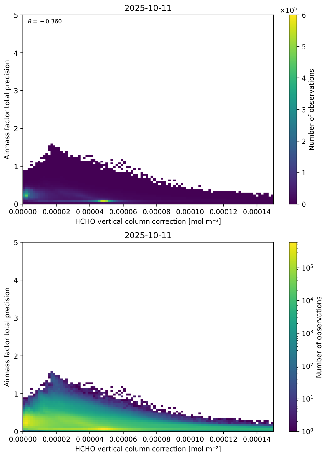
Figure 121: Scatter density plot of “HCHO vertical column correction” against “Airmass factor total precision” for 2025-10-11 to 2025-10-12.
