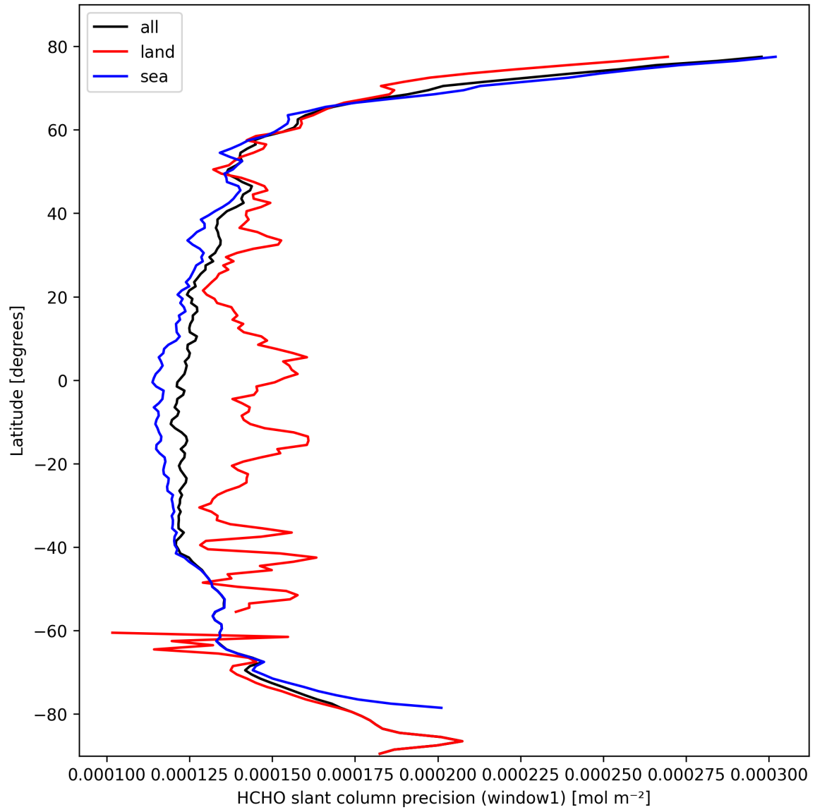
Figure 25: Zonal average of “HCHO slant column precision (window1)” for 2025-10-11 to 2025-10-12.
