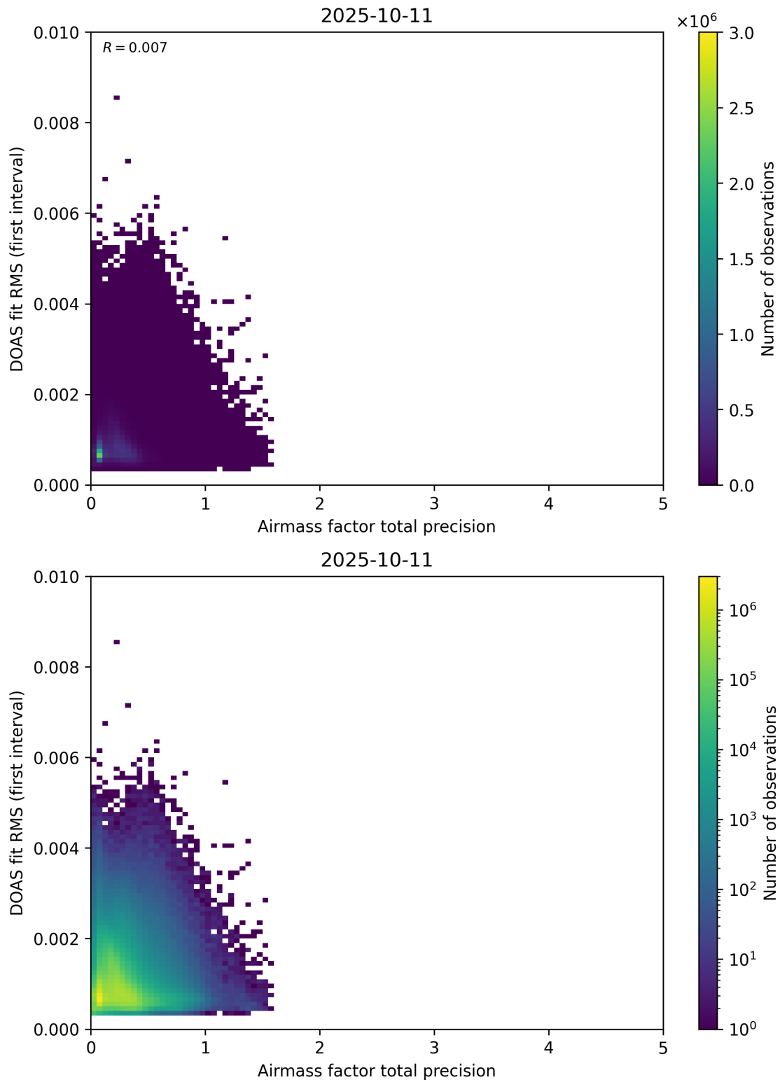
Figure 105: Scatter density plot of “Airmass factor total precision” against “DOAS fit RMS (first interval)” for 2025-10-11 to 2025-10-12.
