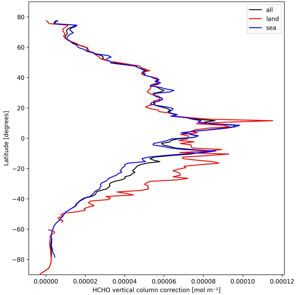
Figure 23: Zonal average of “HCHO vertical column correction” for 2025-10-11 to 2025-10-12.
