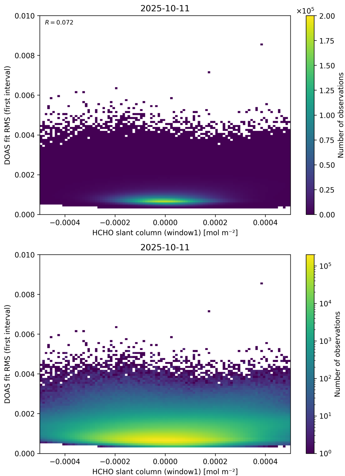
Figure 78: Scatter density plot of “HCHO slant column (window1)” against “DOAS fit RMS (first interval)” for 2025-10-11 to 2025-10-12.
