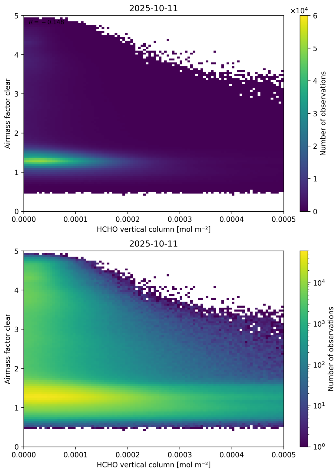
Figure 126: Scatter density plot of “HCHO vertical column” against “Airmass factor clear” for 2025-10-11 to 2025-10-12.
