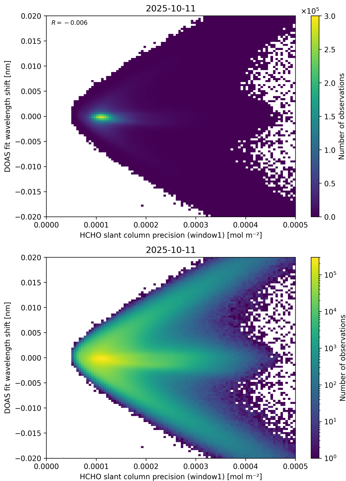
Figure 89: Scatter density plot of “HCHO slant column precision (window1)” against “DOAS fit wavelength shift” for 2025-10-11 to 2025-10-12.
