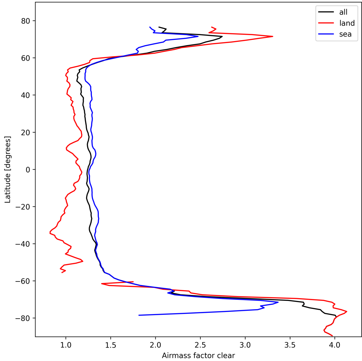
Figure 28: Zonal average of “Airmass factor clear” for 2025-10-13 to 2025-10-15.
