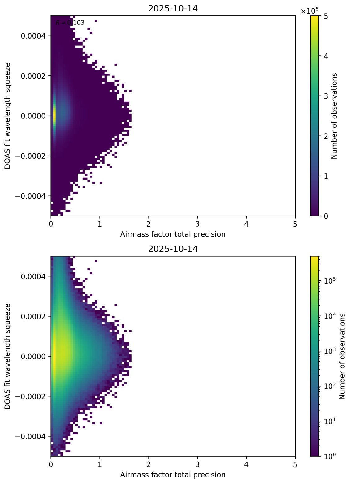
Figure 107: Scatter density plot of “Airmass factor total precision” against “DOAS fit wavelength squeeze” for 2025-10-13 to 2025-10-15.
