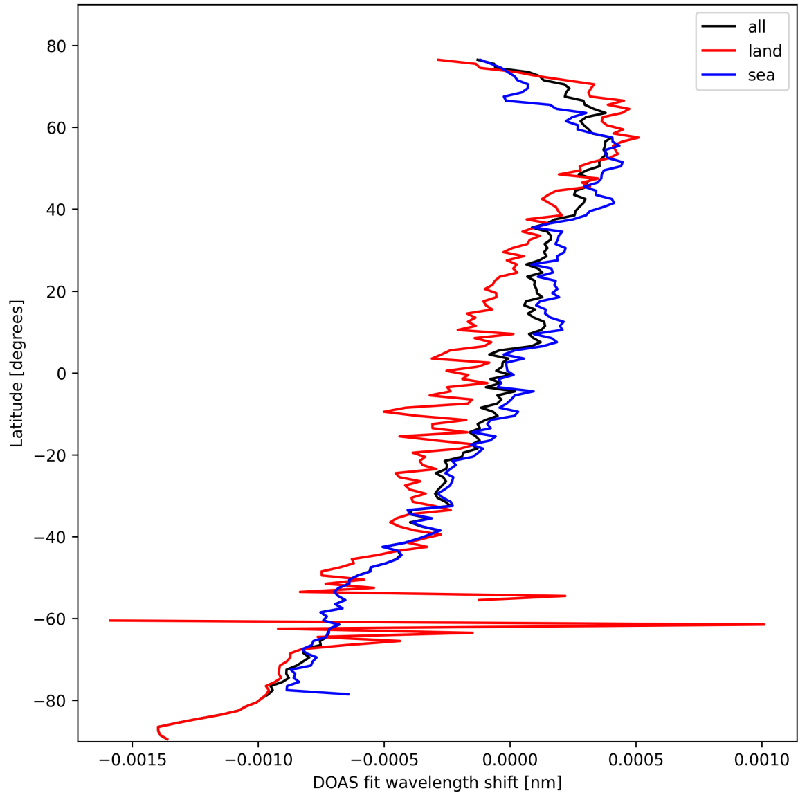
Figure 30: Zonal average of “DOAS fit wavelength shift” for 2025-10-13 to 2025-10-15.
