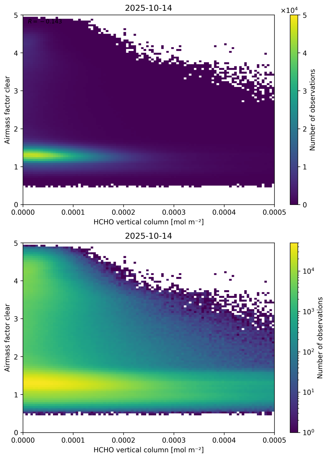
Figure 126: Scatter density plot of “HCHO vertical column” against “Airmass factor clear” for 2025-10-13 to 2025-10-15.
