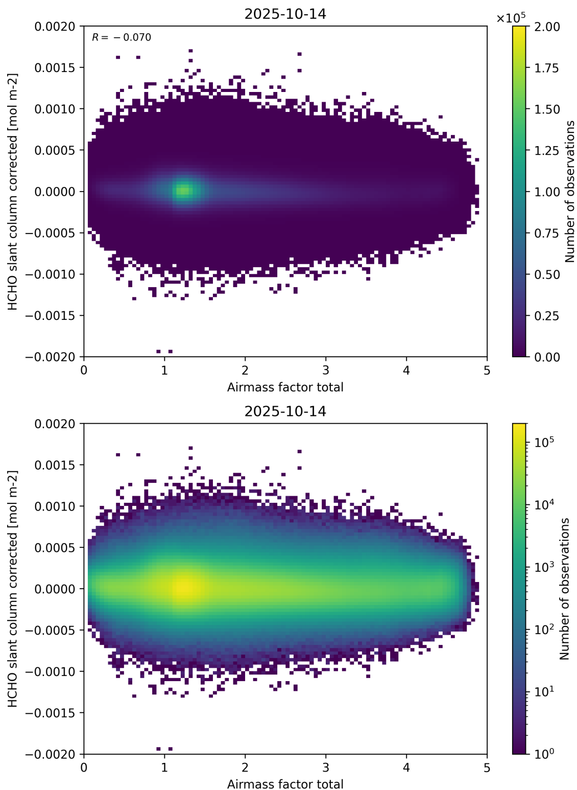
Figure 101: Scatter density plot of “Airmass factor total” against “HCHO slant column corrected” for 2025-10-13 to 2025-10-15.
