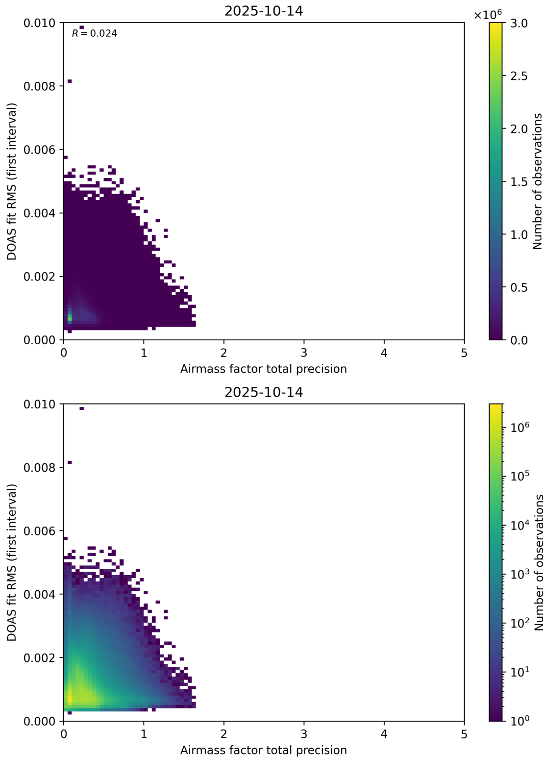
Figure 105: Scatter density plot of “Airmass factor total precision” against “DOAS fit RMS (first interval)” for 2025-10-13 to 2025-10-15.
