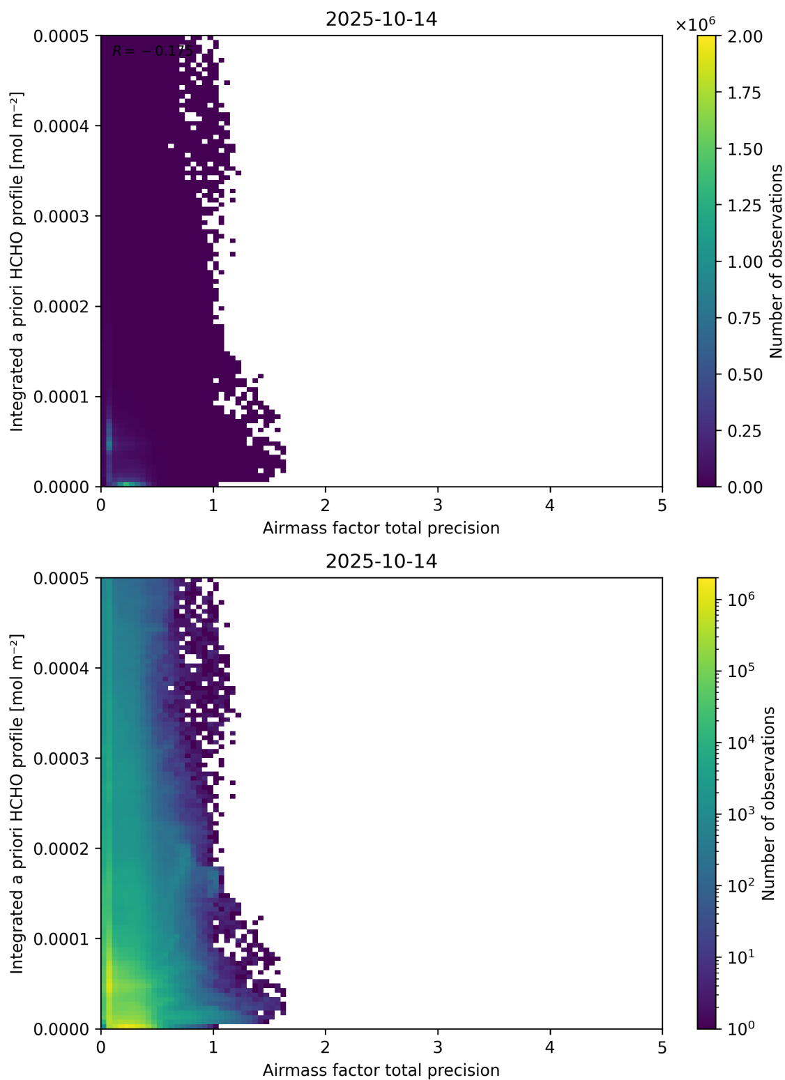
Figure 111: Scatter density plot of “Airmass factor total precision” against “Integrated a priori HCHO profile” for 2025-10-13 to 2025-10-15.
