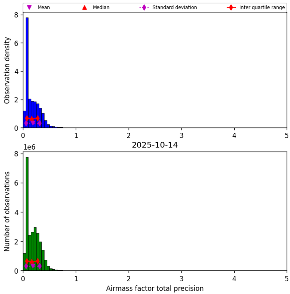
Figure 41: Histogram of “Airmass factor total precision” for 2025-10-13 to 2025-10-15
