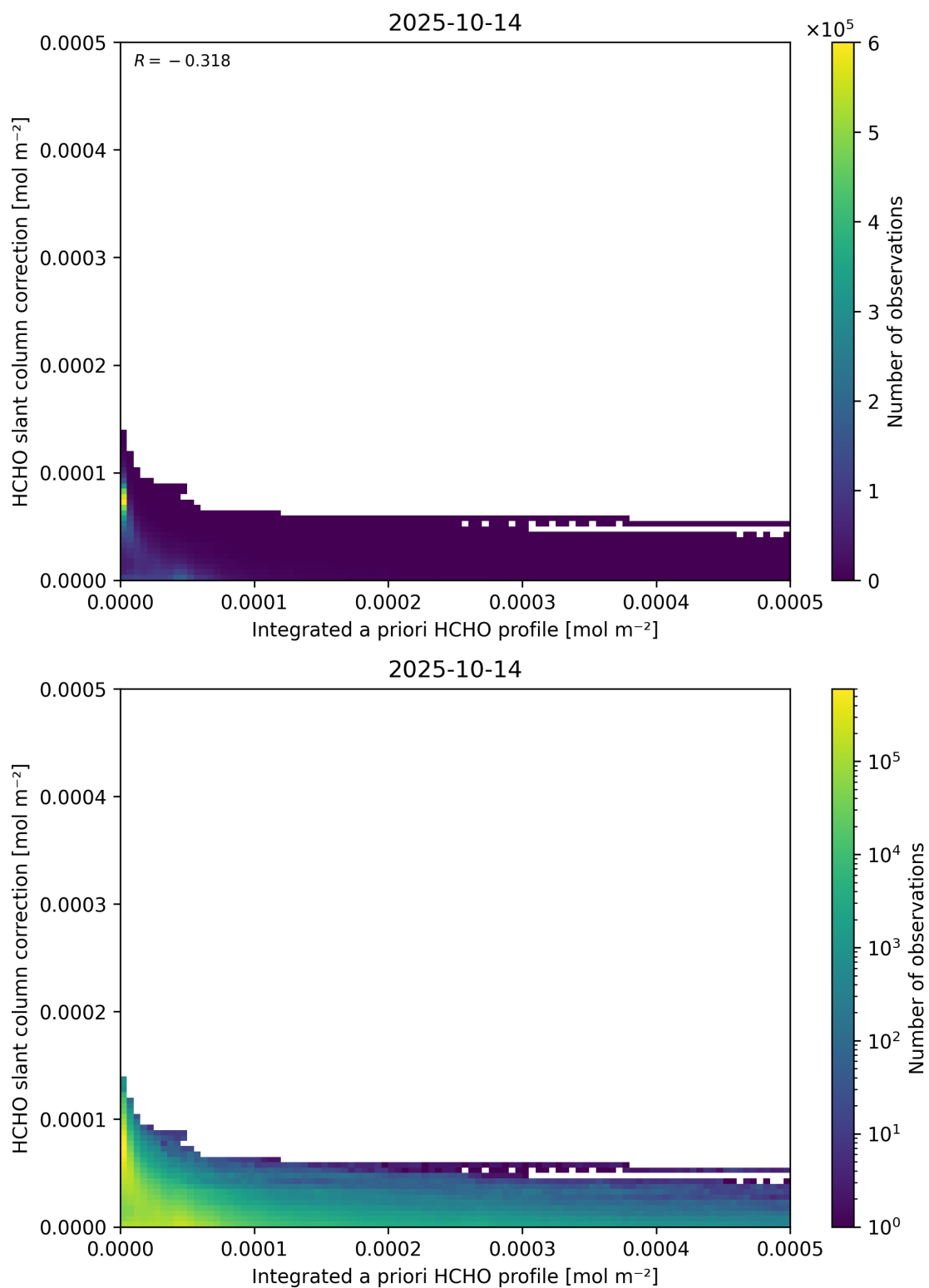
Figure 152: Scatter density plot of “Integrated a priori HCHO profile” against “HCHO slant column correction” for 2025-10-13 to 2025-10-15.
