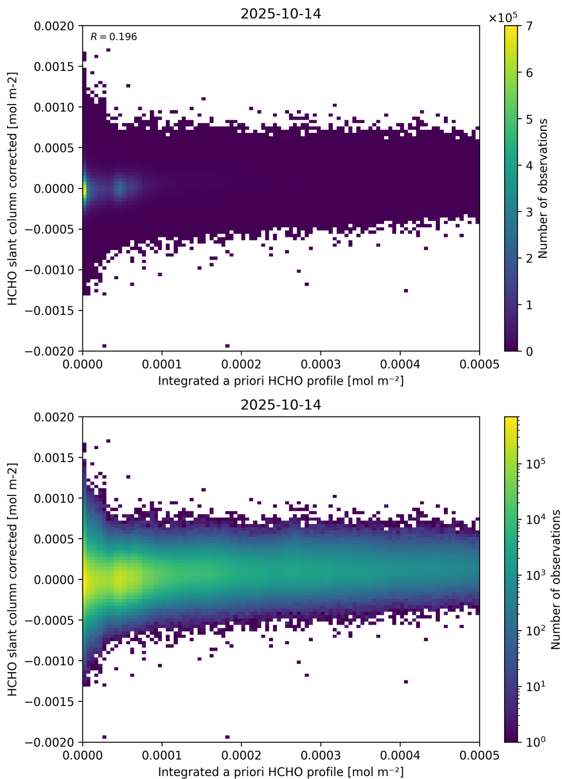
Figure 151: Scatter density plot of “Integrated a priori HCHO profile” against “HCHO slant column corrected” for 2025-10-13 to 2025-10-15.
