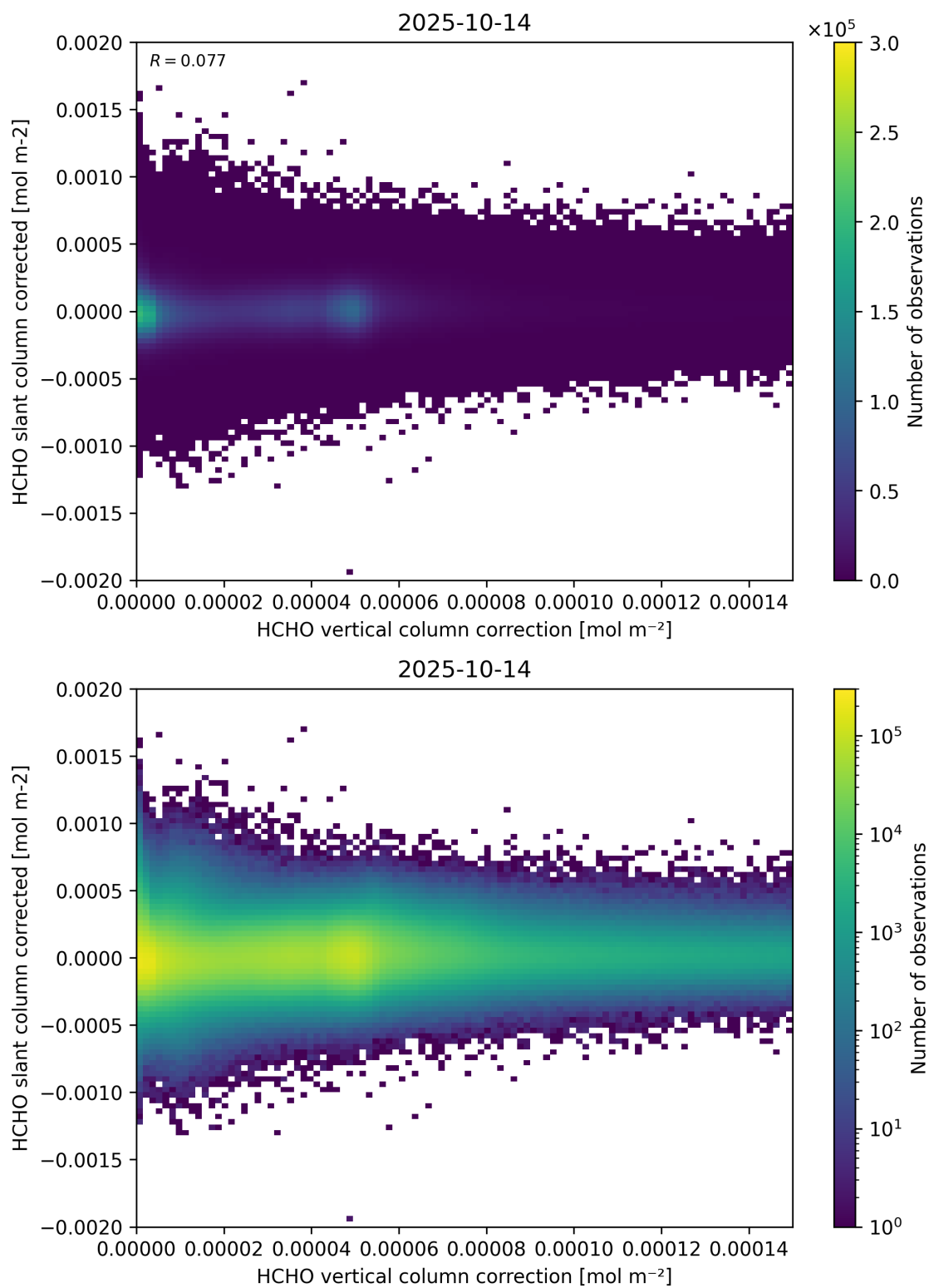
Figure 116: Scatter density plot of “HCHO vertical column correction” against “HCHO slant column corrected” for 2025-10-13 to 2025-10-15.
