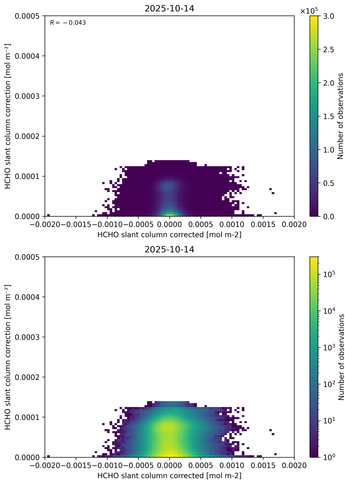
Figure 77: Scatter density plot of “HCHO slant column corrected” against “HCHO slant column correction” for 2025-10-13 to 2025-10-15.
