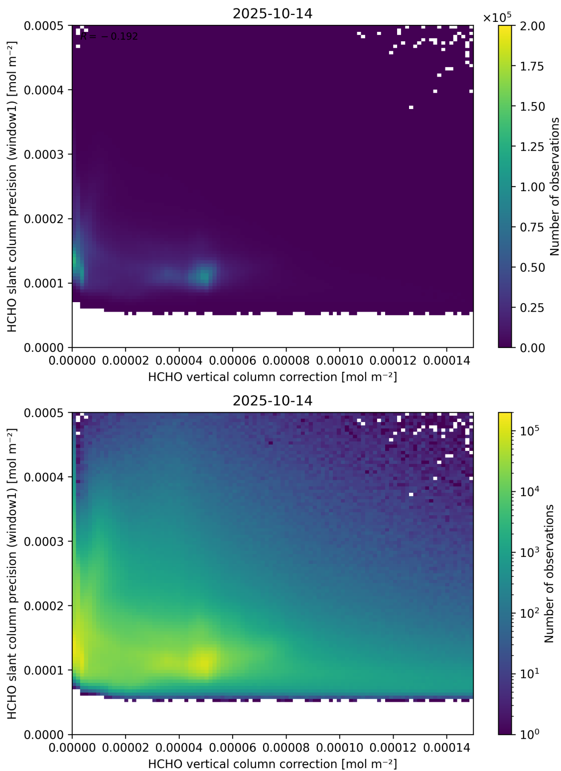
Figure 119: Scatter density plot of “HCHO vertical column correction” against “HCHO slant column precision (window1)” for 2025-10-13 to 2025-10-15.
