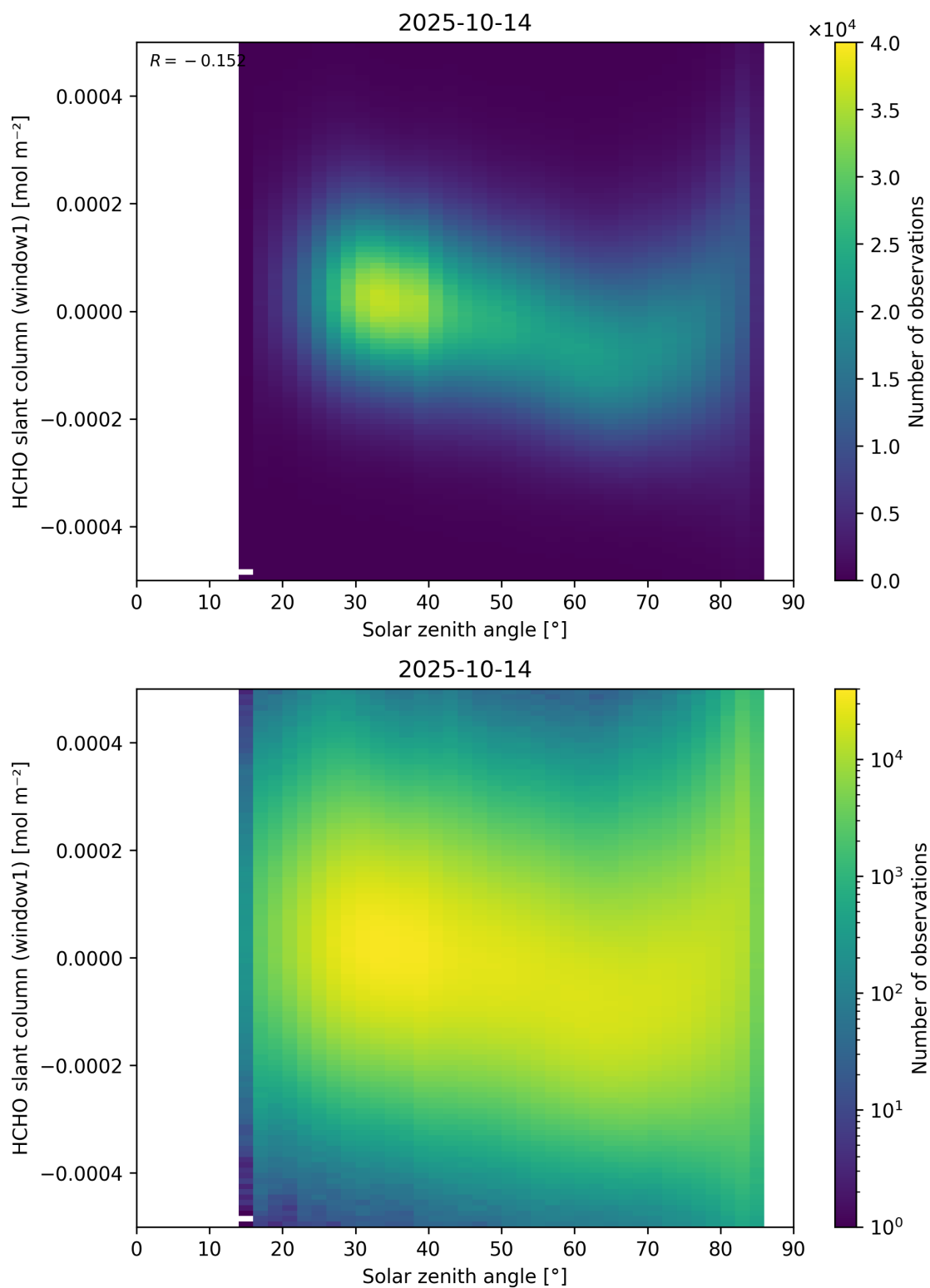
Figure 173: Scatter density plot of “Solar zenith angle” against “HCHO slant column (window1)” for 2025-10-13 to 2025-10-15.
