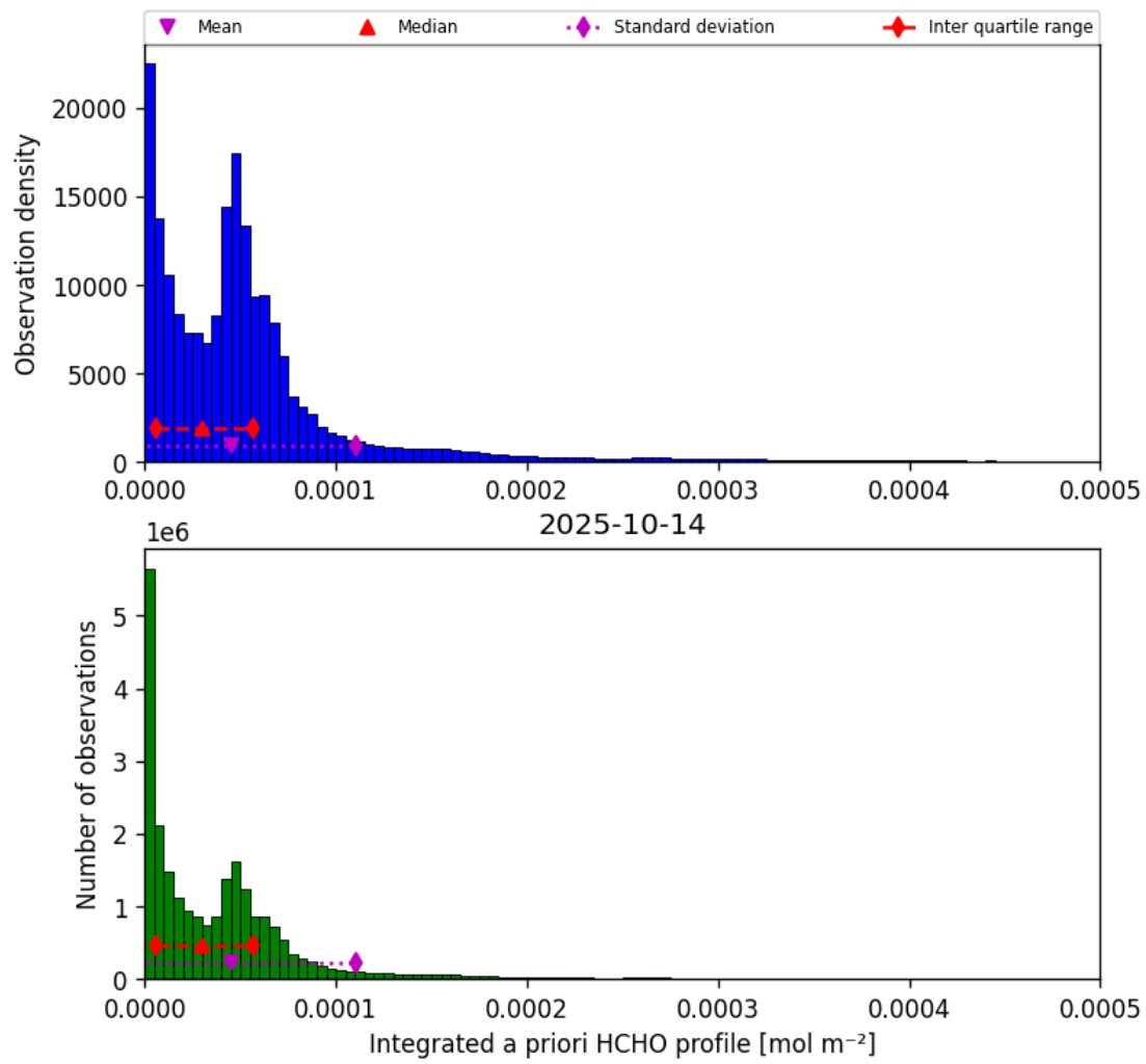
Figure 43: Histogram of “Integrated a priori HCHO profile” for 2025-10-13 to 2025-10-15
