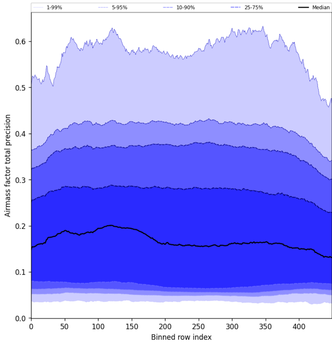
Figure 55: Along track statistics of “Airmass factor total precision” for 2025-10-13 to 2025-10-15
