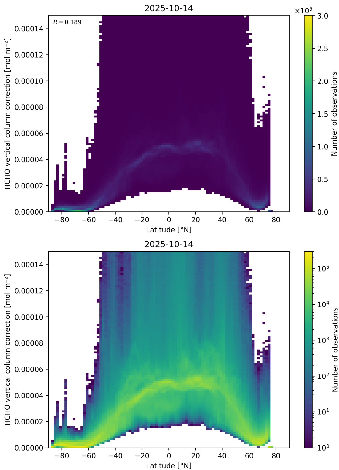
Figure 164: Scatter density plot of “Latitude” against “HCHO vertical column correction” for 2025-10-13 to 2025-10-15.
