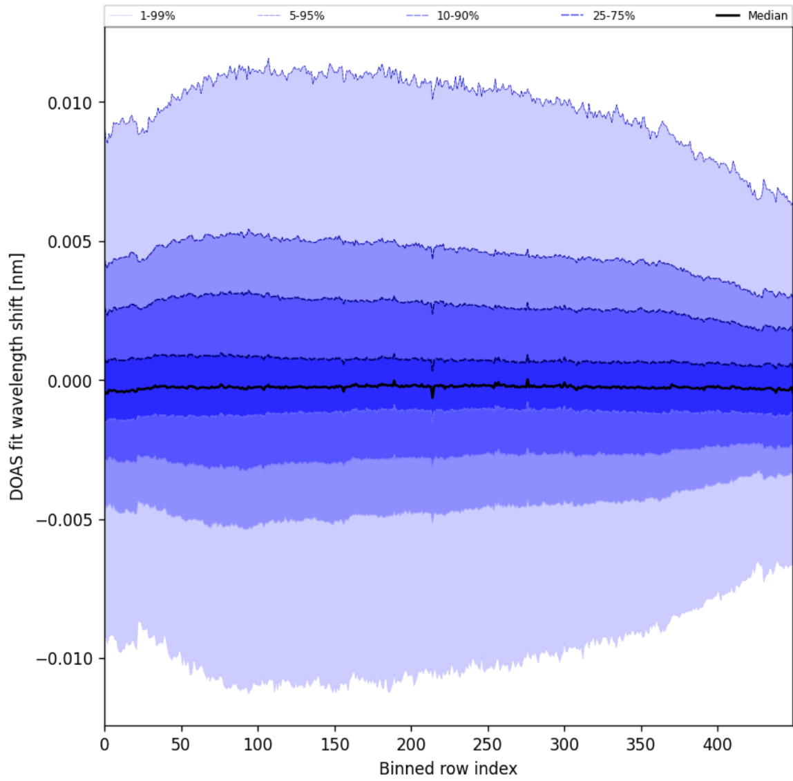
Figure 58: Along track statistics of “DOAS fit wavelength shift” for 2025-10-13 to 2025-10-15
