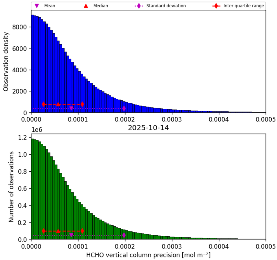
Figure 36: Histogram of “HCHO vertical column precision” for 2025-10-13 to 2025-10-15
