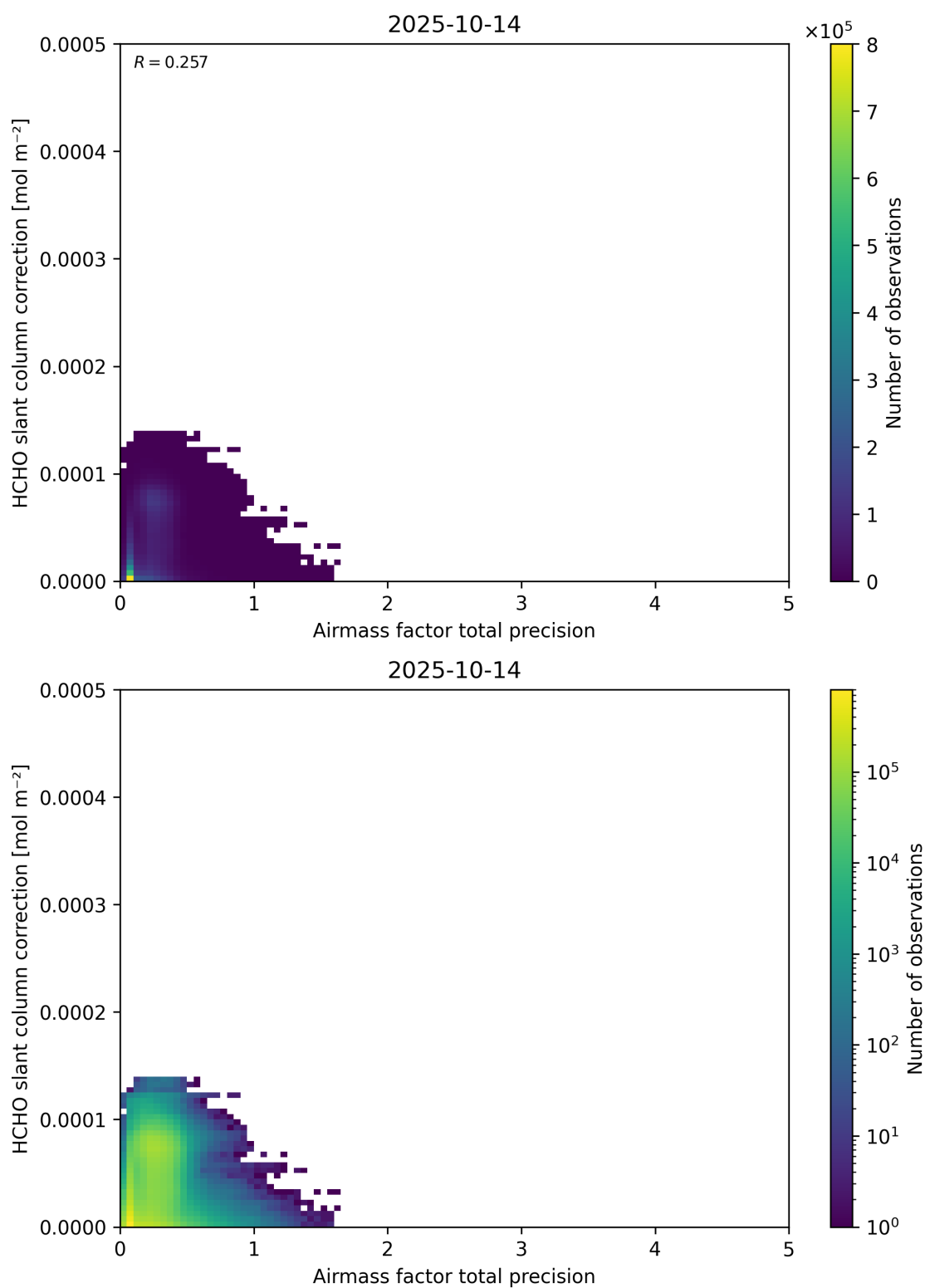
Figure 110: Scatter density plot of “Airmass factor total precision” against “HCHO slant column correction” for 2025-10-13 to 2025-10-15.
