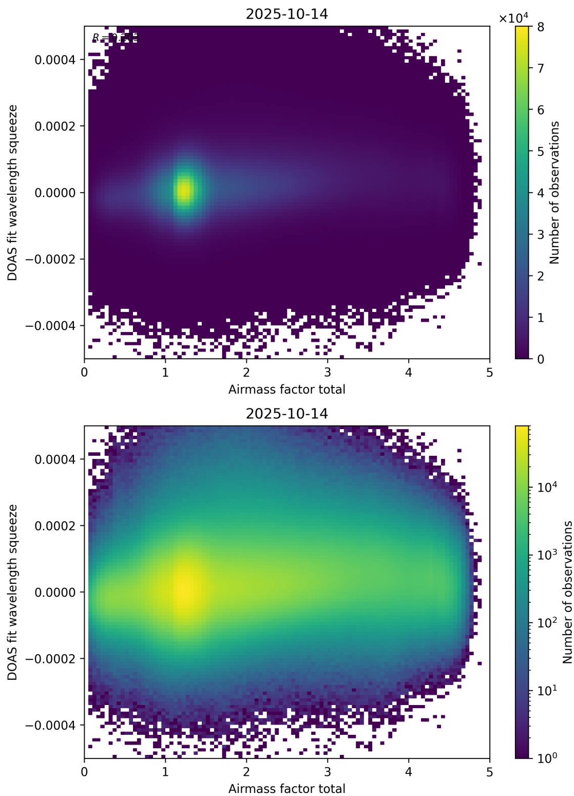
Figure 99: Scatter density plot of “Airmass factor total” against “DOAS fit wavelength squeeze” for 2025-10-13 to 2025-10-15.
