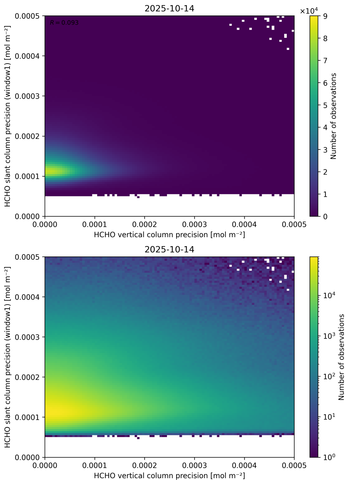
Figure 143: Scatter density plot of “HCHO vertical column precision” against “HCHO slant column precision (window1)” for 2025-10-13 to 2025-10-15.
