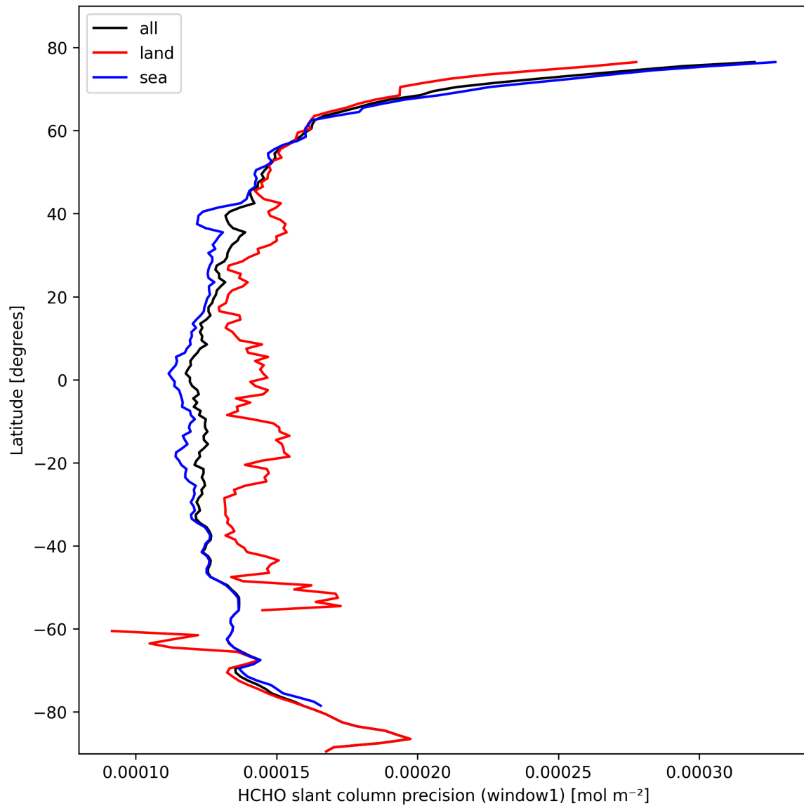
Figure 25: Zonal average of “HCHO slant column precision (window1)” for 2025-10-13 to 2025-10-15.
