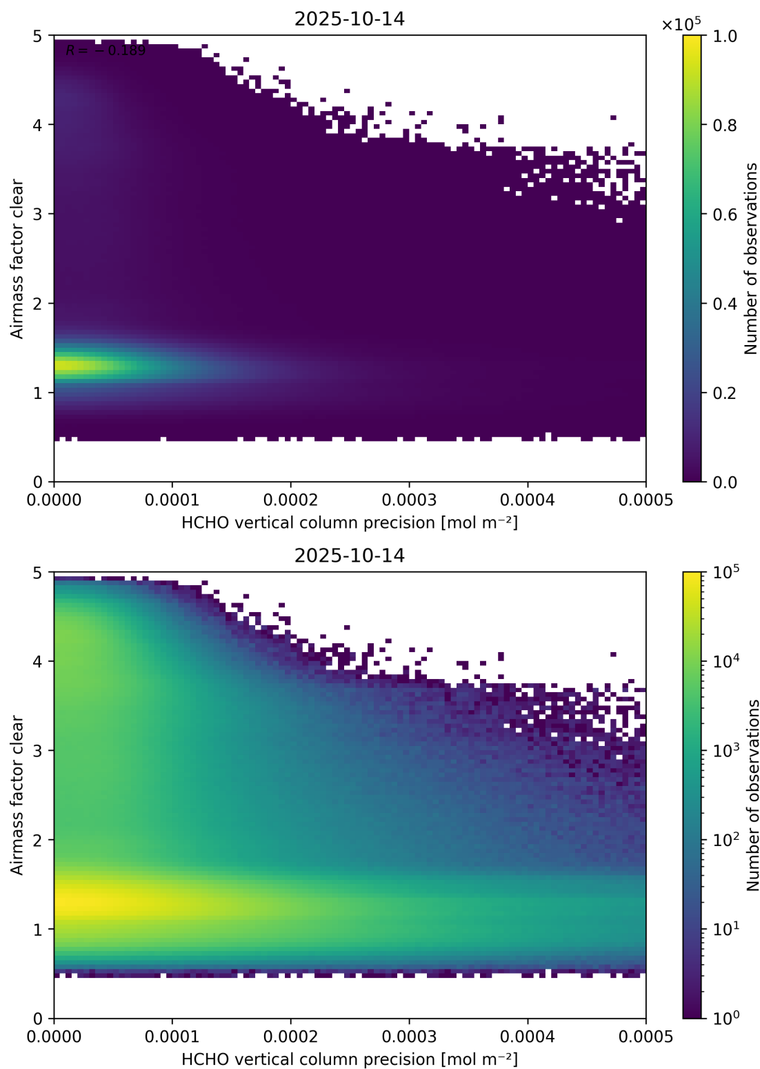
Figure 139: Scatter density plot of “HCHO vertical column precision” against “Airmass factor clear” for 2025-10-13 to 2025-10-15.
