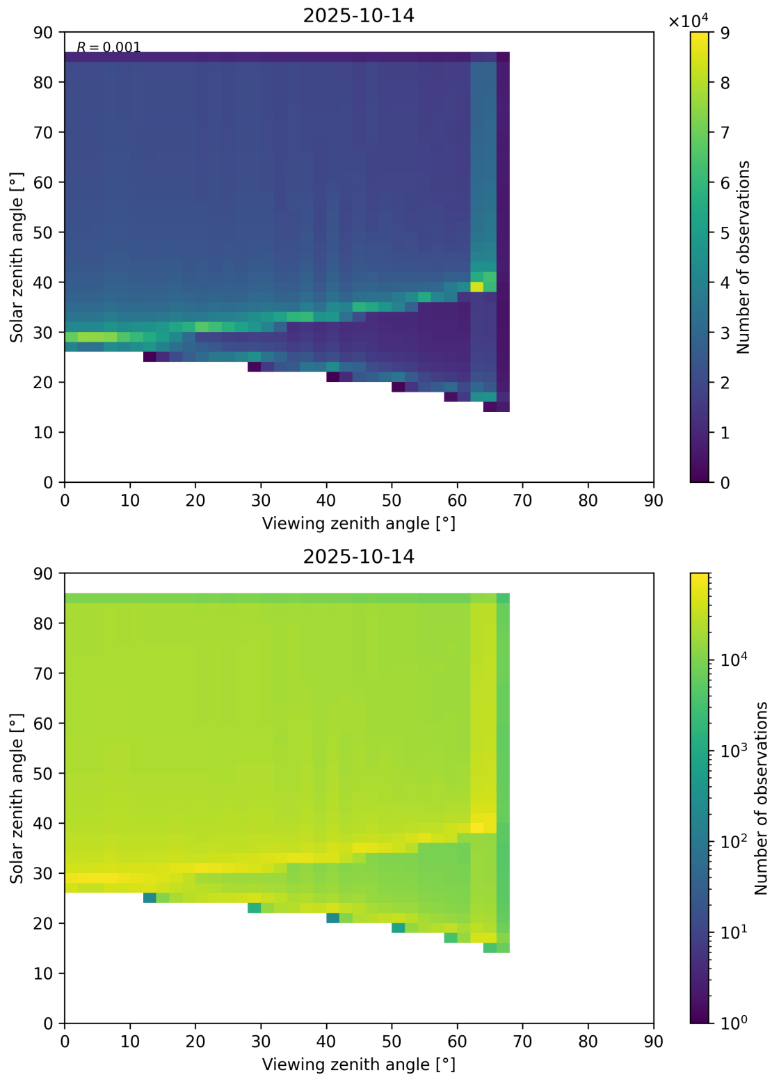
Figure 197: Scatter density plot of “Viewing zenith angle” against “Solar zenith angle” for 2025-10-13 to 2025-10-15.
