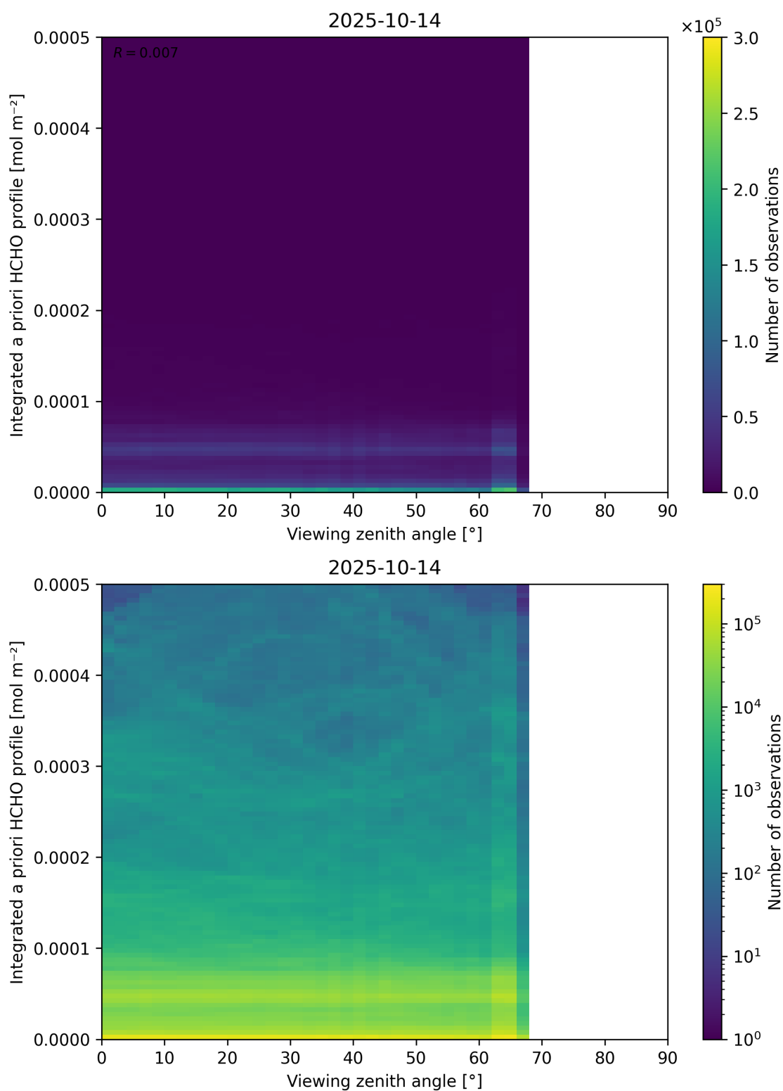
Figure 195: Scatter density plot of “Viewing zenith angle” against “Integrated a priori HCHO profile” for 2025-10-13 to 2025-10-15.
