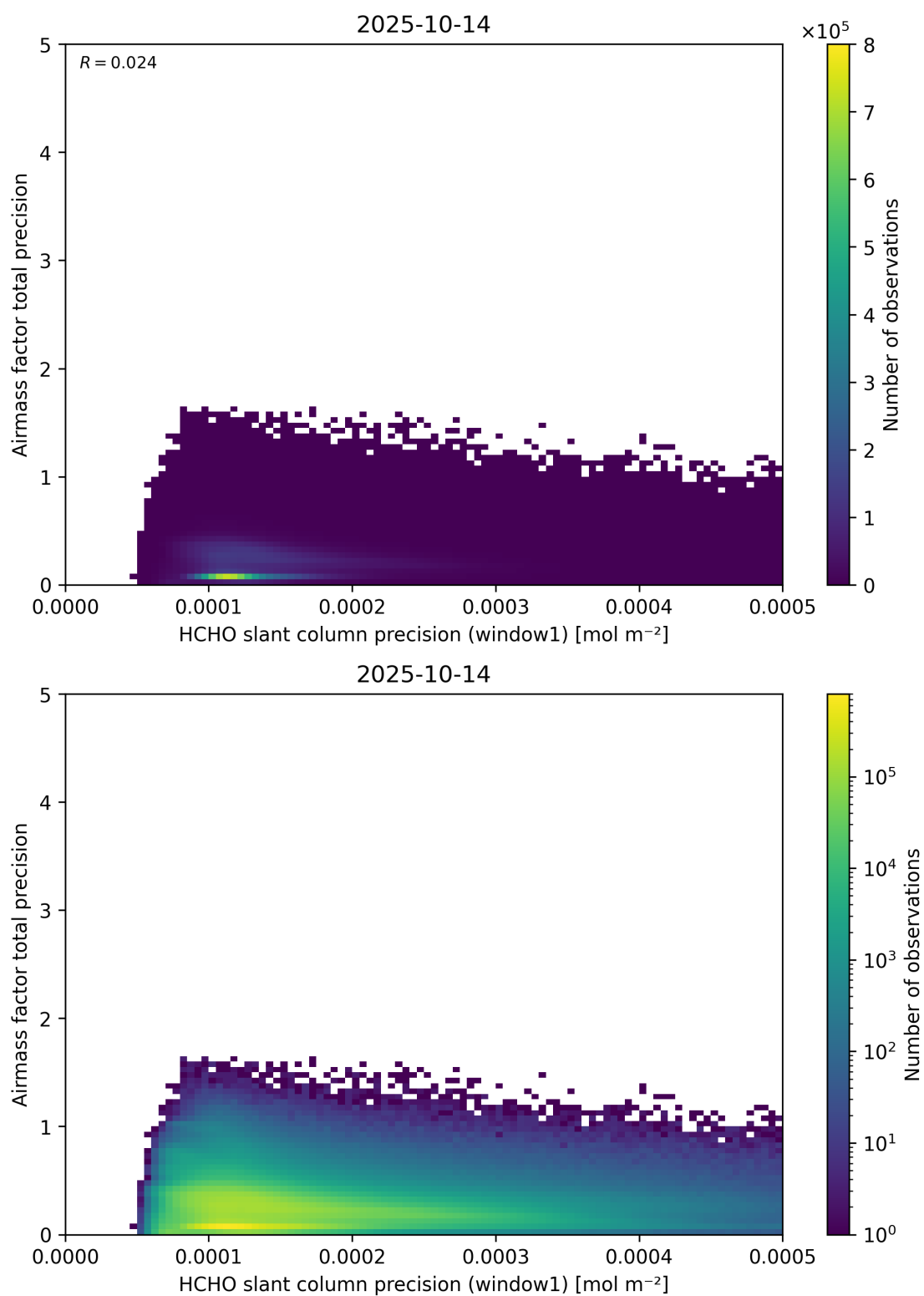
Figure 95: Scatter density plot of “HCHO slant column precision (window1)” against “Airmass factor total precision” for 2025-10-13 to 2025-10-15.
