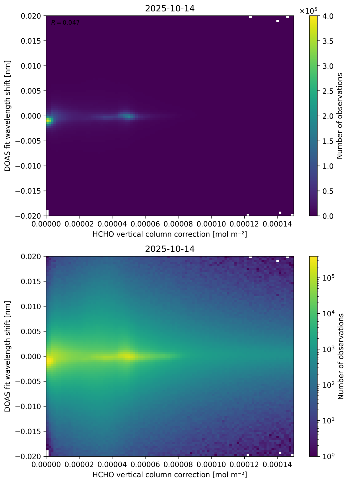
Figure 113: Scatter density plot of “HCHO vertical column correction” against “DOAS fit wavelength shift” for 2025-10-13 to 2025-10-15.
