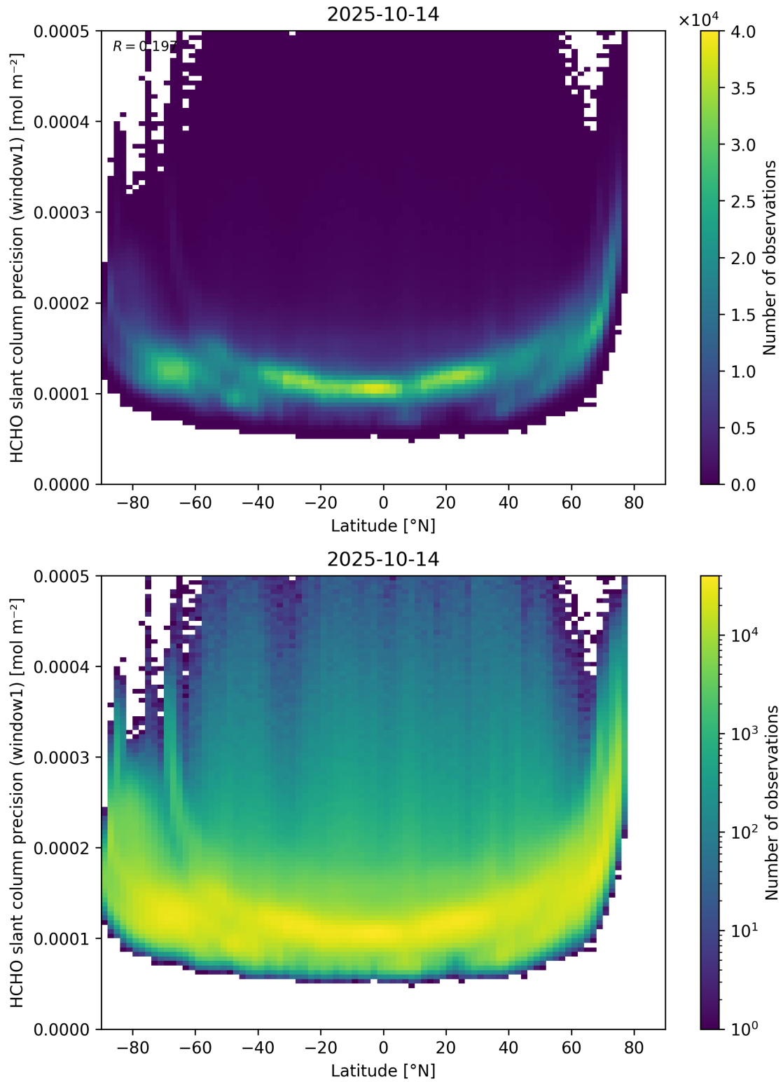
Figure 160: Scatter density plot of “Latitude” against “HCHO slant column precision (window1)” for 2025-10-13 to 2025-10-15.
