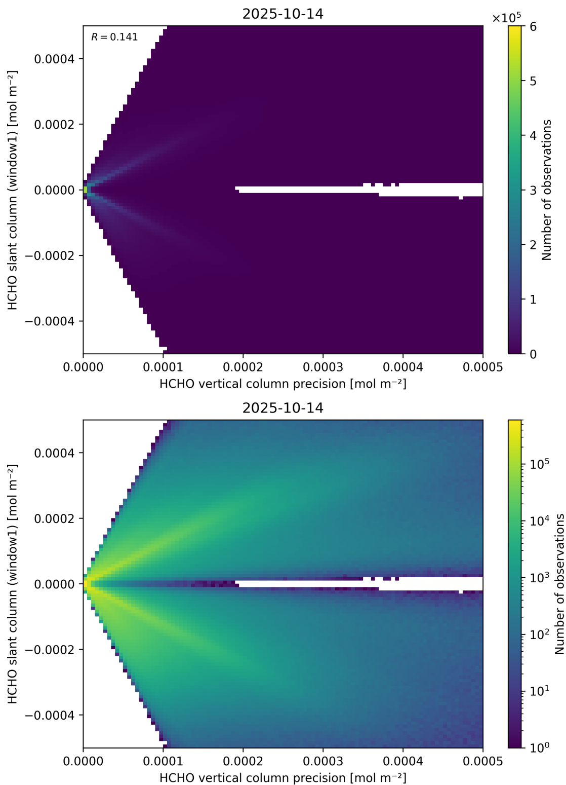
Figure 142: Scatter density plot of “HCHO vertical column precision” against “HCHO slant column (window1)” for 2025-10-13 to 2025-10-15.
