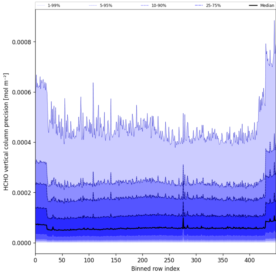
Figure 50: Along track statistics of “HCHO vertical column precision” for 2025-10-13 to 2025-10-15
