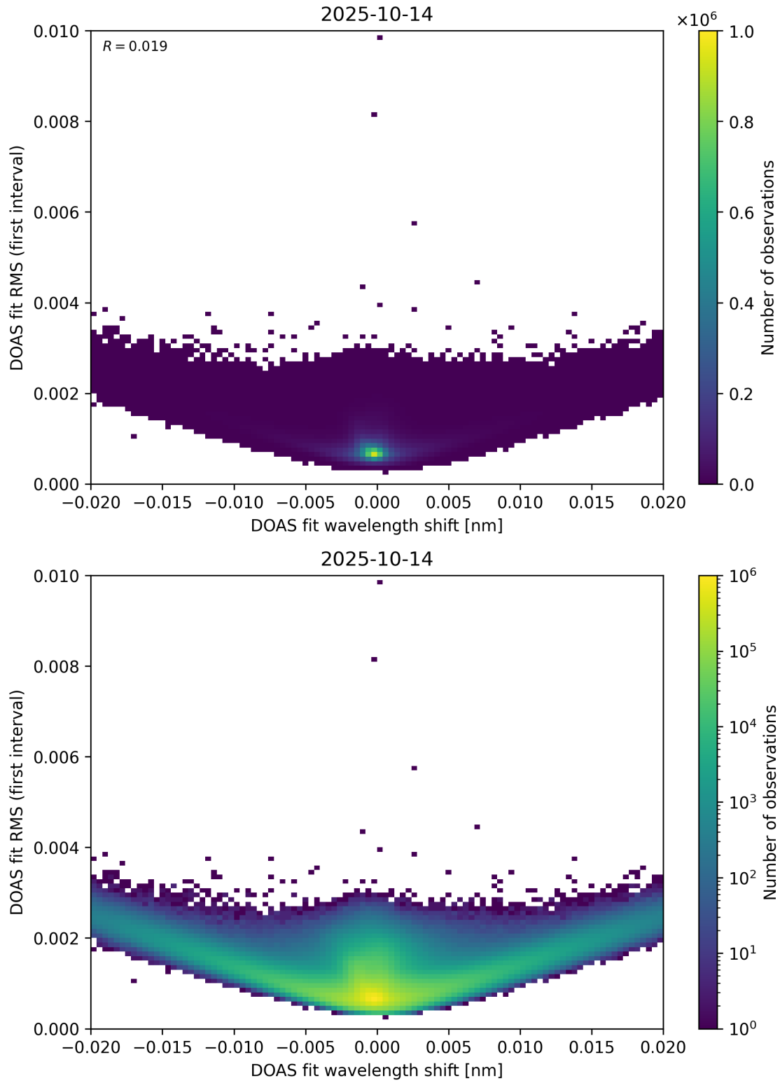
Figure 64: Scatter density plot of “DOAS fit wavelength shift” against “DOAS fit RMS (first interval)” for 2025-10-13 to 2025-10-15.
