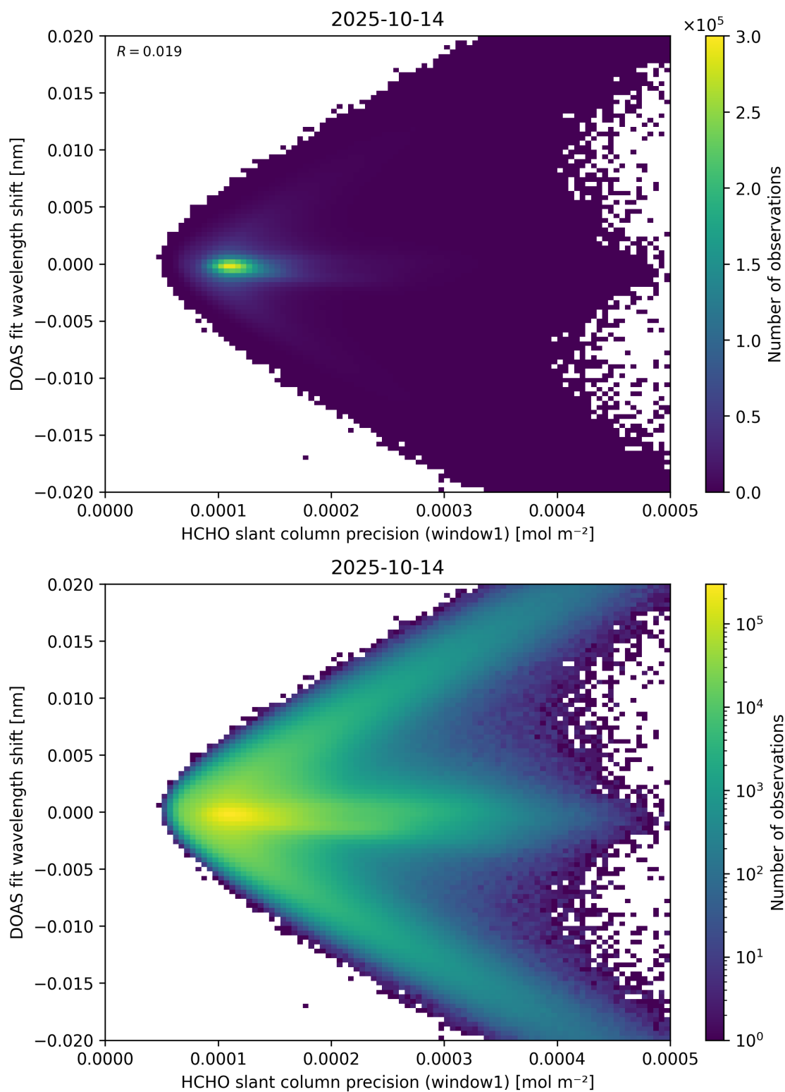
Figure 89: Scatter density plot of “HCHO slant column precision (window1)” against “DOAS fit wavelength shift” for 2025-10-13 to 2025-10-15.
