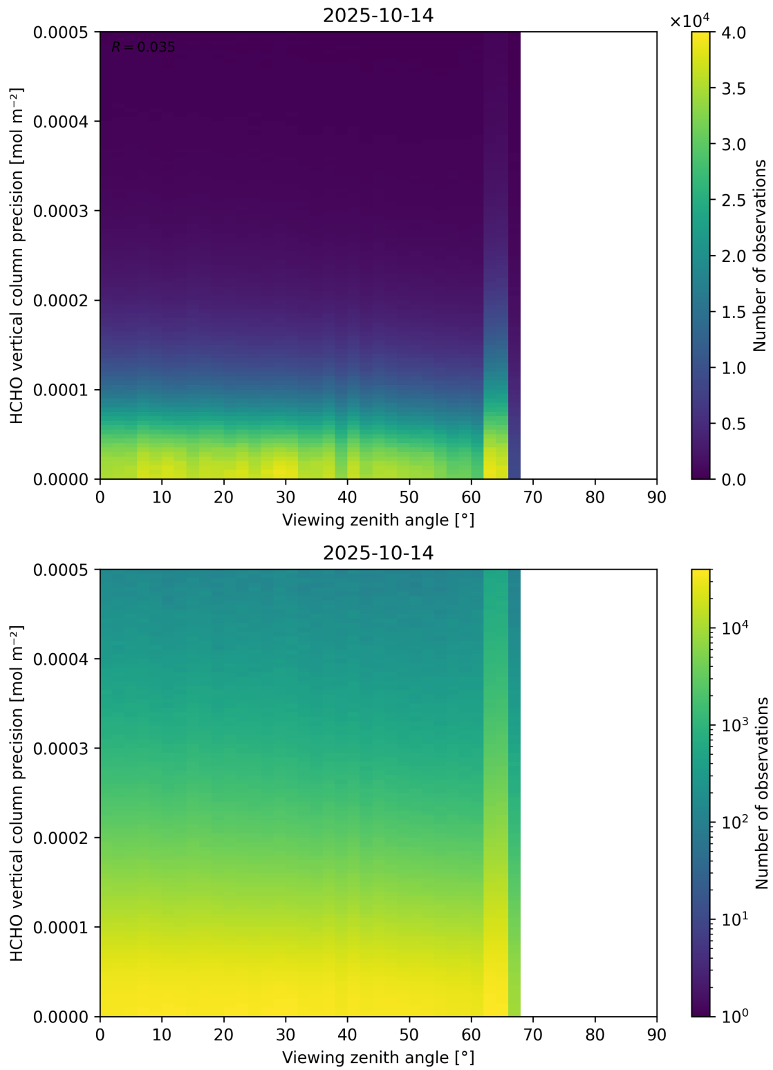
Figure 194: Scatter density plot of “Viewing zenith angle” against “HCHO vertical column precision” for 2025-10-13 to 2025-10-15.
