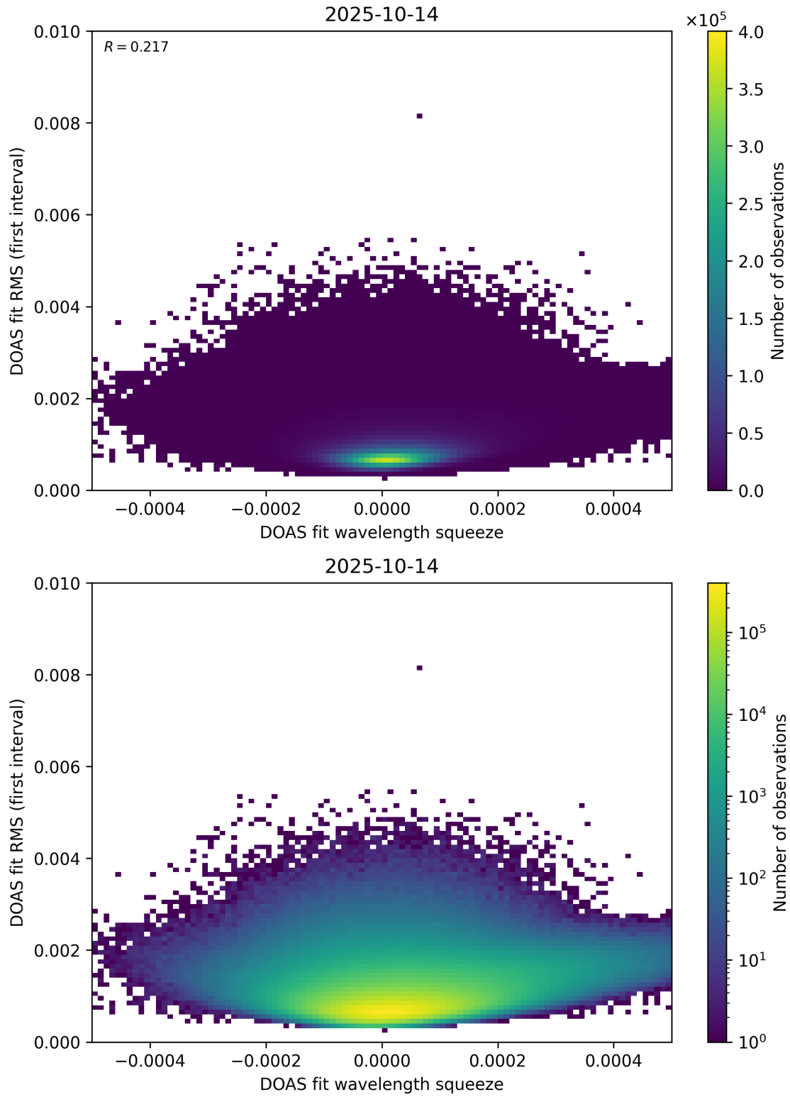
Figure 68: Scatter density plot of “DOAS fit wavelength squeeze” against “DOAS fit RMS (first interval)” for 2025-10-13 to 2025-10-15.
