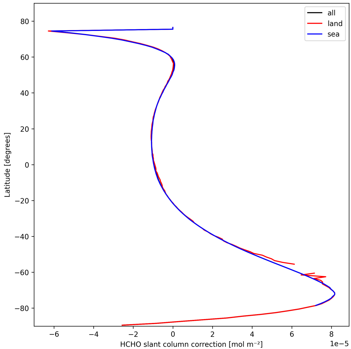
Figure 33: Zonal average of “HCHO slant column correction” for 2025-10-13 to 2025-10-15.
