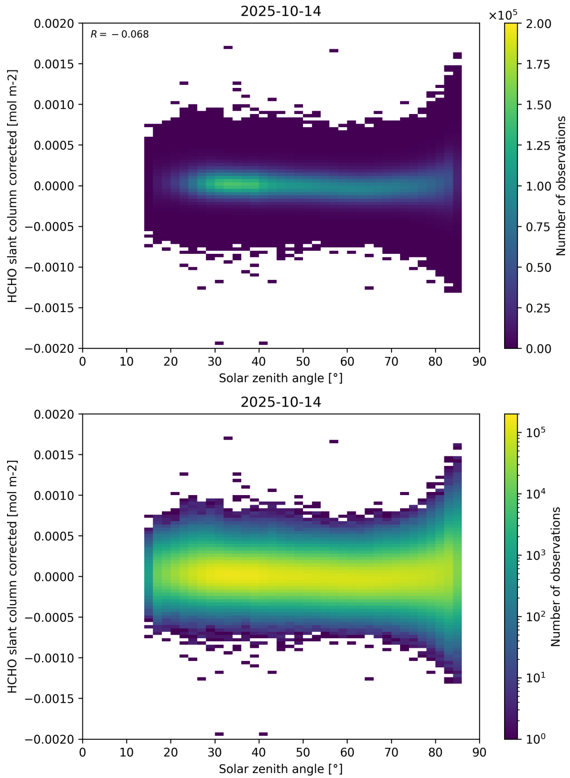
Figure 171: Scatter density plot of “Solar zenith angle” against “HCHO slant column corrected” for 2025-10-13 to 2025-10-15.
