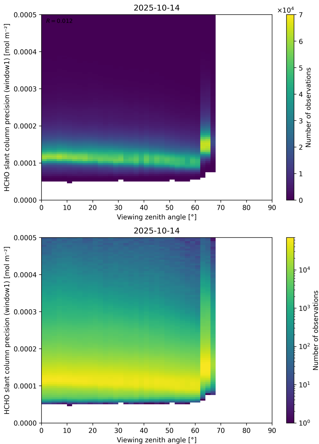
Figure 189: Scatter density plot of “Viewing zenith angle” against “HCHO slant column precision (window1)” for 2025-10-13 to 2025-10-15.
