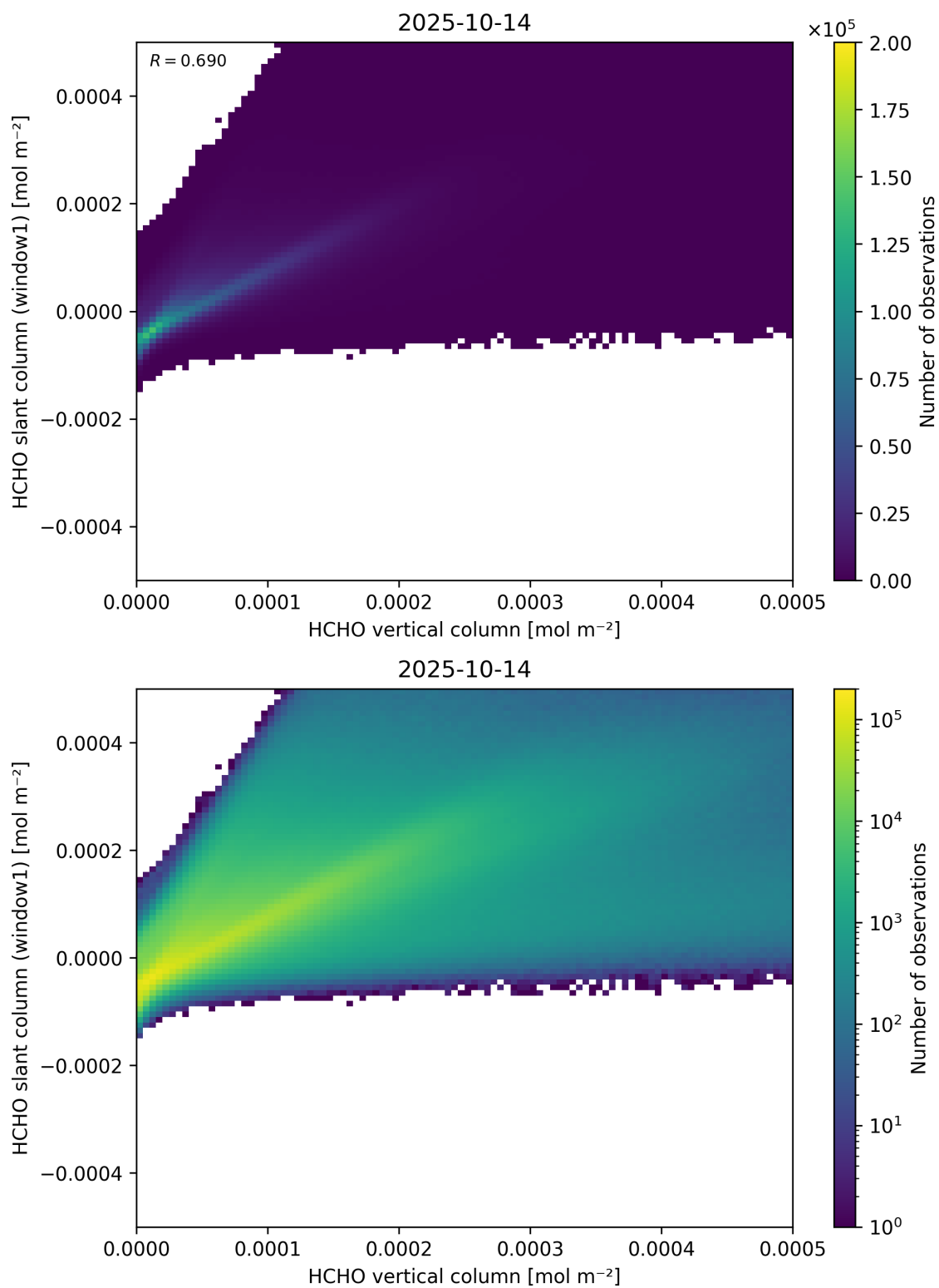
Figure 129: Scatter density plot of “HCHO vertical column” against “HCHO slant column (window1)” for 2025-10-13 to 2025-10-15.
