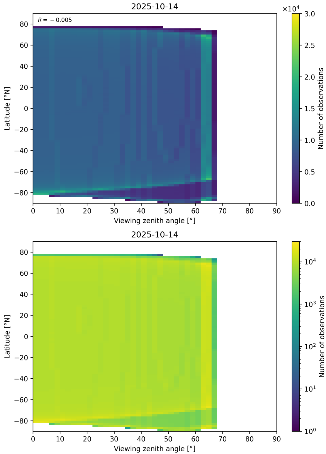
Figure 196: Scatter density plot of “Viewing zenith angle” against “Latitude” for 2025-10-13 to 2025-10-15.
