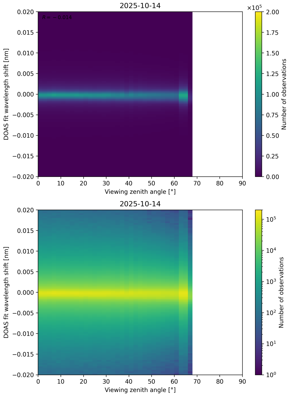
Figure 183: Scatter density plot of “Viewing zenith angle” against “DOAS fit wavelength shift” for 2025-10-13 to 2025-10-15.
