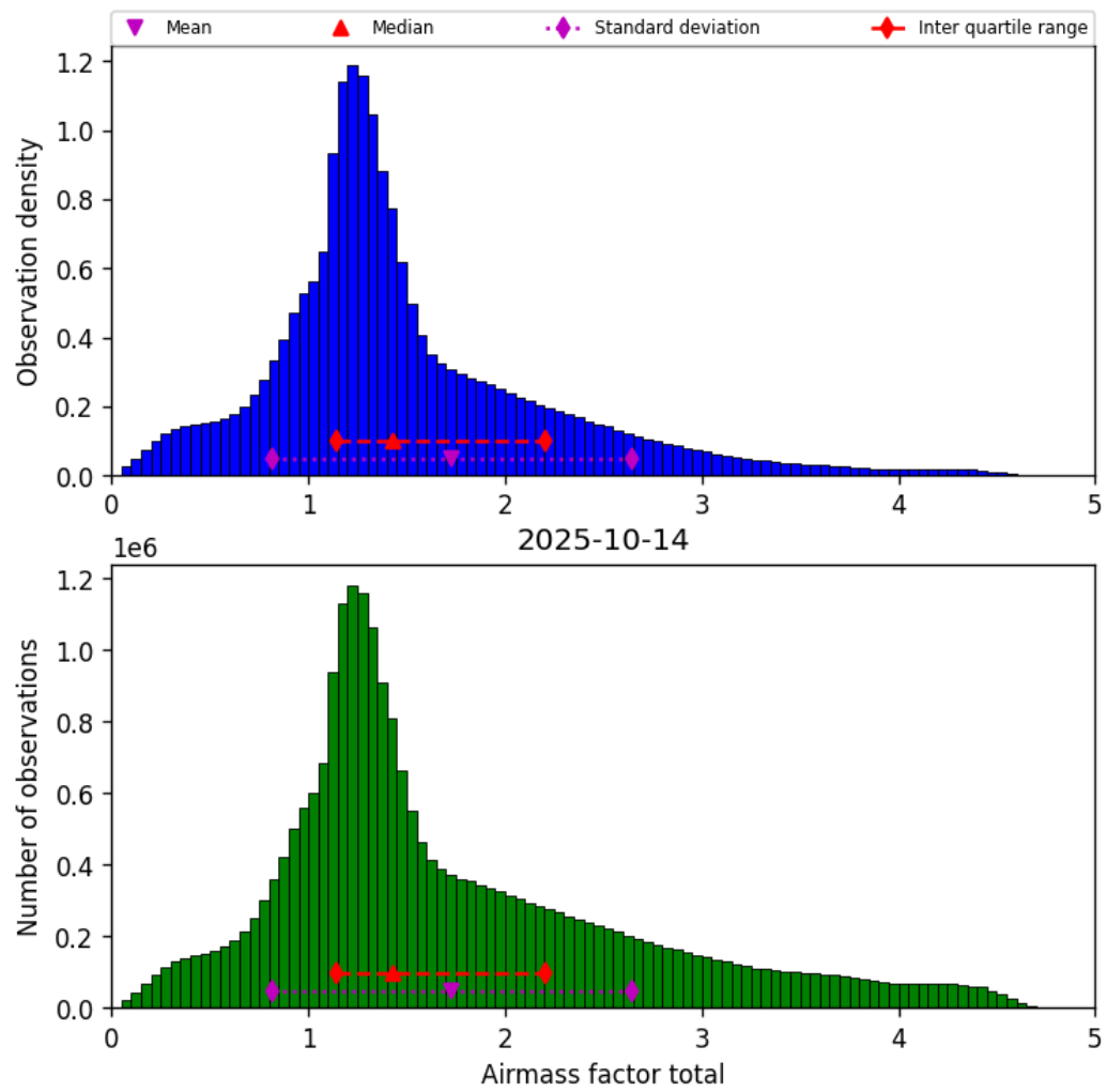
Figure 40: Histogram of “Airmass factor total” for 2025-10-13 to 2025-10-15
