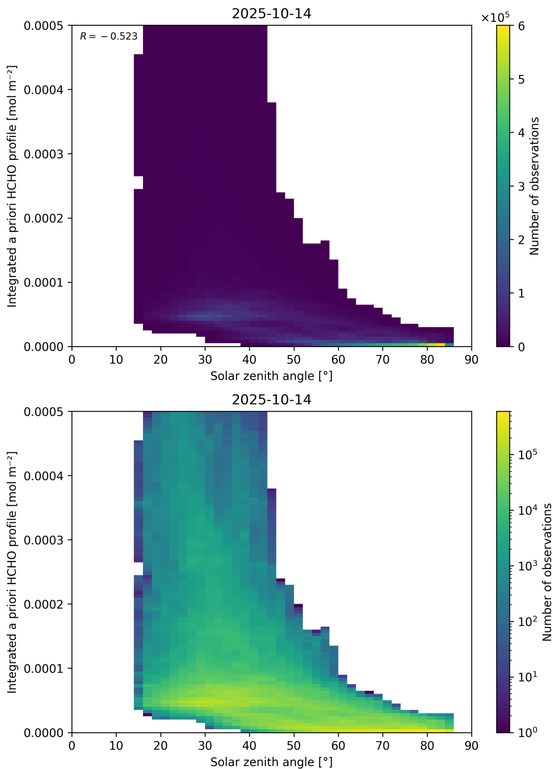
Figure 180: Scatter density plot of “Solar zenith angle” against “Integrated a priori HCHO profile” for 2025-10-13 to 2025-10-15.
