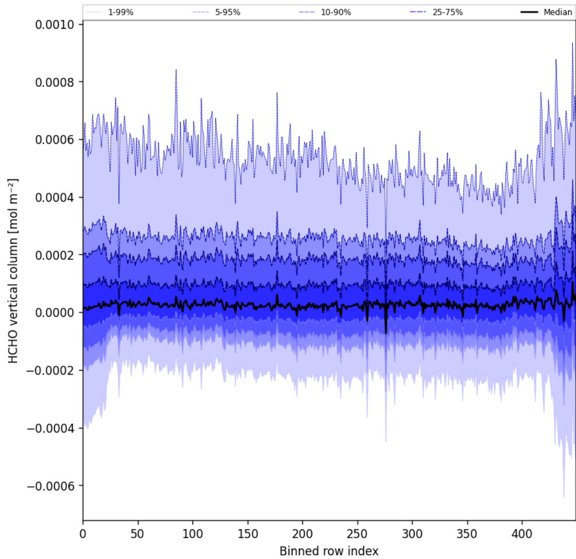
Figure 49: Along track statistics of “HCHO vertical column” for 2025-10-13 to 2025-10-15
