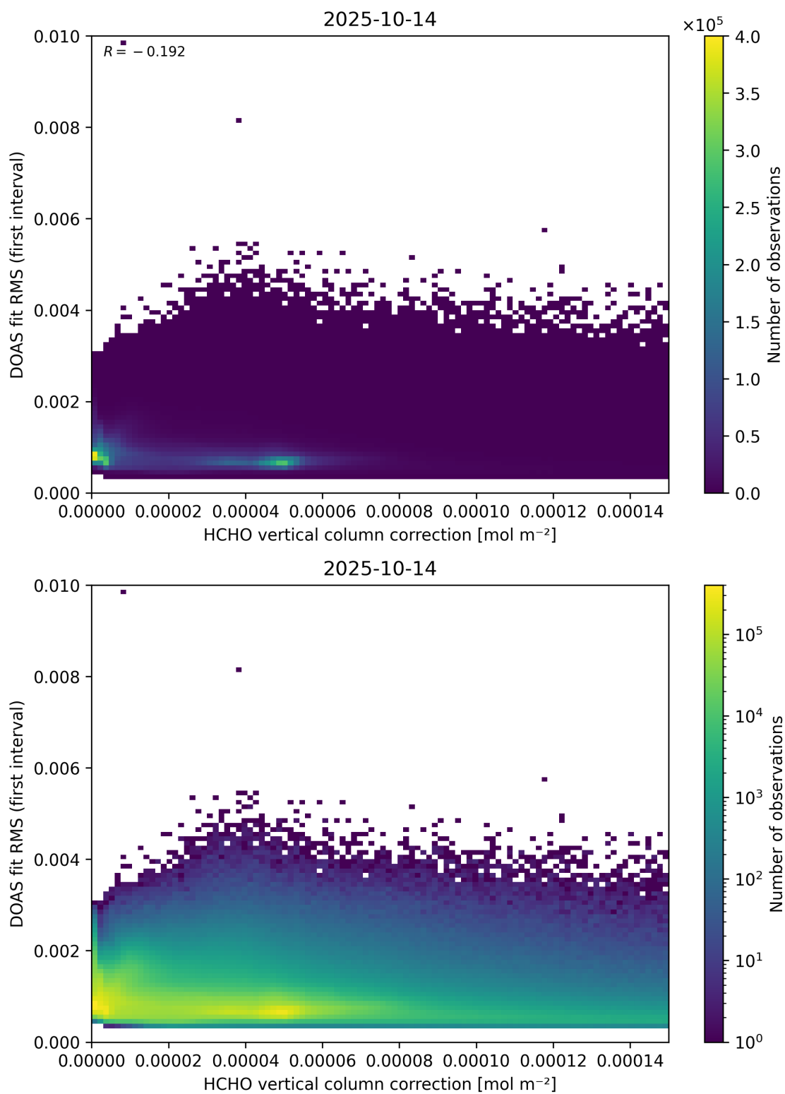
Figure 112: Scatter density plot of “HCHO vertical column correction” against “DOAS fit RMS (first interval)” for 2025-10-13 to 2025-10-15.
