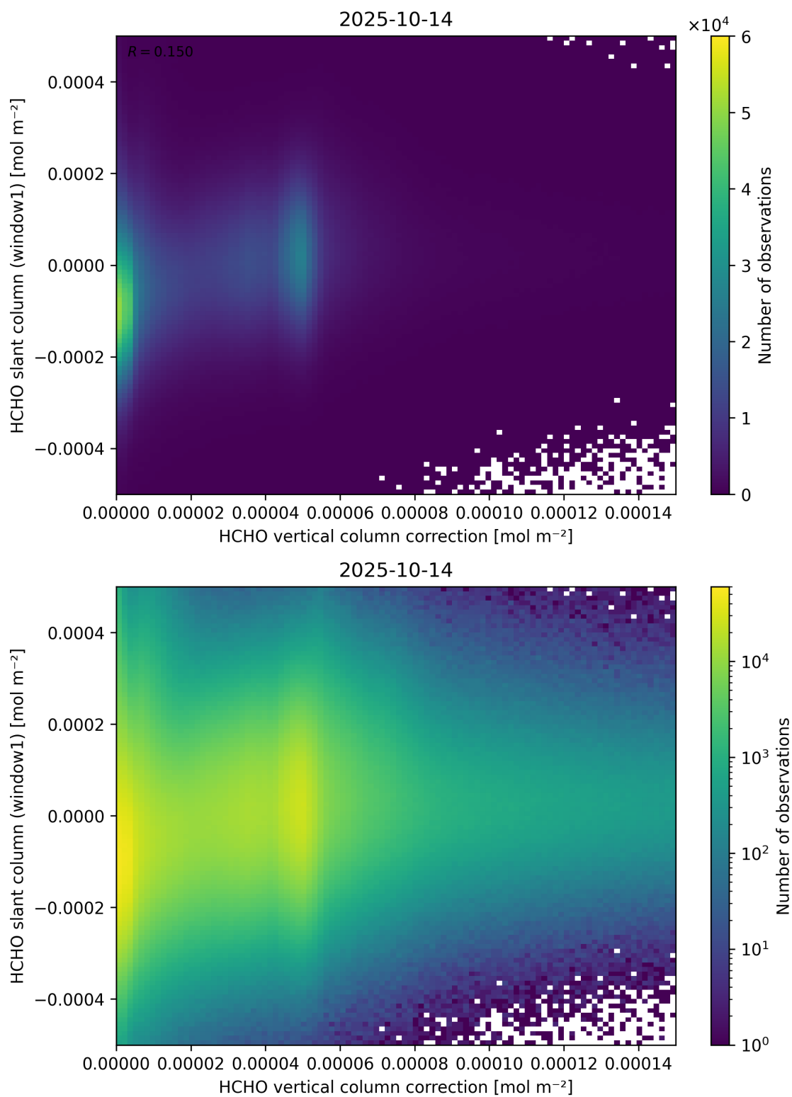
Figure 118: Scatter density plot of “HCHO vertical column correction” against “HCHO slant column (window1)” for 2025-10-13 to 2025-10-15.
