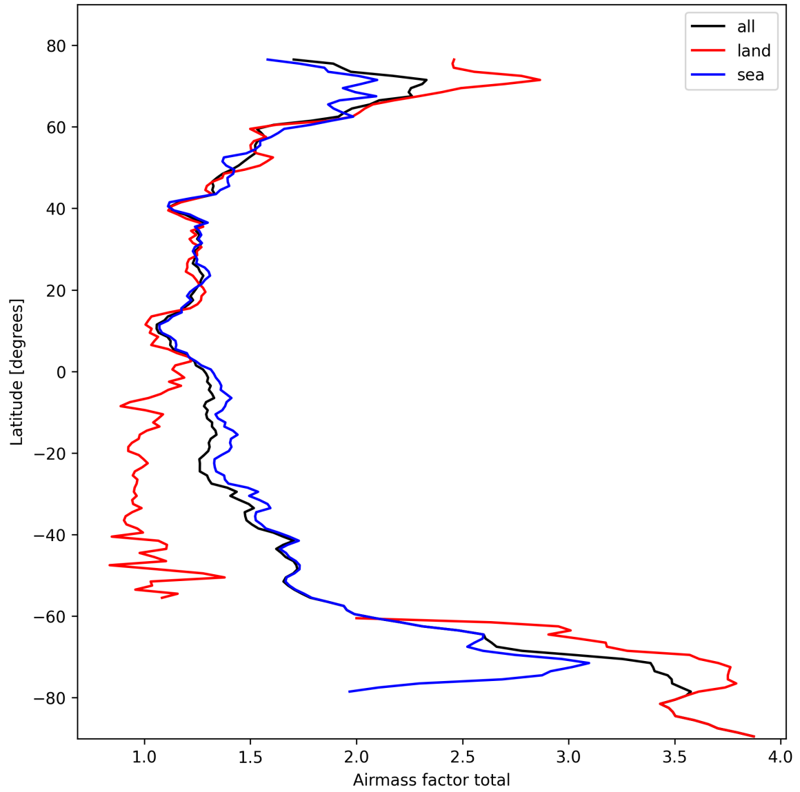
Figure 26: Zonal average of “Airmass factor total” for 2025-10-13 to 2025-10-15.
