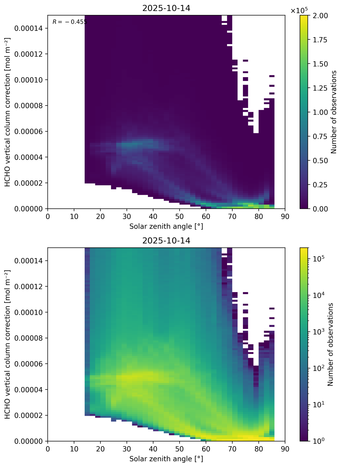
Figure 178: Scatter density plot of “Solar zenith angle” against “HCHO vertical column correction” for 2025-10-13 to 2025-10-15.
