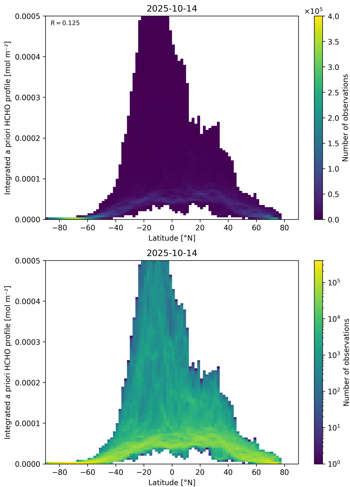
Figure 166: Scatter density plot of “Latitude” against “Integrated a priori HCHO profile” for 2025-10-13 to 2025-10-15.
