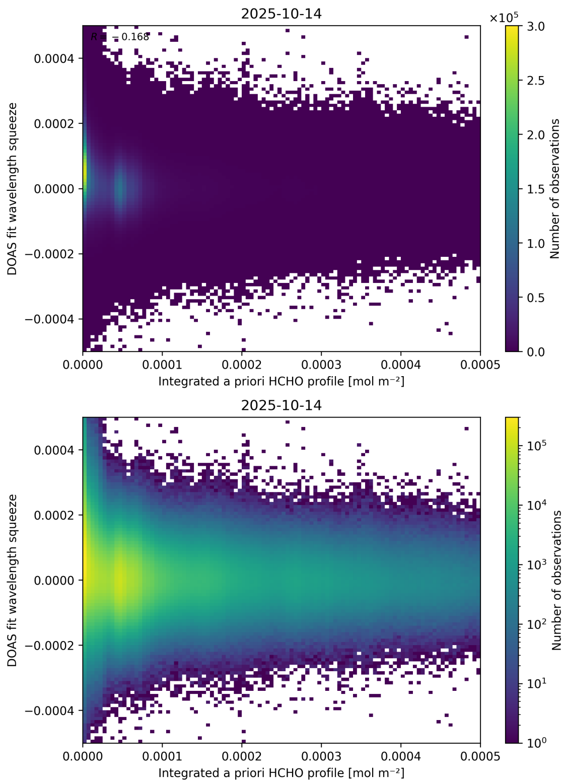
Figure 150: Scatter density plot of “Integrated a priori HCHO profile” against “DOAS fit wavelength squeeze” for 2025-10-13 to 2025-10-15.
