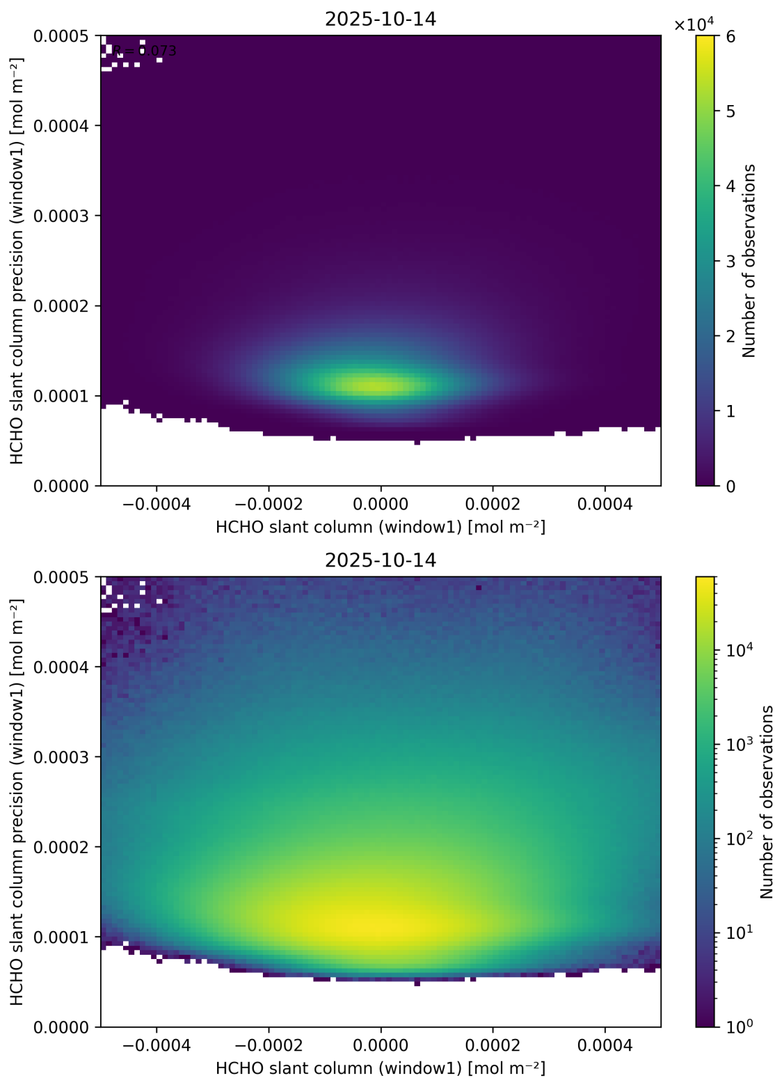
Figure 84: Scatter density plot of “HCHO slant column (window1)” against “HCHO slant column precision (window1)” for 2025-10-13 to 2025-10-15.
