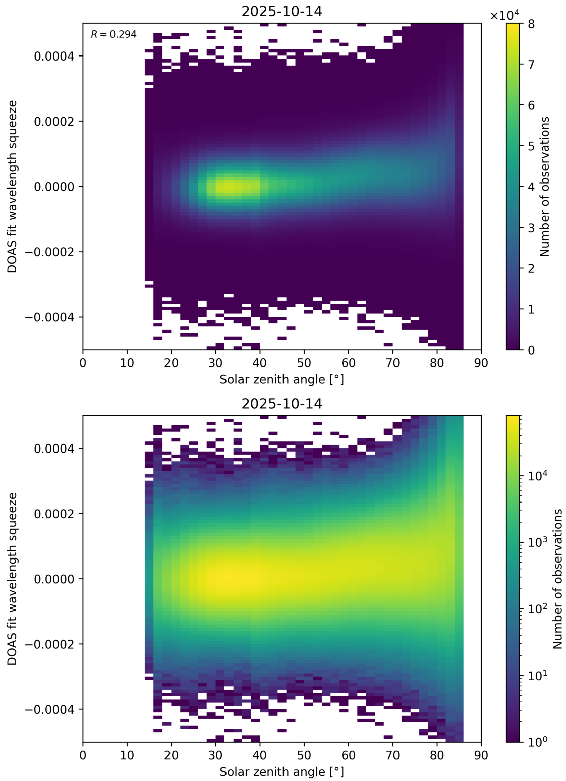
Figure 169: Scatter density plot of “Solar zenith angle” against “DOAS fit wavelength squeeze” for 2025-10-13 to 2025-10-15.
