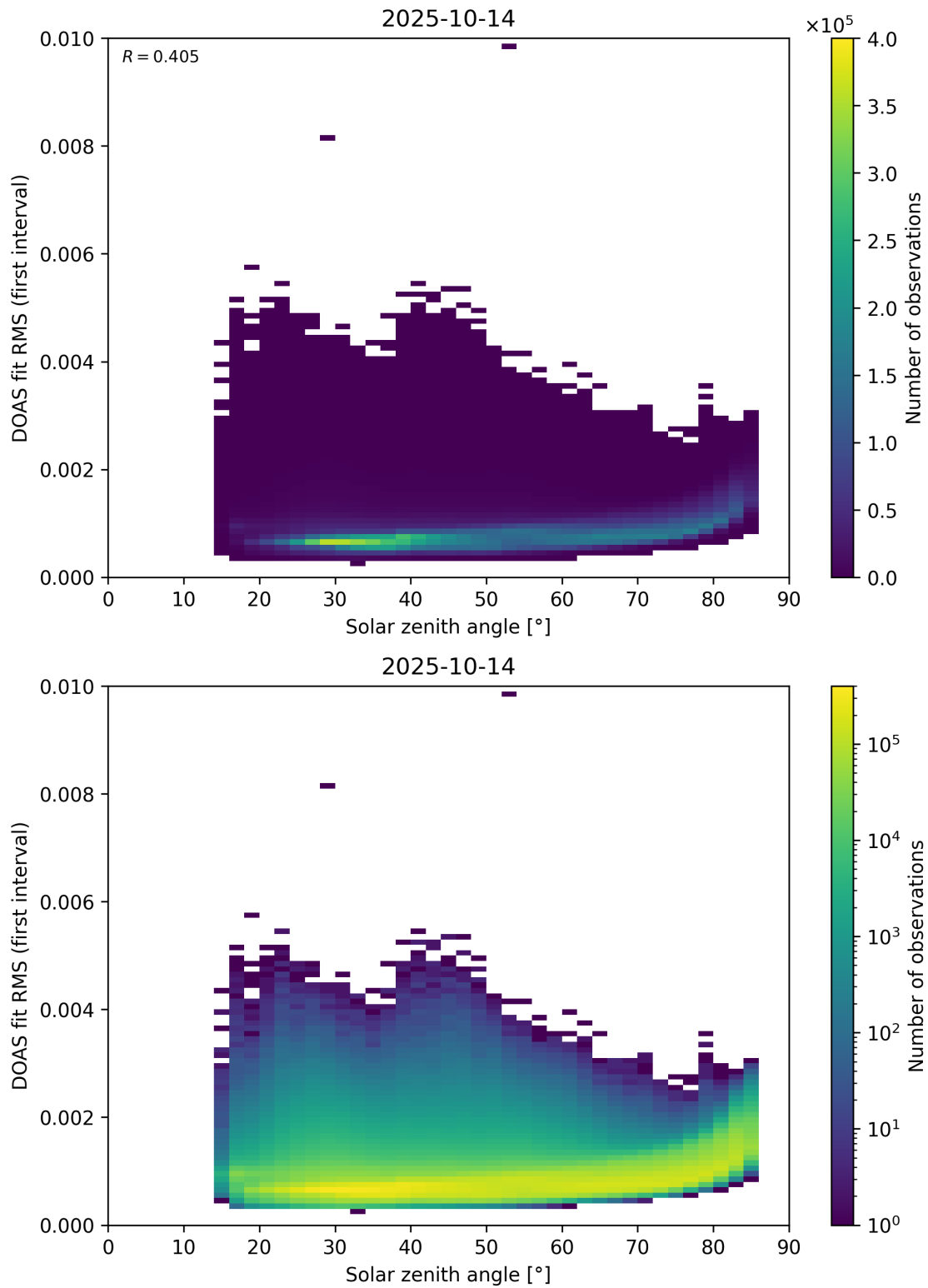
Figure 167: Scatter density plot of “Solar zenith angle” against “DOAS fit RMS (first interval)” for 2025-10-13 to 2025-10-15.
