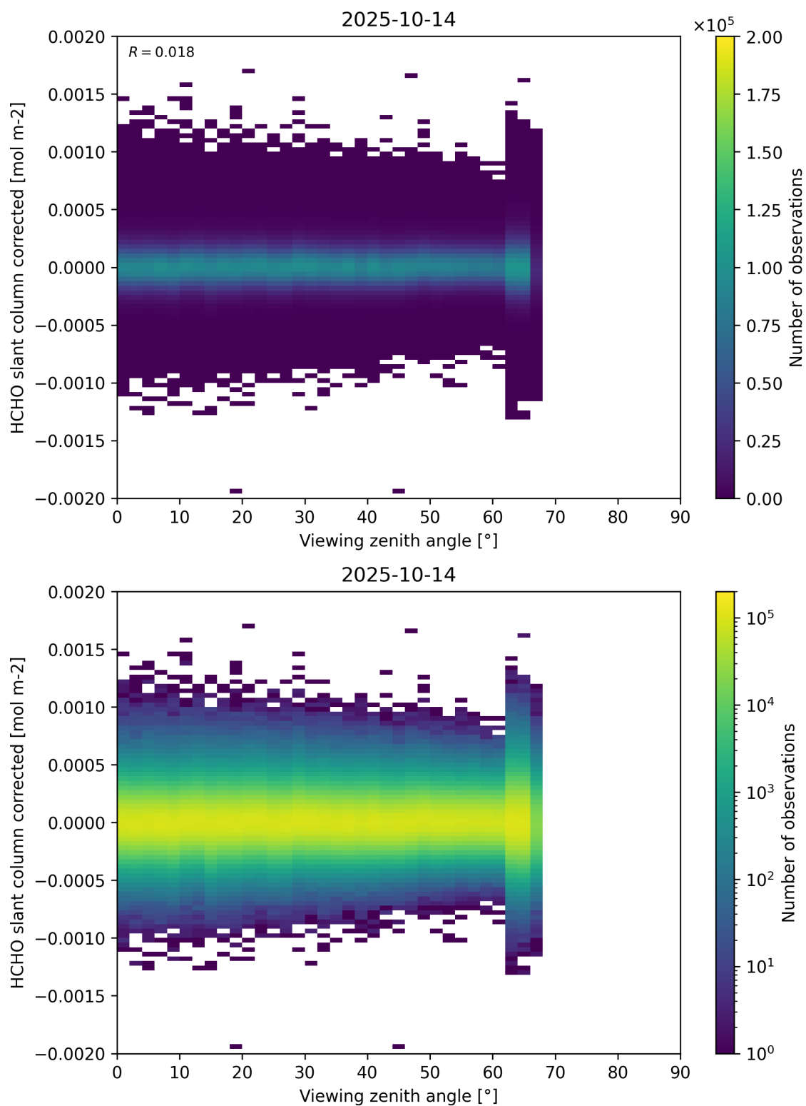
Figure 186: Scatter density plot of “Viewing zenith angle” against “HCHO slant column corrected” for 2025-10-13 to 2025-10-15.
