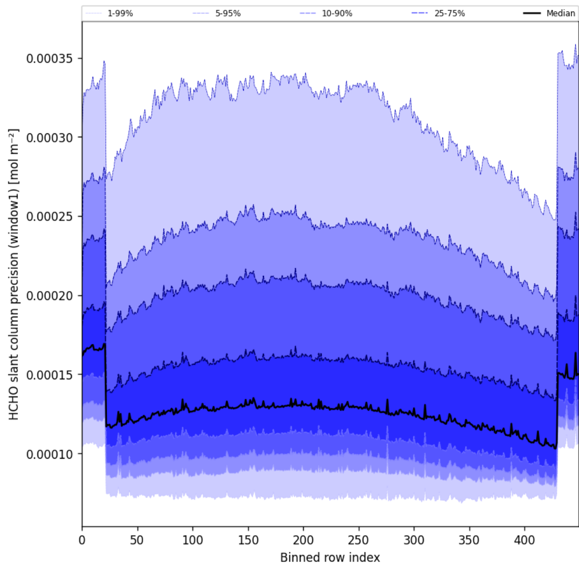
Figure 53: Along track statistics of “HCHO slant column precision (window1)” for 2025-10-13 to 2025-10-15
