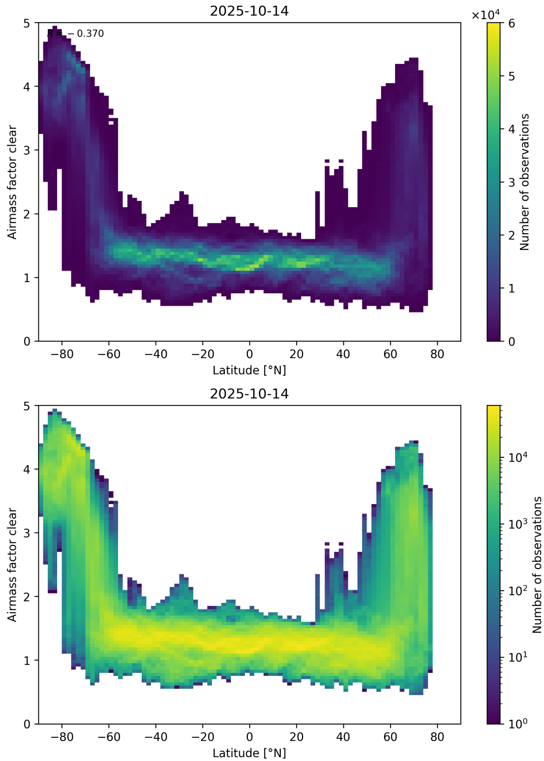
Figure 156: Scatter density plot of “Latitude” against “Airmass factor clear” for 2025-10-13 to 2025-10-15.
