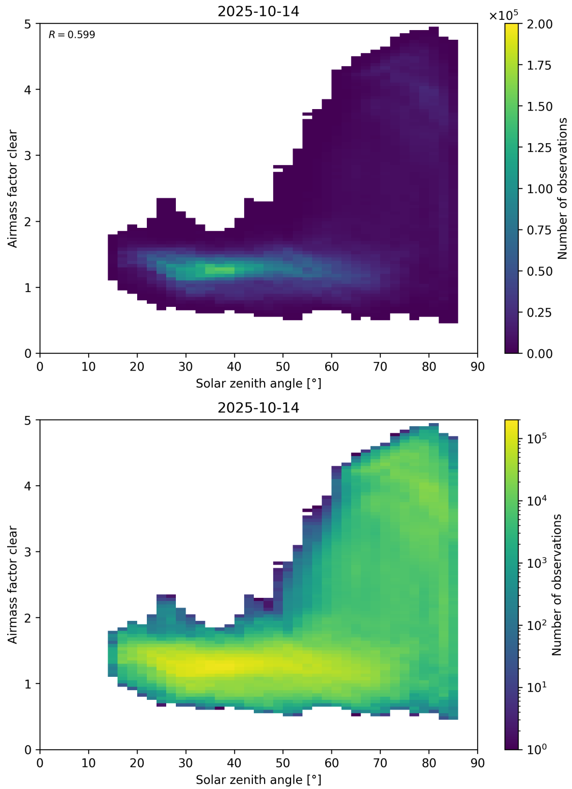
Figure 170: Scatter density plot of “Solar zenith angle” against “Airmass factor clear” for 2025-10-13 to 2025-10-15.
