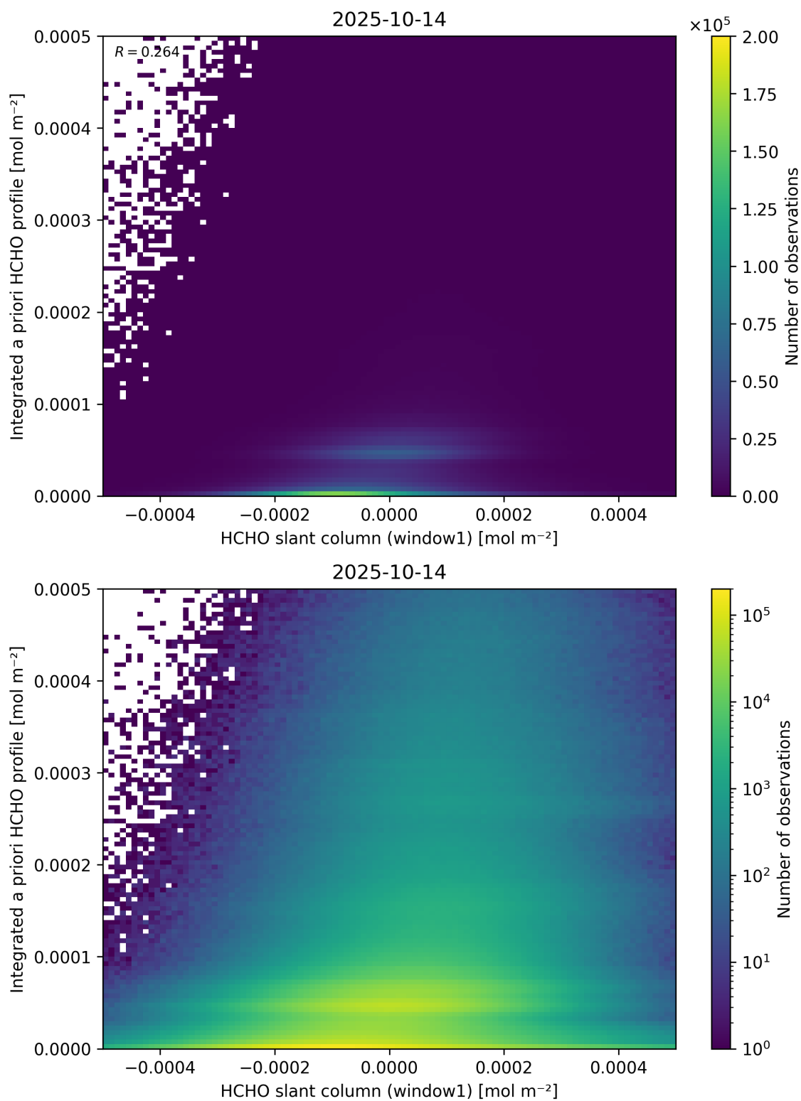
Figure 87: Scatter density plot of “HCHO slant column (window1)” against “Integrated a priori HCHO profile” for 2025-10-13 to 2025-10-15.
