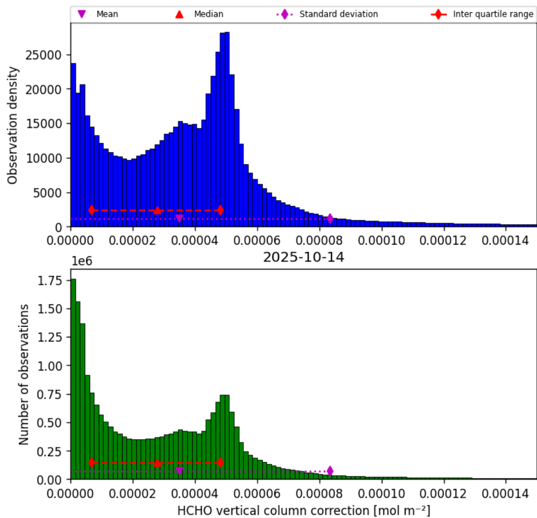
Figure 37: Histogram of “HCHO vertical column correction” for 2025-10-13 to 2025-10-15
