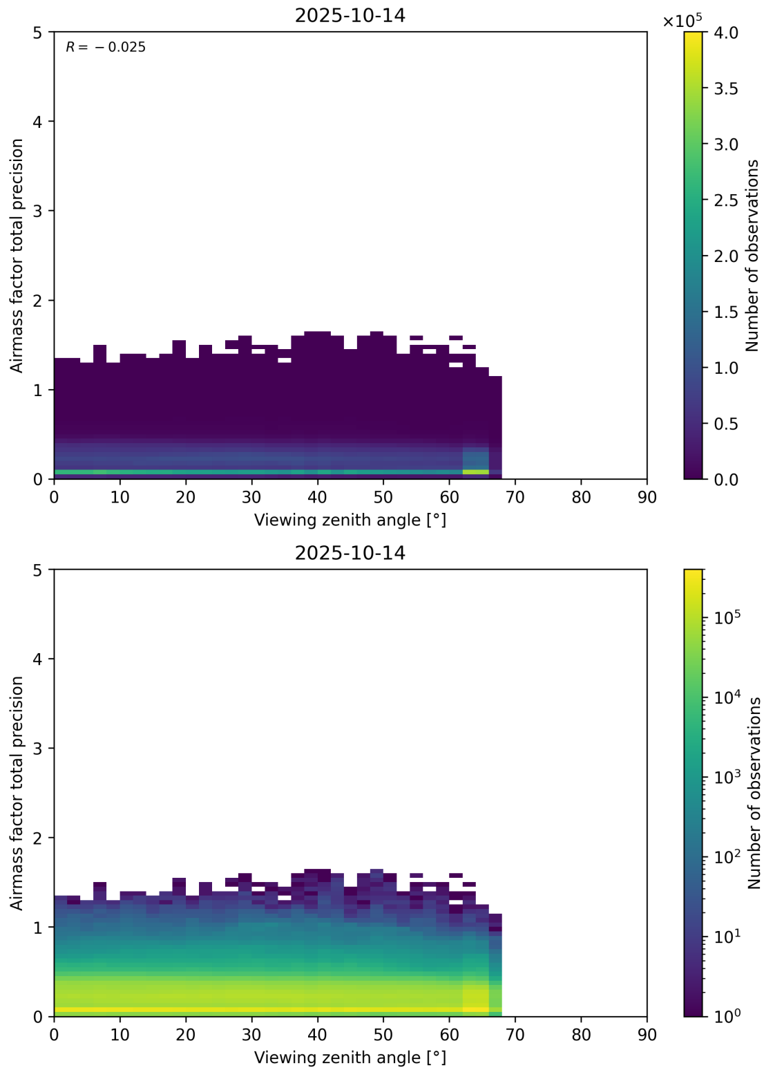
Figure 191: Scatter density plot of “Viewing zenith angle” against “Airmass factor total precision” for 2025-10-13 to 2025-10-15.
