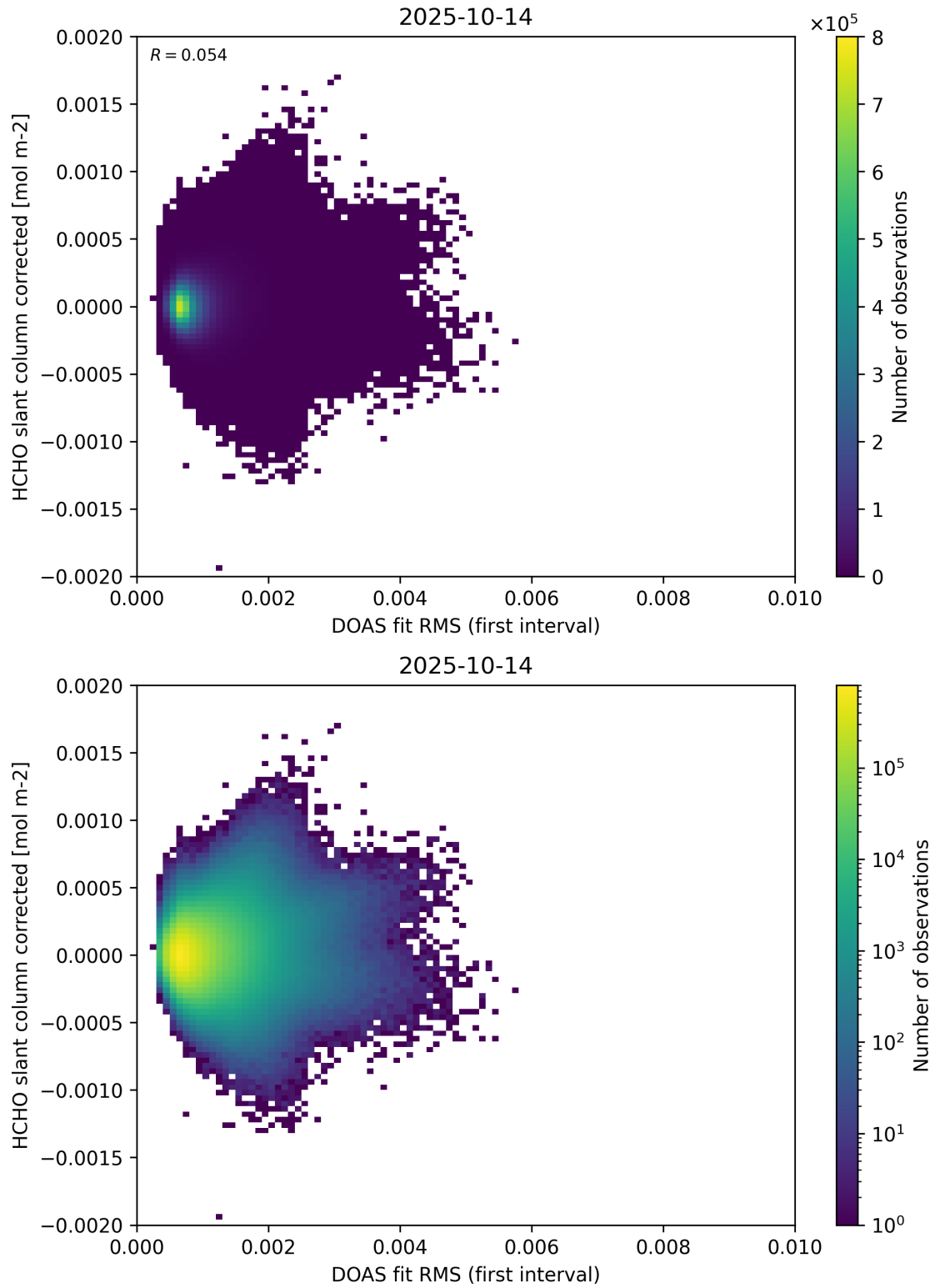
Figure 62: Scatter density plot of “DOAS fit RMS (first interval)” against “HCHO slant column corrected” for 2025-10-13 to 2025-10-15.
