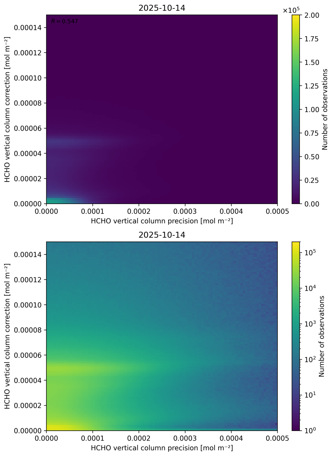
Figure 146: Scatter density plot of “HCHO vertical column precision” against “HCHO vertical column correction” for 2025-10-13 to 2025-10-15.
