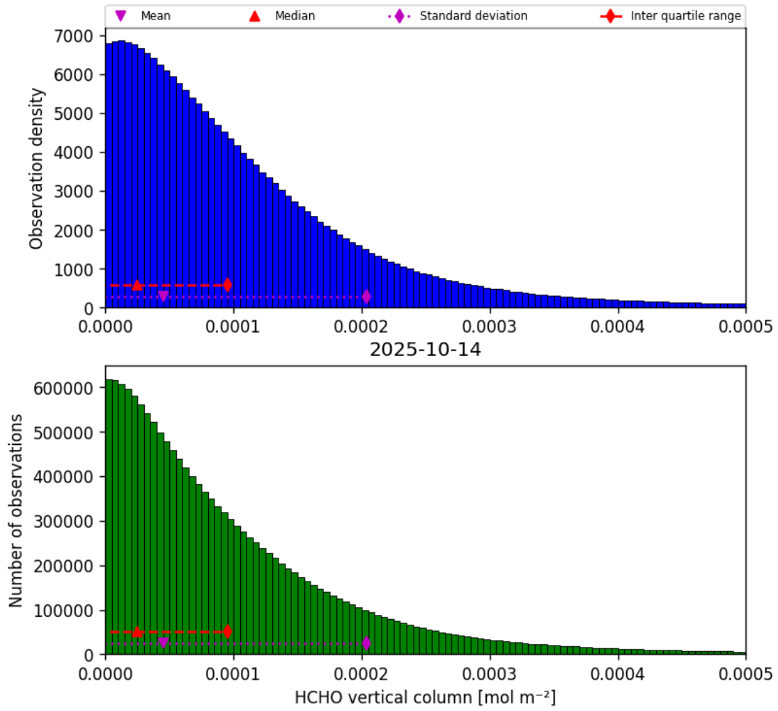
Figure 35: Histogram of “HCHO vertical column” for 2025-10-13 to 2025-10-15
