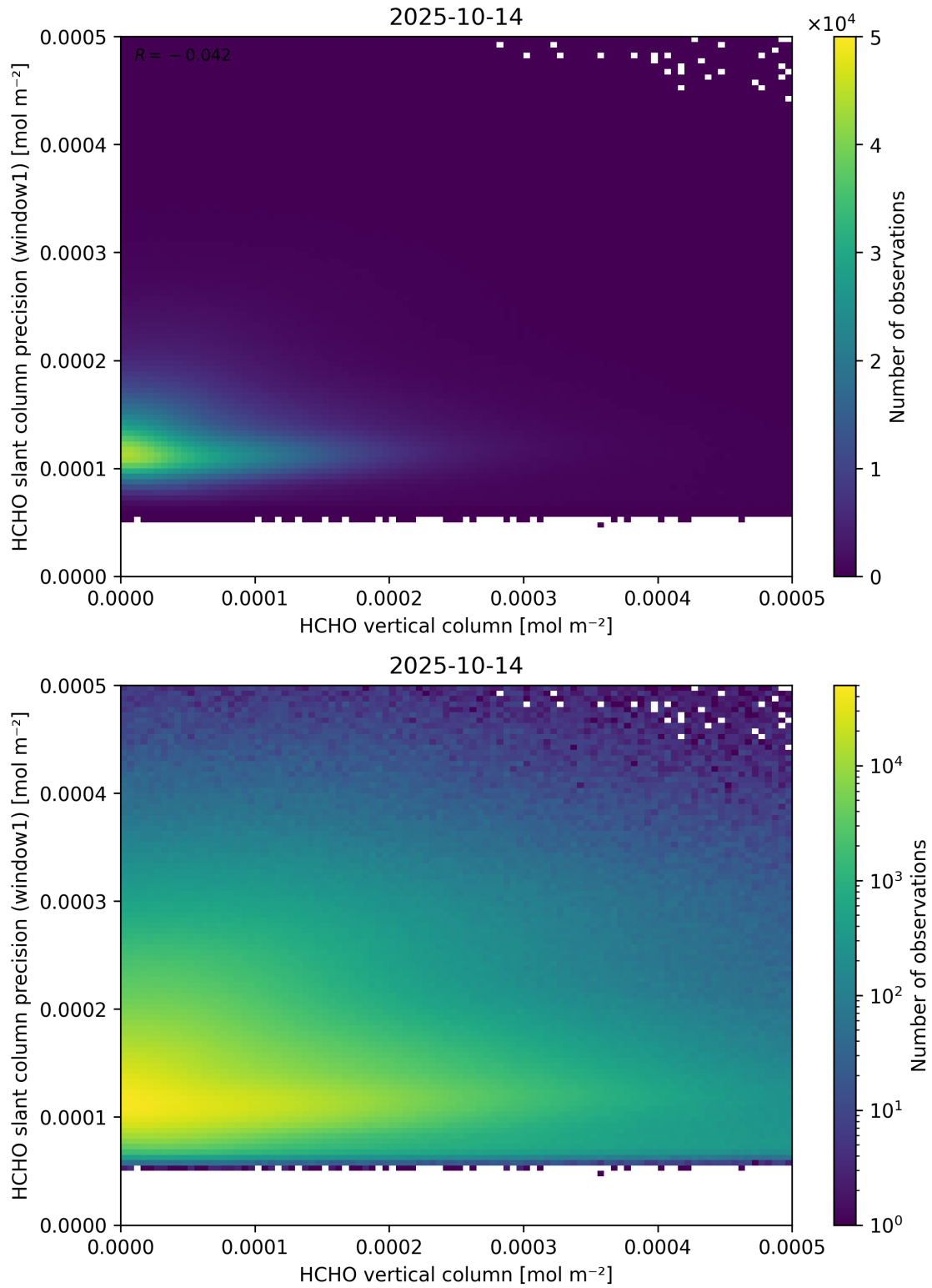
Figure 130: Scatter density plot of “HCHO vertical column” against “HCHO slant column precision (window1)” for 2025-10-13 to 2025-10-15.
