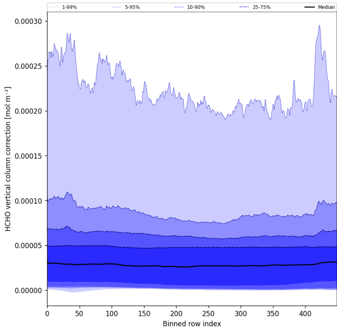
Figure 51: Along track statistics of “HCHO vertical column correction” for 2025-10-13 to 2025-10-15
