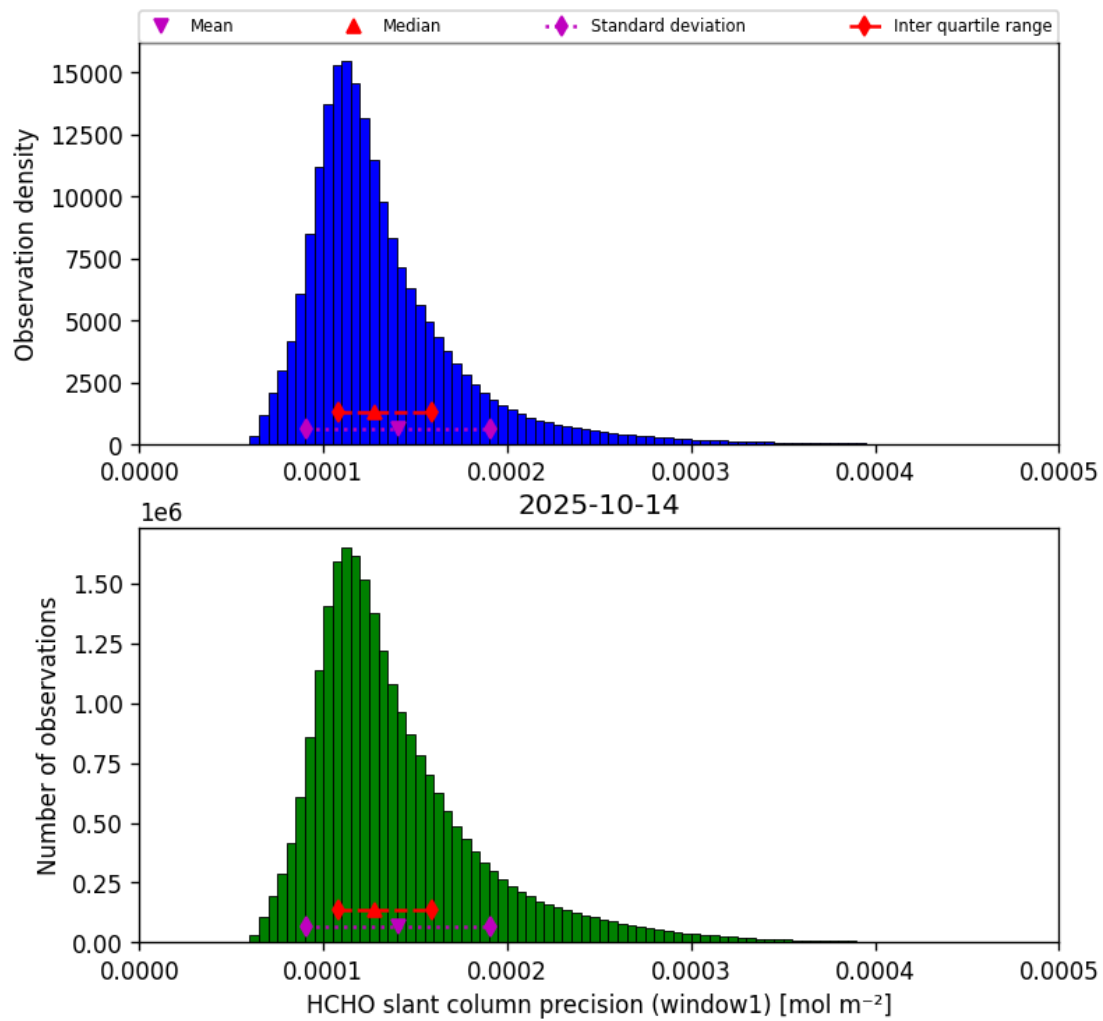
Figure 39: Histogram of “HCHO slant column precision (window1)” for 2025-10-13 to 2025-10-15
