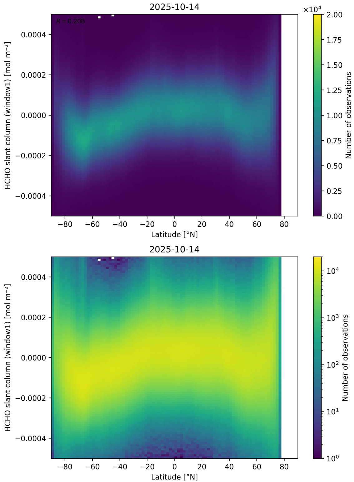
Figure 159: Scatter density plot of “Latitude” against “HCHO slant column (window1)” for 2025-10-13 to 2025-10-15.
