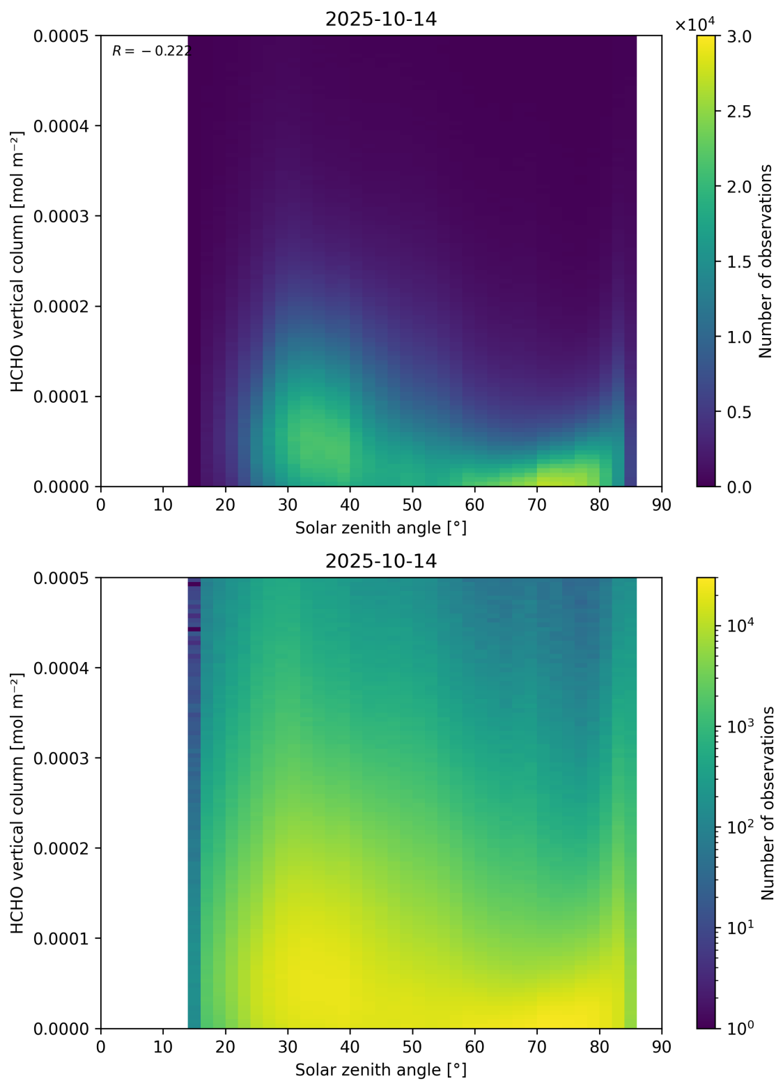
Figure 177: Scatter density plot of “Solar zenith angle” against “HCHO vertical column” for 2025-10-13 to 2025-10-15.
