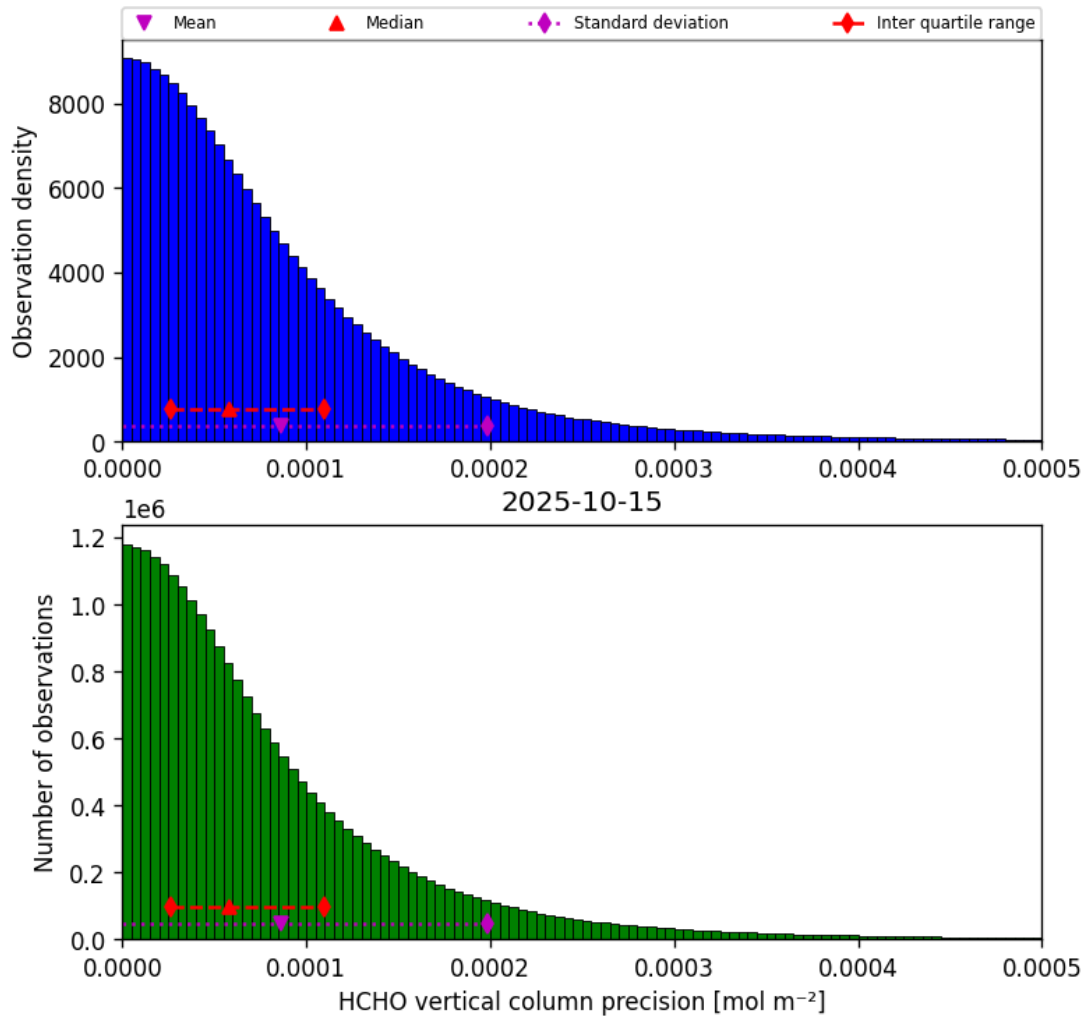
Figure 36: Histogram of “HCHO vertical column precision” for 2025-10-14 to 2025-10-16
