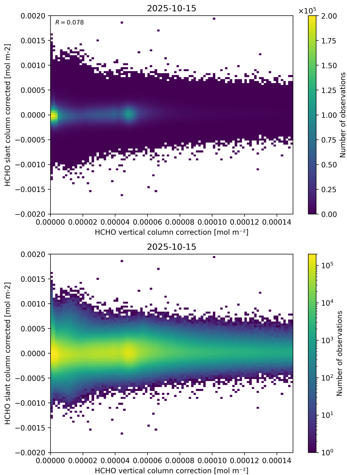
Figure 116: Scatter density plot of “HCHO vertical column correction” against “HCHO slant column corrected” for 2025-10-14 to 2025-10-16.
