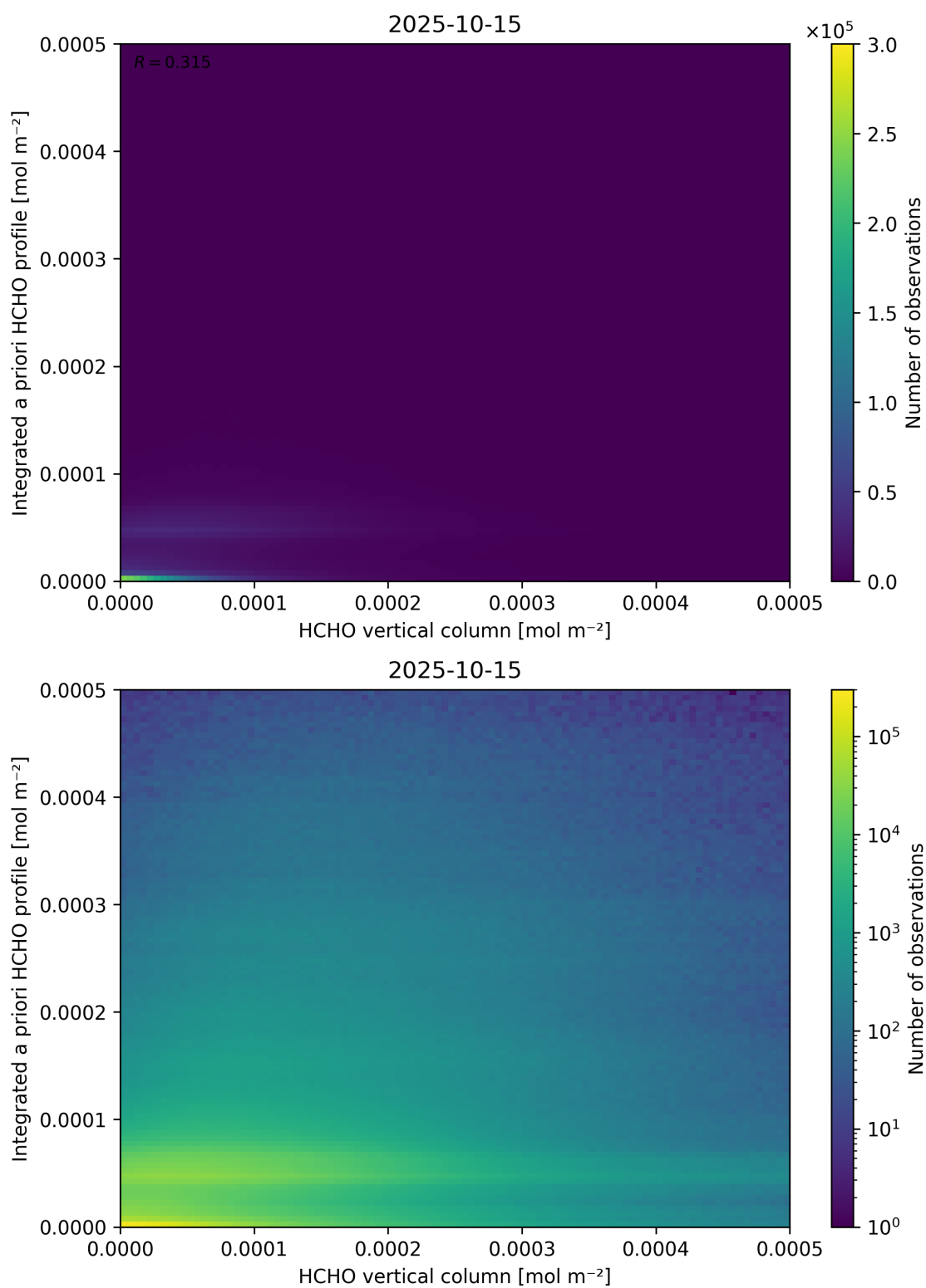
Figure 135: Scatter density plot of “HCHO vertical column” against “Integrated a priori HCHO profile” for 2025-10-14 to 2025-10-16.
