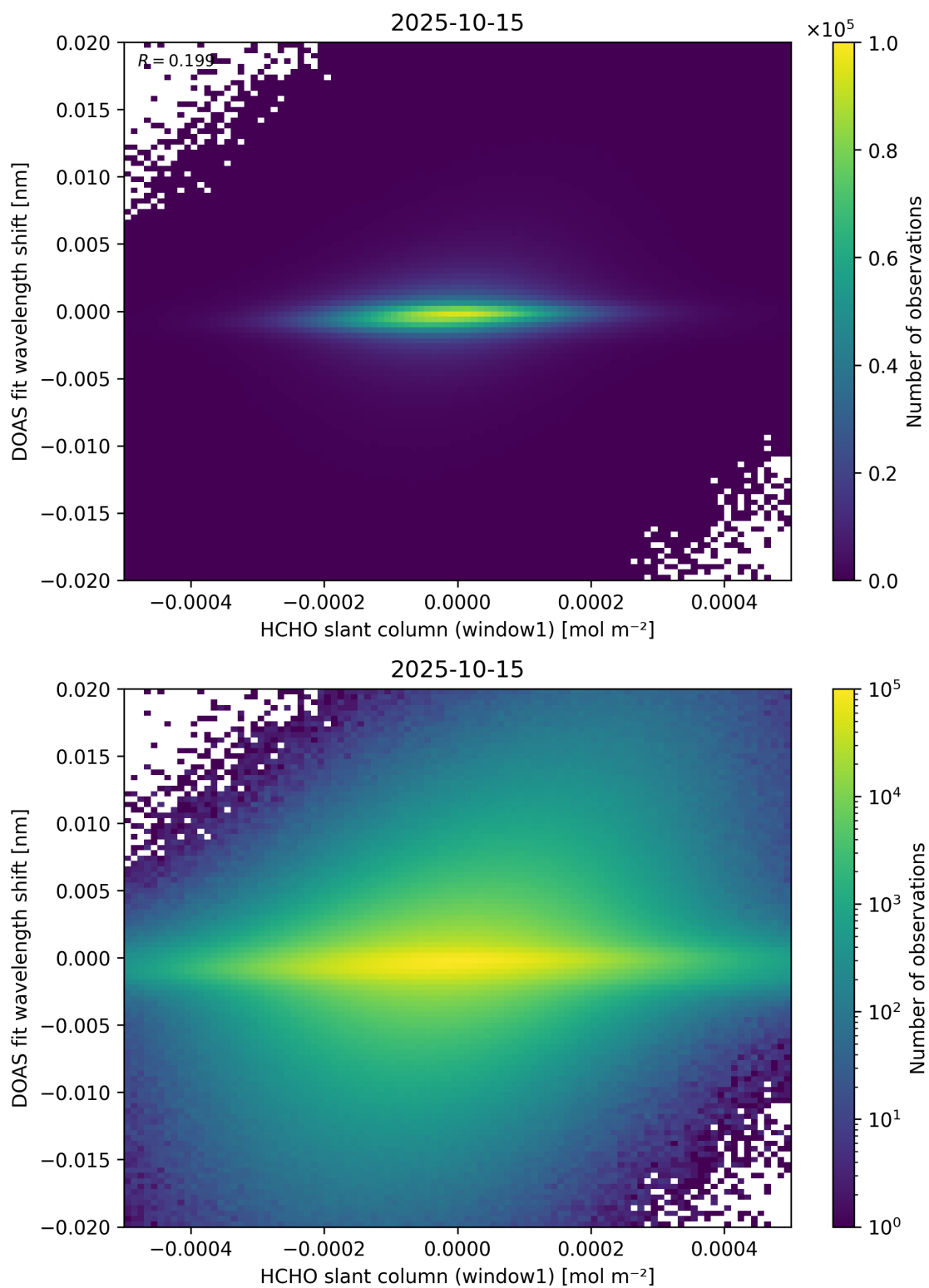
Figure 79: Scatter density plot of “HCHO slant column (window1)” against “DOAS fit wavelength shift” for 2025-10-14 to 2025-10-16.
