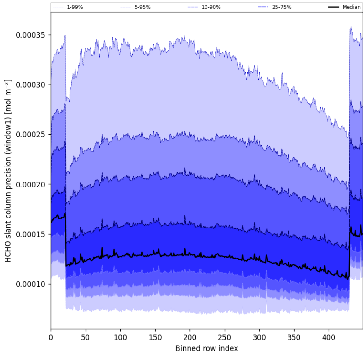
Figure 53: Along track statistics of “HCHO slant column precision (window1)” for 2025-10-14 to 2025-10-16
