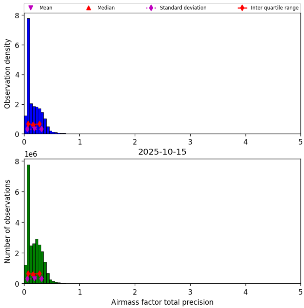
Figure 41: Histogram of “Airmass factor total precision” for 2025-10-14 to 2025-10-16
