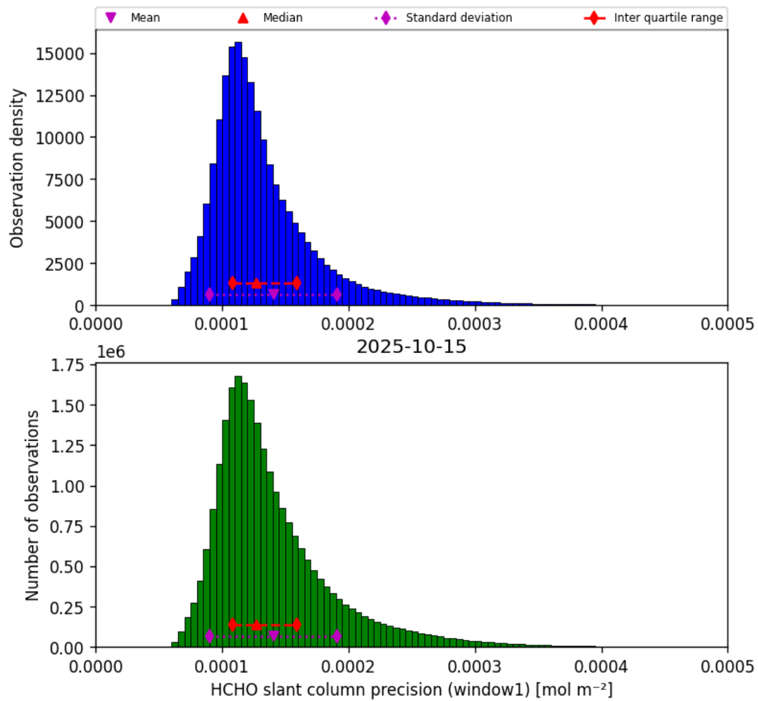
Figure 39: Histogram of “HCHO slant column precision (window1)” for 2025-10-14 to 2025-10-16
