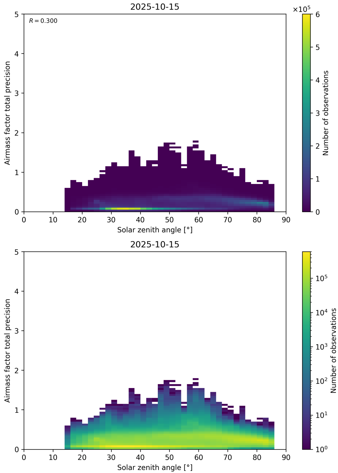
Figure 176: Scatter density plot of “Solar zenith angle” against “Airmass factor total precision” for 2025-10-14 to 2025-10-16.
