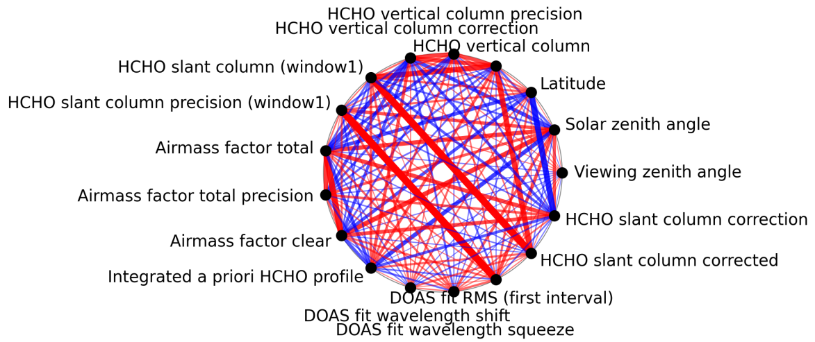
Figure 1: Map of correlation graph for 2025-10-14 to 2025-10-16.
