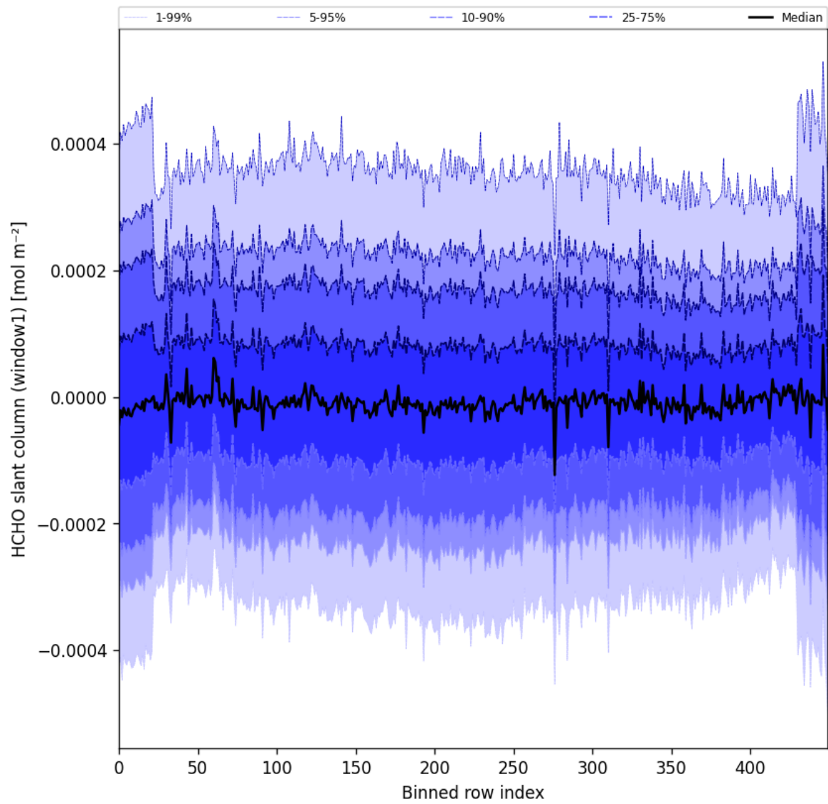
Figure 52: Along track statistics of “HCHO slant column (window1)” for 2025-10-14 to 2025-10-16
