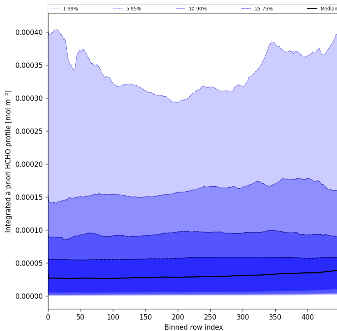
Figure 57: Along track statistics of "Integrated a priori HCHO profile" for 2025-10-14 to 2025-10-16
