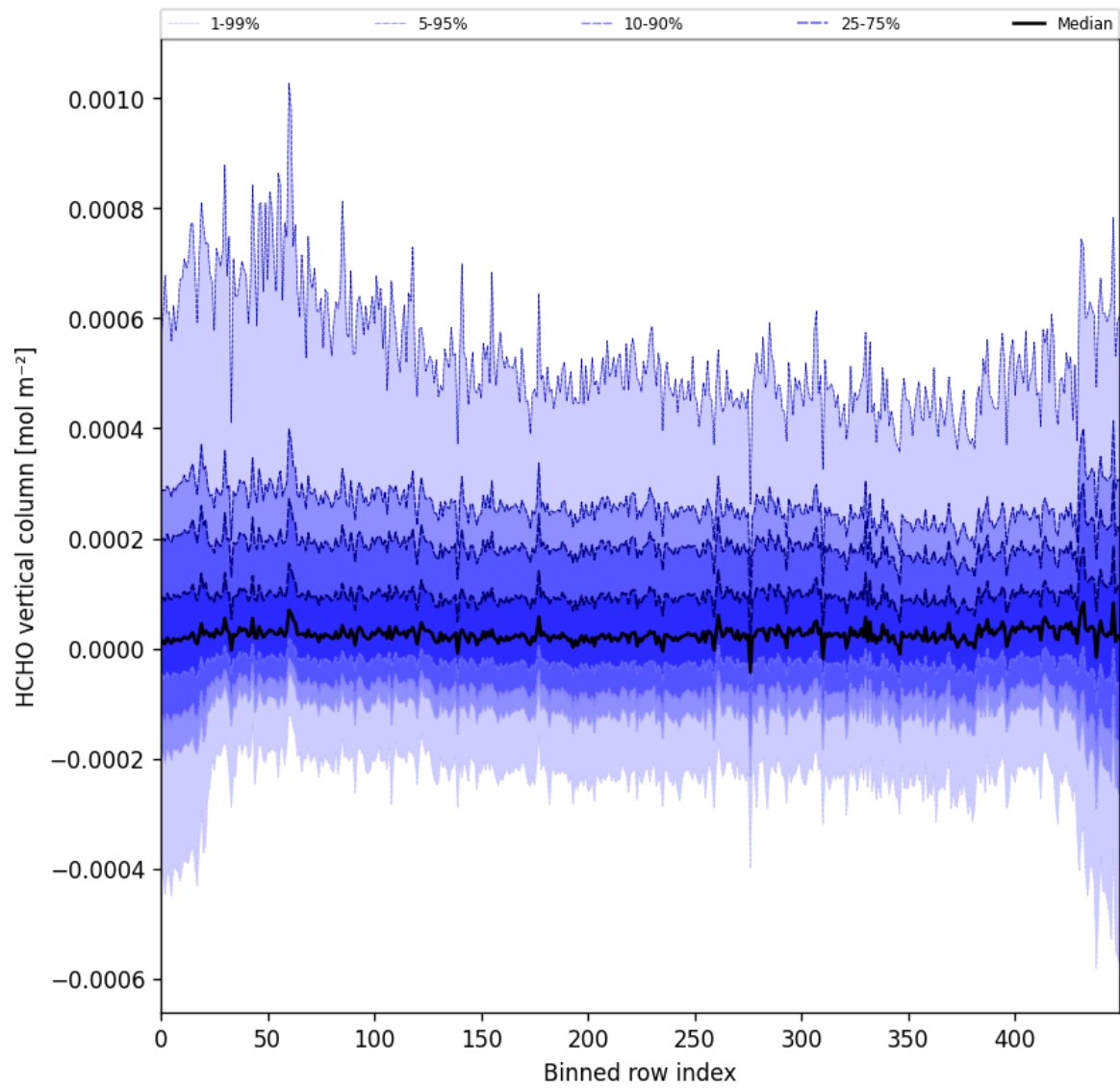
Figure 49: Along track statistics of “HCHO vertical column” for 2025-10-14 to 2025-10-16
