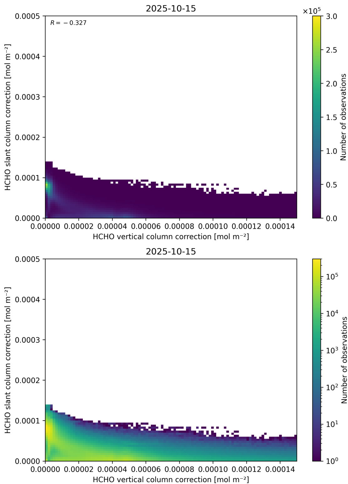
Figure 117: Scatter density plot of “HCHO vertical column correction” against “HCHO slant column correction” for 2025-10-14 to 2025-10-16.
