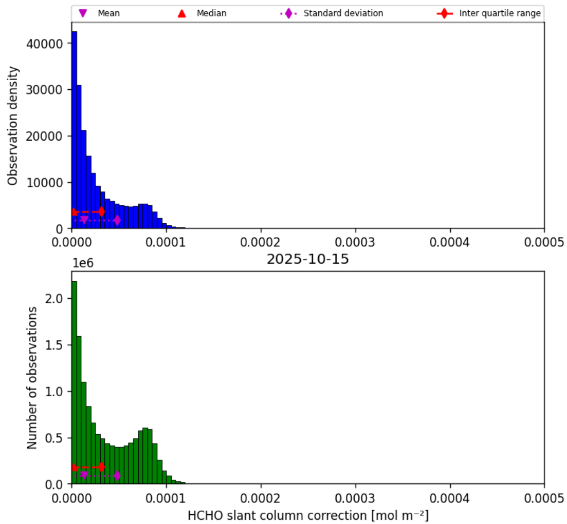
Figure 47: Histogram of “HCHO slant column correction” for 2025-10-14 to 2025-10-16
