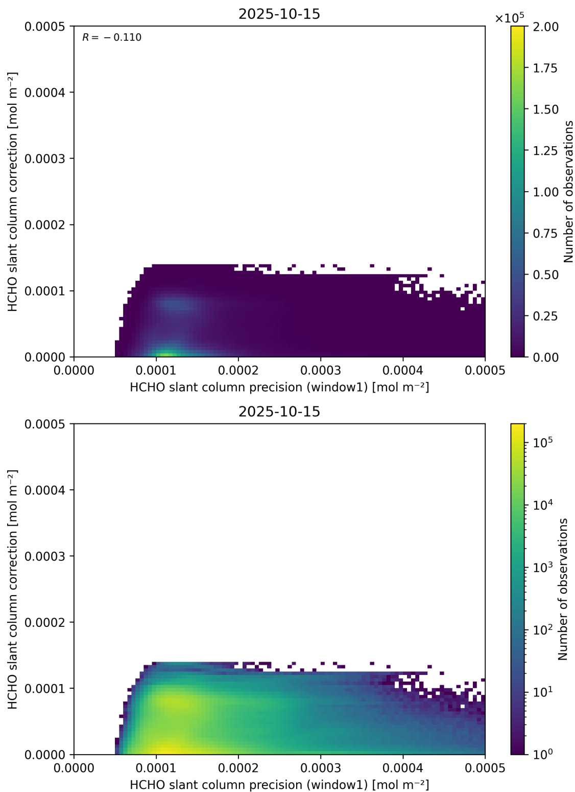
Figure 93: Scatter density plot of “HCHO slant column precision (window1)” against “HCHO slant column correction” for 2025-10-14 to 2025-10-16.
