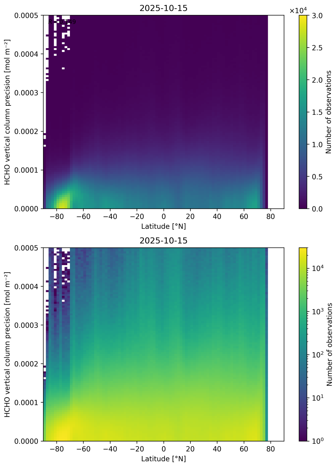
Figure 165: Scatter density plot of “Latitude” against “HCHO vertical column precision” for 2025-10-14 to 2025-10-16.
