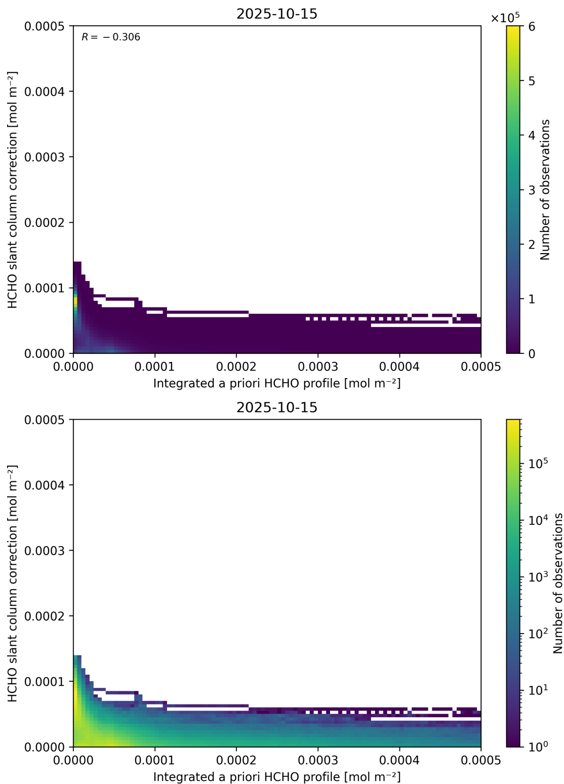
Figure 152: Scatter density plot of “Integrated a priori HCHO profile” against “HCHO slant column correction” for 2025-10-14 to 2025-10-16.
