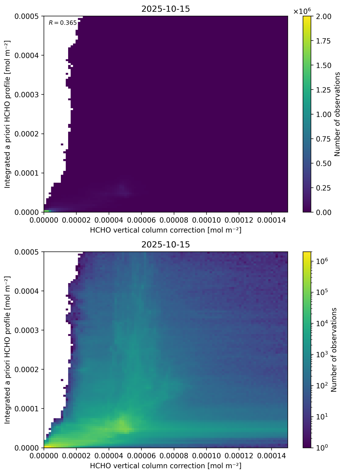
Figure 122: Scatter density plot of “HCHO vertical column correction” against “Integrated a priori HCHO profile” for 2025-10-14 to 2025-10-16.
