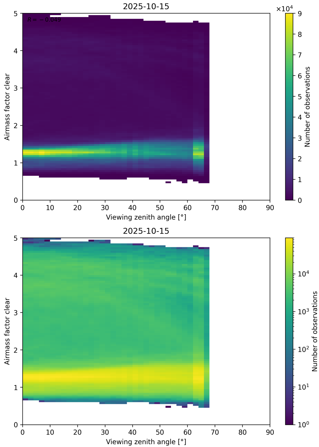
Figure 185: Scatter density plot of “Viewing zenith angle” against “Airmass factor clear” for 2025-10-14 to 2025-10-16.
