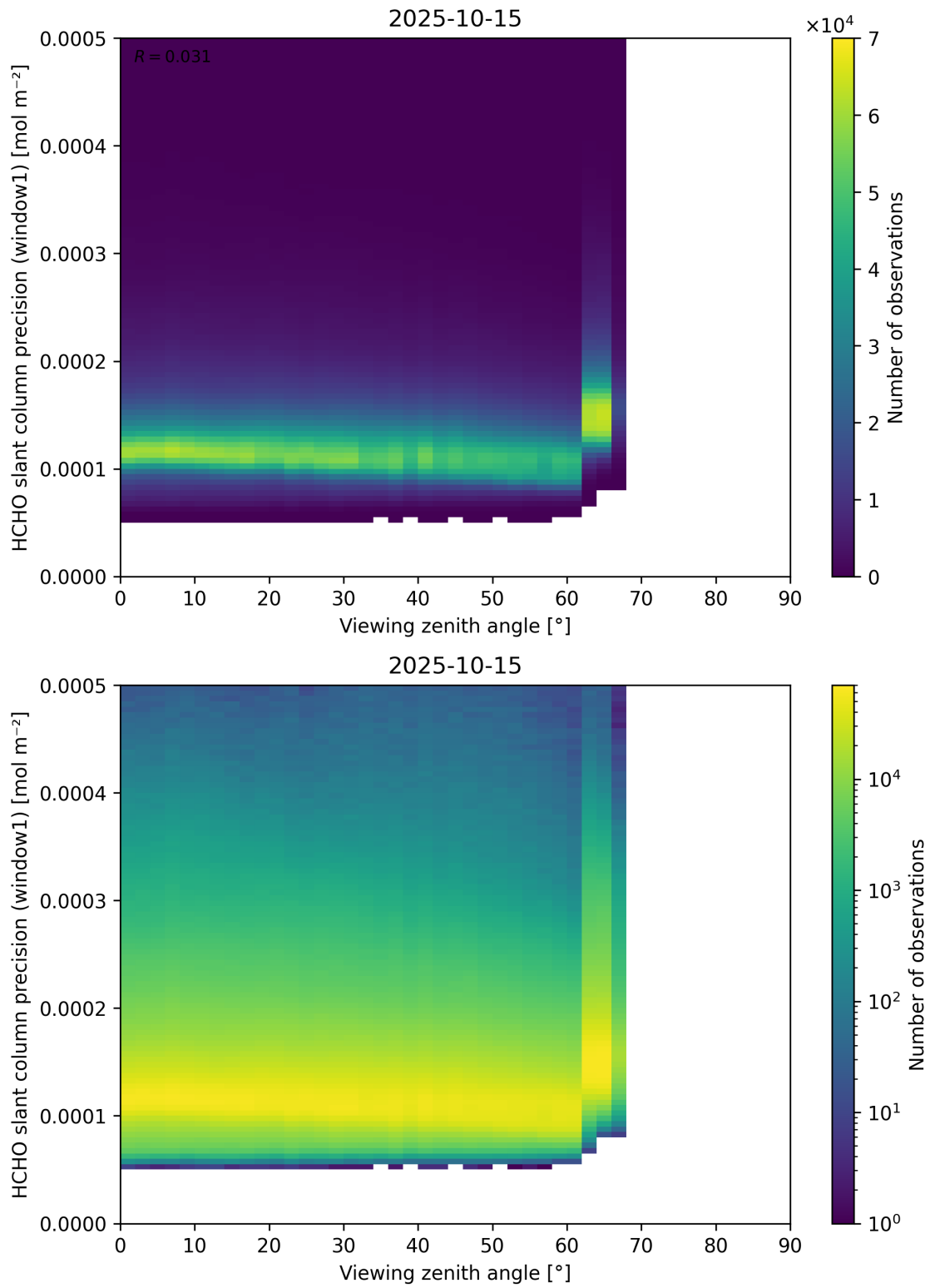
Figure 189: Scatter density plot of “Viewing zenith angle” against “HCHO slant column precision (window1)” for 2025-10-14 to 2025-10-16.
