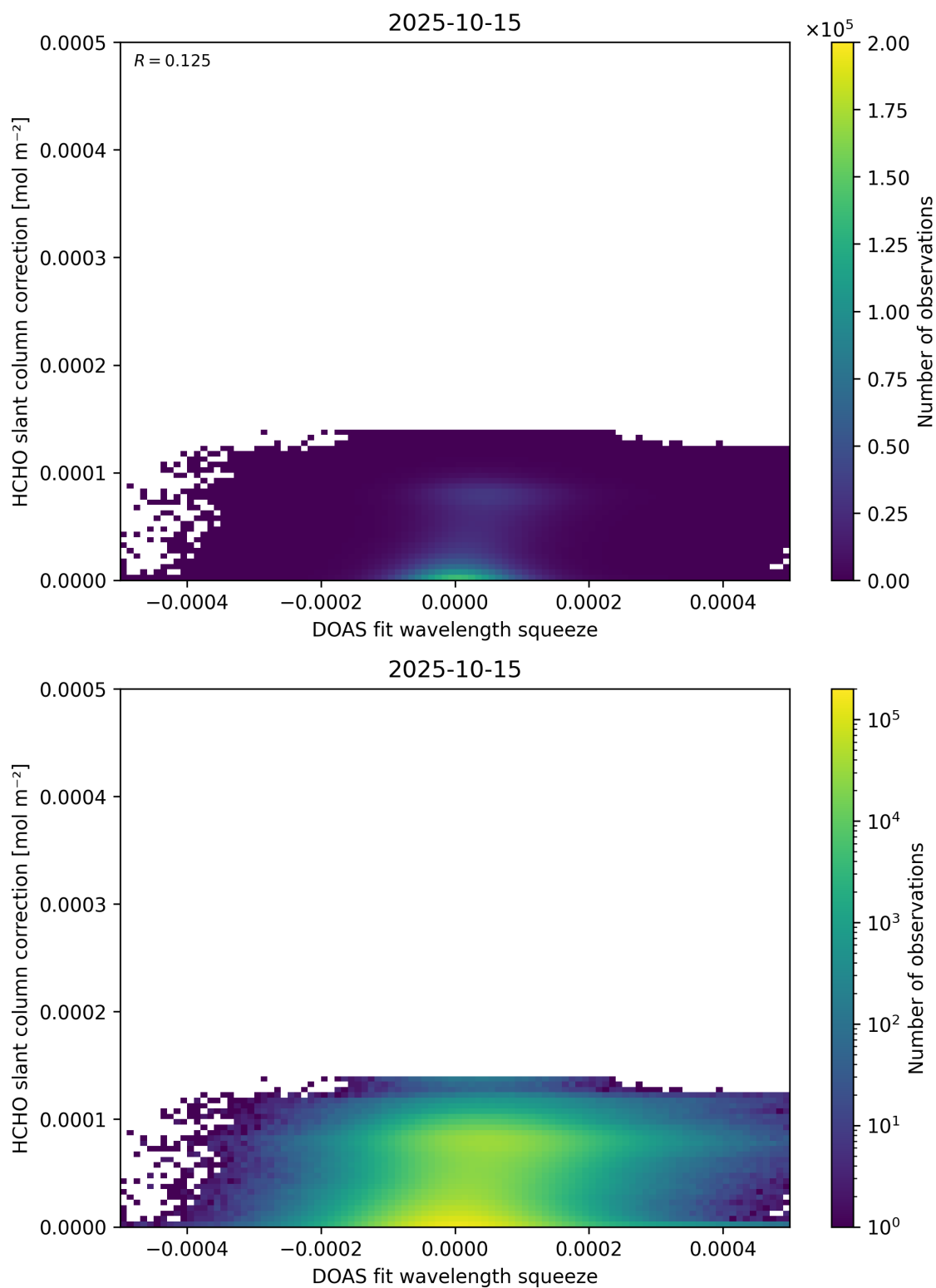
Figure 70: Scatter density plot of “DOAS fit wavelength squeeze” against “HCHO slant column correction” for 2025-10-14 to 2025-10-16.
