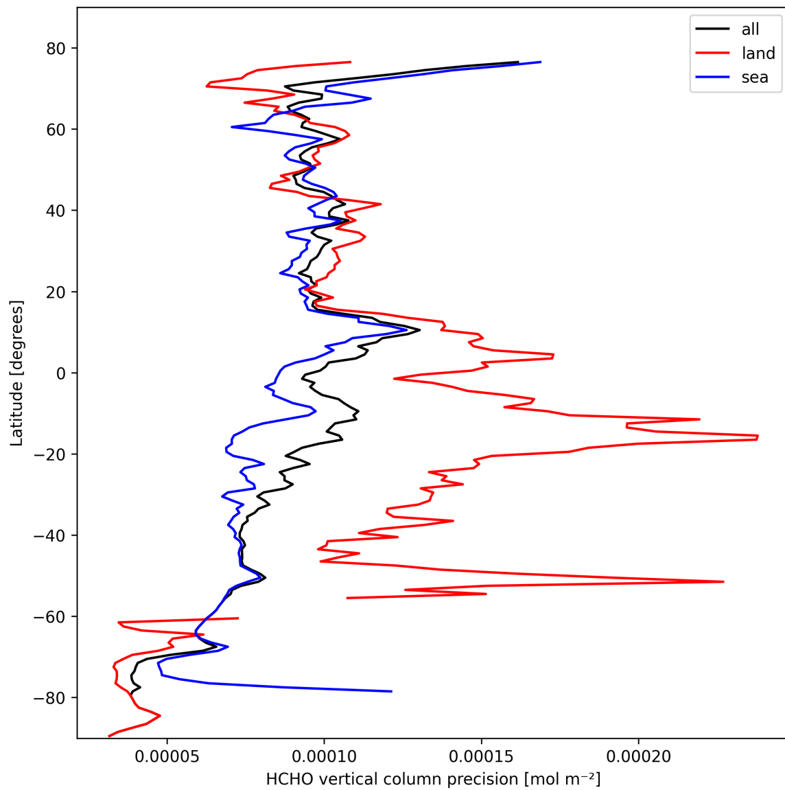
Figure 22: Zonal average of “HCHO vertical column precision” for 2025-10-14 to 2025-10-16.
