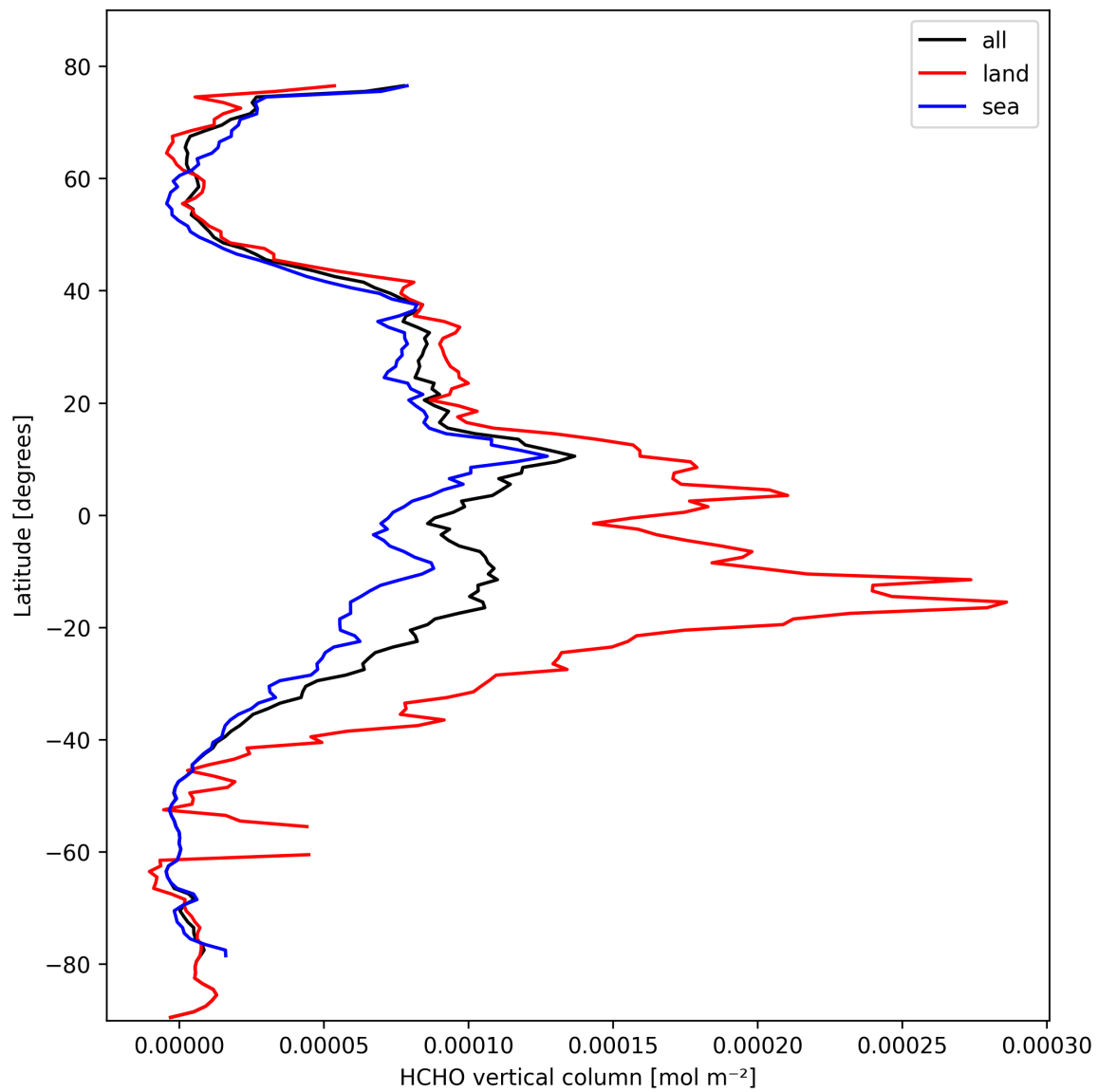
Figure 21: Zonal average of “HCHO vertical column” for 2025-10-14 to 2025-10-16.
