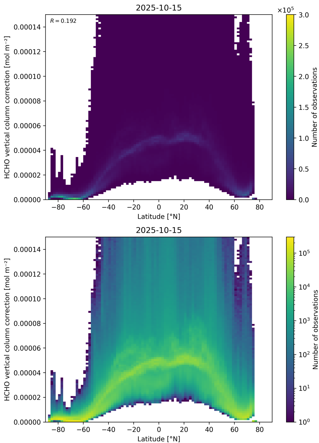
Figure 164: Scatter density plot of “Latitude” against “HCHO vertical column correction” for 2025-10-14 to 2025-10-16.
