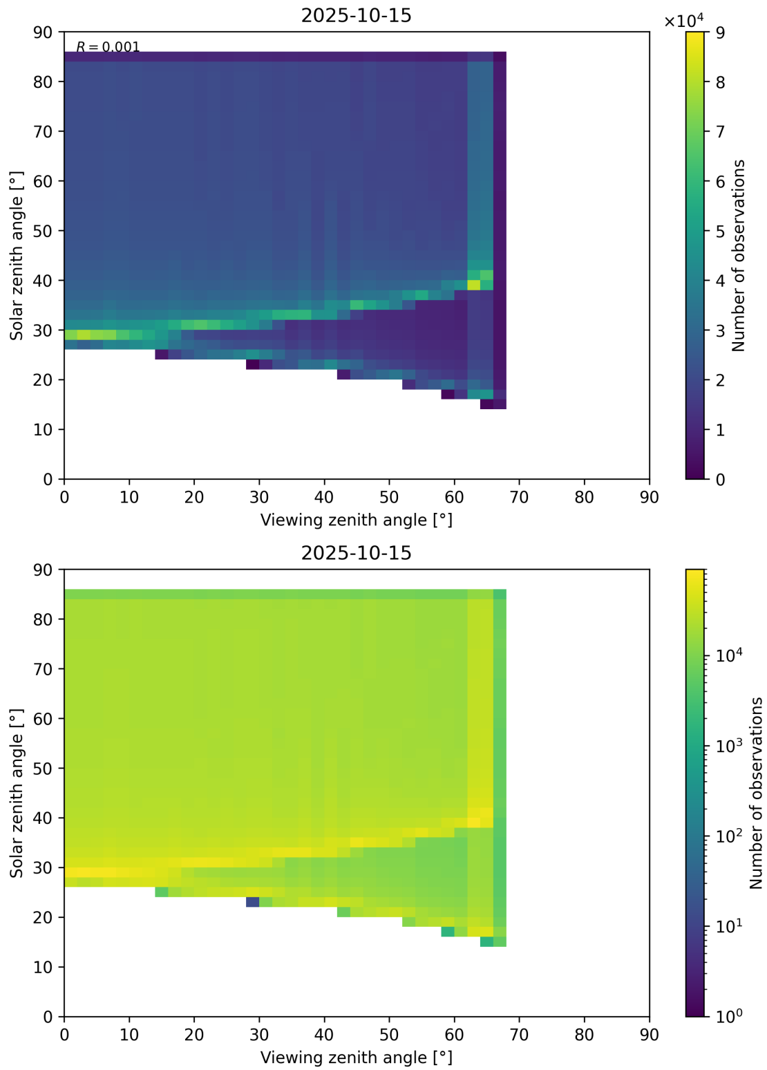
Figure 197: Scatter density plot of “Viewing zenith angle” against “Solar zenith angle” for 2025-10-14 to 2025-10-16.
