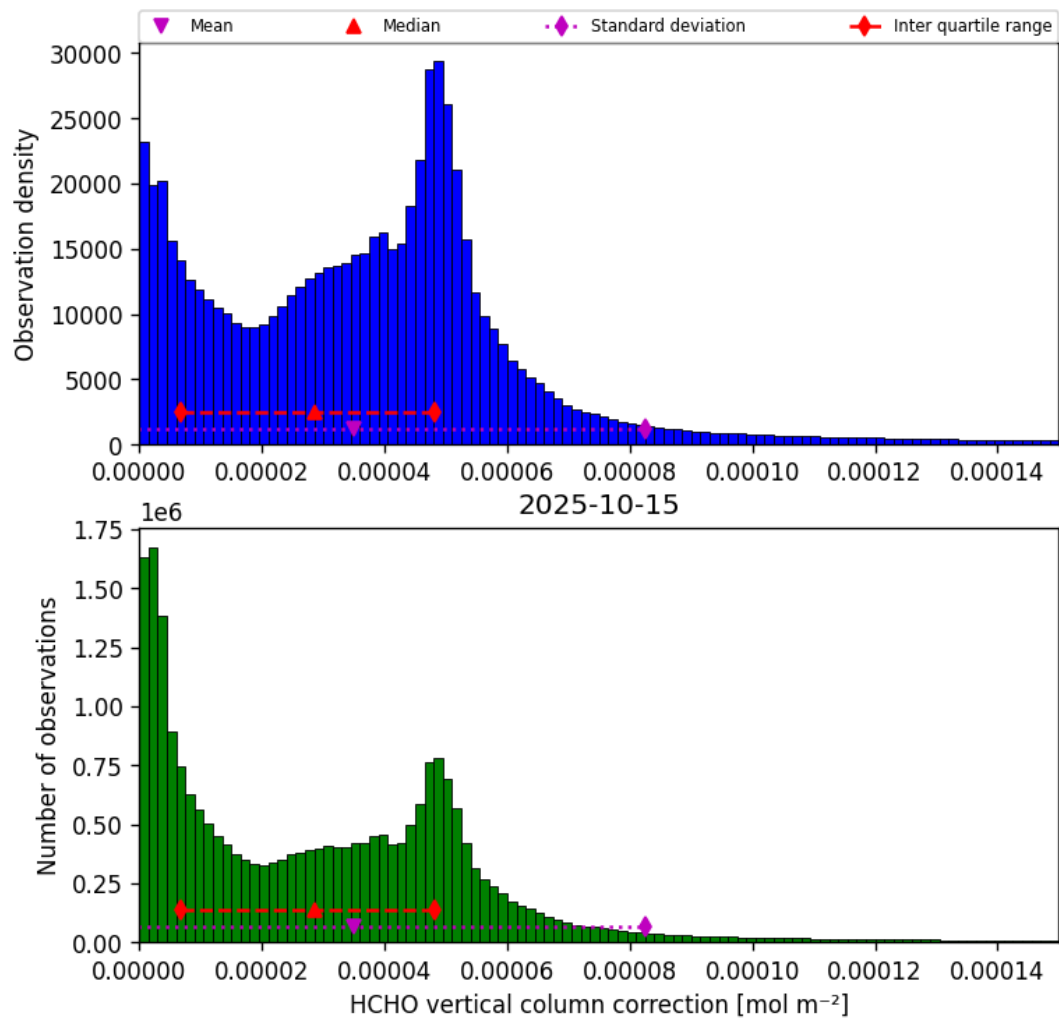
Figure 37: Histogram of “HCHO vertical column correction” for 2025-10-14 to 2025-10-16
