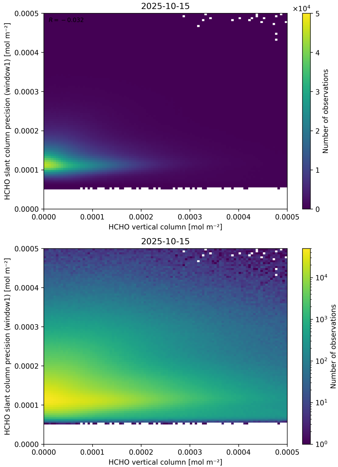
Figure 130: Scatter density plot of “HCHO vertical column” against “HCHO slant column precision (window1)” for 2025-10-14 to 2025-10-16.
