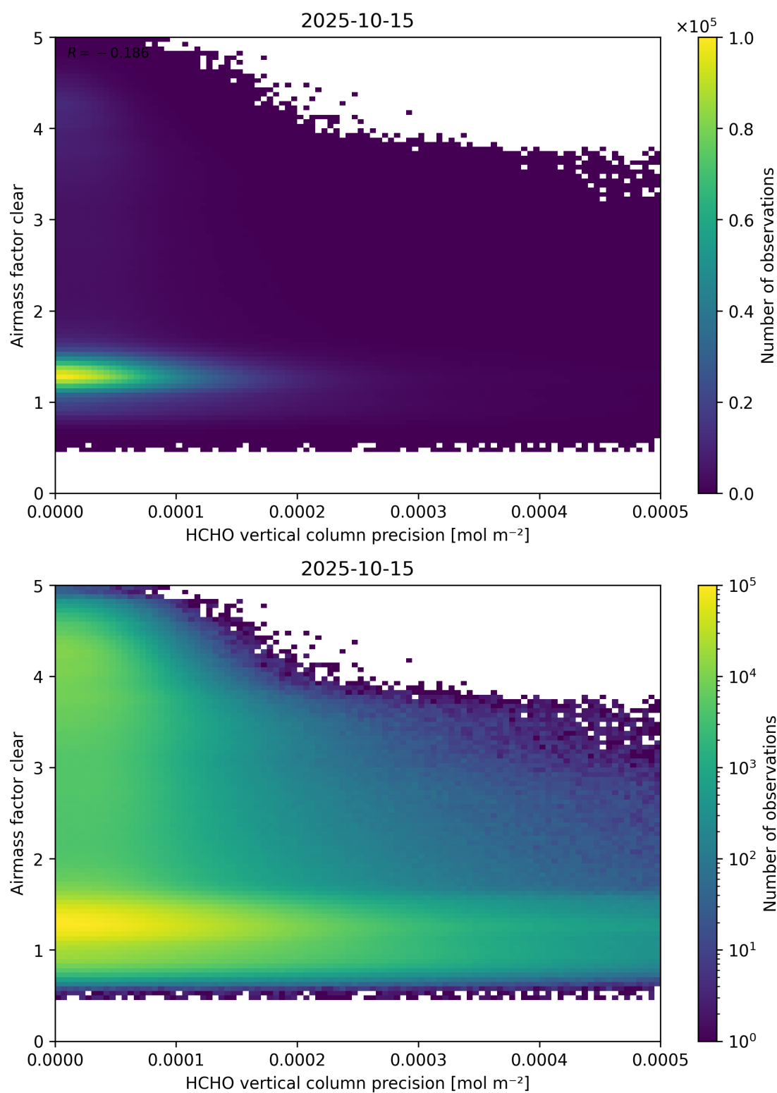
Figure 139: Scatter density plot of “HCHO vertical column precision” against “Airmass factor clear” for 2025-10-14 to 2025-10-16.
