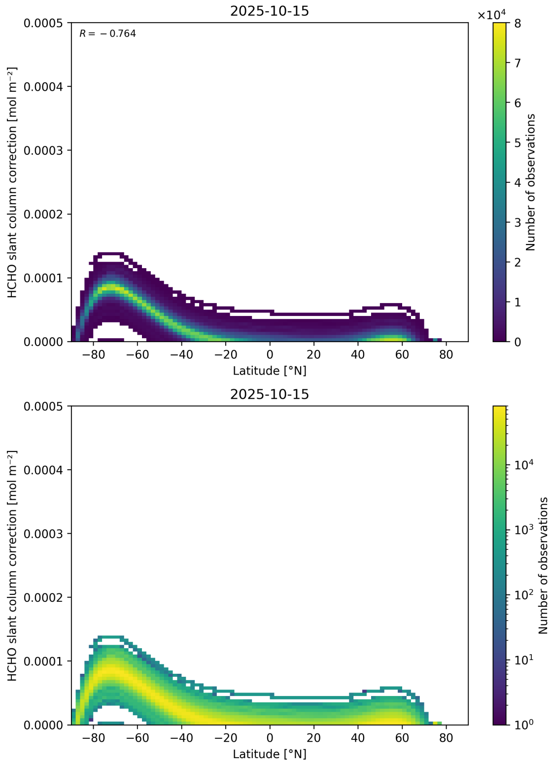
Figure 158: Scatter density plot of “Latitude” against “HCHO slant column correction” for 2025-10-14 to 2025-10-16.
