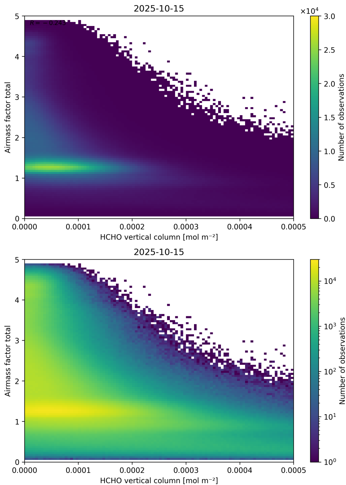
Figure 131: Scatter density plot of “HCHO vertical column” against “Airmass factor total” for 2025-10-14 to 2025-10-16.
