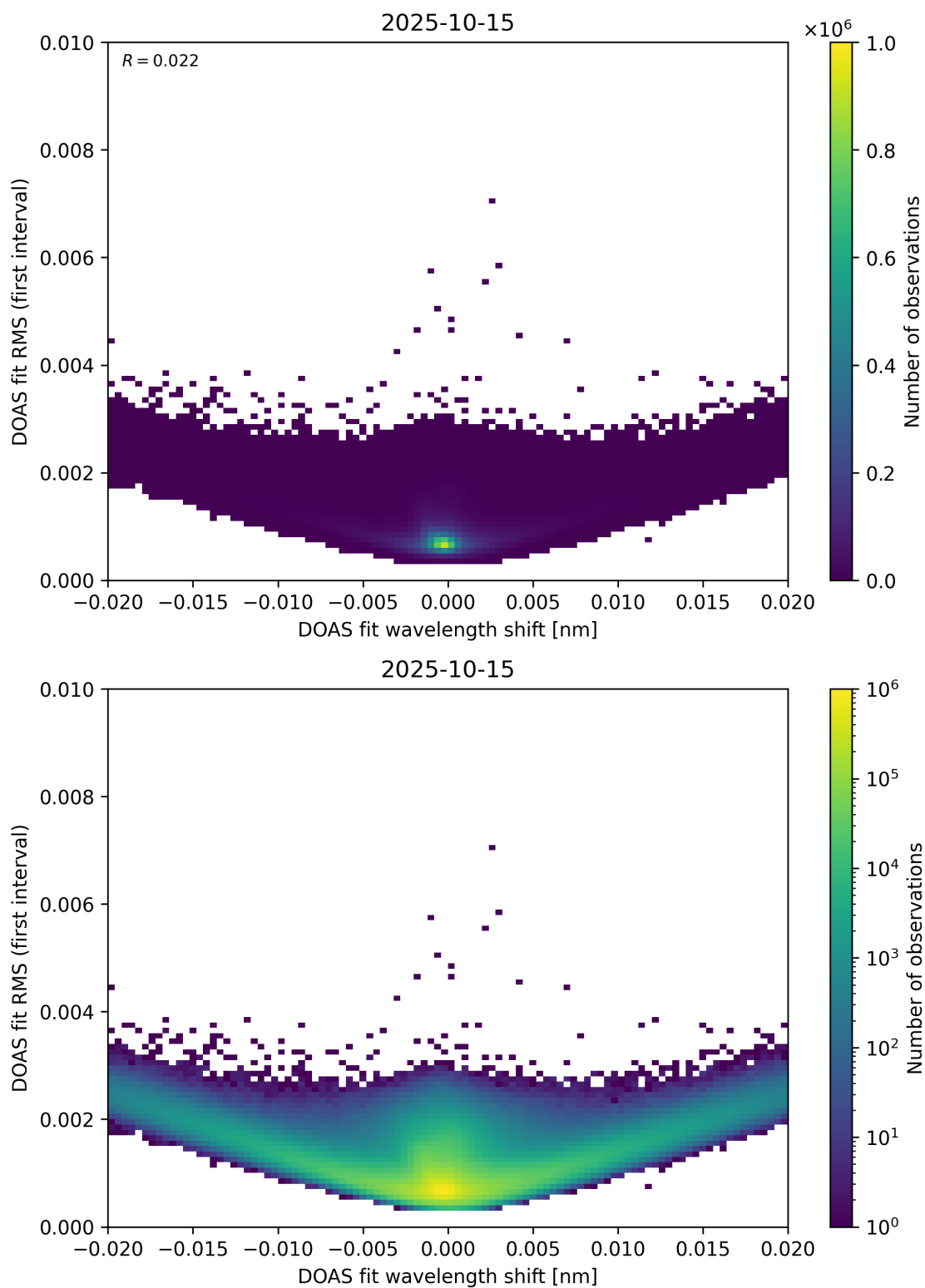
Figure 64: Scatter density plot of “DOAS fit wavelength shift” against “DOAS fit RMS (first interval)” for 2025-10-14 to 2025-10-16.
