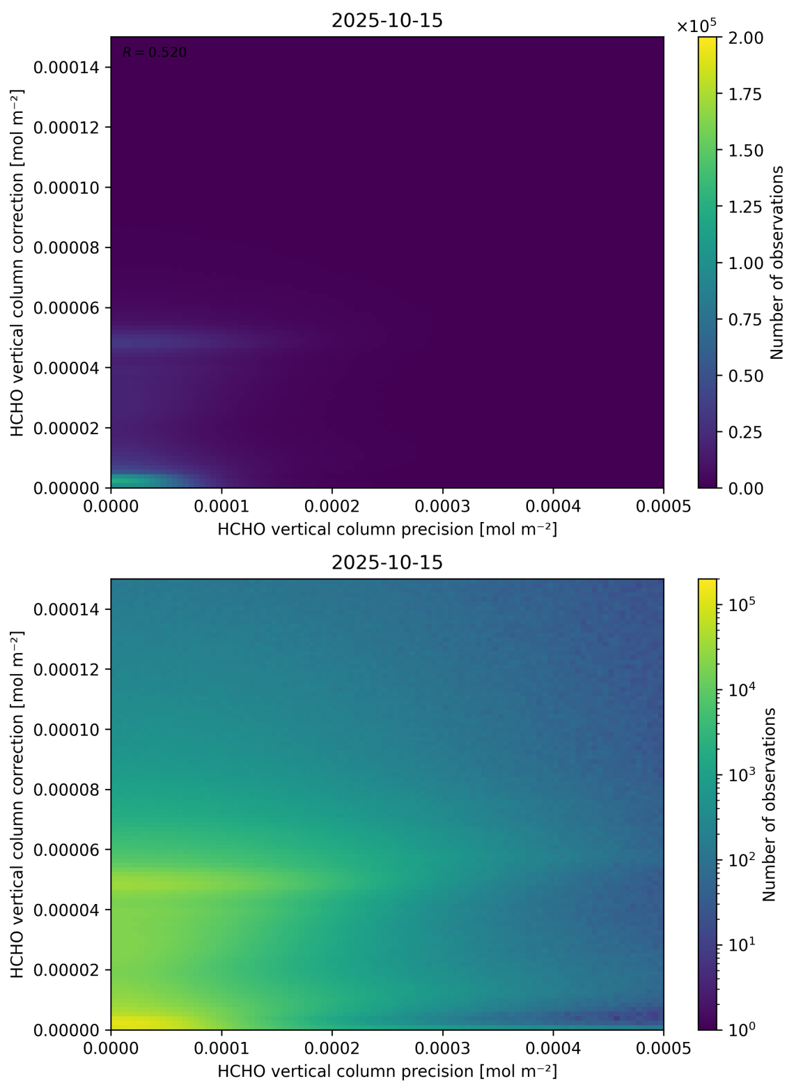
Figure 146: Scatter density plot of “HCHO vertical column precision” against “HCHO vertical column correction” for 2025-10-14 to 2025-10-16.
