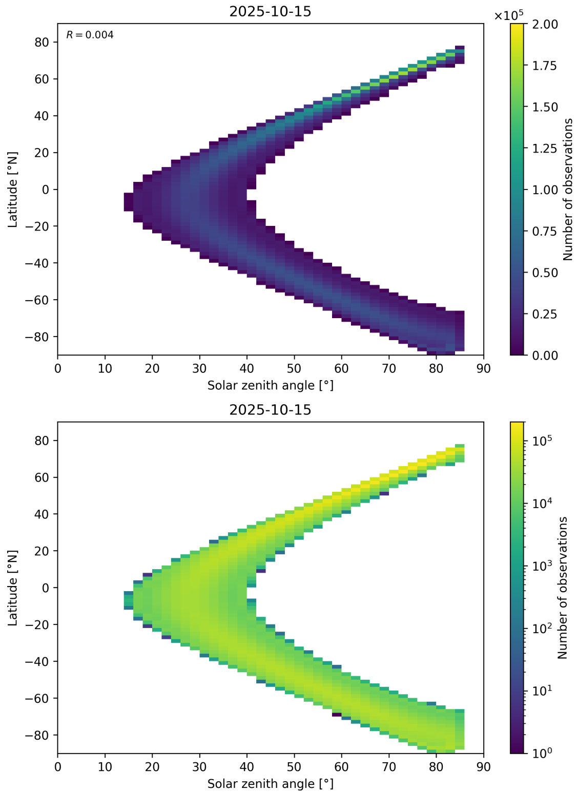
Figure 181: Scatter density plot of “Solar zenith angle” against “Latitude” for 2025-10-14 to 2025-10-16.
