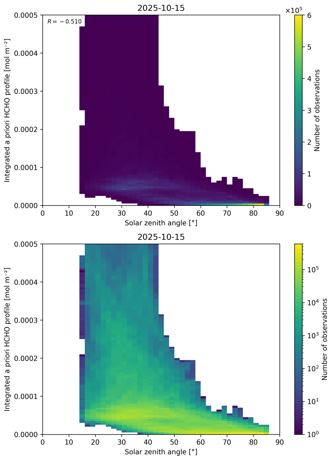
Figure 180: Scatter density plot of “Solar zenith angle” against “Integrated a priori HCHO profile” for 2025-10-14 to 2025-10-16.
