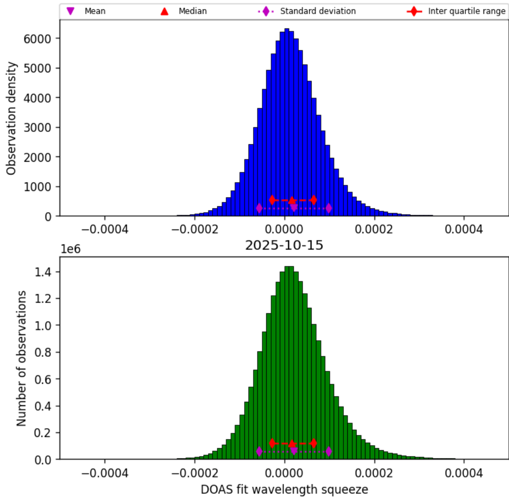
Figure 45: Histogram of “DOAS fit wavelength squeeze” for 2025-10-14 to 2025-10-16
