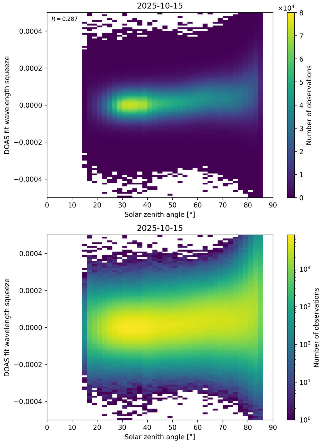
Figure 169: Scatter density plot of “Solar zenith angle” against “DOAS fit wavelength squeeze” for 2025-10-14 to 2025-10-16.
