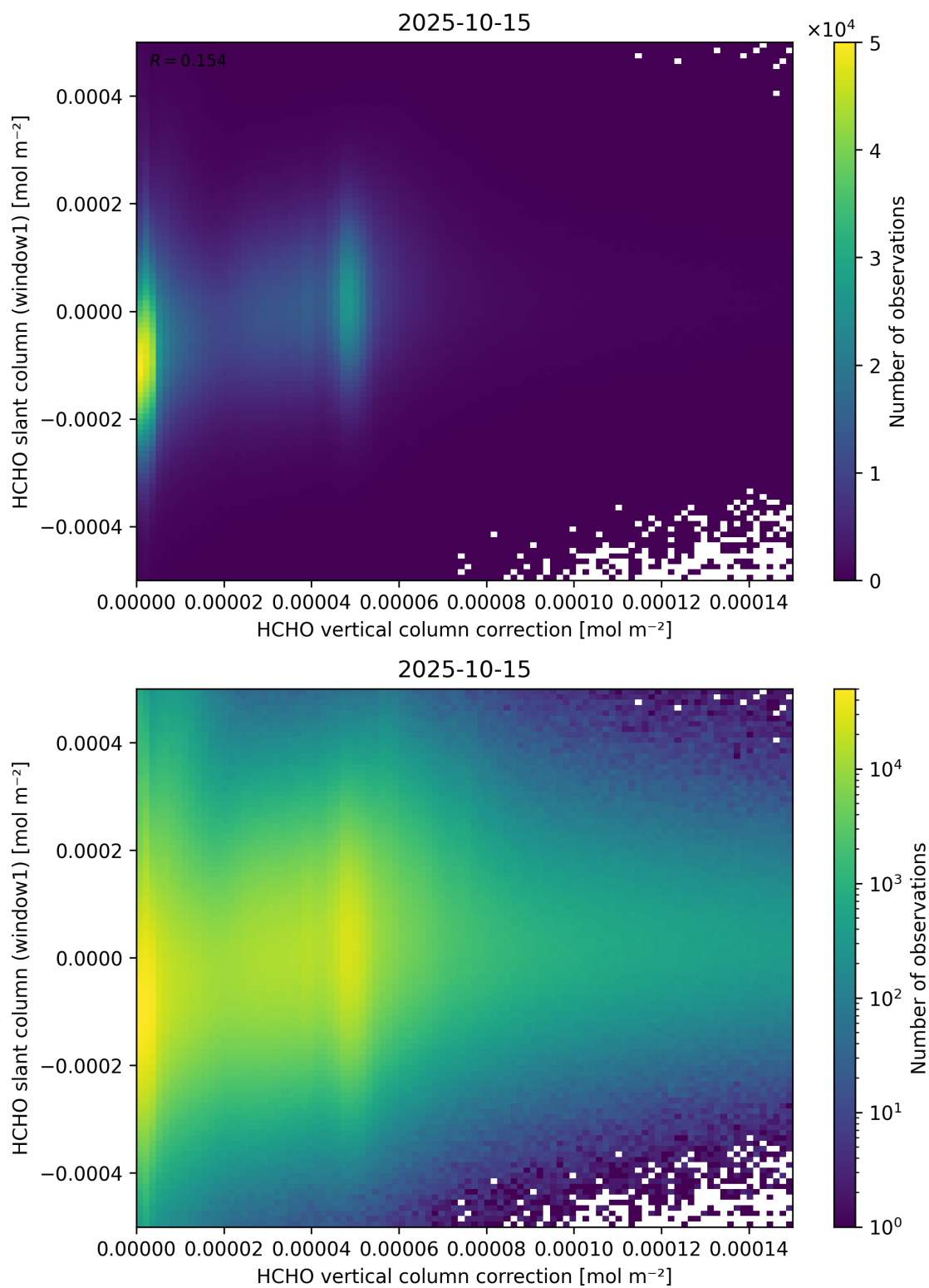
Figure 118: Scatter density plot of “HCHO vertical column correction” against “HCHO slant column (window1)” for 2025-10-14 to 2025-10-16.
