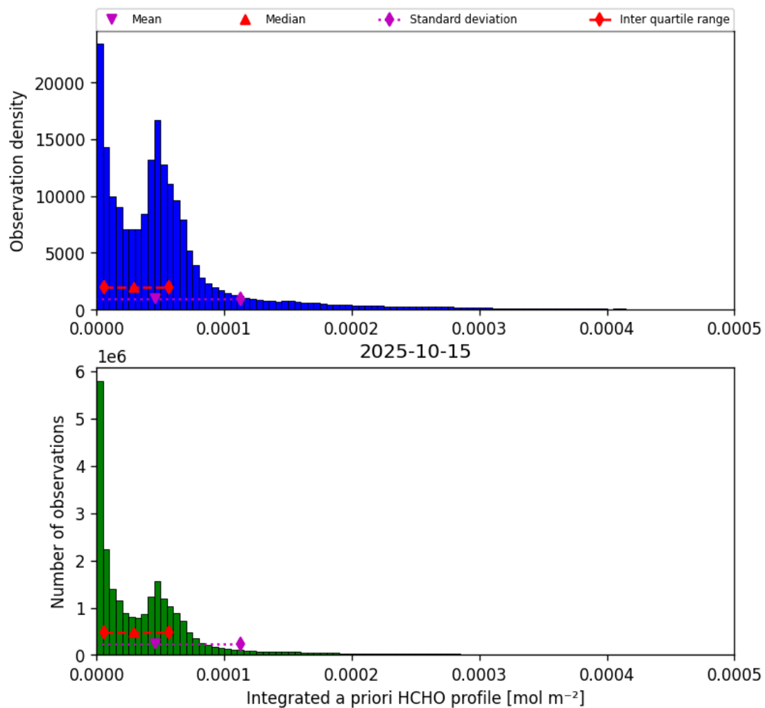
Figure 43: Histogram of “Integrated a priori HCHO profile” for 2025-10-14 to 2025-10-16
