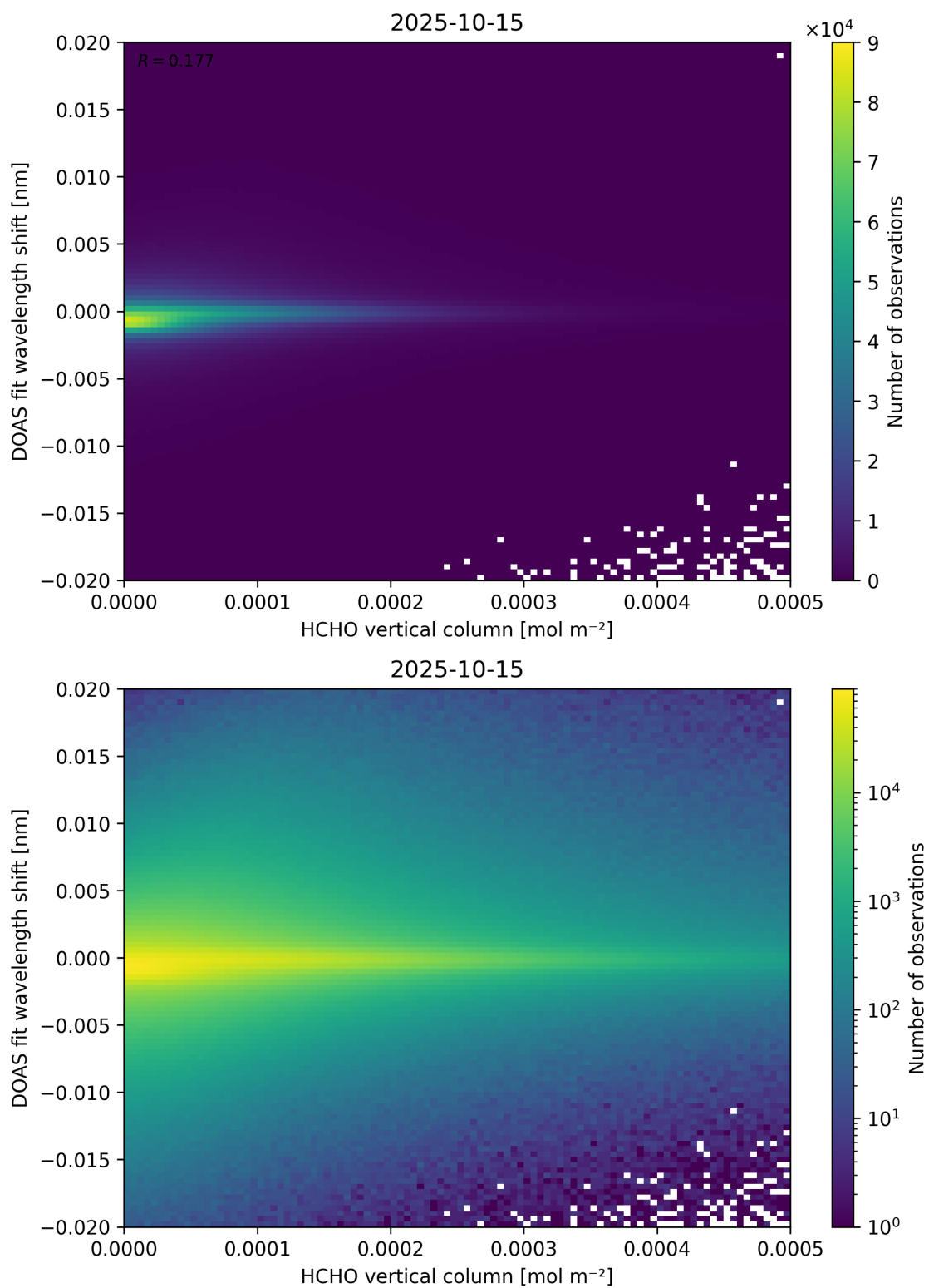
Figure 124: Scatter density plot of “HCHO vertical column” against “DOAS fit wavelength shift” for 2025-10-14 to 2025-10-16.
