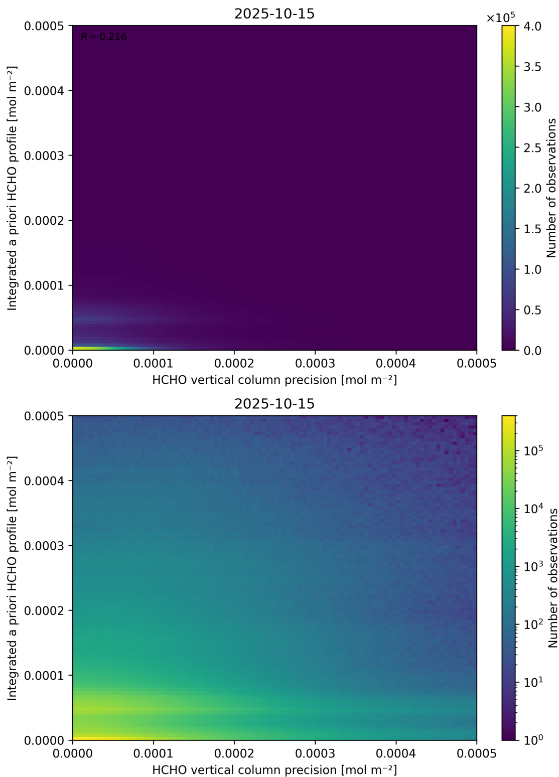
Figure 147: Scatter density plot of “HCHO vertical column precision” against “Integrated a priori HCHO profile” for 2025-10-14 to 2025-10-16.
