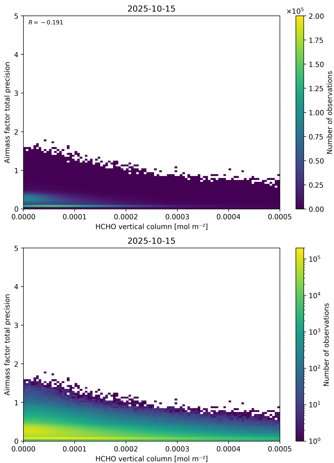
Figure 132: Scatter density plot of “HCHO vertical column” against “Airmass factor total precision” for 2025-10-14 to 2025-10-16.
