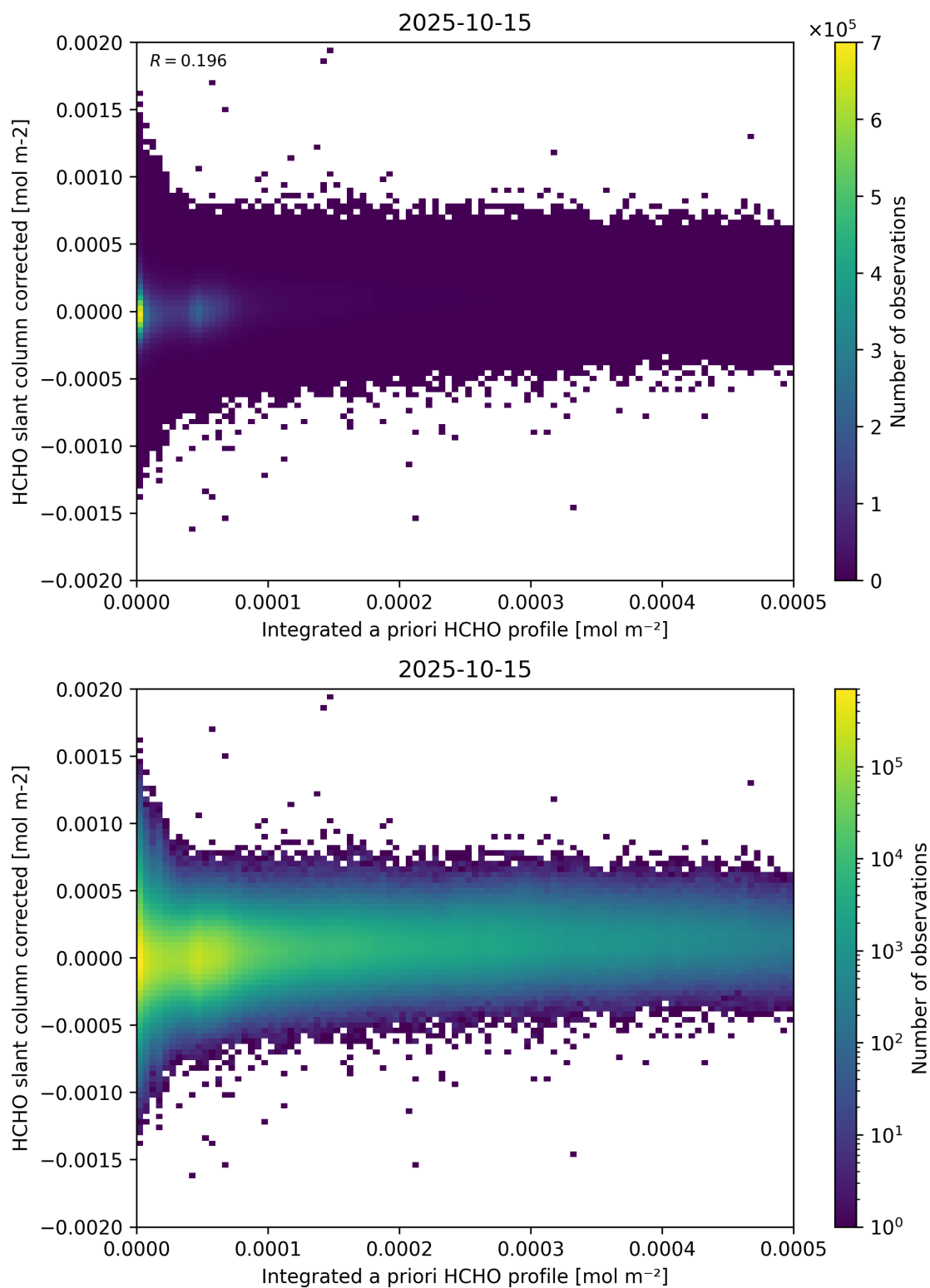
Figure 151: Scatter density plot of “Integrated a priori HCHO profile” against “HCHO slant column corrected” for 2025-10-14 to 2025-10-16.
