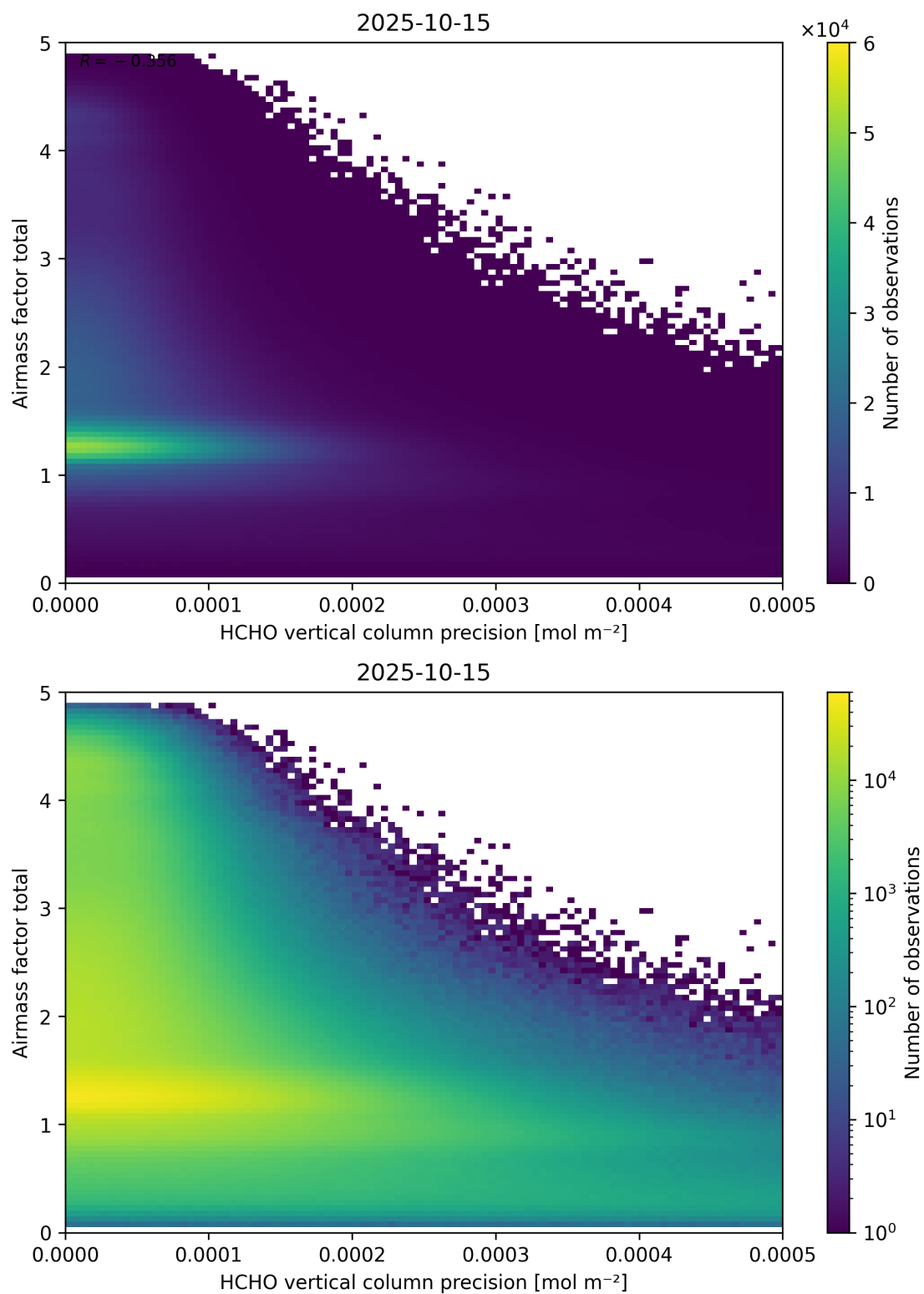
Figure 144: Scatter density plot of “HCHO vertical column precision” against “Airmass factor total” for 2025-10-14 to 2025-10-16.
