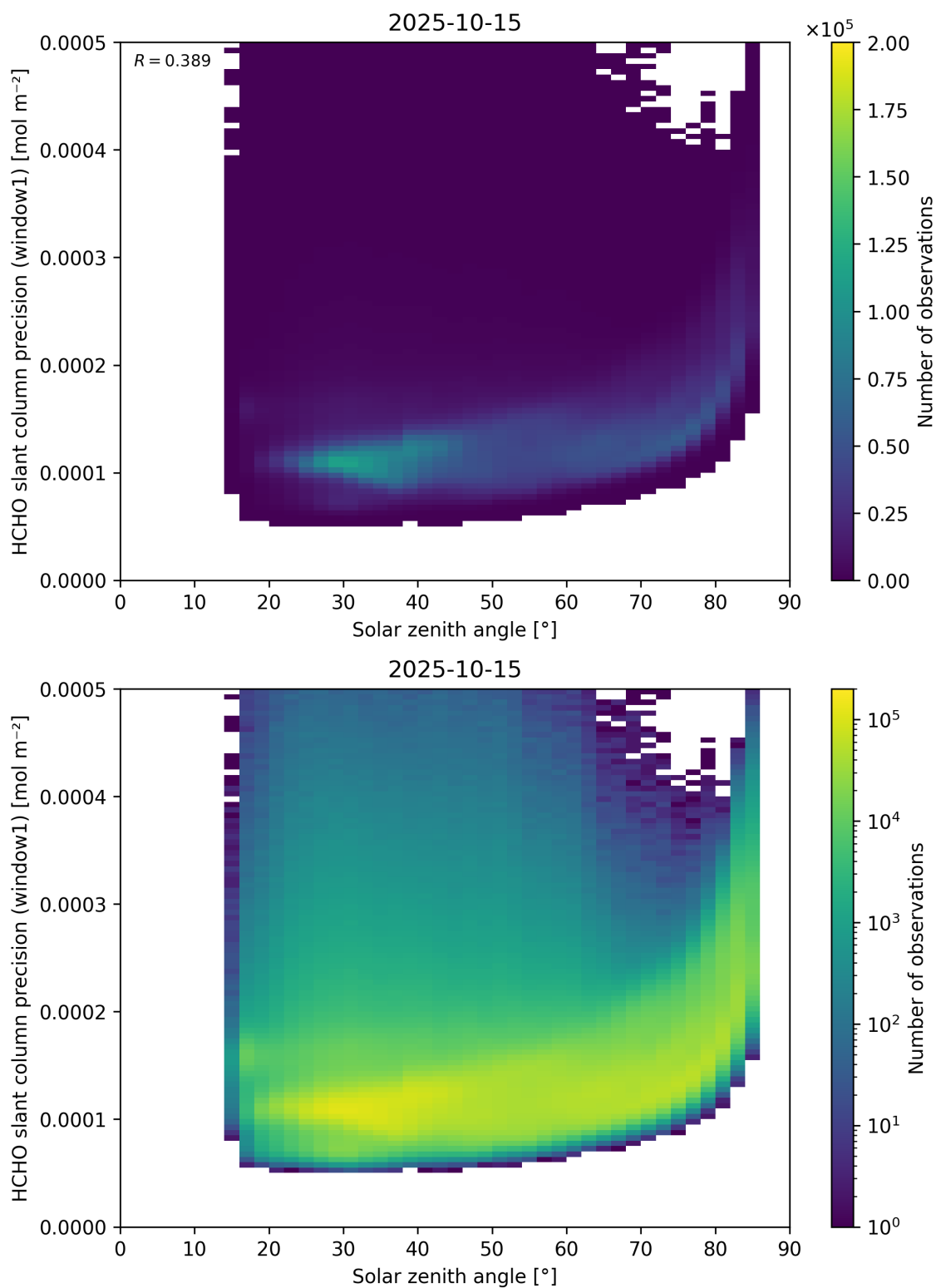
Figure 174: Scatter density plot of “Solar zenith angle” against “HCHO slant column precision (window1)” for 2025-10-14 to 2025-10-16.
