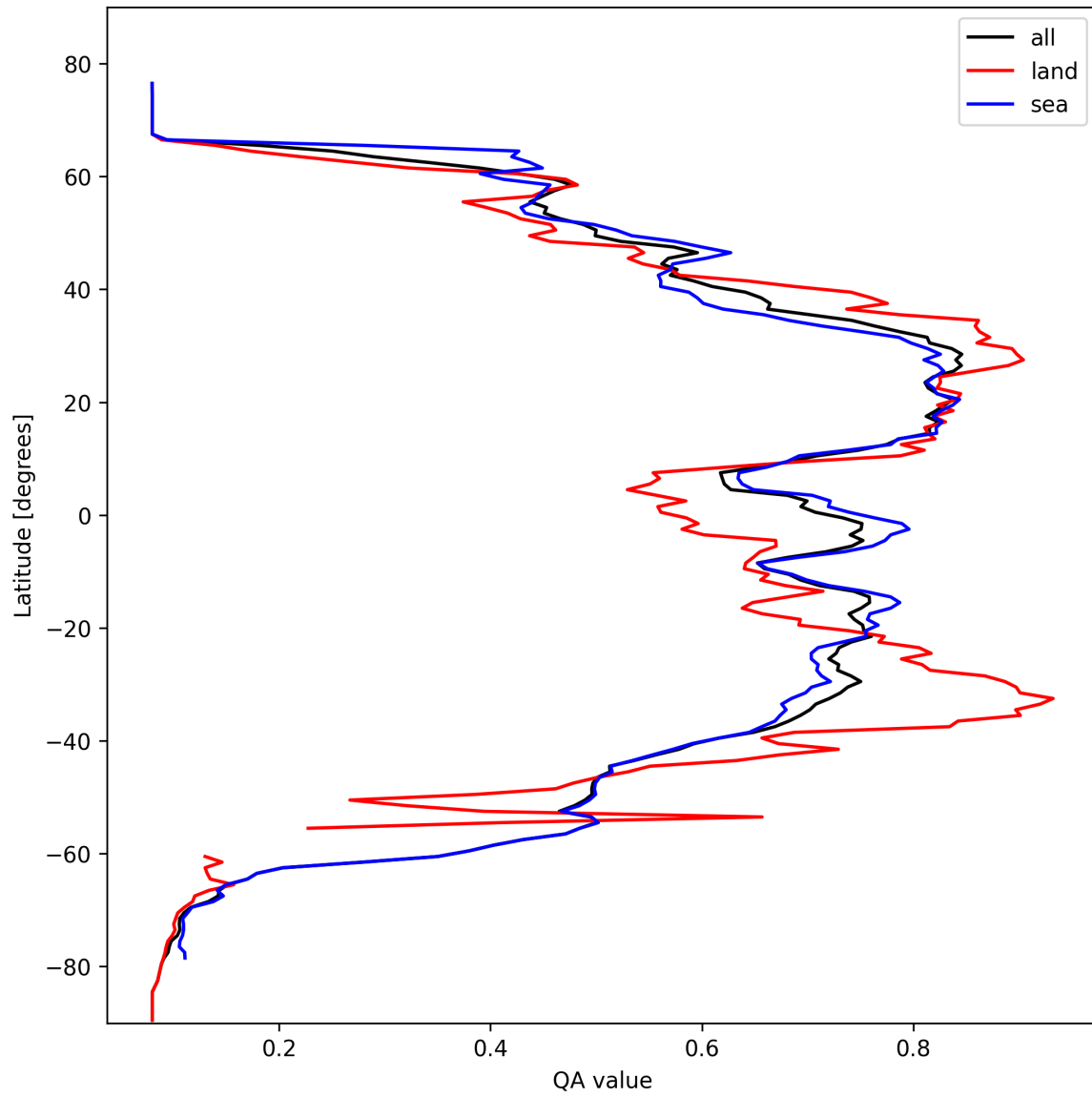
Figure 20: Zonal average of “QA value” for 2025-10-14 to 2025-10-16.
