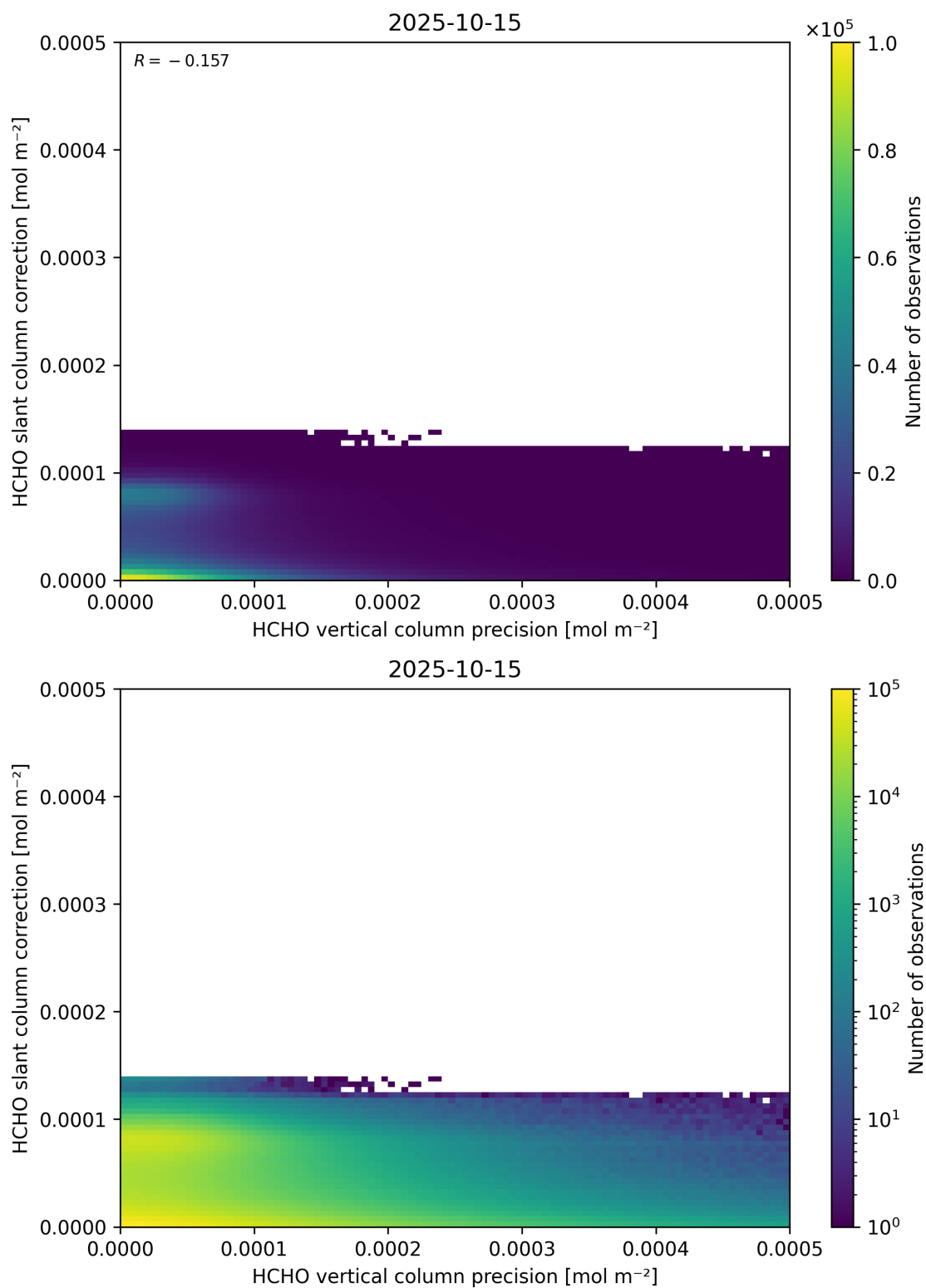
Figure 141: Scatter density plot of “HCHO vertical column precision” against “HCHO slant column correction” for 2025-10-14 to 2025-10-16.
