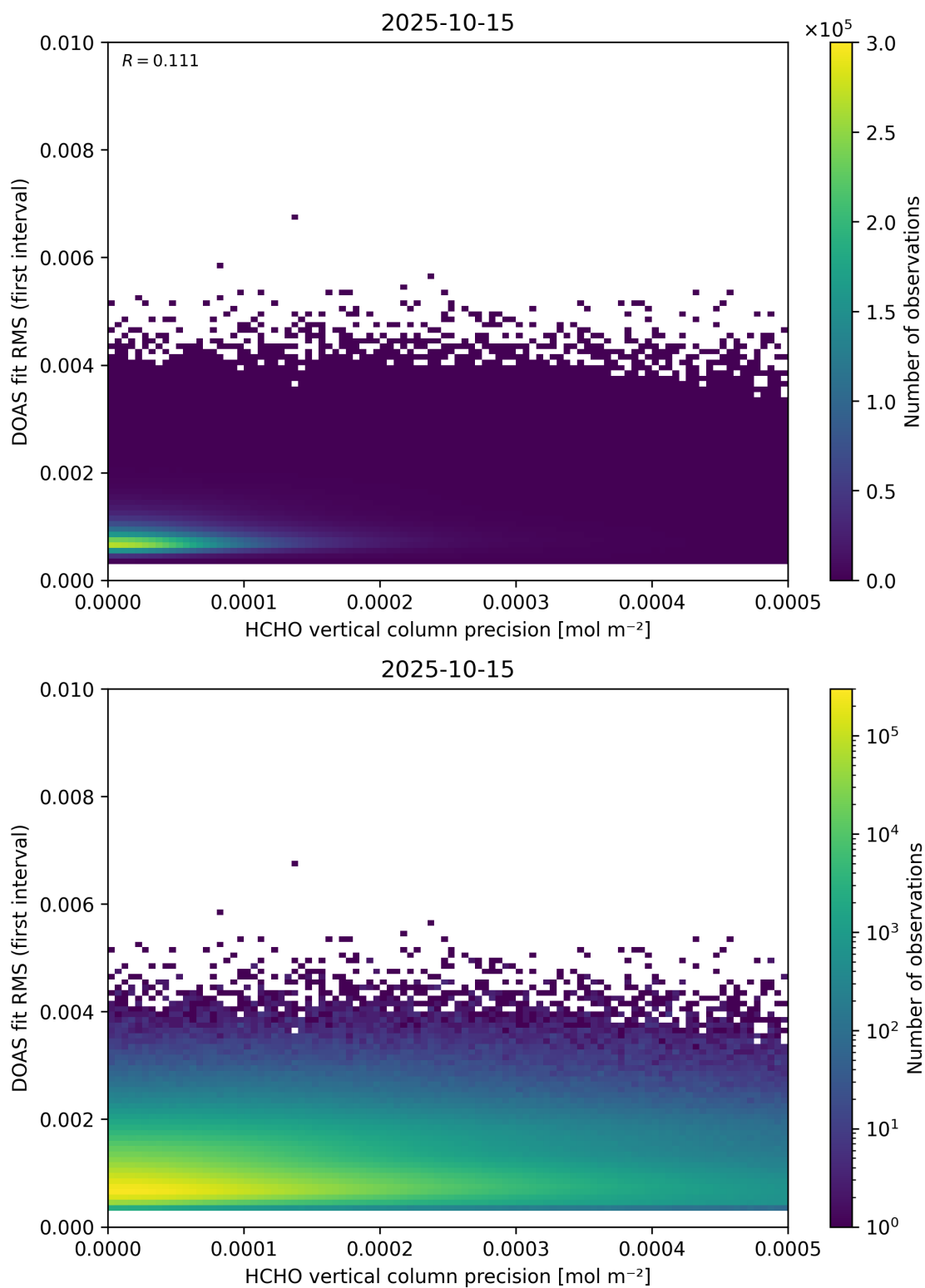
Figure 136: Scatter density plot of “HCHO vertical column precision” against “DOAS fit RMS (first interval)” for 2025-10-14 to 2025-10-16.
