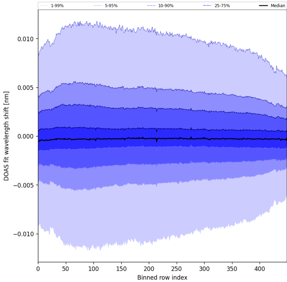
Figure 58: Along track statistics of “DOAS fit wavelength shift” for 2025-10-14 to 2025-10-16
