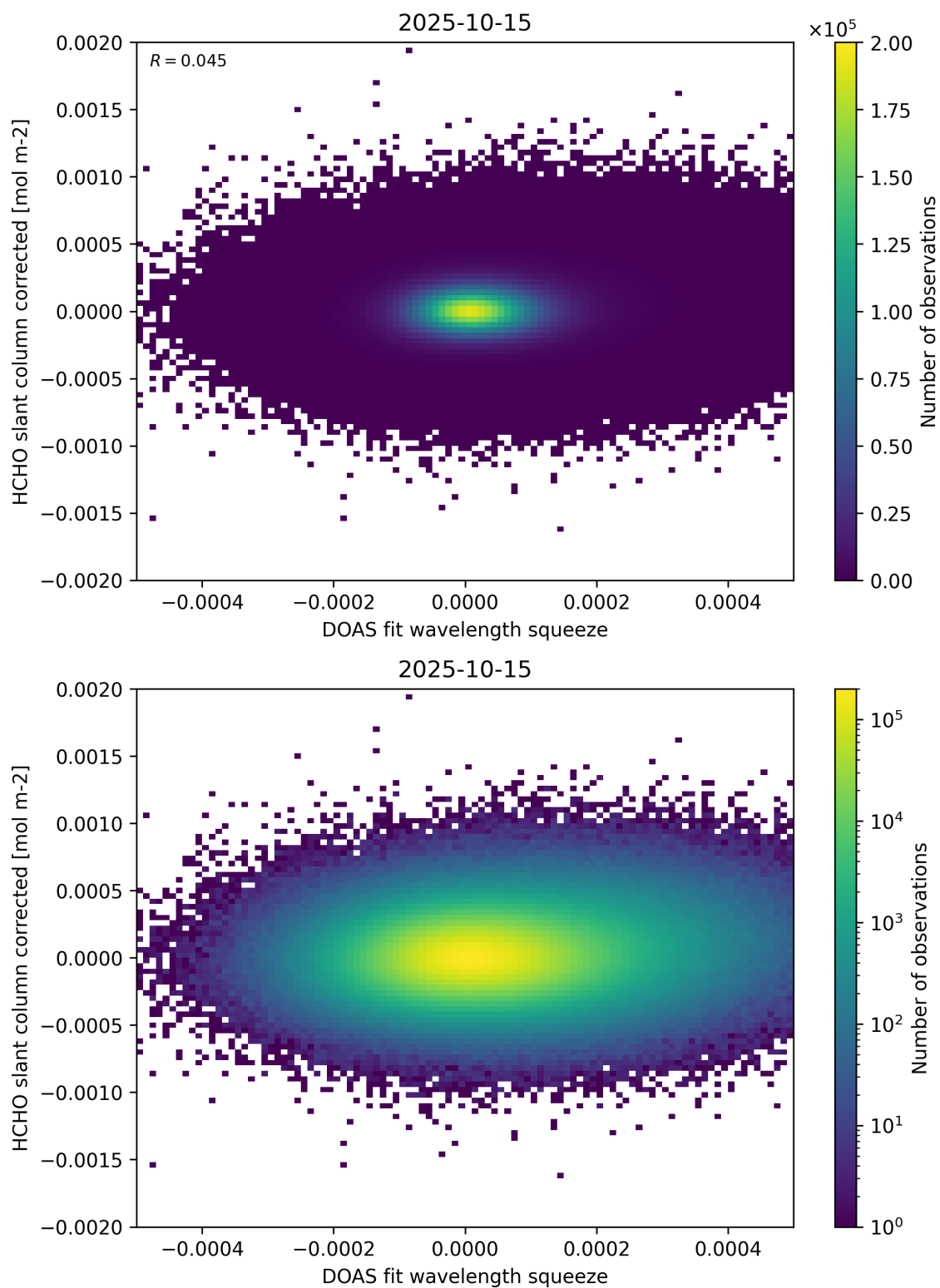
Figure 69: Scatter density plot of “DOAS fit wavelength squeeze” against “HCHO slant column corrected” for 2025-10-14 to 2025-10-16.
