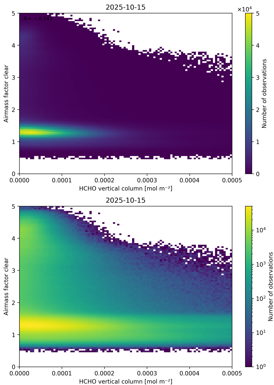
Figure 126: Scatter density plot of “HCHO vertical column” against “Airmass factor clear” for 2025-10-14 to 2025-10-16.
