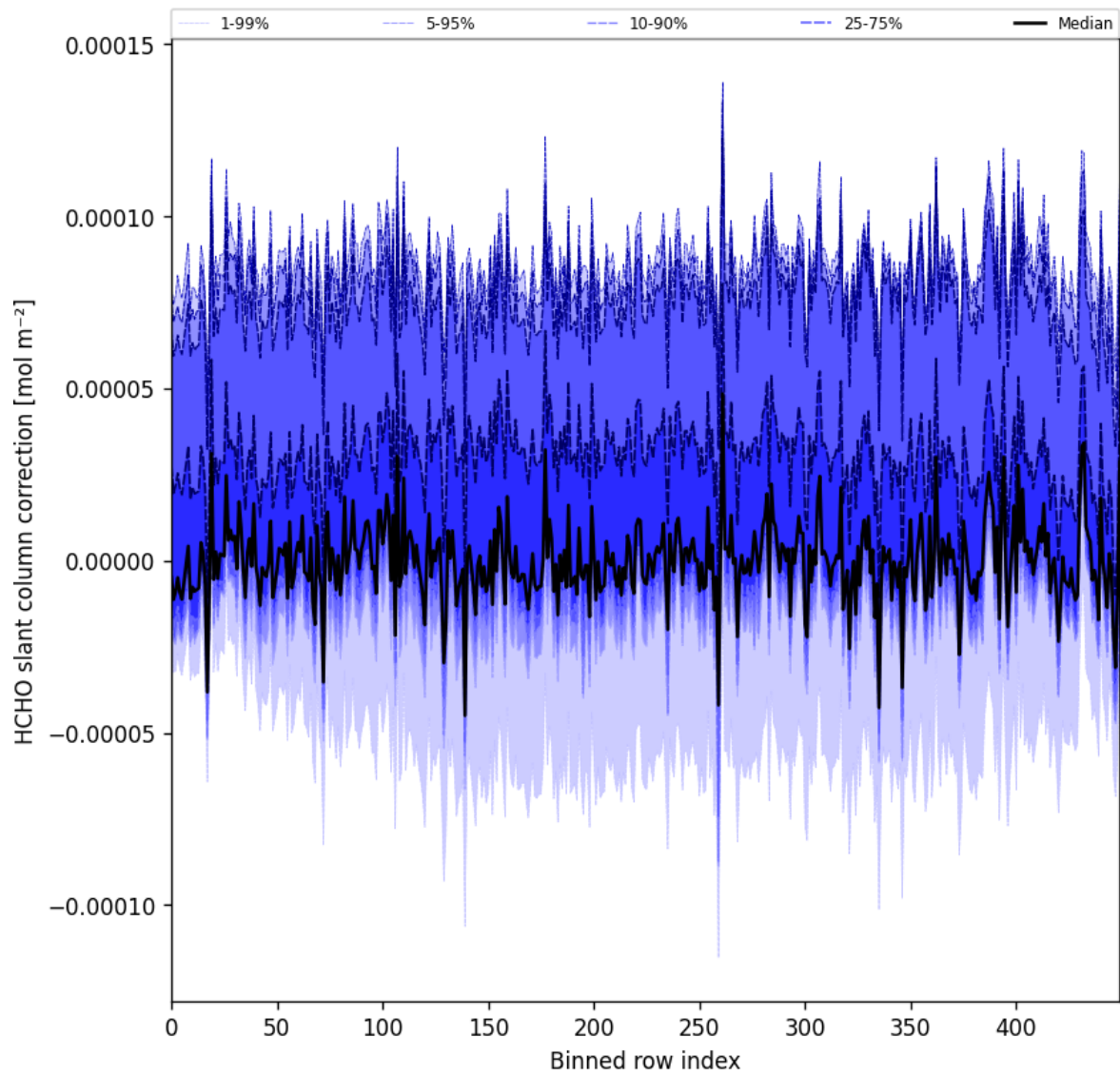
Figure 61: Along track statistics of “HCHO slant column correction” for 2025-10-14 to 2025-10-16
