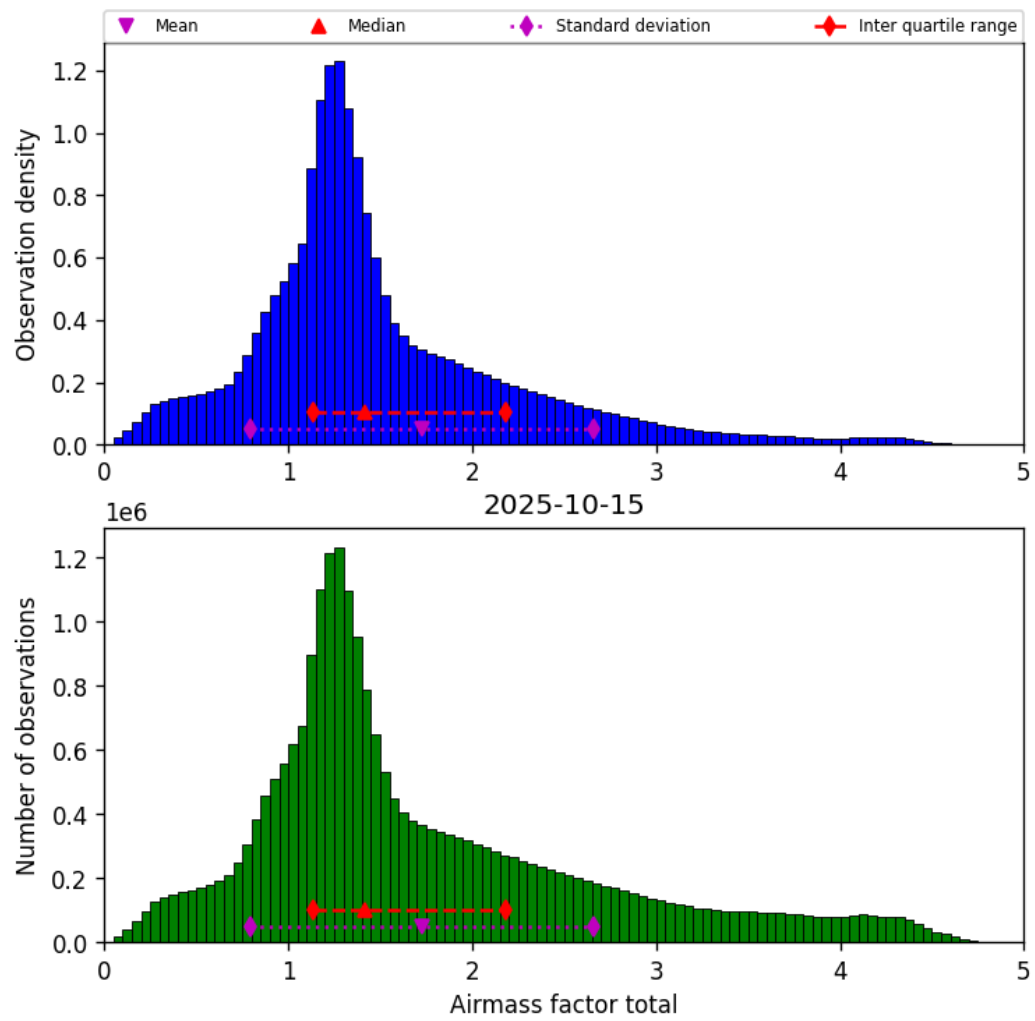
Figure 40: Histogram of “Airmass factor total” for 2025-10-14 to 2025-10-16
