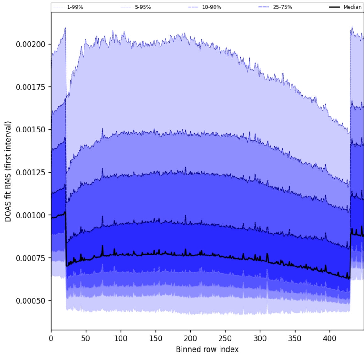
Figure 60: Along track statistics of “DOAS fit RMS (first interval)” for 2025-10-14 to 2025-10-16
