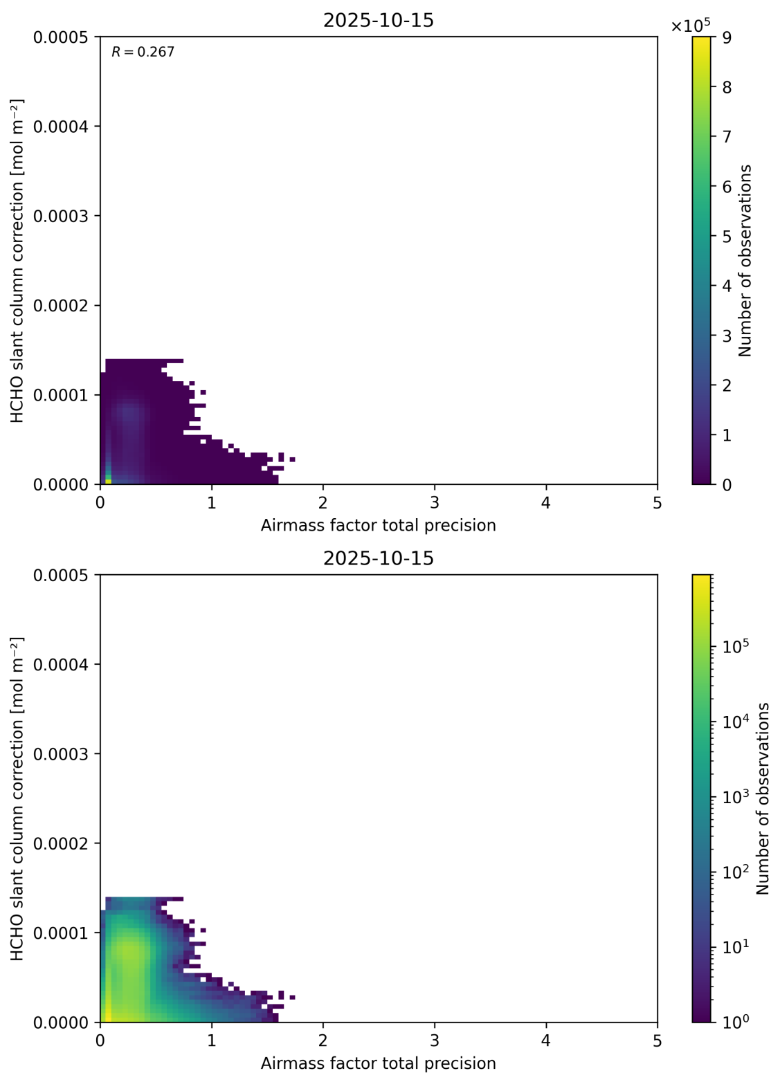
Figure 110: Scatter density plot of “Airmass factor total precision” against “HCHO slant column correction” for 2025-10-14 to 2025-10-16.
