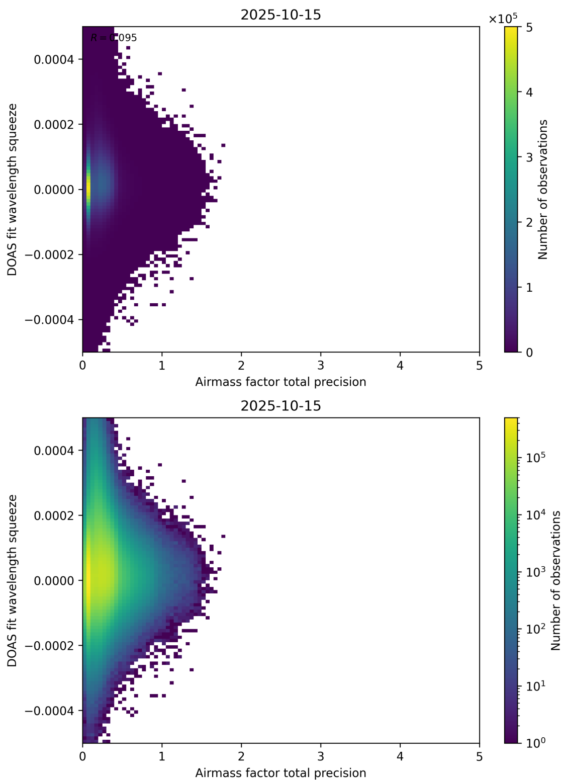
Figure 107: Scatter density plot of “Airmass factor total precision” against “DOAS fit wavelength squeeze” for 2025-10-14 to 2025-10-16.
