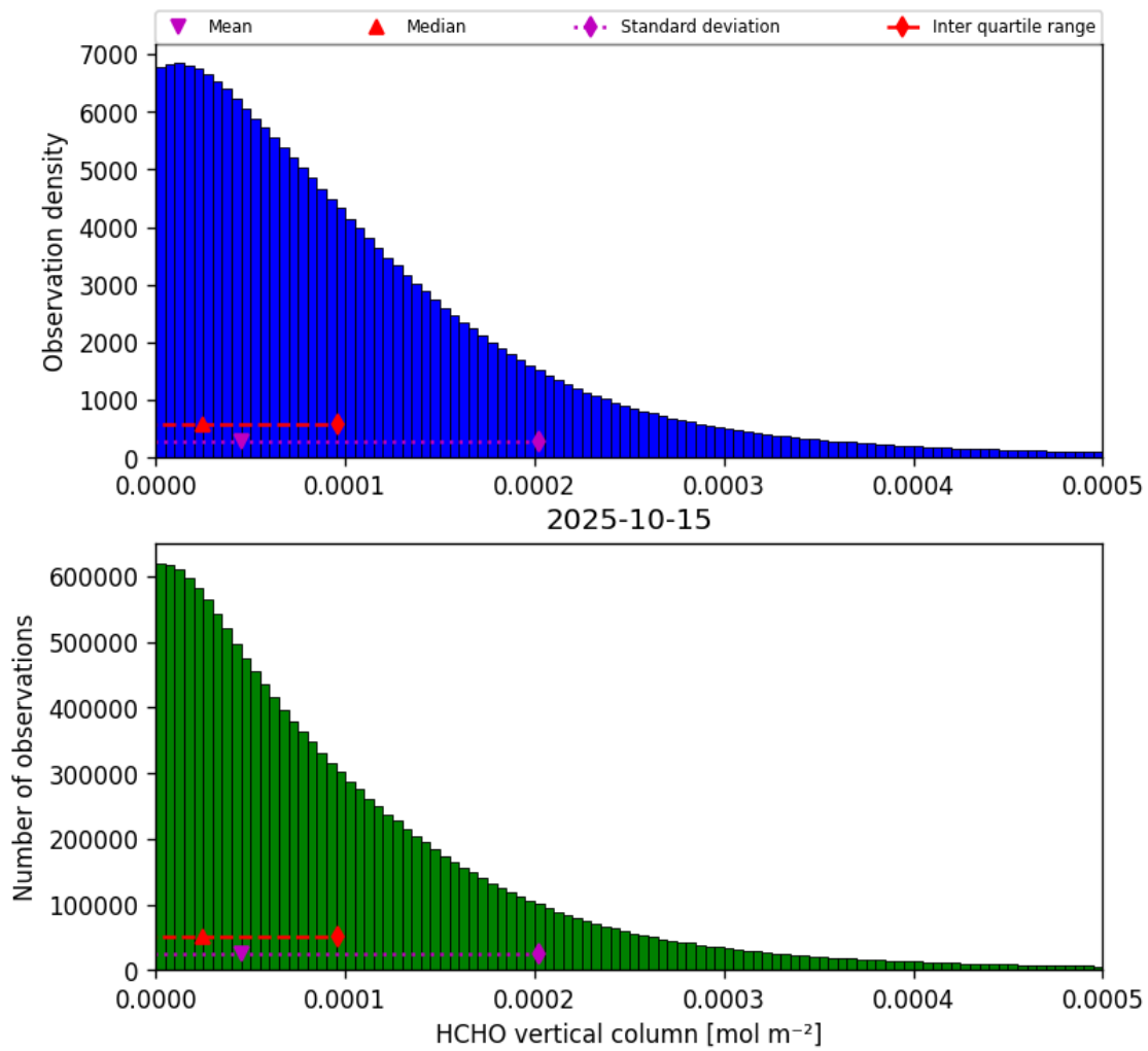
Figure 35: Histogram of “HCHO vertical column” for 2025-10-14 to 2025-10-16
