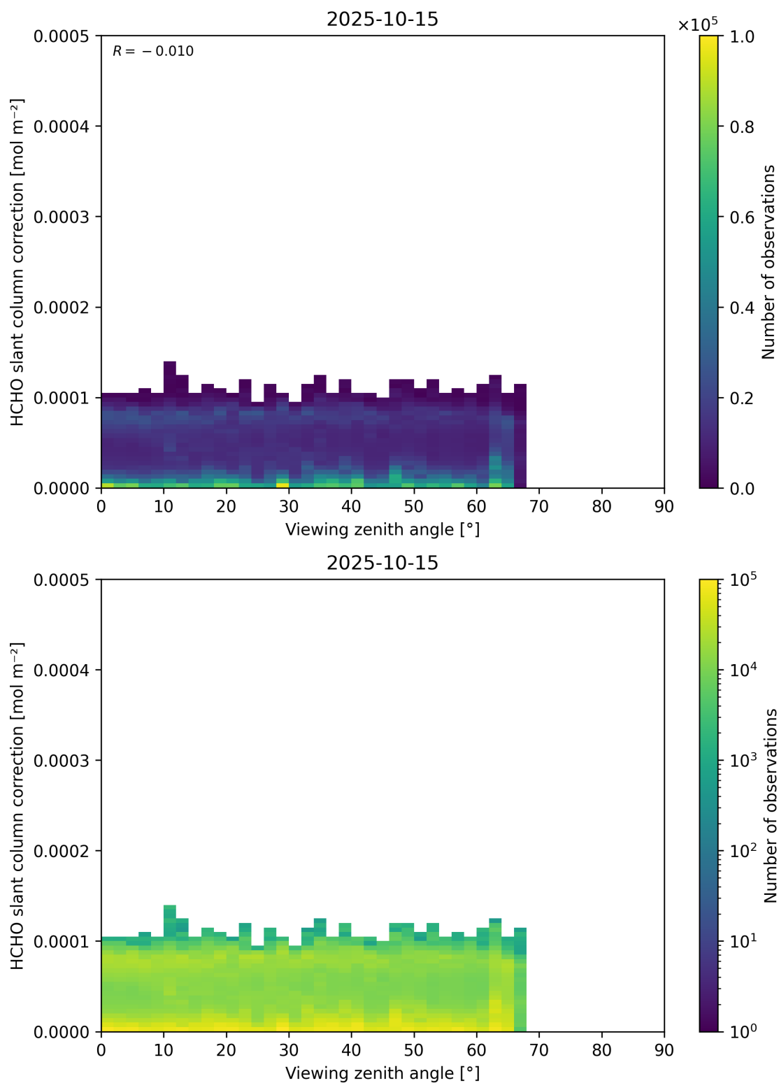
Figure 187: Scatter density plot of “Viewing zenith angle” against “HCHO slant column correction” for 2025-10-14 to 2025-10-16.
