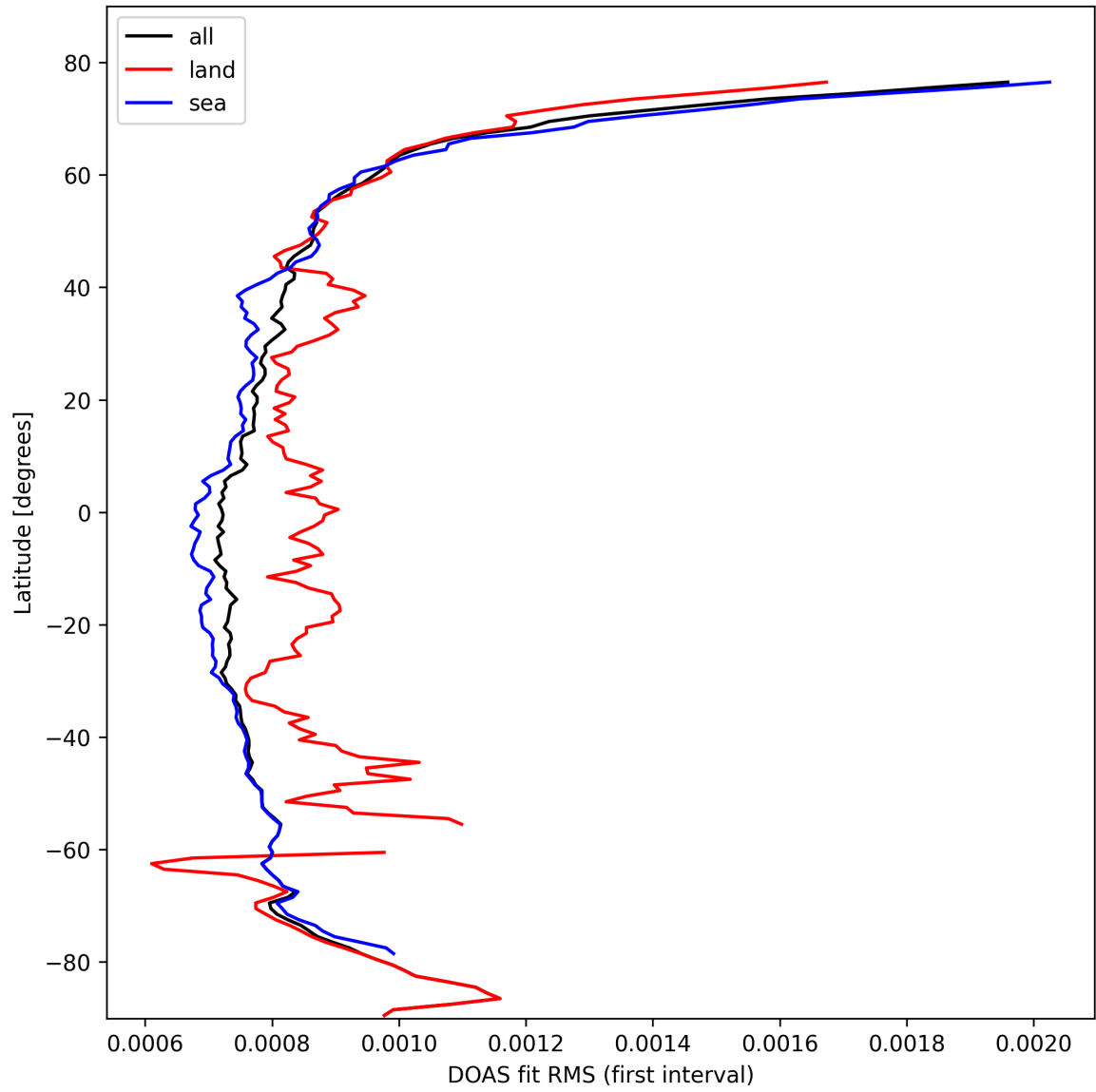
Figure 32: Zonal average of “DOAS fit RMS (first interval)” for 2025-10-14 to 2025-10-16.
