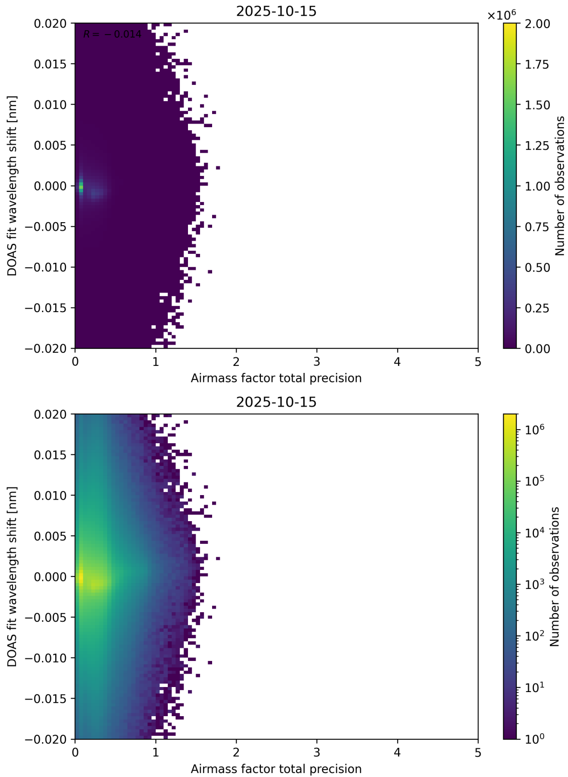
Figure 106: Scatter density plot of “Airmass factor total precision” against “DOAS fit wavelength shift” for 2025-10-14 to 2025-10-16.
