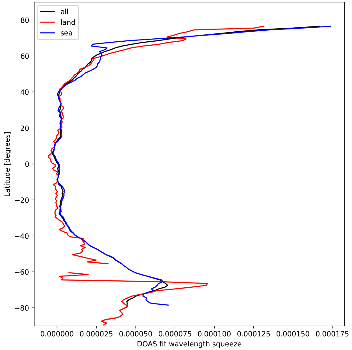
Figure 31: Zonal average of “DOAS fit wavelength squeeze” for 2025-10-14 to 2025-10-16.
