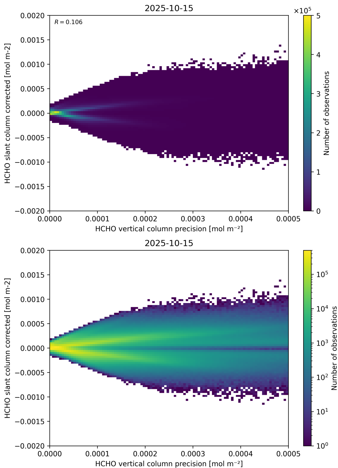
Figure 140: Scatter density plot of “HCHO vertical column precision” against “HCHO slant column corrected” for 2025-10-14 to 2025-10-16.
