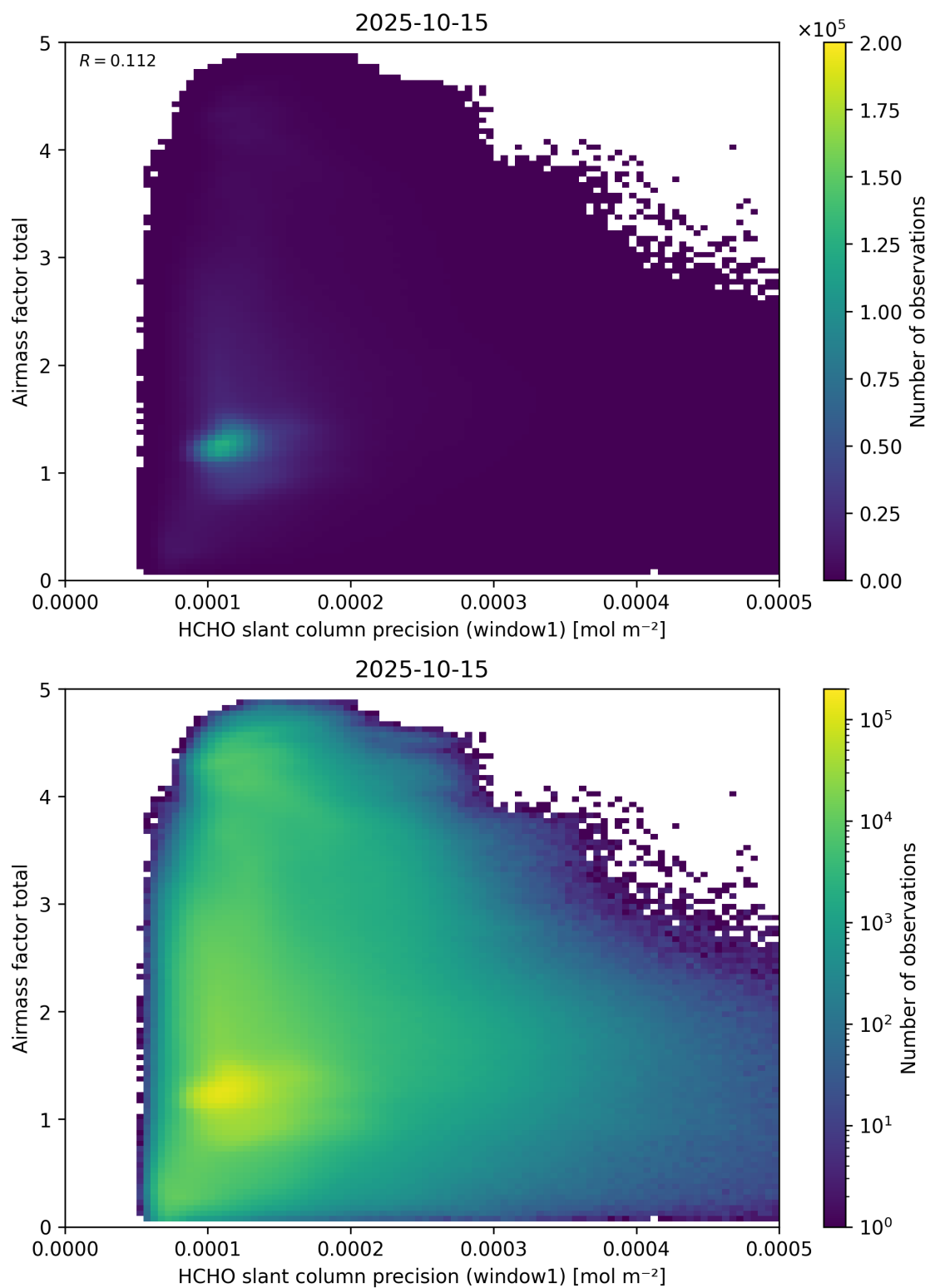
Figure 94: Scatter density plot of “HCHO slant column precision (window1)” against “Airmass factor total” for 2025-10-14 to 2025-10-16.
