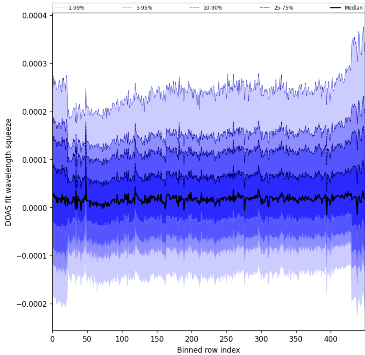
Figure 59: Along track statistics of “DOAS fit wavelength squeeze” for 2025-10-14 to 2025-10-16
