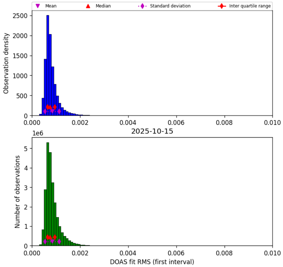
Figure 46: Histogram of “DOAS fit RMS (first interval)” for 2025-10-14 to 2025-10-16
