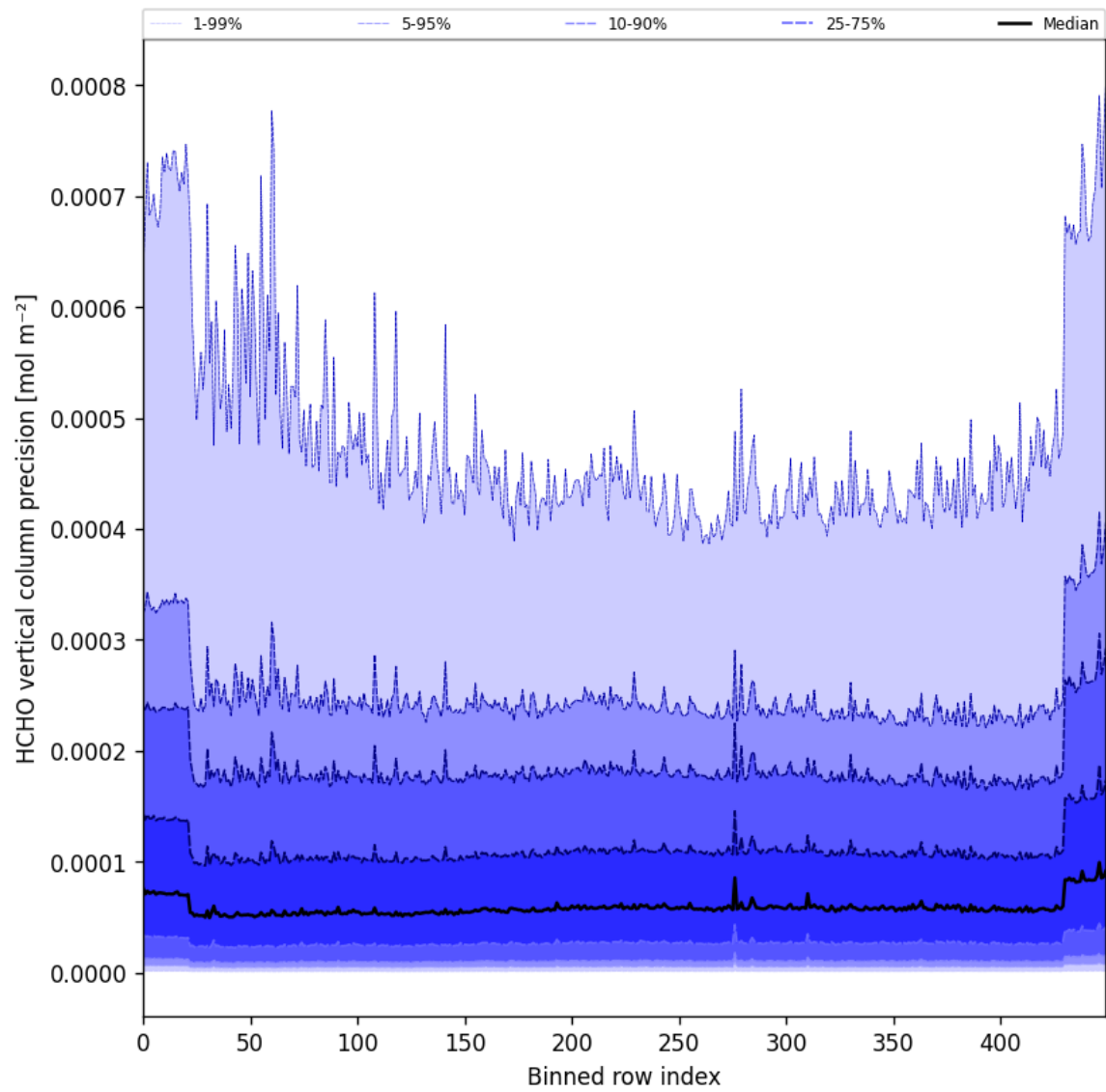
Figure 50: Along track statistics of “HCHO vertical column precision” for 2025-10-14 to 2025-10-16
