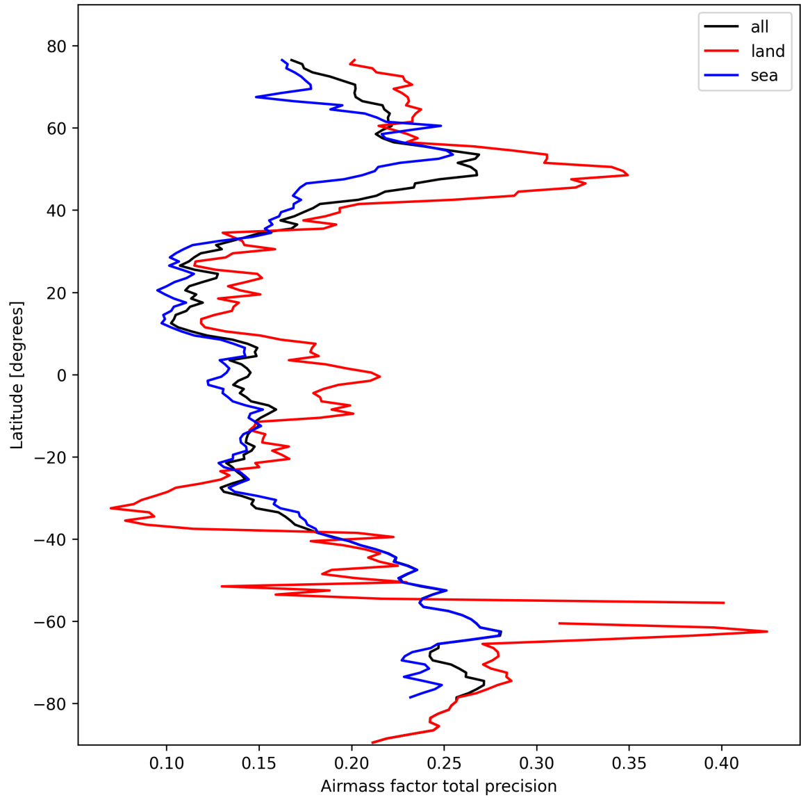
Figure 27: Zonal average of “Airmass factor total precision” for 2025-10-14 to 2025-10-16.
