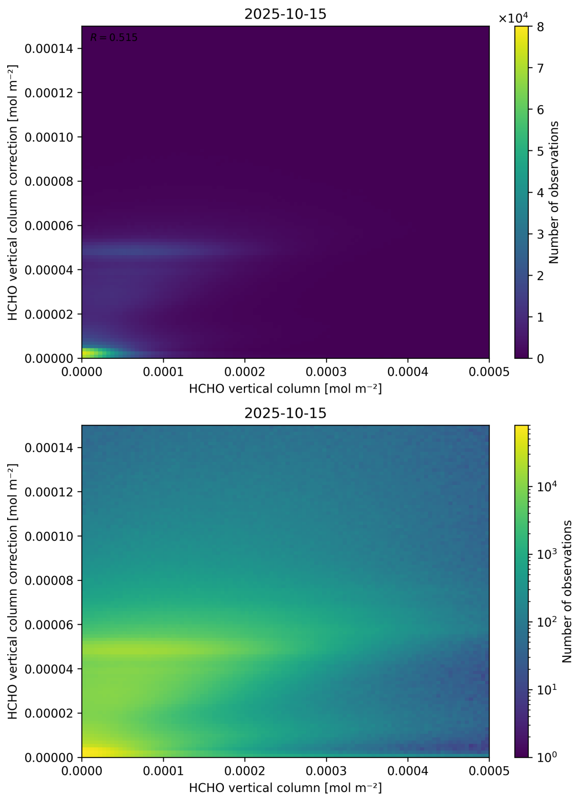
Figure 133: Scatter density plot of “HCHO vertical column” against “HCHO vertical column correction” for 2025-10-14 to 2025-10-16.
