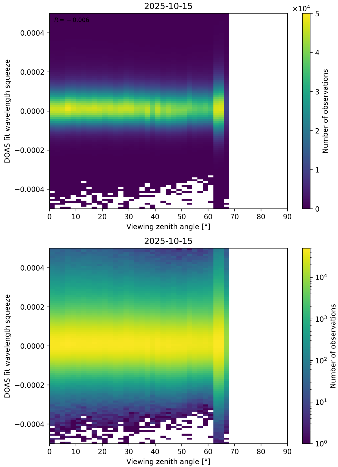
Figure 184: Scatter density plot of “Viewing zenith angle” against “DOAS fit wavelength squeeze” for 2025-10-14 to 2025-10-16.
