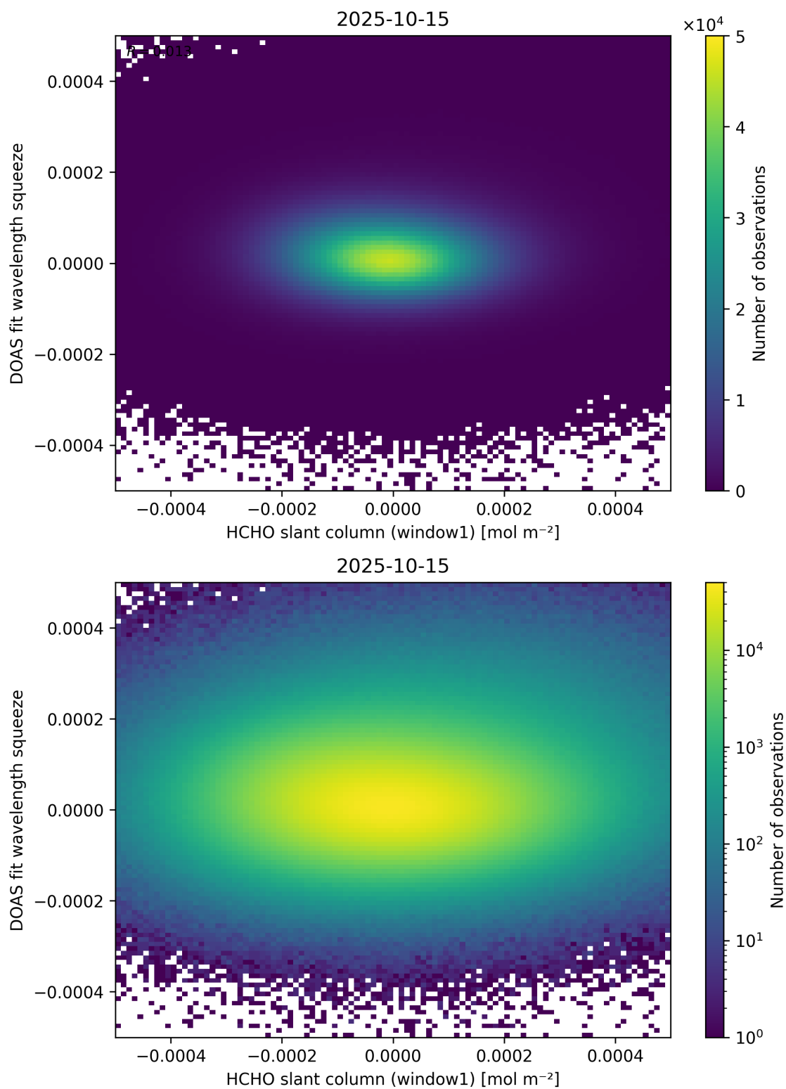
Figure 80: Scatter density plot of “HCHO slant column (window1)” against “DOAS fit wavelength squeeze” for 2025-10-14 to 2025-10-16.
