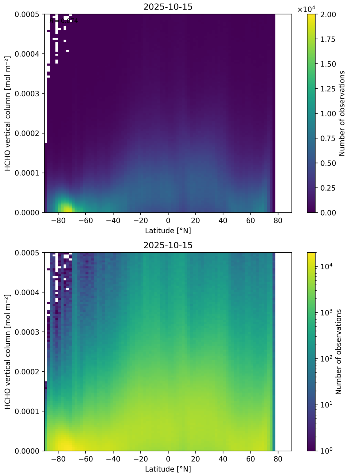
Figure 163: Scatter density plot of “Latitude” against “HCHO vertical column” for 2025-10-14 to 2025-10-16.
