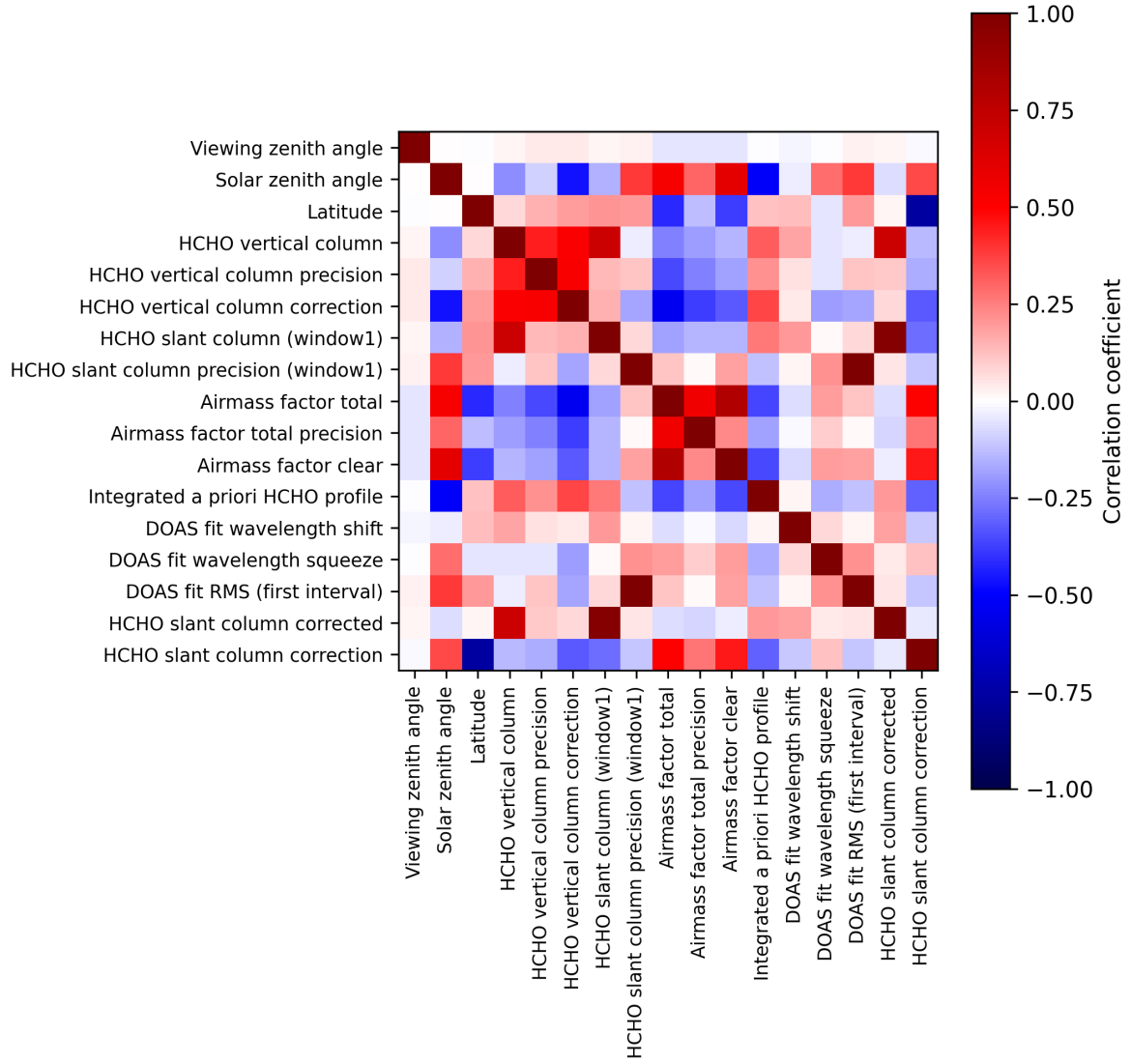
Figure 2: Map of correlation matrix for 2025-10-14 to 2025-10-16.
