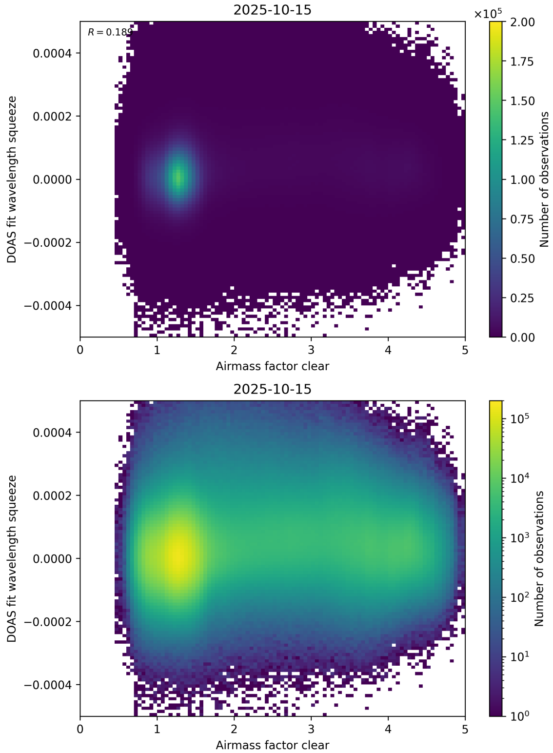
Figure 73: Scatter density plot of “Airmass factor clear” against “DOAS fit wavelength squeeze” for 2025-10-14 to 2025-10-16.
