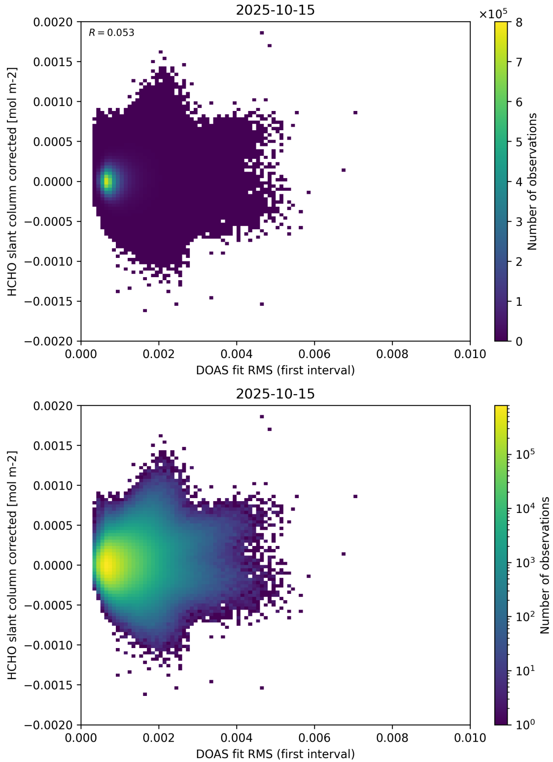
Figure 62: Scatter density plot of “DOAS fit RMS (first interval)” against “HCHO slant column corrected” for 2025-10-14 to 2025-10-16.
