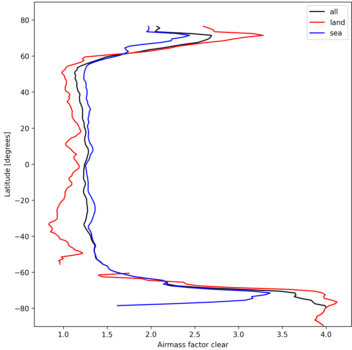
Figure 28: Zonal average of “Airmass factor clear” for 2025-10-14 to 2025-10-16.
