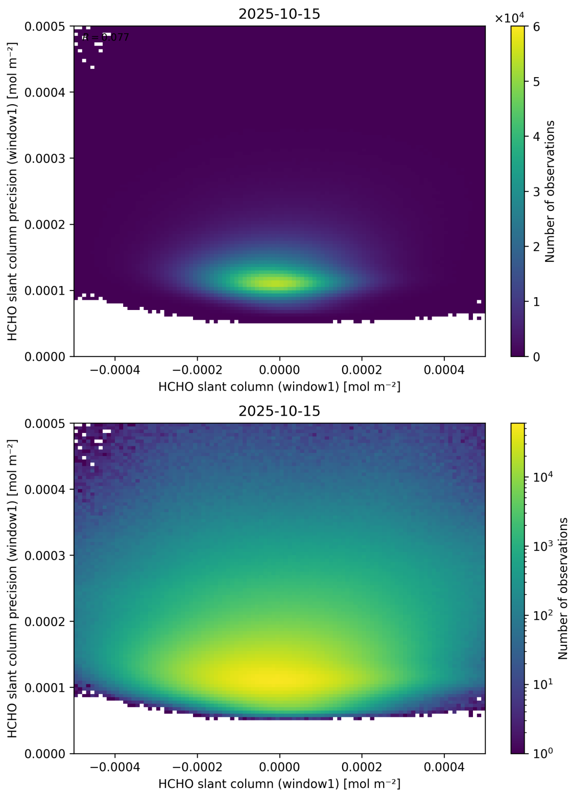
Figure 84: Scatter density plot of “HCHO slant column (window1)” against “HCHO slant column precision (window1)” for 2025-10-14 to 2025-10-16.
