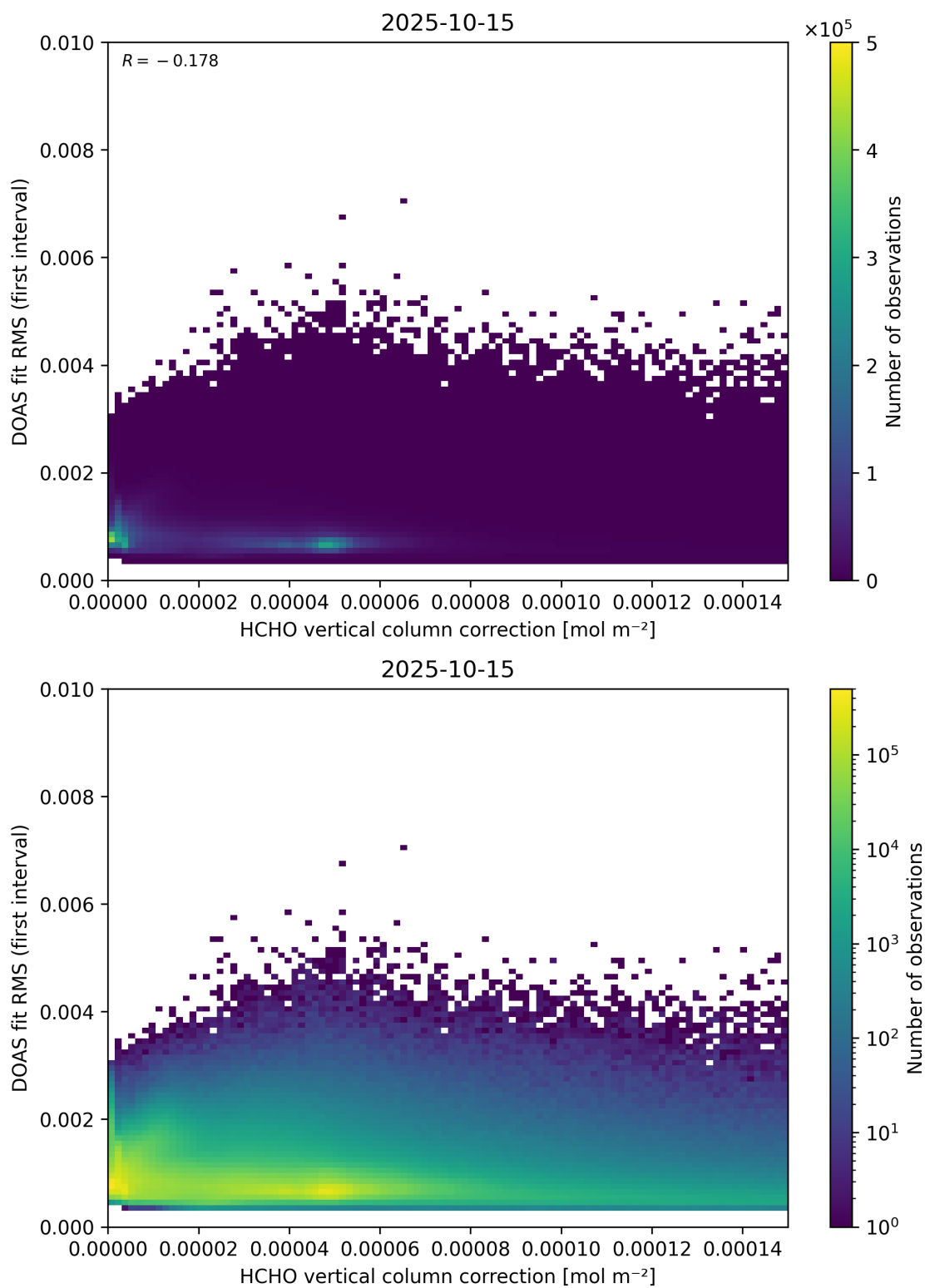
Figure 112: Scatter density plot of “HCHO vertical column correction” against “DOAS fit RMS (first interval)” for 2025-10-14 to 2025-10-16.
