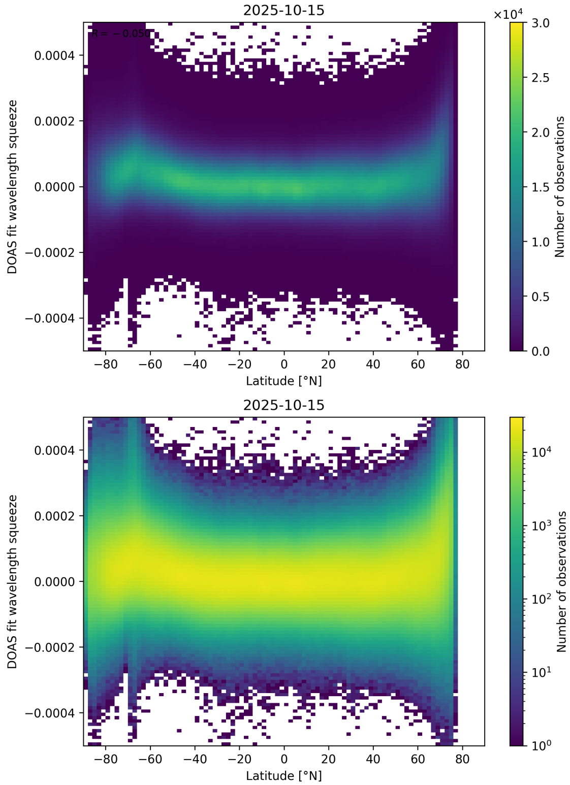
Figure 155: Scatter density plot of “Latitude” against “DOAS fit wavelength squeeze” for 2025-10-14 to 2025-10-16.
