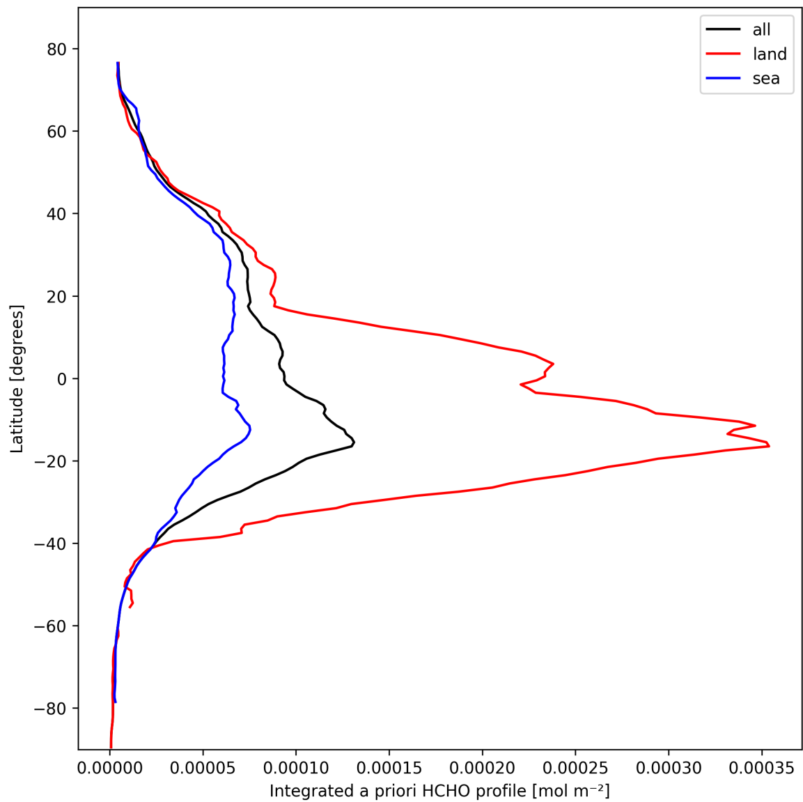
Figure 29: Zonal average of “Integrated a priori HCHO profile” for 2025-10-14 to 2025-10-16.
