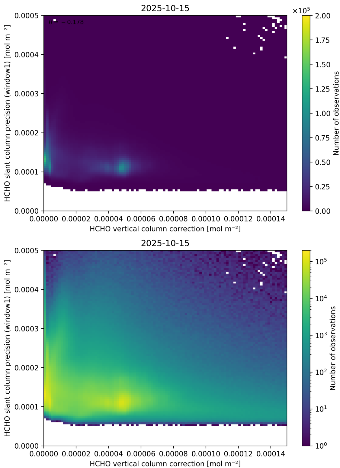
Figure 119: Scatter density plot of “HCHO vertical column correction” against “HCHO slant column precision (window1)” for 2025-10-14 to 2025-10-16.
