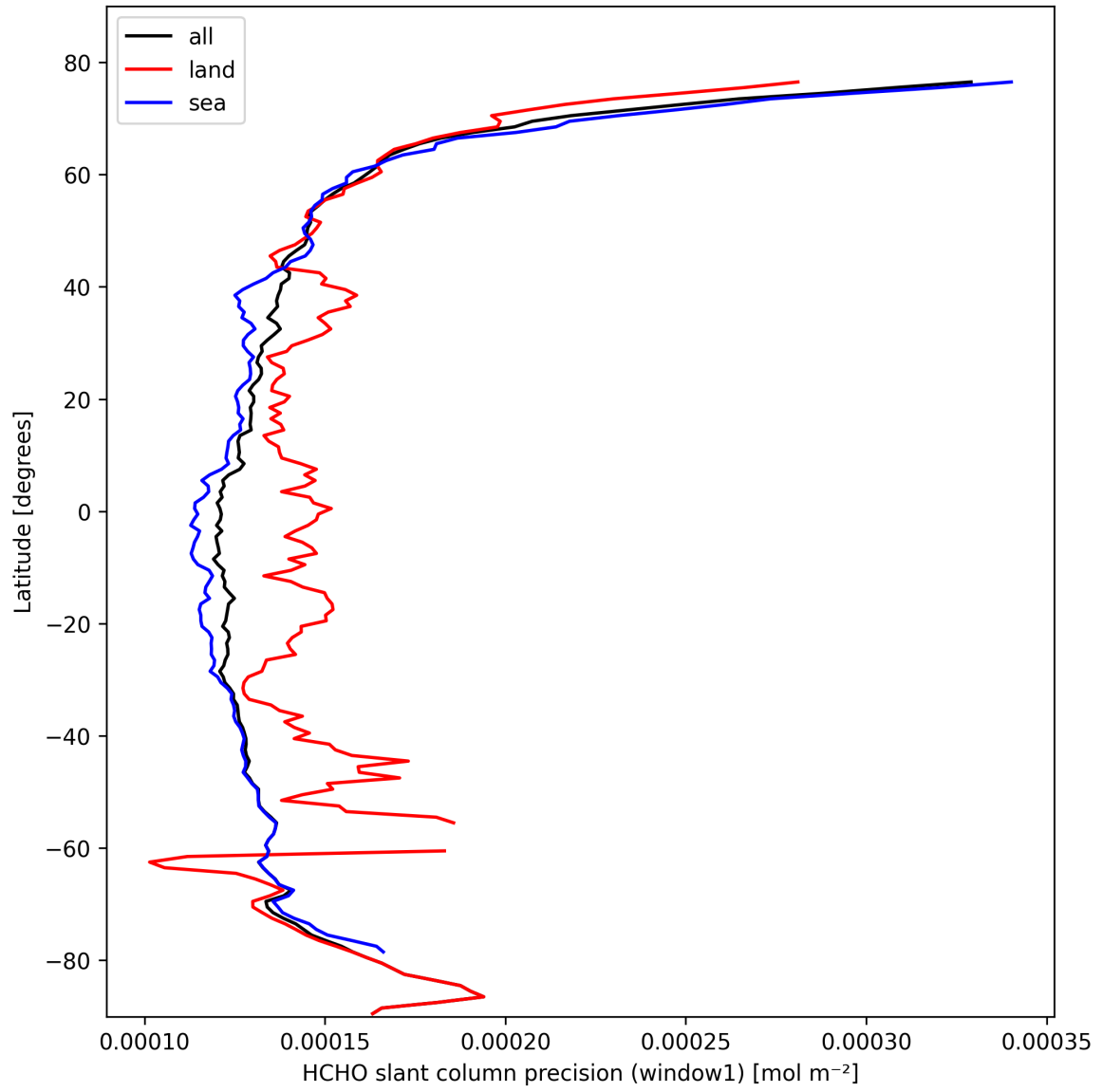
Figure 25: Zonal average of “HCHO slant column precision (window1)” for 2025-10-14 to 2025-10-16.
