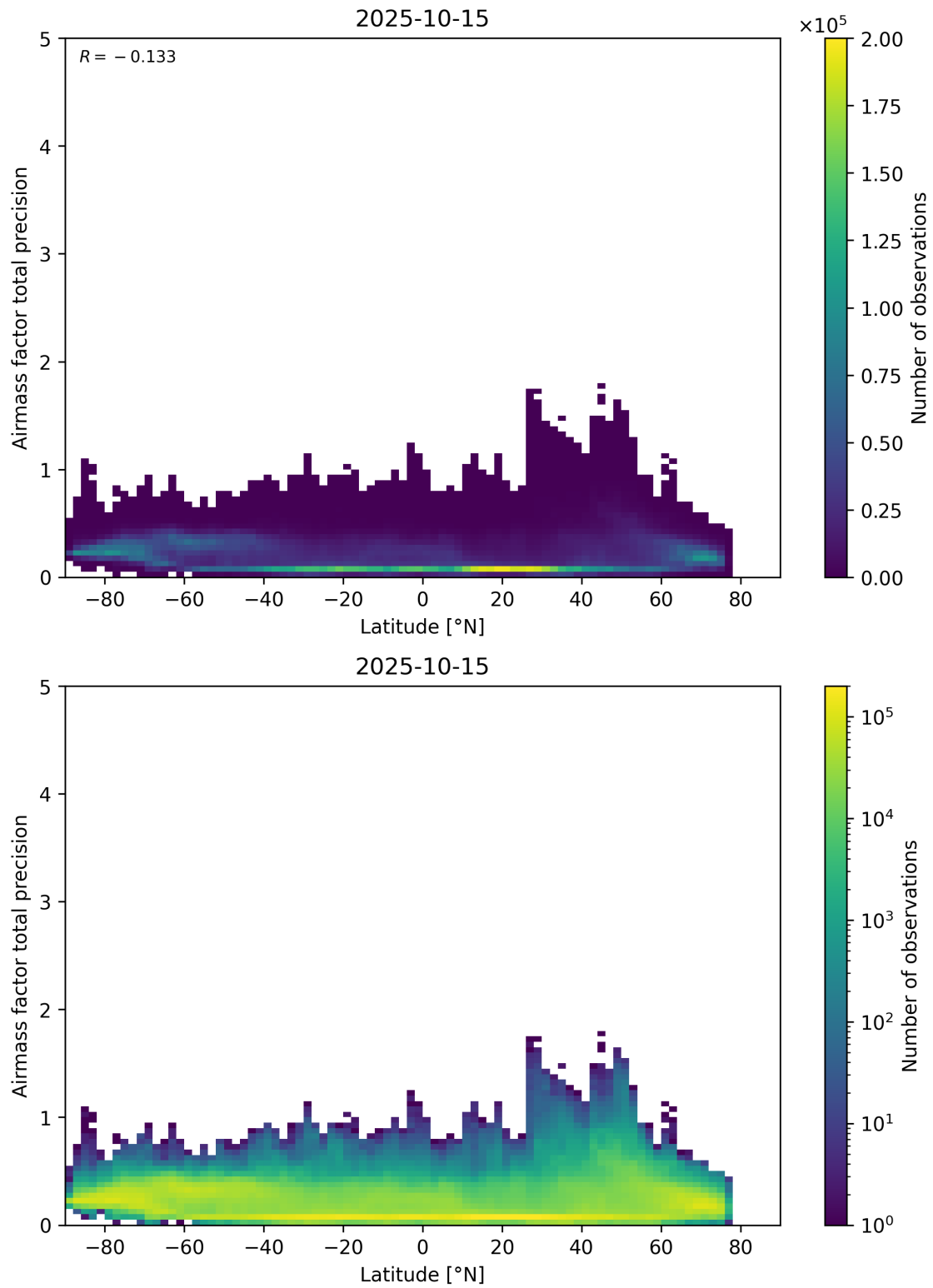
Figure 162: Scatter density plot of “Latitude” against “Airmass factor total precision” for 2025-10-14 to 2025-10-16.
