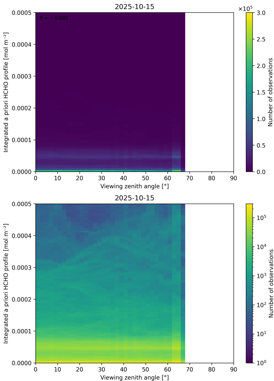
Figure 195: Scatter density plot of “Viewing zenith angle” against “Integrated a priori HCHO profile” for 2025-10-14 to 2025-10-16.
