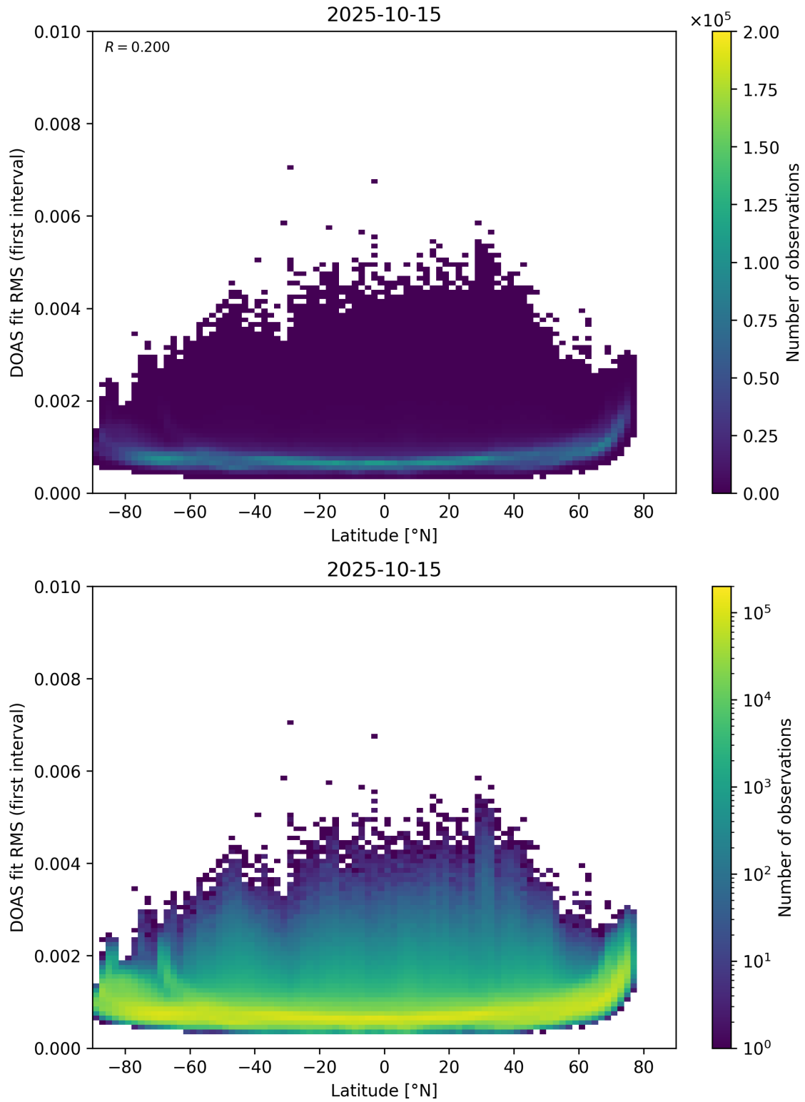
Figure 153: Scatter density plot of “Latitude” against “DOAS fit RMS (first interval)” for 2025-10-14 to 2025-10-16.
