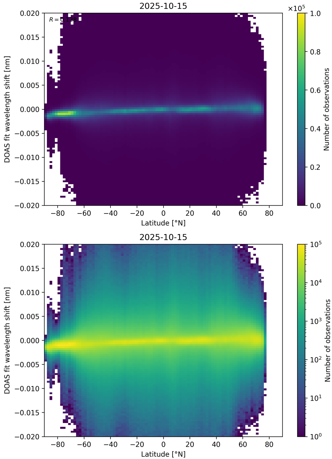
Figure 154: Scatter density plot of “Latitude” against “DOAS fit wavelength shift” for 2025-10-14 to 2025-10-16.
