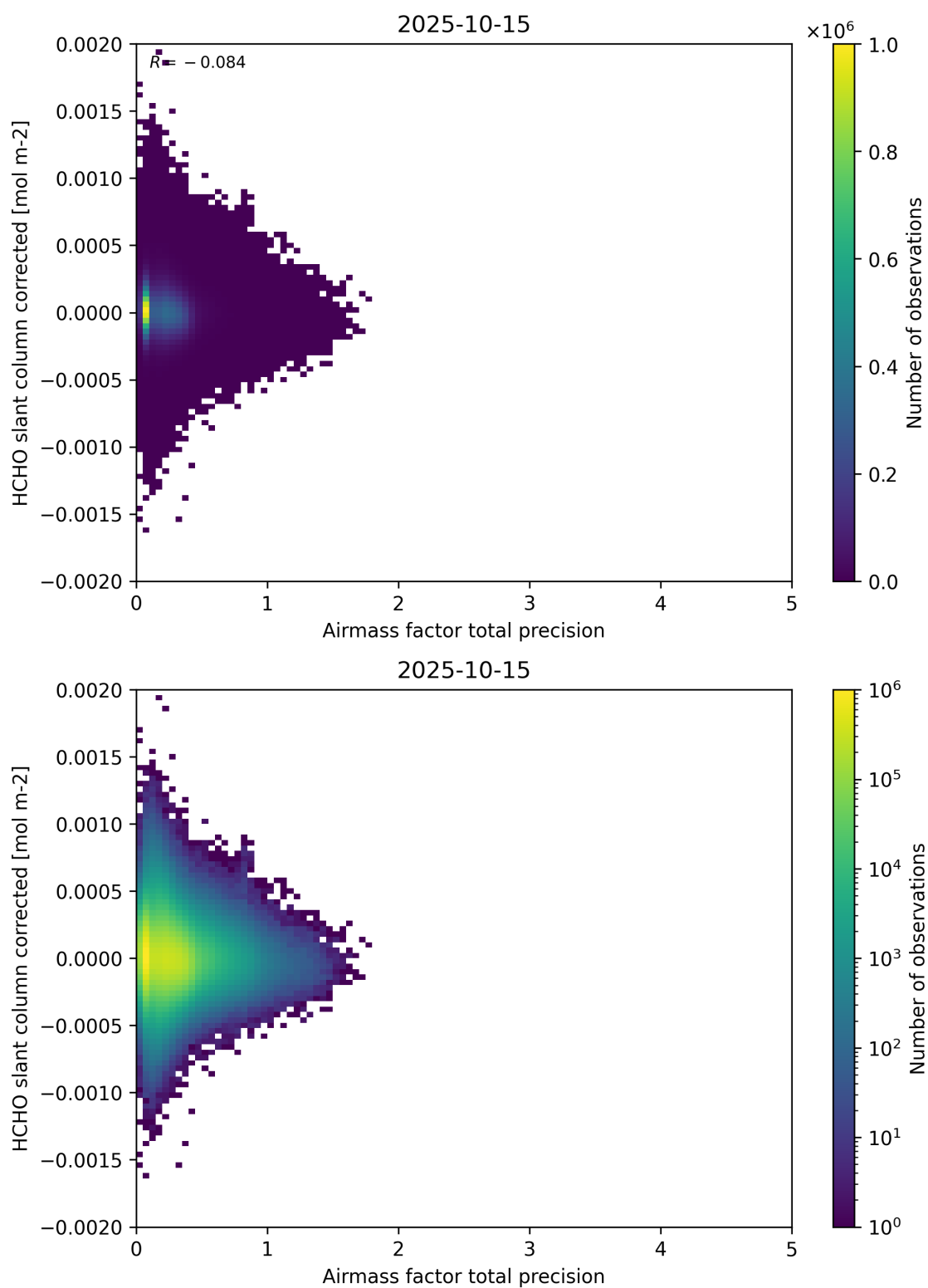
Figure 109: Scatter density plot of “Airmass factor total precision” against “HCHO slant column corrected” for 2025-10-14 to 2025-10-16.
