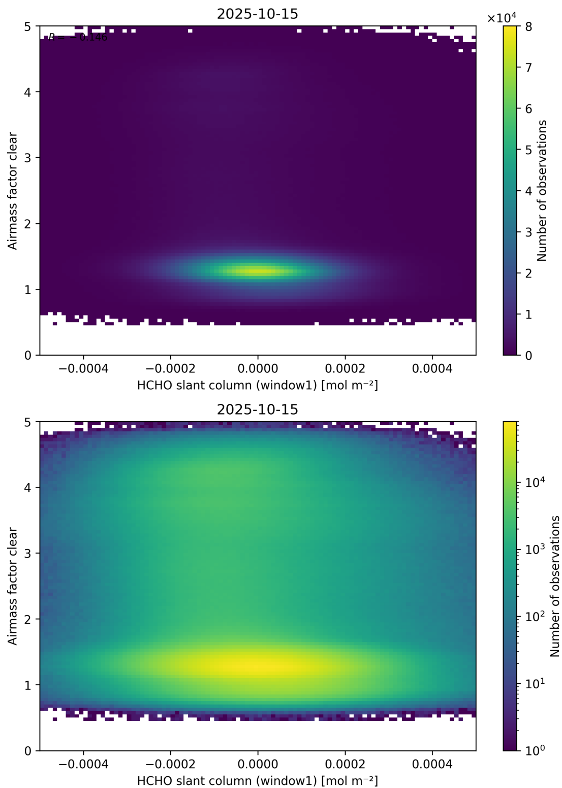
Figure 81: Scatter density plot of “HCHO slant column (window1)” against “Airmass factor clear” for 2025-10-14 to 2025-10-16.
