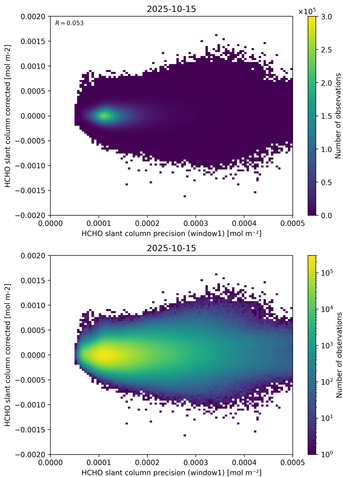
Figure 92: Scatter density plot of “HCHO slant column precision (window1)” against “HCHO slant column corrected” for 2025-10-14 to 2025-10-16.
