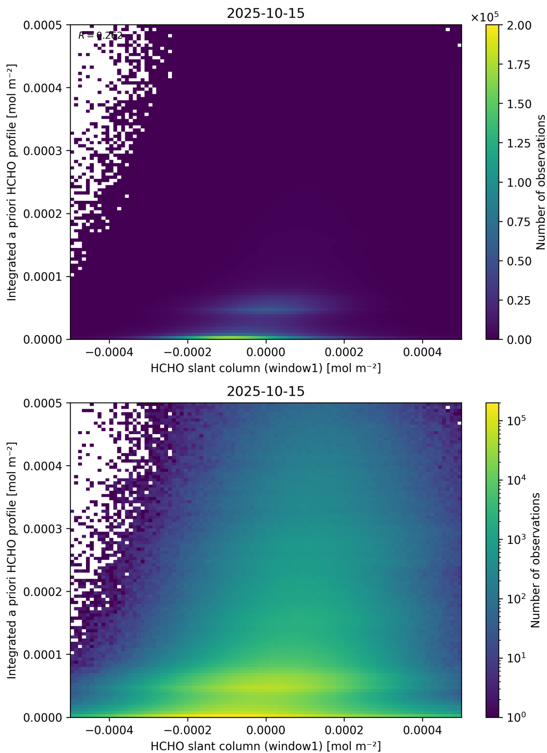
Figure 87: Scatter density plot of “HCHO slant column (window1)” against “Integrated a priori HCHO profile” for 2025-10-14 to 2025-10-16.
