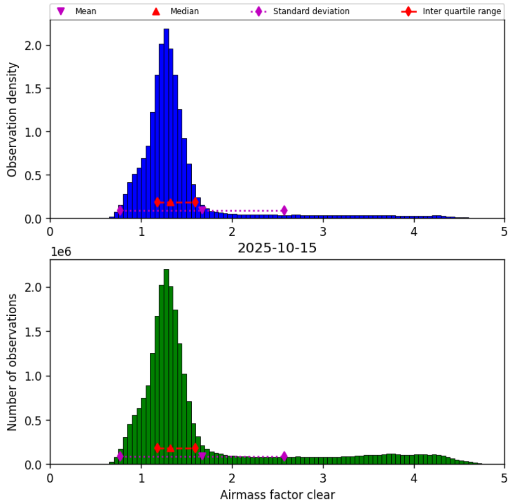
Figure 42: Histogram of “Airmass factor clear” for 2025-10-14 to 2025-10-16
