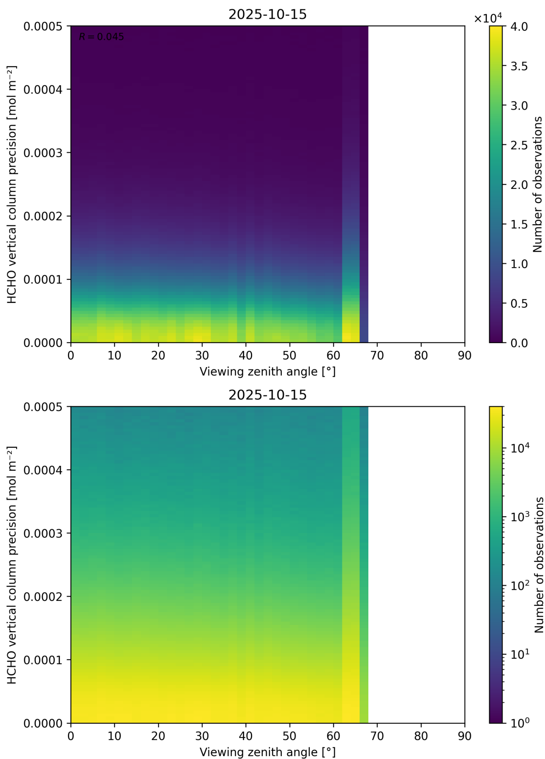
Figure 194: Scatter density plot of “Viewing zenith angle” against “HCHO vertical column precision” for 2025-10-14 to 2025-10-16.
