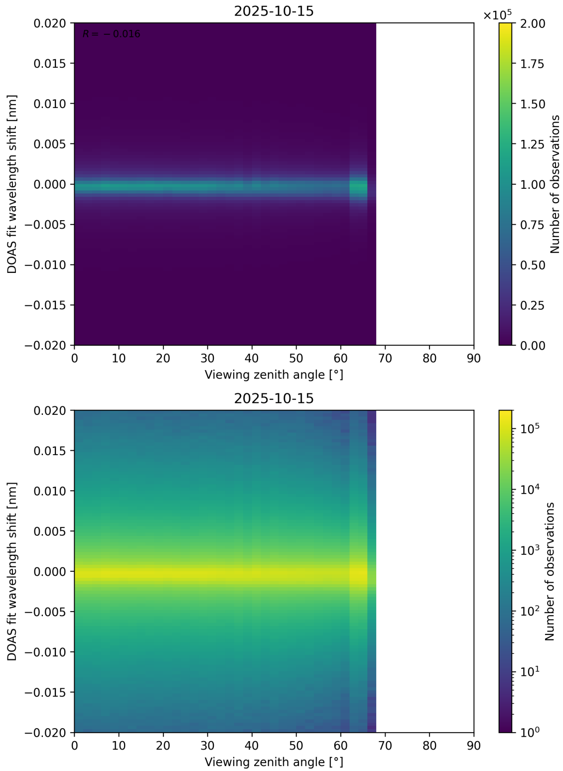
Figure 183: Scatter density plot of “Viewing zenith angle” against “DOAS fit wavelength shift” for 2025-10-14 to 2025-10-16.
