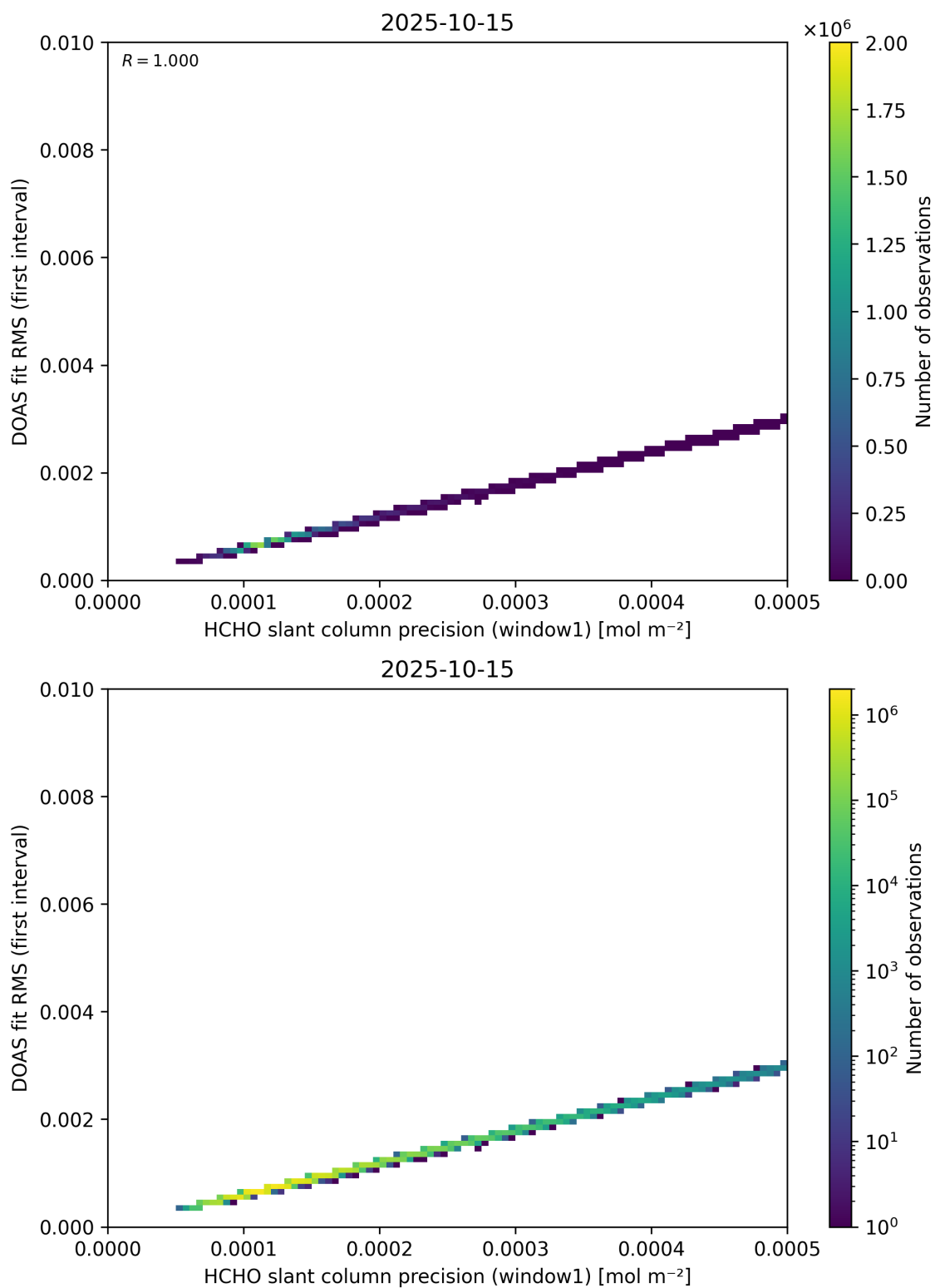
Figure 88: Scatter density plot of “HCHO slant column precision (window1)” against “DOAS fit RMS (first interval)” for 2025-10-14 to 2025-10-16.
