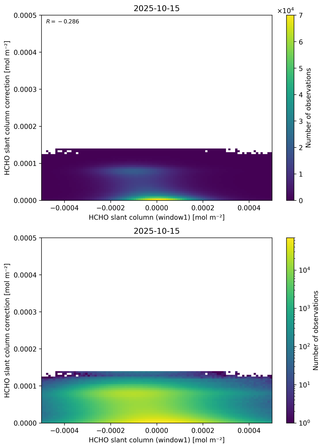
Figure 83: Scatter density plot of “HCHO slant column (window1)” against “HCHO slant column correction” for 2025-10-14 to 2025-10-16.
