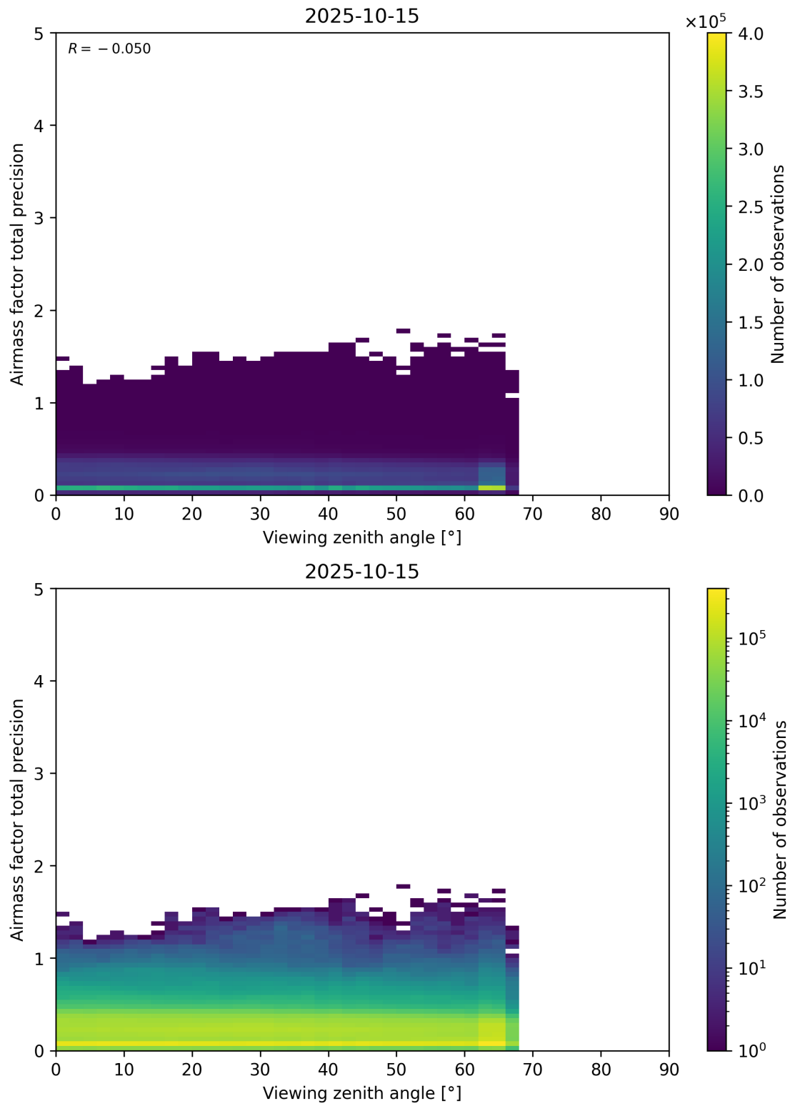
Figure 191: Scatter density plot of “Viewing zenith angle” against “Airmass factor total precision” for 2025-10-14 to 2025-10-16.
