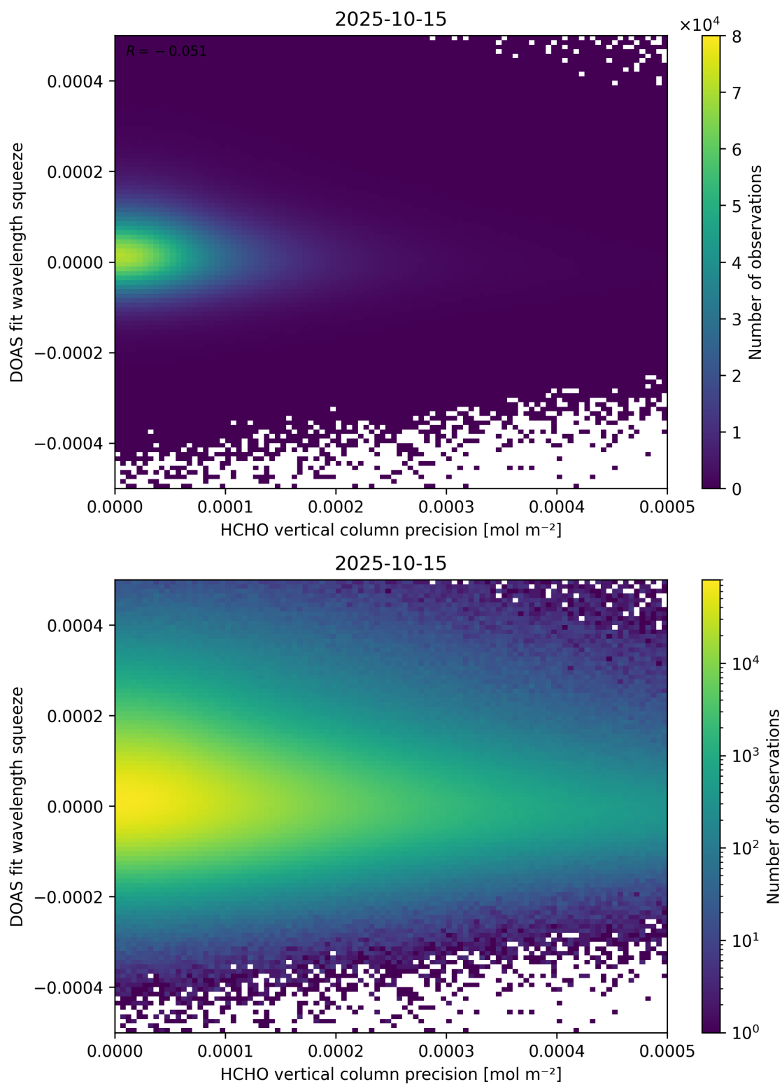
Figure 138: Scatter density plot of “HCHO vertical column precision” against “DOAS fit wavelength squeeze” for 2025-10-14 to 2025-10-16.
