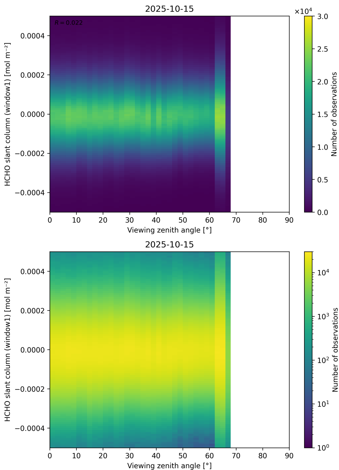
Figure 188: Scatter density plot of “Viewing zenith angle” against “HCHO slant column (window1)” for 2025-10-14 to 2025-10-16.
