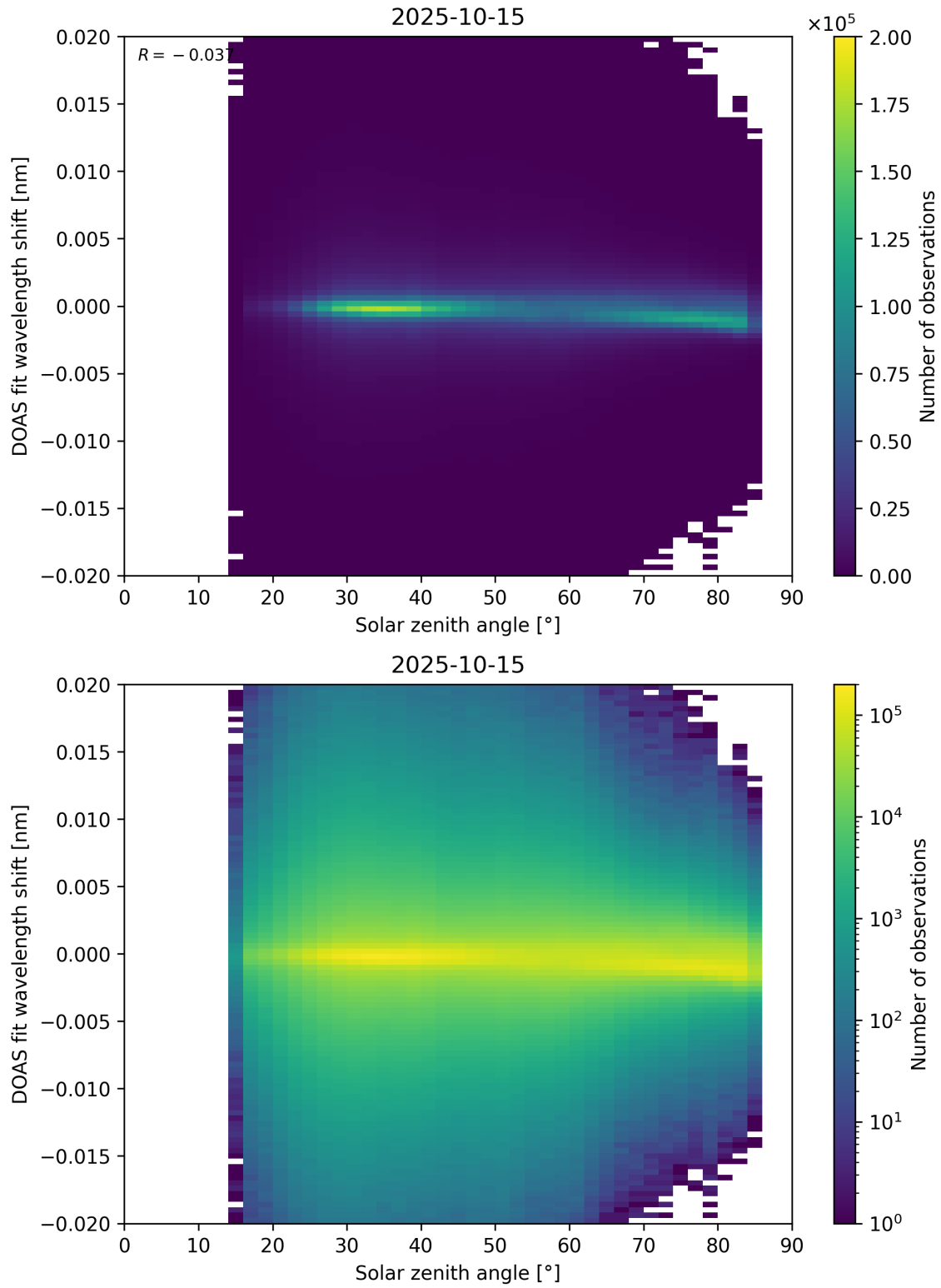
Figure 168: Scatter density plot of “Solar zenith angle” against “DOAS fit wavelength shift” for 2025-10-14 to 2025-10-16.
