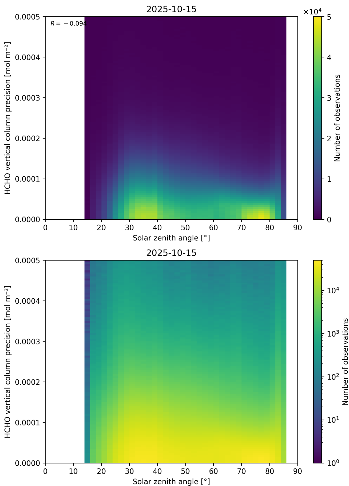
Figure 179: Scatter density plot of “Solar zenith angle” against “HCHO vertical column precision” for 2025-10-14 to 2025-10-16.
