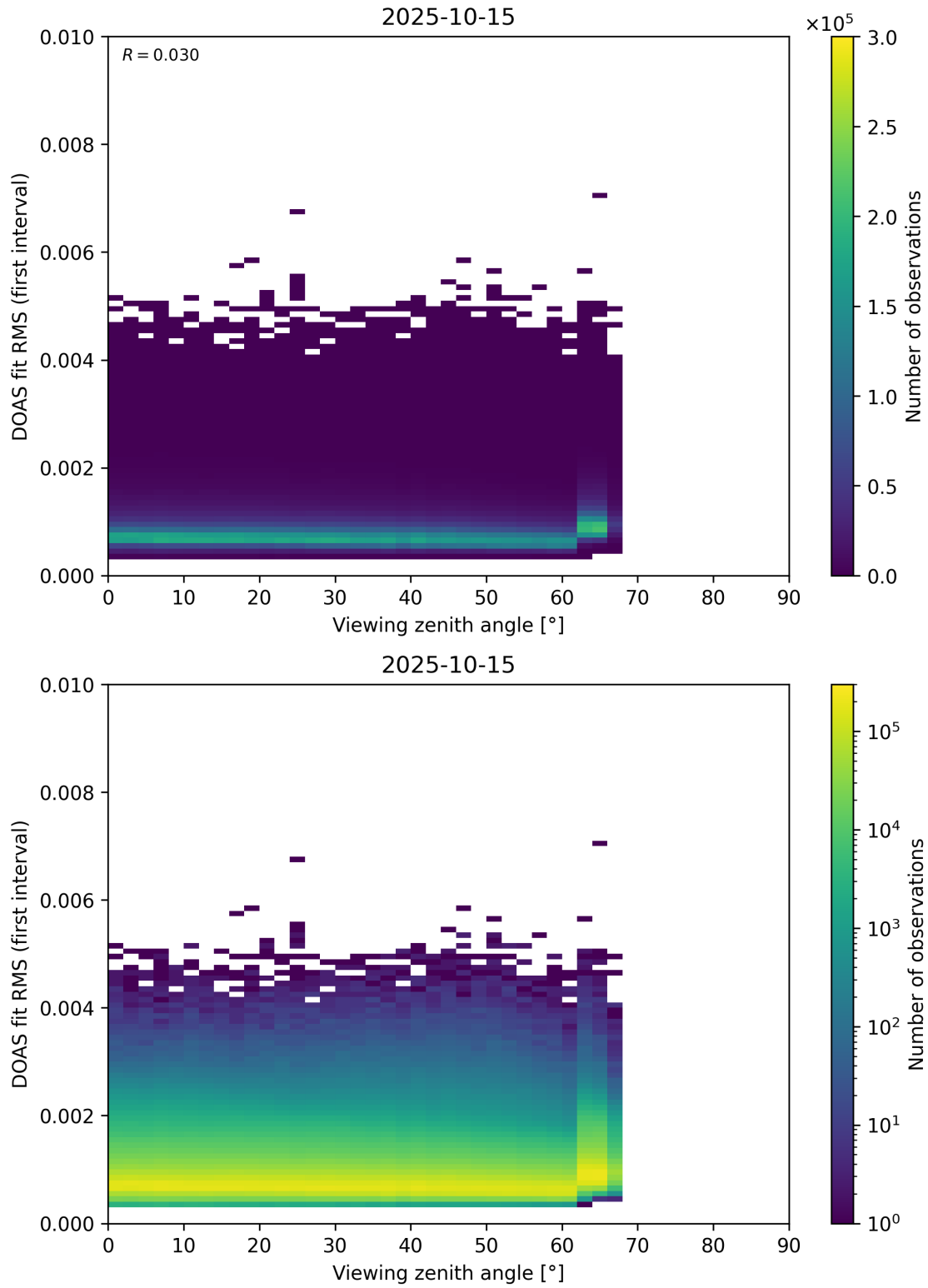
Figure 182: Scatter density plot of “Viewing zenith angle” against “DOAS fit RMS (first interval)” for 2025-10-14 to 2025-10-16.
