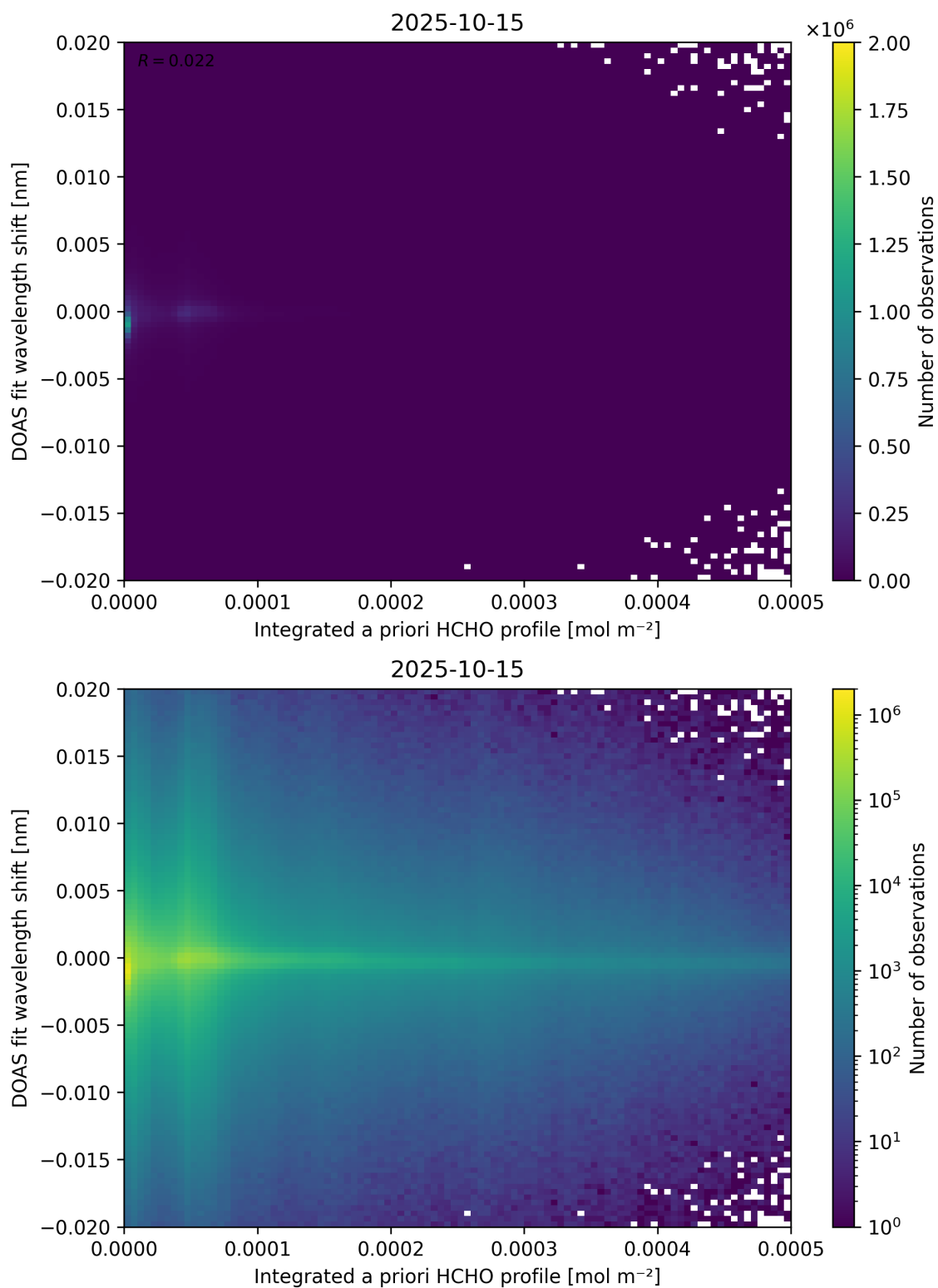
Figure 149: Scatter density plot of “Integrated a priori HCHO profile” against “DOAS fit wavelength shift” for 2025-10-14 to 2025-10-16.
