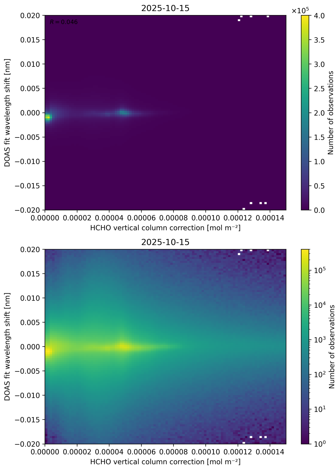
Figure 113: Scatter density plot of “HCHO vertical column correction” against “DOAS fit wavelength shift” for 2025-10-14 to 2025-10-16.
