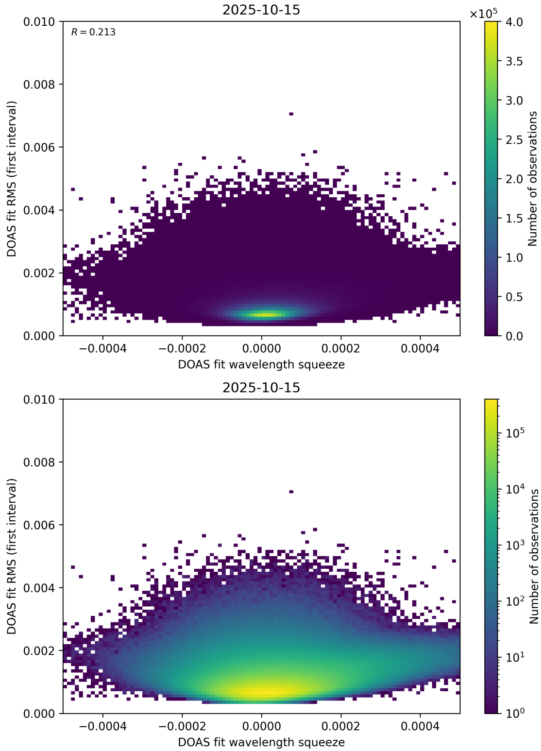
Figure 68: Scatter density plot of “DOAS fit wavelength squeeze” against “DOAS fit RMS (first interval)” for 2025-10-14 to 2025-10-16.
