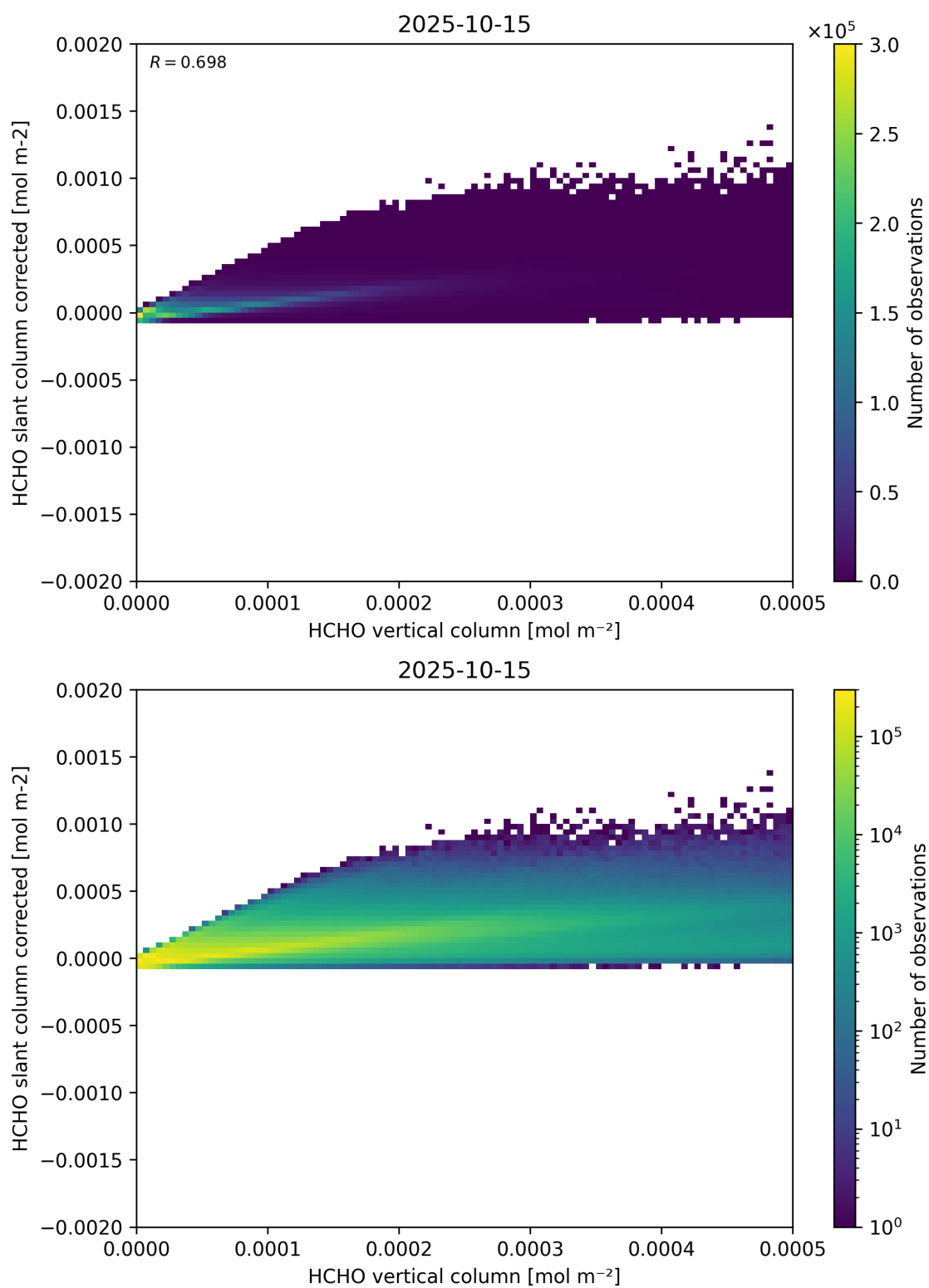
Figure 127: Scatter density plot of “HCHO vertical column” against “HCHO slant column corrected” for 2025-10-14 to 2025-10-16.
