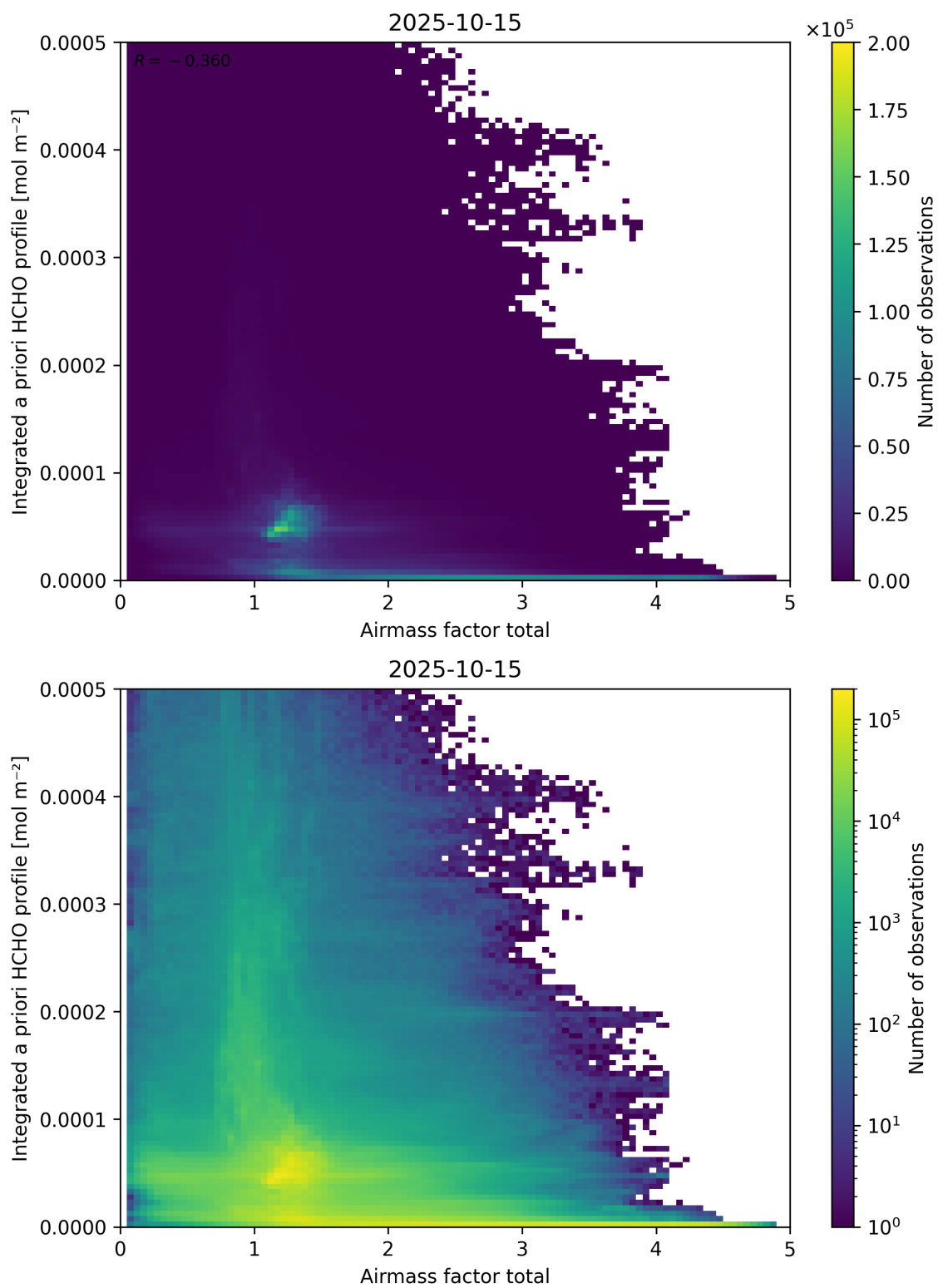
Figure 104: Scatter density plot of “Airmass factor total” against “Integrated a priori HCHO profile” for 2025-10-14 to 2025-10-16.
