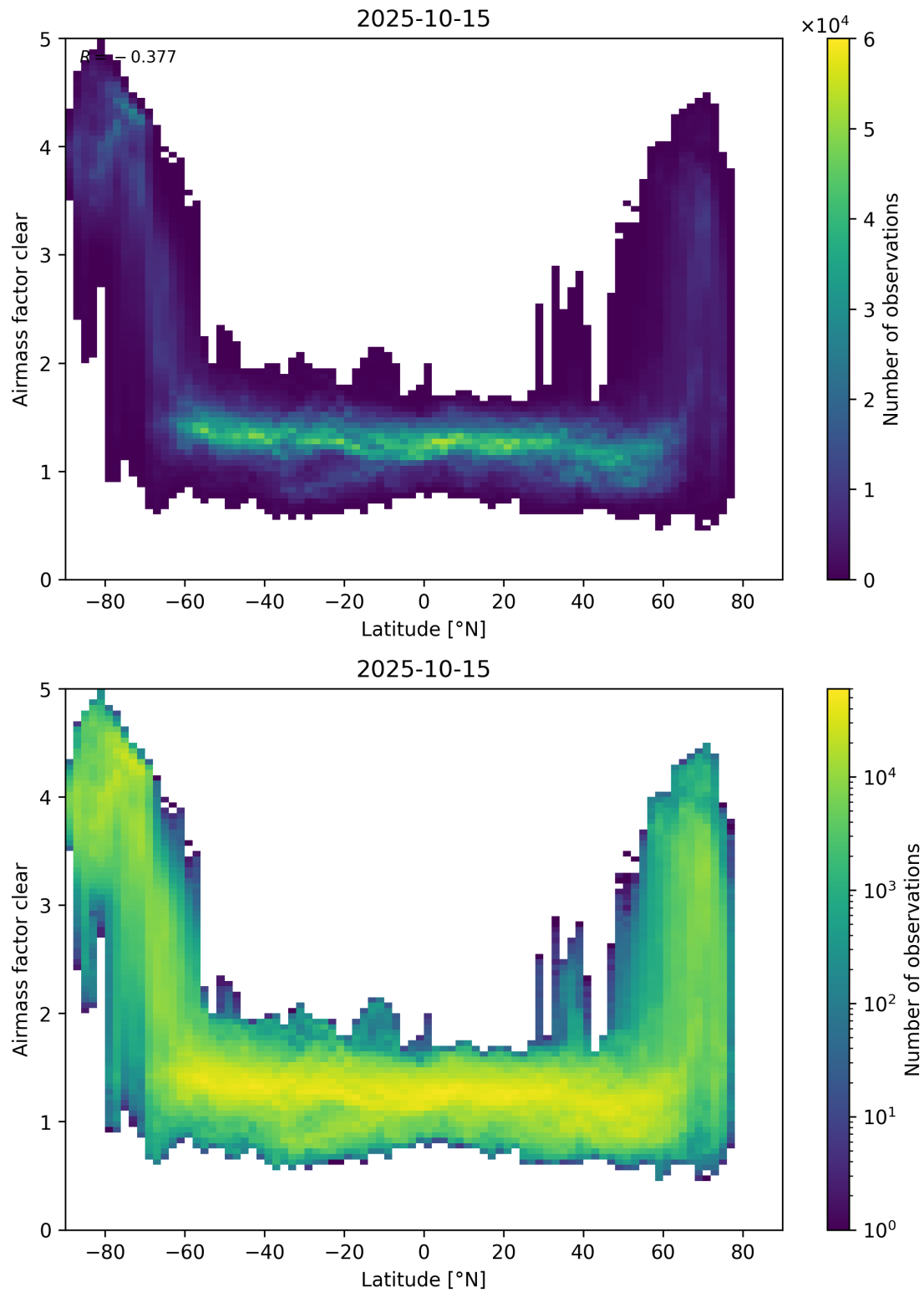
Figure 156: Scatter density plot of “Latitude” against “Airmass factor clear” for 2025-10-14 to 2025-10-16.
