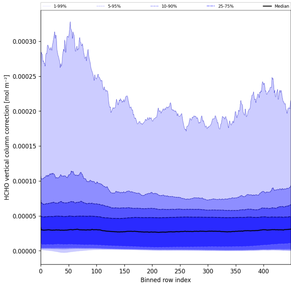
Figure 51: Along track statistics of “HCHO vertical column correction” for 2025-10-14 to 2025-10-16
