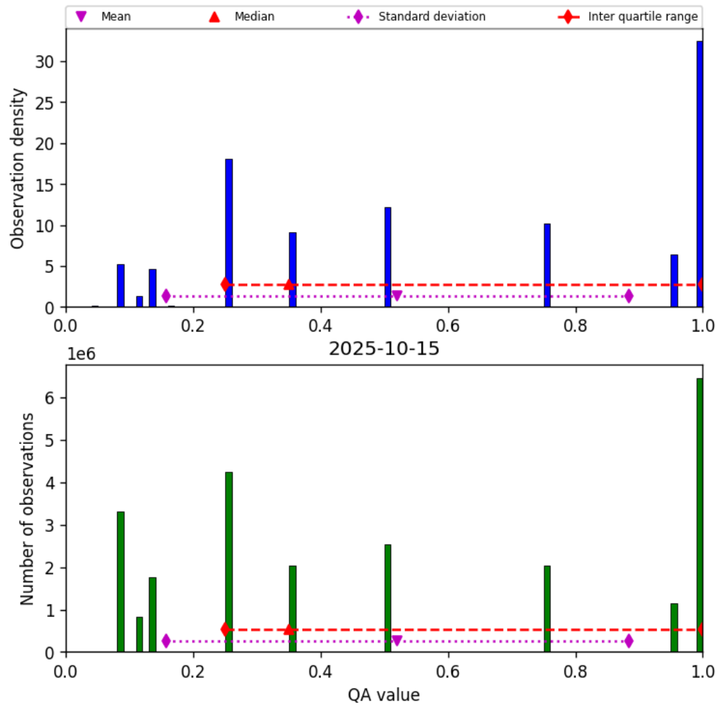
Figure 34: Histogram of “QA value” for 2025-10-14 to 2025-10-16
