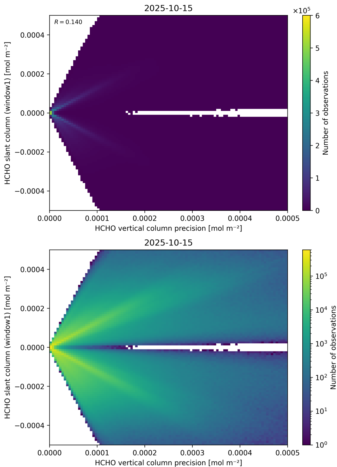
Figure 142: Scatter density plot of “HCHO vertical column precision” against “HCHO slant column (window1)” for 2025-10-14 to 2025-10-16.
