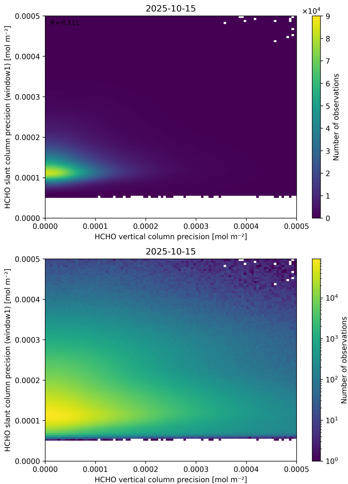
Figure 143: Scatter density plot of “HCHO vertical column precision” against “HCHO slant column precision (window1)” for 2025-10-14 to 2025-10-16.
