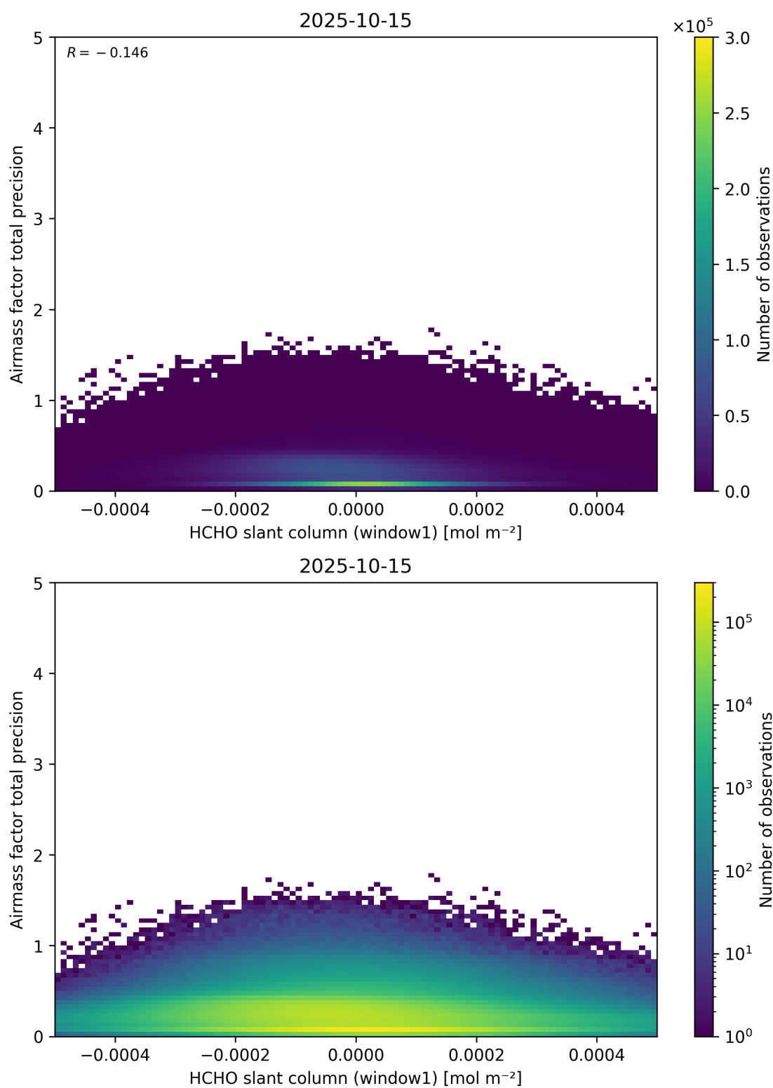
Figure 86: Scatter density plot of “HCHO slant column (window1)” against “Airmass factor total precision” for 2025-10-14 to 2025-10-16.
