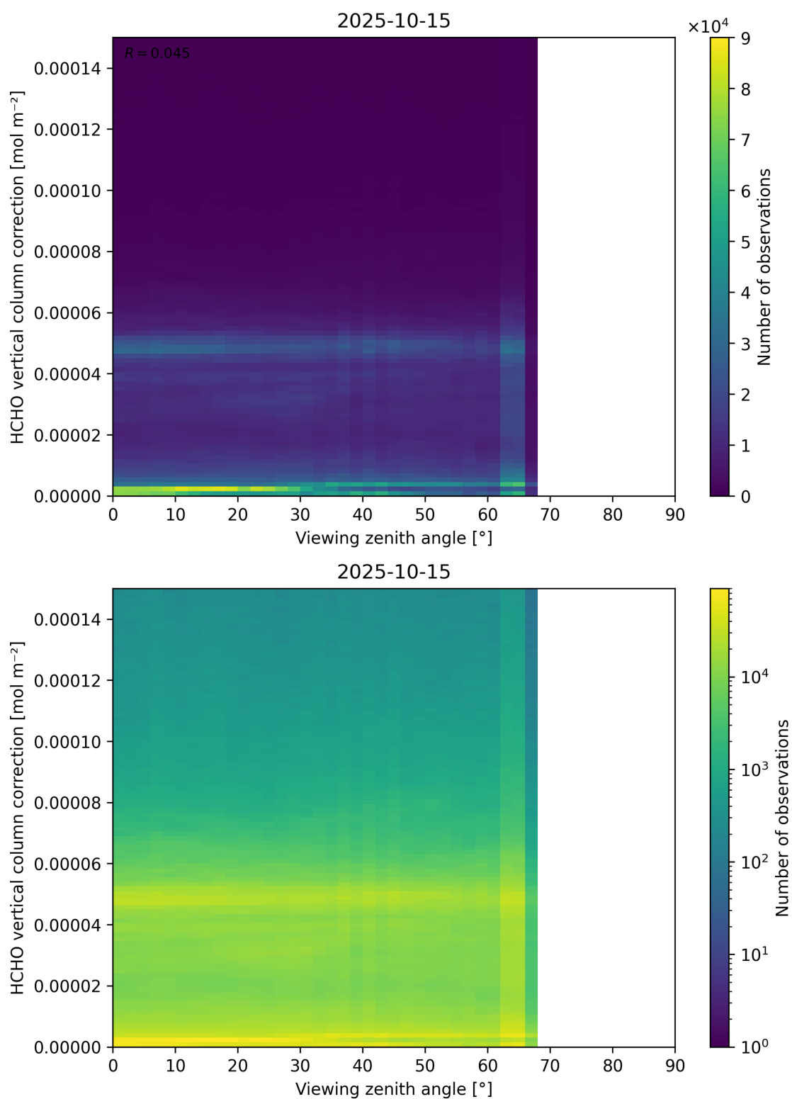
Figure 193: Scatter density plot of “Viewing zenith angle” against “HCHO vertical column correction” for 2025-10-14 to 2025-10-16.
