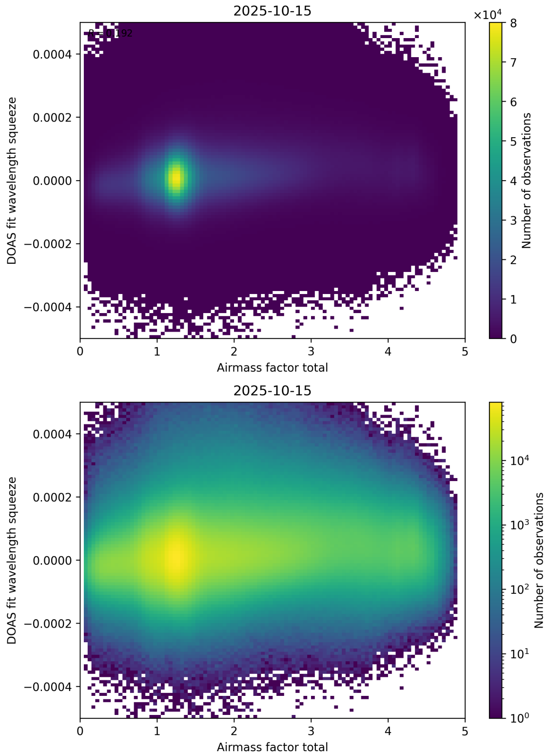
Figure 99: Scatter density plot of “Airmass factor total” against “DOAS fit wavelength squeeze” for 2025-10-14 to 2025-10-16.
