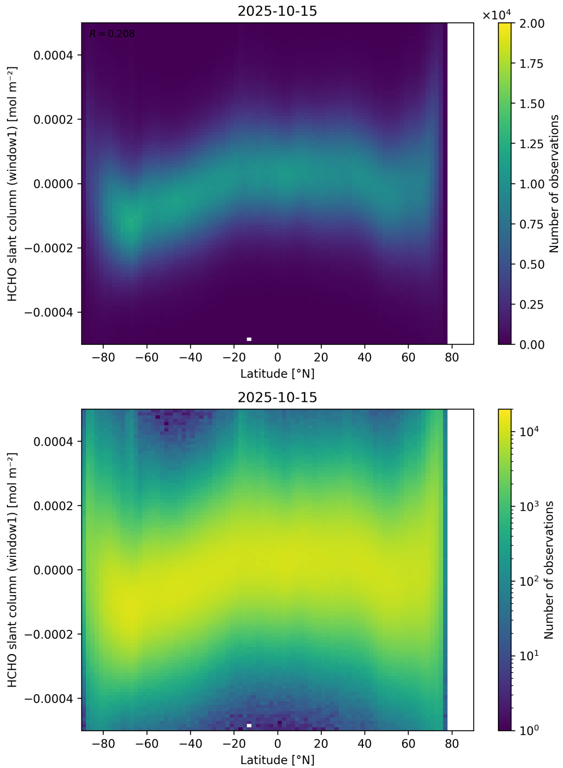
Figure 159: Scatter density plot of “Latitude” against “HCHO slant column (window1)” for 2025-10-14 to 2025-10-16.
