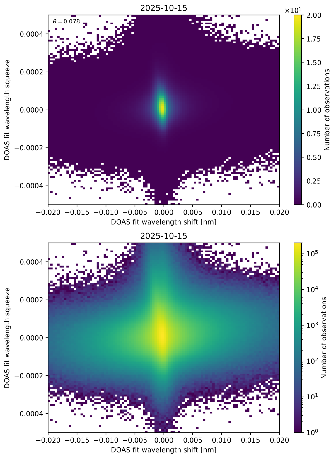
Figure 65: Scatter density plot of “DOAS fit wavelength shift” against “DOAS fit wavelength squeeze” for 2025-10-14 to 2025-10-16.
