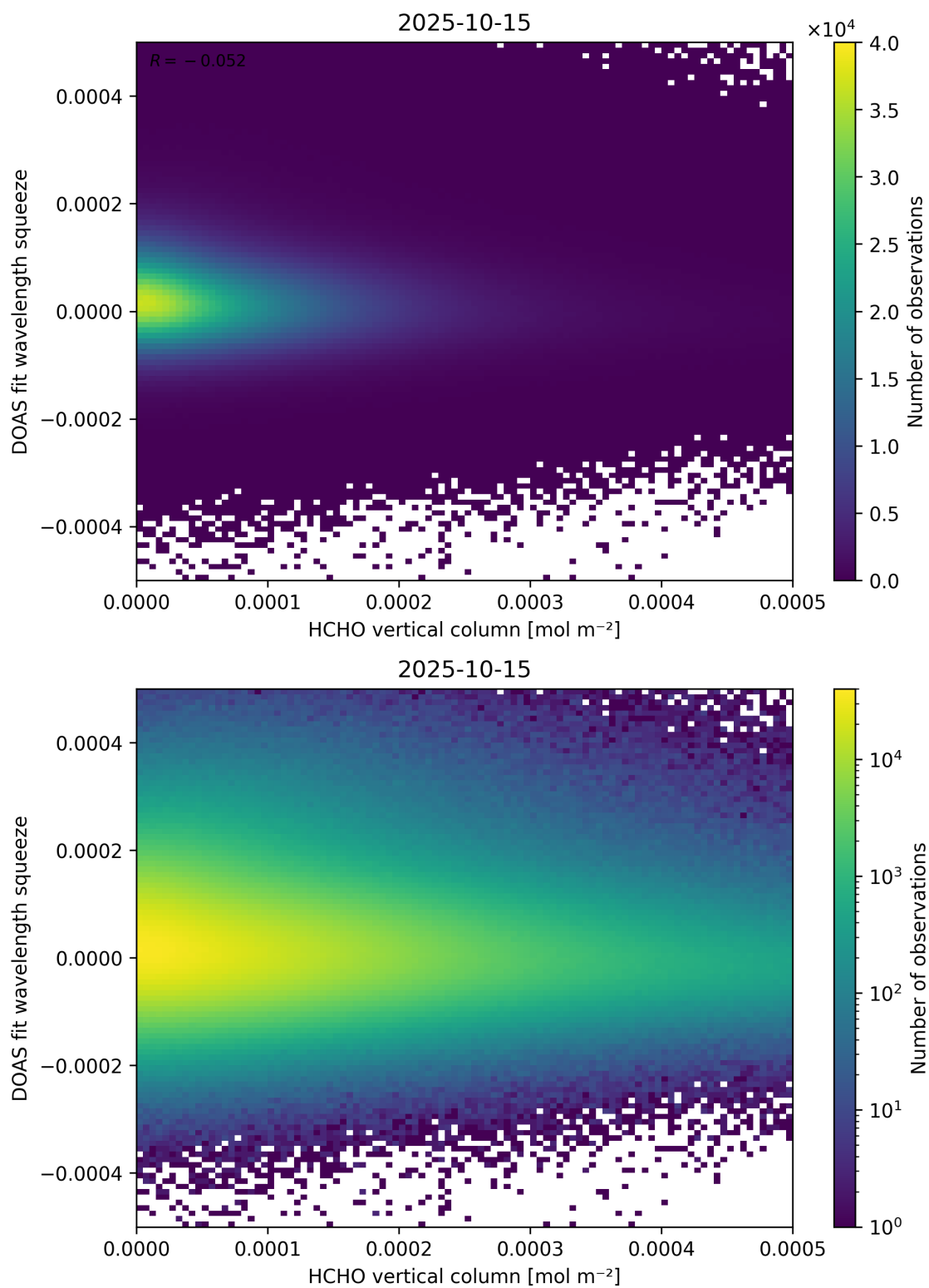
Figure 125: Scatter density plot of “HCHO vertical column” against “DOAS fit wavelength squeeze” for 2025-10-14 to 2025-10-16.
