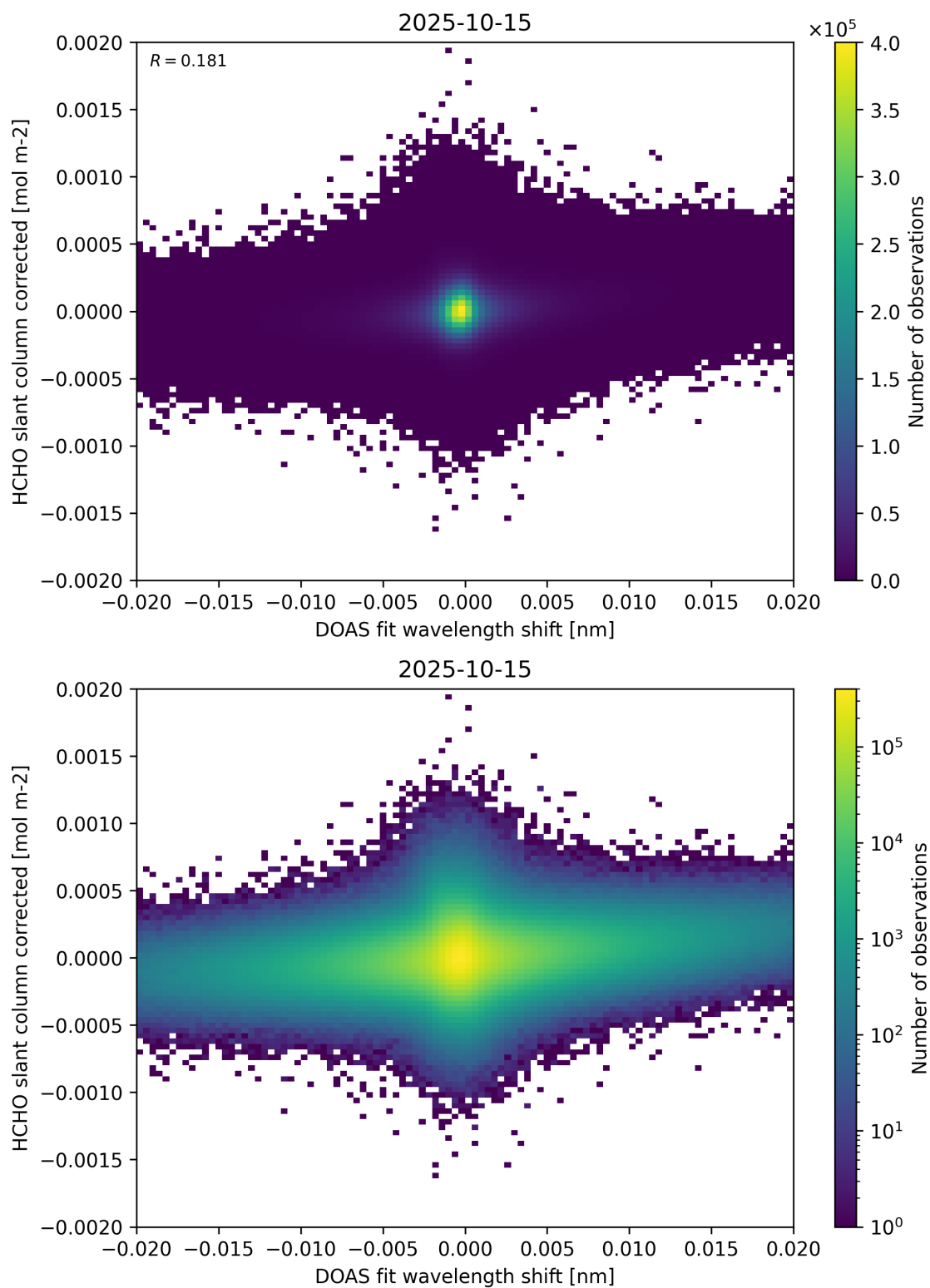
Figure 66: Scatter density plot of “DOAS fit wavelength shift” against “HCHO slant column corrected” for 2025-10-14 to 2025-10-16.
