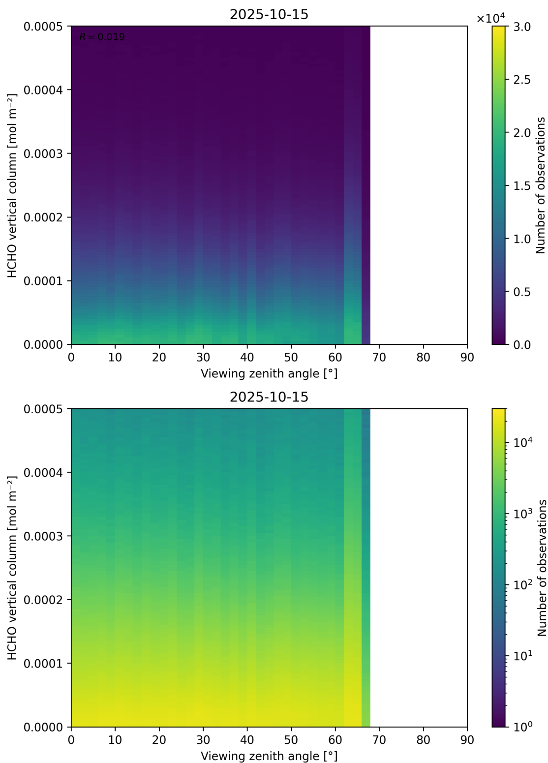
Figure 192: Scatter density plot of “Viewing zenith angle” against “HCHO vertical column” for 2025-10-14 to 2025-10-16.
