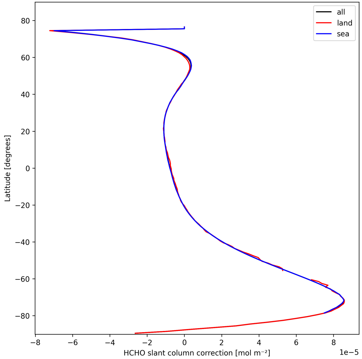
Figure 33: Zonal average of “HCHO slant column correction” for 2025-10-14 to 2025-10-16.
