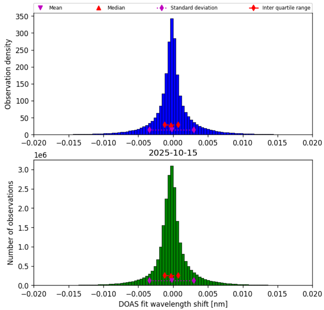
Figure 44: Histogram of “DOAS fit wavelength shift” for 2025-10-14 to 2025-10-16
