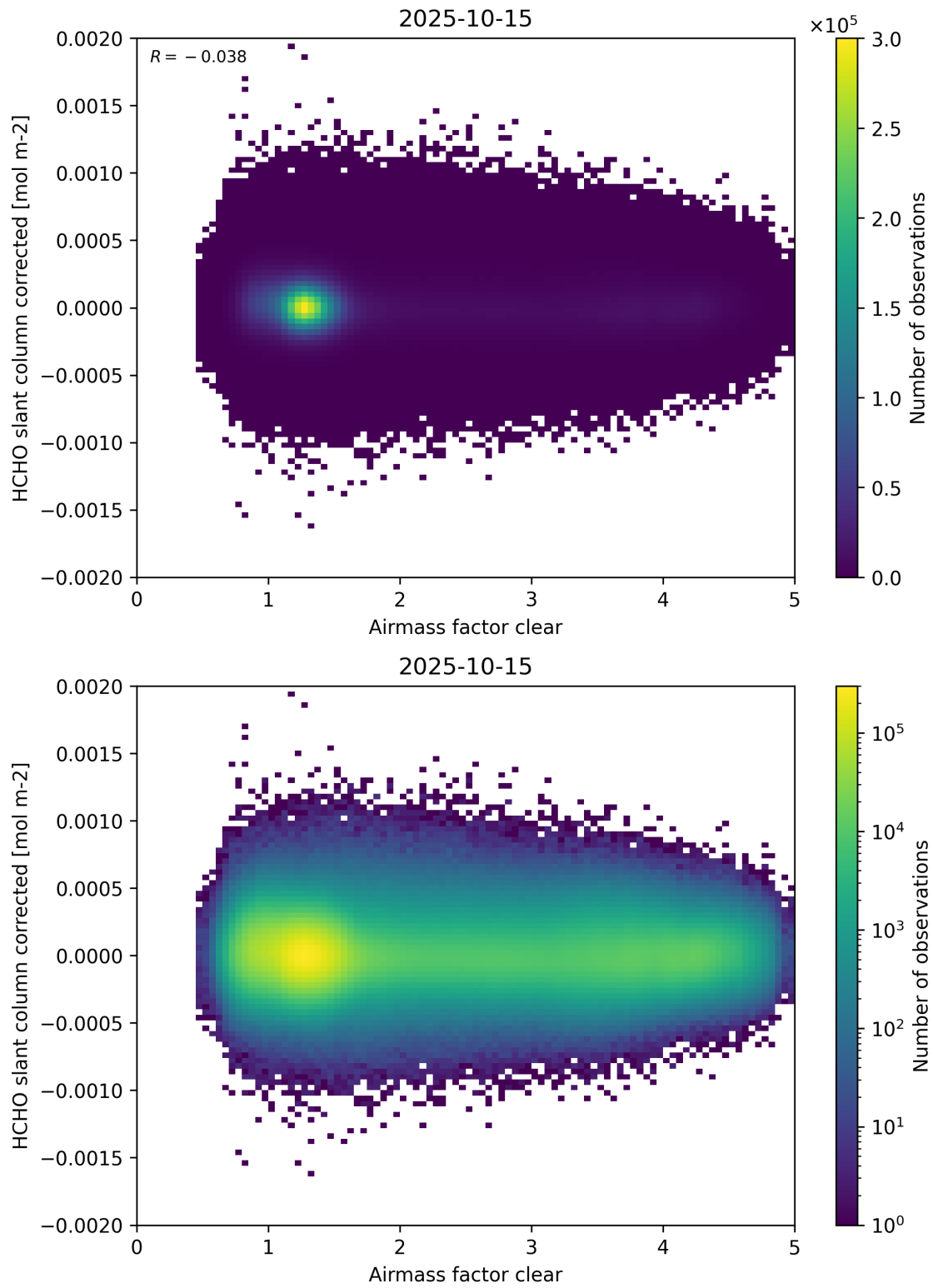
Figure 74: Scatter density plot of “Airmass factor clear” against “HCHO slant column corrected” for 2025-10-14 to 2025-10-16.
