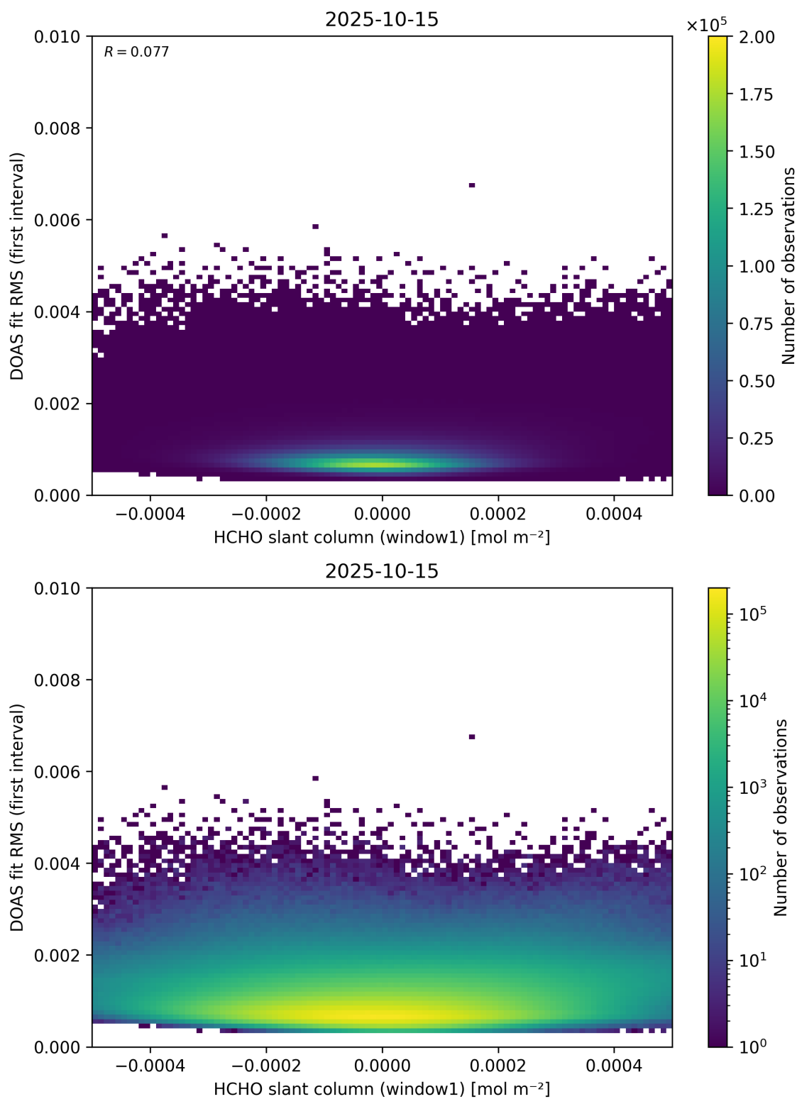
Figure 78: Scatter density plot of “HCHO slant column (window1)” against “DOAS fit RMS (first interval)” for 2025-10-14 to 2025-10-16.
