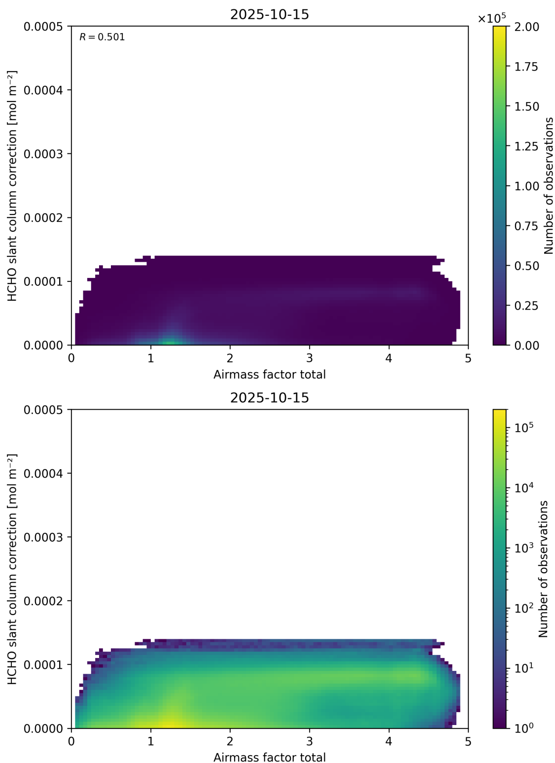
Figure 102: Scatter density plot of “Airmass factor total” against “HCHO slant column correction” for 2025-10-14 to 2025-10-16.
