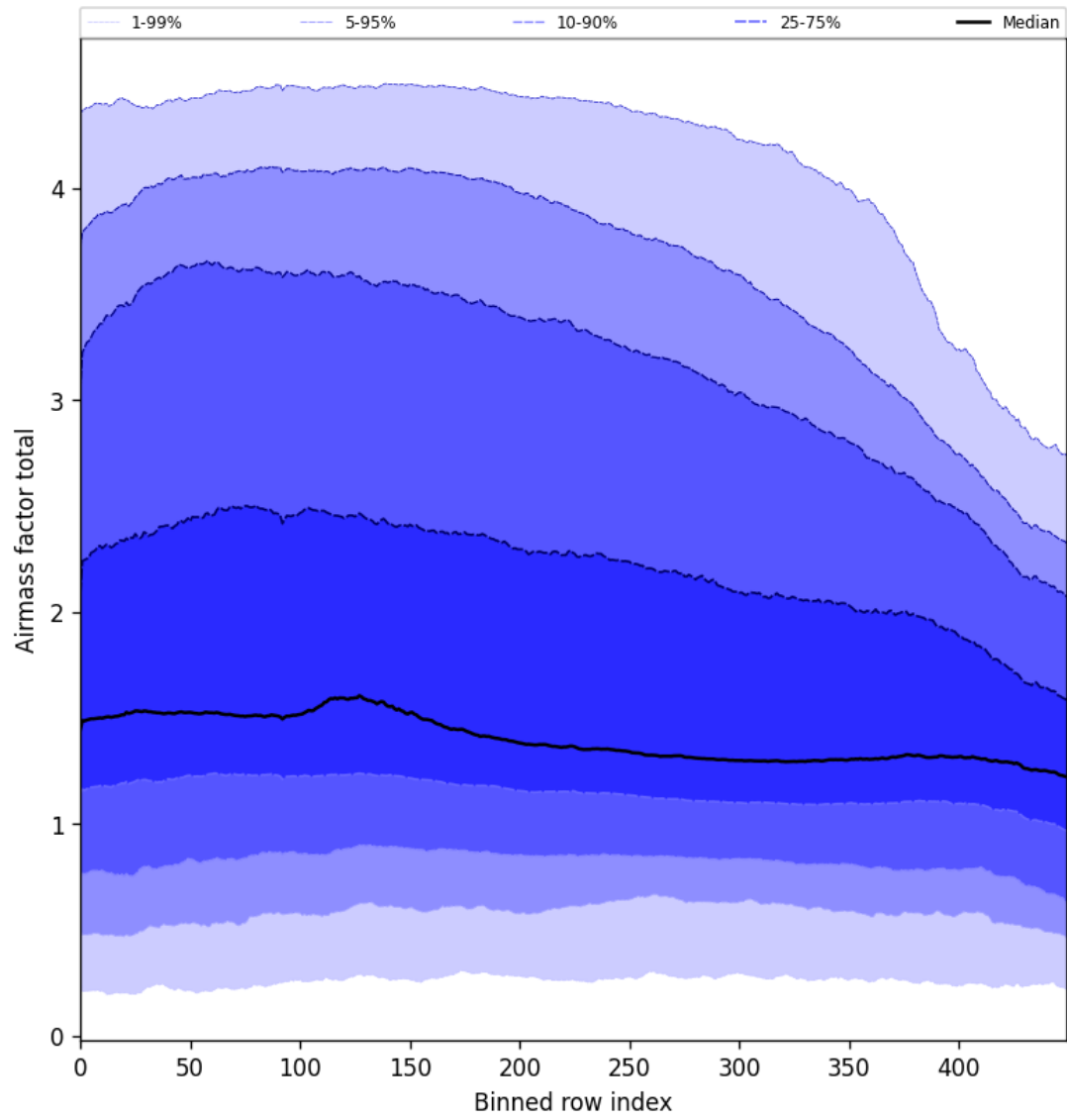
Figure 54: Along track statistics of “Airmass factor total” for 2025-10-14 to 2025-10-16
