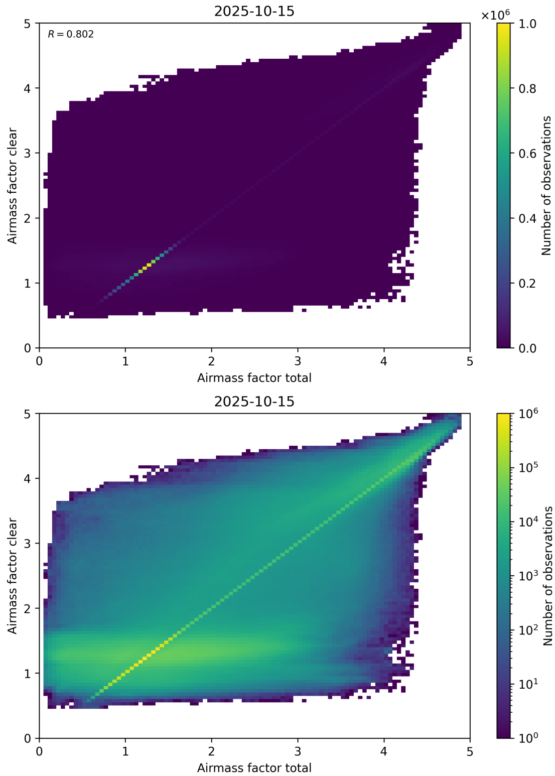
Figure 100: Scatter density plot of “Airmass factor total” against “Airmass factor clear” for 2025-10-14 to 2025-10-16.
