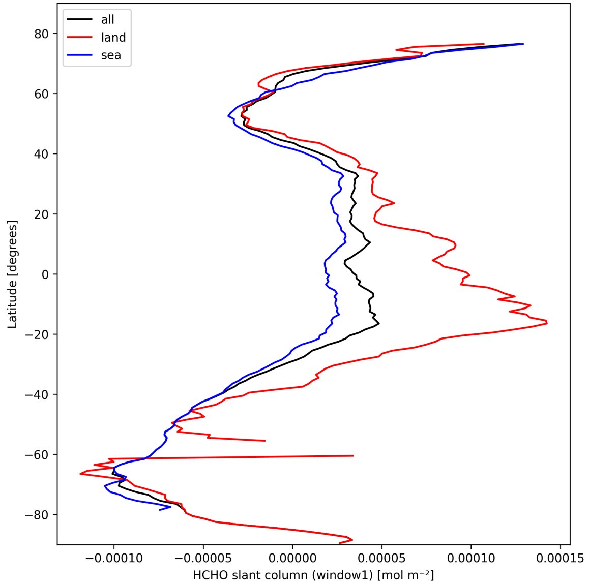
Figure 24: Zonal average of “HCHO slant column (window1)” for 2025-10-14 to 2025-10-16.
