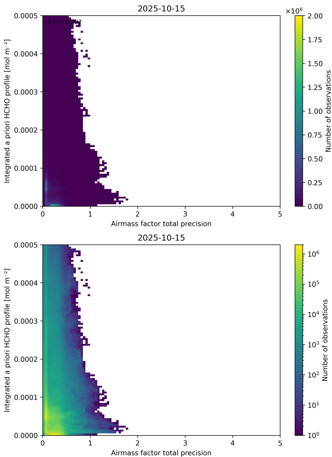
Figure 111: Scatter density plot of “Airmass factor total precision” against “Integrated a priori HCHO profile” for 2025-10-14 to 2025-10-16.
