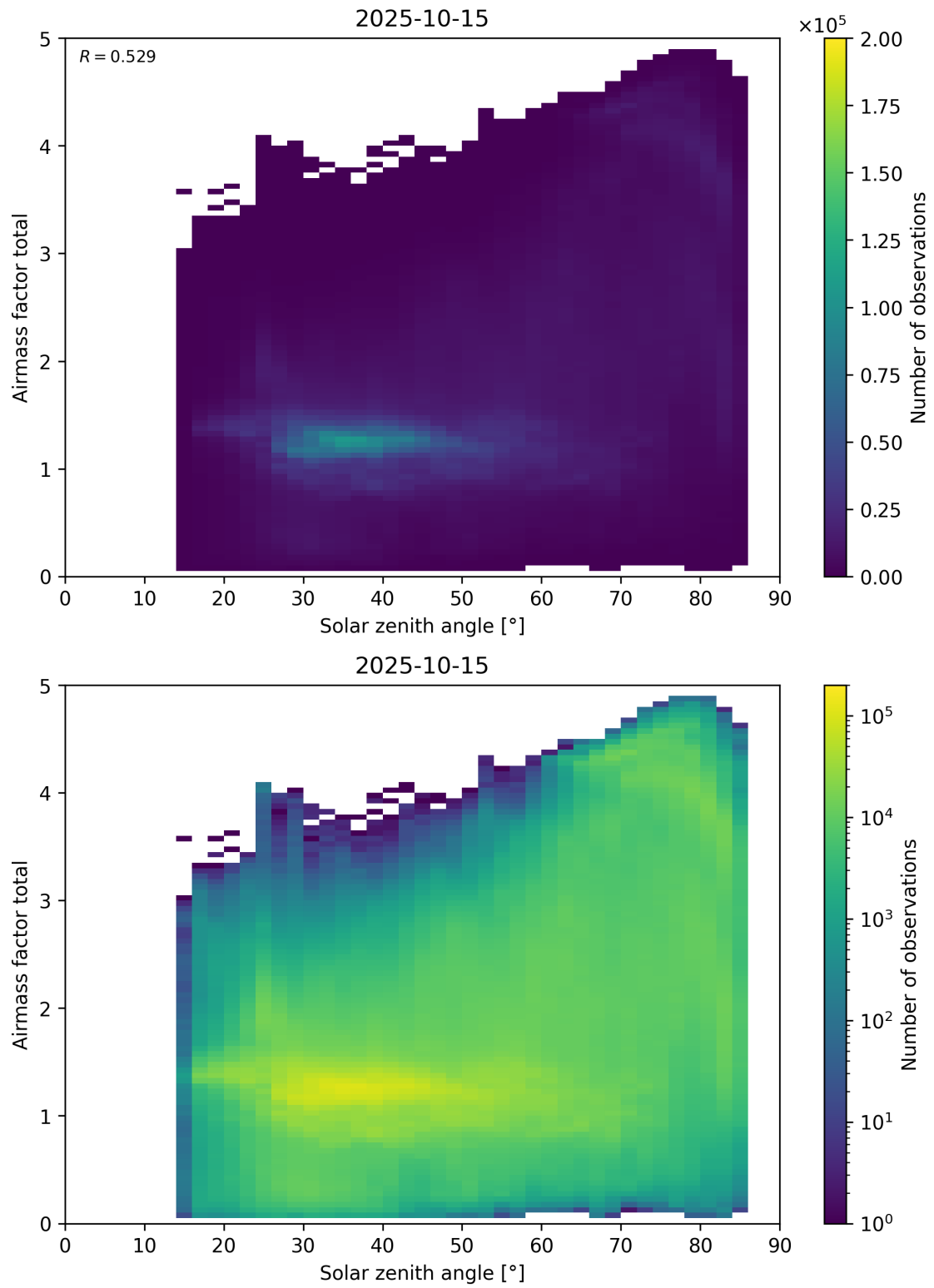
Figure 175: Scatter density plot of “Solar zenith angle” against “Airmass factor total” for 2025-10-14 to 2025-10-16.
