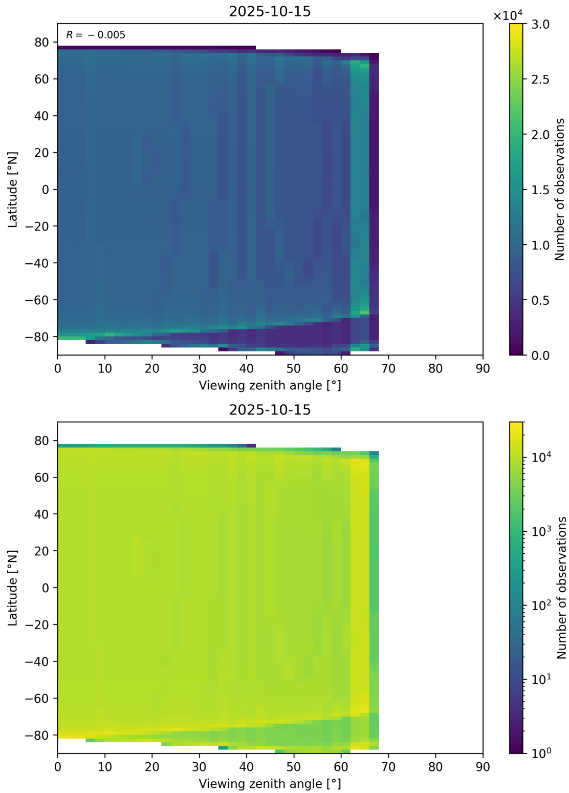
Figure 196: Scatter density plot of “Viewing zenith angle” against “Latitude” for 2025-10-14 to 2025-10-16.
