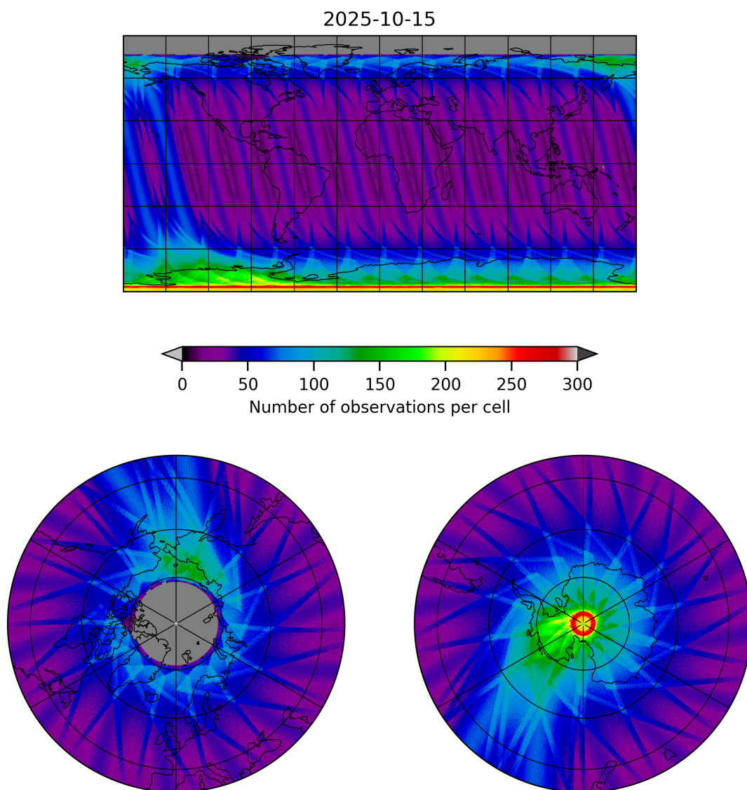
Figure 19: Map of the number of observations for 2025-10-14 to 2025-10-16
