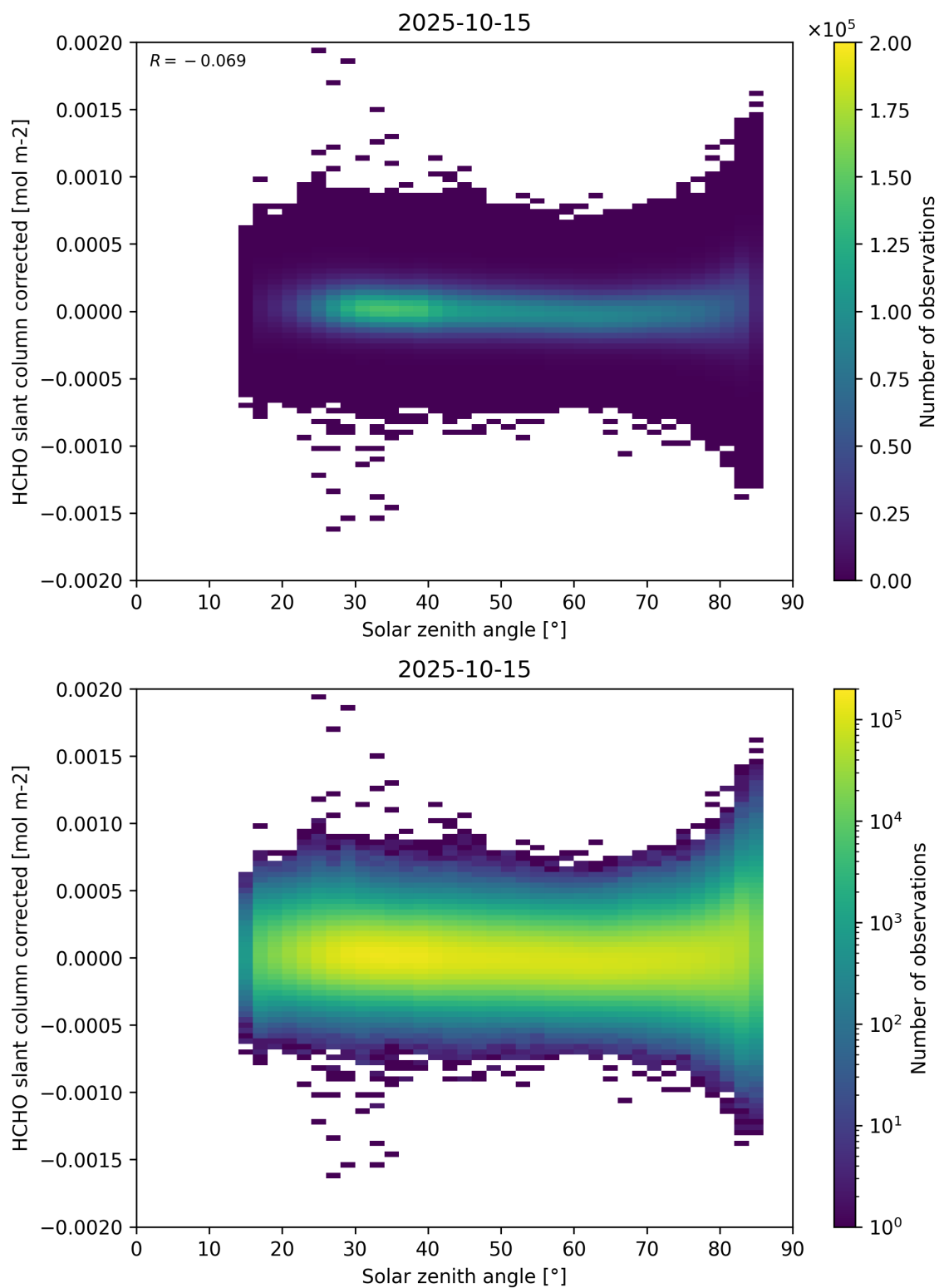
Figure 171: Scatter density plot of “Solar zenith angle” against “HCHO slant column corrected” for 2025-10-14 to 2025-10-16.
