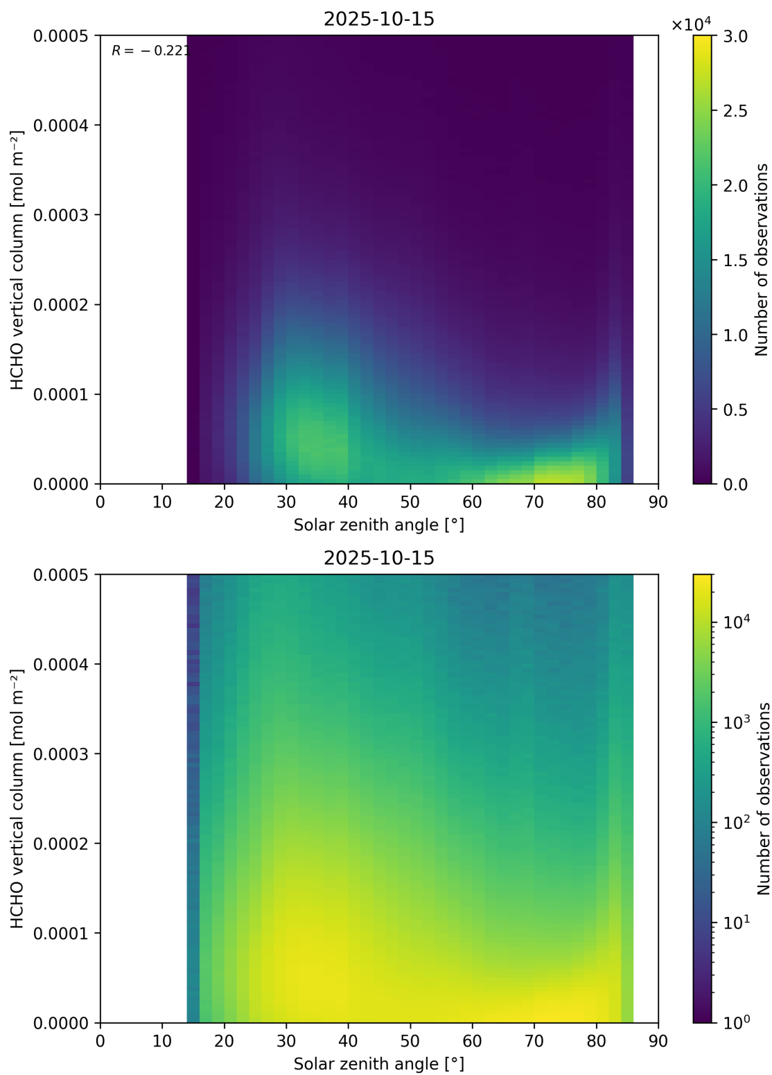
Figure 177: Scatter density plot of “Solar zenith angle” against “HCHO vertical column” for 2025-10-14 to 2025-10-16.
