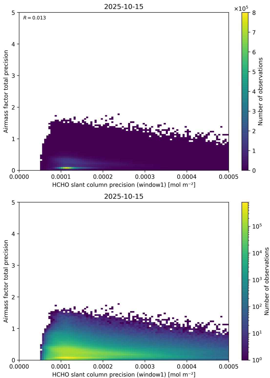
Figure 95: Scatter density plot of “HCHO slant column precision (window1)” against “Airmass factor total precision” for 2025-10-14 to 2025-10-16.
