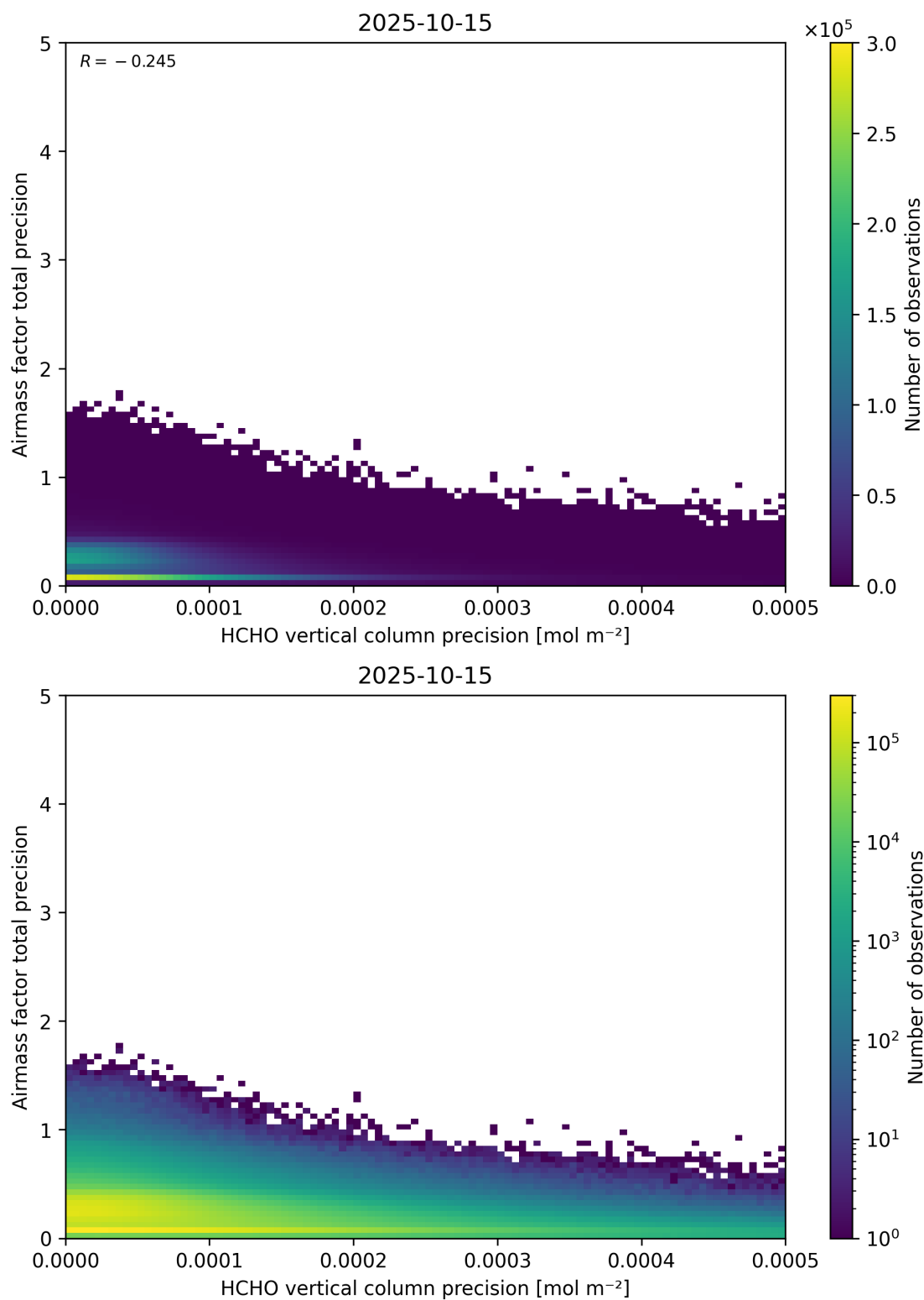
Figure 145: Scatter density plot of “HCHO vertical column precision” against “Airmass factor total precision” for 2025-10-14 to 2025-10-16.
