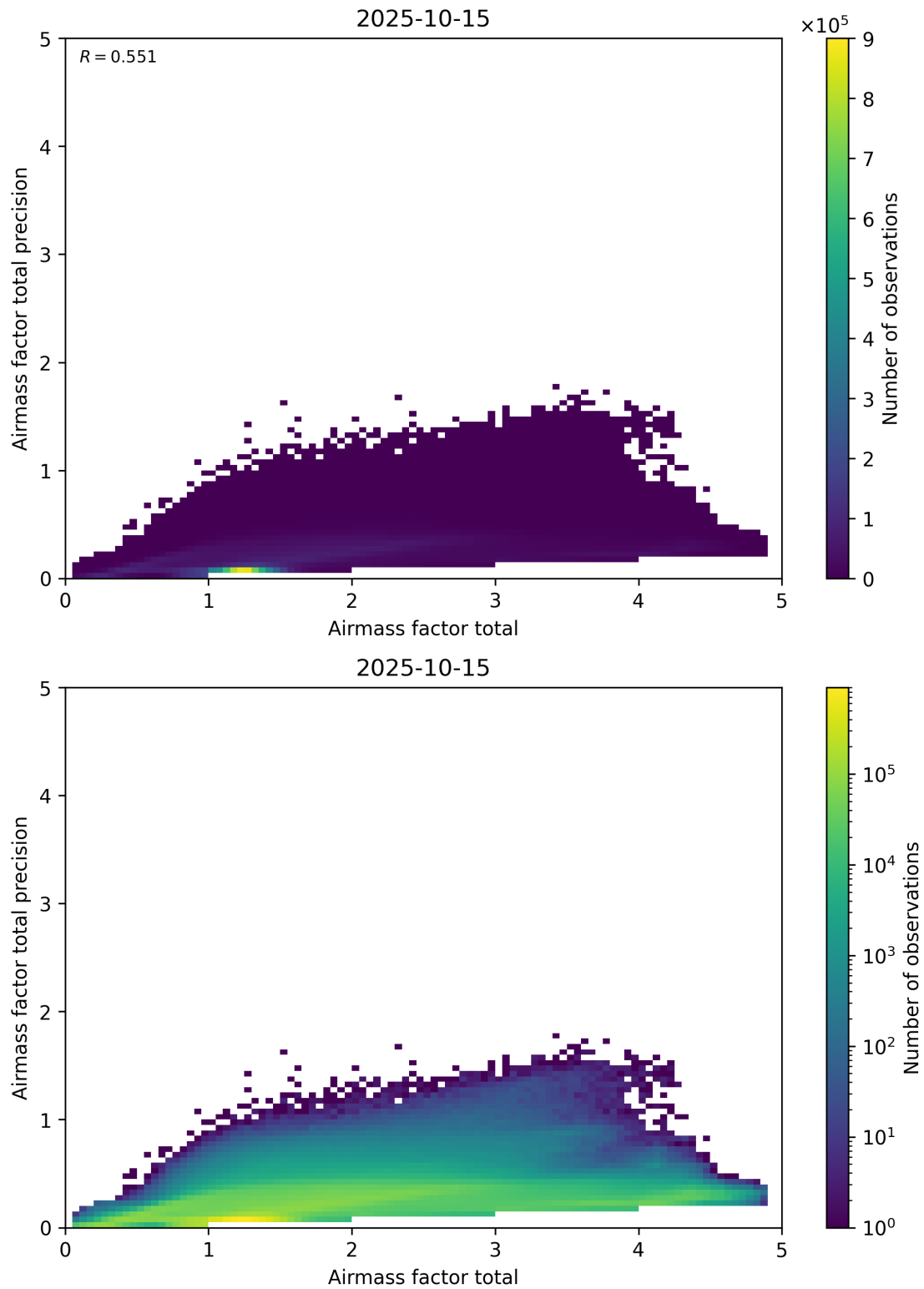
Figure 103: Scatter density plot of “Airmass factor total” against “Airmass factor total precision” for 2025-10-14 to 2025-10-16.
