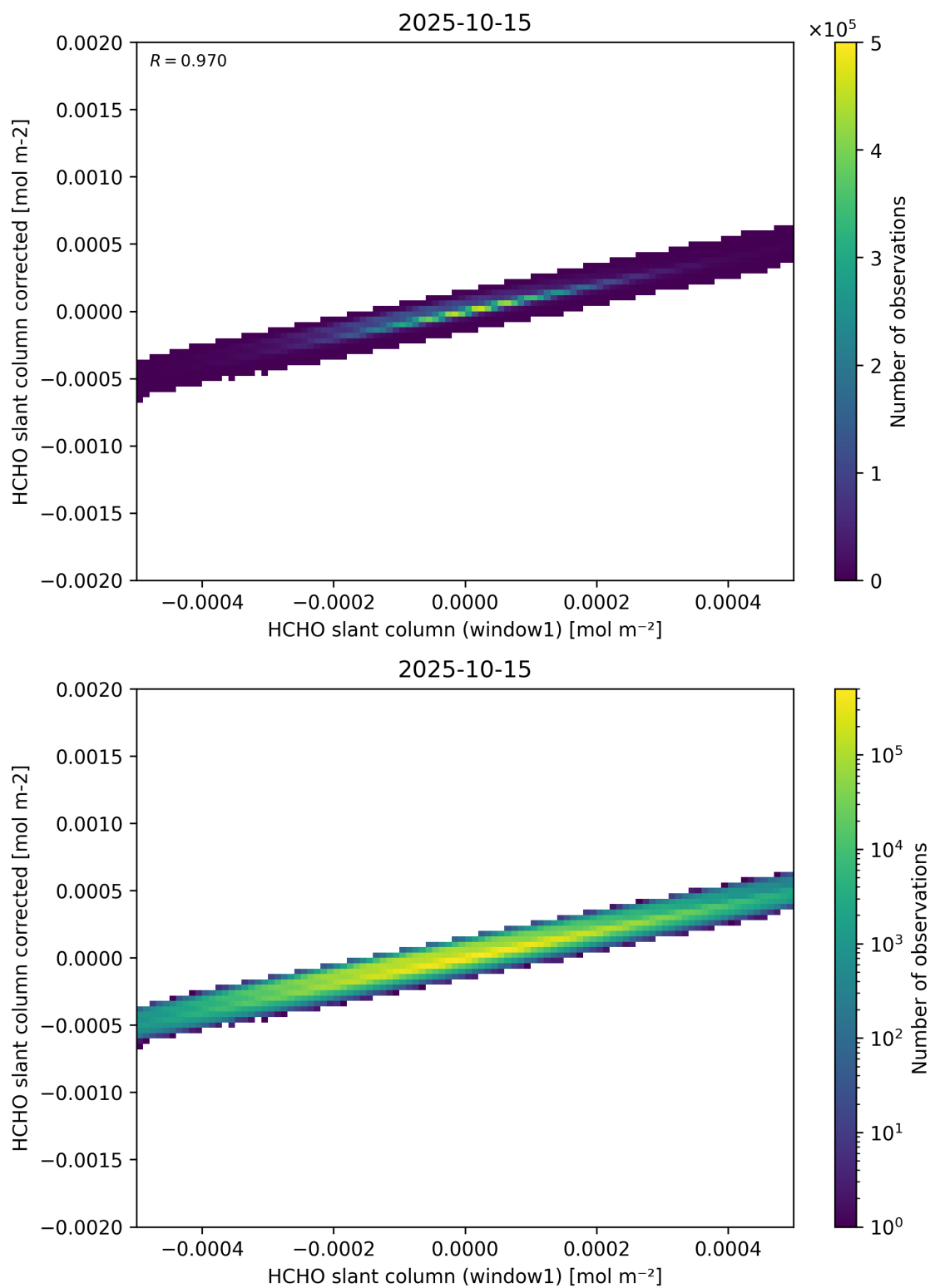
Figure 82: Scatter density plot of “HCHO slant column (window1)” against “HCHO slant column corrected” for 2025-10-14 to 2025-10-16.
