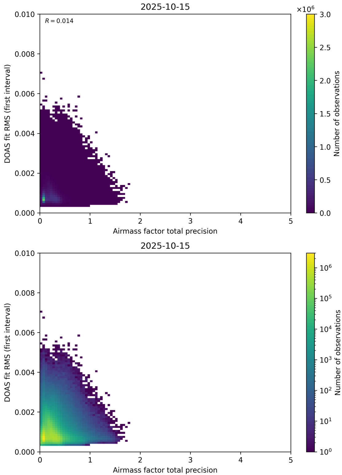
Figure 105: Scatter density plot of “Airmass factor total precision” against “DOAS fit RMS (first interval)” for 2025-10-14 to 2025-10-16.
