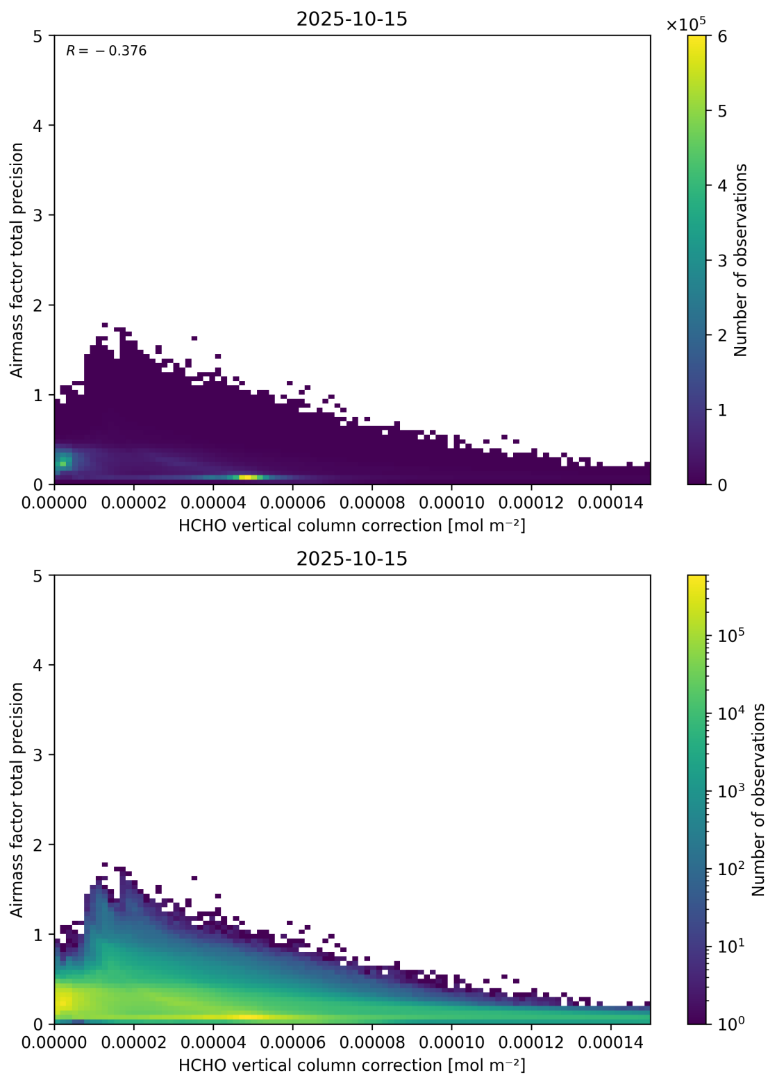
Figure 121: Scatter density plot of “HCHO vertical column correction” against “Airmass factor total precision” for 2025-10-14 to 2025-10-16.
