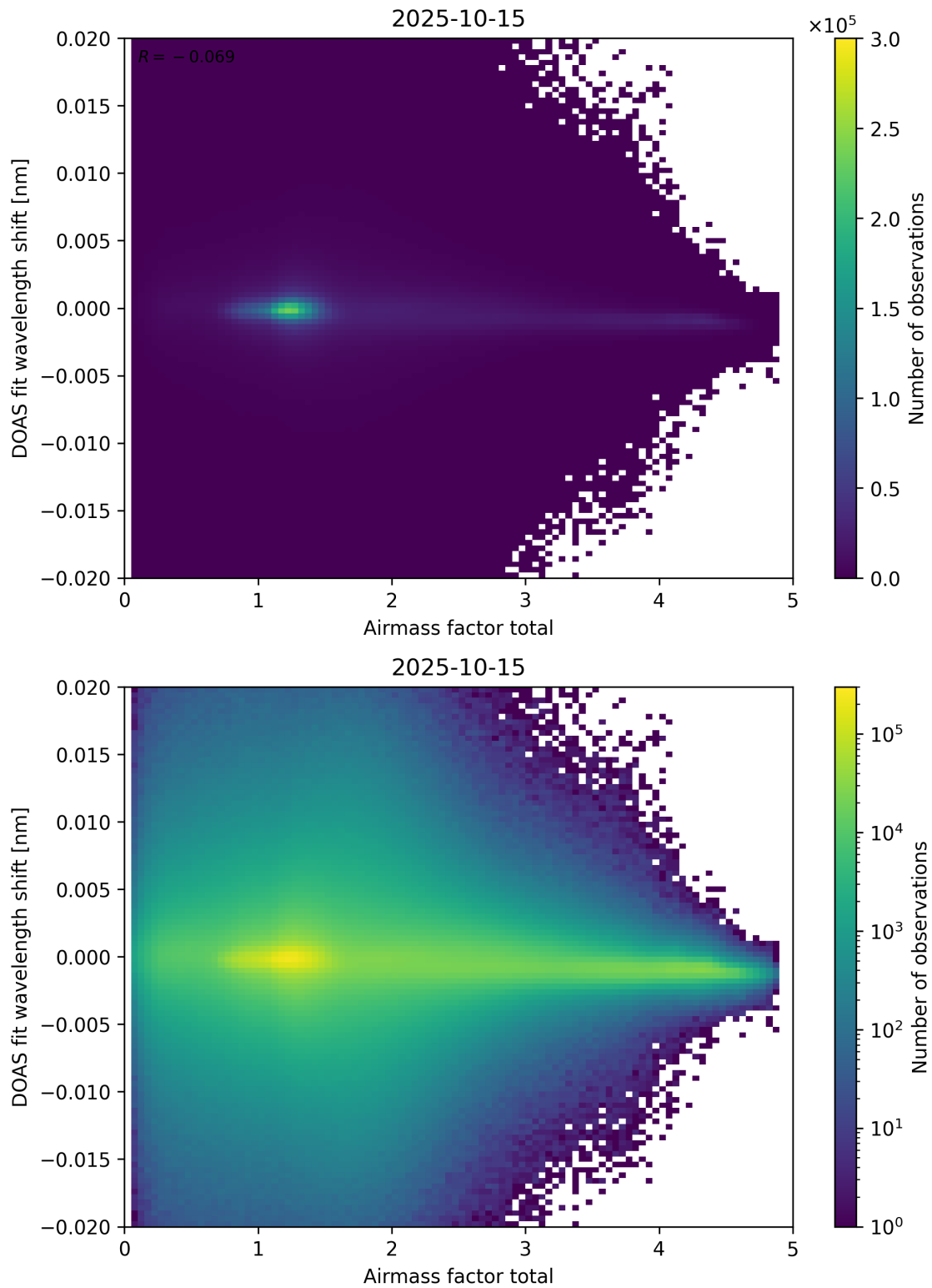
Figure 98: Scatter density plot of “Airmass factor total” against “DOAS fit wavelength shift” for 2025-10-14 to 2025-10-16.
