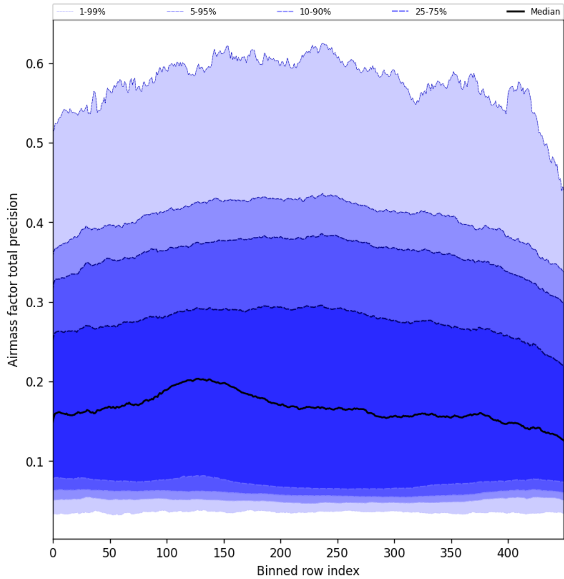
Figure 55: Along track statistics of “Airmass factor total precision” for 2025-10-14 to 2025-10-16
