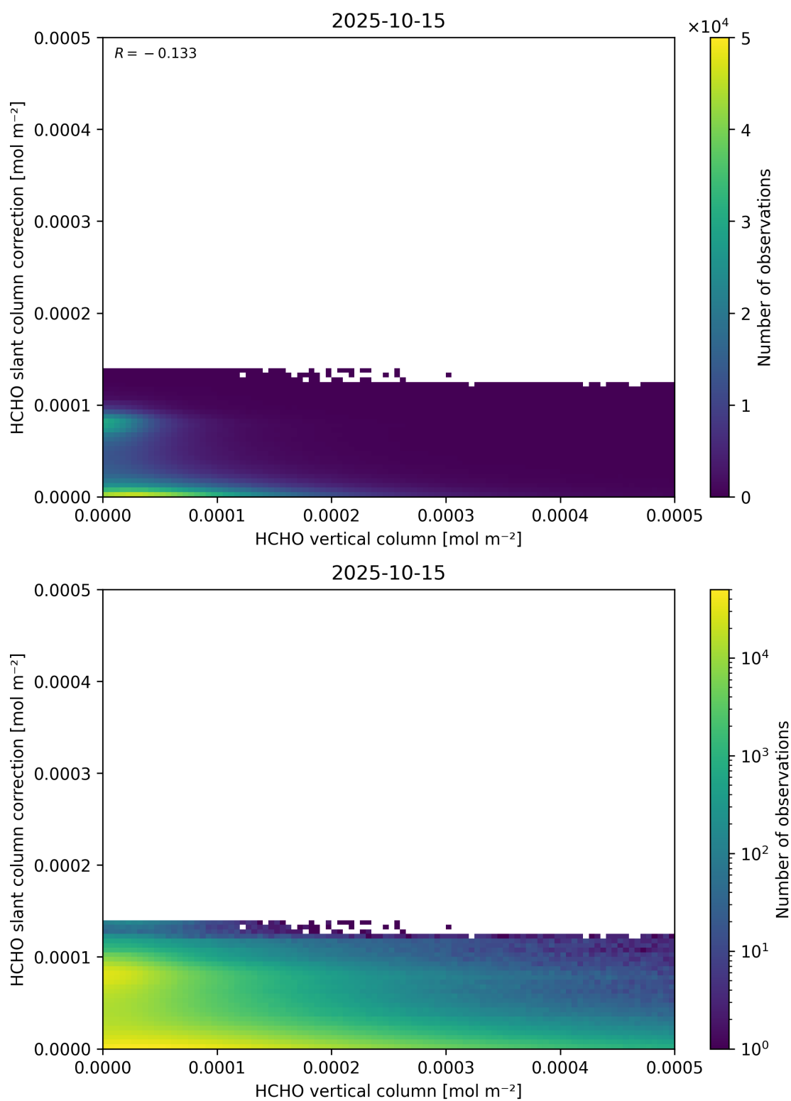
Figure 128: Scatter density plot of “HCHO vertical column” against “HCHO slant column correction” for 2025-10-14 to 2025-10-16.
