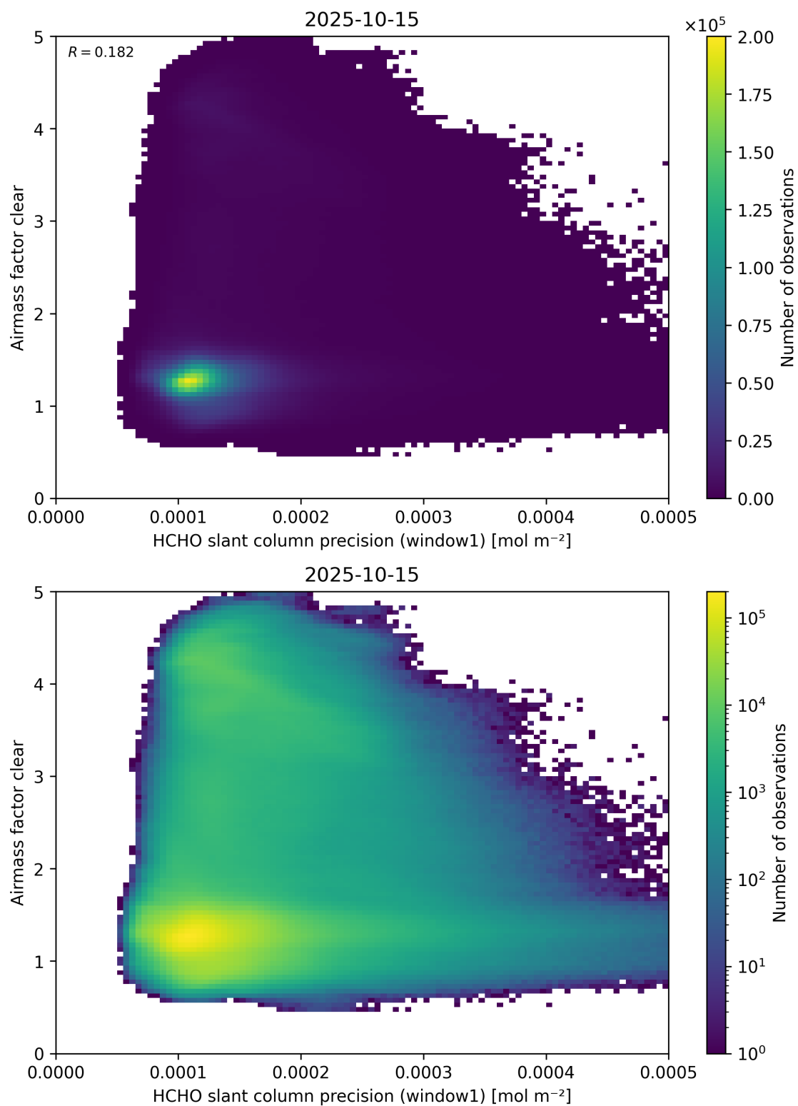
Figure 91: Scatter density plot of “HCHO slant column precision (window1)” against “Airmass factor clear” for 2025-10-14 to 2025-10-16.
