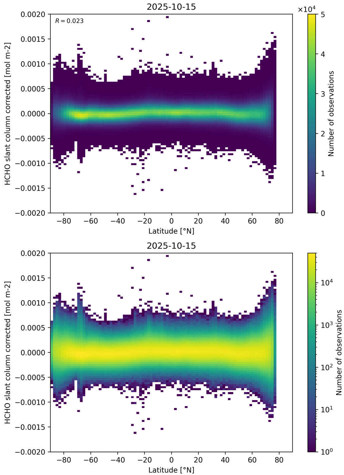
Figure 157: Scatter density plot of “Latitude” against “HCHO slant column corrected” for 2025-10-14 to 2025-10-16.
