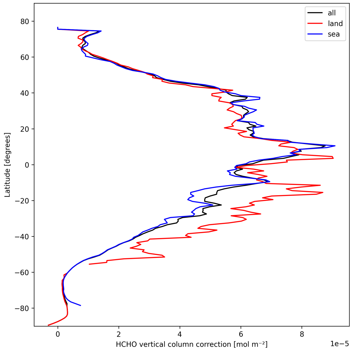
Figure 23: Zonal average of “HCHO vertical column correction” for 2025-10-14 to 2025-10-16.
