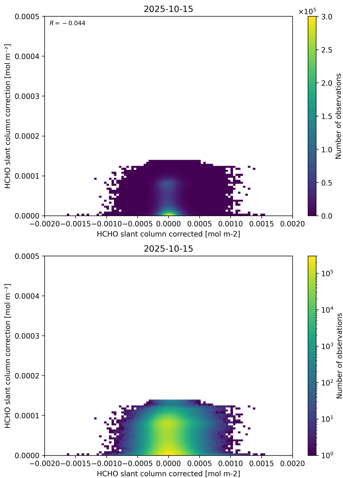
Figure 77: Scatter density plot of “HCHO slant column corrected” against “HCHO slant column correction” for 2025-10-14 to 2025-10-16.
