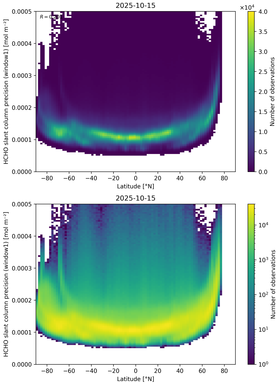
Figure 160: Scatter density plot of “Latitude” against “HCHO slant column precision (window1)” for 2025-10-14 to 2025-10-16.
