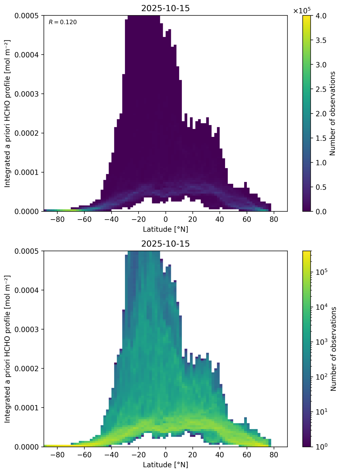
Figure 166: Scatter density plot of “Latitude” against “Integrated a priori HCHO profile” for 2025-10-14 to 2025-10-16.
