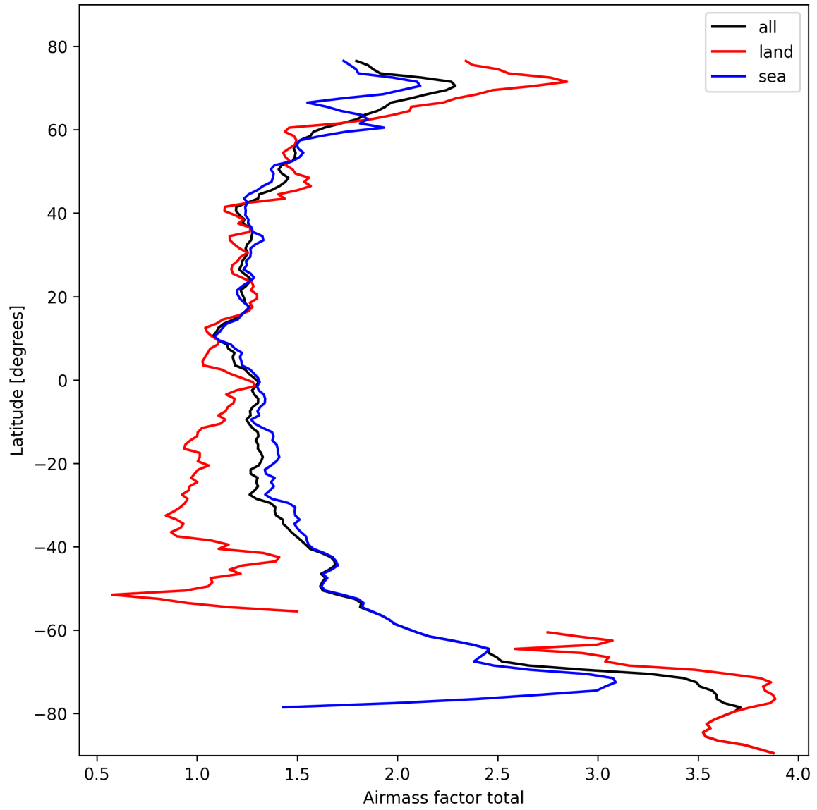
Figure 26: Zonal average of “Airmass factor total” for 2025-10-14 to 2025-10-16.
