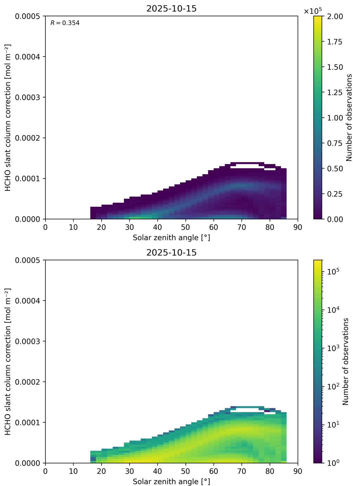
Figure 172: Scatter density plot of “Solar zenith angle” against “HCHO slant column correction” for 2025-10-14 to 2025-10-16.
