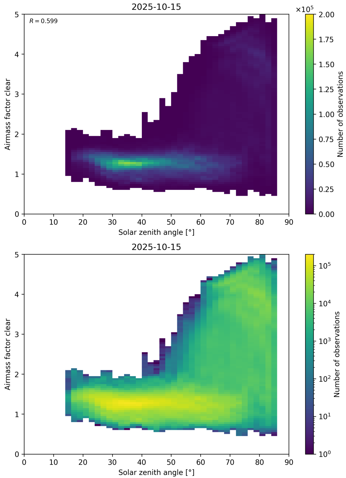
Figure 170: Scatter density plot of “Solar zenith angle” against “Airmass factor clear” for 2025-10-14 to 2025-10-16.
