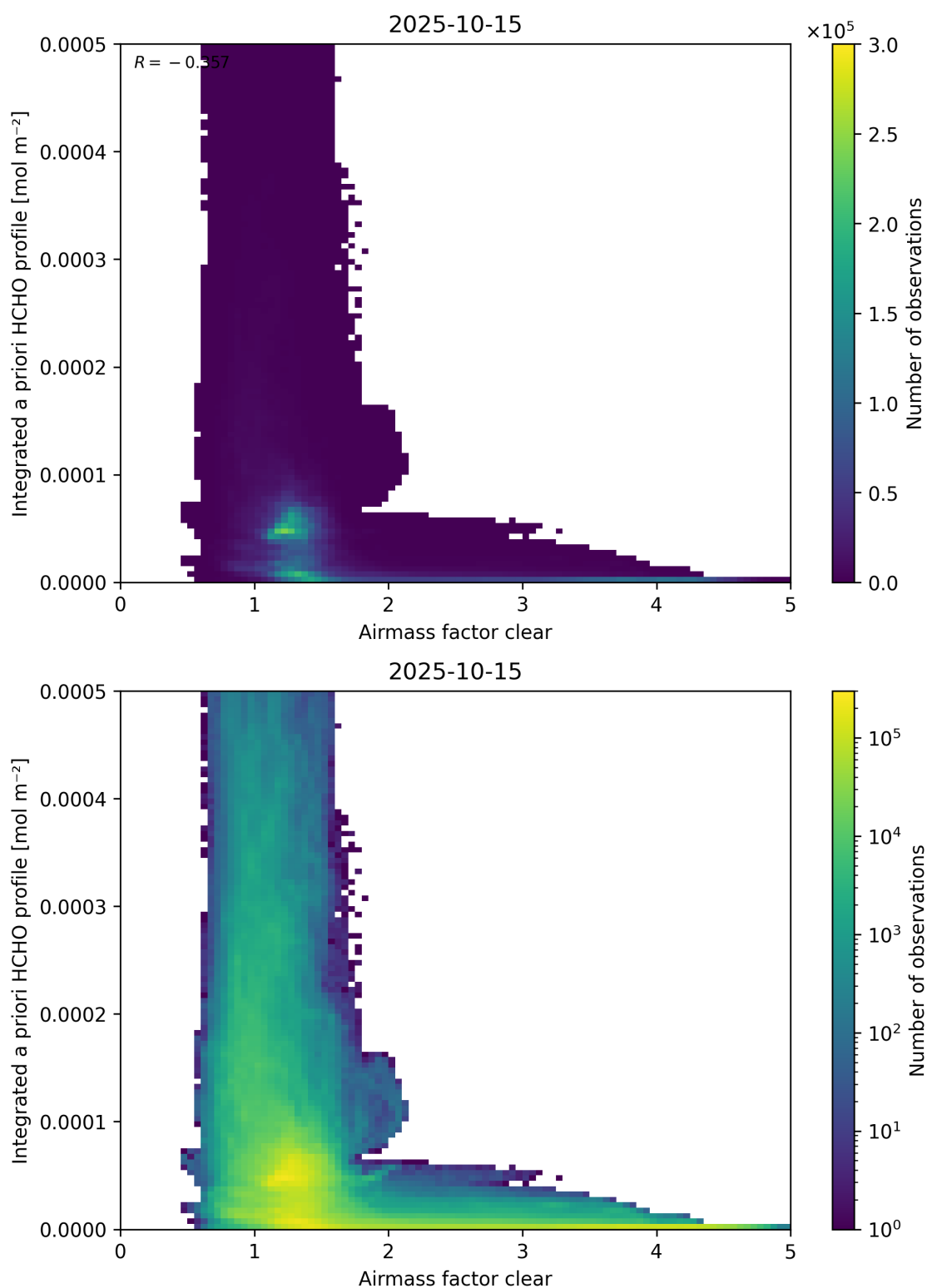
Figure 76: Scatter density plot of “Airmass factor clear” against “Integrated a priori HCHO profile” for 2025-10-14 to 2025-10-16.
