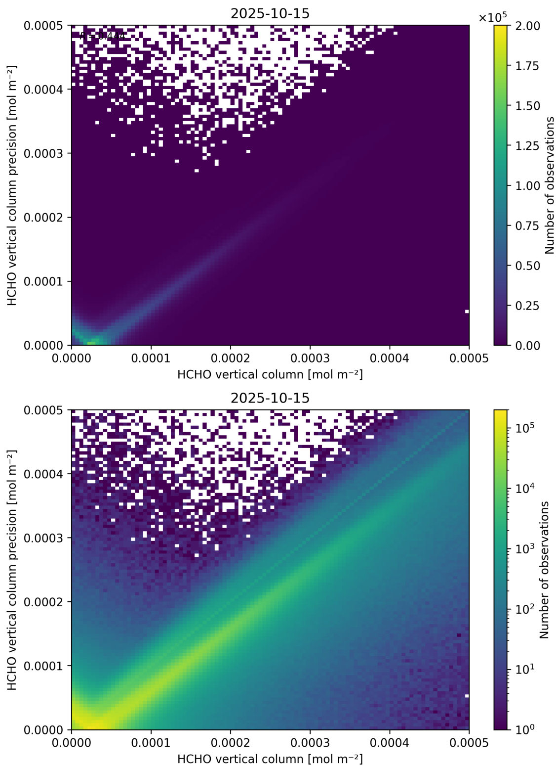
Figure 134: Scatter density plot of “HCHO vertical column” against “HCHO vertical column precision” for 2025-10-14 to 2025-10-16.
