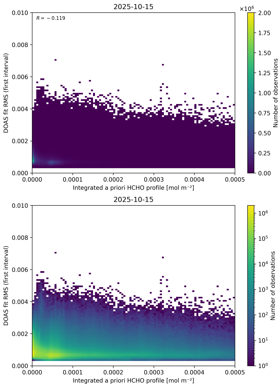
Figure 148: Scatter density plot of “Integrated a priori HCHO profile” against “DOAS fit RMS (first interval)” for 2025-10-14 to 2025-10-16.
