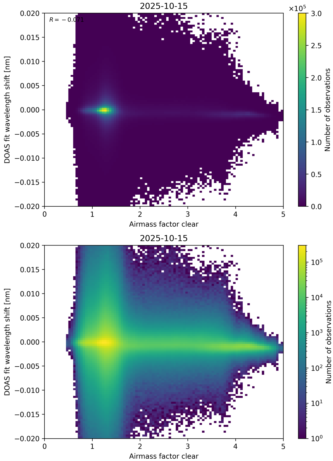
Figure 72: Scatter density plot of “Airmass factor clear” against “DOAS fit wavelength shift” for 2025-10-14 to 2025-10-16.
