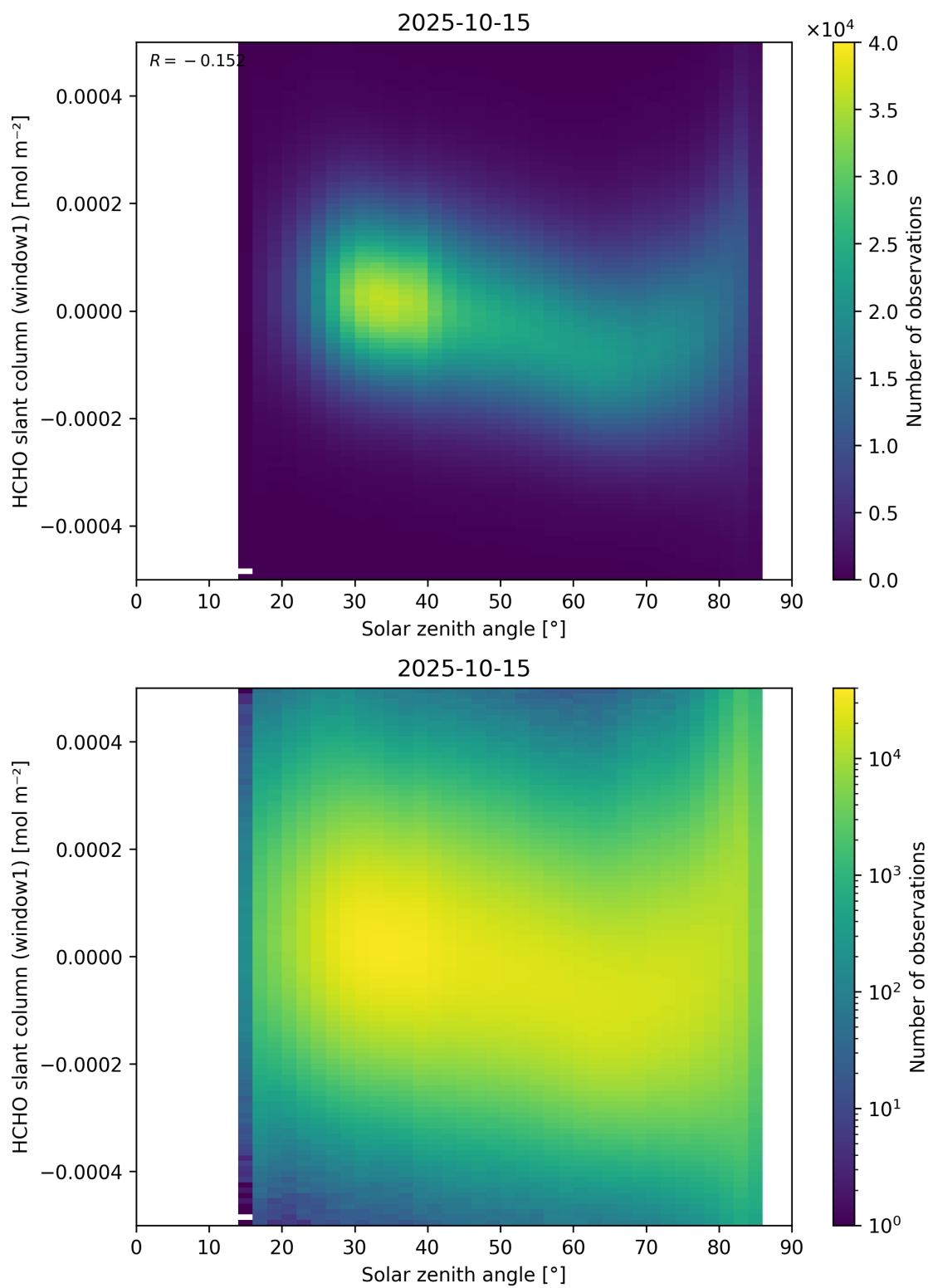
Figure 173: Scatter density plot of “Solar zenith angle” against “HCHO slant column (window1)” for 2025-10-14 to 2025-10-16.
