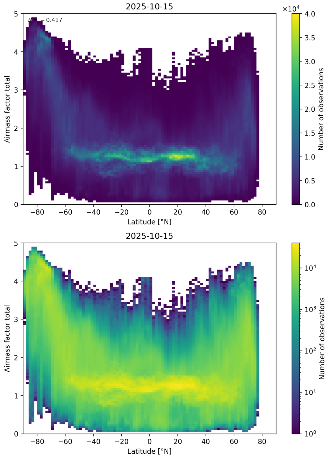
Figure 161: Scatter density plot of “Latitude” against “Airmass factor total” for 2025-10-14 to 2025-10-16.
