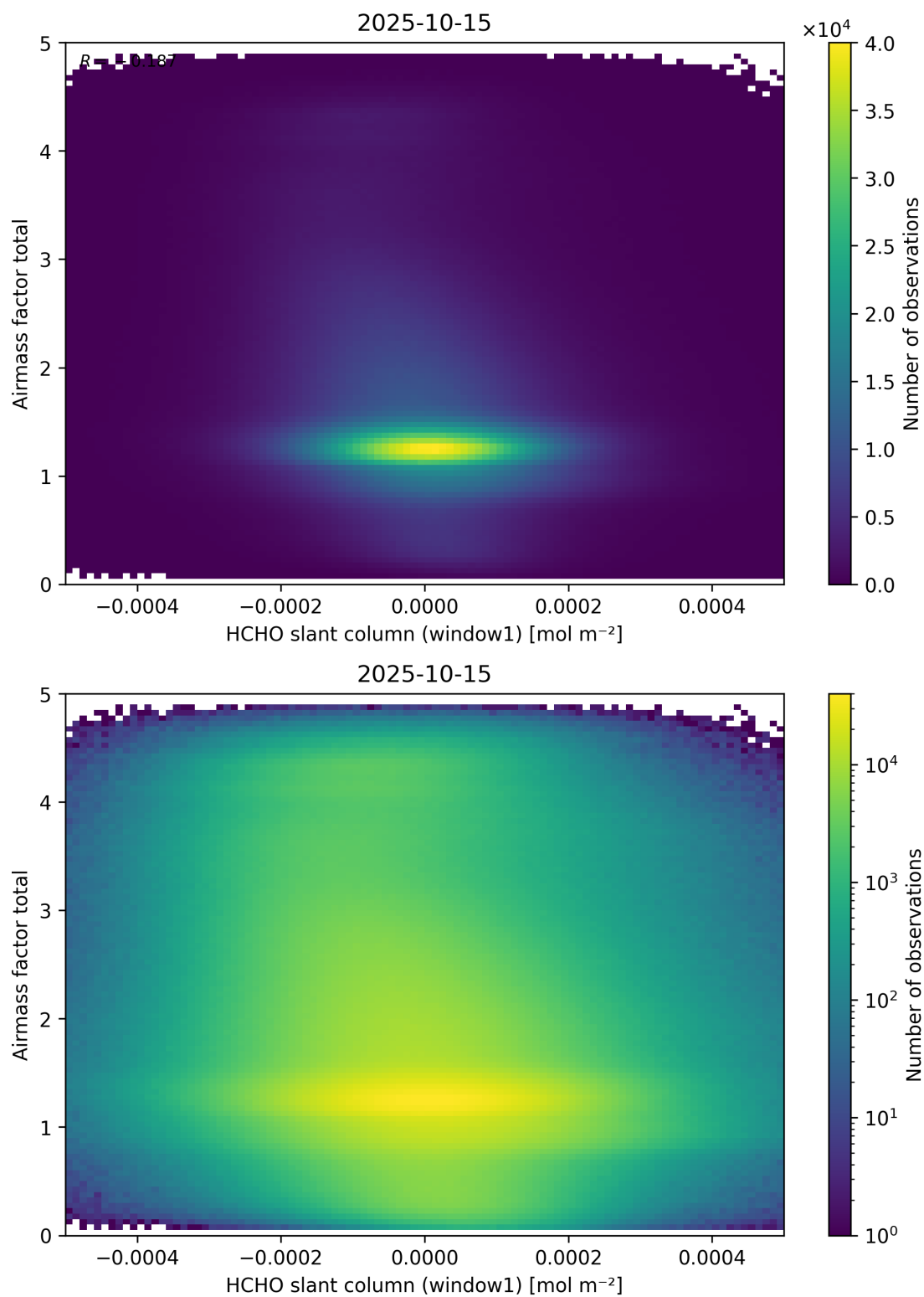
Figure 85: Scatter density plot of “HCHO slant column (window1)” against “Airmass factor total” for 2025-10-14 to 2025-10-16.
