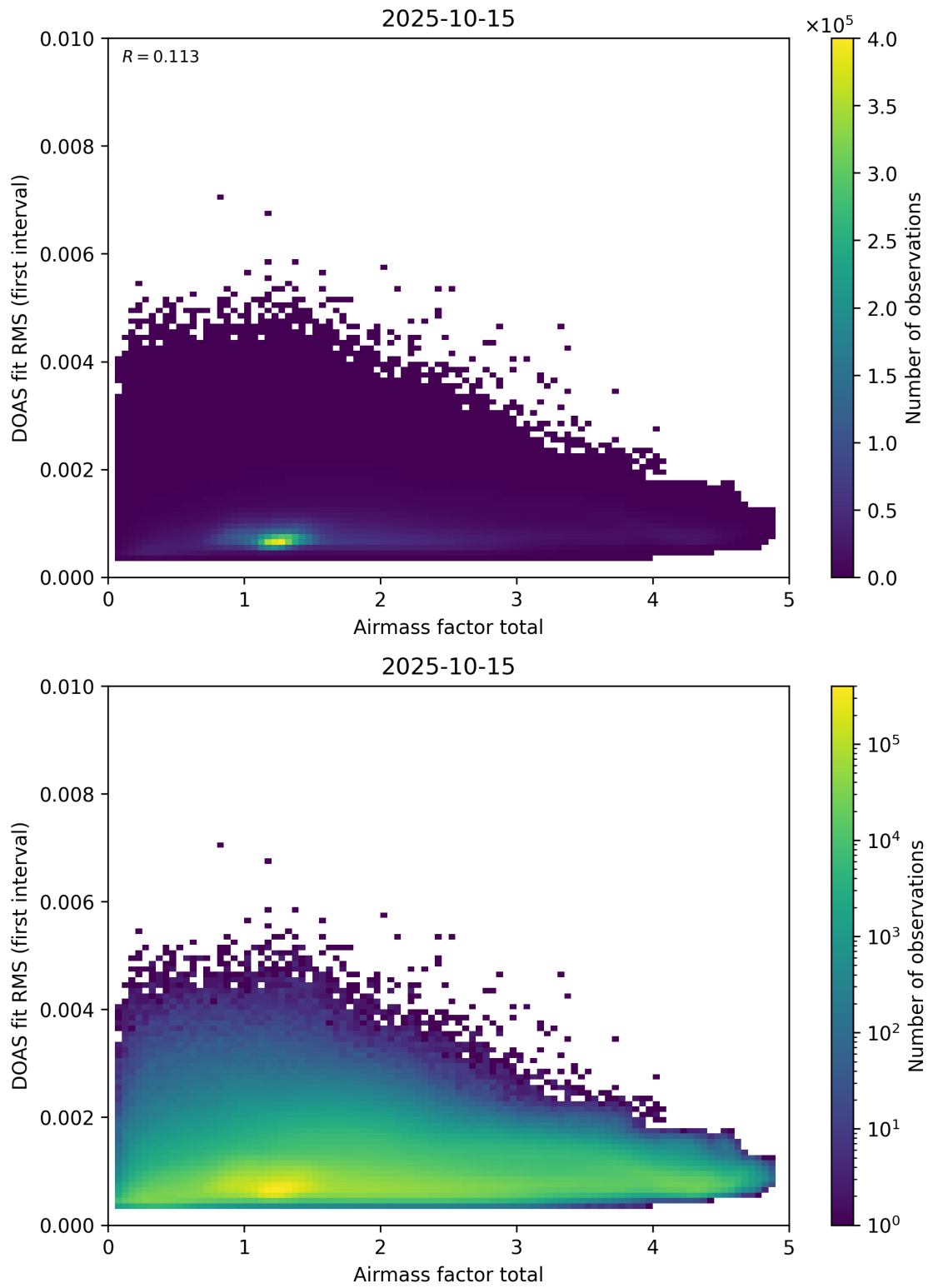
Figure 97: Scatter density plot of “Airmass factor total” against “DOAS fit RMS (first interval)” for 2025-10-14 to 2025-10-16.
