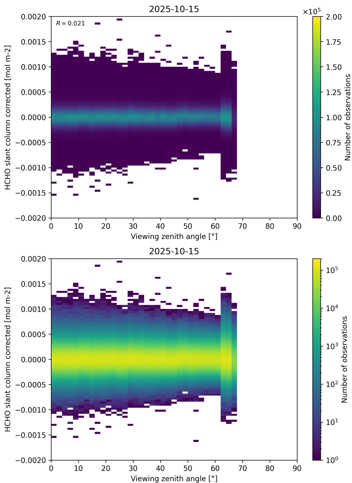
Figure 186: Scatter density plot of “Viewing zenith angle” against “HCHO slant column corrected” for 2025-10-14 to 2025-10-16.
