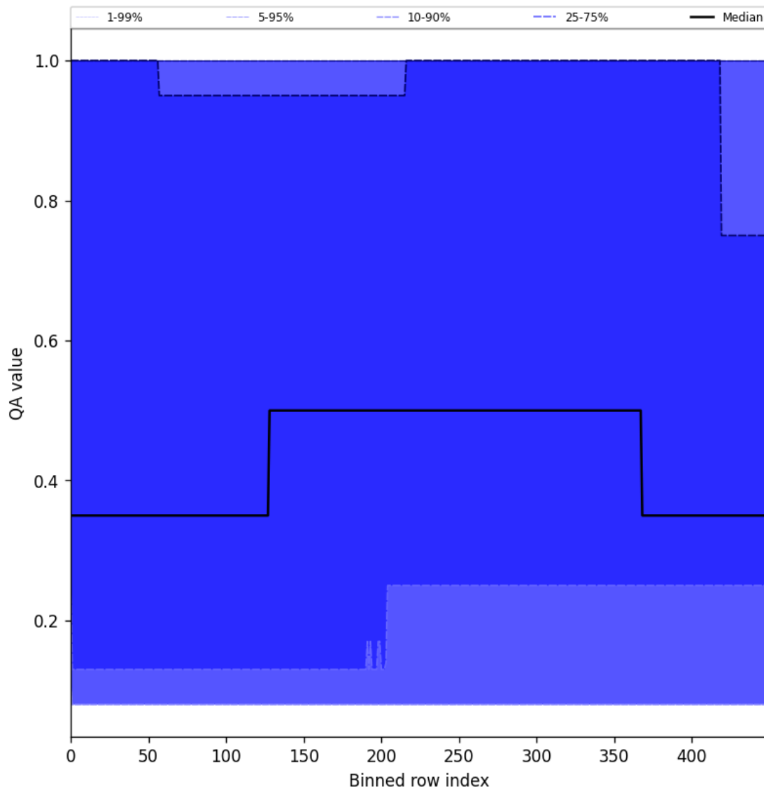
Figure 48: Along track statistics of “QA value” for 2025-10-14 to 2025-10-16
