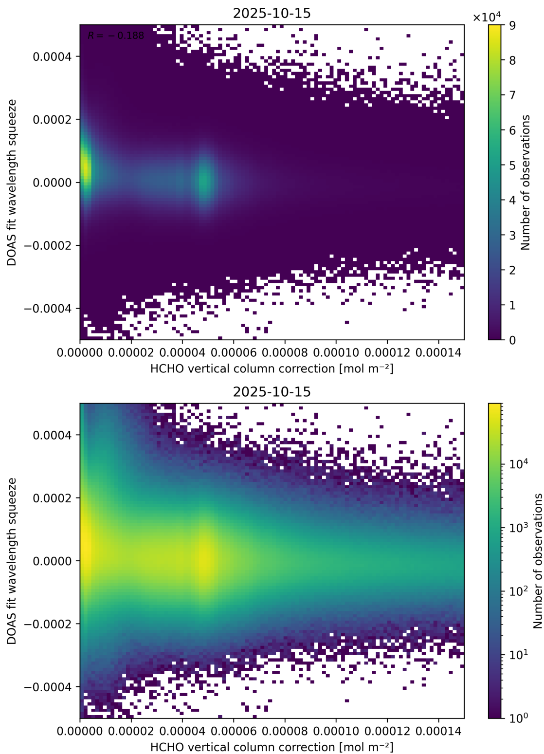
Figure 114: Scatter density plot of “HCHO vertical column correction” against “DOAS fit wavelength squeeze” for 2025-10-14 to 2025-10-16.
