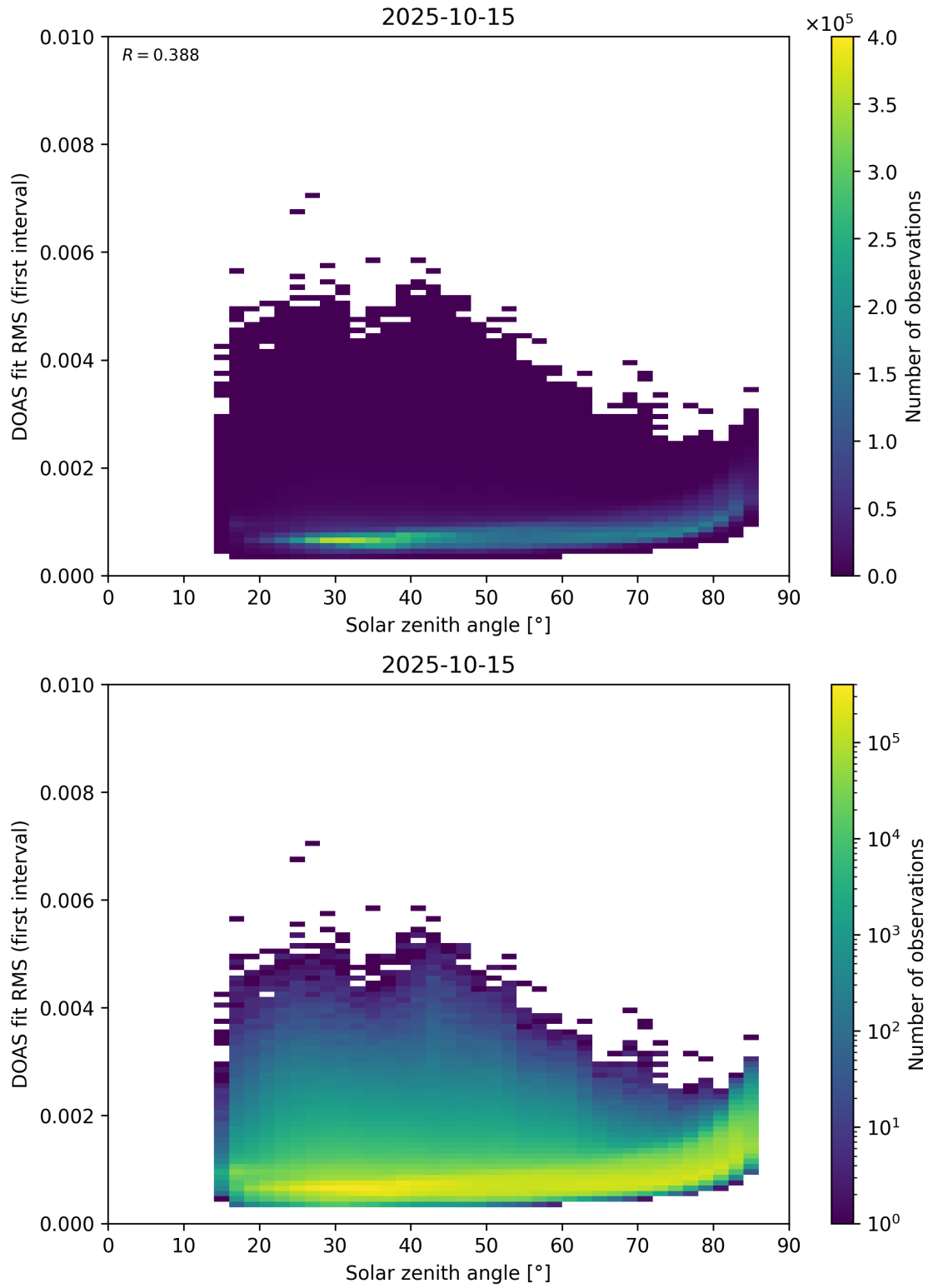
Figure 167: Scatter density plot of “Solar zenith angle” against “DOAS fit RMS (first interval)” for 2025-10-14 to 2025-10-16.
