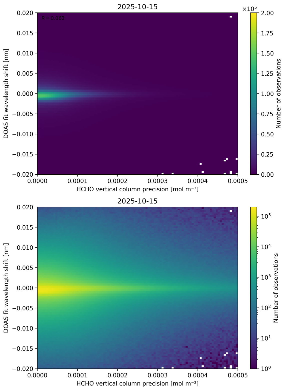
Figure 137: Scatter density plot of “HCHO vertical column precision” against “DOAS fit wavelength shift” for 2025-10-14 to 2025-10-16.
