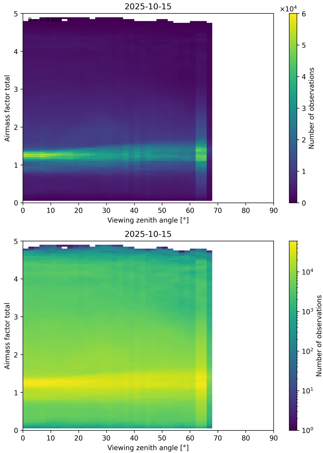
Figure 190: Scatter density plot of “Viewing zenith angle” against “Airmass factor total” for 2025-10-14 to 2025-10-16.
