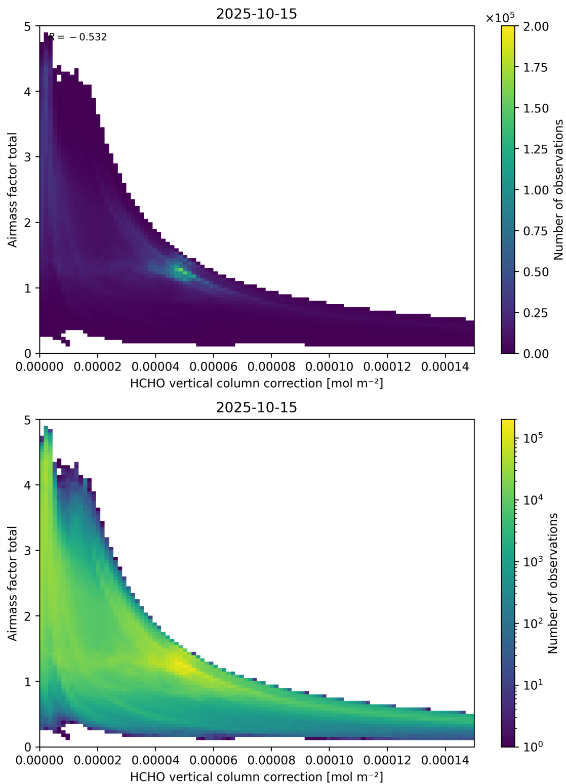
Figure 120: Scatter density plot of “HCHO vertical column correction” against “Airmass factor total” for 2025-10-14 to 2025-10-16.
