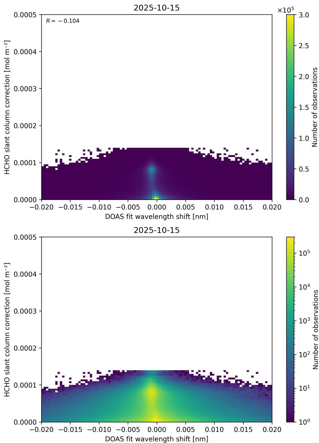
Figure 67: Scatter density plot of “DOAS fit wavelength shift” against “HCHO slant column correction” for 2025-10-14 to 2025-10-16.
