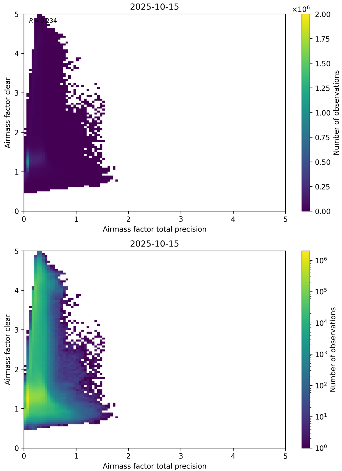
Figure 108: Scatter density plot of “Airmass factor total precision” against “Airmass factor clear” for 2025-10-14 to 2025-10-16.
