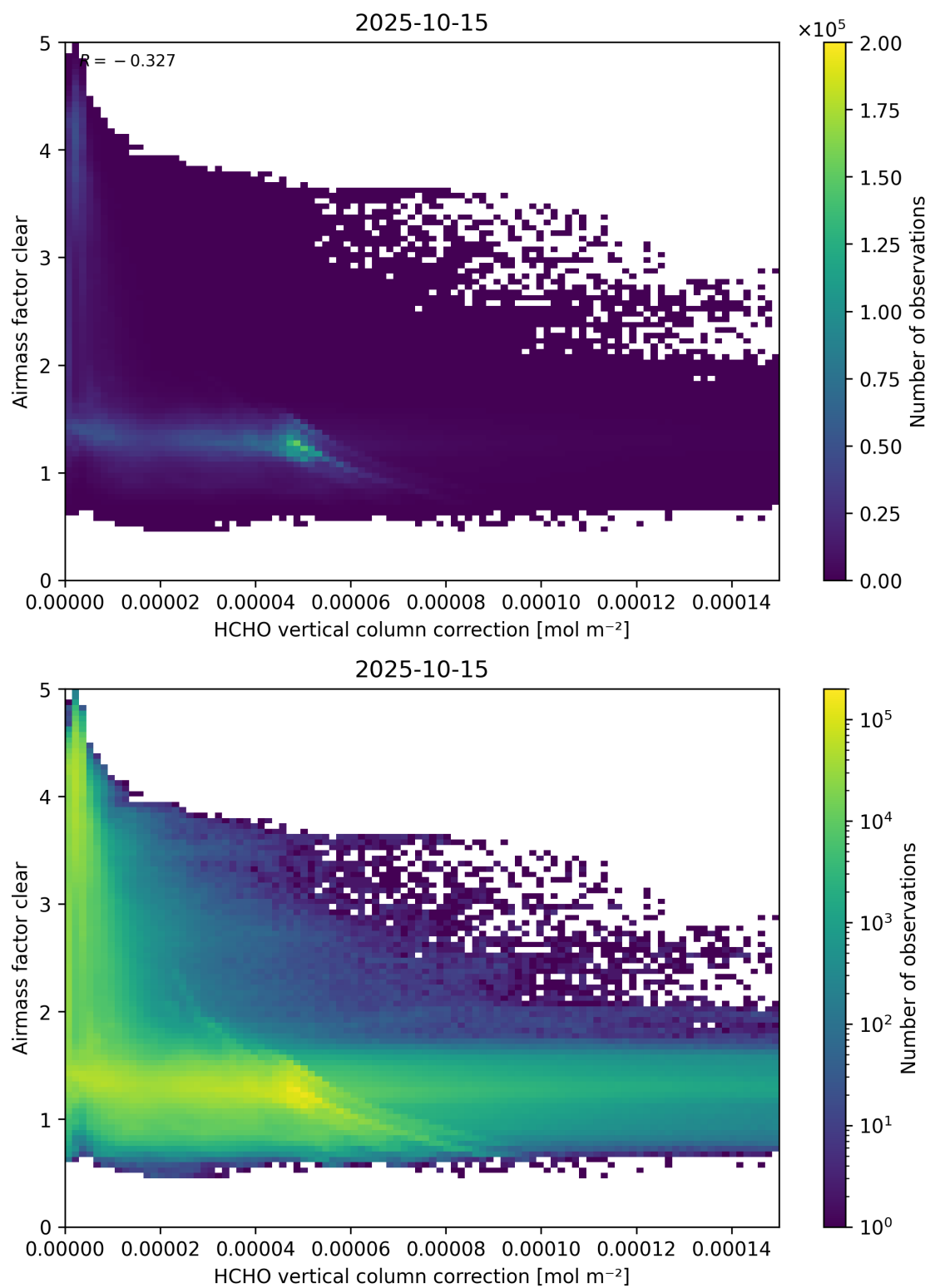
Figure 115: Scatter density plot of “HCHO vertical column correction” against “Airmass factor clear” for 2025-10-14 to 2025-10-16.
