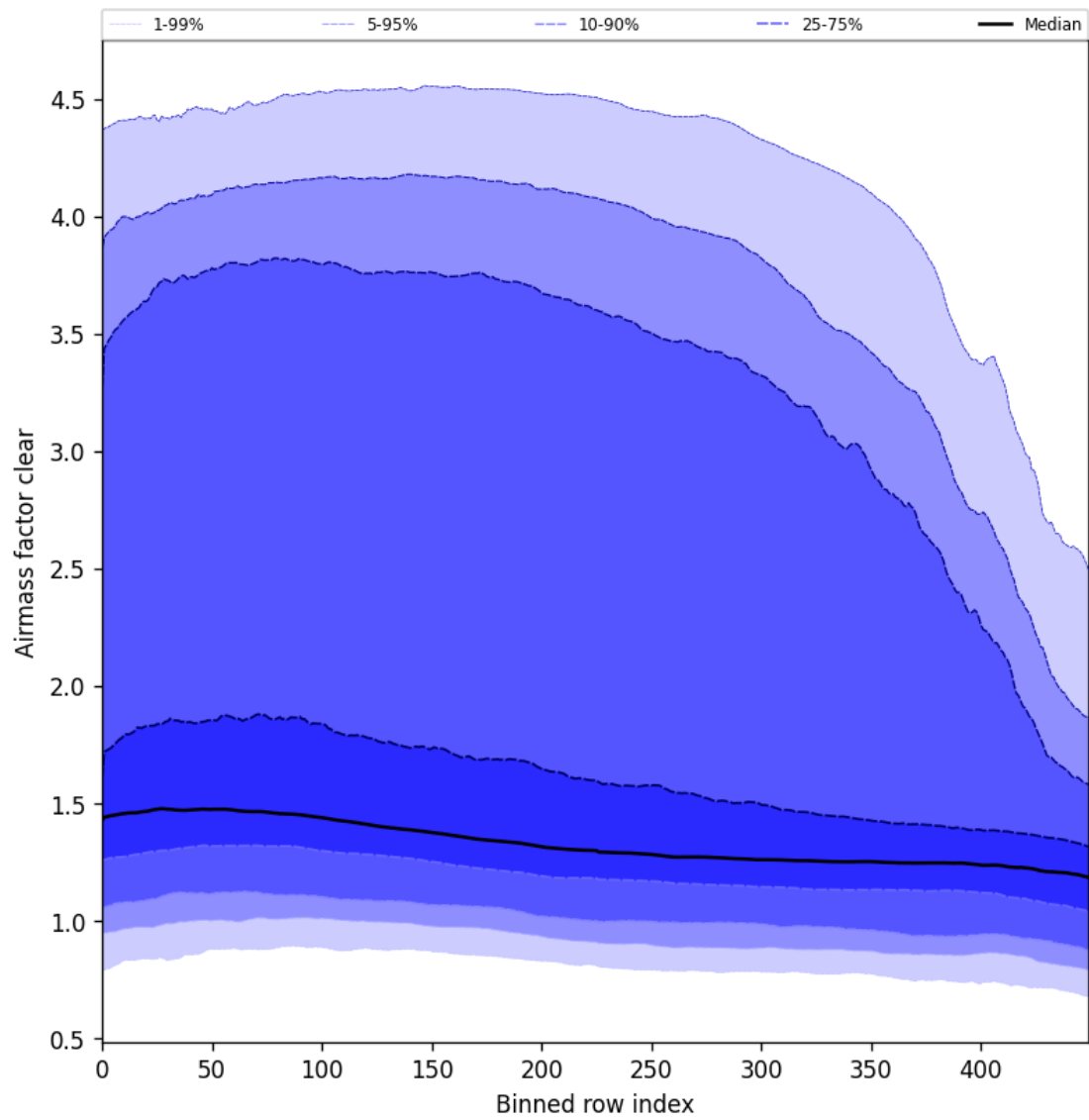
Figure 56: Along track statistics of “Airmass factor clear” for 2025-10-14 to 2025-10-16
