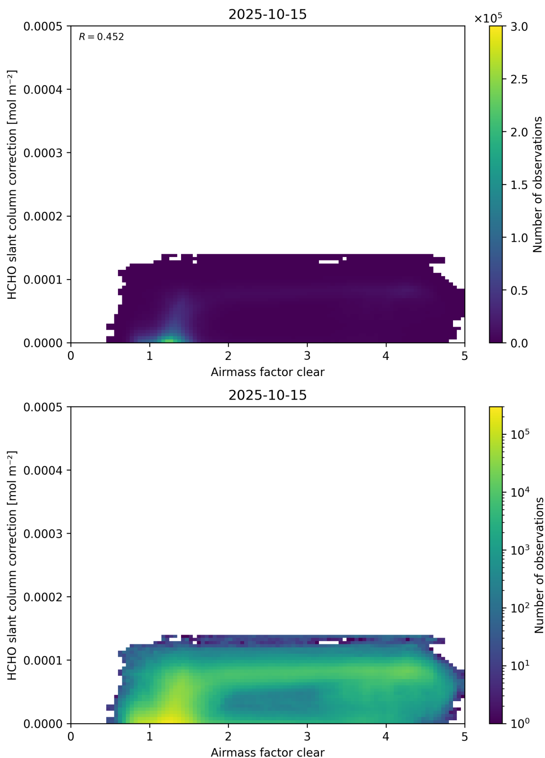
Figure 75: Scatter density plot of “Airmass factor clear” against “HCHO slant column correction” for 2025-10-14 to 2025-10-16.
