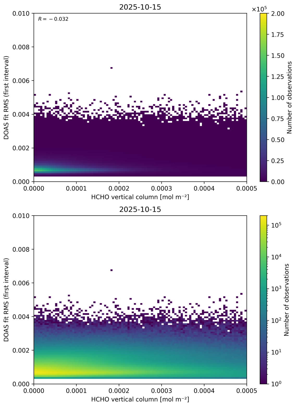
Figure 123: Scatter density plot of “HCHO vertical column” against “DOAS fit RMS (first interval)” for 2025-10-14 to 2025-10-16.
