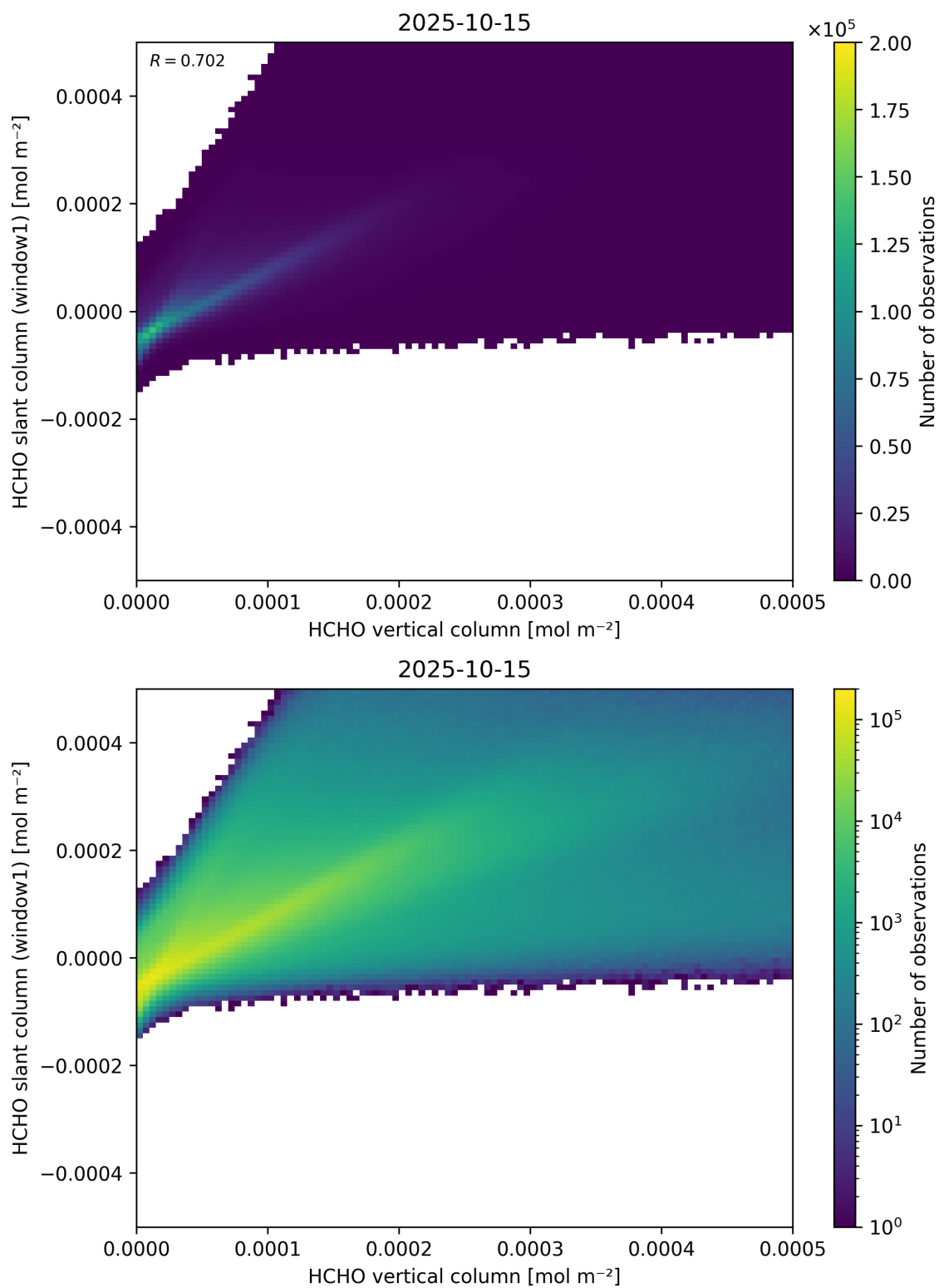
Figure 129: Scatter density plot of “HCHO vertical column” against “HCHO slant column (window1)” for 2025-10-14 to 2025-10-16.
