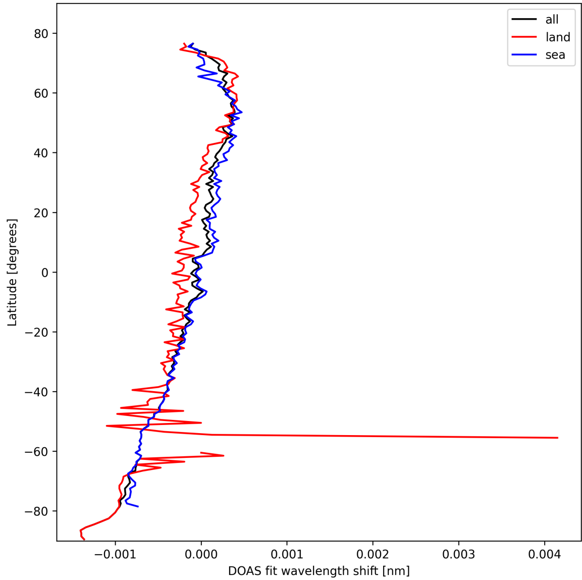
Figure 30: Zonal average of “DOAS fit wavelength shift” for 2025-10-14 to 2025-10-16.
