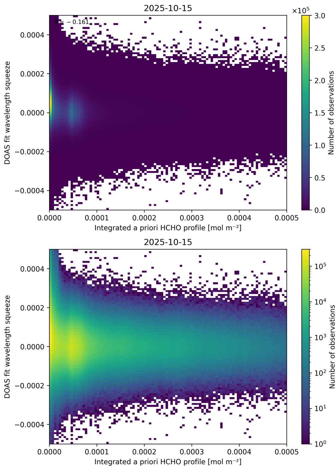
Figure 150: Scatter density plot of “Integrated a priori HCHO profile” against “DOAS fit wavelength squeeze” for 2025-10-14 to 2025-10-16.
