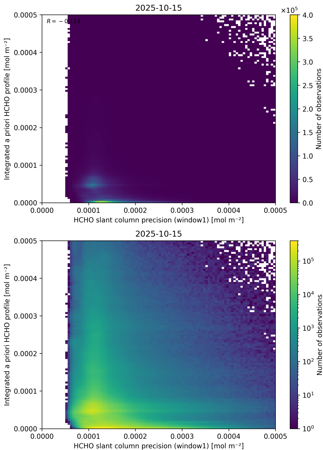
Figure 96: Scatter density plot of “HCHO slant column precision (window1)” against “Integrated a priori HCHO profile” for 2025-10-14 to 2025-10-16.
