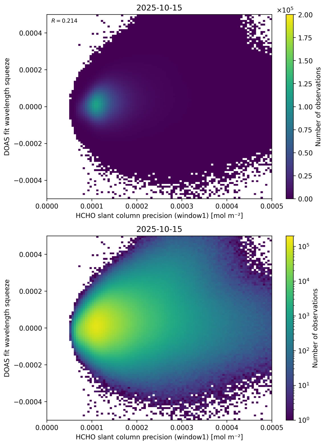
Figure 90: Scatter density plot of “HCHO slant column precision (window1)” against “DOAS fit wavelength squeeze” for 2025-10-14 to 2025-10-16.
