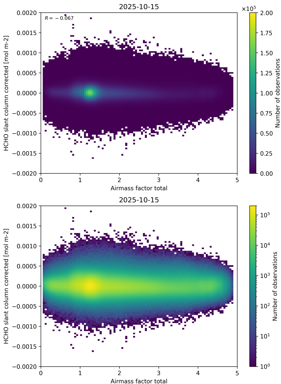
Figure 101: Scatter density plot of “Airmass factor total” against “HCHO slant column corrected” for 2025-10-14 to 2025-10-16.
