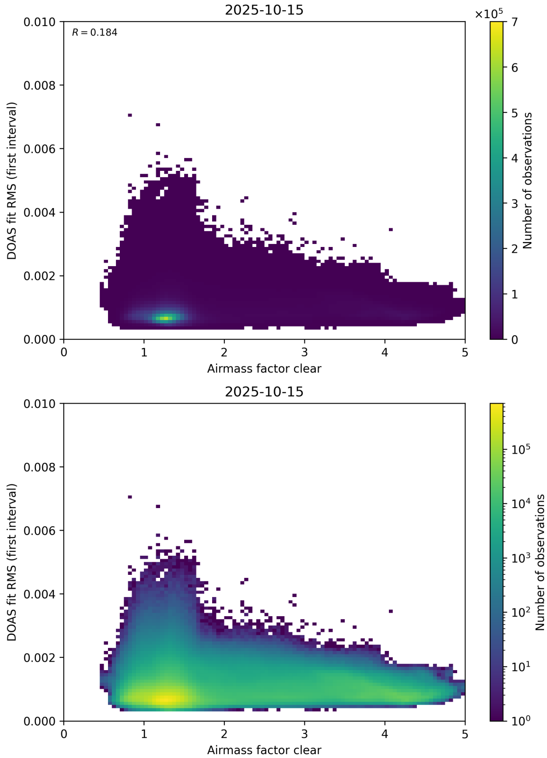
Figure 71: Scatter density plot of “Airmass factor clear” against “DOAS fit RMS (first interval)” for 2025-10-14 to 2025-10-16.
