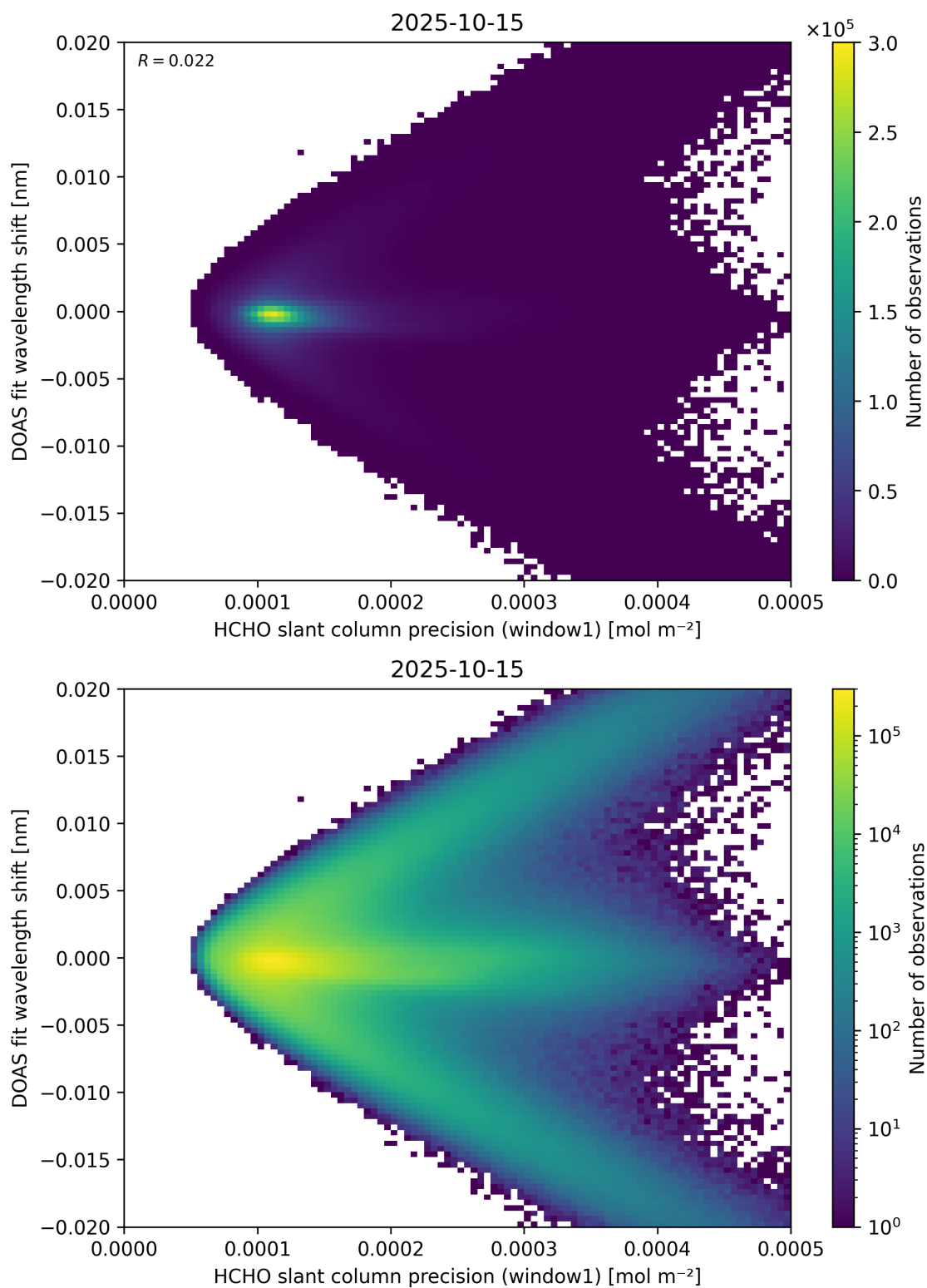
Figure 89: Scatter density plot of “HCHO slant column precision (window1)” against “DOAS fit wavelength shift” for 2025-10-14 to 2025-10-16.
