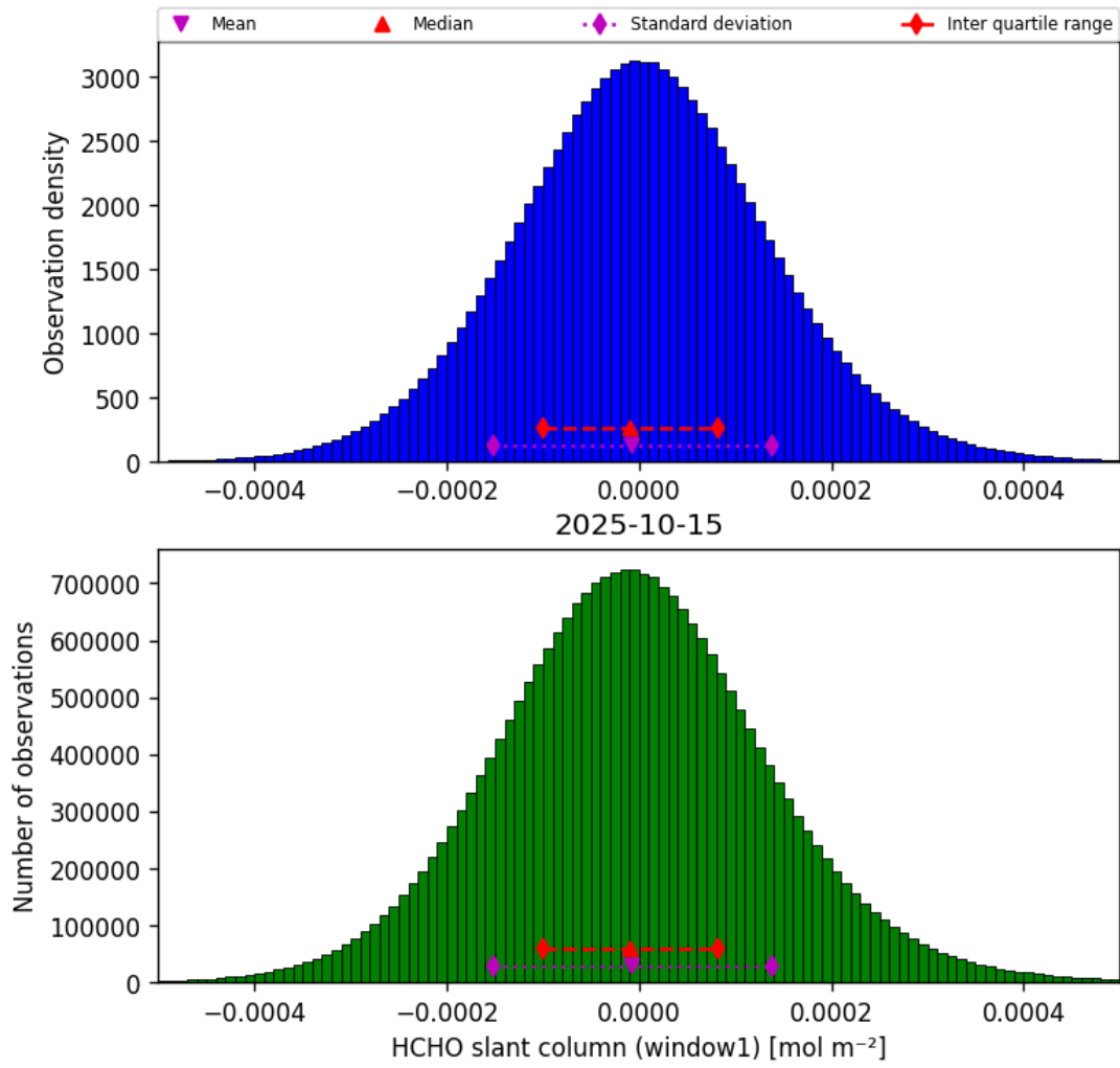
Figure 38: Histogram of “HCHO slant column (window1)” for 2025-10-14 to 2025-10-16
