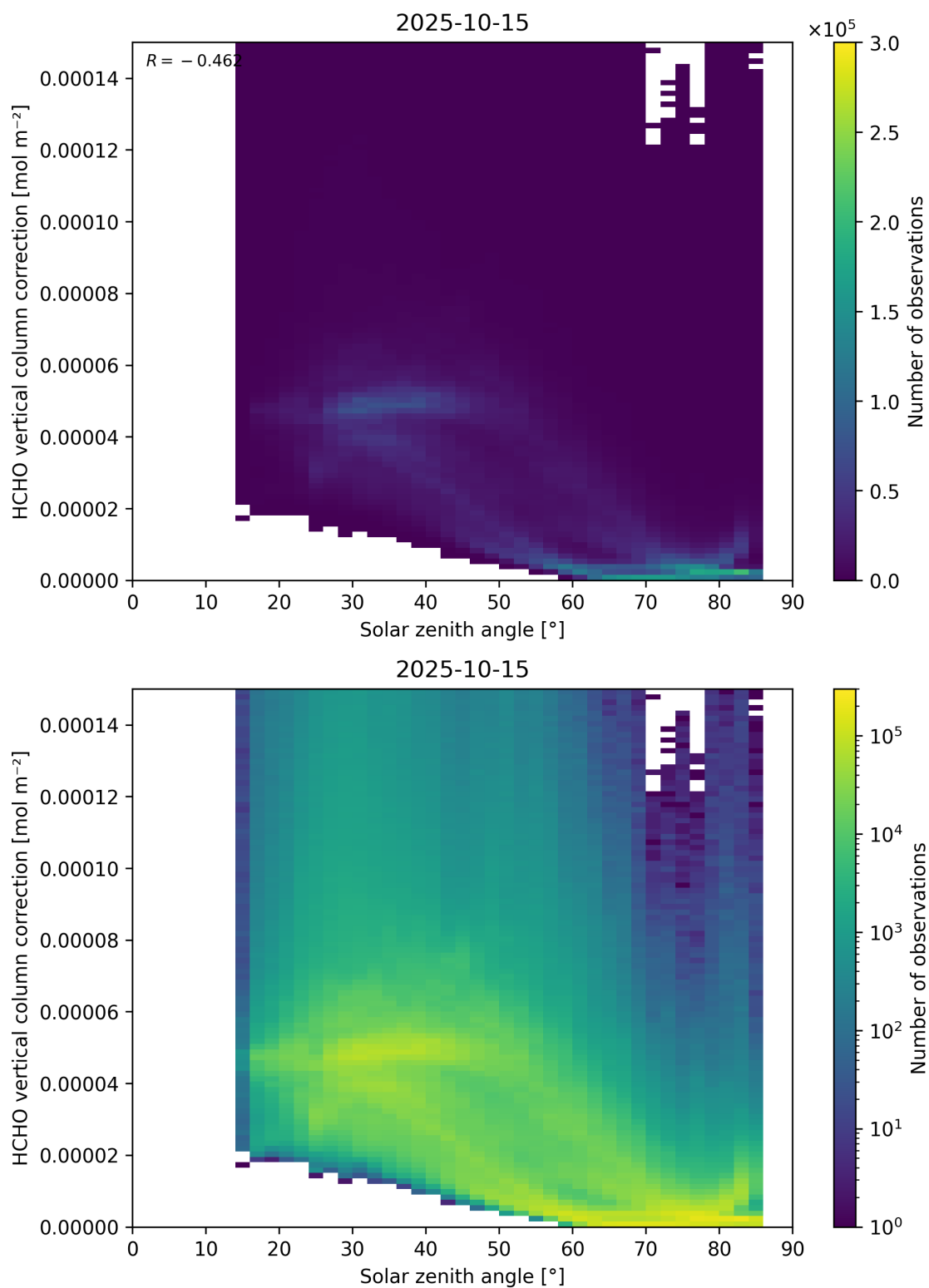
Figure 178: Scatter density plot of “Solar zenith angle” against “HCHO vertical column correction” for 2025-10-14 to 2025-10-16.
