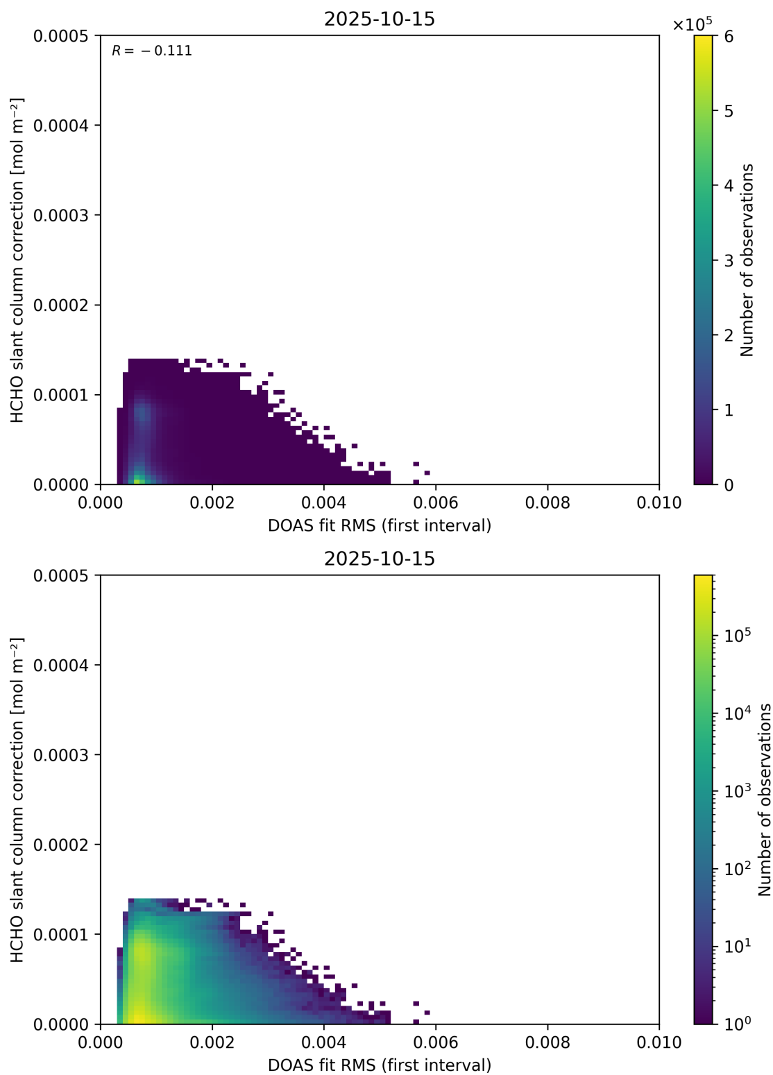
Figure 63: Scatter density plot of “DOAS fit RMS (first interval)” against “HCHO slant column correction” for 2025-10-14 to 2025-10-16.
