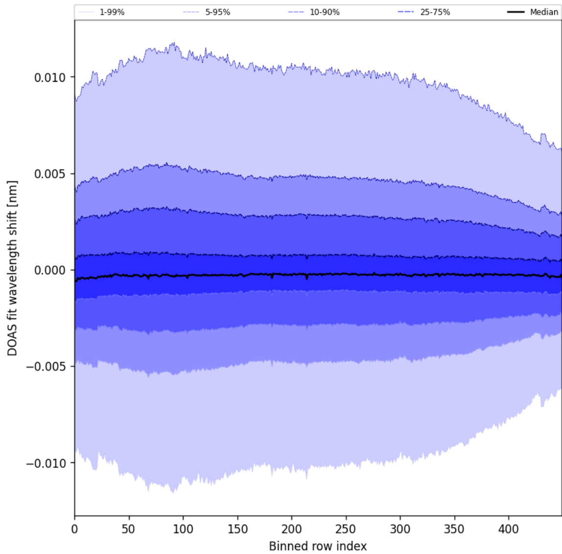
Figure 58: Along track statistics of “DOAS fit wavelength shift” for 2025-10-15 to 2025-10-17
