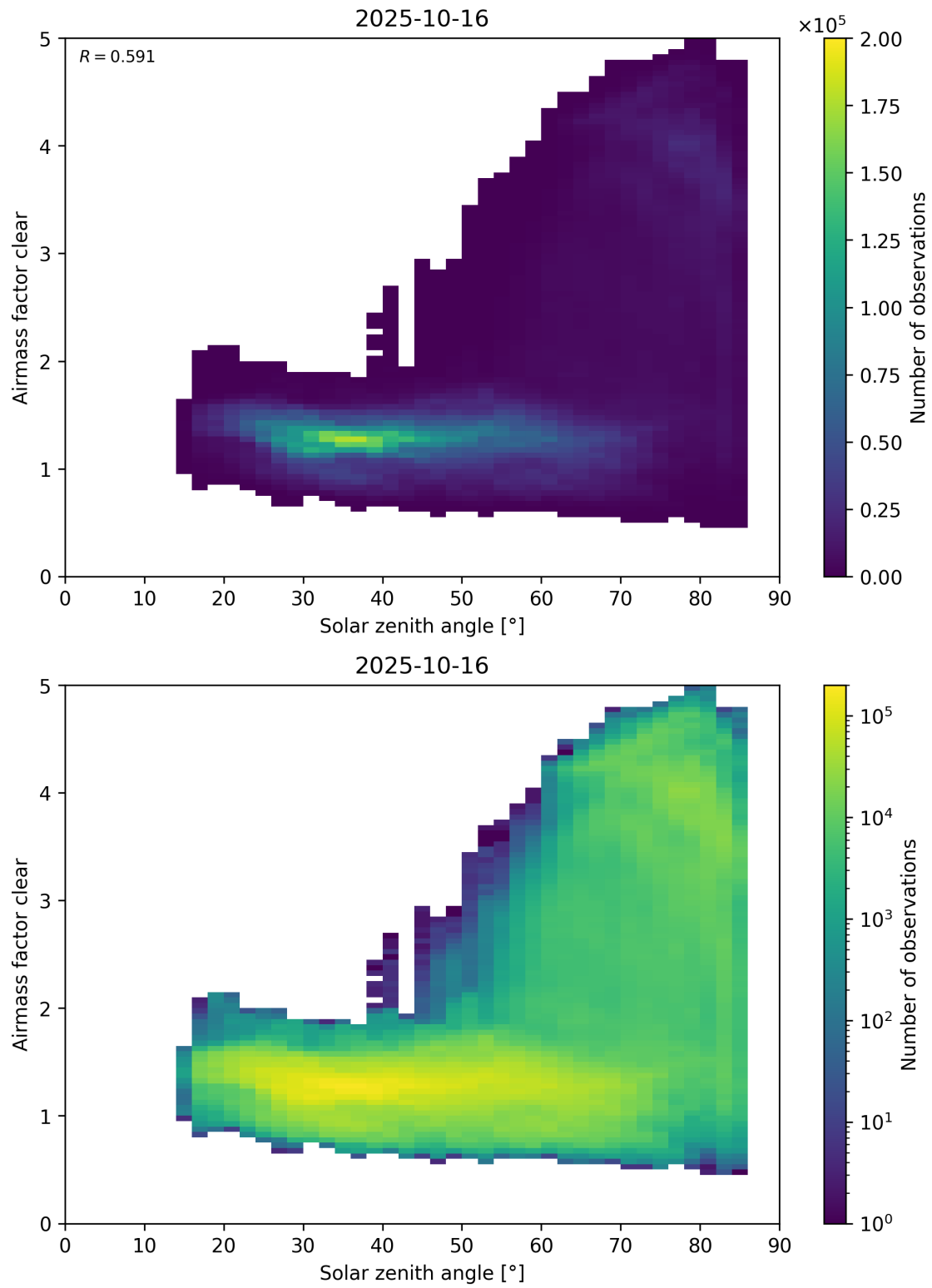
Figure 170: Scatter density plot of “Solar zenith angle” against “Airmass factor clear” for 2025-10-15 to 2025-10-17.
