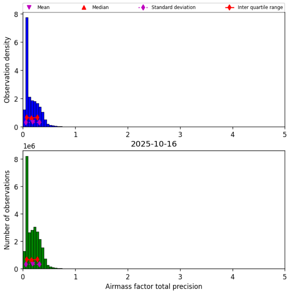
Figure 41: Histogram of “Airmass factor total precision” for 2025-10-15 to 2025-10-17
