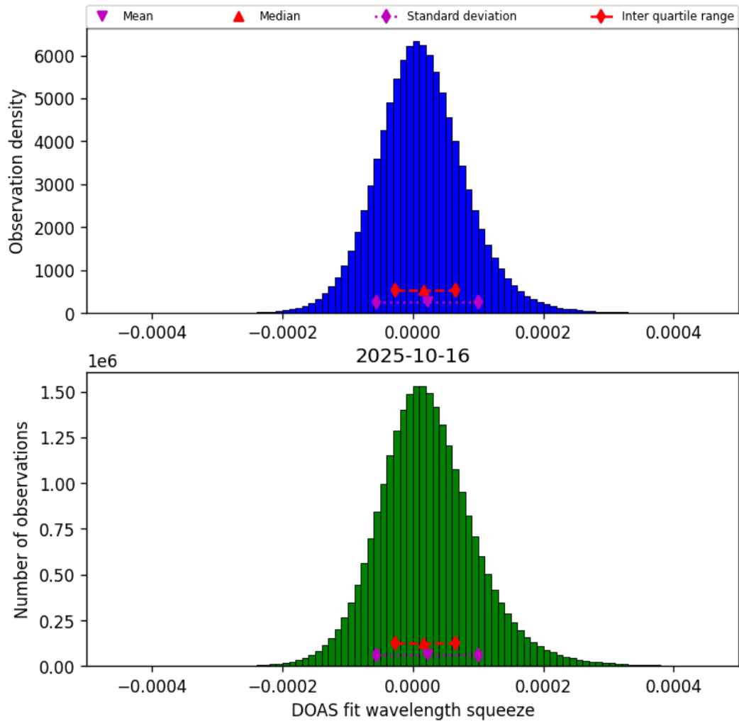
Figure 45: Histogram of “DOAS fit wavelength squeeze” for 2025-10-15 to 2025-10-17
