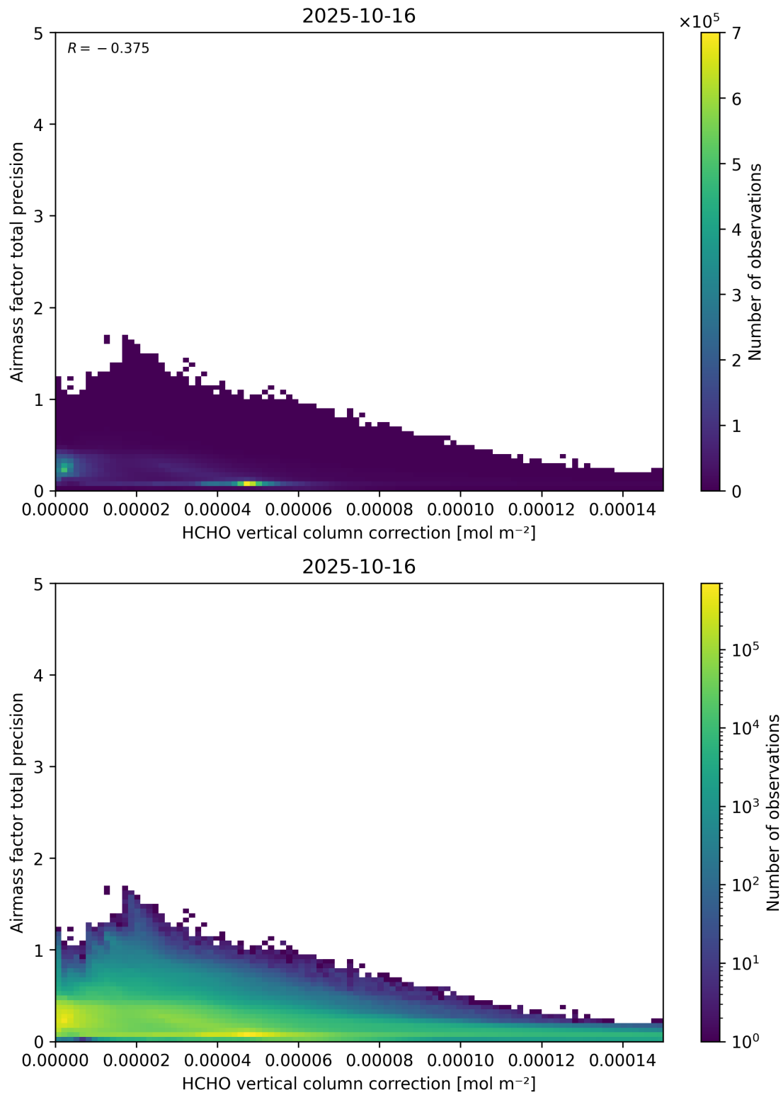
Figure 121: Scatter density plot of “HCHO vertical column correction” against “Airmass factor total precision” for 2025-10-15 to 2025-10-17.
