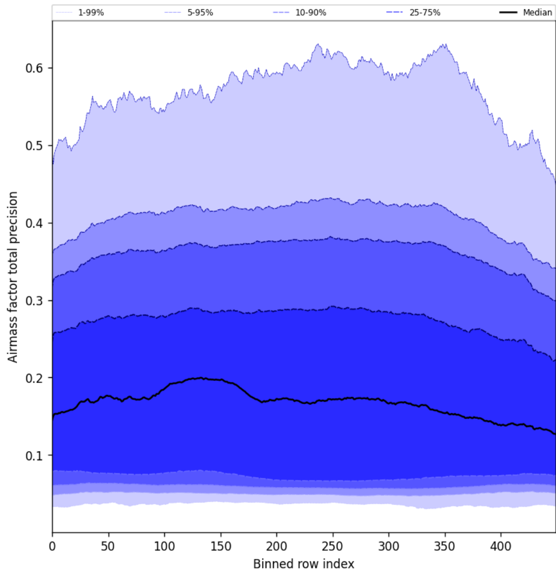
Figure 55: Along track statistics of “Airmass factor total precision” for 2025-10-15 to 2025-10-17
