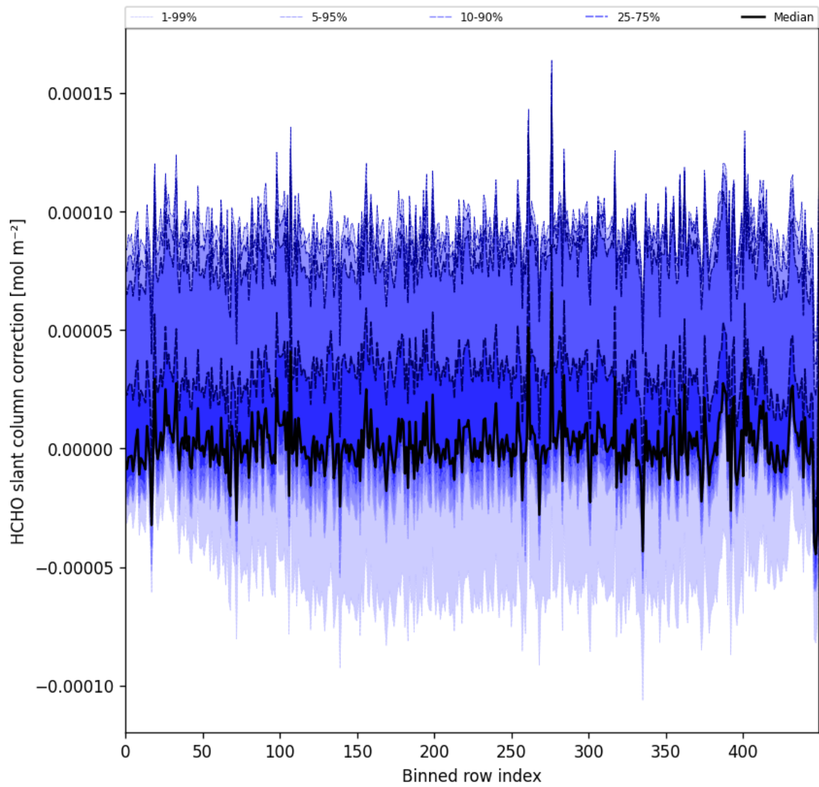
Figure 61: Along track statistics of “HCHO slant column correction” for 2025-10-15 to 2025-10-17
