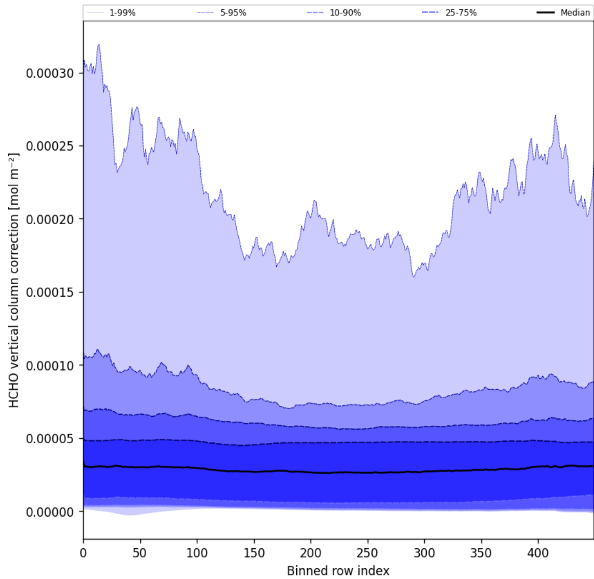
Figure 51: Along track statistics of “HCHO vertical column correction” for 2025-10-15 to 2025-10-17
