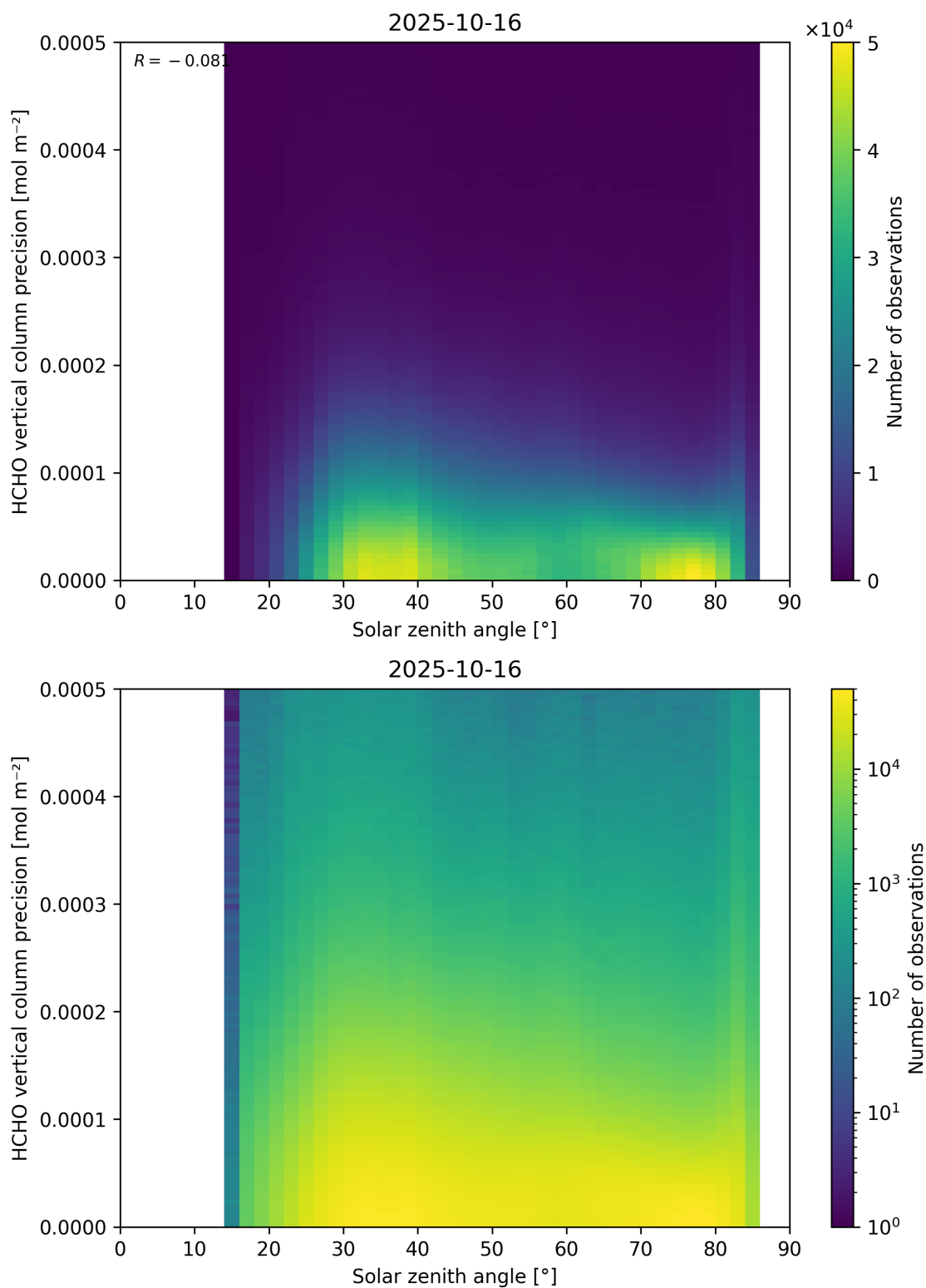
Figure 179: Scatter density plot of “Solar zenith angle” against “HCHO vertical column precision” for 2025-10-15 to 2025-10-17.
