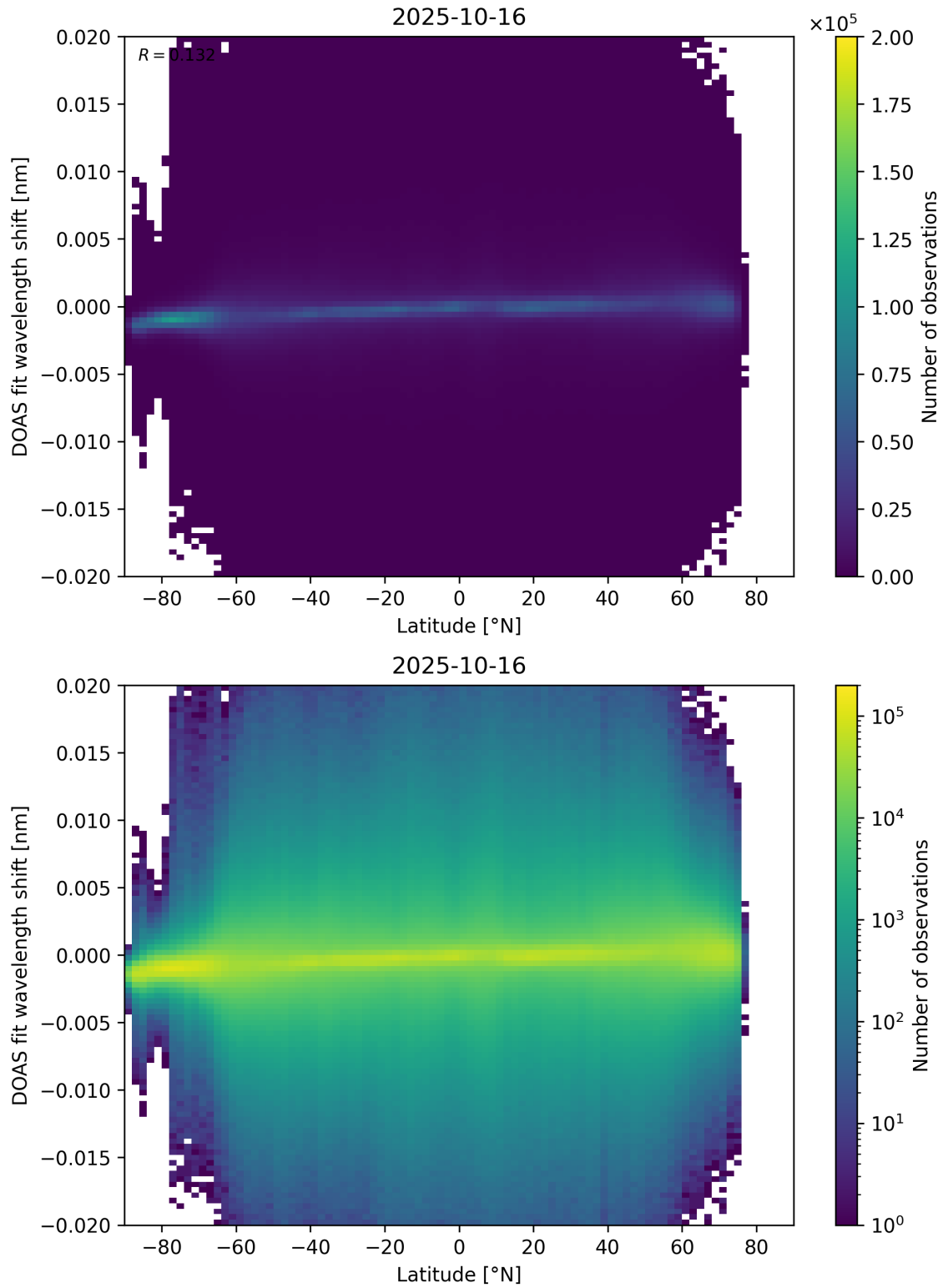
Figure 154: Scatter density plot of “Latitude” against “DOAS fit wavelength shift” for 2025-10-15 to 2025-10-17.
