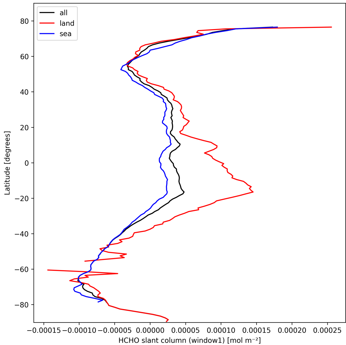
Figure 24: Zonal average of “HCHO slant column (window1)” for 2025-10-15 to 2025-10-17.
