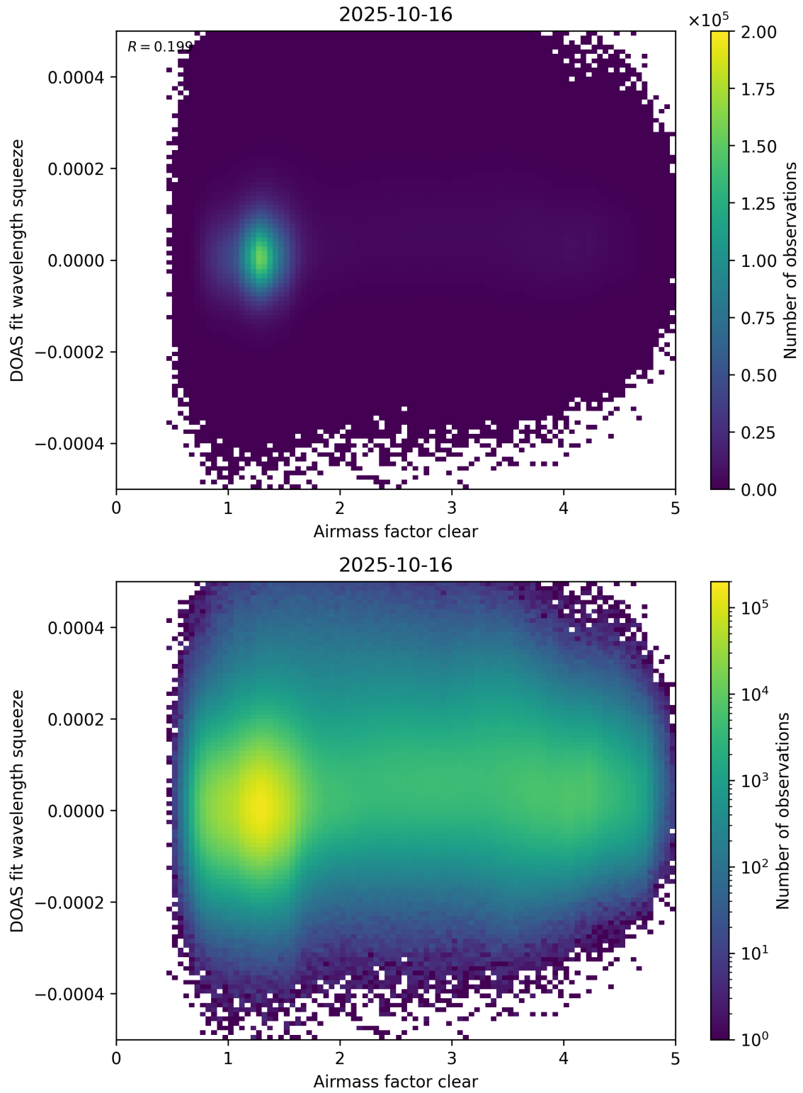
Figure 73: Scatter density plot of “Airmass factor clear” against “DOAS fit wavelength squeeze” for 2025-10-15 to 2025-10-17.
