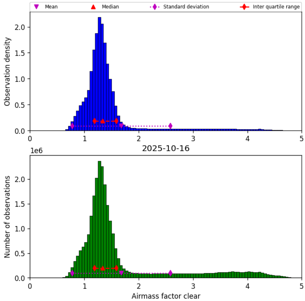
Figure 42: Histogram of “Airmass factor clear” for 2025-10-15 to 2025-10-17
