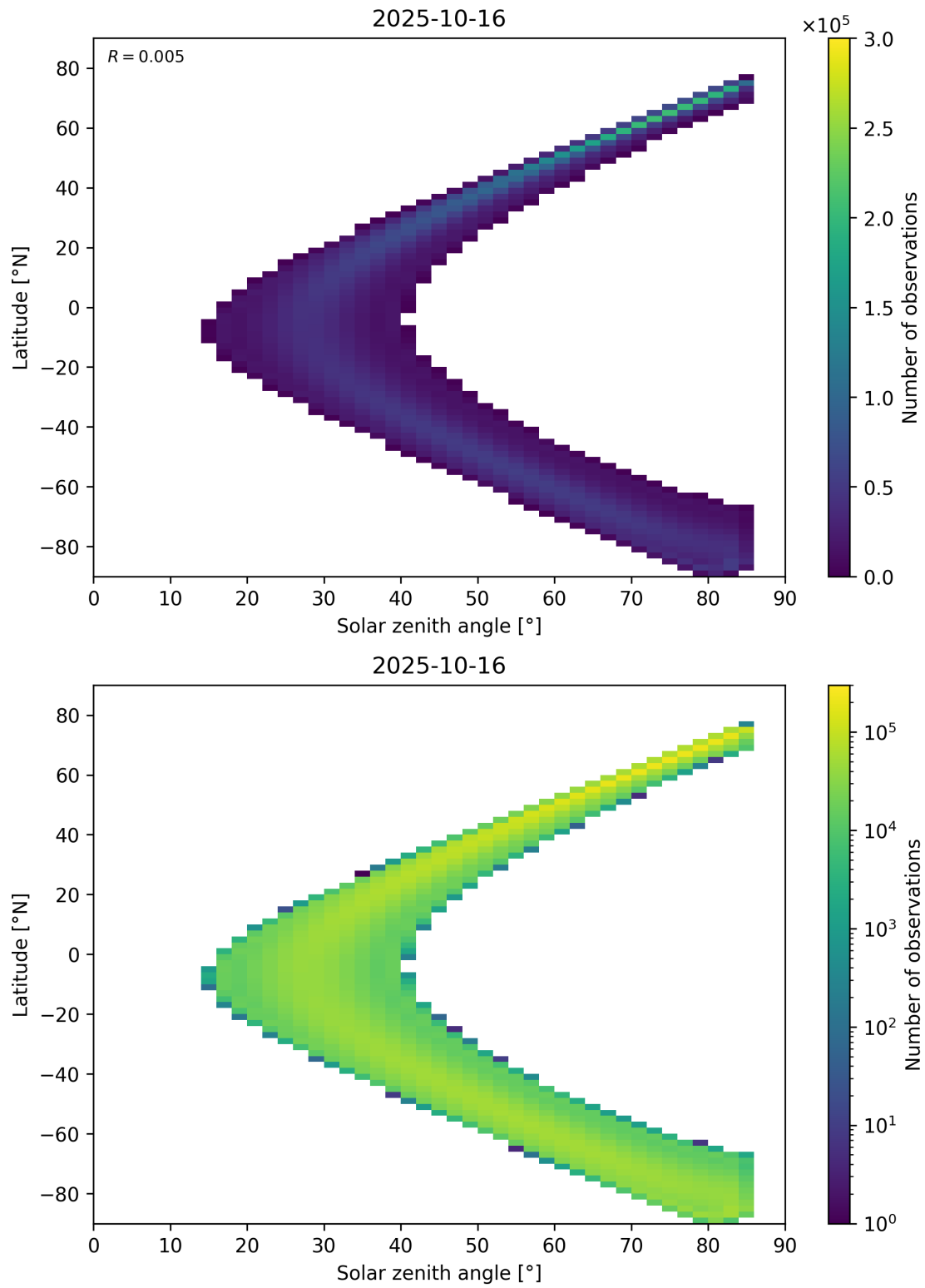
Figure 181: Scatter density plot of “Solar zenith angle” against “Latitude” for 2025-10-15 to 2025-10-17.
