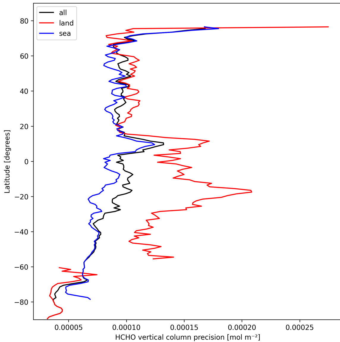
Figure 22: Zonal average of "HCHO vertical column precision" for 2025-10-15 to 2025-10-17.
