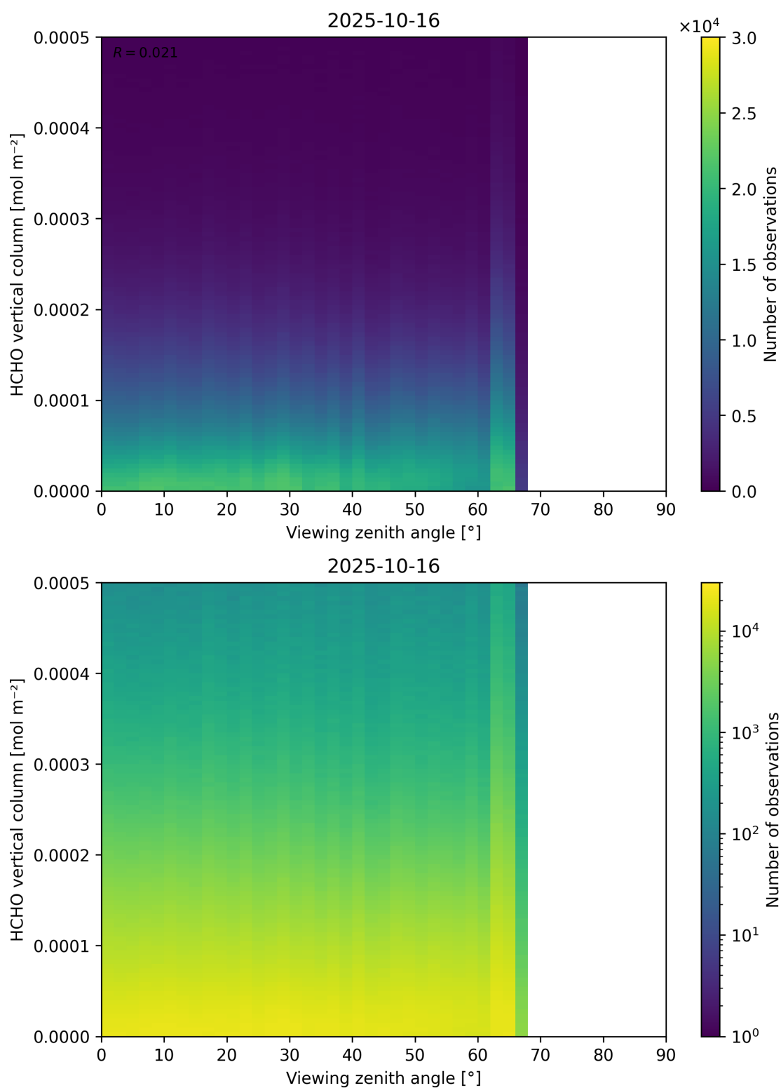
Figure 192: Scatter density plot of “Viewing zenith angle” against “HCHO vertical column” for 2025-10-15 to 2025-10-17.
