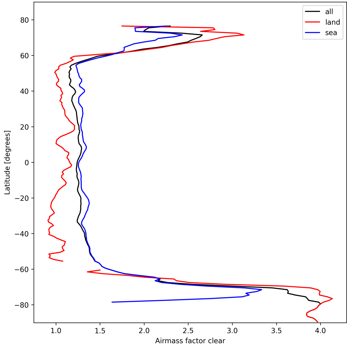
Figure 28: Zonal average of “Airmass factor clear” for 2025-10-15 to 2025-10-17.
