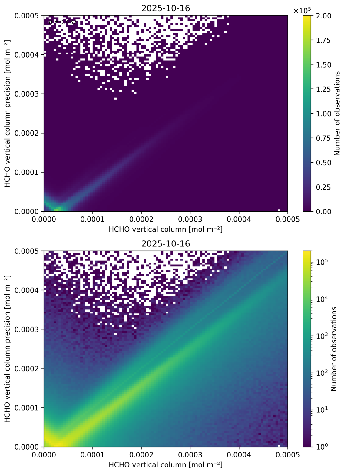
Figure 134: Scatter density plot of “HCHO vertical column” against “HCHO vertical column precision” for 2025-10-15 to 2025-10-17.
