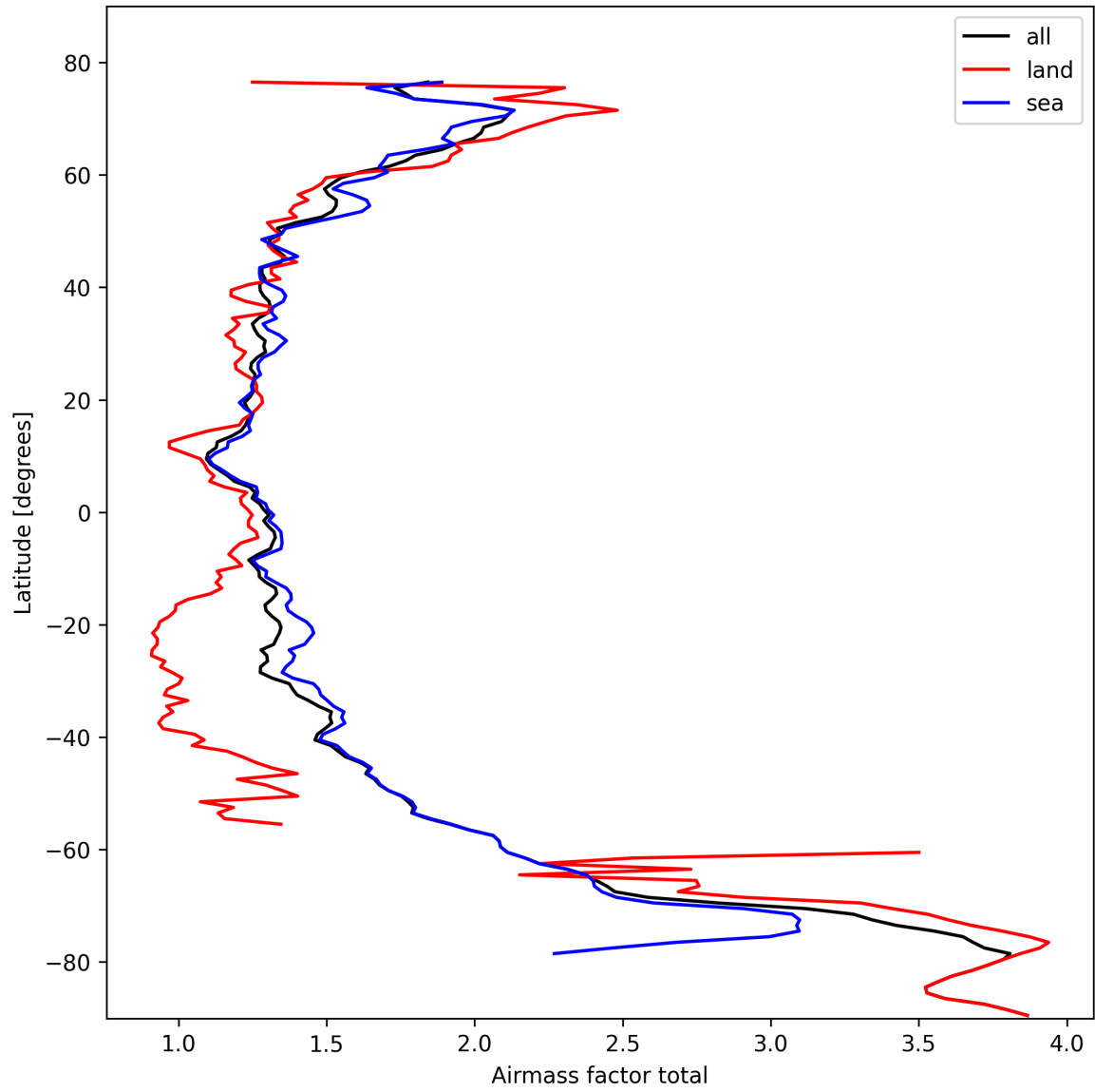
Figure 26: Zonal average of “Airmass factor total” for 2025-10-15 to 2025-10-17.
