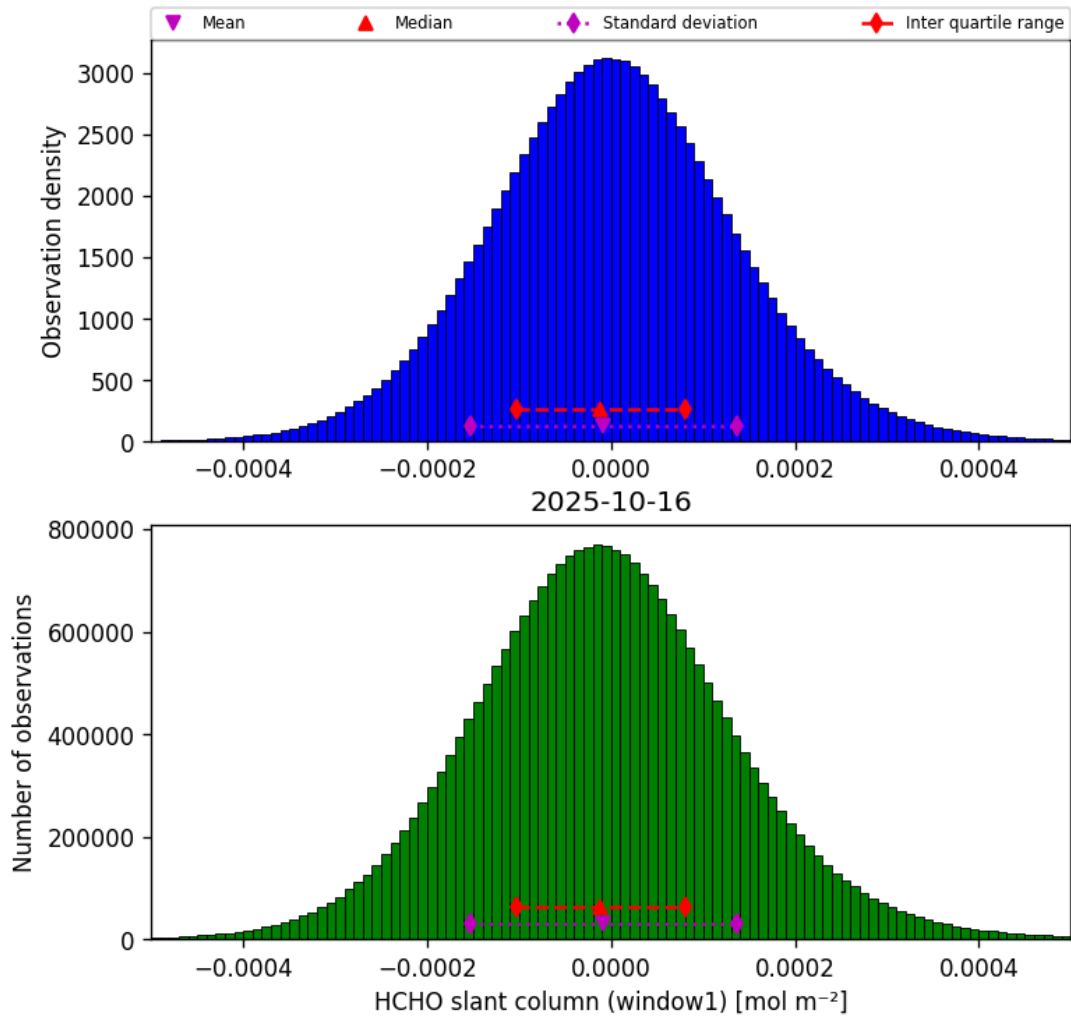
Figure 38: Histogram of “HCHO slant column (window1)” for 2025-10-15 to 2025-10-17
