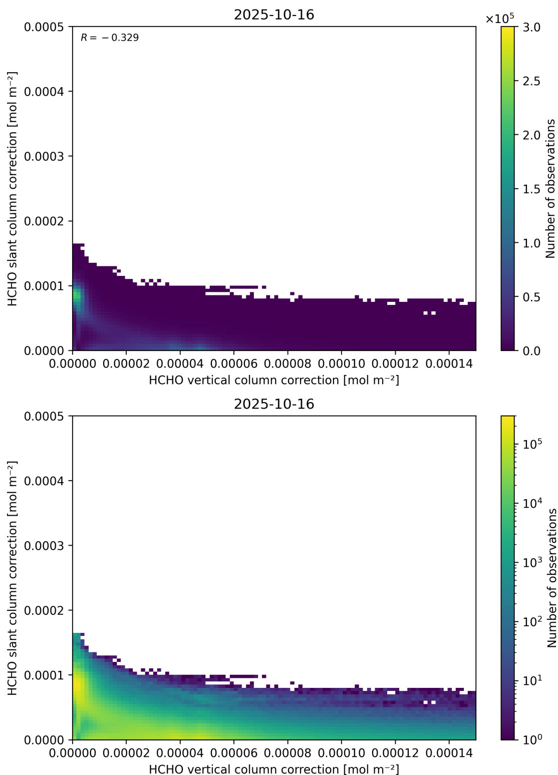
Figure 117: Scatter density plot of “HCHO vertical column correction” against “HCHO slant column correction” for 2025-10-15 to 2025-10-17.
