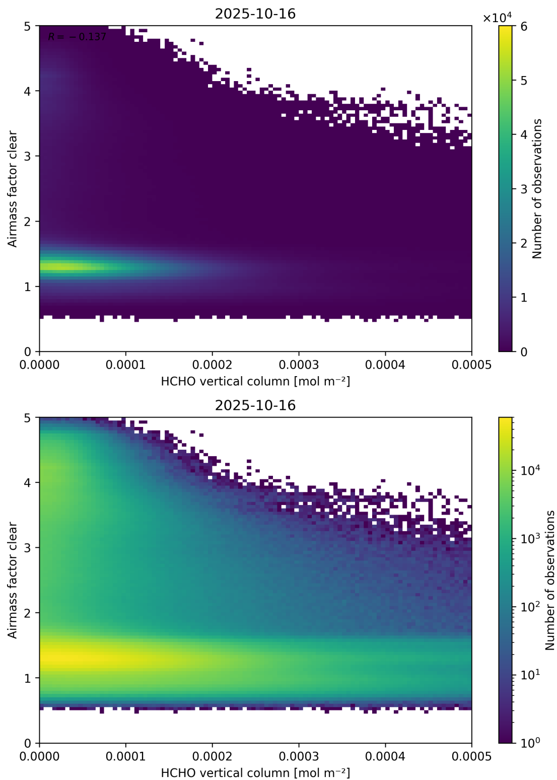
Figure 126: Scatter density plot of “HCHO vertical column” against “Airmass factor clear” for 2025-10-15 to 2025-10-17.
