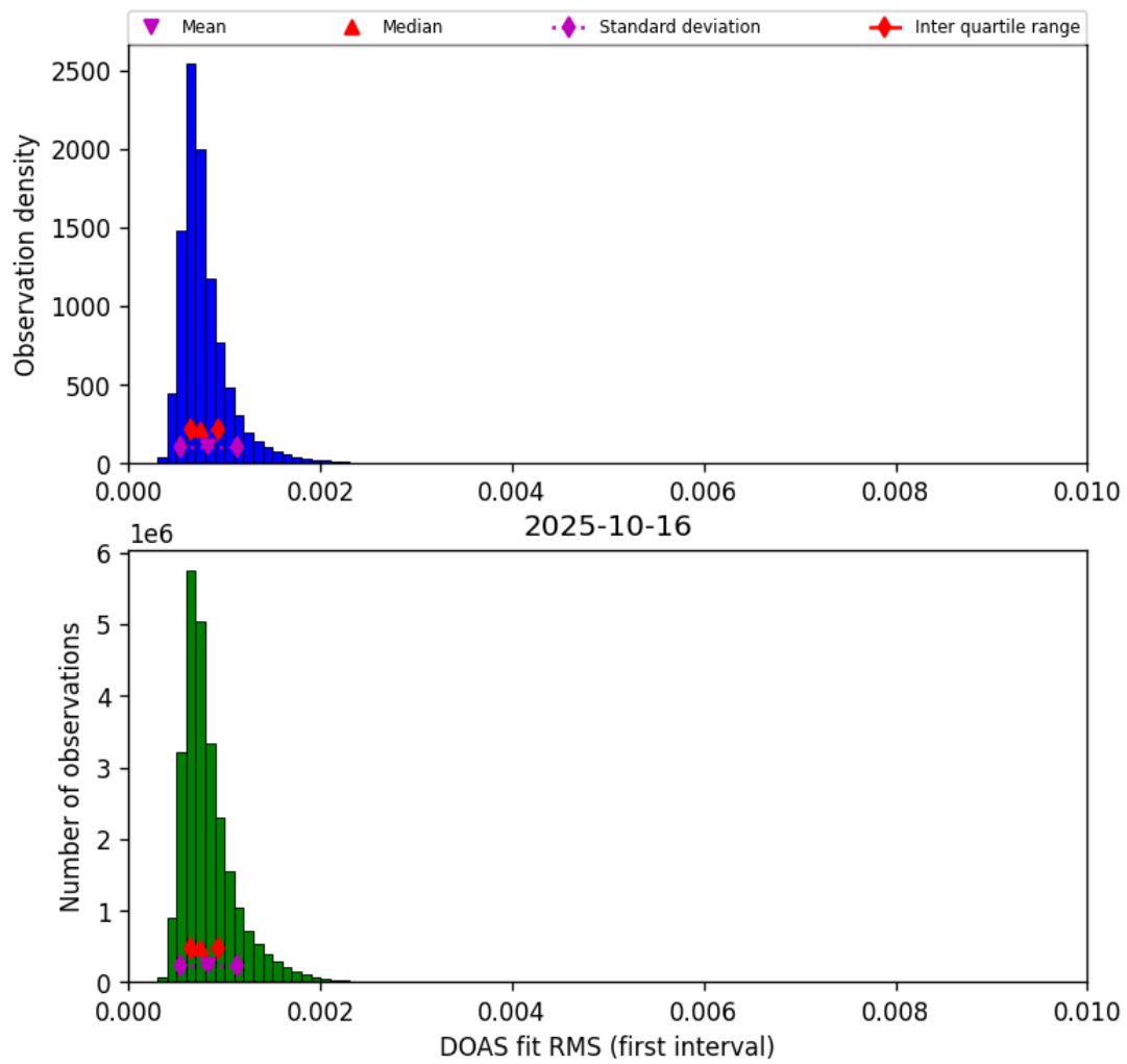
Figure 46: Histogram of “DOAS fit RMS (first interval)” for 2025-10-15 to 2025-10-17
