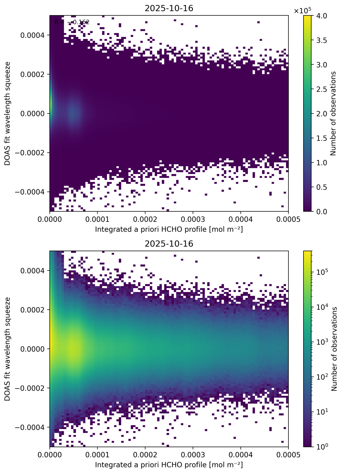
Figure 150: Scatter density plot of “Integrated a priori HCHO profile” against “DOAS fit wavelength squeeze” for 2025-10-15 to 2025-10-17.
