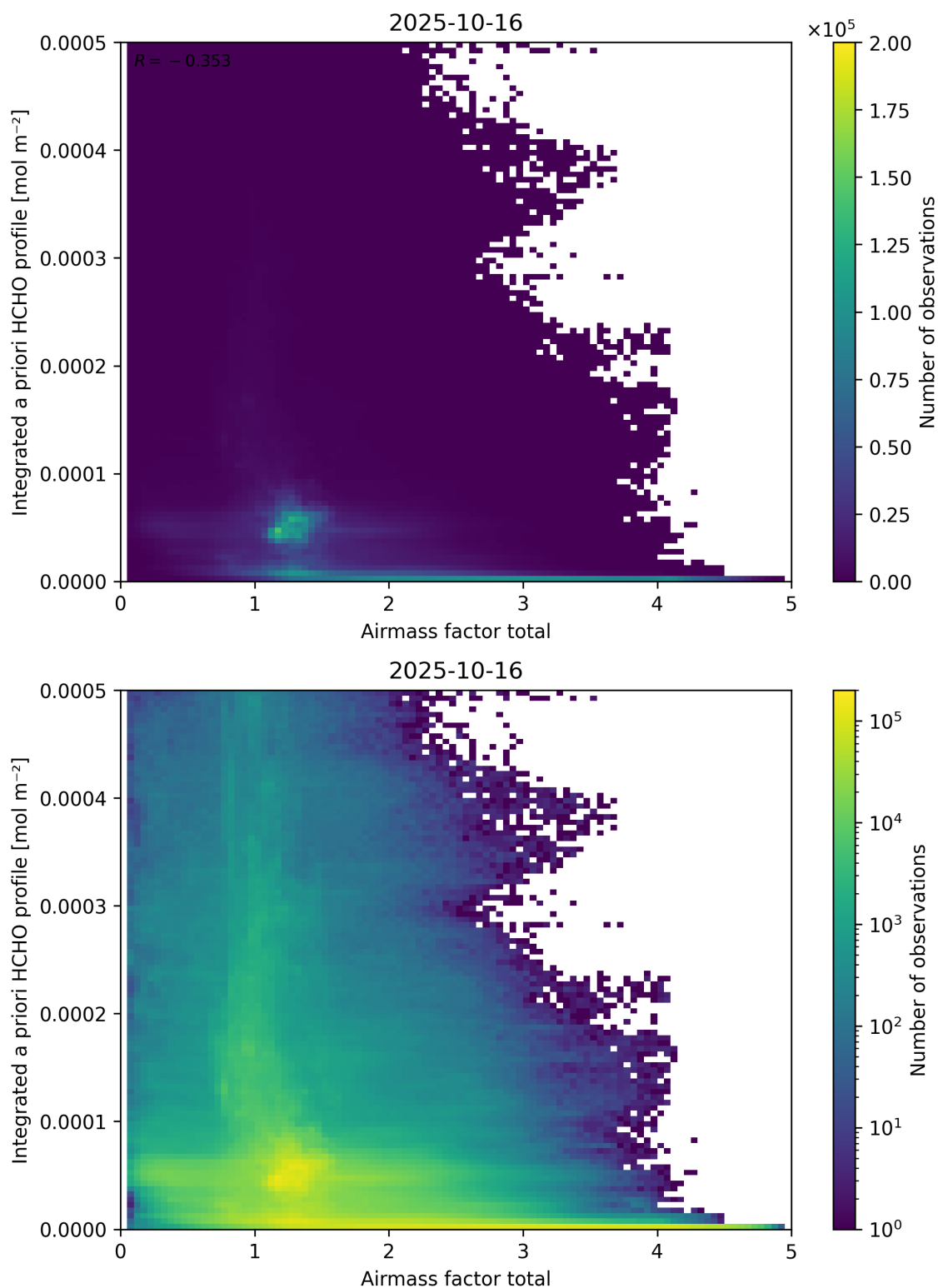
Figure 104: Scatter density plot of “Airmass factor total” against “Integrated a priori HCHO profile” for 2025-10-15 to 2025-10-17.
