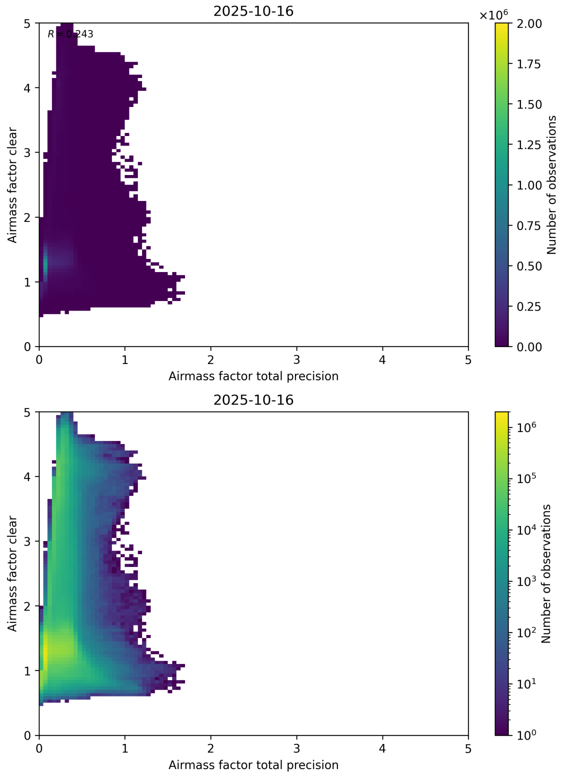
Figure 108: Scatter density plot of “Airmass factor total precision” against “Airmass factor clear” for 2025-10-15 to 2025-10-17.
