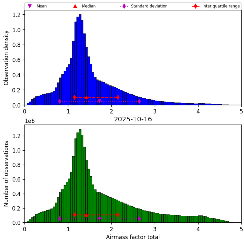
Figure 40: Histogram of “Airmass factor total” for 2025-10-15 to 2025-10-17
