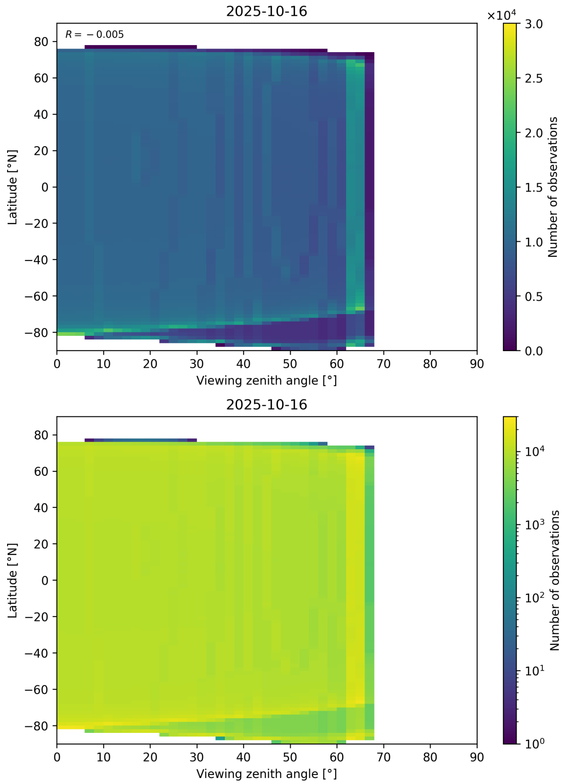
Figure 196: Scatter density plot of “Viewing zenith angle” against “Latitude” for 2025-10-15 to 2025-10-17.
