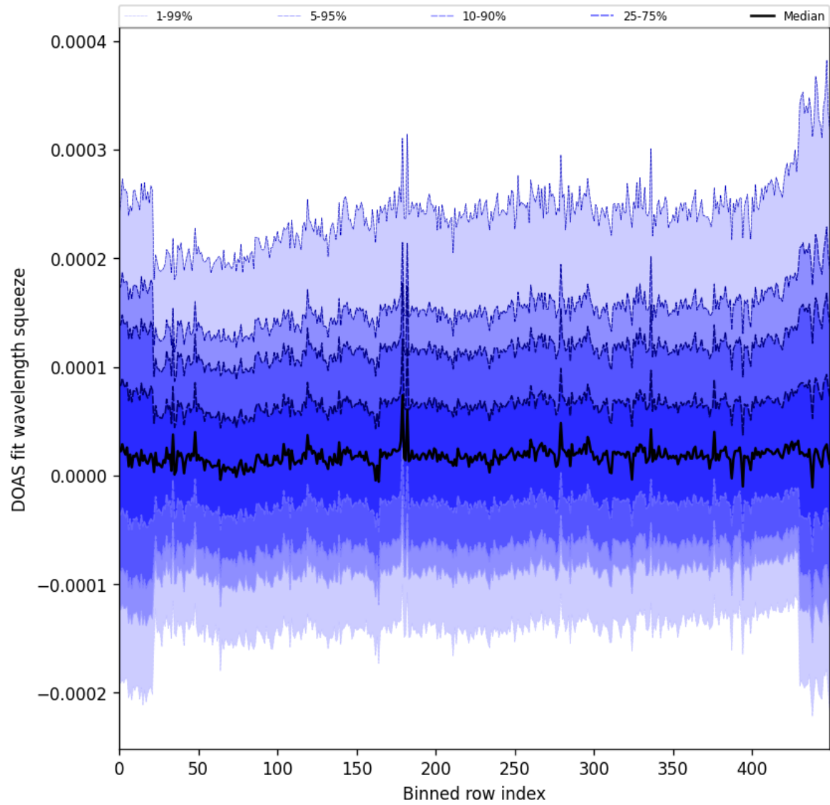
Figure 59: Along track statistics of “DOAS fit wavelength squeeze” for 2025-10-15 to 2025-10-17
