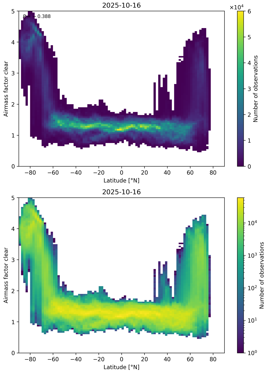
Figure 156: Scatter density plot of “Latitude” against “Airmass factor clear” for 2025-10-15 to 2025-10-17.
