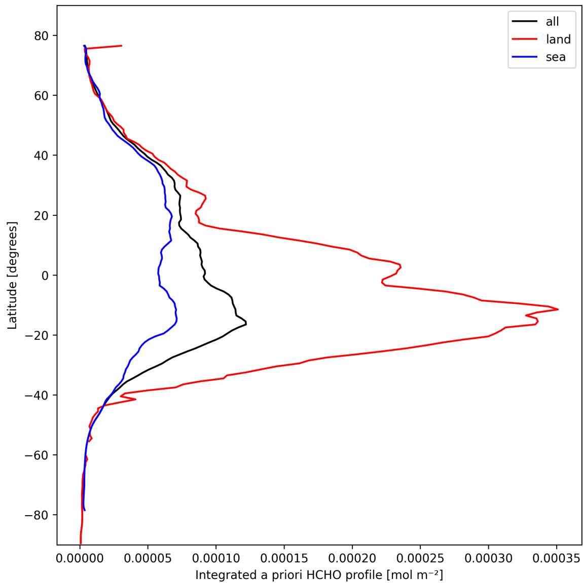
Figure 29: Zonal average of “Integrated a priori HCHO profile” for 2025-10-15 to 2025-10-17.
