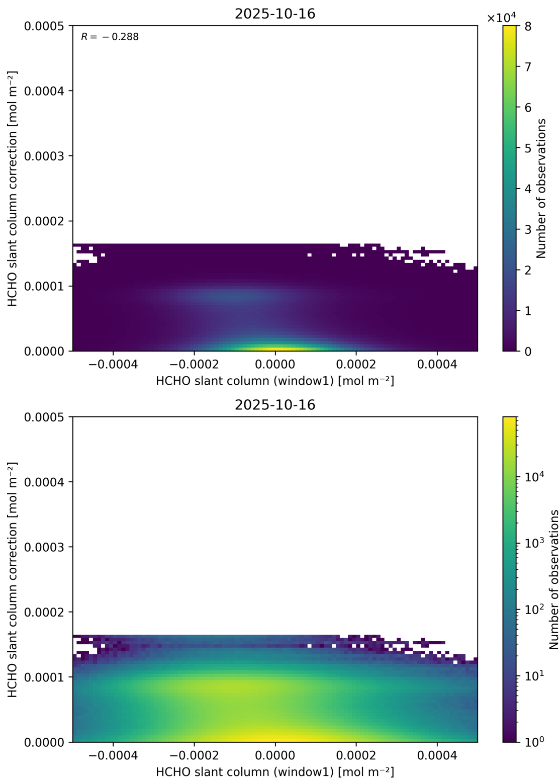
Figure 83: Scatter density plot of “HCHO slant column (window1)” against “HCHO slant column correction” for 2025-10-15 to 2025-10-17.
