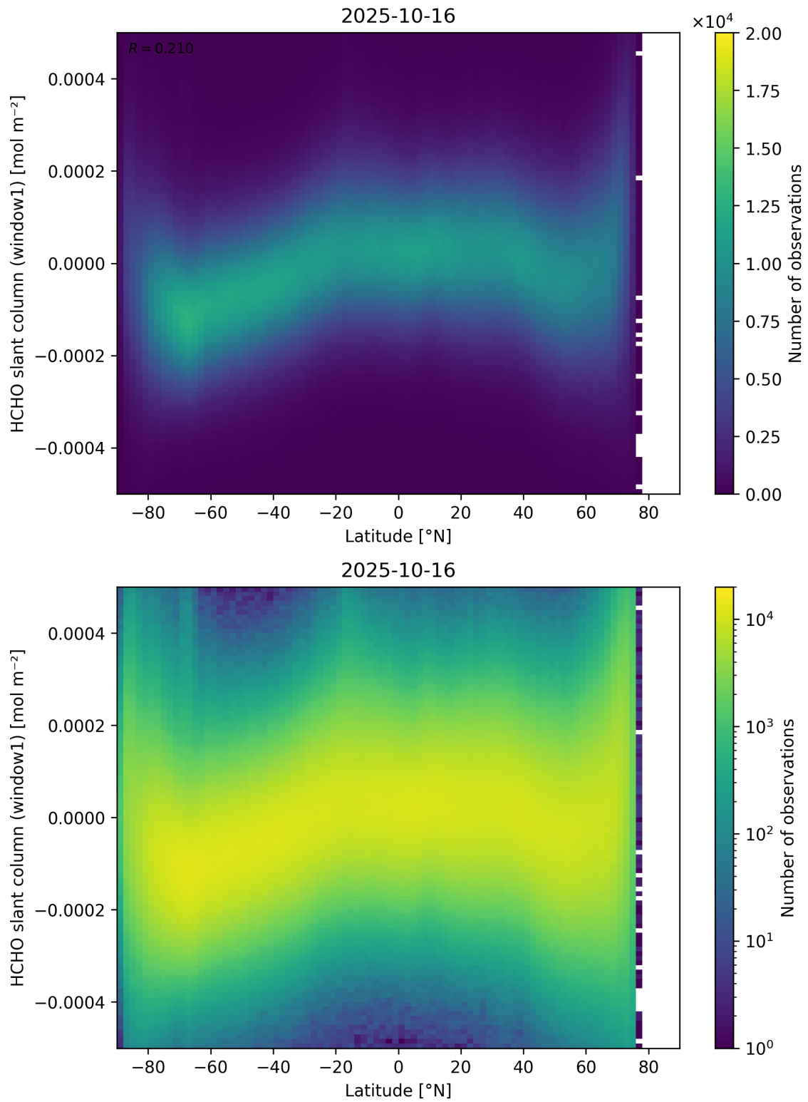
Figure 159: Scatter density plot of “Latitude” against “HCHO slant column (window1)” for 2025-10-15 to 2025-10-17.
