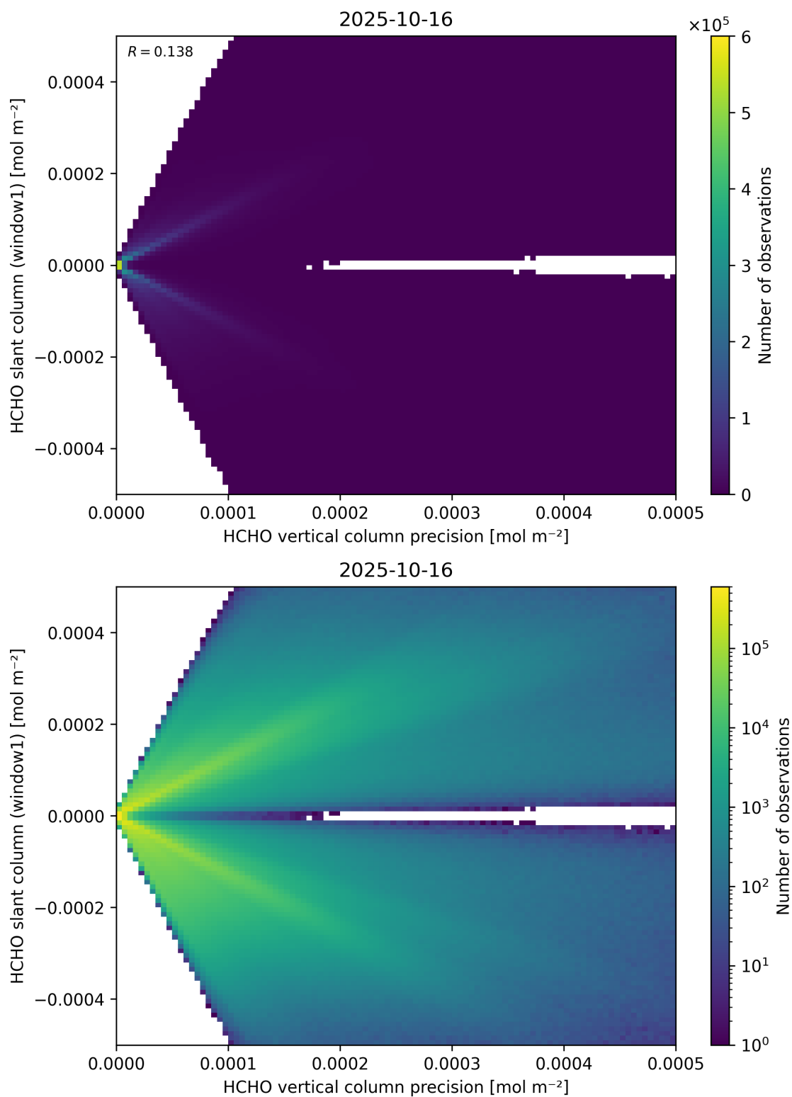
Figure 142: Scatter density plot of “HCHO vertical column precision” against “HCHO slant column (window1)” for 2025-10-15 to 2025-10-17.
