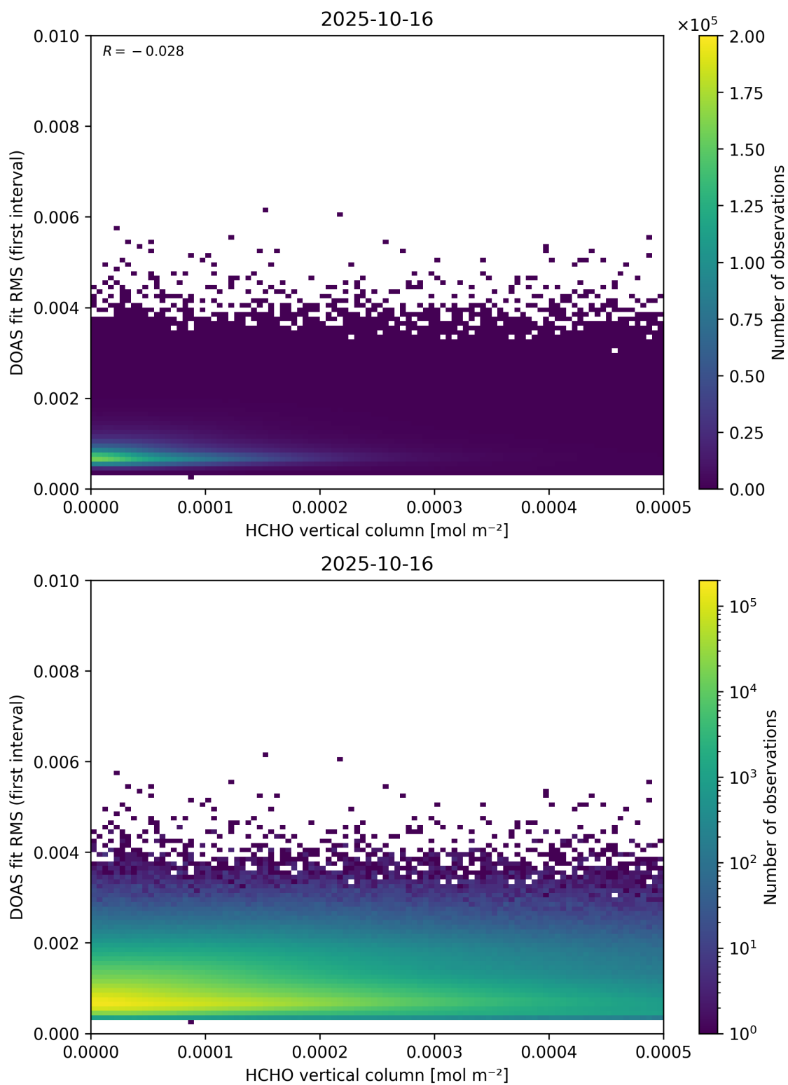
Figure 123: Scatter density plot of “HCHO vertical column” against “DOAS fit RMS (first interval)” for 2025-10-15 to 2025-10-17.
