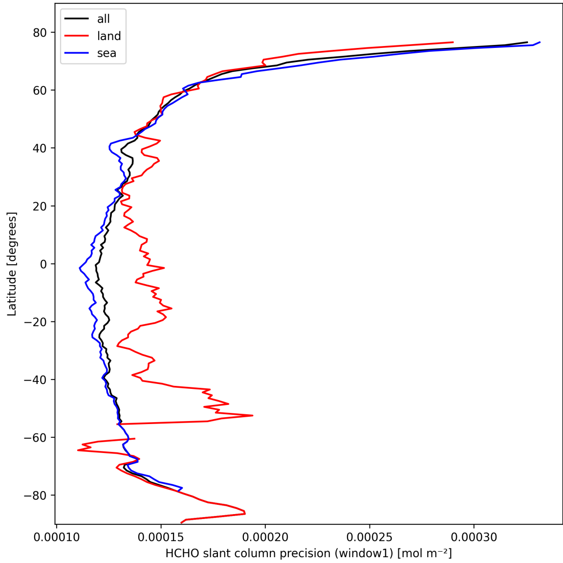
Figure 25: Zonal average of “HCHO slant column precision (window1)” for 2025-10-15 to 2025-10-17.
