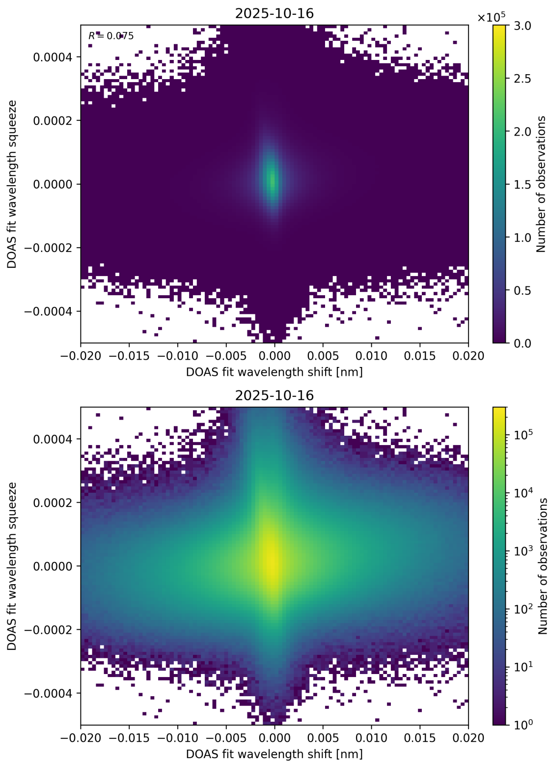
Figure 65: Scatter density plot of “DOAS fit wavelength shift” against “DOAS fit wavelength squeeze” for 2025-10-15 to 2025-10-17.
