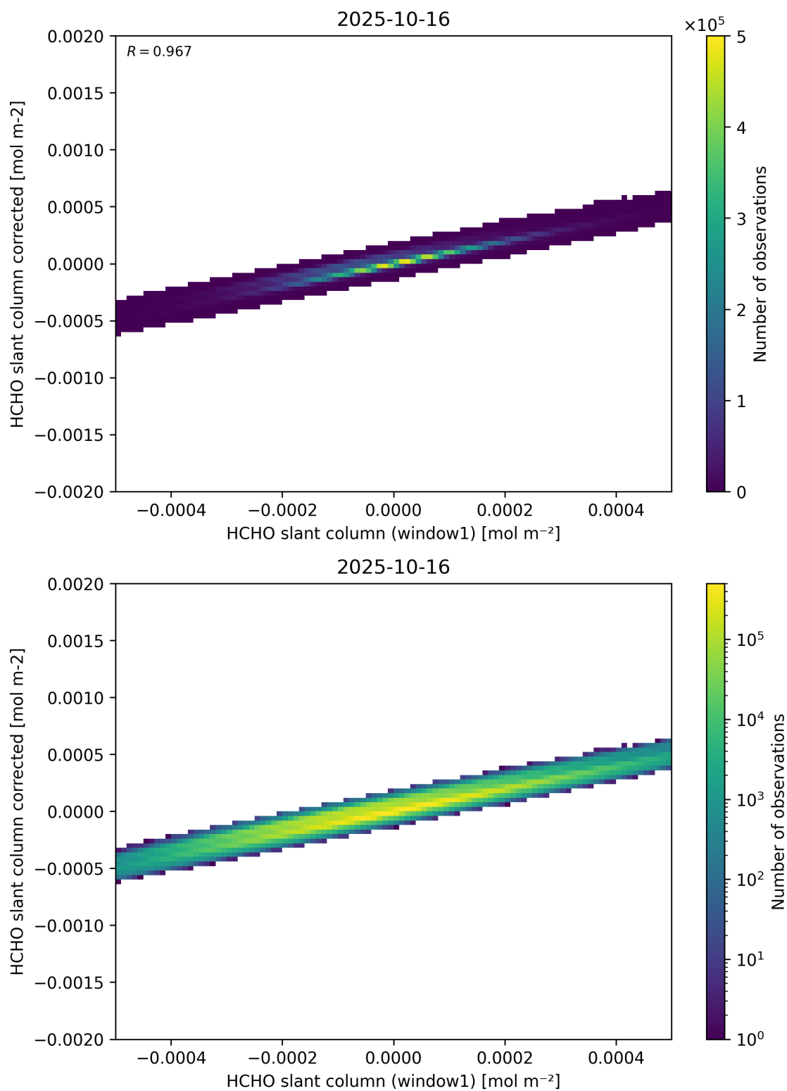
Figure 82: Scatter density plot of “HCHO slant column (window1)” against “HCHO slant column corrected” for 2025-10-15 to 2025-10-17.
