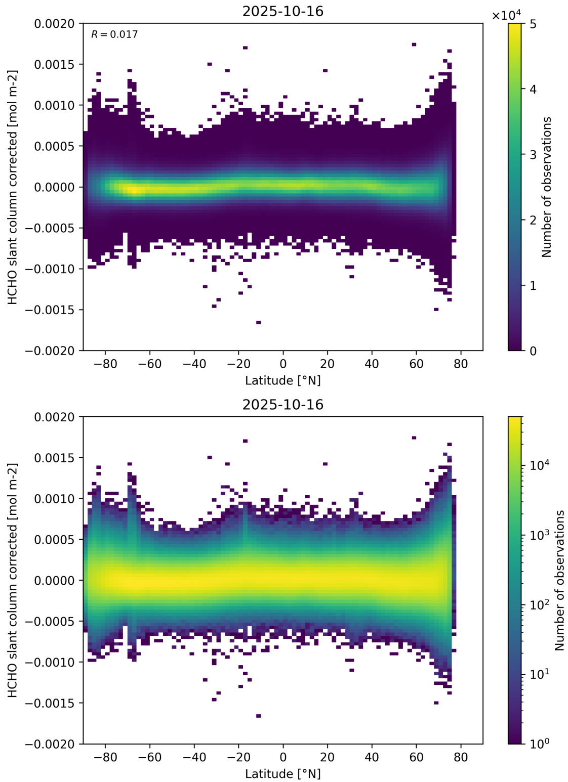
Figure 157: Scatter density plot of “Latitude” against “HCHO slant column corrected” for 2025-10-15 to 2025-10-17.
