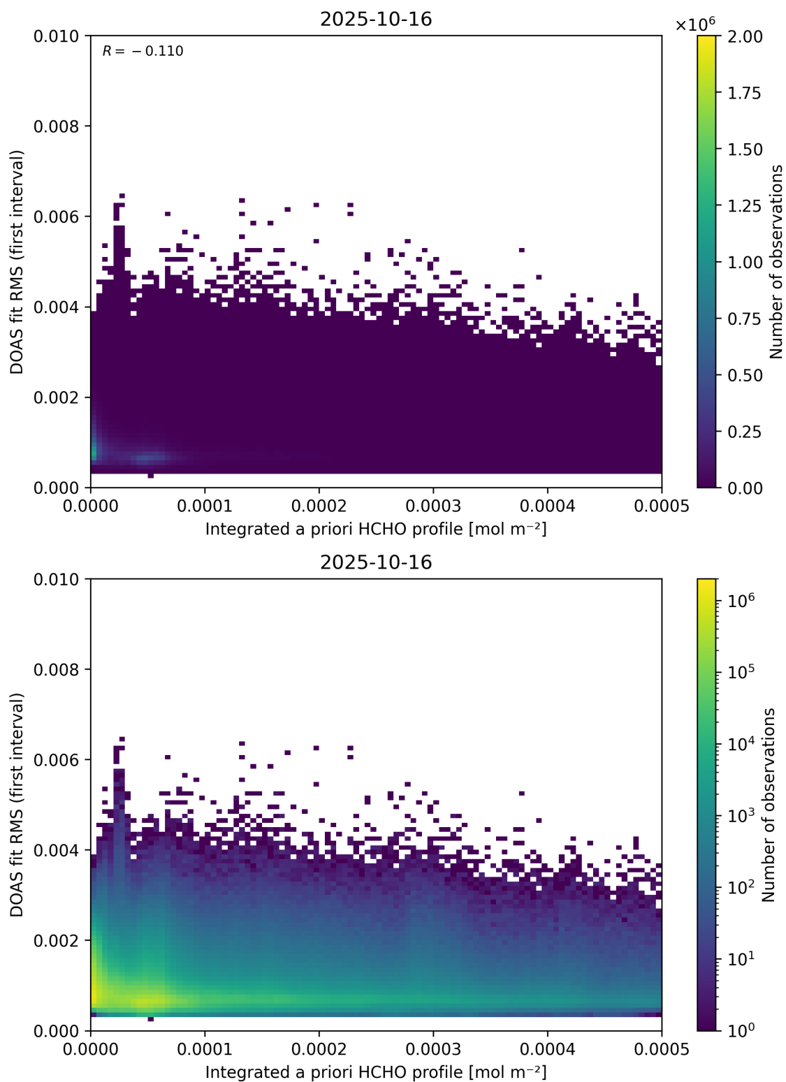
Figure 148: Scatter density plot of “Integrated a priori HCHO profile” against “DOAS fit RMS (first interval)” for 2025-10-15 to 2025-10-17.
