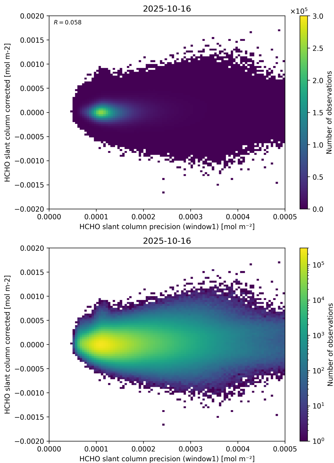
Figure 92: Scatter density plot of “HCHO slant column precision (window1)” against “HCHO slant column corrected” for 2025-10-15 to 2025-10-17.
