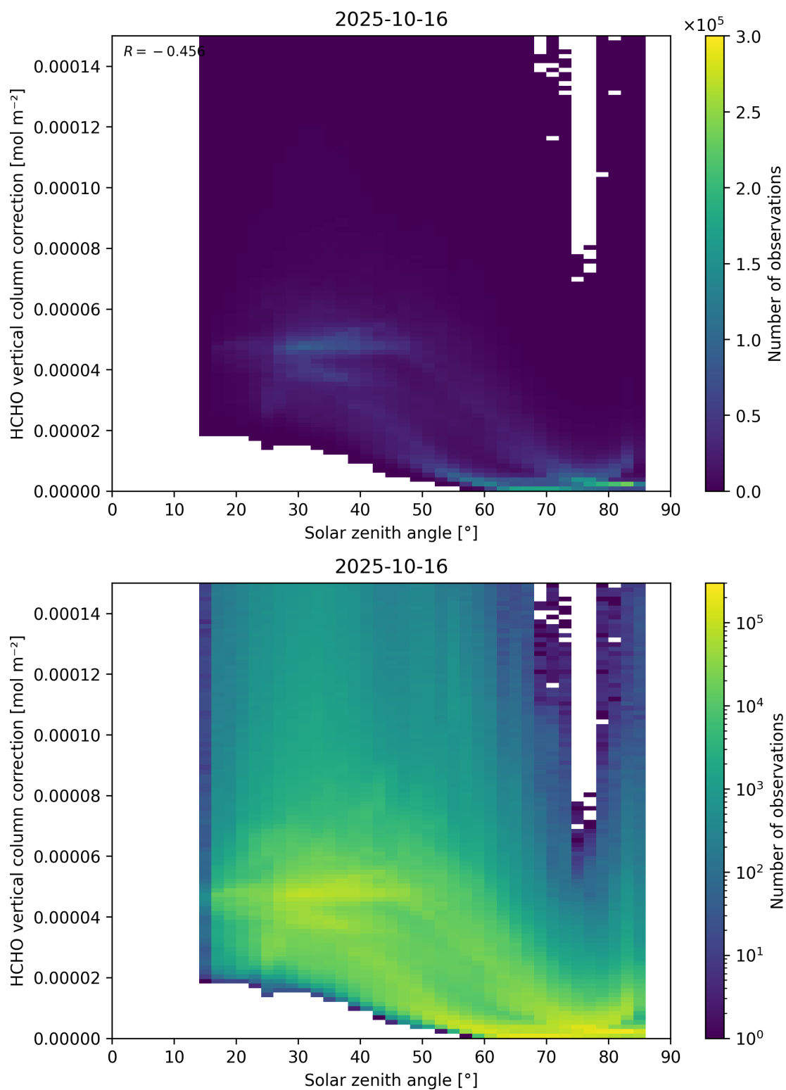
Figure 178: Scatter density plot of “Solar zenith angle” against “HCHO vertical column correction” for 2025-10-15 to 2025-10-17.
