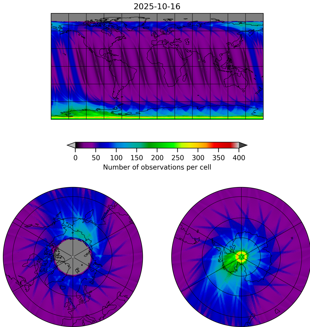
Figure 19: Map of the number of observations for 2025-10-15 to 2025-10-17
