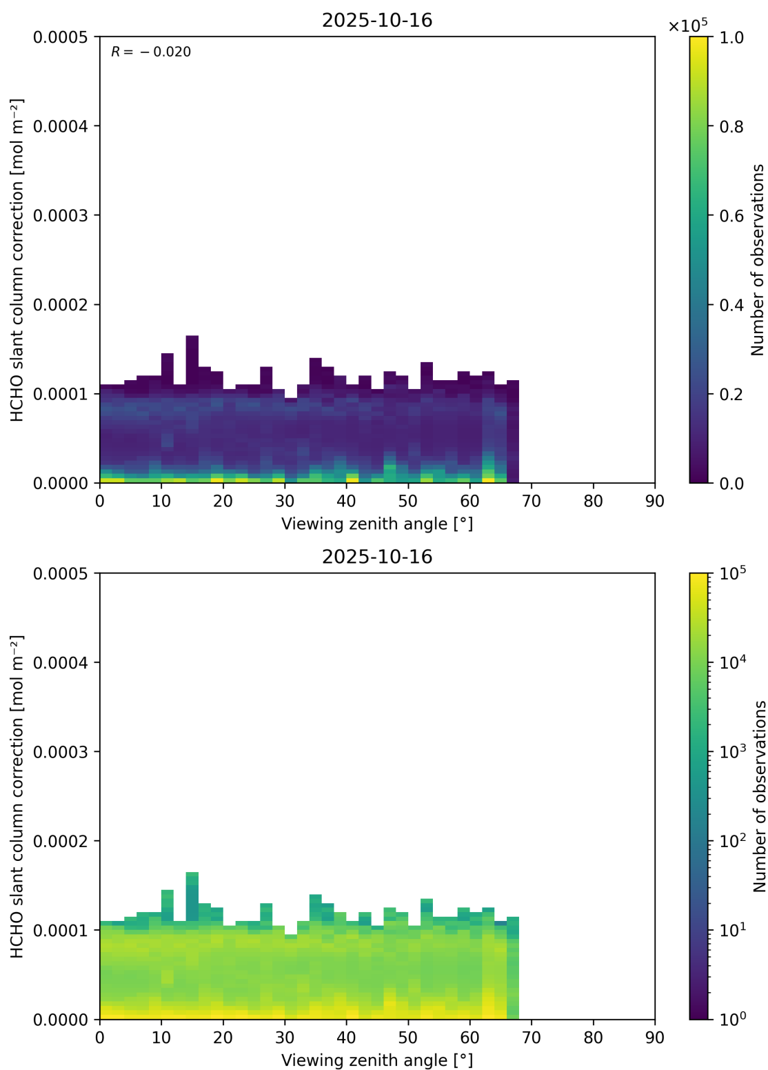
Figure 187: Scatter density plot of “Viewing zenith angle” against “HCHO slant column correction” for 2025-10-15 to 2025-10-17.
