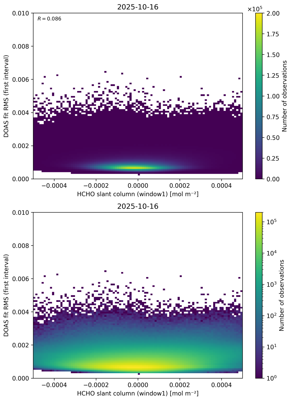
Figure 78: Scatter density plot of “HCHO slant column (window1)” against “DOAS fit RMS (first interval)” for 2025-10-15 to 2025-10-17.
