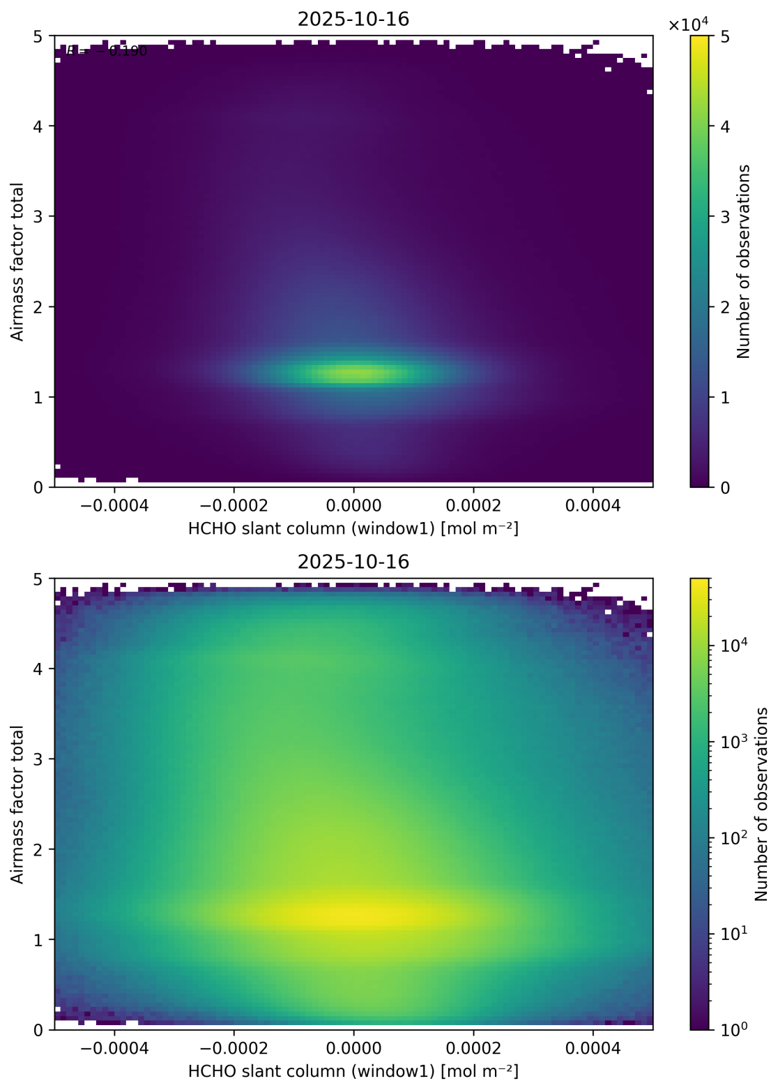
Figure 85: Scatter density plot of “HCHO slant column (window1)” against “Airmass factor total” for 2025-10-15 to 2025-10-17.
