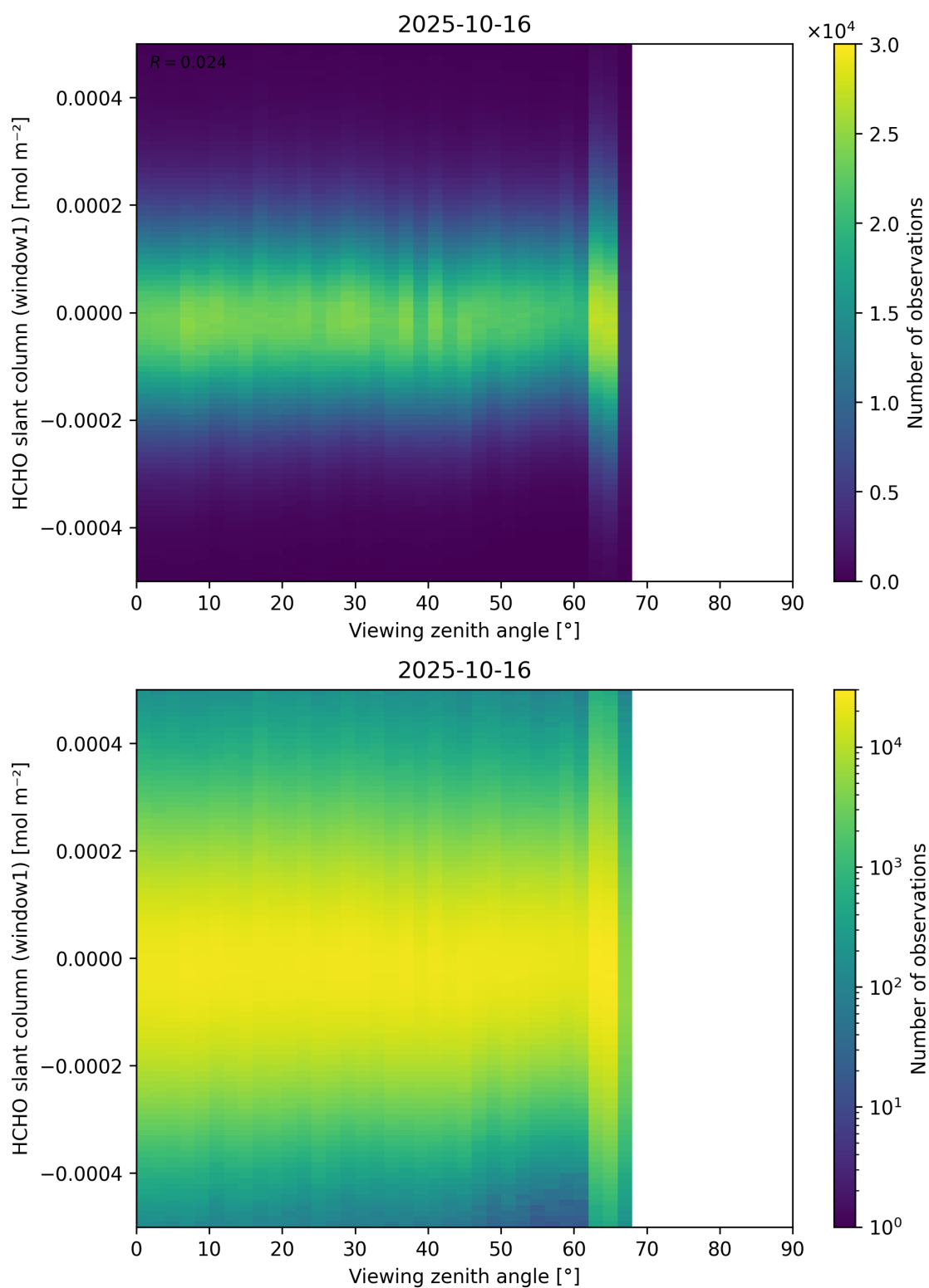
Figure 188: Scatter density plot of “Viewing zenith angle” against “HCHO slant column (window1)” for 2025-10-15 to 2025-10-17.
