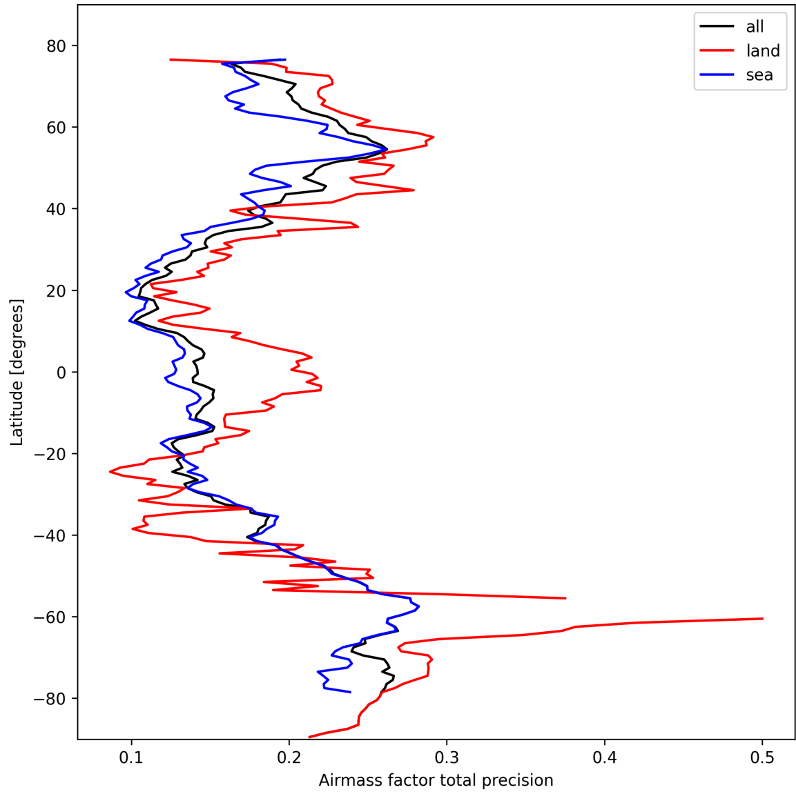
Figure 27: Zonal average of “Airmass factor total precision” for 2025-10-15 to 2025-10-17.
