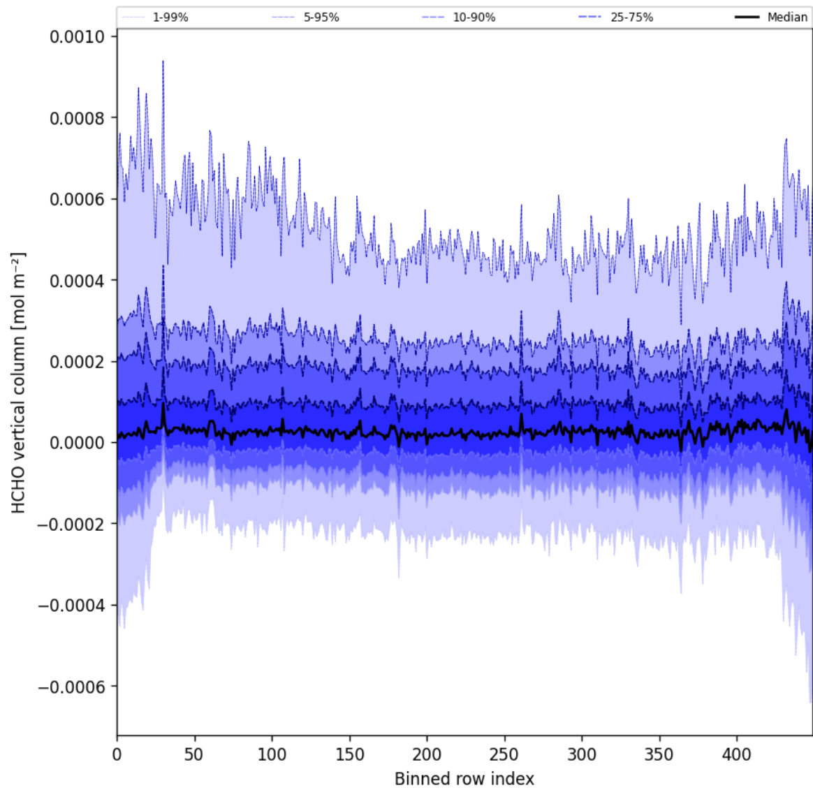
Figure 49: Along track statistics of “HCHO vertical column” for 2025-10-15 to 2025-10-17
