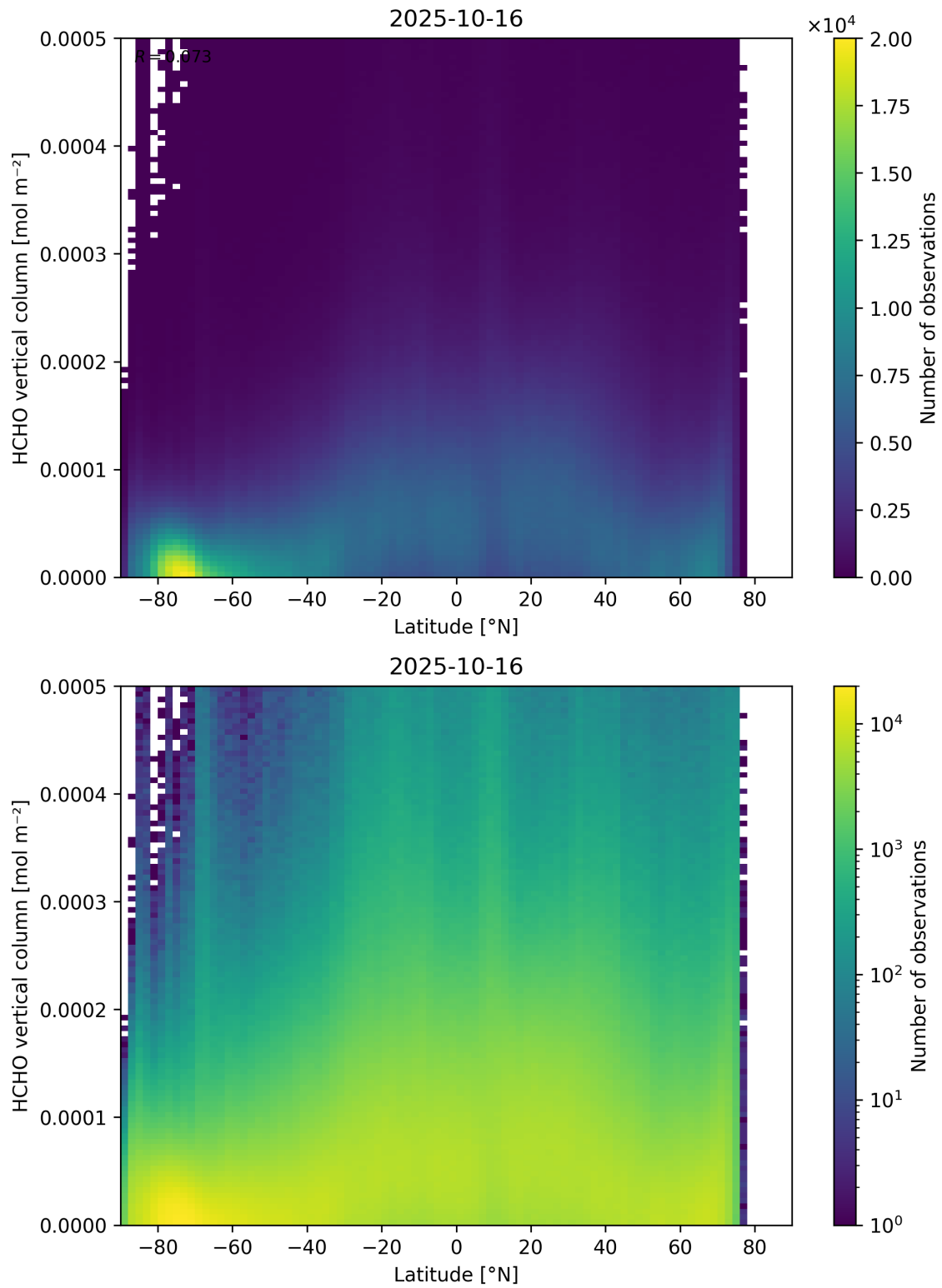
Figure 163: Scatter density plot of “Latitude” against “HCHO vertical column” for 2025-10-15 to 2025-10-17.
