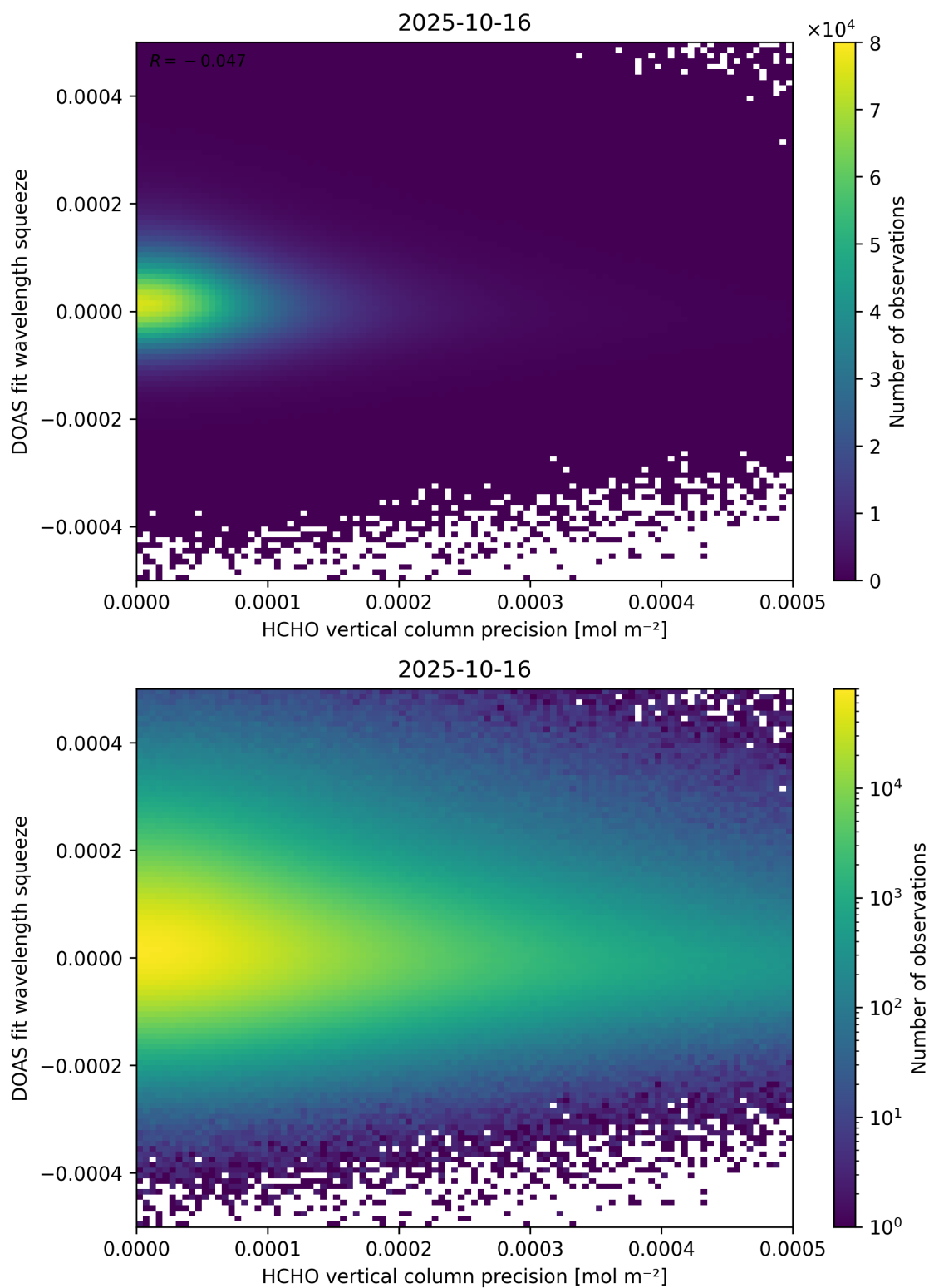
Figure 138: Scatter density plot of “HCHO vertical column precision” against “DOAS fit wavelength squeeze” for 2025-10-15 to 2025-10-17.
