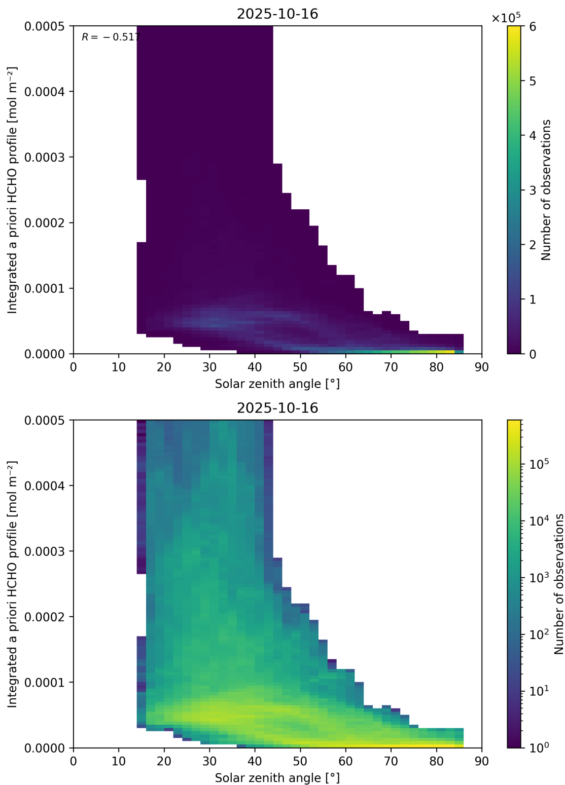
Figure 180: Scatter density plot of “Solar zenith angle” against “Integrated a priori HCHO profile” for 2025-10-15 to 2025-10-17.
