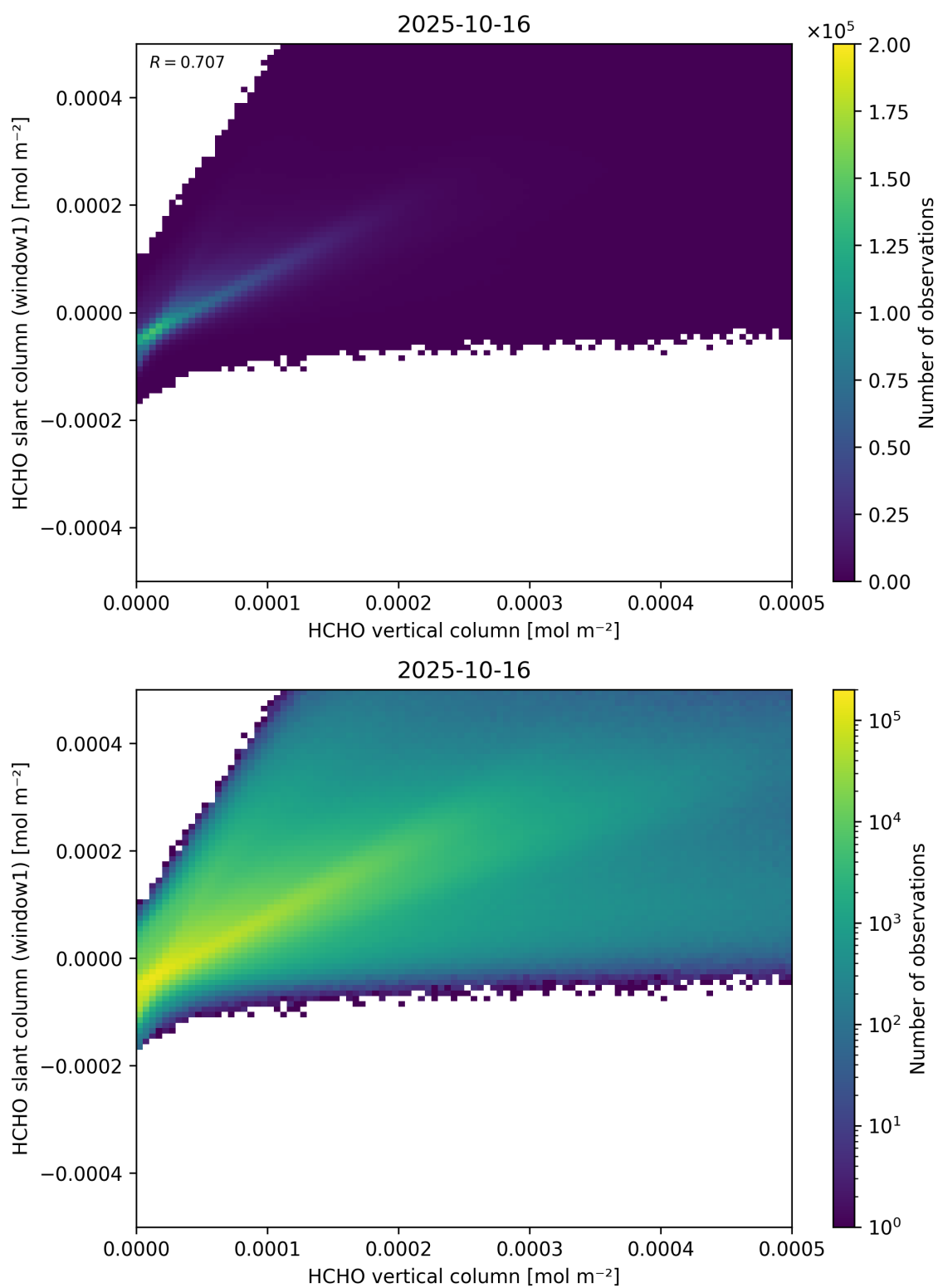
Figure 129: Scatter density plot of “HCHO vertical column” against “HCHO slant column (window1)” for 2025-10-15 to 2025-10-17.
