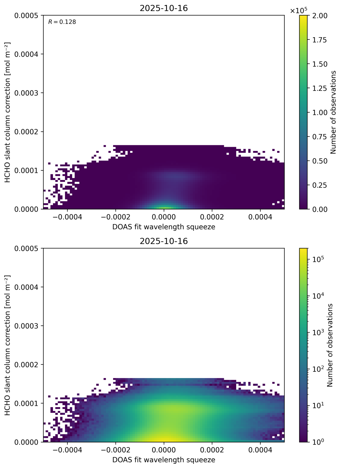
Figure 70: Scatter density plot of “DOAS fit wavelength squeeze” against “HCHO slant column correction” for 2025-10-15 to 2025-10-17.
