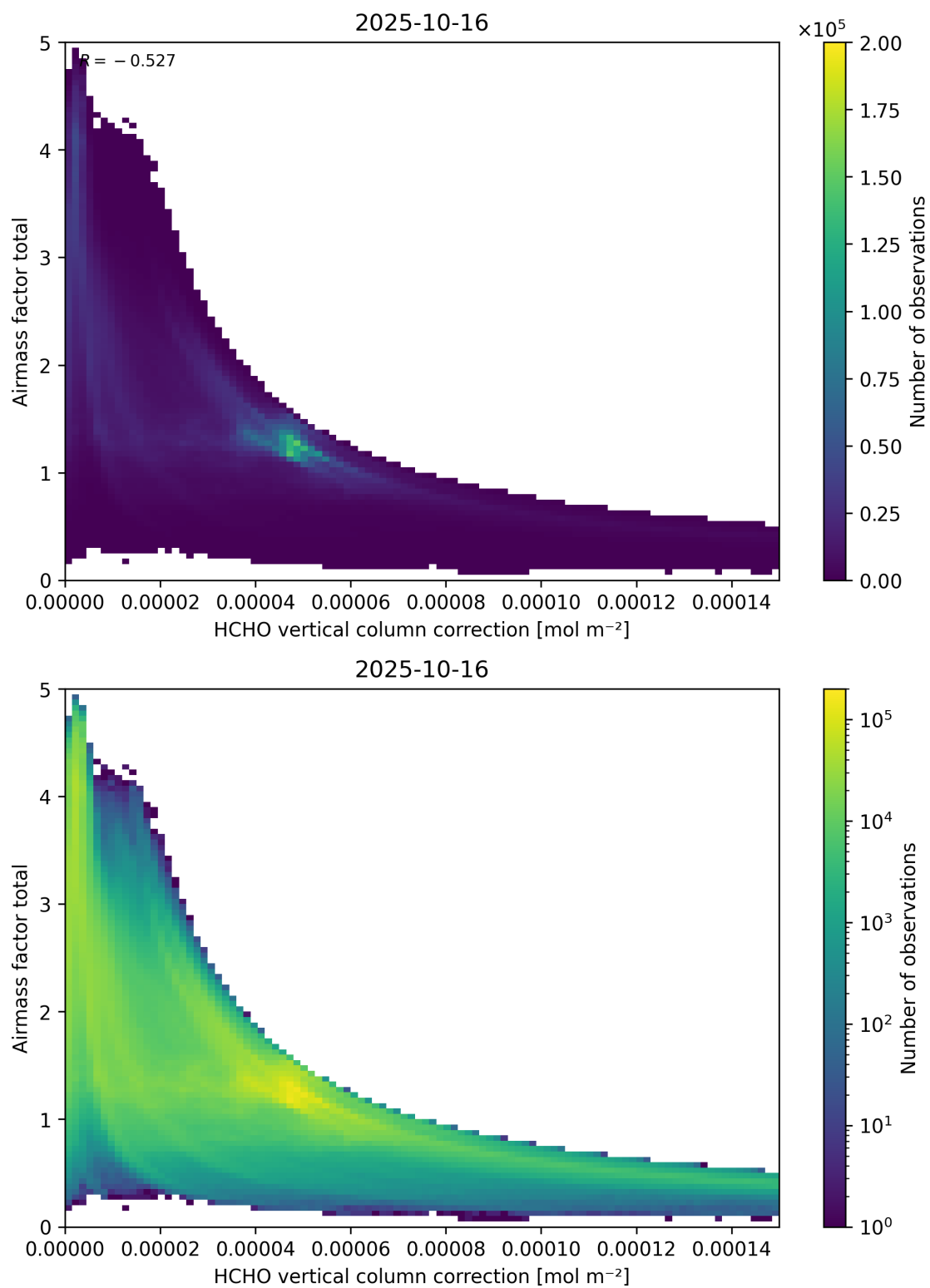
Figure 120: Scatter density plot of “HCHO vertical column correction” against “Airmass factor total” for 2025-10-15 to 2025-10-17.
