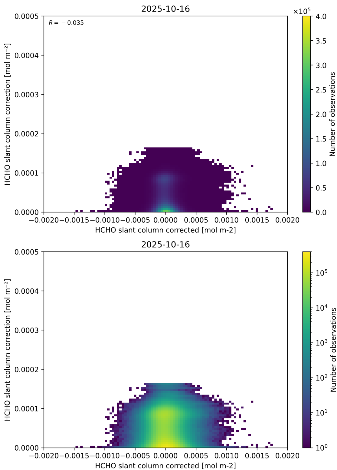
Figure 77: Scatter density plot of “HCHO slant column corrected” against “HCHO slant column correction” for 2025-10-15 to 2025-10-17.
