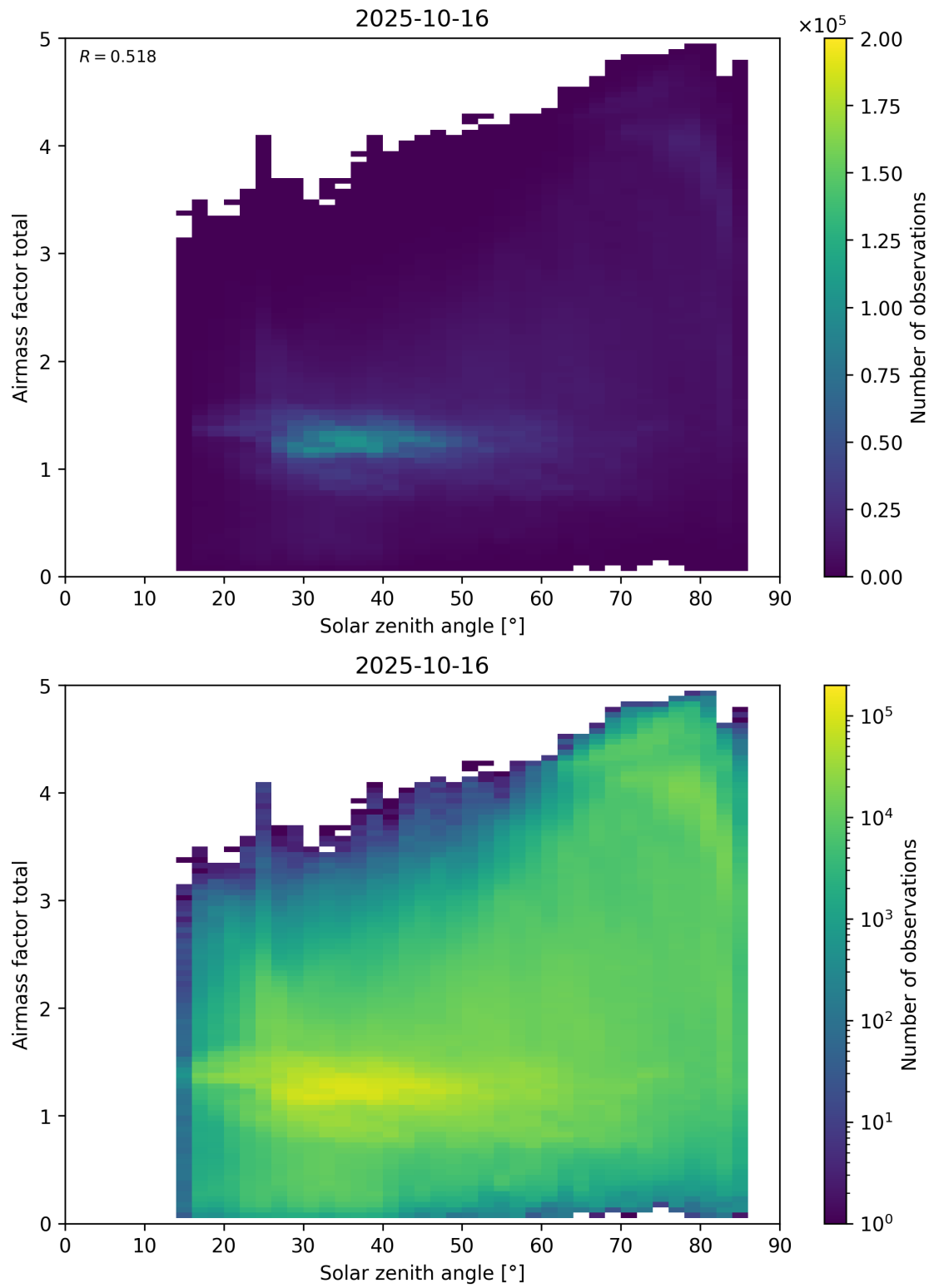
Figure 175: Scatter density plot of “Solar zenith angle” against “Airmass factor total” for 2025-10-15 to 2025-10-17.
