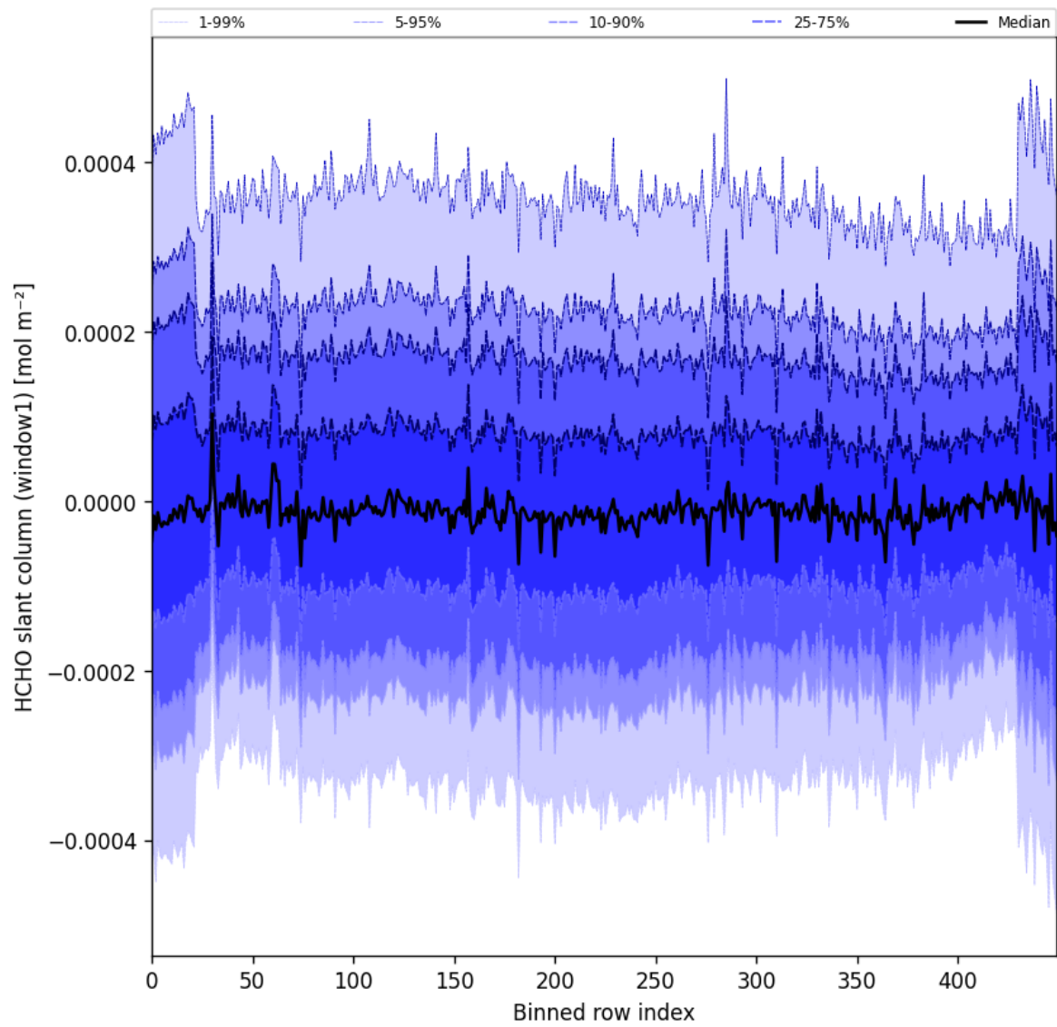
Figure 52: Along track statistics of “HCHO slant column (window1)” for 2025-10-15 to 2025-10-17
