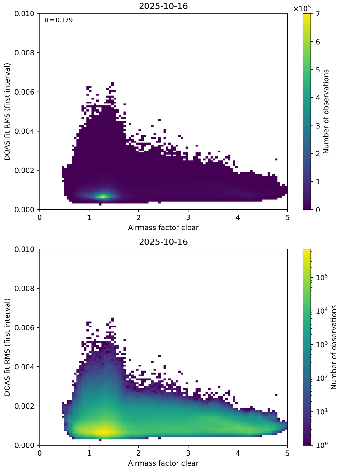
Figure 71: Scatter density plot of “Airmass factor clear” against “DOAS fit RMS (first interval)” for 2025-10-15 to 2025-10-17.
