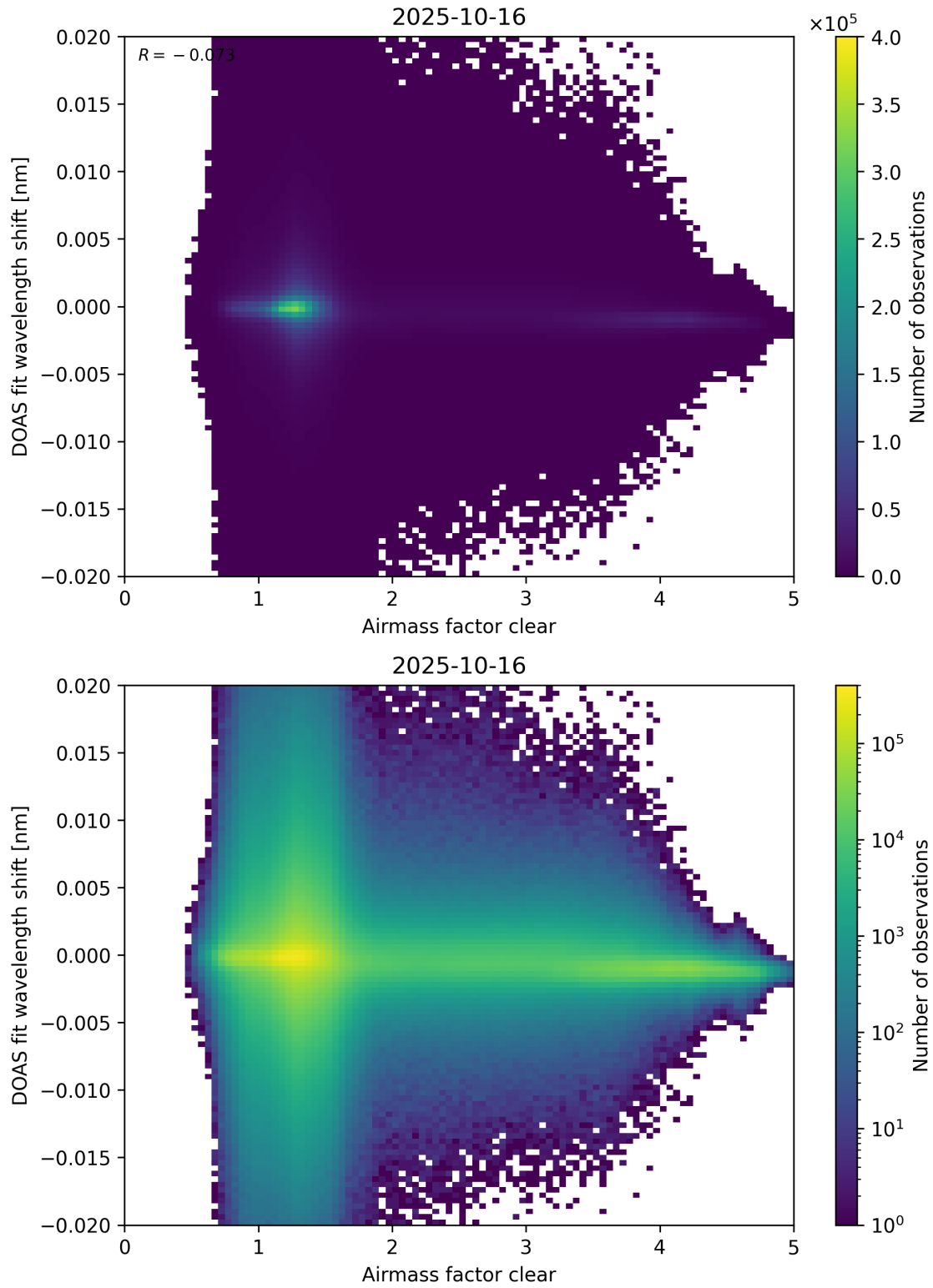
Figure 72: Scatter density plot of “Airmass factor clear” against “DOAS fit wavelength shift” for 2025-10-15 to 2025-10-17.
