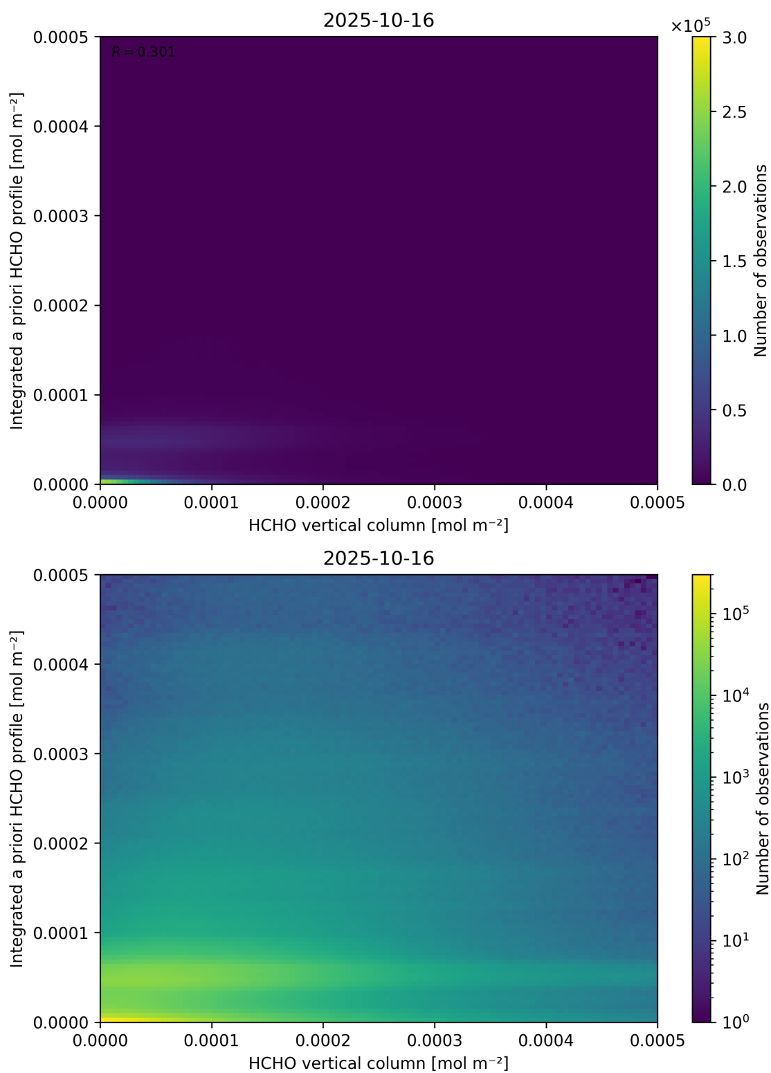
Figure 135: Scatter density plot of “HCHO vertical column” against “Integrated a priori HCHO profile” for 2025-10-15 to 2025-10-17.
