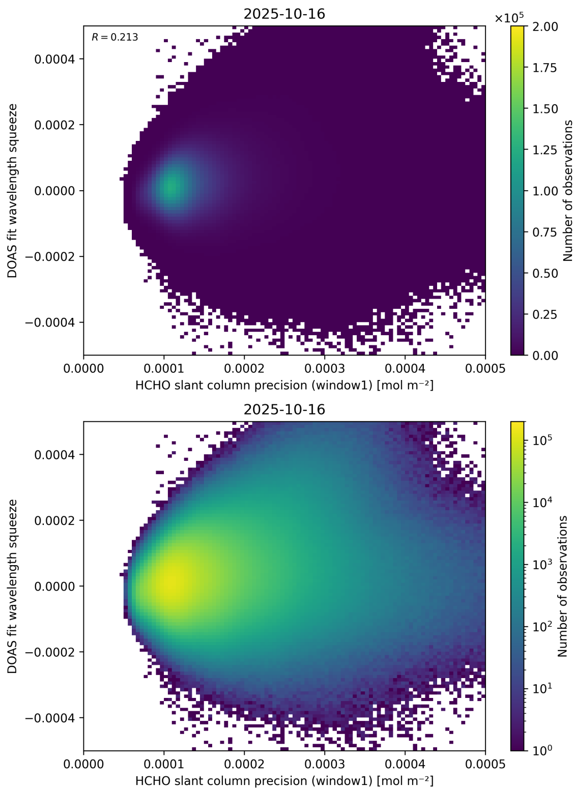
Figure 90: Scatter density plot of “HCHO slant column precision (window1)” against “DOAS fit wavelength squeeze” for 2025-10-15 to 2025-10-17.
