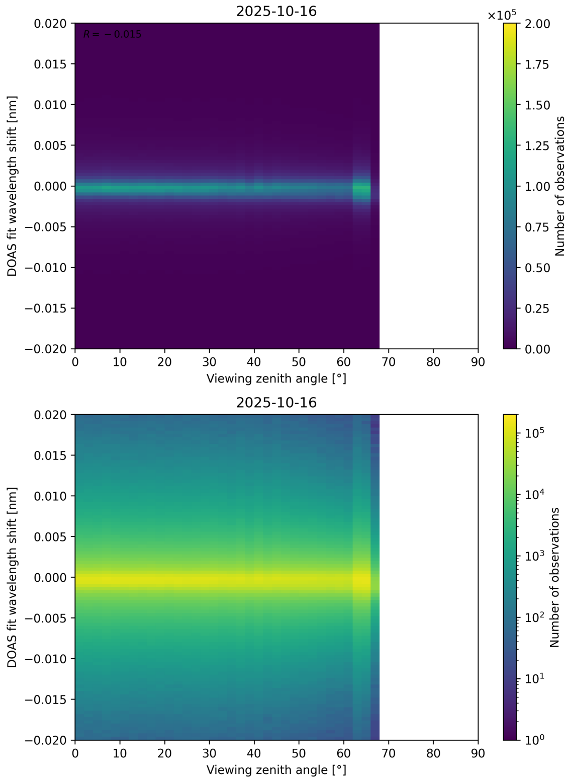
Figure 183: Scatter density plot of “Viewing zenith angle” against “DOAS fit wavelength shift” for 2025-10-15 to 2025-10-17.
