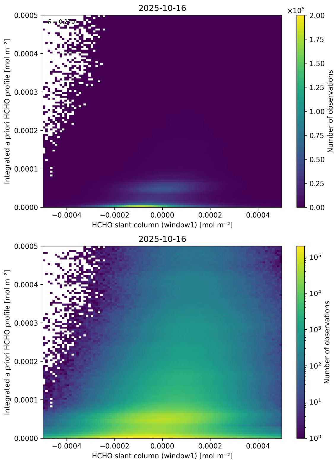
Figure 87: Scatter density plot of “HCHO slant column (window1)” against “Integrated a priori HCHO profile” for 2025-10-15 to 2025-10-17.
