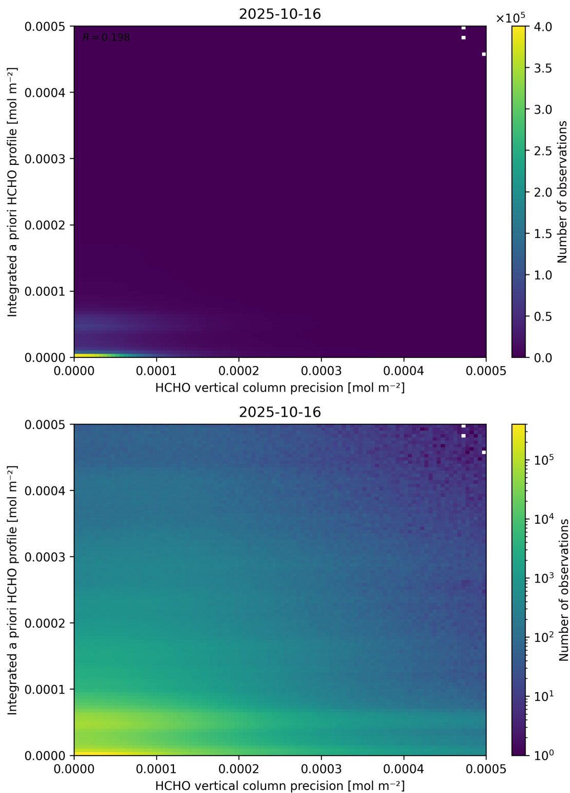
Figure 147: Scatter density plot of “HCHO vertical column precision” against “Integrated a priori HCHO profile” for 2025-10-15 to 2025-10-17.
