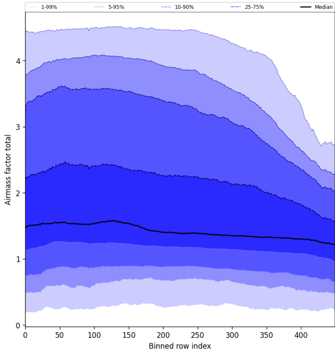
Figure 54: Along track statistics of “Airmass factor total” for 2025-10-15 to 2025-10-17
