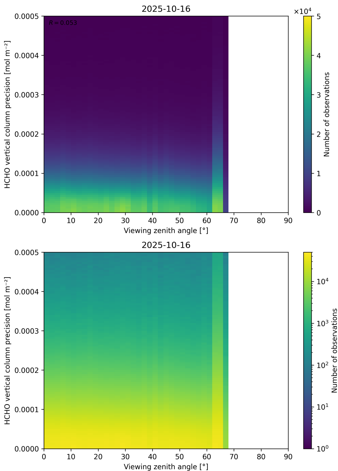
Figure 194: Scatter density plot of “Viewing zenith angle” against “HCHO vertical column precision” for 2025-10-15 to 2025-10-17.
