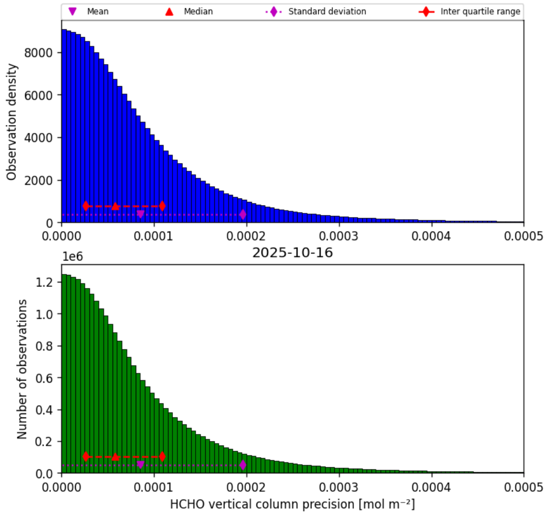
Figure 36: Histogram of “HCHO vertical column precision” for 2025-10-15 to 2025-10-17
