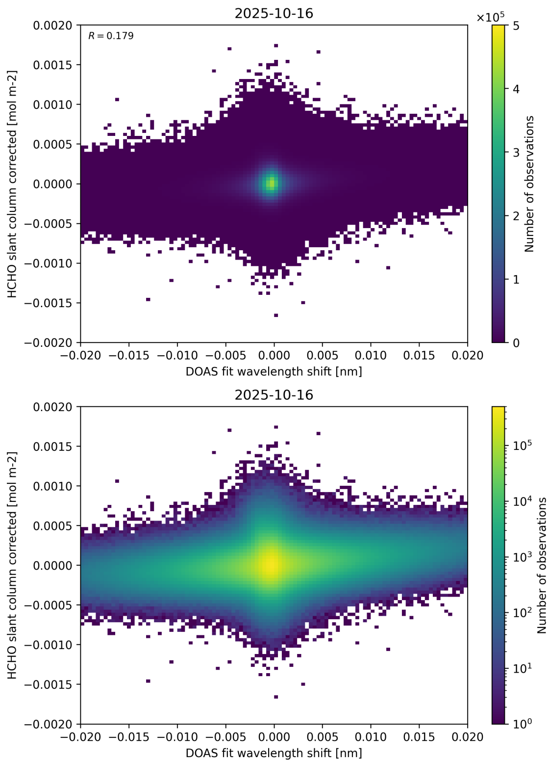
Figure 66: Scatter density plot of “DOAS fit wavelength shift” against “HCHO slant column corrected” for 2025-10-15 to 2025-10-17.
