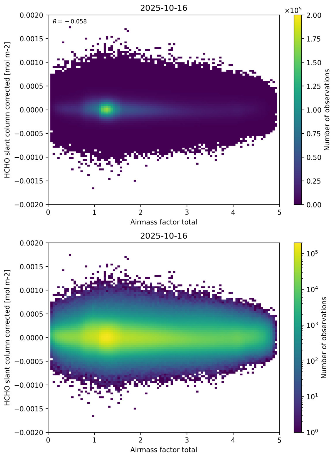
Figure 101: Scatter density plot of “Airmass factor total” against “HCHO slant column corrected” for 2025-10-15 to 2025-10-17.
