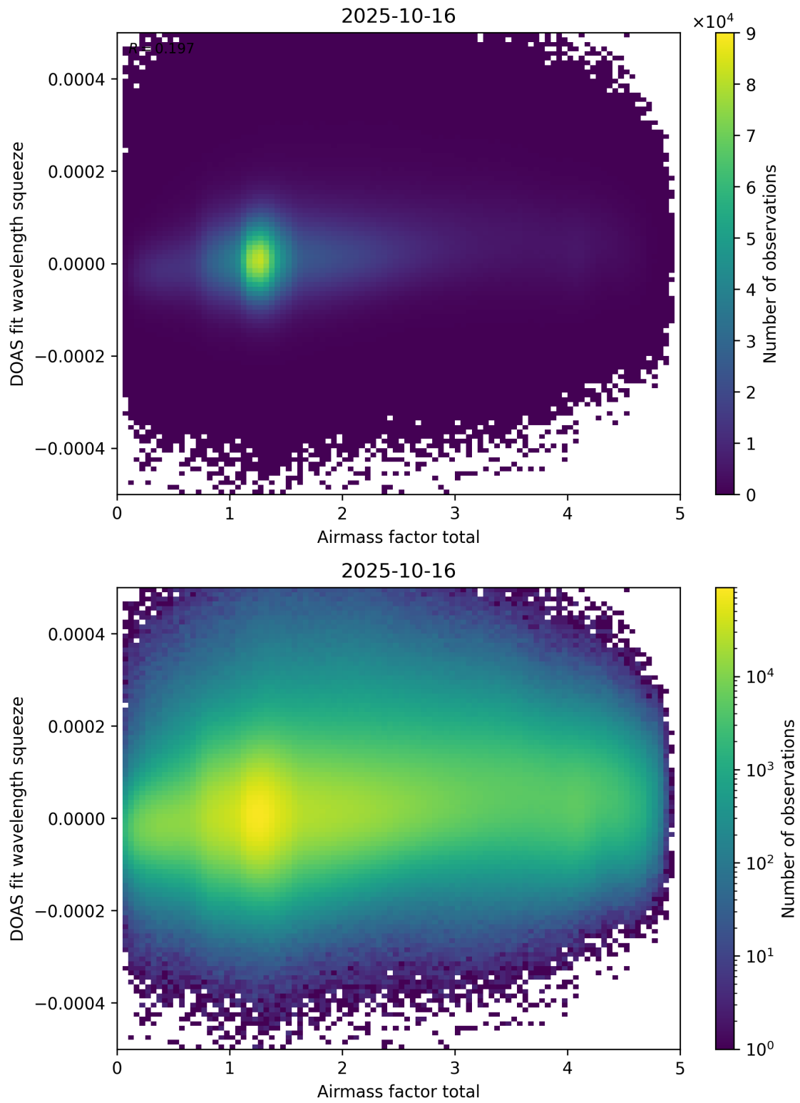
Figure 99: Scatter density plot of “Airmass factor total” against “DOAS fit wavelength squeeze” for 2025-10-15 to 2025-10-17.
