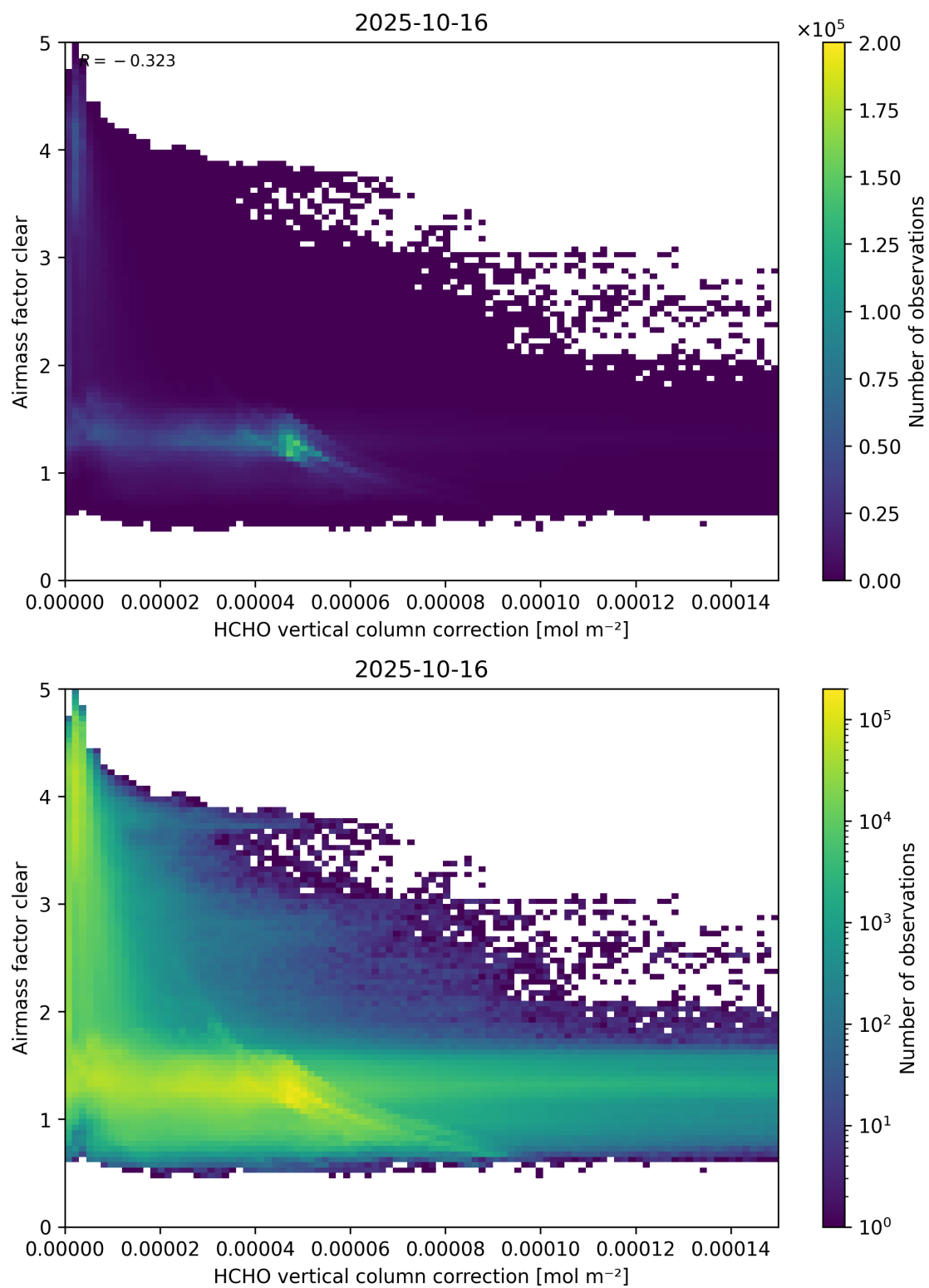
Figure 115: Scatter density plot of “HCHO vertical column correction” against “Airmass factor clear” for 2025-10-15 to 2025-10-17.
