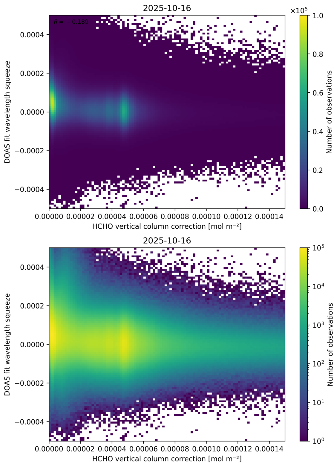
Figure 114: Scatter density plot of “HCHO vertical column correction” against “DOAS fit wavelength squeeze” for 2025-10-15 to 2025-10-17.
