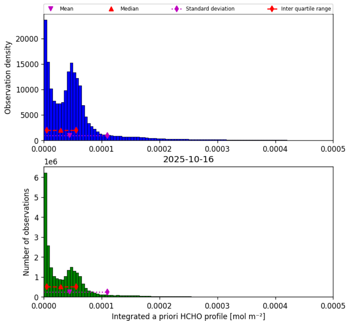
Figure 43: Histogram of “Integrated a priori HCHO profile” for 2025-10-15 to 2025-10-17
