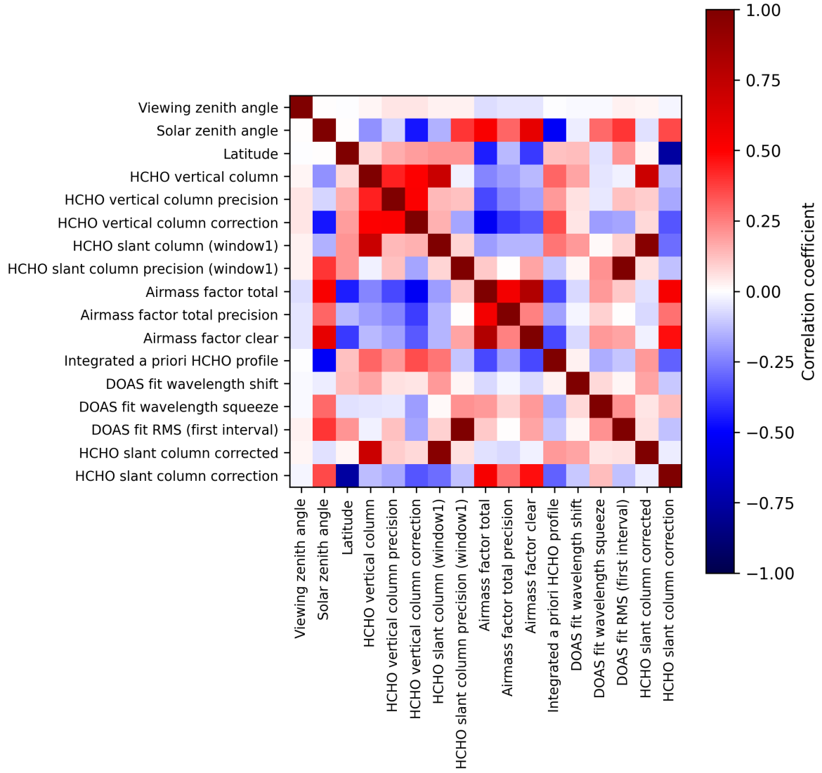
Figure 2: Map of correlation matrix for 2025-10-15 to 2025-10-17.
