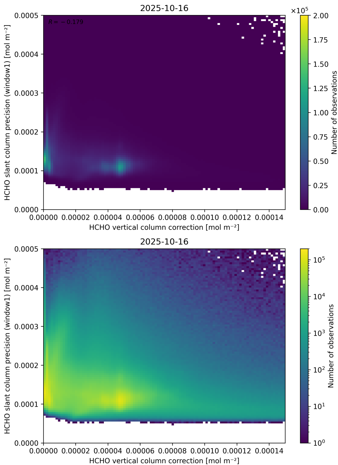
Figure 119: Scatter density plot of “HCHO vertical column correction” against “HCHO slant column precision (window1)” for 2025-10-15 to 2025-10-17.
