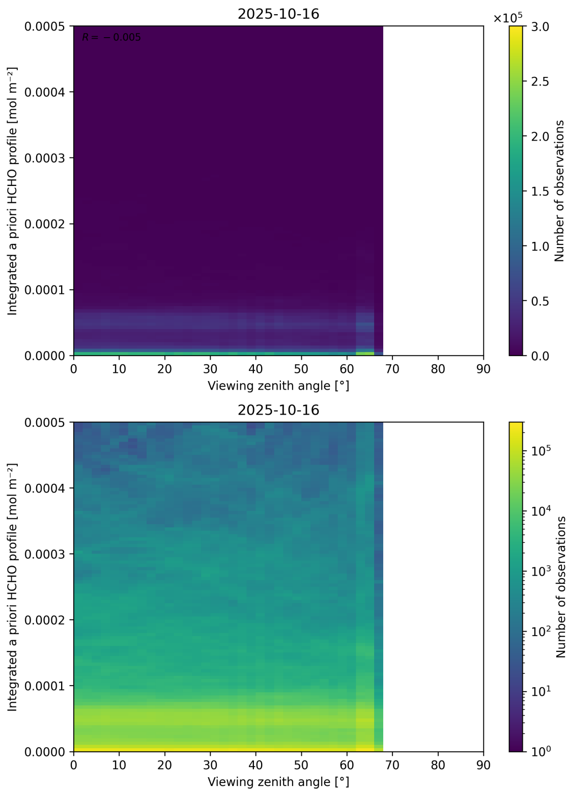
Figure 195: Scatter density plot of “Viewing zenith angle” against “Integrated a priori HCHO profile” for 2025-10-15 to 2025-10-17.
