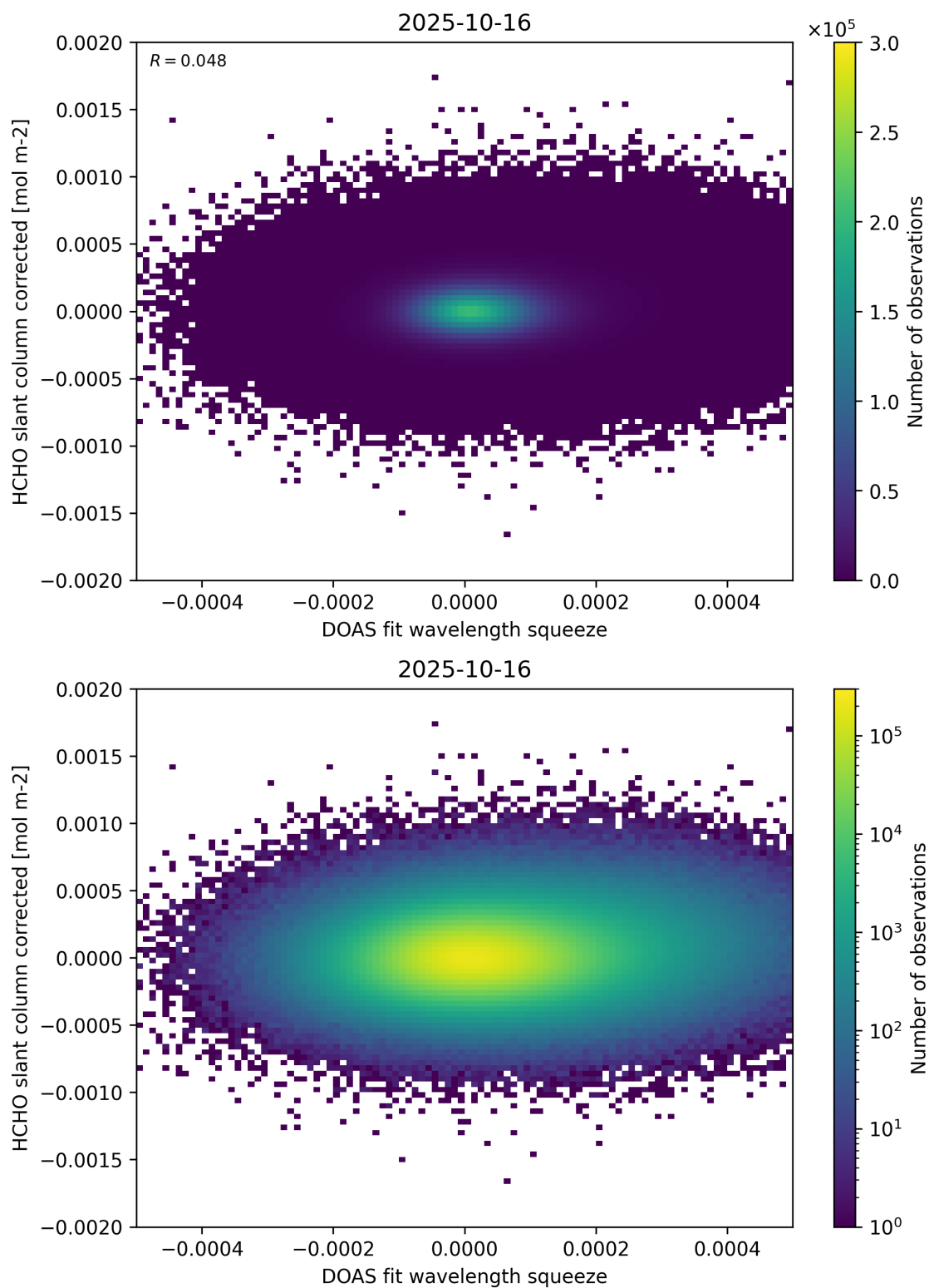
Figure 69: Scatter density plot of “DOAS fit wavelength squeeze” against “HCHO slant column corrected” for 2025-10-15 to 2025-10-17.
