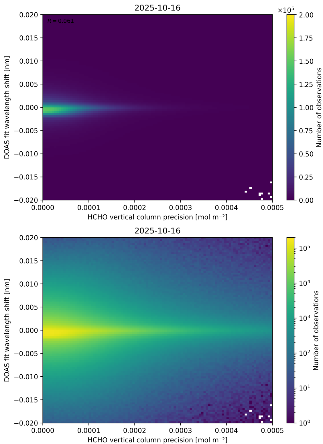
Figure 137: Scatter density plot of “HCHO vertical column precision” against “DOAS fit wavelength shift” for 2025-10-15 to 2025-10-17.
