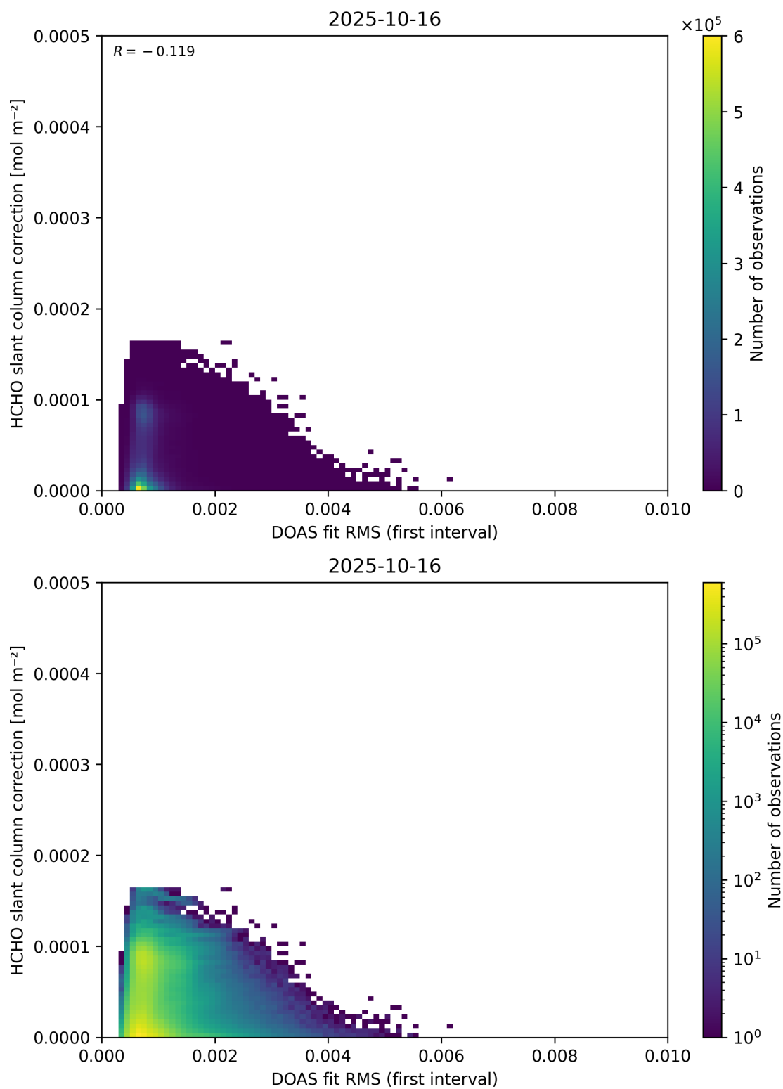
Figure 63: Scatter density plot of “DOAS fit RMS (first interval)” against “HCHO slant column correction” for 2025-10-15 to 2025-10-17.
