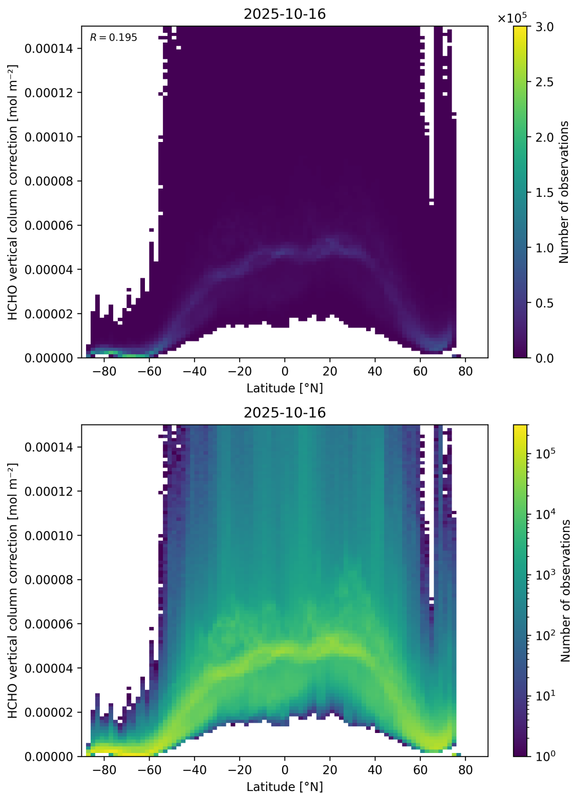
Figure 164: Scatter density plot of “Latitude” against “HCHO vertical column correction” for 2025-10-15 to 2025-10-17.
