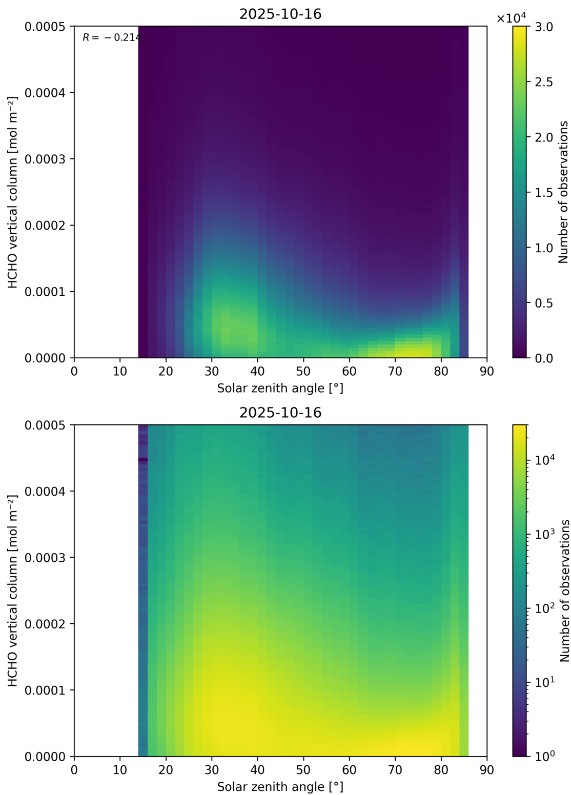
Figure 177: Scatter density plot of “Solar zenith angle” against “HCHO vertical column” for 2025-10-15 to 2025-10-17.
