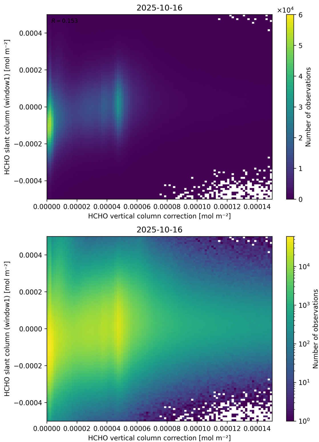
Figure 118: Scatter density plot of “HCHO vertical column correction” against “HCHO slant column (window1)” for 2025-10-15 to 2025-10-17.
