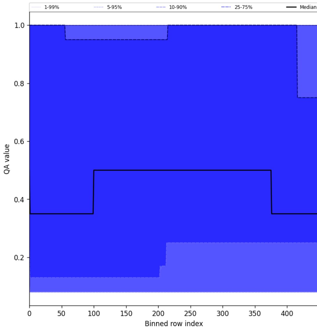
Figure 48: Along track statistics of “QA value” for 2025-10-15 to 2025-10-17
