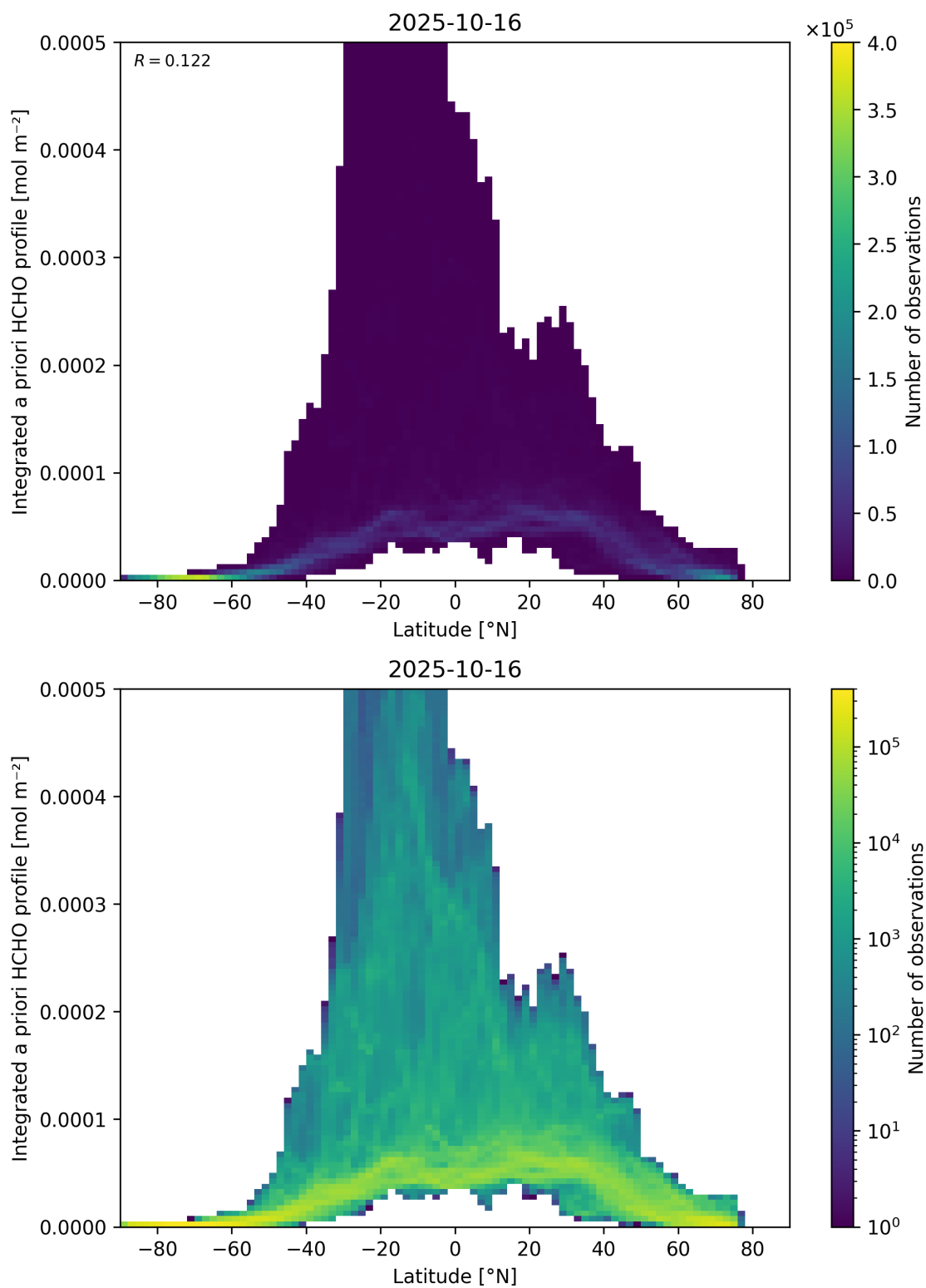
Figure 166: Scatter density plot of “Latitude” against “Integrated a priori HCHO profile” for 2025-10-15 to 2025-10-17.
