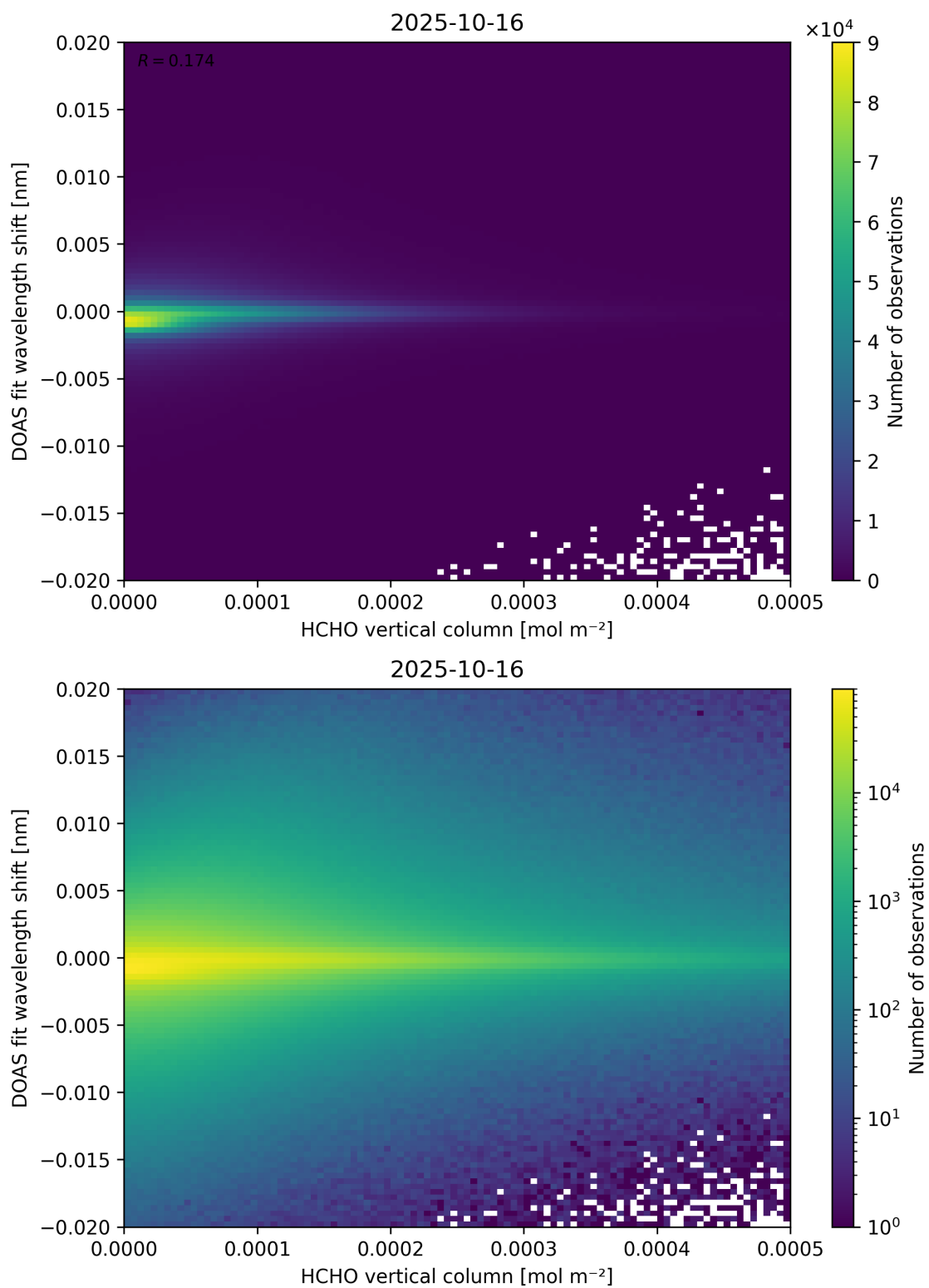
Figure 124: Scatter density plot of “HCHO vertical column” against “DOAS fit wavelength shift” for 2025-10-15 to 2025-10-17.
