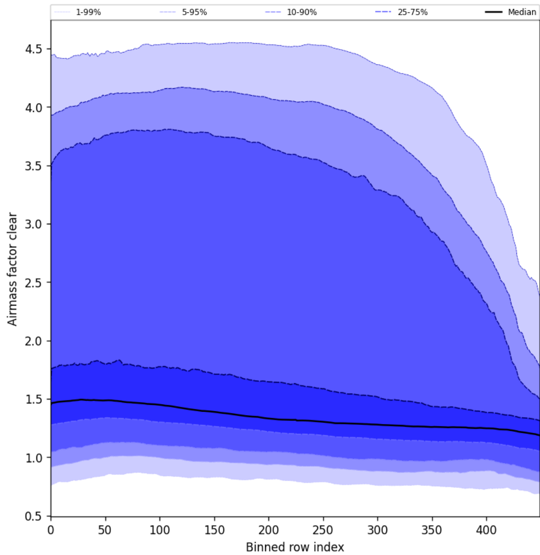
Figure 56: Along track statistics of “Airmass factor clear” for 2025-10-15 to 2025-10-17
