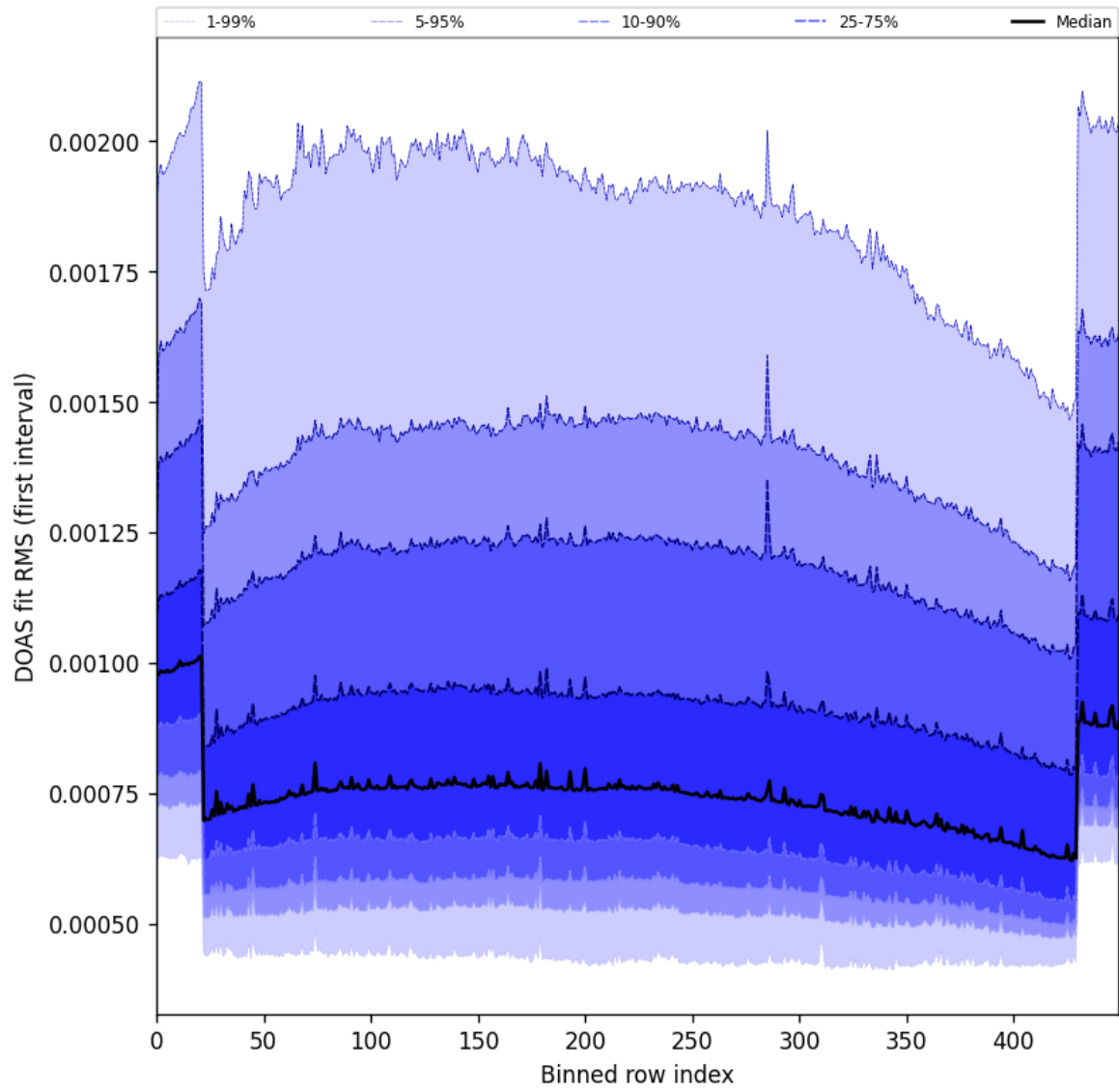
Figure 60: Along track statistics of “DOAS fit RMS (first interval)” for 2025-10-15 to 2025-10-17
