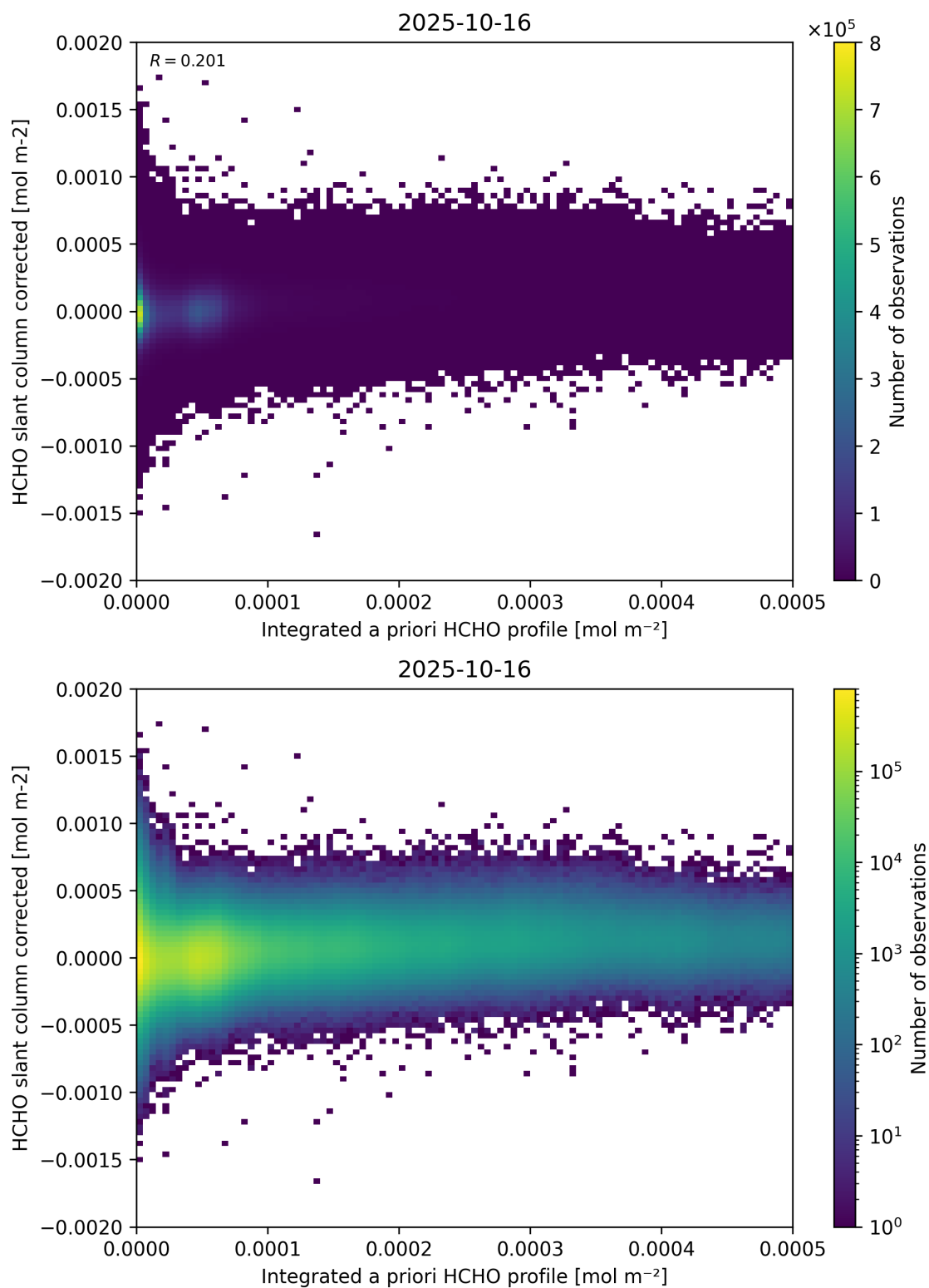
Figure 151: Scatter density plot of “Integrated a priori HCHO profile” against “HCHO slant column corrected” for 2025-10-15 to 2025-10-17.
