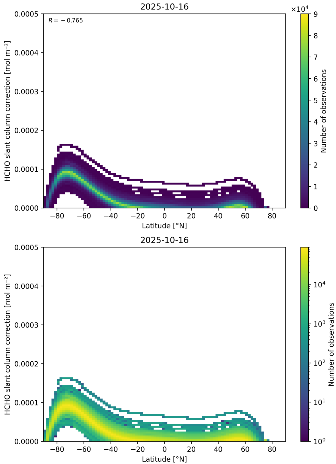
Figure 158: Scatter density plot of “Latitude” against “HCHO slant column correction” for 2025-10-15 to 2025-10-17.
