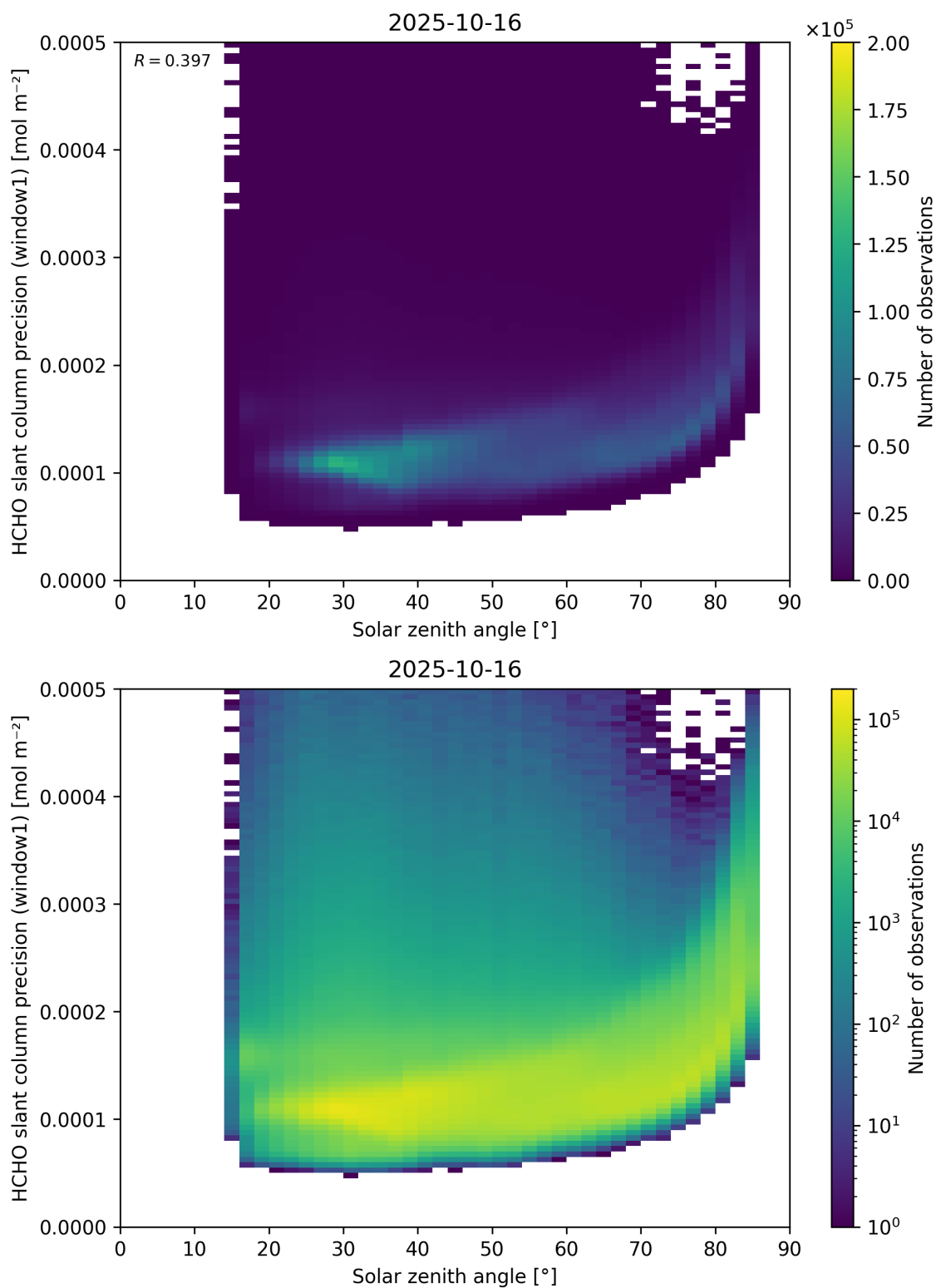
Figure 174: Scatter density plot of “Solar zenith angle” against “HCHO slant column precision (window1)” for 2025-10-15 to 2025-10-17.
