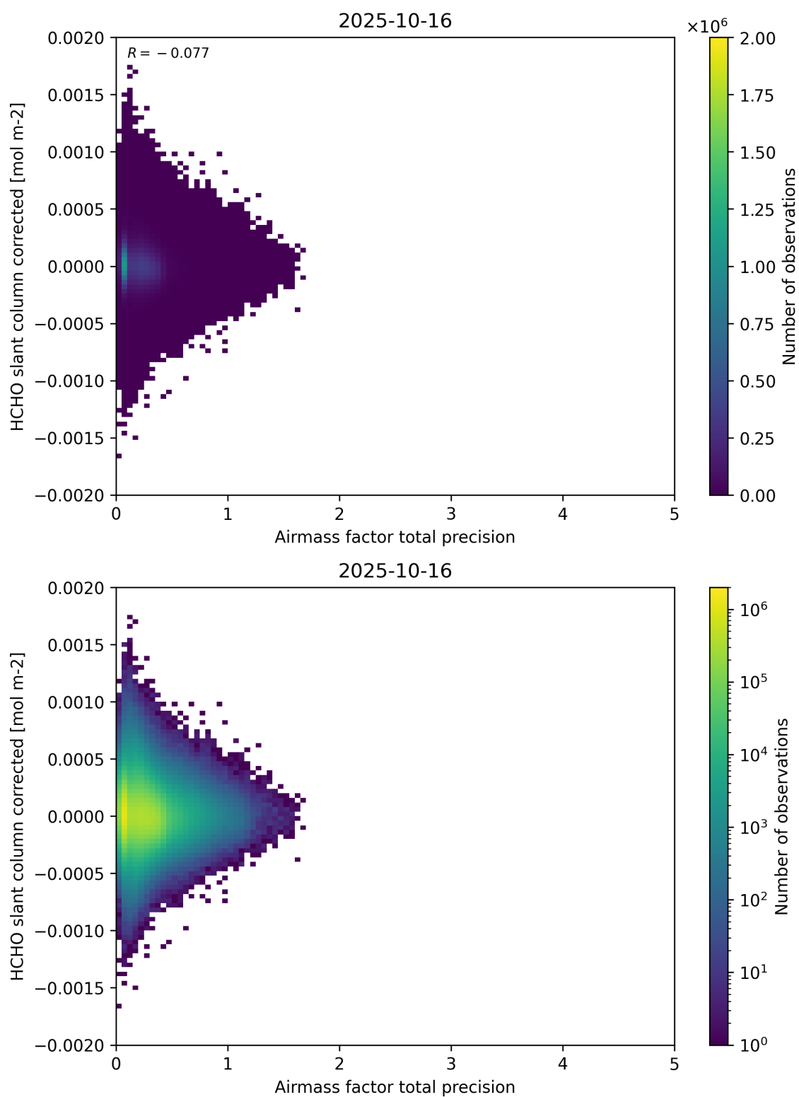
Figure 109: Scatter density plot of “Airmass factor total precision” against “HCHO slant column corrected” for 2025-10-15 to 2025-10-17.
