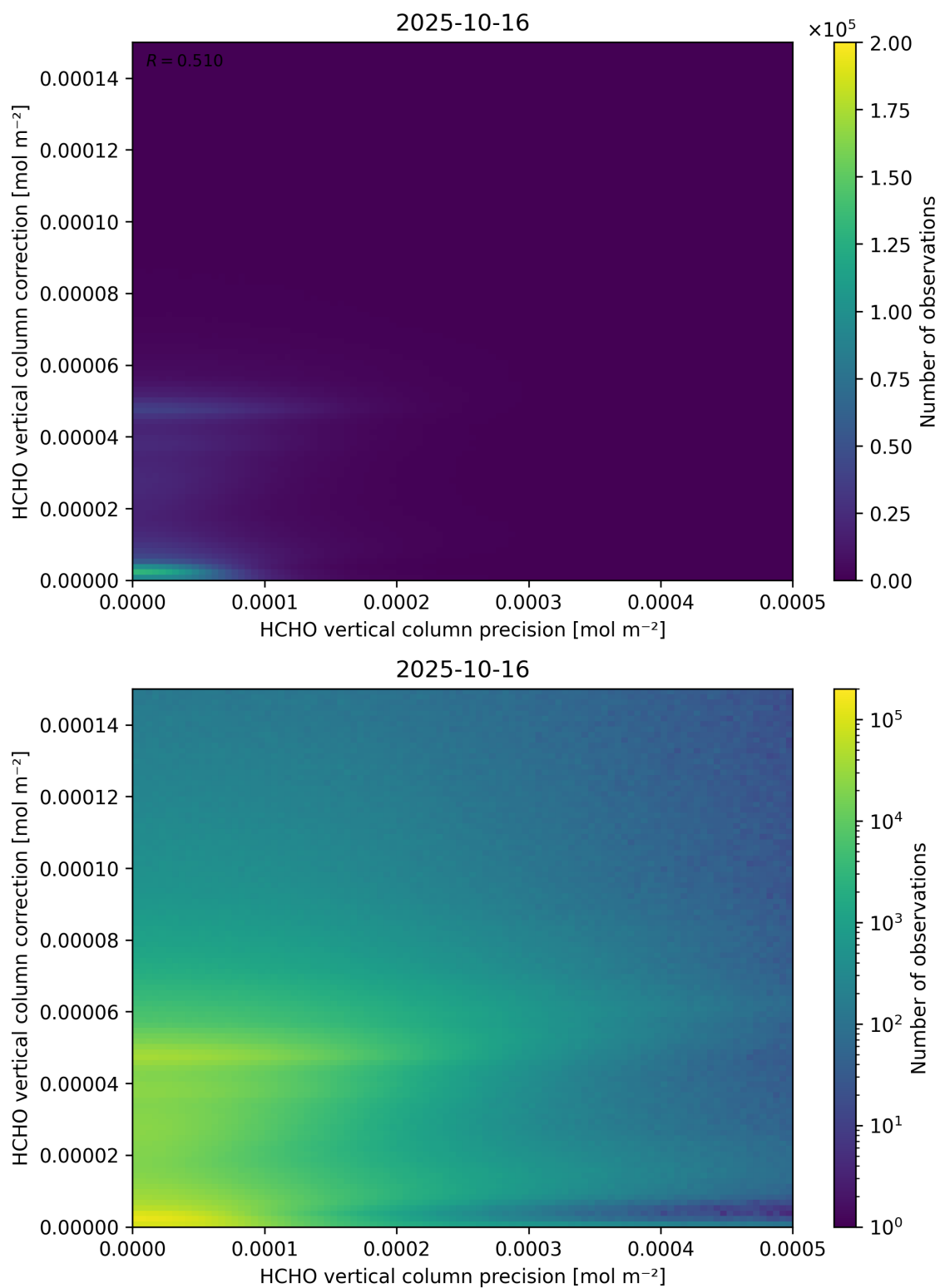
Figure 146: Scatter density plot of “HCHO vertical column precision” against “HCHO vertical column correction” for 2025-10-15 to 2025-10-17.
