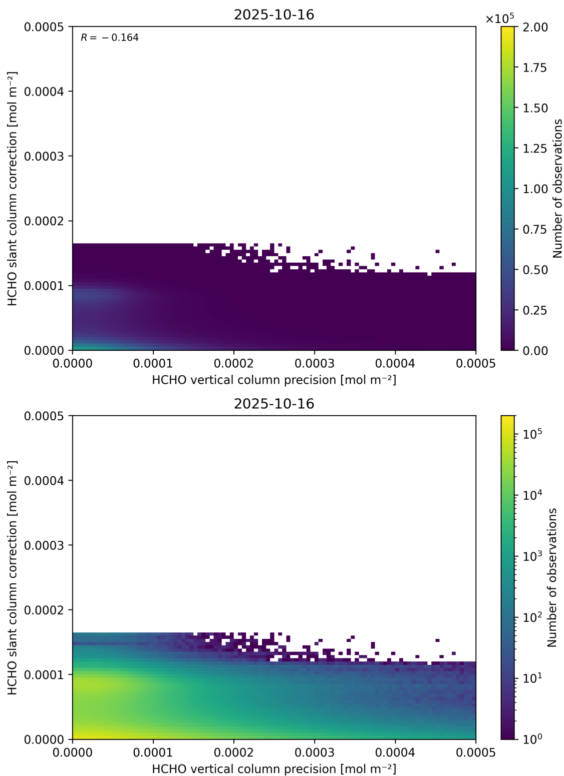
Figure 141: Scatter density plot of “HCHO vertical column precision” against “HCHO slant column correction” for 2025-10-15 to 2025-10-17.
