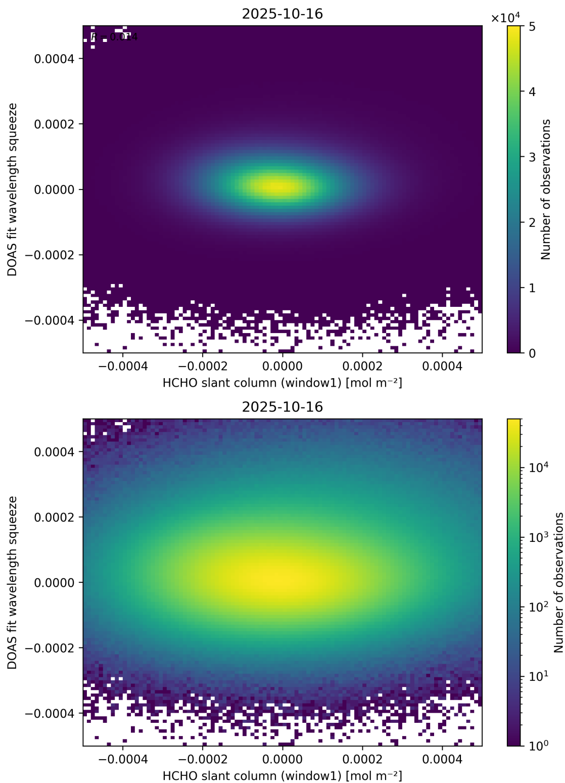
Figure 80: Scatter density plot of “HCHO slant column (window1)” against “DOAS fit wavelength squeeze” for 2025-10-15 to 2025-10-17.
