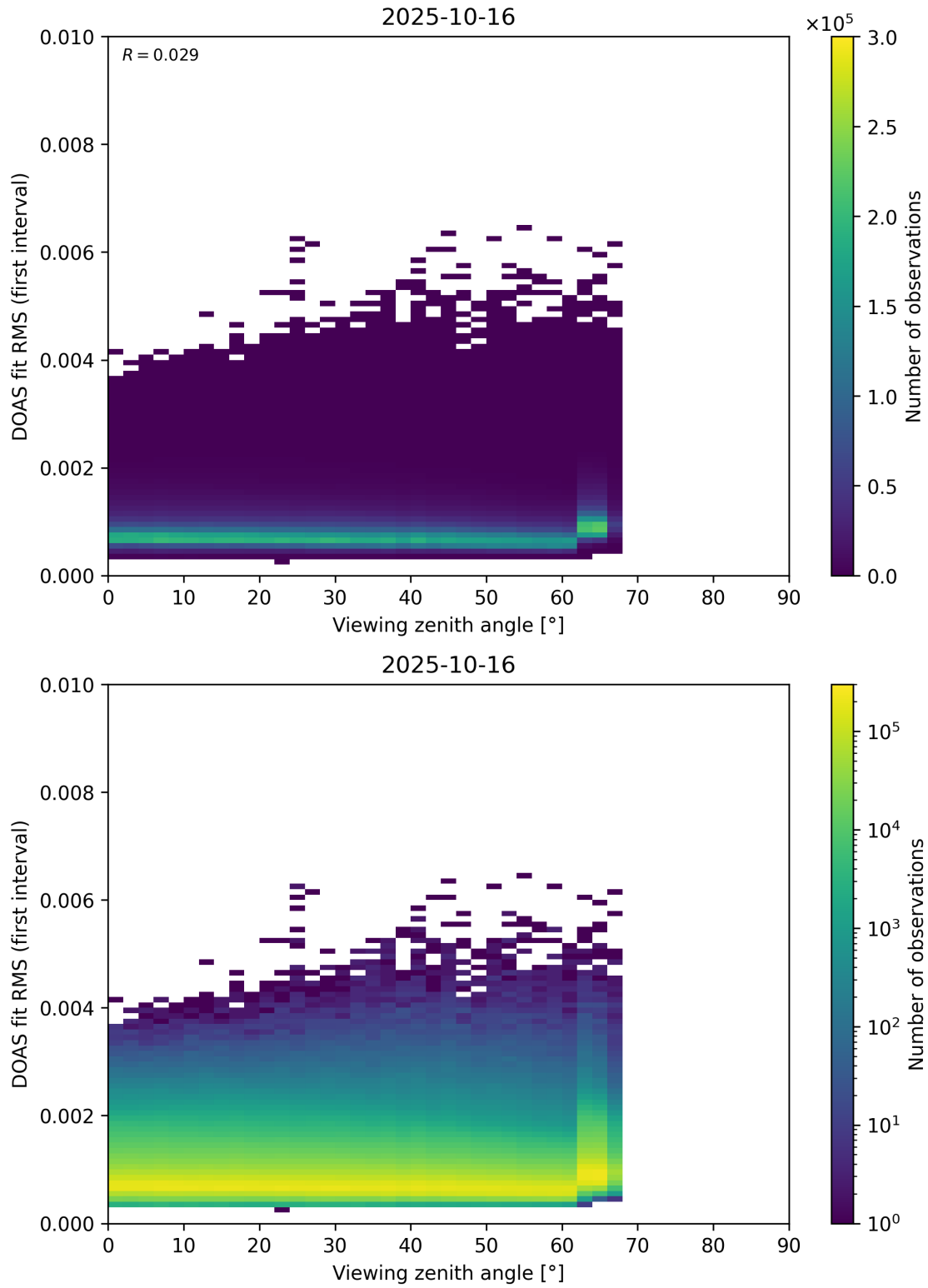
Figure 182: Scatter density plot of “Viewing zenith angle” against “DOAS fit RMS (first interval)” for 2025-10-15 to 2025-10-17.
