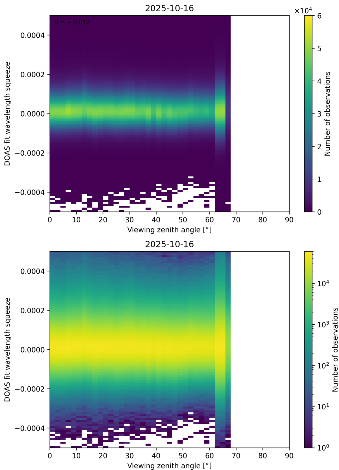
Figure 184: Scatter density plot of “Viewing zenith angle” against “DOAS fit wavelength squeeze” for 2025-10-15 to 2025-10-17.
