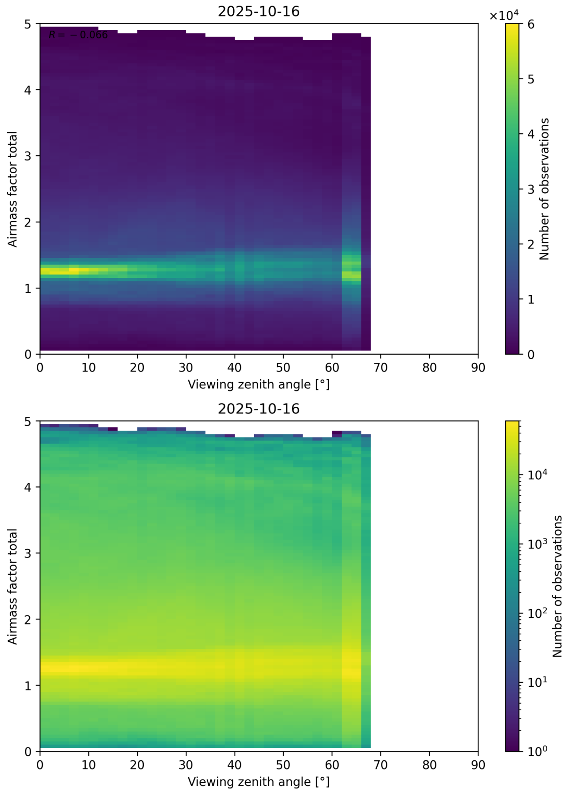
Figure 190: Scatter density plot of “Viewing zenith angle” against “Airmass factor total” for 2025-10-15 to 2025-10-17.
