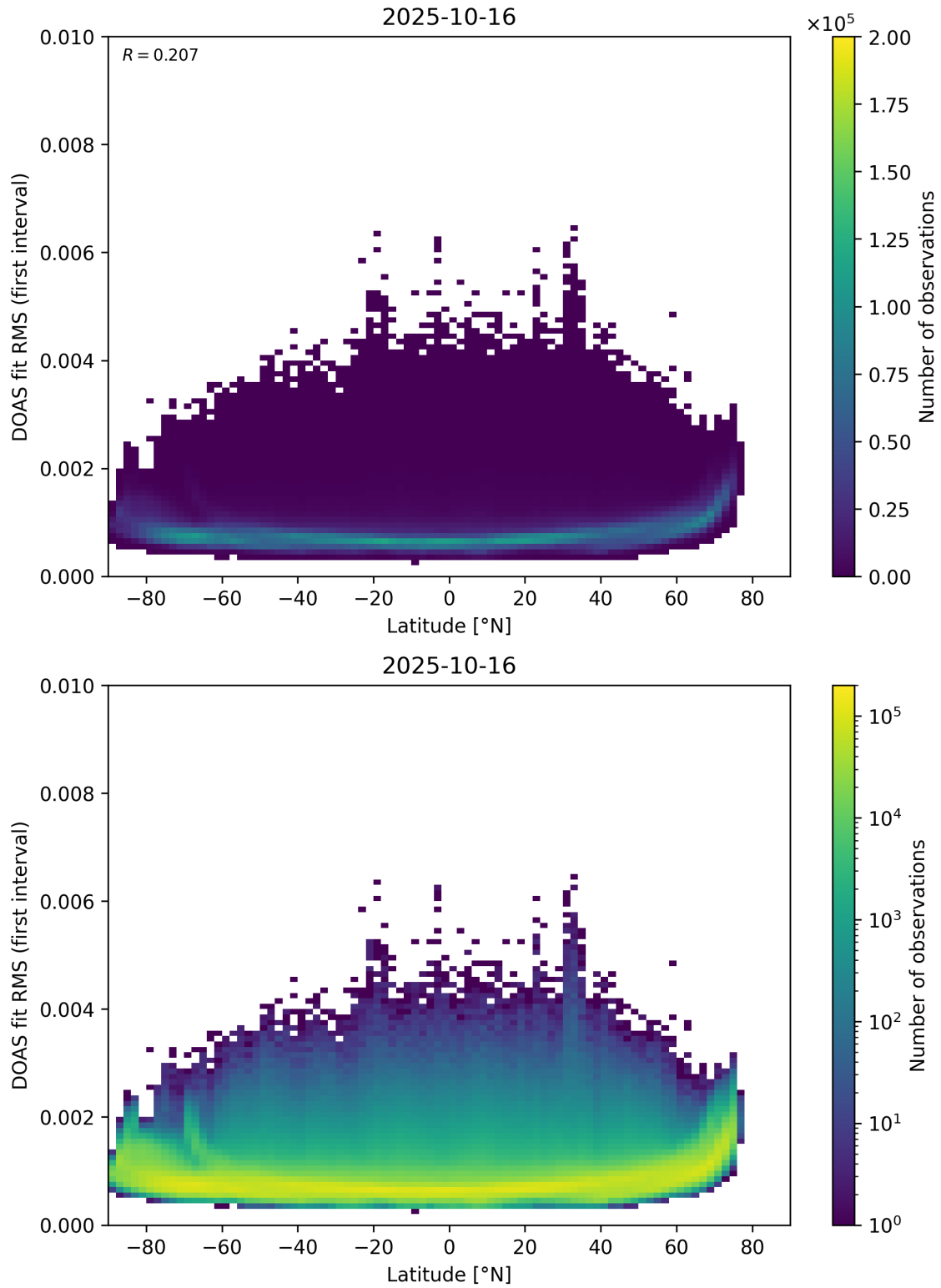
Figure 153: Scatter density plot of “Latitude” against “DOAS fit RMS (first interval)” for 2025-10-15 to 2025-10-17.
