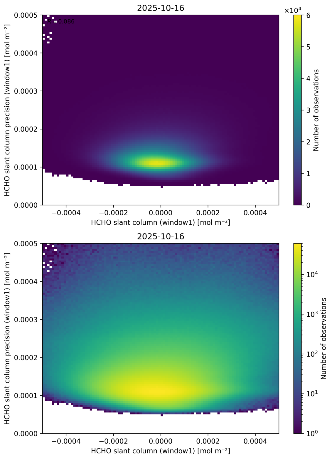
Figure 84: Scatter density plot of “HCHO slant column (window1)” against “HCHO slant column precision (window1)” for 2025-10-15 to 2025-10-17.
