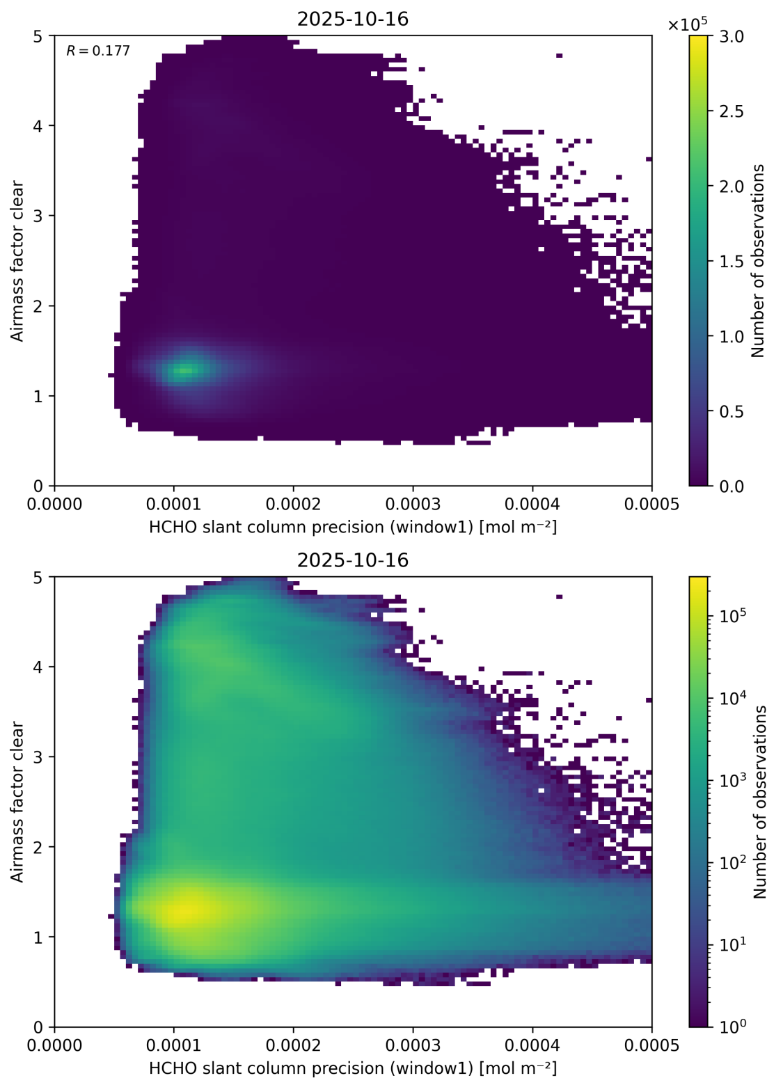
Figure 91: Scatter density plot of “HCHO slant column precision (window1)” against “Airmass factor clear” for 2025-10-15 to 2025-10-17.
