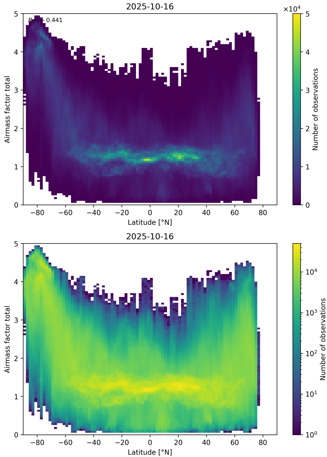
Figure 161: Scatter density plot of “Latitude” against “Airmass factor total” for 2025-10-15 to 2025-10-17.
