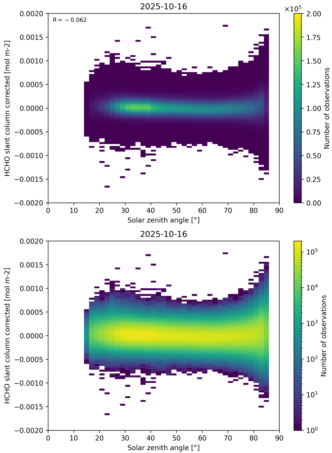
Figure 171: Scatter density plot of “Solar zenith angle” against “HCHO slant column corrected” for 2025-10-15 to 2025-10-17.
