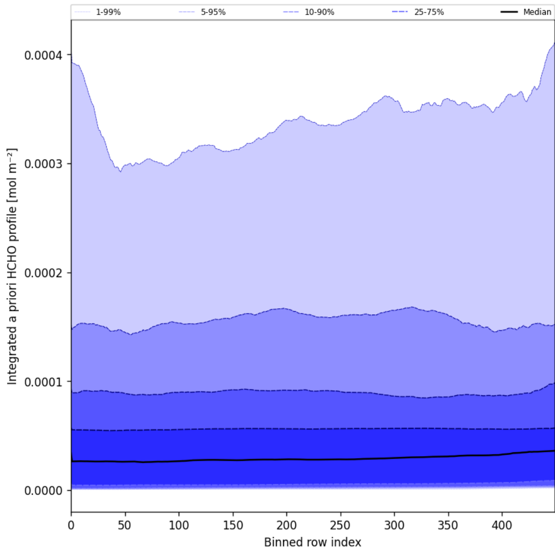
Figure 57: Along track statistics of “Integrated a priori HCHO profile” for 2025-10-15 to 2025-10-17
