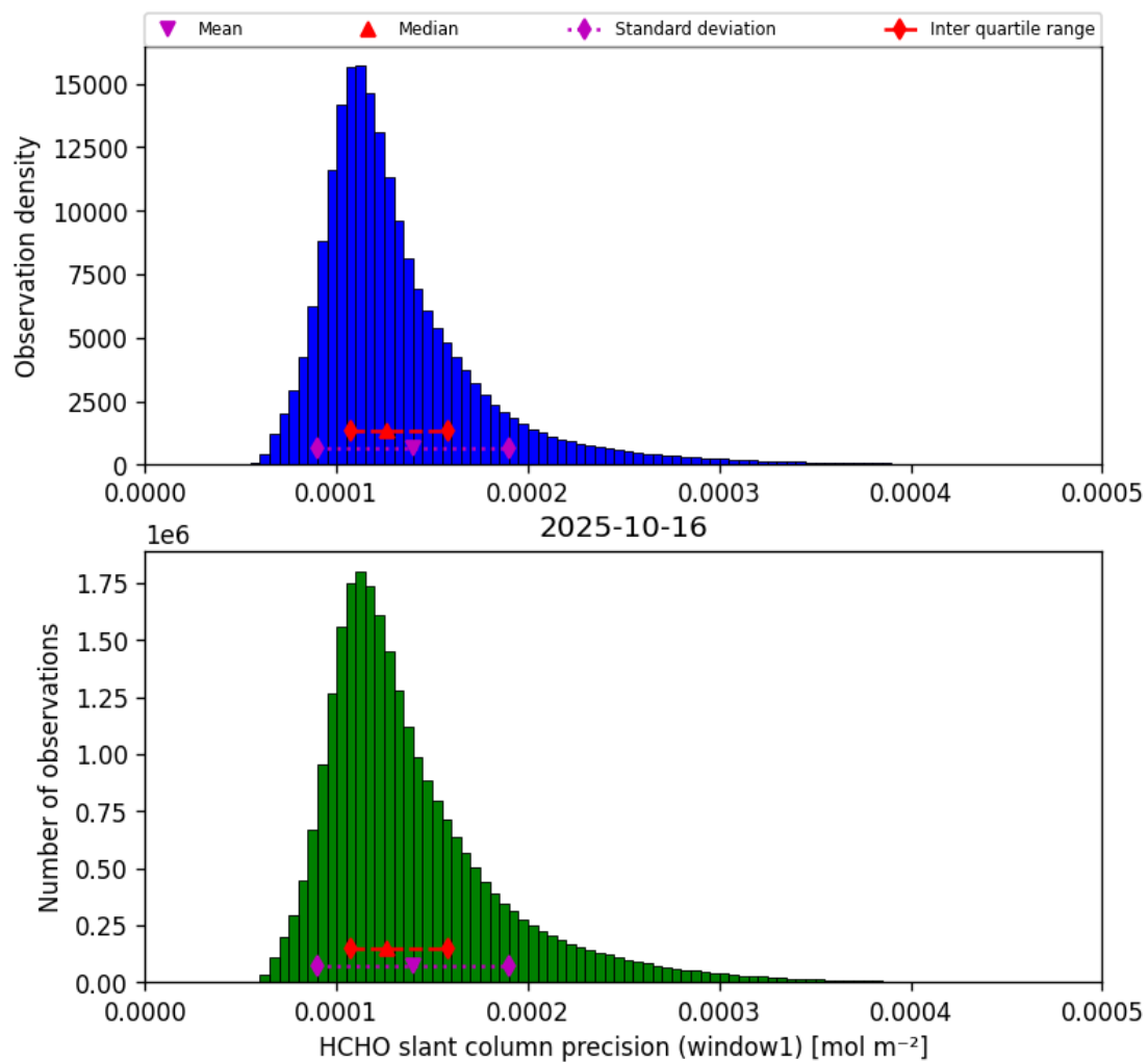
Figure 39: Histogram of “HCHO slant column precision (window1)” for 2025-10-15 to 2025-10-17
