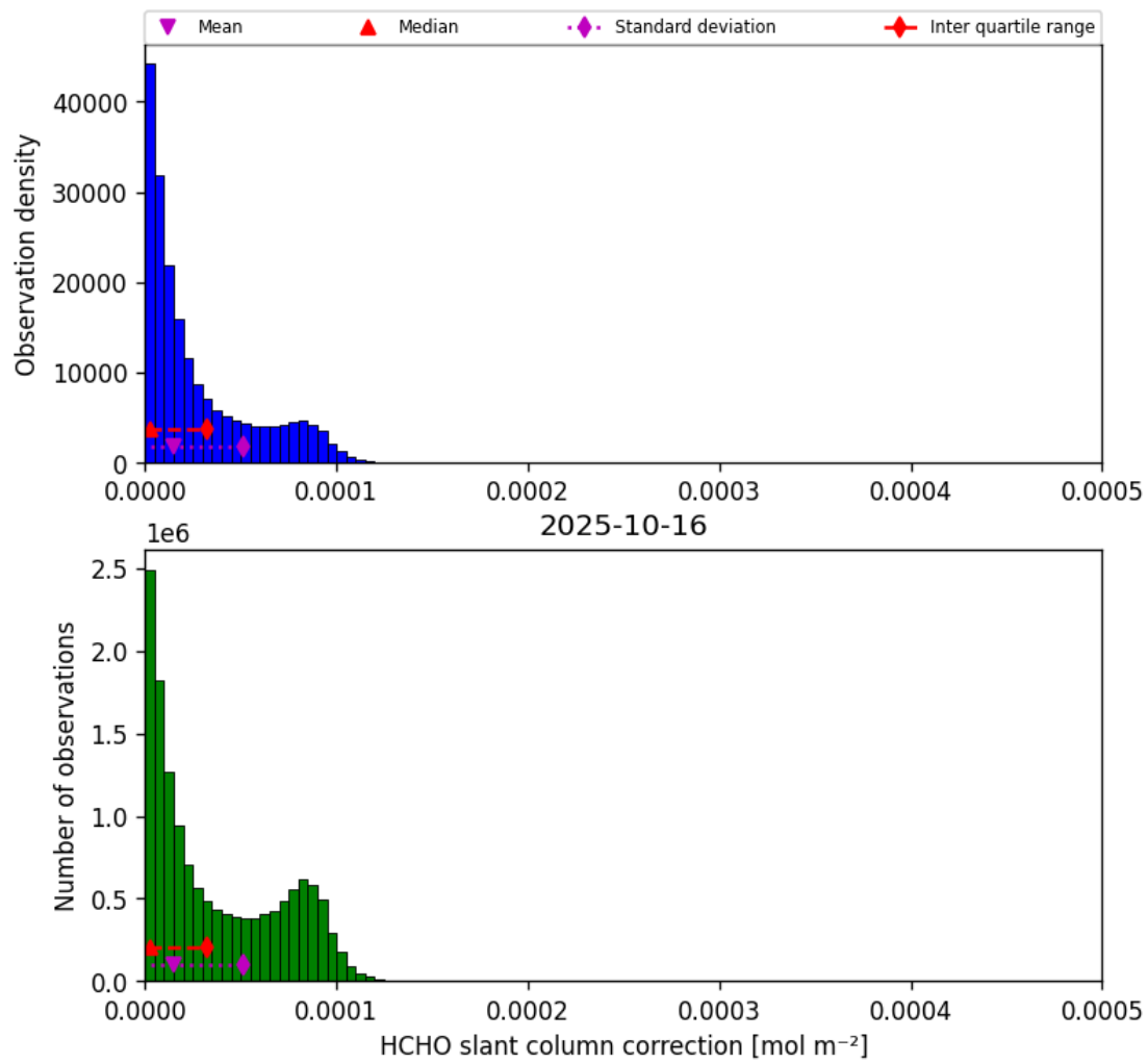
Figure 47: Histogram of “HCHO slant column correction” for 2025-10-15 to 2025-10-17
