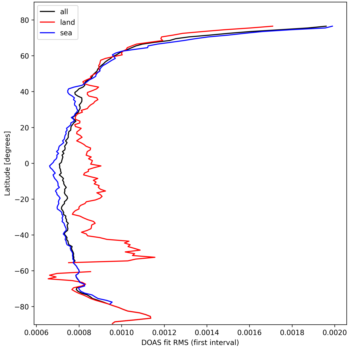
Figure 32: Zonal average of “DOAS fit RMS (first interval)” for 2025-10-15 to 2025-10-17.
