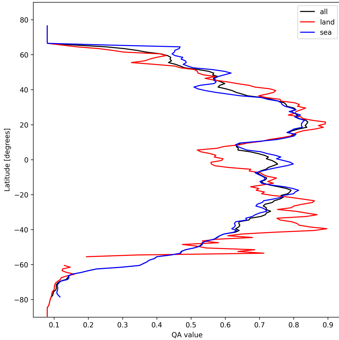
Figure 20: Zonal average of “QA value” for 2025-10-15 to 2025-10-17.
