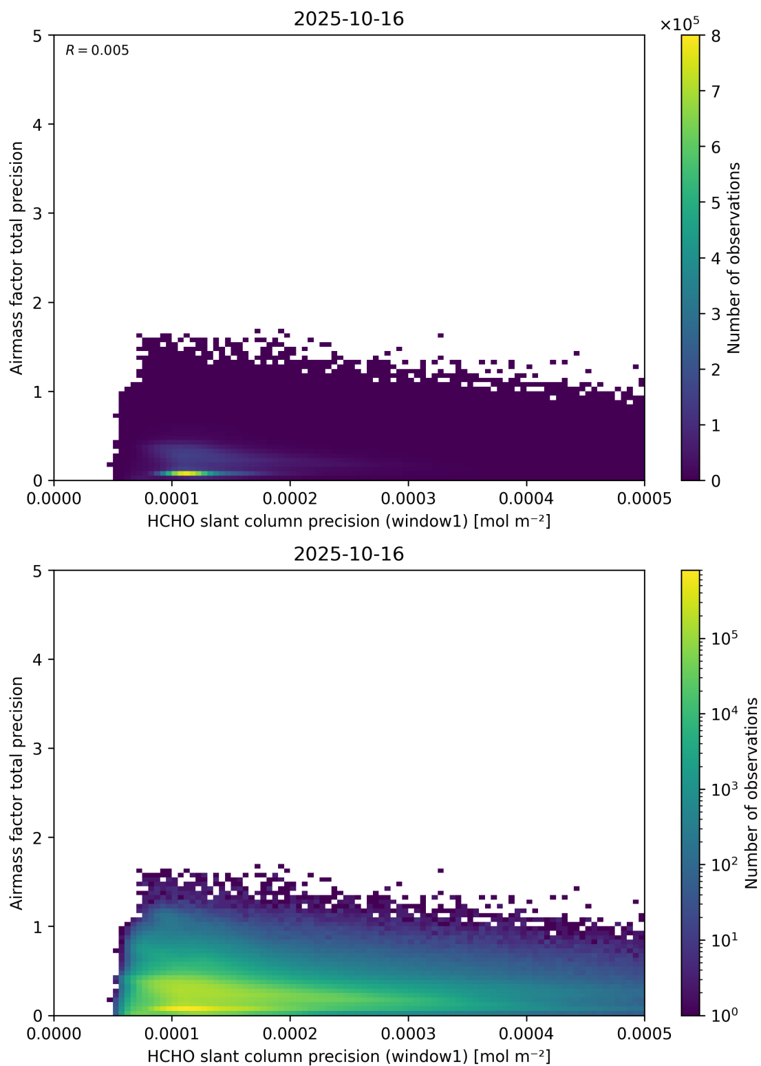
Figure 95: Scatter density plot of “HCHO slant column precision (window1)” against “Airmass factor total precision” for 2025-10-15 to 2025-10-17.
