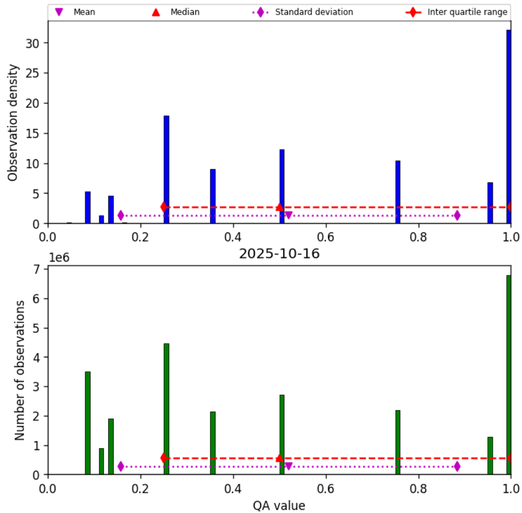
Figure 34: Histogram of “QA value” for 2025-10-15 to 2025-10-17
