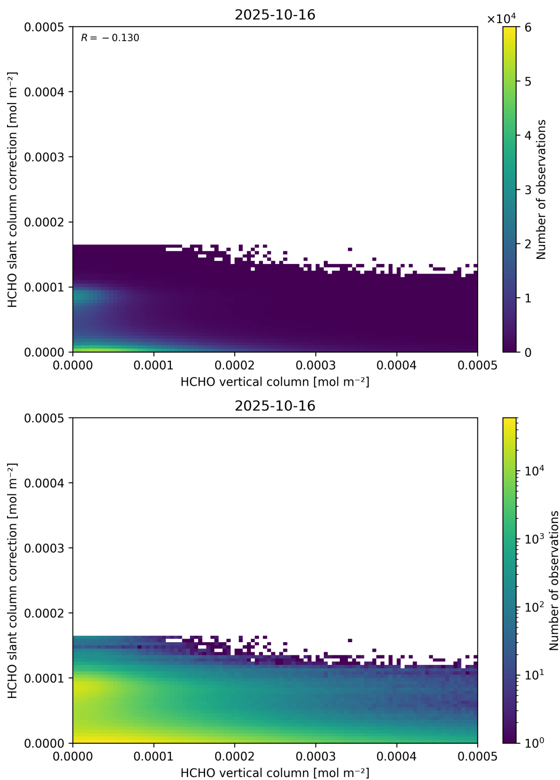
Figure 128: Scatter density plot of “HCHO vertical column” against “HCHO slant column correction” for 2025-10-15 to 2025-10-17.
