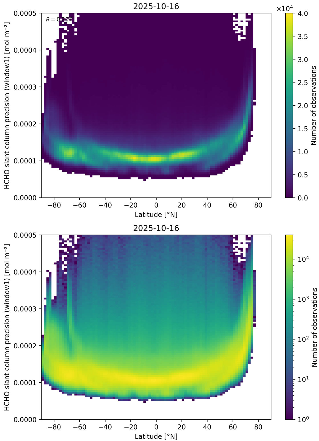
Figure 160: Scatter density plot of “Latitude” against “HCHO slant column precision (window1)” for 2025-10-15 to 2025-10-17.
