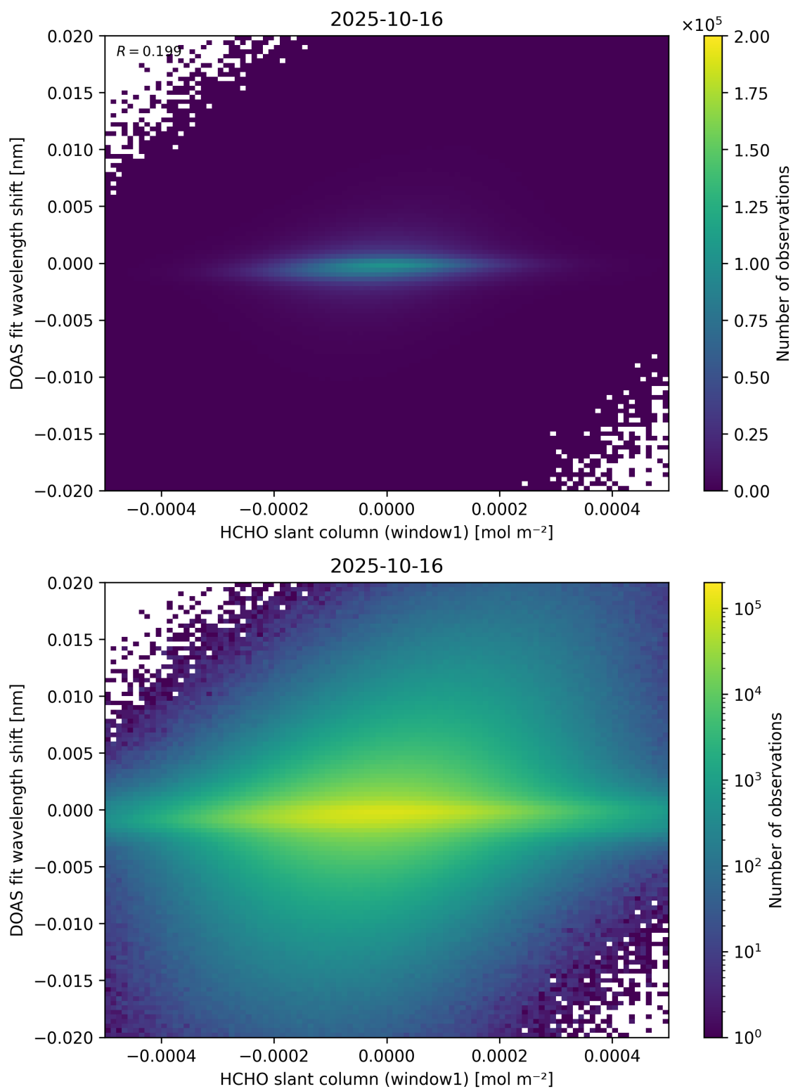
Figure 79: Scatter density plot of “HCHO slant column (window1)” against “DOAS fit wavelength shift” for 2025-10-15 to 2025-10-17.
