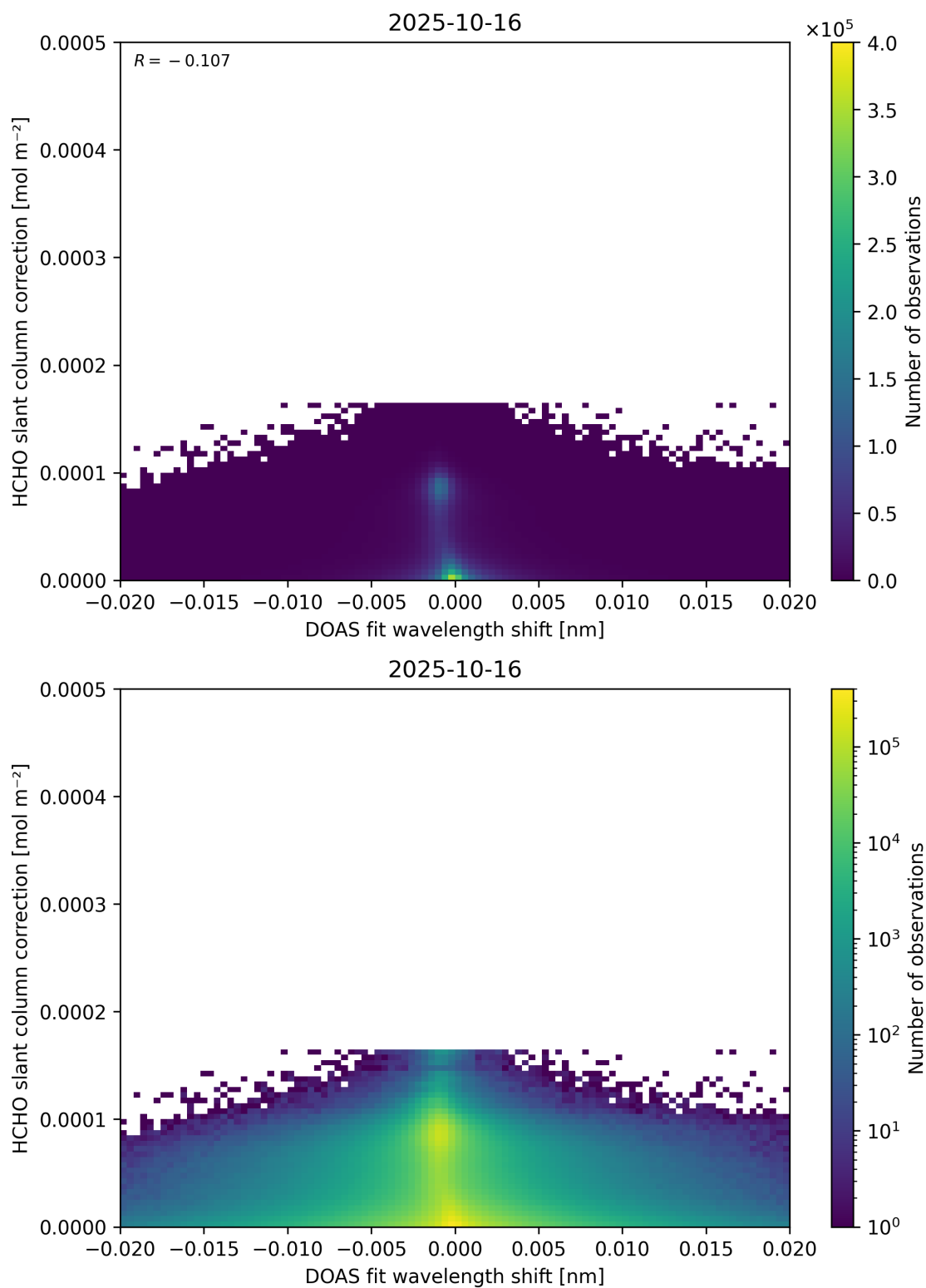
Figure 67: Scatter density plot of “DOAS fit wavelength shift” against “HCHO slant column correction” for 2025-10-15 to 2025-10-17.
