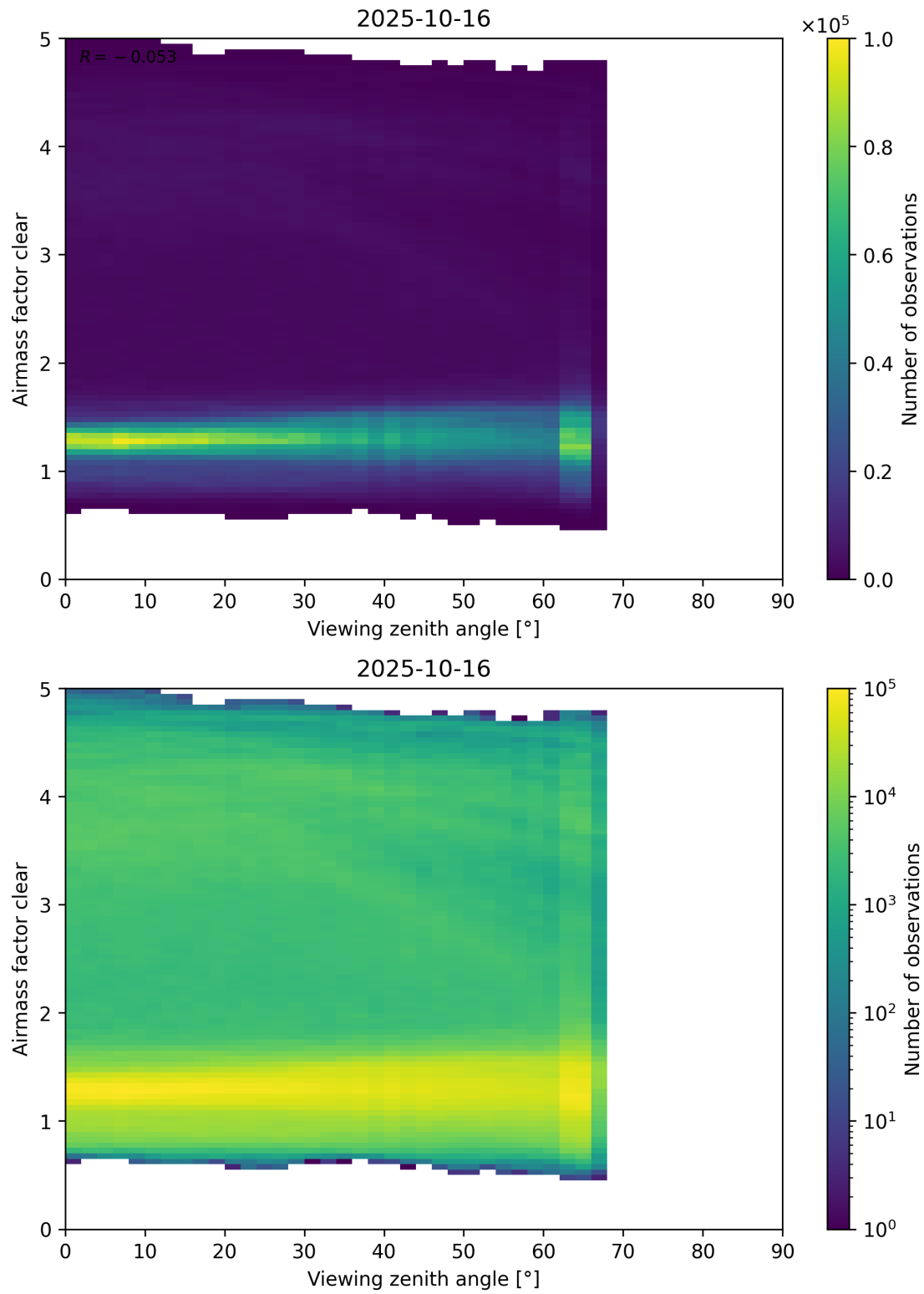
Figure 185: Scatter density plot of “Viewing zenith angle” against “Airmass factor clear” for 2025-10-15 to 2025-10-17.
