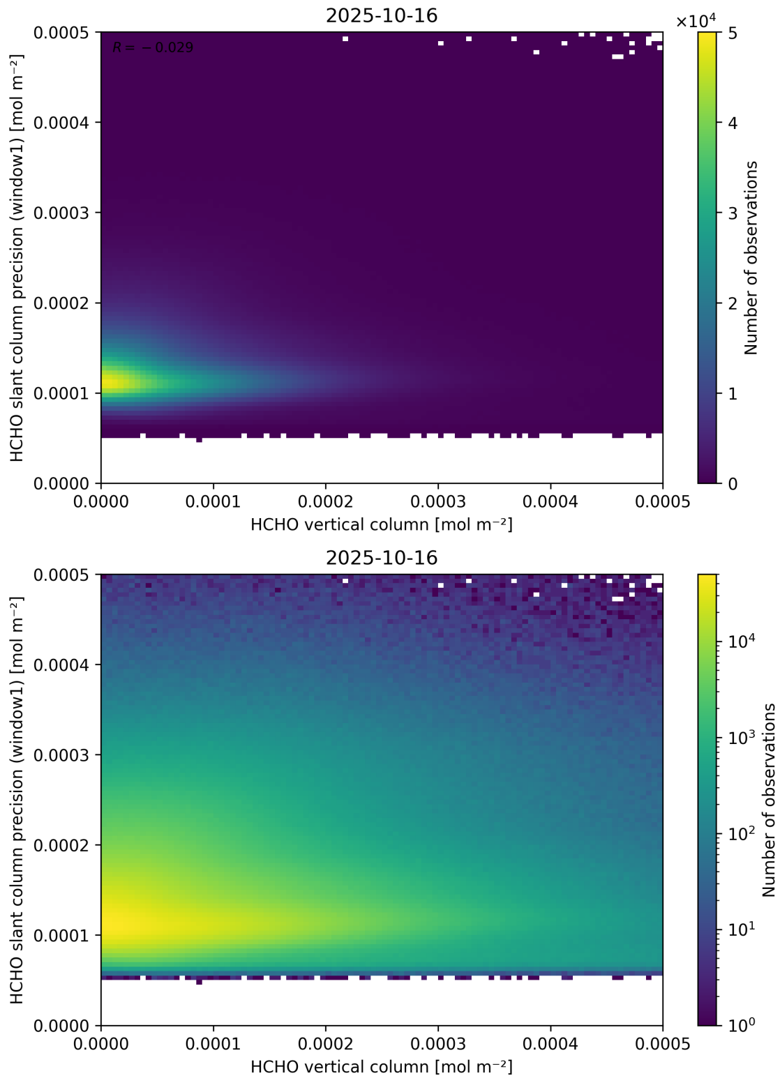
Figure 130: Scatter density plot of “HCHO vertical column” against “HCHO slant column precision (window1)” for 2025-10-15 to 2025-10-17.
