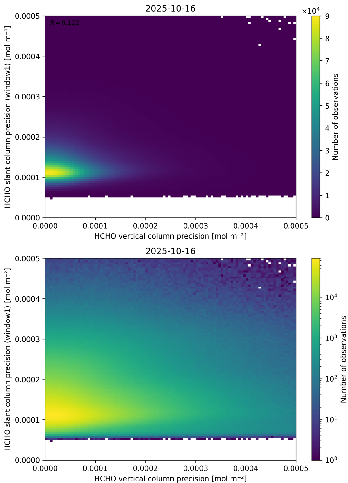
Figure 143: Scatter density plot of “HCHO vertical column precision” against “HCHO slant column precision (window1)” for 2025-10-15 to 2025-10-17.
