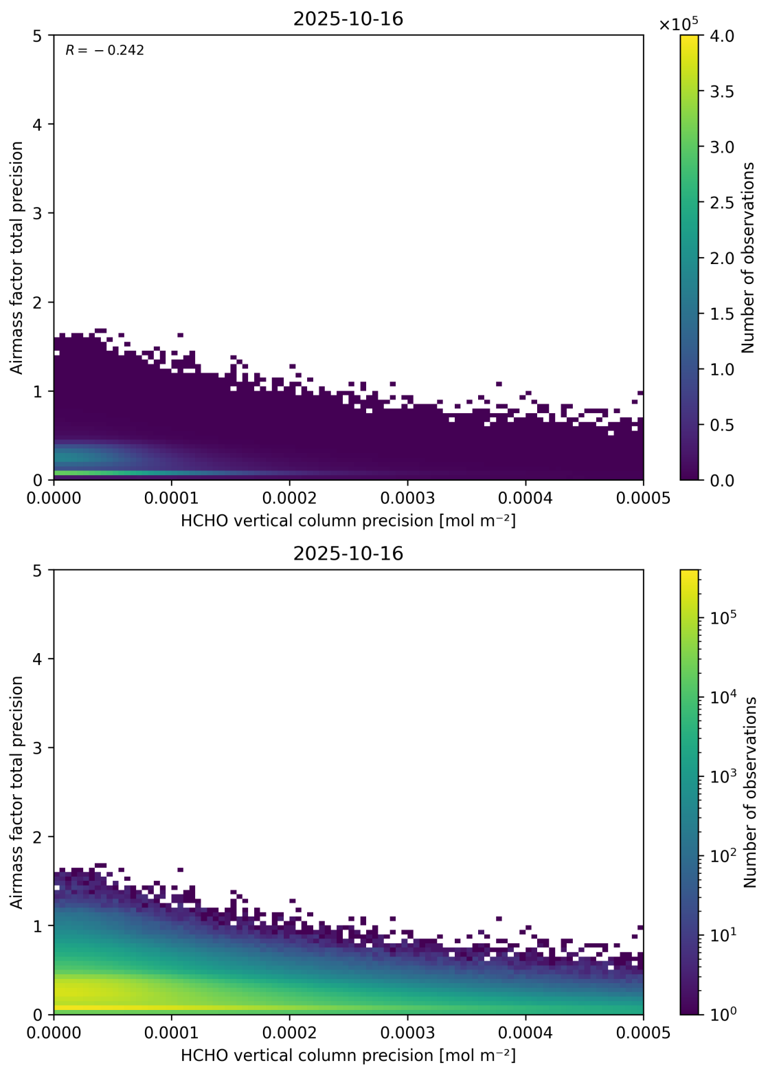
Figure 145: Scatter density plot of “HCHO vertical column precision” against “Airmass factor total precision” for 2025-10-15 to 2025-10-17.
