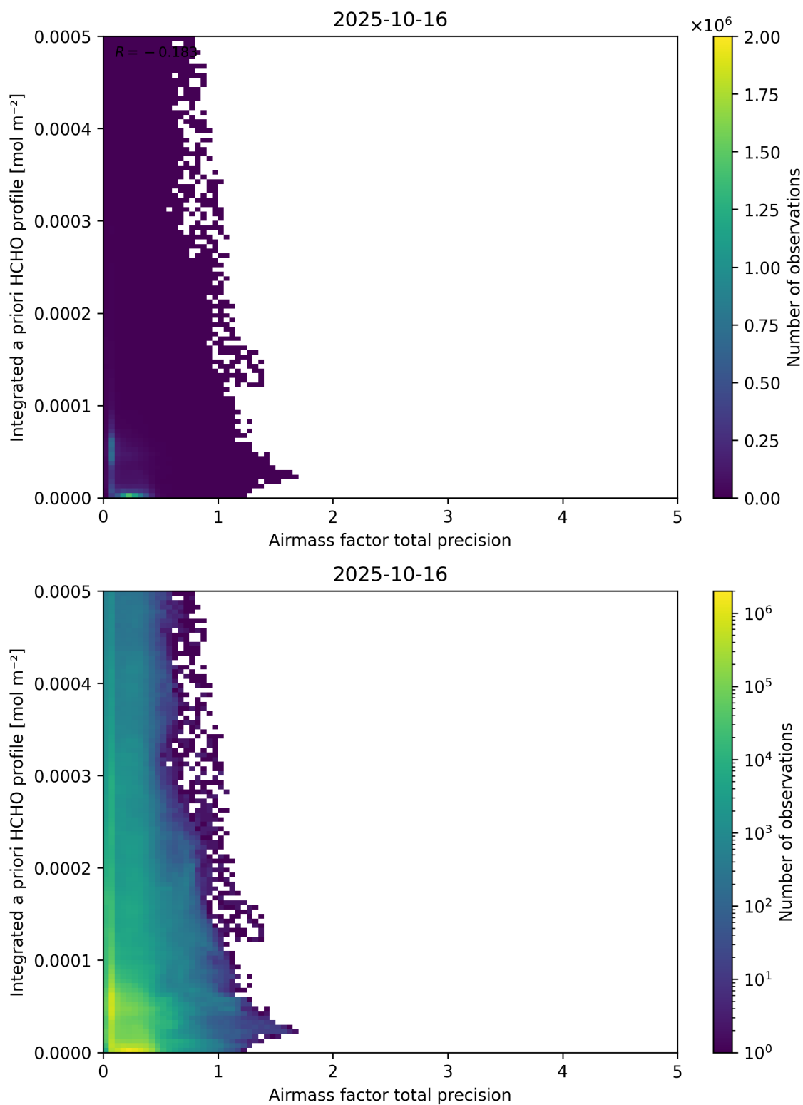
Figure 111: Scatter density plot of “Airmass factor total precision” against “Integrated a priori HCHO profile” for 2025-10-15 to 2025-10-17.
