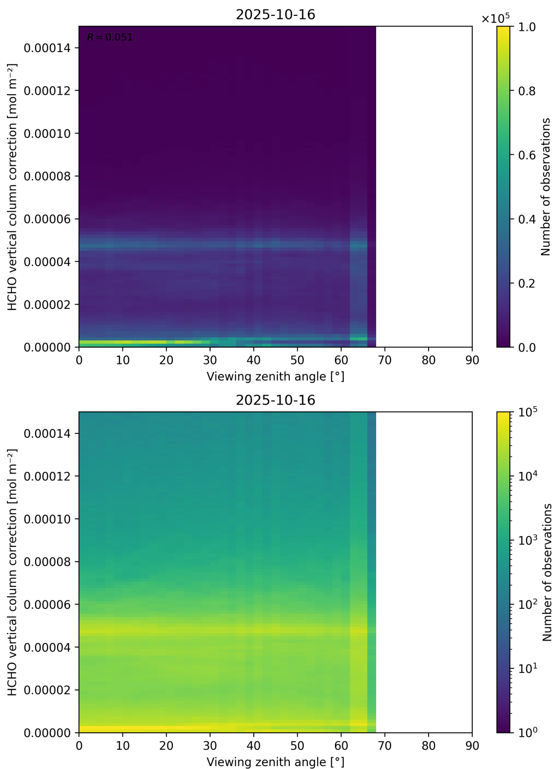
Figure 193: Scatter density plot of “Viewing zenith angle” against “HCHO vertical column correction” for 2025-10-15 to 2025-10-17.
