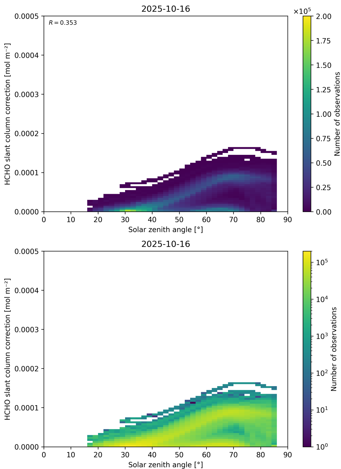
Figure 172: Scatter density plot of “Solar zenith angle” against “HCHO slant column correction” for 2025-10-15 to 2025-10-17.
