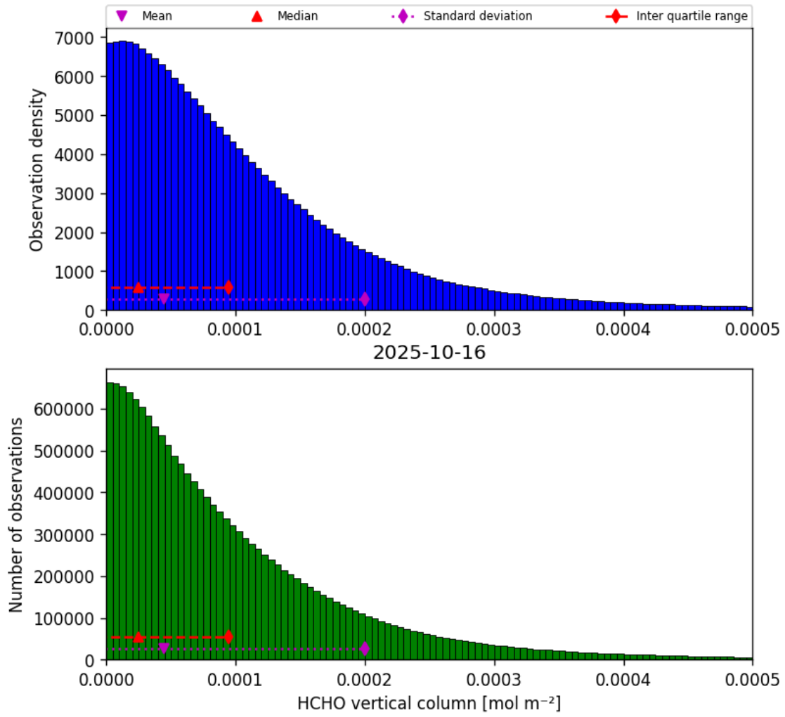
Figure 35: Histogram of “HCHO vertical column” for 2025-10-15 to 2025-10-17
