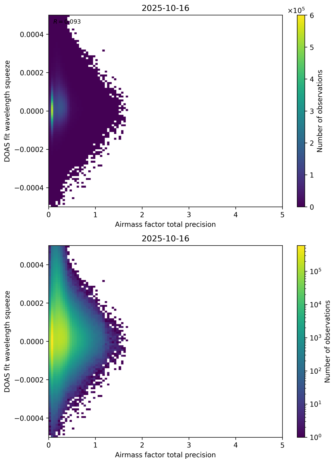
Figure 107: Scatter density plot of “Airmass factor total precision” against “DOAS fit wavelength squeeze” for 2025-10-15 to 2025-10-17.
