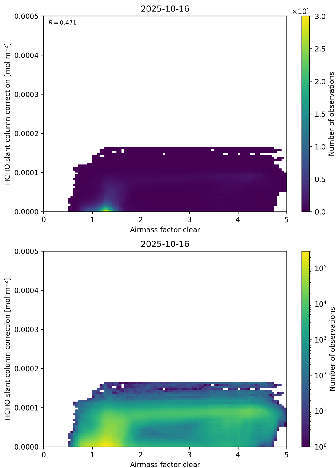
Figure 75: Scatter density plot of “Airmass factor clear” against “HCHO slant column correction” for 2025-10-15 to 2025-10-17.
