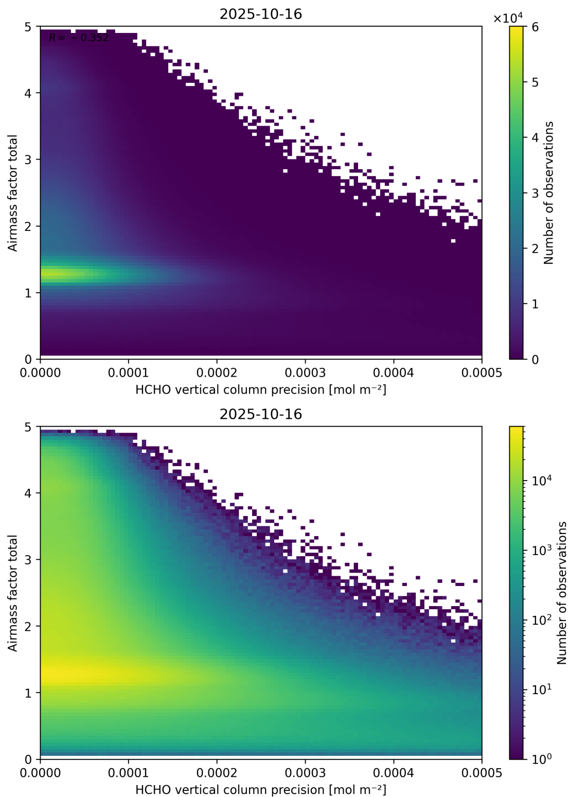
Figure 144: Scatter density plot of “HCHO vertical column precision” against “Airmass factor total” for 2025-10-15 to 2025-10-17.
