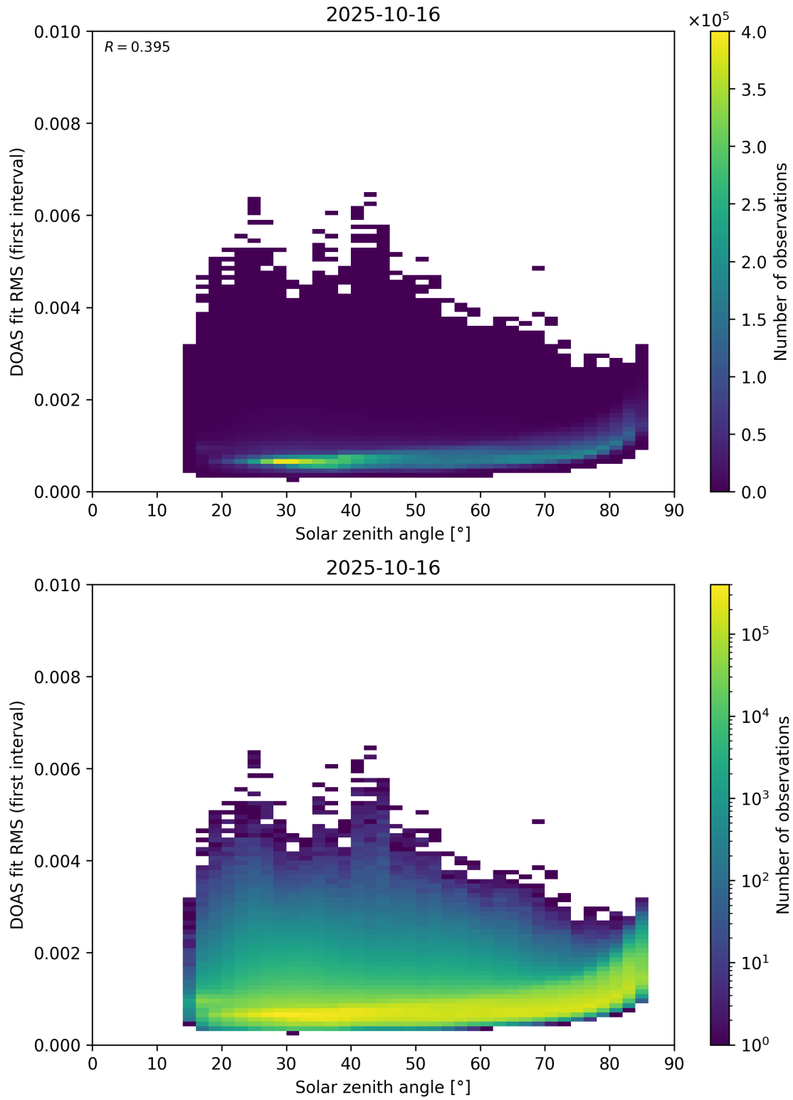
Figure 167: Scatter density plot of “Solar zenith angle” against “DOAS fit RMS (first interval)” for 2025-10-15 to 2025-10-17.
