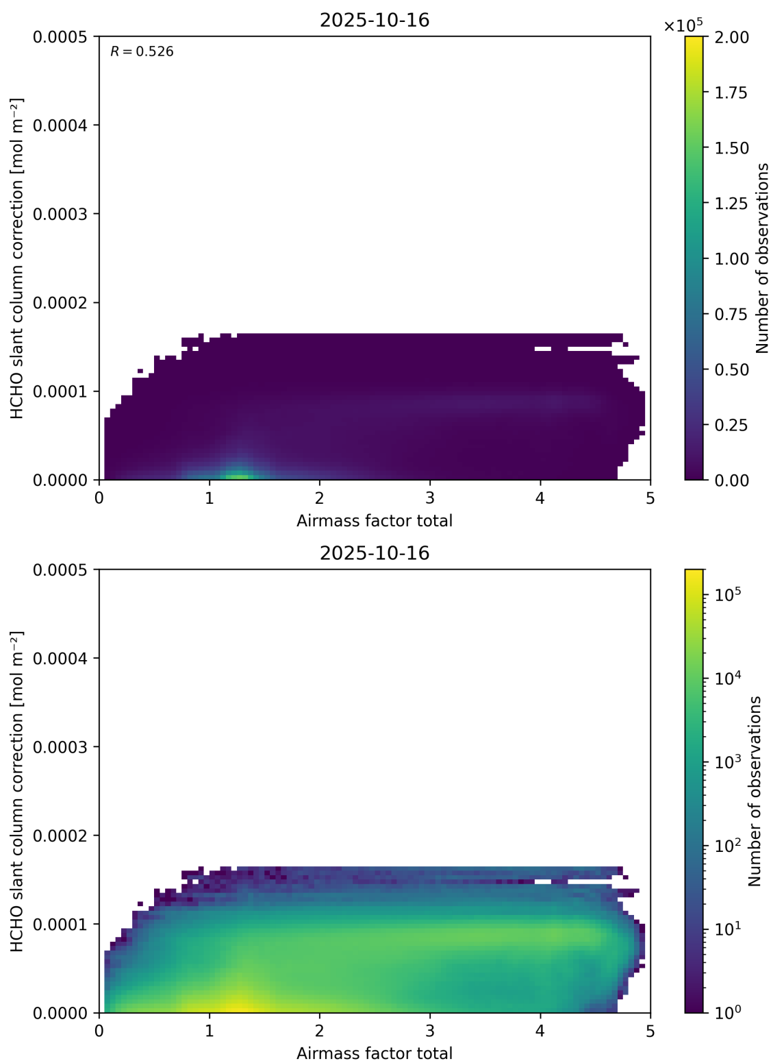
Figure 102: Scatter density plot of “Airmass factor total” against “HCHO slant column correction” for 2025-10-15 to 2025-10-17.
