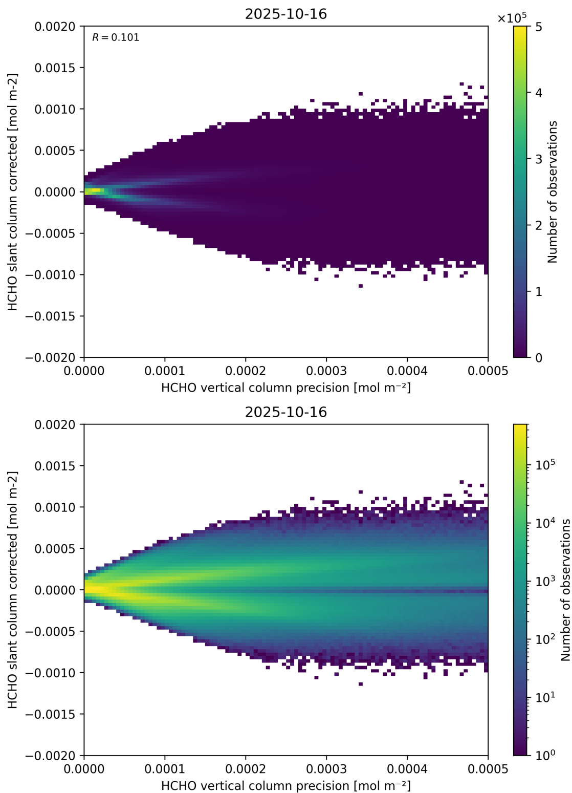
Figure 140: Scatter density plot of “HCHO vertical column precision” against “HCHO slant column corrected” for 2025-10-15 to 2025-10-17.
