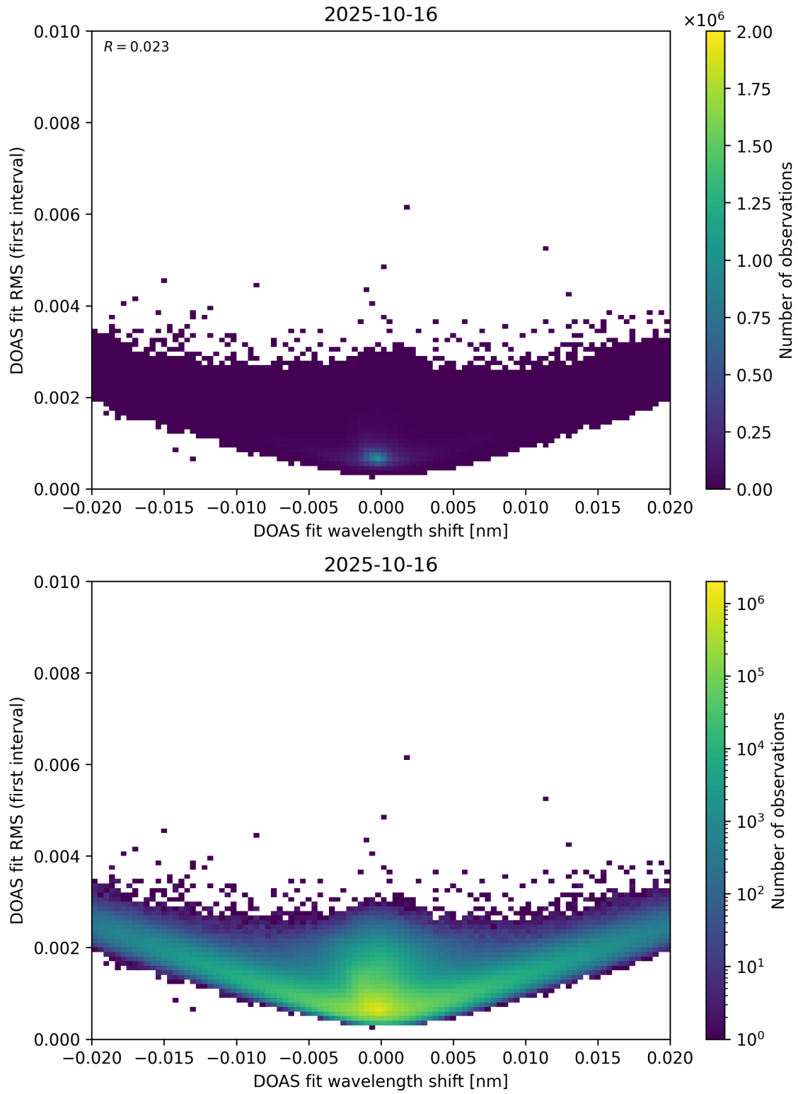
Figure 64: Scatter density plot of “DOAS fit wavelength shift” against “DOAS fit RMS (first interval)” for 2025-10-15 to 2025-10-17.
