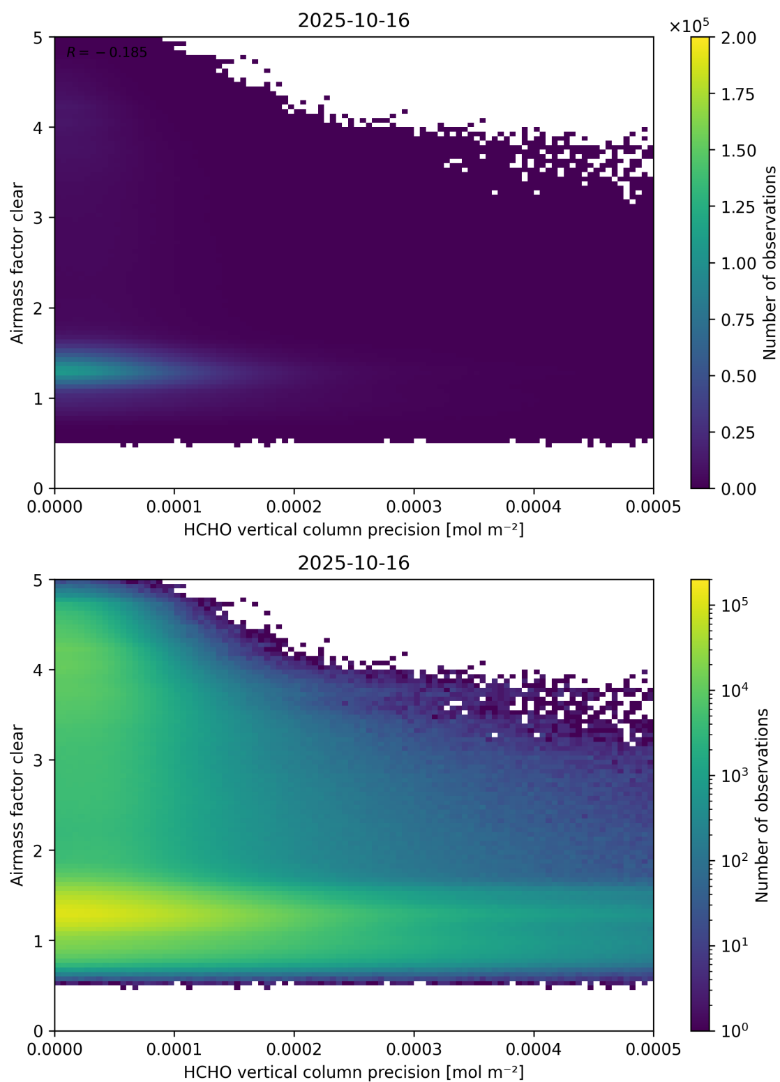
Figure 139: Scatter density plot of “HCHO vertical column precision” against “Airmass factor clear” for 2025-10-15 to 2025-10-17.
