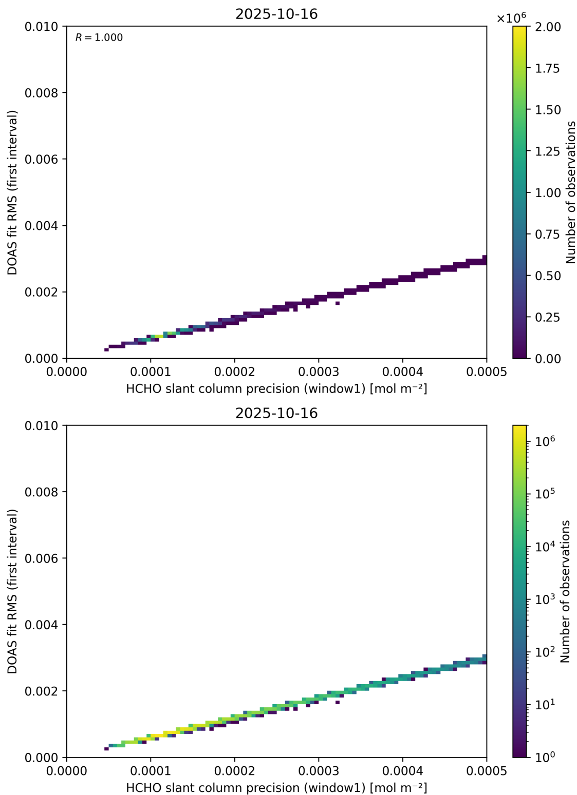
Figure 88: Scatter density plot of “HCHO slant column precision (window1)” against “DOAS fit RMS (first interval)” for 2025-10-15 to 2025-10-17.
