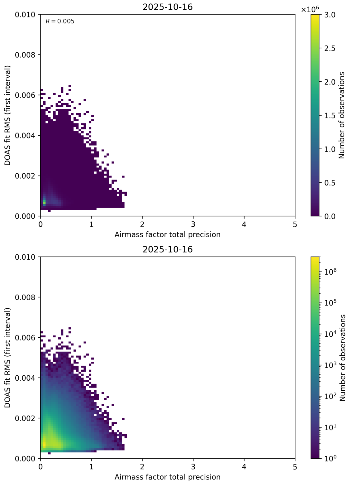
Figure 105: Scatter density plot of “Airmass factor total precision” against “DOAS fit RMS (first interval)” for 2025-10-15 to 2025-10-17.
