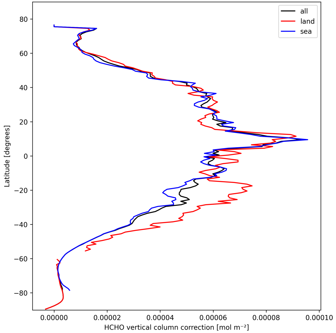
Figure 23: Zonal average of “HCHO vertical column correction” for 2025-10-15 to 2025-10-17.
