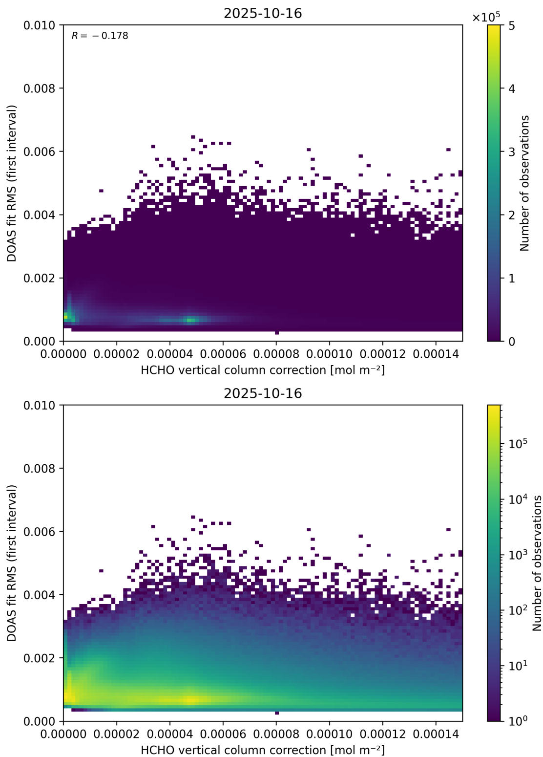
Figure 112: Scatter density plot of “HCHO vertical column correction” against “DOAS fit RMS (first interval)” for 2025-10-15 to 2025-10-17.
