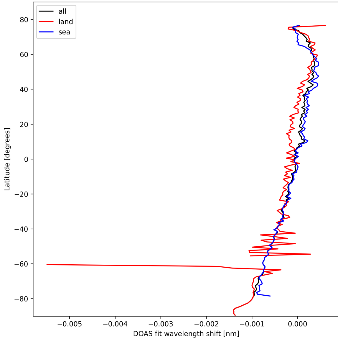
Figure 30: Zonal average of “DOAS fit wavelength shift” for 2025-10-15 to 2025-10-17.
