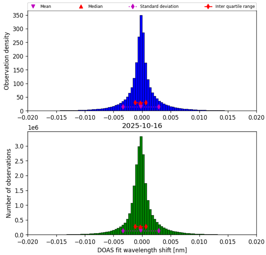
Figure 44: Histogram of “DOAS fit wavelength shift” for 2025-10-15 to 2025-10-17
