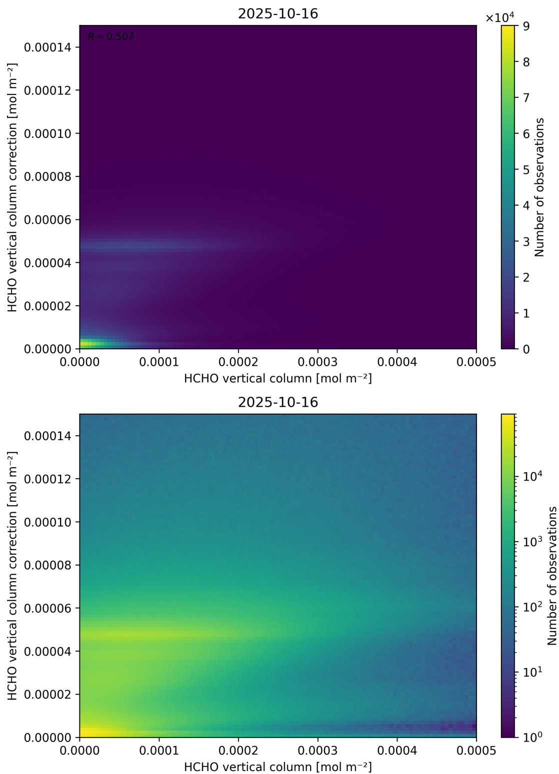
Figure 133: Scatter density plot of “HCHO vertical column” against “HCHO vertical column correction” for 2025-10-15 to 2025-10-17.
