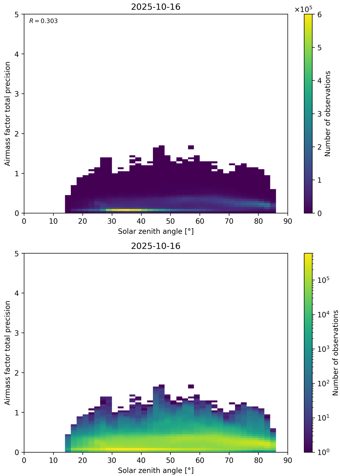
Figure 176: Scatter density plot of “Solar zenith angle” against “Airmass factor total precision” for 2025-10-15 to 2025-10-17.
