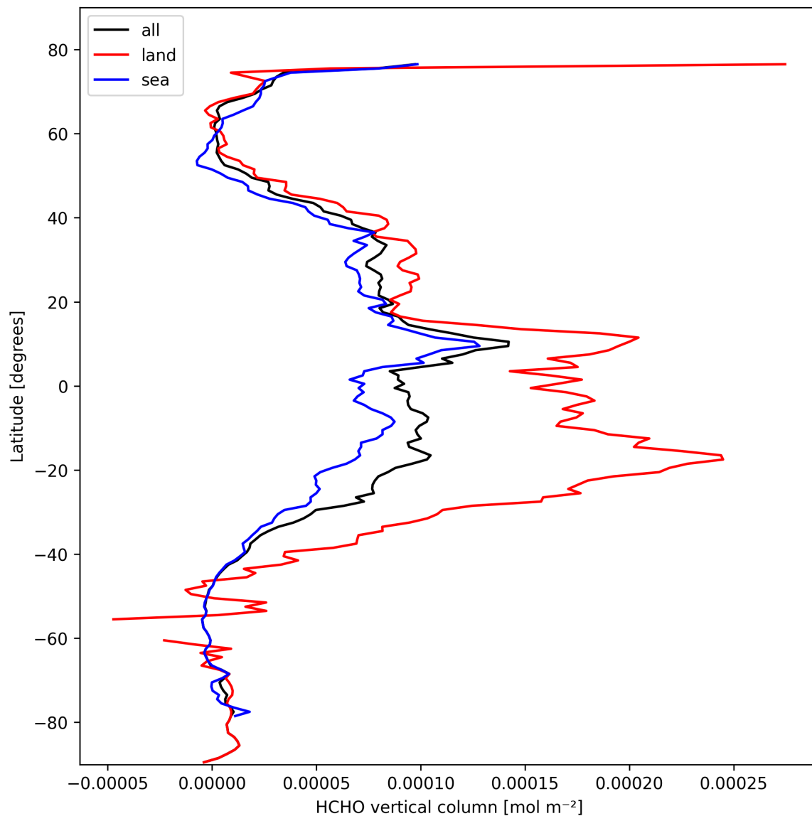
Figure 21: Zonal average of “HCHO vertical column” for 2025-10-15 to 2025-10-17.
