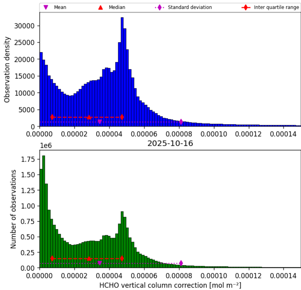
Figure 37: Histogram of “HCHO vertical column correction” for 2025-10-15 to 2025-10-17
