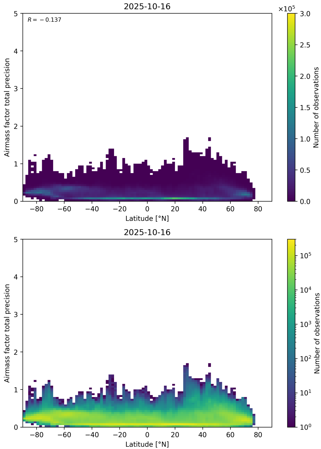
Figure 162: Scatter density plot of “Latitude” against “Airmass factor total precision” for 2025-10-15 to 2025-10-17.
