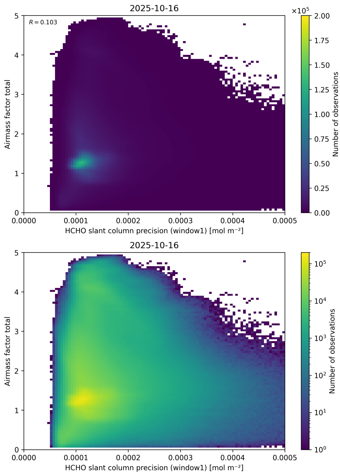
Figure 94: Scatter density plot of “HCHO slant column precision (window1)” against “Airmass factor total” for 2025-10-15 to 2025-10-17.
