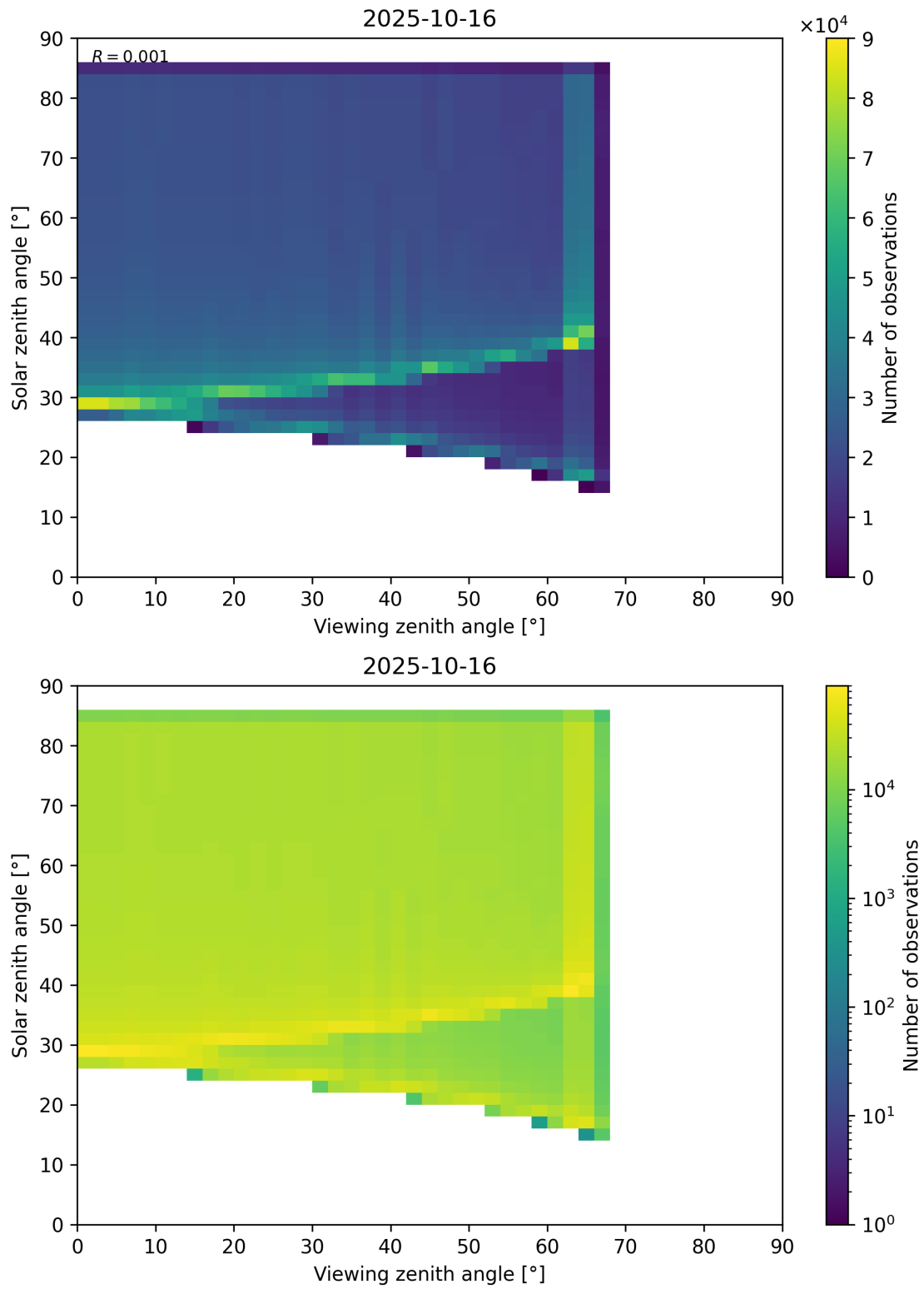
Figure 197: Scatter density plot of “Viewing zenith angle” against “Solar zenith angle” for 2025-10-15 to 2025-10-17.
