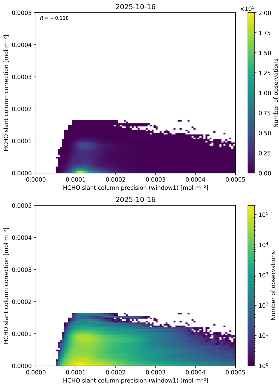
Figure 93: Scatter density plot of “HCHO slant column precision (window1)” against “HCHO slant column correction” for 2025-10-15 to 2025-10-17.
