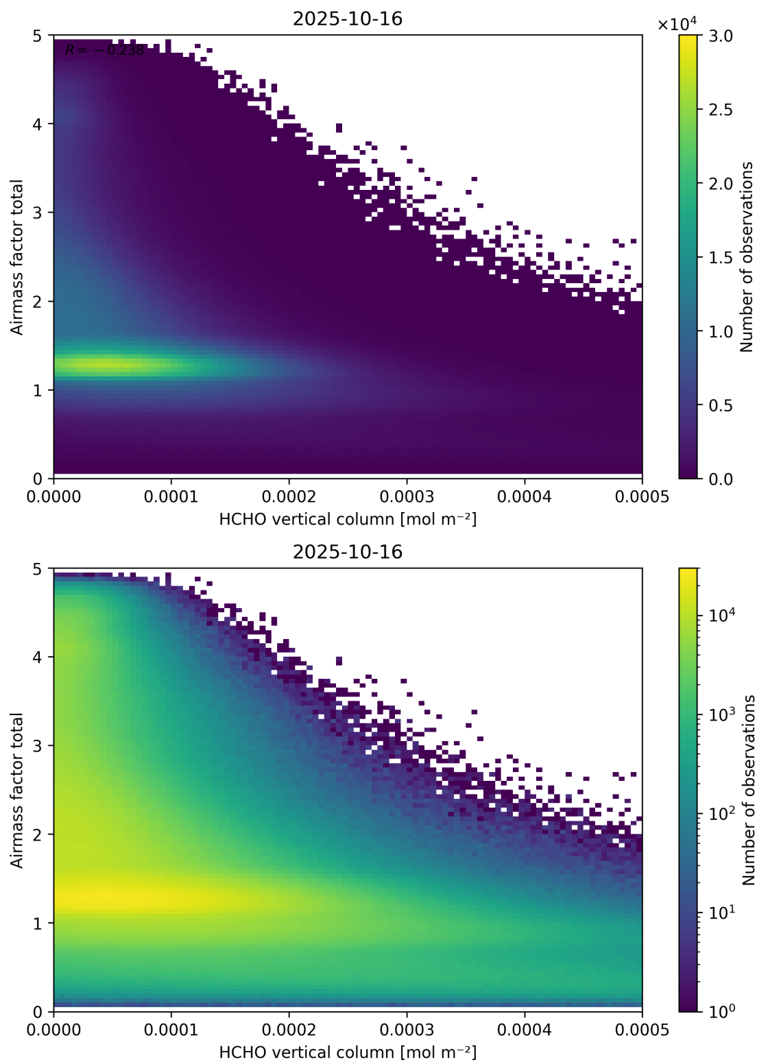
Figure 131: Scatter density plot of “HCHO vertical column” against “Airmass factor total” for 2025-10-15 to 2025-10-17.
