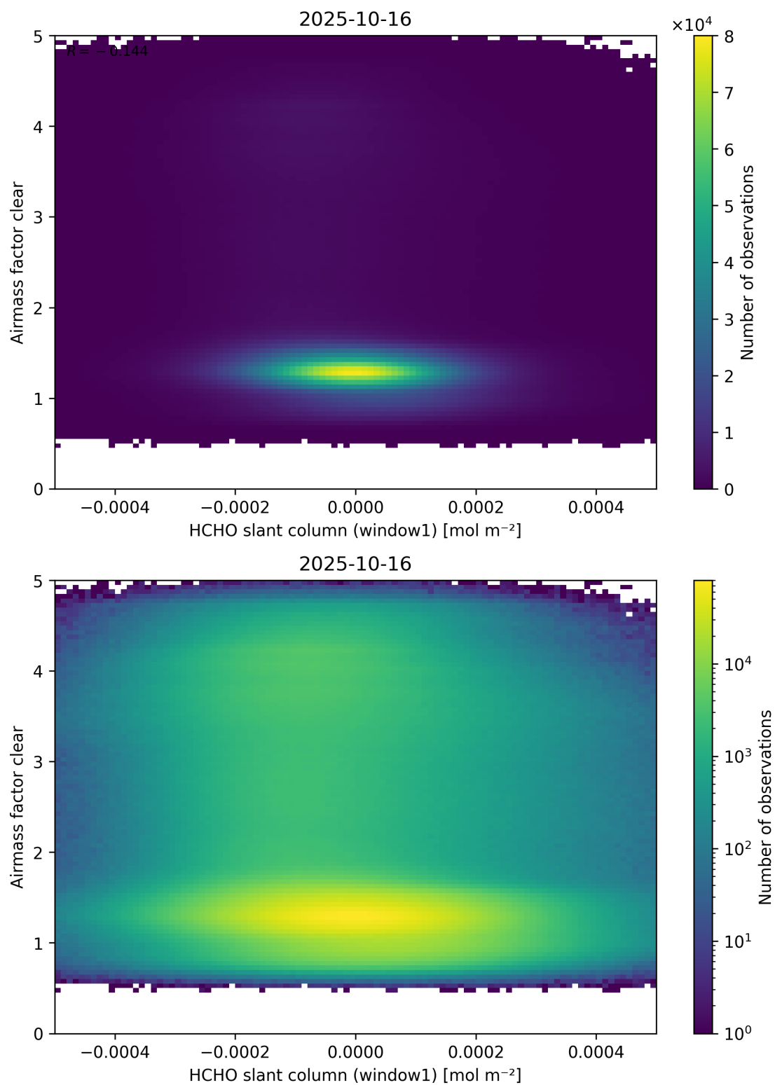
Figure 81: Scatter density plot of “HCHO slant column (window1)” against “Airmass factor clear” for 2025-10-15 to 2025-10-17.
