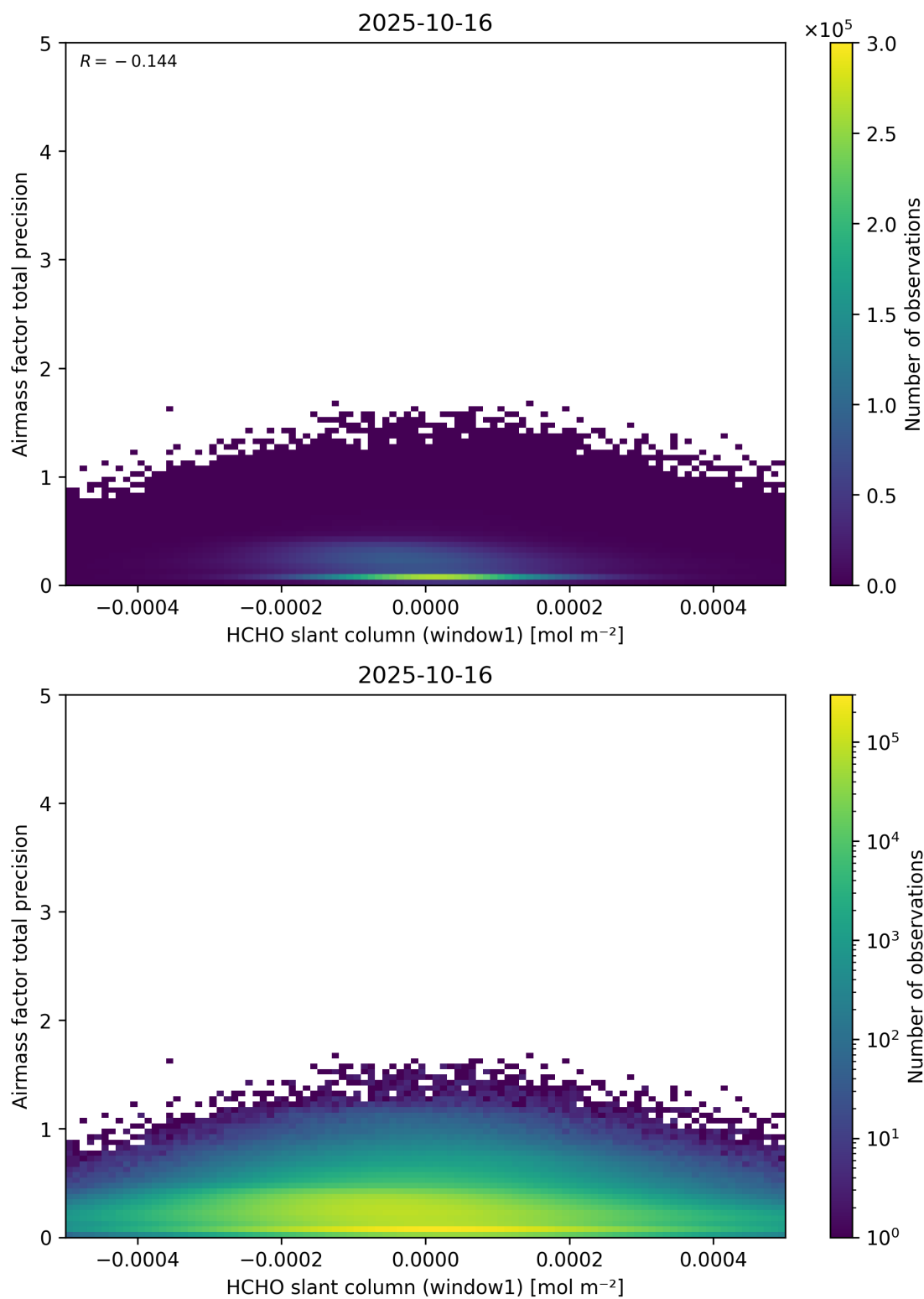
Figure 86: Scatter density plot of “HCHO slant column (window1)” against “Airmass factor total precision” for 2025-10-15 to 2025-10-17.
