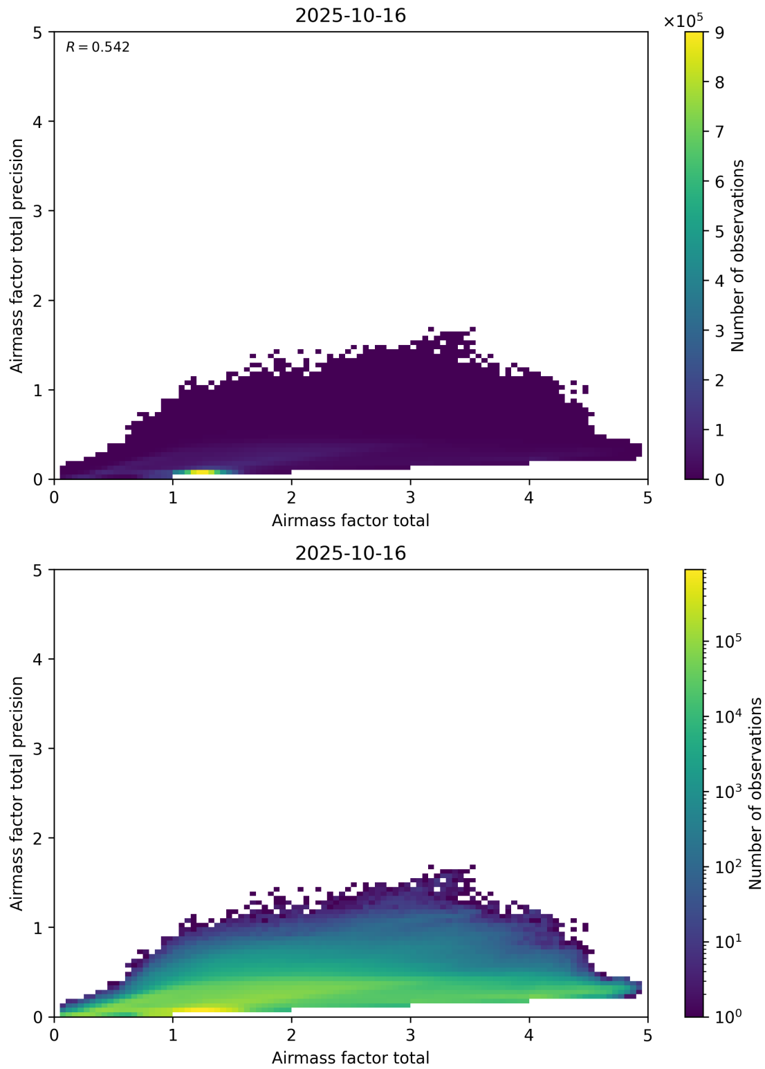
Figure 103: Scatter density plot of “Airmass factor total” against “Airmass factor total precision” for 2025-10-15 to 2025-10-17.
