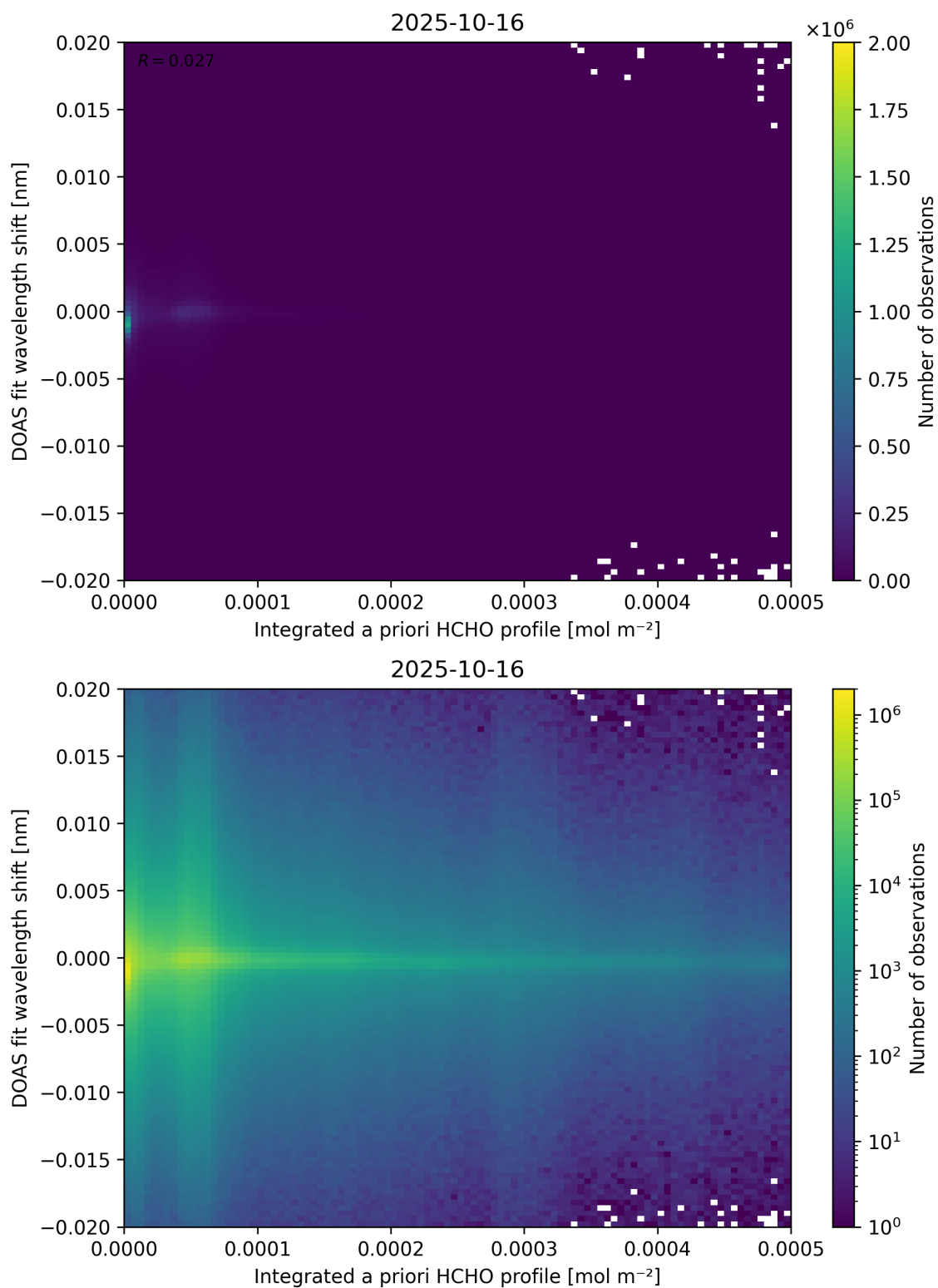
Figure 149: Scatter density plot of “Integrated a priori HCHO profile” against “DOAS fit wavelength shift” for 2025-10-15 to 2025-10-17.
