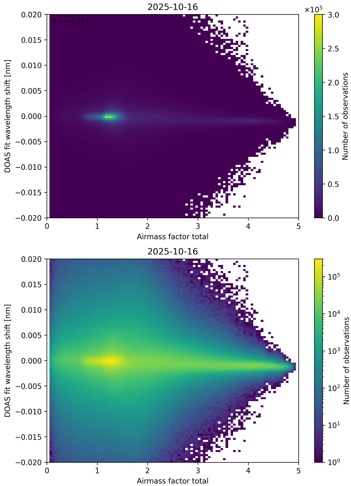
Figure 98: Scatter density plot of “Airmass factor total” against “DOAS fit wavelength shift” for 2025-10-15 to 2025-10-17.
