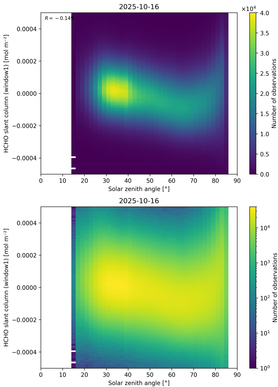
Figure 173: Scatter density plot of “Solar zenith angle” against “HCHO slant column (window1)” for 2025-10-15 to 2025-10-17.
