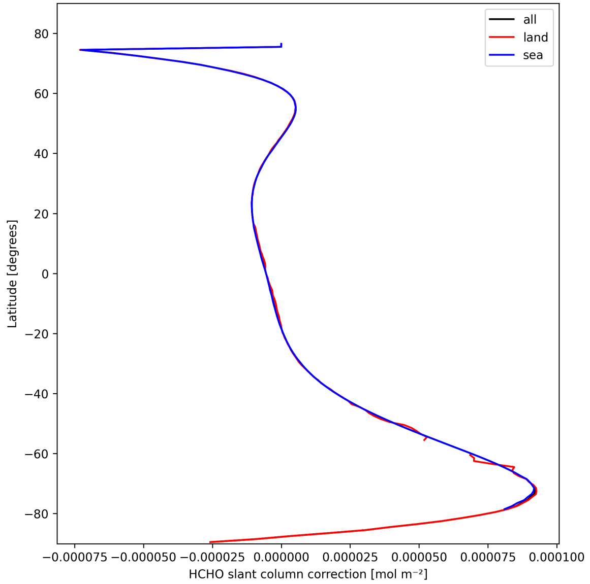
Figure 33: Zonal average of “HCHO slant column correction” for 2025-10-15 to 2025-10-17.
