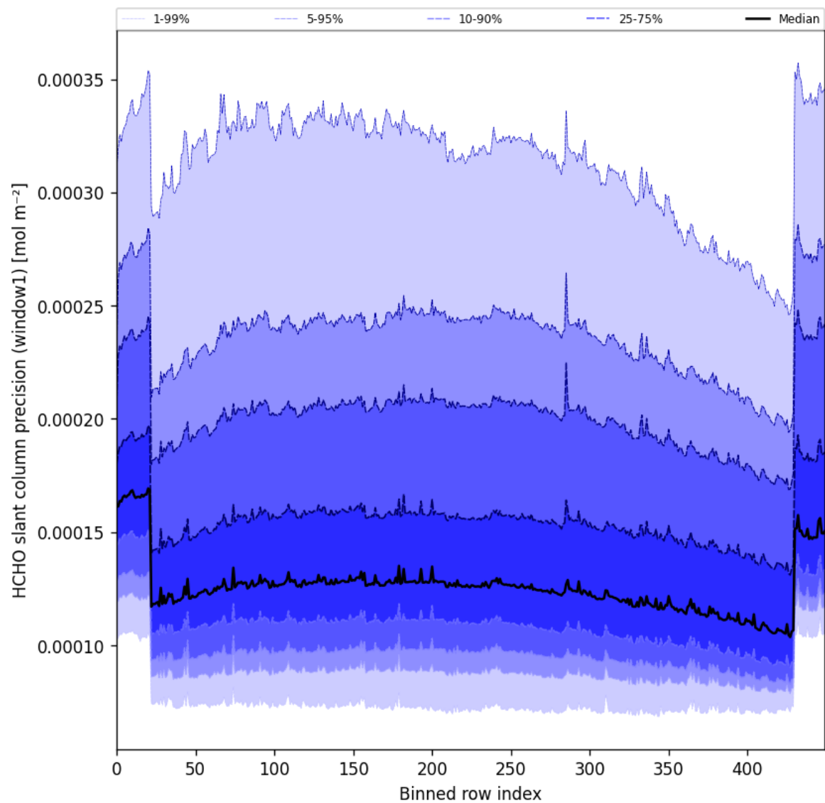
Figure 53: Along track statistics of “HCHO slant column precision (window1)” for 2025-10-15 to 2025-10-17
