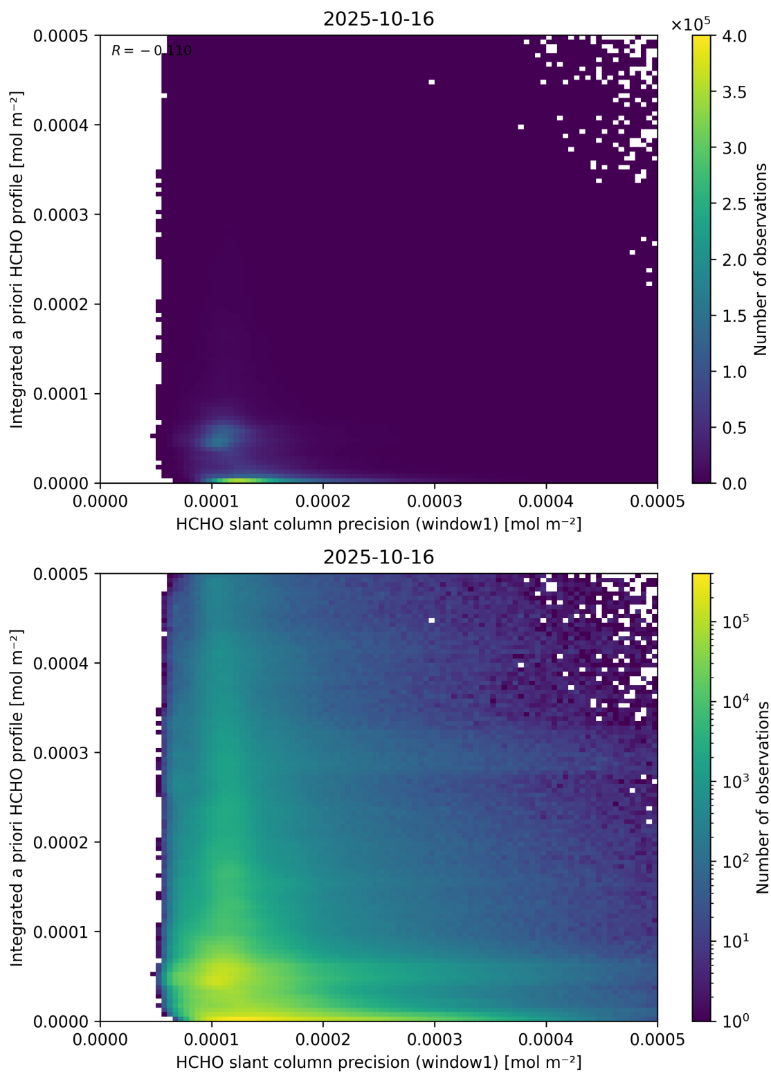
Figure 96: Scatter density plot of “HCHO slant column precision (window1)” against “Integrated a priori HCHO profile” for 2025-10-15 to 2025-10-17.
