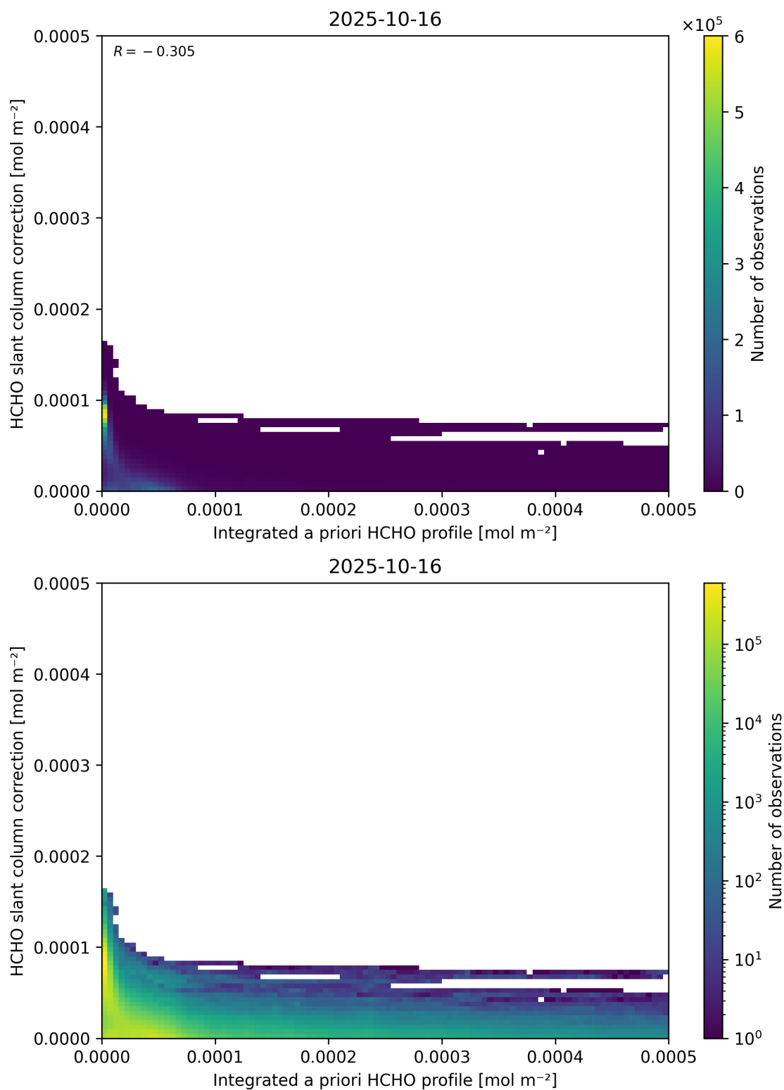
Figure 152: Scatter density plot of “Integrated a priori HCHO profile” against “HCHO slant column correction” for 2025-10-15 to 2025-10-17.
