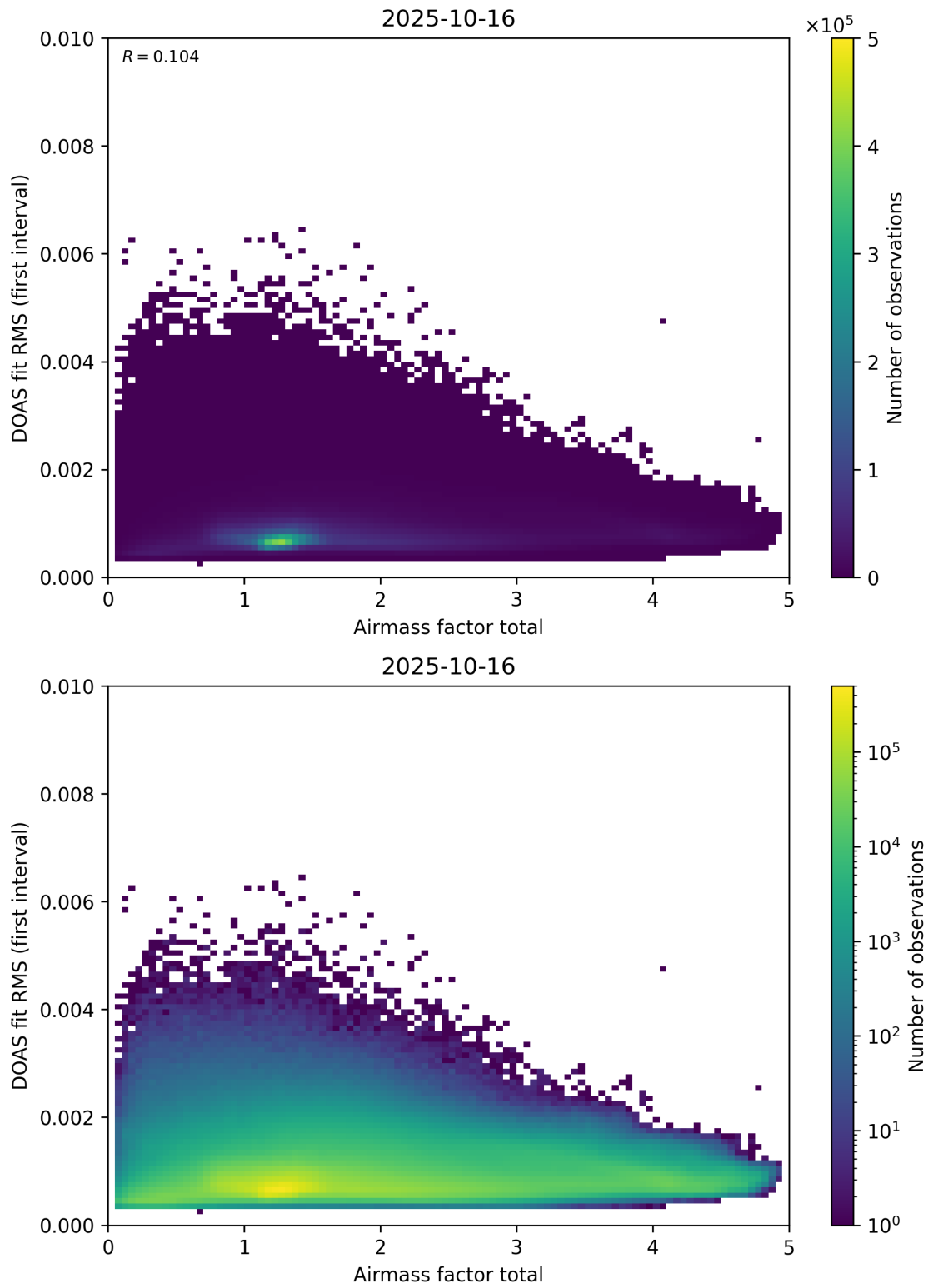
Figure 97: Scatter density plot of “Airmass factor total” against “DOAS fit RMS (first interval)” for 2025-10-15 to 2025-10-17.
