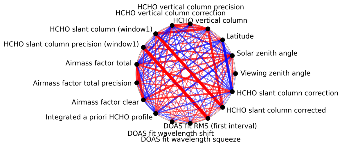
Figure 1: Map of correlation graph for 2025-10-15 to 2025-10-17.
