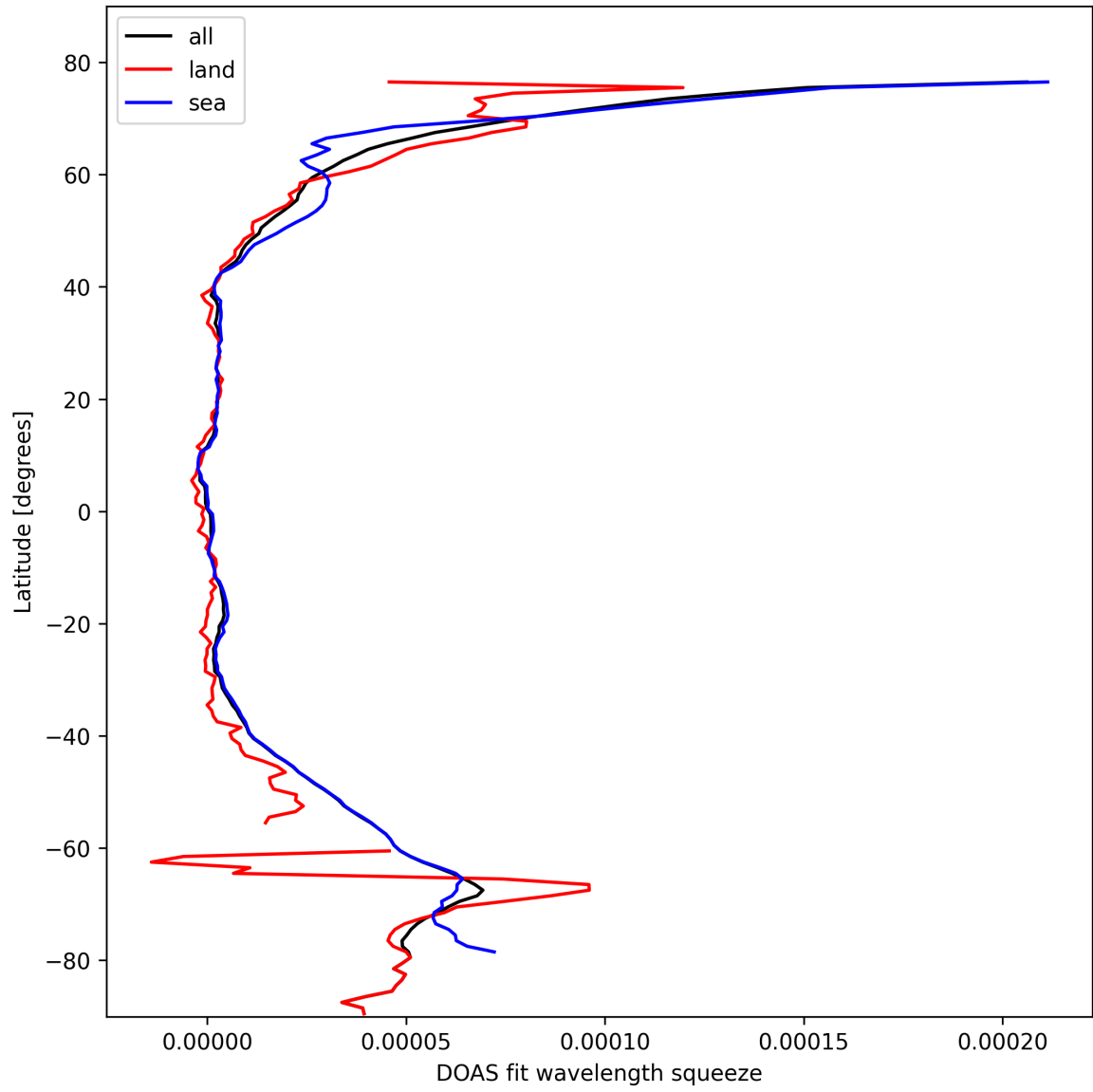
Figure 31: Zonal average of “DOAS fit wavelength squeeze” for 2025-10-15 to 2025-10-17.
