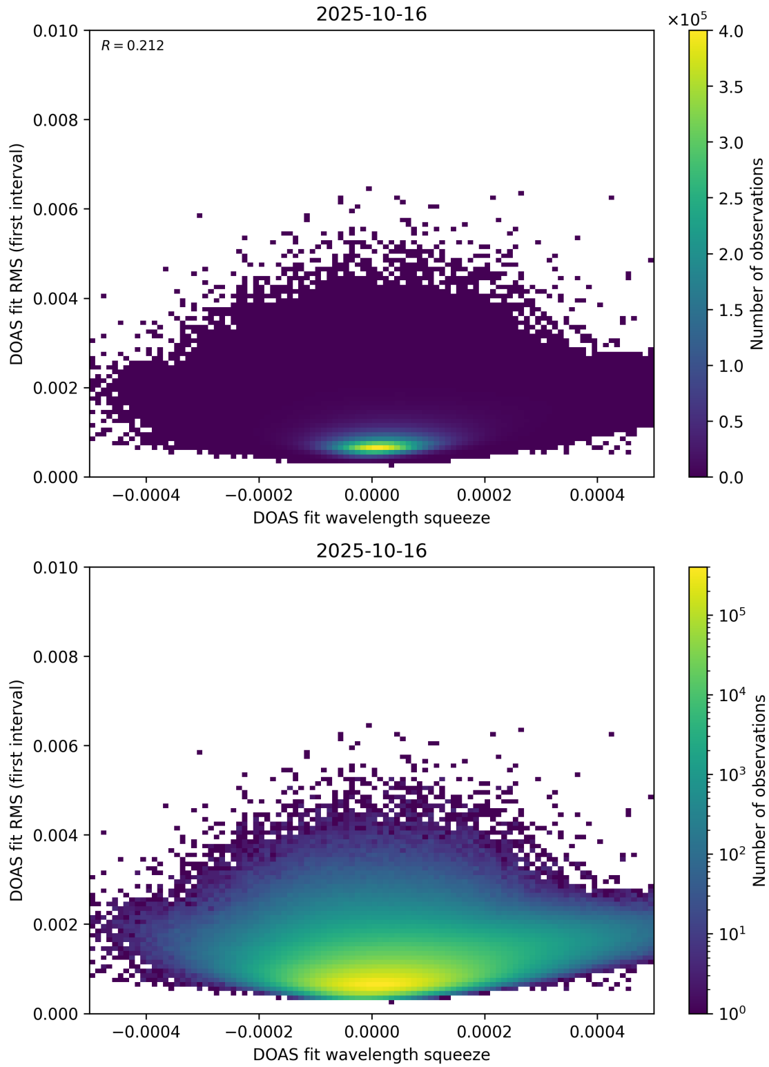
Figure 68: Scatter density plot of “DOAS fit wavelength squeeze” against “DOAS fit RMS (first interval)” for 2025-10-15 to 2025-10-17.
