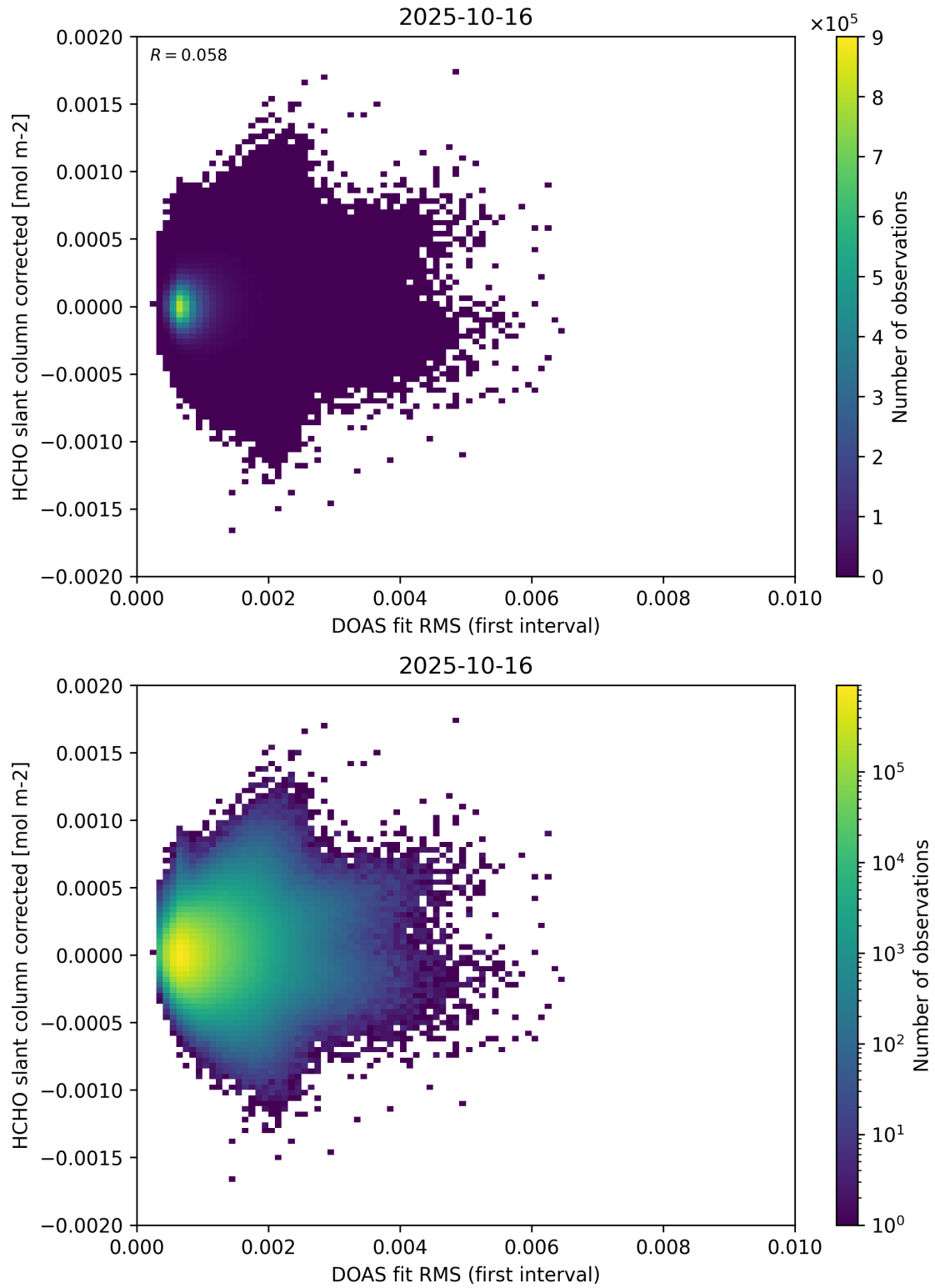
Figure 62: Scatter density plot of “DOAS fit RMS (first interval)” against “HCHO slant column corrected” for 2025-10-15 to 2025-10-17.
