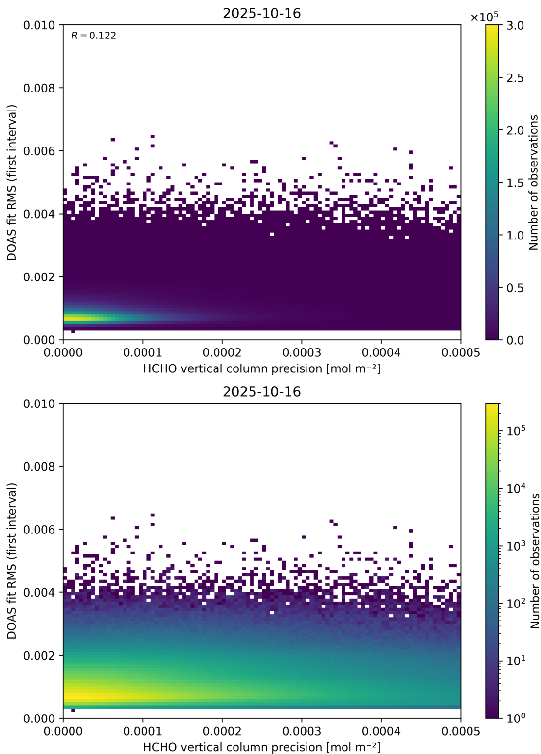
Figure 136: Scatter density plot of “HCHO vertical column precision” against “DOAS fit RMS (first interval)” for 2025-10-15 to 2025-10-17.
