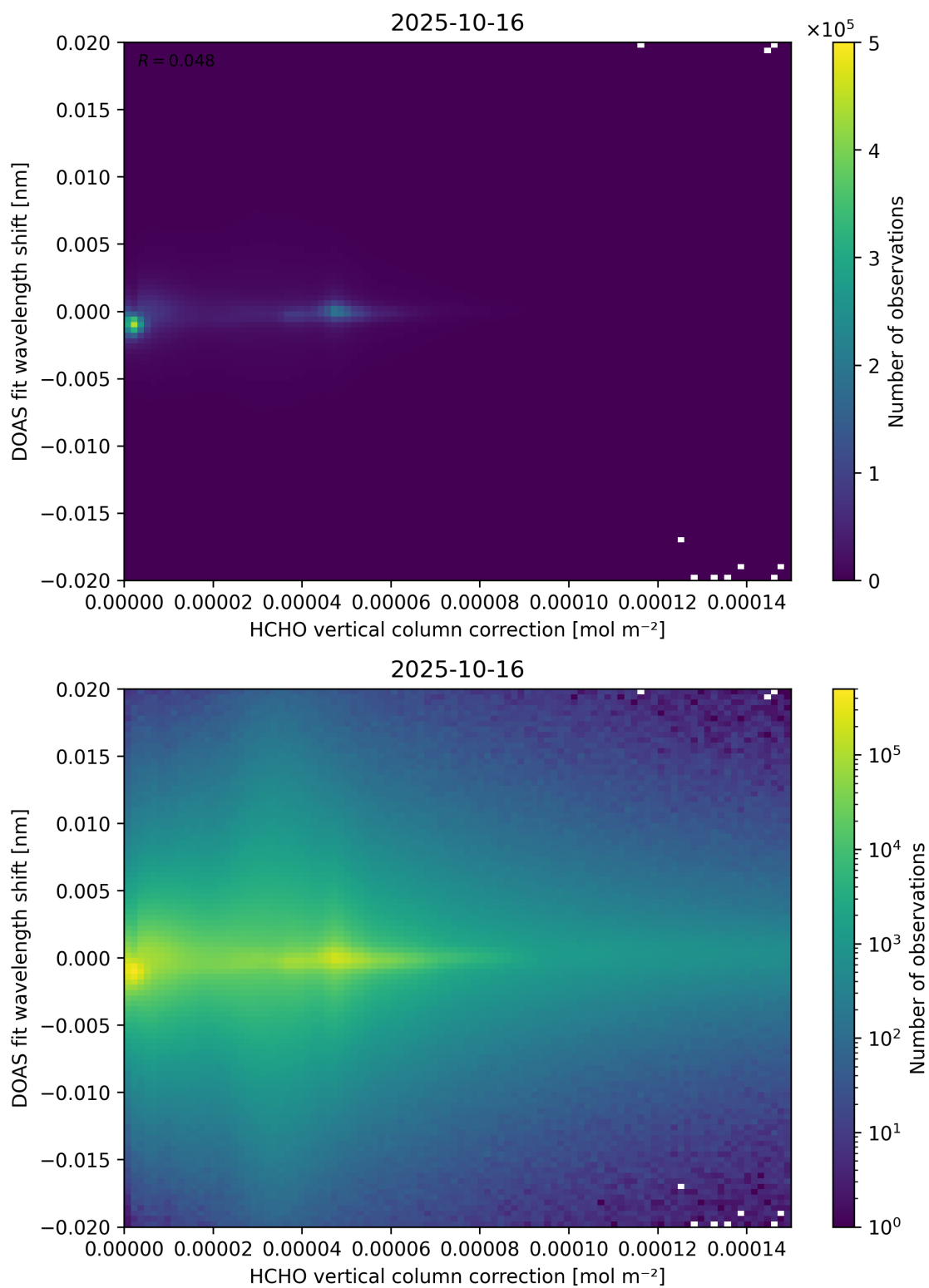
Figure 113: Scatter density plot of “HCHO vertical column correction” against “DOAS fit wavelength shift” for 2025-10-15 to 2025-10-17.
