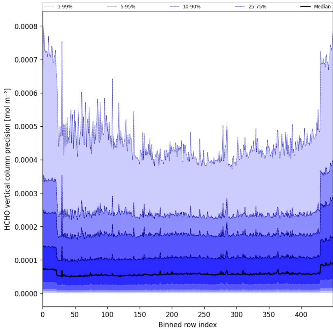
Figure 50: Along track statistics of “HCHO vertical column precision” for 2025-10-15 to 2025-10-17
