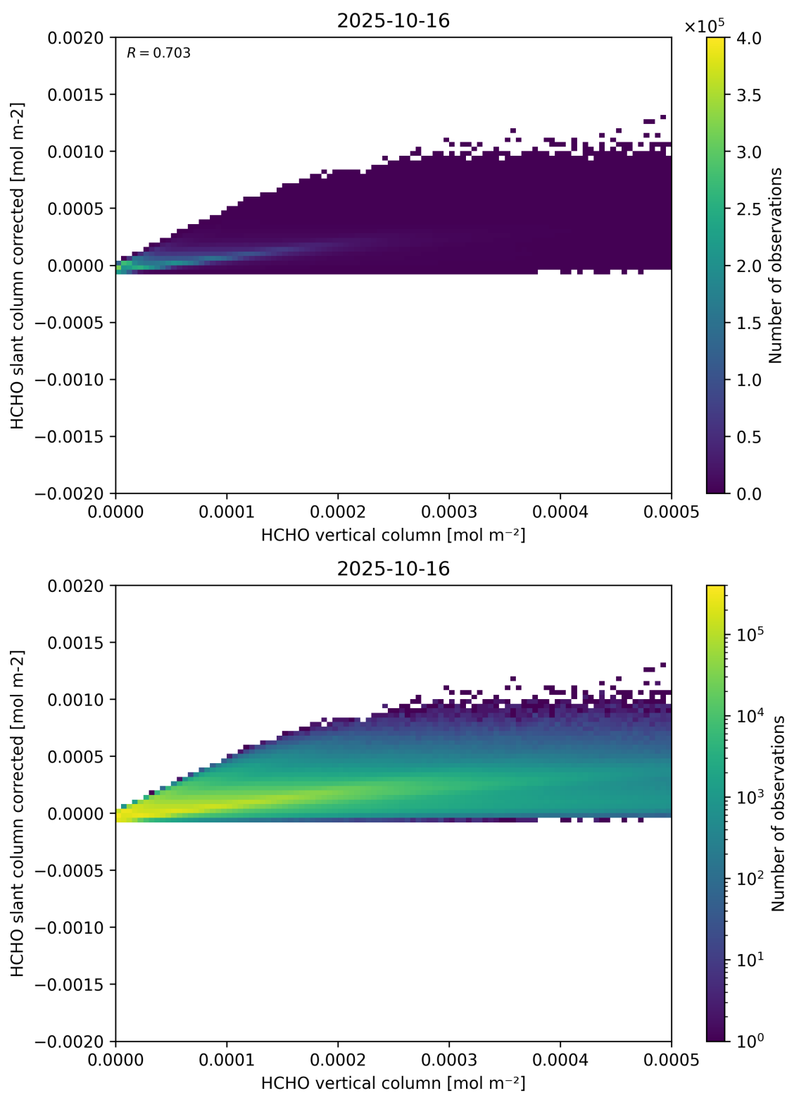
Figure 127: Scatter density plot of “HCHO vertical column” against “HCHO slant column corrected” for 2025-10-15 to 2025-10-17.
