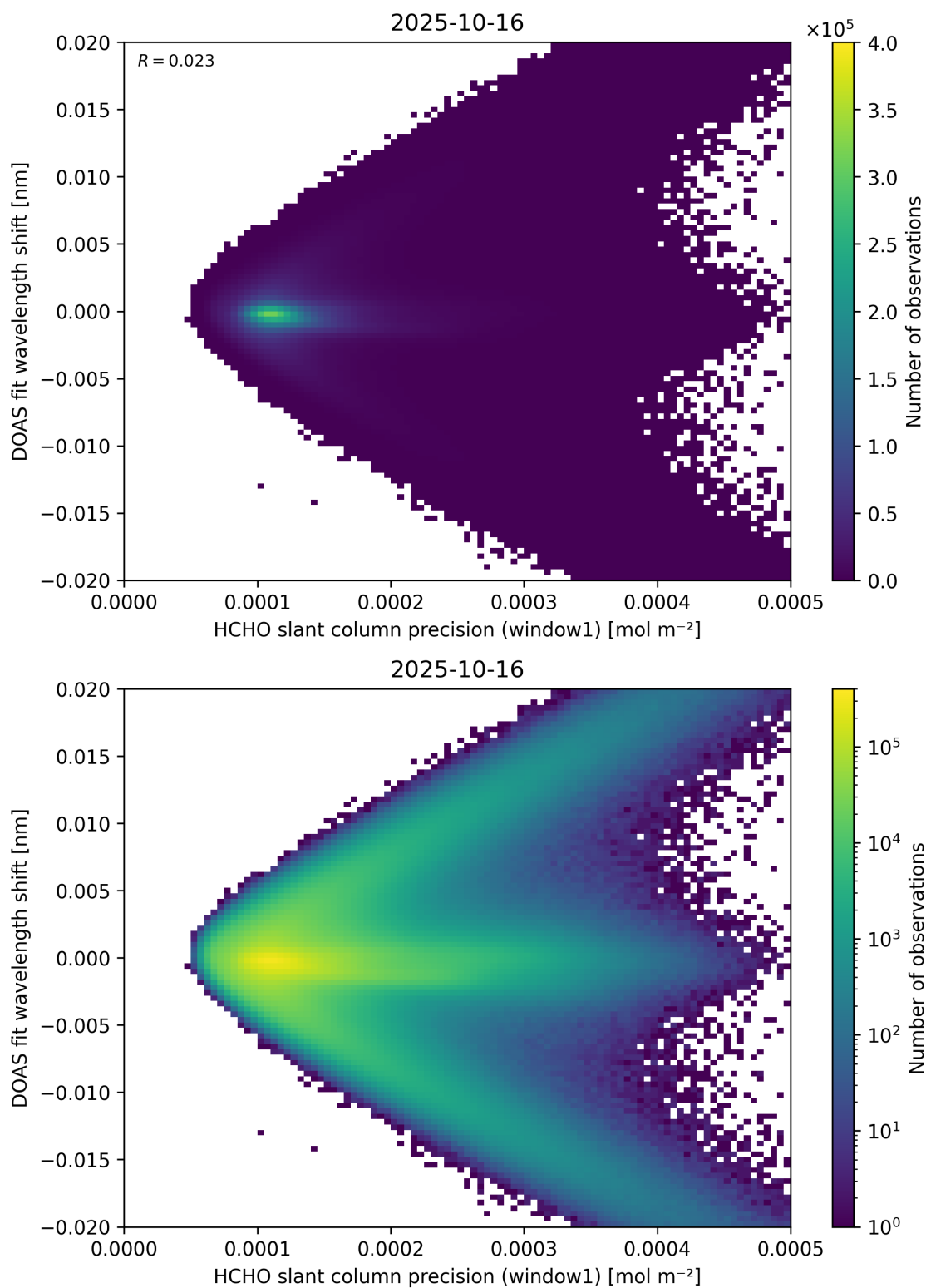
Figure 89: Scatter density plot of “HCHO slant column precision (window1)” against “DOAS fit wavelength shift” for 2025-10-15 to 2025-10-17.
