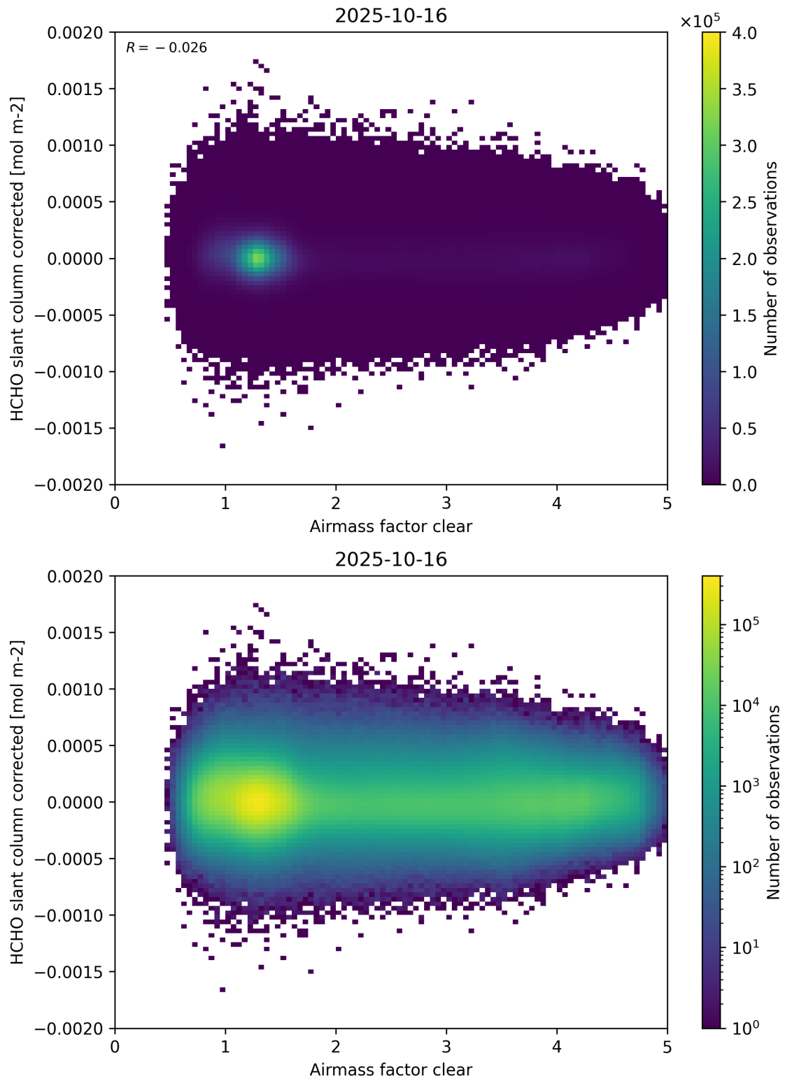
Figure 74: Scatter density plot of “Airmass factor clear” against “HCHO slant column corrected” for 2025-10-15 to 2025-10-17.
