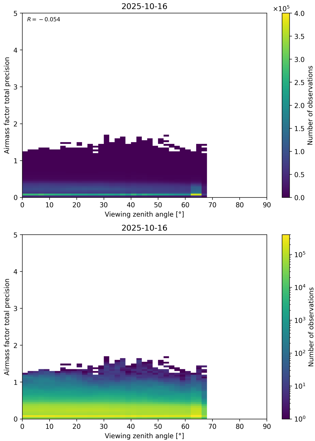
Figure 191: Scatter density plot of “Viewing zenith angle” against “Airmass factor total precision” for 2025-10-15 to 2025-10-17.
