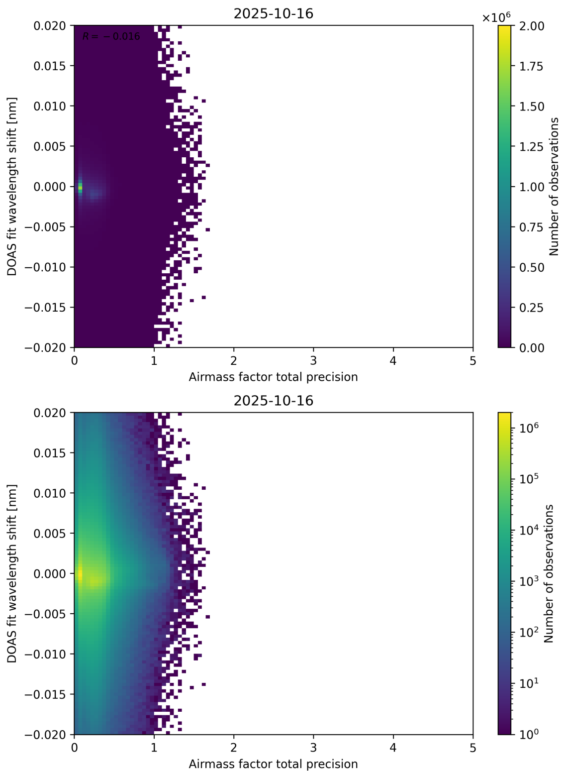
Figure 106: Scatter density plot of “Airmass factor total precision” against “DOAS fit wavelength shift” for 2025-10-15 to 2025-10-17.
