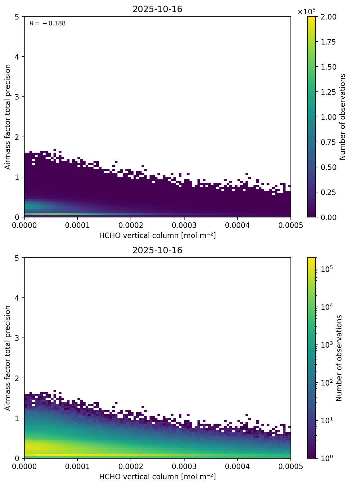
Figure 132: Scatter density plot of “HCHO vertical column” against “Airmass factor total precision” for 2025-10-15 to 2025-10-17.
