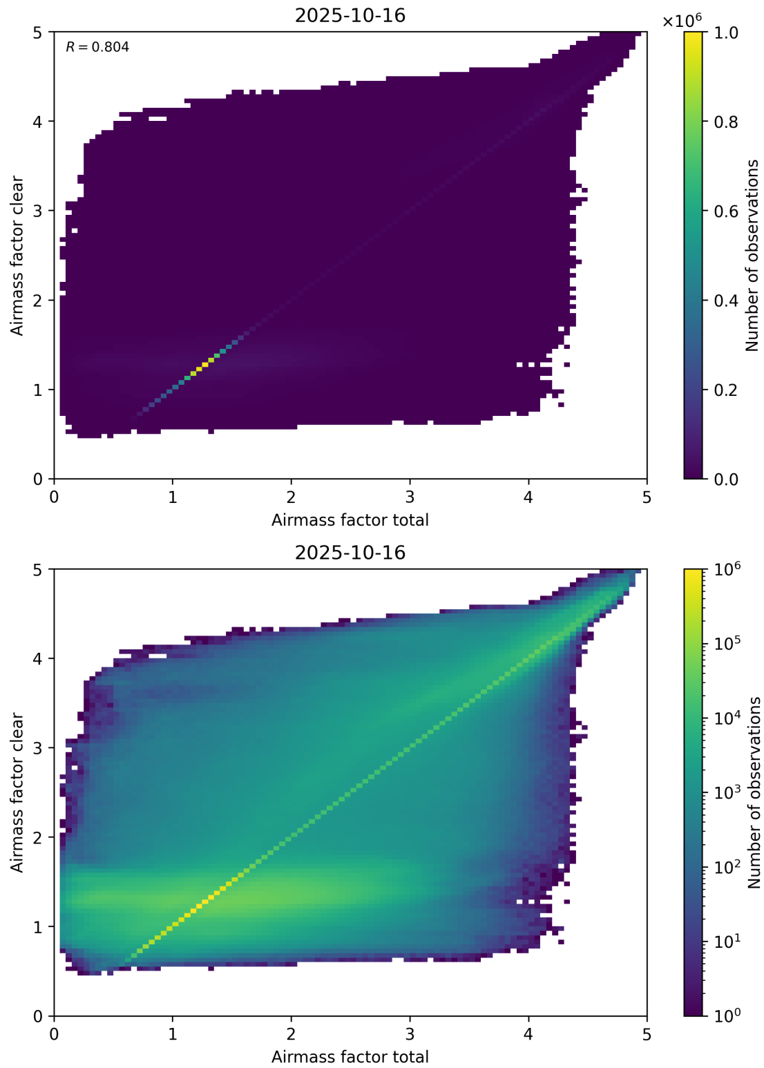
Figure 100: Scatter density plot of “Airmass factor total” against “Airmass factor clear” for 2025-10-15 to 2025-10-17.
