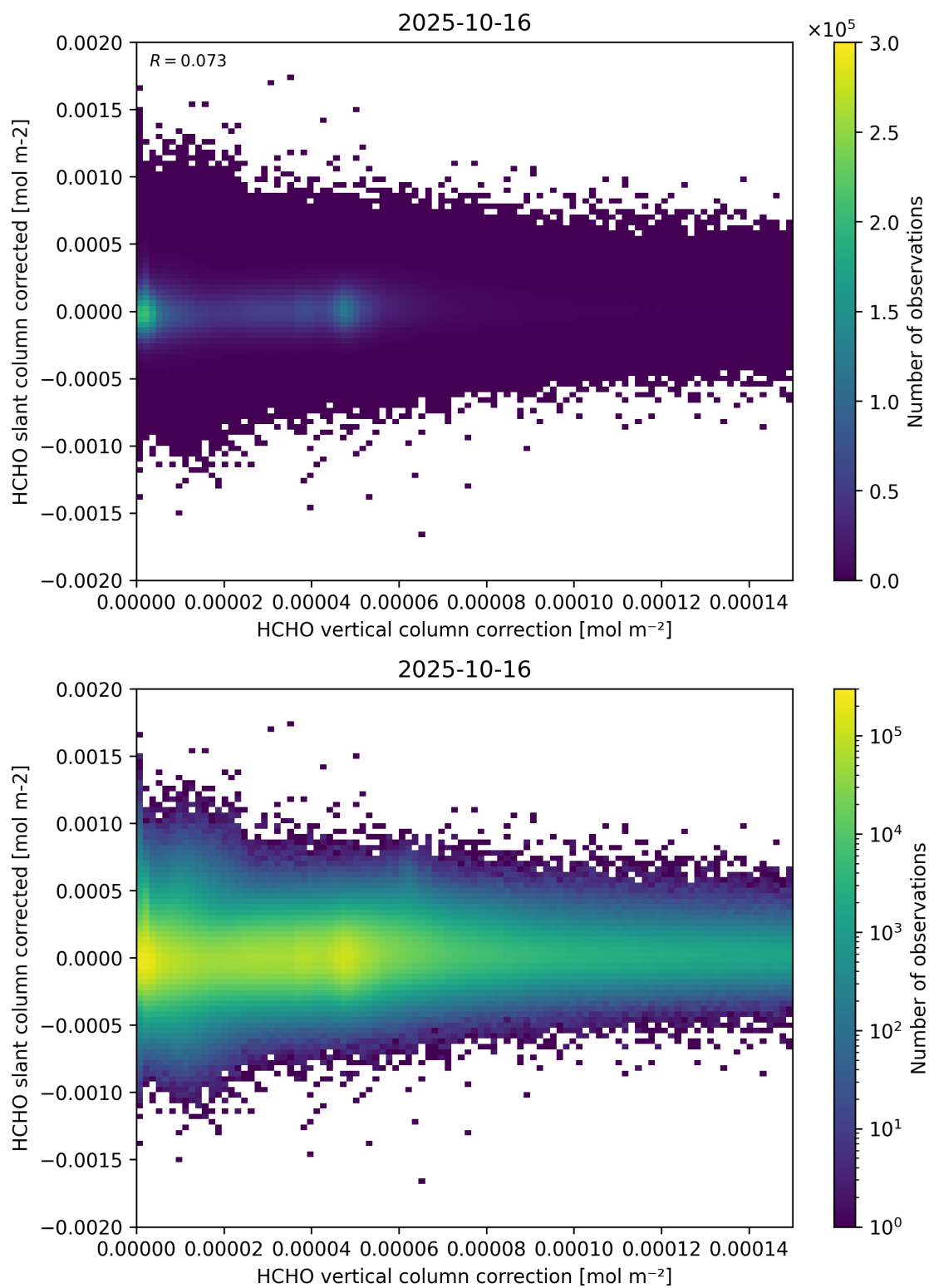
Figure 116: Scatter density plot of “HCHO vertical column correction” against “HCHO slant column corrected” for 2025-10-15 to 2025-10-17.
