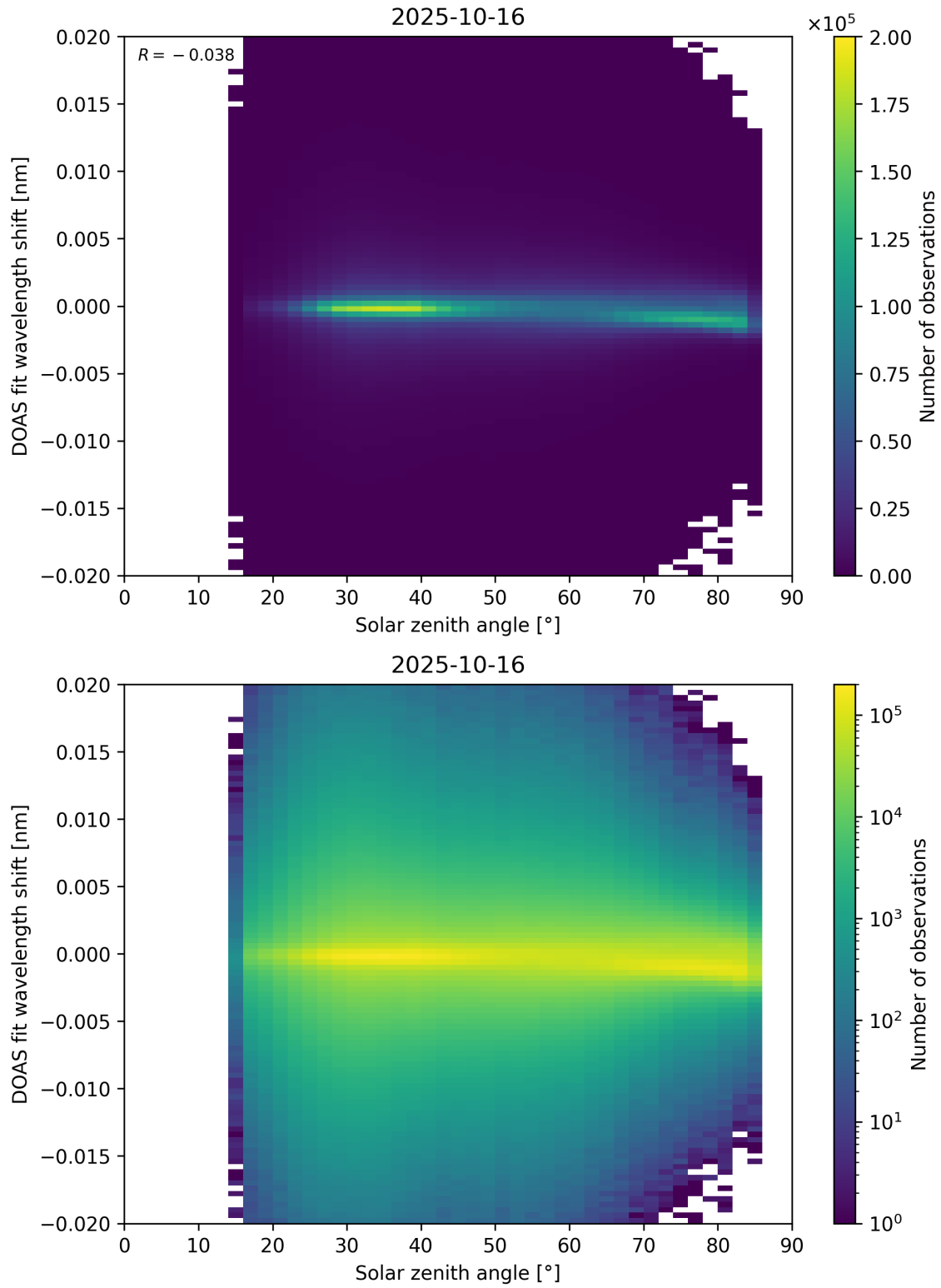
Figure 168: Scatter density plot of “Solar zenith angle” against “DOAS fit wavelength shift” for 2025-10-15 to 2025-10-17.
