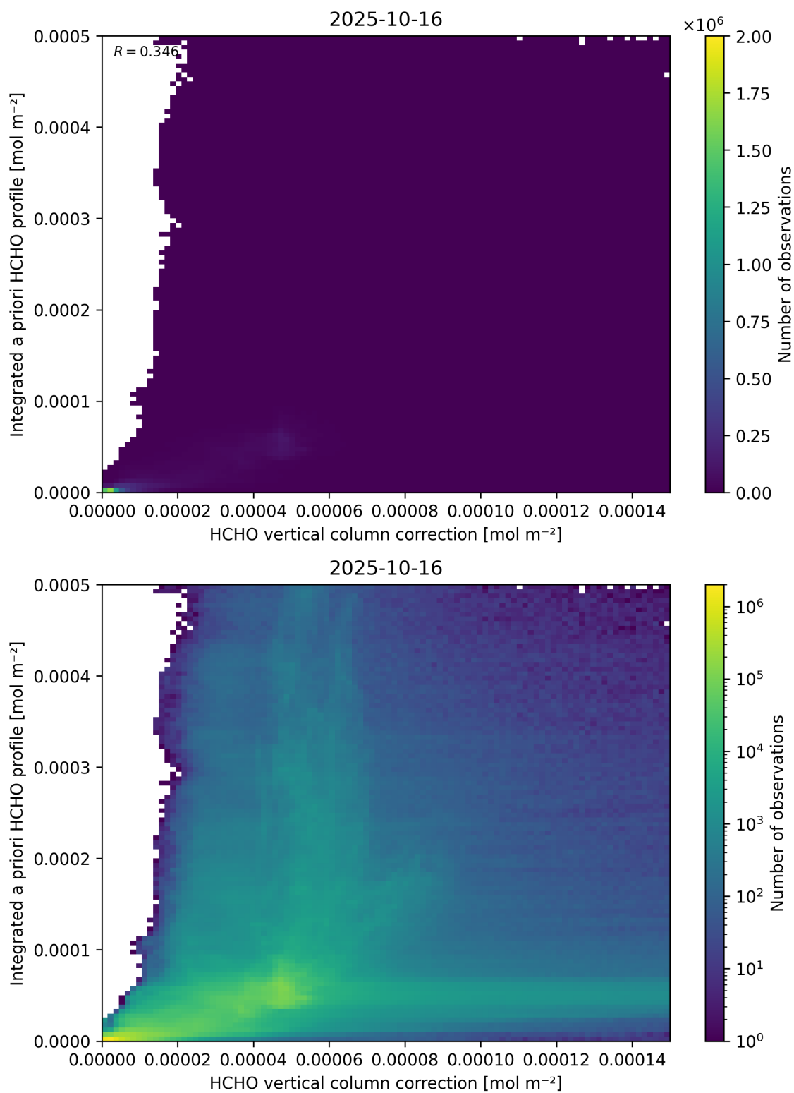
Figure 122: Scatter density plot of “HCHO vertical column correction” against “Integrated a priori HCHO profile” for 2025-10-15 to 2025-10-17.
