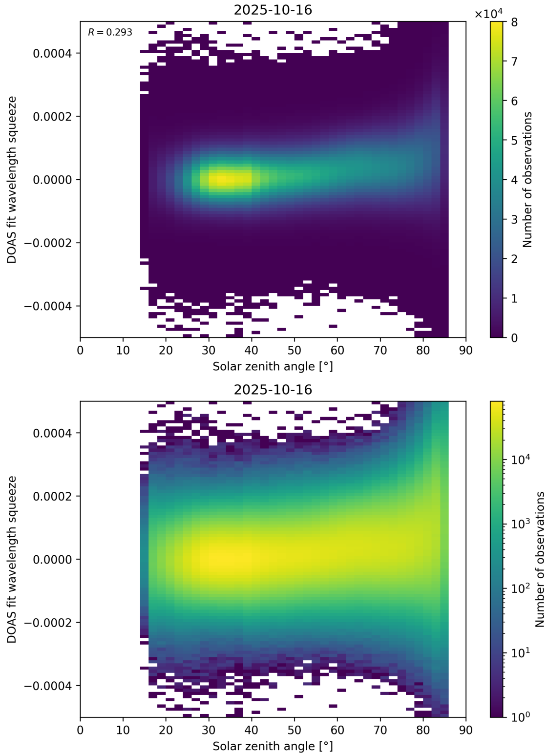
Figure 169: Scatter density plot of “Solar zenith angle” against “DOAS fit wavelength squeeze” for 2025-10-15 to 2025-10-17.
