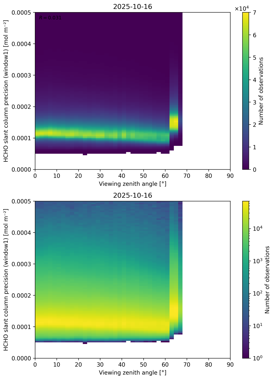
Figure 189: Scatter density plot of “Viewing zenith angle” against “HCHO slant column precision (window1)” for 2025-10-15 to 2025-10-17.
