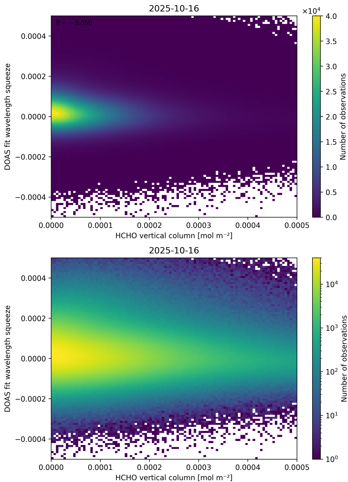
Figure 125: Scatter density plot of “HCHO vertical column” against “DOAS fit wavelength squeeze” for 2025-10-15 to 2025-10-17.
