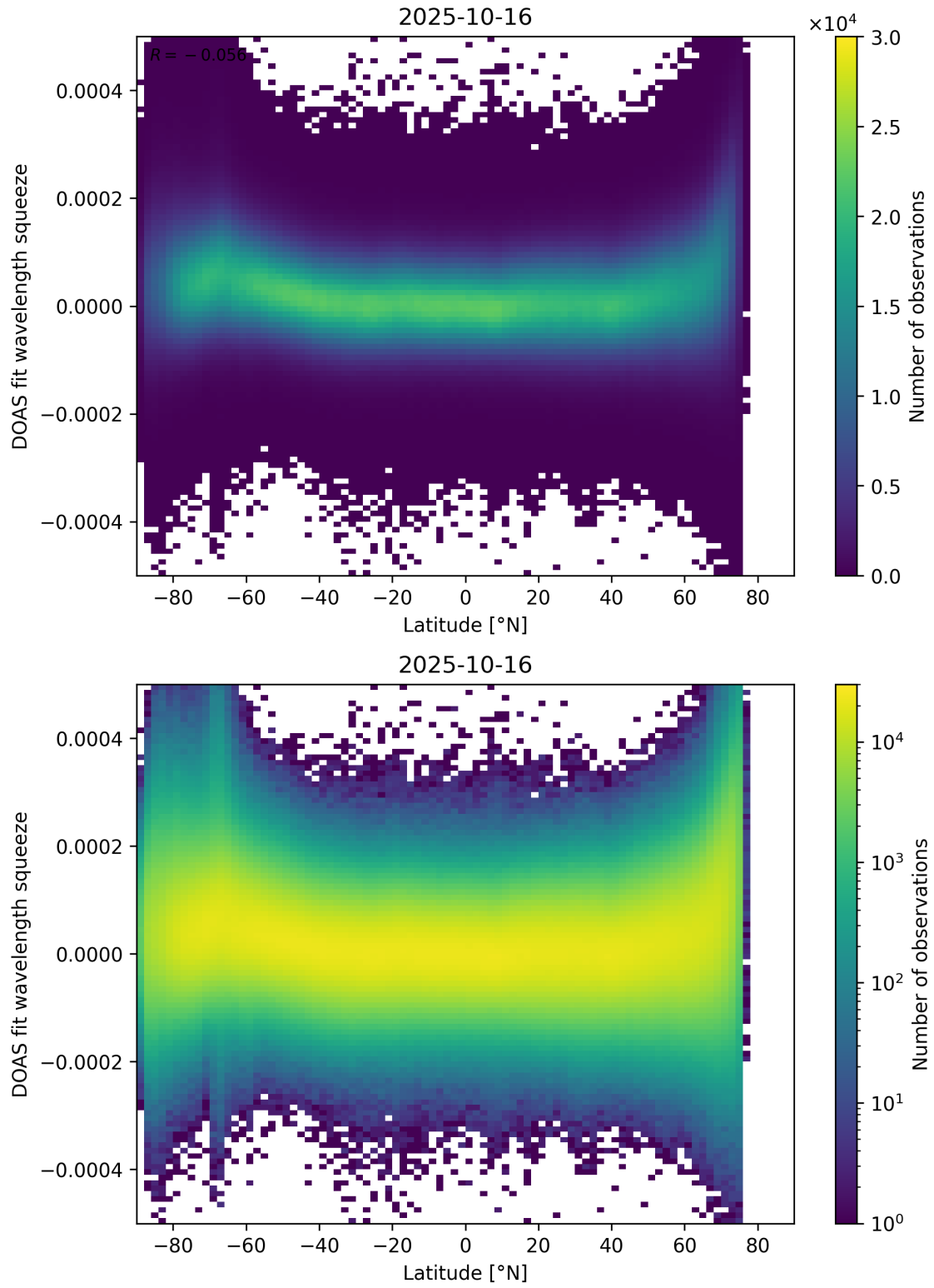
Figure 155: Scatter density plot of “Latitude” against “DOAS fit wavelength squeeze” for 2025-10-15 to 2025-10-17.
