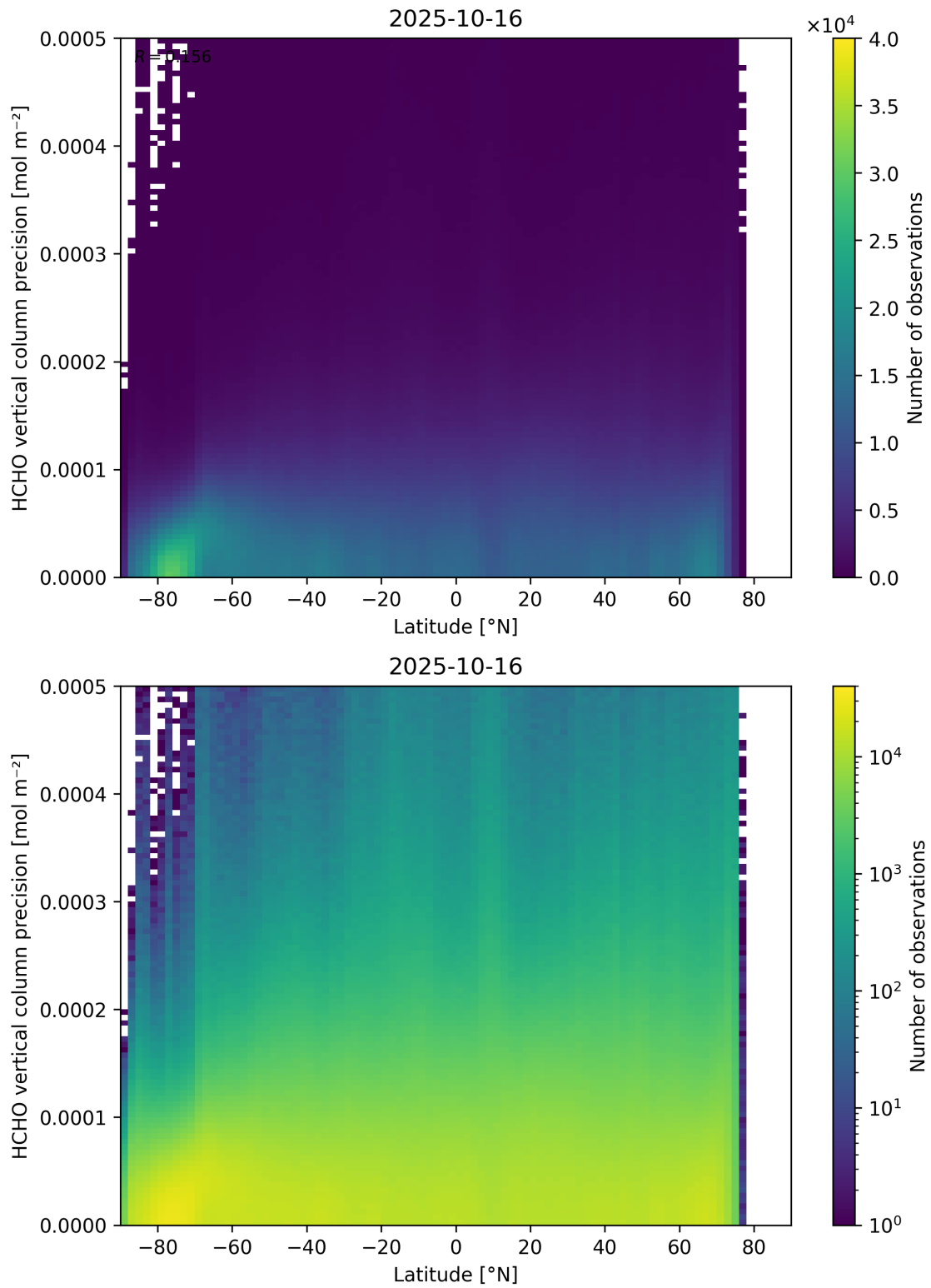
Figure 165: Scatter density plot of “Latitude” against “HCHO vertical column precision” for 2025-10-15 to 2025-10-17.
