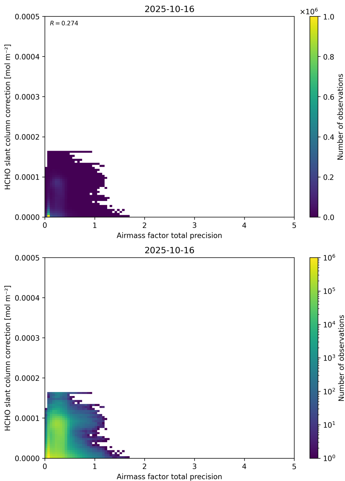
Figure 110: Scatter density plot of “Airmass factor total precision” against “HCHO slant column correction” for 2025-10-15 to 2025-10-17.
