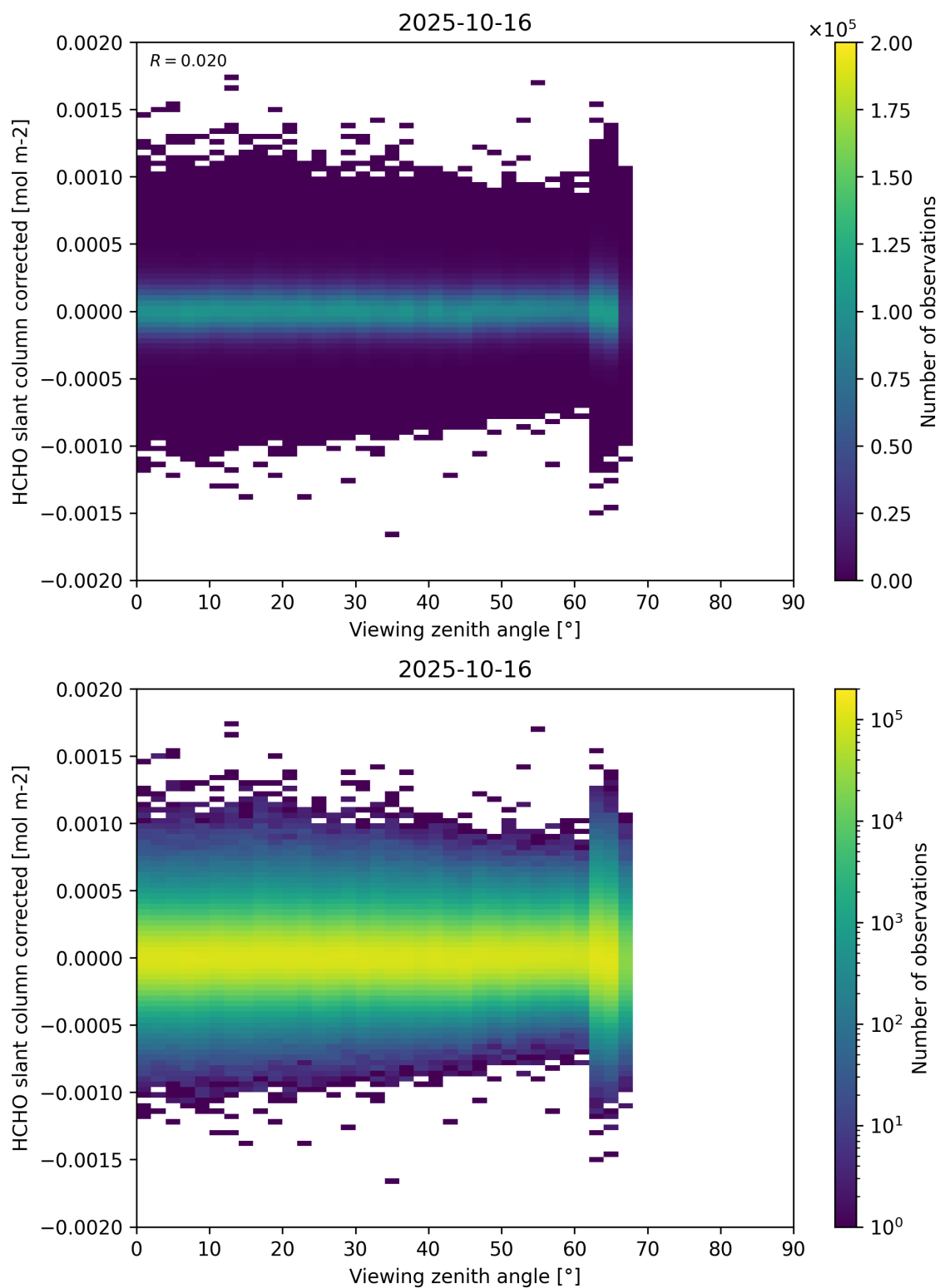
Figure 186: Scatter density plot of “Viewing zenith angle” against “HCHO slant column corrected” for 2025-10-15 to 2025-10-17.
