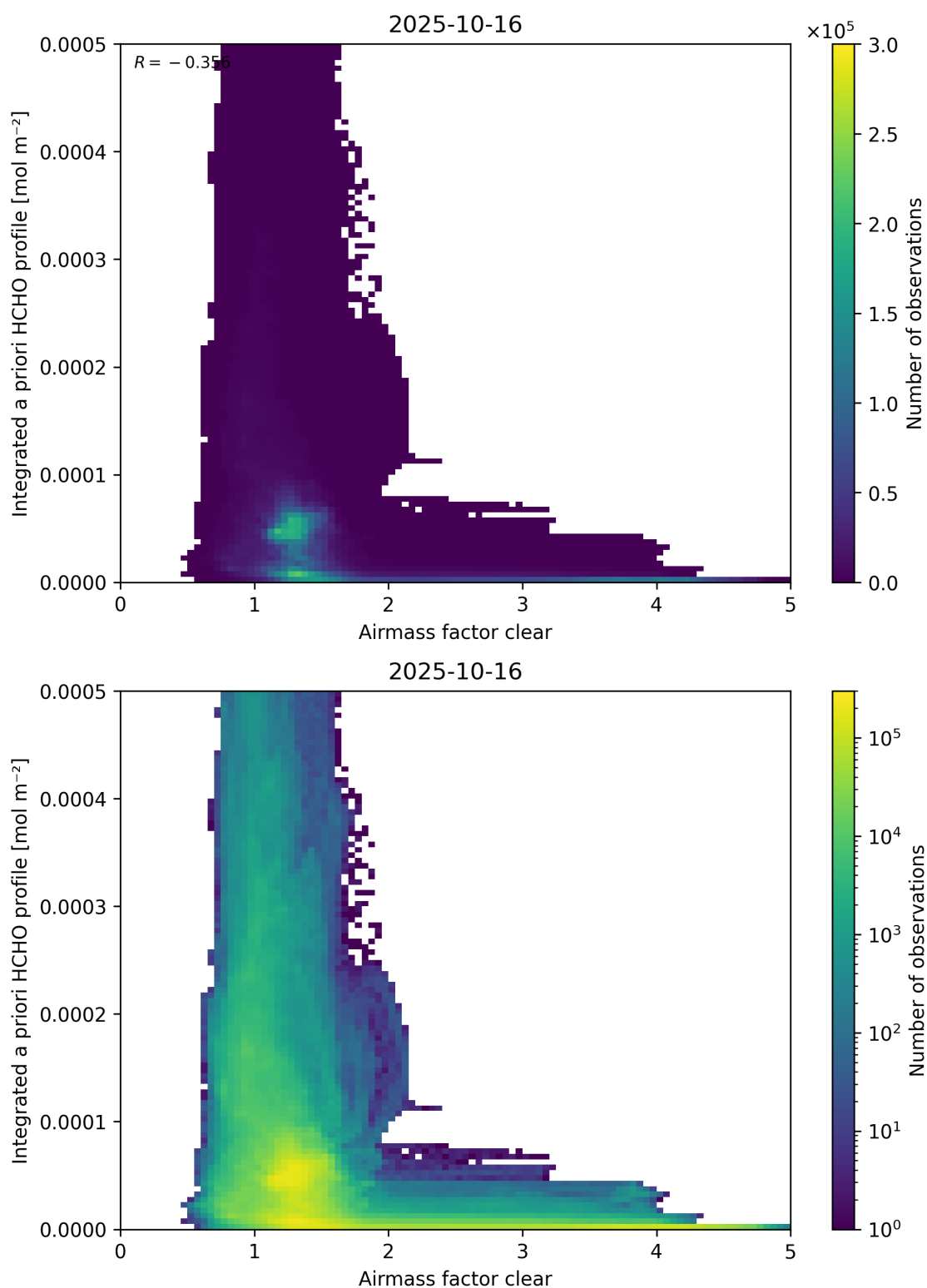
Figure 76: Scatter density plot of “Airmass factor clear” against “Integrated a priori HCHO profile” for 2025-10-15 to 2025-10-17.
