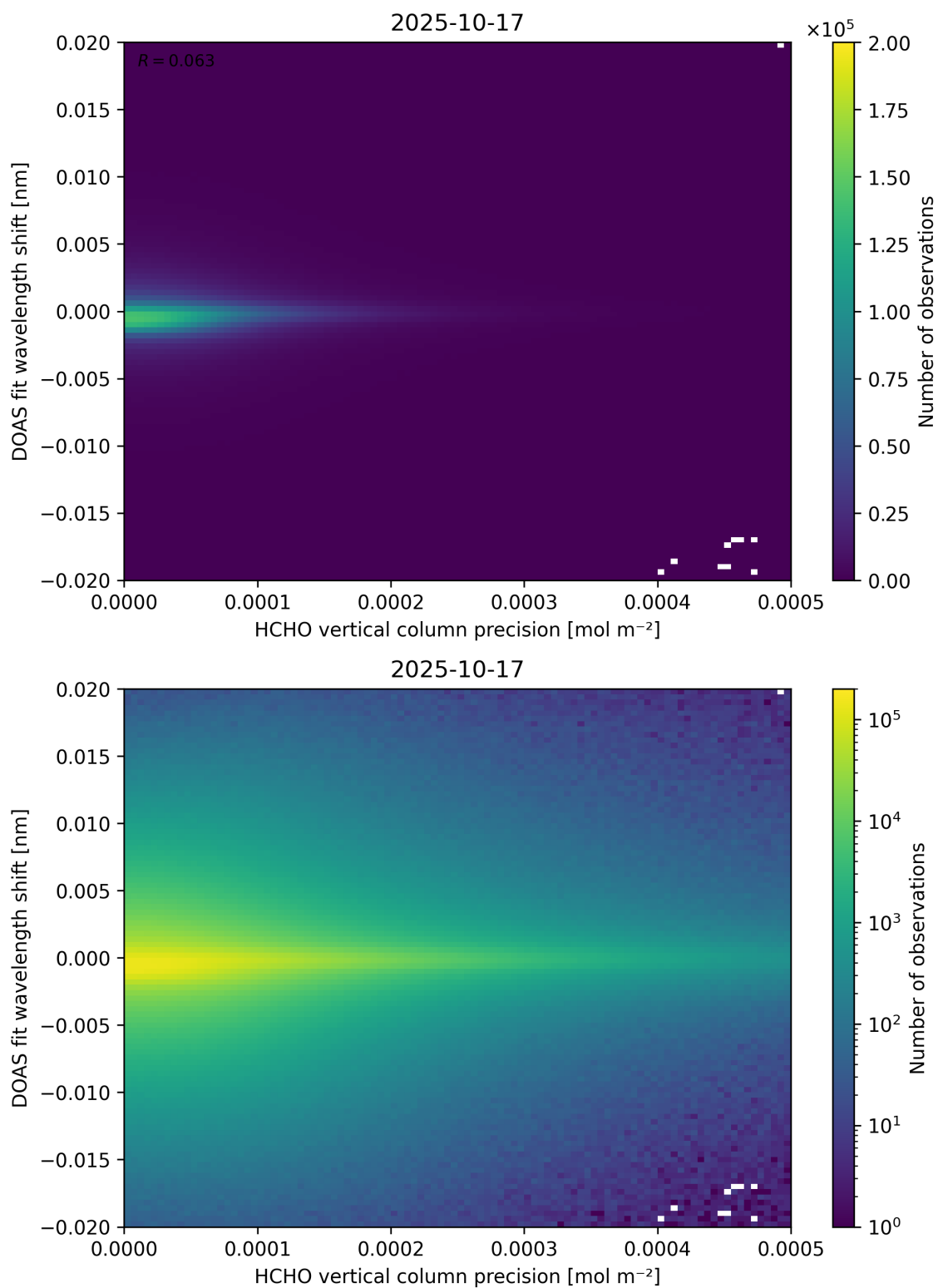
Figure 137: Scatter density plot of “HCHO vertical column precision” against “DOAS fit wavelength shift” for 2025-10-17 to 2025-10-18.
