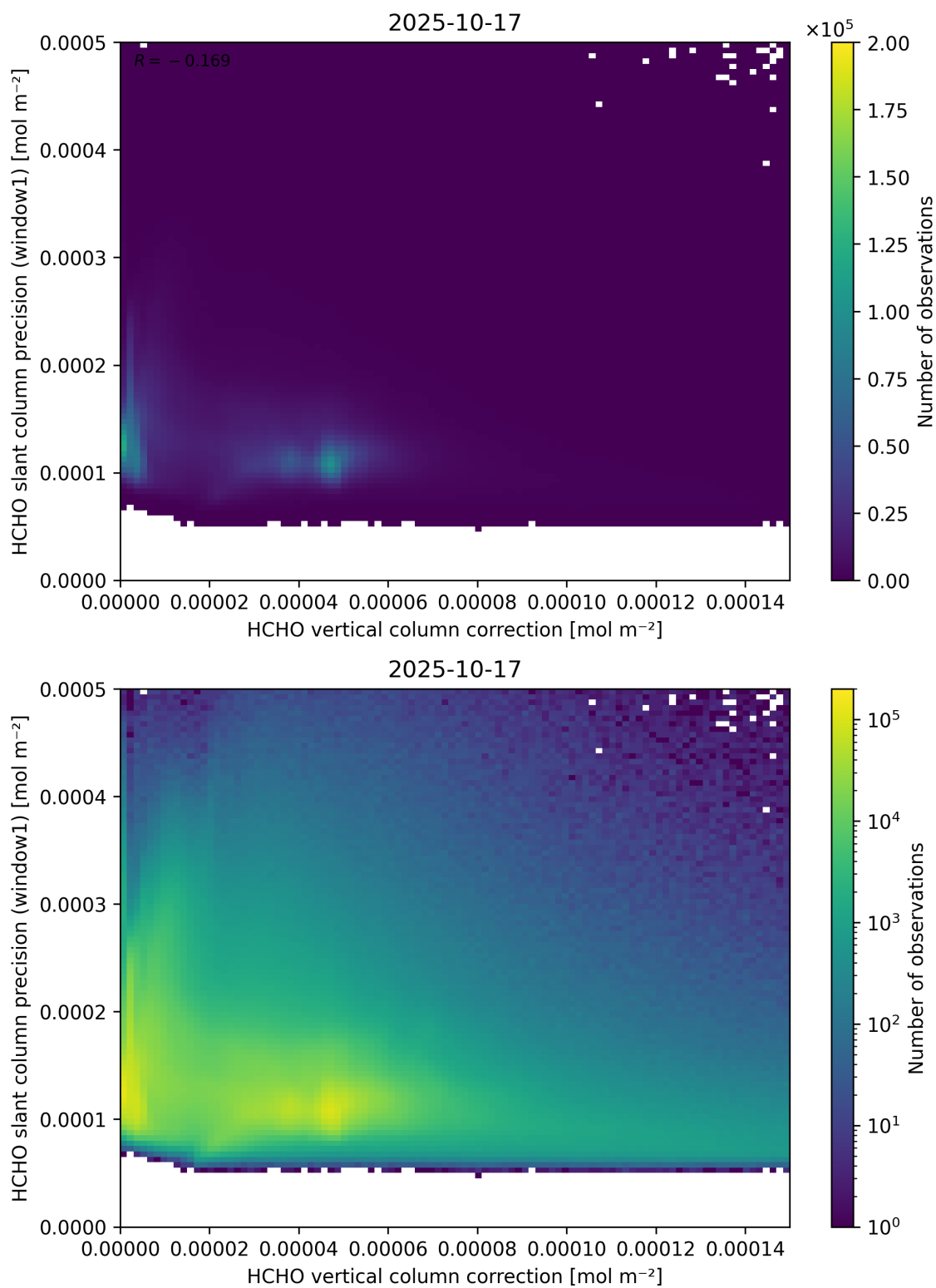
Figure 119: Scatter density plot of “HCHO vertical column correction” against “HCHO slant column precision (window1)” for 2025-10-17 to 2025-10-18.
