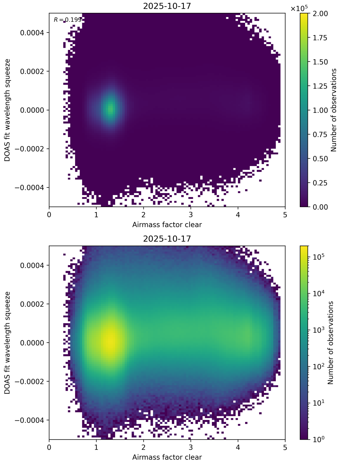
Figure 73: Scatter density plot of “Airmass factor clear” against “DOAS fit wavelength squeeze” for 2025-10-17 to 2025-10-18.
