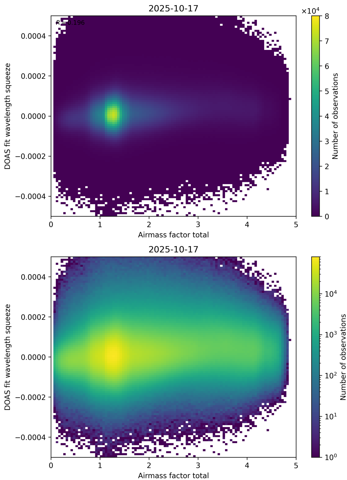
Figure 99: Scatter density plot of “Airmass factor total” against “DOAS fit wavelength squeeze” for 2025-10-17 to 2025-10-18.
