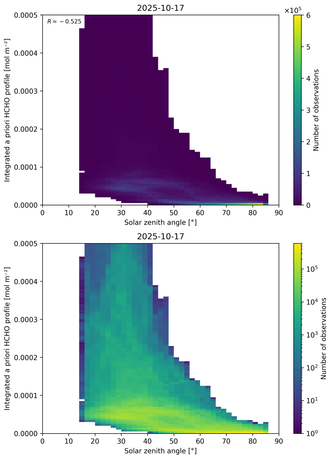
Figure 180: Scatter density plot of “Solar zenith angle” against “Integrated a priori HCHO profile” for 2025-10-17 to 2025-10-18.
