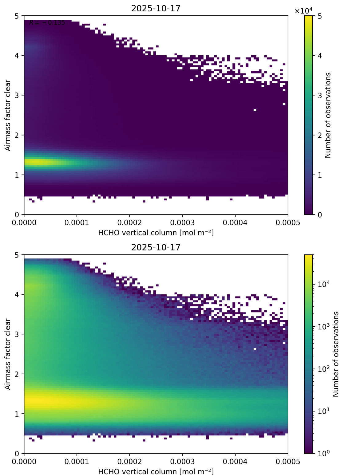
Figure 126: Scatter density plot of “HCHO vertical column” against “Airmass factor clear” for 2025-10-17 to 2025-10-18.
