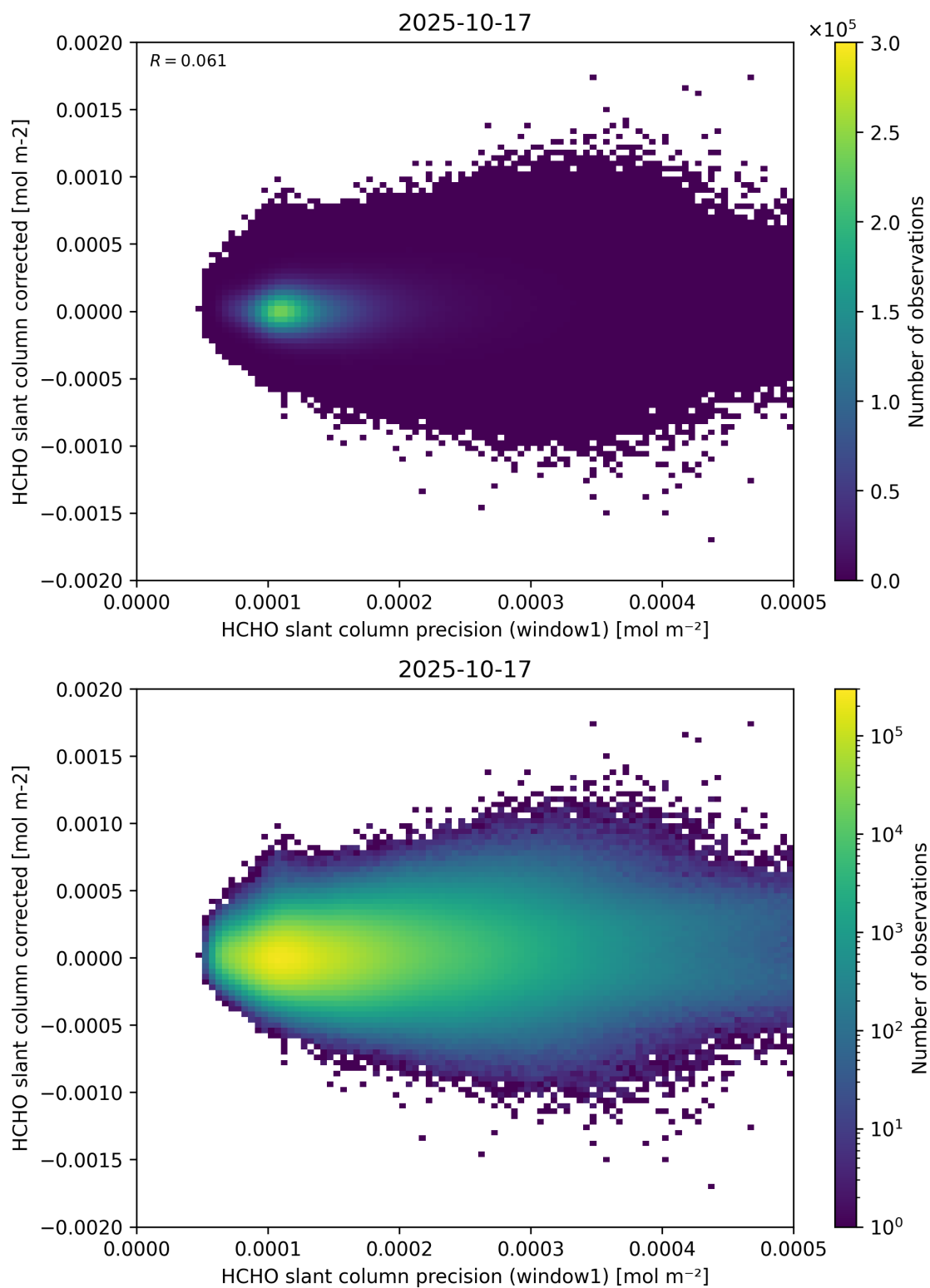
Figure 92: Scatter density plot of “HCHO slant column precision (window1)” against “HCHO slant column corrected” for 2025-10-17 to 2025-10-18.
