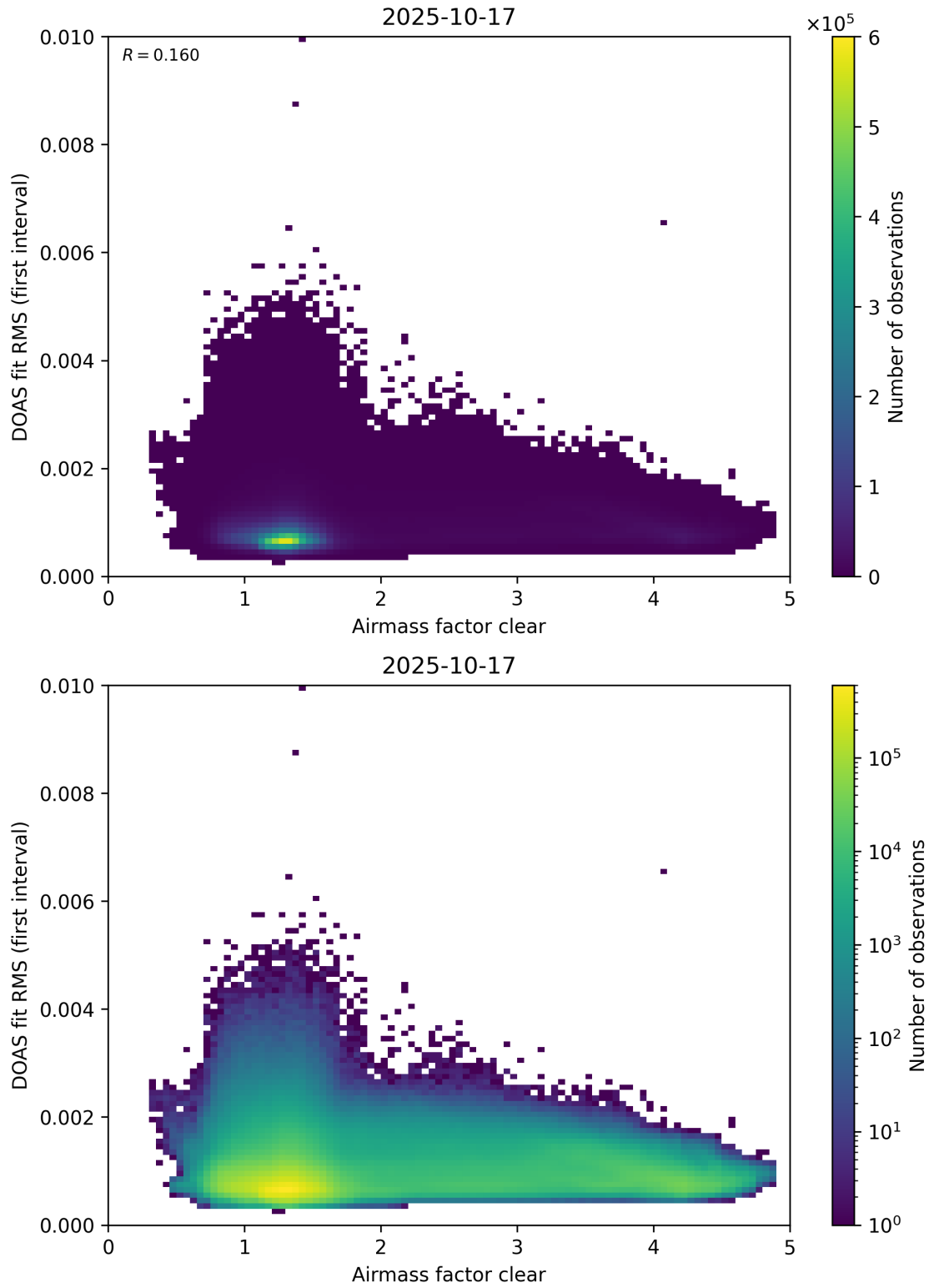
Figure 71: Scatter density plot of “Airmass factor clear” against “DOAS fit RMS (first interval)” for 2025-10-17 to 2025-10-18.
