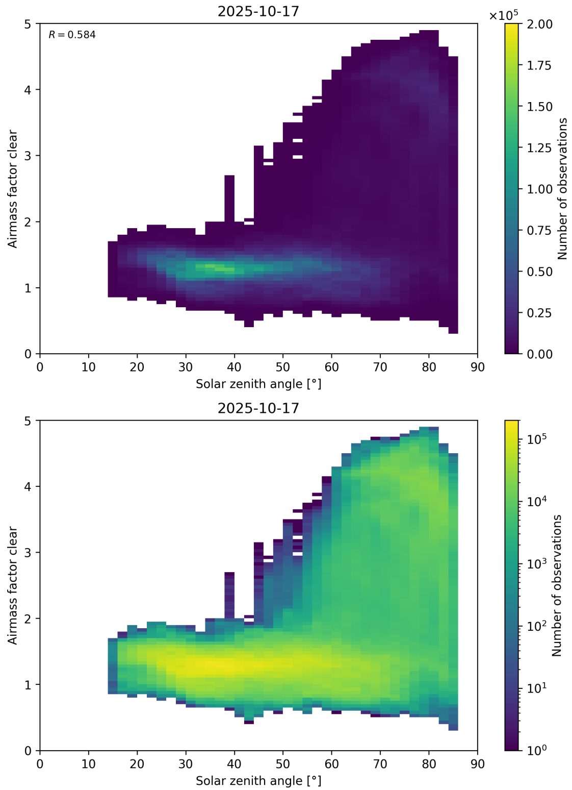
Figure 170: Scatter density plot of “Solar zenith angle” against “Airmass factor clear” for 2025-10-17 to 2025-10-18.
