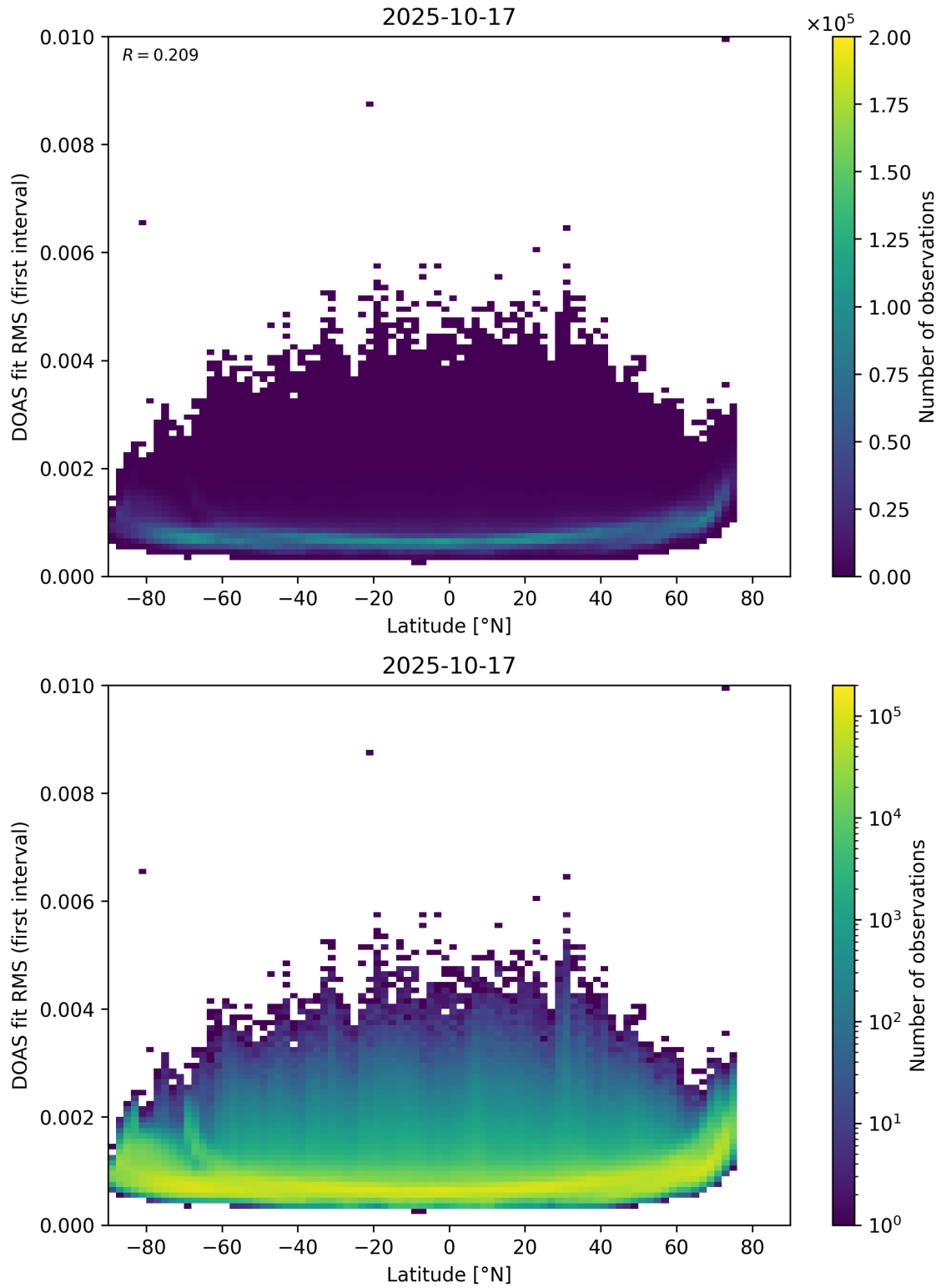
Figure 153: Scatter density plot of “Latitude” against “DOAS fit RMS (first interval)” for 2025-10-17 to 2025-10-18.
