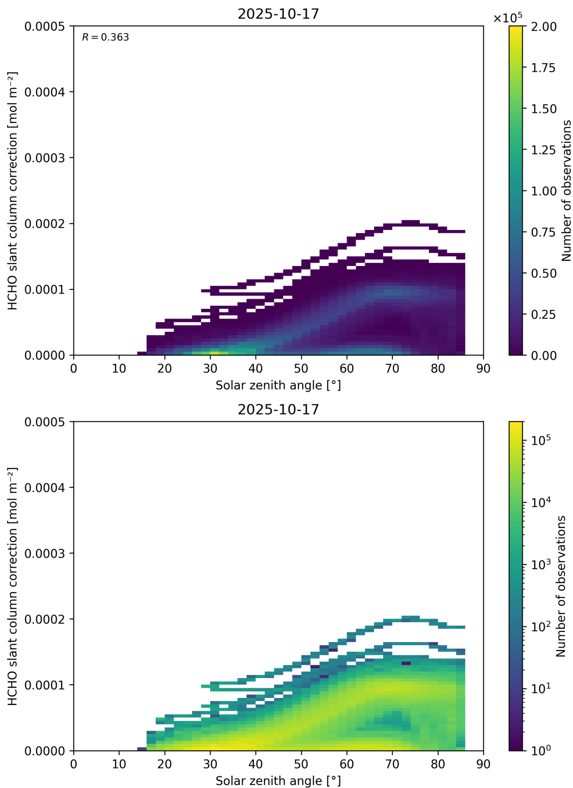
Figure 172: Scatter density plot of “Solar zenith angle” against “HCHO slant column correction” for 2025-10-17 to 2025-10-18.
