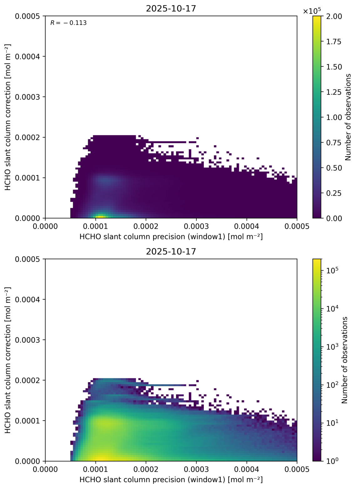
Figure 93: Scatter density plot of “HCHO slant column precision (window1)” against “HCHO slant column correction” for 2025-10-17 to 2025-10-18.
