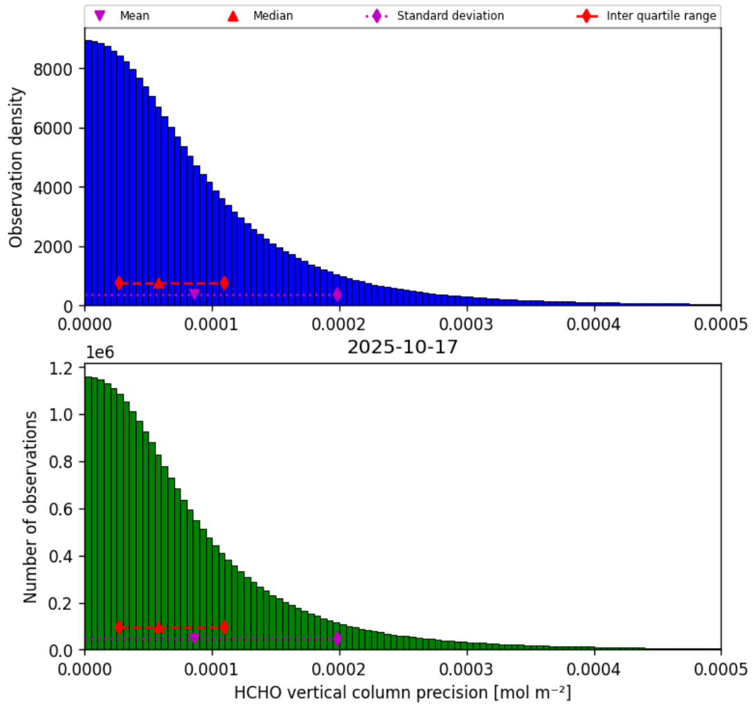
Figure 36: Histogram of “HCHO vertical column precision” for 2025-10-17 to 2025-10-18
