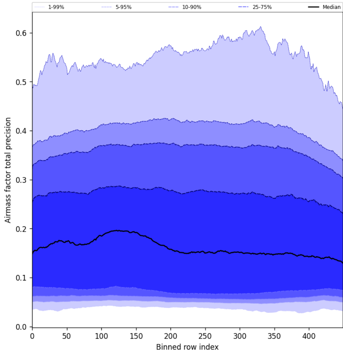
Figure 55: Along track statistics of “Airmass factor total precision” for 2025-10-17 to 2025-10-18
