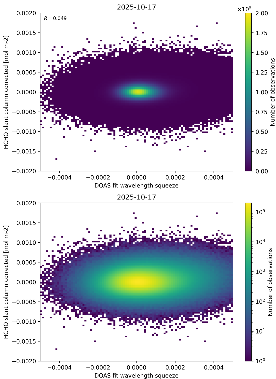
Figure 69: Scatter density plot of “DOAS fit wavelength squeeze” against “HCHO slant column corrected” for 2025-10-17 to 2025-10-18.
