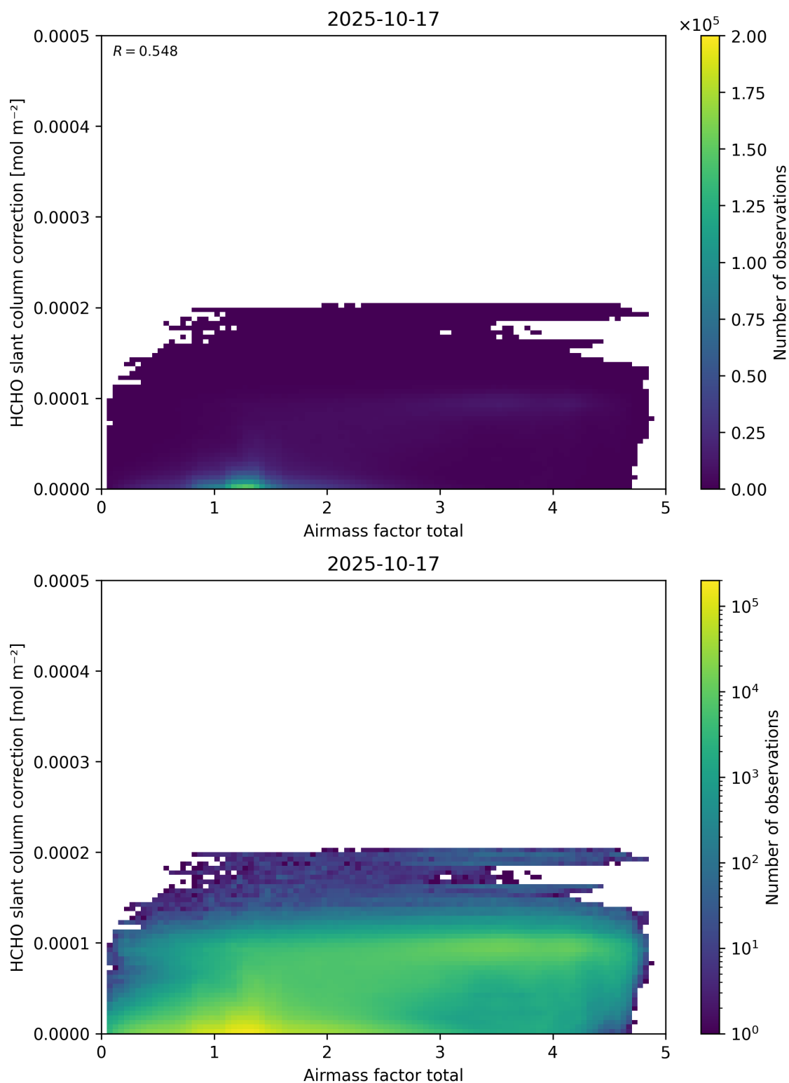
Figure 102: Scatter density plot of “Airmass factor total” against “HCHO slant column correction” for 2025-10-17 to 2025-10-18.
