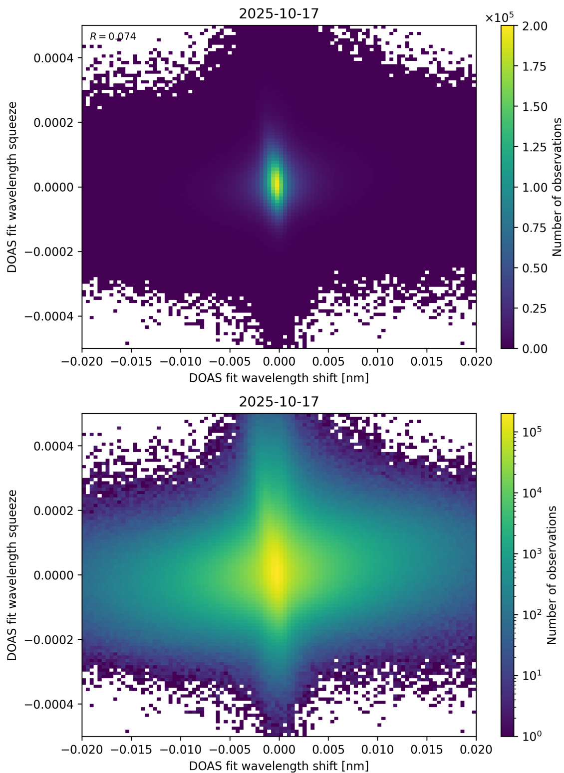
Figure 65: Scatter density plot of “DOAS fit wavelength shift” against “DOAS fit wavelength squeeze” for 2025-10-17 to 2025-10-18.
