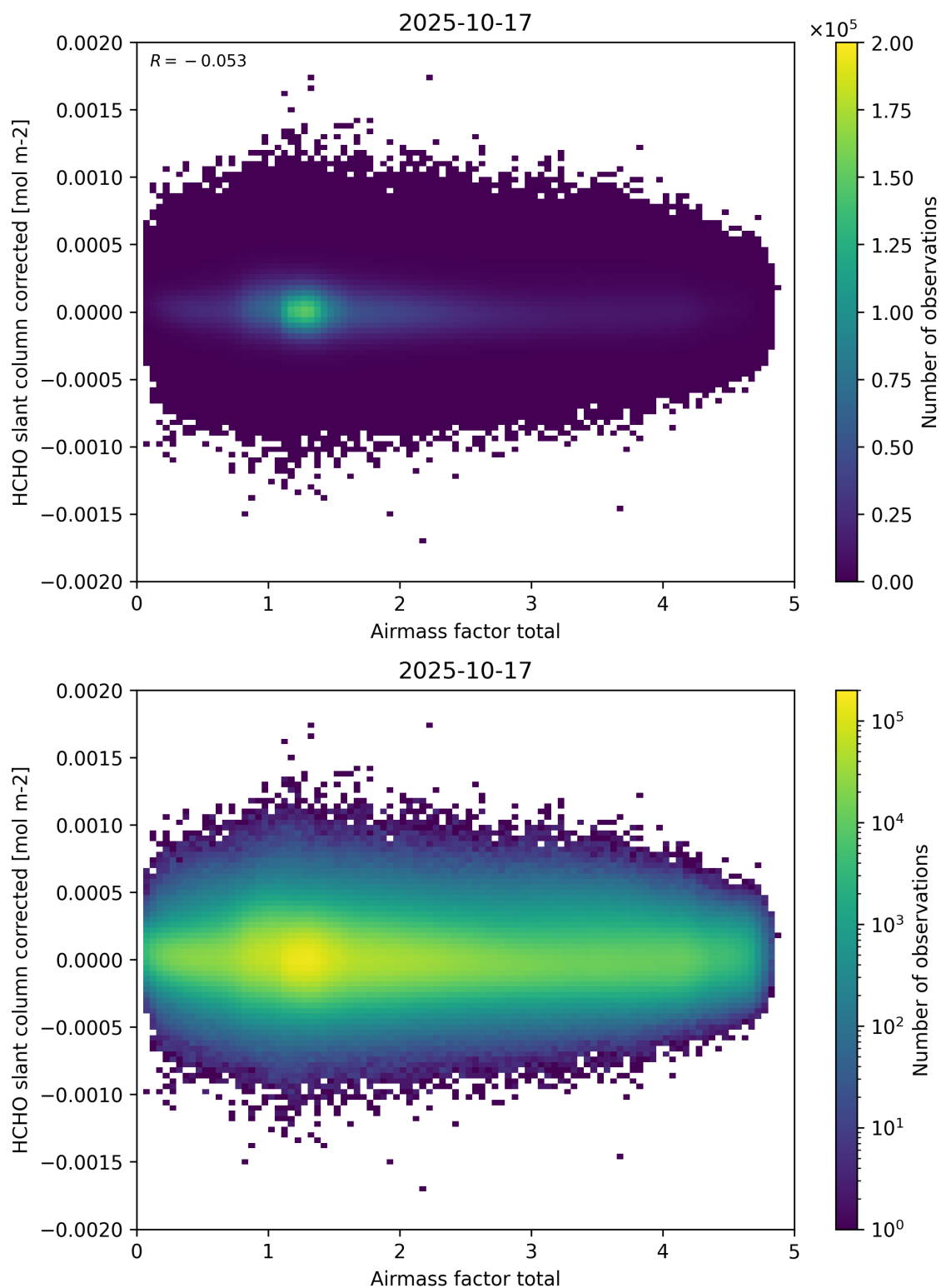
Figure 101: Scatter density plot of “Airmass factor total” against “HCHO slant column corrected” for 2025-10-17 to 2025-10-18.
