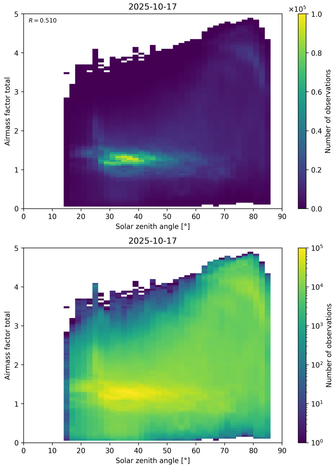
Figure 175: Scatter density plot of “Solar zenith angle” against “Airmass factor total” for 2025-10-17 to 2025-10-18.
