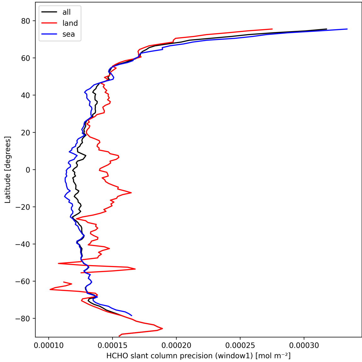
Figure 25: Zonal average of "HCHO slant column precision (window1)" for 2025-10-17 to 2025-10-18.
