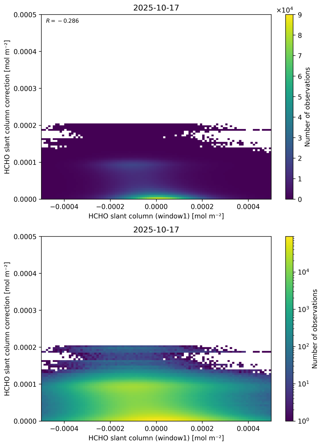
Figure 83: Scatter density plot of “HCHO slant column (window1)” against “HCHO slant column correction” for 2025-10-17 to 2025-10-18.
