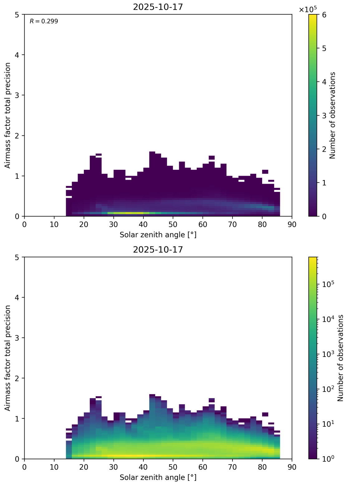
Figure 176: Scatter density plot of “Solar zenith angle” against “Airmass factor total precision” for 2025-10-17 to 2025-10-18.
