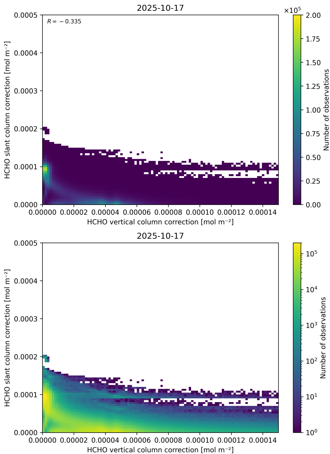
Figure 117: Scatter density plot of “HCHO vertical column correction” against “HCHO slant column correction” for 2025-10-17 to 2025-10-18.
