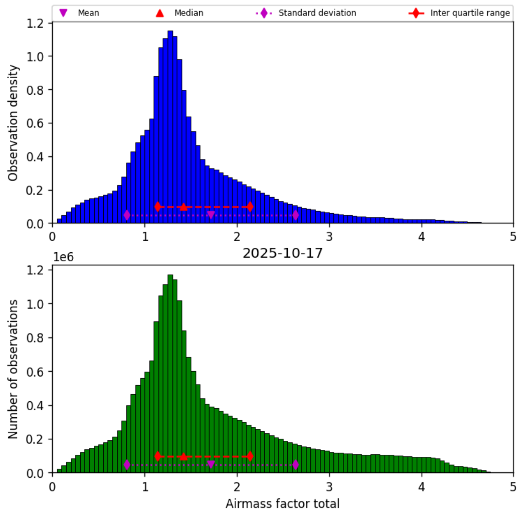
Figure 40: Histogram of “Airmass factor total” for 2025-10-17 to 2025-10-18
