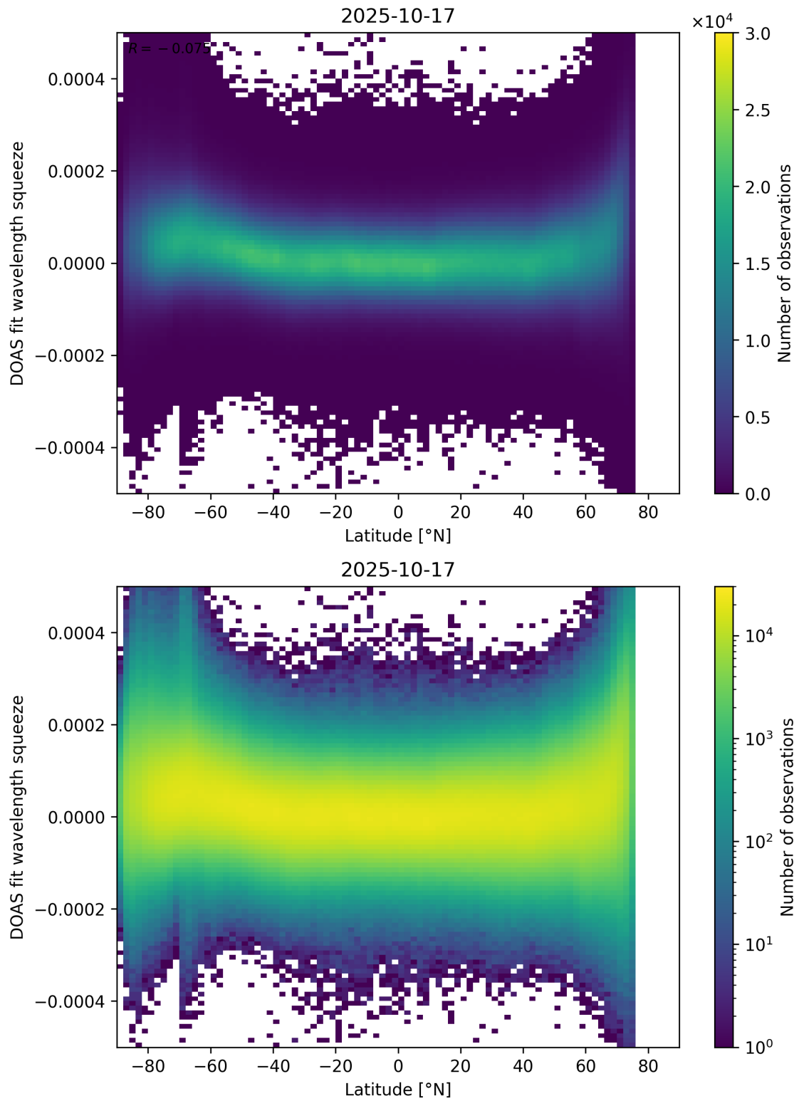
Figure 155: Scatter density plot of “Latitude” against “DOAS fit wavelength squeeze” for 2025-10-17 to 2025-10-18.
