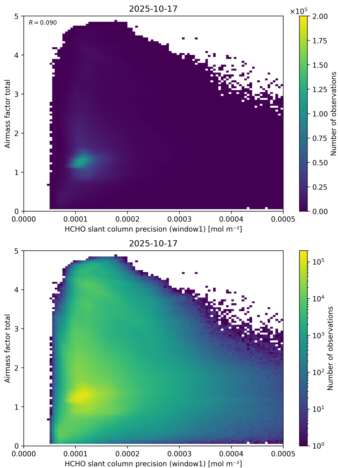
Figure 94: Scatter density plot of “HCHO slant column precision (window1)” against “Airmass factor total” for 2025-10-17 to 2025-10-18.
