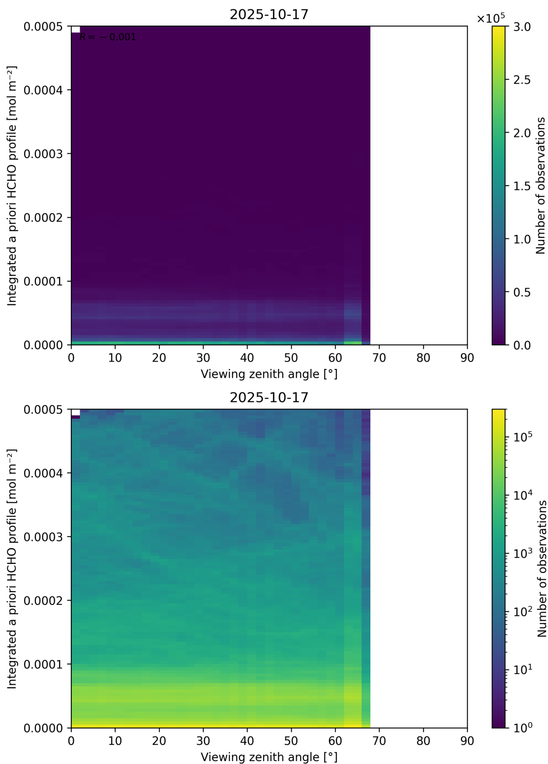
Figure 195: Scatter density plot of “Viewing zenith angle” against “Integrated a priori HCHO profile” for 2025-10-17 to 2025-10-18.
