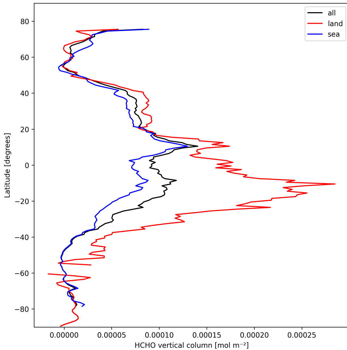
Figure 21: Zonal average of “HCHO vertical column” for 2025-10-17 to 2025-10-18.
