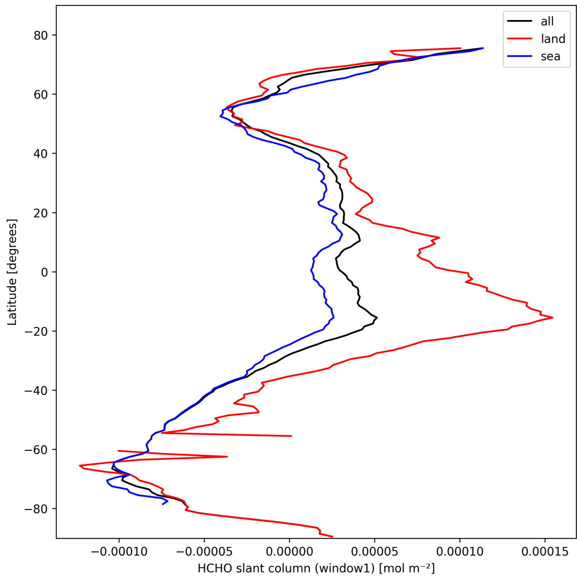
Figure 24: Zonal average of “HCHO slant column (window1)” for 2025-10-17 to 2025-10-18.
