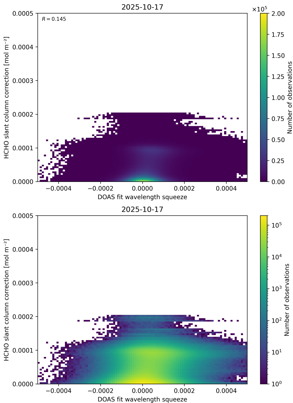
Figure 70: Scatter density plot of “DOAS fit wavelength squeeze” against “HCHO slant column correction” for 2025-10-17 to 2025-10-18.
