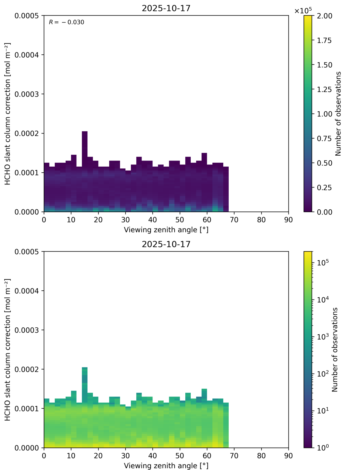
Figure 187: Scatter density plot of “Viewing zenith angle” against “HCHO slant column correction” for 2025-10-17 to 2025-10-18.
