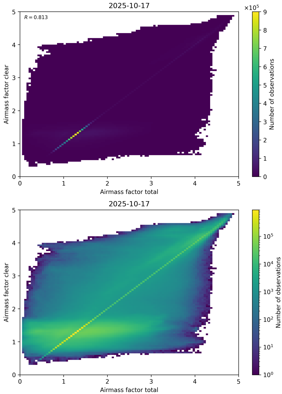
Figure 100: Scatter density plot of “Airmass factor total” against “Airmass factor clear” for 2025-10-17 to 2025-10-18.
