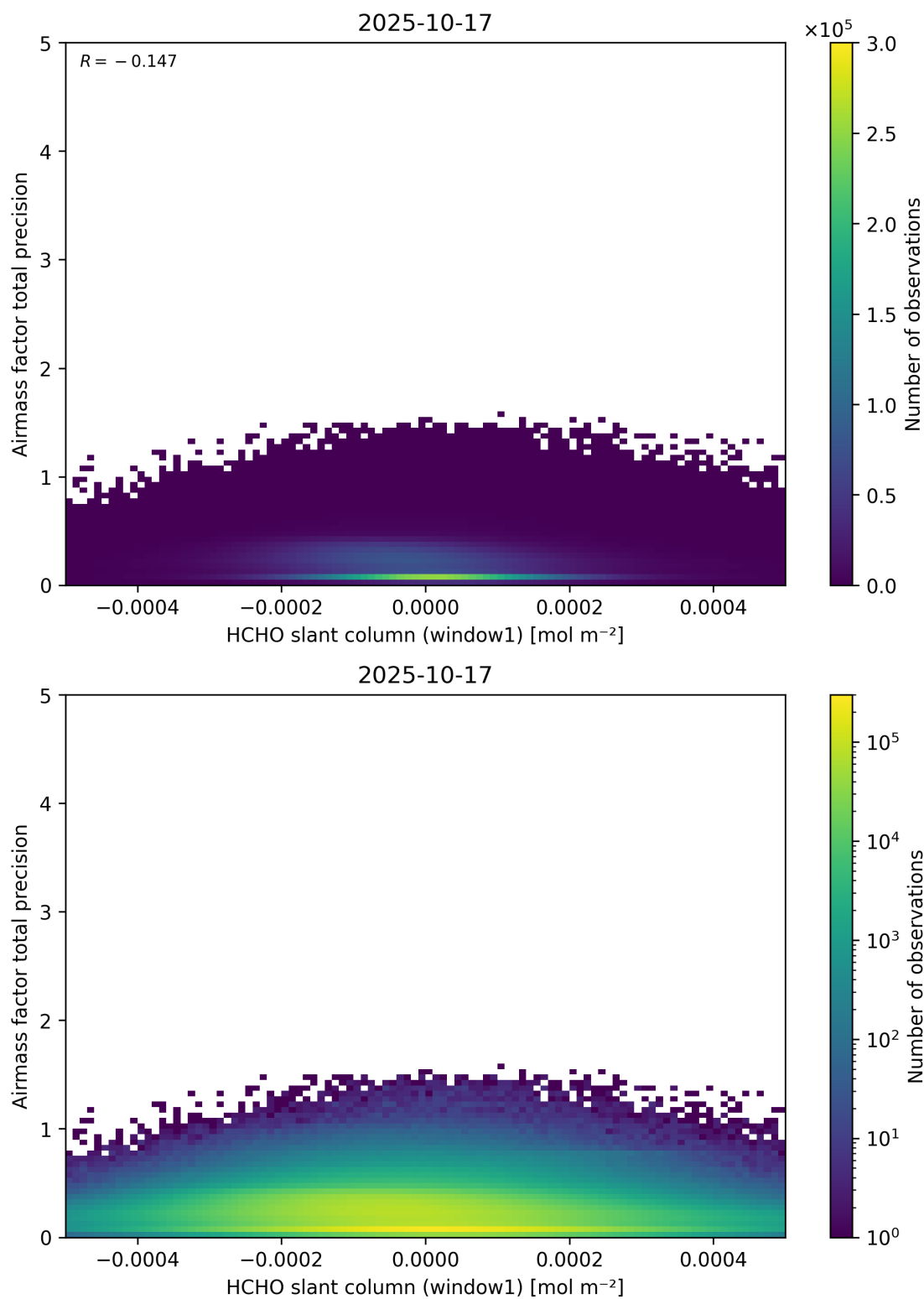
Figure 86: Scatter density plot of “HCHO slant column (window1)” against “Airmass factor total precision” for 2025-10-17 to 2025-10-18.
