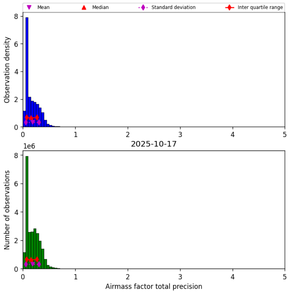
Figure 41: Histogram of “Airmass factor total precision” for 2025-10-17 to 2025-10-18
