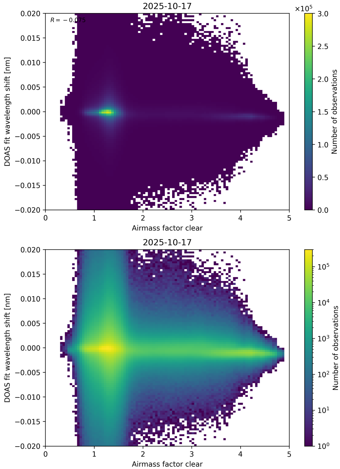
Figure 72: Scatter density plot of “Airmass factor clear” against “DOAS fit wavelength shift” for 2025-10-17 to 2025-10-18.
