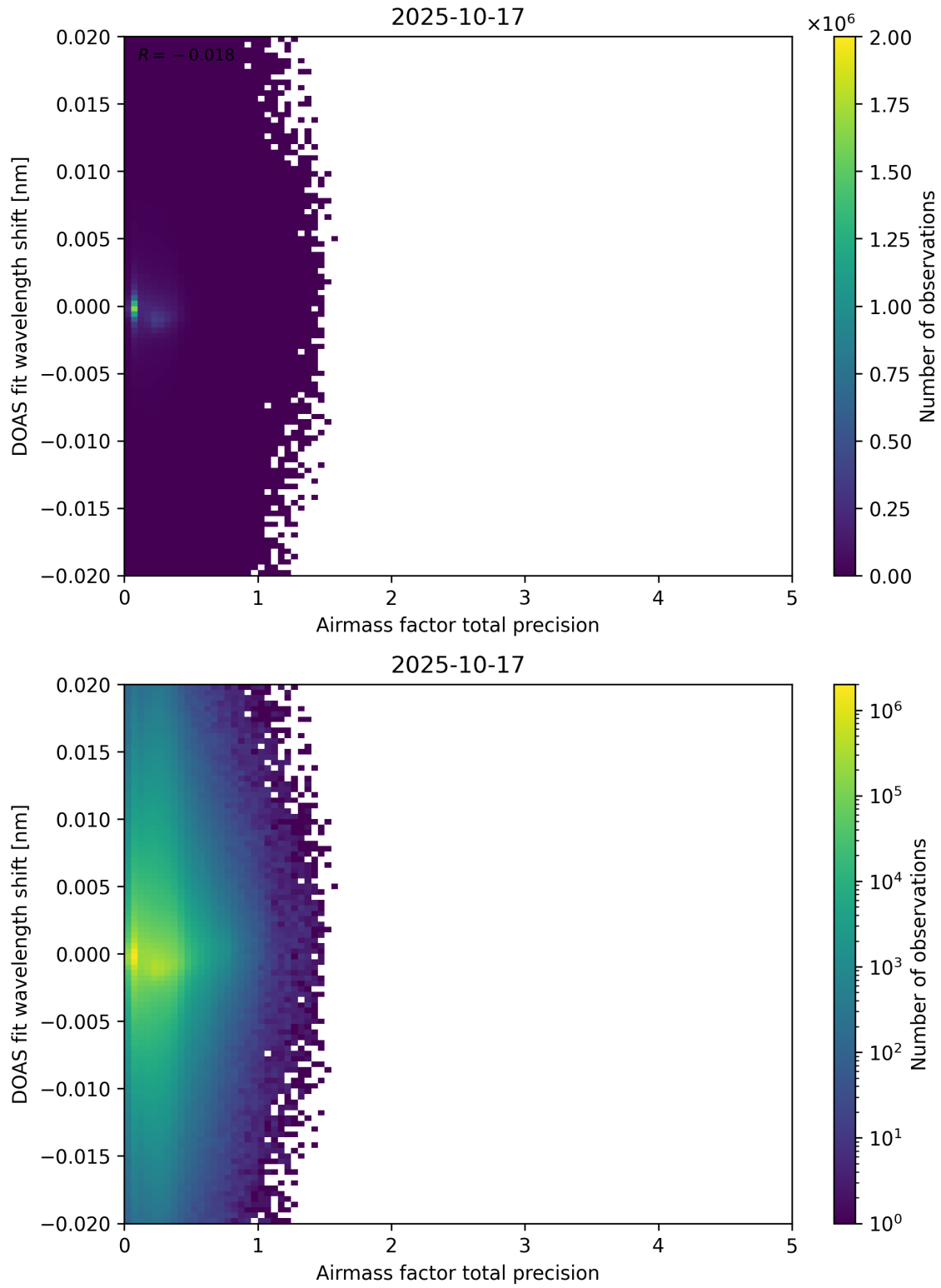
Figure 106: Scatter density plot of “Airmass factor total precision” against “DOAS fit wavelength shift” for 2025-10-17 to 2025-10-18.
