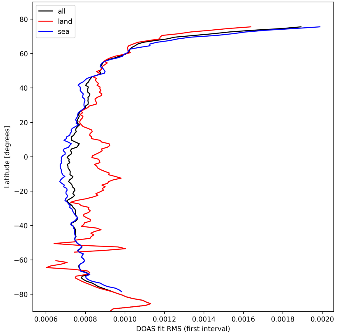
Figure 32: Zonal average of “DOAS fit RMS (first interval)” for 2025-10-17 to 2025-10-18.
