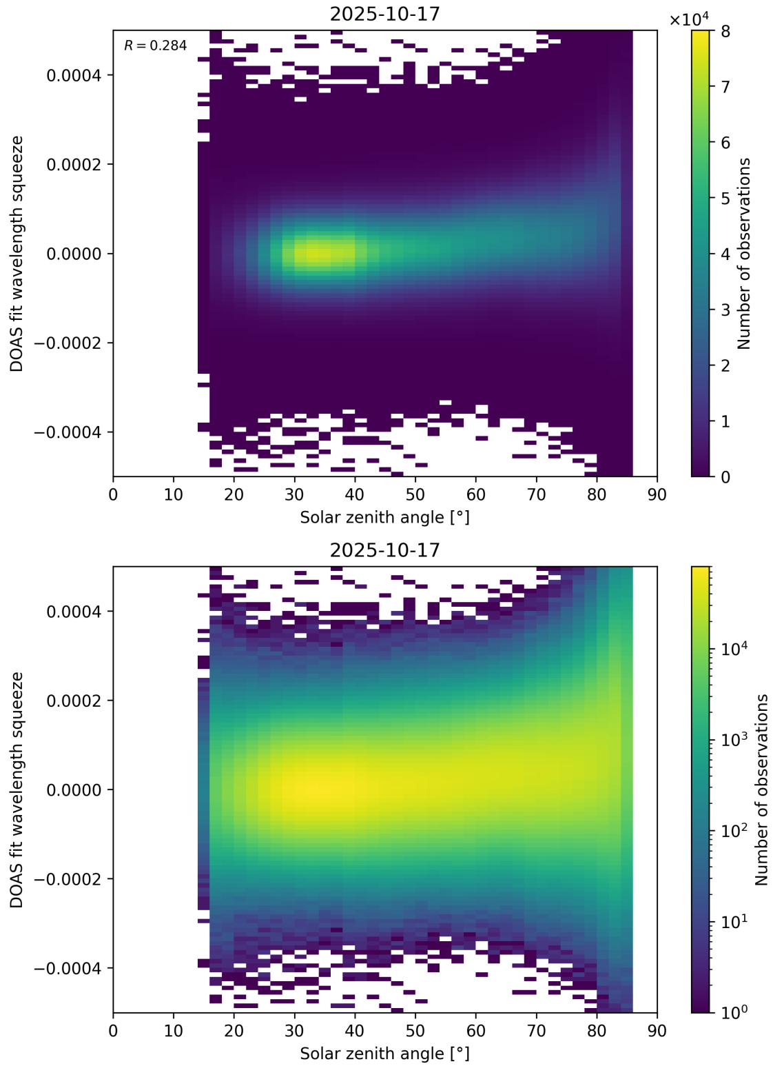
Figure 169: Scatter density plot of “Solar zenith angle” against “DOAS fit wavelength squeeze” for 2025-10-17 to 2025-10-18.
