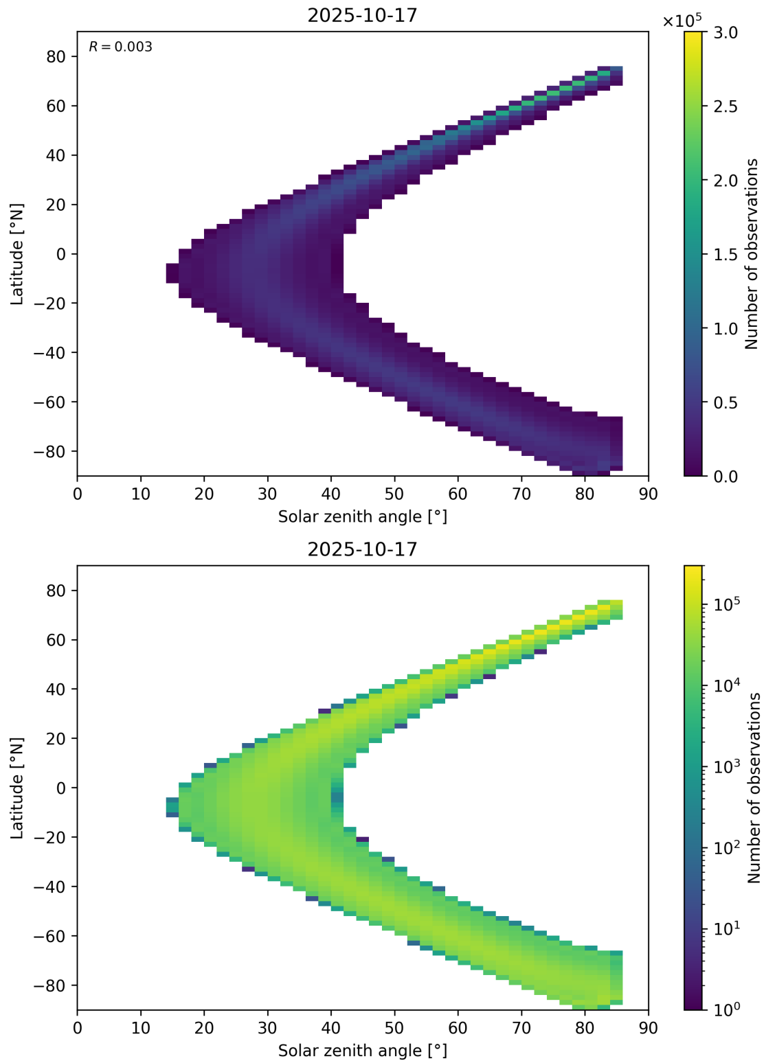
Figure 181: Scatter density plot of “Solar zenith angle” against “Latitude” for 2025-10-17 to 2025-10-18.
