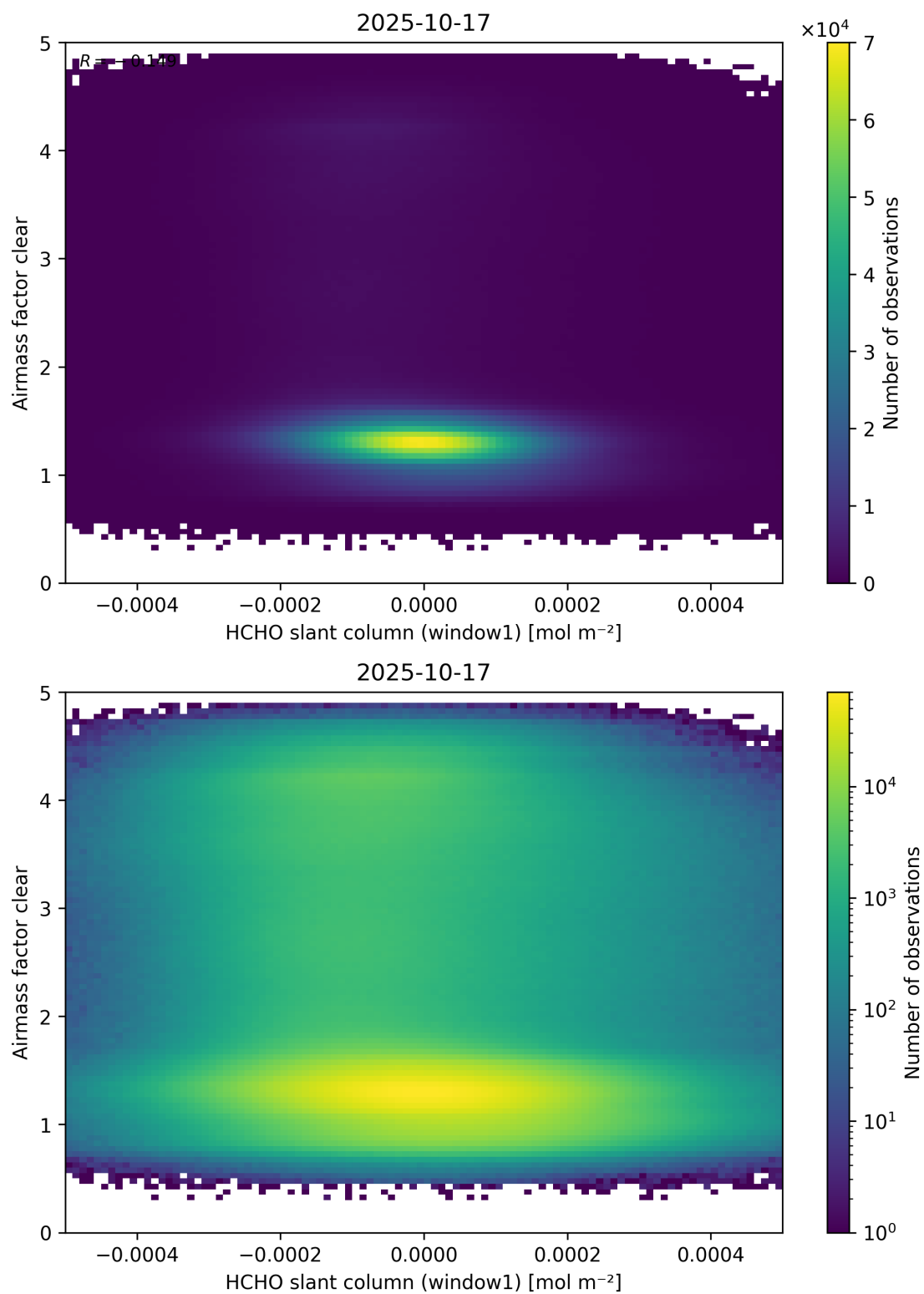
Figure 81: Scatter density plot of “HCHO slant column (window1)” against “Airmass factor clear” for 2025-10-17 to 2025-10-18.
