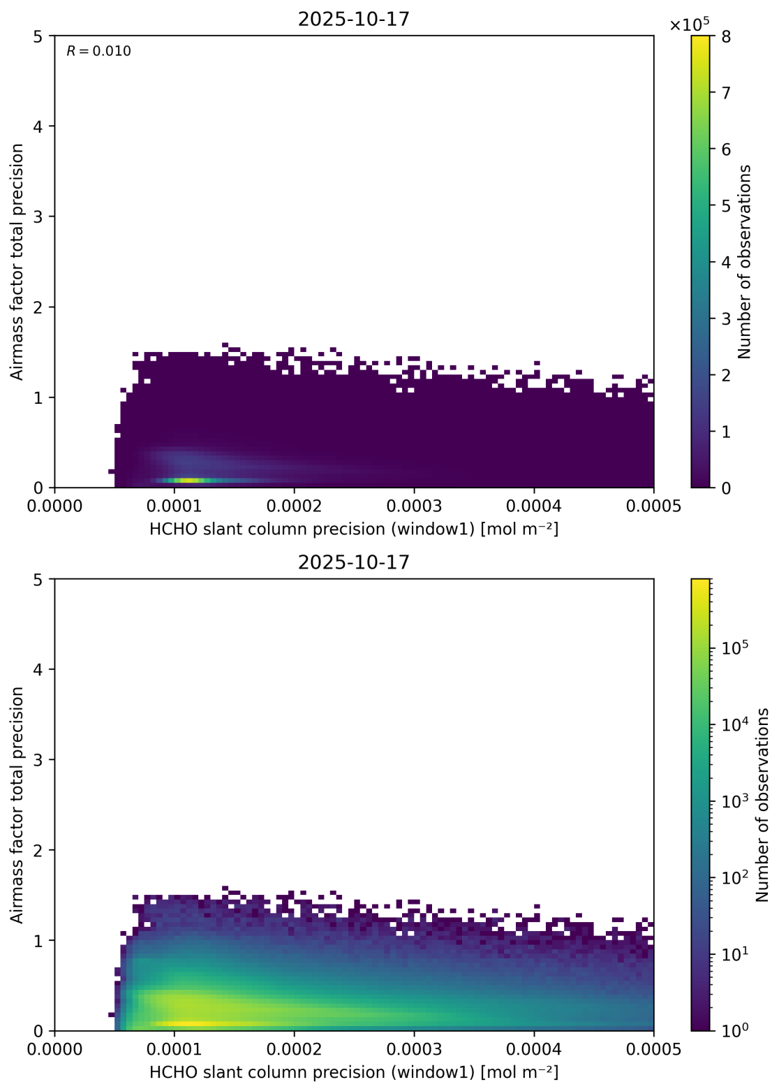
Figure 95: Scatter density plot of “HCHO slant column precision (window1)” against “Airmass factor total precision” for 2025-10-17 to 2025-10-18.
