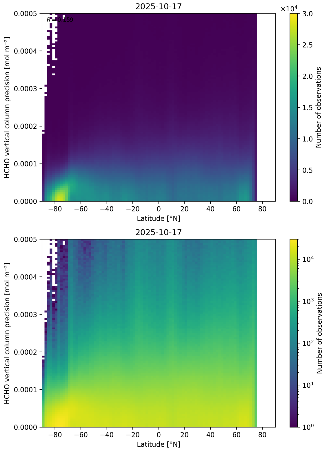
Figure 165: Scatter density plot of “Latitude” against “HCHO vertical column precision” for 2025-10-17 to 2025-10-18.
