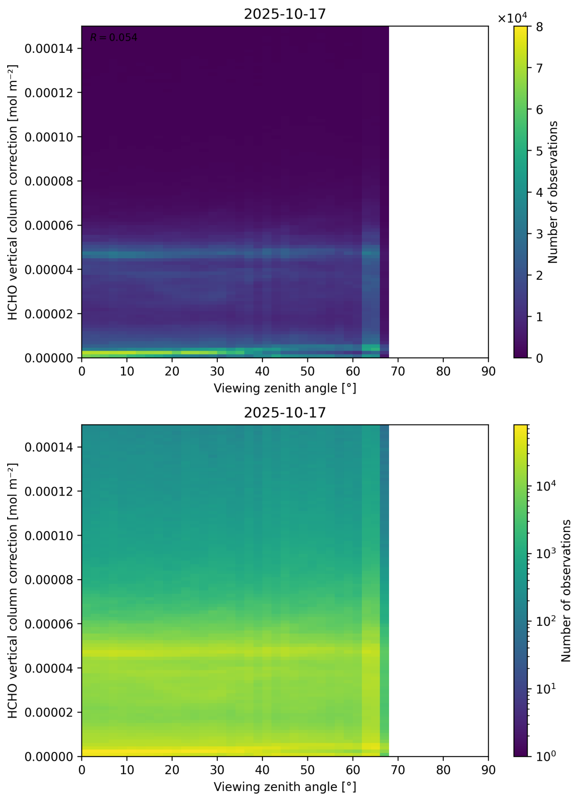
Figure 193: Scatter density plot of “Viewing zenith angle” against “HCHO vertical column correction” for 2025-10-17 to 2025-10-18.
