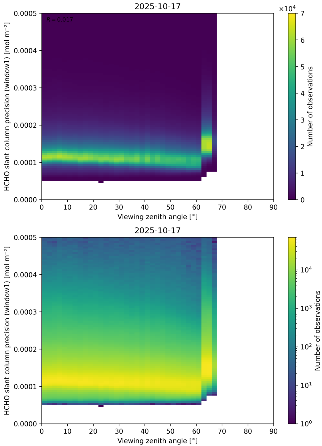
Figure 189: Scatter density plot of “Viewing zenith angle” against “HCHO slant column precision (window1)” for 2025-10-17 to 2025-10-18.
