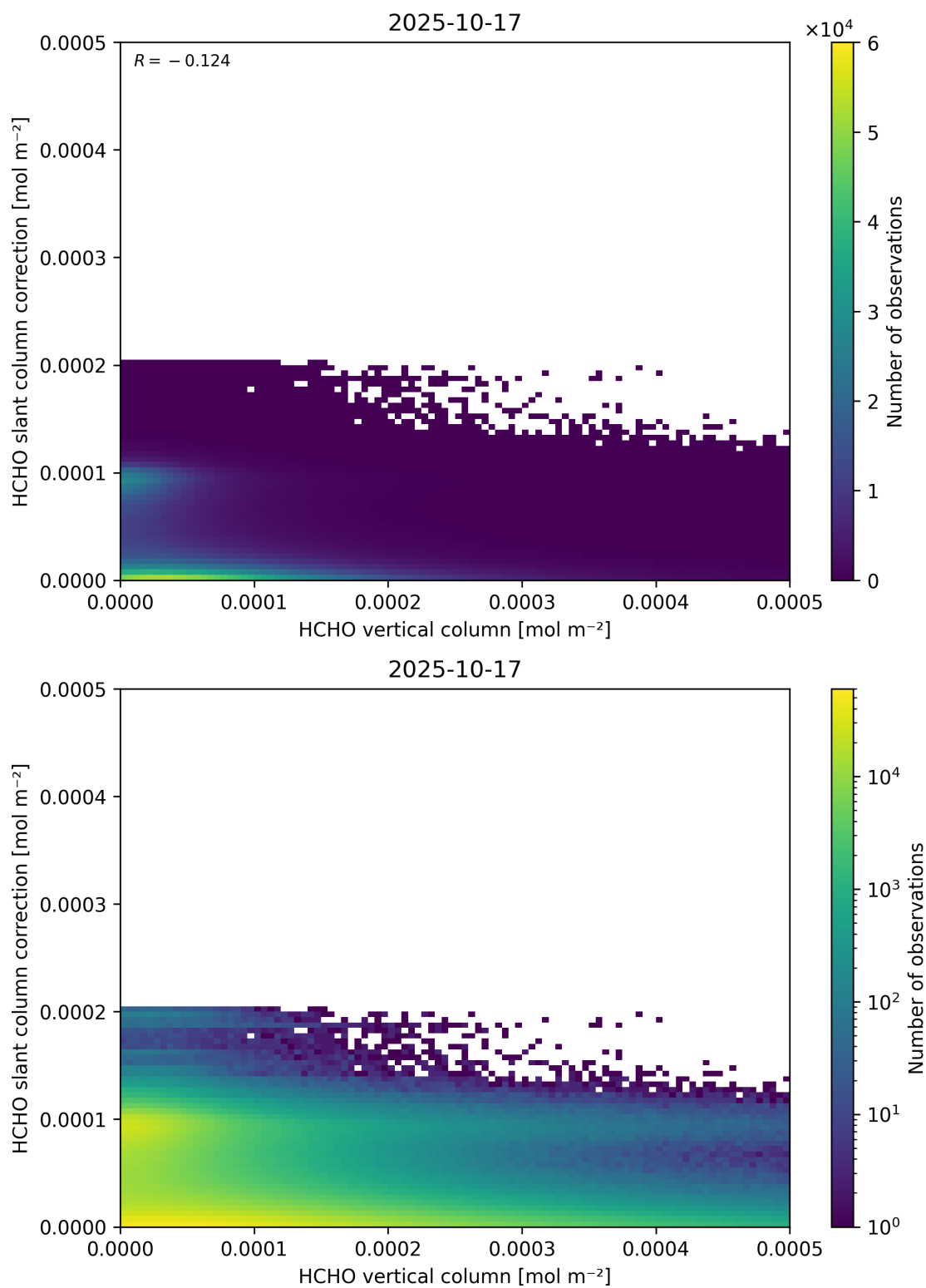
Figure 128: Scatter density plot of “HCHO vertical column” against “HCHO slant column correction” for 2025-10-17 to 2025-10-18.
