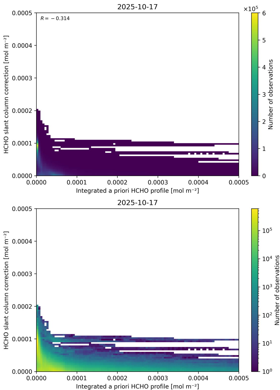
Figure 152: Scatter density plot of “Integrated a priori HCHO profile” against “HCHO slant column correction” for 2025-10-17 to 2025-10-18.
