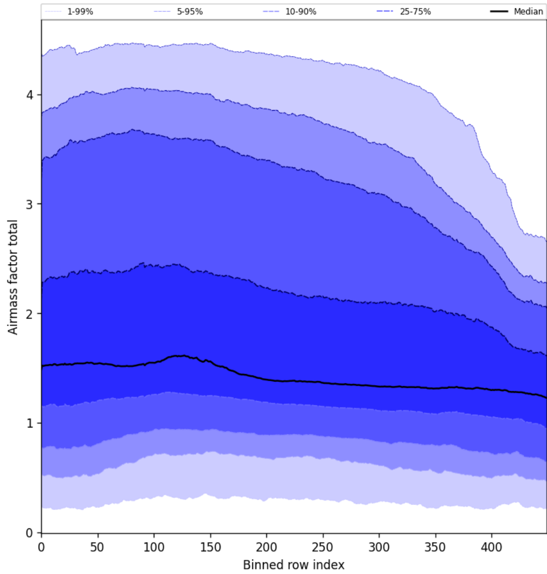
Figure 54: Along track statistics of “Airmass factor total” for 2025-10-17 to 2025-10-18
