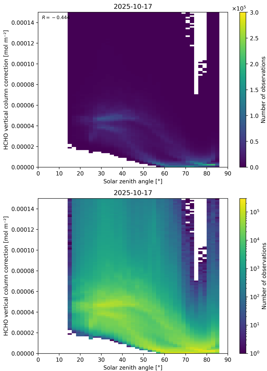
Figure 178: Scatter density plot of “Solar zenith angle” against “HCHO vertical column correction” for 2025-10-17 to 2025-10-18.
