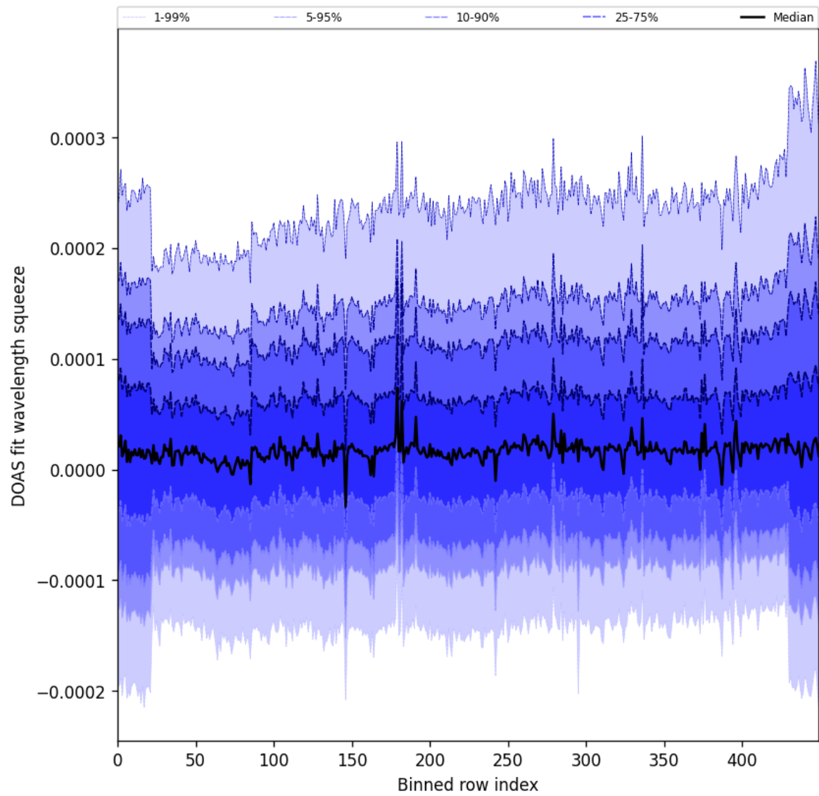
Figure 59: Along track statistics of “DOAS fit wavelength squeeze” for 2025-10-17 to 2025-10-18
