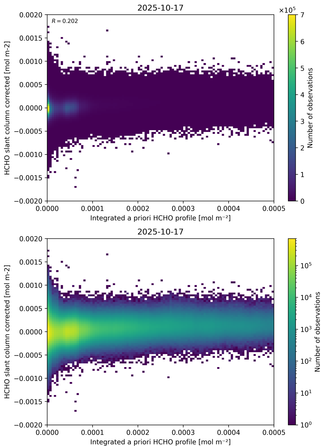
Figure 151: Scatter density plot of “Integrated a priori HCHO profile” against “HCHO slant column corrected” for 2025-10-17 to 2025-10-18.
