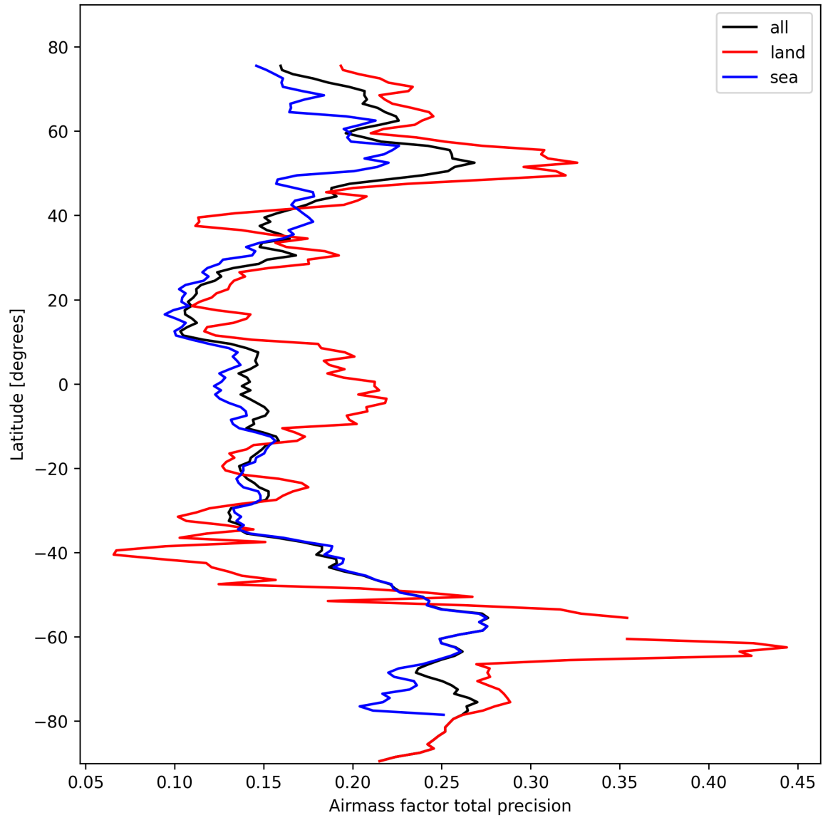
Figure 27: Zonal average of “Airmass factor total precision” for 2025-10-17 to 2025-10-18.
