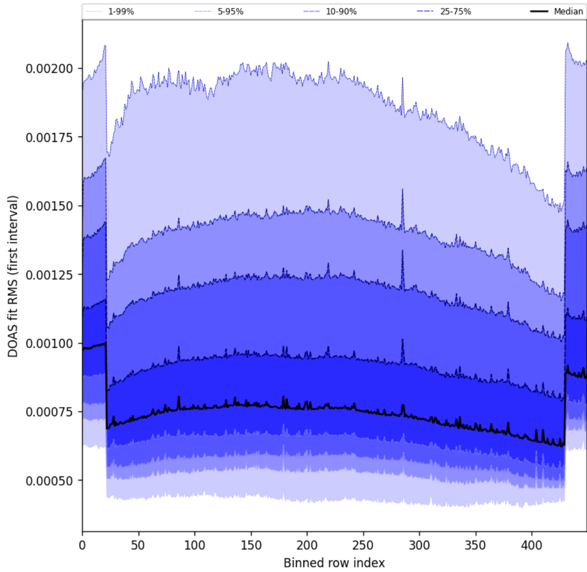
Figure 60: Along track statistics of “DOAS fit RMS (first interval)” for 2025-10-17 to 2025-10-18
