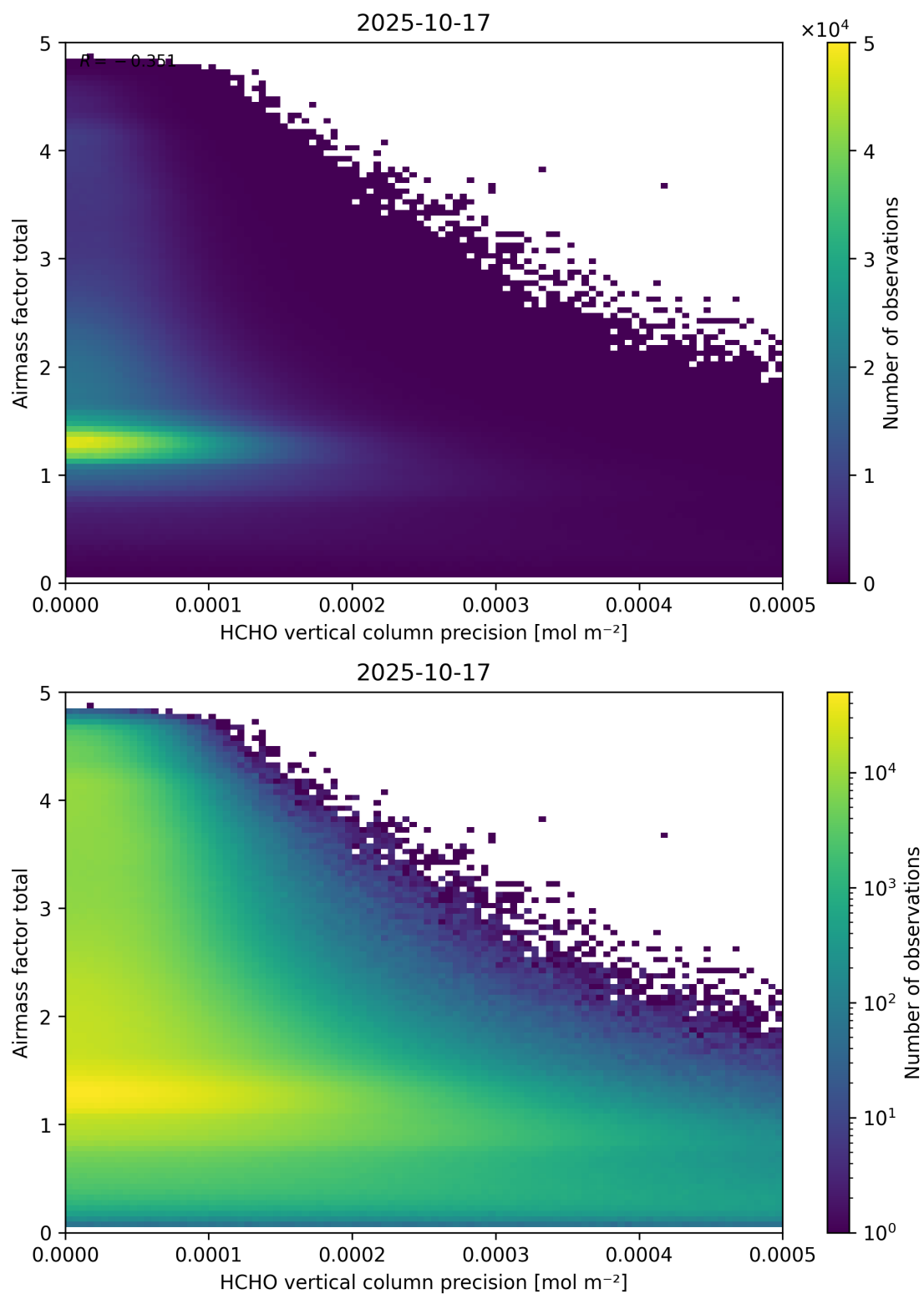
Figure 144: Scatter density plot of “HCHO vertical column precision” against “Airmass factor total” for 2025-10-17 to 2025-10-18.
