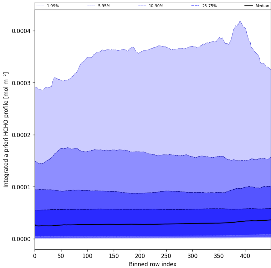
Figure 57: Along track statistics of “Integrated a priori HCHO profile” for 2025-10-17 to 2025-10-18
