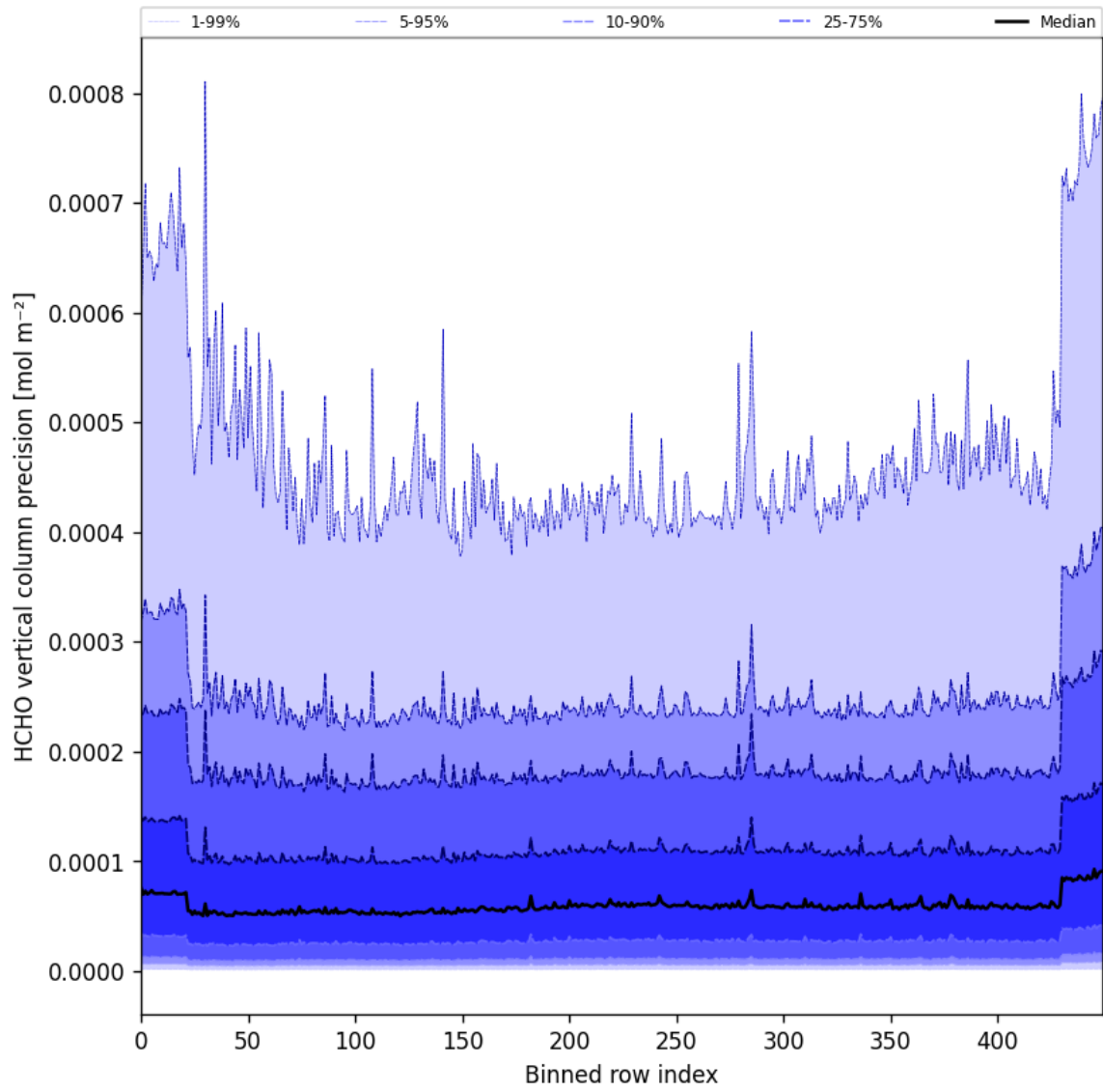
Figure 50: Along track statistics of "HCHO vertical column precision" for 2025-10-17 to 2025-10-18
