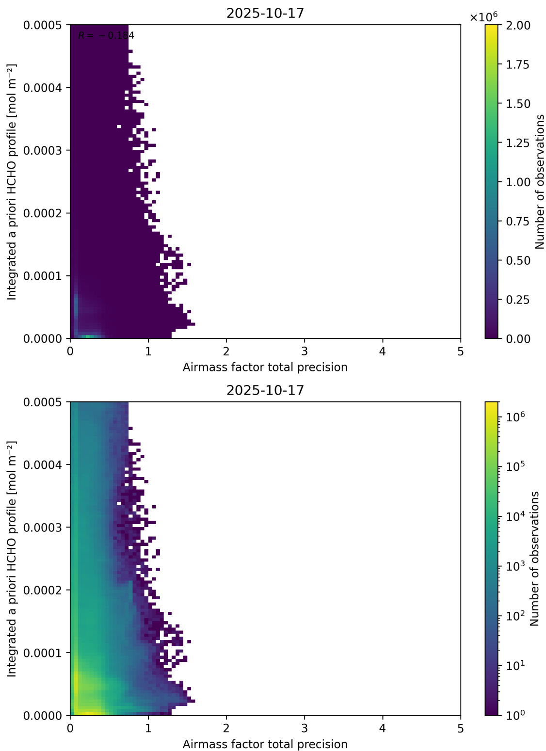
Figure 111: Scatter density plot of “Airmass factor total precision” against “Integrated a priori HCHO profile” for 2025-10-17 to 2025-10-18.
