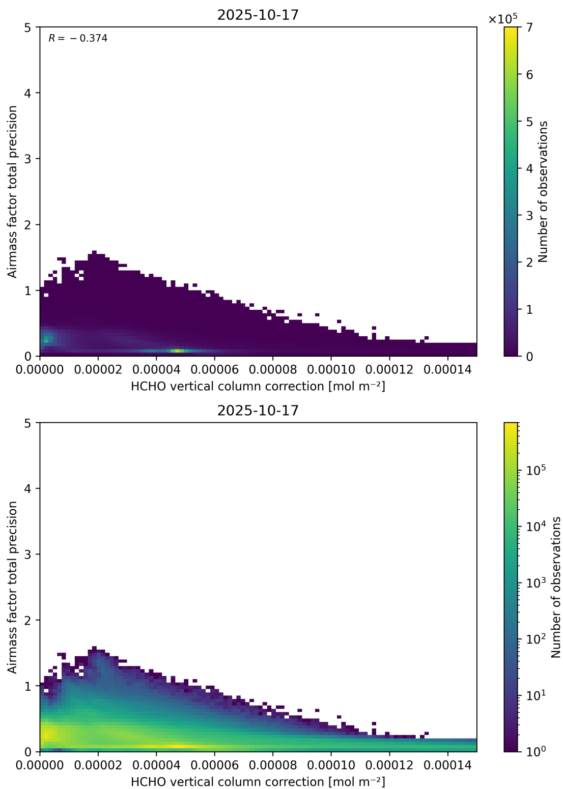
Figure 121: Scatter density plot of “HCHO vertical column correction” against “Airmass factor total precision” for 2025-10-17 to 2025-10-18.
