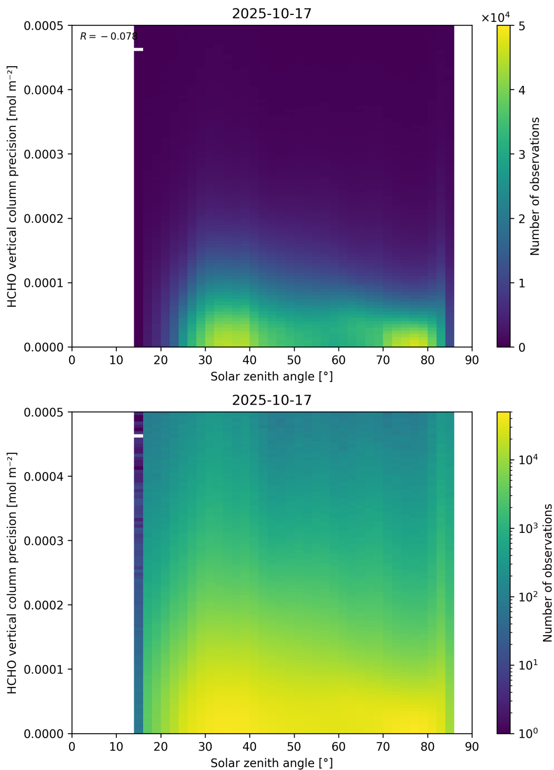
Figure 179: Scatter density plot of “Solar zenith angle” against “HCHO vertical column precision” for 2025-10-17 to 2025-10-18.
