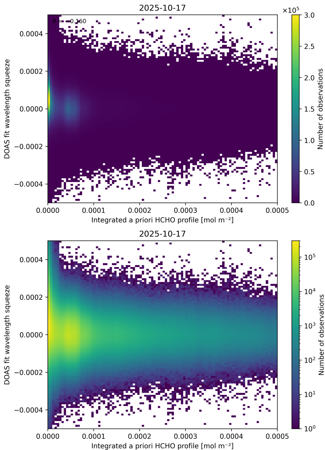
Figure 150: Scatter density plot of “Integrated a priori HCHO profile” against “DOAS fit wavelength squeeze” for 2025-10-17 to 2025-10-18.
