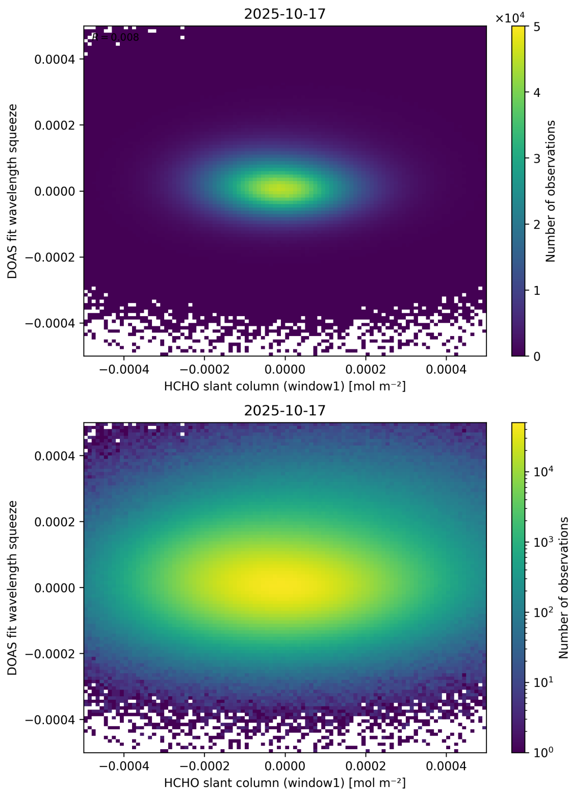
Figure 80: Scatter density plot of “HCHO slant column (window1)” against “DOAS fit wavelength squeeze” for 2025-10-17 to 2025-10-18.
