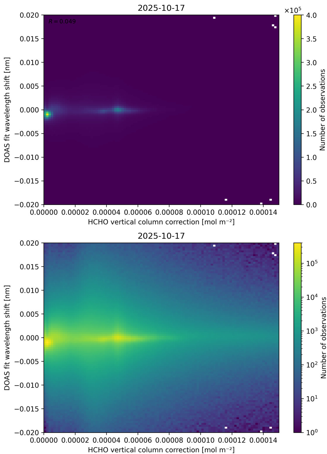
Figure 113: Scatter density plot of “HCHO vertical column correction” against “DOAS fit wavelength shift” for 2025-10-17 to 2025-10-18.
