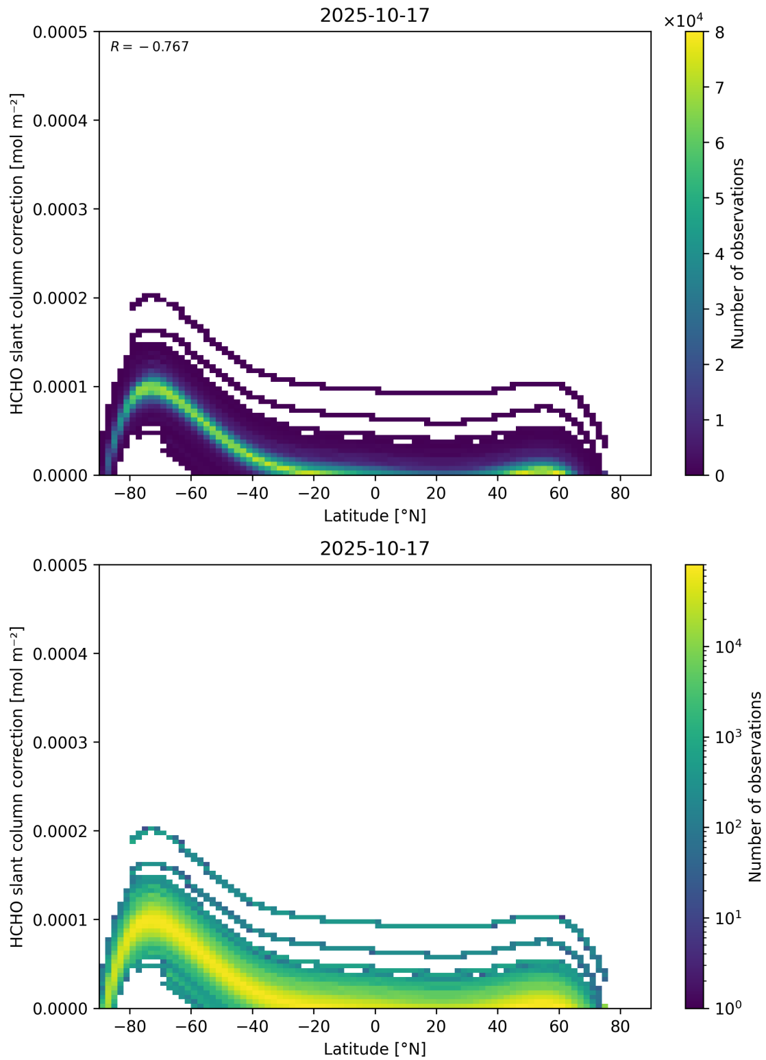
Figure 158: Scatter density plot of “Latitude” against “HCHO slant column correction” for 2025-10-17 to 2025-10-18.
