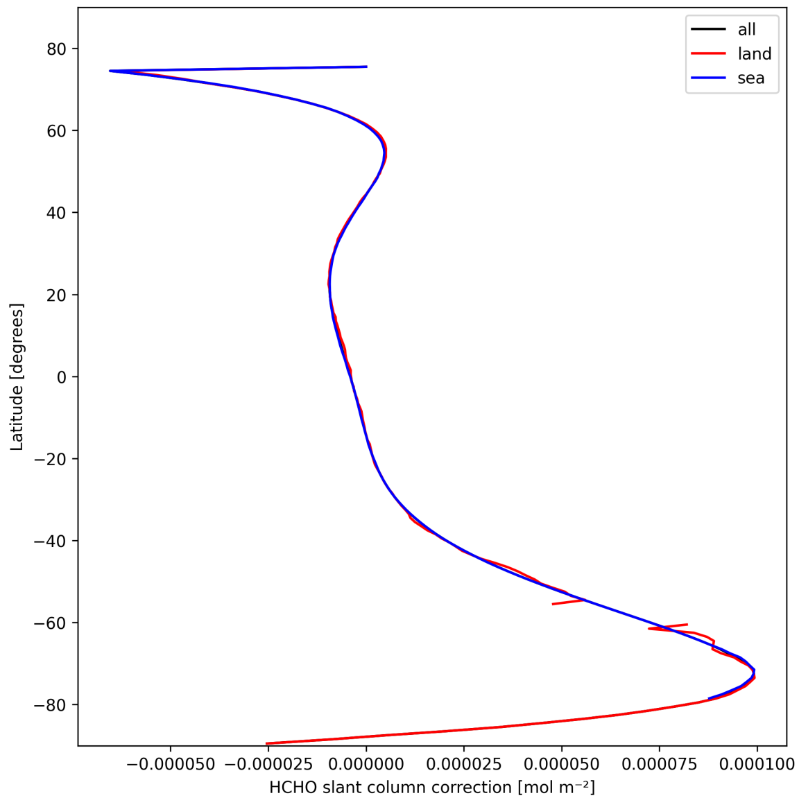
Figure 33: Zonal average of “HCHO slant column correction” for 2025-10-17 to 2025-10-18.
