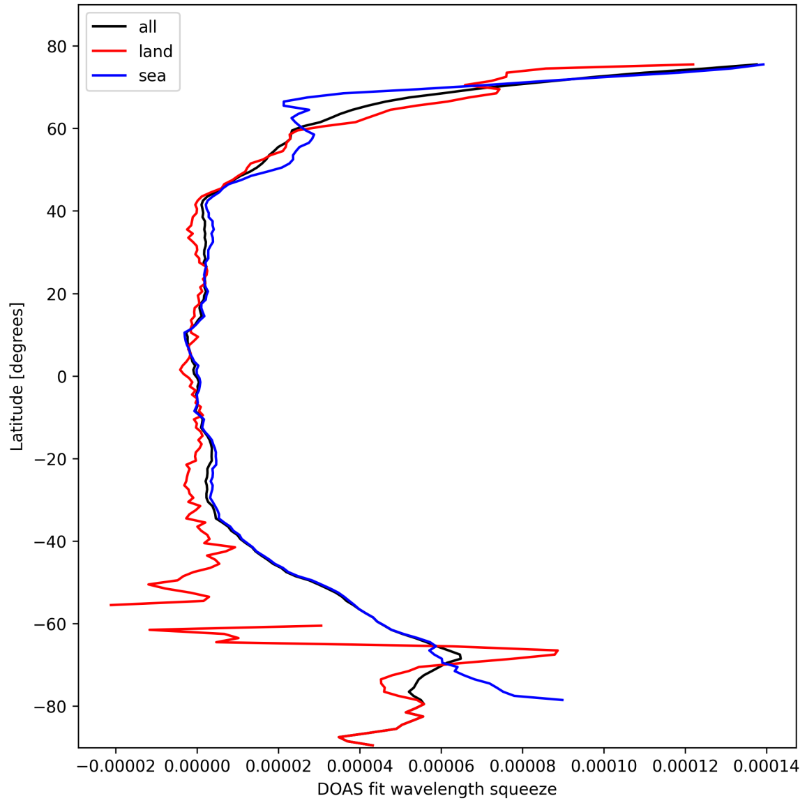
Figure 31: Zonal average of “DOAS fit wavelength squeeze” for 2025-10-17 to 2025-10-18.
