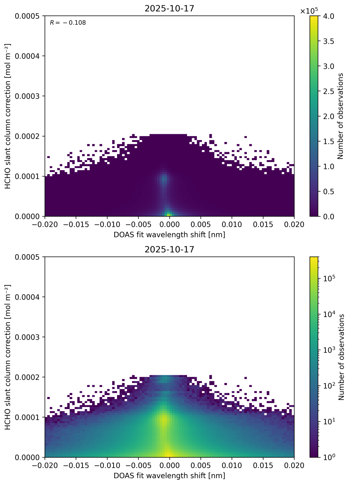
Figure 67: Scatter density plot of “DOAS fit wavelength shift” against “HCHO slant column correction” for 2025-10-17 to 2025-10-18.
