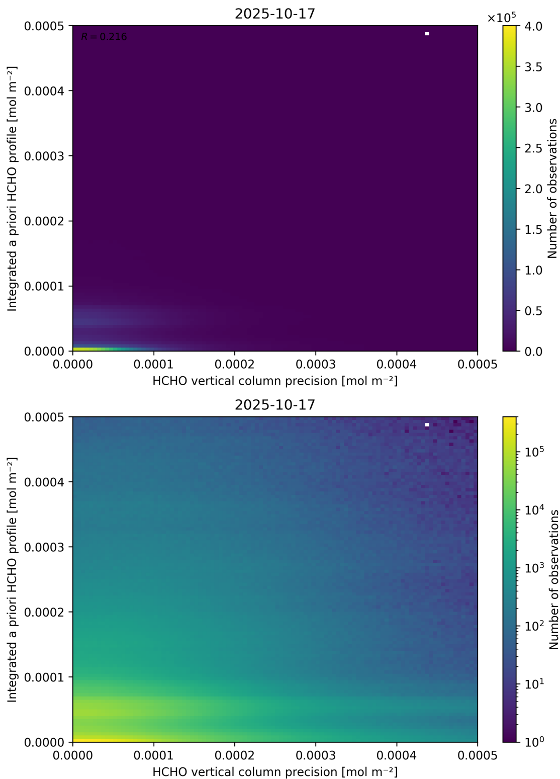
Figure 147: Scatter density plot of “HCHO vertical column precision” against “Integrated a priori HCHO profile” for 2025-10-17 to 2025-10-18.
