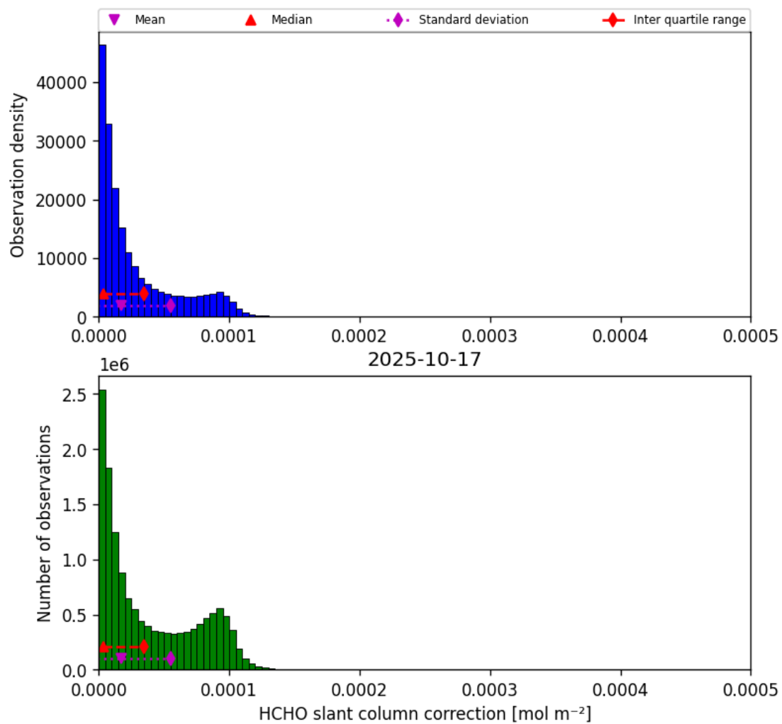
Figure 47: Histogram of “HCHO slant column correction” for 2025-10-17 to 2025-10-18
