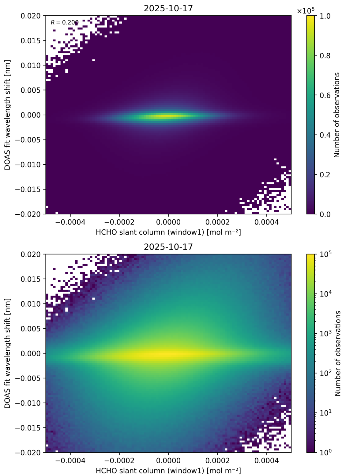
Figure 79: Scatter density plot of “HCHO slant column (window1)” against “DOAS fit wavelength shift” for 2025-10-17 to 2025-10-18.
