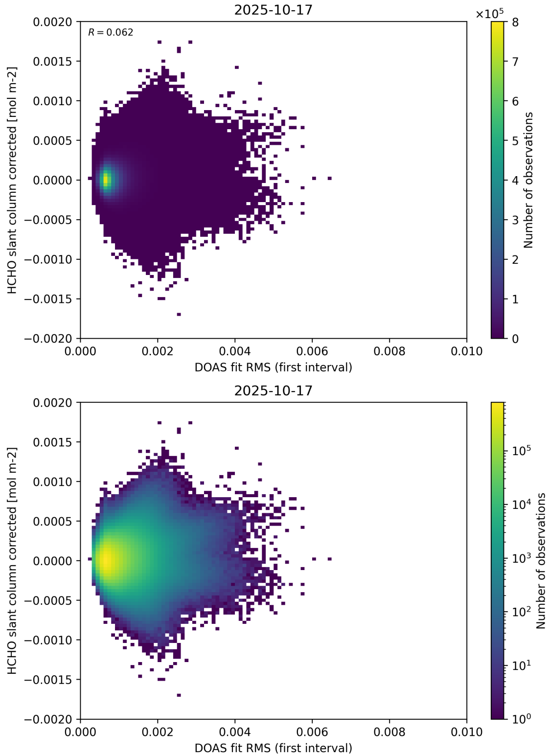
Figure 62: Scatter density plot of “DOAS fit RMS (first interval)” against “HCHO slant column corrected” for 2025-10-17 to 2025-10-18.
