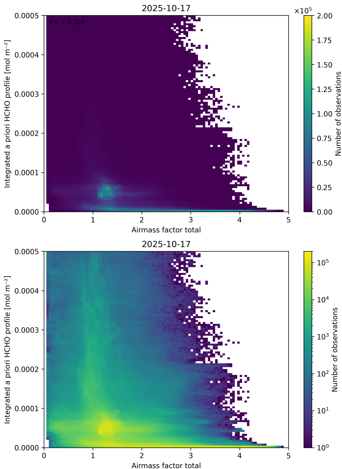
Figure 104: Scatter density plot of “Airmass factor total” against “Integrated a priori HCHO profile” for 2025-10-17 to 2025-10-18.
