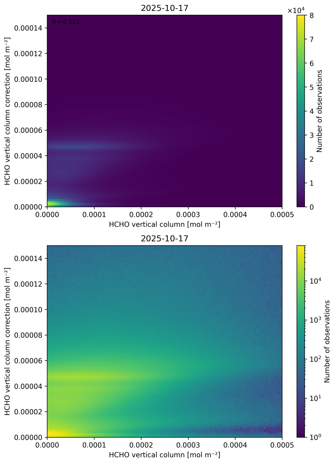
Figure 133: Scatter density plot of “HCHO vertical column” against “HCHO vertical column correction” for 2025-10-17 to 2025-10-18.
