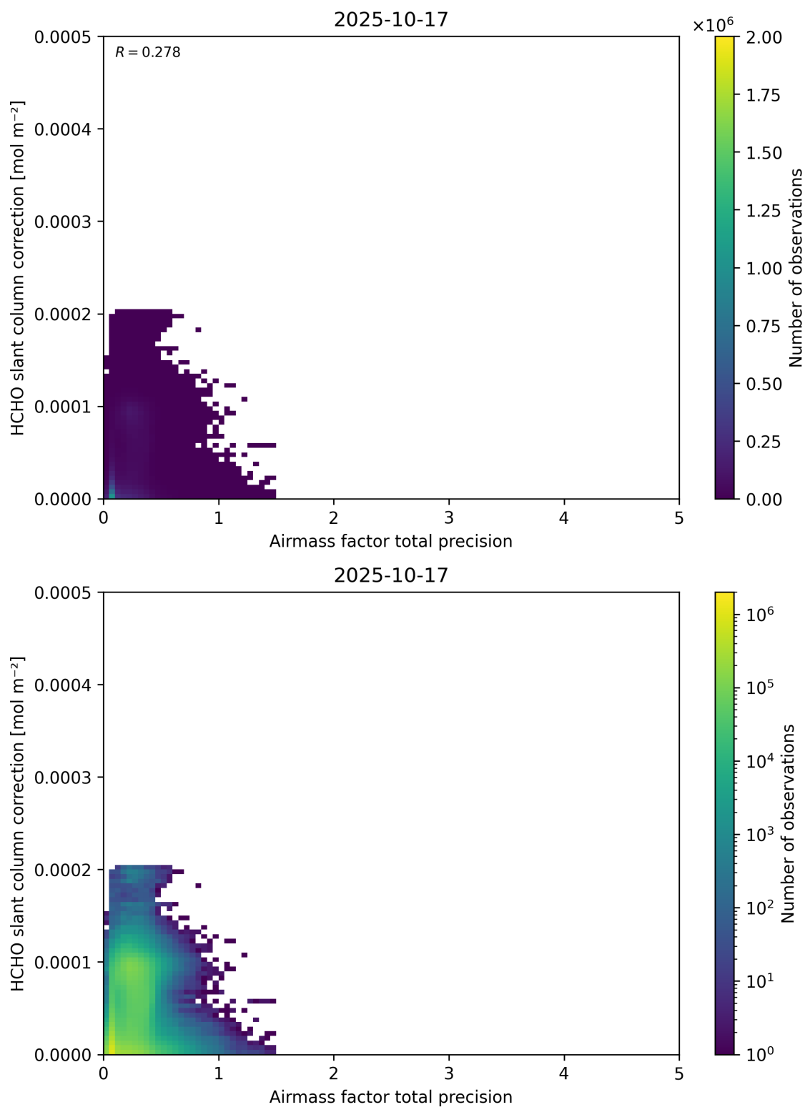
Figure 110: Scatter density plot of “Airmass factor total precision” against “HCHO slant column correction” for 2025-10-17 to 2025-10-18.
