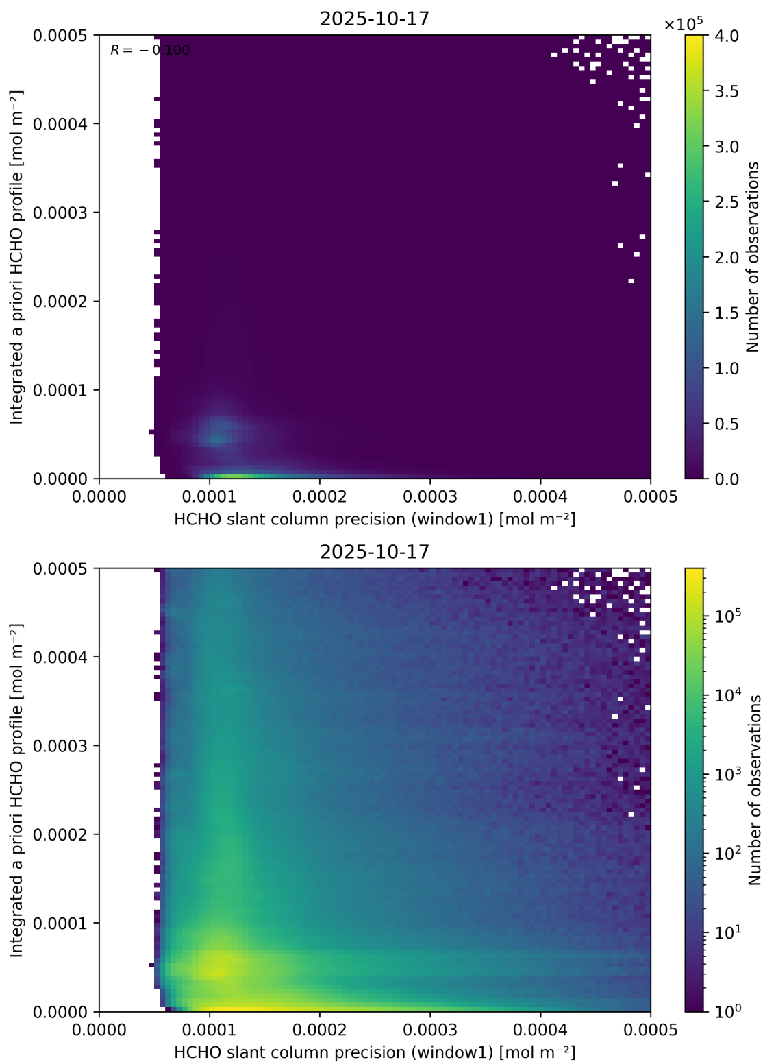
Figure 96: Scatter density plot of “HCHO slant column precision (window1)” against “Integrated a priori HCHO profile” for 2025-10-17 to 2025-10-18.
