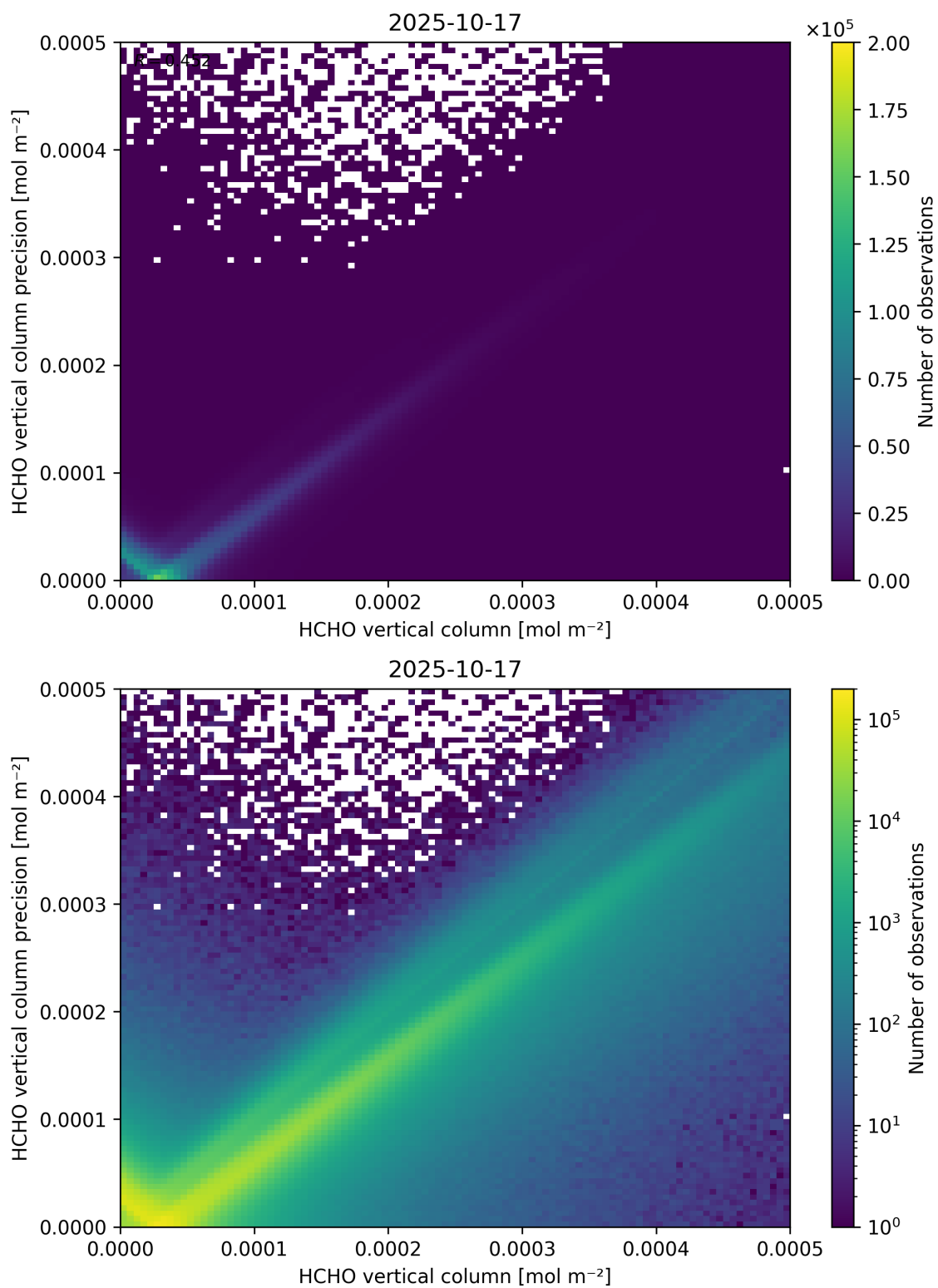
Figure 134: Scatter density plot of “HCHO vertical column” against “HCHO vertical column precision” for 2025-10-17 to 2025-10-18.
