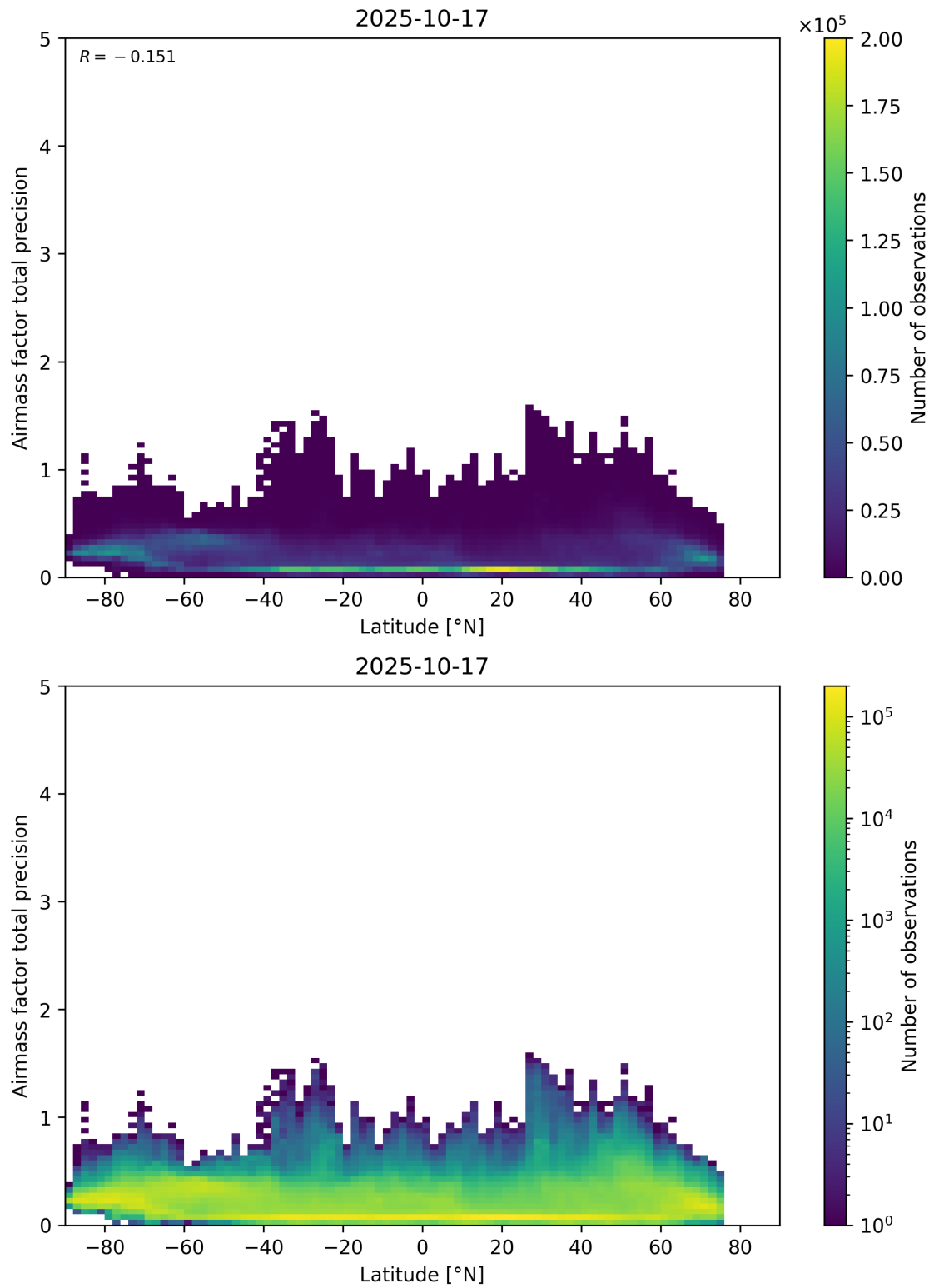
Figure 162: Scatter density plot of “Latitude” against “Airmass factor total precision” for 2025-10-17 to 2025-10-18.
