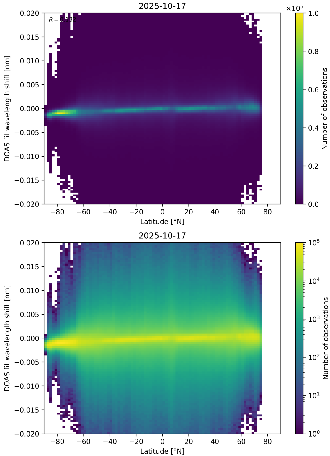
Figure 154: Scatter density plot of “Latitude” against “DOAS fit wavelength shift” for 2025-10-17 to 2025-10-18.
