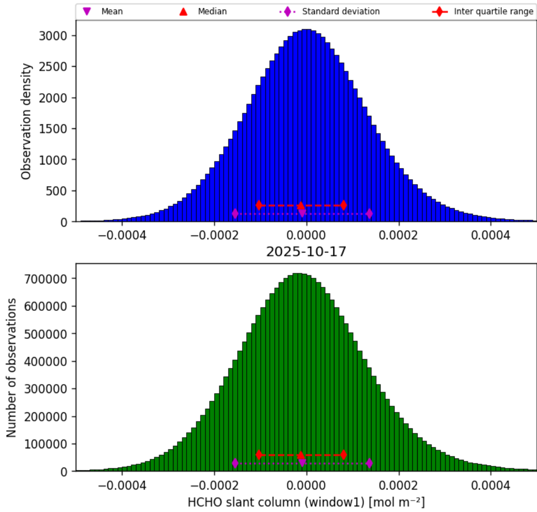
Figure 38: Histogram of “HCHO slant column (window1)” for 2025-10-17 to 2025-10-18
