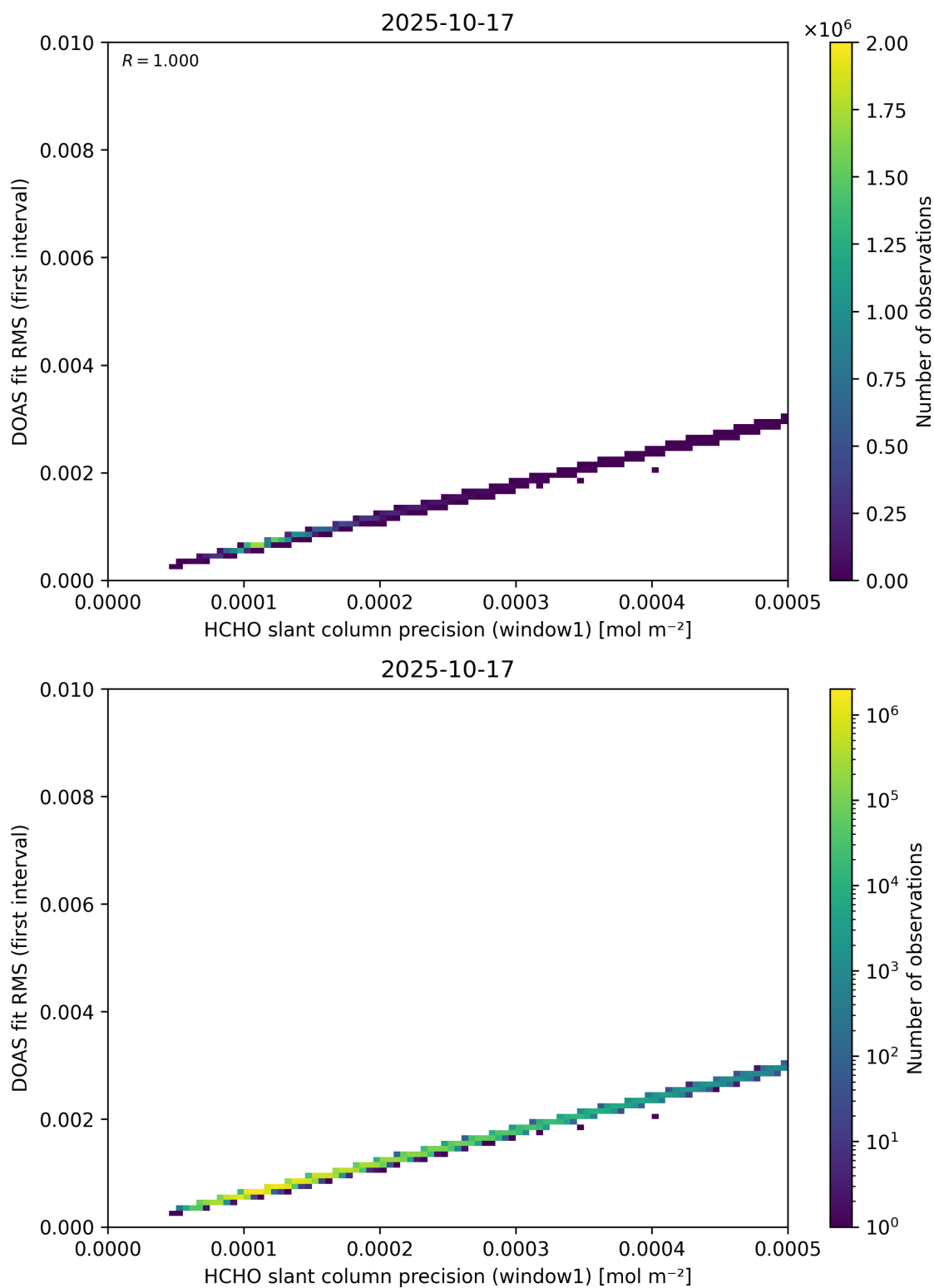
Figure 88: Scatter density plot of “HCHO slant column precision (window1)” against “DOAS fit RMS (first interval)” for 2025-10-17 to 2025-10-18.
