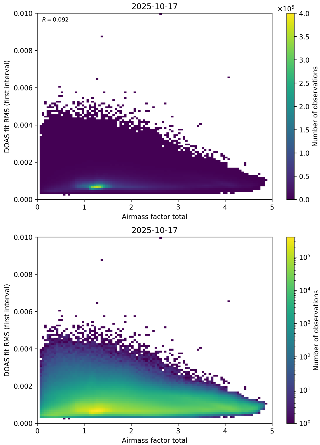
Figure 97: Scatter density plot of “Airmass factor total” against “DOAS fit RMS (first interval)” for 2025-10-17 to 2025-10-18.
