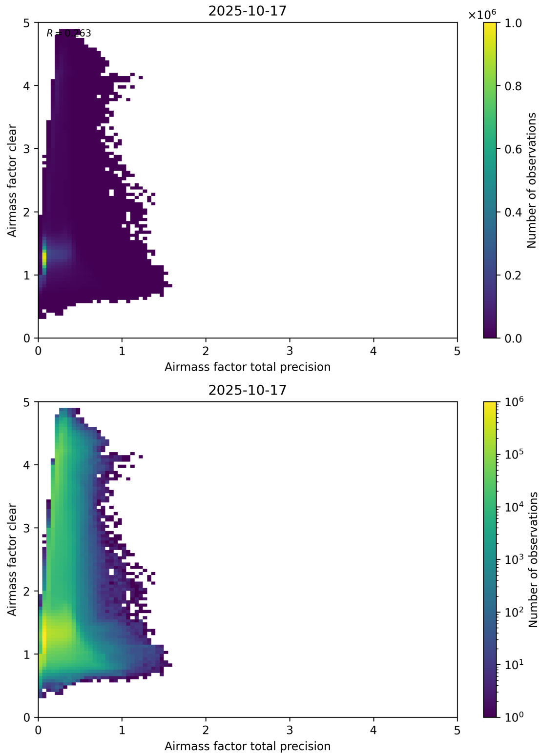
Figure 108: Scatter density plot of “Airmass factor total precision” against “Airmass factor clear” for 2025-10-17 to 2025-10-18.
