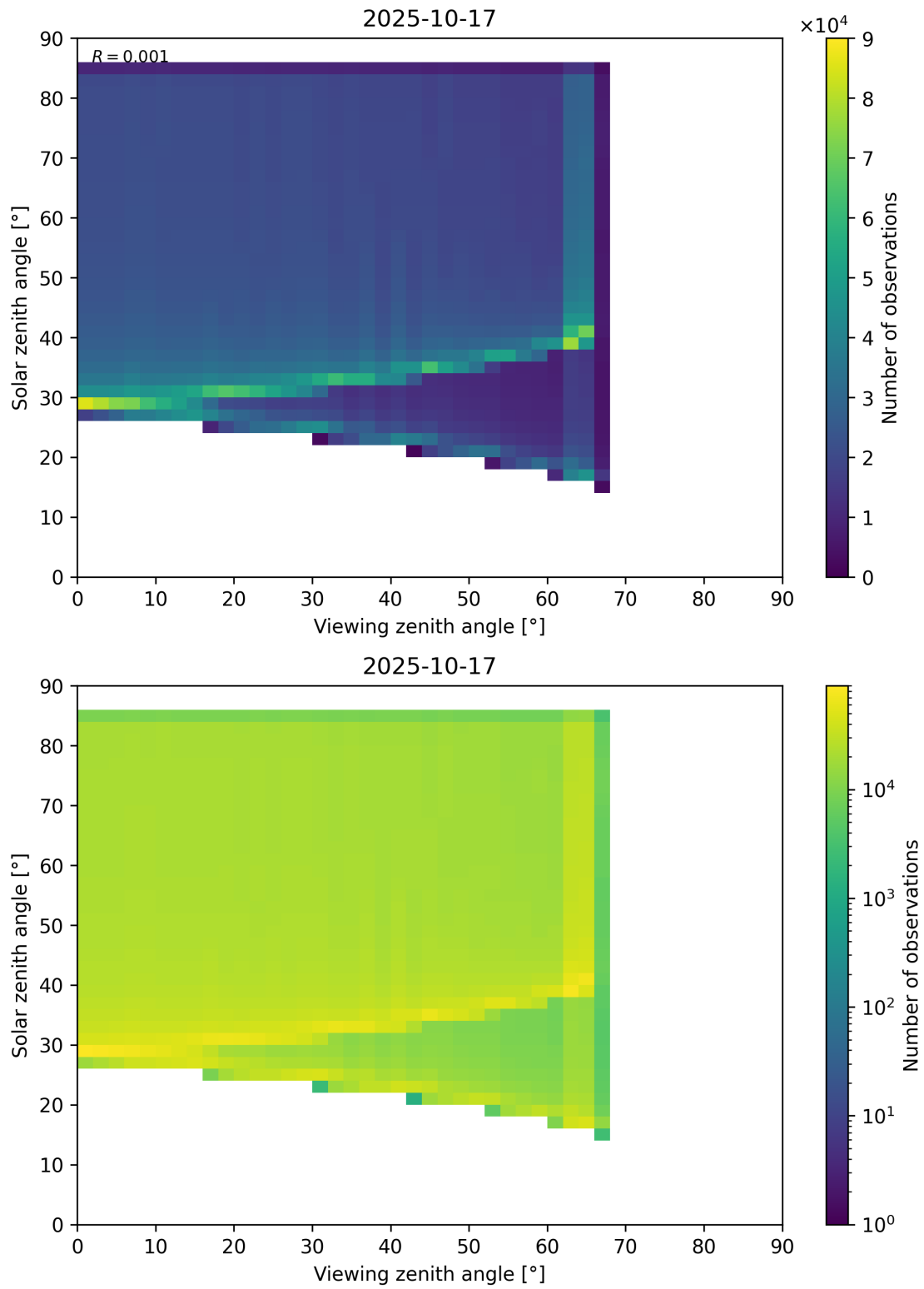
Figure 197: Scatter density plot of “Viewing zenith angle” against “Solar zenith angle” for 2025-10-17 to 2025-10-18.
