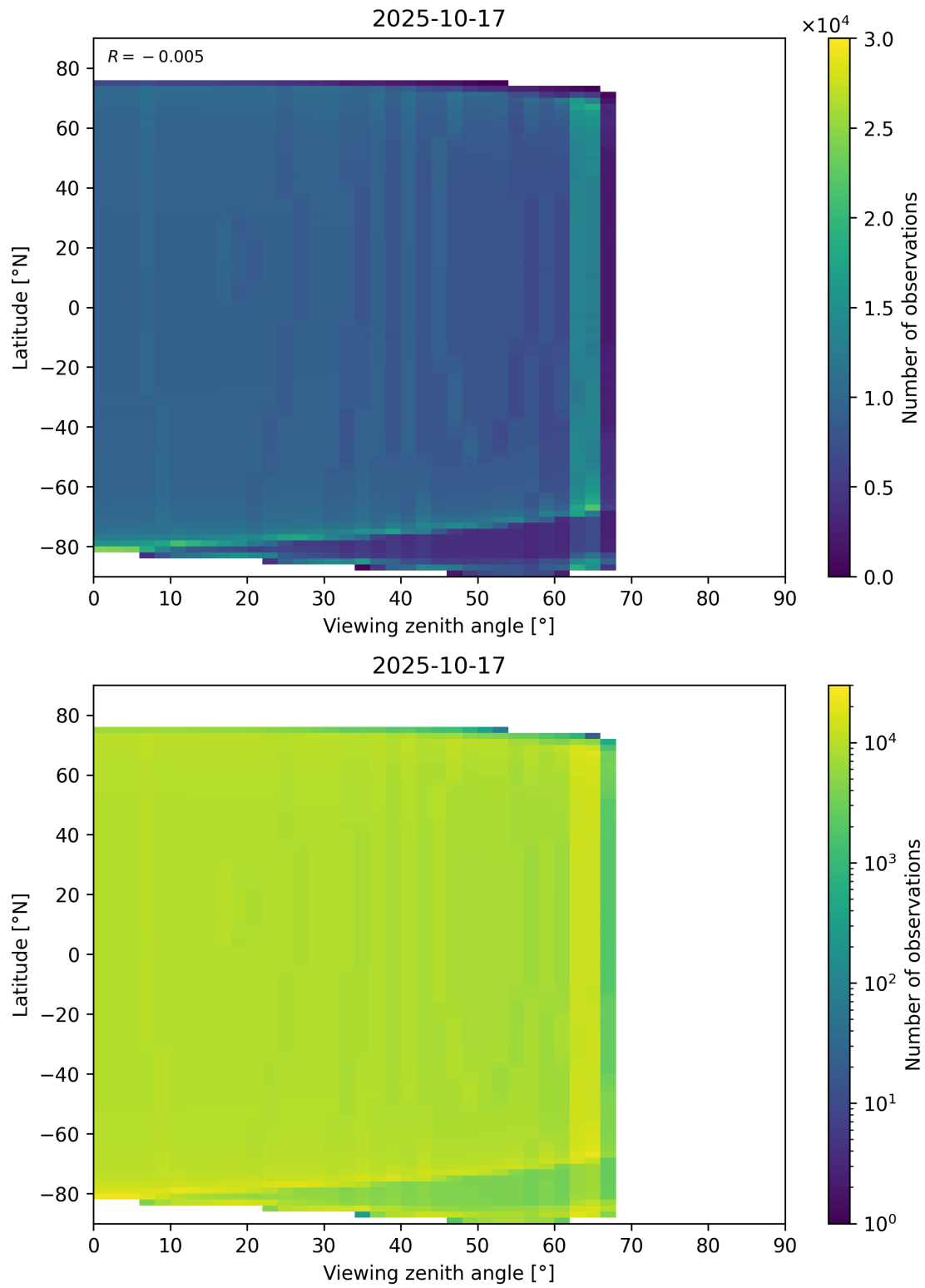
Figure 196: Scatter density plot of “Viewing zenith angle” against “Latitude” for 2025-10-17 to 2025-10-18.
