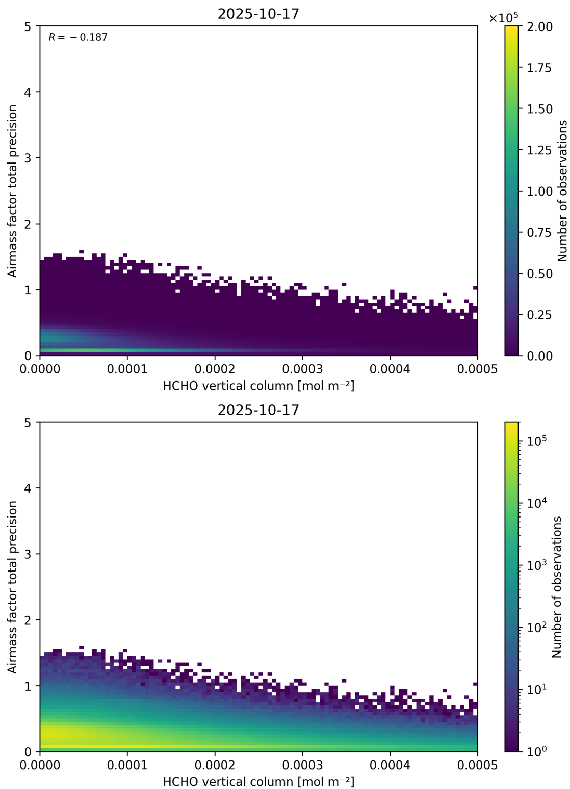
Figure 132: Scatter density plot of “HCHO vertical column” against “Airmass factor total precision” for 2025-10-17 to 2025-10-18.
