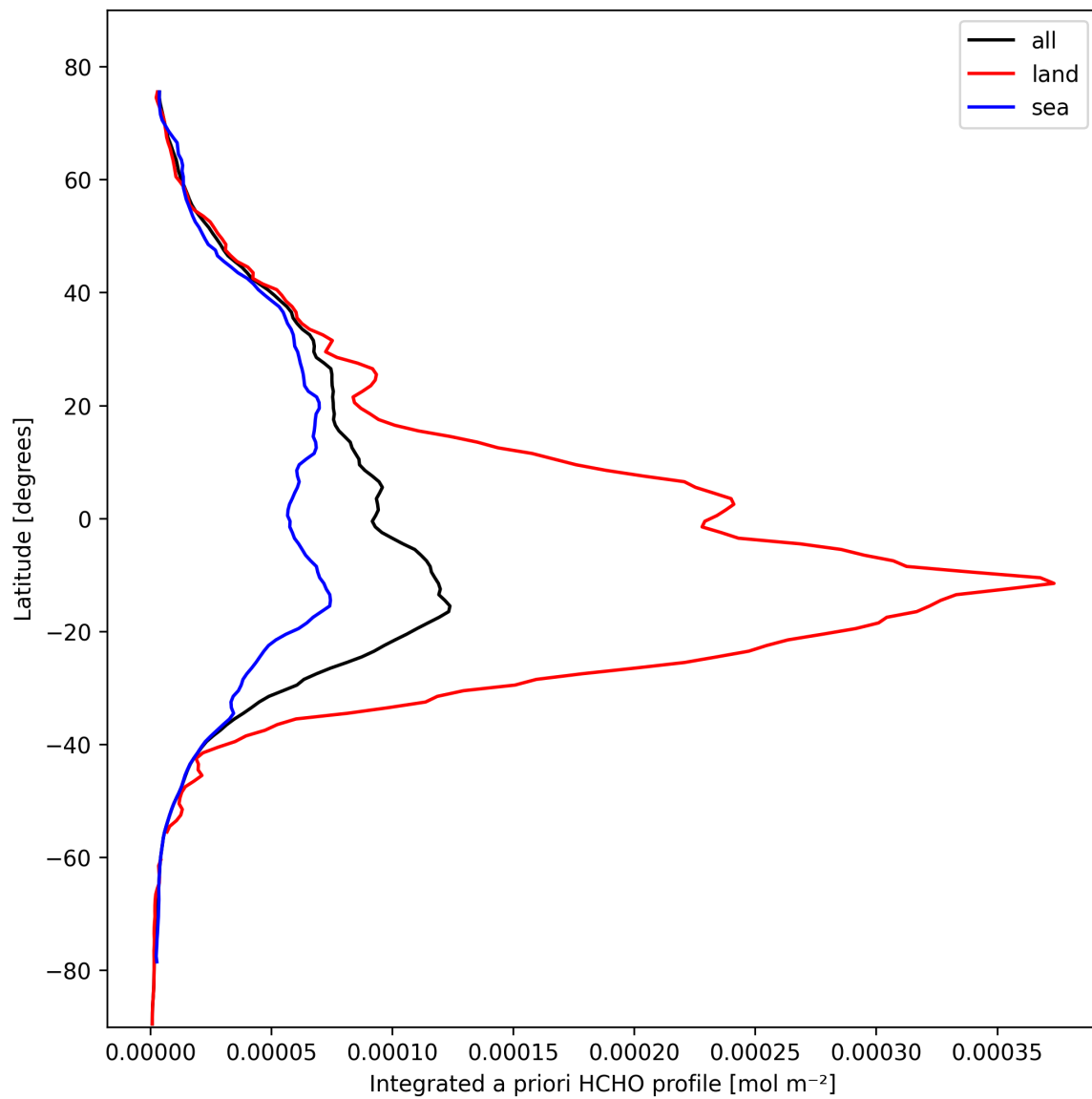
Figure 29: Zonal average of “Integrated a priori HCHO profile” for 2025-10-17 to 2025-10-18.
