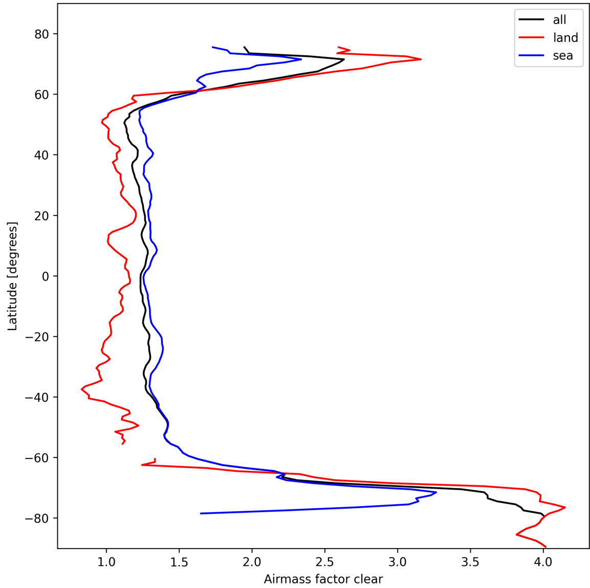
Figure 28: Zonal average of “Airmass factor clear” for 2025-10-17 to 2025-10-18.
