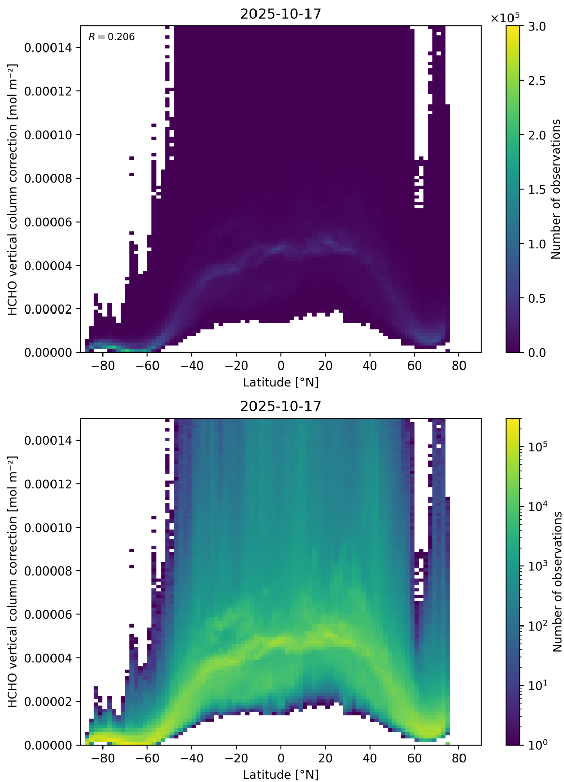
Figure 164: Scatter density plot of “Latitude” against “HCHO vertical column correction” for 2025-10-17 to 2025-10-18.
