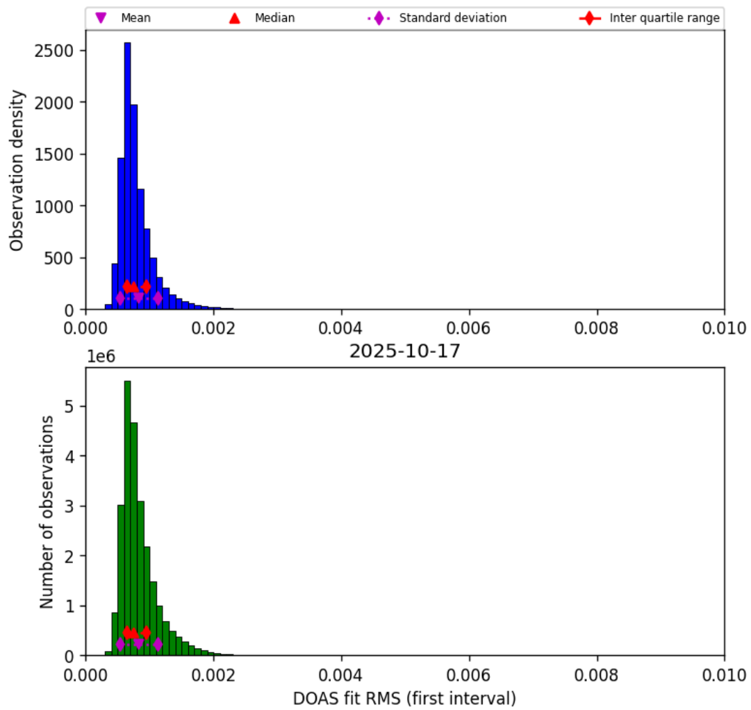
Figure 46: Histogram of “DOAS fit RMS (first interval)” for 2025-10-17 to 2025-10-18
