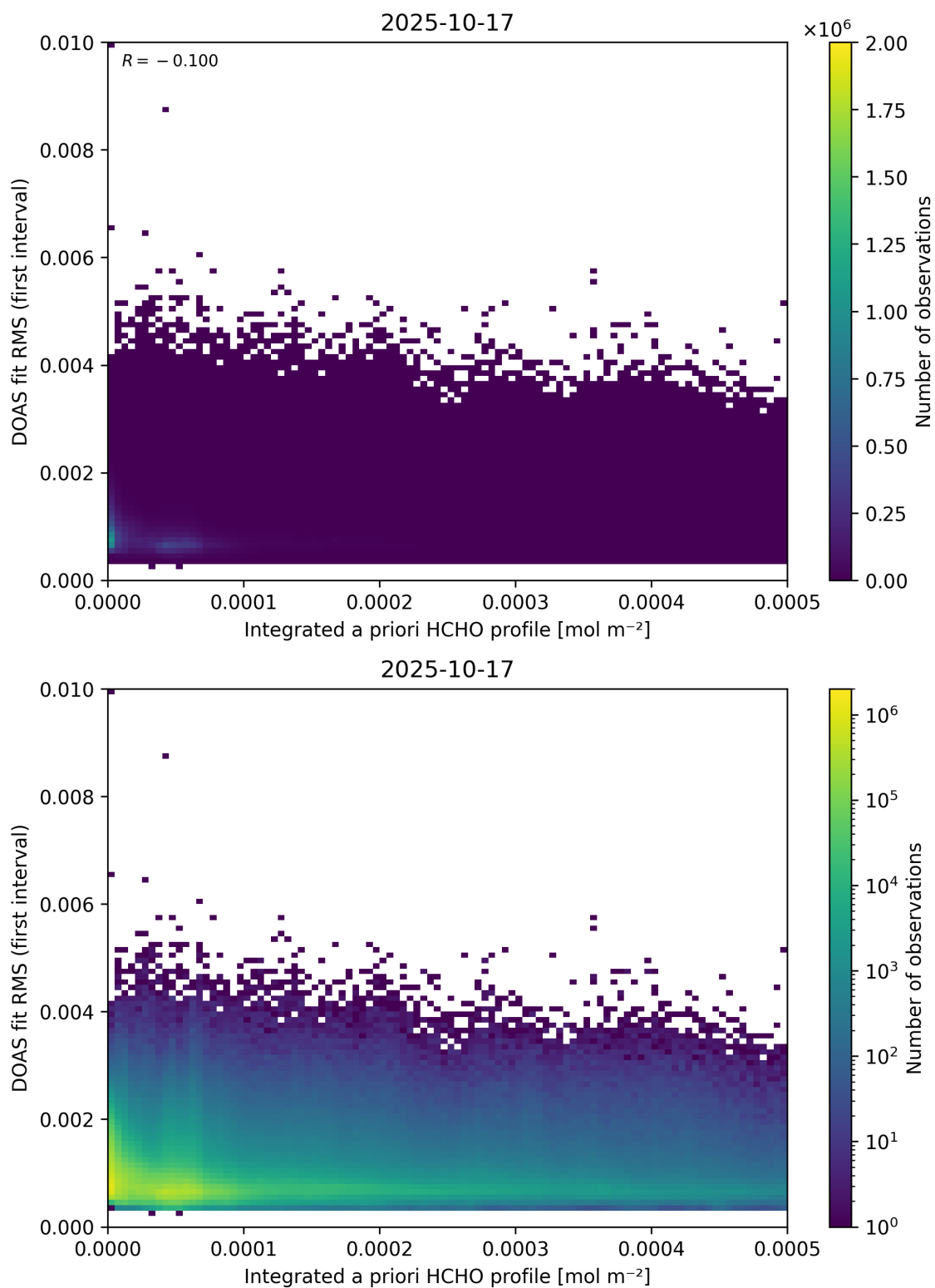
Figure 148: Scatter density plot of “Integrated a priori HCHO profile” against “DOAS fit RMS (first interval)” for 2025-10-17 to 2025-10-18.
