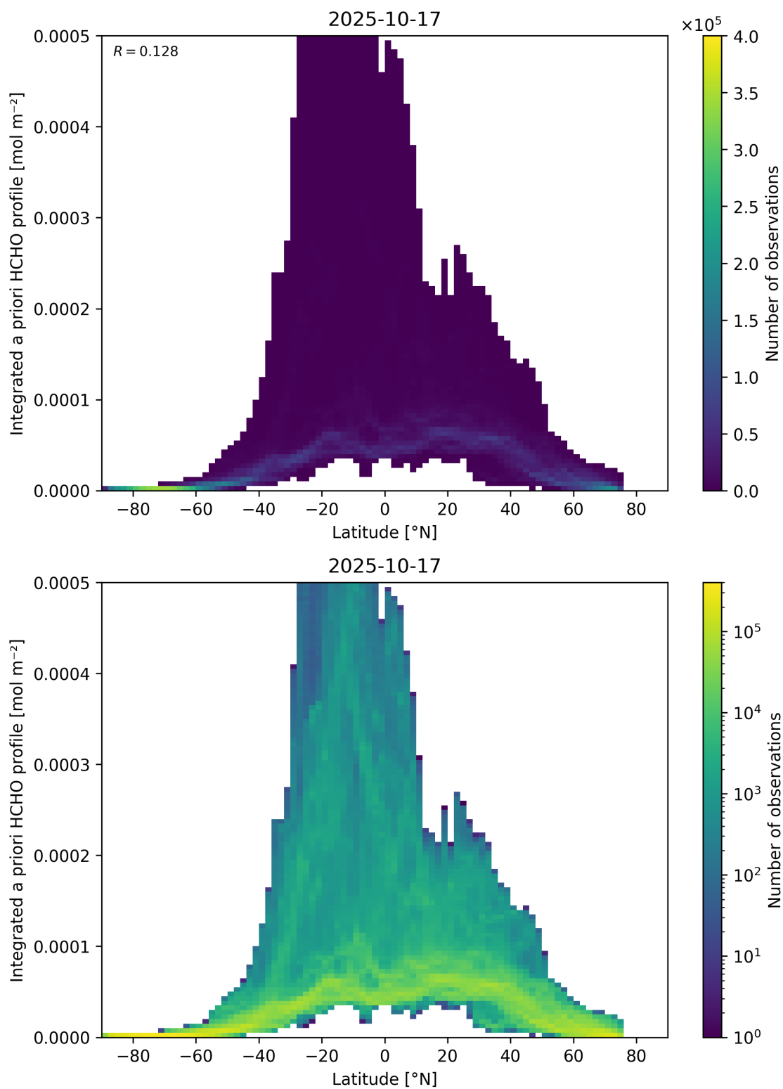
Figure 166: Scatter density plot of “Latitude” against “Integrated a priori HCHO profile” for 2025-10-17 to 2025-10-18.
