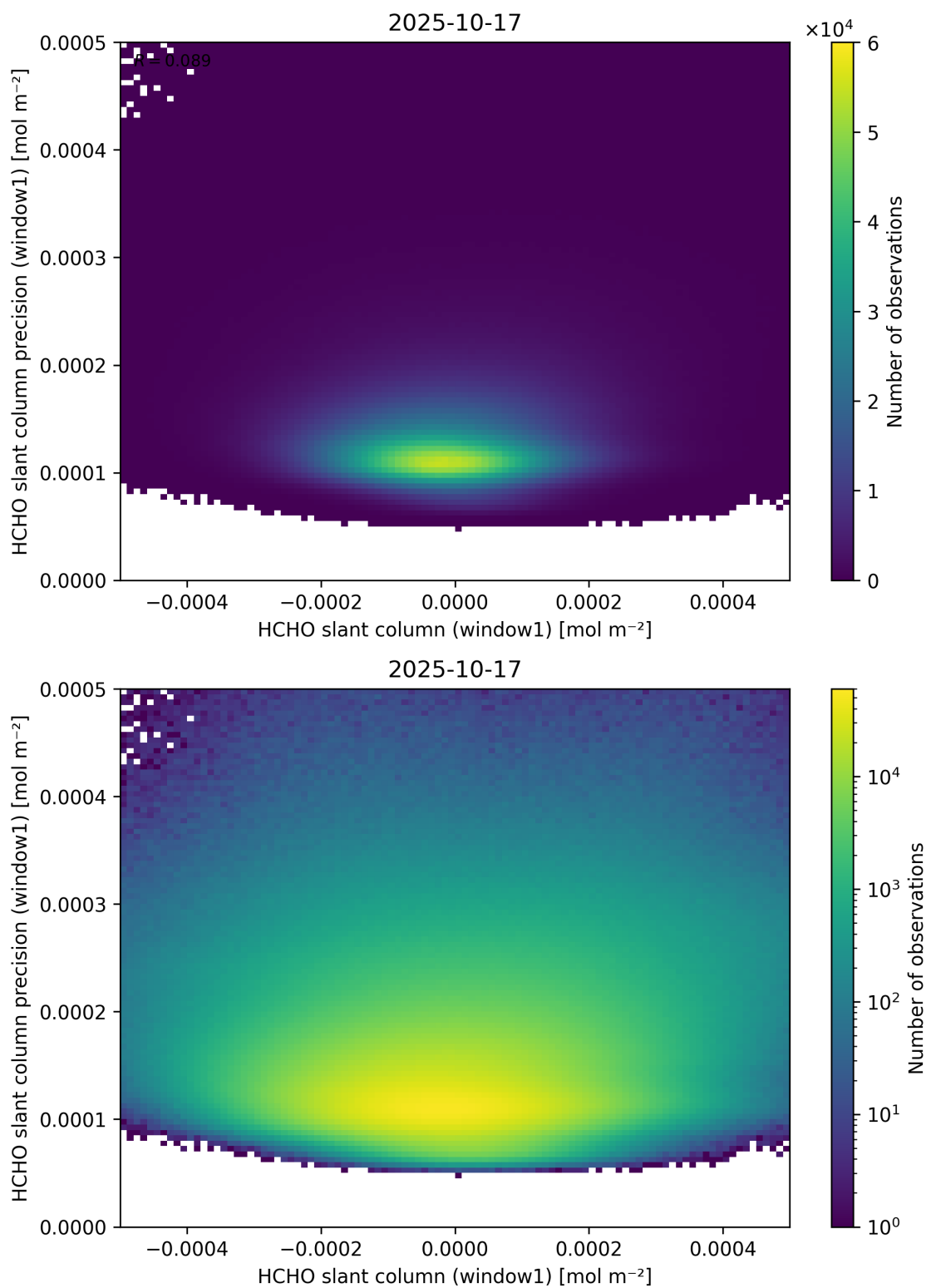
Figure 84: Scatter density plot of “HCHO slant column (window1)” against “HCHO slant column precision (window1)” for 2025-10-17 to 2025-10-18.
