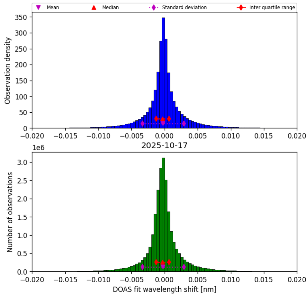
Figure 44: Histogram of “DOAS fit wavelength shift” for 2025-10-17 to 2025-10-18
