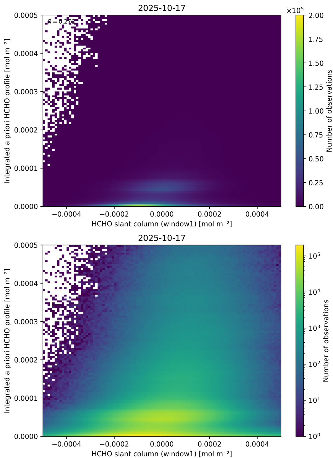
Figure 87: Scatter density plot of “HCHO slant column (window1)” against “Integrated a priori HCHO profile” for 2025-10-17 to 2025-10-18.
