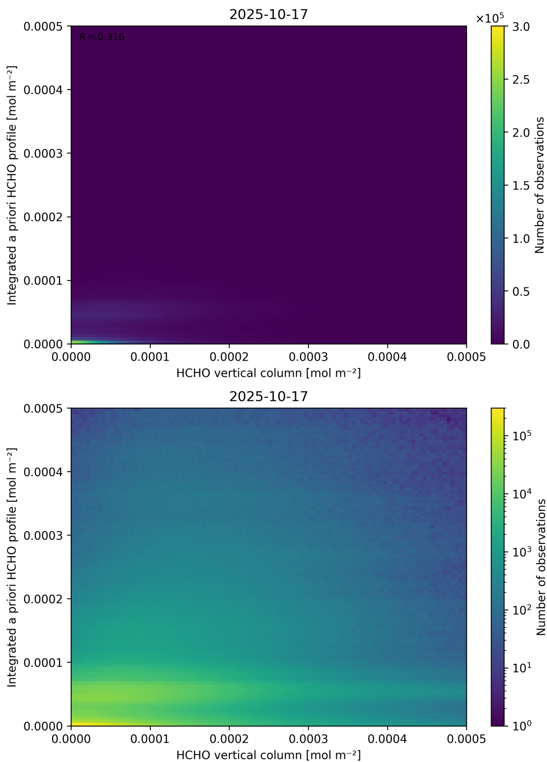
Figure 135: Scatter density plot of “HCHO vertical column” against “Integrated a priori HCHO profile” for 2025-10-17 to 2025-10-18.
