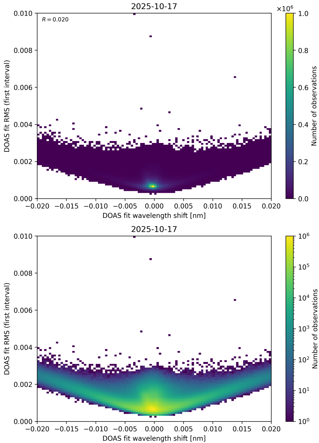
Figure 64: Scatter density plot of “DOAS fit wavelength shift” against “DOAS fit RMS (first interval)” for 2025-10-17 to 2025-10-18.
