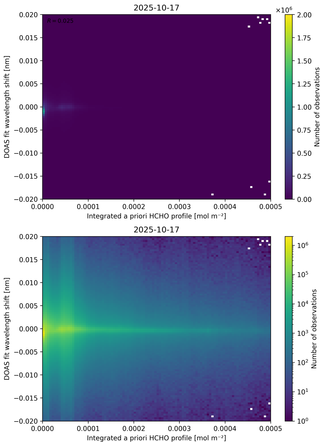
Figure 149: Scatter density plot of “Integrated a priori HCHO profile” against “DOAS fit wavelength shift” for 2025-10-17 to 2025-10-18.
