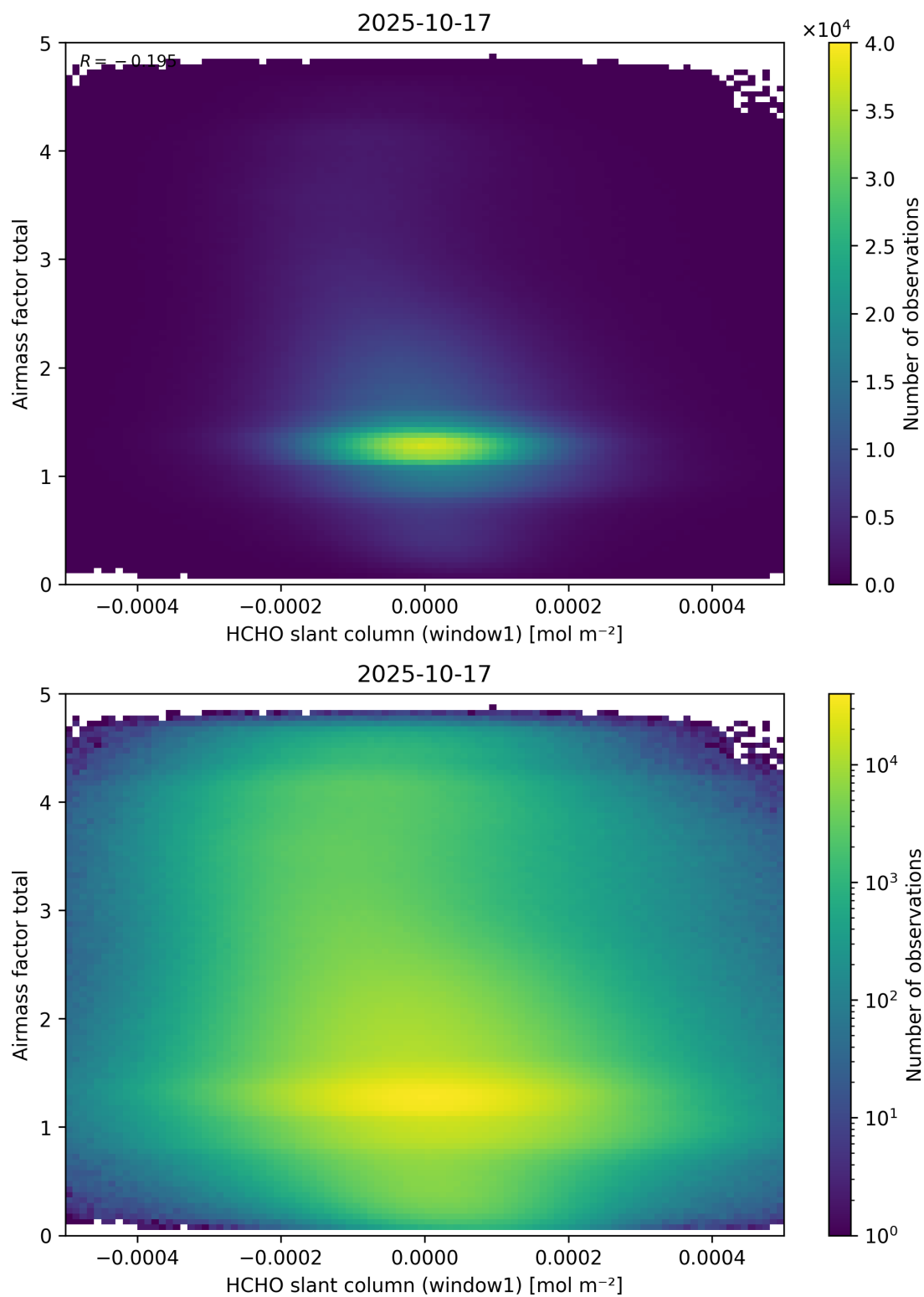
Figure 85: Scatter density plot of “HCHO slant column (window1)” against “Airmass factor total” for 2025-10-17 to 2025-10-18.
