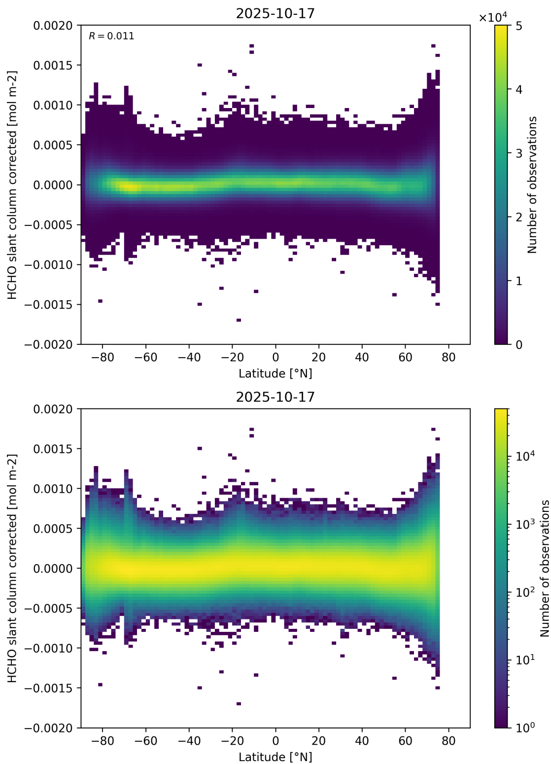
Figure 157: Scatter density plot of “Latitude” against “HCHO slant column corrected” for 2025-10-17 to 2025-10-18.
