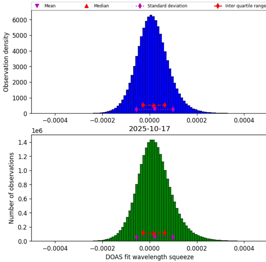
Figure 45: Histogram of “DOAS fit wavelength squeeze” for 2025-10-17 to 2025-10-18
