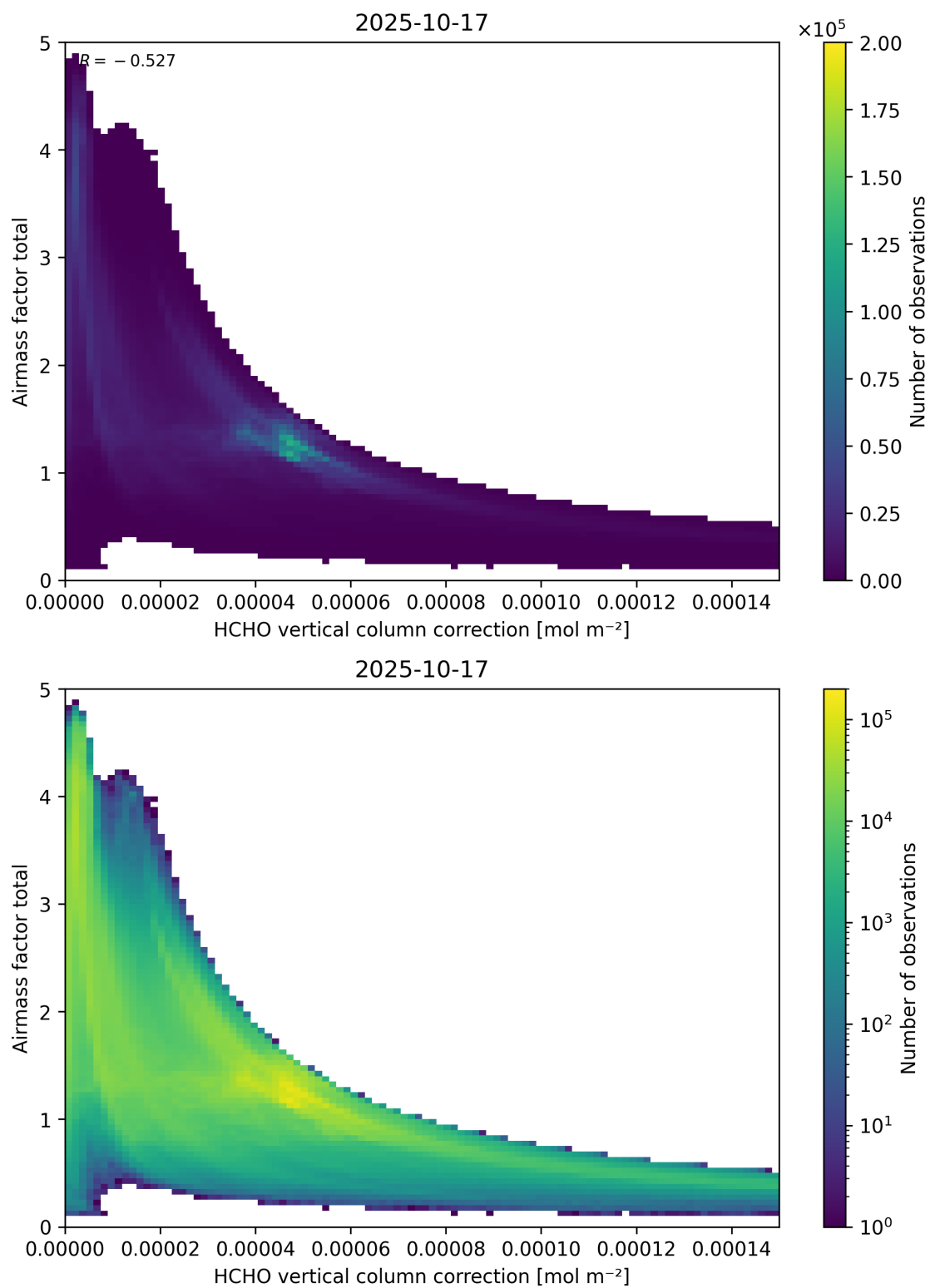
Figure 120: Scatter density plot of “HCHO vertical column correction” against “Airmass factor total” for 2025-10-17 to 2025-10-18.
