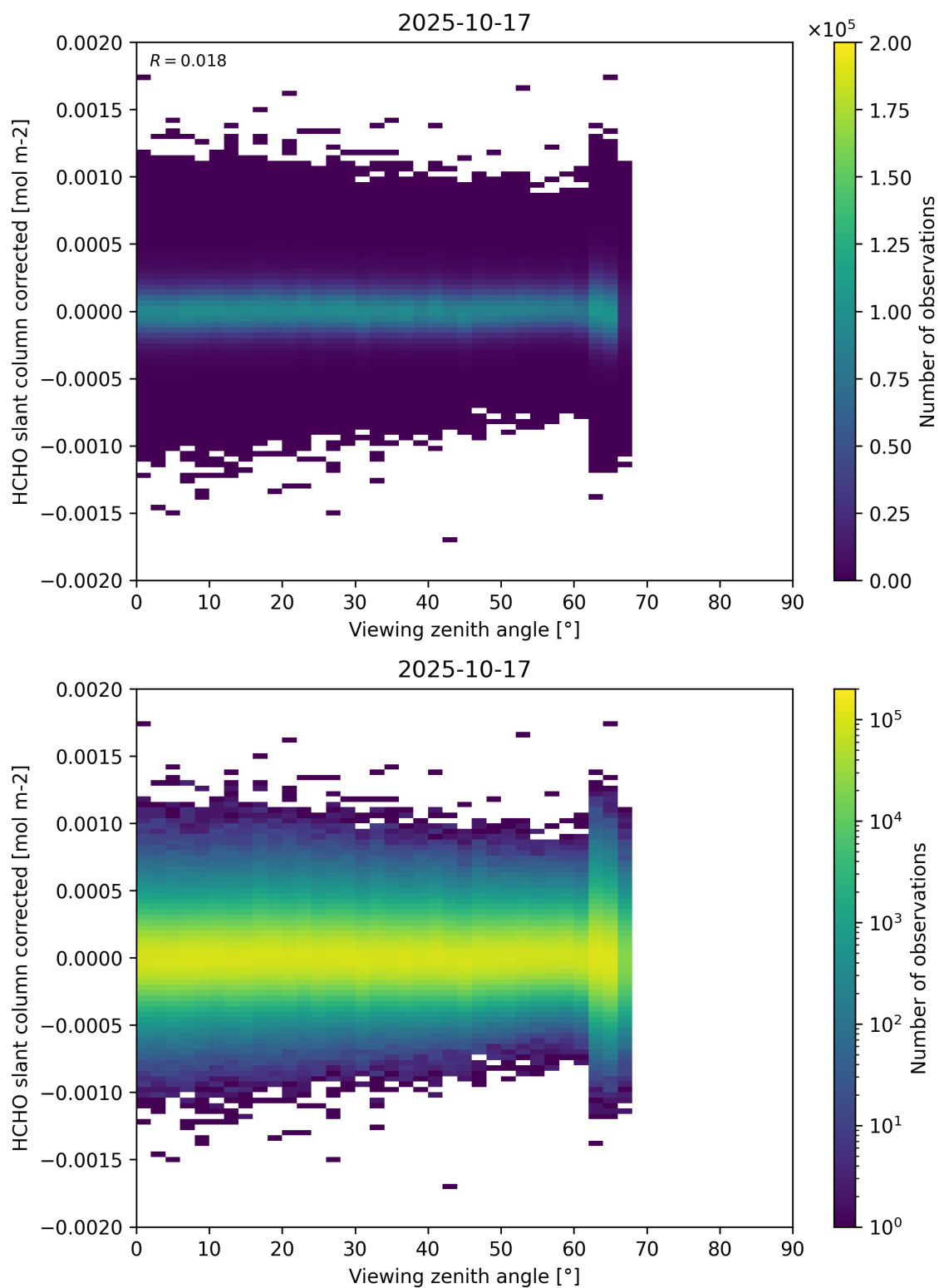
Figure 186: Scatter density plot of “Viewing zenith angle” against “HCHO slant column corrected” for 2025-10-17 to 2025-10-18.
