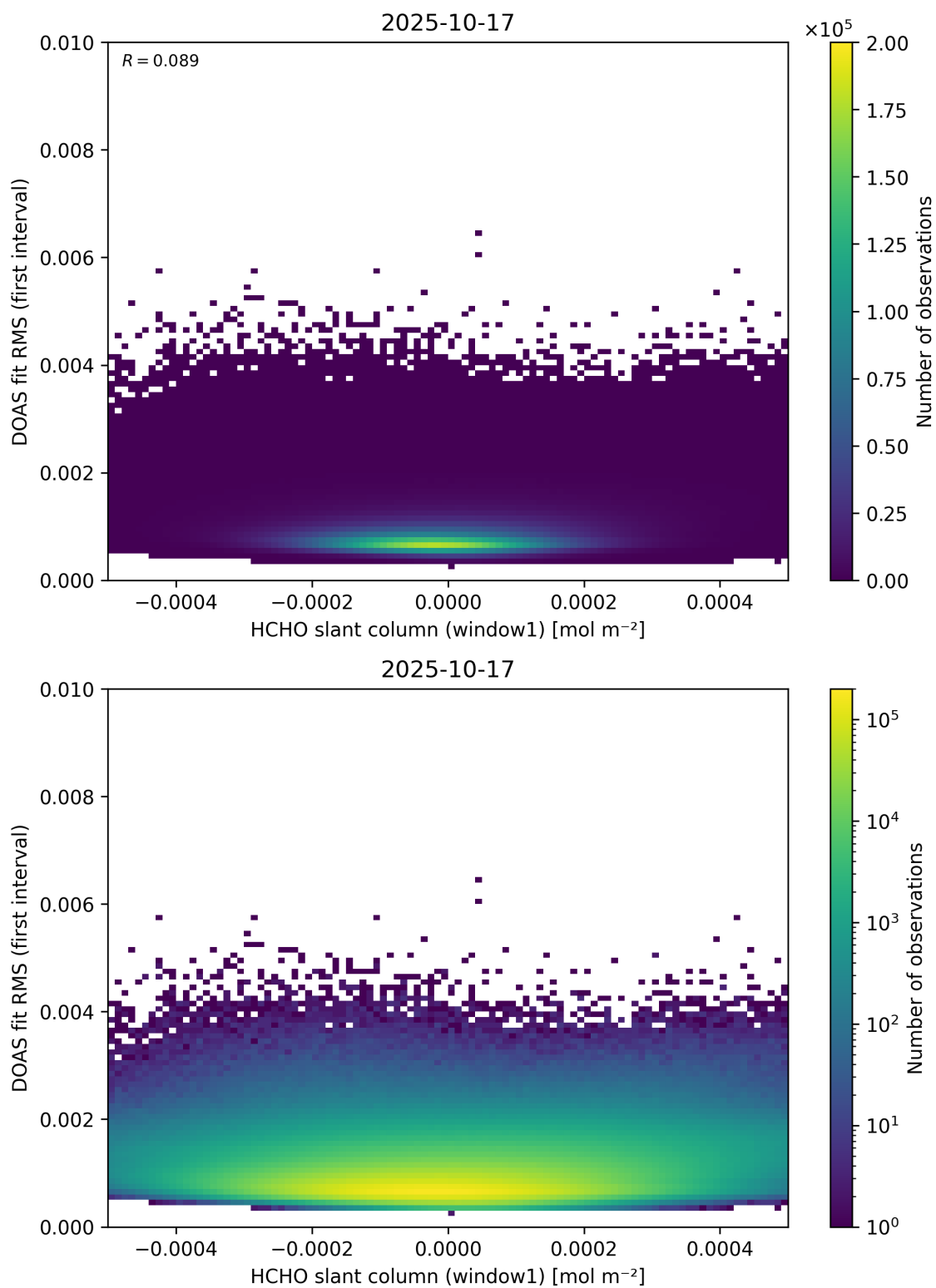
Figure 78: Scatter density plot of “HCHO slant column (window1)” against “DOAS fit RMS (first interval)” for 2025-10-17 to 2025-10-18.
