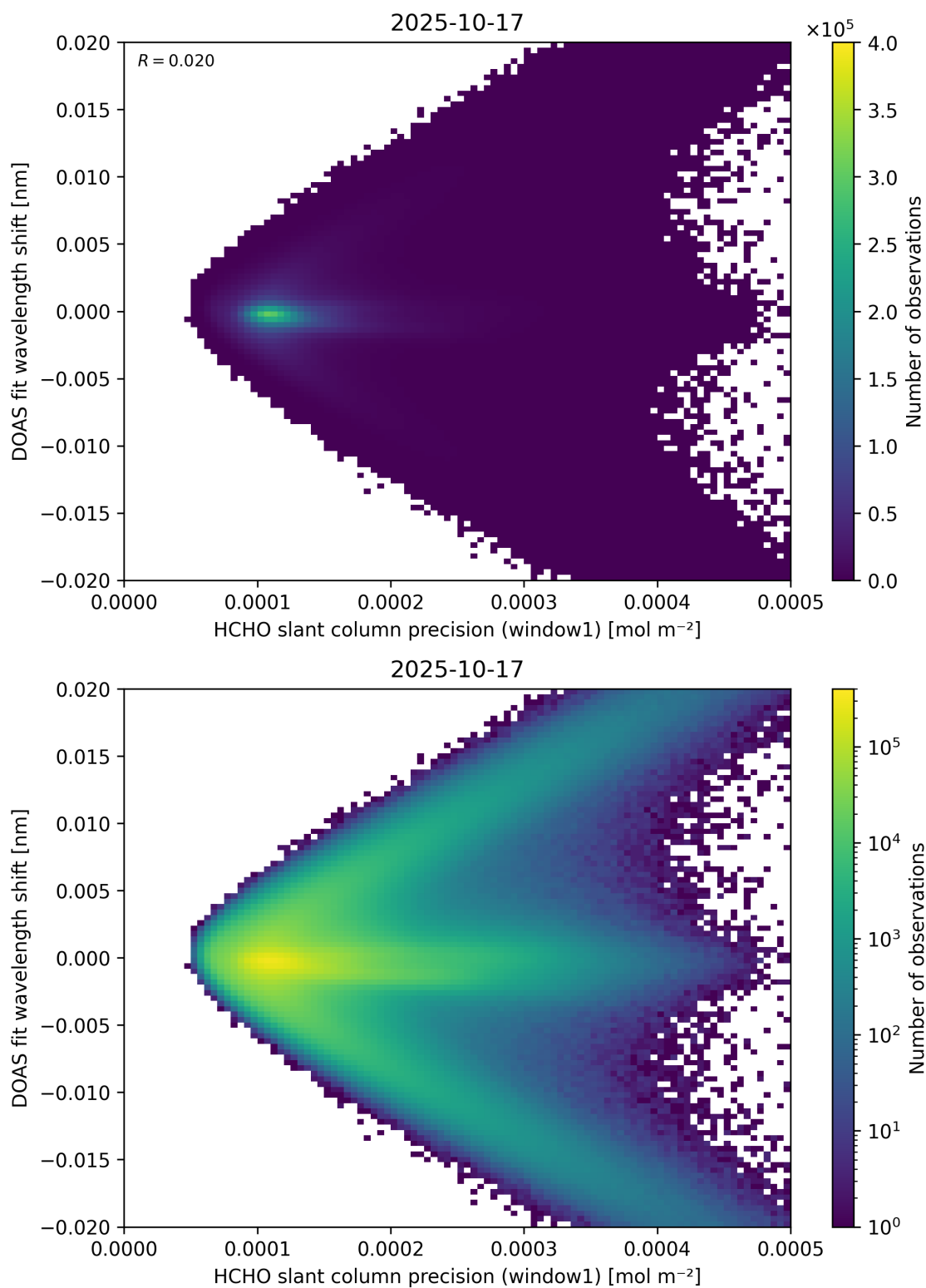
Figure 89: Scatter density plot of “HCHO slant column precision (window1)” against “DOAS fit wavelength shift” for 2025-10-17 to 2025-10-18.
