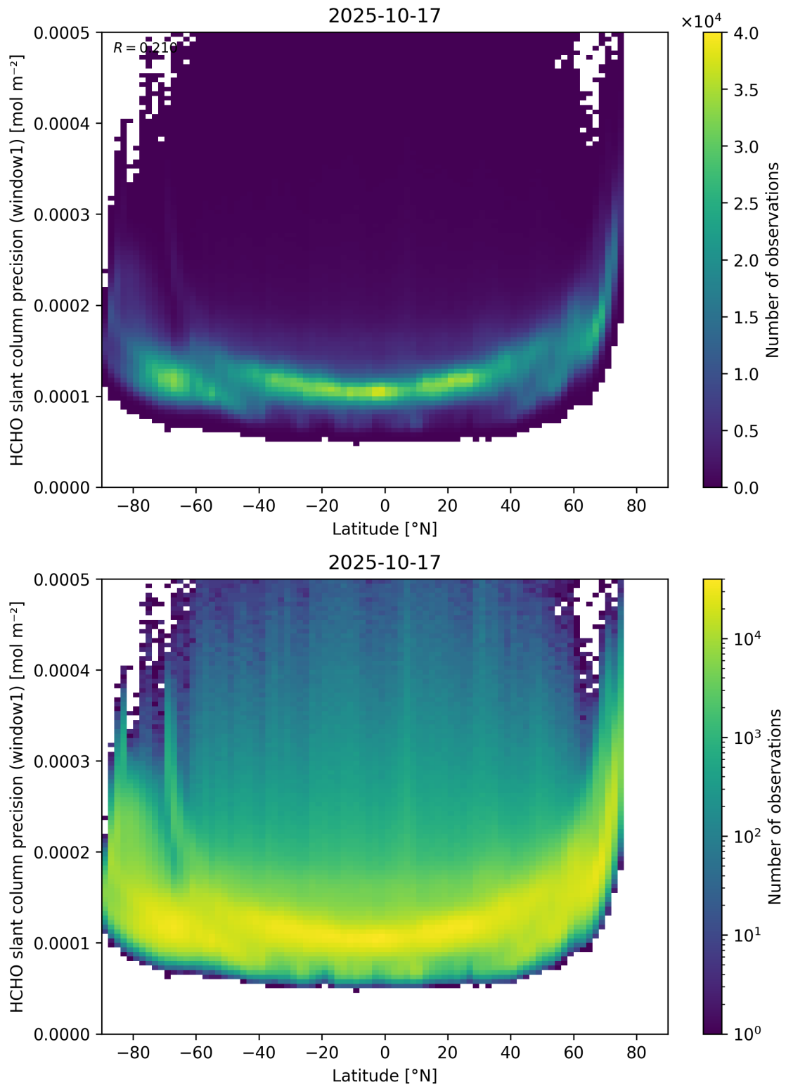
Figure 160: Scatter density plot of “Latitude” against “HCHO slant column precision (window1)” for 2025-10-17 to 2025-10-18.
