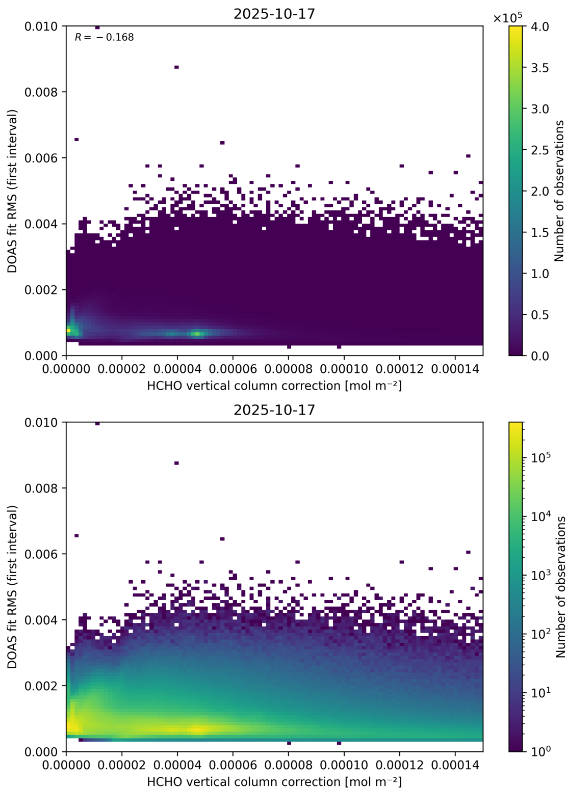
Figure 112: Scatter density plot of “HCHO vertical column correction” against “DOAS fit RMS (first interval)” for 2025-10-17 to 2025-10-18.
