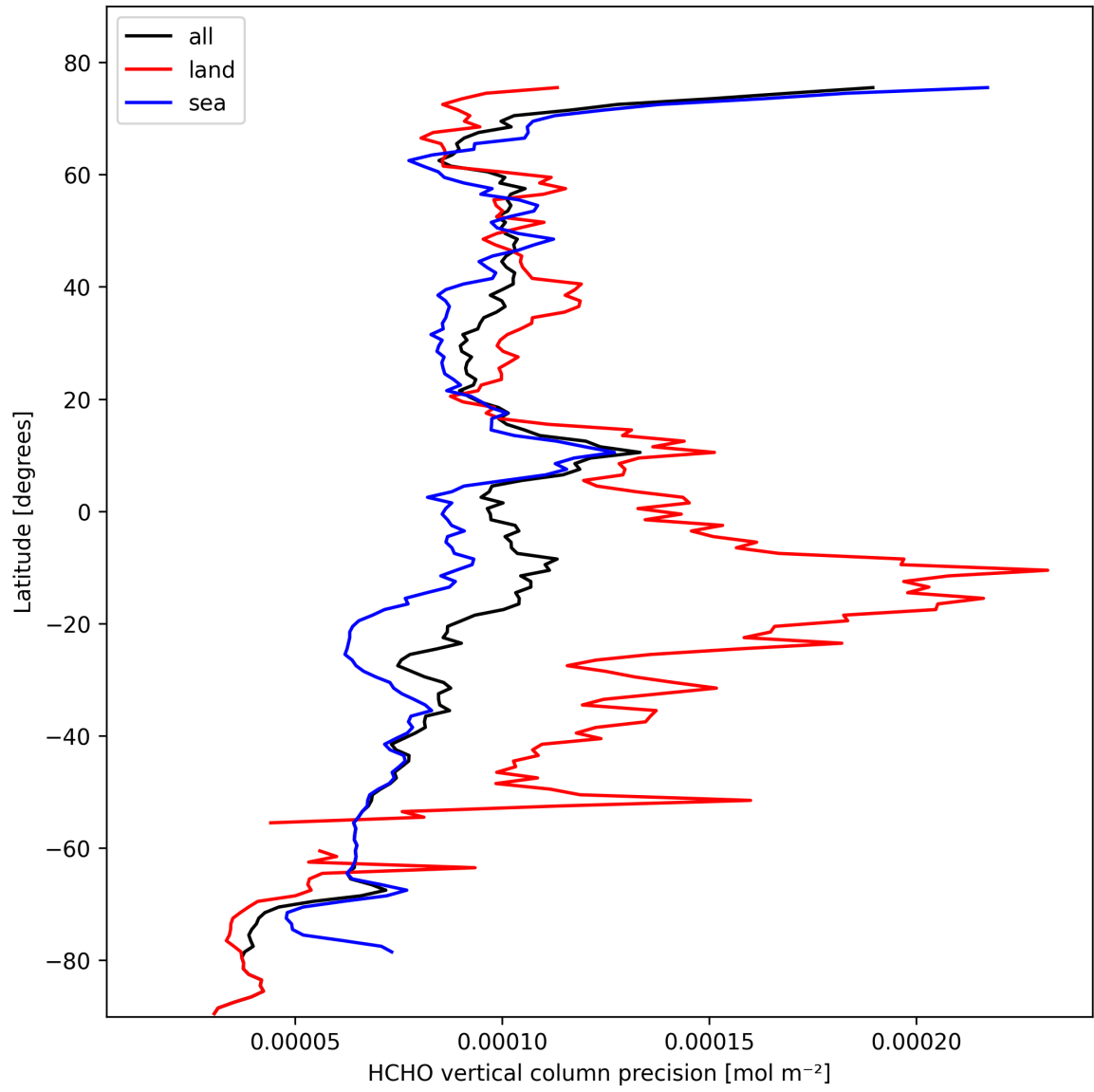
Figure 22: Zonal average of “HCHO vertical column precision” for 2025-10-17 to 2025-10-18.
