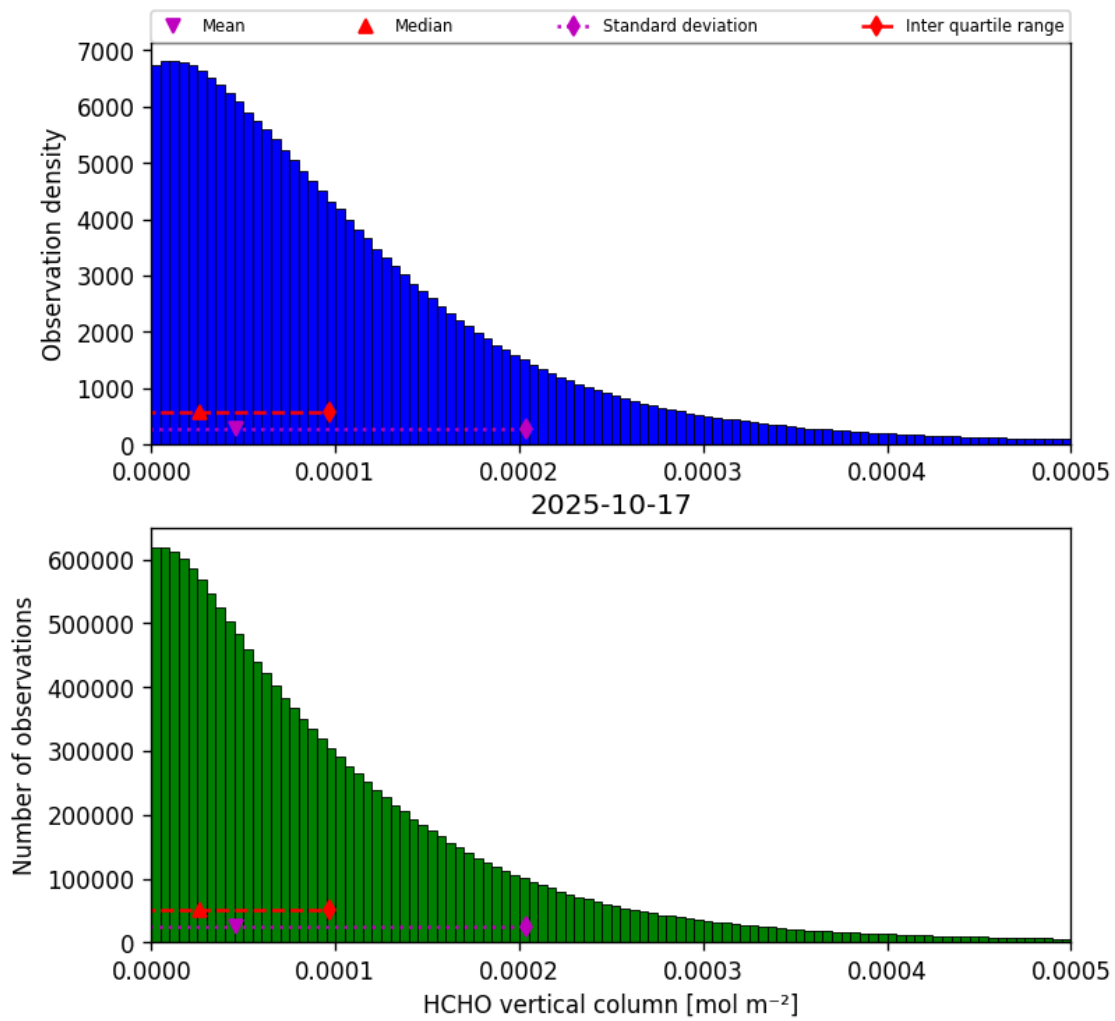
Figure 35: Histogram of “HCHO vertical column” for 2025-10-17 to 2025-10-18
