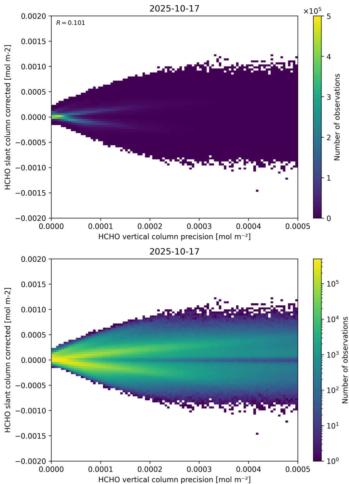
Figure 140: Scatter density plot of “HCHO vertical column precision” against “HCHO slant column corrected” for 2025-10-17 to 2025-10-18.
