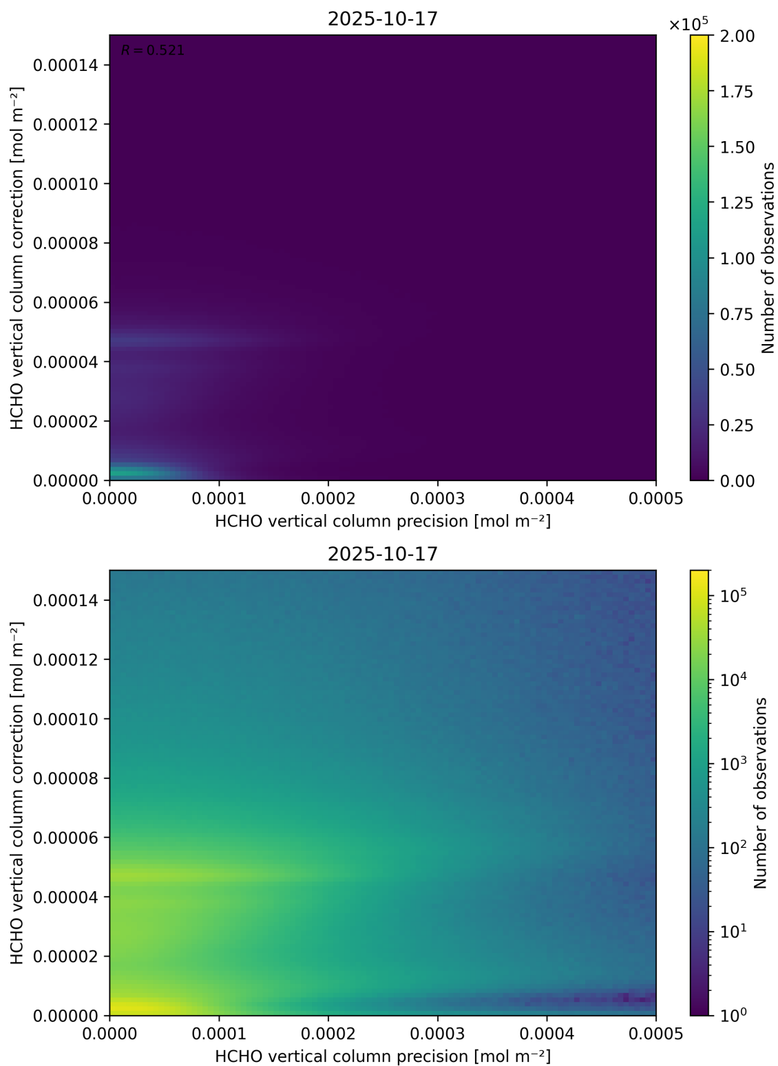
Figure 146: Scatter density plot of “HCHO vertical column precision” against “HCHO vertical column correction” for 2025-10-17 to 2025-10-18.
