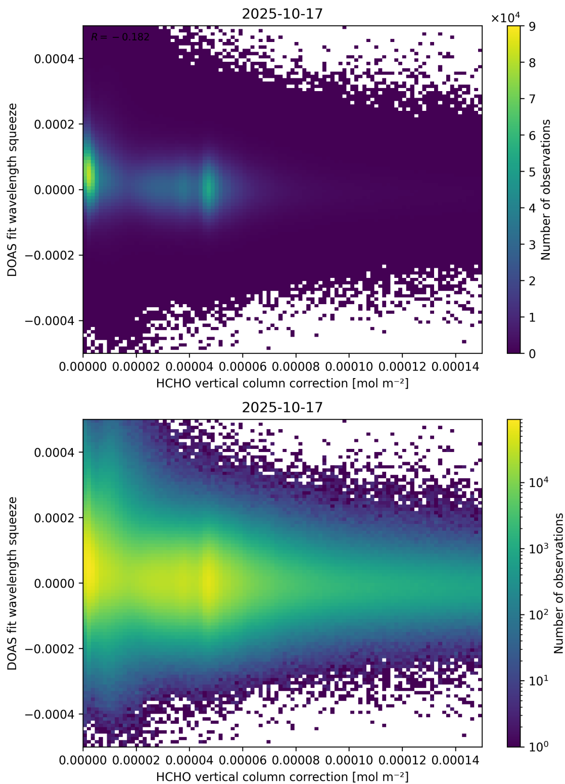
Figure 114: Scatter density plot of “HCHO vertical column correction” against “DOAS fit wavelength squeeze” for 2025-10-17 to 2025-10-18.
