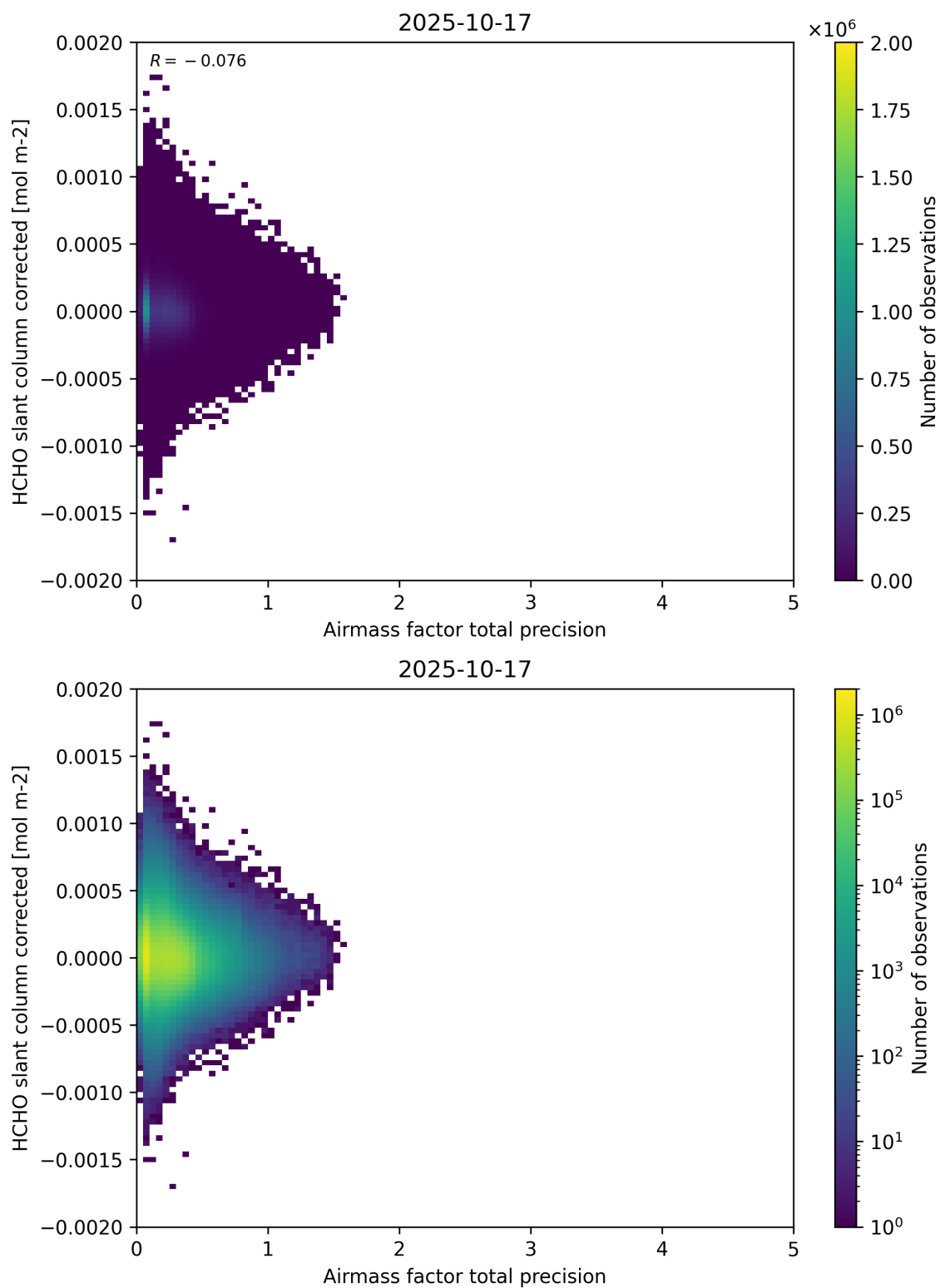
Figure 109: Scatter density plot of “Airmass factor total precision” against “HCHO slant column corrected” for 2025-10-17 to 2025-10-18.
