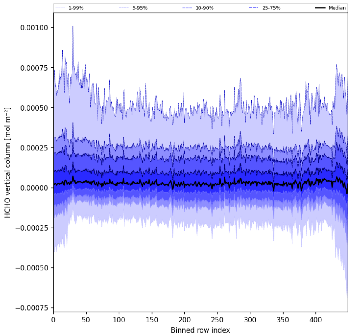
Figure 49: Along track statistics of “HCHO vertical column” for 2025-10-17 to 2025-10-18
