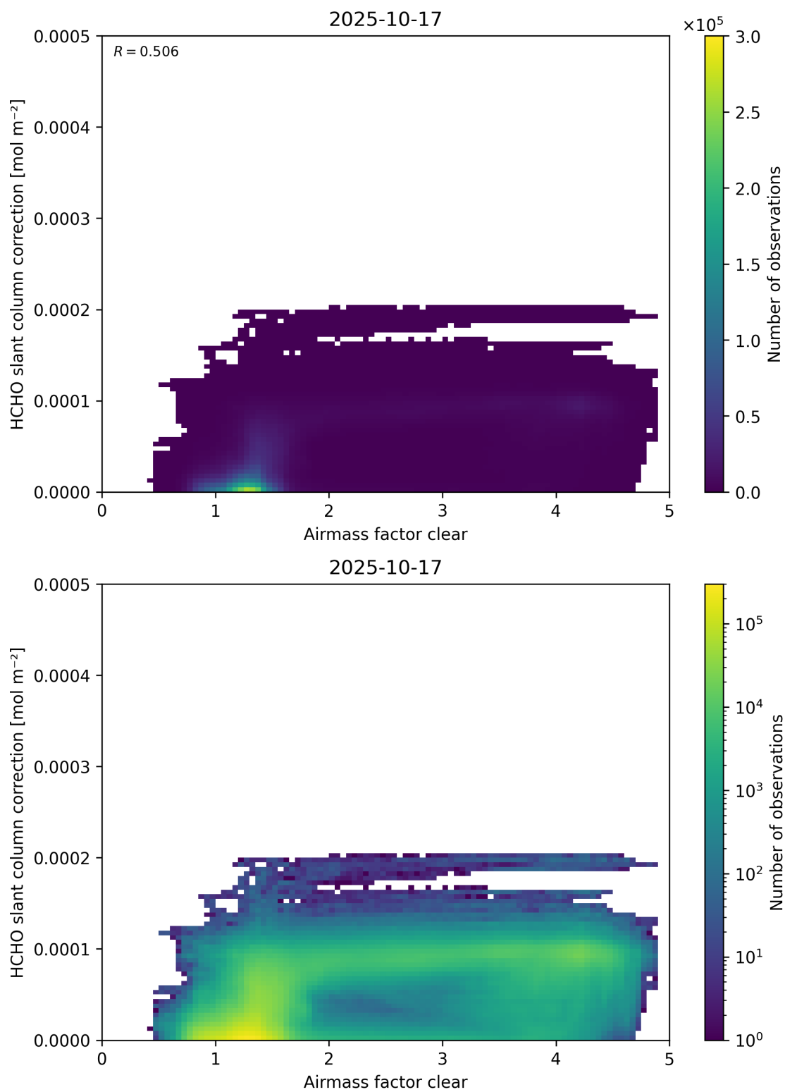
Figure 75: Scatter density plot of “Airmass factor clear” against “HCHO slant column correction” for 2025-10-17 to 2025-10-18.
