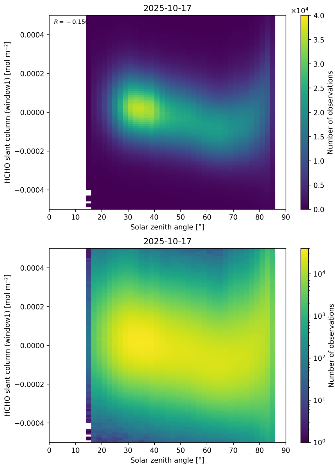
Figure 173: Scatter density plot of “Solar zenith angle” against “HCHO slant column (window1)” for 2025-10-17 to 2025-10-18.
