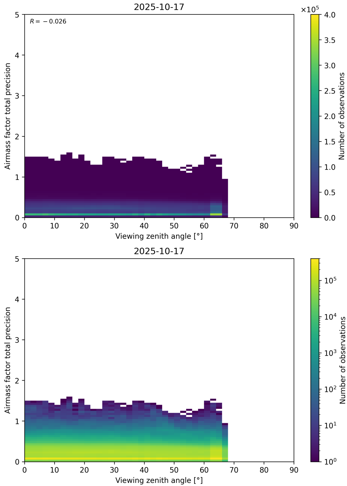
Figure 191: Scatter density plot of “Viewing zenith angle” against “Airmass factor total precision” for 2025-10-17 to 2025-10-18.
