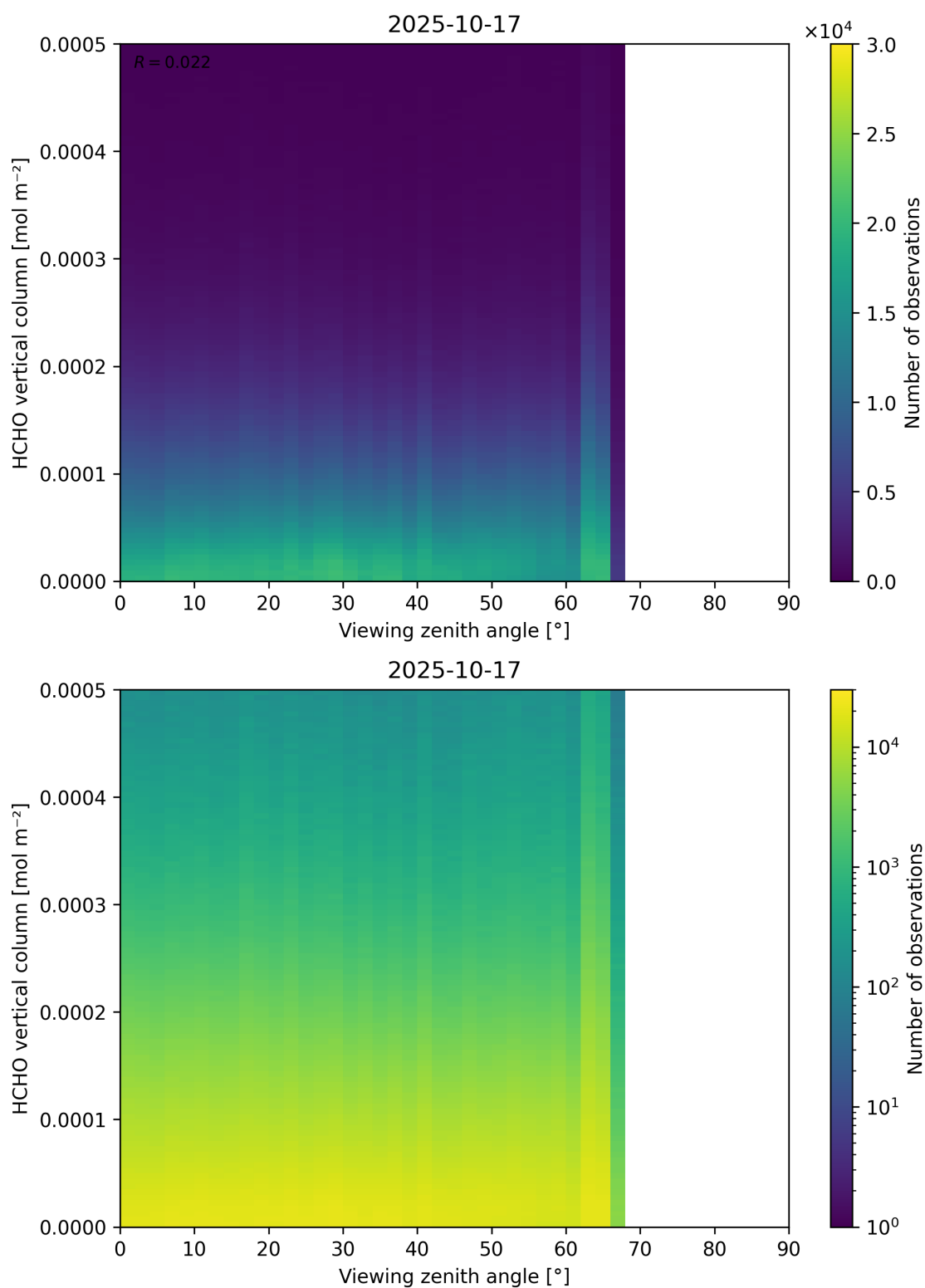
Figure 192: Scatter density plot of “Viewing zenith angle” against “HCHO vertical column” for 2025-10-17 to 2025-10-18.
