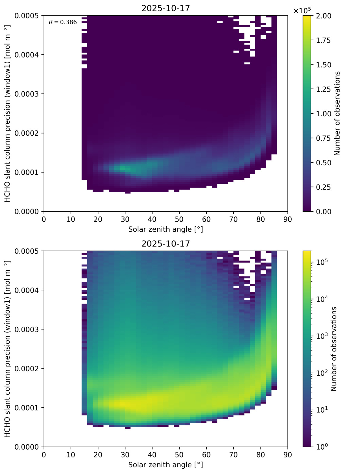
Figure 174: Scatter density plot of “Solar zenith angle” against “HCHO slant column precision (window1)” for 2025-10-17 to 2025-10-18.
