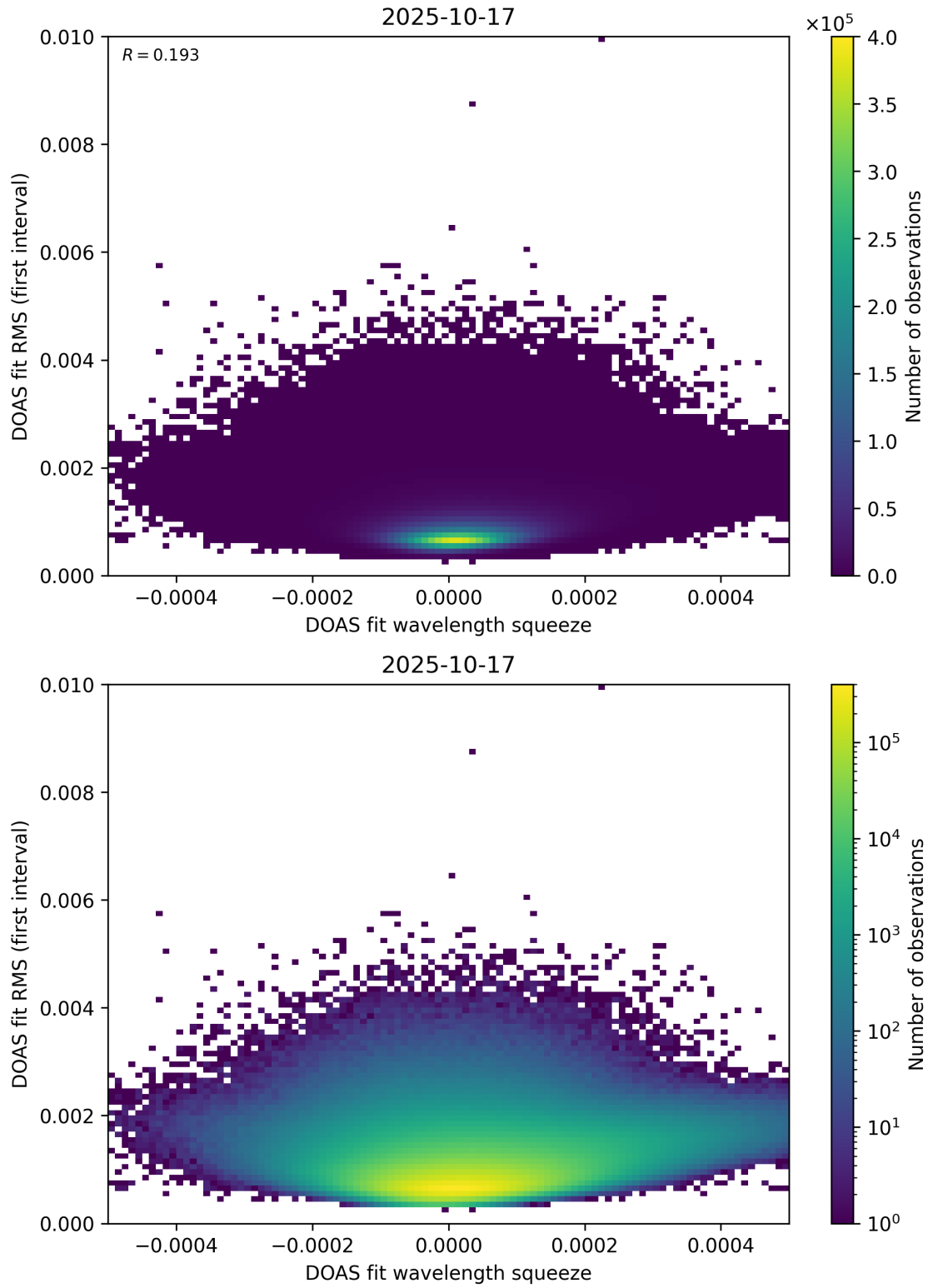
Figure 68: Scatter density plot of “DOAS fit wavelength squeeze” against “DOAS fit RMS (first interval)” for 2025-10-17 to 2025-10-18.
