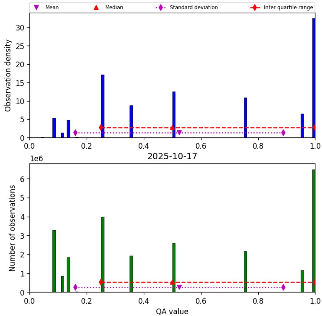
Figure 34: Histogram of “QA value” for 2025-10-17 to 2025-10-18
