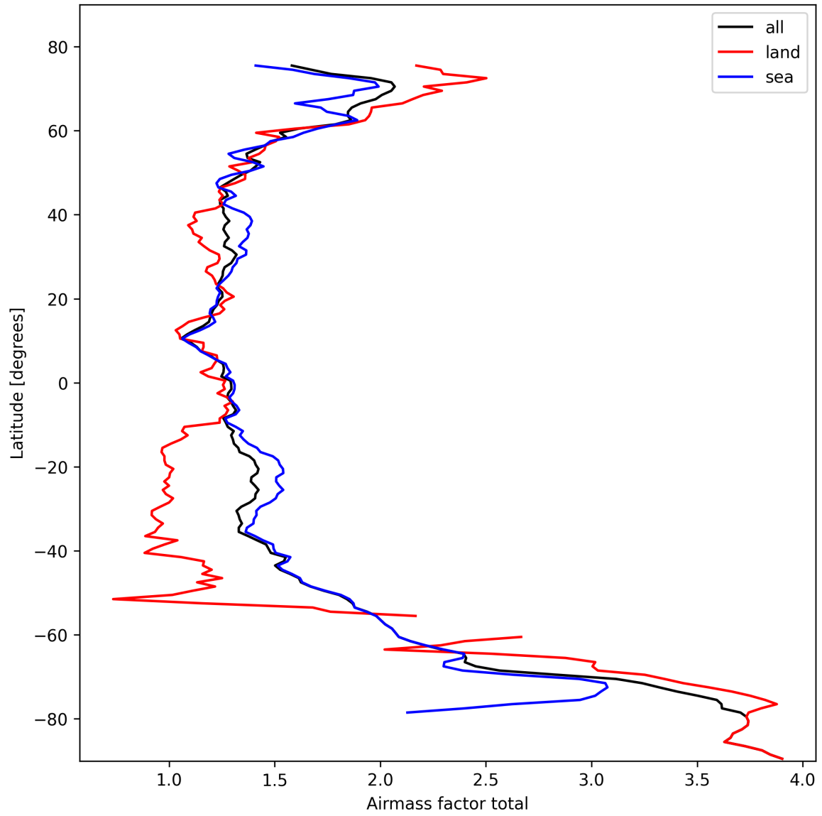
Figure 26: Zonal average of “Airmass factor total” for 2025-10-17 to 2025-10-18.
