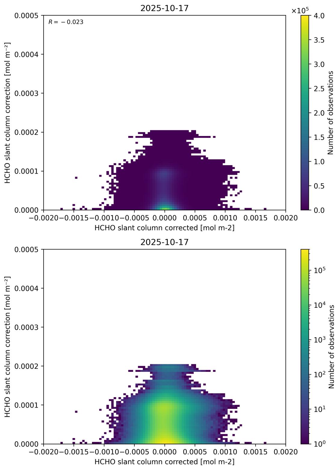
Figure 77: Scatter density plot of “HCHO slant column corrected” against “HCHO slant column correction” for 2025-10-17 to 2025-10-18.
