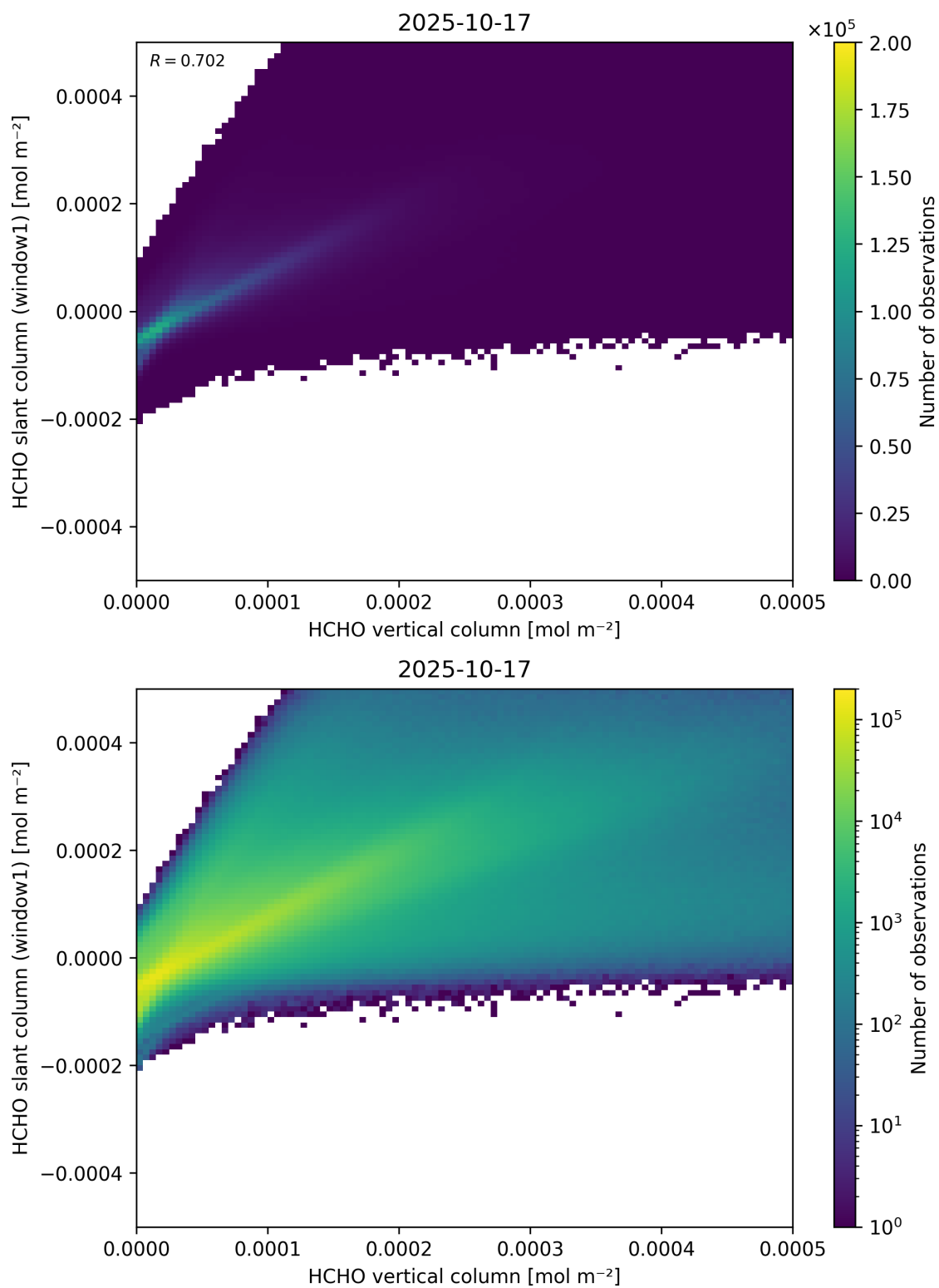
Figure 129: Scatter density plot of “HCHO vertical column” against “HCHO slant column (window1)” for 2025-10-17 to 2025-10-18.
