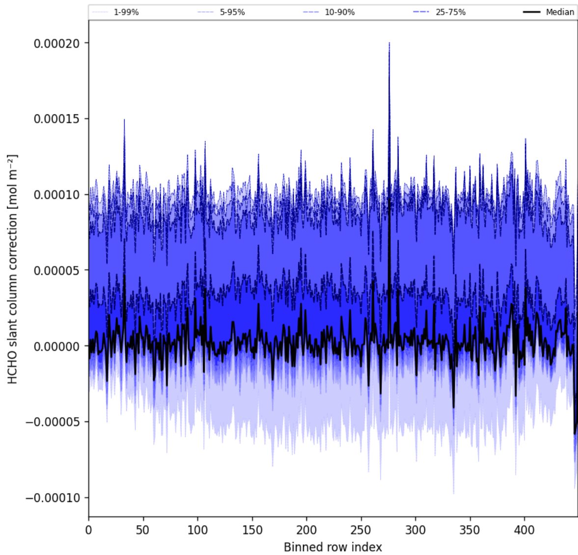
Figure 61: Along track statistics of “HCHO slant column correction” for 2025-10-17 to 2025-10-18
