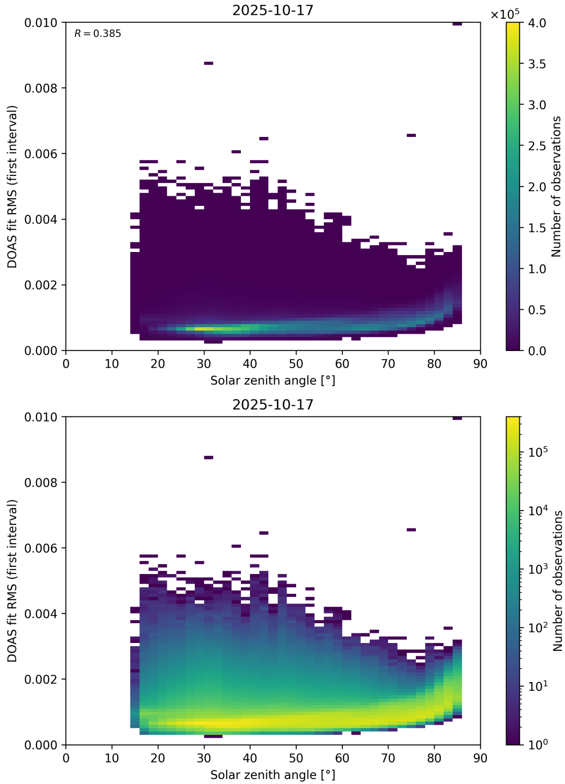
Figure 167: Scatter density plot of “Solar zenith angle” against “DOAS fit RMS (first interval)” for 2025-10-17 to 2025-10-18.
