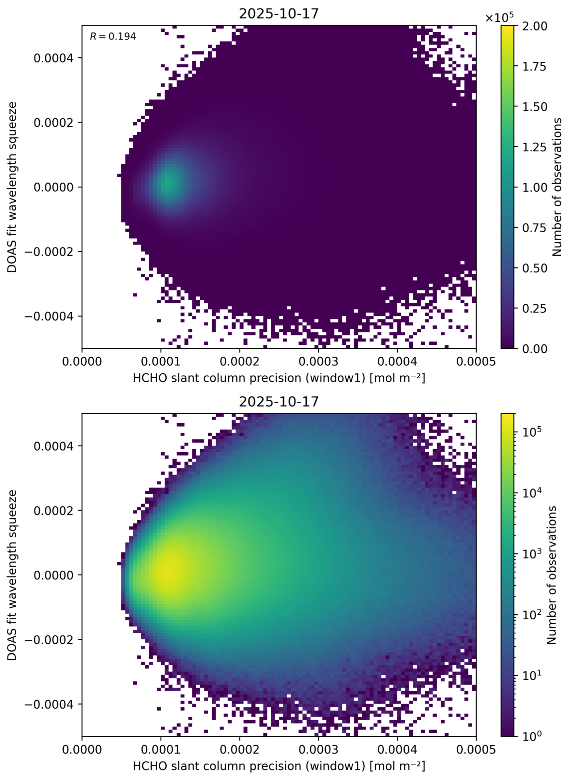
Figure 90: Scatter density plot of “HCHO slant column precision (window1)” against “DOAS fit wavelength squeeze” for 2025-10-17 to 2025-10-18.
