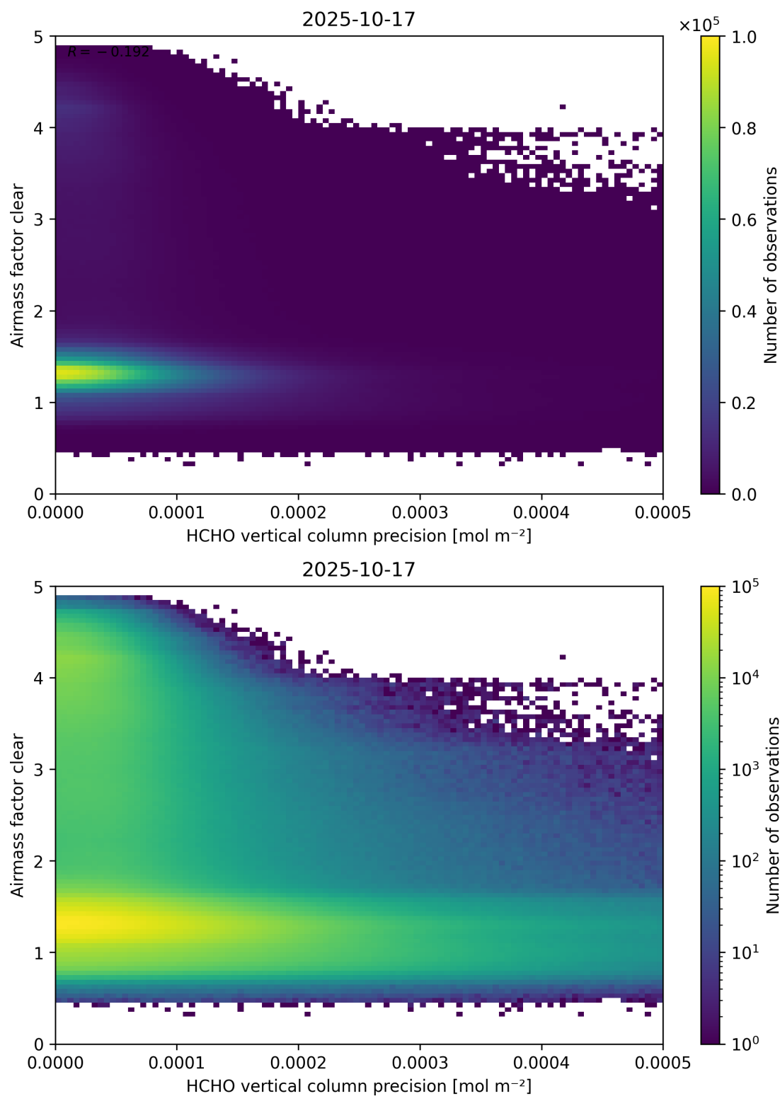
Figure 139: Scatter density plot of “HCHO vertical column precision” against “Airmass factor clear” for 2025-10-17 to 2025-10-18.
