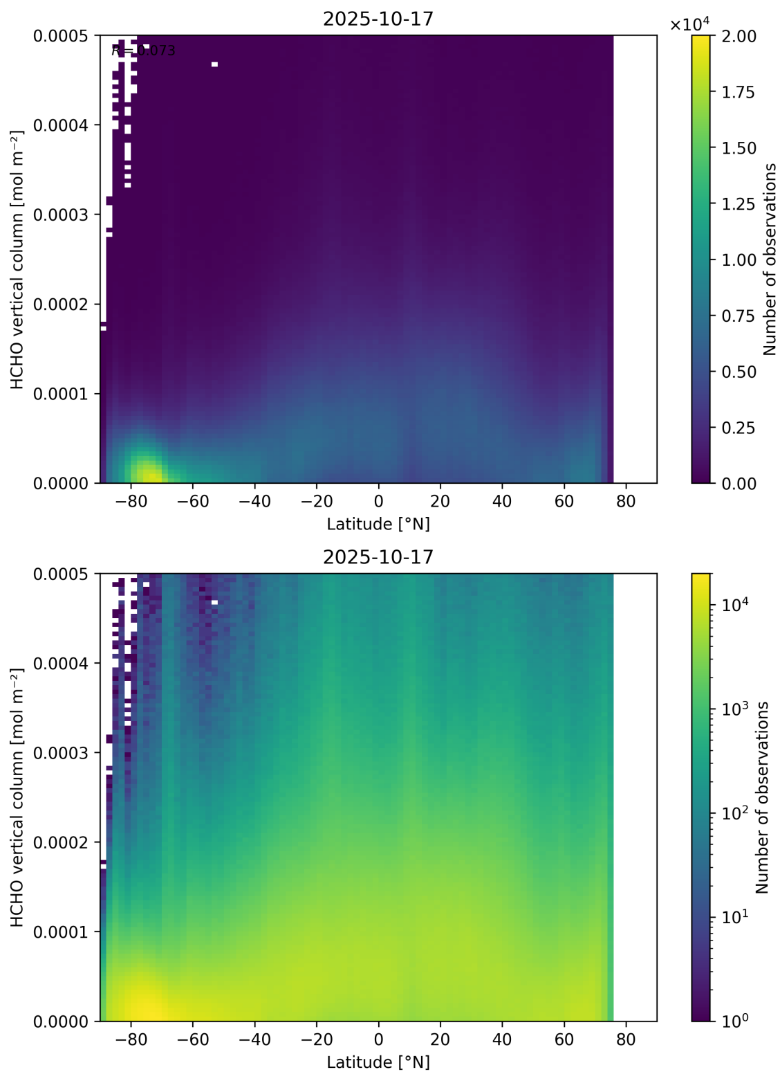
Figure 163: Scatter density plot of “Latitude” against “HCHO vertical column” for 2025-10-17 to 2025-10-18.
