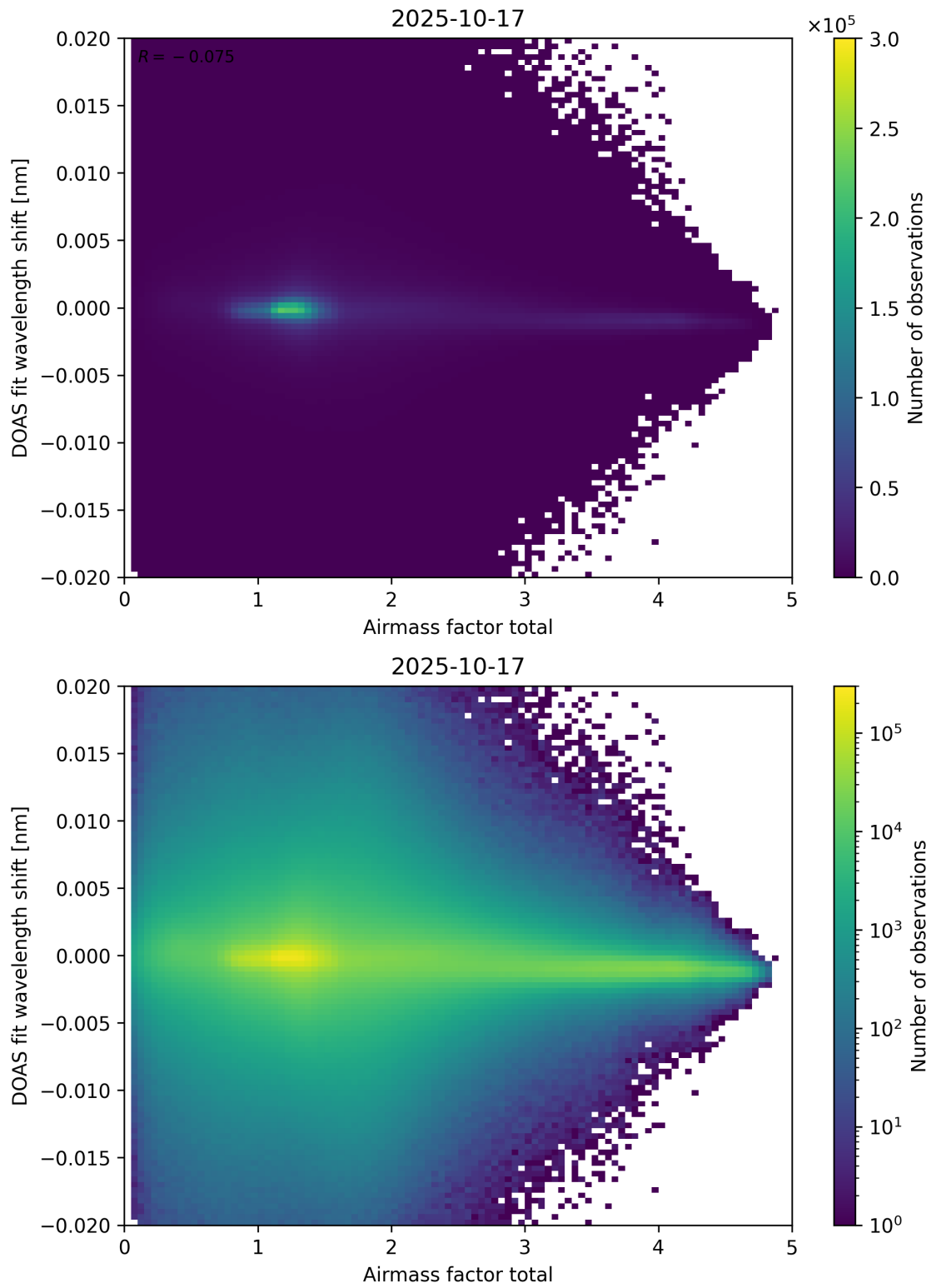
Figure 98: Scatter density plot of “Airmass factor total” against “DOAS fit wavelength shift” for 2025-10-17 to 2025-10-18.
