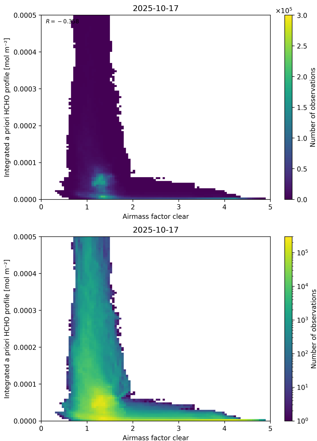
Figure 76: Scatter density plot of “Airmass factor clear” against “Integrated a priori HCHO profile” for 2025-10-17 to 2025-10-18.
