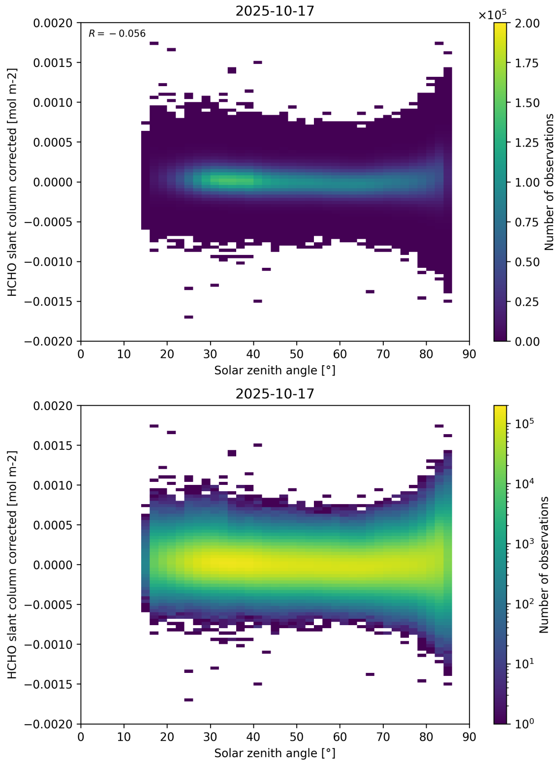
Figure 171: Scatter density plot of “Solar zenith angle” against “HCHO slant column corrected” for 2025-10-17 to 2025-10-18.
