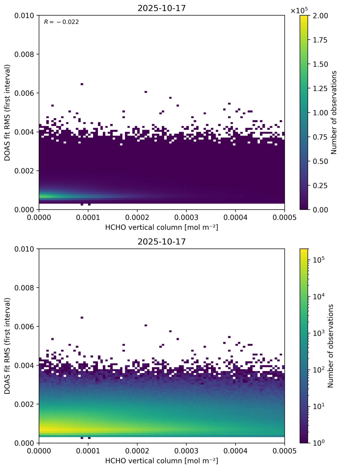
Figure 123: Scatter density plot of “HCHO vertical column” against “DOAS fit RMS (first interval)” for 2025-10-17 to 2025-10-18.
