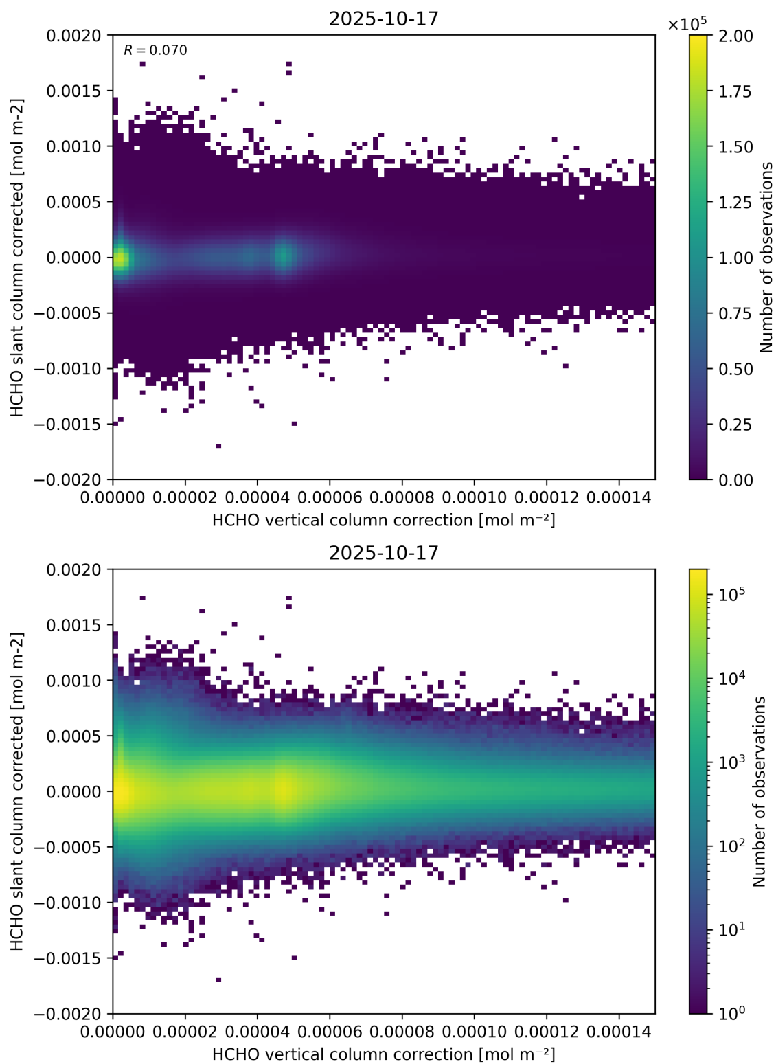
Figure 116: Scatter density plot of “HCHO vertical column correction” against “HCHO slant column corrected” for 2025-10-17 to 2025-10-18.
