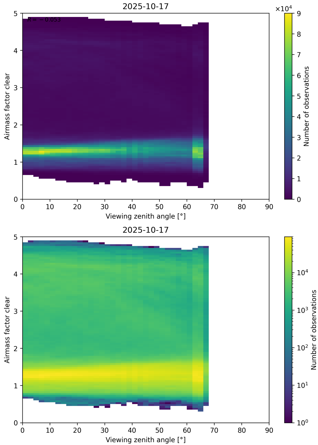
Figure 185: Scatter density plot of “Viewing zenith angle” against “Airmass factor clear” for 2025-10-17 to 2025-10-18.
