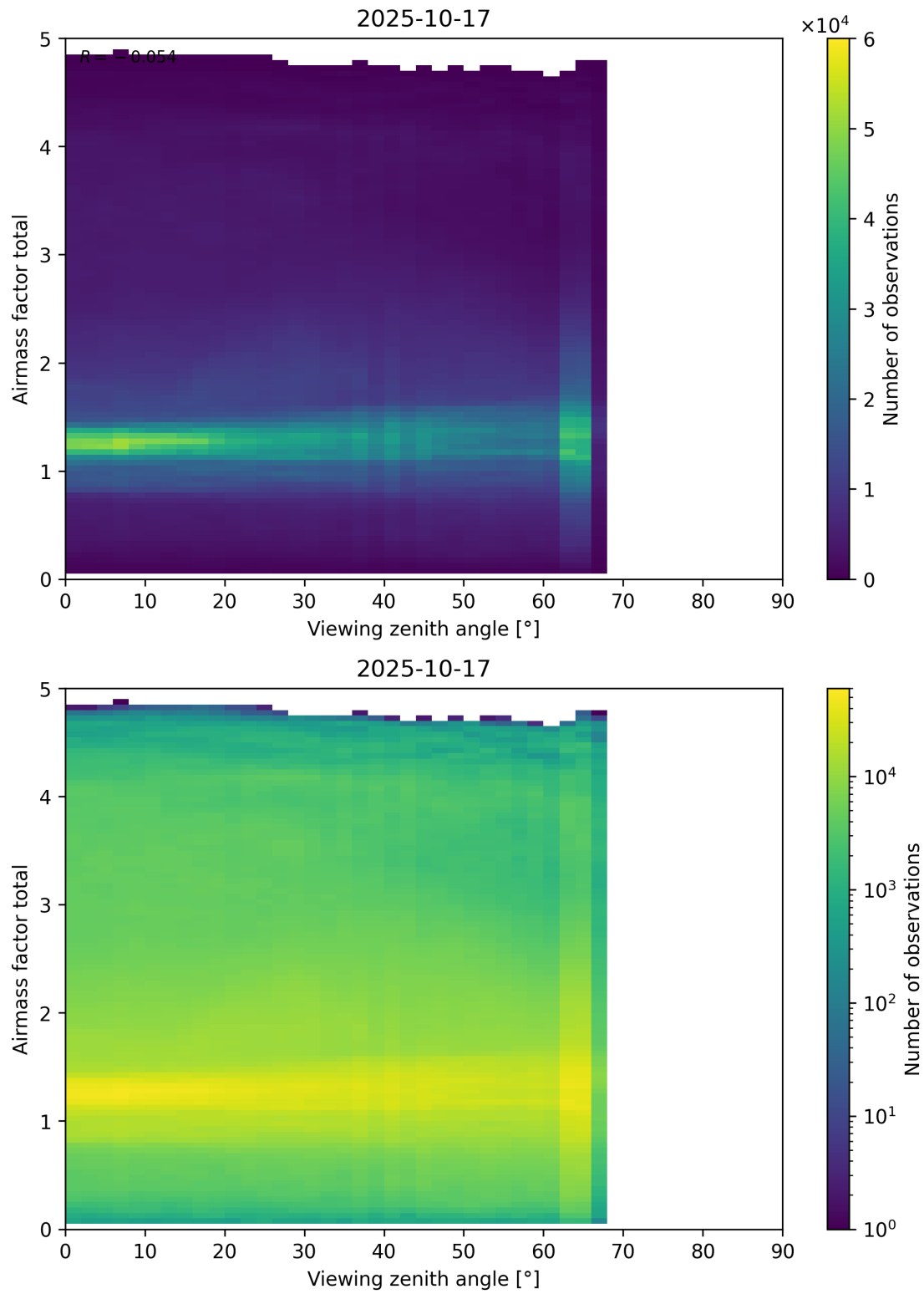
Figure 190: Scatter density plot of “Viewing zenith angle” against “Airmass factor total” for 2025-10-17 to 2025-10-18.
