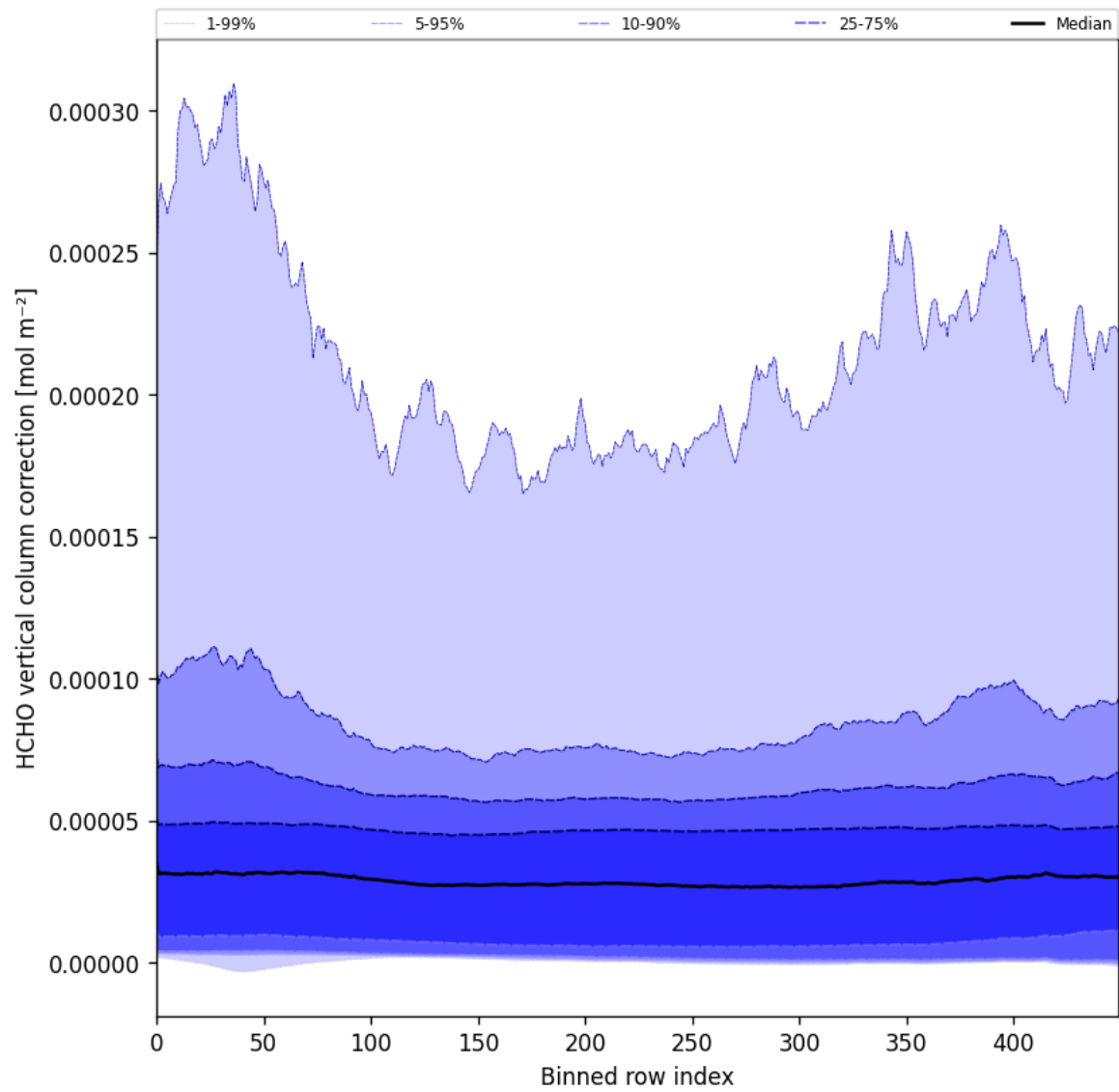
Figure 51: Along track statistics of “HCHO vertical column correction” for 2025-10-17 to 2025-10-18
