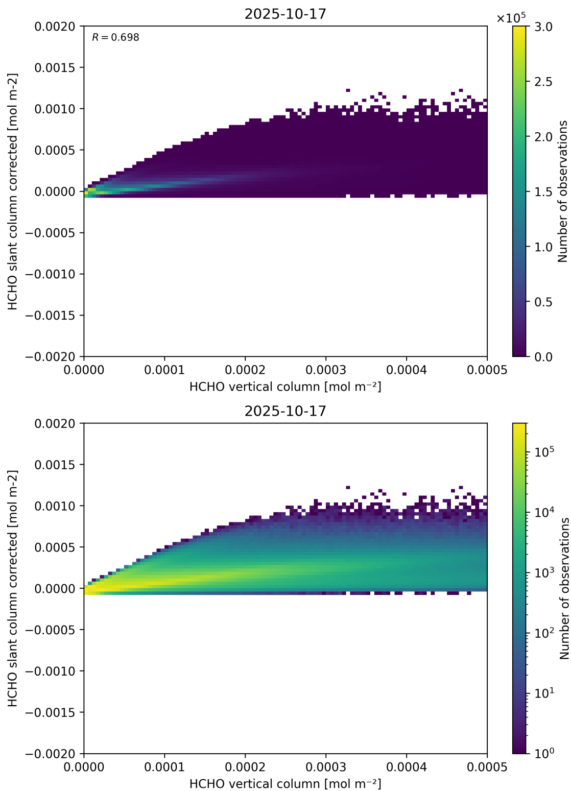
Figure 127: Scatter density plot of “HCHO vertical column” against “HCHO slant column corrected” for 2025-10-17 to 2025-10-18.
