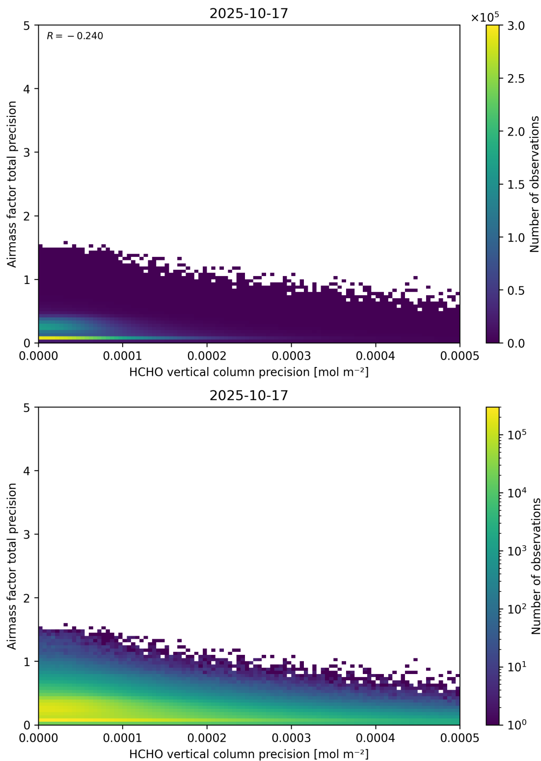
Figure 145: Scatter density plot of “HCHO vertical column precision” against “Airmass factor total precision” for 2025-10-17 to 2025-10-18.
