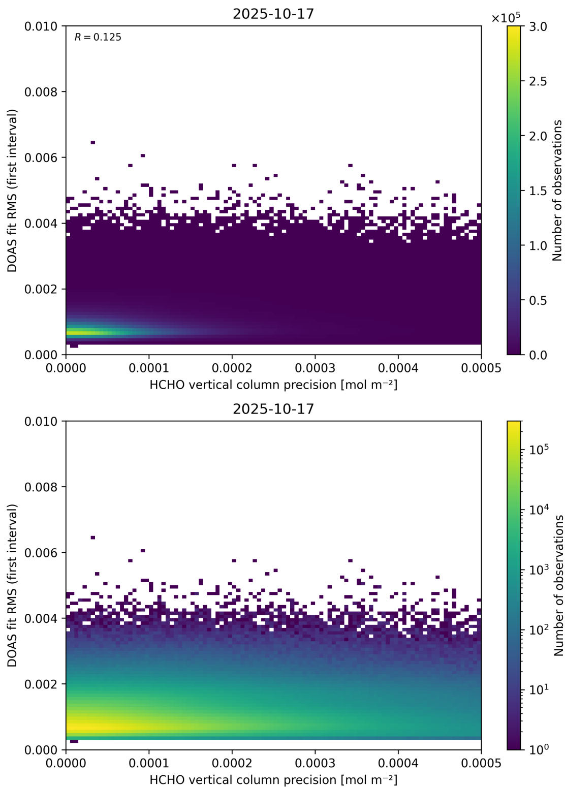
Figure 136: Scatter density plot of “HCHO vertical column precision” against “DOAS fit RMS (first interval)” for 2025-10-17 to 2025-10-18.
