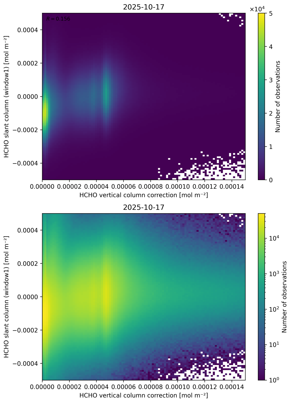
Figure 118: Scatter density plot of “HCHO vertical column correction” against “HCHO slant column (window1)” for 2025-10-17 to 2025-10-18.
