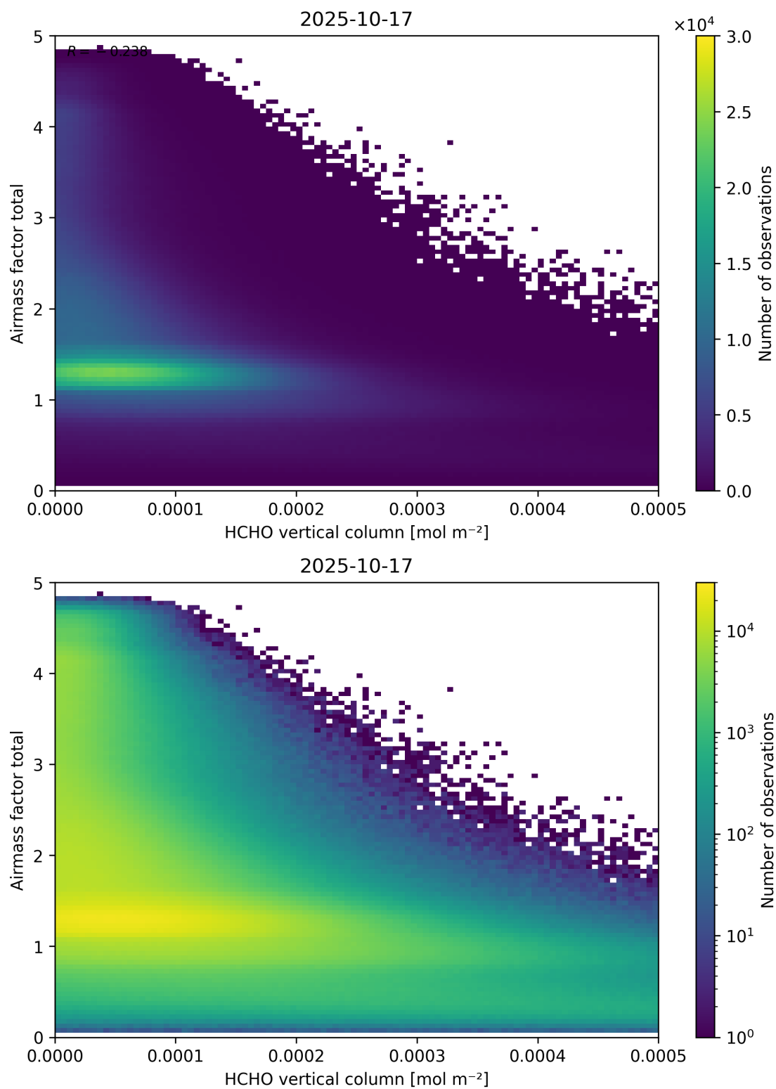
Figure 131: Scatter density plot of “HCHO vertical column” against “Airmass factor total” for 2025-10-17 to 2025-10-18.
