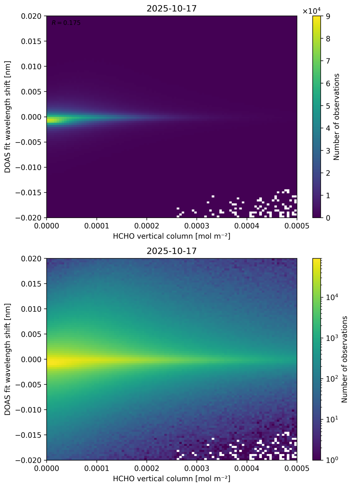
Figure 124: Scatter density plot of “HCHO vertical column” against “DOAS fit wavelength shift” for 2025-10-17 to 2025-10-18.
