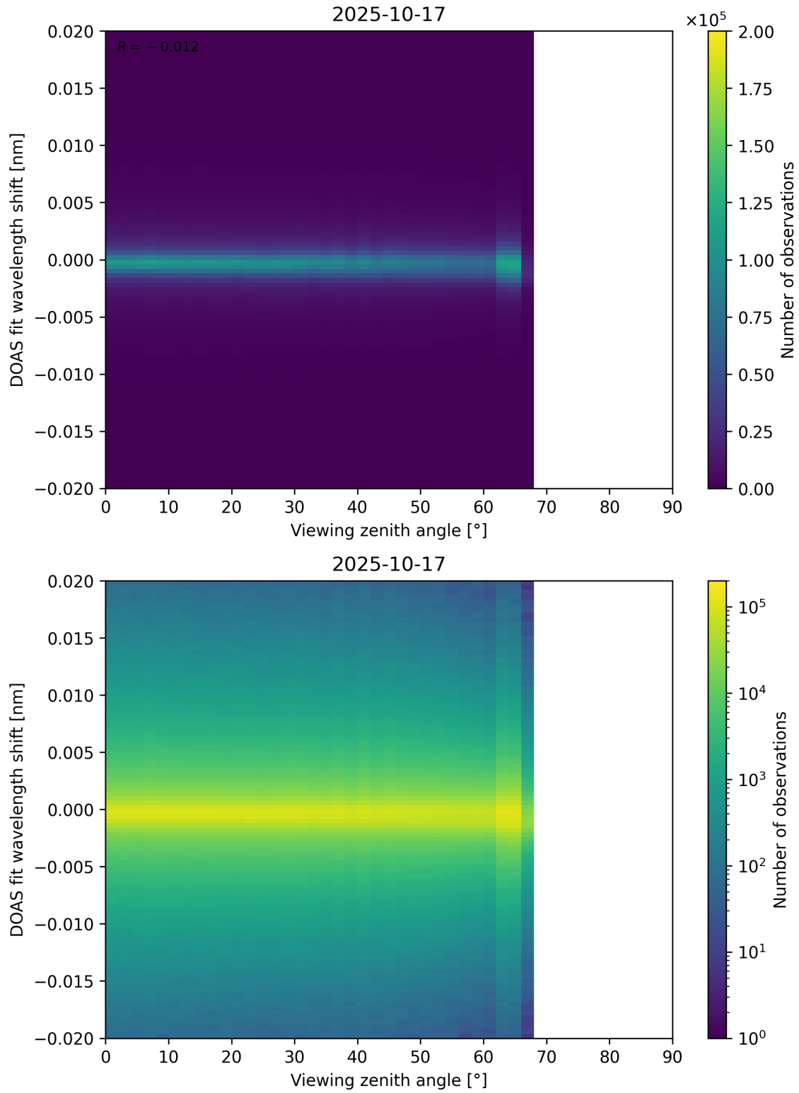
Figure 183: Scatter density plot of “Viewing zenith angle” against “DOAS fit wavelength shift” for 2025-10-17 to 2025-10-18.
