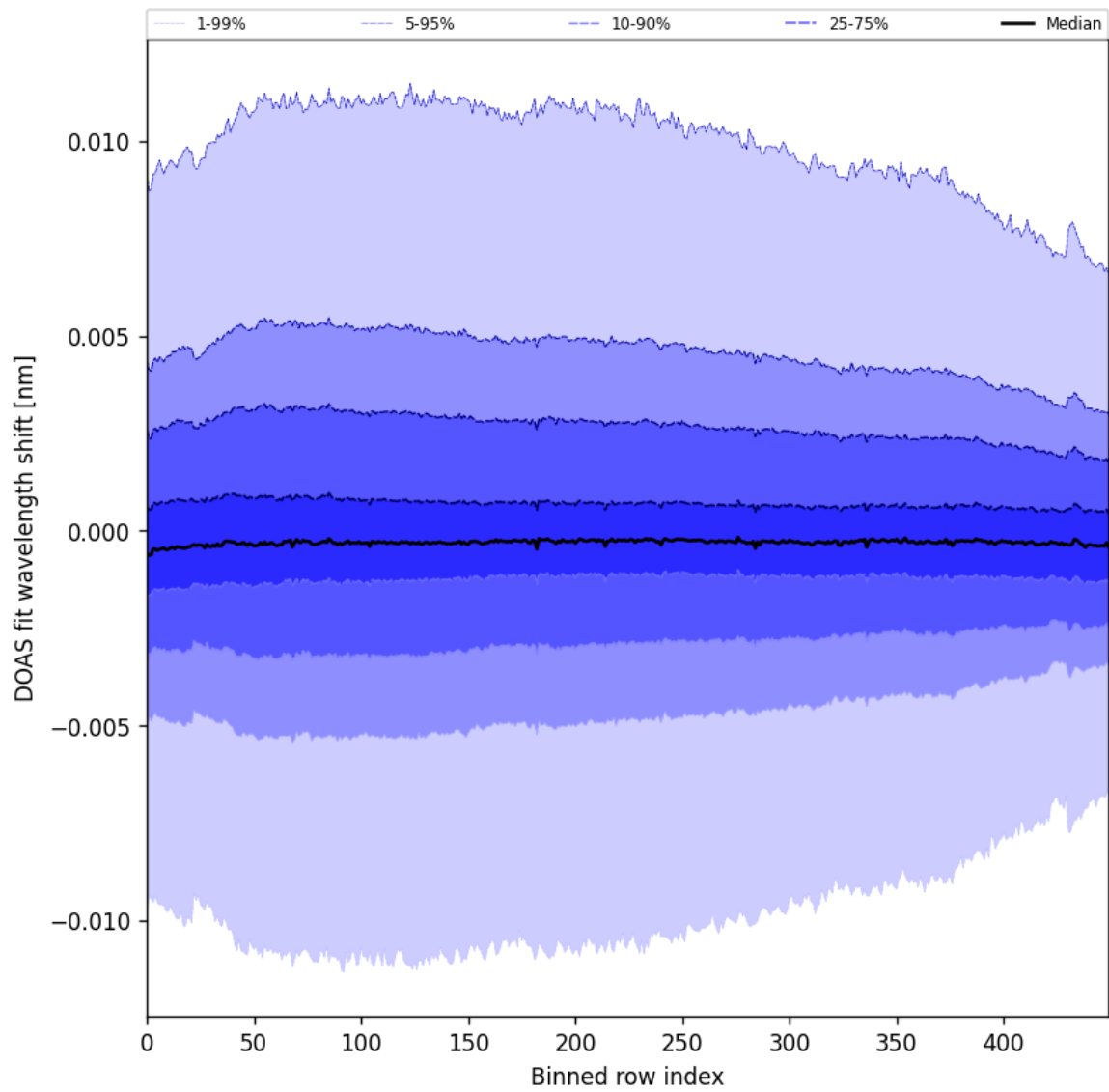
Figure 58: Along track statistics of “DOAS fit wavelength shift” for 2025-10-17 to 2025-10-18
