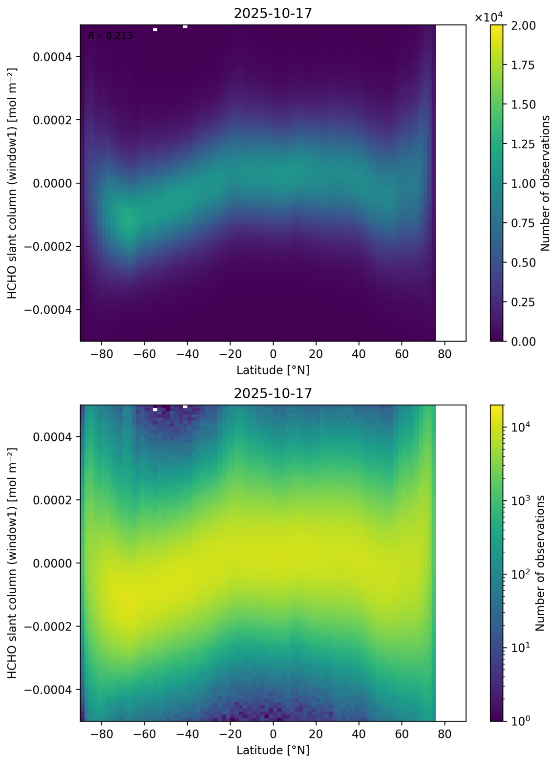
Figure 159: Scatter density plot of “Latitude” against “HCHO slant column (window1)” for 2025-10-17 to 2025-10-18.
