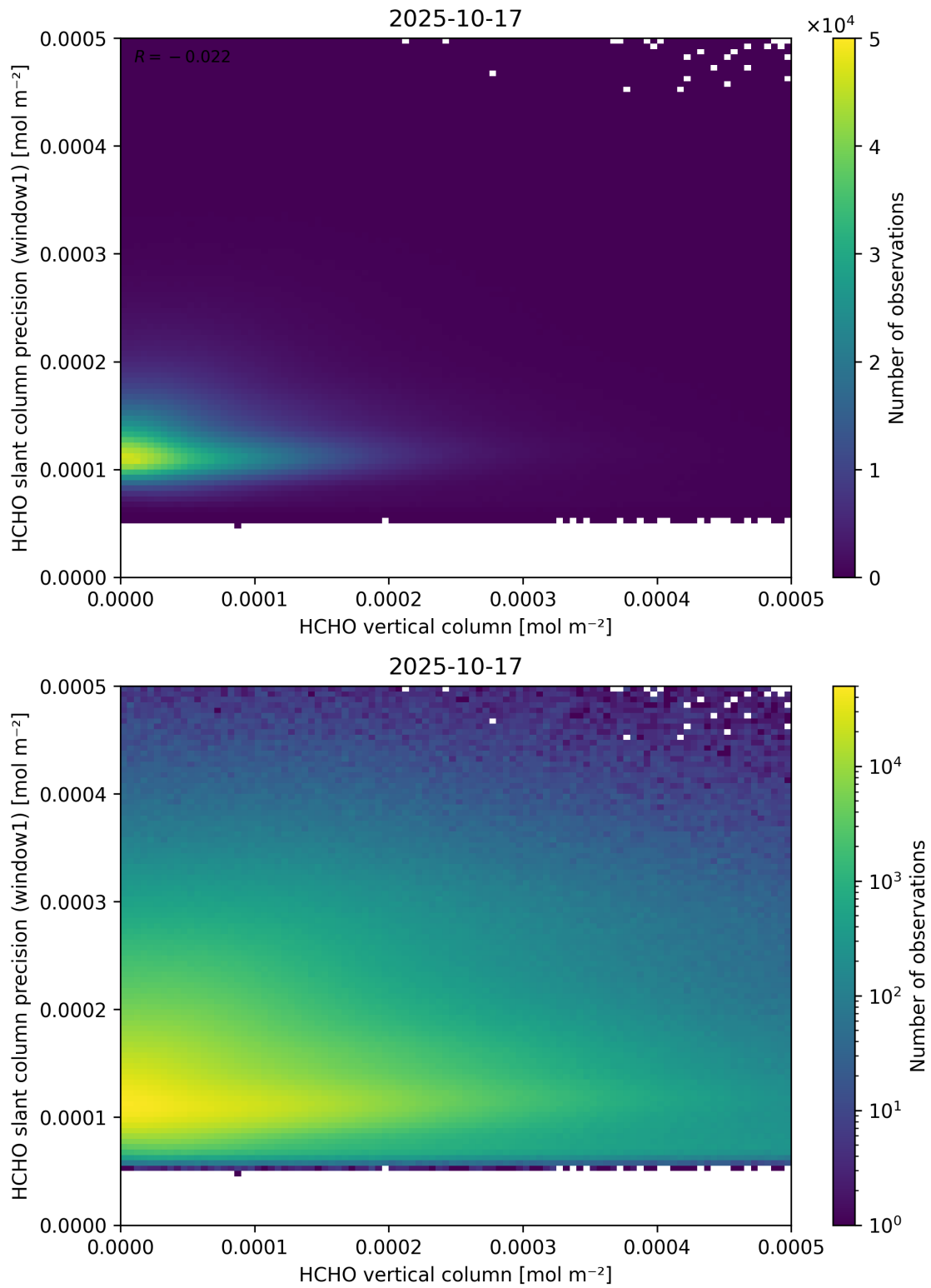
Figure 130: Scatter density plot of “HCHO vertical column” against “HCHO slant column precision (window1)” for 2025-10-17 to 2025-10-18.
