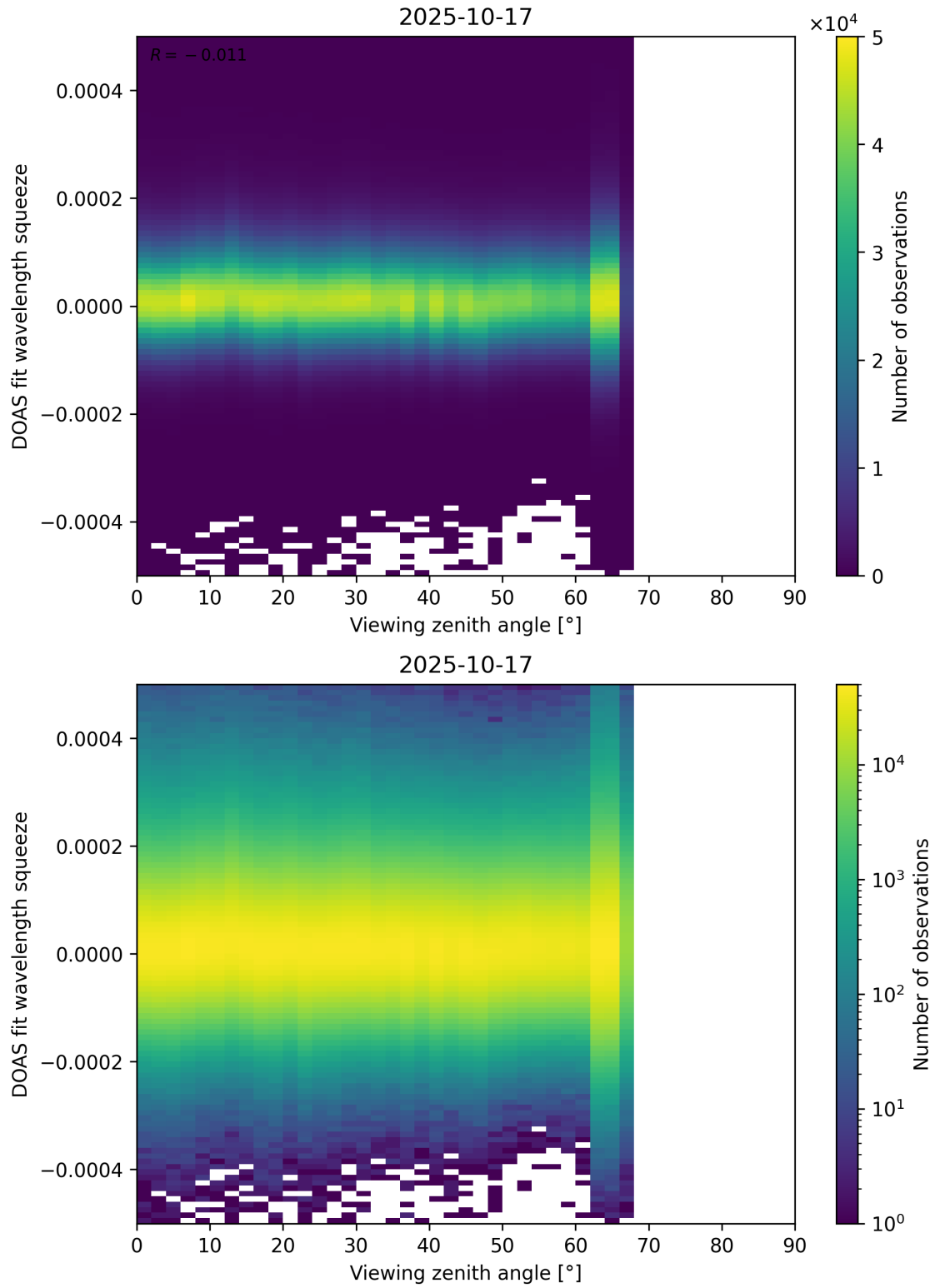
Figure 184: Scatter density plot of “Viewing zenith angle” against “DOAS fit wavelength squeeze” for 2025-10-17 to 2025-10-18.
