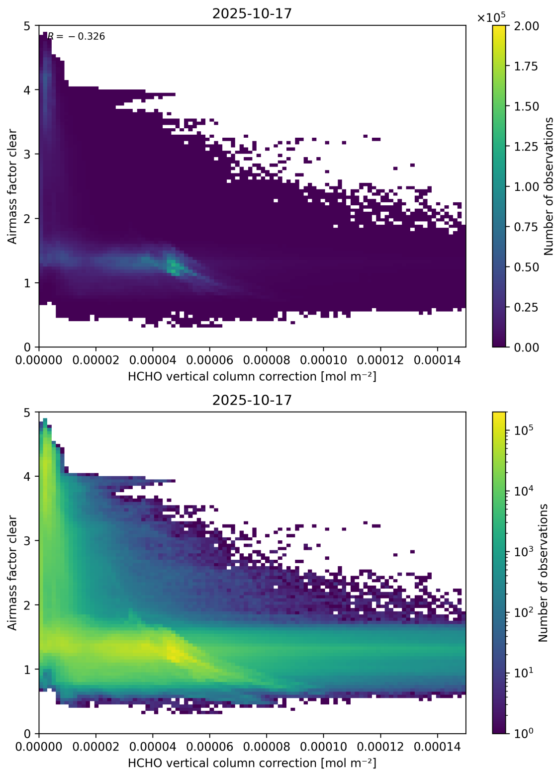
Figure 115: Scatter density plot of “HCHO vertical column correction” against “Airmass factor clear” for 2025-10-17 to 2025-10-18.
