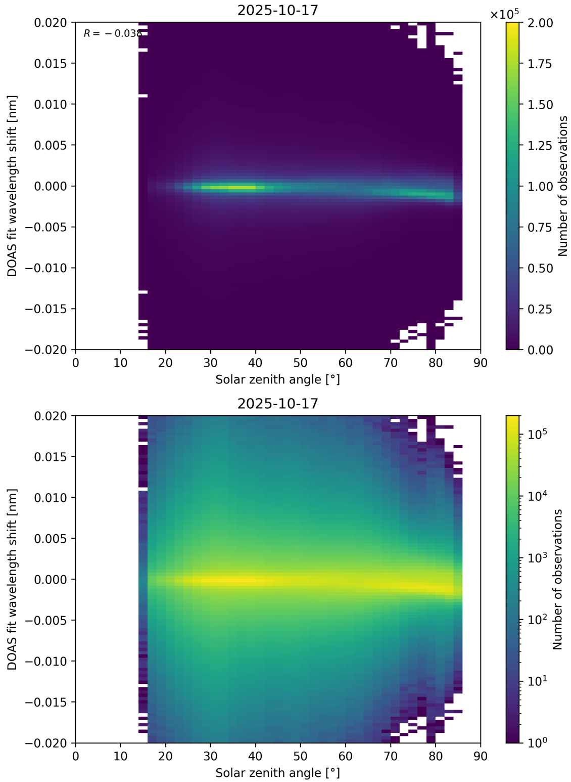
Figure 168: Scatter density plot of “Solar zenith angle” against “DOAS fit wavelength shift” for 2025-10-17 to 2025-10-18.
