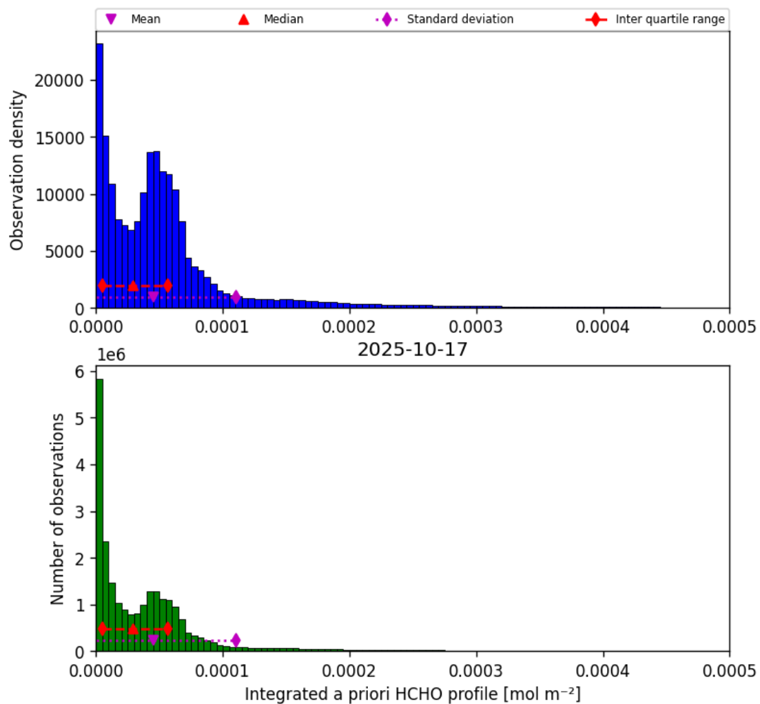
Figure 43: Histogram of “Integrated a priori HCHO profile” for 2025-10-17 to 2025-10-18
