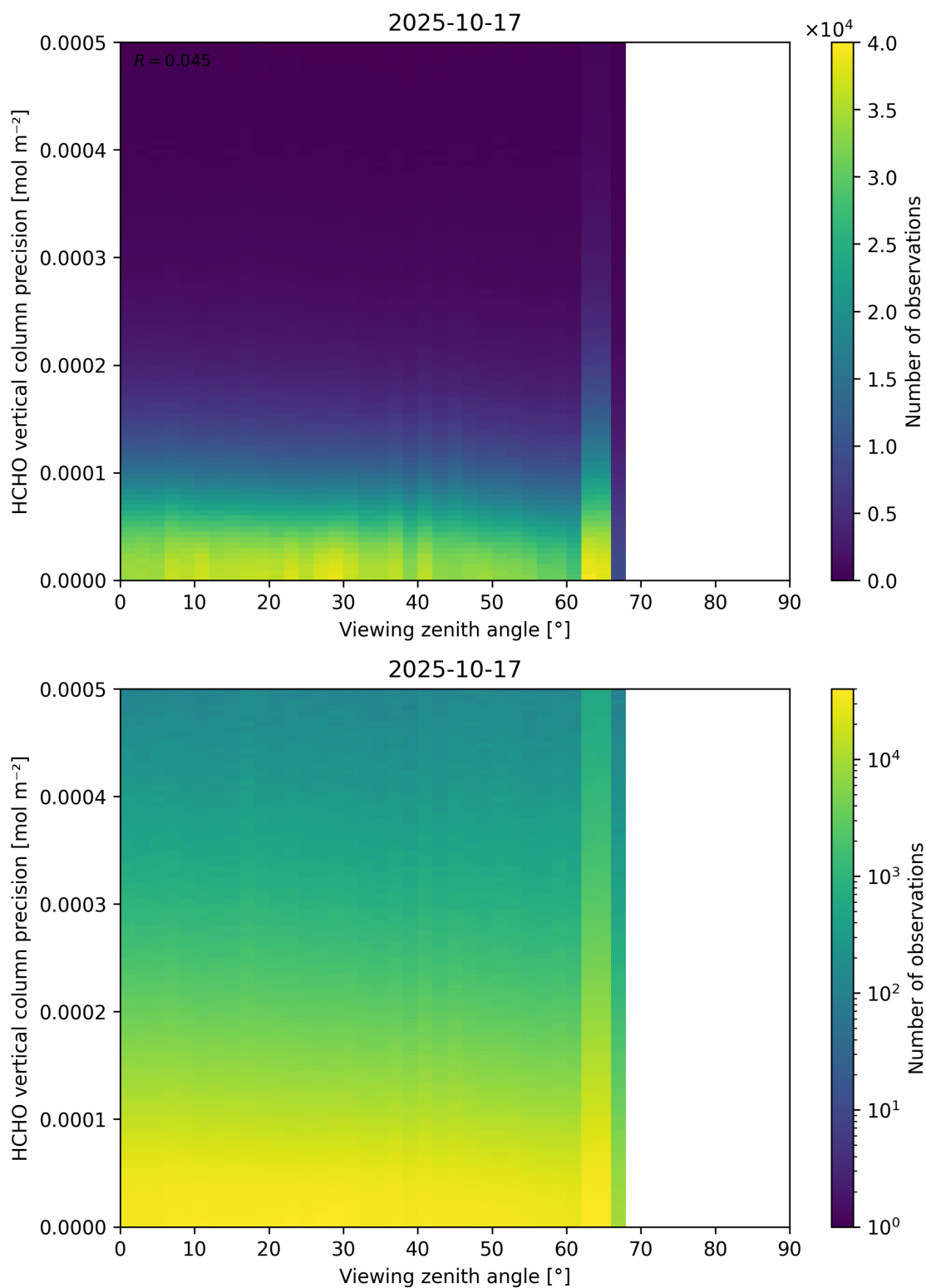
Figure 194: Scatter density plot of “Viewing zenith angle” against “HCHO vertical column precision” for 2025-10-17 to 2025-10-18.
