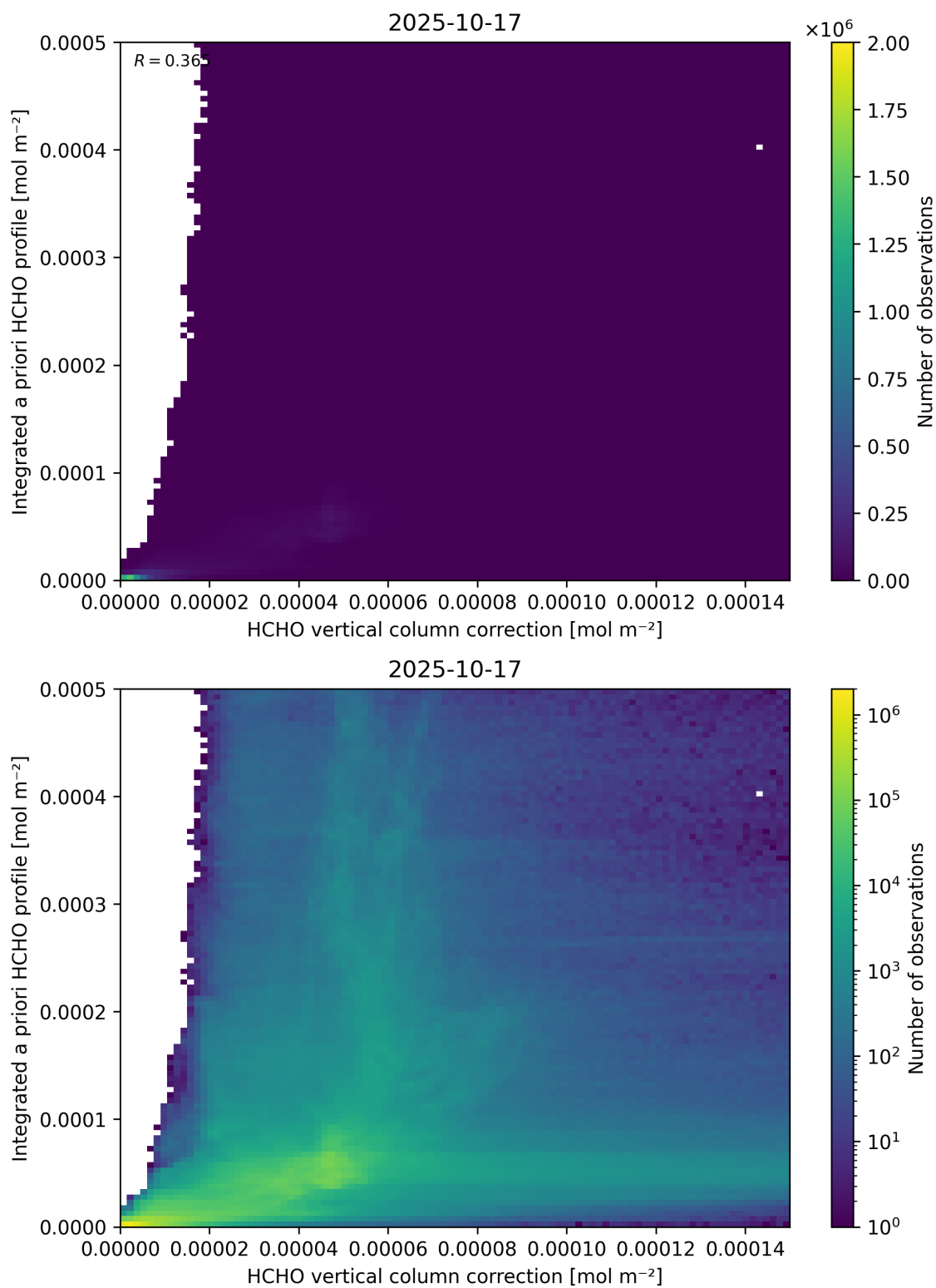
Figure 122: Scatter density plot of “HCHO vertical column correction” against “Integrated a priori HCHO profile” for 2025-10-17 to 2025-10-18.
