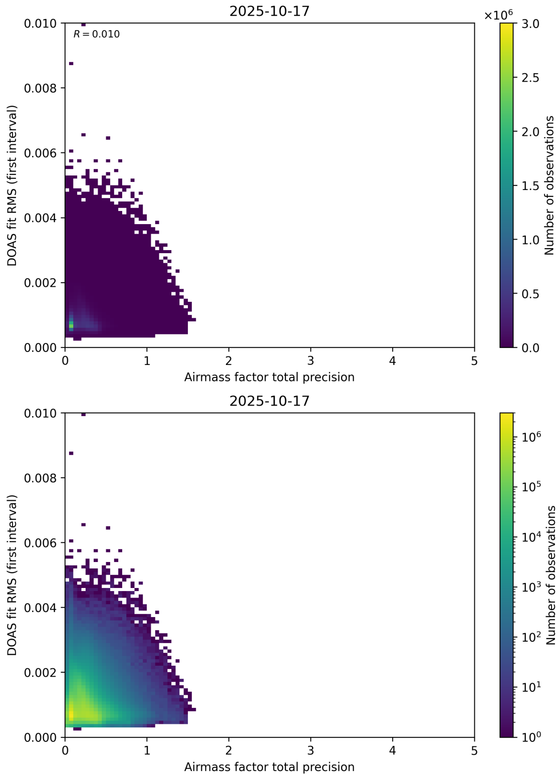
Figure 105: Scatter density plot of “Airmass factor total precision” against “DOAS fit RMS (first interval)” for 2025-10-17 to 2025-10-18.
