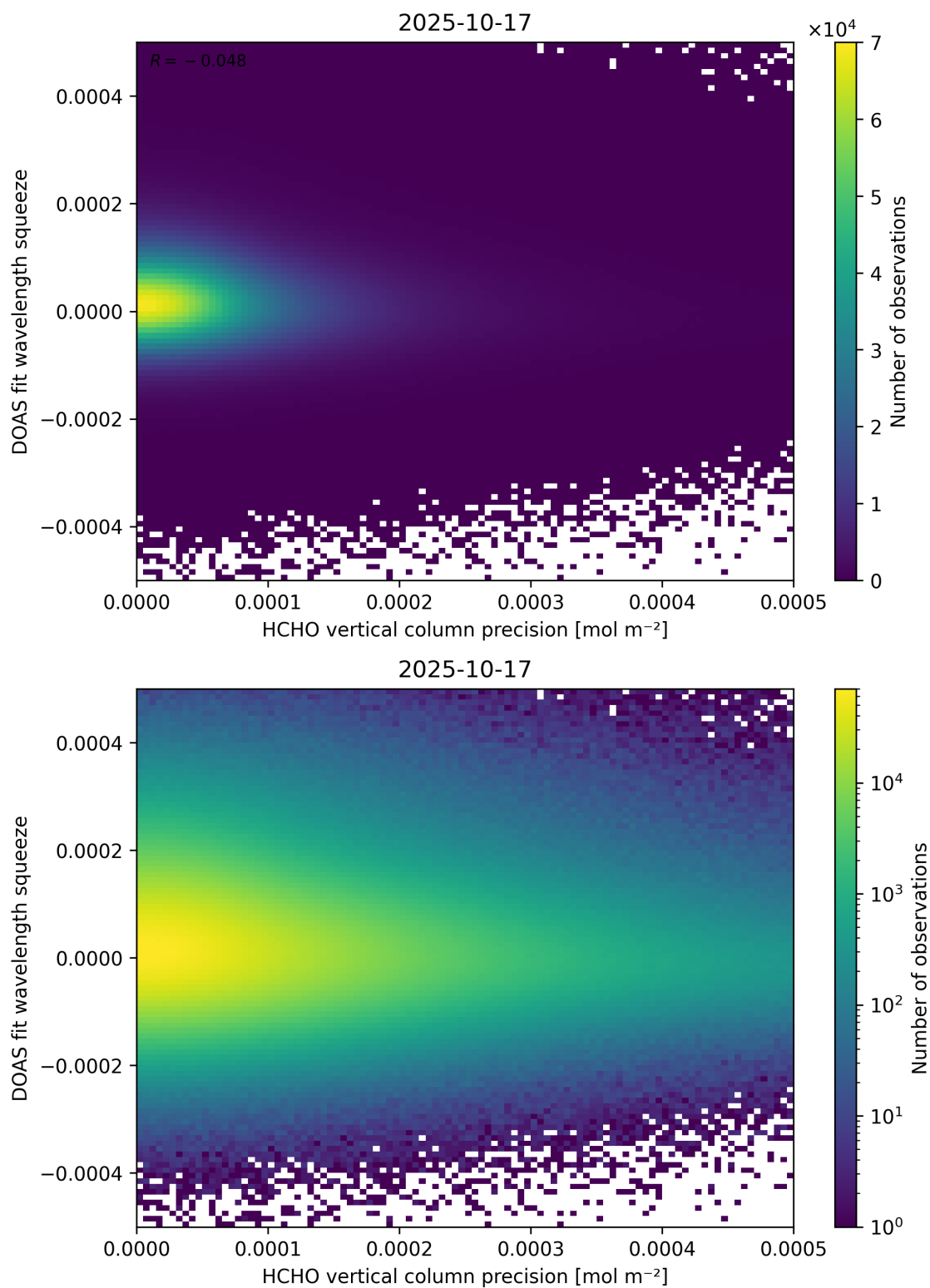
Figure 138: Scatter density plot of “HCHO vertical column precision” against “DOAS fit wavelength squeeze” for 2025-10-17 to 2025-10-18.
