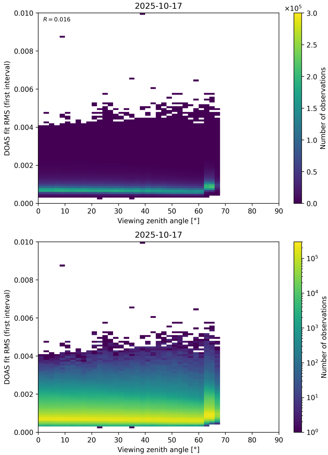
Figure 182: Scatter density plot of “Viewing zenith angle” against “DOAS fit RMS (first interval)” for 2025-10-17 to 2025-10-18.
