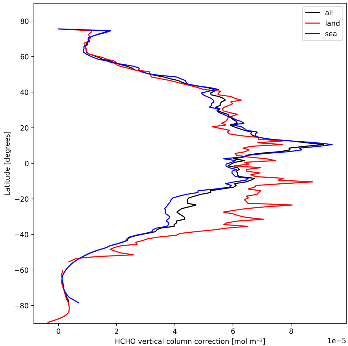
Figure 23: Zonal average of “HCHO vertical column correction” for 2025-10-17 to 2025-10-18.
