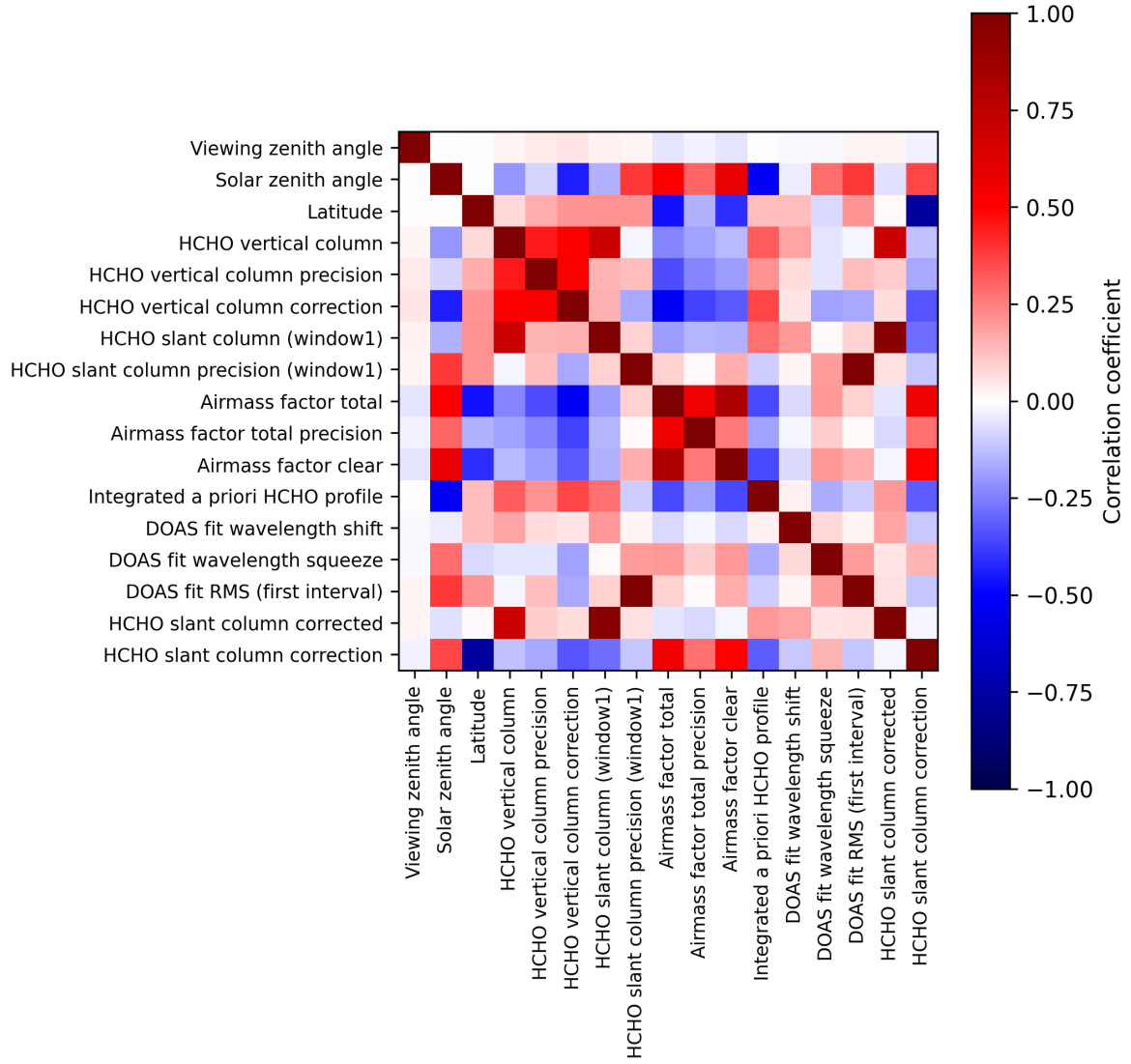
Figure 2: Map of correlation matrix for 2025-10-17 to 2025-10-18.
