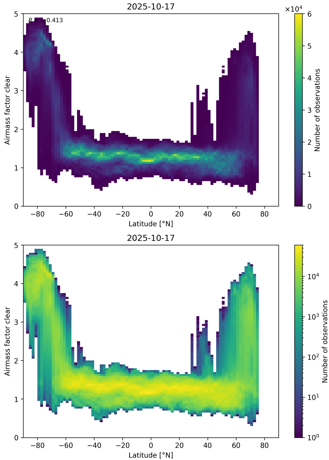
Figure 156: Scatter density plot of “Latitude” against “Airmass factor clear” for 2025-10-17 to 2025-10-18.
