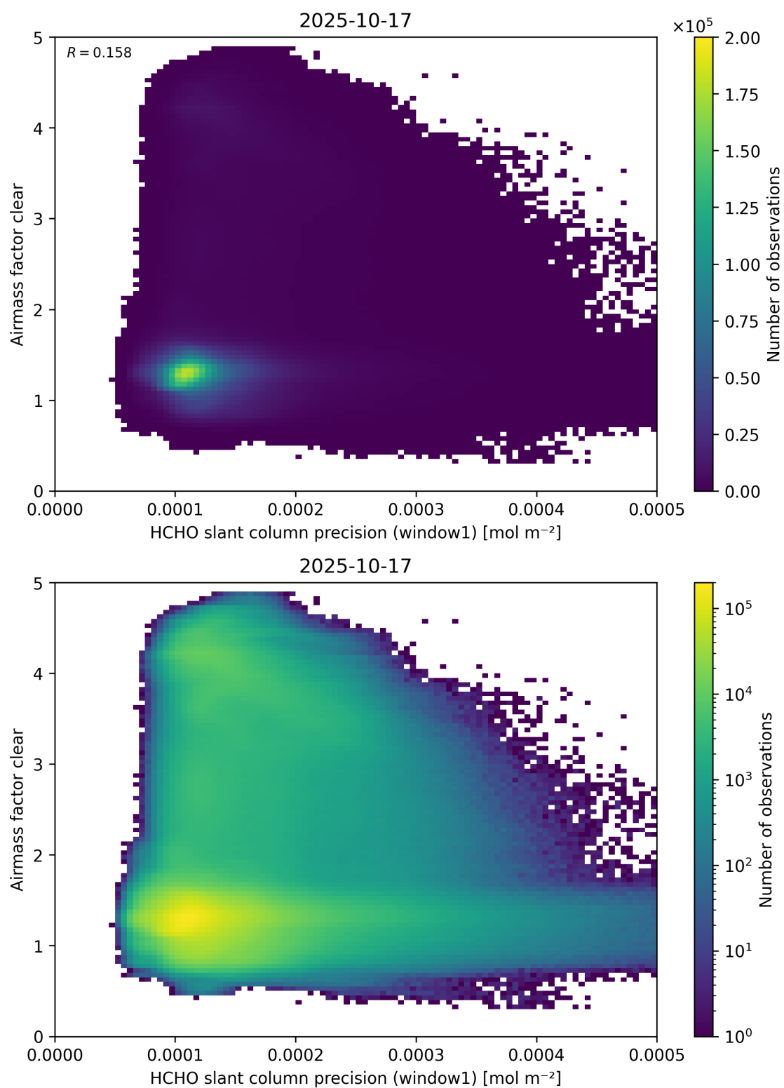
Figure 91: Scatter density plot of “HCHO slant column precision (window1)” against “Airmass factor clear” for 2025-10-17 to 2025-10-18.
