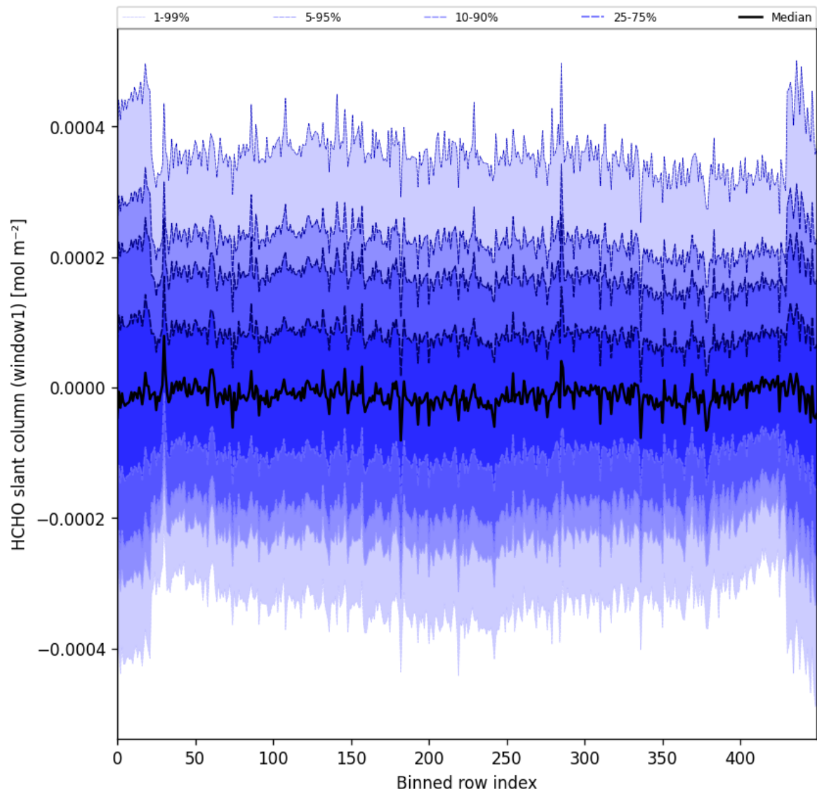
Figure 52: Along track statistics of “HCHO slant column (window1)” for 2025-10-17 to 2025-10-18
