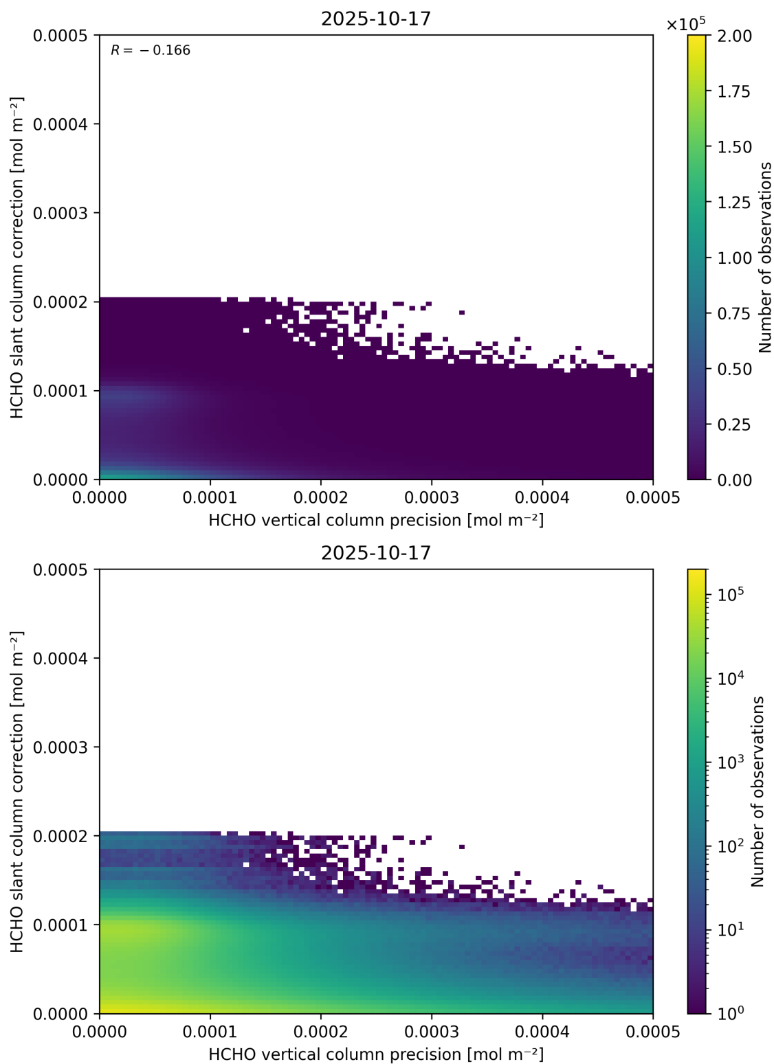
Figure 141: Scatter density plot of “HCHO vertical column precision” against “HCHO slant column correction” for 2025-10-17 to 2025-10-18.
