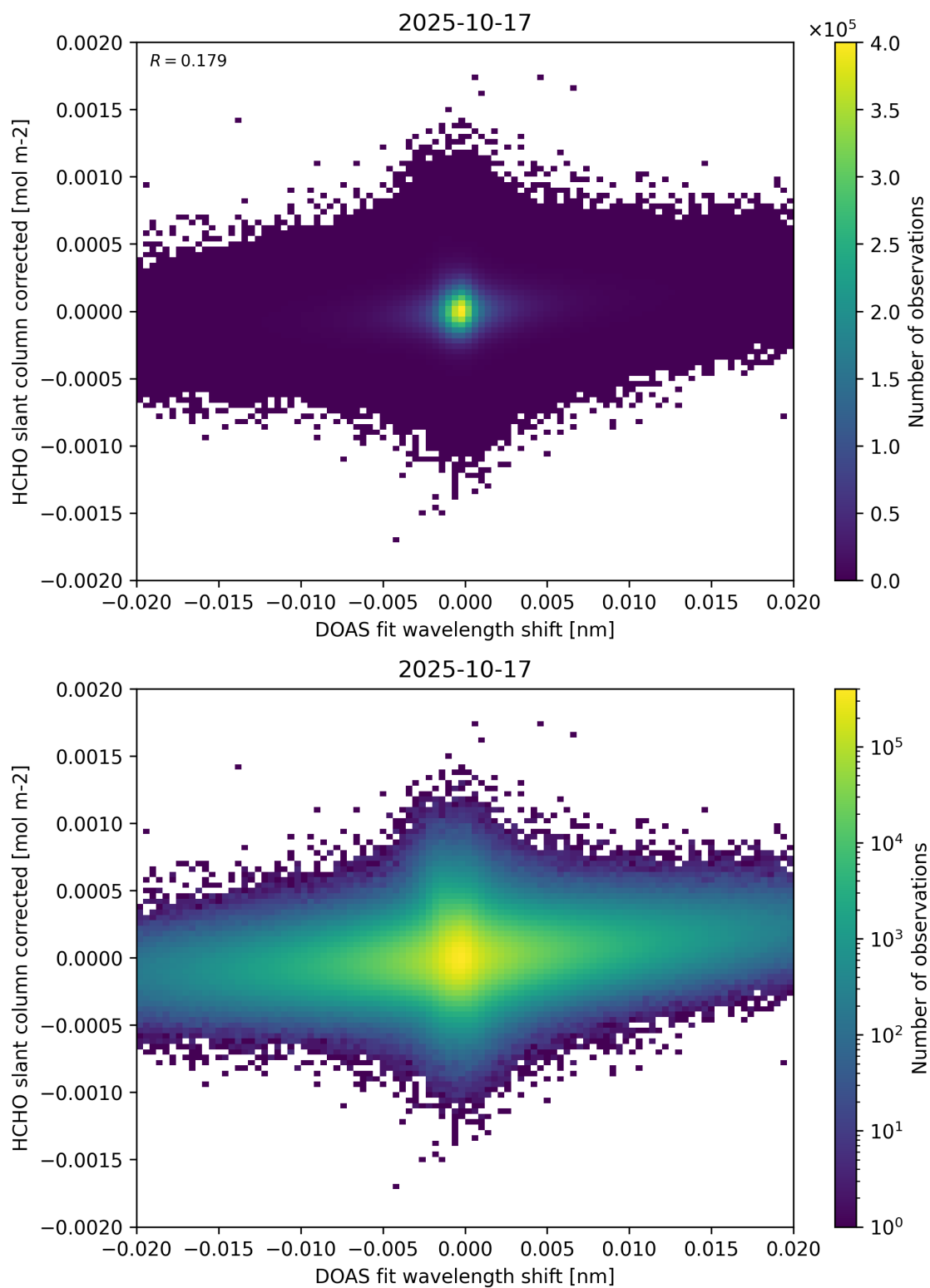
Figure 66: Scatter density plot of “DOAS fit wavelength shift” against “HCHO slant column corrected” for 2025-10-17 to 2025-10-18.
