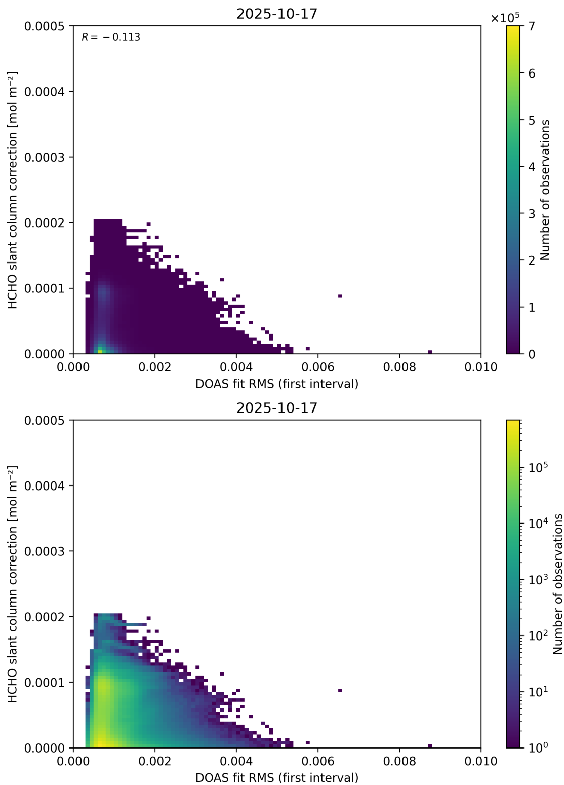
Figure 63: Scatter density plot of “DOAS fit RMS (first interval)” against “HCHO slant column correction” for 2025-10-17 to 2025-10-18.
