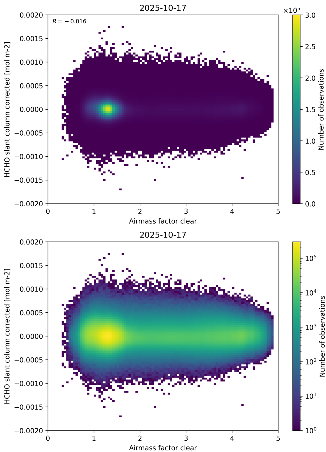
Figure 74: Scatter density plot of “Airmass factor clear” against “HCHO slant column corrected” for 2025-10-17 to 2025-10-18.
