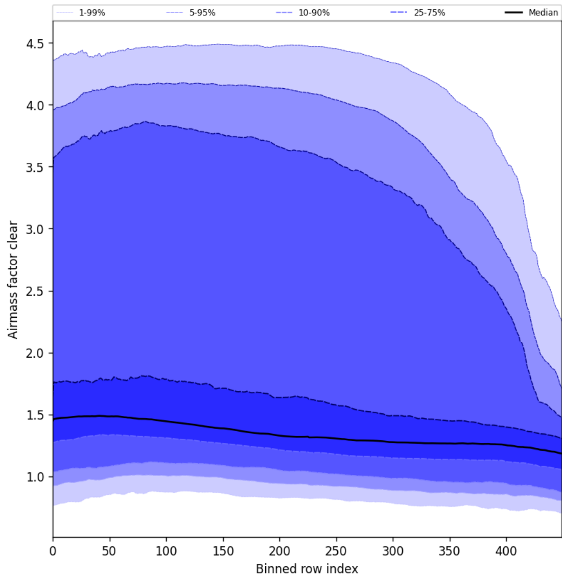
Figure 56: Along track statistics of “Airmass factor clear” for 2025-10-17 to 2025-10-18
