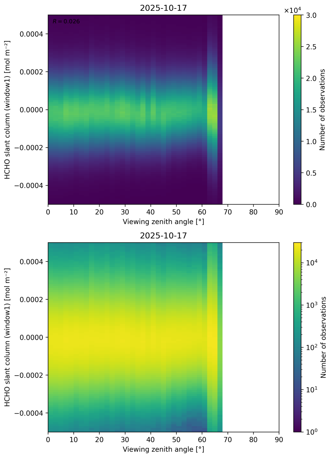
Figure 188: Scatter density plot of “Viewing zenith angle” against “HCHO slant column (window1)” for 2025-10-17 to 2025-10-18.
