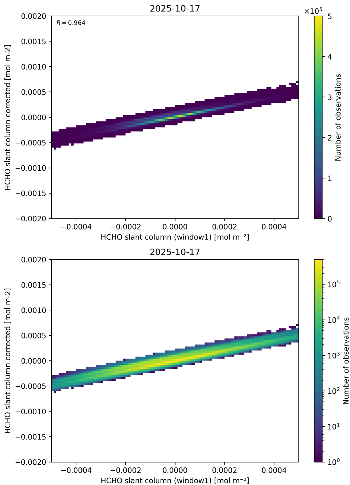
Figure 82: Scatter density plot of “HCHO slant column (window1)” against “HCHO slant column corrected” for 2025-10-17 to 2025-10-18.
