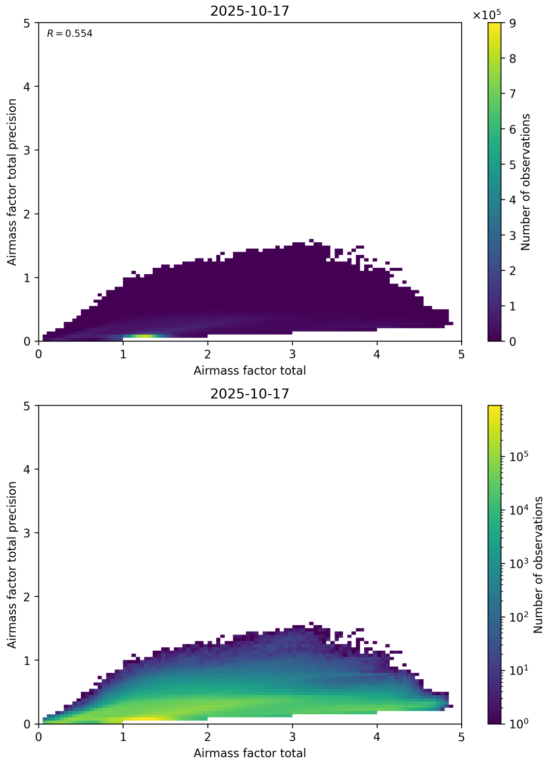
Figure 103: Scatter density plot of “Airmass factor total” against “Airmass factor total precision” for 2025-10-17 to 2025-10-18.
