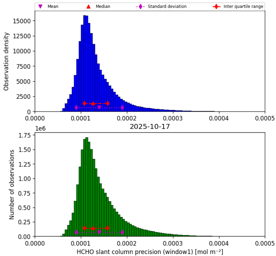
Figure 39: Histogram of “HCHO slant column precision (window1)” for 2025-10-17 to 2025-10-18
