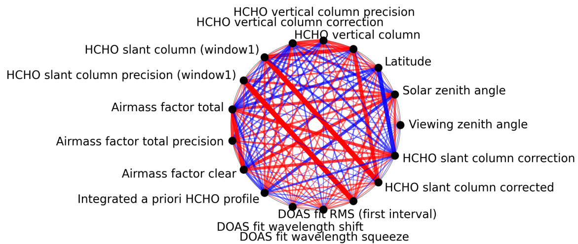
Figure 1: Map of correlation graph for 2025-10-17 to 2025-10-18.
