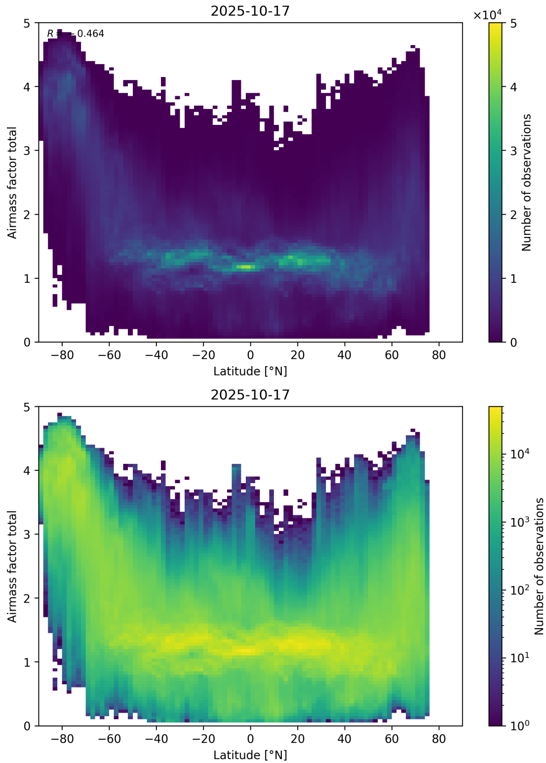
Figure 161: Scatter density plot of “Latitude” against “Airmass factor total” for 2025-10-17 to 2025-10-18.
