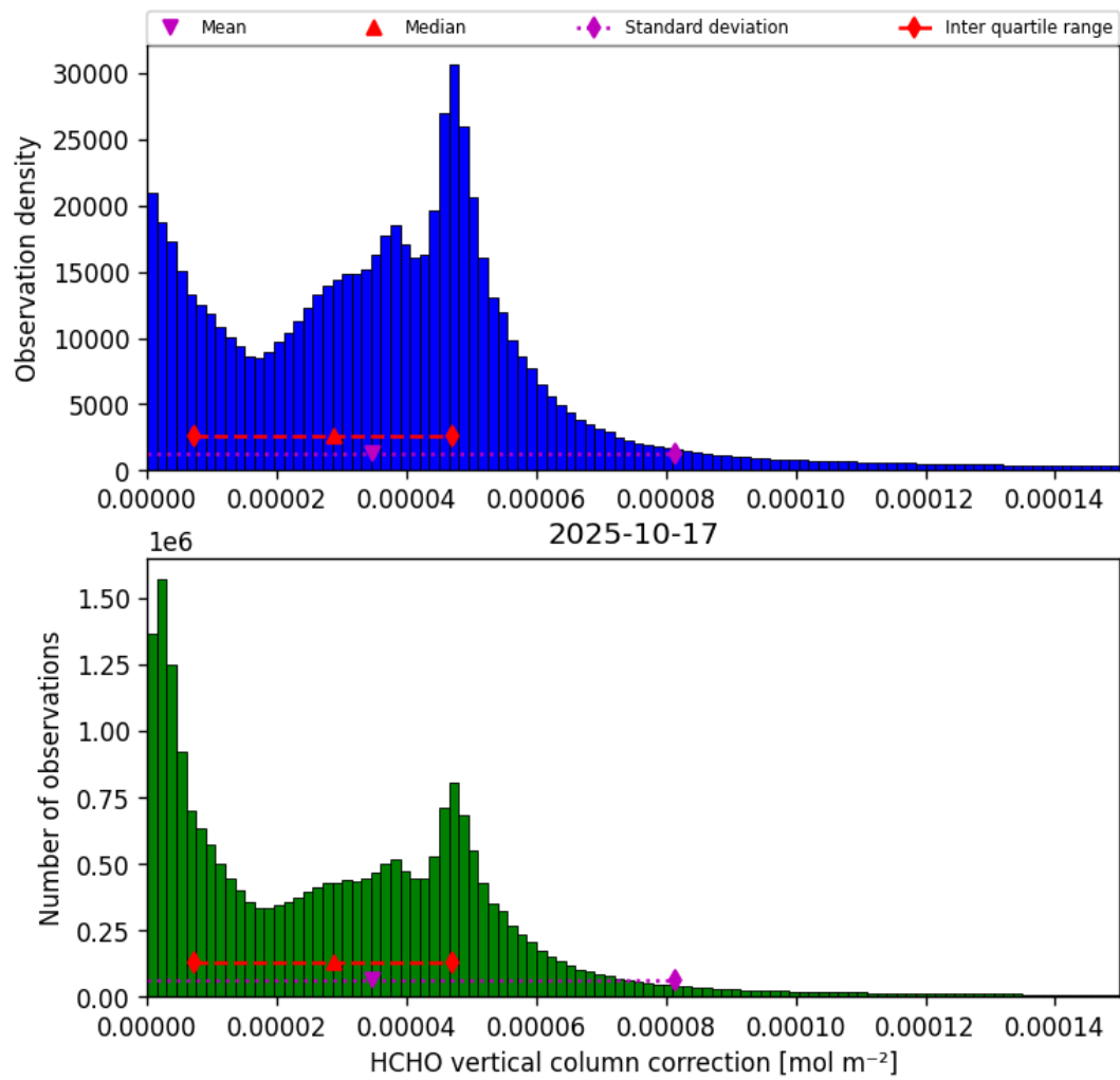
Figure 37: Histogram of “HCHO vertical column correction” for 2025-10-17 to 2025-10-18
