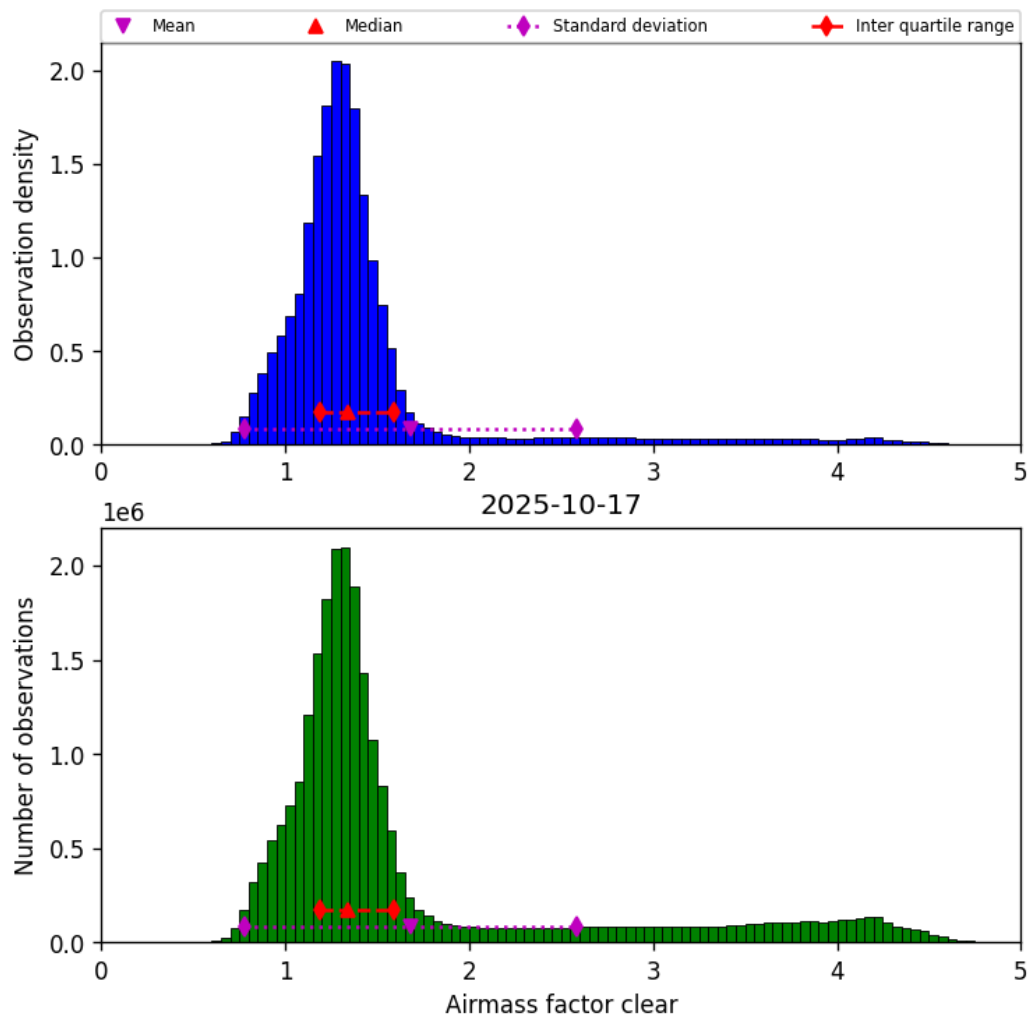
Figure 42: Histogram of “Airmass factor clear” for 2025-10-17 to 2025-10-18
