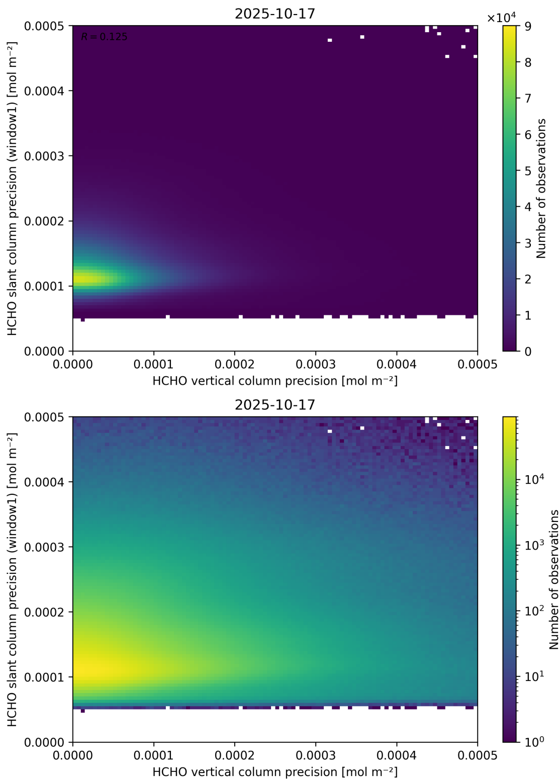
Figure 143: Scatter density plot of “HCHO vertical column precision” against “HCHO slant column precision (window1)” for 2025-10-17 to 2025-10-18.
