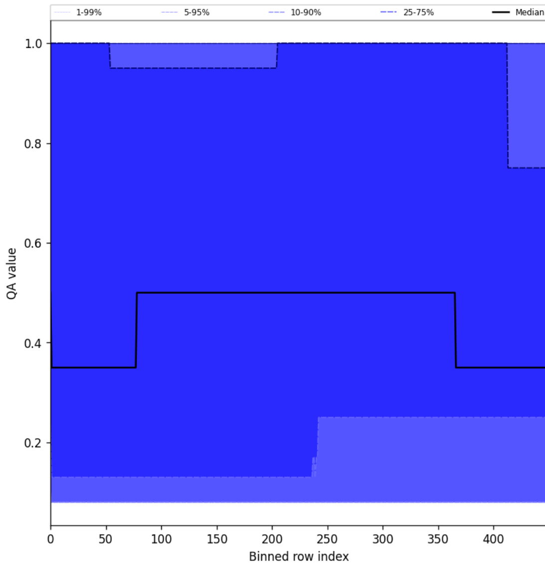
Figure 48: Along track statistics of “QA value” for 2025-10-17 to 2025-10-18
