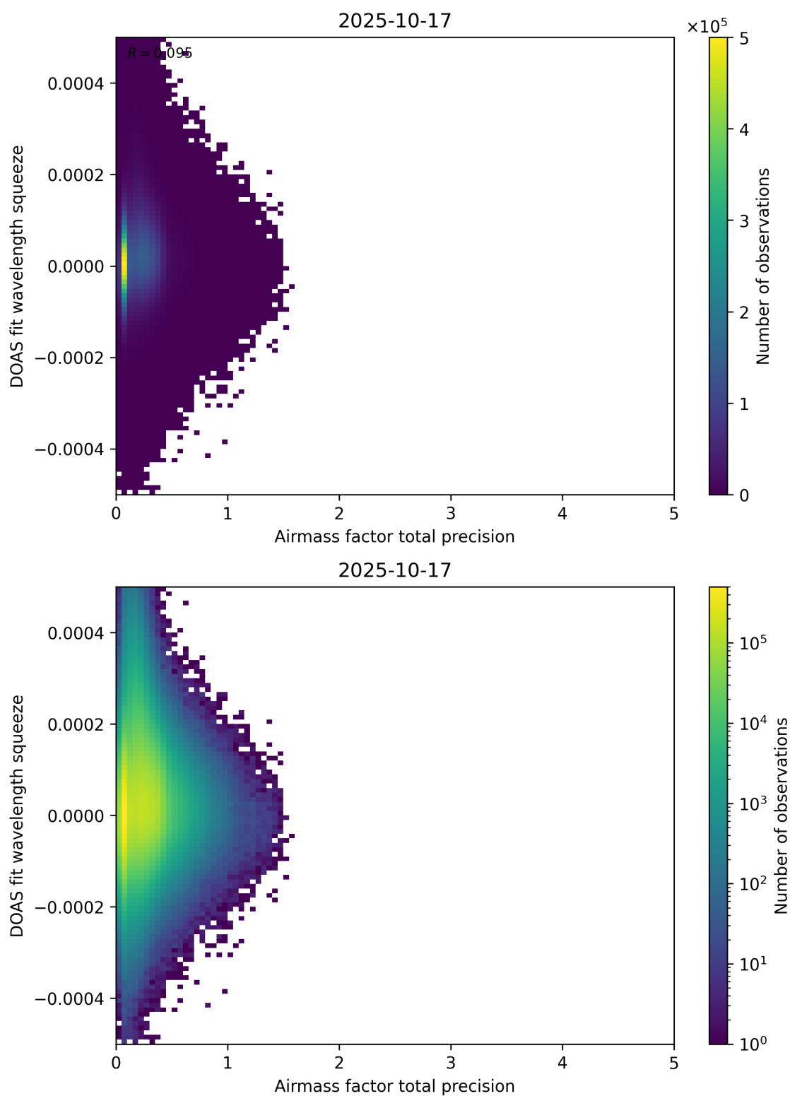
Figure 107: Scatter density plot of “Airmass factor total precision” against “DOAS fit wavelength squeeze” for 2025-10-17 to 2025-10-18.
