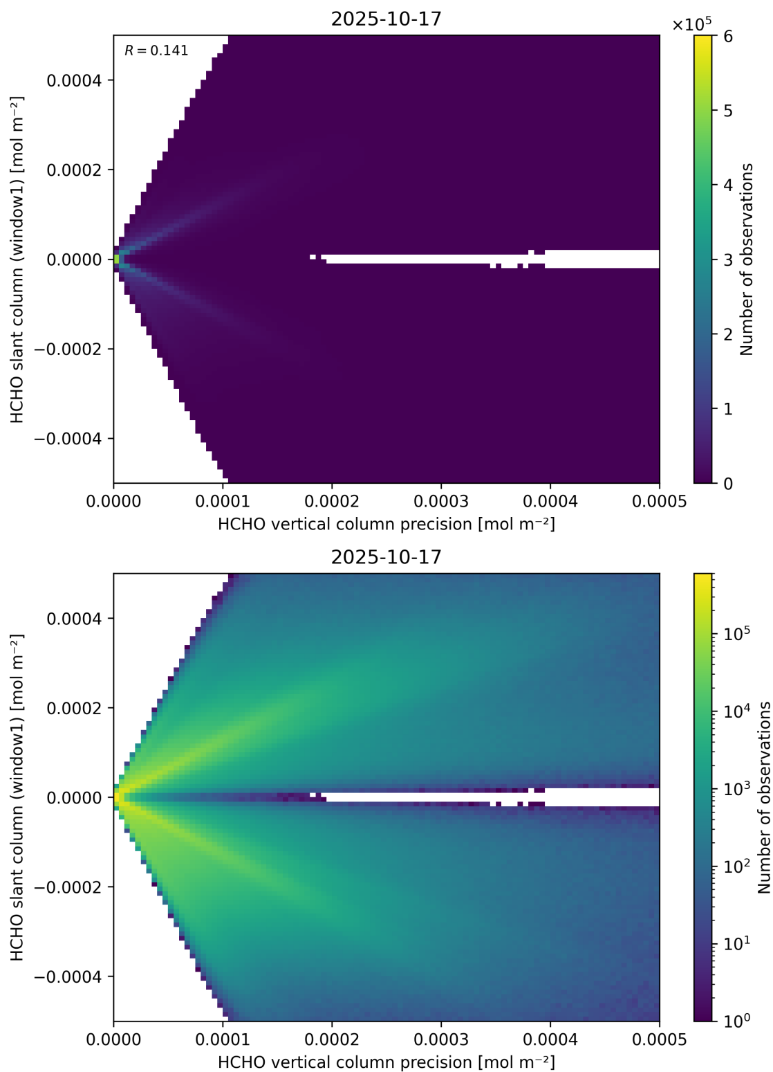
Figure 142: Scatter density plot of “HCHO vertical column precision” against “HCHO slant column (window1)” for 2025-10-17 to 2025-10-18.
