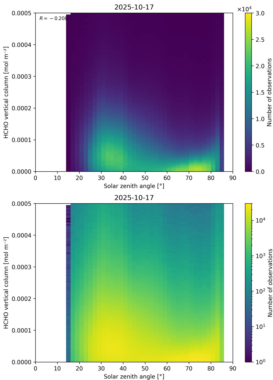
Figure 177: Scatter density plot of “Solar zenith angle” against “HCHO vertical column” for 2025-10-17 to 2025-10-18.
