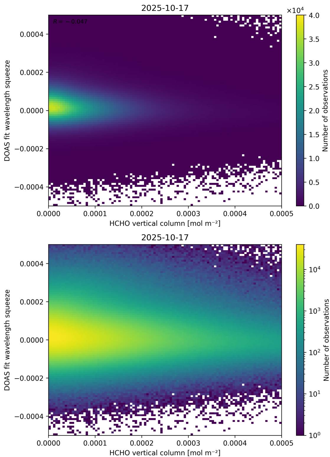
Figure 125: Scatter density plot of “HCHO vertical column” against “DOAS fit wavelength squeeze” for 2025-10-17 to 2025-10-18.
