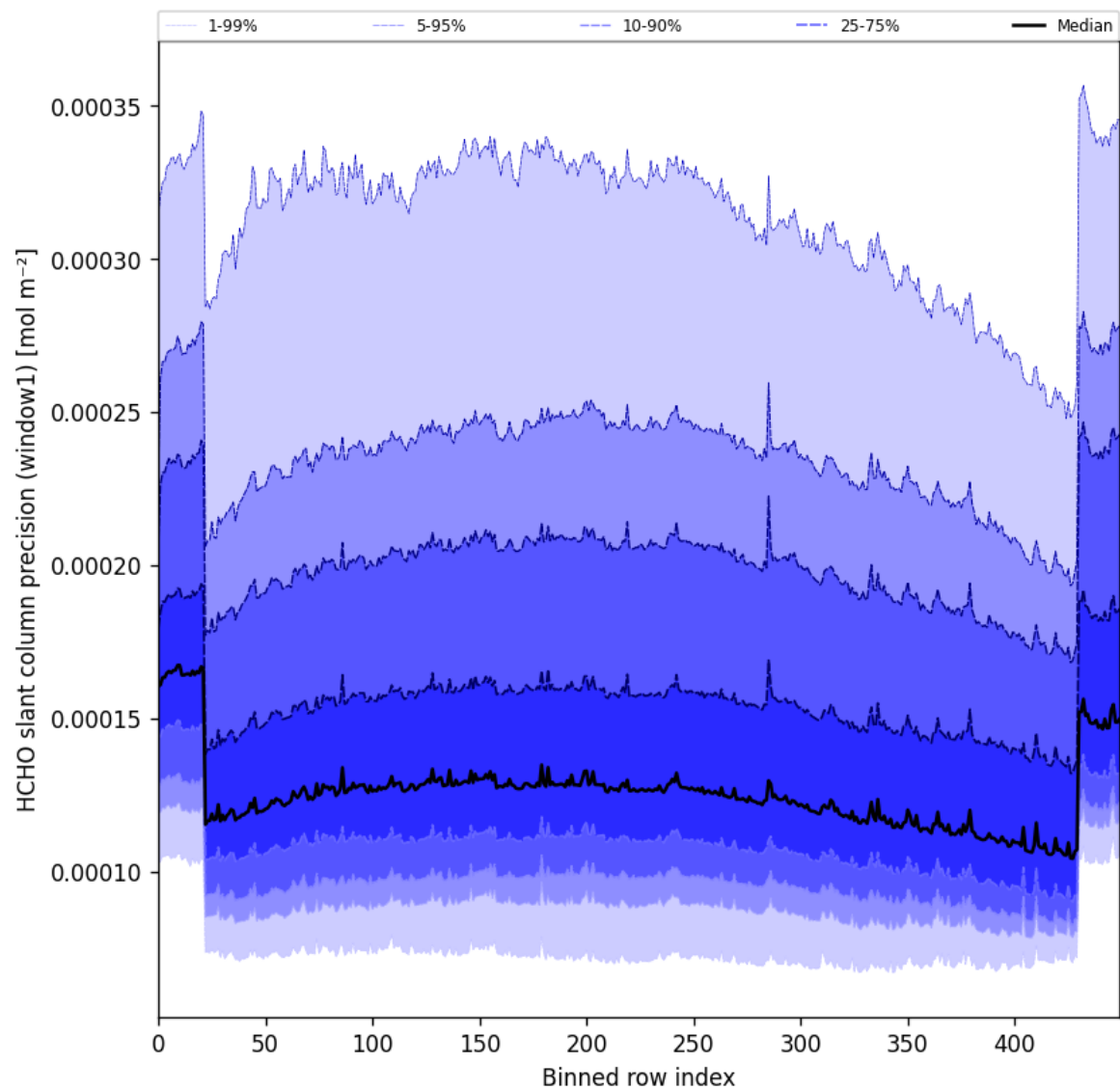
Figure 53: Along track statistics of “HCHO slant column precision (window1)” for 2025-10-17 to 2025-10-18
