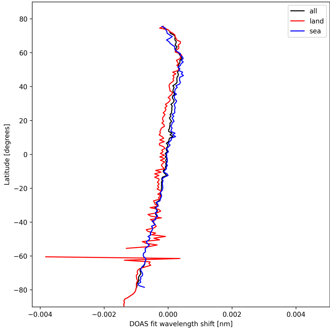
Figure 30: Zonal average of “DOAS fit wavelength shift” for 2025-10-17 to 2025-10-18.
