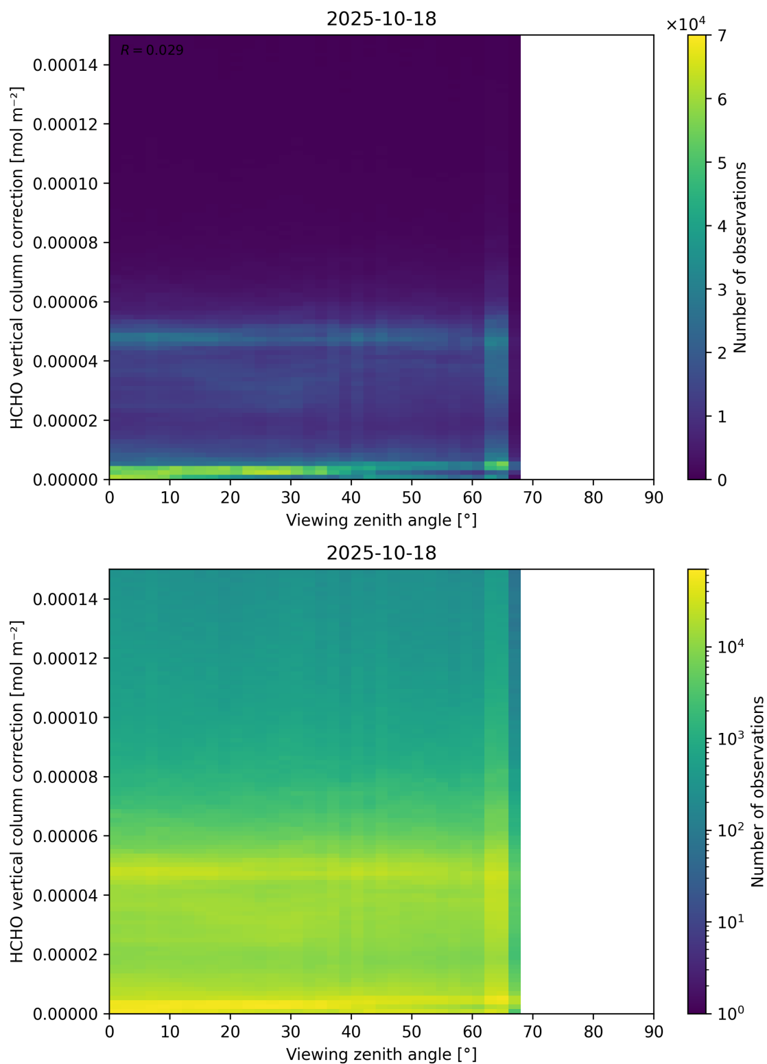
Figure 193: Scatter density plot of “Viewing zenith angle” against “HCHO vertical column correction” for 2025-10-17 to 2025-10-19.
