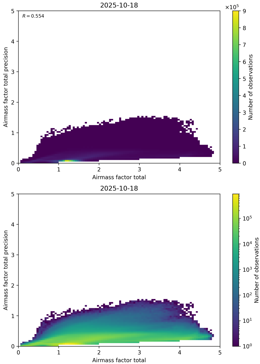
Figure 103: Scatter density plot of “Airmass factor total” against “Airmass factor total precision” for 2025-10-17 to 2025-10-19.
