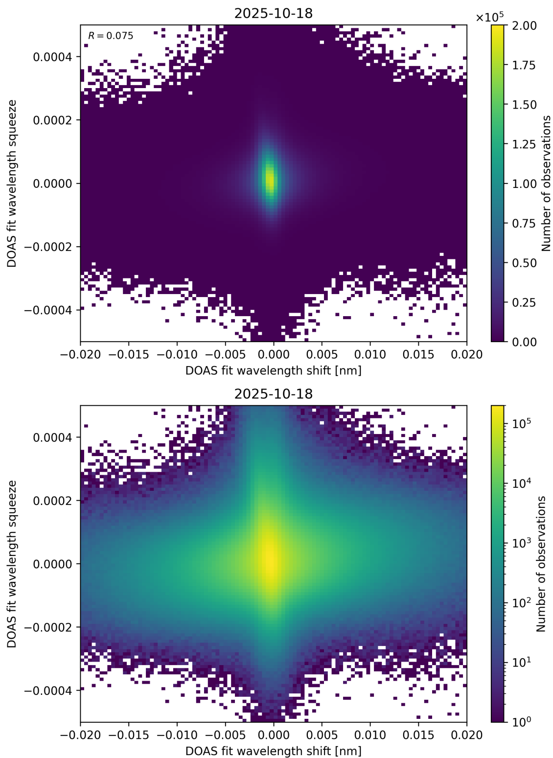
Figure 65: Scatter density plot of “DOAS fit wavelength shift” against “DOAS fit wavelength squeeze” for 2025-10-17 to 2025-10-19.
