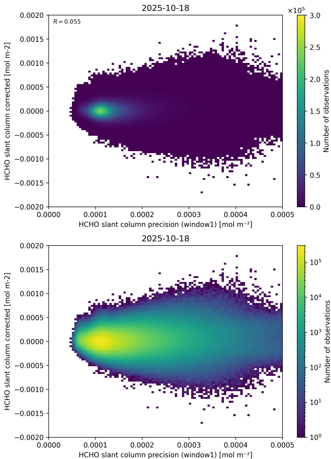
Figure 92: Scatter density plot of “HCHO slant column precision (window1)” against “HCHO slant column corrected” for 2025-10-17 to 2025-10-19.
