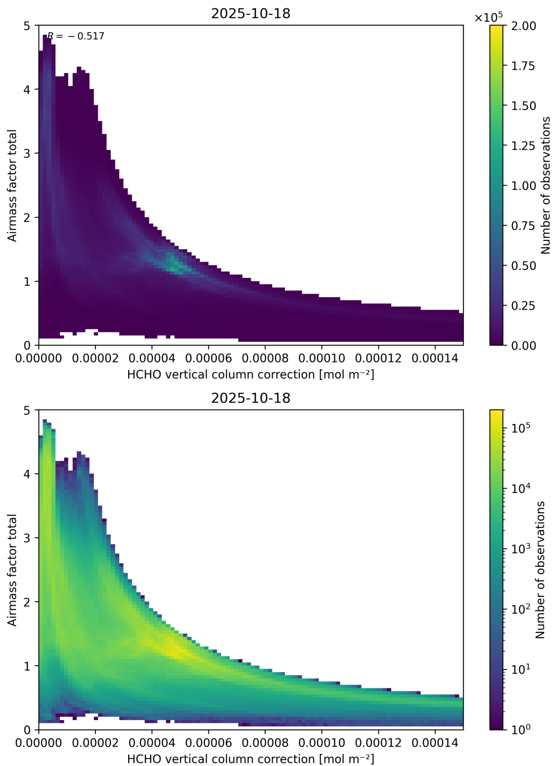
Figure 120: Scatter density plot of “HCHO vertical column correction” against “Airmass factor total” for 2025-10-17 to 2025-10-19.
