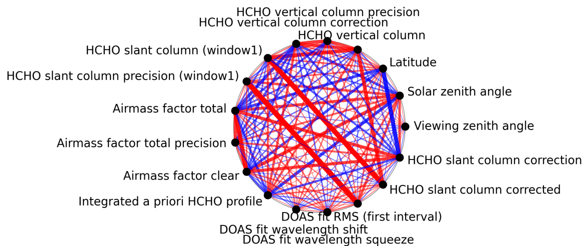
Figure 1: Map of correlation graph for 2025-10-17 to 2025-10-19.
