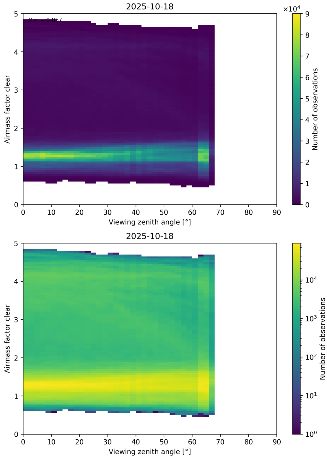
Figure 185: Scatter density plot of “Viewing zenith angle” against “Airmass factor clear” for 2025-10-17 to 2025-10-19.
