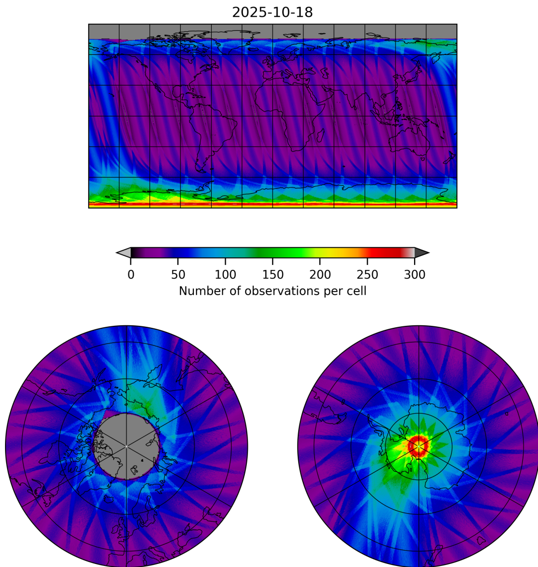
Figure 19: Map of the number of observations for 2025-10-17 to 2025-10-19
