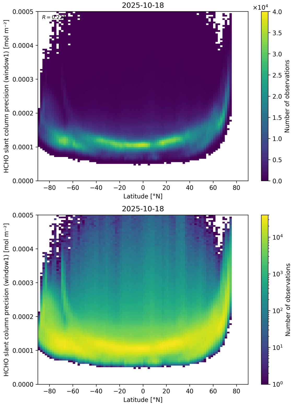
Figure 160: Scatter density plot of “Latitude” against “HCHO slant column precision (window1)” for 2025-10-17 to 2025-10-19.
