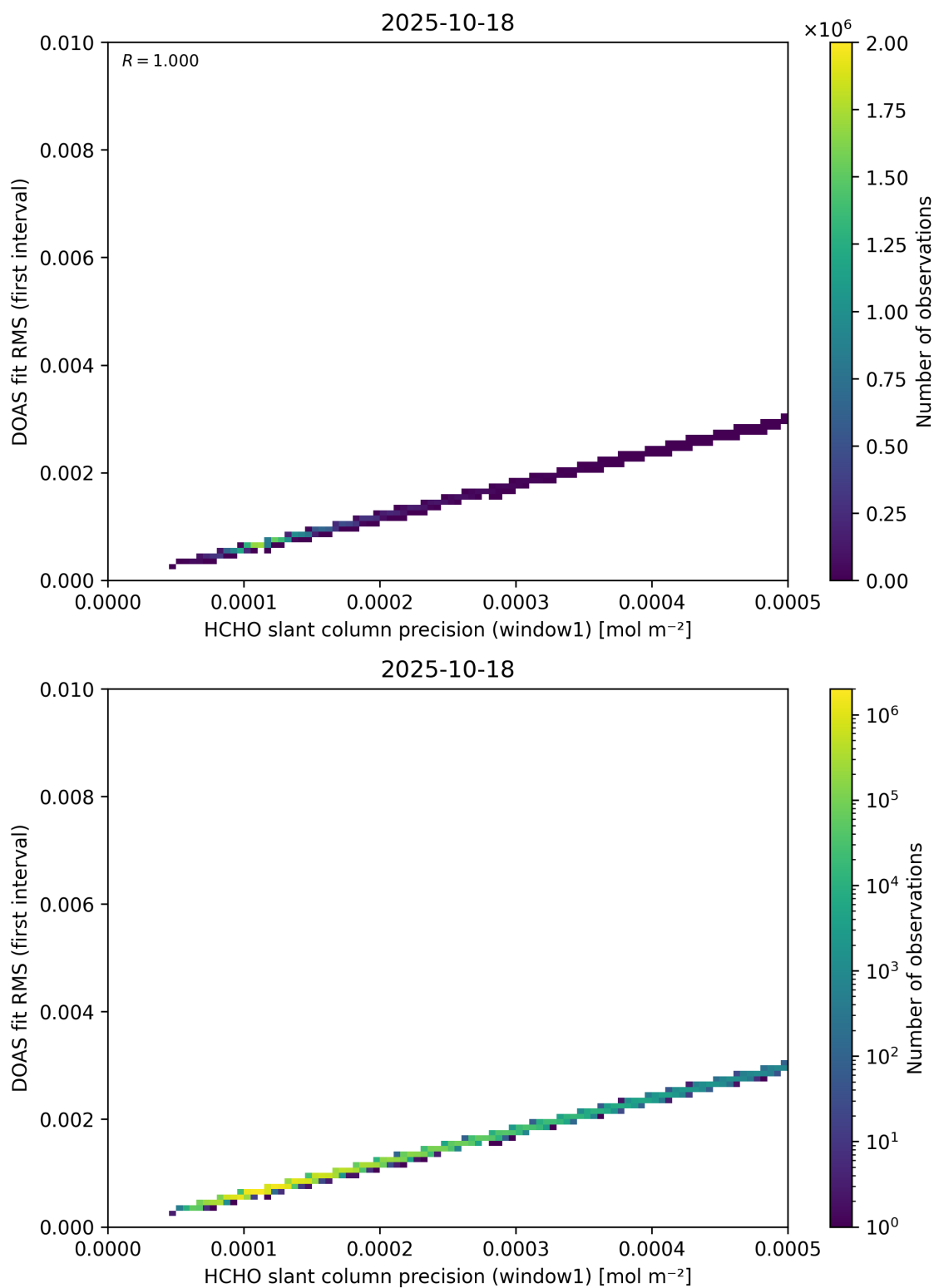
Figure 88: Scatter density plot of “HCHO slant column precision (window1)” against “DOAS fit RMS (first interval)” for 2025-10-17 to 2025-10-19.
