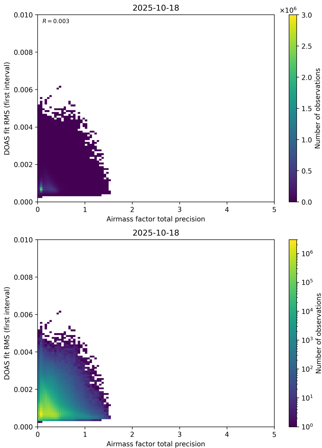
Figure 105: Scatter density plot of “Airmass factor total precision” against “DOAS fit RMS (first interval)” for 2025-10-17 to 2025-10-19.
