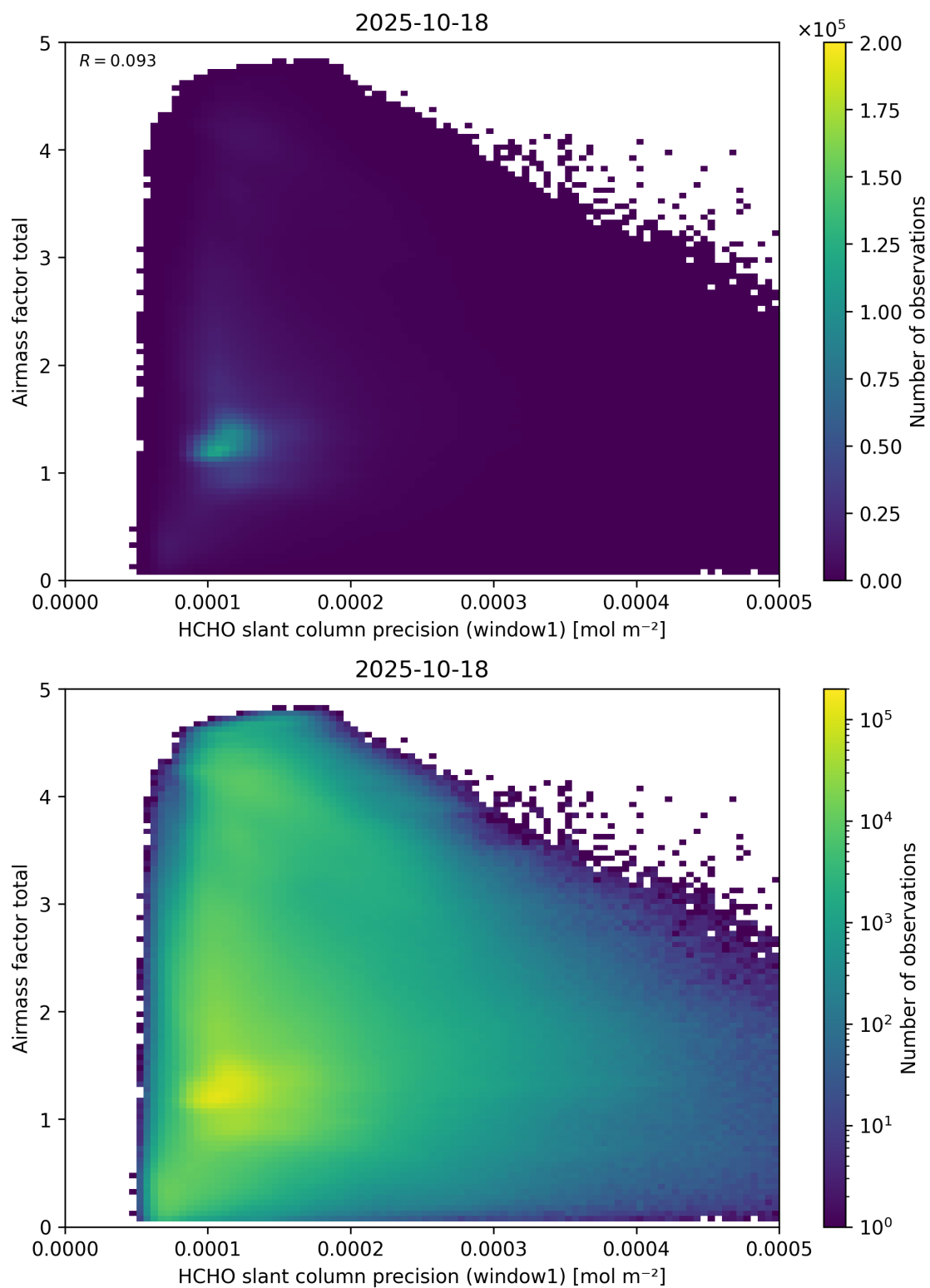
Figure 94: Scatter density plot of “HCHO slant column precision (window1)” against “Airmass factor total” for 2025-10-17 to 2025-10-19.
