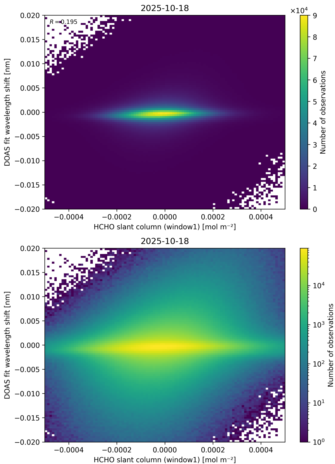
Figure 79: Scatter density plot of “HCHO slant column (window1)” against “DOAS fit wavelength shift” for 2025-10-17 to 2025-10-19.
