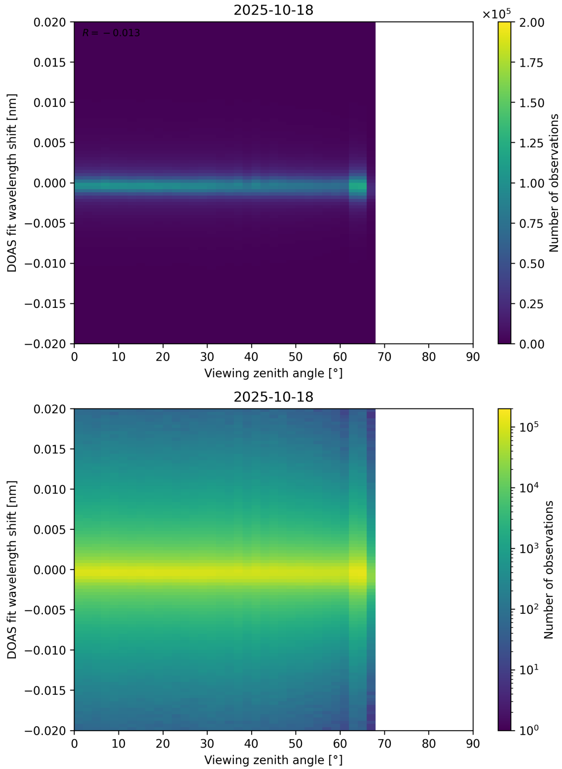
Figure 183: Scatter density plot of “Viewing zenith angle” against “DOAS fit wavelength shift” for 2025-10-17 to 2025-10-19.
