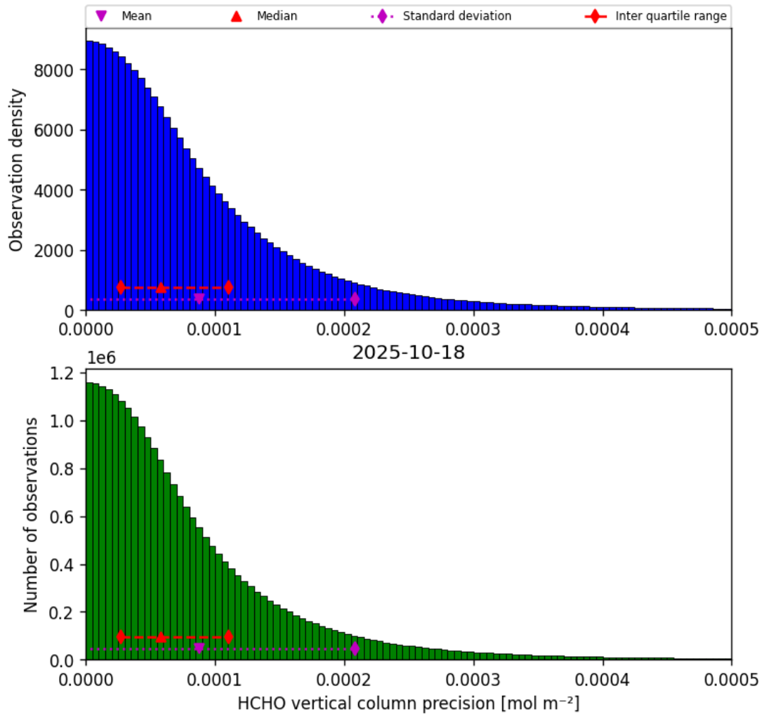
Figure 36: Histogram of “HCHO vertical column precision” for 2025-10-17 to 2025-10-19
