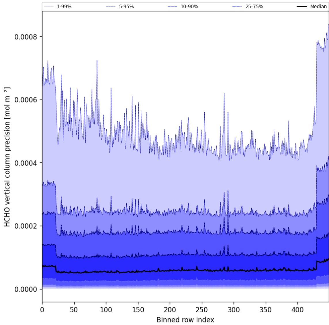
Figure 50: Along track statistics of “HCHO vertical column precision” for 2025-10-17 to 2025-10-19
