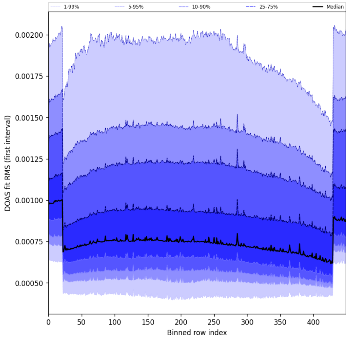
Figure 60: Along track statistics of “DOAS fit RMS (first interval)” for 2025-10-17 to 2025-10-19
