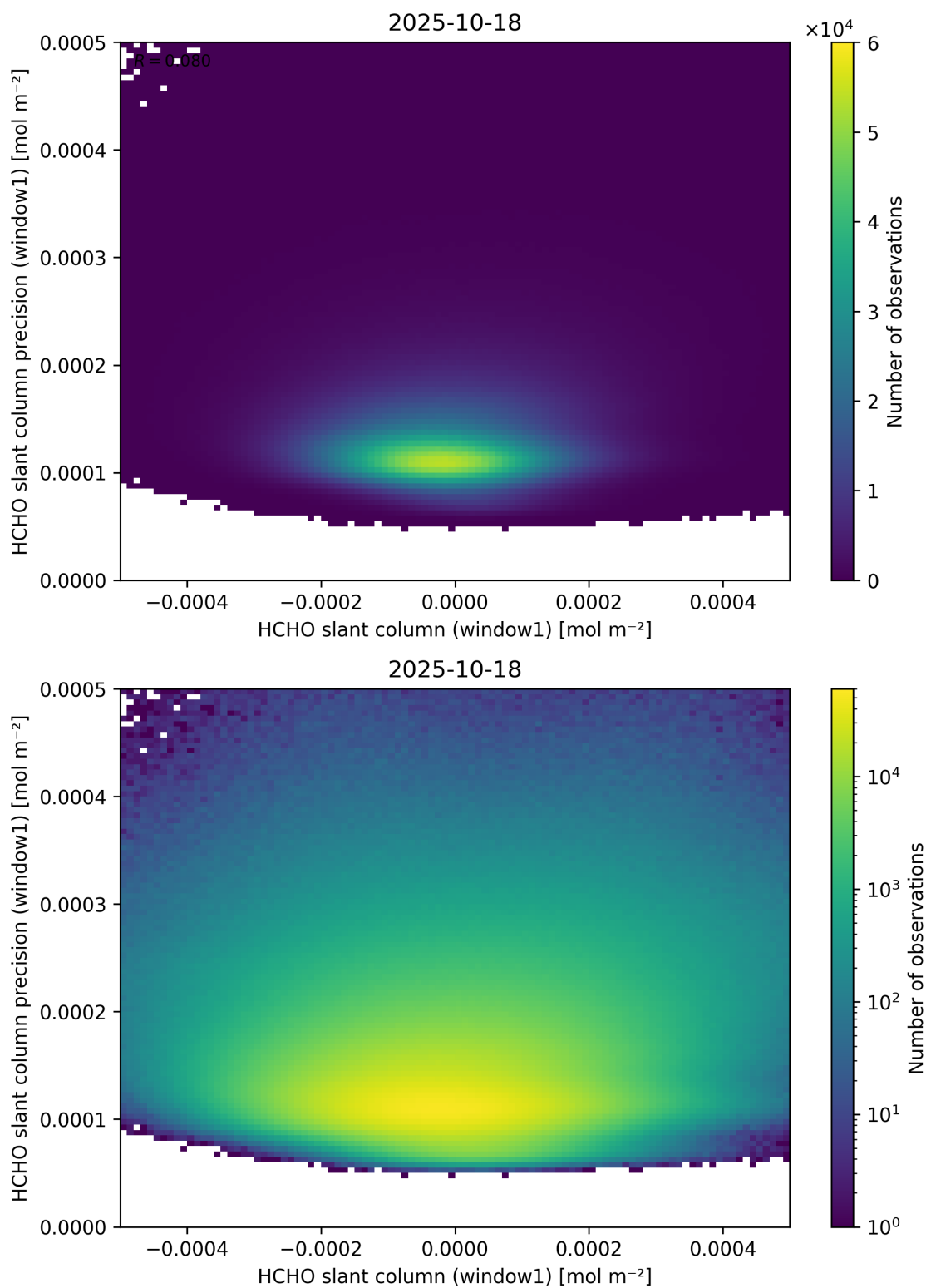
Figure 84: Scatter density plot of “HCHO slant column (window1)” against “HCHO slant column precision (window1)” for 2025-10-17 to 2025-10-19.
