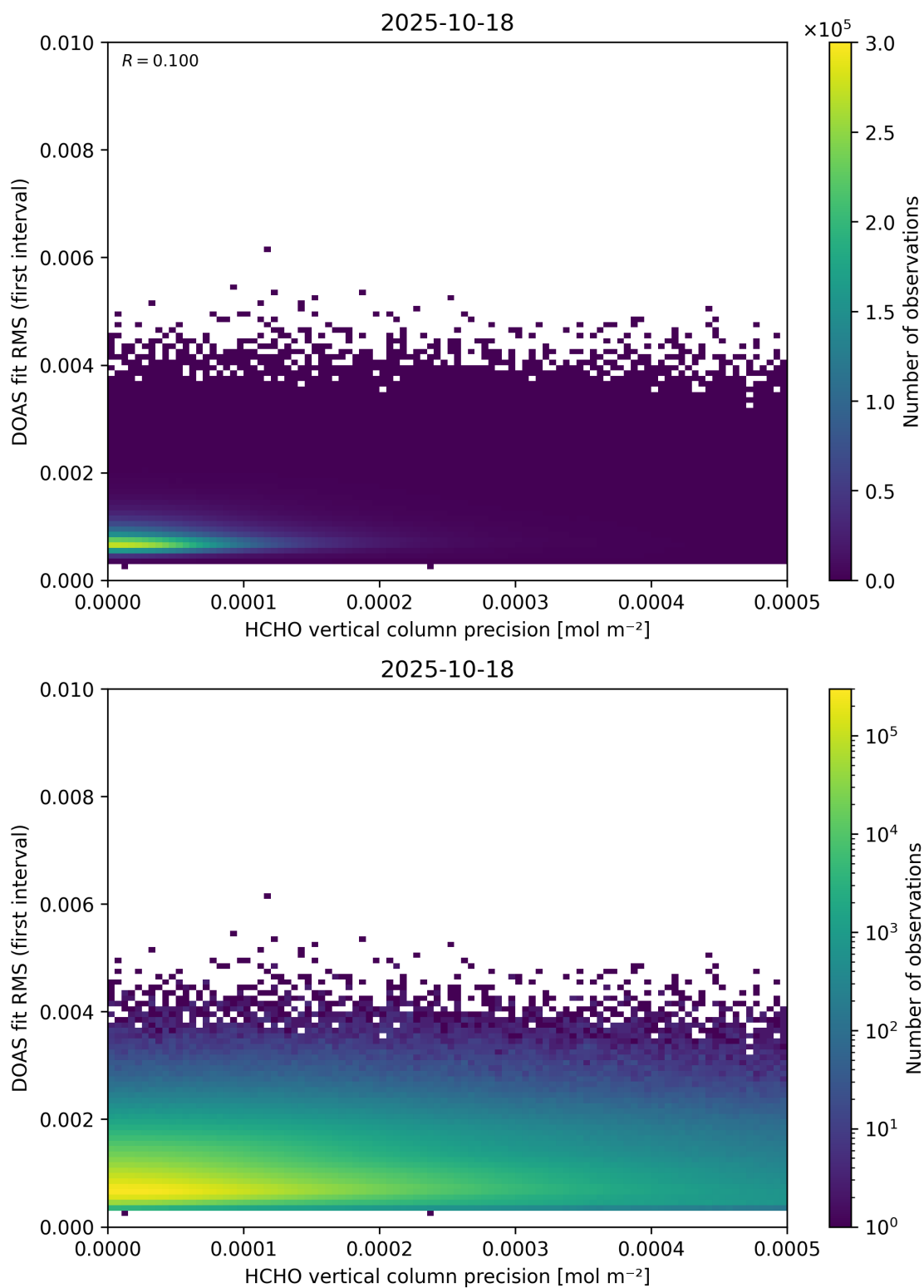
Figure 136: Scatter density plot of “HCHO vertical column precision” against “DOAS fit RMS (first interval)” for 2025-10-17 to 2025-10-19.
