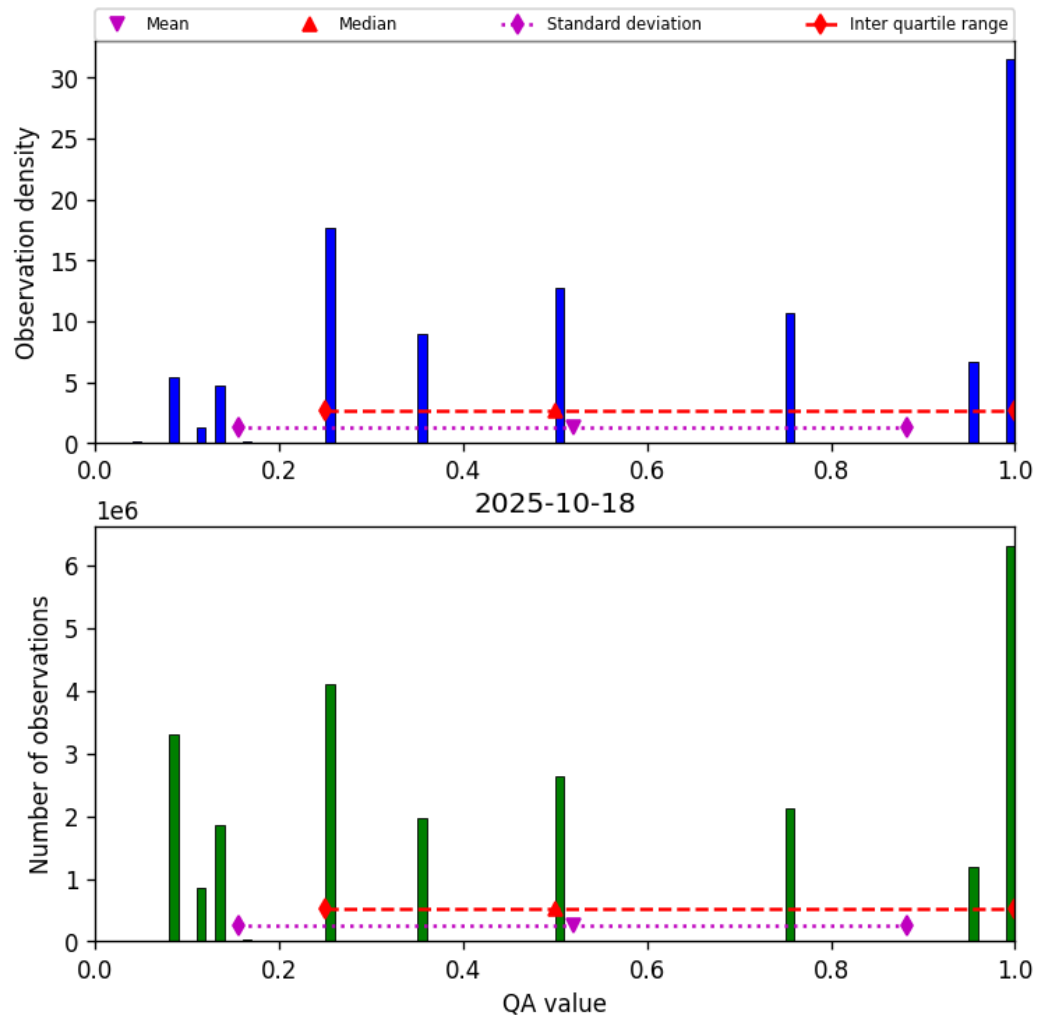
Figure 34: Histogram of “QA value” for 2025-10-17 to 2025-10-19
