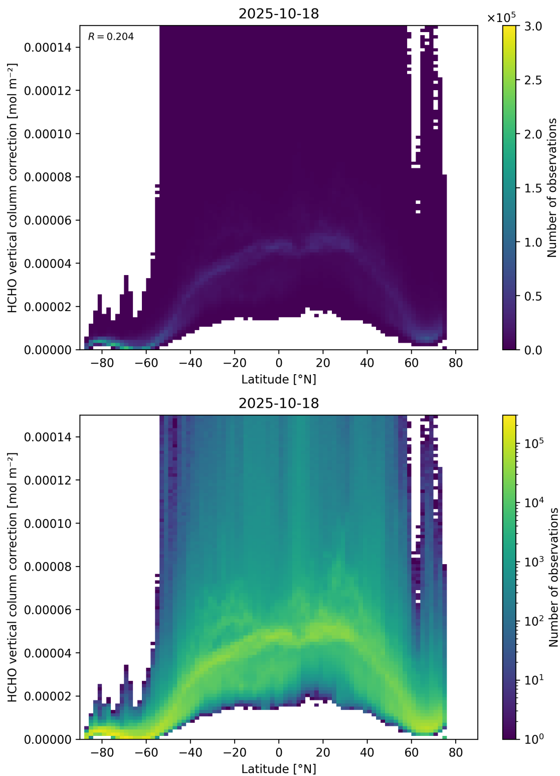
Figure 164: Scatter density plot of “Latitude” against “HCHO vertical column correction” for 2025-10-17 to 2025-10-19.
