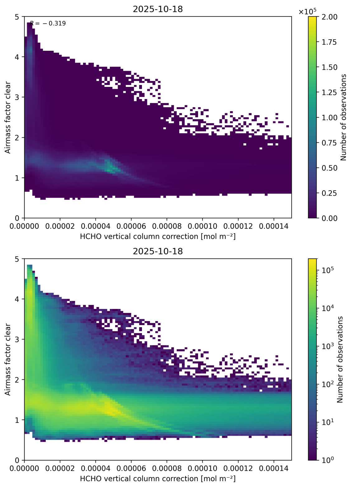
Figure 115: Scatter density plot of “HCHO vertical column correction” against “Airmass factor clear” for 2025-10-17 to 2025-10-19.
