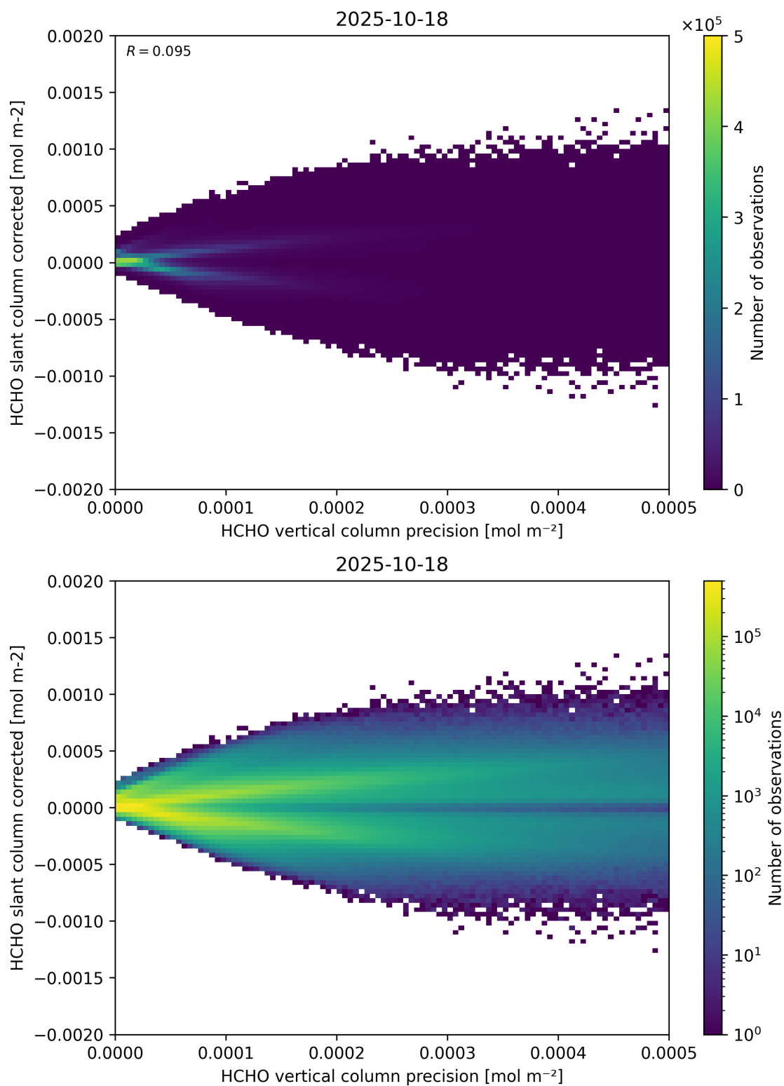
Figure 140: Scatter density plot of “HCHO vertical column precision” against “HCHO slant column corrected” for 2025-10-17 to 2025-10-19.
