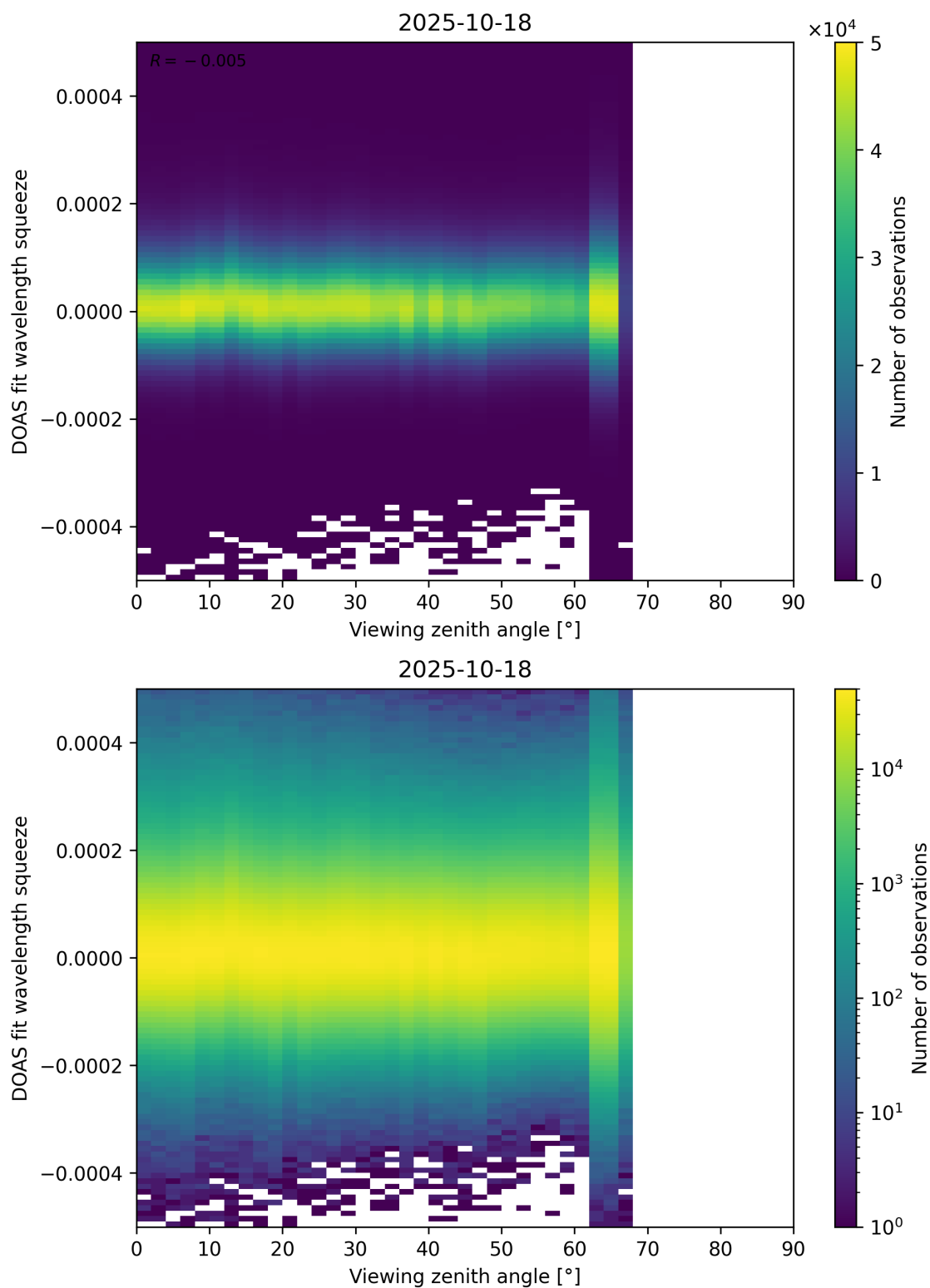
Figure 184: Scatter density plot of “Viewing zenith angle” against “DOAS fit wavelength squeeze” for 2025-10-17 to 2025-10-19.
