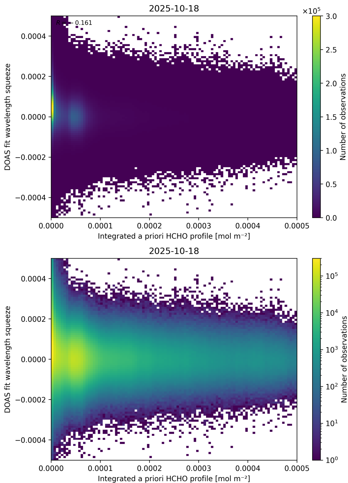
Figure 150: Scatter density plot of “Integrated a priori HCHO profile” against “DOAS fit wavelength squeeze” for 2025-10-17 to 2025-10-19.
