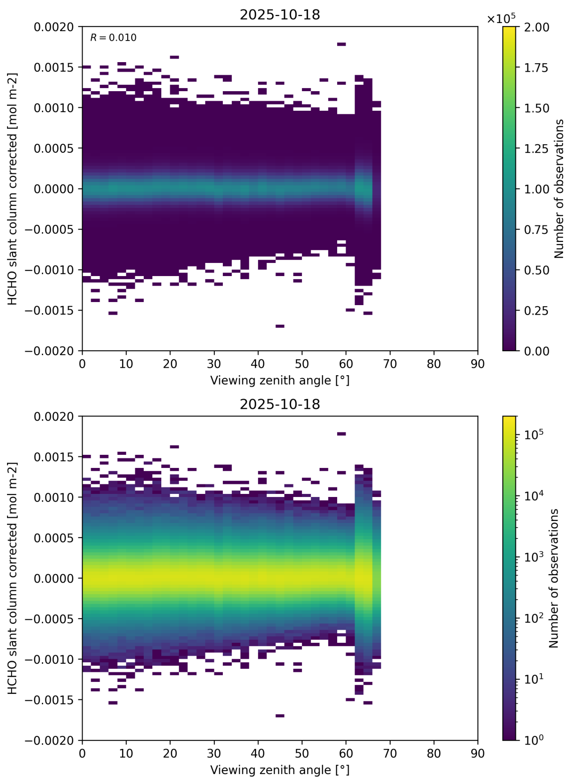
Figure 186: Scatter density plot of “Viewing zenith angle” against “HCHO slant column corrected” for 2025-10-17 to 2025-10-19.
