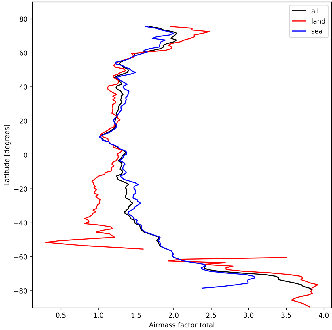
Figure 26: Zonal average of “Airmass factor total” for 2025-10-17 to 2025-10-19.
