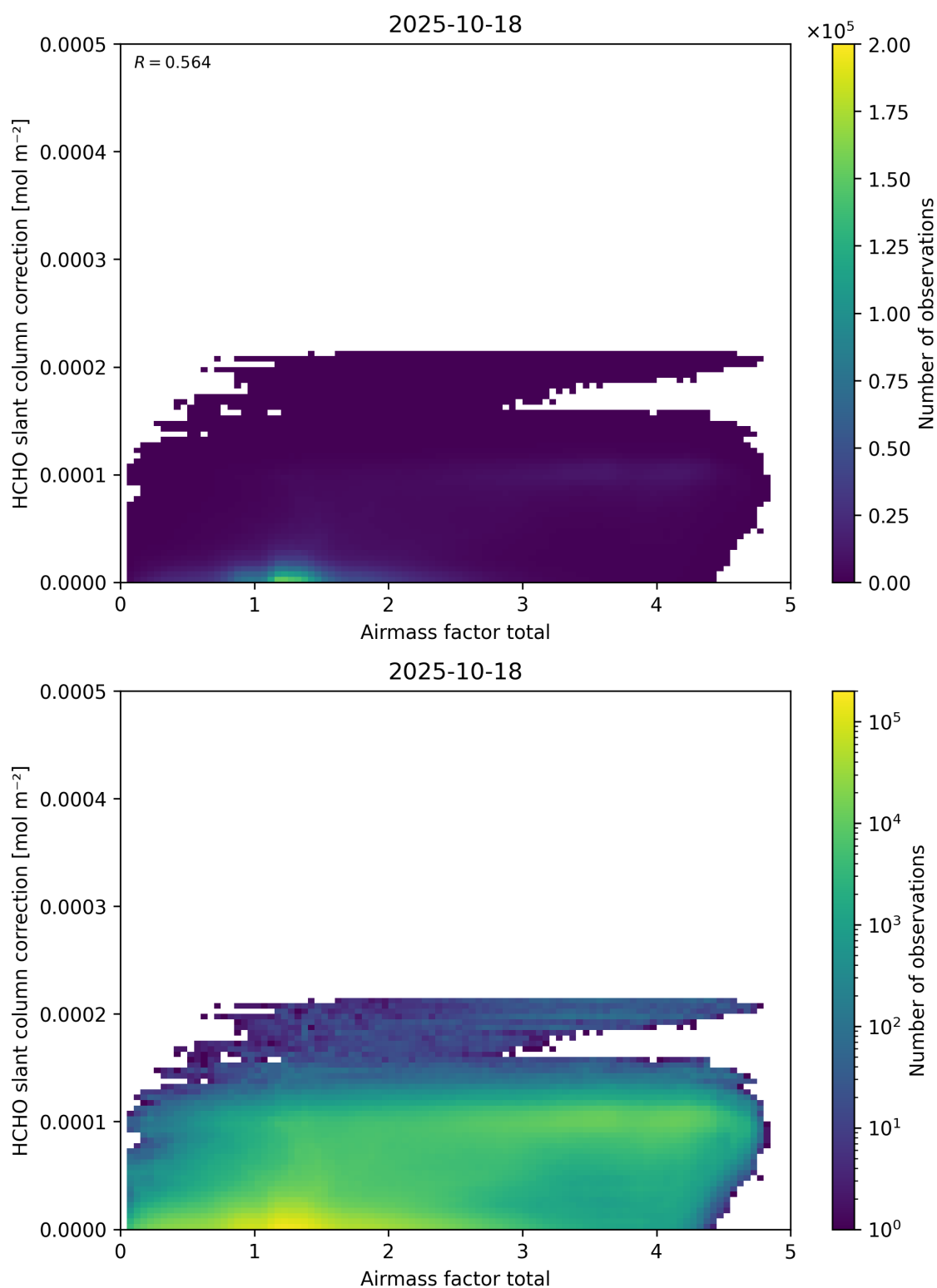
Figure 102: Scatter density plot of “Airmass factor total” against “HCHO slant column correction” for 2025-10-17 to 2025-10-19.
