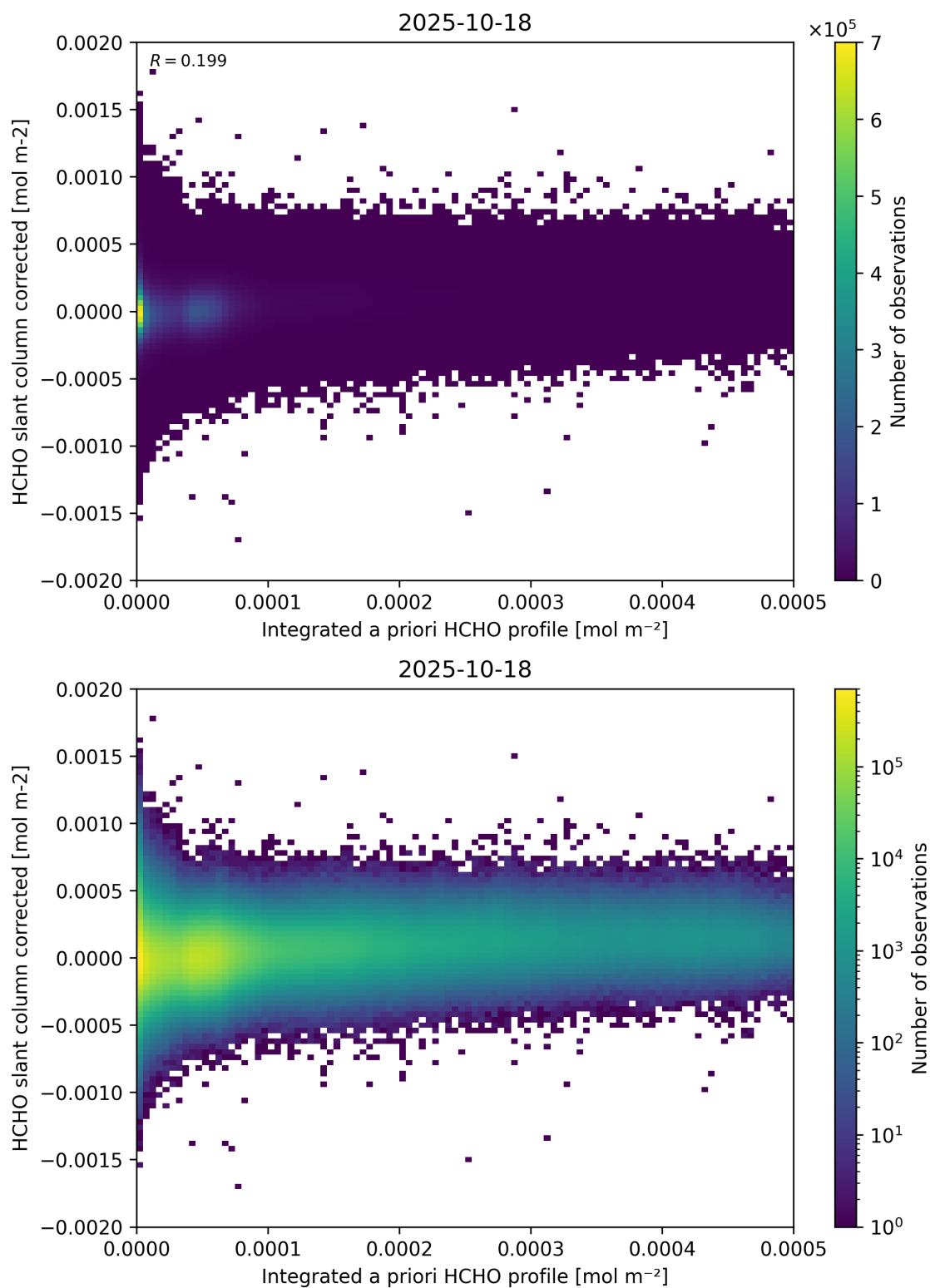
Figure 151: Scatter density plot of “Integrated a priori HCHO profile” against “HCHO slant column corrected” for 2025-10-17 to 2025-10-19.
