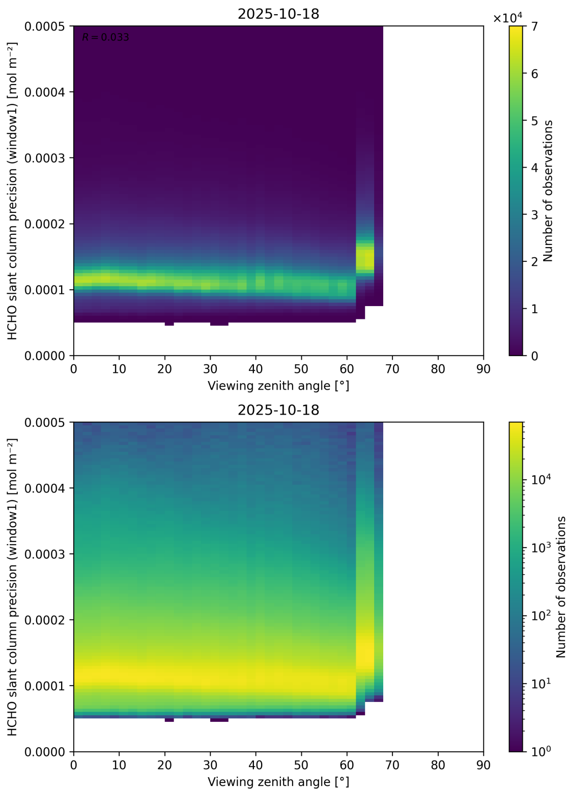
Figure 189: Scatter density plot of “Viewing zenith angle” against “HCHO slant column precision (window1)” for 2025-10-17 to 2025-10-19.
