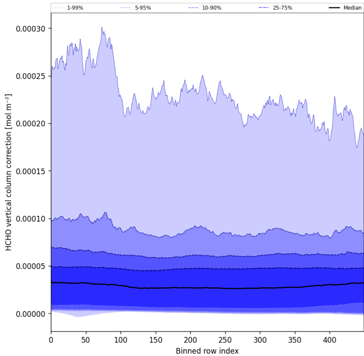
Figure 51: Along track statistics of “HCHO vertical column correction” for 2025-10-17 to 2025-10-19
