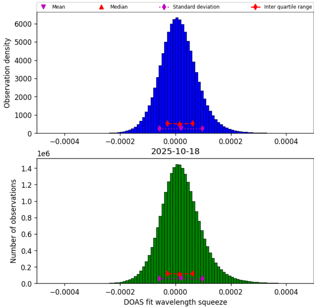
Figure 45: Histogram of “DOAS fit wavelength squeeze” for 2025-10-17 to 2025-10-19
