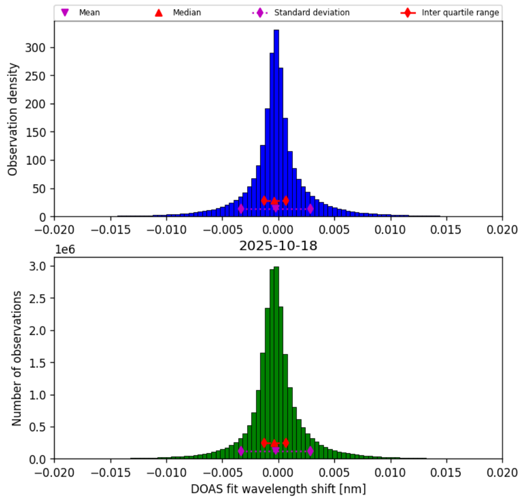
Figure 44: Histogram of “DOAS fit wavelength shift” for 2025-10-17 to 2025-10-19
