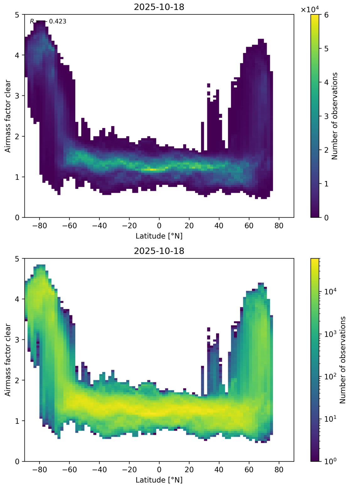
Figure 156: Scatter density plot of “Latitude” against “Airmass factor clear” for 2025-10-17 to 2025-10-19.
