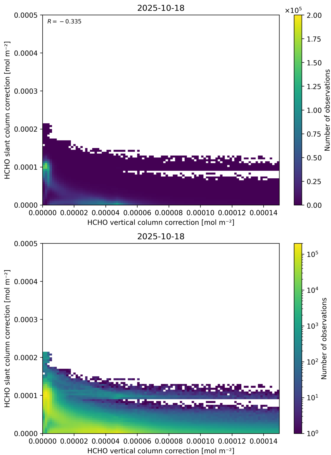
Figure 117: Scatter density plot of “HCHO vertical column correction” against “HCHO slant column correction” for 2025-10-17 to 2025-10-19.
