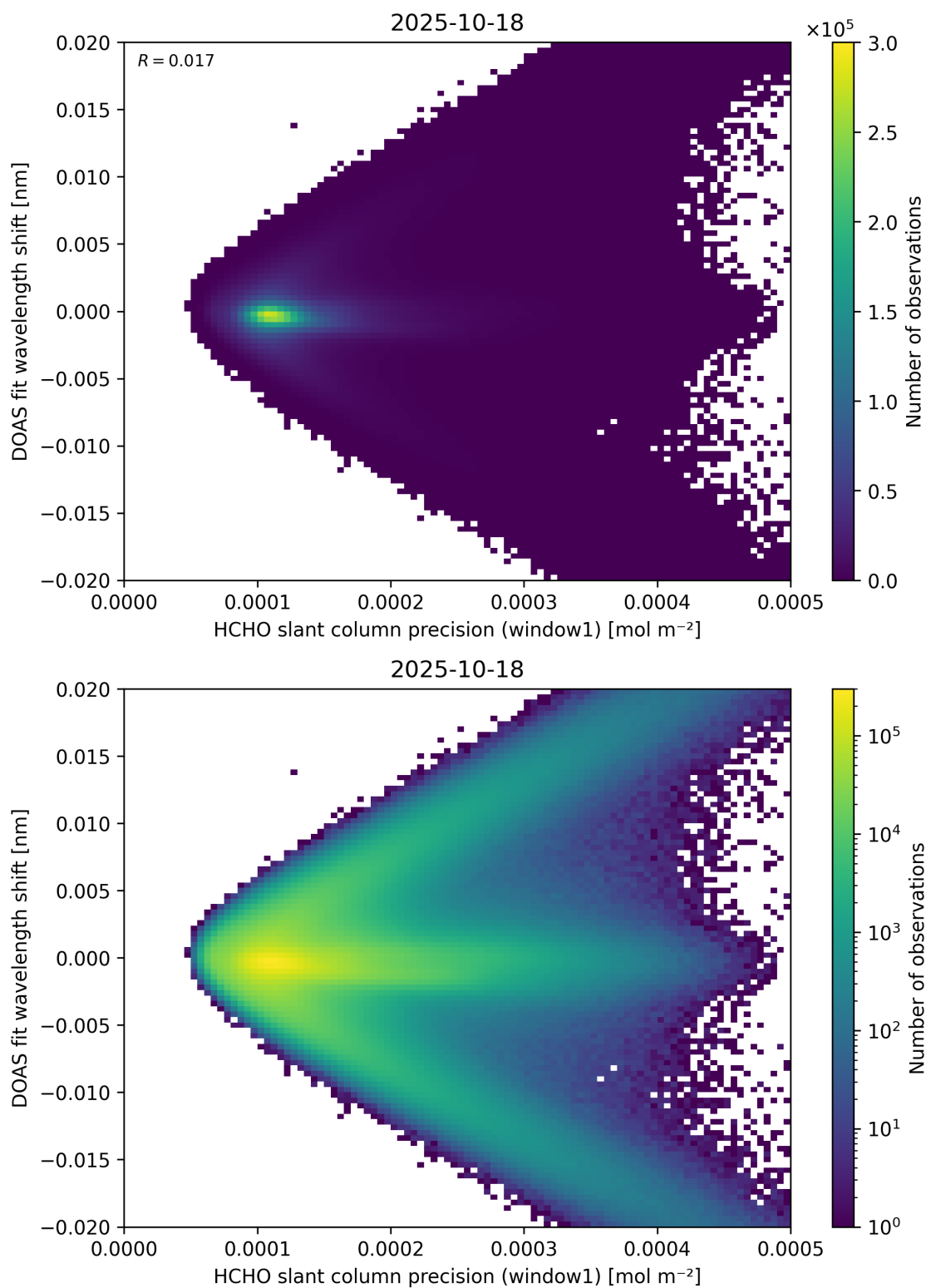
Figure 89: Scatter density plot of “HCHO slant column precision (window1)” against “DOAS fit wavelength shift” for 2025-10-17 to 2025-10-19.
