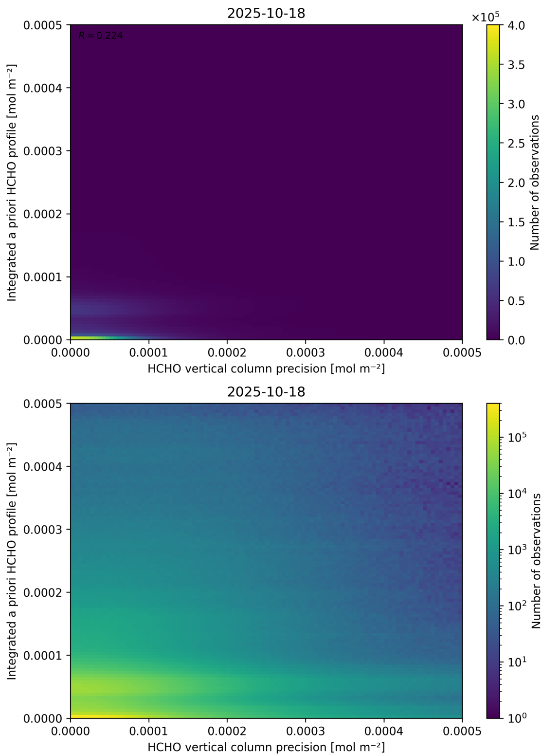
Figure 147: Scatter density plot of “HCHO vertical column precision” against “Integrated a priori HCHO profile” for 2025-10-17 to 2025-10-19.
