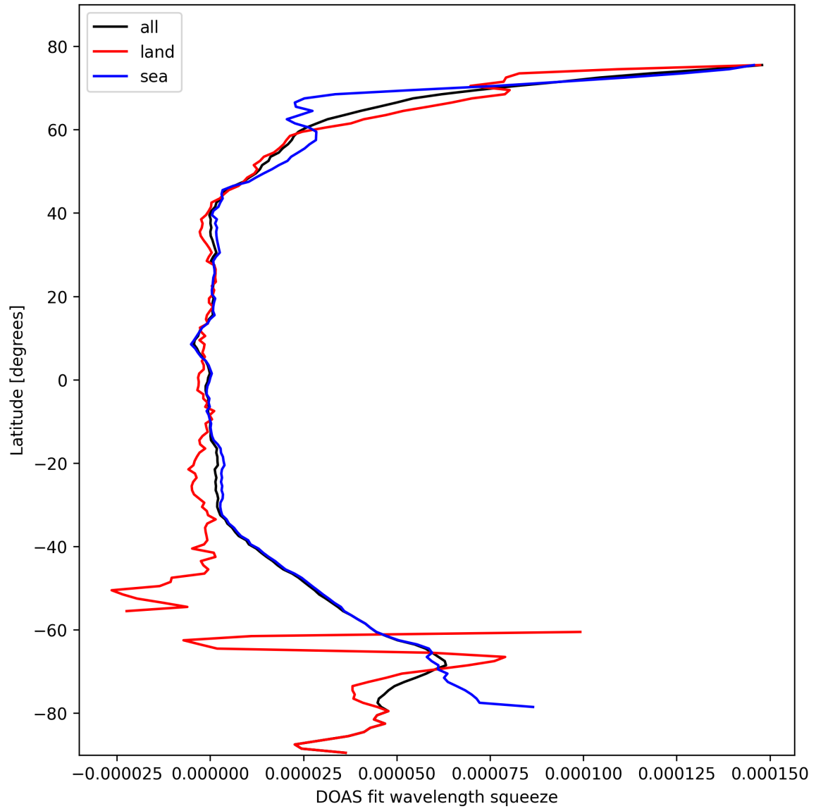
Figure 31: Zonal average of “DOAS fit wavelength squeeze” for 2025-10-17 to 2025-10-19.
