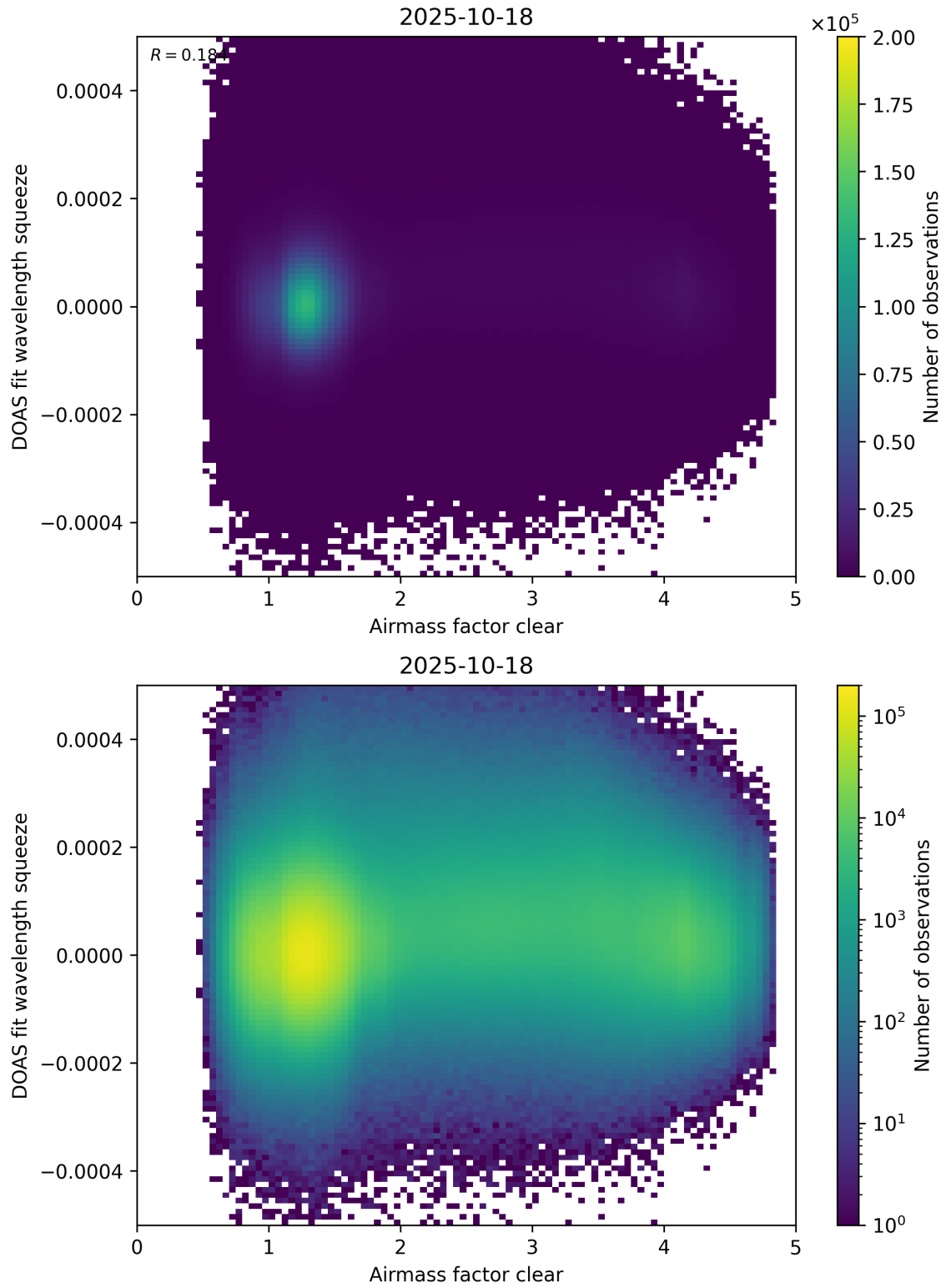
Figure 73: Scatter density plot of “Airmass factor clear” against “DOAS fit wavelength squeeze” for 2025-10-17 to 2025-10-19.
