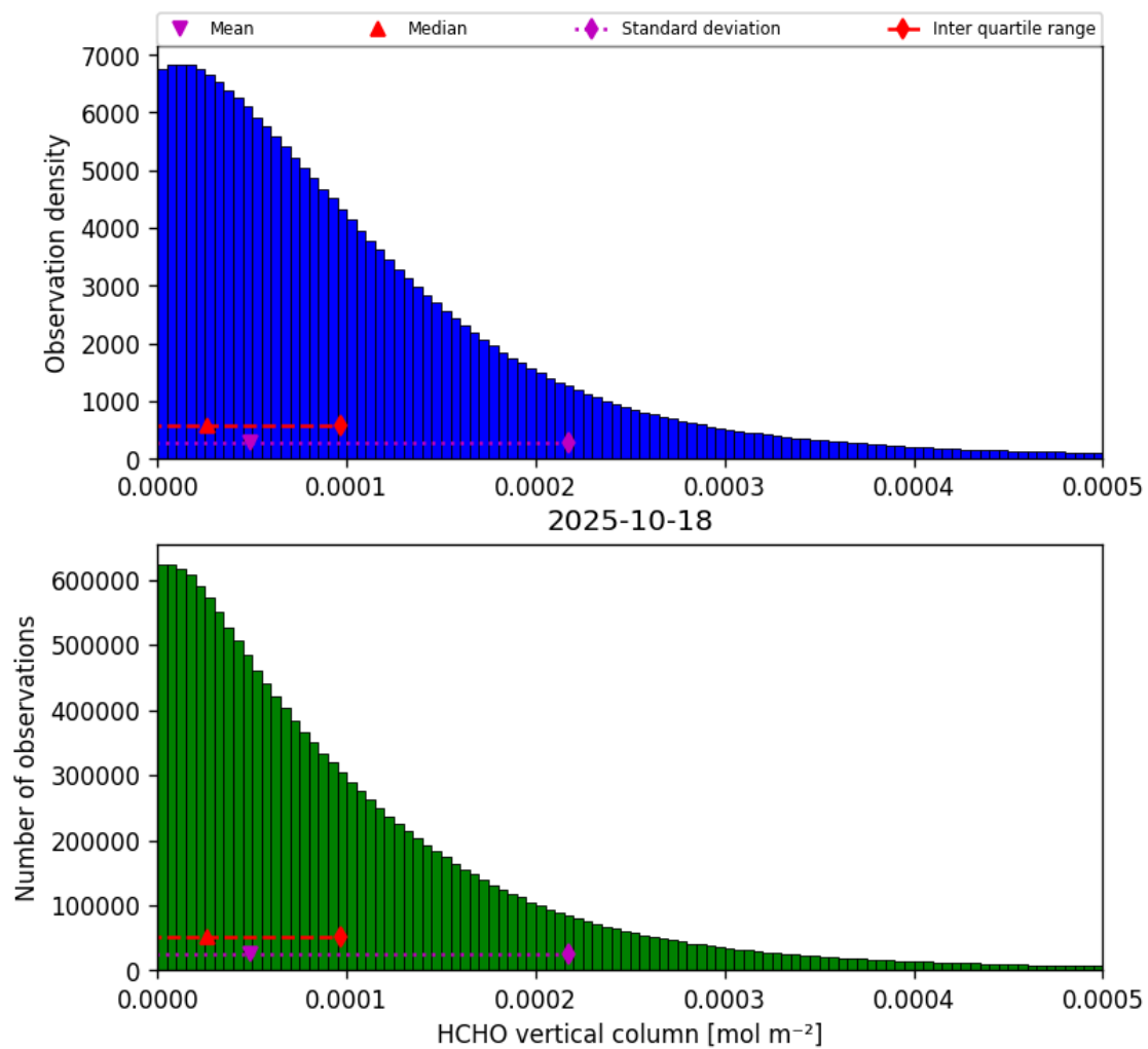
Figure 35: Histogram of “HCHO vertical column” for 2025-10-17 to 2025-10-19
