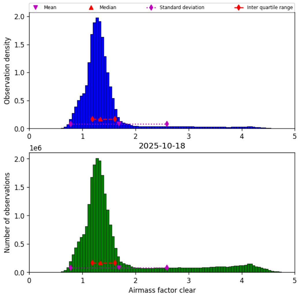
Figure 42: Histogram of “Airmass factor clear” for 2025-10-17 to 2025-10-19
