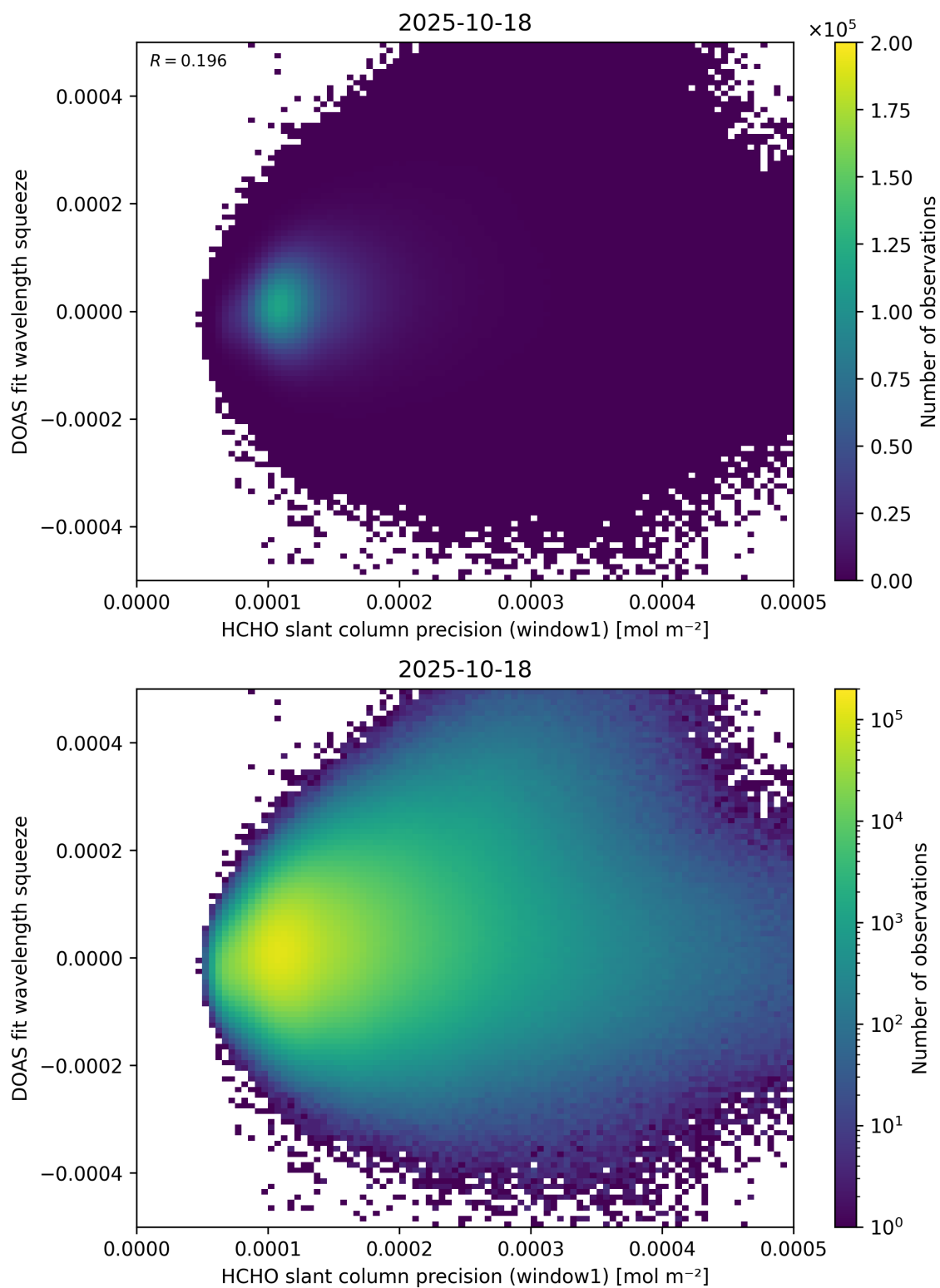
Figure 90: Scatter density plot of “HCHO slant column precision (window1)” against “DOAS fit wavelength squeeze” for 2025-10-17 to 2025-10-19.
