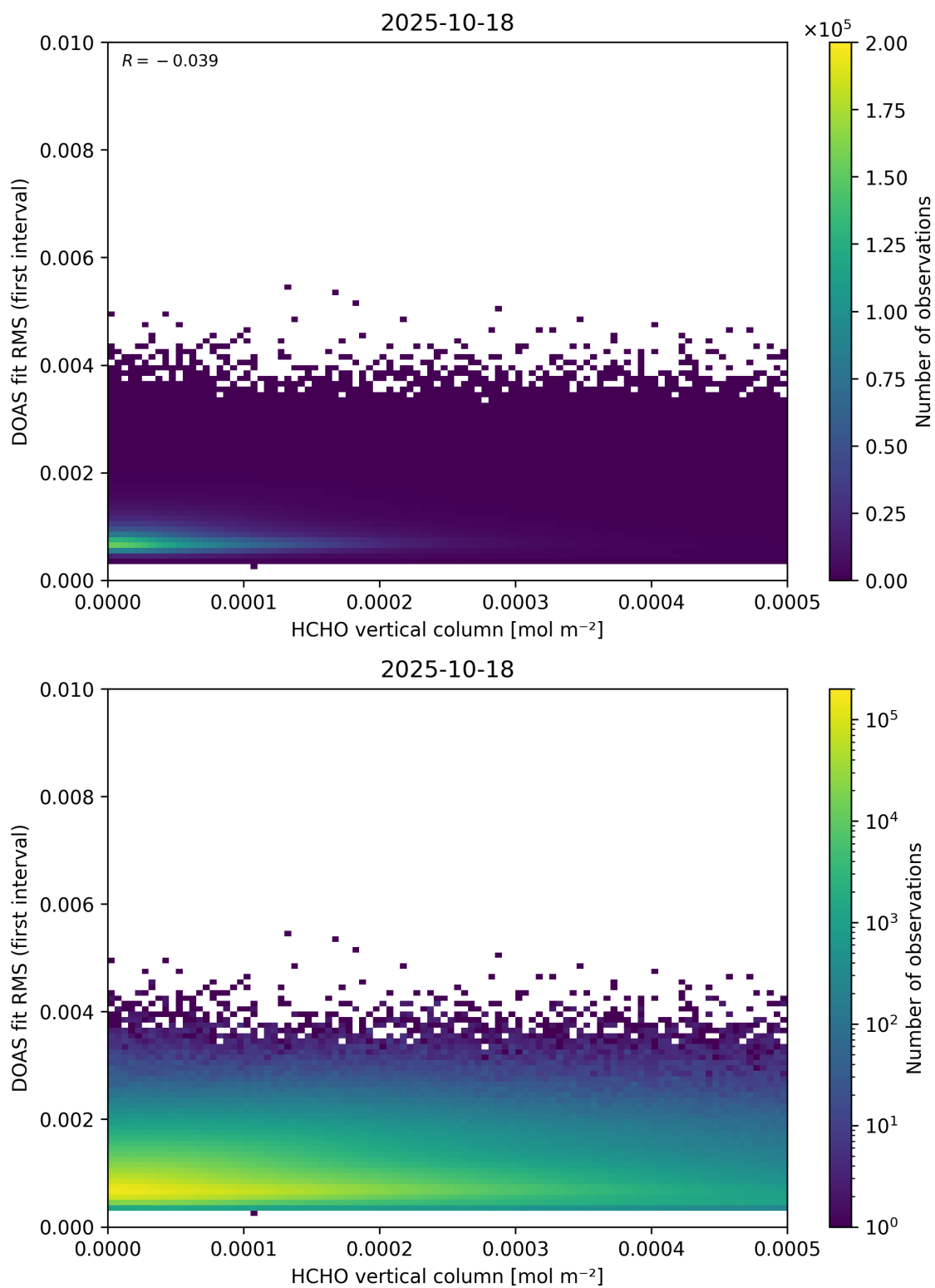
Figure 123: Scatter density plot of “HCHO vertical column” against “DOAS fit RMS (first interval)” for 2025-10-17 to 2025-10-19.
