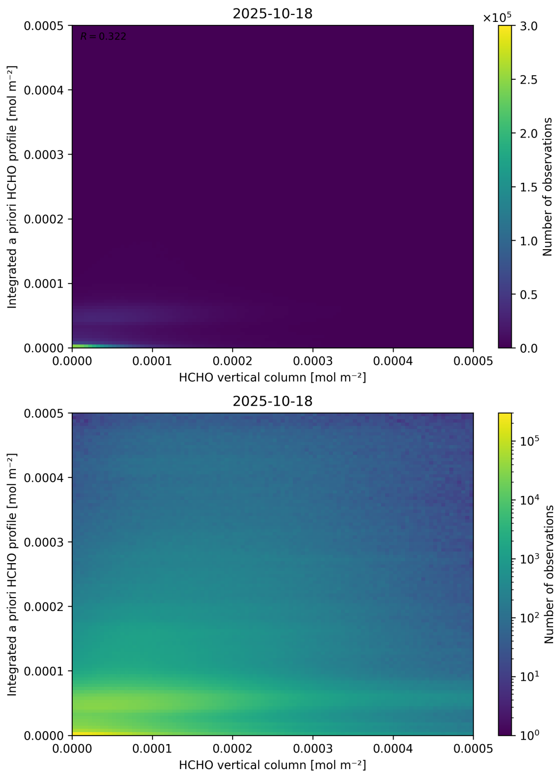
Figure 135: Scatter density plot of “HCHO vertical column” against “Integrated a priori HCHO profile” for 2025-10-17 to 2025-10-19.
