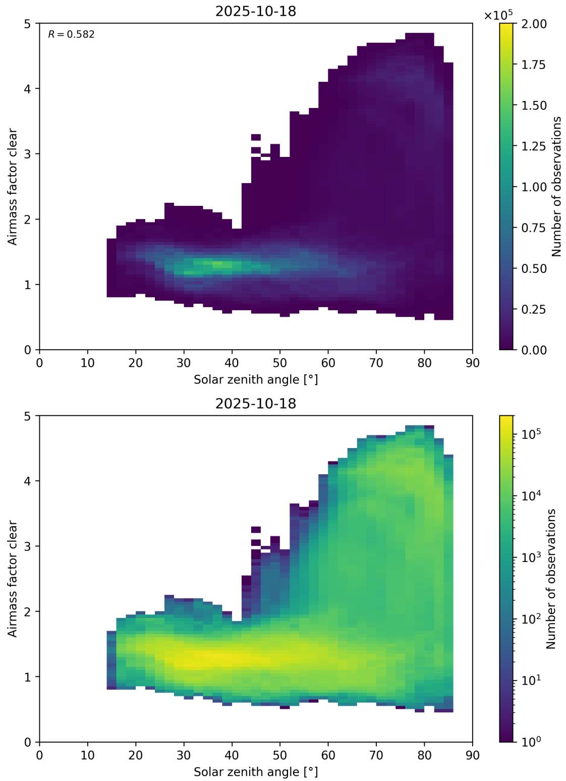
Figure 170: Scatter density plot of “Solar zenith angle” against “Airmass factor clear” for 2025-10-17 to 2025-10-19.
