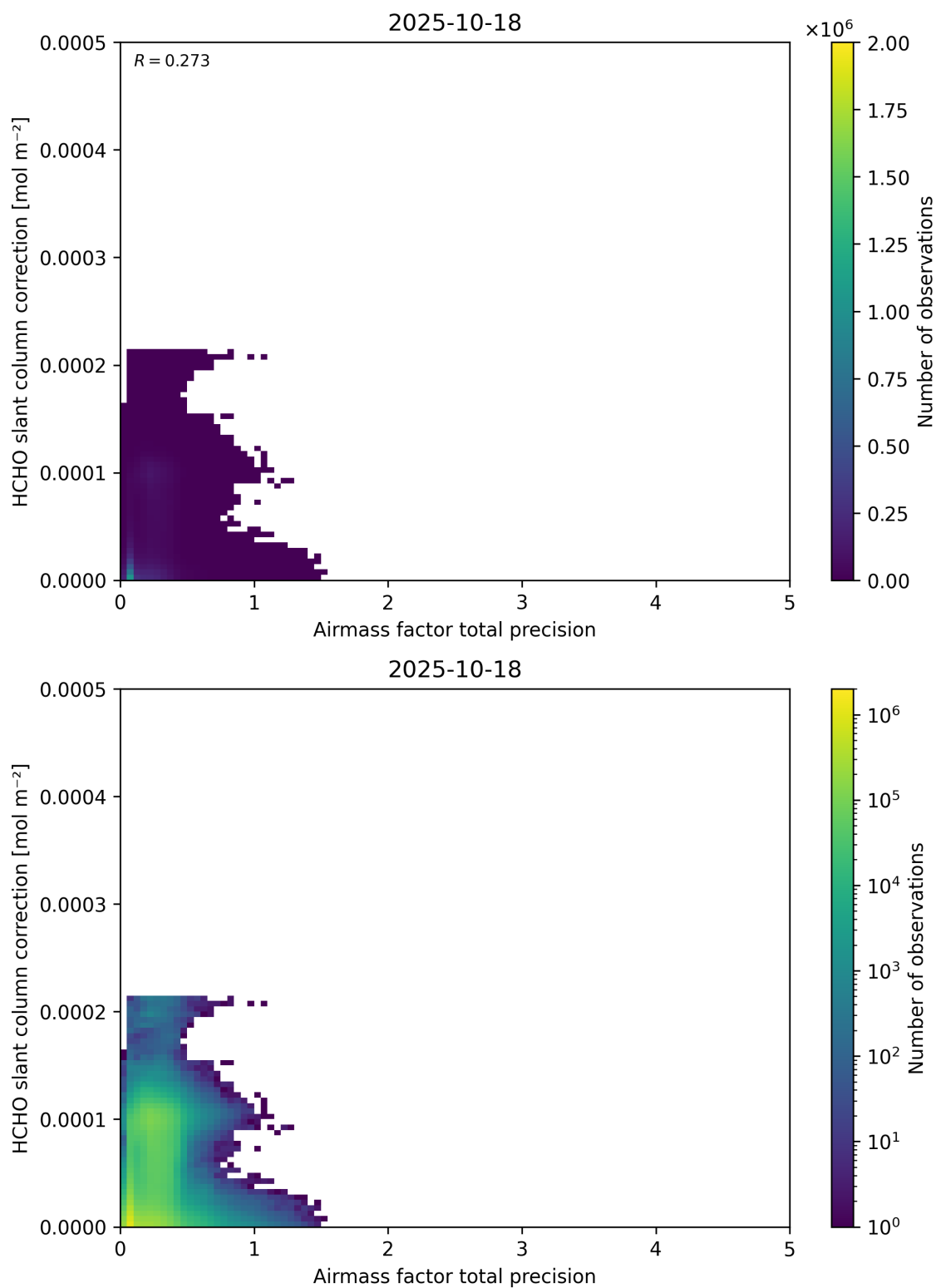
Figure 110: Scatter density plot of “Airmass factor total precision” against “HCHO slant column correction” for 2025-10-17 to 2025-10-19.
