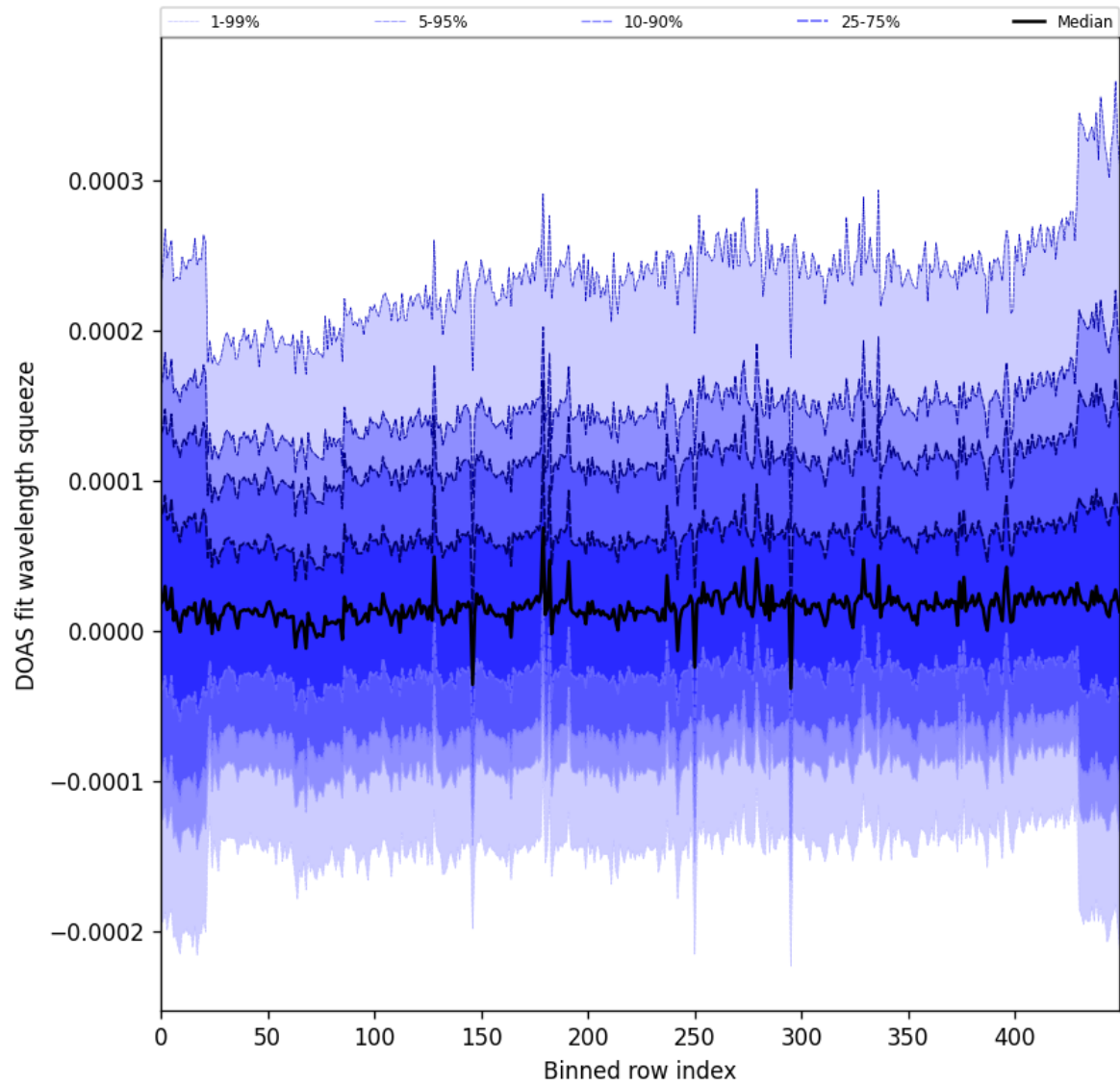
Figure 59: Along track statistics of “DOAS fit wavelength squeeze” for 2025-10-17 to 2025-10-19
