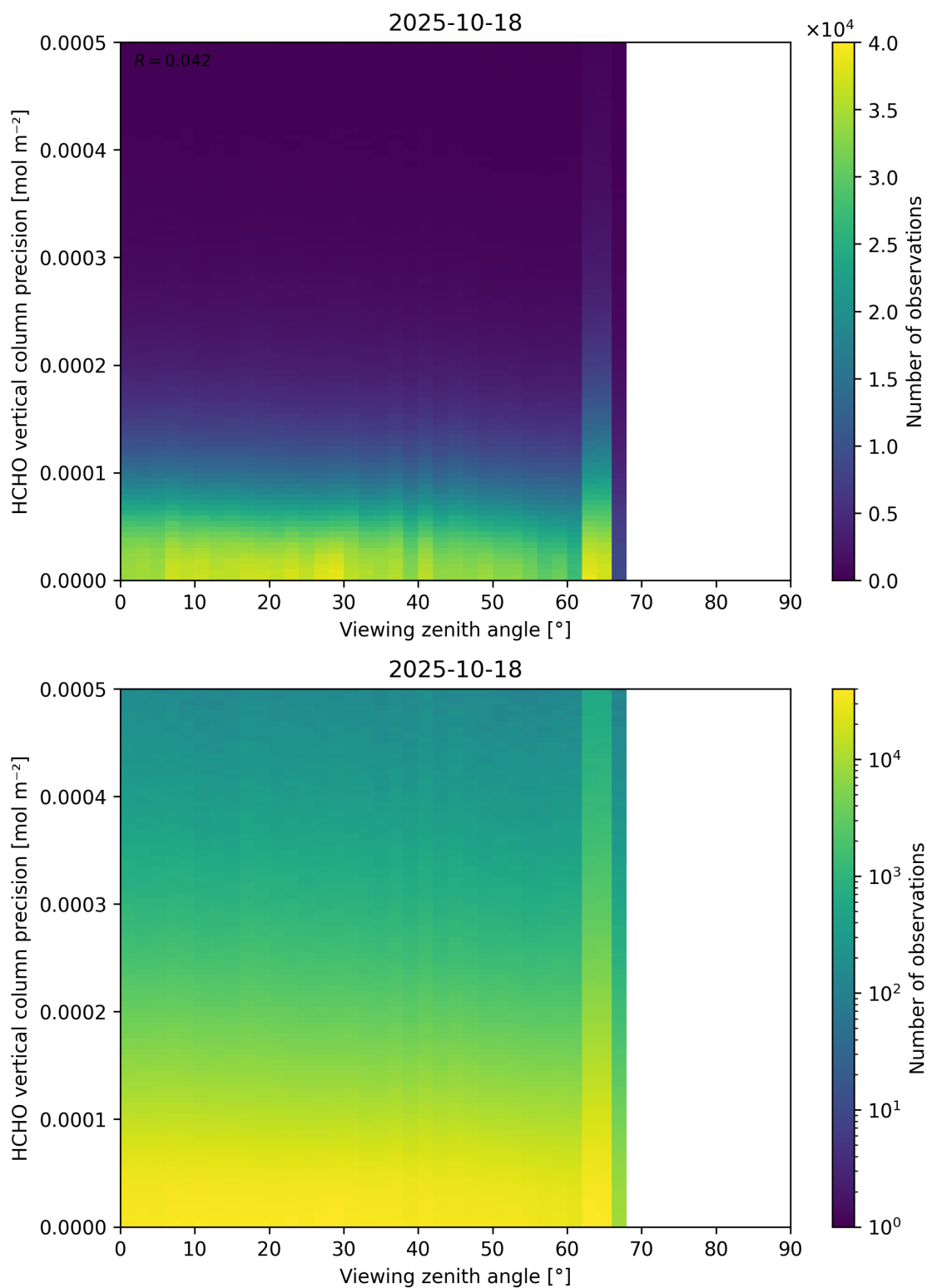
Figure 194: Scatter density plot of “Viewing zenith angle” against “HCHO vertical column precision” for 2025-10-17 to 2025-10-19.
