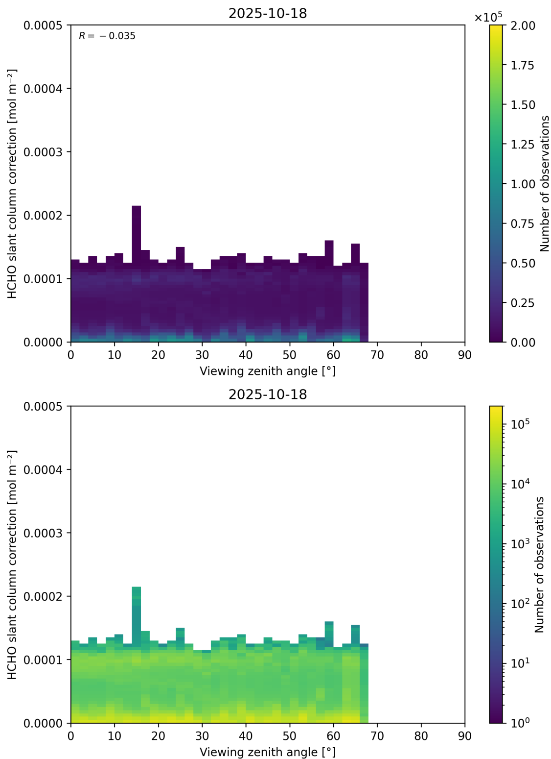
Figure 187: Scatter density plot of “Viewing zenith angle” against “HCHO slant column correction” for 2025-10-17 to 2025-10-19.
