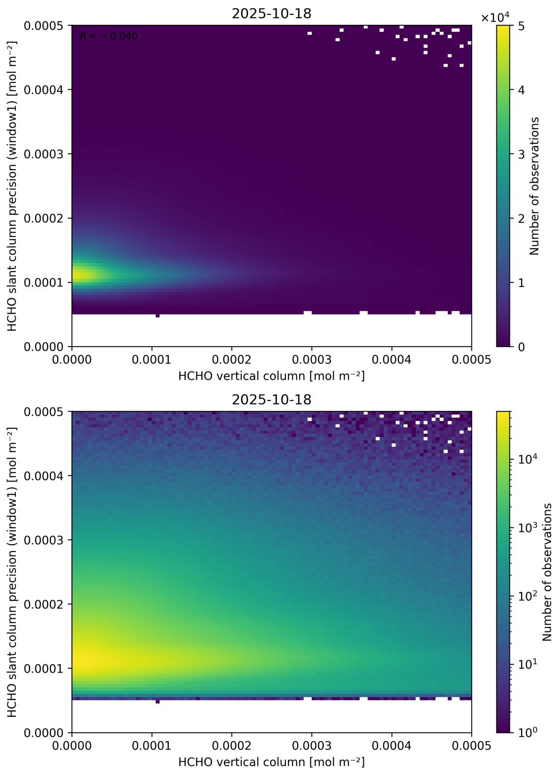
Figure 130: Scatter density plot of “HCHO vertical column” against “HCHO slant column precision (window1)” for 2025-10-17 to 2025-10-19.
