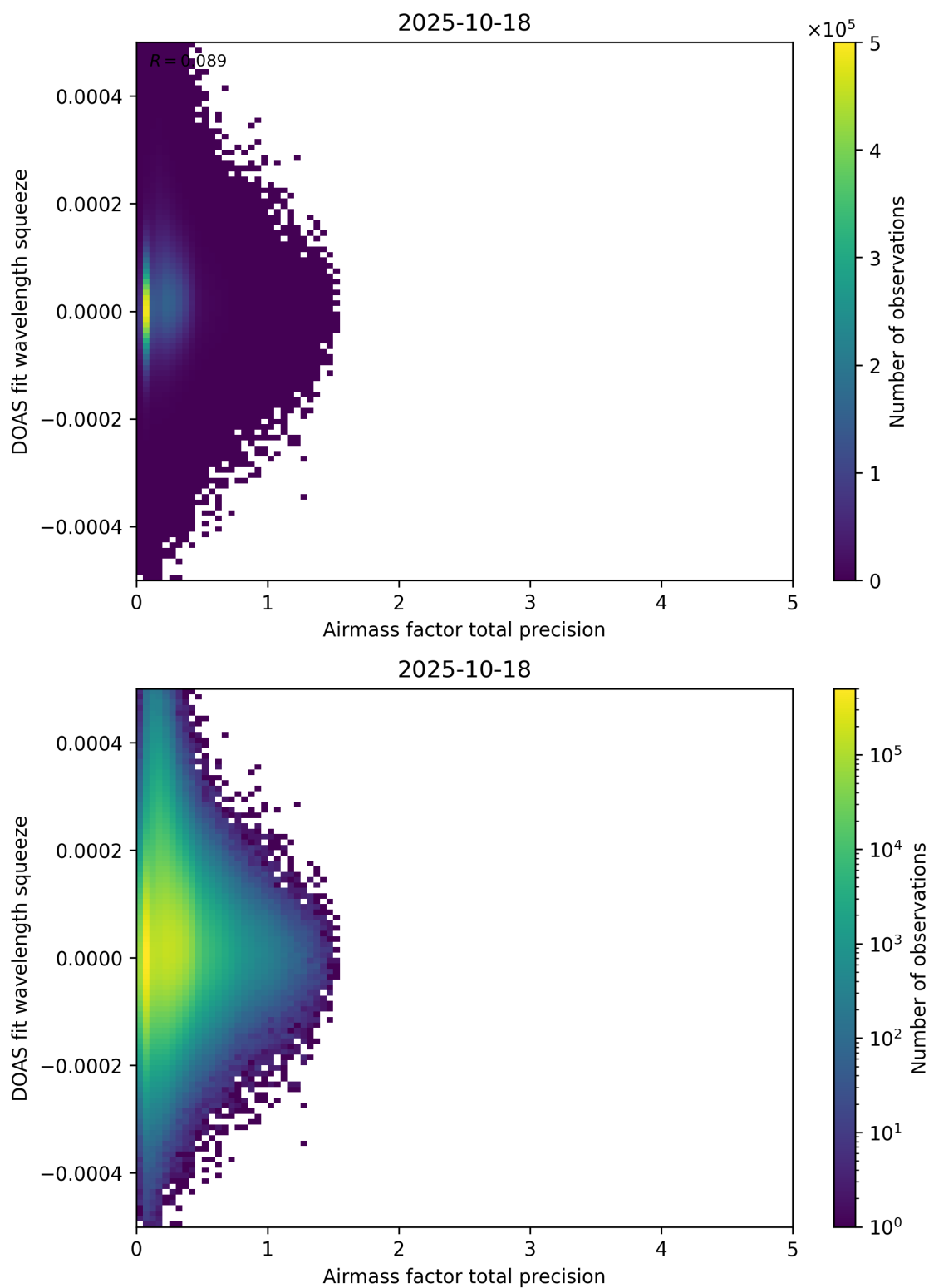
Figure 107: Scatter density plot of “Airmass factor total precision” against “DOAS fit wavelength squeeze” for 2025-10-17 to 2025-10-19.
