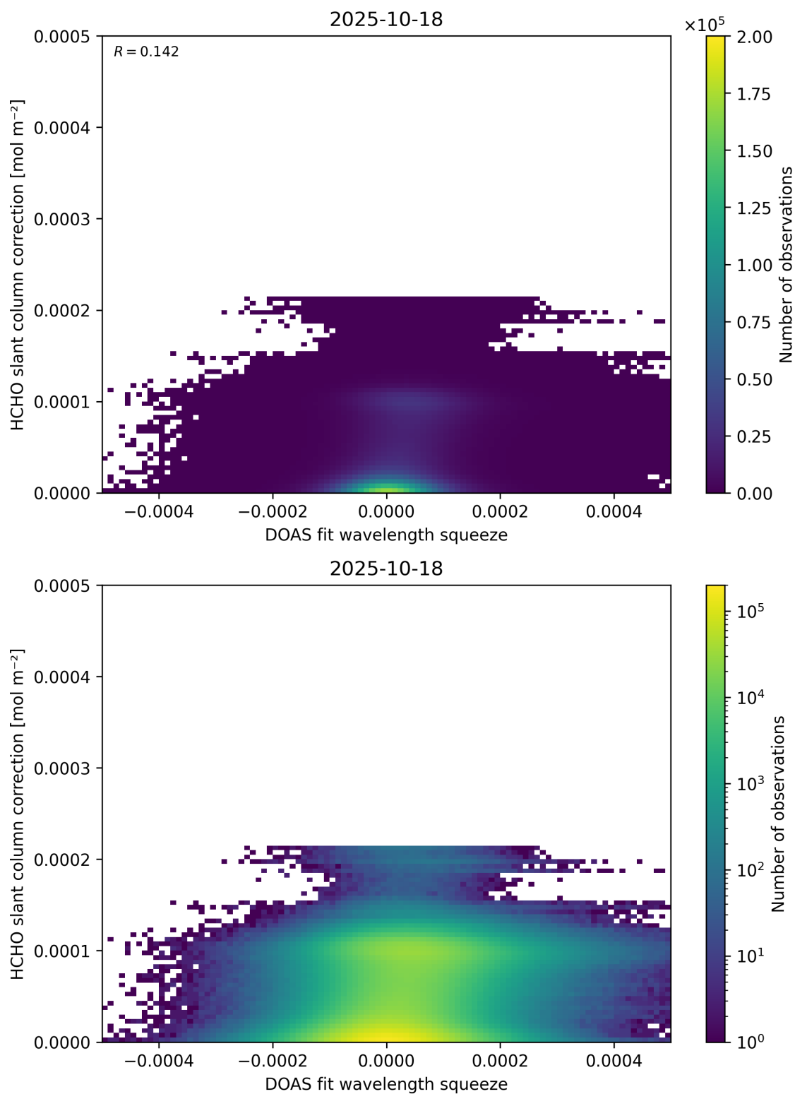
Figure 70: Scatter density plot of “DOAS fit wavelength squeeze” against “HCHO slant column correction” for 2025-10-17 to 2025-10-19.
