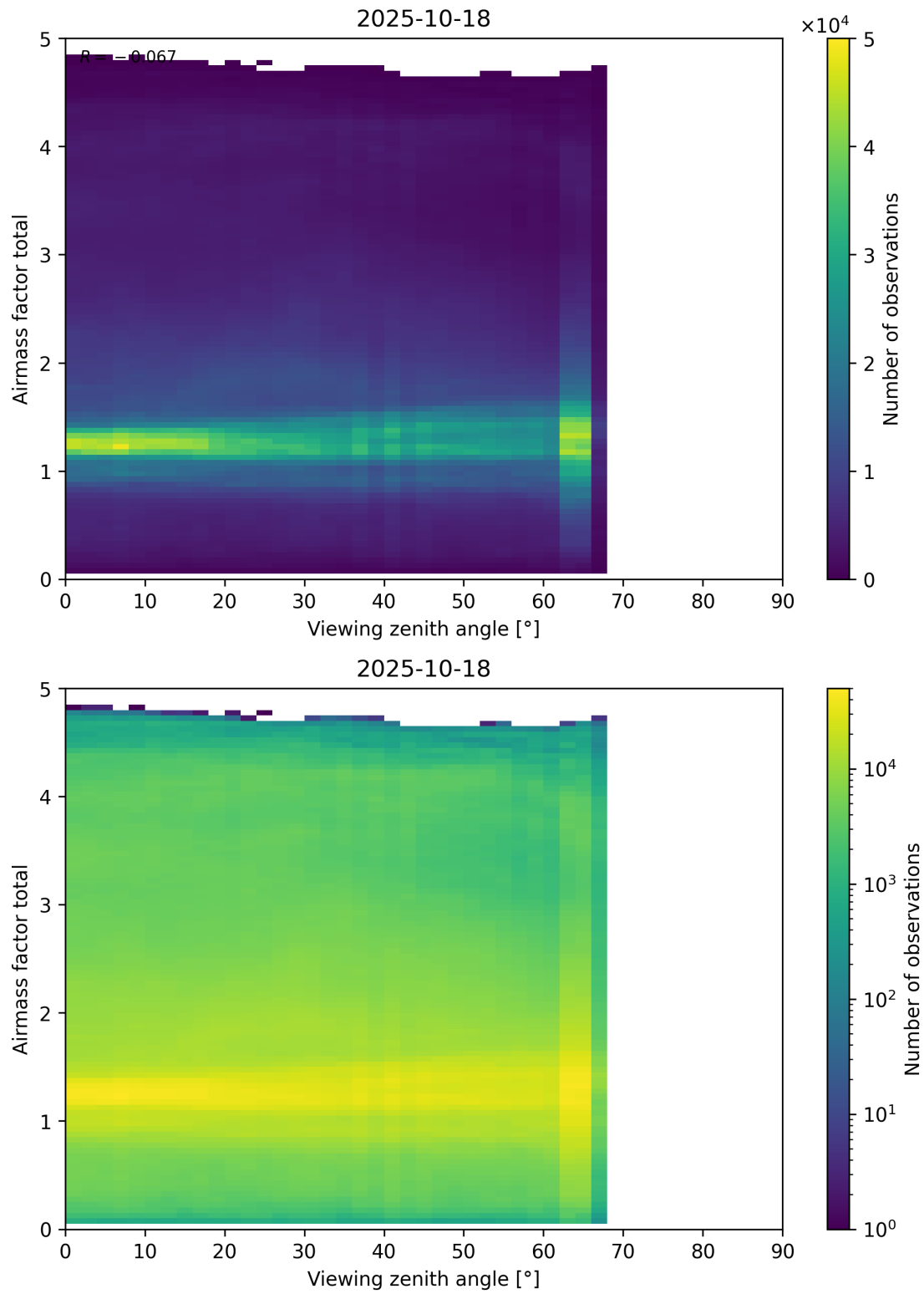
Figure 190: Scatter density plot of “Viewing zenith angle” against “Airmass factor total” for 2025-10-17 to 2025-10-19.
