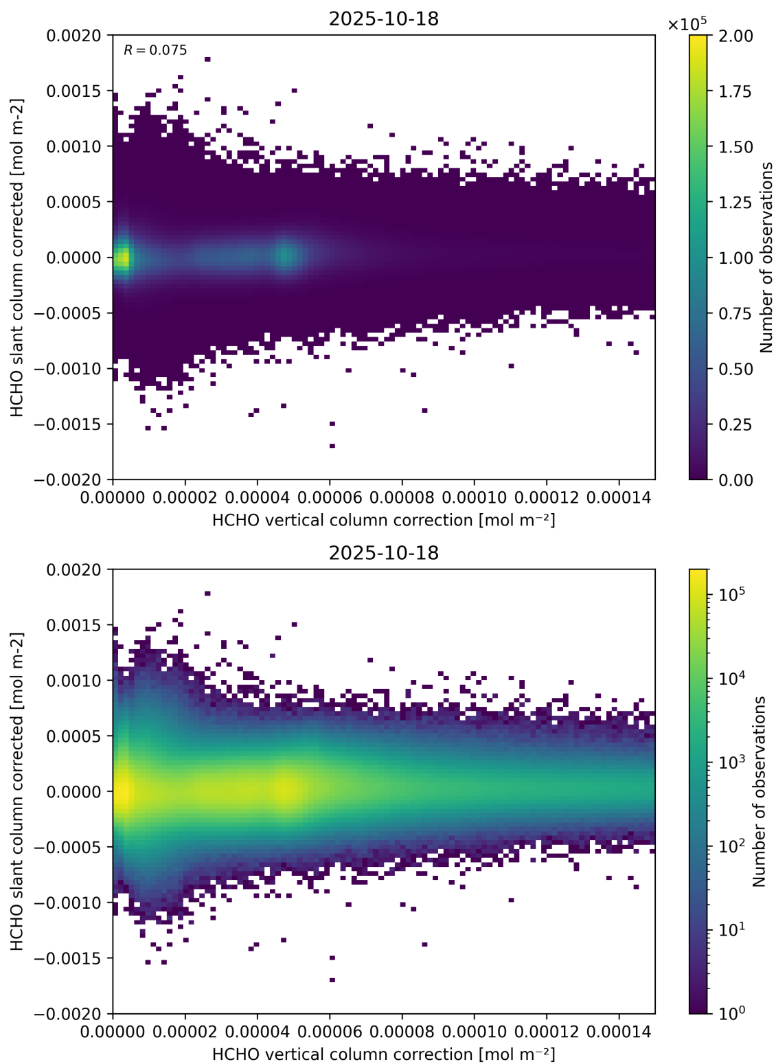
Figure 116: Scatter density plot of “HCHO vertical column correction” against “HCHO slant column corrected” for 2025-10-17 to 2025-10-19.
