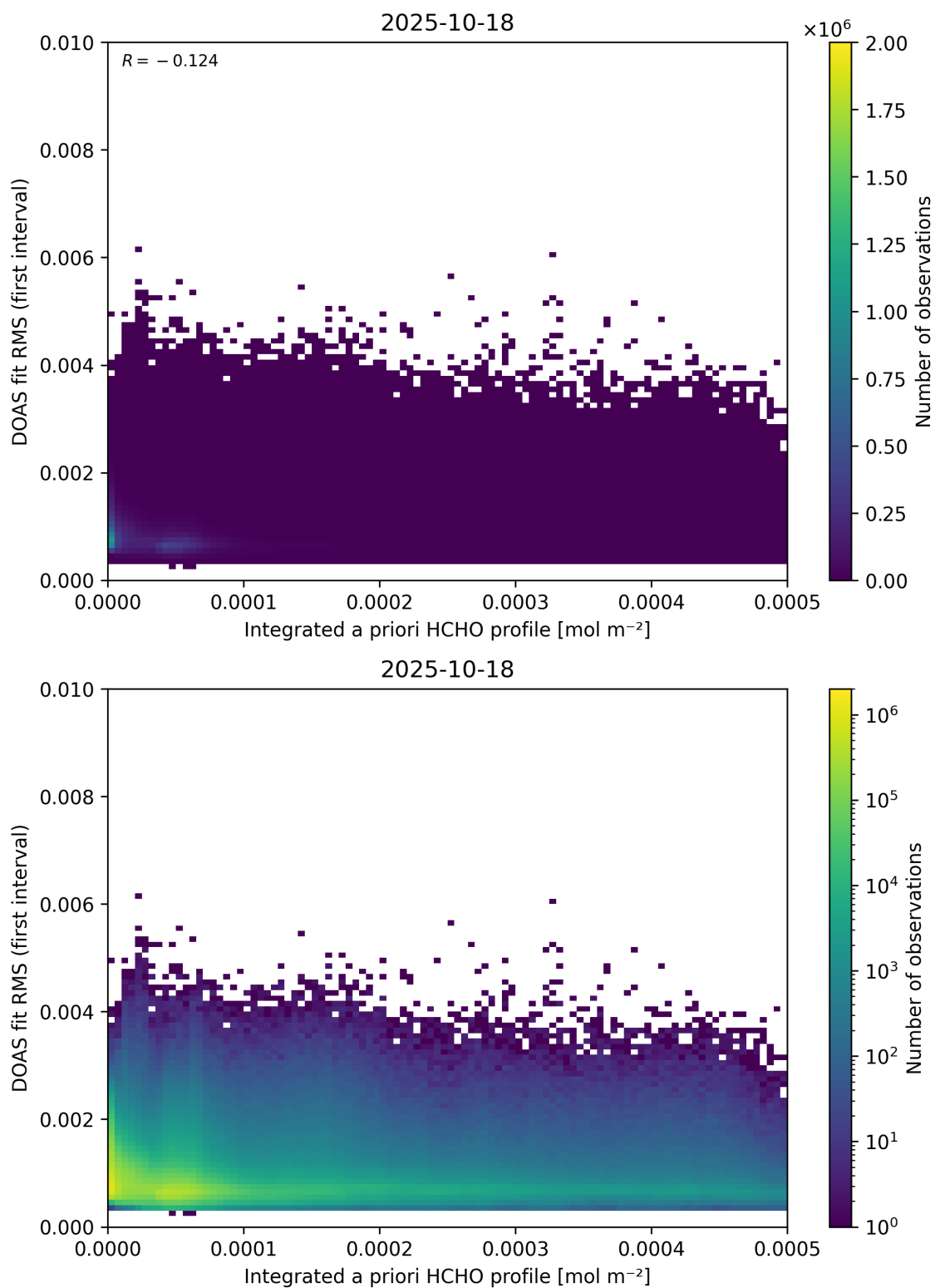
Figure 148: Scatter density plot of “Integrated a priori HCHO profile” against “DOAS fit RMS (first interval)” for 2025-10-17 to 2025-10-19.
