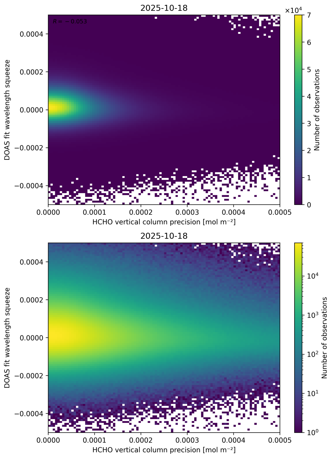
Figure 138: Scatter density plot of “HCHO vertical column precision” against “DOAS fit wavelength squeeze” for 2025-10-17 to 2025-10-19.
