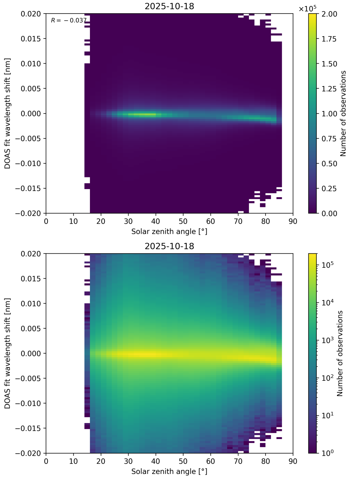
Figure 168: Scatter density plot of “Solar zenith angle” against “DOAS fit wavelength shift” for 2025-10-17 to 2025-10-19.
