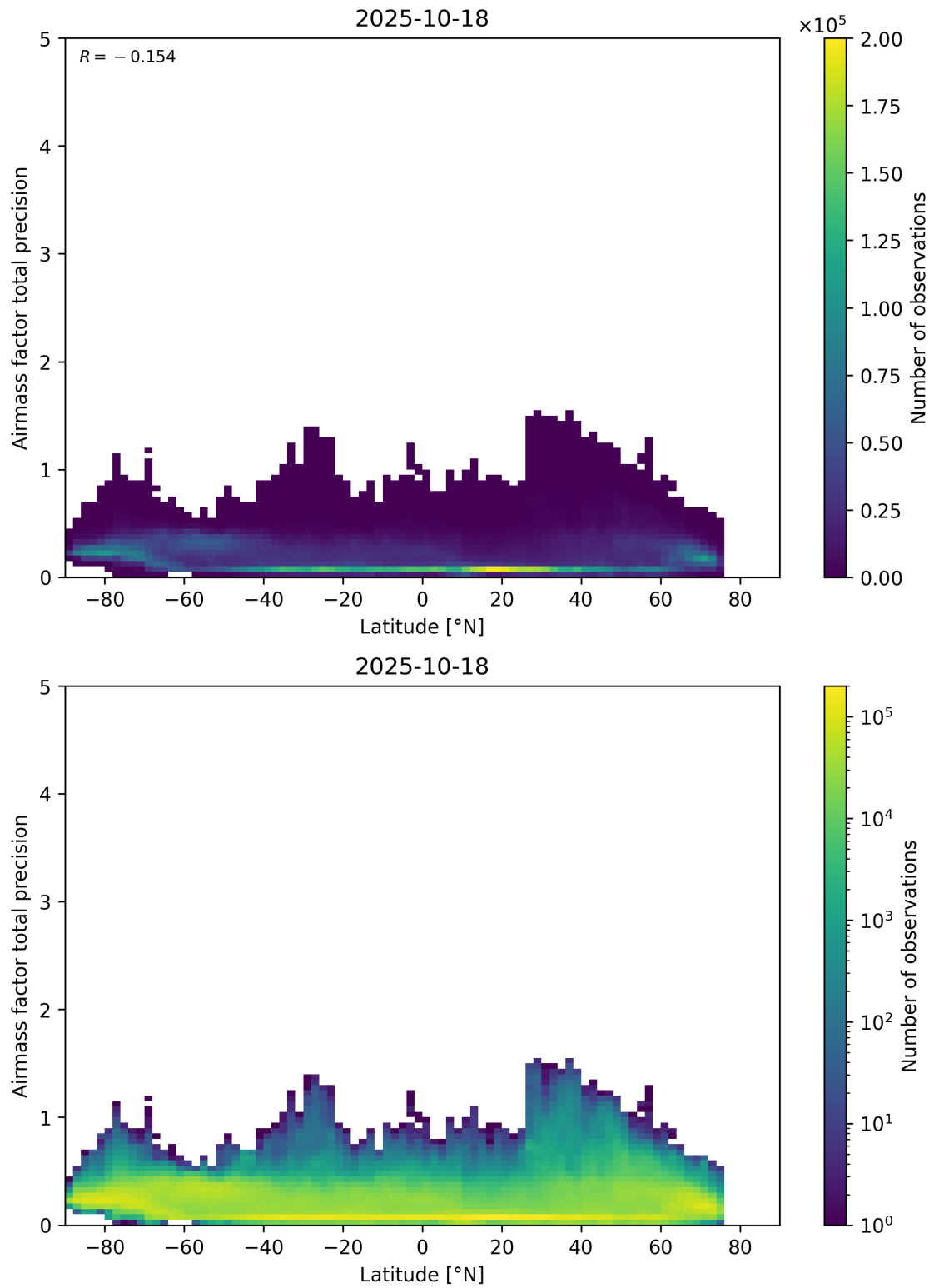
Figure 162: Scatter density plot of “Latitude” against “Airmass factor total precision” for 2025-10-17 to 2025-10-19.
