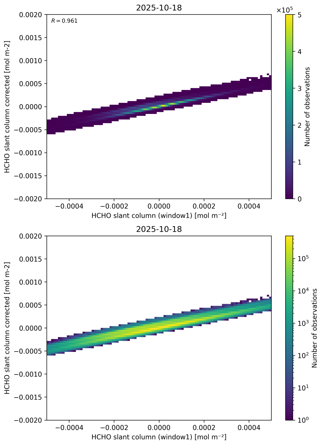
Figure 82: Scatter density plot of “HCHO slant column (window1)” against “HCHO slant column corrected” for 2025-10-17 to 2025-10-19.
