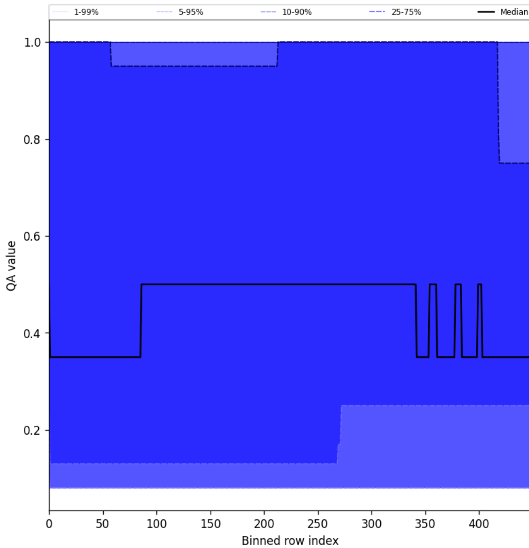
Figure 48: Along track statistics of “QA value” for 2025-10-17 to 2025-10-19
