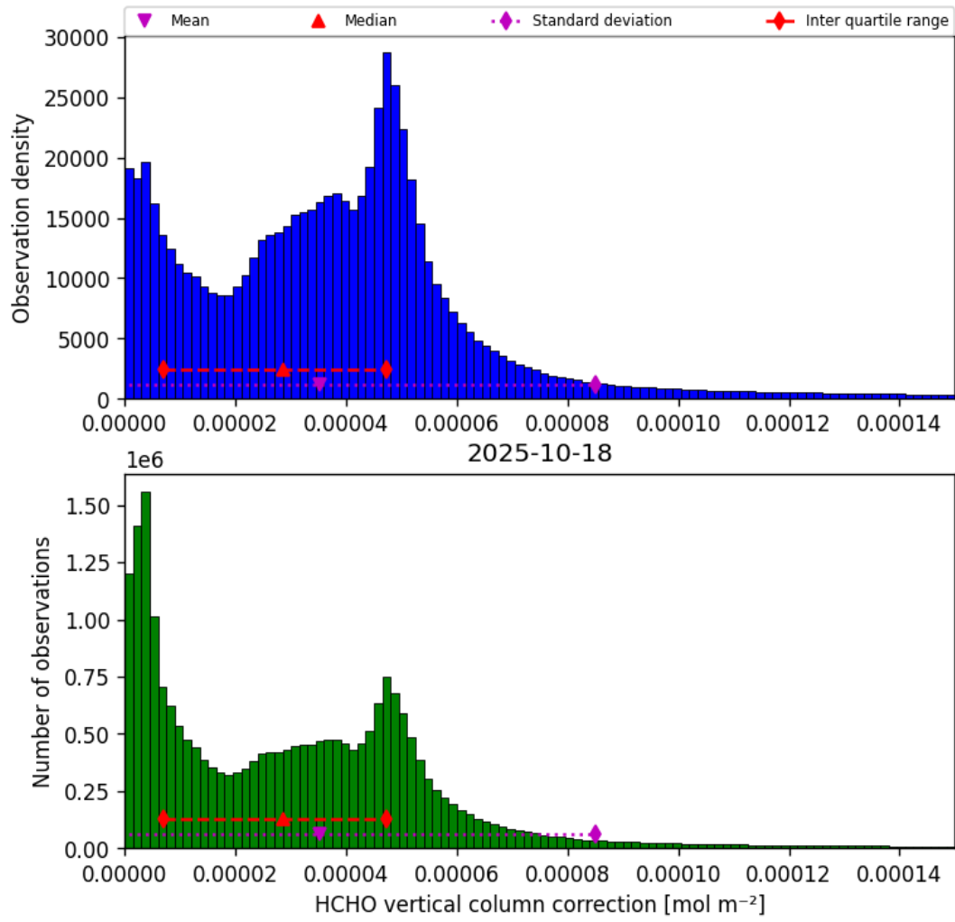
Figure 37: Histogram of “HCHO vertical column correction” for 2025-10-17 to 2025-10-19
