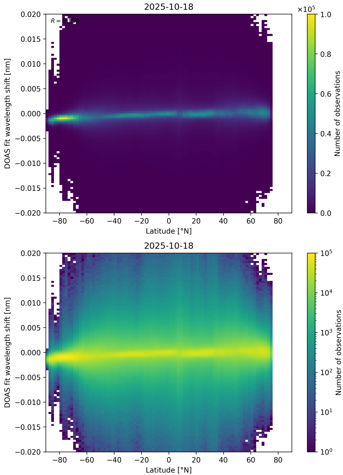
Figure 154: Scatter density plot of “Latitude” against “DOAS fit wavelength shift” for 2025-10-17 to 2025-10-19.
