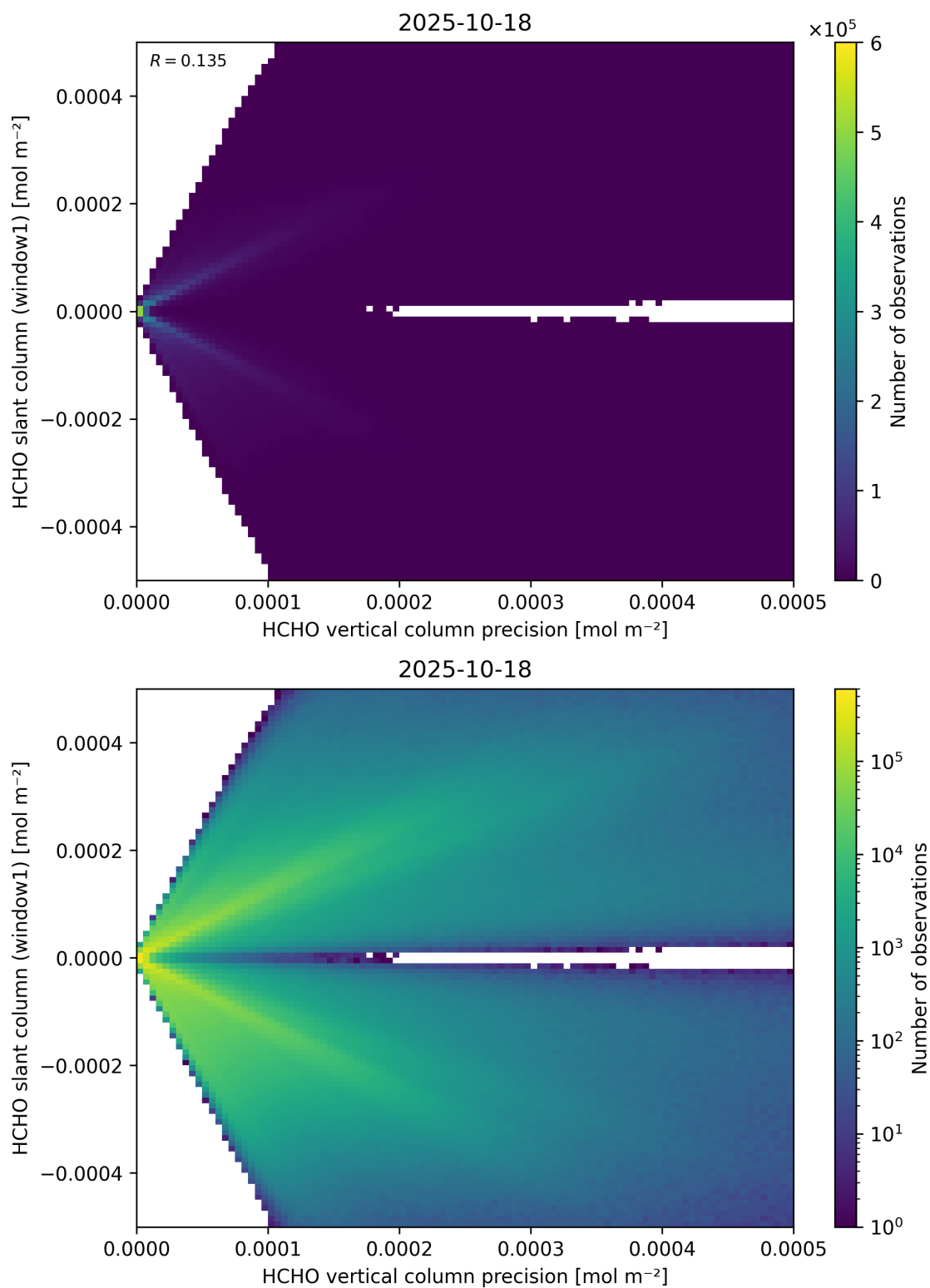
Figure 142: Scatter density plot of “HCHO vertical column precision” against “HCHO slant column (window1)” for 2025-10-17 to 2025-10-19.
