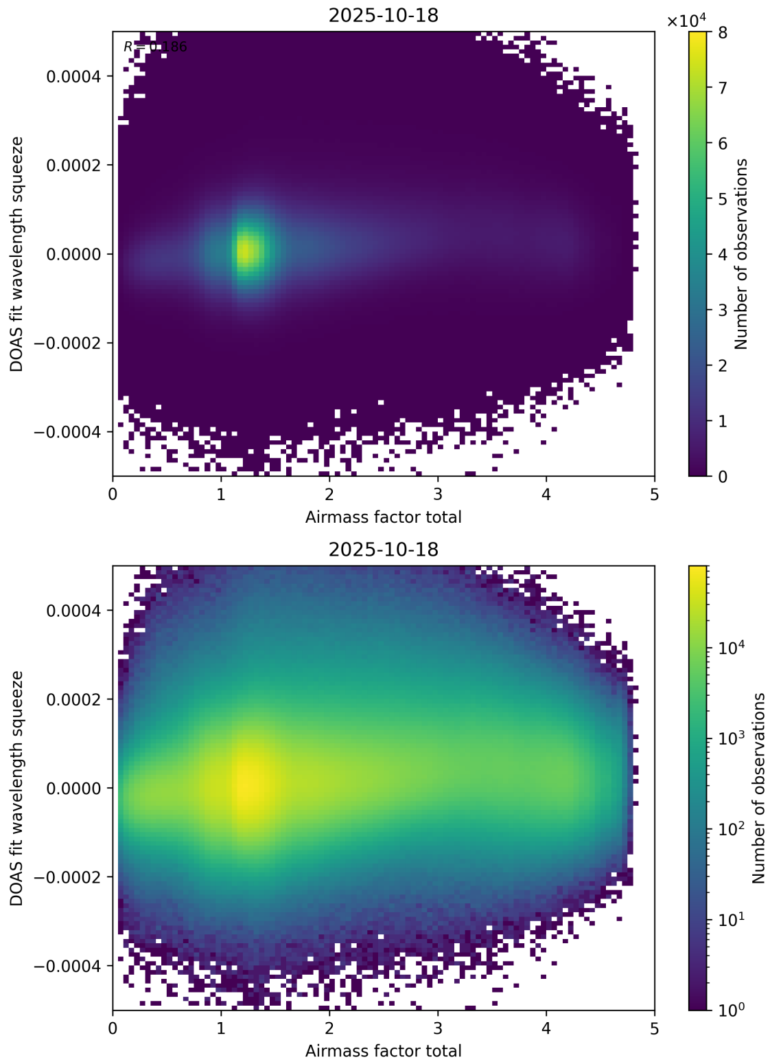
Figure 99: Scatter density plot of “Airmass factor total” against “DOAS fit wavelength squeeze” for 2025-10-17 to 2025-10-19.
