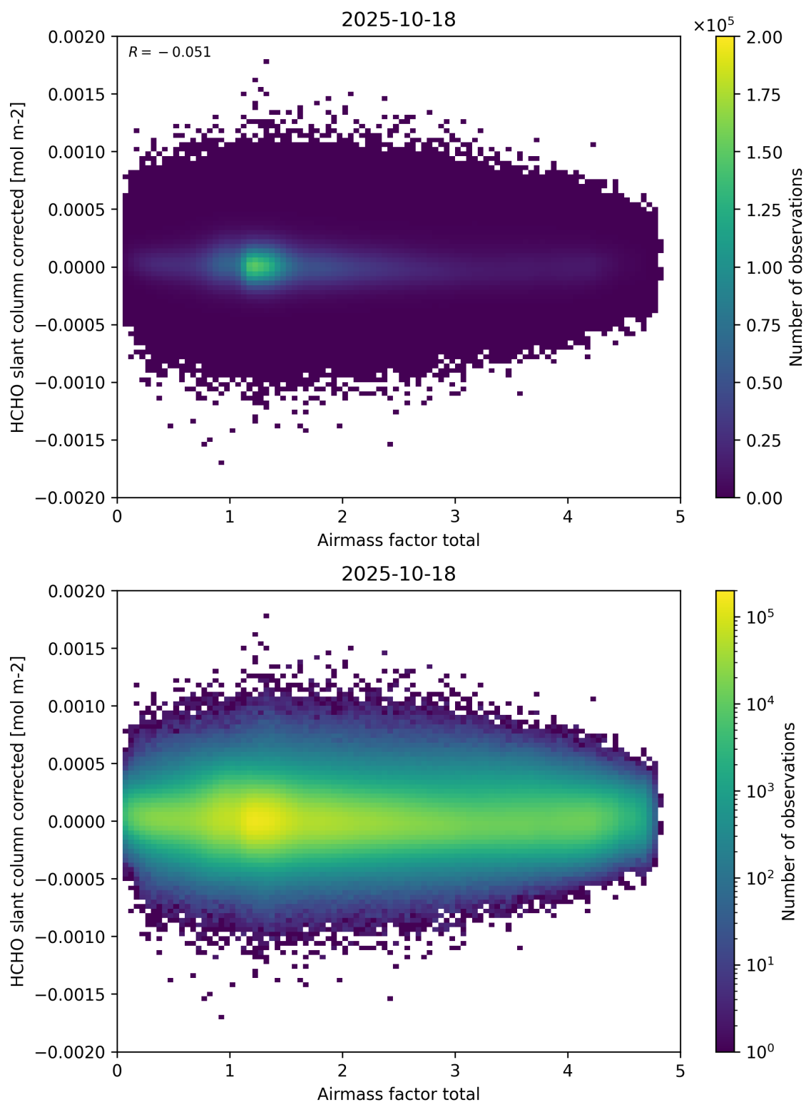
Figure 101: Scatter density plot of “Airmass factor total” against “HCHO slant column corrected” for 2025-10-17 to 2025-10-19.
