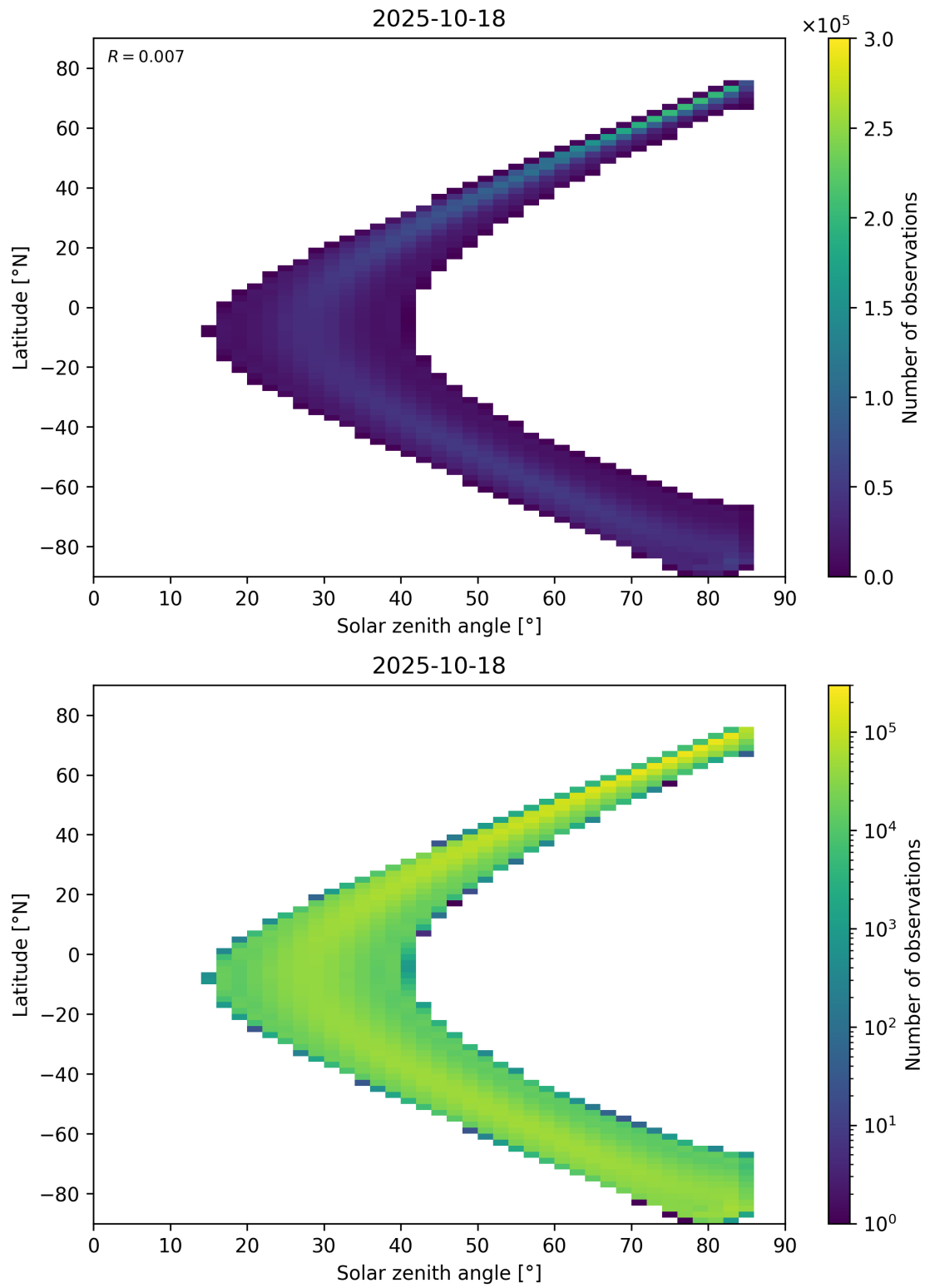
Figure 181: Scatter density plot of “Solar zenith angle” against “Latitude” for 2025-10-17 to 2025-10-19.
