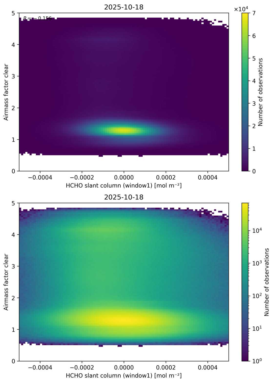
Figure 81: Scatter density plot of “HCHO slant column (window1)” against “Airmass factor clear” for 2025-10-17 to 2025-10-19.
