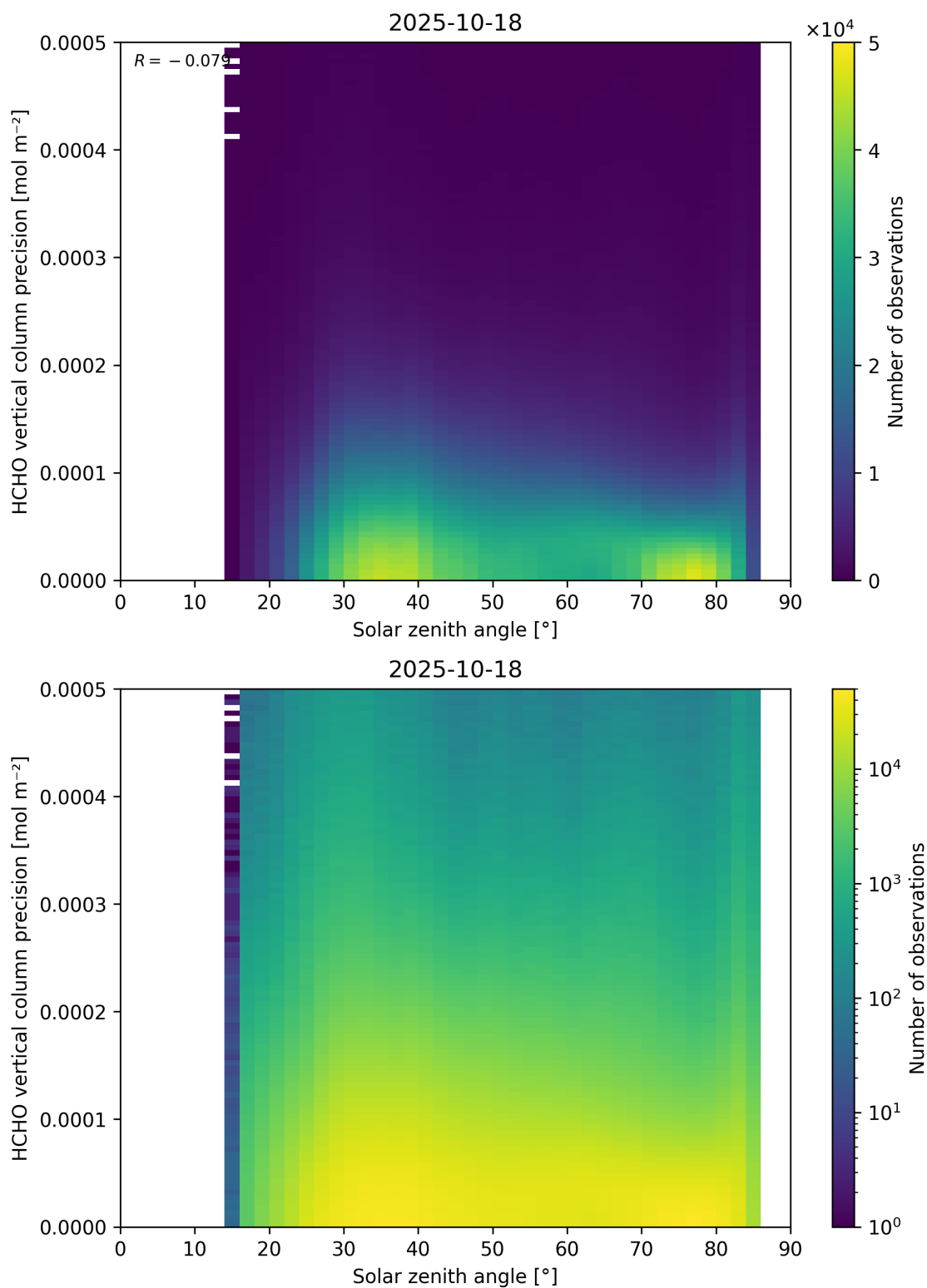
Figure 179: Scatter density plot of “Solar zenith angle” against “HCHO vertical column precision” for 2025-10-17 to 2025-10-19.
