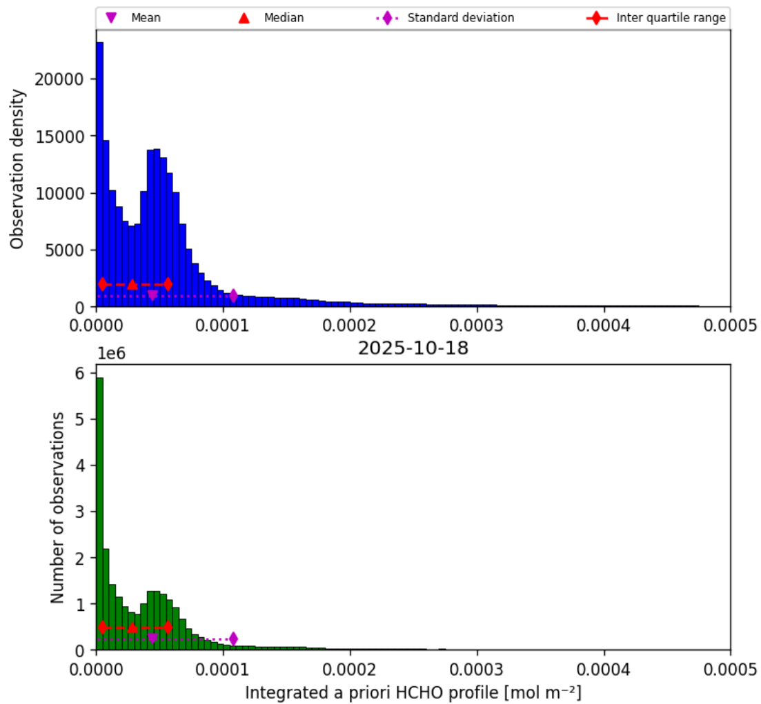
Figure 43: Histogram of “Integrated a priori HCHO profile” for 2025-10-17 to 2025-10-19
