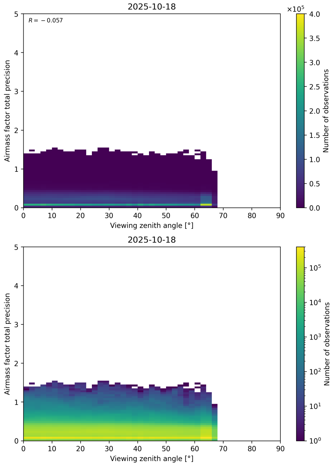
Figure 191: Scatter density plot of “Viewing zenith angle” against “Airmass factor total precision” for 2025-10-17 to 2025-10-19.
