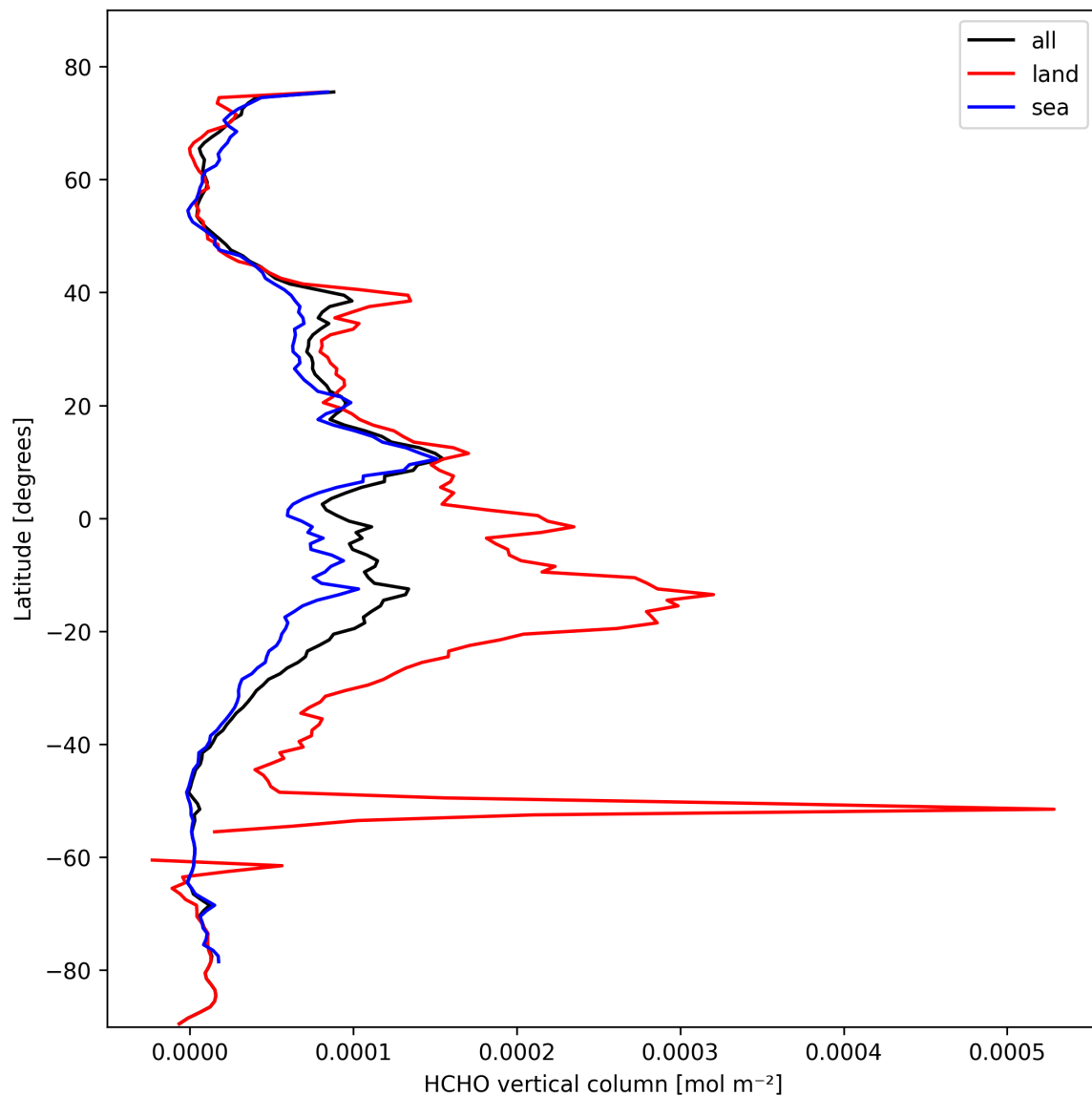
Figure 21: Zonal average of “HCHO vertical column” for 2025-10-17 to 2025-10-19.
