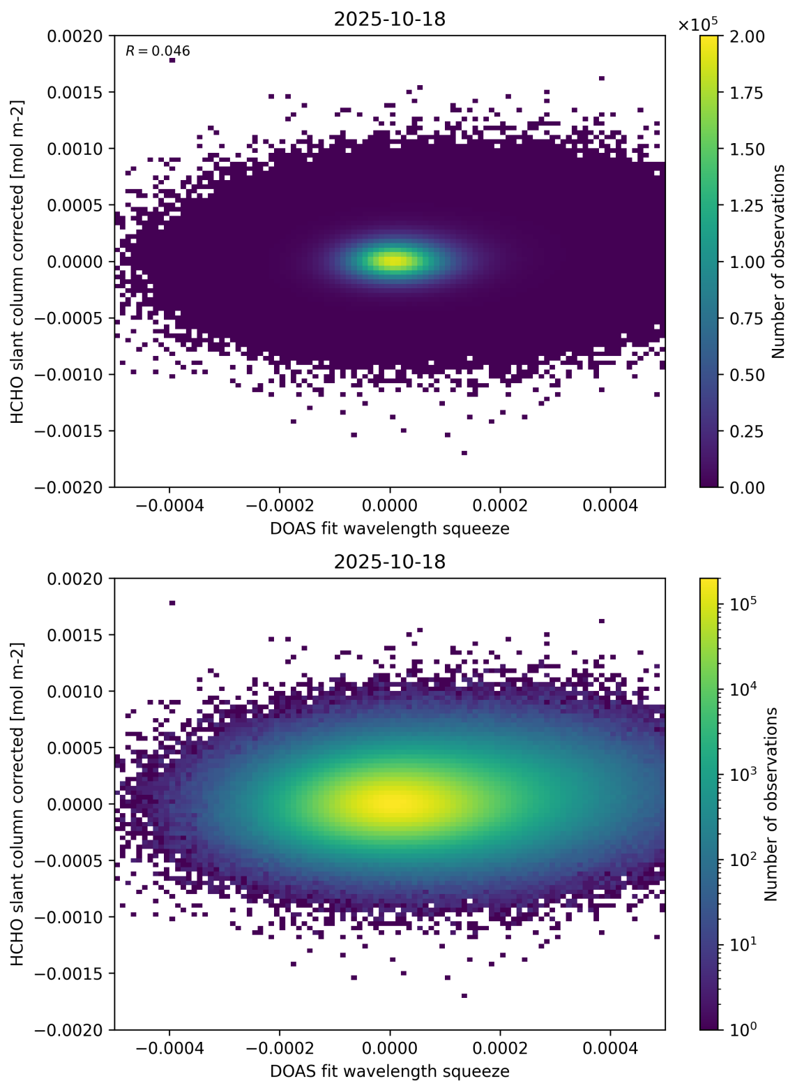
Figure 69: Scatter density plot of “DOAS fit wavelength squeeze” against “HCHO slant column corrected” for 2025-10-17 to 2025-10-19.
