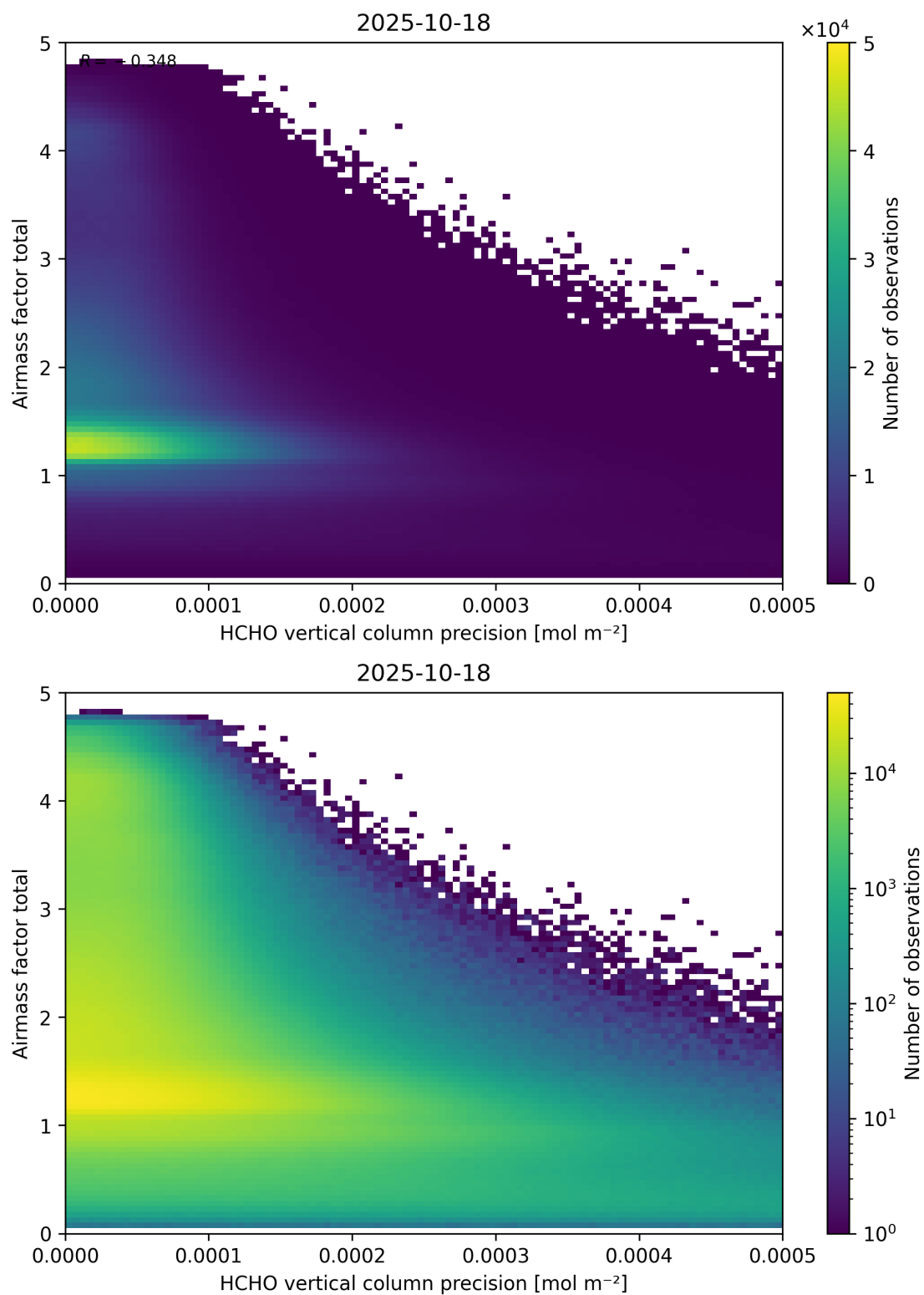
Figure 144: Scatter density plot of “HCHO vertical column precision” against “Airmass factor total” for 2025-10-17 to 2025-10-19.
