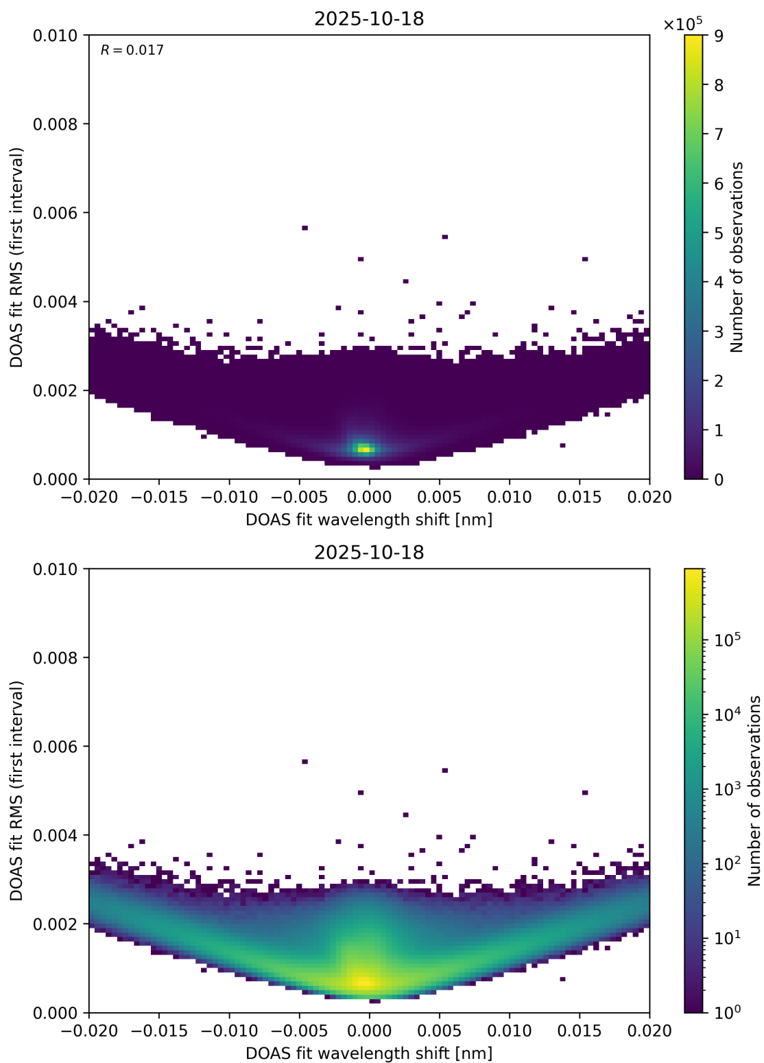
Figure 64: Scatter density plot of “DOAS fit wavelength shift” against “DOAS fit RMS (first interval)” for 2025-10-17 to 2025-10-19.
