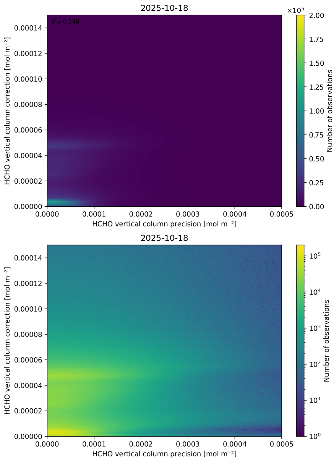
Figure 146: Scatter density plot of “HCHO vertical column precision” against “HCHO vertical column correction” for 2025-10-17 to 2025-10-19.
