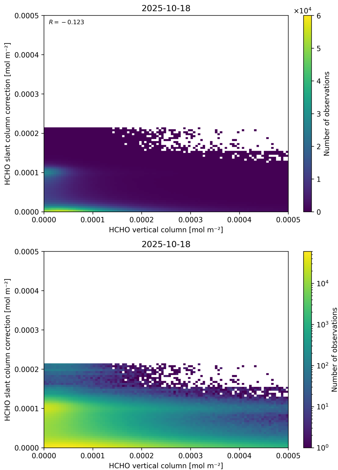
Figure 128: Scatter density plot of “HCHO vertical column” against “HCHO slant column correction” for 2025-10-17 to 2025-10-19.
