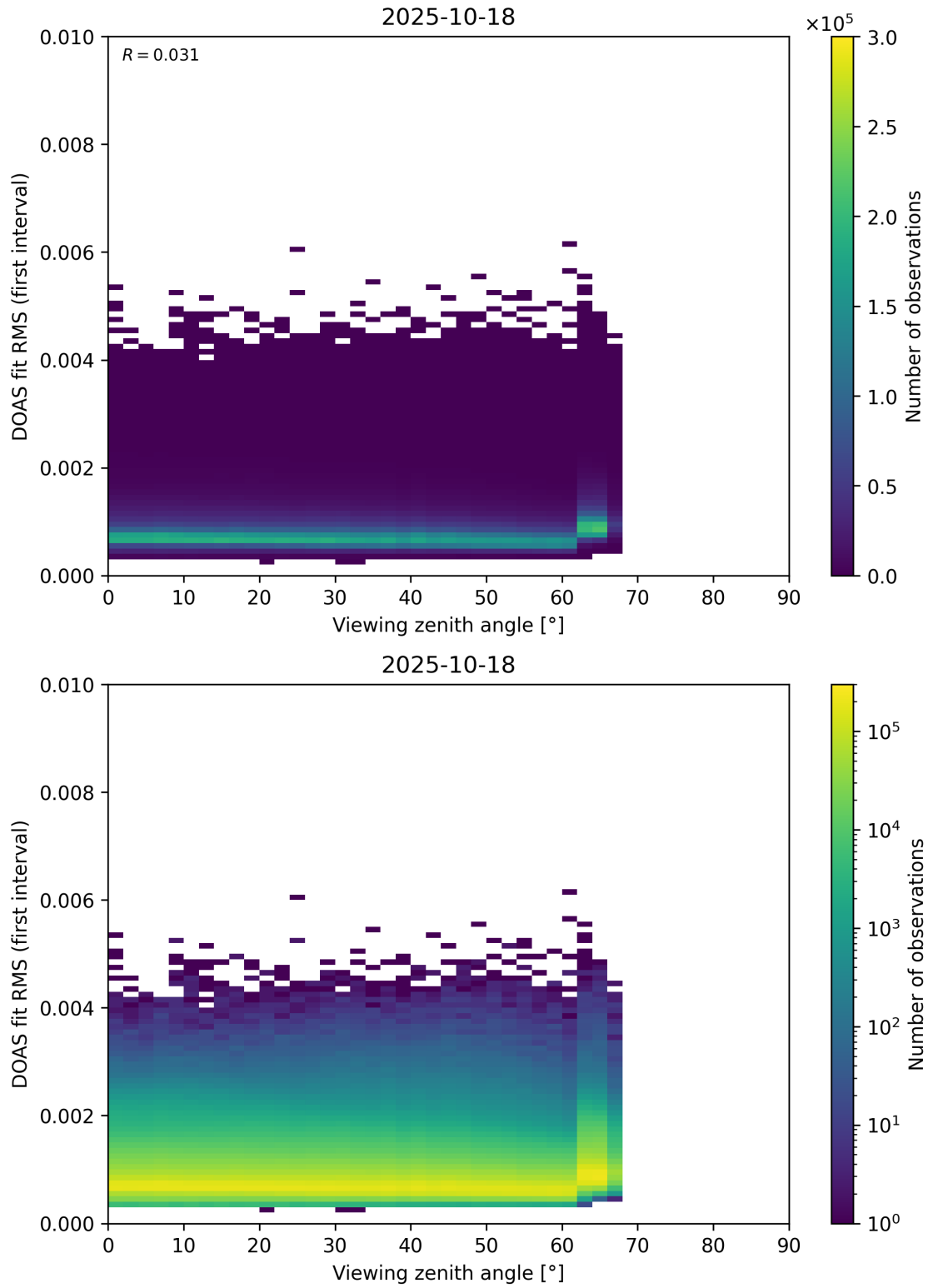
Figure 182: Scatter density plot of “Viewing zenith angle” against “DOAS fit RMS (first interval)” for 2025-10-17 to 2025-10-19.
