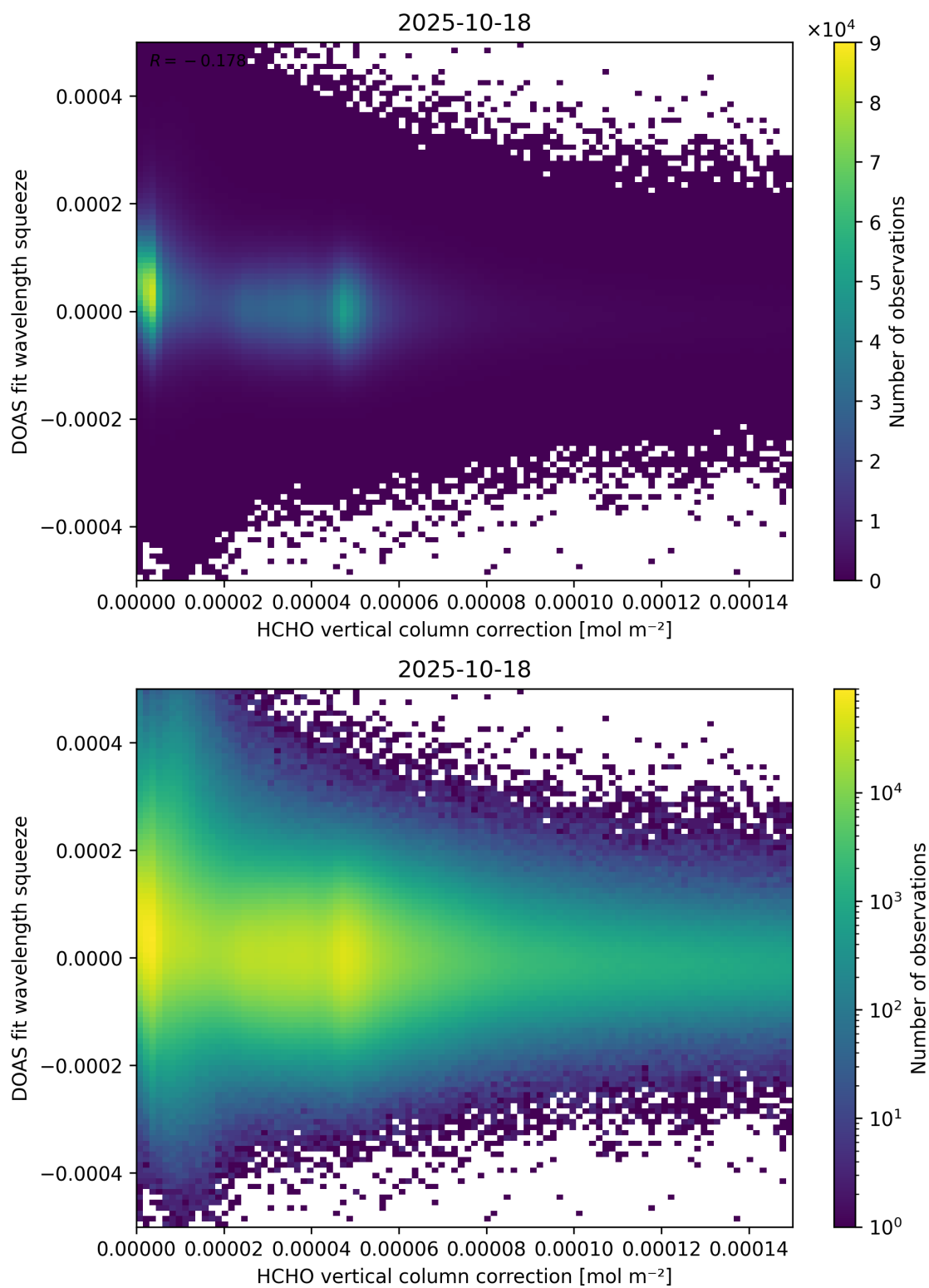
Figure 114: Scatter density plot of “HCHO vertical column correction” against “DOAS fit wavelength squeeze” for 2025-10-17 to 2025-10-19.
