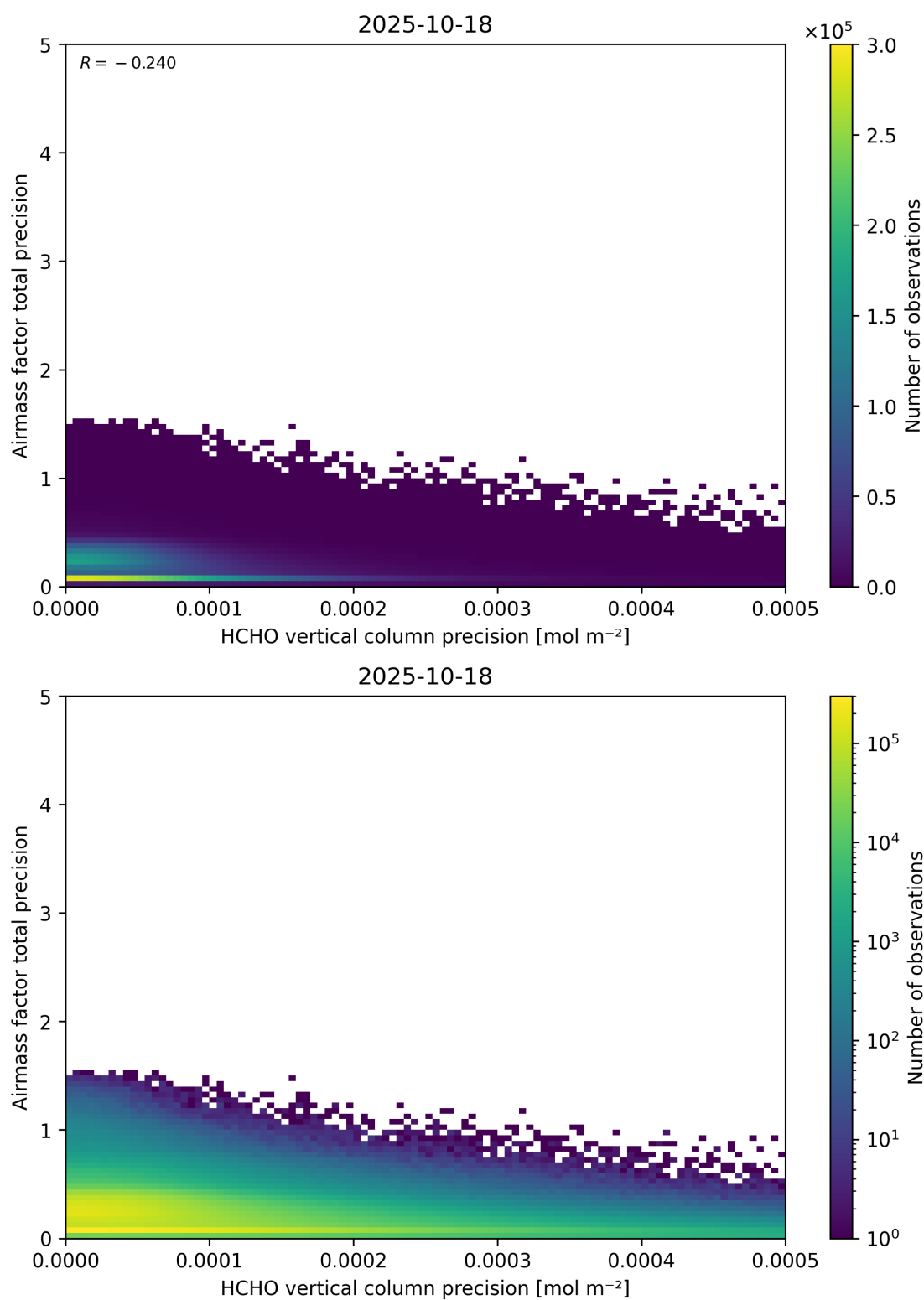
Figure 145: Scatter density plot of “HCHO vertical column precision” against “Airmass factor total precision” for 2025-10-17 to 2025-10-19.
