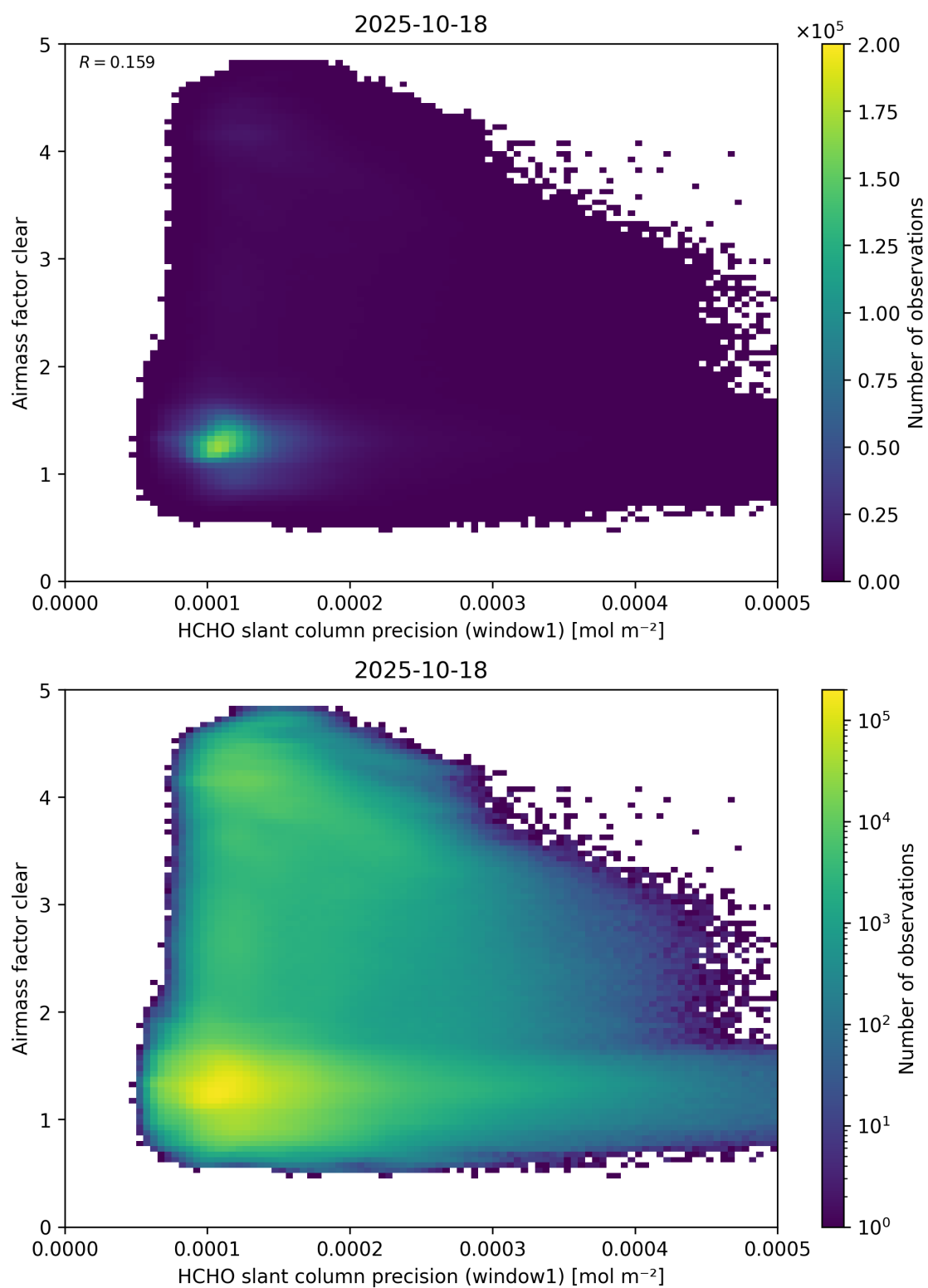
Figure 91: Scatter density plot of “HCHO slant column precision (window1)” against “Airmass factor clear” for 2025-10-17 to 2025-10-19.
