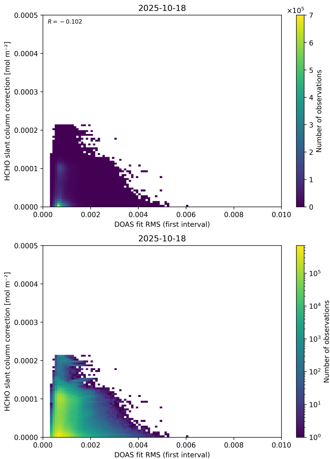
Figure 63: Scatter density plot of “DOAS fit RMS (first interval)” against “HCHO slant column correction” for 2025-10-17 to 2025-10-19.
