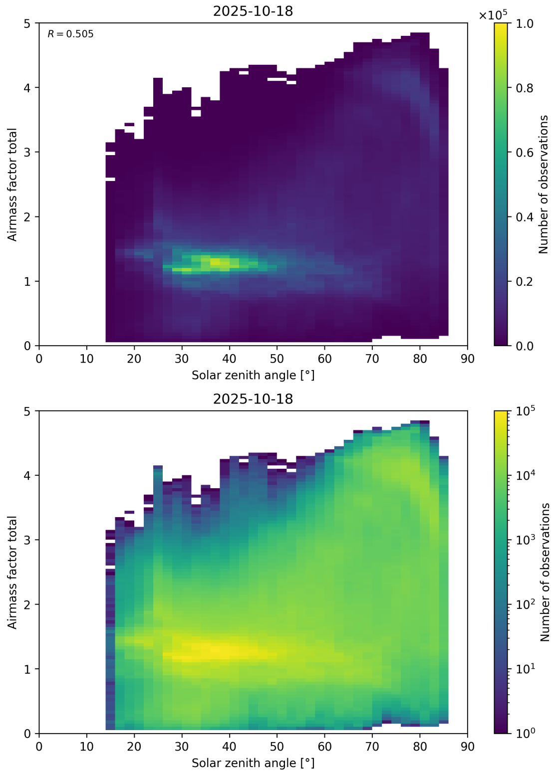
Figure 175: Scatter density plot of “Solar zenith angle” against “Airmass factor total” for 2025-10-17 to 2025-10-19.
