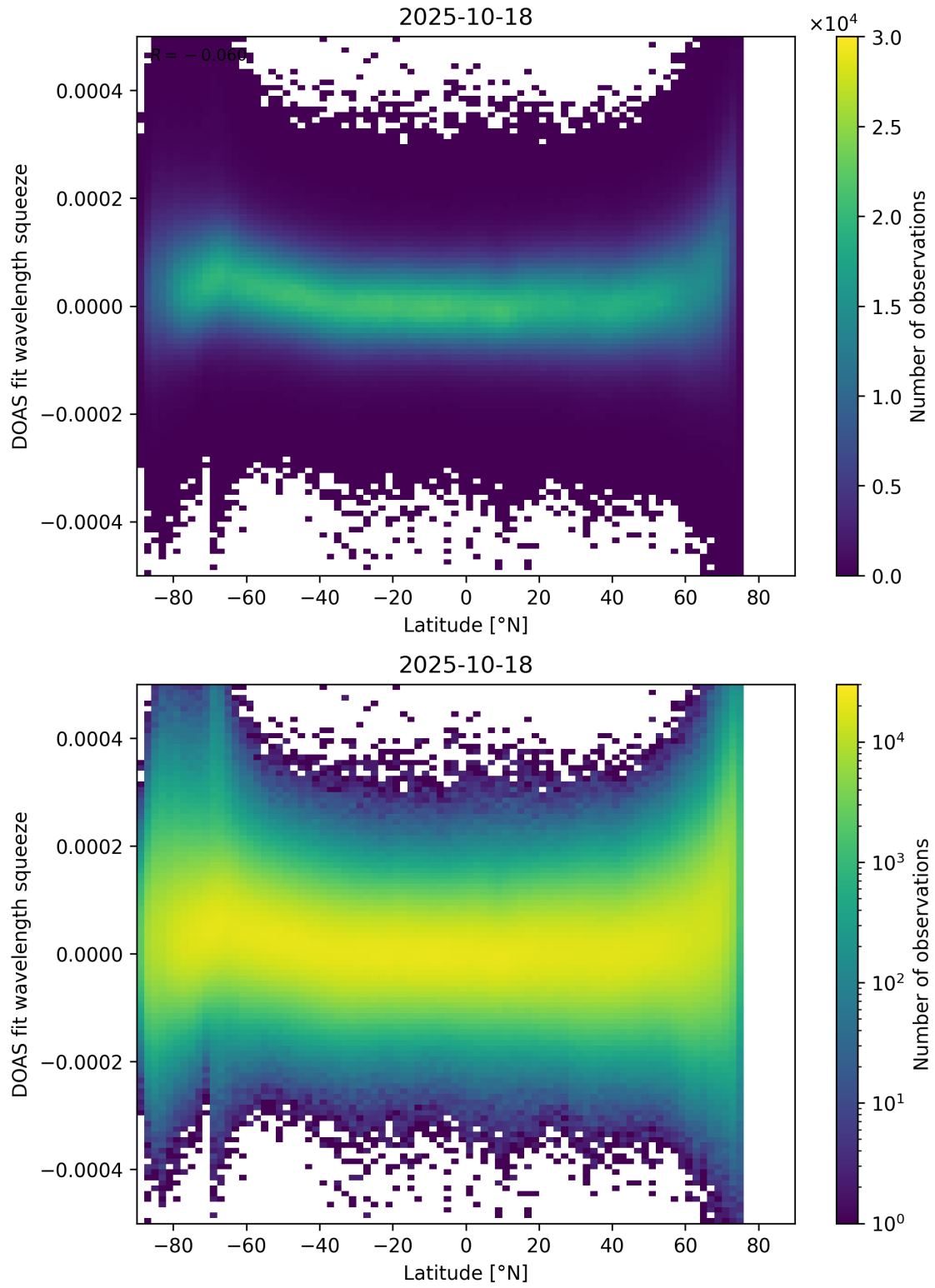
Figure 155: Scatter density plot of “Latitude” against “DOAS fit wavelength squeeze” for 2025-10-17 to 2025-10-19.
