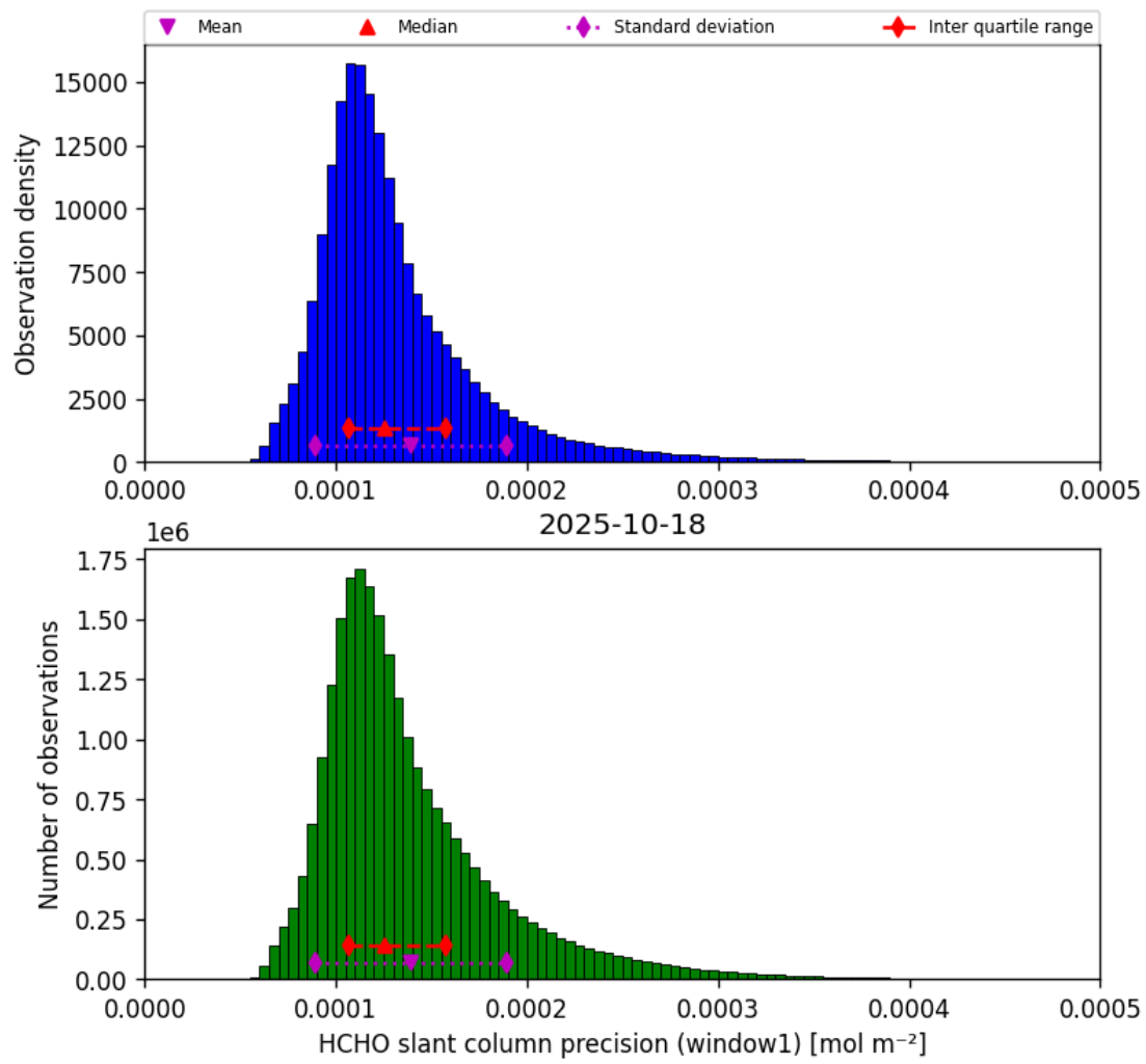
Figure 39: Histogram of “HCHO slant column precision (window1)” for 2025-10-17 to 2025-10-19
