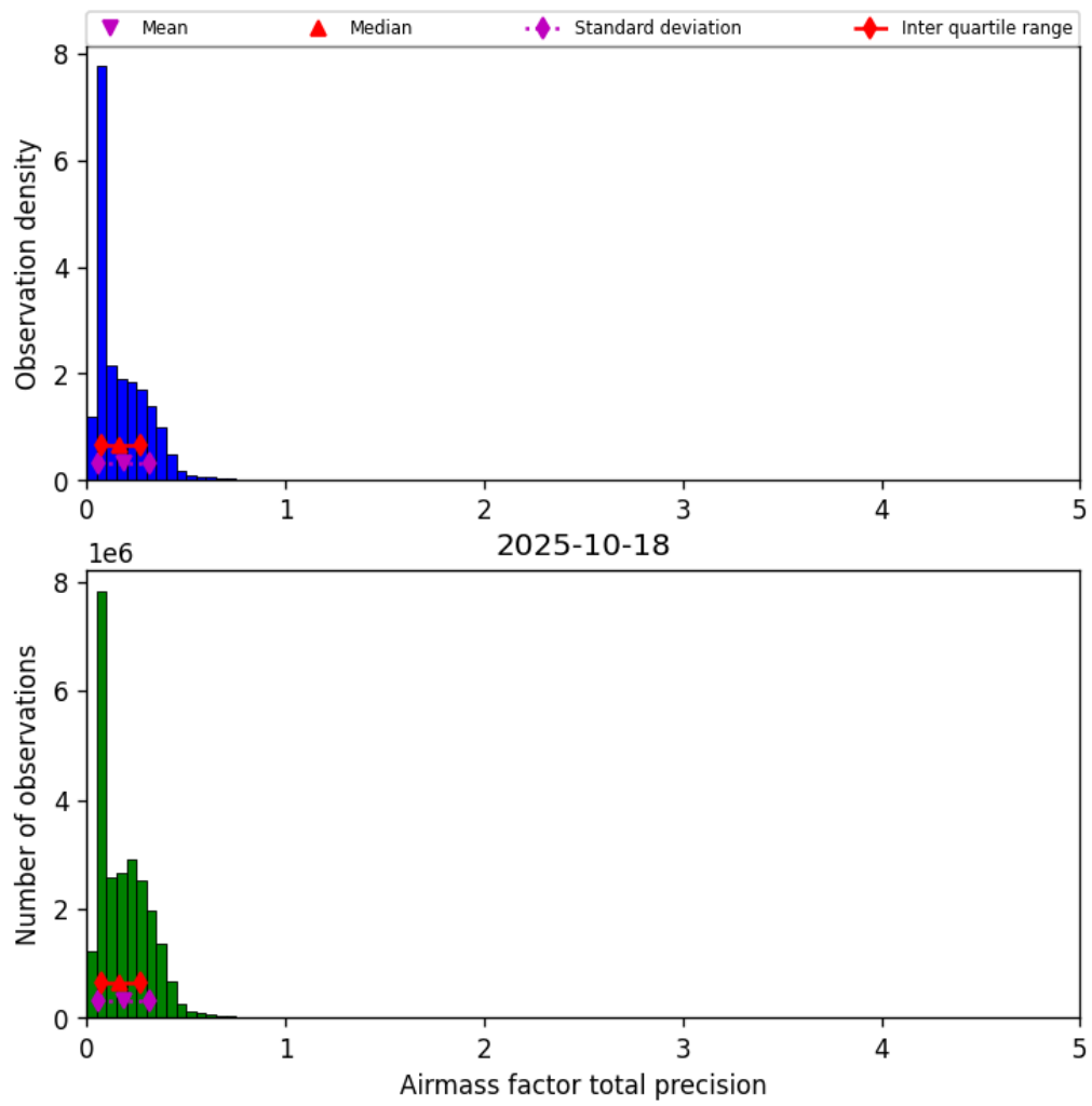
Figure 41: Histogram of “Airmass factor total precision” for 2025-10-17 to 2025-10-19
