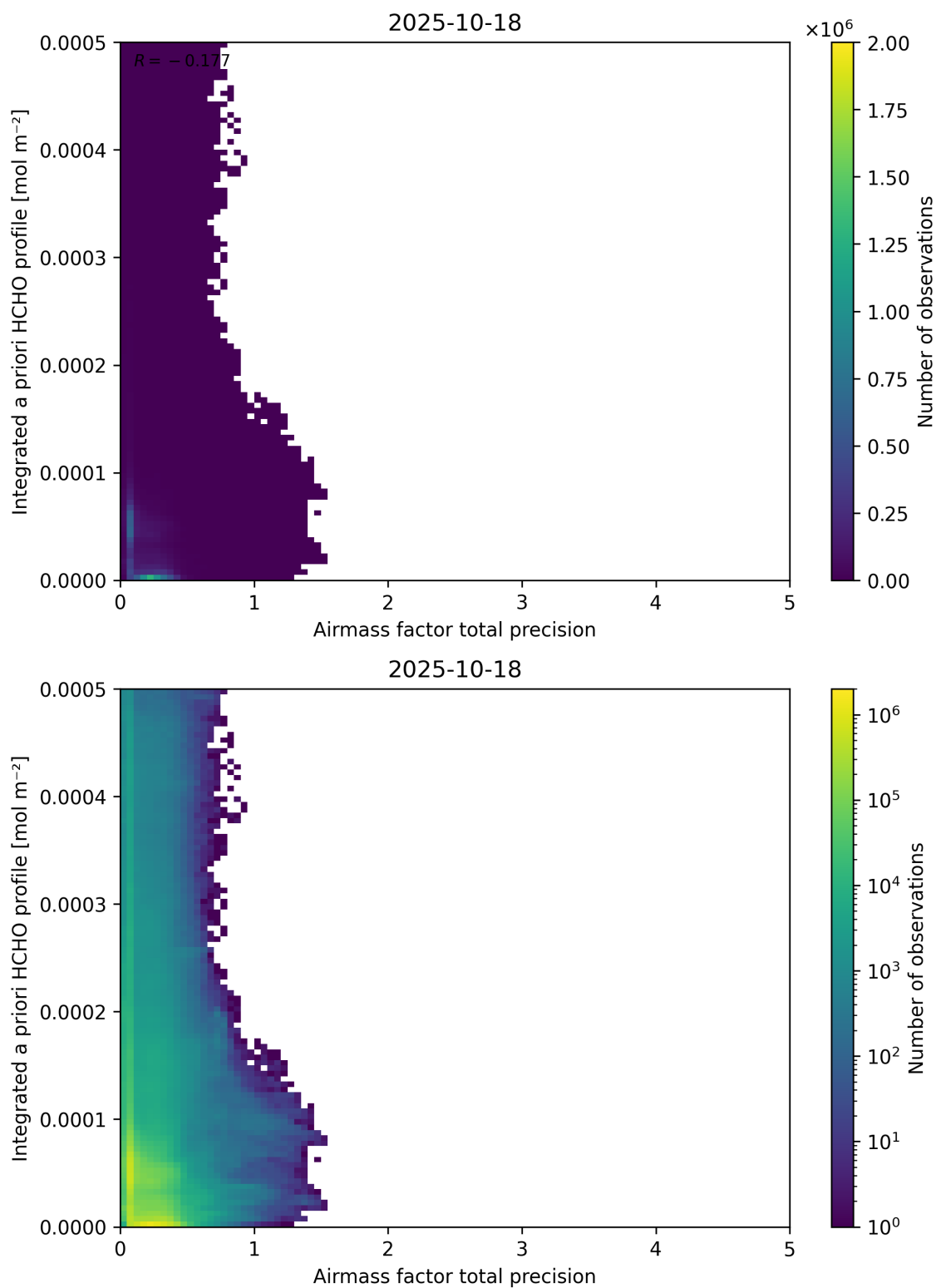
Figure 111: Scatter density plot of “Airmass factor total precision” against “Integrated a priori HCHO profile” for 2025-10-17 to 2025-10-19.
