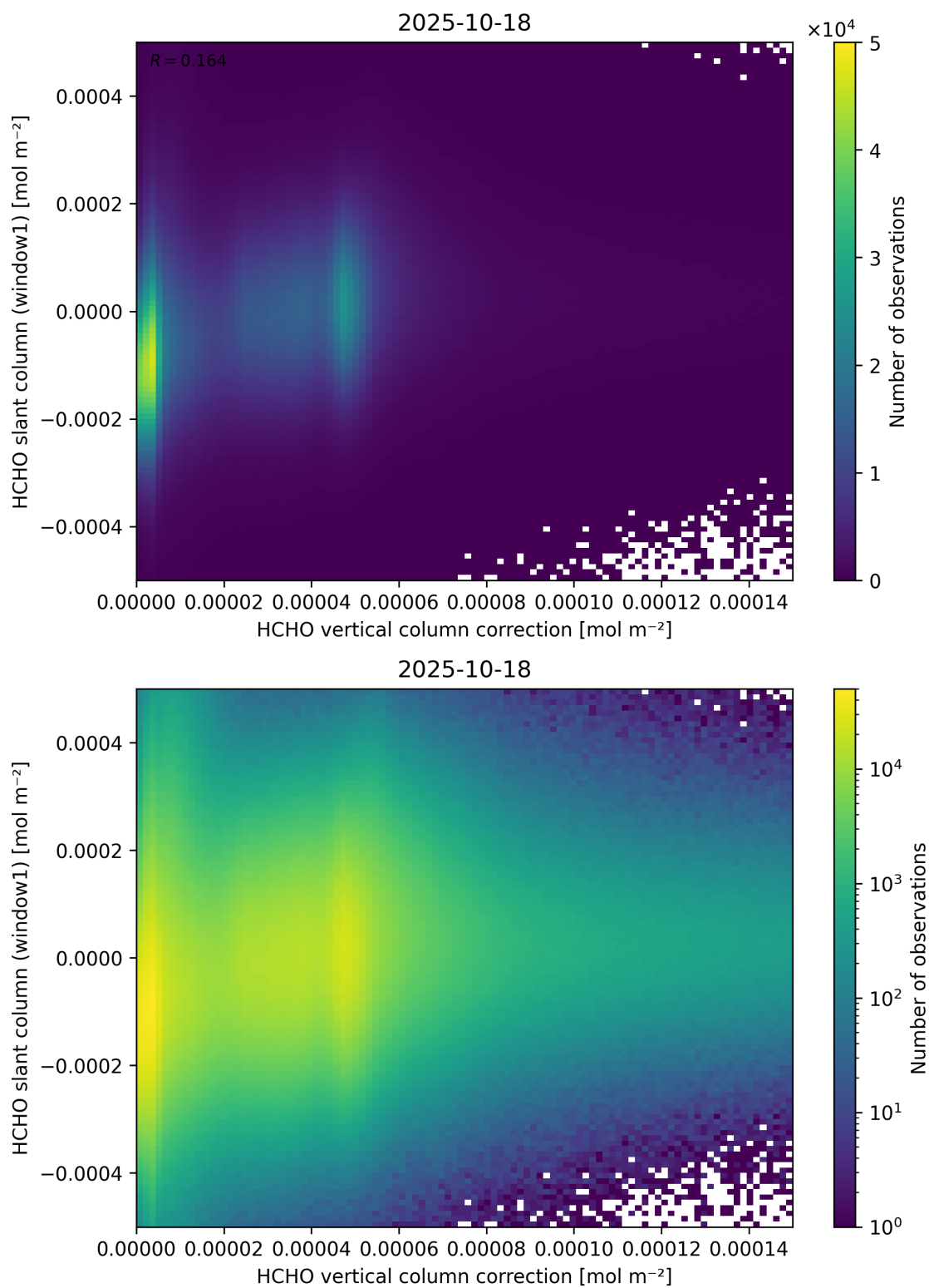
Figure 118: Scatter density plot of “HCHO vertical column correction” against “HCHO slant column (window1)” for 2025-10-17 to 2025-10-19.
