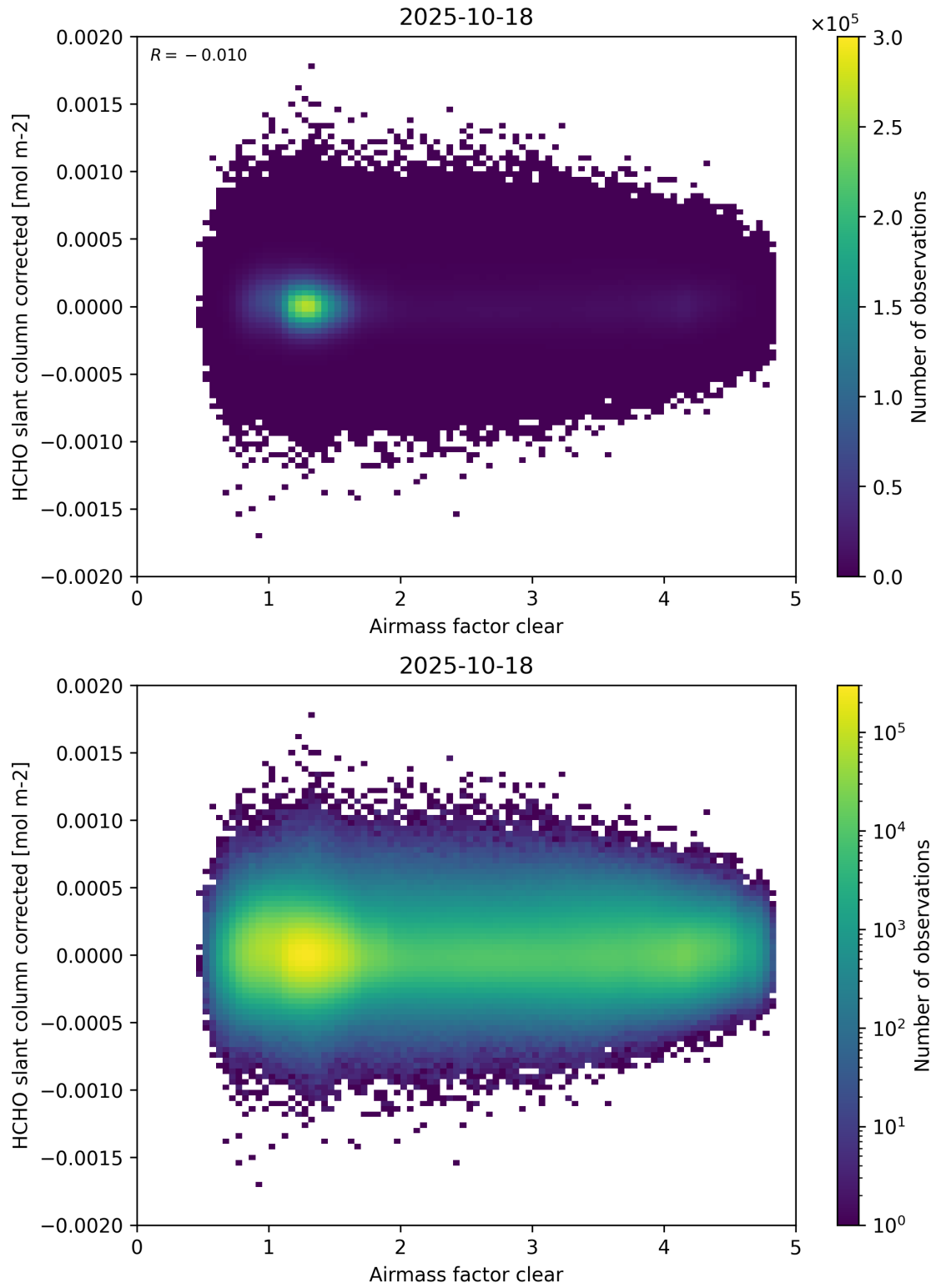
Figure 74: Scatter density plot of “Airmass factor clear” against “HCHO slant column corrected” for 2025-10-17 to 2025-10-19.
