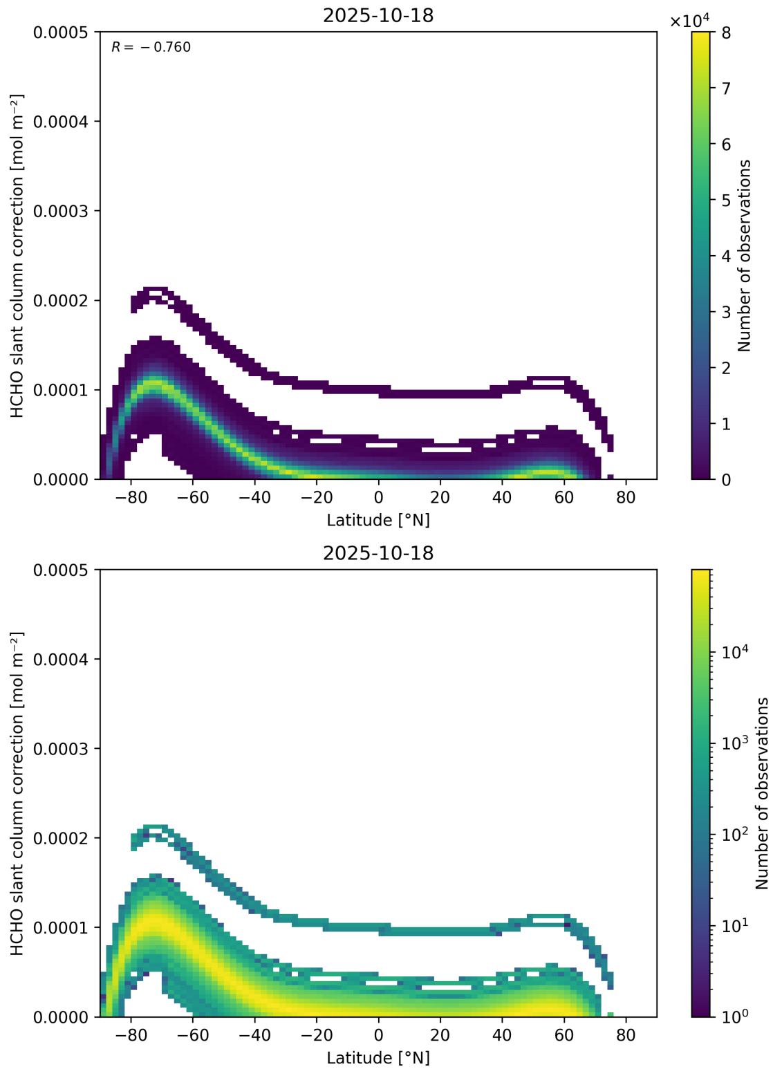
Figure 158: Scatter density plot of “Latitude” against “HCHO slant column correction” for 2025-10-17 to 2025-10-19.
