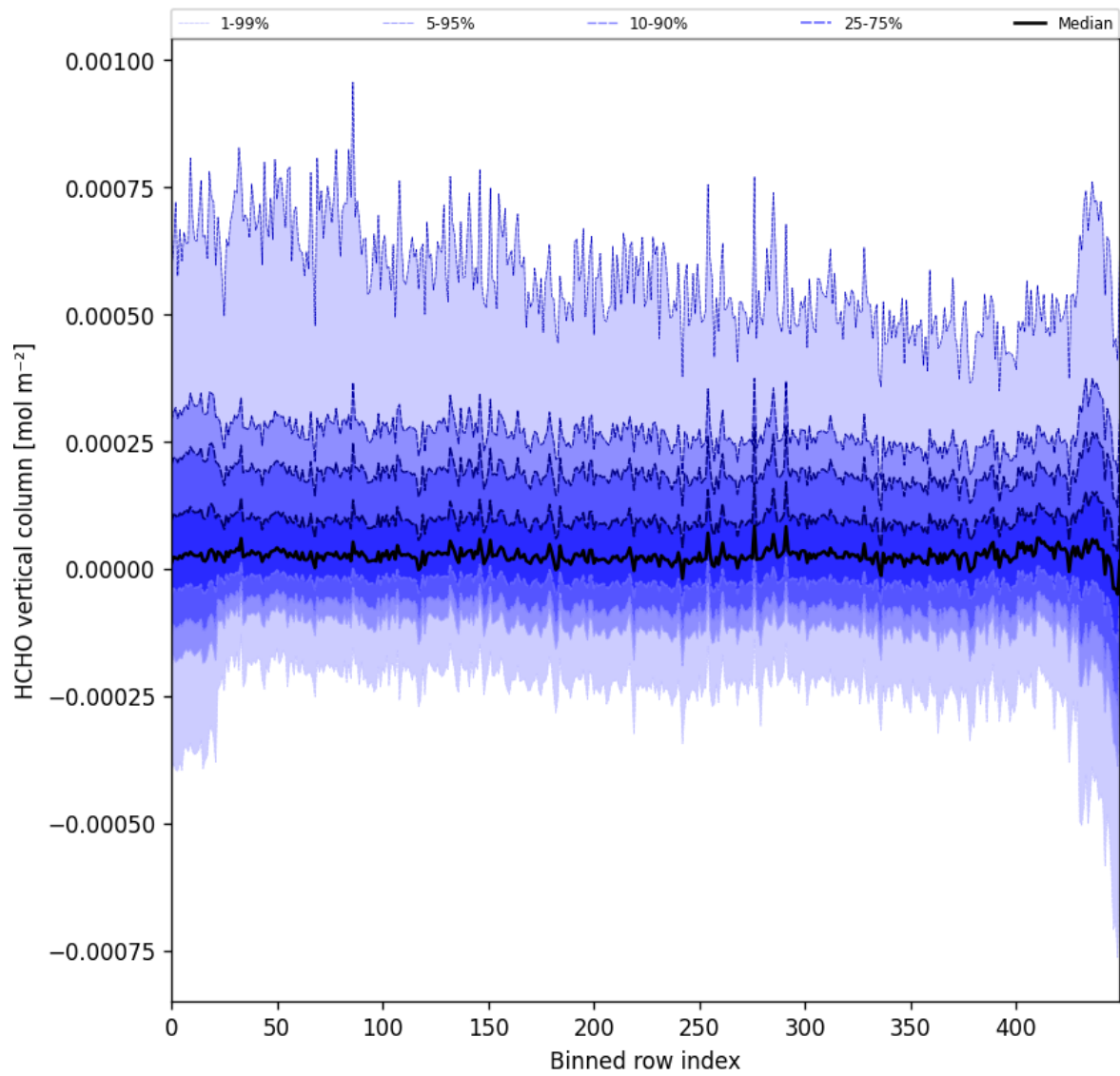
Figure 49: Along track statistics of “HCHO vertical column” for 2025-10-17 to 2025-10-19
