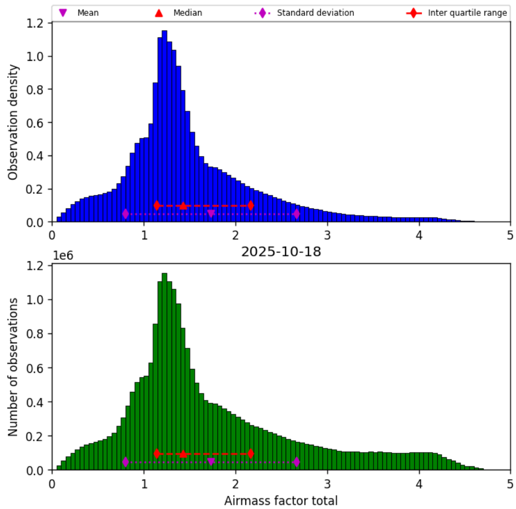
Figure 40: Histogram of “Airmass factor total” for 2025-10-17 to 2025-10-19
