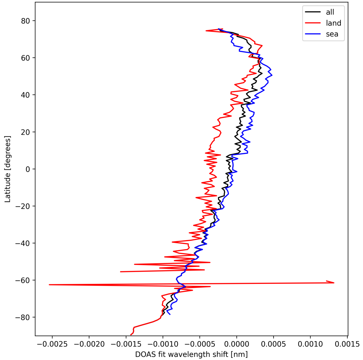
Figure 30: Zonal average of “DOAS fit wavelength shift” for 2025-10-17 to 2025-10-19.
