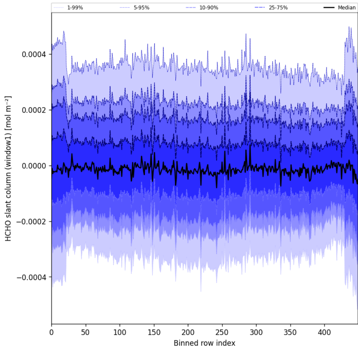
Figure 52: Along track statistics of "HCHO slant column (window1)" for 2025-10-17 to 2025-10-19
