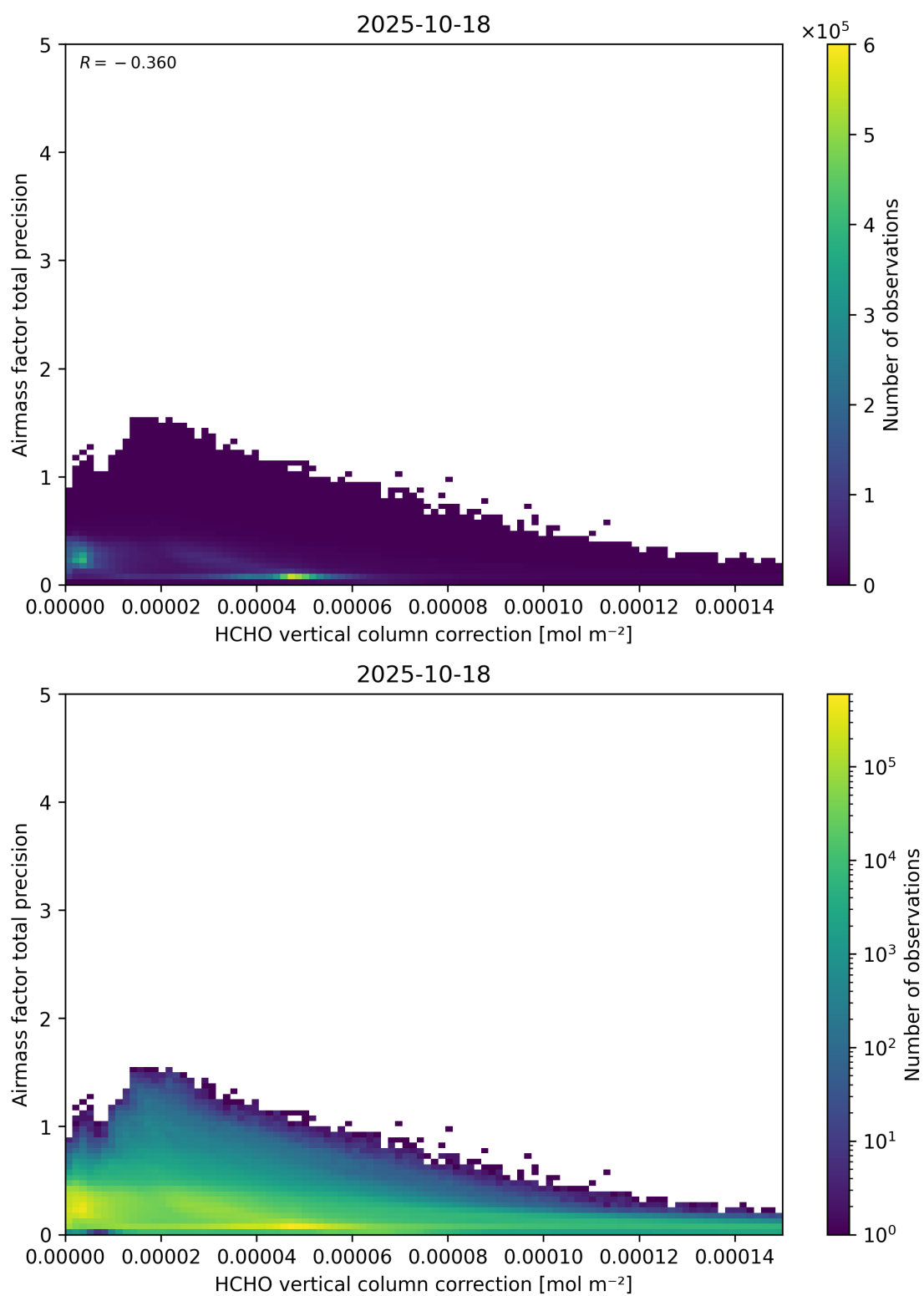
Figure 121: Scatter density plot of “HCHO vertical column correction” against “Airmass factor total precision” for 2025-10-17 to 2025-10-19.
