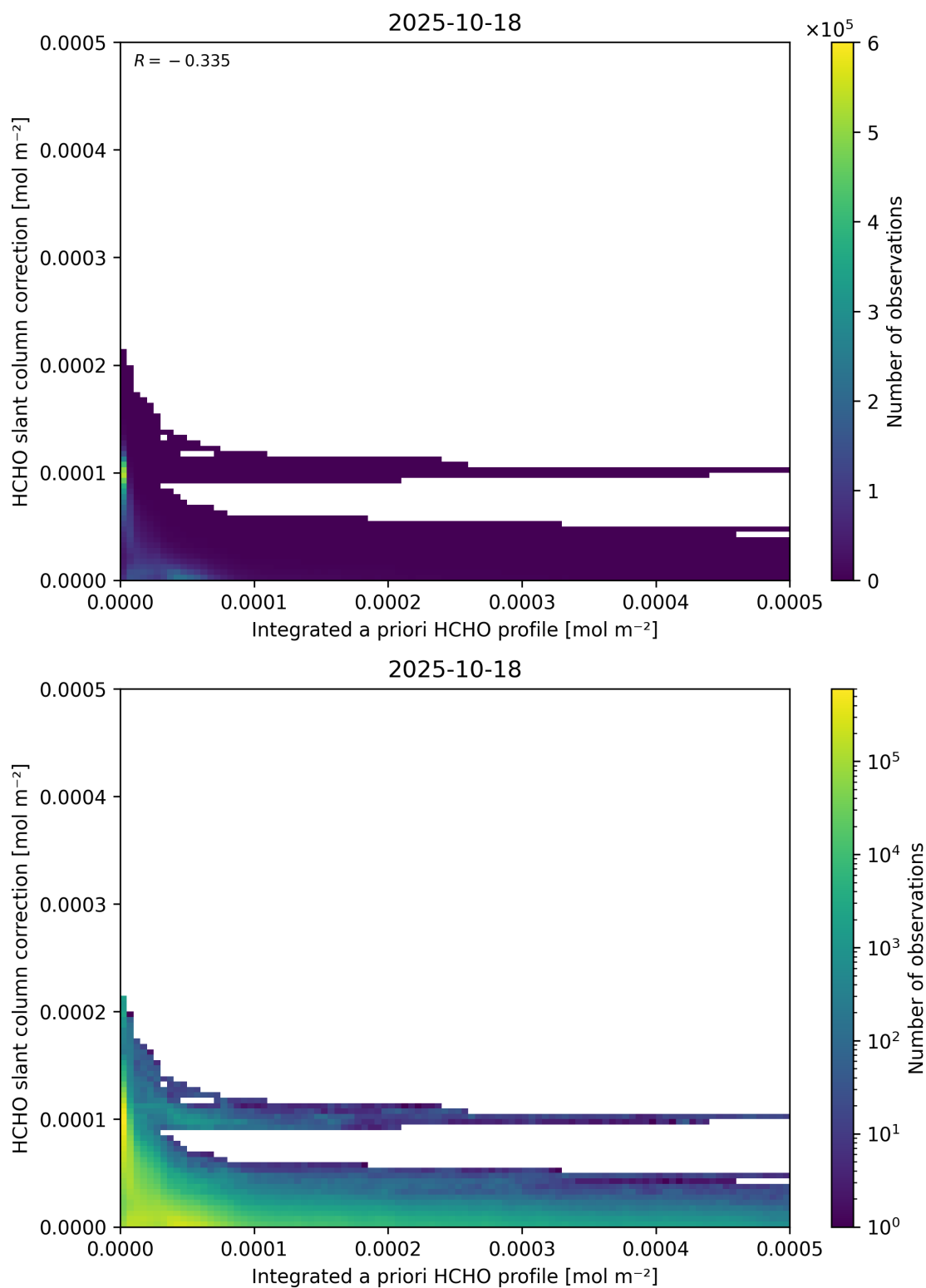
Figure 152: Scatter density plot of “Integrated a priori HCHO profile” against “HCHO slant column correction” for 2025-10-17 to 2025-10-19.
