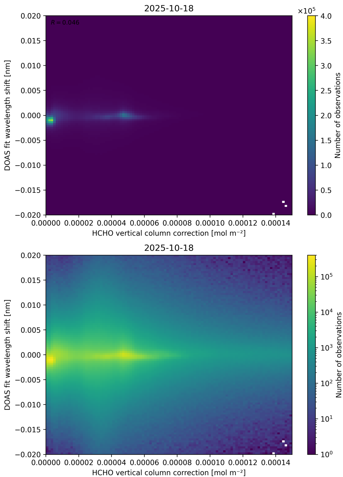
Figure 113: Scatter density plot of “HCHO vertical column correction” against “DOAS fit wavelength shift” for 2025-10-17 to 2025-10-19.
