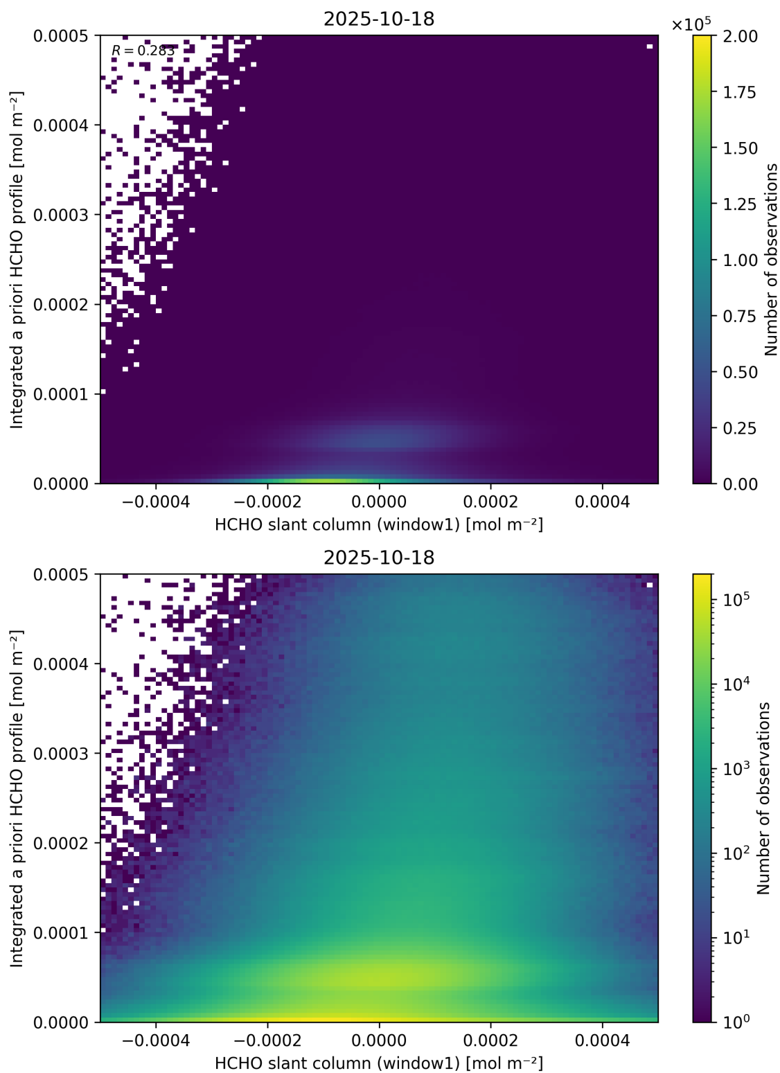
Figure 87: Scatter density plot of “HCHO slant column (window1)” against “Integrated a priori HCHO profile” for 2025-10-17 to 2025-10-19.
