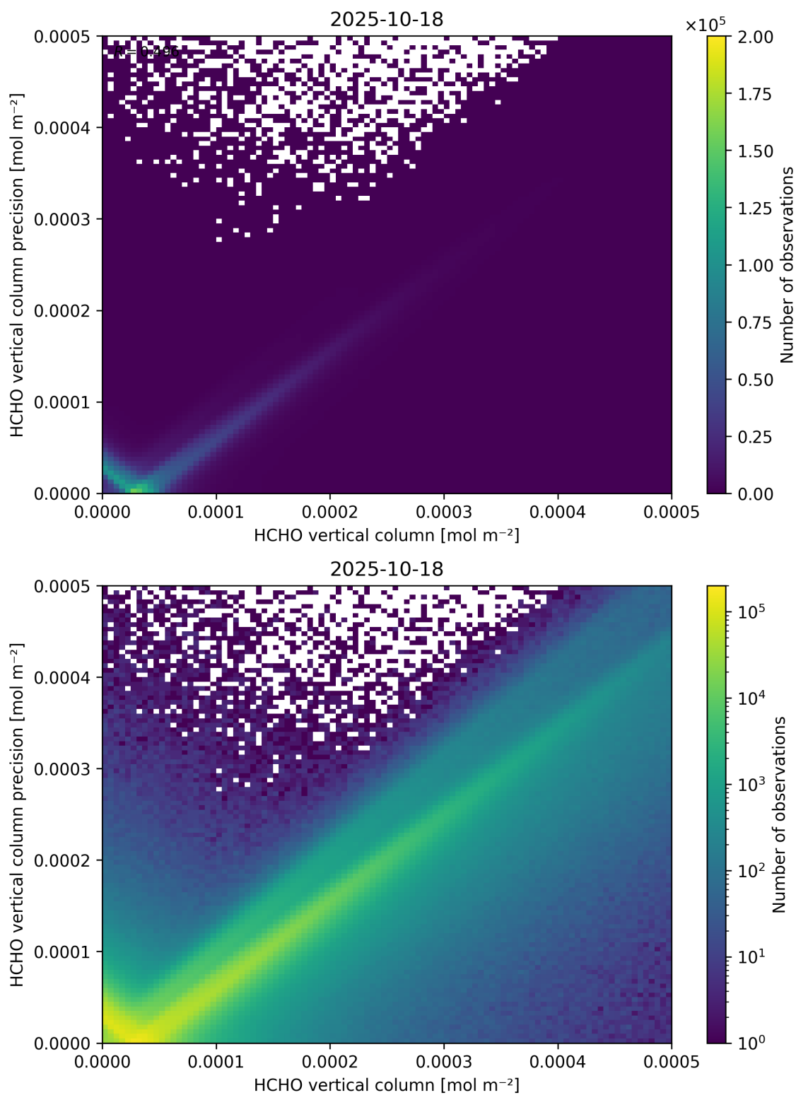
Figure 134: Scatter density plot of “HCHO vertical column” against “HCHO vertical column precision” for 2025-10-17 to 2025-10-19.
