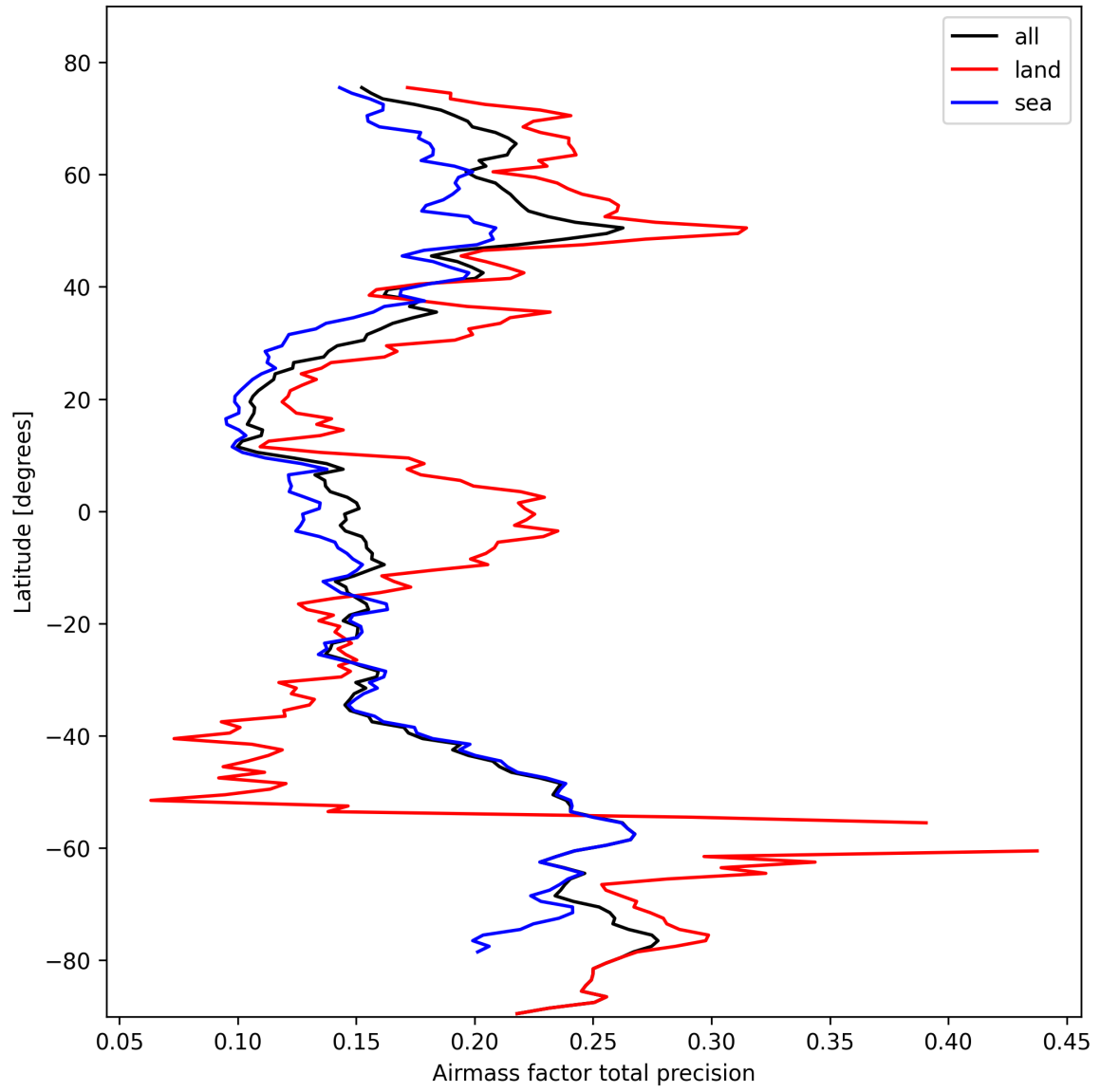
Figure 27: Zonal average of “Airmass factor total precision” for 2025-10-17 to 2025-10-19.
