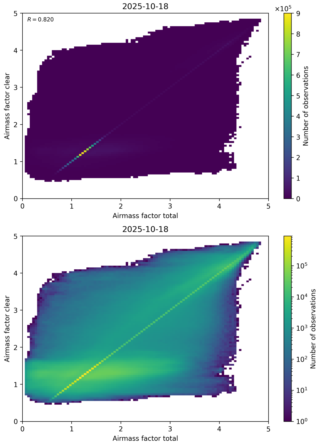
Figure 100: Scatter density plot of “Airmass factor total” against “Airmass factor clear” for 2025-10-17 to 2025-10-19.
