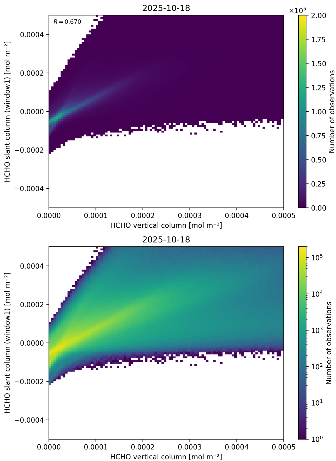
Figure 129: Scatter density plot of “HCHO vertical column” against “HCHO slant column (window1)” for 2025-10-17 to 2025-10-19.
