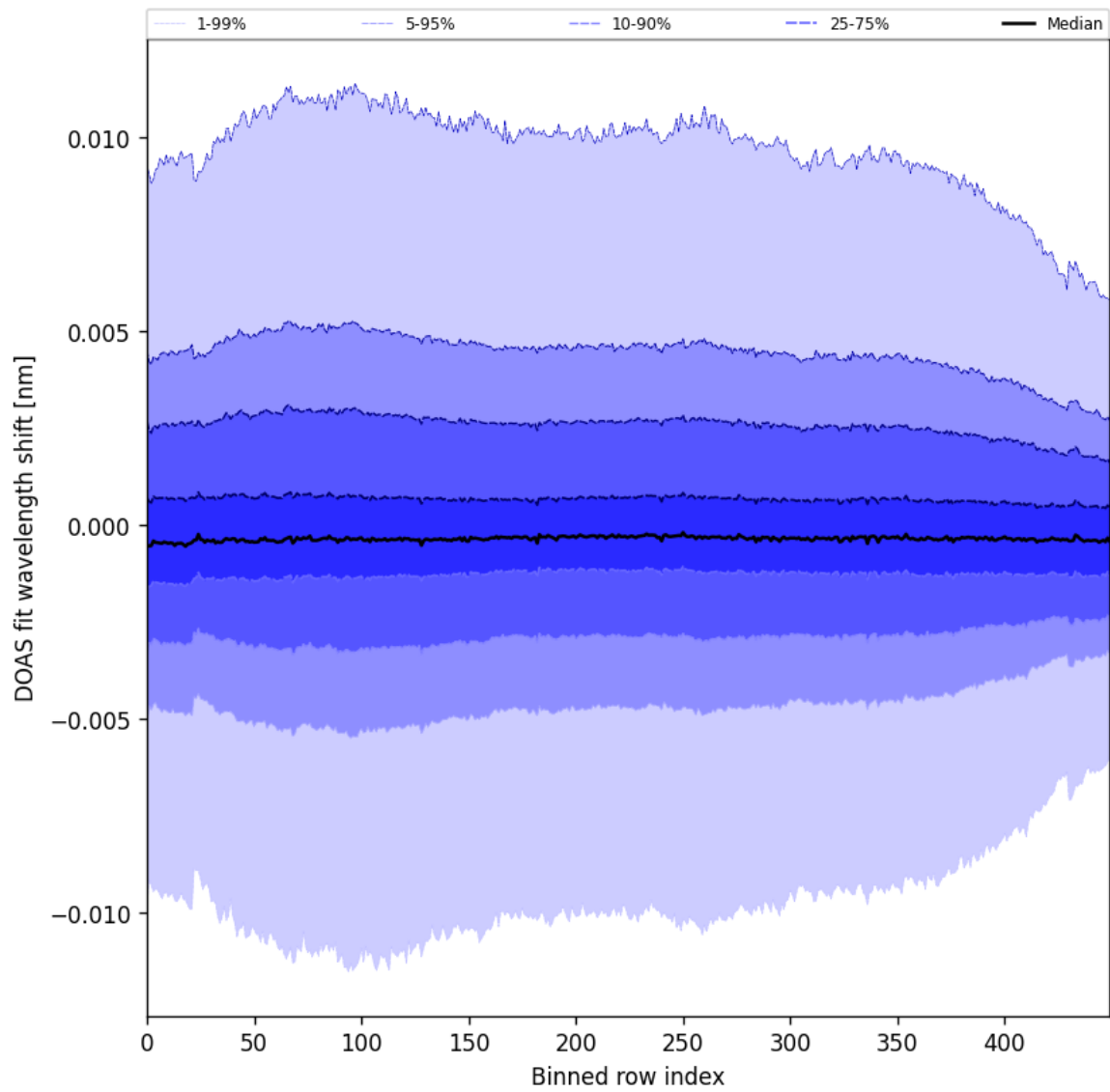
Figure 58: Along track statistics of “DOAS fit wavelength shift” for 2025-10-17 to 2025-10-19
