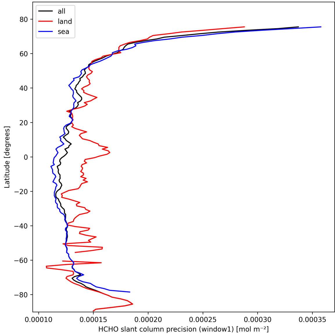
Figure 25: Zonal average of “HCHO slant column precision (window1)” for 2025-10-17 to 2025-10-19.
