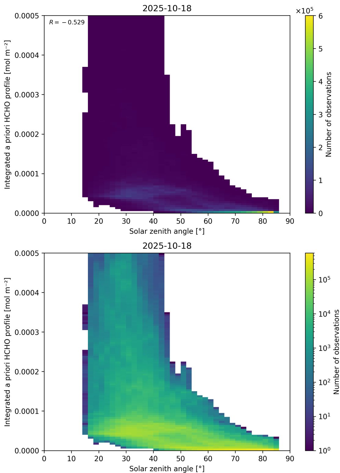
Figure 180: Scatter density plot of “Solar zenith angle” against “Integrated a priori HCHO profile” for 2025-10-17 to 2025-10-19.
