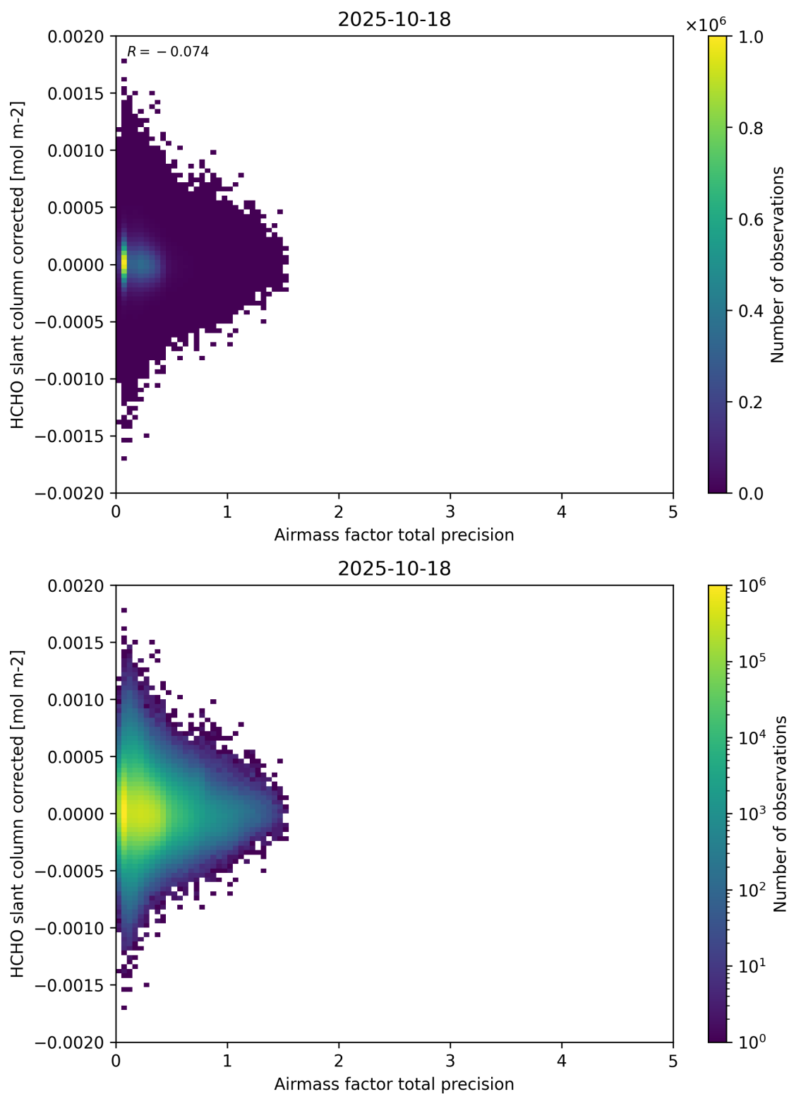
Figure 109: Scatter density plot of “Airmass factor total precision” against “HCHO slant column corrected” for 2025-10-17 to 2025-10-19.
