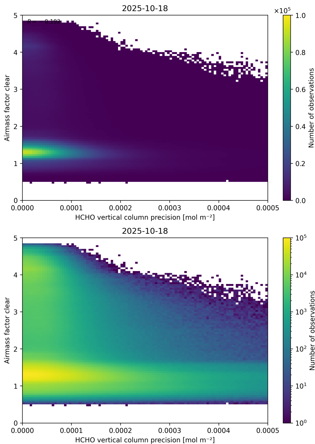
Figure 139: Scatter density plot of “HCHO vertical column precision” against “Airmass factor clear” for 2025-10-17 to 2025-10-19.
