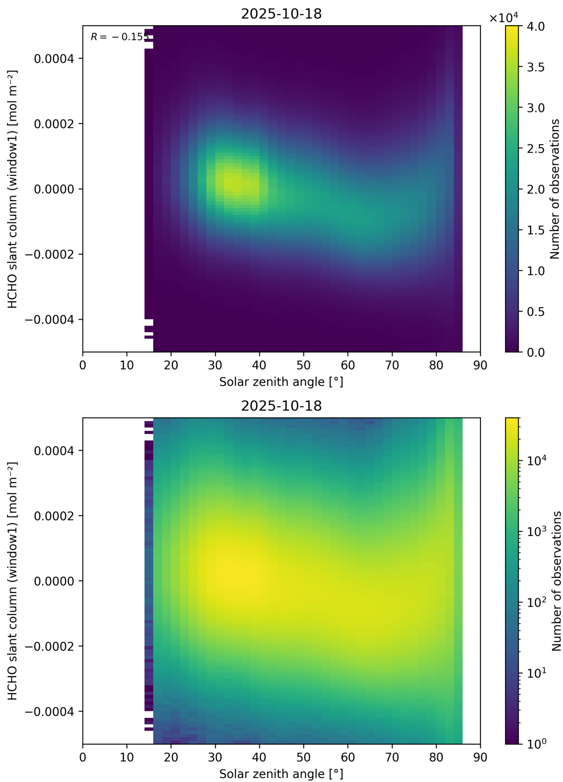
Figure 173: Scatter density plot of “Solar zenith angle” against “HCHO slant column (window1)” for 2025-10-17 to 2025-10-19.
