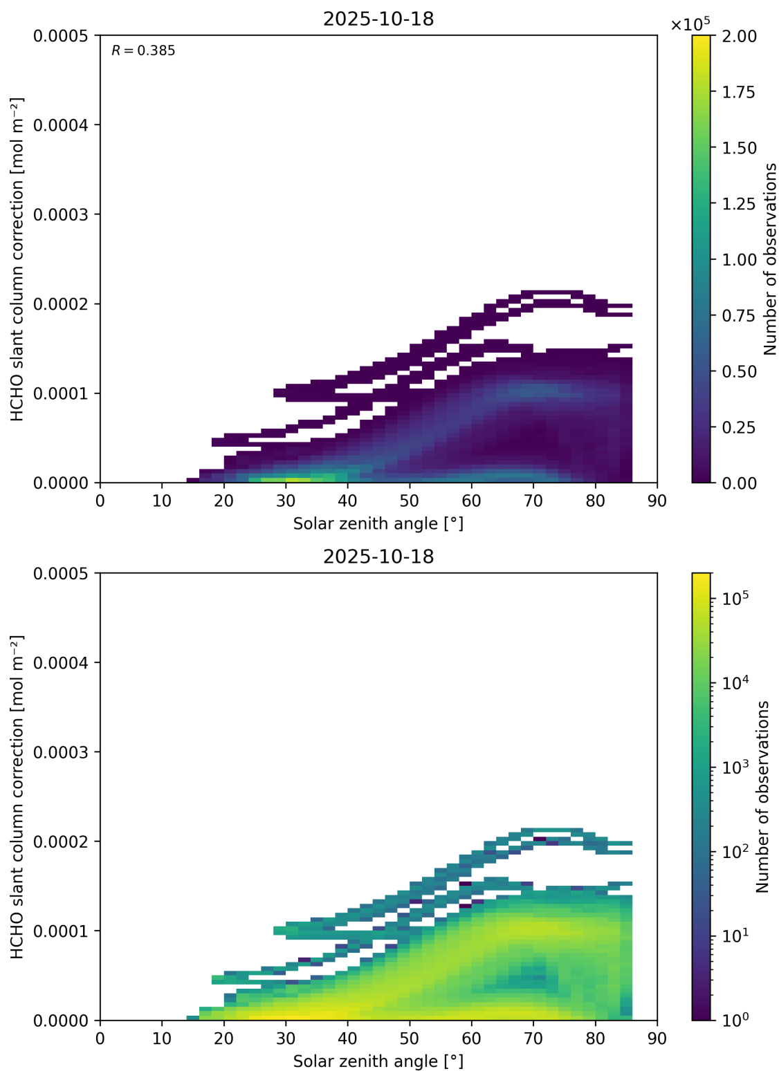
Figure 172: Scatter density plot of “Solar zenith angle” against “HCHO slant column correction” for 2025-10-17 to 2025-10-19.
