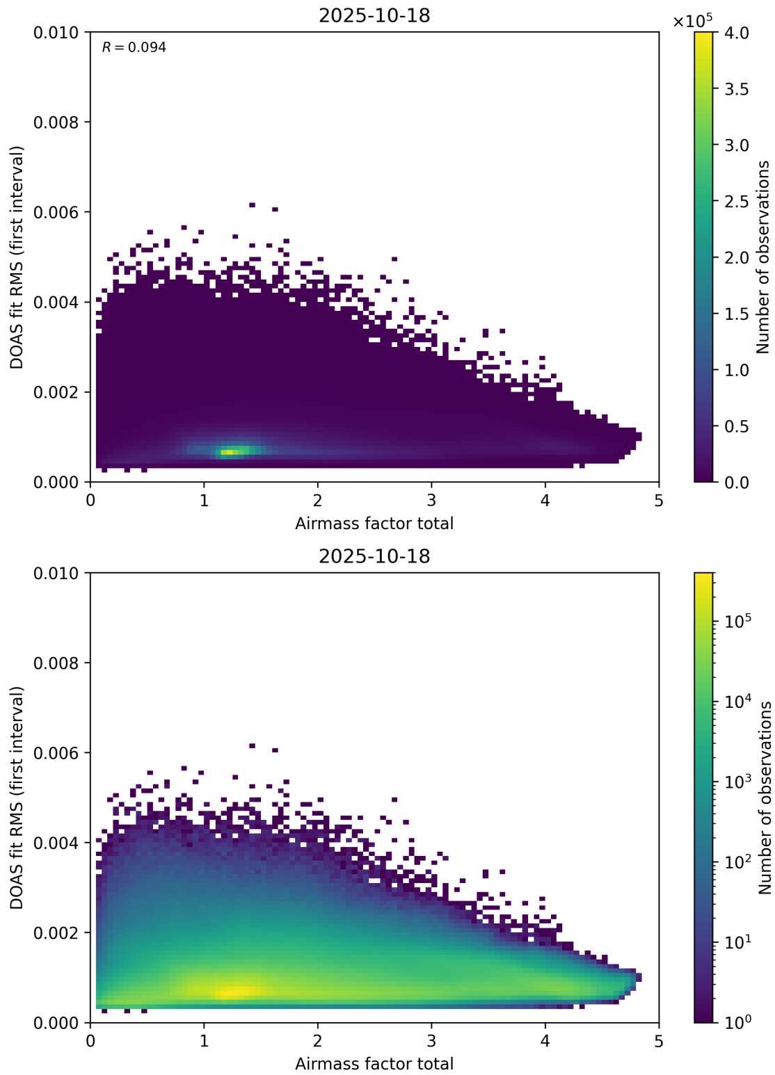
Figure 97: Scatter density plot of “Airmass factor total” against “DOAS fit RMS (first interval)” for 2025-10-17 to 2025-10-19.
