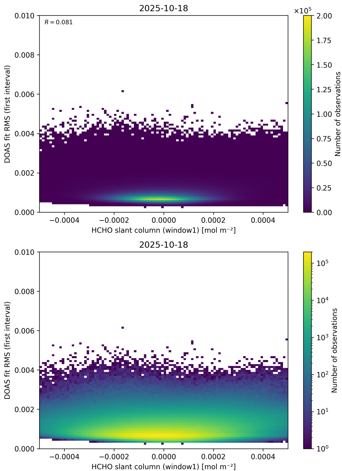
Figure 78: Scatter density plot of “HCHO slant column (window1)” against “DOAS fit RMS (first interval)” for 2025-10-17 to 2025-10-19.
