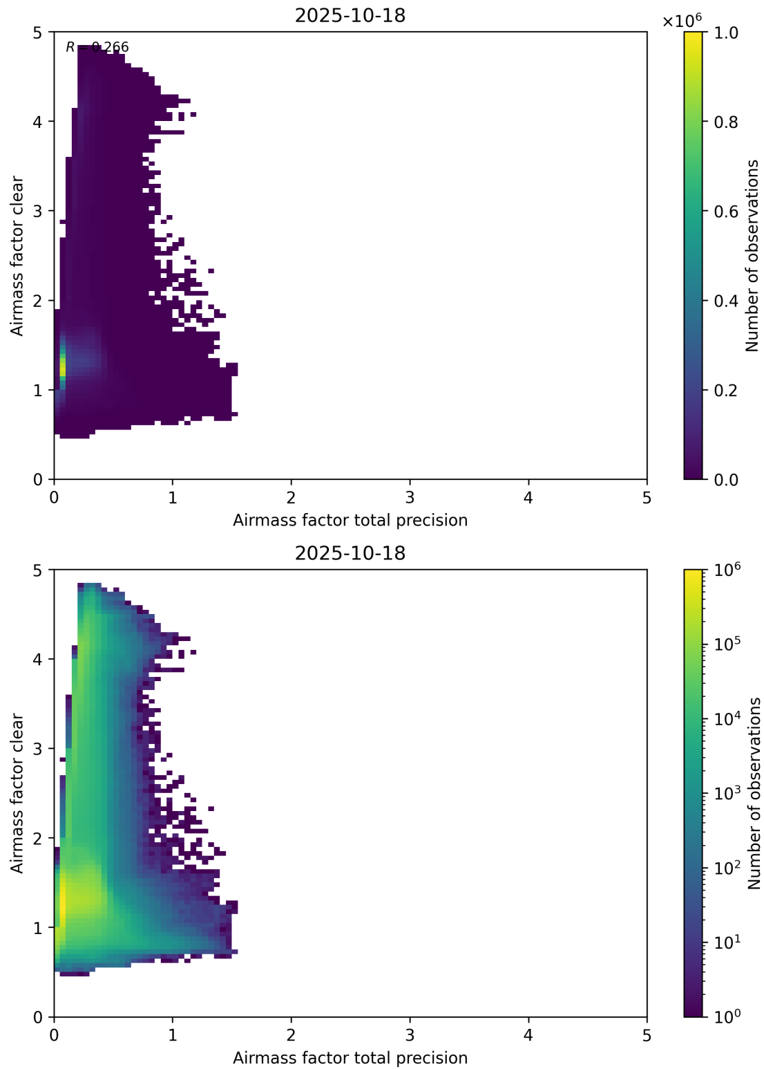
Figure 108: Scatter density plot of “Airmass factor total precision” against “Airmass factor clear” for 2025-10-17 to 2025-10-19.
