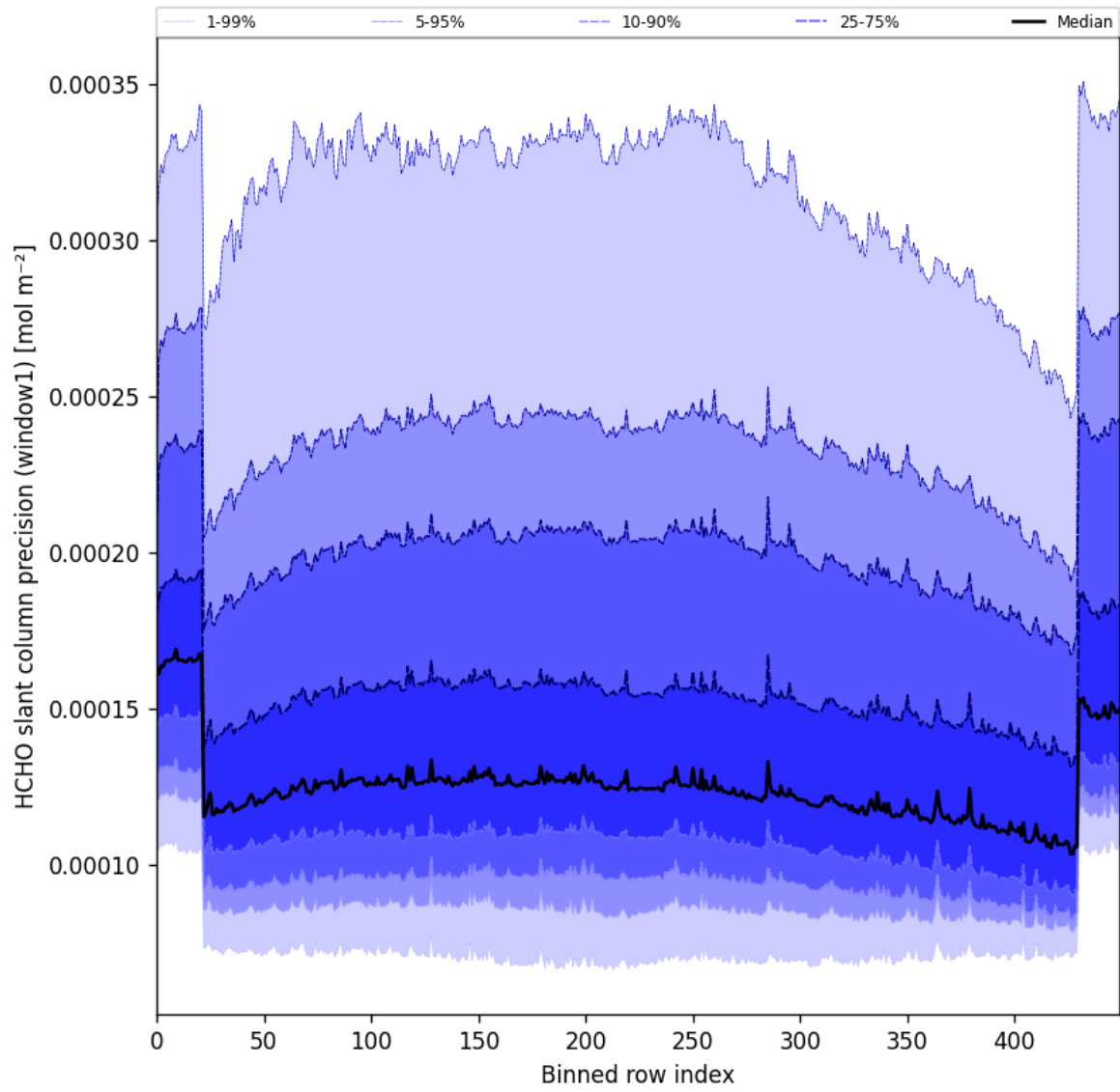
Figure 53: Along track statistics of “HCHO slant column precision (window1)” for 2025-10-17 to 2025-10-19
