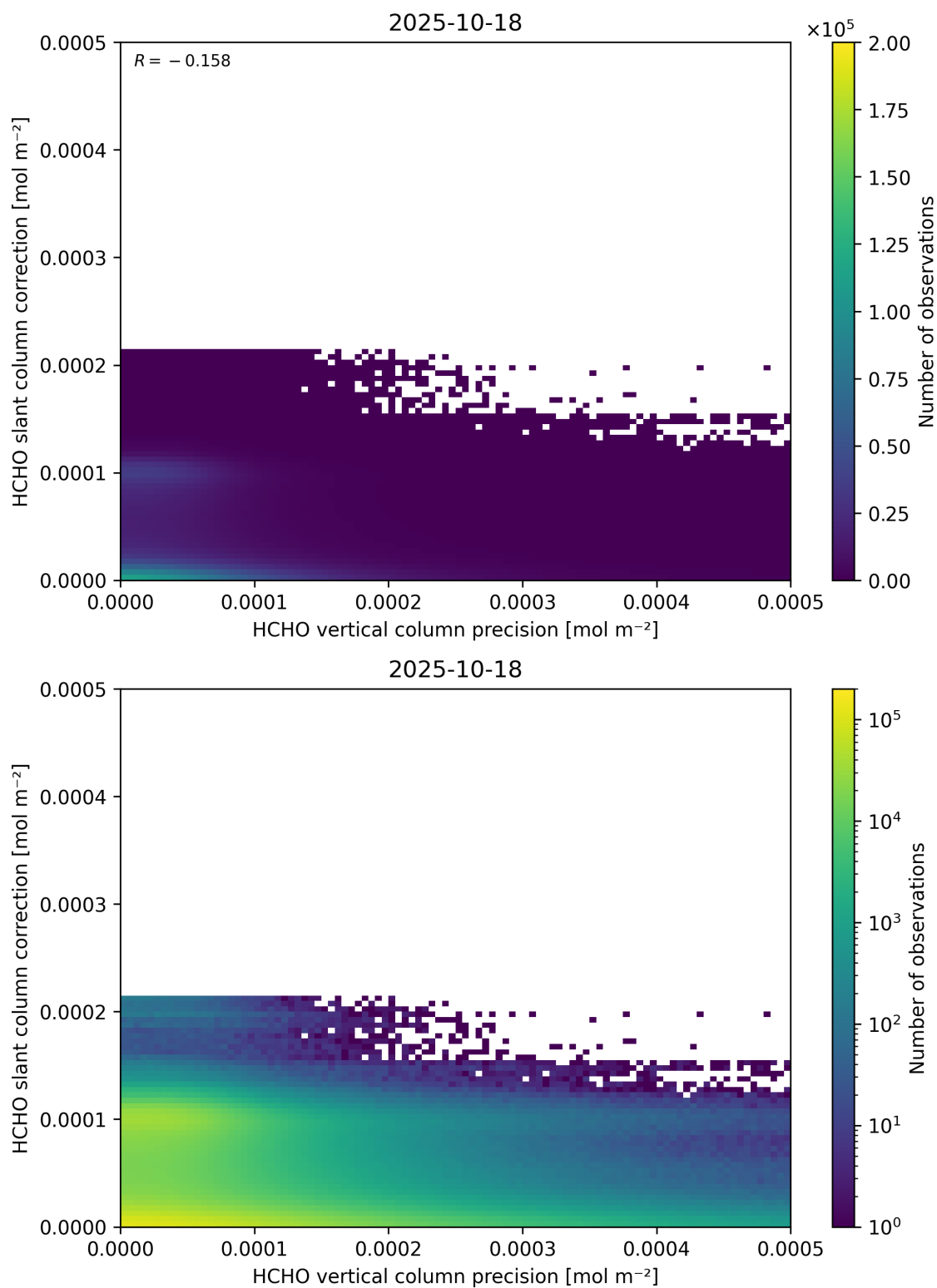
Figure 141: Scatter density plot of “HCHO vertical column precision” against “HCHO slant column correction” for 2025-10-17 to 2025-10-19.
