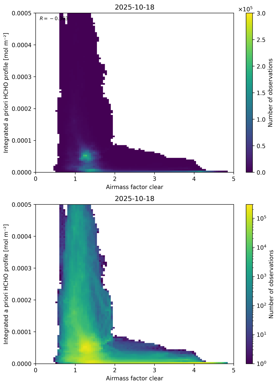
Figure 76: Scatter density plot of “Airmass factor clear” against “Integrated a priori HCHO profile” for 2025-10-17 to 2025-10-19.
