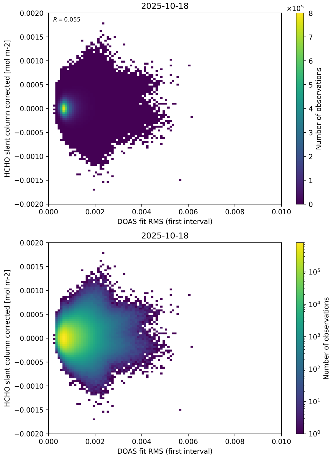
Figure 62: Scatter density plot of “DOAS fit RMS (first interval)” against “HCHO slant column corrected” for 2025-10-17 to 2025-10-19.
