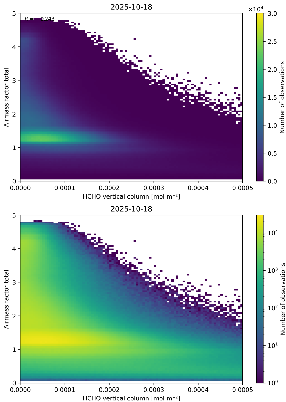
Figure 131: Scatter density plot of “HCHO vertical column” against “Airmass factor total” for 2025-10-17 to 2025-10-19.
