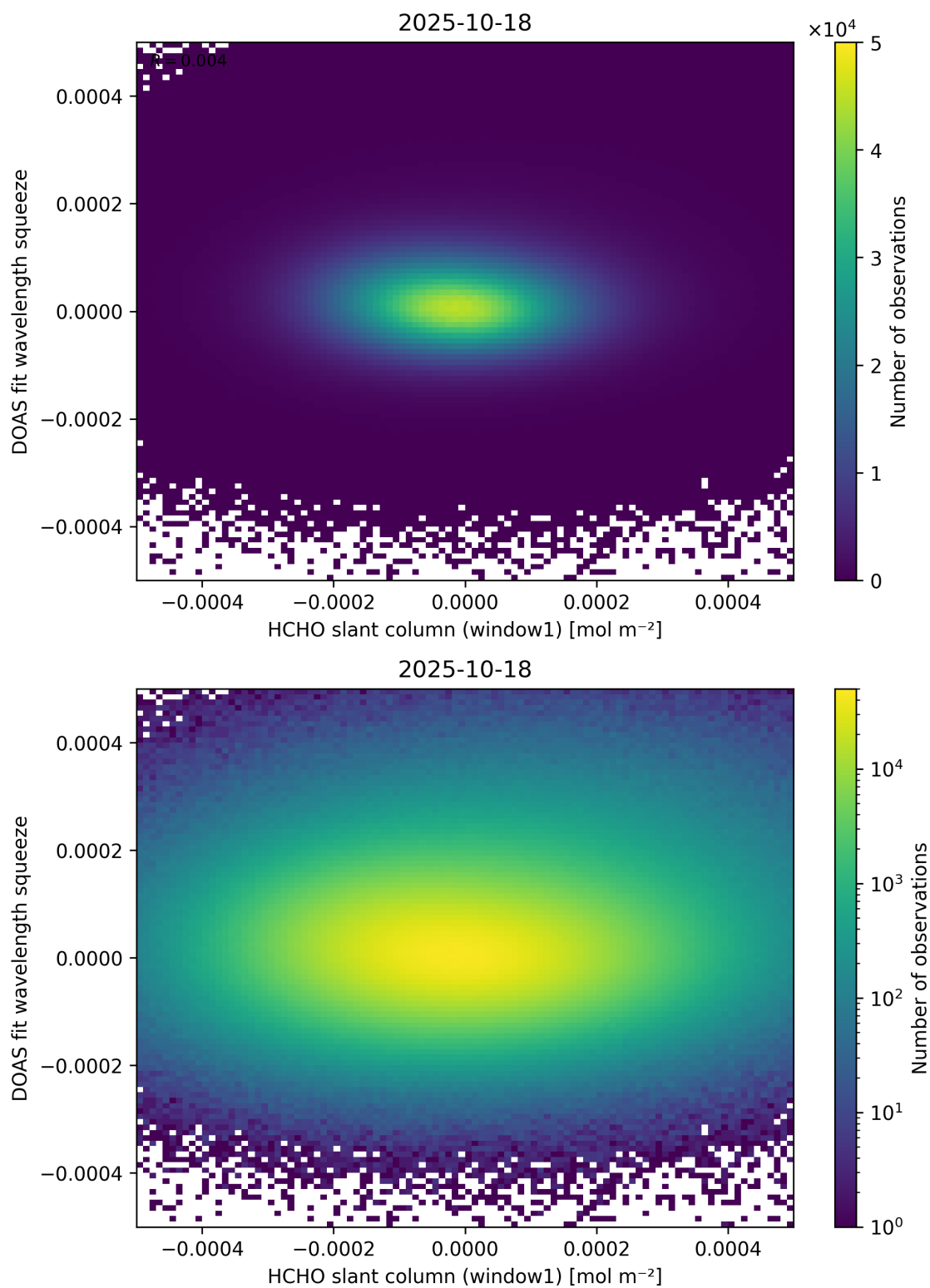
Figure 80: Scatter density plot of “HCHO slant column (window1)” against “DOAS fit wavelength squeeze” for 2025-10-17 to 2025-10-19.
