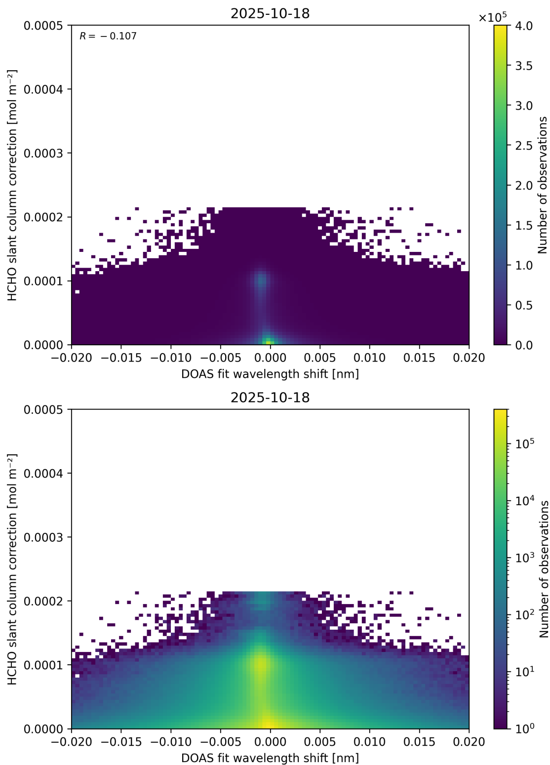
Figure 67: Scatter density plot of “DOAS fit wavelength shift” against “HCHO slant column correction” for 2025-10-17 to 2025-10-19.
