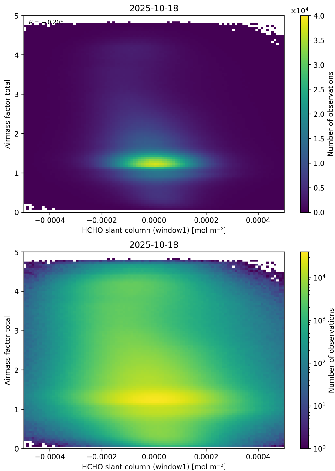
Figure 85: Scatter density plot of “HCHO slant column (window1)” against “Airmass factor total” for 2025-10-17 to 2025-10-19.
