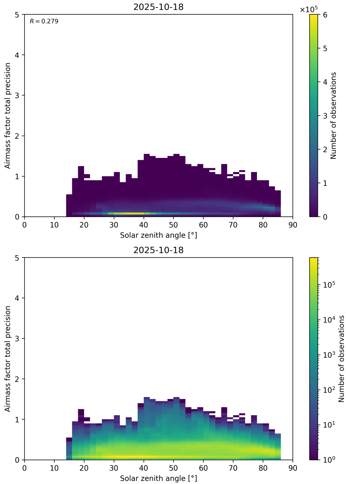
Figure 176: Scatter density plot of “Solar zenith angle” against “Airmass factor total precision” for 2025-10-17 to 2025-10-19.
