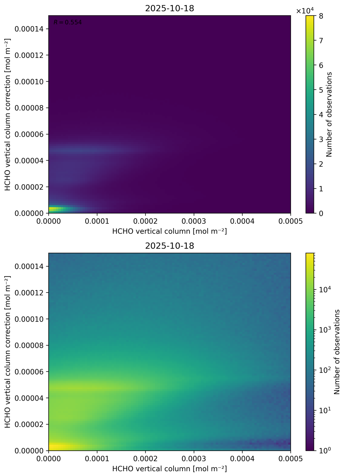
Figure 133: Scatter density plot of “HCHO vertical column” against “HCHO vertical column correction” for 2025-10-17 to 2025-10-19.
