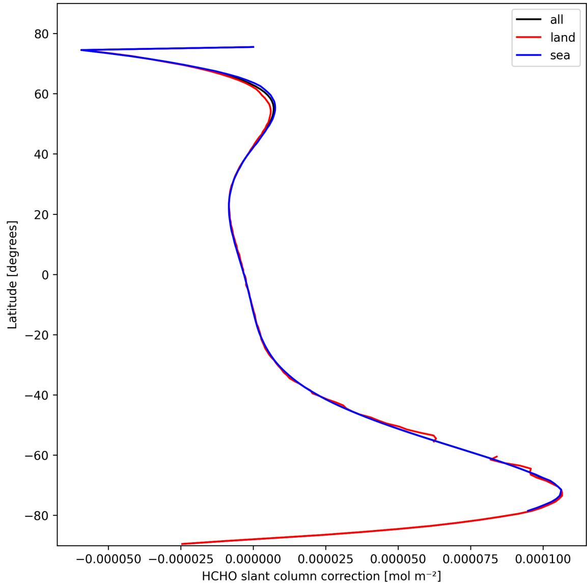
Figure 33: Zonal average of “HCHO slant column correction” for 2025-10-17 to 2025-10-19.
