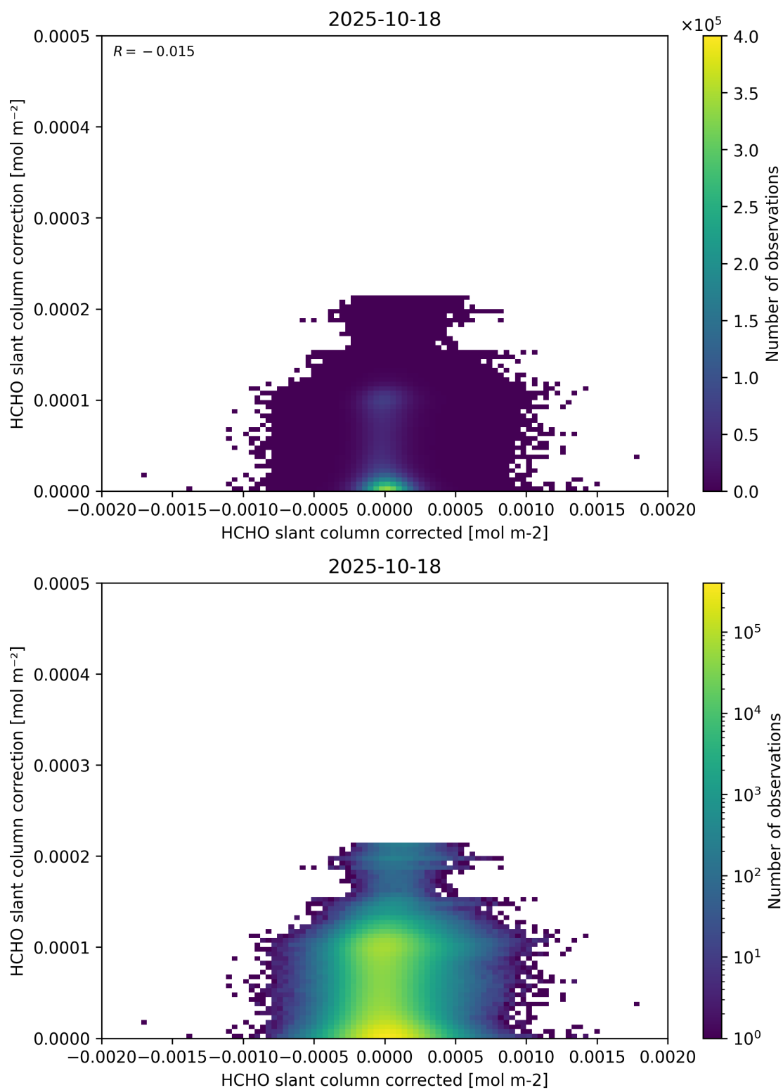
Figure 77: Scatter density plot of “HCHO slant column corrected” against “HCHO slant column correction” for 2025-10-17 to 2025-10-19.
