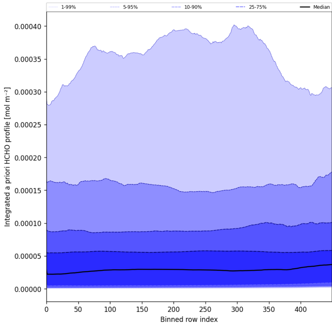
Figure 57: Along track statistics of “Integrated a priori HCHO profile” for 2025-10-17 to 2025-10-19
