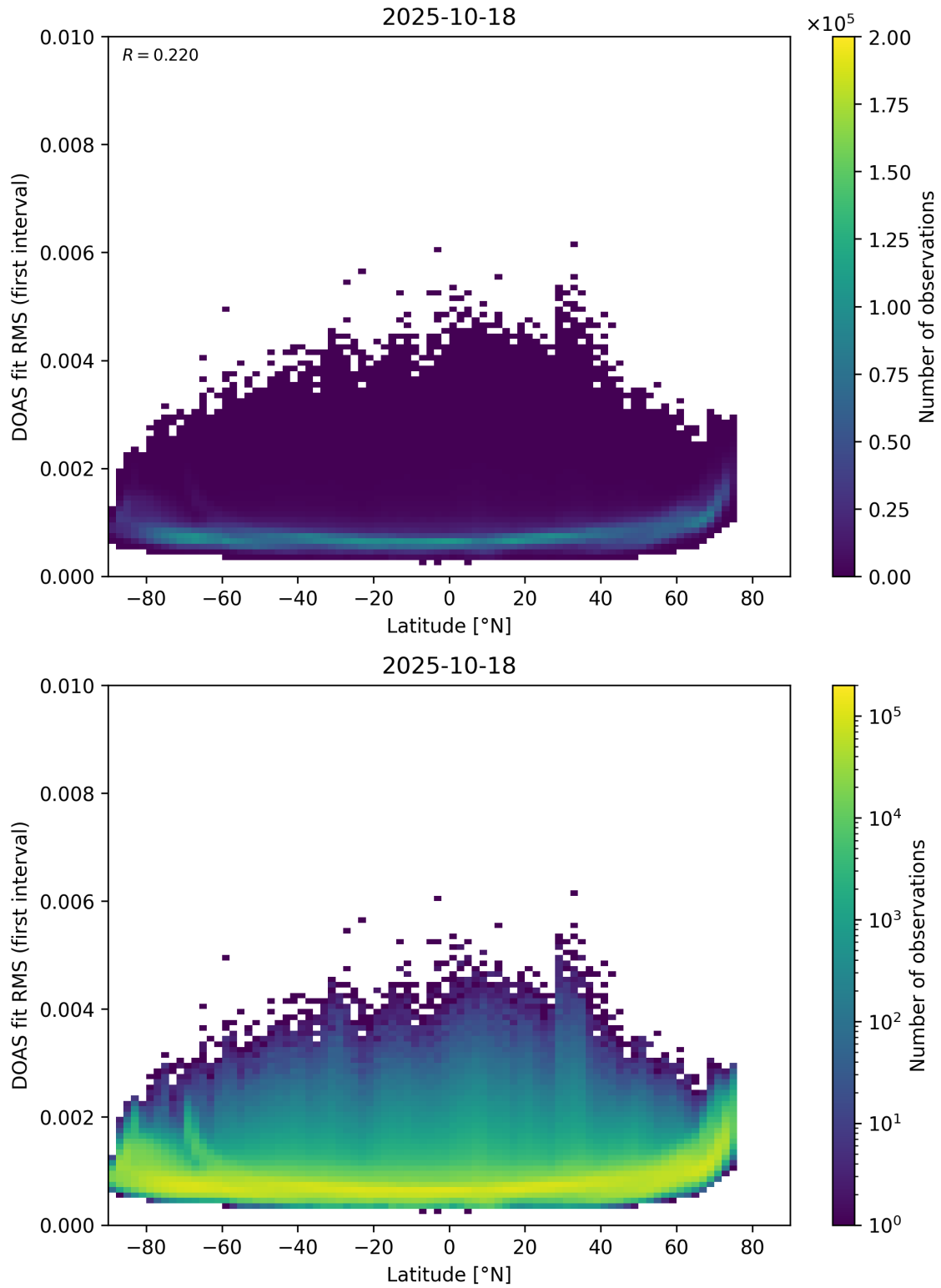
Figure 153: Scatter density plot of “Latitude” against “DOAS fit RMS (first interval)” for 2025-10-17 to 2025-10-19.
