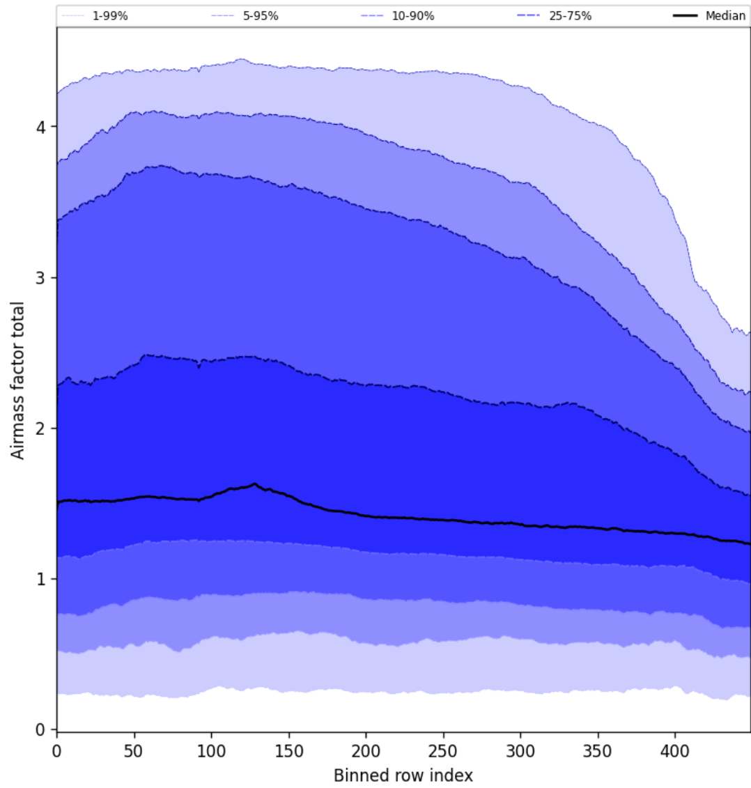
Figure 54: Along track statistics of “Airmass factor total” for 2025-10-17 to 2025-10-19
