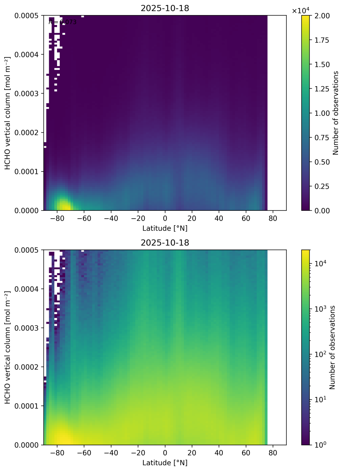
Figure 163: Scatter density plot of “Latitude” against “HCHO vertical column” for 2025-10-17 to 2025-10-19.
