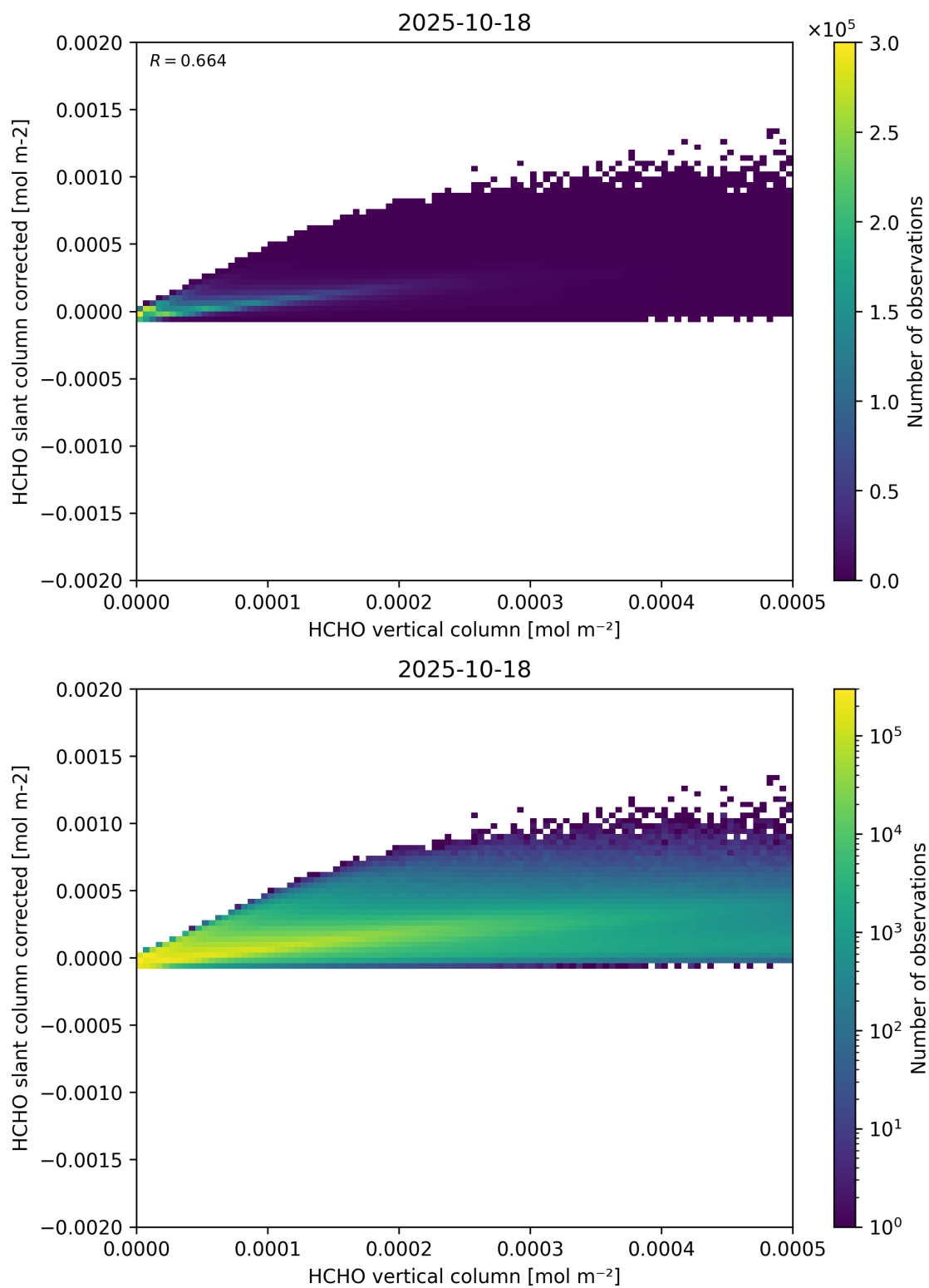
Figure 127: Scatter density plot of “HCHO vertical column” against “HCHO slant column corrected” for 2025-10-17 to 2025-10-19.
