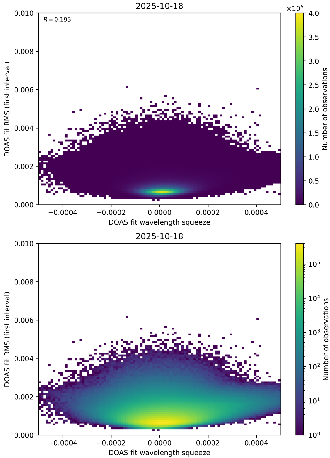
Figure 68: Scatter density plot of “DOAS fit wavelength squeeze” against “DOAS fit RMS (first interval)” for 2025-10-17 to 2025-10-19.
