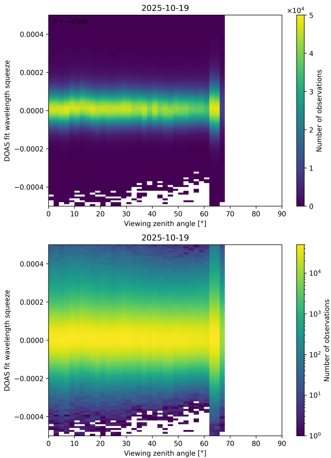
Figure 184: Scatter density plot of “Viewing zenith angle” against “DOAS fit wavelength squeeze” for 2025-10-18 to 2025-10-20.
