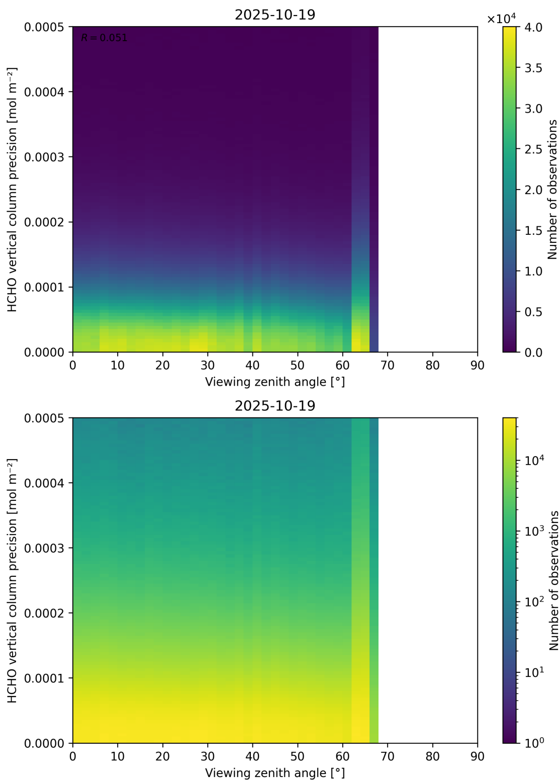
Figure 194: Scatter density plot of “Viewing zenith angle” against “HCHO vertical column precision” for 2025-10-18 to 2025-10-20.
