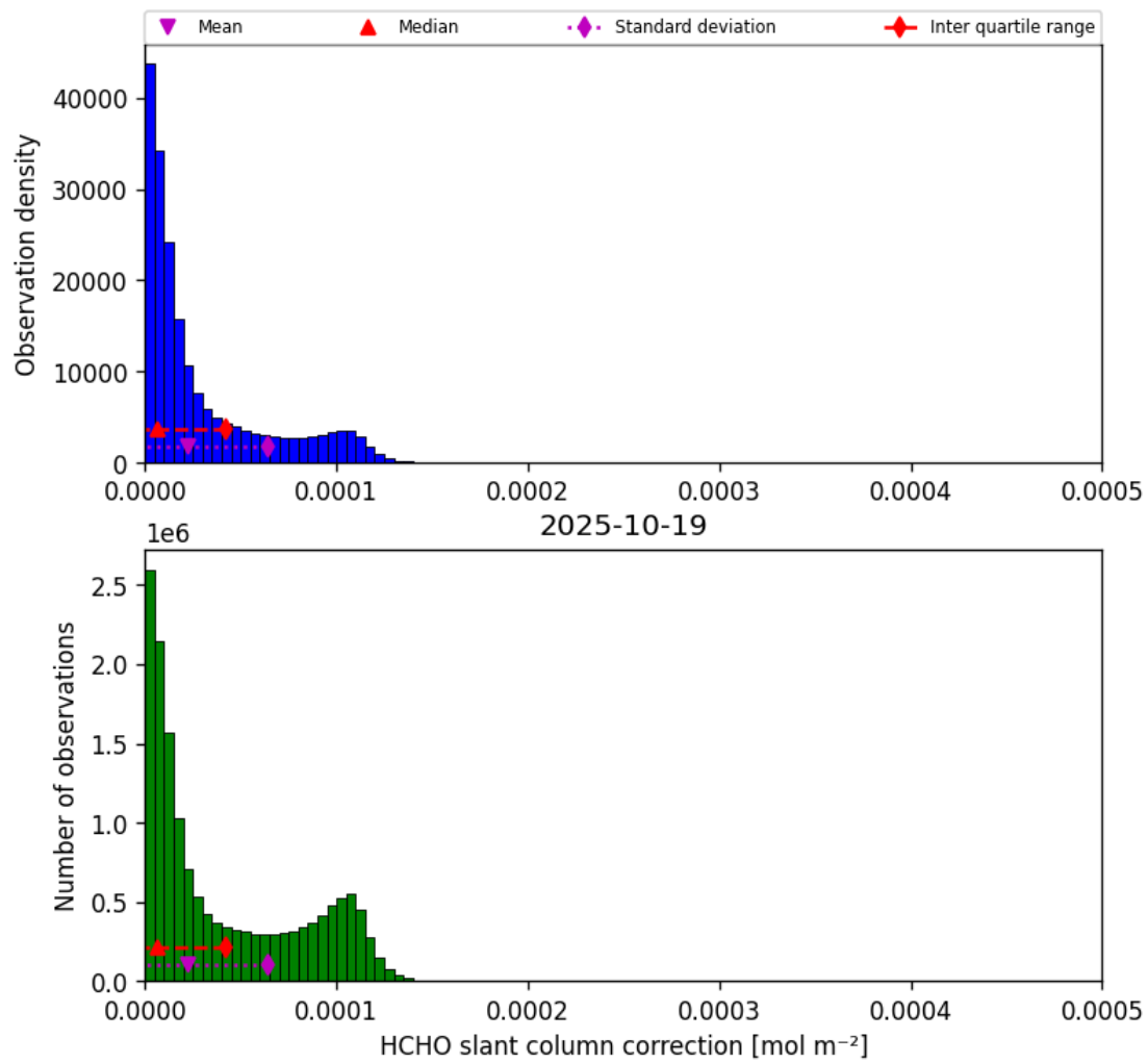
Figure 47: Histogram of “HCHO slant column correction” for 2025-10-18 to 2025-10-20
