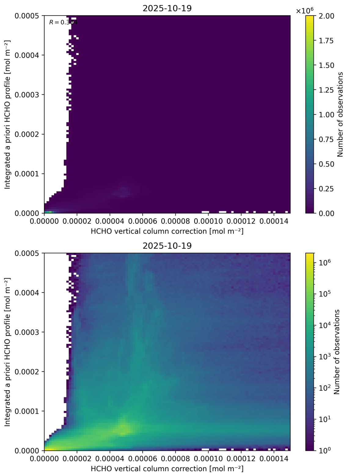
Figure 122: Scatter density plot of “HCHO vertical column correction” against “Integrated a priori HCHO profile” for 2025-10-18 to 2025-10-20.
