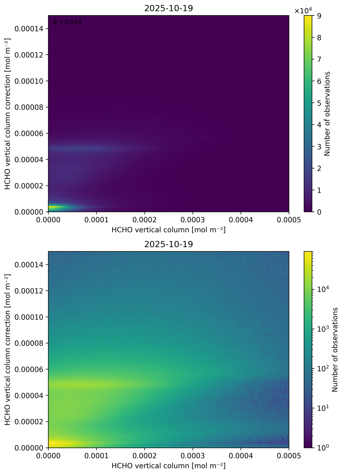
Figure 133: Scatter density plot of “HCHO vertical column” against “HCHO vertical column correction” for 2025-10-18 to 2025-10-20.
