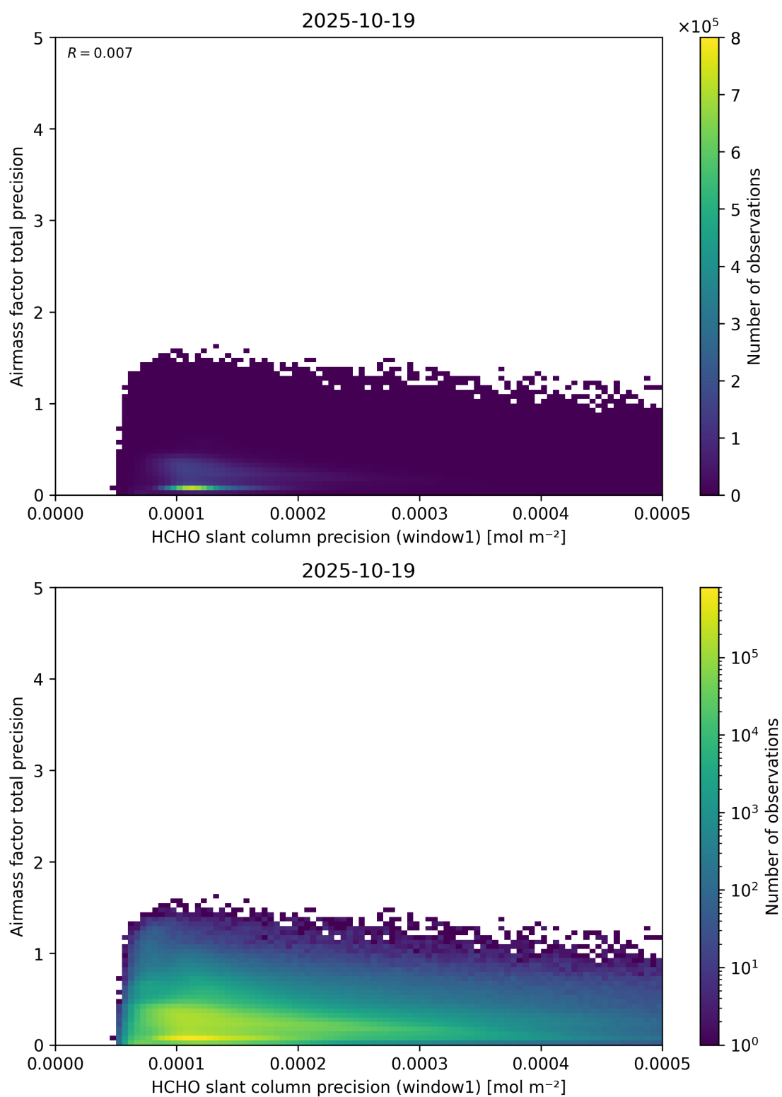
Figure 95: Scatter density plot of “HCHO slant column precision (window1)” against “Airmass factor total precision” for 2025-10-18 to 2025-10-20.
