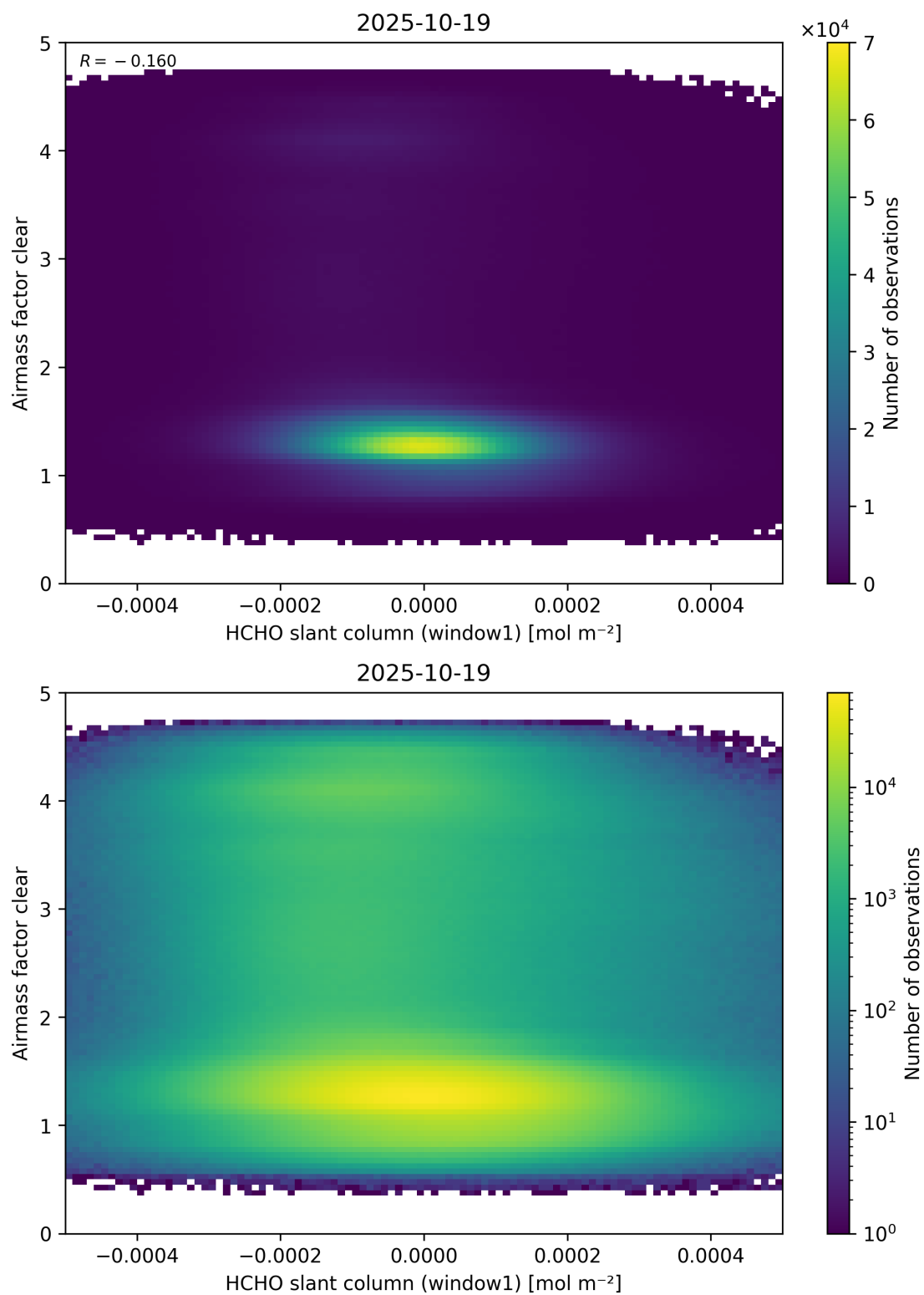
Figure 81: Scatter density plot of “HCHO slant column (window1)” against “Airmass factor clear” for 2025-10-18 to 2025-10-20.
