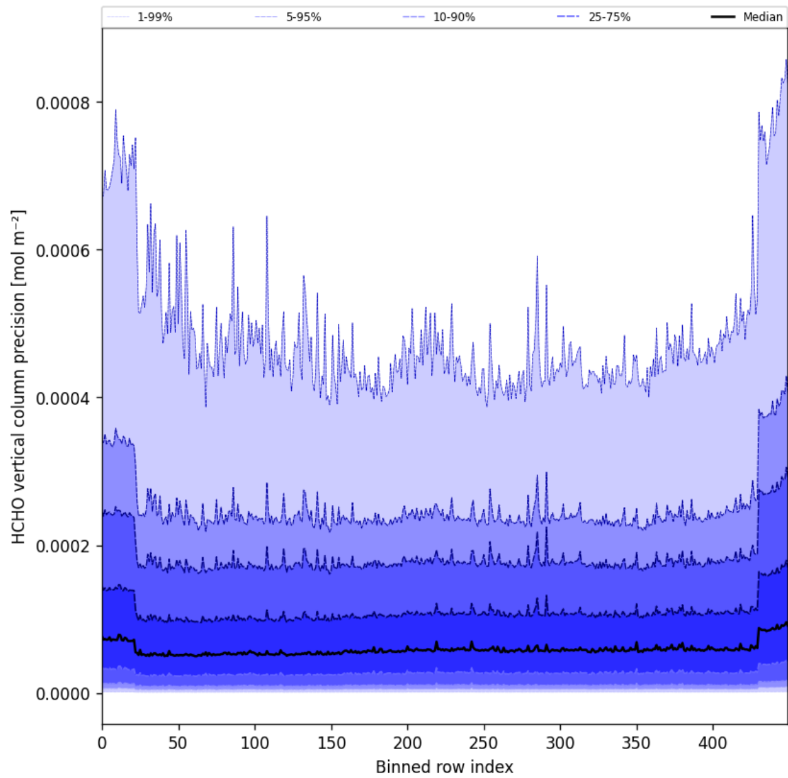
Figure 50: Along track statistics of “HCHO vertical column precision” for 2025-10-18 to 2025-10-20
