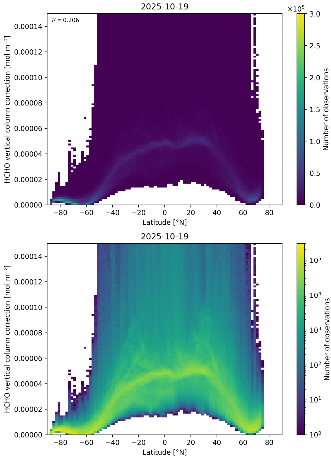
Figure 164: Scatter density plot of “Latitude” against “HCHO vertical column correction” for 2025-10-18 to 2025-10-20.
