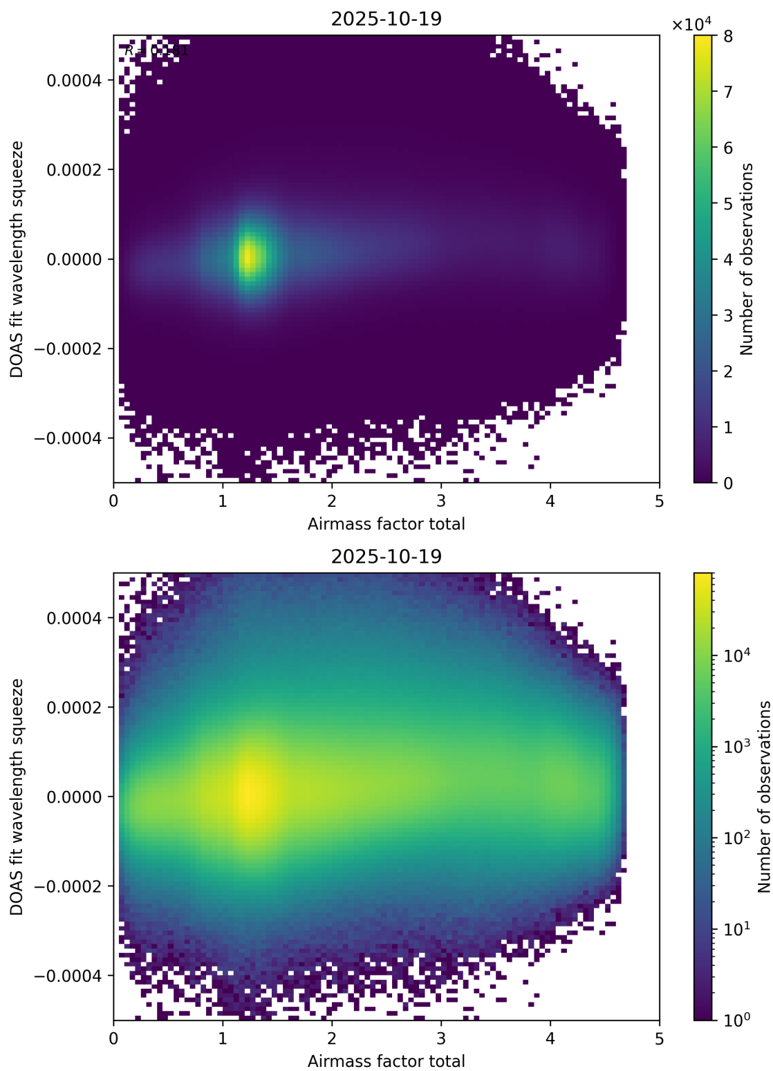
Figure 99: Scatter density plot of “Airmass factor total” against “DOAS fit wavelength squeeze” for 2025-10-18 to 2025-10-20.
