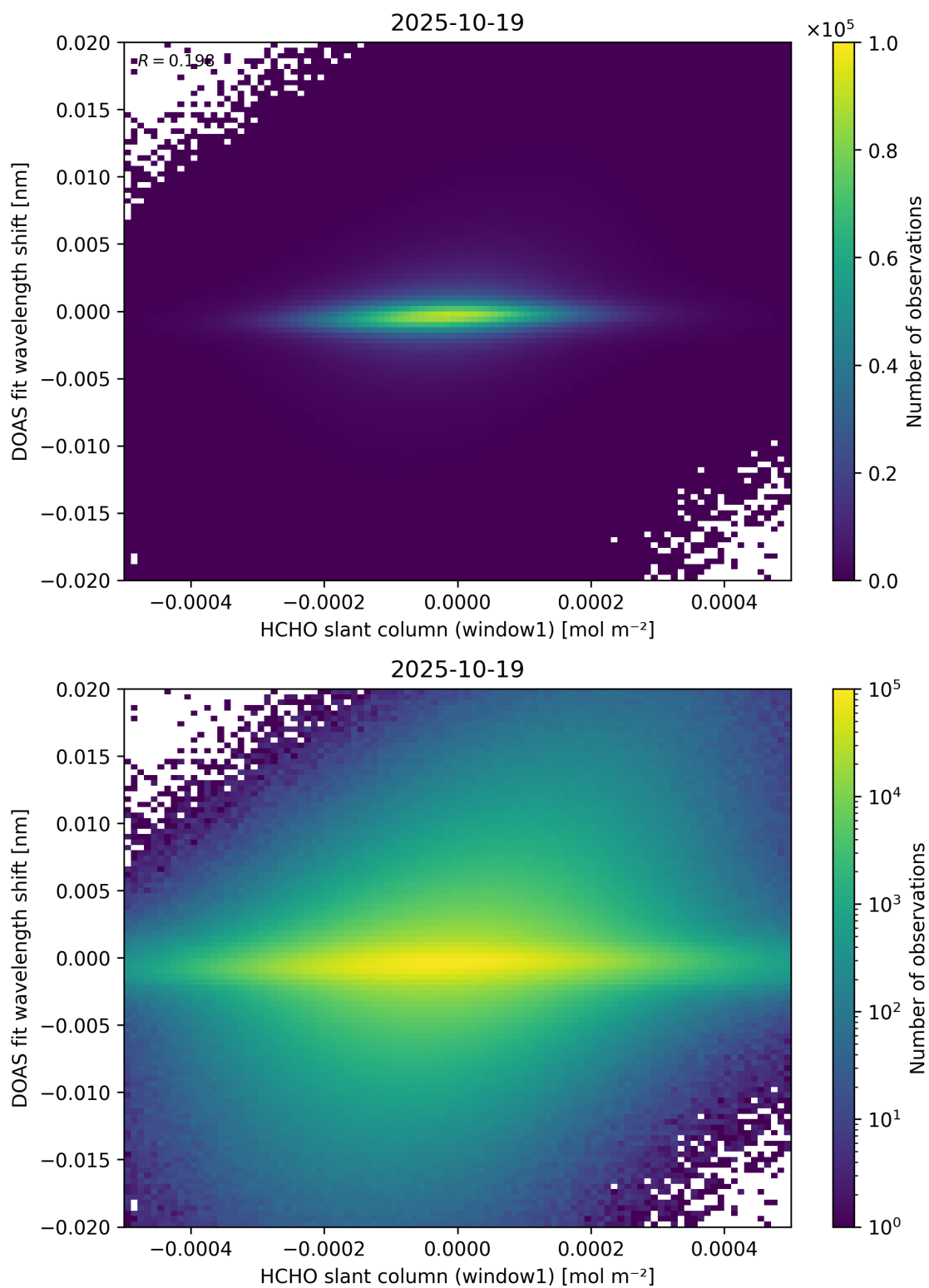
Figure 79: Scatter density plot of “HCHO slant column (window1)” against “DOAS fit wavelength shift” for 2025-10-18 to 2025-10-20.
