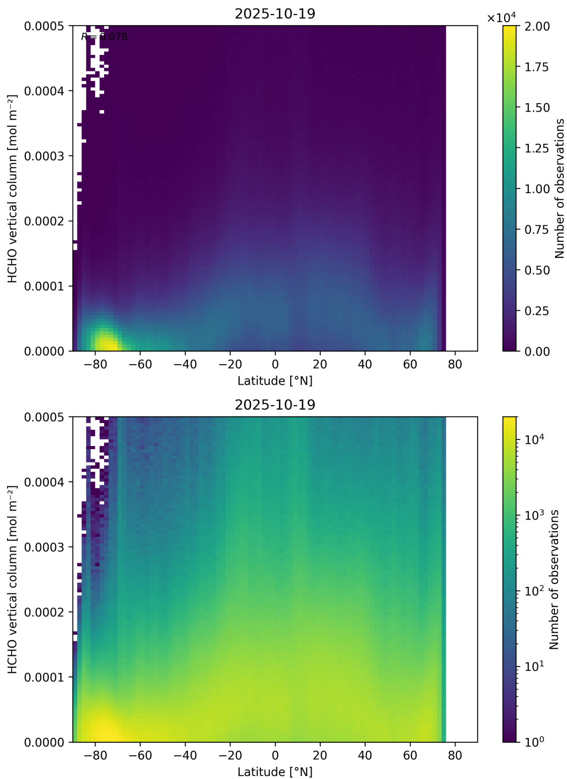
Figure 163: Scatter density plot of “Latitude” against “HCHO vertical column” for 2025-10-18 to 2025-10-20.
