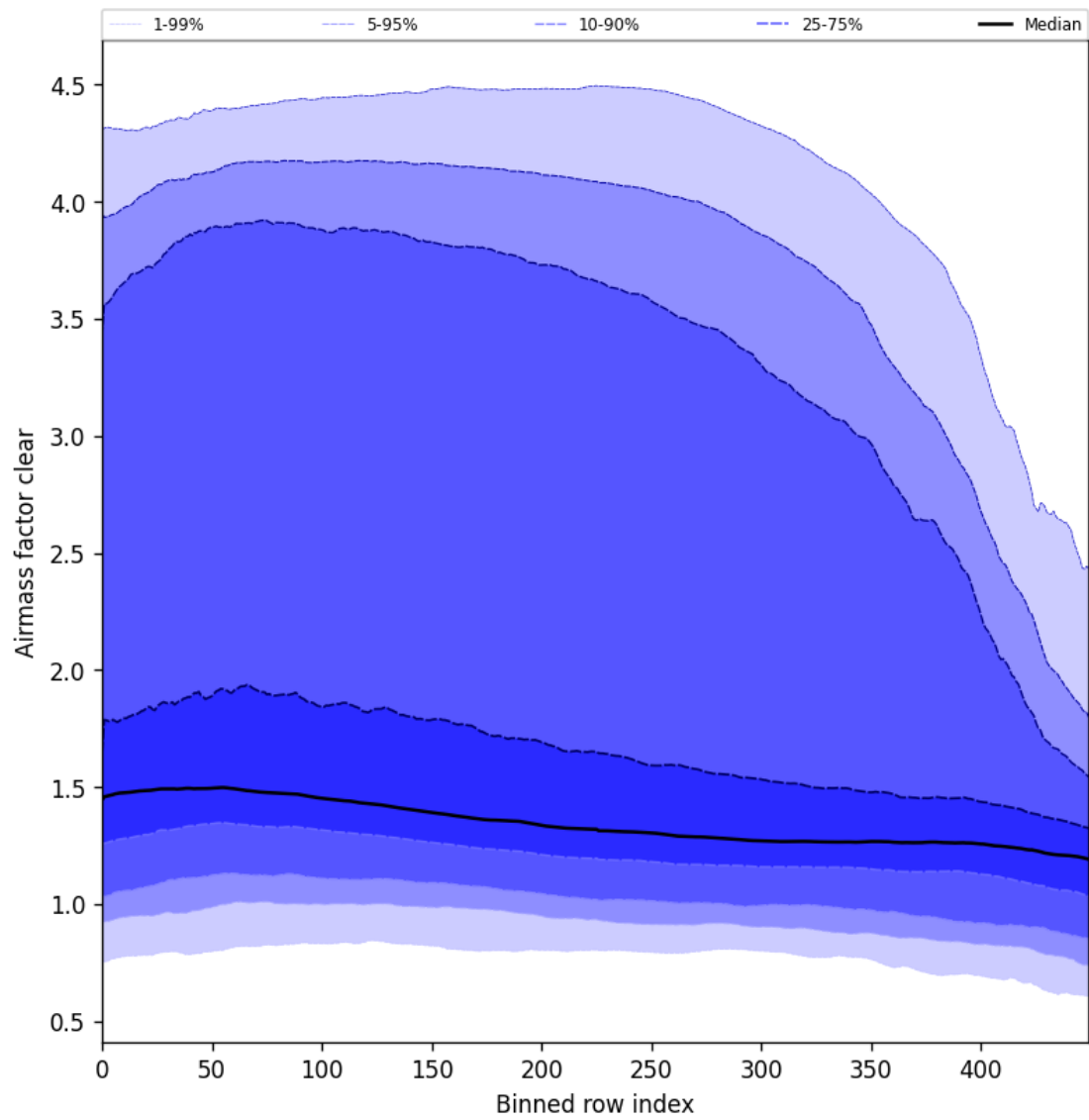
Figure 56: Along track statistics of “Air mass factor clear” for 2025-10-18 to 2025-10-20
