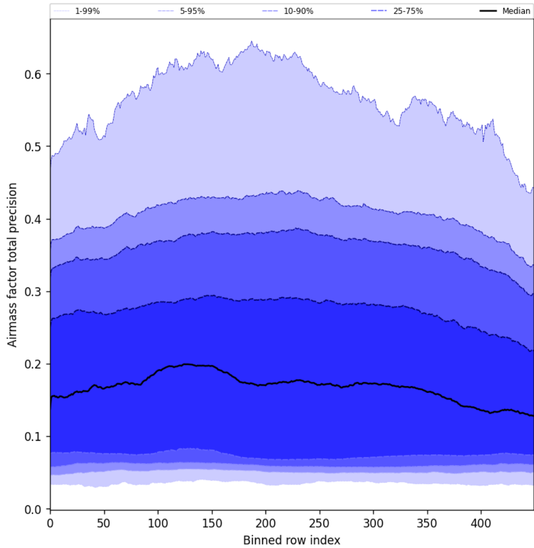
Figure 55: Along track statistics of “Airmass factor total precision” for 2025-10-18 to 2025-10-20
