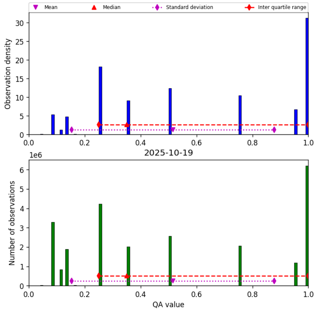
Figure 34: Histogram of “QA value” for 2025-10-18 to 2025-10-20
