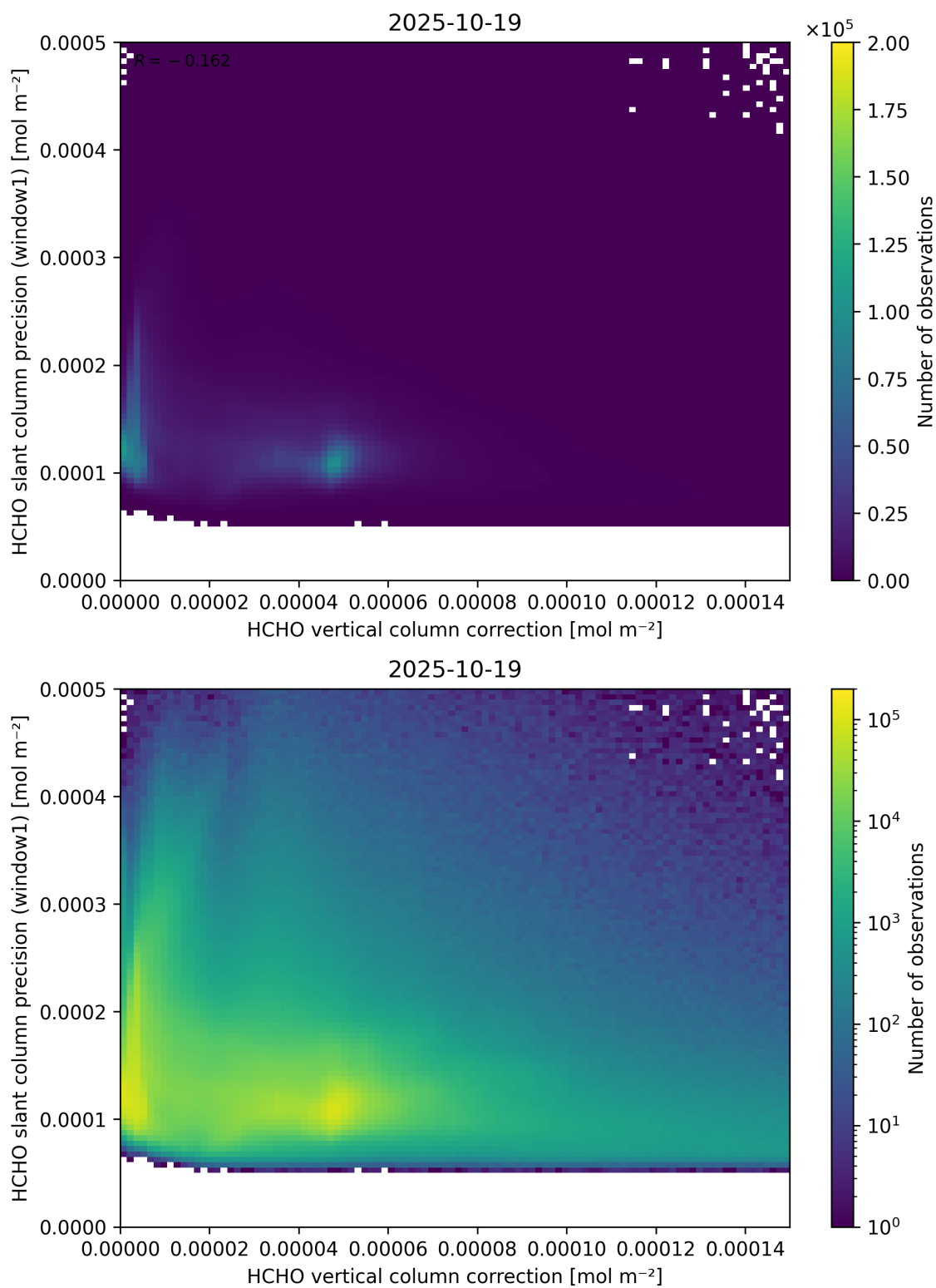
Figure 119: Scatter density plot of “HCHO vertical column correction” against “HCHO slant column precision (window1)” for 2025-10-18 to 2025-10-20.
