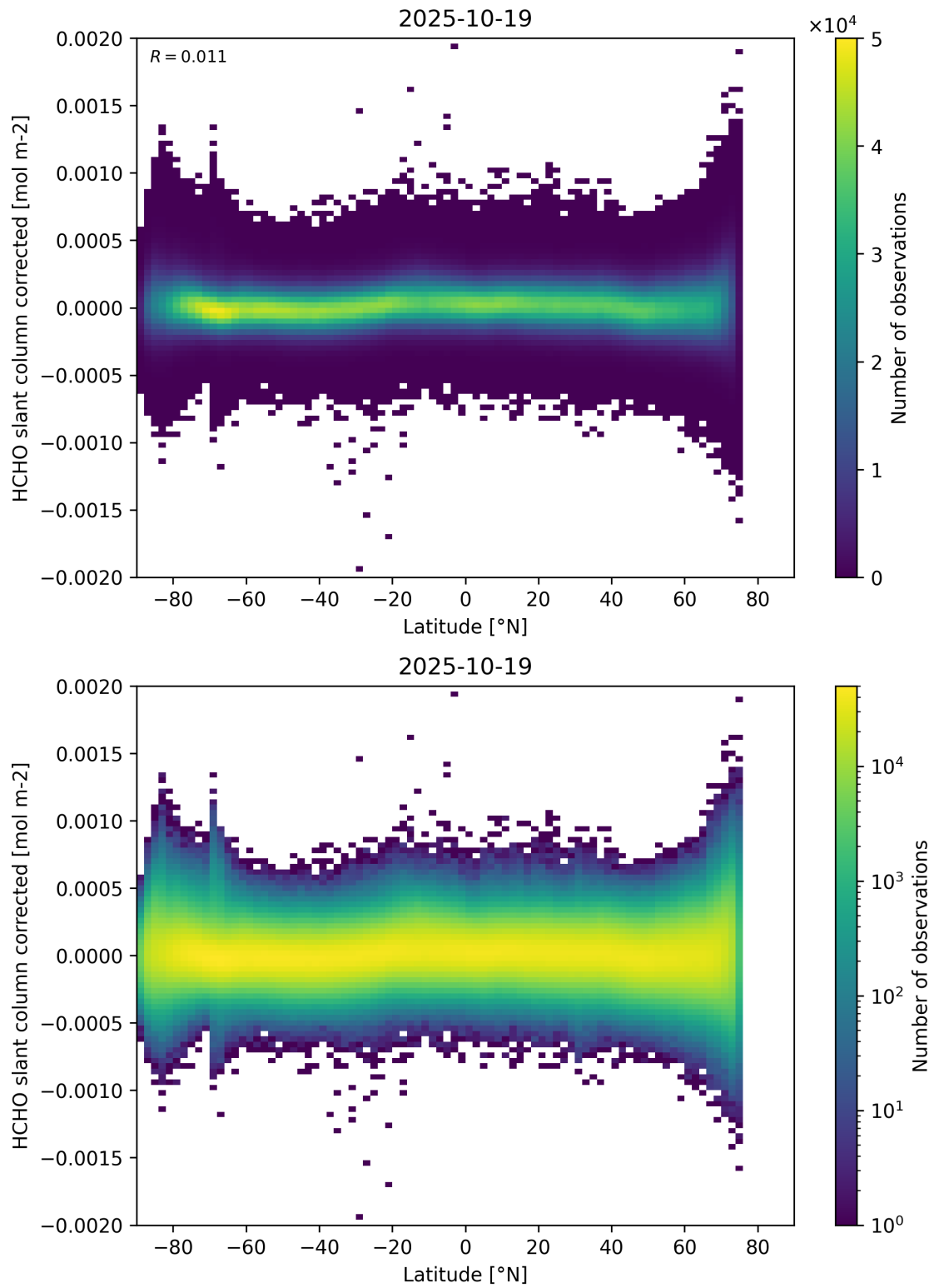
Figure 157: Scatter density plot of “Latitude” against “HCHO slant column corrected” for 2025-10-18 to 2025-10-20.
