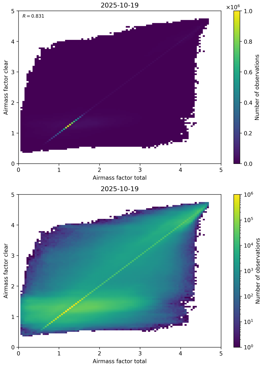
Figure 100: Scatter density plot of “Airmass factor total” against “Airmass factor clear” for 2025-10-18 to 2025-10-20.
