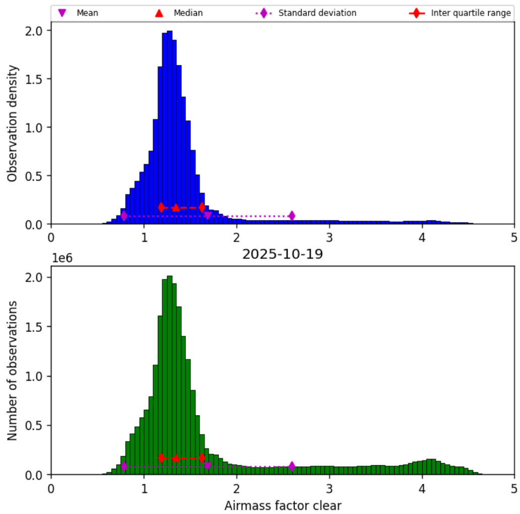
Figure 42: Histogram of “Airmass factor clear” for 2025-10-18 to 2025-10-20
