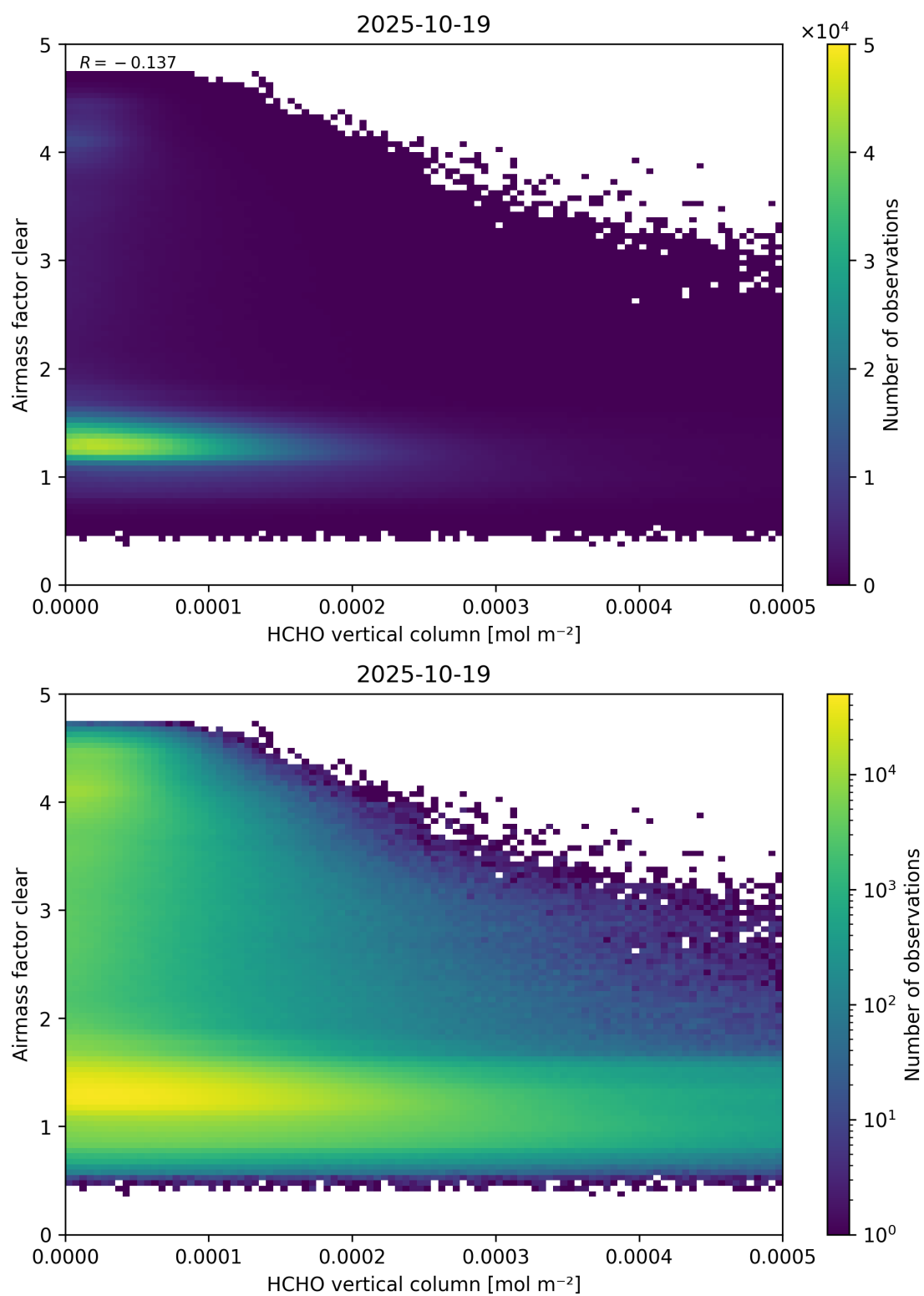
Figure 126: Scatter density plot of “HCHO vertical column” against “Airmass factor clear” for 2025-10-18 to 2025-10-20.
