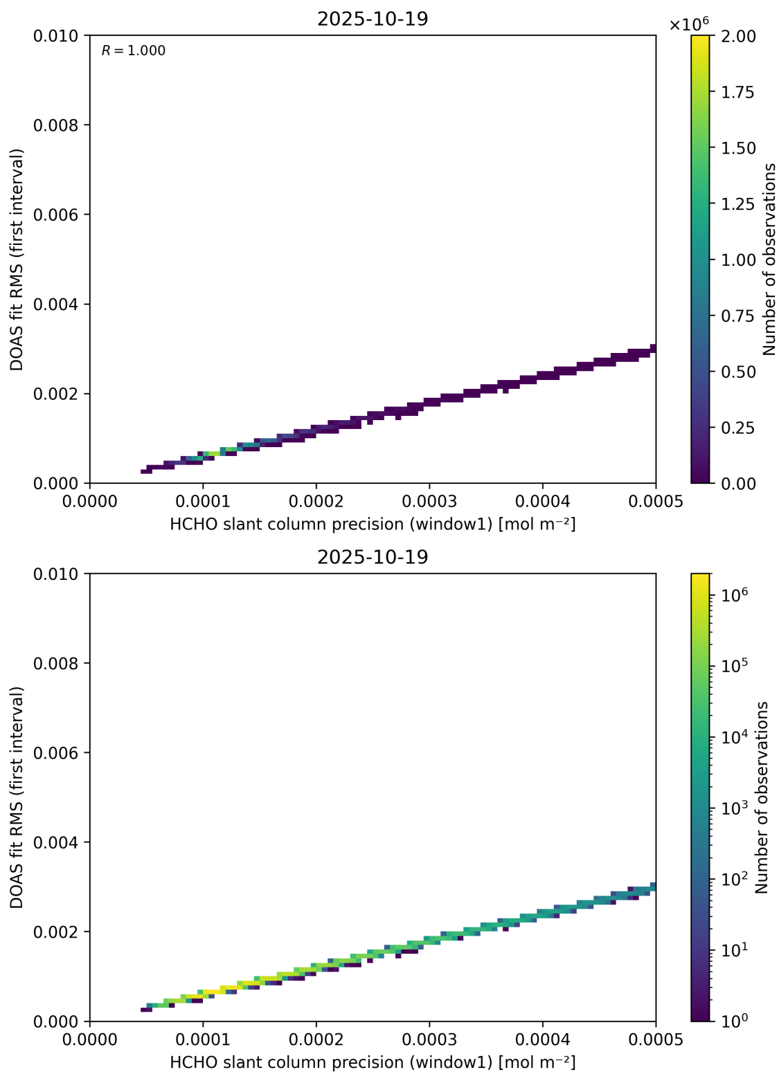
Figure 88: Scatter density plot of “HCHO slant column precision (window1)” against “DOAS fit RMS (first interval)” for 2025-10-18 to 2025-10-20.
