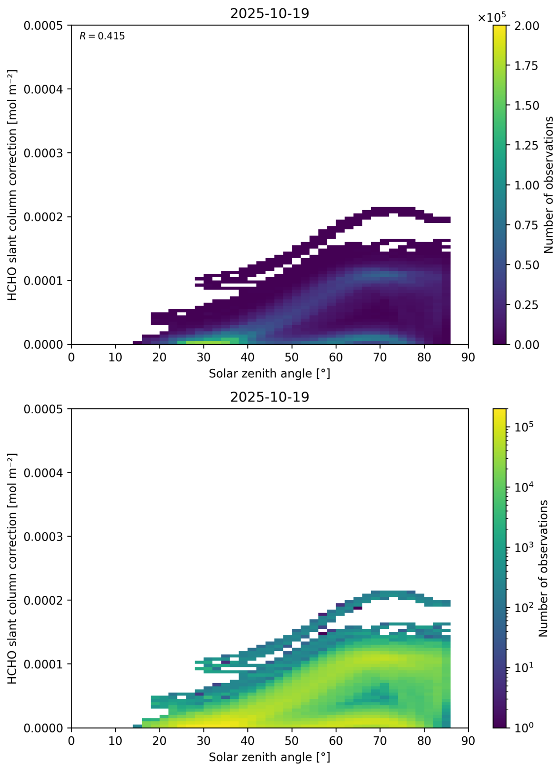
Figure 172: Scatter density plot of “Solar zenith angle” against “HCHO slant column correction” for 2025-10-18 to 2025-10-20.
