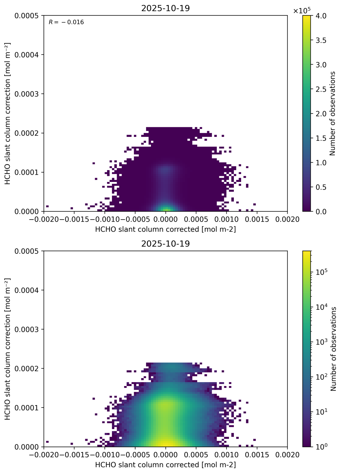
Figure 77: Scatter density plot of “HCHO slant column corrected” against “HCHO slant column correction” for 2025-10-18 to 2025-10-20.
