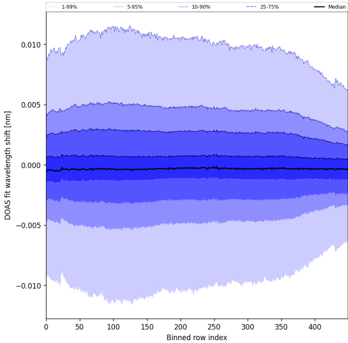
Figure 58: Along track statistics of “DOAS fit wavelength shift” for 2025-10-18 to 2025-10-20
