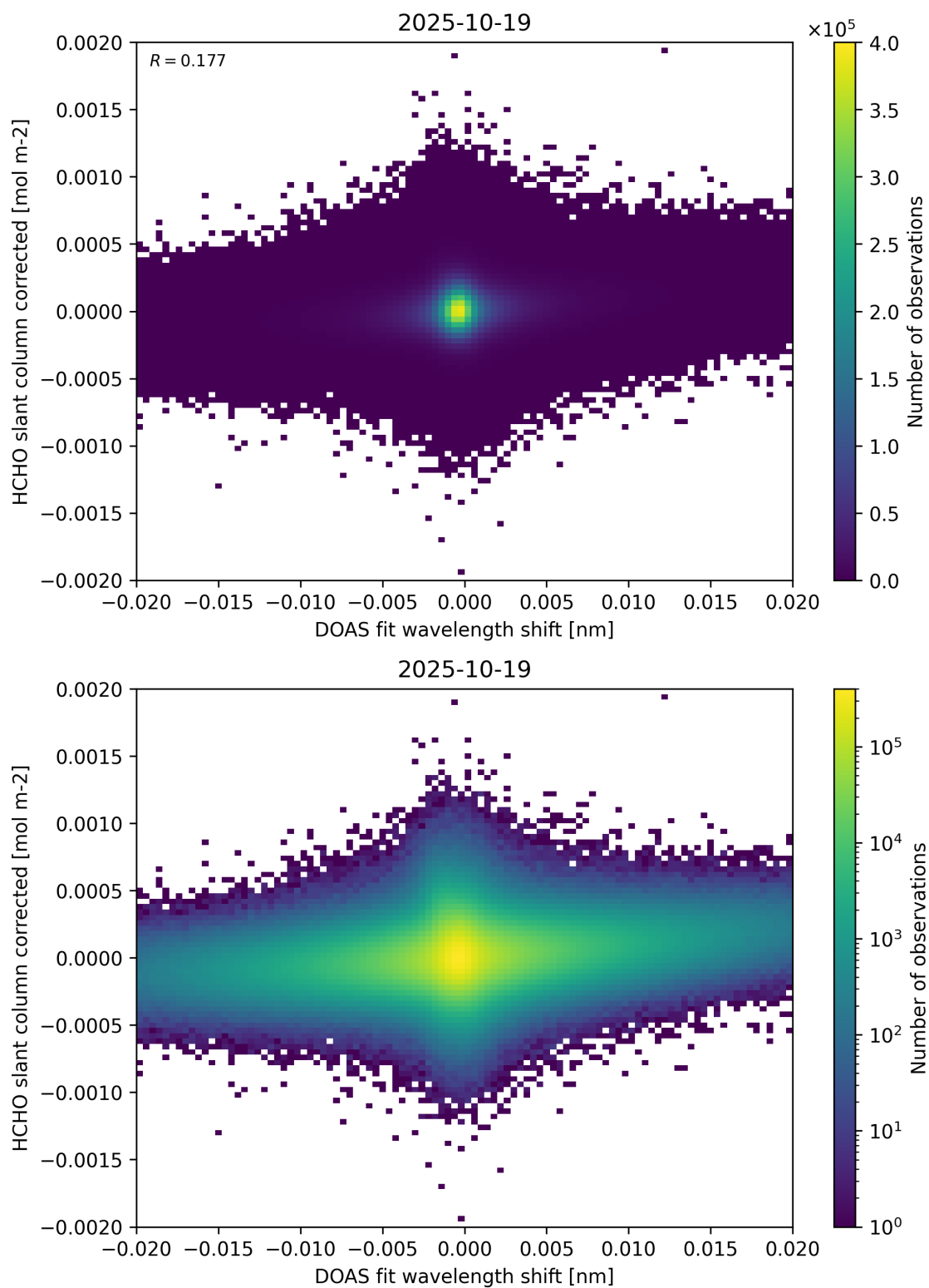
Figure 66: Scatter density plot of “DOAS fit wavelength shift” against “HCHO slant column corrected” for 2025-10-18 to 2025-10-20.
