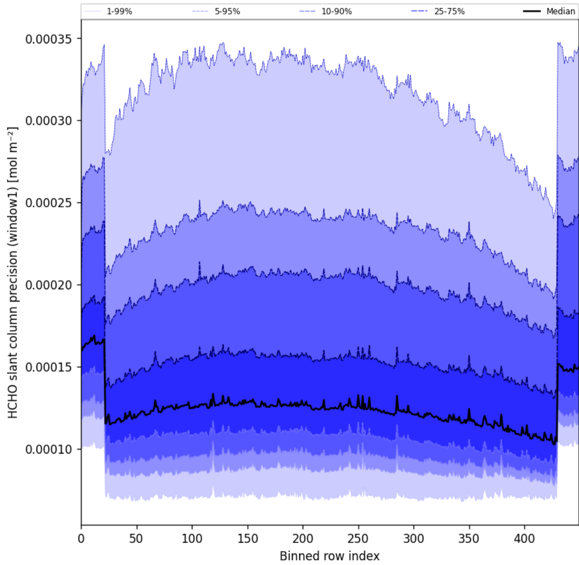
Figure 53: Along track statistics of “HCHO slant column precision (window1)” for 2025-10-18 to 2025-10-20
