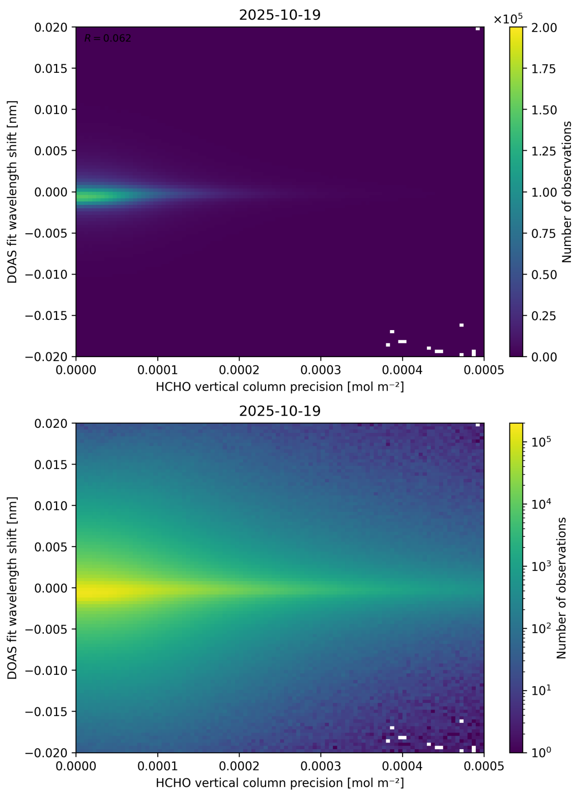
Figure 137: Scatter density plot of “HCHO vertical column precision” against “DOAS fit wavelength shift” for 2025-10-18 to 2025-10-20.
