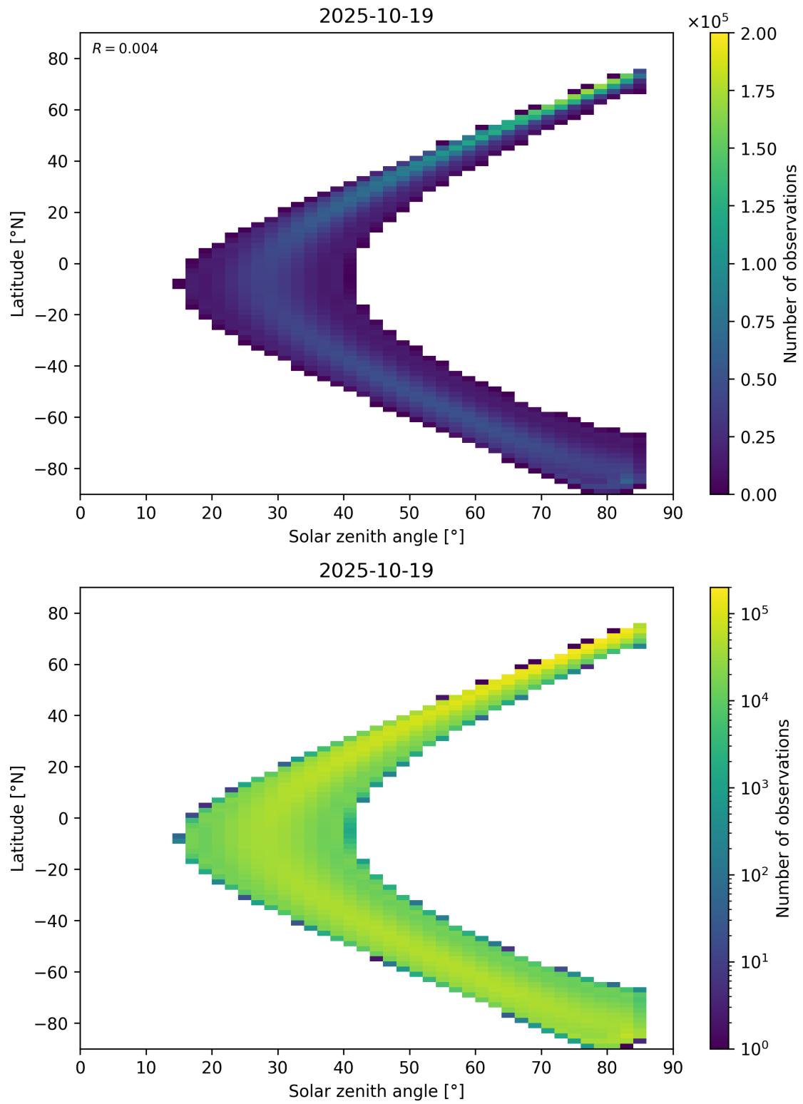
Figure 181: Scatter density plot of “Solar zenith angle” against “Latitude” for 2025-10-18 to 2025-10-20.
