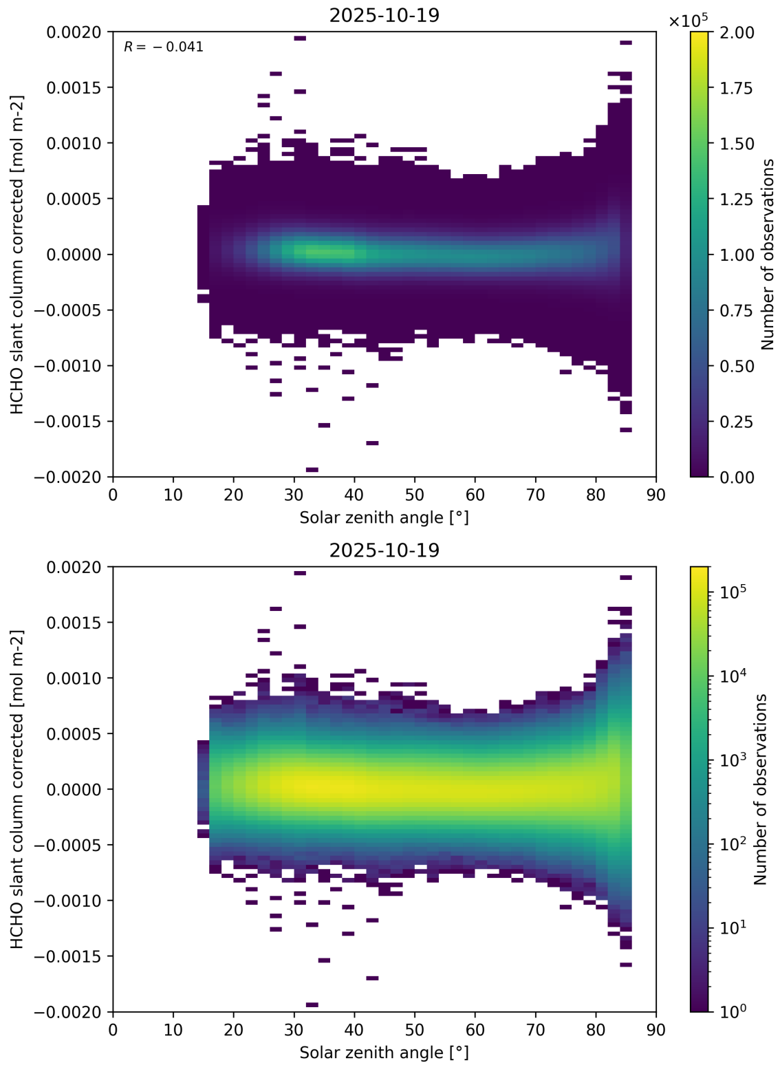
Figure 171: Scatter density plot of “Solar zenith angle” against “HCHO slant column corrected” for 2025-10-18 to 2025-10-20.
