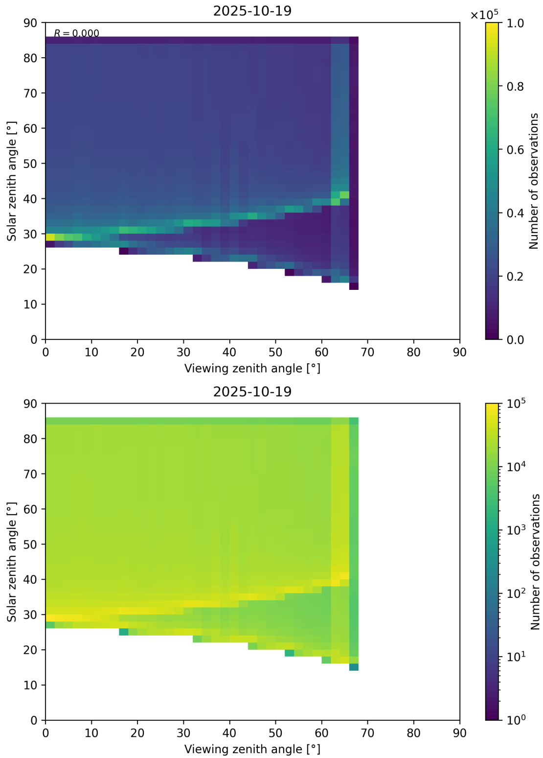
Figure 197: Scatter density plot of “Viewing zenith angle” against “Solar zenith angle” for 2025-10-18 to 2025-10-20.
