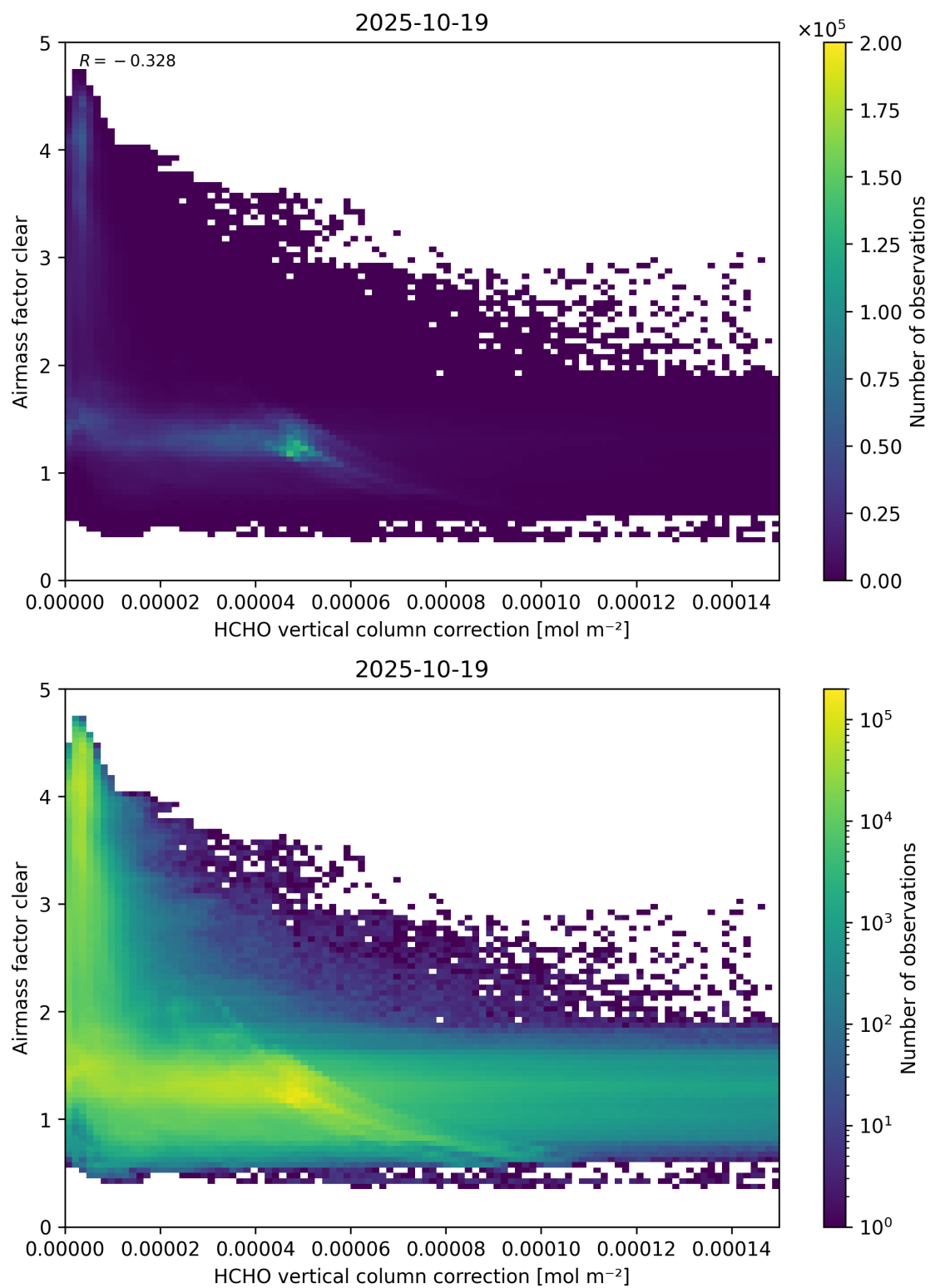
Figure 115: Scatter density plot of “HCHO vertical column correction” against “Air mass factor clear” for 2025-10-18 to 2025-10-20.
