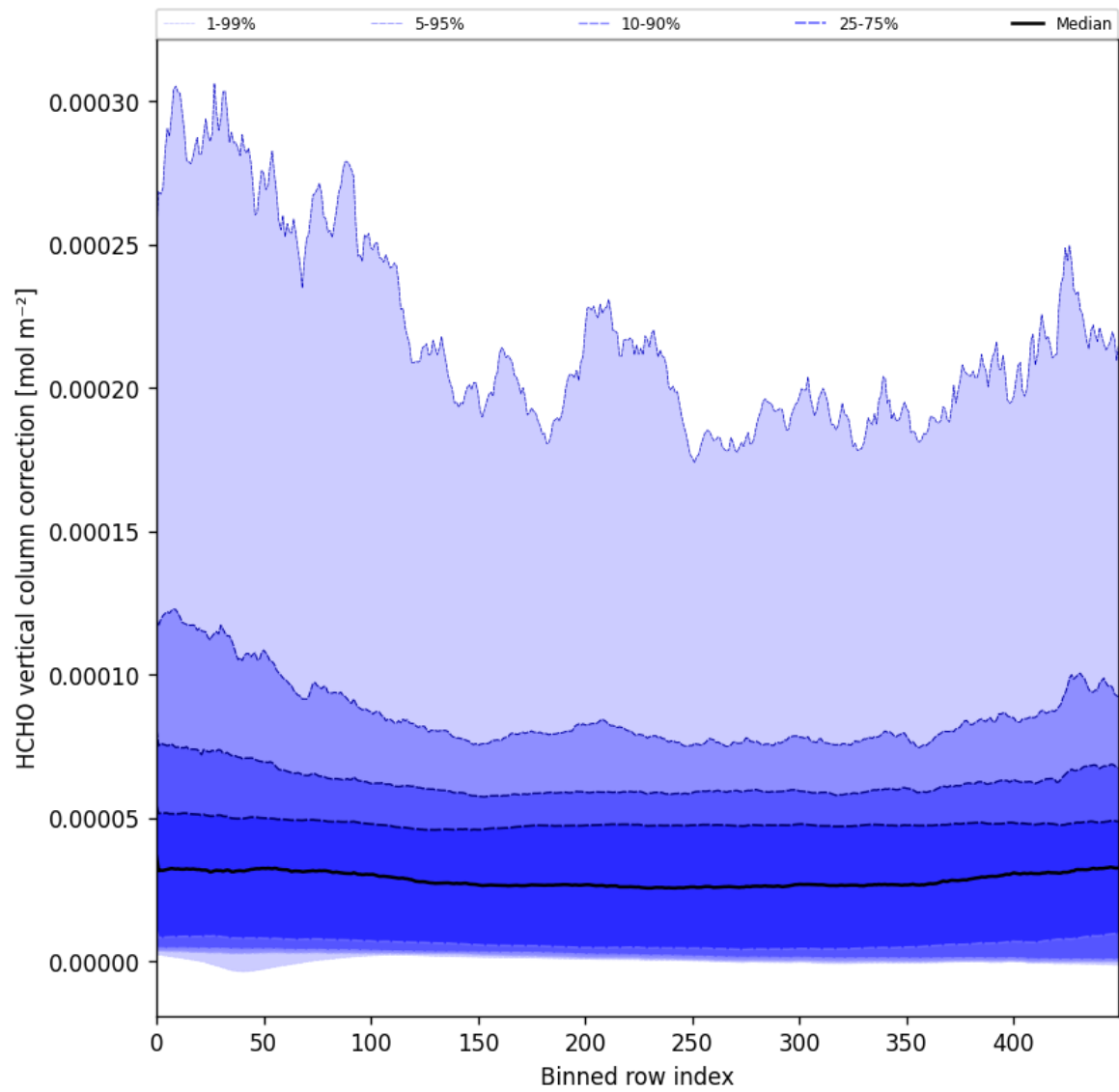
Figure 51: Along track statistics of “HCHO vertical column correction” for 2025-10-18 to 2025-10-20
