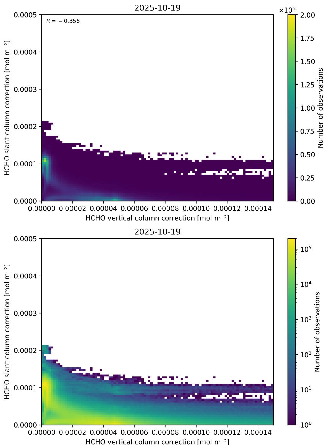
Figure 117: Scatter density plot of “HCHO vertical column correction” against “HCHO slant column correction” for 2025-10-18 to 2025-10-20.
