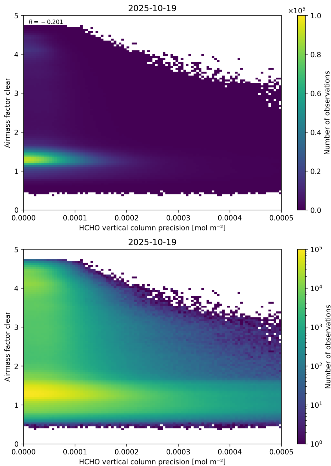
Figure 139: Scatter density plot of “HCHO vertical column precision” against “Airmass factor clear” for 2025-10-18 to 2025-10-20.
