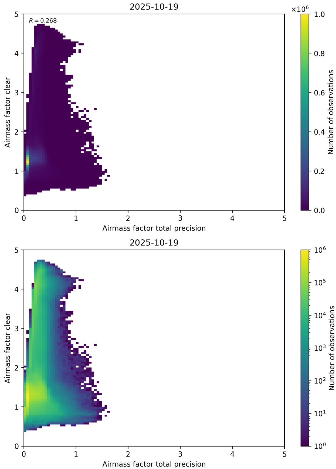
Figure 108: Scatter density plot of “Airmass factor total precision” against “Airmass factor clear” for 2025-10-18 to 2025-10-20.
