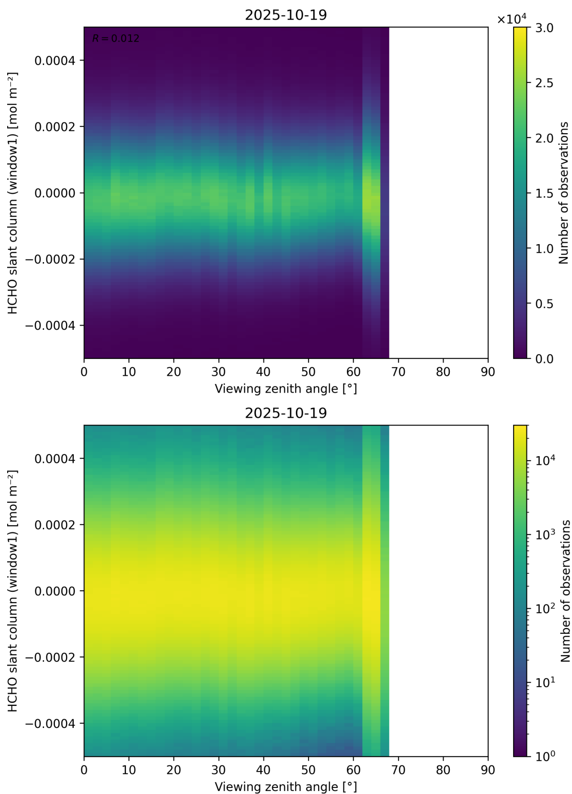
Figure 188: Scatter density plot of “Viewing zenith angle” against “HCHO slant column (window1)” for 2025-10-18 to 2025-10-20.
