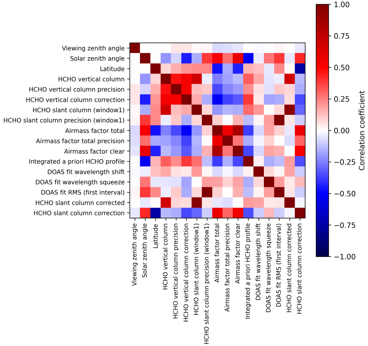
Figure 2: Map of correlation matrix for 2025-10-18 to 2025-10-20.
