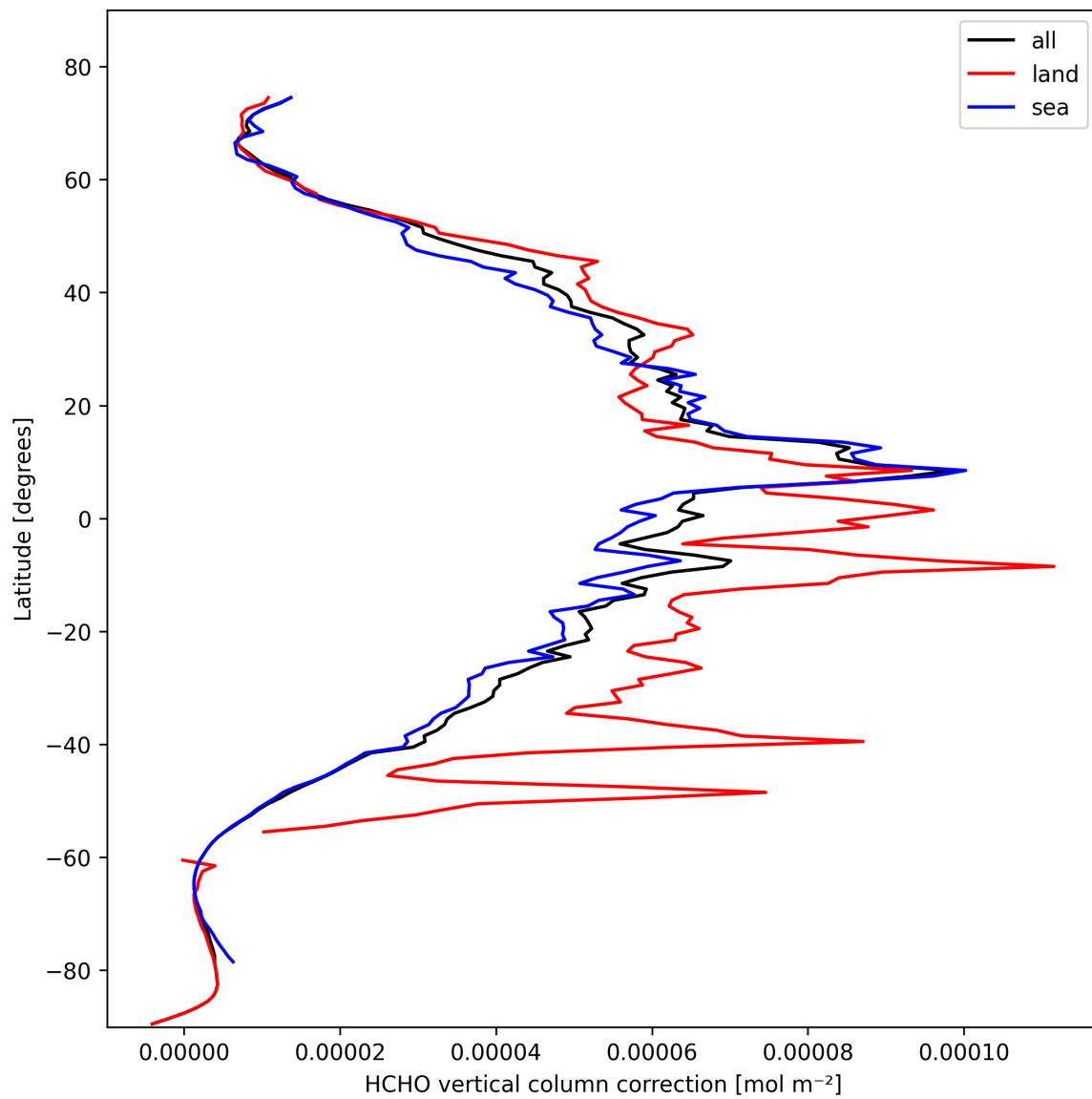
Figure 23: Zonal average of “HCHO vertical column correction” for 2025-10-18 to 2025-10-20.
