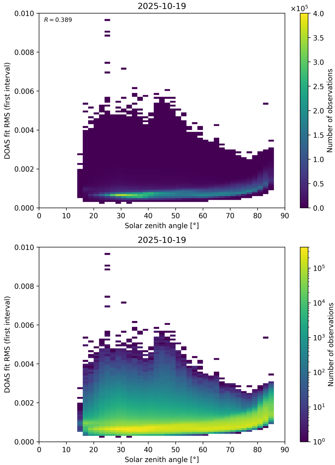
Figure 167: Scatter density plot of “Solar zenith angle” against “DOAS fit RMS (first interval)” for 2025-10-18 to 2025-10-20.
