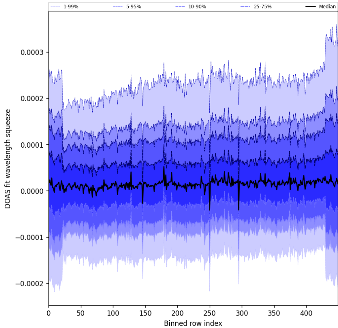
Figure 59: Along track statistics of “DOAS fit wavelength squeeze” for 2025-10-18 to 2025-10-20
