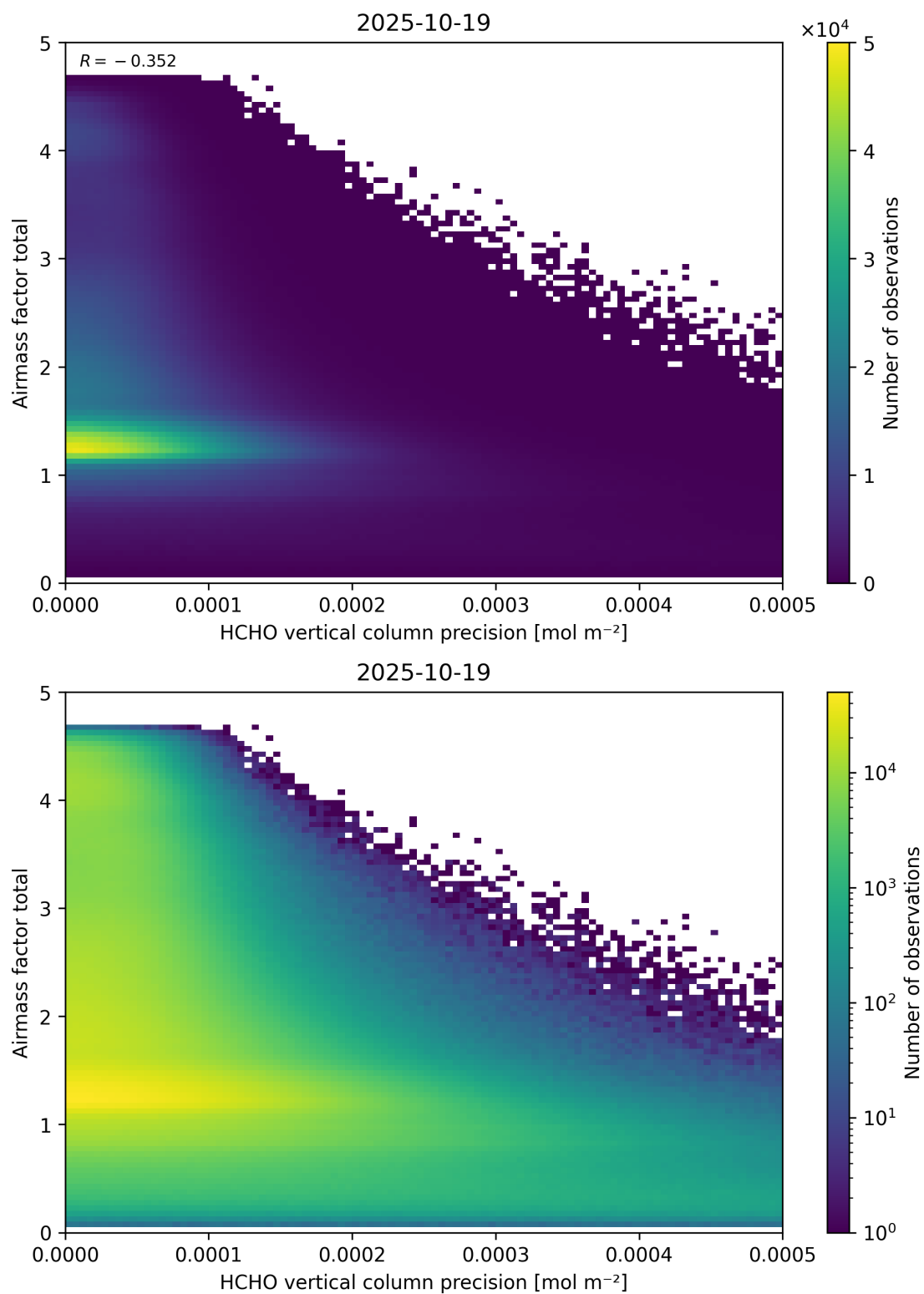
Figure 144: Scatter density plot of “HCHO vertical column precision” against “Airmass factor total” for 2025-10-18 to 2025-10-20.
