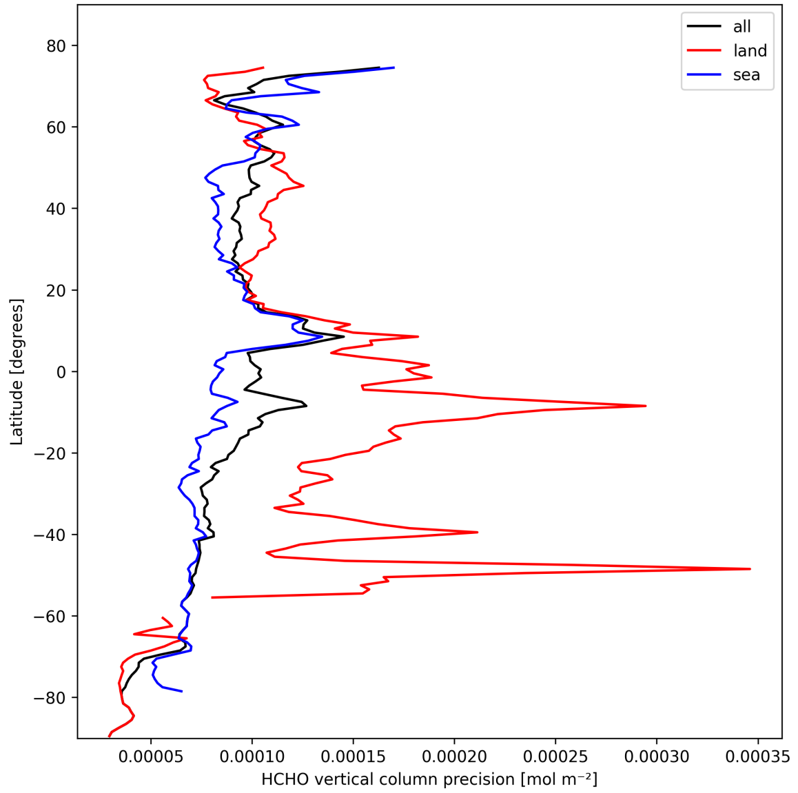
Figure 22: Zonal average of “HCHO vertical column precision” for 2025-10-18 to 2025-10-20.
