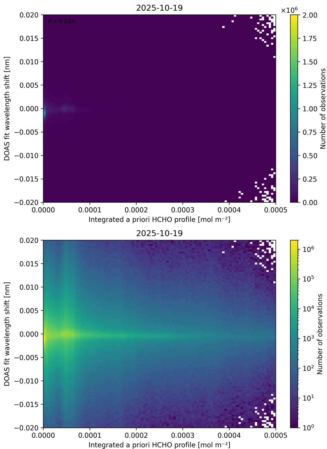
Figure 149: Scatter density plot of “Integrated a priori HCHO profile” against “DOAS fit wavelength shift” for 2025-10-18 to 2025-10-20.
