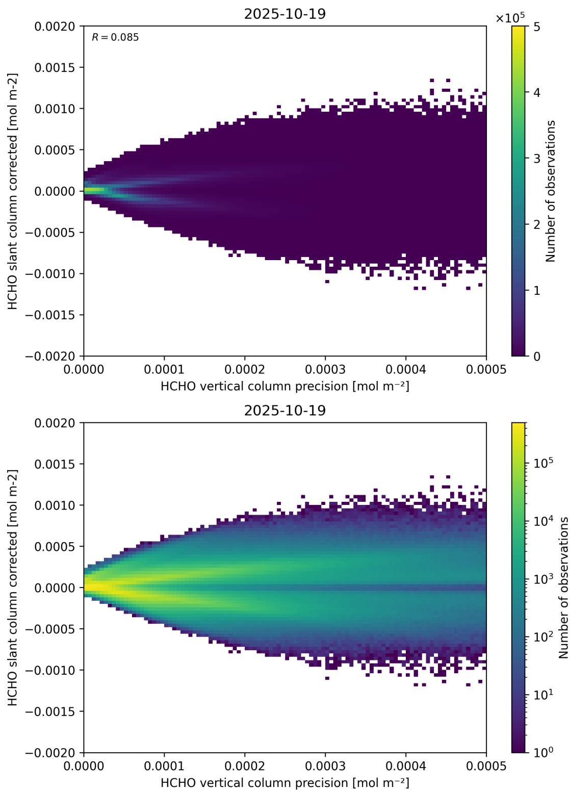
Figure 140: Scatter density plot of “HCHO vertical column precision” against “HCHO slant column corrected” for 2025-10-18 to 2025-10-20.
