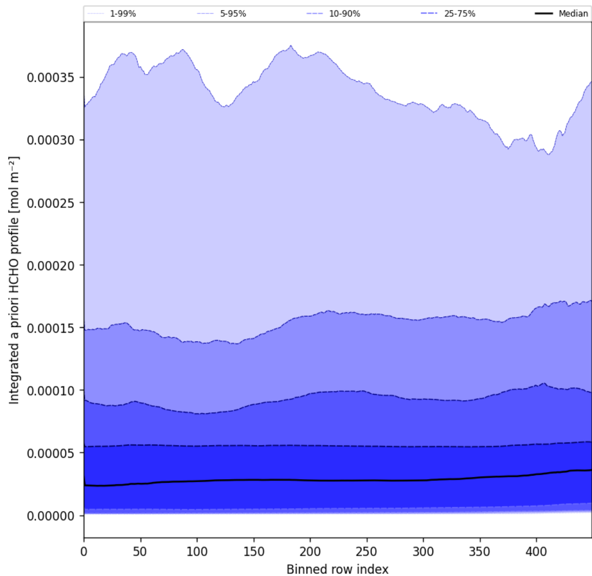
Figure 57: Along track statistics of “Integrated a priori HCHO profile” for 2025-10-18 to 2025-10-20
