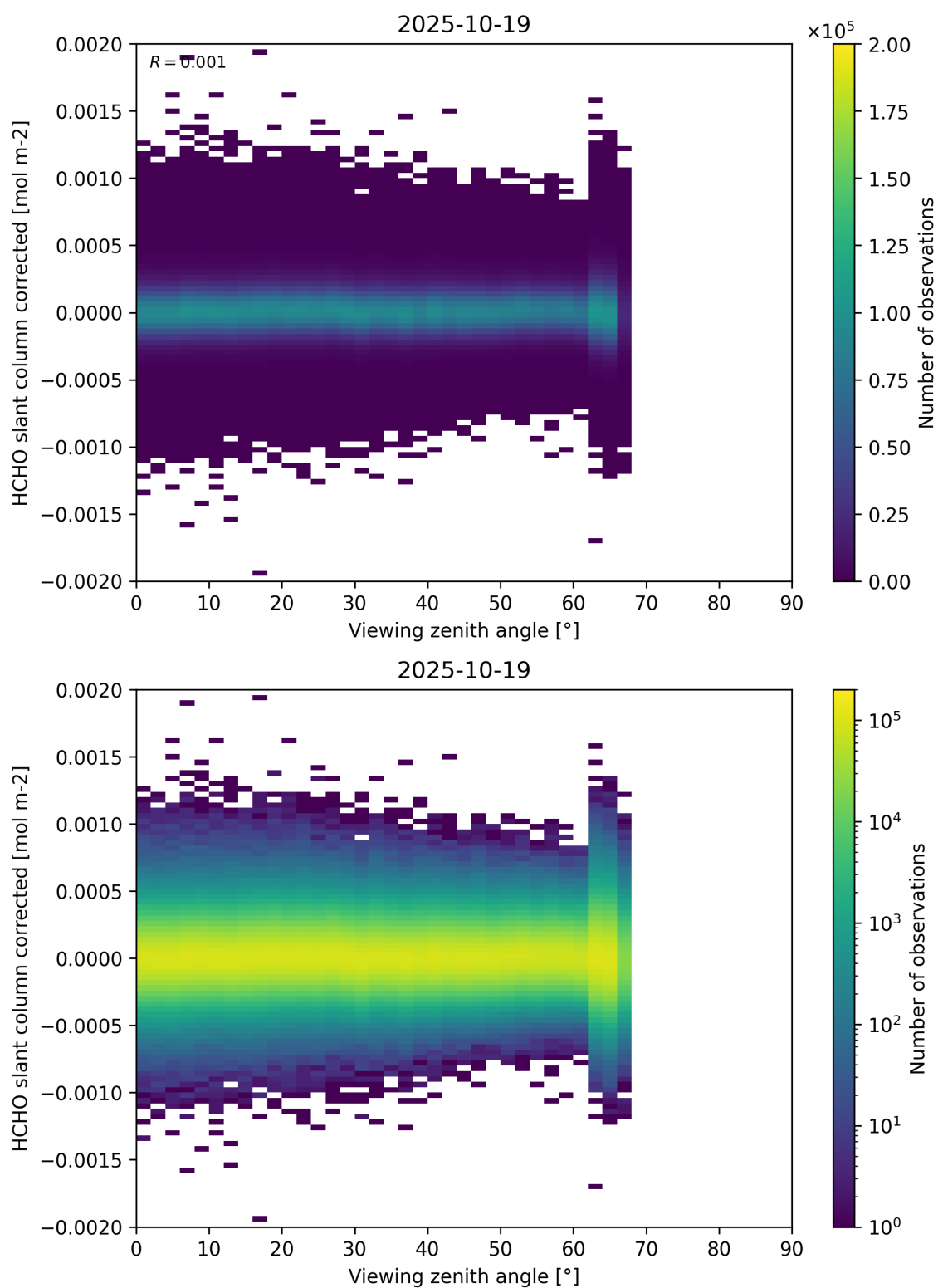
Figure 186: Scatter density plot of “Viewing zenith angle” against “HCHO slant column corrected” for 2025-10-18 to 2025-10-20.
