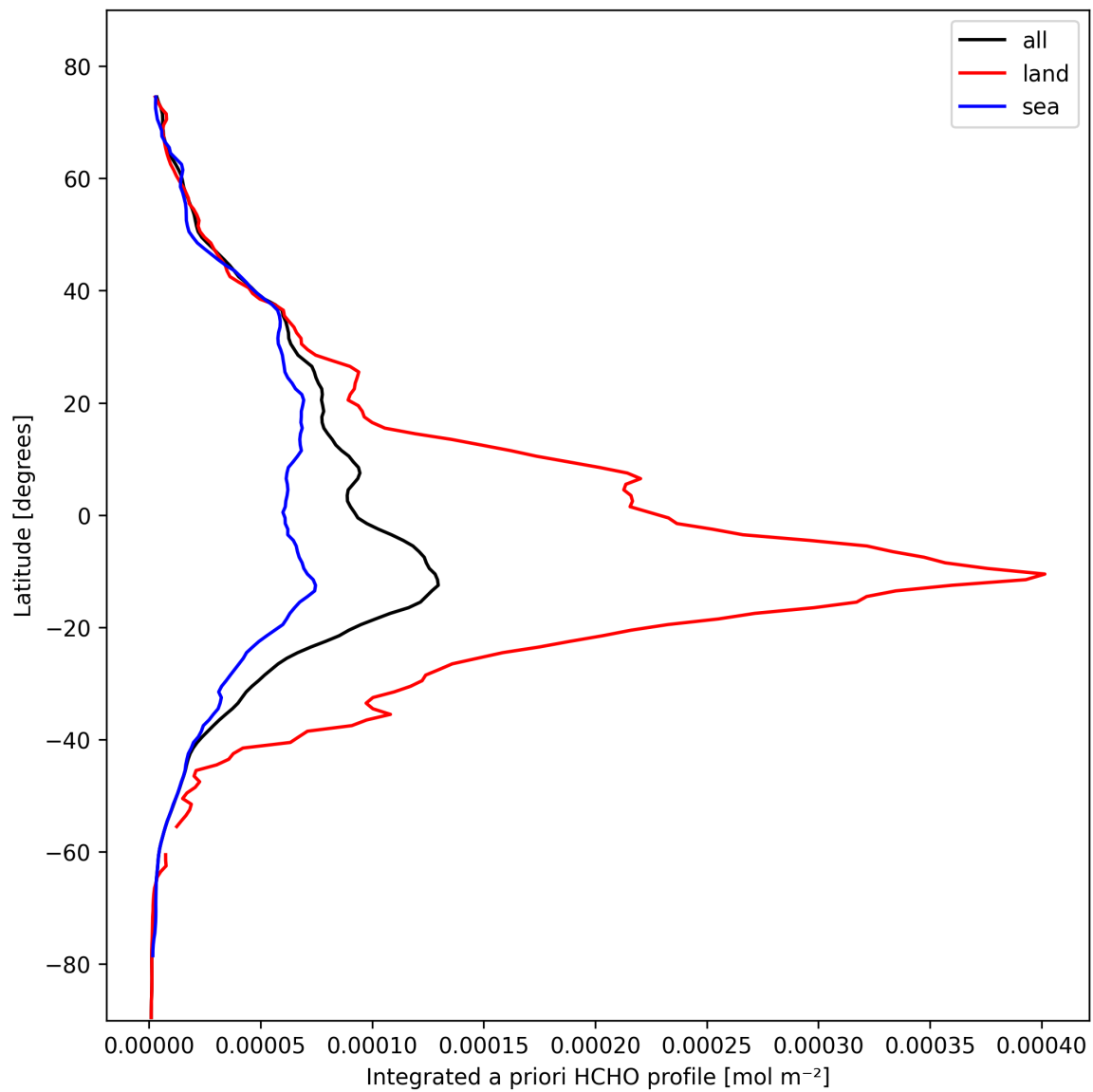
Figure 29: Zonal average of “Integrated a priori HCHO profile” for 2025-10-18 to 2025-10-20.
