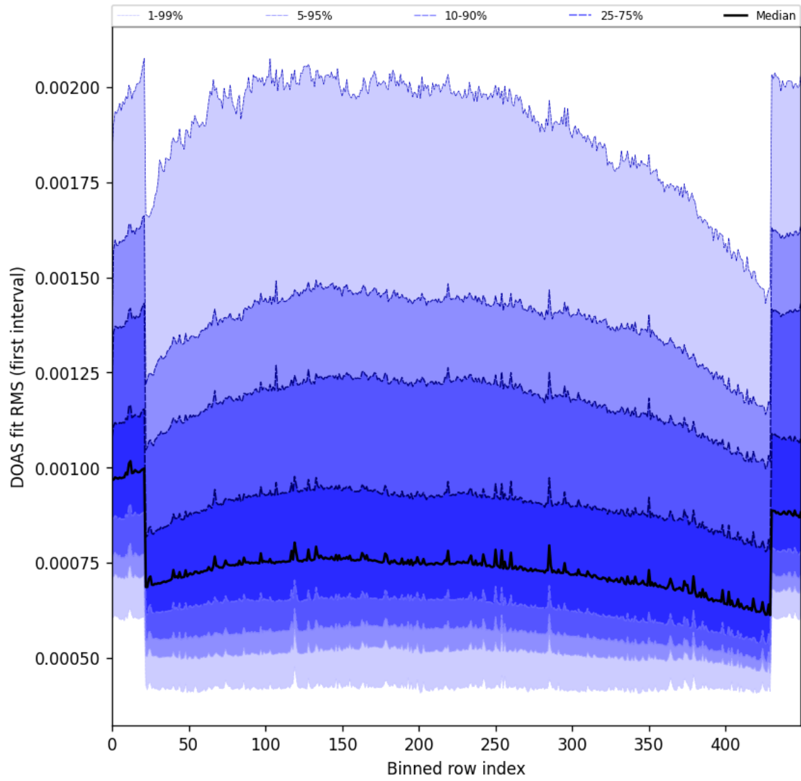
Figure 60: Along track statistics of “DOAS fit RMS (first interval)” for 2025-10-18 to 2025-10-20
