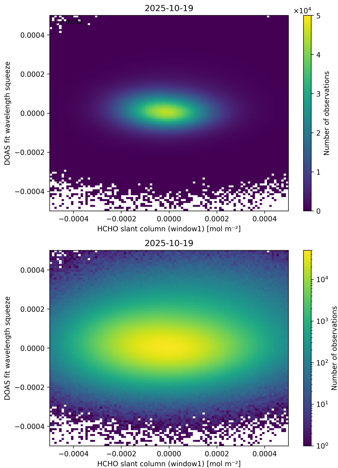
Figure 80: Scatter density plot of “HCHO slant column (window1)” against “DOAS fit wavelength squeeze” for 2025-10-18 to 2025-10-20.
