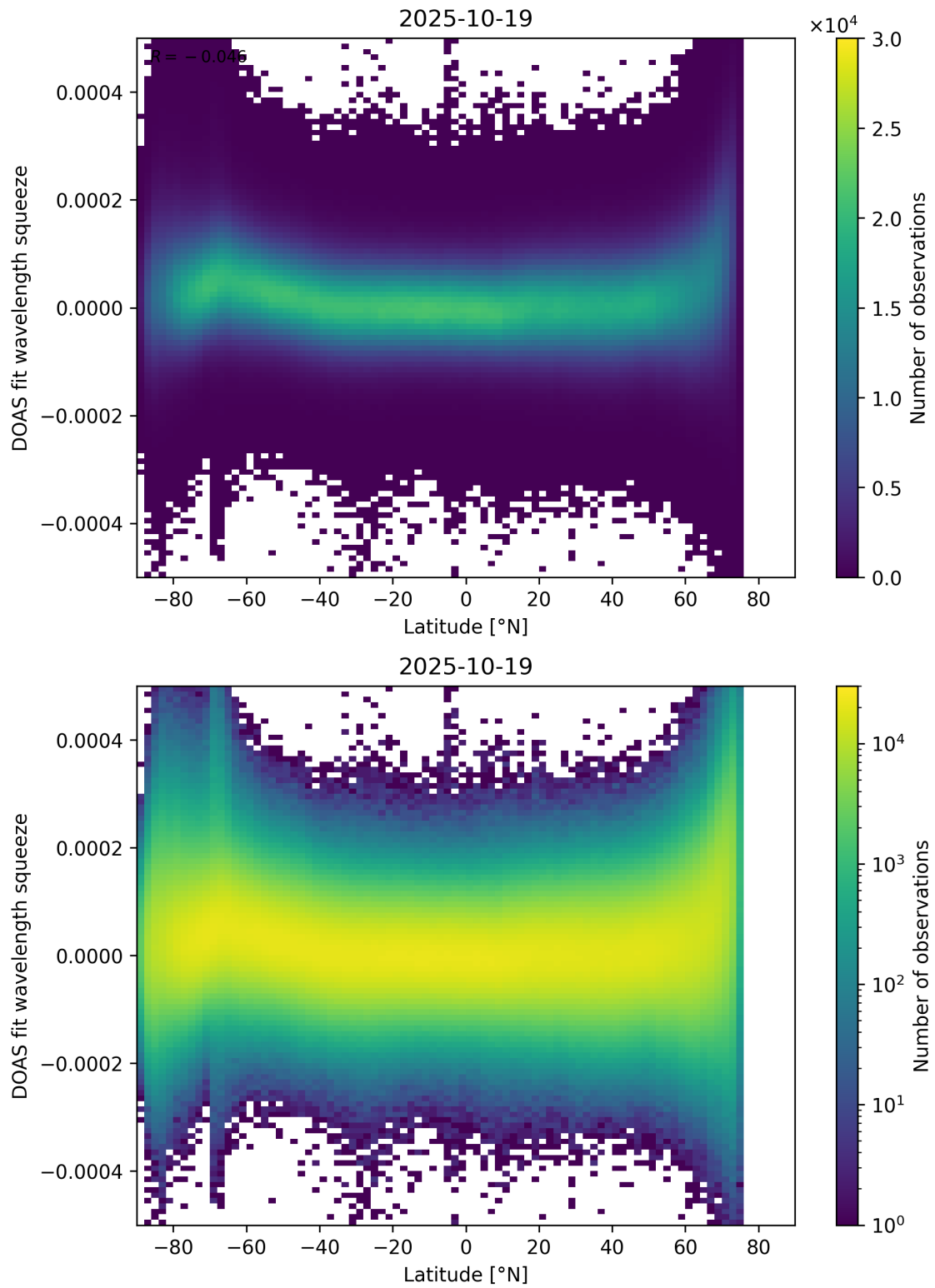
Figure 155: Scatter density plot of “Latitude” against “DOAS fit wavelength squeeze” for 2025-10-18 to 2025-10-20.
