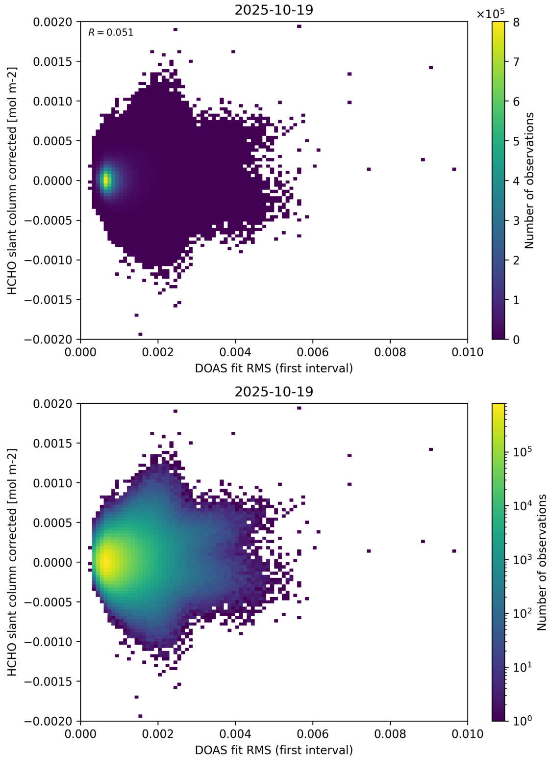
Figure 62: Scatter density plot of “DOAS fit RMS (first interval)” against “HCHO slant column corrected” for 2025-10-18 to 2025-10-20.
