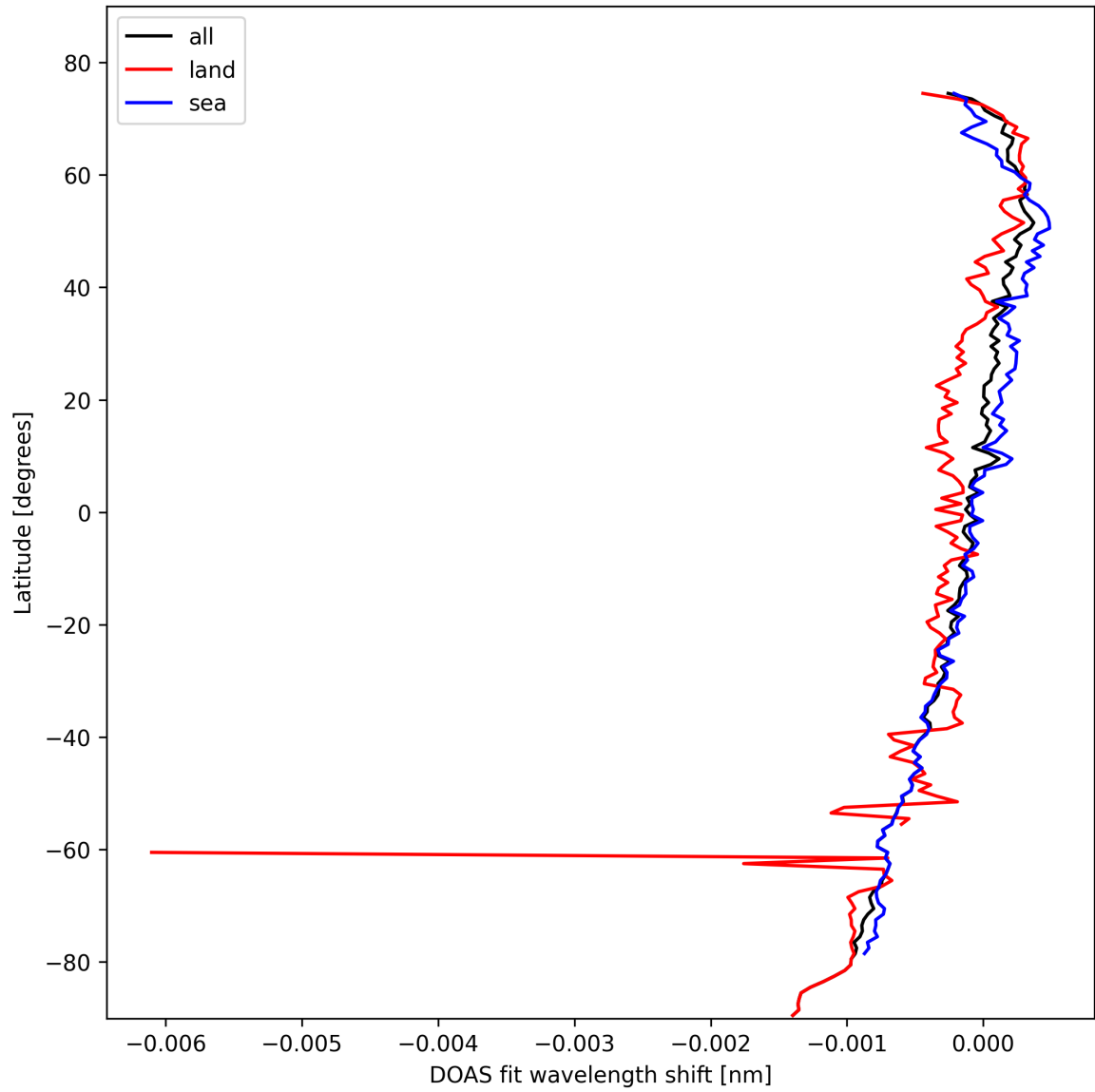
Figure 30: Zonal average of “DOAS fit wavelength shift” for 2025-10-18 to 2025-10-20.
