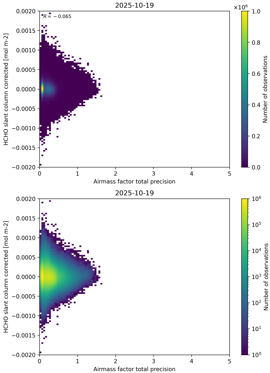
Figure 109: Scatter density plot of “Airmass factor total precision” against “HCHO slant column corrected” for 2025-10-18 to 2025-10-20.
