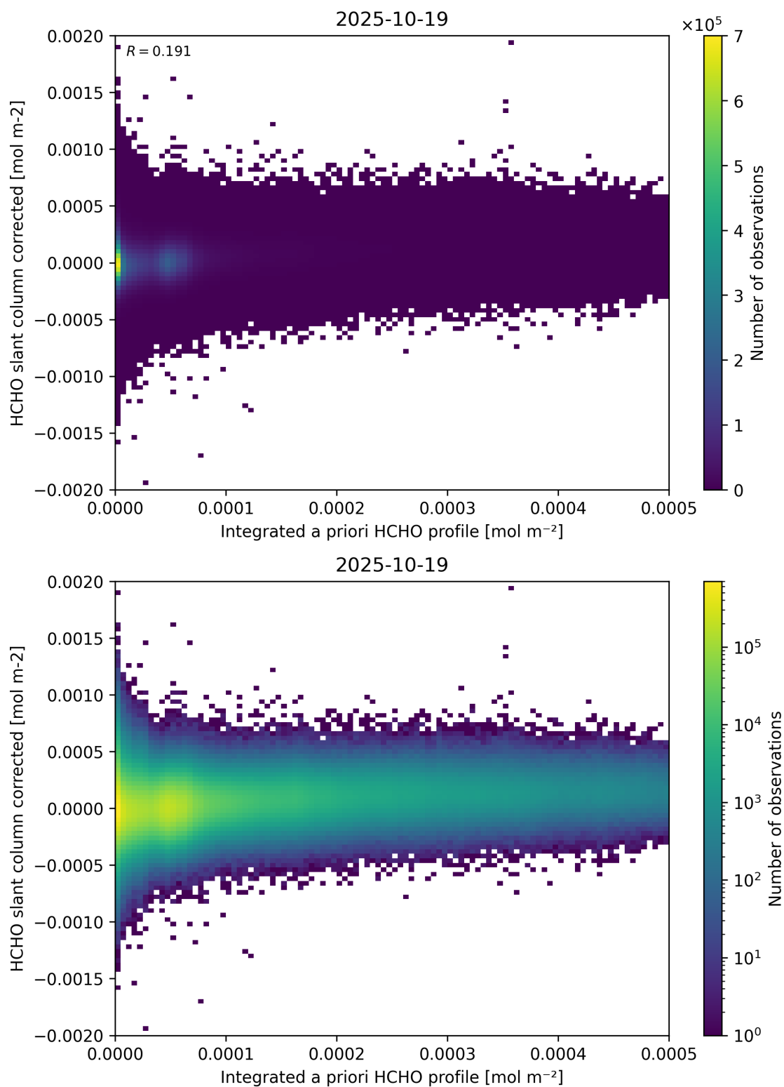
Figure 151: Scatter density plot of “Integrated a priori HCHO profile” against “HCHO slant column corrected” for 2025-10-18 to 2025-10-20.
