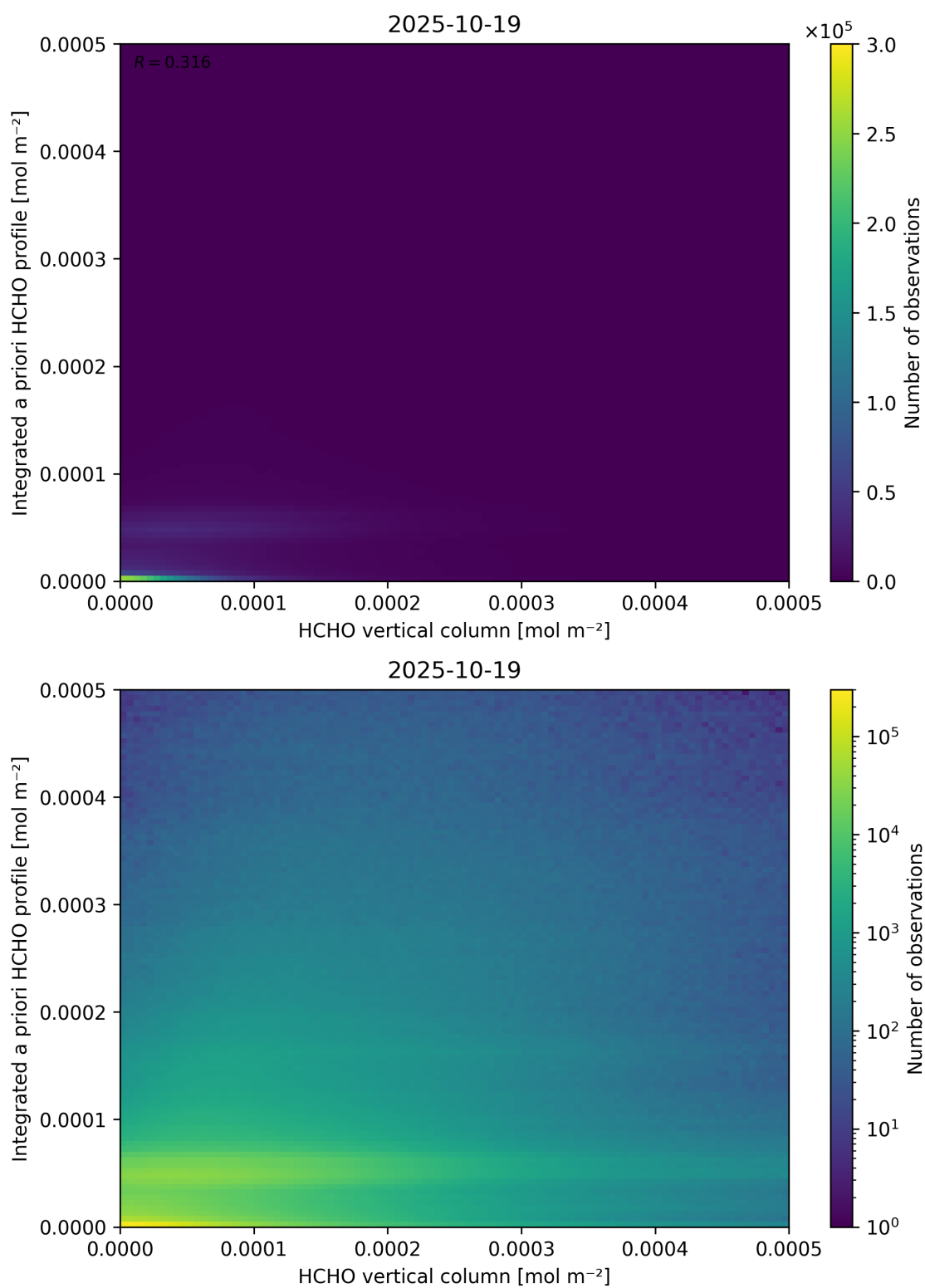
Figure 135: Scatter density plot of “HCHO vertical column” against “Integrated a priori HCHO profile” for 2025-10-18 to 2025-10-20.
