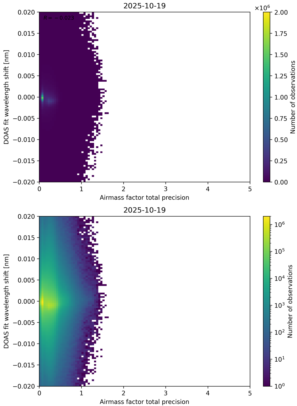
Figure 106: Scatter density plot of “Airmass factor total precision” against “DOAS fit wavelength shift” for 2025-10-18 to 2025-10-20.
