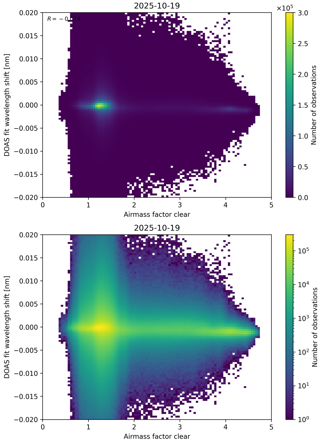
Figure 72: Scatter density plot of “Airmass factor clear” against “DOAS fit wavelength shift” for 2025-10-18 to 2025-10-20.
