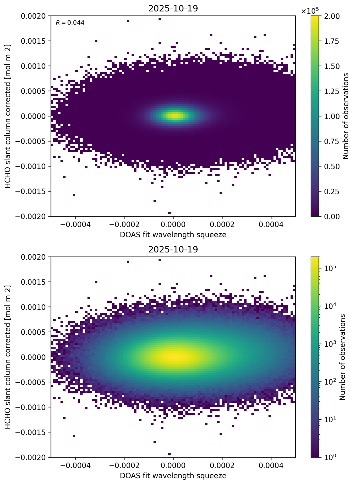
Figure 69: Scatter density plot of “DOAS fit wavelength squeeze” against “HCHO slant column corrected” for 2025-10-18 to 2025-10-20.
