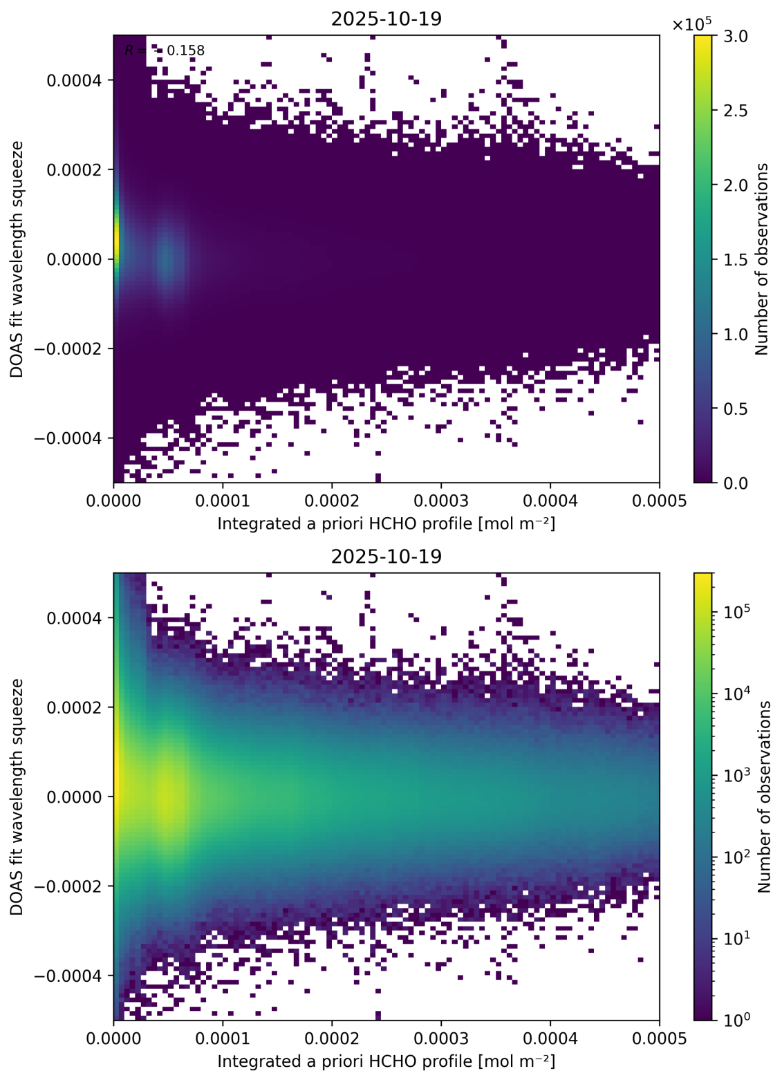
Figure 150: Scatter density plot of “Integrated a priori HCHO profile” against “DOAS fit wavelength squeeze” for 2025-10-18 to 2025-10-20.
