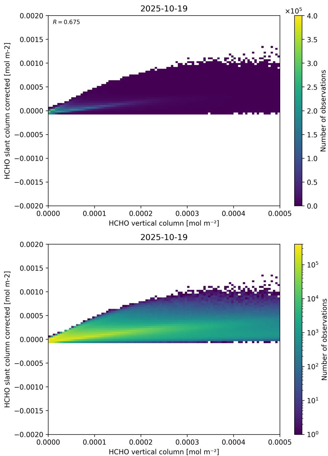
Figure 127: Scatter density plot of “HCHO vertical column” against “HCHO slant column corrected” for 2025-10-18 to 2025-10-20.
