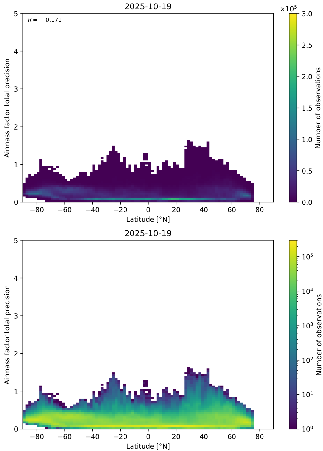
Figure 162: Scatter density plot of “Latitude” against “Airmass factor total precision” for 2025-10-18 to 2025-10-20.
