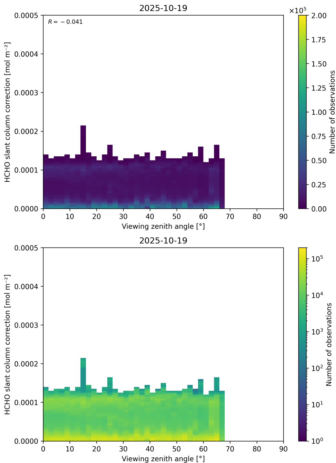
Figure 187: Scatter density plot of “Viewing zenith angle” against “HCHO slant column correction” for 2025-10-18 to 2025-10-20.
