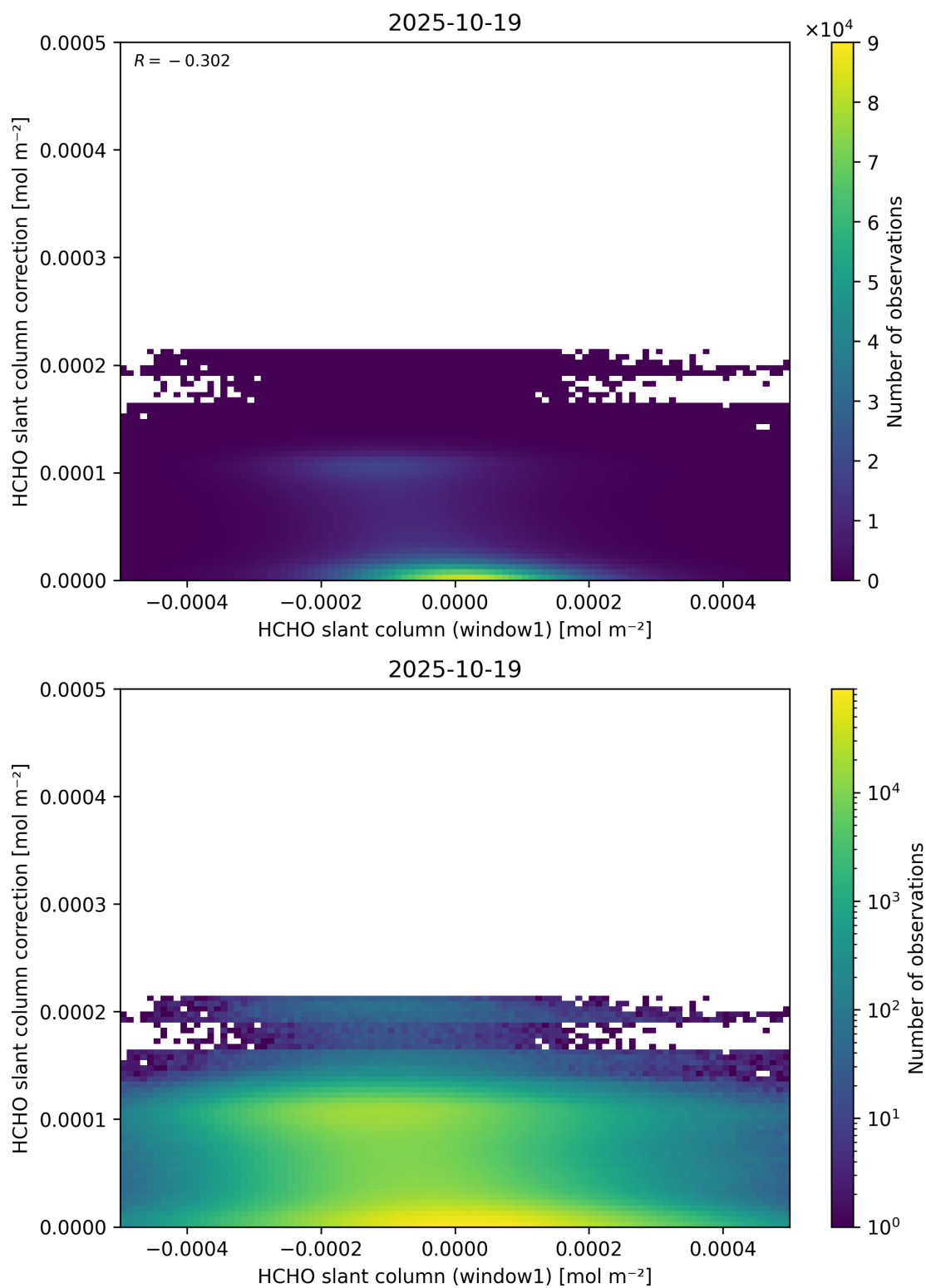
Figure 83: Scatter density plot of “HCHO slant column (window1)” against “HCHO slant column correction” for 2025-10-18 to 2025-10-20.
