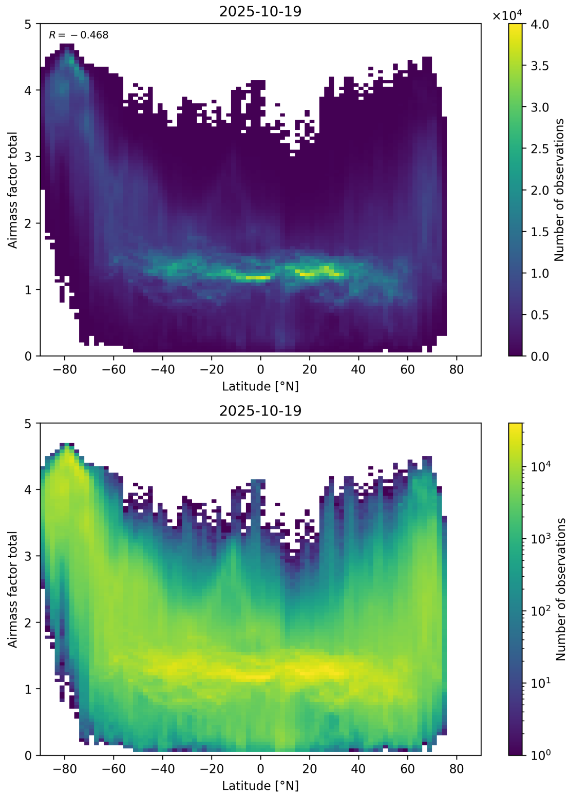
Figure 161: Scatter density plot of “Latitude” against “Airmass factor total” for 2025-10-18 to 2025-10-20.
