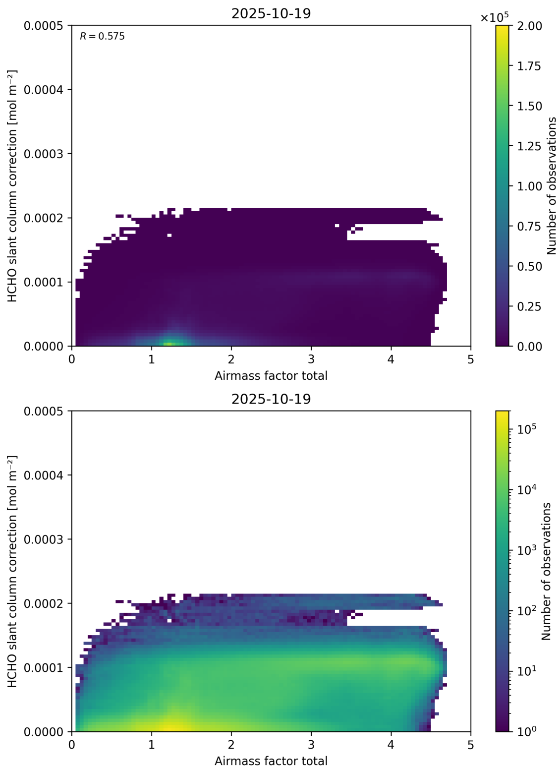
Figure 102: Scatter density plot of “Airmass factor total” against “HCHO slant column correction” for 2025-10-18 to 2025-10-20.
