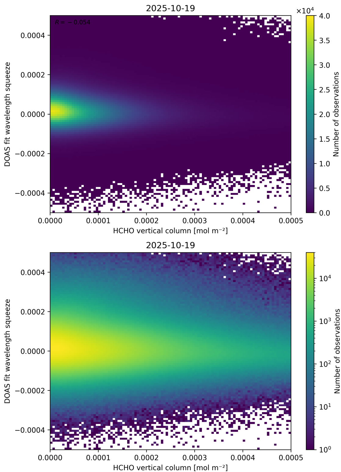
Figure 125: Scatter density plot of “HCHO vertical column” against “DOAS fit wavelength squeeze” for 2025-10-18 to 2025-10-20.
