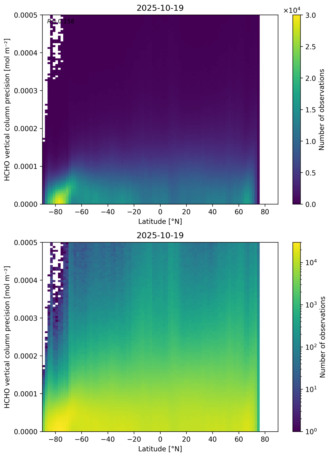
Figure 165: Scatter density plot of “Latitude” against “HCHO vertical column precision” for 2025-10-18 to 2025-10-20.
