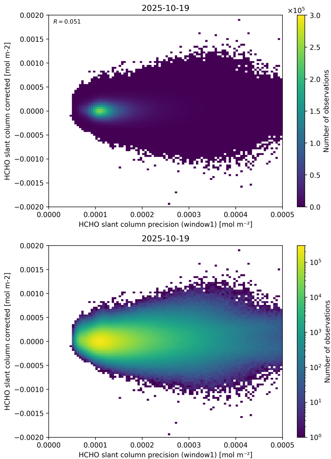
Figure 92: Scatter density plot of “HCHO slant column precision (window1)” against “HCHO slant column corrected” for 2025-10-18 to 2025-10-20.
