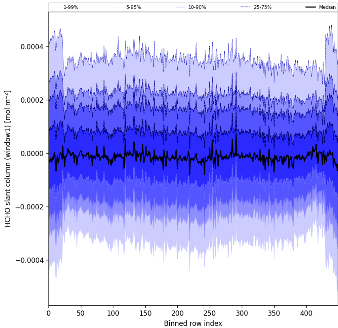
Figure 52: Along track statistics of “HCHO slant column (window1)” for 2025-10-18 to 2025-10-20
