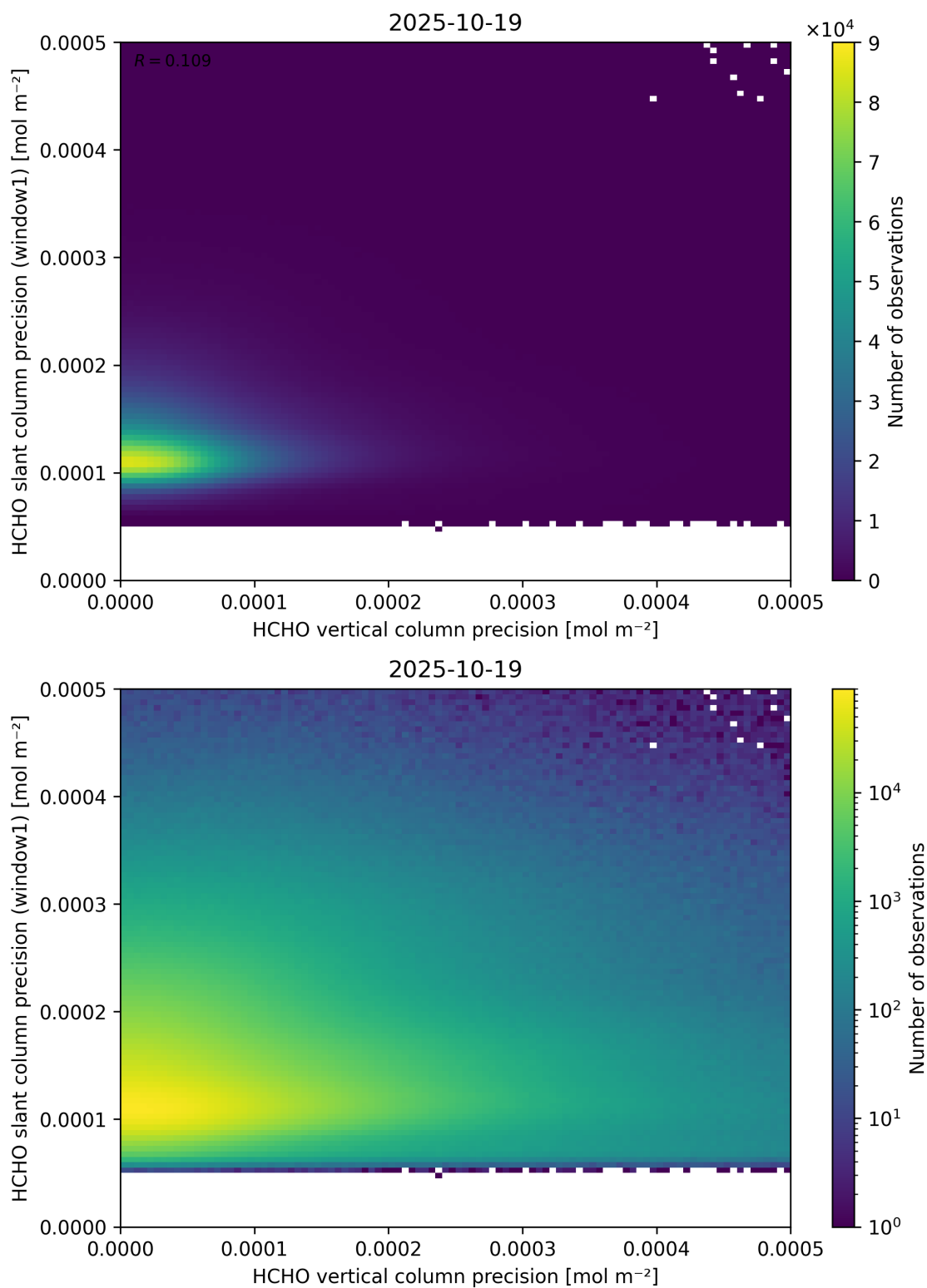
Figure 143: Scatter density plot of “HCHO vertical column precision” against “HCHO slant column precision (window1)” for 2025-10-18 to 2025-10-20.
