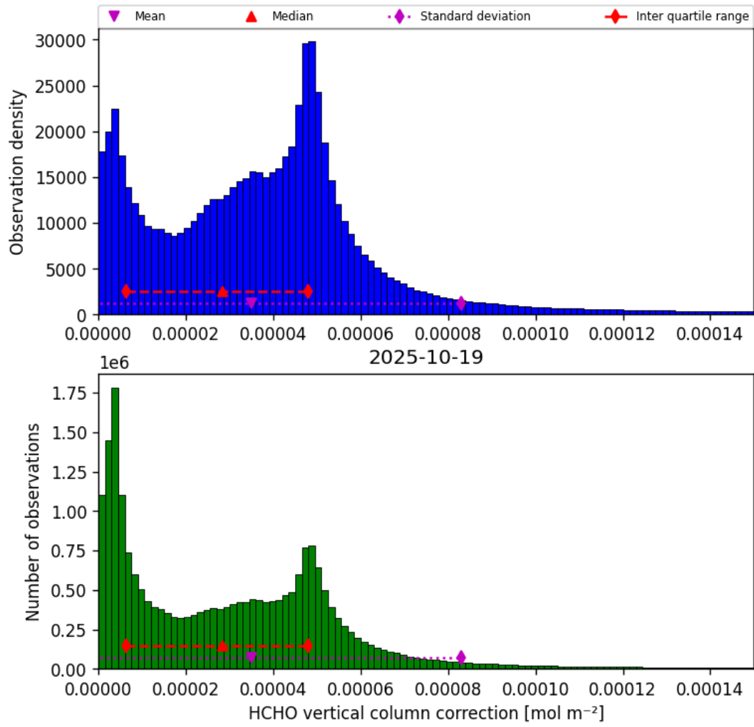
Figure 37: Histogram of “HCHO vertical column correction” for 2025-10-18 to 2025-10-20
