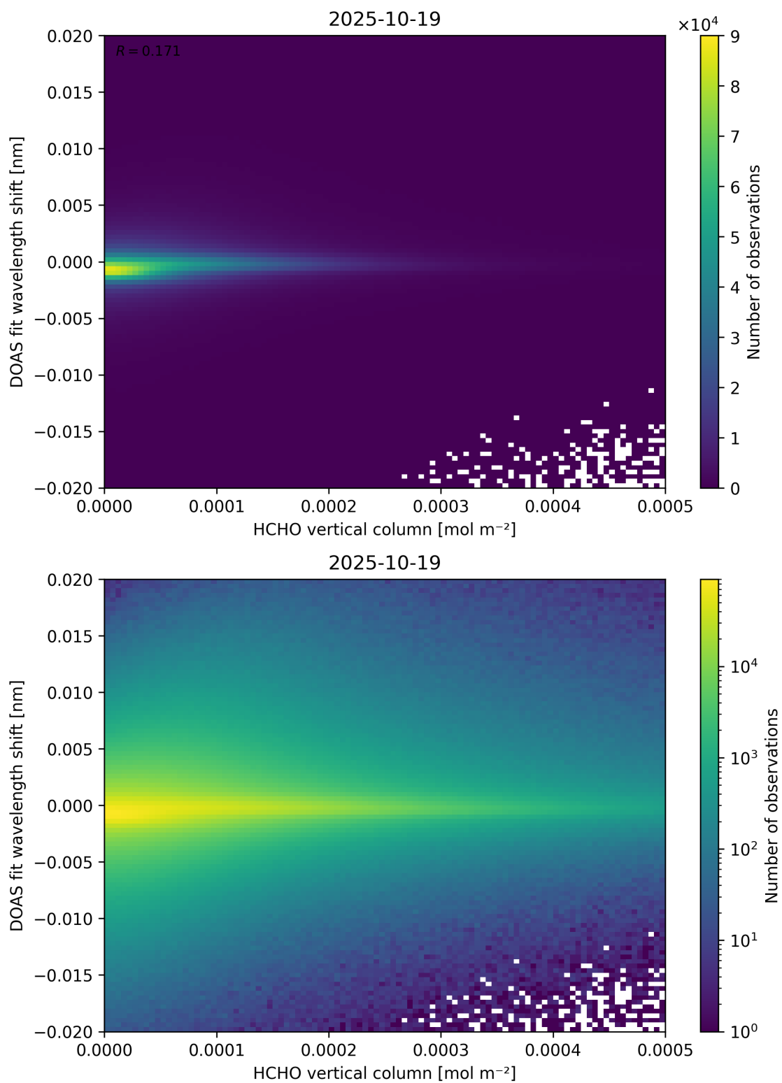
Figure 124: Scatter density plot of “HCHO vertical column” against “DOAS fit wavelength shift” for 2025-10-18 to 2025-10-20.
