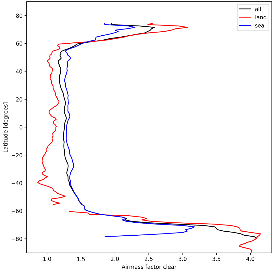
Figure 28: Zonal average of “Airmass factor clear” for 2025-10-18 to 2025-10-20.
