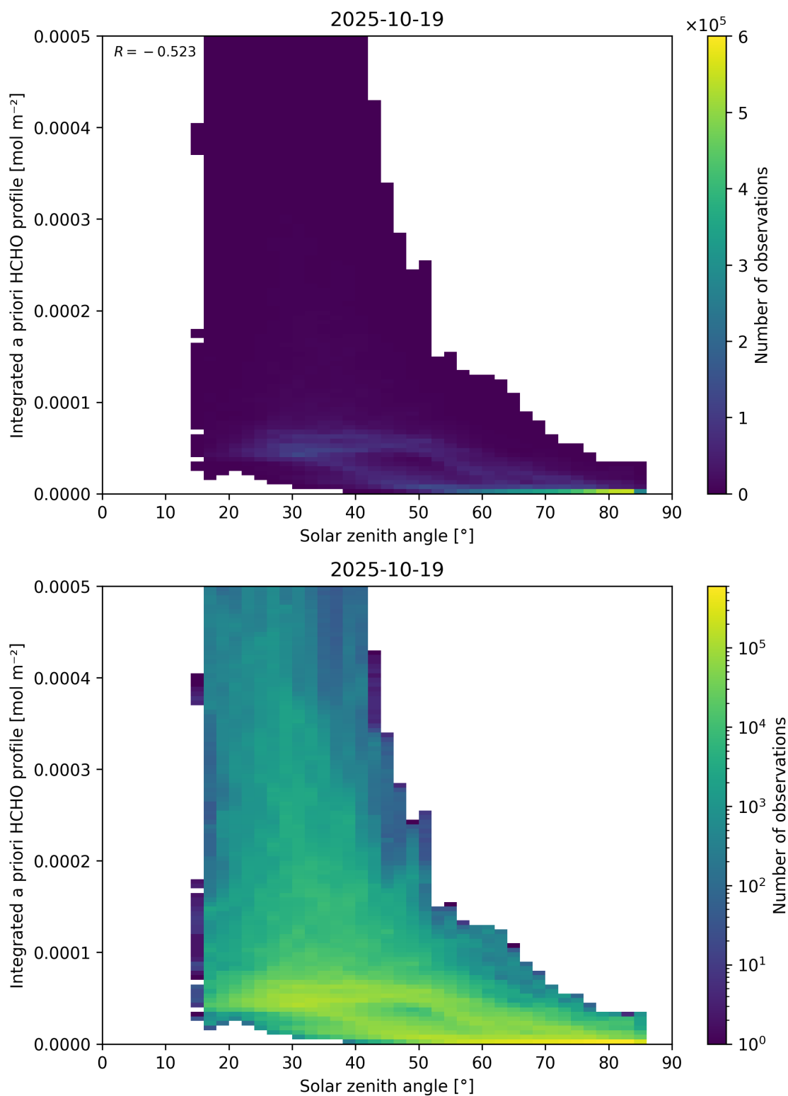
Figure 180: Scatter density plot of “Solar zenith angle” against “Integrated a priori HCHO profile” for 2025-10-18 to 2025-10-20.
