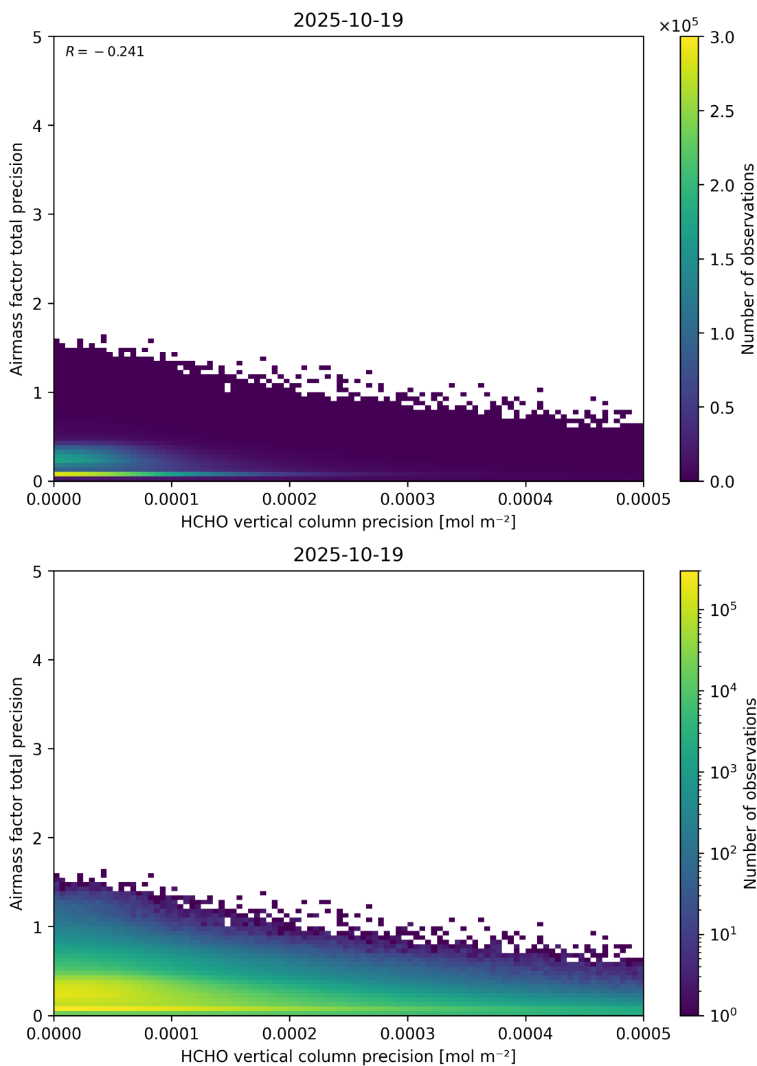
Figure 145: Scatter density plot of “HCHO vertical column precision” against “Airmass factor total precision” for 2025-10-18 to 2025-10-20.
