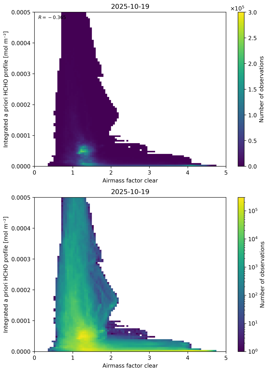
Figure 76: Scatter density plot of “Airmass factor clear” against “Integrated a priori HCHO profile” for 2025-10-18 to 2025-10-20.
