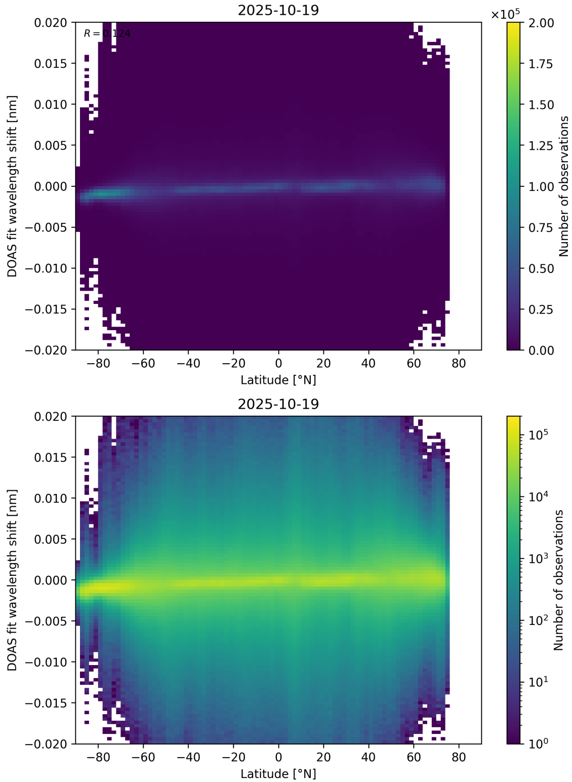
Figure 154: Scatter density plot of “Latitude” against “DOAS fit wavelength shift” for 2025-10-18 to 2025-10-20.
