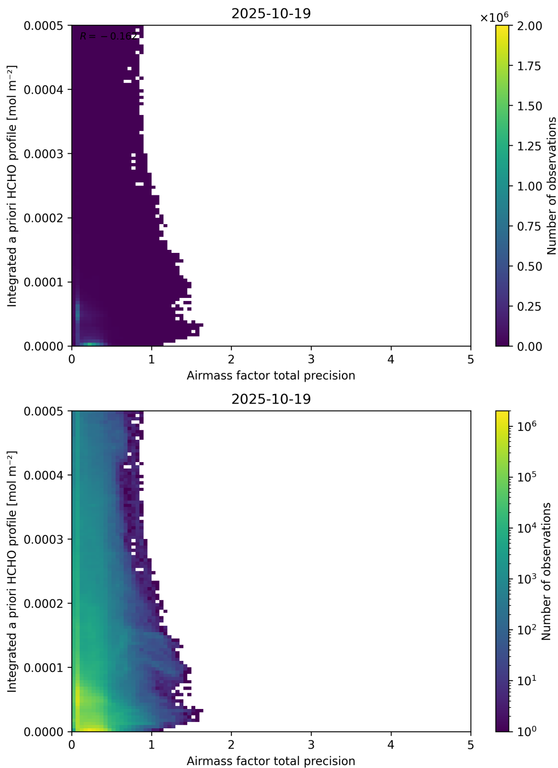
Figure 111: Scatter density plot of “Airmass factor total precision” against “Integrated a priori HCHO profile” for 2025-10-18 to 2025-10-20.
