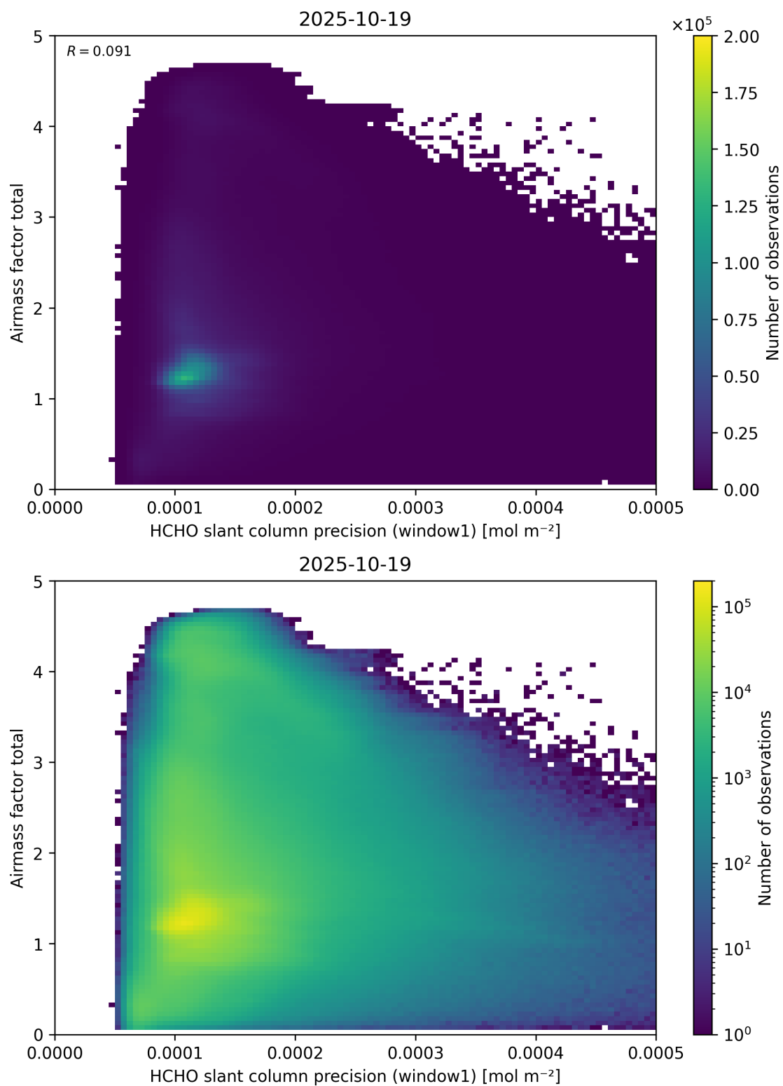
Figure 94: Scatter density plot of “HCHO slant column precision (window1)” against “Airmass factor total” for 2025-10-18 to 2025-10-20.
