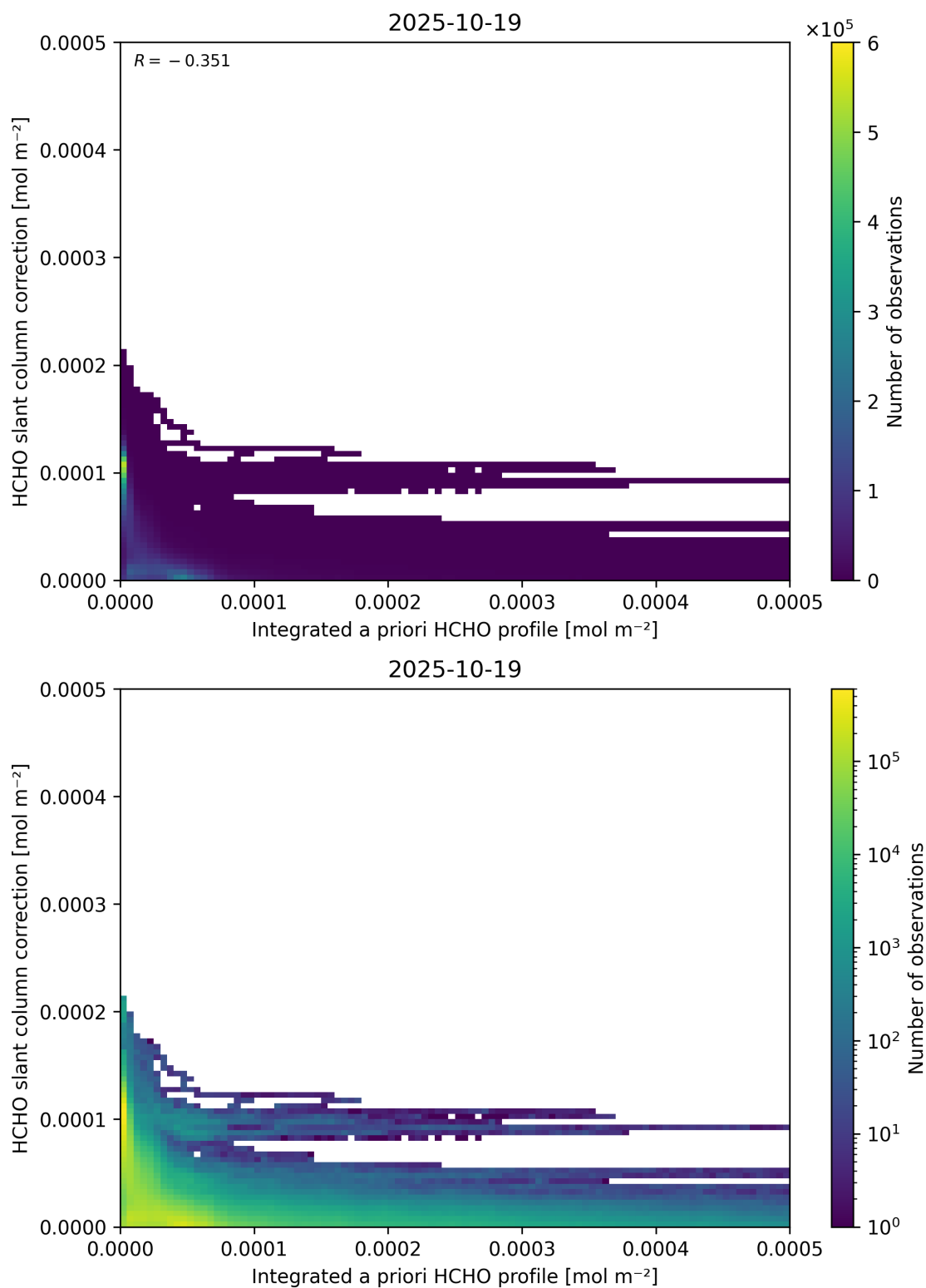
Figure 152: Scatter density plot of “Integrated a priori HCHO profile” against “HCHO slant column correction” for 2025-10-18 to 2025-10-20.
