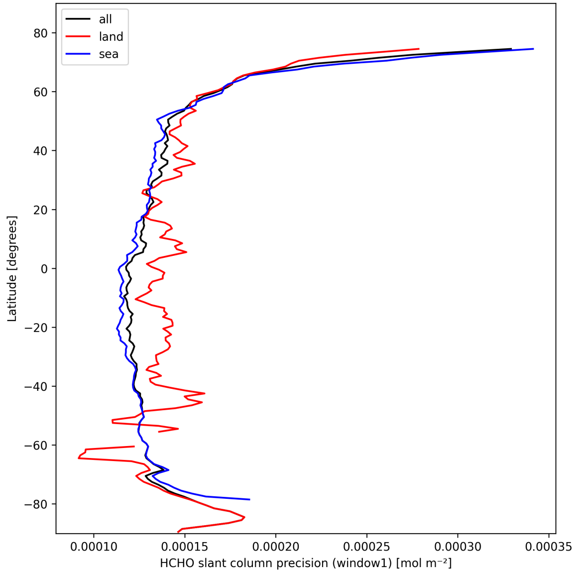
Figure 25: Zonal average of “HCHO slant column precision (window1)” for 2025-10-18 to 2025-10-20.
