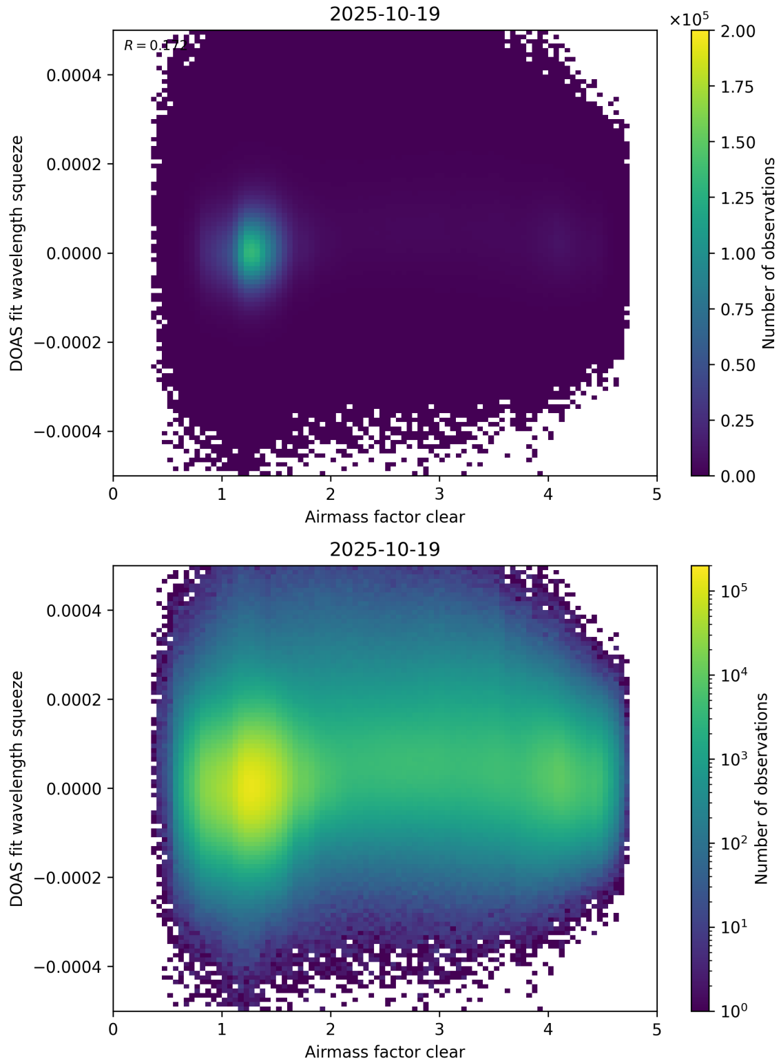
Figure 73: Scatter density plot of “Airmass factor clear” against “DOAS fit wavelength squeeze” for 2025-10-18 to 2025-10-20.
