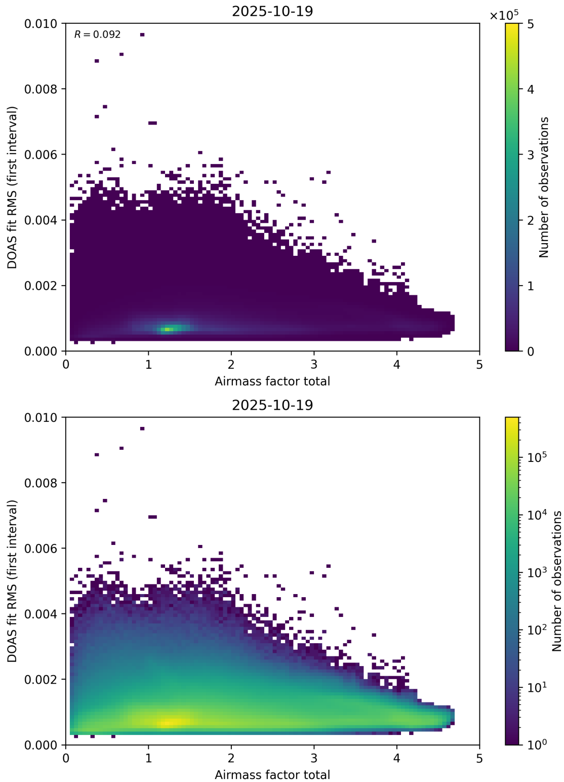
Figure 97: Scatter density plot of “Airmass factor total” against “DOAS fit RMS (first interval)” for 2025-10-18 to 2025-10-20.
