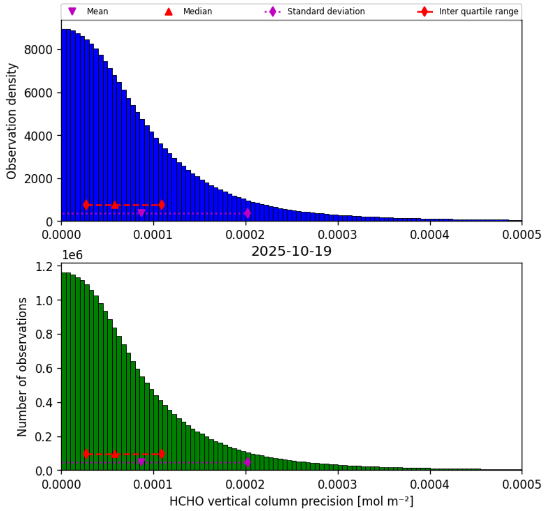
Figure 36: Histogram of “HCHO vertical column precision” for 2025-10-18 to 2025-10-20
