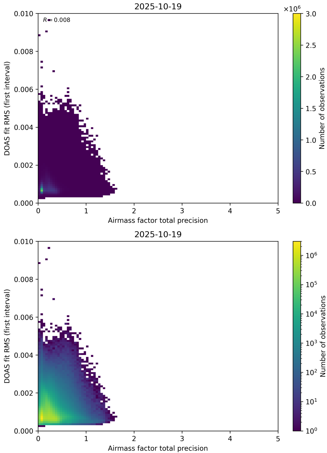
Figure 105: Scatter density plot of “Airmass factor total precision” against “DOAS fit RMS (first interval)” for 2025-10-18 to 2025-10-20.
