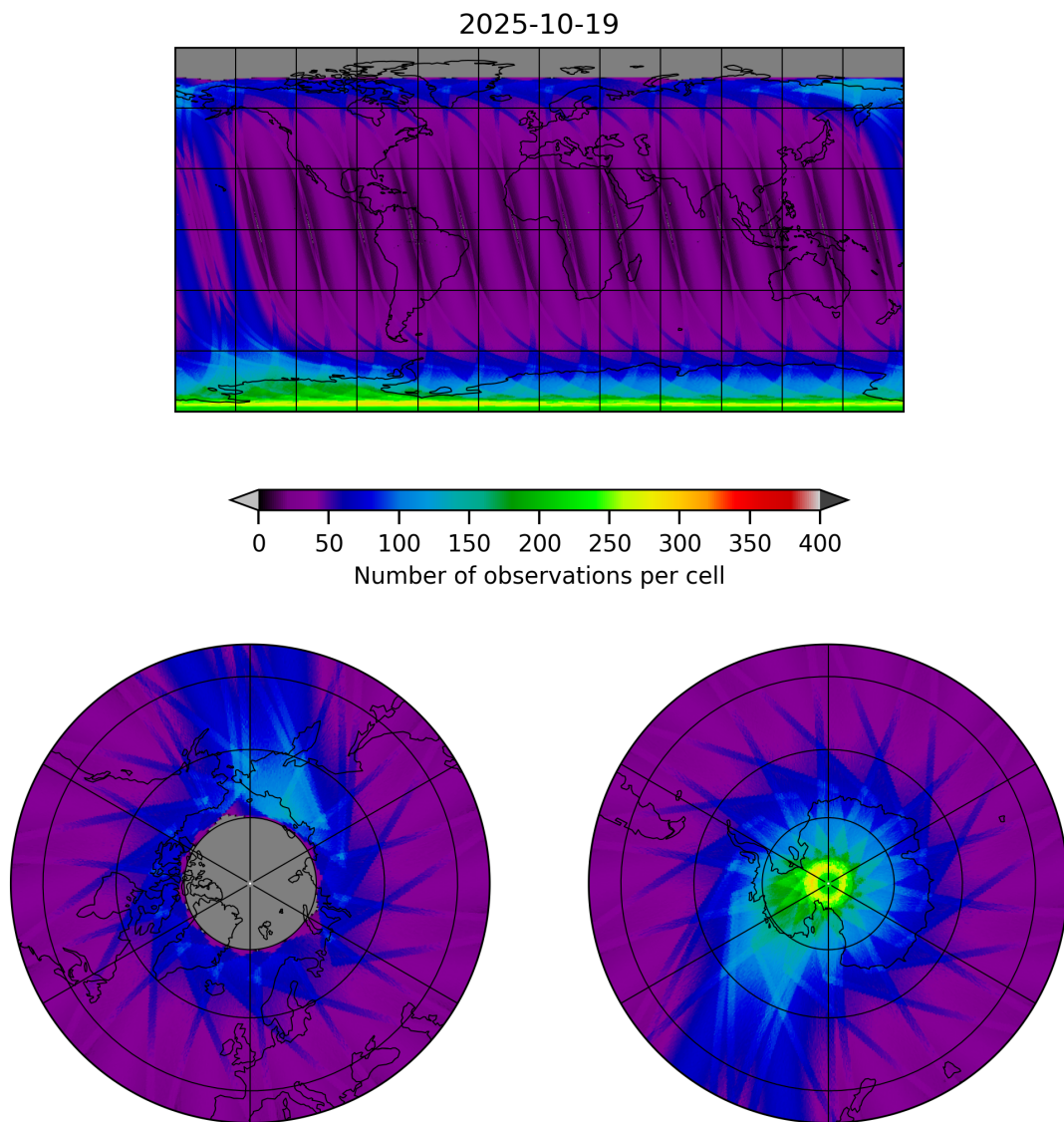
Figure 19: Map of the number of observations for 2025-10-18 to 2025-10-20
