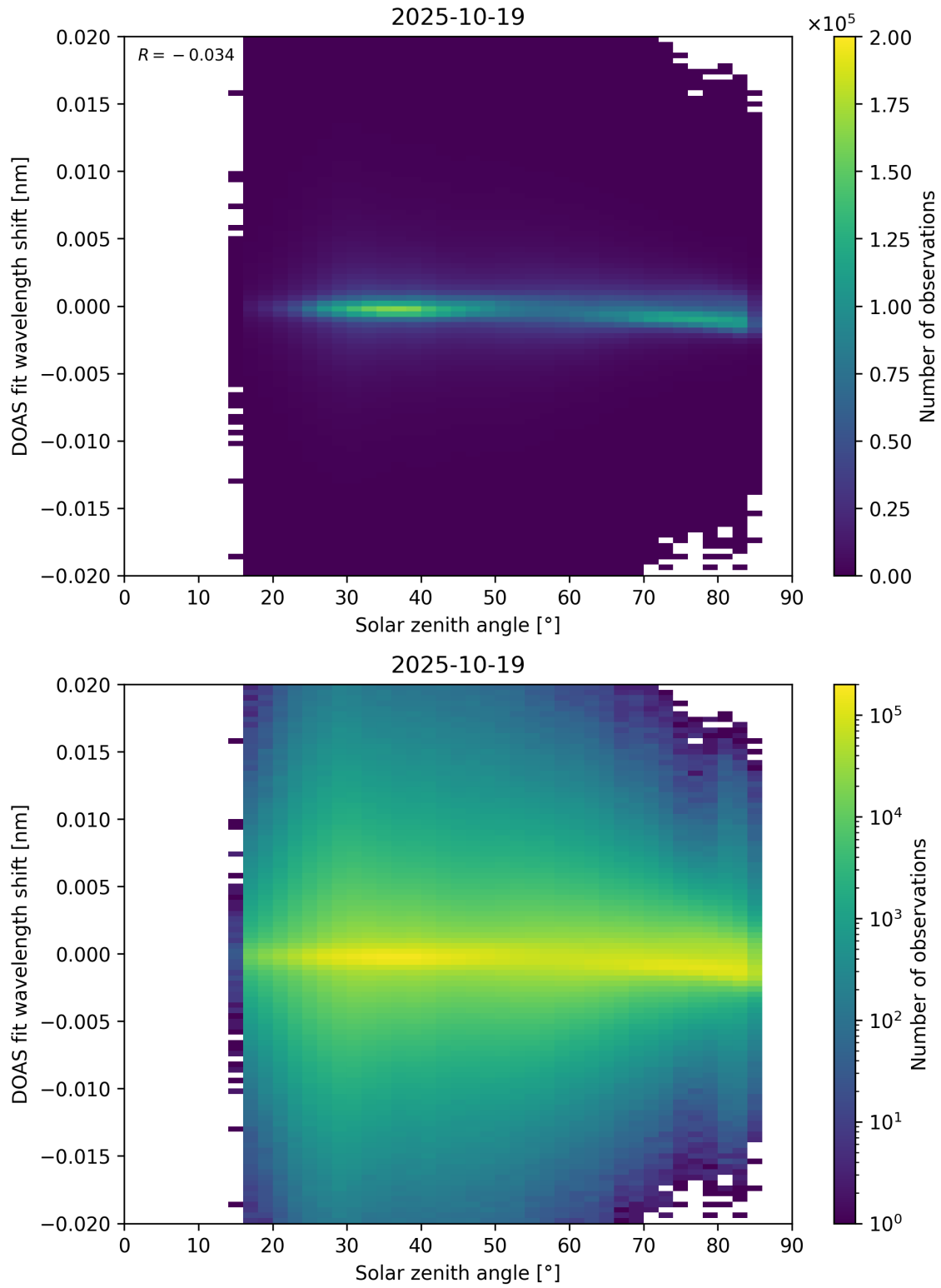
Figure 168: Scatter density plot of “Solar zenith angle” against “DOAS fit wavelength shift” for 2025-10-18 to 2025-10-20.
