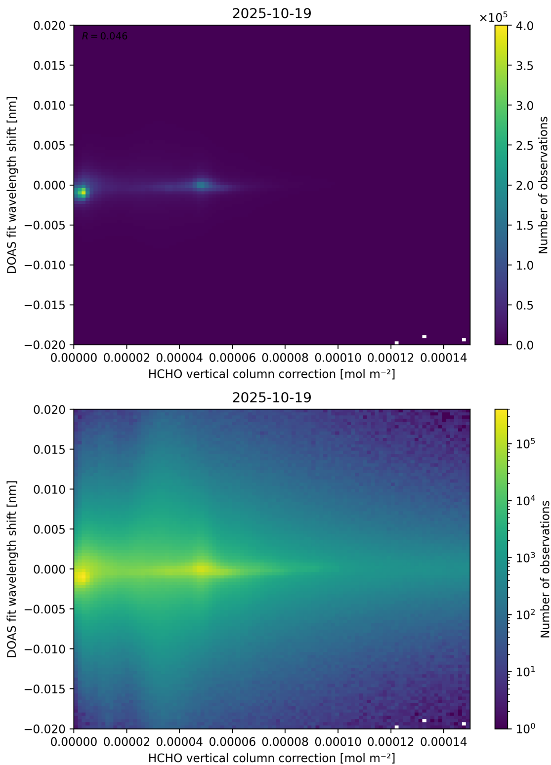
Figure 113: Scatter density plot of “HCHO vertical column correction” against “DOAS fit wavelength shift” for 2025-10-18 to 2025-10-20.
