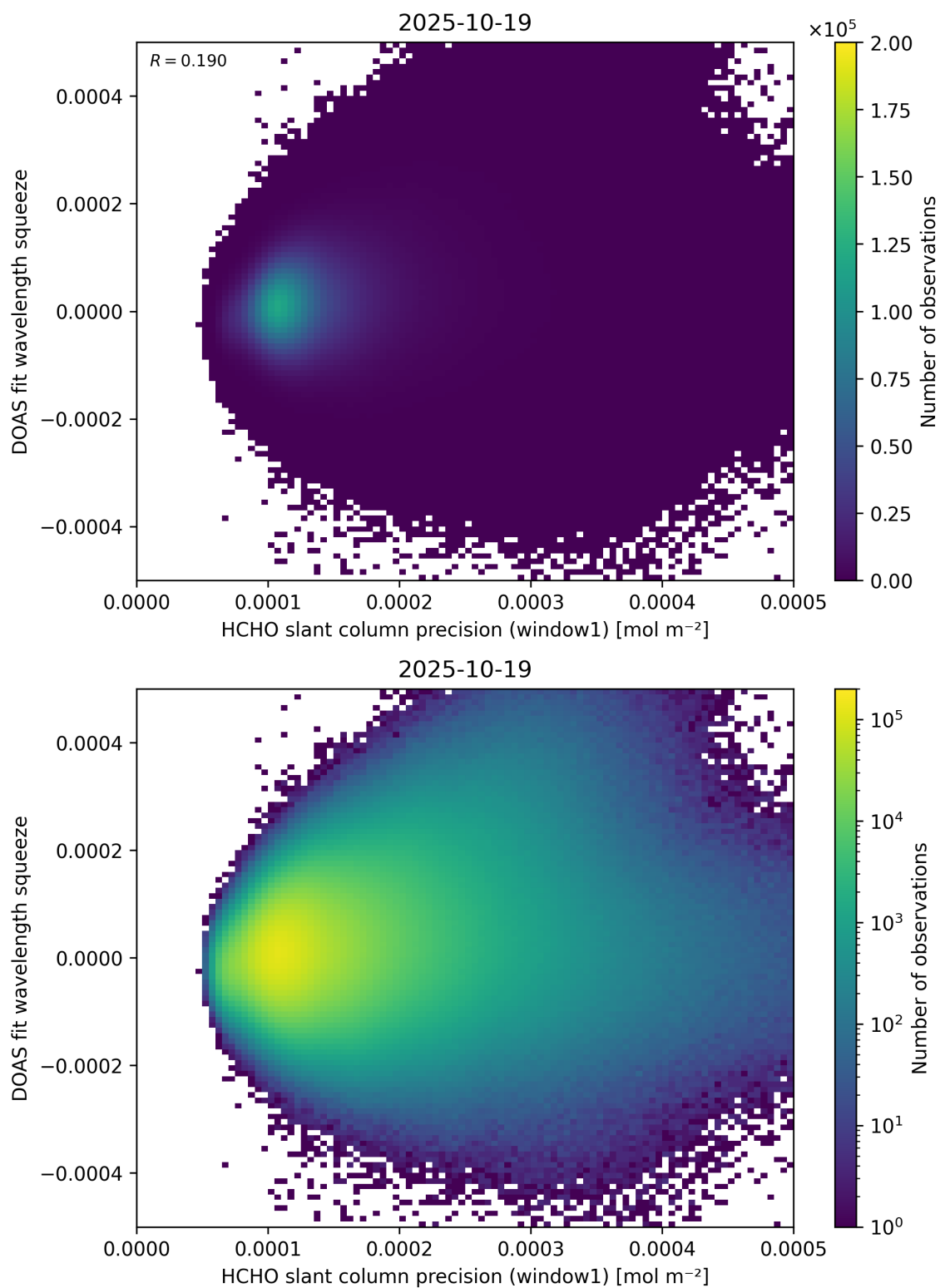
Figure 90: Scatter density plot of “HCHO slant column precision (window1)” against “DOAS fit wavelength squeeze” for 2025-10-18 to 2025-10-20.
