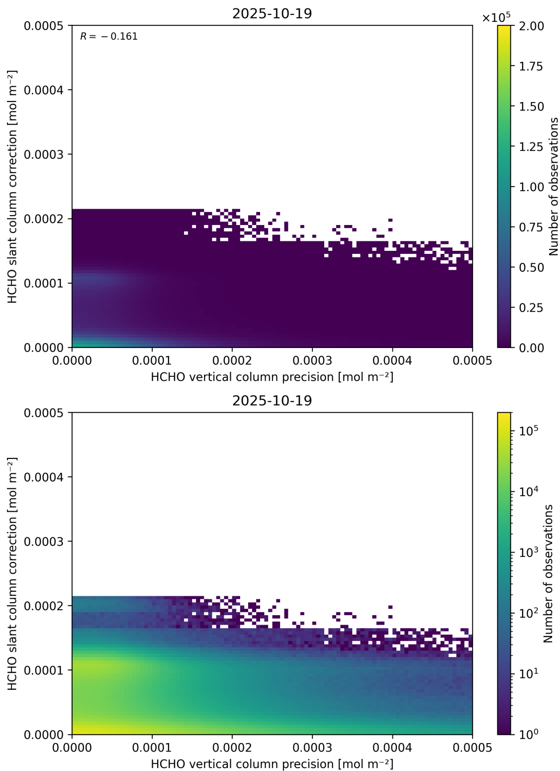
Figure 141: Scatter density plot of “HCHO vertical column precision” against “HCHO slant column correction” for 2025-10-18 to 2025-10-20.
