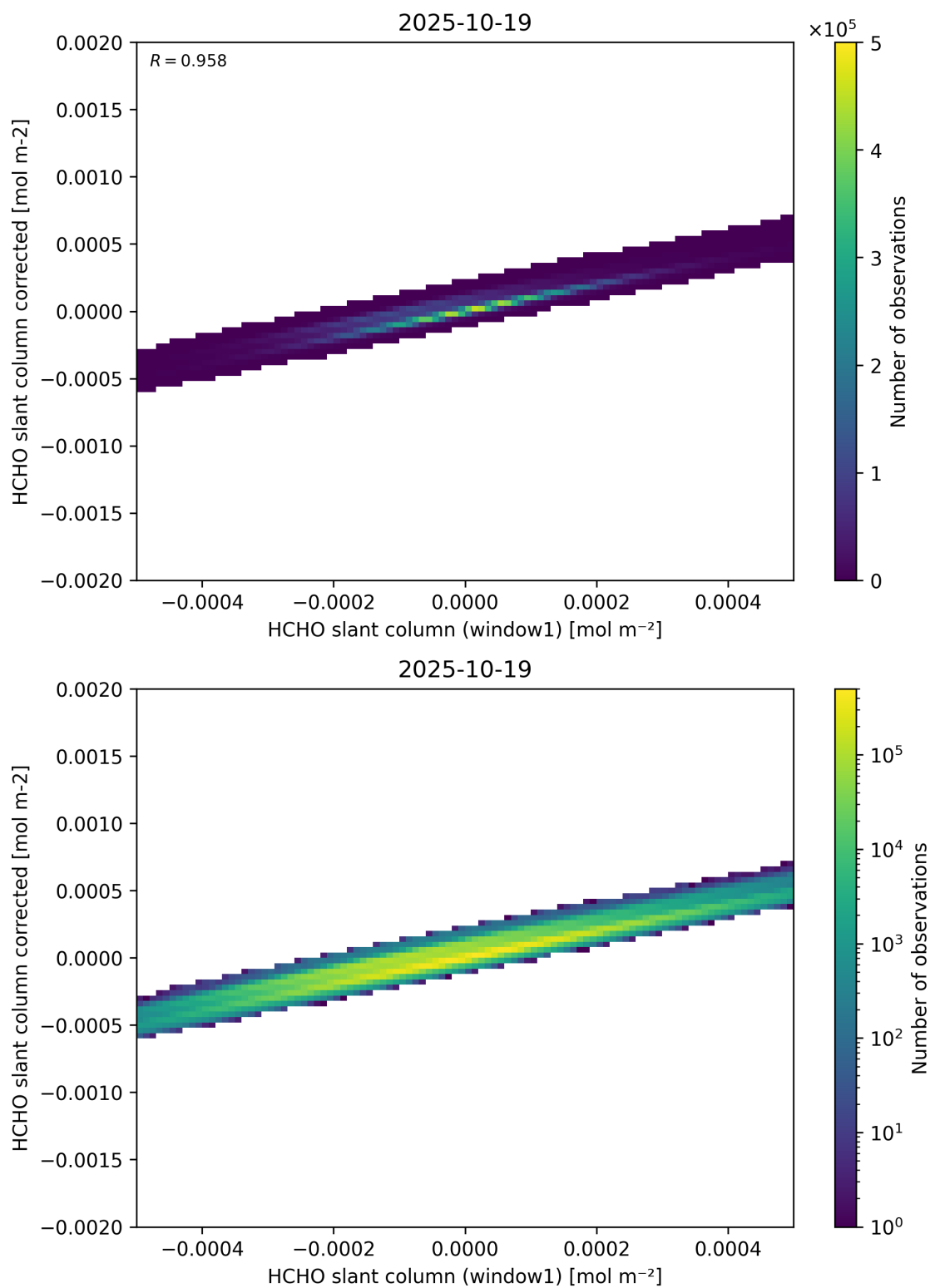
Figure 82: Scatter density plot of “HCHO slant column (window1)” against “HCHO slant column corrected” for 2025-10-18 to 2025-10-20.
