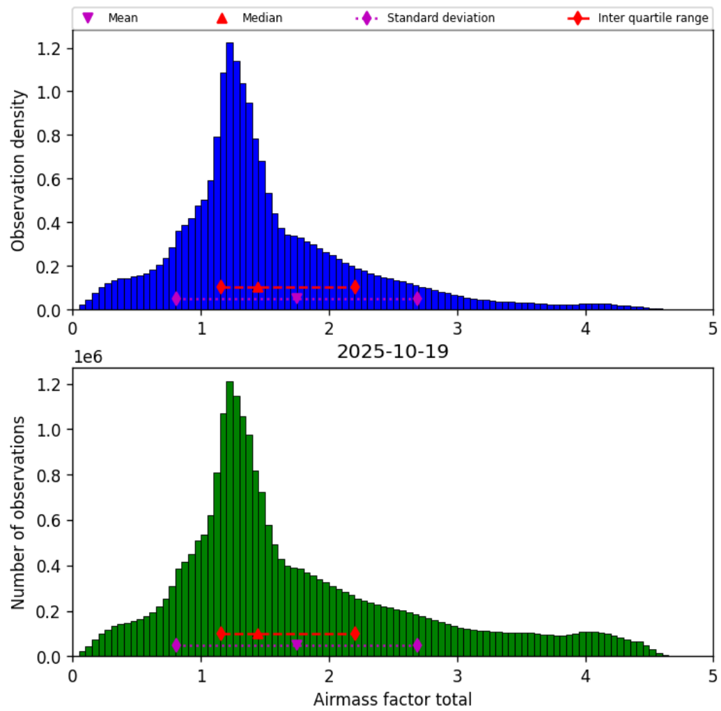
Figure 40: Histogram of “Airmass factor total” for 2025-10-18 to 2025-10-20
