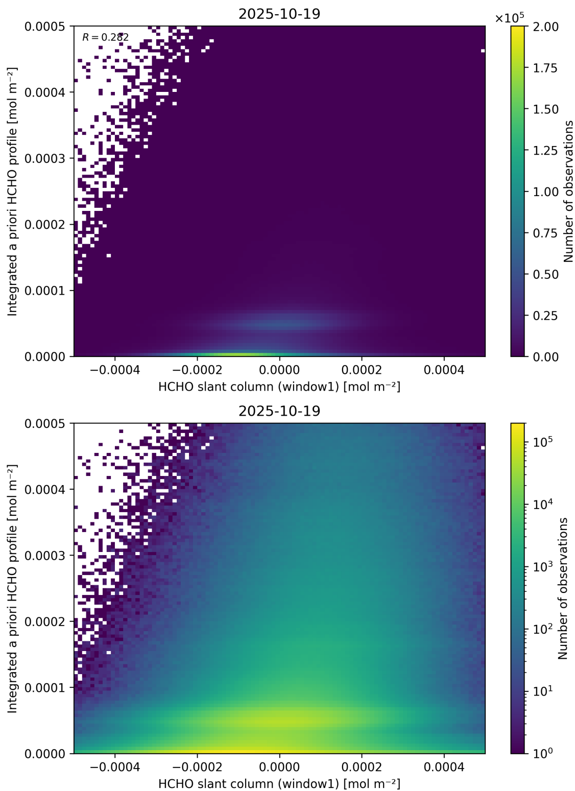
Figure 87: Scatter density plot of “HCHO slant column (window1)” against “Integrated a priori HCHO profile” for 2025-10-18 to 2025-10-20.
