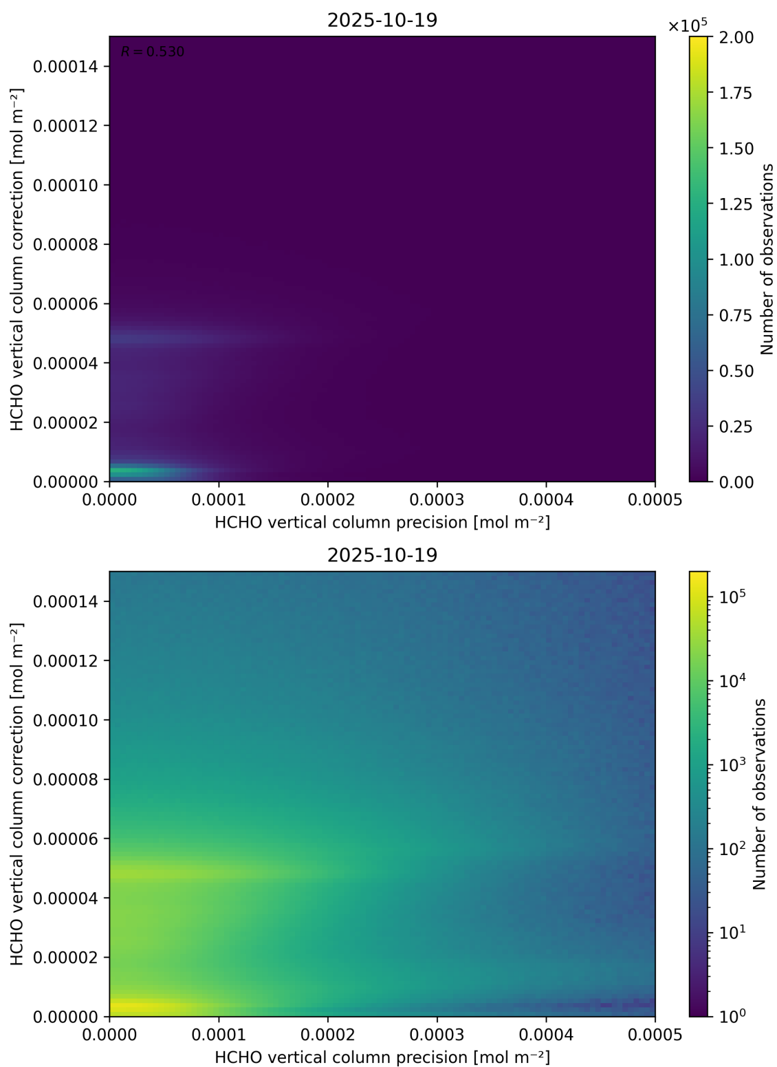
Figure 146: Scatter density plot of “HCHO vertical column precision” against “HCHO vertical column correction” for 2025-10-18 to 2025-10-20.
