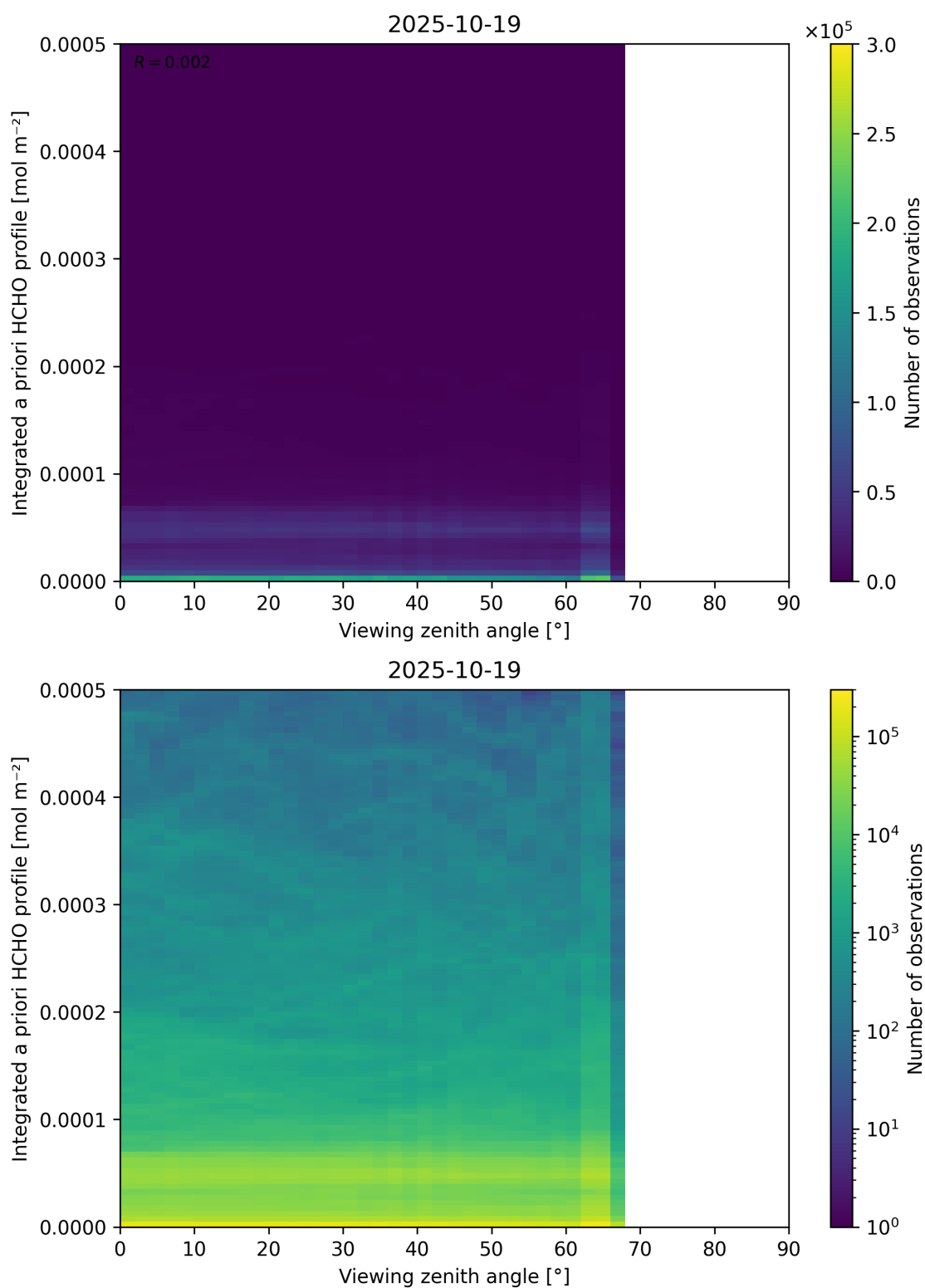
Figure 195: Scatter density plot of “Viewing zenith angle” against “Integrated a priori HCHO profile” for 2025-10-18 to 2025-10-20.
