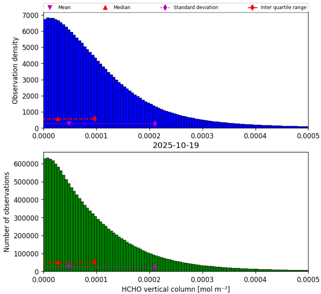
Figure 35: Histogram of “HCHO vertical column” for 2025-10-18 to 2025-10-20
