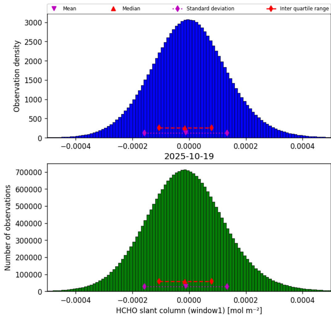
Figure 38: Histogram of “HCHO slant column (window1)” for 2025-10-18 to 2025-10-20
