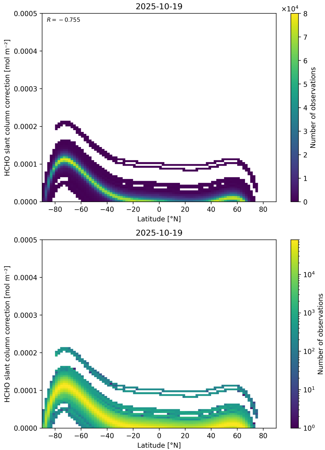
Figure 158: Scatter density plot of “Latitude” against “HCHO slant column correction” for 2025-10-18 to 2025-10-20.
