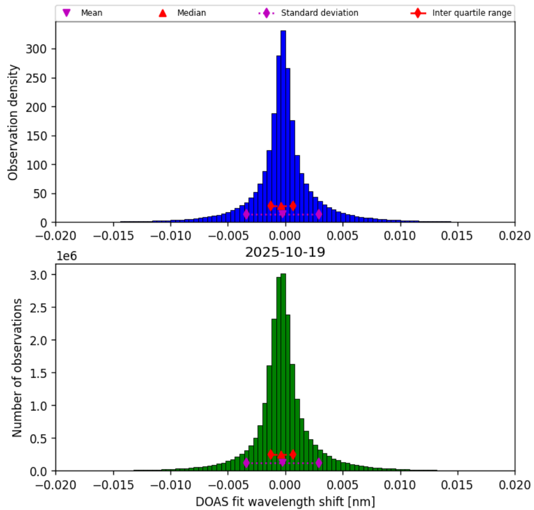
Figure 44: Histogram of “DOAS fit wavelength shift” for 2025-10-18 to 2025-10-20
