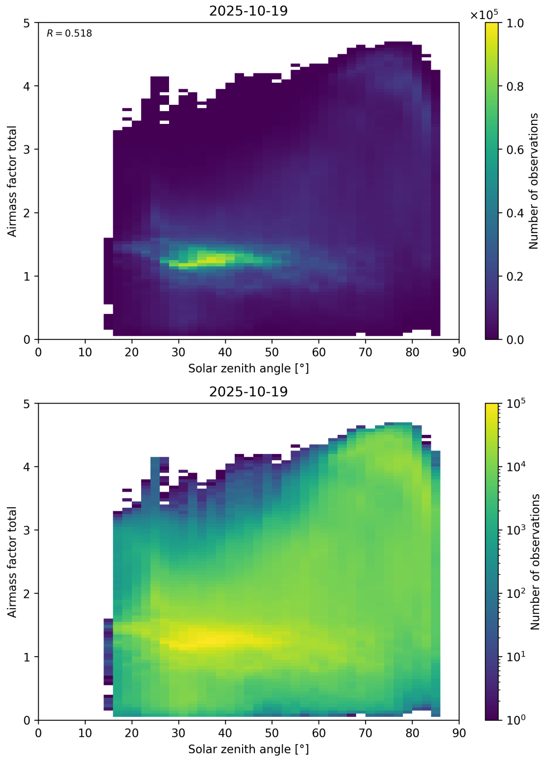
Figure 175: Scatter density plot of “Solar zenith angle” against “Airmass factor total” for 2025-10-18 to 2025-10-20.
