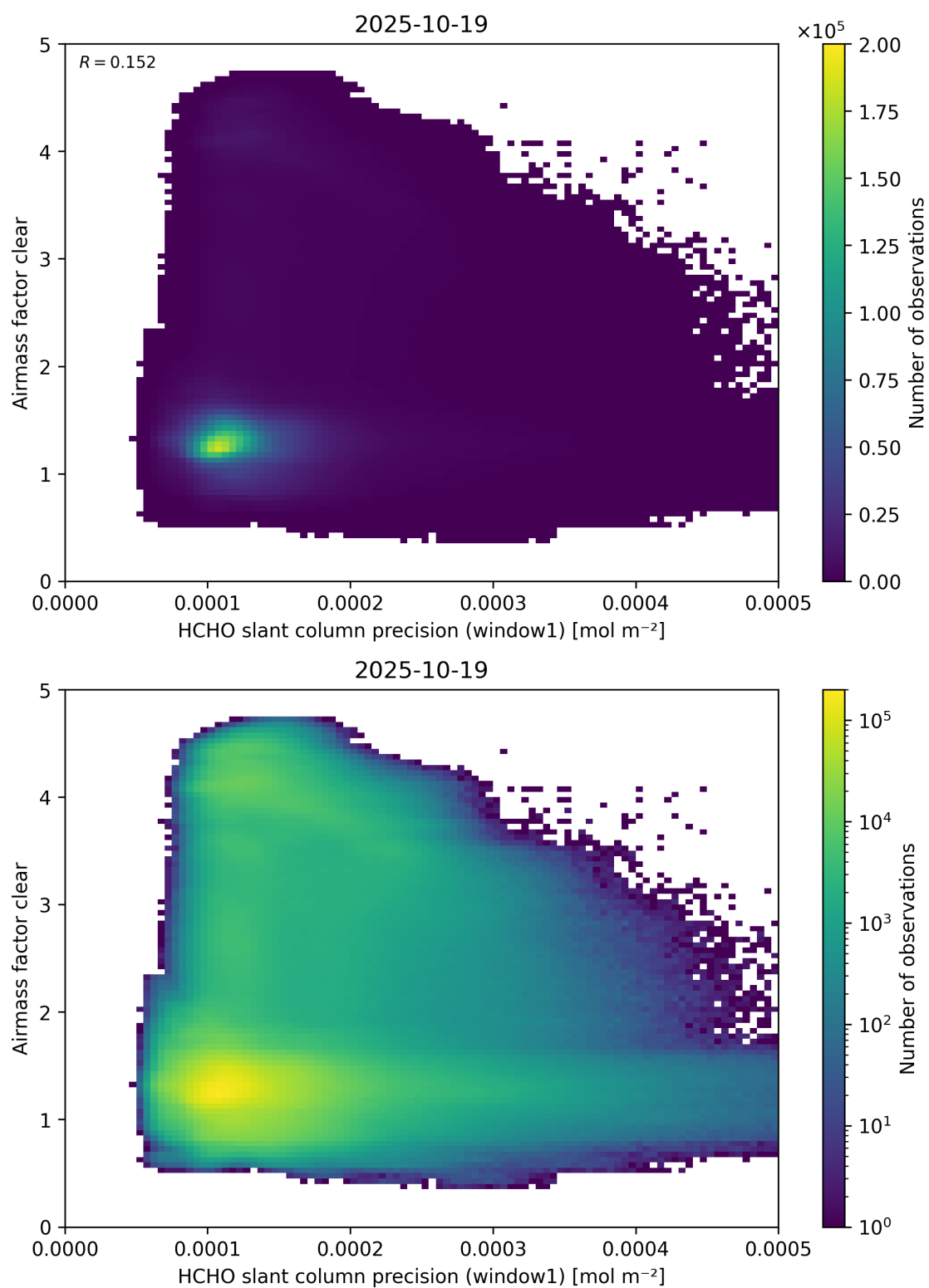
Figure 91: Scatter density plot of “HCHO slant column precision (window1)” against “Airmass factor clear” for 2025-10-18 to 2025-10-20.
