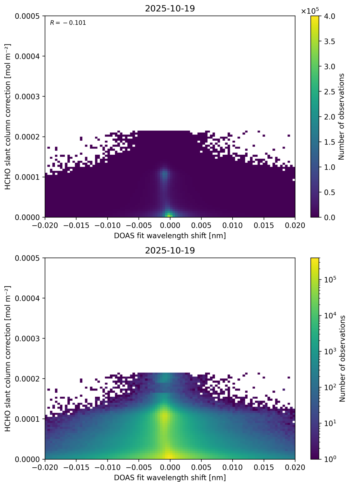
Figure 67: Scatter density plot of “DOAS fit wavelength shift” against “HCHO slant column correction” for 2025-10-18 to 2025-10-20.
