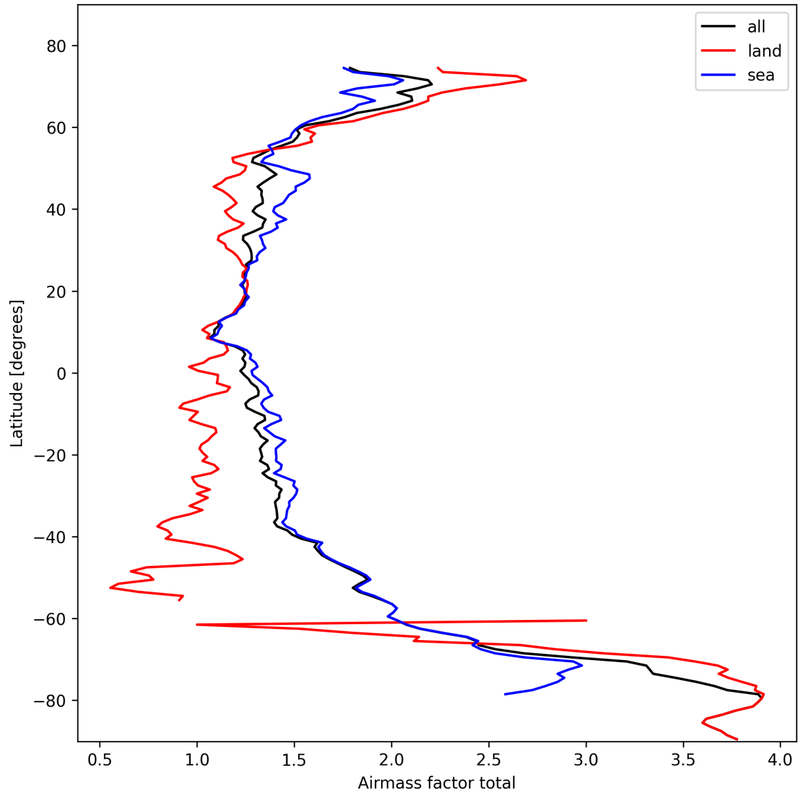
Figure 26: Zonal average of “Airmass factor total” for 2025-10-18 to 2025-10-20.
