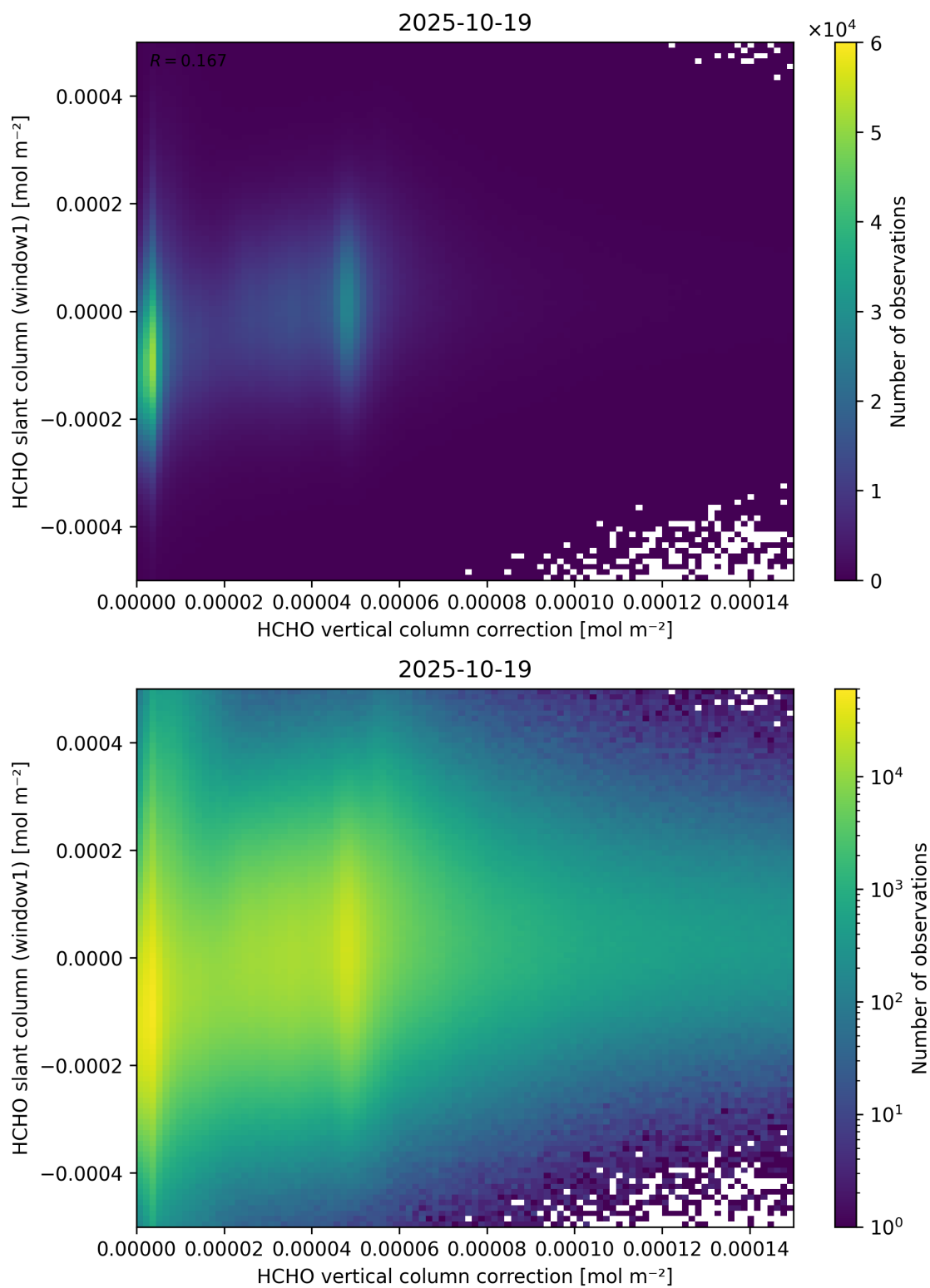
Figure 118: Scatter density plot of “HCHO vertical column correction” against “HCHO slant column (window1)” for 2025-10-18 to 2025-10-20.
