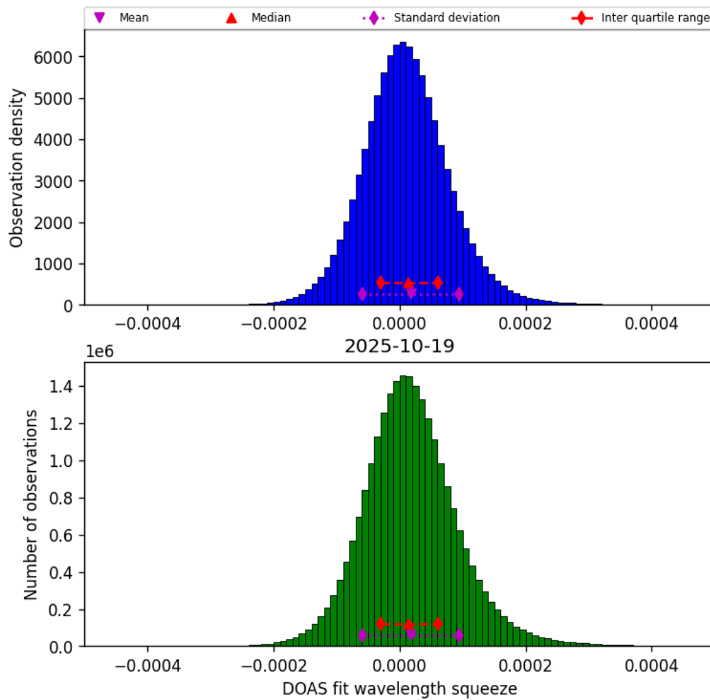
Figure 45: Histogram of “DOAS fit wavelength squeeze” for 2025-10-18 to 2025-10-20
