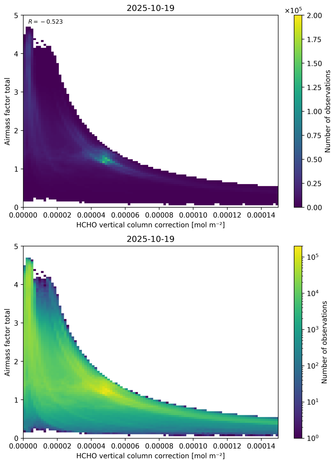
Figure 120: Scatter density plot of “HCHO vertical column correction” against “Airmass factor total” for 2025-10-18 to 2025-10-20.
