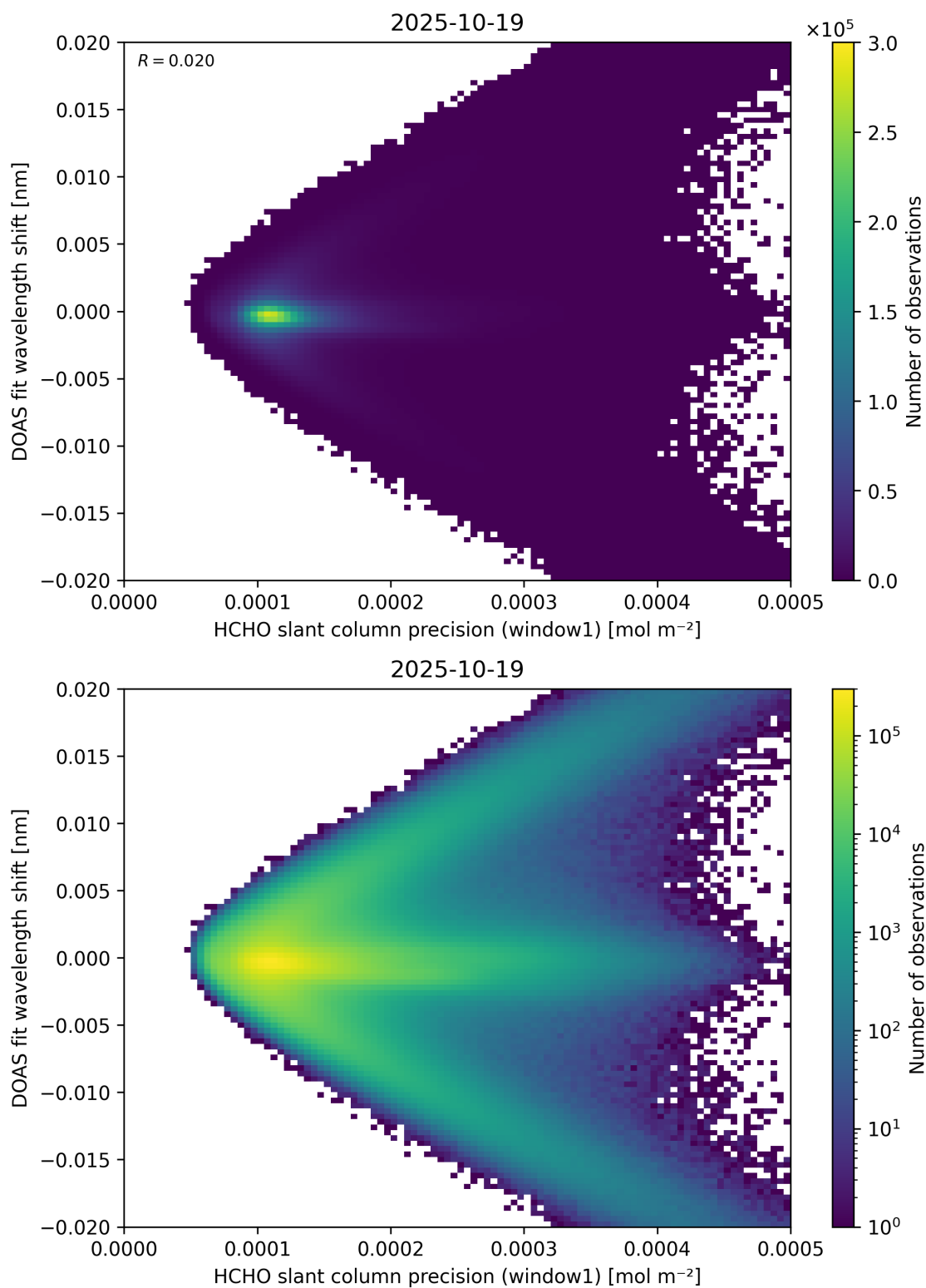
Figure 89: Scatter density plot of “HCHO slant column precision (window1)” against “DOAS fit wavelength shift” for 2025-10-18 to 2025-10-20.
