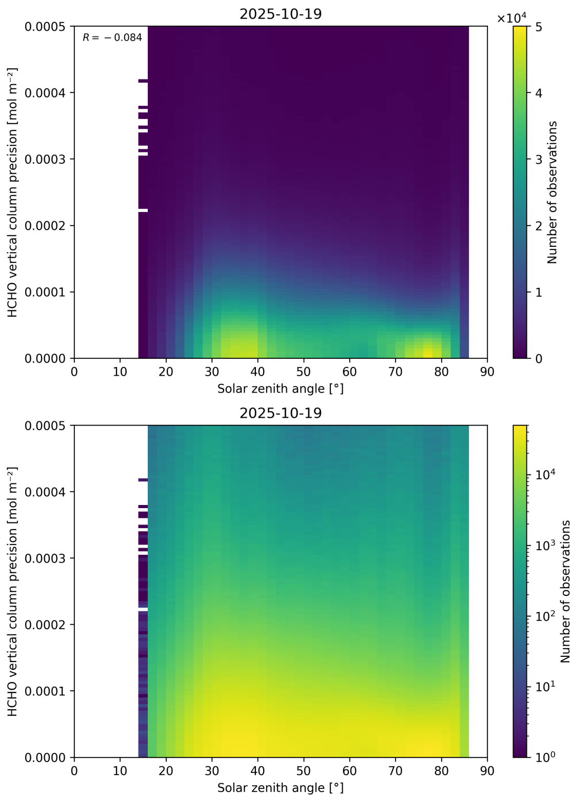
Figure 179: Scatter density plot of “Solar zenith angle” against “HCHO vertical column precision” for 2025-10-18 to 2025-10-20.
