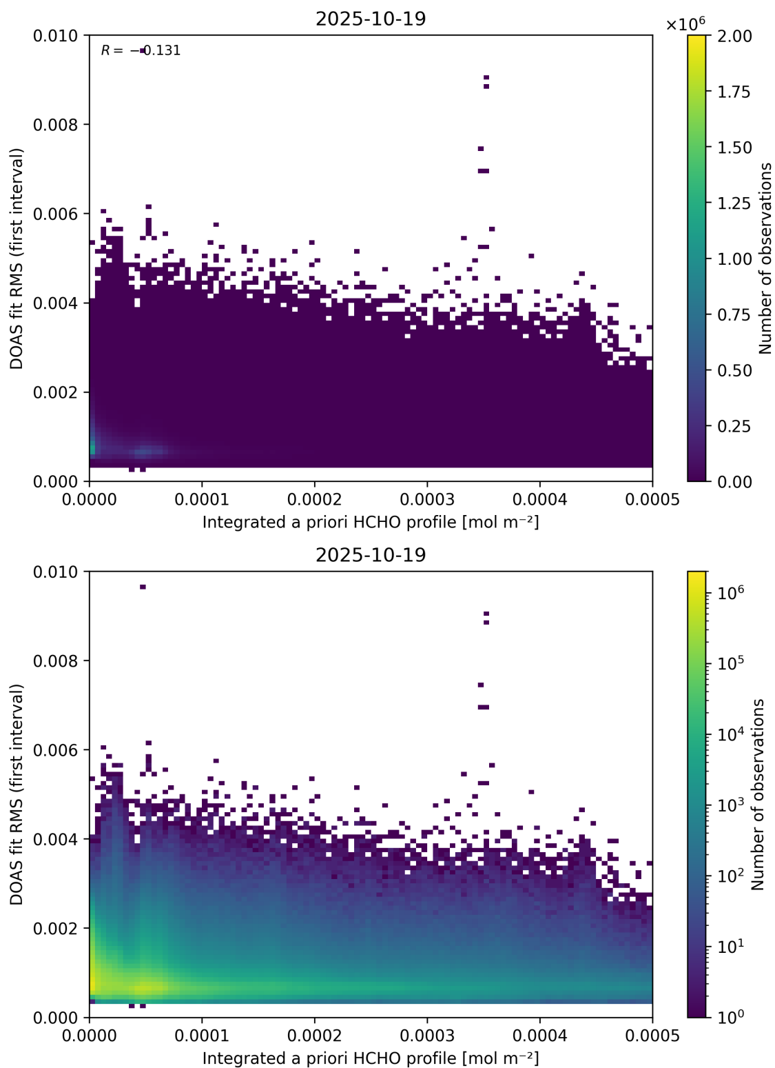
Figure 148: Scatter density plot of “Integrated a priori HCHO profile” against “DOAS fit RMS (first interval)” for 2025-10-18 to 2025-10-20.
