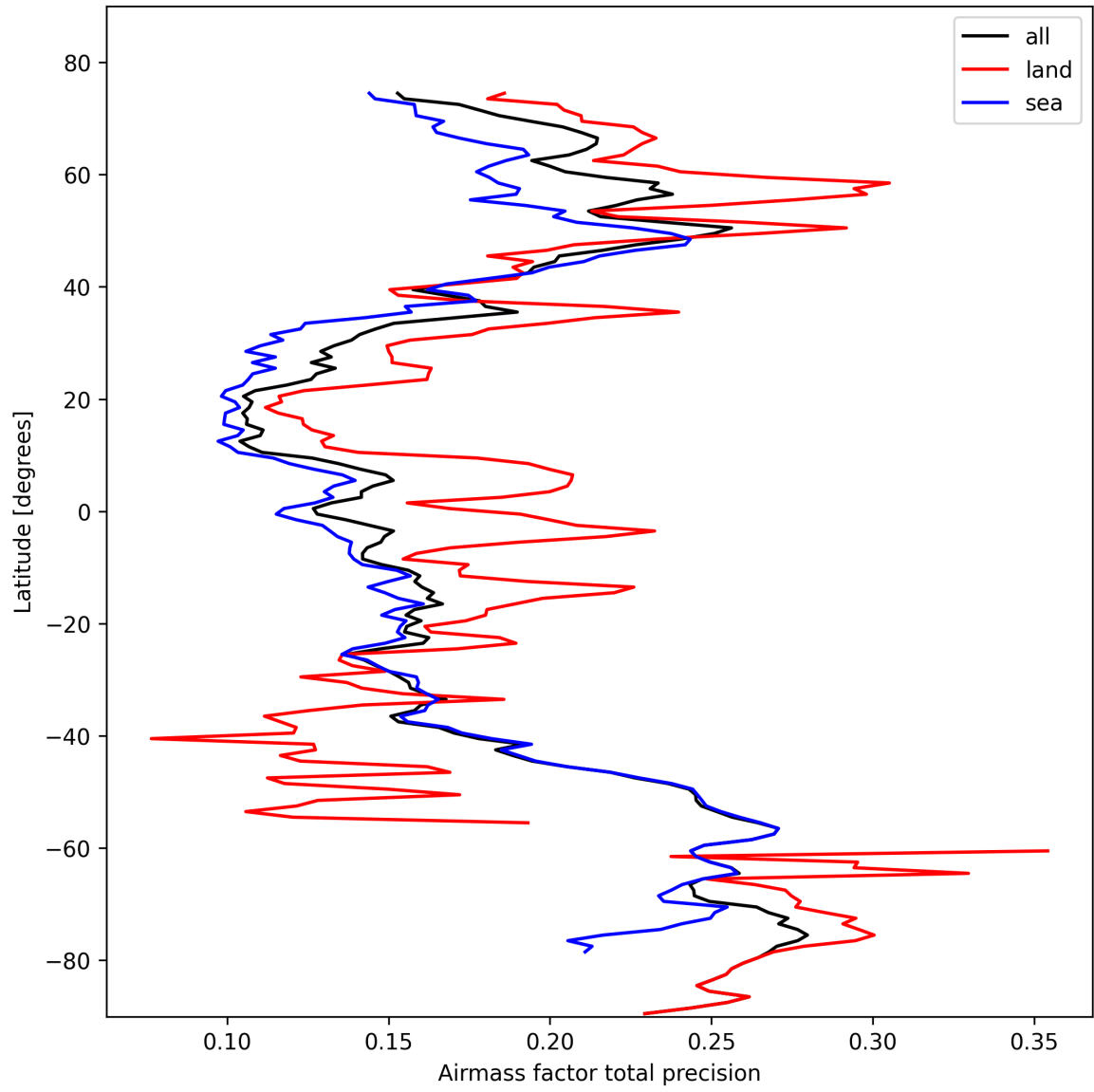
Figure 27: Zonal average of “Airmass factor total precision” for 2025-10-18 to 2025-10-20.
