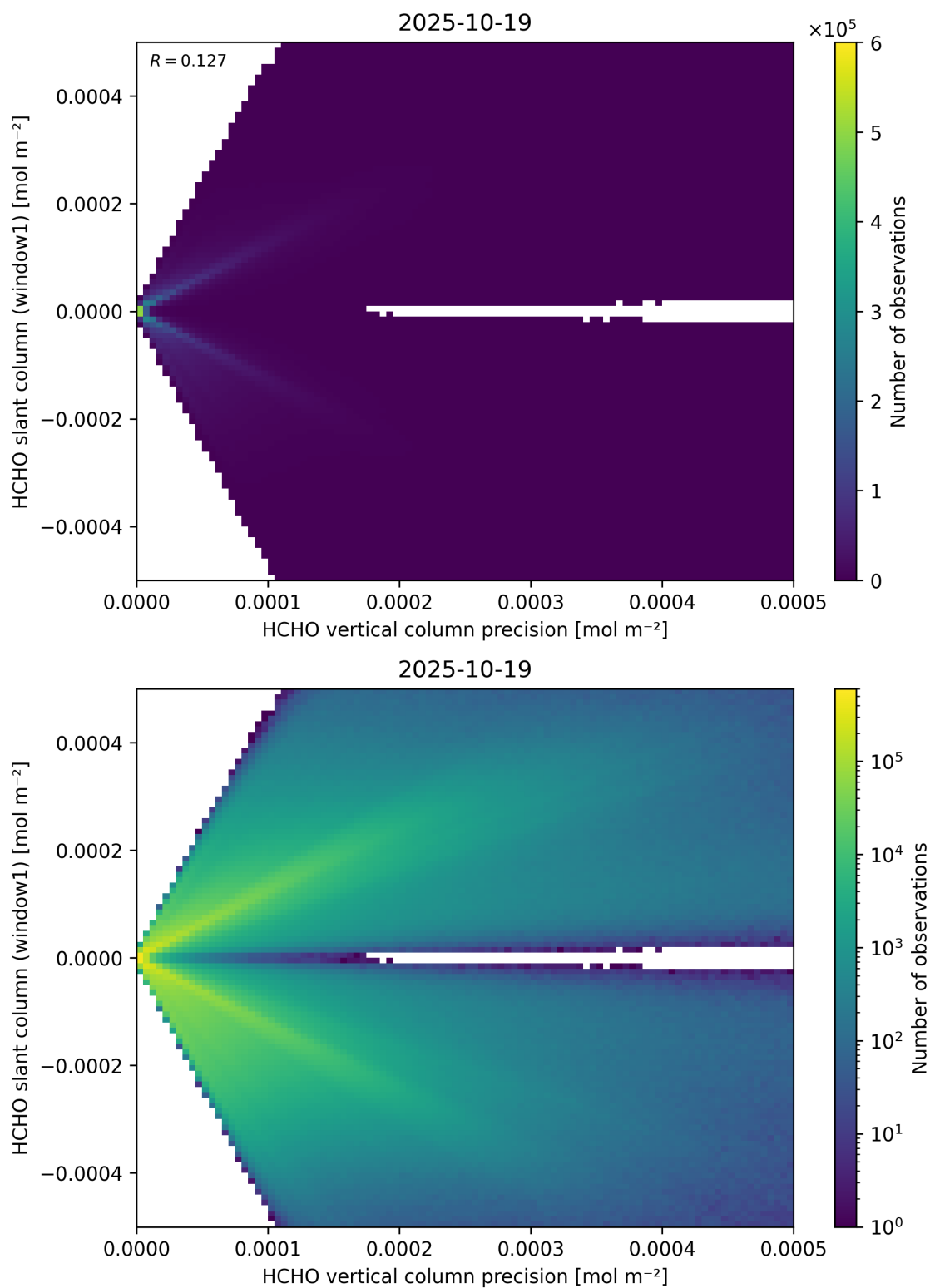
Figure 142: Scatter density plot of “HCHO vertical column precision” against “HCHO slant column (window1)” for 2025-10-18 to 2025-10-20.
