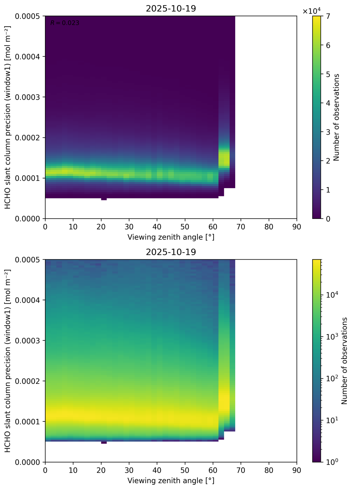
Figure 189: Scatter density plot of “Viewing zenith angle” against “HCHO slant column precision (window1)” for 2025-10-18 to 2025-10-20.
