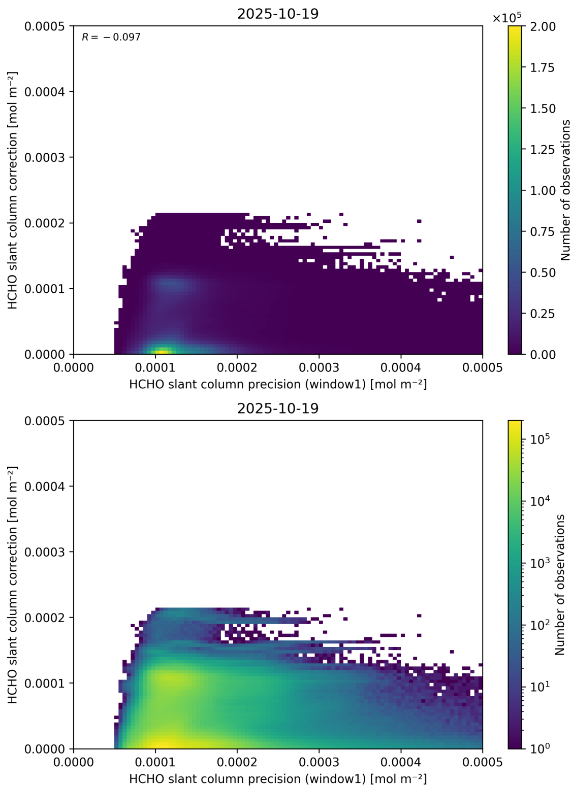
Figure 93: Scatter density plot of “HCHO slant column precision (window1)” against “HCHO slant column correction” for 2025-10-18 to 2025-10-20.
