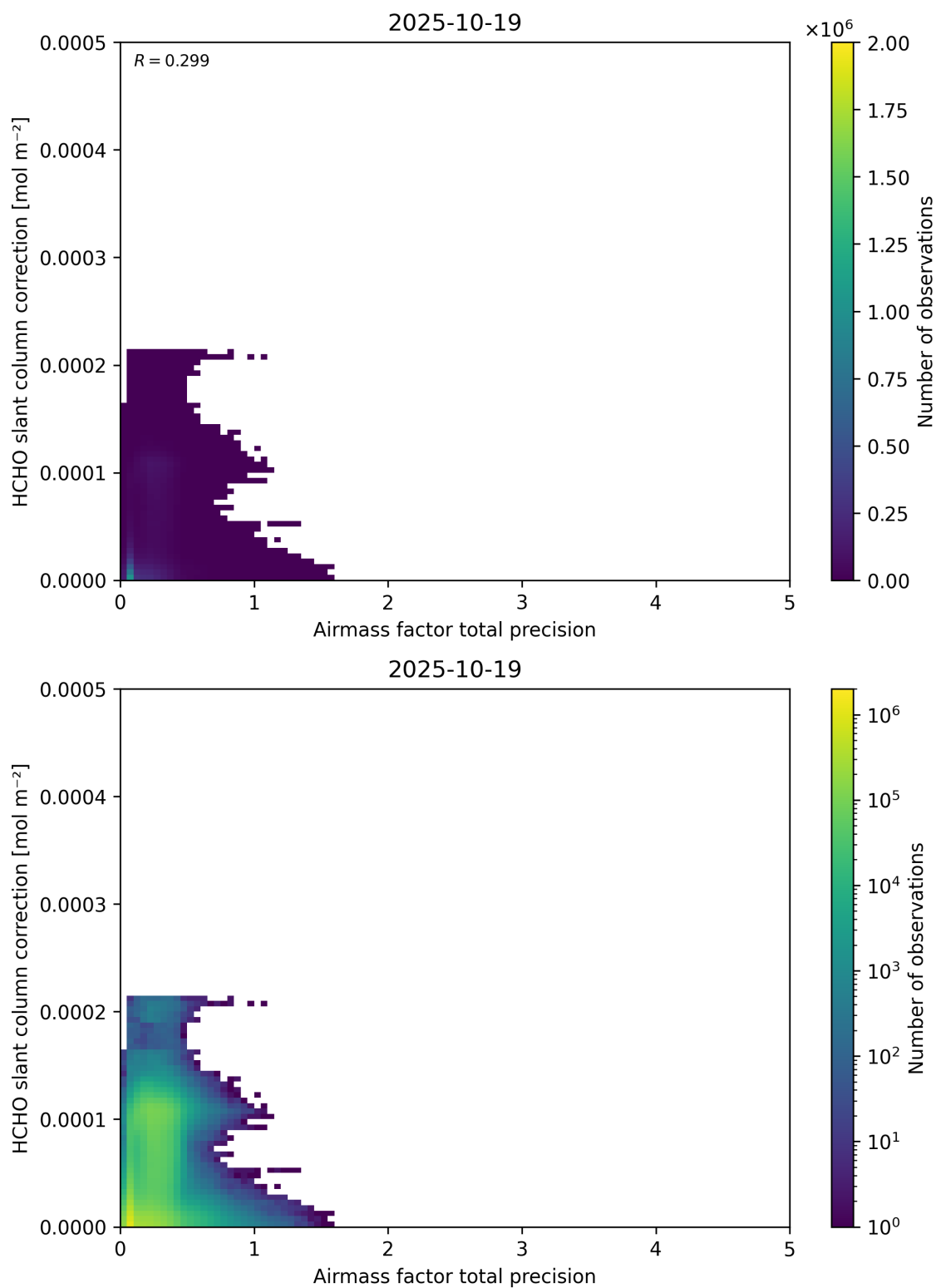
Figure 110: Scatter density plot of “Airmass factor total precision” against “HCHO slant column correction” for 2025-10-18 to 2025-10-20.
