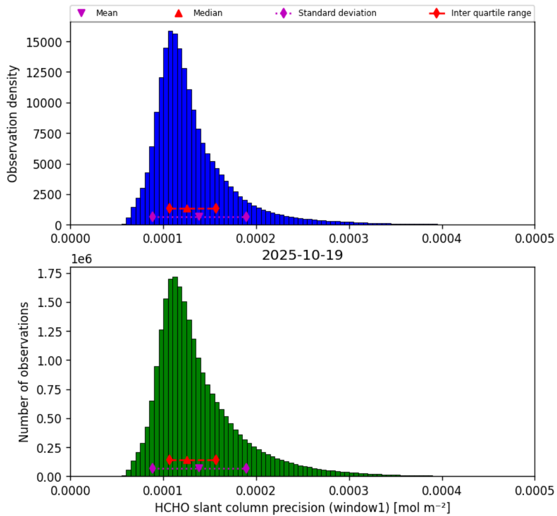
Figure 39: Histogram of “HCHO slant column precision (window1)” for 2025-10-18 to 2025-10-20
