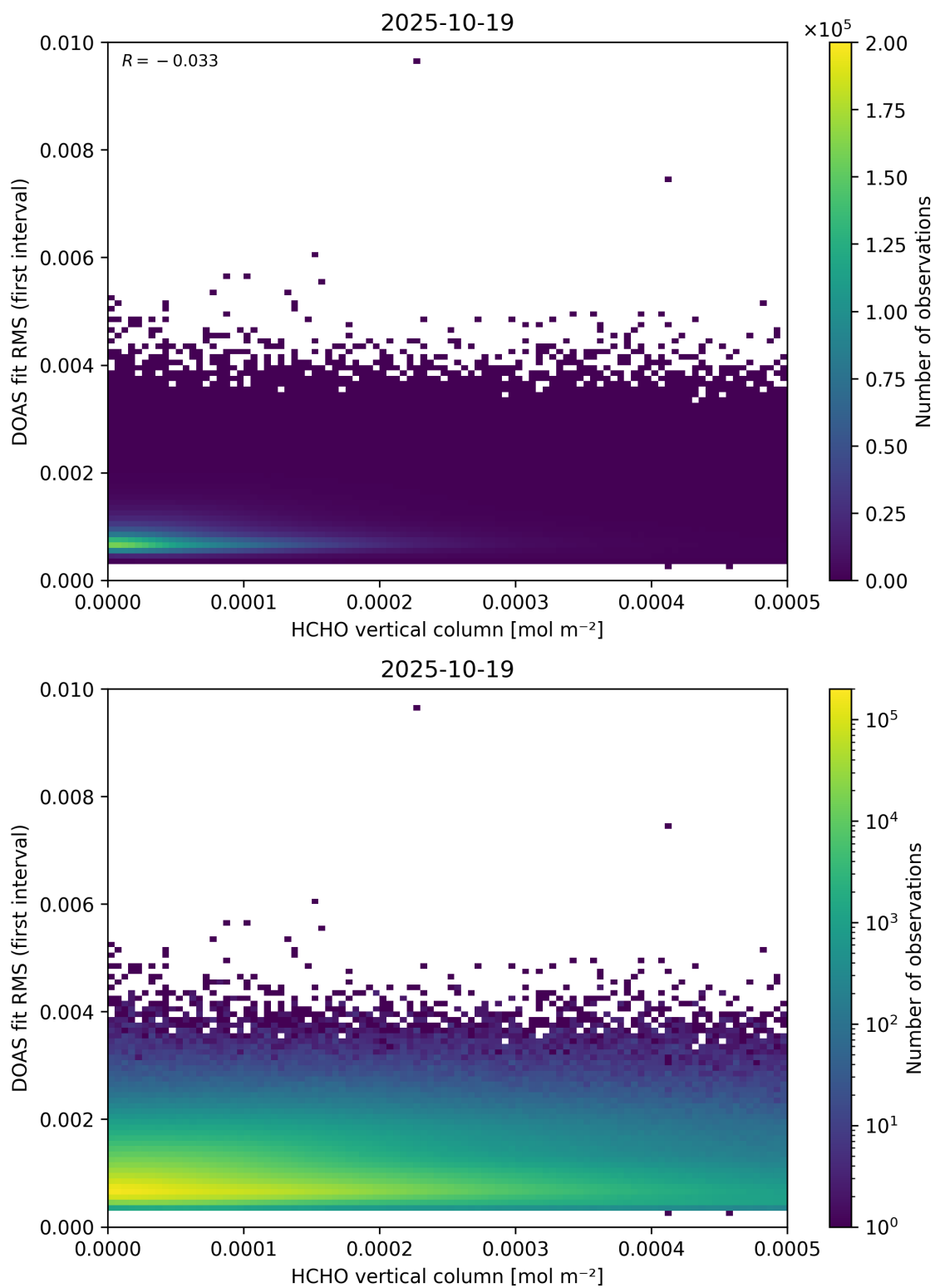
Figure 123: Scatter density plot of “HCHO vertical column” against “DOAS fit RMS (first interval)” for 2025-10-18 to 2025-10-20.
