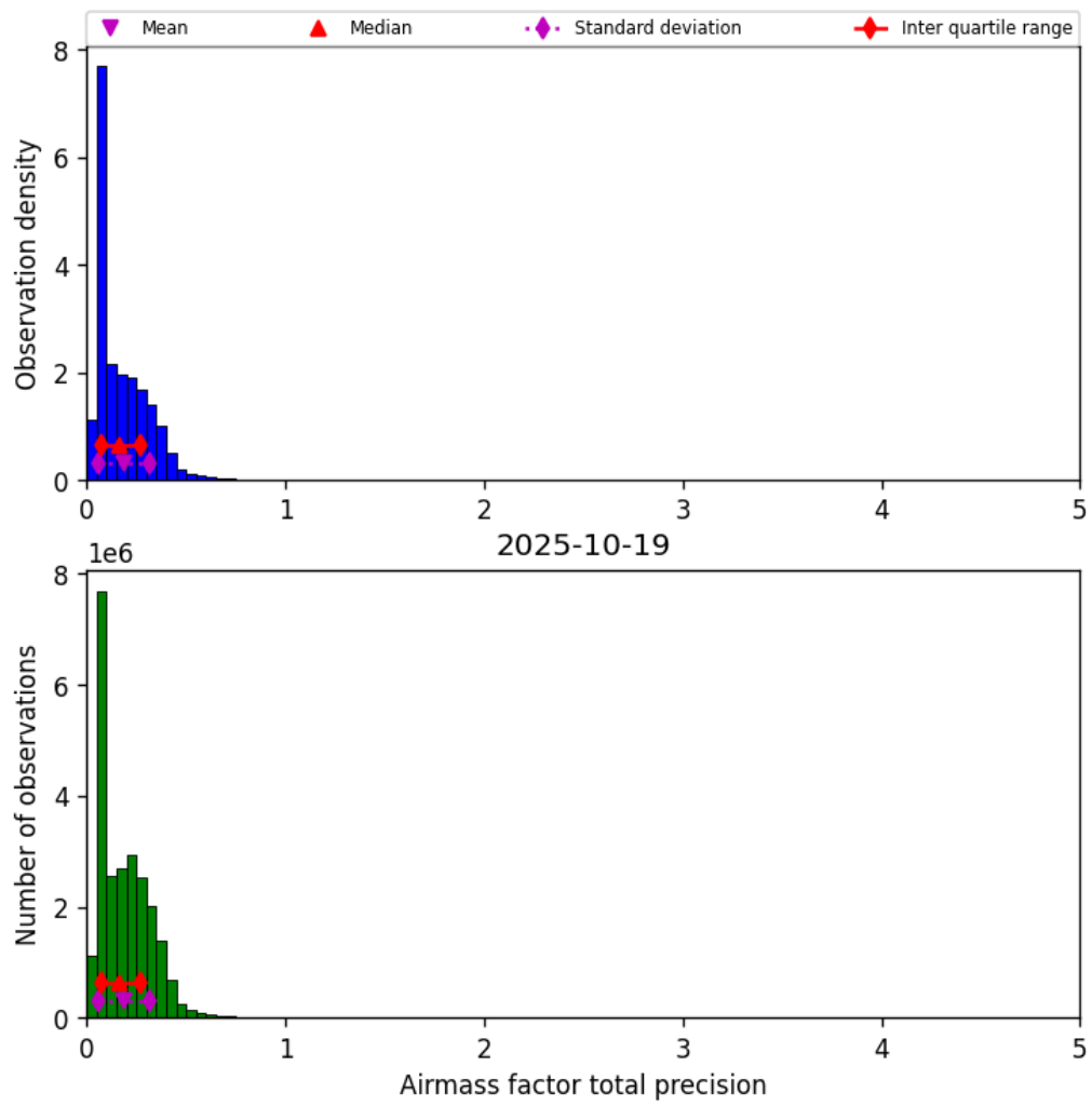
Figure 41: Histogram of “Airmass factor total precision” for 2025-10-18 to 2025-10-20
