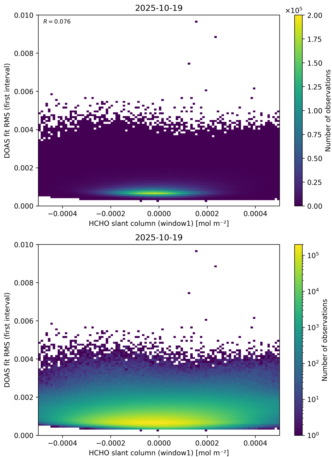
Figure 78: Scatter density plot of “HCHO slant column (window1)” against “DOAS fit RMS (first interval)” for 2025-10-18 to 2025-10-20.
