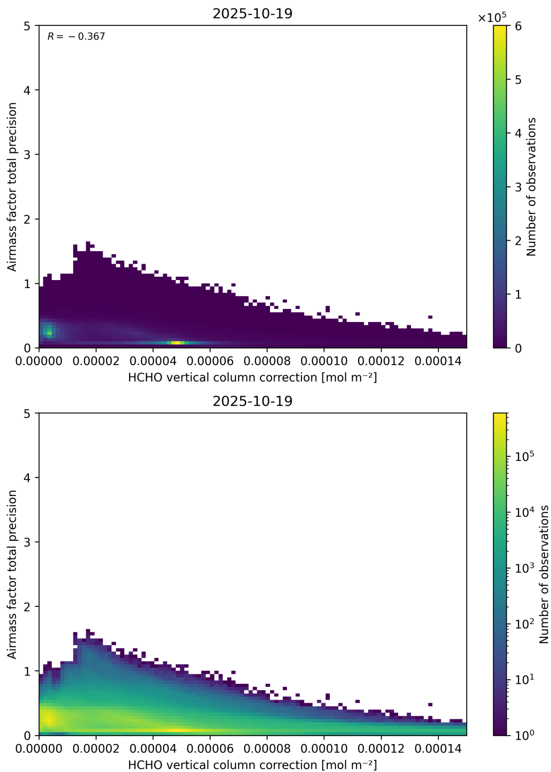
Figure 121: Scatter density plot of “HCHO vertical column correction” against “Airmass factor total precision” for 2025-10-18 to 2025-10-20.
