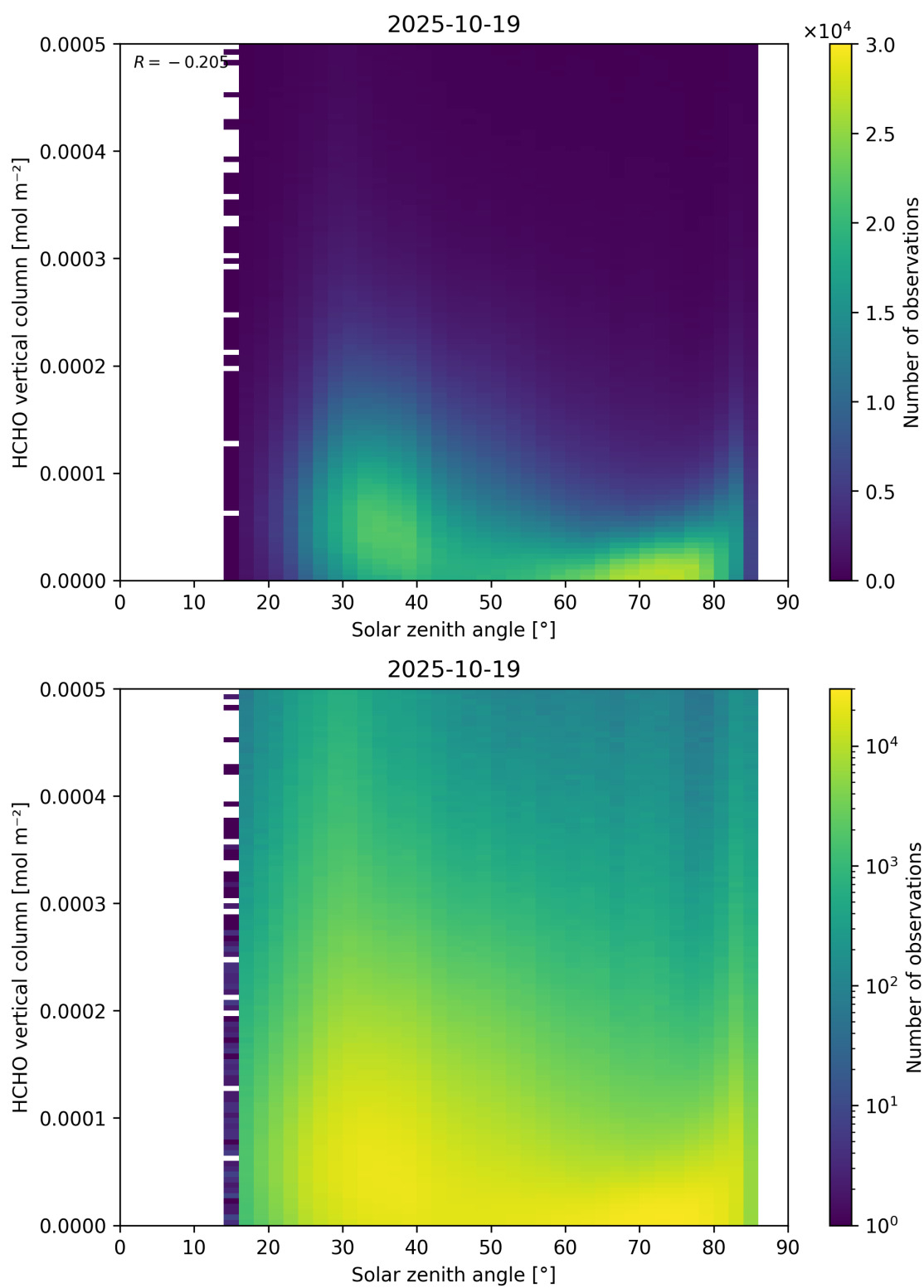
Figure 177: Scatter density plot of “Solar zenith angle” against “HCHO vertical column” for 2025-10-18 to 2025-10-20.
