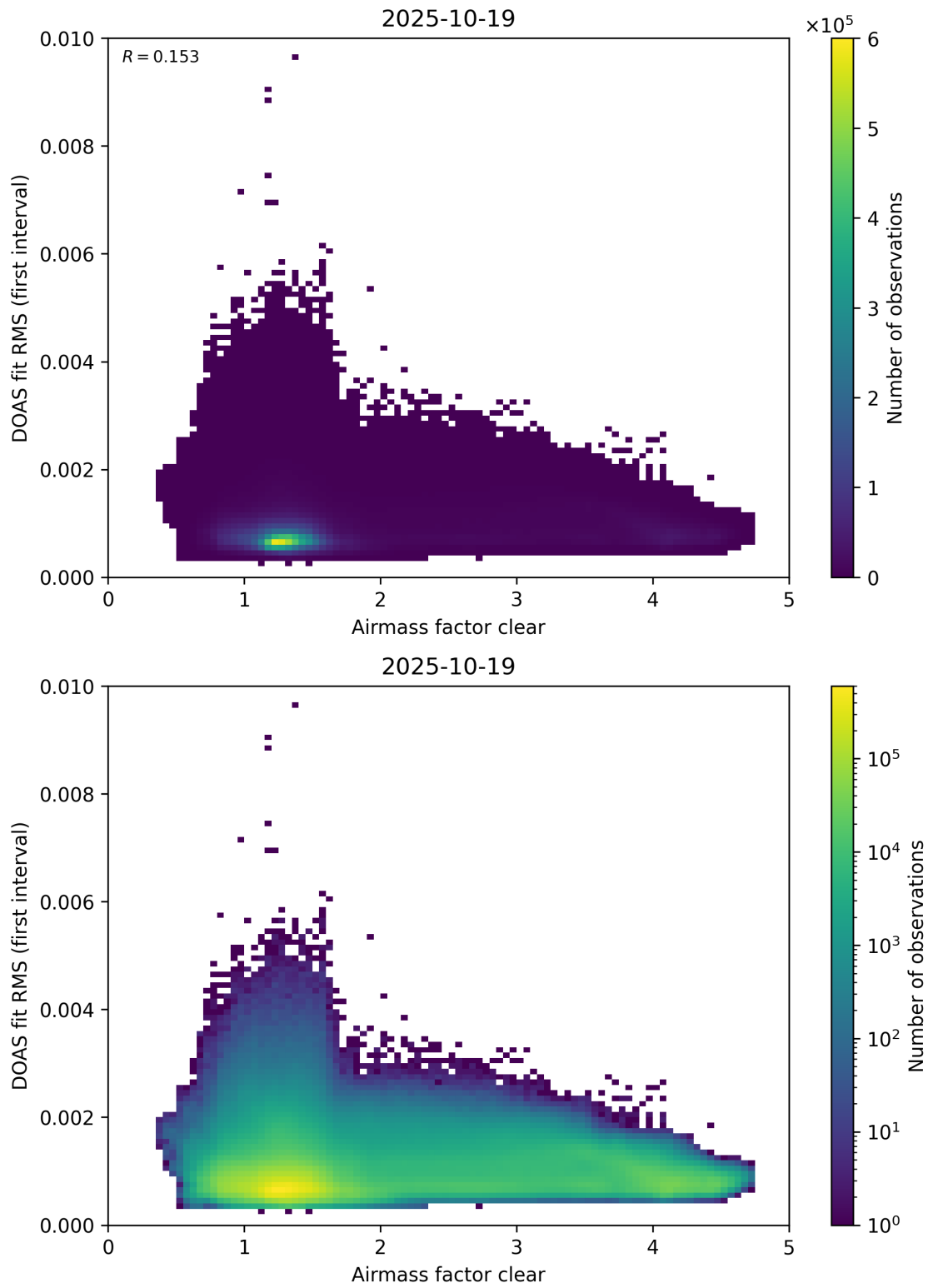
Figure 71: Scatter density plot of “Airmass factor clear” against “DOAS fit RMS (first interval)” for 2025-10-18 to 2025-10-20.
