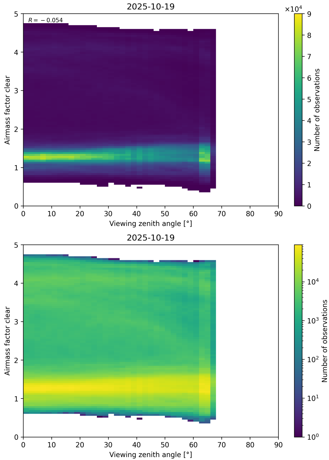
Figure 185: Scatter density plot of “Viewing zenith angle” against “Airmass factor clear” for 2025-10-18 to 2025-10-20.
