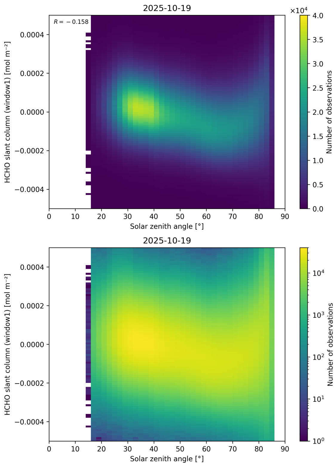
Figure 173: Scatter density plot of “Solar zenith angle” against “HCHO slant column (window1)” for 2025-10-18 to 2025-10-20.
