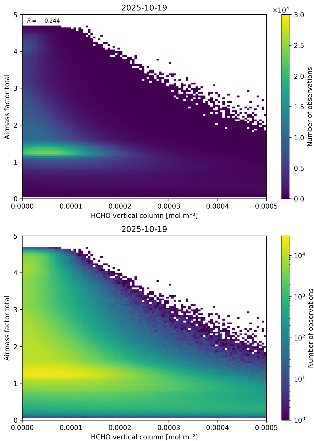
Figure 131: Scatter density plot of “HCHO vertical column” against “Airmass factor total” for 2025-10-18 to 2025-10-20.
