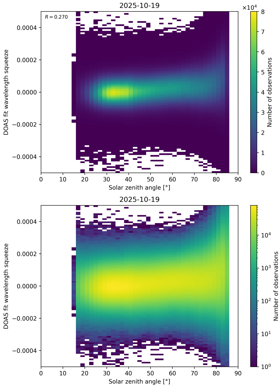
Figure 169: Scatter density plot of “Solar zenith angle” against “DOAS fit wavelength squeeze” for 2025-10-18 to 2025-10-20.
