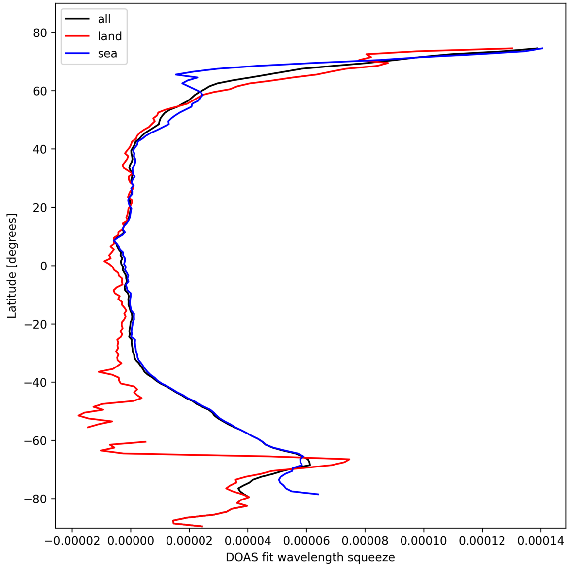
Figure 31: Zonal average of “DOAS fit wavelength squeeze” for 2025-10-18 to 2025-10-20.
