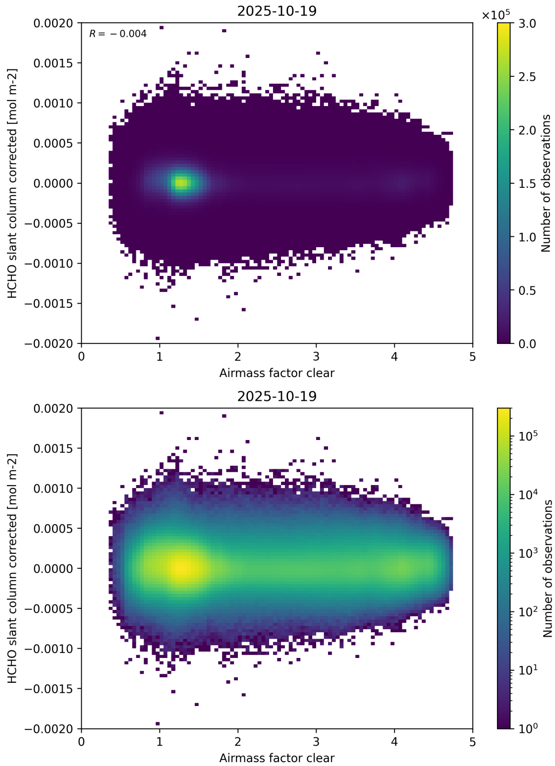
Figure 74: Scatter density plot of “Airmass factor clear” against “HCHO slant column corrected” for 2025-10-18 to 2025-10-20.
