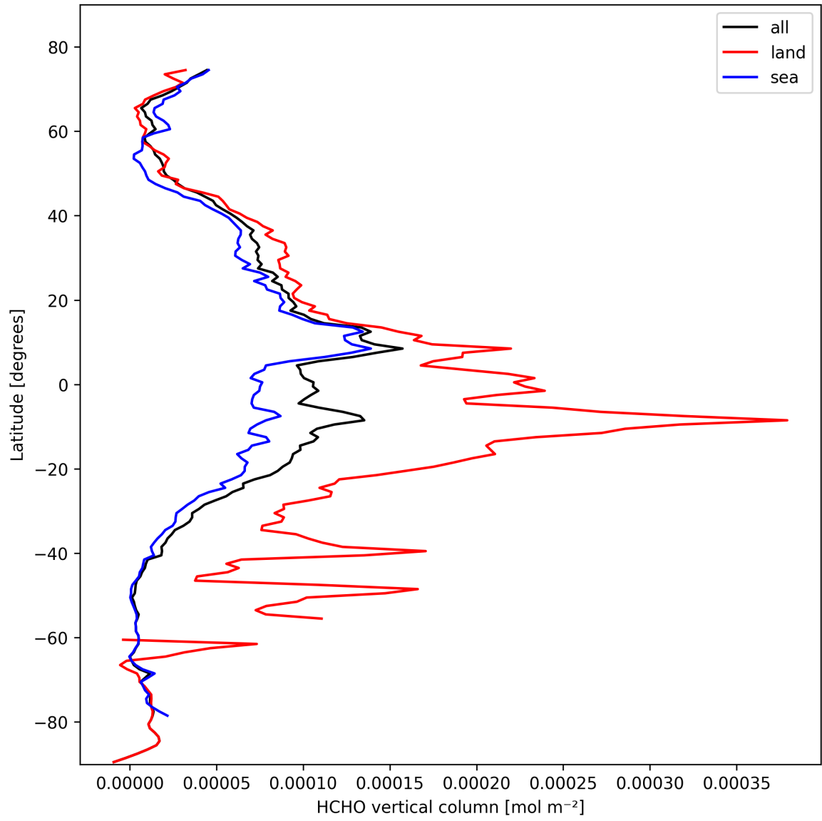
Figure 21: Zonal average of “HCHO vertical column” for 2025-10-18 to 2025-10-20.
