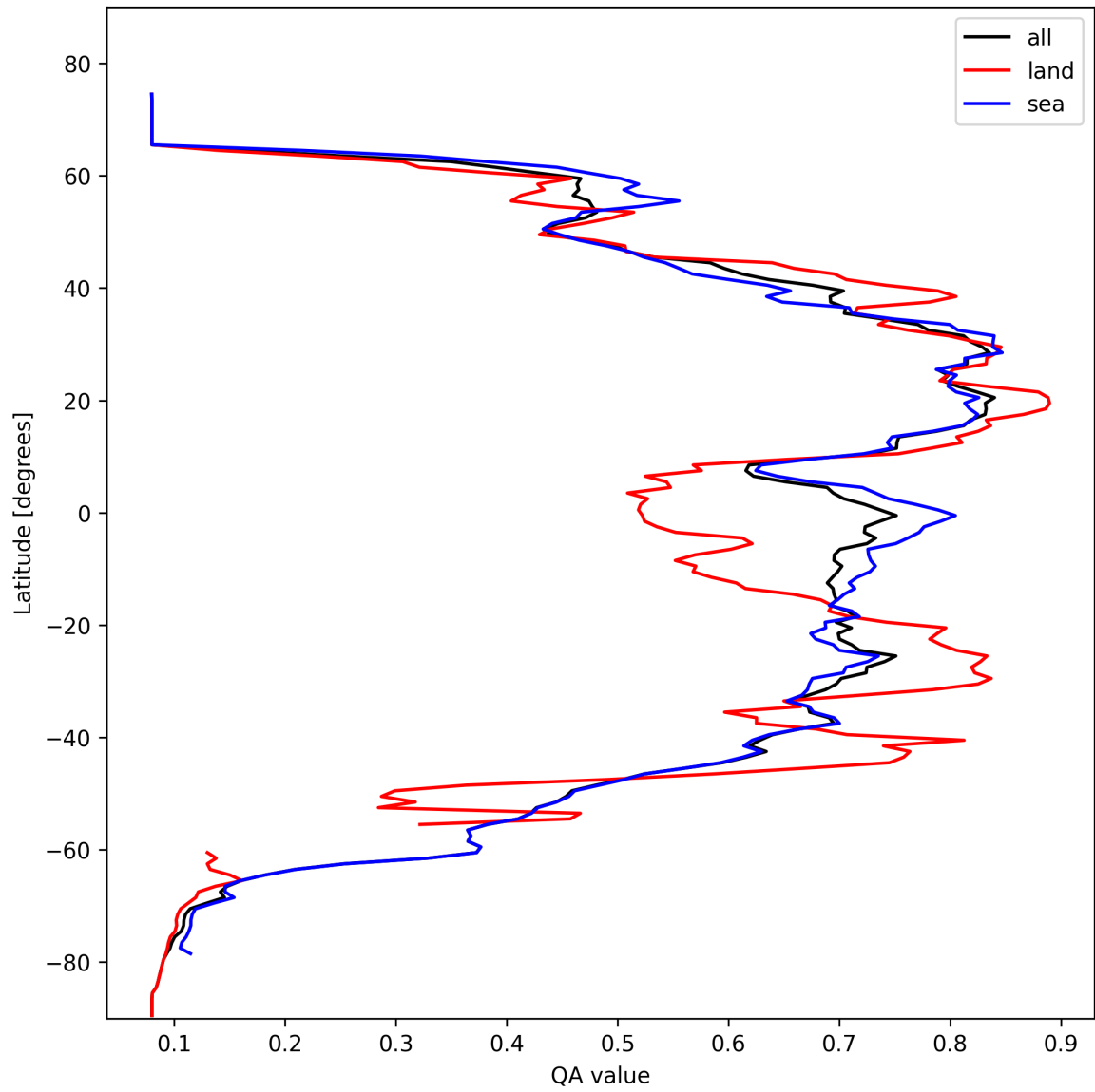
Figure 20: Zonal average of “QA value” for 2025-10-18 to 2025-10-20.
