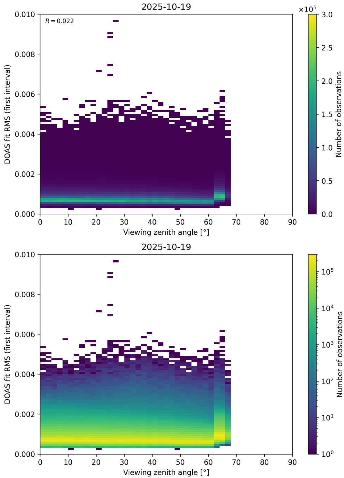
Figure 182: Scatter density plot of “Viewing zenith angle” against “DOAS fit RMS (first interval)” for 2025-10-18 to 2025-10-20.
