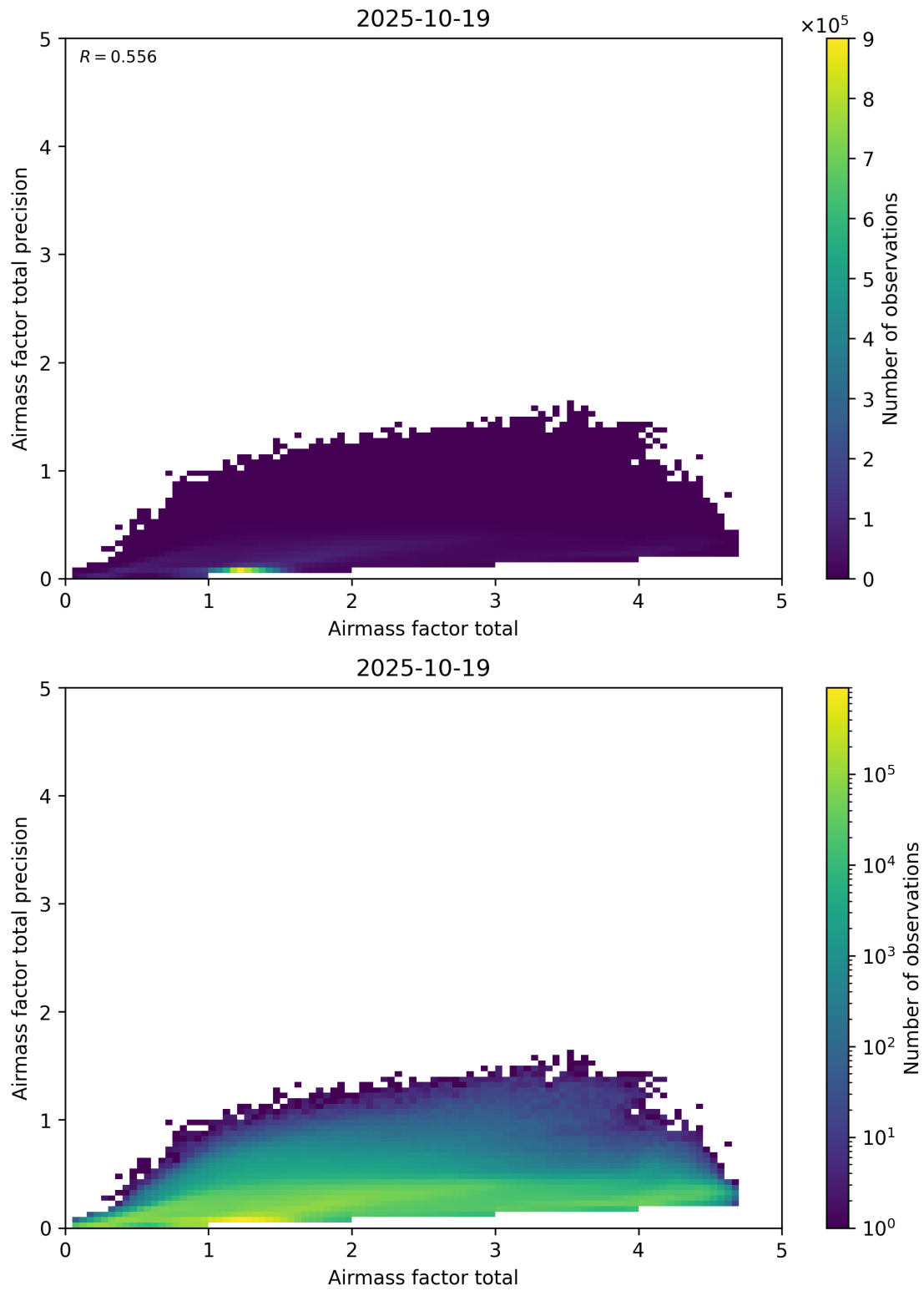
Figure 103: Scatter density plot of “Airmass factor total” against “Airmass factor total precision” for 2025-10-18 to 2025-10-20.
