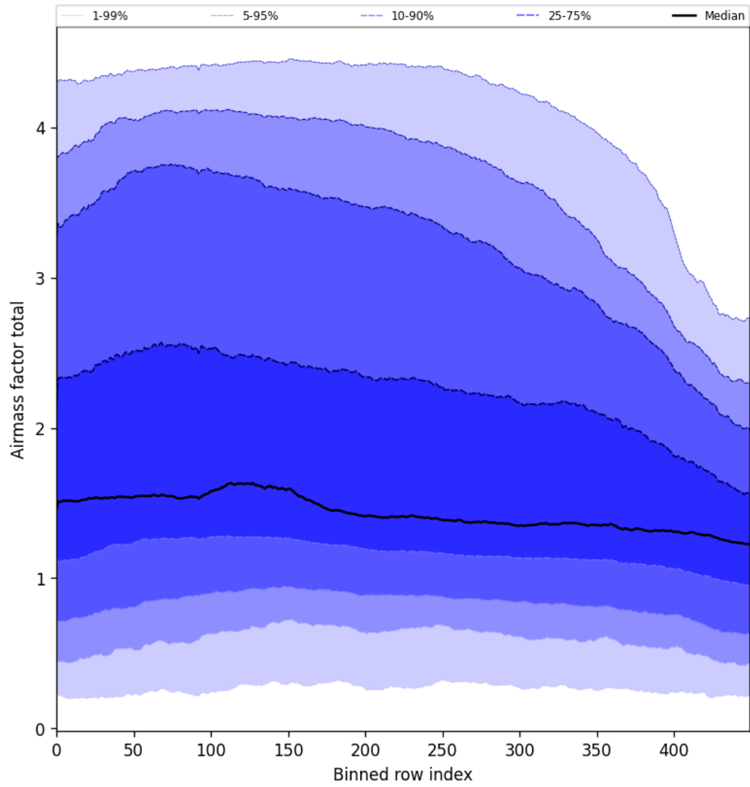
Figure 54: Along track statistics of “Airmass factor total” for 2025-10-18 to 2025-10-20
