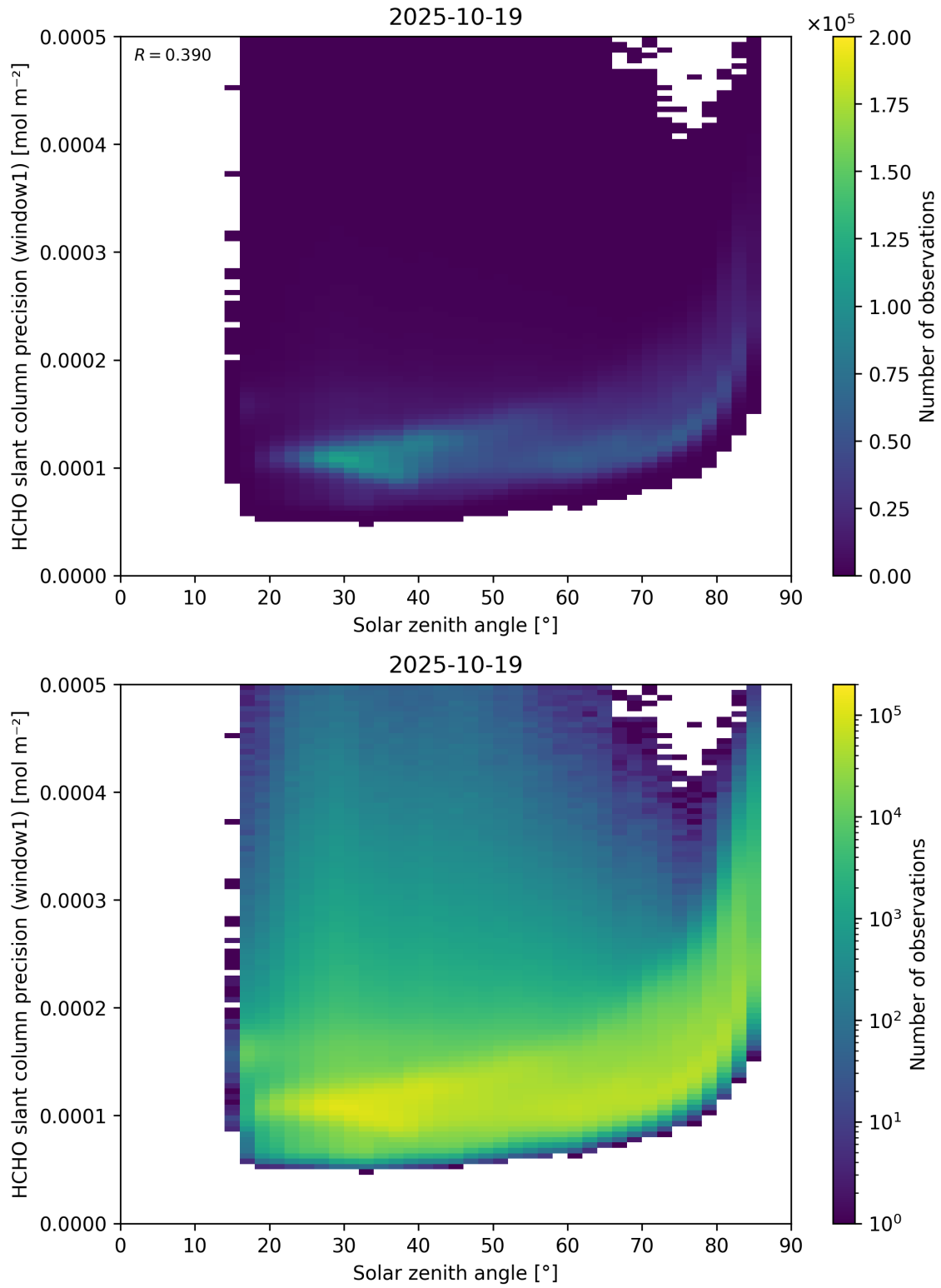
Figure 174: Scatter density plot of “Solar zenith angle” against “HCHO slant column precision (window1)” for 2025-10-18 to 2025-10-20.
