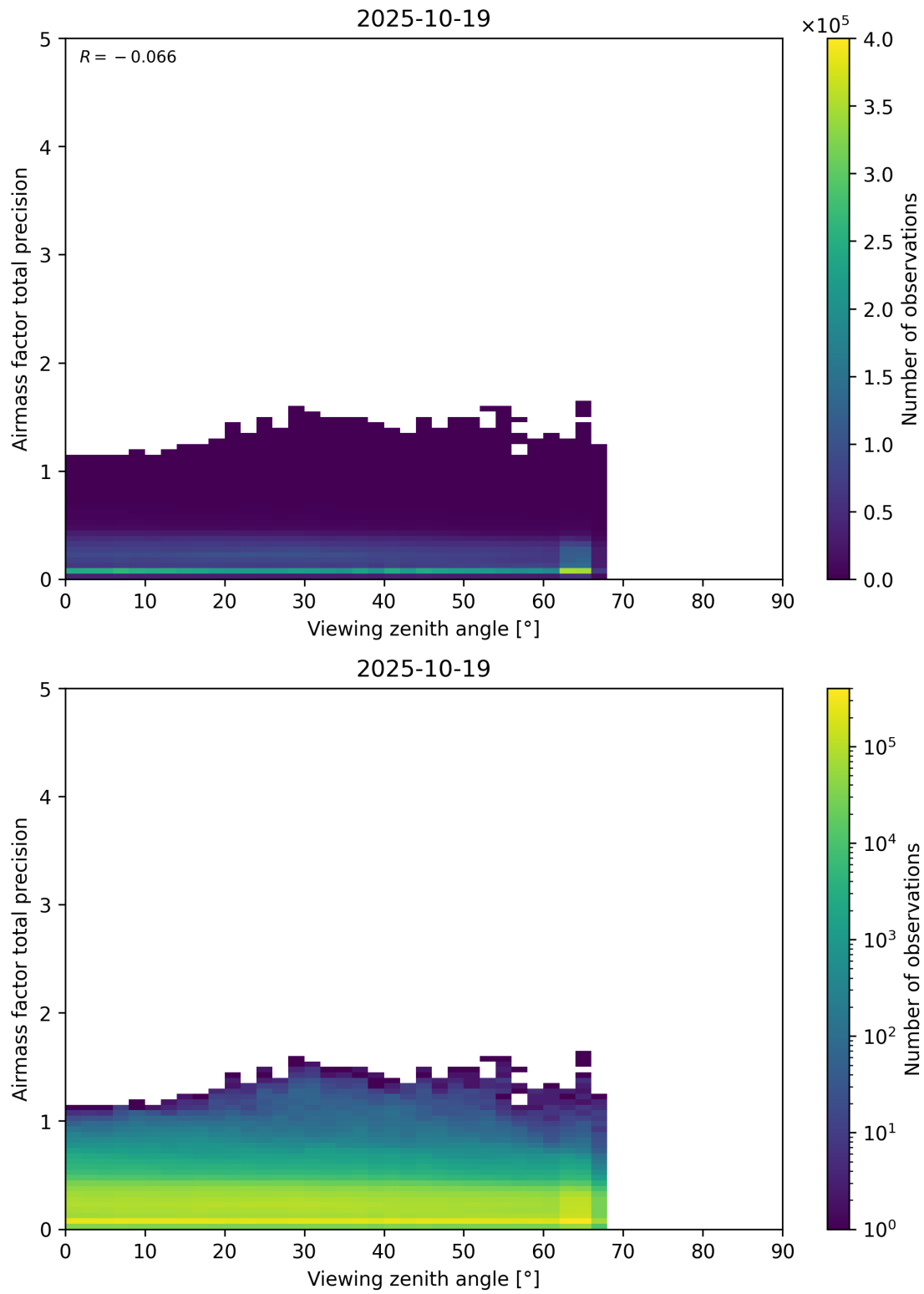
Figure 191: Scatter density plot of “Viewing zenith angle” against “Airmass factor total precision” for 2025-10-18 to 2025-10-20.
