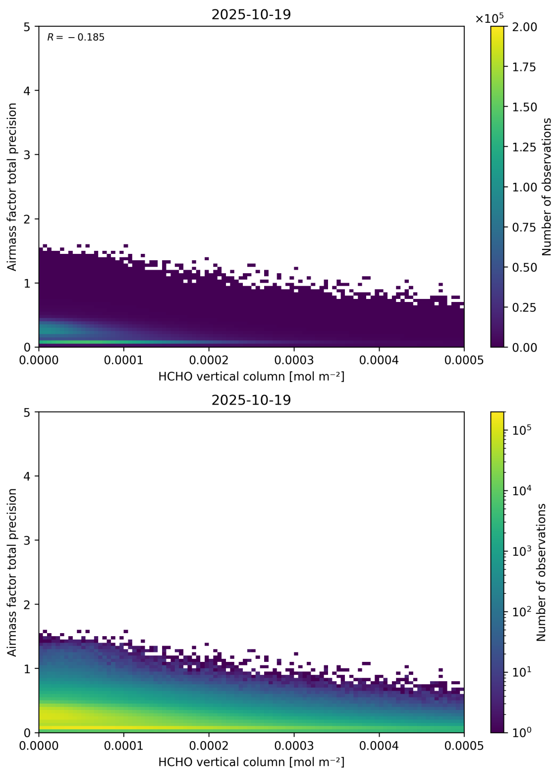
Figure 132: Scatter density plot of “HCHO vertical column” against “Airmass factor total precision” for 2025-10-18 to 2025-10-20.
