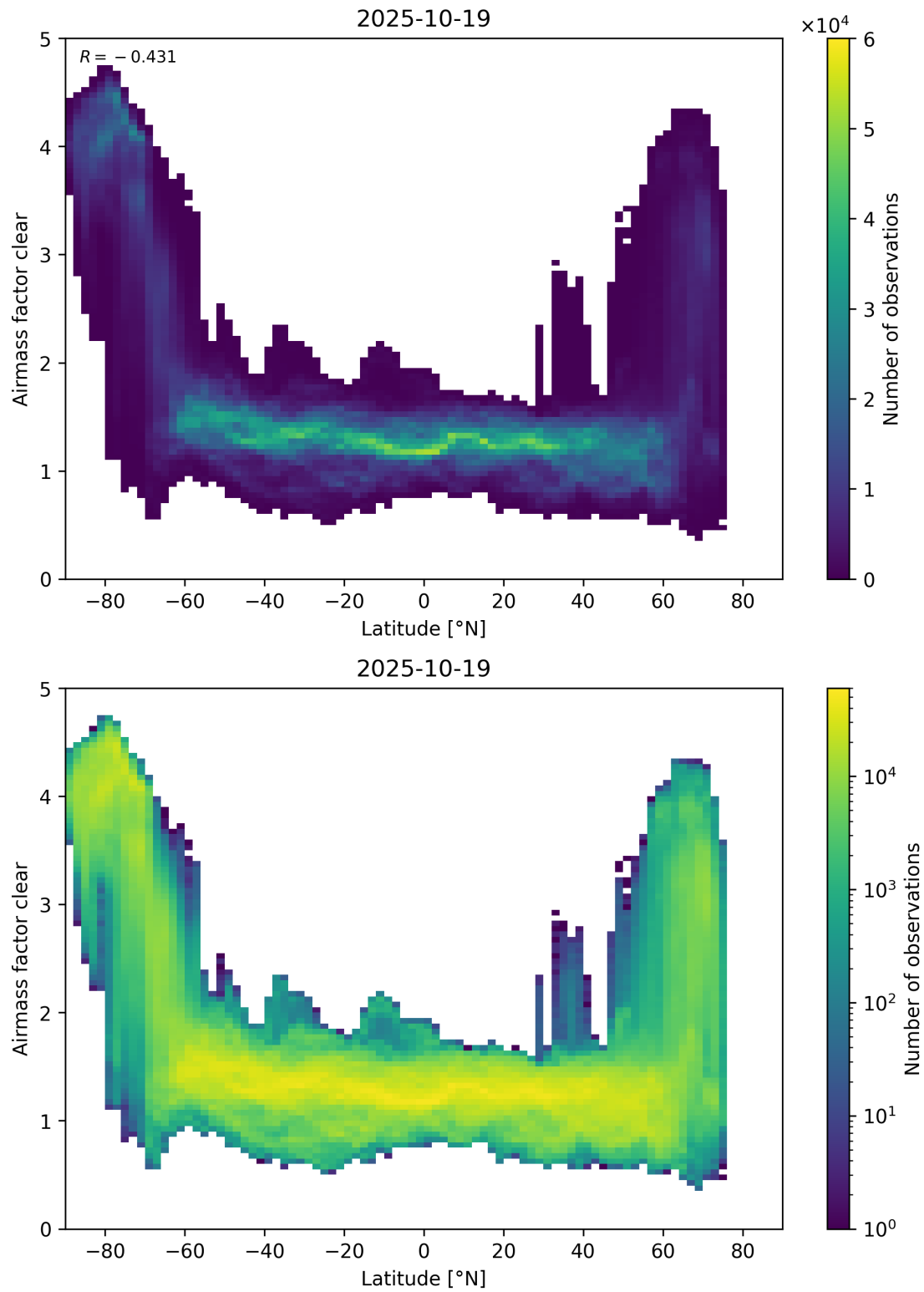
Figure 156: Scatter density plot of “Latitude” against “Airmass factor clear” for 2025-10-18 to 2025-10-20.
