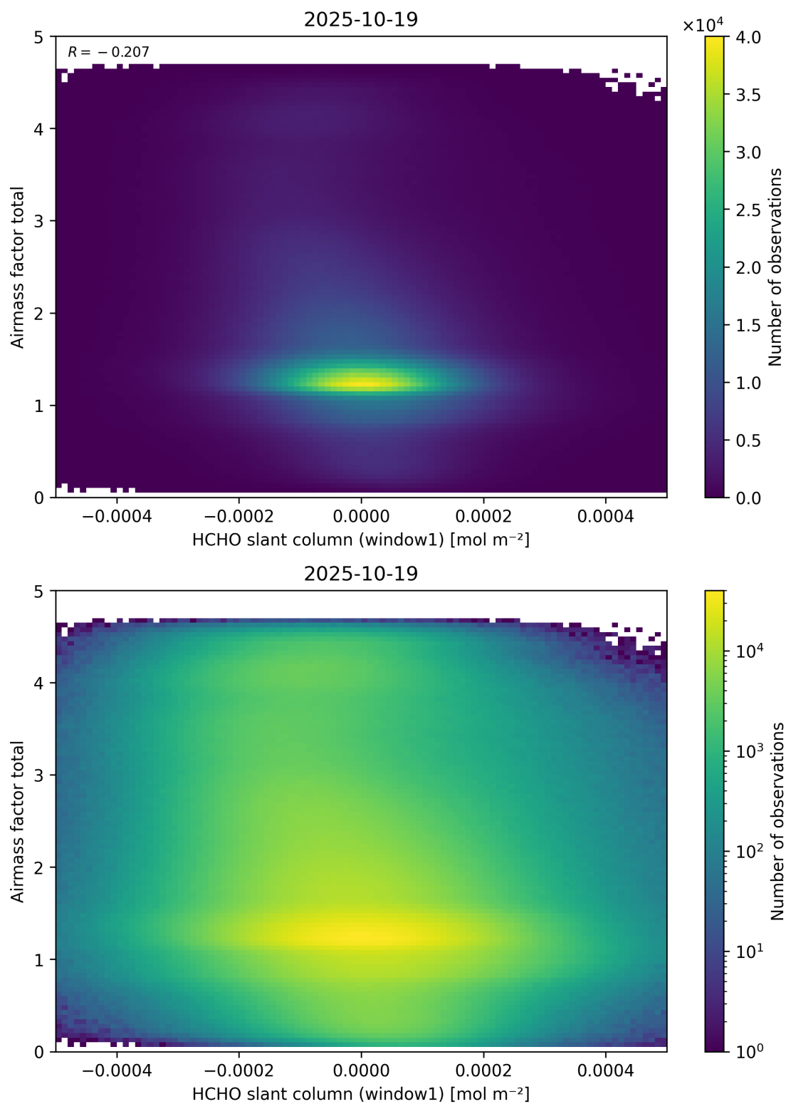
Figure 85: Scatter density plot of “HCHO slant column (window1)” against “Airmass factor total” for 2025-10-18 to 2025-10-20.
