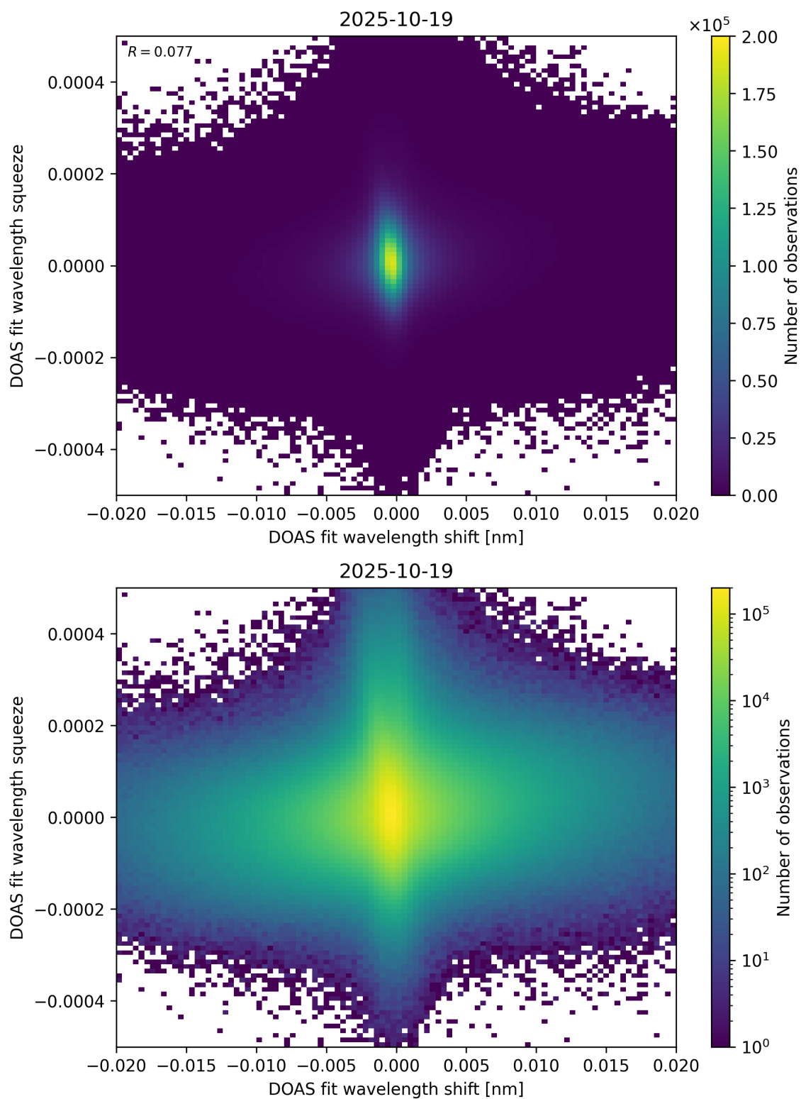
Figure 65: Scatter density plot of “DOAS fit wavelength shift” against “DOAS fit wavelength squeeze” for 2025-10-18 to 2025-10-20.
