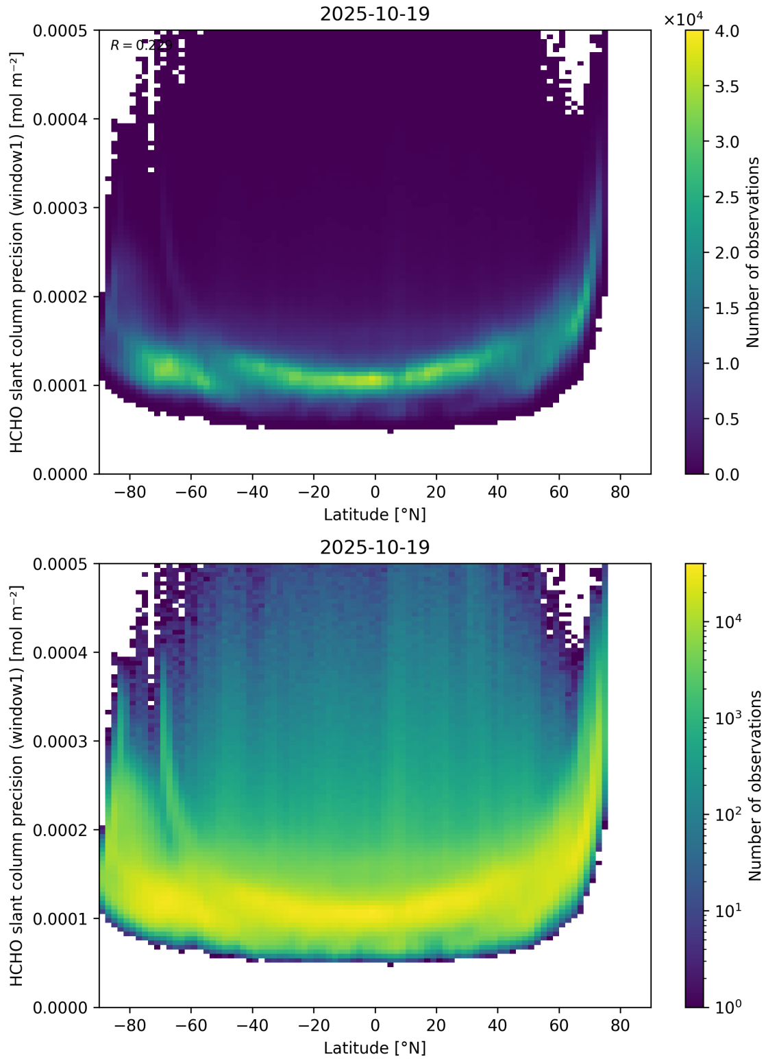
Figure 160: Scatter density plot of “Latitude” against “HCHO slant column precision (window1)” for 2025-10-18 to 2025-10-20.
