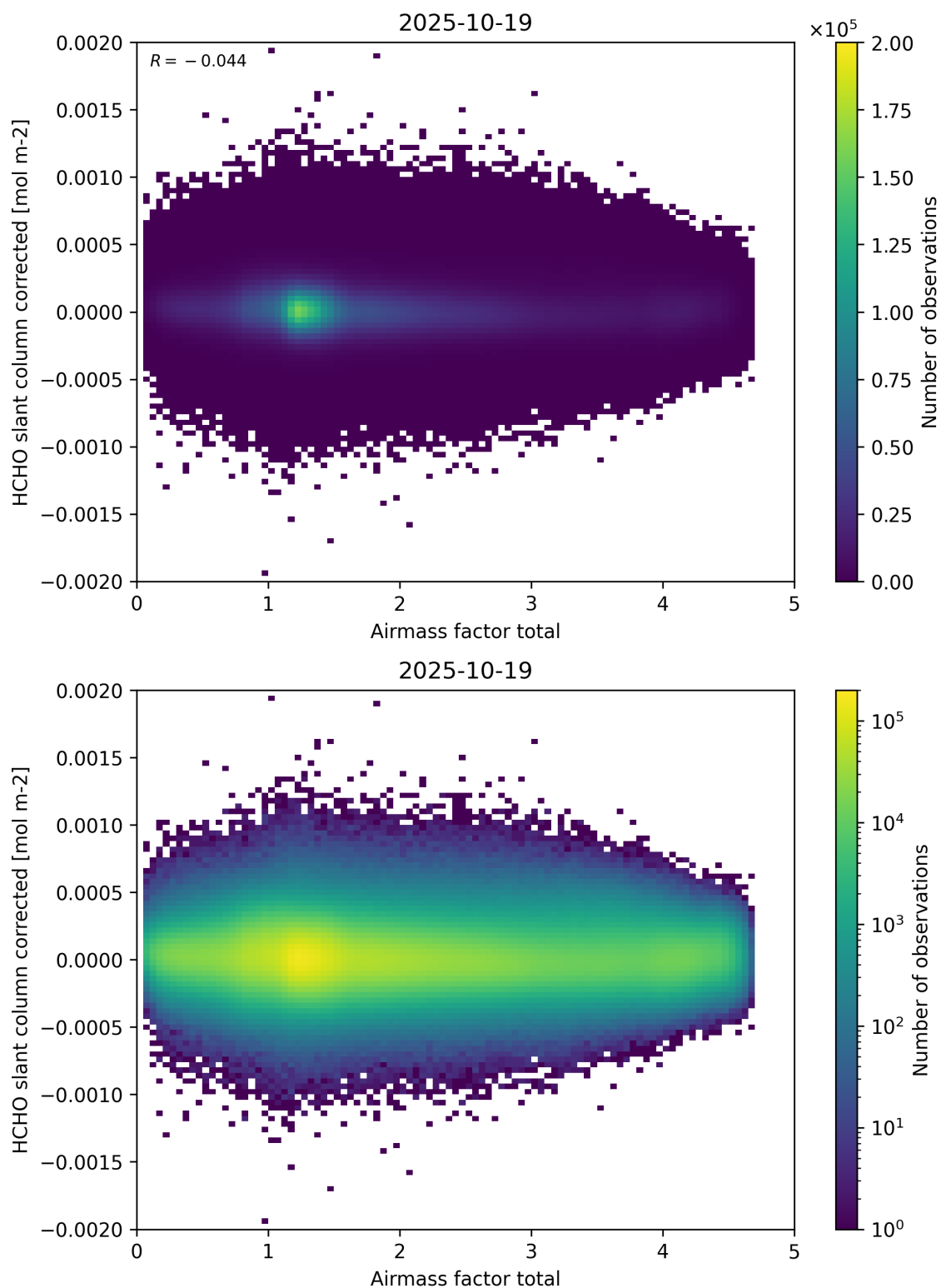
Figure 101: Scatter density plot of “Airmass factor total” against “HCHO slant column corrected” for 2025-10-18 to 2025-10-20.
