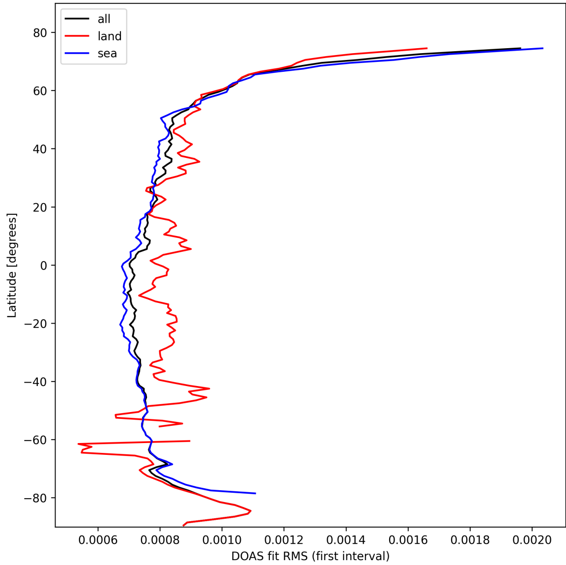
Figure 32: Zonal average of “DOAS fit RMS (first interval)” for 2025-10-18 to 2025-10-20.
