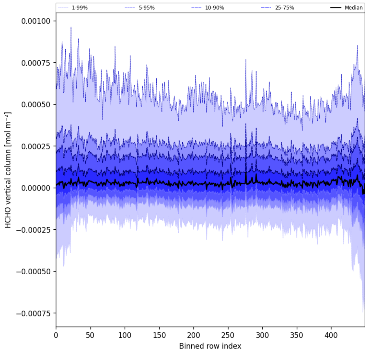
Figure 49: Along track statistics of “HCHO vertical column” for 2025-10-18 to 2025-10-20
