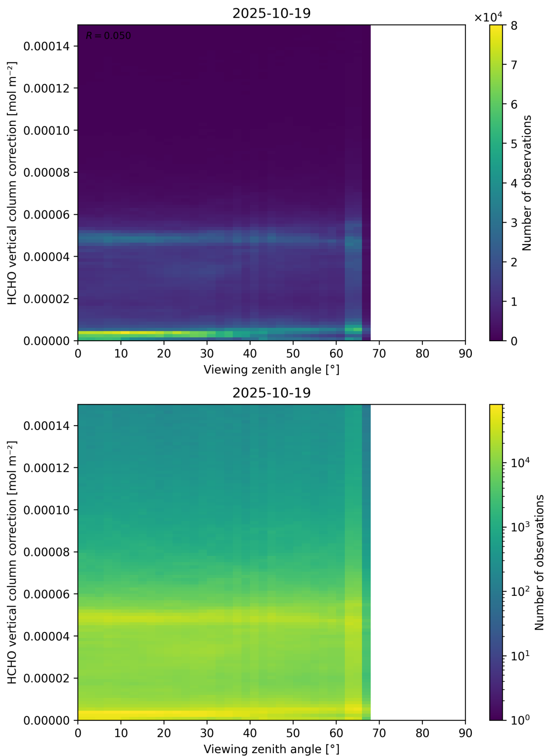
Figure 193: Scatter density plot of “Viewing zenith angle” against “HCHO vertical column correction” for 2025-10-18 to 2025-10-20.
