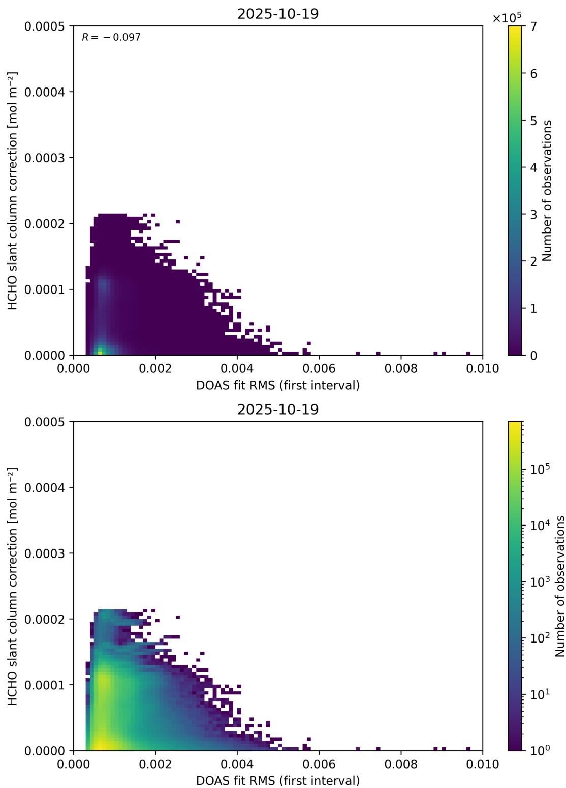
Figure 63: Scatter density plot of “DOAS fit RMS (first interval)” against “HCHO slant column correction” for 2025-10-18 to 2025-10-20.
