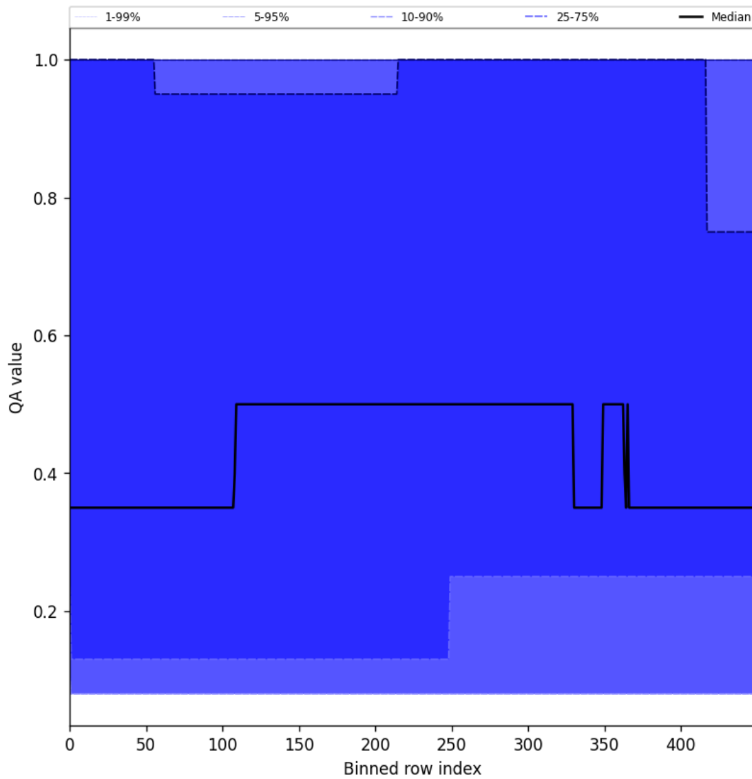
Figure 48: Along track statistics of “QA value” for 2025-10-18 to 2025-10-20
