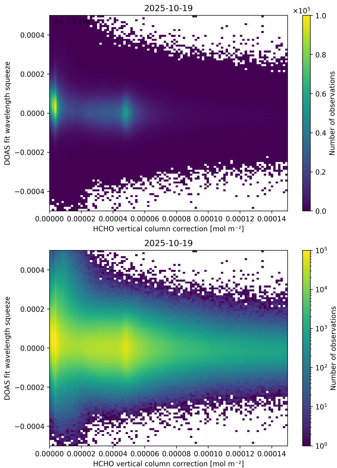
Figure 114: Scatter density plot of “HCHO vertical column correction” against “DOAS fit wavelength squeeze” for 2025-10-18 to 2025-10-20.
