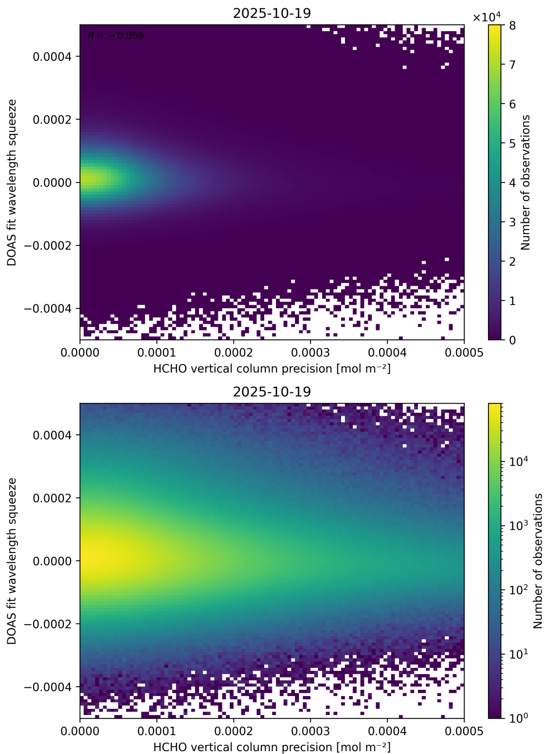
Figure 138: Scatter density plot of “HCHO vertical column precision” against “DOAS fit wavelength squeeze” for 2025-10-18 to 2025-10-20.
