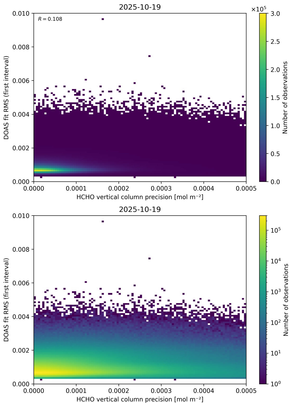
Figure 136: Scatter density plot of “HCHO vertical column precision” against “DOAS fit RMS (first interval)” for 2025-10-18 to 2025-10-20.
