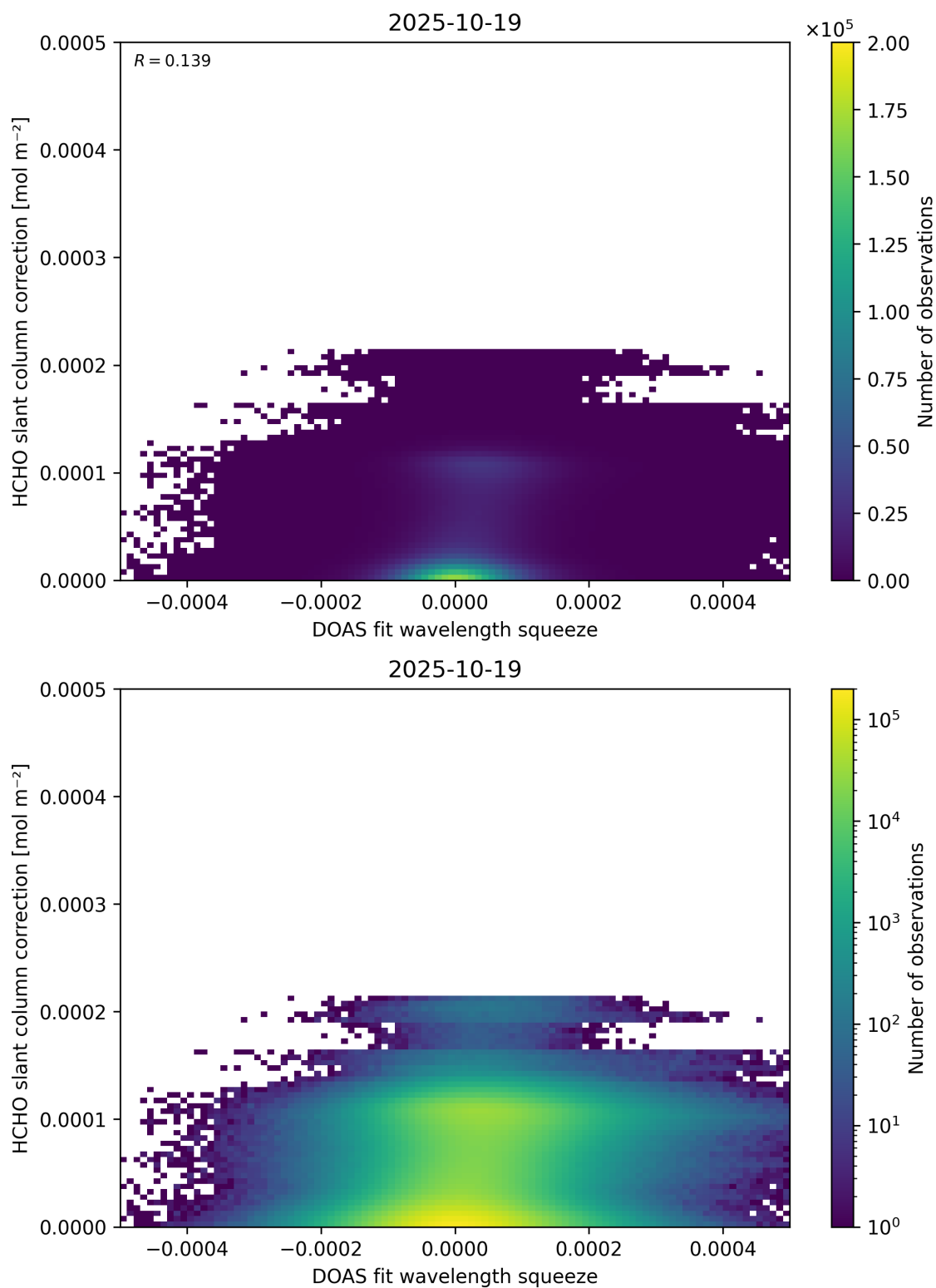
Figure 70: Scatter density plot of “DOAS fit wavelength squeeze” against “HCHO slant column correction” for 2025-10-18 to 2025-10-20.
