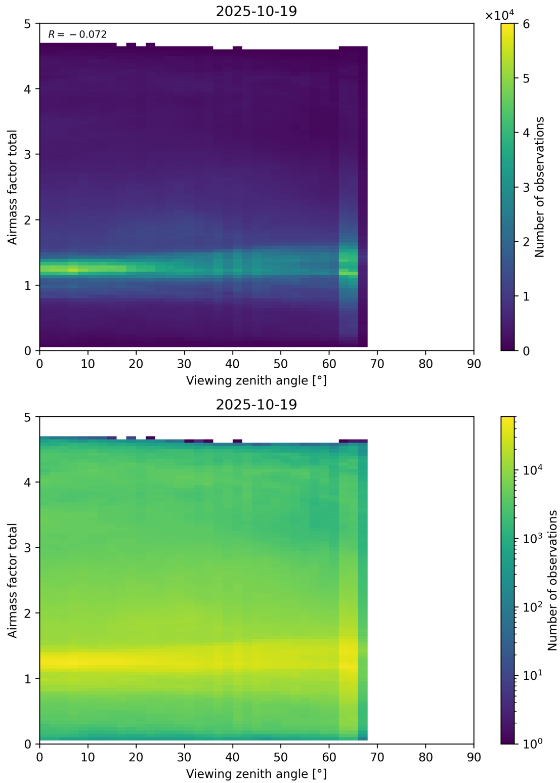
Figure 190: Scatter density plot of “Viewing zenith angle” against “Airmass factor total” for 2025-10-18 to 2025-10-20.
