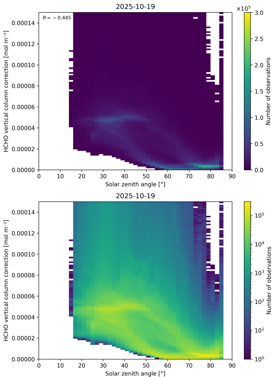
Figure 178: Scatter density plot of “Solar zenith angle” against “HCHO vertical column correction” for 2025-10-18 to 2025-10-20.
