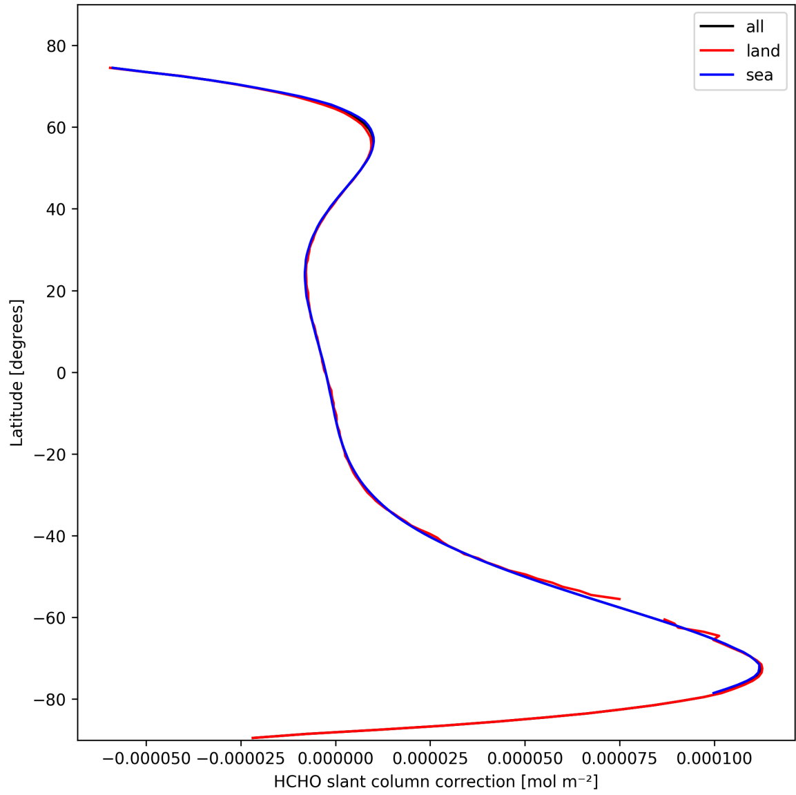
Figure 33: Zonal average of “HCHO slant column correction” for 2025-10-18 to 2025-10-20.
