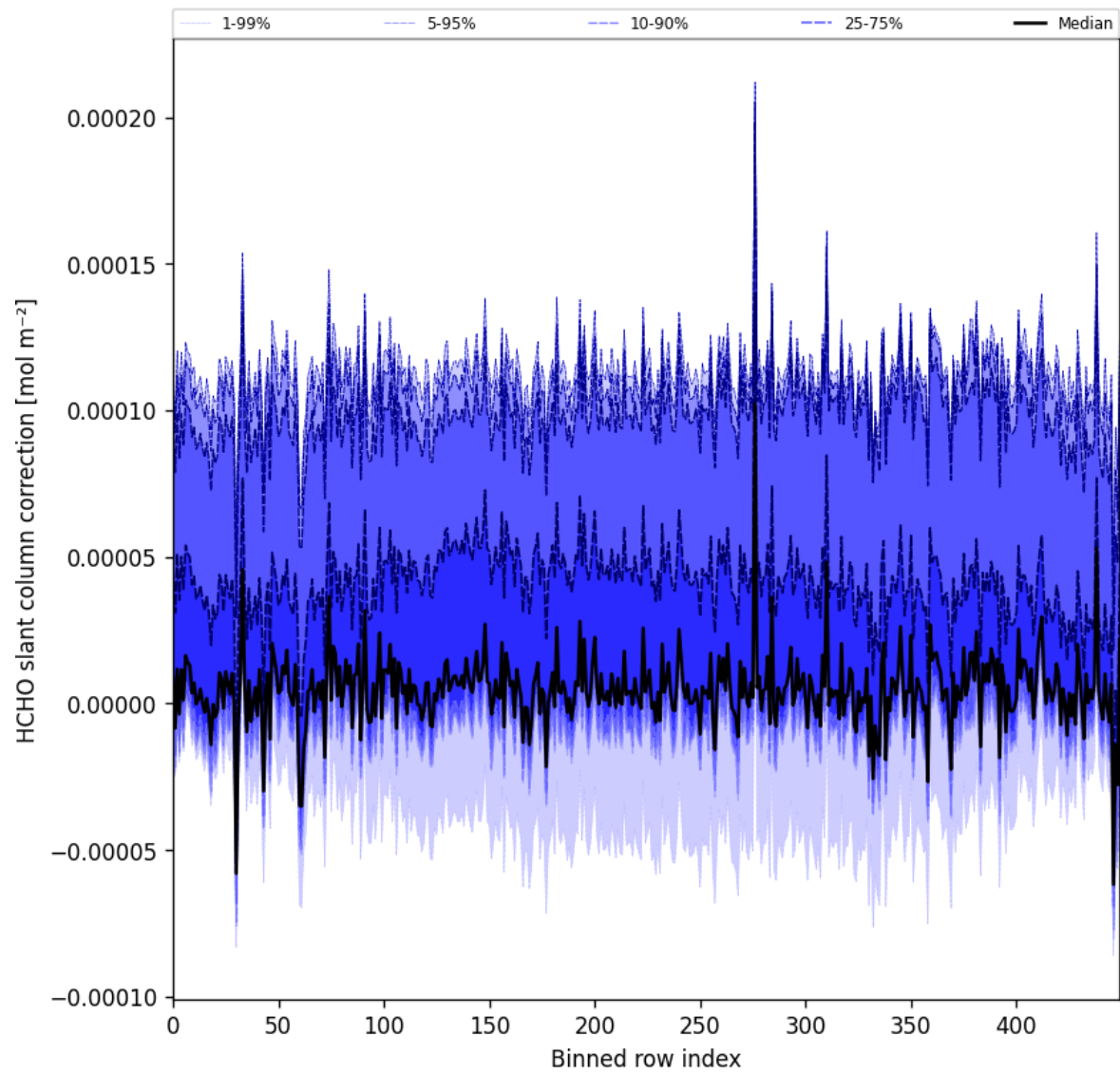
Figure 61: Along track statistics of “HCHO slant column correction” for 2025-10-18 to 2025-10-20
