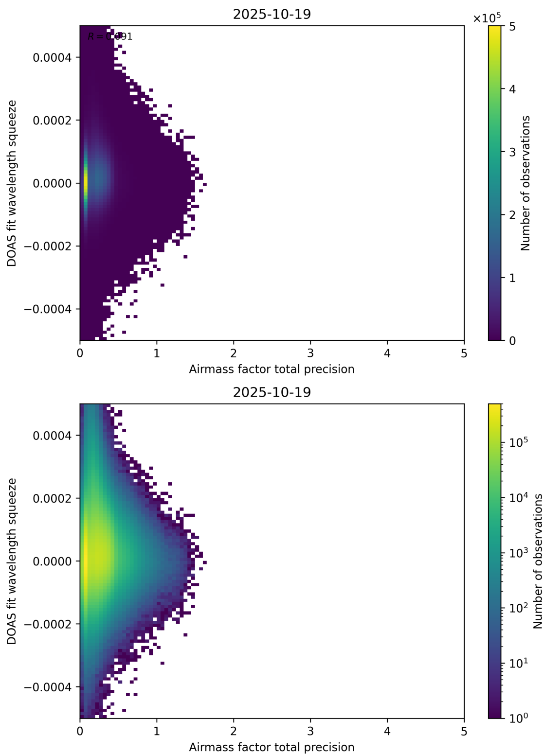
Figure 107: Scatter density plot of “Airmass factor total precision” against “DOAS fit wavelength squeeze” for 2025-10-18 to 2025-10-20.
