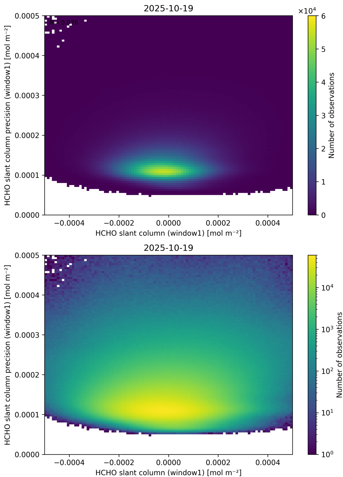
Figure 84: Scatter density plot of “HCHO slant column (window1)” against “HCHO slant column precision (window1)” for 2025-10-18 to 2025-10-20.
