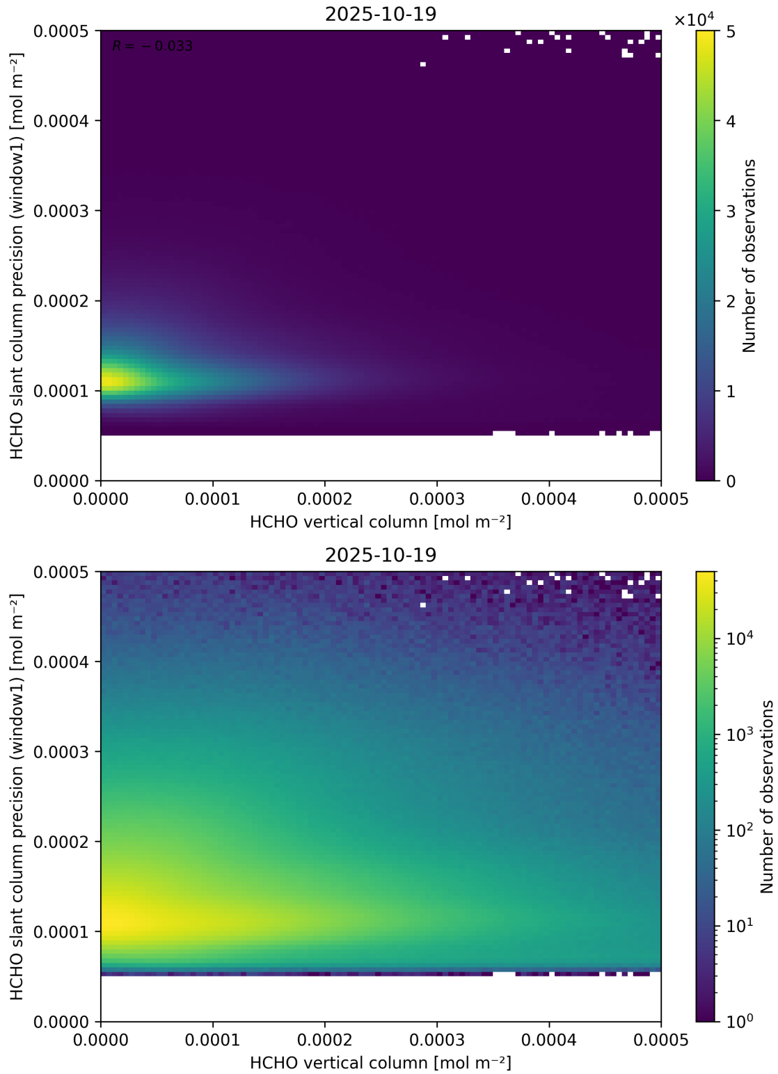
Figure 130: Scatter density plot of “HCHO vertical column” against “HCHO slant column precision (window1)” for 2025-10-18 to 2025-10-20.
