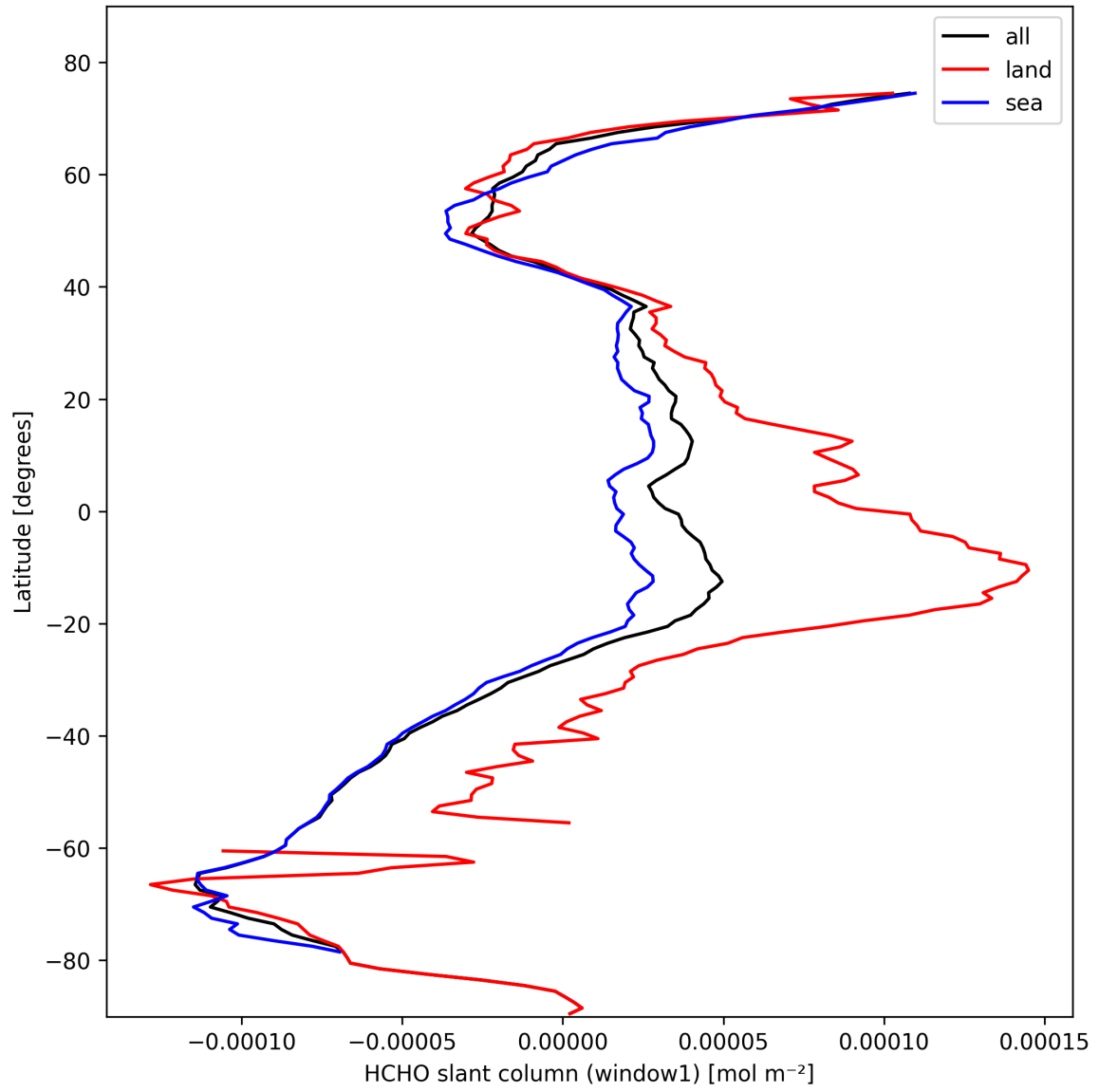
Figure 24: Zonal average of “HCHO slant column (window1)” for 2025-10-18 to 2025-10-20.
