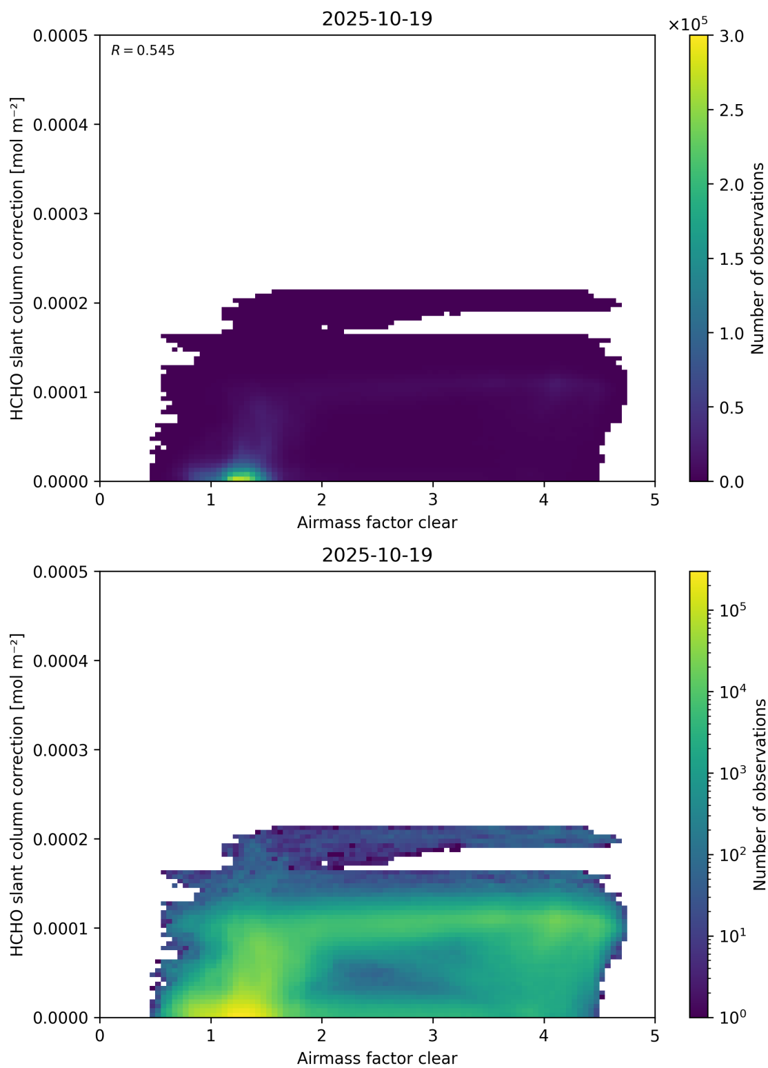
Figure 75: Scatter density plot of “Airmass factor clear” against “HCHO slant column correction” for 2025-10-18 to 2025-10-20.
