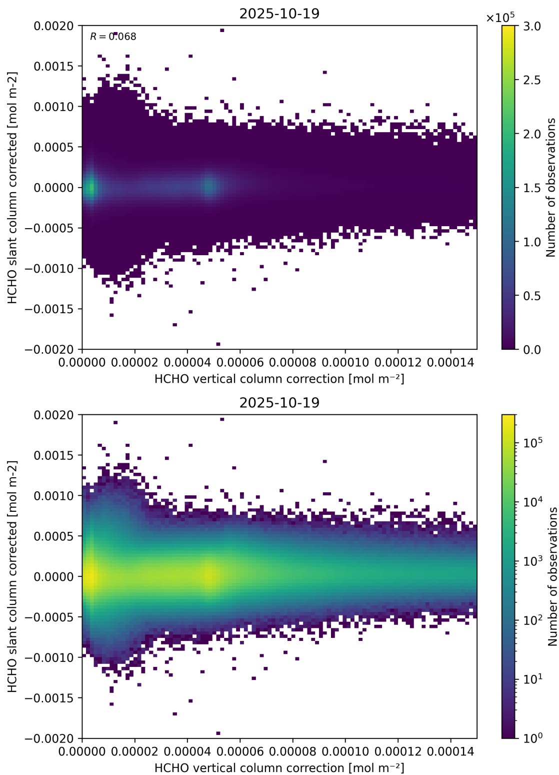
Figure 116: Scatter density plot of “HCHO vertical column correction” against “HCHO slant column corrected” for 2025-10-18 to 2025-10-20.
