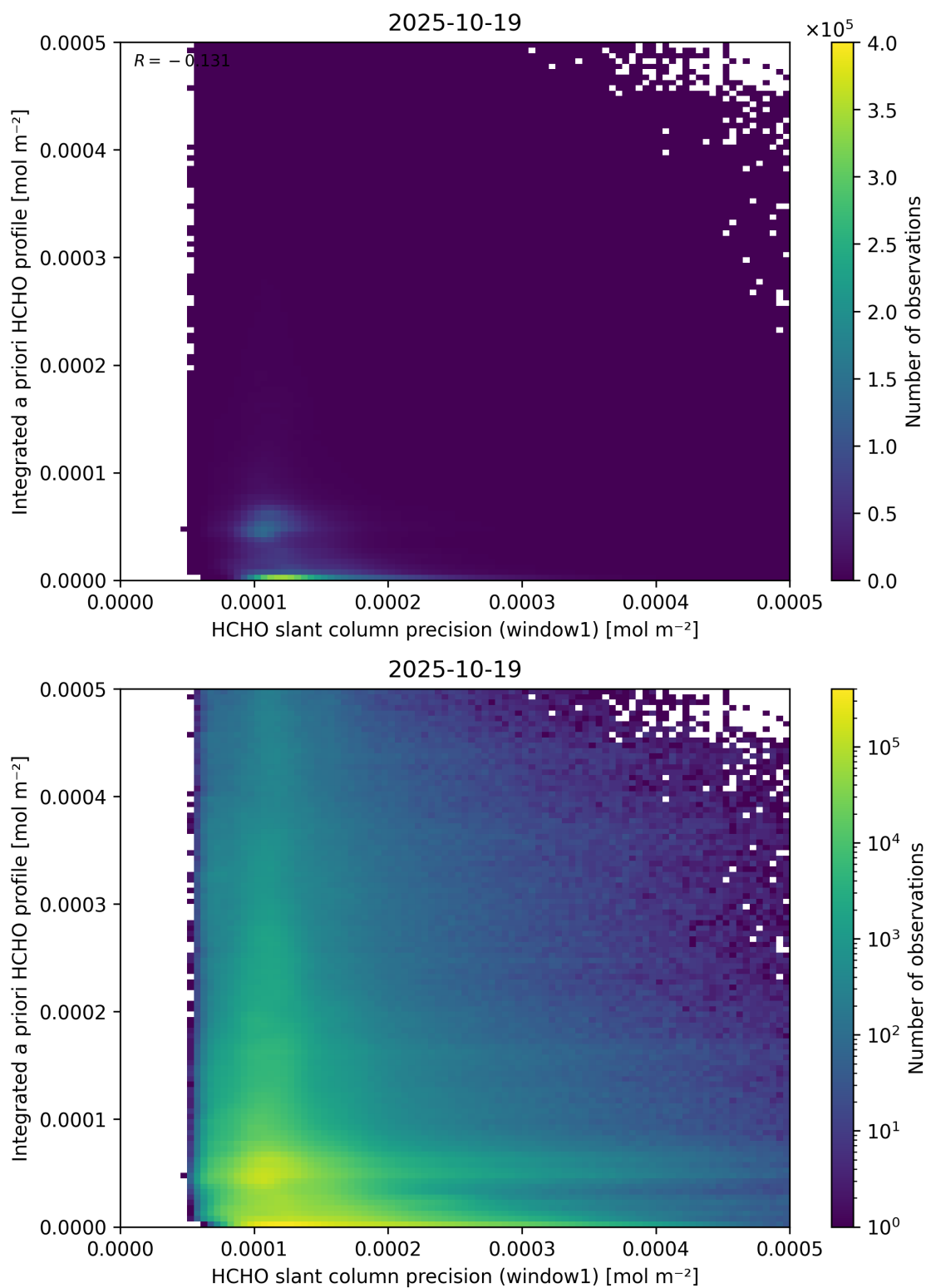
Figure 96: Scatter density plot of “HCHO slant column precision (window1)” against “Integrated a priori HCHO profile” for 2025-10-18 to 2025-10-20.
