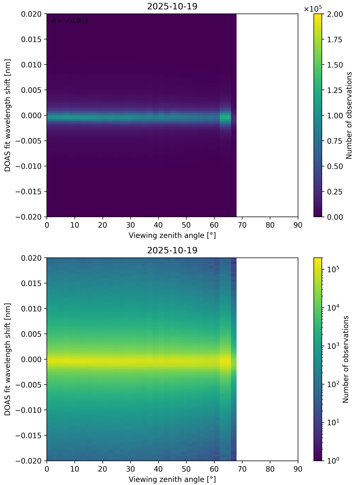
Figure 183: Scatter density plot of “Viewing zenith angle” against “DOAS fit wavelength shift” for 2025-10-18 to 2025-10-20.
