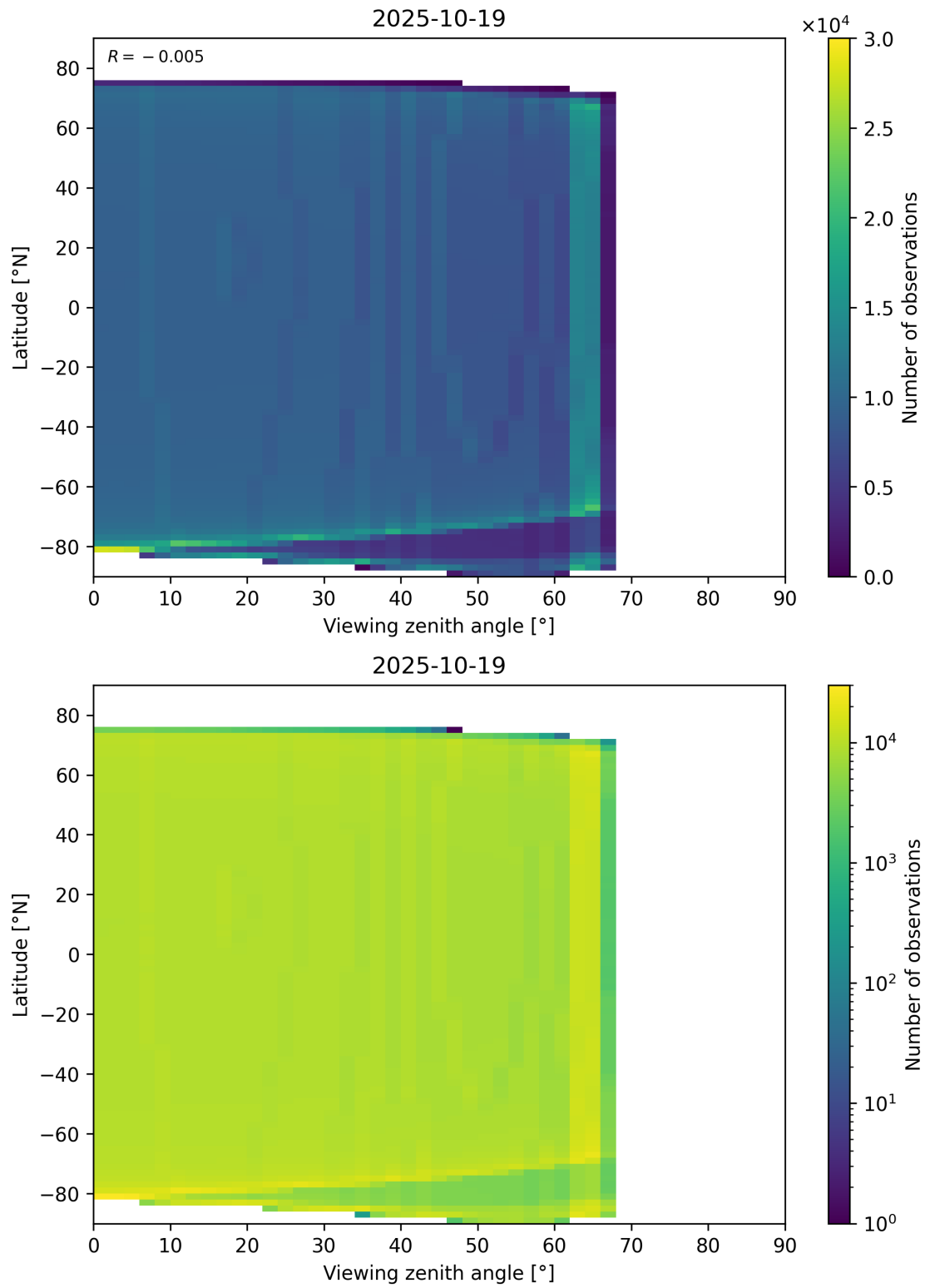
Figure 196: Scatter density plot of “Viewing zenith angle” against “Latitude” for 2025-10-18 to 2025-10-20.
