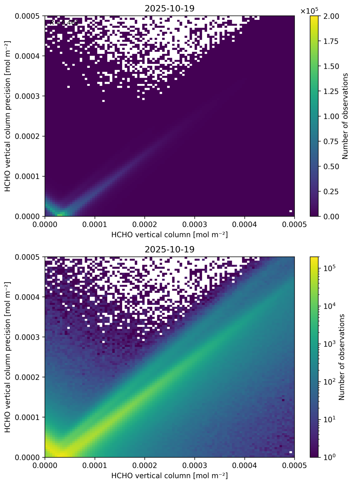
Figure 134: Scatter density plot of “HCHO vertical column” against “HCHO vertical column precision” for 2025-10-18 to 2025-10-20.
