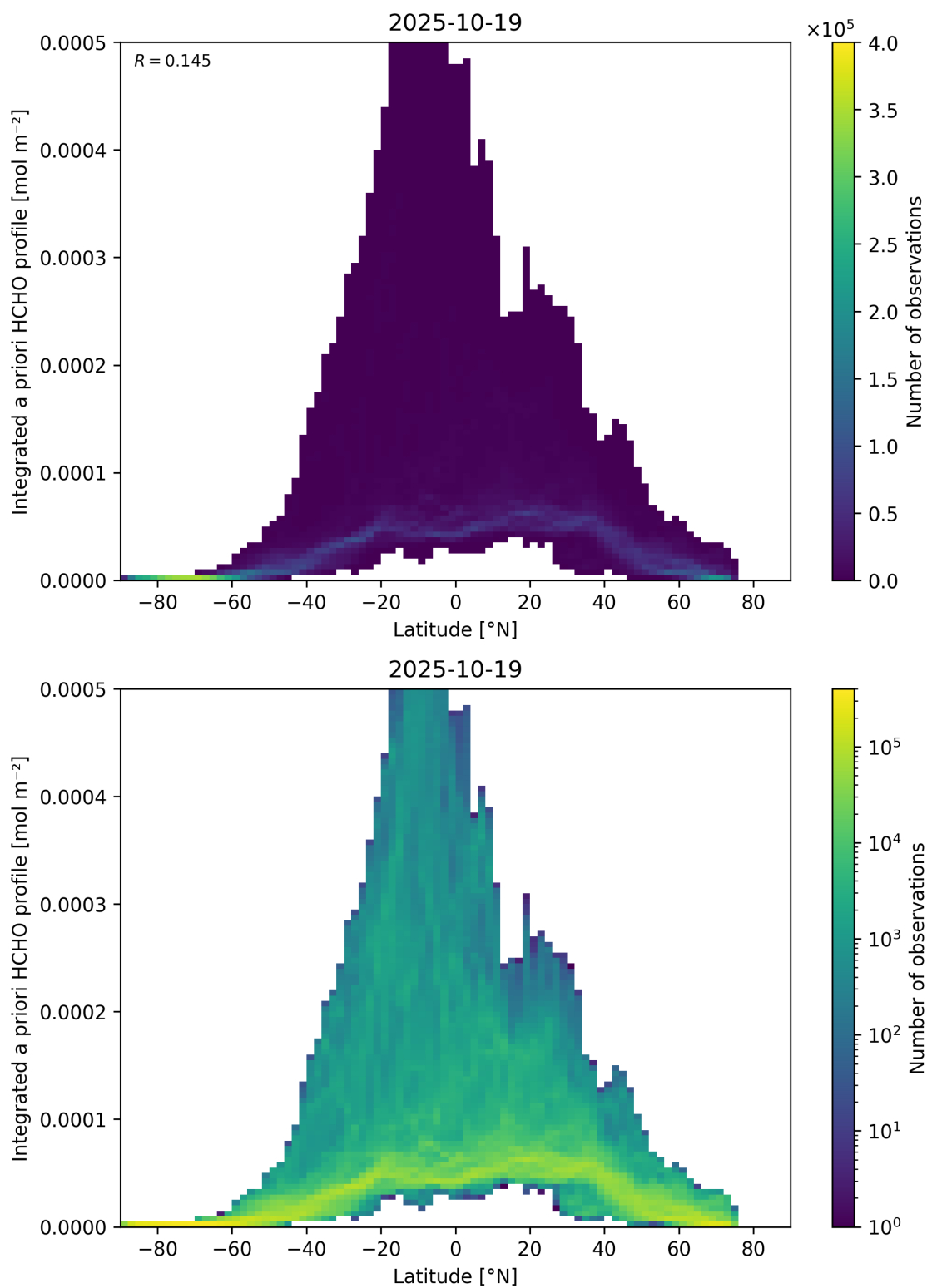
Figure 166: Scatter density plot of “Latitude” against “Integrated a priori HCHO profile” for 2025-10-18 to 2025-10-20.
