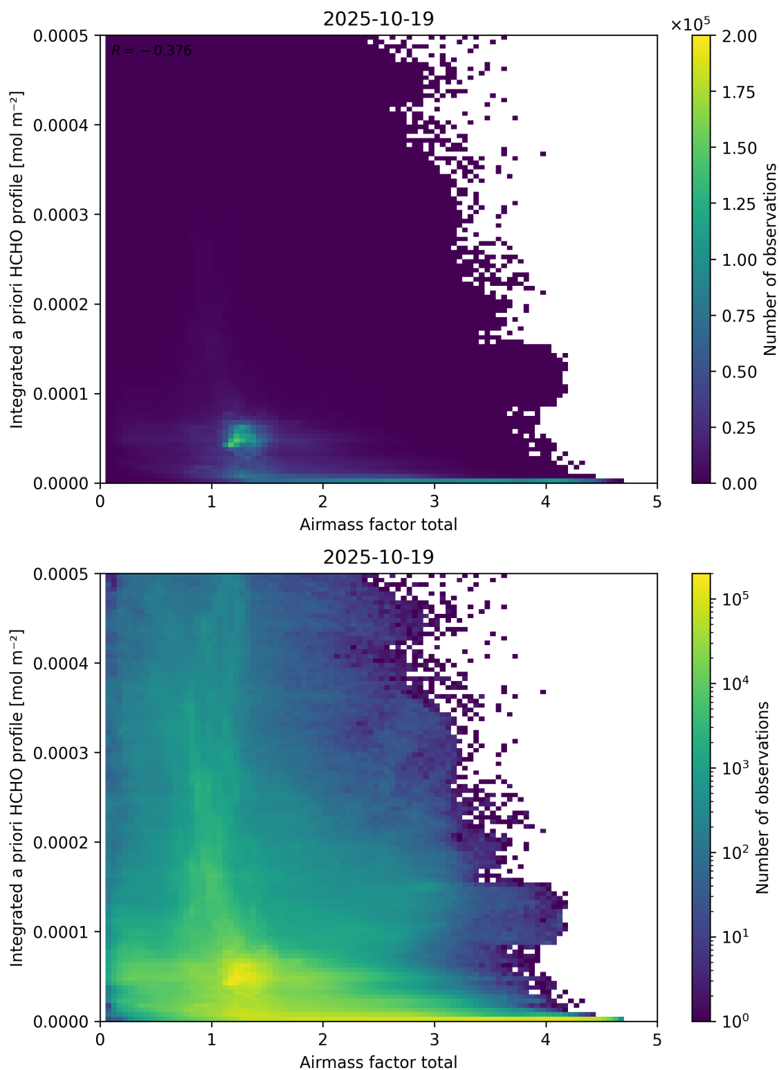
Figure 104: Scatter density plot of “Airmass factor total” against “Integrated a priori HCHO profile” for 2025-10-18 to 2025-10-20.
