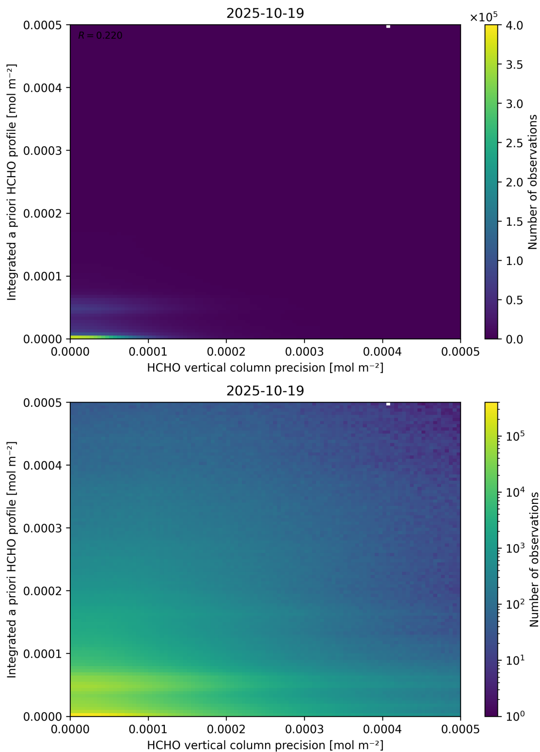
Figure 147: Scatter density plot of “HCHO vertical column precision” against “Integrated a priori HCHO profile” for 2025-10-18 to 2025-10-20.
