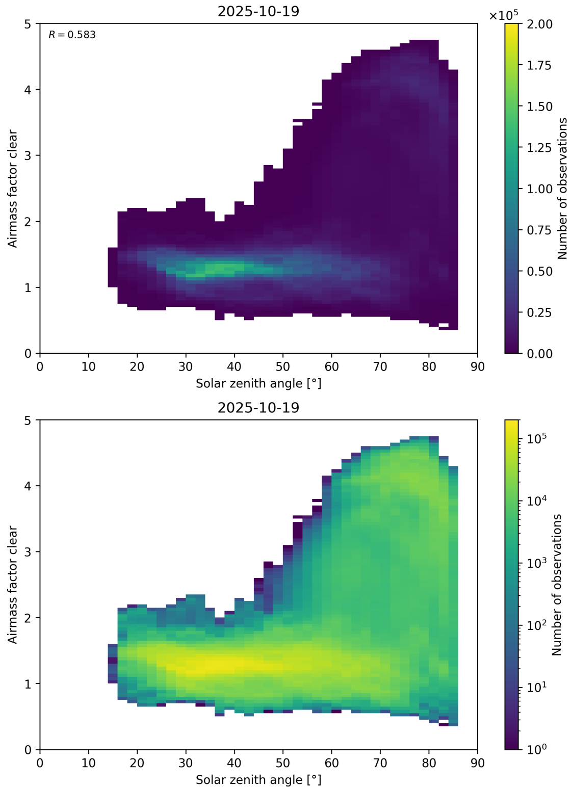
Figure 170: Scatter density plot of “Solar zenith angle” against “Airmass factor clear” for 2025-10-18 to 2025-10-20.
