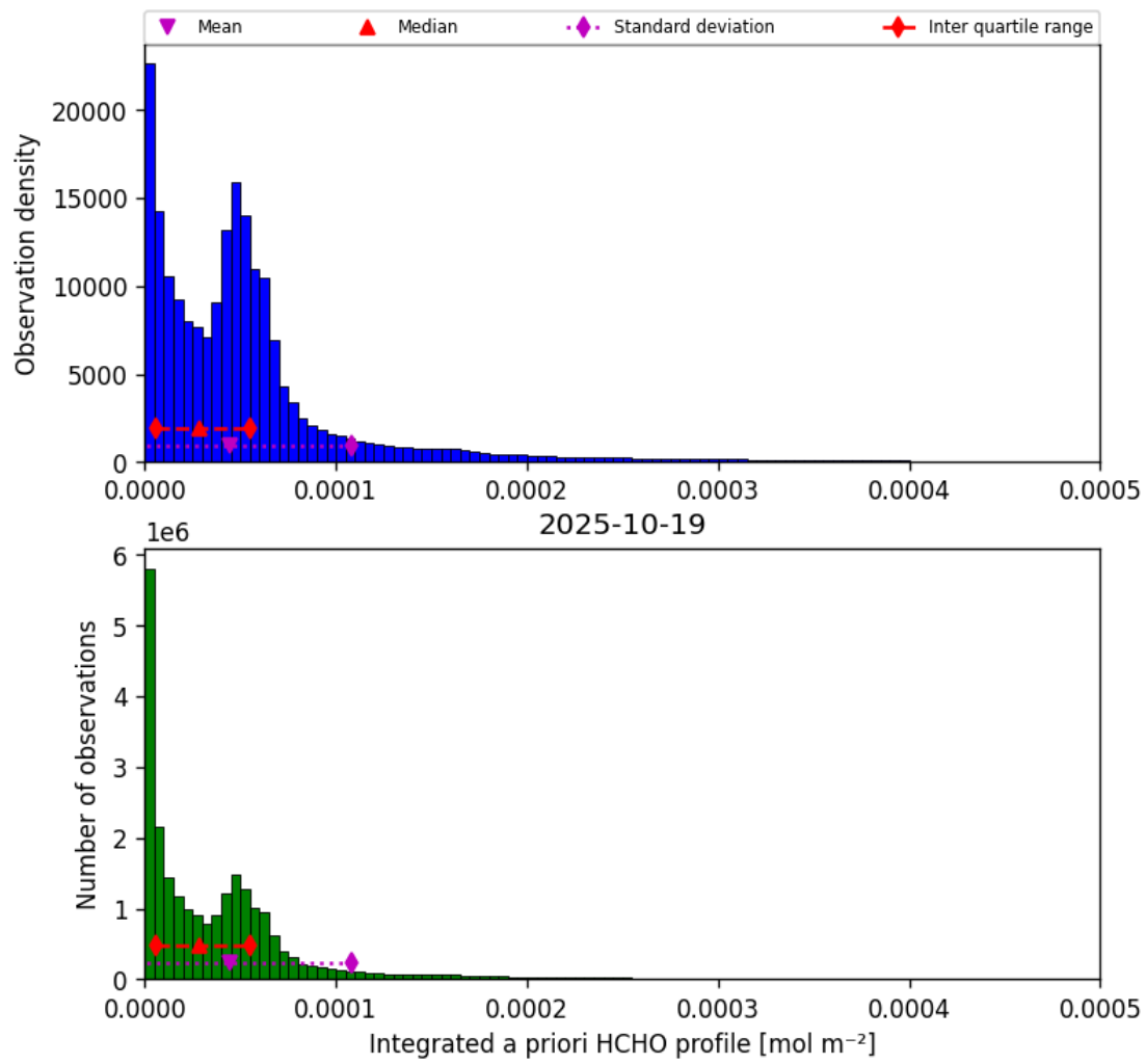
Figure 43: Histogram of “Integrated a priori HCHO profile” for 2025-10-18 to 2025-10-20
