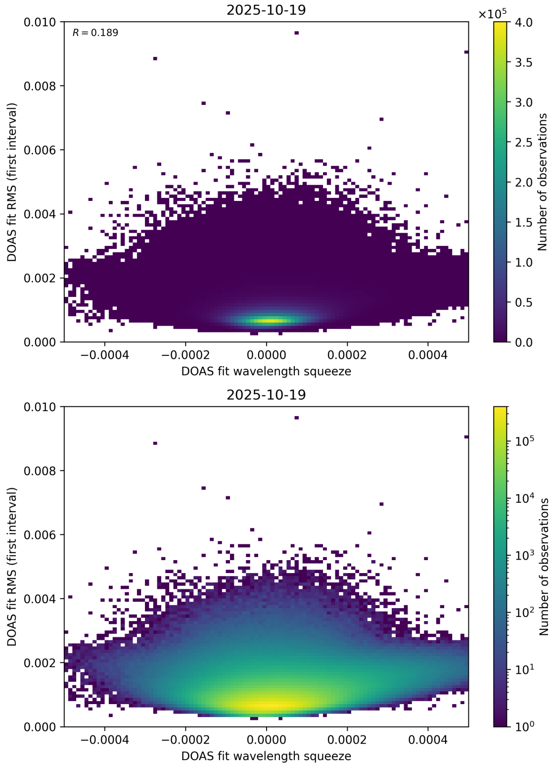
Figure 68: Scatter density plot of “DOAS fit wavelength squeeze” against “DOAS fit RMS (first interval)” for 2025-10-18 to 2025-10-20.
