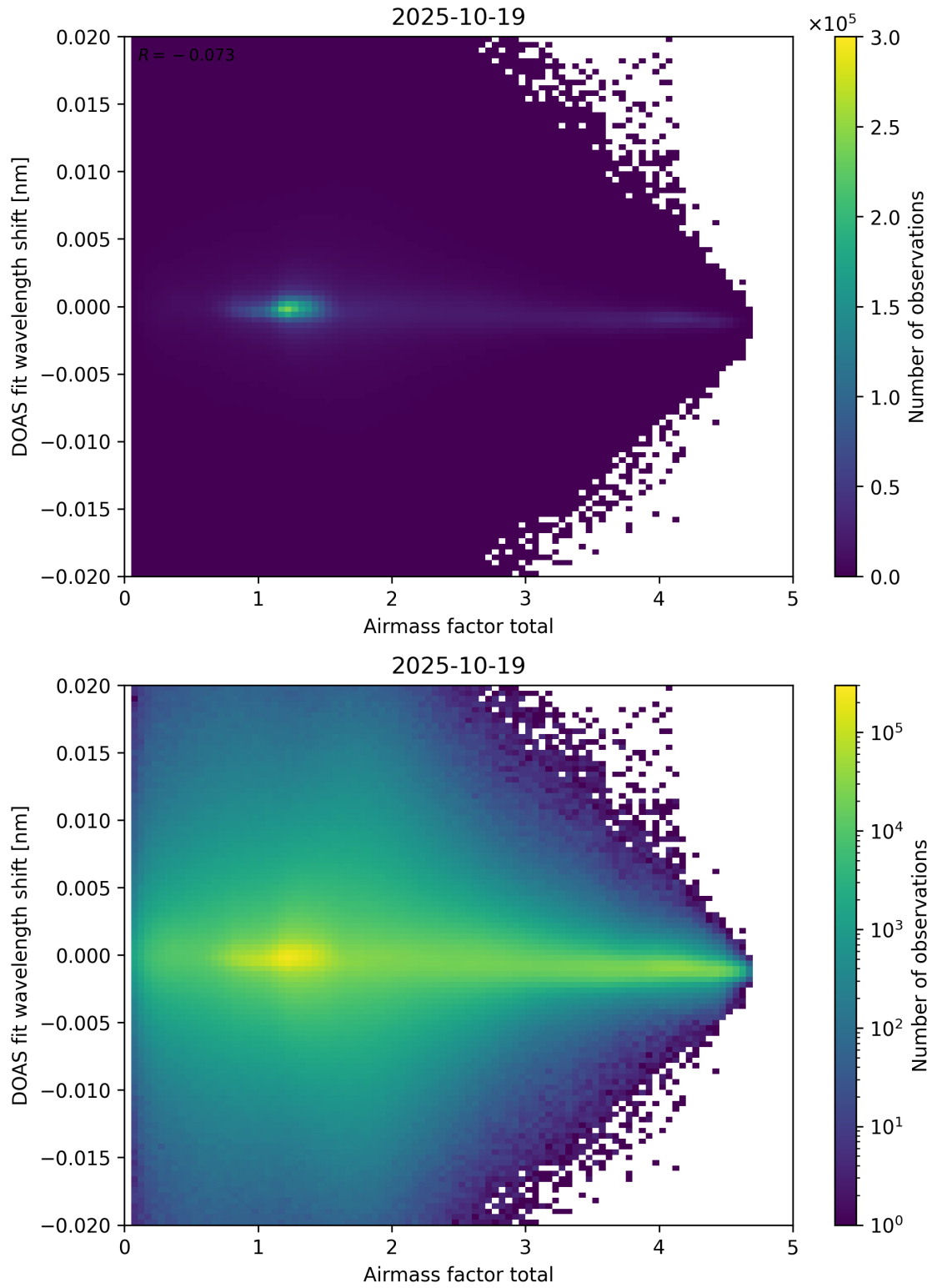
Figure 98: Scatter density plot of “Airmass factor total” against “DOAS fit wavelength shift” for 2025-10-18 to 2025-10-20.
