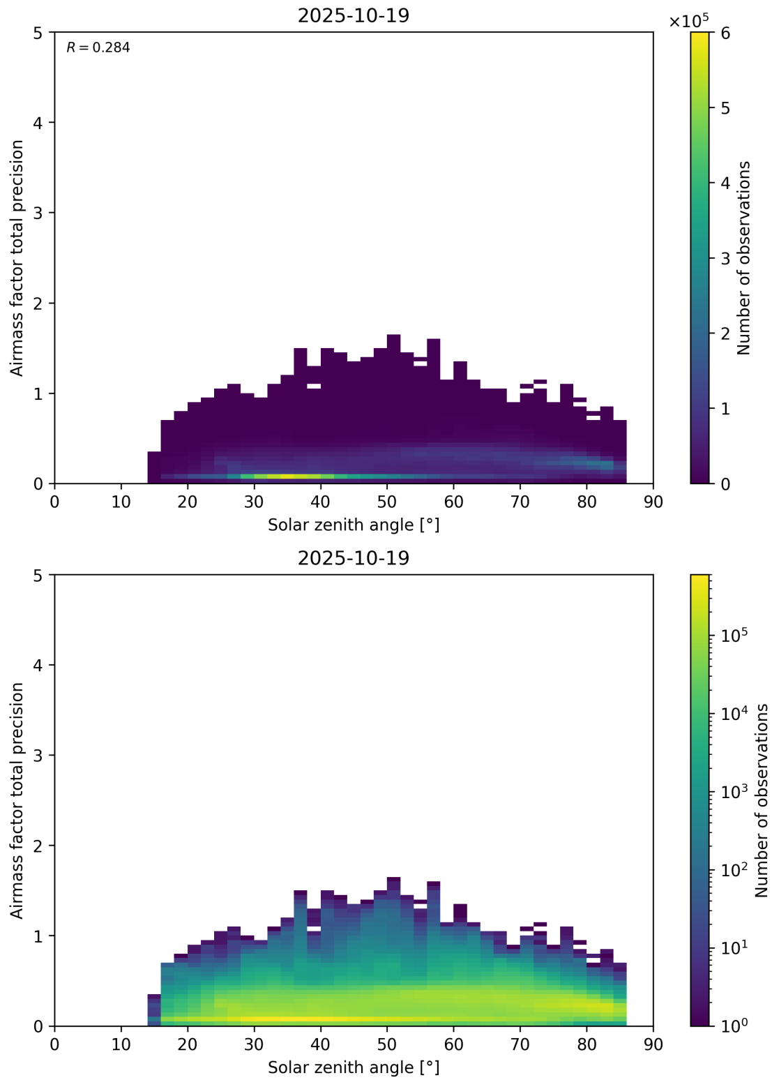
Figure 176: Scatter density plot of “Solar zenith angle” against “Airmass factor total precision” for 2025-10-18 to 2025-10-20.
