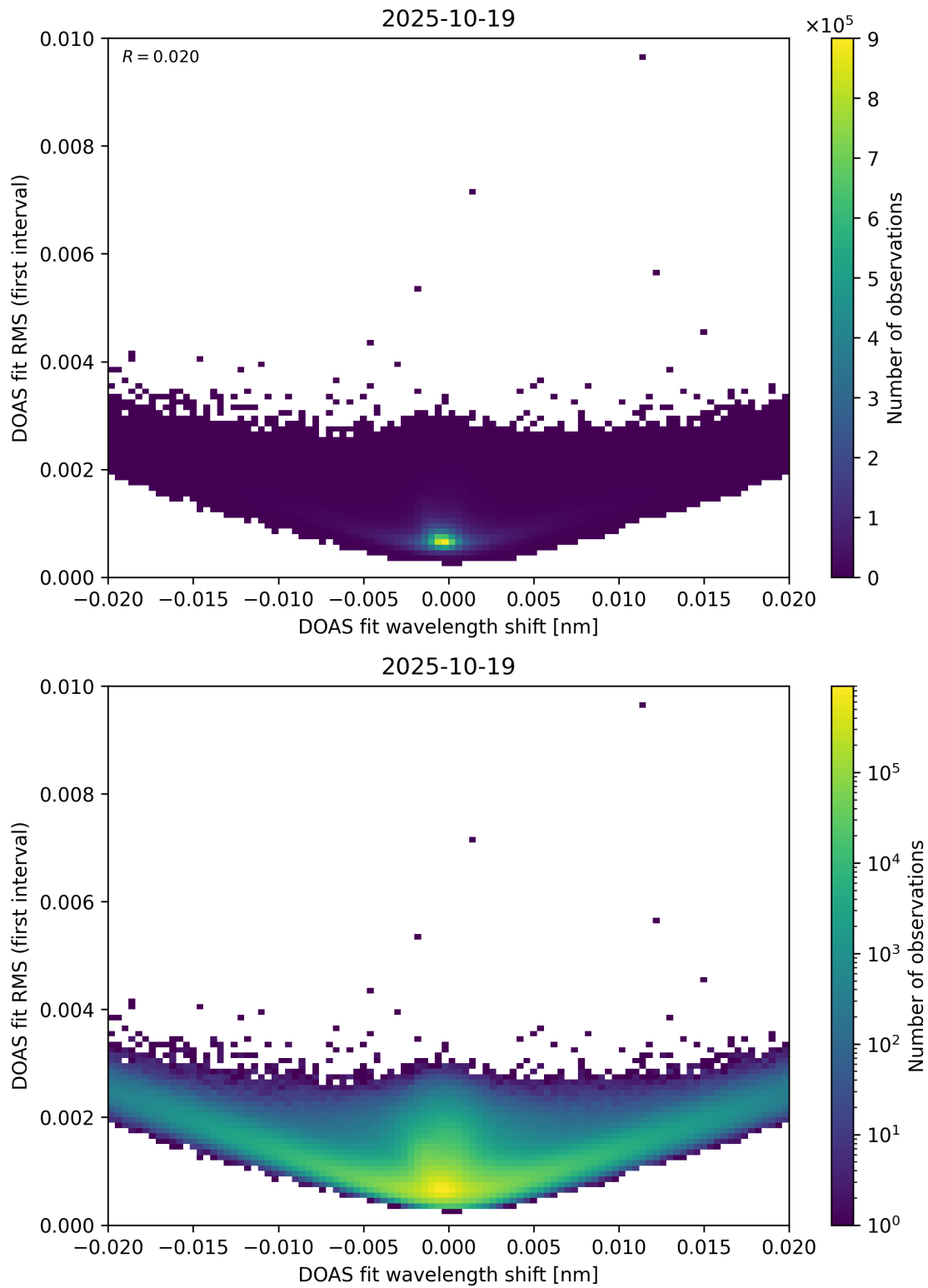
Figure 64: Scatter density plot of “DOAS fit wavelength shift” against “DOAS fit RMS (first interval)” for 2025-10-18 to 2025-10-20.
