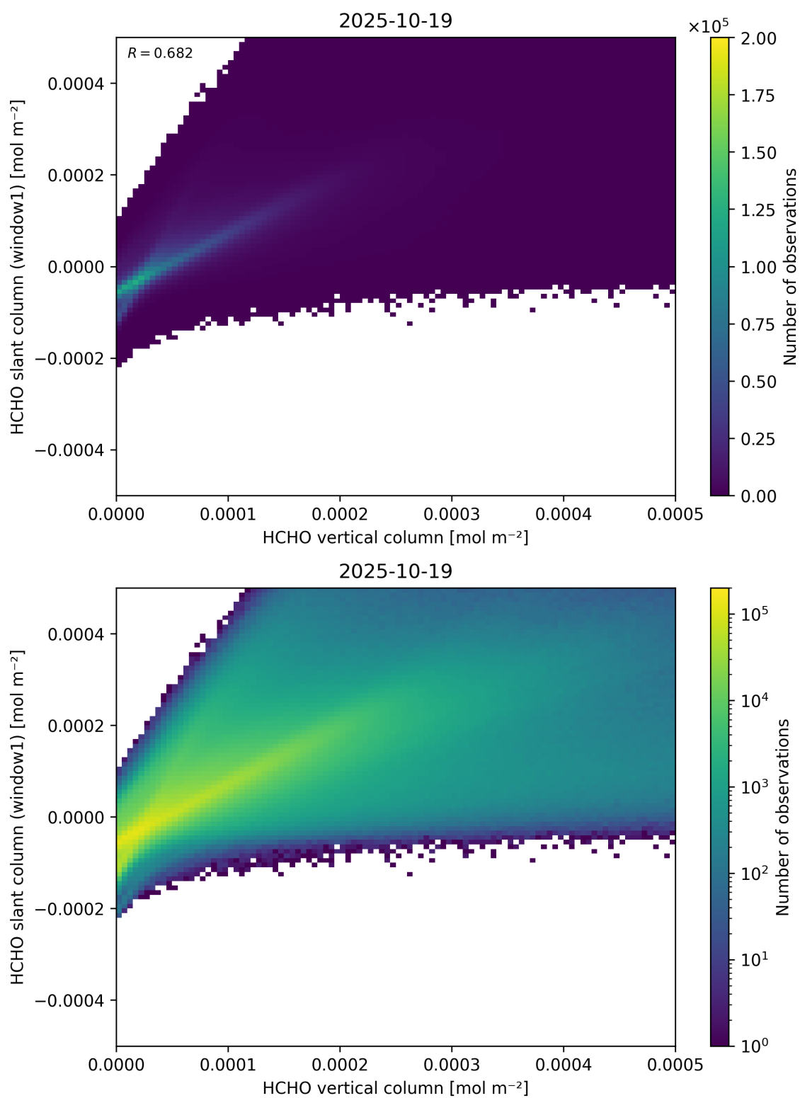
Figure 129: Scatter density plot of “HCHO vertical column” against “HCHO slant column (window1)” for 2025-10-18 to 2025-10-20.
