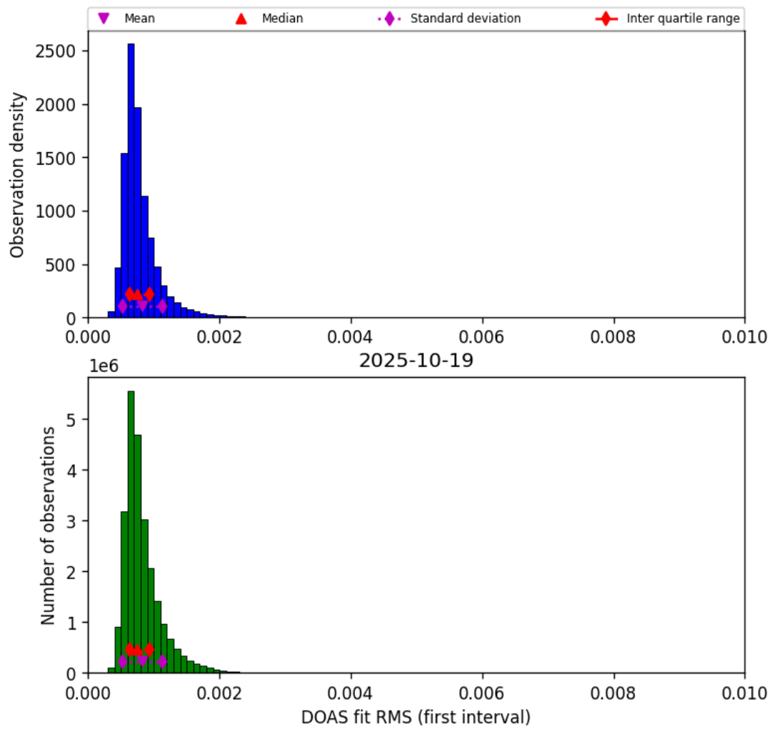
Figure 46: Histogram of “DOAS fit RMS (first interval)” for 2025-10-18 to 2025-10-20
