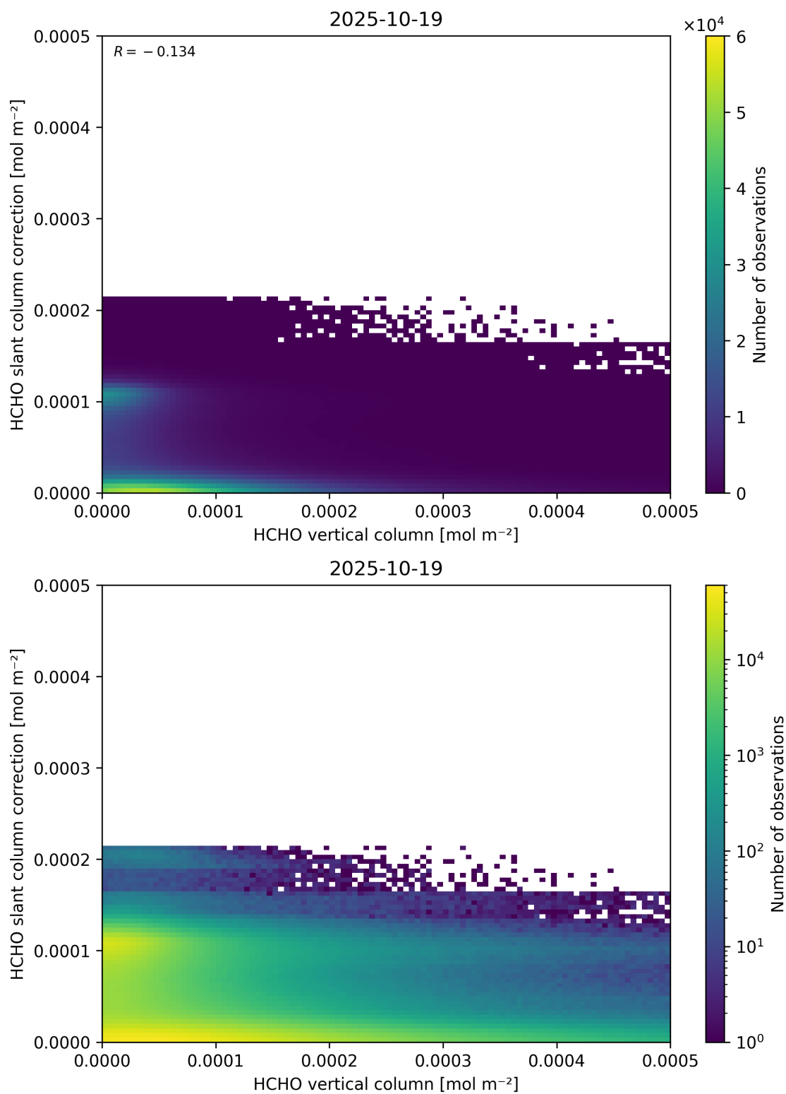
Figure 128: Scatter density plot of “HCHO vertical column” against “HCHO slant column correction” for 2025-10-18 to 2025-10-20.
