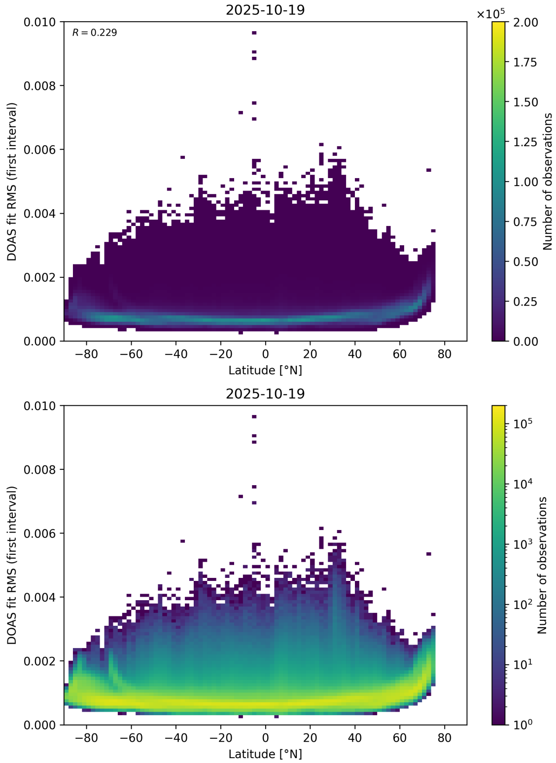
Figure 153: Scatter density plot of “Latitude” against “DOAS fit RMS (first interval)” for 2025-10-18 to 2025-10-20.
