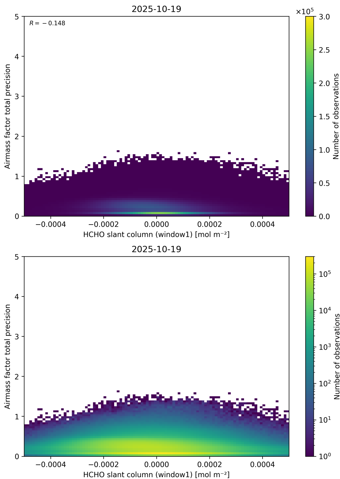
Figure 86: Scatter density plot of “HCHO slant column (window1)” against “Airmass factor total precision” for 2025-10-18 to 2025-10-20.
