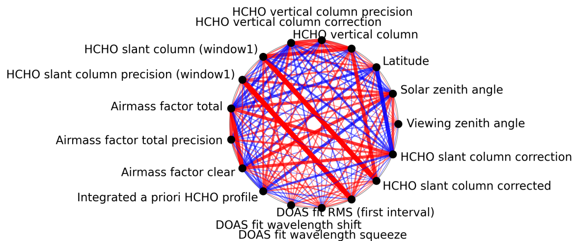
Figure 1: Map of correlation graph for 2025-10-18 to 2025-10-20.
