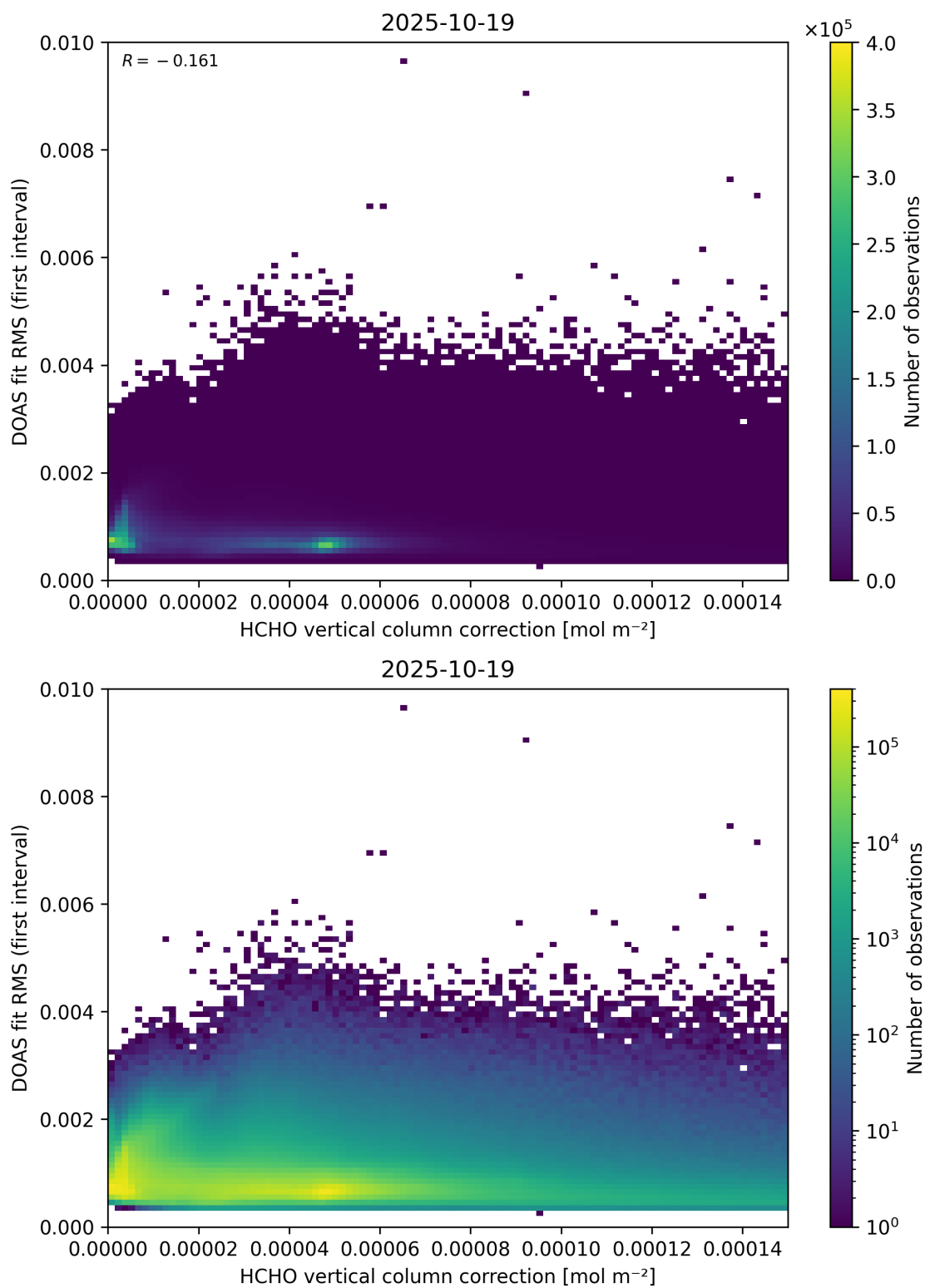
Figure 112: Scatter density plot of “HCHO vertical column correction” against “DOAS fit RMS (first interval)” for 2025-10-18 to 2025-10-20.
