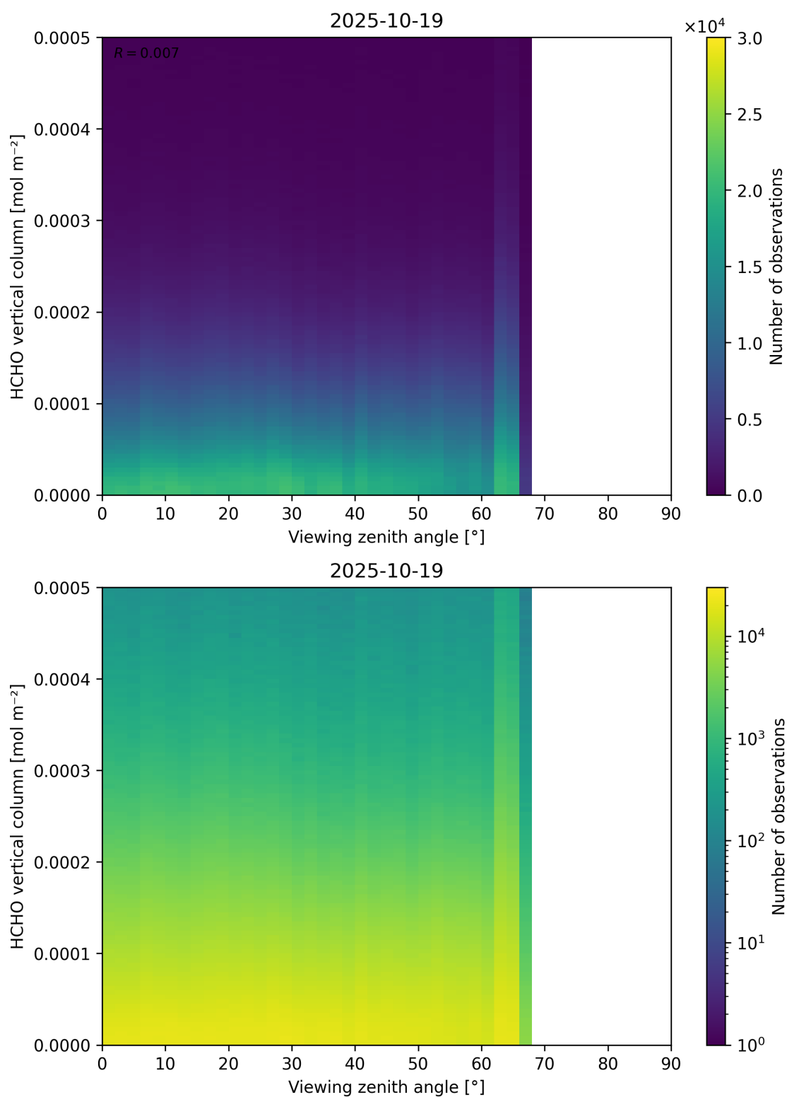
Figure 192: Scatter density plot of “Viewing zenith angle” against “HCHO vertical column” for 2025-10-18 to 2025-10-20.
