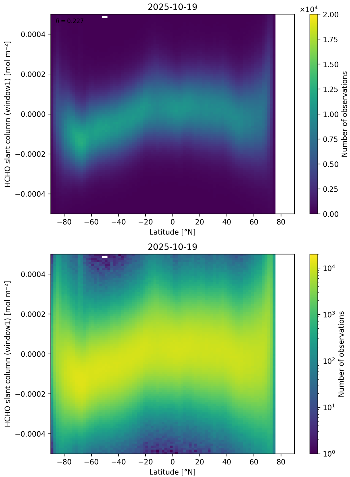
Figure 159: Scatter density plot of “Latitude” against “HCHO slant column (window1)” for 2025-10-18 to 2025-10-20.
