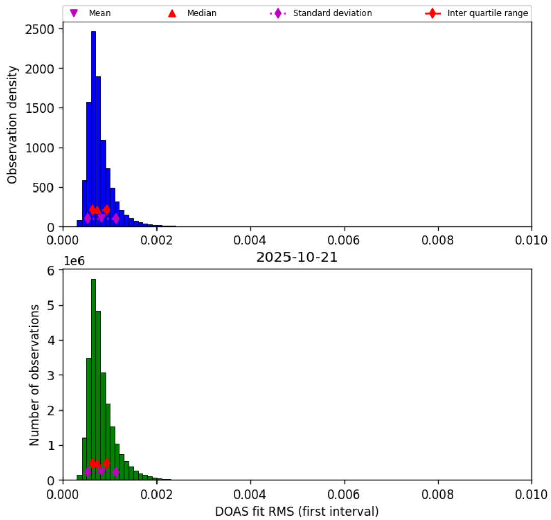
Figure 46: Histogram of “DOAS fit RMS (first interval)” for 2025-10-20 to 2025-10-22
