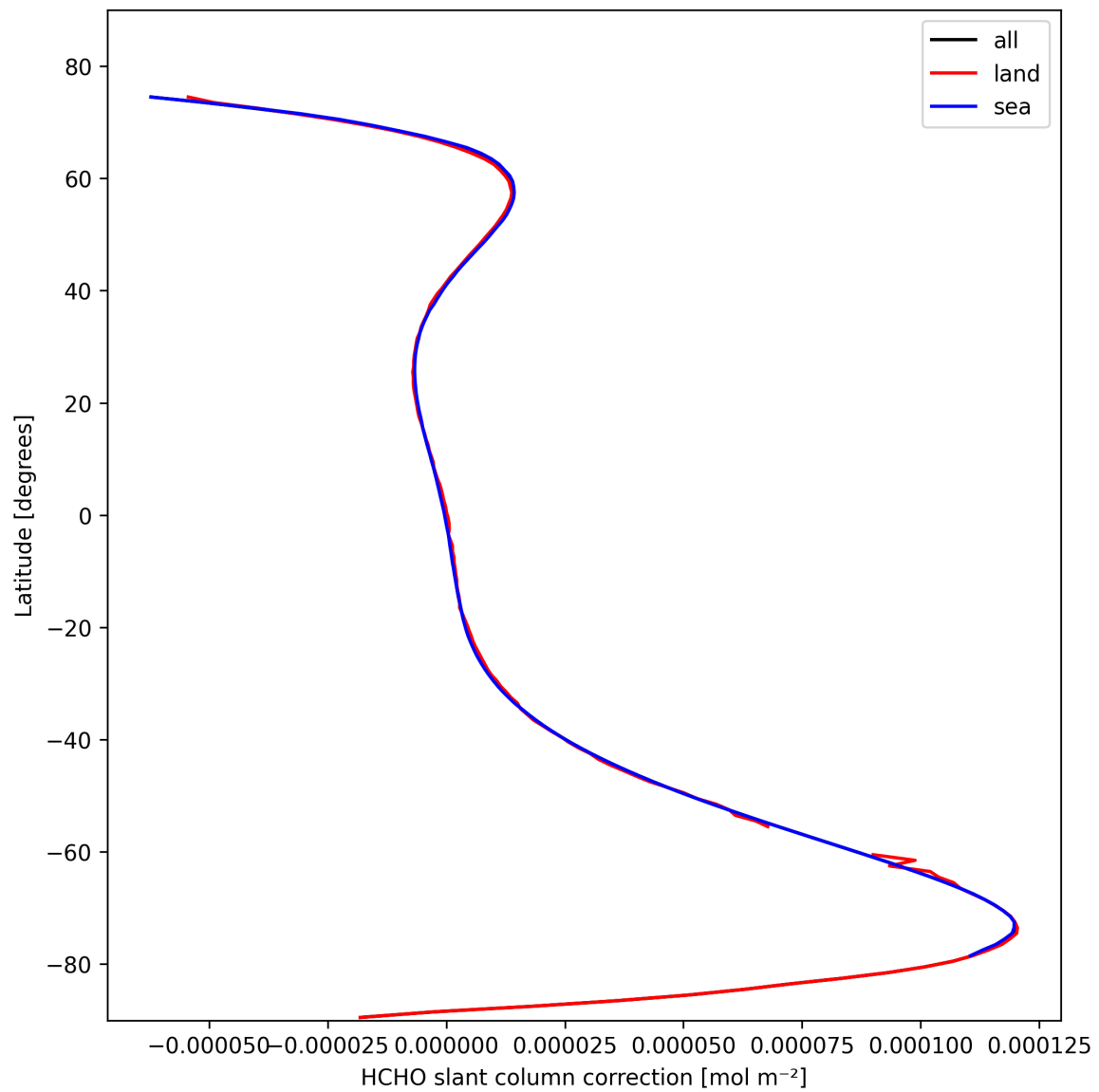
Figure 33: Zonal average of “HCHO slant column correction” for 2025-10-20 to 2025-10-22.
