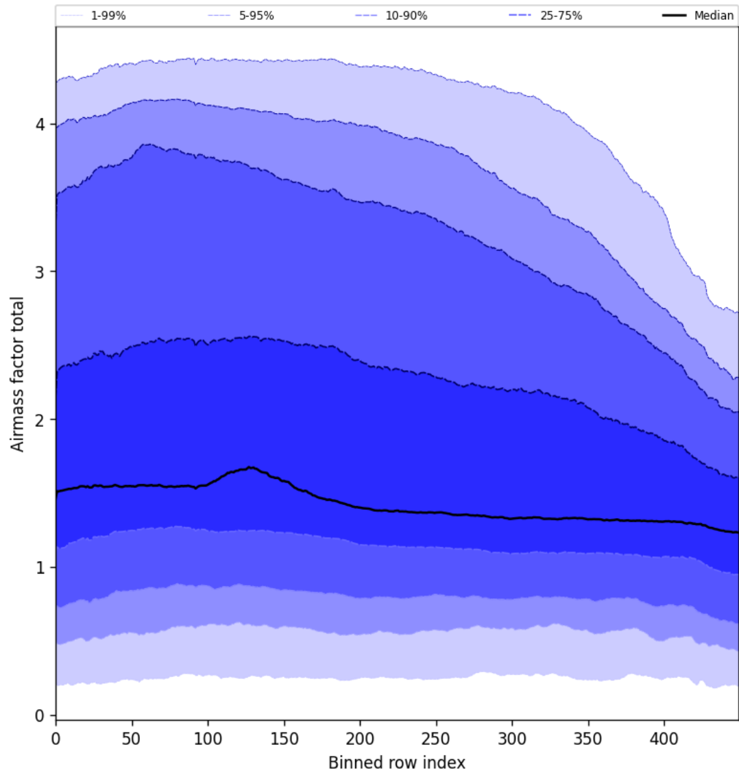
Figure 54: Along track statistics of “Airmass factor total” for 2025-10-20 to 2025-10-22
