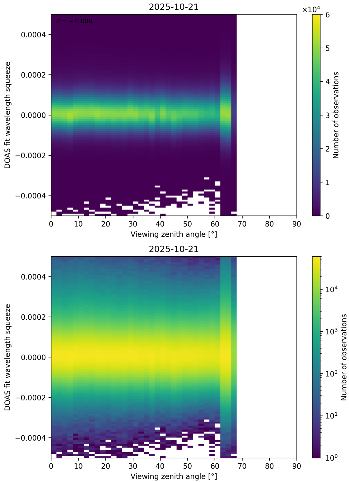
Figure 184: Scatter density plot of “Viewing zenith angle” against “DOAS fit wavelength squeeze” for 2025-10-20 to 2025-10-22.
