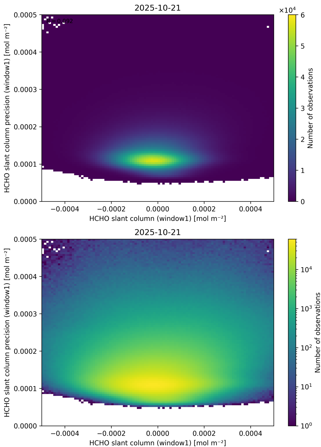
Figure 84: Scatter density plot of “HCHO slant column (window1)” against “HCHO slant column precision (window1)” for 2025-10-20 to 2025-10-22.
