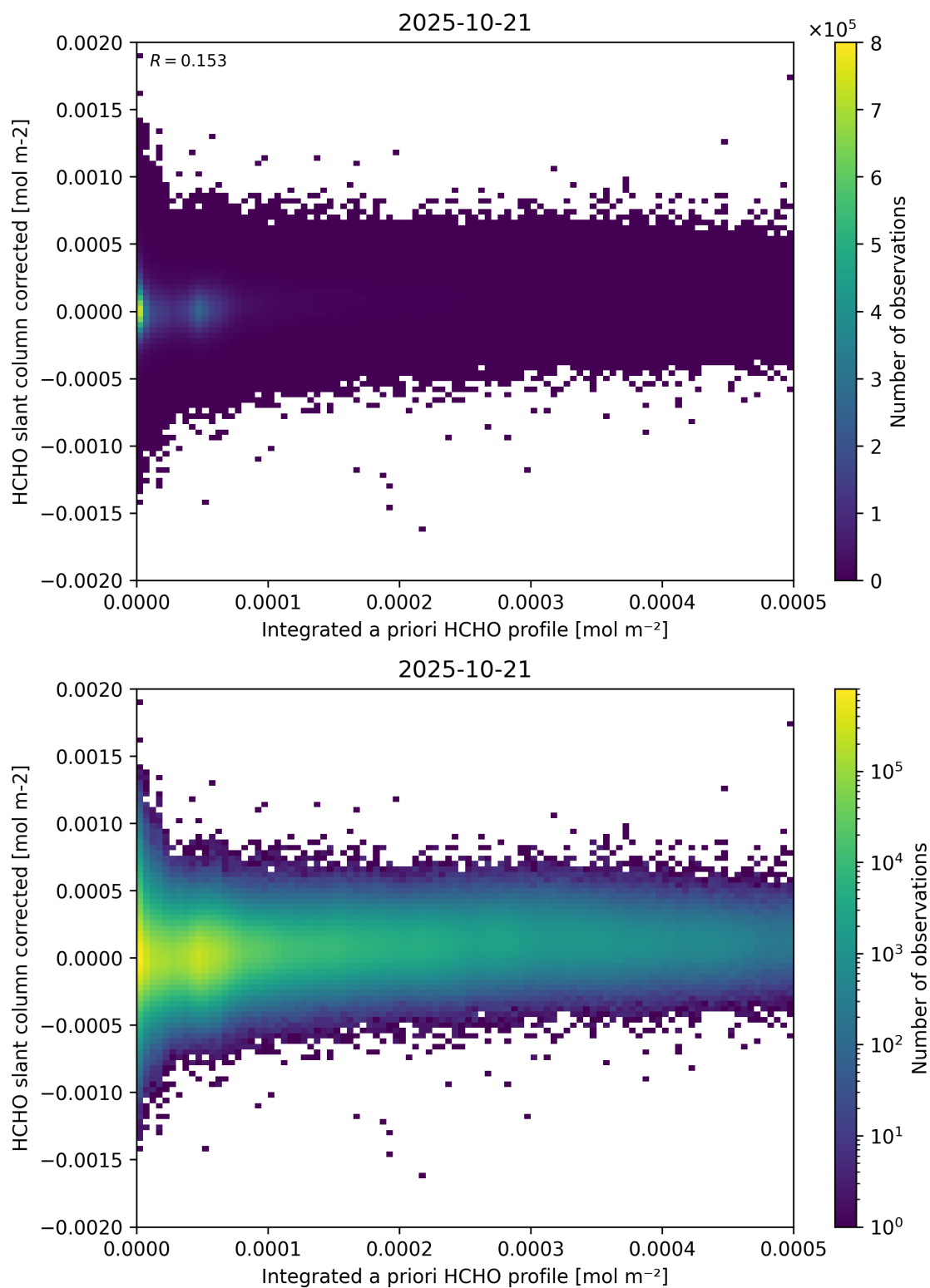
Figure 151: Scatter density plot of “Integrated a priori HCHO profile” against “HCHO slant column corrected” for 2025-10-20 to 2025-10-22.
