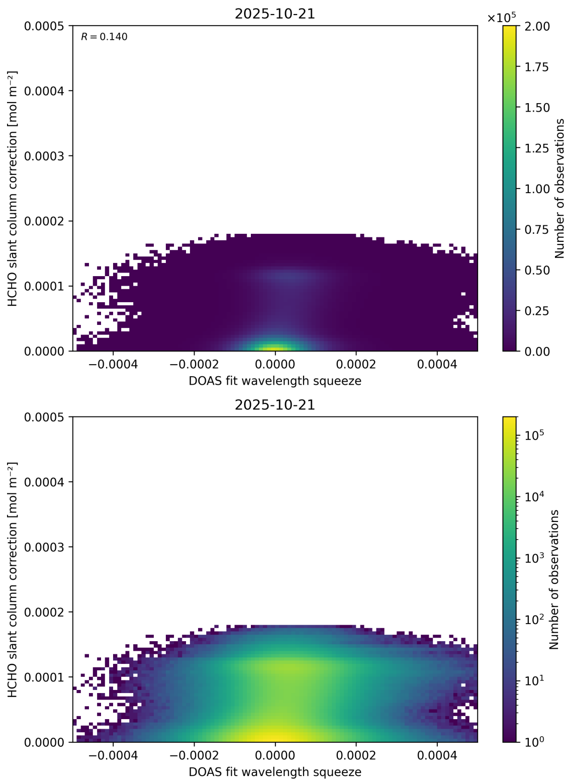
Figure 70: Scatter density plot of “DOAS fit wavelength squeeze” against “HCHO slant column correction” for 2025-10-20 to 2025-10-22.
