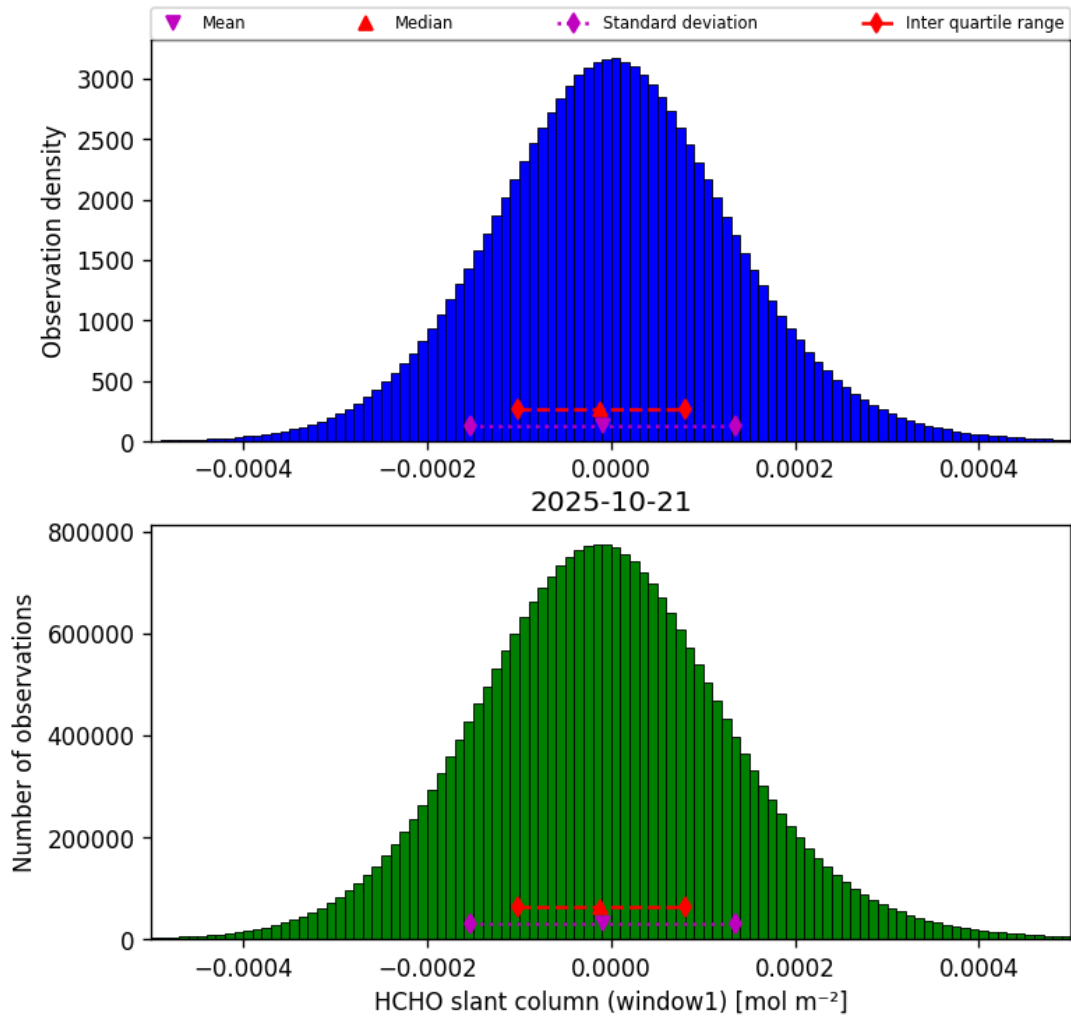
Figure 38: Histogram of “HCHO slant column (window1)” for 2025-10-20 to 2025-10-22
