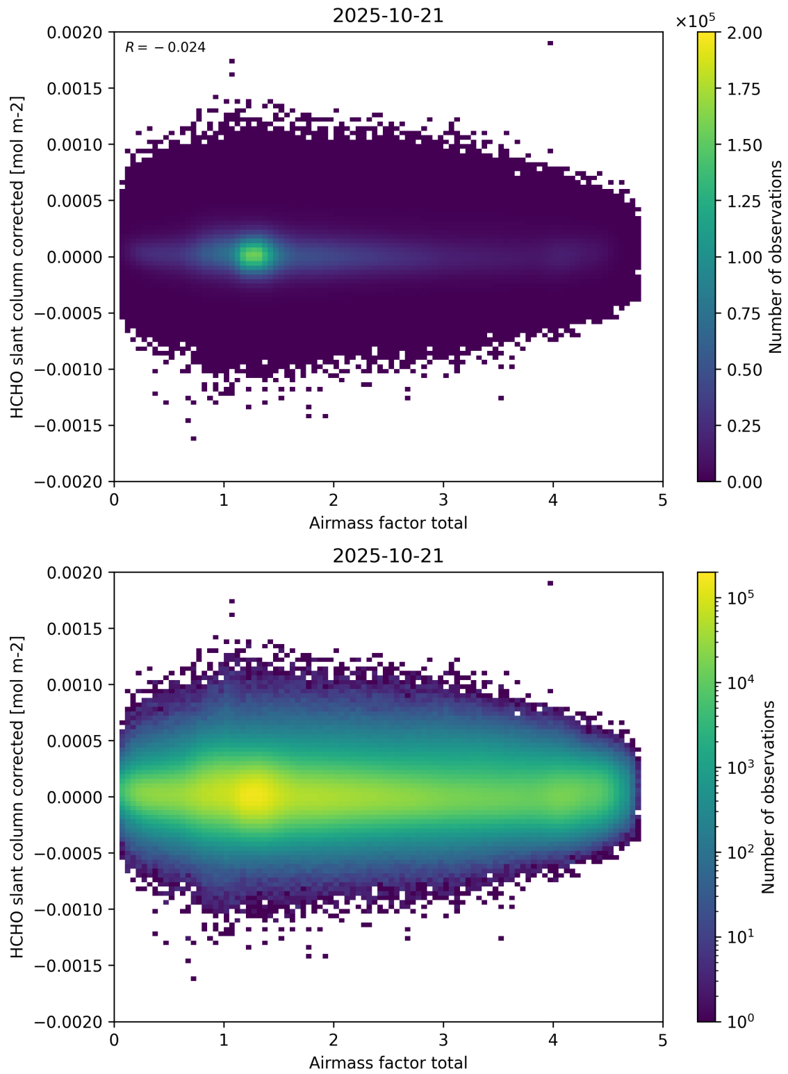
Figure 101: Scatter density plot of “Airmass factor total” against “HCHO slant column corrected” for 2025-10-20 to 2025-10-22.
