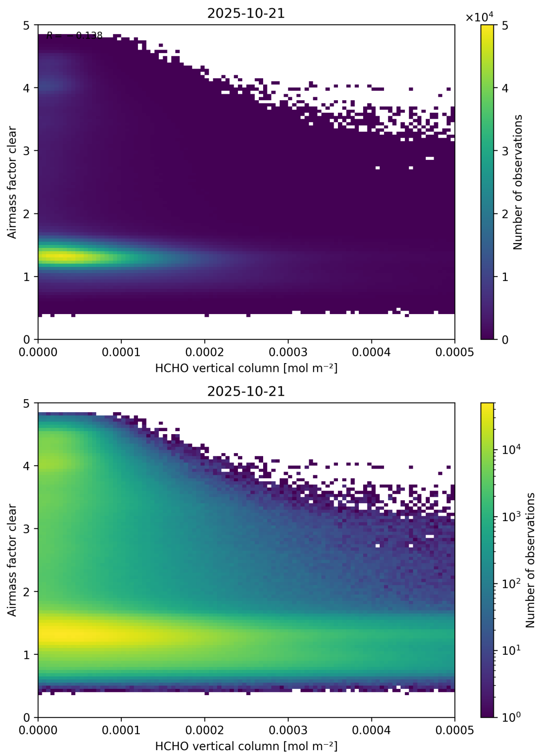
Figure 126: Scatter density plot of “HCHO vertical column” against “Airmass factor clear” for 2025-10-20 to 2025-10-22.
