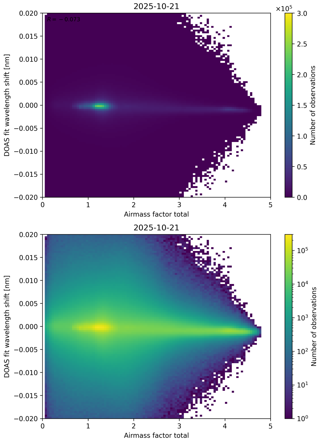
Figure 98: Scatter density plot of “Airmass factor total” against “DOAS fit wavelength shift” for 2025-10-20 to 2025-10-22.
