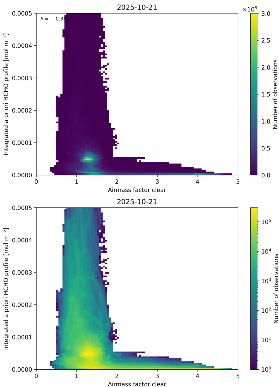
Figure 76: Scatter density plot of “Airmass factor clear” against “Integrated a priori HCHO profile” for 2025-10-20 to 2025-10-22.
