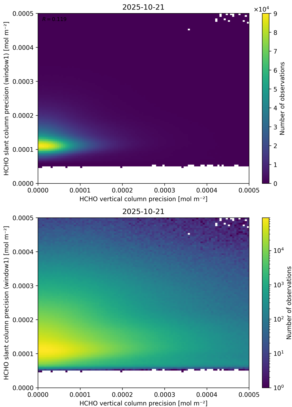
Figure 143: Scatter density plot of “HCHO vertical column precision” against “HCHO slant column precision (window1)” for 2025-10-20 to 2025-10-22.
