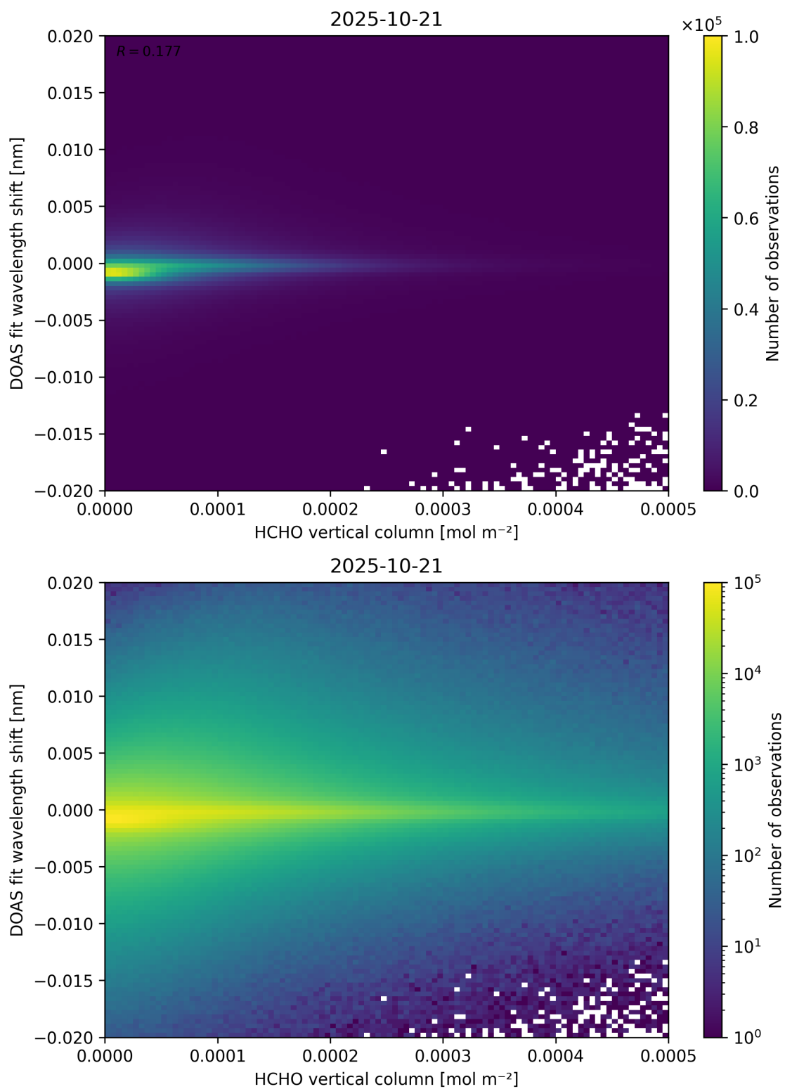
Figure 124: Scatter density plot of “HCHO vertical column” against “DOAS fit wavelength shift” for 2025-10-20 to 2025-10-22.
