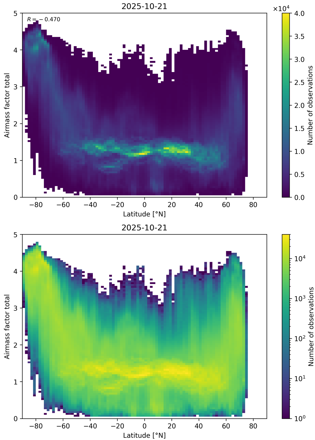
Figure 161: Scatter density plot of “Latitude” against “Airmass factor total” for 2025-10-20 to 2025-10-22.
