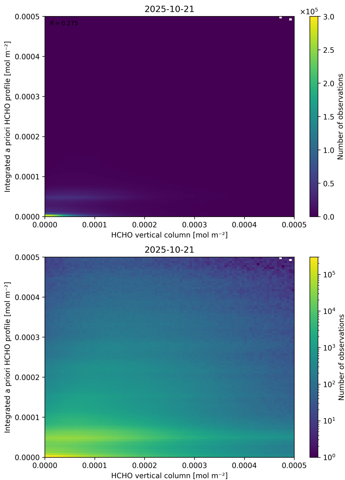
Figure 135: Scatter density plot of “HCHO vertical column” against “Integrated a priori HCHO profile” for 2025-10-20 to 2025-10-22.
