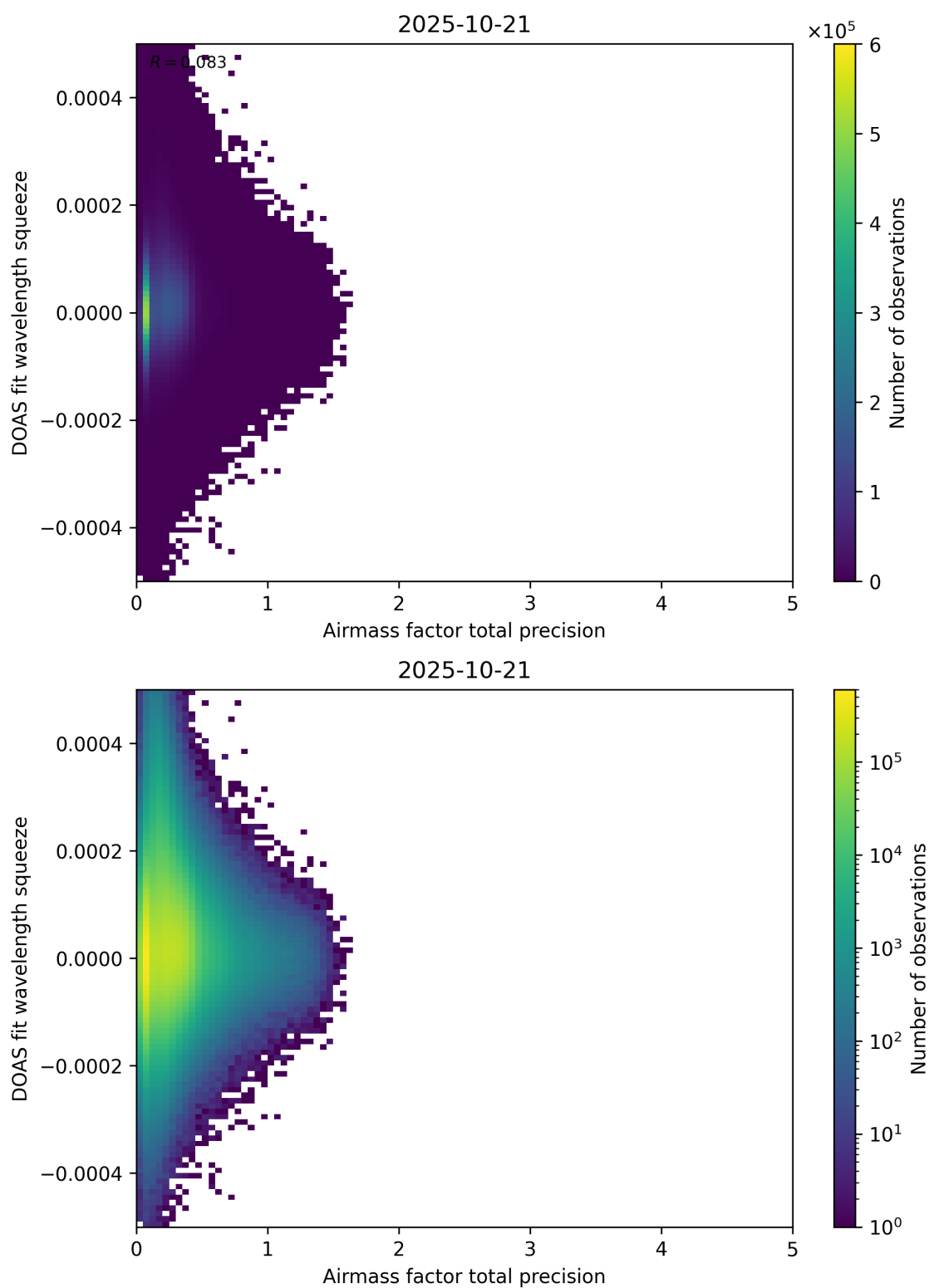
Figure 107: Scatter density plot of “Airmass factor total precision” against “DOAS fit wavelength squeeze” for 2025-10-20 to 2025-10-22.
