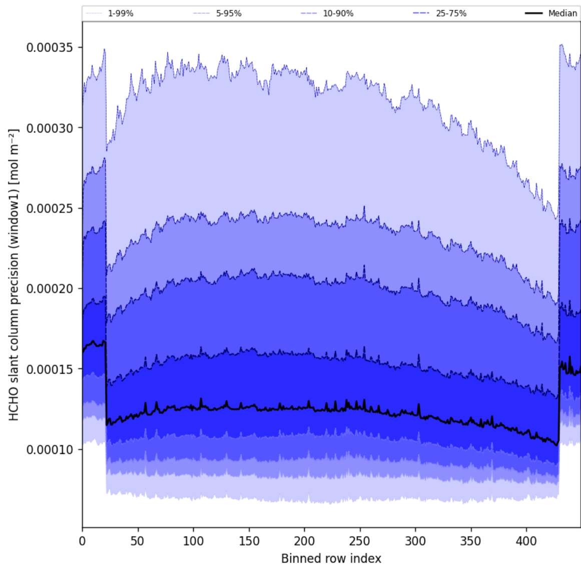
Figure 53: Along track statistics of “HCHO slant column precision (window1)” for 2025-10-20 to 2025-10-22
