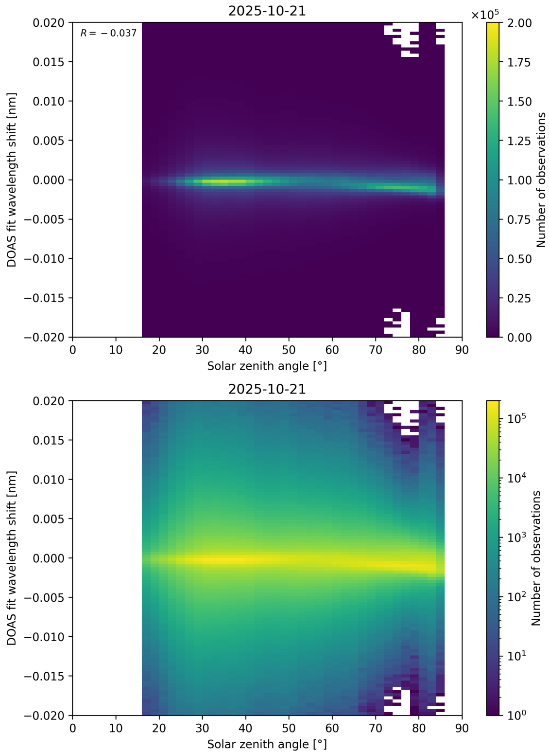
Figure 168: Scatter density plot of “Solar zenith angle” against “DOAS fit wavelength shift” for 2025-10-20 to 2025-10-22.
