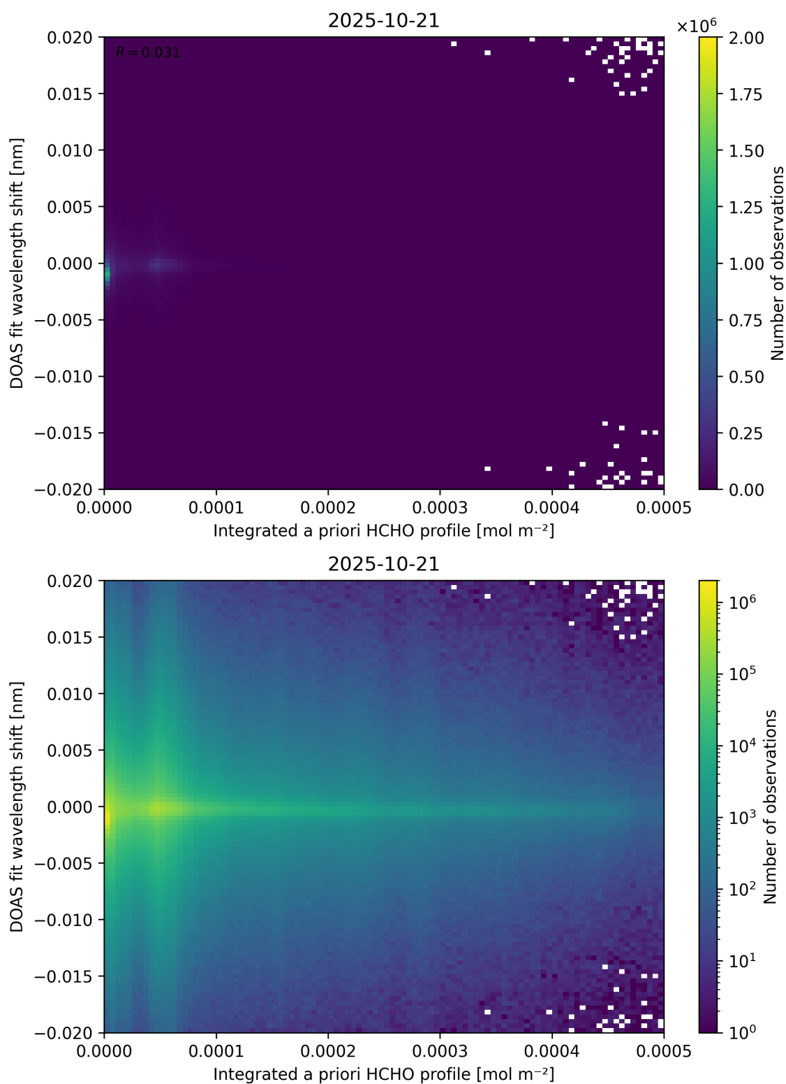
Figure 149: Scatter density plot of “Integrated a priori HCHO profile” against “DOAS fit wavelength shift” for 2025-10-20 to 2025-10-22.
