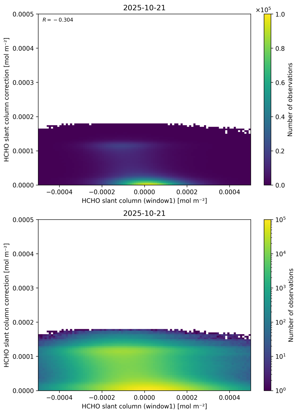
Figure 83: Scatter density plot of “HCHO slant column (window1)” against “HCHO slant column correction” for 2025-10-20 to 2025-10-22.
