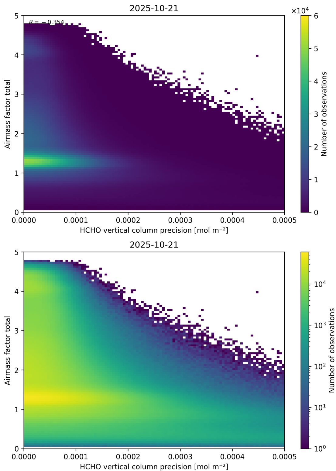
Figure 144: Scatter density plot of “HCHO vertical column precision” against “Airmass factor total” for 2025-10-20 to 2025-10-22.
