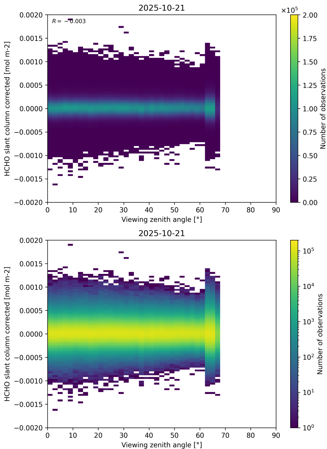
Figure 186: Scatter density plot of “Viewing zenith angle” against “HCHO slant column corrected” for 2025-10-20 to 2025-10-22.
