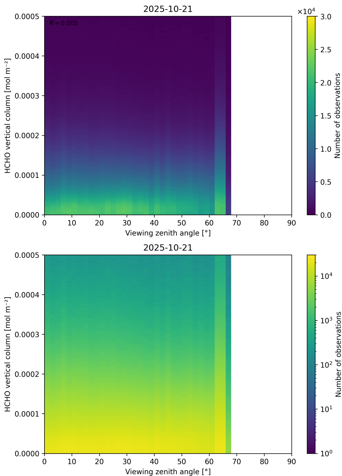
Figure 192: Scatter density plot of “Viewing zenith angle” against “HCHO vertical column” for 2025-10-20 to 2025-10-22.
