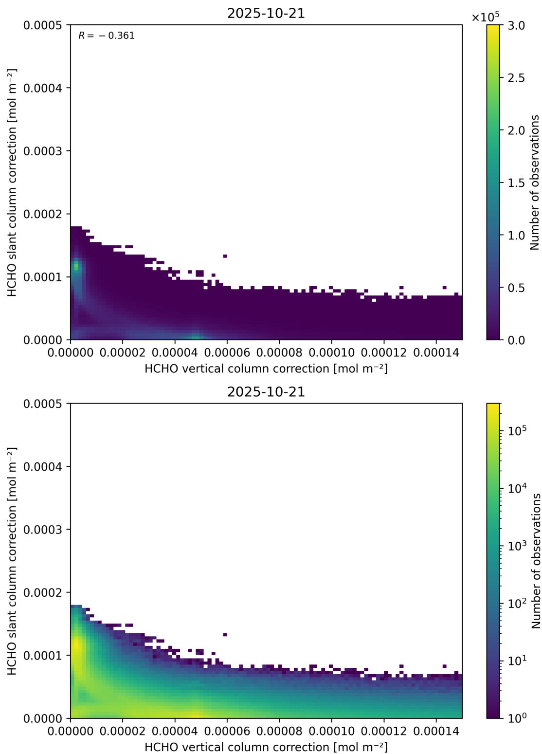
Figure 117: Scatter density plot of “HCHO vertical column correction” against “HCHO slant column correction” for 2025-10-20 to 2025-10-22.
