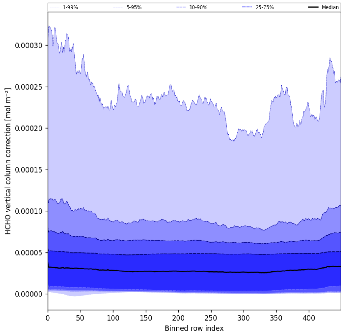
Figure 51: Along track statistics of “HCHO vertical column correction” for 2025-10-20 to 2025-10-22
