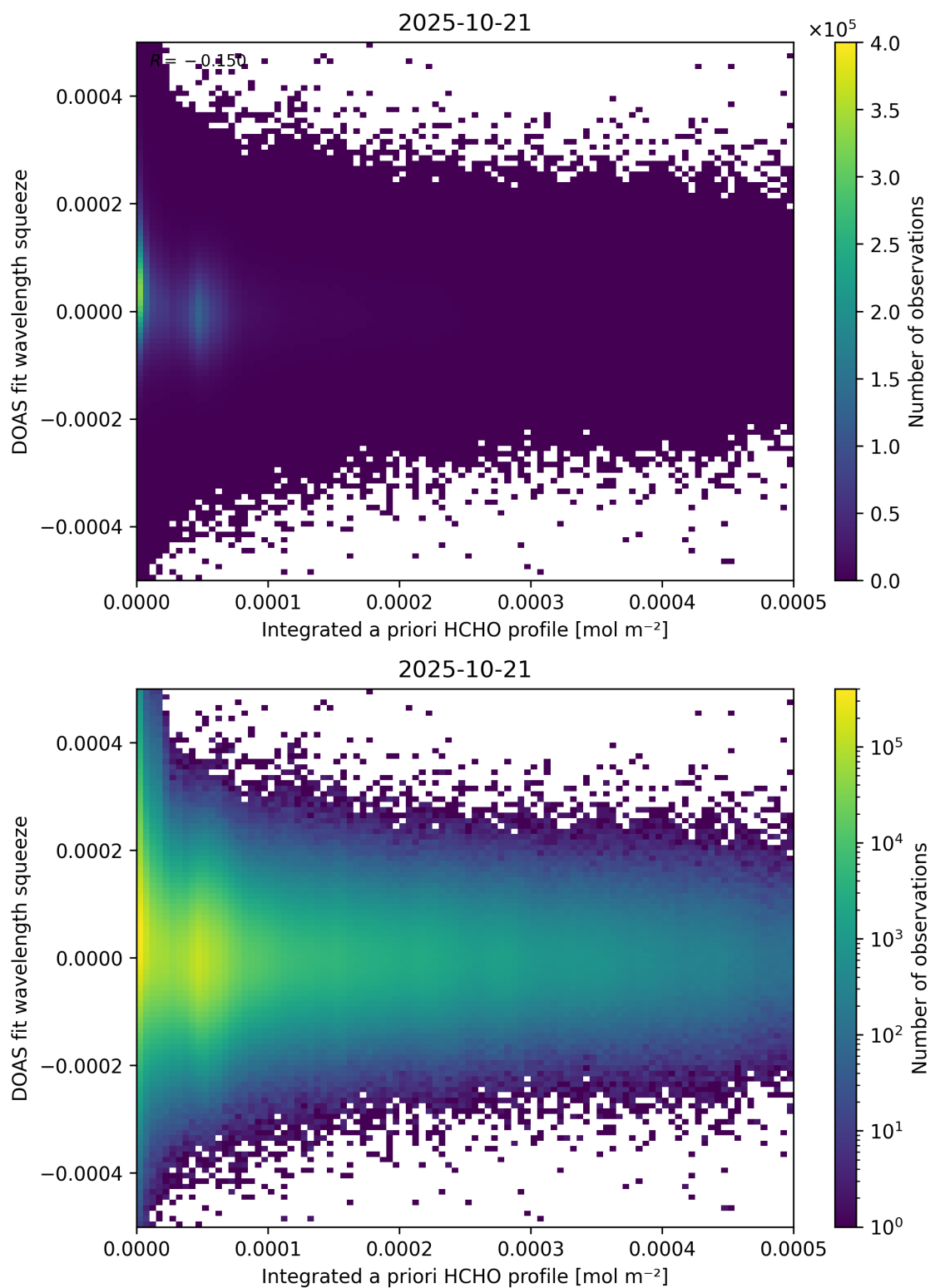
Figure 150: Scatter density plot of “Integrated a priori HCHO profile” against “DOAS fit wavelength squeeze” for 2025-10-20 to 2025-10-22.
