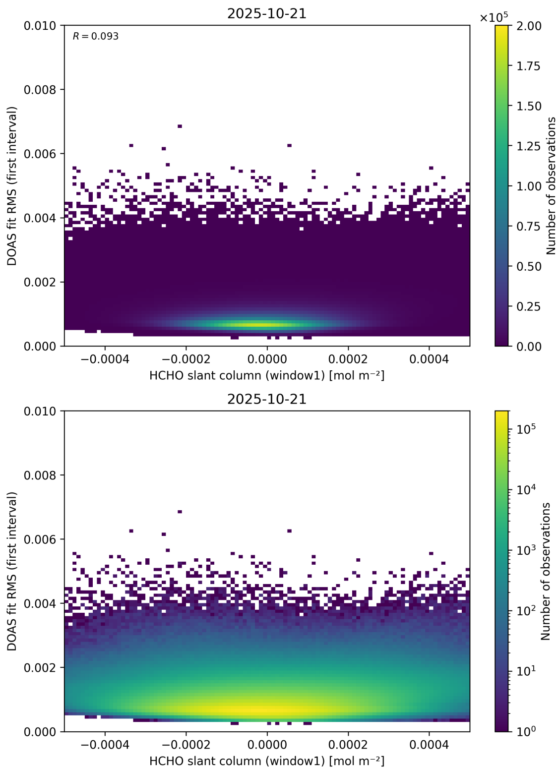
Figure 78: Scatter density plot of “HCHO slant column (window1)” against “DOAS fit RMS (first interval)” for 2025-10-20 to 2025-10-22.
