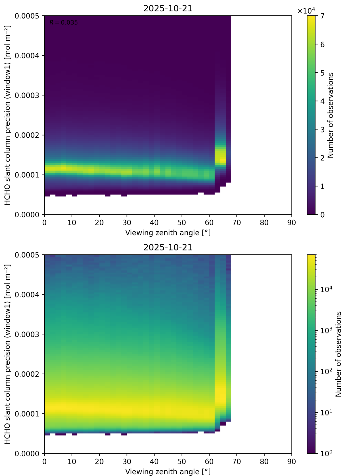
Figure 189: Scatter density plot of “Viewing zenith angle” against “HCHO slant column precision (window1)” for 2025-10-20 to 2025-10-22.
