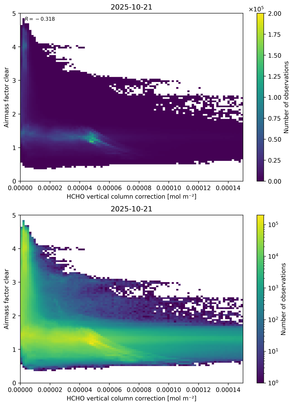
Figure 115: Scatter density plot of “HCHO vertical column correction” against “Airmass factor clear” for 2025-10-20 to 2025-10-22.
