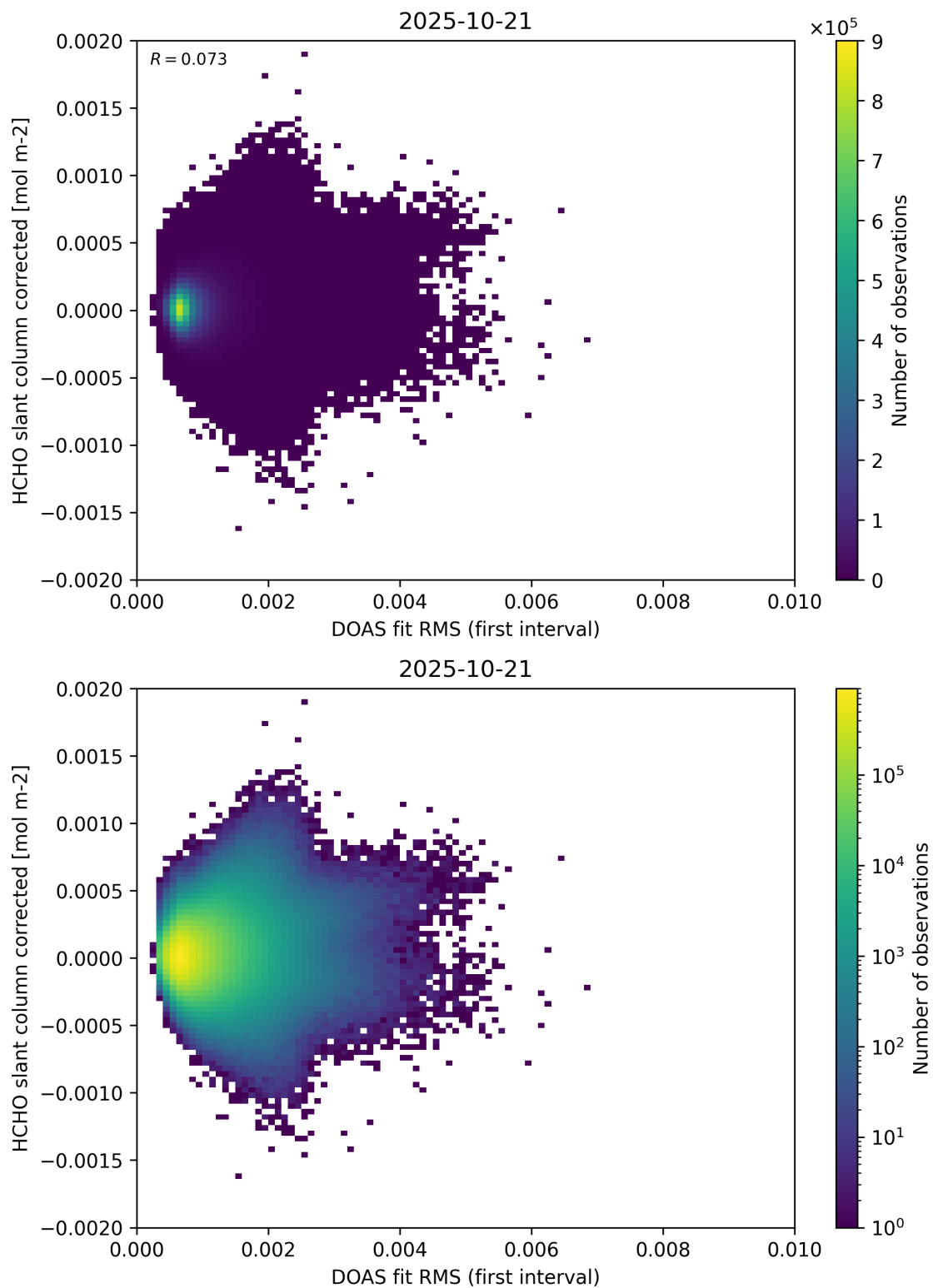
Figure 62: Scatter density plot of “DOAS fit RMS (first interval)” against “HCHO slant column corrected” for 2025-10-20 to 2025-10-22.
