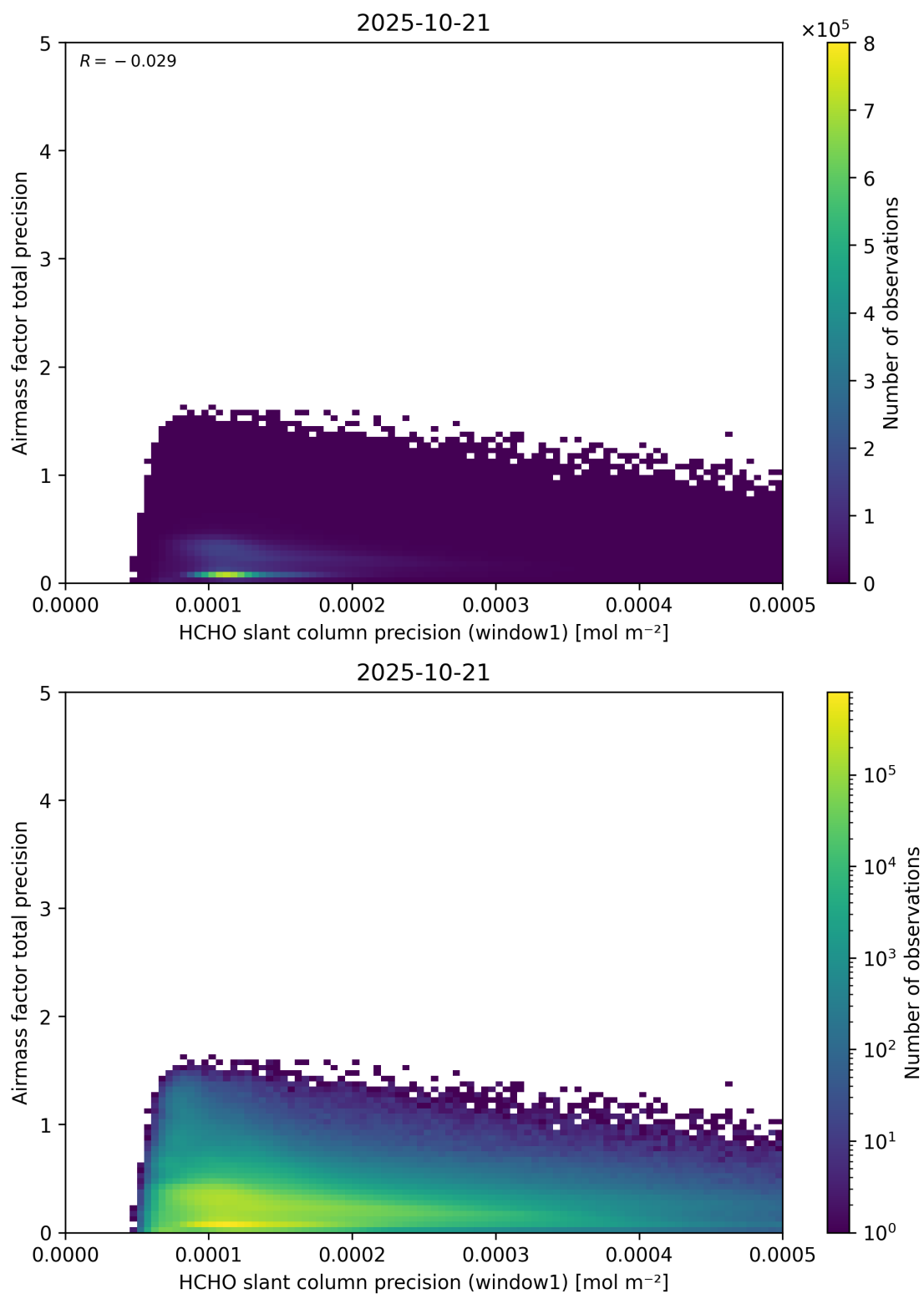
Figure 95: Scatter density plot of “HCHO slant column precision (window1)” against “Airmass factor total precision” for 2025-10-20 to 2025-10-22.
