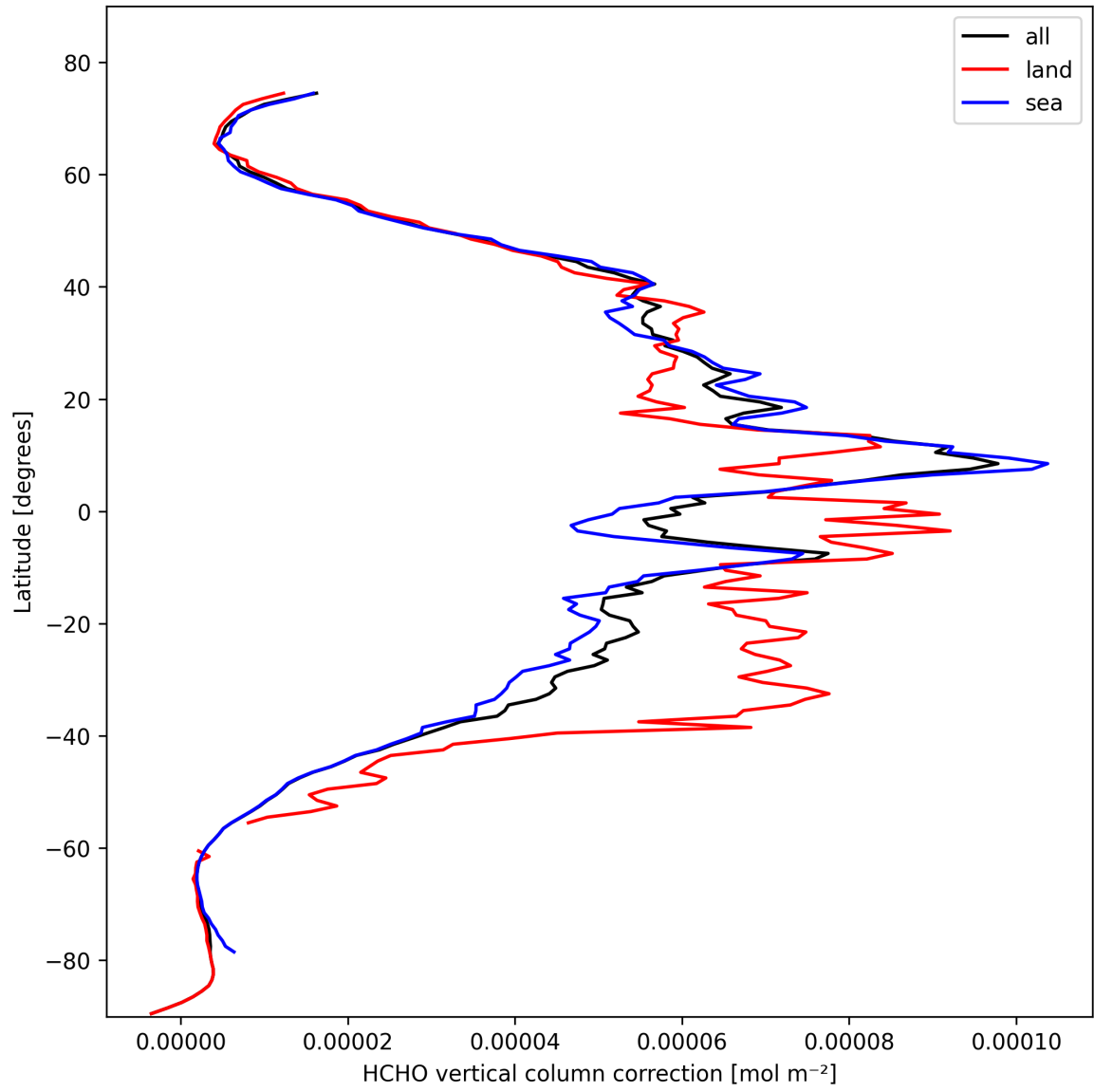
Figure 23: Zonal average of “HCHO vertical column correction” for 2025-10-20 to 2025-10-22.
