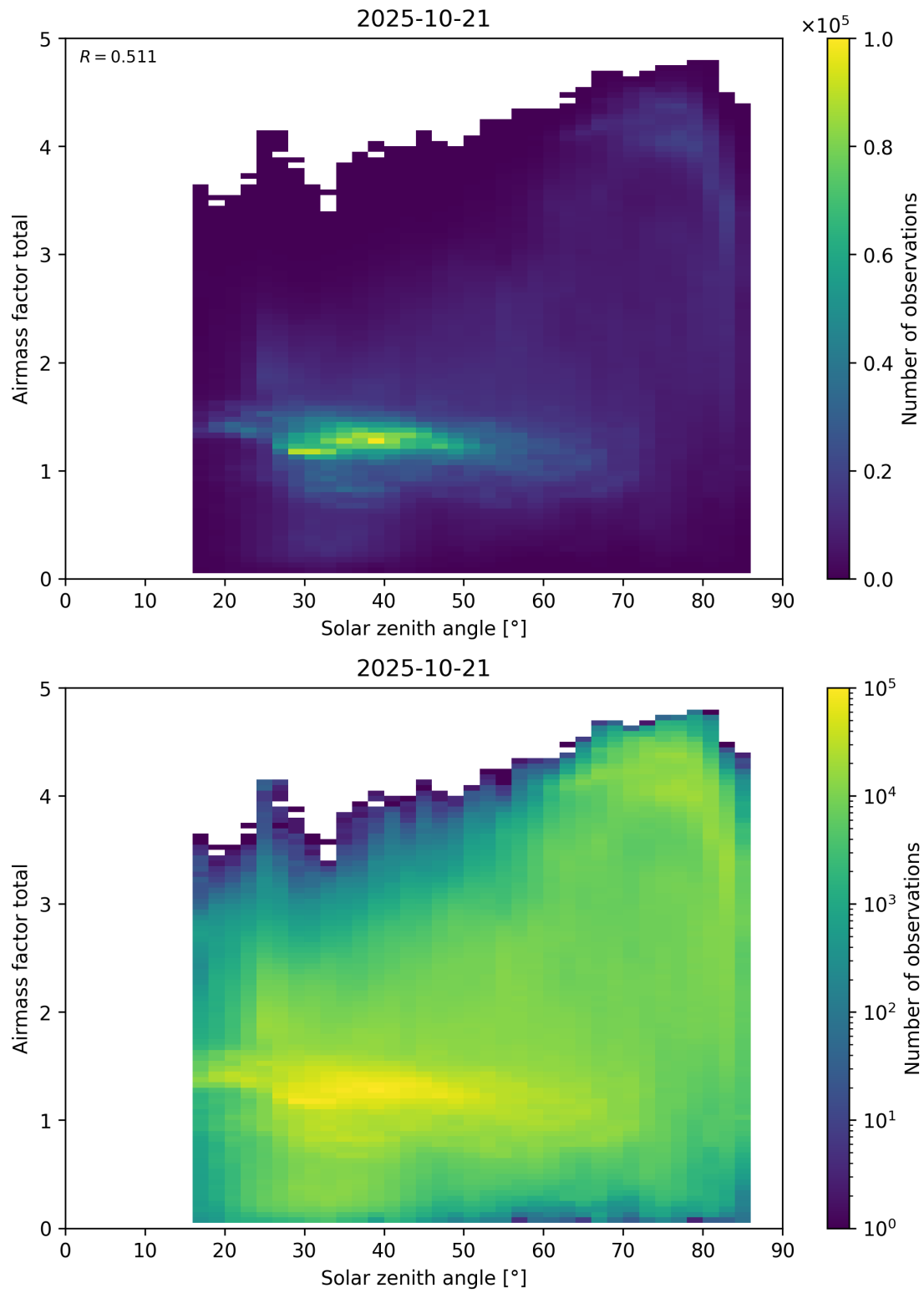
Figure 175: Scatter density plot of “Solar zenith angle” against “Airmass factor total” for 2025-10-20 to 2025-10-22.
