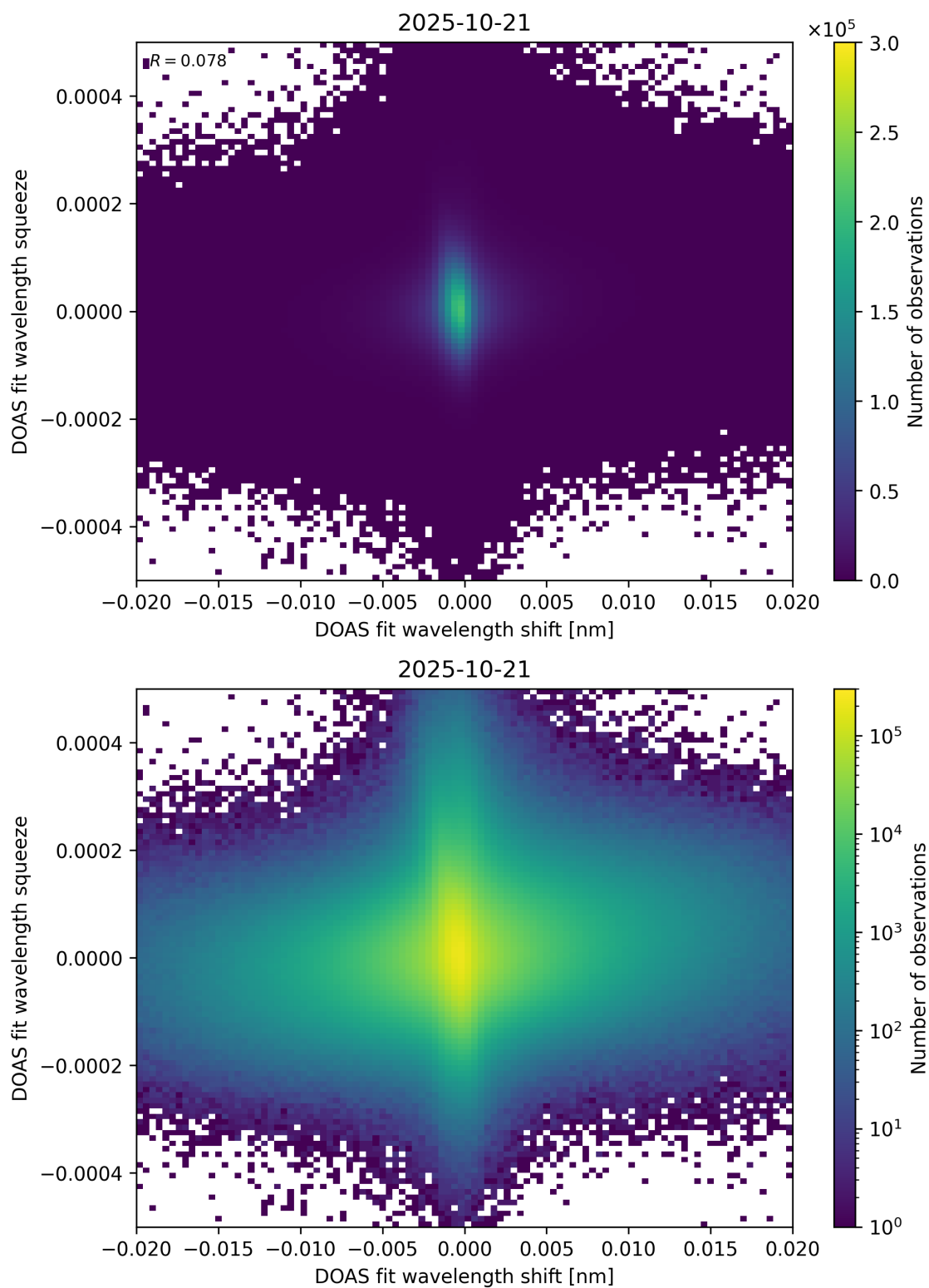
Figure 65: Scatter density plot of “DOAS fit wavelength shift” against “DOAS fit wavelength squeeze” for 2025-10-20 to 2025-10-22.
