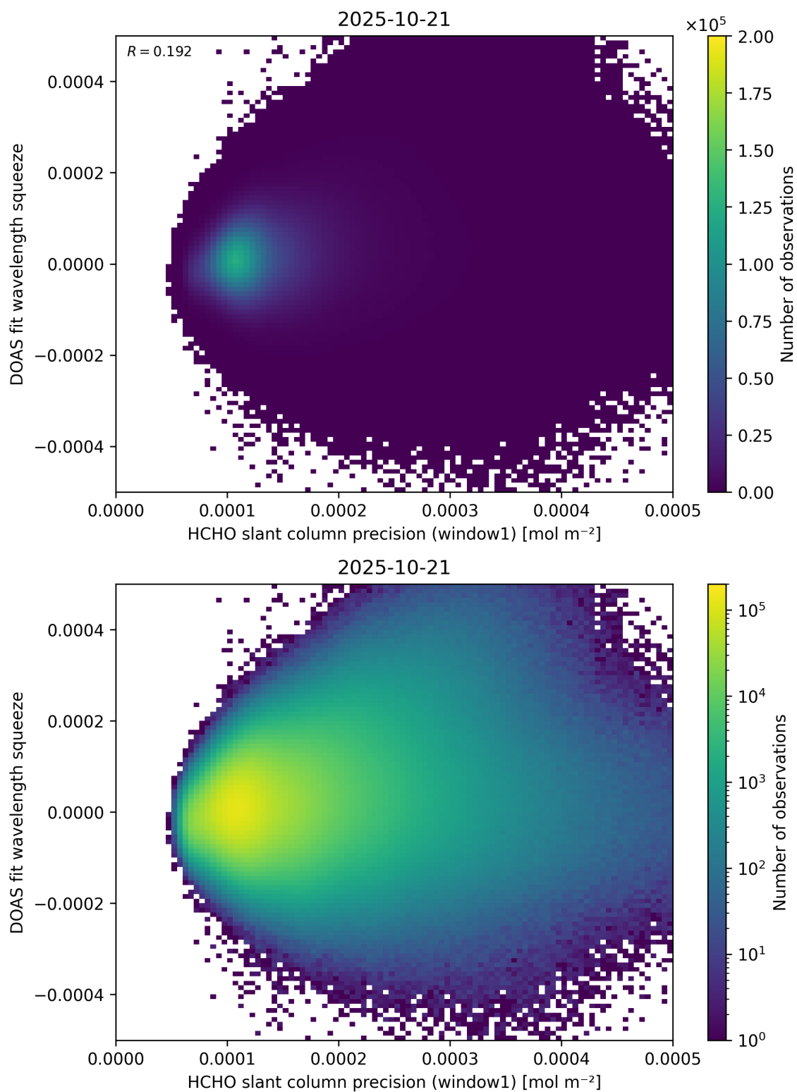
Figure 90: Scatter density plot of “HCHO slant column precision (window1)” against “DOAS fit wavelength squeeze” for 2025-10-20 to 2025-10-22.
