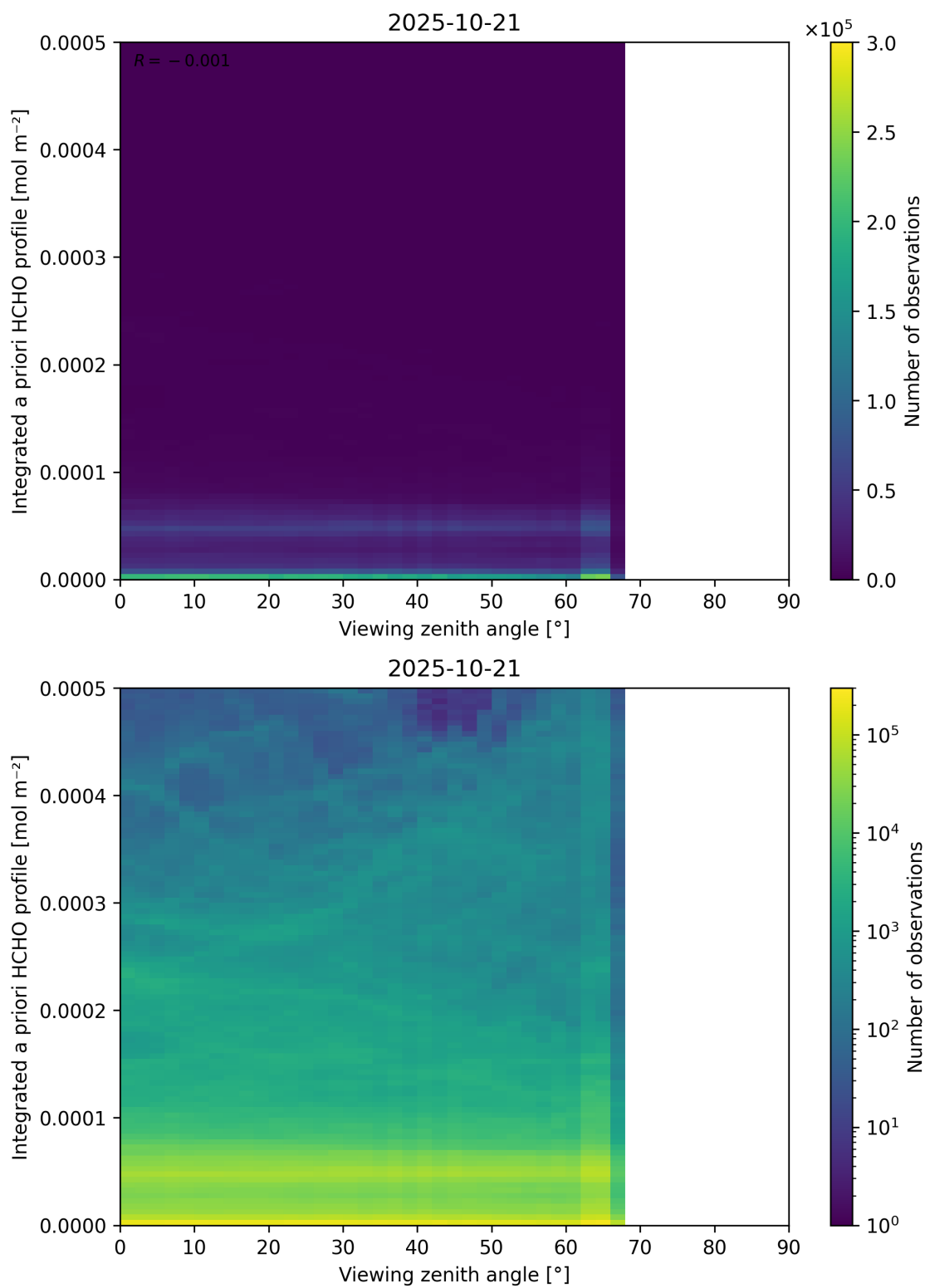
Figure 195: Scatter density plot of “Viewing zenith angle” against “Integrated a priori HCHO profile” for 2025-10-20 to 2025-10-22.
