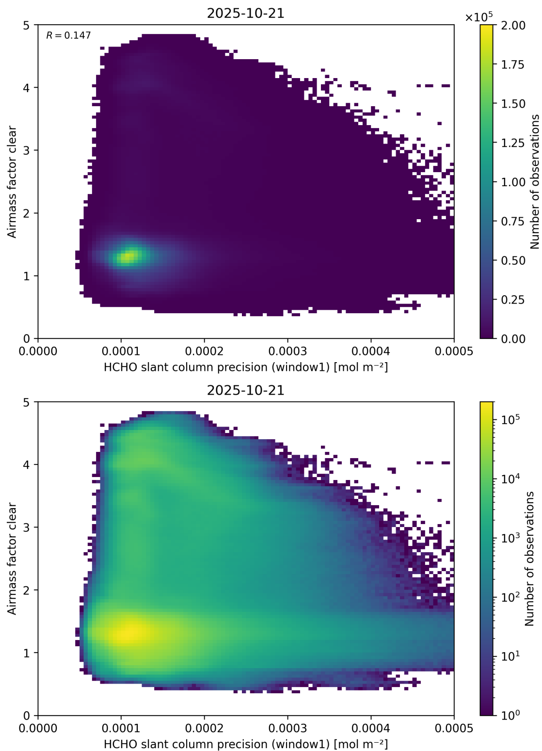
Figure 91: Scatter density plot of “HCHO slant column precision (window1)” against “Airmass factor clear” for 2025-10-20 to 2025-10-22.
