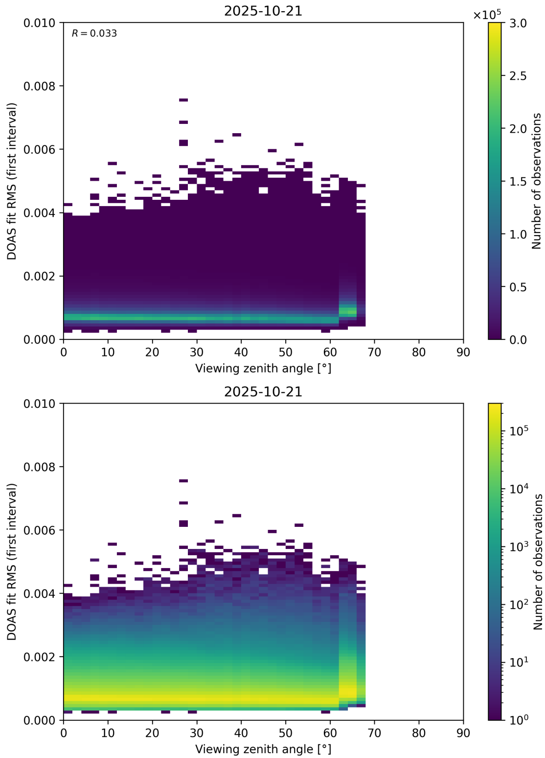
Figure 182: Scatter density plot of “Viewing zenith angle” against “DOAS fit RMS (first interval)” for 2025-10-20 to 2025-10-22.
