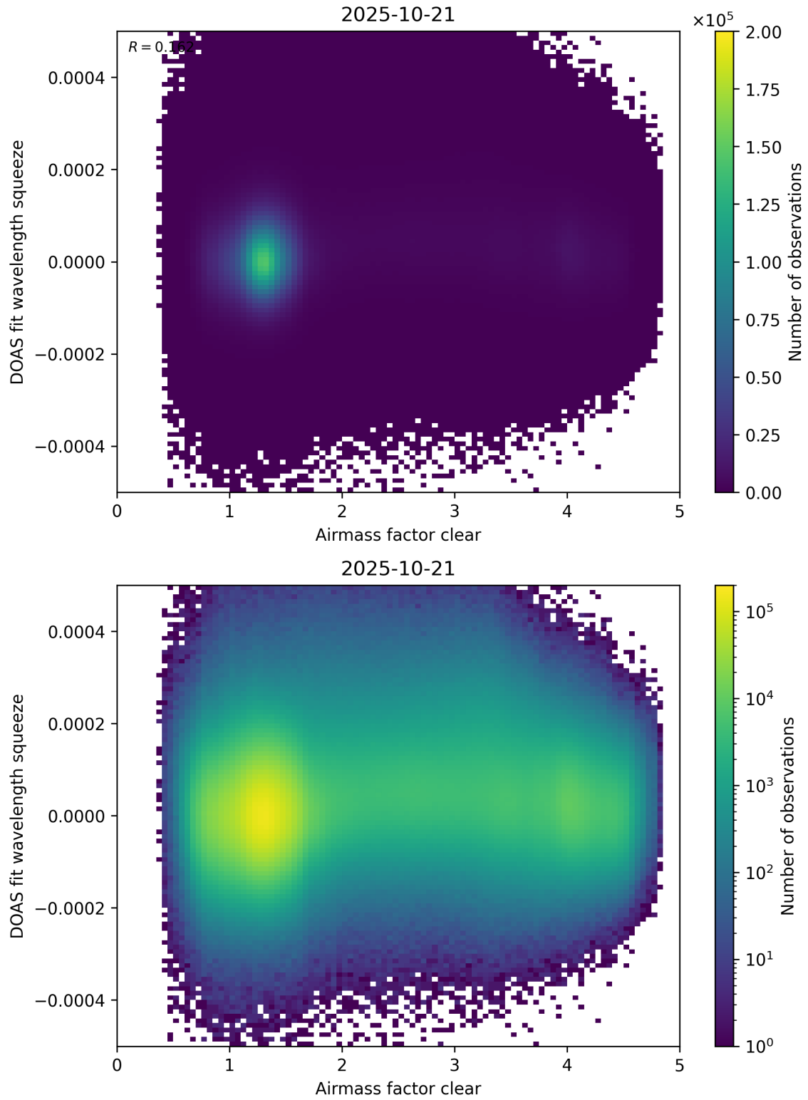
Figure 73: Scatter density plot of “Airmass factor clear” against “DOAS fit wavelength squeeze” for 2025-10-20 to 2025-10-22.
