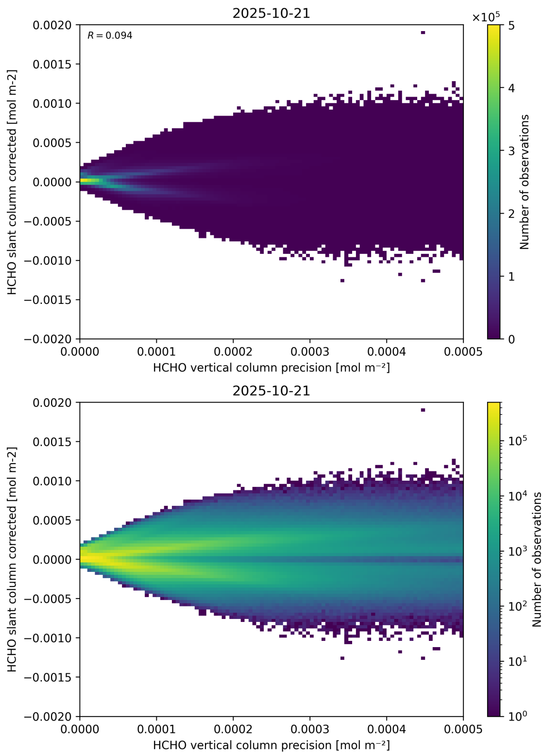
Figure 140: Scatter density plot of “HCHO vertical column precision” against “HCHO slant column corrected” for 2025-10-20 to 2025-10-22.
