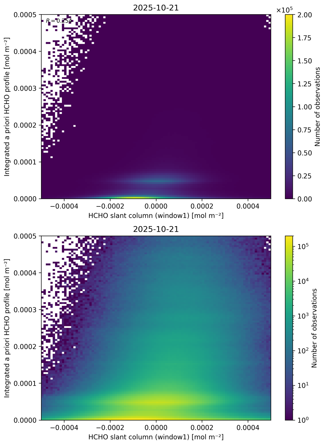
Figure 87: Scatter density plot of “HCHO slant column (window1)” against “Integrated a priori HCHO profile” for 2025-10-20 to 2025-10-22.
