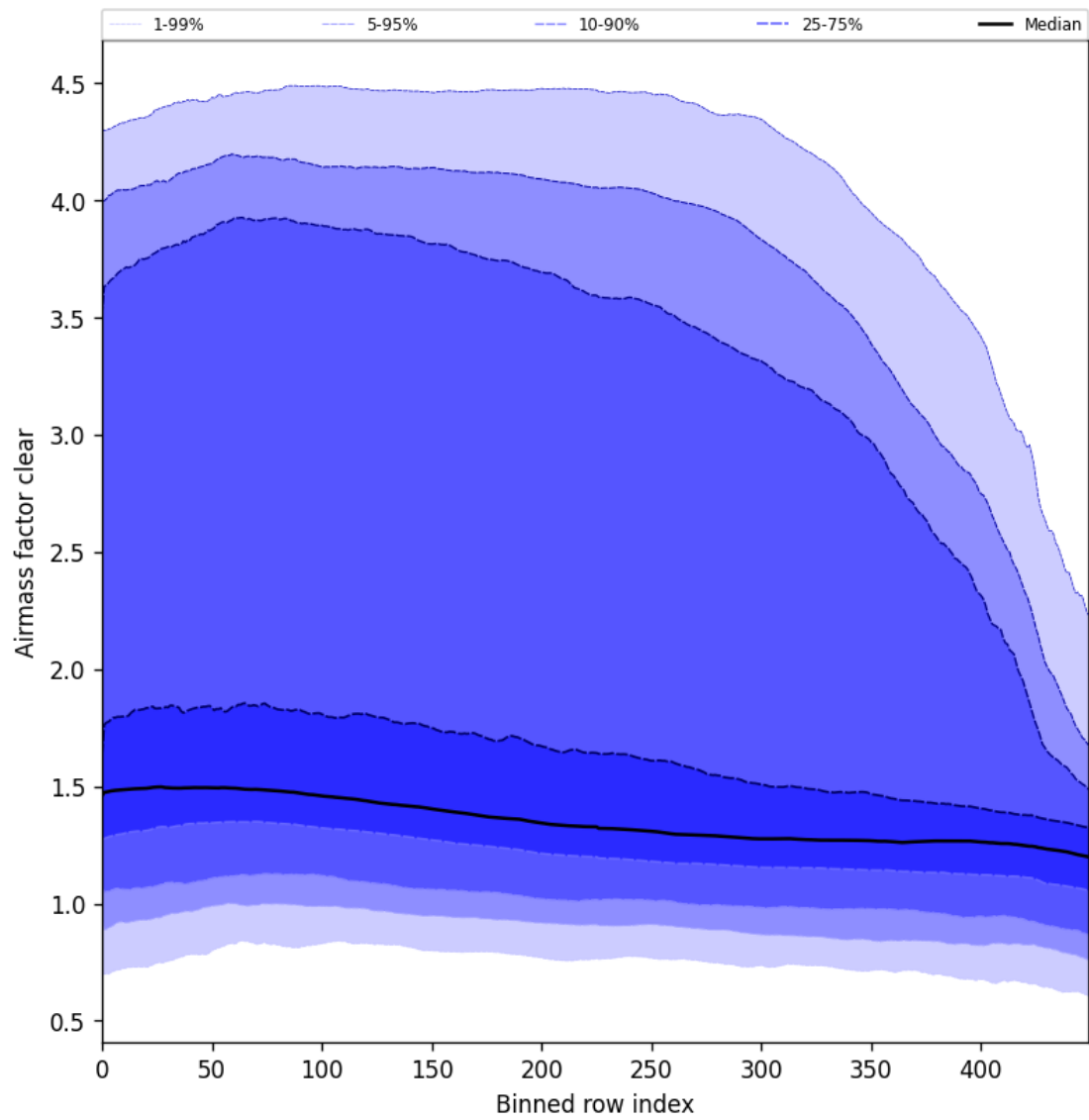
Figure 56: Along track statistics of “Airmass factor clear” for 2025-10-20 to 2025-10-22
