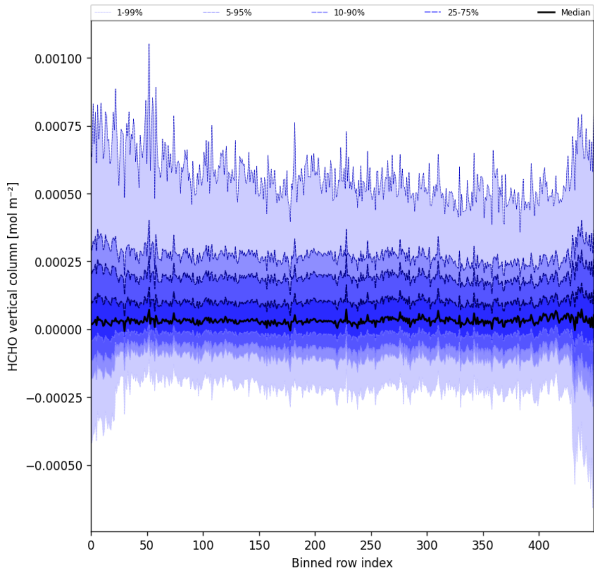
Figure 49: Along track statistics of “HCHO vertical column” for 2025-10-20 to 2025-10-22
