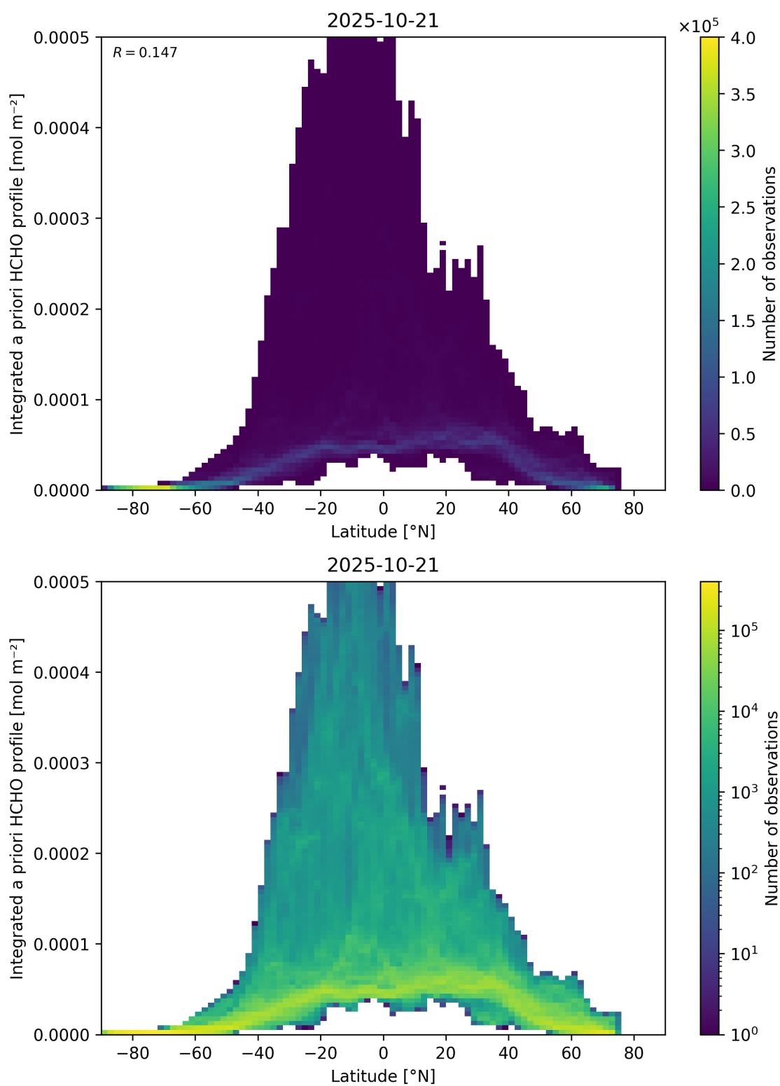
Figure 166: Scatter density plot of “Latitude” against “Integrated a priori HCHO profile” for 2025-10-20 to 2025-10-22.
