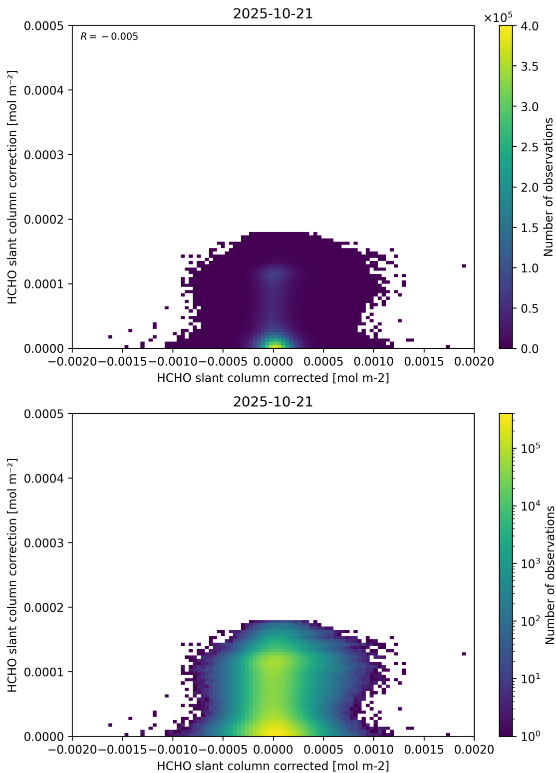
Figure 77: Scatter density plot of “HCHO slant column corrected” against “HCHO slant column correction” for 2025-10-20 to 2025-10-22.
