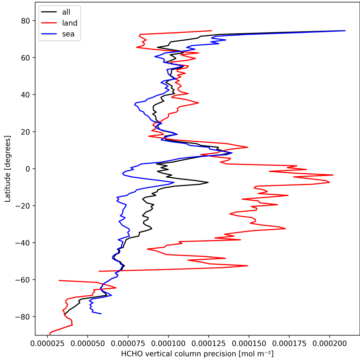
Figure 22: Zonal average of “HCHO vertical column precision” for 2025-10-20 to 2025-10-22.
