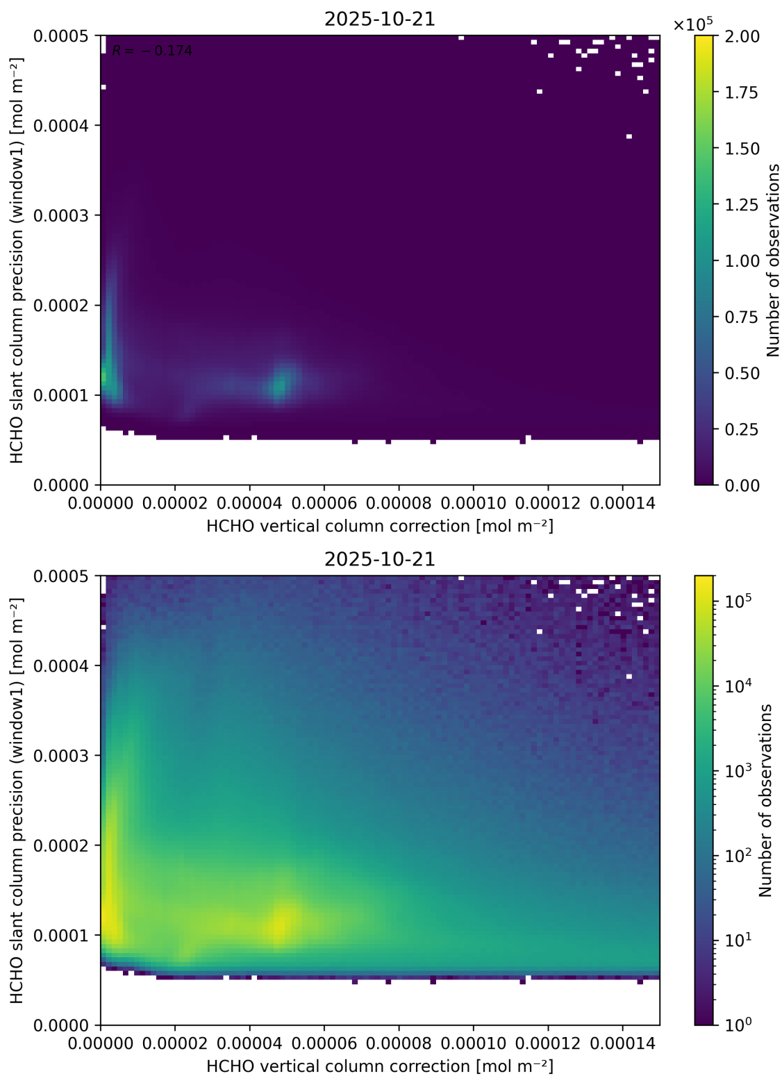
Figure 119: Scatter density plot of “HCHO vertical column correction” against “HCHO slant column precision (window1)” for 2025-10-20 to 2025-10-22.
