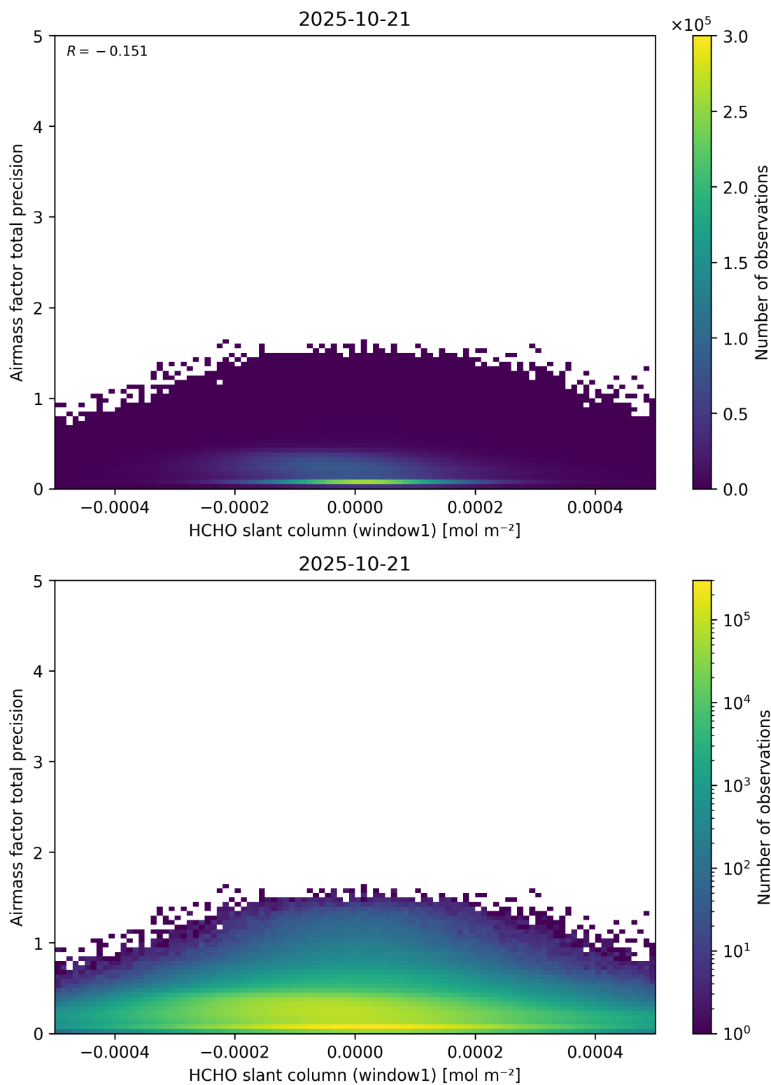
Figure 86: Scatter density plot of “HCHO slant column (window1)” against “Airmass factor total precision” for 2025-10-20 to 2025-10-22.
