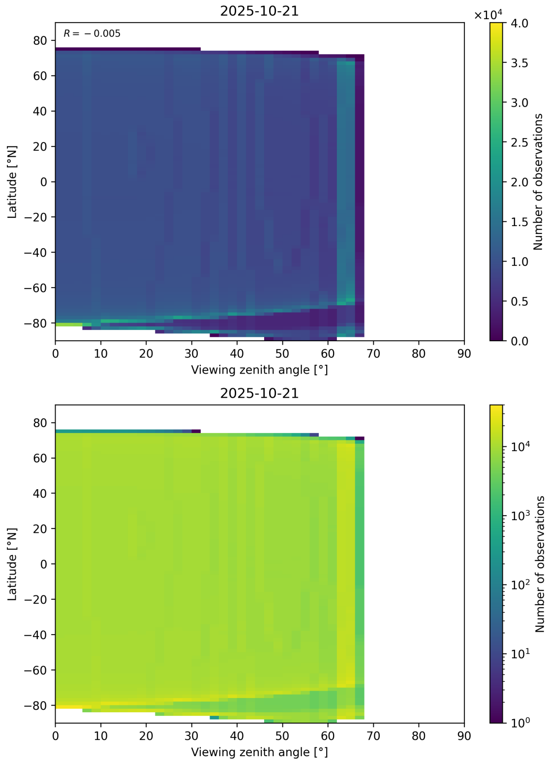
Figure 196: Scatter density plot of “Viewing zenith angle” against “Latitude” for 2025-10-20 to 2025-10-22.
