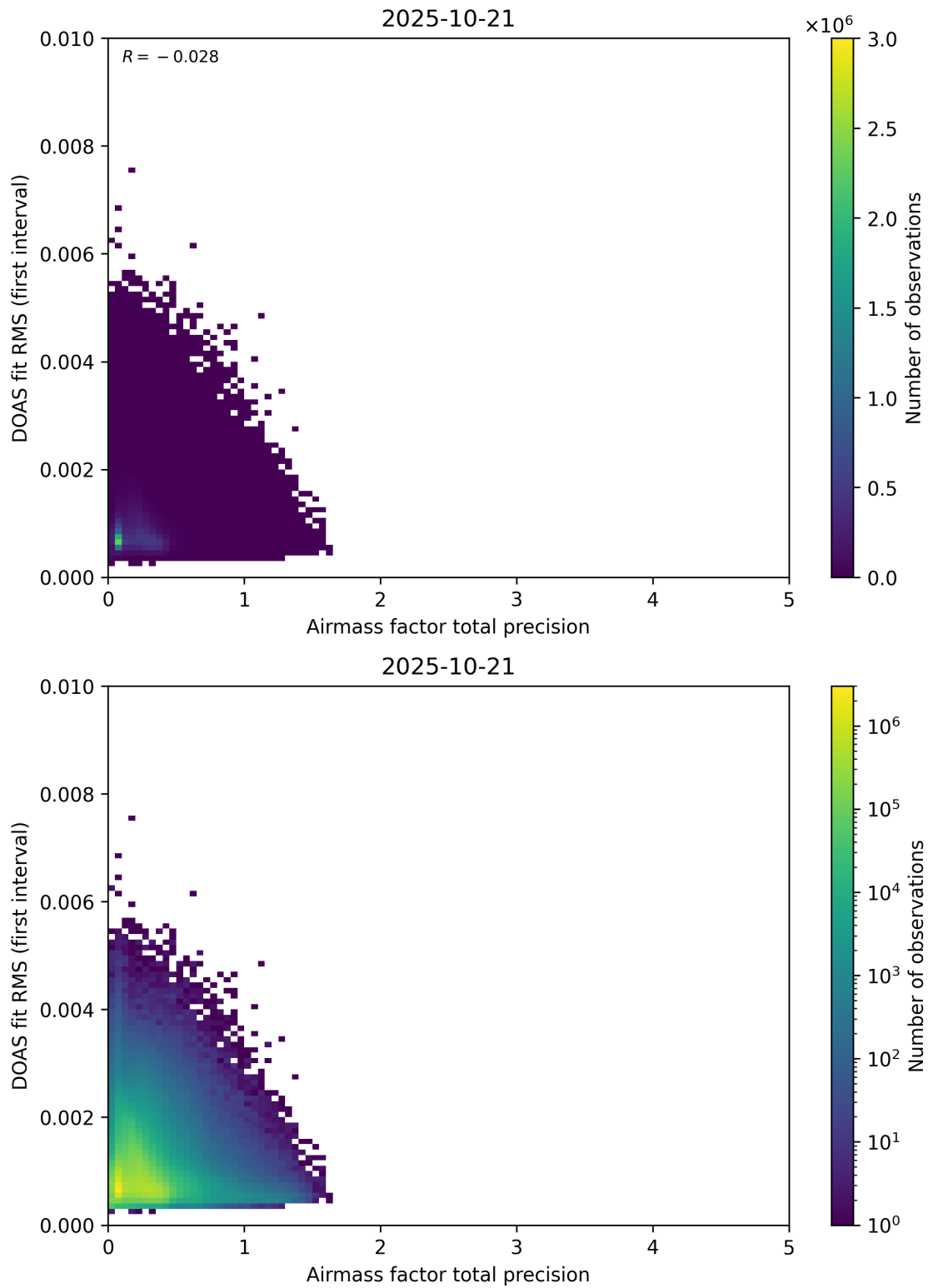
Figure 105: Scatter density plot of “Airmass factor total precision” against “DOAS fit RMS (first interval)” for 2025-10-20 to 2025-10-22.
