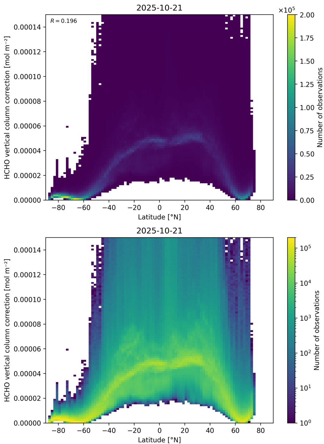
Figure 164: Scatter density plot of “Latitude” against “HCHO vertical column correction” for 2025-10-20 to 2025-10-22.
