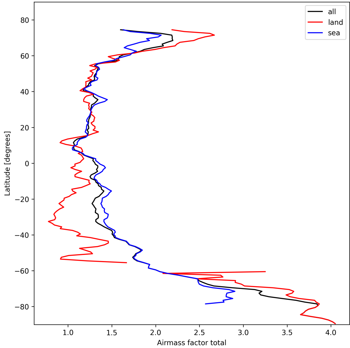
Figure 26: Zonal average of “Airmass factor total” for 2025-10-20 to 2025-10-22.
