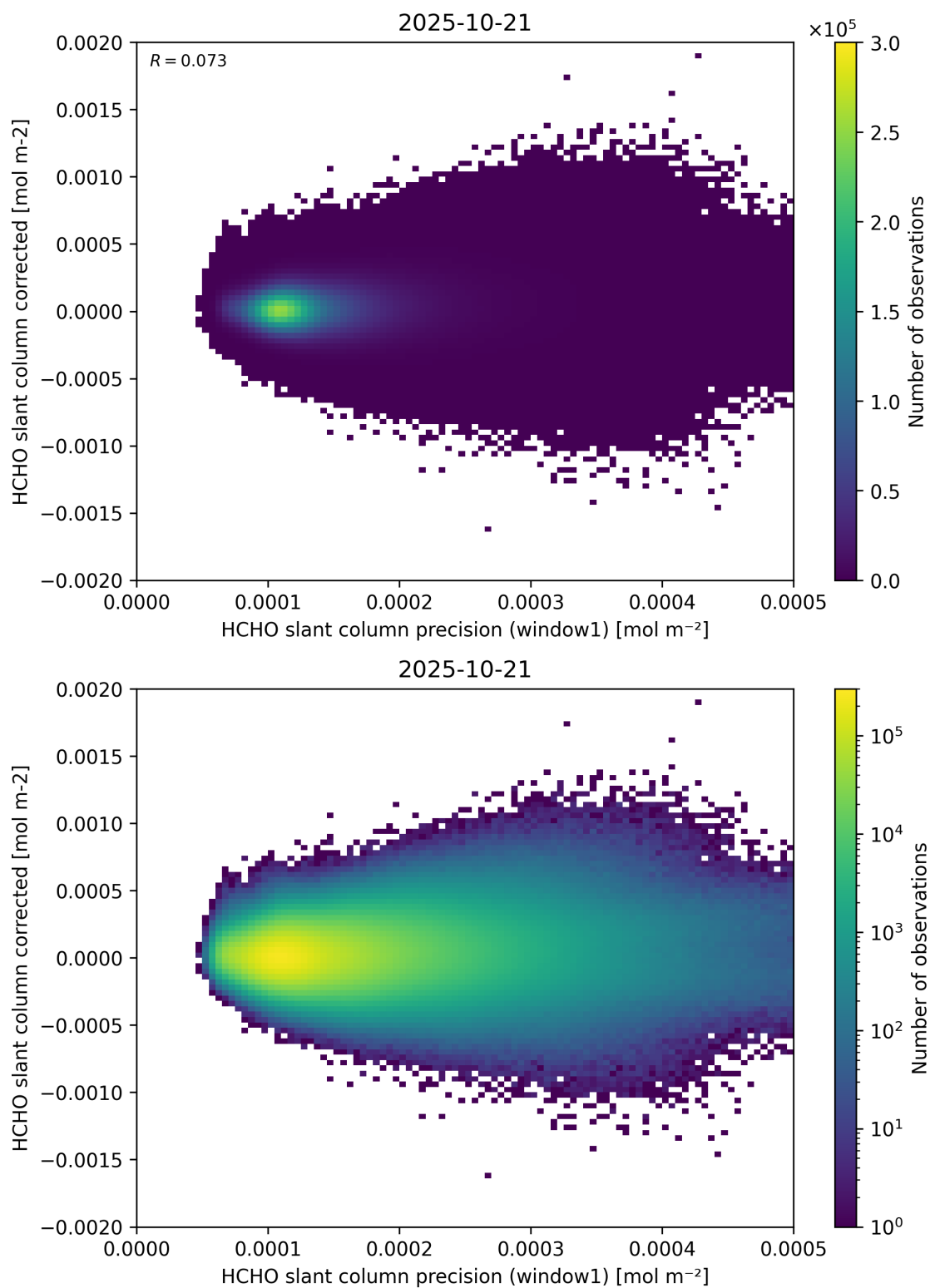
Figure 92: Scatter density plot of “HCHO slant column precision (window1)” against “HCHO slant column corrected” for 2025-10-20 to 2025-10-22.
