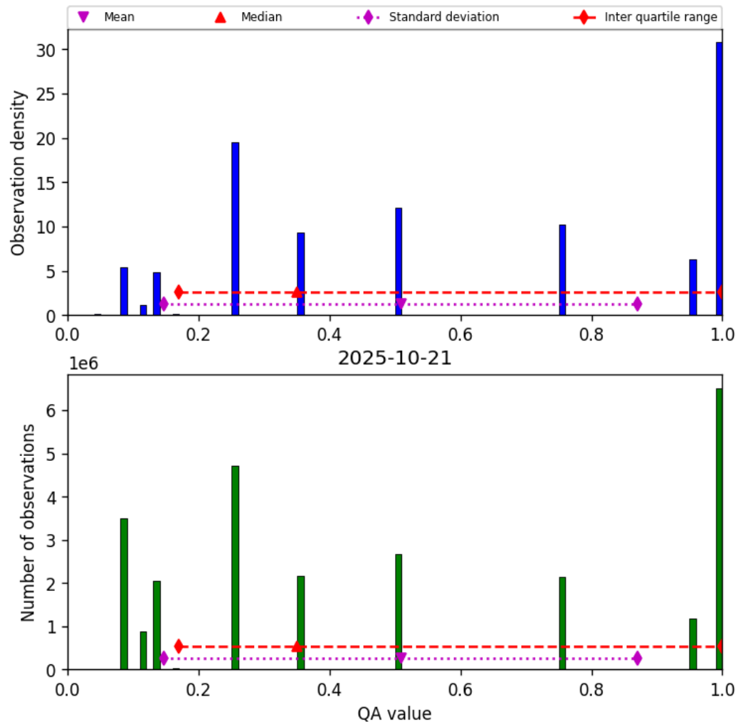
Figure 34: Histogram of “QA value” for 2025-10-20 to 2025-10-22
