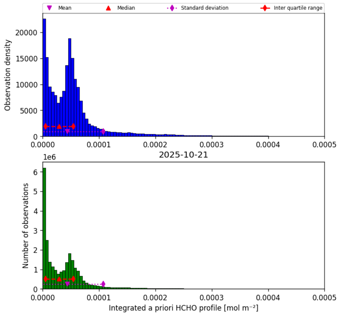
Figure 43: Histogram of “Integrated a priori HCHO profile” for 2025-10-20 to 2025-10-22
