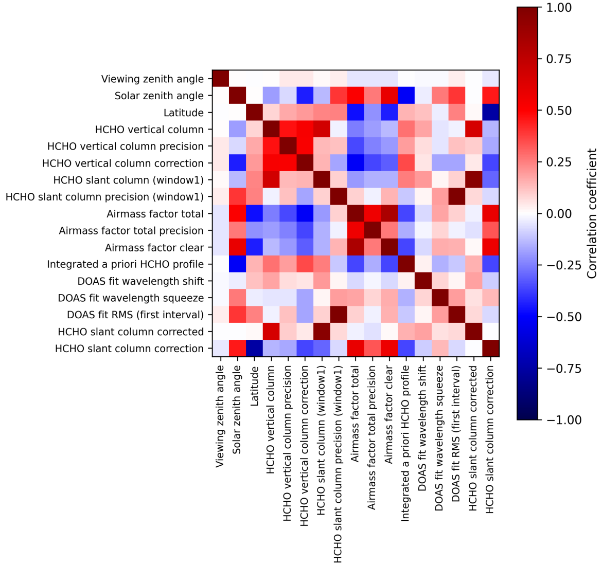
Figure 2: Map of correlation matrix for 2025-10-20 to 2025-10-22.
