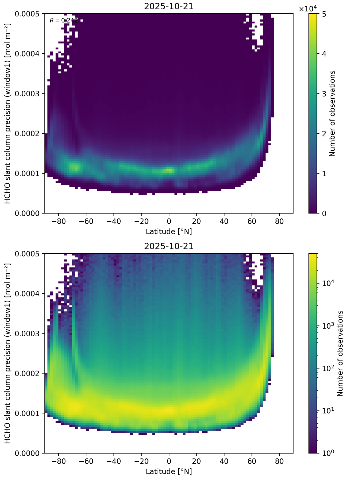
Figure 160: Scatter density plot of “Latitude” against “HCHO slant column precision (window1)” for 2025-10-20 to 2025-10-22.
