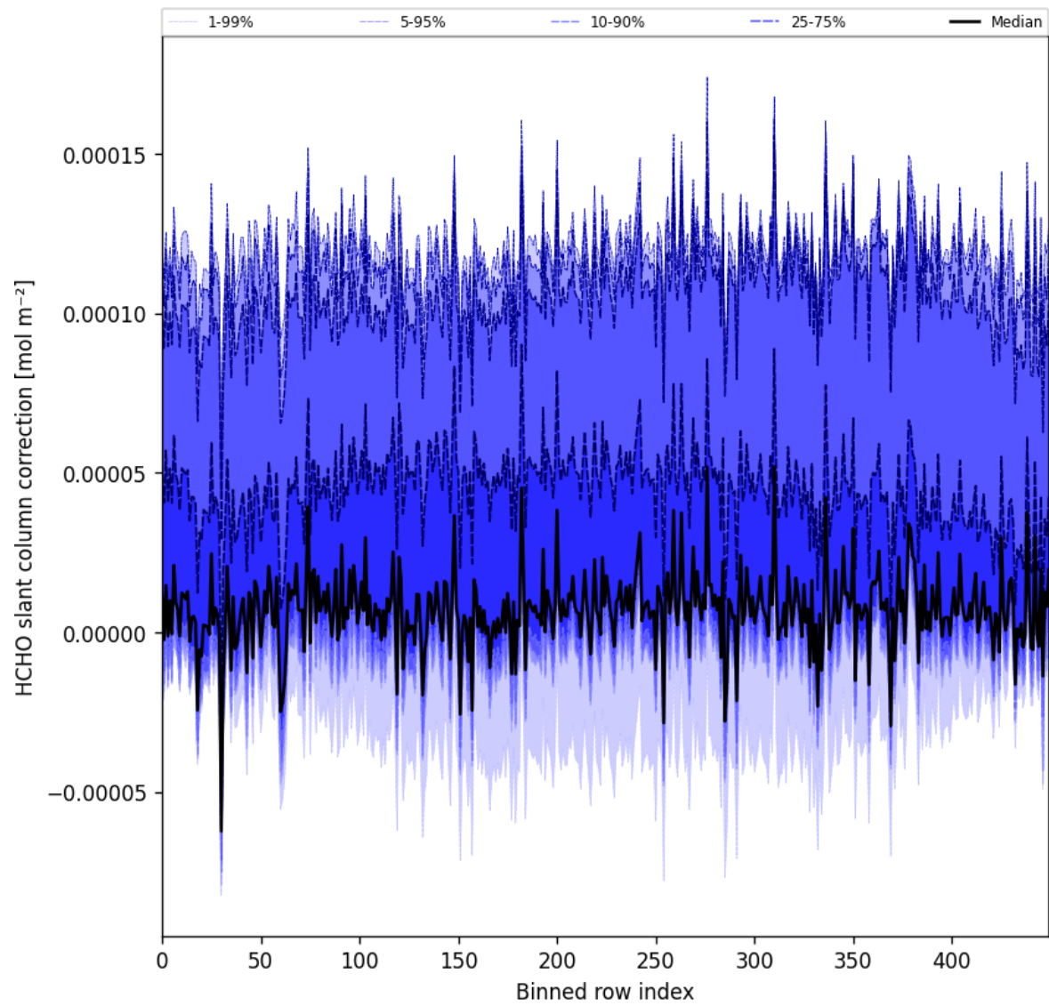
Figure 61: Along track statistics of “HCHO slant column correction” for 2025-10-20 to 2025-10-22
