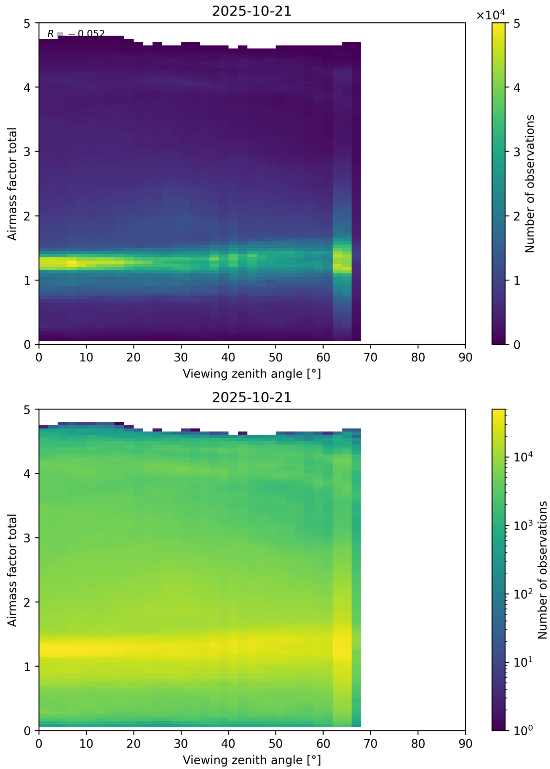
Figure 190: Scatter density plot of “Viewing zenith angle” against “Airmass factor total” for 2025-10-20 to 2025-10-22.
