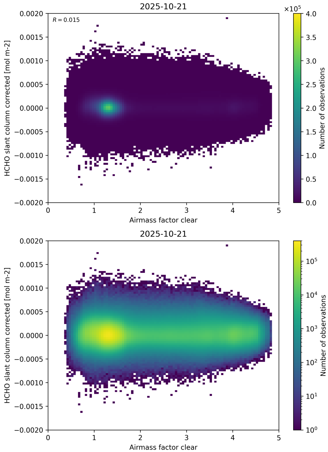
Figure 74: Scatter density plot of “Airmass factor clear” against “HCHO slant column corrected” for 2025-10-20 to 2025-10-22.
