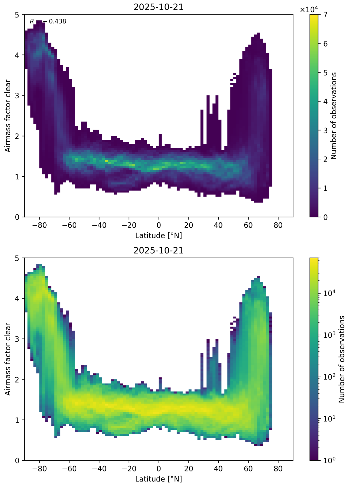
Figure 156: Scatter density plot of “Latitude” against “Airmass factor clear” for 2025-10-20 to 2025-10-22.
