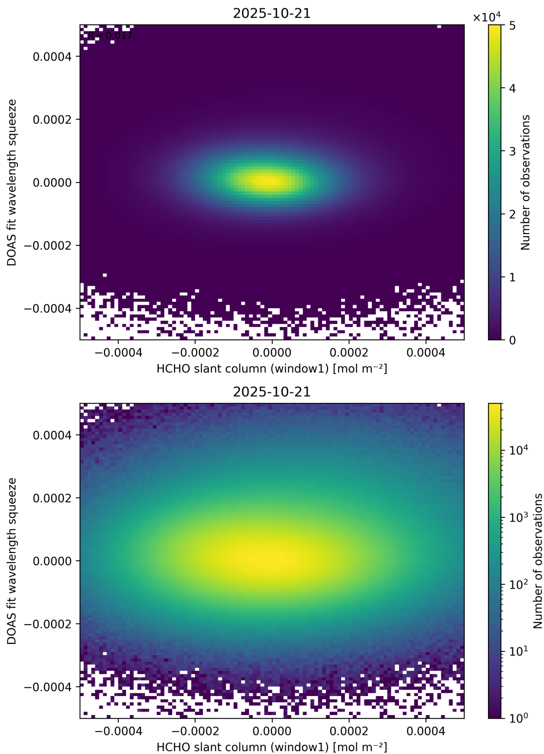
Figure 80: Scatter density plot of “HCHO slant column (window1)” against “DOAS fit wavelength squeeze” for 2025-10-20 to 2025-10-22.
