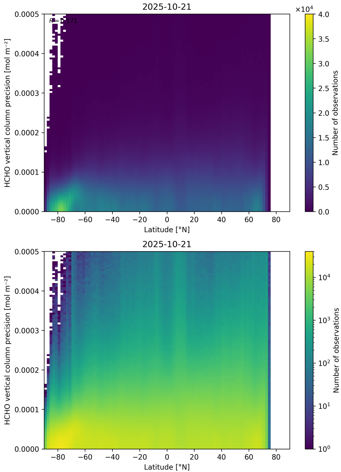
Figure 165: Scatter density plot of “Latitude” against “HCHO vertical column precision” for 2025-10-20 to 2025-10-22.
