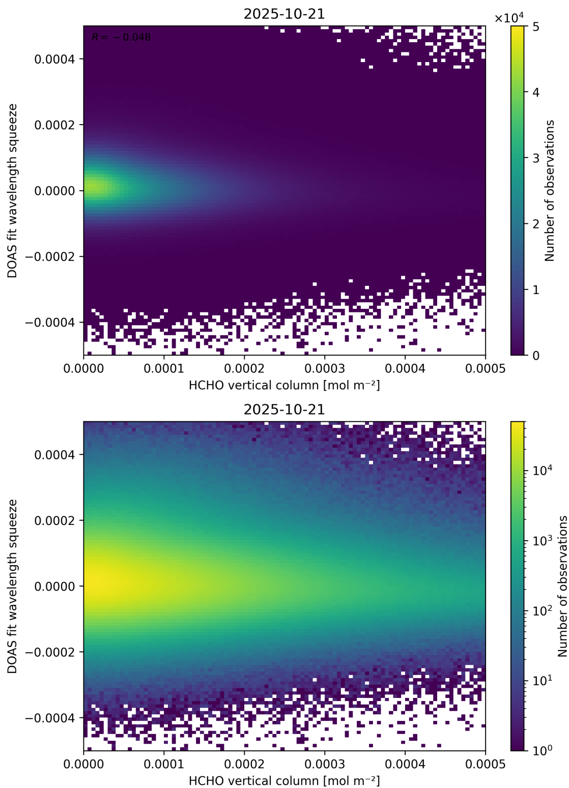
Figure 125: Scatter density plot of “HCHO vertical column” against “DOAS fit wavelength squeeze” for 2025-10-20 to 2025-10-22.
