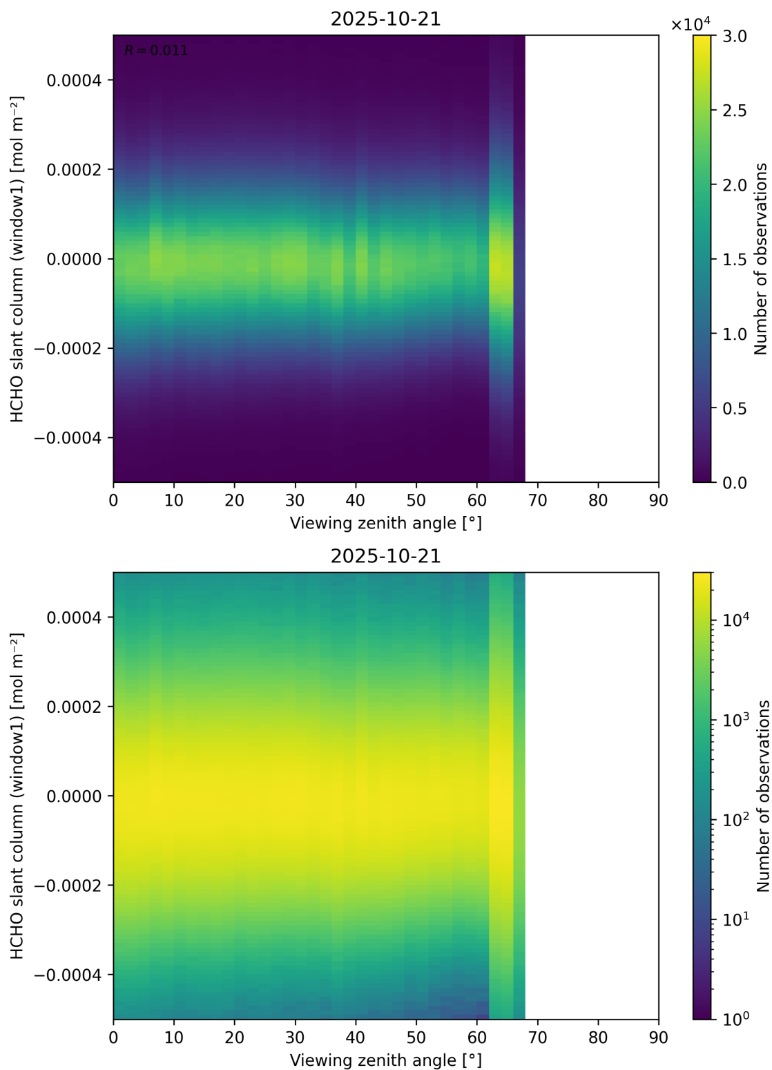
Figure 188: Scatter density plot of “Viewing zenith angle” against “HCHO slant column (window1)” for 2025-10-20 to 2025-10-22.
