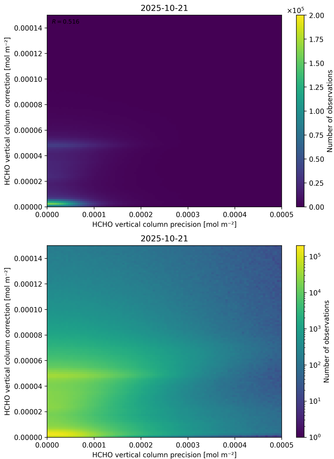
Figure 146: Scatter density plot of “HCHO vertical column precision” against “HCHO vertical column correction” for 2025-10-20 to 2025-10-22.
