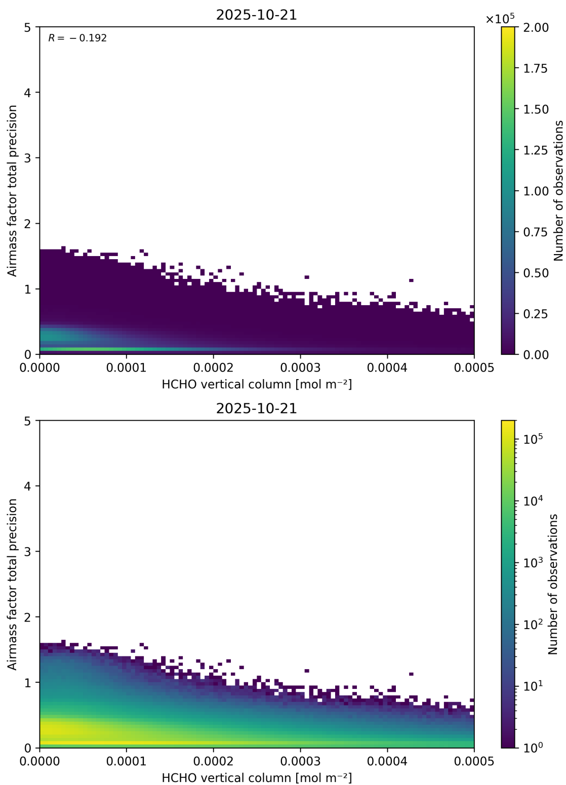
Figure 132: Scatter density plot of “HCHO vertical column” against “Airmass factor total precision” for 2025-10-20 to 2025-10-22.
