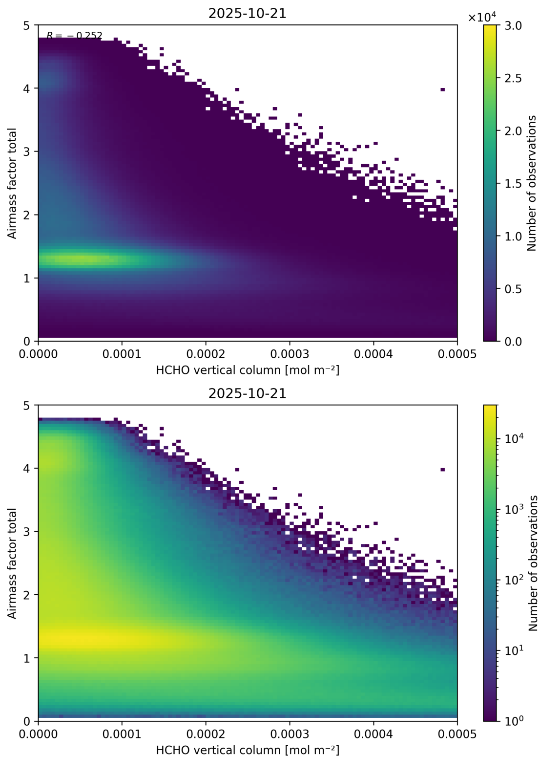
Figure 131: Scatter density plot of “HCHO vertical column” against “Airmass factor total” for 2025-10-20 to 2025-10-22.
