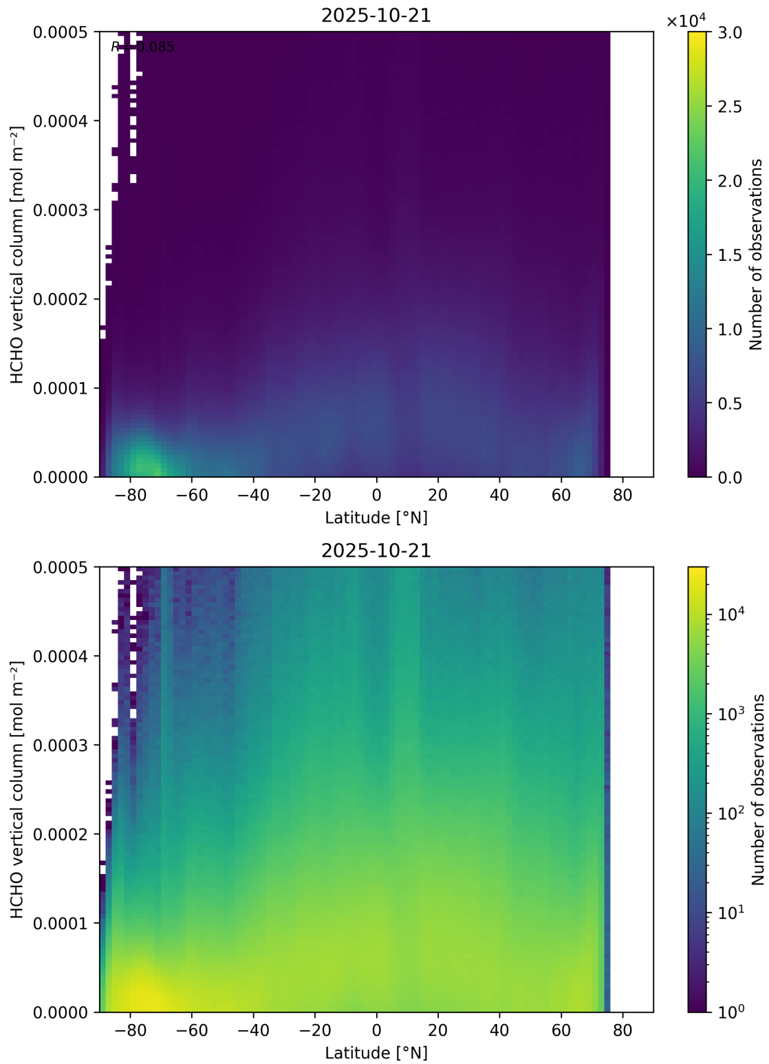
Figure 163: Scatter density plot of “Latitude” against “HCHO vertical column” for 2025-10-20 to 2025-10-22.
