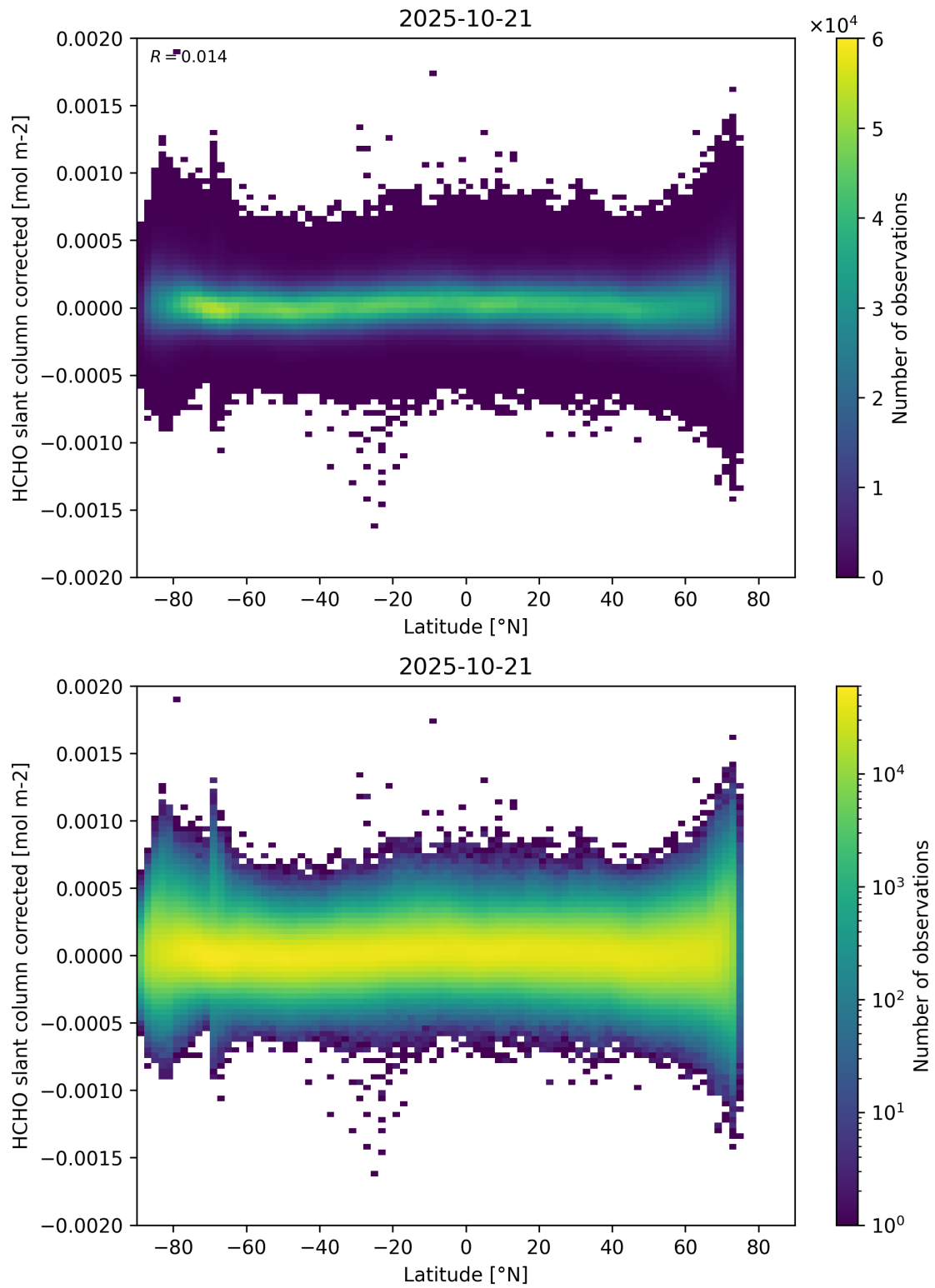
Figure 157: Scatter density plot of “Latitude” against “HCHO slant column corrected” for 2025-10-20 to 2025-10-22.
