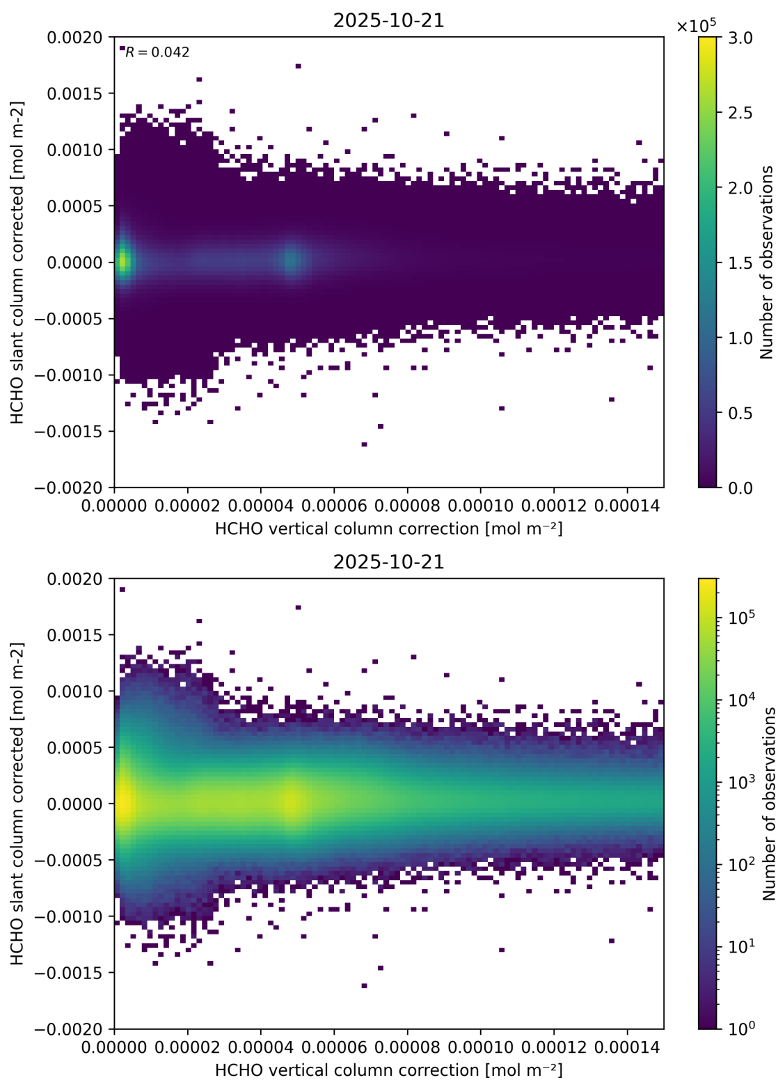
Figure 116: Scatter density plot of “HCHO vertical column correction” against “HCHO slant column corrected” for 2025-10-20 to 2025-10-22.
