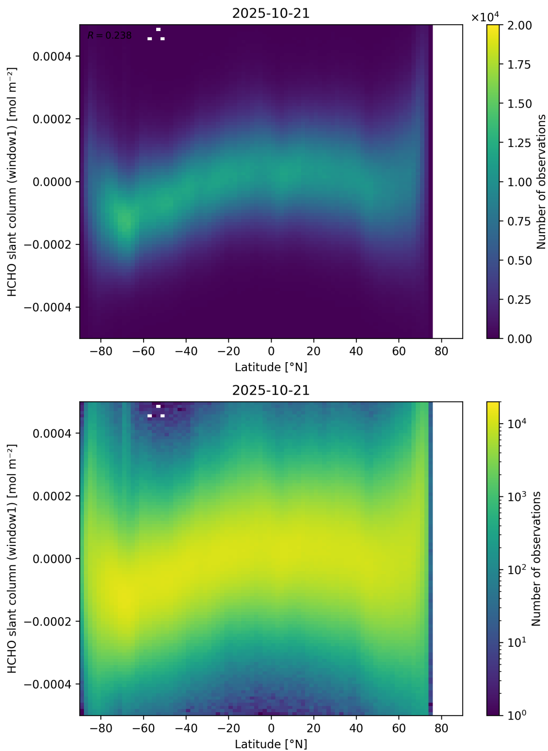
Figure 159: Scatter density plot of “Latitude” against “HCHO slant column (window1)” for 2025-10-20 to 2025-10-22.
