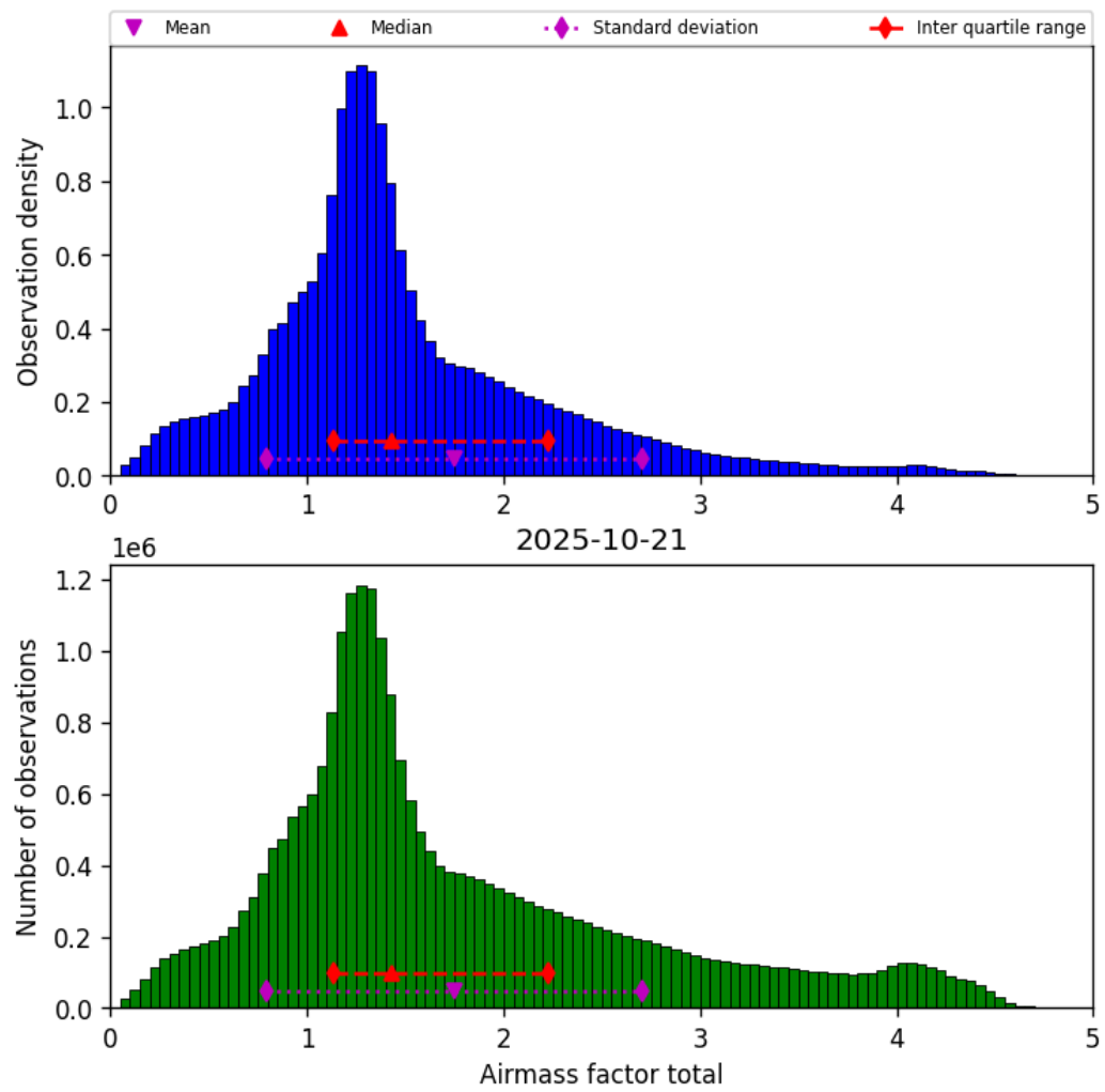
Figure 40: Histogram of “Airmass factor total” for 2025-10-20 to 2025-10-22
