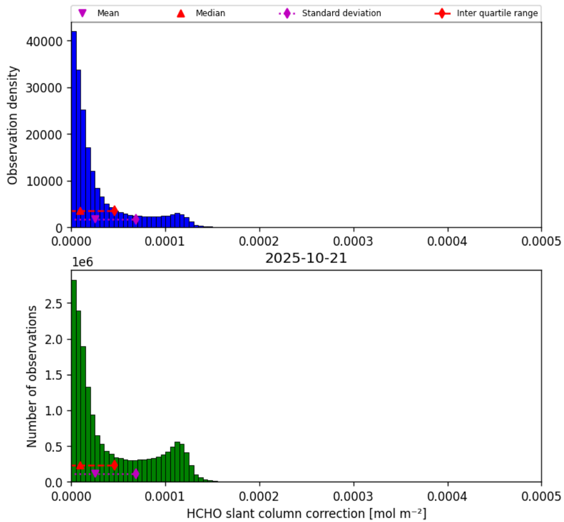
Figure 47: Histogram of “HCHO slant column correction” for 2025-10-20 to 2025-10-22
