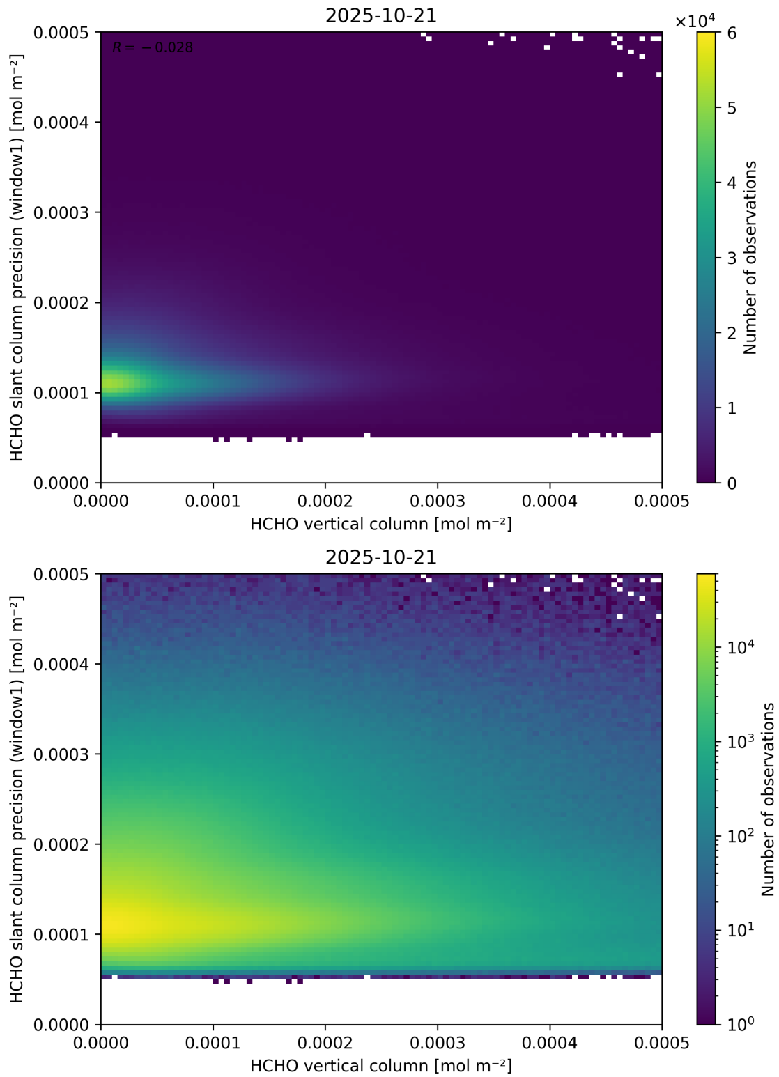
Figure 130: Scatter density plot of “HCHO vertical column” against “HCHO slant column precision (window1)” for 2025-10-20 to 2025-10-22.
