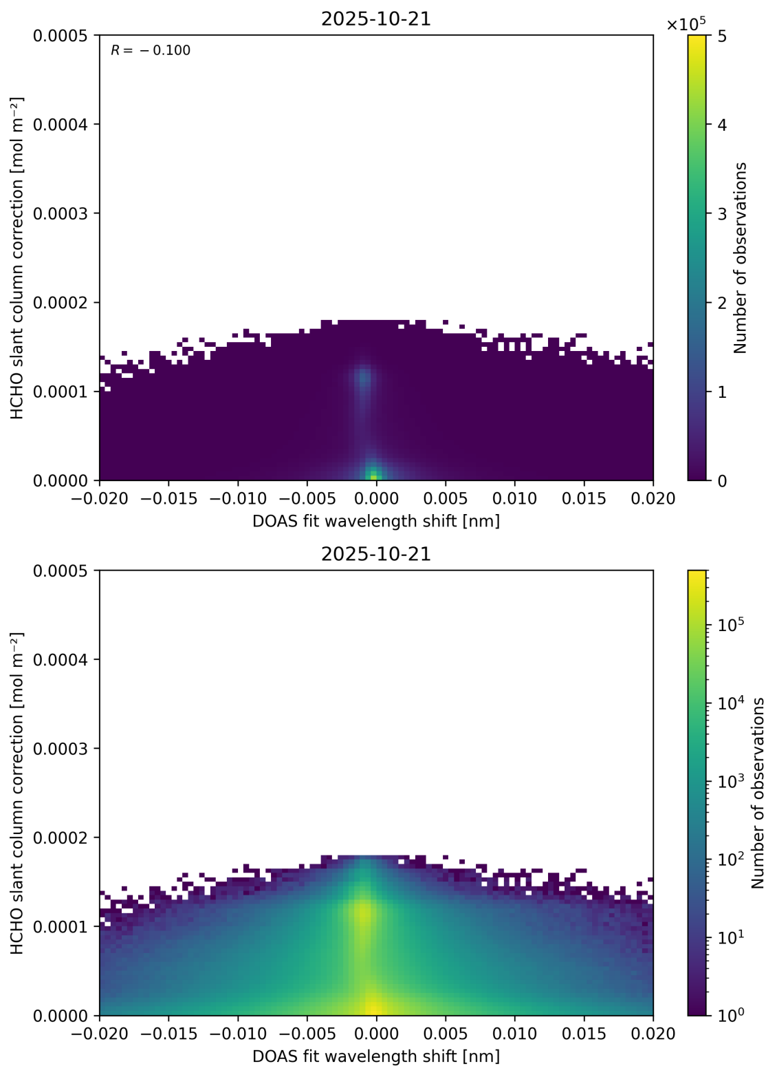
Figure 67: Scatter density plot of “DOAS fit wavelength shift” against “HCHO slant column correction” for 2025-10-20 to 2025-10-22.
