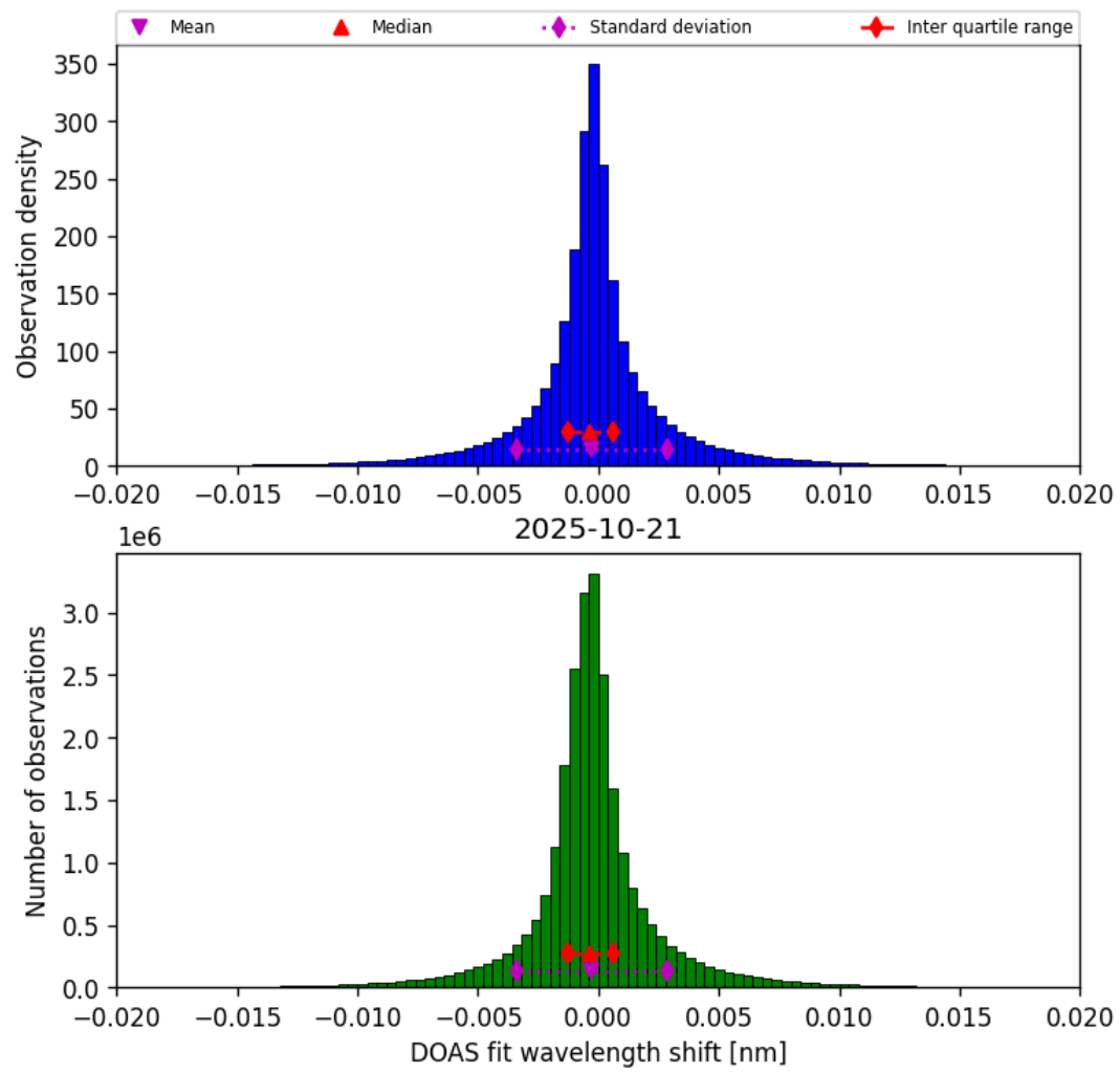
Figure 44: Histogram of “DOAS fit wavelength shift” for 2025-10-20 to 2025-10-22
