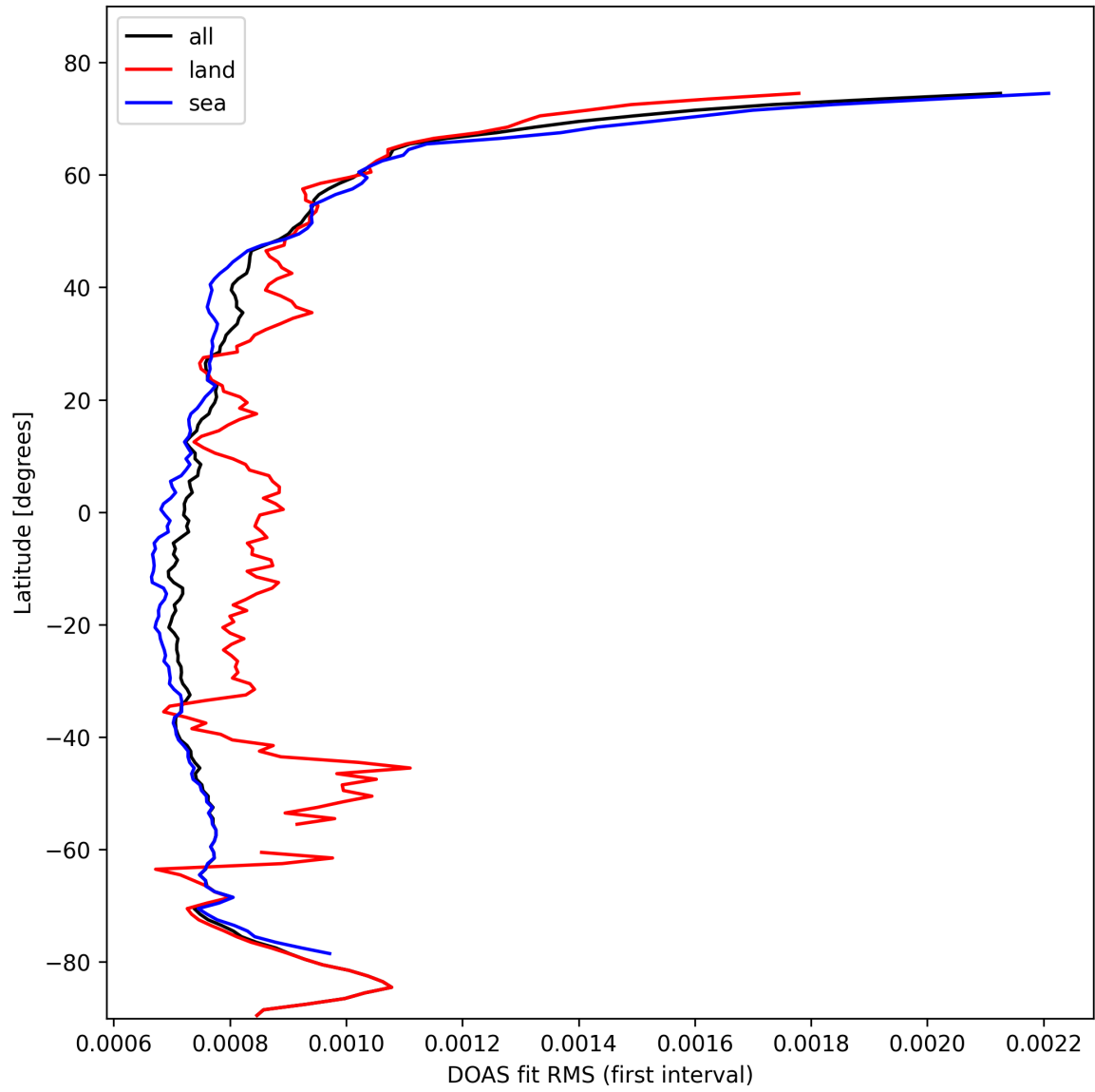
Figure 32: Zonal average of “DOAS fit RMS (first interval)” for 2025-10-20 to 2025-10-22.
