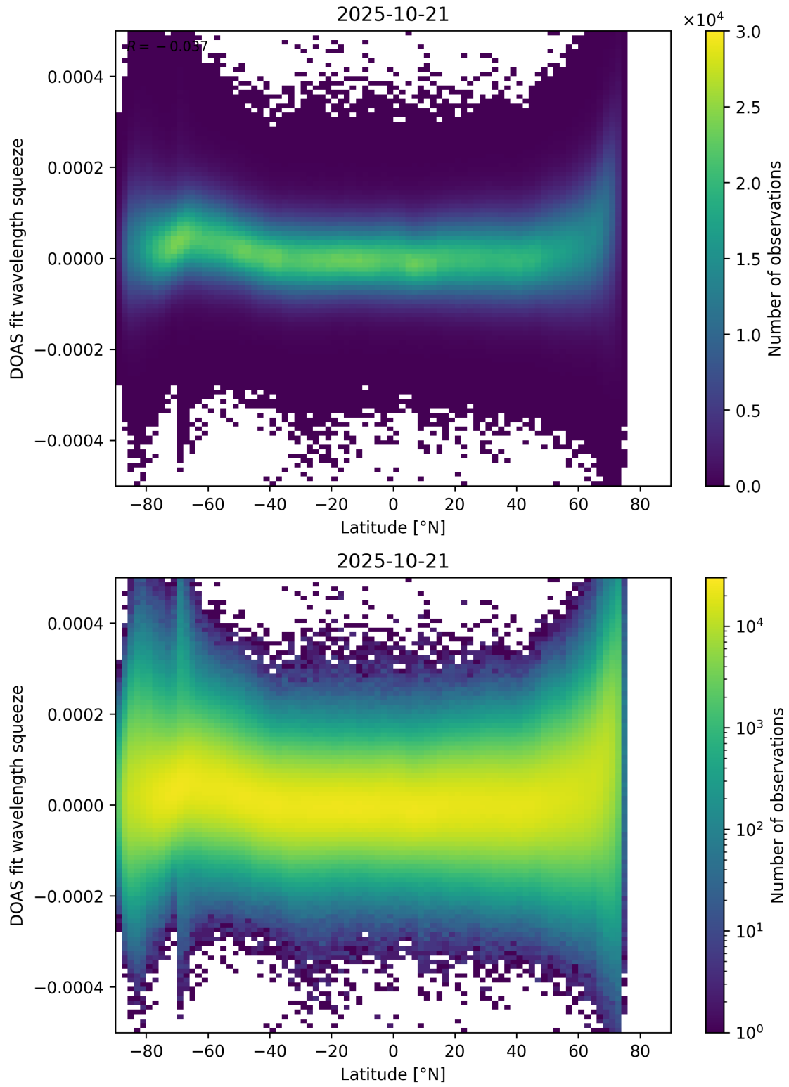
Figure 155: Scatter density plot of “Latitude” against “DOAS fit wavelength squeeze” for 2025-10-20 to 2025-10-22.
