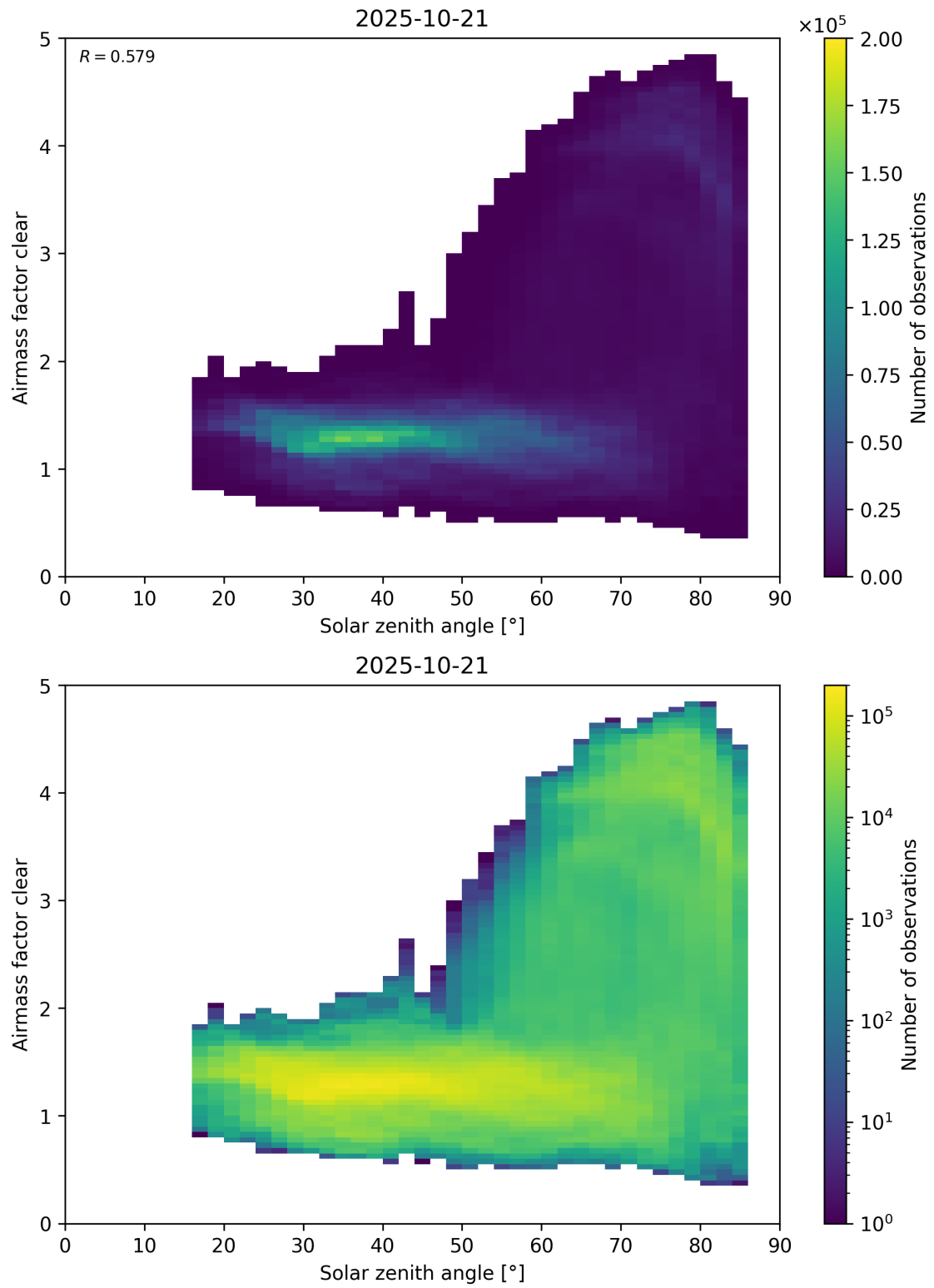
Figure 170: Scatter density plot of “Solar zenith angle” against “Airmass factor clear” for 2025-10-20 to 2025-10-22.
