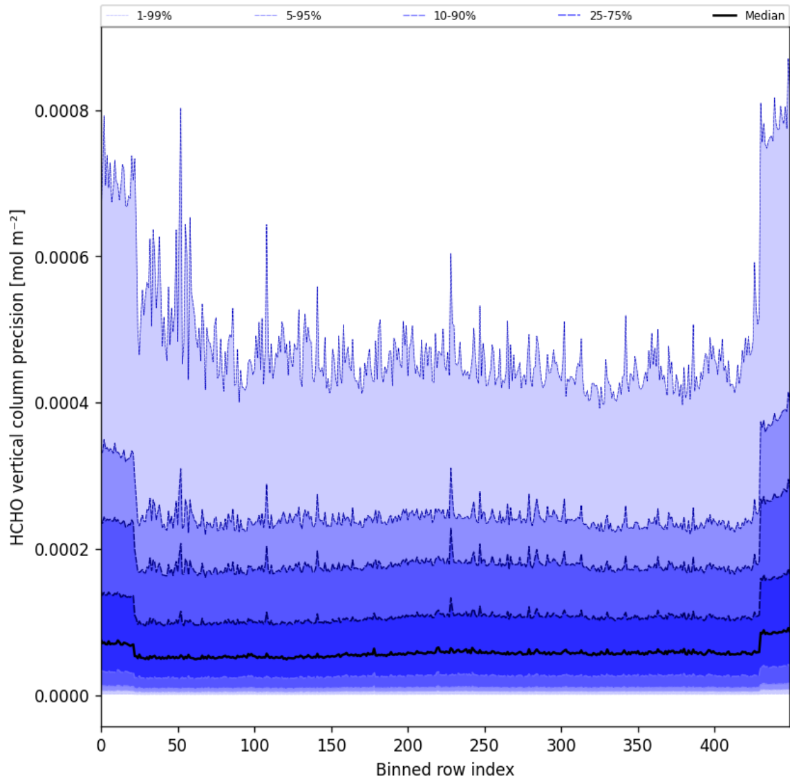
Figure 50: Along track statistics of “HCHO vertical column precision” for 2025-10-20 to 2025-10-22
