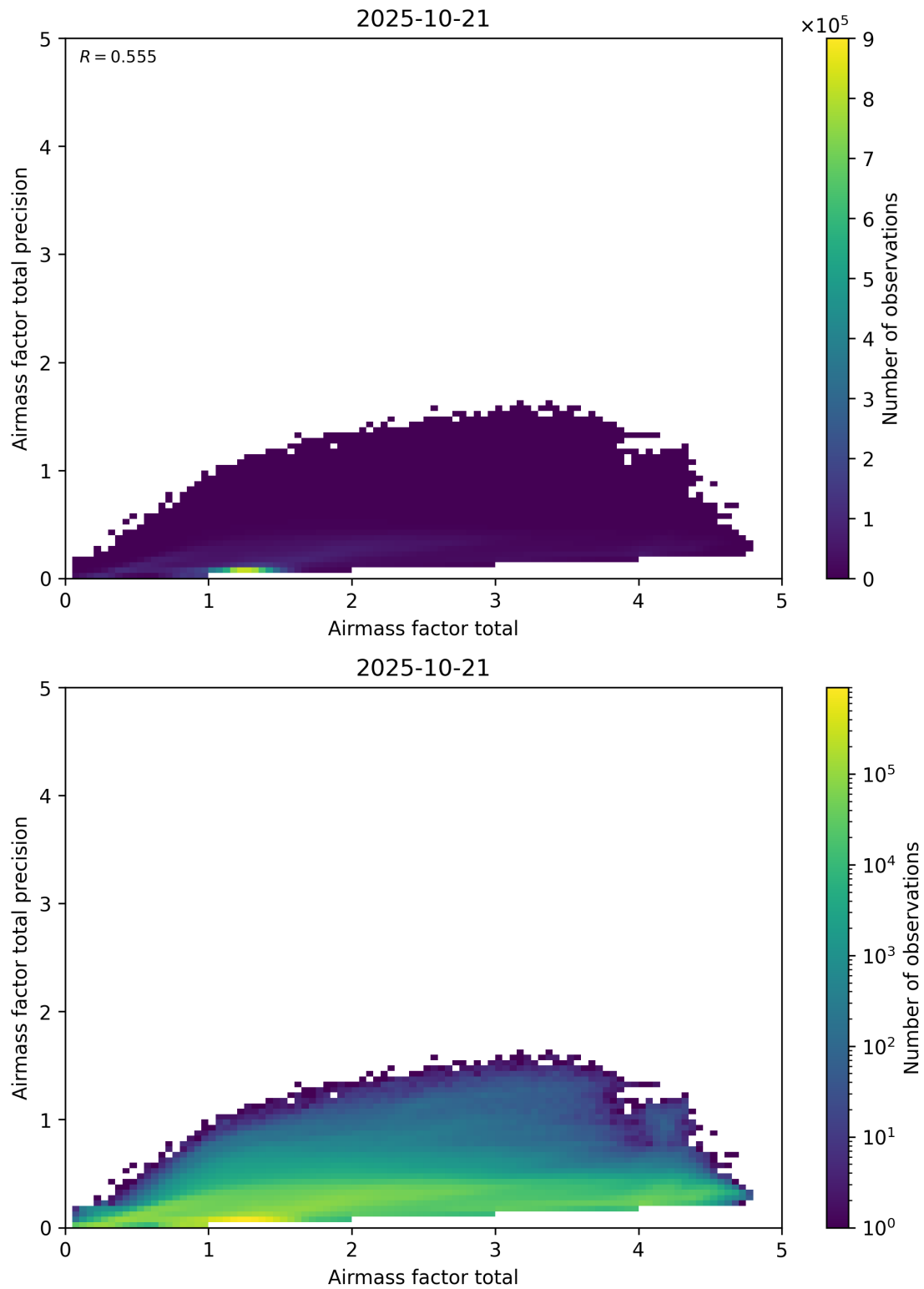
Figure 103: Scatter density plot of “Airmass factor total” against “Airmass factor total precision” for 2025-10-20 to 2025-10-22.
