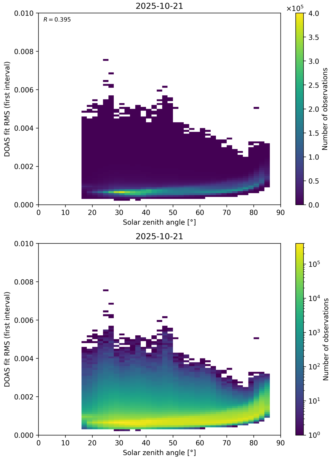
Figure 167: Scatter density plot of “Solar zenith angle” against “DOAS fit RMS (first interval)” for 2025-10-20 to 2025-10-22.
