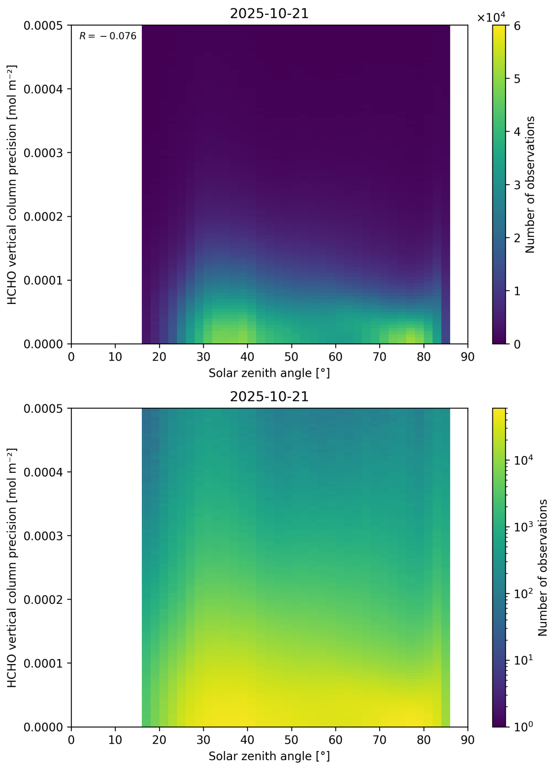
Figure 179: Scatter density plot of “Solar zenith angle” against “HCHO vertical column precision” for 2025-10-20 to 2025-10-22.
