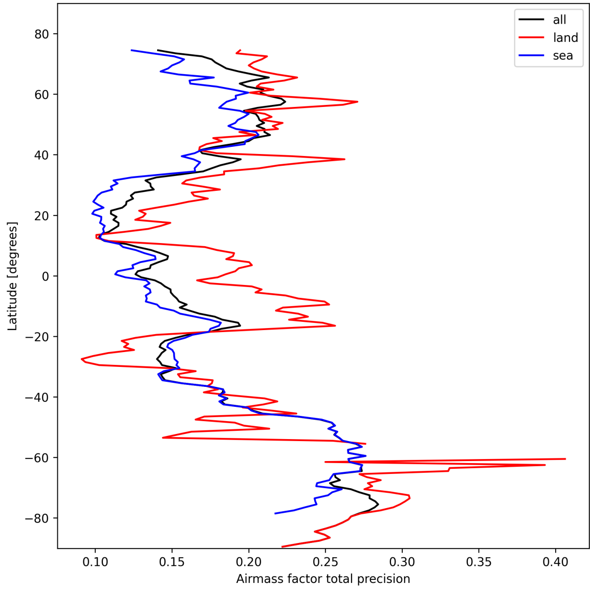
Figure 27: Zonal average of “Airmass factor total precision” for 2025-10-20 to 2025-10-22.
