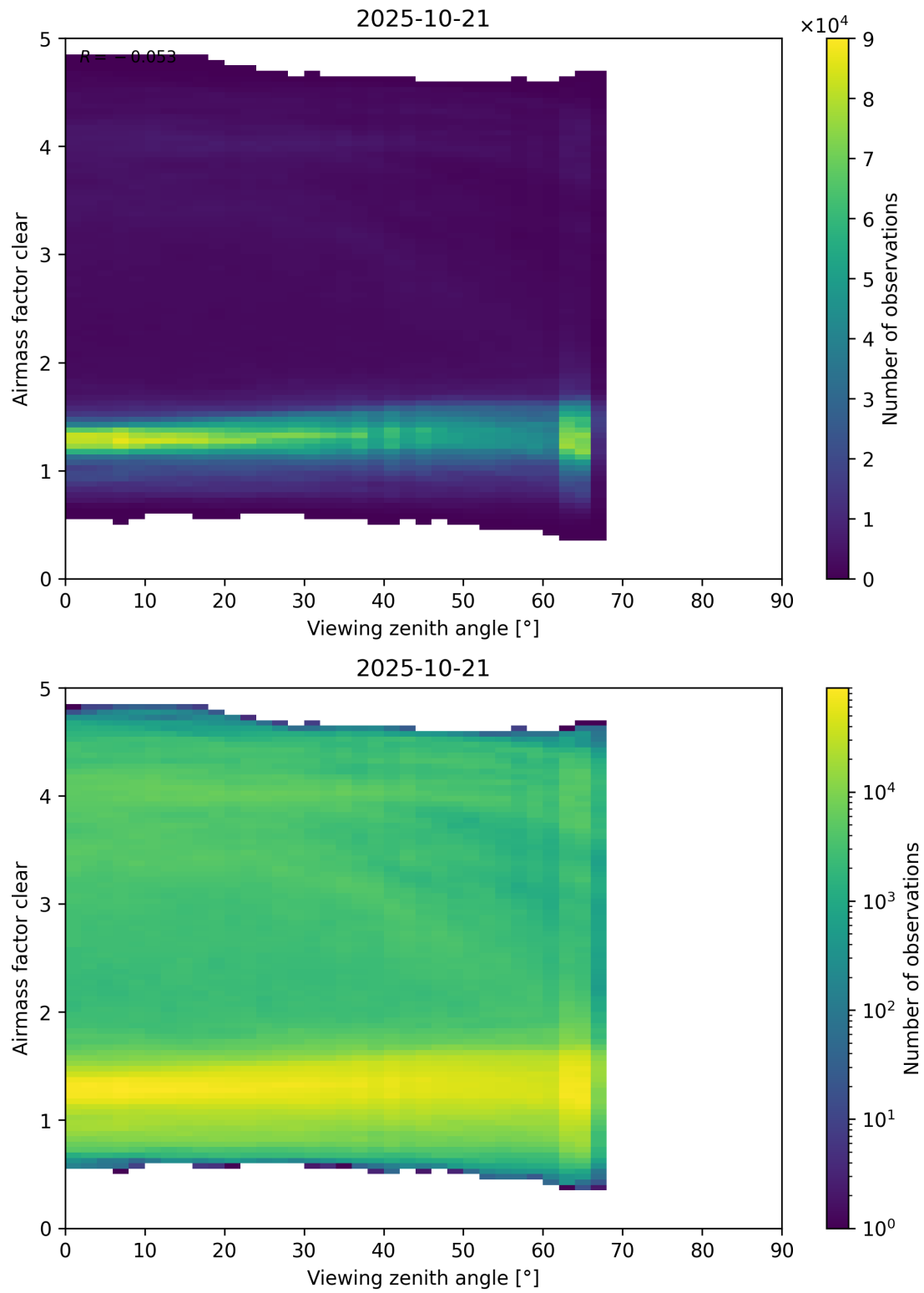
Figure 185: Scatter density plot of “Viewing zenith angle” against “Airmass factor clear” for 2025-10-20 to 2025-10-22.
