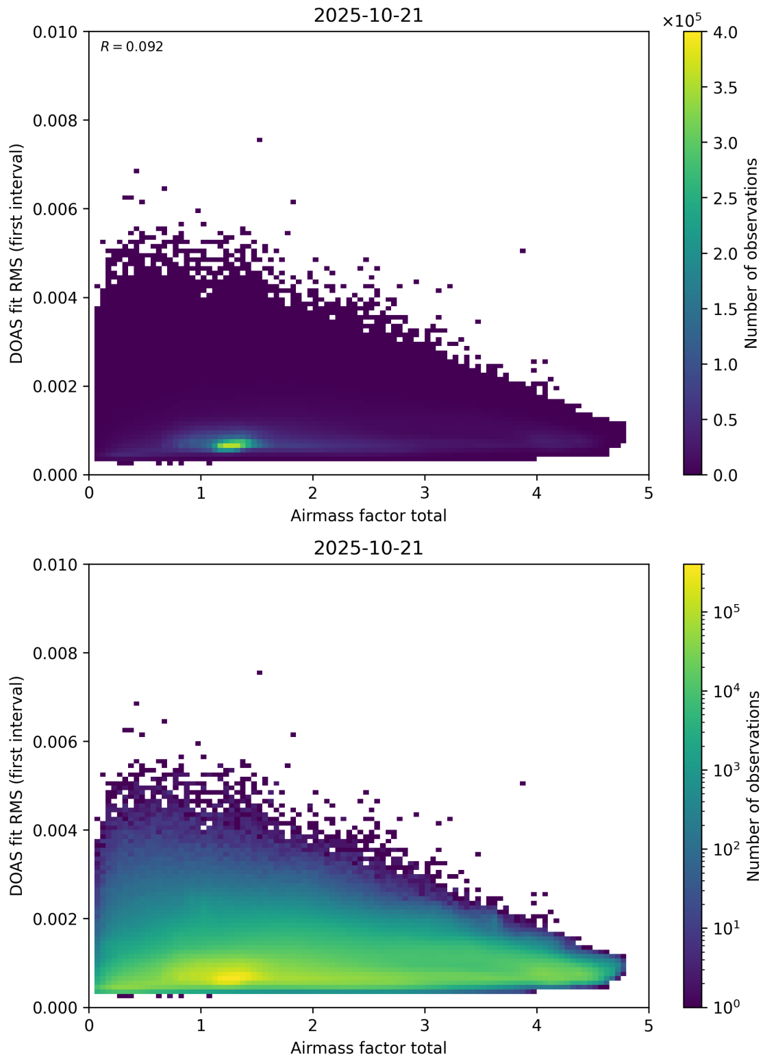
Figure 97: Scatter density plot of “Airmass factor total” against “DOAS fit RMS (first interval)” for 2025-10-20 to 2025-10-22.
