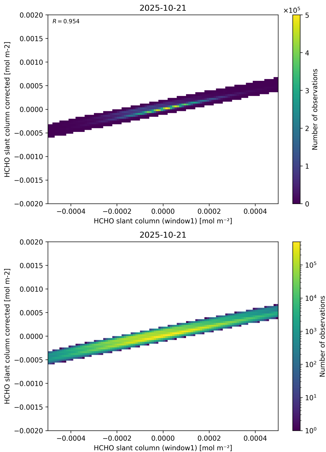
Figure 82: Scatter density plot of “HCHO slant column (window1)” against “HCHO slant column corrected” for 2025-10-20 to 2025-10-22.
