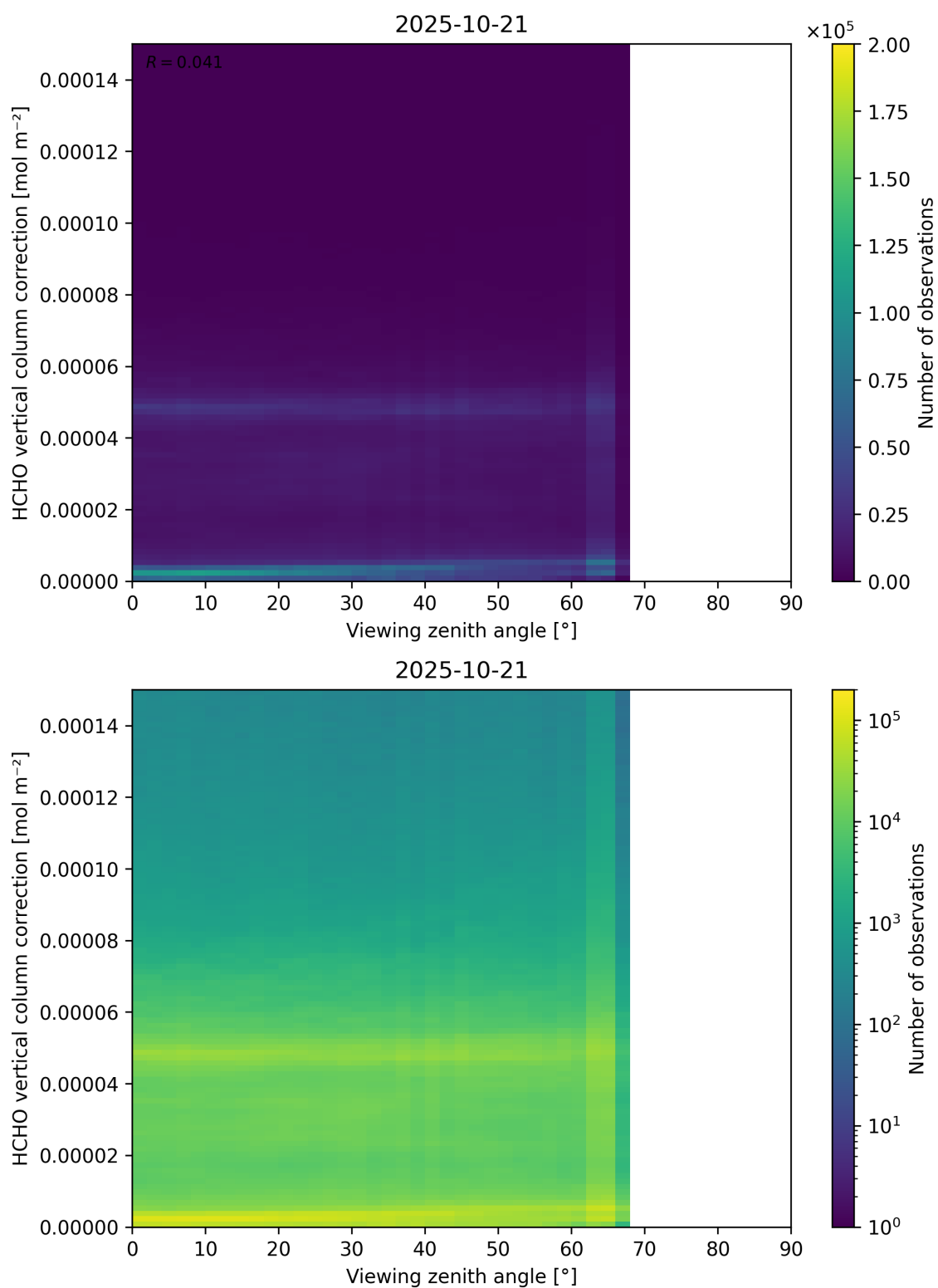
Figure 193: Scatter density plot of “Viewing zenith angle” against “HCHO vertical column correction” for 2025-10-20 to 2025-10-22.
