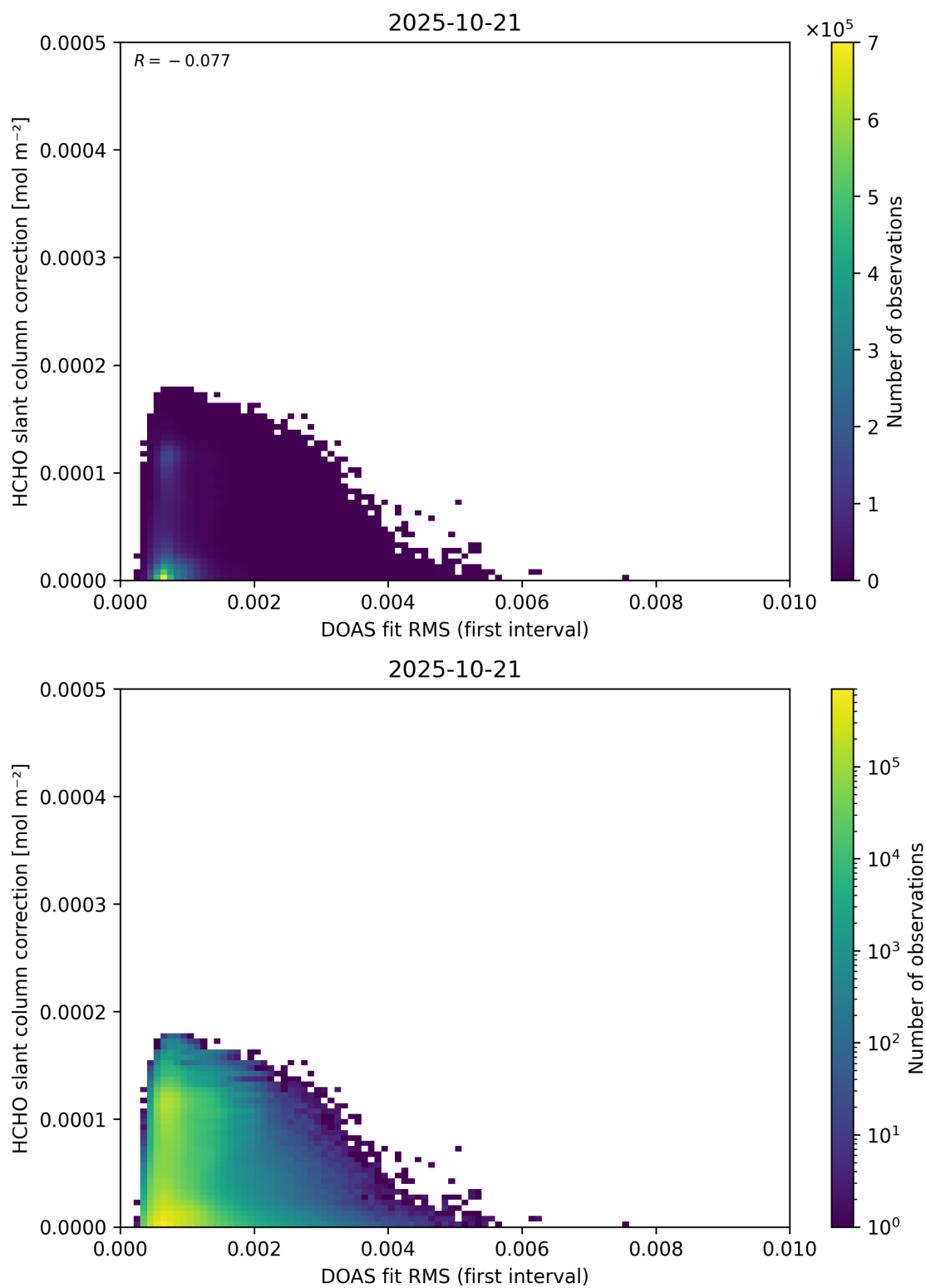
Figure 63: Scatter density plot of “DOAS fit RMS (first interval)” against “HCHO slant column correction” for 2025-10-20 to 2025-10-22.
