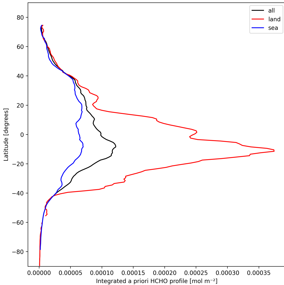
Figure 29: Zonal average of “Integrated a priori HCHO profile” for 2025-10-20 to 2025-10-22.
