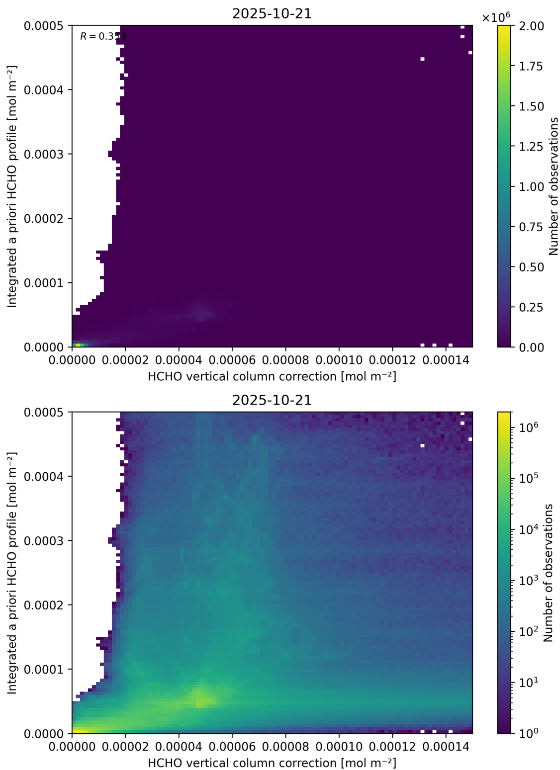
Figure 122: Scatter density plot of “HCHO vertical column correction” against “Integrated a priori HCHO profile” for 2025-10-20 to 2025-10-22.
