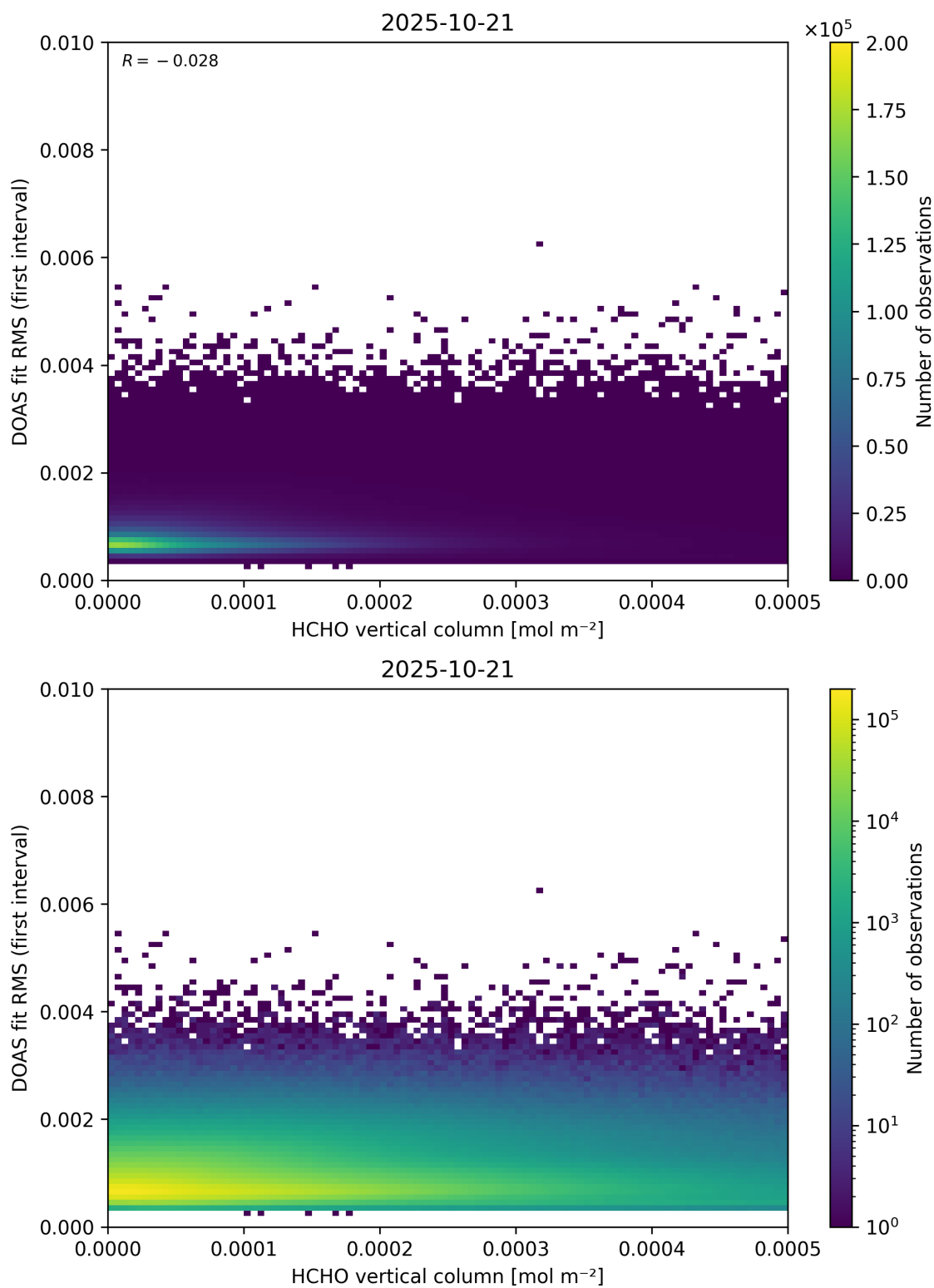
Figure 123: Scatter density plot of “HCHO vertical column” against “DOAS fit RMS (first interval)” for 2025-10-20 to 2025-10-22.
