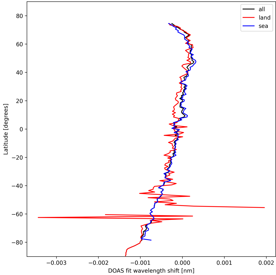
Figure 30: Zonal average of “DOAS fit wavelength shift” for 2025-10-20 to 2025-10-22.
