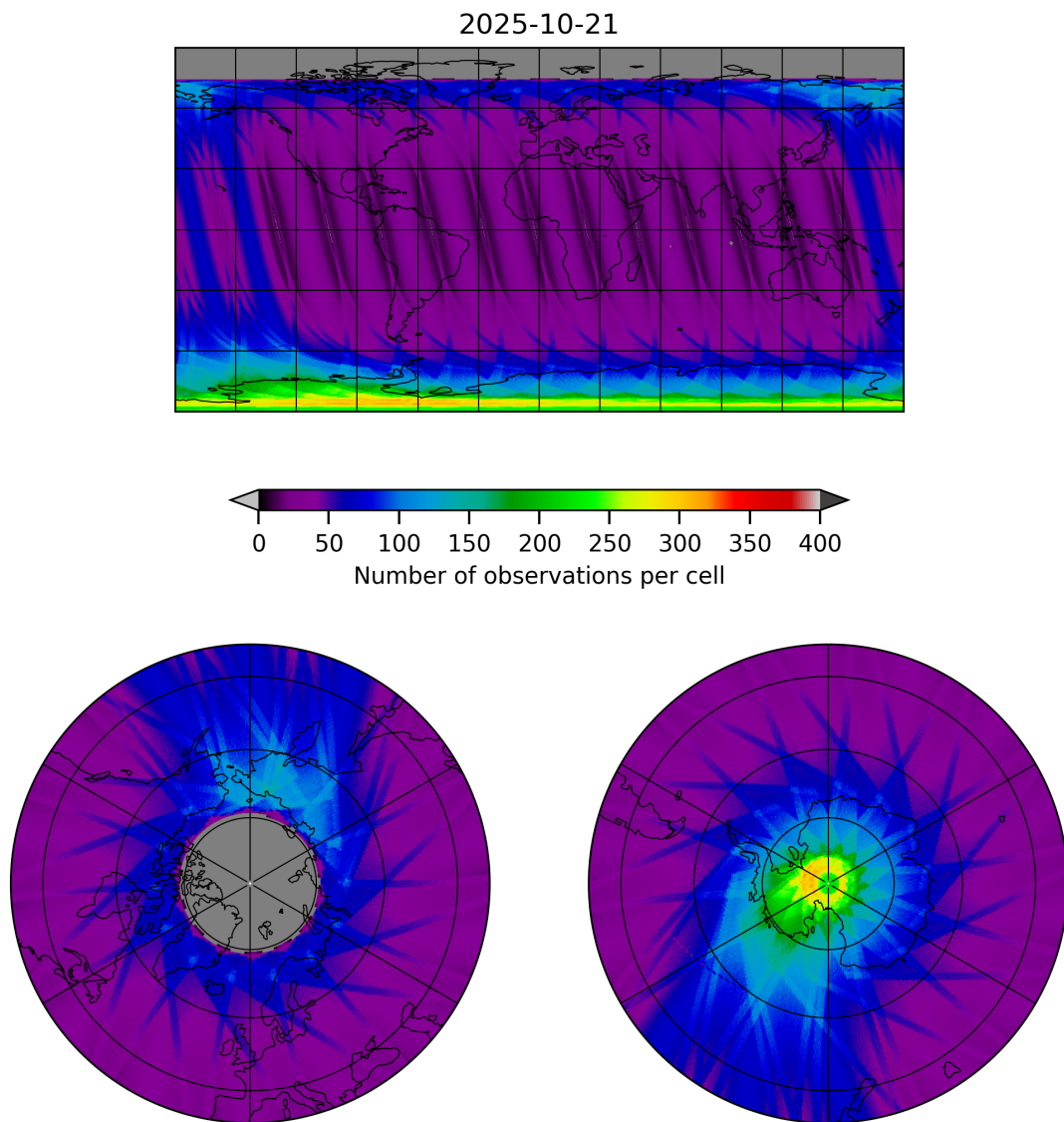
Figure 19: Map of the number of observations for 2025-10-20 to 2025-10-22
