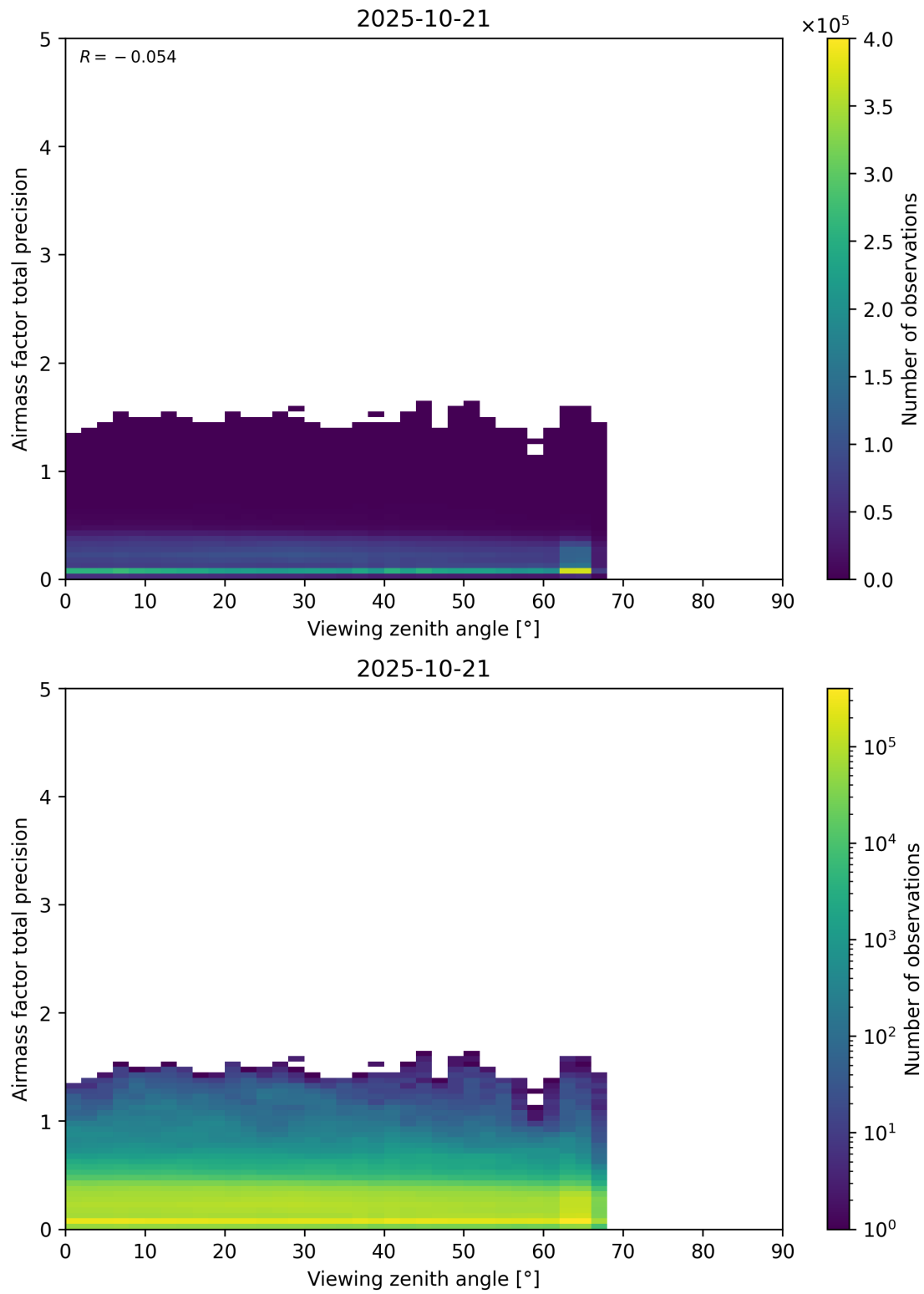
Figure 191: Scatter density plot of “Viewing zenith angle” against “Airmass factor total precision” for 2025-10-20 to 2025-10-22.
