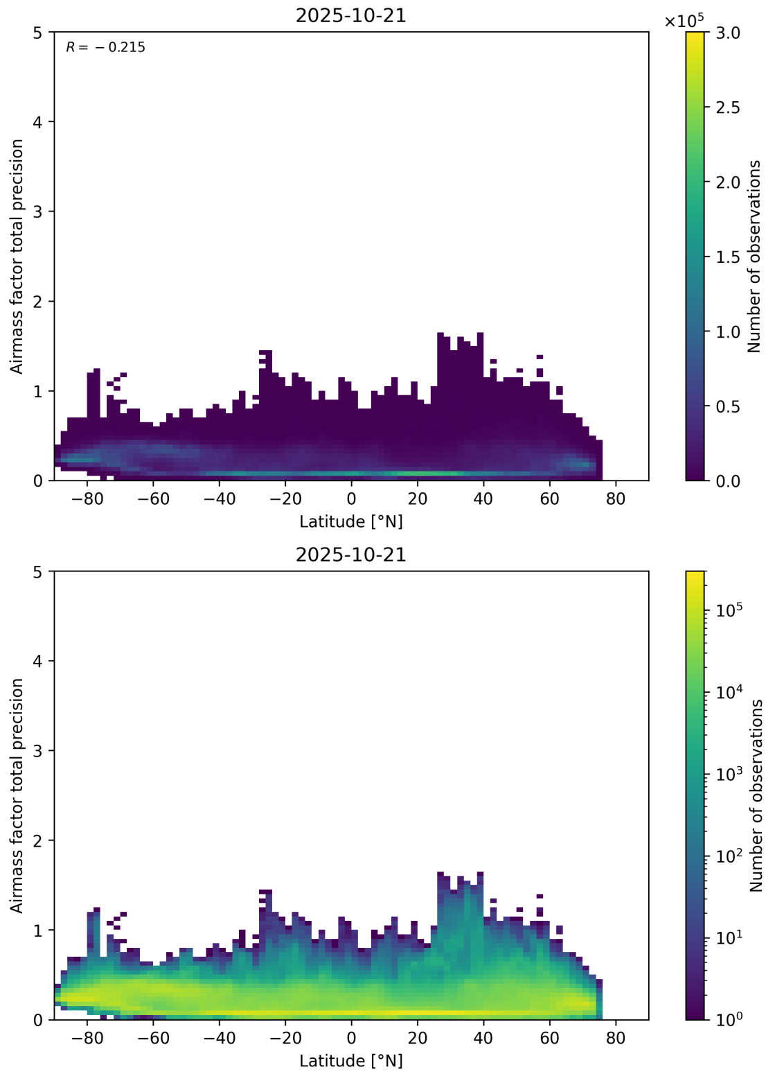
Figure 162: Scatter density plot of “Latitude” against “Airmass factor total precision” for 2025-10-20 to 2025-10-22.
