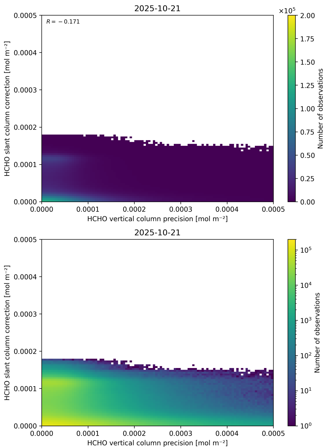
Figure 141: Scatter density plot of “HCHO vertical column precision” against “HCHO slant column correction” for 2025-10-20 to 2025-10-22.
