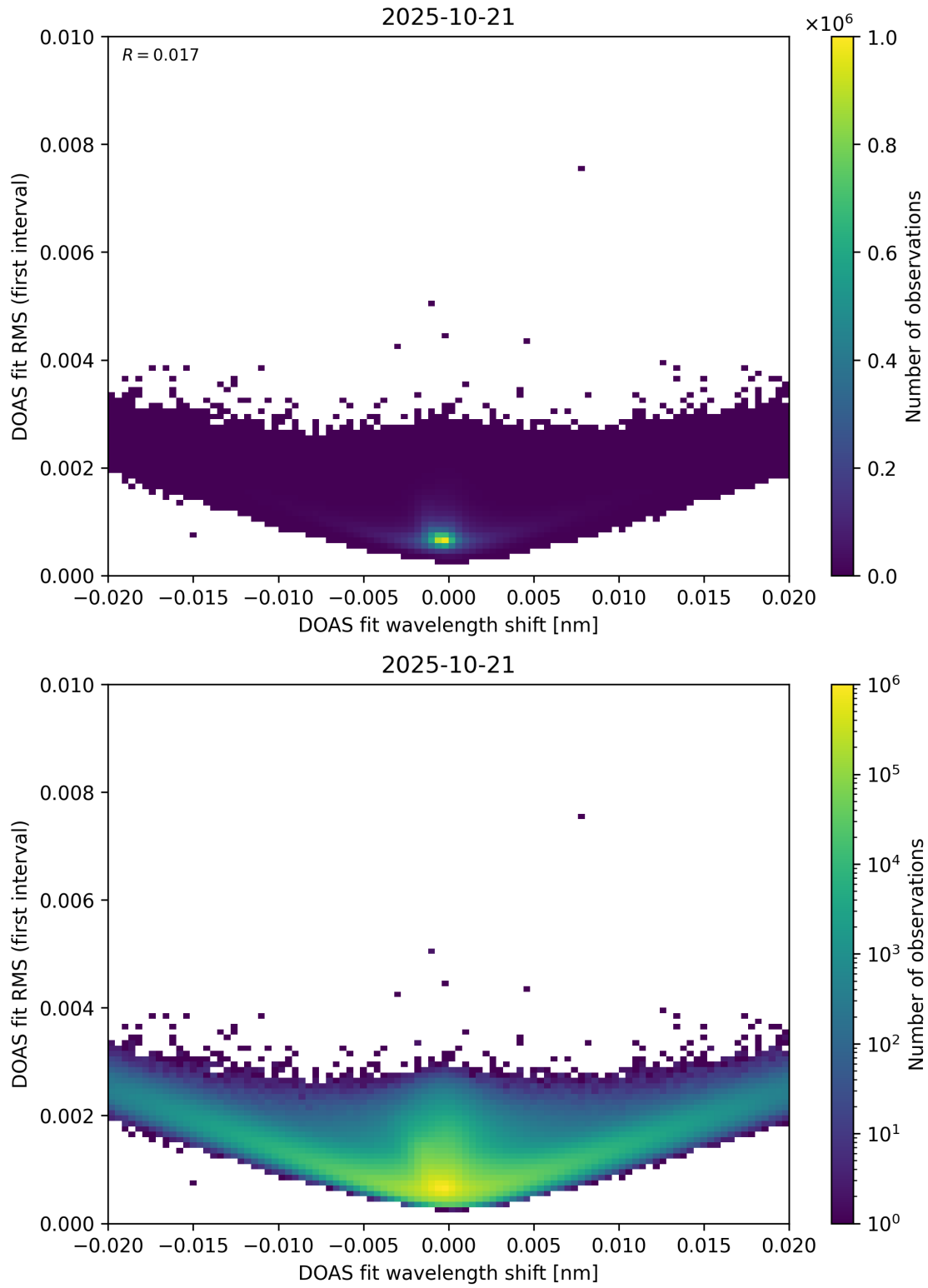
Figure 64: Scatter density plot of “DOAS fit wavelength shift” against “DOAS fit RMS (first interval)” for 2025-10-20 to 2025-10-22.
