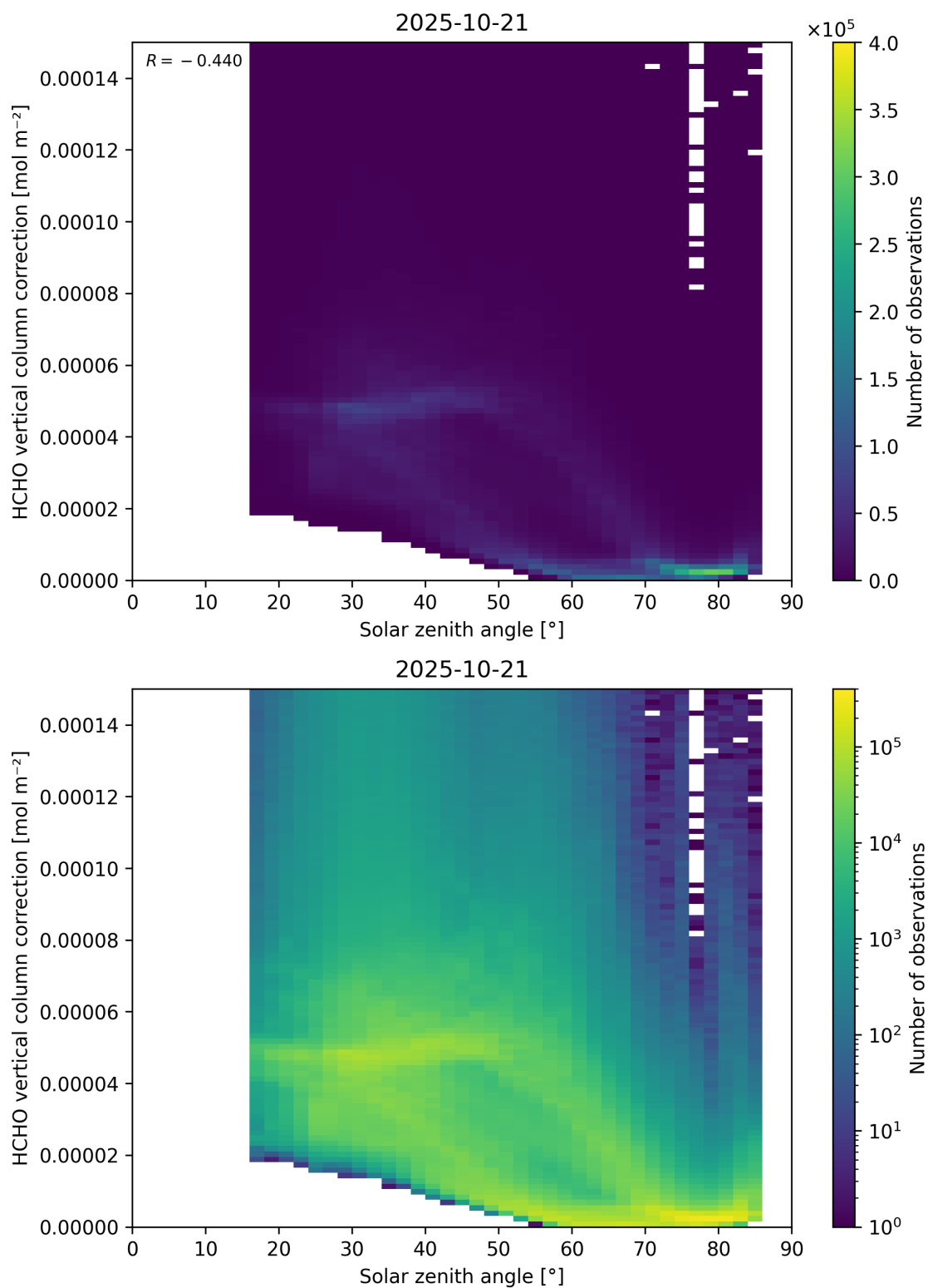
Figure 178: Scatter density plot of “Solar zenith angle” against “HCHO vertical column correction” for 2025-10-20 to 2025-10-22.
