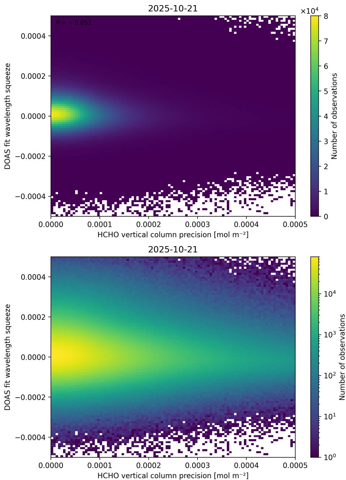
Figure 138: Scatter density plot of “HCHO vertical column precision” against “DOAS fit wavelength squeeze” for 2025-10-20 to 2025-10-22.
