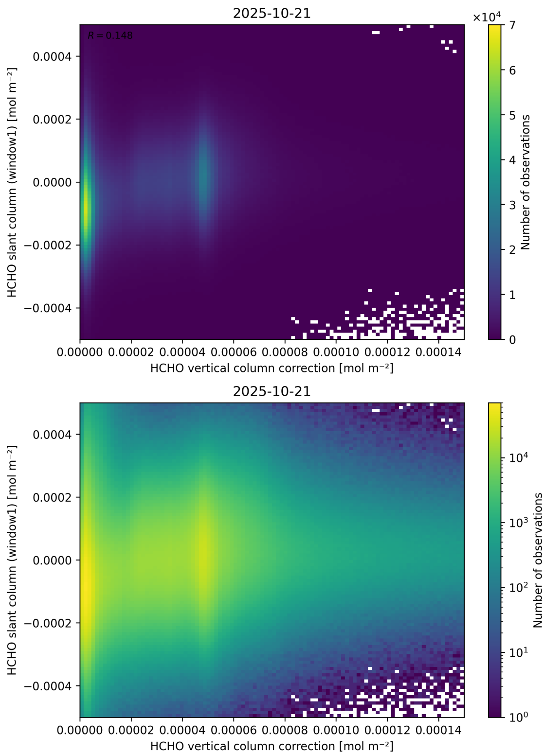
Figure 118: Scatter density plot of “HCHO vertical column correction” against “HCHO slant column (window1)” for 2025-10-20 to 2025-10-22.
