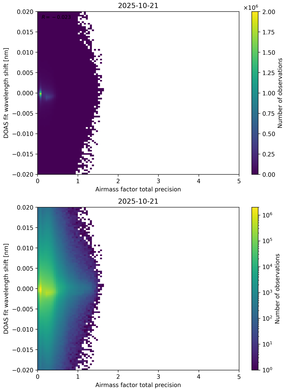
Figure 106: Scatter density plot of “Airmass factor total precision” against “DOAS fit wavelength shift” for 2025-10-20 to 2025-10-22.
