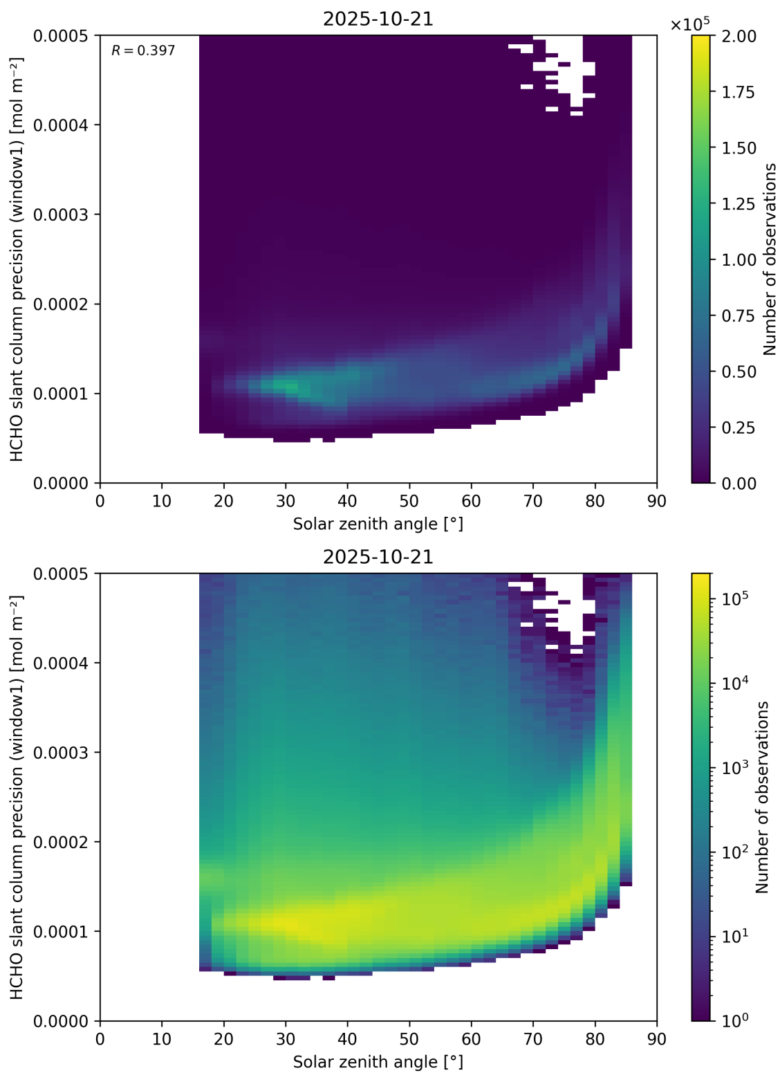
Figure 174: Scatter density plot of “Solar zenith angle” against “HCHO slant column precision (window1)” for 2025-10-20 to 2025-10-22.
