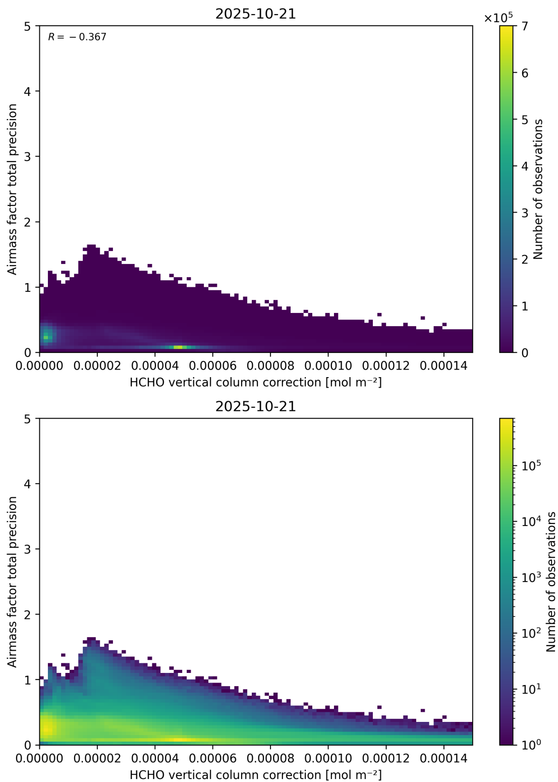
Figure 121: Scatter density plot of “HCHO vertical column correction” against “Airmass factor total precision” for 2025-10-20 to 2025-10-22.
