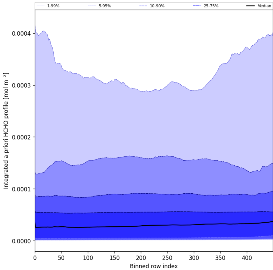
Figure 57: Along track statistics of "Integrated a priori HCHO profile" for 2025-10-20 to 2025-10-22
