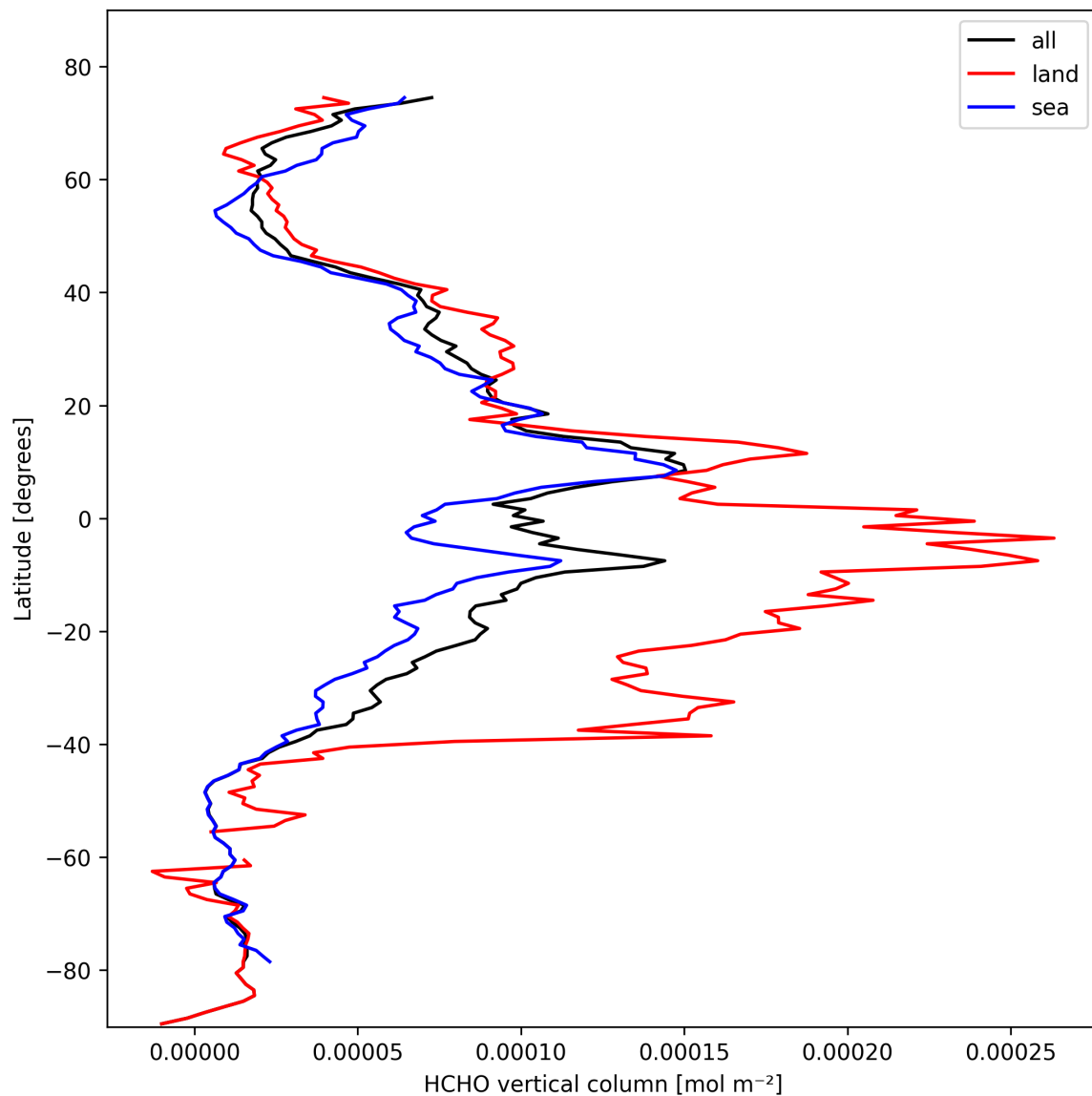
Figure 21: Zonal average of “HCHO vertical column” for 2025-10-20 to 2025-10-22.
