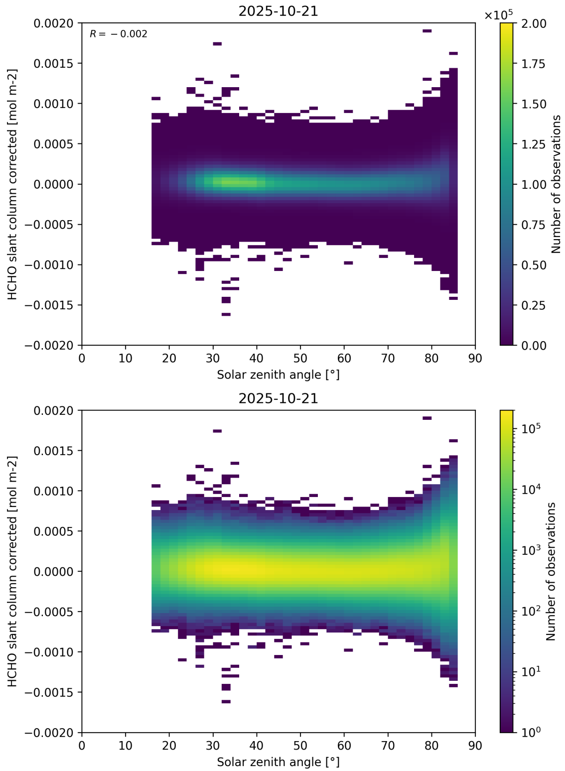
Figure 171: Scatter density plot of “Solar zenith angle” against “HCHO slant column corrected” for 2025-10-20 to 2025-10-22.
