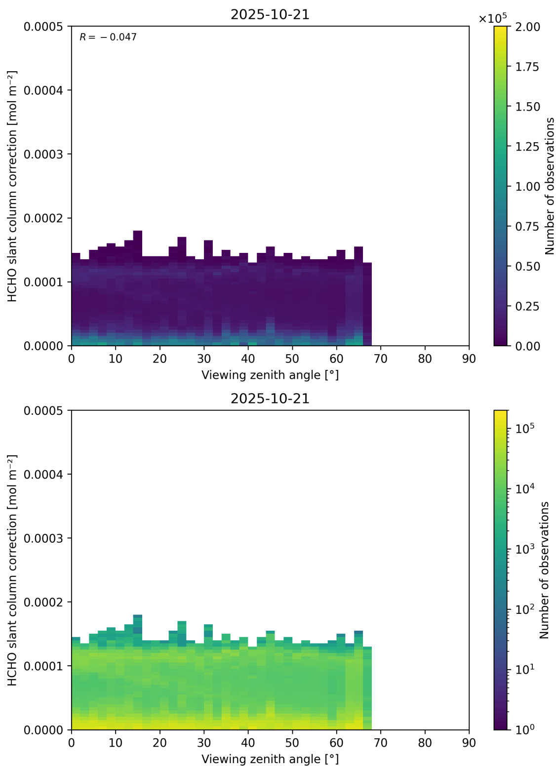
Figure 187: Scatter density plot of “Viewing zenith angle” against “HCHO slant column correction” for 2025-10-20 to 2025-10-22.
