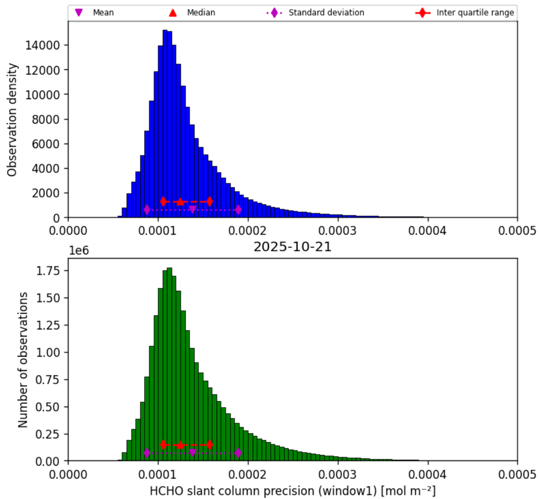
Figure 39: Histogram of “HCHO slant column precision (window1)” for 2025-10-20 to 2025-10-22
