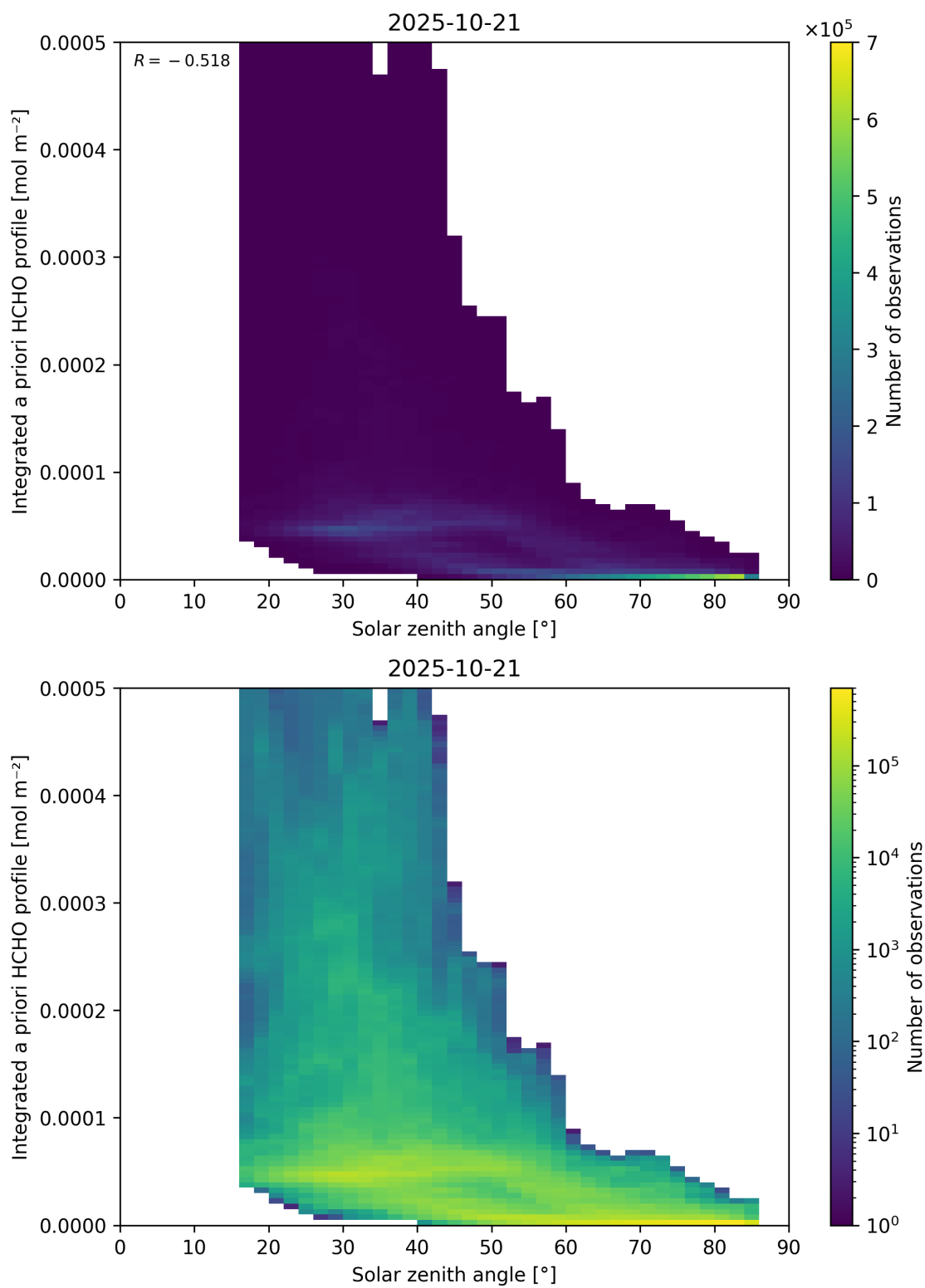
Figure 180: Scatter density plot of “Solar zenith angle” against “Integrated a priori HCHO profile” for 2025-10-20 to 2025-10-22.
