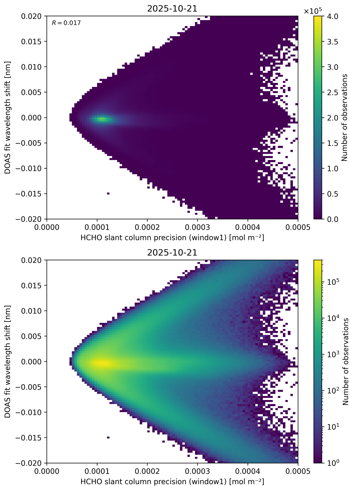
Figure 89: Scatter density plot of “HCHO slant column precision (window1)” against “DOAS fit wavelength shift” for 2025-10-20 to 2025-10-22.
