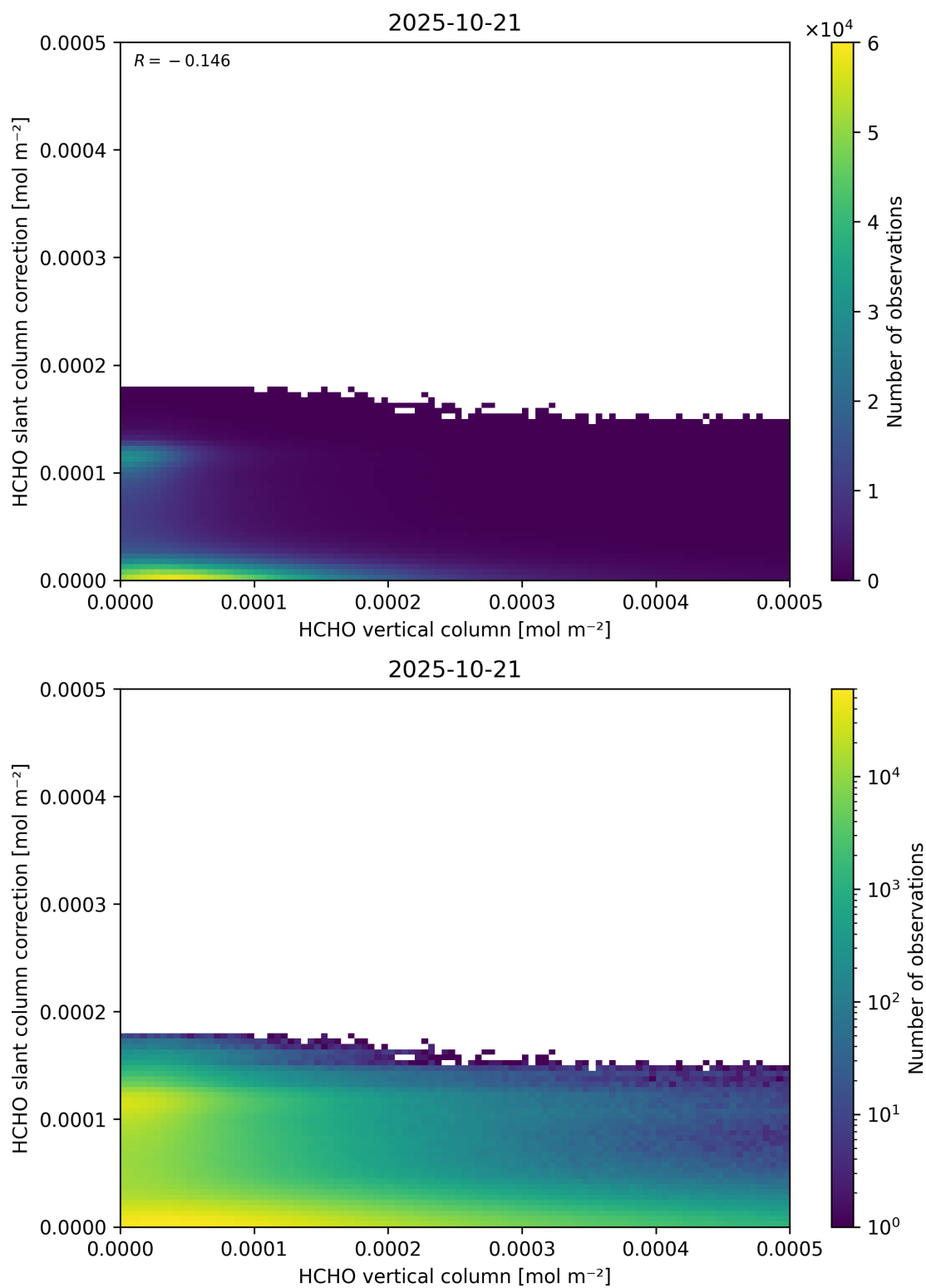
Figure 128: Scatter density plot of “HCHO vertical column” against “HCHO slant column correction” for 2025-10-20 to 2025-10-22.
