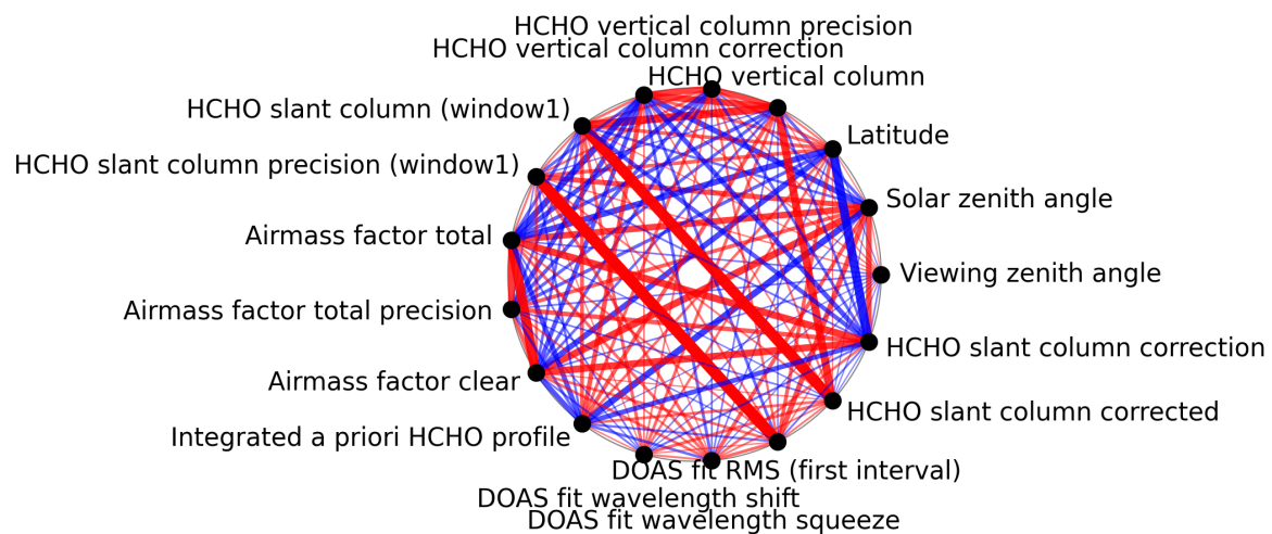
Figure 1: Map of correlation graph for 2025-10-20 to 2025-10-22.
