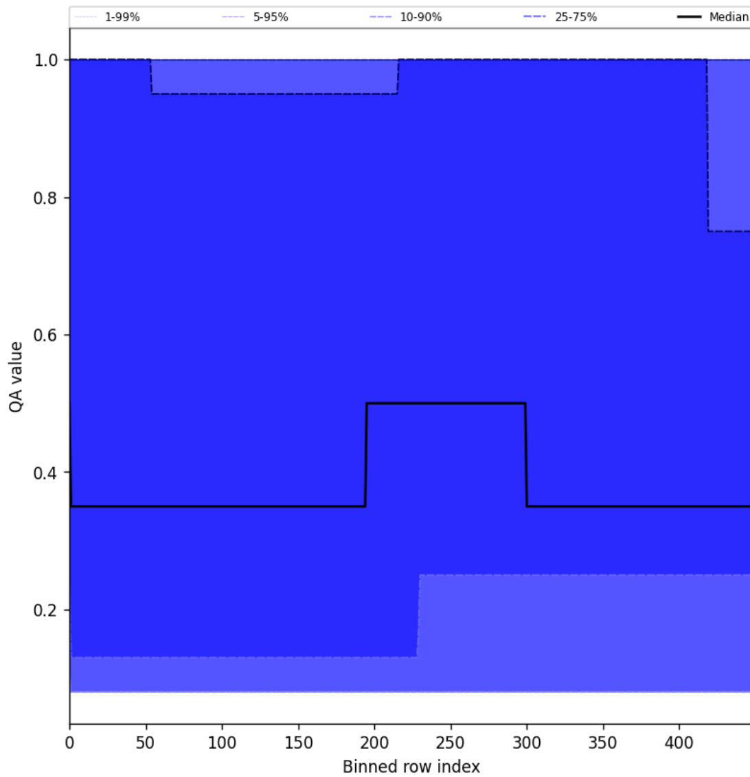
Figure 48: Along track statistics of “QA value” for 2025-10-20 to 2025-10-22
