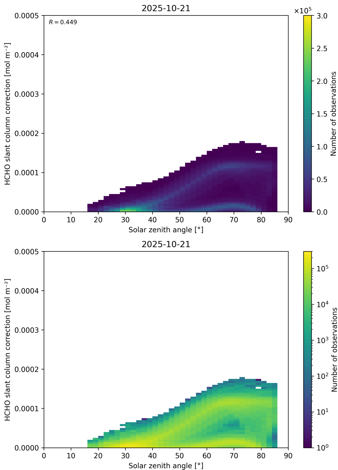
Figure 172: Scatter density plot of “Solar zenith angle” against “HCHO slant column correction” for 2025-10-20 to 2025-10-22.
