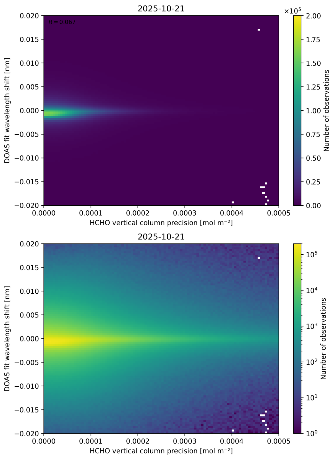
Figure 137: Scatter density plot of “HCHO vertical column precision” against “DOAS fit wavelength shift” for 2025-10-20 to 2025-10-22.
