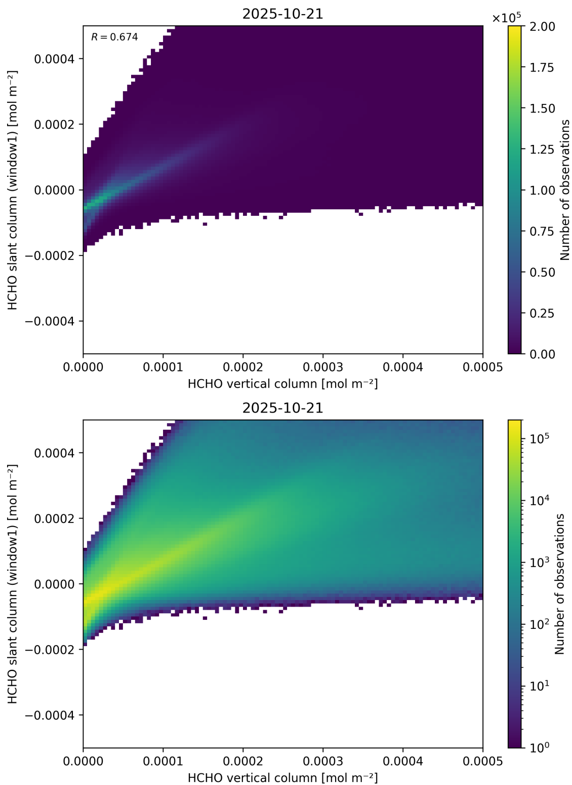
Figure 129: Scatter density plot of “HCHO vertical column” against “HCHO slant column (window1)” for 2025-10-20 to 2025-10-22.
