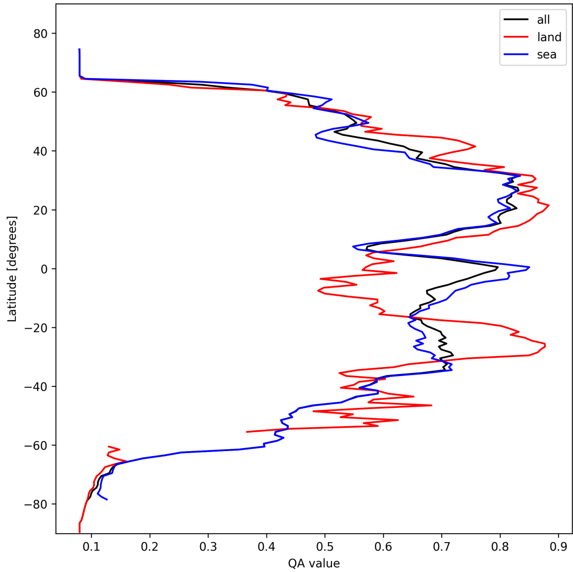
Figure 20: Zonal average of “QA value” for 2025-10-20 to 2025-10-22.
