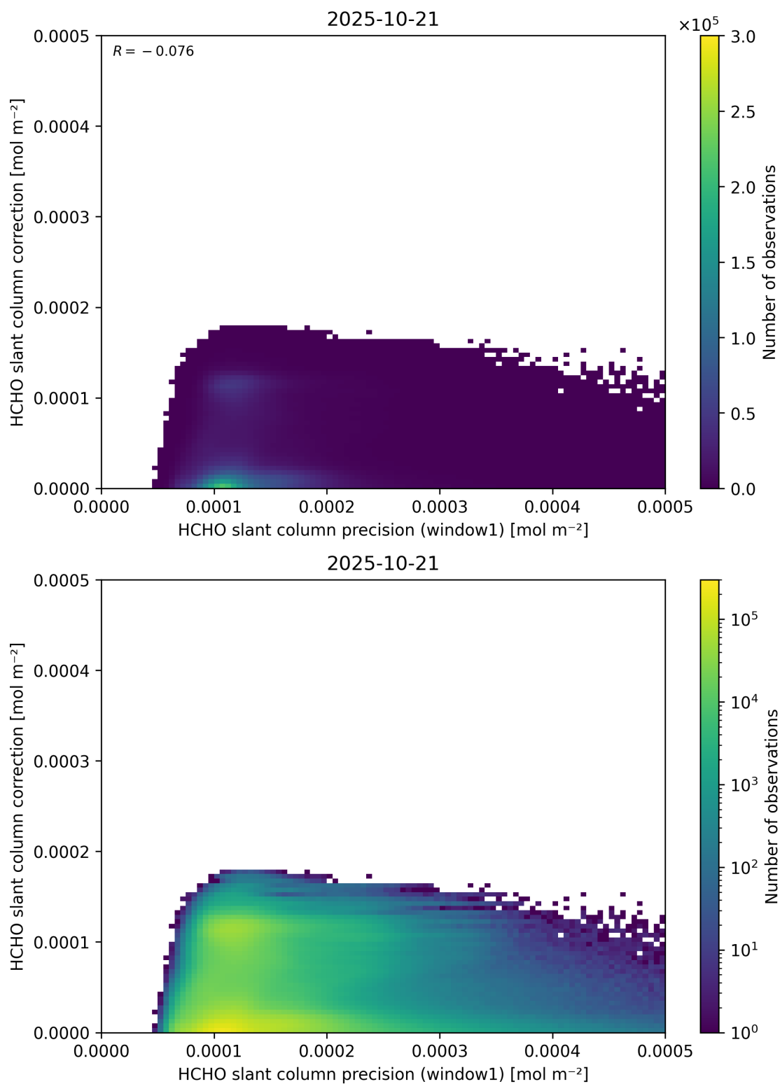
Figure 93: Scatter density plot of “HCHO slant column precision (window1)” against “HCHO slant column correction” for 2025-10-20 to 2025-10-22.
