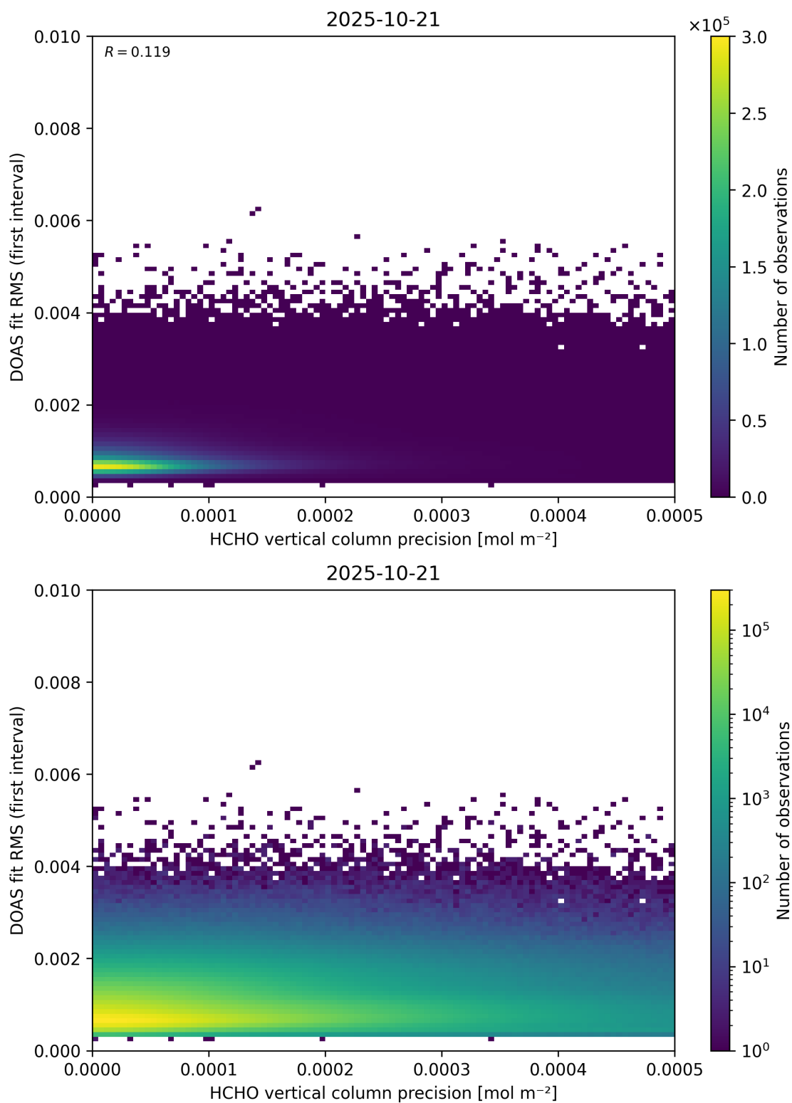
Figure 136: Scatter density plot of “HCHO vertical column precision” against “DOAS fit RMS (first interval)” for 2025-10-20 to 2025-10-22.
