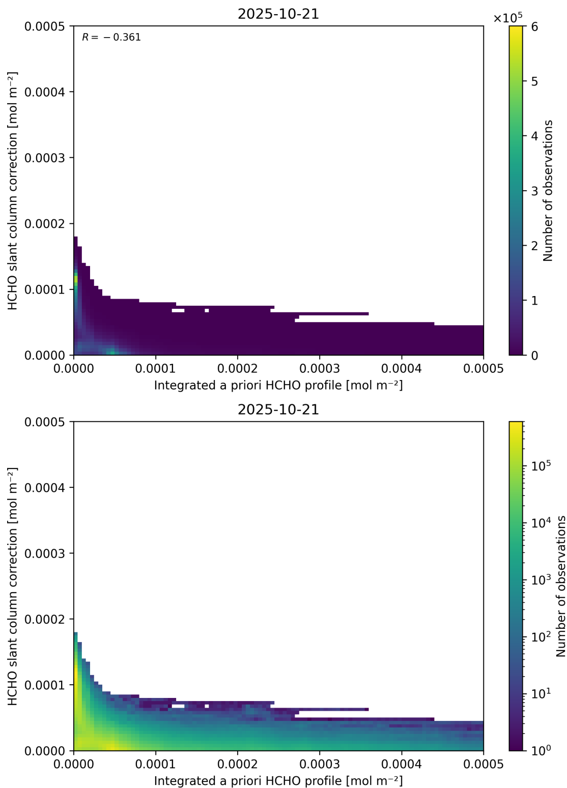
Figure 152: Scatter density plot of “Integrated a priori HCHO profile” against “HCHO slant column correction” for 2025-10-20 to 2025-10-22.
