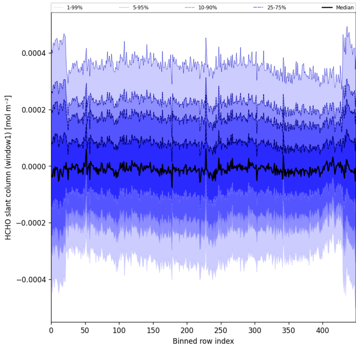
Figure 52: Along track statistics of “HCHO slant column (window1)” for 2025-10-20 to 2025-10-22
