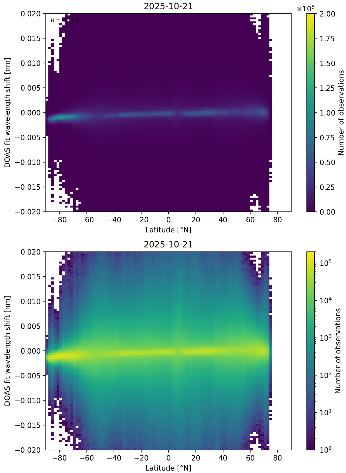
Figure 154: Scatter density plot of “Latitude” against “DOAS fit wavelength shift” for 2025-10-20 to 2025-10-22.
