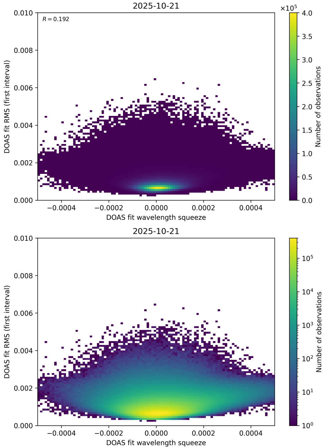
Figure 68: Scatter density plot of “DOAS fit wavelength squeeze” against “DOAS fit RMS (first interval)” for 2025-10-20 to 2025-10-22.
