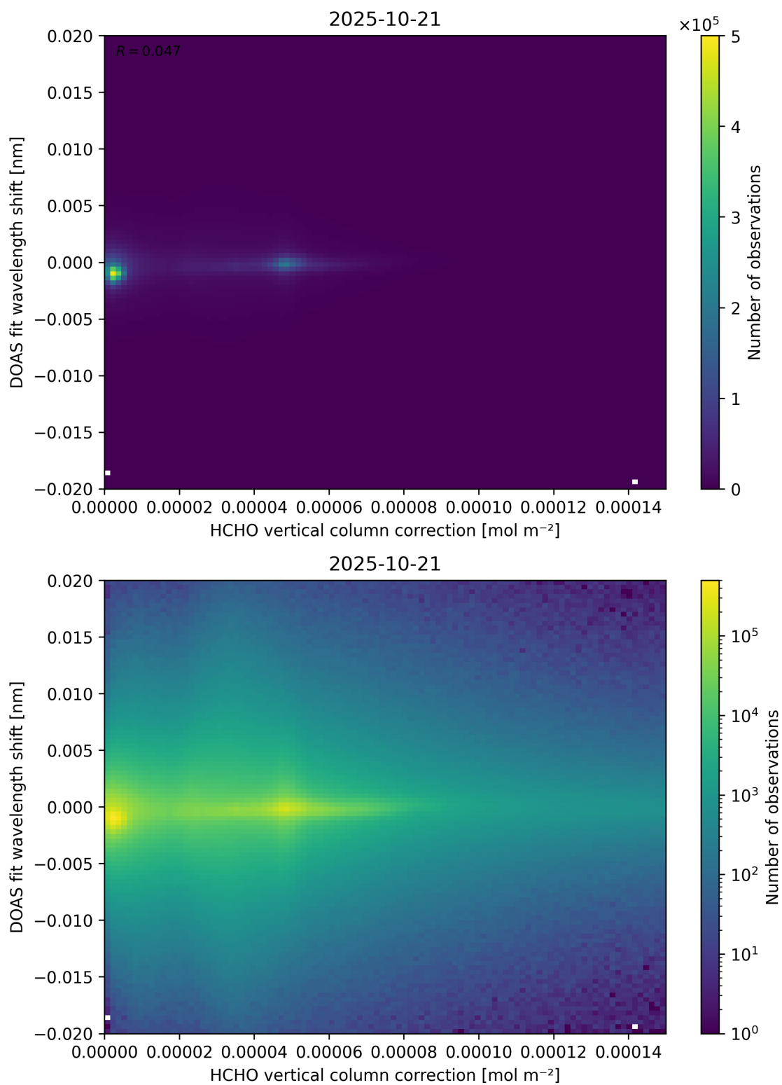
Figure 113: Scatter density plot of “HCHO vertical column correction” against “DOAS fit wavelength shift” for 2025-10-20 to 2025-10-22.
