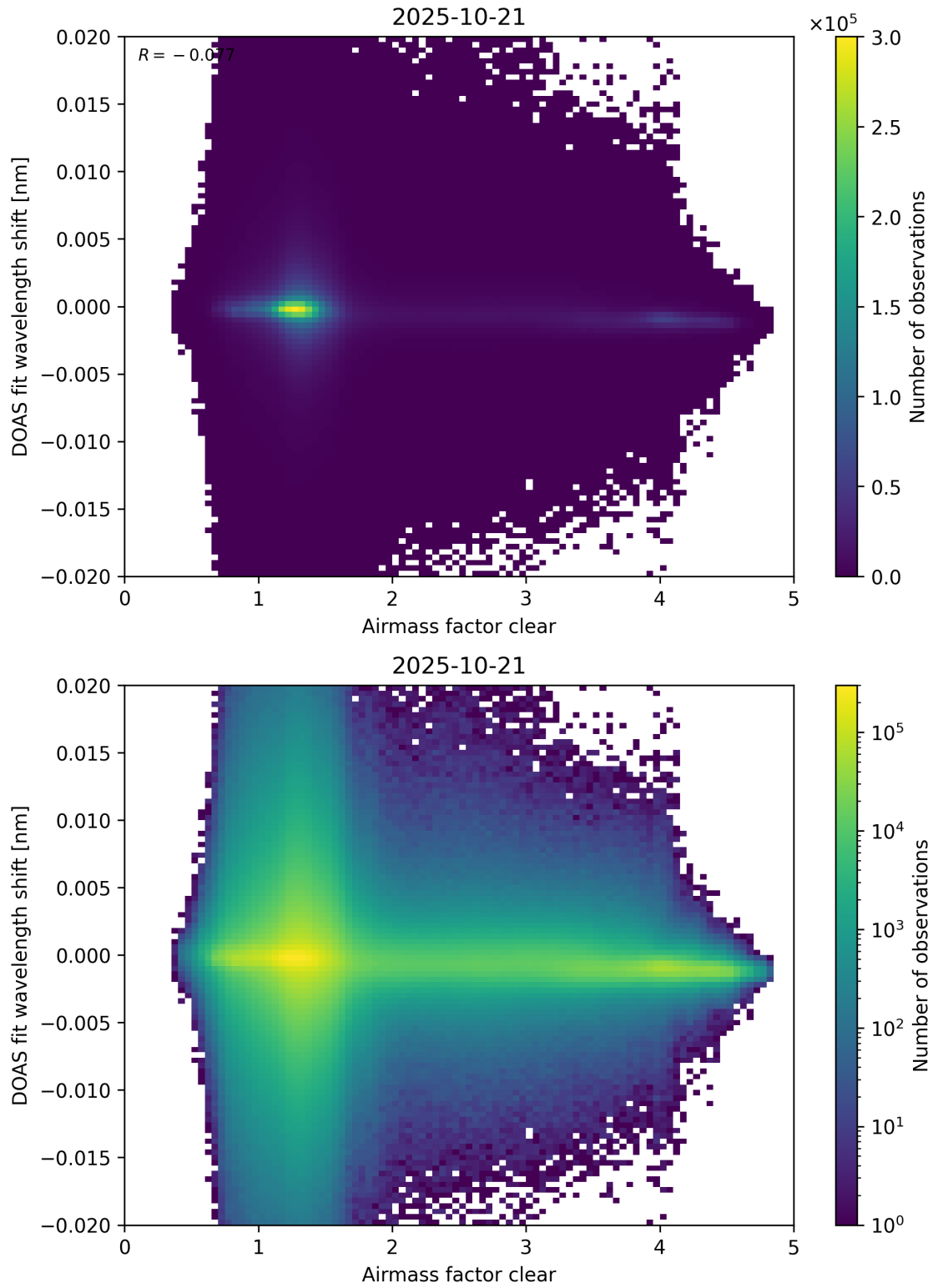
Figure 72: Scatter density plot of “Airmass factor clear” against “DOAS fit wavelength shift” for 2025-10-20 to 2025-10-22.
