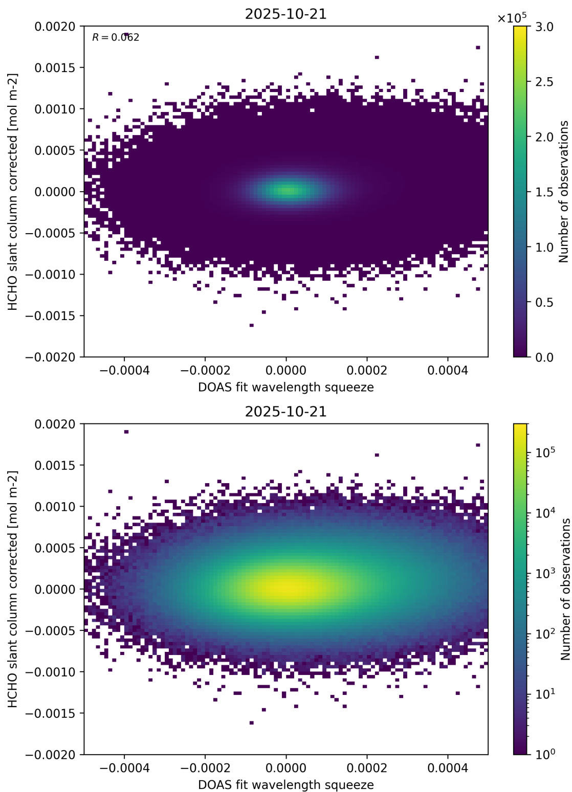
Figure 69: Scatter density plot of “DOAS fit wavelength squeeze” against “HCHO slant column corrected” for 2025-10-20 to 2025-10-22.
