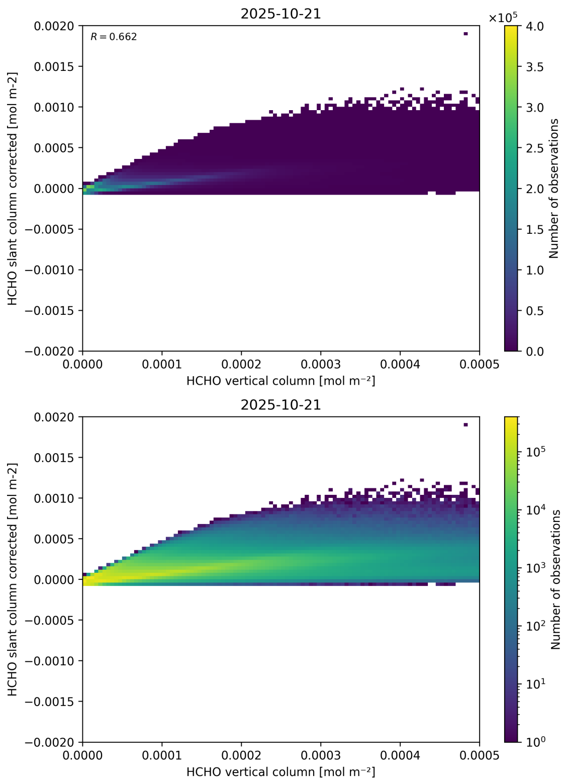
Figure 127: Scatter density plot of “HCHO vertical column” against “HCHO slant column corrected” for 2025-10-20 to 2025-10-22.
