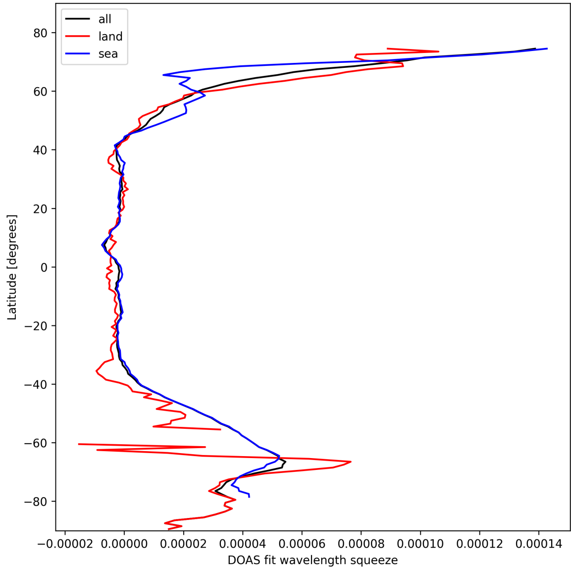
Figure 31: Zonal average of “DOAS fit wavelength squeeze” for 2025-10-20 to 2025-10-22.
