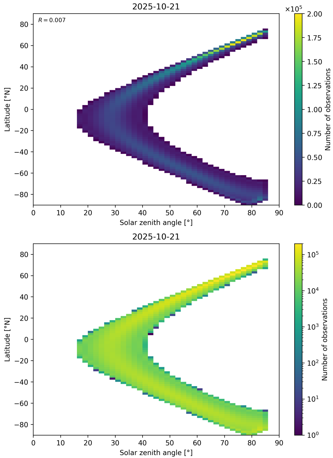
Figure 181: Scatter density plot of “Solar zenith angle” against “Latitude” for 2025-10-20 to 2025-10-22.
