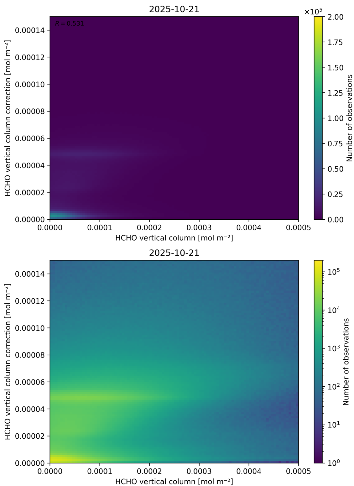
Figure 133: Scatter density plot of “HCHO vertical column” against “HCHO vertical column correction” for 2025-10-20 to 2025-10-22.
