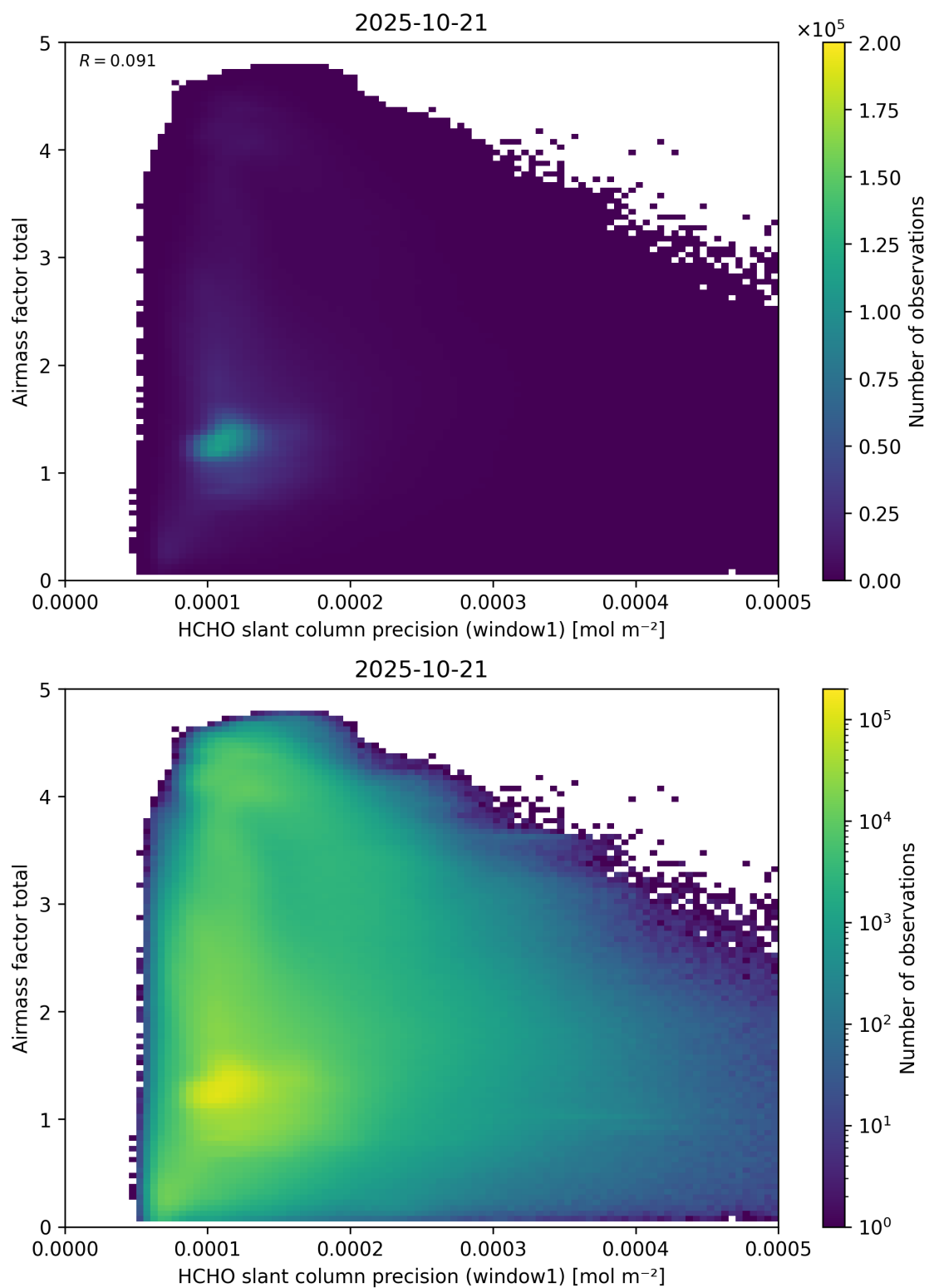
Figure 94: Scatter density plot of “HCHO slant column precision (window1)” against “Airmass factor total” for 2025-10-20 to 2025-10-22.
