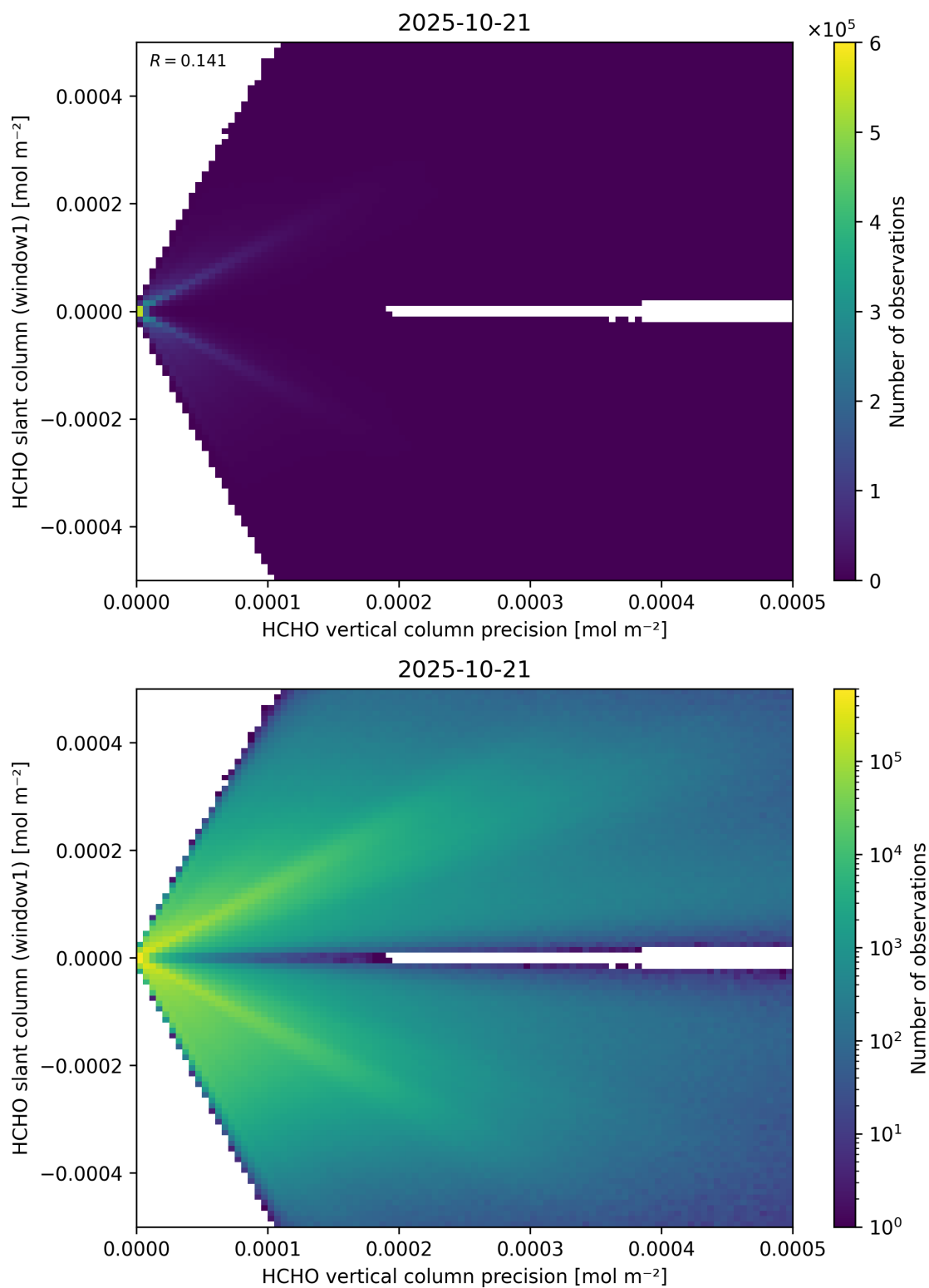
Figure 142: Scatter density plot of “HCHO vertical column precision” against “HCHO slant column (window1)” for 2025-10-20 to 2025-10-22.
