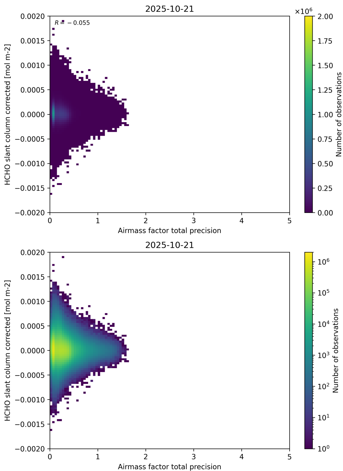
Figure 109: Scatter density plot of “Airmass factor total precision” against “HCHO slant column corrected” for 2025-10-20 to 2025-10-22.
