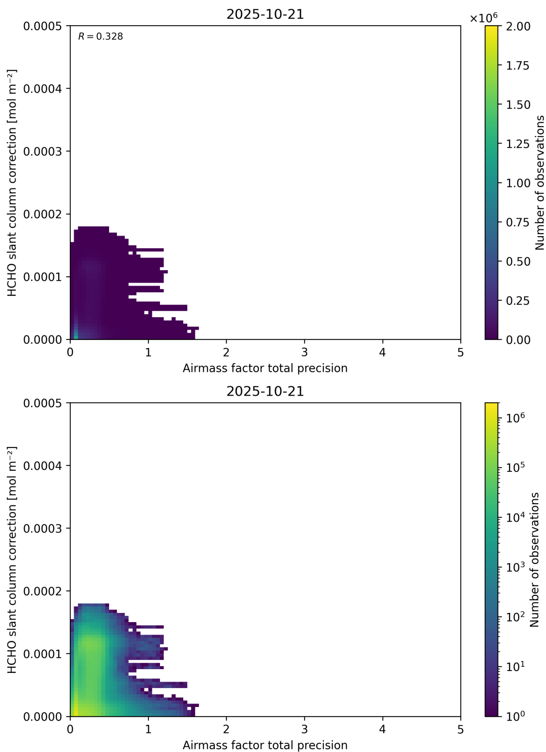
Figure 110: Scatter density plot of “Airmass factor total precision” against “HCHO slant column correction” for 2025-10-20 to 2025-10-22.
