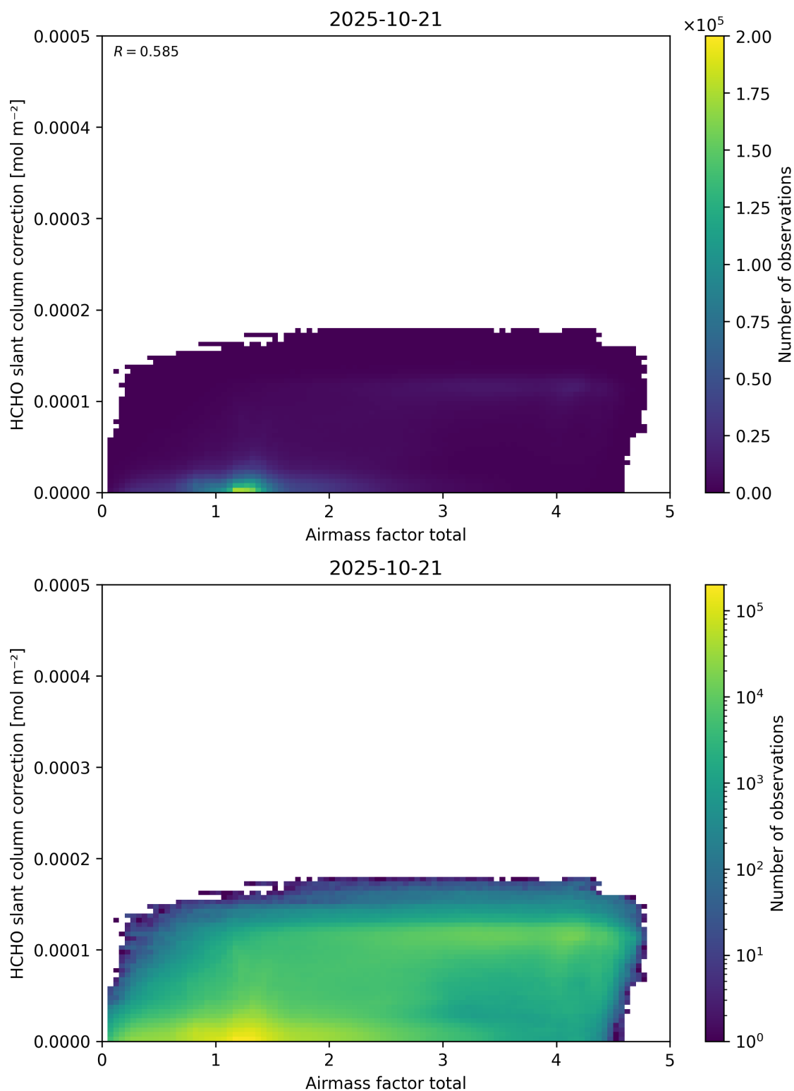
Figure 102: Scatter density plot of “Airmass factor total” against “HCHO slant column correction” for 2025-10-20 to 2025-10-22.
