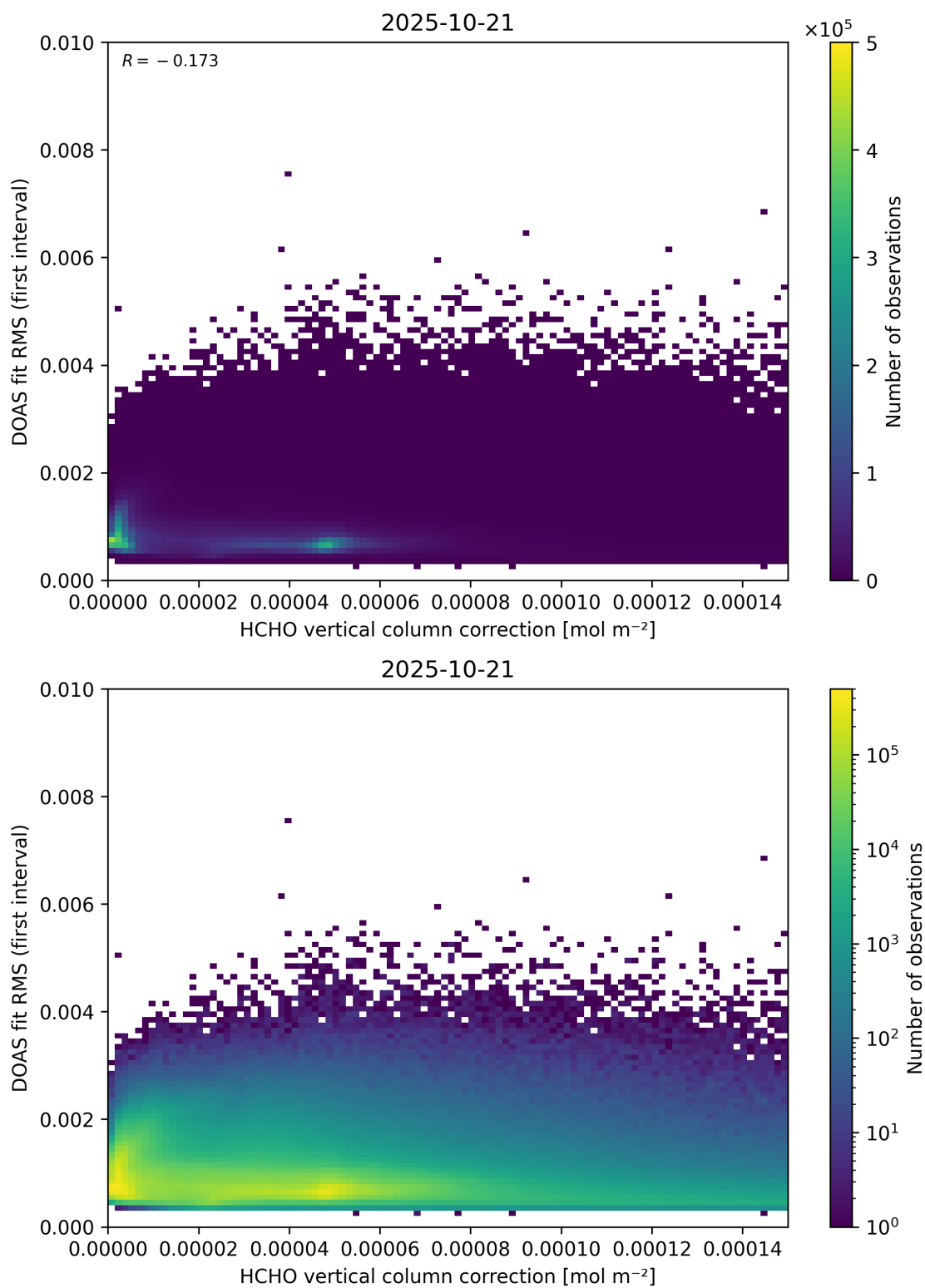
Figure 112: Scatter density plot of “HCHO vertical column correction” against “DOAS fit RMS (first interval)” for 2025-10-20 to 2025-10-22.
