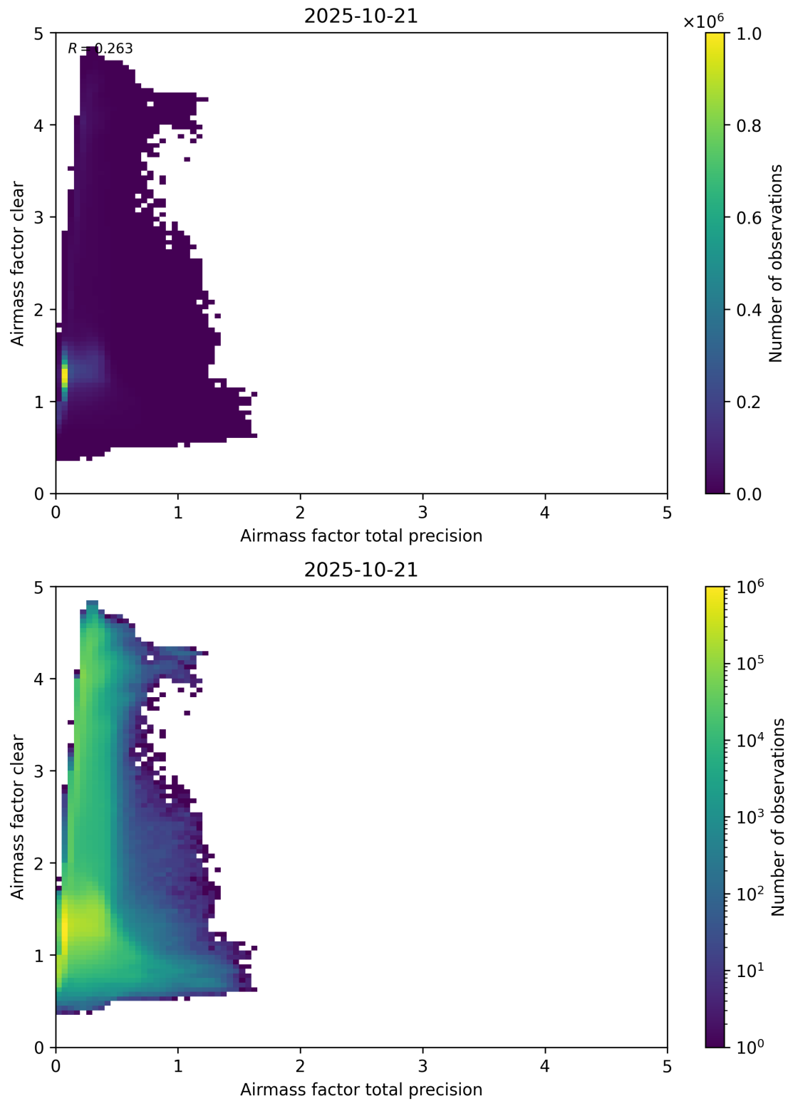
Figure 108: Scatter density plot of “Airmass factor total precision” against “Airmass factor clear” for 2025-10-20 to 2025-10-22.
