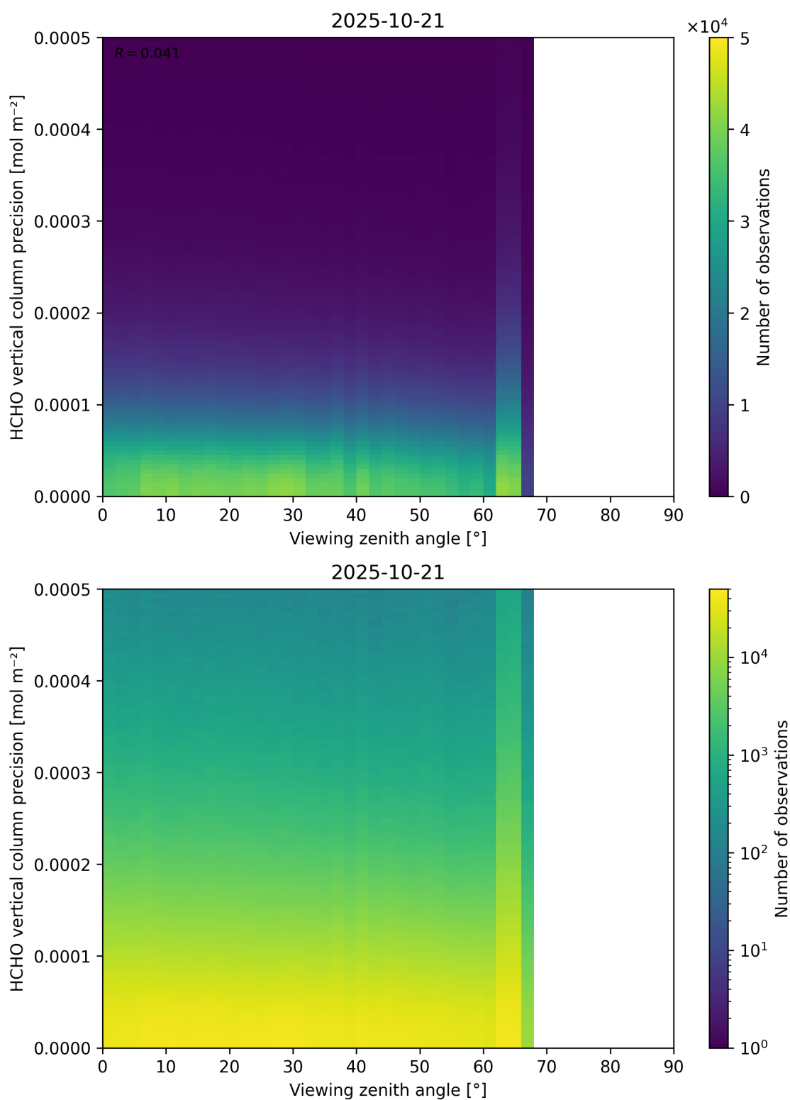
Figure 194: Scatter density plot of “Viewing zenith angle” against “HCHO vertical column precision” for 2025-10-20 to 2025-10-22.
