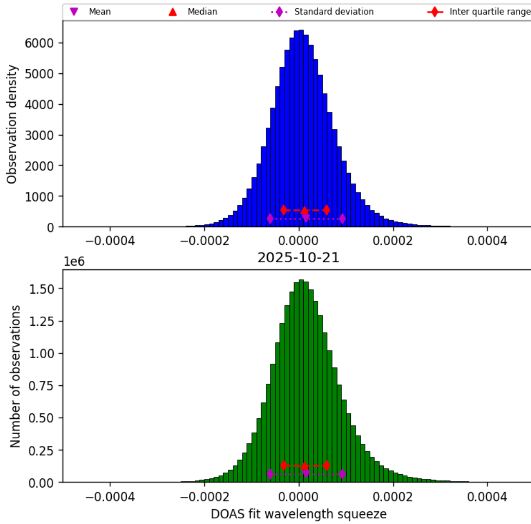
Figure 45: Histogram of “DOAS fit wavelength squeeze” for 2025-10-20 to 2025-10-22
