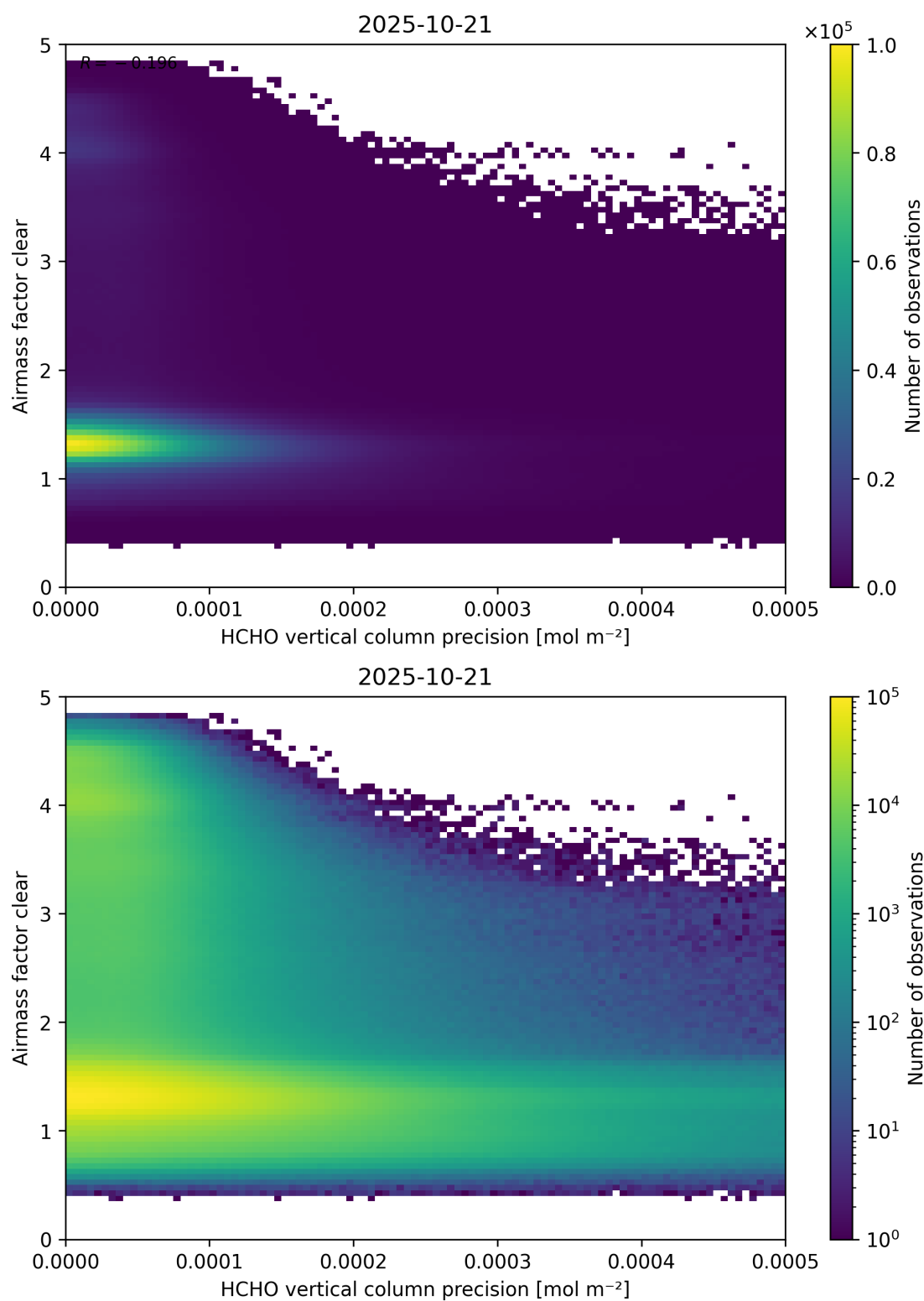
Figure 139: Scatter density plot of “HCHO vertical column precision” against “Airmass factor clear” for 2025-10-20 to 2025-10-22.
