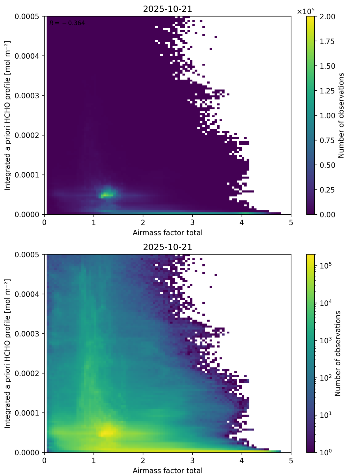
Figure 104: Scatter density plot of “Airmass factor total” against “Integrated a priori HCHO profile” for 2025-10-20 to 2025-10-22.
