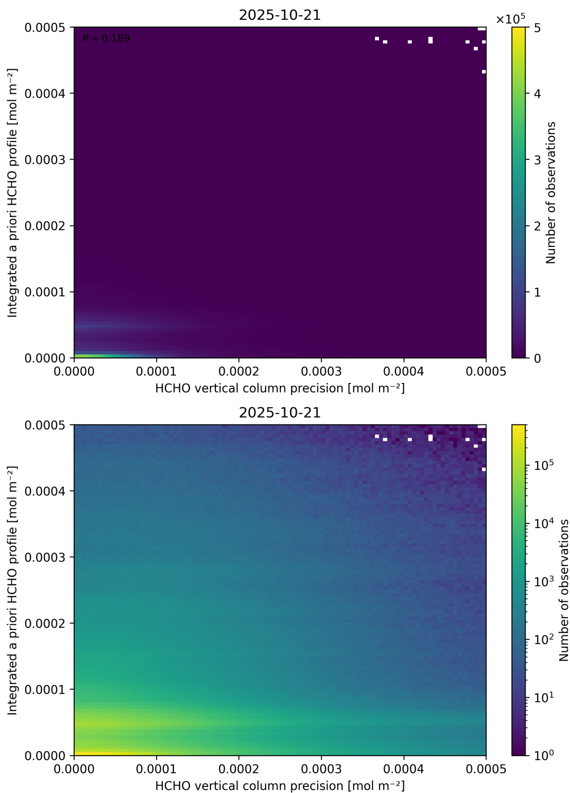
Figure 147: Scatter density plot of “HCHO vertical column precision” against “Integrated a priori HCHO profile” for 2025-10-20 to 2025-10-22.
