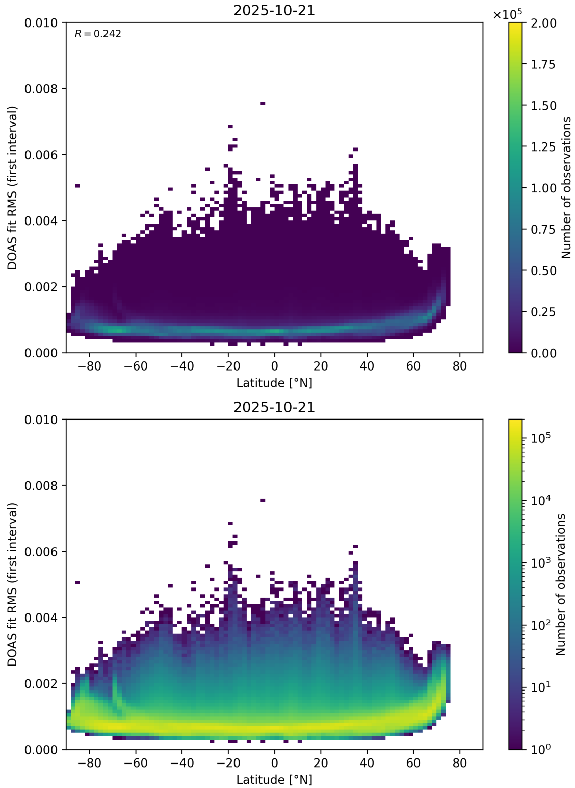
Figure 153: Scatter density plot of “Latitude” against “DOAS fit RMS (first interval)” for 2025-10-20 to 2025-10-22.
