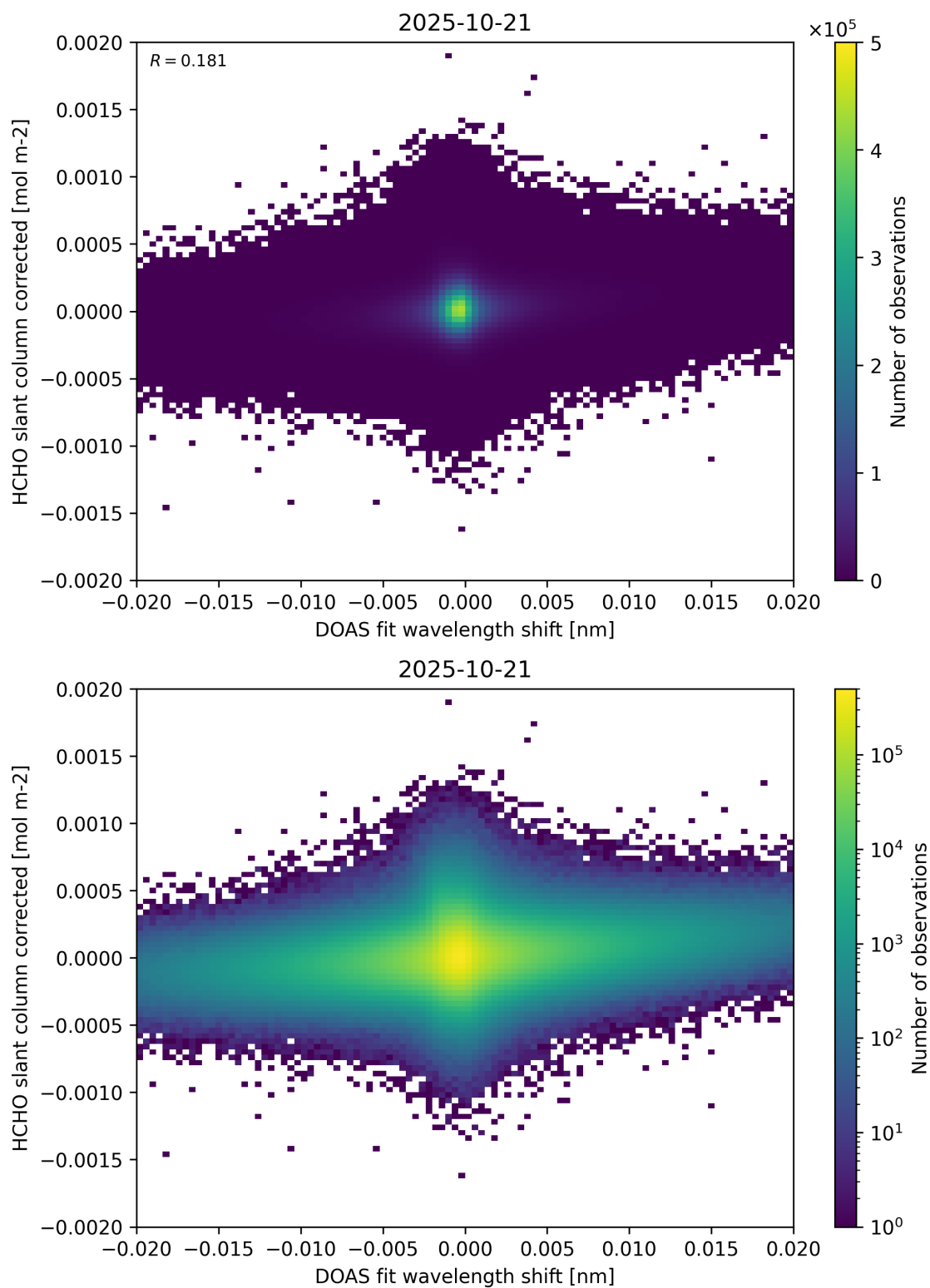
Figure 66: Scatter density plot of “DOAS fit wavelength shift” against “HCHO slant column corrected” for 2025-10-20 to 2025-10-22.
