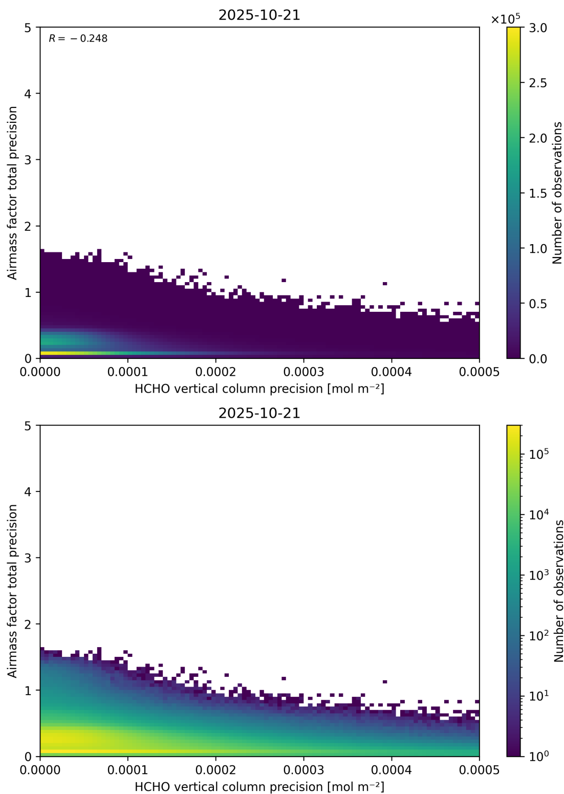
Figure 145: Scatter density plot of “HCHO vertical column precision” against “Airmass factor total precision” for 2025-10-20 to 2025-10-22.
