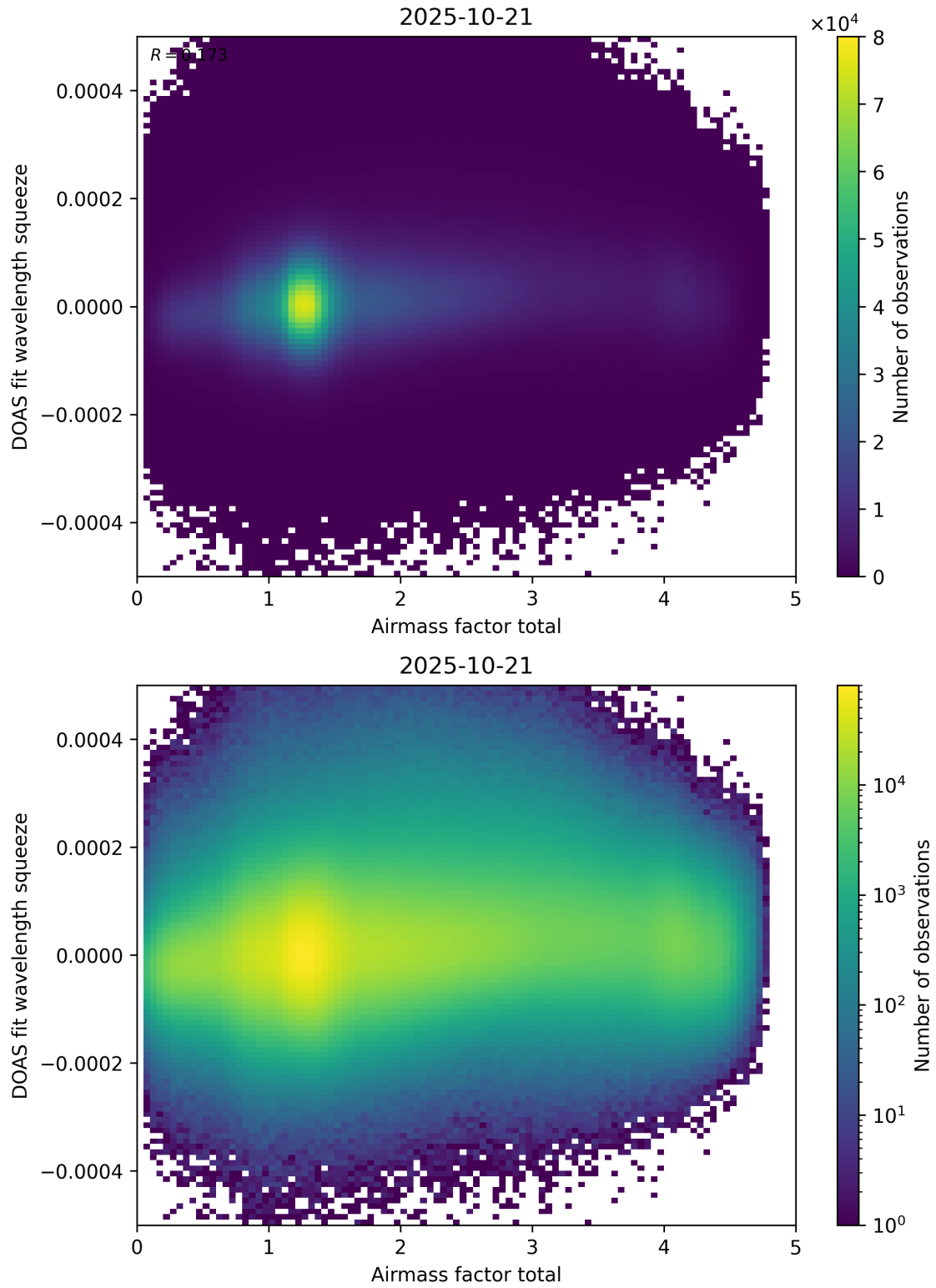
Figure 99: Scatter density plot of “Airmass factor total” against “DOAS fit wavelength squeeze” for 2025-10-20 to 2025-10-22.
