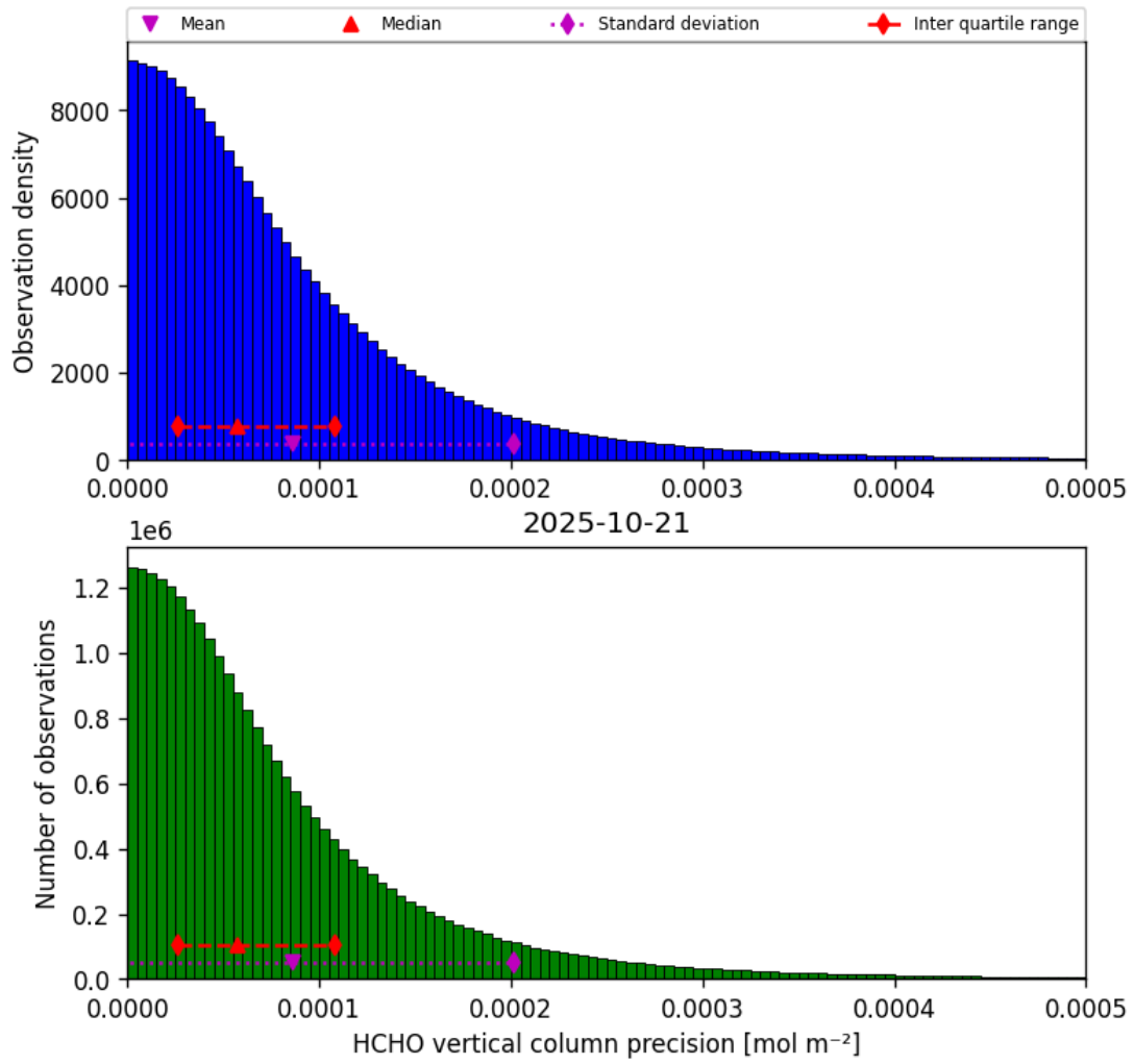
Figure 36: Histogram of “HCHO vertical column precision” for 2025-10-20 to 2025-10-22
