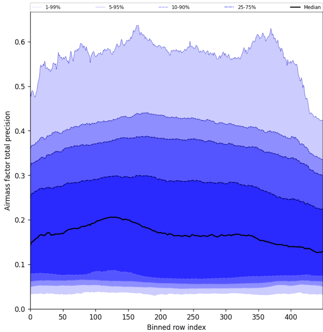
Figure 55: Along track statistics of “Airmass factor total precision” for 2025-10-20 to 2025-10-22
