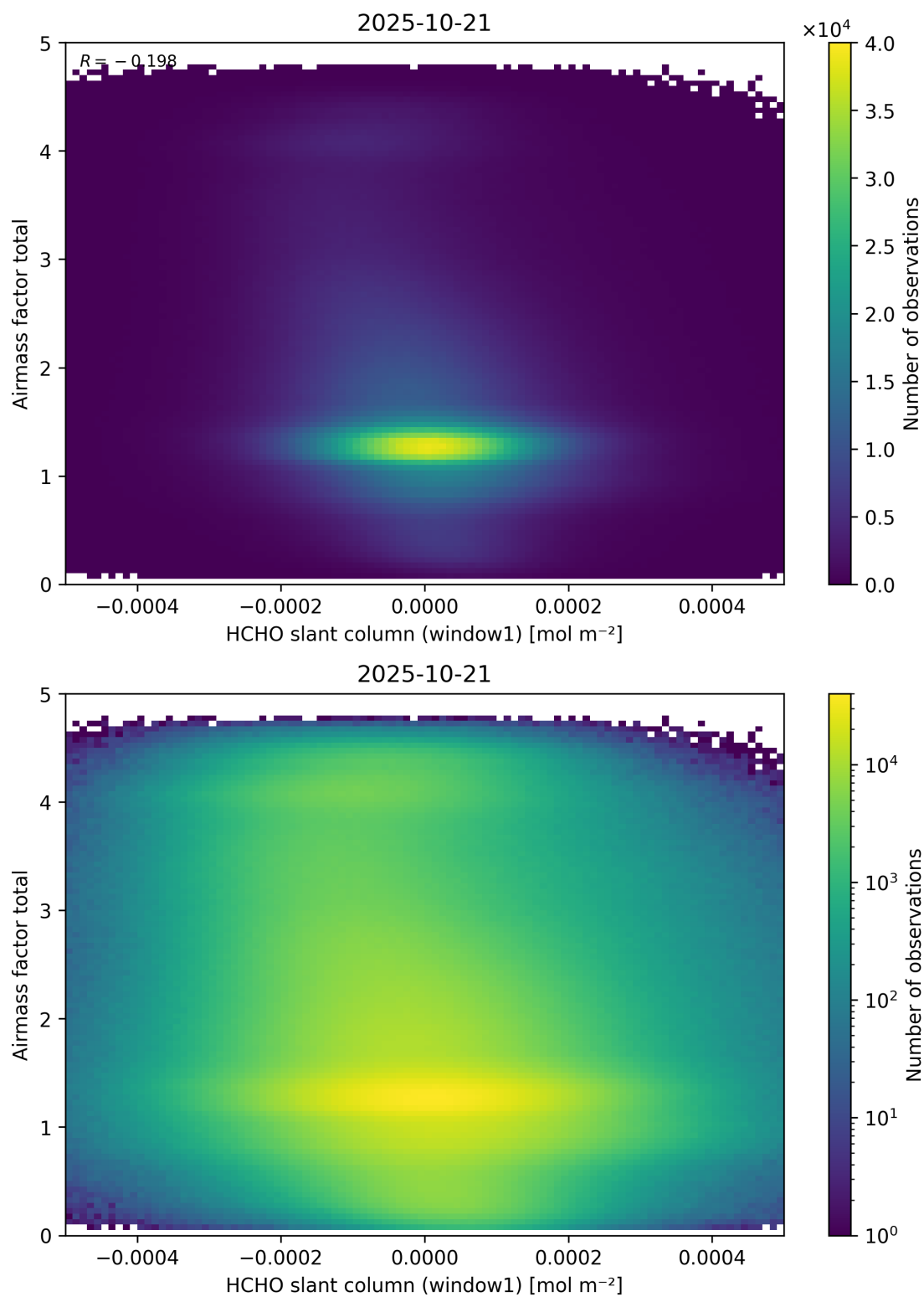
Figure 85: Scatter density plot of “HCHO slant column (window1)” against “Airmass factor total” for 2025-10-20 to 2025-10-22.
