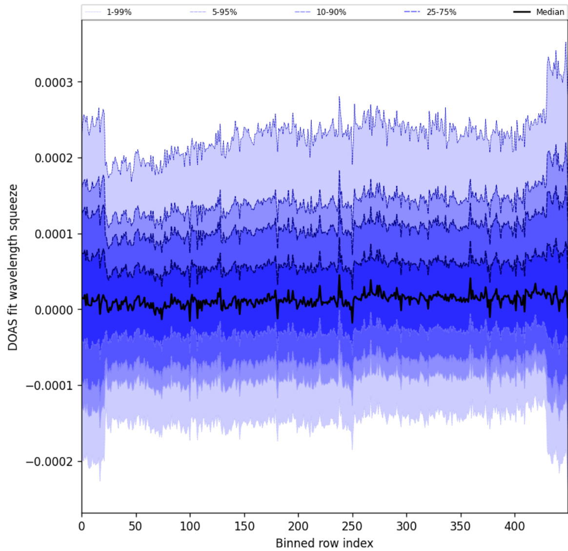
Figure 59: Along track statistics of “DOAS fit wavelength squeeze” for 2025-10-20 to 2025-10-22
