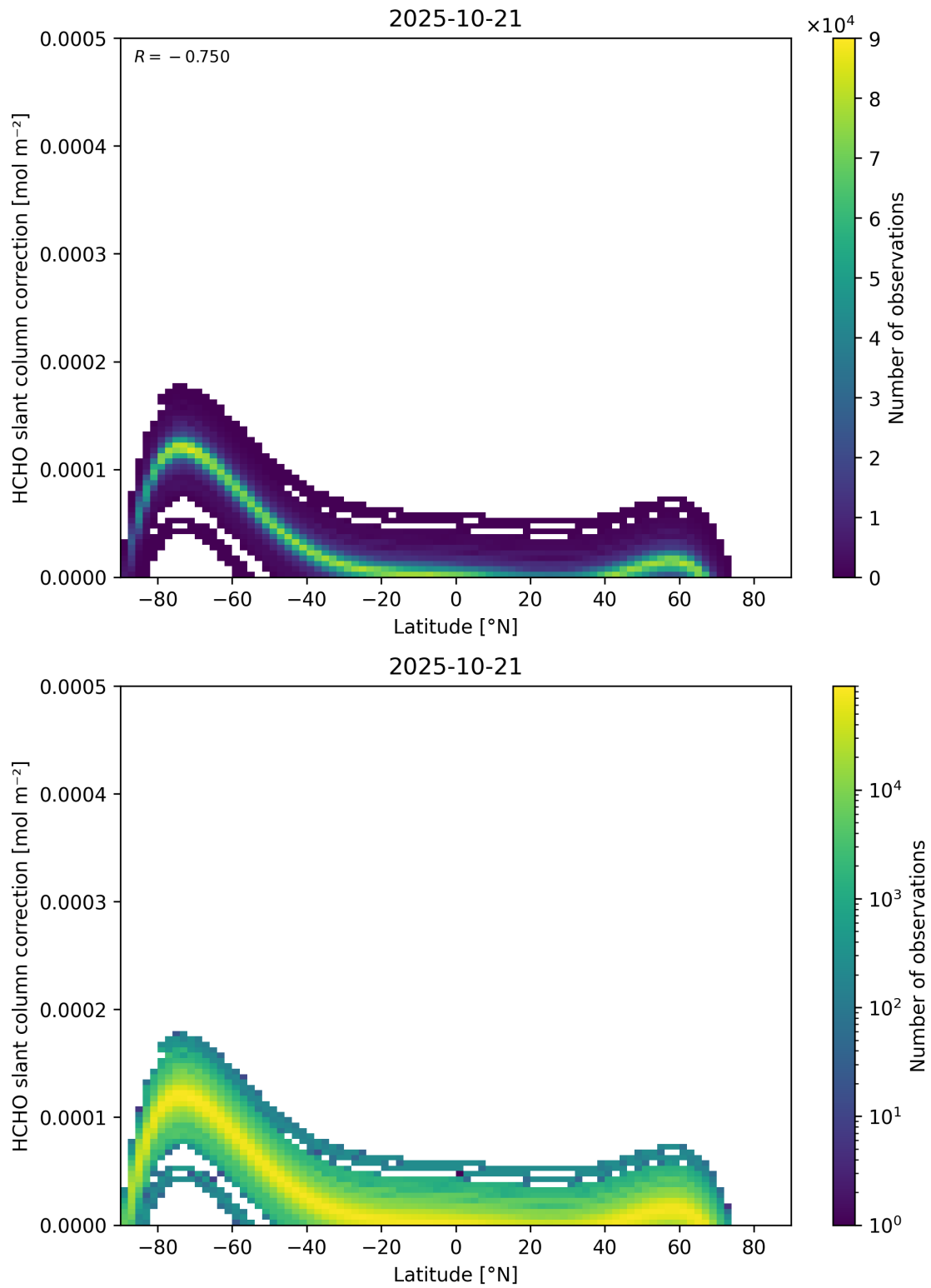
Figure 158: Scatter density plot of “Latitude” against “HCHO slant column correction” for 2025-10-20 to 2025-10-22.
