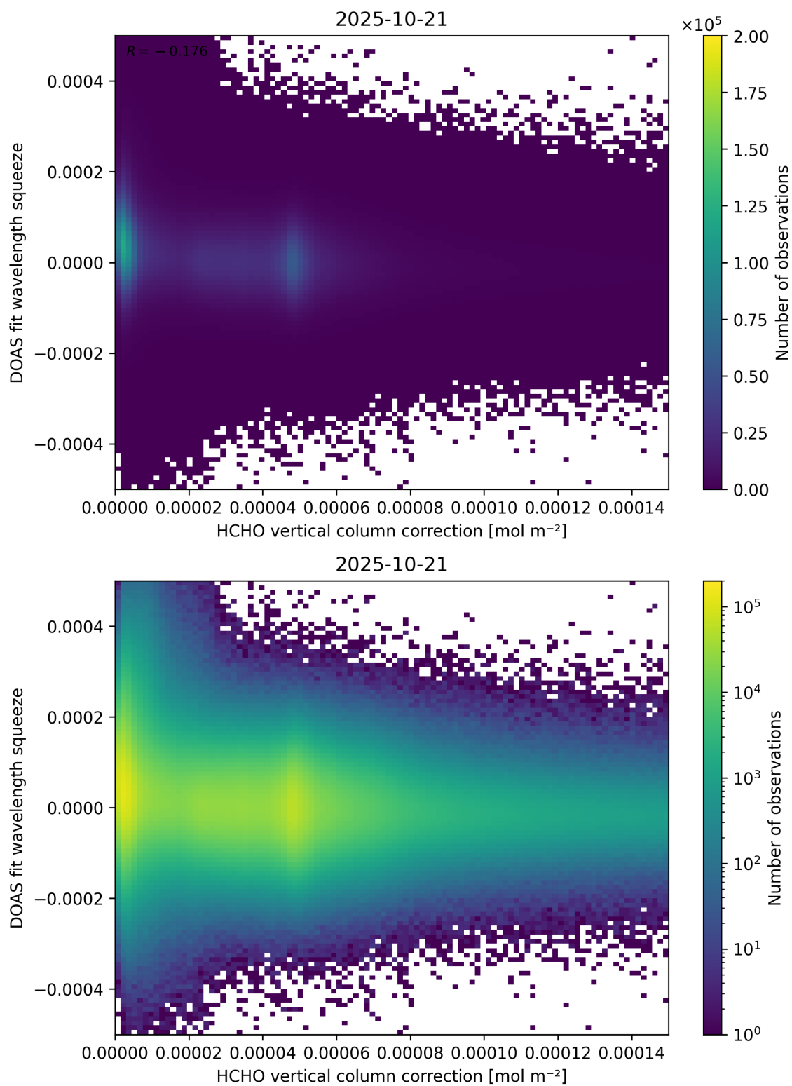
Figure 114: Scatter density plot of “HCHO vertical column correction” against “DOAS fit wavelength squeeze” for 2025-10-20 to 2025-10-22.
