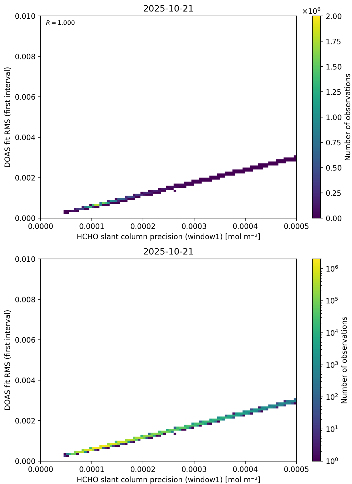
Figure 88: Scatter density plot of “HCHO slant column precision (window1)” against “DOAS fit RMS (first interval)” for 2025-10-20 to 2025-10-22.
