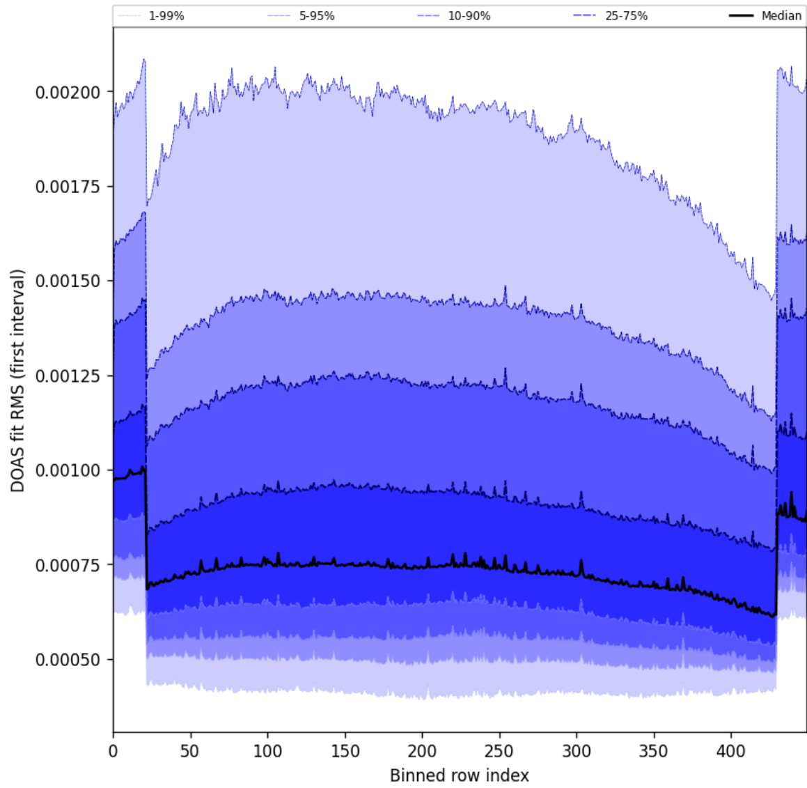
Figure 60: Along track statistics of “DOAS fit RMS (first interval)” for 2025-10-20 to 2025-10-22
