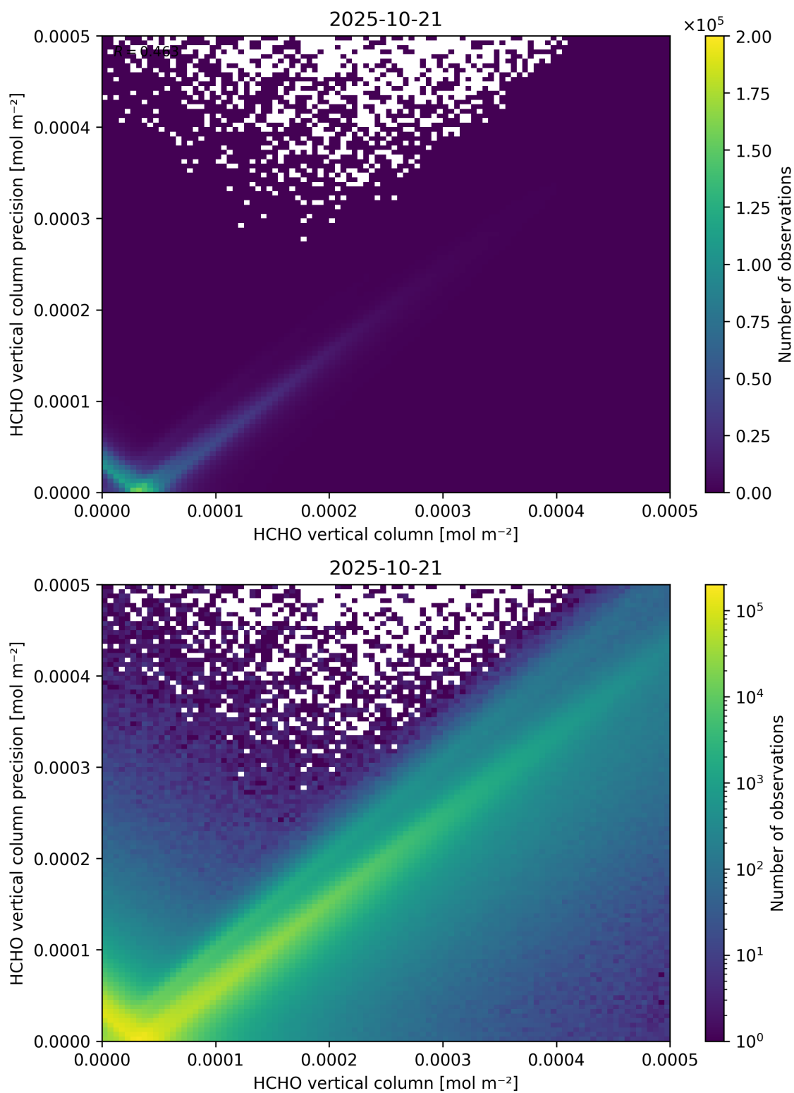
Figure 134: Scatter density plot of “HCHO vertical column” against “HCHO vertical column precision” for 2025-10-20 to 2025-10-22.
