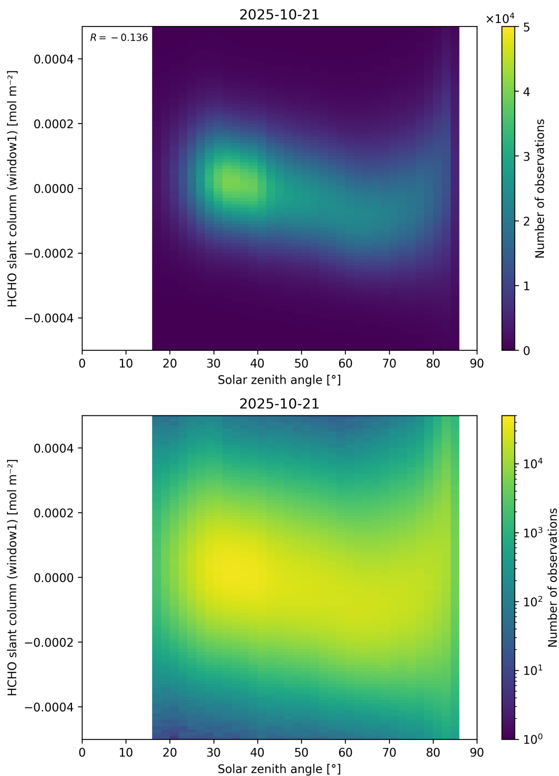
Figure 173: Scatter density plot of “Solar zenith angle” against “HCHO slant column (window1)” for 2025-10-20 to 2025-10-22.
