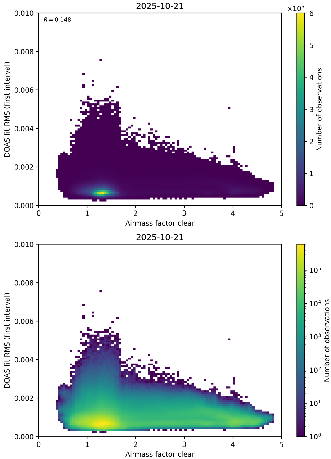
Figure 71: Scatter density plot of “Airmass factor clear” against “DOAS fit RMS (first interval)” for 2025-10-20 to 2025-10-22.
