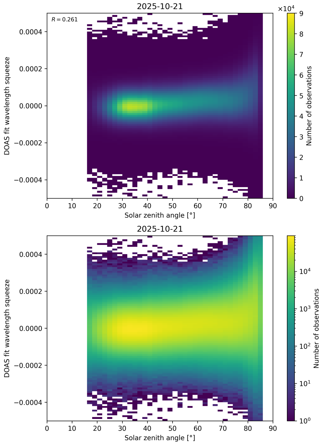
Figure 169: Scatter density plot of “Solar zenith angle” against “DOAS fit wavelength squeeze” for 2025-10-20 to 2025-10-22.
