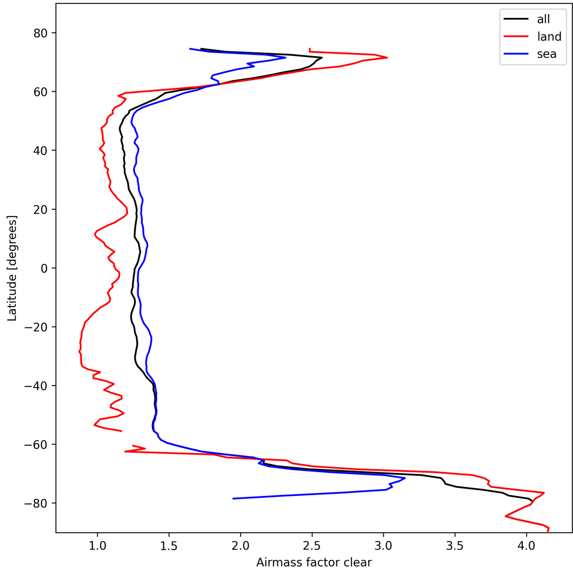
Figure 28: Zonal average of “Airmass factor clear” for 2025-10-20 to 2025-10-22.
