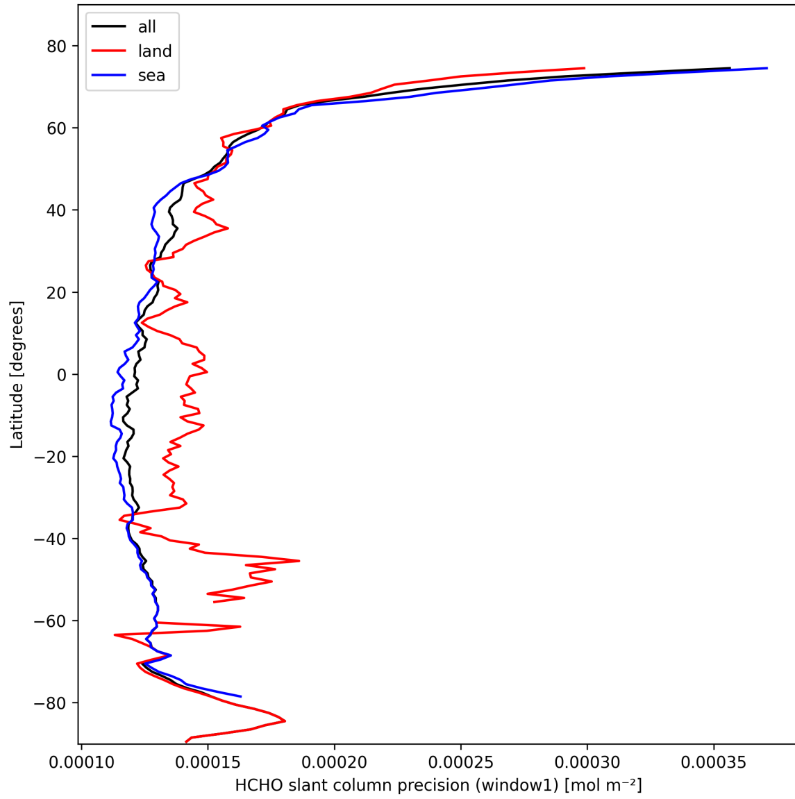
Figure 25: Zonal average of "HCHO slant column precision (window1)" for 2025-10-20 to 2025-10-22.
