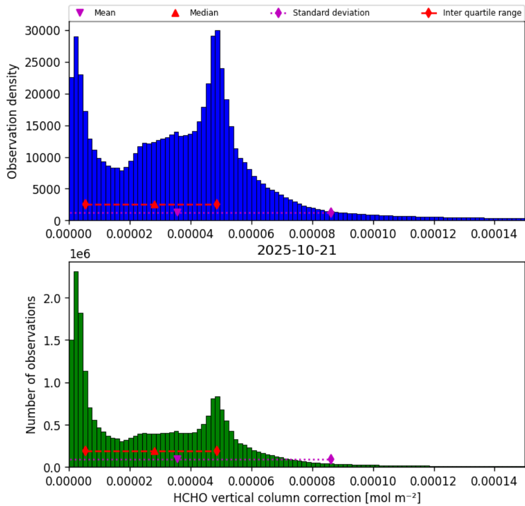
Figure 37: Histogram of “HCHO vertical column correction” for 2025-10-20 to 2025-10-22
