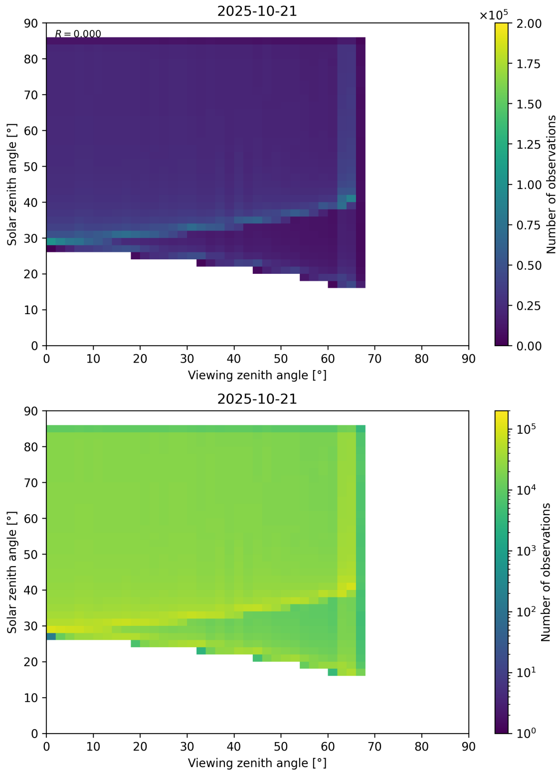
Figure 197: Scatter density plot of “Viewing zenith angle” against “Solar zenith angle” for 2025-10-20 to 2025-10-22.
