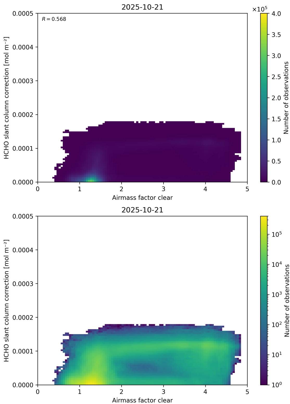
Figure 75: Scatter density plot of “Airmass factor clear” against “HCHO slant column correction” for 2025-10-20 to 2025-10-22.
