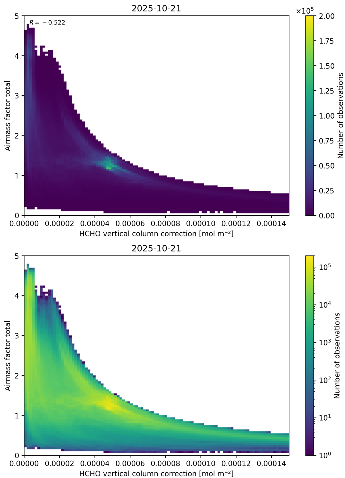
Figure 120: Scatter density plot of “HCHO vertical column correction” against “Airmass factor total” for 2025-10-20 to 2025-10-22.
