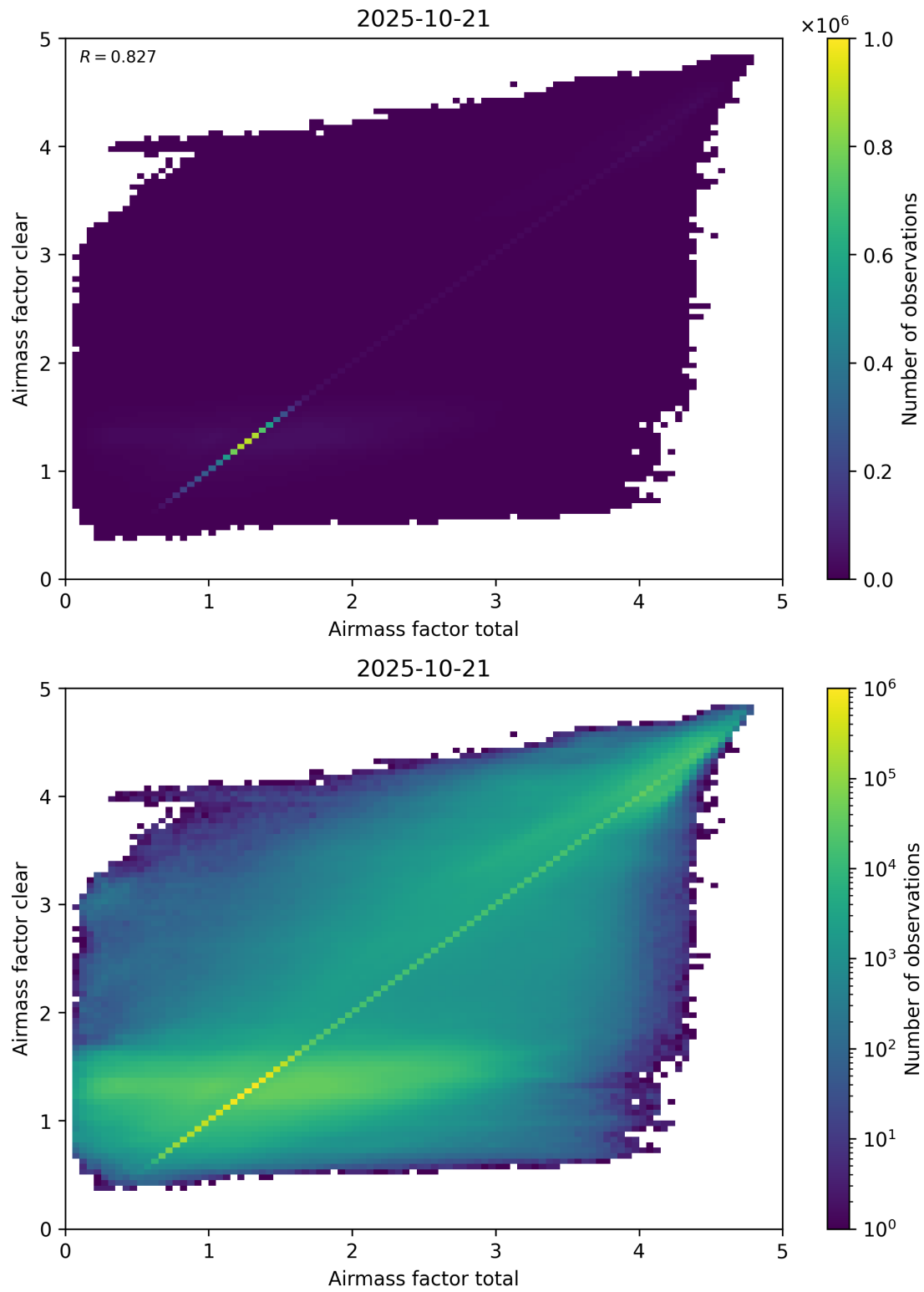
Figure 100: Scatter density plot of “Airmass factor total” against “Airmass factor clear” for 2025-10-20 to 2025-10-22.
