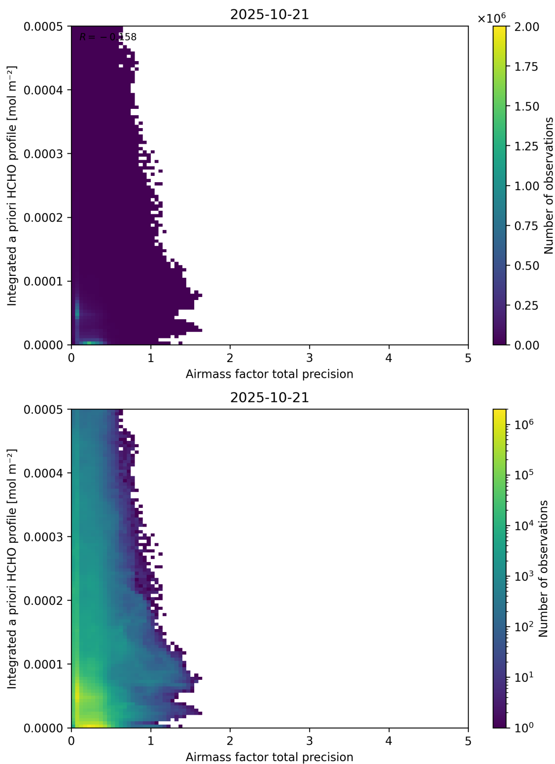
Figure 111: Scatter density plot of “Airmass factor total precision” against “Integrated a priori HCHO profile” for 2025-10-20 to 2025-10-22.
