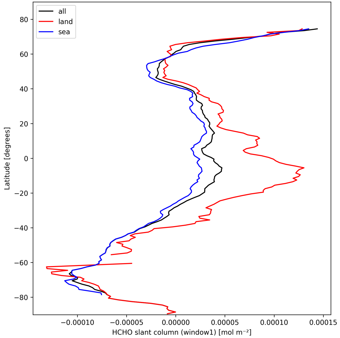
Figure 24: Zonal average of “HCHO slant column (window1)” for 2025-10-20 to 2025-10-22.
