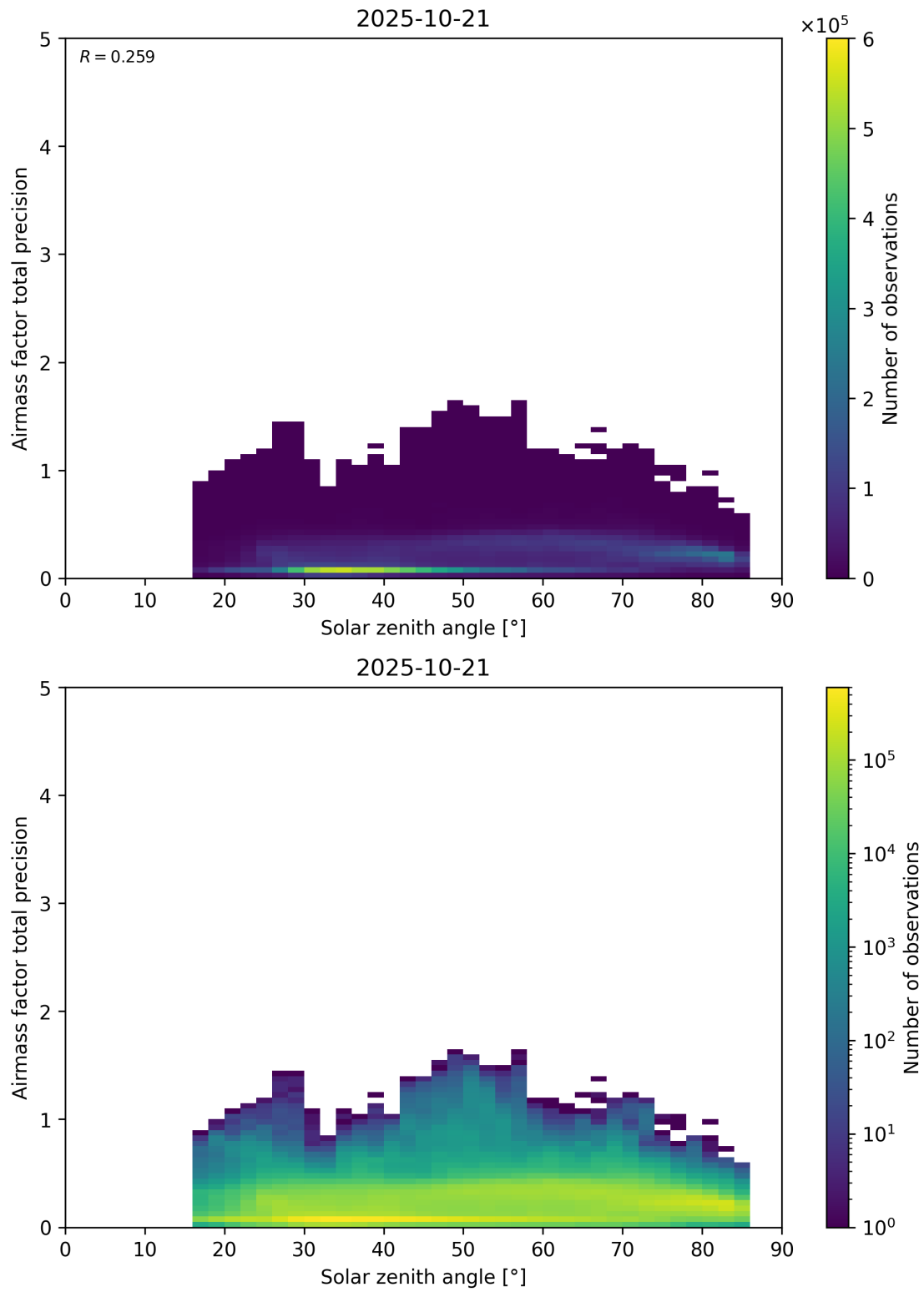
Figure 176: Scatter density plot of “Solar zenith angle” against “Airmass factor total precision” for 2025-10-20 to 2025-10-22.
