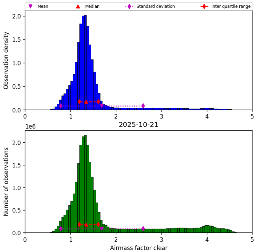
Figure 42: Histogram of “Airmass factor clear” for 2025-10-20 to 2025-10-22
