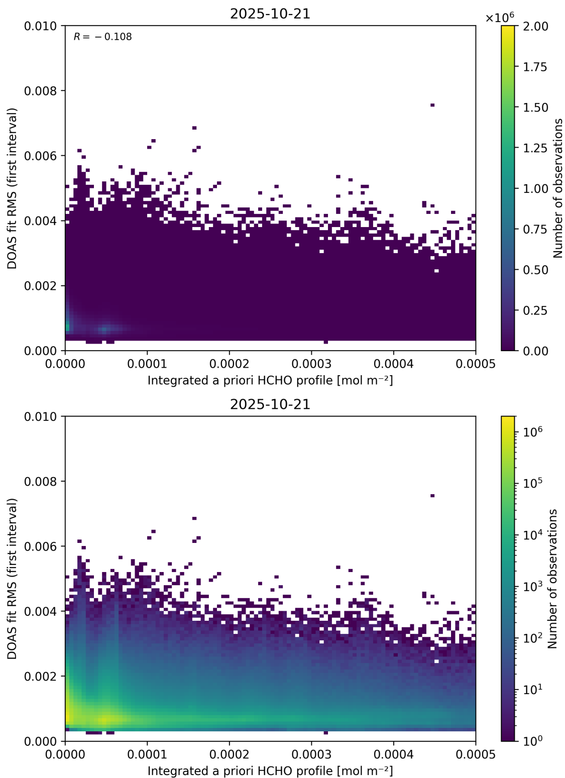
Figure 148: Scatter density plot of “Integrated a priori HCHO profile” against “DOAS fit RMS (first interval)” for 2025-10-20 to 2025-10-22.
