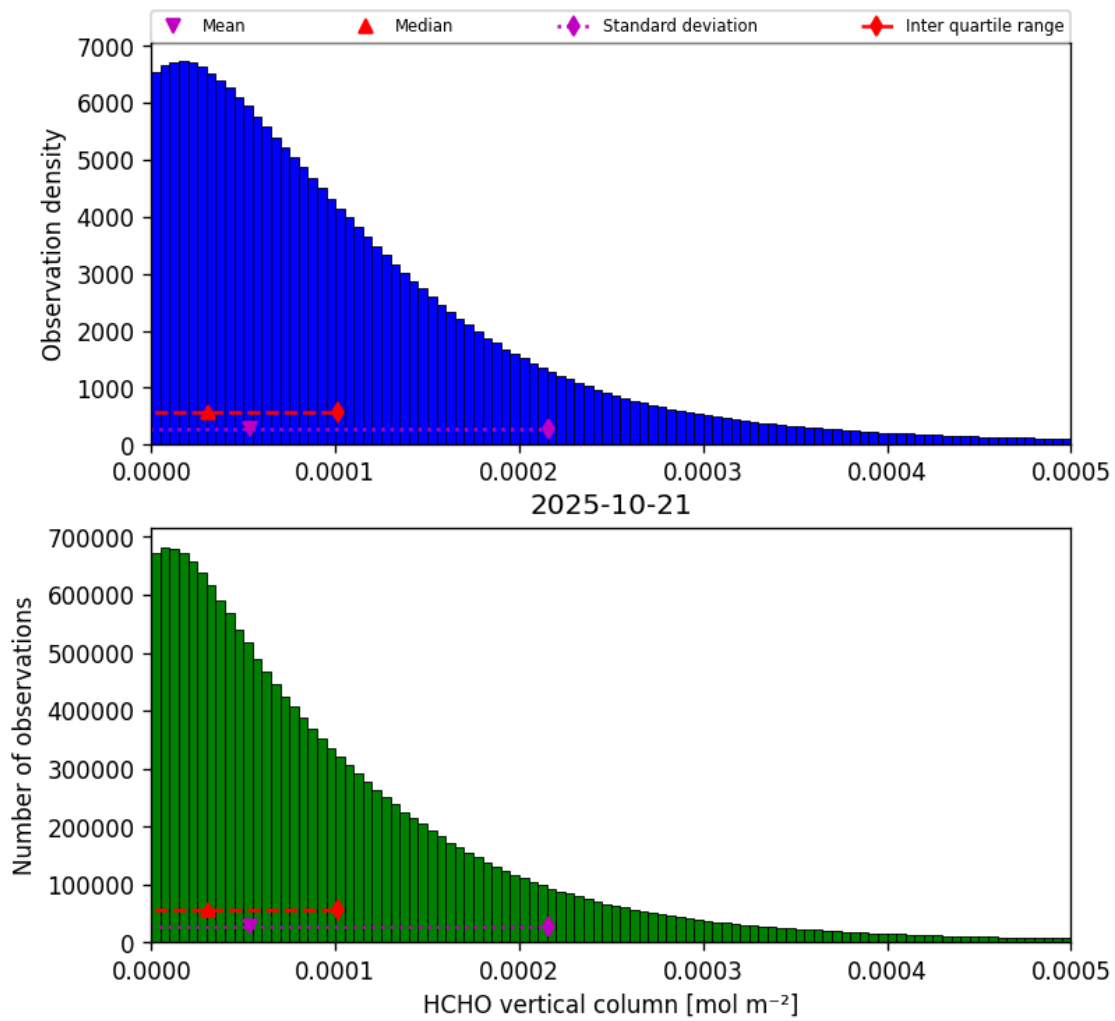
Figure 35: Histogram of “HCHO vertical column” for 2025-10-20 to 2025-10-22
