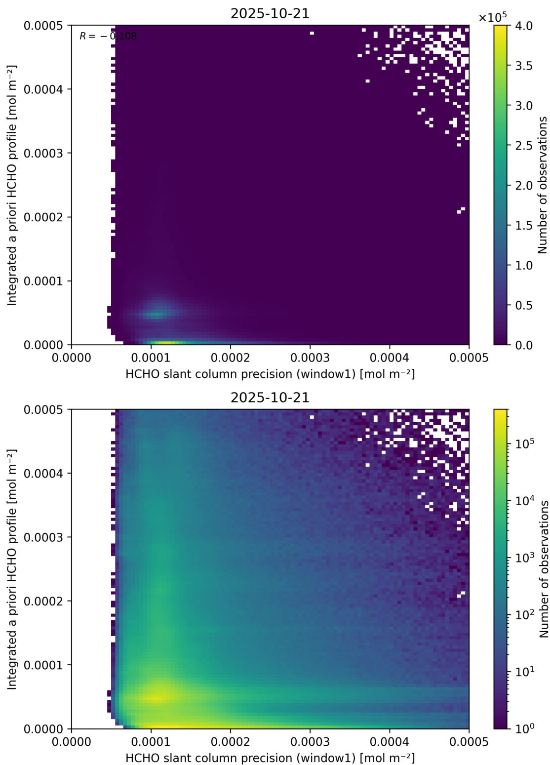
Figure 96: Scatter density plot of “HCHO slant column precision (window1)” against “Integrated a priori HCHO profile” for 2025-10-20 to 2025-10-22.
