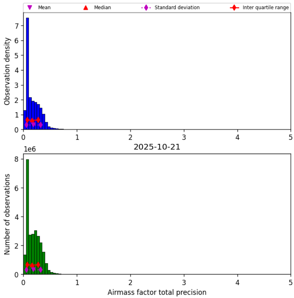
Figure 41: Histogram of “Airmass factor total precision” for 2025-10-20 to 2025-10-22
