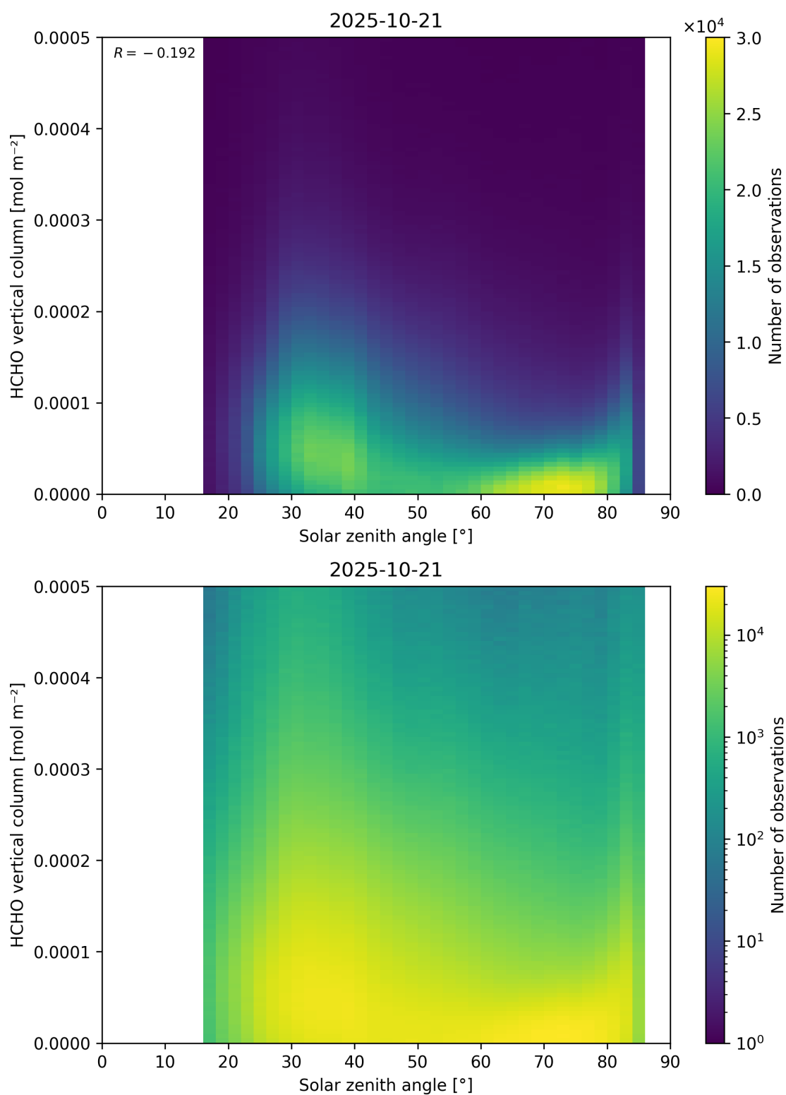
Figure 177: Scatter density plot of “Solar zenith angle” against “HCHO vertical column” for 2025-10-20 to 2025-10-22.
