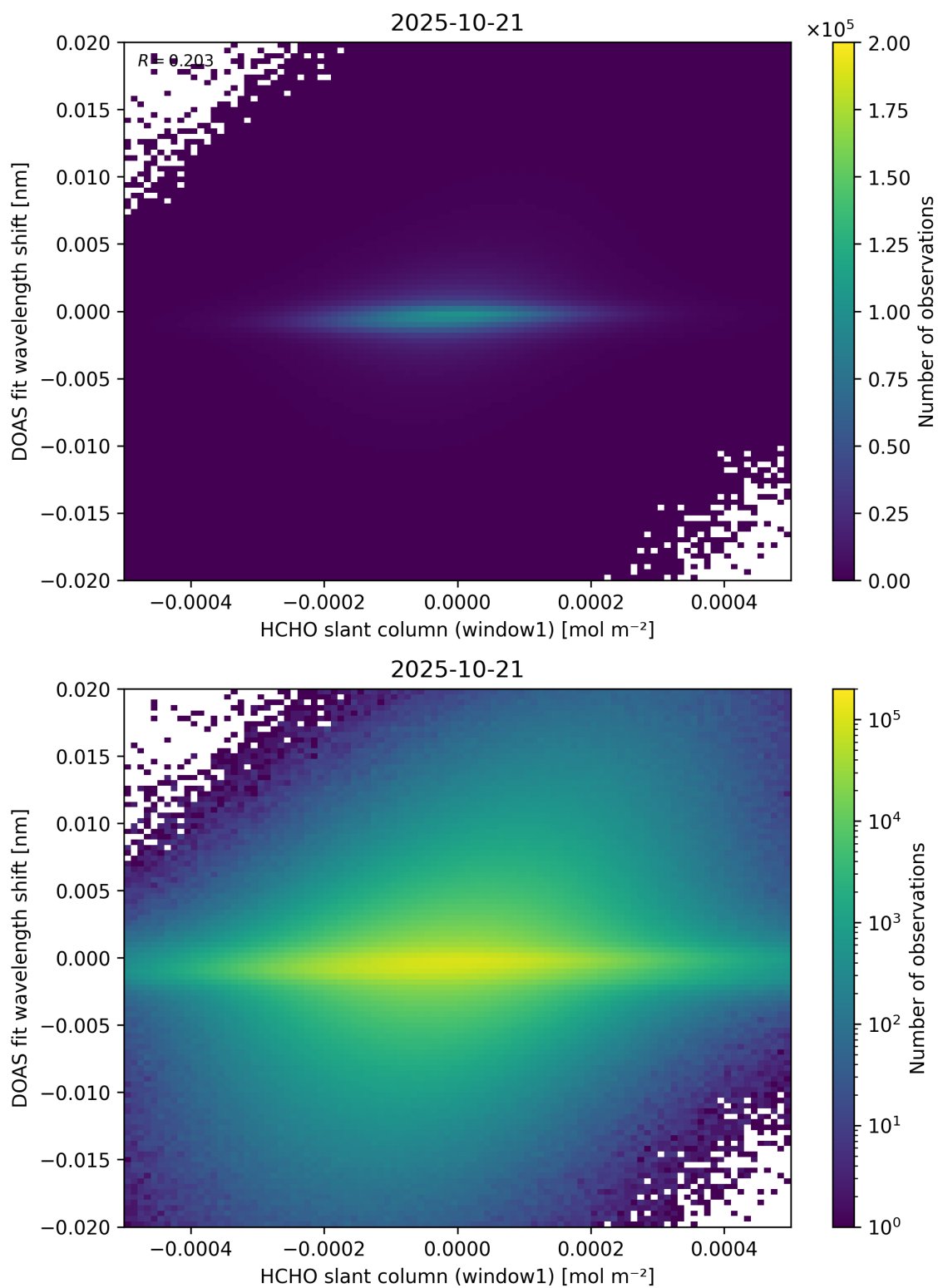
Figure 79: Scatter density plot of “HCHO slant column (window1)” against “DOAS fit wavelength shift” for 2025-10-20 to 2025-10-22.
