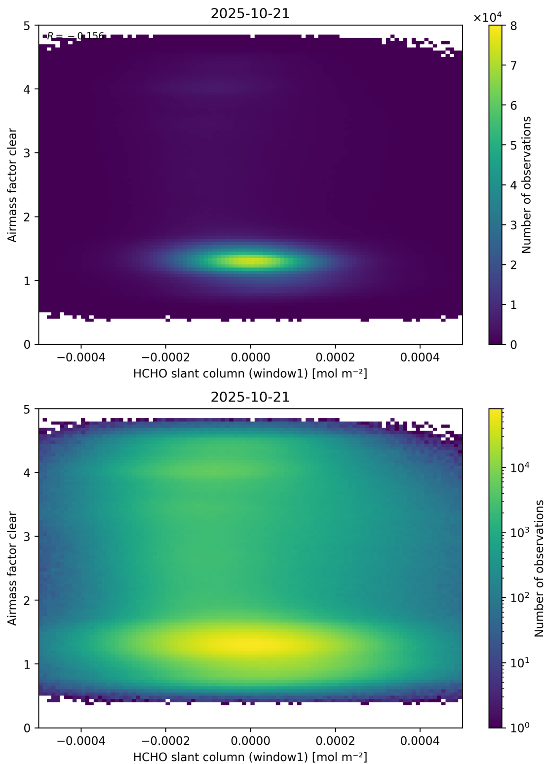
Figure 81: Scatter density plot of “HCHO slant column (window1)” against “Airmass factor clear” for 2025-10-20 to 2025-10-22.
