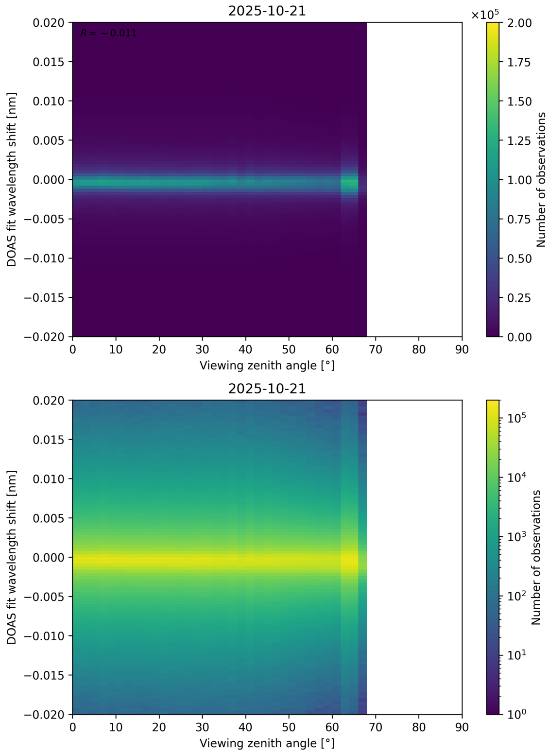
Figure 183: Scatter density plot of “Viewing zenith angle” against “DOAS fit wavelength shift” for 2025-10-20 to 2025-10-22.
