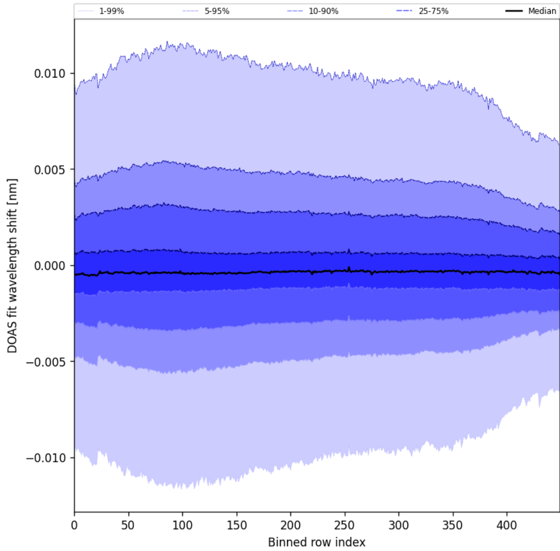
Figure 58: Along track statistics of “DOAS fit wavelength shift” for 2025-10-20 to 2025-10-22
