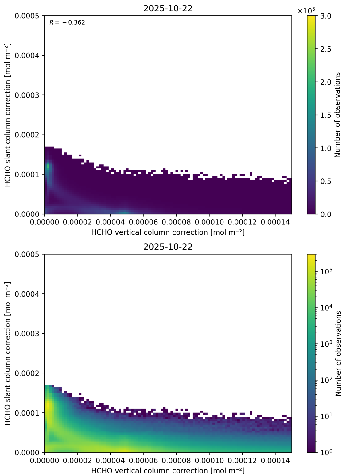
Figure 117: Scatter density plot of “HCHO vertical column correction” against “HCHO slant column correction” for 2025-10-22 to 2025-10-23.
