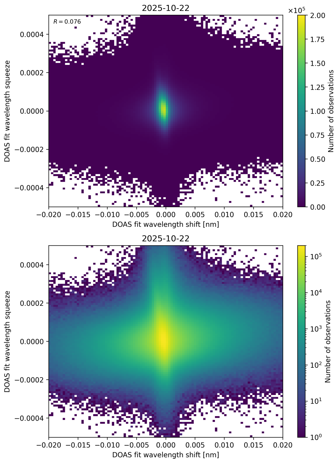
Figure 65: Scatter density plot of “DOAS fit wavelength shift” against “DOAS fit wavelength squeeze” for 2025-10-22 to 2025-10-23.
