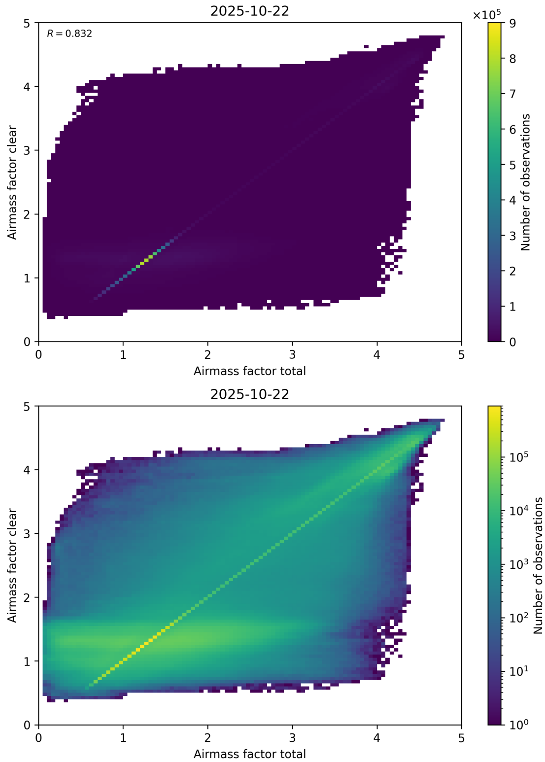
Figure 100: Scatter density plot of “Airmass factor total” against “Airmass factor clear” for 2025-10-22 to 2025-10-23.
