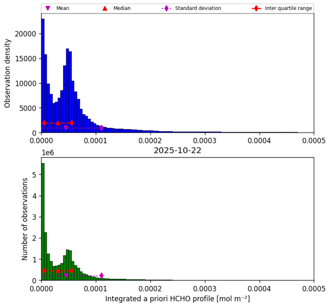
Figure 43: Histogram of “Integrated a priori HCHO profile” for 2025-10-22 to 2025-10-23
