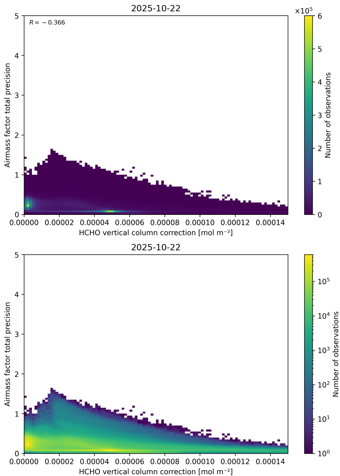
Figure 121: Scatter density plot of “HCHO vertical column correction” against “Airmass factor total precision” for 2025-10-22 to 2025-10-23.
