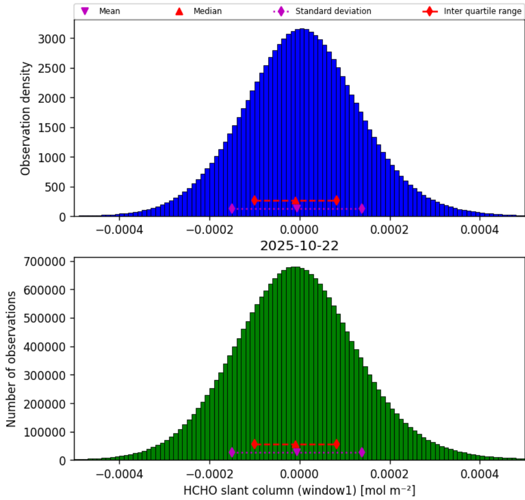
Figure 38: Histogram of “HCHO slant column (window1)” for 2025-10-22 to 2025-10-23
