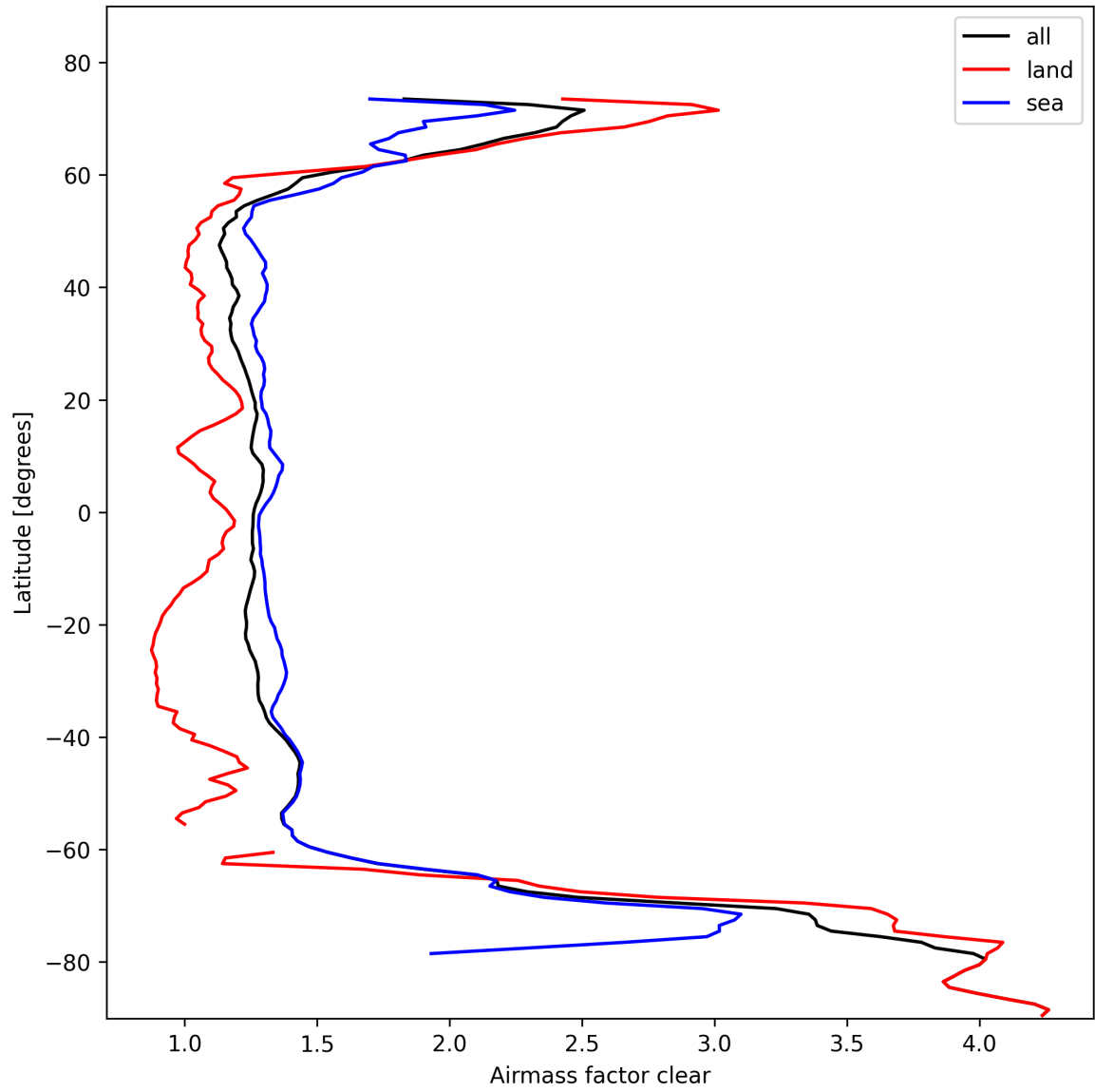
Figure 28: Zonal average of “Airmass factor clear” for 2025-10-22 to 2025-10-23.
