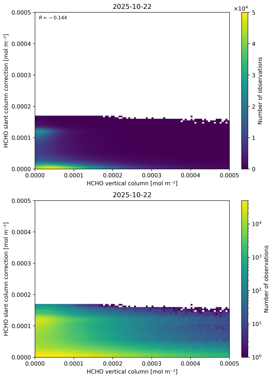
Figure 128: Scatter density plot of “HCHO vertical column” against “HCHO slant column correction” for 2025-10-22 to 2025-10-23.
