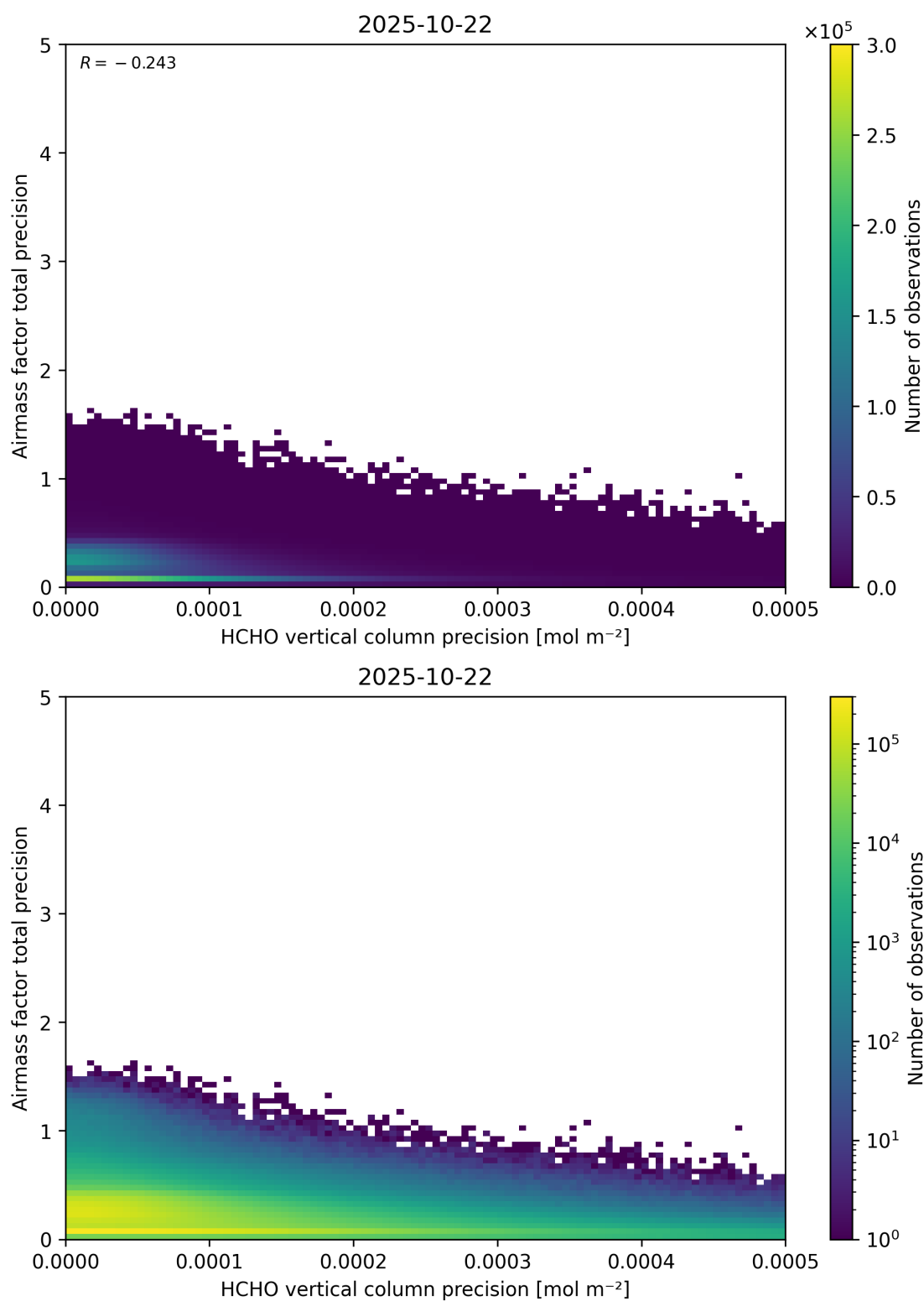
Figure 145: Scatter density plot of “HCHO vertical column precision” against “Airmass factor total precision” for 2025-10-22 to 2025-10-23.
