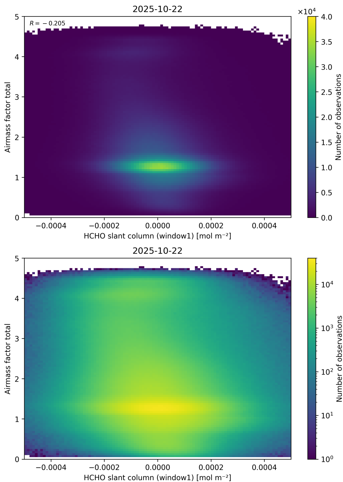
Figure 85: Scatter density plot of “HCHO slant column (window1)” against “Airmass factor total” for 2025-10-22 to 2025-10-23.
