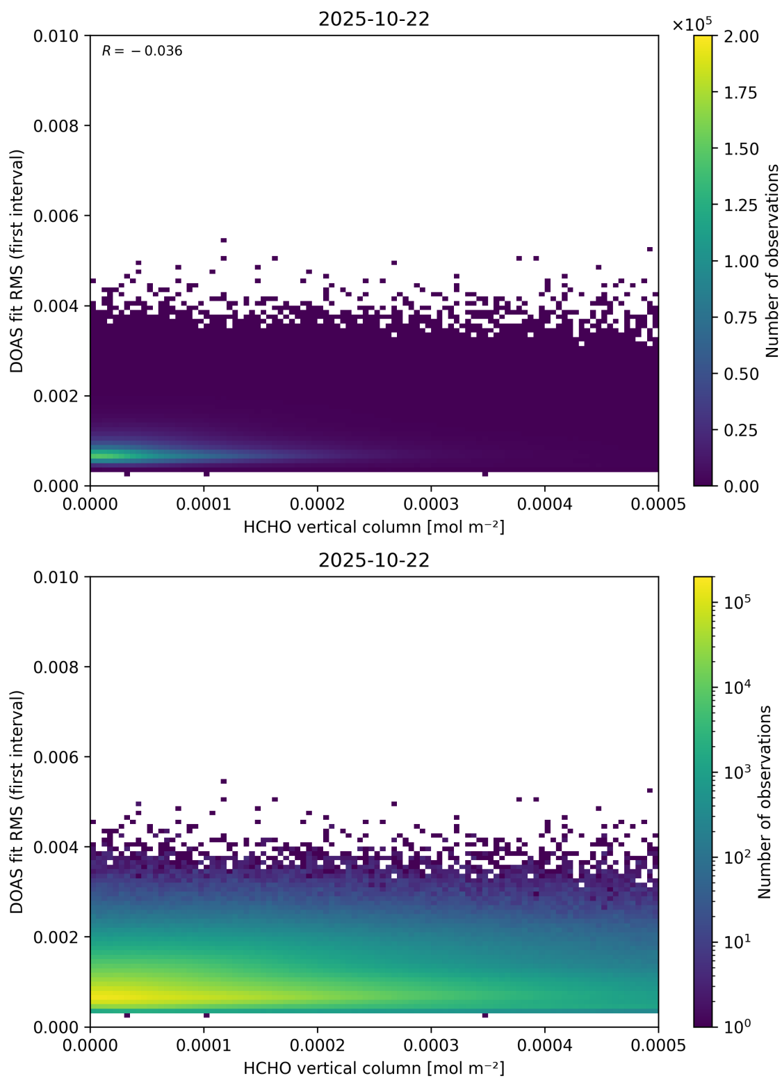
Figure 123: Scatter density plot of “HCHO vertical column” against “DOAS fit RMS (first interval)” for 2025-10-22 to 2025-10-23.
