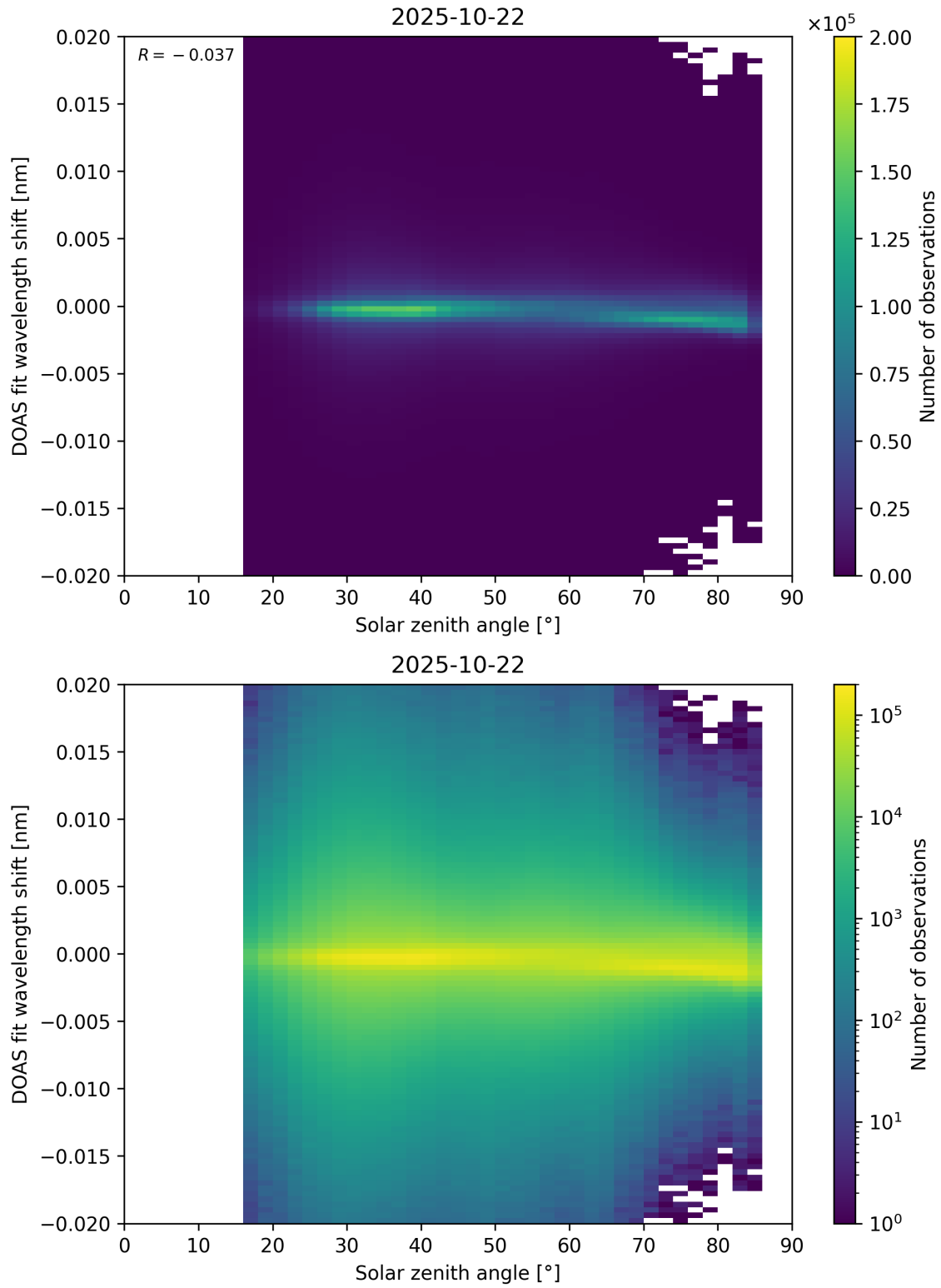
Figure 168: Scatter density plot of “Solar zenith angle” against “DOAS fit wavelength shift” for 2025-10-22 to 2025-10-23.
