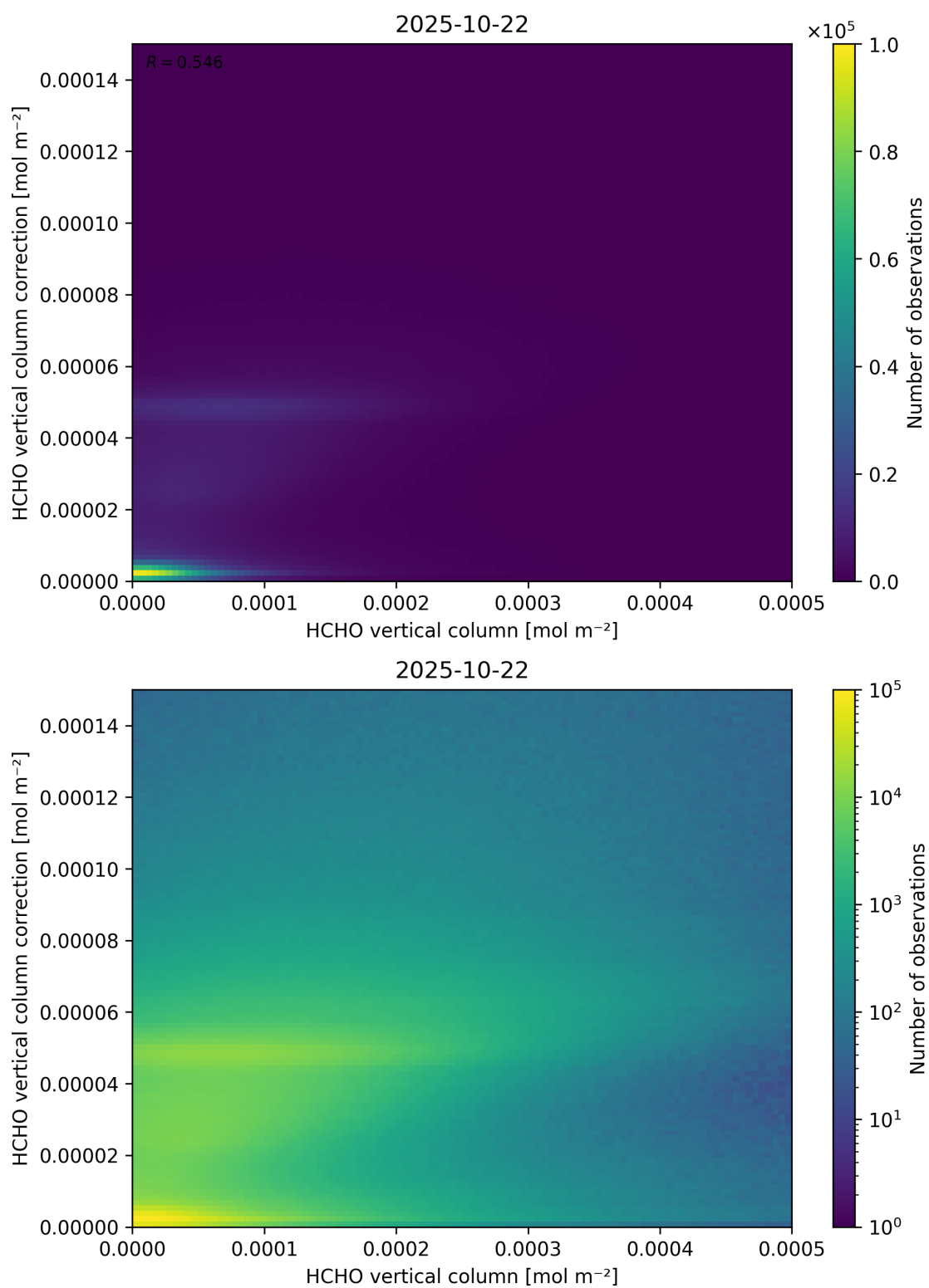
Figure 133: Scatter density plot of “HCHO vertical column” against “HCHO vertical column correction” for 2025-10-22 to 2025-10-23.
