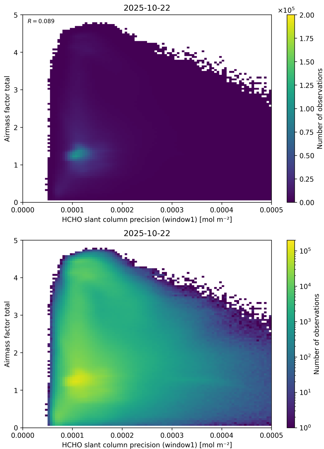
Figure 94: Scatter density plot of “HCHO slant column precision (window1)” against “Airmass factor total” for 2025-10-22 to 2025-10-23.
