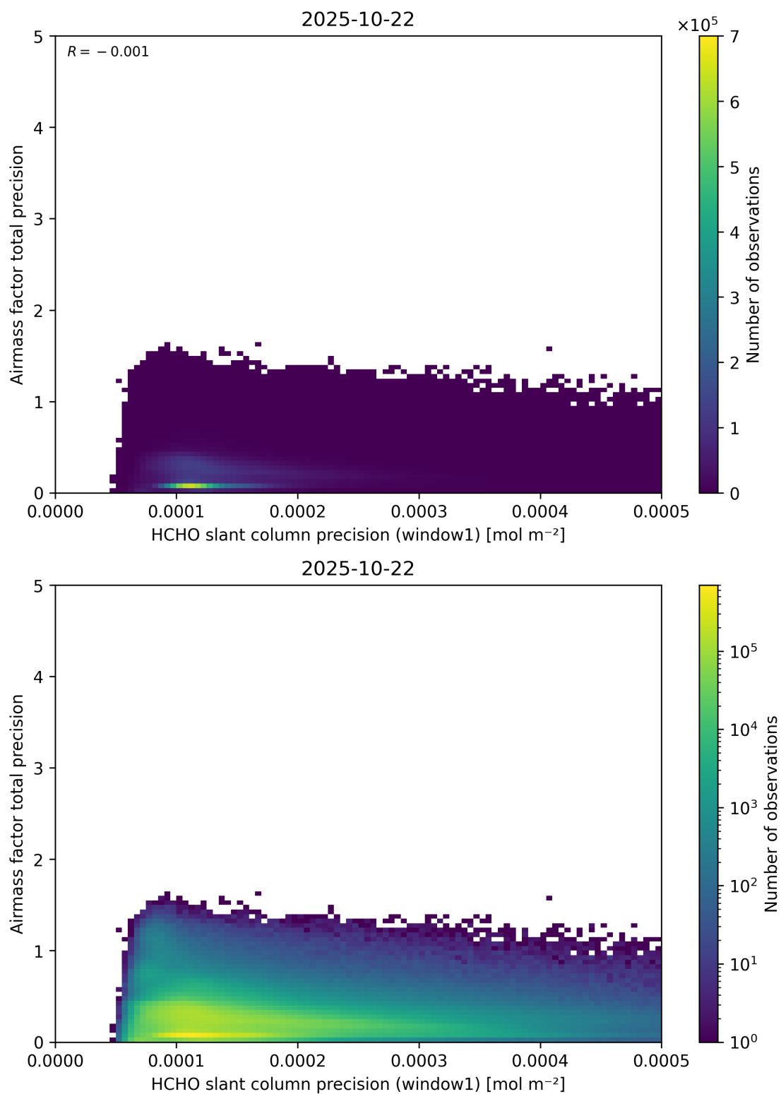
Figure 95: Scatter density plot of “HCHO slant column precision (window1)” against “Airmass factor total precision” for 2025-10-22 to 2025-10-23.
