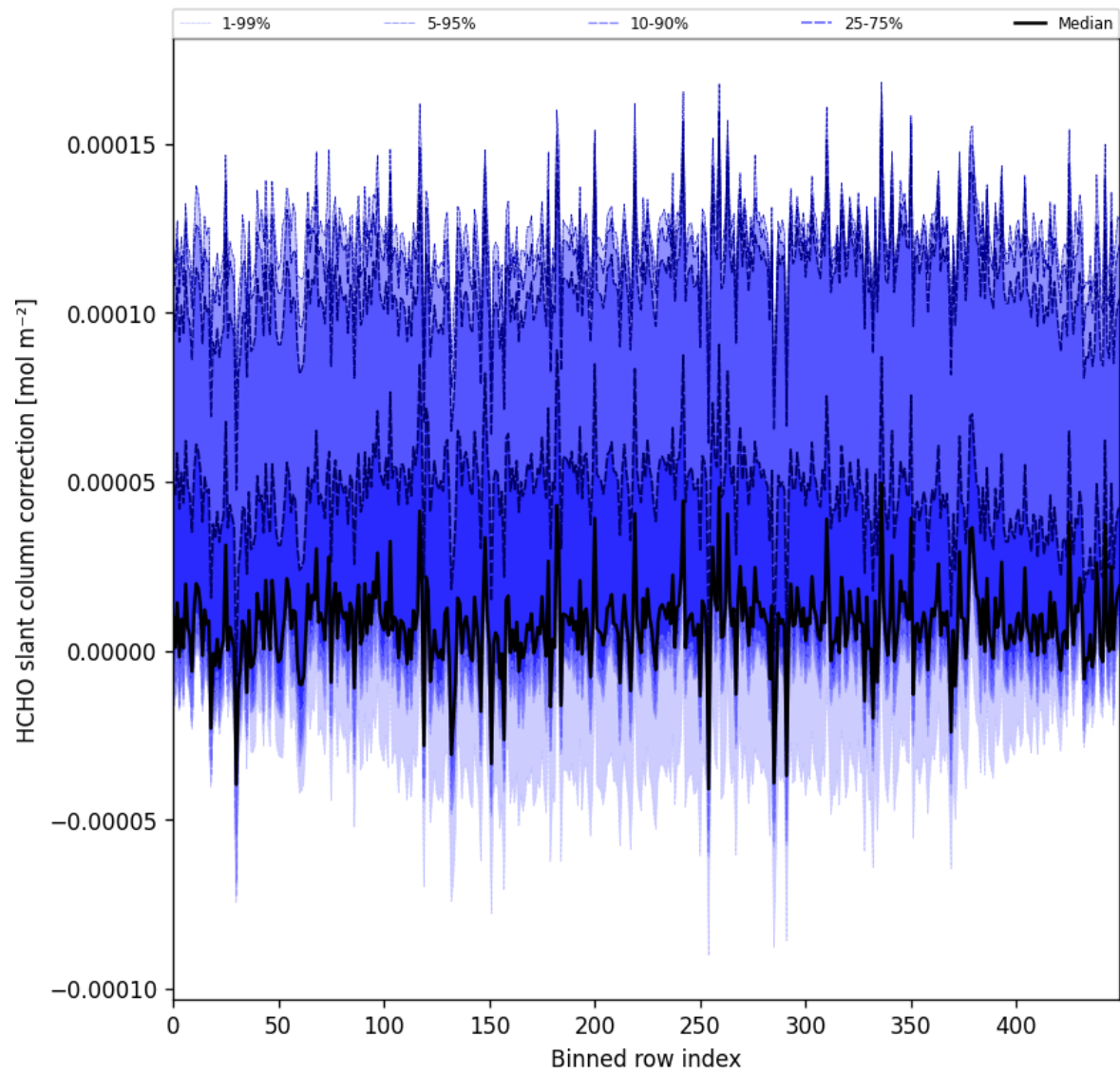
Figure 61: Along track statistics of “HCHO slant column correction” for 2025-10-22 to 2025-10-23
