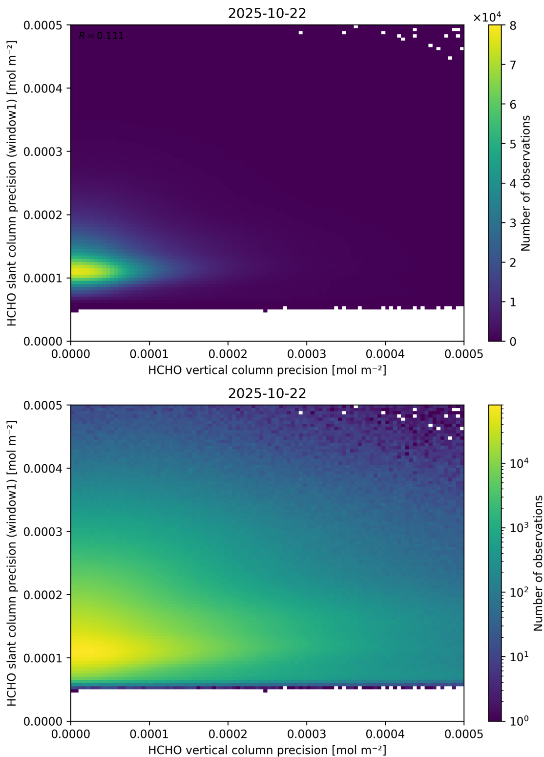
Figure 143: Scatter density plot of “HCHO vertical column precision” against “HCHO slant column precision (window1)” for 2025-10-22 to 2025-10-23.
