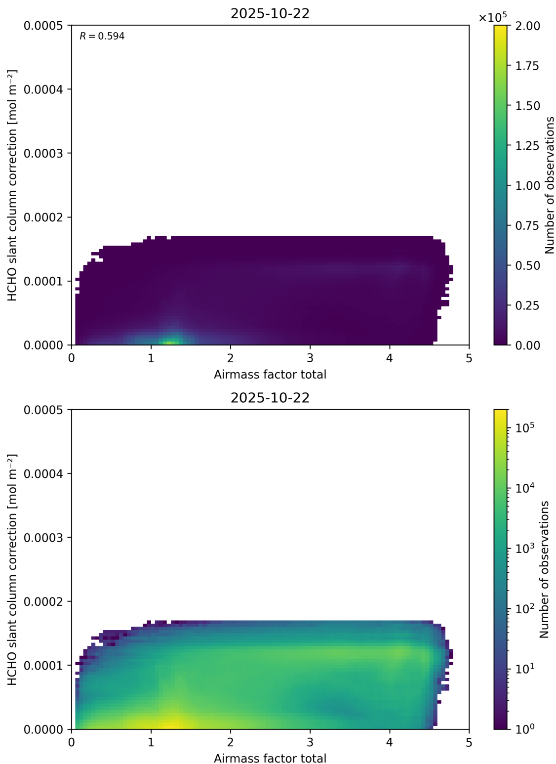
Figure 102: Scatter density plot of “Airmass factor total” against “HCHO slant column correction” for 2025-10-22 to 2025-10-23.
