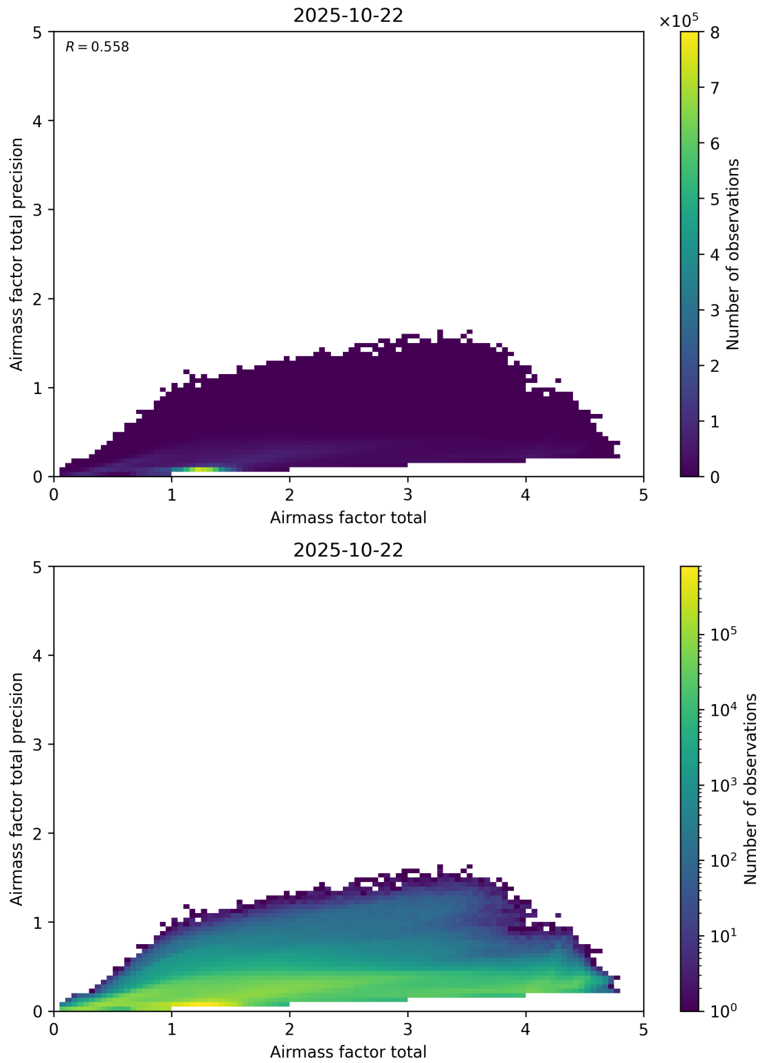
Figure 103: Scatter density plot of “Airmass factor total” against “Airmass factor total precision” for 2025-10-22 to 2025-10-23.
