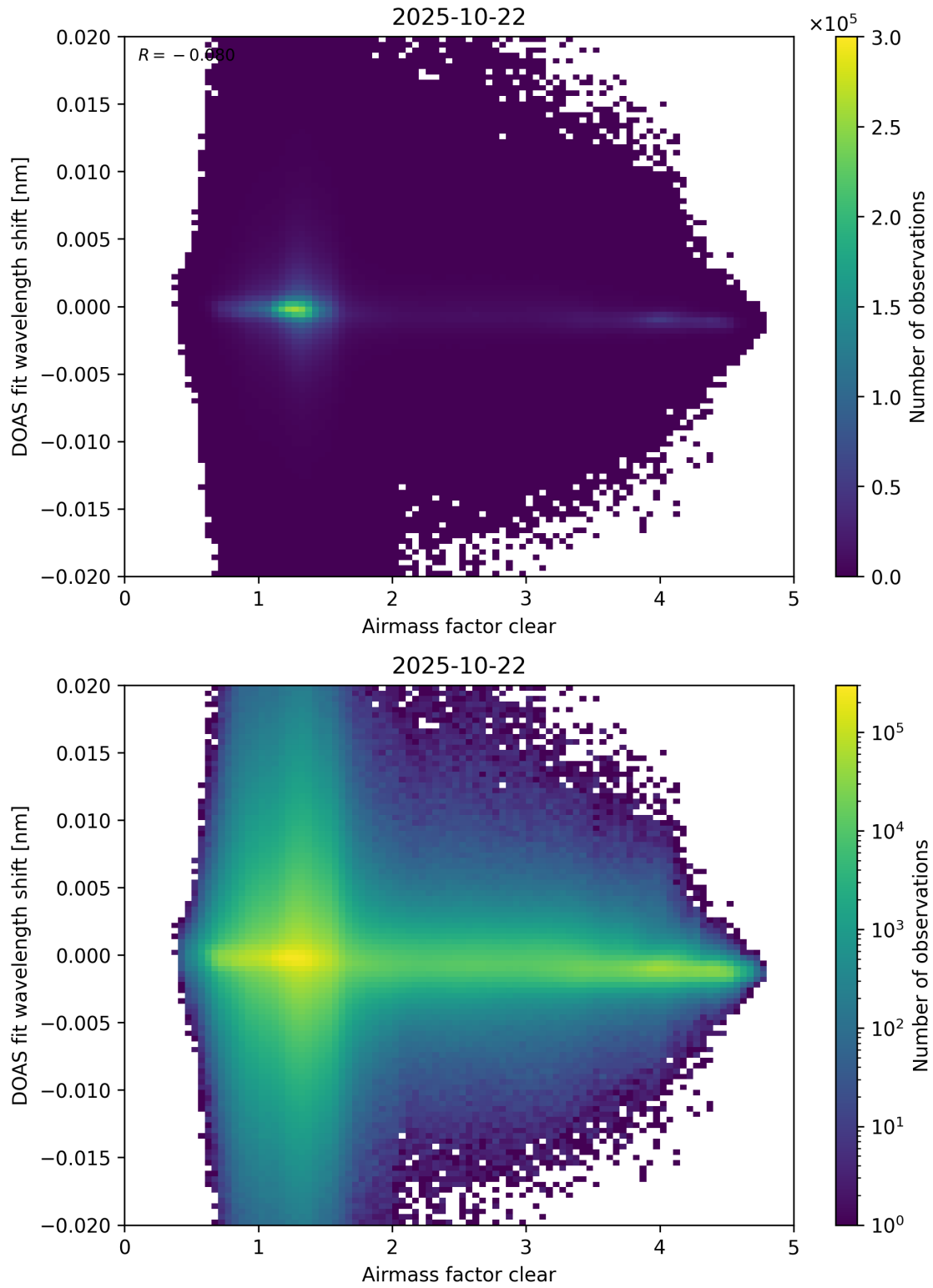
Figure 72: Scatter density plot of “Airmass factor clear” against “DOAS fit wavelength shift” for 2025-10-22 to 2025-10-23.
