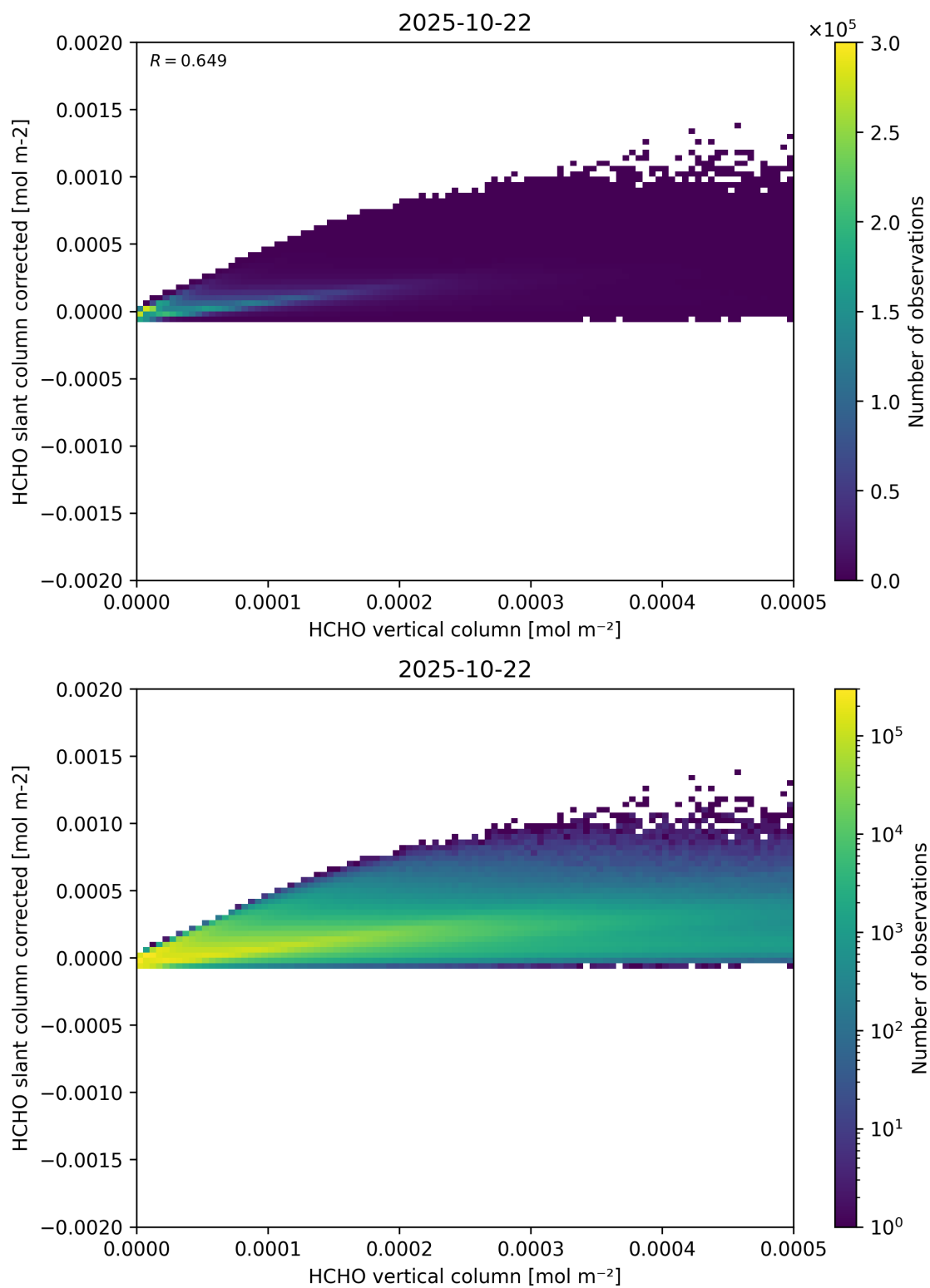
Figure 127: Scatter density plot of “HCHO vertical column” against “HCHO slant column corrected” for 2025-10-22 to 2025-10-23.
