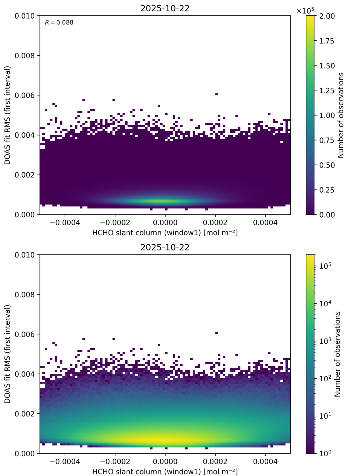
Figure 78: Scatter density plot of “HCHO slant column (window1)” against “DOAS fit RMS (first interval)” for 2025-10-22 to 2025-10-23.
