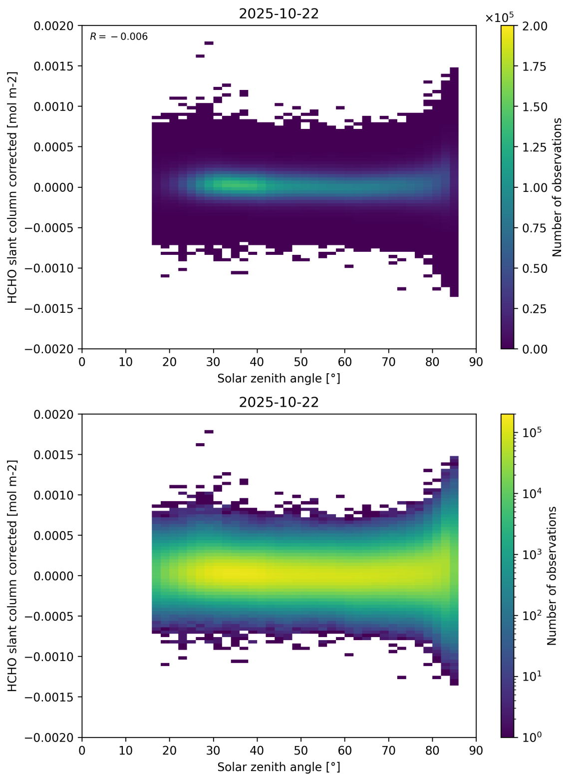
Figure 171: Scatter density plot of “Solar zenith angle” against “HCHO slant column corrected” for 2025-10-22 to 2025-10-23.
