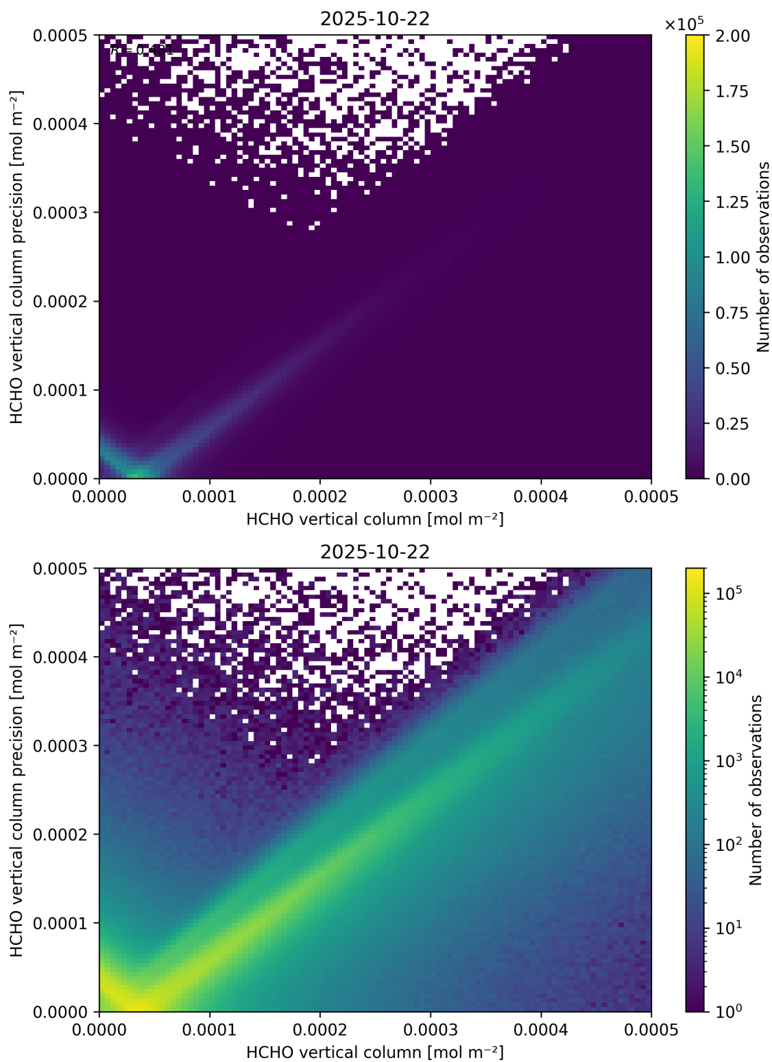
Figure 134: Scatter density plot of “HCHO vertical column” against “HCHO vertical column precision” for 2025-10-22 to 2025-10-23.
