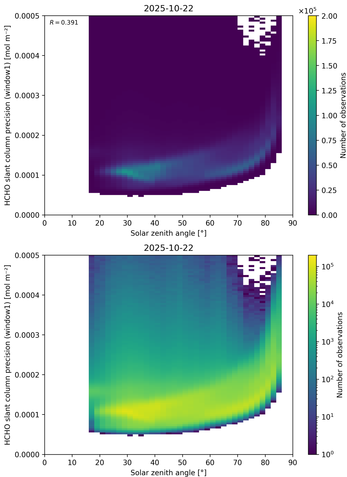
Figure 174: Scatter density plot of “Solar zenith angle” against “HCHO slant column precision (window1)” for 2025-10-22 to 2025-10-23.
