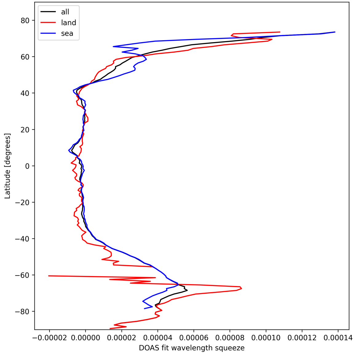
Figure 31: Zonal average of “DOAS fit wavelength squeeze” for 2025-10-22 to 2025-10-23.
