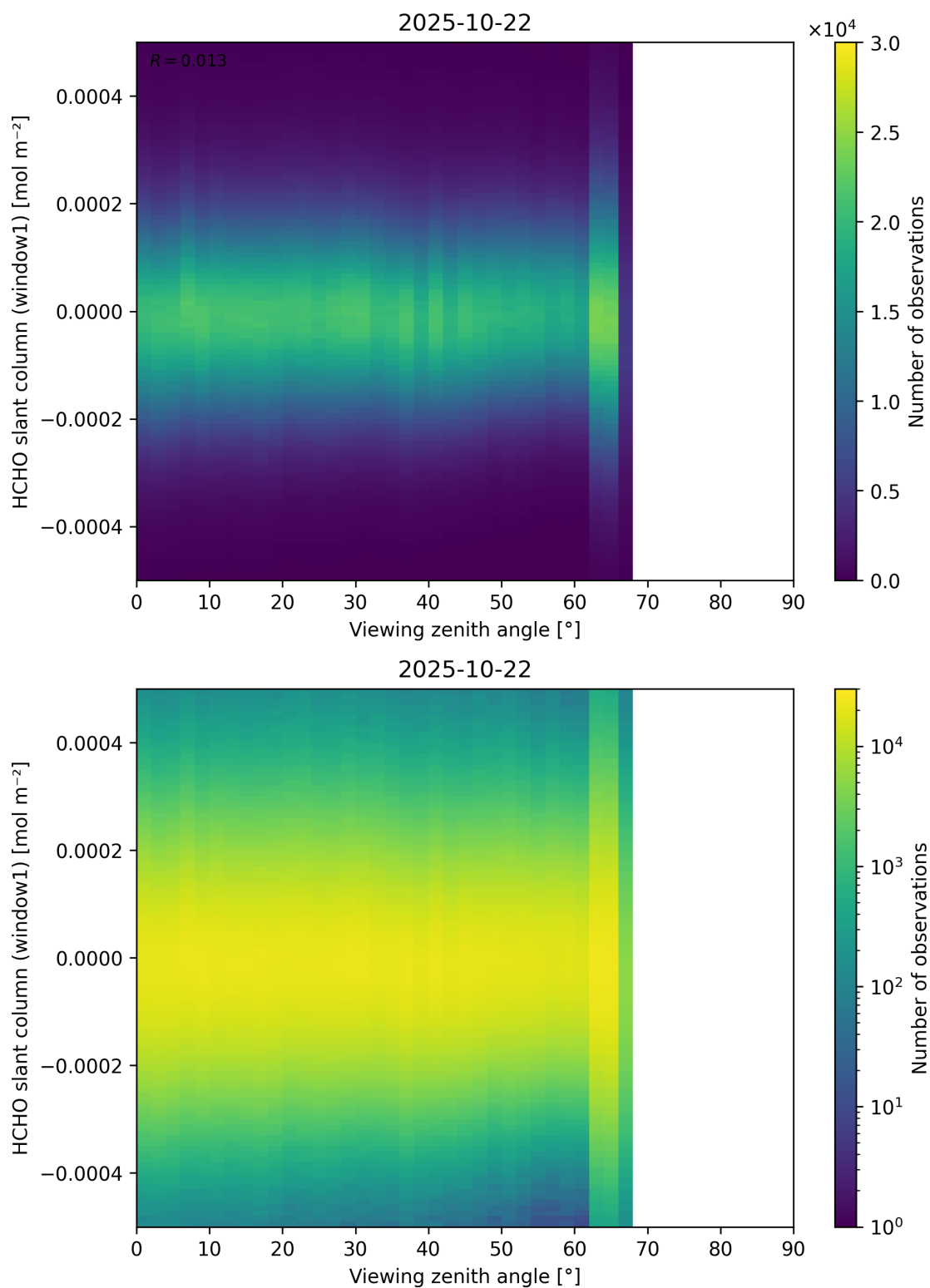
Figure 188: Scatter density plot of “Viewing zenith angle” against “HCHO slant column (window1)” for 2025-10-22 to 2025-10-23.
