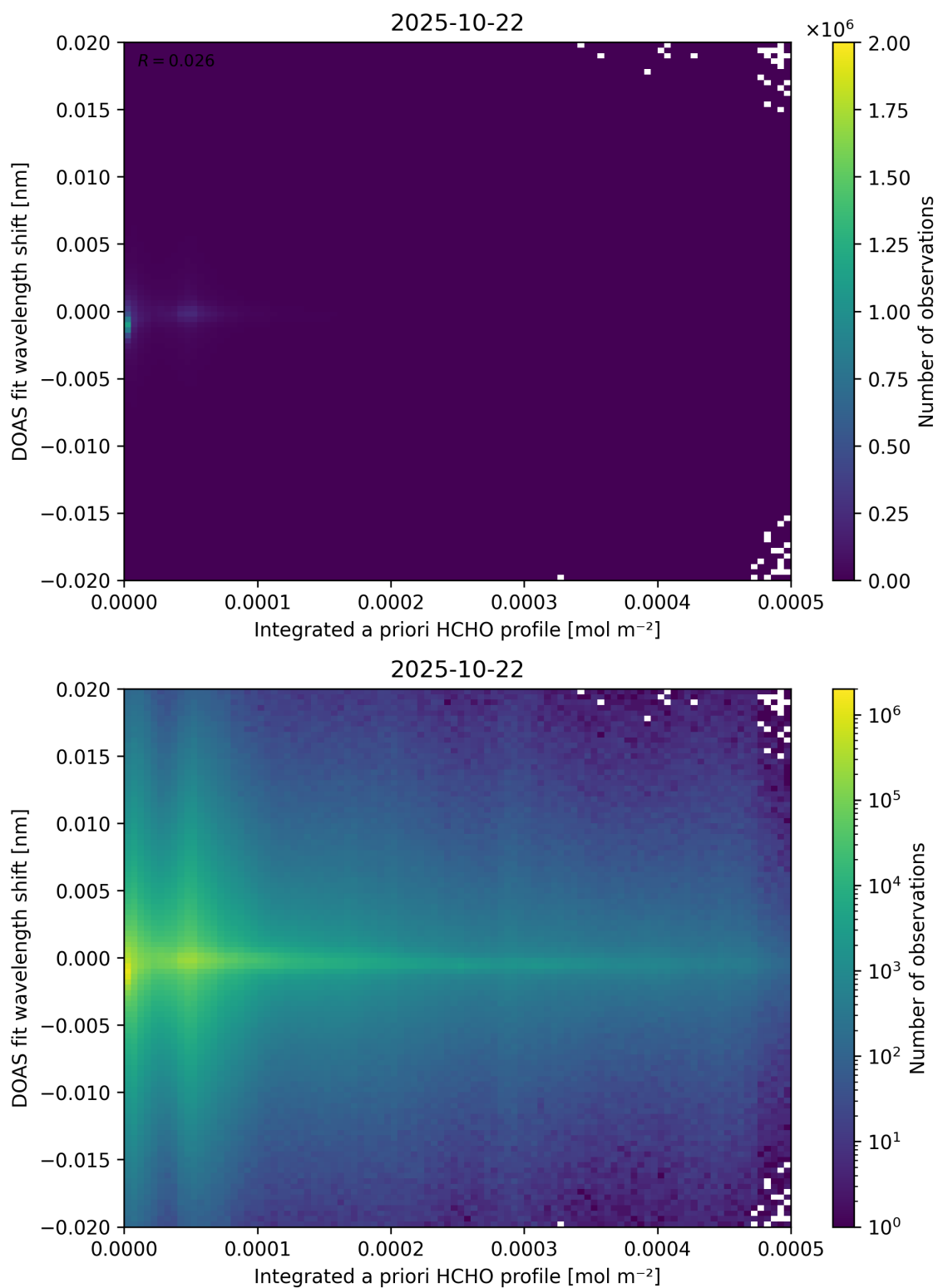
Figure 149: Scatter density plot of “Integrated a priori HCHO profile” against “DOAS fit wavelength shift” for 2025-10-22 to 2025-10-23.
