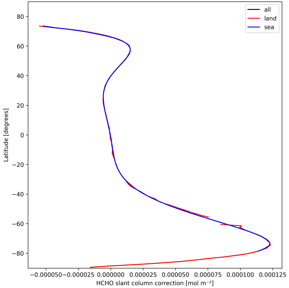
Figure 33: Zonal average of “HCHO slant column correction” for 2025-10-22 to 2025-10-23.
