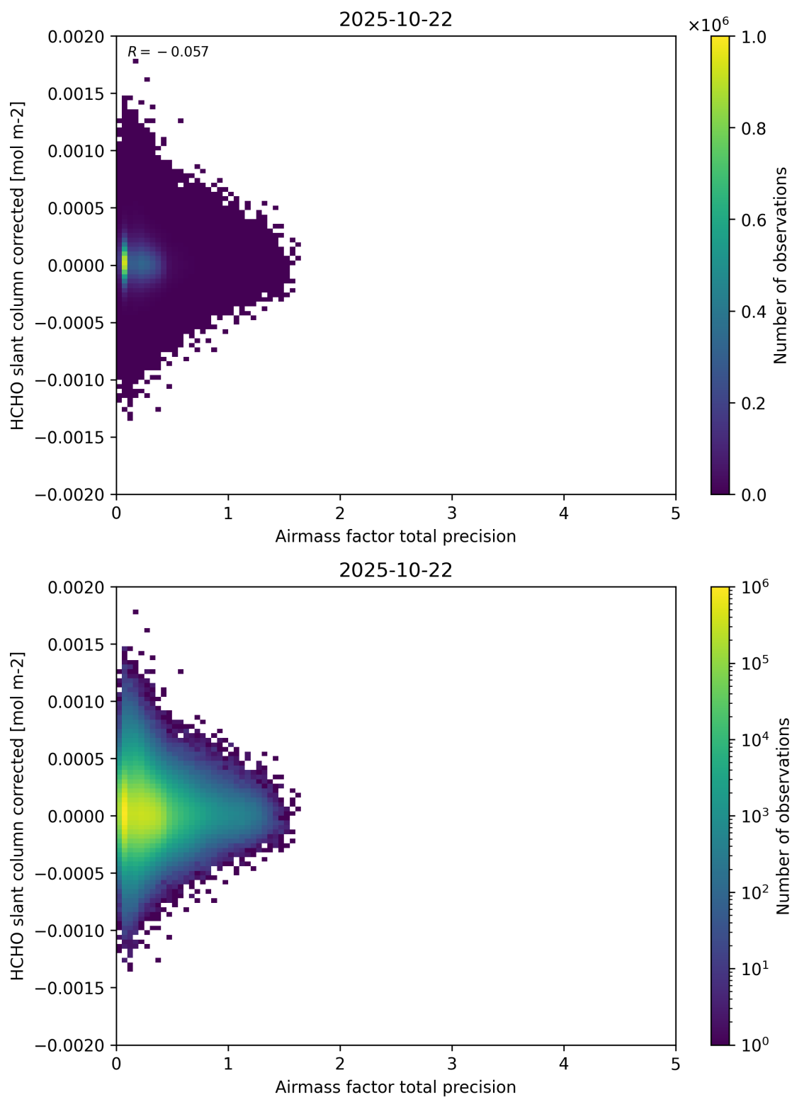
Figure 109: Scatter density plot of “Airmass factor total precision” against “HCHO slant column corrected” for 2025-10-22 to 2025-10-23.
