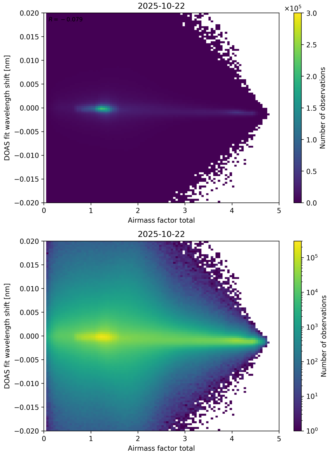
Figure 98: Scatter density plot of “Airmass factor total” against “DOAS fit wavelength shift” for 2025-10-22 to 2025-10-23.
