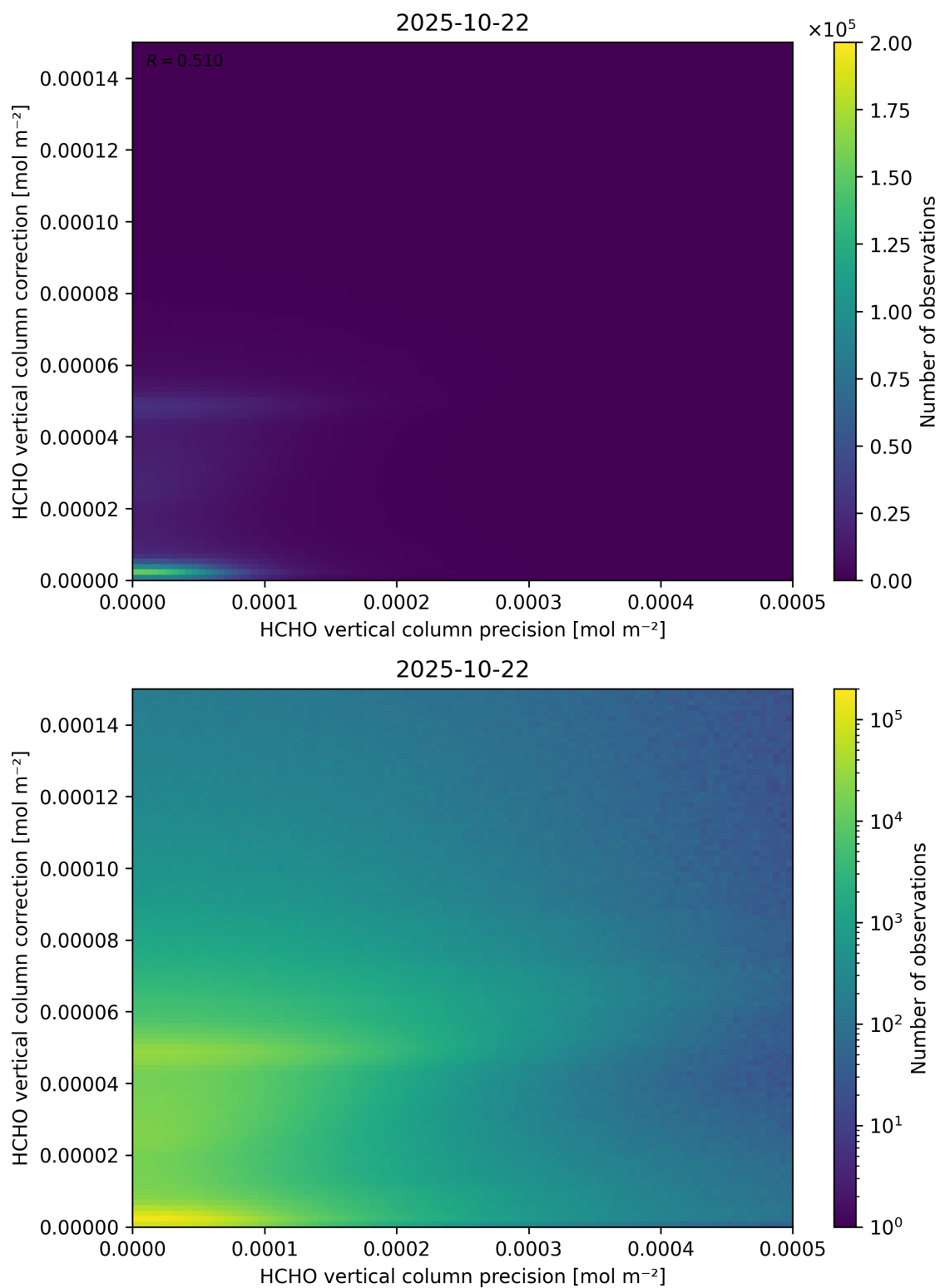
Figure 146: Scatter density plot of “HCHO vertical column precision” against “HCHO vertical column correction” for 2025-10-22 to 2025-10-23.
