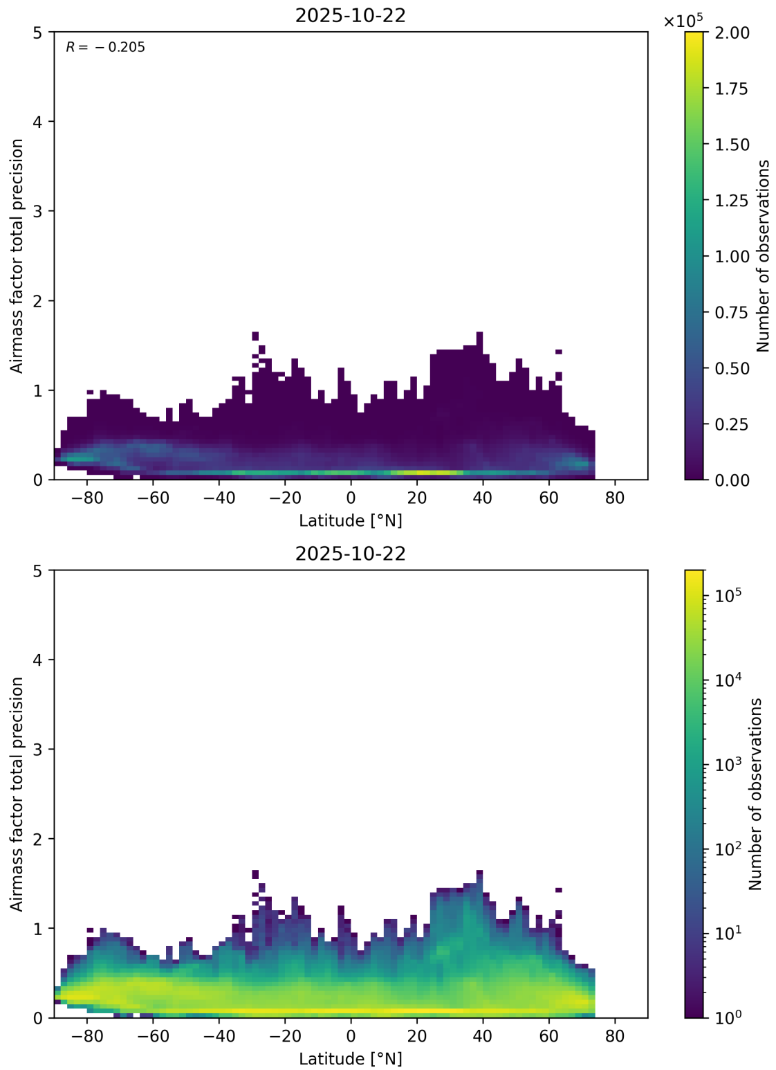
Figure 162: Scatter density plot of “Latitude” against “Airmass factor total precision” for 2025-10-22 to 2025-10-23.
