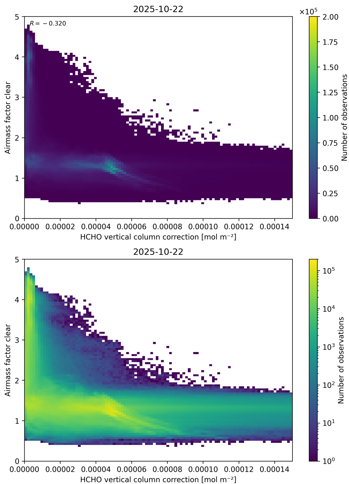
Figure 115: Scatter density plot of “HCHO vertical column correction” against “Airmass factor clear” for 2025-10-22 to 2025-10-23.
