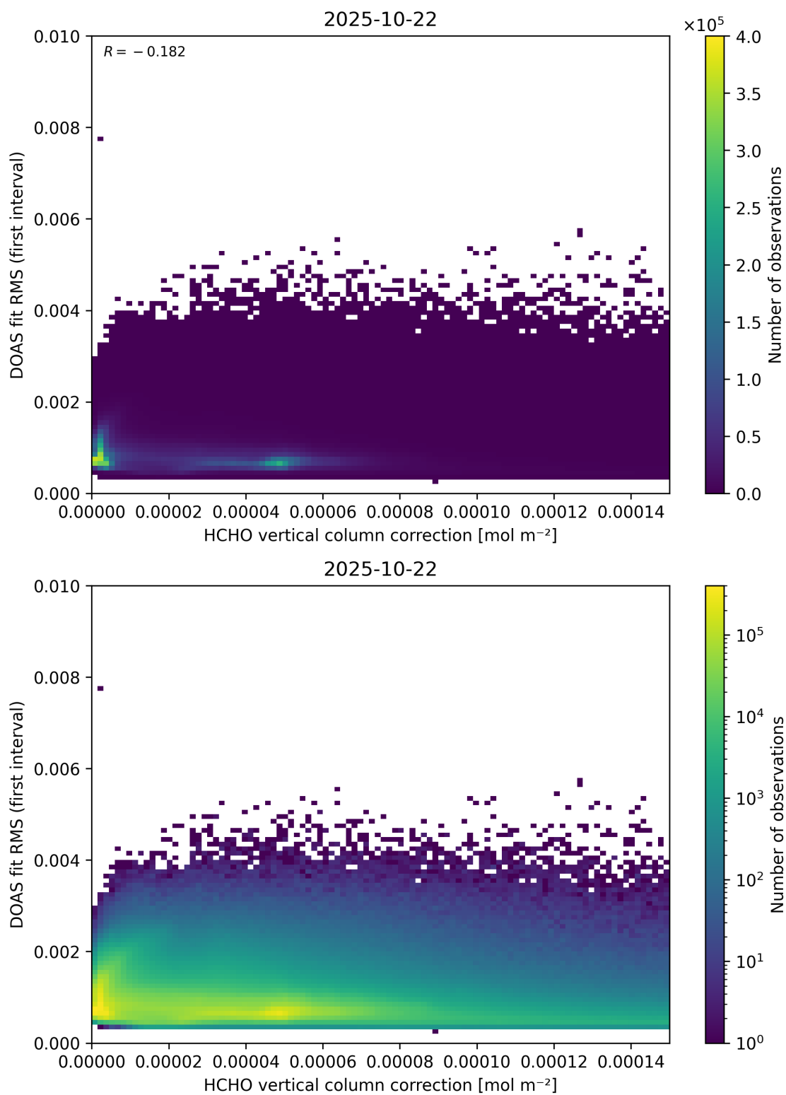
Figure 112: Scatter density plot of “HCHO vertical column correction” against “DOAS fit RMS (first interval)” for 2025-10-22 to 2025-10-23.
