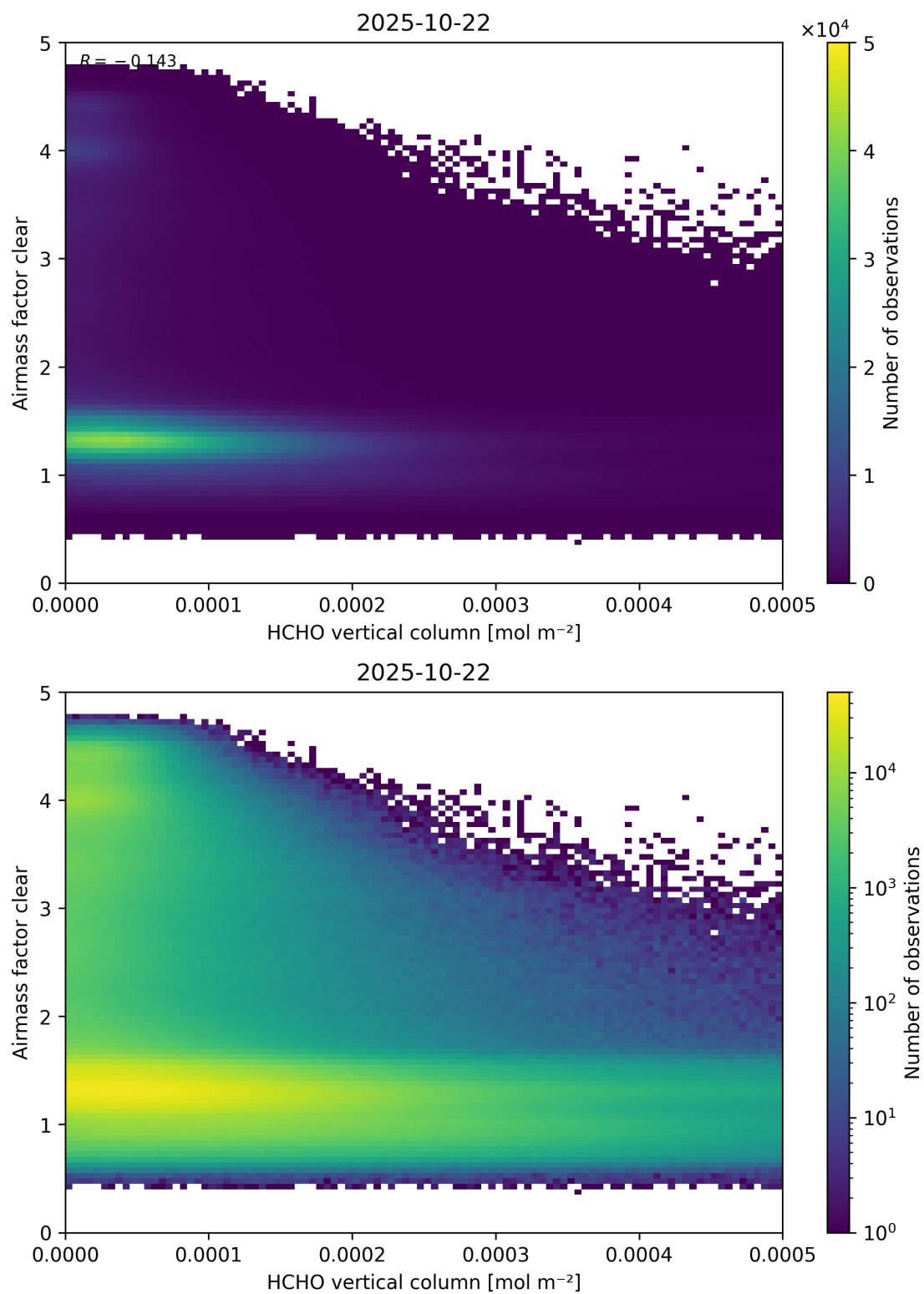
Figure 126: Scatter density plot of “HCHO vertical column” against “Airmass factor clear” for 2025-10-22 to 2025-10-23.
