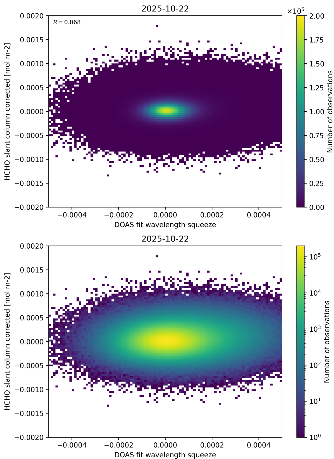
Figure 69: Scatter density plot of “DOAS fit wavelength squeeze” against “HCHO slant column corrected” for 2025-10-22 to 2025-10-23.
