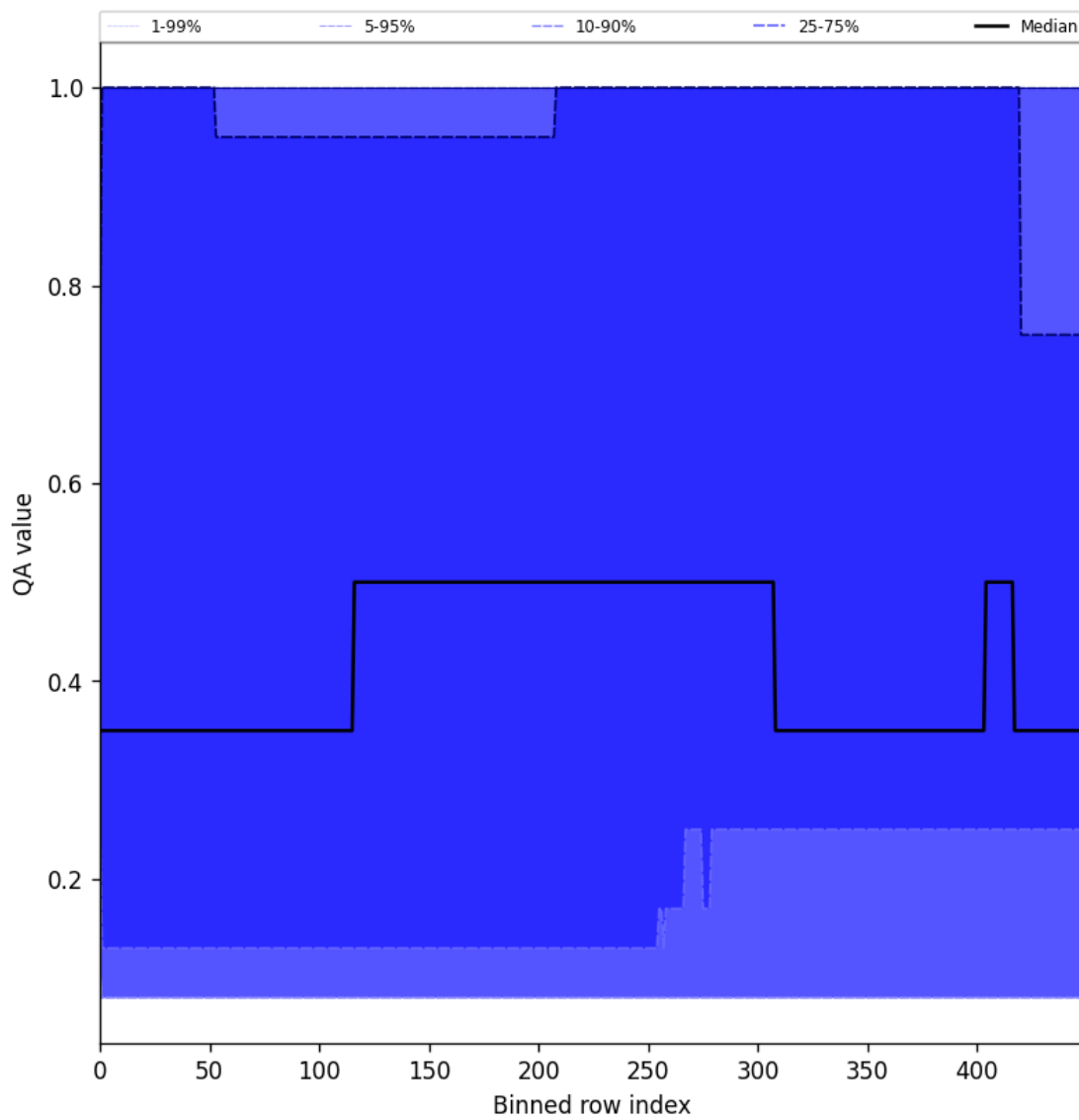
Figure 48: Along track statistics of “QA value” for 2025-10-22 to 2025-10-23
