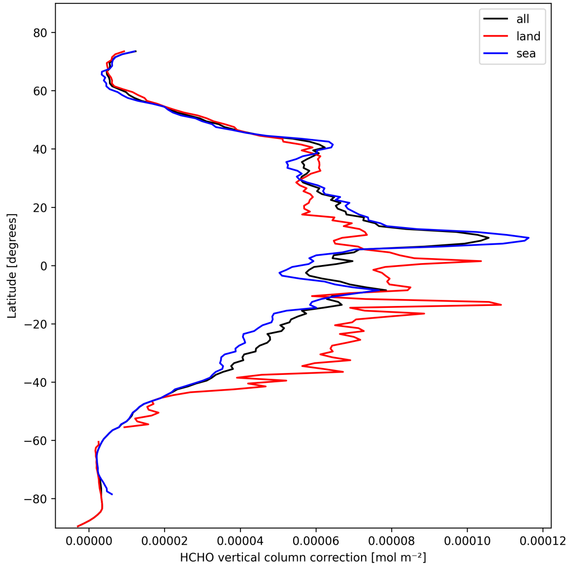
Figure 23: Zonal average of “HCHO vertical column correction” for 2025-10-22 to 2025-10-23.
