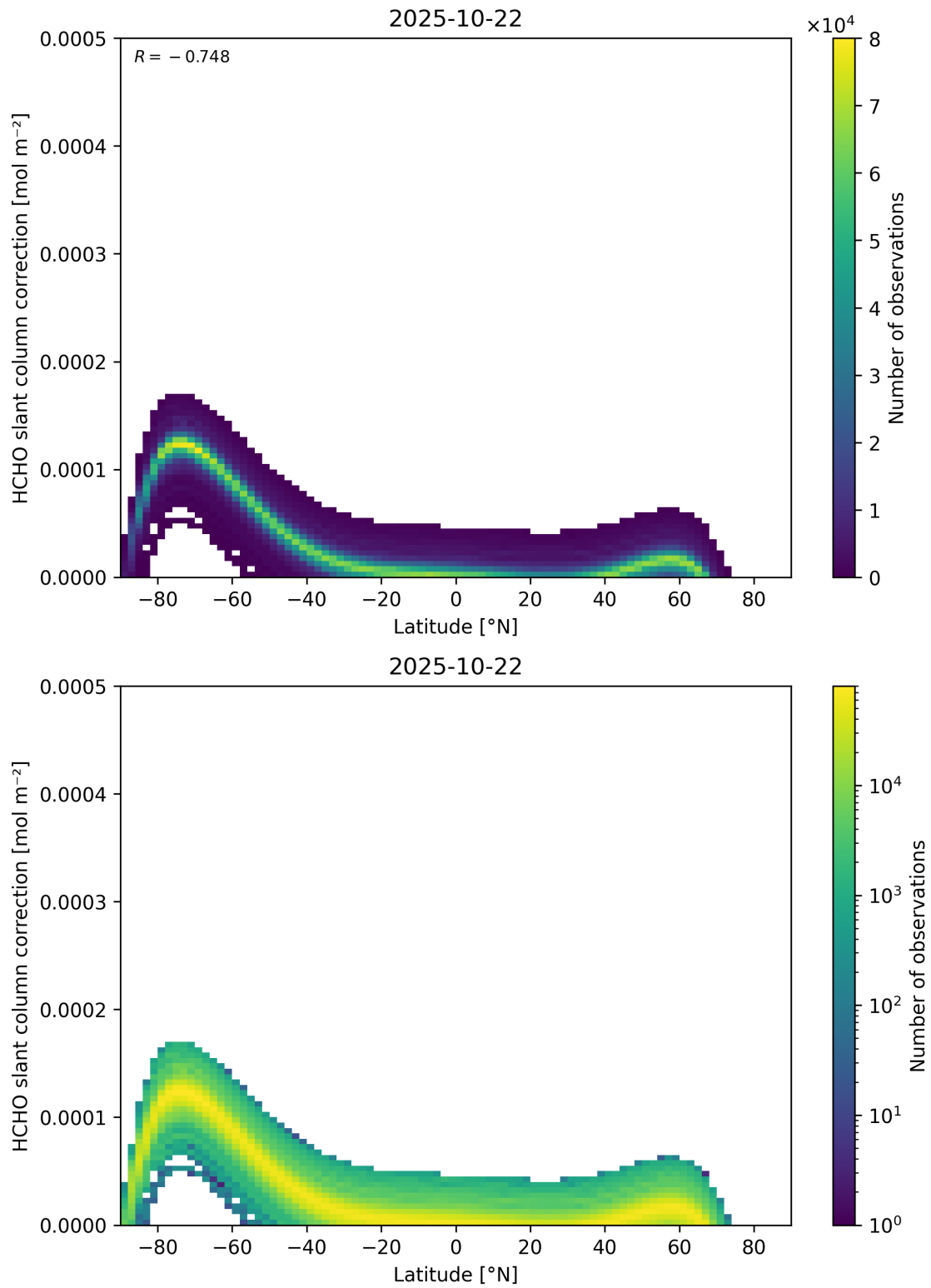
Figure 158: Scatter density plot of “Latitude” against “HCHO slant column correction” for 2025-10-22 to 2025-10-23.
