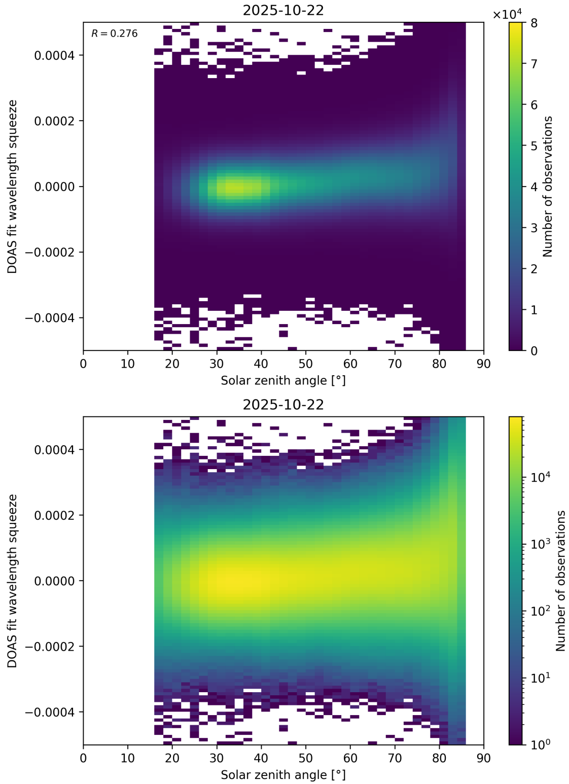
Figure 169: Scatter density plot of “Solar zenith angle” against “DOAS fit wavelength squeeze” for 2025-10-22 to 2025-10-23.
