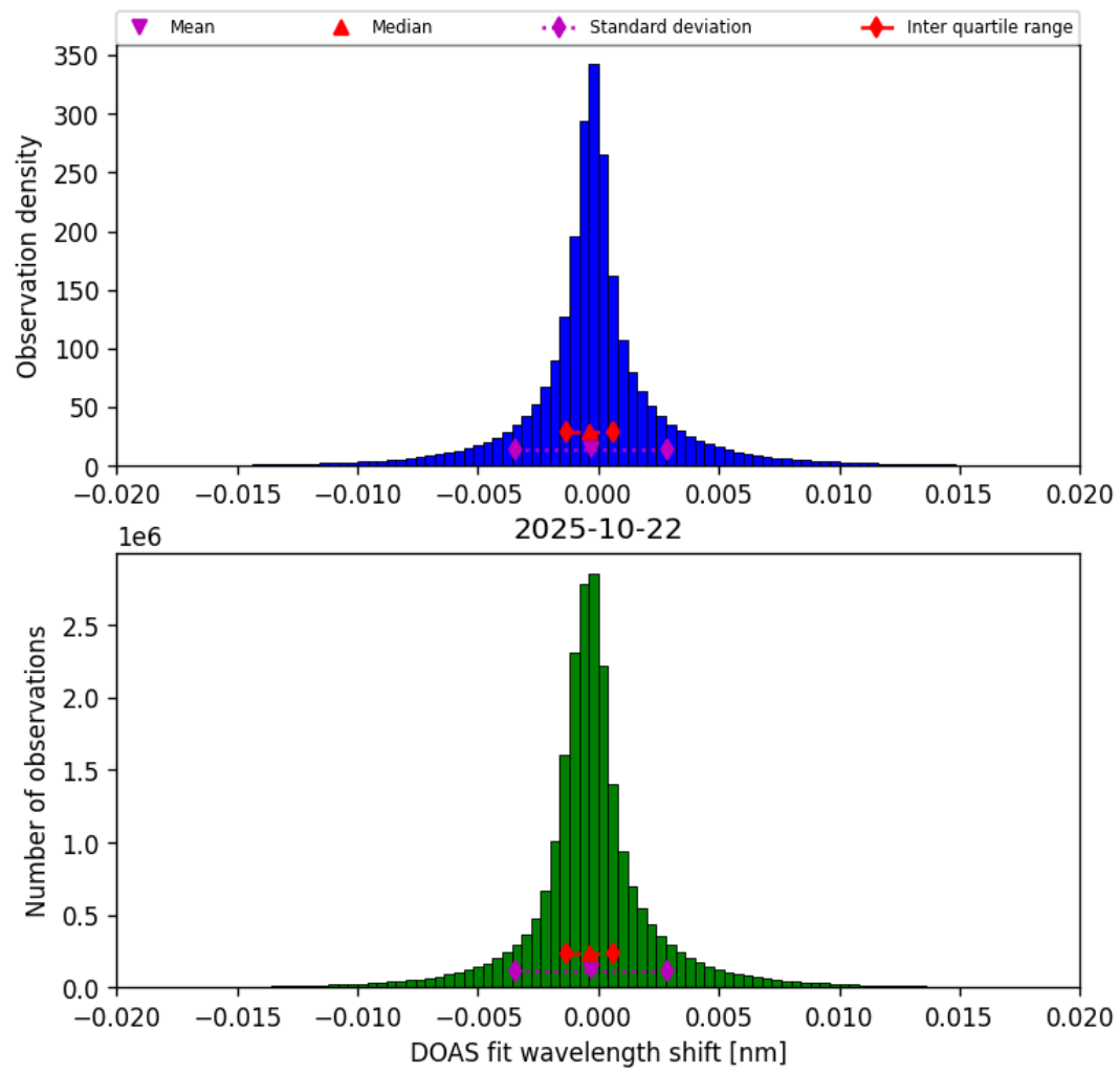
Figure 44: Histogram of “DOAS fit wavelength shift” for 2025-10-22 to 2025-10-23
