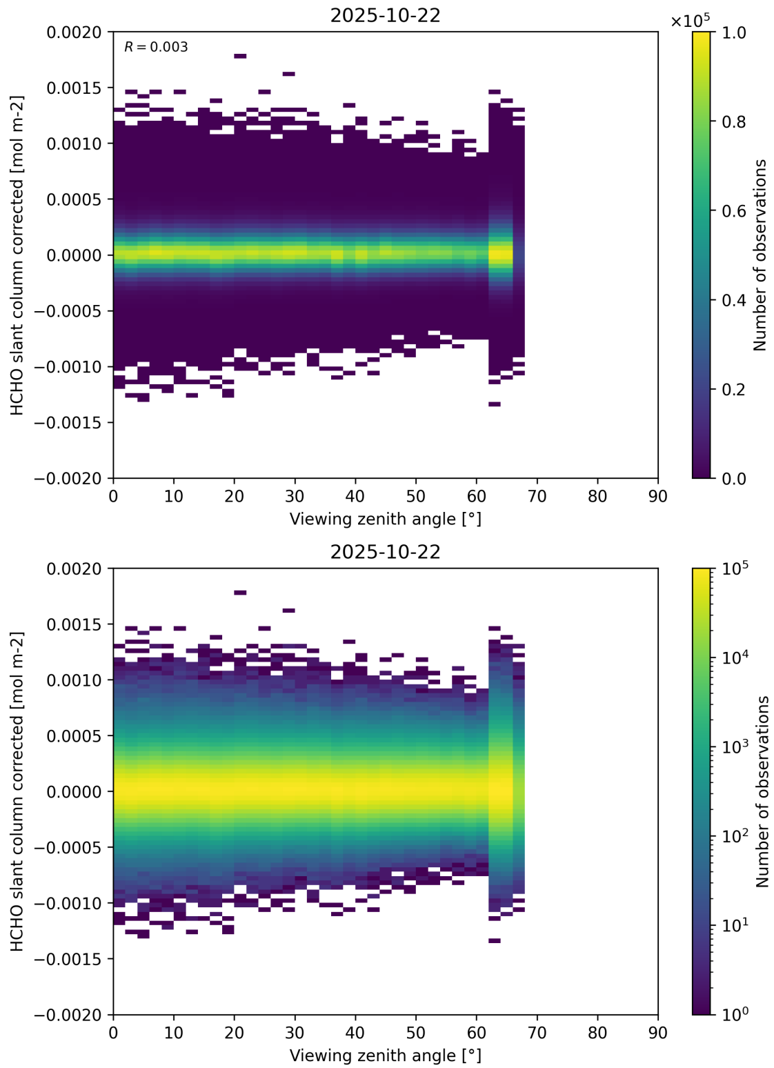
Figure 186: Scatter density plot of “Viewing zenith angle” against “HCHO slant column corrected” for 2025-10-22 to 2025-10-23.
