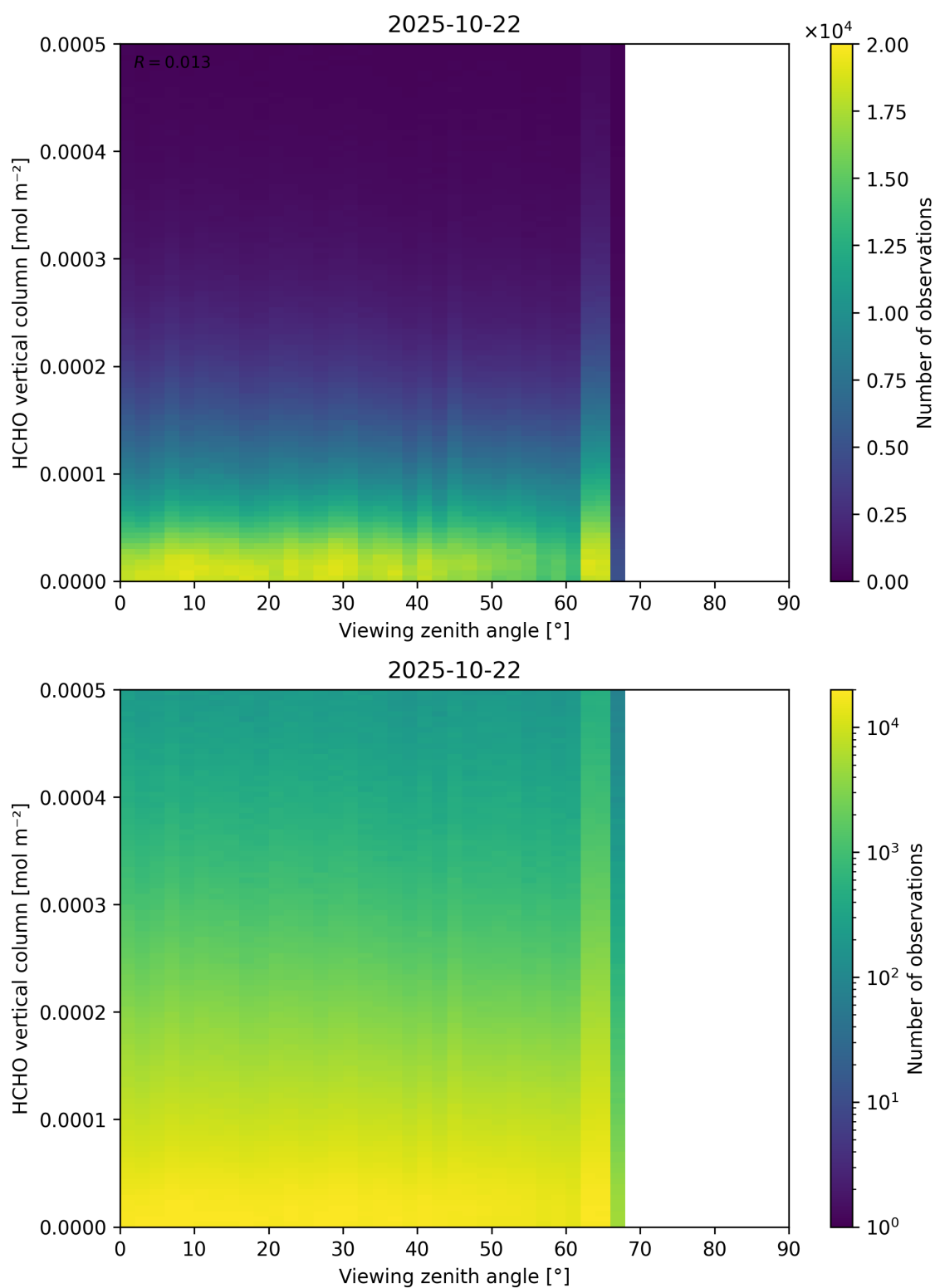
Figure 192: Scatter density plot of “Viewing zenith angle” against “HCHO vertical column” for 2025-10-22 to 2025-10-23.
