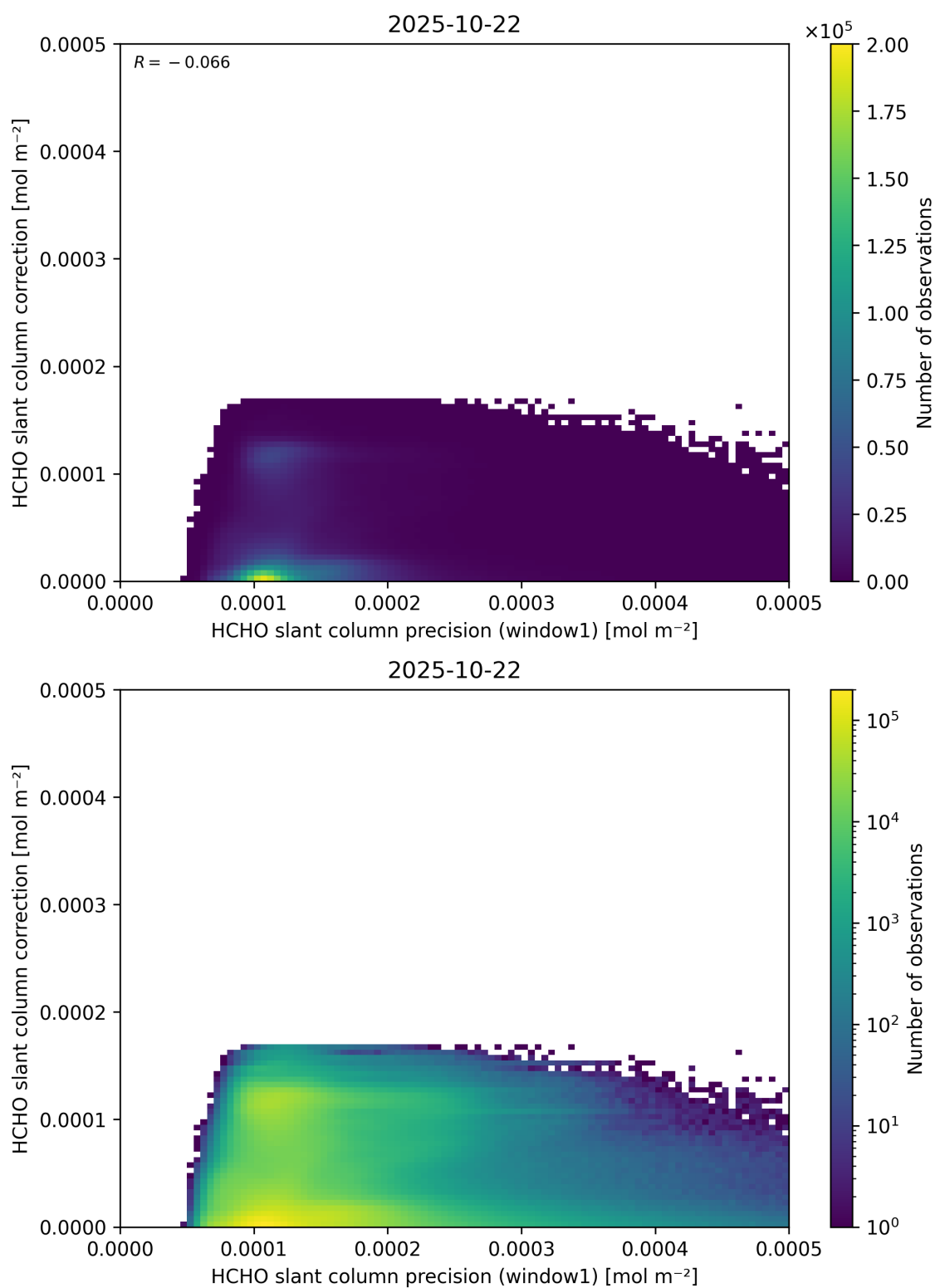
Figure 93: Scatter density plot of “HCHO slant column precision (window1)” against “HCHO slant column correction” for 2025-10-22 to 2025-10-23.
