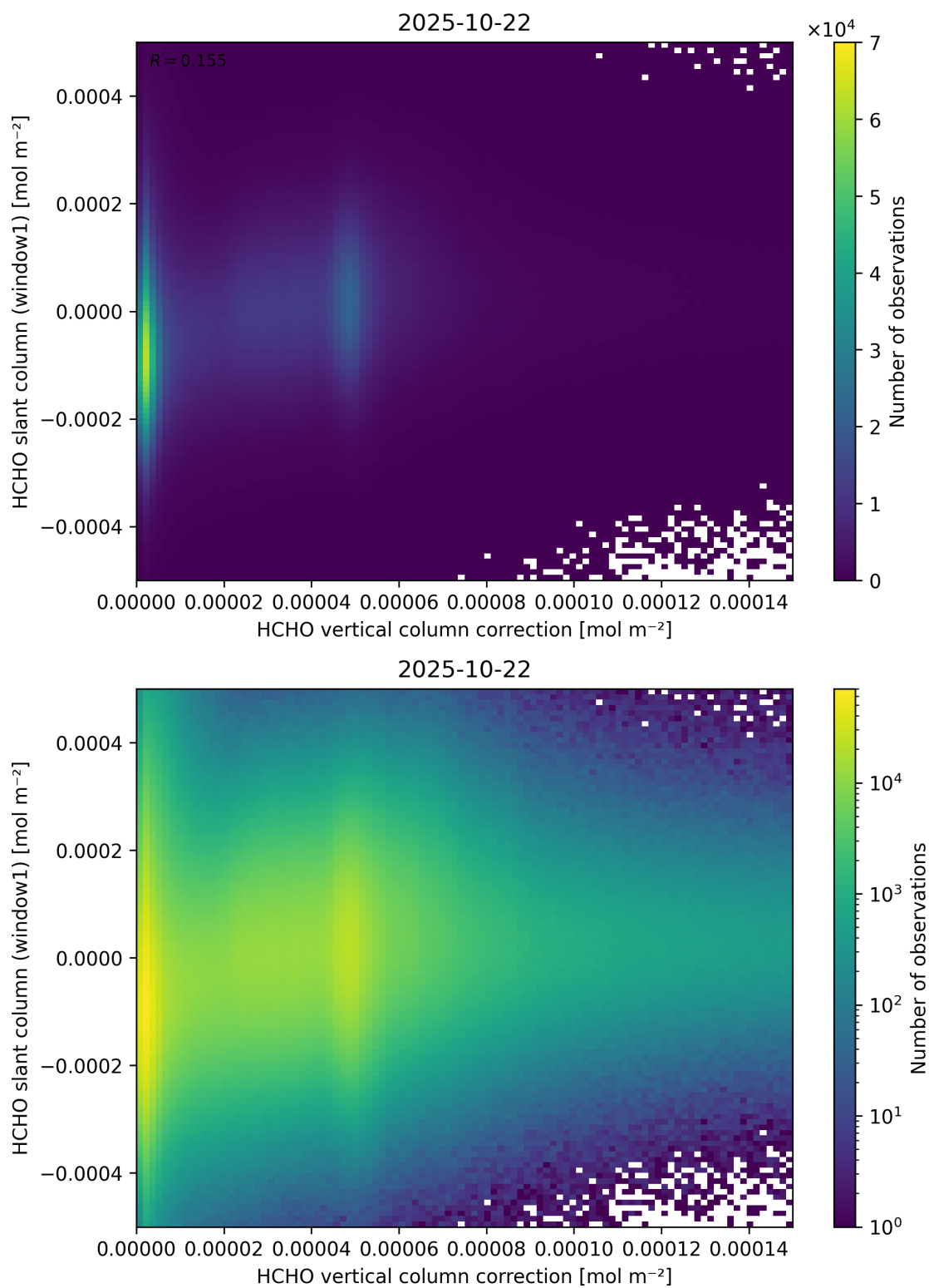
Figure 118: Scatter density plot of “HCHO vertical column correction” against “HCHO slant column (window1)” for 2025-10-22 to 2025-10-23.
