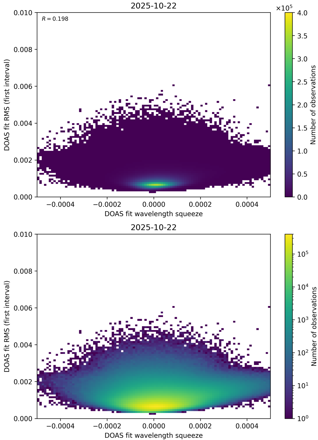
Figure 68: Scatter density plot of “DOAS fit wavelength squeeze” against “DOAS fit RMS (first interval)” for 2025-10-22 to 2025-10-23.
