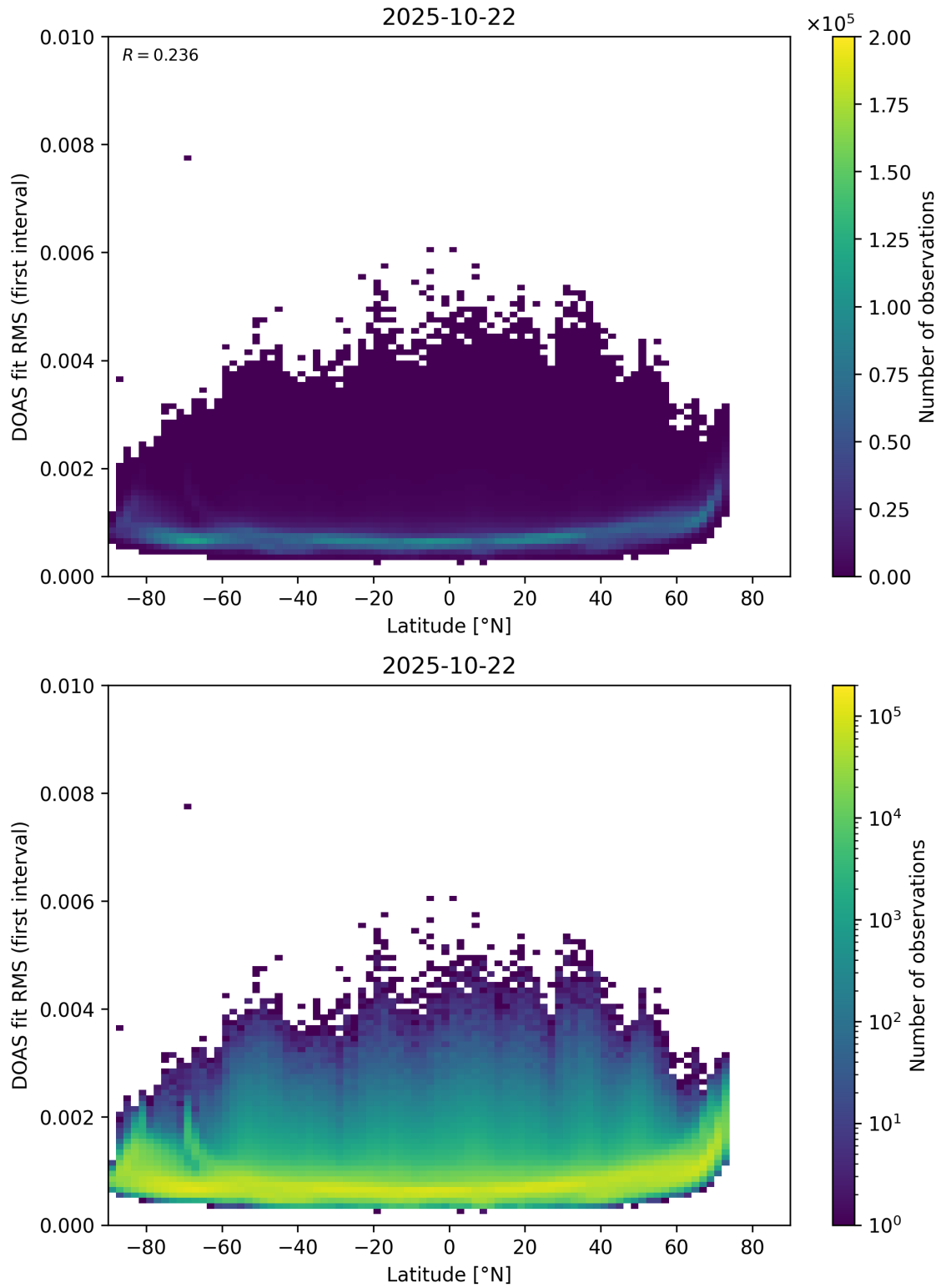
Figure 153: Scatter density plot of “Latitude” against “DOAS fit RMS (first interval)” for 2025-10-22 to 2025-10-23.
