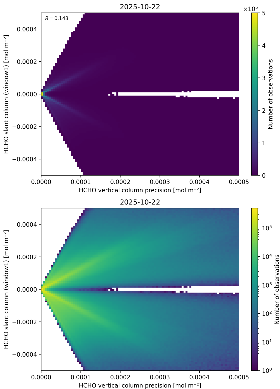
Figure 142: Scatter density plot of “HCHO vertical column precision” against “HCHO slant column (window1)” for 2025-10-22 to 2025-10-23.
