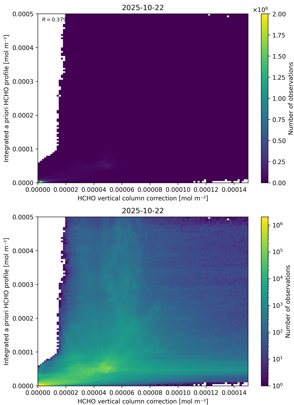
Figure 122: Scatter density plot of “HCHO vertical column correction” against “Integrated a priori HCHO profile” for 2025-10-22 to 2025-10-23.
