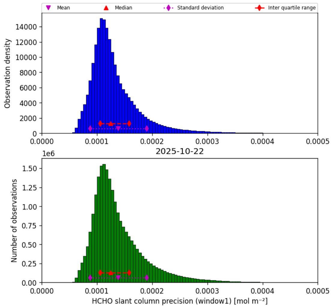
Figure 39: Histogram of “HCHO slant column precision (window1)” for 2025-10-22 to 2025-10-23
