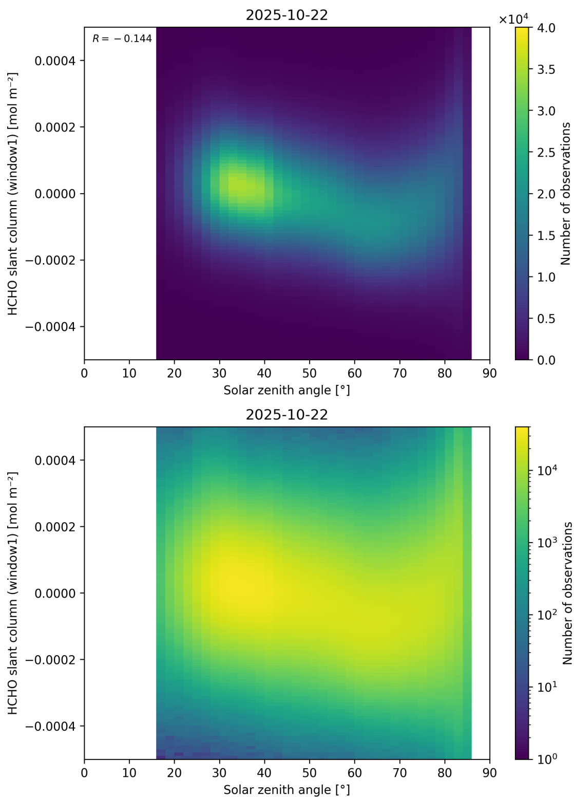
Figure 173: Scatter density plot of “Solar zenith angle” against “HCHO slant column (window1)” for 2025-10-22 to 2025-10-23.
