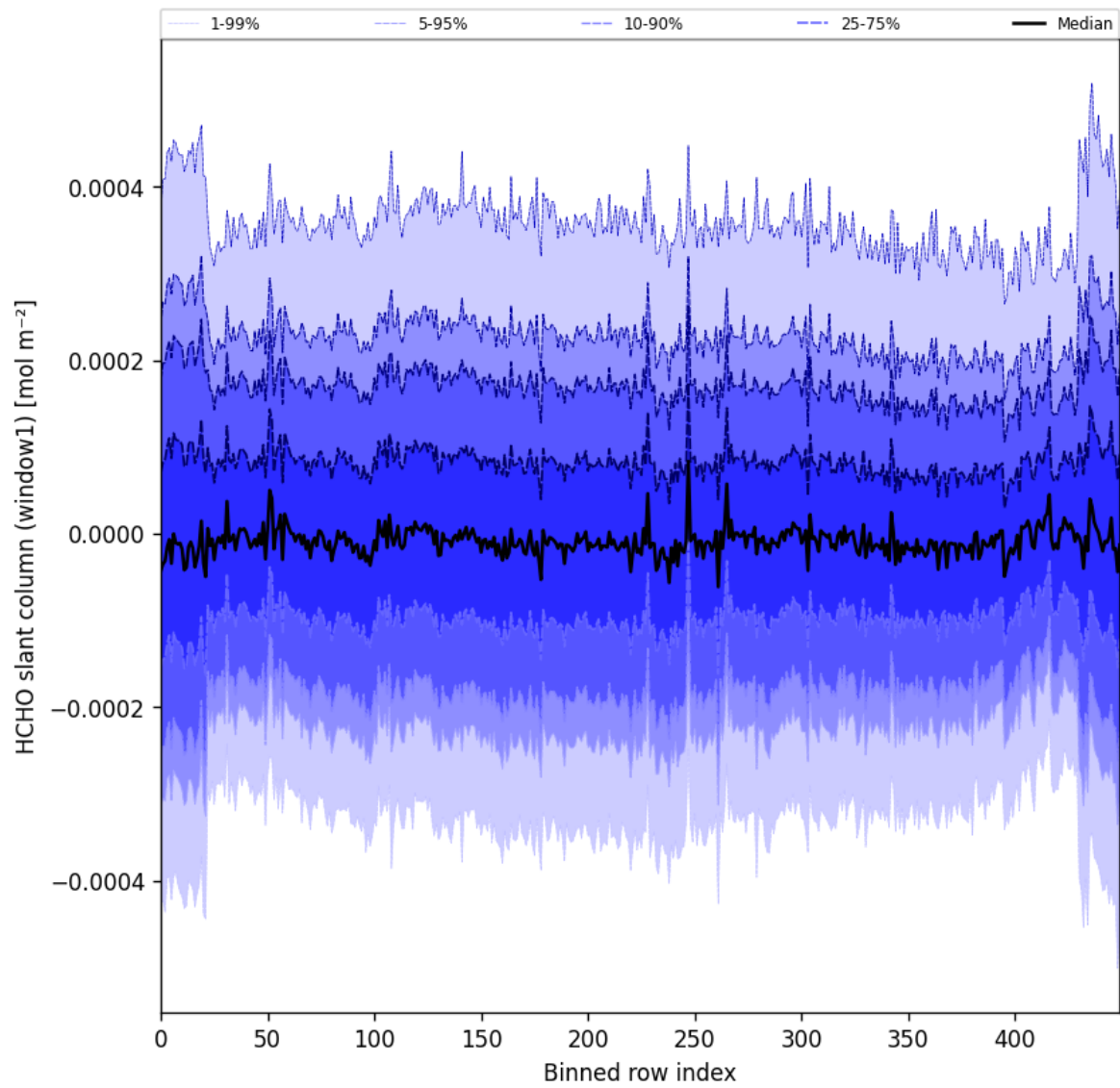
Figure 52: Along track statistics of “HCHO slant column (window1)” for 2025-10-22 to 2025-10-23
