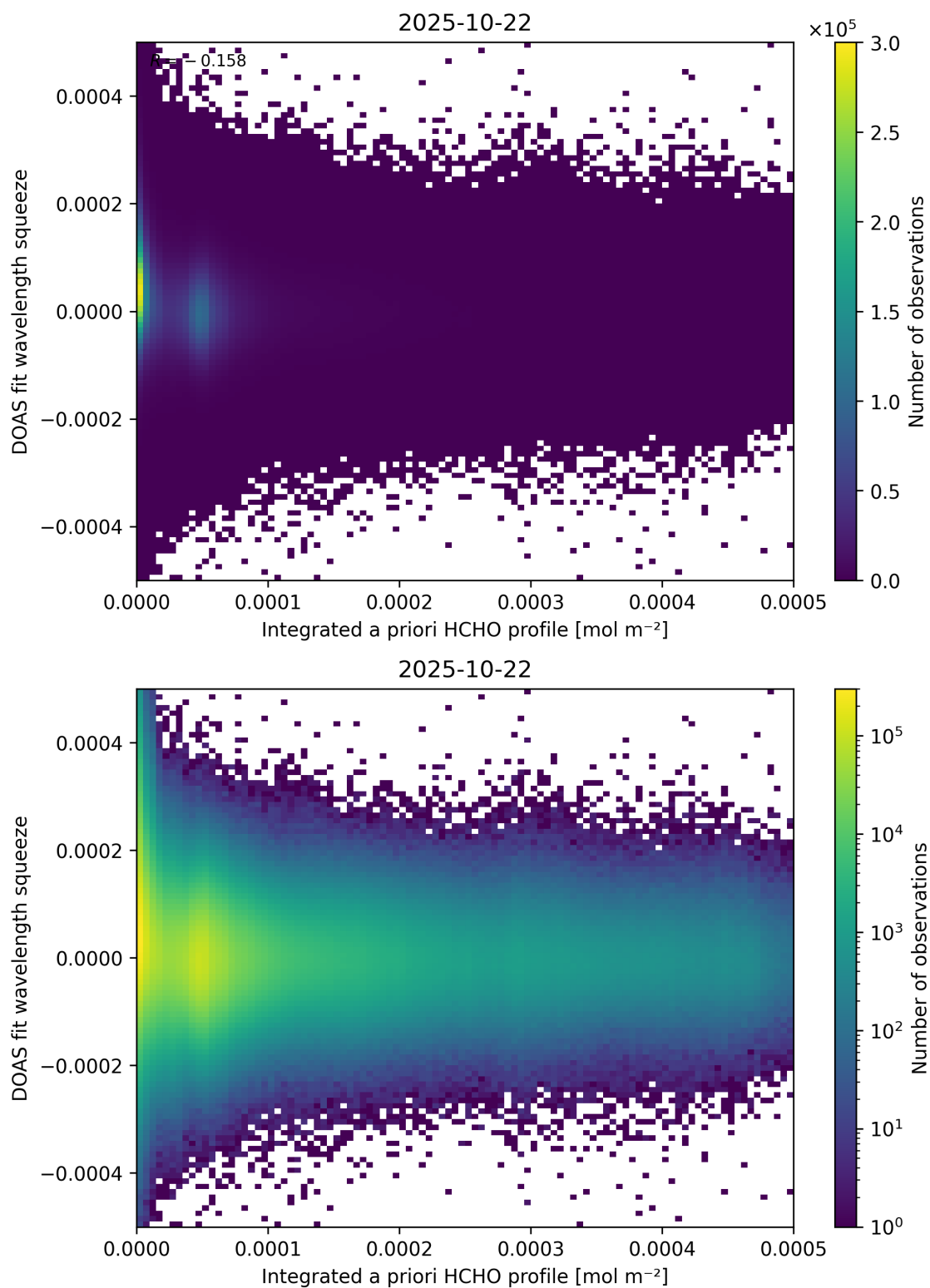
Figure 150: Scatter density plot of “Integrated a priori HCHO profile” against “DOAS fit wavelength squeeze” for 2025-10-22 to 2025-10-23.
