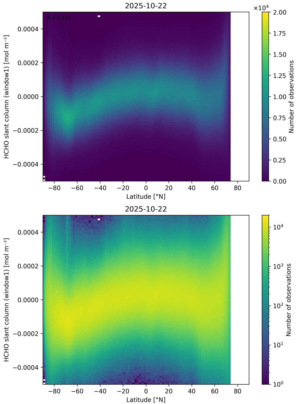
Figure 159: Scatter density plot of “Latitude” against “HCHO slant column (window1)” for 2025-10-22 to 2025-10-23.
