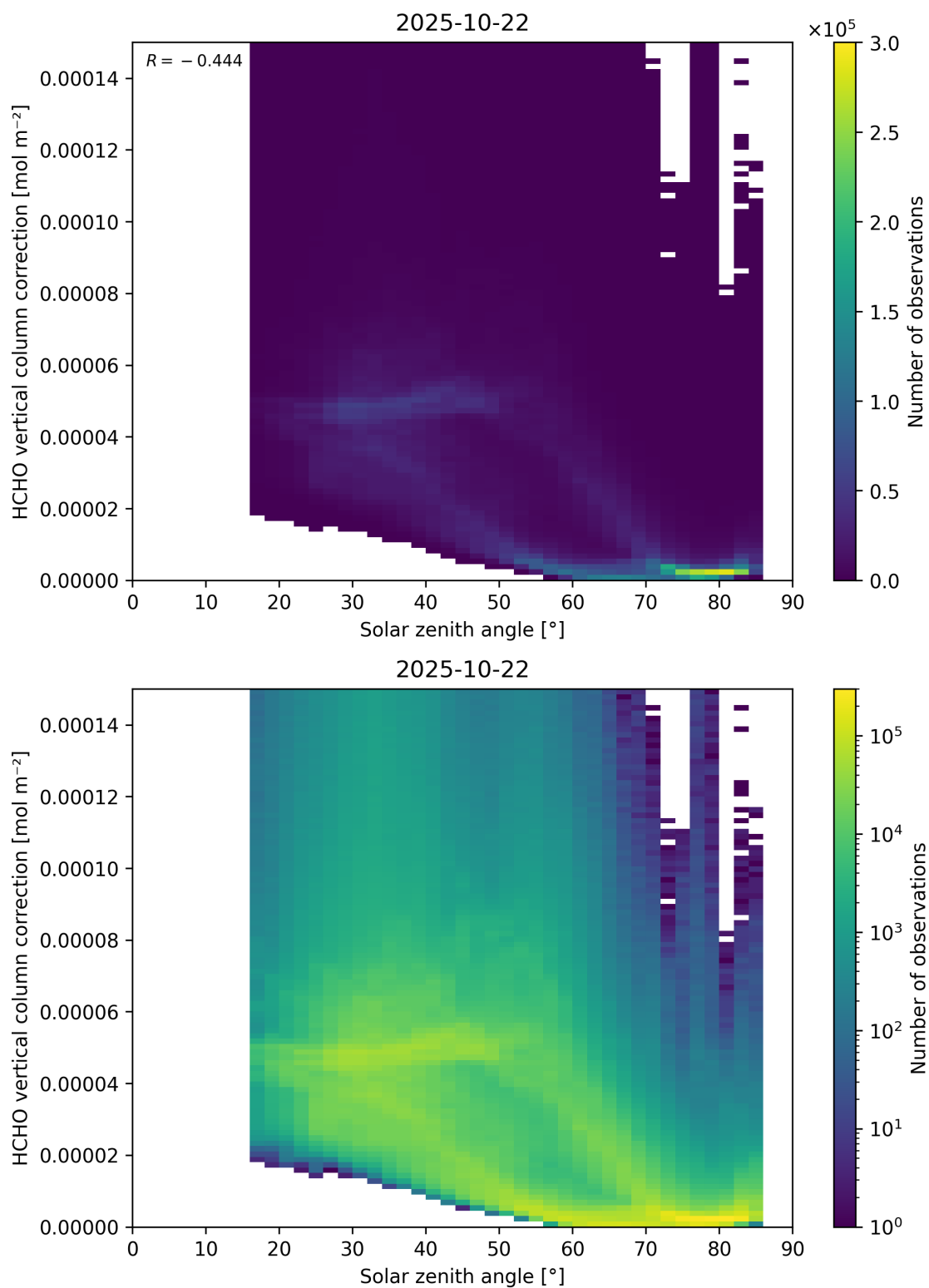
Figure 178: Scatter density plot of “Solar zenith angle” against “HCHO vertical column correction” for 2025-10-22 to 2025-10-23.
