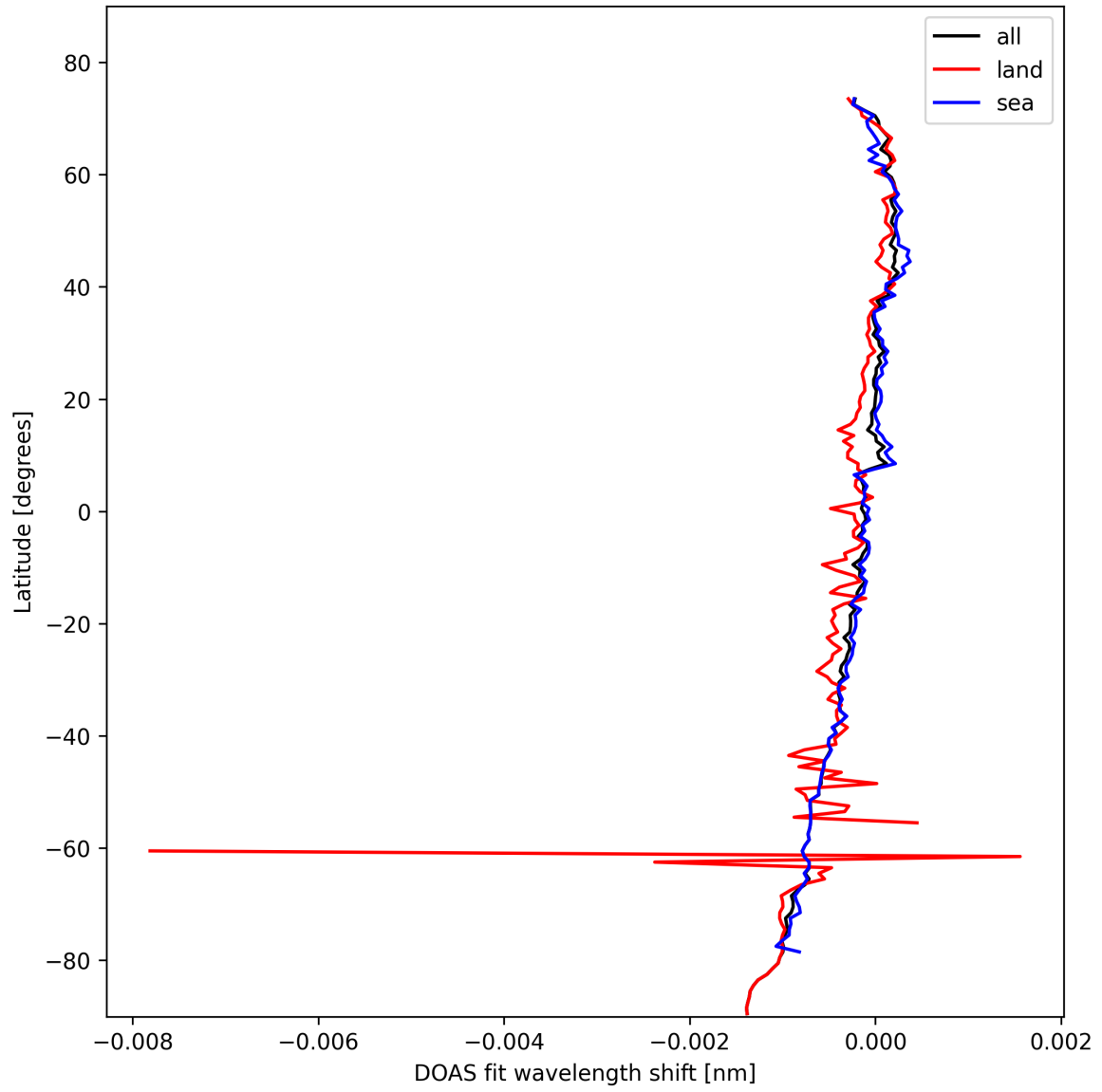
Figure 30: Zonal average of “DOAS fit wavelength shift” for 2025-10-22 to 2025-10-23.
