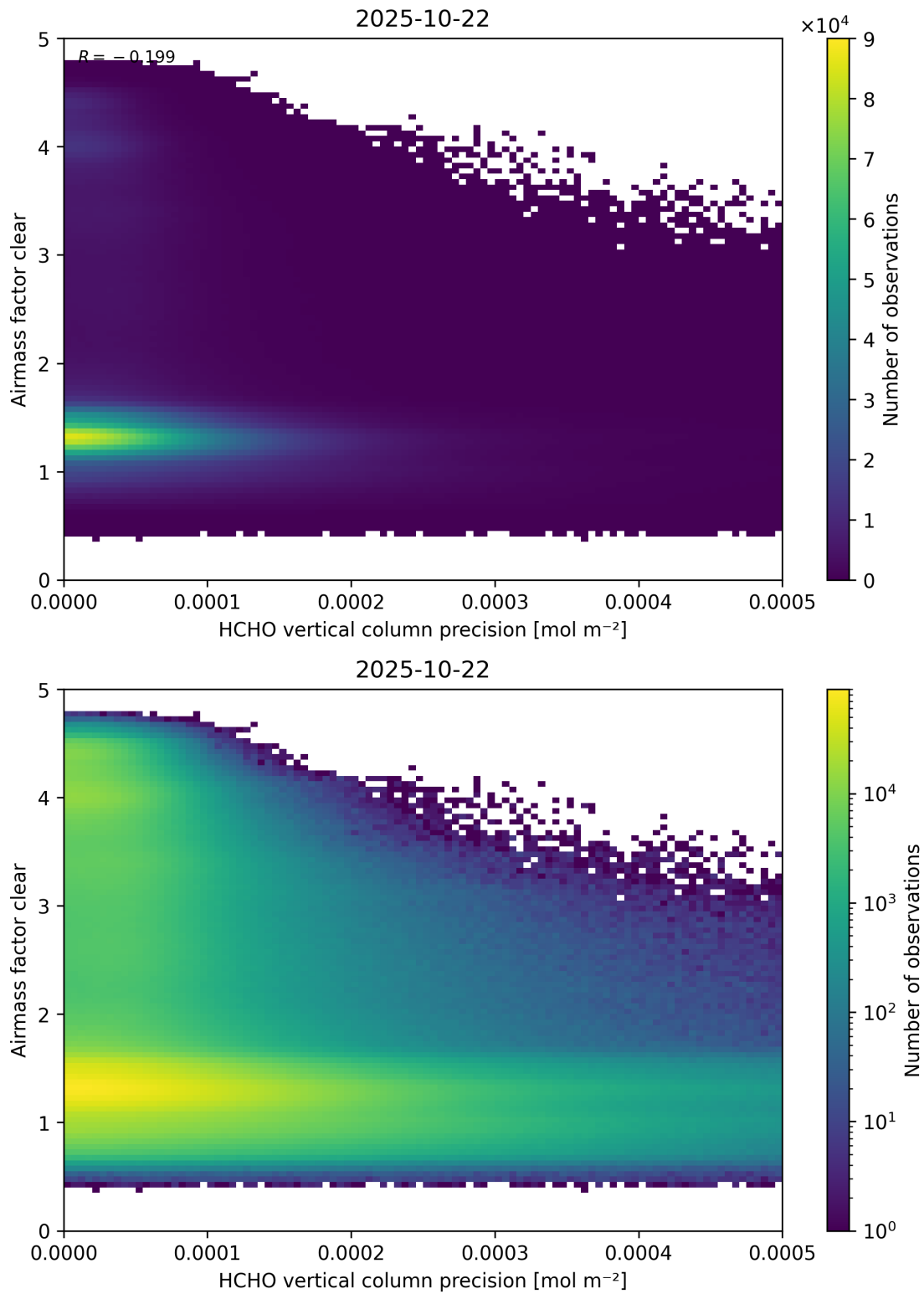
Figure 139: Scatter density plot of “HCHO vertical column precision” against “Airmass factor clear” for 2025-10-22 to 2025-10-23.
