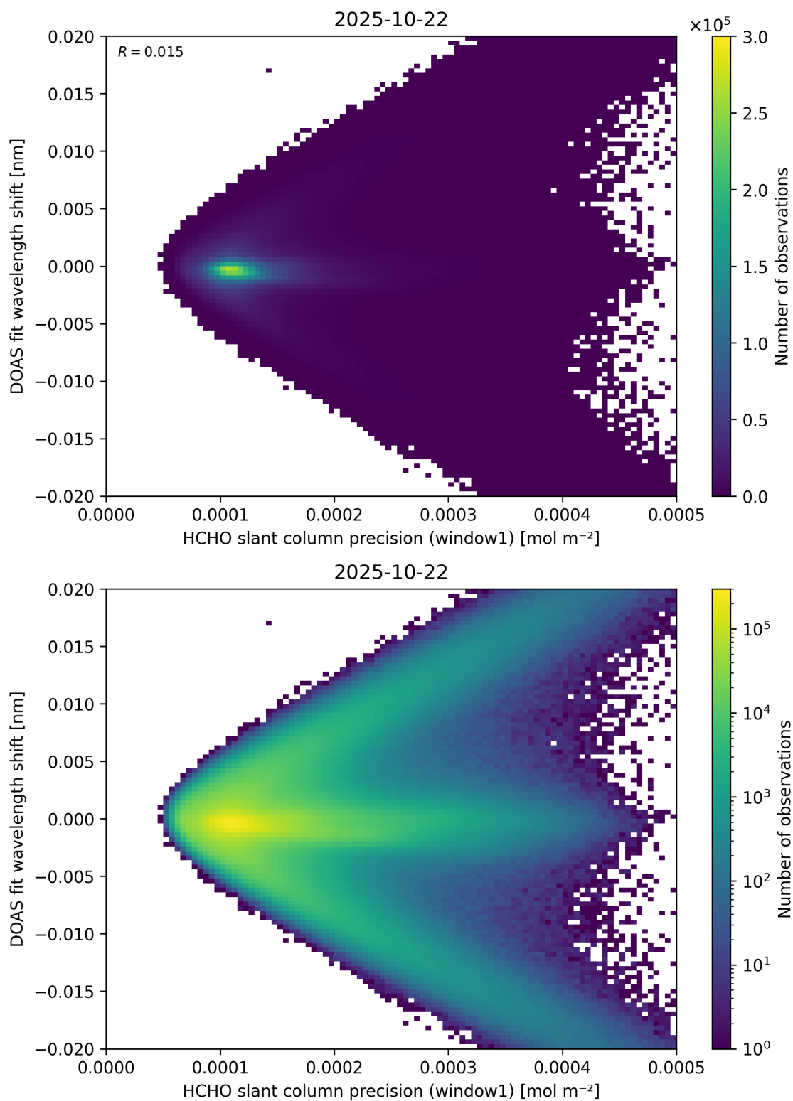
Figure 89: Scatter density plot of “HCHO slant column precision (window1)” against “DOAS fit wavelength shift” for 2025-10-22 to 2025-10-23.
