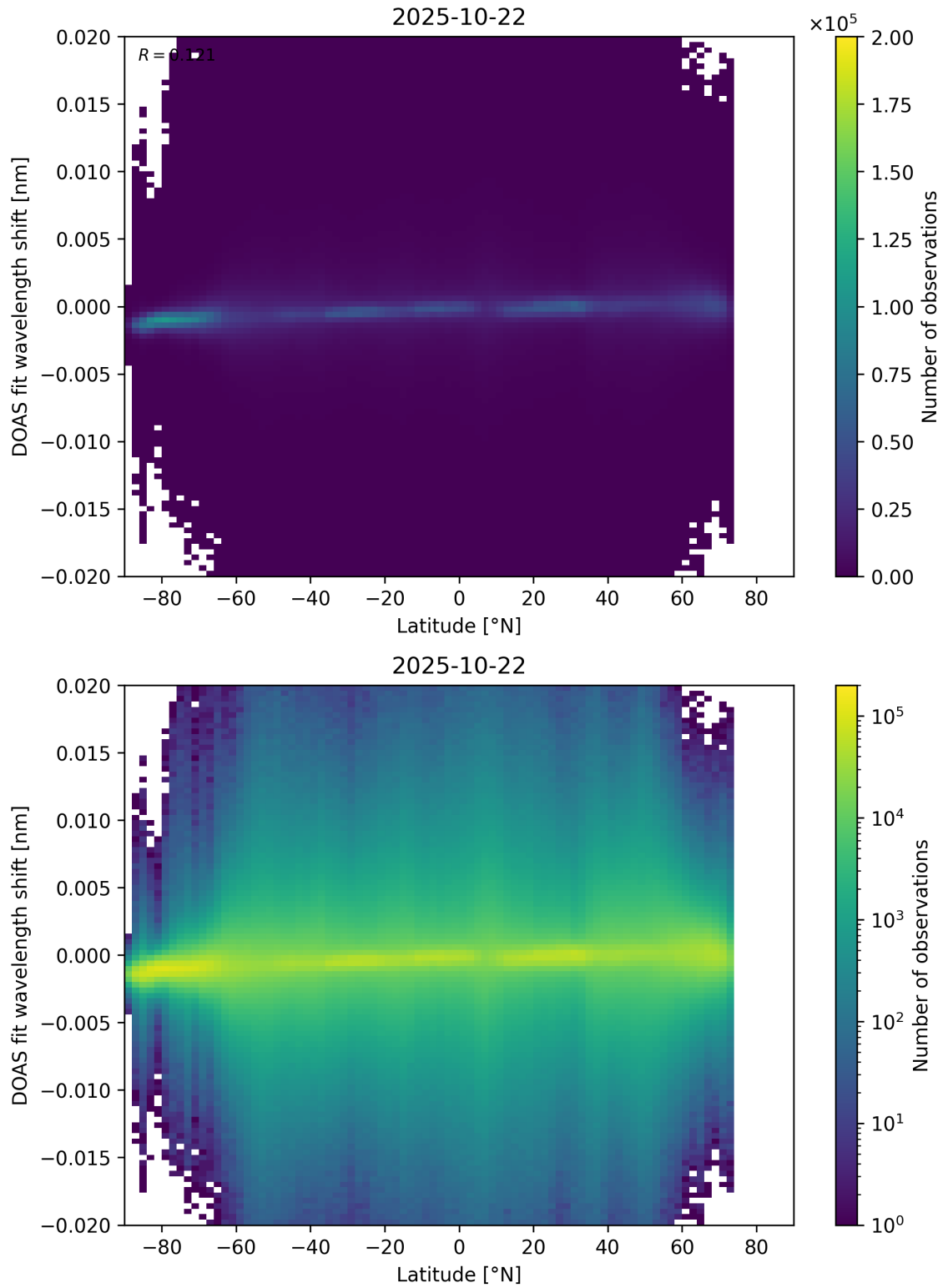
Figure 154: Scatter density plot of “Latitude” against “DOAS fit wavelength shift” for 2025-10-22 to 2025-10-23.
