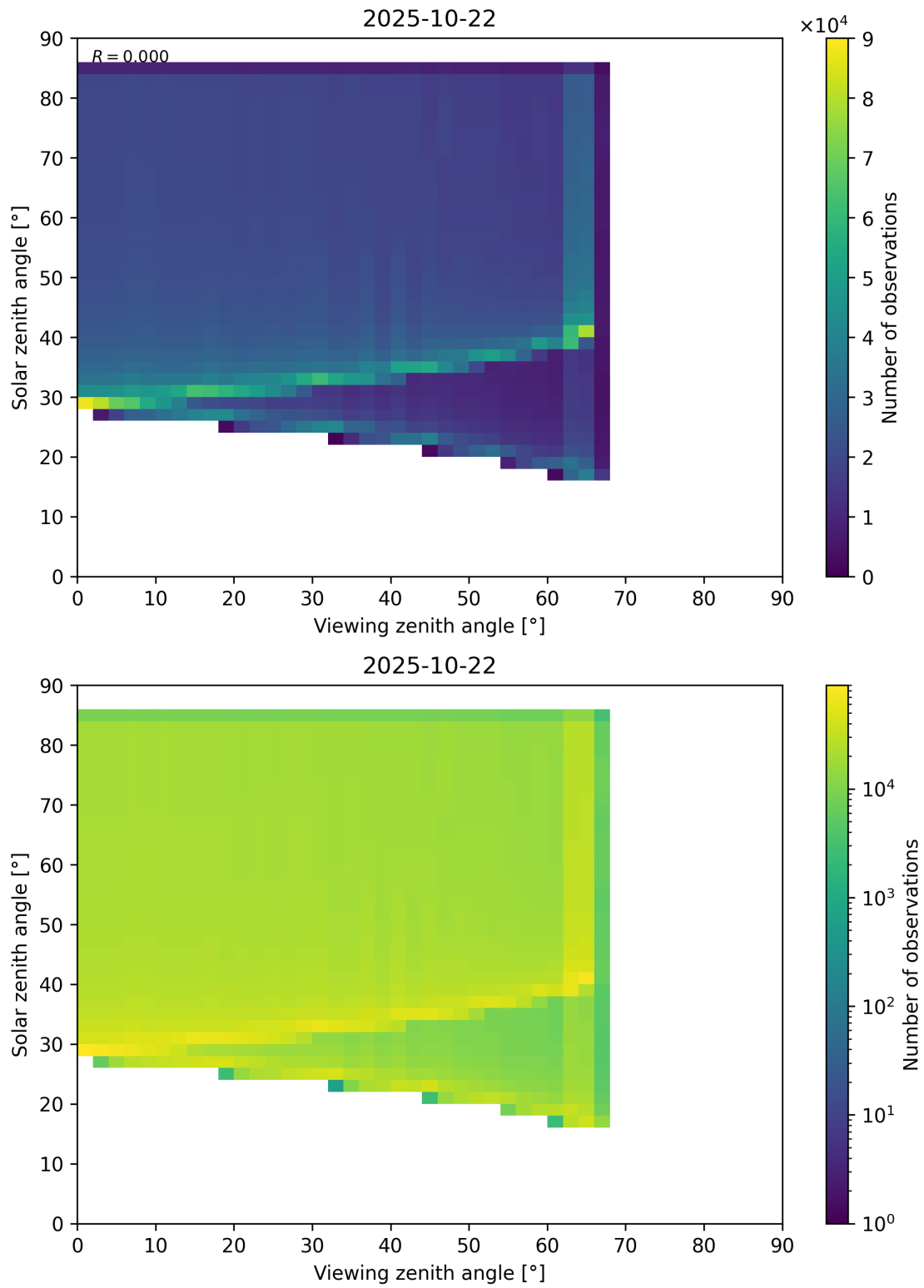
Figure 197: Scatter density plot of “Viewing zenith angle” against “Solar zenith angle” for 2025-10-22 to 2025-10-23.
