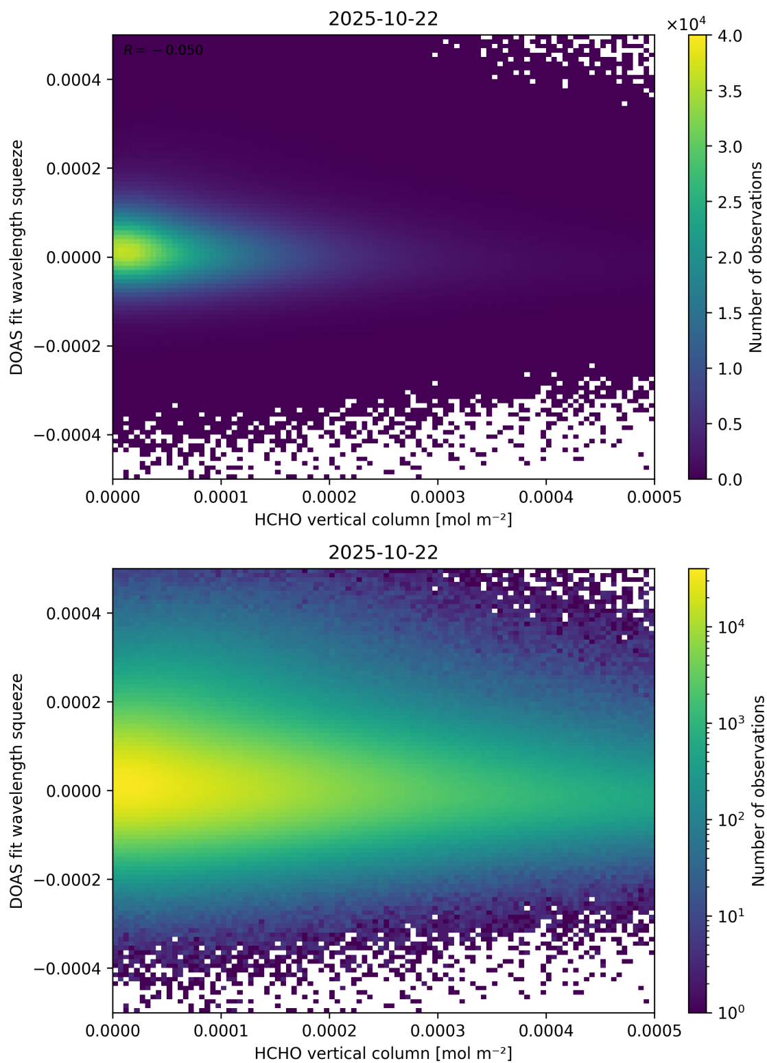
Figure 125: Scatter density plot of “HCHO vertical column” against “DOAS fit wavelength squeeze” for 2025-10-22 to 2025-10-23.
