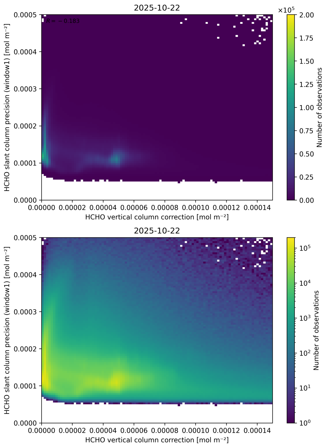
Figure 119: Scatter density plot of “HCHO vertical column correction” against “HCHO slant column precision (window1)” for 2025-10-22 to 2025-10-23.
