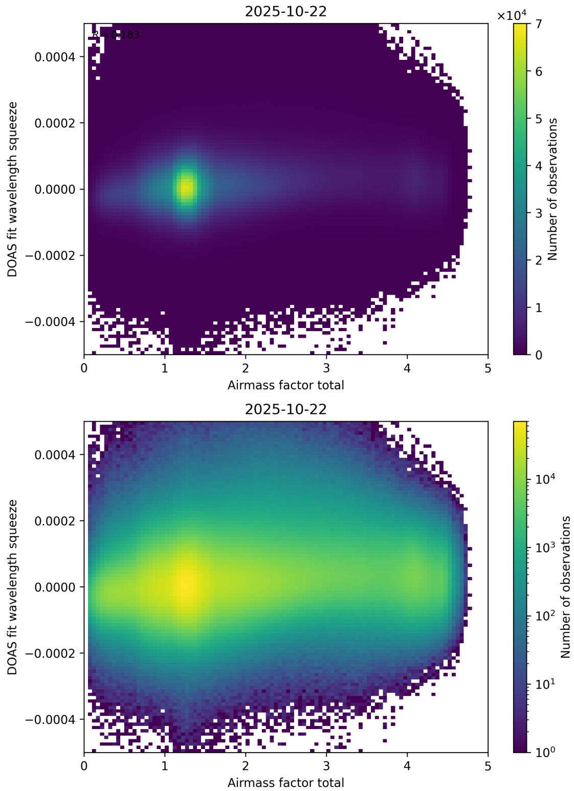
Figure 99: Scatter density plot of “Airmass factor total” against “DOAS fit wavelength squeeze” for 2025-10-22 to 2025-10-23.
