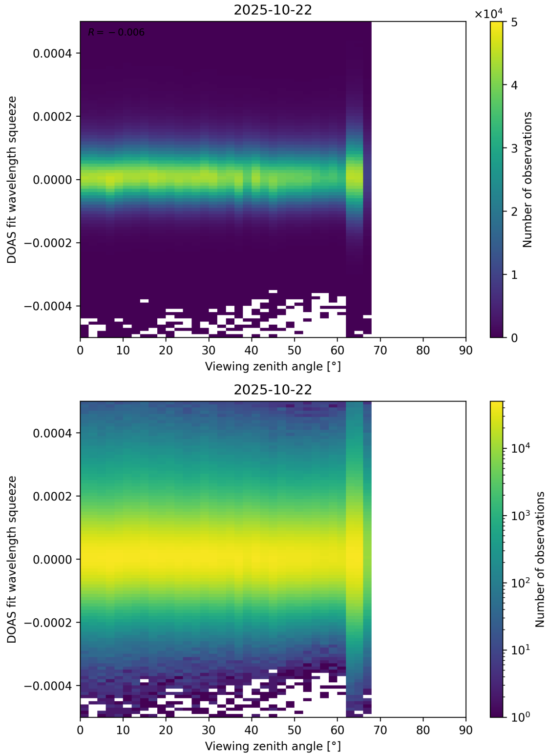
Figure 184: Scatter density plot of “Viewing zenith angle” against “DOAS fit wavelength squeeze” for 2025-10-22 to 2025-10-23.
