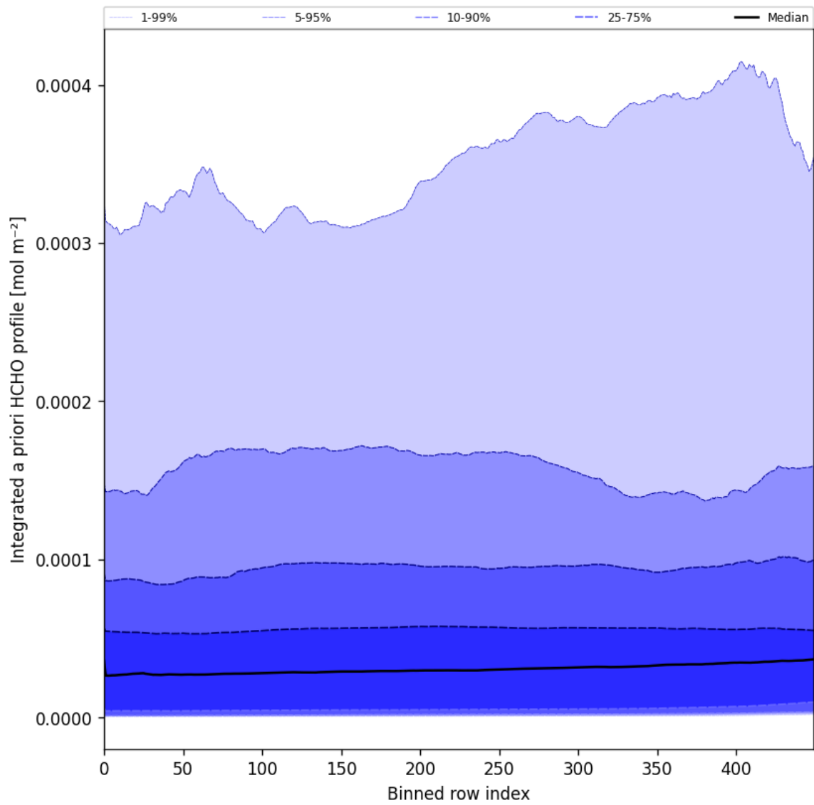
Figure 57: Along track statistics of "Integrated a priori HCHO profile" for 2025-10-22 to 2025-10-23
