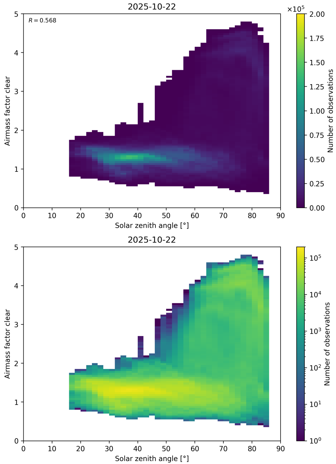
Figure 170: Scatter density plot of “Solar zenith angle” against “Airmass factor clear” for 2025-10-22 to 2025-10-23.
