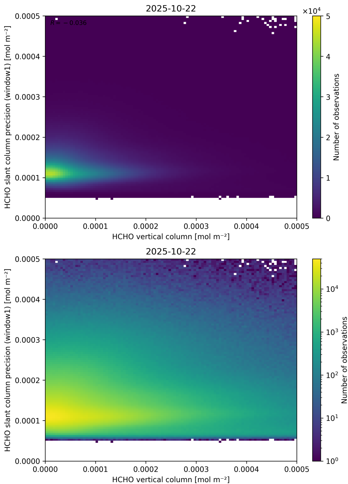
Figure 130: Scatter density plot of “HCHO vertical column” against “HCHO slant column precision (window1)” for 2025-10-22 to 2025-10-23.
