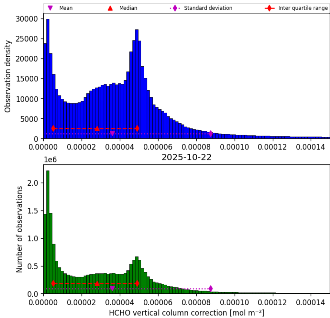
Figure 37: Histogram of “HCHO vertical column correction” for 2025-10-22 to 2025-10-23
