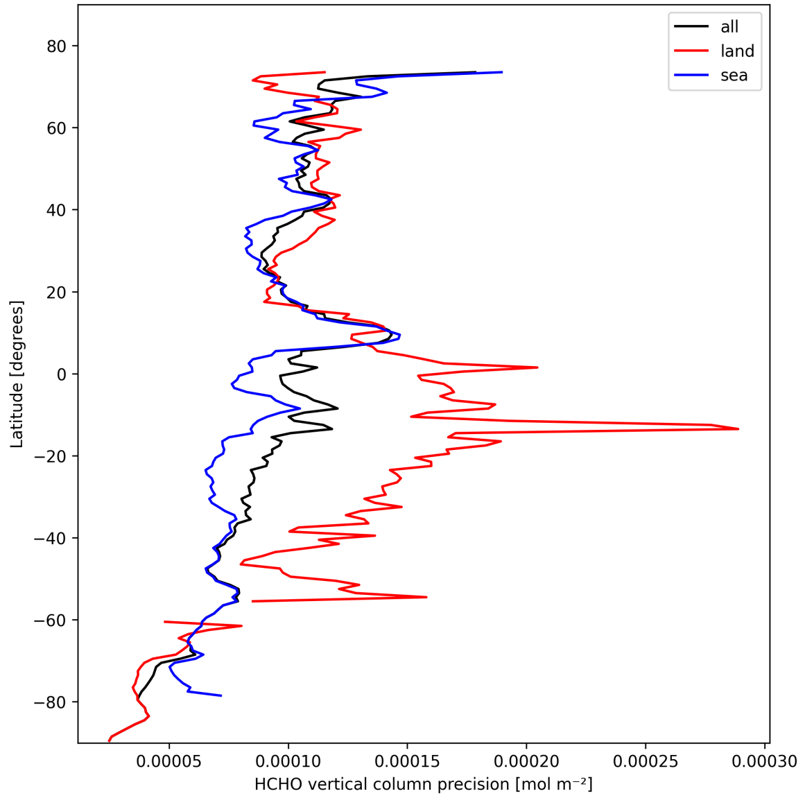
Figure 22: Zonal average of “HCHO vertical column precision” for 2025-10-22 to 2025-10-23.
