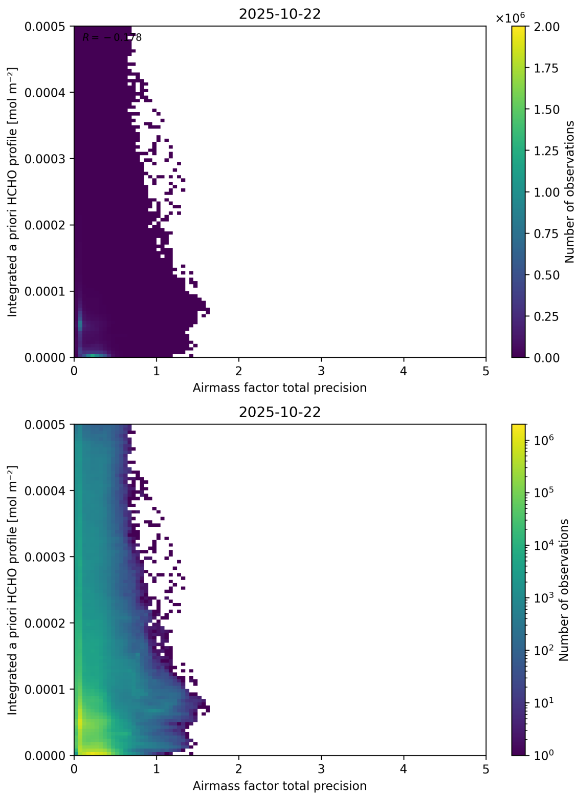
Figure 111: Scatter density plot of “Airmass factor total precision” against “Integrated a priori HCHO profile” for 2025-10-22 to 2025-10-23.
