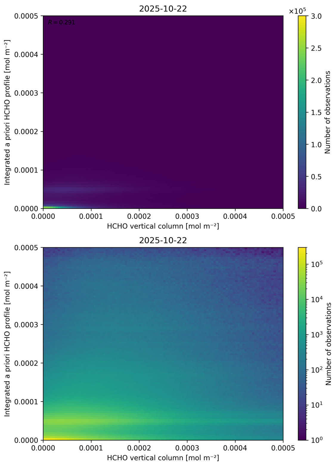
Figure 135: Scatter density plot of “HCHO vertical column” against “Integrated a priori HCHO profile” for 2025-10-22 to 2025-10-23.
