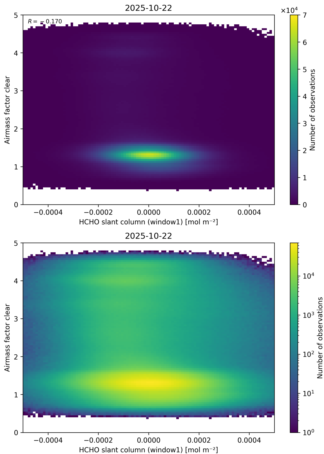
Figure 81: Scatter density plot of “HCHO slant column (window1)” against “Airmass factor clear” for 2025-10-22 to 2025-10-23.
