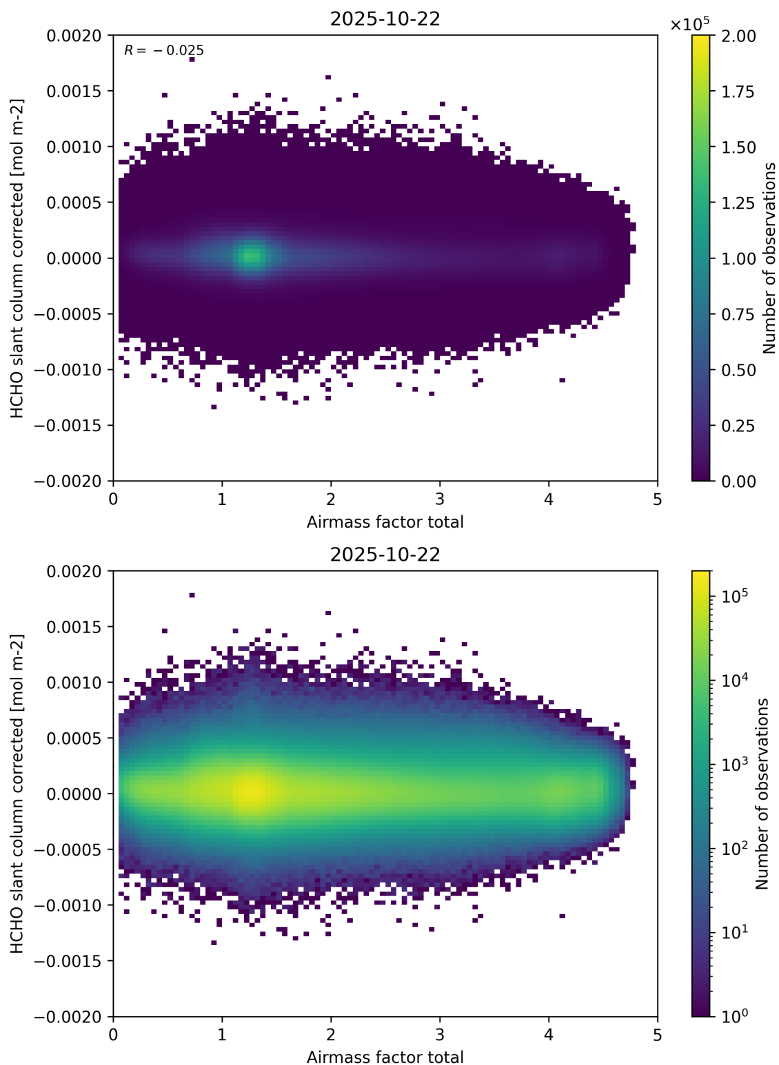
Figure 101: Scatter density plot of “Airmass factor total” against “HCHO slant column corrected” for 2025-10-22 to 2025-10-23.
