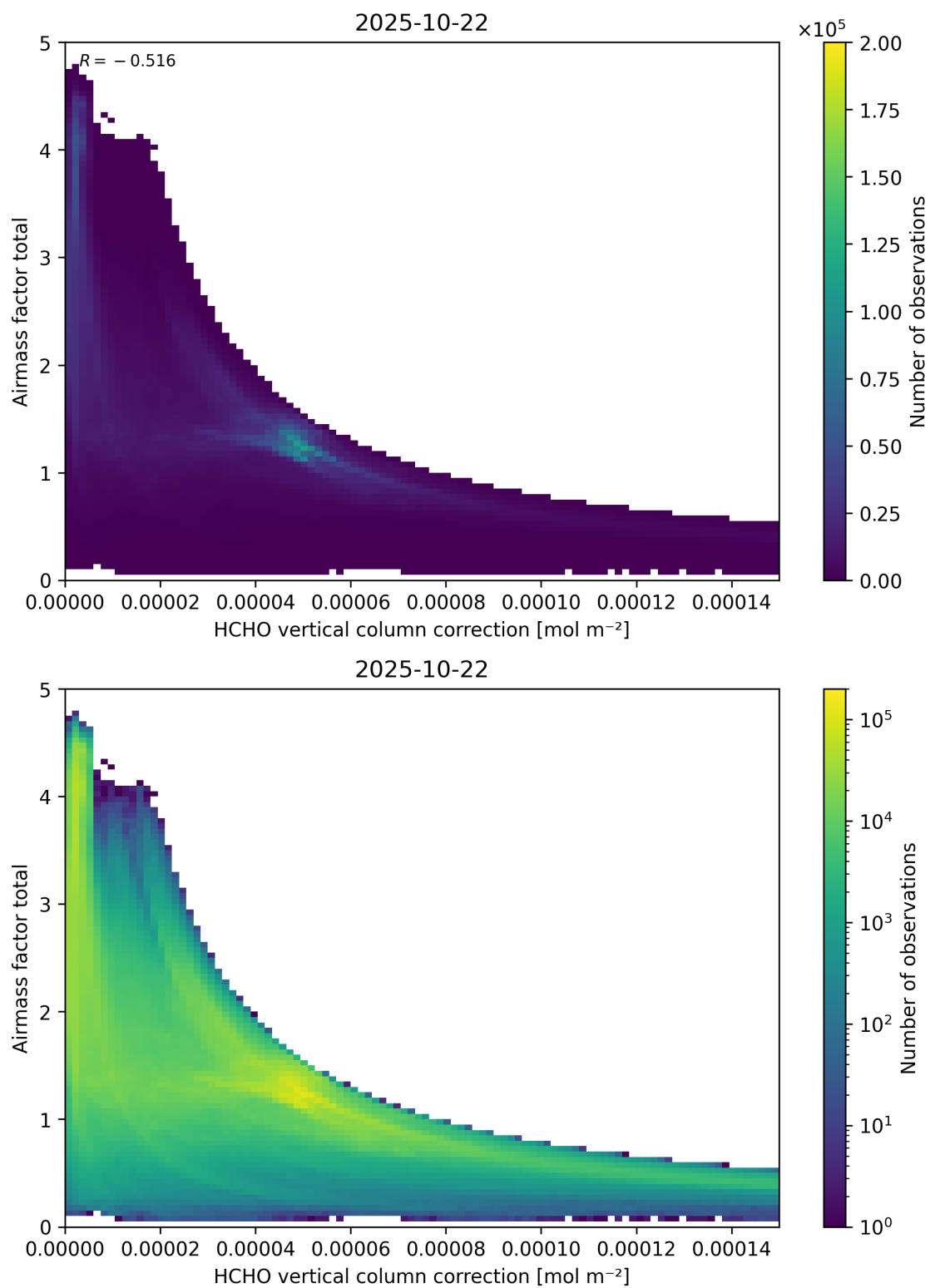
Figure 120: Scatter density plot of “HCHO vertical column correction” against “Airmass factor total” for 2025-10-22 to 2025-10-23.
