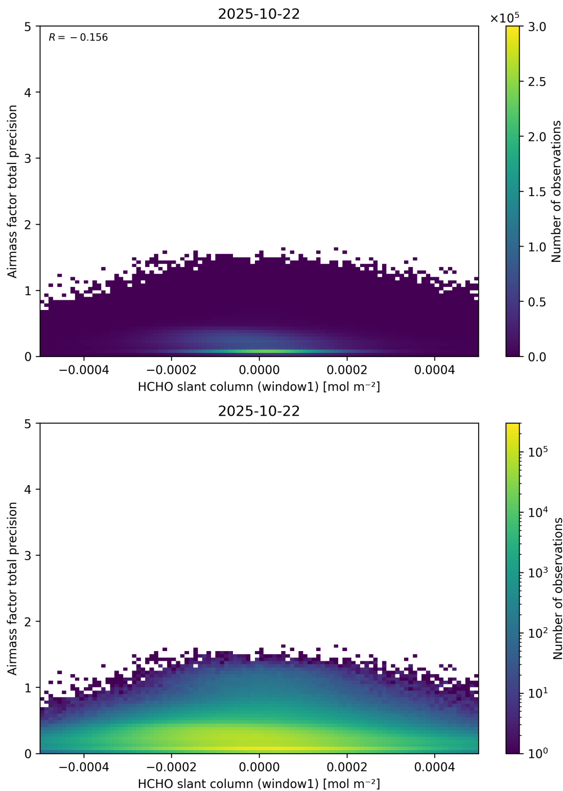
Figure 86: Scatter density plot of “HCHO slant column (window1)” against “Airmass factor total precision” for 2025-10-22 to 2025-10-23.
