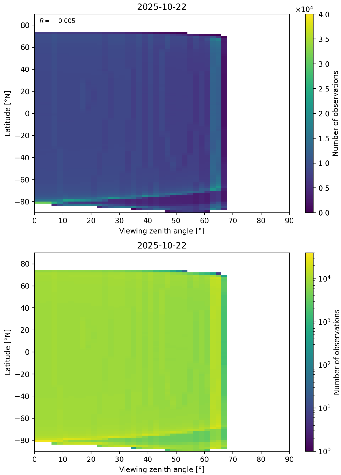
Figure 196: Scatter density plot of “Viewing zenith angle” against “Latitude” for 2025-10-22 to 2025-10-23.
