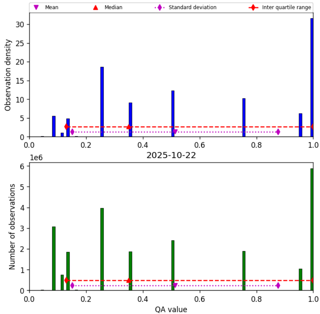
Figure 34: Histogram of “QA value” for 2025-10-22 to 2025-10-23
