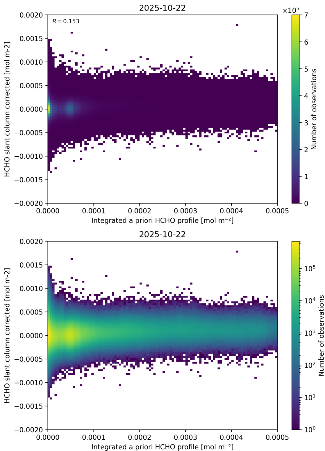
Figure 151: Scatter density plot of “Integrated a priori HCHO profile” against “HCHO slant column corrected” for 2025-10-22 to 2025-10-23.
