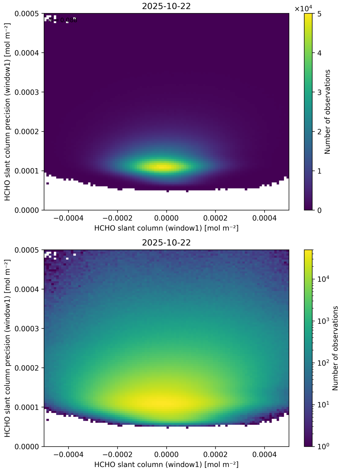
Figure 84: Scatter density plot of “HCHO slant column (window1)” against “HCHO slant column precision (window1)” for 2025-10-22 to 2025-10-23.
