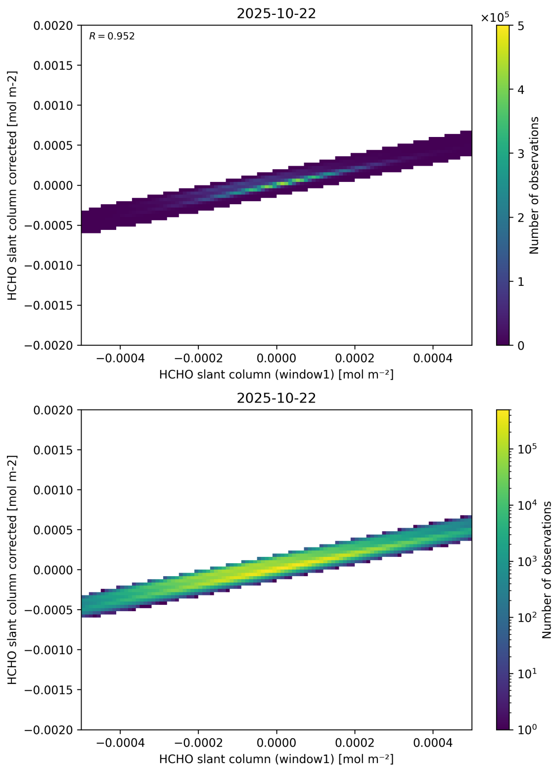
Figure 82: Scatter density plot of “HCHO slant column (window1)” against “HCHO slant column corrected” for 2025-10-22 to 2025-10-23.
