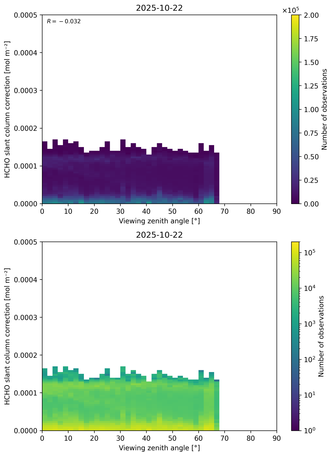
Figure 187: Scatter density plot of “Viewing zenith angle” against “HCHO slant column correction” for 2025-10-22 to 2025-10-23.
