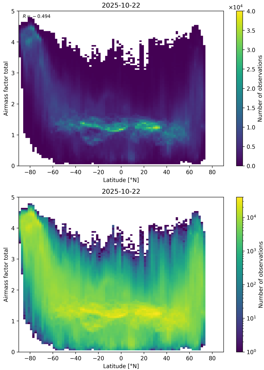
Figure 161: Scatter density plot of “Latitude” against “Airmass factor total” for 2025-10-22 to 2025-10-23.
