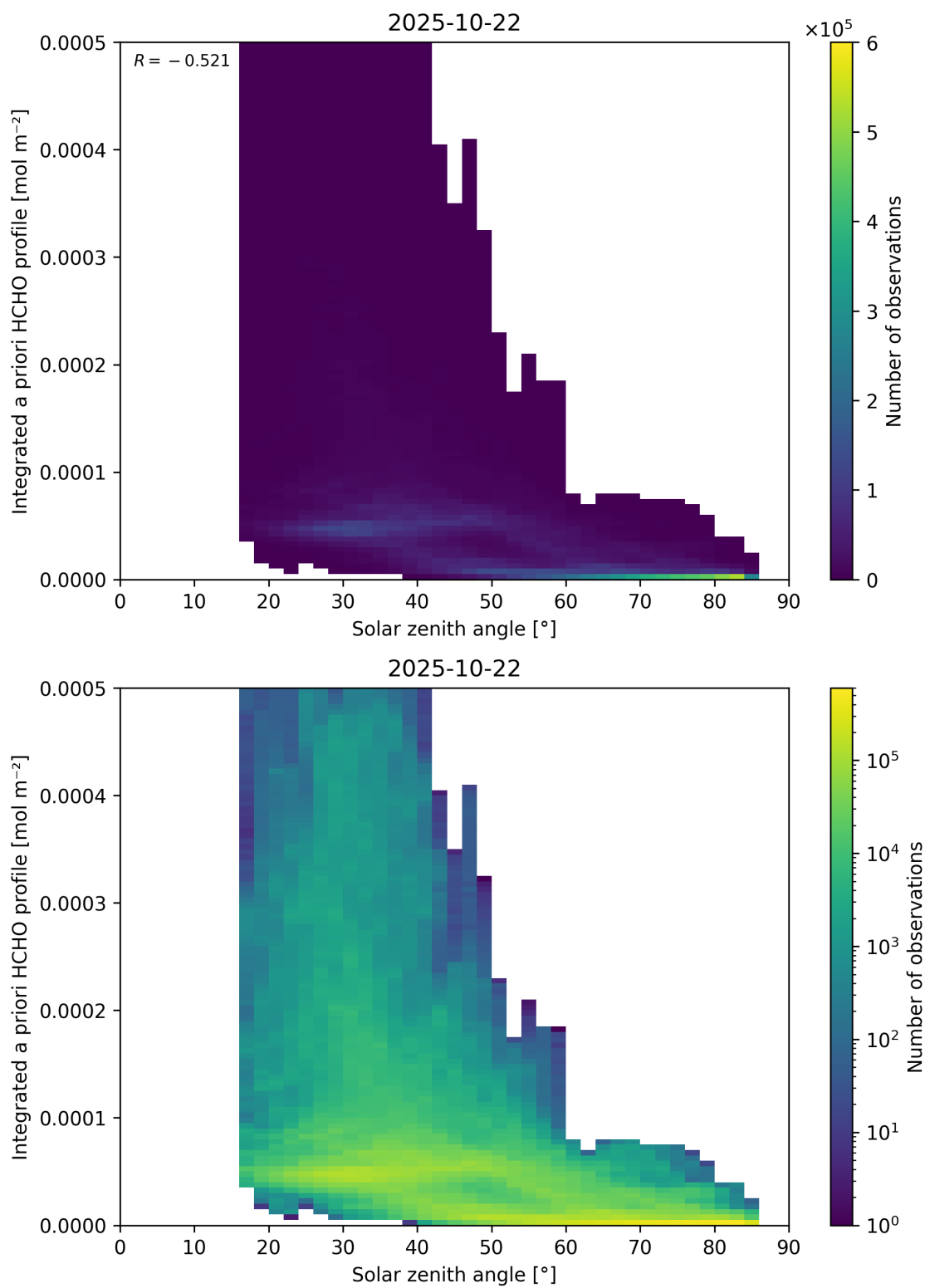
Figure 180: Scatter density plot of “Solar zenith angle” against “Integrated a priori HCHO profile” for 2025-10-22 to 2025-10-23.
