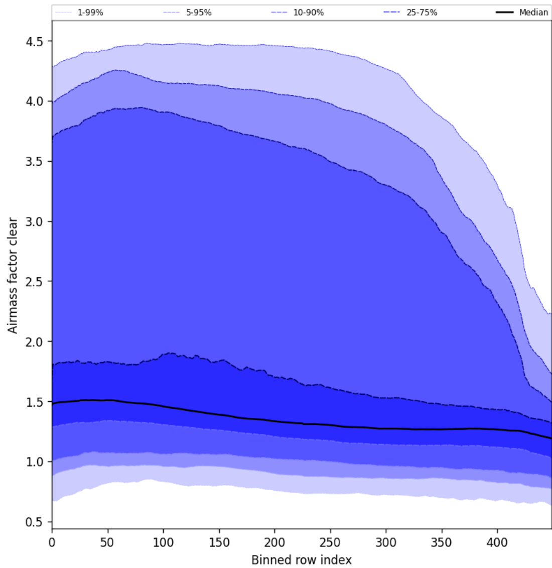
Figure 56: Along track statistics of “Airmass factor clear” for 2025-10-22 to 2025-10-23
