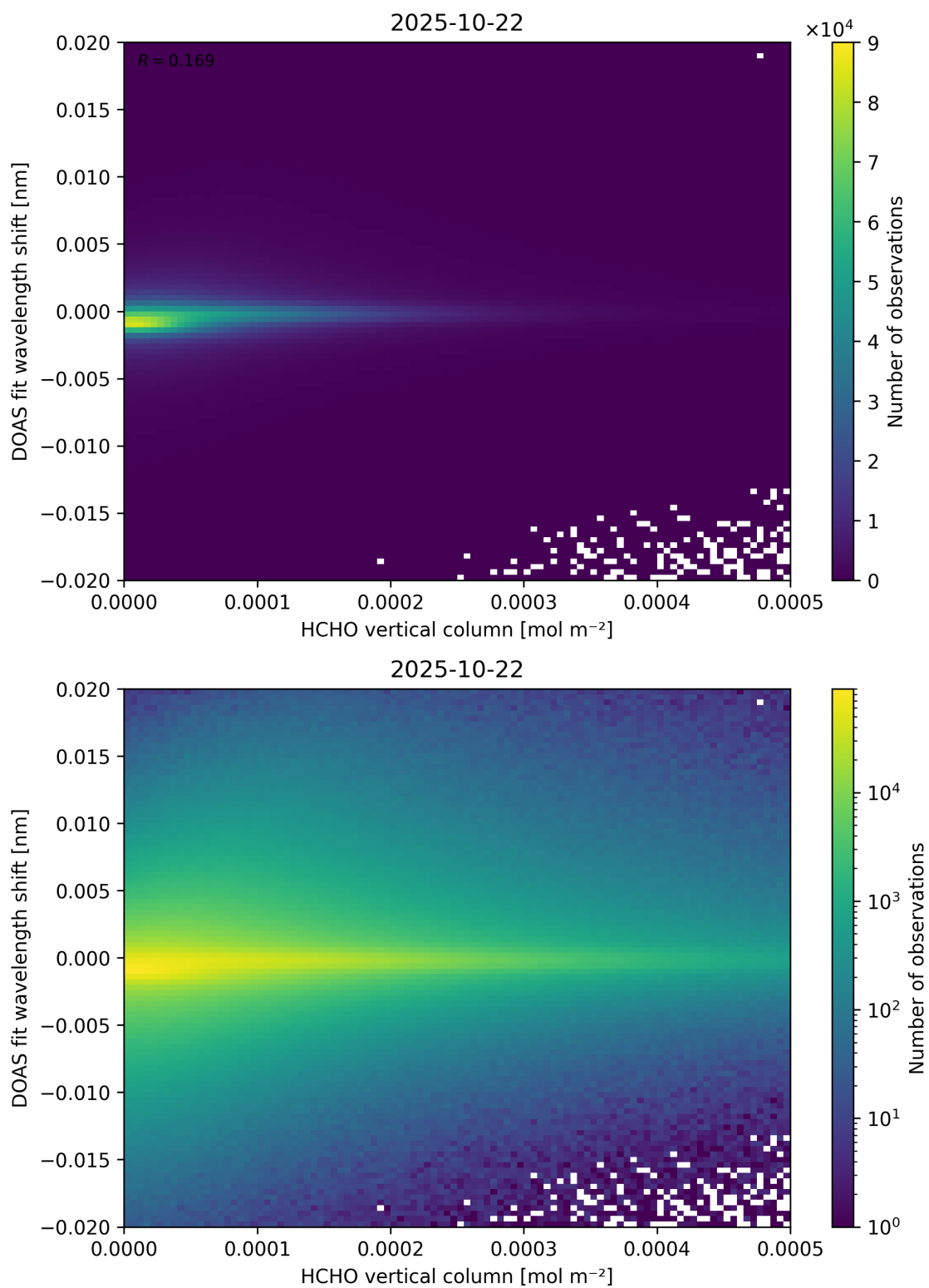
Figure 124: Scatter density plot of “HCHO vertical column” against “DOAS fit wavelength shift” for 2025-10-22 to 2025-10-23.
