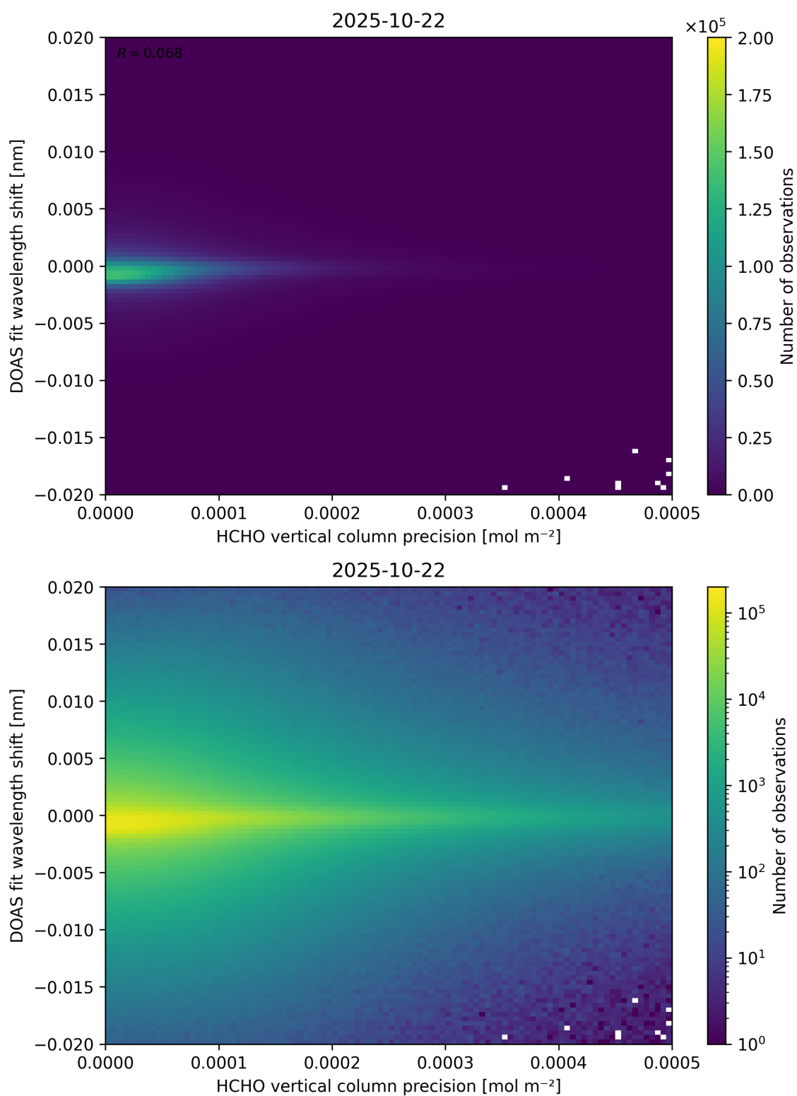
Figure 137: Scatter density plot of “HCHO vertical column precision” against “DOAS fit wavelength shift” for 2025-10-22 to 2025-10-23.
